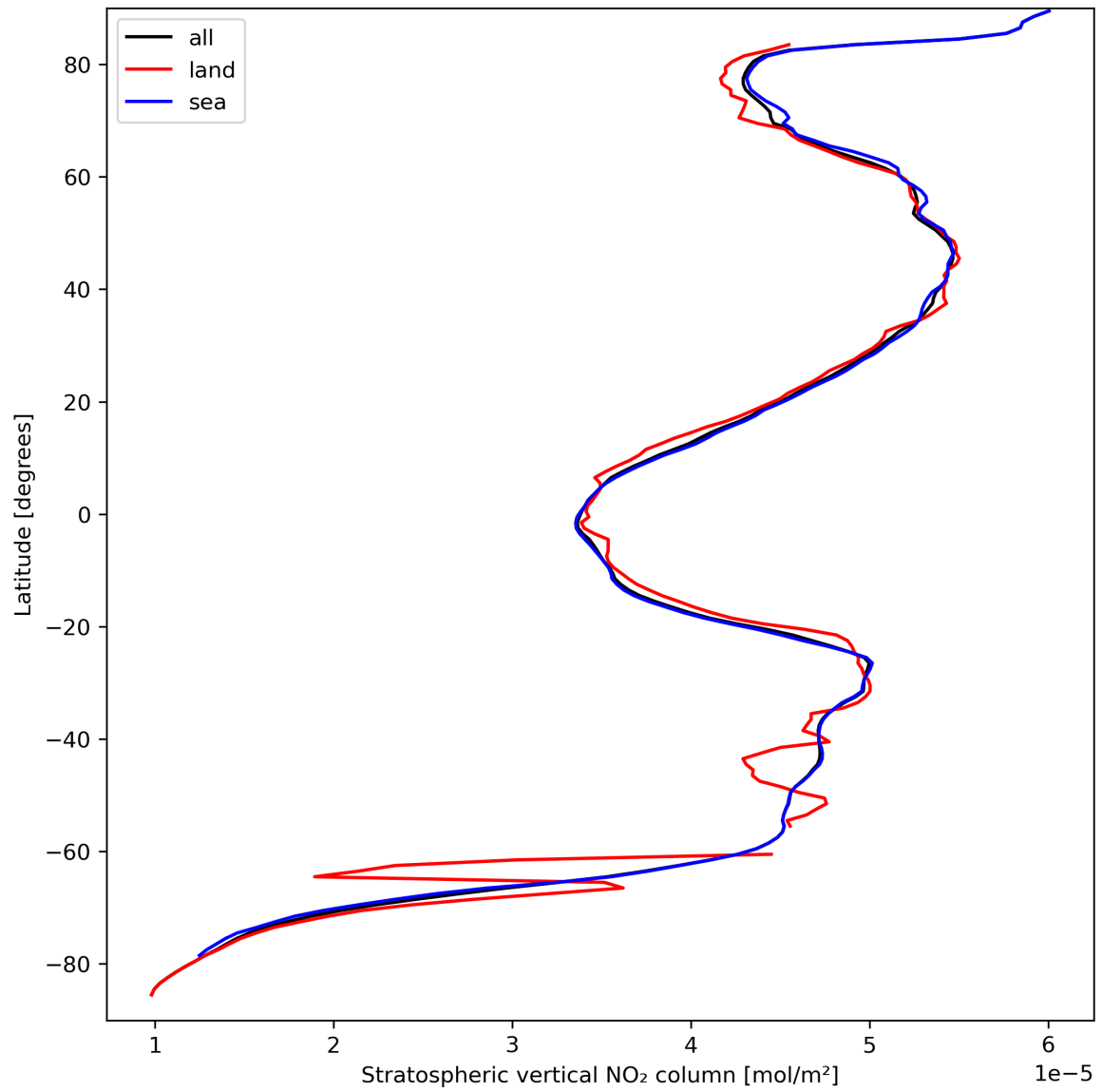
Figure 19: Zonal average of “Stratospheric vertical NO 2 column” for 2023-09-16 to 2023-09-18.
