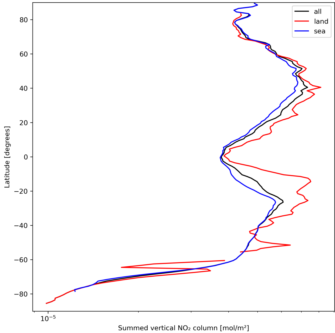
Figure 23: Zonal average of “Summed vertical NO 2 column” for 2023-09-16 to 2023-09-18.
