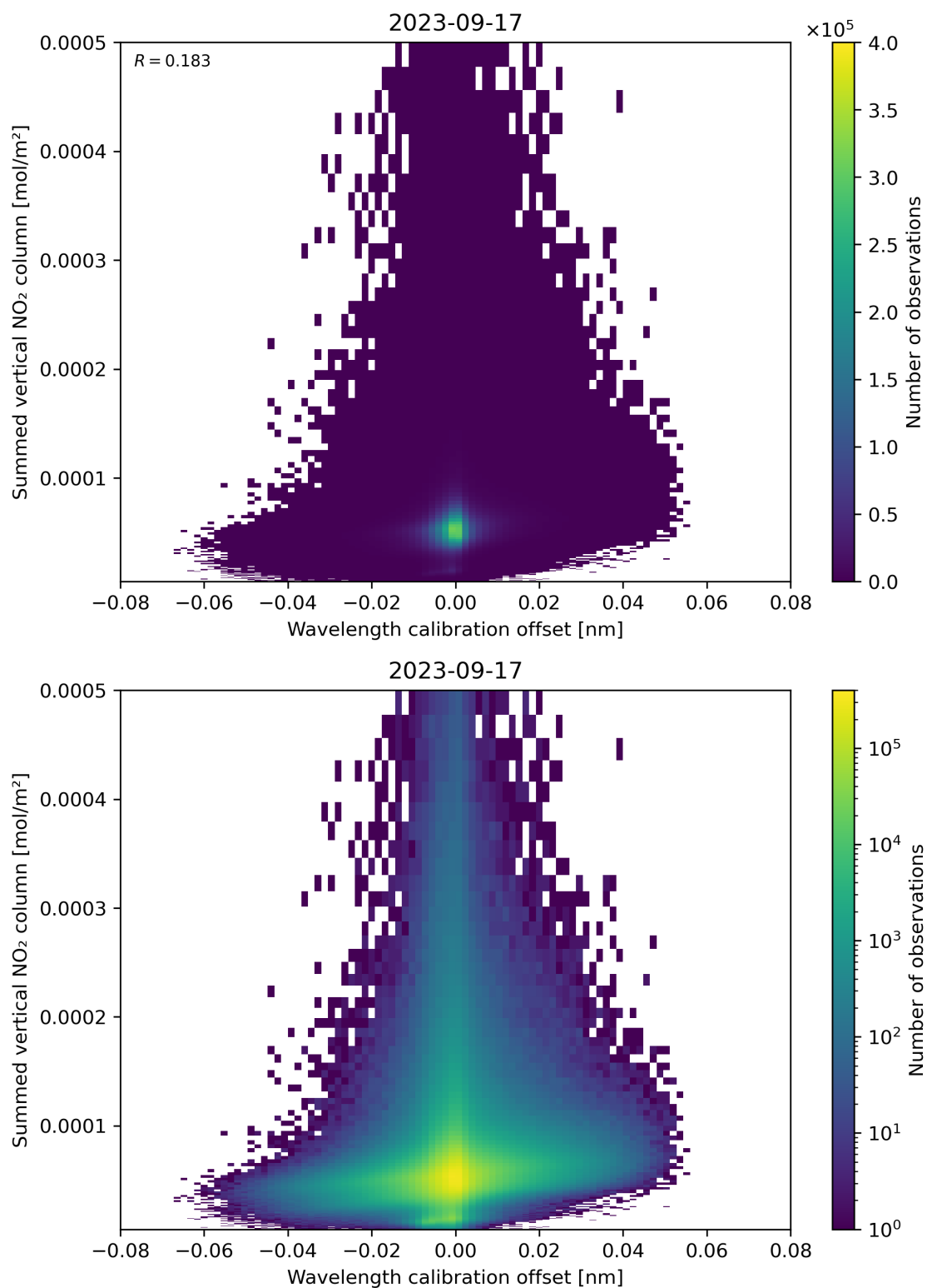
Figure 177: Scatter density plot of “Wavelength calibration offset” against “Summed vertical NO 2 column” for 2023-09-16 to 2023-09-18.
