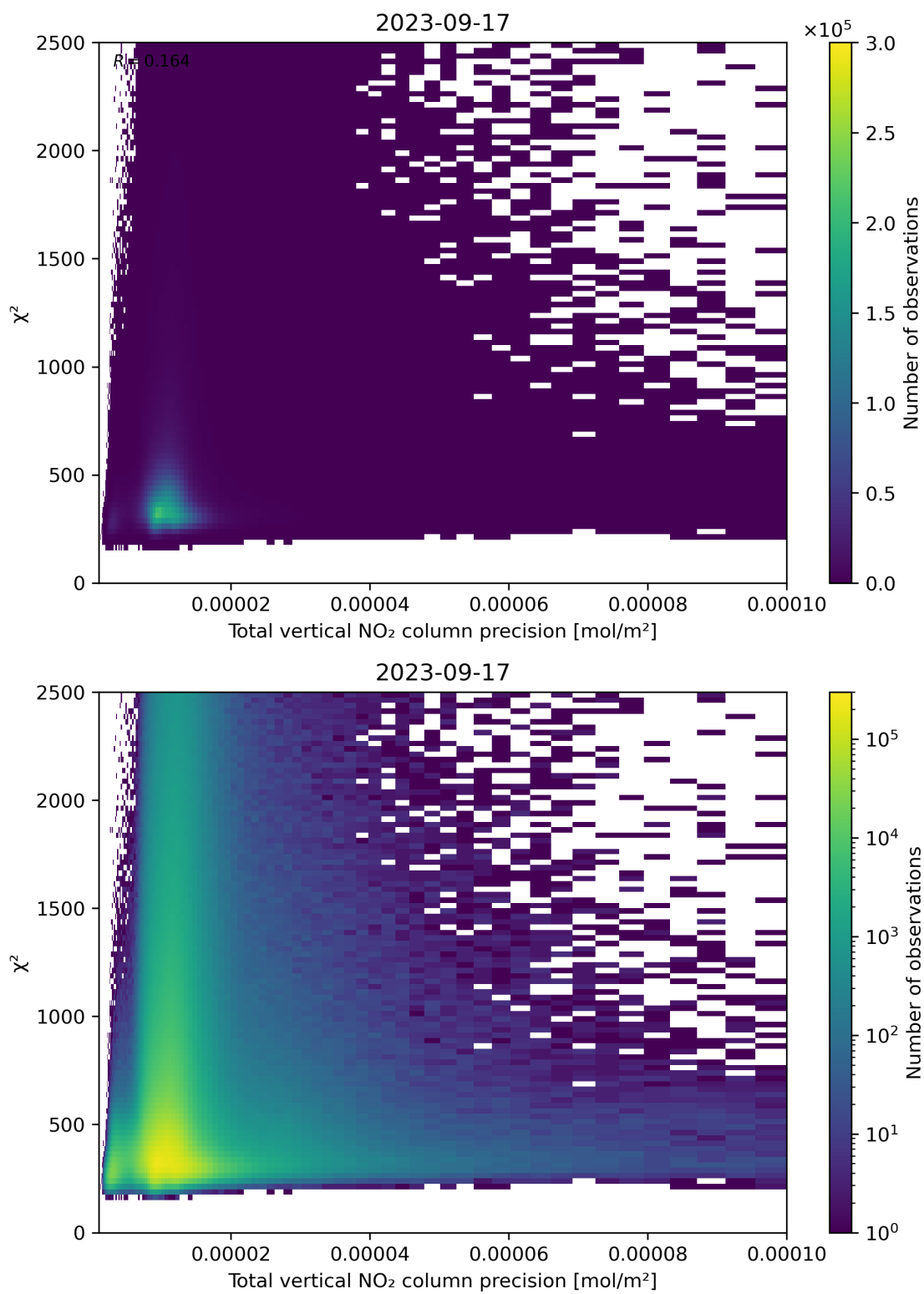
Figure 116: Scatter density plot of “Total vertical NO 2 column precision” against “ \chi^2 ” for 2023-09-16 to 2023-09-18.
