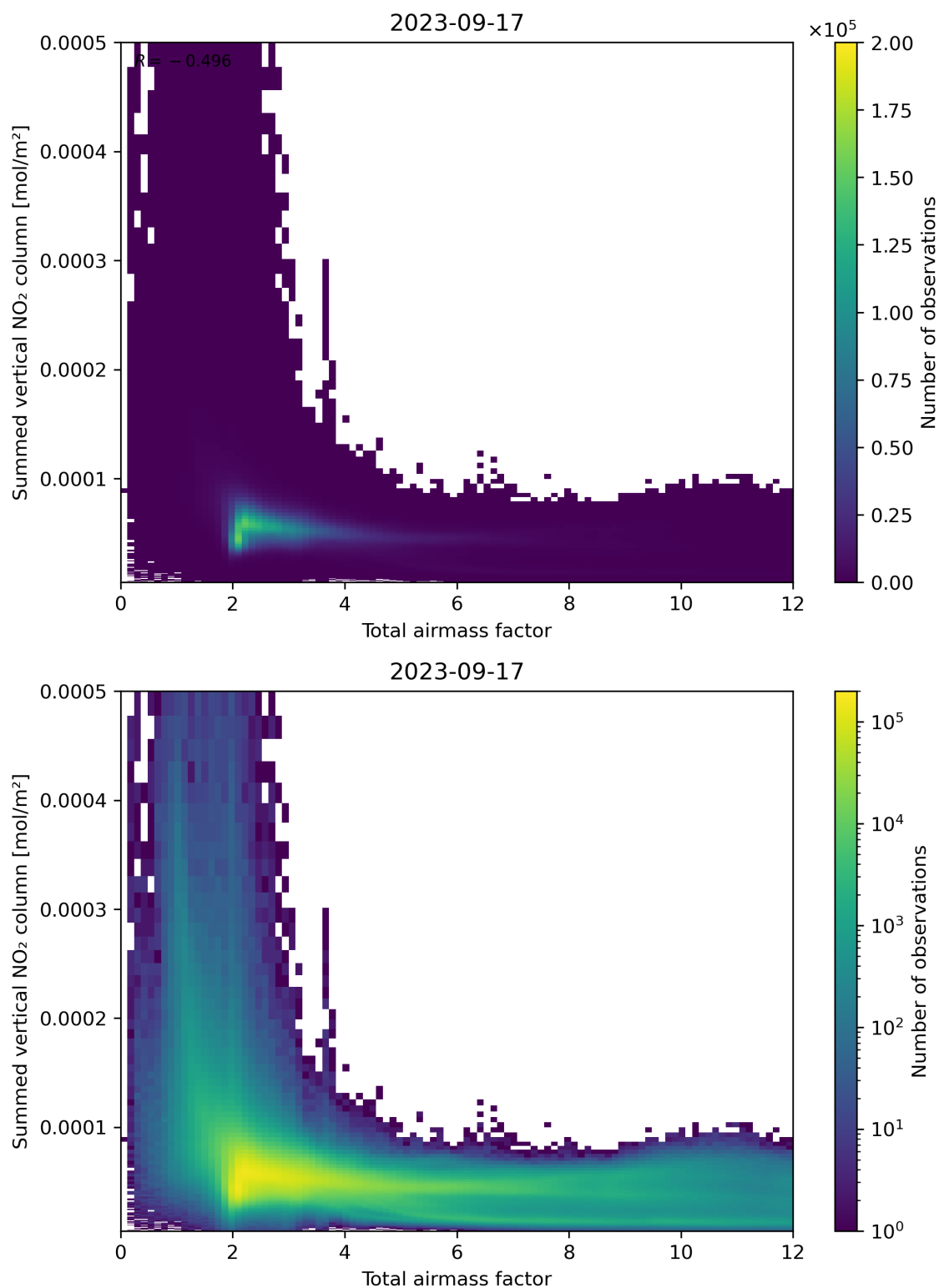
Figure 65: Scatter density plot of “Total airmass factor” against “Summed vertical NO 2 column” for 2023-09-16 to 2023-09-18.
