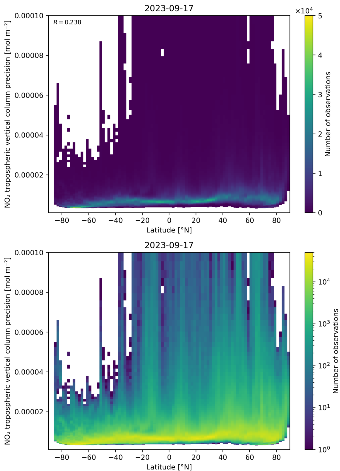
Figure 93: Scatter density plot of “Latitude” against “NO 2 tropospheric vertical column precision” for 2023-09-16 to 2023-09-18.
