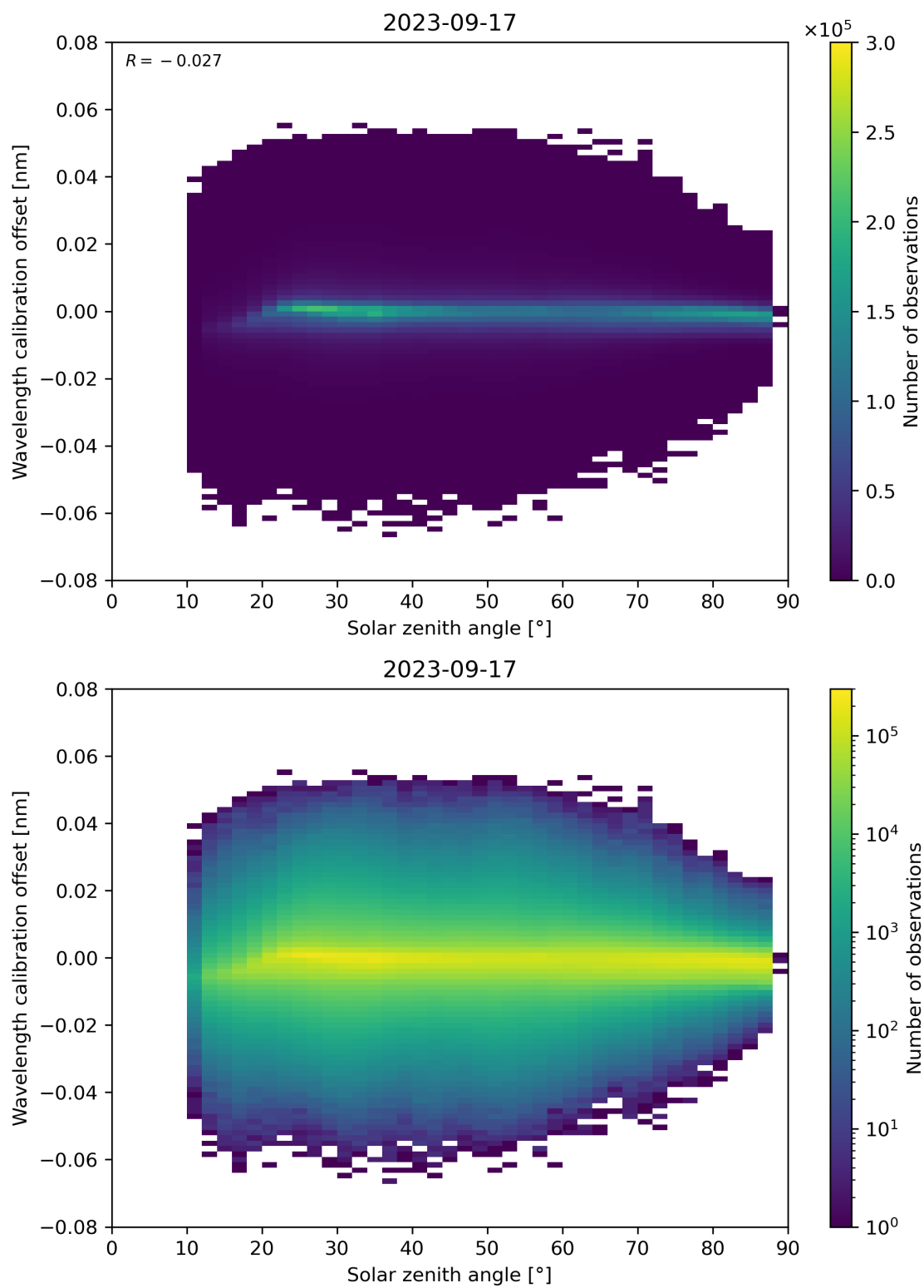
Figure 158: Scatter density plot of “Solar zenith angle” against “Wavelength calibration offset” for 2023-09-16 to 2023-09-18.
