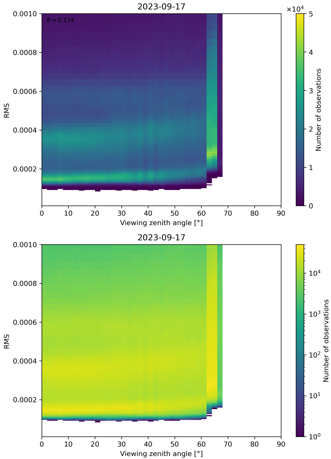
Figure 171: Scatter density plot of “Viewing zenith angle” against “RMS” for 2023-09-16 to 2023-09-18.
