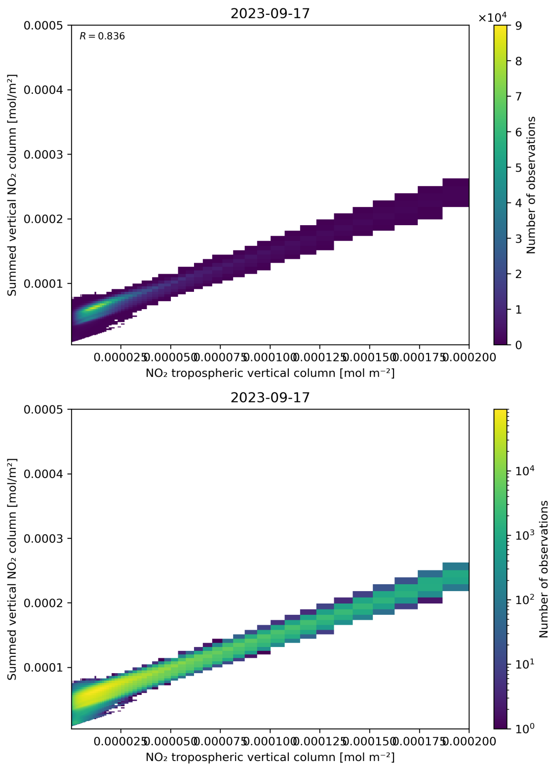
Figure 126: Scatter density plot of “NO 2 tropospheric vertical column” against “Summed vertical NO 2 column” for 2023-09-16 to 2023-09-18.
