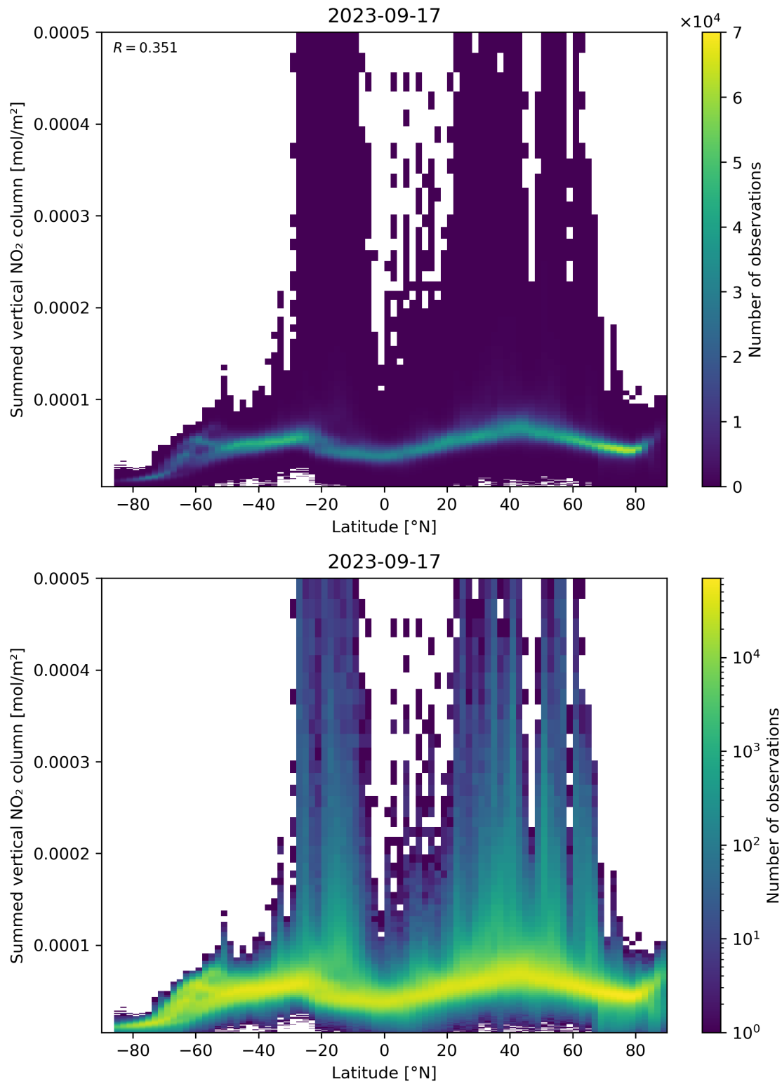
Figure 88: Scatter density plot of “Latitude” against “Summed vertical NO 2 column” for 2023-09-16 to 2023-09-18.
