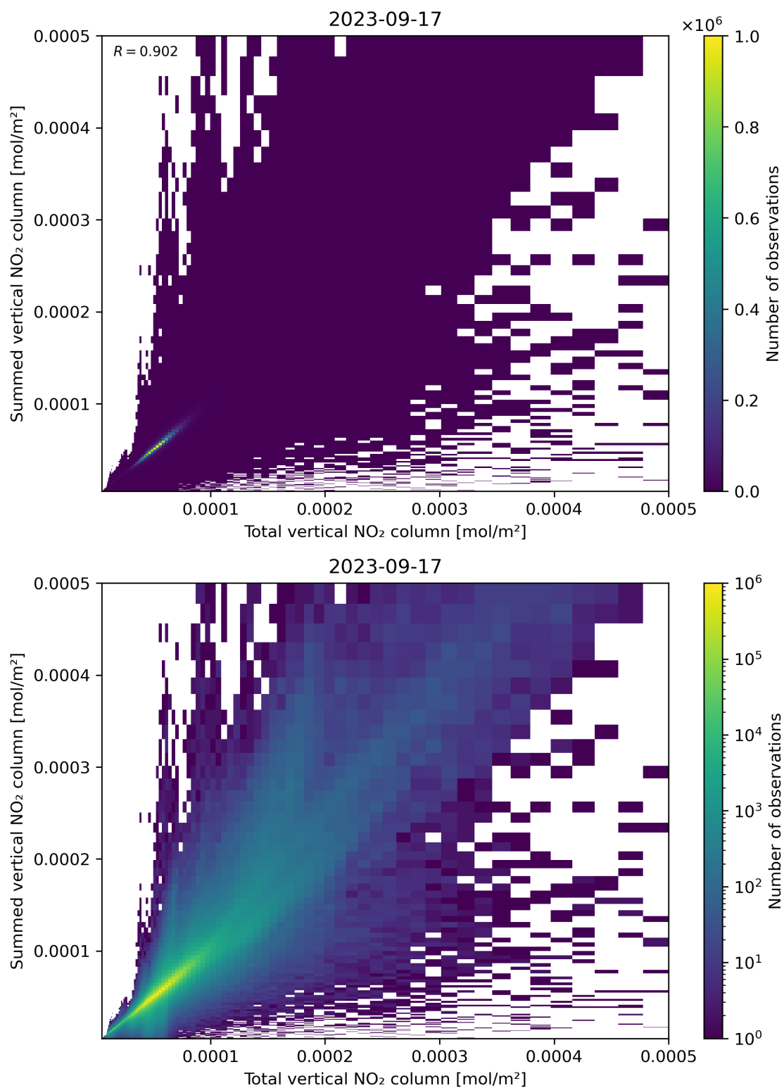
Figure 112: Scatter density plot of “Total vertical NO 2 column” against “Summed vertical NO 2 column” for 2023-09-16 to 2023-09-18.
