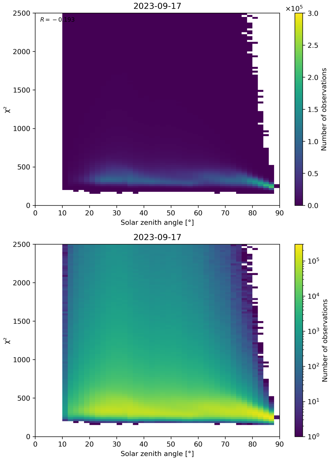
Figure 148: Scatter density plot of “Solar zenith angle” against “ \chi^2 ” for 2023-09-16 to 2023-09-18.
