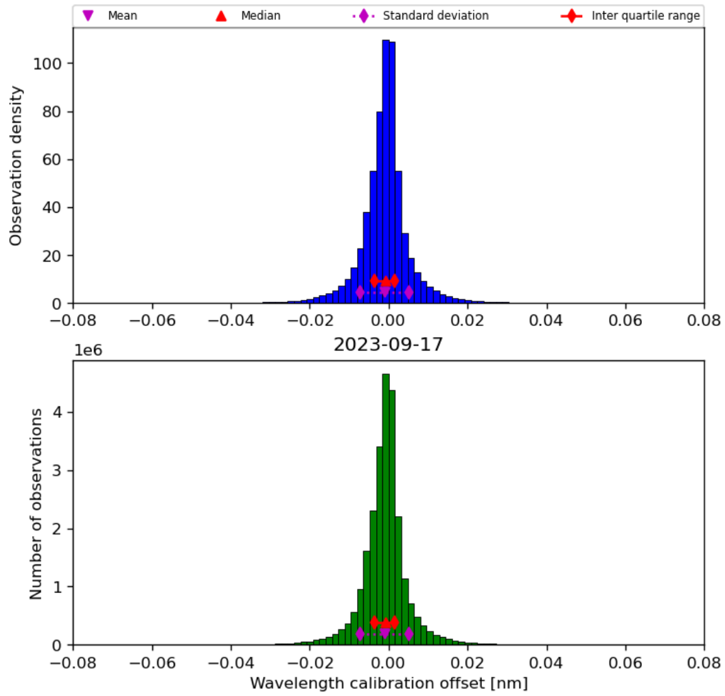
Figure 35: Histogram of “Wavelength calibration offset” for 2023-09-16 to 2023-09-18
