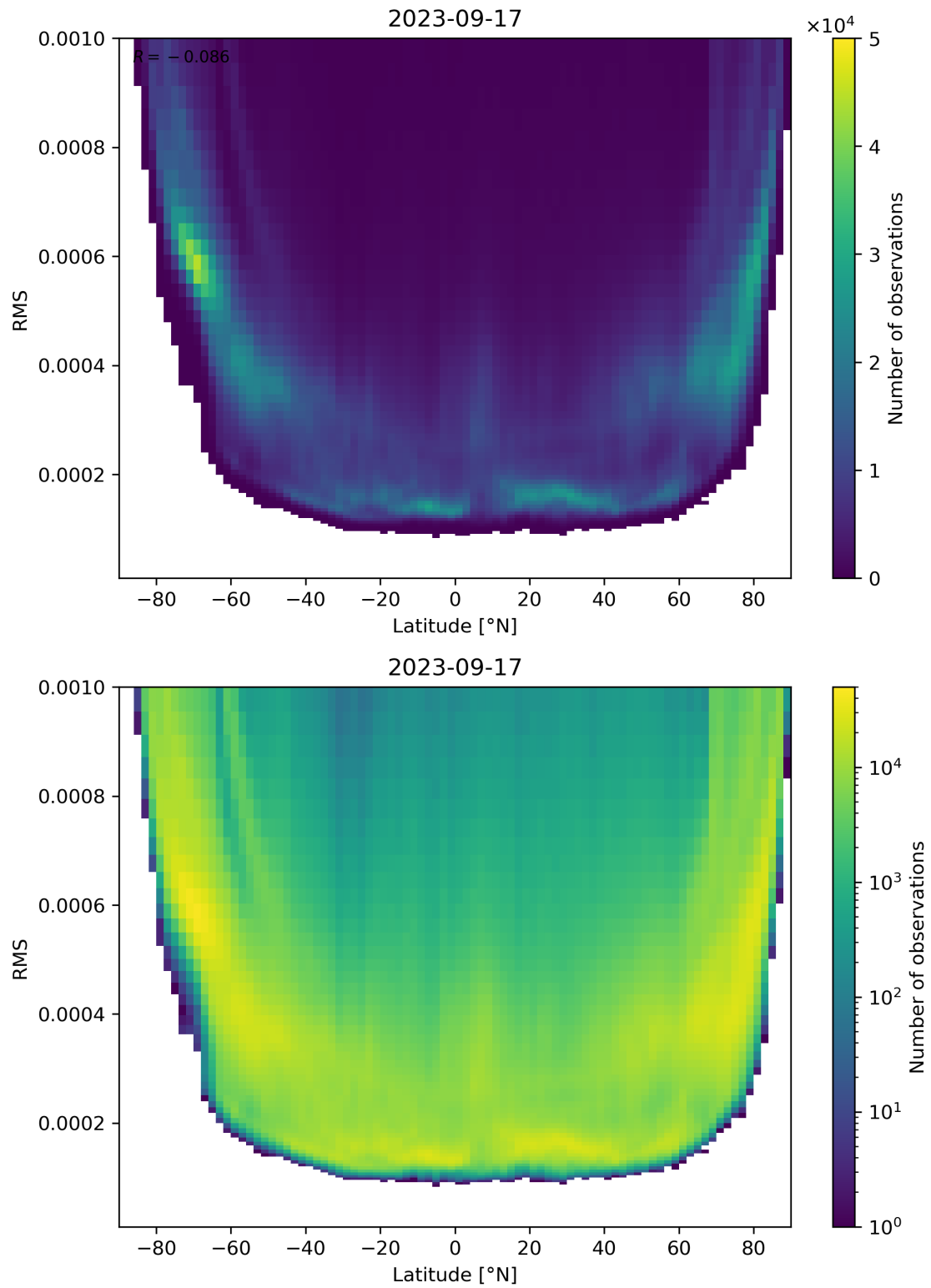
Figure 94: Scatter density plot of “Latitude” against “RMS” for 2023-09-16 to 2023-09-18.
