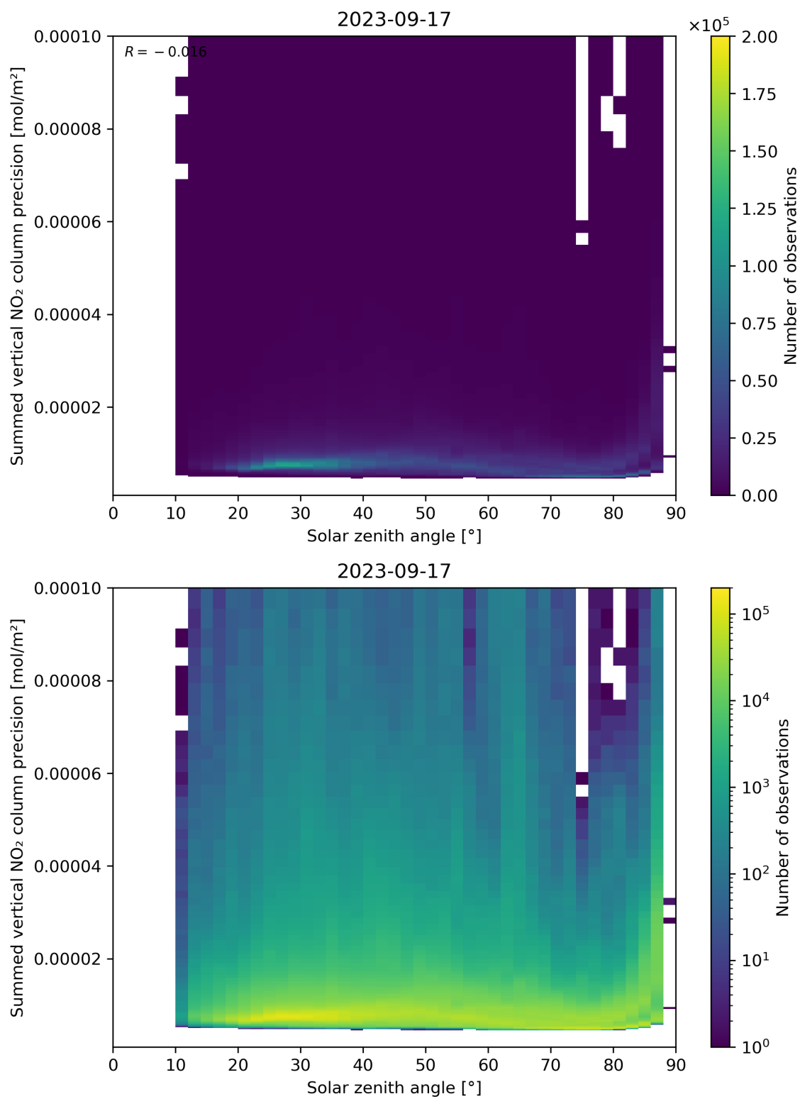
Figure 152: Scatter density plot of “Solar zenith angle” against “Summed vertical NO 2 column precision” for 2023-09-16 to 2023-09-18.
