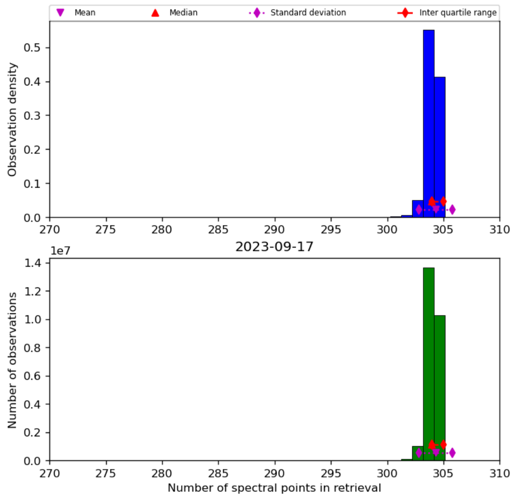
Figure 33: Histogram of “Number of spectral points in retrieval” for 2023-09-16 to 2023-09-18
