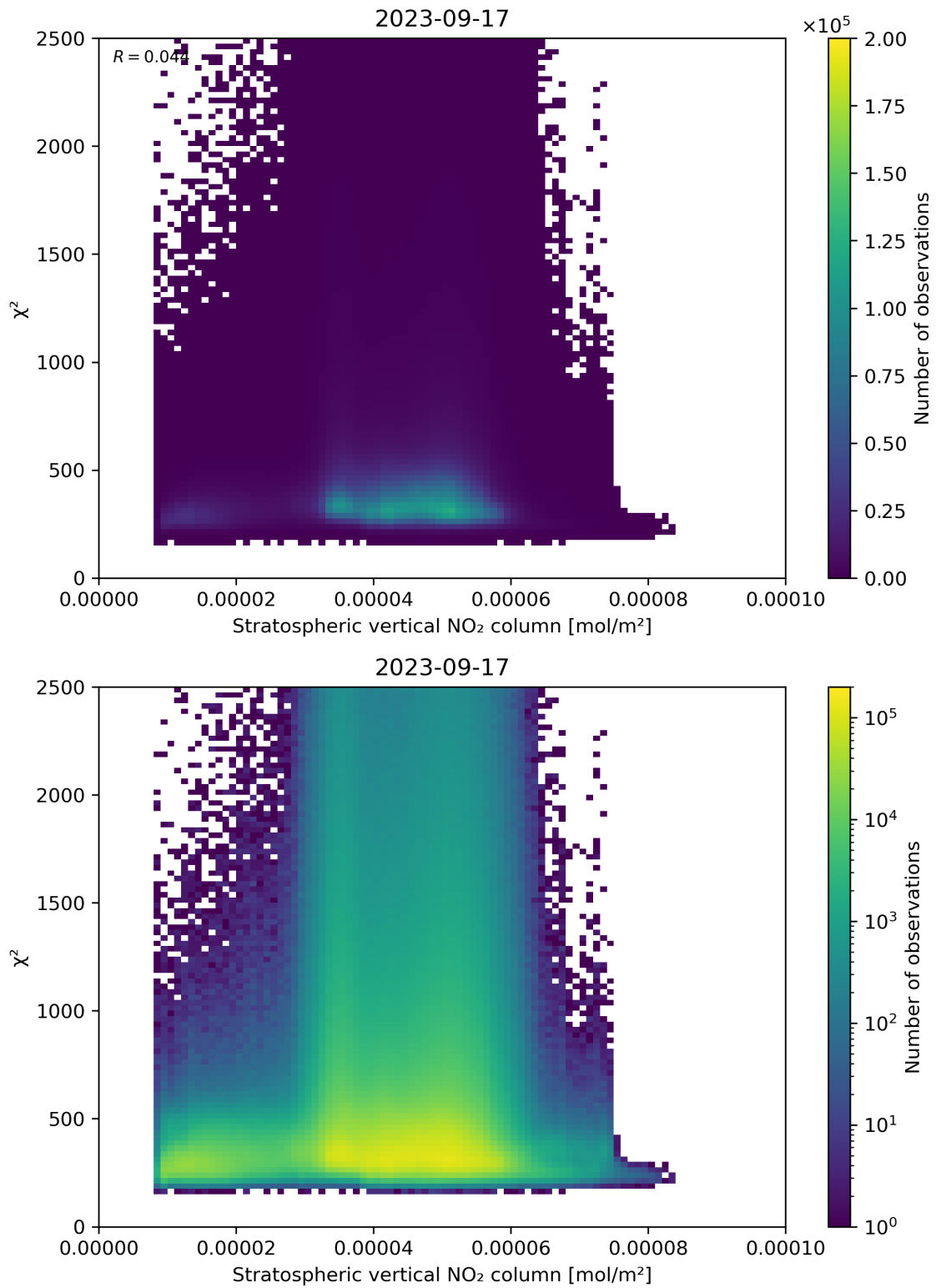
Figure 97: Scatter density plot of “Stratospheric vertical NO 2 column” against “ \chi^2 ” for 2023-09-16 to 2023-09-18.
