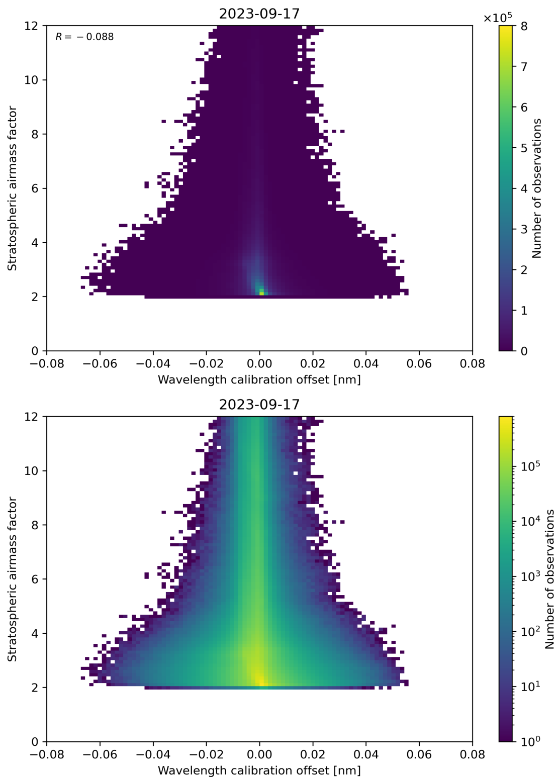
Figure 174: Scatter density plot of “Wavelength calibration offset” against “Stratospheric airmass factor” for 2023-09-16 to 2023-09-18.
