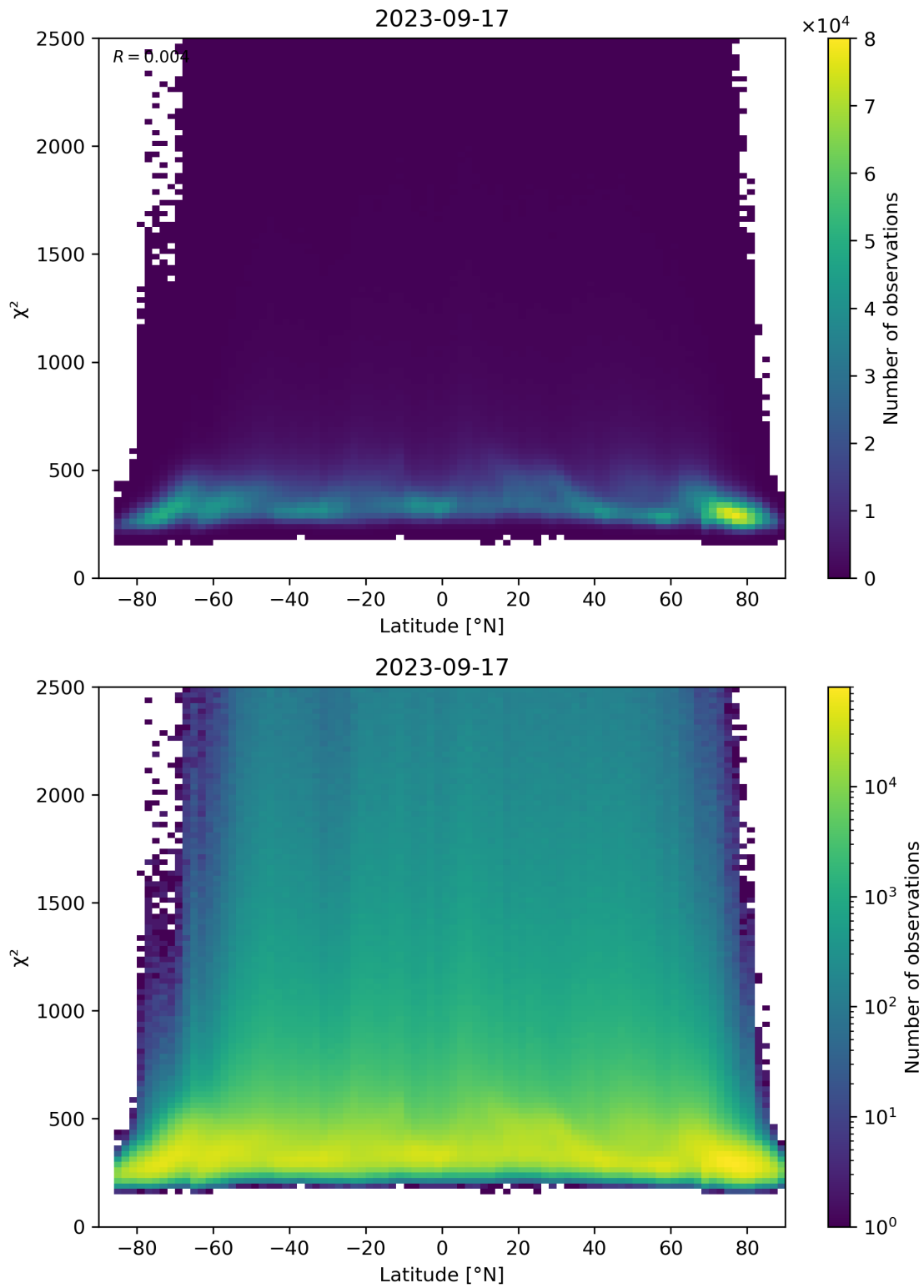
Figure 86: Scatter density plot of “Latitude” against “ \chi^2 ” for 2023-09-16 to 2023-09-18.
