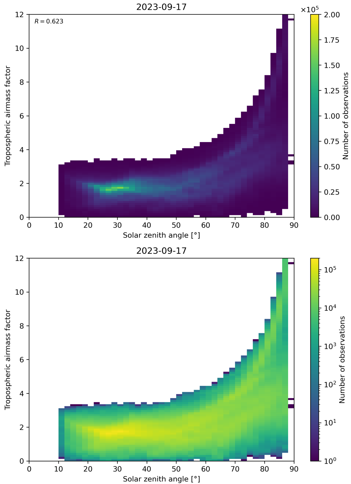
Figure 147: Scatter density plot of “Solar zenith angle” against “Tropospheric airmass factor” for 2023-09-16 to 2023-09-18.
