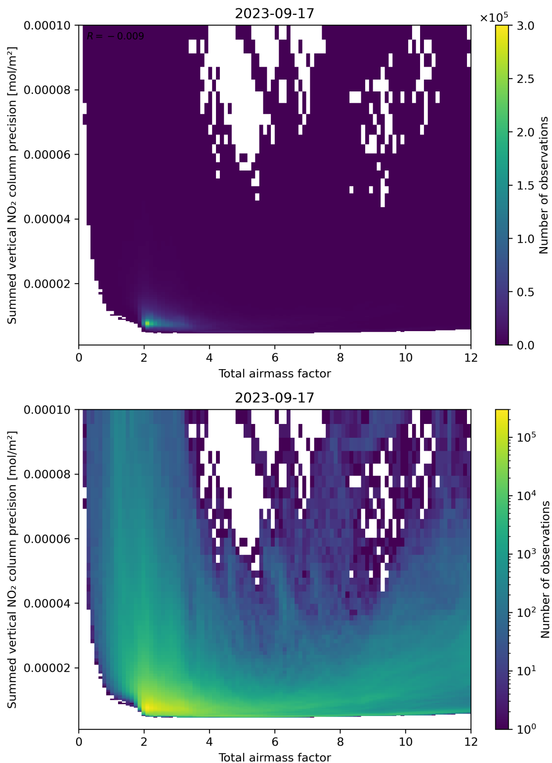
Figure 66: Scatter density plot of “Total airmass factor” against “Summed vertical NO 2 column precision” for 2023-09-16 to 2023-09-18.
