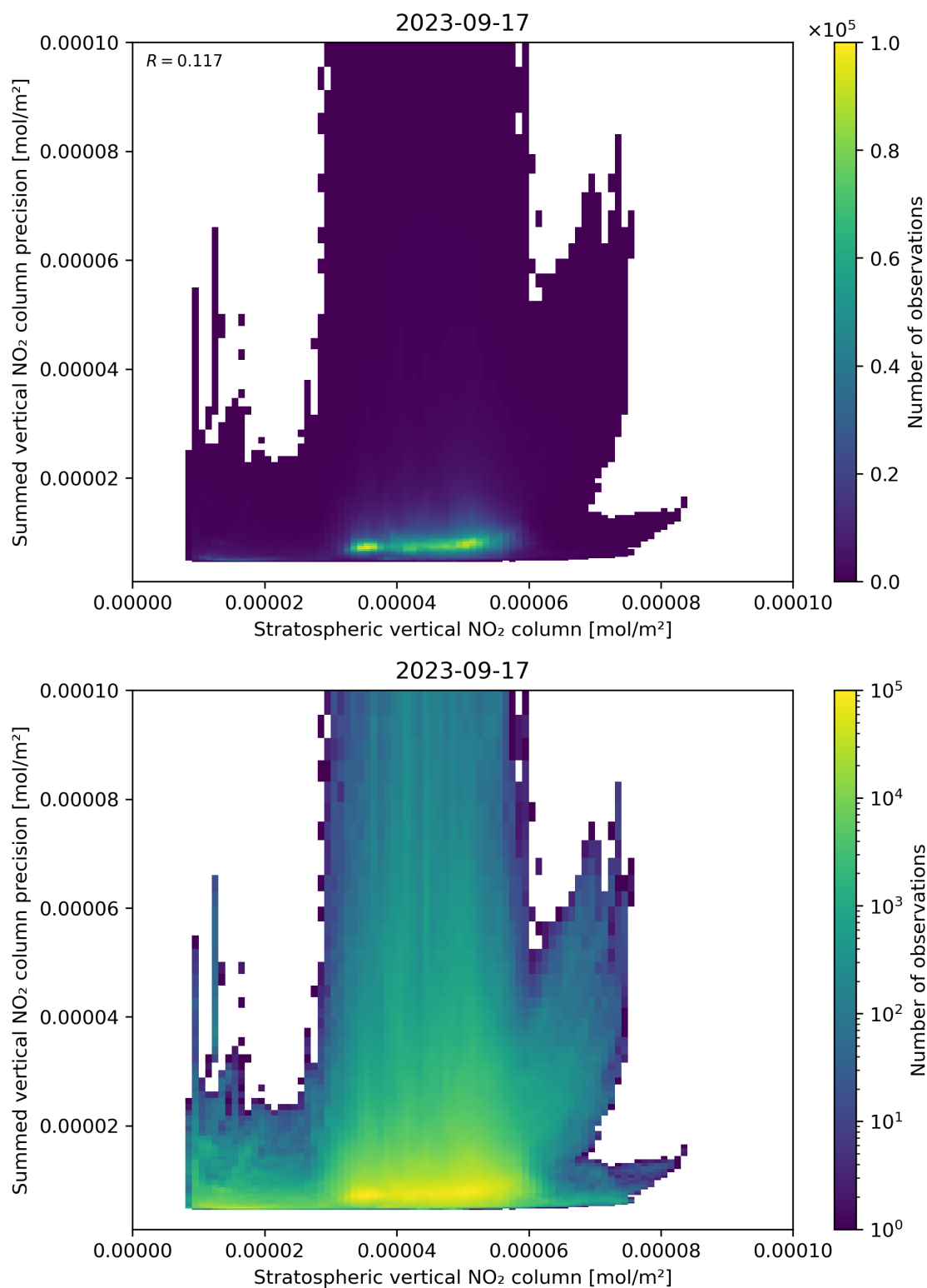
Figure 99: Scatter density plot of “Stratospheric vertical NO 2 column” against “Summed vertical NO 2 column precision” for 2023-09-16 to 2023-09-18.
