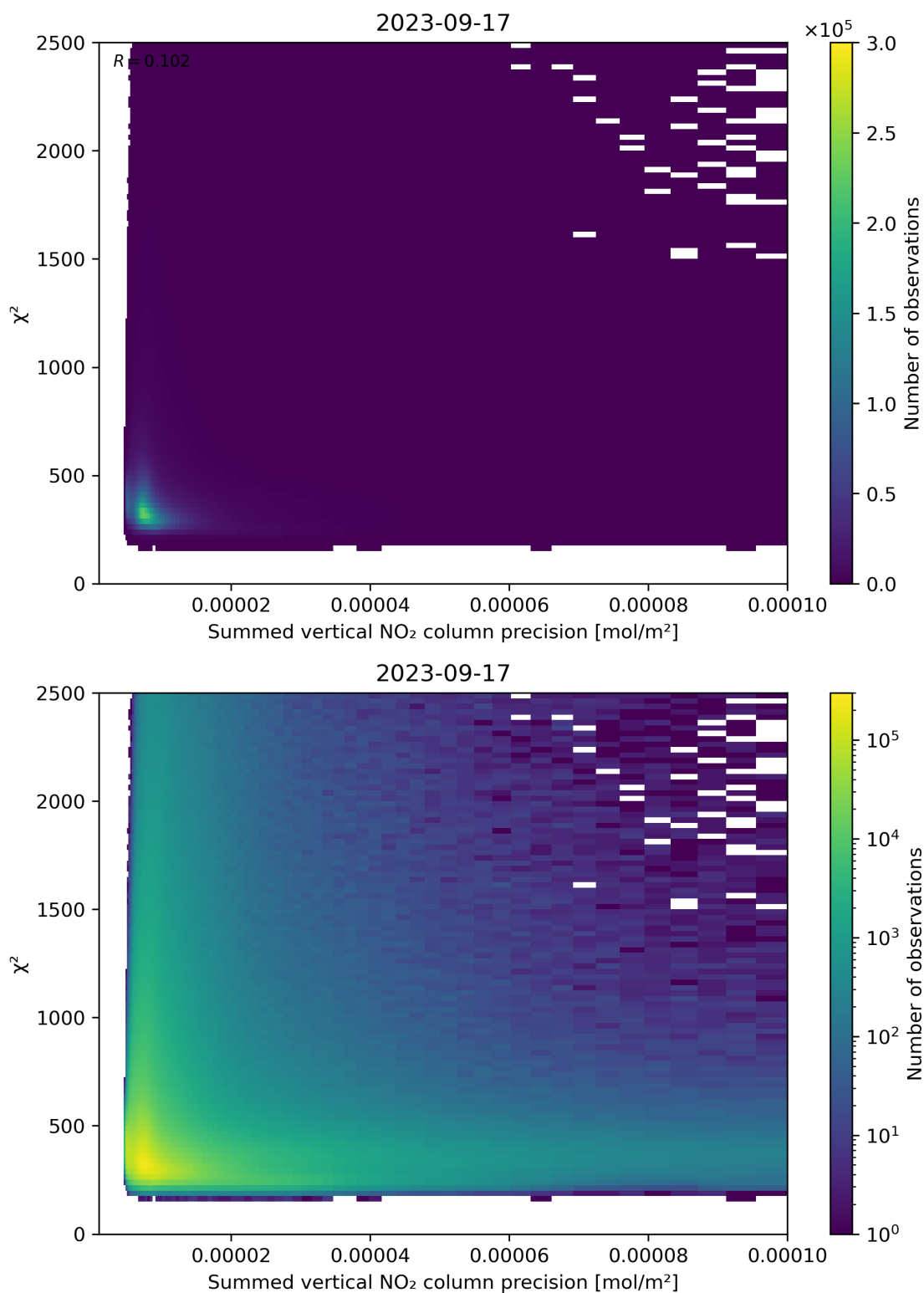
Figure 107: Scatter density plot of “Summed vertical NO 2 column precision” against “ \chi^2 ” for 2023-09-16 to 2023-09-18.
