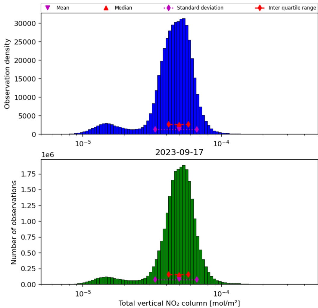
Figure 38: Histogram of “Total vertical NO 2 column” for 2023-09-16 to 2023-09-18
