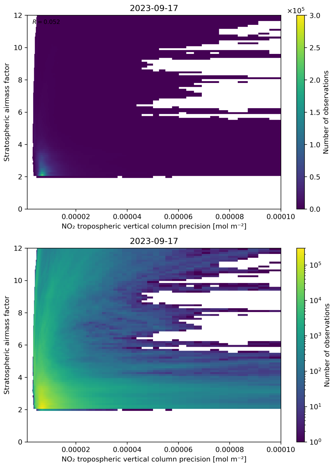
Figure 131: Scatter density plot of “NO 2 tropospheric vertical column precision” against “Stratospheric airmass factor” for 2023-09-16 to 2023-09-18.
