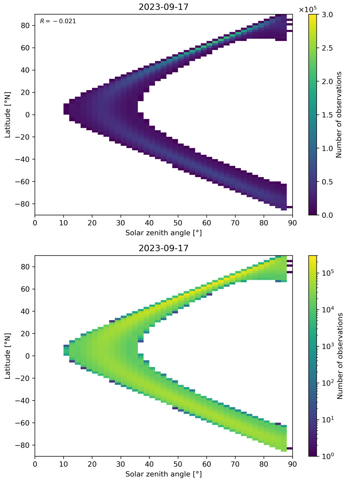
Figure 149: Scatter density plot of “Solar zenith angle” against “Latitude” for 2023-09-16 to 2023-09-18.
