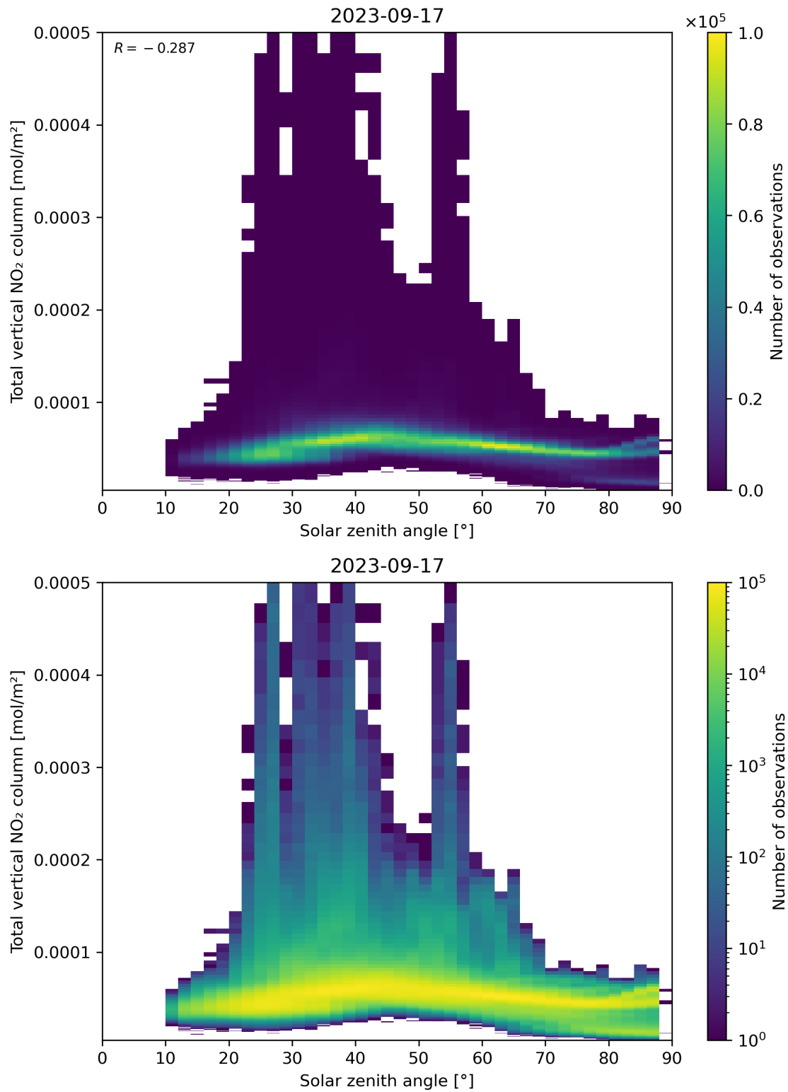
Figure 153: Scatter density plot of “Solar zenith angle” against “Total vertical NO 2 column” for 2023-09-16 to 2023-09-18.
