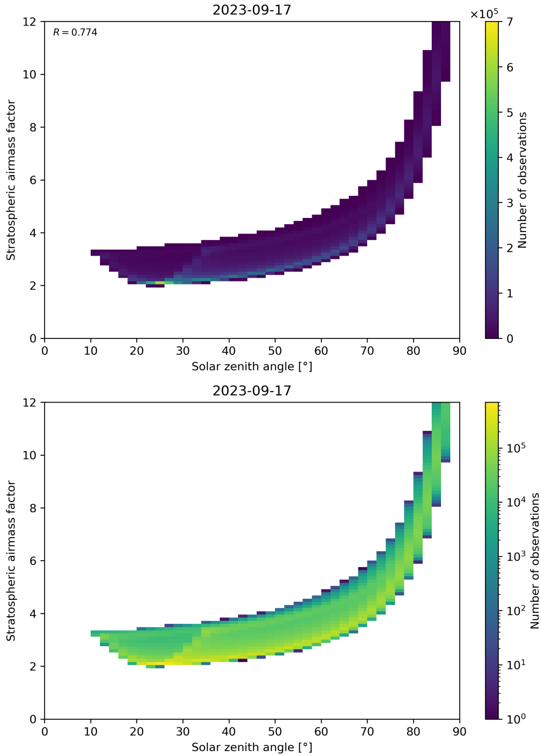
Figure 145: Scatter density plot of “Solar zenith angle” against “Stratospheric airmass factor” for 2023-09-16 to 2023-09-18.
