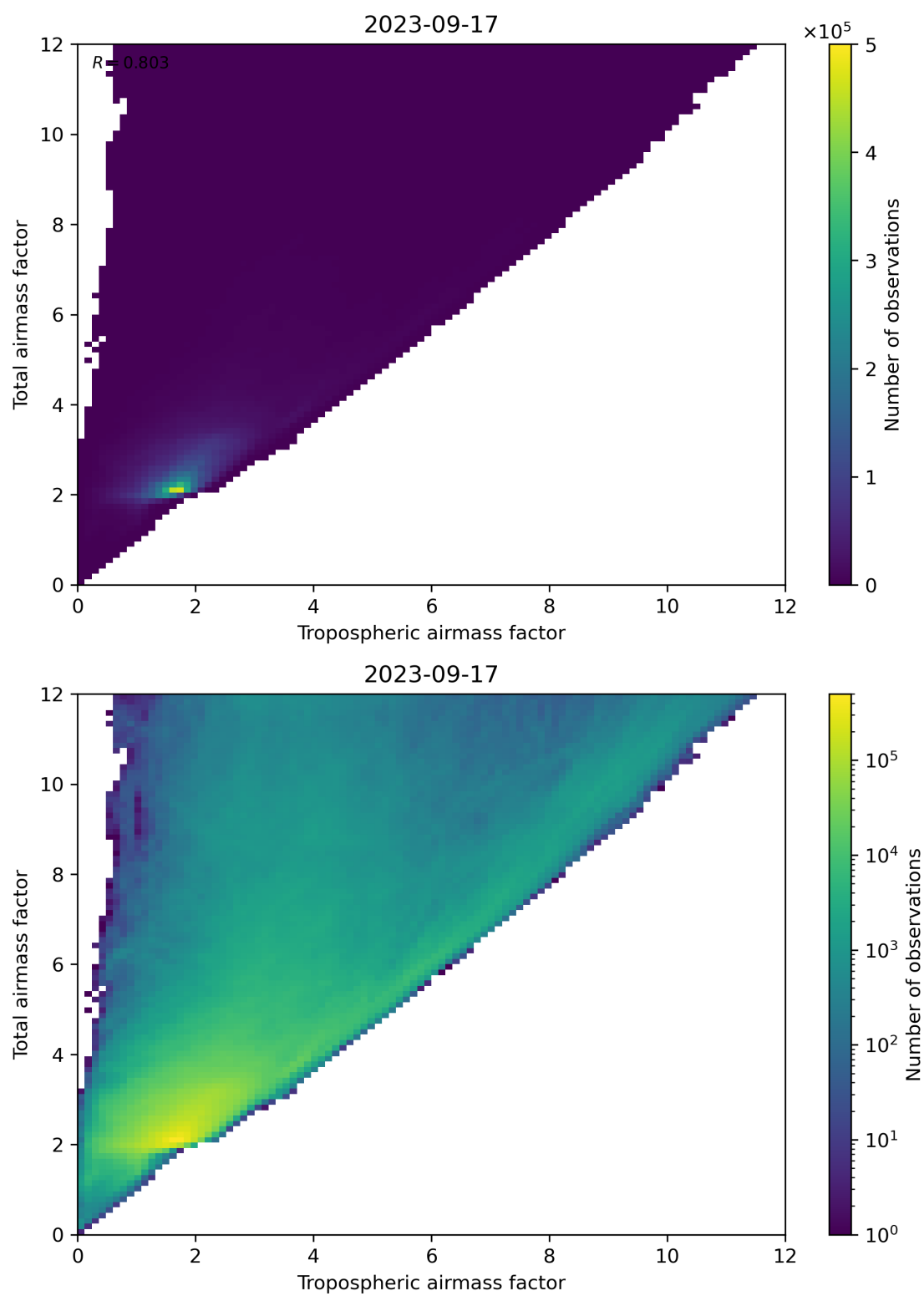
Figure 72: Scatter density plot of “Tropospheric airmass factor” against “Total airmass factor” for 2023-09-16 to 2023-09-18.
