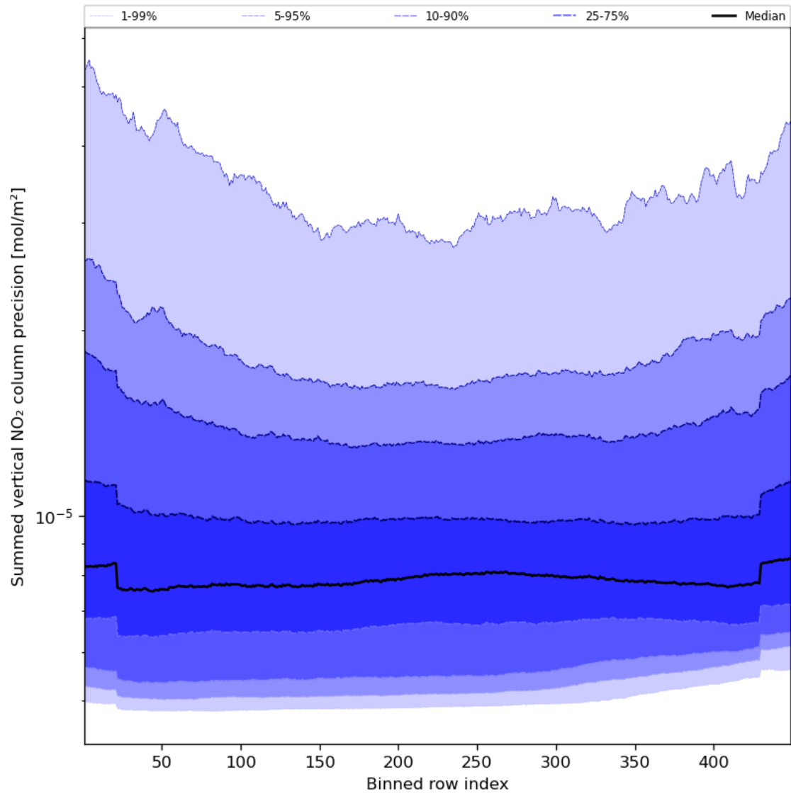
Figure 58: Along track statistics of “Summed vertical NO 2 column precision” for 2023-09-16 to 2023-09-18
