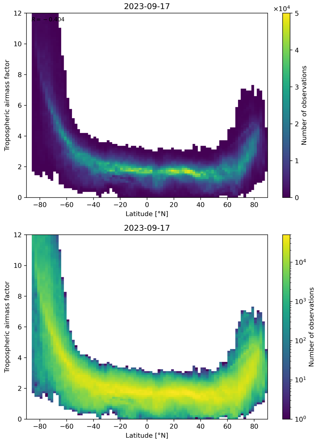
Figure 85: Scatter density plot of “Latitude” against “Tropospheric airmass factor” for 2023-09-16 to 2023-09-18.
