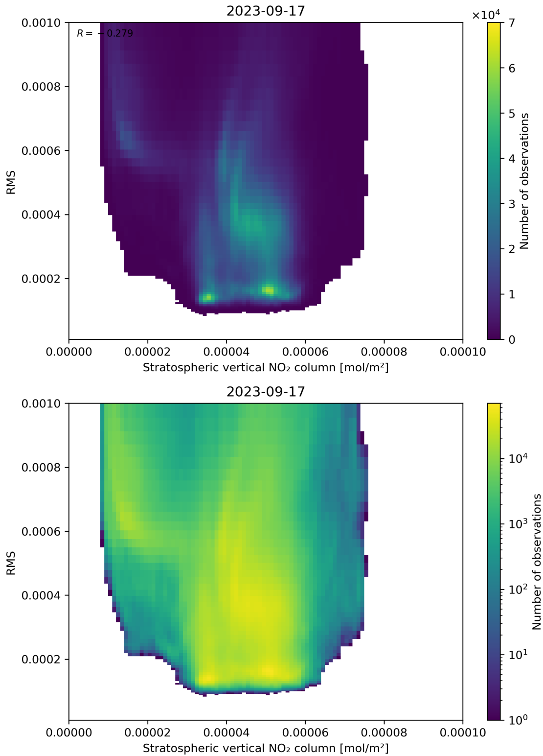
Figure 102: Scatter density plot of “Stratospheric vertical NO 2 column” against “RMS” for 2023-09-16 to 2023-09-18.
