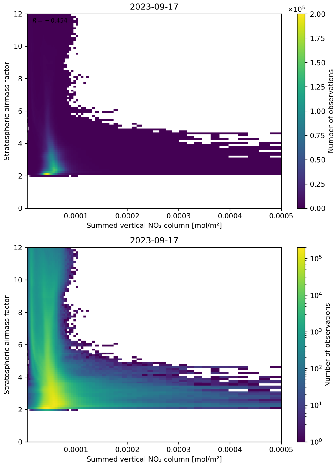
Figure 103: Scatter density plot of “Summed vertical NO 2 column” against “Stratospheric air mass factor” for 2023-09-16 to 2023-09-18.
