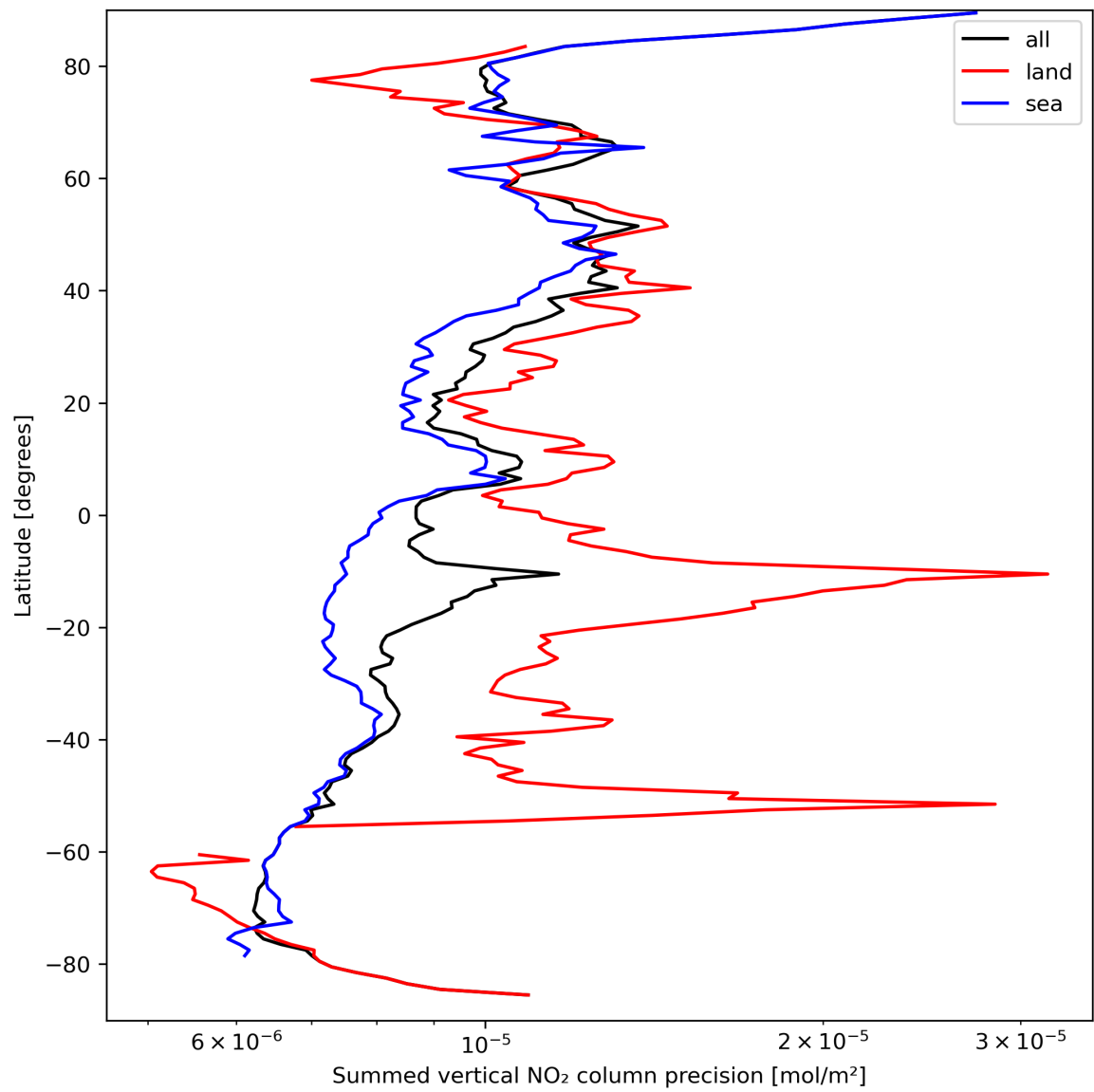
Figure 24: Zonal average of “Summed vertical NO 2 column precision” for 2023-09-16 to 2023-09-18.
