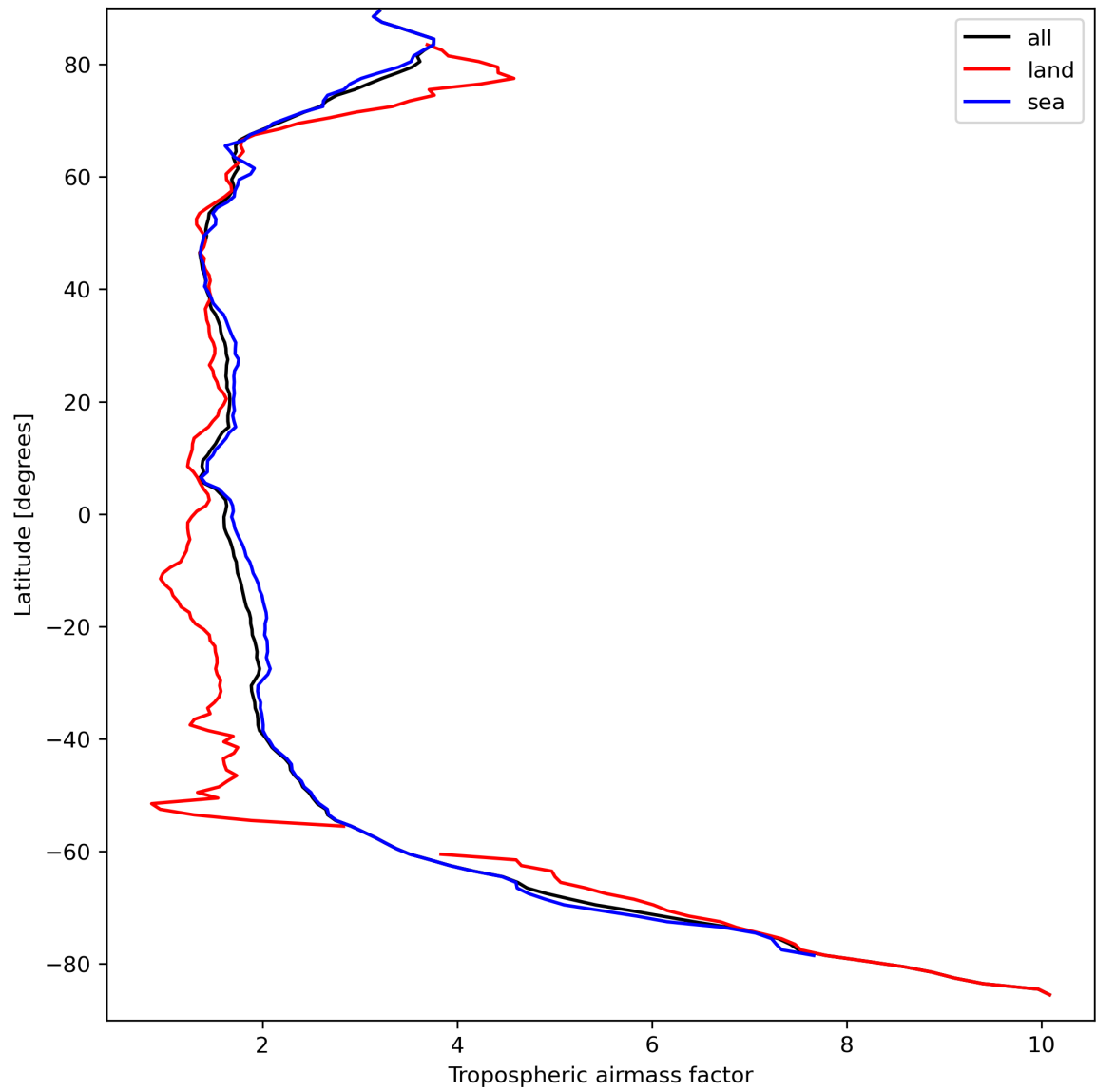
Figure 14: Zonal average of “Tropospheric airmass factor” for 2023-09-16 to 2023-09-18.
