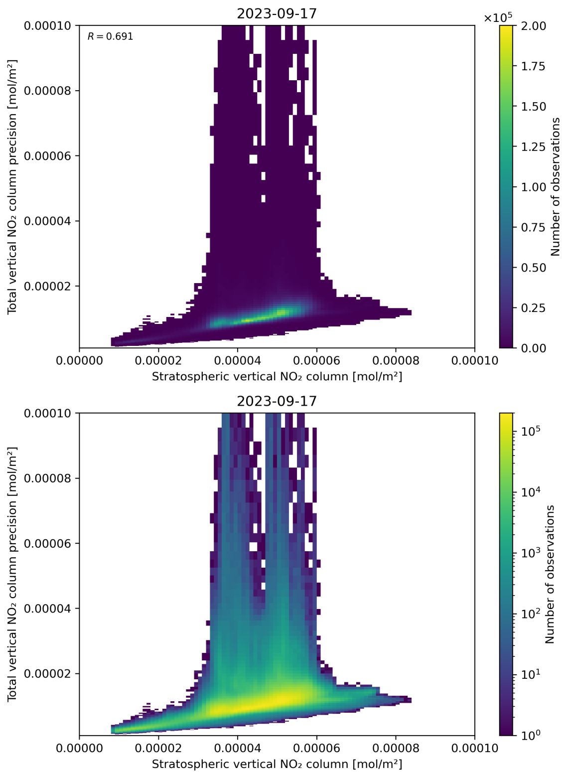
Figure 101: Scatter density plot of “Stratospheric vertical NO 2 column” against “Total vertical NO 2 column precision” for 2023-09-16 to 2023-09-18.
