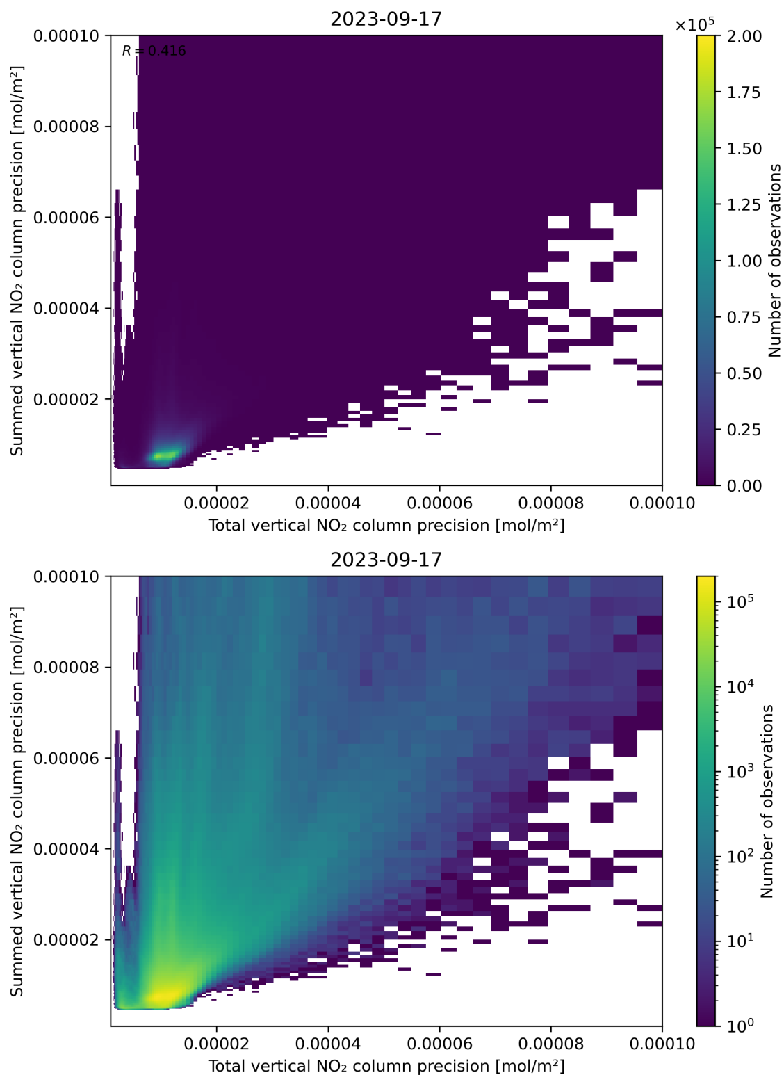
Figure 118: Scatter density plot of “Total vertical NO 2 column precision” against “Summed vertical NO 2 column precision” for 2023-09-16 to 2023-09-18.
