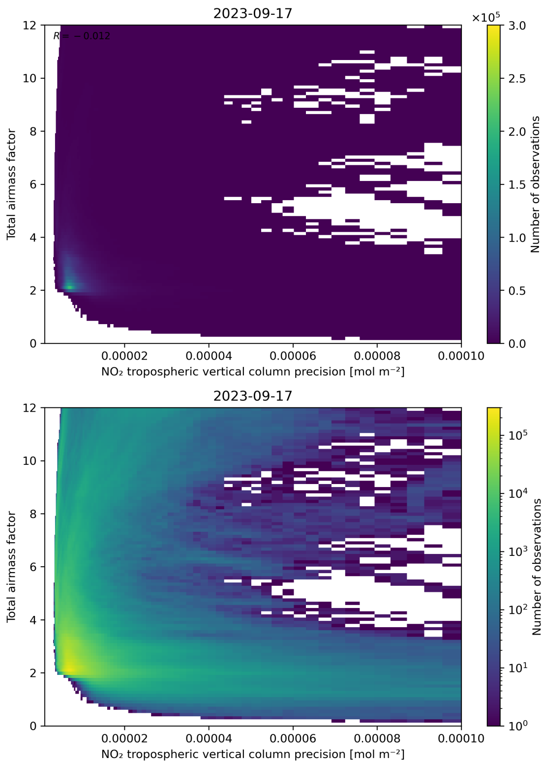
Figure 132: Scatter density plot of “NO 2 tropospheric vertical column precision” against “Total air mass factor” for 2023-09-16 to 2023-09-18.
