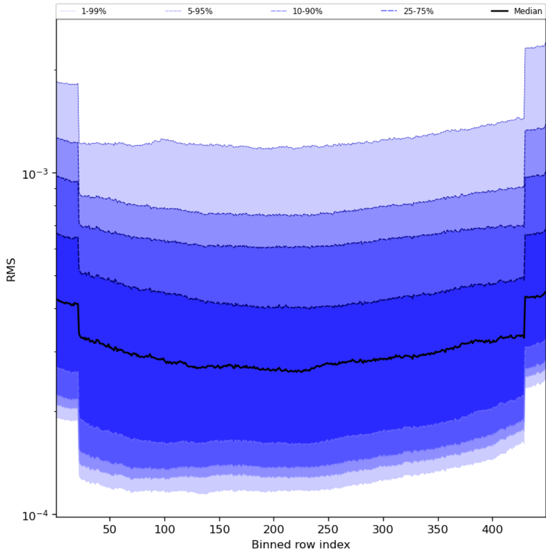
Figure 60: Along track statistics of “RMS” for 2023-09-16 to 2023-09-18
