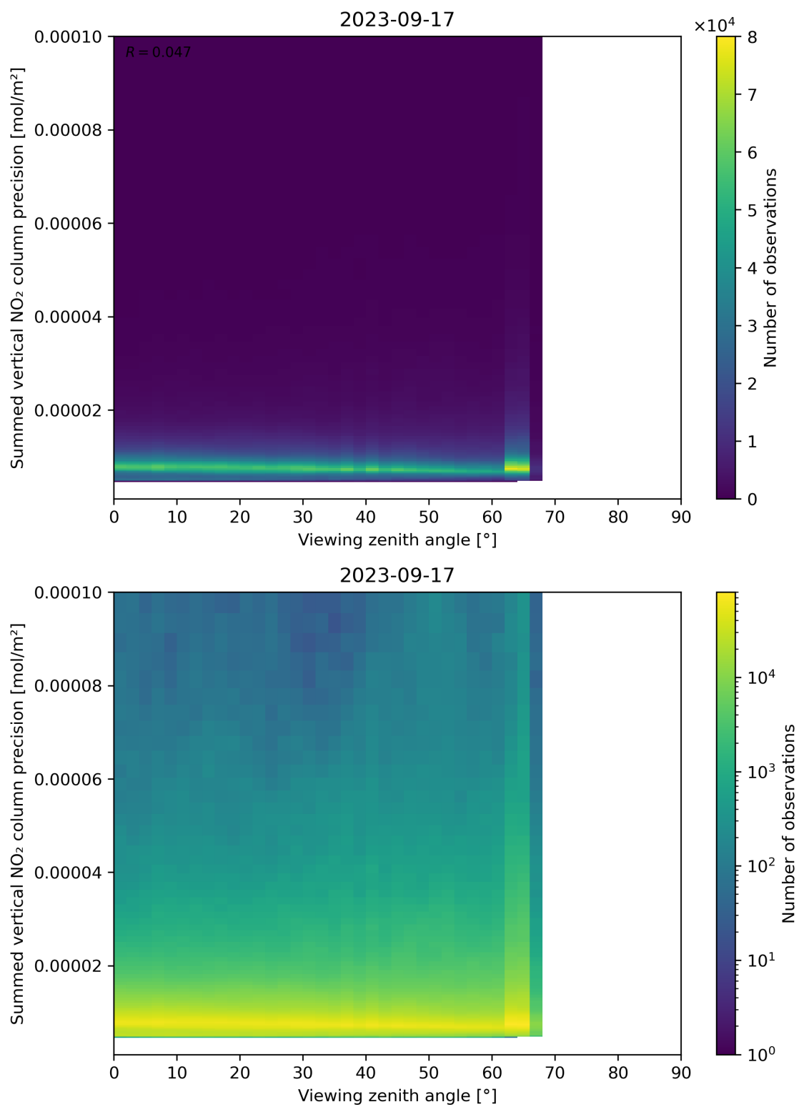
Figure 166: Scatter density plot of “Viewing zenith angle” against “Summed vertical NO 2 column precision” for 2023-09-16 to 2023-09-18.
