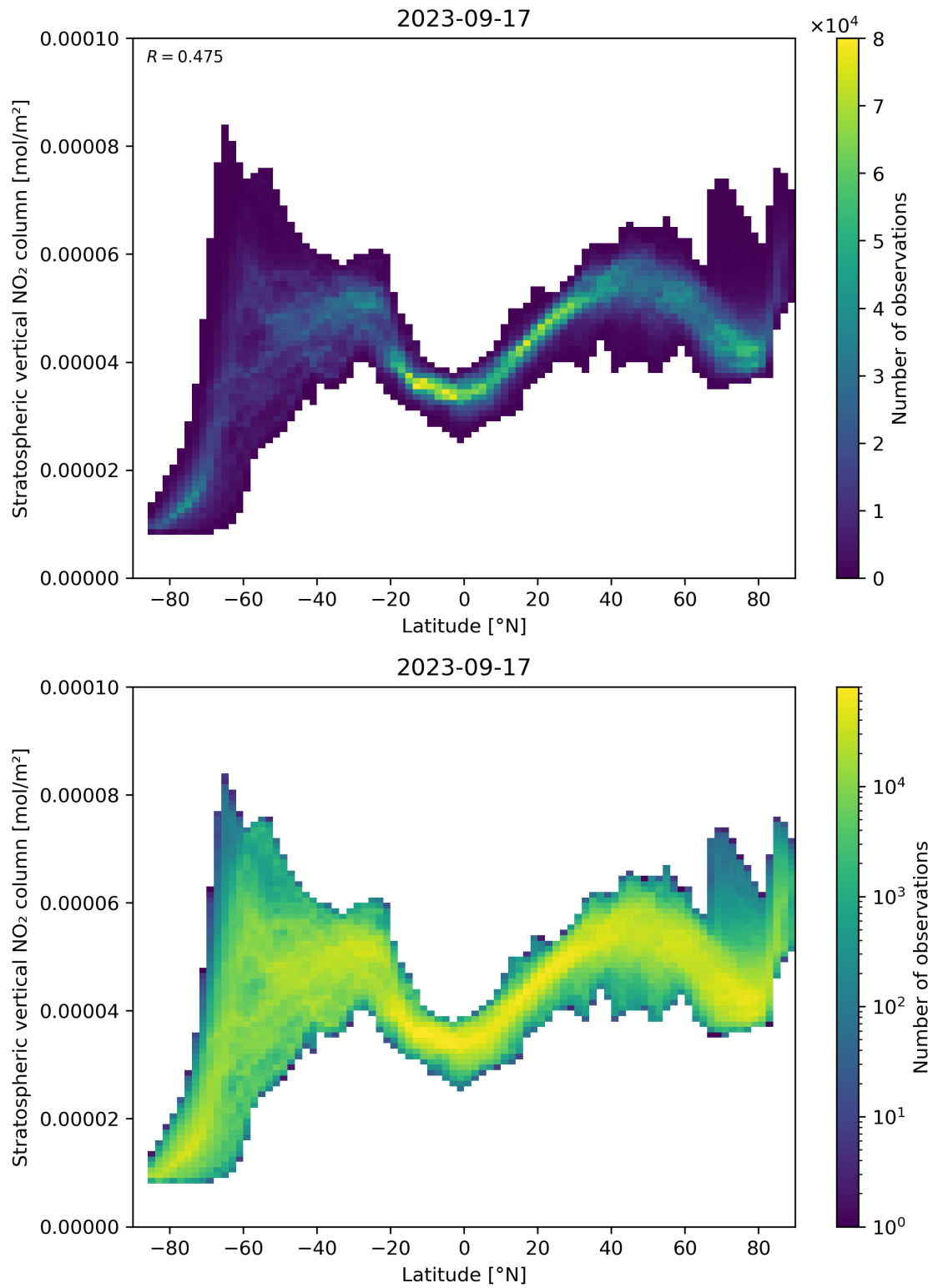
Figure 87: Scatter density plot of “Latitude” against “Stratospheric vertical NO 2 column” for 2023-09-16 to 2023-09-18.
