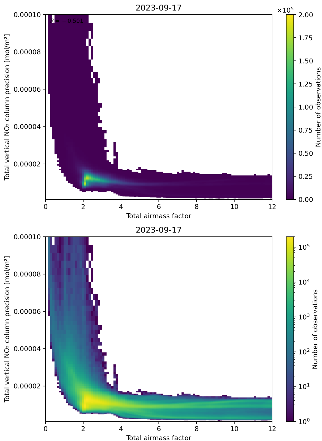
Figure 68: Scatter density plot of “Total airmass factor” against “Total vertical NO 2 column precision” for 2023-09-16 to 2023-09-18.
