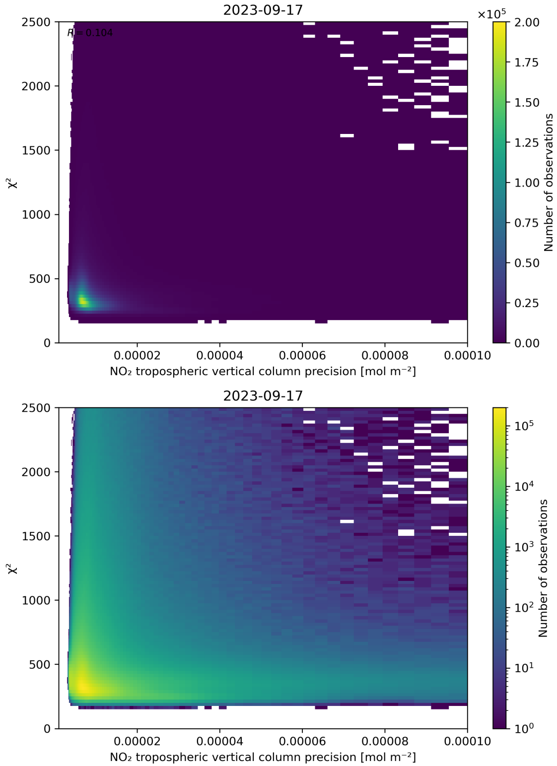
Figure 134: Scatter density plot of “NO 2 tropospheric vertical column precision” against “ \chi^2 ” for 2023-09-16 to 2023-09-18.
