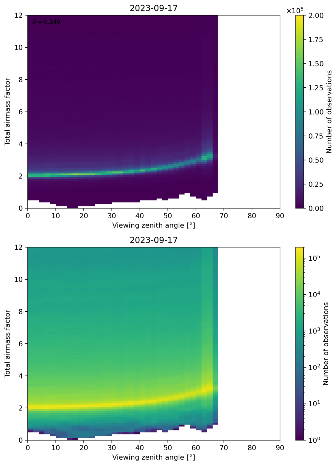
Figure 160: Scatter density plot of “Viewing zenith angle” against “Total airmass factor” for 2023-09-16 to 2023-09-18.
