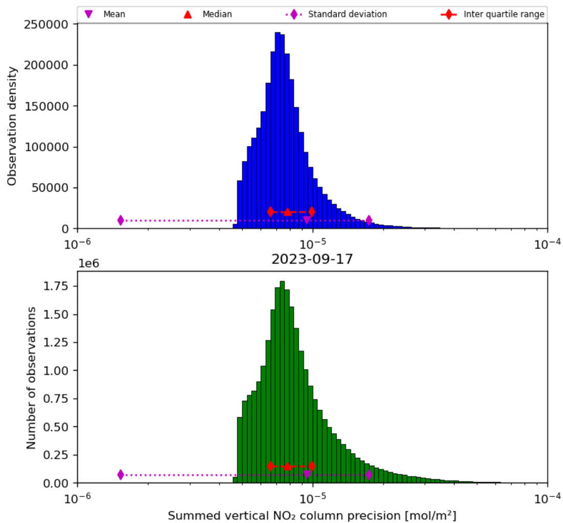
Figure 41: Histogram of “Summed vertical NO 2 column precision” for 2023-09-16 to 2023-09-18
