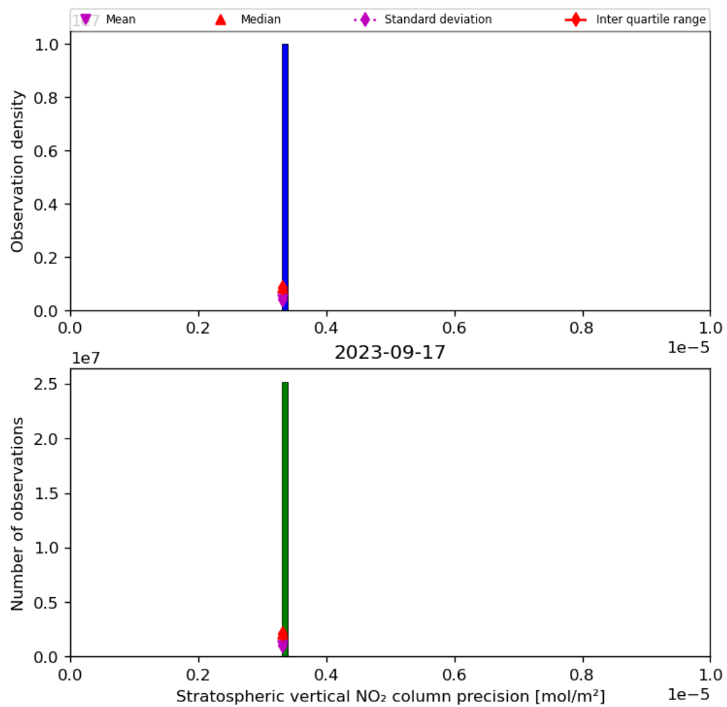
Figure 37: Histogram of “Stratospheric vertical NO 2 column precision” for 2023-09-16 to 2023-09-18
