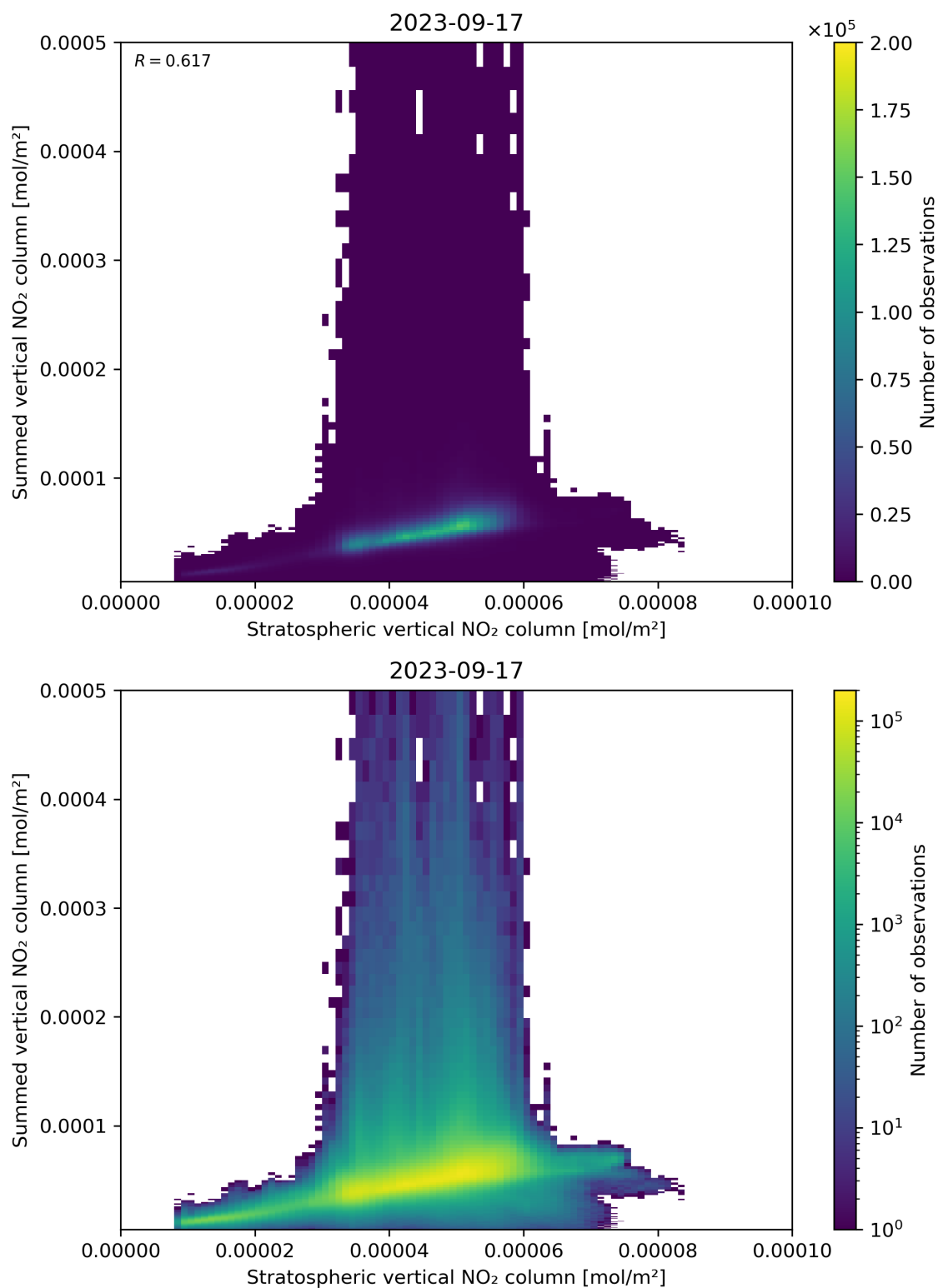
Figure 98: Scatter density plot of “Stratospheric vertical NO 2 column” against “Summed vertical NO 2 column” for 2023-09-16 to 2023-09-18.
