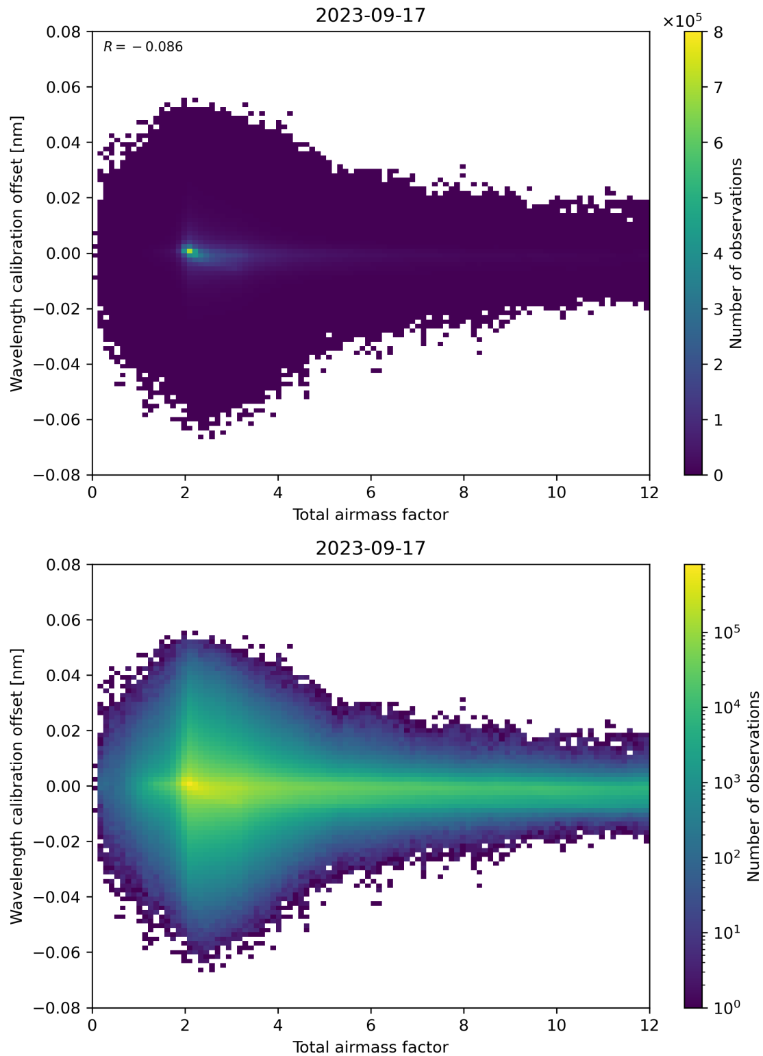
Figure 70: Scatter density plot of “Total airmass factor” against “Wavelength calibration offset” for 2023-09-16 to 2023-09-18.
