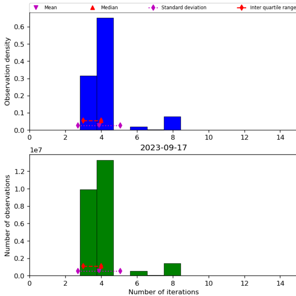
Figure 34: Histogram of “Number of iterations” for 2023-09-16 to 2023-09-18
