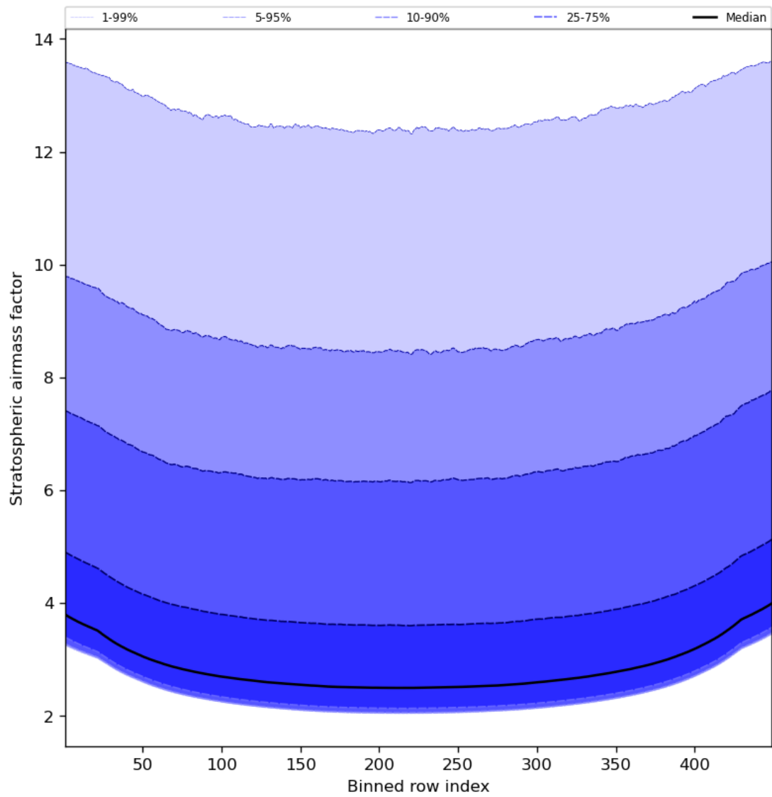
Figure 61: Along track statistics of “Stratospheric airmass factor” for 2023-09-16 to 2023-09-18
