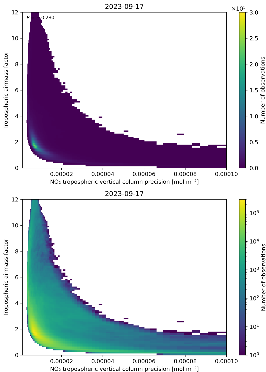
Figure 133: Scatter density plot of “NO 2 tropospheric vertical column precision” against “Tropospheric airmass factor” for 2023-09-16 to 2023-09-18.
