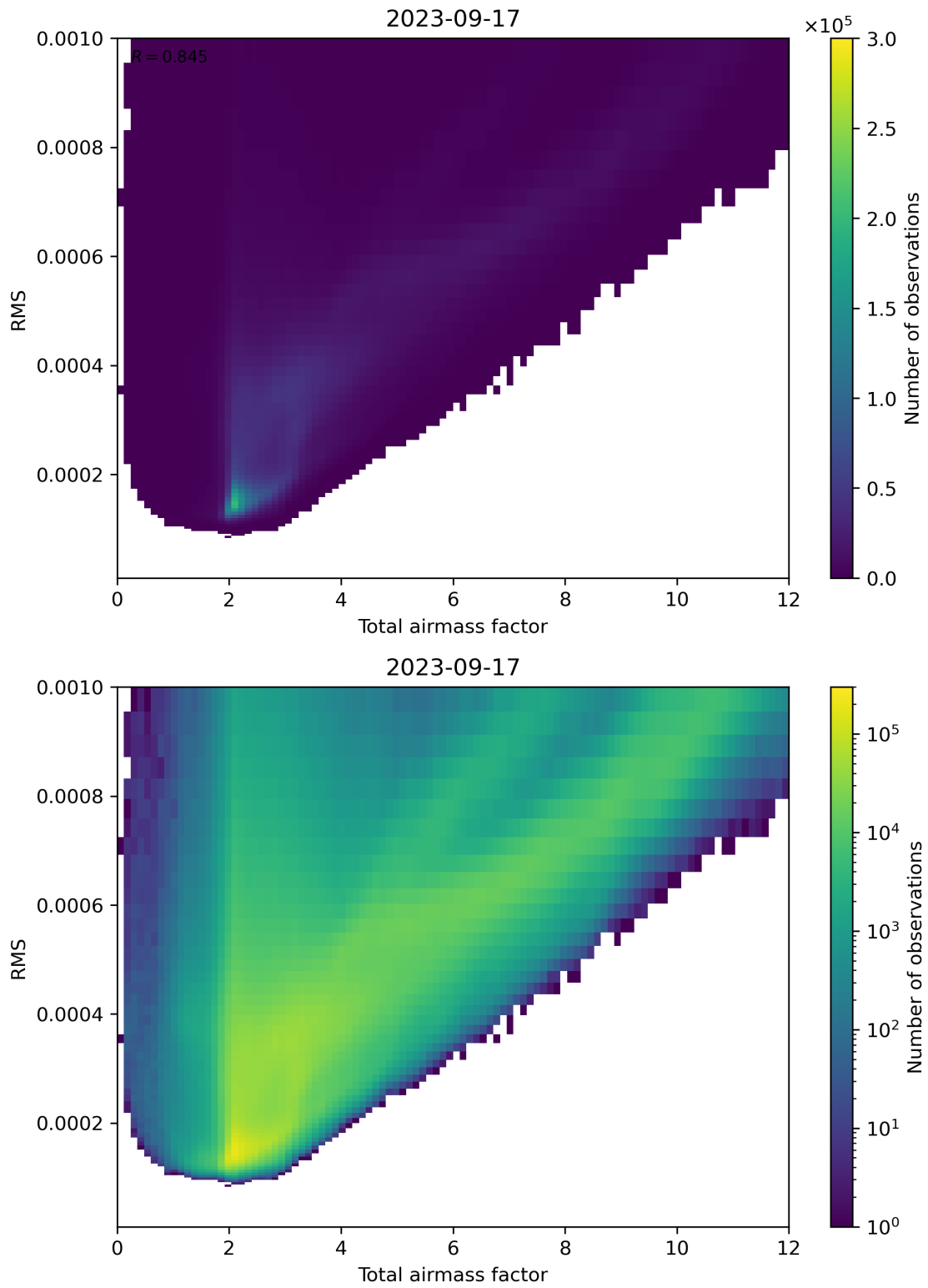
Figure 69: Scatter density plot of “Total airmass factor” against “RMS” for 2023-09-16 to 2023-09-18.
