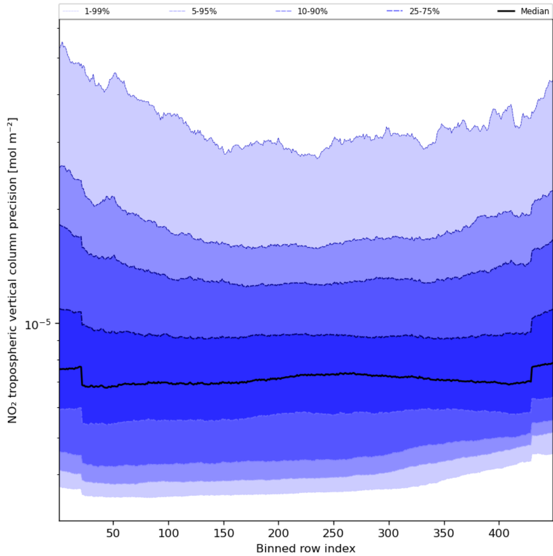
Figure 47: Along track statistics of “NO 2 tropospheric vertical column precision” for 2023-09-16 to 2023-09-18
