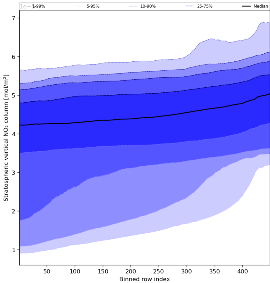
Figure 53: Along track statistics of “Stratospheric vertical NO 2 column” for 2023-09-16 to 2023-09-18
