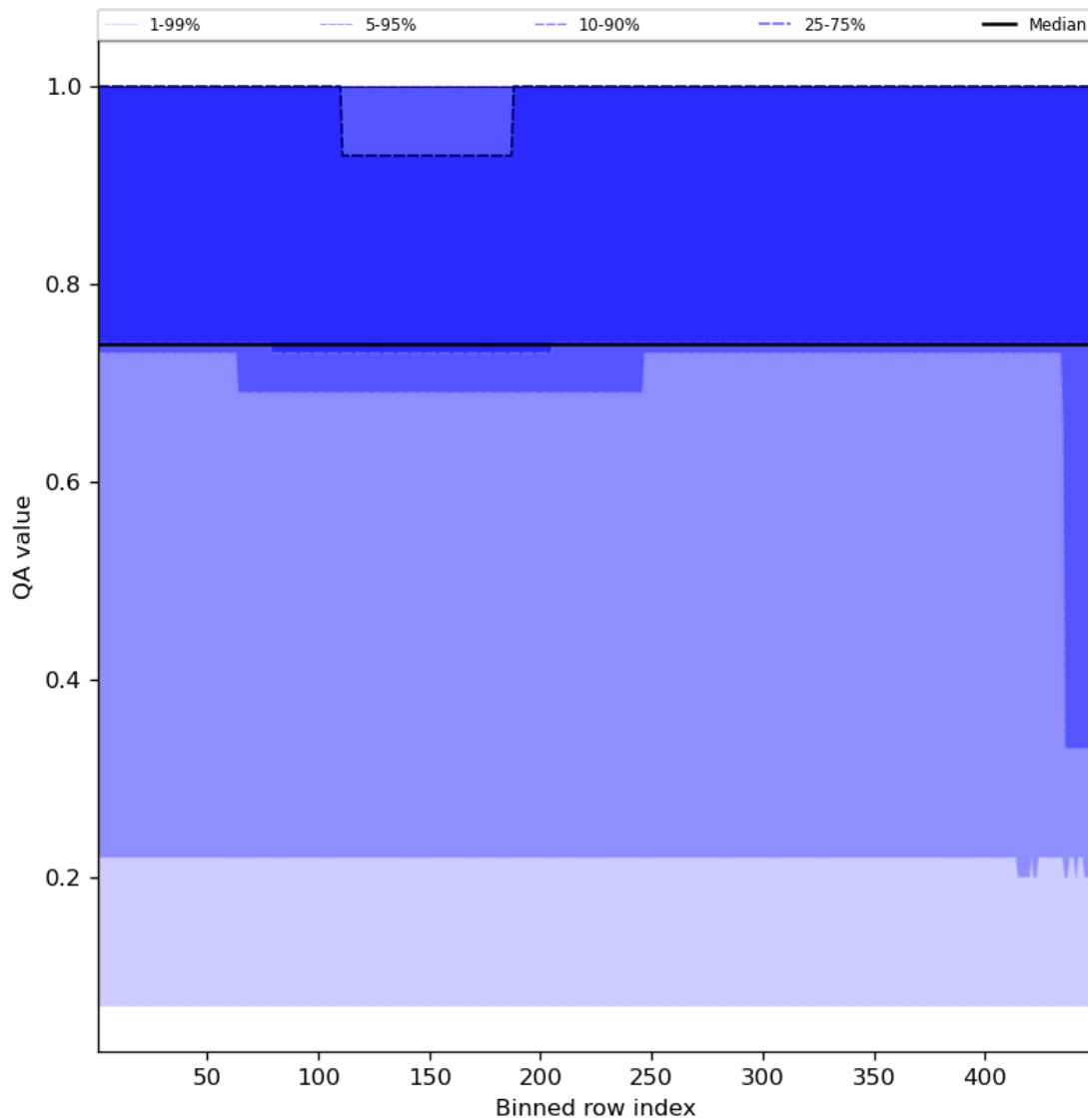
Figure 45: Along track statistics of “QA value” for 2023-09-16 to 2023-09-18
