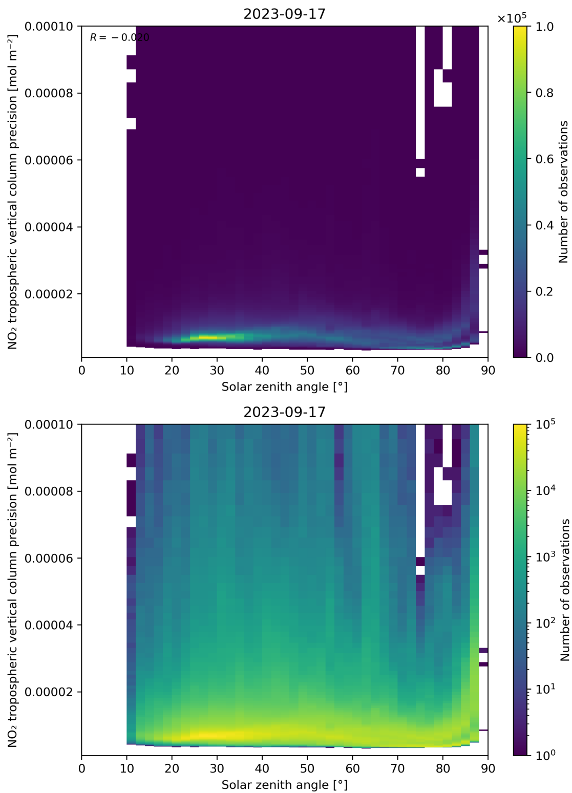
Figure 156: Scatter density plot of “Solar zenith angle” against “NO 2 tropospheric vertical column precision” for 2023-09-16 to 2023-09-18.
