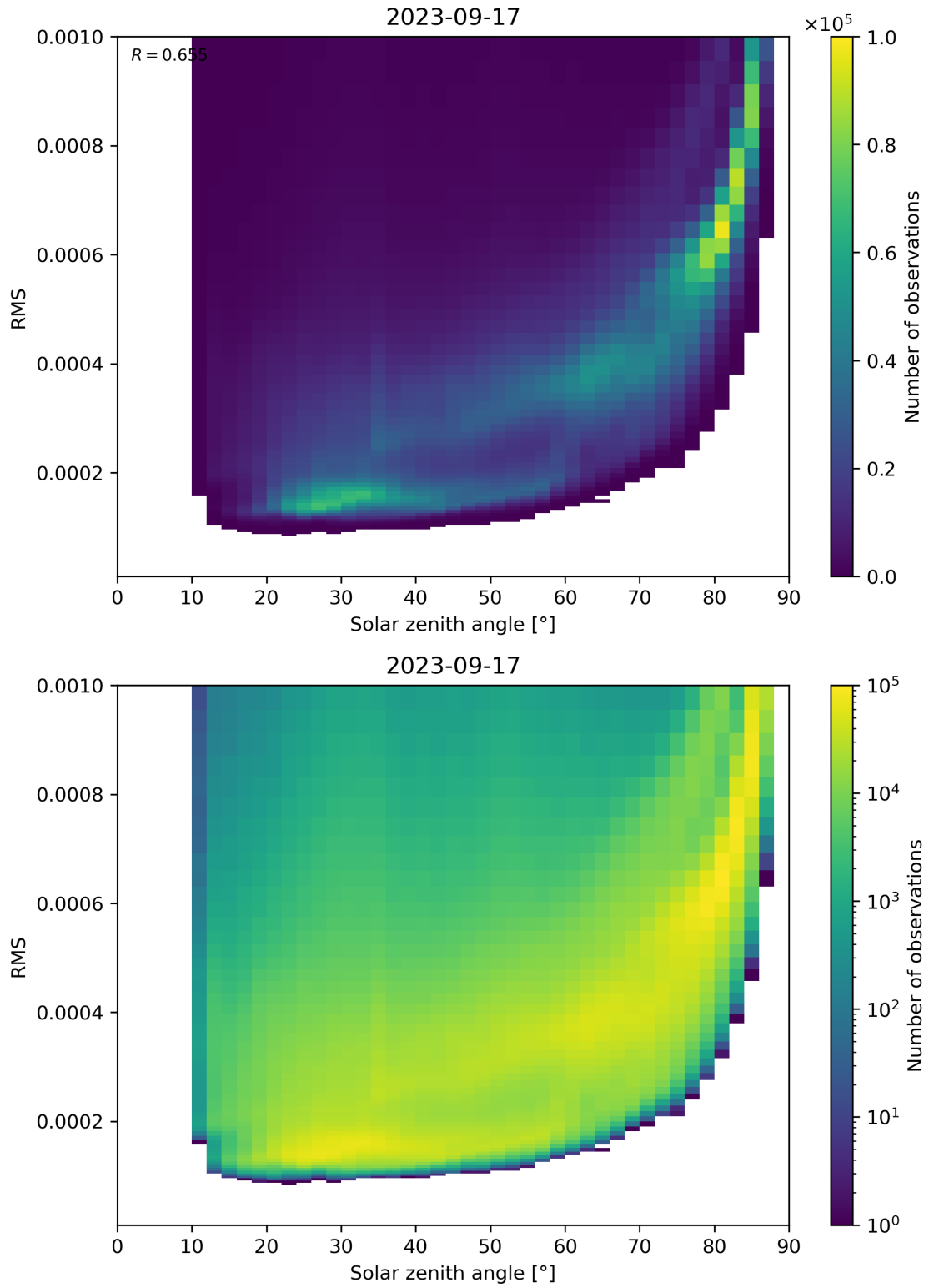
Figure 157: Scatter density plot of “Solar zenith angle” against “RMS” for 2023-09-16 to 2023-09-18.
