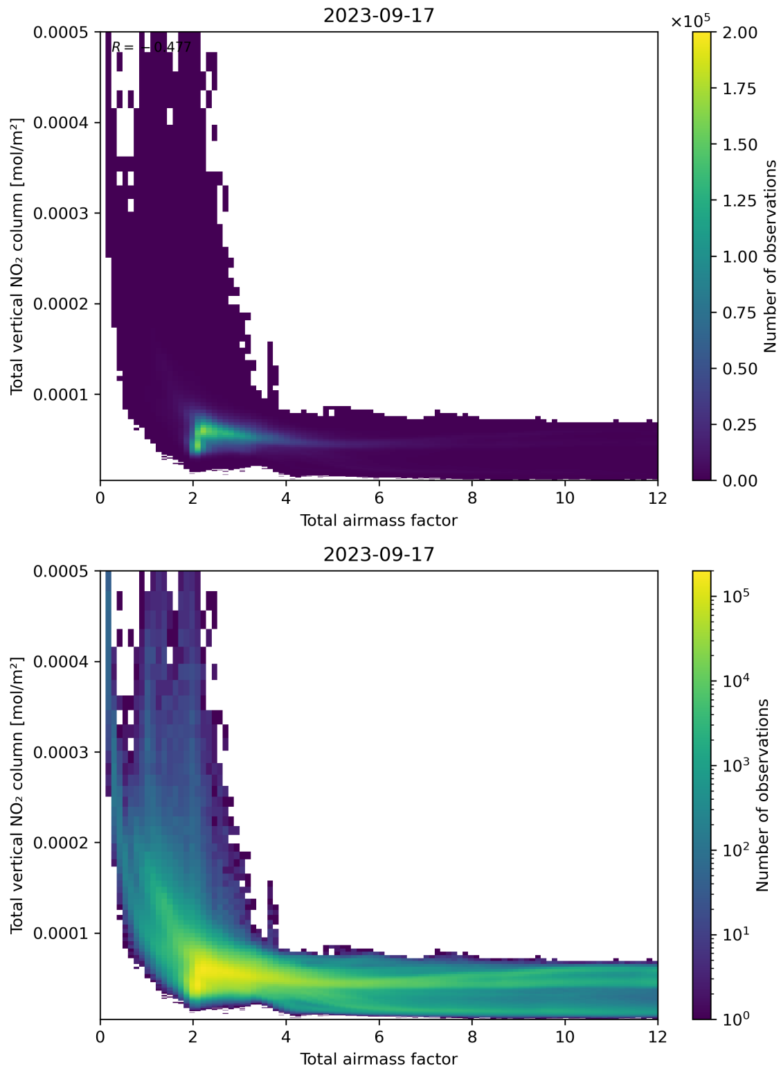
Figure 67: Scatter density plot of “Total airmass factor” against “Total vertical NO 2 column” for 2023-09-16 to 2023-09-18.
