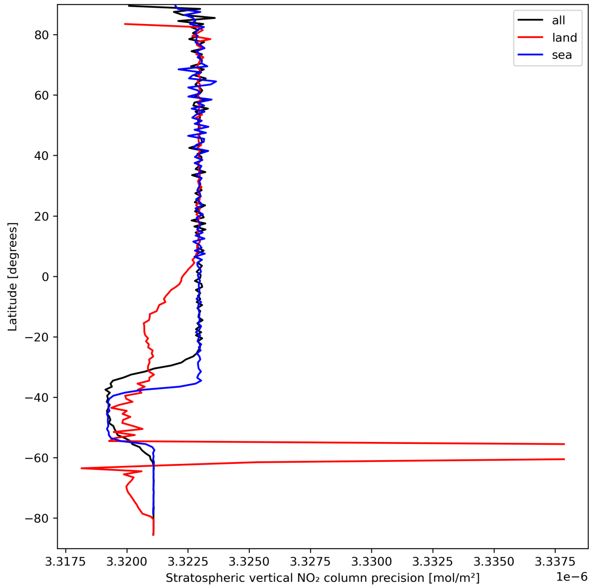
Figure 20: Zonal average of “Stratospheric vertical NO 2 column precision” for 2023-09-16 to 2023-09-18.
