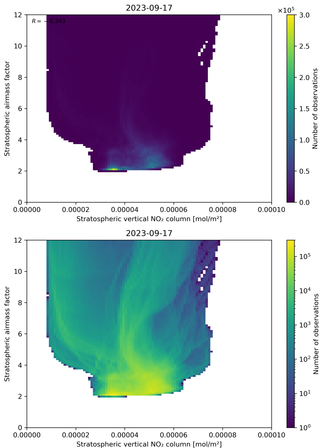
Figure 96: Scatter density plot of “Stratospheric vertical NO 2 column” against “Stratospheric airmass factor” for 2023-09-16 to 2023-09-18.
