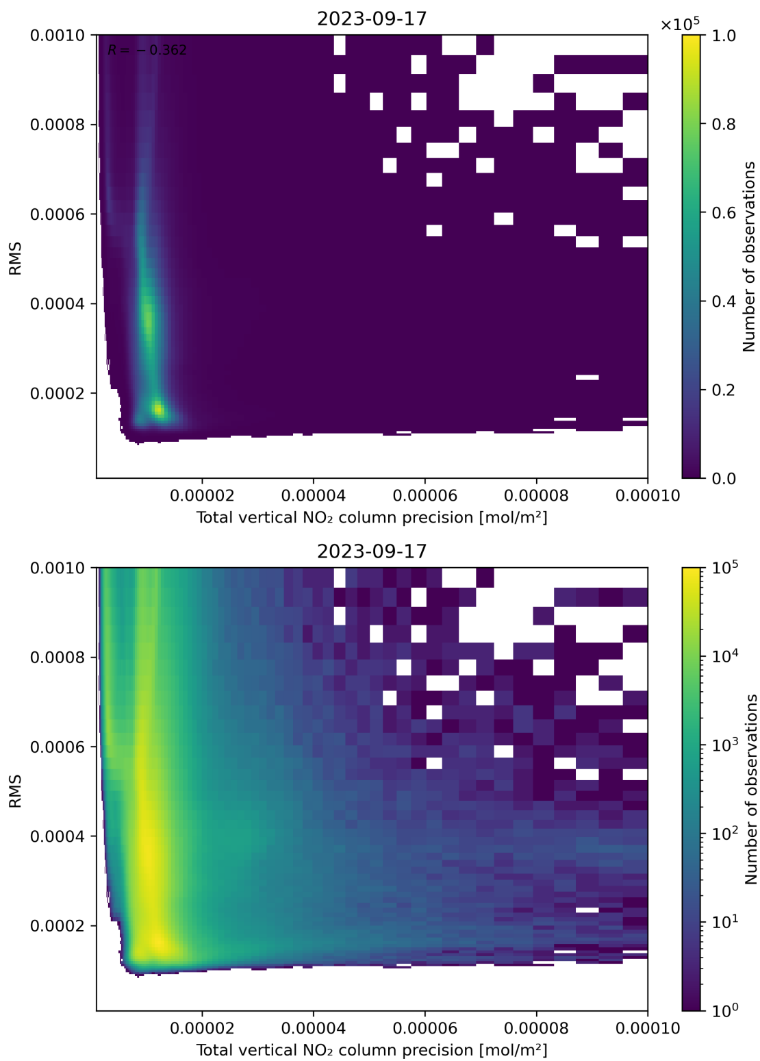
Figure 119: Scatter density plot of “Total vertical NO 2 column precision” against “RMS” for 2023-09-16 to 2023-09-18.
