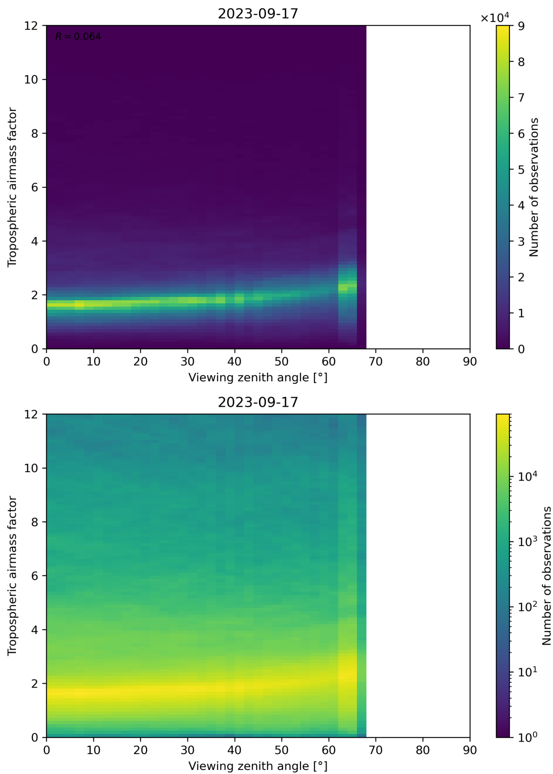
Figure 161: Scatter density plot of “Viewing zenith angle” against “Tropospheric airmass factor” for 2023-09-16 to 2023-09-18.
