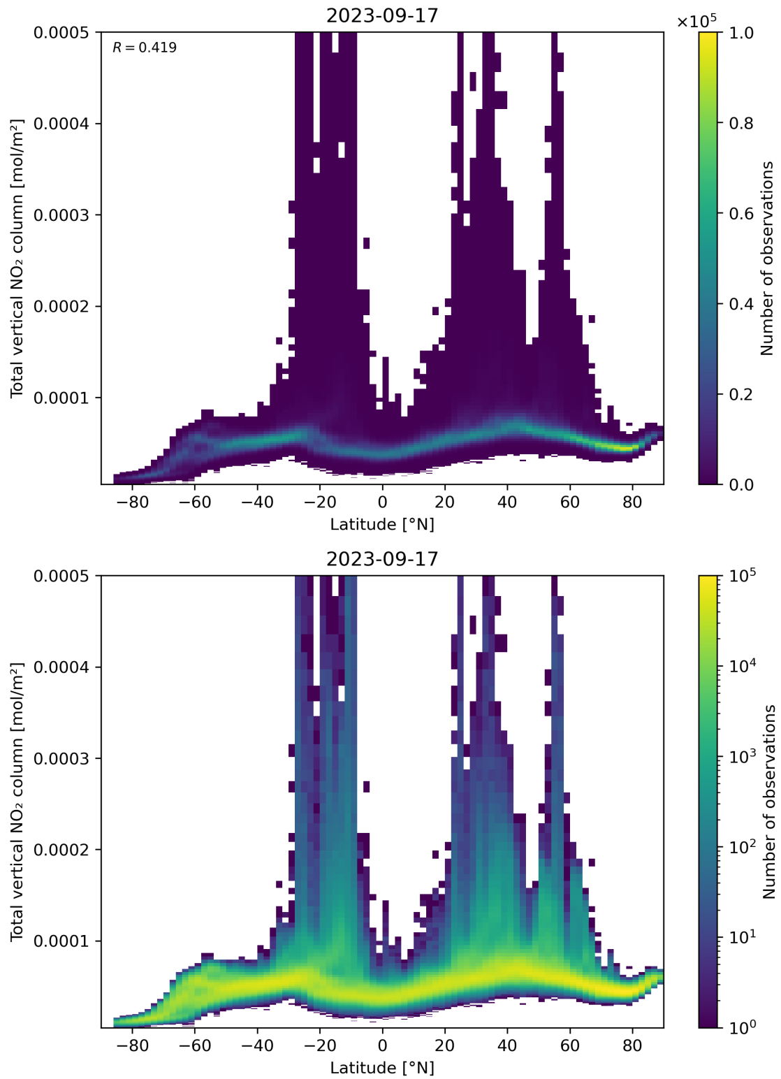
Figure 90: Scatter density plot of “Latitude” against “Total vertical NO 2 column” for 2023-09-16 to 2023-09-18.
