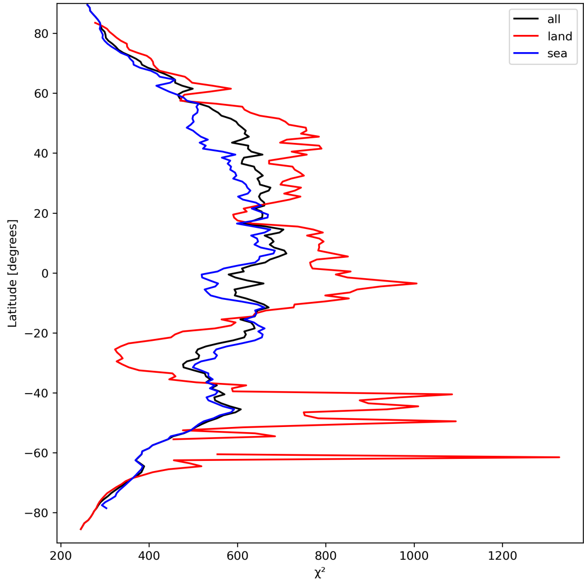
Figure 25: Zonal average of “ \chi^2 ” for 2023-09-16 to 2023-09-18.
