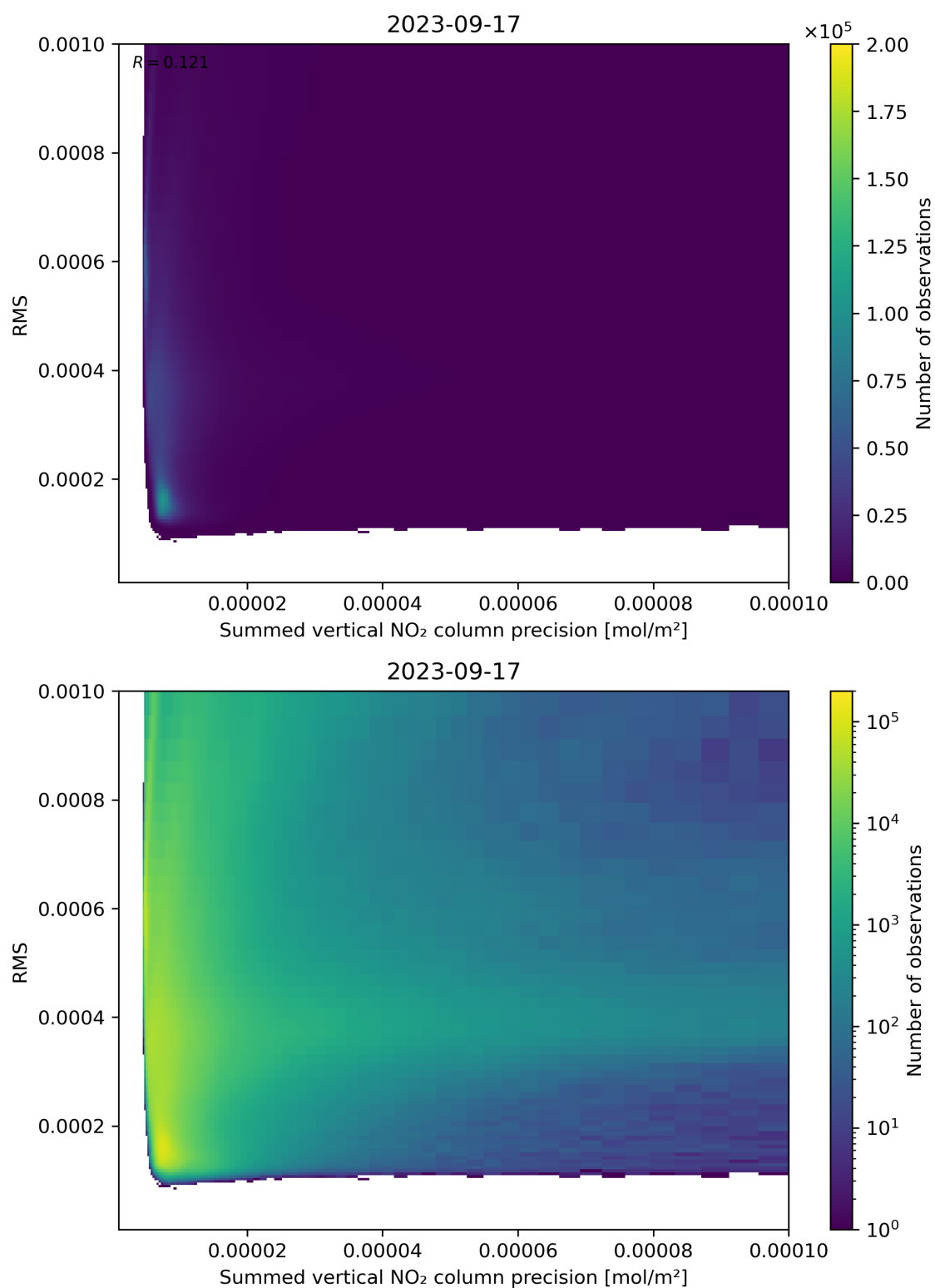
Figure 108: Scatter density plot of “Summed vertical NO 2 column precision” against “RMS” for 2023-09-16 to 2023-09-18.
