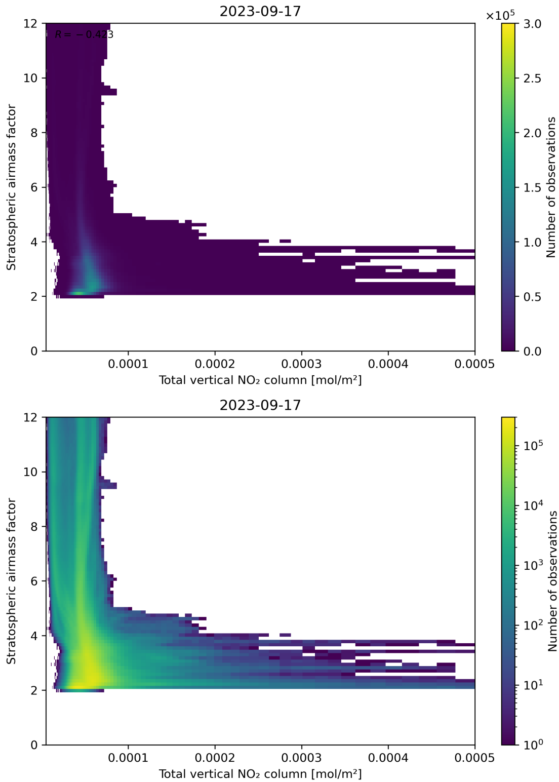
Figure 110: Scatter density plot of “Total vertical NO 2 column” against “Stratospheric airmass factor” for 2023-09-16 to 2023-09-18.
