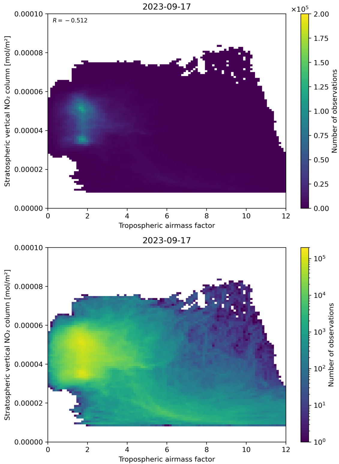
Figure 74: Scatter density plot of “Tropospheric air mass factor” against “Stratospheric vertical NO 2 column” for 2023-09-16 to 2023-09-18.
