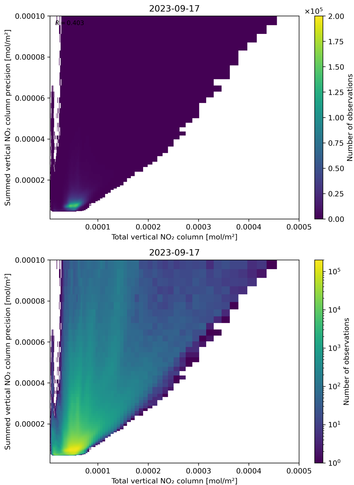
Figure 113: Scatter density plot of “Total vertical NO 2 column” against “Summed vertical NO 2 column precision” for 2023-09-16 to 2023-09-18.
