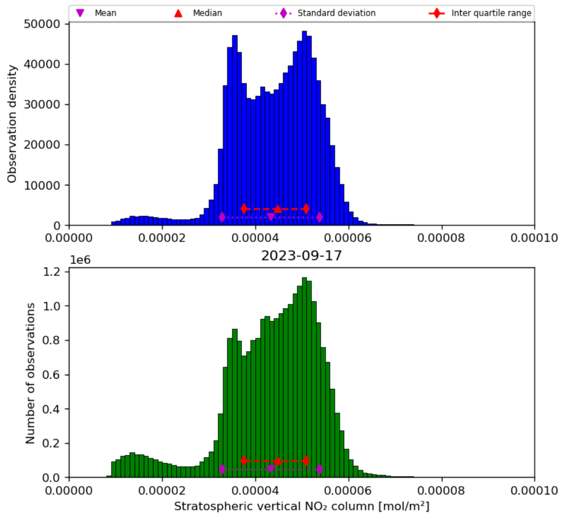
Figure 36: Histogram of “Stratospheric vertical NO 2 column” for 2023-09-16 to 2023-09-18
