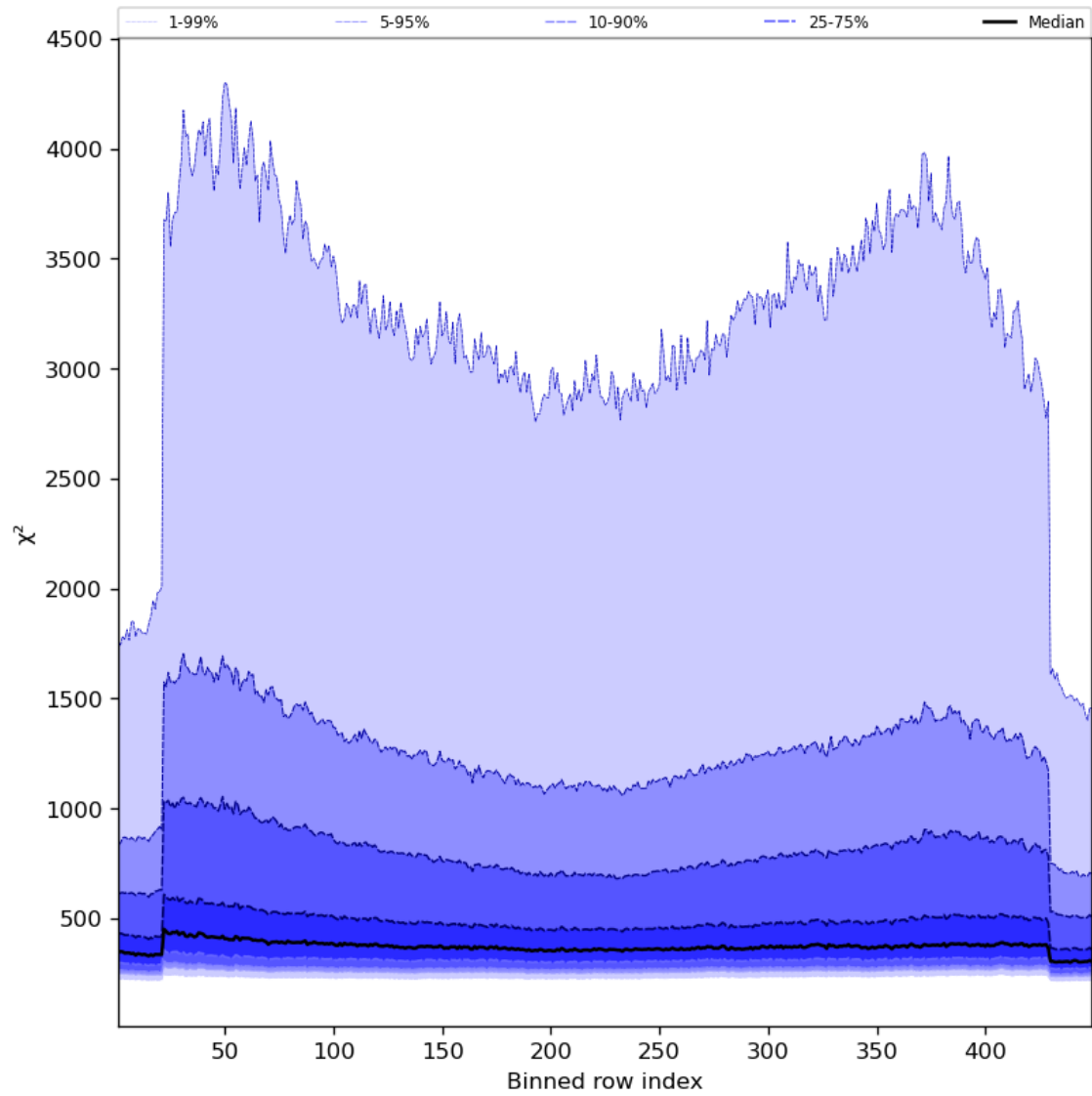
Figure 59: Along track statistics of “ \chi^2 ” for 2023-09-16 to 2023-09-18
