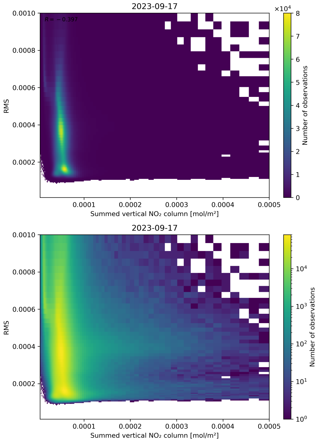
Figure 109: Scatter density plot of “Summed vertical NO 2 column” against “RMS” for 2023-09-16 to 2023-09-18.
