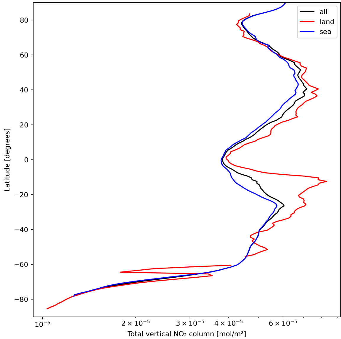
Figure 21: Zonal average of “Total vertical NO 2 column” for 2023-09-16 to 2023-09-18.
