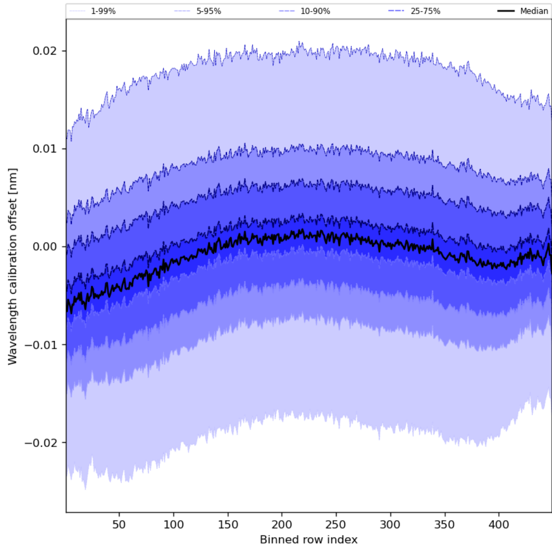
Figure 52: Along track statistics of “Wavelength calibration offset” for 2023-09-16 to 2023-09-18
