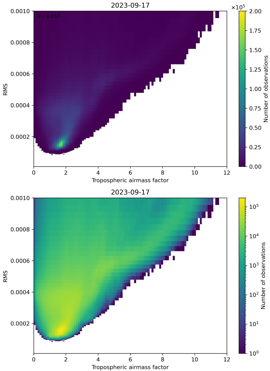
Figure 79: Scatter density plot of “Tropospheric airmass factor” against “RMS” for 2023-09-16 to 2023-09-18.
