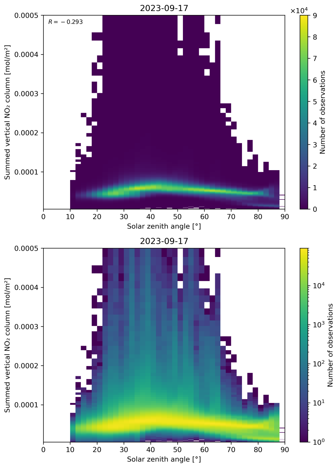
Figure 151: Scatter density plot of “Solar zenith angle” against “Summed vertical NO 2 column” for 2023-09-16 to 2023-09-18.
