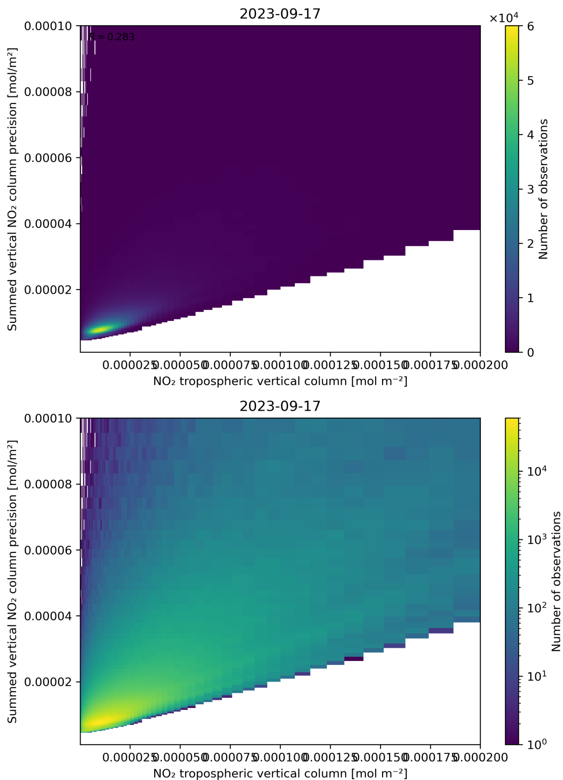
Figure 127: Scatter density plot of “NO 2 tropospheric vertical column” against “Summed vertical NO 2 column precision” for 2023-09-16 to 2023-09-18.
