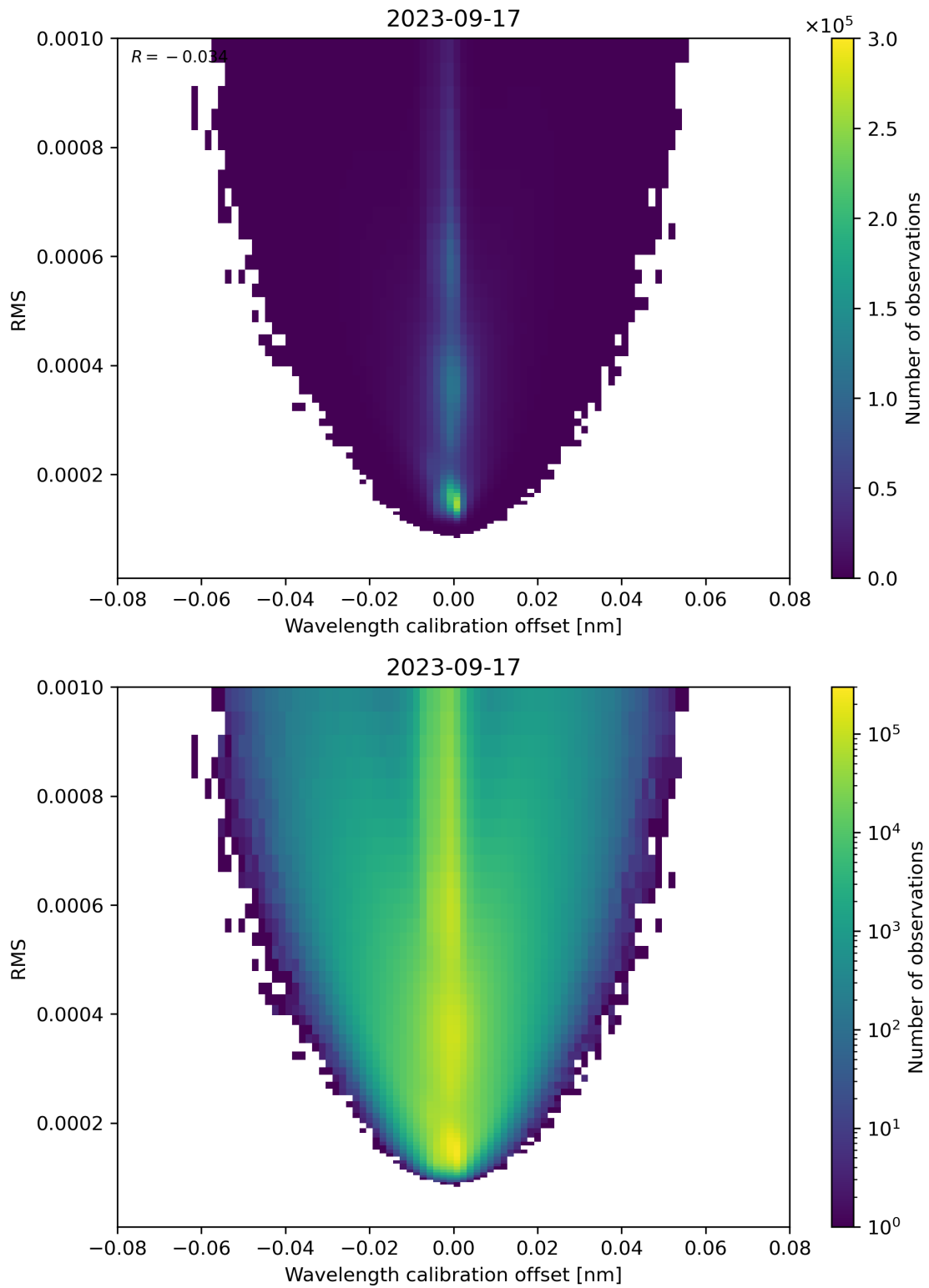
Figure 181: Scatter density plot of “Wavelength calibration offset” against “RMS” for 2023-09-16 to 2023-09-18.
