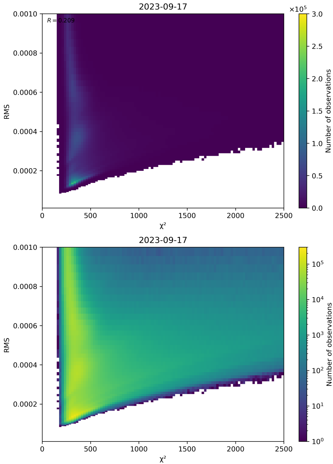
Figure 82: Scatter density plot of “ \chi^2 ” against “RMS” for 2023-09-16 to 2023-09-18.
