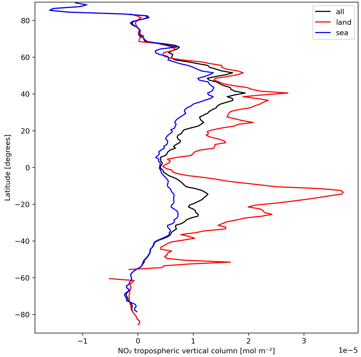
Figure 12: Zonal average of “NO 2 tropospheric vertical column” for 2023-09-16 to 2023-09-18.
