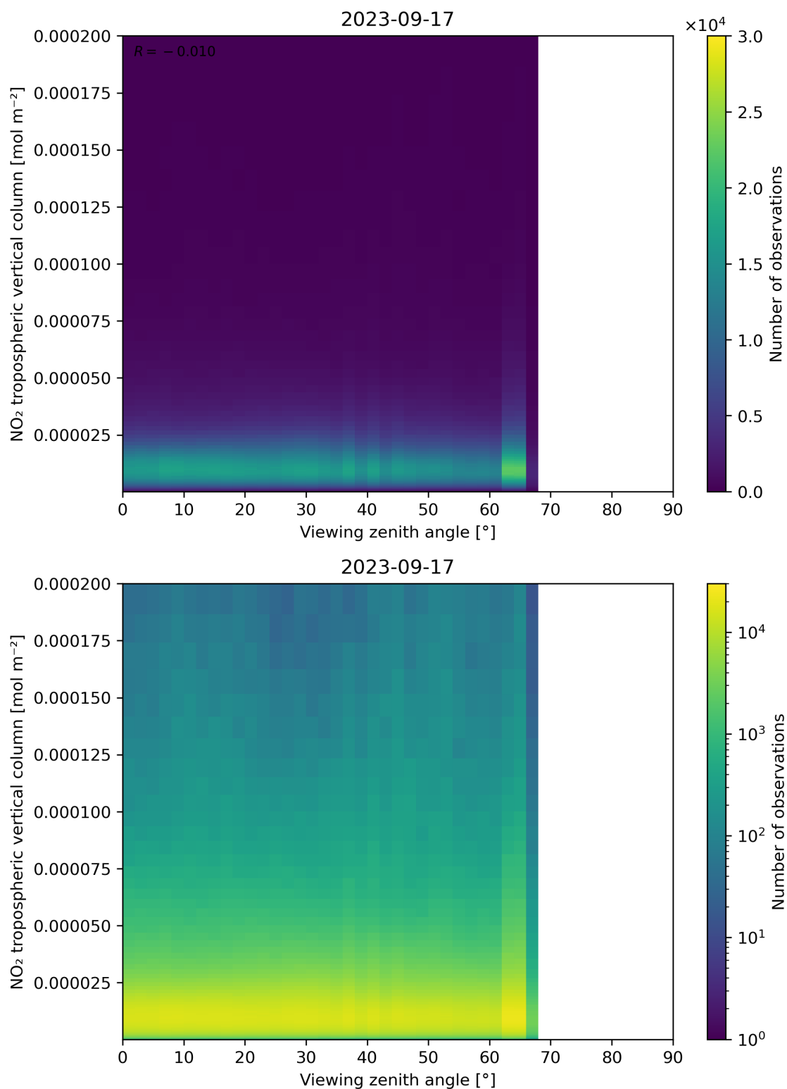
Figure 169: Scatter density plot of “Viewing zenith angle” against “NO 2 tropospheric vertical column” for 2023-09-16 to 2023-09-18.
