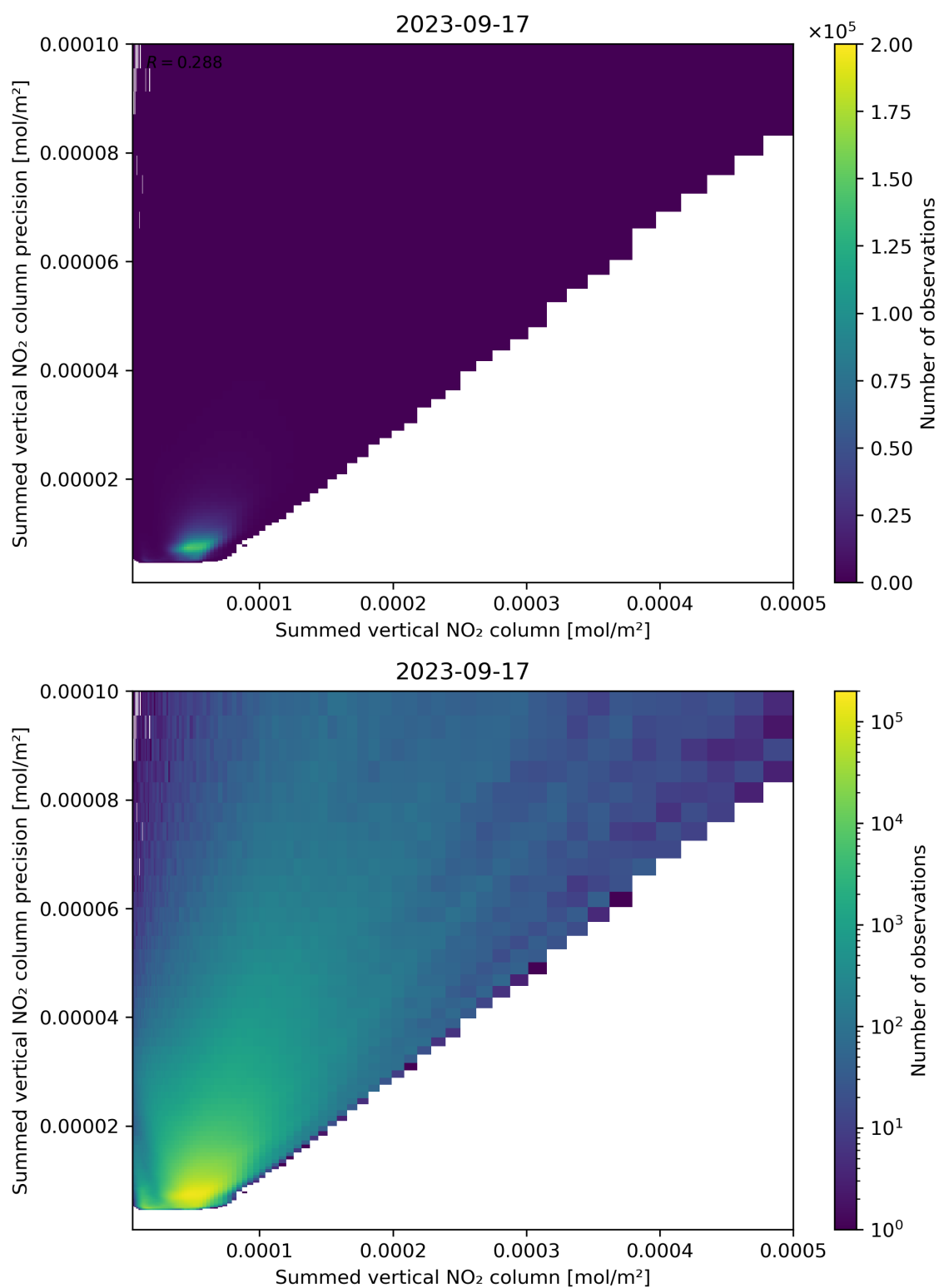
Figure 105: Scatter density plot of “Summed vertical NO 2 column” against “Summed vertical NO 2 column precision” for 2023-09-16 to 2023-09-18.
