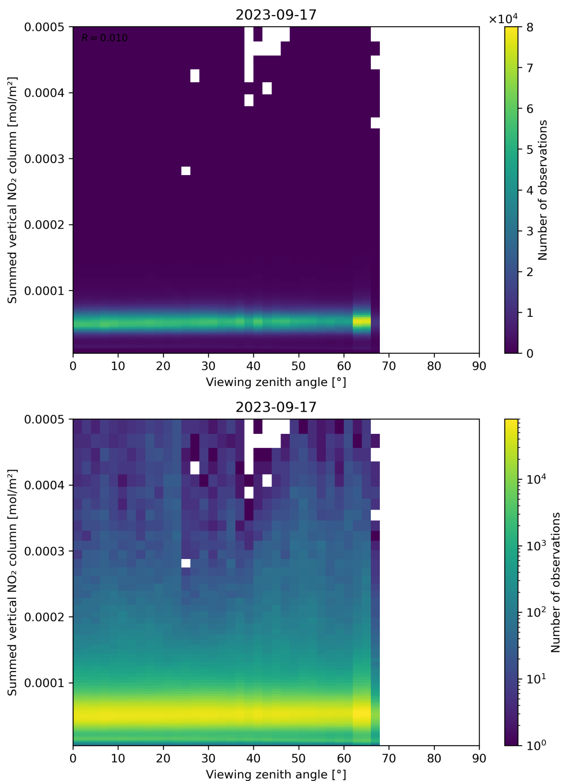
Figure 165: Scatter density plot of “Viewing zenith angle” against “Summed vertical NO 2 column” for 2023-09-16 to 2023-09-18.
