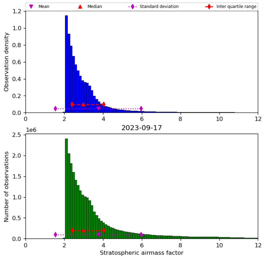
Figure 44: Histogram of “Stratospheric air mass factor” for 2023-09-16 to 2023-09-18
