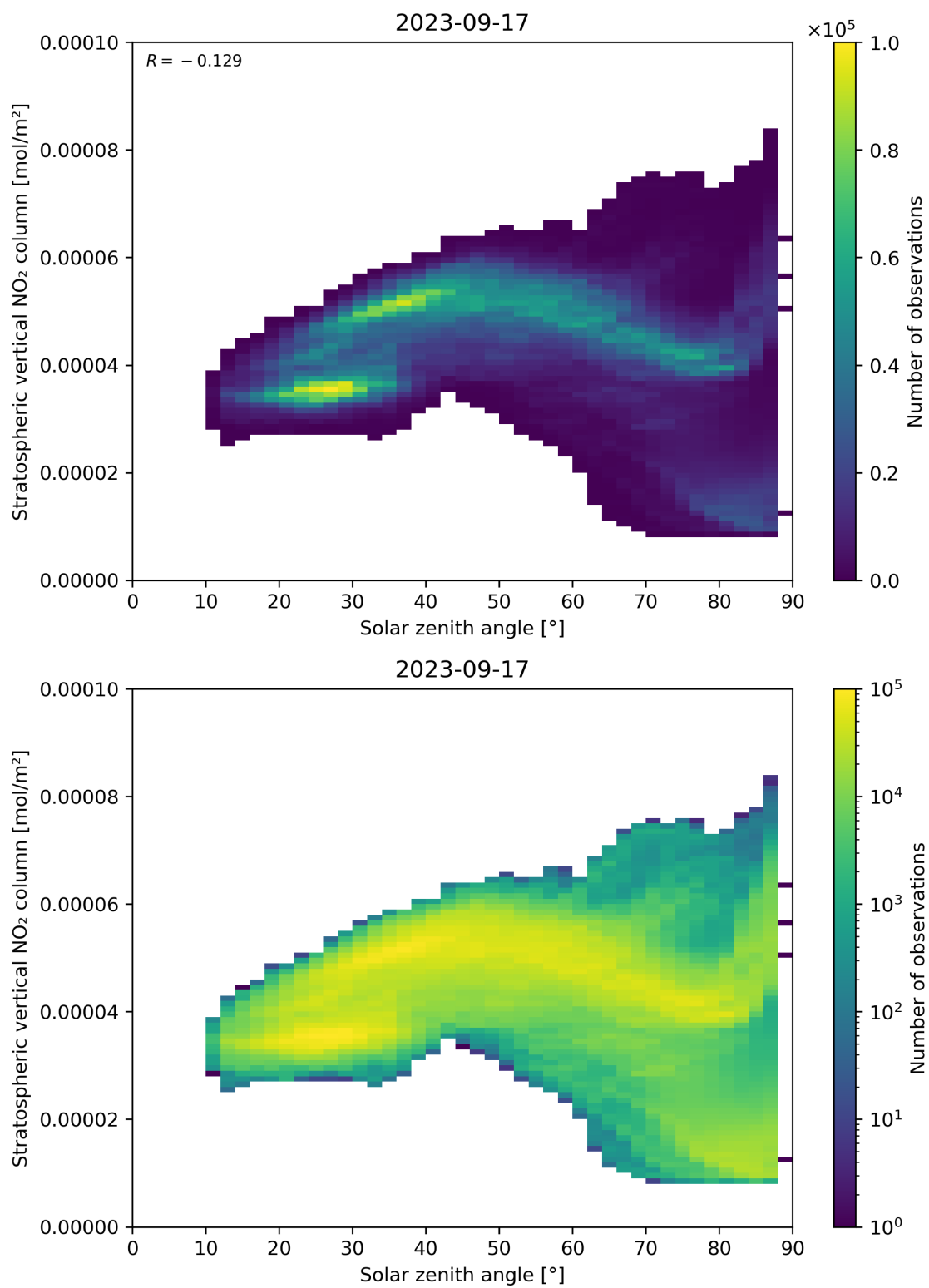
Figure 150: Scatter density plot of “Solar zenith angle” against “Stratospheric vertical NO 2 column” for 2023-09-16 to 2023-09-18.
