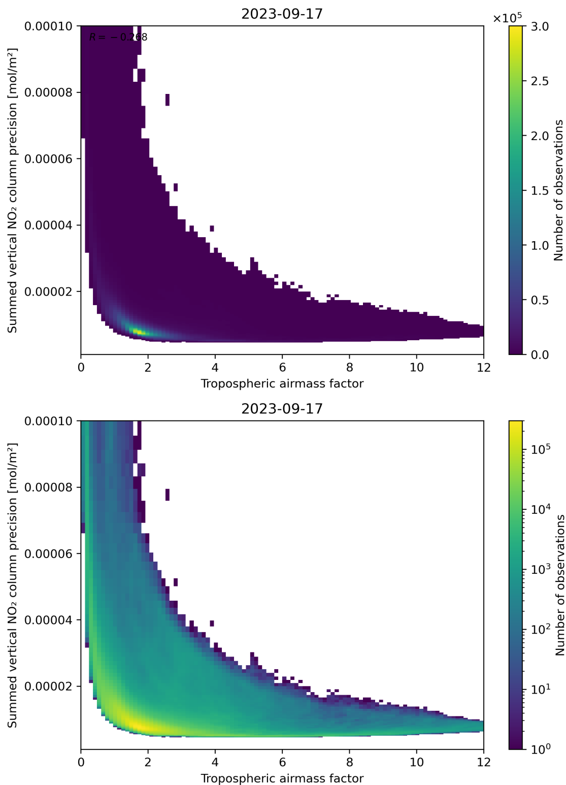
Figure 76: Scatter density plot of “Tropospheric air mass factor” against “Summed vertical NO 2 column precision” for 2023-09-16 to 2023-09-18.
