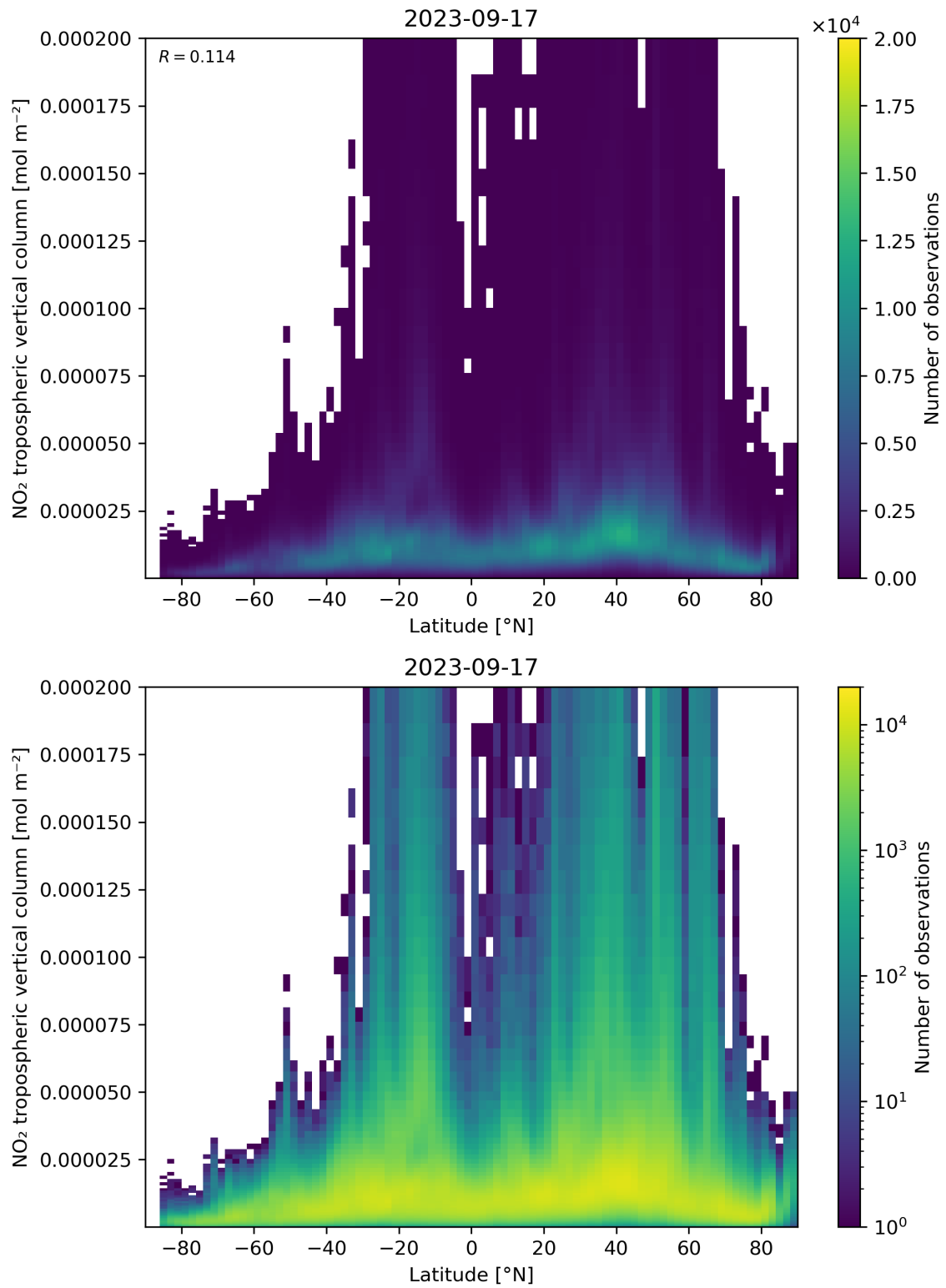
Figure 92: Scatter density plot of “Latitude” against “NO 2 tropospheric vertical column” for 2023-09-16 to 2023-09-18.
