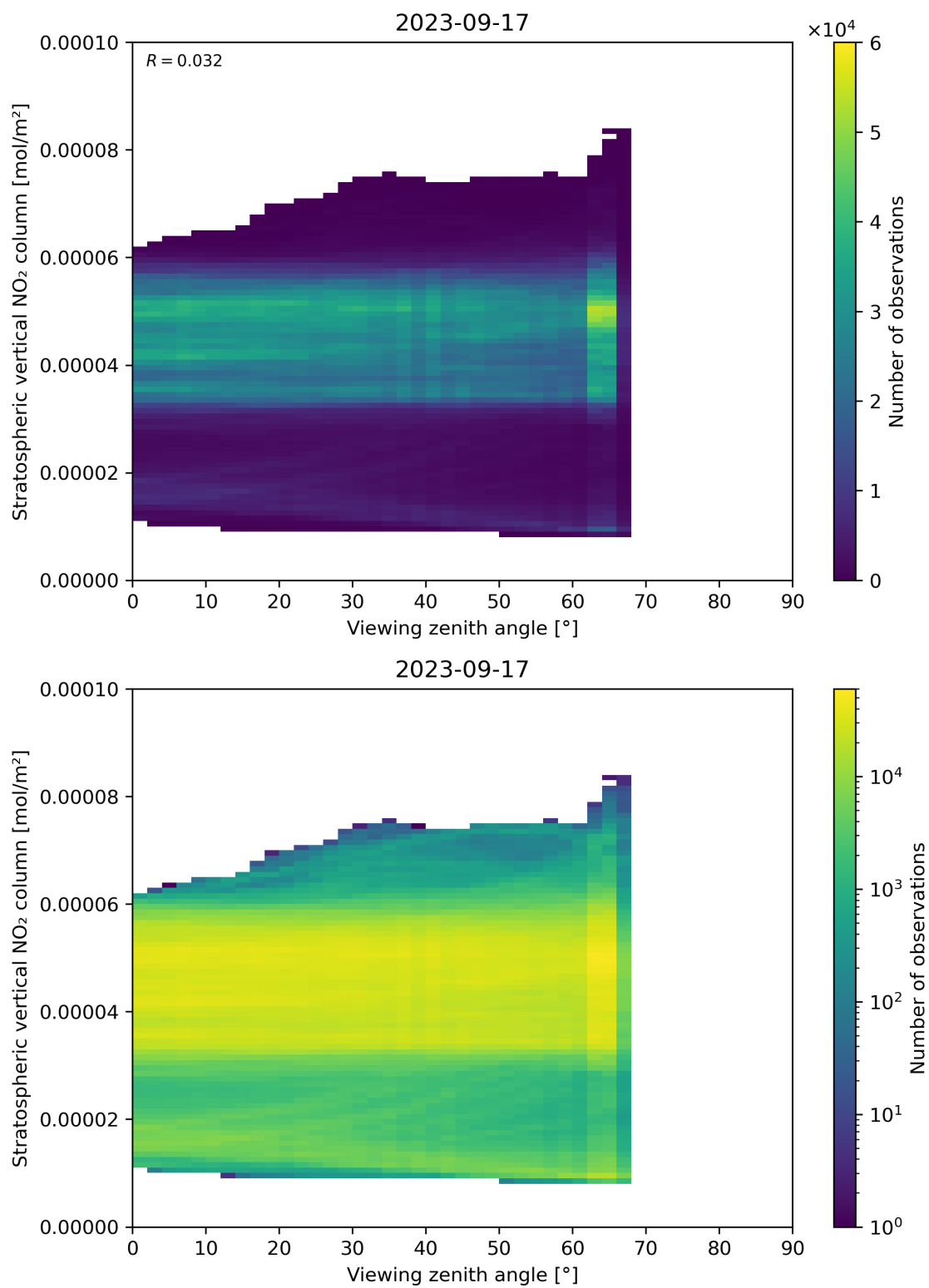
Figure 164: Scatter density plot of “Viewing zenith angle” against “Stratospheric vertical NO 2 column” for 2023-09-16 to 2023-09-18.
