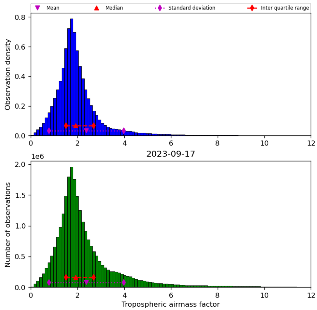
Figure 31: Histogram of “Tropospheric airmass factor” for 2023-09-16 to 2023-09-18
