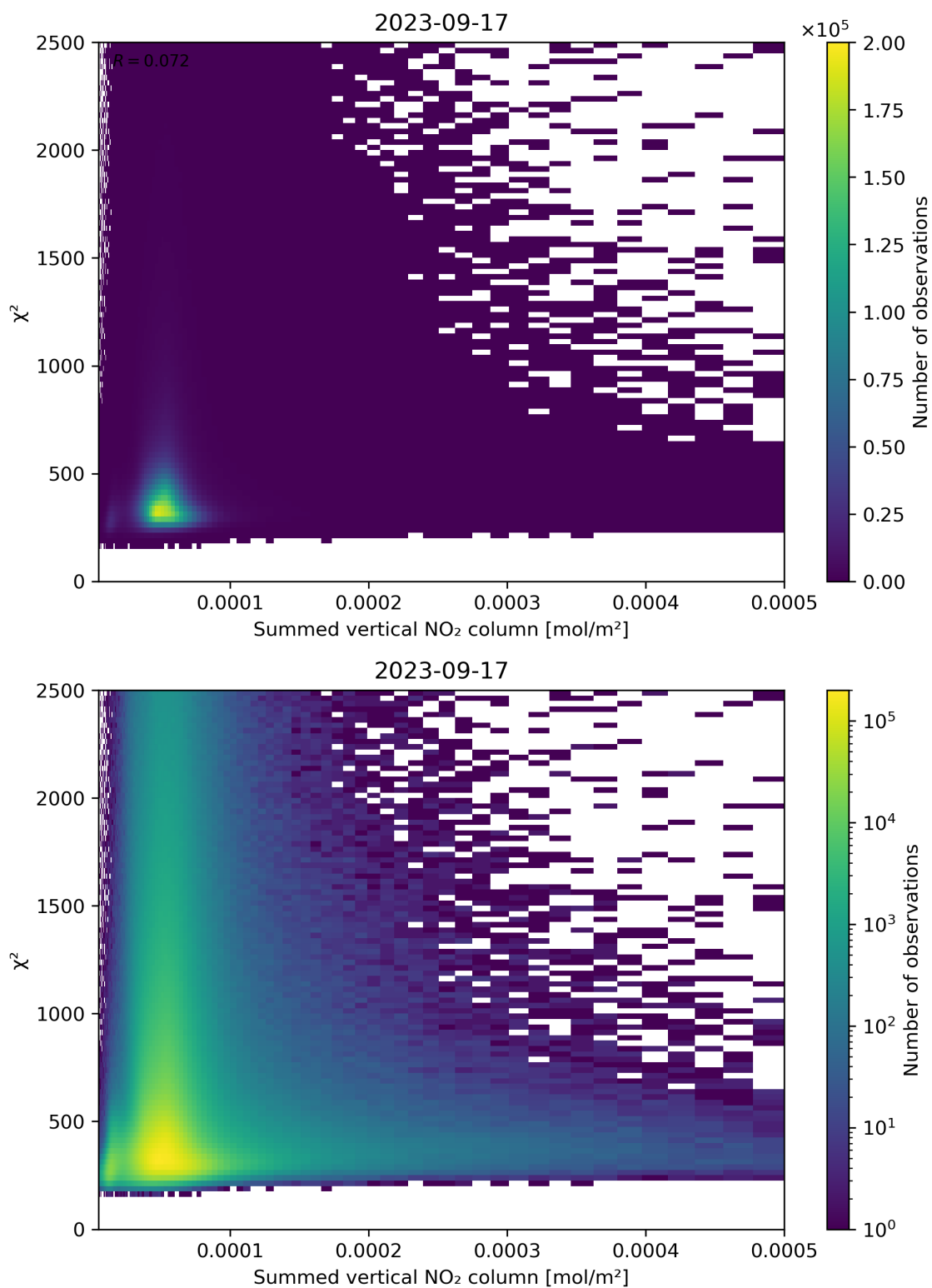
Figure 104: Scatter density plot of “Summed vertical NO 2 column” against “ \chi^2 ” for 2023-09-16 to 2023-09-18.
