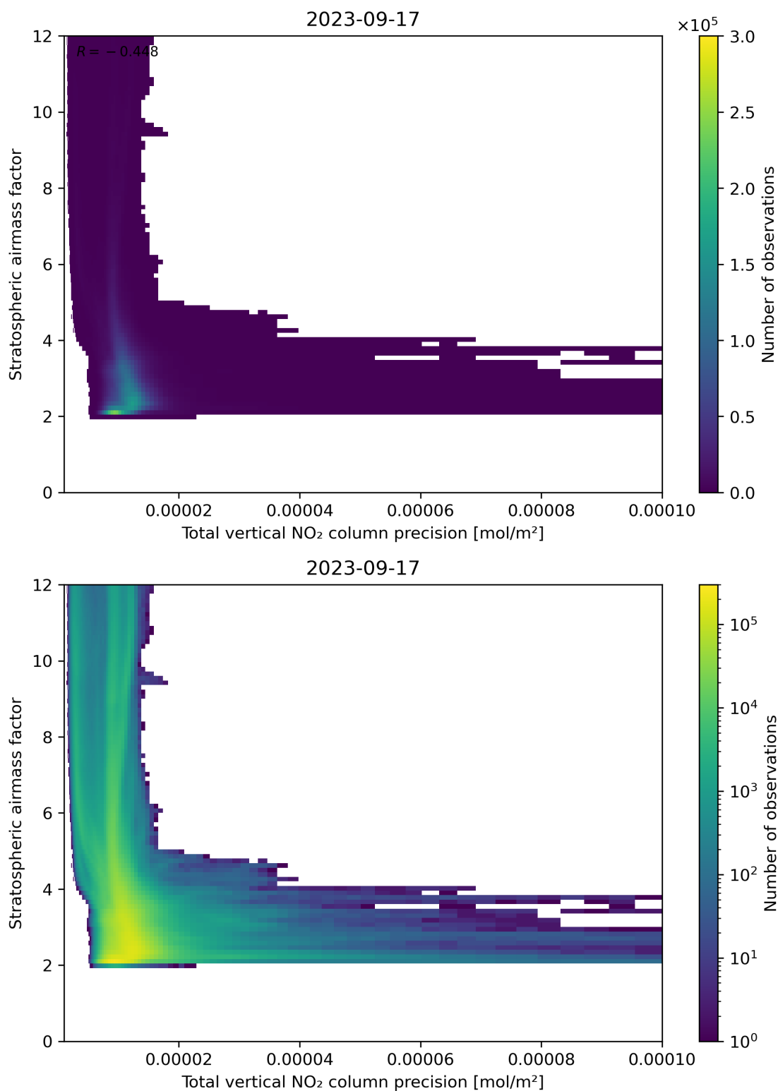
Figure 115: Scatter density plot of “Total vertical NO 2 column precision” against “Stratospheric air mass factor” for 2023-09-16 to 2023-09-18.
