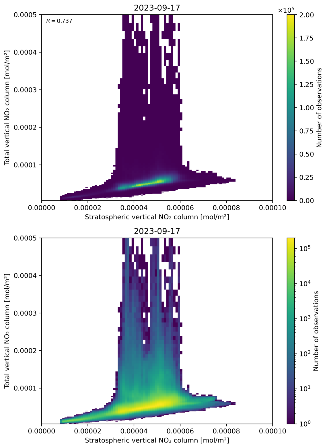
Figure 100: Scatter density plot of “Stratospheric vertical NO 2 column” against “Total vertical NO 2 column” for 2023-09-16 to 2023-09-18.
