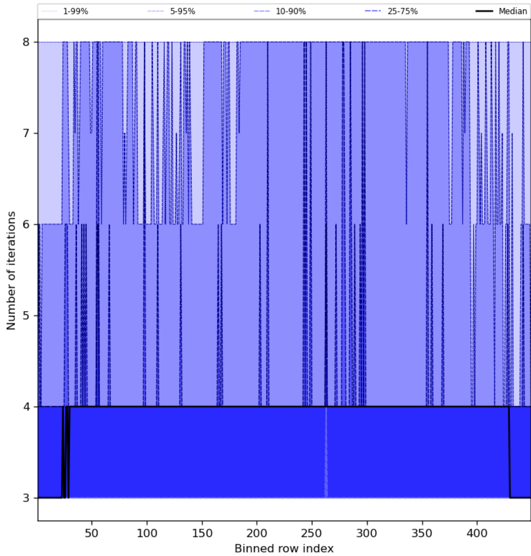
Figure 51: Along track statistics of “Number of iterations” for 2023-09-16 to 2023-09-18
