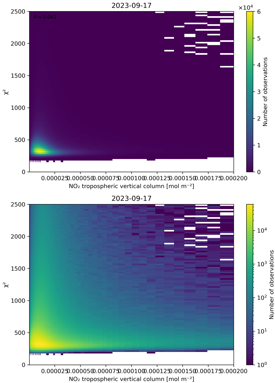
Figure 124: Scatter density plot of “NO 2 tropospheric vertical column” against “ \chi^2 ” for 2023-09-16 to 2023-09-18.
