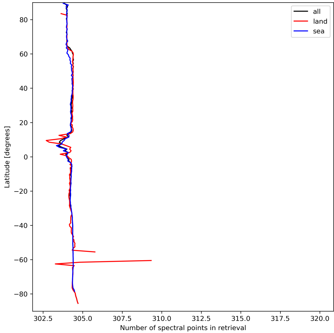
Figure 16: Zonal average of “Number of spectral points in retrieval” for 2023-09-16 to 2023-09-18.
