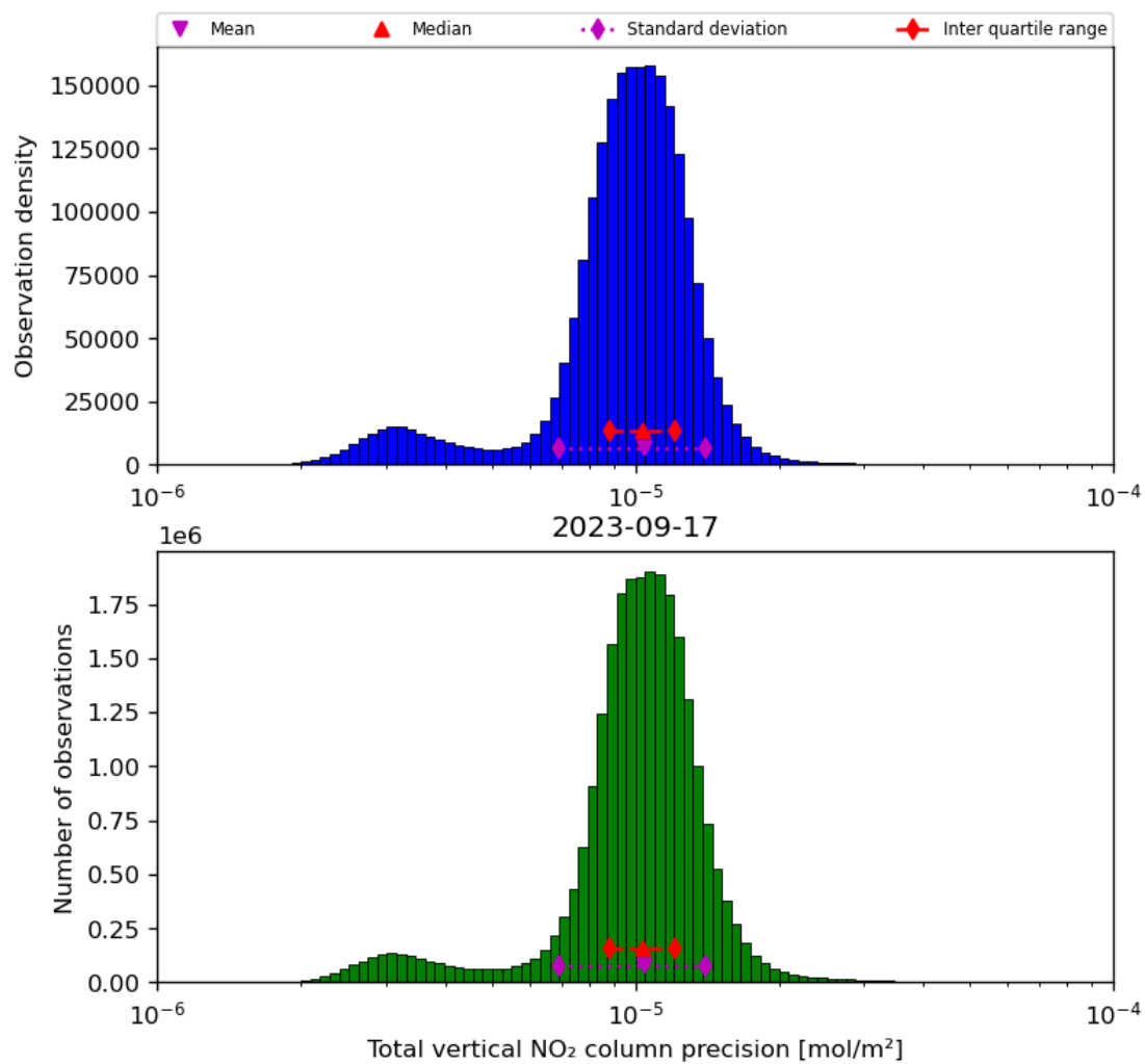
Figure 39: Histogram of “Total vertical NO 2 column precision” for 2023-09-16 to 2023-09-18
