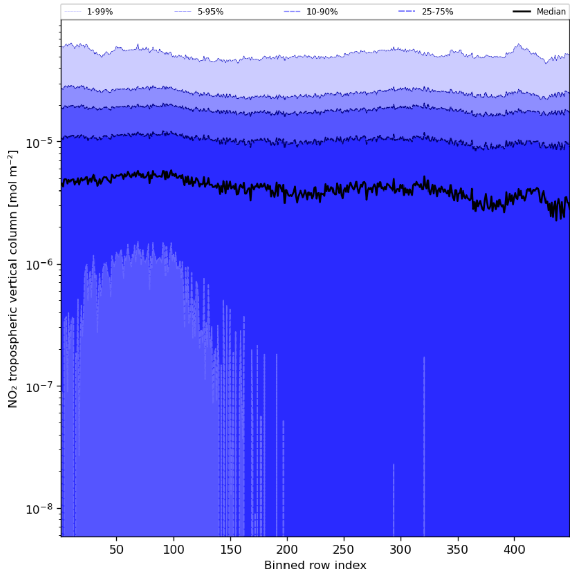
Figure 46: Along track statistics of “NO 2 tropospheric vertical column” for 2023-09-16 to 2023-09-18
