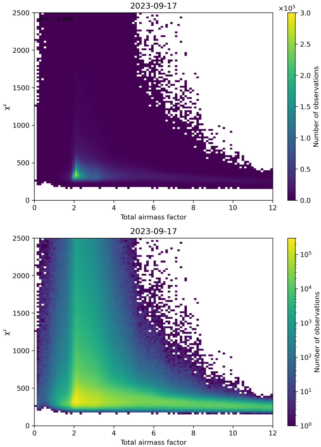
Figure 63: Scatter density plot of “Total airmass factor” against “ \chi^2 ” for 2023-09-16 to 2023-09-18.
