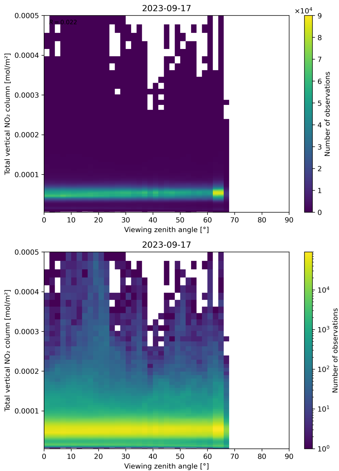
Figure 167: Scatter density plot of “Viewing zenith angle” against “Total vertical NO 2 column” for 2023-09-16 to 2023-09-18.
