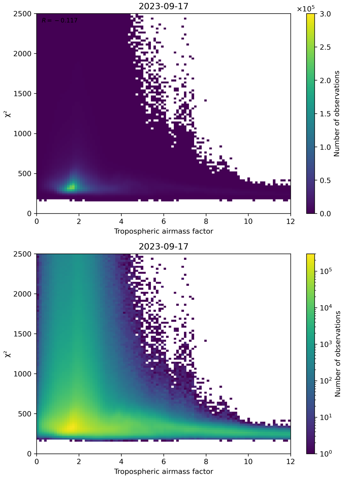
Figure 73: Scatter density plot of “Tropospheric airmass factor” against “ \chi^2 ” for 2023-09-16 to 2023-09-18.
