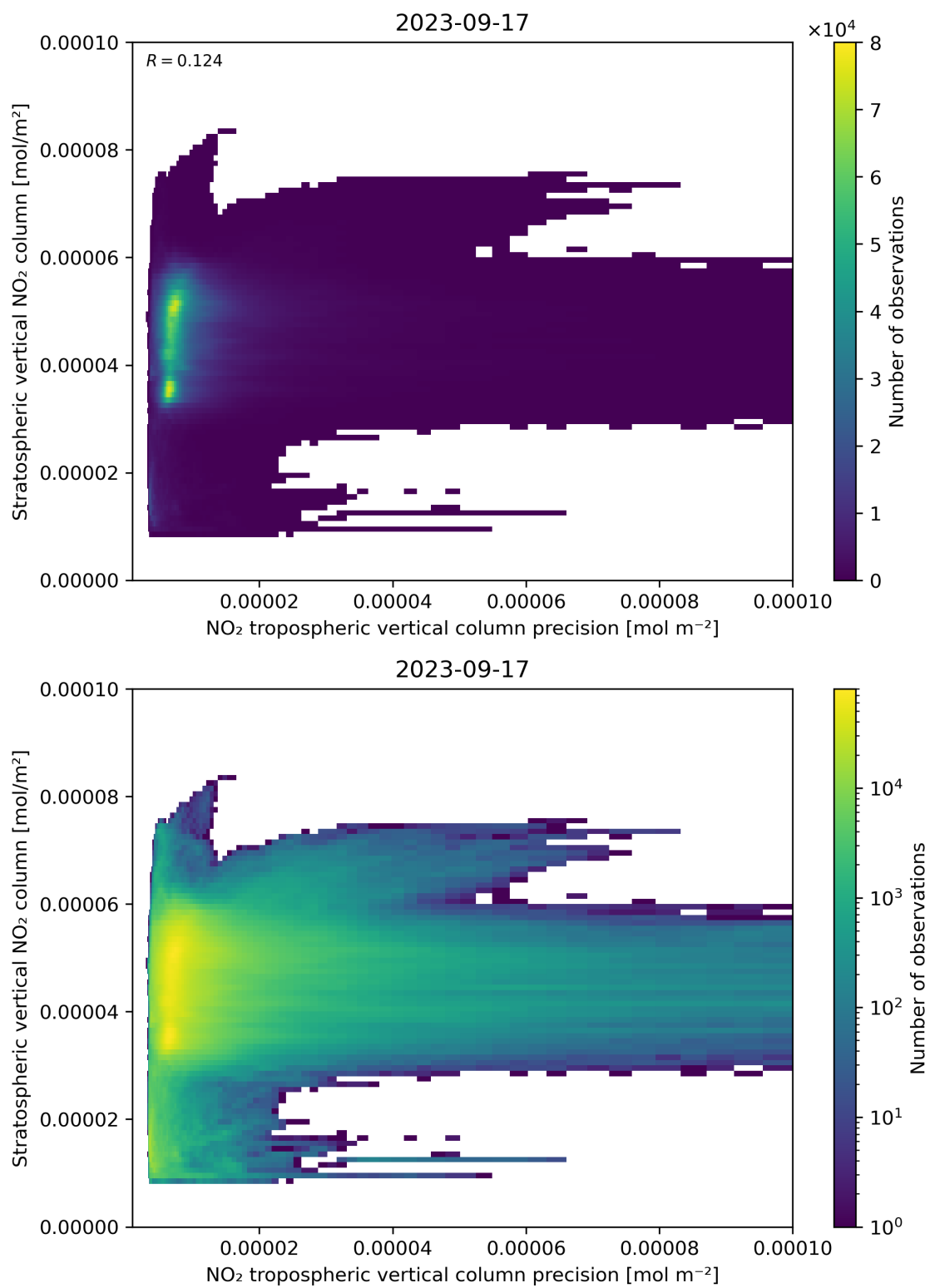
Figure 135: Scatter density plot of “NO 2 tropospheric vertical column precision” against “Stratospheric vertical NO 2 column” for 2023-09-16 to 2023-09-18.
