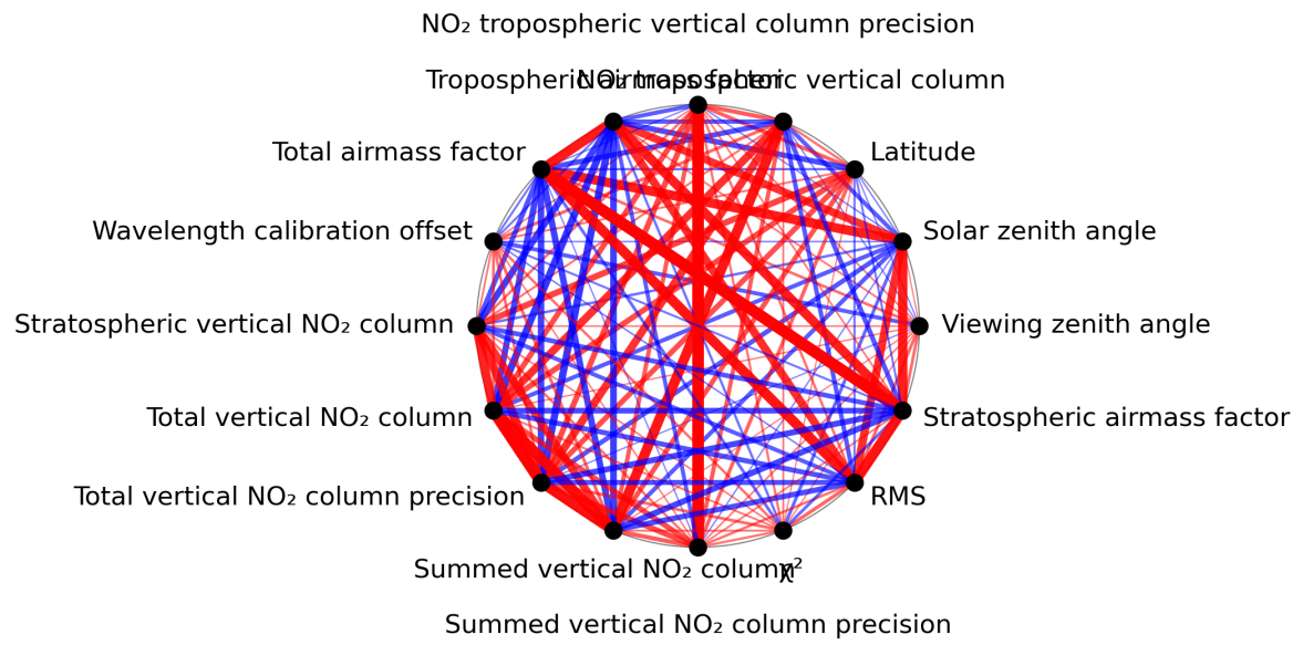
Figure 1: Map of correlation graph for 2023-09-16 to 2023-09-18.
