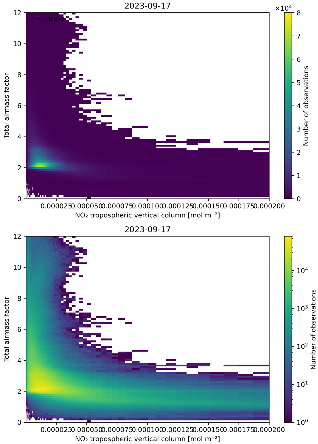
Figure 122: Scatter density plot of “NO 2 tropospheric vertical column” against “Total air mass factor” for 2023-09-16 to 2023-09-18.
