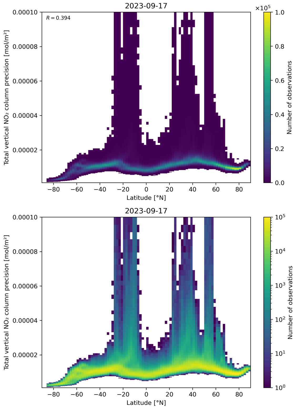
Figure 91: Scatter density plot of “Latitude” against “Total vertical NO 2 column precision” for 2023-09-16 to 2023-09-18.
