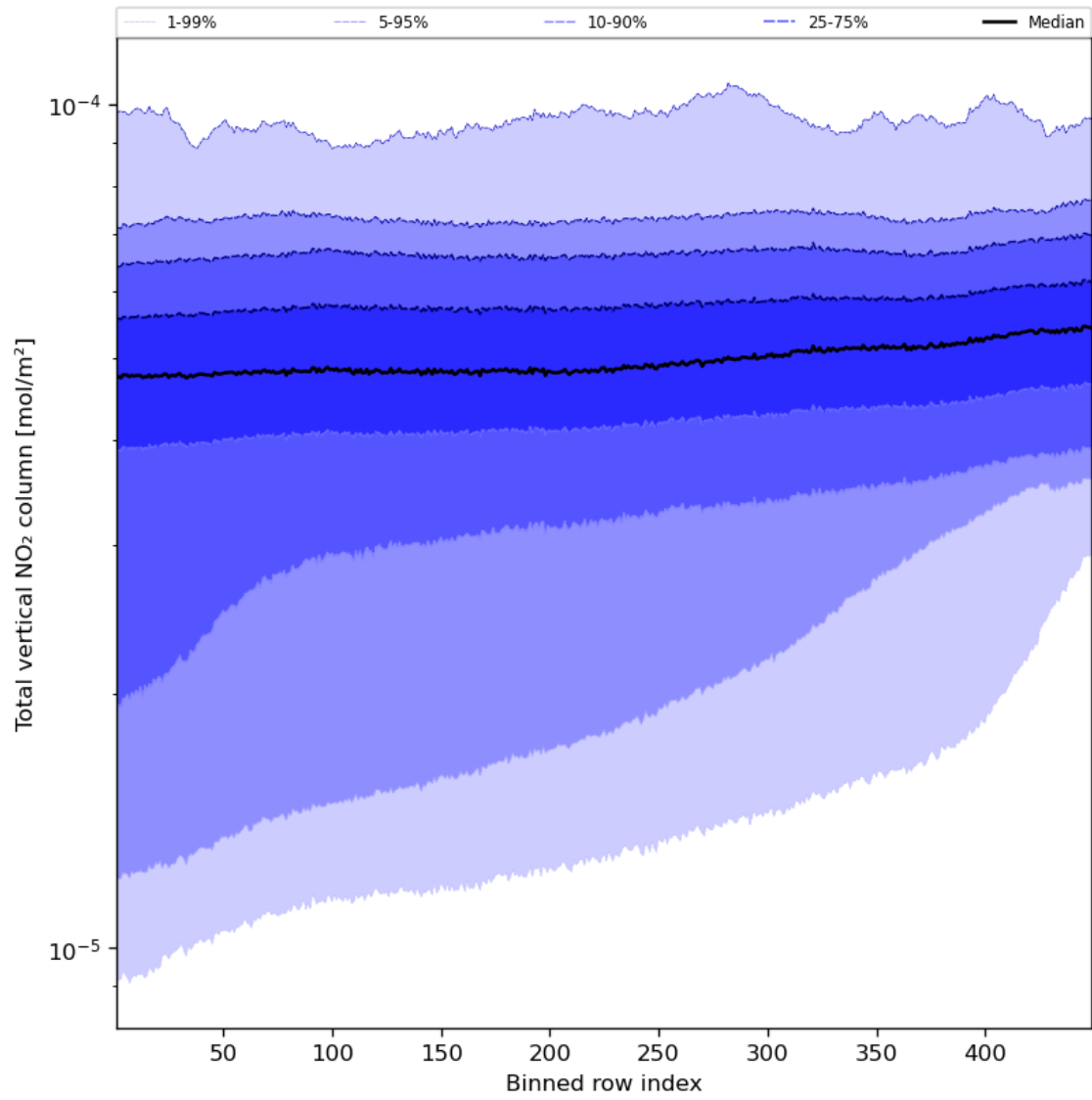
Figure 55: Along track statistics of “Total vertical NO 2 column” for 2023-09-16 to 2023-09-18
