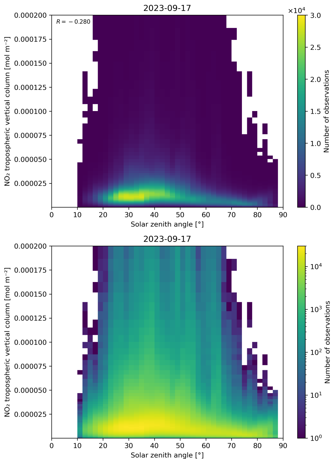
Figure 155: Scatter density plot of “Solar zenith angle” against “NO 2 tropospheric vertical column” for 2023-09-16 to 2023-09-18.
