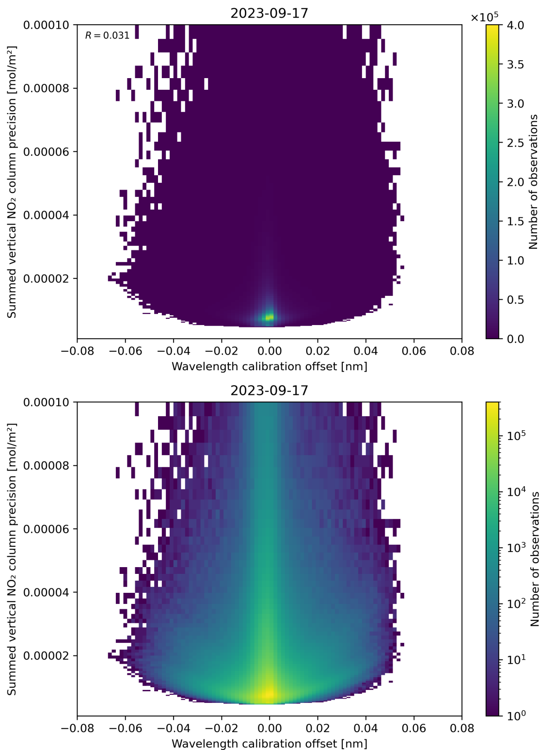
Figure 178: Scatter density plot of “Wavelength calibration offset” against “Summed vertical NO 2 column precision” for 2023-09-16 to 2023-09-18.
