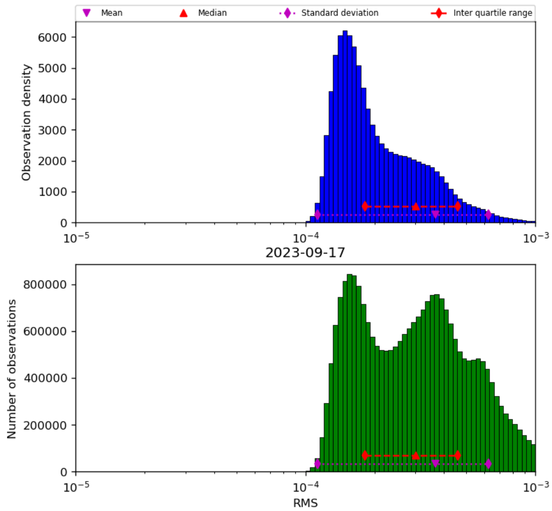
Figure 43: Histogram of “RMS” for 2023-09-16 to 2023-09-18
