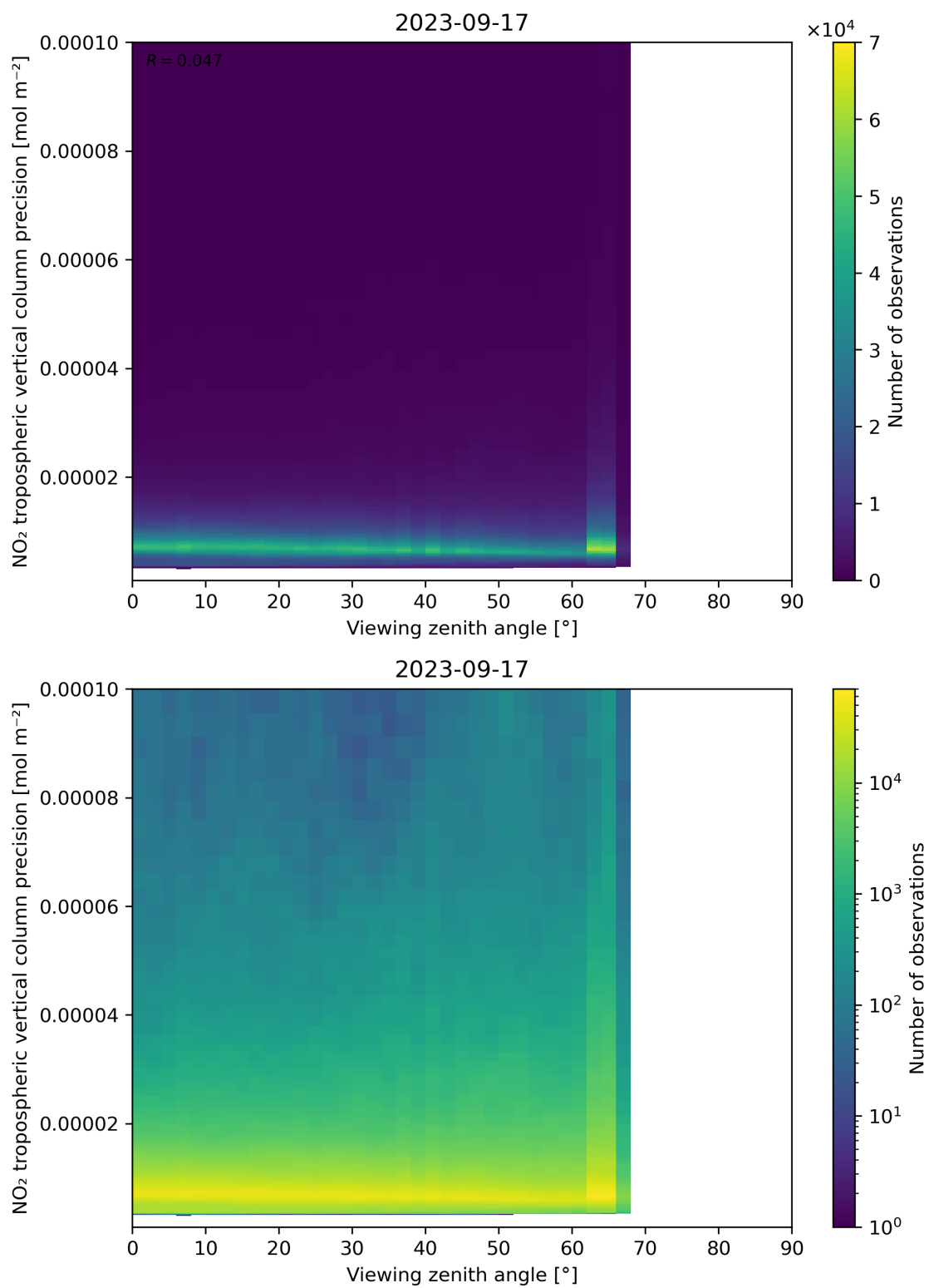
Figure 170: Scatter density plot of “Viewing zenith angle” against “NO 2 tropospheric vertical column precision” for 2023-09-16 to 2023-09-18.
