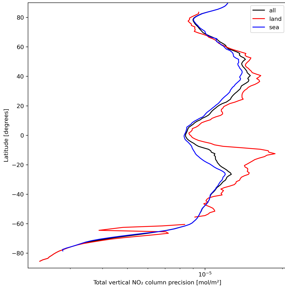
Figure 22: Zonal average of “Total vertical NO 2 column precision” for 2023-09-16 to 2023-09-18.
