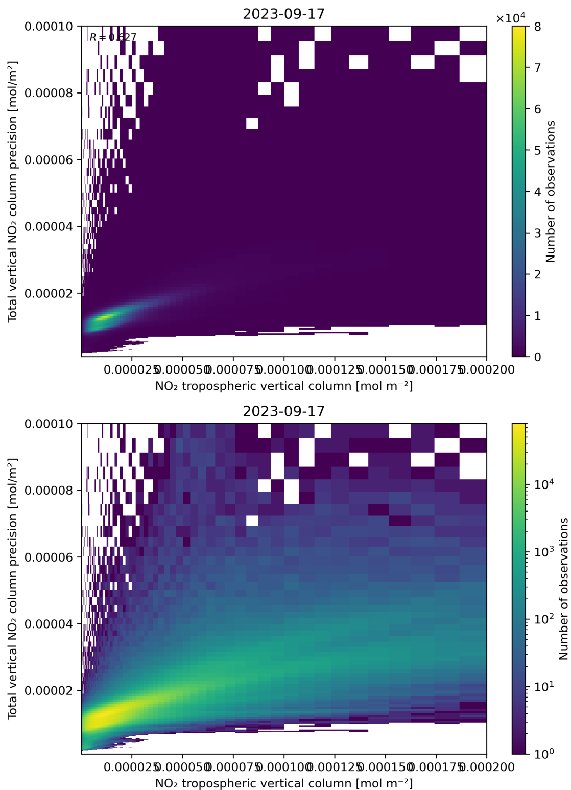
Figure 129: Scatter density plot of “NO 2 tropospheric vertical column” against “Total vertical NO 2 column precision” for 2023-09-16 to 2023-09-18.
