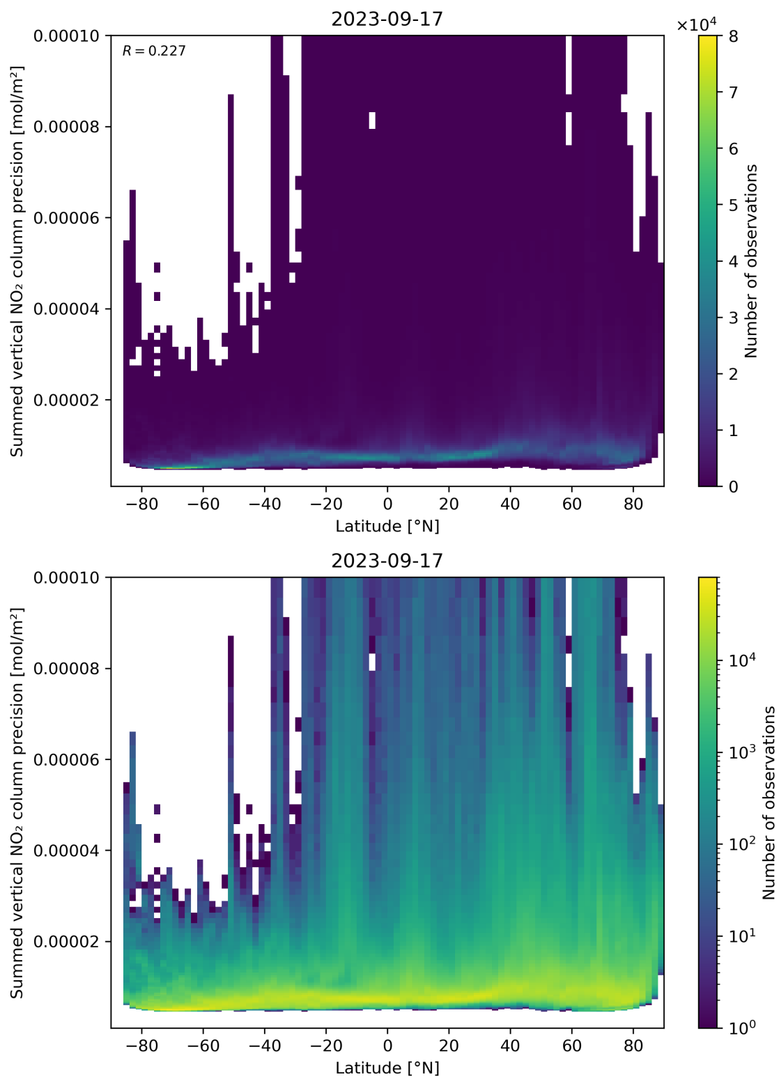
Figure 89: Scatter density plot of “Latitude” against “Summed vertical NO 2 column precision” for 2023-09-16 to 2023-09-18.
