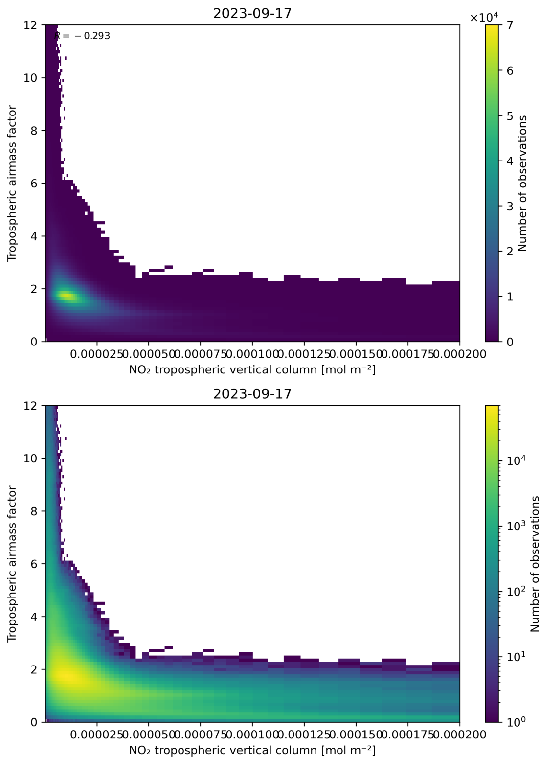
Figure 123: Scatter density plot of “NO 2 tropospheric vertical column” against “Tropospheric air mass factor” for 2023-09-16 to 2023-09-18.
