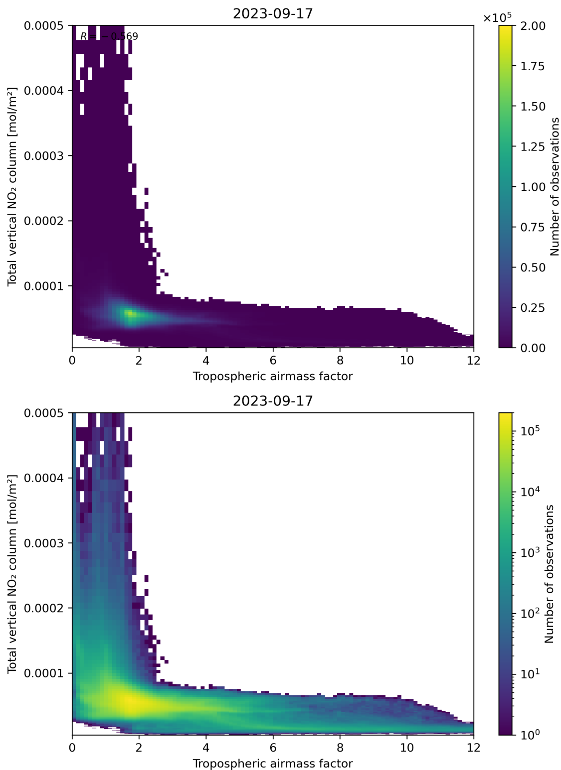
Figure 77: Scatter density plot of “Tropospheric airmass factor” against “Total vertical NO 2 column” for 2023-09-16 to 2023-09-18.
