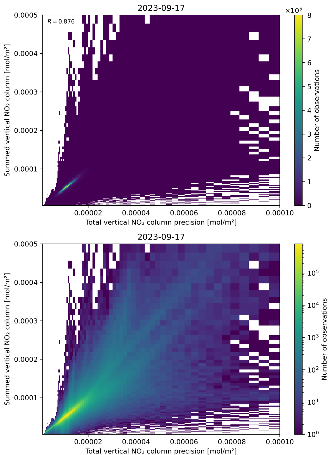
Figure 117: Scatter density plot of “Total vertical NO 2 column precision” against “Summed vertical NO 2 column” for 2023-09-16 to 2023-09-18.
