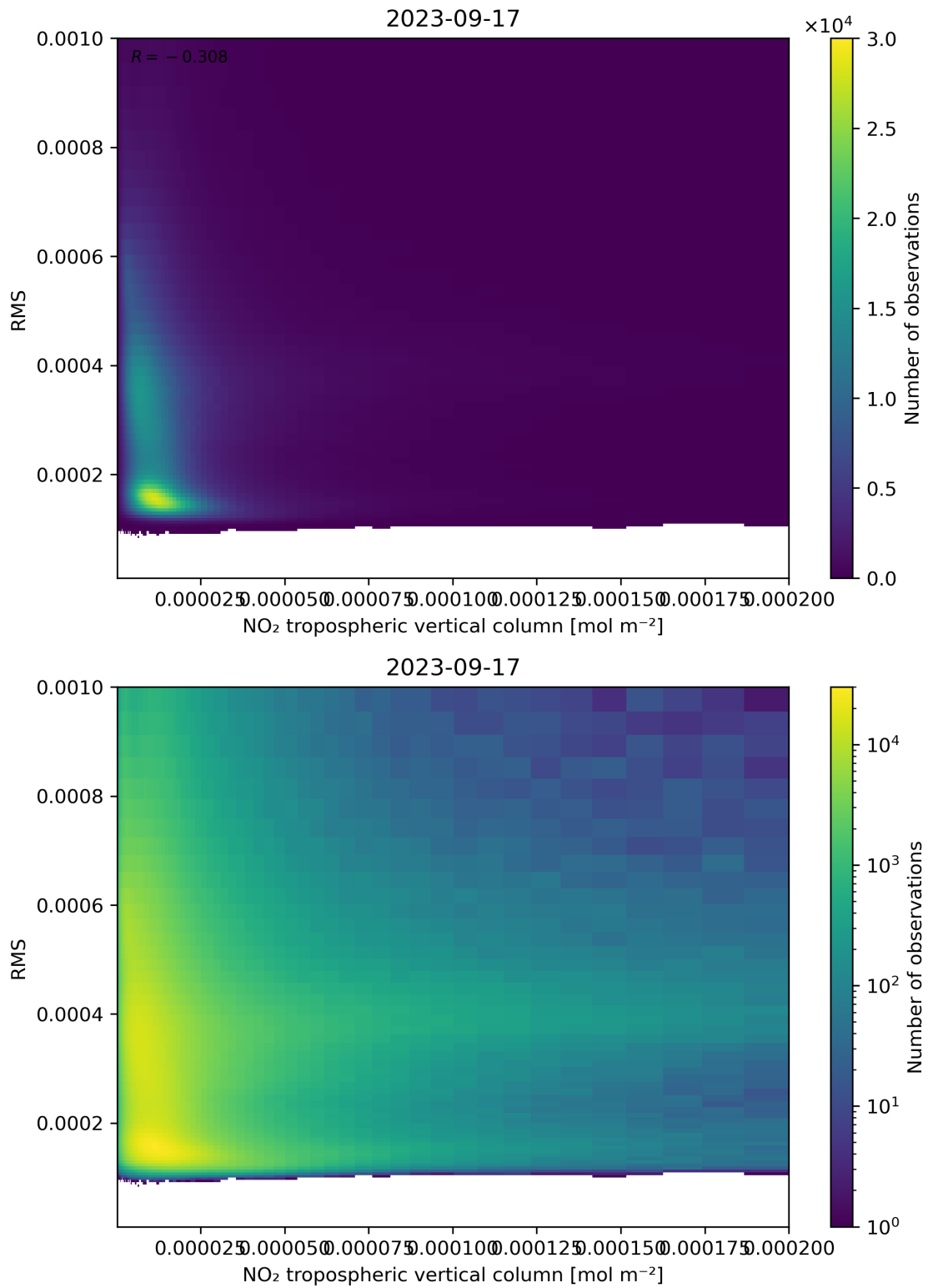
Figure 142: Scatter density plot of “NO 2 tropospheric vertical column” against “RMS” for 2023-09-16 to 2023-09-18.
