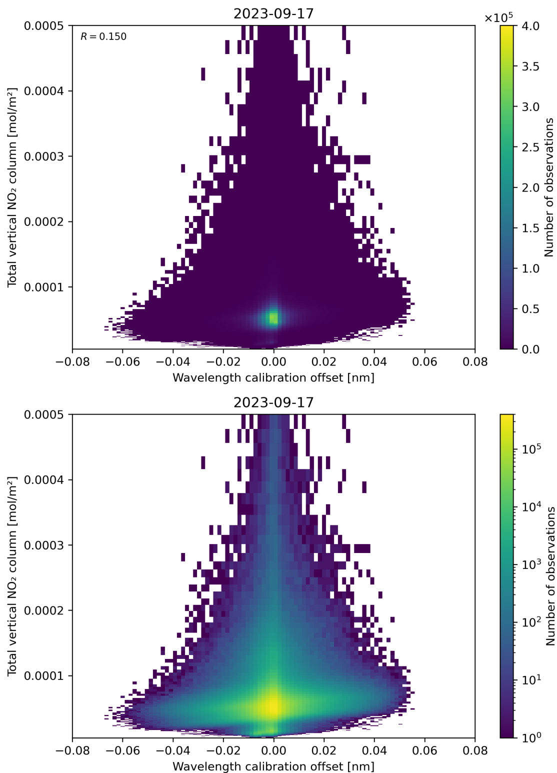
Figure 179: Scatter density plot of “Wavelength calibration offset” against “Total vertical NO 2 column” for 2023-09-16 to 2023-09-18.
