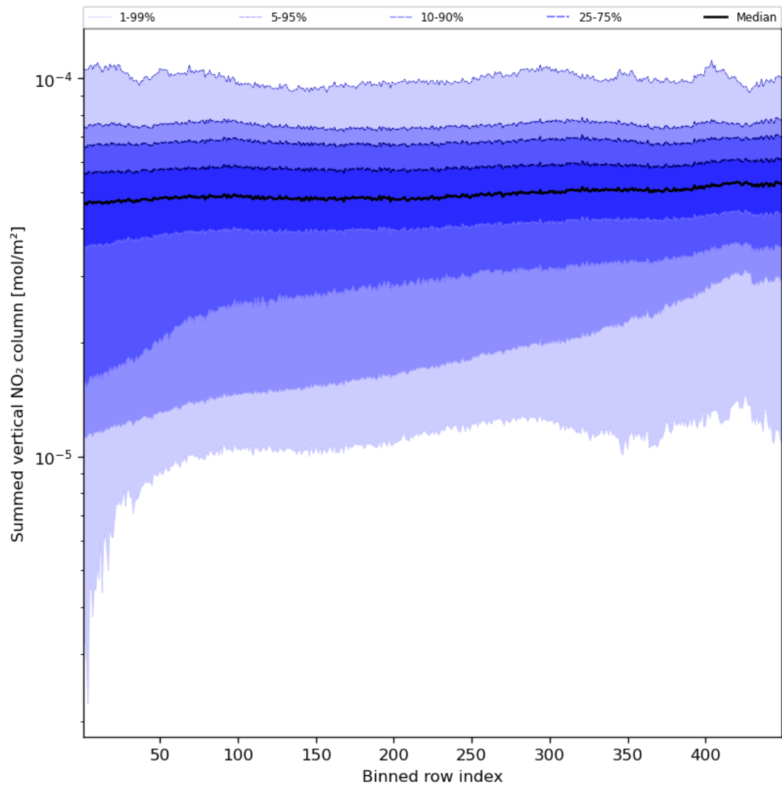
Figure 57: Along track statistics of “Summed vertical NO 2 column” for 2023-09-16 to 2023-09-18
