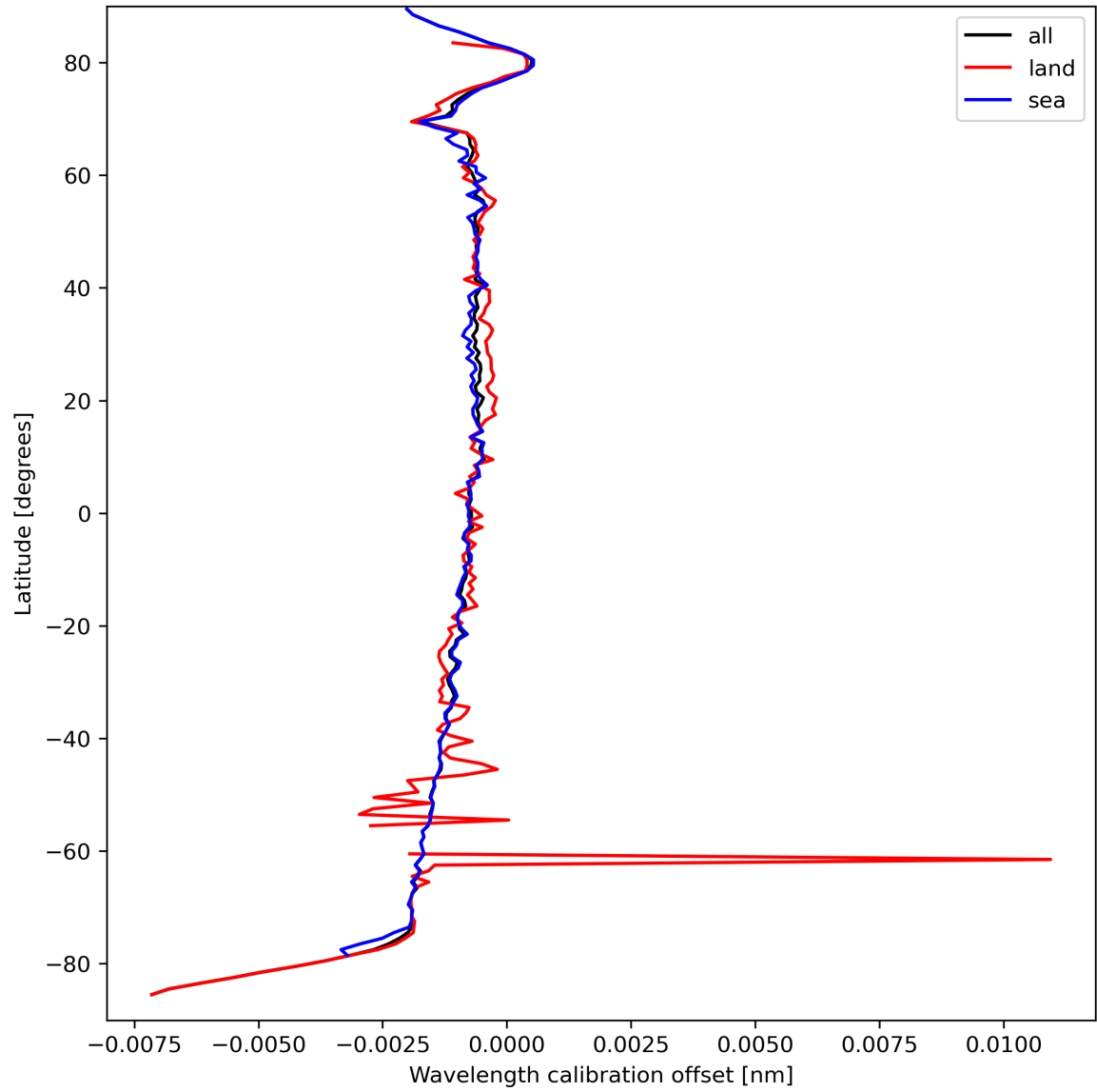
Figure 18: Zonal average of “Wavelength calibration offset” for 2023-09-16 to 2023-09-18.
