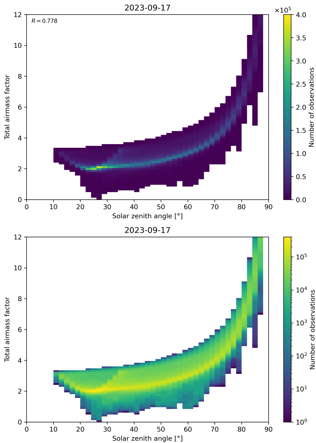
Figure 146: Scatter density plot of “Solar zenith angle” against “Total air mass factor” for 2023-09-16 to 2023-09-18.
