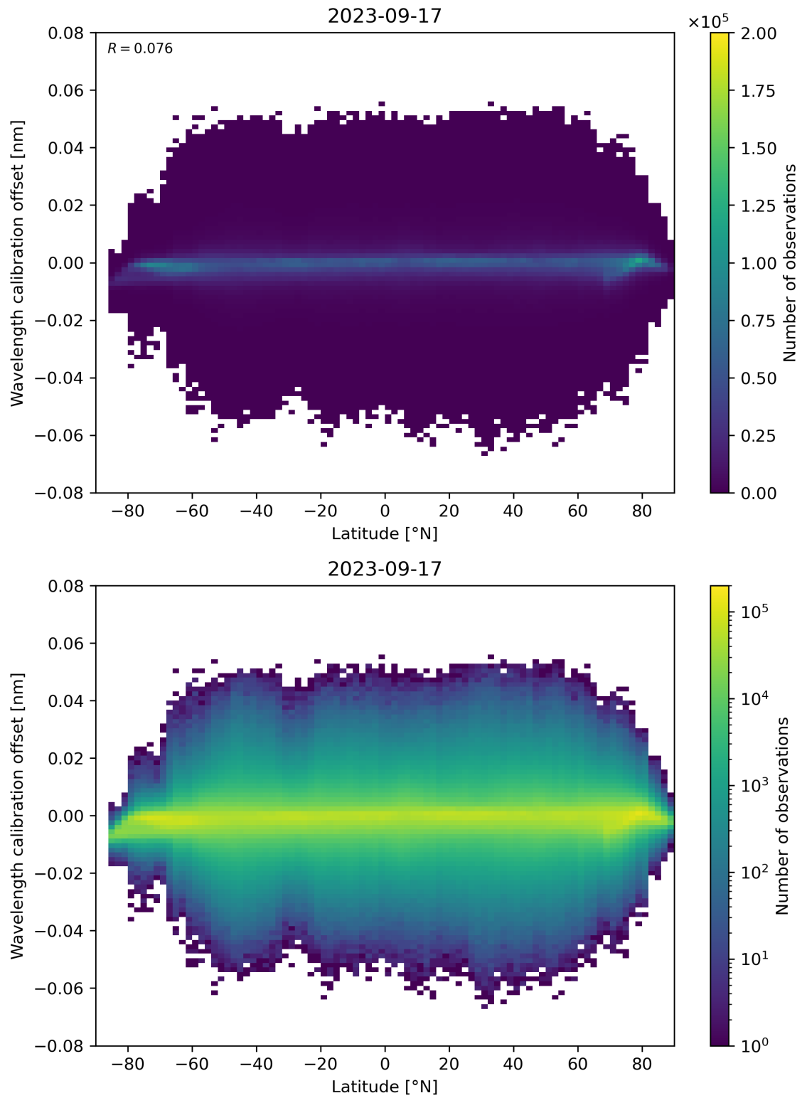
Figure 95: Scatter density plot of “Latitude” against “Wavelength calibration offset” for 2023-09-16 to 2023-09-18.
