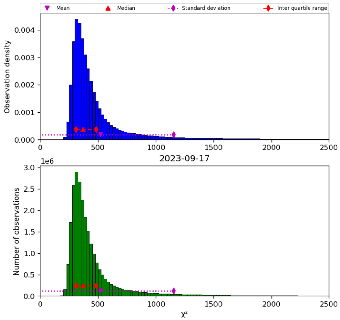
Figure 42: Histogram of “ \chi^2 ” for 2023-09-16 to 2023-09-18
