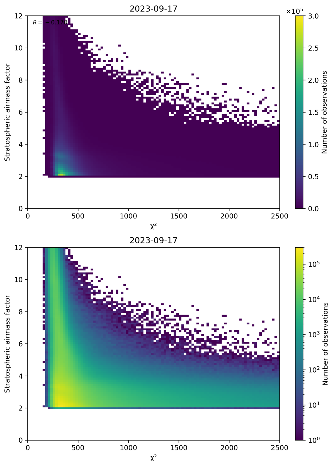
Figure 81: Scatter density plot of “ \chi^2 ” against “Stratospheric airmass factor” for 2023-09-16 to 2023-09-18.
