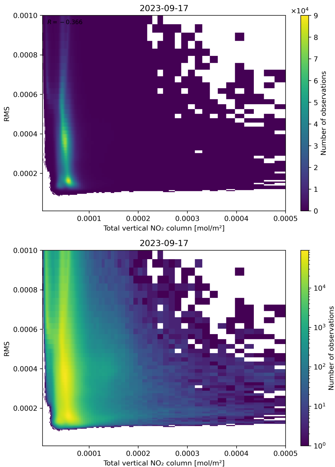
Figure 120: Scatter density plot of “Total vertical NO 2 column” against “RMS” for 2023-09-16 to 2023-09-18.
