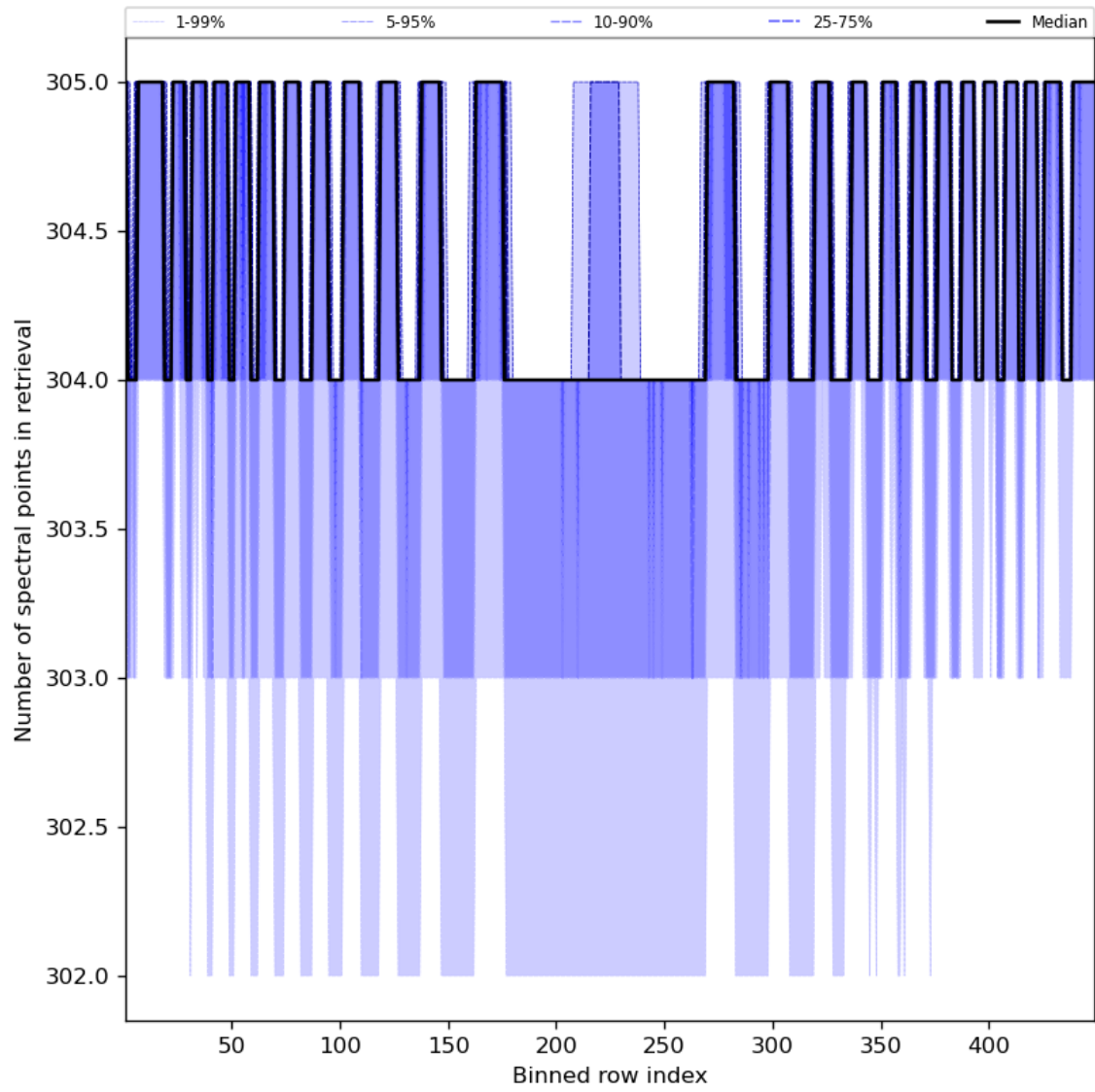
Figure 50: Along track statistics of “Number of spectral points in retrieval” for 2023-09-16 to 2023-09-18
