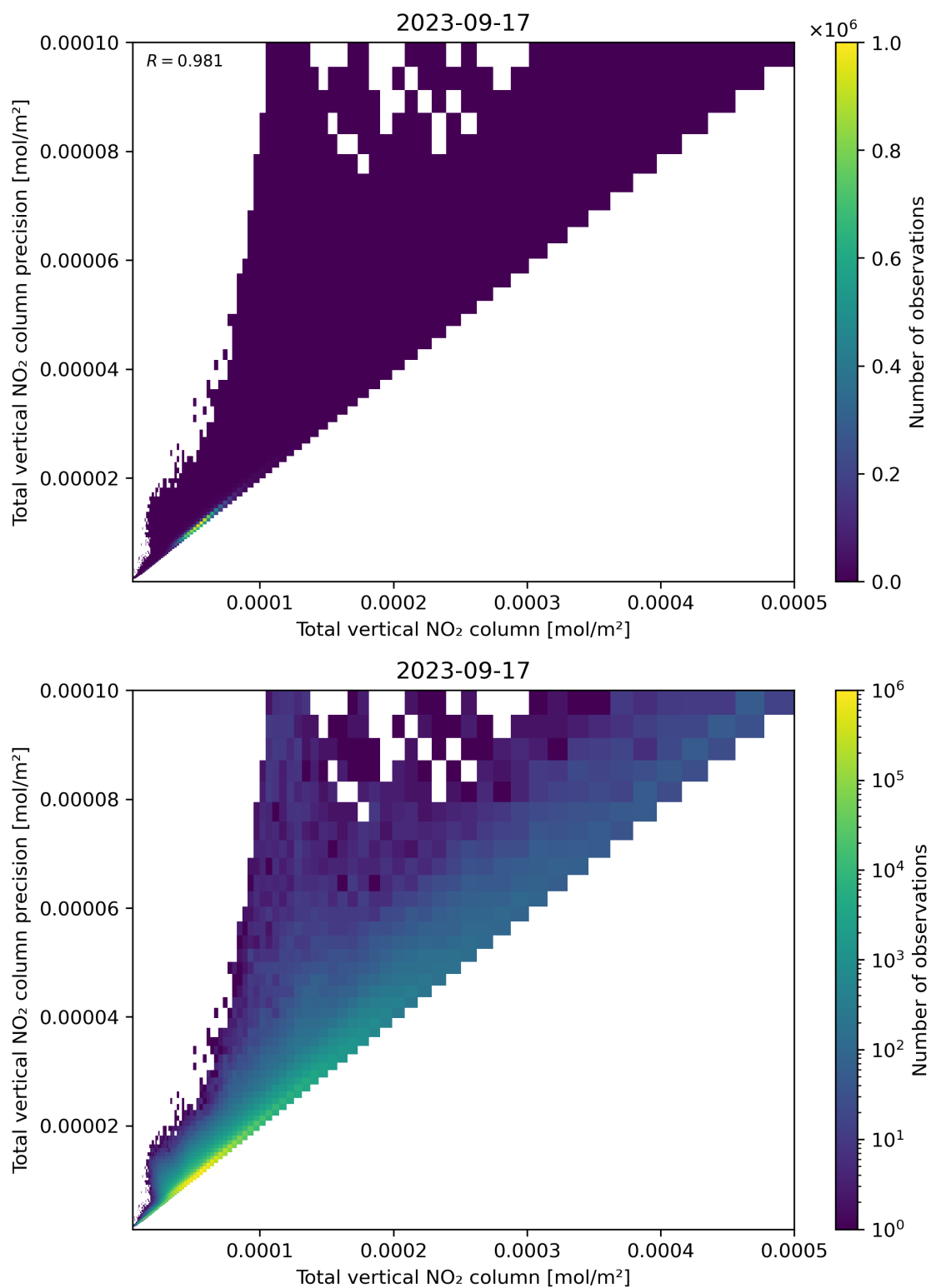
Figure 114: Scatter density plot of “Total vertical NO 2 column” against “Total vertical NO 2 column precision” for 2023-09-16 to 2023-09-18.
