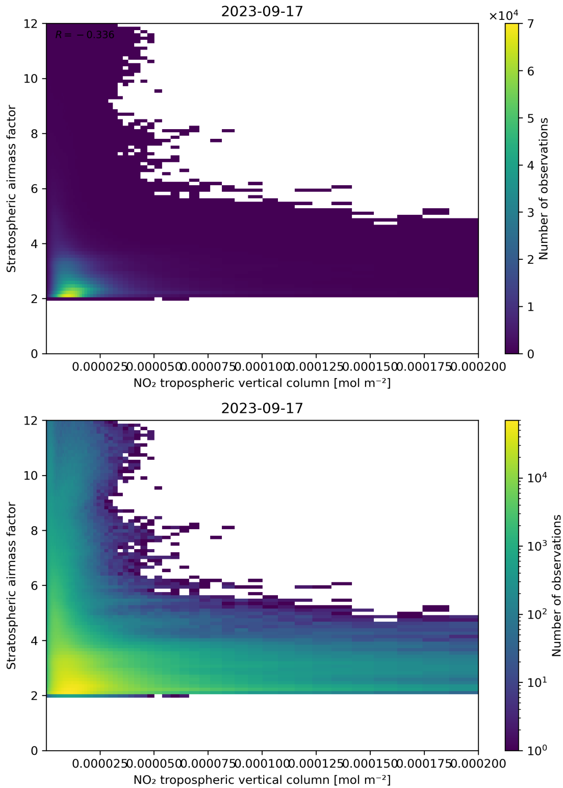
Figure 121: Scatter density plot of “NO 2 tropospheric vertical column” against “Stratospheric air mass factor” for 2023-09-16 to 2023-09-18.
