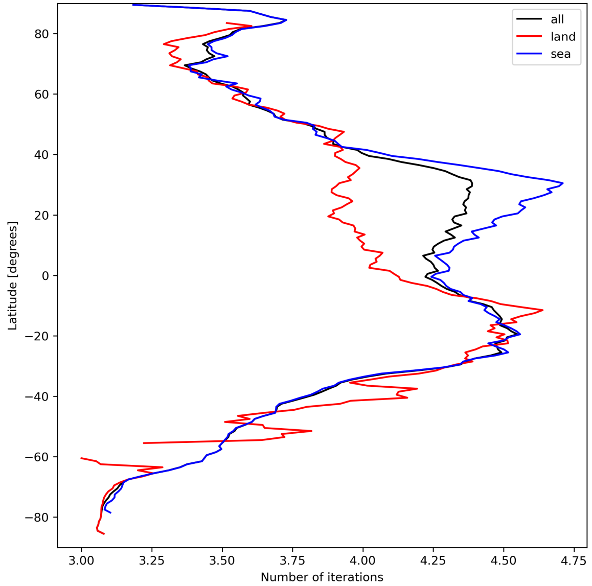
Figure 17: Zonal average of “Number of iterations” for 2023-09-16 to 2023-09-18.
