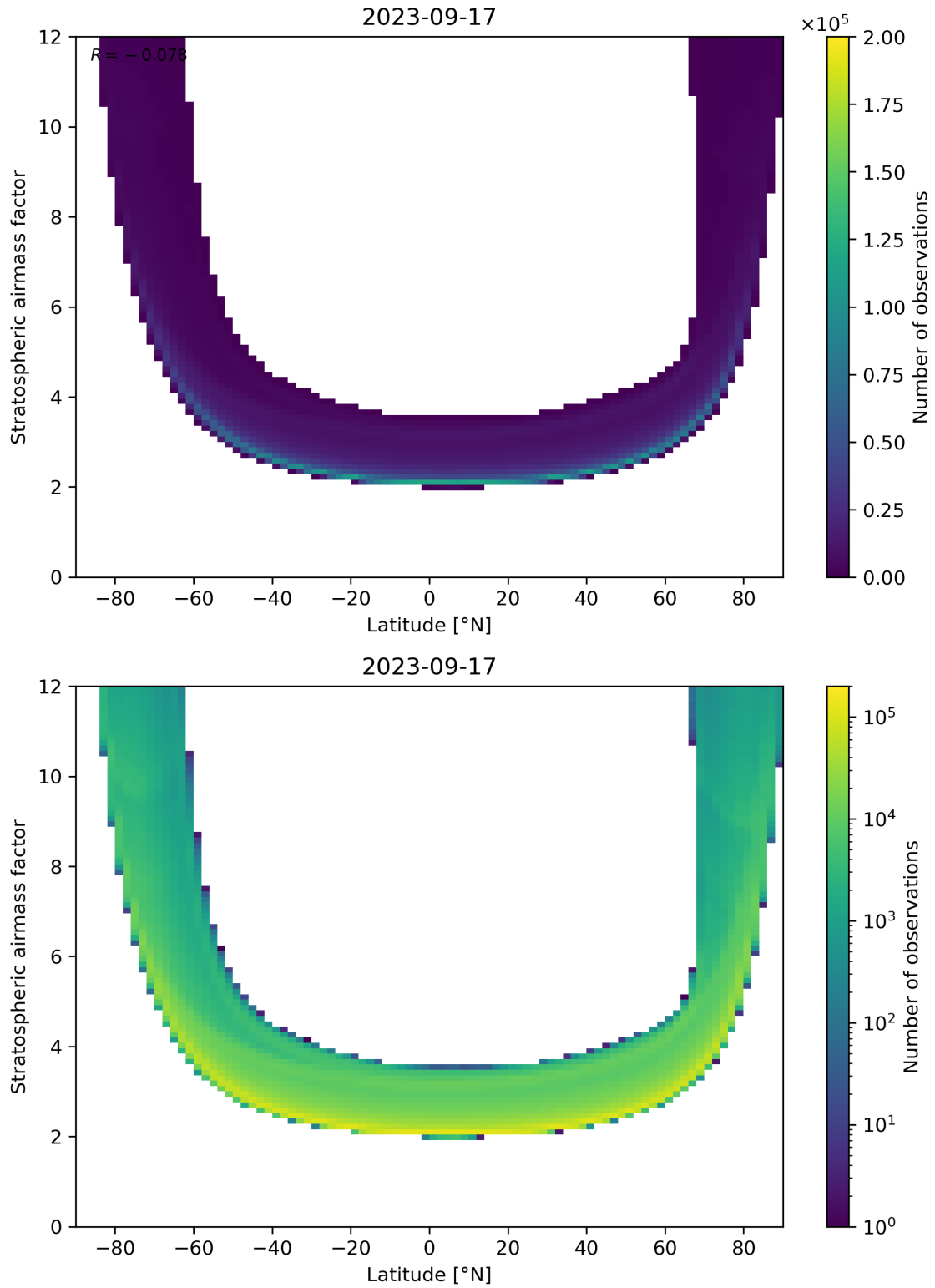
Figure 83: Scatter density plot of “Latitude” against “Stratospheric air mass factor” for 2023-09-16 to 2023-09-18.
