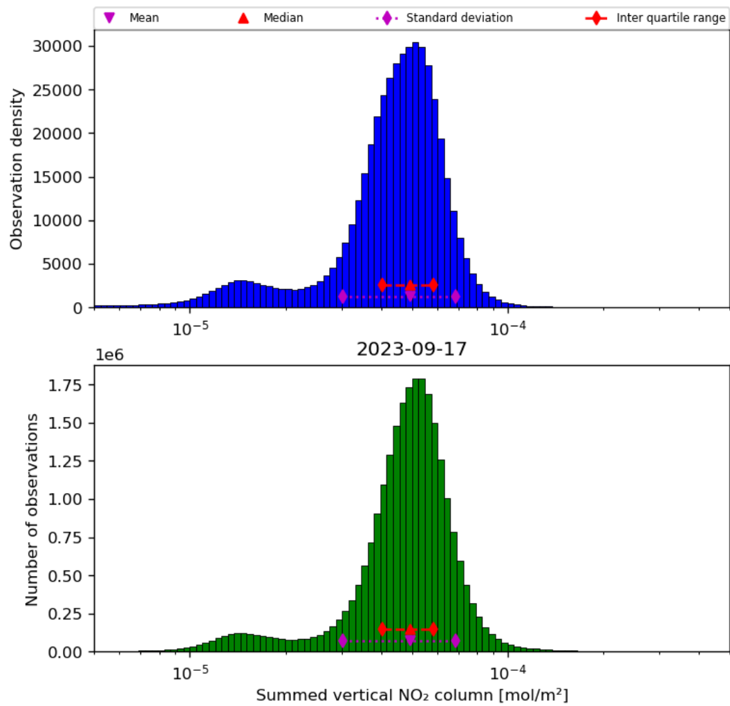
Figure 40: Histogram of "Summed vertical NO 2 column" for 2023-09-16 to 2023-09-18
