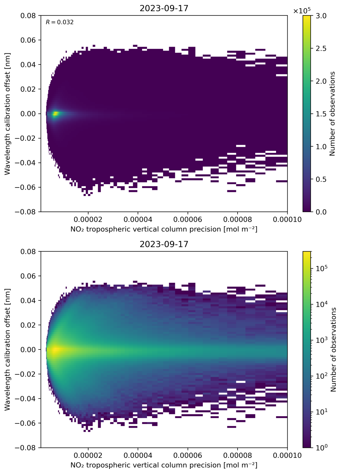
Figure 141: Scatter density plot of “NO 2 tropospheric vertical column precision” against “Wavelength calibration offset” for 2023-09-16 to 2023-09-18.
