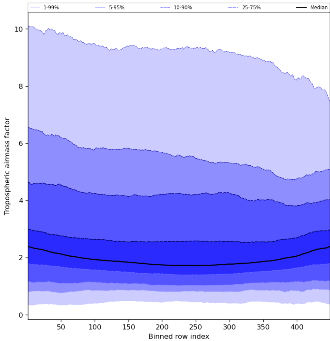
Figure 48: Along track statistics of “Tropospheric airmass factor” for 2023-09-16 to 2023-09-18
