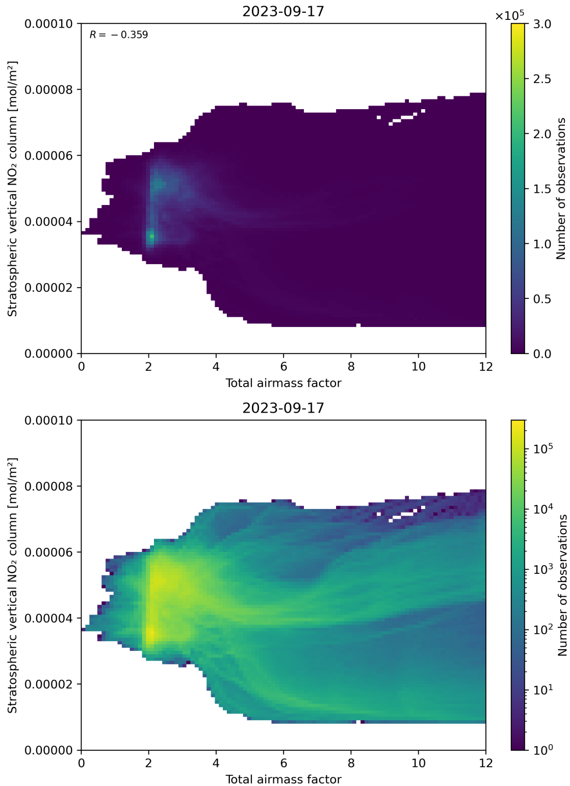
Figure 64: Scatter density plot of “Total airmass factor” against “Stratospheric vertical NO 2 column” for 2023-09-16 to 2023-09-18.
