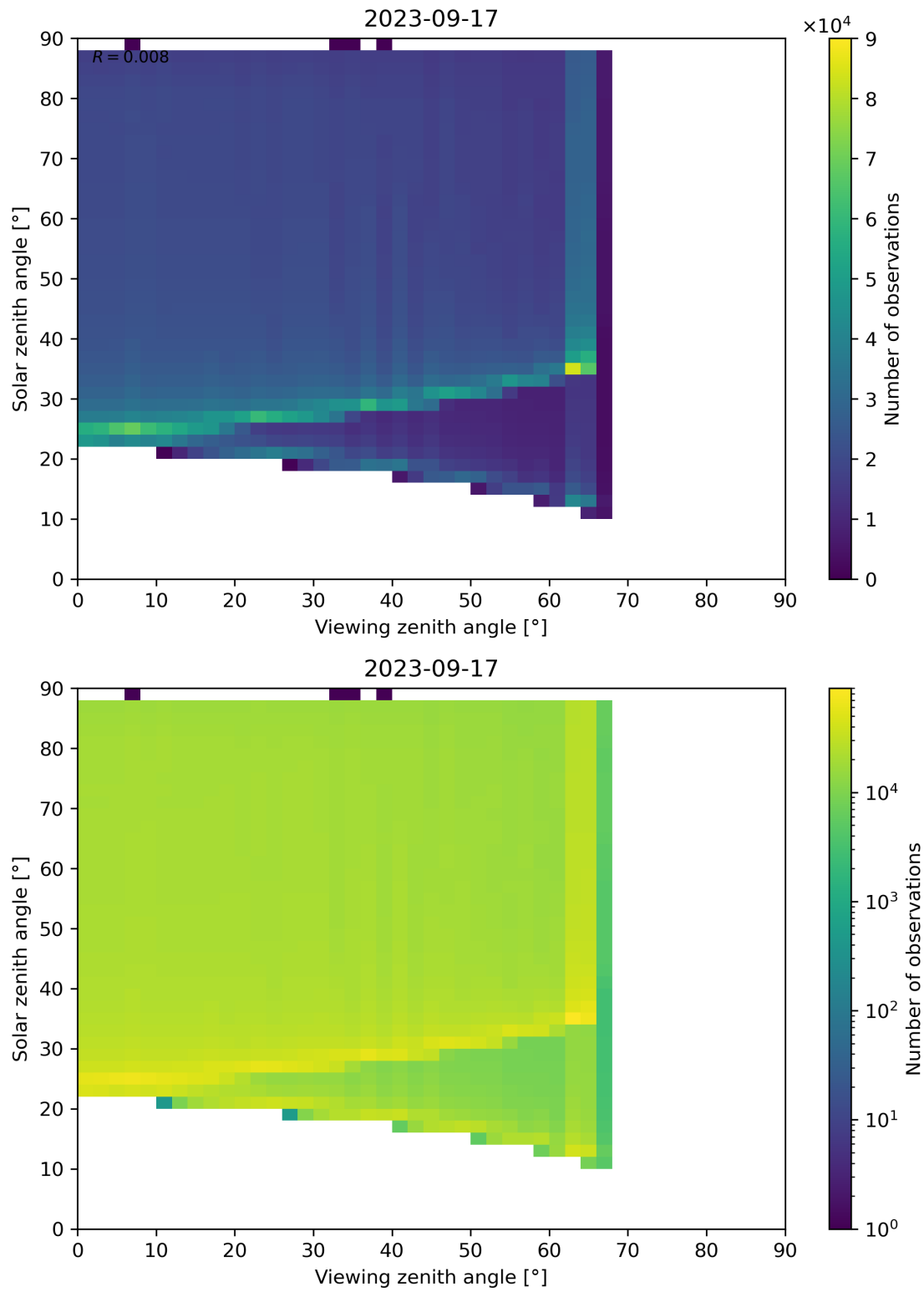
Figure 172: Scatter density plot of “Viewing zenith angle” against “Solar zenith angle” for 2023-09-16 to 2023-09-18.
