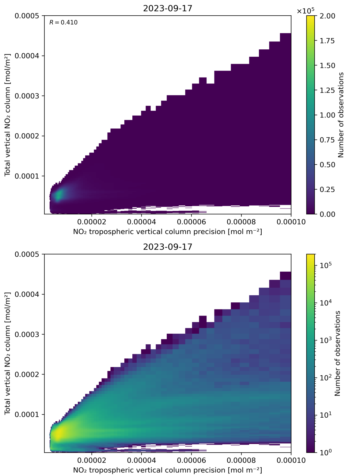
Figure 138: Scatter density plot of “NO 2 tropospheric vertical column precision” against “Total vertical NO 2 column” for 2023-09-16 to 2023-09-18.
