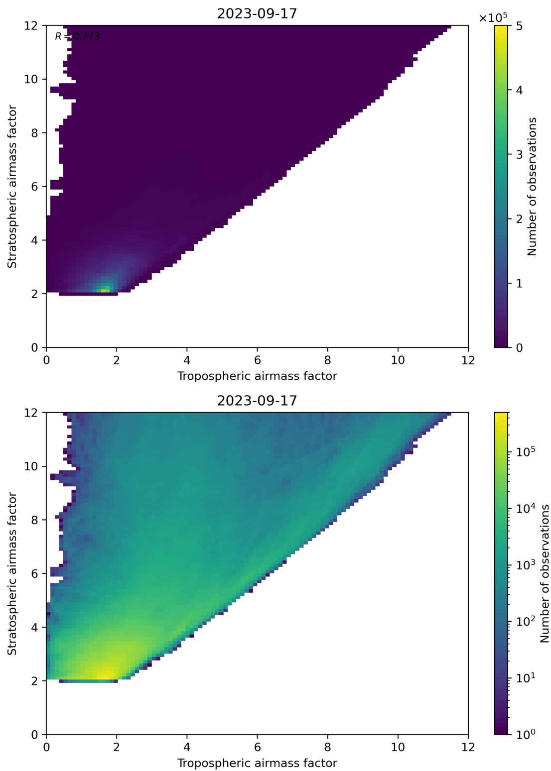
Figure 71: Scatter density plot of “Tropospheric airmass factor” against “Stratospheric airmass factor” for 2023-09-16 to 2023-09-18.
