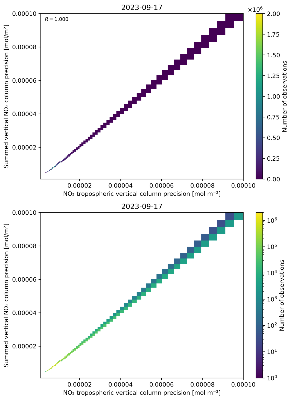
Figure 137: Scatter density plot of “NO 2 tropospheric vertical column precision” against “Summed vertical NO 2 column precision” for 2023-09-16 to 2023-09-18.
