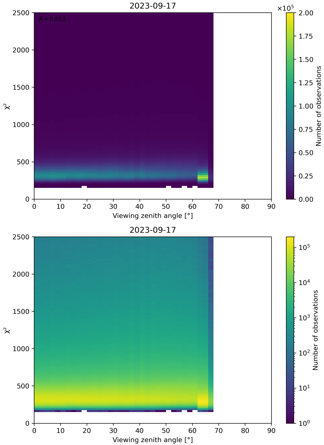
Figure 162: Scatter density plot of “Viewing zenith angle” against “ \chi^2 ” for 2023-09-16 to 2023-09-18.
