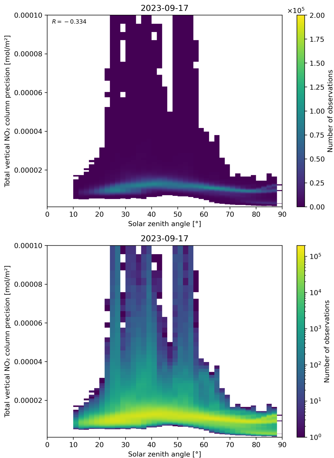
Figure 154: Scatter density plot of “Solar zenith angle” against “Total vertical NO 2 column precision” for 2023-09-16 to 2023-09-18.
