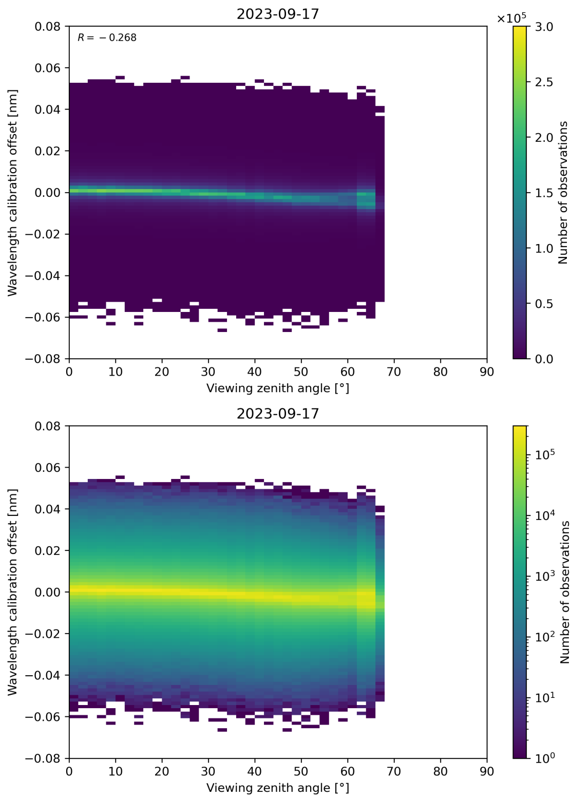
Figure 173: Scatter density plot of “Viewing zenith angle” against “Wavelength calibration offset” for 2023-09-16 to 2023-09-18.
