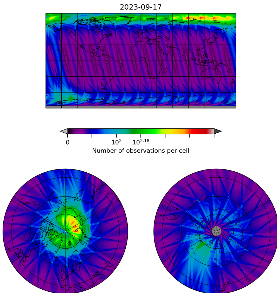
Figure 10: Map of the number of observations for 2023-09-16 to 2023-09-18
