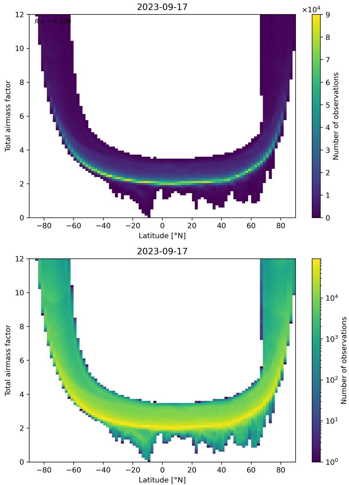
Figure 84: Scatter density plot of “Latitude” against “Total airmass factor” for 2023-09-16 to 2023-09-18.
