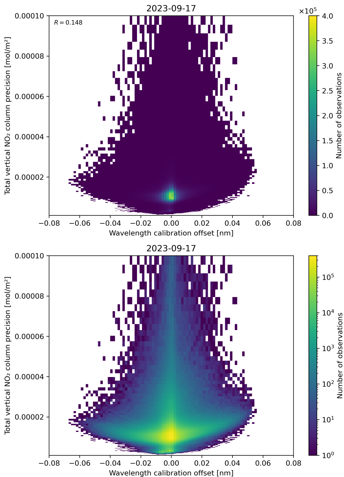
Figure 180: Scatter density plot of “Wavelength calibration offset” against “Total vertical NO 2 column precision” for 2023-09-16 to 2023-09-18.
