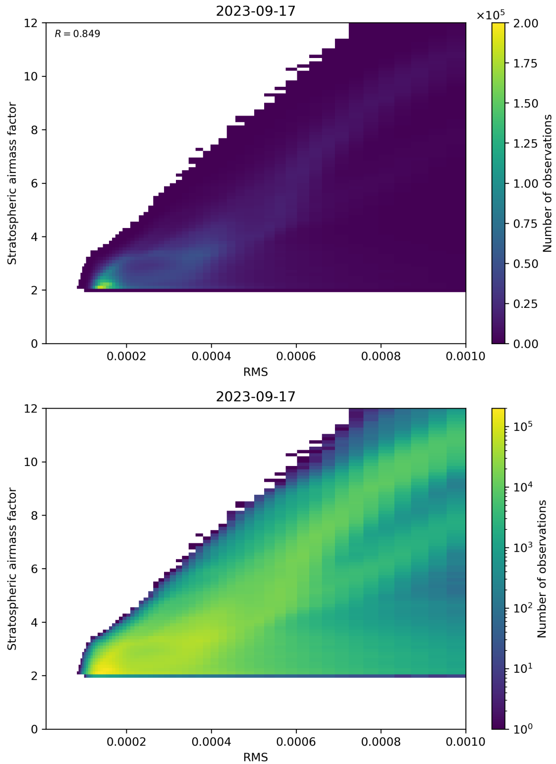
Figure 144: Scatter density plot of “RMS” against “Stratospheric airmass factor” for 2023-09-16 to 2023-09-18.
