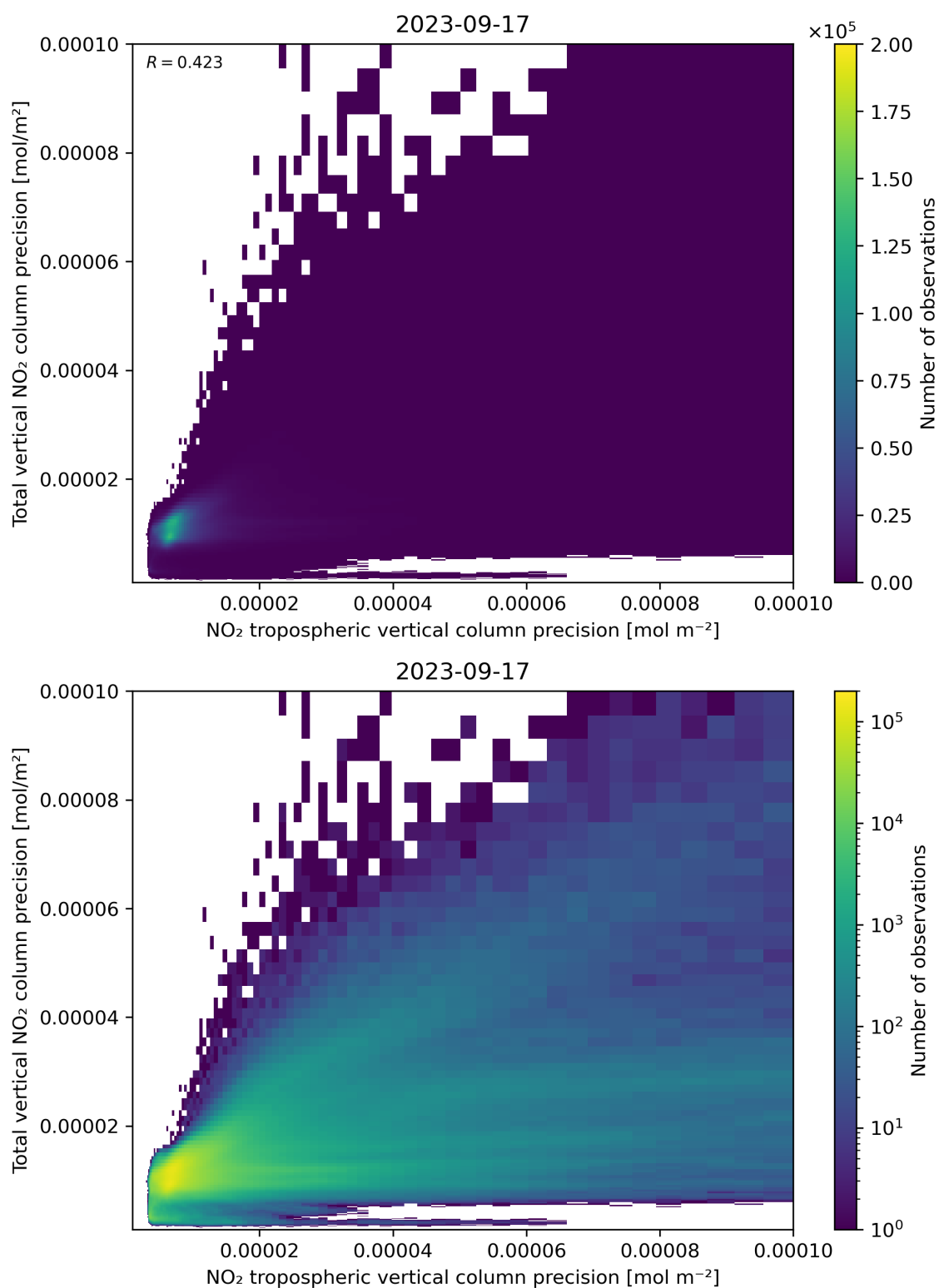
Figure 139: Scatter density plot of “NO 2 tropospheric vertical column precision” against “Total vertical NO 2 column precision” for 2023-09-16 to 2023-09-18.
