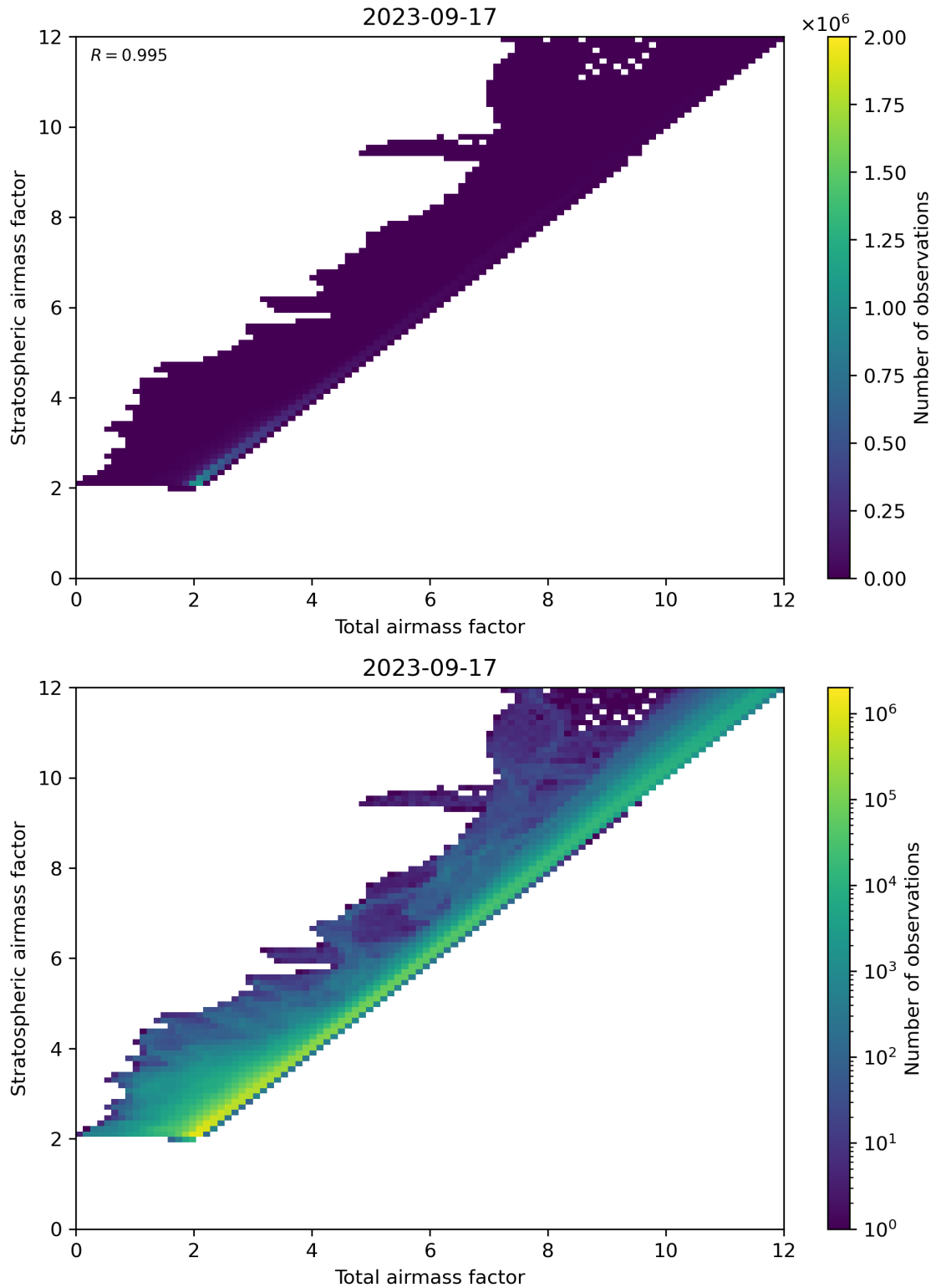
Figure 62: Scatter density plot of “Total air mass factor” against “Stratospheric air mass factor” for 2023-09-16 to 2023-09-18.
