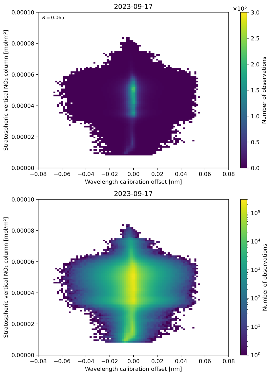
Figure 176: Scatter density plot of “Wavelength calibration offset” against “Stratospheric vertical NO 2 column” for 2023-09-16 to 2023-09-18.
