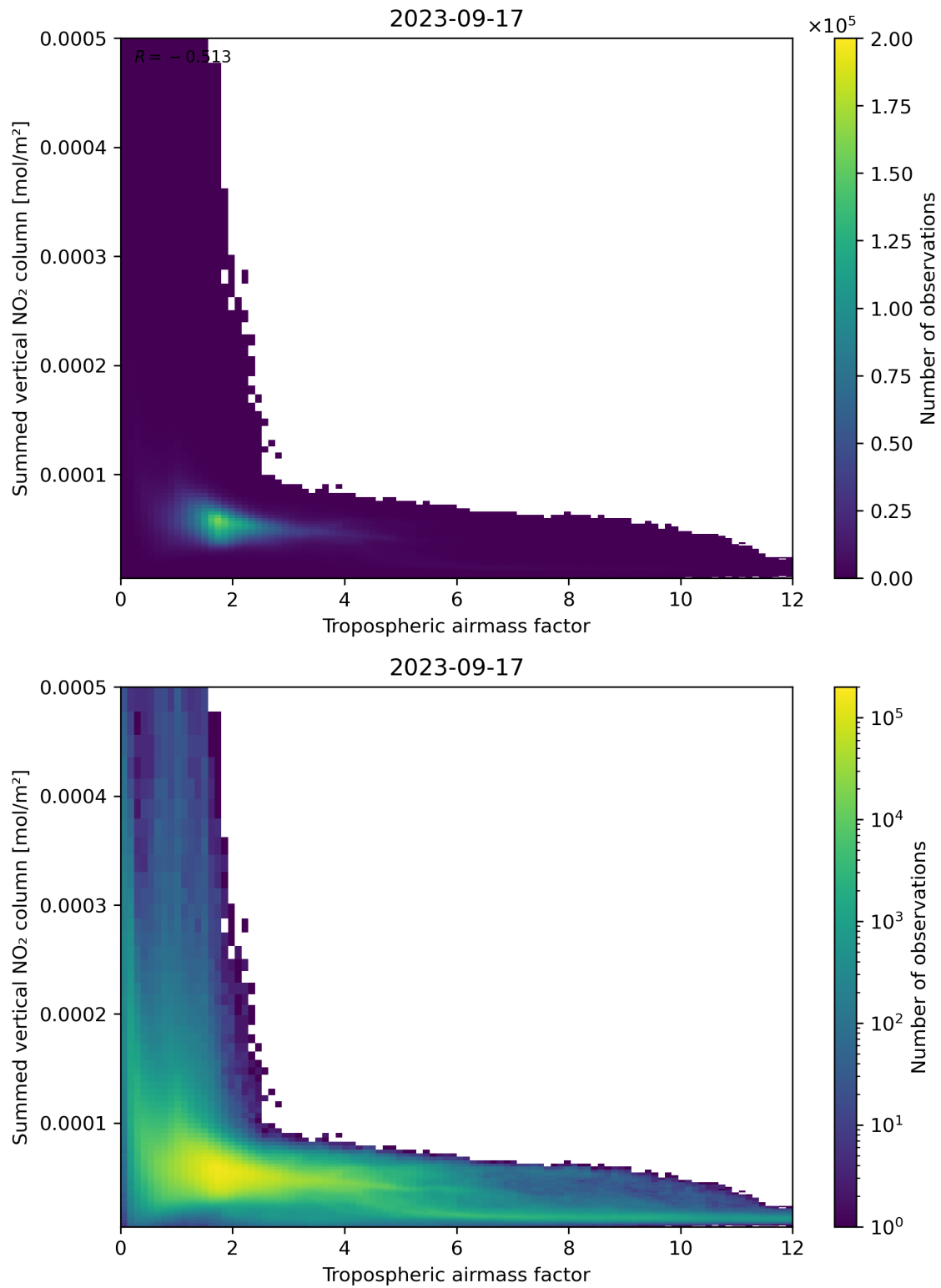
Figure 75: Scatter density plot of “Tropospheric air mass factor” against “Summed vertical NO 2 column” for 2023-09-16 to 2023-09-18.
