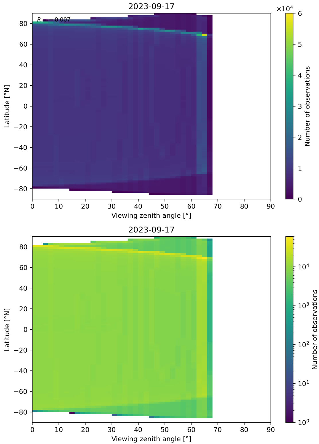
Figure 163: Scatter density plot of “Viewing zenith angle” against “Latitude” for 2023-09-16 to 2023-09-18.
