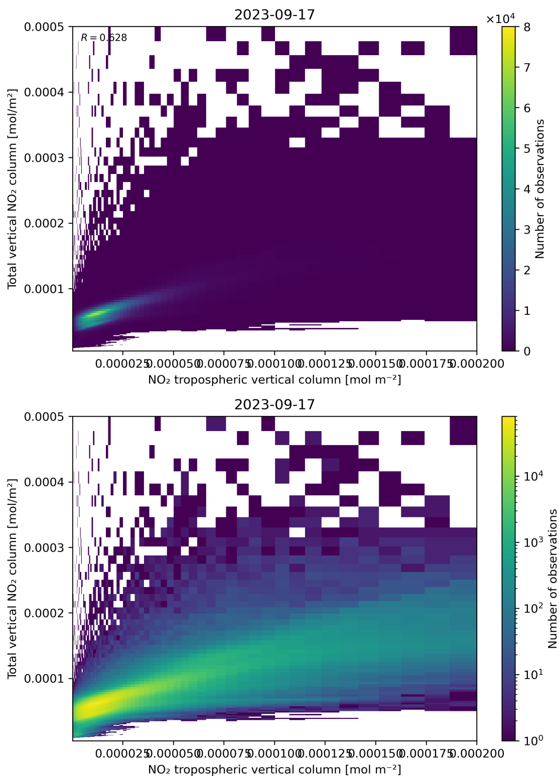
Figure 128: Scatter density plot of “NO 2 tropospheric vertical column” against “Total vertical NO 2 column” for 2023-09-16 to 2023-09-18.
