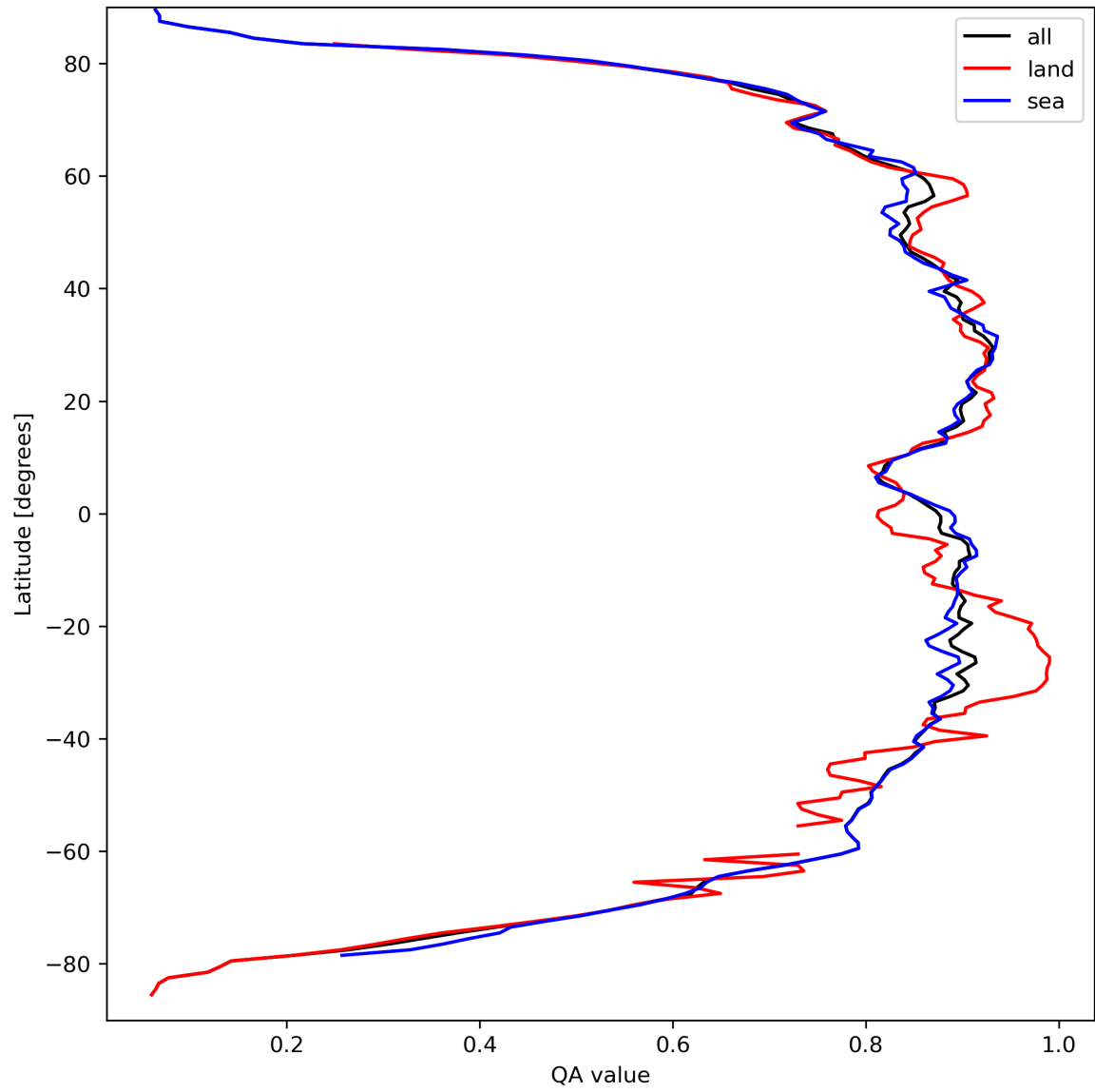
Figure 11: Zonal average of “QA value” for 2023-09-16 to 2023-09-18.
