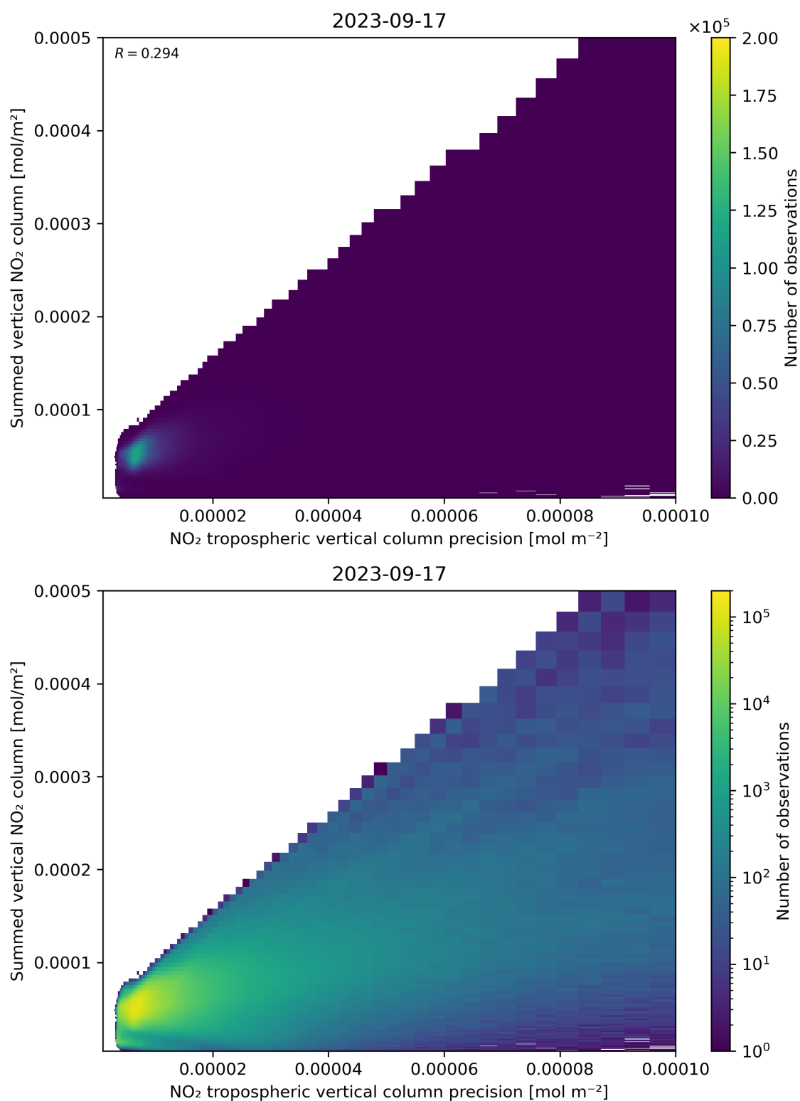
Figure 136: Scatter density plot of “NO 2 tropospheric vertical column precision” against “Summed vertical NO 2 column” for 2023-09-16 to 2023-09-18.
