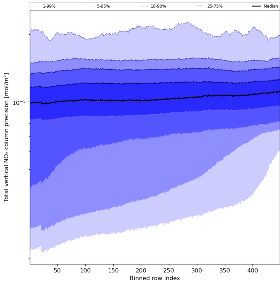
Figure 56: Along track statistics of “Total vertical NO 2 column precision” for 2023-09-16 to 2023-09-18
