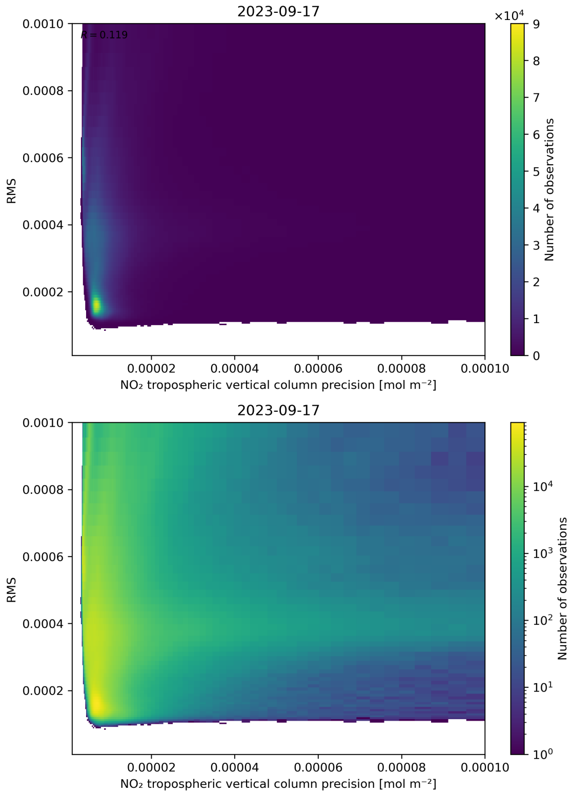
Figure 140: Scatter density plot of “NO 2 tropospheric vertical column precision” against “RMS” for 2023-09-16 to 2023-09-18.
