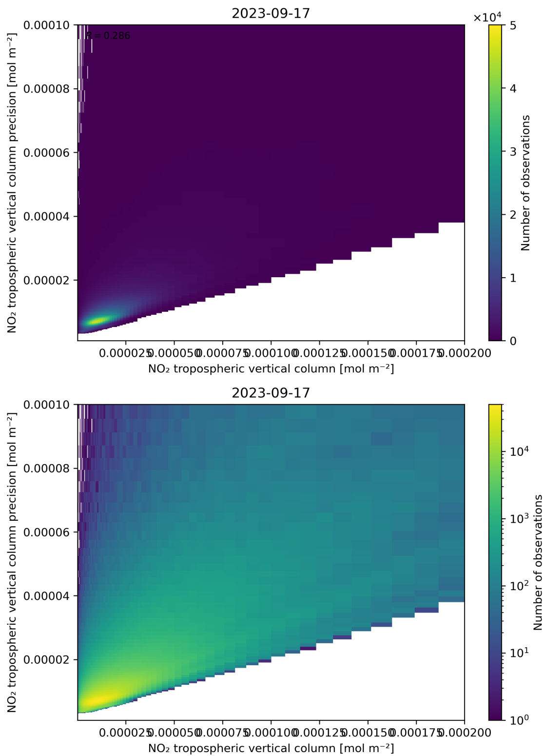
Figure 130: Scatter density plot of “NO 2 tropospheric vertical column” against “NO 2 tropospheric vertical column precision” for 2023-09-16 to 2023-09-18.
