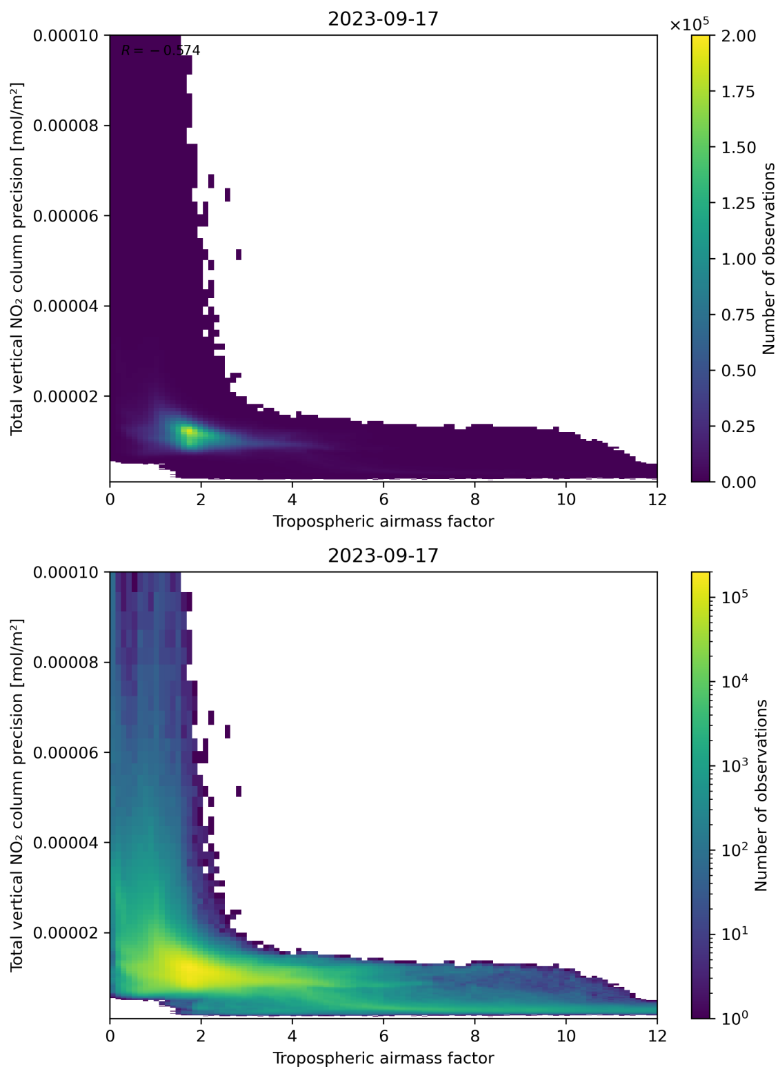
Figure 78: Scatter density plot of “Tropospheric air mass factor” against “Total vertical NO 2 column precision” for 2023-09-16 to 2023-09-18.
