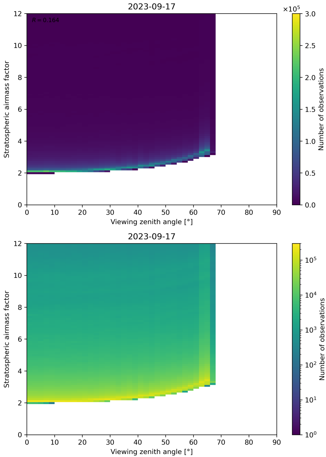
Figure 159: Scatter density plot of “Viewing zenith angle” against “Stratospheric airmass factor” for 2023-09-16 to 2023-09-18.
