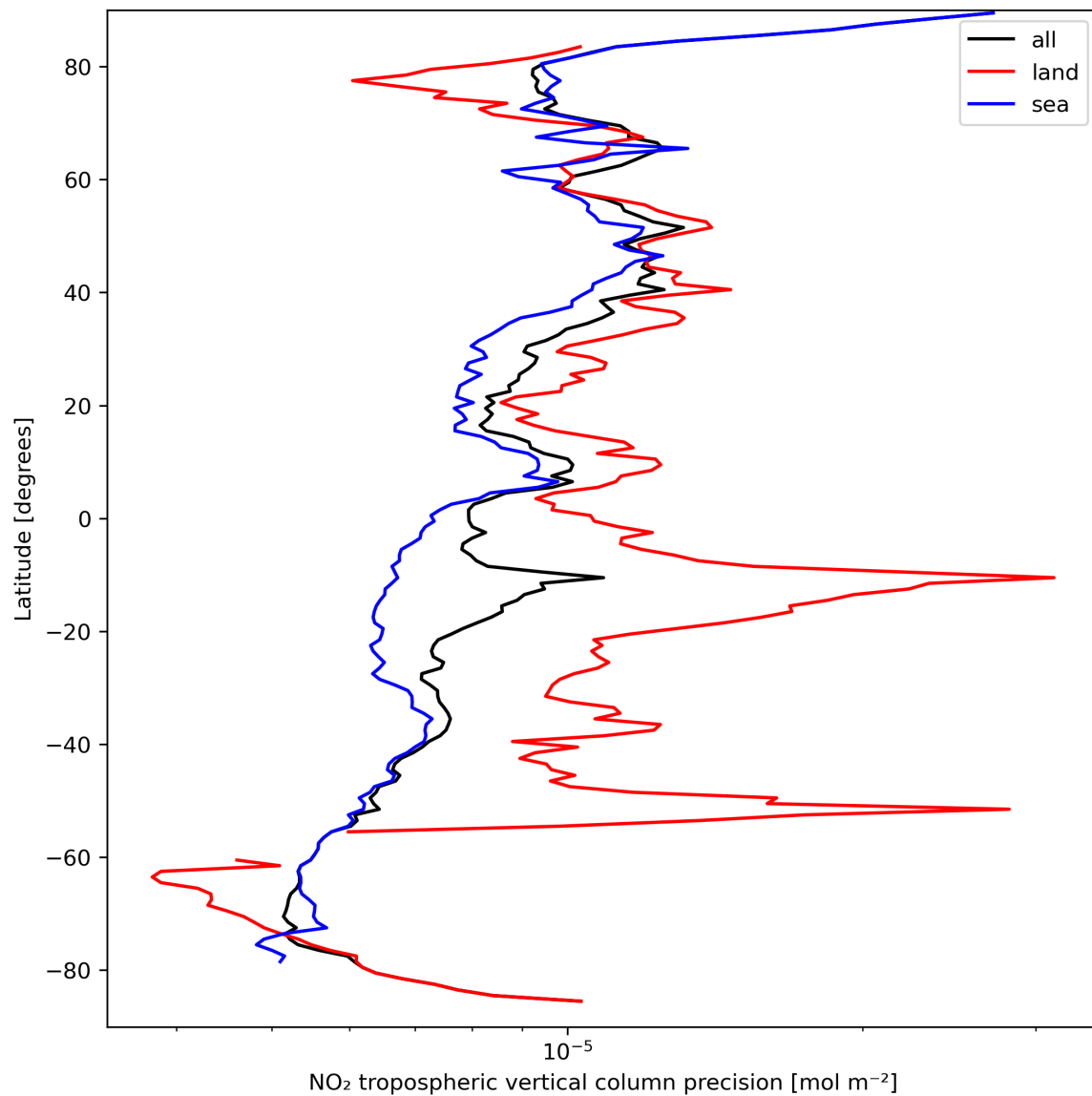
Figure 13: Zonal average of “NO 2 tropospheric vertical column precision” for 2023-09-16 to 2023-09-18.
