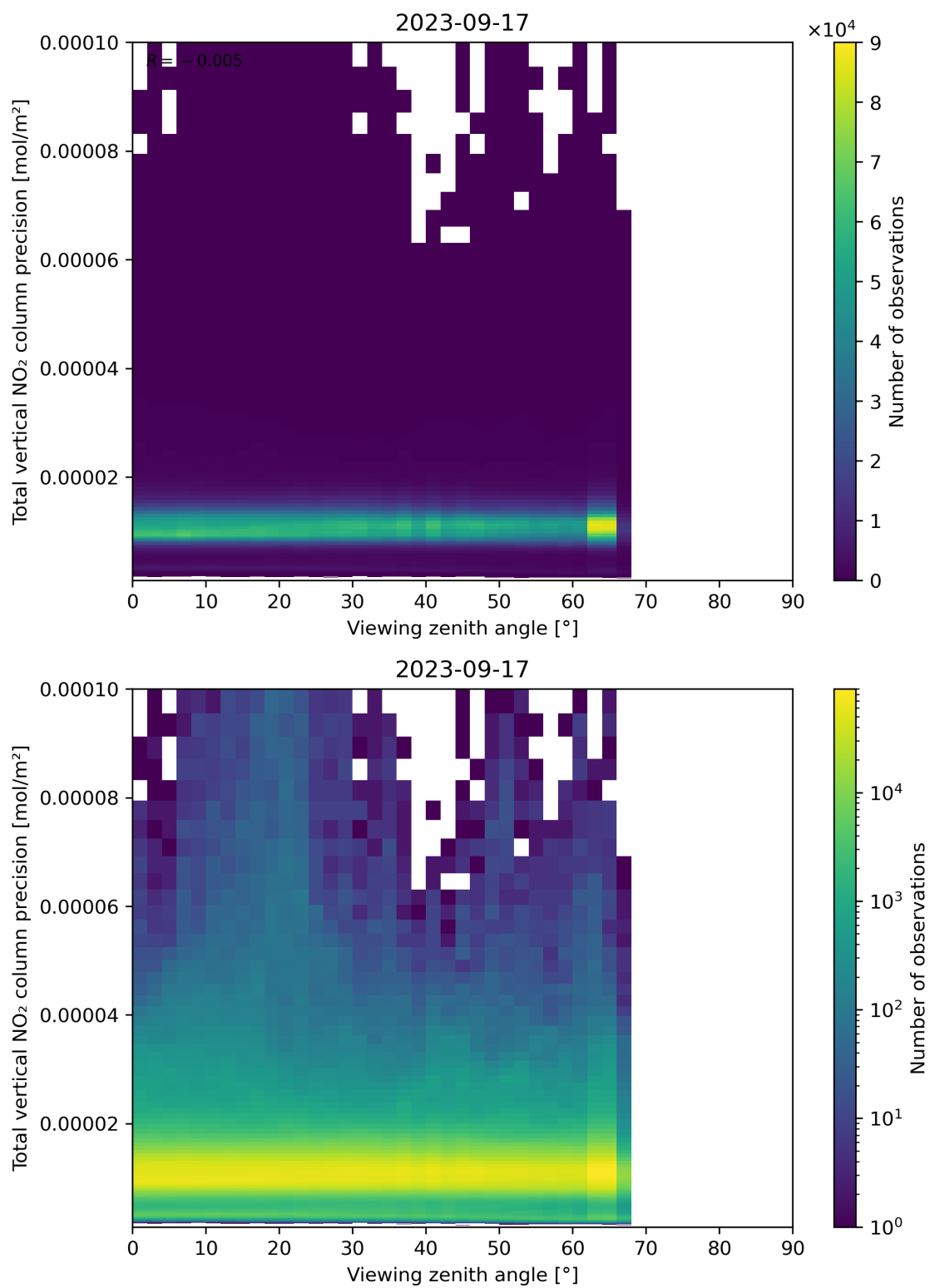
Figure 168: Scatter density plot of “Viewing zenith angle” against “Total vertical NO 2 column precision” for 2023-09-16 to 2023-09-18.
