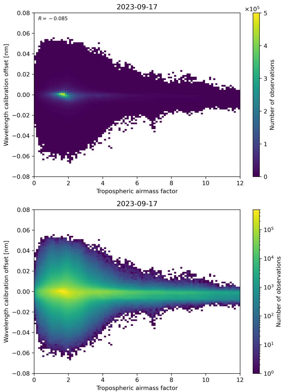
Figure 80: Scatter density plot of “Tropospheric airmass factor” against “Wavelength calibration offset” for 2023-09-16 to 2023-09-18.
