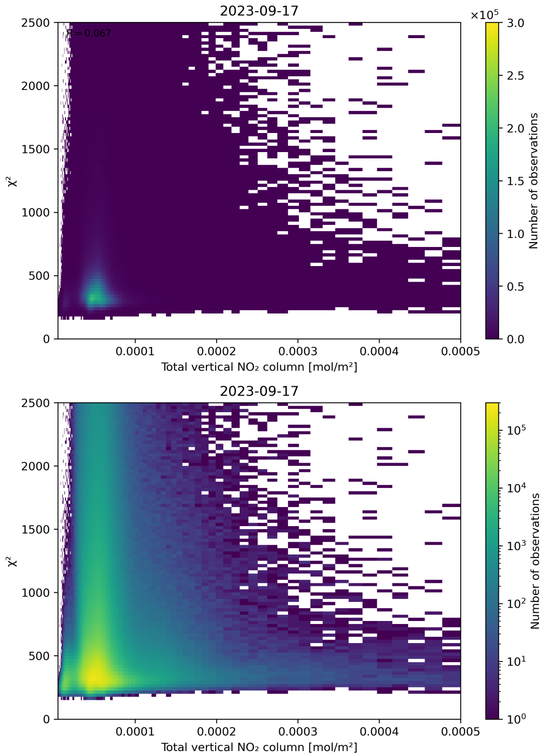
Figure 111: Scatter density plot of “Total vertical NO 2 column” against “ \chi^2 ” for 2023-09-16 to 2023-09-18.
