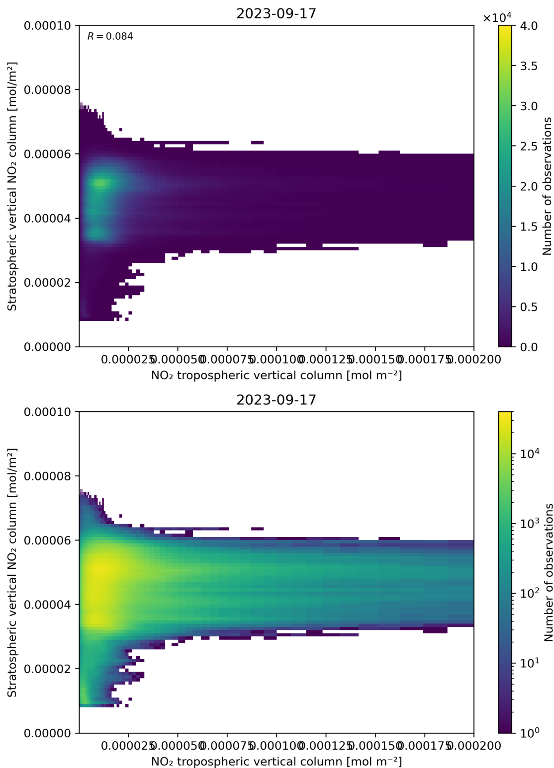
Figure 125: Scatter density plot of “NO 2 tropospheric vertical column” against “Stratospheric vertical NO 2 column” for 2023-09-16 to 2023-09-18.
