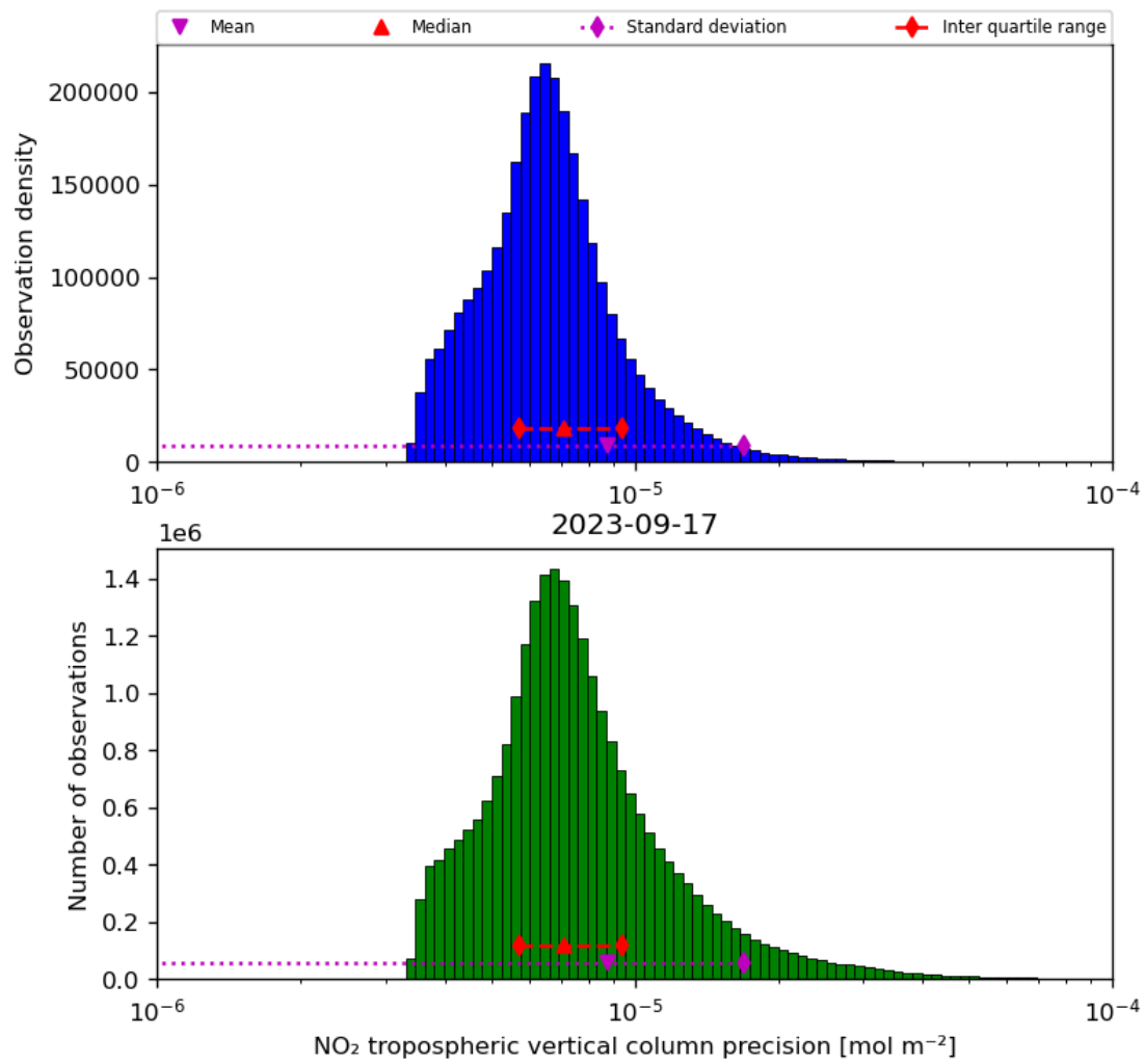
Figure 30: Histogram of “NO 2 tropospheric vertical column precision” for 2023-09-16 to 2023-09-18
