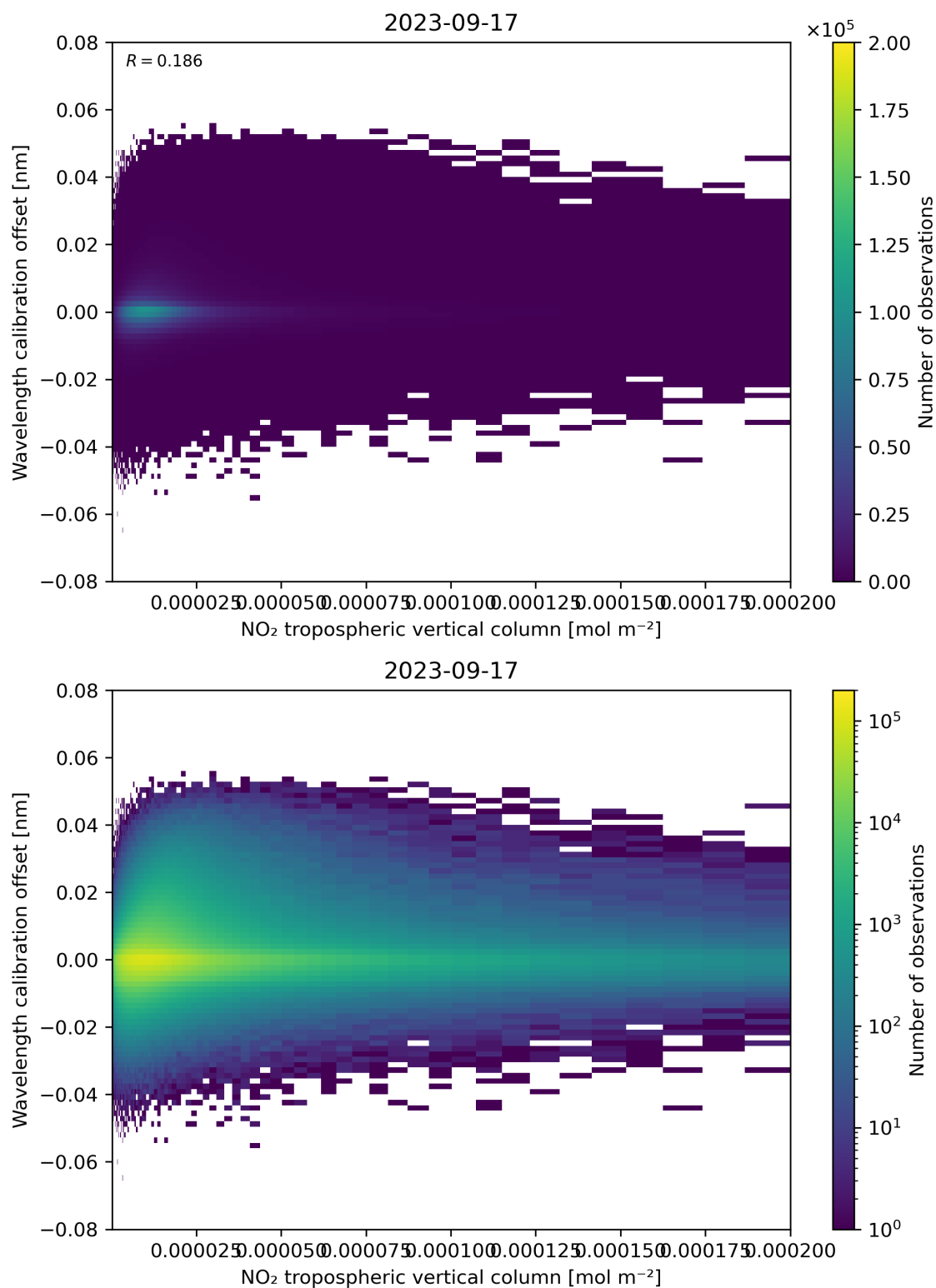
Figure 143: Scatter density plot of “NO 2 tropospheric vertical column” against “Wavelength calibration offset” for 2023-09-16 to 2023-09-18.
