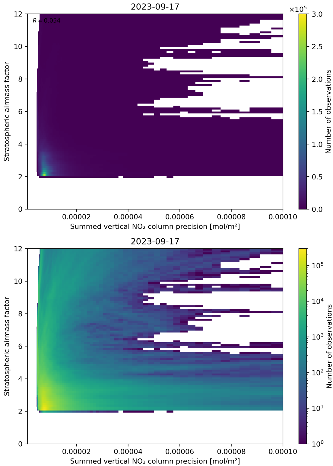
Figure 106: Scatter density plot of “Summed vertical NO 2 column precision” against “Stratospheric airmass factor” for 2023-09-16 to 2023-09-18.
