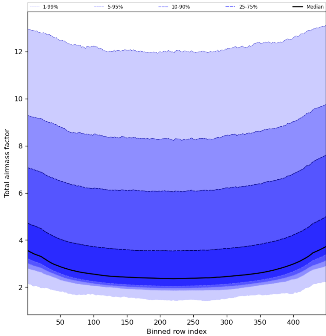
Figure 49: Along track statistics of “Total airmass factor” for 2023-09-16 to 2023-09-18
