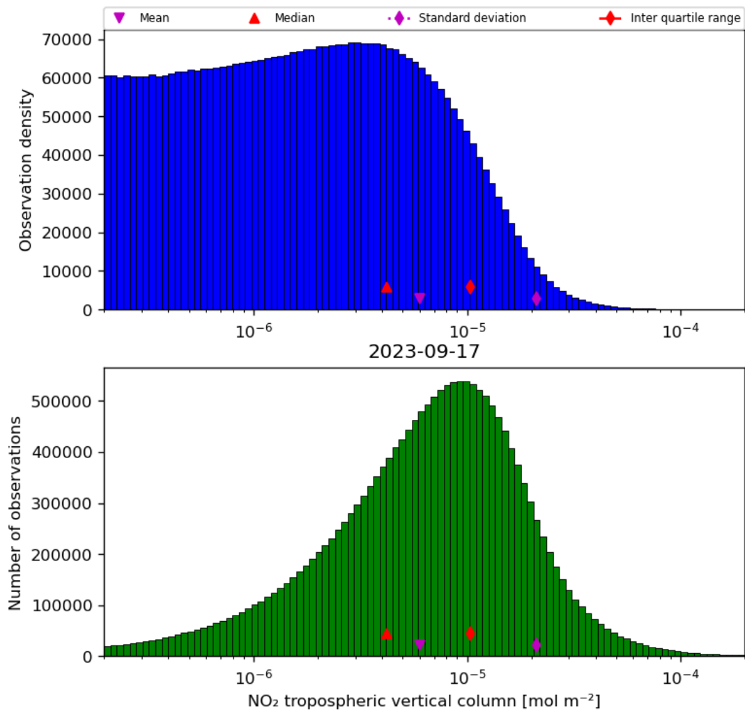
Figure 29: Histogram of “NO 2 tropospheric vertical column” for 2023-09-16 to 2023-09-18
