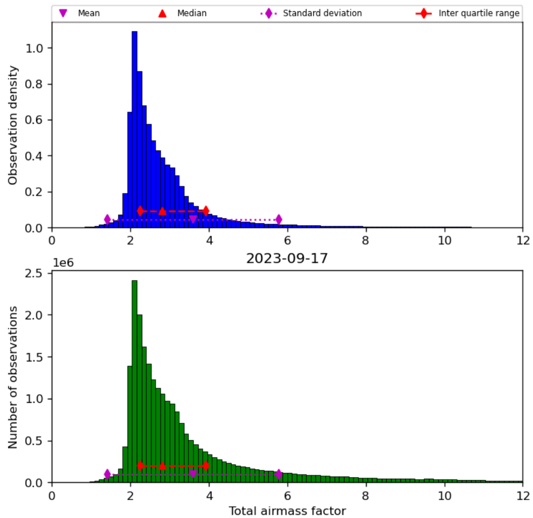
Figure 32: Histogram of “Total airmass factor” for 2023-09-16 to 2023-09-18
