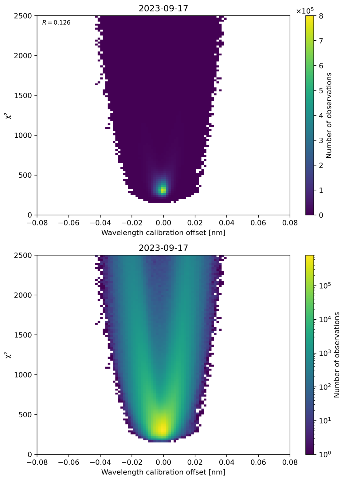
Figure 175: Scatter density plot of “Wavelength calibration offset” against “ \chi^2 ” for 2023-09-16 to 2023-09-18.
