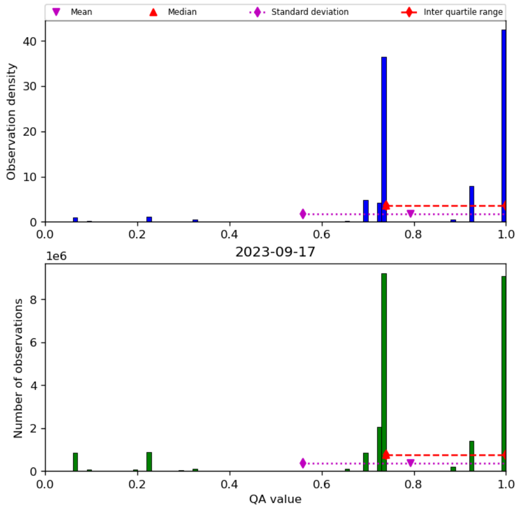
Figure 28: Histogram of “QA value” for 2023-09-16 to 2023-09-18
