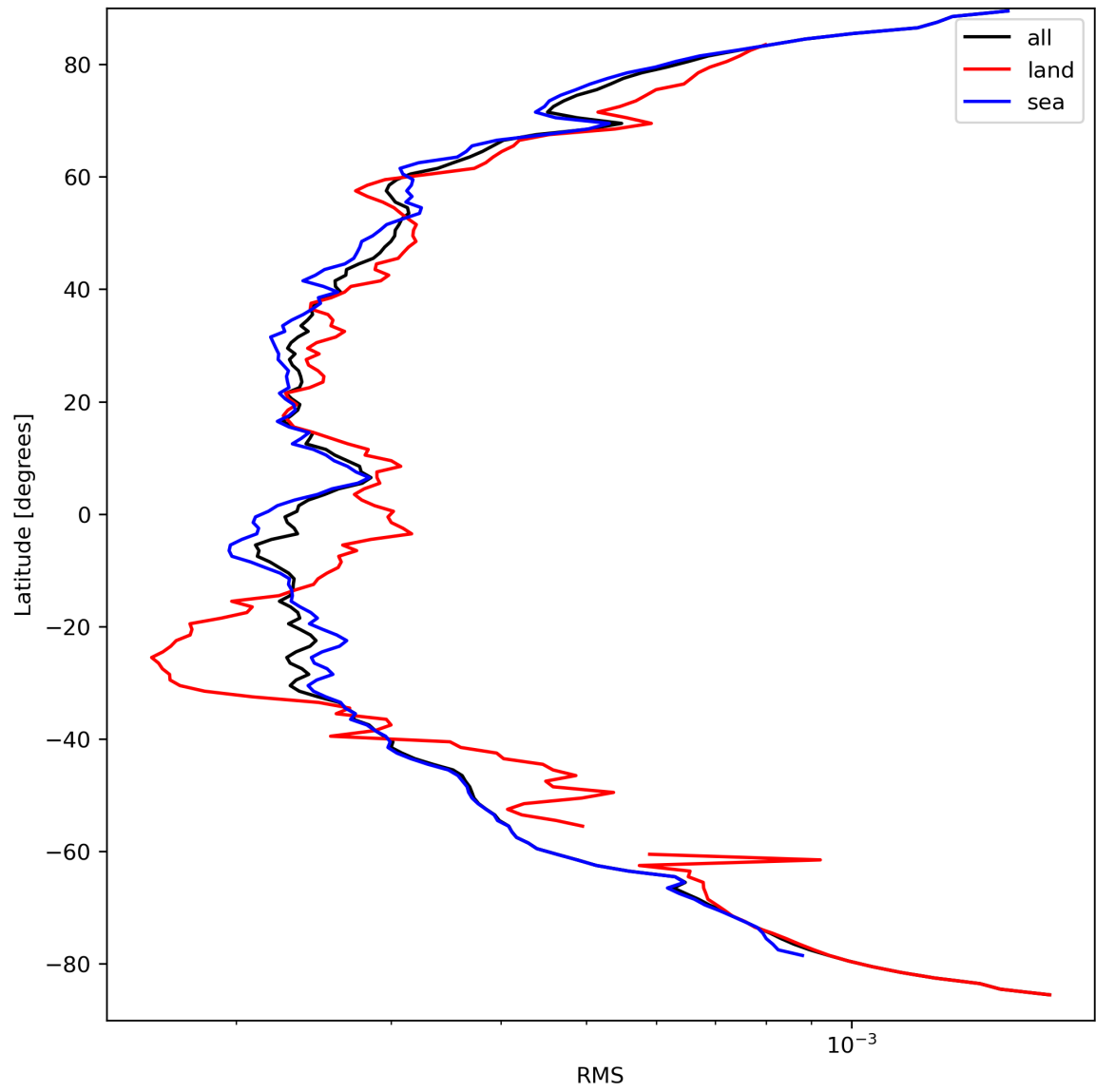
Figure 26: Zonal average of “RMS” for 2023-09-16 to 2023-09-18.
