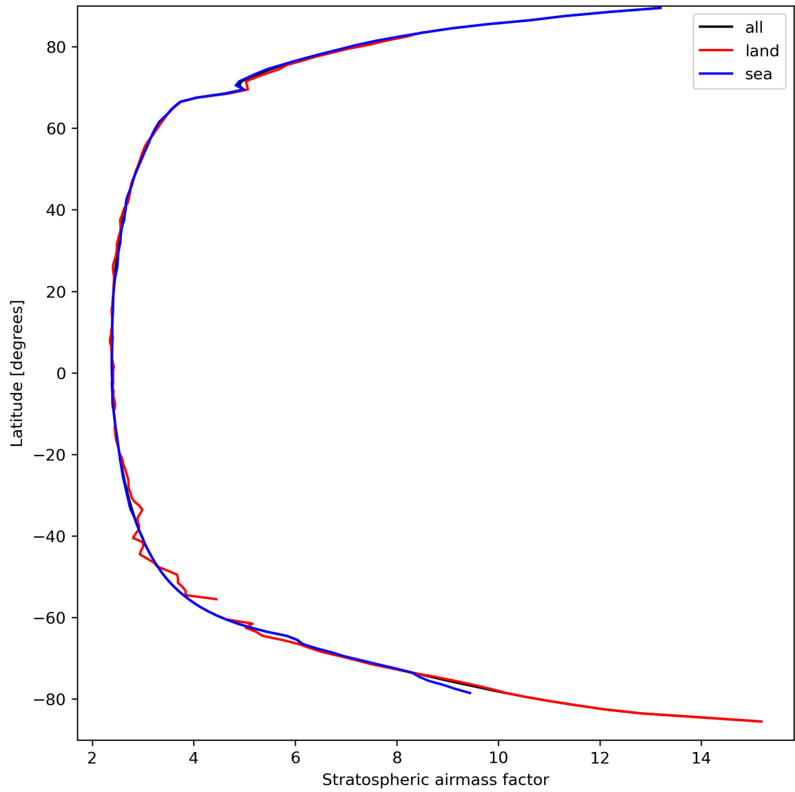
Figure 27: Zonal average of “Stratospheric airmass factor” for 2023-09-16 to 2023-09-18.
