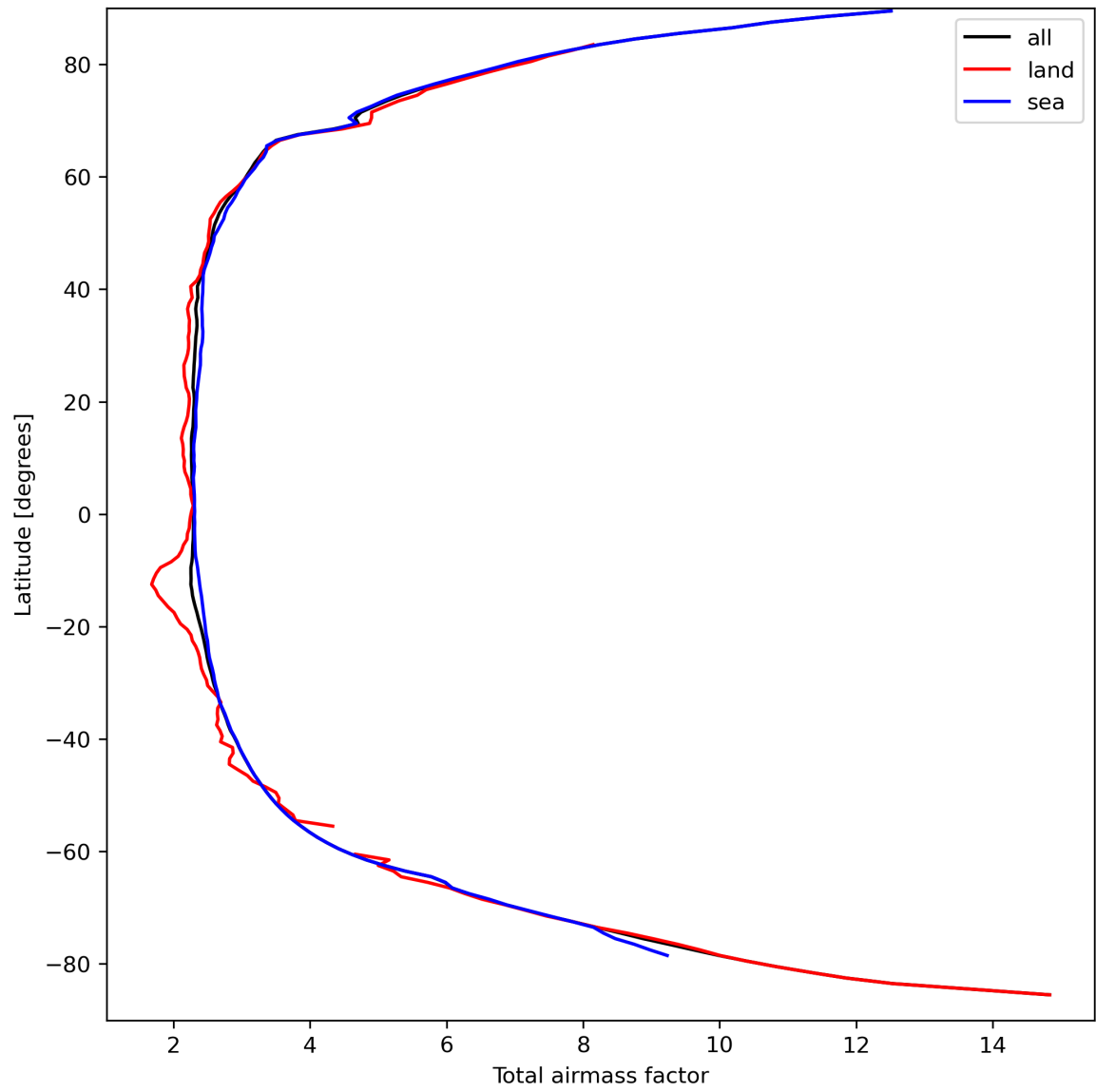
Figure 15: Zonal average of “Total airmass factor” for 2023-09-16 to 2023-09-18.
