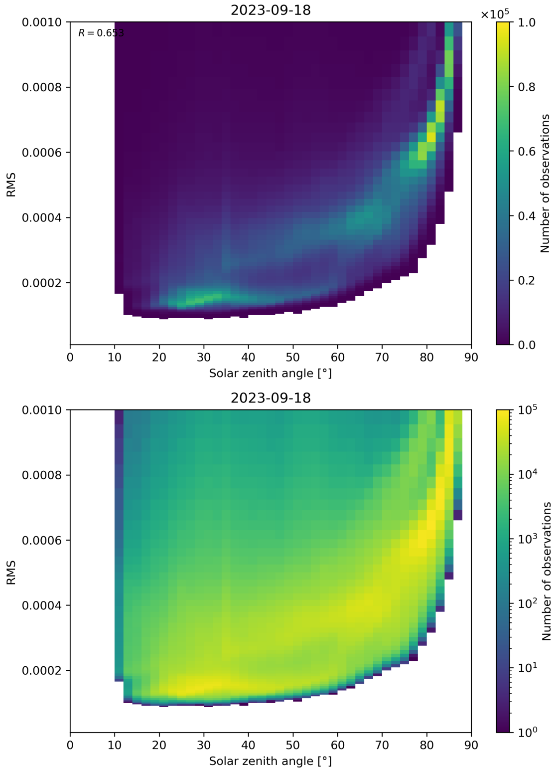
Figure 157: Scatter density plot of “Solar zenith angle” against “RMS” for 2023-09-17 to 2023-09-19.
