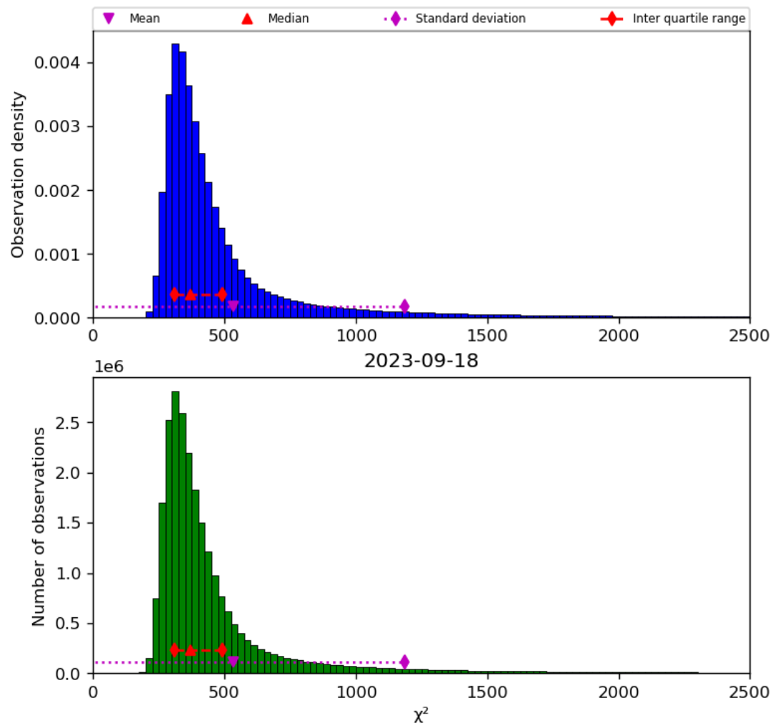
Figure 42: Histogram of " \chi^2 " for 2023-09-17 to 2023-09-19
