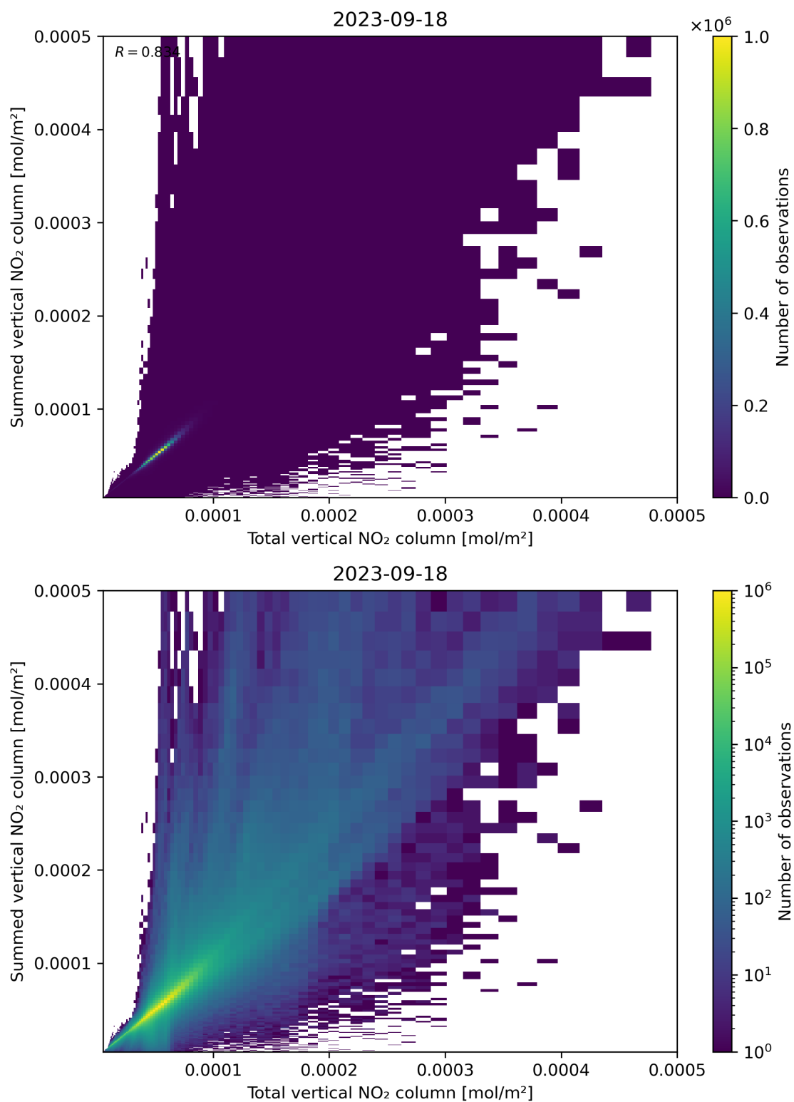
Figure 112: Scatter density plot of “Total vertical NO 2 column” against “Summed vertical NO 2 column” for 2023-09-17 to 2023-09-19.
