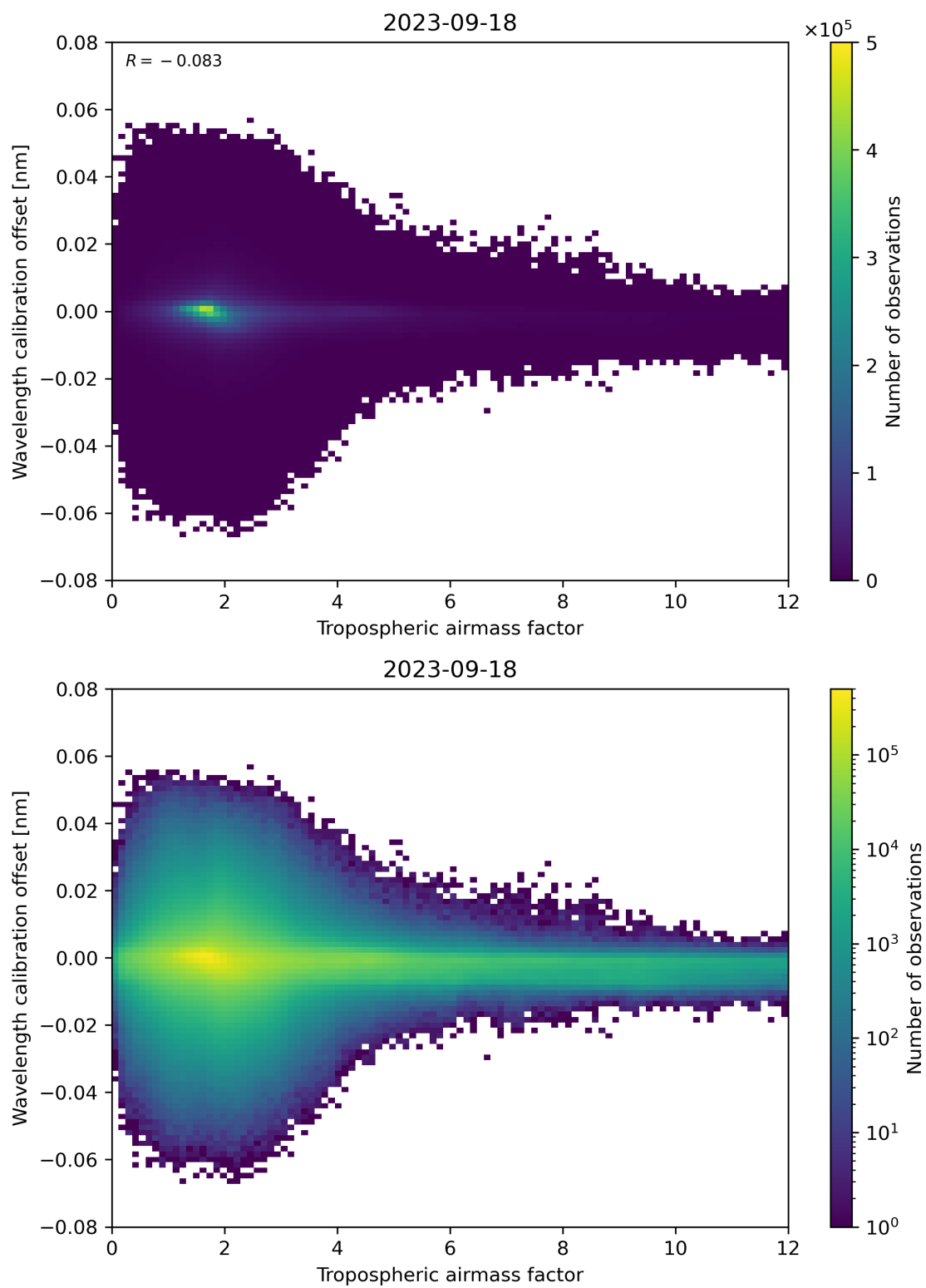
Figure 80: Scatter density plot of “Tropospheric airmass factor” against “Wavelength calibration offset” for 2023-09-17 to 2023-09-19.
