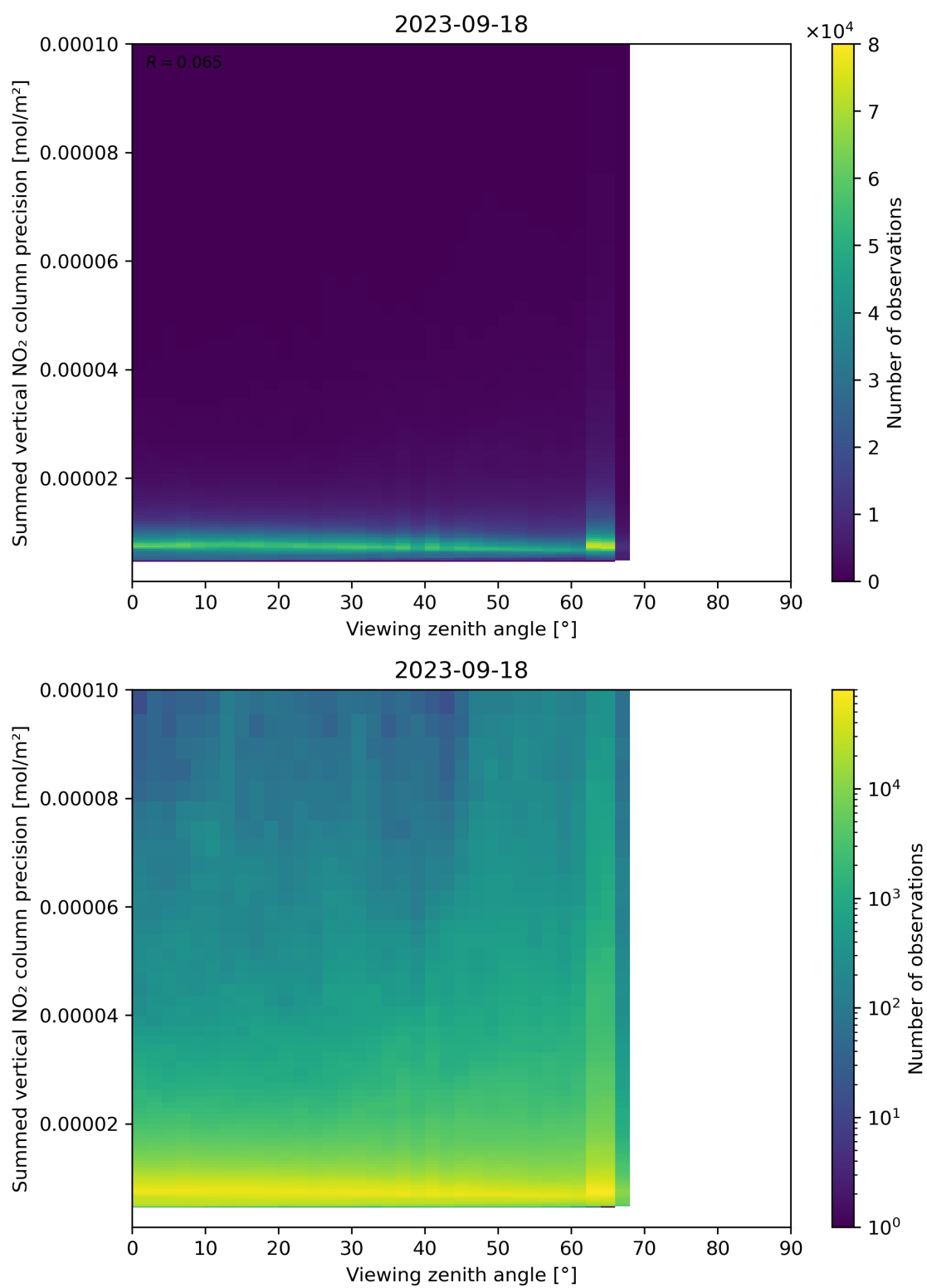
Figure 166: Scatter density plot of “Viewing zenith angle” against “Summed vertical NO 2 column precision” for 2023-09-17 to 2023-09-19.
