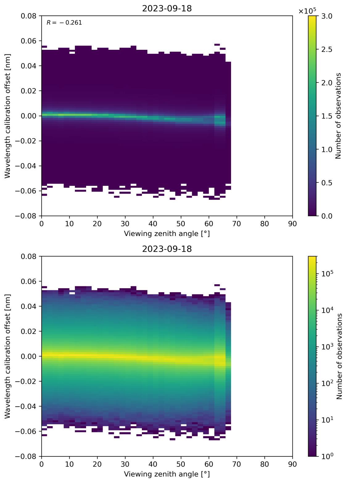
Figure 173: Scatter density plot of “Viewing zenith angle” against “Wavelength calibration offset” for 2023-09-17 to 2023-09-19.
