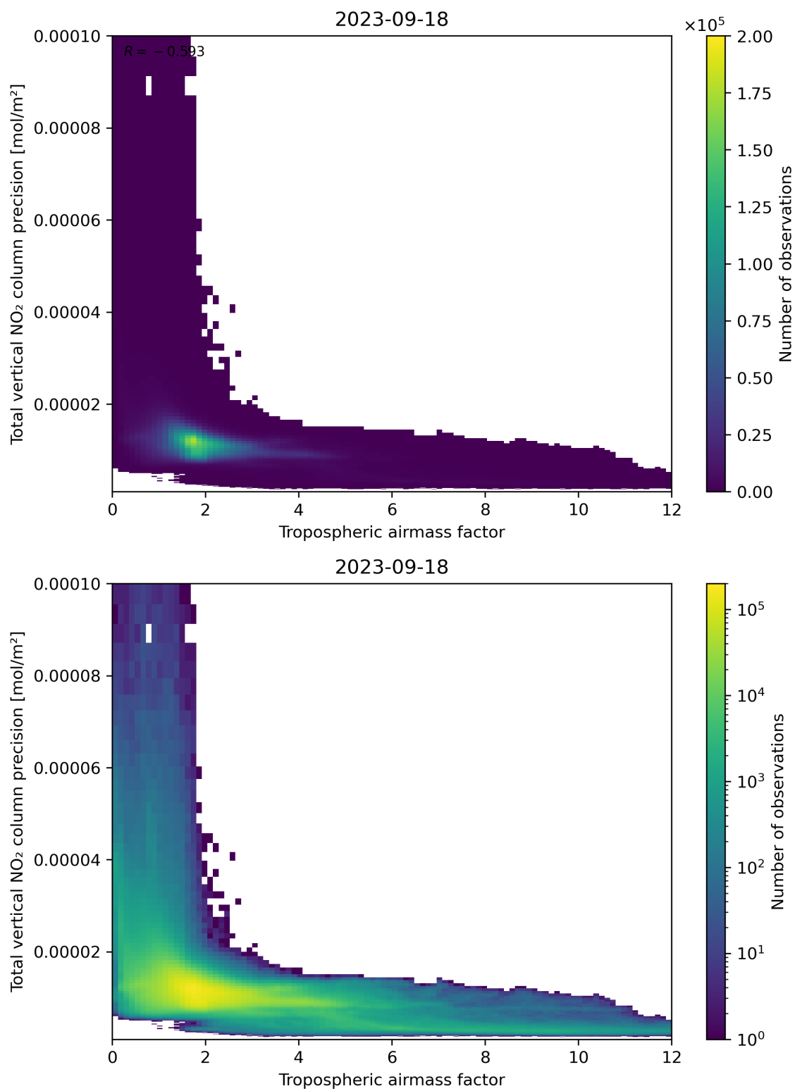
Figure 78: Scatter density plot of “Tropospheric air mass factor” against “Total vertical NO 2 column precision” for 2023-09-17 to 2023-09-19.
