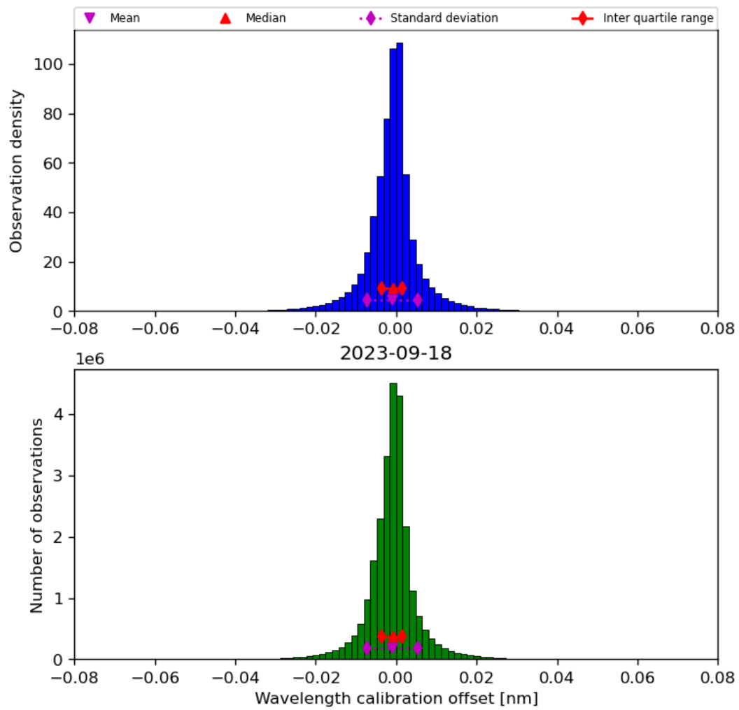
Figure 35: Histogram of “Wavelength calibration offset” for 2023-09-17 to 2023-09-19
