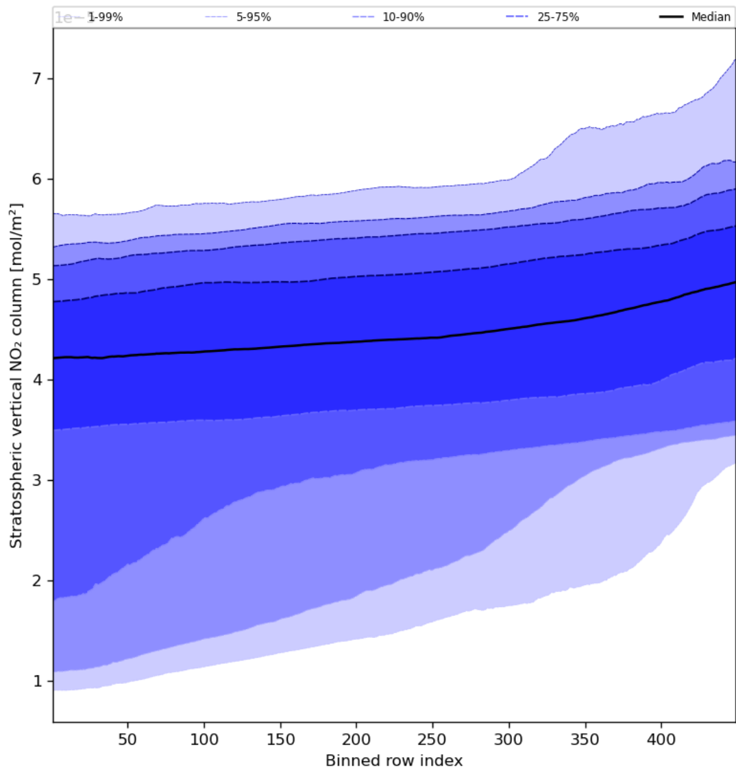
Figure 53: Along track statistics of “Stratospheric vertical NO 2 column” for 2023-09-17 to 2023-09-19
