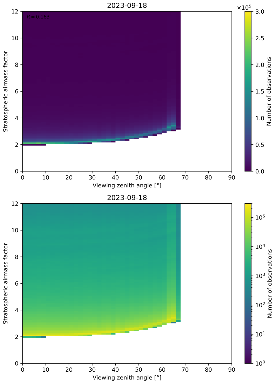
Figure 159: Scatter density plot of “Viewing zenith angle” against “Stratospheric airmass factor” for 2023-09-17 to 2023-09-19.
