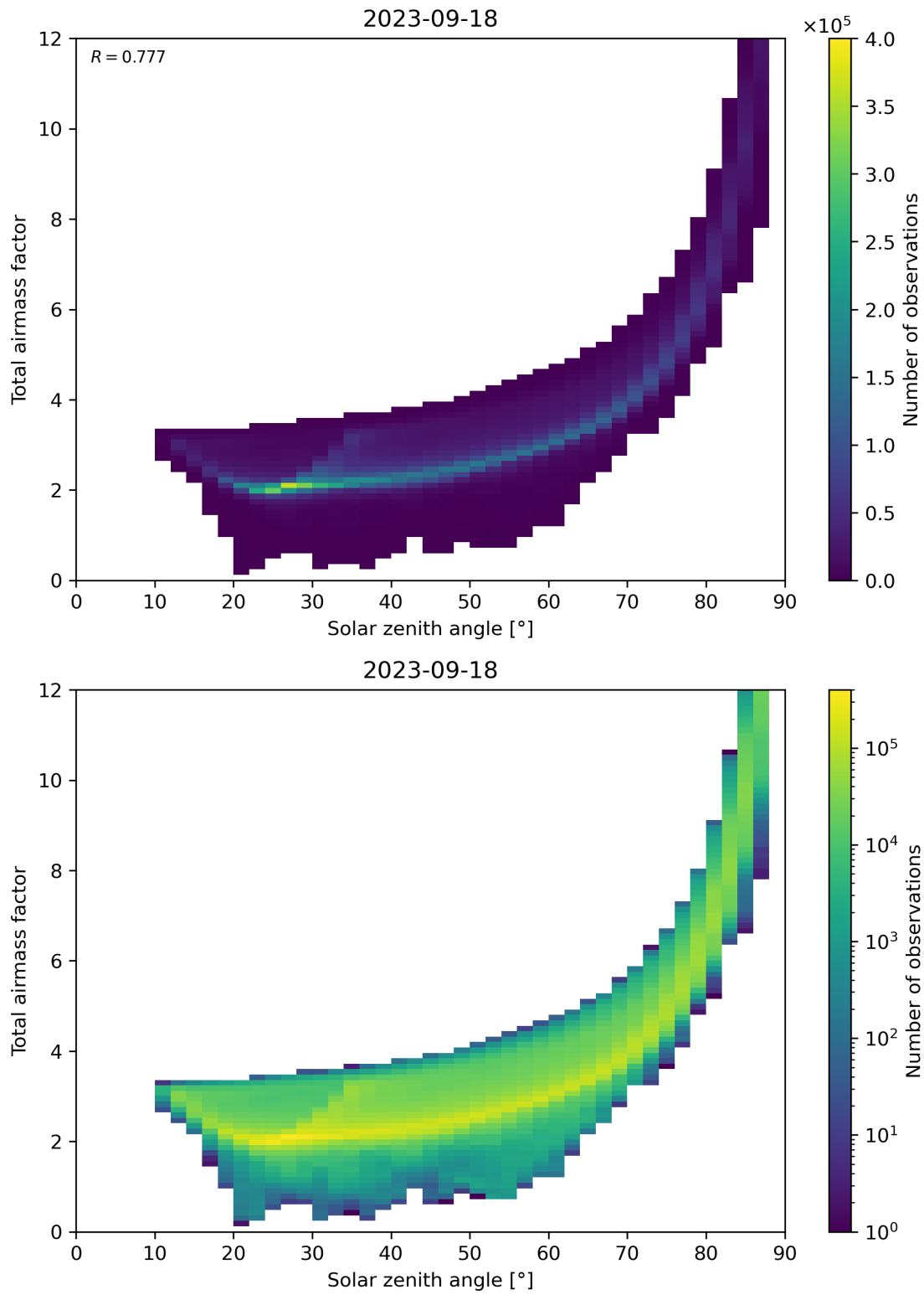
Figure 146: Scatter density plot of “Solar zenith angle” against “Total air mass factor” for 2023-09-17 to 2023-09-19.
