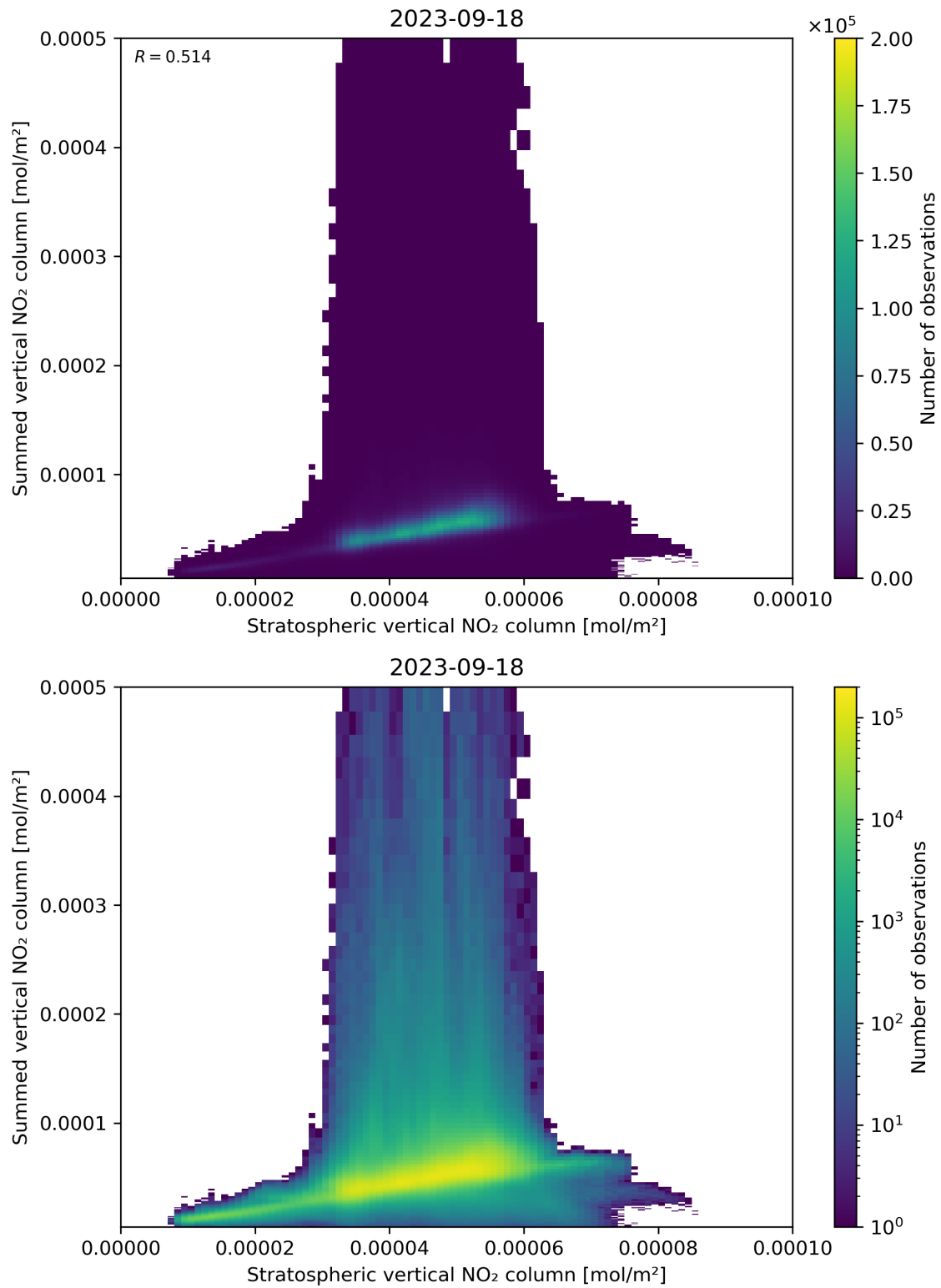
Figure 98: Scatter density plot of “Stratospheric vertical NO 2 column” against “Summed vertical NO 2 column” for 2023-09-17 to 2023-09-19.
