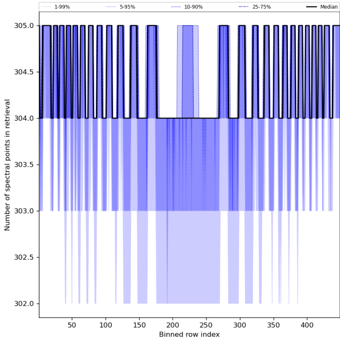
Figure 50: Along track statistics of “Number of spectral points in retrieval” for 2023-09-17 to 2023-09-19
