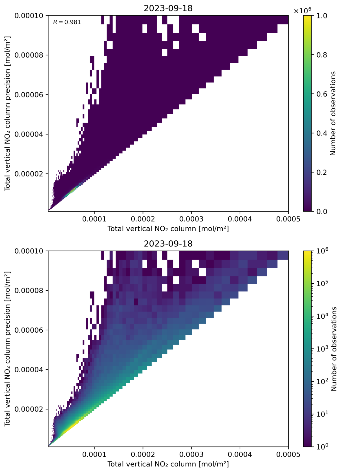
Figure 114: Scatter density plot of “Total vertical NO 2 column” against “Total vertical NO 2 column precision” for 2023-09-17 to 2023-09-19.
