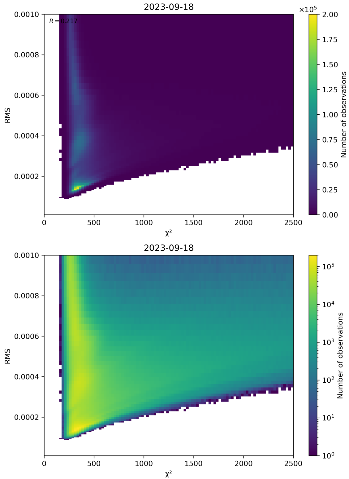
Figure 82: Scatter density plot of “ \chi^2 ” against “RMS” for 2023-09-17 to 2023-09-19.
