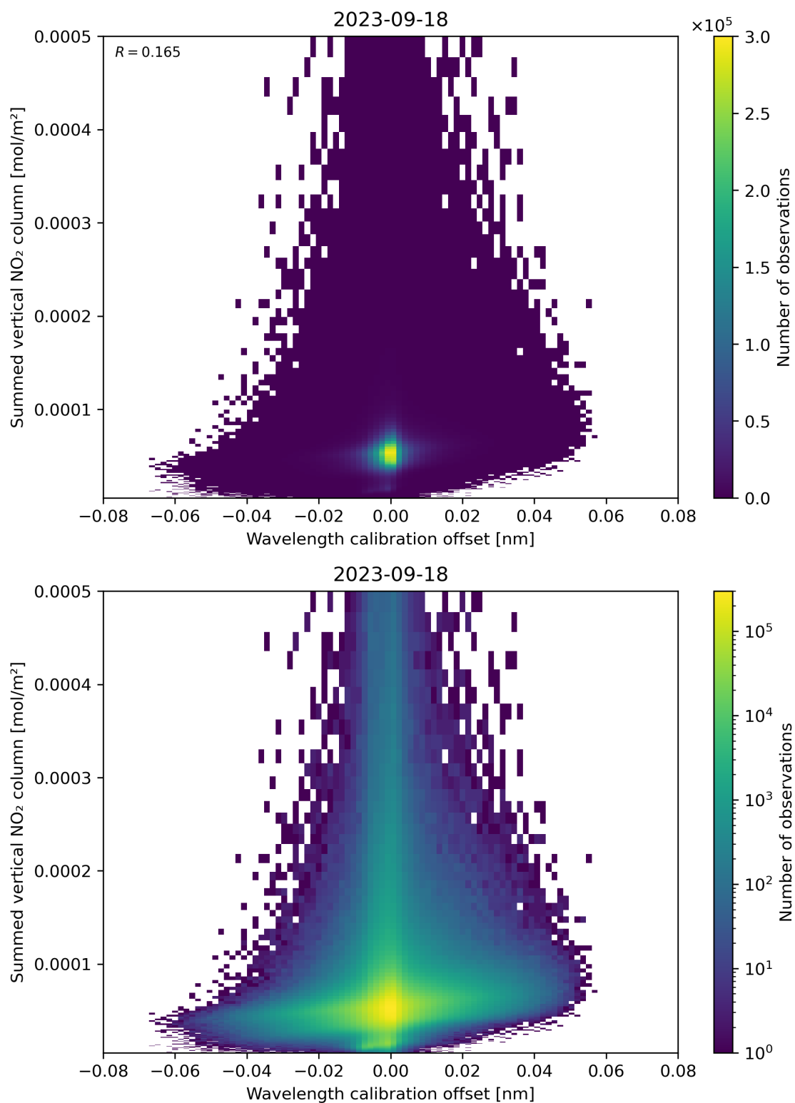
Figure 177: Scatter density plot of “Wavelength calibration offset” against “Summed vertical NO 2 column” for 2023-09-17 to 2023-09-19.
