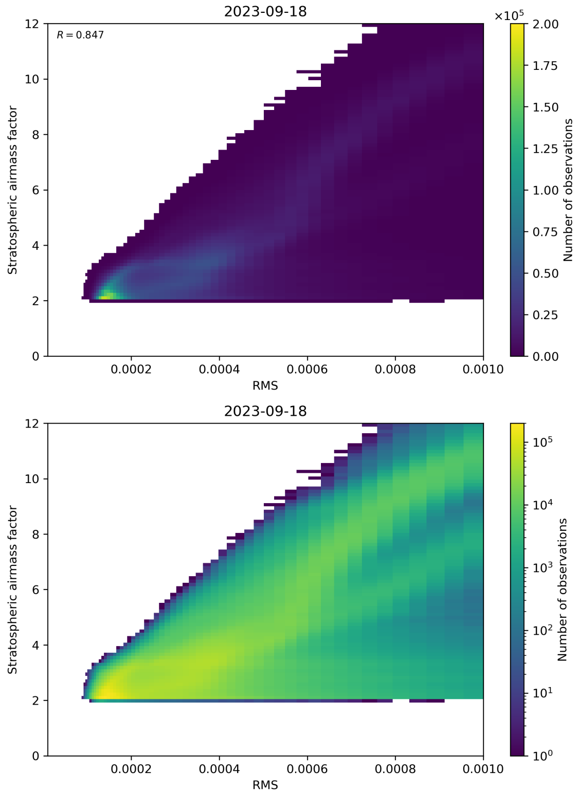
Figure 144: Scatter density plot of “RMS” against “Stratospheric airmass factor” for 2023-09-17 to 2023-09-19.
