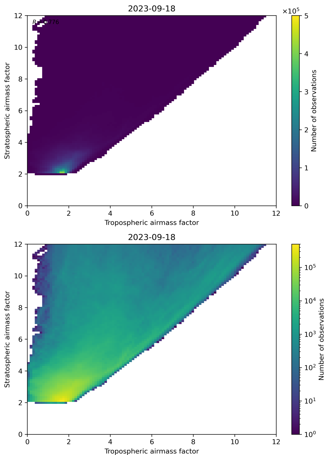
Figure 71: Scatter density plot of “Tropospheric airmass factor” against “Stratospheric airmass factor” for 2023-09-17 to 2023-09-19.
