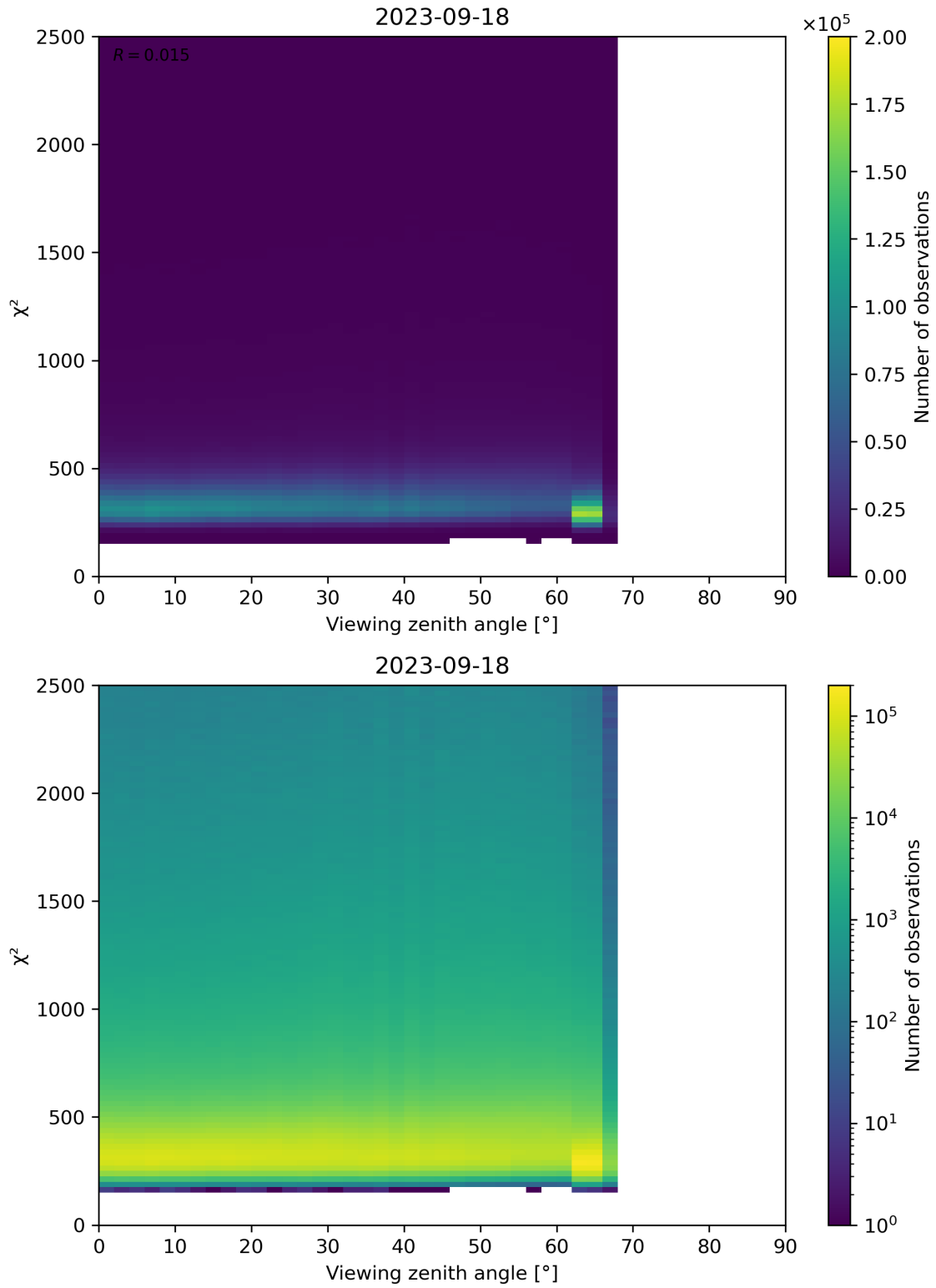
Figure 162: Scatter density plot of “Viewing zenith angle” against “ \chi^2 ” for 2023-09-17 to 2023-09-19.
