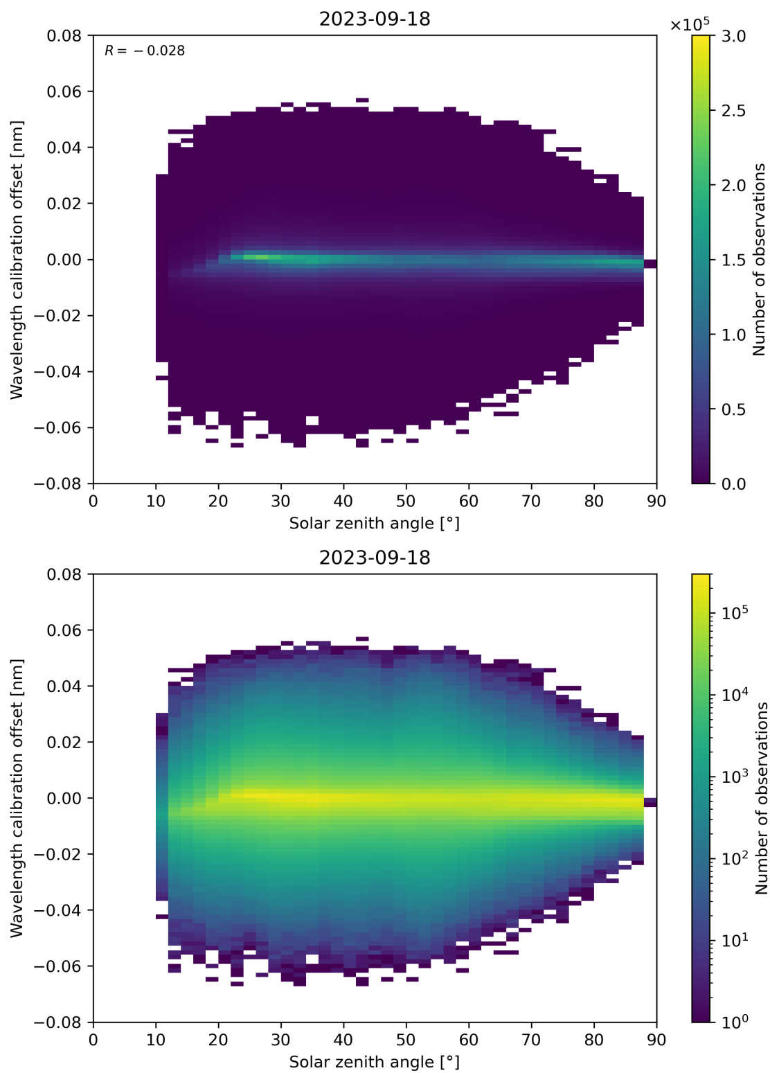
Figure 158: Scatter density plot of “Solar zenith angle” against “Wavelength calibration offset” for 2023-09-17 to 2023-09-19.
