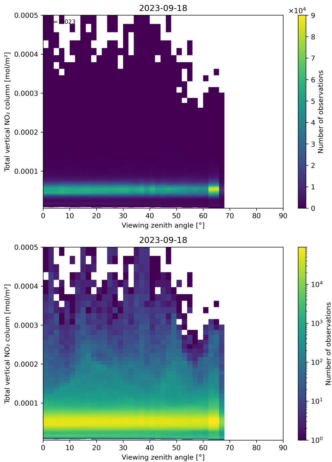
Figure 167: Scatter density plot of “Viewing zenith angle” against “Total vertical NO 2 column” for 2023-09-17 to 2023-09-19.
