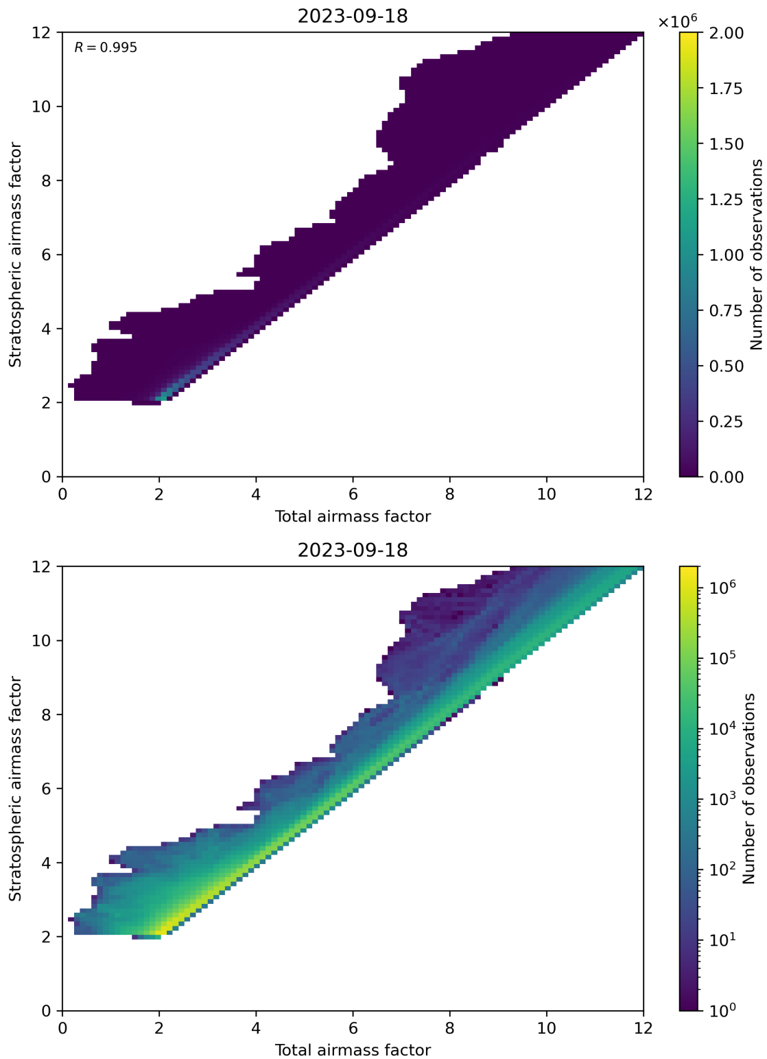
Figure 62: Scatter density plot of “Total airmass factor” against “Stratospheric airmass factor” for 2023-09-17 to 2023-09-19.
