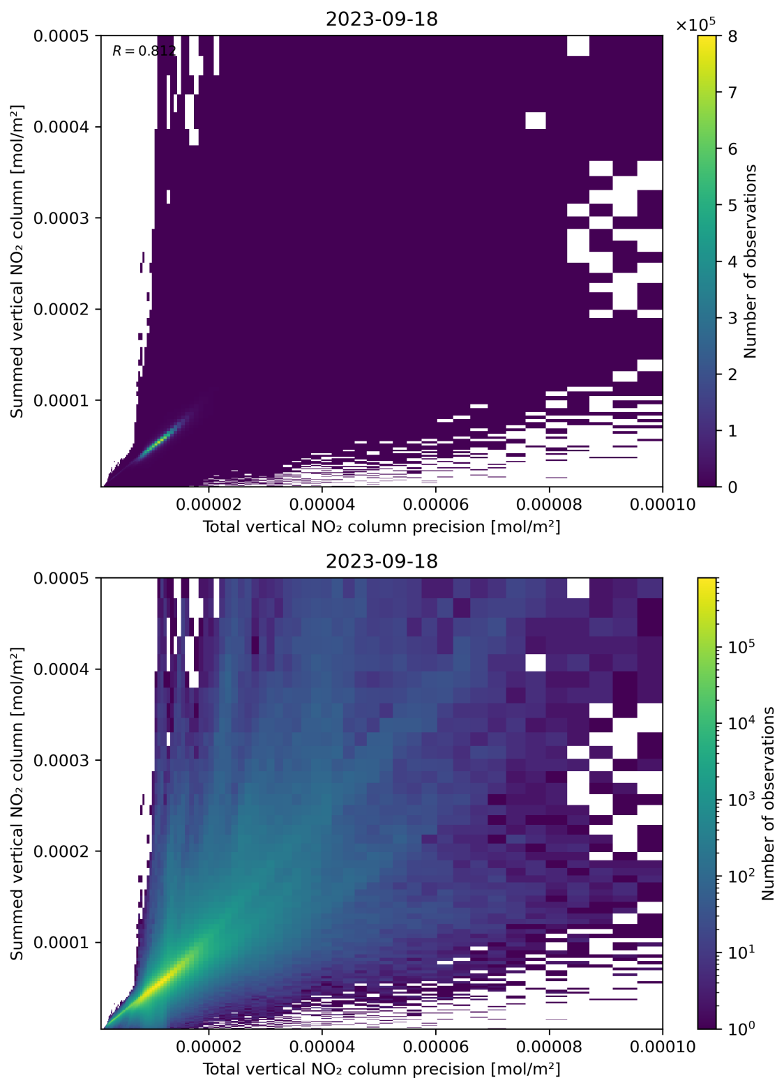
Figure 117: Scatter density plot of “Total vertical NO 2 column precision” against “Summed vertical NO 2 column” for 2023-09-17 to 2023-09-19.
