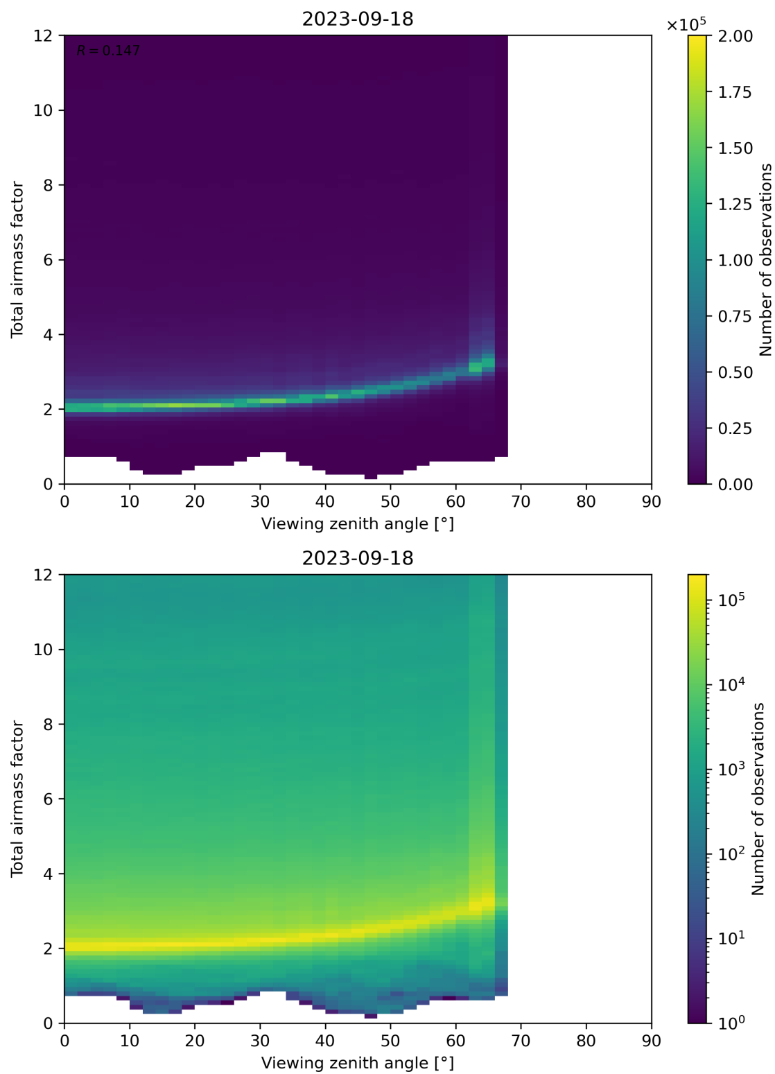
Figure 160: Scatter density plot of “Viewing zenith angle” against “Total airmass factor” for 2023-09-17 to 2023-09-19.
