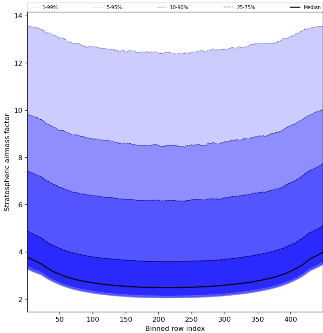
Figure 61: Along track statistics of “Stratospheric air mass factor” for 2023-09-17 to 2023-09-19
