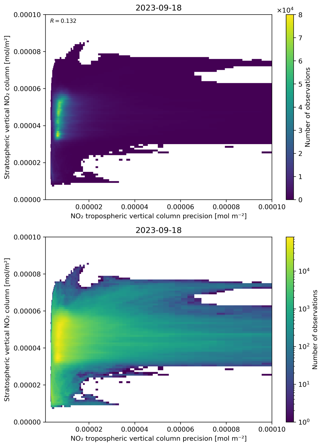
Figure 135: Scatter density plot of “NO 2 tropospheric vertical column precision” against “Stratospheric vertical NO 2 column” for 2023-09-17 to 2023-09-19.
