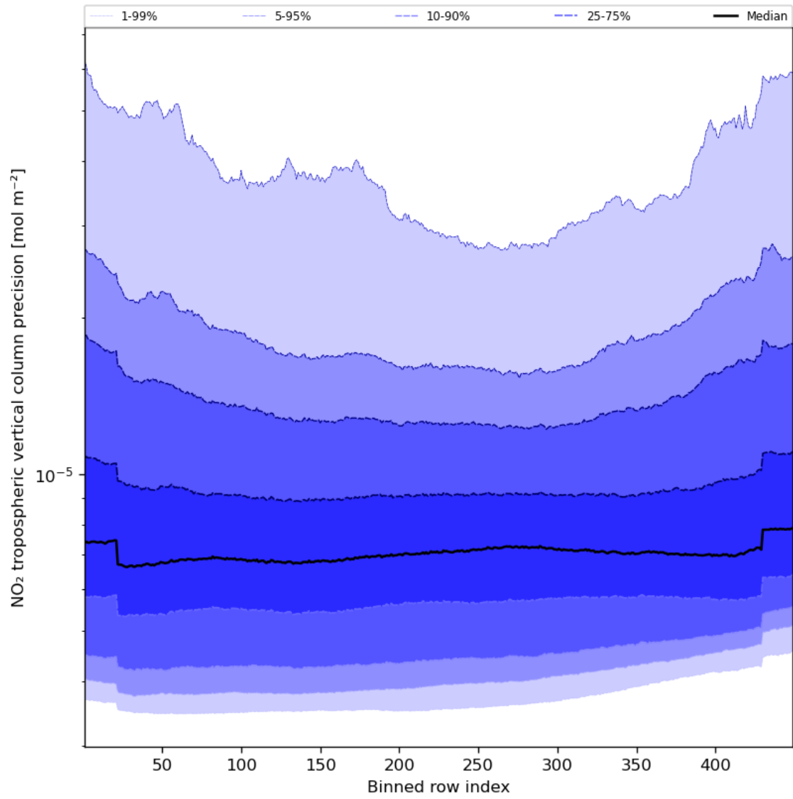
Figure 47: Along track statistics of “NO 2 tropospheric vertical column precision” for 2023-09-17 to 2023-09-19
