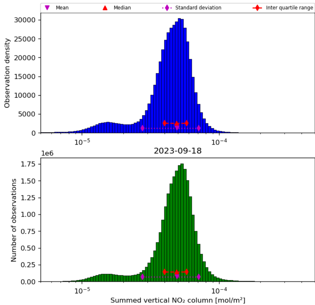
Figure 40: Histogram of “Summed vertical NO 2 column” for 2023-09-17 to 2023-09-19
