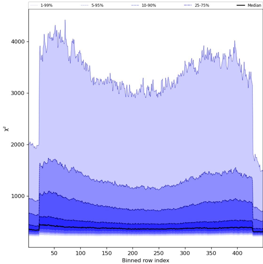
Figure 59: Along track statistics of “ \chi^2 ” for 2023-09-17 to 2023-09-19
