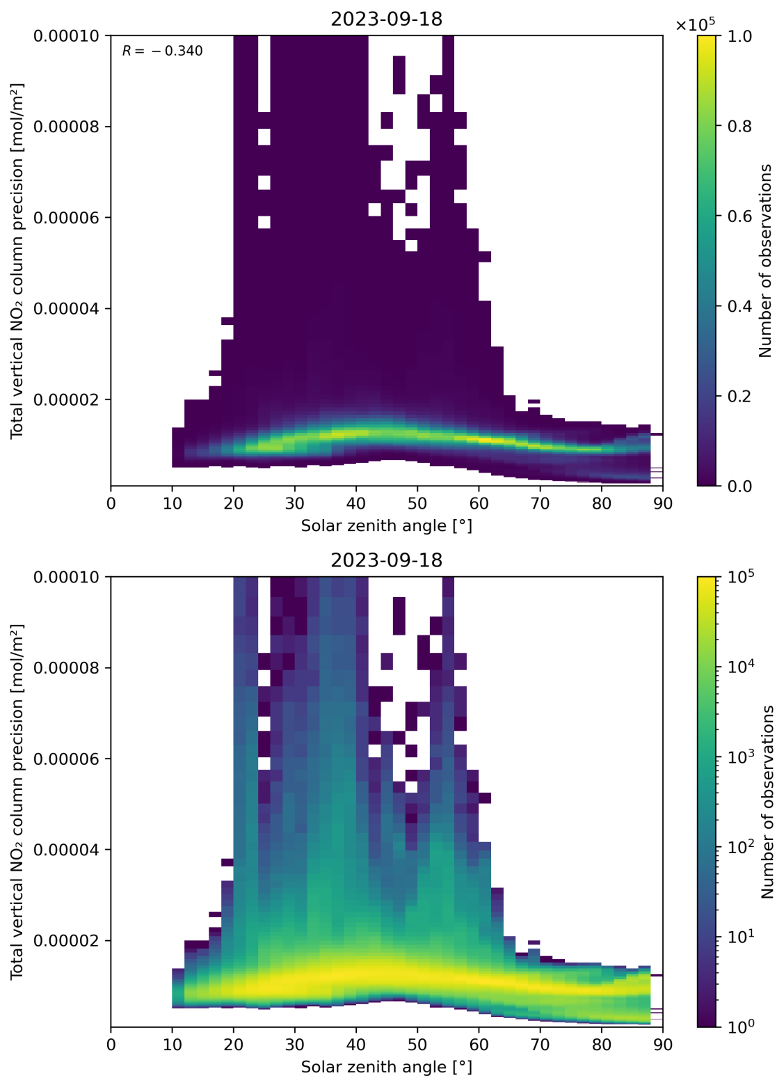
Figure 154: Scatter density plot of “Solar zenith angle” against “Total vertical NO 2 column precision” for 2023-09-17 to 2023-09-19.
