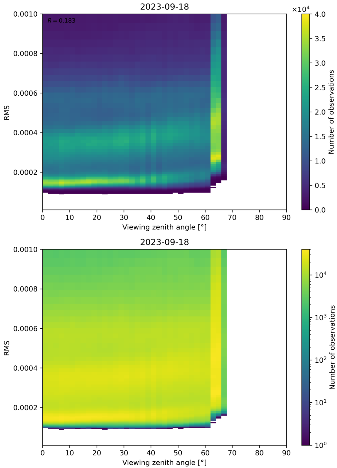
Figure 171: Scatter density plot of “Viewing zenith angle” against “RMS” for 2023-09-17 to 2023-09-19.
