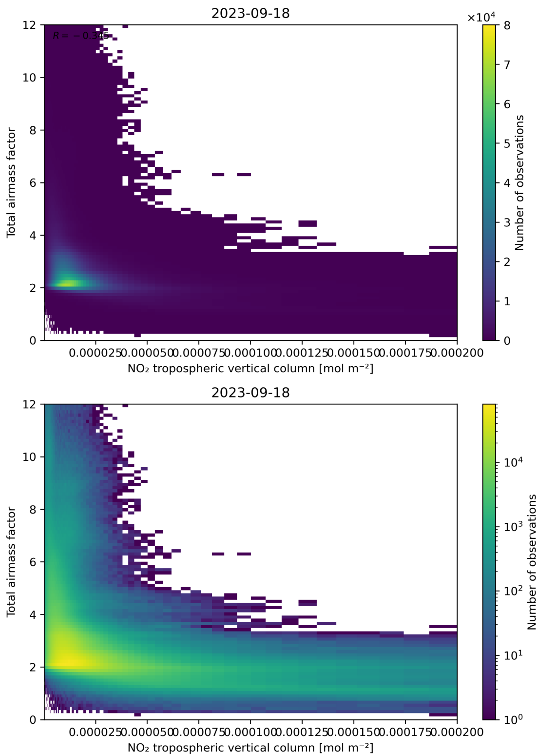
Figure 122: Scatter density plot of “NO 2 tropospheric vertical column” against “Total air mass factor” for 2023-09-17 to 2023-09-19.
