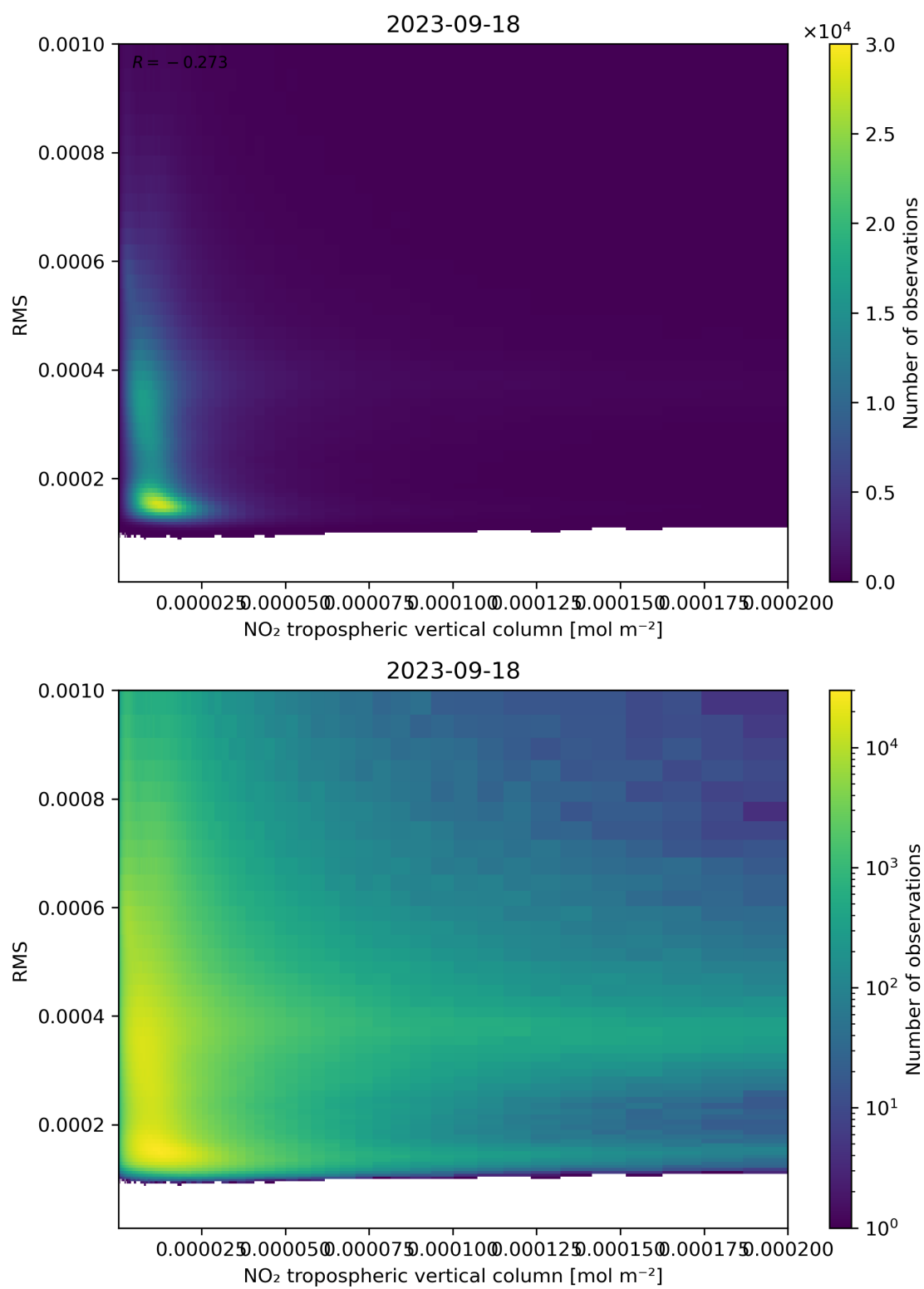
Figure 142: Scatter density plot of “NO 2 tropospheric vertical column” against “RMS” for 2023-09-17 to 2023-09-19.
