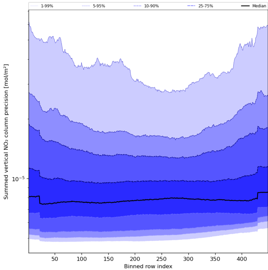
Figure 58: Along track statistics of “Summed vertical NO 2 column precision” for 2023-09-17 to 2023-09-19
