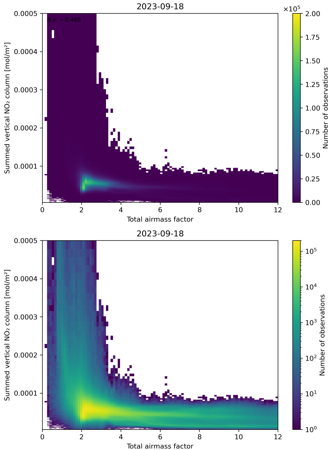
Figure 65: Scatter density plot of “Total airmass factor” against “Summed vertical NO 2 column” for 2023-09-17 to 2023-09-19.
