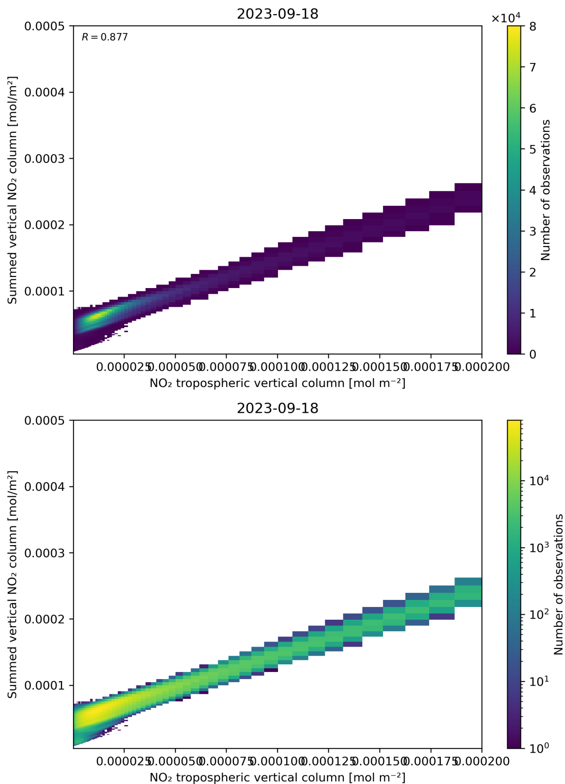
Figure 126: Scatter density plot of “NO 2 tropospheric vertical column” against “Summed vertical NO 2 column” for 2023-09-17 to 2023-09-19.
