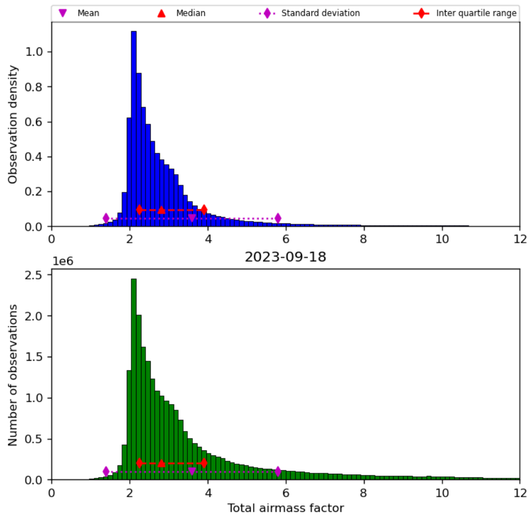
Figure 32: Histogram of “Total airmass factor” for 2023-09-17 to 2023-09-19
