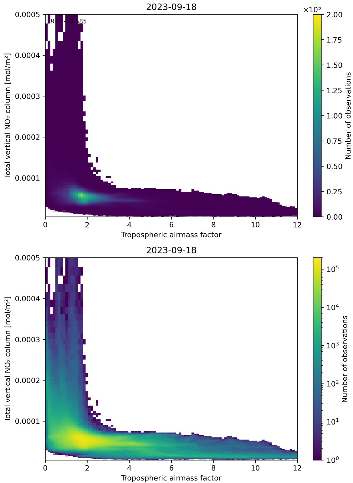
Figure 77: Scatter density plot of “Tropospheric airmass factor” against “Total vertical NO 2 column” for 2023-09-17 to 2023-09-19.
