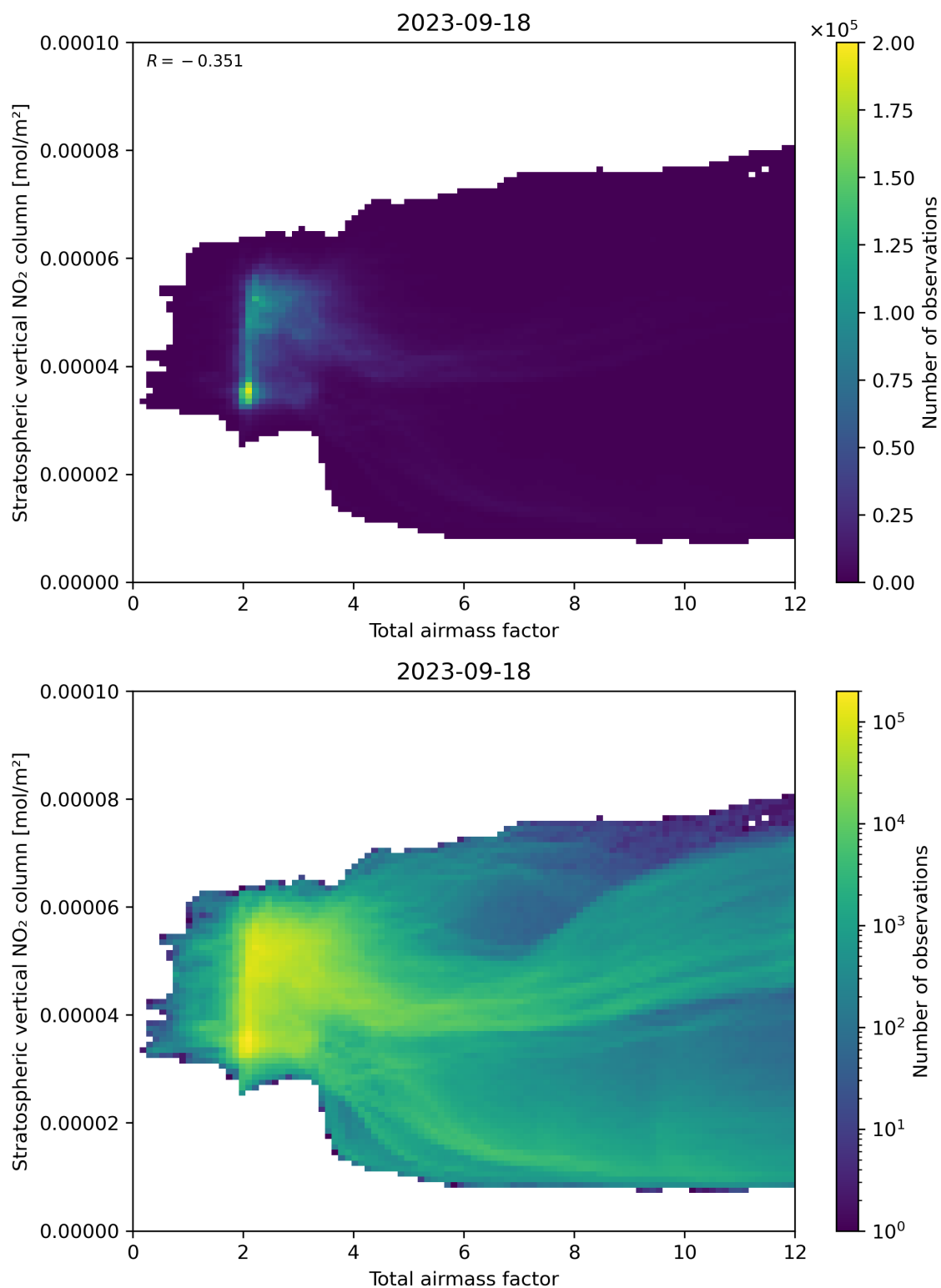
Figure 64: Scatter density plot of “Total airmass factor” against “Stratospheric vertical NO 2 column” for 2023-09-17 to 2023-09-19.
