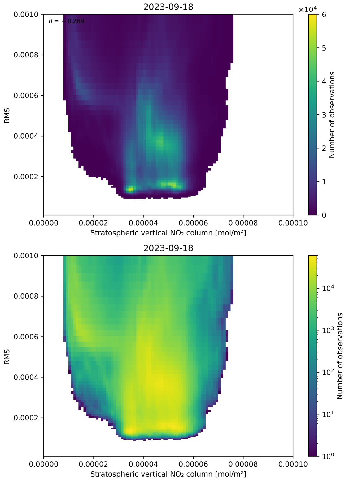
Figure 102: Scatter density plot of “Stratospheric vertical NO 2 column” against “RMS” for 2023-09-17 to 2023-09-19.
