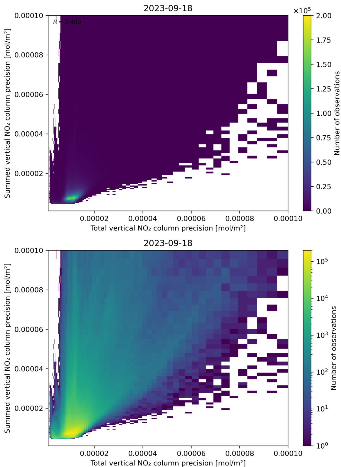
Figure 118: Scatter density plot of “Total vertical NO 2 column precision” against “Summed vertical NO 2 column precision” for 2023-09-17 to 2023-09-19.
