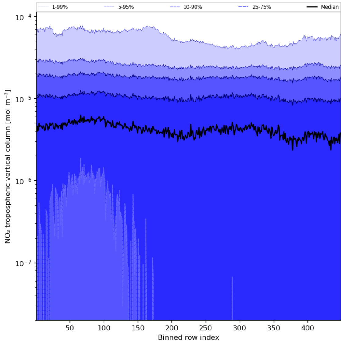
Figure 46: Along track statistics of “NO 2 tropospheric vertical column” for 2023-09-17 to 2023-09-19
