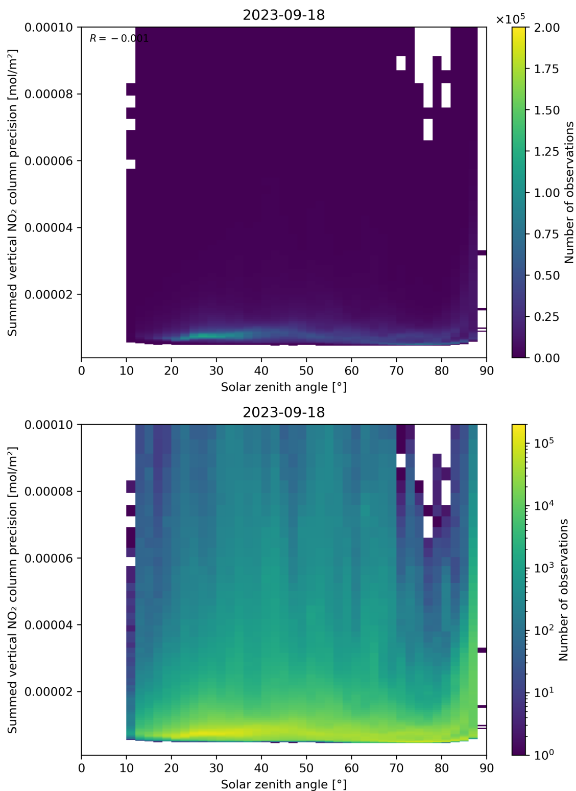
Figure 152: Scatter density plot of “Solar zenith angle” against “Summed vertical NO 2 column precision” for 2023-09-17 to 2023-09-19.
