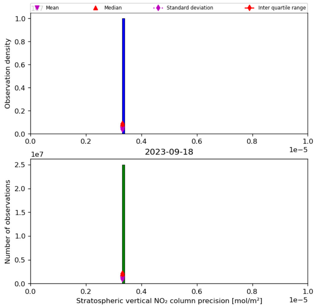
Figure 37: Histogram of “Stratospheric vertical NO 2 column precision” for 2023-09-17 to 2023-09-19
