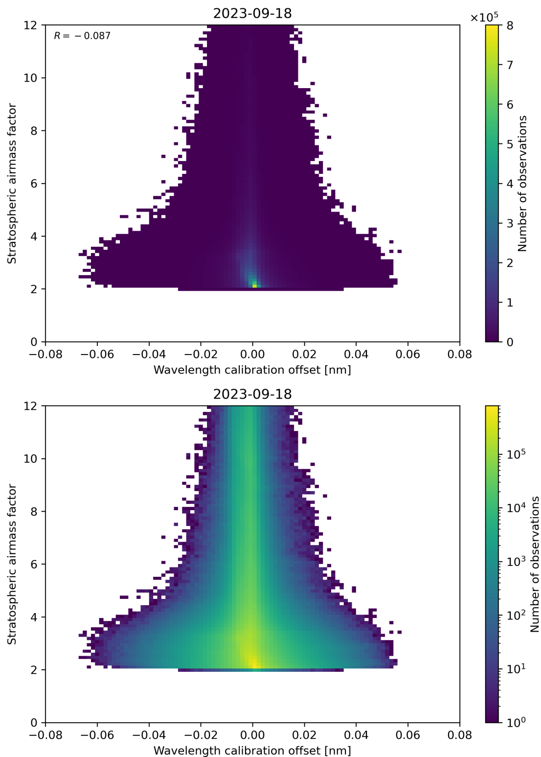
Figure 174: Scatter density plot of “Wavelength calibration offset” against “Stratospheric airmass factor” for 2023-09-17 to 2023-09-19.
