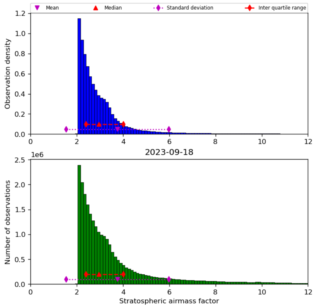
Figure 44: Histogram of “Stratospheric airmass factor” for 2023-09-17 to 2023-09-19
