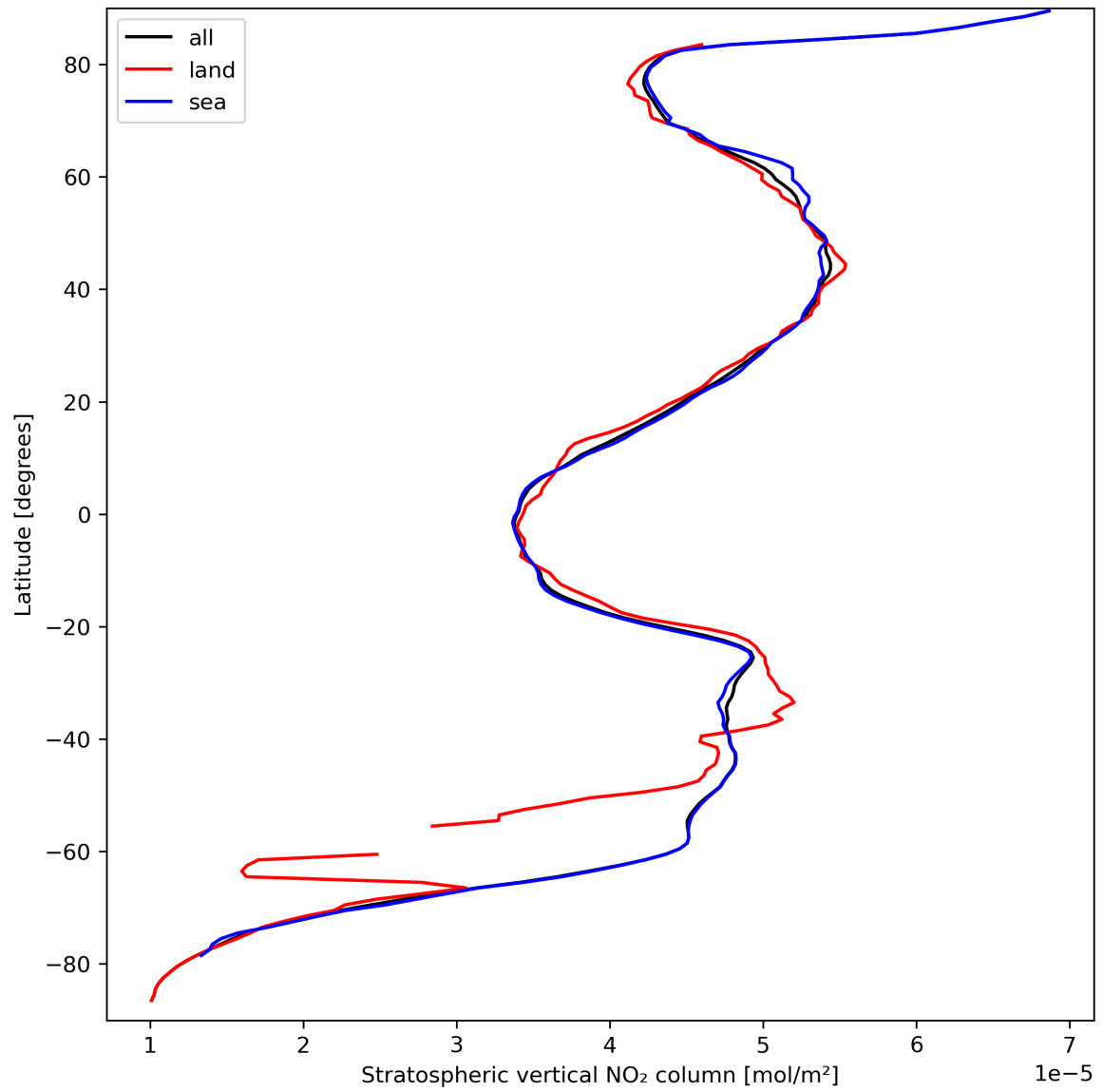
Figure 19: Zonal average of “Stratospheric vertical NO 2 column” for 2023-09-17 to 2023-09-19.
