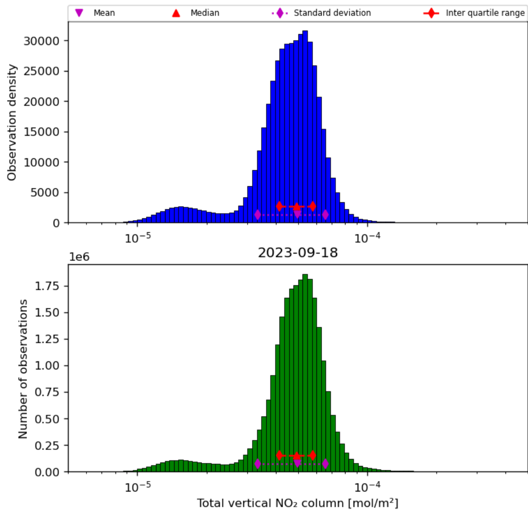
Figure 38: Histogram of “Total vertical NO 2 column” for 2023-09-17 to 2023-09-19
