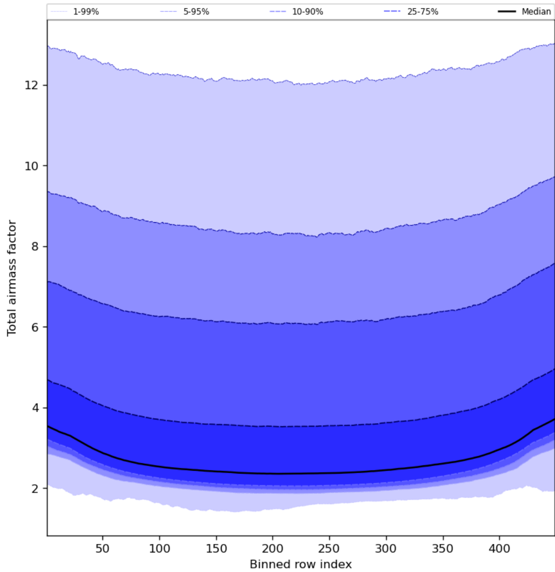
Figure 49: Along track statistics of “Total airmass factor” for 2023-09-17 to 2023-09-19
