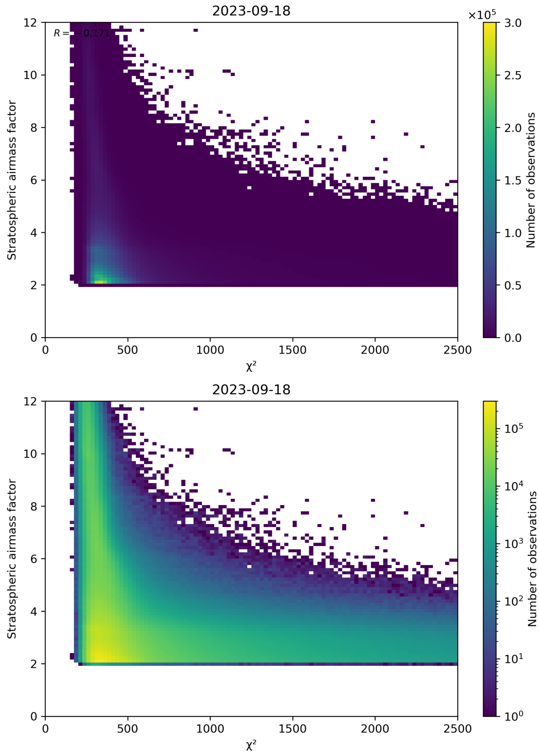
Figure 81: Scatter density plot of “ \chi^2 ” against “Stratospheric airmass factor” for 2023-09-17 to 2023-09-19.
