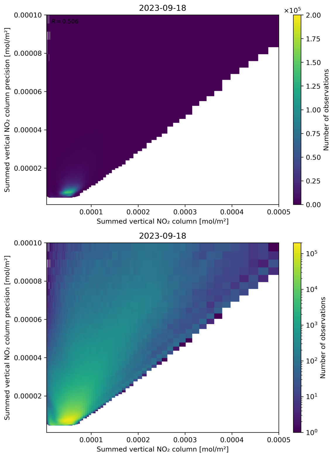
Figure 105: Scatter density plot of “Summed vertical NO 2 column” against “Summed vertical NO 2 column precision” for 2023-09-17 to 2023-09-19.
