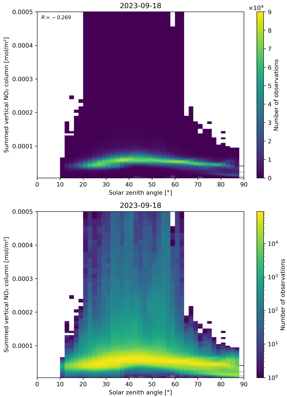
Figure 151: Scatter density plot of “Solar zenith angle” against “Summed vertical NO 2 column” for 2023-09-17 to 2023-09-19.
