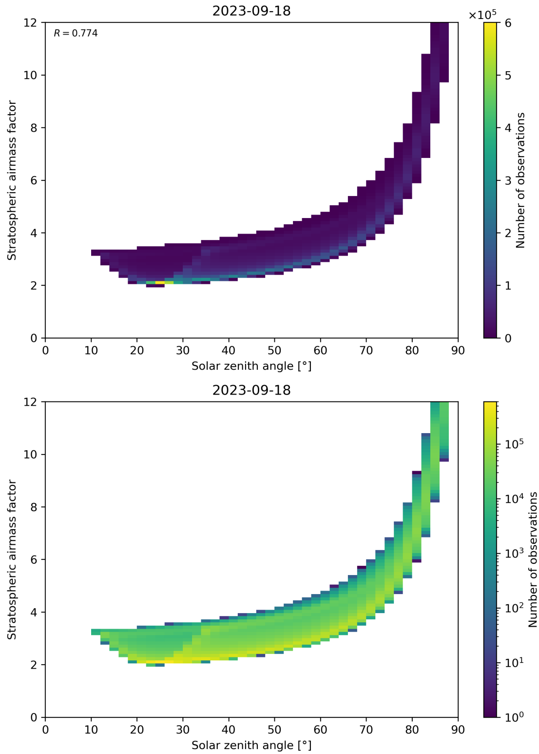
Figure 145: Scatter density plot of “Solar zenith angle” against “Stratospheric airmass factor” for 2023-09-17 to 2023-09-19.
