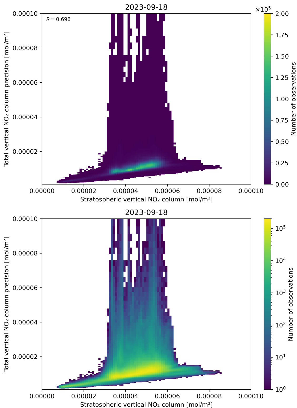
Figure 101: Scatter density plot of “Stratospheric vertical NO 2 column” against “Total vertical NO 2 column precision” for 2023-09-17 to 2023-09-19.
