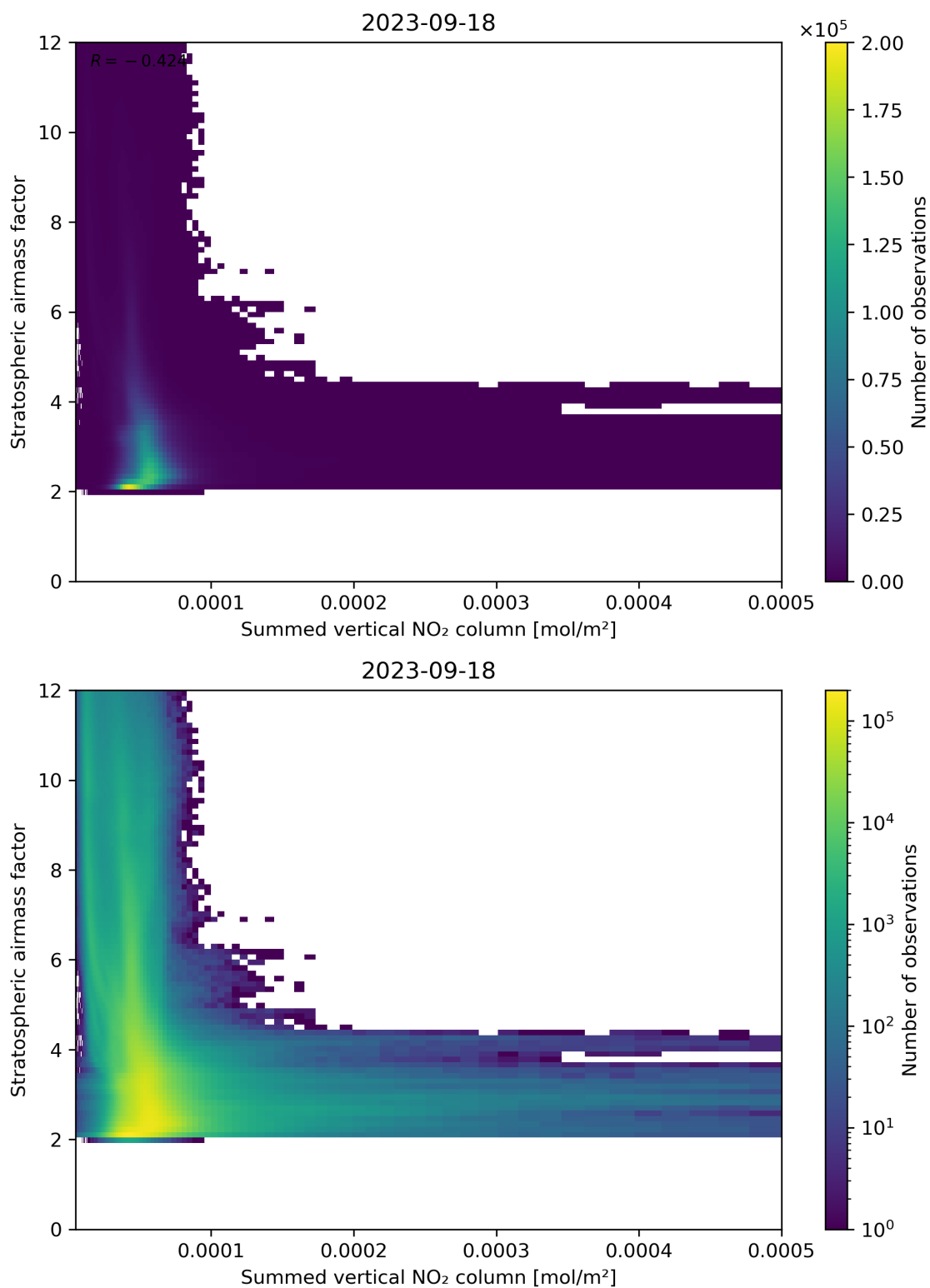
Figure 103: Scatter density plot of “Summed vertical NO 2 column” against “Stratospheric air mass factor” for 2023-09-17 to 2023-09-19.
