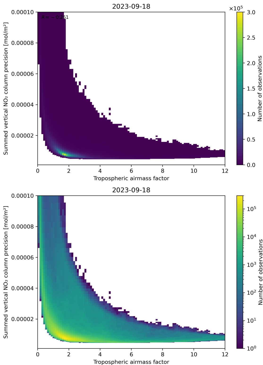
Figure 76: Scatter density plot of “Tropospheric air mass factor” against “Summed vertical NO 2 column precision” for 2023-09-17 to 2023-09-19.
