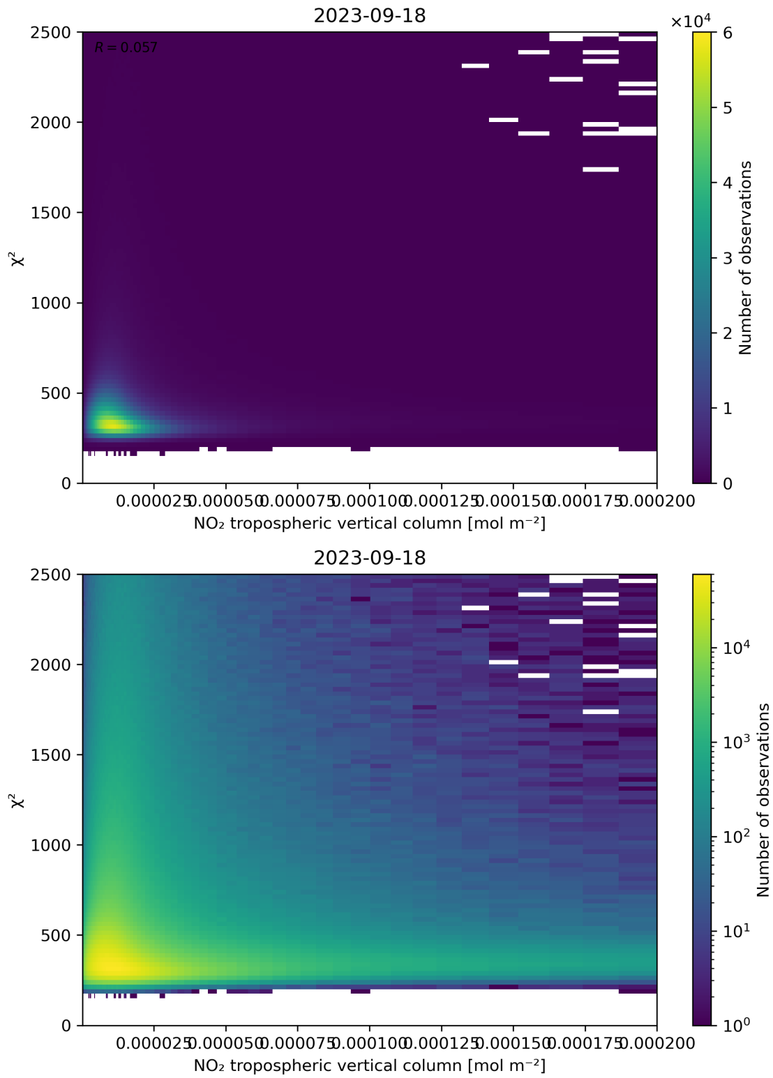
Figure 124: Scatter density plot of “NO 2 tropospheric vertical column” against “ \chi^2 ” for 2023-09-17 to 2023-09-19.
