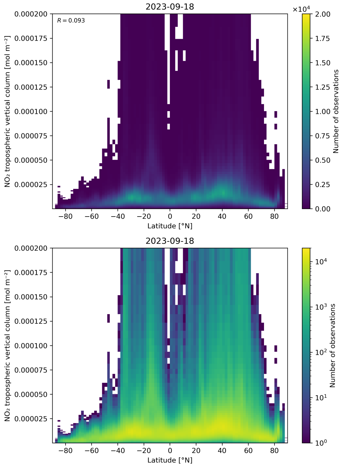
Figure 92: Scatter density plot of “Latitude” against “NO 2 tropospheric vertical column” for 2023-09-17 to 2023-09-19.
