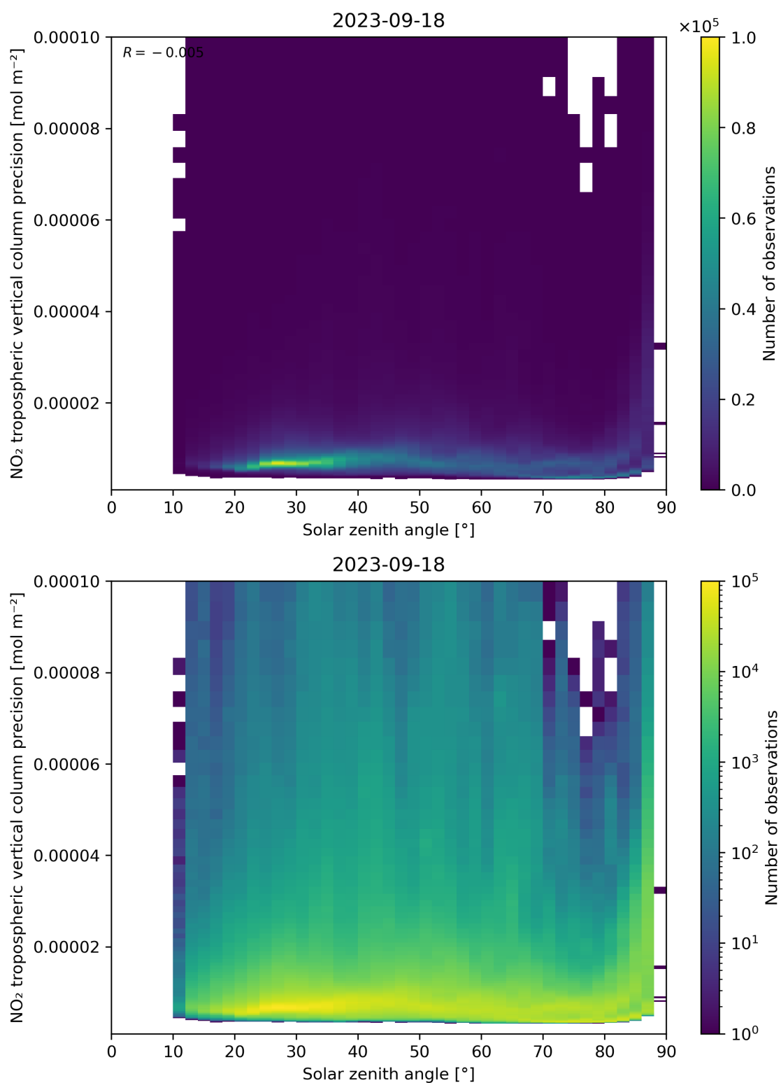
Figure 156: Scatter density plot of “Solar zenith angle” against “NO 2 tropospheric vertical column precision” for 2023-09-17 to 2023-09-19.
