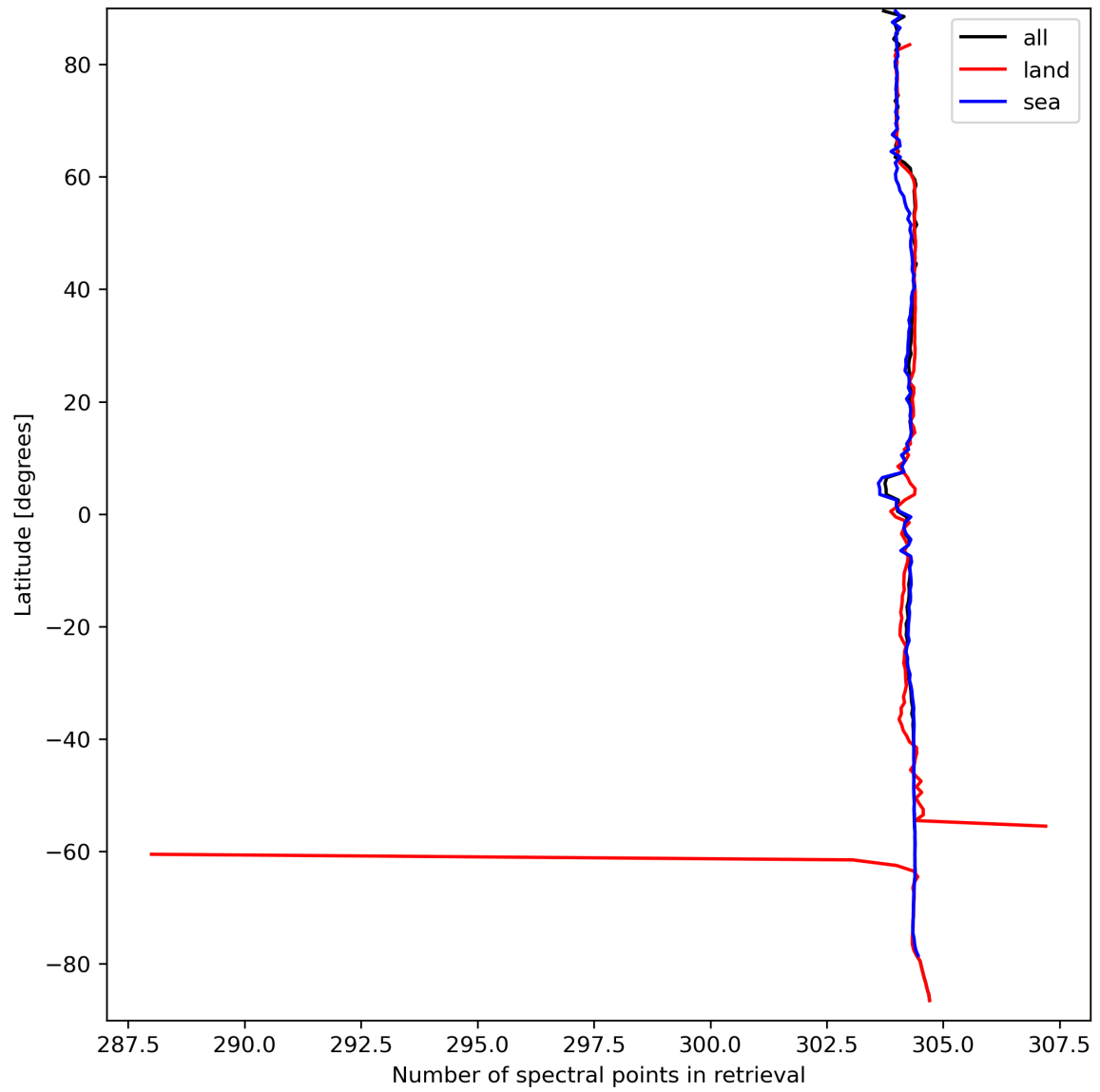
Figure 16: Zonal average of “Number of spectral points in retrieval” for 2023-09-17 to 2023-09-19.
