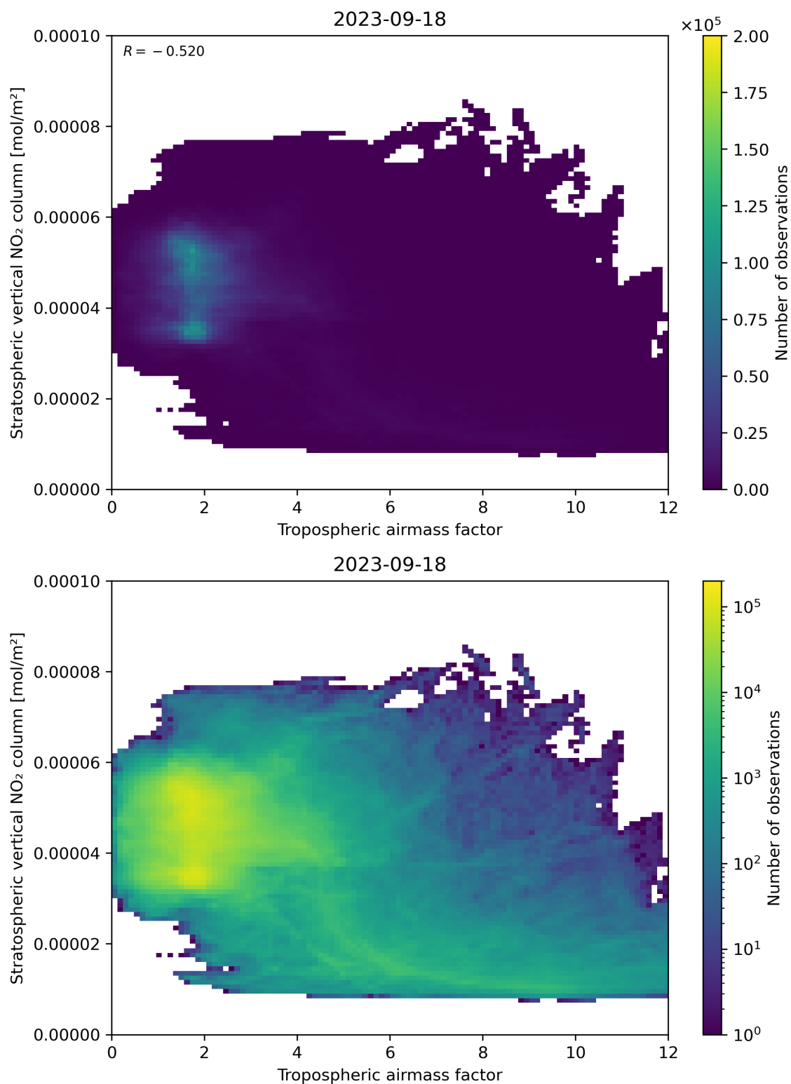
Figure 74: Scatter density plot of “Tropospheric air mass factor” against “Stratospheric vertical NO 2 column” for 2023-09-17 to 2023-09-19.
