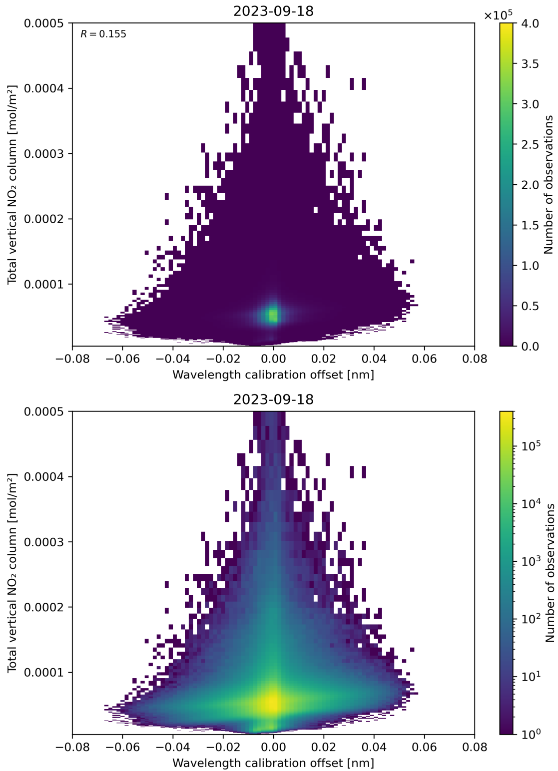
Figure 179: Scatter density plot of “Wavelength calibration offset” against “Total vertical NO 2 column” for 2023-09-17 to 2023-09-19.
