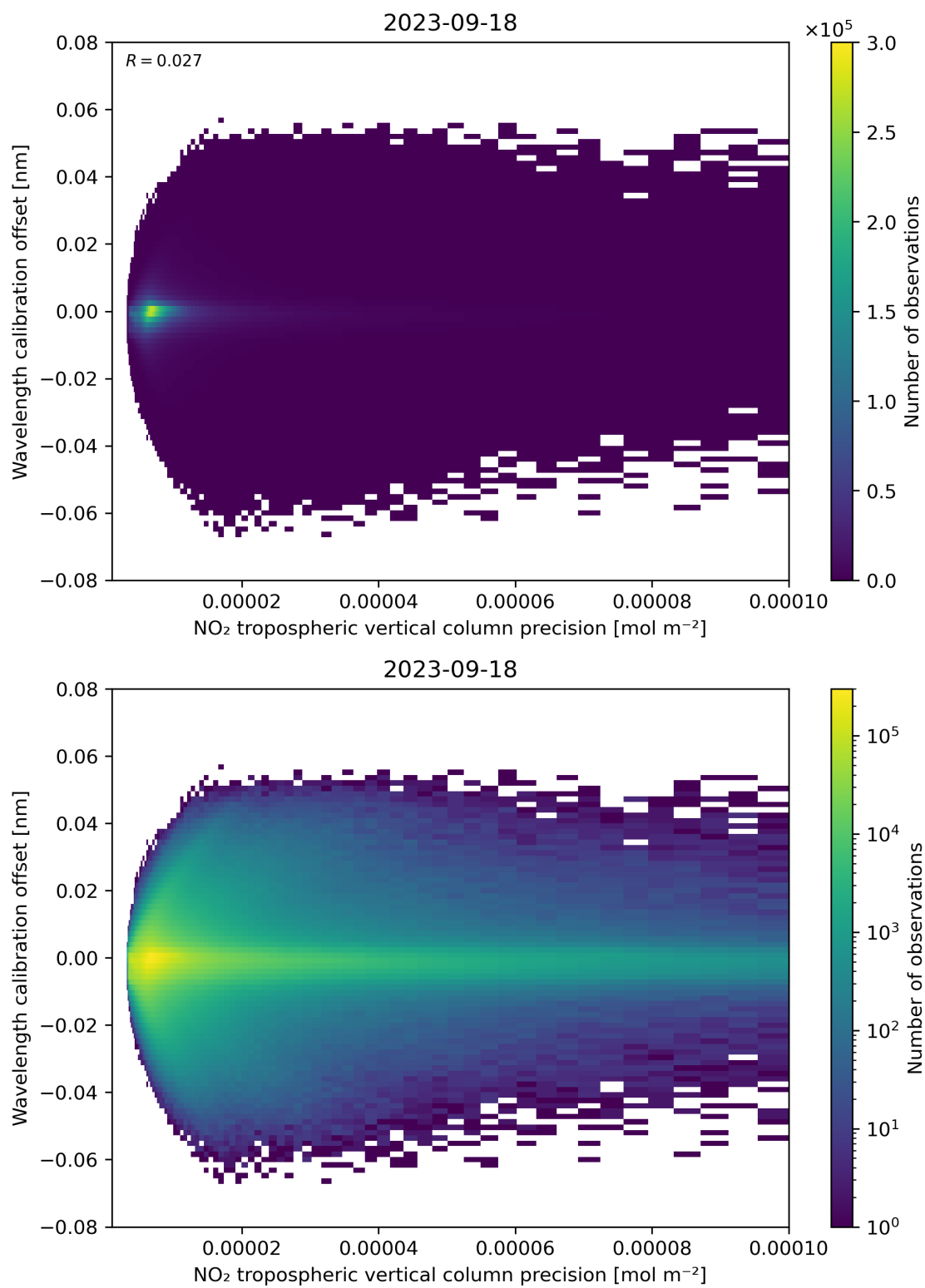
Figure 141: Scatter density plot of “NO 2 tropospheric vertical column precision” against “Wavelength calibration offset” for 2023-09-17 to 2023-09-19.
