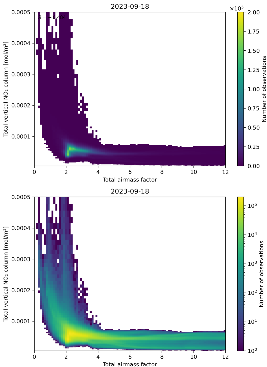
Figure 67: Scatter density plot of “Total airmass factor” against “Total vertical NO 2 column” for 2023-09-17 to 2023-09-19.
