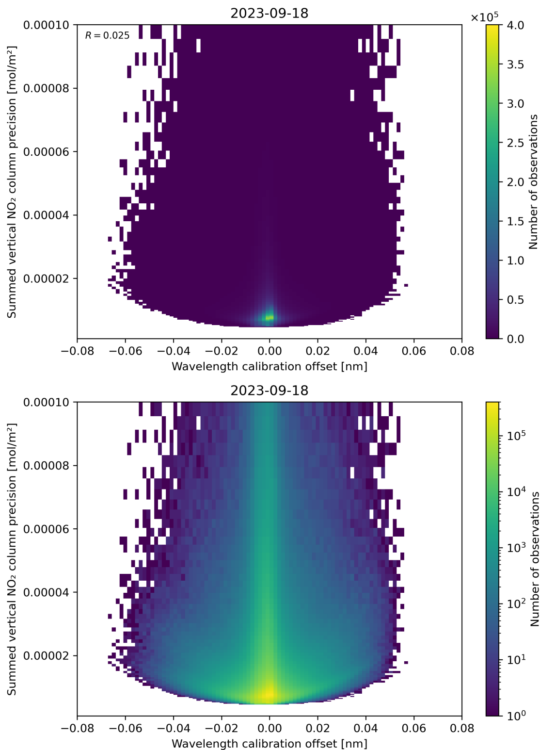
Figure 178: Scatter density plot of “Wavelength calibration offset” against “Summed vertical NO 2 column precision” for 2023-09-17 to 2023-09-19.
