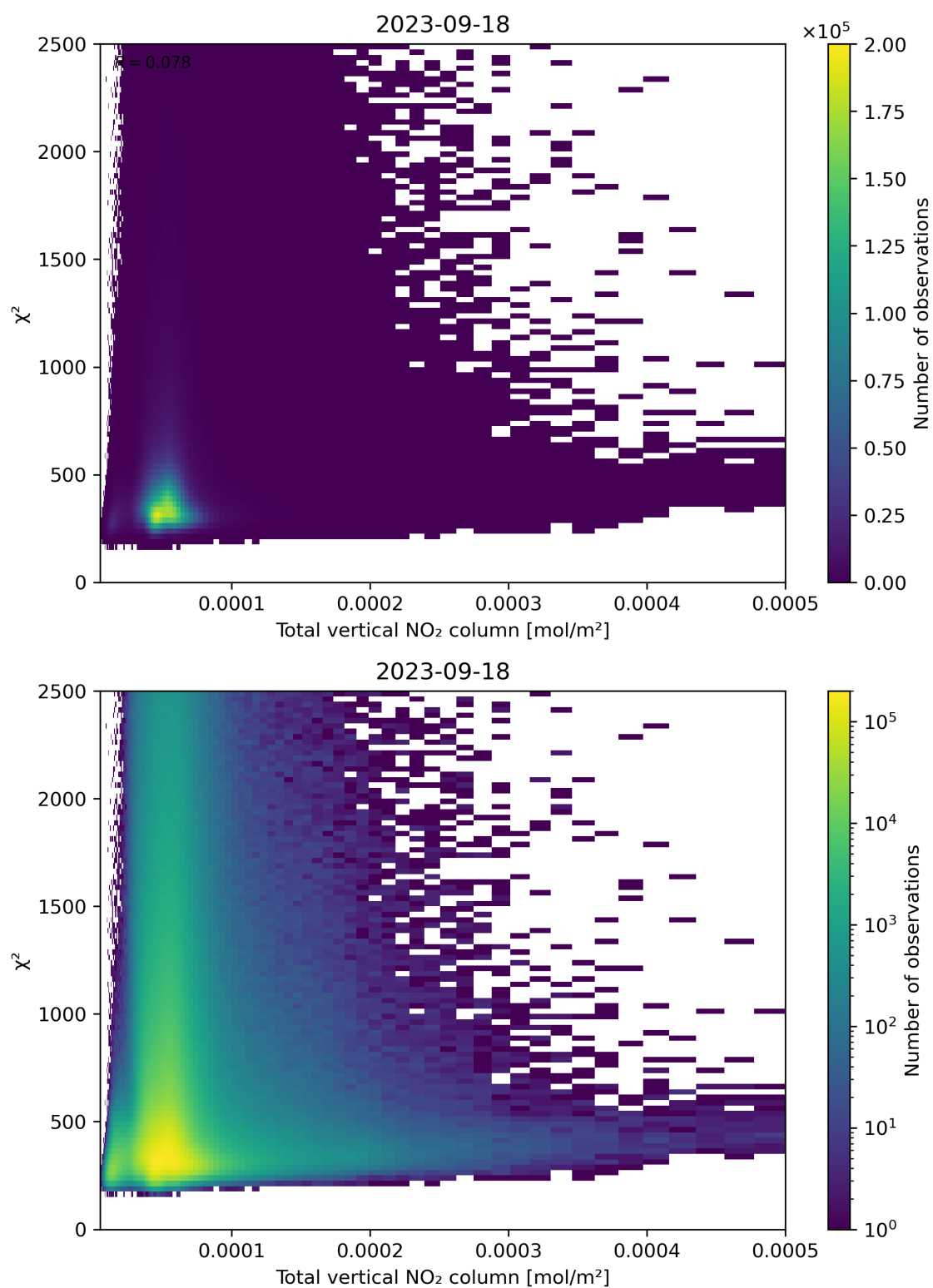
Figure 111: Scatter density plot of “Total vertical NO 2 column” against “ \chi^2 ” for 2023-09-17 to 2023-09-19.
