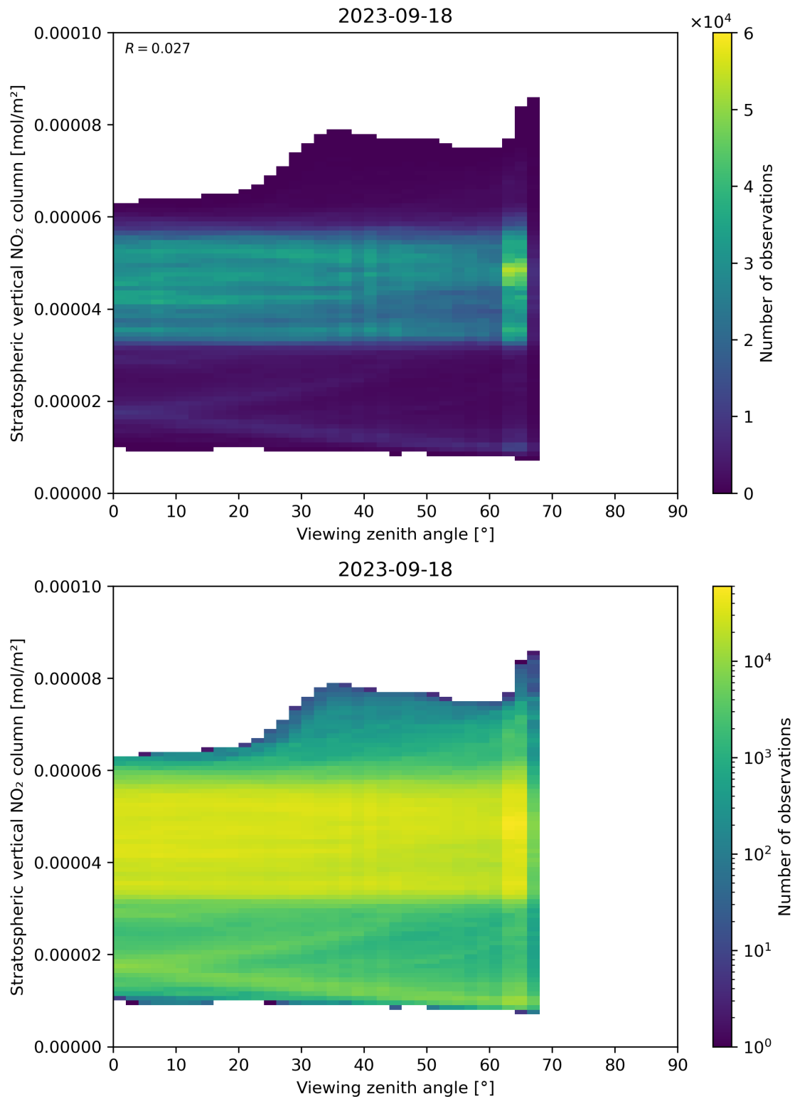
Figure 164: Scatter density plot of “Viewing zenith angle” against “Stratospheric vertical NO 2 column” for 2023-09-17 to 2023-09-19.
