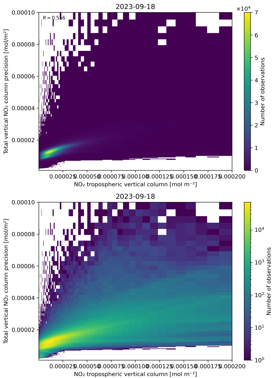
Figure 129: Scatter density plot of “NO 2 tropospheric vertical column” against “Total vertical NO 2 column precision” for 2023-09-17 to 2023-09-19.
