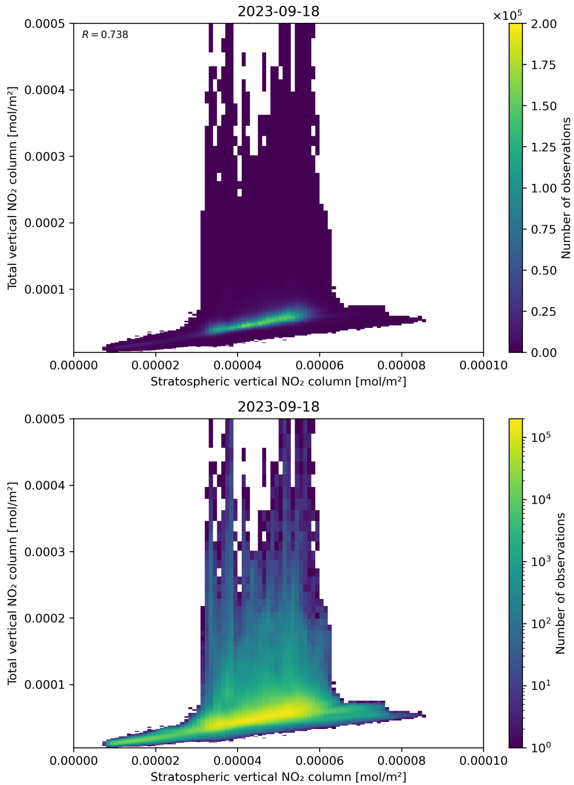
Figure 100: Scatter density plot of “Stratospheric vertical NO 2 column” against “Total vertical NO 2 column” for 2023-09-17 to 2023-09-19.
