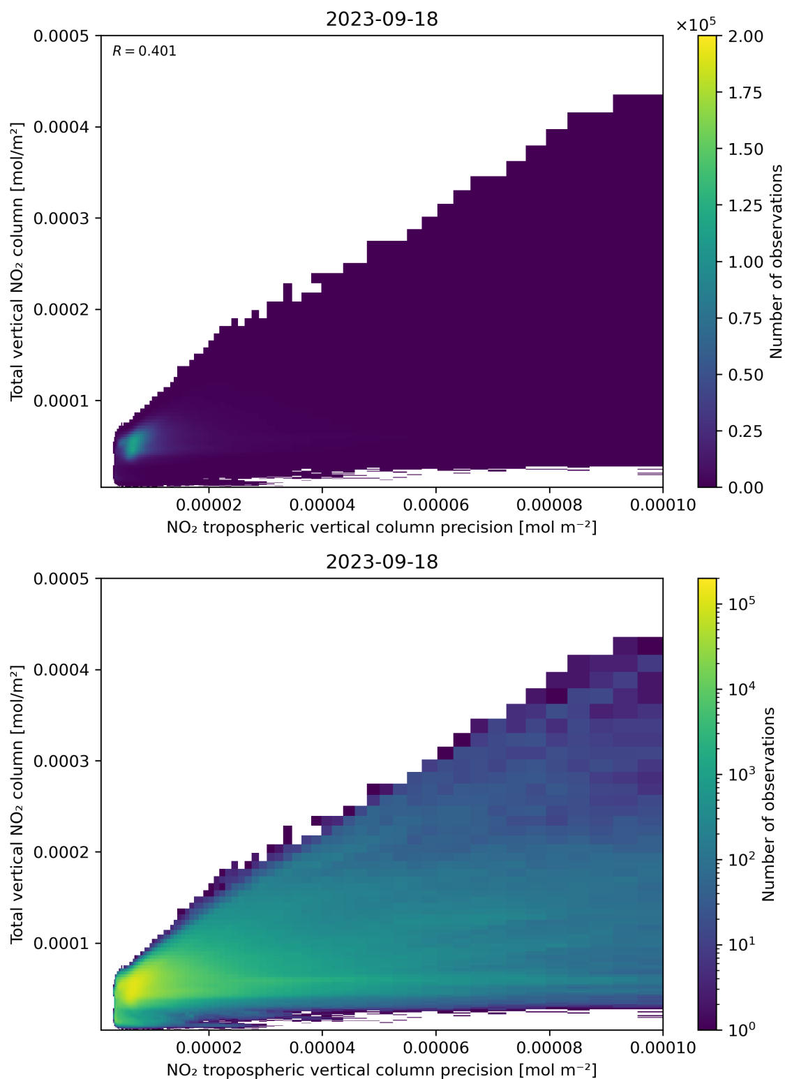
Figure 138: Scatter density plot of “NO 2 tropospheric vertical column precision” against “Total vertical NO 2 column” for 2023-09-17 to 2023-09-19.
