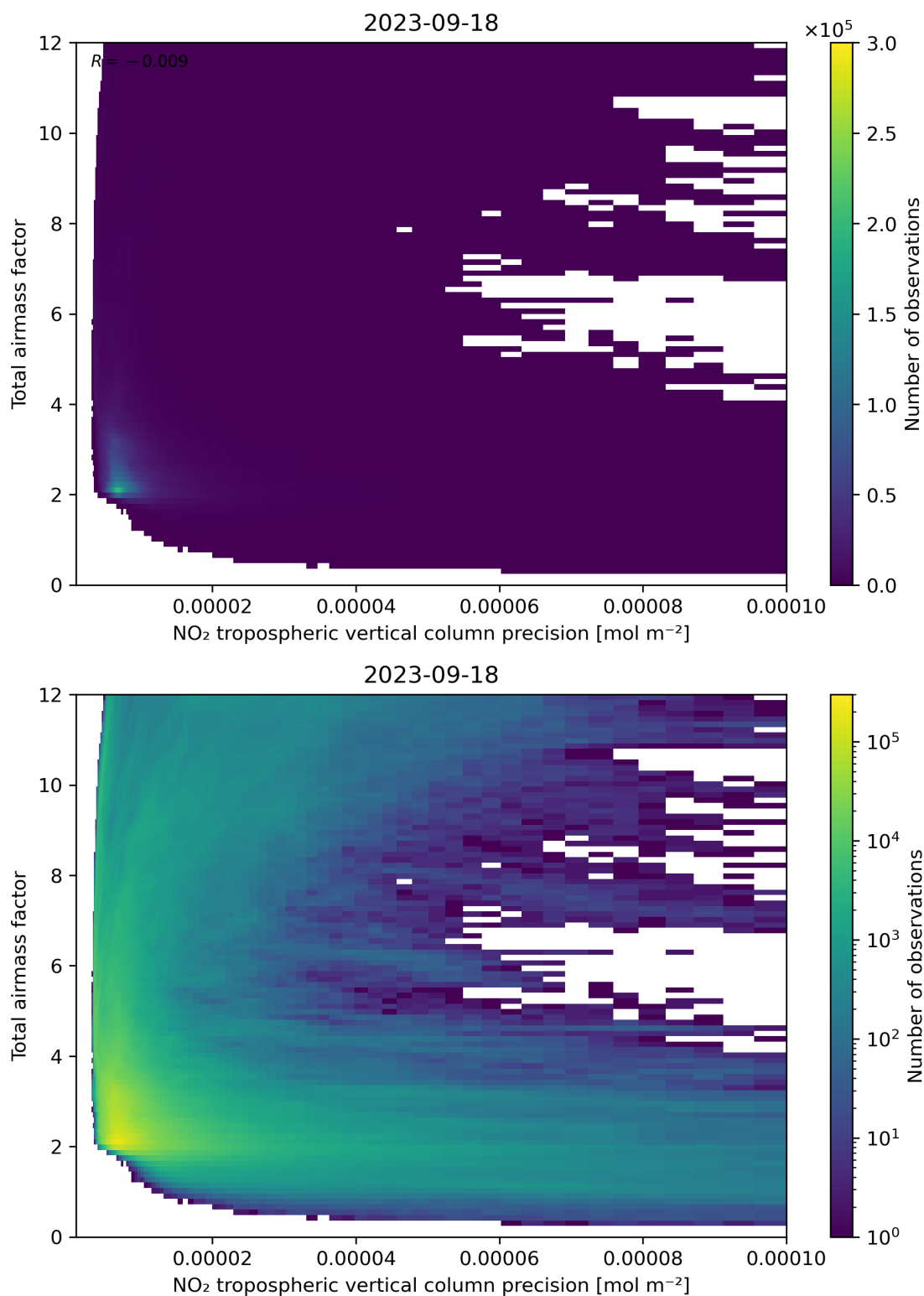
Figure 132: Scatter density plot of “NO 2 tropospheric vertical column precision” against “Total air mass factor” for 2023-09-17 to 2023-09-19.
