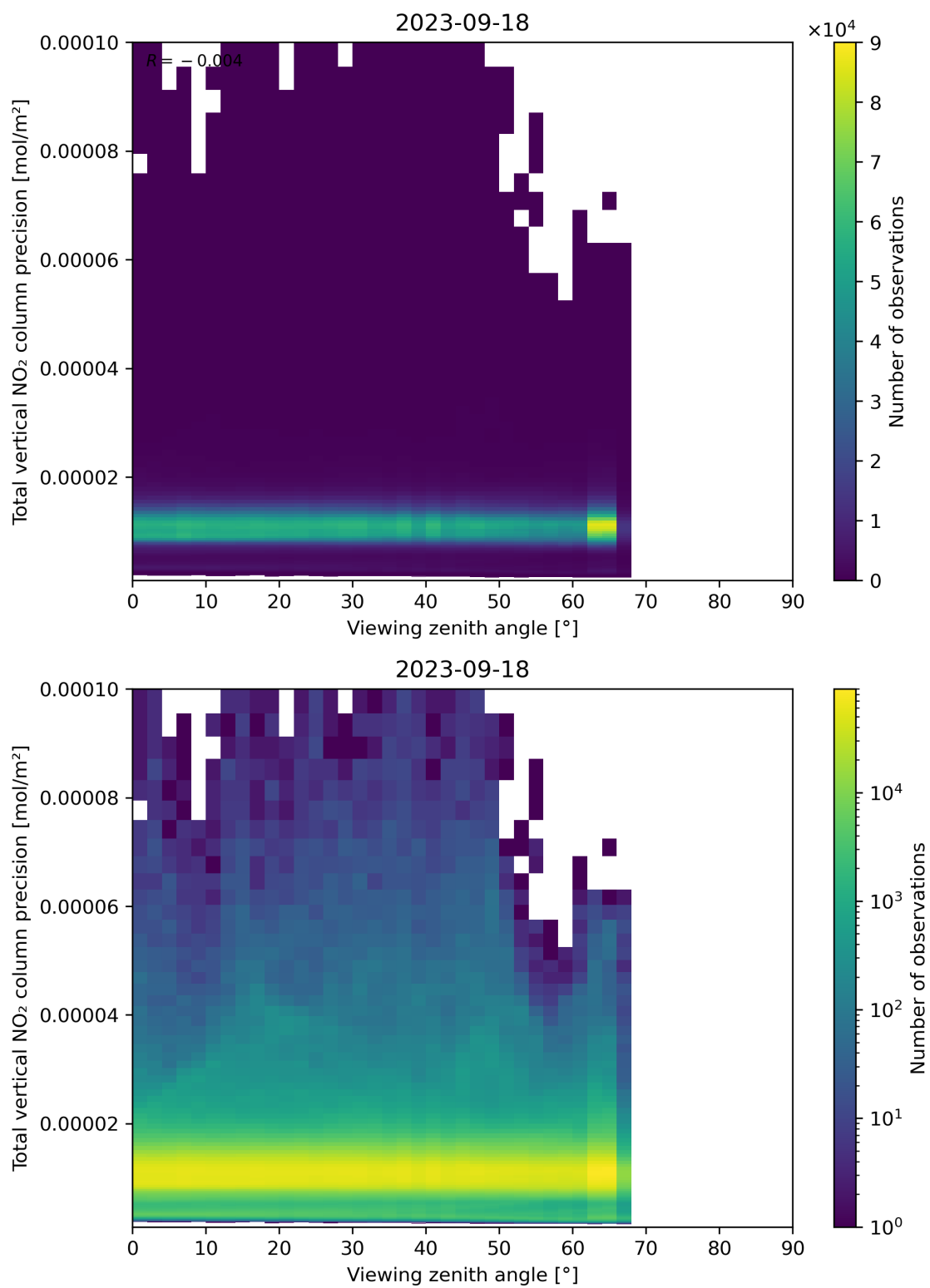
Figure 168: Scatter density plot of “Viewing zenith angle” against “Total vertical NO 2 column precision” for 2023-09-17 to 2023-09-19.
