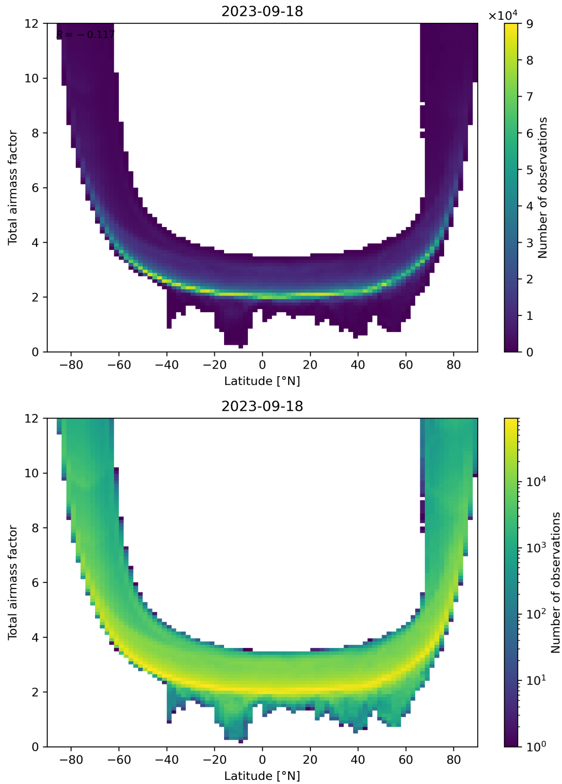
Figure 84: Scatter density plot of “Latitude” against “Total airmass factor” for 2023-09-17 to 2023-09-19.
