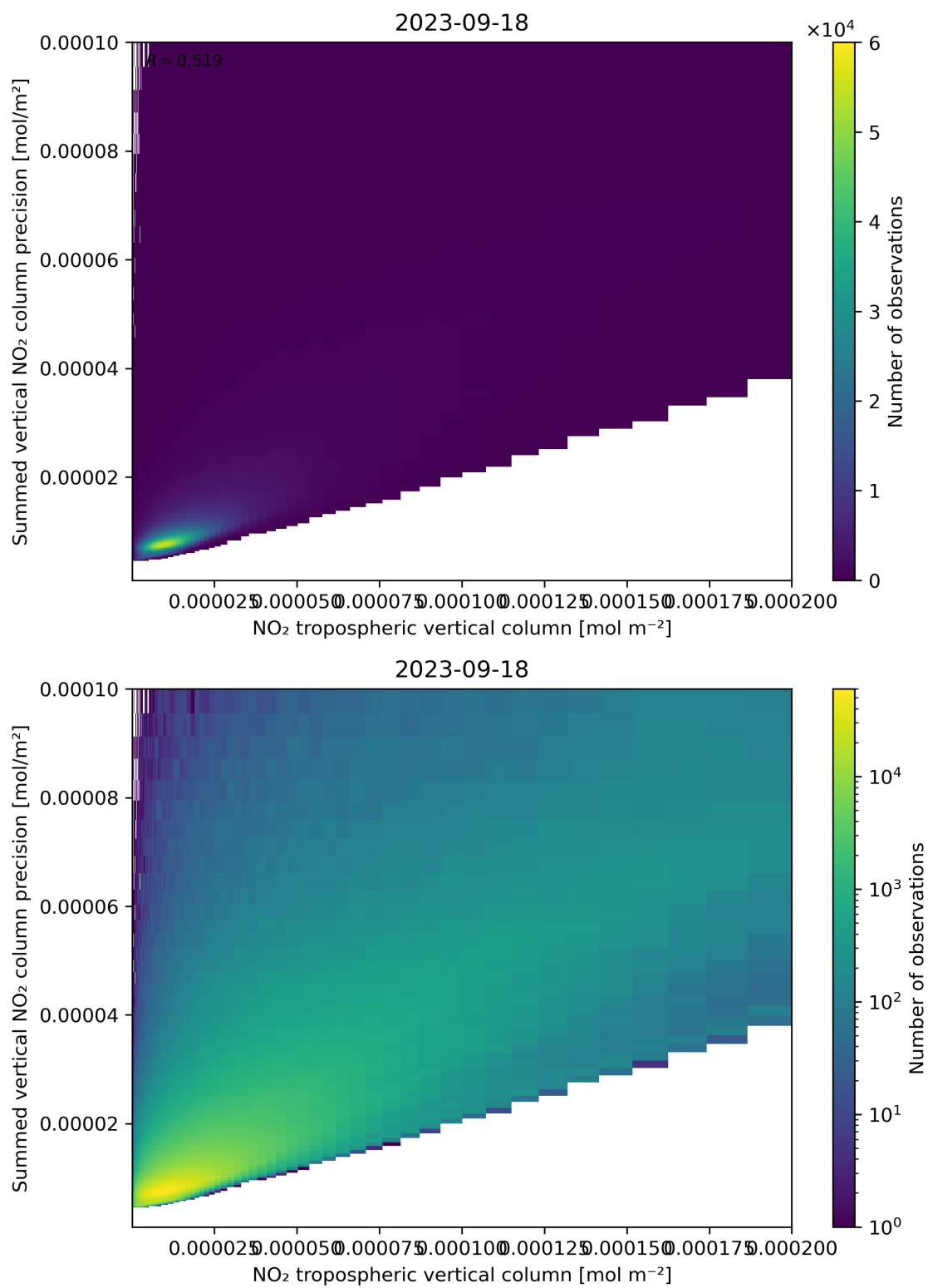
Figure 127: Scatter density plot of “NO 2 tropospheric vertical column” against “Summed vertical NO 2 column precision” for 2023-09-17 to 2023-09-19.
