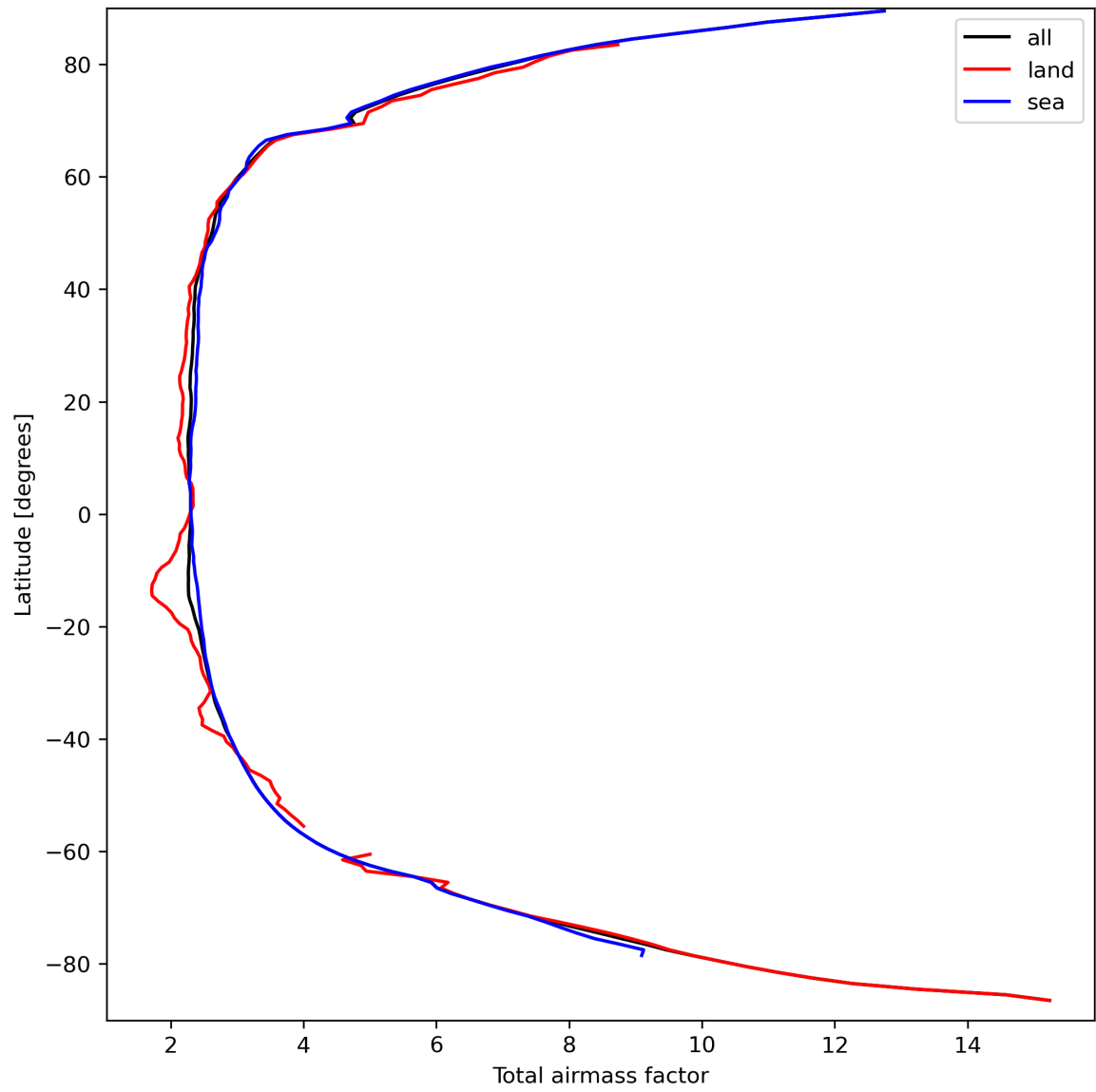
Figure 15: Zonal average of “Total airmass factor” for 2023-09-17 to 2023-09-19.
