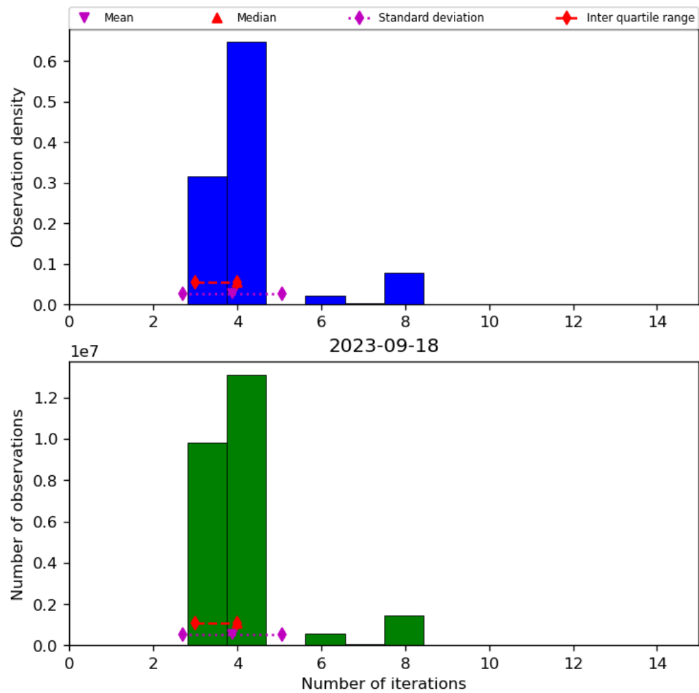
Figure 34: Histogram of “Number of iterations” for 2023-09-17 to 2023-09-19
