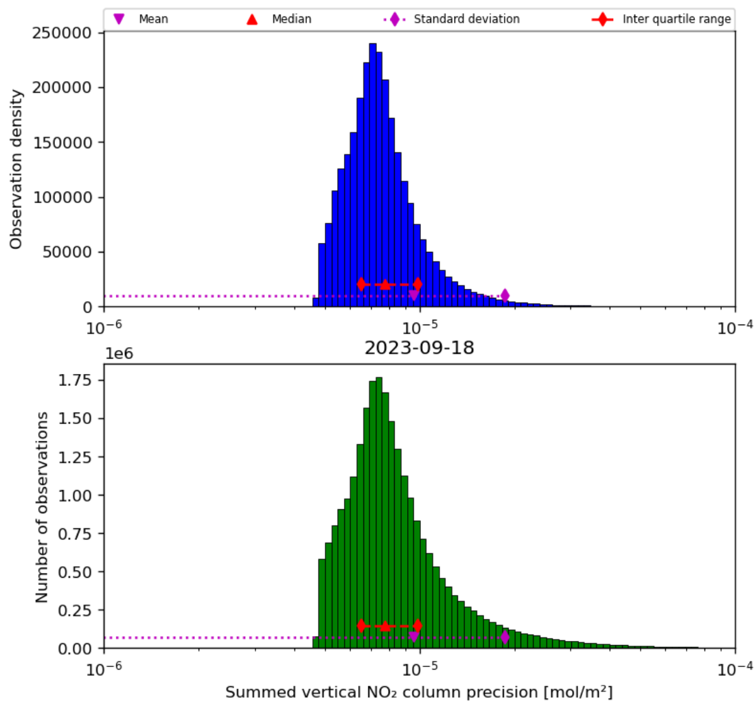
Figure 41: Histogram of "Summed vertical NO 2 column precision" for 2023-09-17 to 2023-09-19
