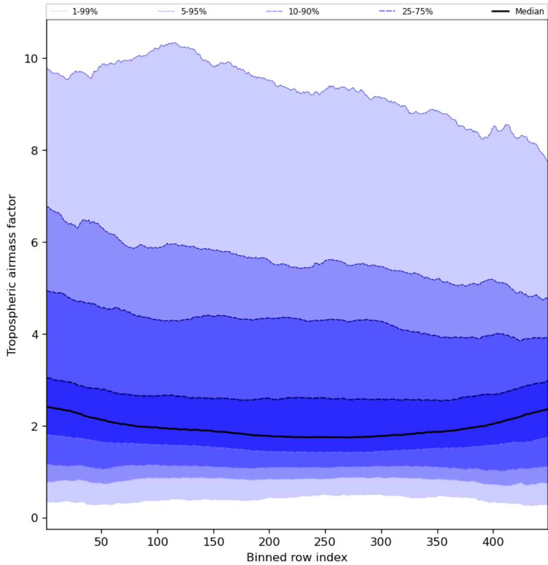
Figure 48: Along track statistics of “Tropospheric airmass factor” for 2023-09-17 to 2023-09-19
