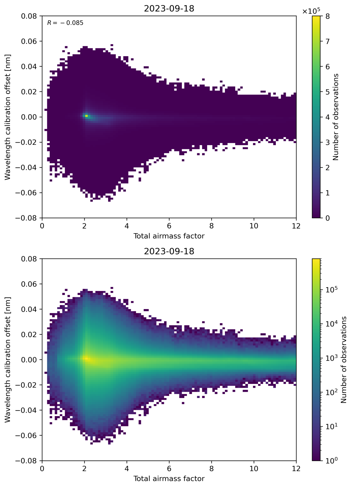
Figure 70: Scatter density plot of “Total airmass factor” against “Wavelength calibration offset” for 2023-09-17 to 2023-09-19.
