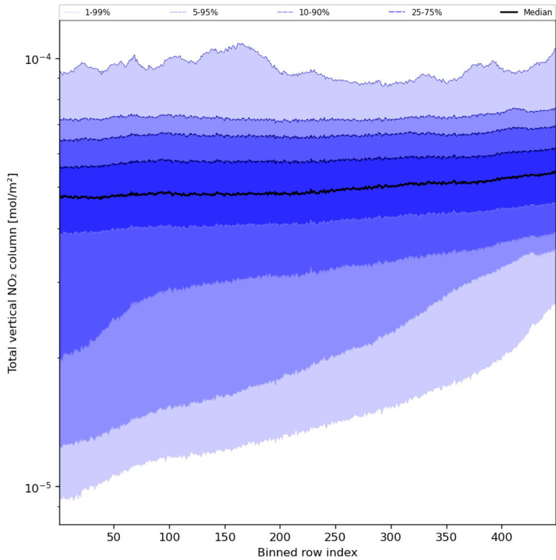
Figure 55: Along track statistics of “Total vertical NO 2 column” for 2023-09-17 to 2023-09-19
