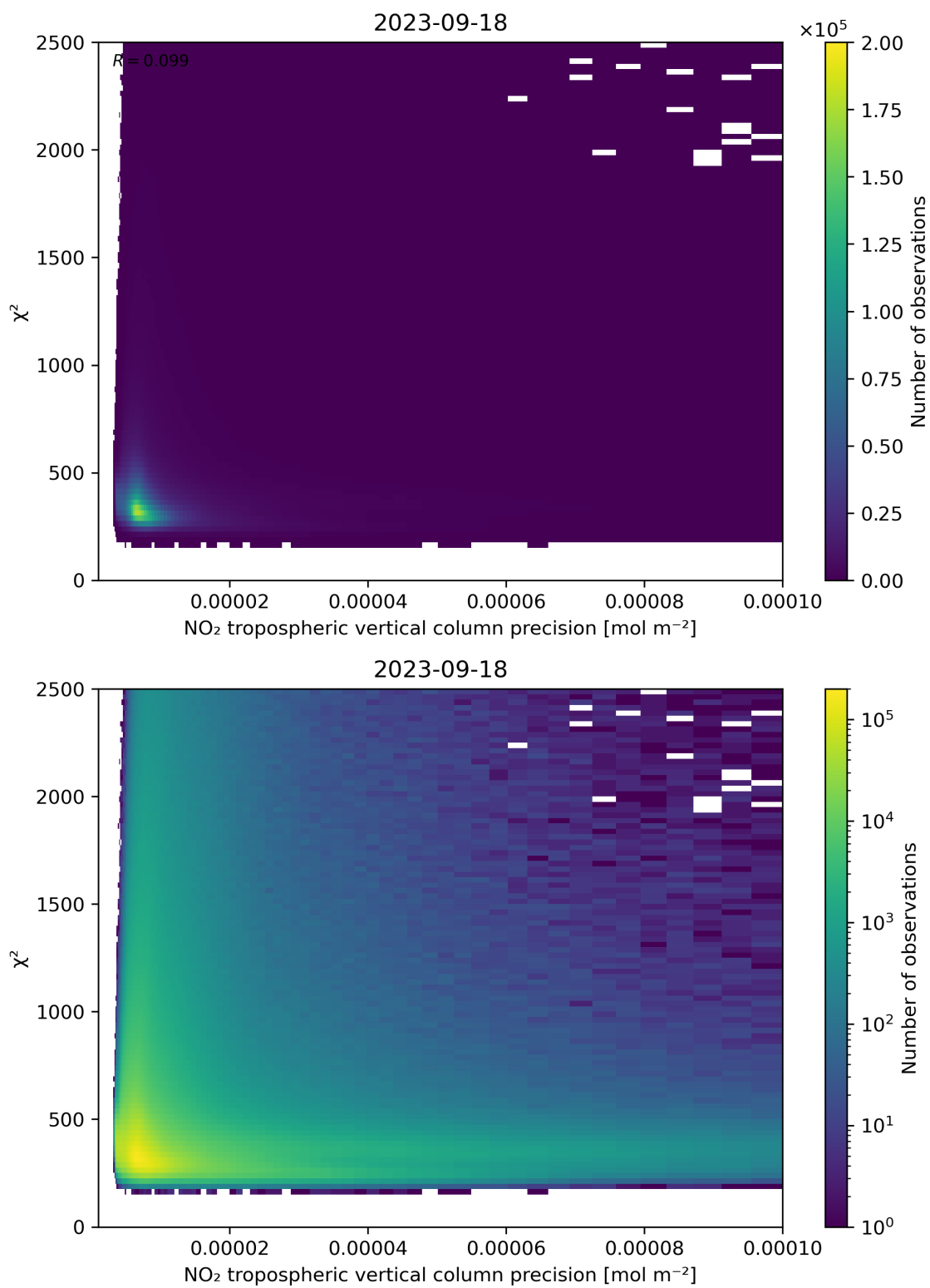
Figure 134: Scatter density plot of “NO 2 tropospheric vertical column precision” against “ \chi^2 ” for 2023-09-17 to 2023-09-19.
