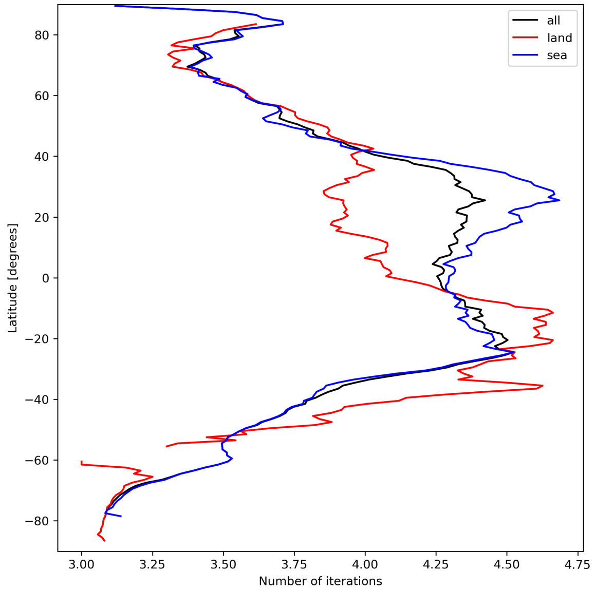
Figure 17: Zonal average of “Number of iterations” for 2023-09-17 to 2023-09-19.
