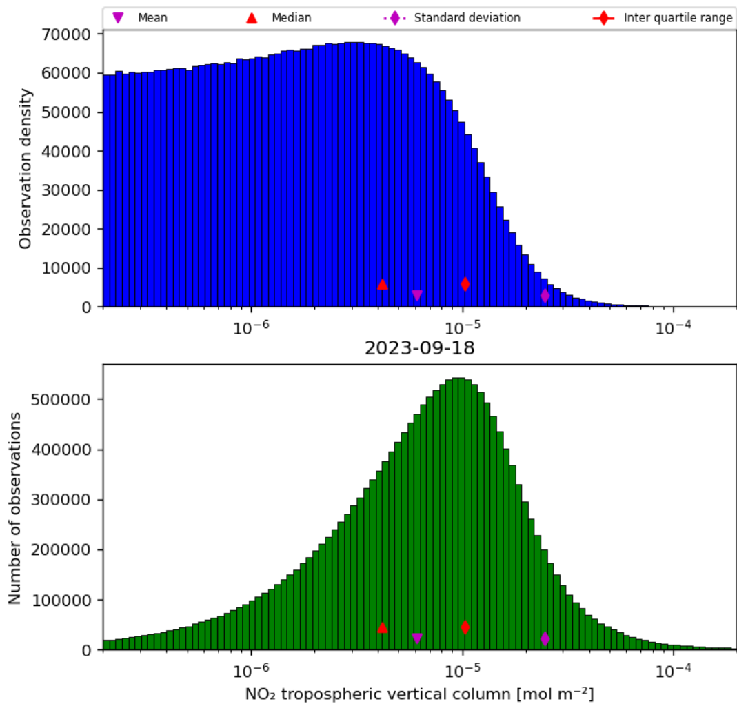
Figure 29: Histogram of “NO 2 tropospheric vertical column” for 2023-09-17 to 2023-09-19
