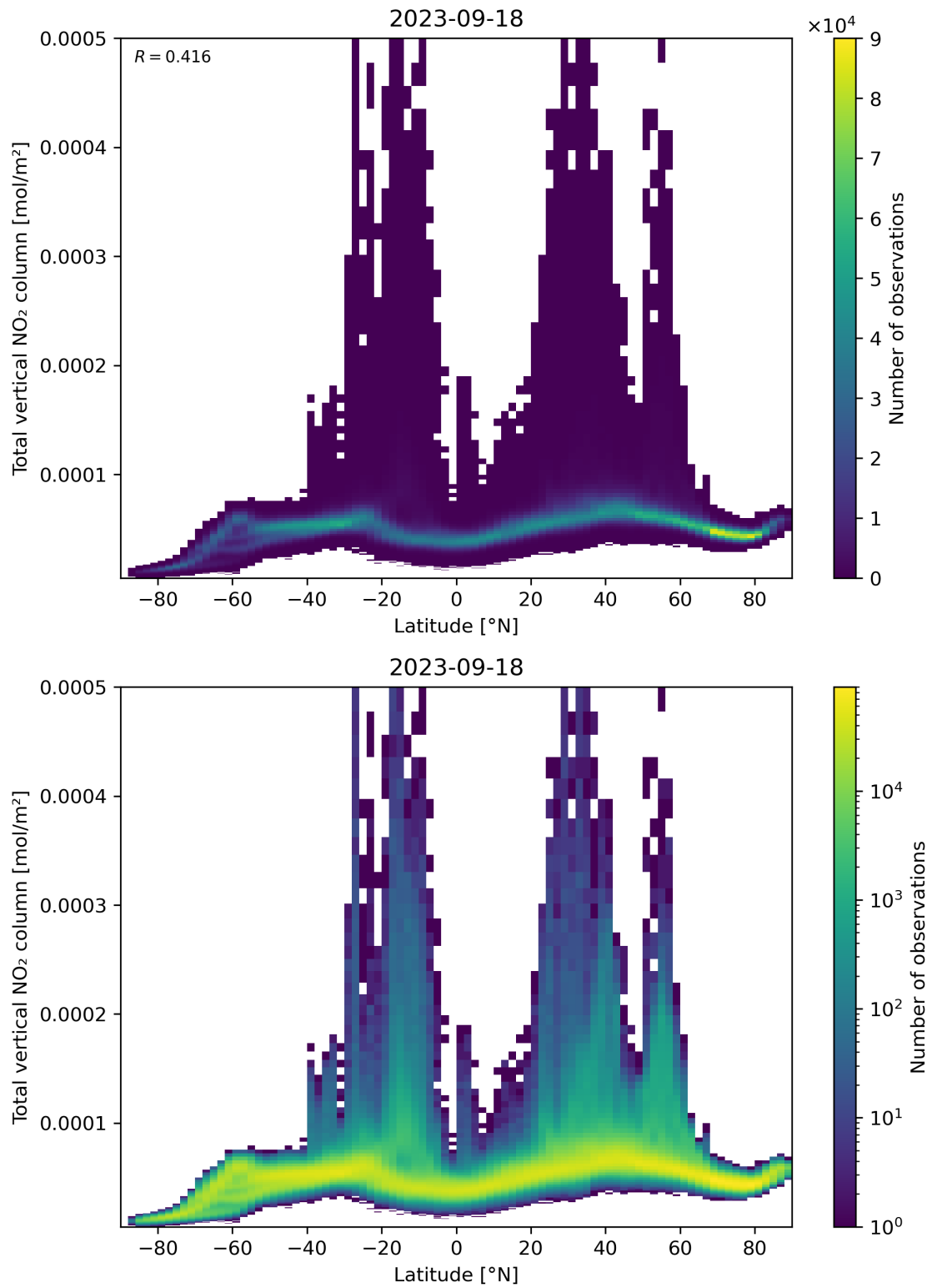
Figure 90: Scatter density plot of “Latitude” against “Total vertical NO 2 column” for 2023-09-17 to 2023-09-19.
