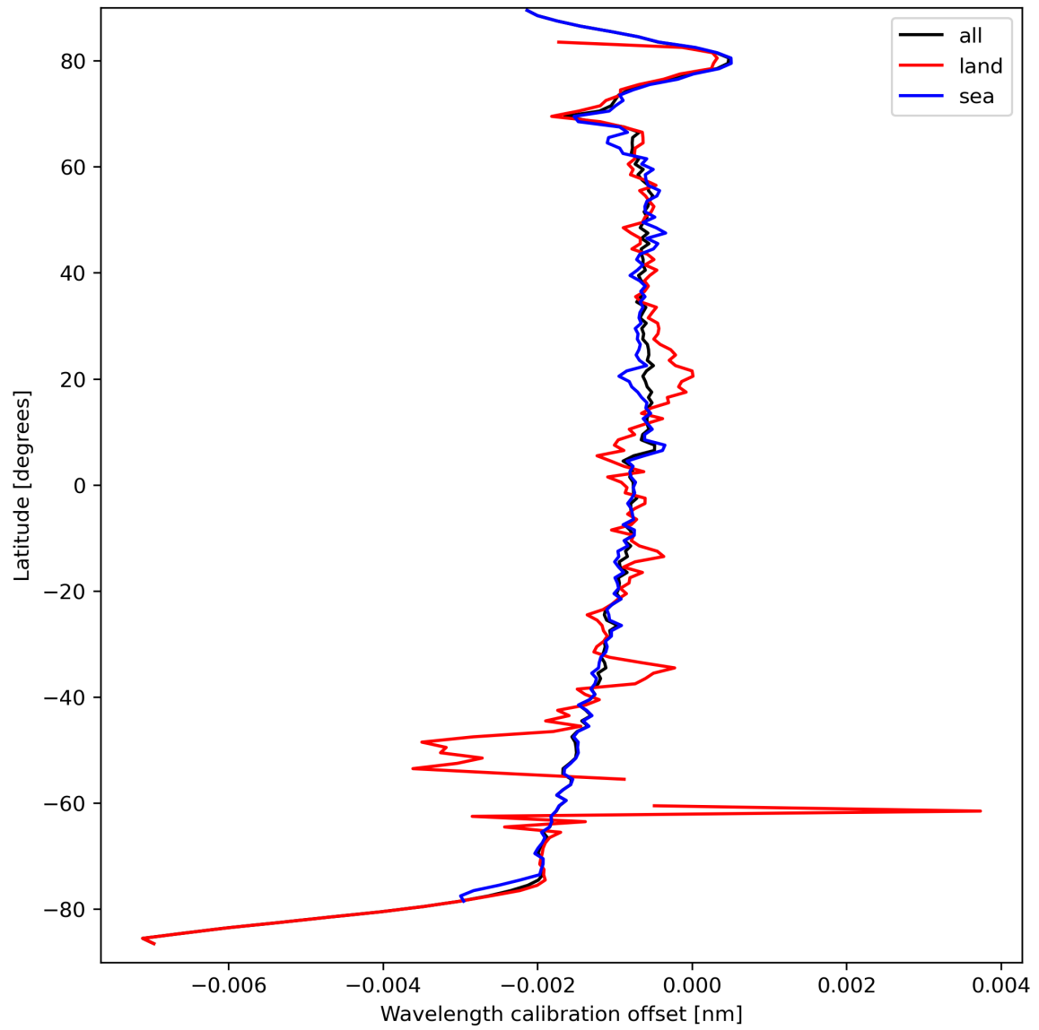
Figure 18: Zonal average of “Wavelength calibration offset” for 2023-09-17 to 2023-09-19.
