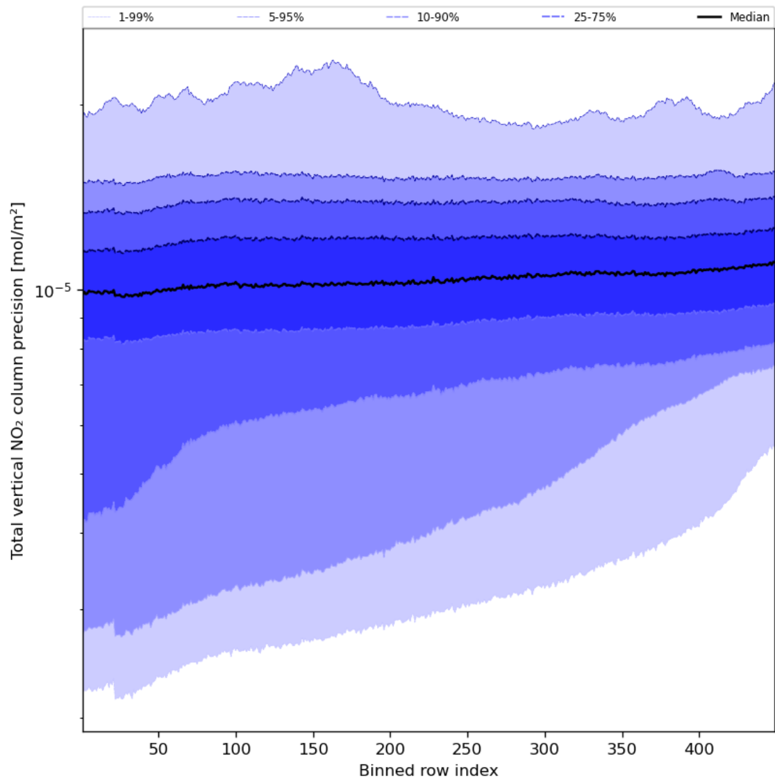
Figure 56: Along track statistics of “Total vertical NO 2 column precision” for 2023-09-17 to 2023-09-19
