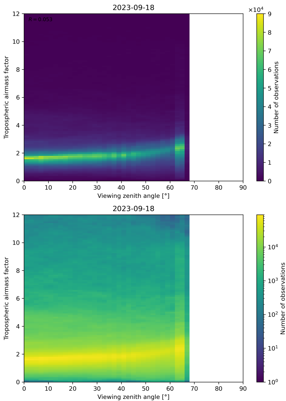
Figure 161: Scatter density plot of “Viewing zenith angle” against “Tropospheric airmass factor” for 2023-09-17 to 2023-09-19.
