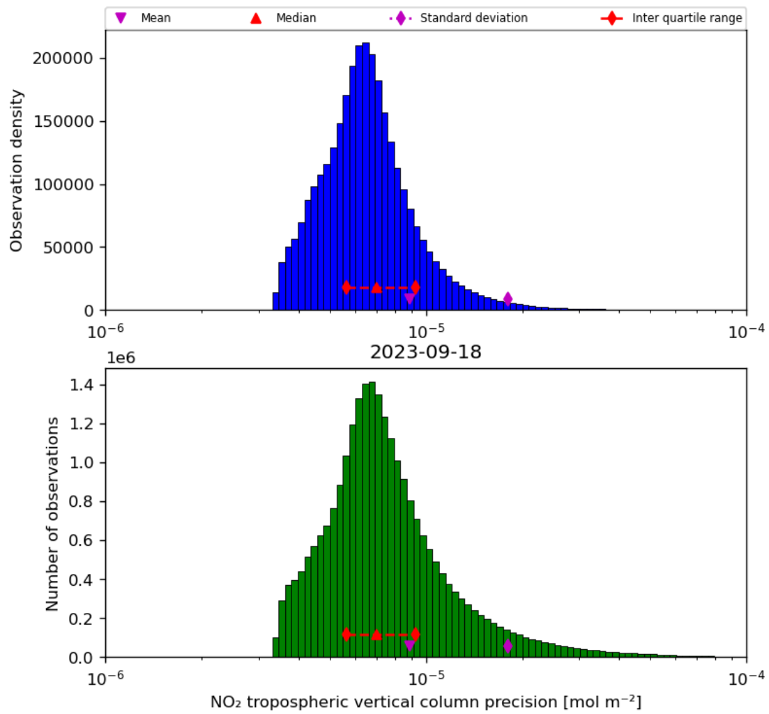
Figure 30: Histogram of “NO 2 tropospheric vertical column precision” for 2023-09-17 to 2023-09-19
