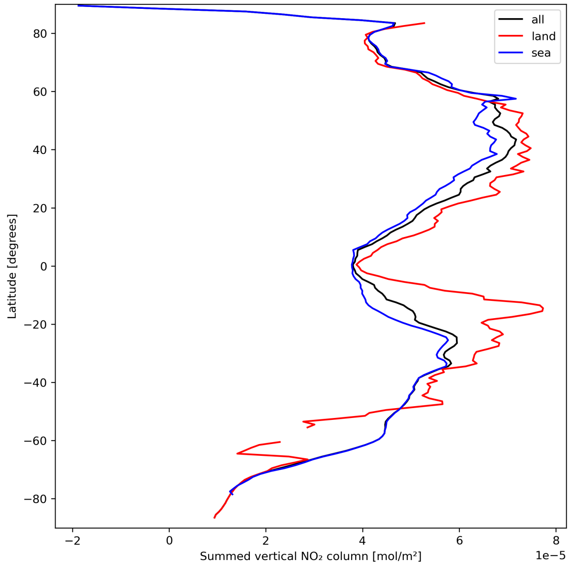
Figure 23: Zonal average of “Summed vertical NO 2 column” for 2023-09-17 to 2023-09-19.
