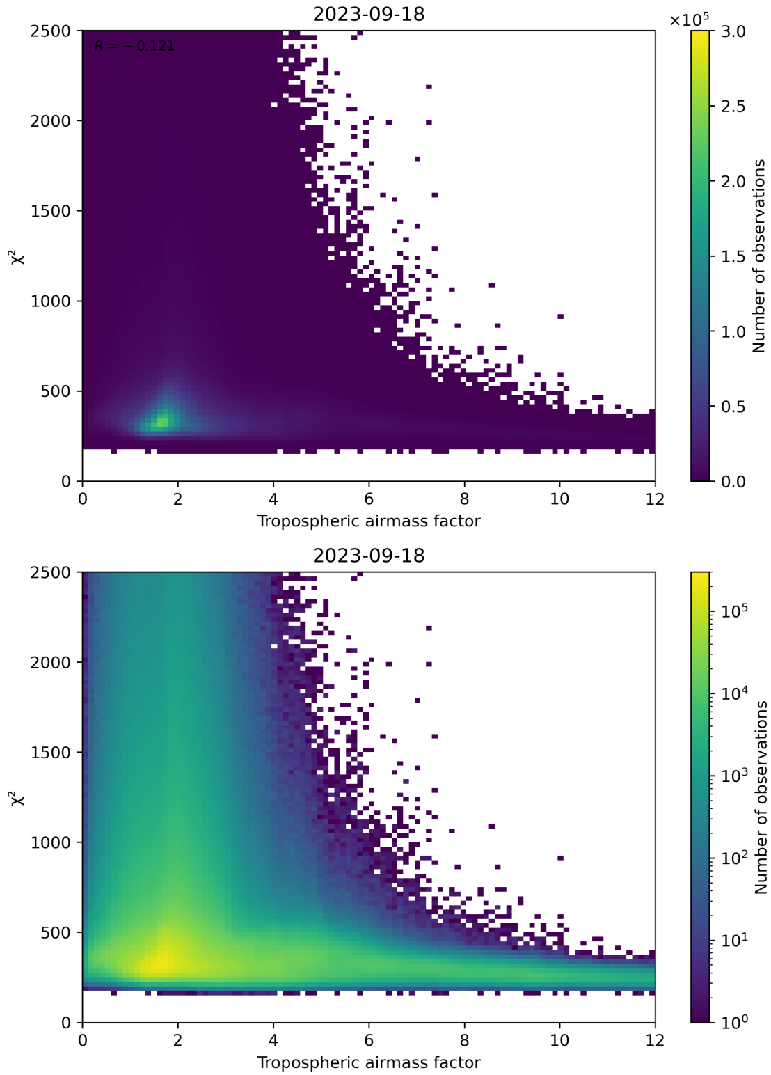
Figure 73: Scatter density plot of “Tropospheric airmass factor” against “ \chi^2 ” for 2023-09-17 to 2023-09-19.
