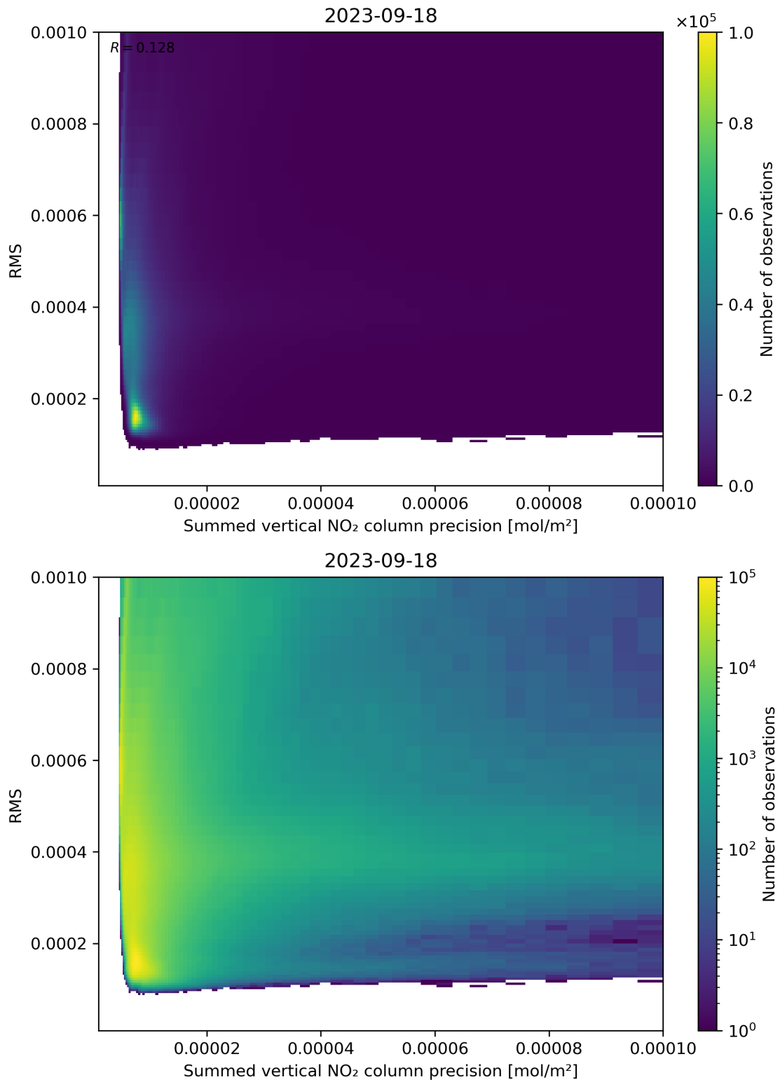
Figure 108: Scatter density plot of “Summed vertical NO 2 column precision” against “RMS” for 2023-09-17 to 2023-09-19.
