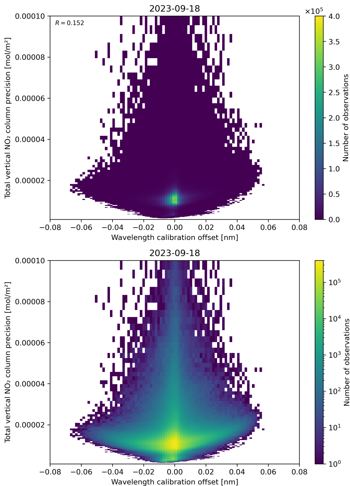
Figure 180: Scatter density plot of “Wavelength calibration offset” against “Total vertical NO 2 column precision” for 2023-09-17 to 2023-09-19.
