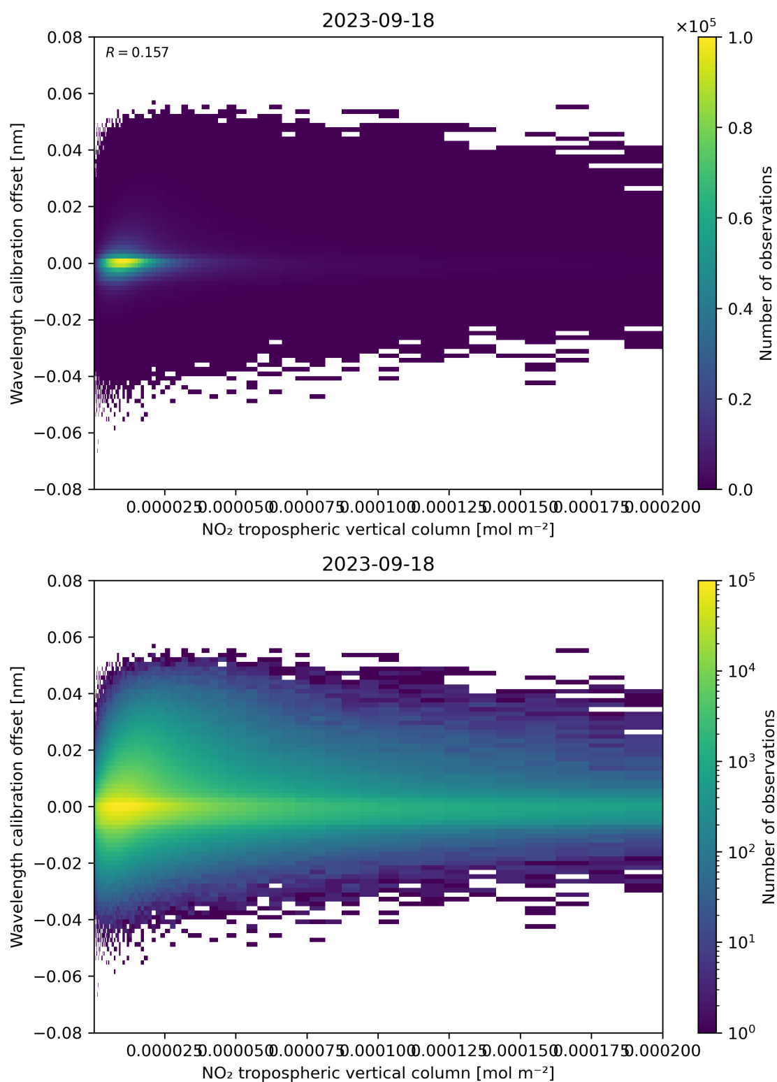
Figure 143: Scatter density plot of “NO 2 tropospheric vertical column” against “Wavelength calibration offset” for 2023-09-17 to 2023-09-19.
