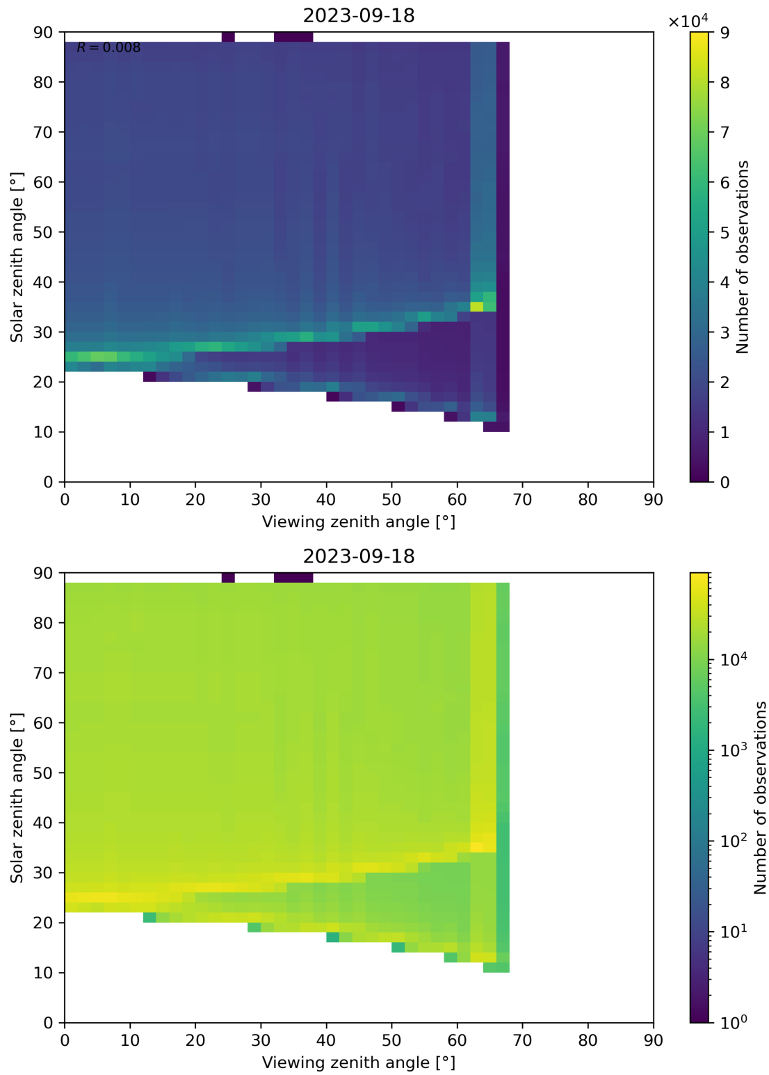
Figure 172: Scatter density plot of “Viewing zenith angle” against “Solar zenith angle” for 2023-09-17 to 2023-09-19.
