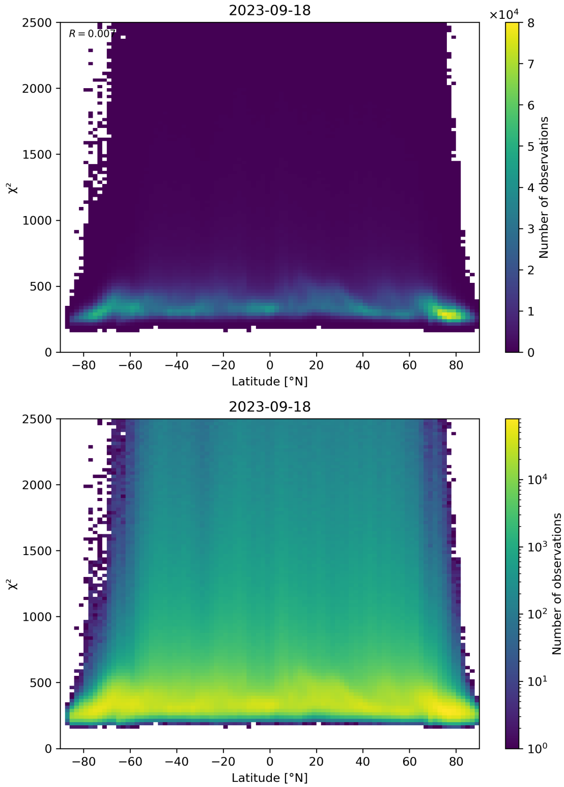
Figure 86: Scatter density plot of “Latitude” against “ \chi^2 ” for 2023-09-17 to 2023-09-19.
