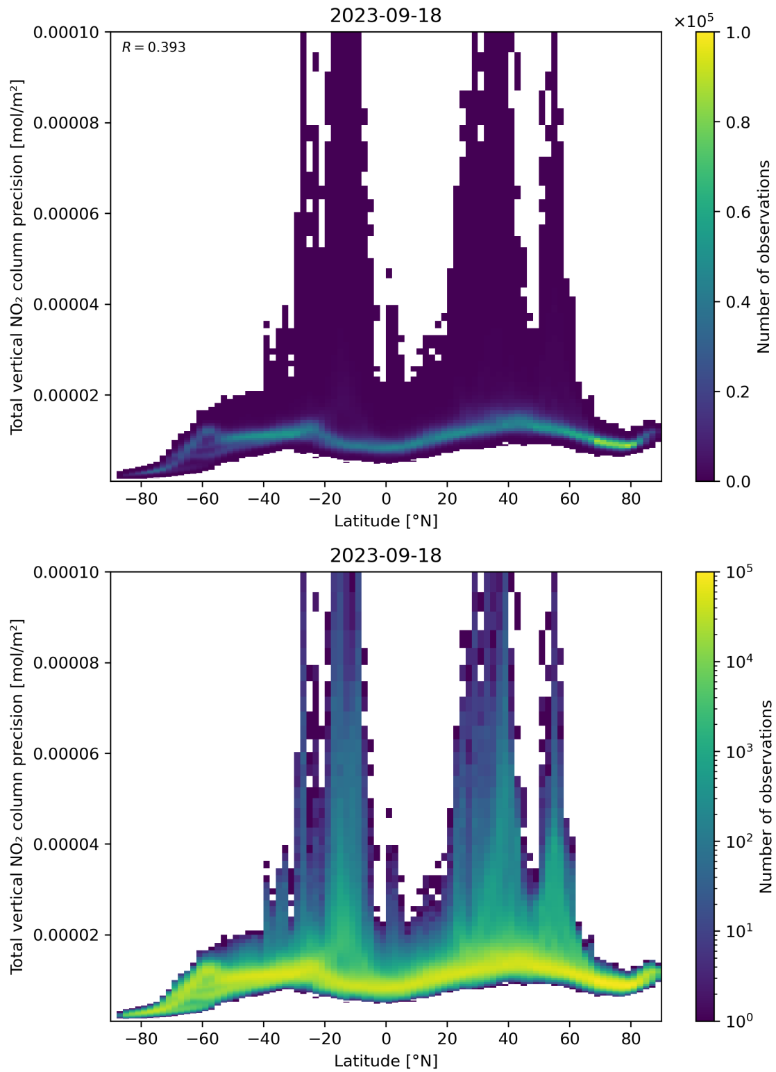
Figure 91: Scatter density plot of “Latitude” against “Total vertical NO 2 column precision” for 2023-09-17 to 2023-09-19.
