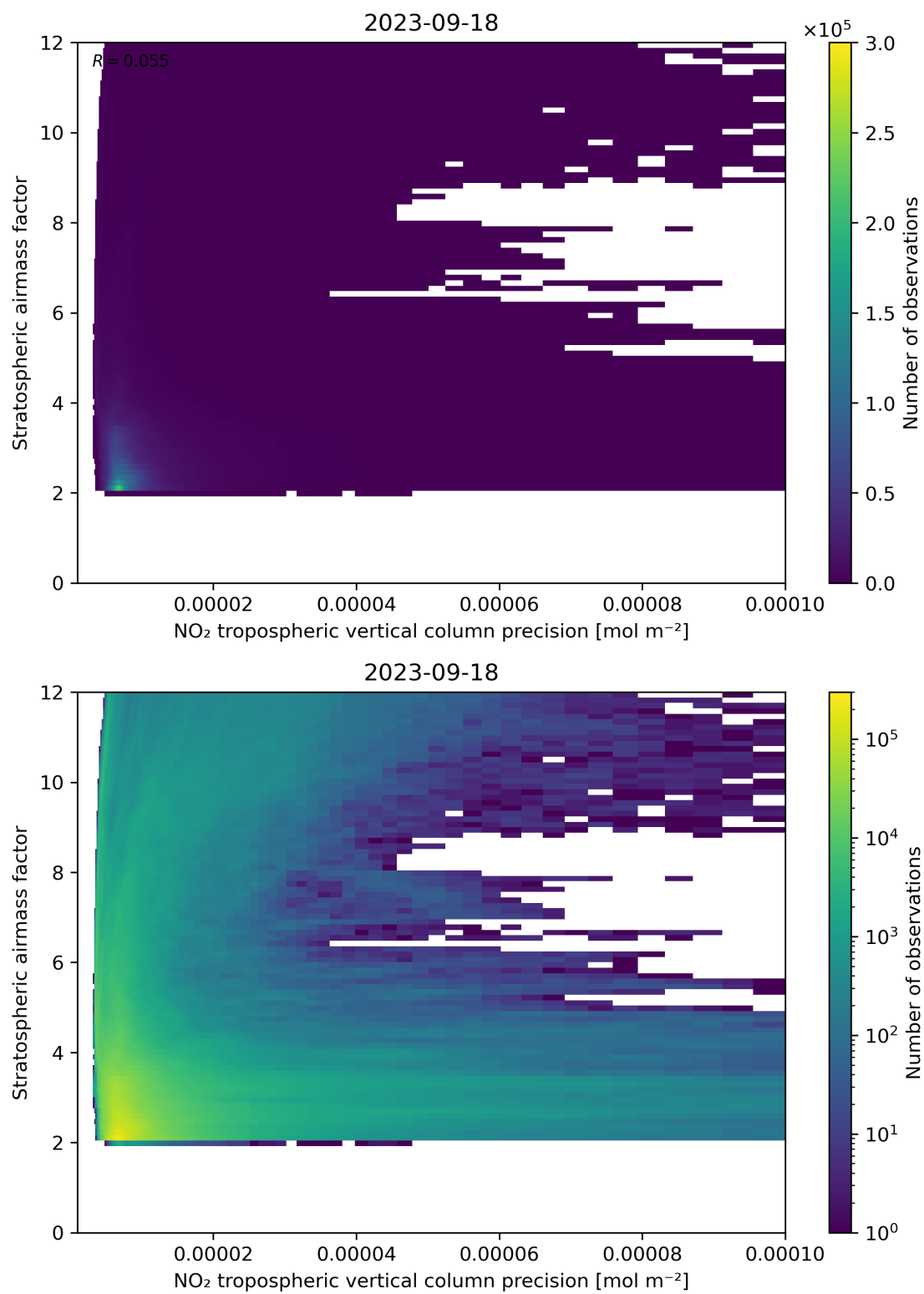
Figure 131: Scatter density plot of “NO 2 tropospheric vertical column precision” against “Stratospheric airmass factor” for 2023-09-17 to 2023-09-19.
