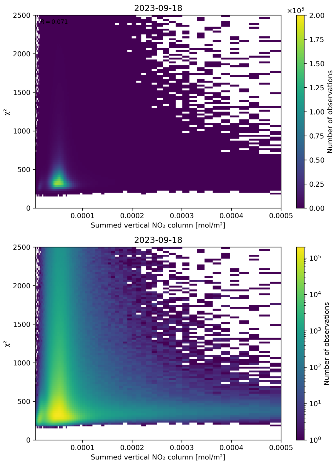
Figure 104: Scatter density plot of “Summed vertical NO 2 column” against “ \chi^2 ” for 2023-09-17 to 2023-09-19.
