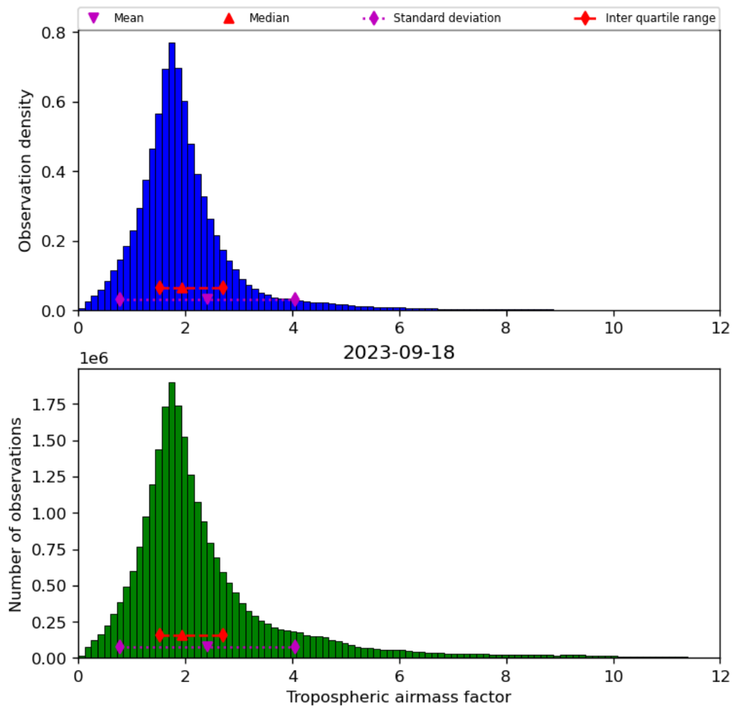
Figure 31: Histogram of “Tropospheric airmass factor” for 2023-09-17 to 2023-09-19
