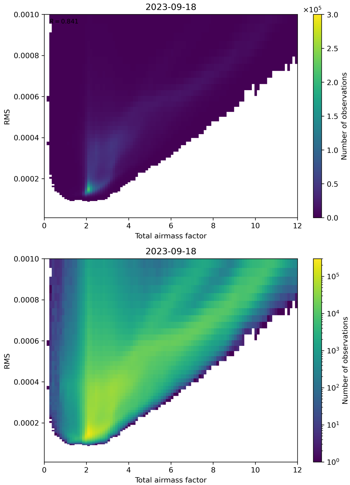
Figure 69: Scatter density plot of “Total airmass factor” against “RMS” for 2023-09-17 to 2023-09-19.
