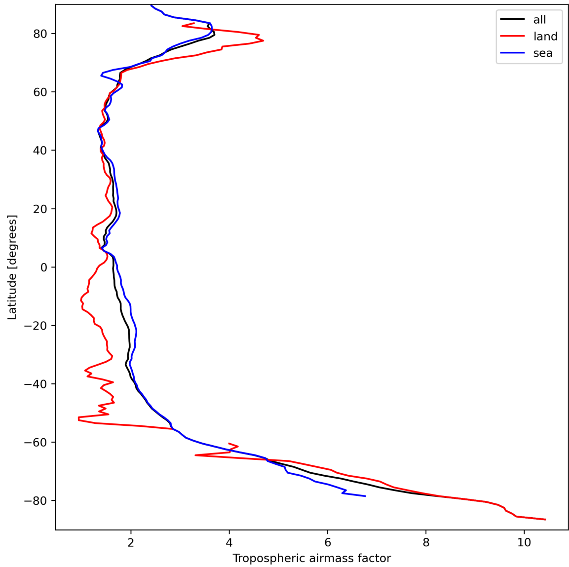
Figure 14: Zonal average of “Tropospheric airmass factor” for 2023-09-17 to 2023-09-19.
