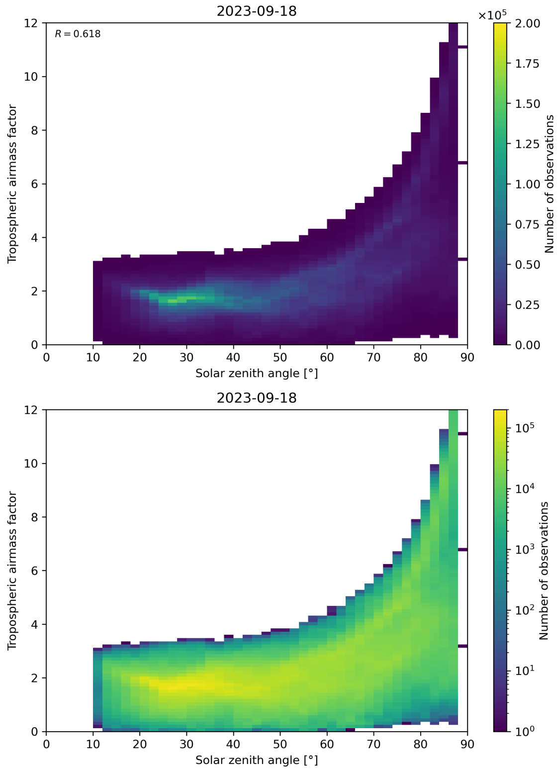
Figure 147: Scatter density plot of “Solar zenith angle” against “Tropospheric airmass factor” for 2023-09-17 to 2023-09-19.
