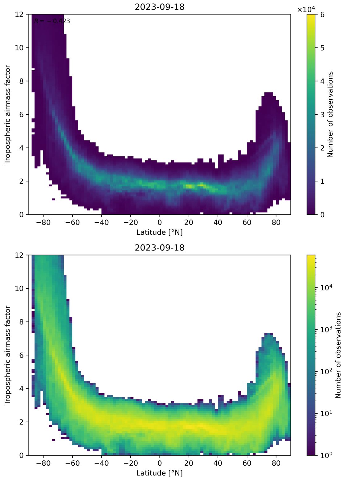
Figure 85: Scatter density plot of “Latitude” against “Tropospheric airmass factor” for 2023-09-17 to 2023-09-19.
