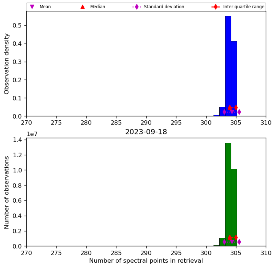
Figure 33: Histogram of “Number of spectral points in retrieval” for 2023-09-17 to 2023-09-19
