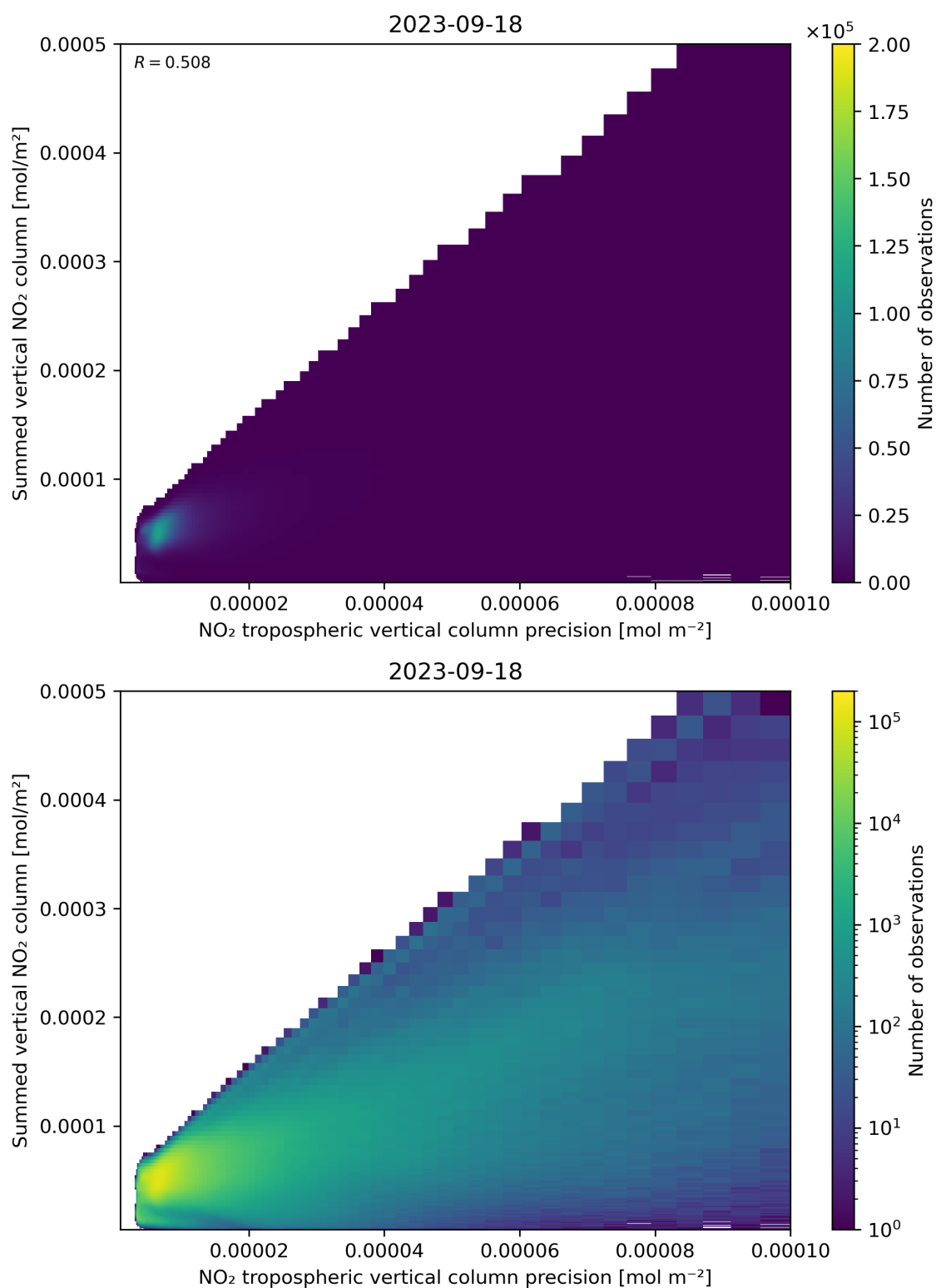
Figure 136: Scatter density plot of “NO 2 tropospheric vertical column precision” against “Summed vertical NO 2 column” for 2023-09-17 to 2023-09-19.
