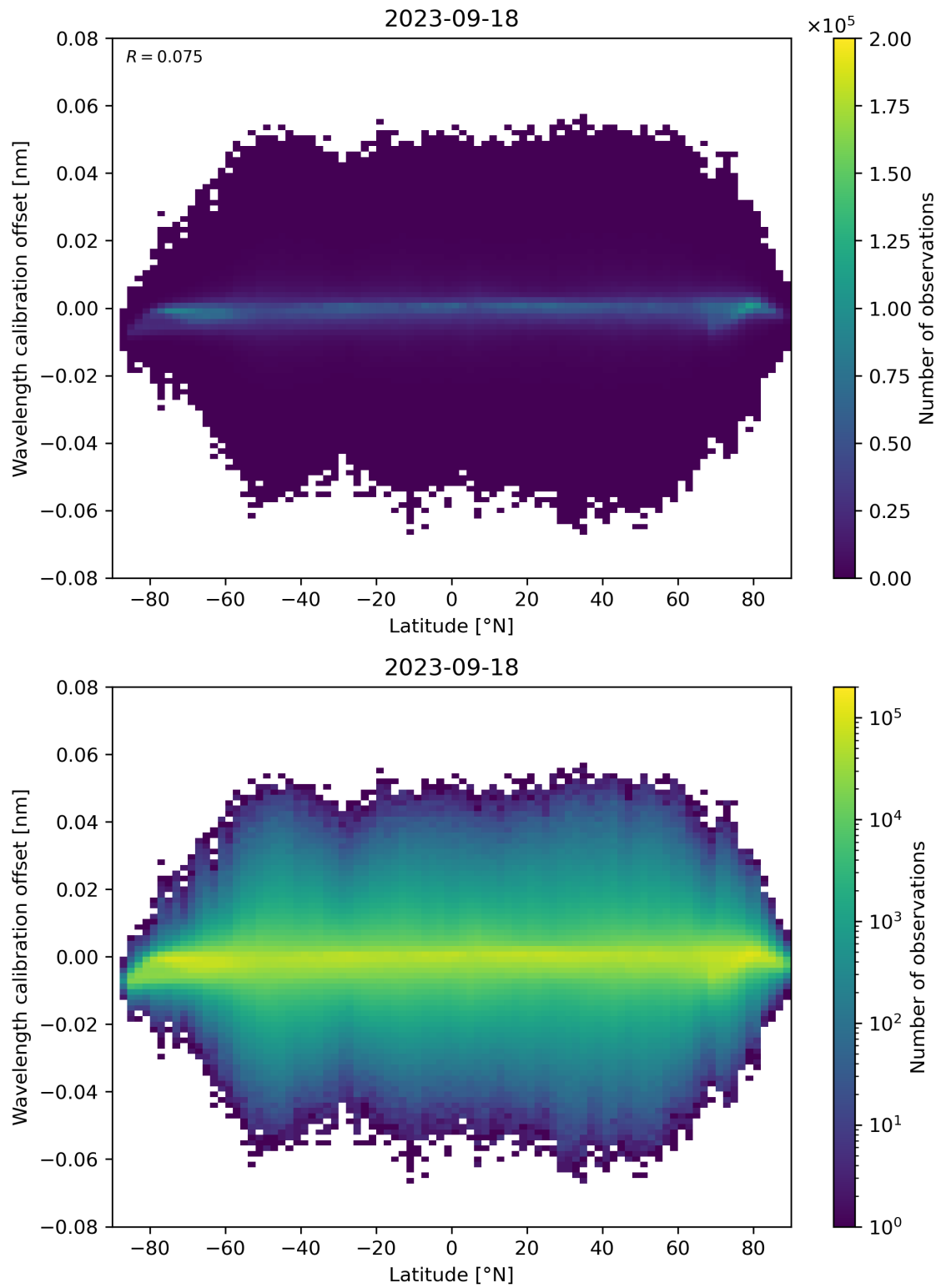
Figure 95: Scatter density plot of “Latitude” against “Wavelength calibration offset” for 2023-09-17 to 2023-09-19.
