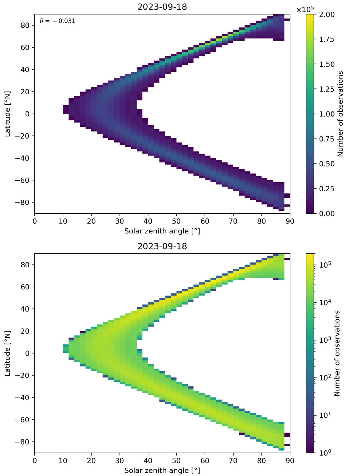
Figure 149: Scatter density plot of “Solar zenith angle” against “Latitude” for 2023-09-17 to 2023-09-19.
