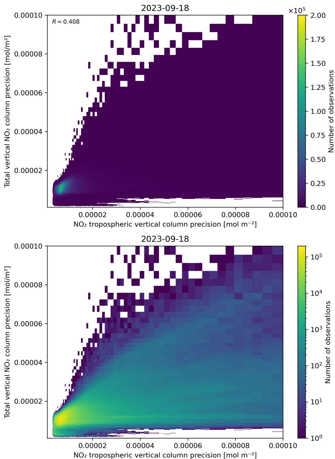
Figure 139: Scatter density plot of “NO 2 tropospheric vertical column precision” against “Total vertical NO 2 column precision” for 2023-09-17 to 2023-09-19.
