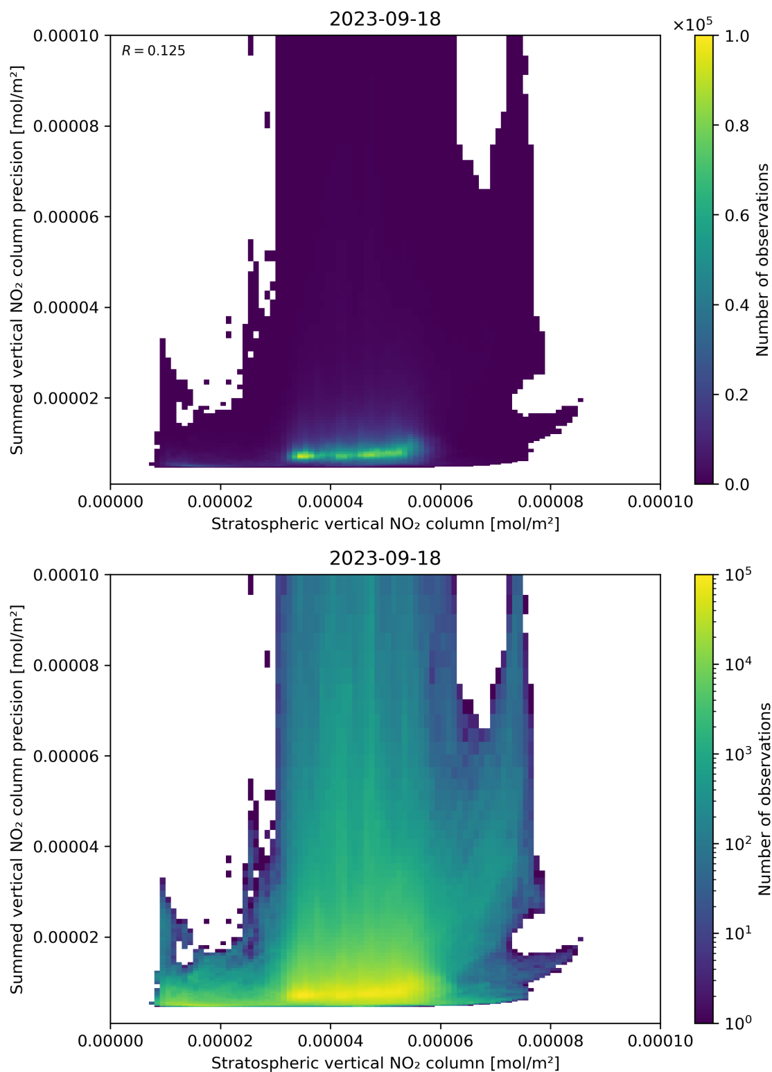
Figure 99: Scatter density plot of “Stratospheric vertical NO 2 column” against “Summed vertical NO 2 column precision” for 2023-09-17 to 2023-09-19.
