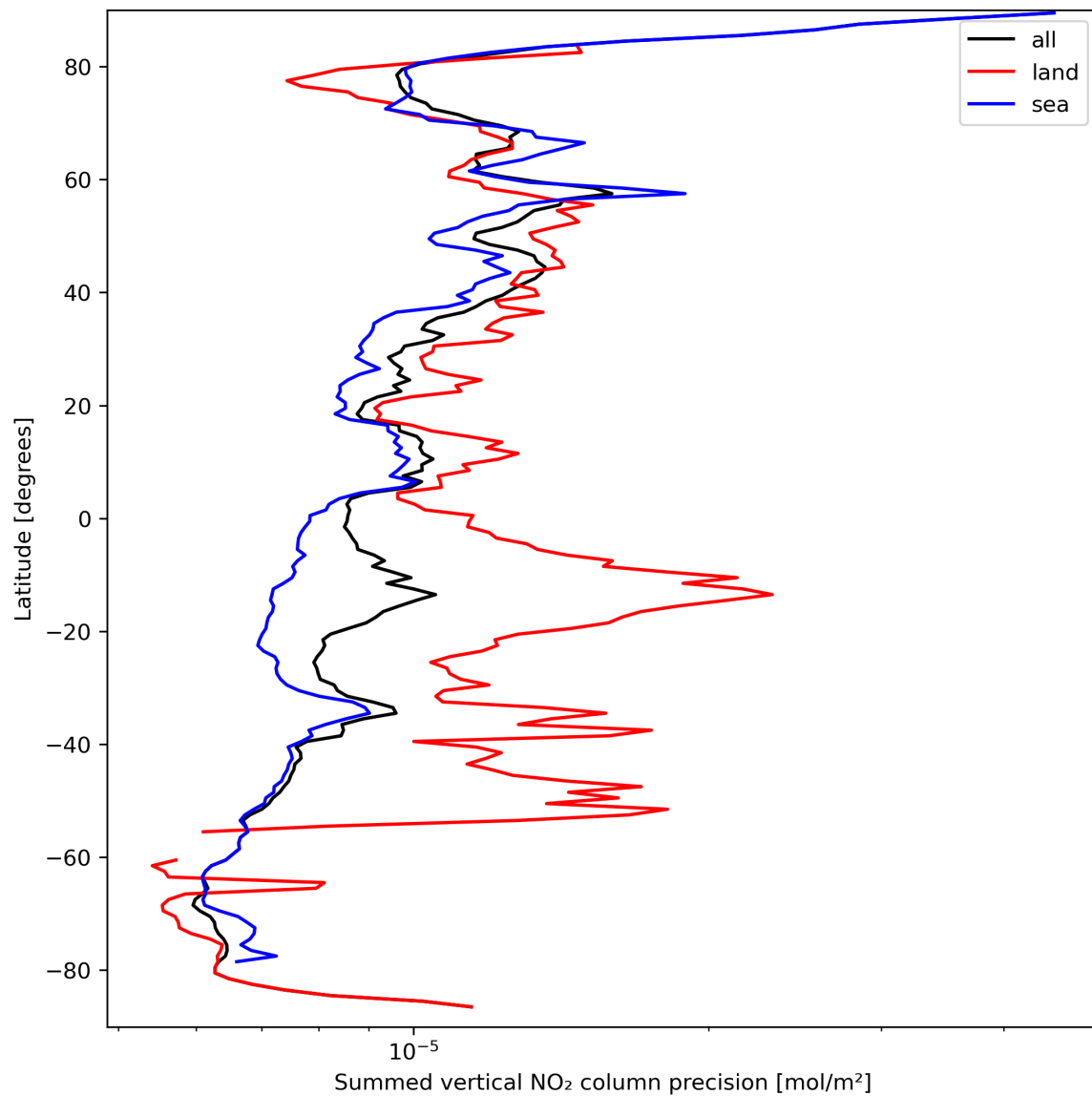
Figure 24: Zonal average of “Summed vertical NO 2 column precision” for 2023-09-17 to 2023-09-19.
