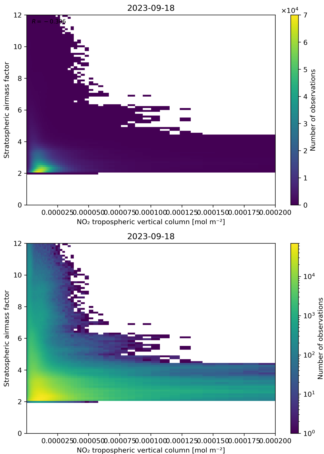
Figure 121: Scatter density plot of “NO 2 tropospheric vertical column” against “Stratospheric air mass factor” for 2023-09-17 to 2023-09-19.
