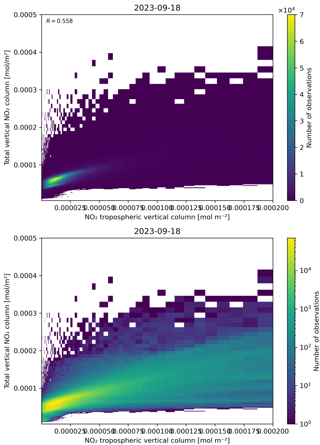
Figure 128: Scatter density plot of “NO 2 tropospheric vertical column” against “Total vertical NO 2 column” for 2023-09-17 to 2023-09-19.
