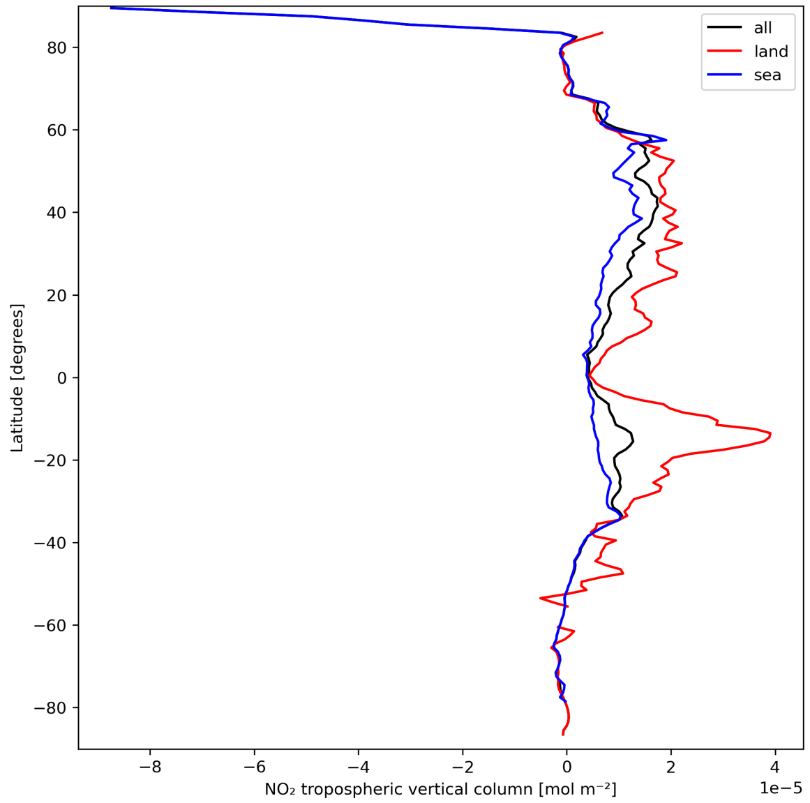
Figure 12: Zonal average of “NO 2 tropospheric vertical column” for 2023-09-17 to 2023-09-19.
