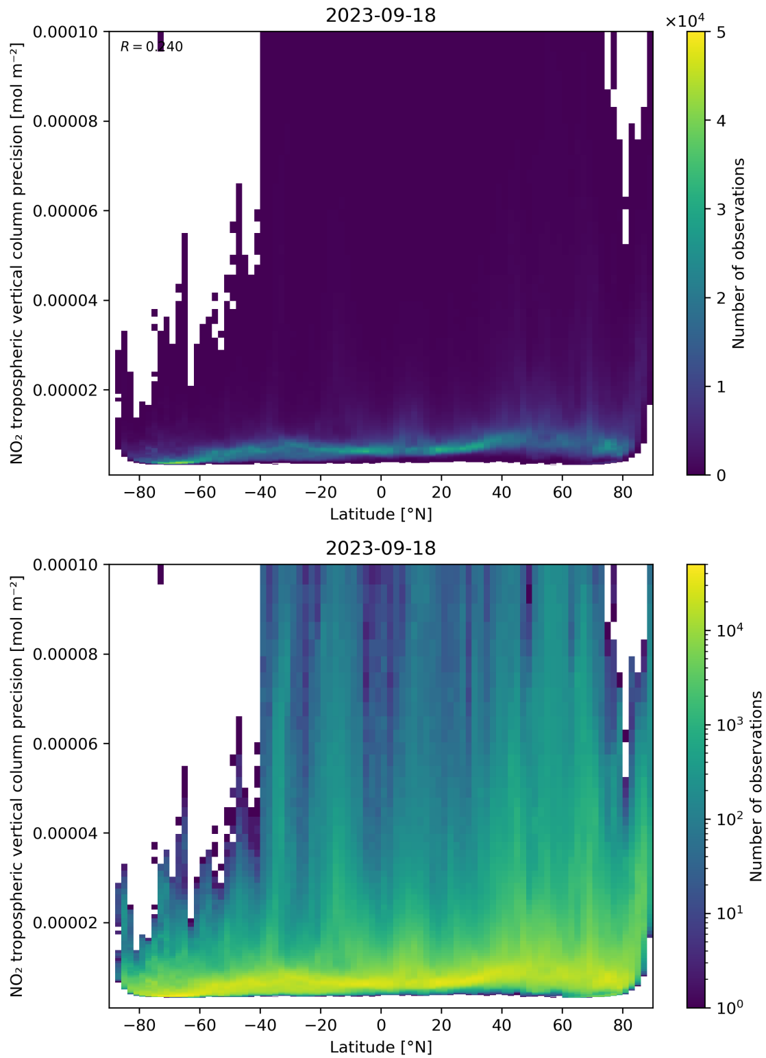
Figure 93: Scatter density plot of “Latitude” against “NO 2 tropospheric vertical column precision” for 2023-09-17 to 2023-09-19.
