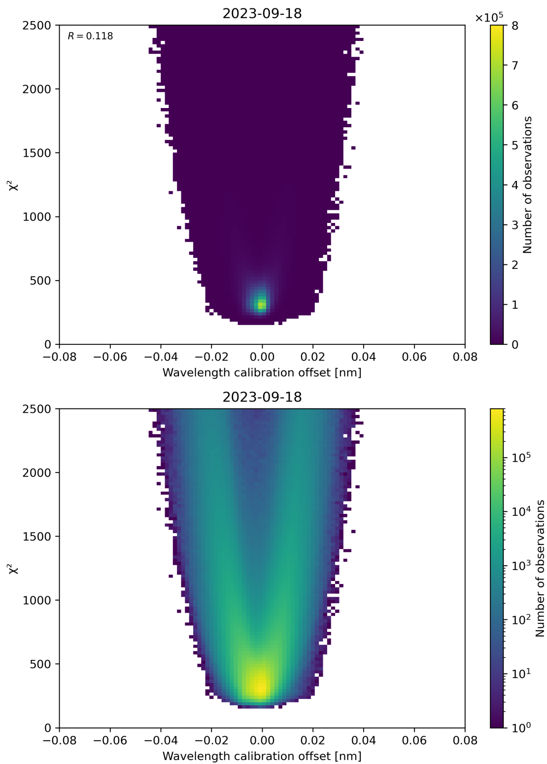
Figure 175: Scatter density plot of “Wavelength calibration offset” against “ \chi^2 ” for 2023-09-17 to 2023-09-19.
