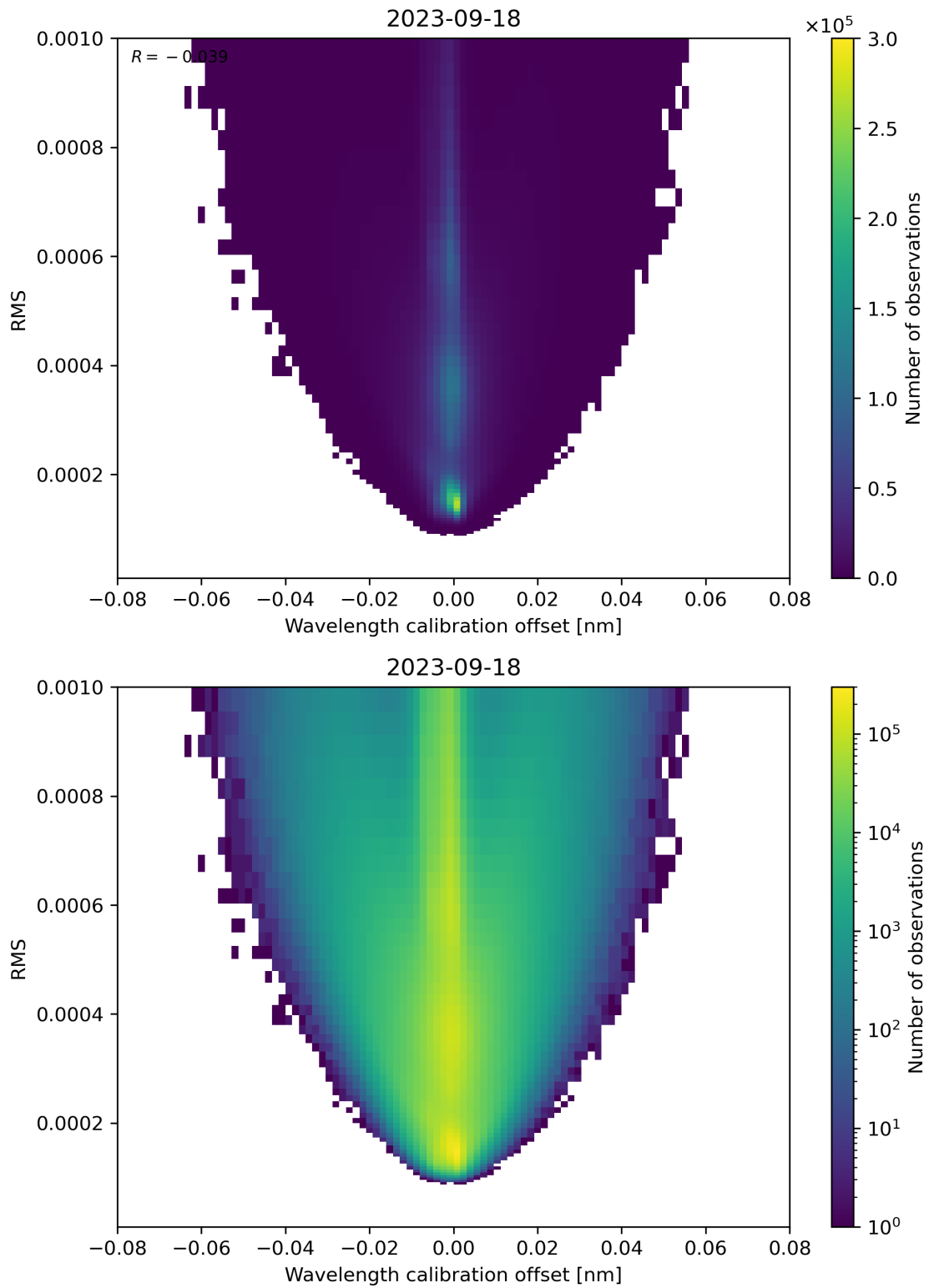
Figure 181: Scatter density plot of “Wavelength calibration offset” against “RMS” for 2023-09-17 to 2023-09-19.
