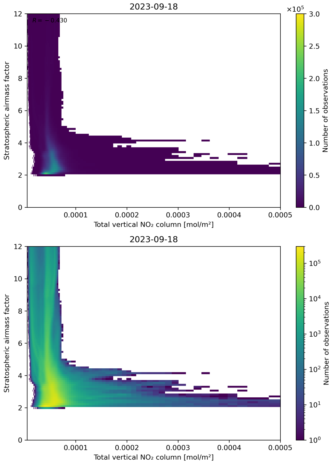
Figure 110: Scatter density plot of “Total vertical NO 2 column” against “Stratospheric airmass factor” for 2023-09-17 to 2023-09-19.
