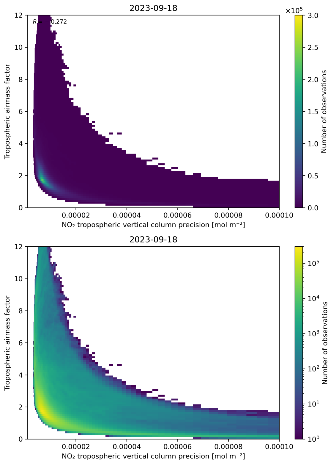
Figure 133: Scatter density plot of “NO 2 tropospheric vertical column precision” against “Tropospheric airmass factor” for 2023-09-17 to 2023-09-19.
