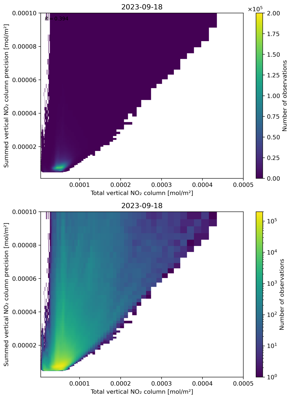
Figure 113: Scatter density plot of “Total vertical NO 2 column” against “Summed vertical NO 2 column precision” for 2023-09-17 to 2023-09-19.
