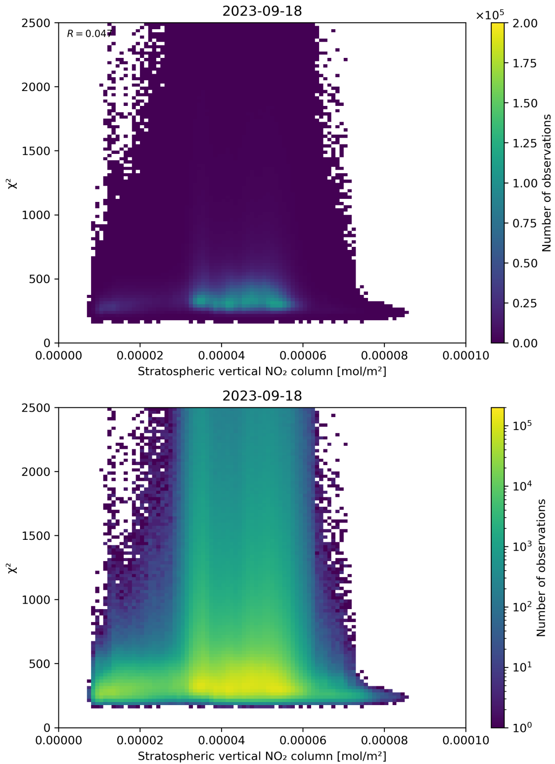
Figure 97: Scatter density plot of “Stratospheric vertical NO 2 column” against “ \chi^2 ” for 2023-09-17 to 2023-09-19.
