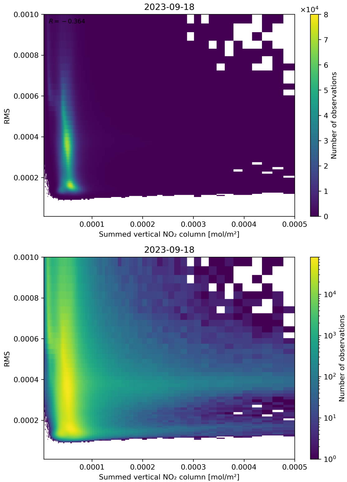
Figure 109: Scatter density plot of “Summed vertical NO 2 column” against “RMS” for 2023-09-17 to 2023-09-19.
