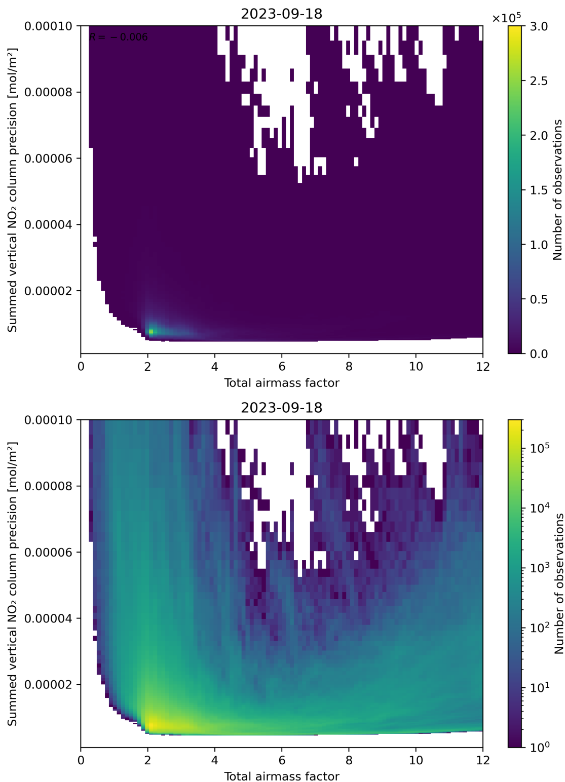
Figure 66: Scatter density plot of “Total airmass factor” against “Summed vertical NO 2 column precision” for 2023-09-17 to 2023-09-19.
