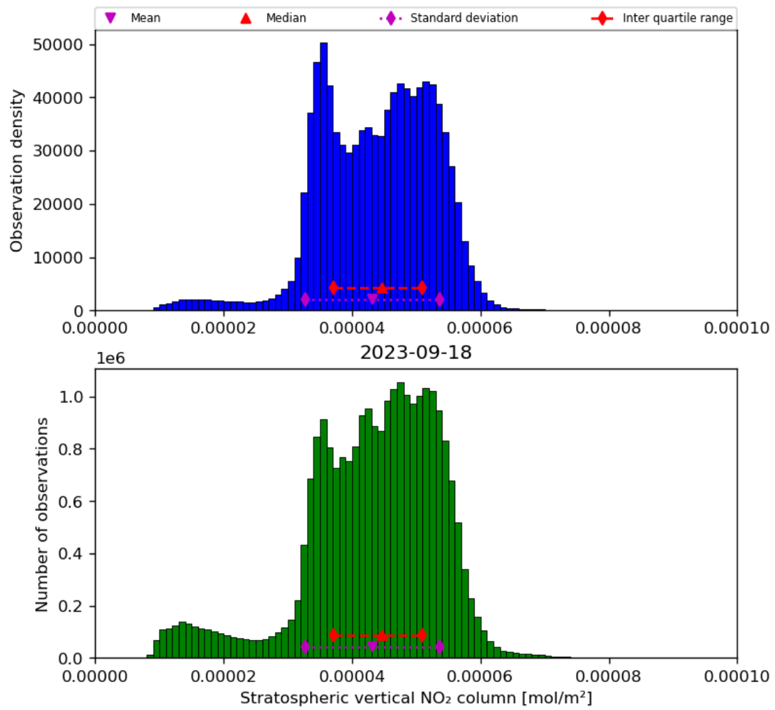
Figure 36: Histogram of “Stratospheric vertical NO 2 column” for 2023-09-17 to 2023-09-19
