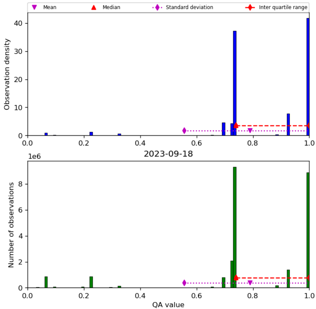
Figure 28: Histogram of “QA value” for 2023-09-17 to 2023-09-19
