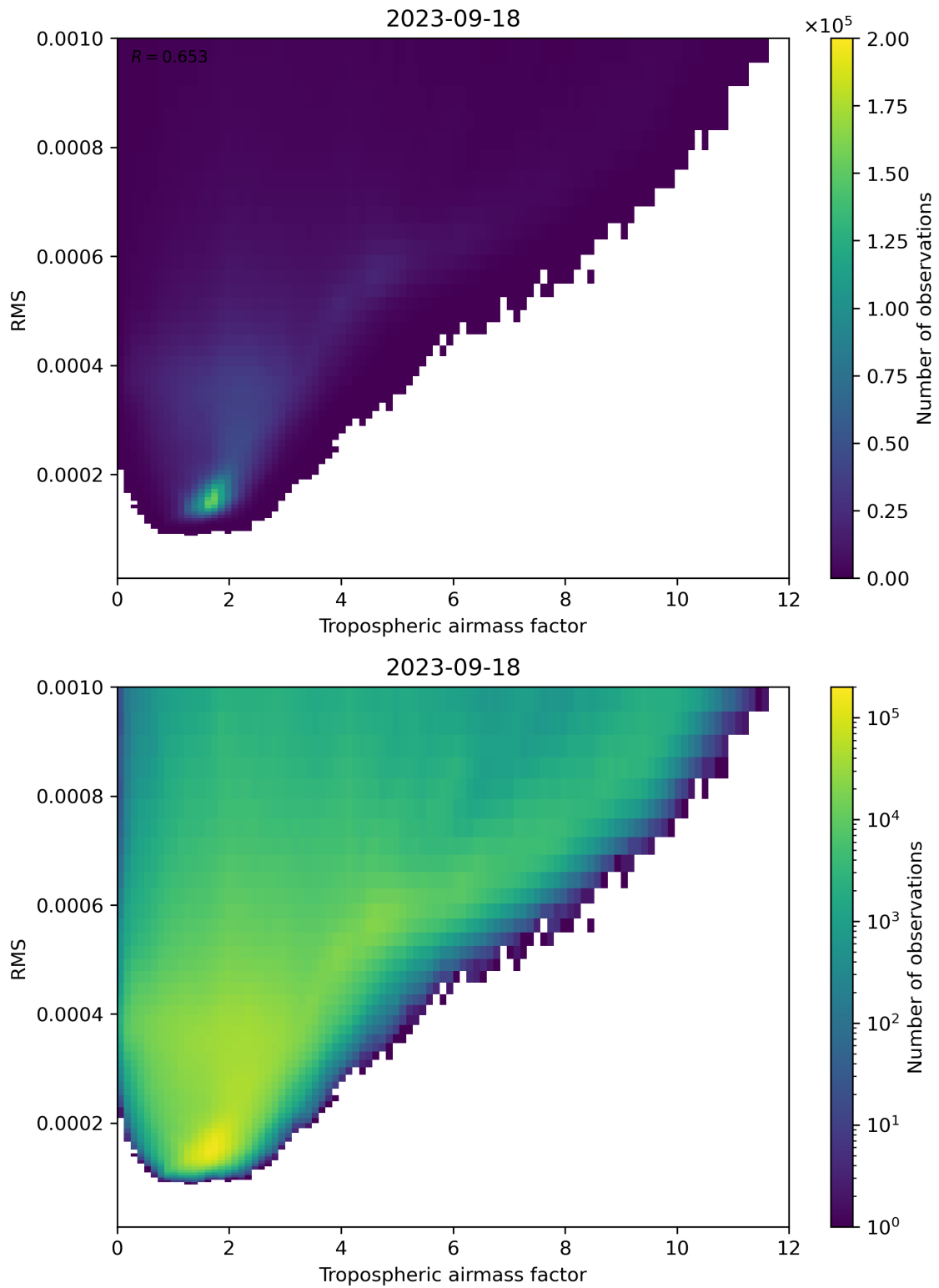
Figure 79: Scatter density plot of “Tropospheric airmass factor” against “RMS” for 2023-09-17 to 2023-09-19.
