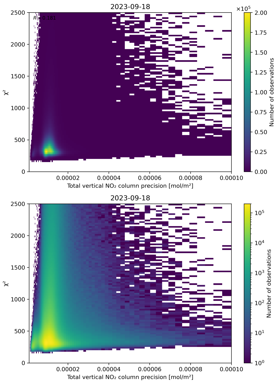
Figure 116: Scatter density plot of “Total vertical NO 2 column precision” against “ \chi^2 ” for 2023-09-17 to 2023-09-19.
