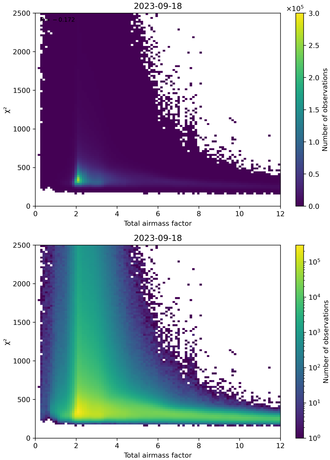
Figure 63: Scatter density plot of “Total airmass factor” against “ \chi^2 ” for 2023-09-17 to 2023-09-19.
