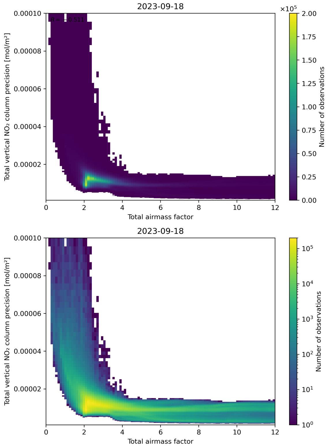
Figure 68: Scatter density plot of “Total airmass factor” against “Total vertical NO 2 column precision” for 2023-09-17 to 2023-09-19.
