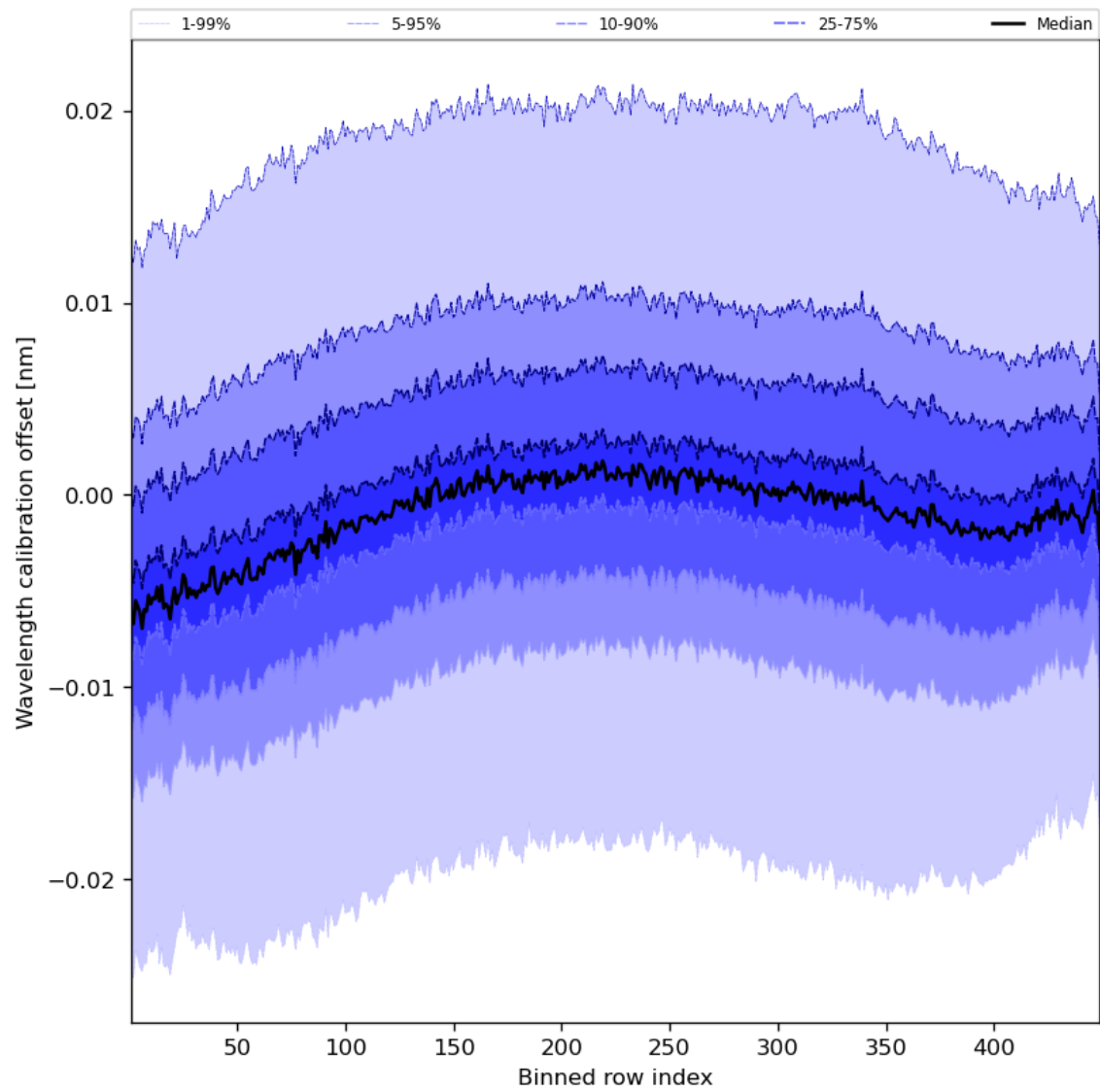
Figure 52: Along track statistics of “Wavelength calibration offset” for 2023-09-17 to 2023-09-19
