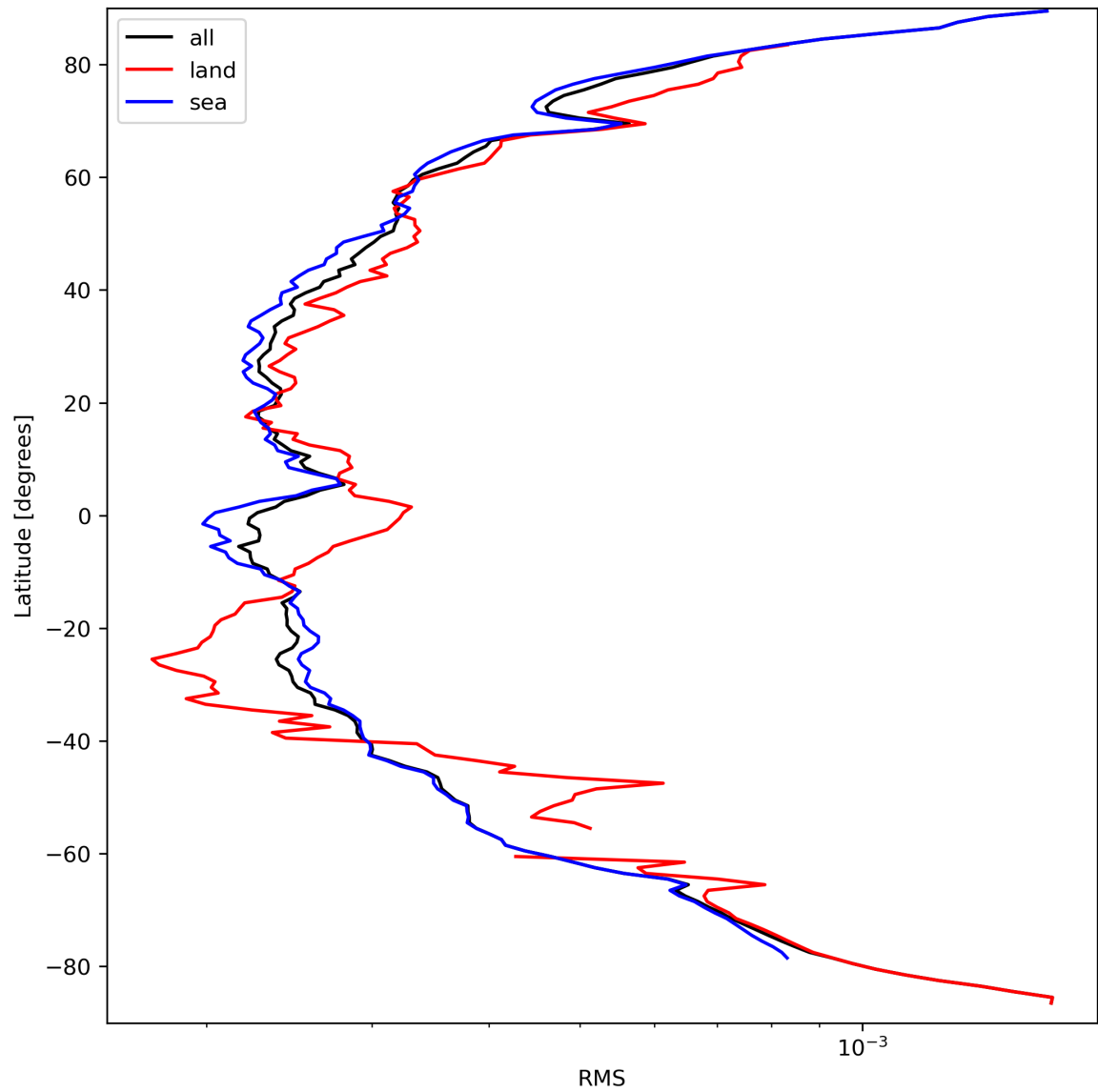
Figure 26: Zonal average of “RMS” for 2023-09-17 to 2023-09-19.
