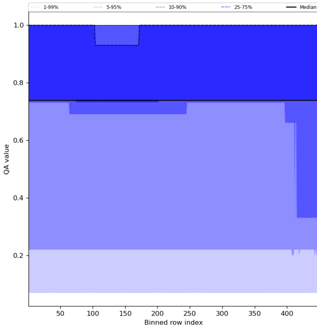
Figure 45: Along track statistics of “QA value” for 2023-09-17 to 2023-09-19
