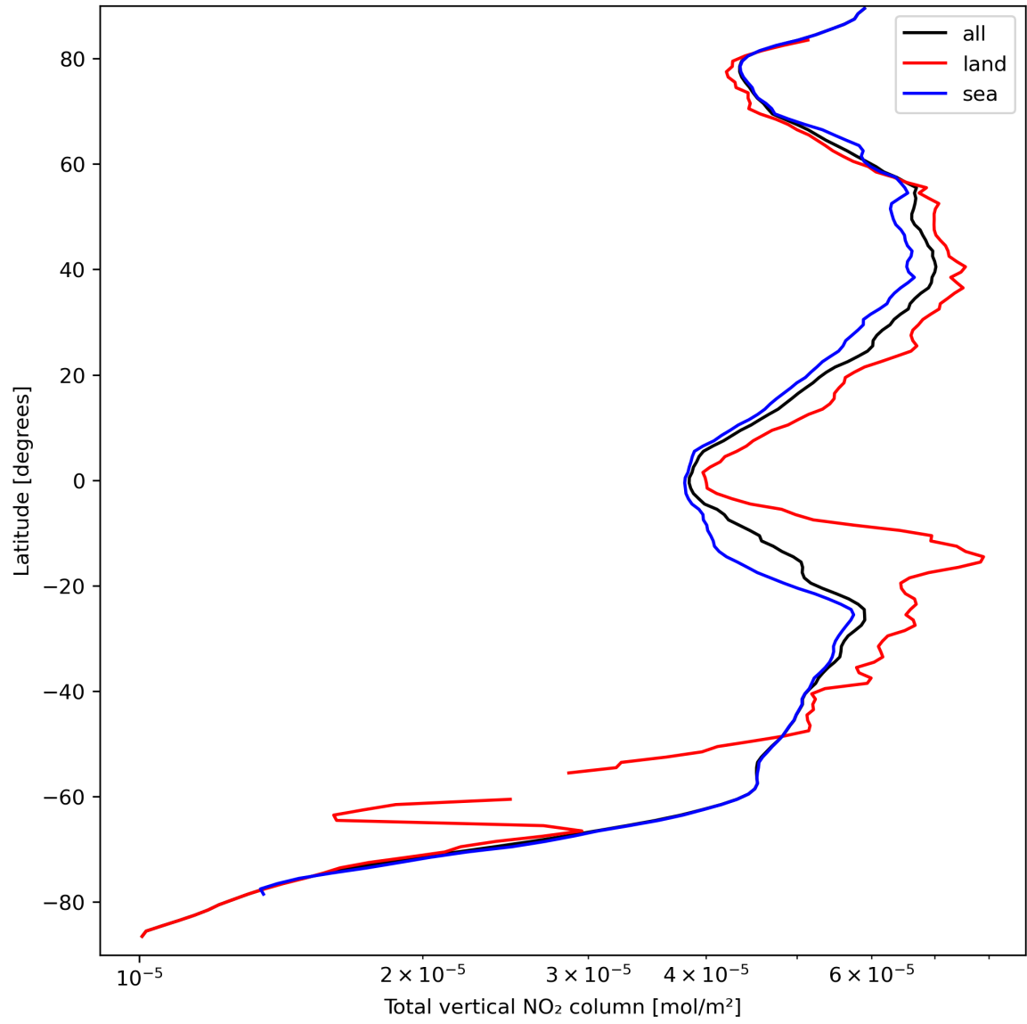
Figure 21: Zonal average of “Total vertical NO 2 column” for 2023-09-17 to 2023-09-19.
