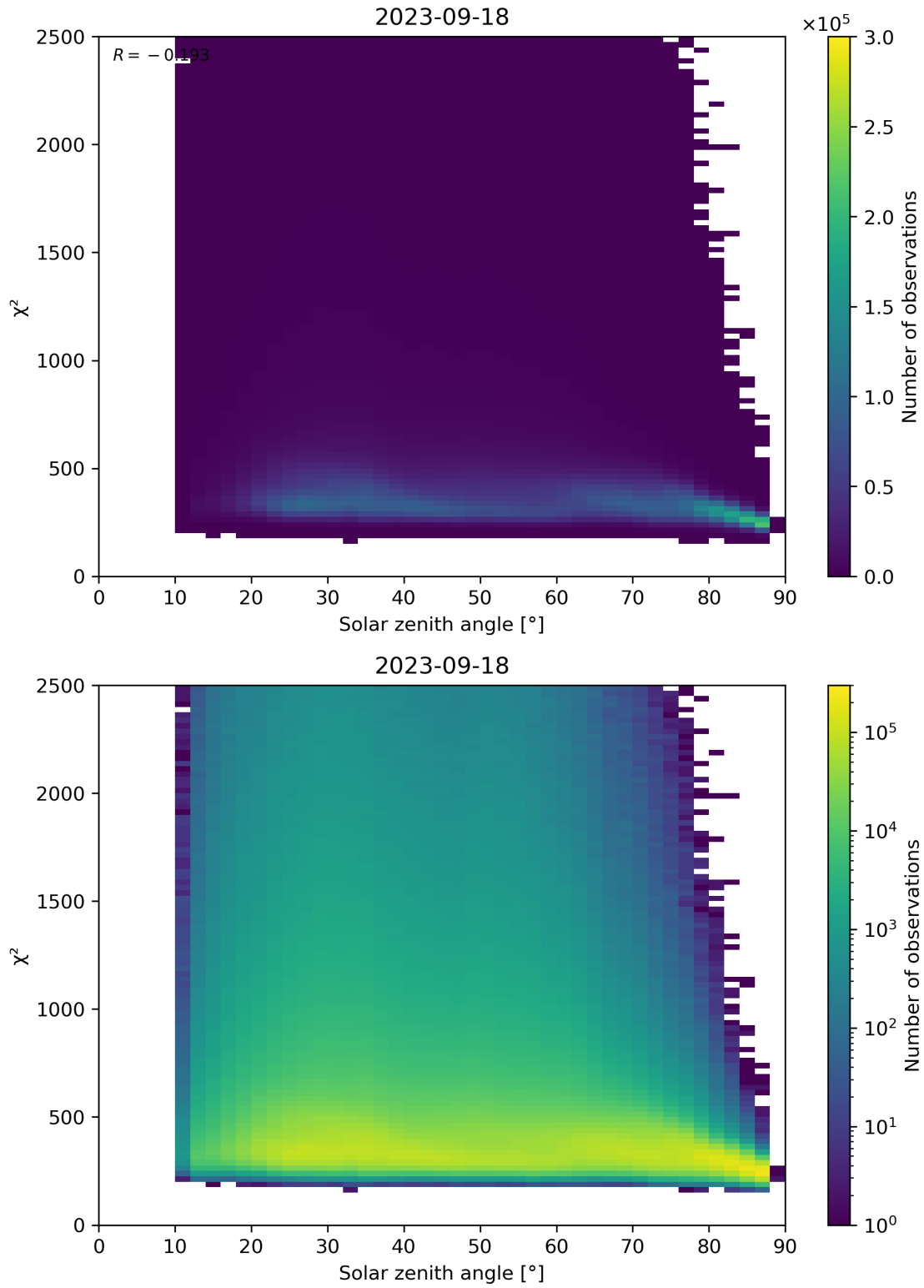
Figure 148: Scatter density plot of “Solar zenith angle” against “ \chi^2 ” for 2023-09-17 to 2023-09-19.
