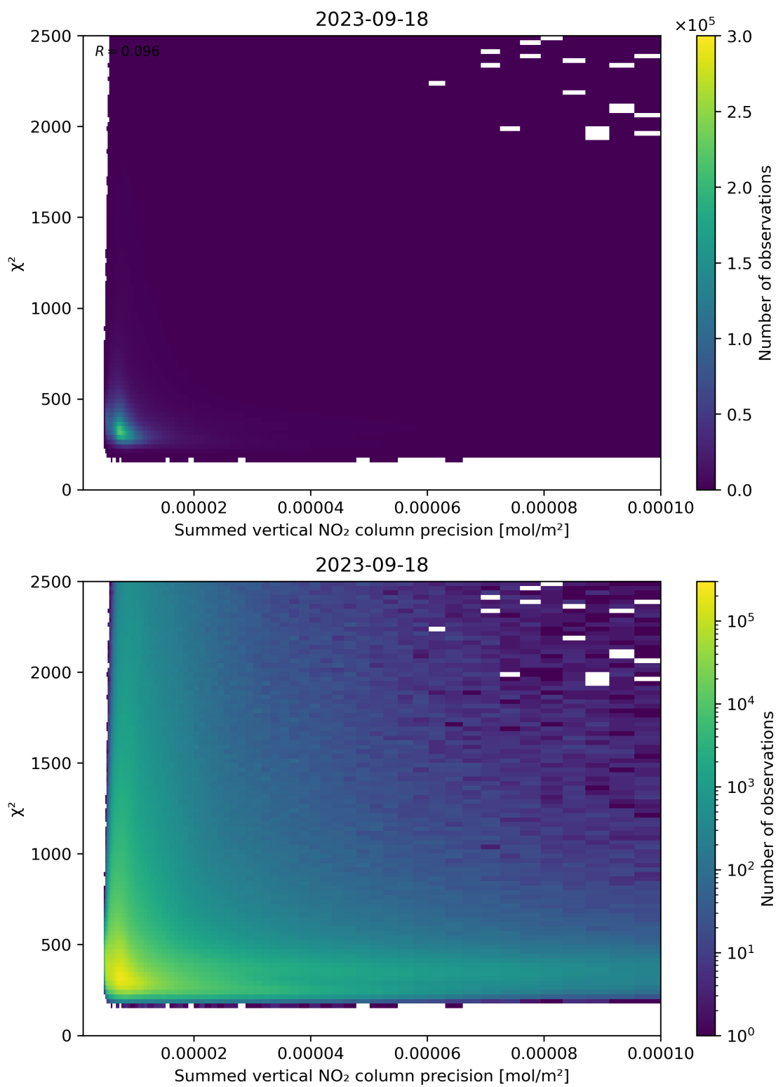
Figure 107: Scatter density plot of “Summed vertical NO 2 column precision” against “ \chi^2 ” for 2023-09-17 to 2023-09-19.
