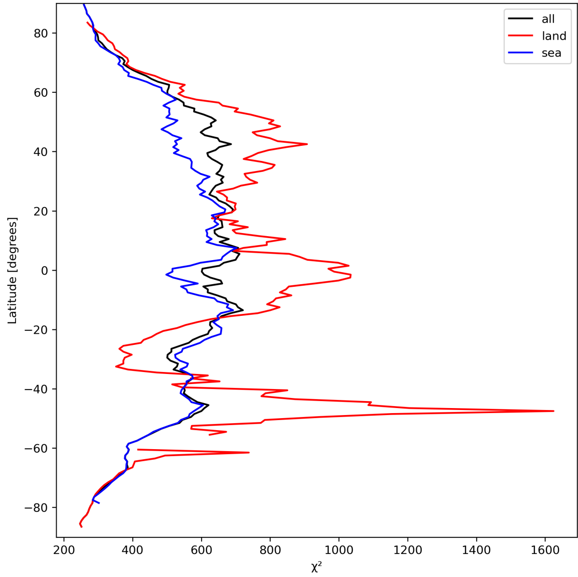
Figure 25: Zonal average of “ \chi^2 ” for 2023-09-17 to 2023-09-19.
