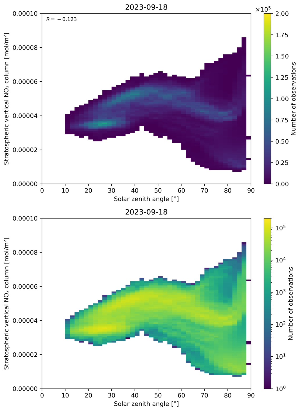
Figure 150: Scatter density plot of “Solar zenith angle” against “Stratospheric vertical NO 2 column” for 2023-09-17 to 2023-09-19.
