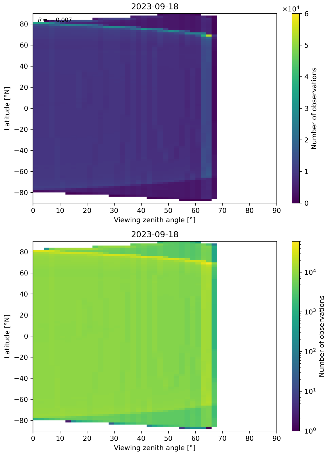
Figure 163: Scatter density plot of “Viewing zenith angle” against “Latitude” for 2023-09-17 to 2023-09-19.
