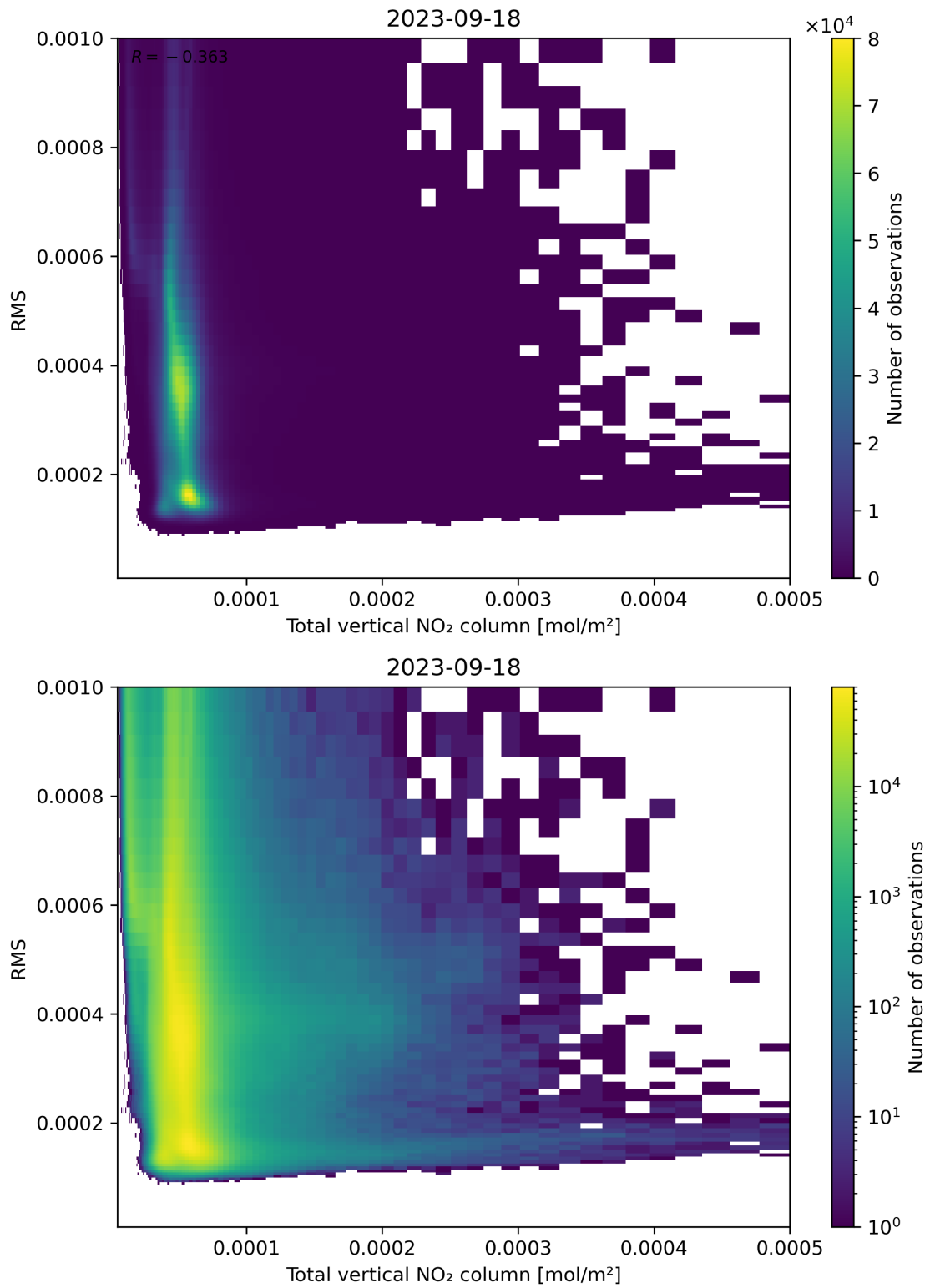
Figure 120: Scatter density plot of “Total vertical NO 2 column” against “RMS” for 2023-09-17 to 2023-09-19.
