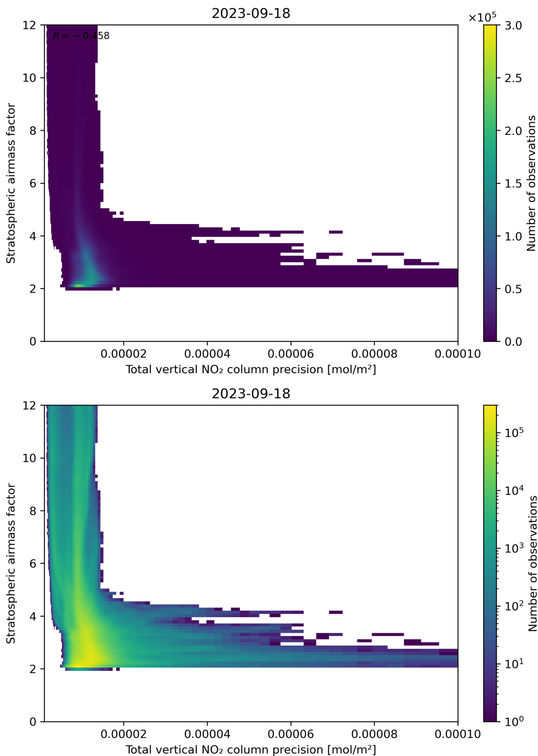
Figure 115: Scatter density plot of “Total vertical NO 2 column precision” against “Stratospheric air mass factor” for 2023-09-17 to 2023-09-19.
