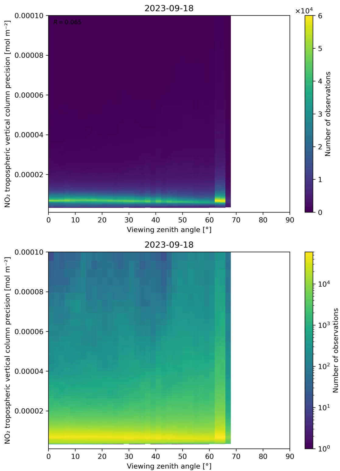
Figure 170: Scatter density plot of “Viewing zenith angle” against “NO 2 tropospheric vertical column precision” for 2023-09-17 to 2023-09-19.
