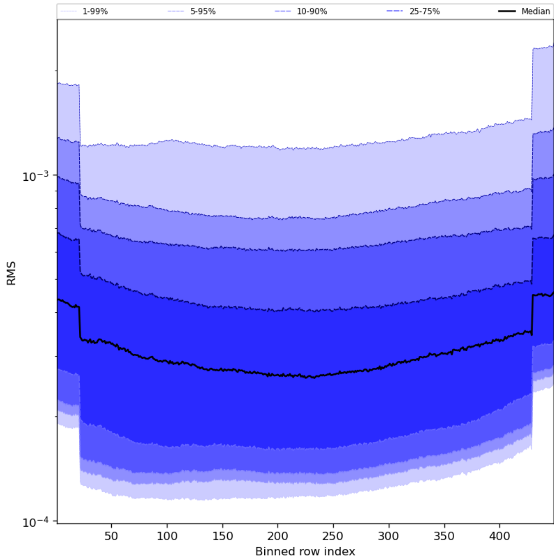
Figure 60: Along track statistics of “RMS” for 2023-09-17 to 2023-09-19
