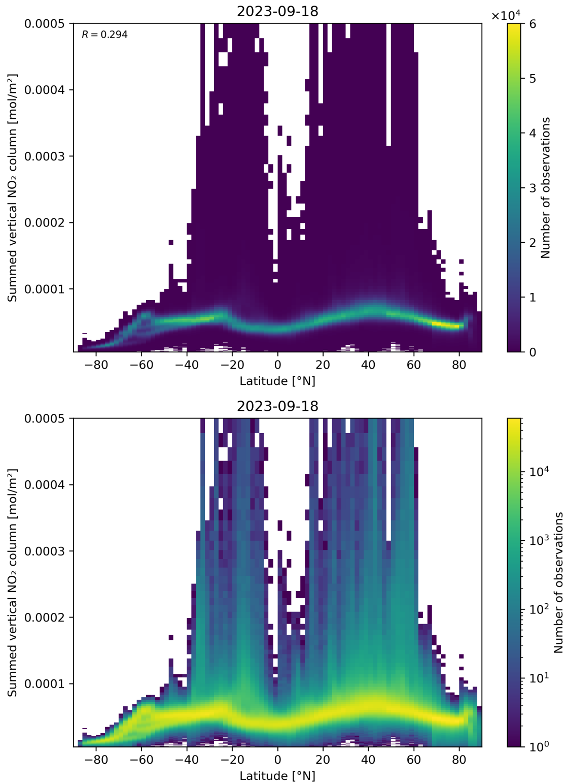
Figure 88: Scatter density plot of “Latitude” against “Summed vertical NO 2 column” for 2023-09-17 to 2023-09-19.
