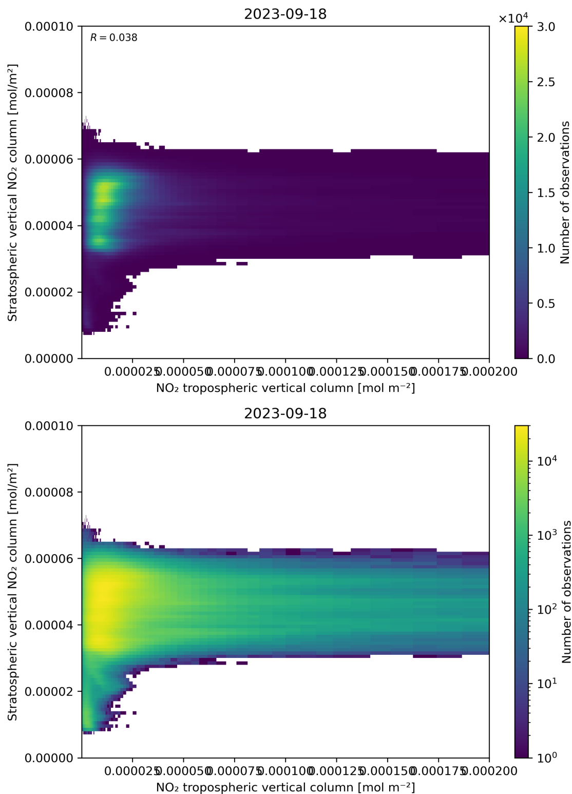
Figure 125: Scatter density plot of “NO 2 tropospheric vertical column” against “Stratospheric vertical NO 2 column” for 2023-09-17 to 2023-09-19.
