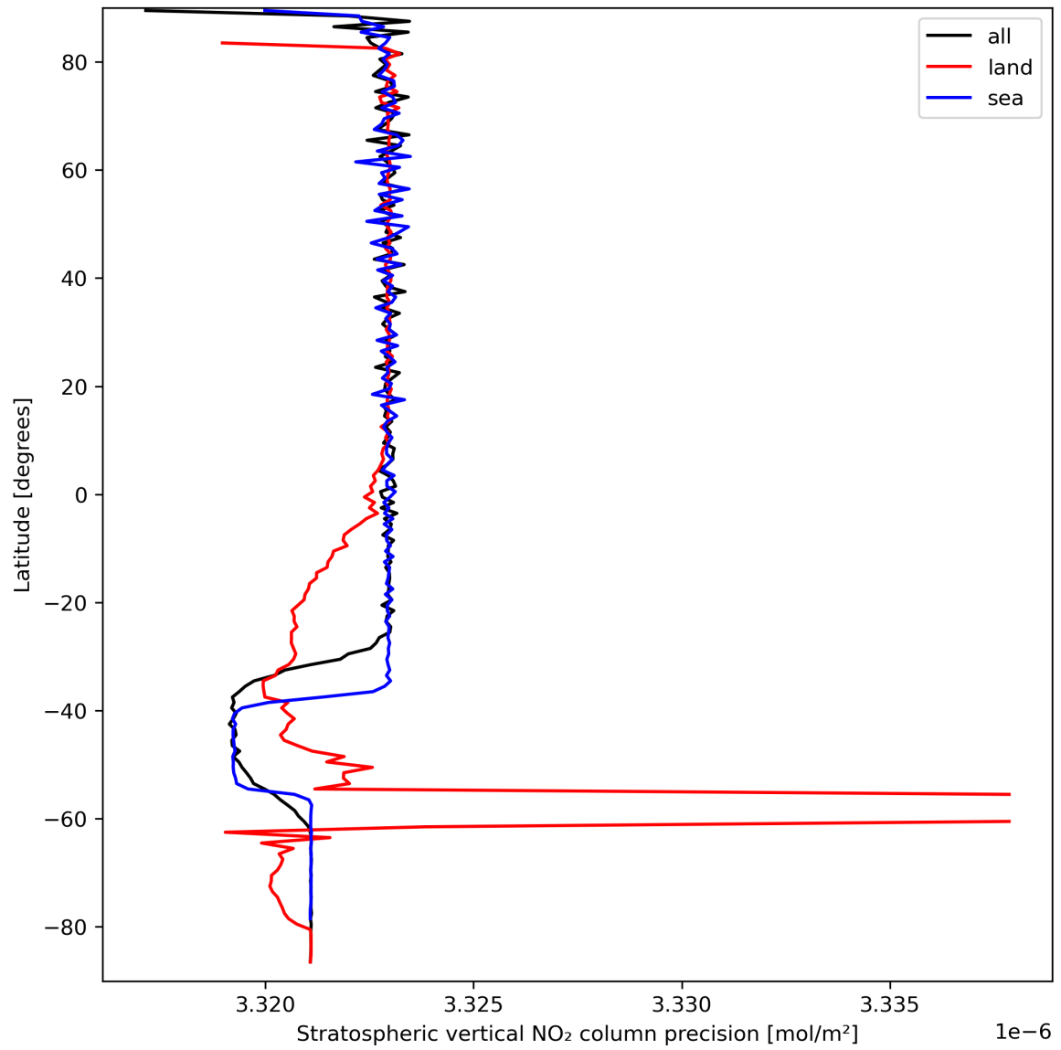
Figure 20: Zonal average of “Stratospheric vertical NO 2 column precision” for 2023-09-17 to 2023-09-19.
