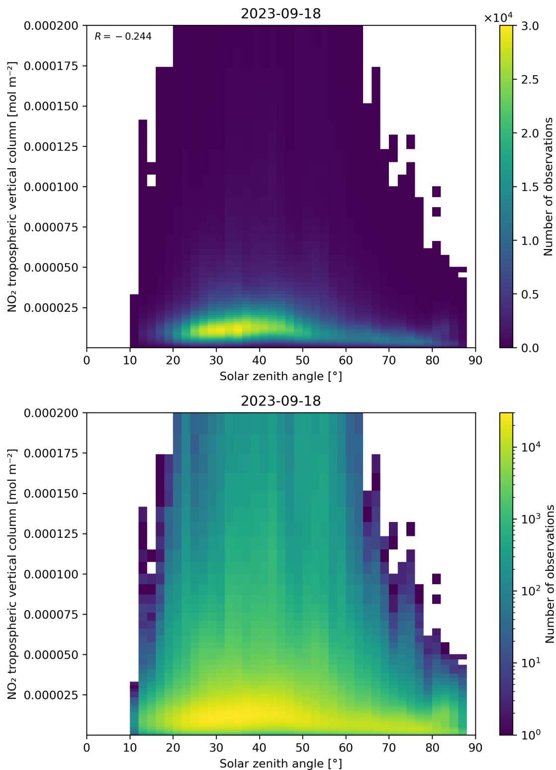
Figure 155: Scatter density plot of “Solar zenith angle” against “NO 2 tropospheric vertical column” for 2023-09-17 to 2023-09-19.
