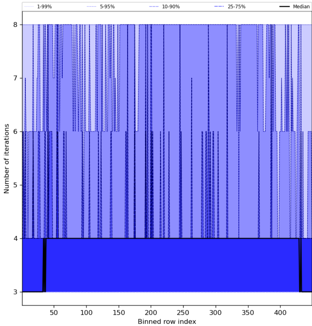
Figure 51: Along track statistics of “Number of iterations” for 2023-09-17 to 2023-09-19
