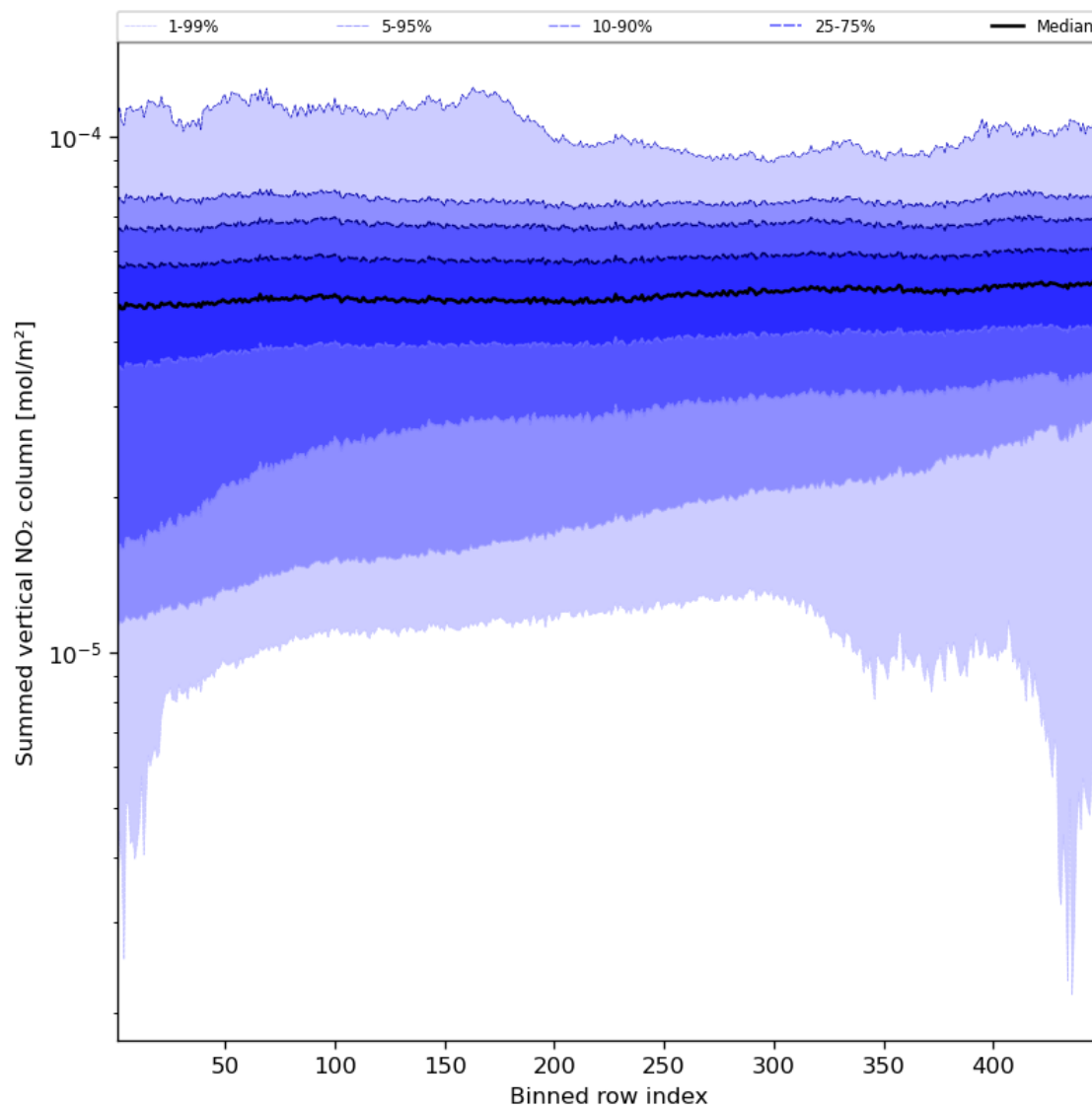
Figure 57: Along track statistics of “Summed vertical NO 2 column” for 2023-09-17 to 2023-09-19
