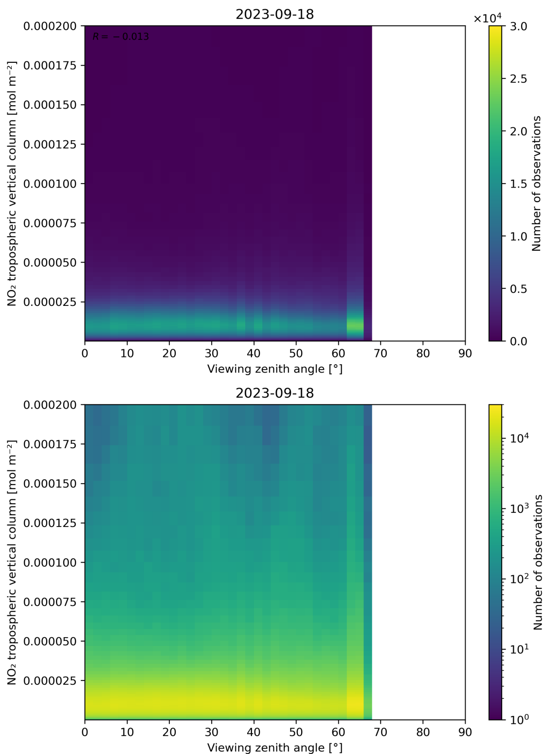
Figure 169: Scatter density plot of “Viewing zenith angle” against “NO 2 tropospheric vertical column” for 2023-09-17 to 2023-09-19.
