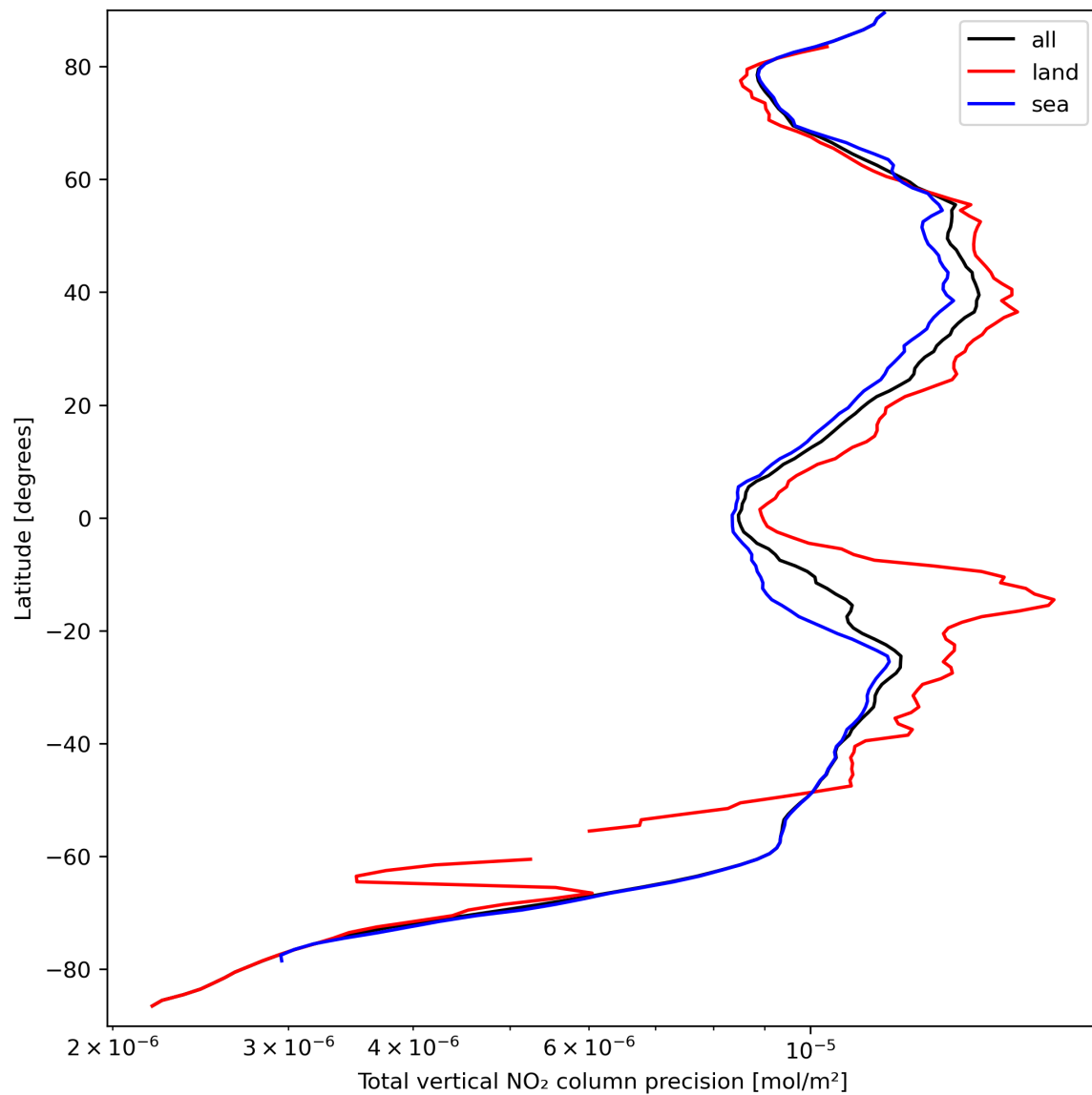
Figure 22: Zonal average of “Total vertical NO 2 column precision” for 2023-09-17 to 2023-09-19.
