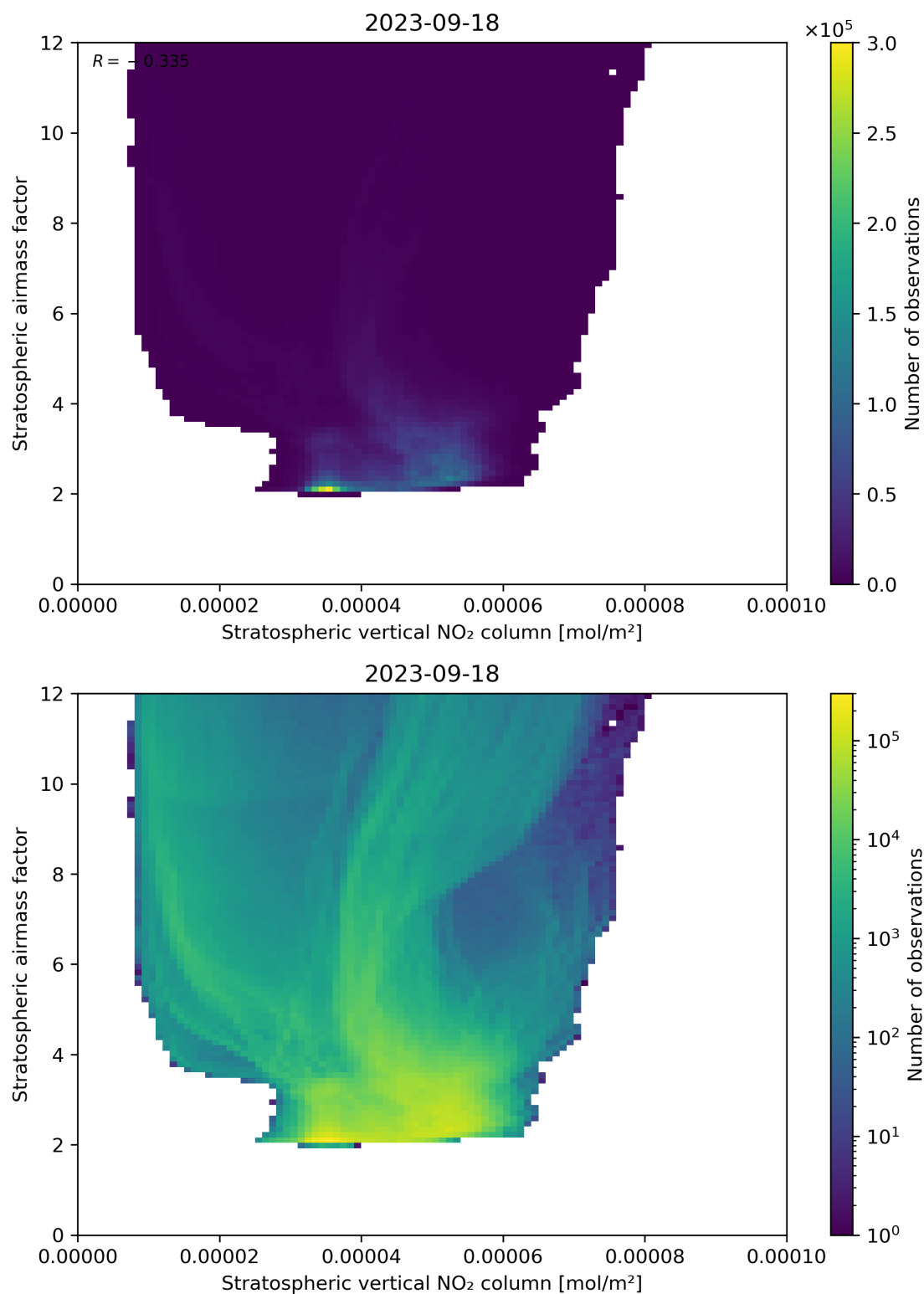
Figure 96: Scatter density plot of “Stratospheric vertical NO 2 column” against “Stratospheric airmass factor” for 2023-09-17 to 2023-09-19.
