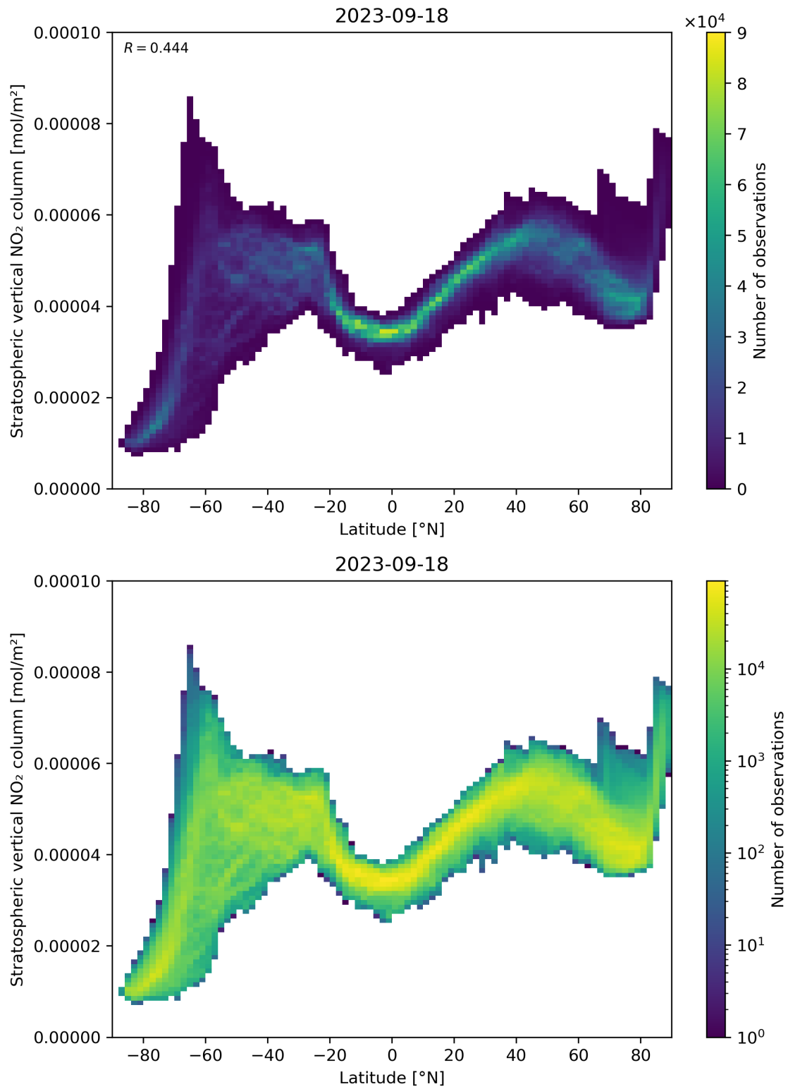
Figure 87: Scatter density plot of “Latitude” against “Stratospheric vertical NO 2 column” for 2023-09-17 to 2023-09-19.
