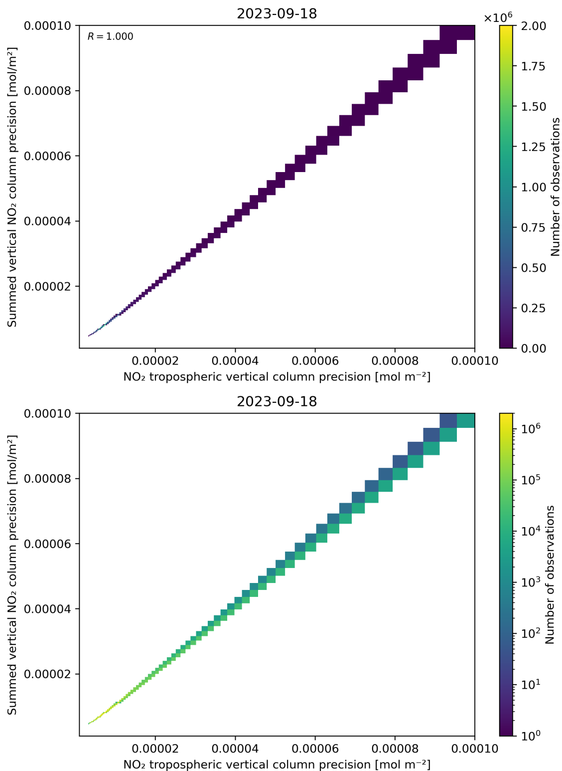
Figure 137: Scatter density plot of “NO 2 tropospheric vertical column precision” against “Summed vertical NO 2 column precision” for 2023-09-17 to 2023-09-19.
