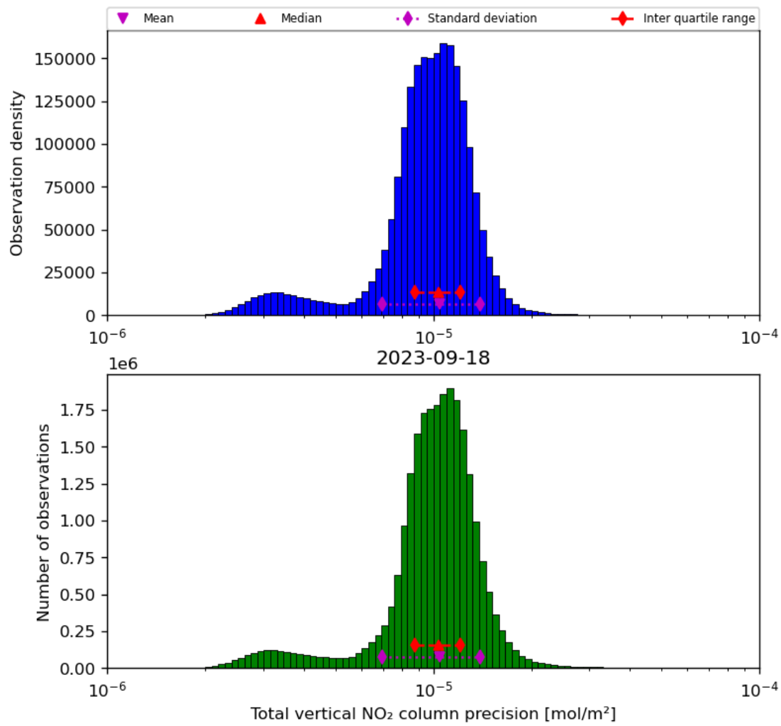
Figure 39: Histogram of "Total vertical NO 2 column precision" for 2023-09-17 to 2023-09-19
