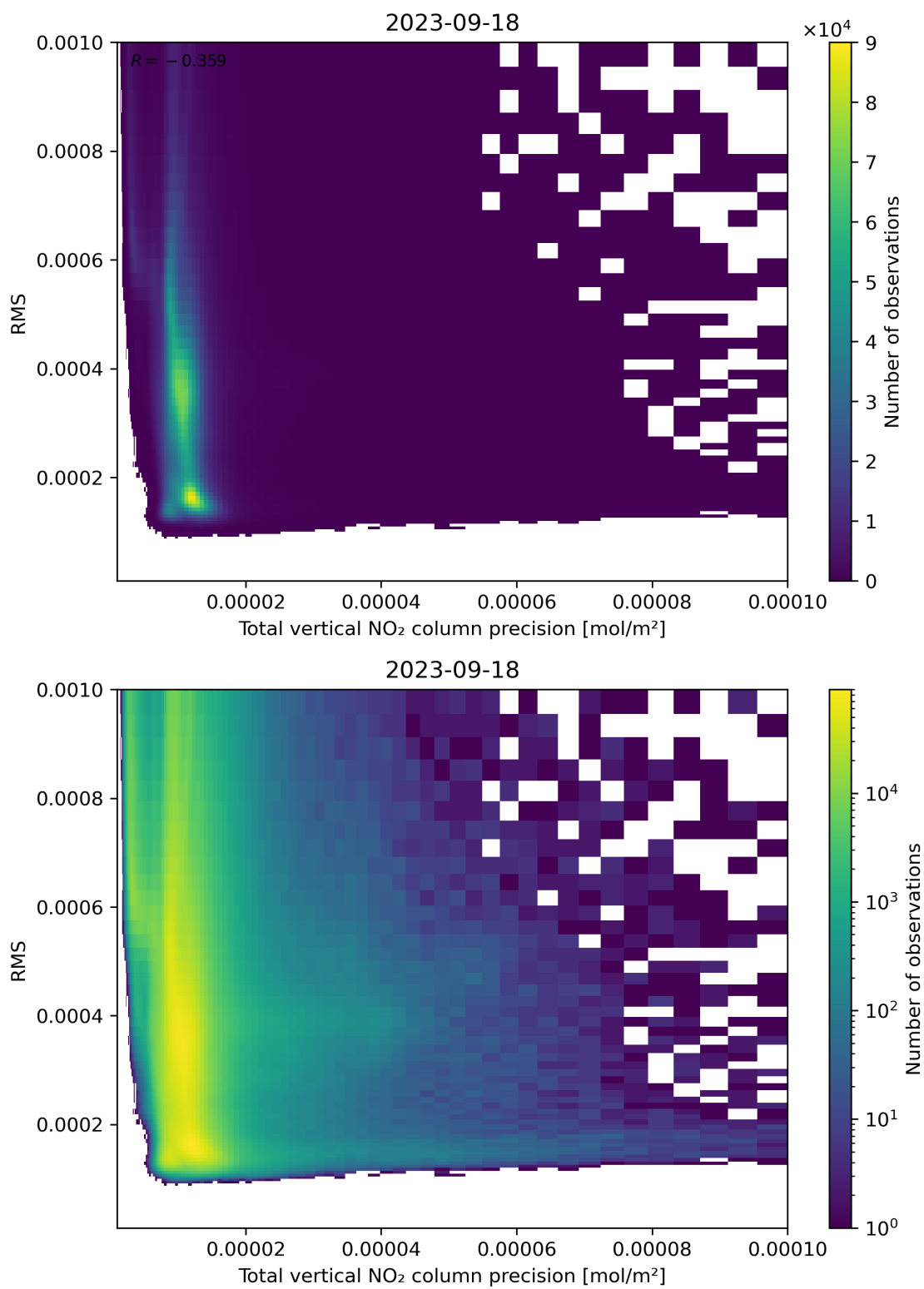
Figure 119: Scatter density plot of “Total vertical NO 2 column precision” against “RMS” for 2023-09-17 to 2023-09-19.
