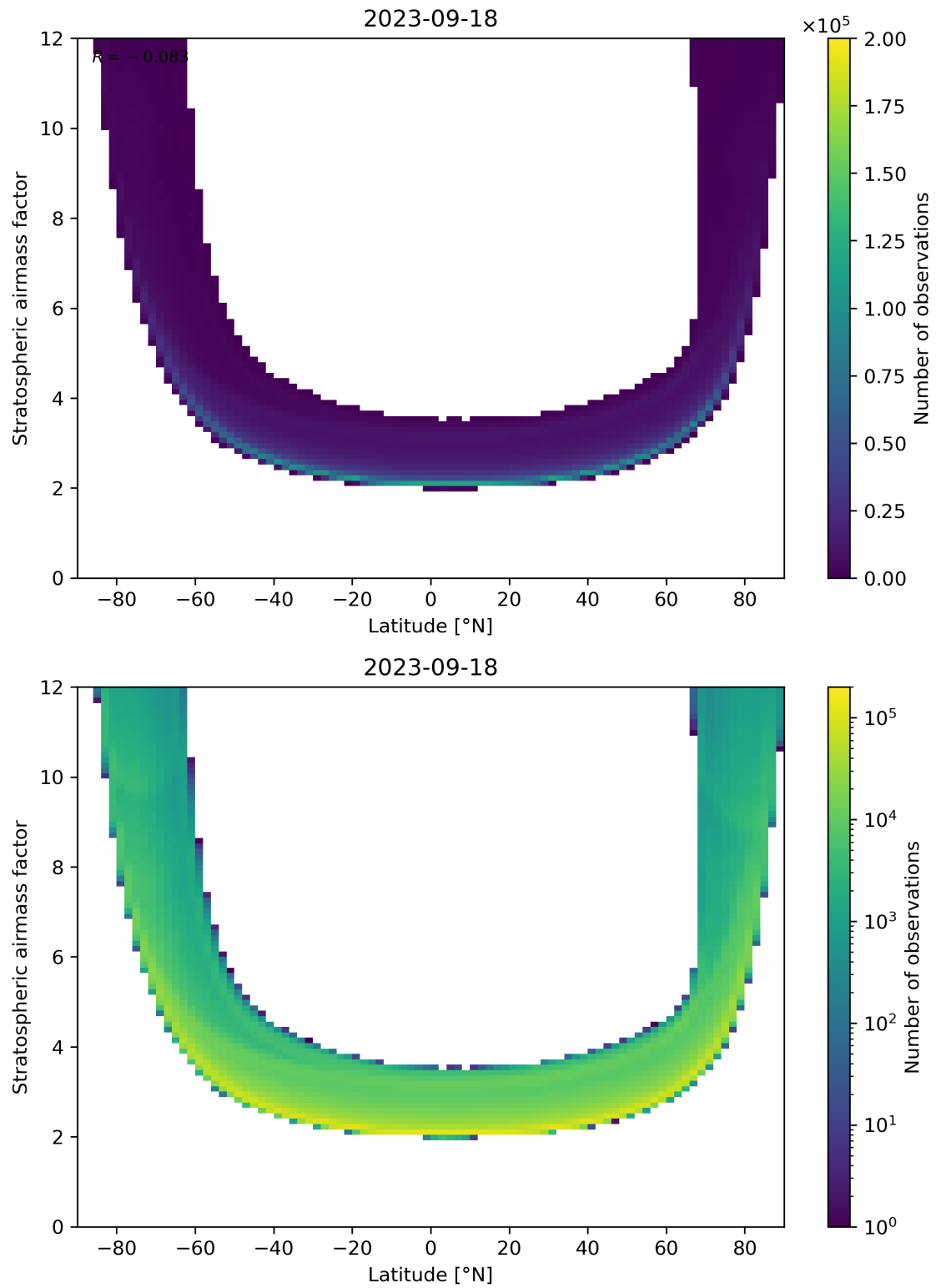
Figure 83: Scatter density plot of “Latitude” against “Stratospheric air mass factor” for 2023-09-17 to 2023-09-19.
