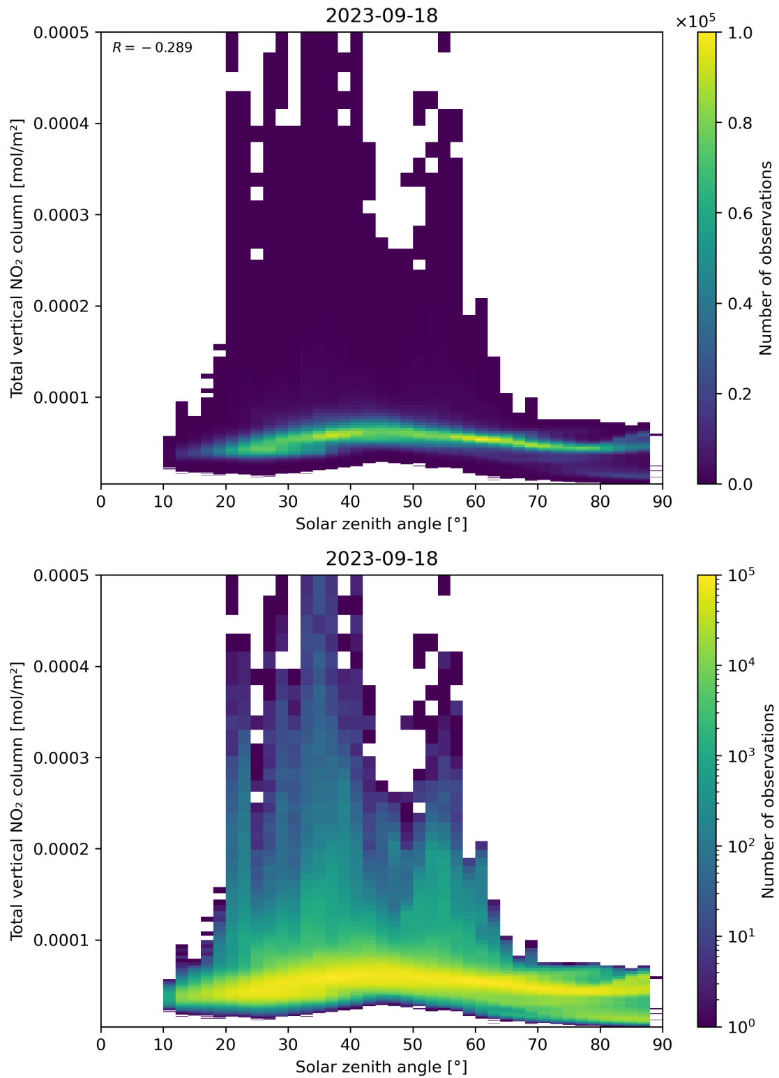
Figure 153: Scatter density plot of “Solar zenith angle” against “Total vertical NO 2 column” for 2023-09-17 to 2023-09-19.
