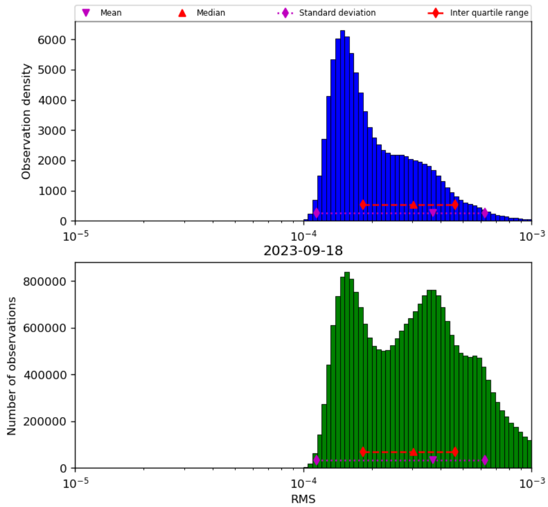
Figure 43: Histogram of “RMS” for 2023-09-17 to 2023-09-19
