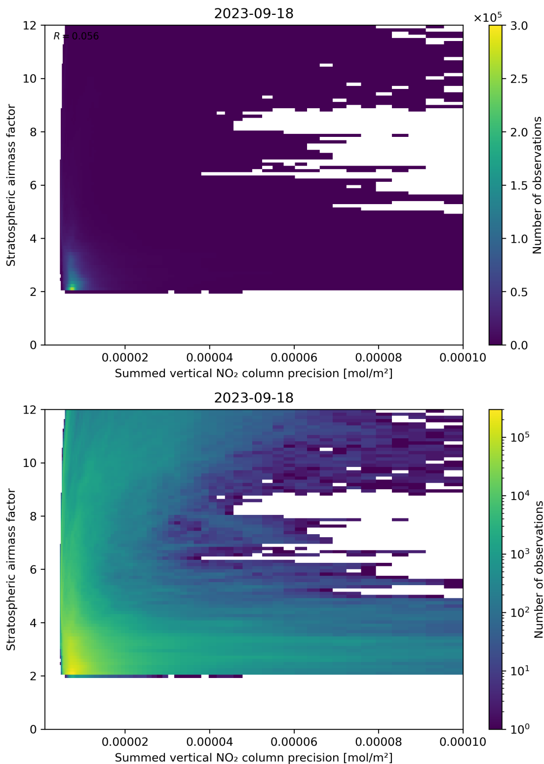
Figure 106: Scatter density plot of “Summed vertical NO 2 column precision” against “Stratospheric airmass factor” for 2023-09-17 to 2023-09-19.
