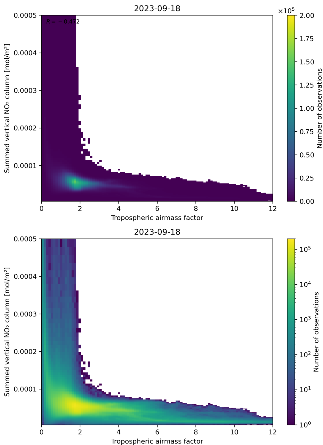
Figure 75: Scatter density plot of “Tropospheric air mass factor” against “Summed vertical NO 2 column” for 2023-09-17 to 2023-09-19.
