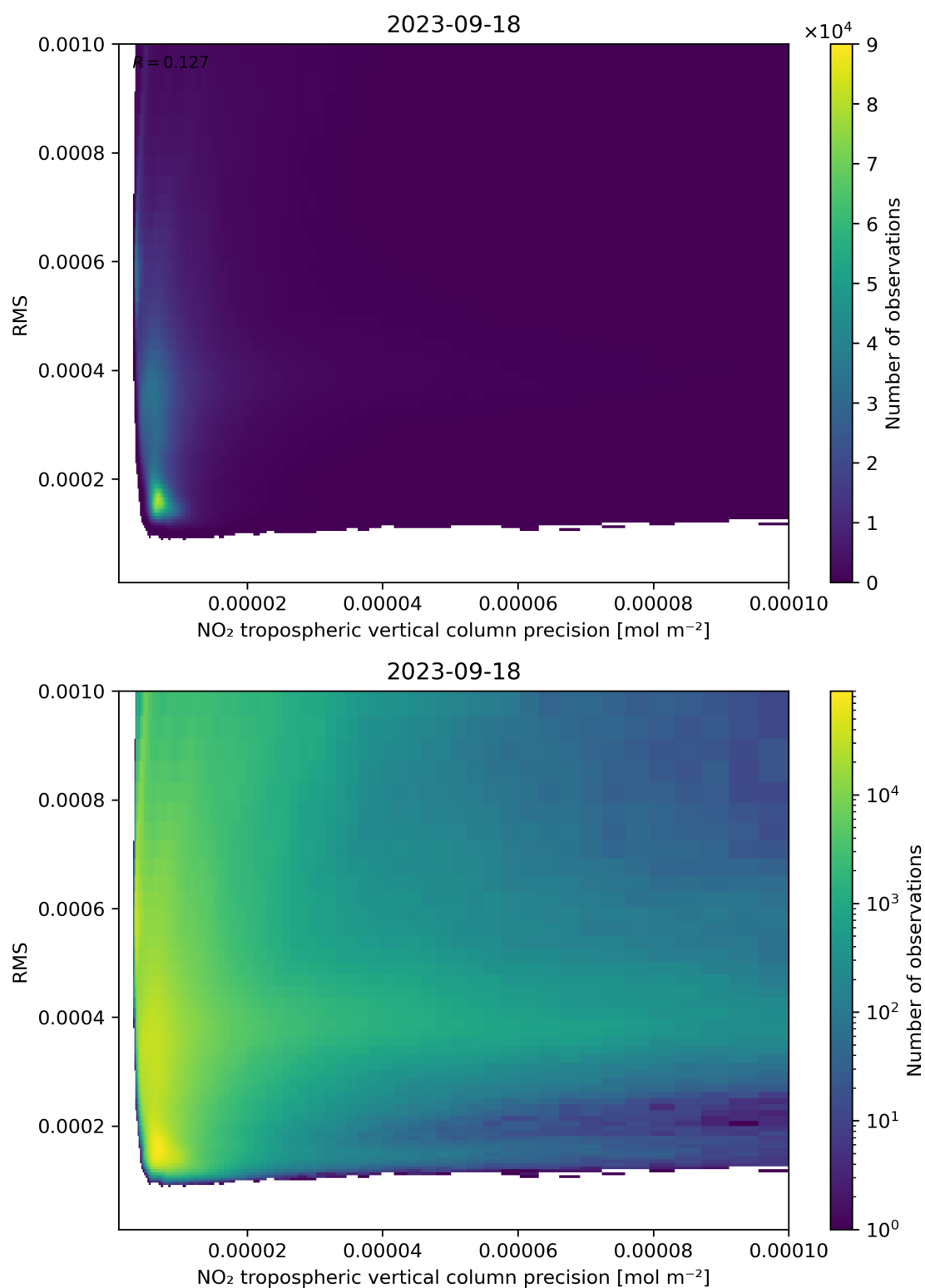
Figure 140: Scatter density plot of “NO 2 tropospheric vertical column precision” against “RMS” for 2023-09-17 to 2023-09-19.
