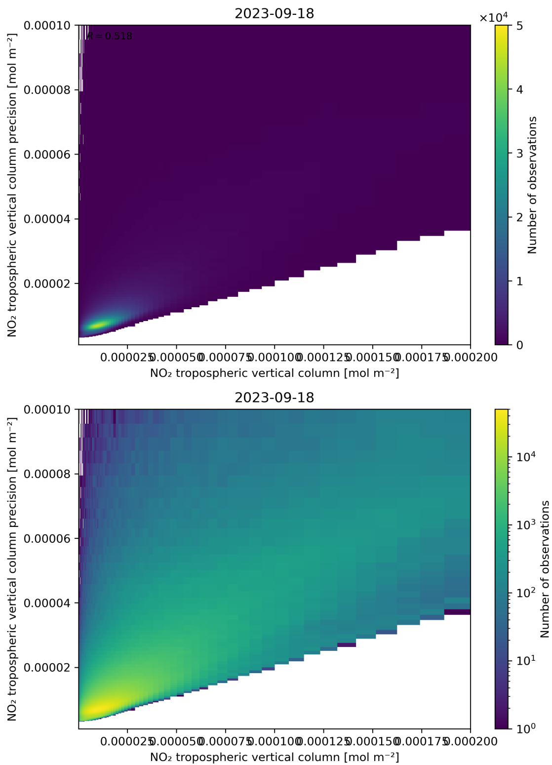
Figure 130: Scatter density plot of “NO 2 tropospheric vertical column” against “NO 2 tropospheric vertical column precision” for 2023-09-17 to 2023-09-19.
