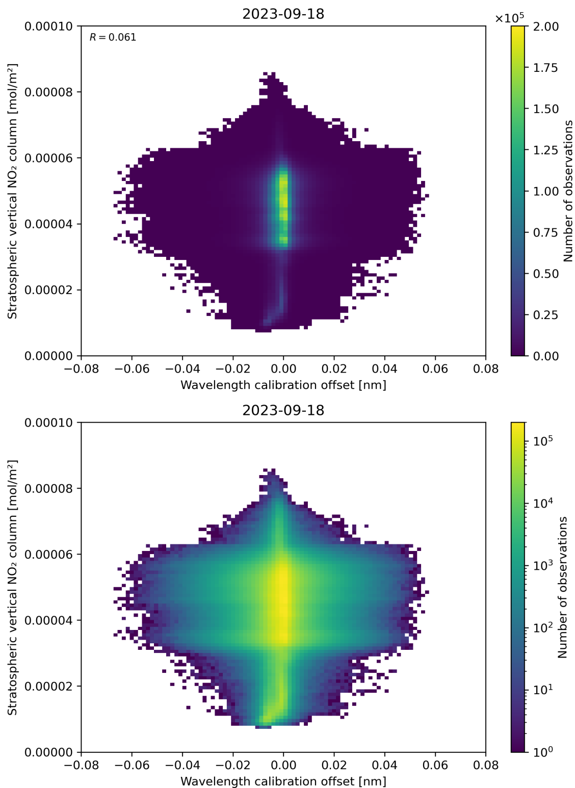
Figure 176: Scatter density plot of “Wavelength calibration offset” against “Stratospheric vertical NO 2 column” for 2023-09-17 to 2023-09-19.
