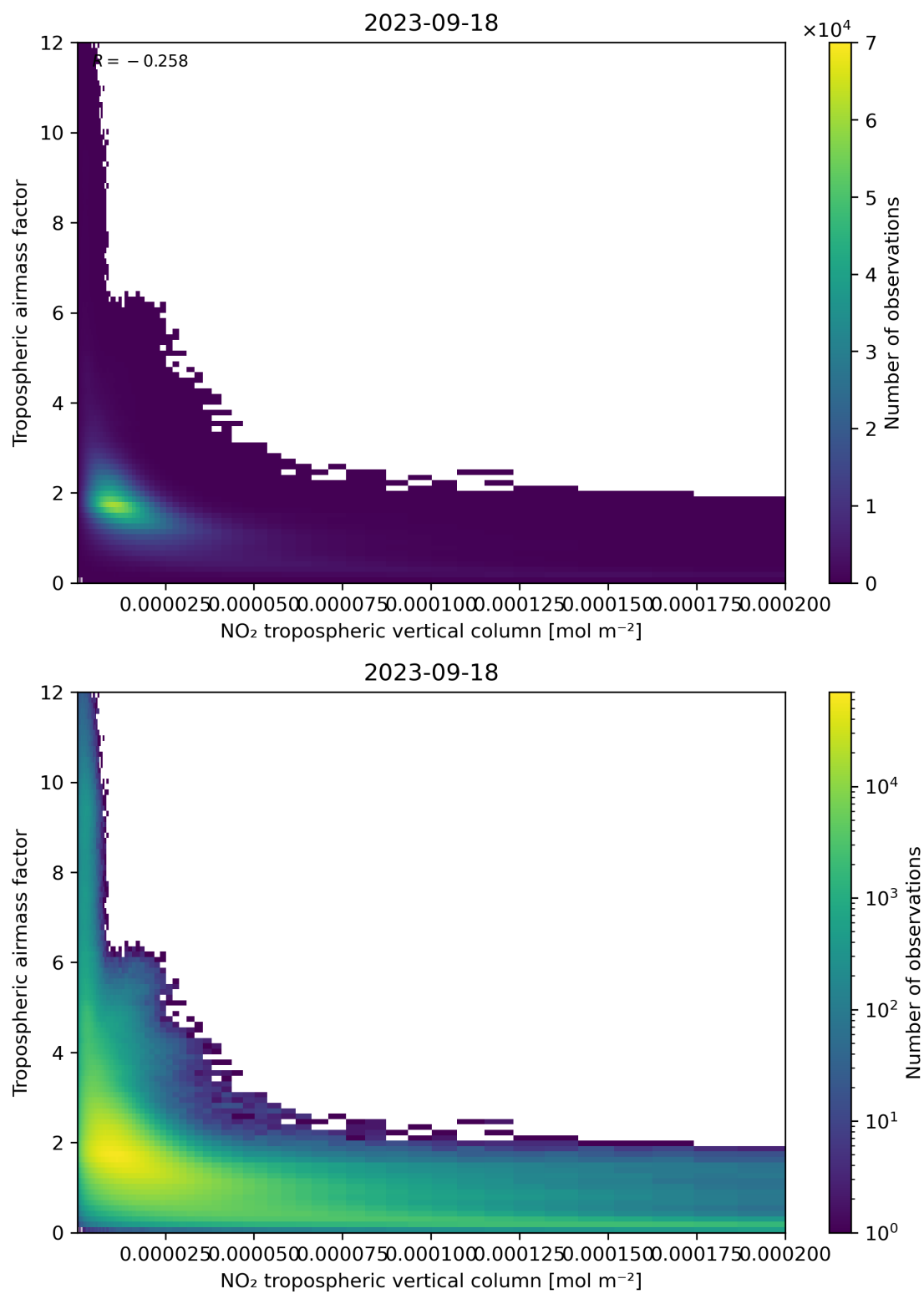
Figure 123: Scatter density plot of “NO 2 tropospheric vertical column” against “Tropospheric air mass factor” for 2023-09-17 to 2023-09-19.
