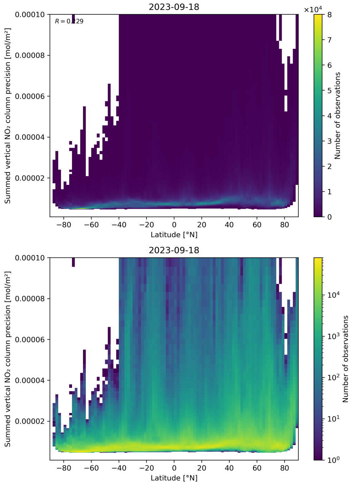
Figure 89: Scatter density plot of “Latitude” against “Summed vertical NO 2 column precision” for 2023-09-17 to 2023-09-19.
