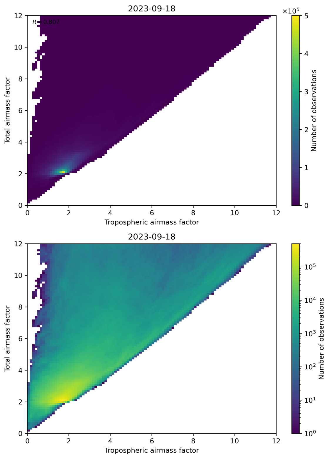
Figure 72: Scatter density plot of “Tropospheric airmass factor” against “Total airmass factor” for 2023-09-17 to 2023-09-19.
