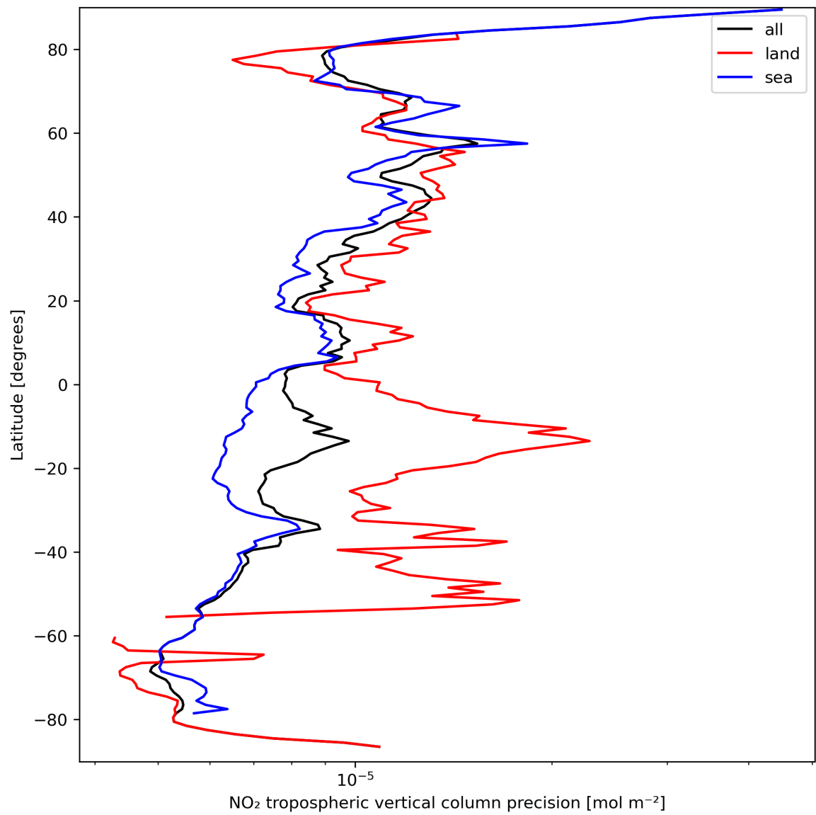
Figure 13: Zonal average of “NO 2 tropospheric vertical column precision” for 2023-09-17 to 2023-09-19.
