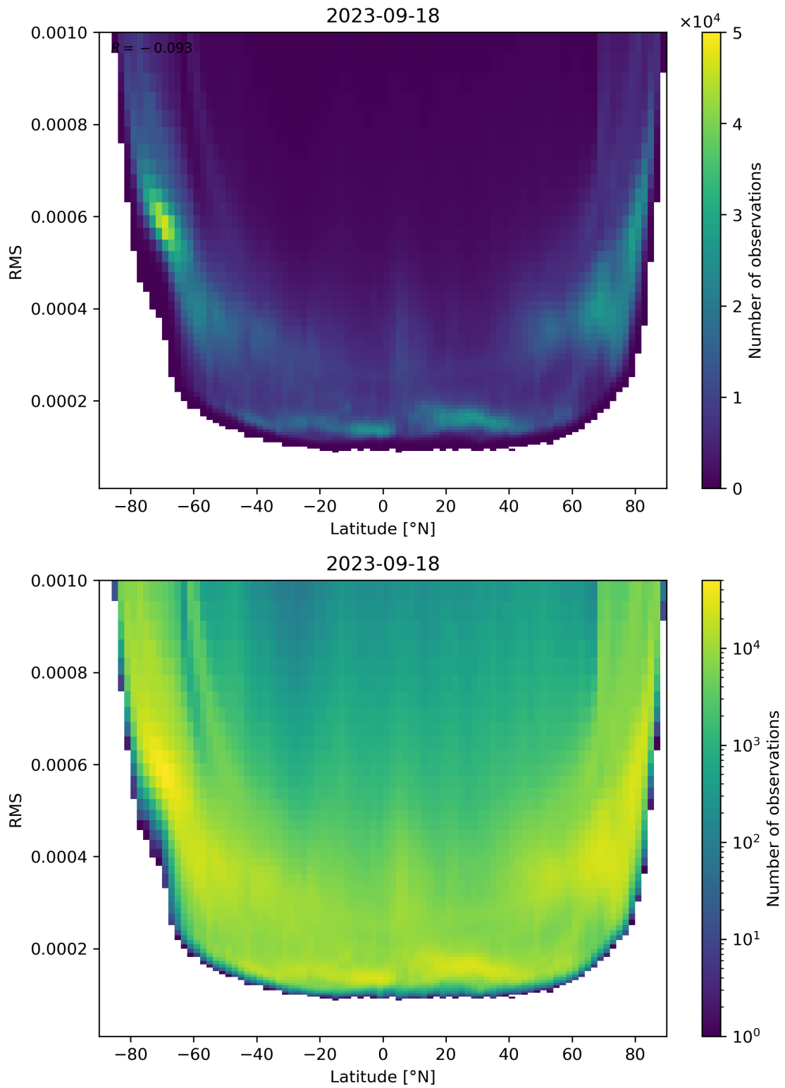
Figure 94: Scatter density plot of “Latitude” against “RMS” for 2023-09-17 to 2023-09-19.
