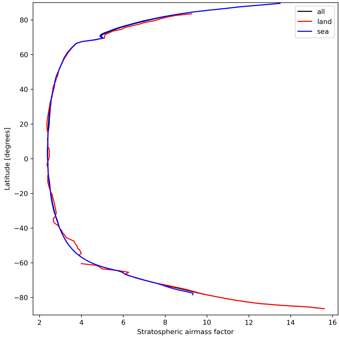
Figure 27: Zonal average of “Stratospheric airmass factor” for 2023-09-17 to 2023-09-19.
