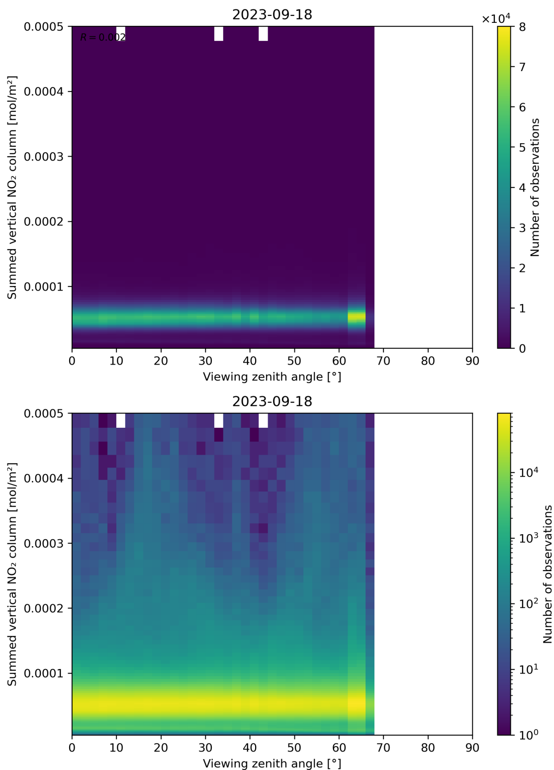
Figure 165: Scatter density plot of “Viewing zenith angle” against “Summed vertical NO 2 column” for 2023-09-17 to 2023-09-19.
