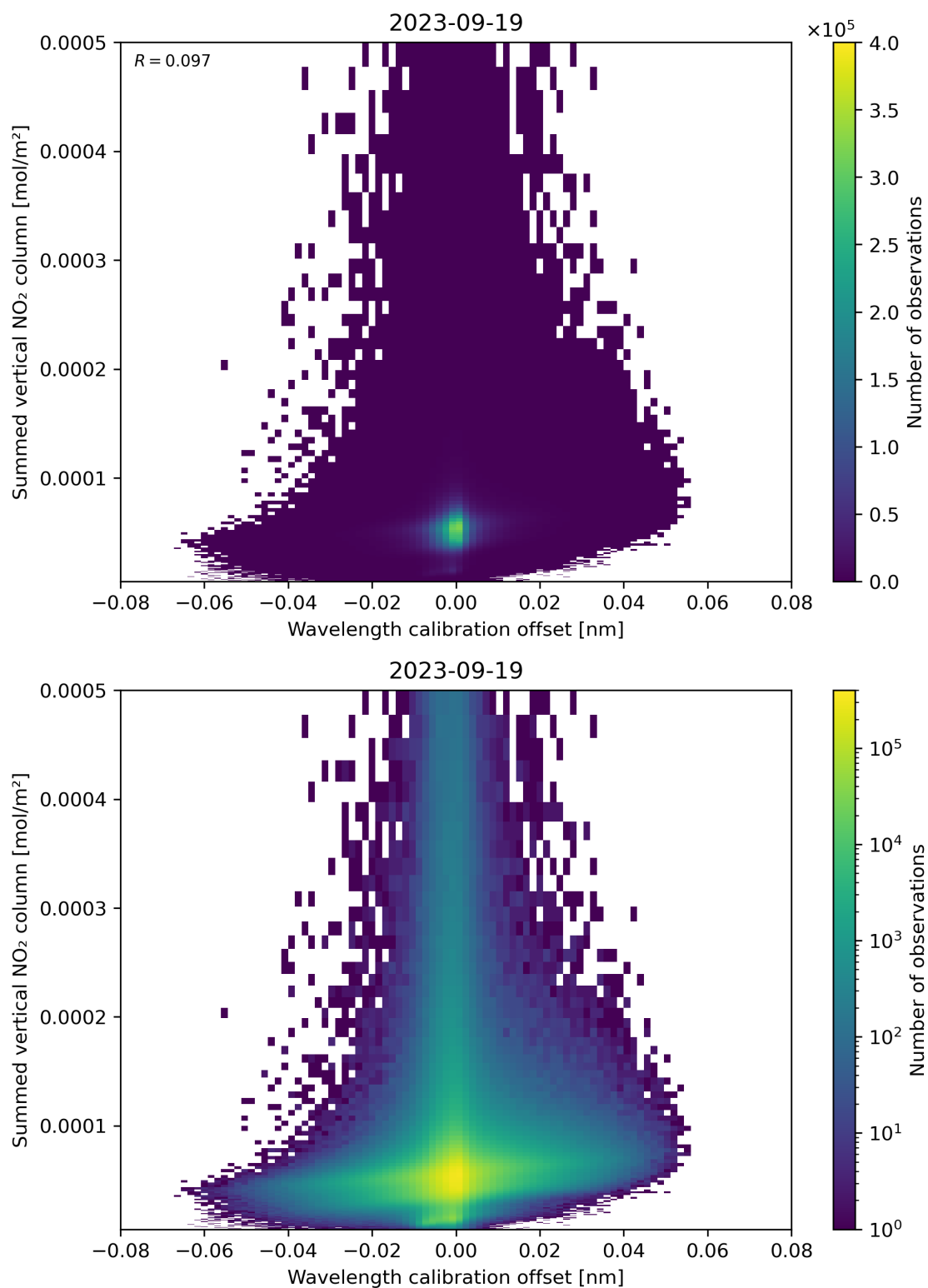
Figure 177: Scatter density plot of “Wavelength calibration offset” against “Summed vertical NO 2 column” for 2023-09-18 to 2023-09-20.
