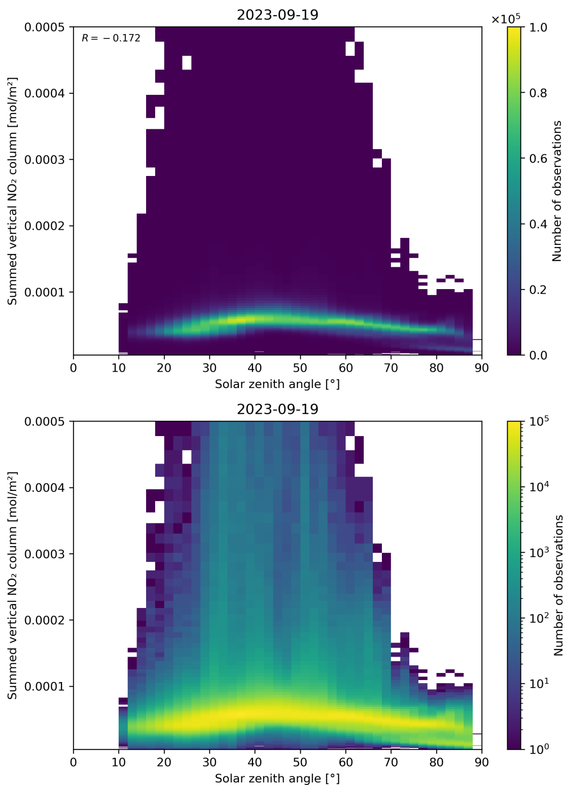
Figure 151: Scatter density plot of “Solar zenith angle” against “Summed vertical NO 2 column” for 2023-09-18 to 2023-09-20.
