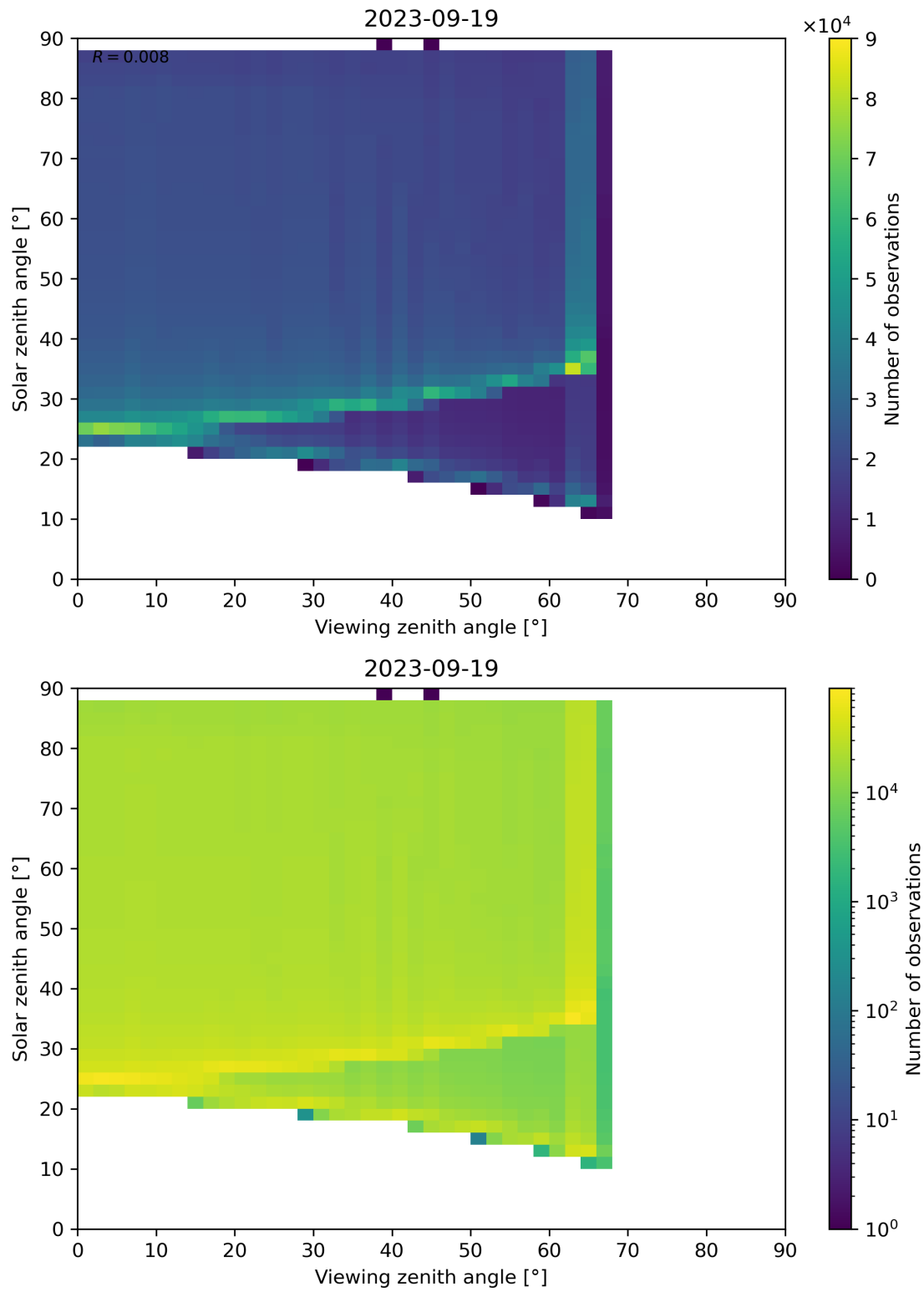
Figure 172: Scatter density plot of “Viewing zenith angle” against “Solar zenith angle” for 2023-09-18 to 2023-09-20.
