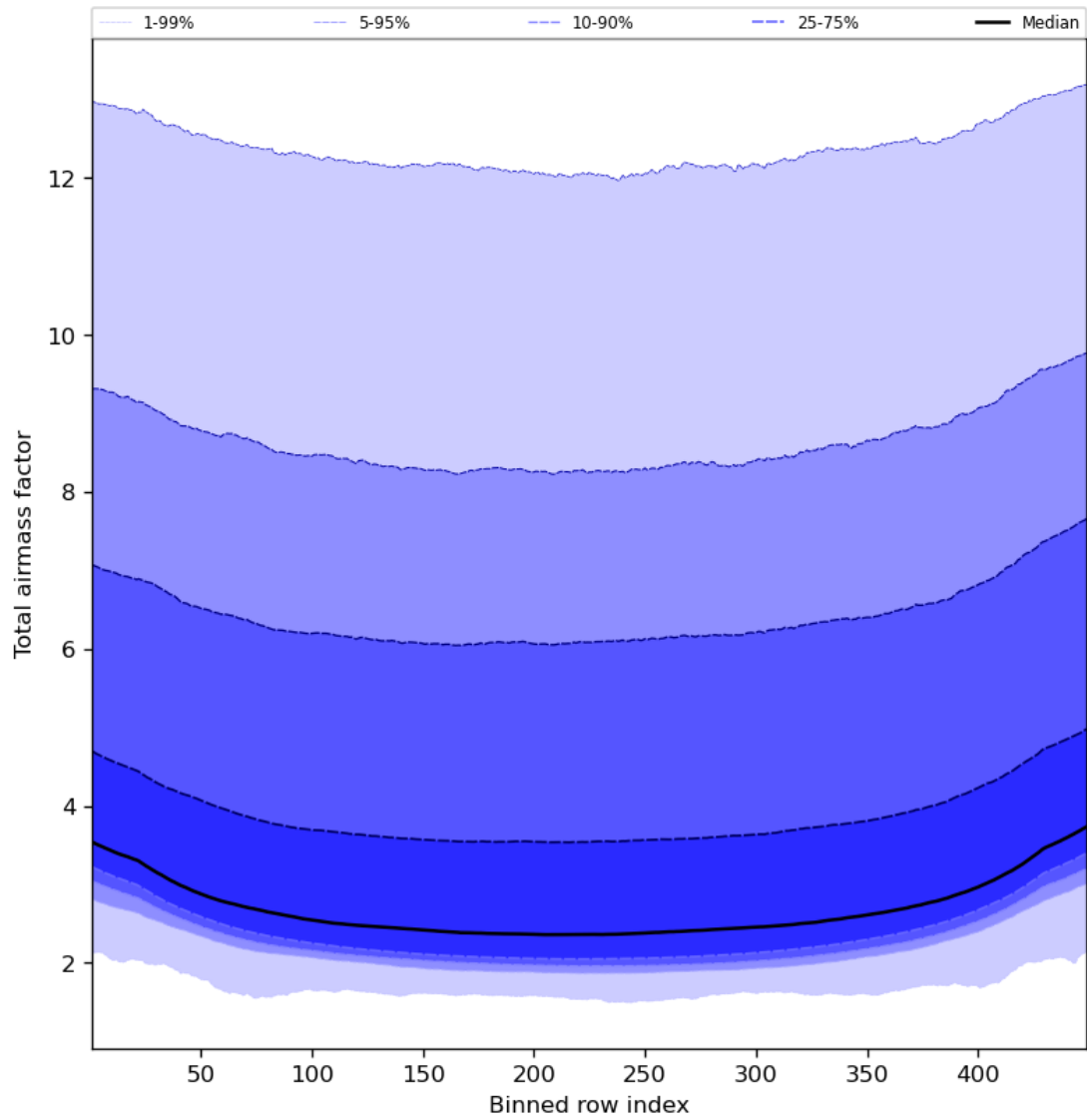
Figure 49: Along track statistics of “Total airmass factor” for 2023-09-18 to 2023-09-20
