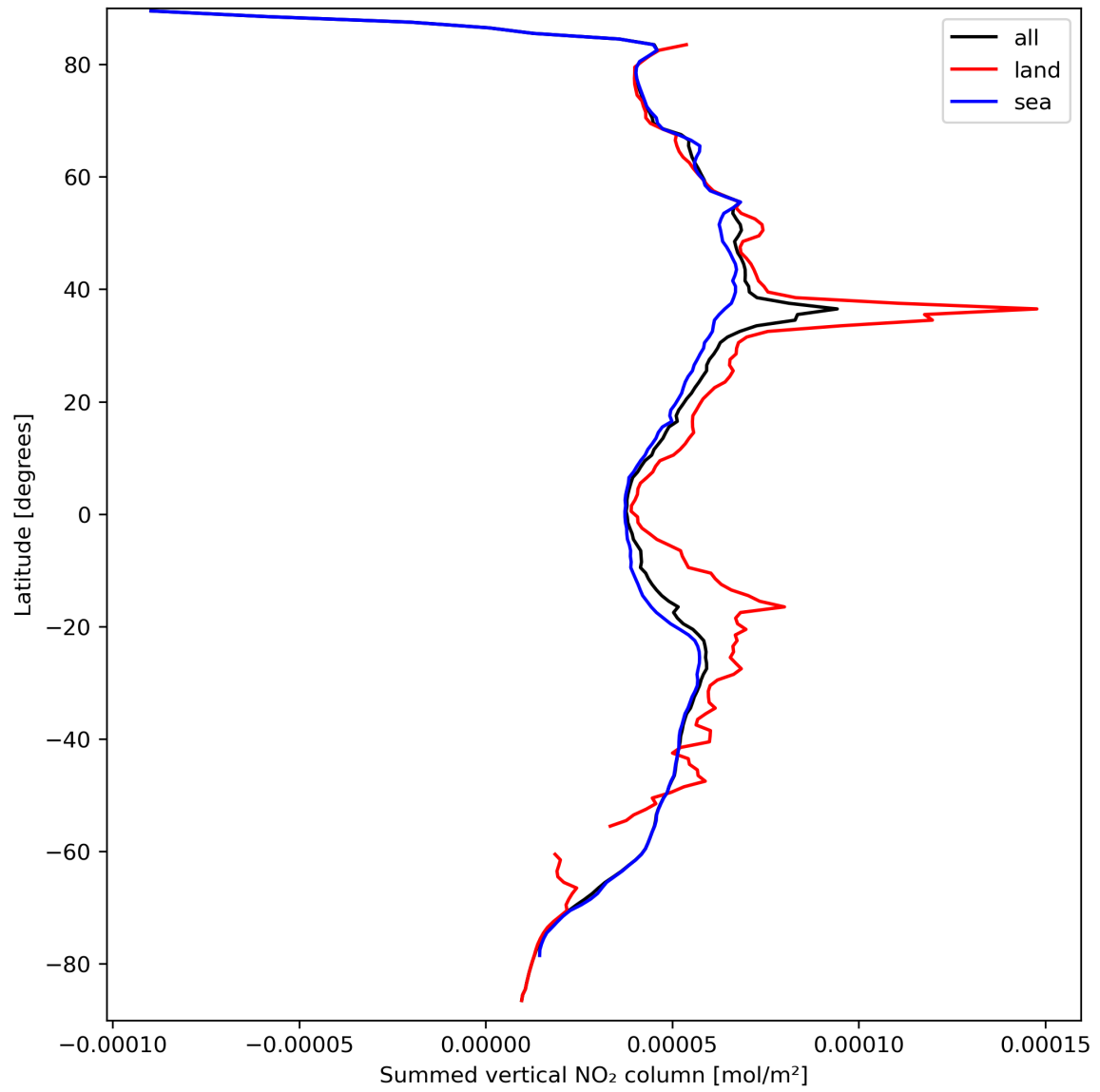
Figure 23: Zonal average of “Summed vertical NO 2 column” for 2023-09-18 to 2023-09-20.
