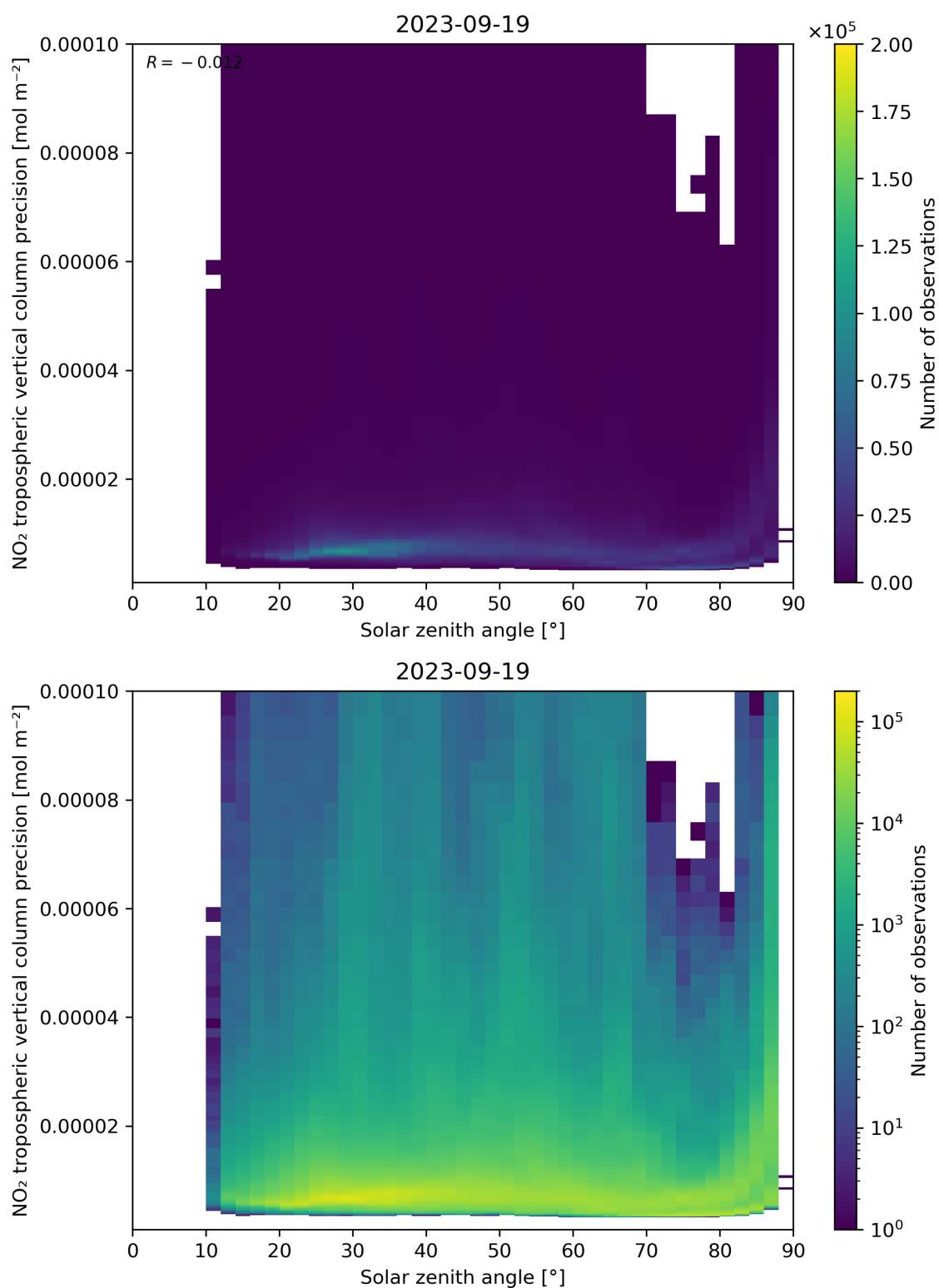
Figure 156: Scatter density plot of “Solar zenith angle” against “NO 2 tropospheric vertical column precision” for 2023-09-18 to 2023-09-20.
