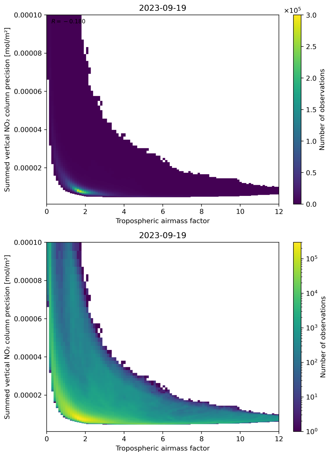
Figure 76: Scatter density plot of “Tropospheric airmass factor” against “Summed vertical NO 2 column precision” for 2023-09-18 to 2023-09-20.
