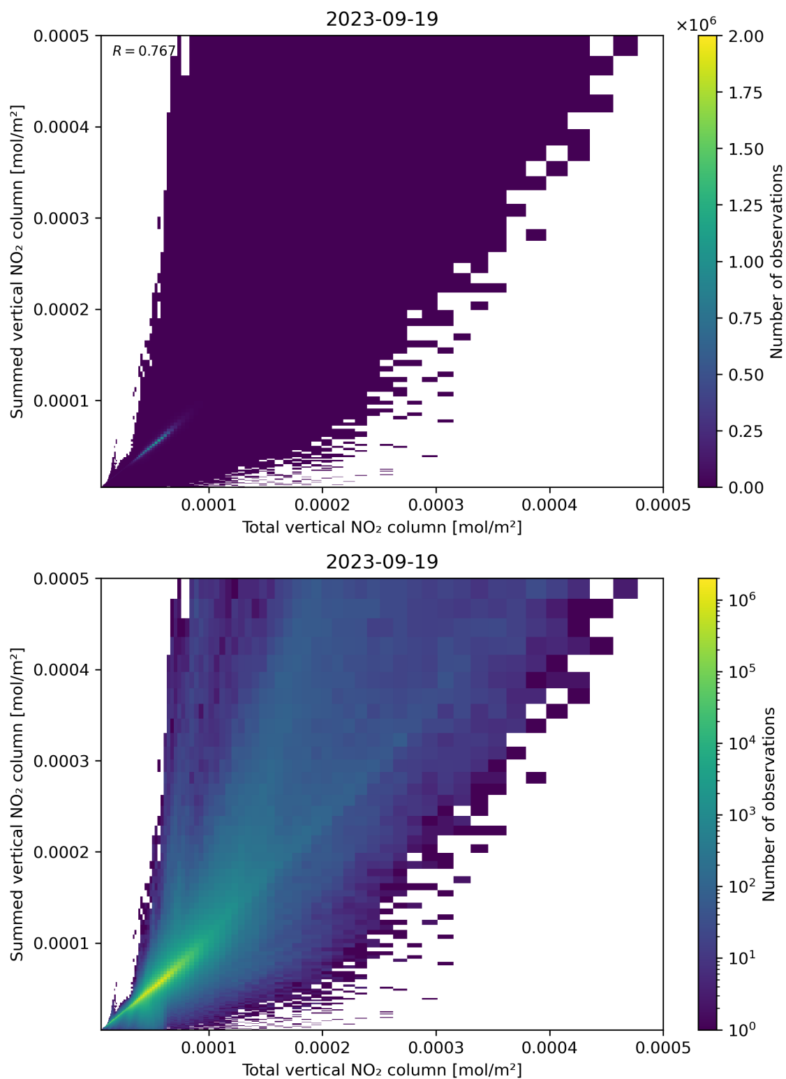
Figure 112: Scatter density plot of “Total vertical NO 2 column” against “Summed vertical NO 2 column” for 2023-09-18 to 2023-09-20.
