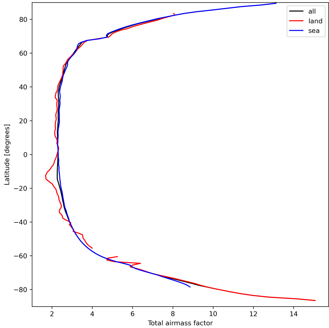
Figure 15: Zonal average of “Total airmass factor” for 2023-09-18 to 2023-09-20.
