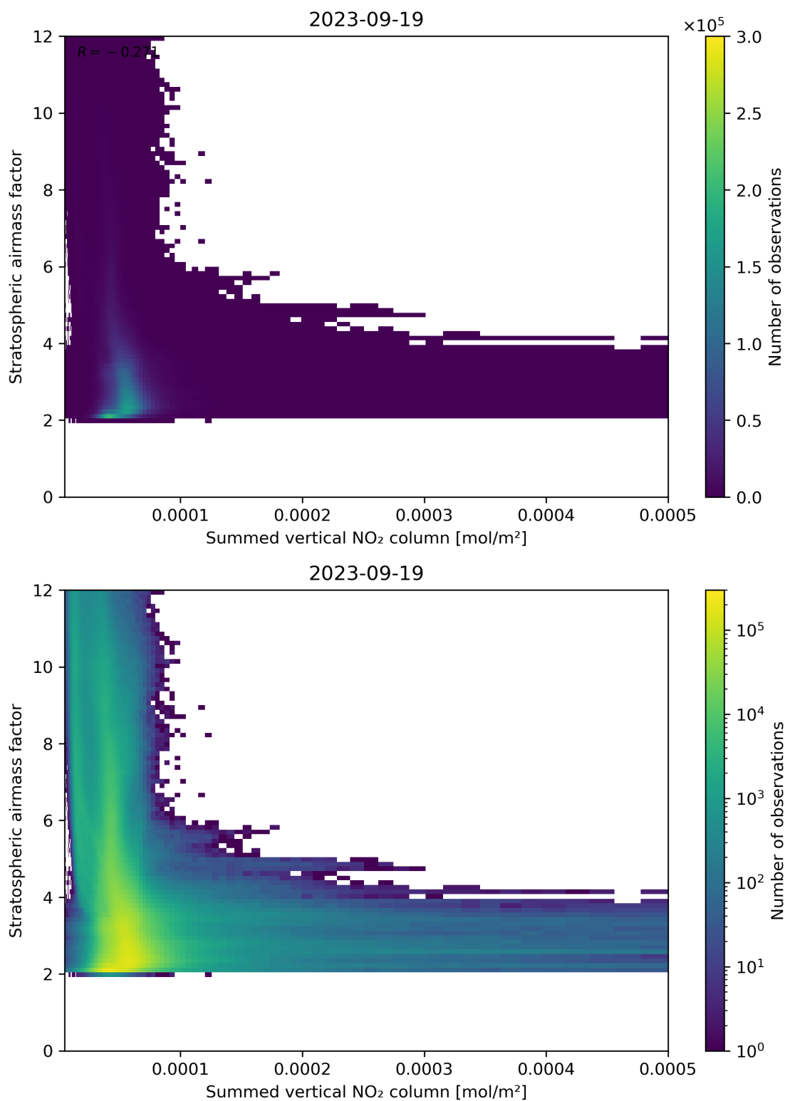
Figure 103: Scatter density plot of “Summed vertical NO 2 column” against “Stratospheric airmass factor” for 2023-09-18 to 2023-09-20.
