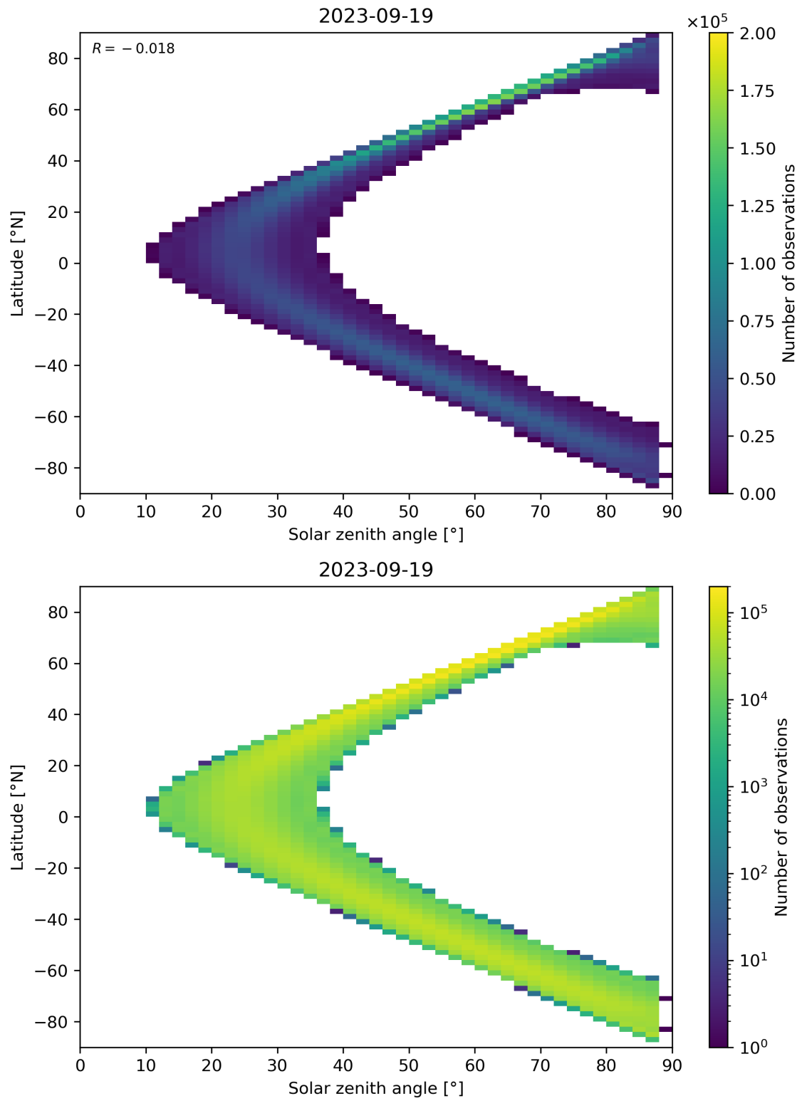
Figure 149: Scatter density plot of “Solar zenith angle” against “Latitude” for 2023-09-18 to 2023-09-20.
