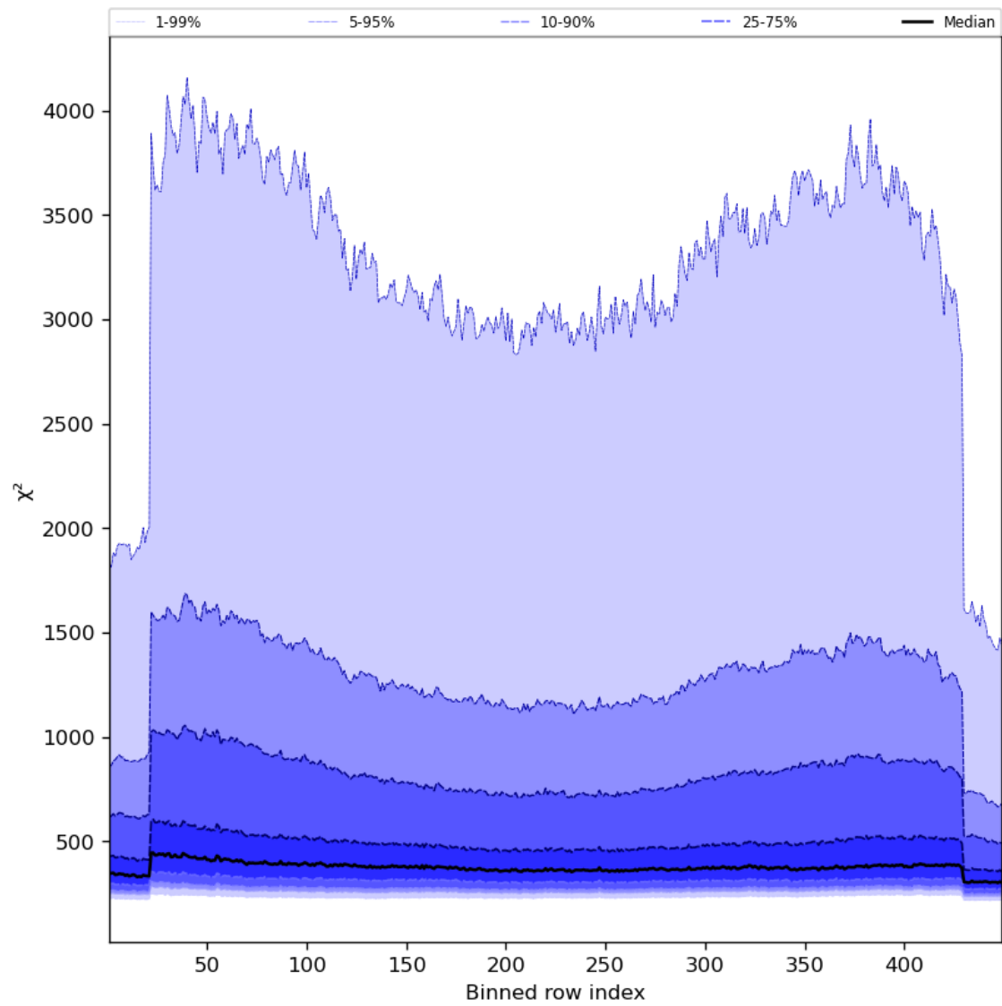
Figure 59: Along track statistics of “ \chi^2 ” for 2023-09-18 to 2023-09-20
