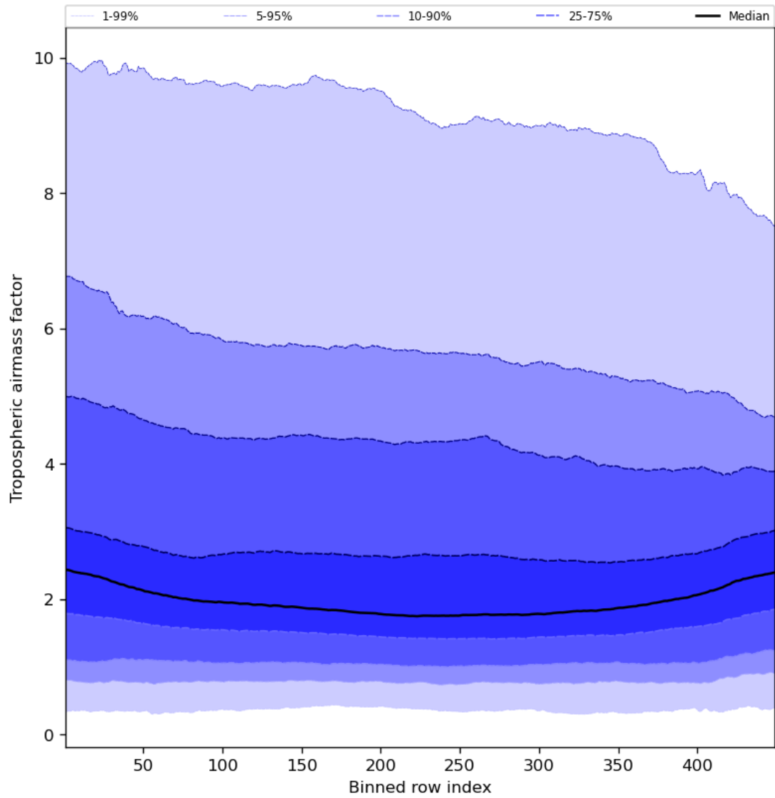
Figure 48: Along track statistics of “Tropospheric air mass factor” for 2023-09-18 to 2023-09-20
