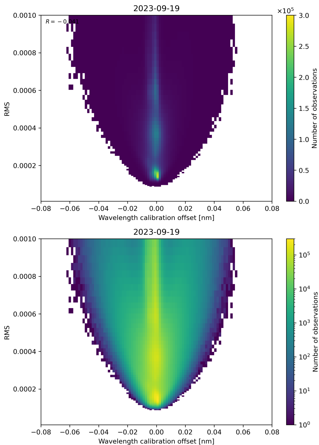
Figure 181: Scatter density plot of “Wavelength calibration offset” against “RMS” for 2023-09-18 to 2023-09-20.
