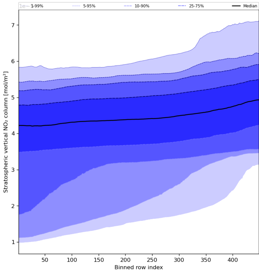
Figure 53: Along track statistics of “Stratospheric vertical NO 2 column” for 2023-09-18 to 2023-09-20
