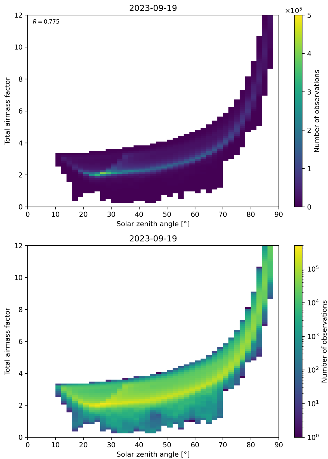
Figure 146: Scatter density plot of “Solar zenith angle” against “Total air mass factor” for 2023-09-18 to 2023-09-20.
