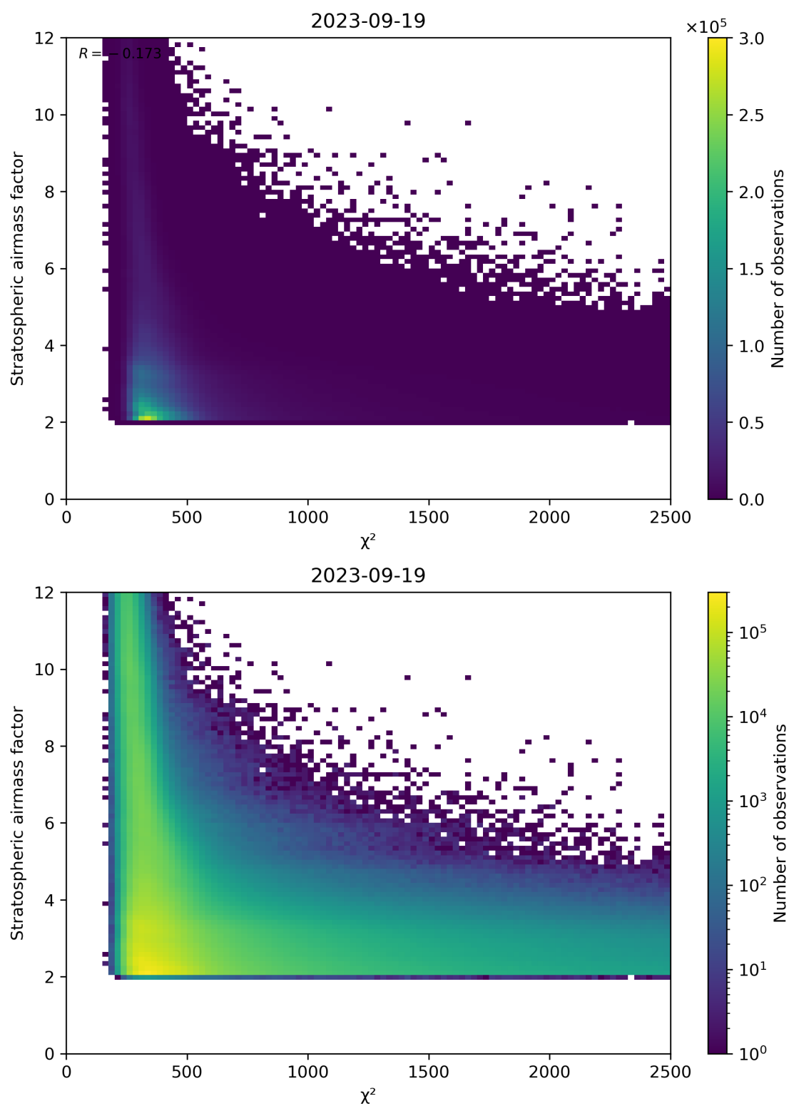
Figure 81: Scatter density plot of “ \chi^2 ” against “Stratospheric airmass factor” for 2023-09-18 to 2023-09-20.
