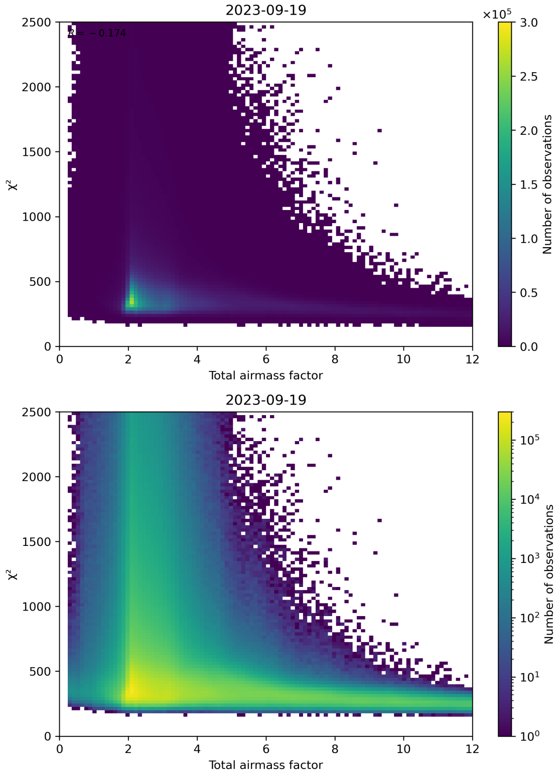
Figure 63: Scatter density plot of “Total airmass factor” against “ \chi^2 ” for 2023-09-18 to 2023-09-20.
