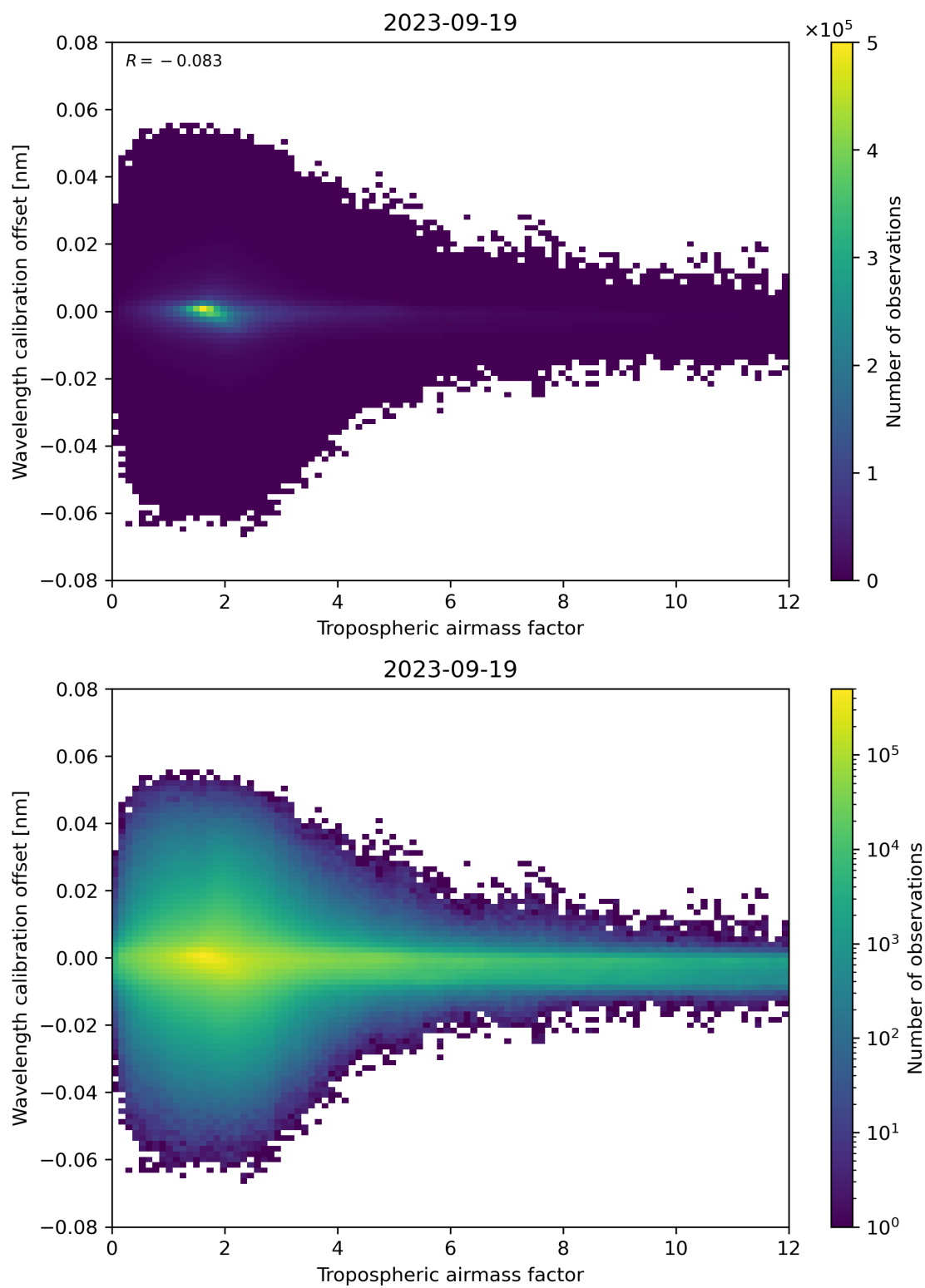
Figure 80: Scatter density plot of “Tropospheric airmass factor” against “Wavelength calibration offset” for 2023-09-18 to 2023-09-20.
