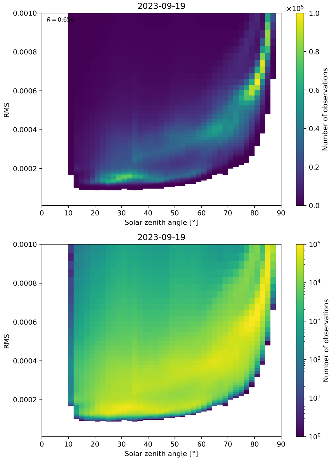
Figure 157: Scatter density plot of “Solar zenith angle” against “RMS” for 2023-09-18 to 2023-09-20.
