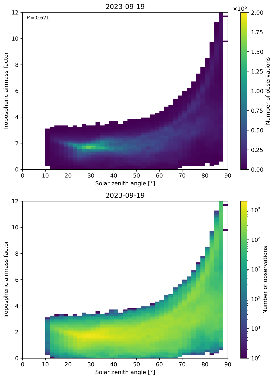
Figure 147: Scatter density plot of “Solar zenith angle” against “Tropospheric airmass factor” for 2023-09-18 to 2023-09-20.
