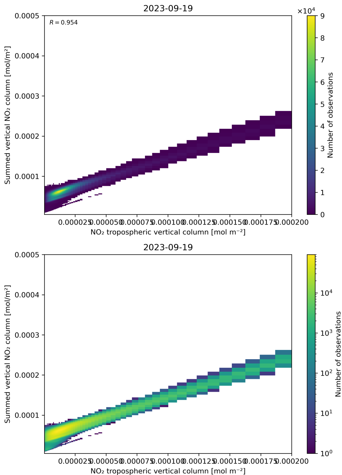
Figure 126: Scatter density plot of “NO 2 tropospheric vertical column” against “Summed vertical NO 2 column” for 2023-09-18 to 2023-09-20.
