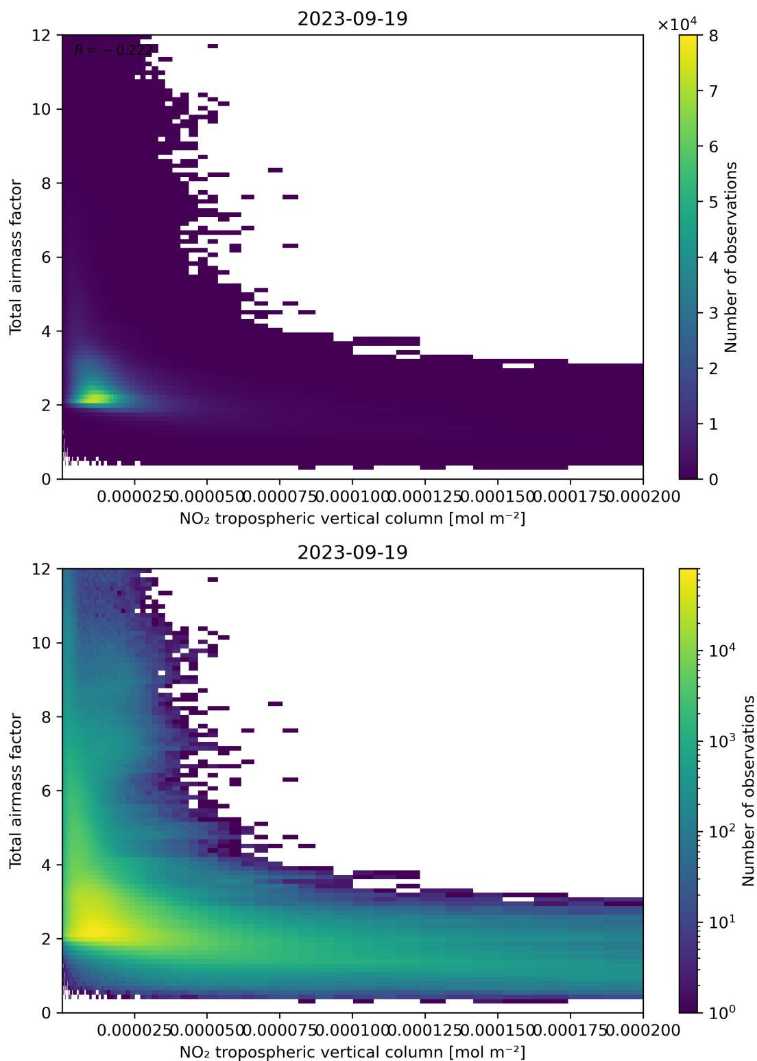
Figure 122: Scatter density plot of “NO 2 tropospheric vertical column” against “Total air mass factor” for 2023-09-18 to 2023-09-20.
