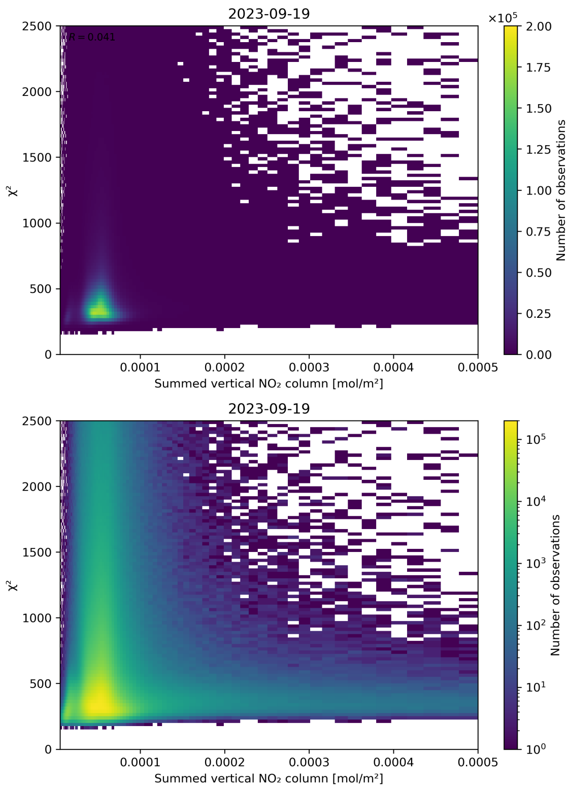
Figure 104: Scatter density plot of “Summed vertical NO 2 column” against “ \chi^2 ” for 2023-09-18 to 2023-09-20.
