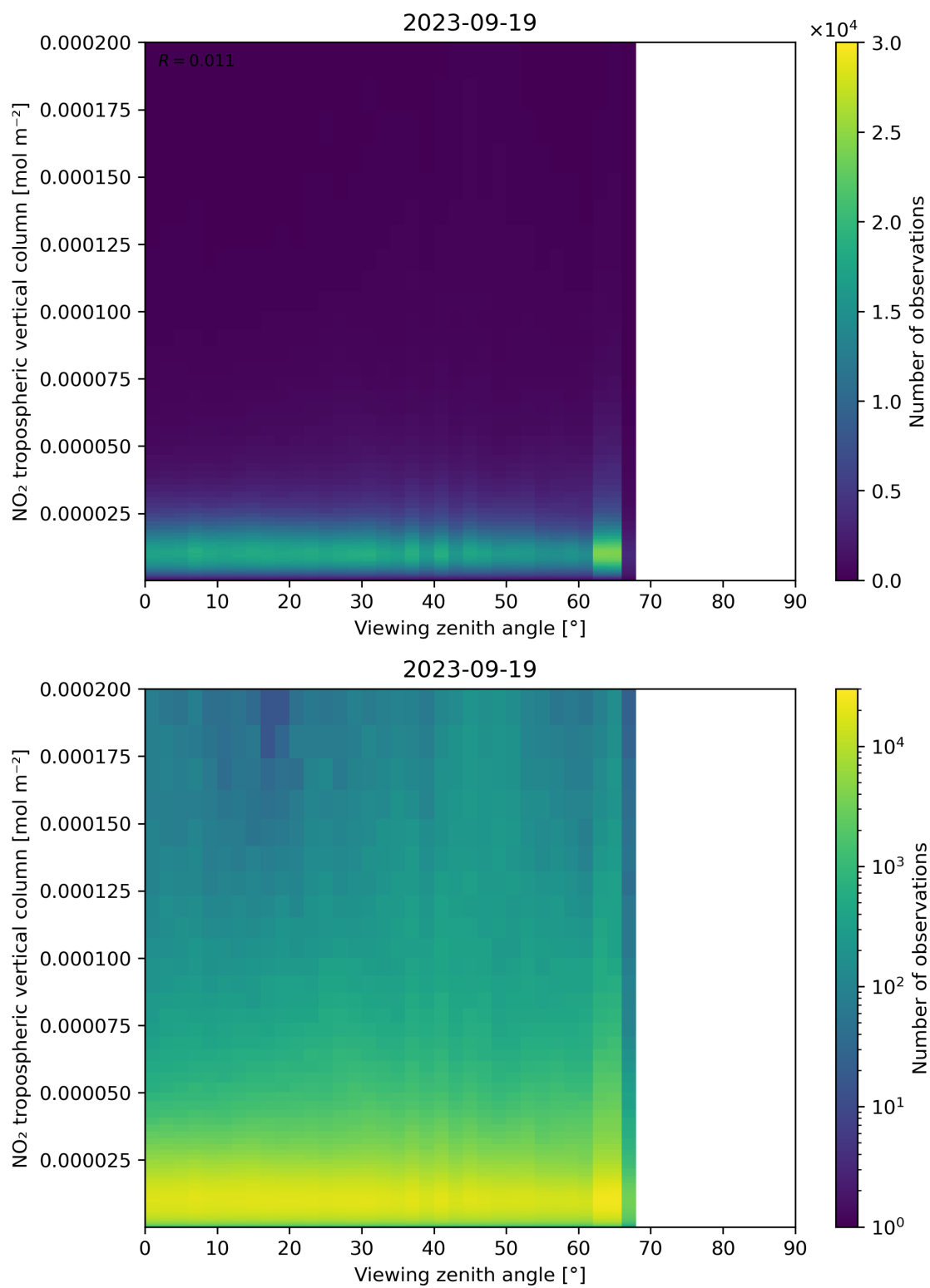
Figure 169: Scatter density plot of “Viewing zenith angle” against “NO 2 tropospheric vertical column” for 2023-09-18 to 2023-09-20.
