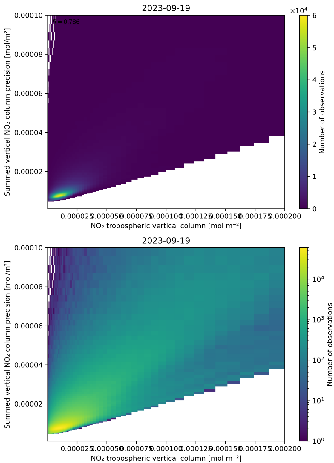
Figure 127: Scatter density plot of “NO 2 tropospheric vertical column” against “Summed vertical NO 2 column precision” for 2023-09-18 to 2023-09-20.
