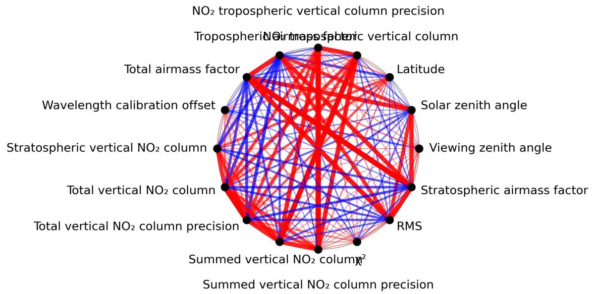
Figure 1: Map of correlation graph for 2023-09-18 to 2023-09-20.
