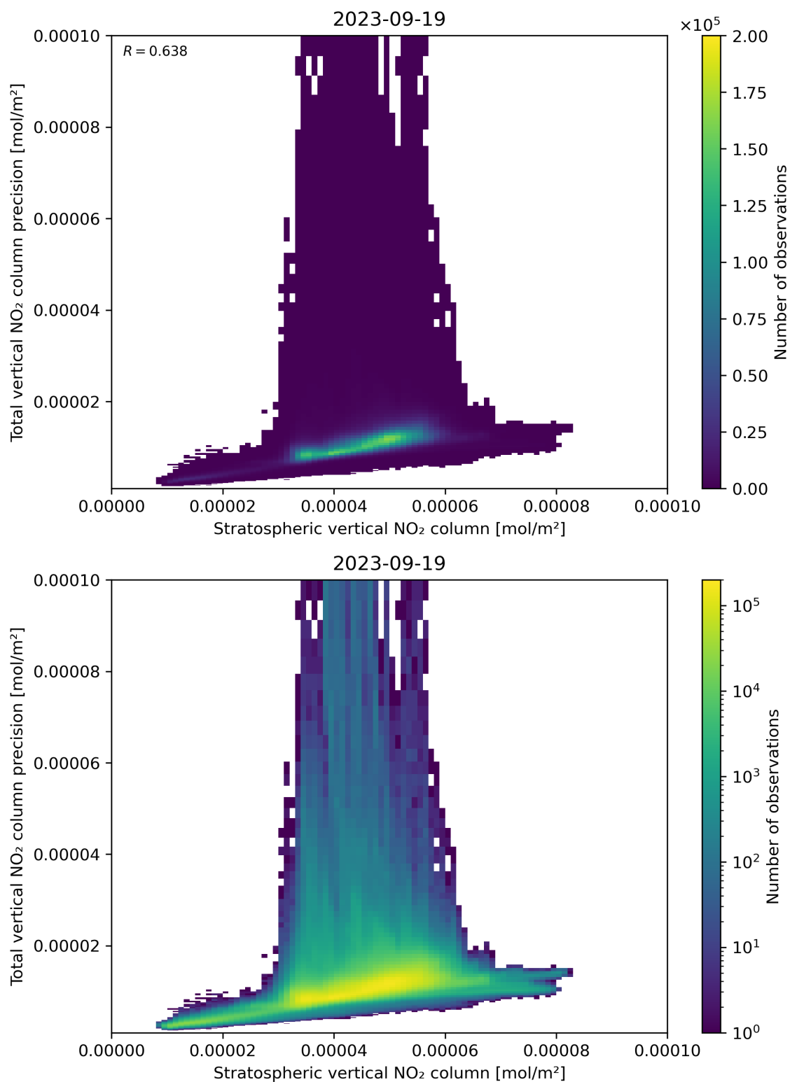
Figure 101: Scatter density plot of “Stratospheric vertical NO 2 column” against “Total vertical NO 2 column precision” for 2023-09-18 to 2023-09-20.
