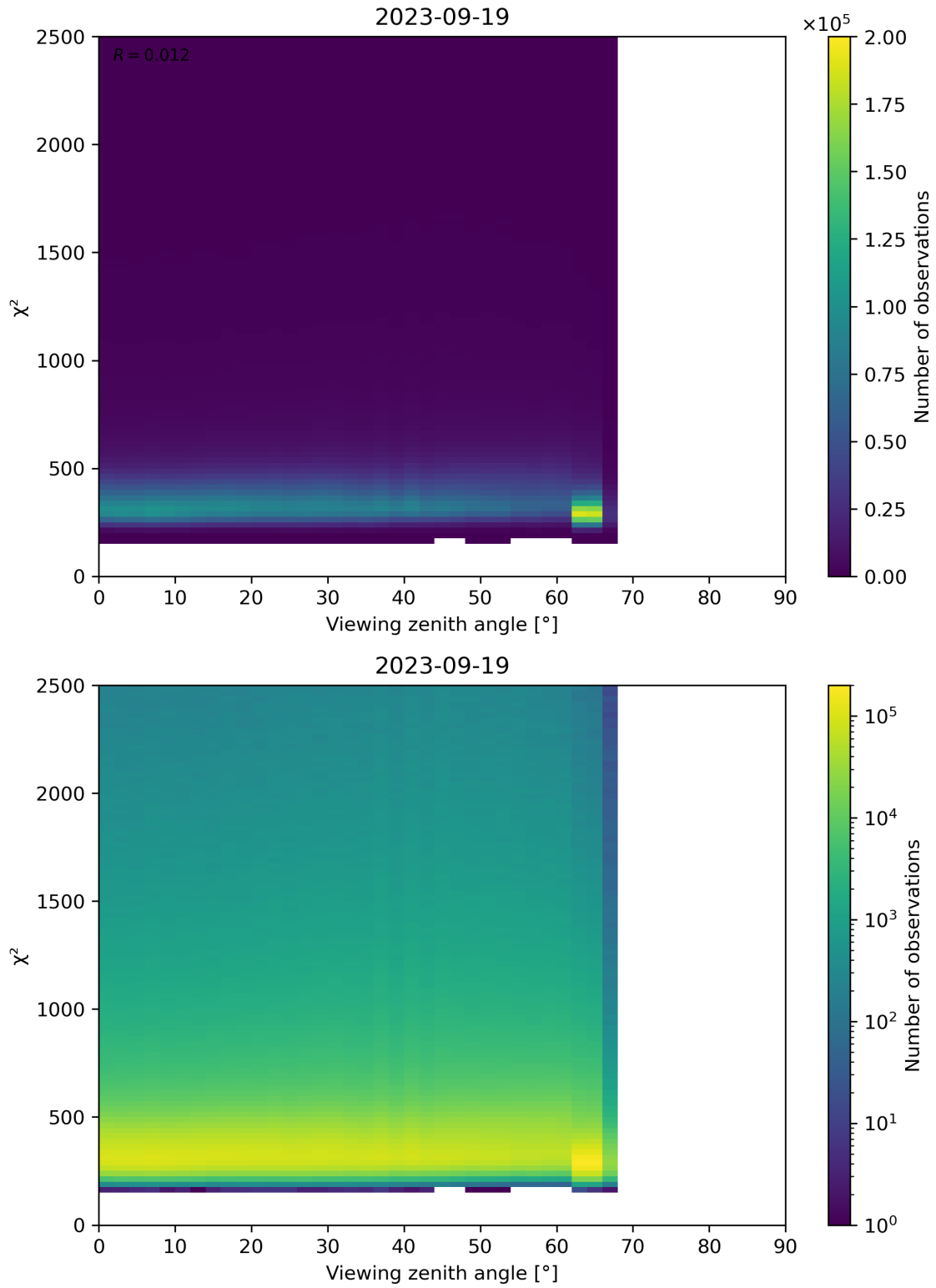
Figure 162: Scatter density plot of “Viewing zenith angle” against “ \chi^2 ” for 2023-09-18 to 2023-09-20.
