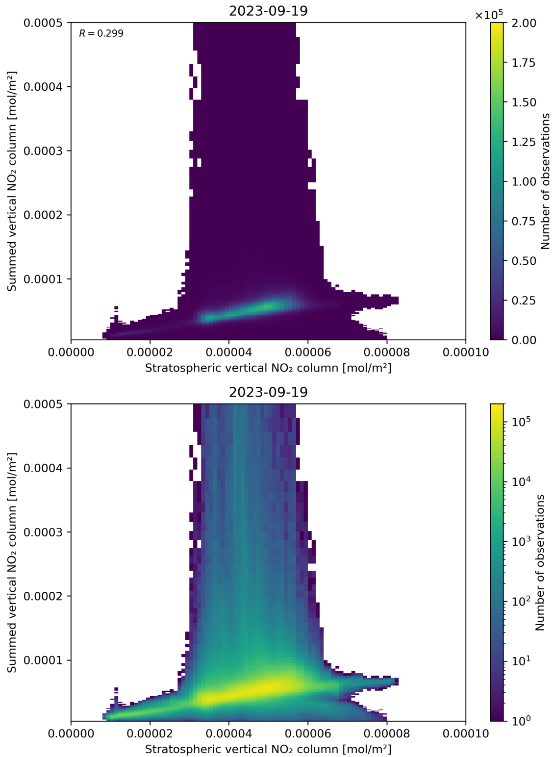
Figure 98: Scatter density plot of “Stratospheric vertical NO 2 column” against “Summed vertical NO 2 column” for 2023-09-18 to 2023-09-20.
