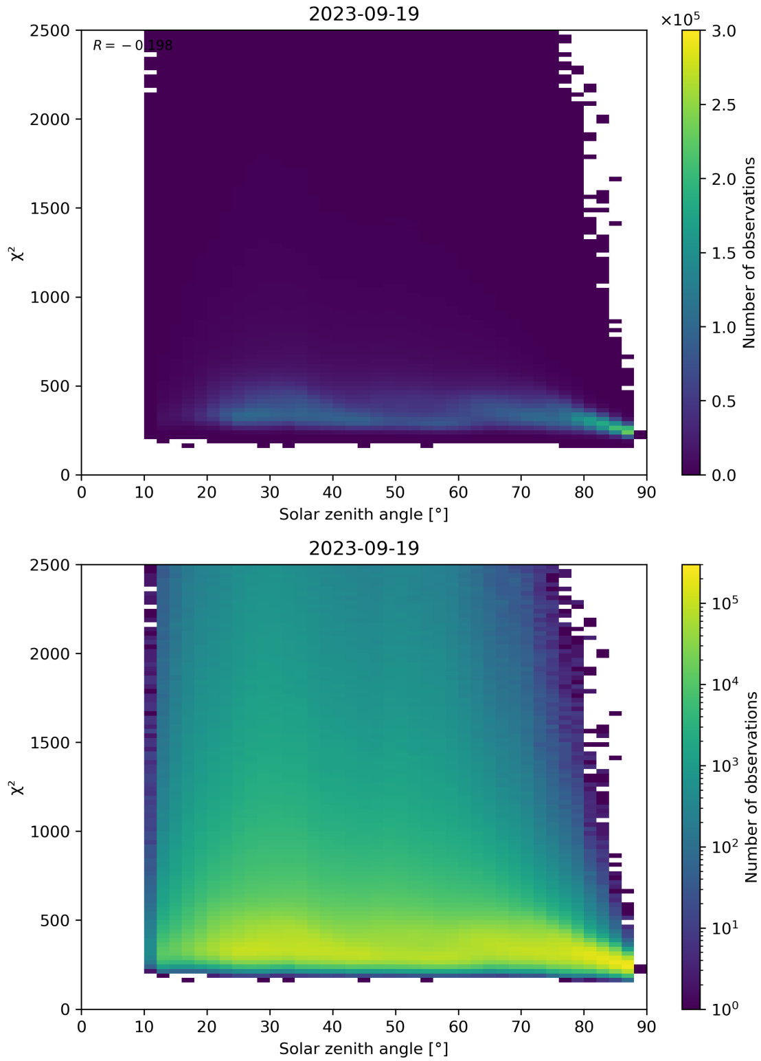
Figure 148: Scatter density plot of “Solar zenith angle” against “ \chi^2 ” for 2023-09-18 to 2023-09-20.
