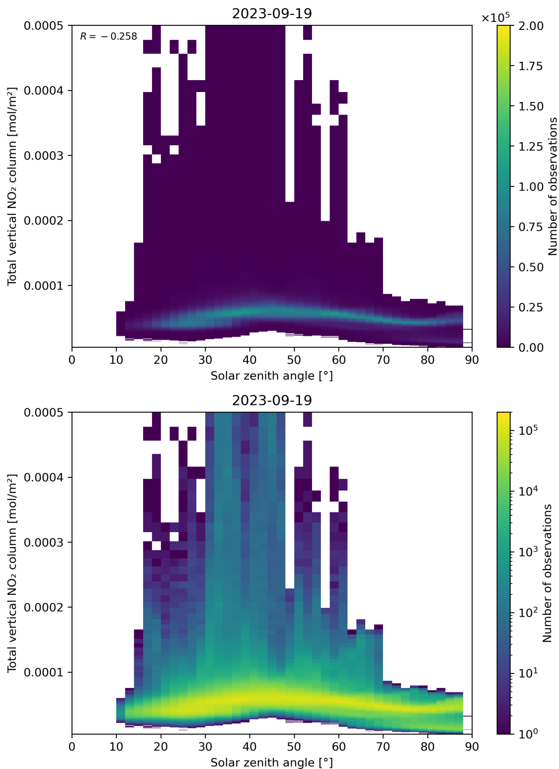
Figure 153: Scatter density plot of “Solar zenith angle” against “Total vertical NO 2 column” for 2023-09-18 to 2023-09-20.
