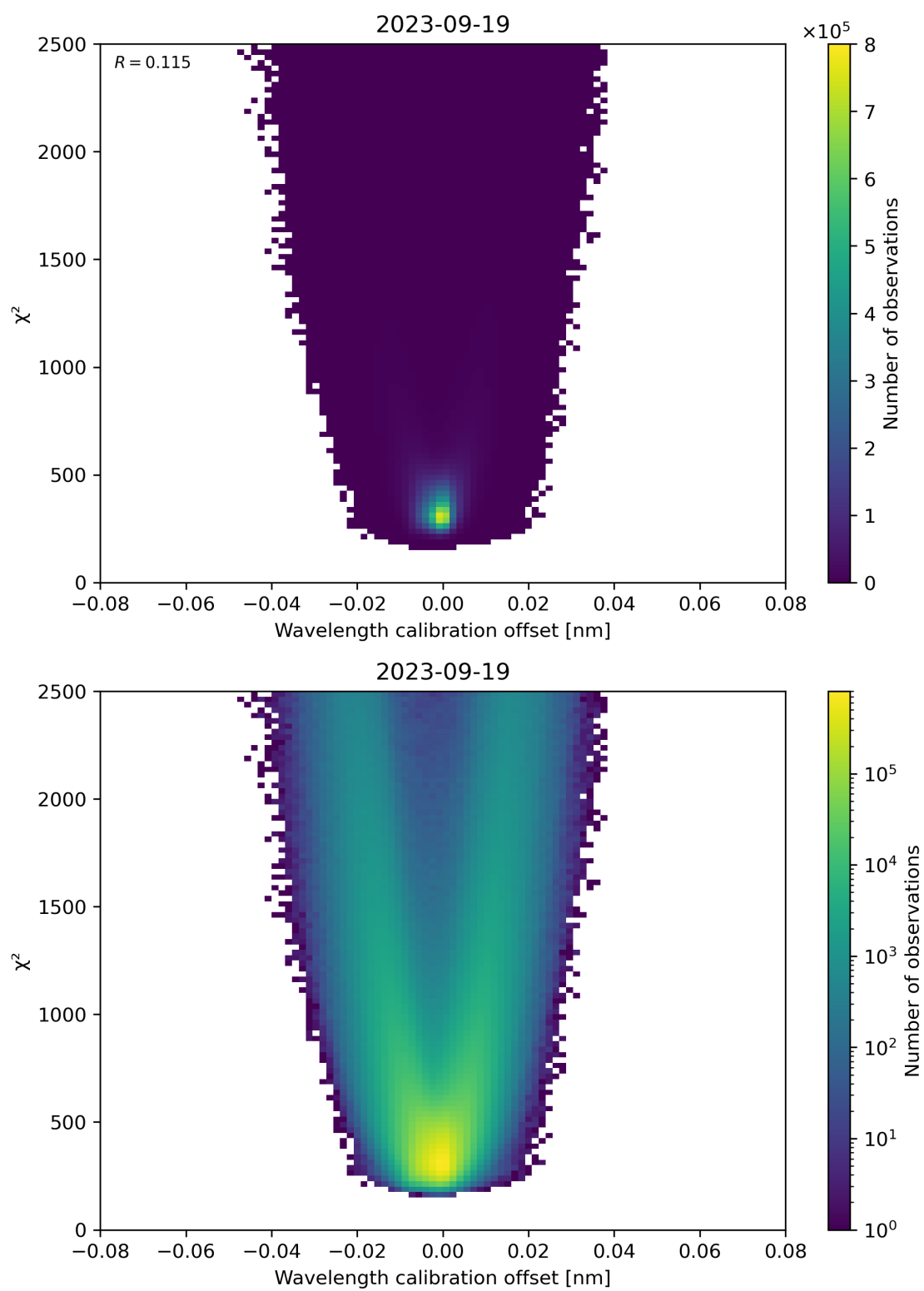
Figure 175: Scatter density plot of “Wavelength calibration offset” against “ \chi^2 ” for 2023-09-18 to 2023-09-20.
