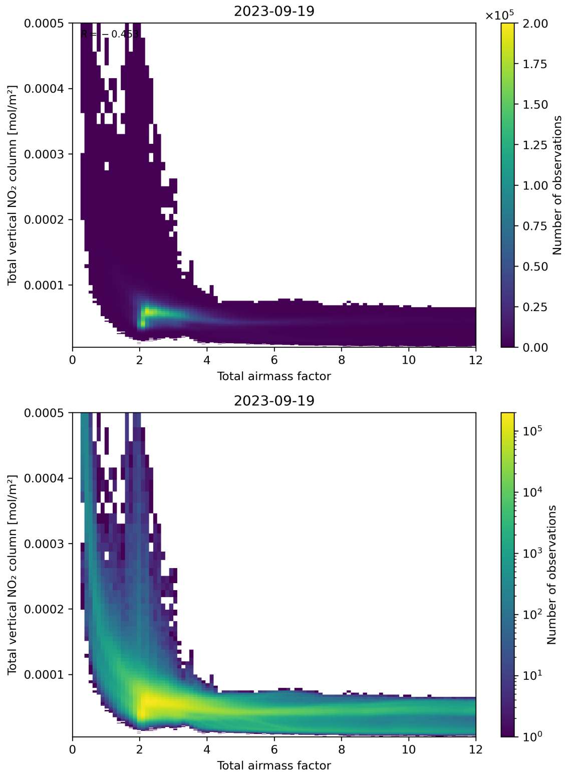
Figure 67: Scatter density plot of “Total airmass factor” against “Total vertical NO 2 column” for 2023-09-18 to 2023-09-20.
