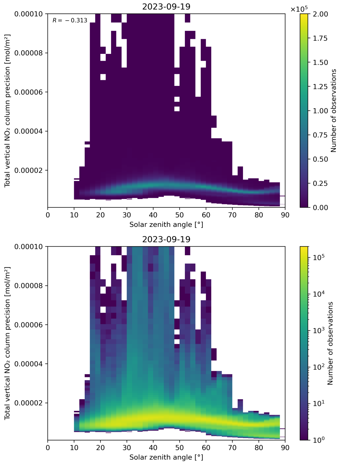
Figure 154: Scatter density plot of “Solar zenith angle” against “Total vertical NO 2 column precision” for 2023-09-18 to 2023-09-20.
