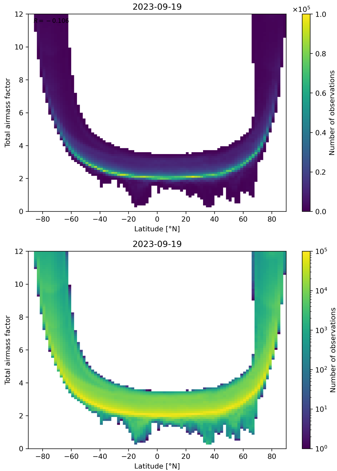
Figure 84: Scatter density plot of “Latitude” against “Total airmass factor” for 2023-09-18 to 2023-09-20.
