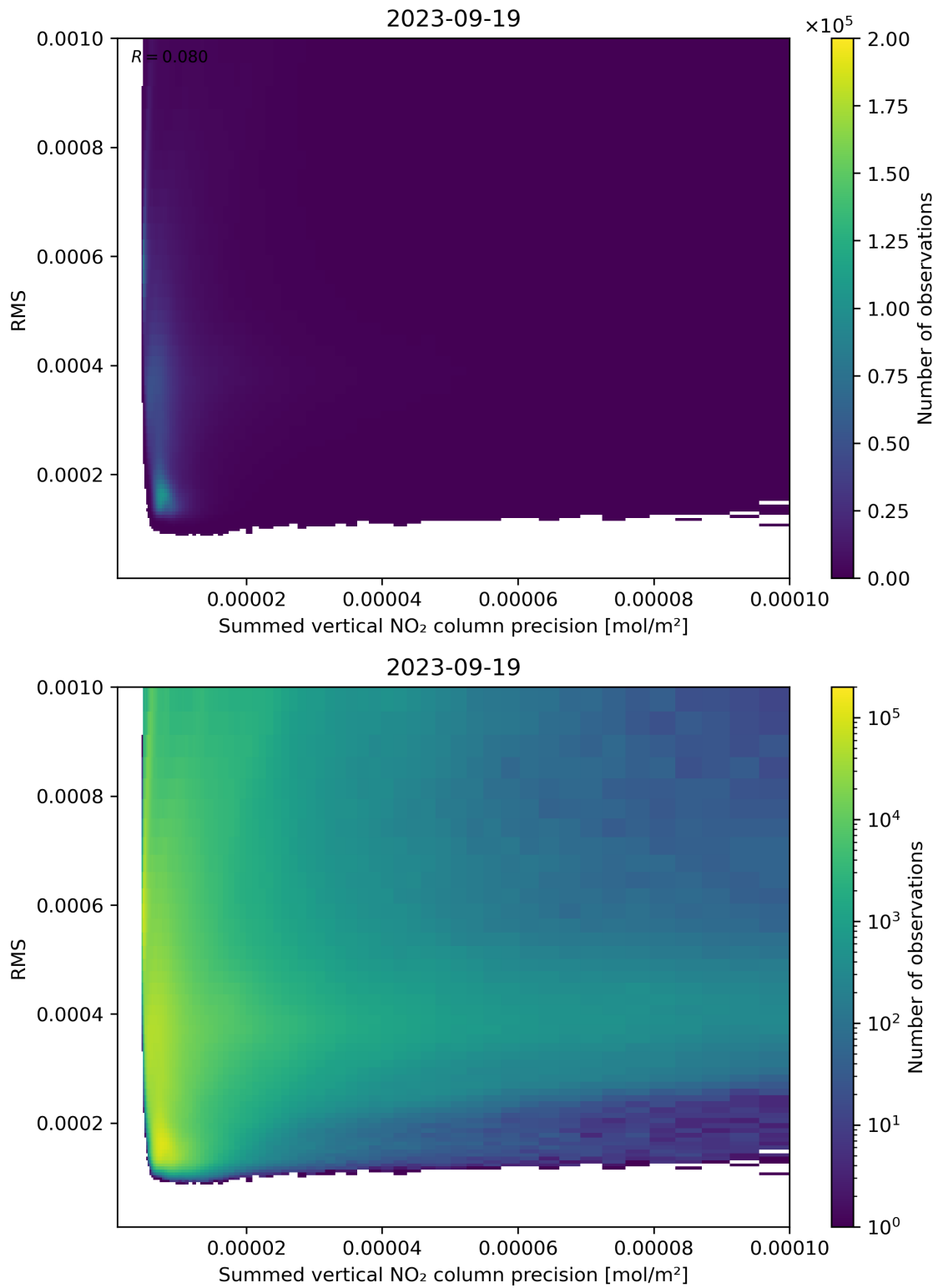
Figure 108: Scatter density plot of “Summed vertical NO 2 column precision” against “RMS” for 2023-09-18 to 2023-09-20.
