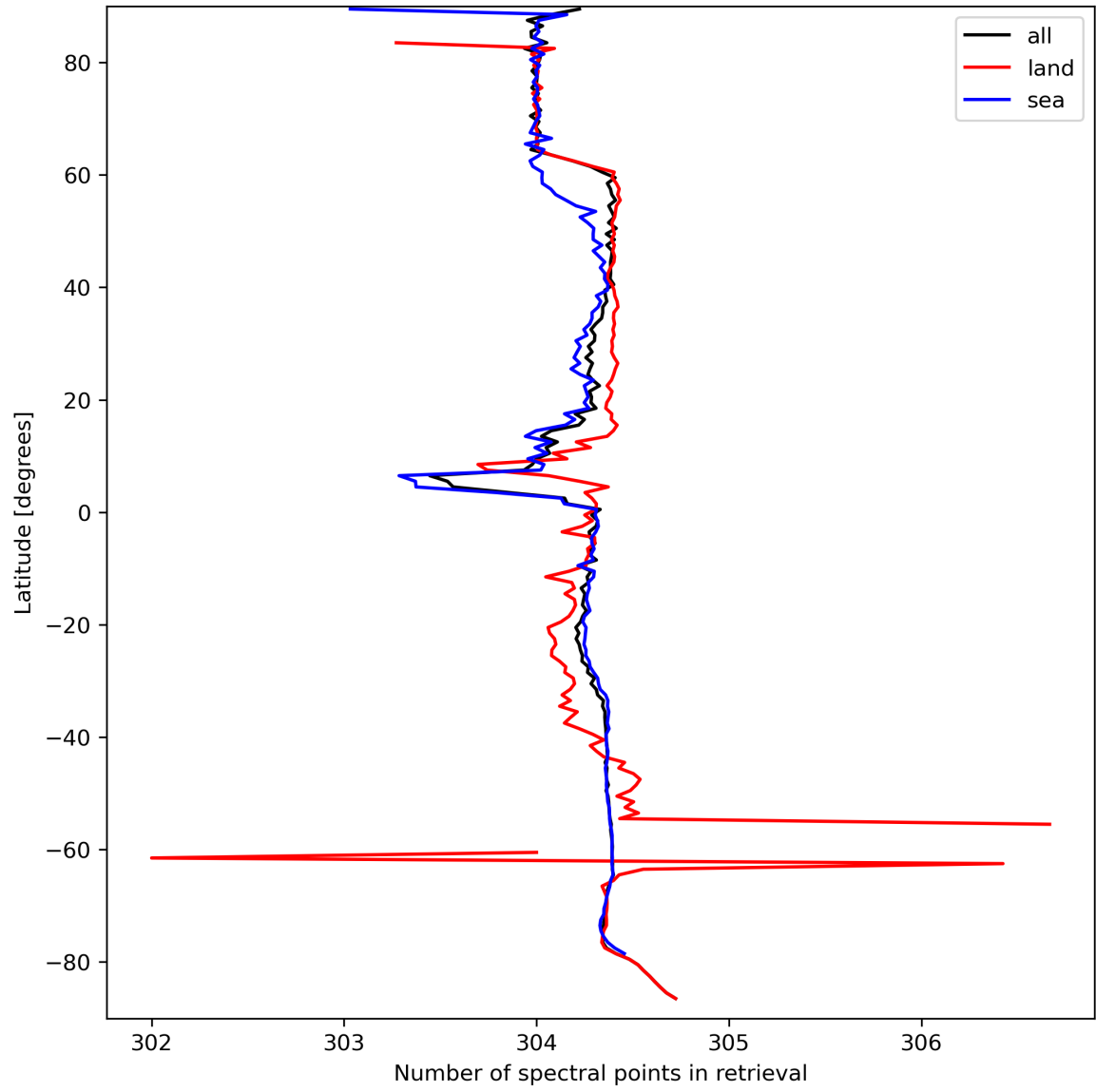
Figure 16: Zonal average of “Number of spectral points in retrieval” for 2023-09-18 to 2023-09-20.
