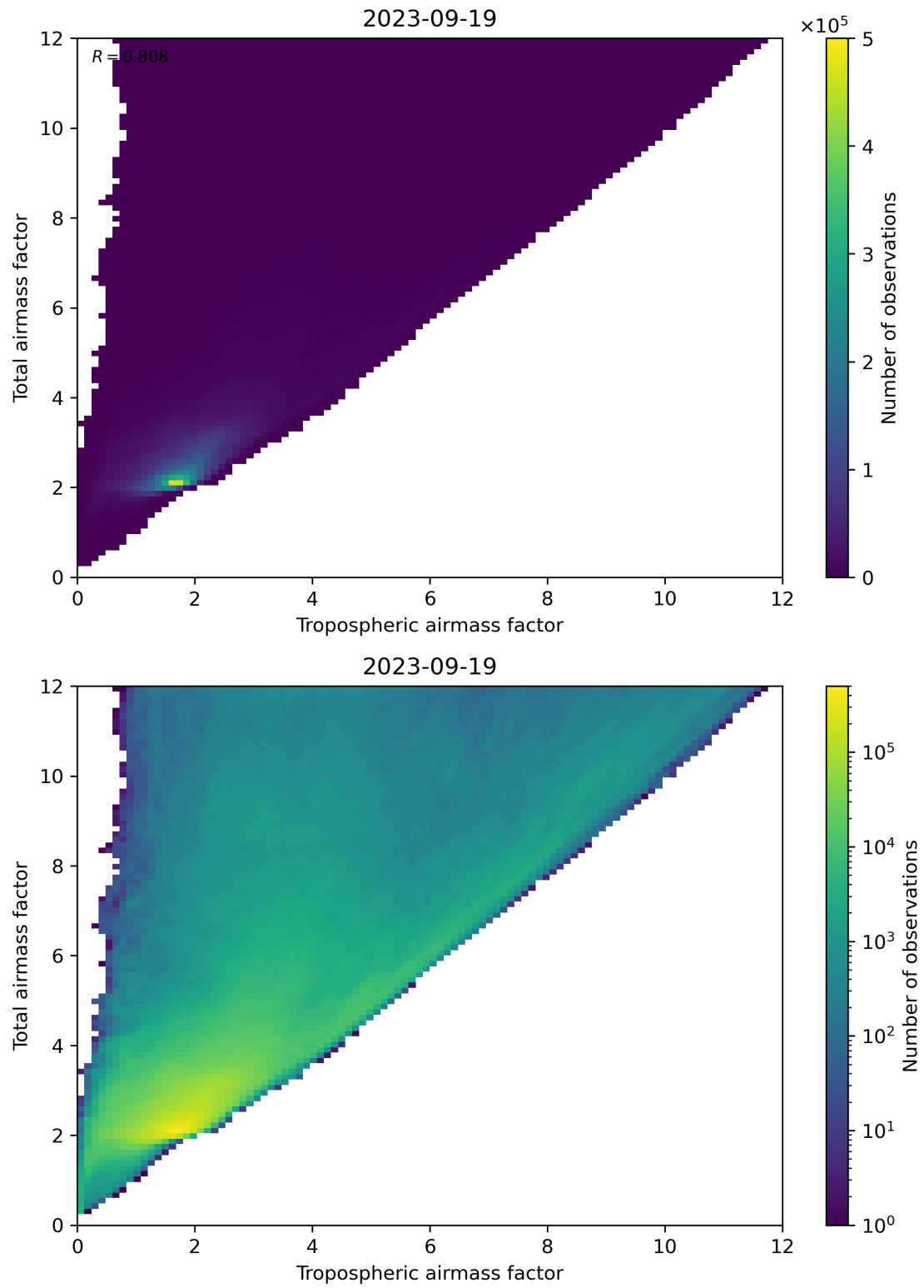
Figure 72: Scatter density plot of “Tropospheric airmass factor” against “Total airmass factor” for 2023-09-18 to 2023-09-20.
