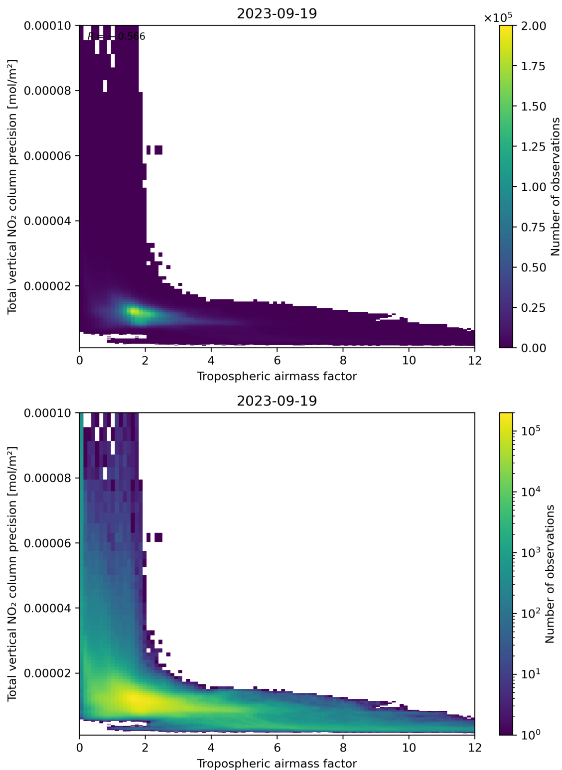
Figure 78: Scatter density plot of “Tropospheric air mass factor” against “Total vertical NO 2 column precision” for 2023-09-18 to 2023-09-20.
