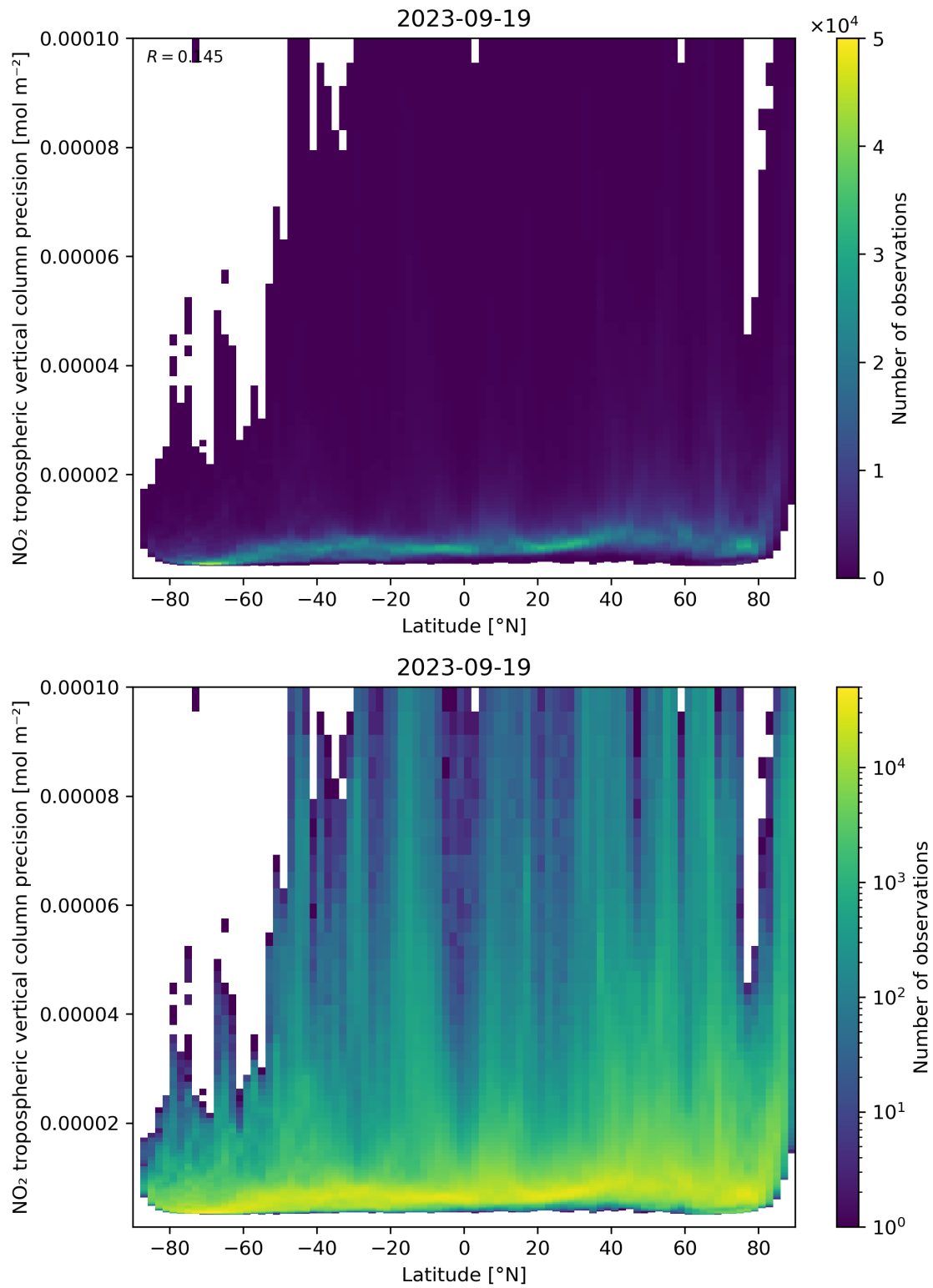
Figure 93: Scatter density plot of “Latitude” against “NO 2 tropospheric vertical column precision” for 2023-09-18 to 2023-09-20.
