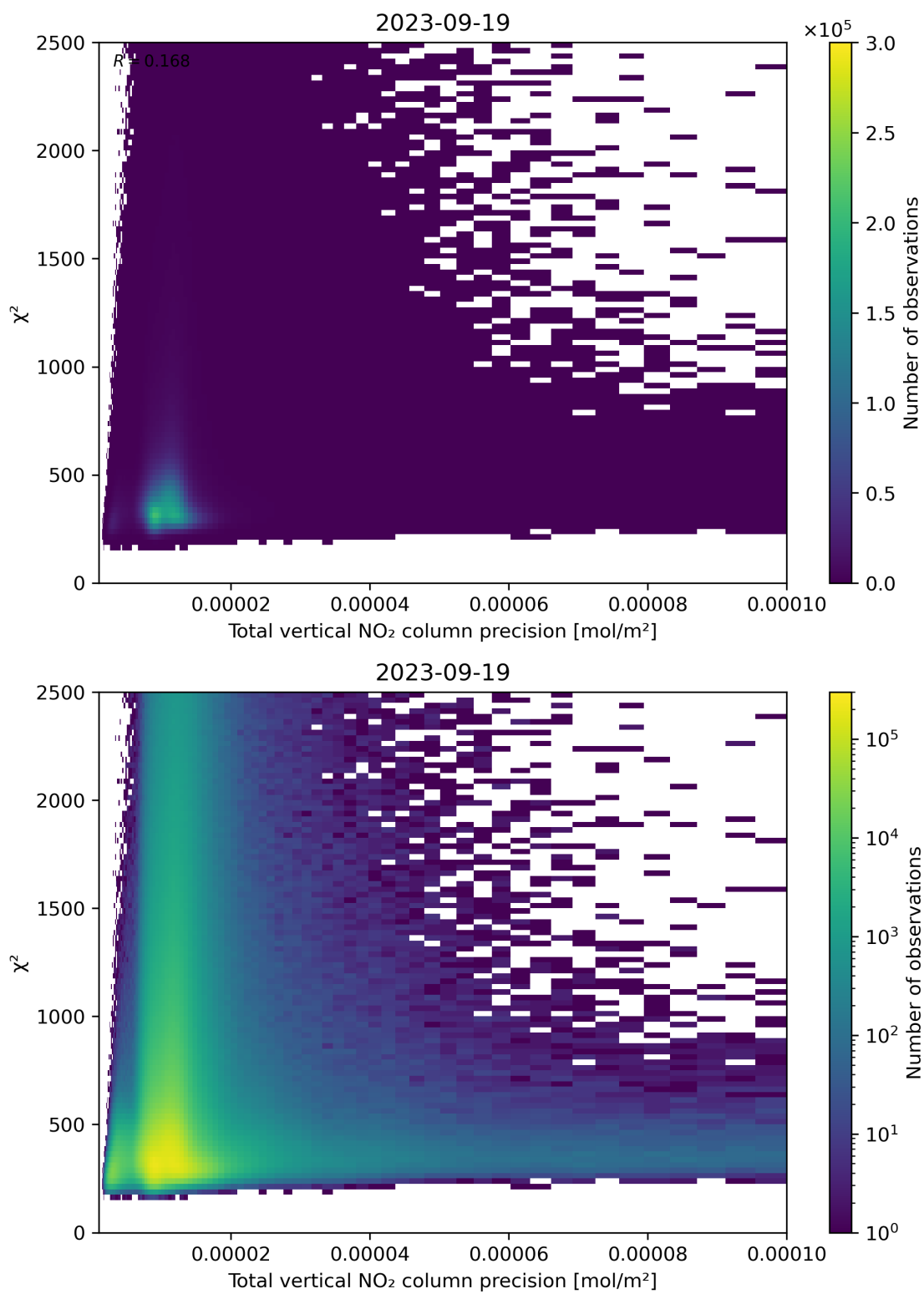
Figure 116: Scatter density plot of “Total vertical NO 2 column precision” against “ \chi^2 ” for 2023-09-18 to 2023-09-20.
