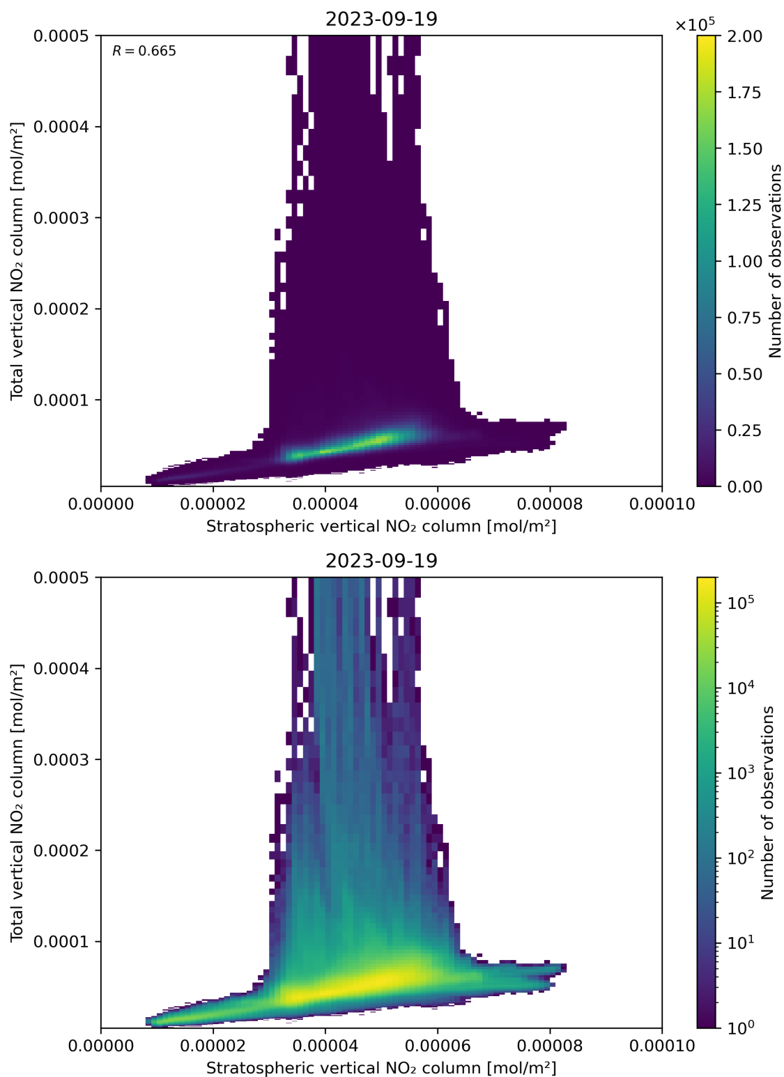
Figure 100: Scatter density plot of “Stratospheric vertical NO 2 column” against “Total vertical NO 2 column” for 2023-09-18 to 2023-09-20.
