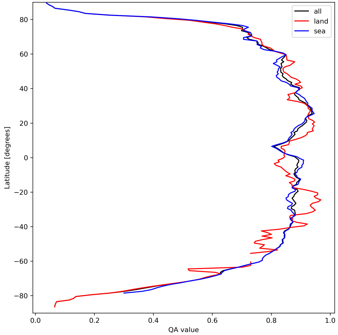
Figure 11: Zonal average of “QA value” for 2023-09-18 to 2023-09-20.
