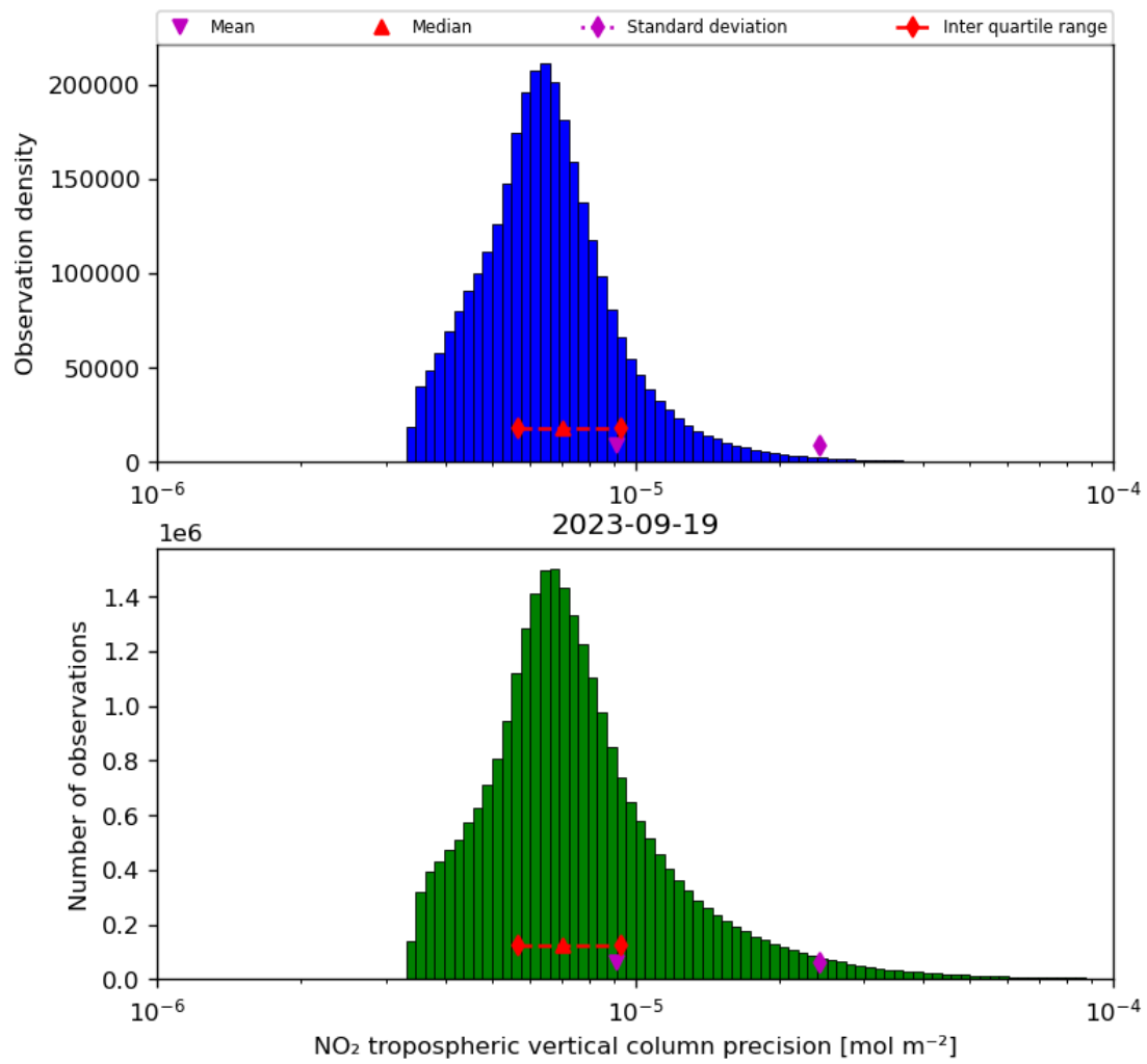
Figure 30: Histogram of “NO 2 tropospheric vertical column precision” for 2023-09-18 to 2023-09-20
