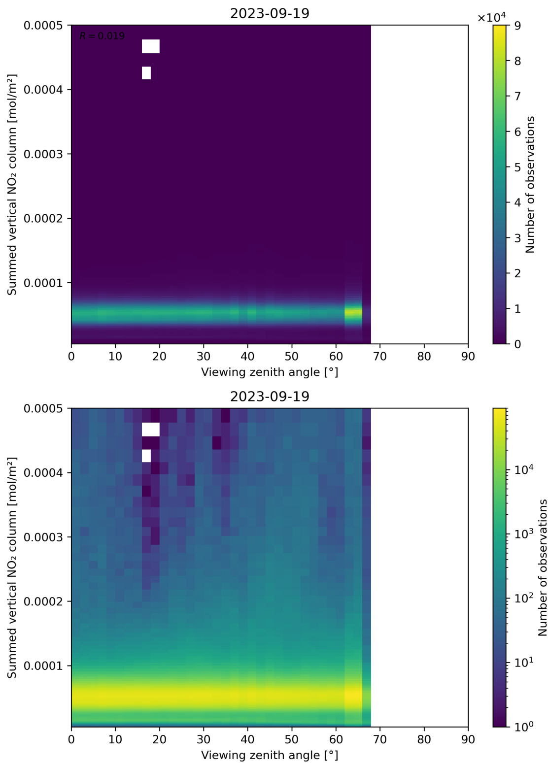
Figure 165: Scatter density plot of “Viewing zenith angle” against “Summed vertical NO 2 column” for 2023-09-18 to 2023-09-20.
