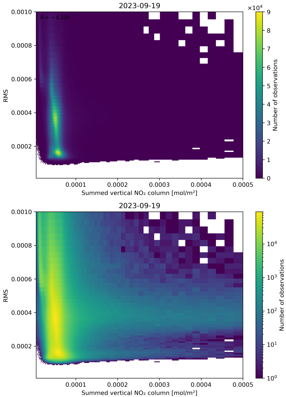
Figure 109: Scatter density plot of “Summed vertical NO 2 column” against “RMS” for 2023-09-18 to 2023-09-20.
