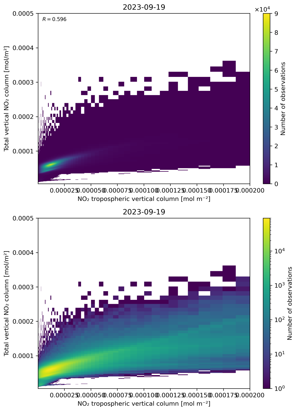
Figure 128: Scatter density plot of “NO 2 tropospheric vertical column” against “Total vertical NO 2 column” for 2023-09-18 to 2023-09-20.
