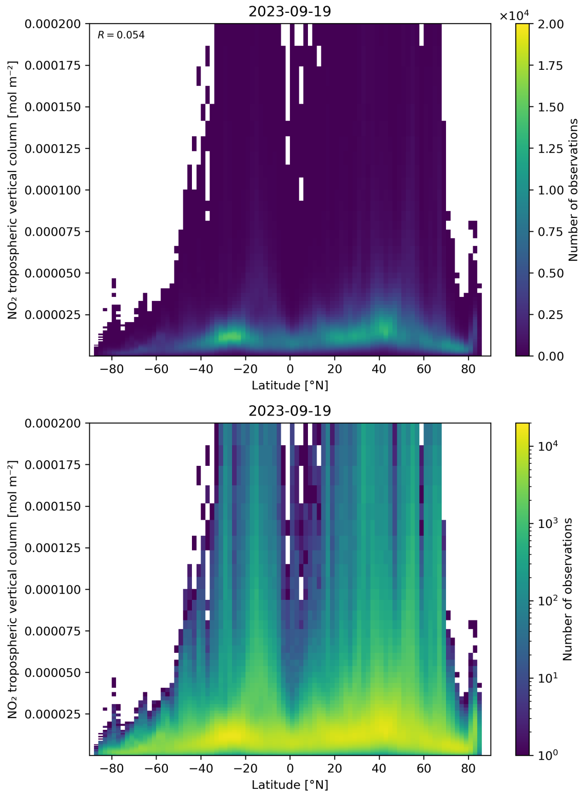
Figure 92: Scatter density plot of “Latitude” against “NO 2 tropospheric vertical column” for 2023-09-18 to 2023-09-20.
