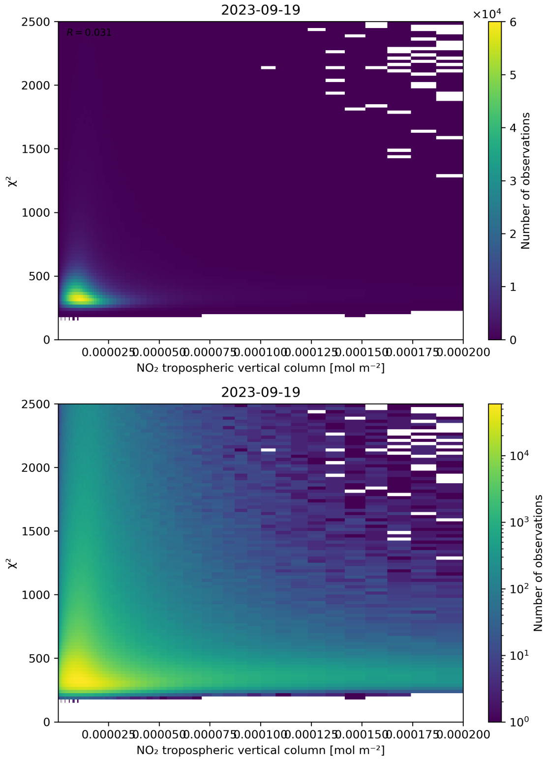
Figure 124: Scatter density plot of “NO 2 tropospheric vertical column” against “ \chi^2 ” for 2023-09-18 to 2023-09-20.
