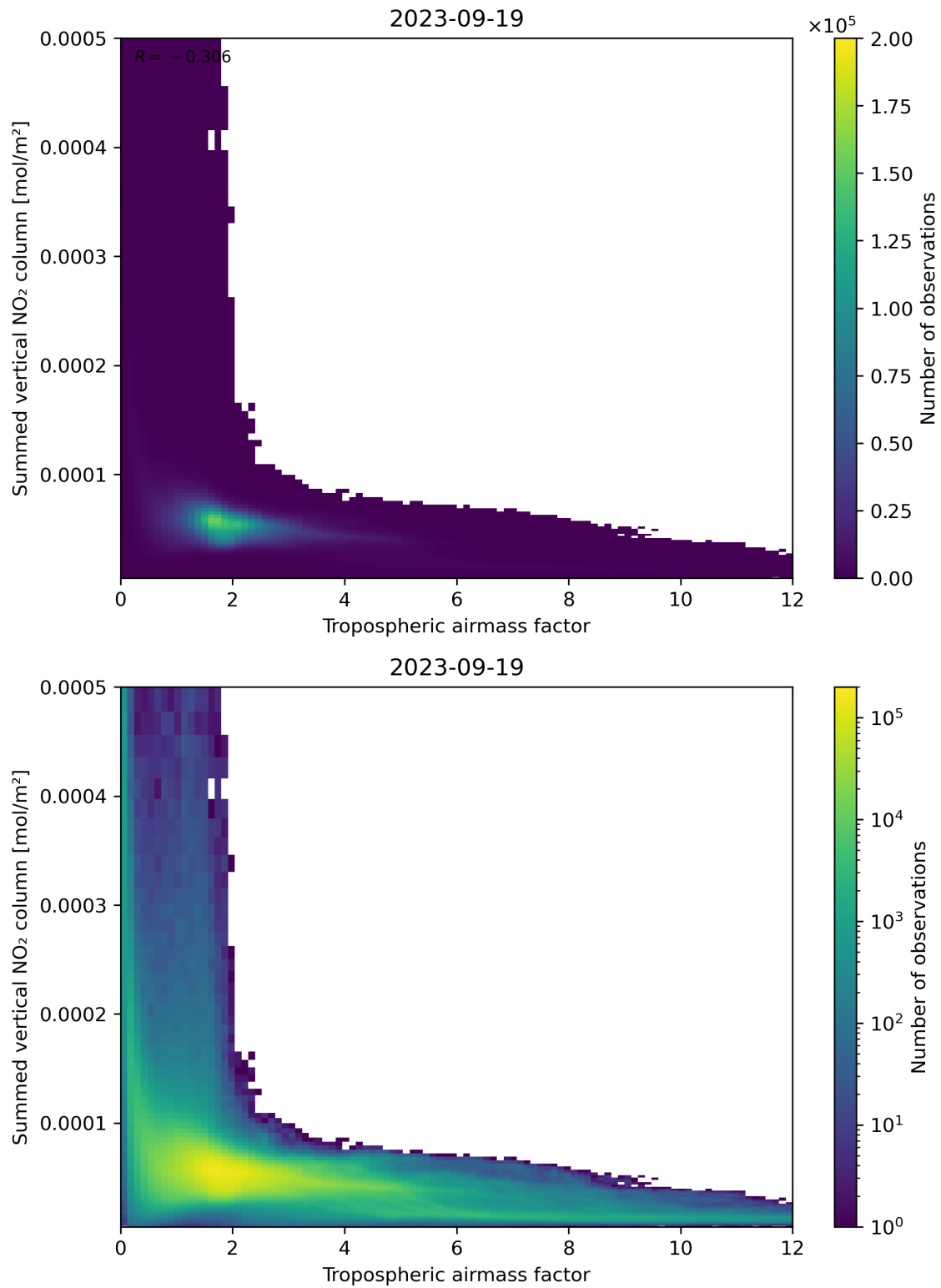
Figure 75: Scatter density plot of “Tropospheric airmass factor” against “Summed vertical NO 2 column” for 2023-09-18 to 2023-09-20.
