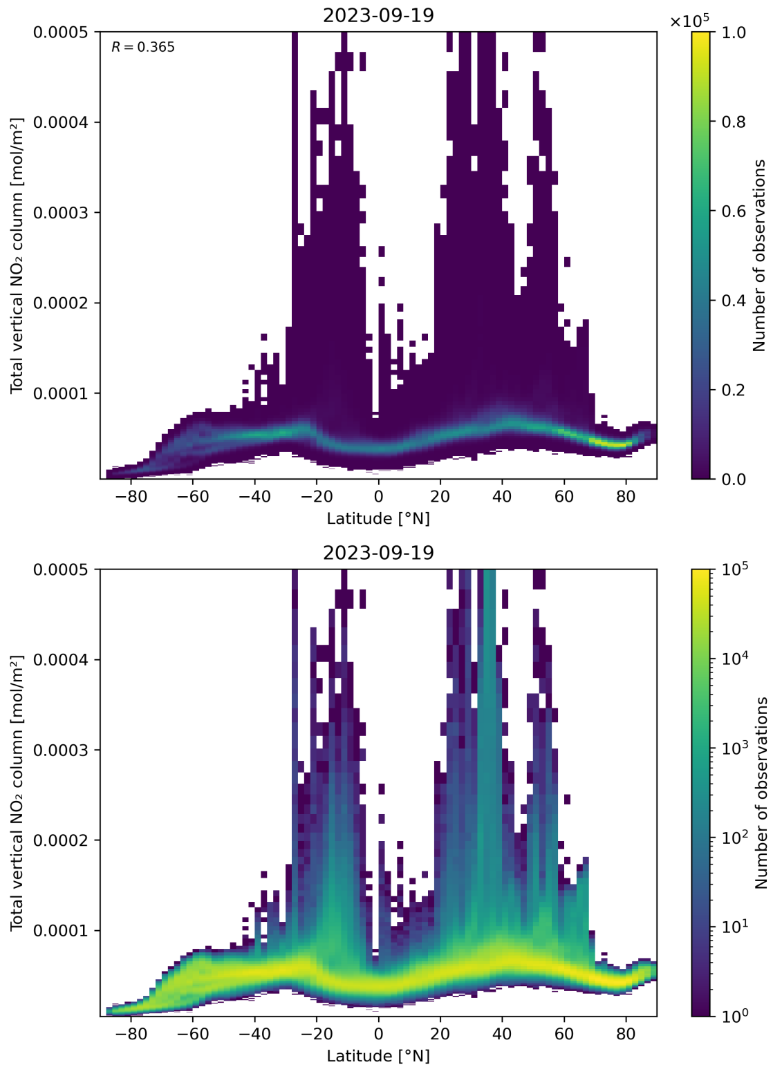
Figure 90: Scatter density plot of “Latitude” against “Total vertical NO 2 column” for 2023-09-18 to 2023-09-20.
