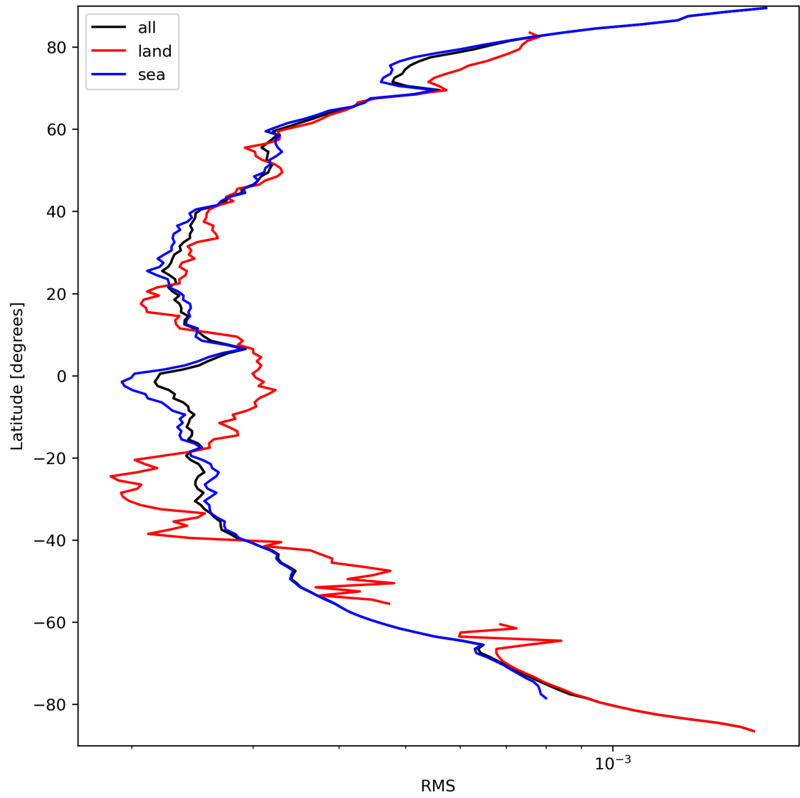
Figure 26: Zonal average of “RMS” for 2023-09-18 to 2023-09-20.
