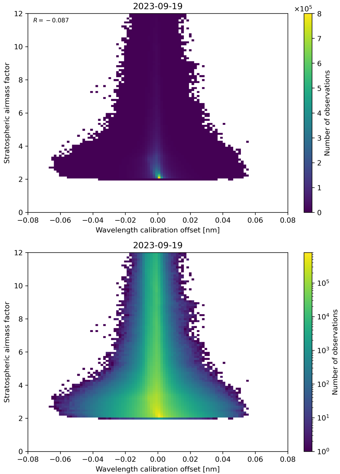
Figure 174: Scatter density plot of “Wavelength calibration offset” against “Stratospheric airmass factor” for 2023-09-18 to 2023-09-20.
