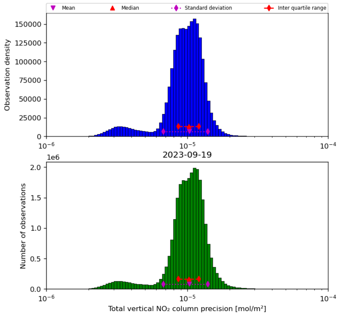
Figure 39: Histogram of “Total vertical NO 2 column precision” for 2023-09-18 to 2023-09-20
