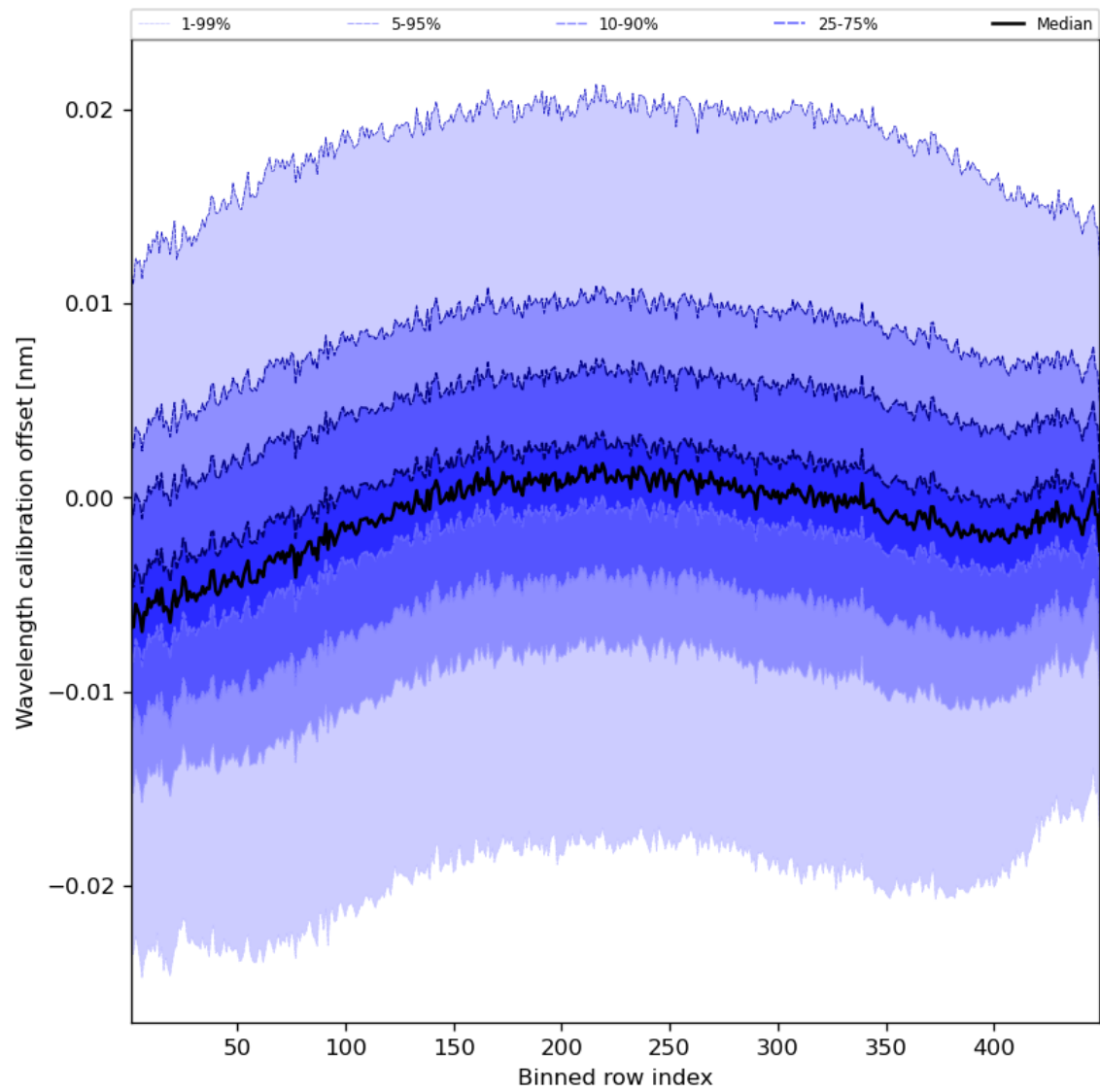
Figure 52: Along track statistics of “Wavelength calibration offset” for 2023-09-18 to 2023-09-20
