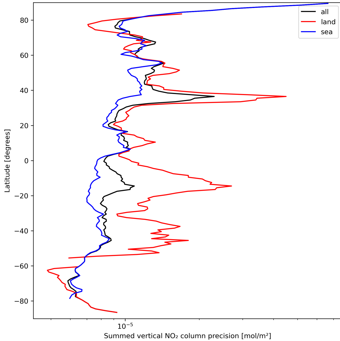
Figure 24: Zonal average of “Summed vertical NO 2 column precision” for 2023-09-18 to 2023-09-20.
