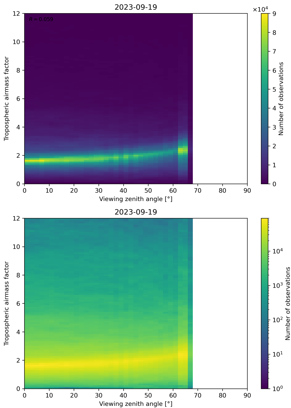
Figure 161: Scatter density plot of “Viewing zenith angle” against “Tropospheric air mass factor” for 2023-09-18 to 2023-09-20.
