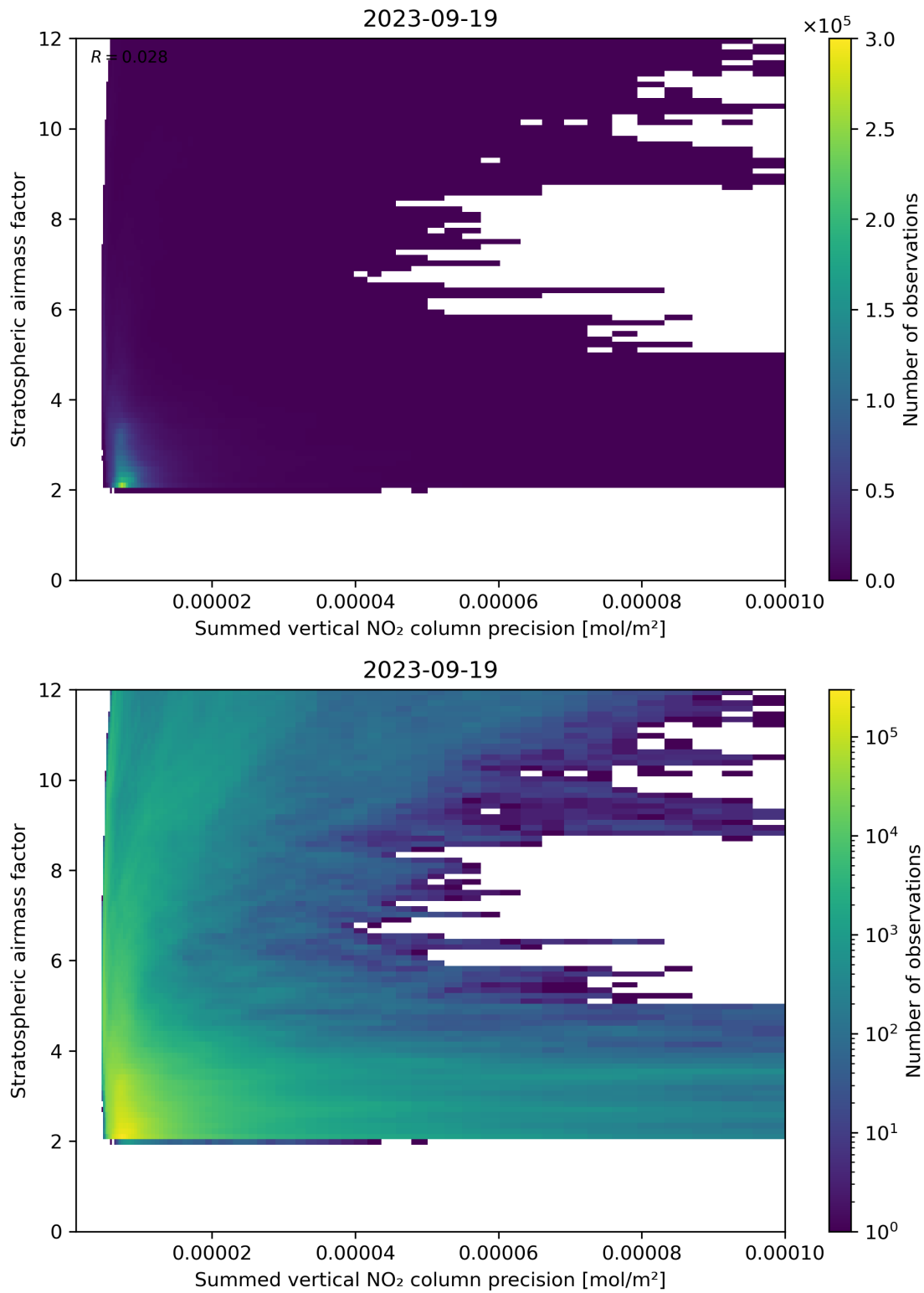
Figure 106: Scatter density plot of “Summed vertical NO 2 column precision” against “Stratospheric airmass factor” for 2023-09-18 to 2023-09-20.
