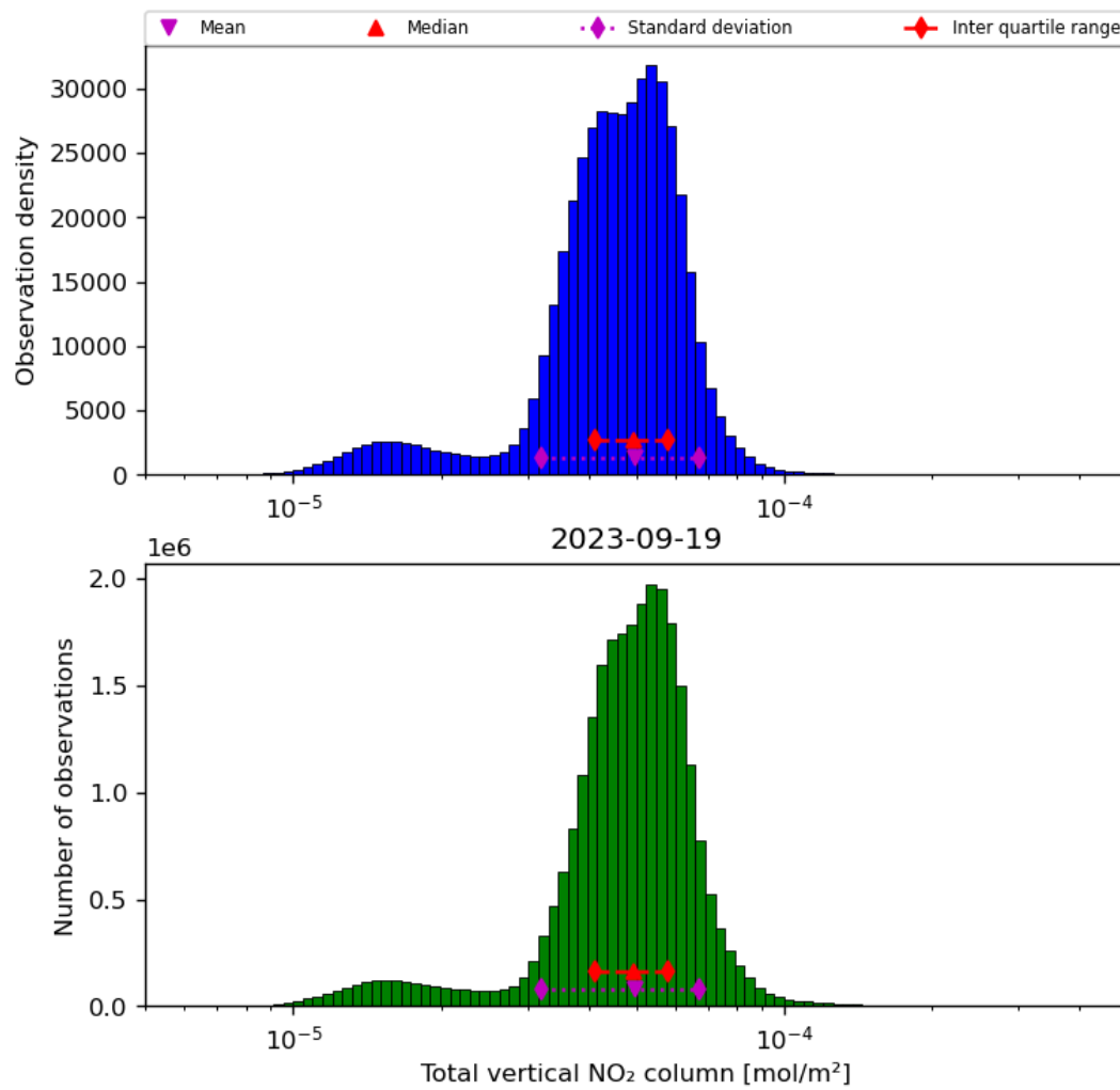
Figure 38: Histogram of "Total vertical NO 2 column" for 2023-09-18 to 2023-09-20
