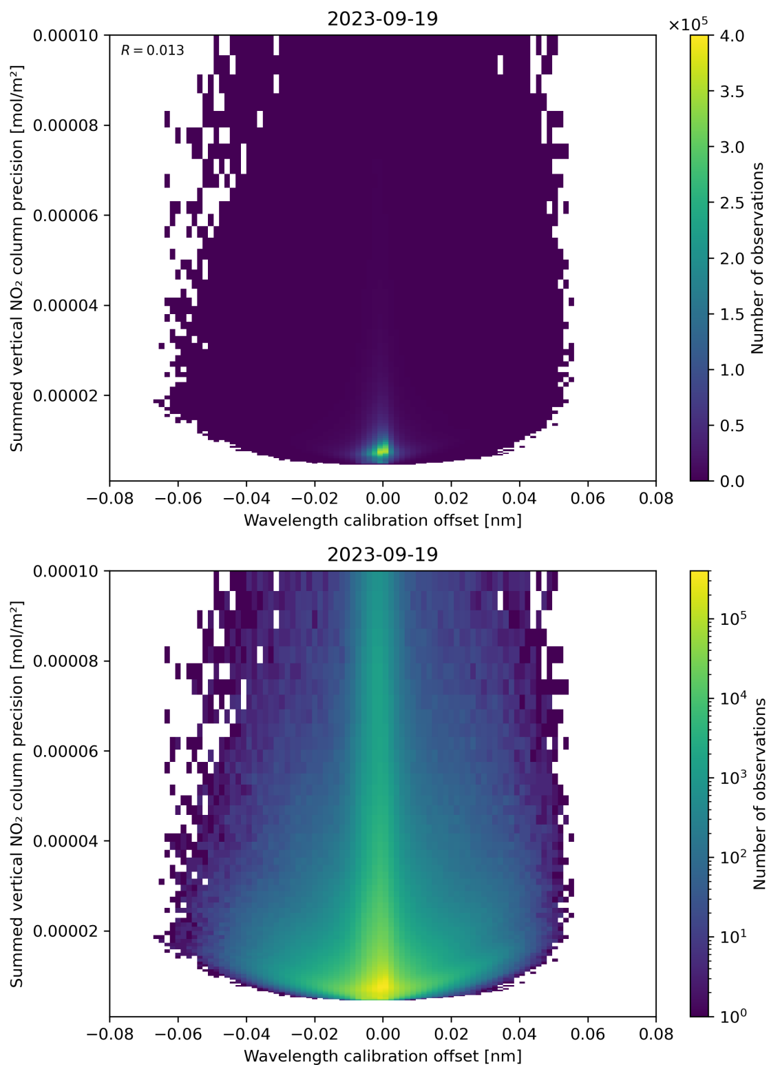
Figure 178: Scatter density plot of “Wavelength calibration offset” against “Summed vertical NO 2 column precision” for 2023-09-18 to 2023-09-20.
