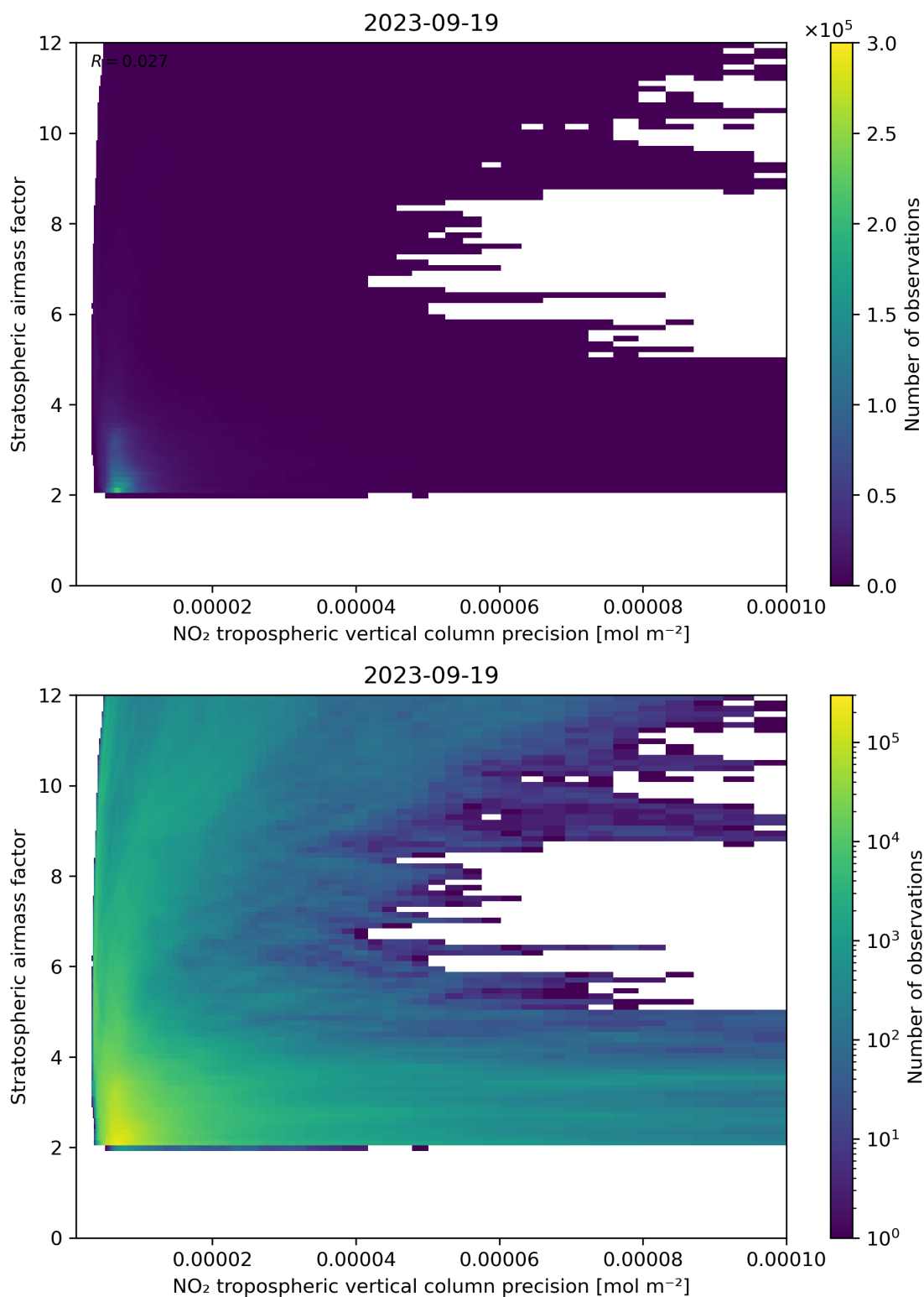
Figure 131: Scatter density plot of “NO 2 tropospheric vertical column precision” against “Stratospheric airmass factor” for 2023-09-18 to 2023-09-20.
