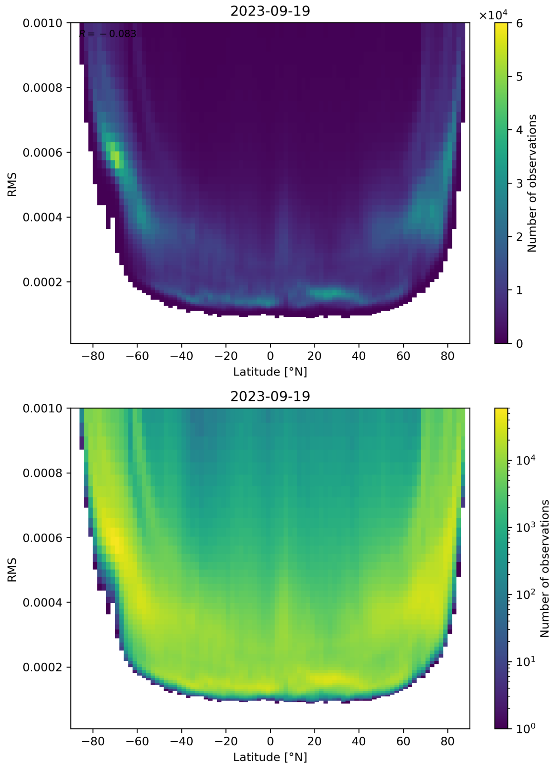
Figure 94: Scatter density plot of “Latitude” against “RMS” for 2023-09-18 to 2023-09-20.
