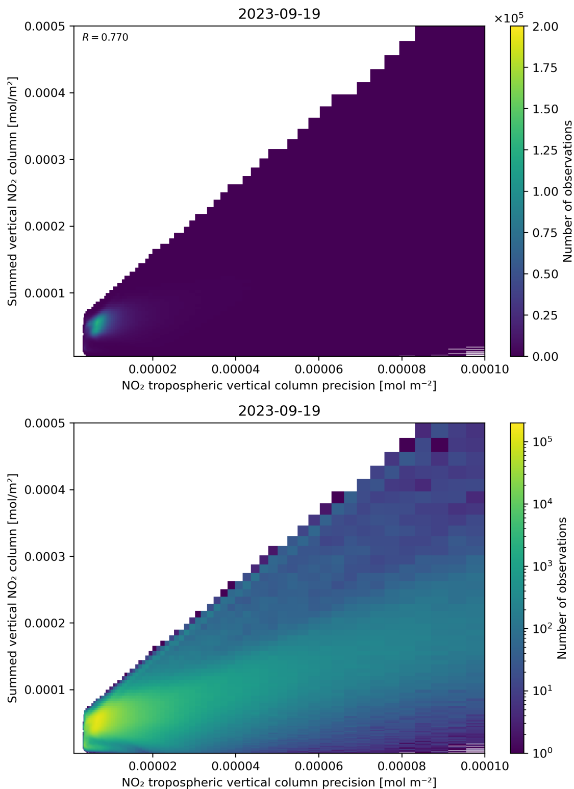
Figure 136: Scatter density plot of “NO 2 tropospheric vertical column precision” against “Summed vertical NO 2 column” for 2023-09-18 to 2023-09-20.
