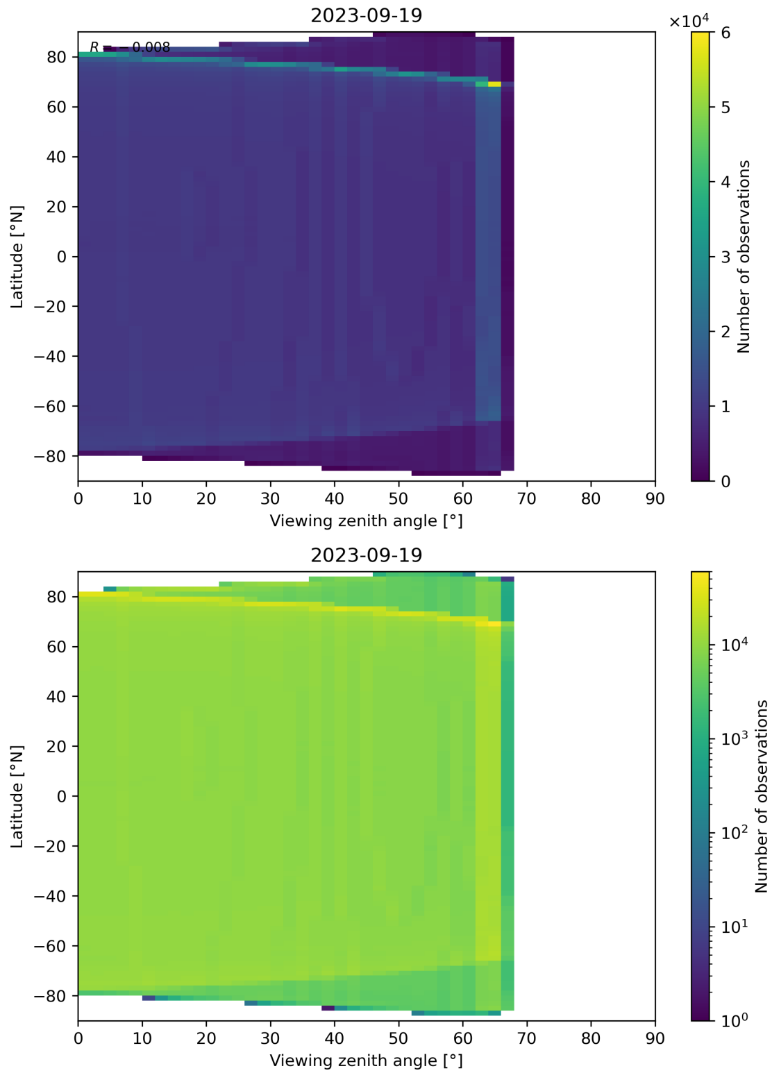
Figure 163: Scatter density plot of “Viewing zenith angle” against “Latitude” for 2023-09-18 to 2023-09-20.
