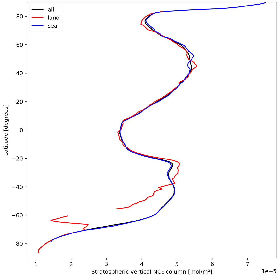
Figure 19: Zonal average of “Stratospheric vertical NO 2 column” for 2023-09-18 to 2023-09-20.
