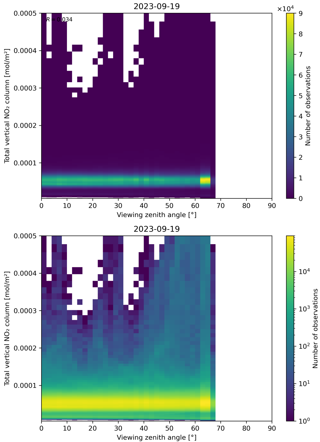
Figure 167: Scatter density plot of “Viewing zenith angle” against “Total vertical NO 2 column” for 2023-09-18 to 2023-09-20.
