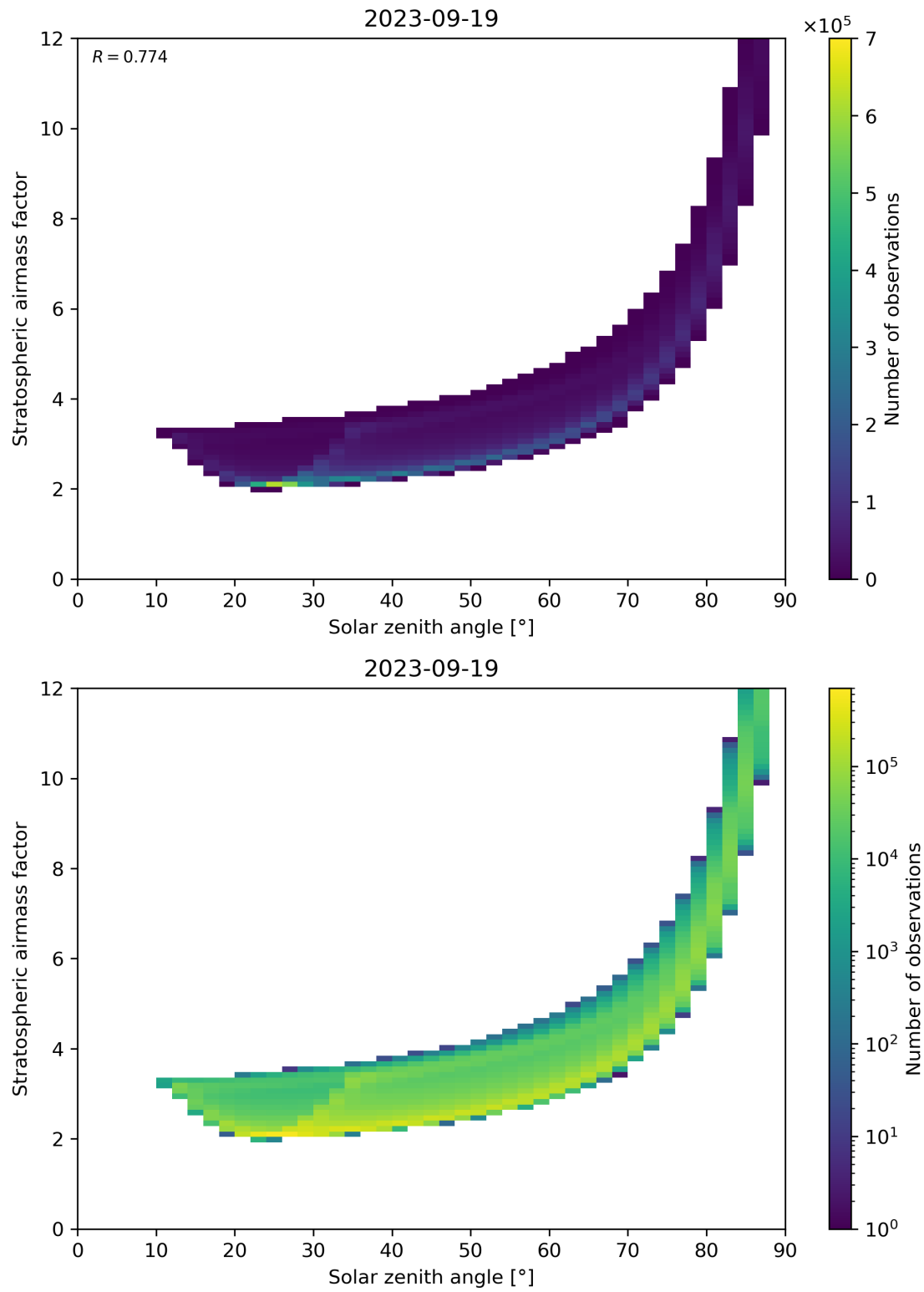
Figure 145: Scatter density plot of “Solar zenith angle” against “Stratospheric airmass factor” for 2023-09-18 to 2023-09-20.
