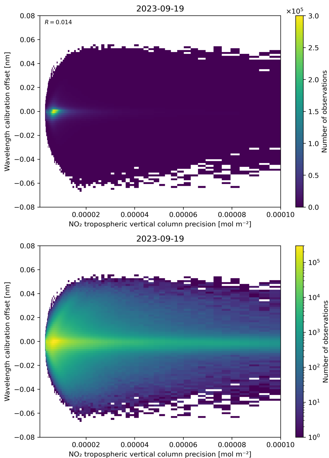
Figure 141: Scatter density plot of “NO 2 tropospheric vertical column precision” against “Wavelength calibration offset” for 2023-09-18 to 2023-09-20.
