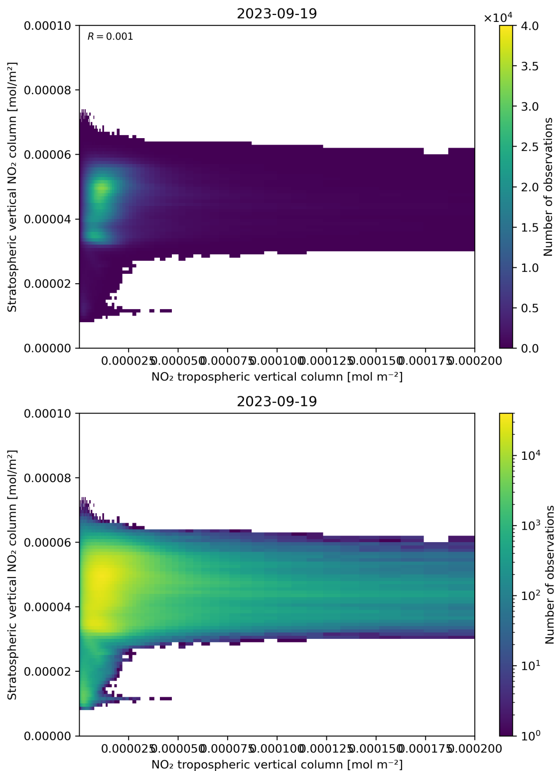
Figure 125: Scatter density plot of “NO 2 tropospheric vertical column” against “Stratospheric vertical NO 2 column” for 2023-09-18 to 2023-09-20.
