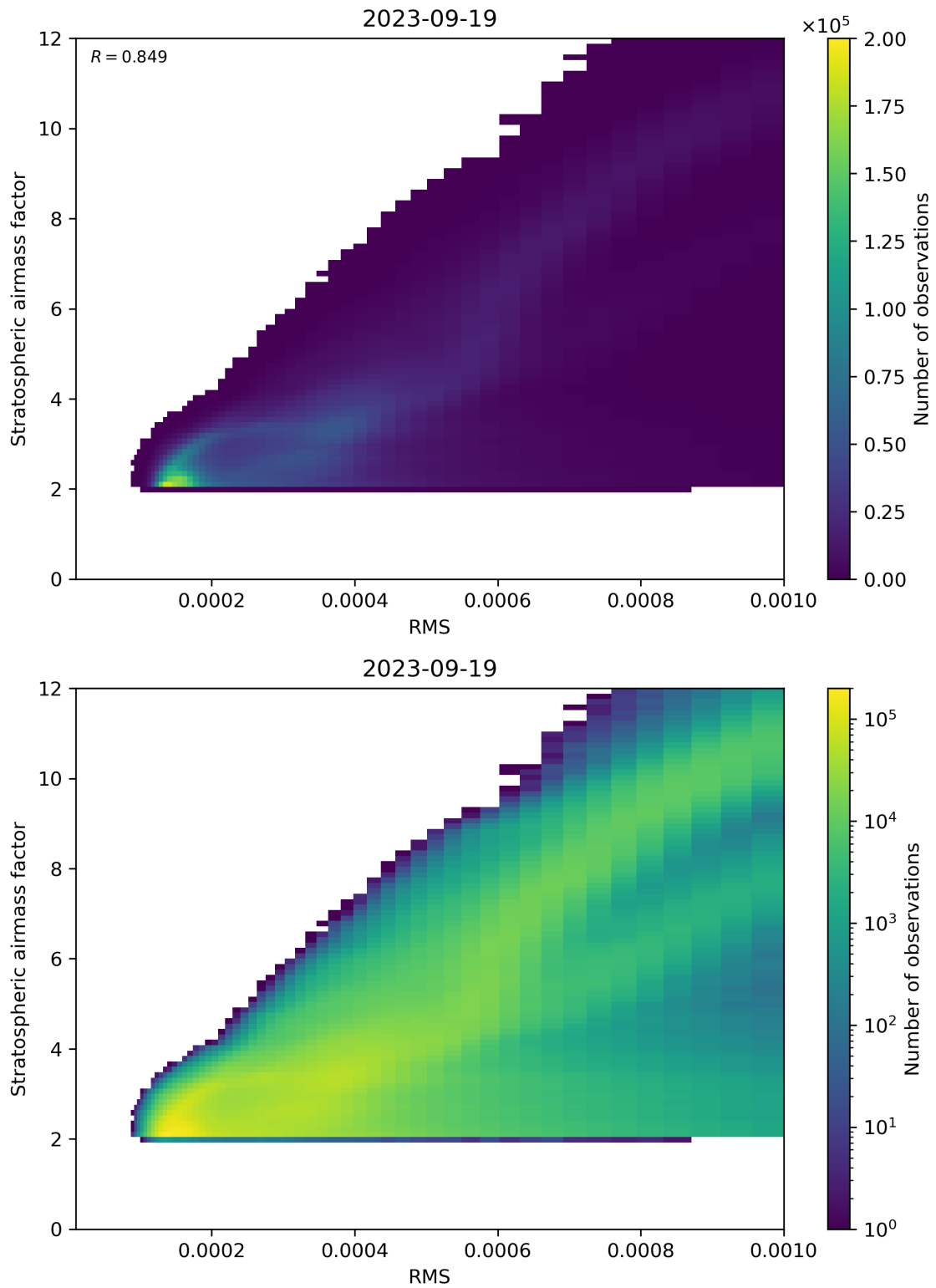
Figure 144: Scatter density plot of “RMS” against “Stratospheric airmass factor” for 2023-09-18 to 2023-09-20.
