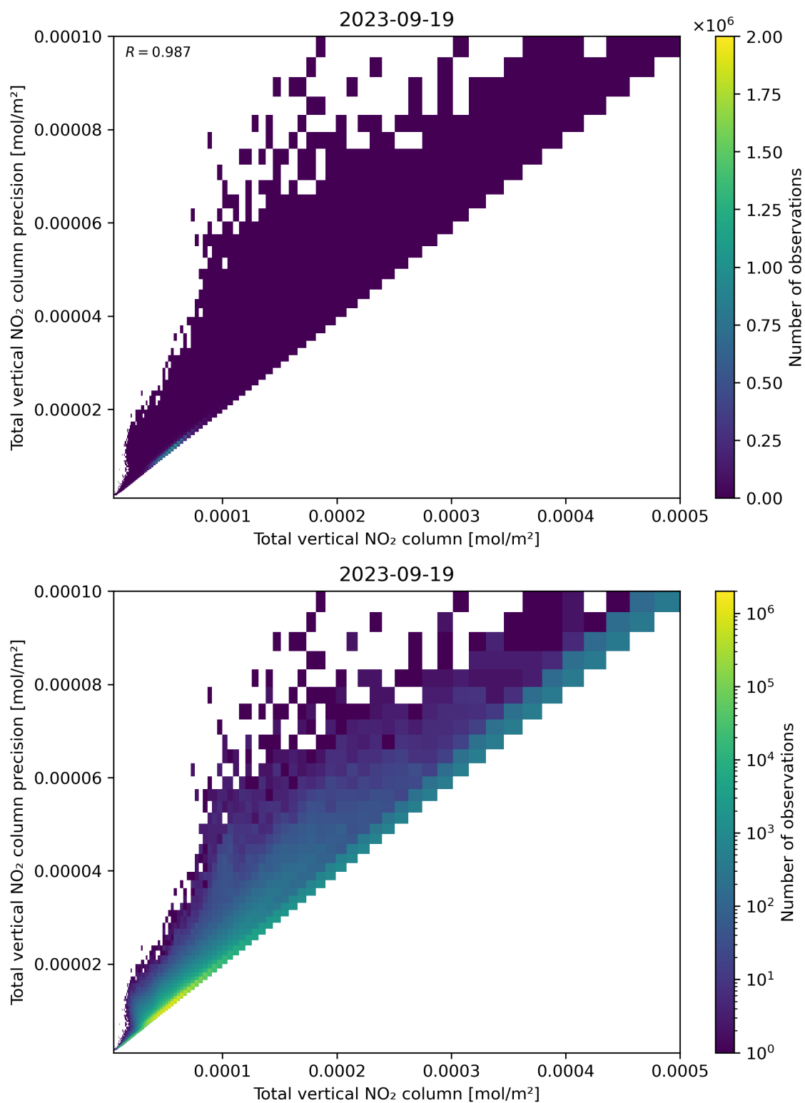
Figure 114: Scatter density plot of “Total vertical NO 2 column” against “Total vertical NO 2 column precision” for 2023-09-18 to 2023-09-20.
