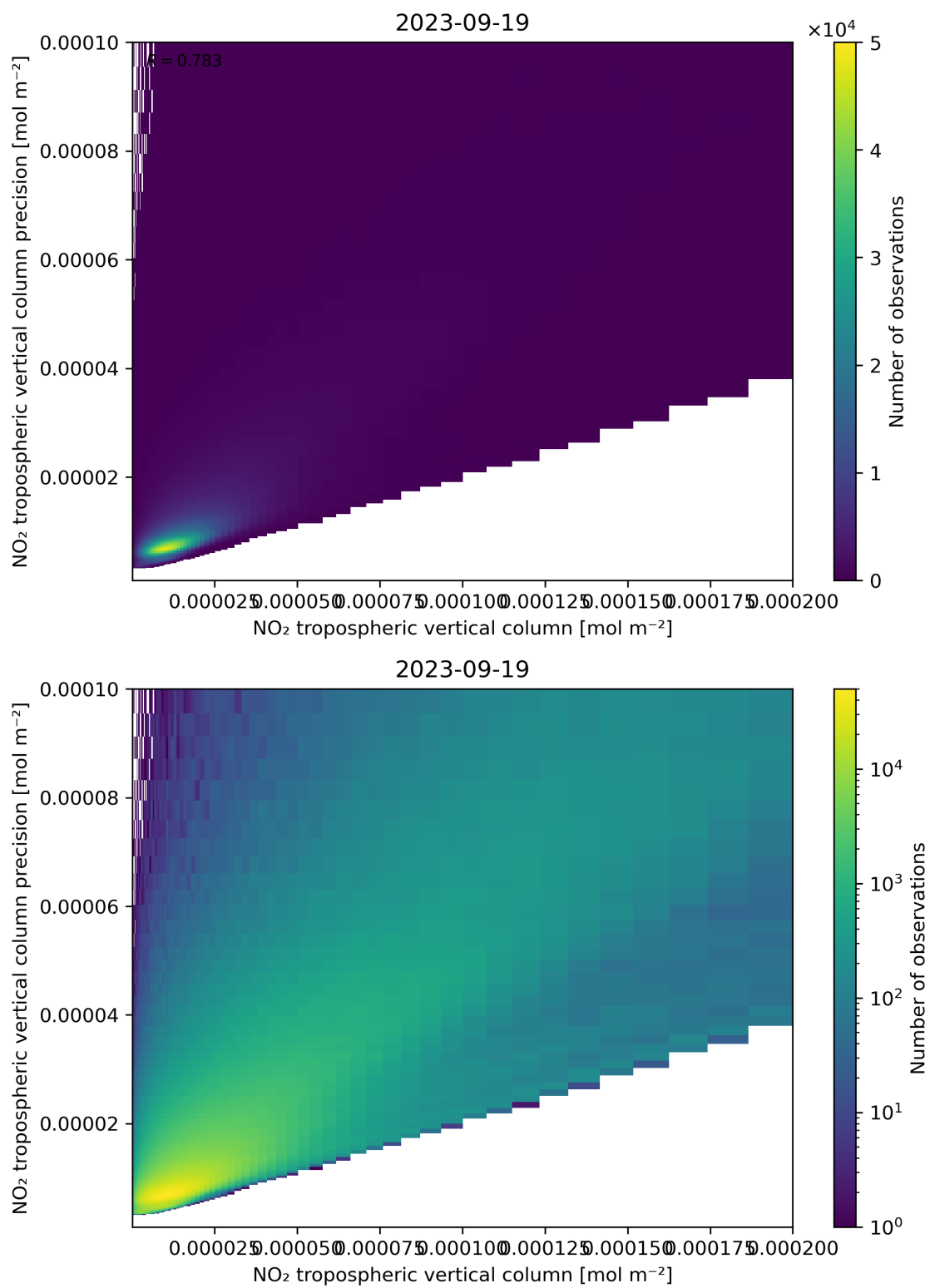
Figure 130: Scatter density plot of “NO 2 tropospheric vertical column” against “NO 2 tropospheric vertical column precision” for 2023-09-18 to 2023-09-20.
