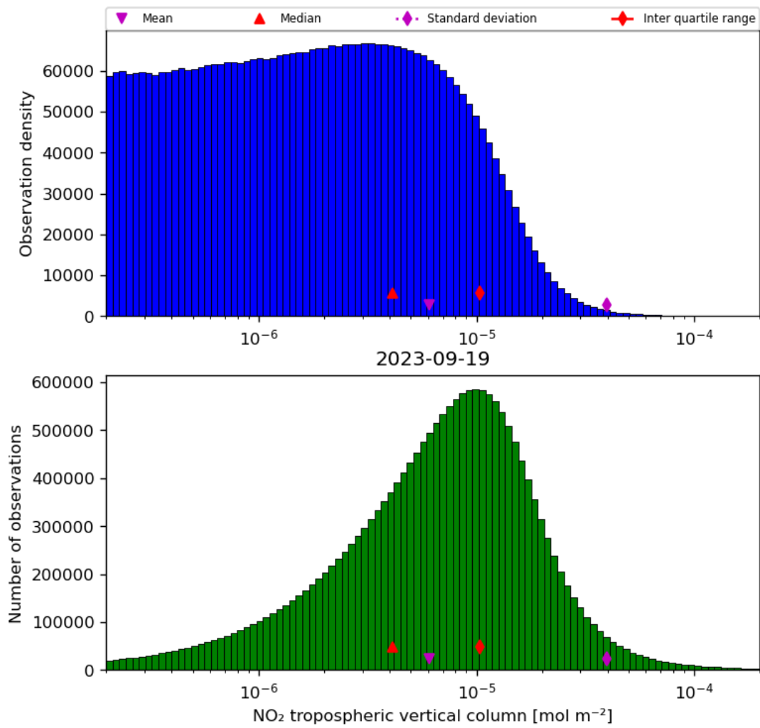
Figure 29: Histogram of “NO 2 tropospheric vertical column” for 2023-09-18 to 2023-09-20
