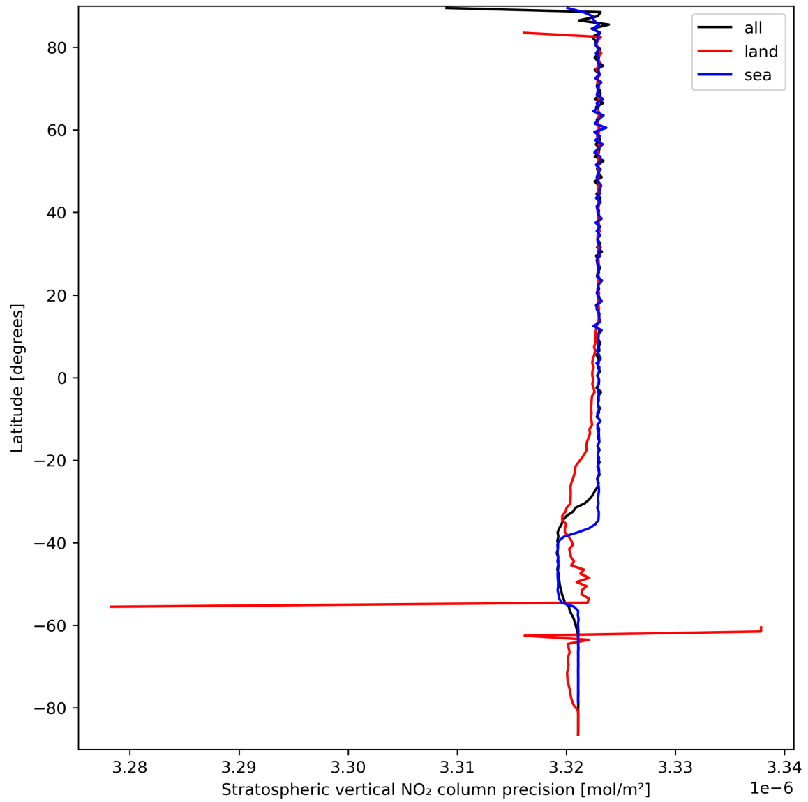
Figure 20: Zonal average of “Stratospheric vertical NO 2 column precision” for 2023-09-18 to 2023-09-20.
