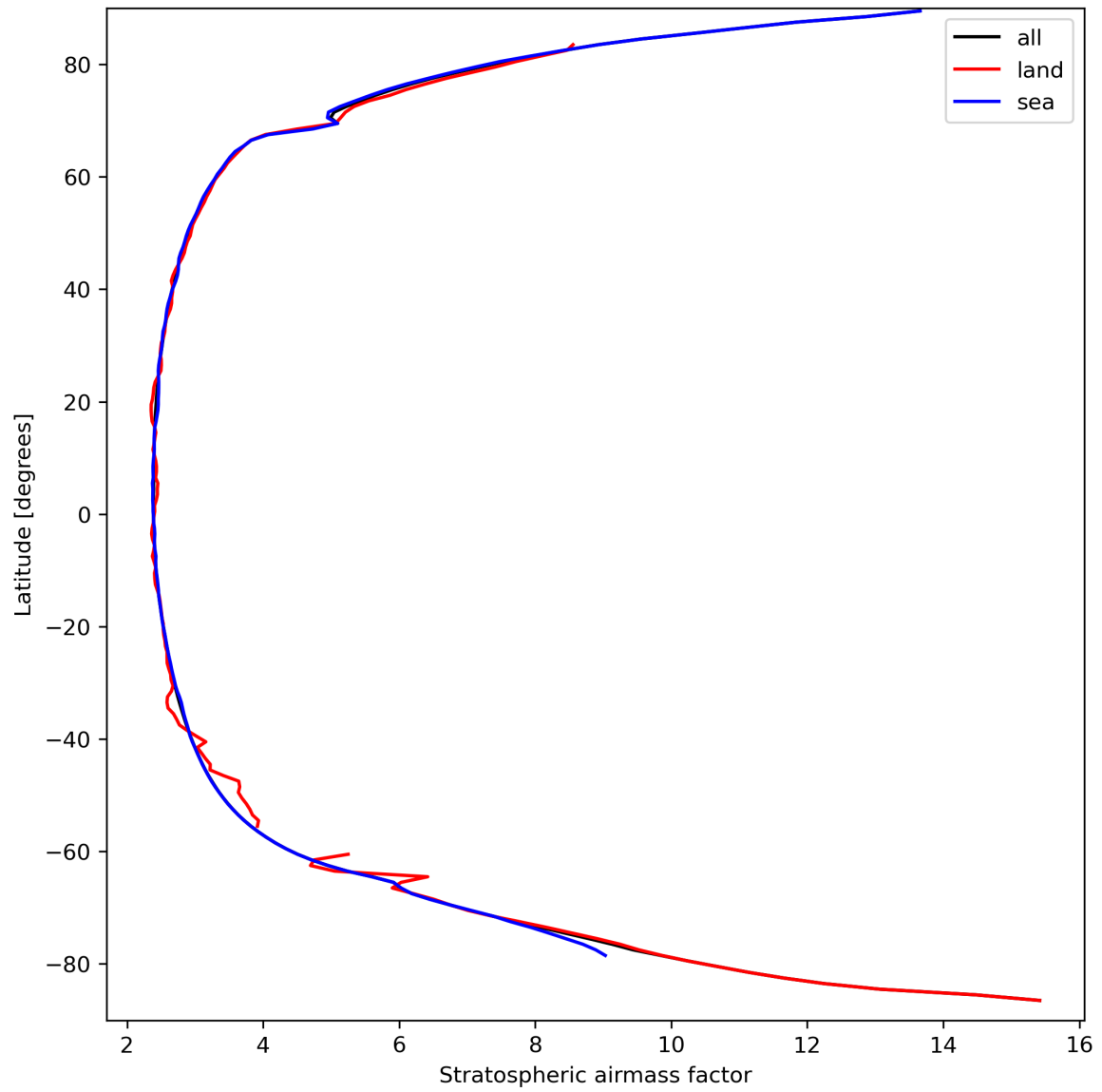
Figure 27: Zonal average of “Stratospheric airmass factor” for 2023-09-18 to 2023-09-20.
