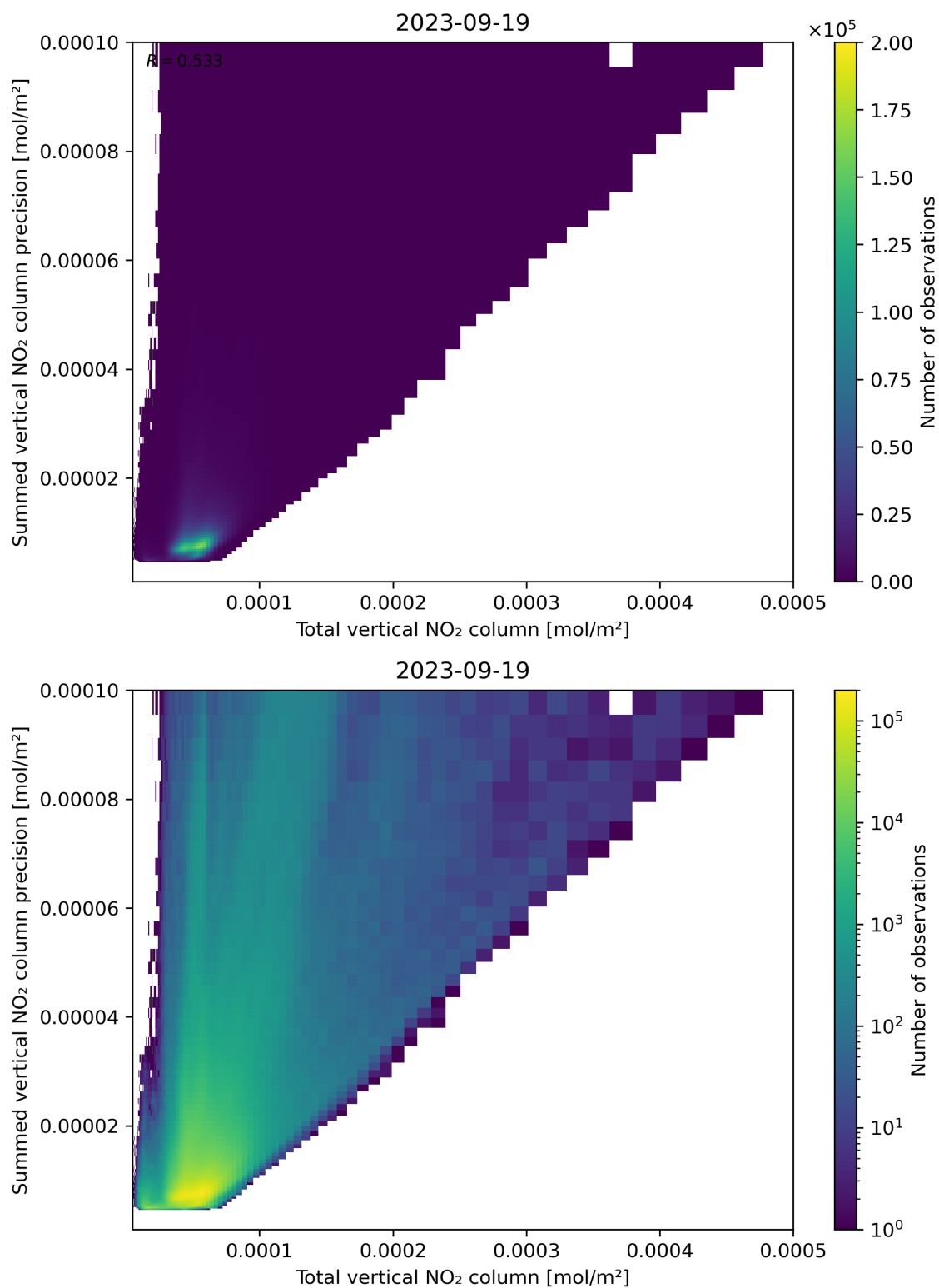
Figure 113: Scatter density plot of “Total vertical NO 2 column” against “Summed vertical NO 2 column precision” for 2023-09-18 to 2023-09-20.
