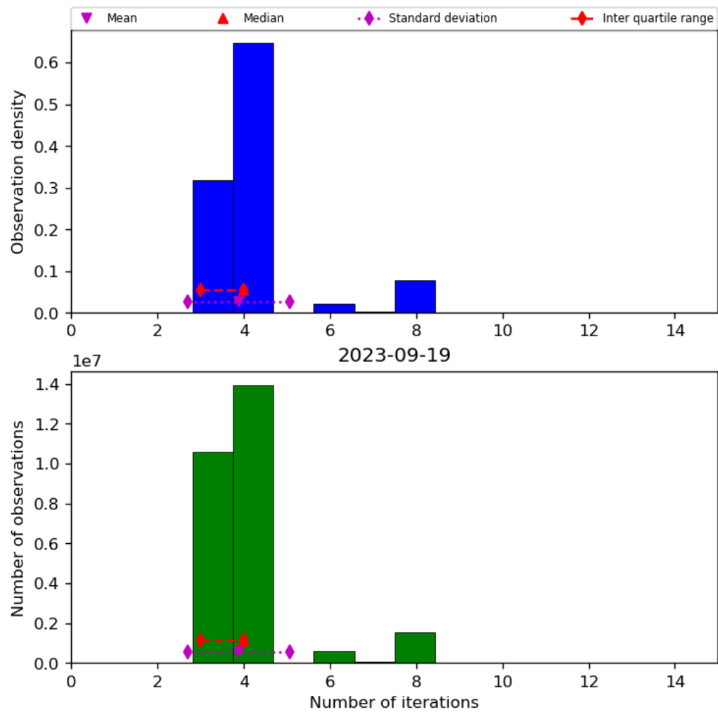
Figure 34: Histogram of “Number of iterations” for 2023-09-18 to 2023-09-20
