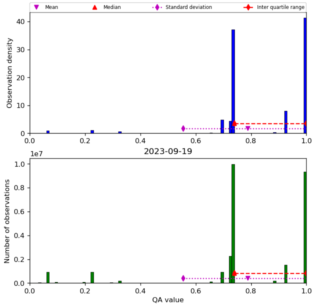
Figure 28: Histogram of “QA value” for 2023-09-18 to 2023-09-20
