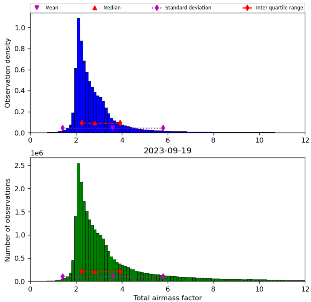
Figure 32: Histogram of “Total airmass factor” for 2023-09-18 to 2023-09-20
