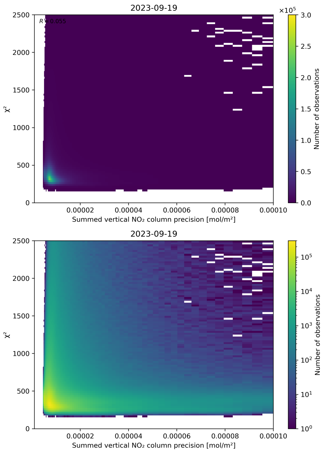
Figure 107: Scatter density plot of “Summed vertical NO 2 column precision” against “ \chi^2 ” for 2023-09-18 to 2023-09-20.
