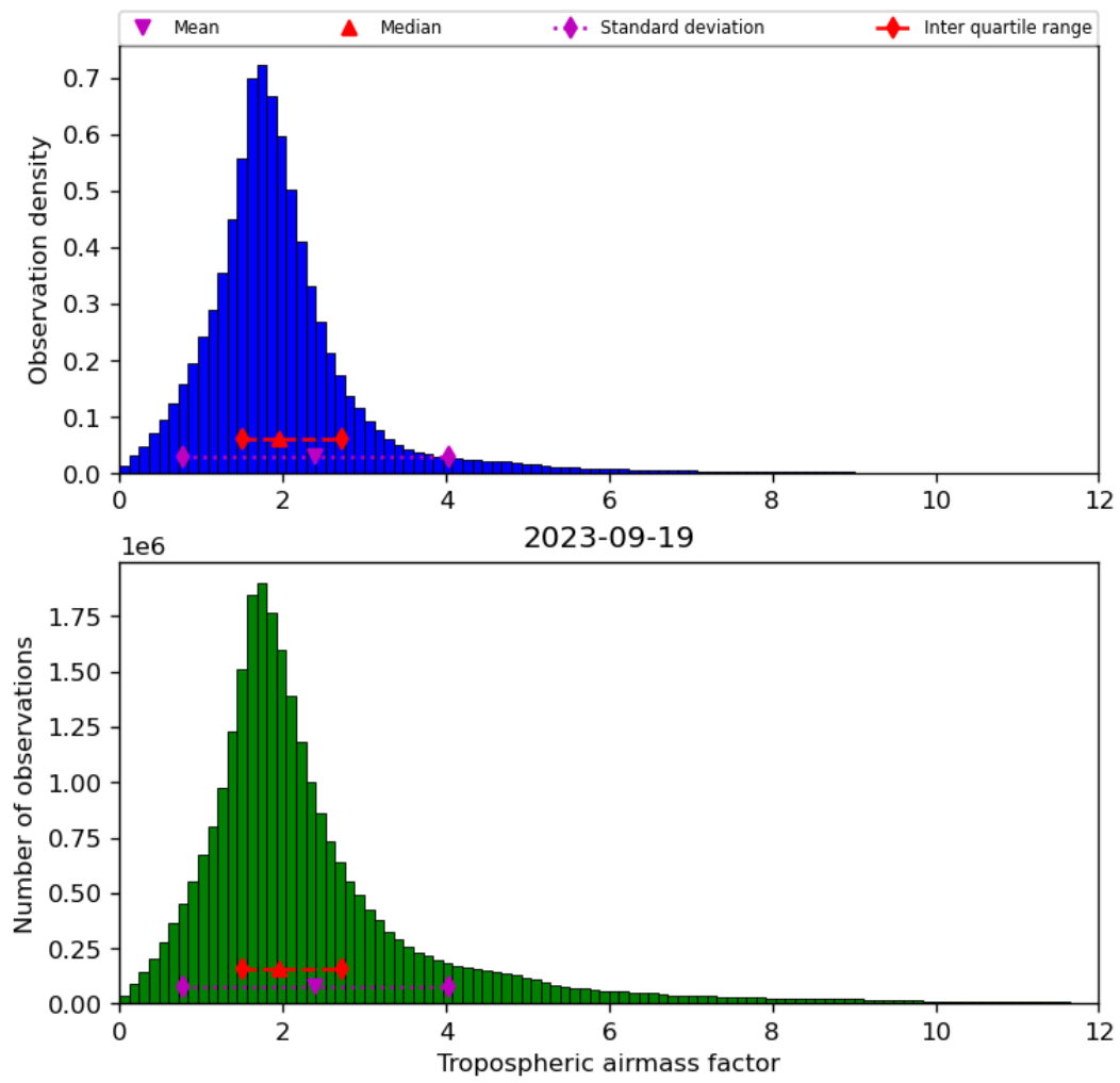
Figure 31: Histogram of “Tropospheric airmass factor” for 2023-09-18 to 2023-09-20
