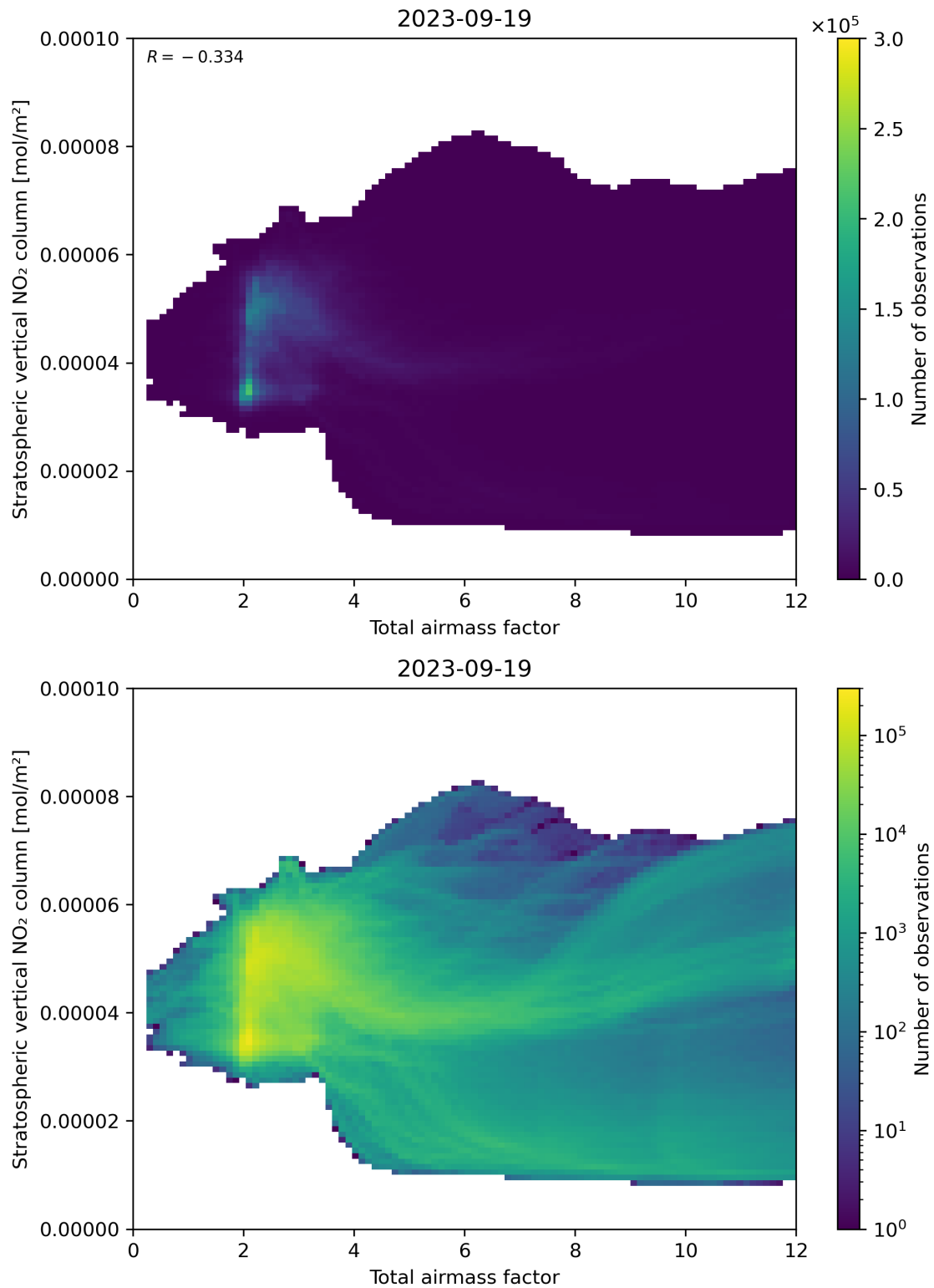
Figure 64: Scatter density plot of “Total airmass factor” against “Stratospheric vertical \text{NO}_2 column” for 2023-09-18 to 2023-09-20.
