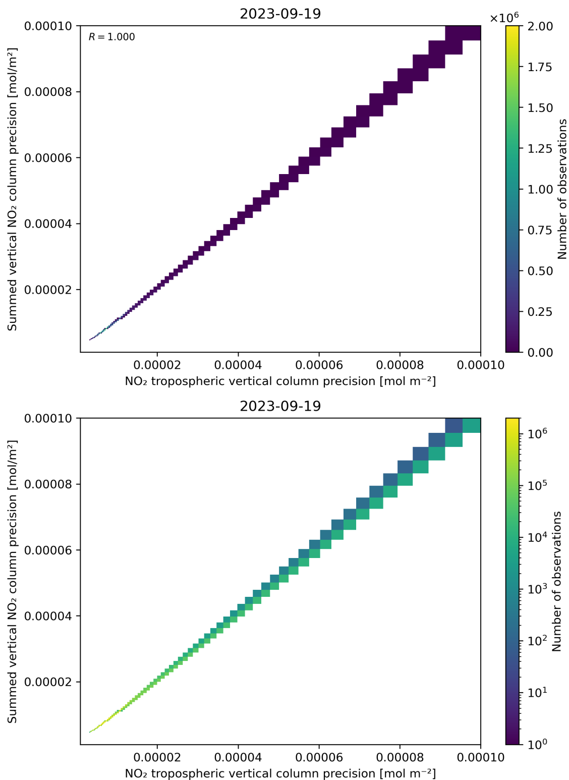
Figure 137: Scatter density plot of “NO 2 tropospheric vertical column precision” against “Summed vertical NO 2 column precision” for 2023-09-18 to 2023-09-20.
