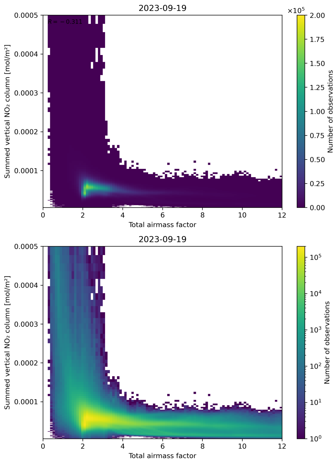
Figure 65: Scatter density plot of “Total airmass factor” against “Summed vertical NO 2 column” for 2023-09-18 to 2023-09-20.
