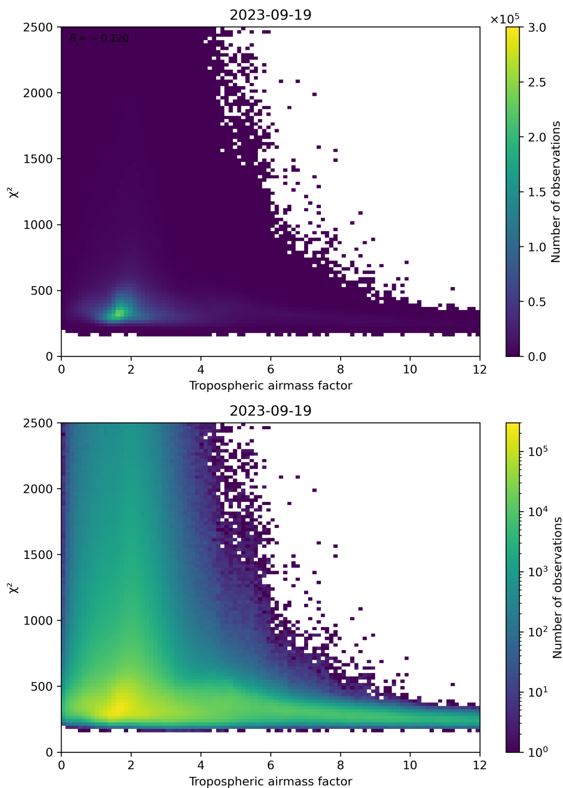
Figure 73: Scatter density plot of “Tropospheric airmass factor” against “ \chi^2 ” for 2023-09-18 to 2023-09-20.
