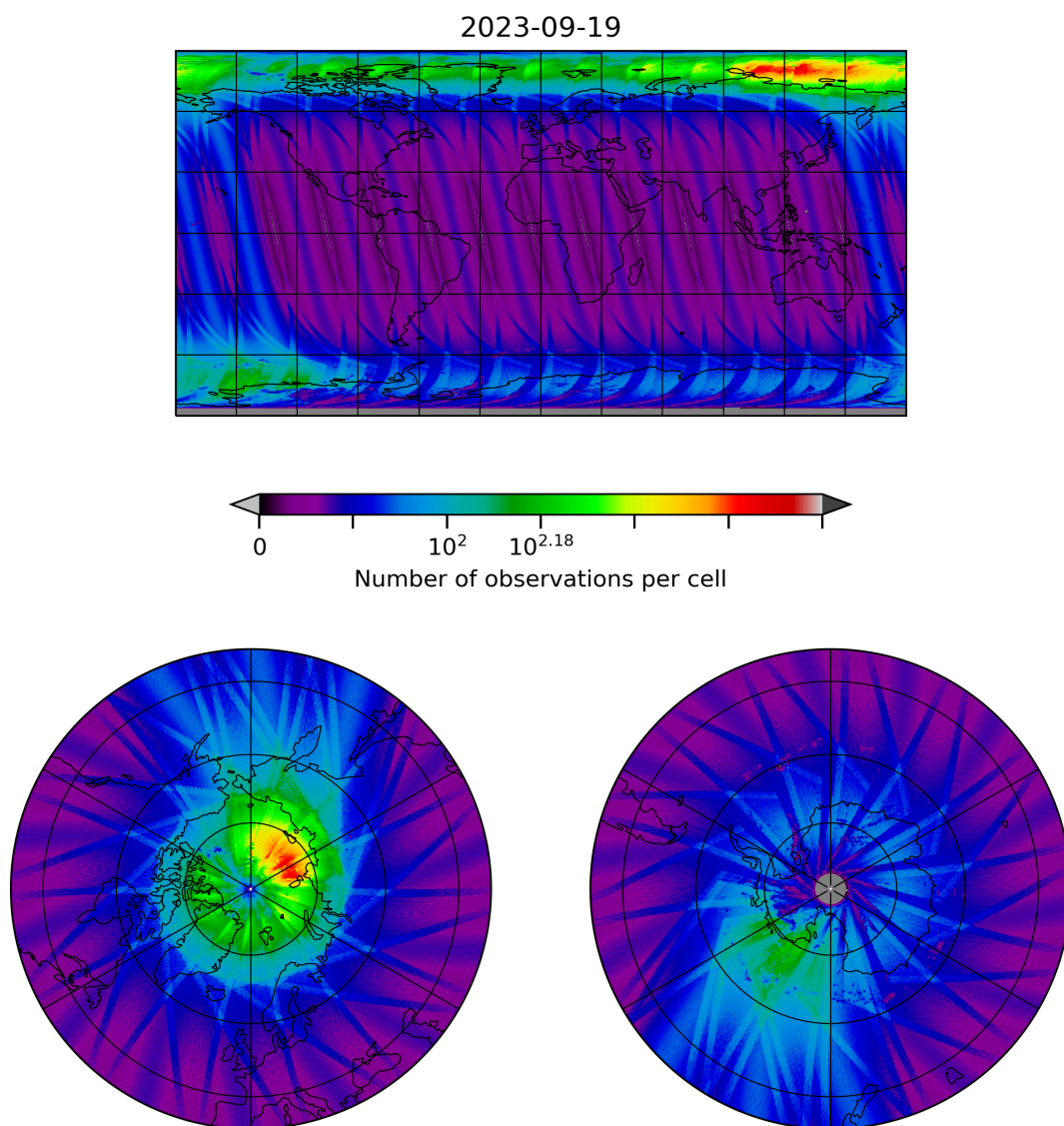
Figure 10: Map of the number of observations for 2023-09-18 to 2023-09-20
