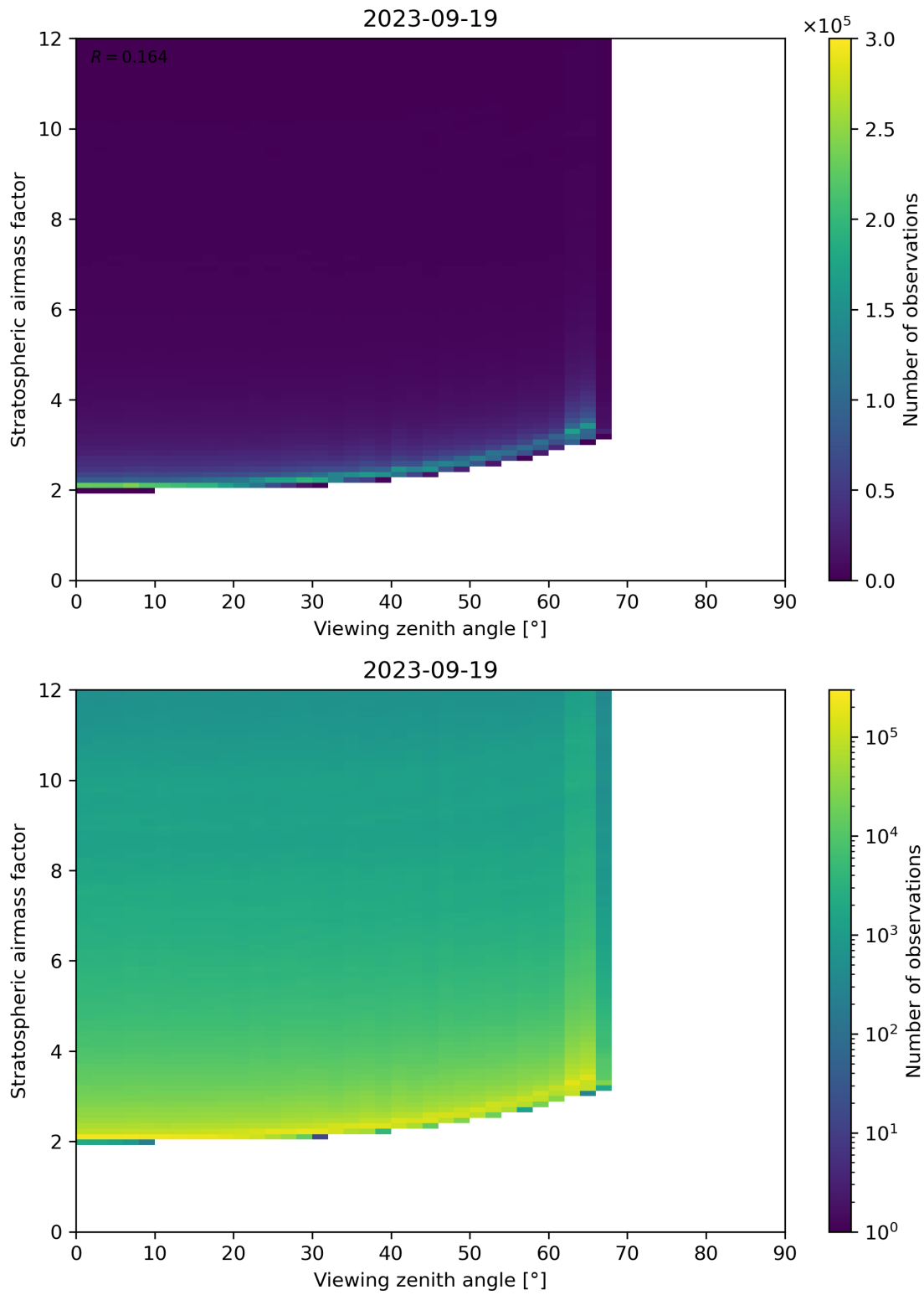
Figure 159: Scatter density plot of “Viewing zenith angle” against “Stratospheric airmass factor” for 2023-09-18 to 2023-09-20.
