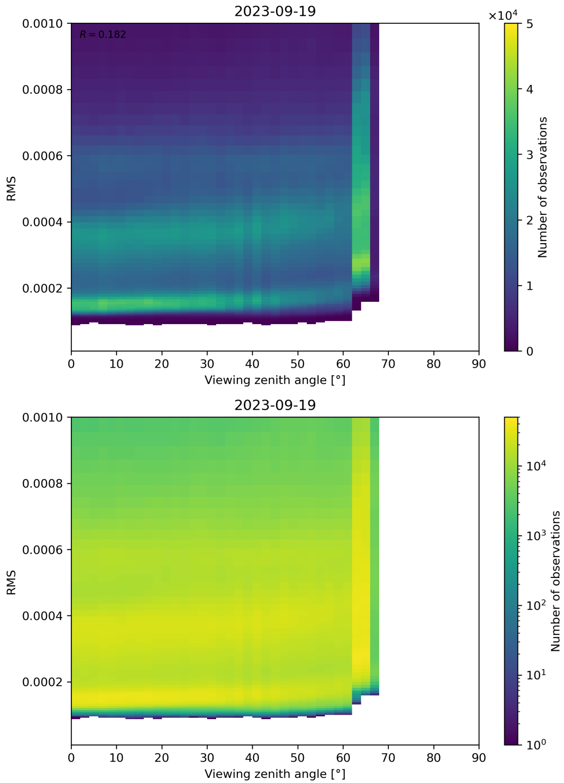
Figure 171: Scatter density plot of “Viewing zenith angle” against “RMS” for 2023-09-18 to 2023-09-20.
