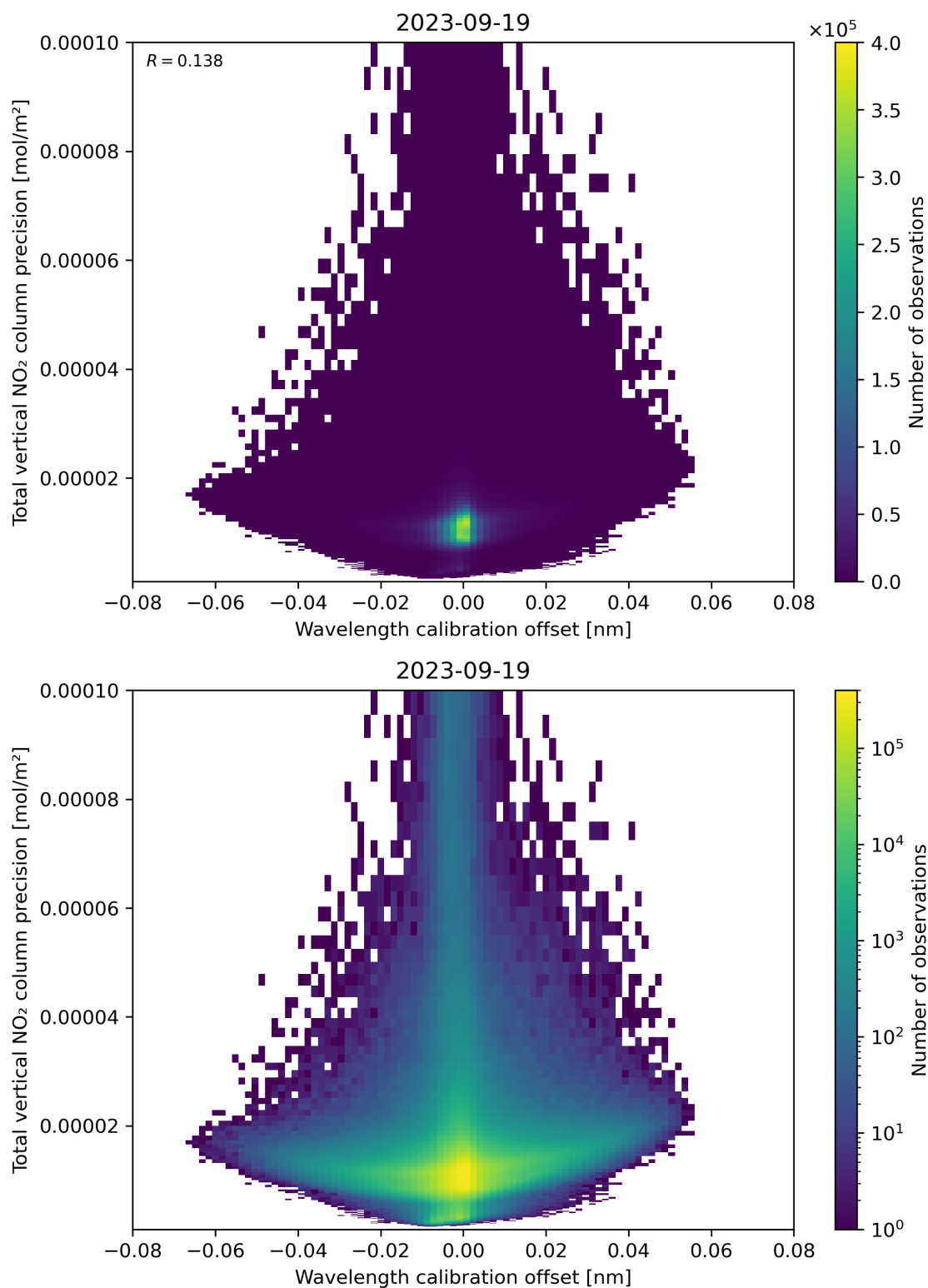
Figure 180: Scatter density plot of “Wavelength calibration offset” against “Total vertical NO 2 column precision” for 2023-09-18 to 2023-09-20.
