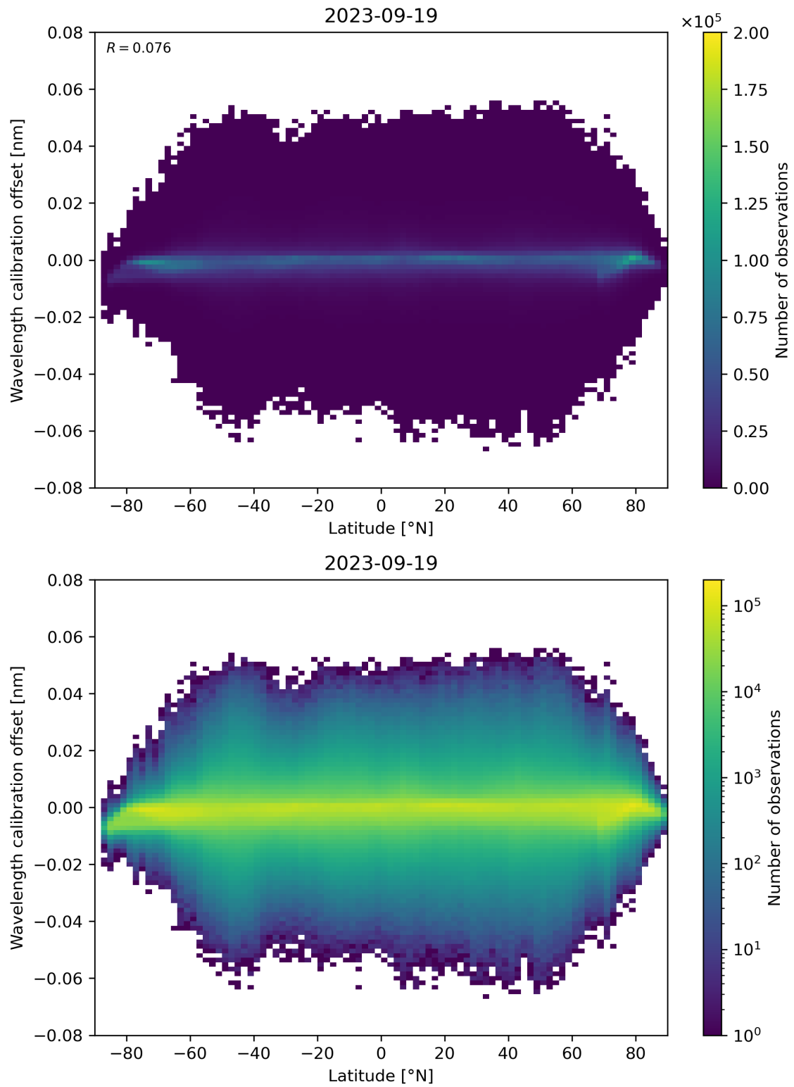
Figure 95: Scatter density plot of “Latitude” against “Wavelength calibration offset” for 2023-09-18 to 2023-09-20.
