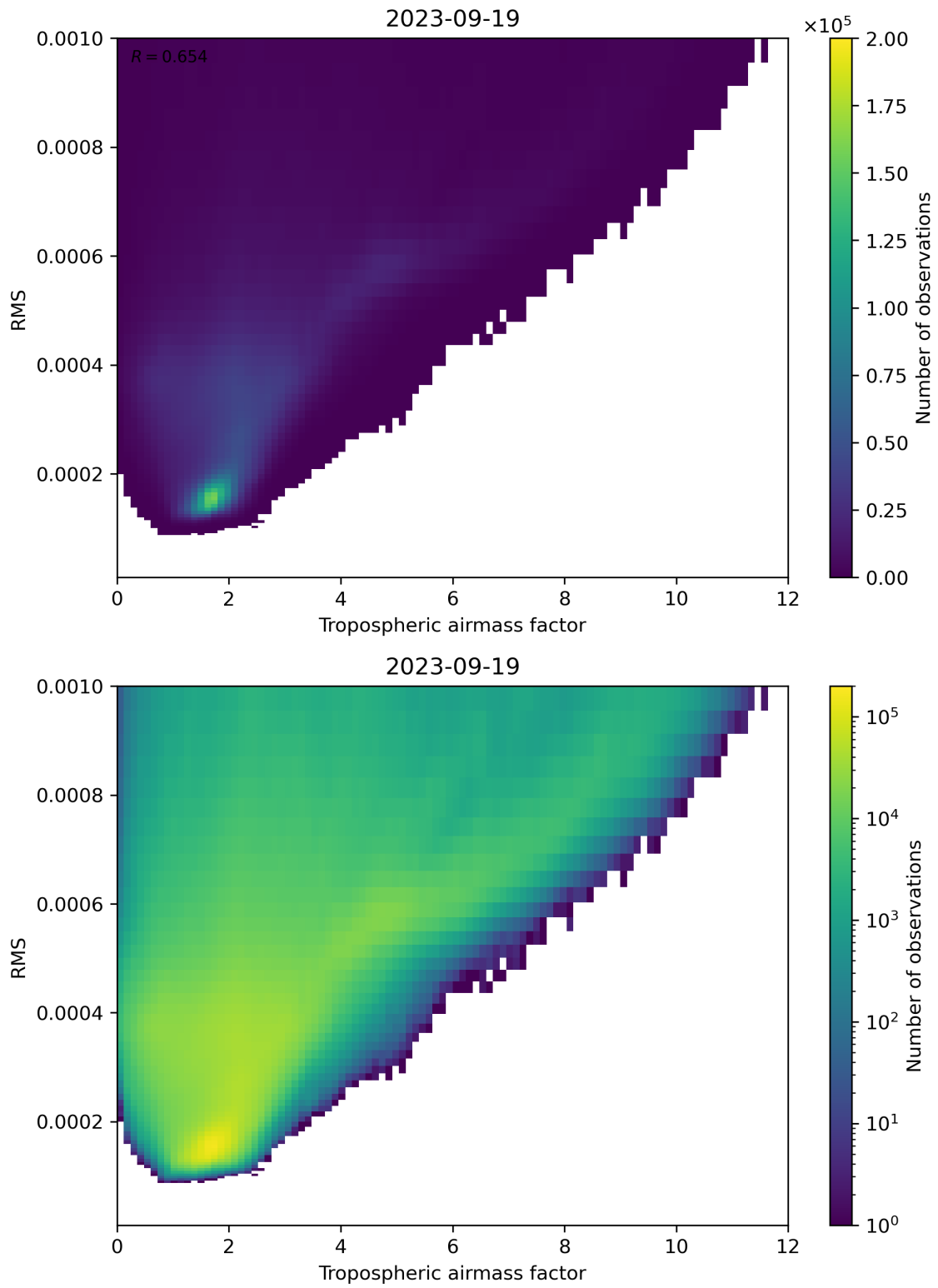
Figure 79: Scatter density plot of “Tropospheric airmass factor” against “RMS” for 2023-09-18 to 2023-09-20.
