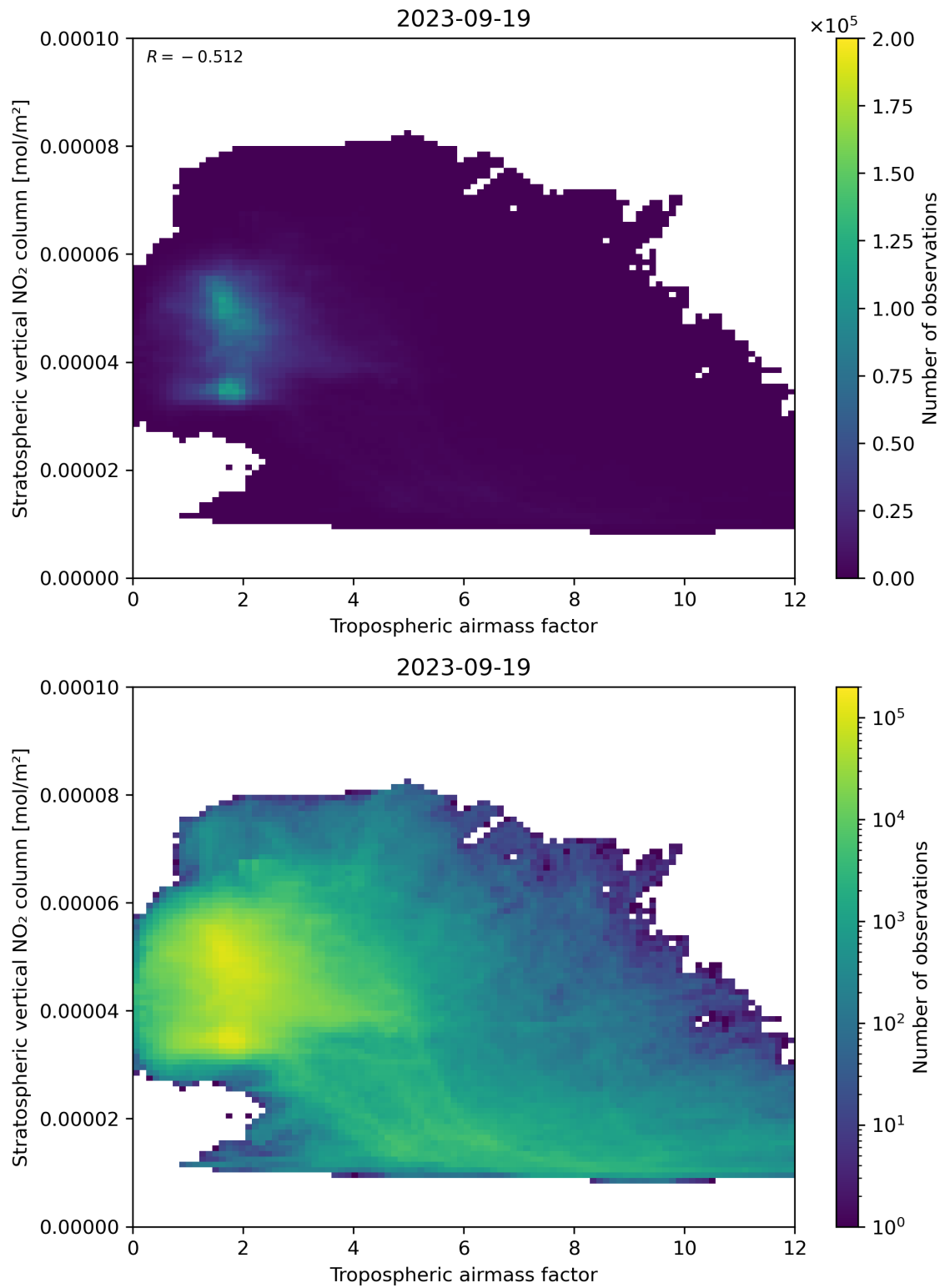
Figure 74: Scatter density plot of “Tropospheric air mass factor” against “Stratospheric vertical NO 2 column” for 2023-09-18 to 2023-09-20.
