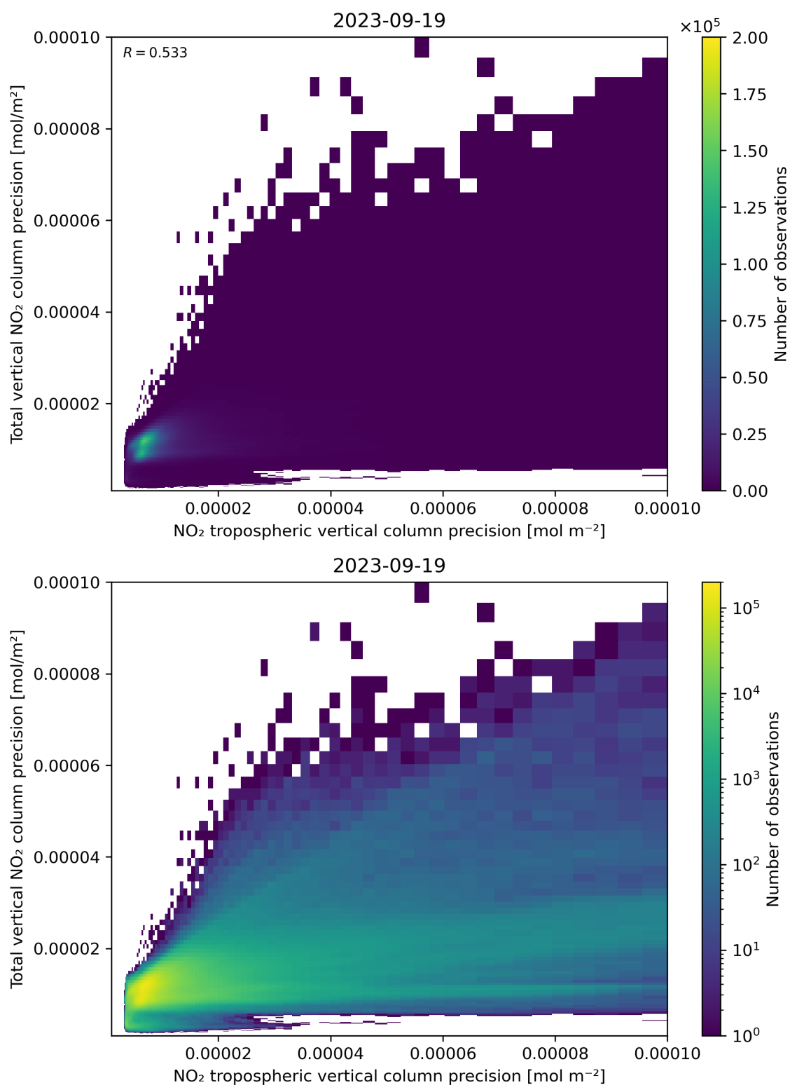
Figure 139: Scatter density plot of “NO 2 tropospheric vertical column precision” against “Total vertical NO 2 column precision” for 2023-09-18 to 2023-09-20.
