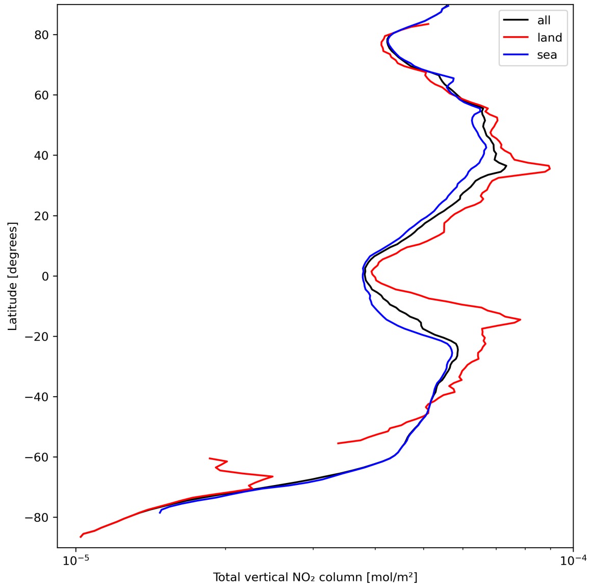
Figure 21: Zonal average of “Total vertical NO 2 column” for 2023-09-18 to 2023-09-20.
