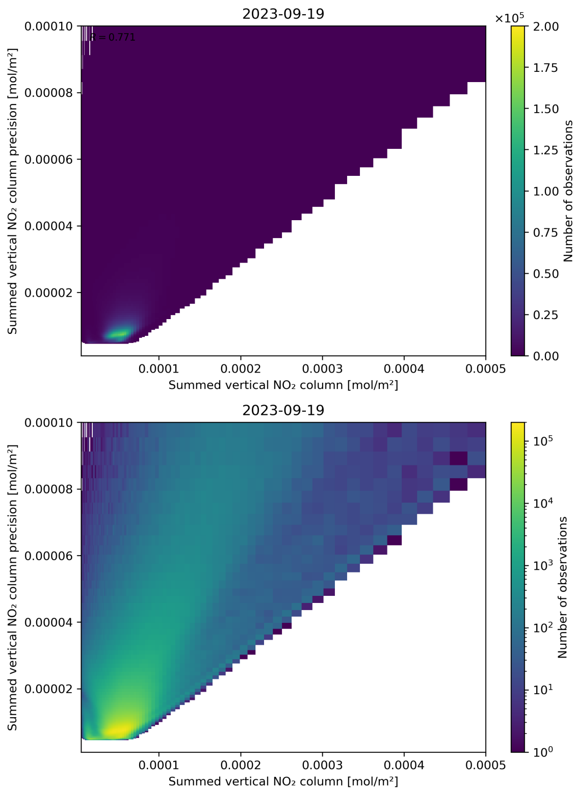
Figure 105: Scatter density plot of “Summed vertical NO 2 column” against “Summed vertical NO 2 column precision” for 2023-09-18 to 2023-09-20.
