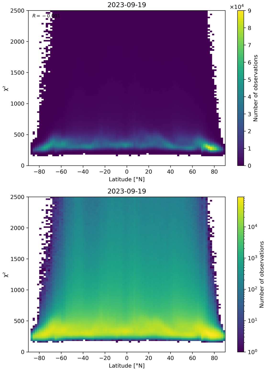
Figure 86: Scatter density plot of “Latitude” against “ \chi^2 ” for 2023-09-18 to 2023-09-20.
