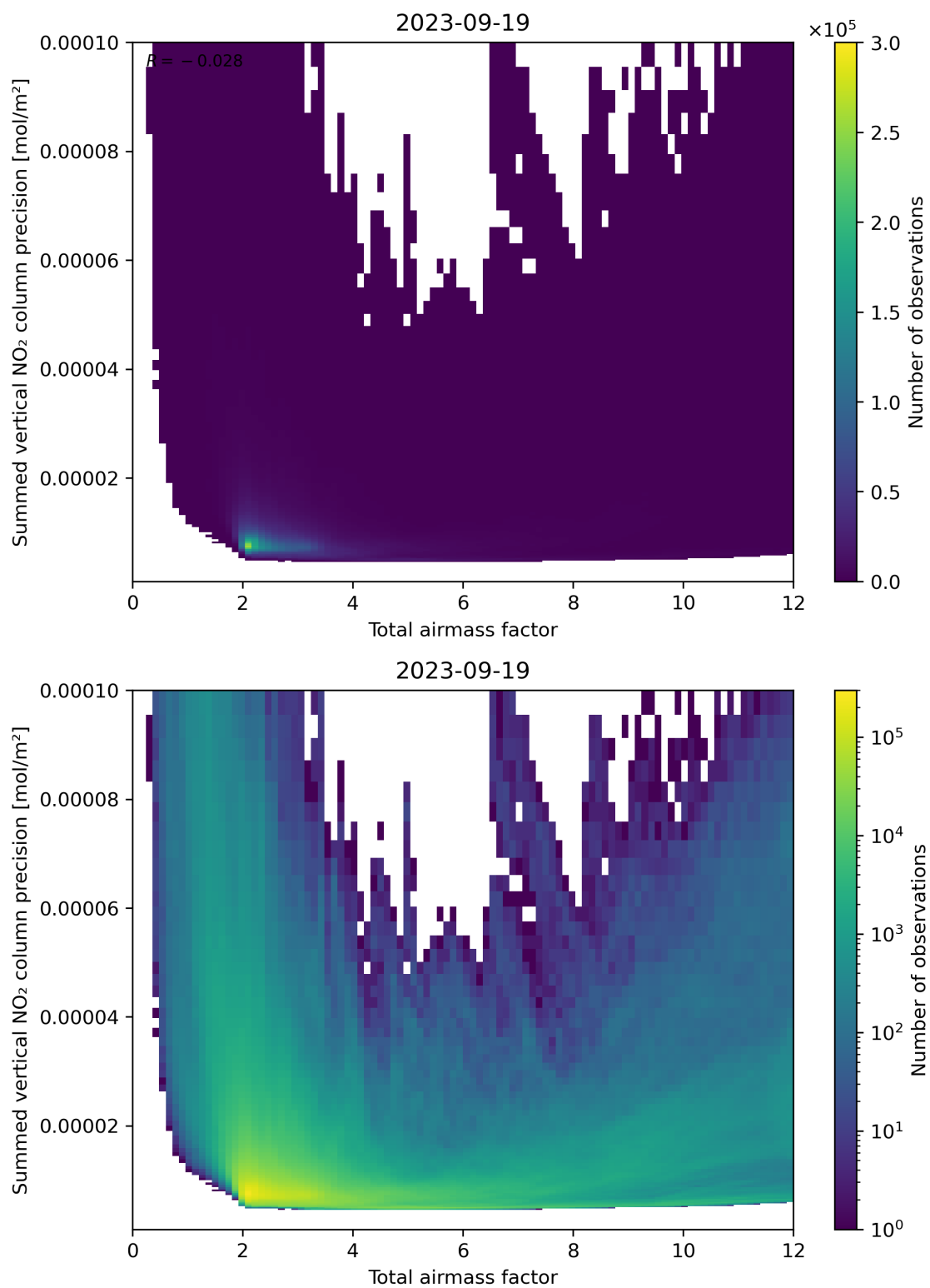
Figure 66: Scatter density plot of “Total airmass factor” against “Summed vertical NO 2 column precision” for 2023-09-18 to 2023-09-20.
