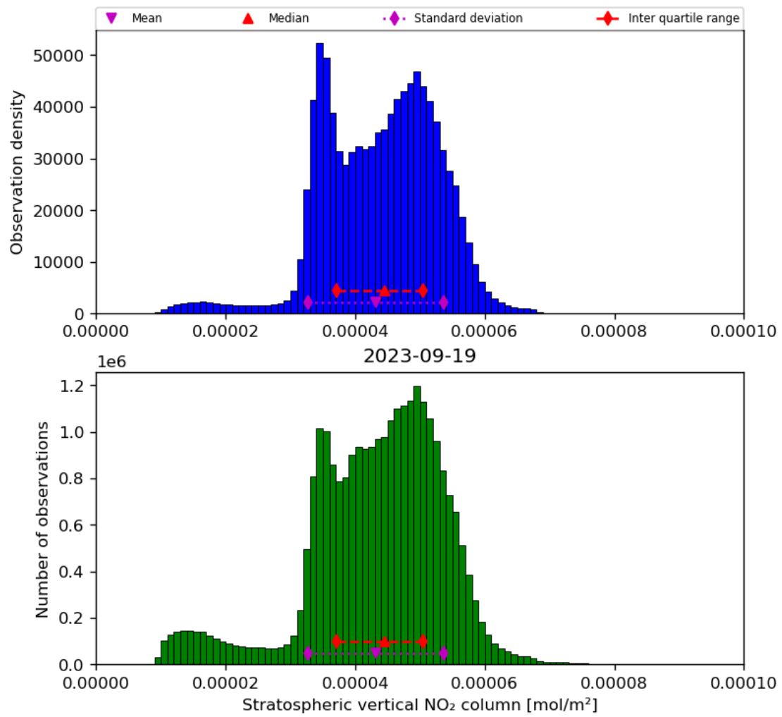
Figure 36: Histogram of “Stratospheric vertical NO 2 column” for 2023-09-18 to 2023-09-20
