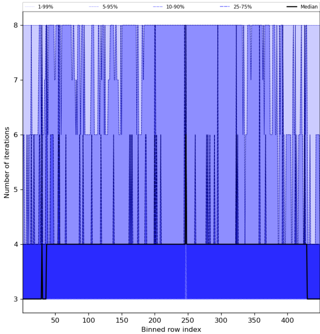
Figure 51: Along track statistics of “Number of iterations” for 2023-09-18 to 2023-09-20
