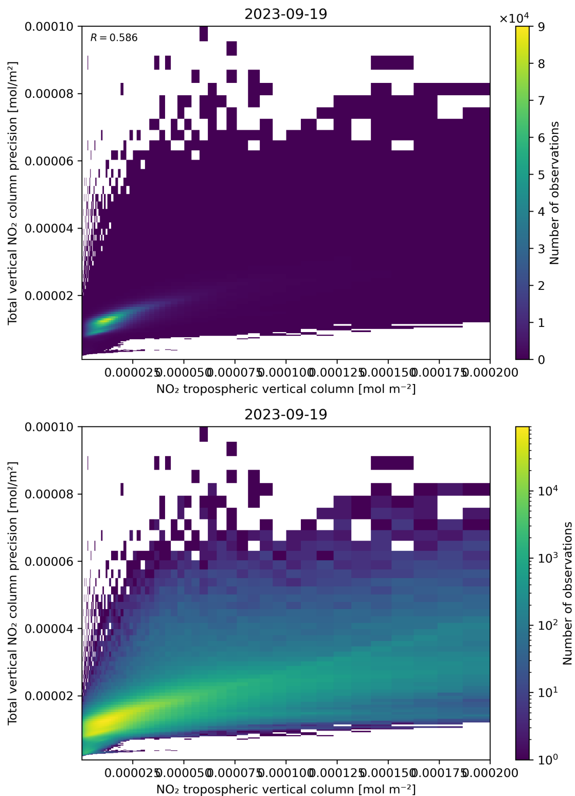
Figure 129: Scatter density plot of “NO 2 tropospheric vertical column” against “Total vertical NO 2 column precision” for 2023-09-18 to 2023-09-20.
