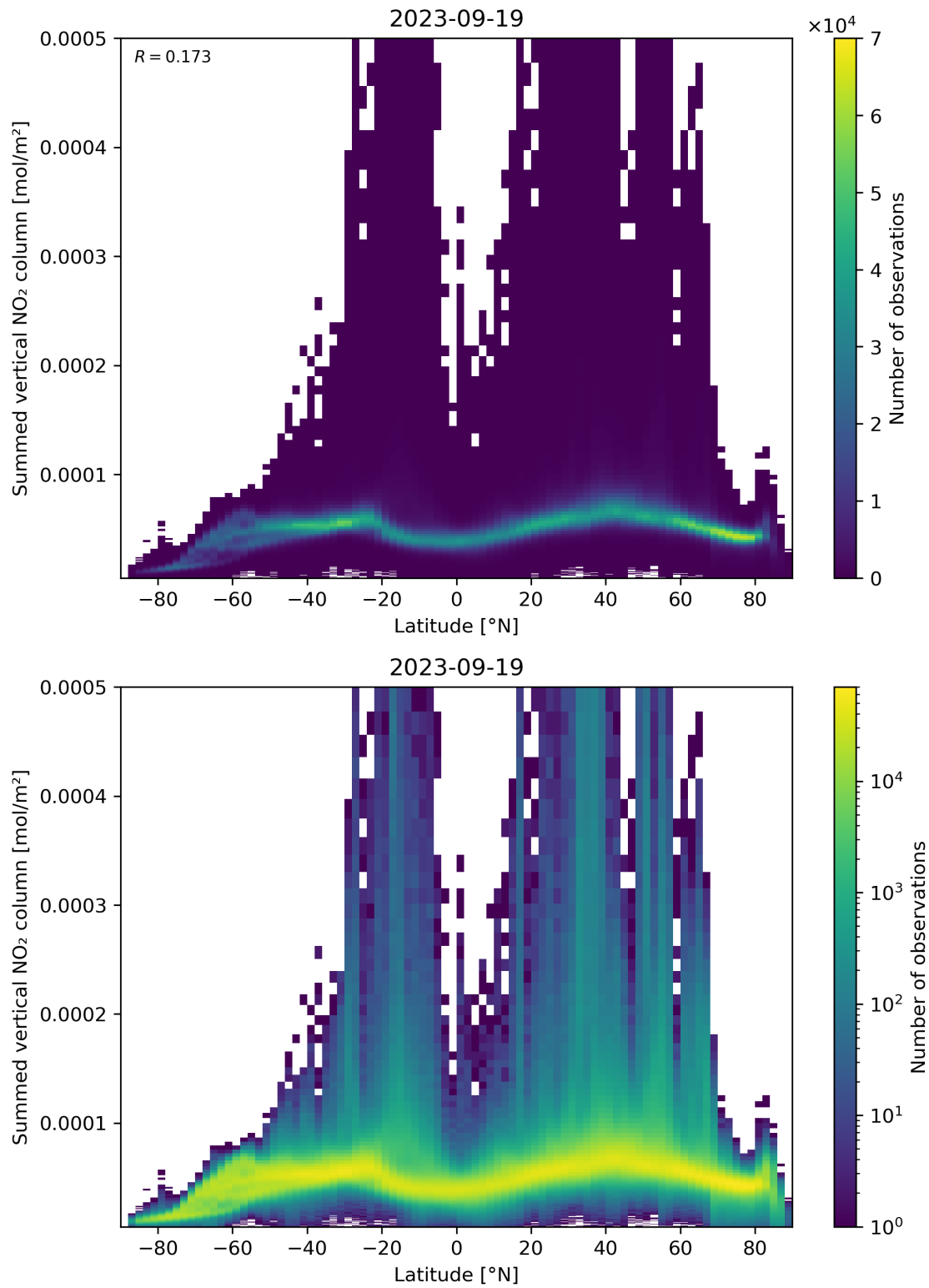
Figure 88: Scatter density plot of “Latitude” against “Summed vertical NO 2 column” for 2023-09-18 to 2023-09-20.
