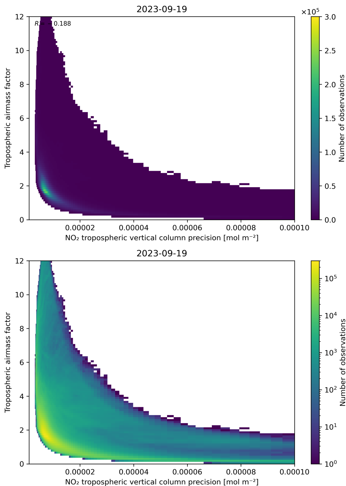
Figure 133: Scatter density plot of “NO 2 tropospheric vertical column precision” against “Tropospheric airmass factor” for 2023-09-18 to 2023-09-20.
