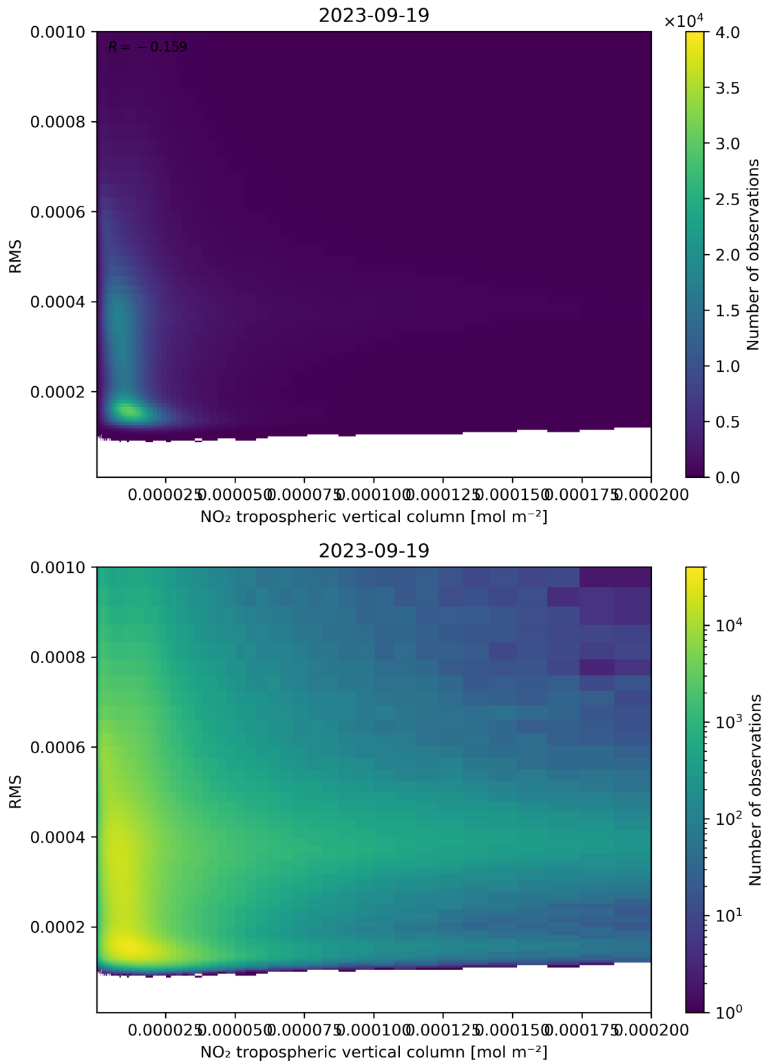
Figure 142: Scatter density plot of “NO 2 tropospheric vertical column” against “RMS” for 2023-09-18 to 2023-09-20.
