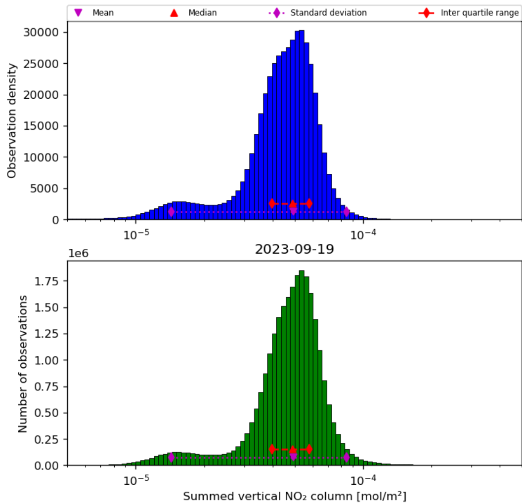
Figure 40: Histogram of “Summed vertical NO 2 column” for 2023-09-18 to 2023-09-20
