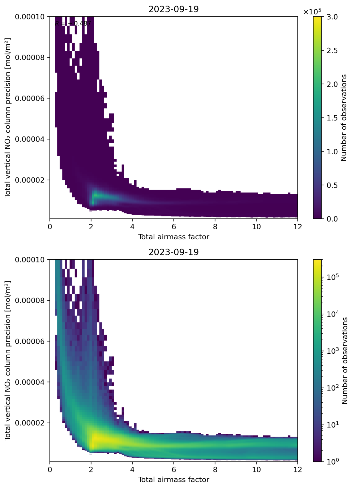
Figure 68: Scatter density plot of “Total airmass factor” against “Total vertical NO 2 column precision” for 2023-09-18 to 2023-09-20.
