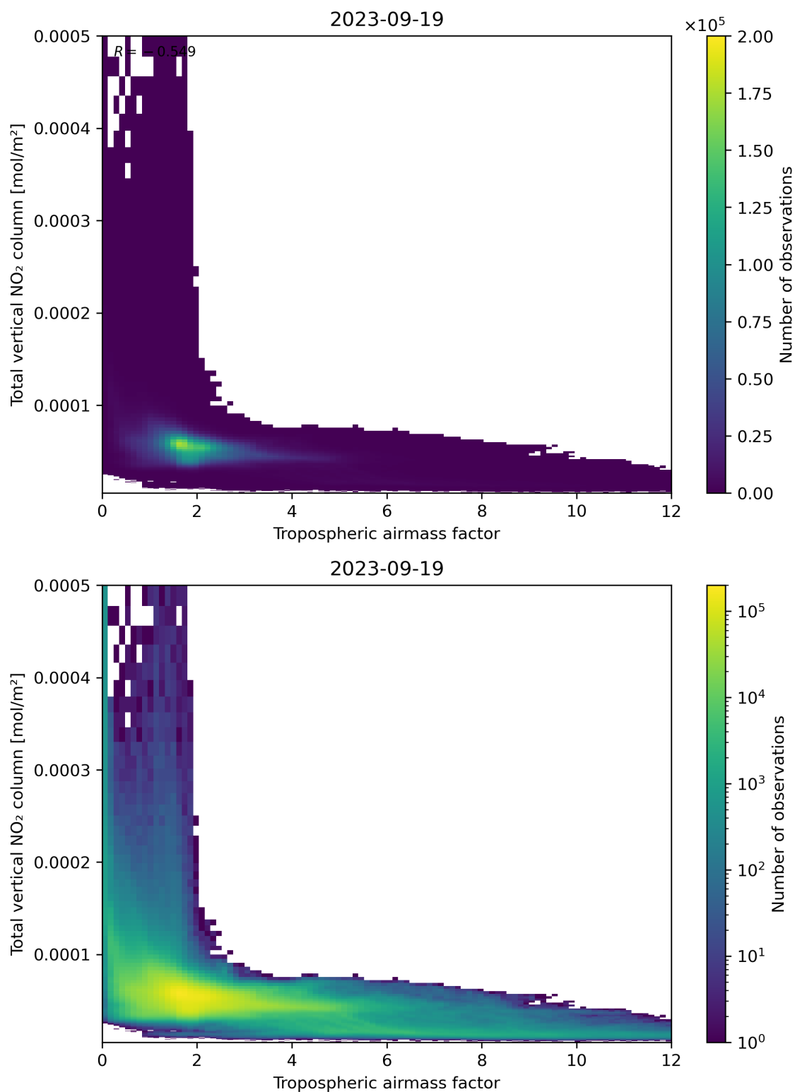
Figure 77: Scatter density plot of “Tropospheric airmass factor” against “Total vertical NO 2 column” for 2023-09-18 to 2023-09-20.
