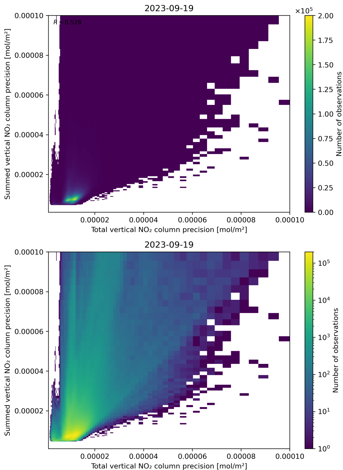
Figure 118: Scatter density plot of “Total vertical NO 2 column precision” against “Summed vertical NO 2 column precision” for 2023-09-18 to 2023-09-20.
