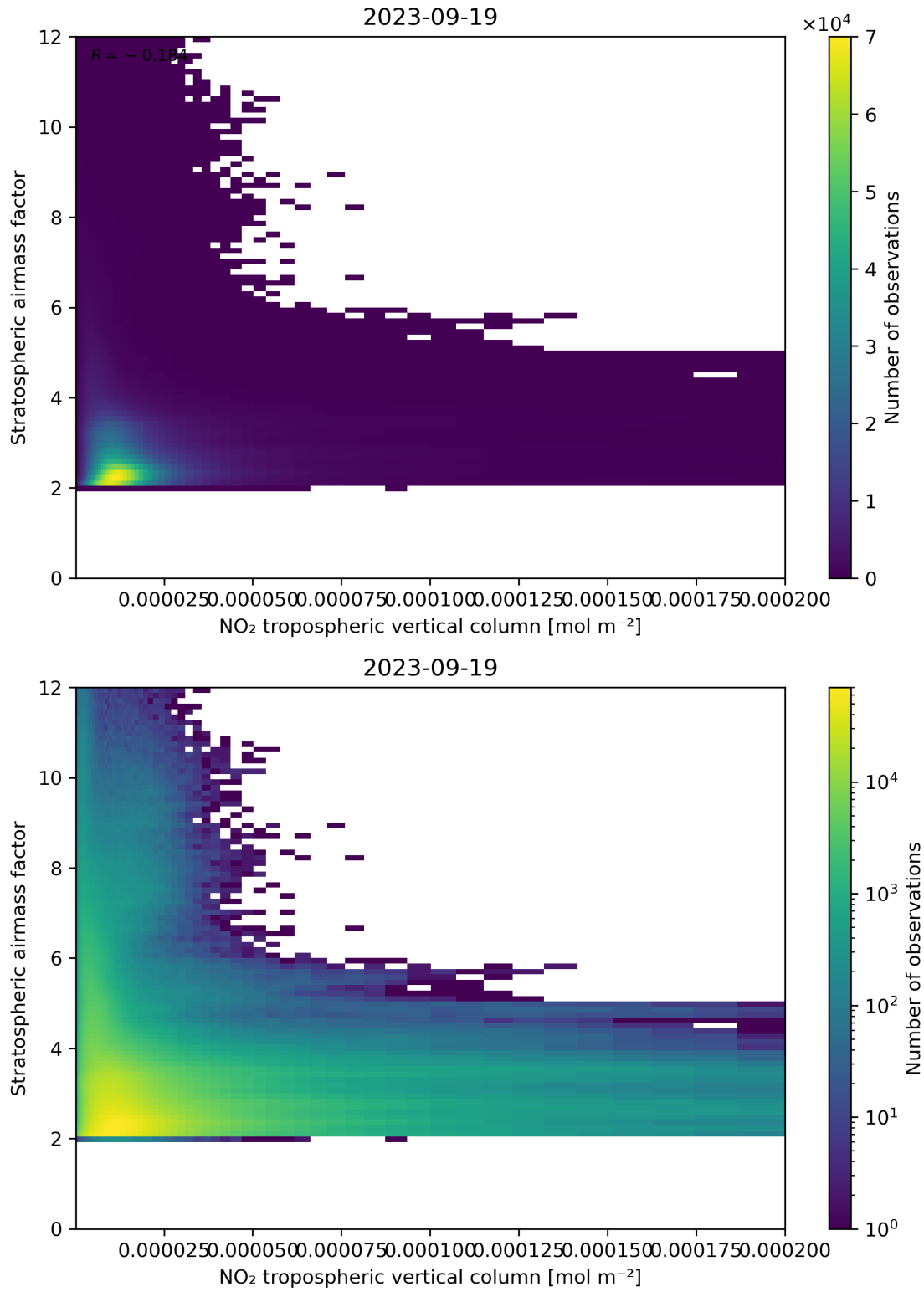
Figure 121: Scatter density plot of “NO 2 tropospheric vertical column” against “Stratospheric air mass factor” for 2023-09-18 to 2023-09-20.
