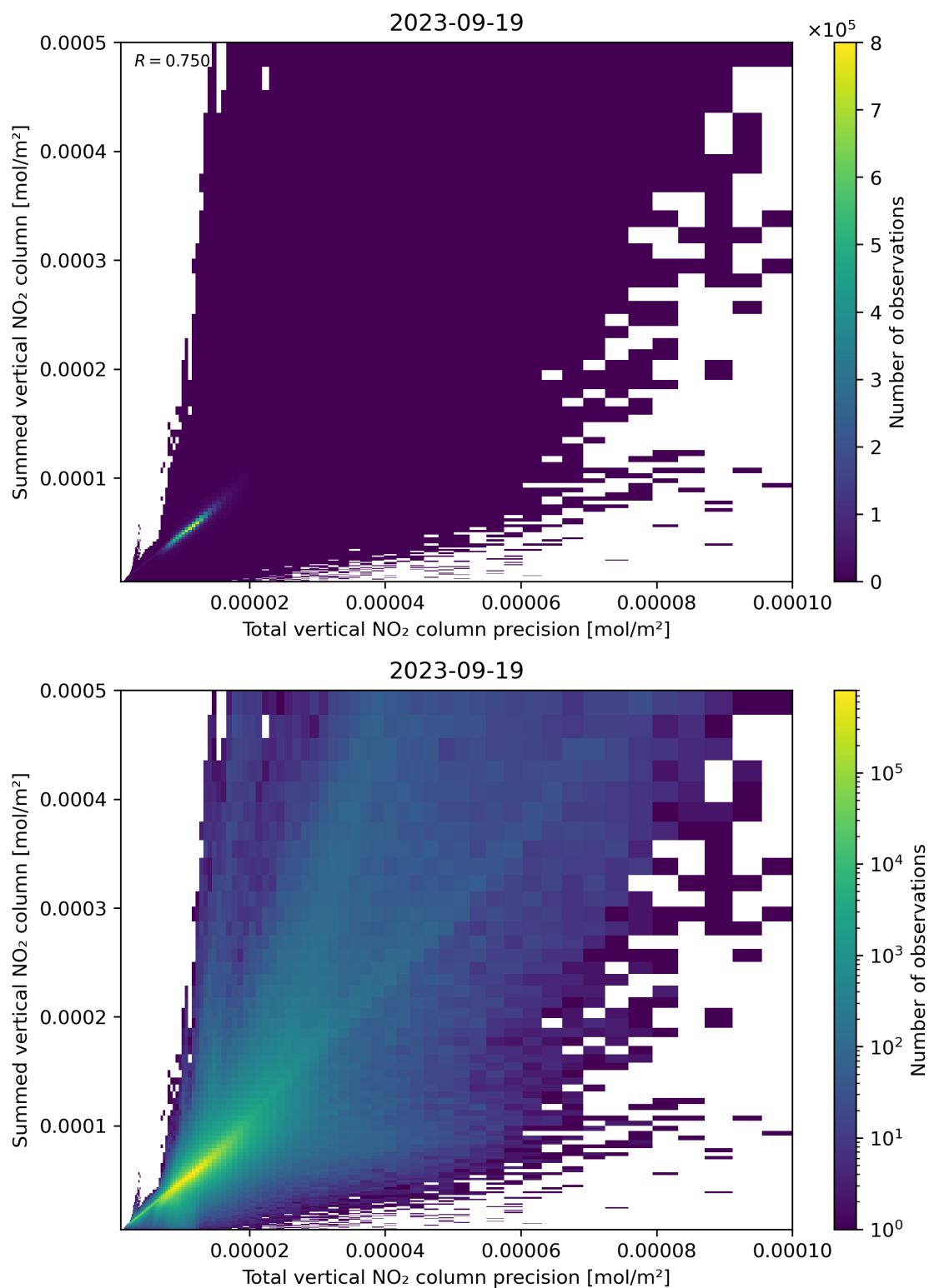
Figure 117: Scatter density plot of “Total vertical NO 2 column precision” against “Summed vertical NO 2 column” for 2023-09-18 to 2023-09-20.
