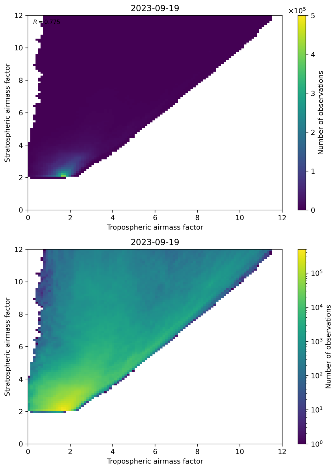
Figure 71: Scatter density plot of “Tropospheric airmass factor” against “Stratospheric airmass factor” for 2023-09-18 to 2023-09-20.
