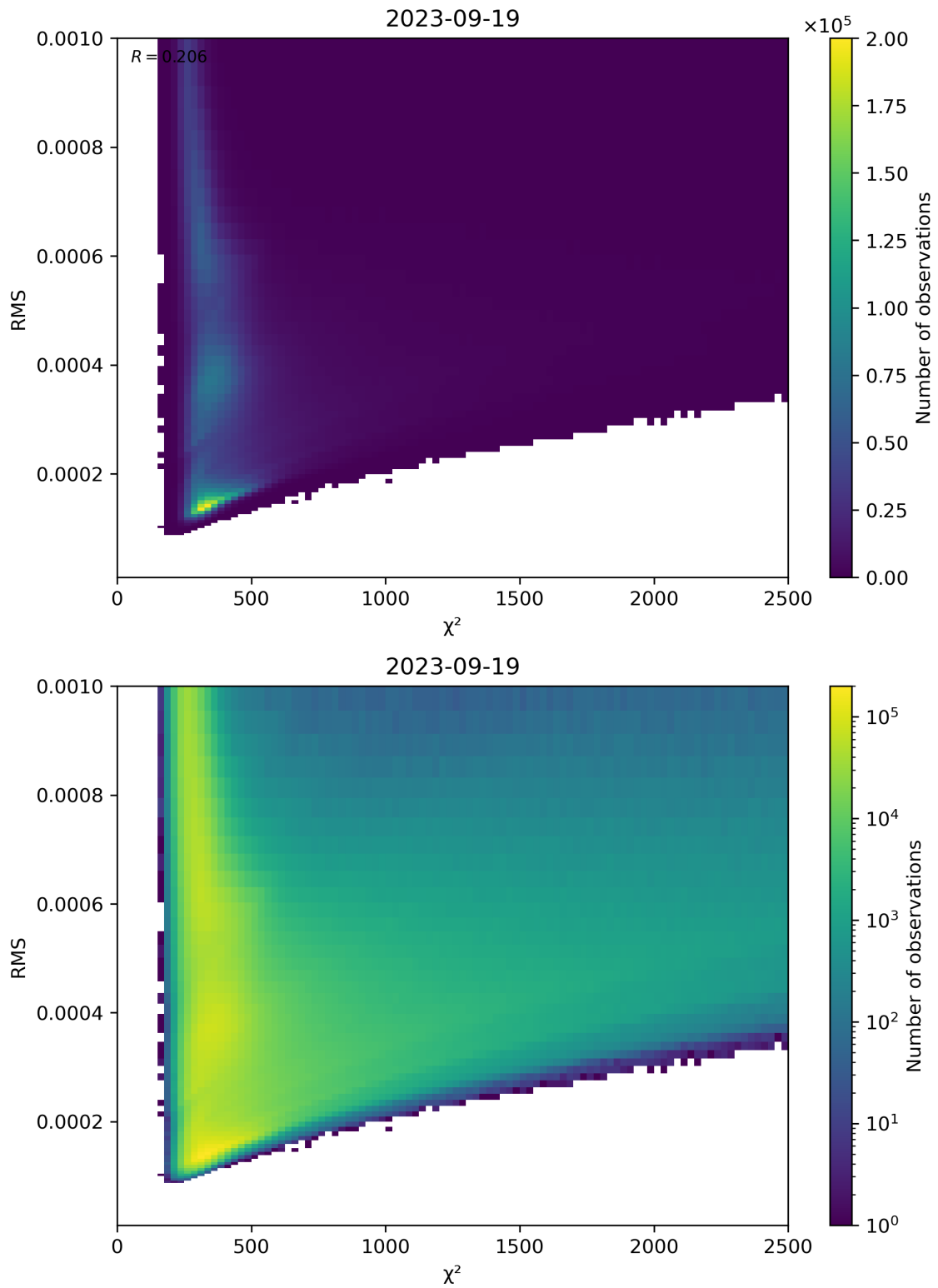
Figure 82: Scatter density plot of “ \chi^2 ” against “RMS” for 2023-09-18 to 2023-09-20.
