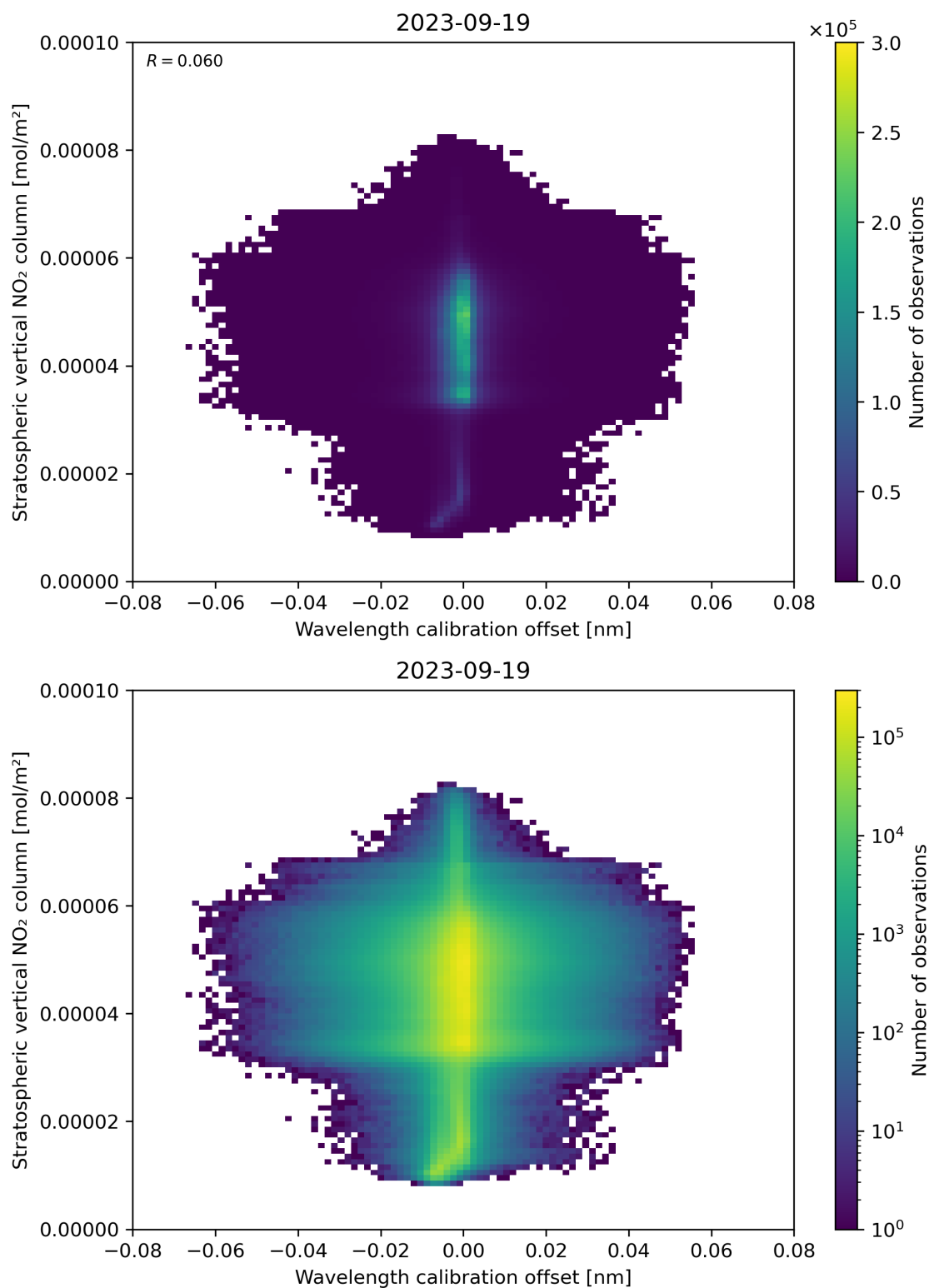
Figure 176: Scatter density plot of “Wavelength calibration offset” against “Stratospheric vertical NO 2 column” for 2023-09-18 to 2023-09-20.
