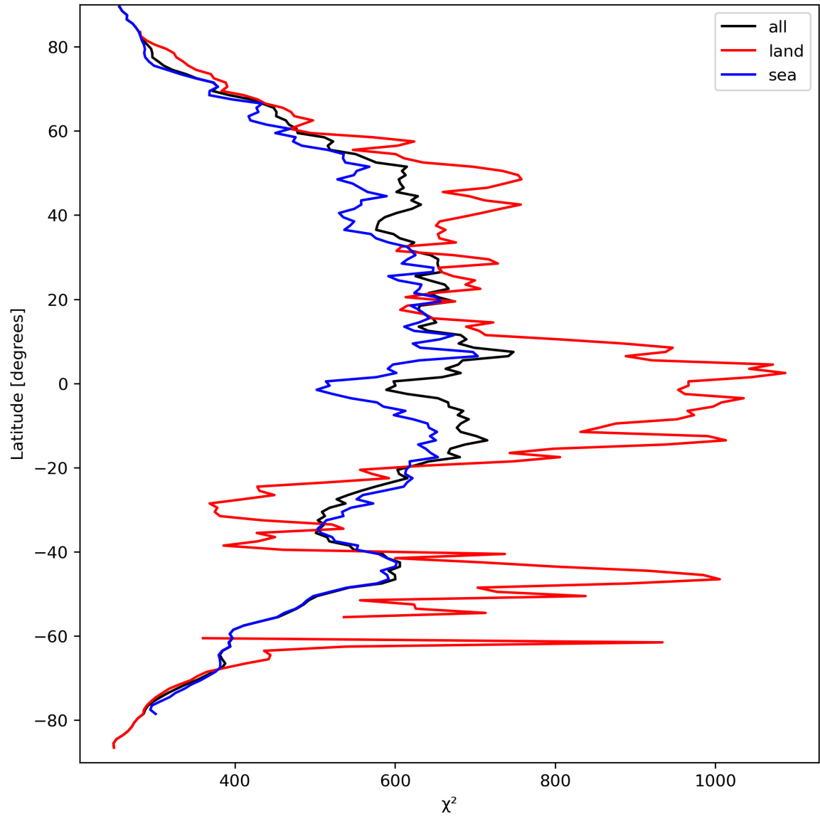
Figure 25: Zonal average of “ \chi^2 ” for 2023-09-18 to 2023-09-20.
