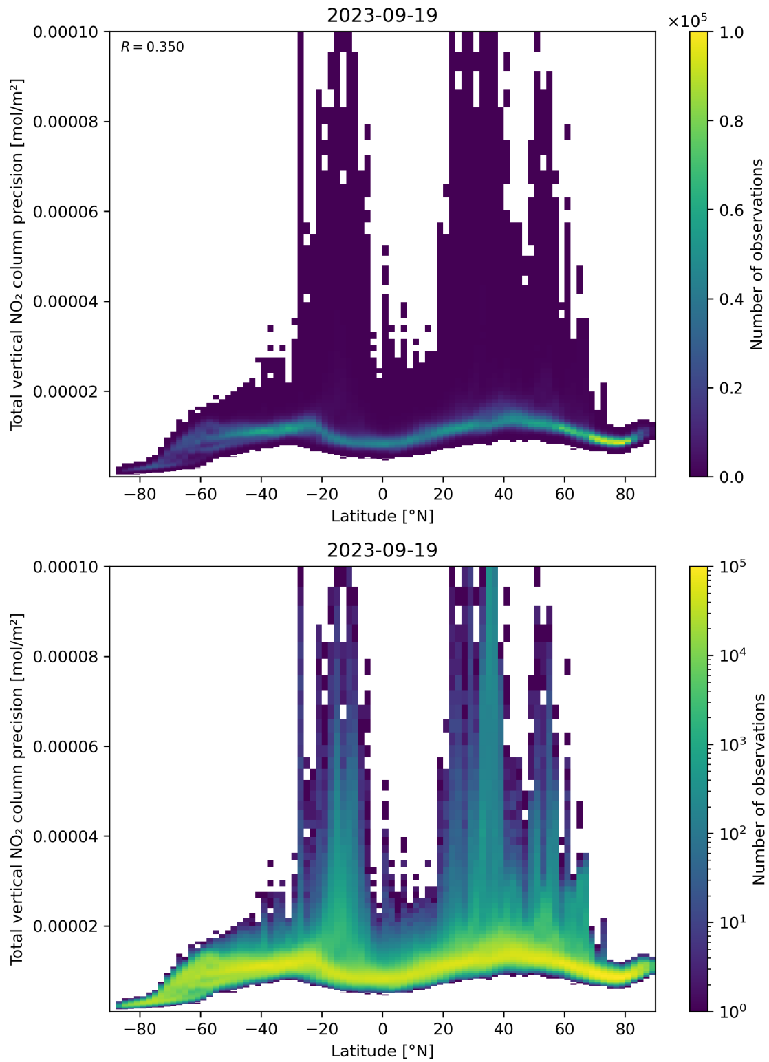
Figure 91: Scatter density plot of “Latitude” against “Total vertical NO 2 column precision” for 2023-09-18 to 2023-09-20.
