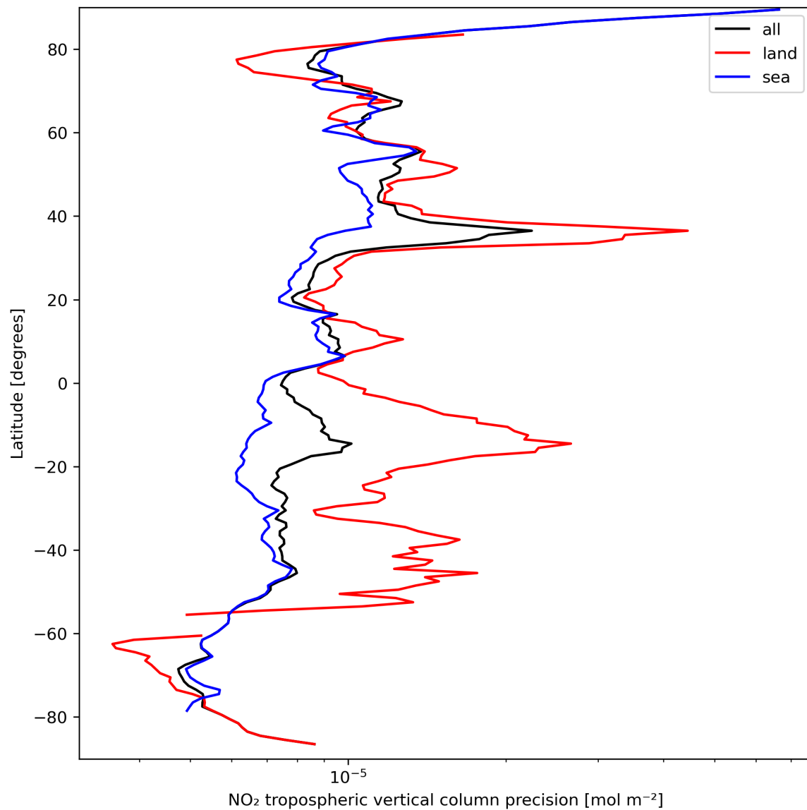
Figure 13: Zonal average of “NO 2 tropospheric vertical column precision” for 2023-09-18 to 2023-09-20.
