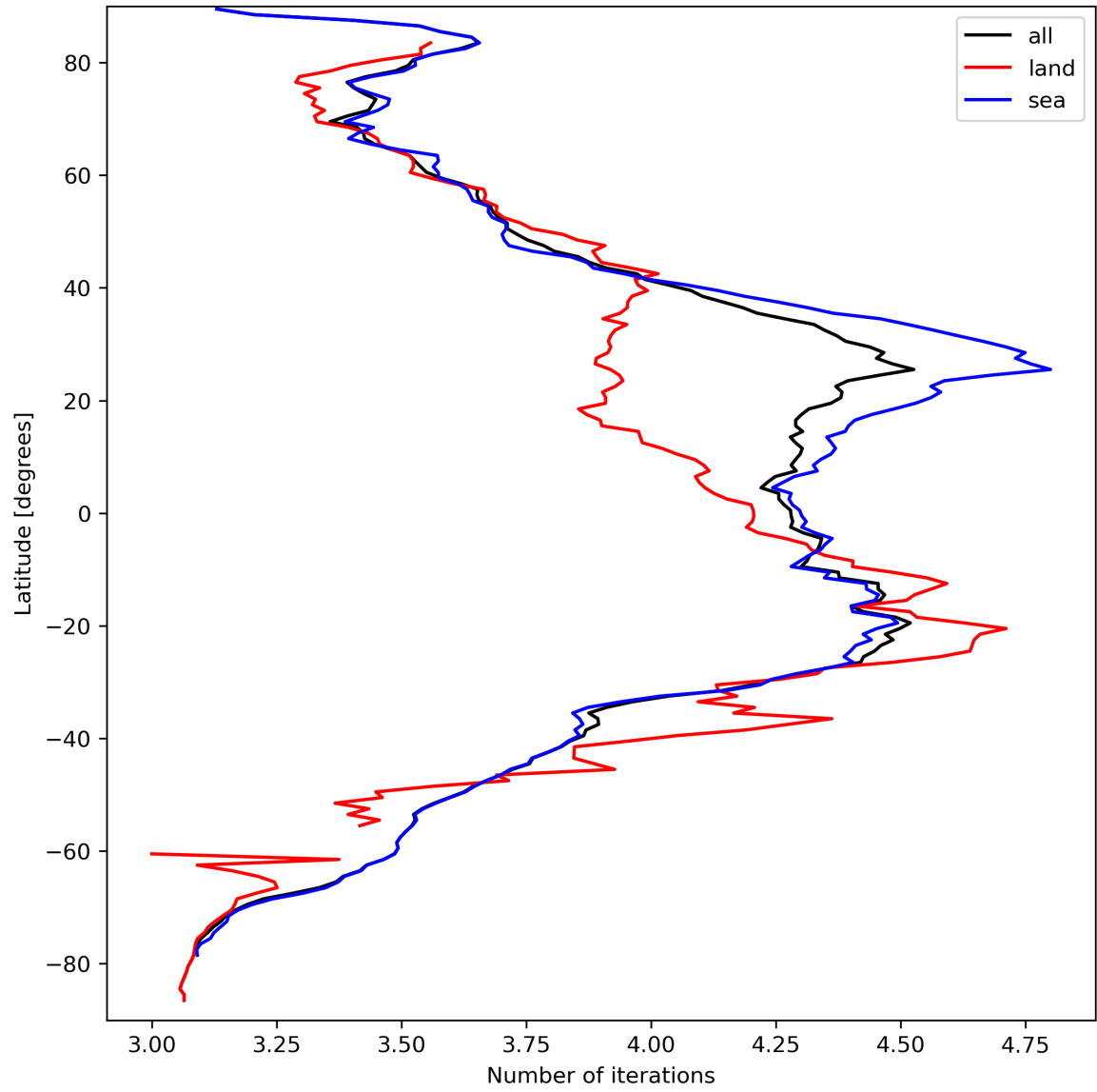
Figure 17: Zonal average of “Number of iterations” for 2023-09-18 to 2023-09-20.
