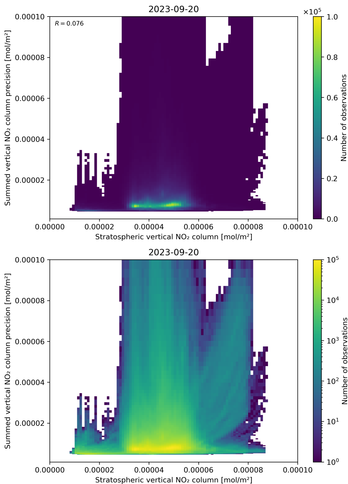
Figure 99: Scatter density plot of “Stratospheric vertical NO 2 column” against “Summed vertical NO 2 column precision” for 2023-09-20 to 2023-09-21.
