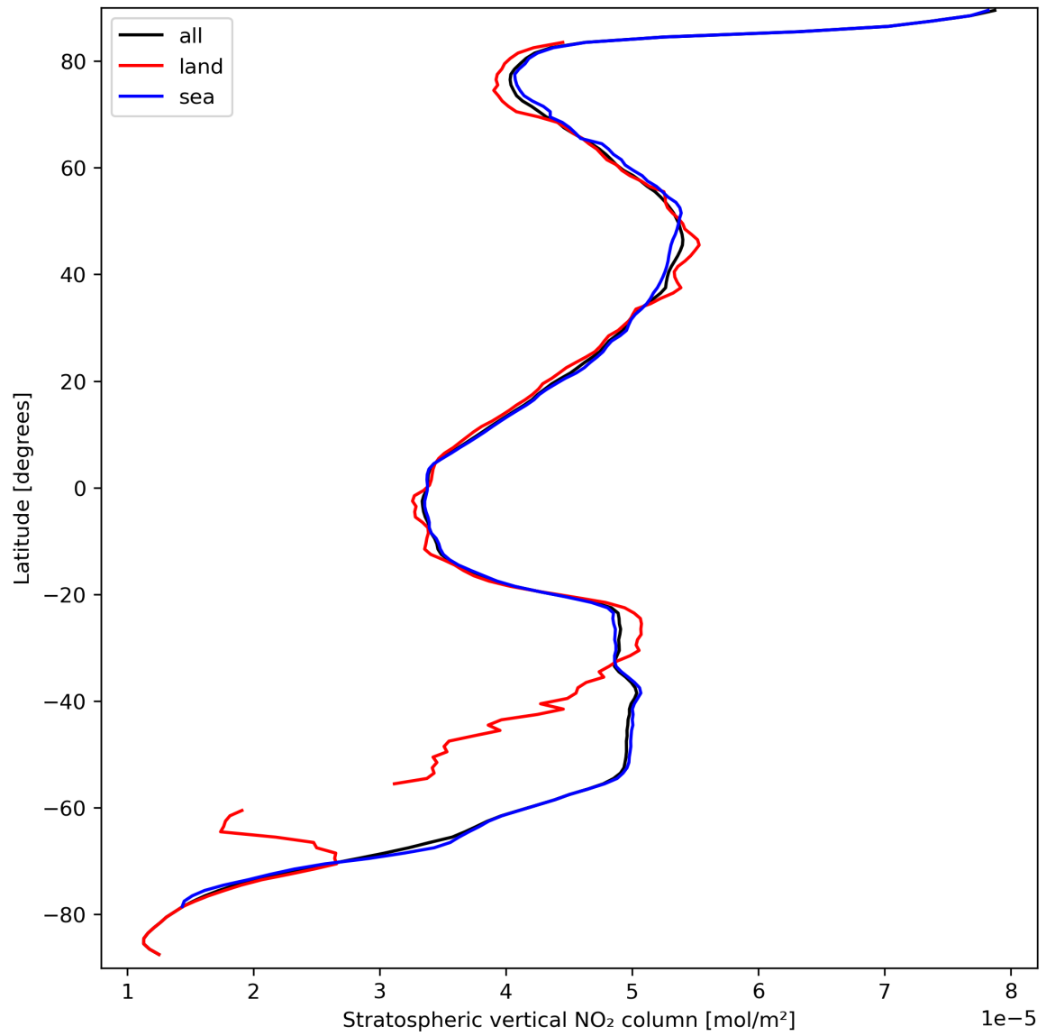
Figure 19: Zonal average of “Stratospheric vertical NO 2 column” for 2023-09-20 to 2023-09-21.
