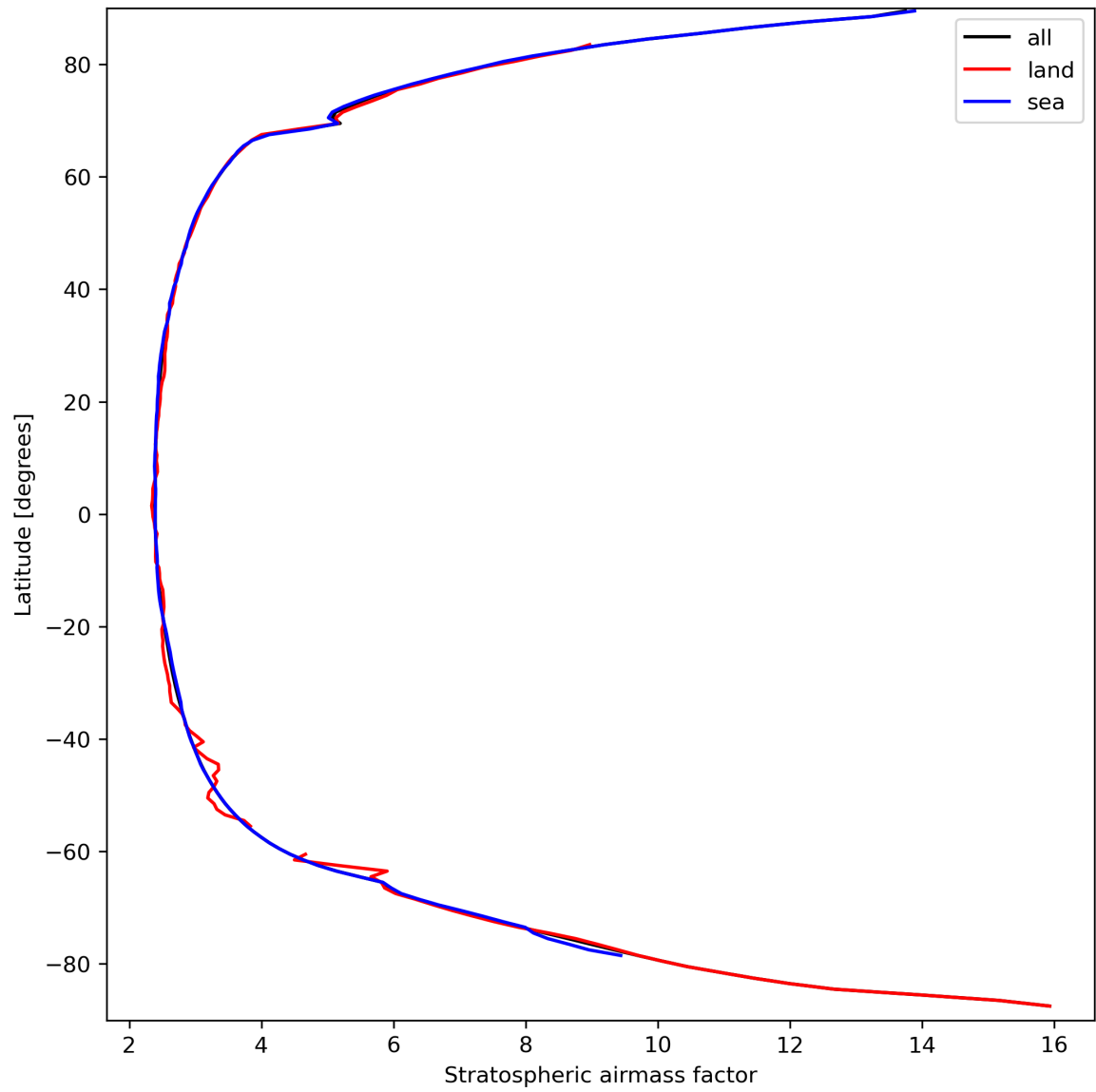
Figure 27: Zonal average of “Stratospheric air mass factor” for 2023-09-20 to 2023-09-21.
