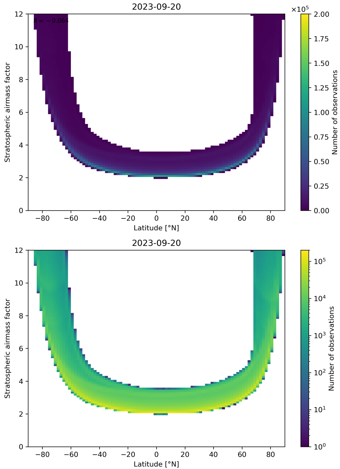
Figure 83: Scatter density plot of “Latitude” against “Stratospheric air mass factor” for 2023-09-20 to 2023-09-21.
