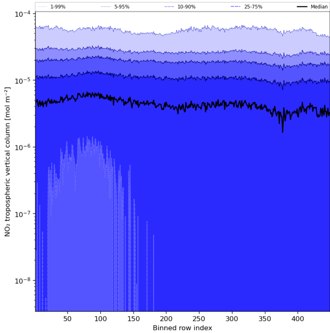
Figure 46: Along track statistics of “NO 2 tropospheric vertical column” for 2023-09-20 to 2023-09-21
