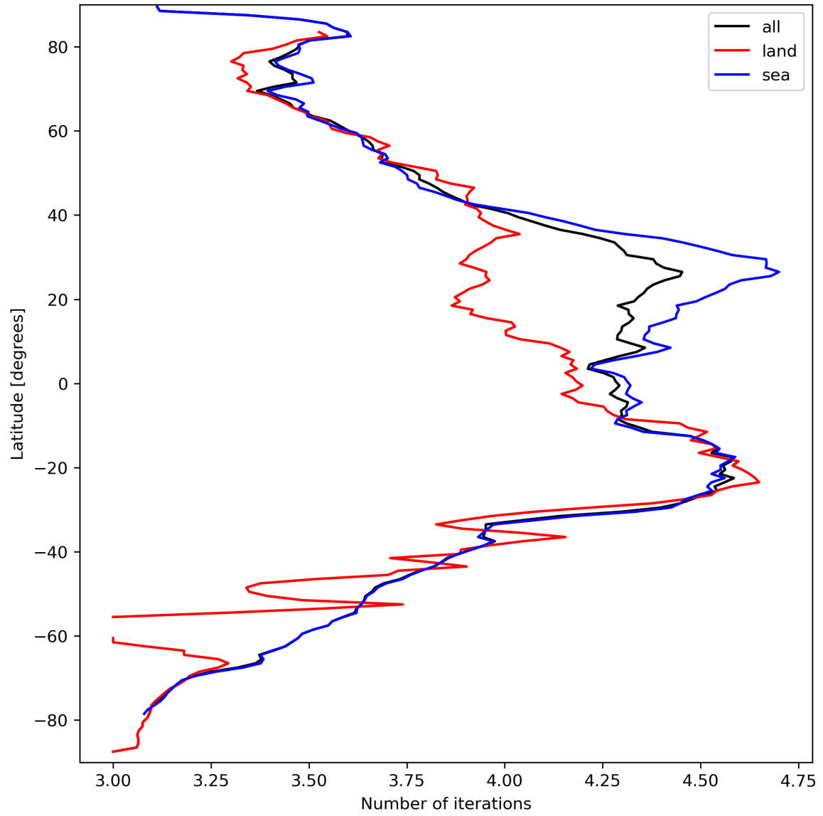
Figure 17: Zonal average of “Number of iterations” for 2023-09-20 to 2023-09-21.
