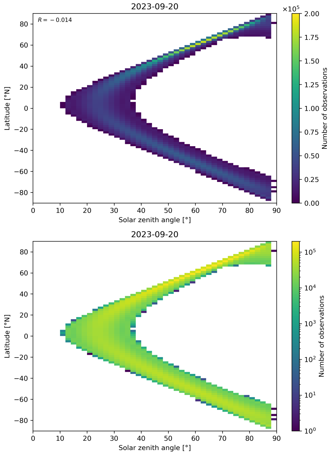
Figure 149: Scatter density plot of “Solar zenith angle” against “Latitude” for 2023-09-20 to 2023-09-21.
