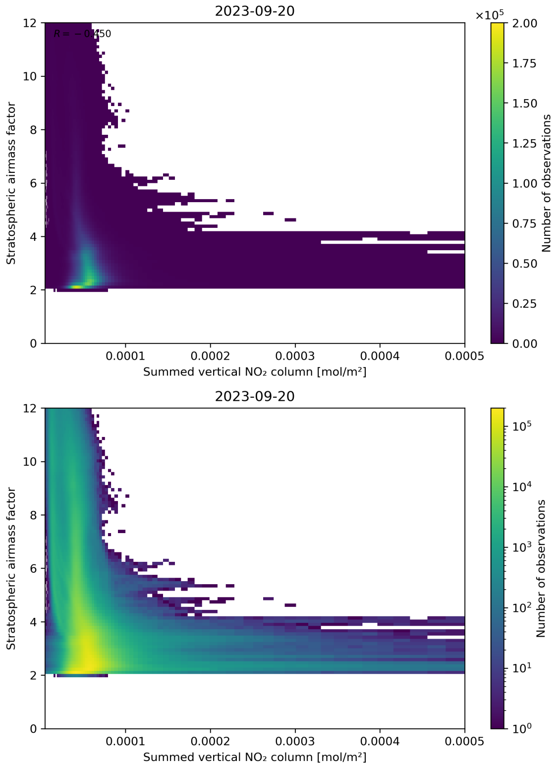
Figure 103: Scatter density plot of “Summed vertical NO 2 column” against “Stratospheric air mass factor” for 2023-09-20 to 2023-09-21.
