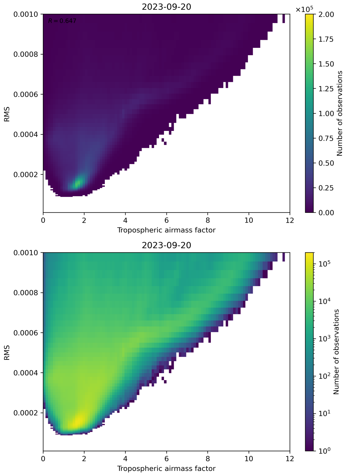
Figure 79: Scatter density plot of “Tropospheric airmass factor” against “RMS” for 2023-09-20 to 2023-09-21.
