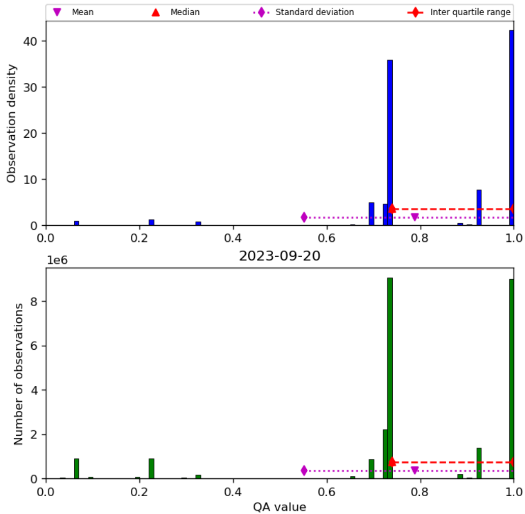
Figure 28: Histogram of “QA value” for 2023-09-20 to 2023-09-21
