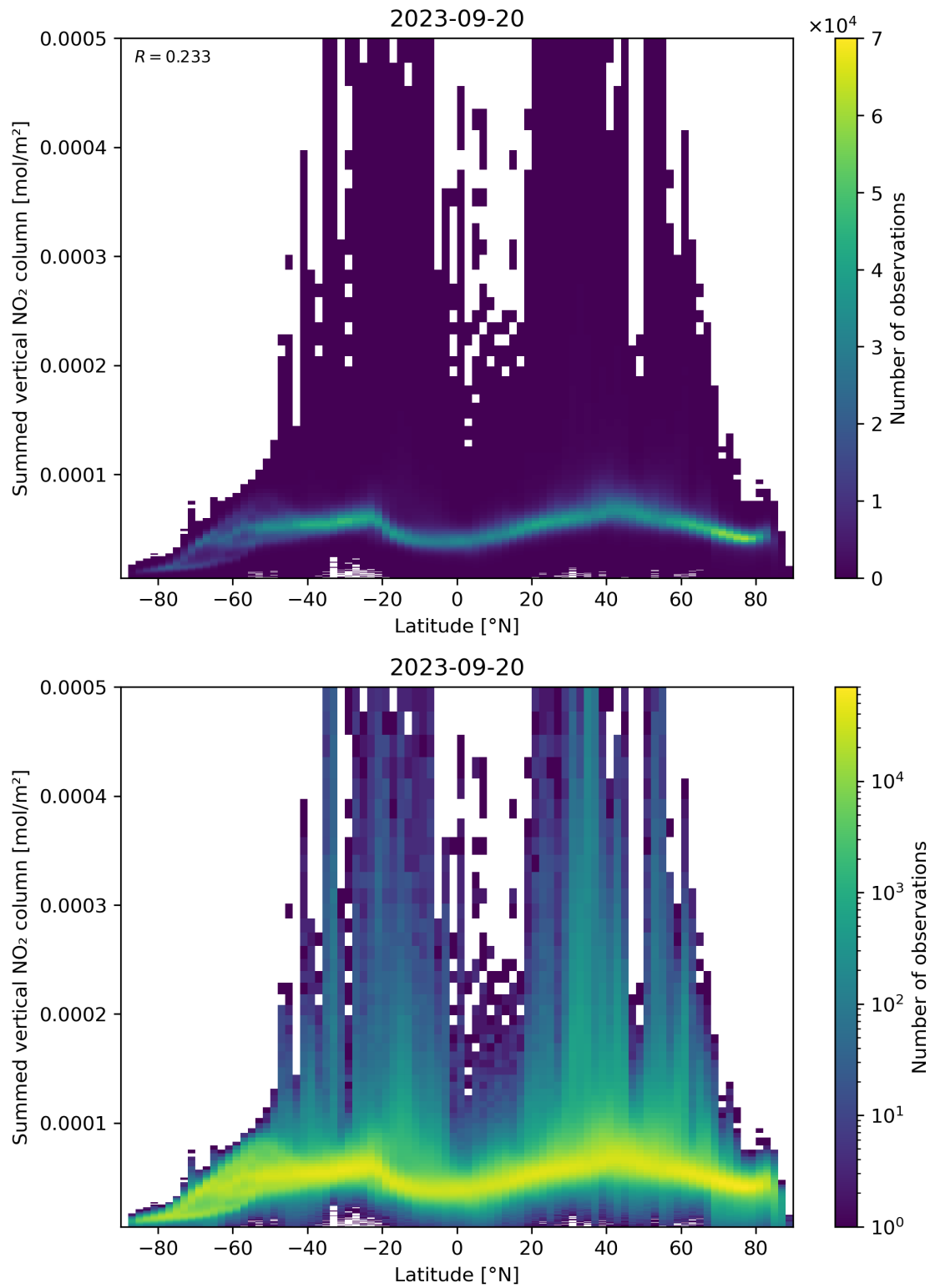
Figure 88: Scatter density plot of “Latitude” against “Summed vertical NO 2 column” for 2023-09-20 to 2023-09-21.
