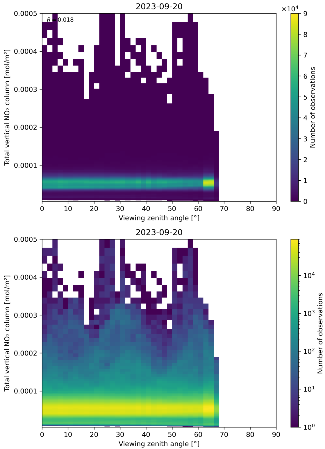
Figure 167: Scatter density plot of “Viewing zenith angle” against “Total vertical NO 2 column” for 2023-09-20 to 2023-09-21.
