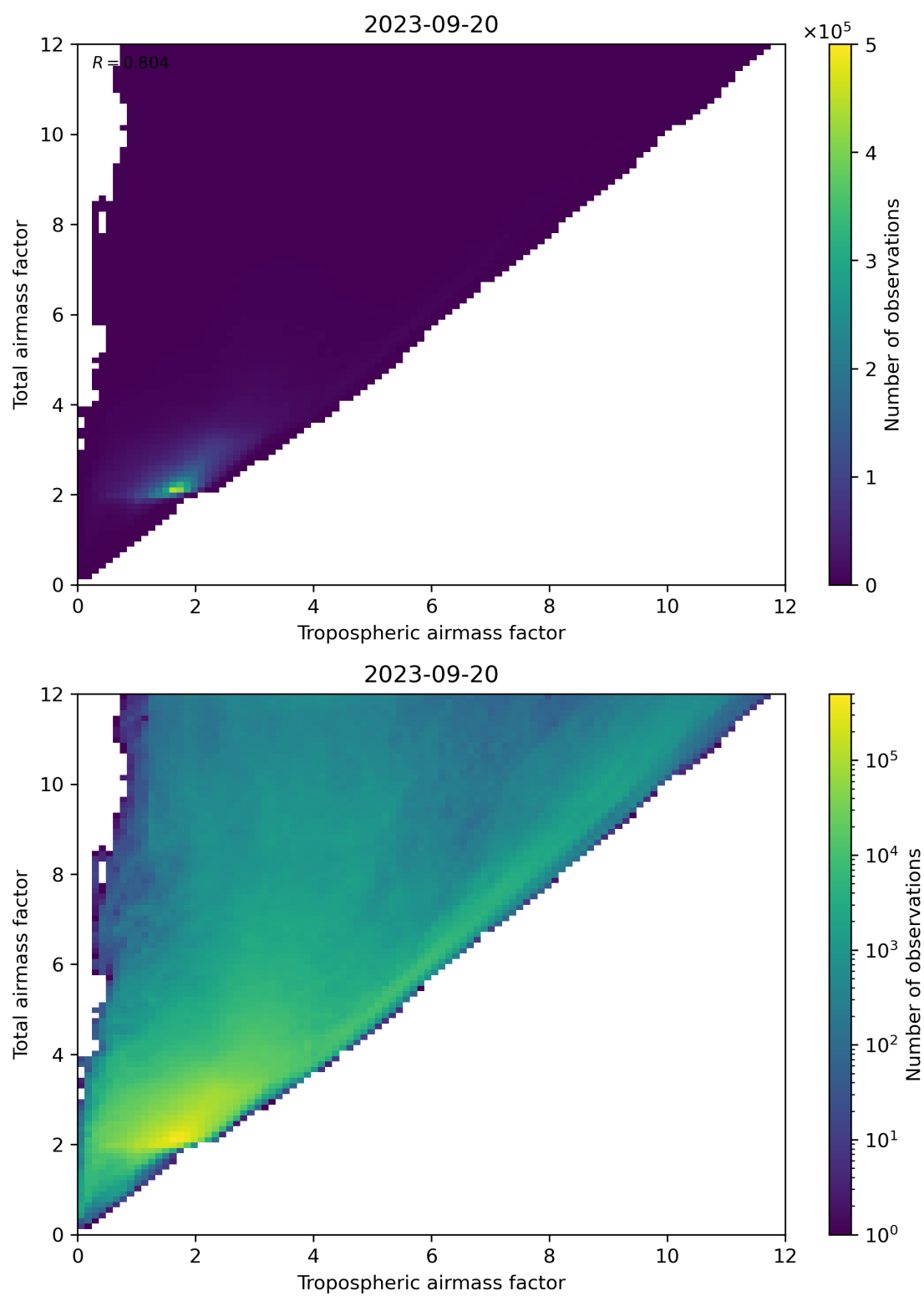
Figure 72: Scatter density plot of “Tropospheric airmass factor” against “Total airmass factor” for 2023-09-20 to 2023-09-21.
