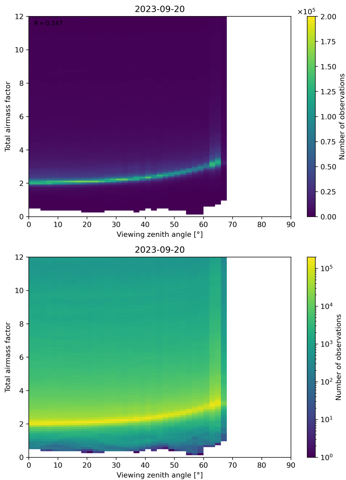
Figure 160: Scatter density plot of “Viewing zenith angle” against “Total airmass factor” for 2023-09-20 to 2023-09-21.
