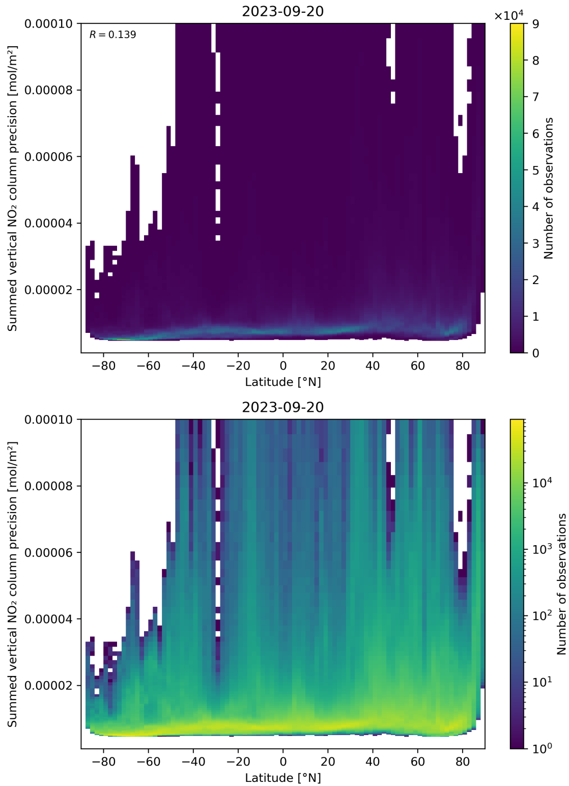
Figure 89: Scatter density plot of “Latitude” against “Summed vertical NO 2 column precision” for 2023-09-20 to 2023-09-21.
