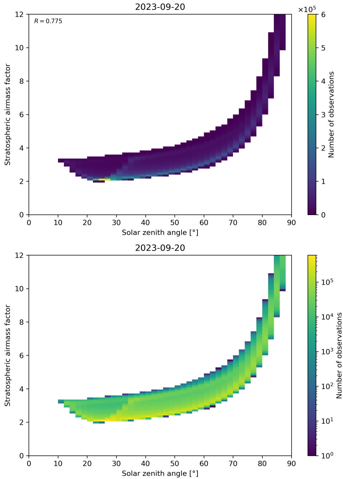
Figure 145: Scatter density plot of “Solar zenith angle” against “Stratospheric airmass factor” for 2023-09-20 to 2023-09-21.
