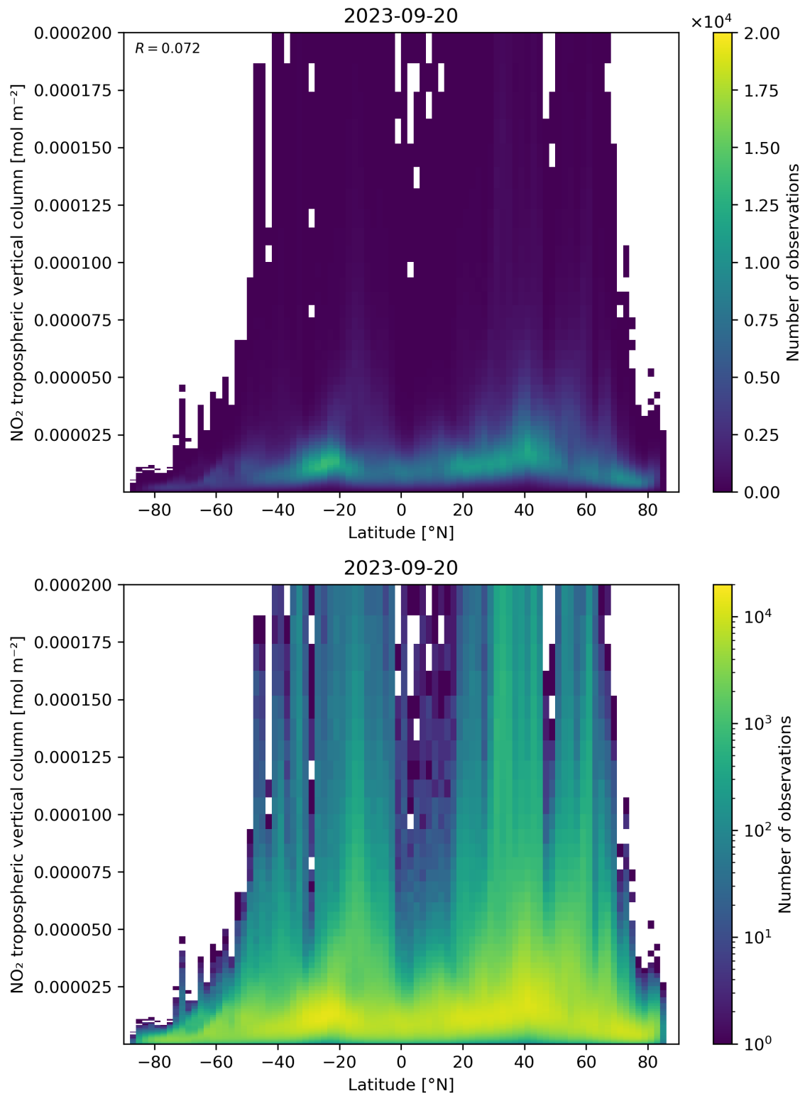
Figure 92: Scatter density plot of “Latitude” against “NO 2 tropospheric vertical column” for 2023-09-20 to 2023-09-21.
