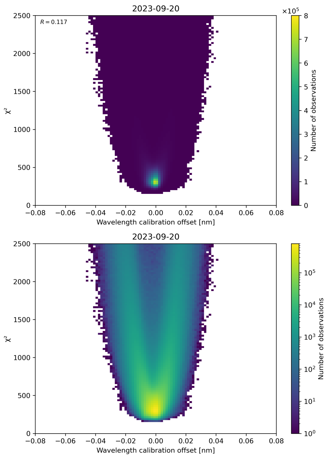
Figure 175: Scatter density plot of “Wavelength calibration offset” against “ \chi^2 ” for 2023-09-20 to 2023-09-21.
