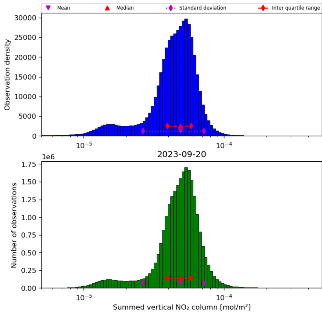
Figure 40: Histogram of “Summed vertical NO 2 column” for 2023-09-20 to 2023-09-21
