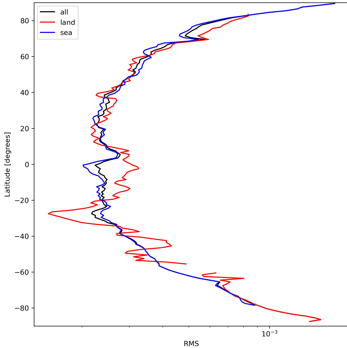
Figure 26: Zonal average of “RMS” for 2023-09-20 to 2023-09-21.
