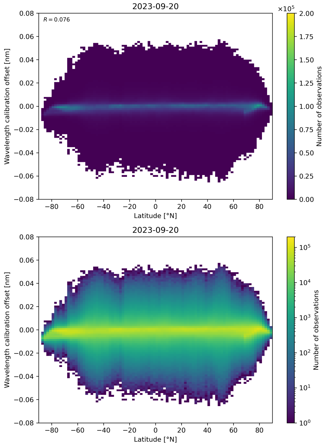
Figure 95: Scatter density plot of “Latitude” against “Wavelength calibration offset” for 2023-09-20 to 2023-09-21.
