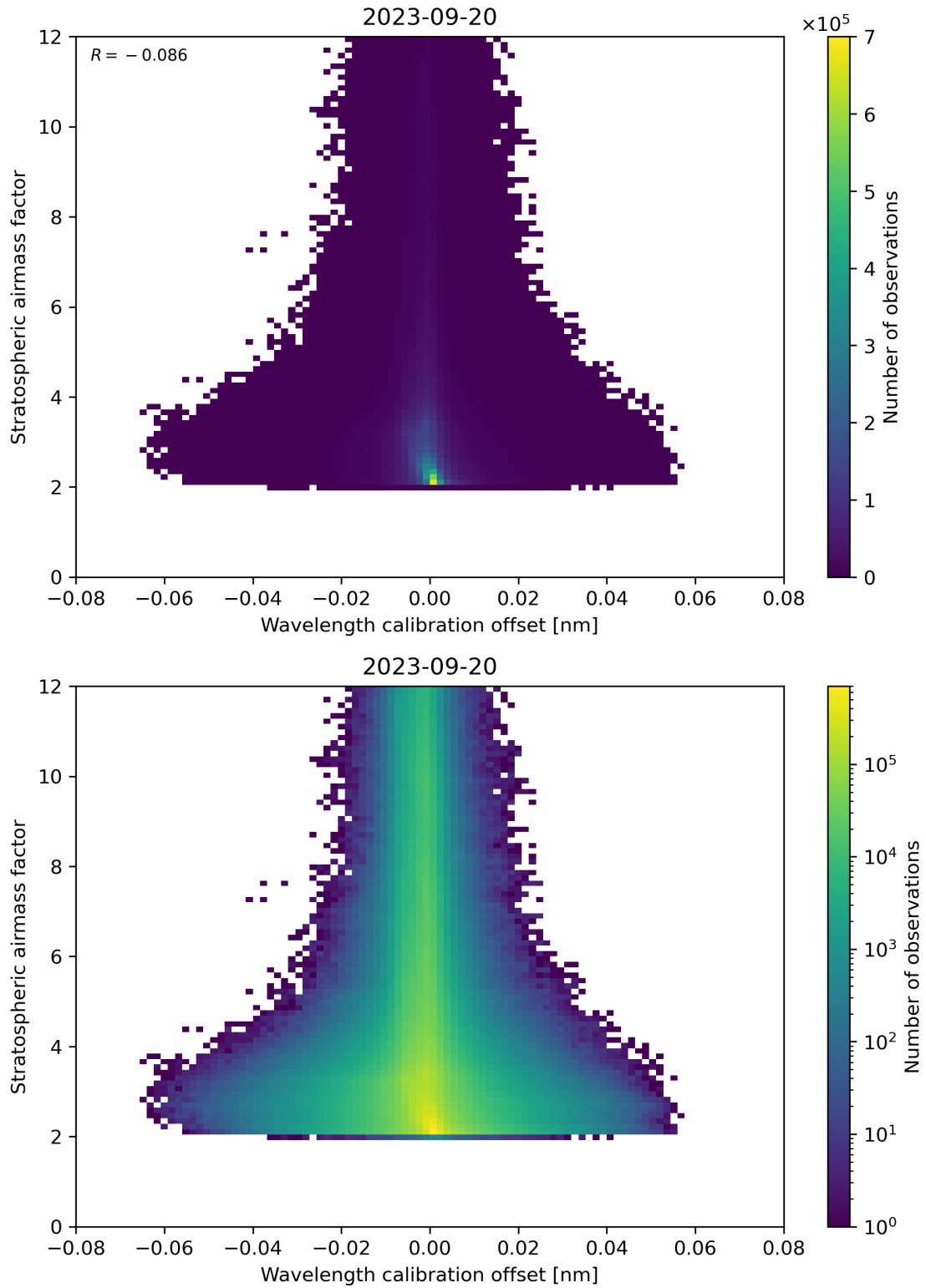
Figure 174: Scatter density plot of “Wavelength calibration offset” against “Stratospheric airmass factor” for 2023-09-20 to 2023-09-21.
