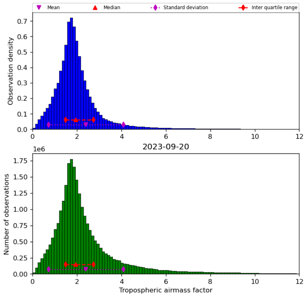
Figure 31: Histogram of “Tropospheric airmass factor” for 2023-09-20 to 2023-09-21
