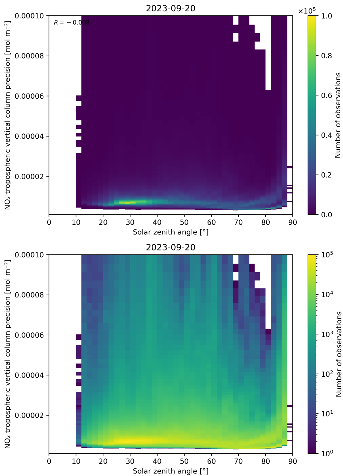
Figure 156: Scatter density plot of “Solar zenith angle” against “NO 2 tropospheric vertical column precision” for 2023-09-20 to 2023-09-21.
