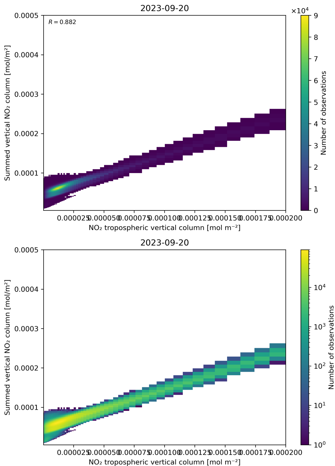
Figure 126: Scatter density plot of “NO 2 tropospheric vertical column” against “Summed vertical NO 2 column” for 2023-09-20 to 2023-09-21.
