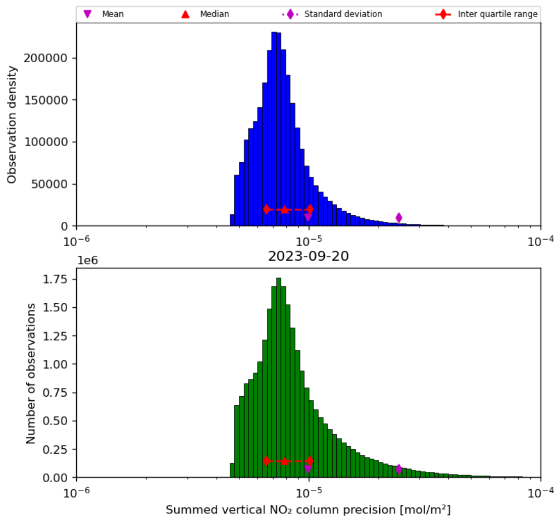
Figure 41: Histogram of “Summed vertical NO 2 column precision” for 2023-09-20 to 2023-09-21
