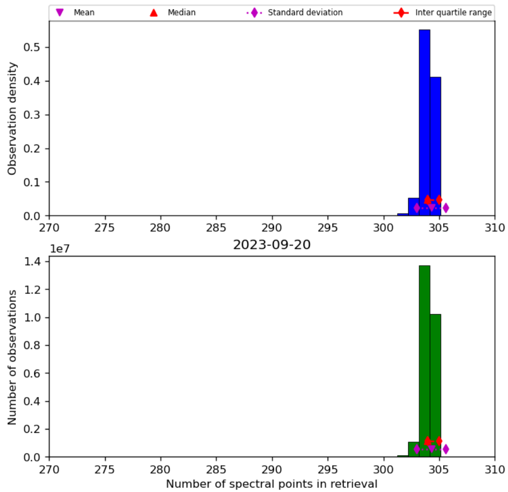
Figure 33: Histogram of “Number of spectral points in retrieval” for 2023-09-20 to 2023-09-21
