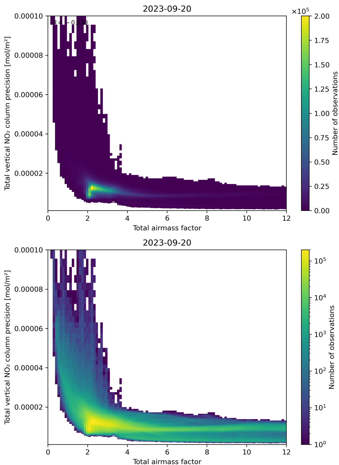
Figure 68: Scatter density plot of “Total airmass factor” against “Total vertical NO 2 column precision” for 2023-09-20 to 2023-09-21.
