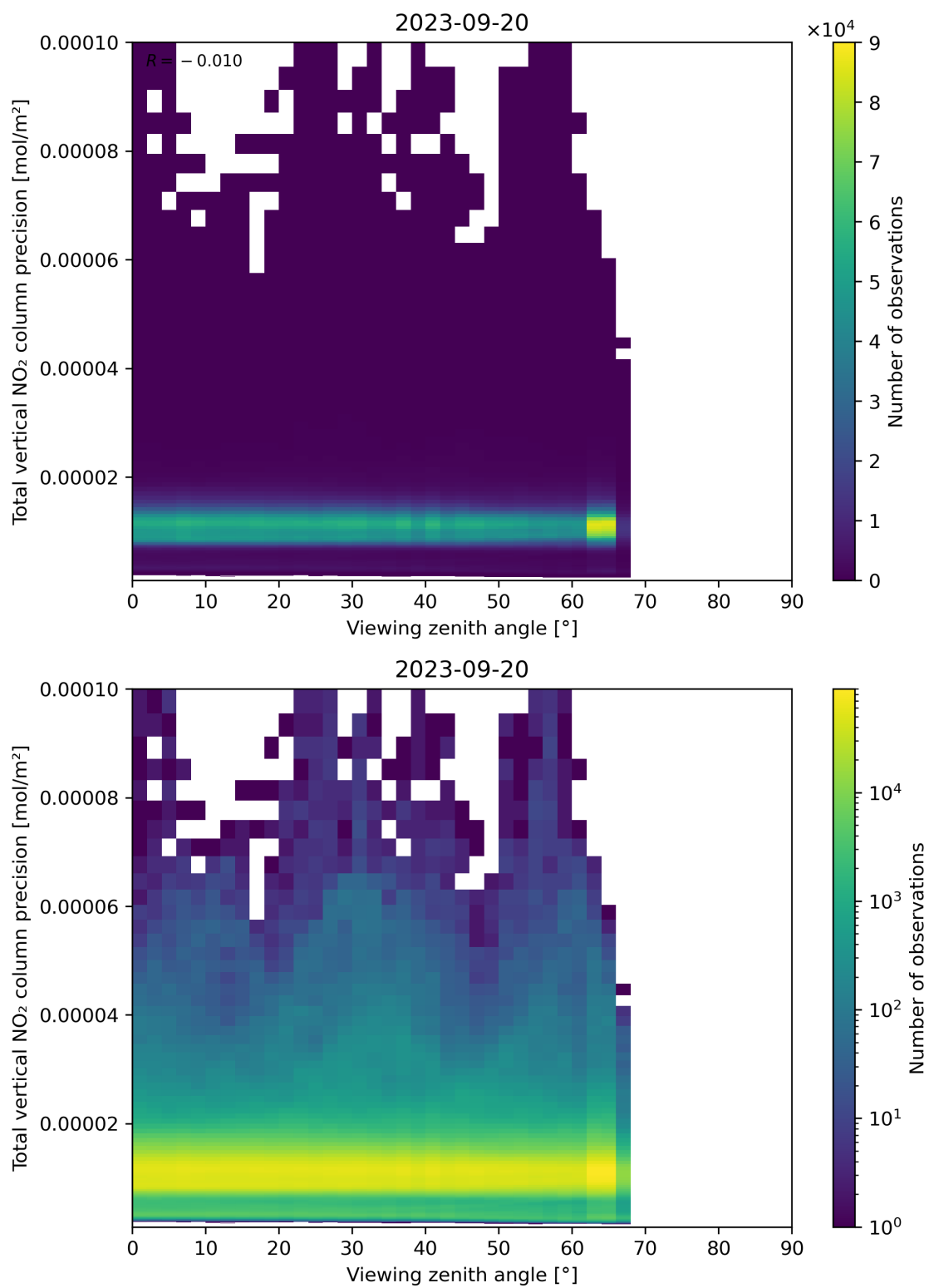
Figure 168: Scatter density plot of “Viewing zenith angle” against “Total vertical NO 2 column precision” for 2023-09-20 to 2023-09-21.
