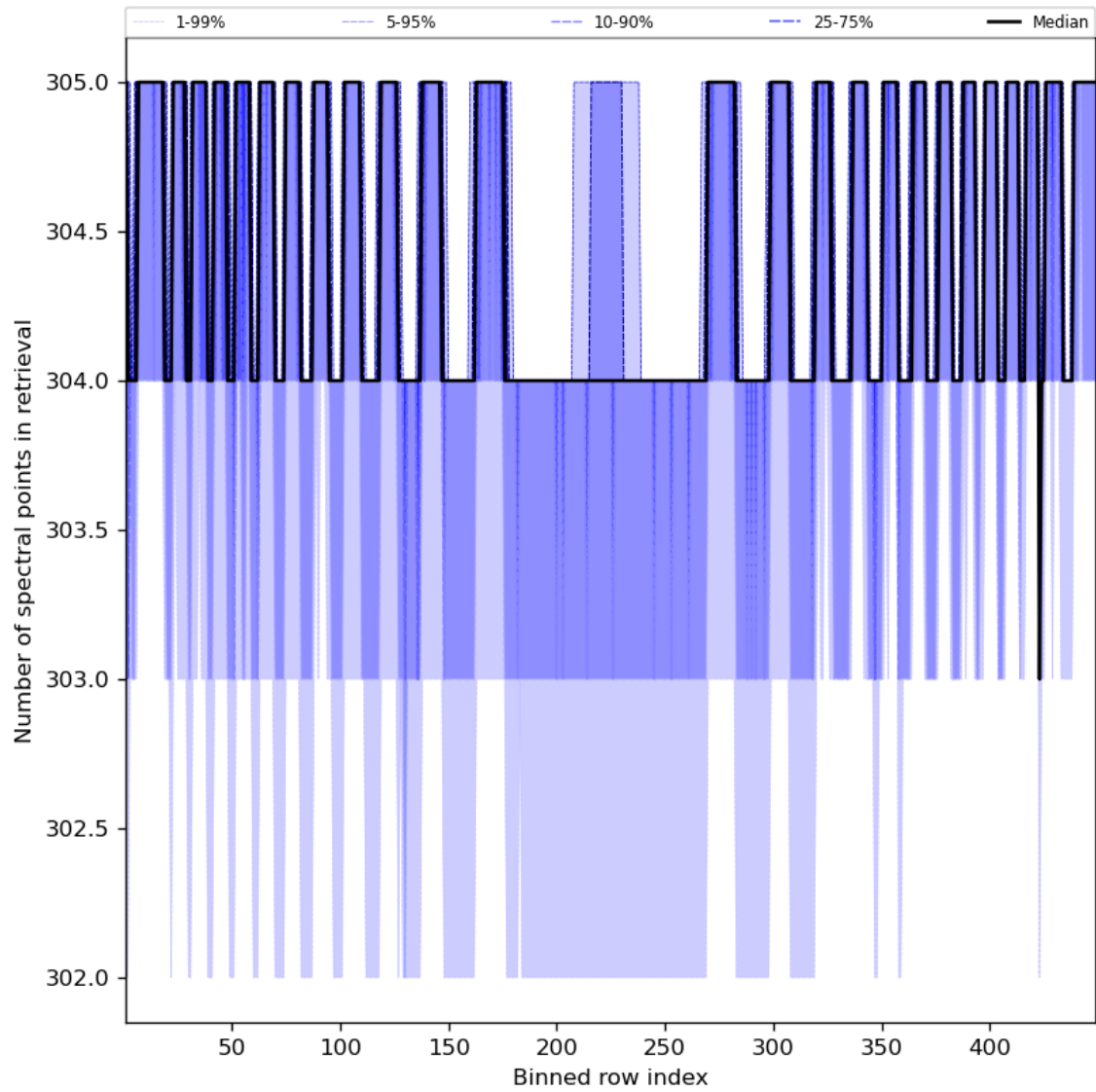
Figure 50: Along track statistics of “Number of spectral points in retrieval” for 2023-09-20 to 2023-09-21
