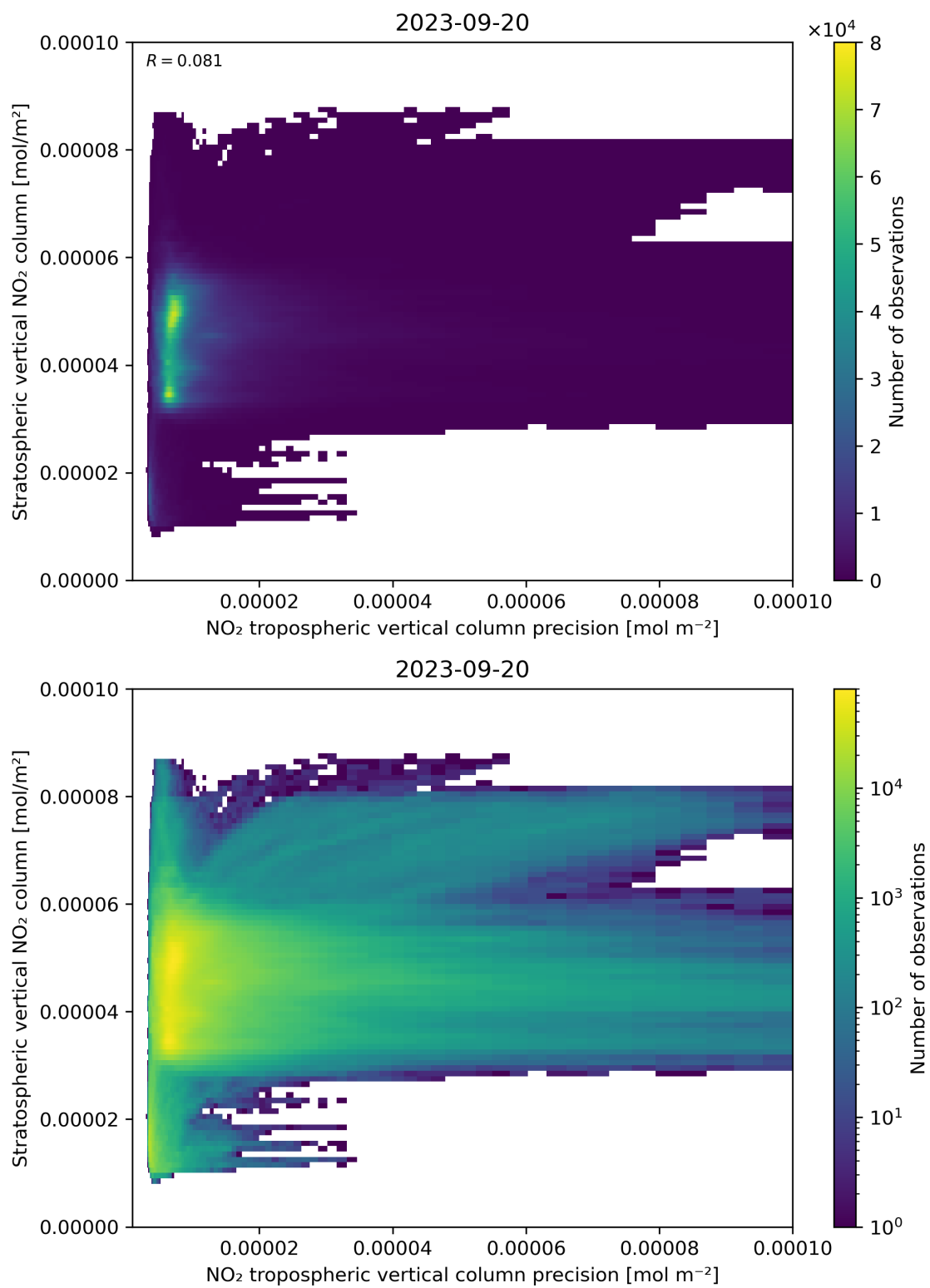
Figure 135: Scatter density plot of “NO 2 tropospheric vertical column precision” against “Stratospheric vertical NO 2 column” for 2023-09-20 to 2023-09-21.
