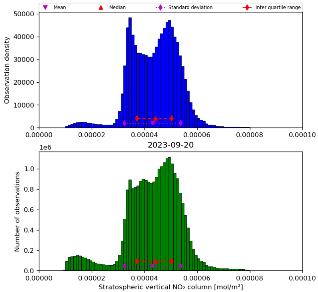
Figure 36: Histogram of “Stratospheric vertical NO 2 column” for 2023-09-20 to 2023-09-21
