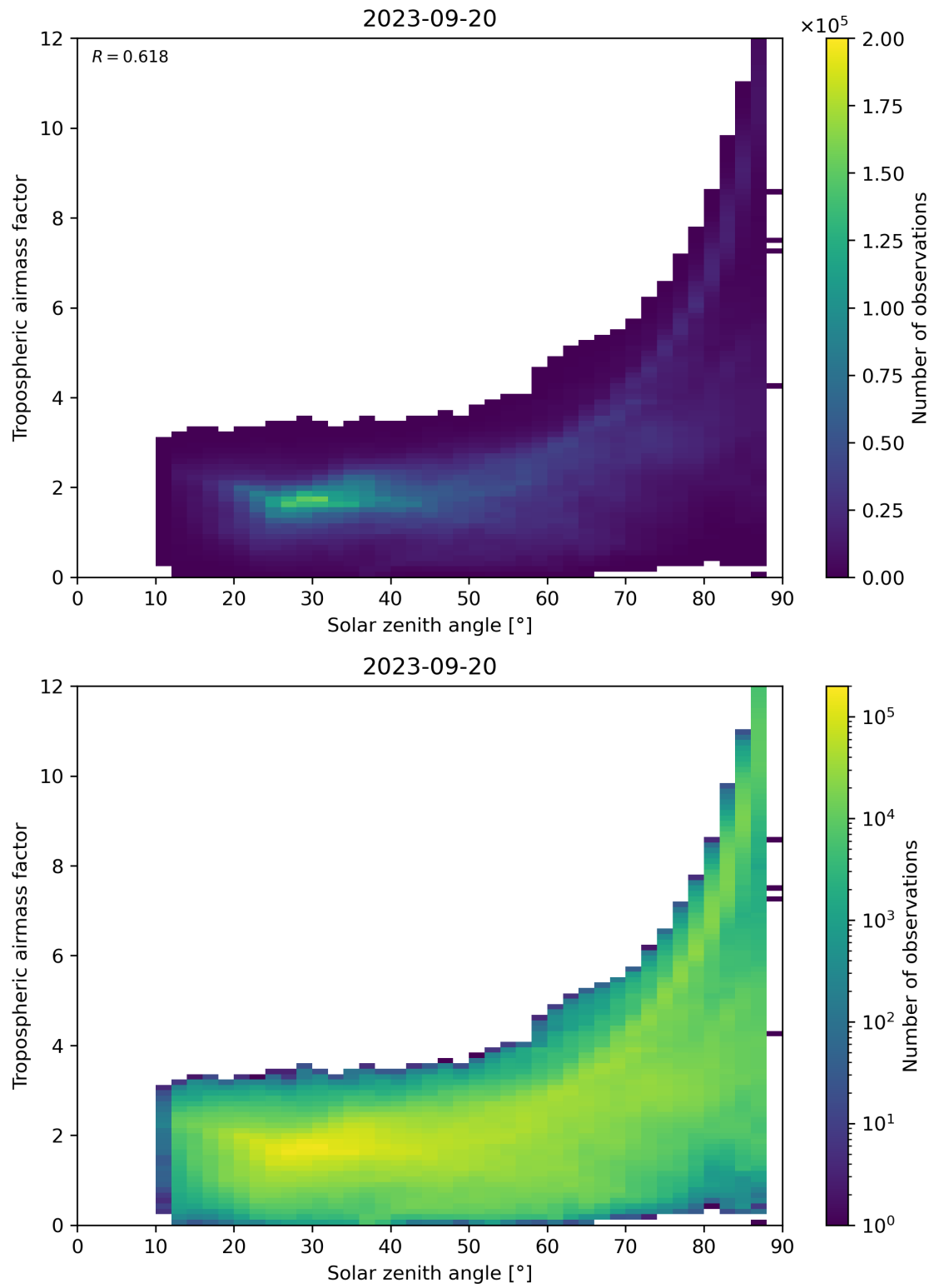
Figure 147: Scatter density plot of “Solar zenith angle” against “Tropospheric airmass factor” for 2023-09-20 to 2023-09-21.
