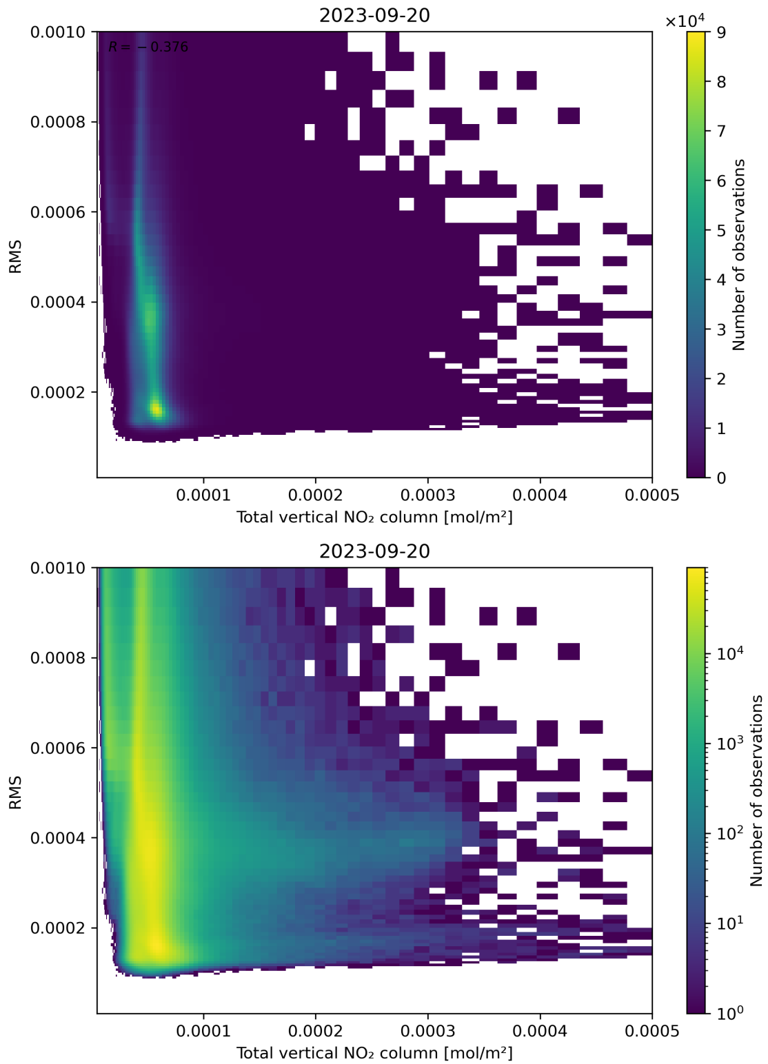
Figure 120: Scatter density plot of “Total vertical NO 2 column” against “RMS” for 2023-09-20 to 2023-09-21.
