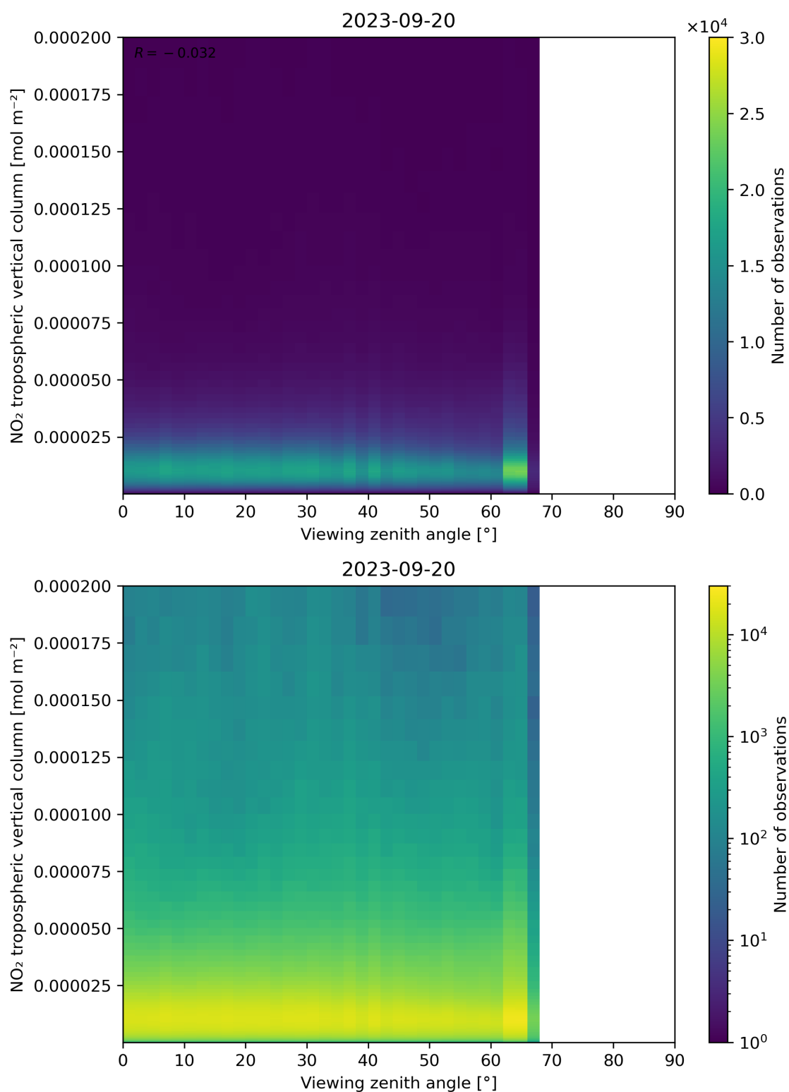
Figure 169: Scatter density plot of “Viewing zenith angle” against “NO 2 tropospheric vertical column” for 2023-09-20 to 2023-09-21.
