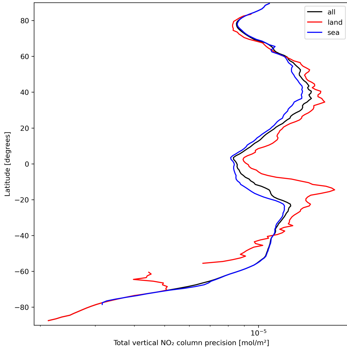
Figure 22: Zonal average of “Total vertical NO 2 column precision” for 2023-09-20 to 2023-09-21.
