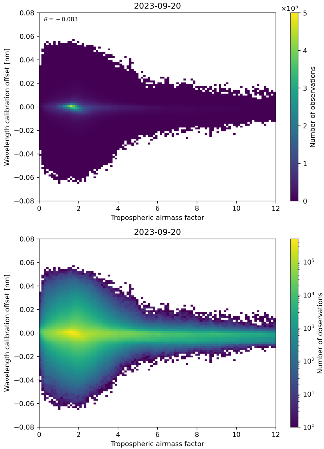
Figure 80: Scatter density plot of “Tropospheric airmass factor” against “Wavelength calibration offset” for 2023-09-20 to 2023-09-21.
