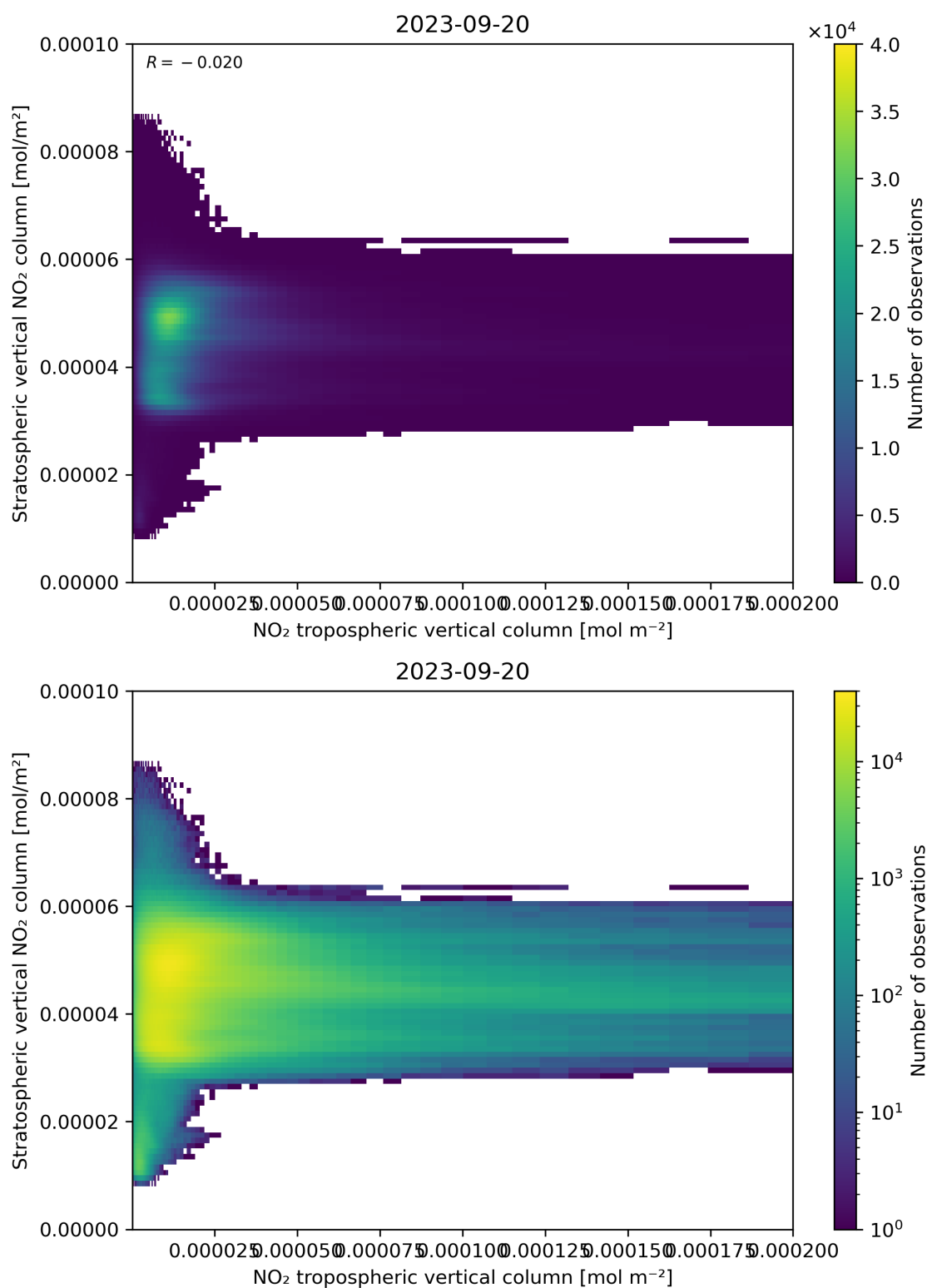
Figure 125: Scatter density plot of “NO 2 tropospheric vertical column” against “Stratospheric vertical NO 2 column” for 2023-09-20 to 2023-09-21.
