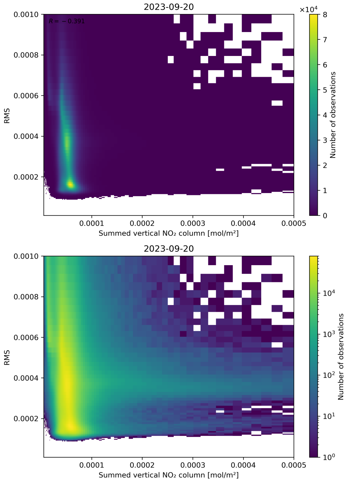
Figure 109: Scatter density plot of “Summed vertical NO 2 column” against “RMS” for 2023-09-20 to 2023-09-21.
