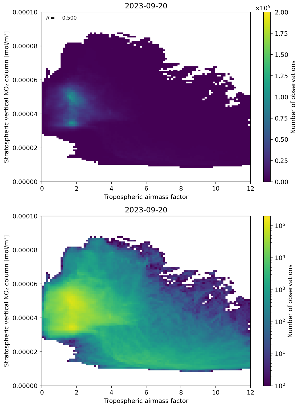
Figure 74: Scatter density plot of “Tropospheric air mass factor” against “Stratospheric vertical NO 2 column” for 2023-09-20 to 2023-09-21.
