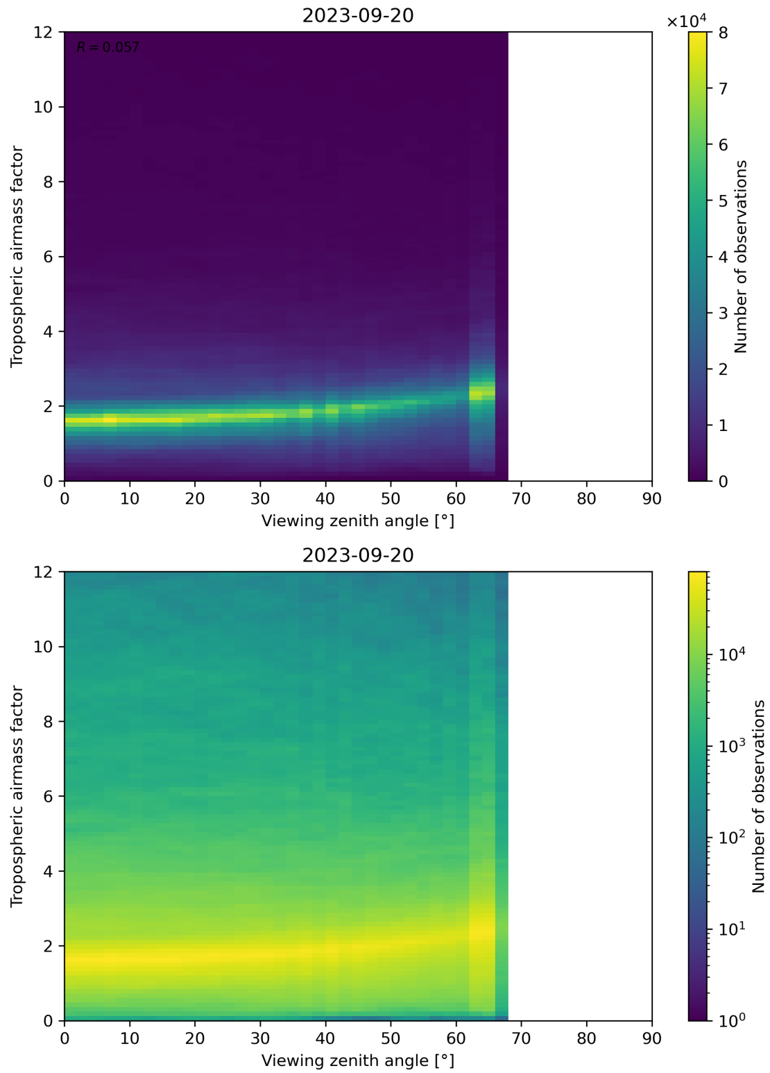
Figure 161: Scatter density plot of “Viewing zenith angle” against “Tropospheric airmass factor” for 2023-09-20 to 2023-09-21.
