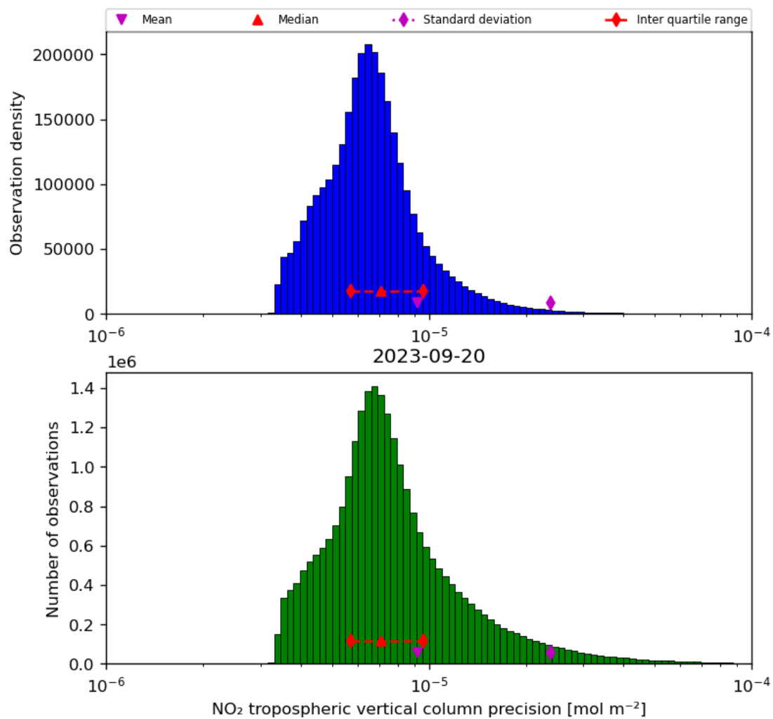
Figure 30: Histogram of “NO 2 tropospheric vertical column precision” for 2023-09-20 to 2023-09-21
