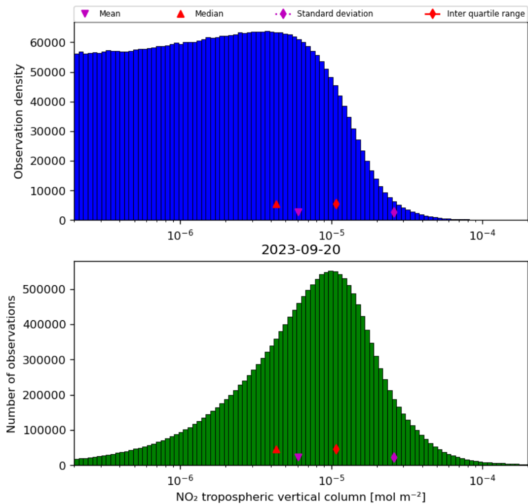
Figure 29: Histogram of “NO 2 tropospheric vertical column” for 2023-09-20 to 2023-09-21
