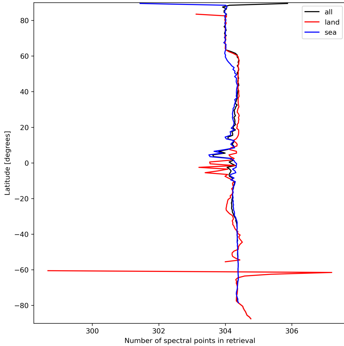
Figure 16: Zonal average of “Number of spectral points in retrieval” for 2023-09-20 to 2023-09-21.
