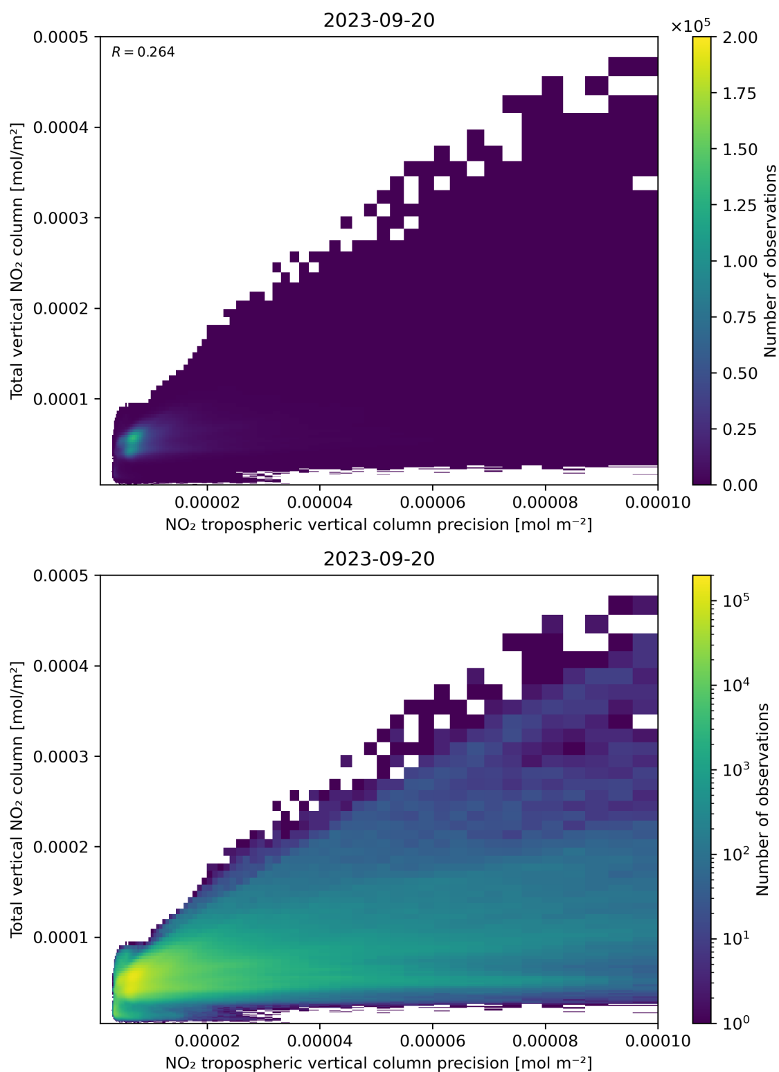
Figure 138: Scatter density plot of “NO 2 tropospheric vertical column precision” against “Total vertical NO 2 column” for 2023-09-20 to 2023-09-21.
