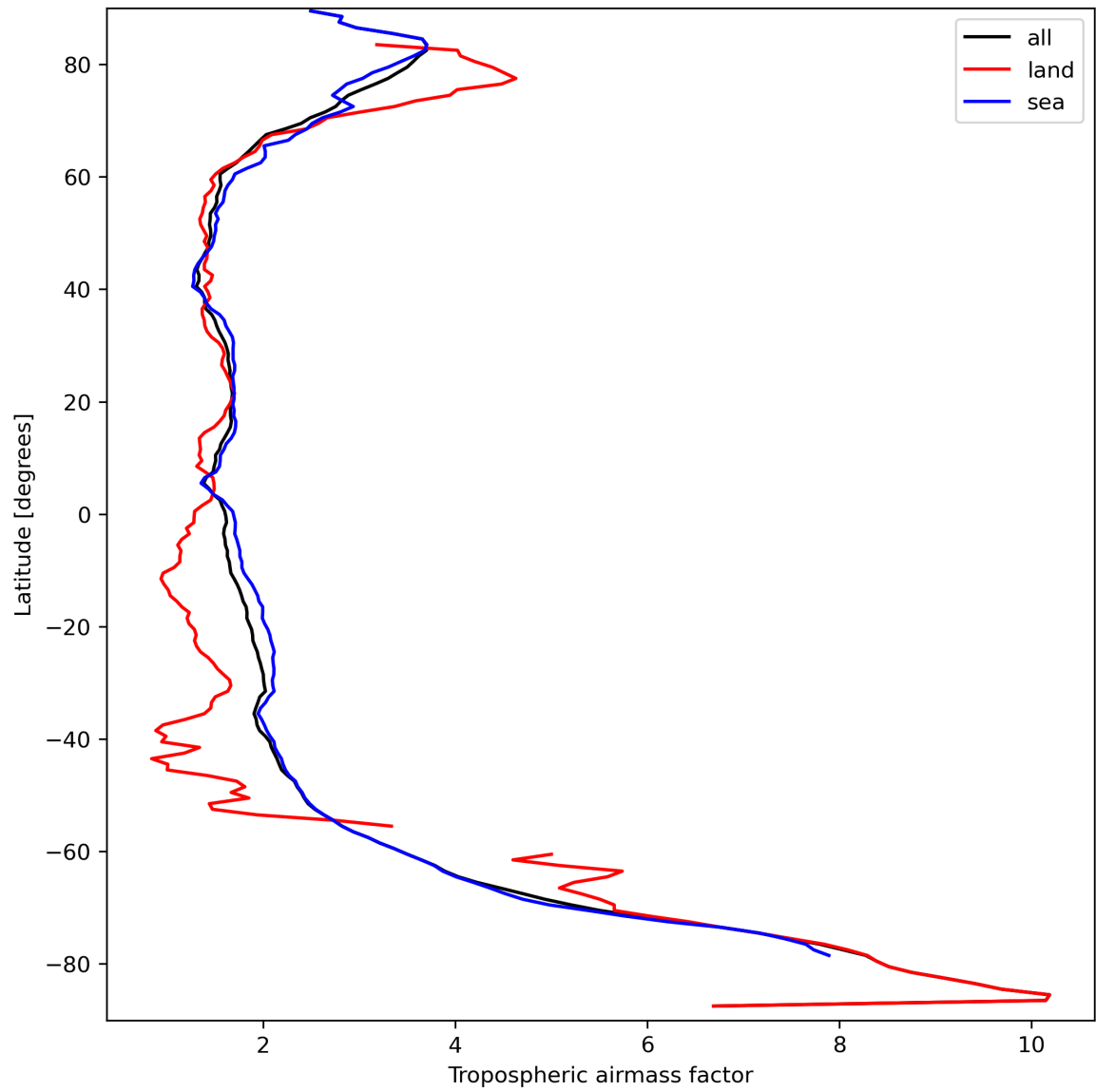
Figure 14: Zonal average of “Tropospheric airmass factor” for 2023-09-20 to 2023-09-21.
