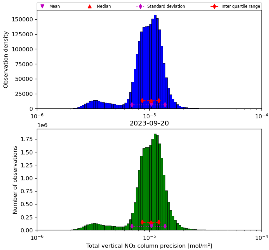
Figure 39: Histogram of “Total vertical NO 2 column precision” for 2023-09-20 to 2023-09-21
