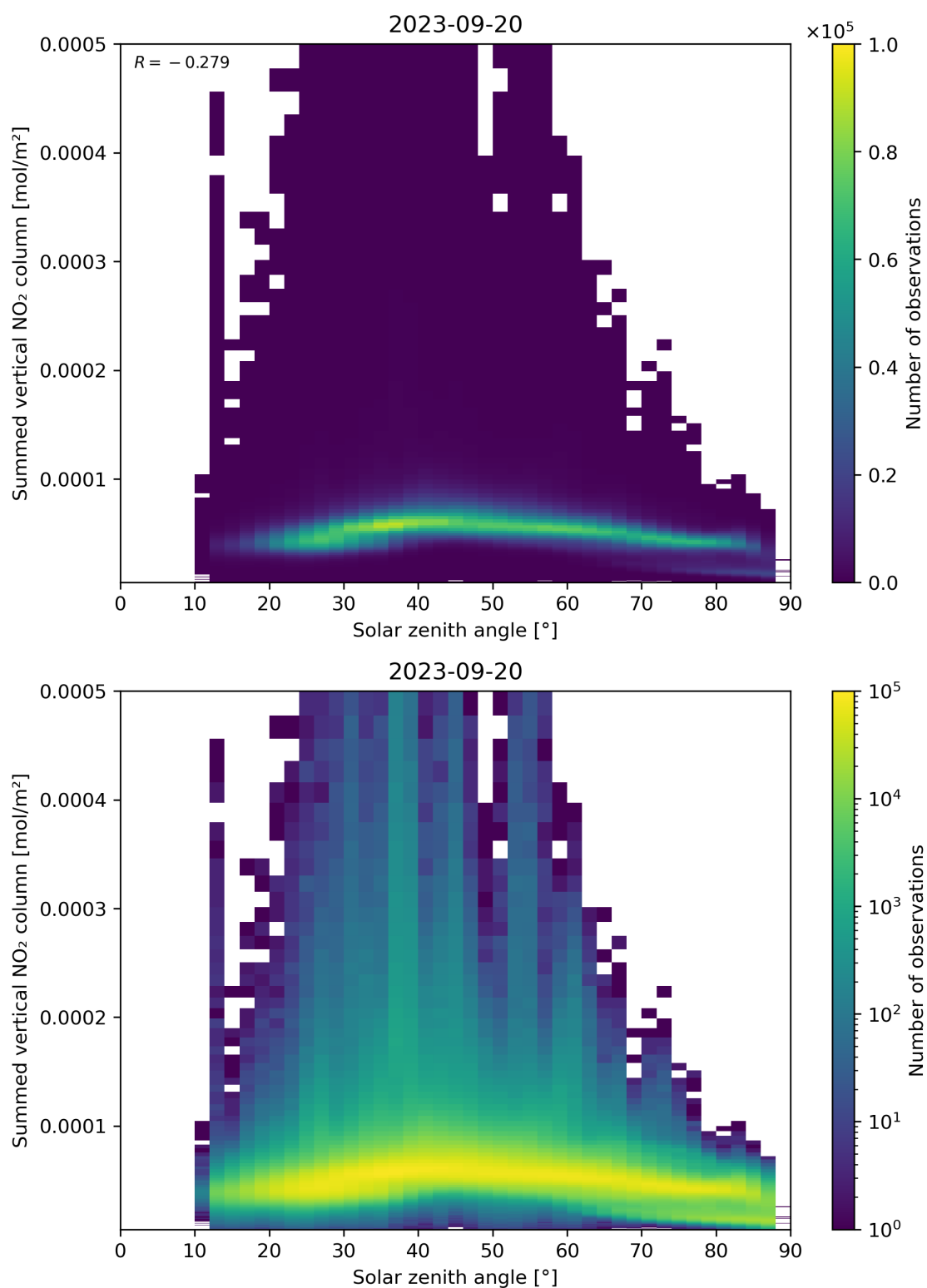
Figure 151: Scatter density plot of “Solar zenith angle” against “Summed vertical NO 2 column” for 2023-09-20 to 2023-09-21.
