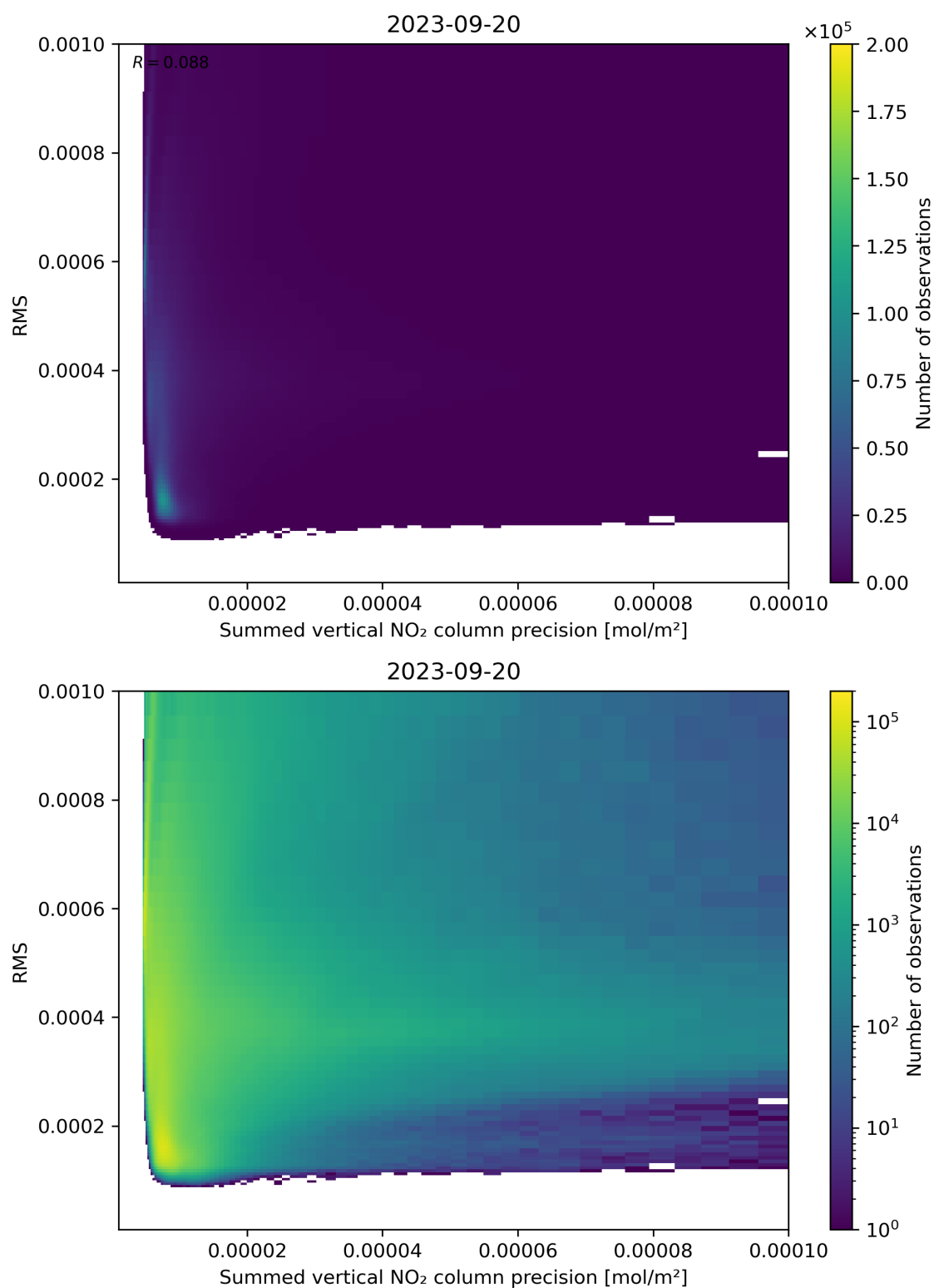
Figure 108: Scatter density plot of “Summed vertical NO 2 column precision” against “RMS” for 2023-09-20 to 2023-09-21.
