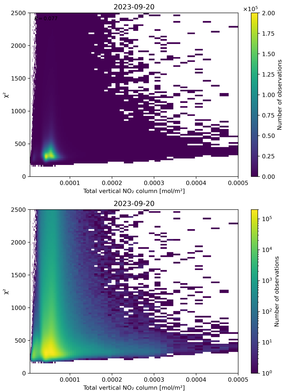
Figure 111: Scatter density plot of “Total vertical NO 2 column” against “ \chi^2 ” for 2023-09-20 to 2023-09-21.
