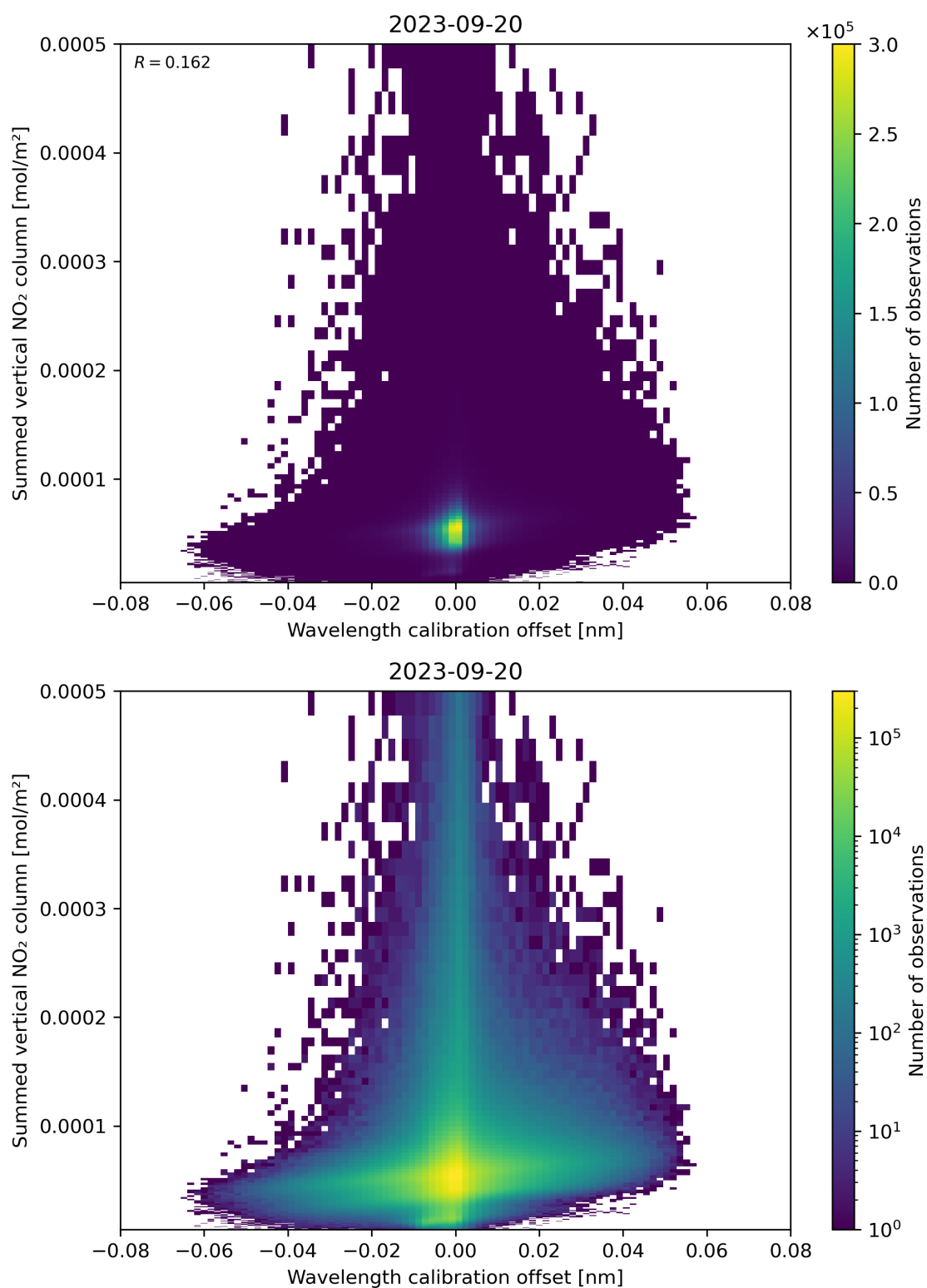
Figure 177: Scatter density plot of “Wavelength calibration offset” against “Summed vertical NO 2 column” for 2023-09-20 to 2023-09-21.
