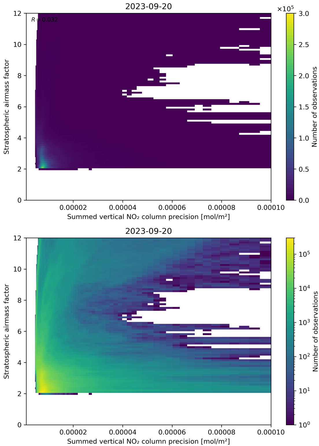
Figure 106: Scatter density plot of “Summed vertical NO 2 column precision” against “Stratospheric airmass factor” for 2023-09-20 to 2023-09-21.
