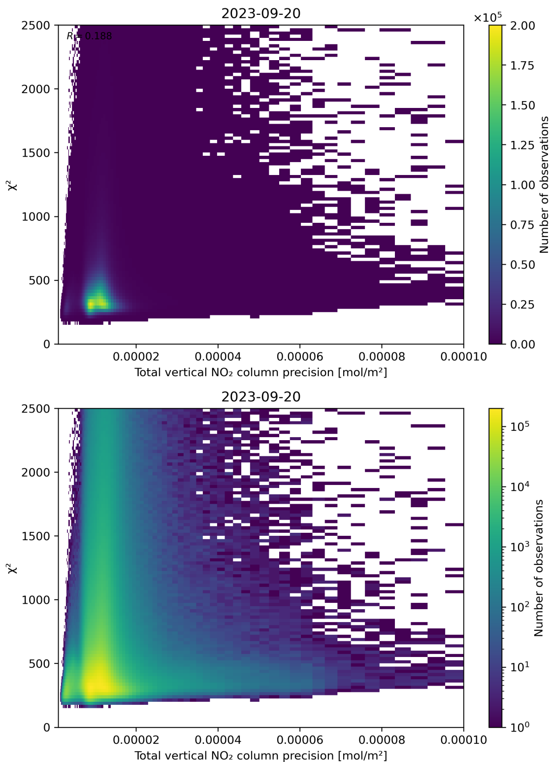
Figure 116: Scatter density plot of “Total vertical NO 2 column precision” against “ \chi^2 ” for 2023-09-20 to 2023-09-21.
