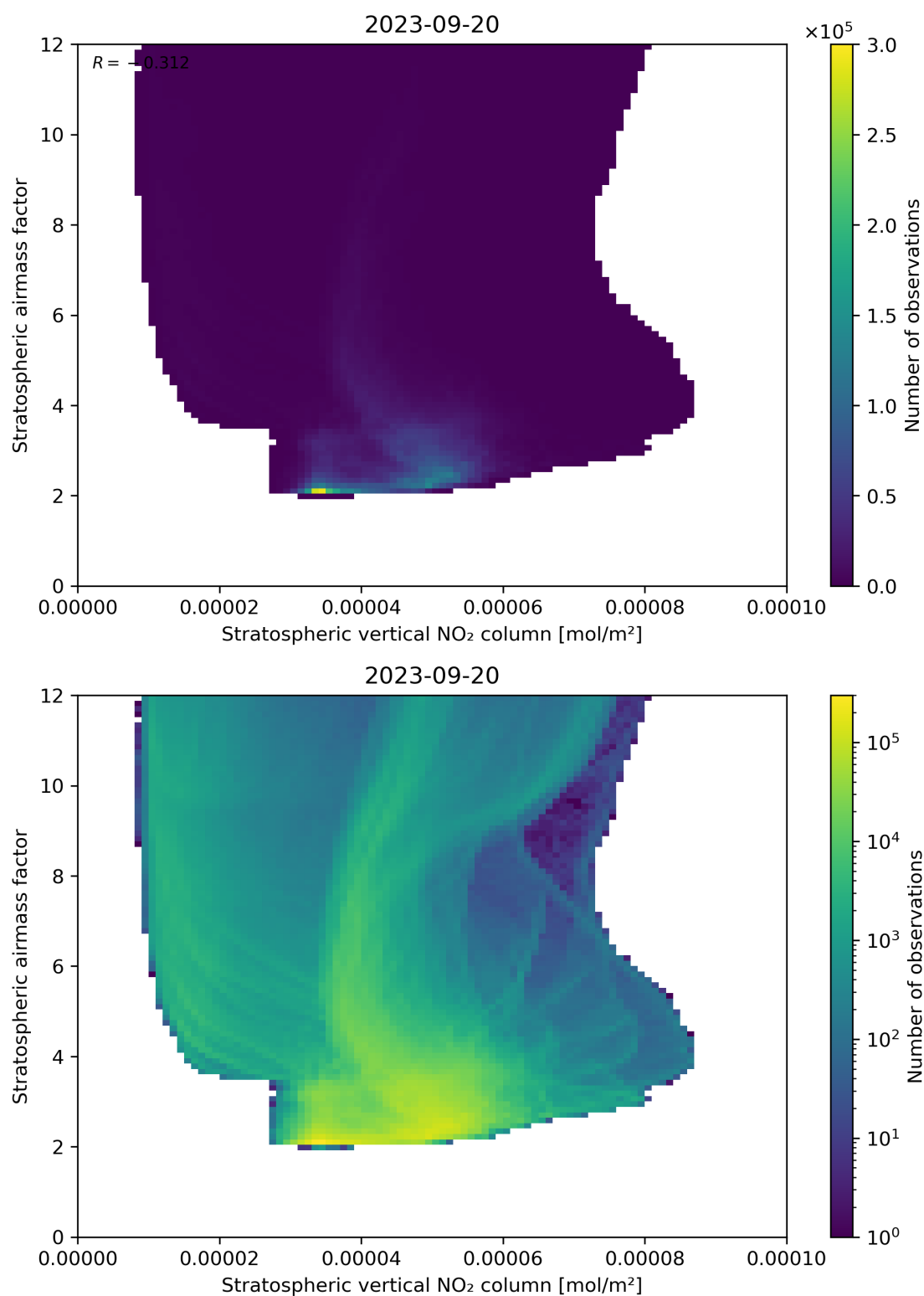
Figure 96: Scatter density plot of “Stratospheric vertical NO 2 column” against “Stratospheric airmass factor” for 2023-09-20 to 2023-09-21.
