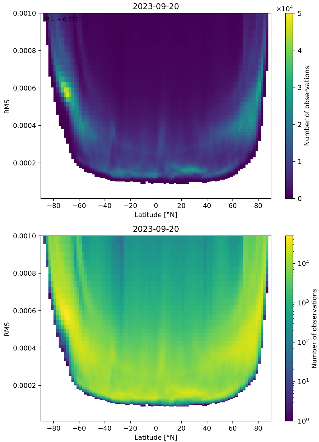
Figure 94: Scatter density plot of “Latitude” against “RMS” for 2023-09-20 to 2023-09-21.
