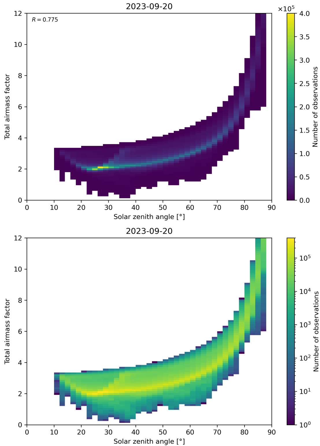
Figure 146: Scatter density plot of “Solar zenith angle” against “Total air mass factor” for 2023-09-20 to 2023-09-21.
