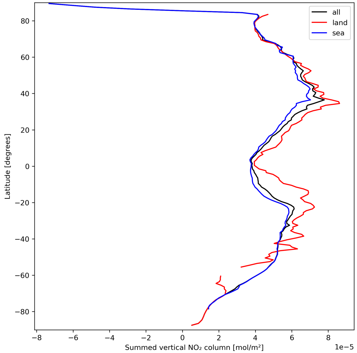
Figure 23: Zonal average of “Summed vertical NO 2 column” for 2023-09-20 to 2023-09-21.
