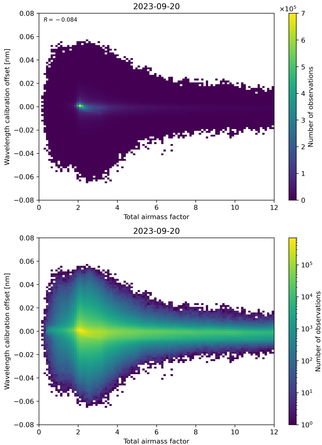
Figure 70: Scatter density plot of “Total airmass factor” against “Wavelength calibration offset” for 2023-09-20 to 2023-09-21.
