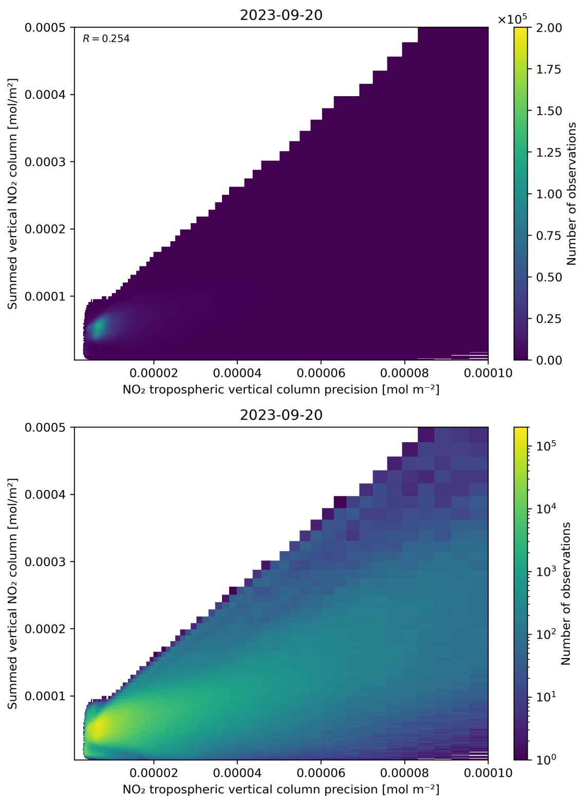
Figure 136: Scatter density plot of “NO 2 tropospheric vertical column precision” against “Summed vertical NO 2 column” for 2023-09-20 to 2023-09-21.
