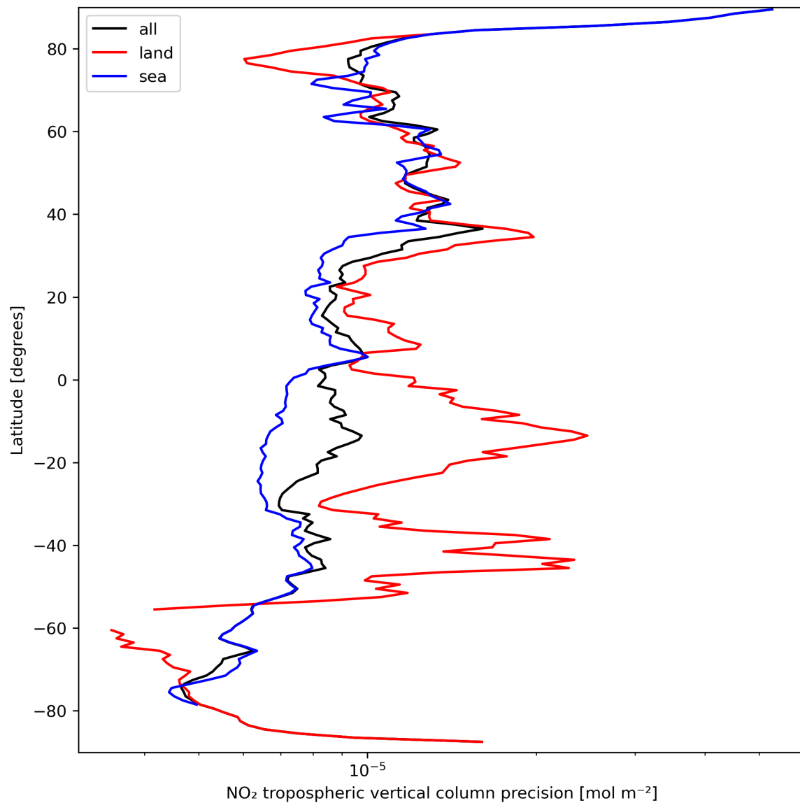
Figure 13: Zonal average of “NO 2 tropospheric vertical column precision” for 2023-09-20 to 2023-09-21.
