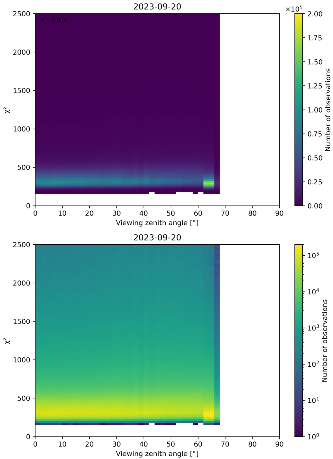
Figure 162: Scatter density plot of “Viewing zenith angle” against “ \chi^2 ” for 2023-09-20 to 2023-09-21.
