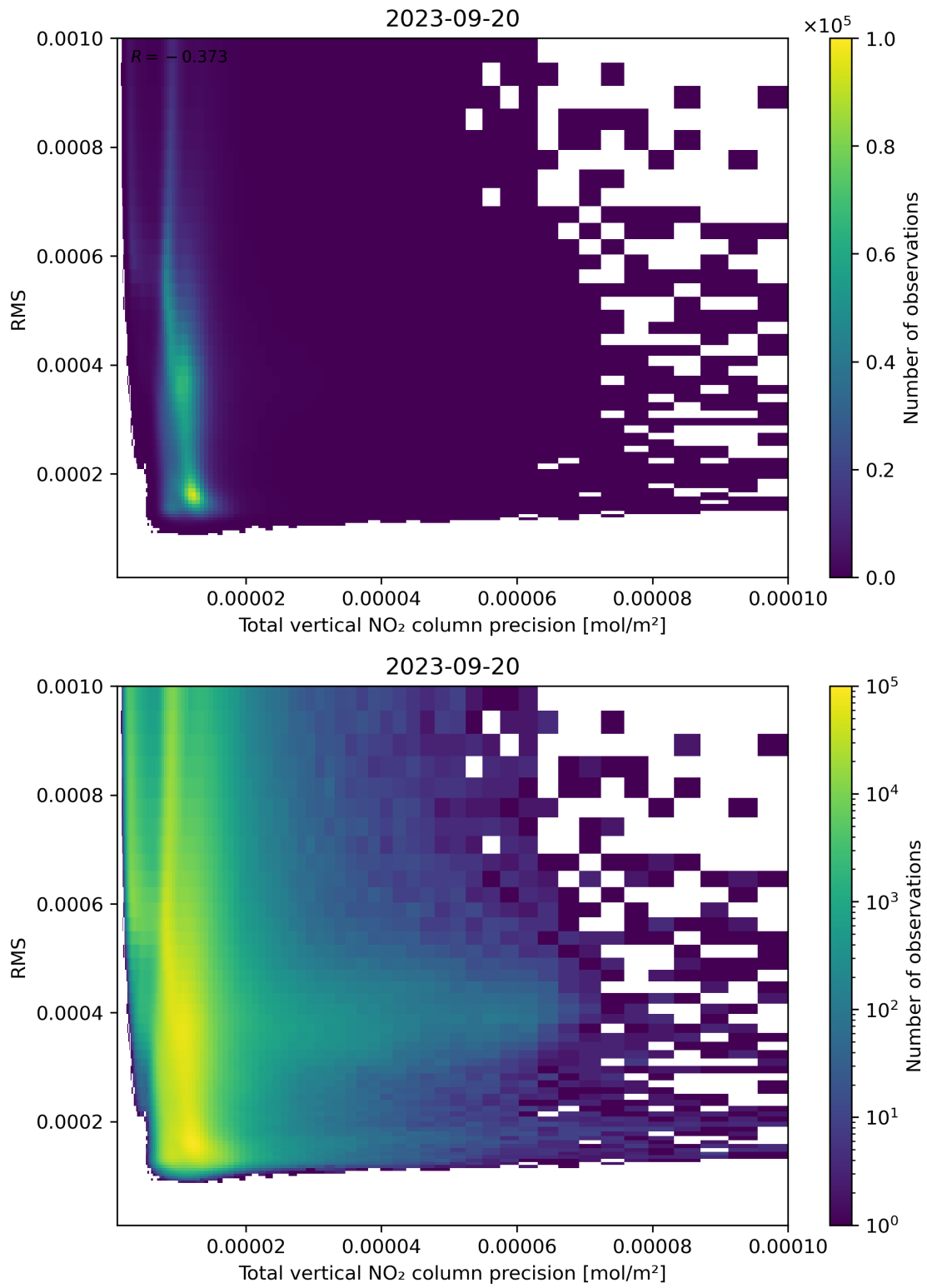
Figure 119: Scatter density plot of “Total vertical NO 2 column precision” against “RMS” for 2023-09-20 to 2023-09-21.
