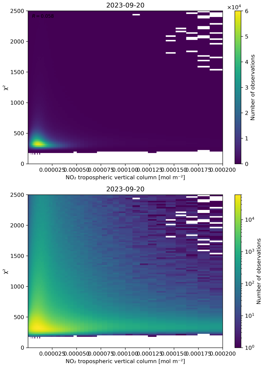
Figure 124: Scatter density plot of “NO 2 tropospheric vertical column” against “ \chi^2 ” for 2023-09-20 to 2023-09-21.
