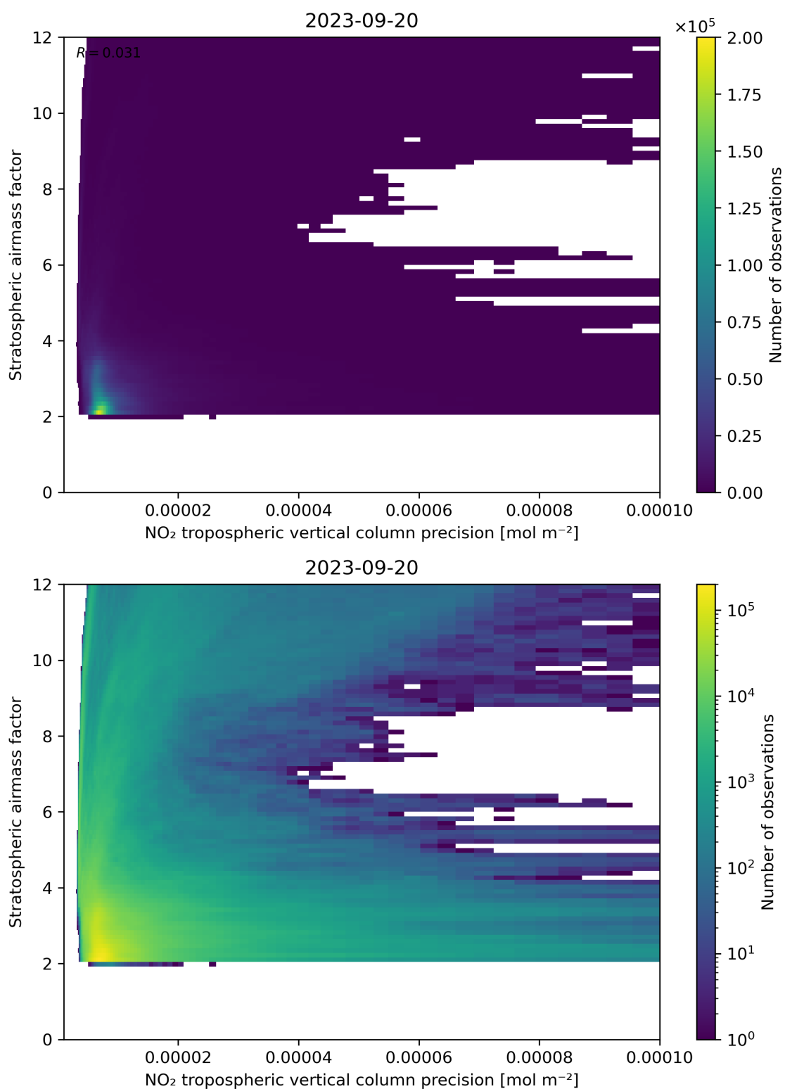
Figure 131: Scatter density plot of “NO 2 tropospheric vertical column precision” against “Stratospheric airmass factor” for 2023-09-20 to 2023-09-21.
