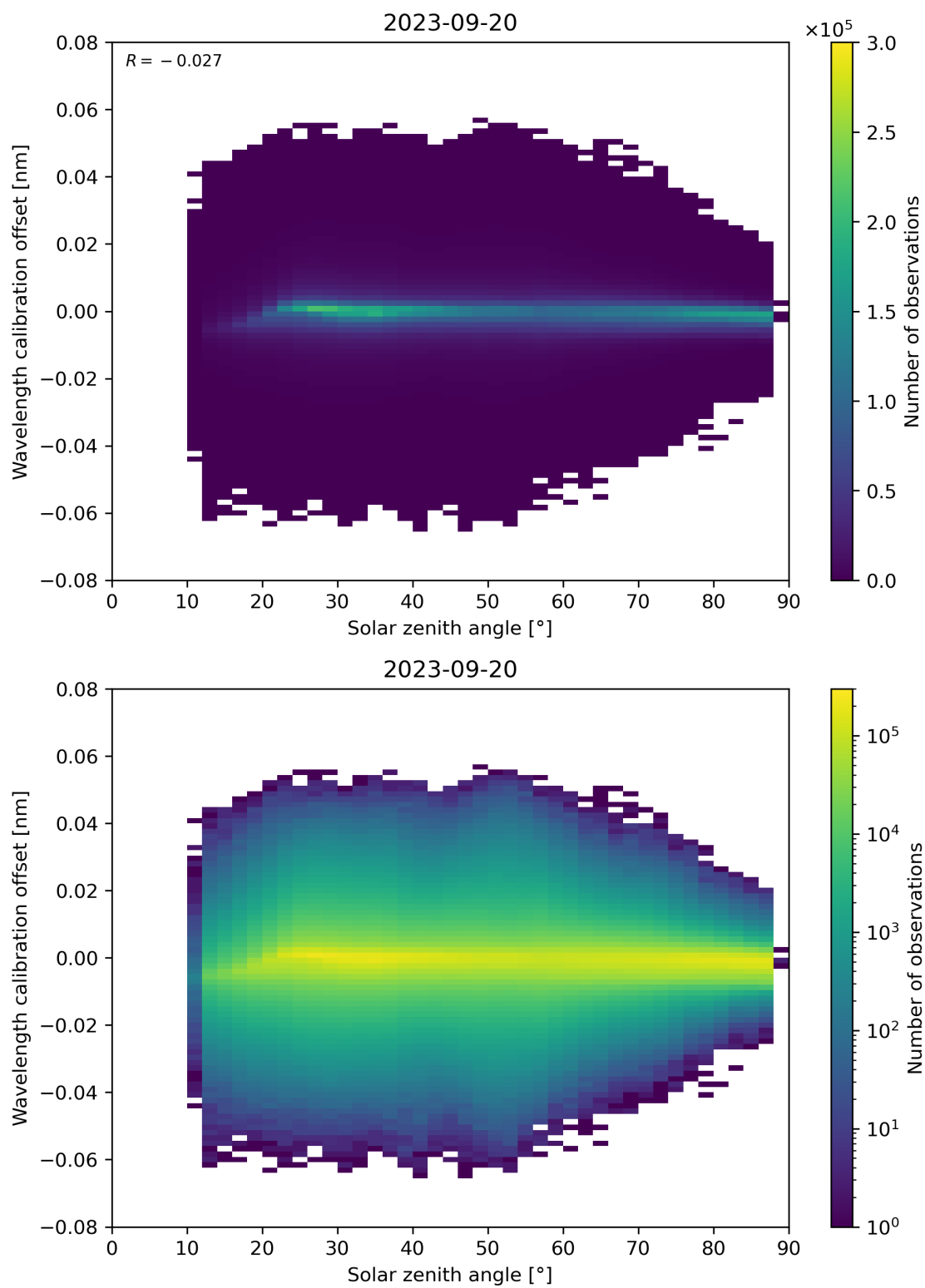
Figure 158: Scatter density plot of “Solar zenith angle” against “Wavelength calibration offset” for 2023-09-20 to 2023-09-21.
