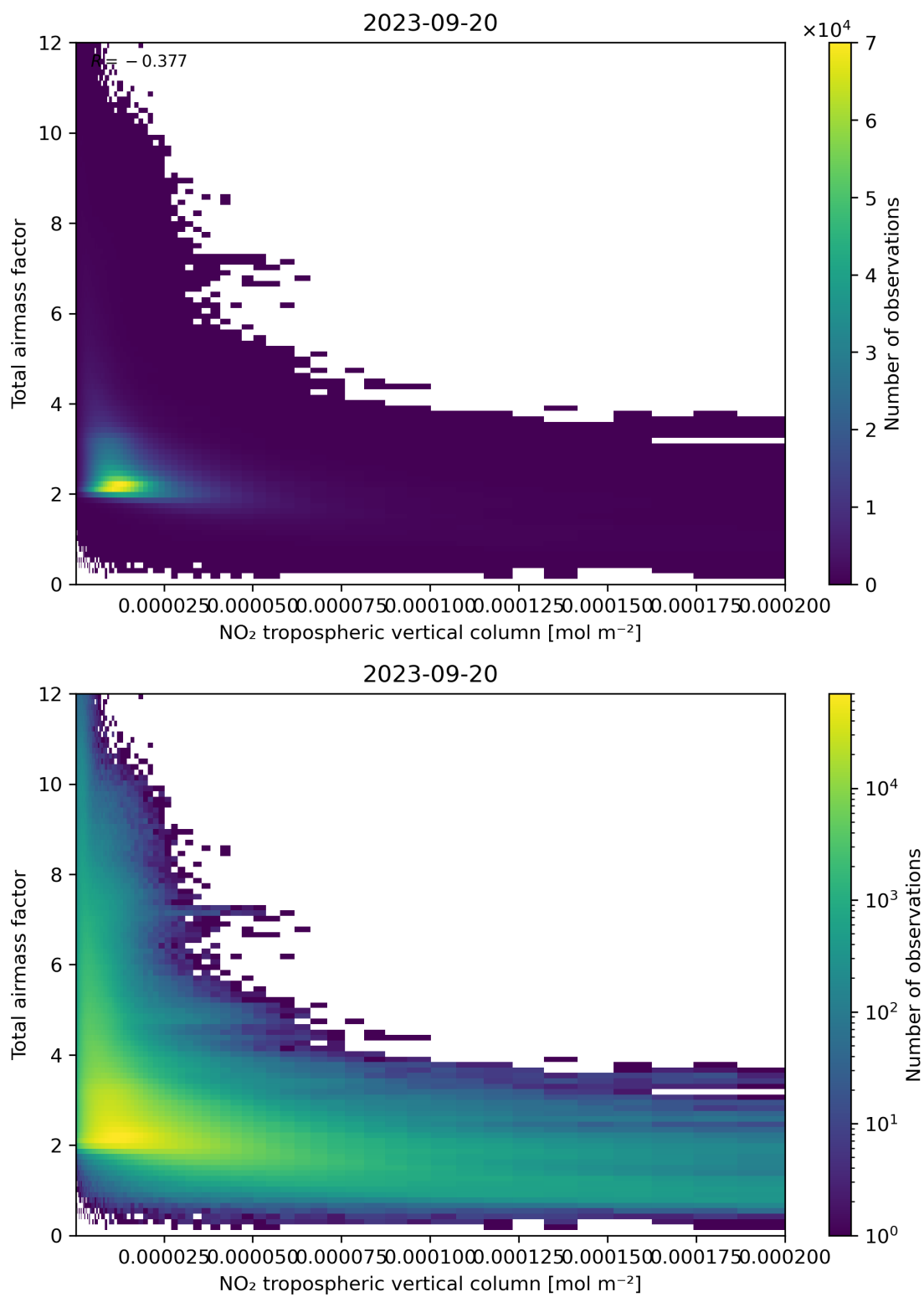
Figure 122: Scatter density plot of “NO 2 tropospheric vertical column” against “Total airmass factor” for 2023-09-20 to 2023-09-21.
