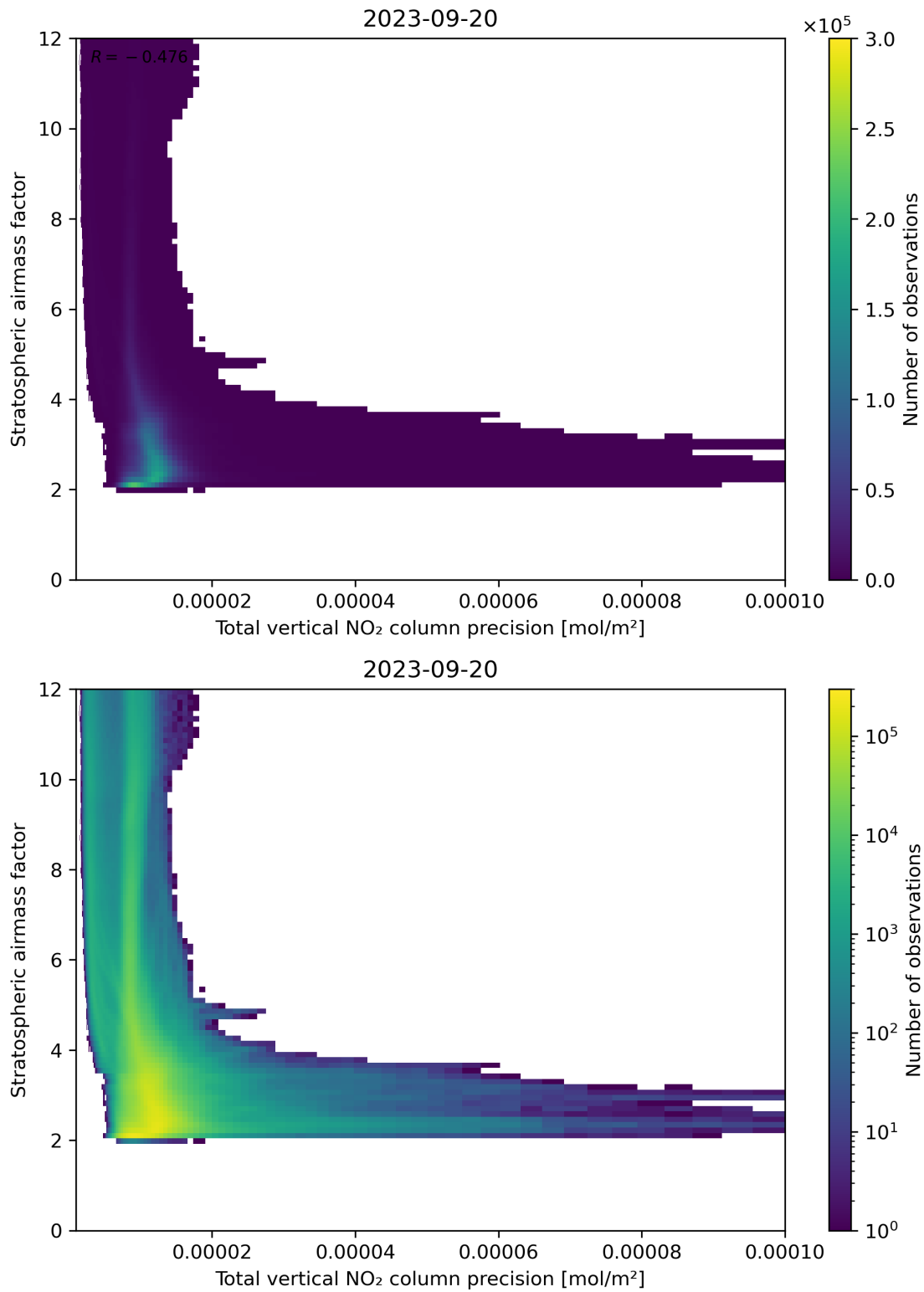
Figure 115: Scatter density plot of “Total vertical NO 2 column precision” against “Stratospheric air mass factor” for 2023-09-20 to 2023-09-21.
