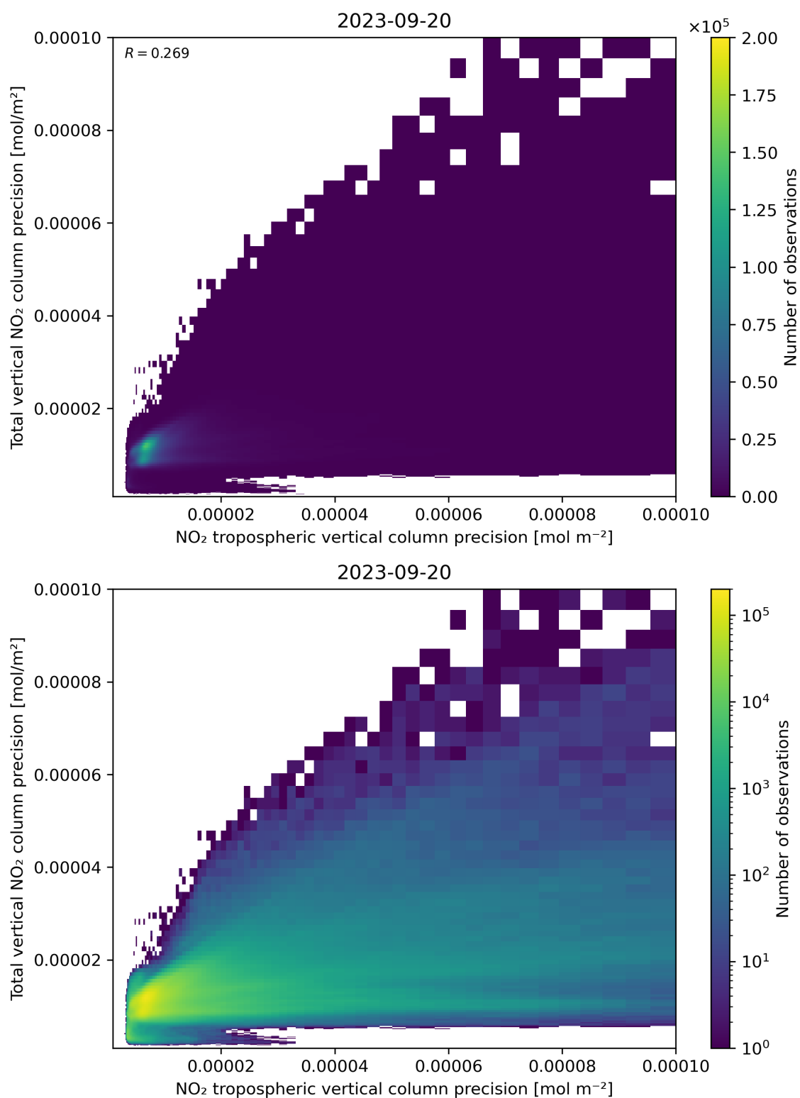
Figure 139: Scatter density plot of “NO 2 tropospheric vertical column precision” against “Total vertical NO 2 column precision” for 2023-09-20 to 2023-09-21.
