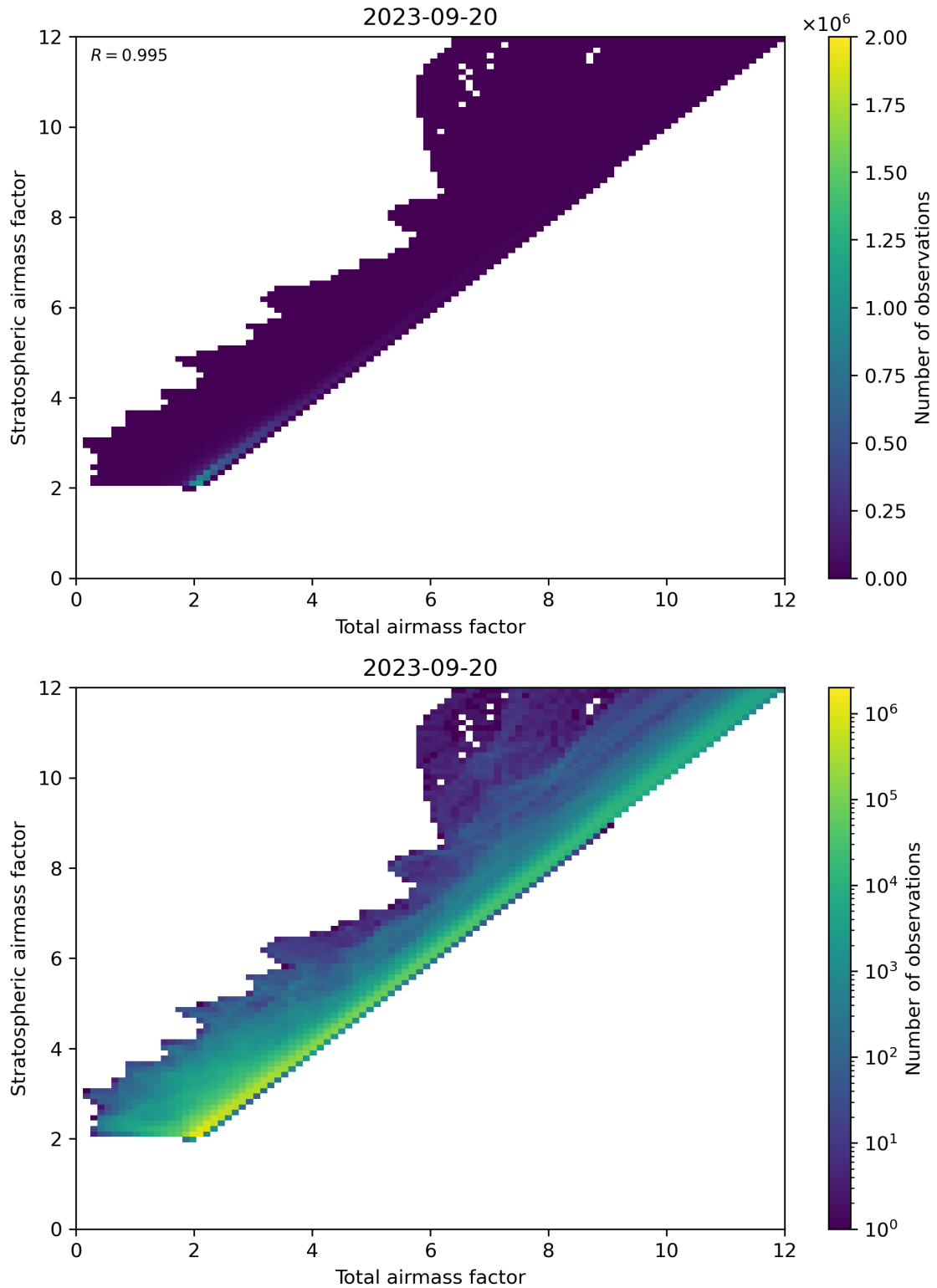
Figure 62: Scatter density plot of “Total airmass factor” against “Stratospheric airmass factor” for 2023-09-20 to 2023-09-21.
