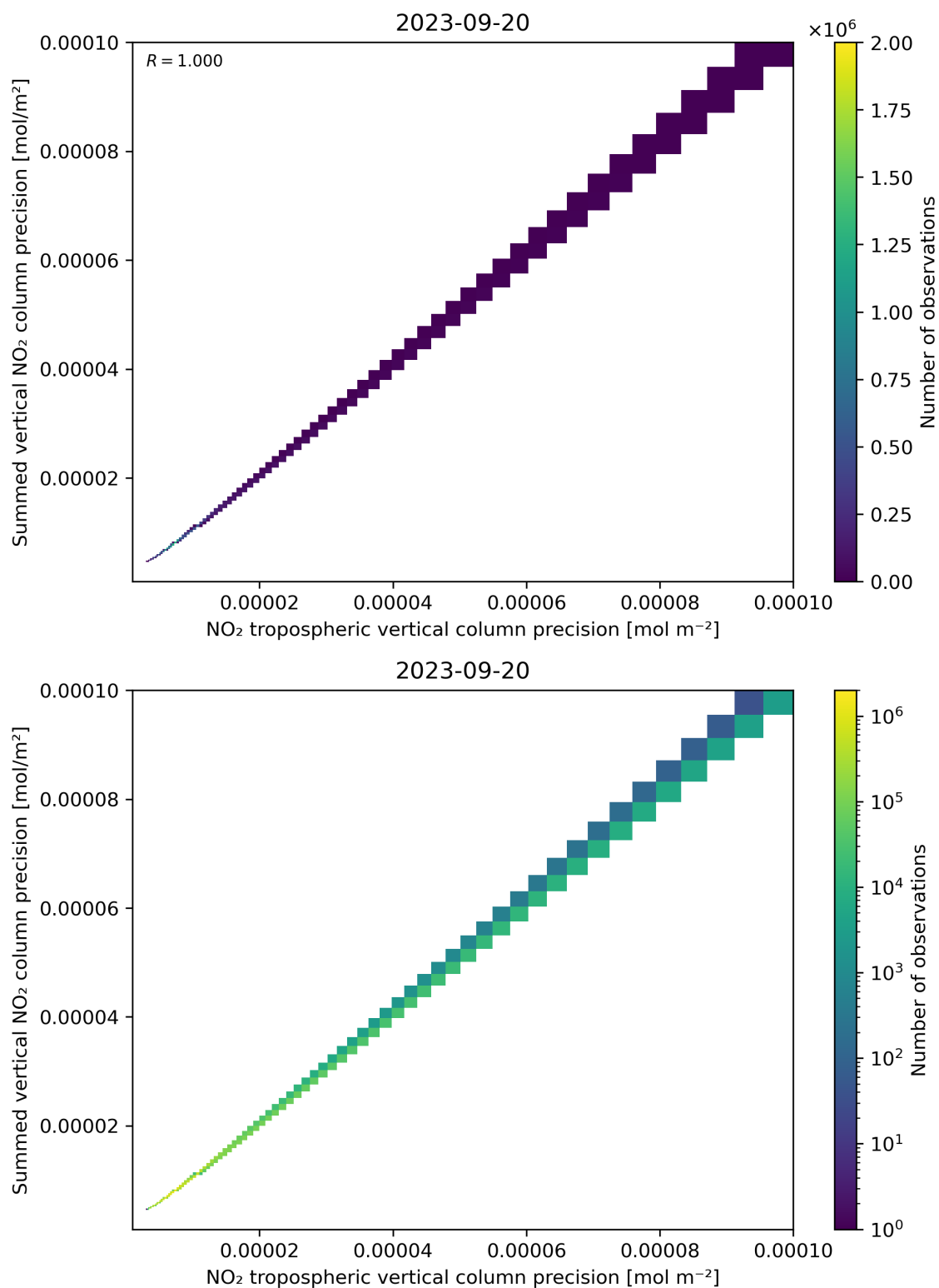
Figure 137: Scatter density plot of “NO 2 tropospheric vertical column precision” against “Summed vertical NO 2 column precision” for 2023-09-20 to 2023-09-21.
