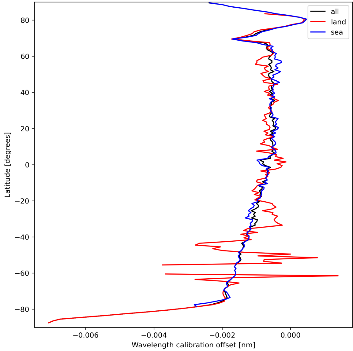
Figure 18: Zonal average of “Wavelength calibration offset” for 2023-09-20 to 2023-09-21.
