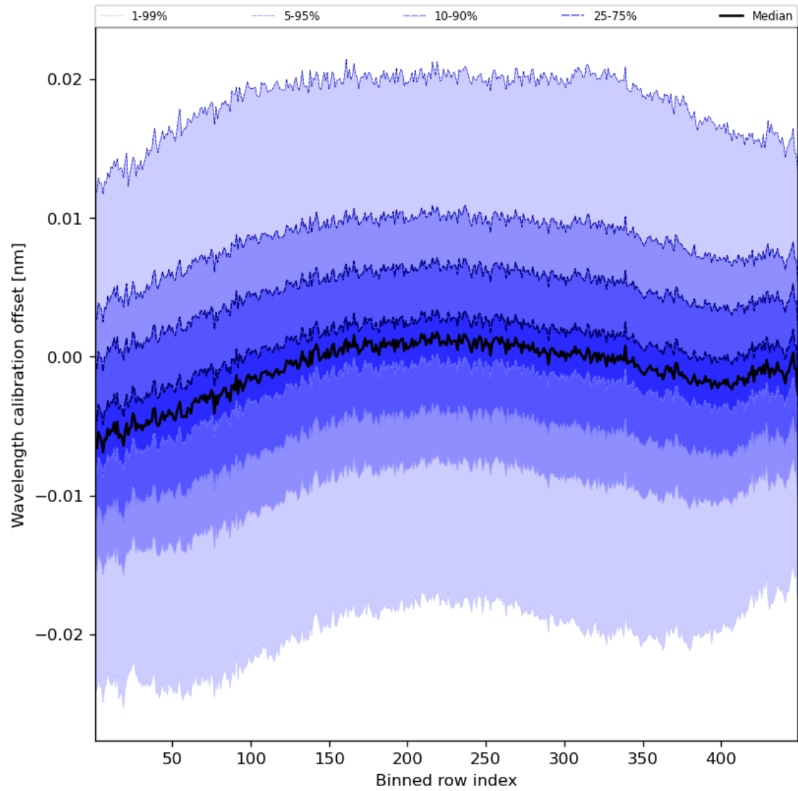
Figure 52: Along track statistics of “Wavelength calibration offset” for 2023-09-20 to 2023-09-21
