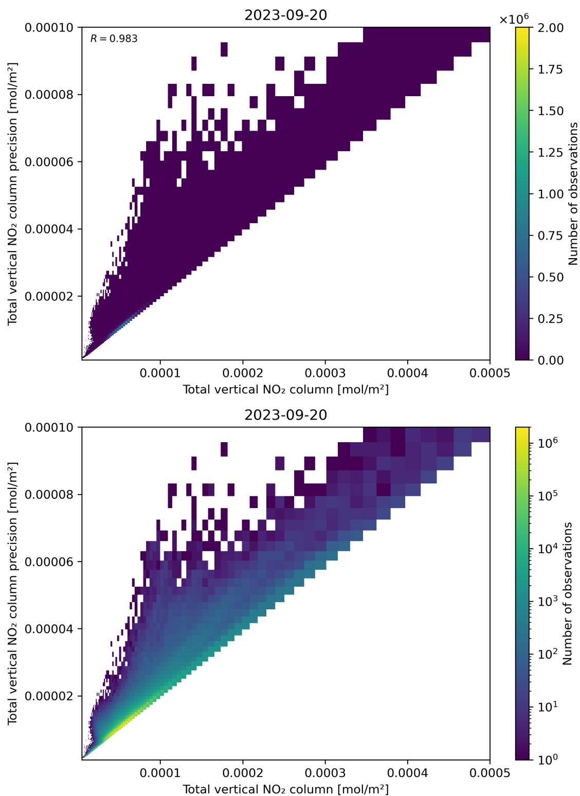
Figure 114: Scatter density plot of “Total vertical NO 2 column” against “Total vertical NO 2 column precision” for 2023-09-20 to 2023-09-21.
