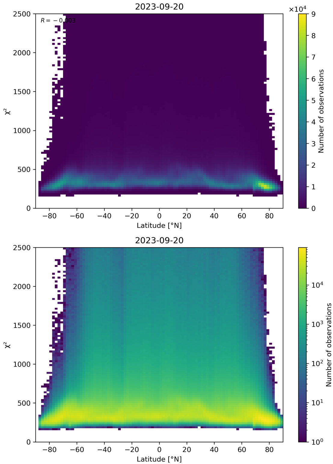
Figure 86: Scatter density plot of “Latitude” against “ \chi^2 ” for 2023-09-20 to 2023-09-21.
