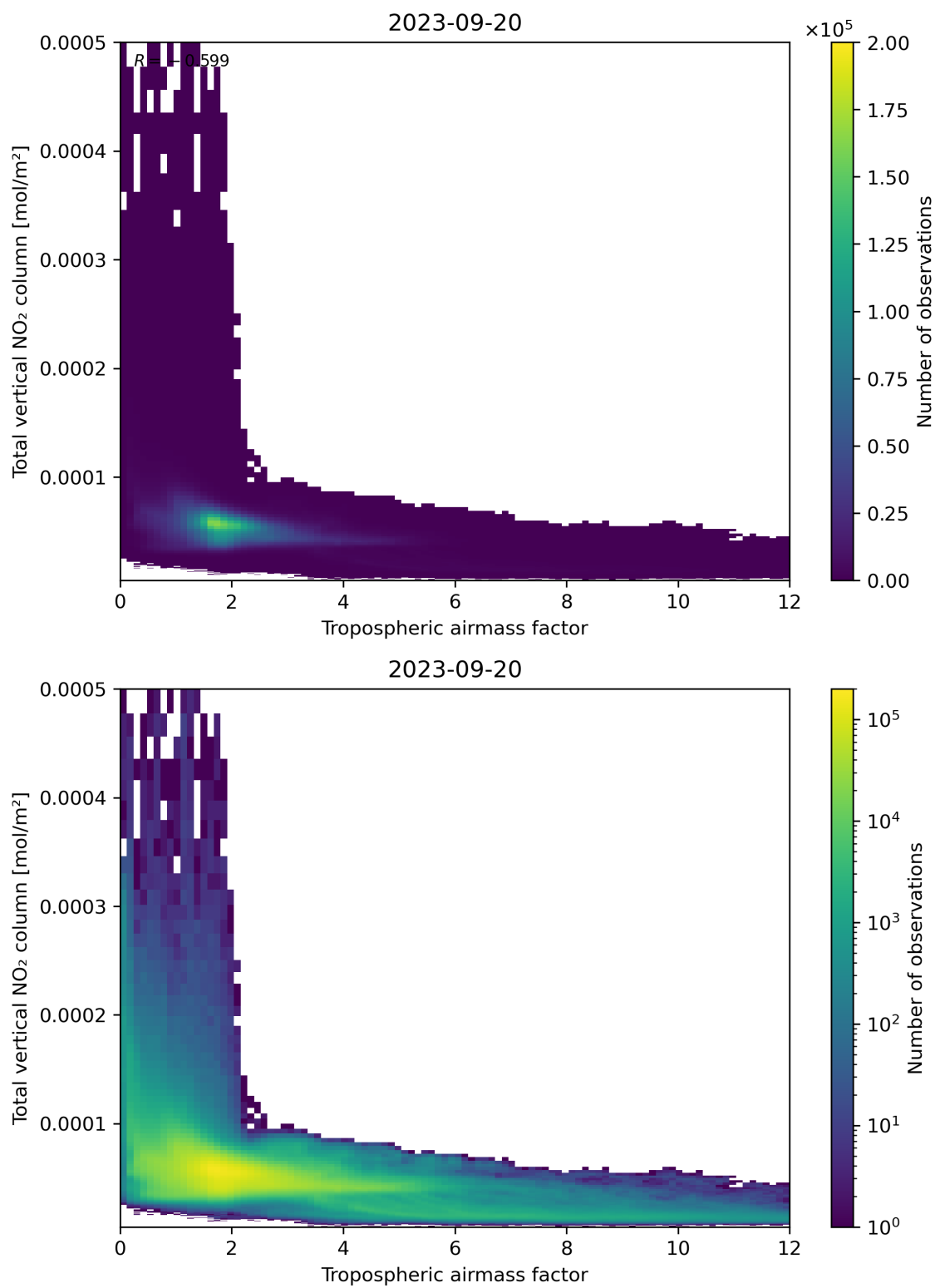
Figure 77: Scatter density plot of “Tropospheric airmass factor” against “Total vertical NO 2 column” for 2023-09-20 to 2023-09-21.
