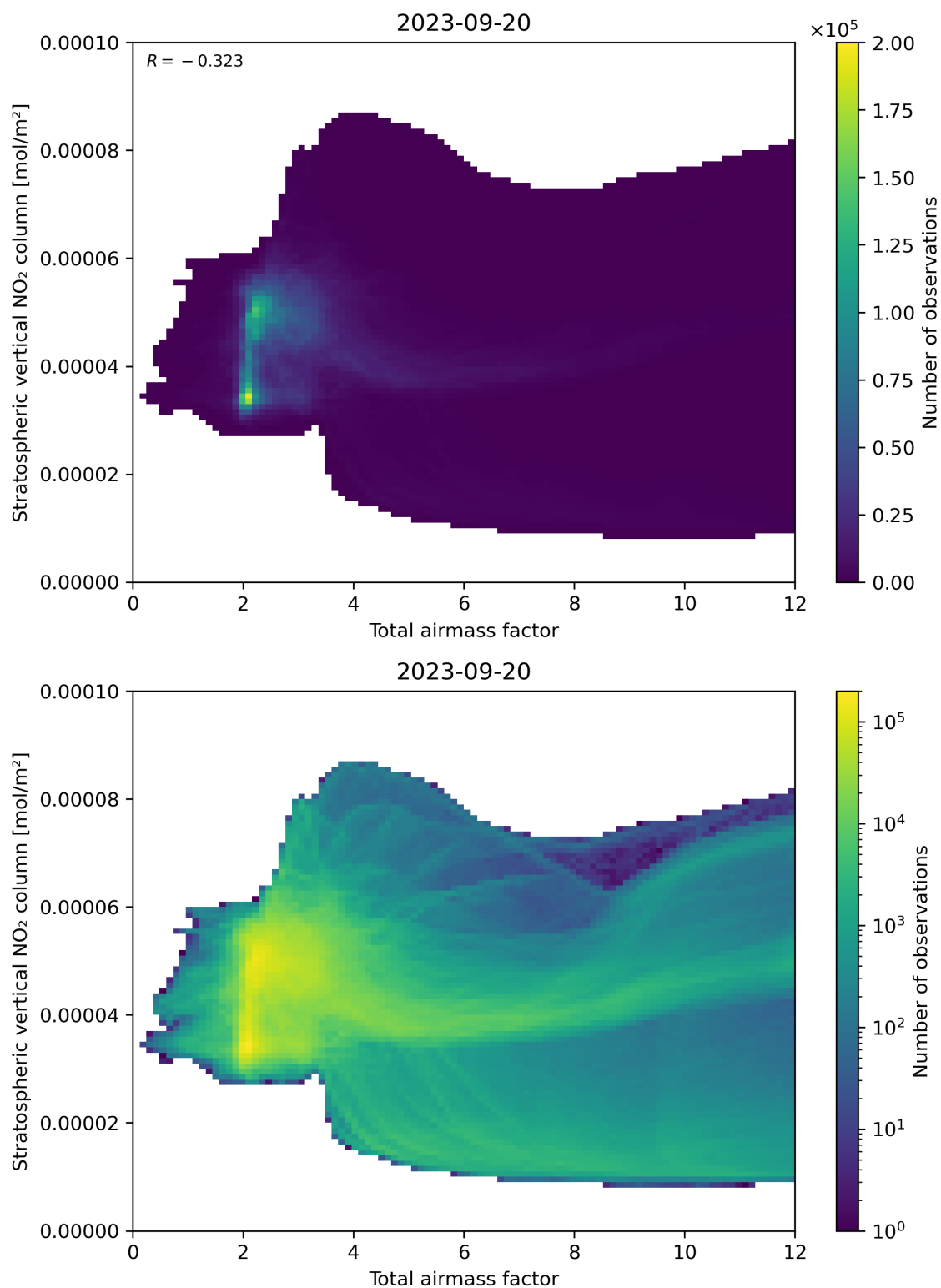
Figure 64: Scatter density plot of “Total airmass factor” against “Stratospheric vertical NO 2 column” for 2023-09-20 to 2023-09-21.
