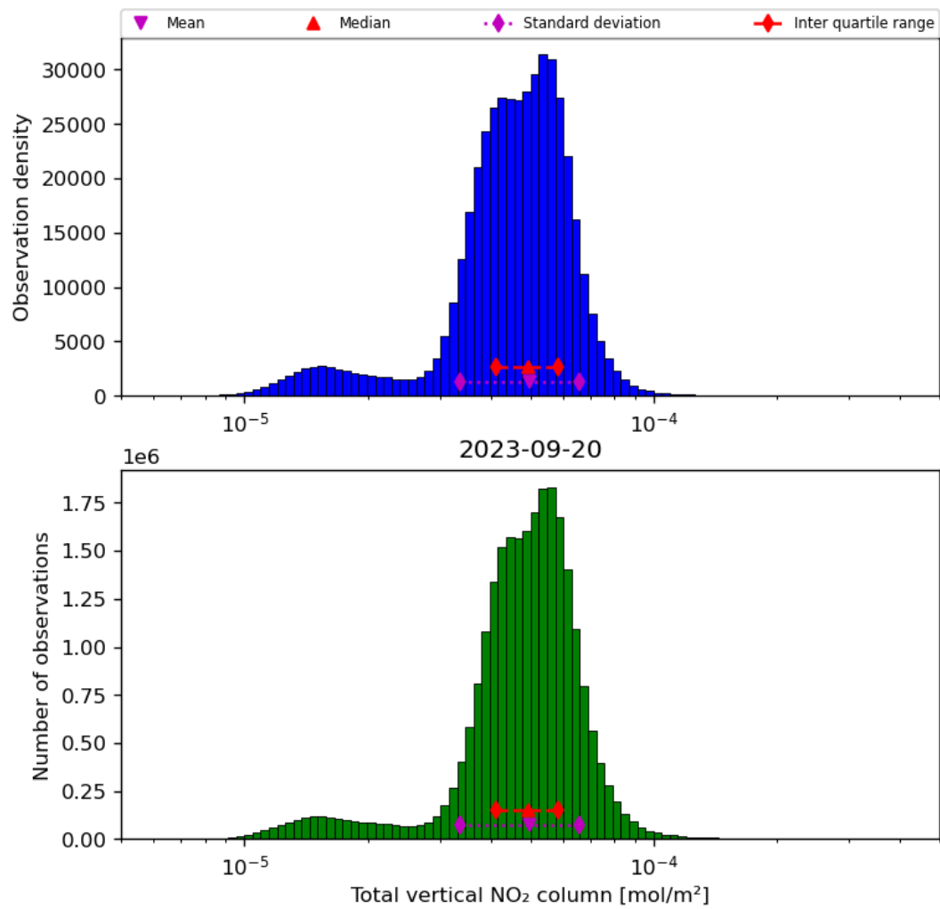
Figure 38: Histogram of “Total vertical NO 2 column” for 2023-09-20 to 2023-09-21
