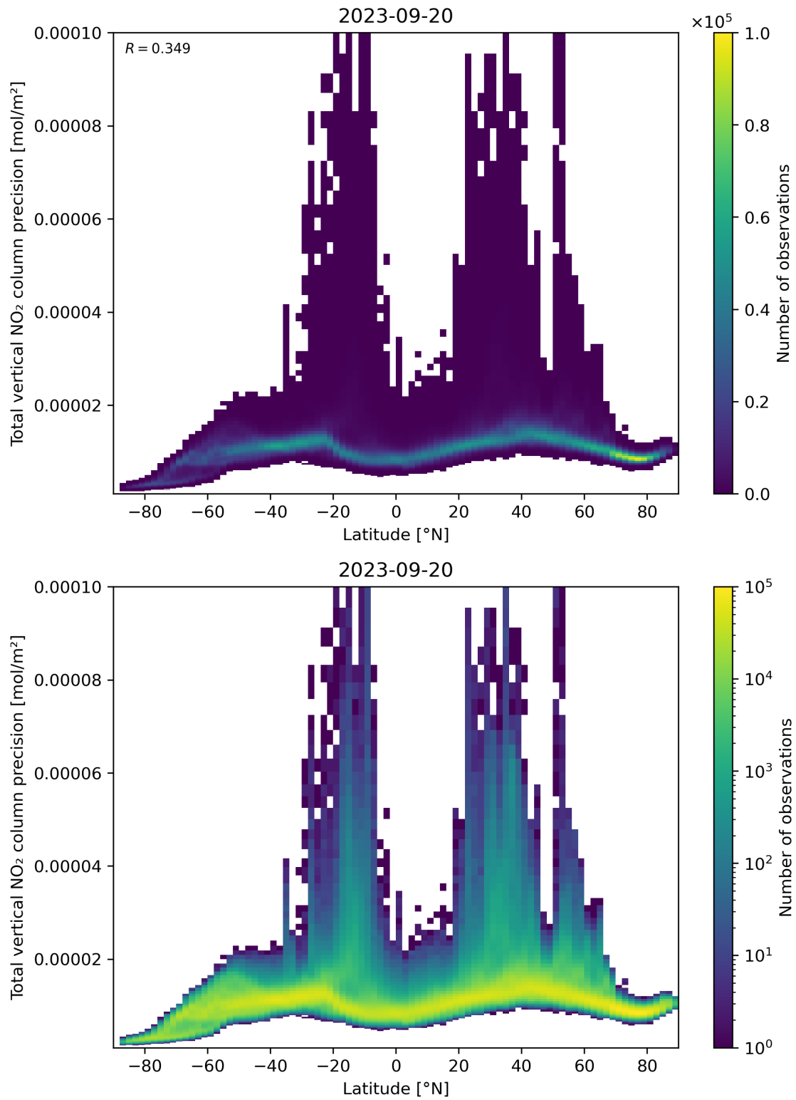
Figure 91: Scatter density plot of “Latitude” against “Total vertical NO 2 column precision” for 2023-09-20 to 2023-09-21.
