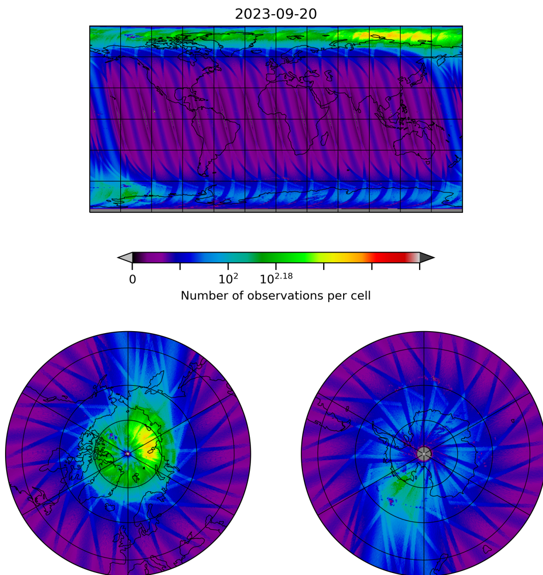
Figure 10: Map of the number of observations for 2023-09-20 to 2023-09-21
