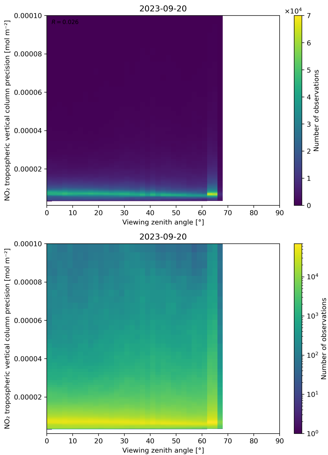
Figure 170: Scatter density plot of “Viewing zenith angle” against “NO 2 tropospheric vertical column precision” for 2023-09-20 to 2023-09-21.
