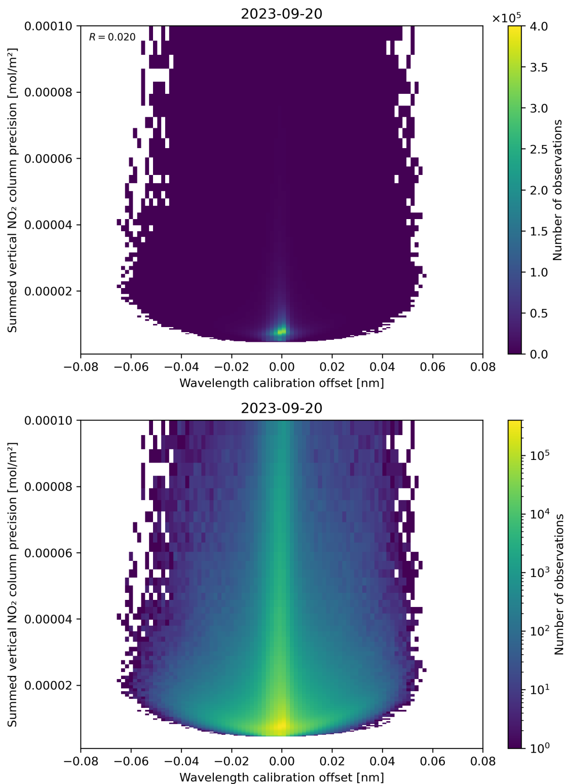
Figure 178: Scatter density plot of “Wavelength calibration offset” against “Summed vertical NO 2 column precision” for 2023-09-20 to 2023-09-21.
