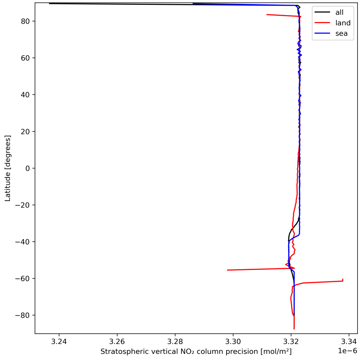
Figure 20: Zonal average of “Stratospheric vertical NO 2 column precision” for 2023-09-20 to 2023-09-21.
