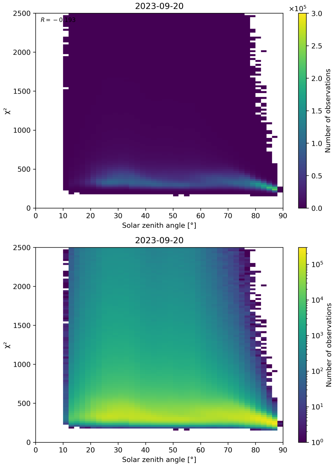
Figure 148: Scatter density plot of “Solar zenith angle” against “ \chi^2 ” for 2023-09-20 to 2023-09-21.
