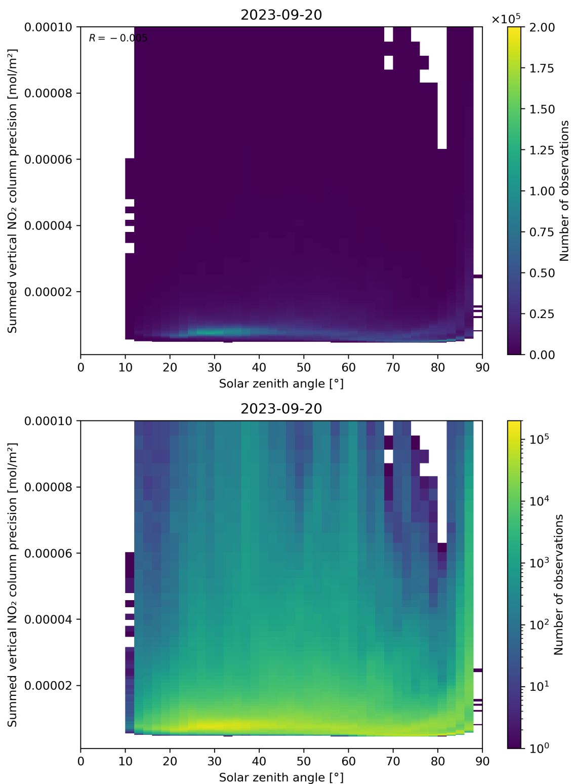
Figure 152: Scatter density plot of “Solar zenith angle” against “Summed vertical NO 2 column precision” for 2023-09-20 to 2023-09-21.
