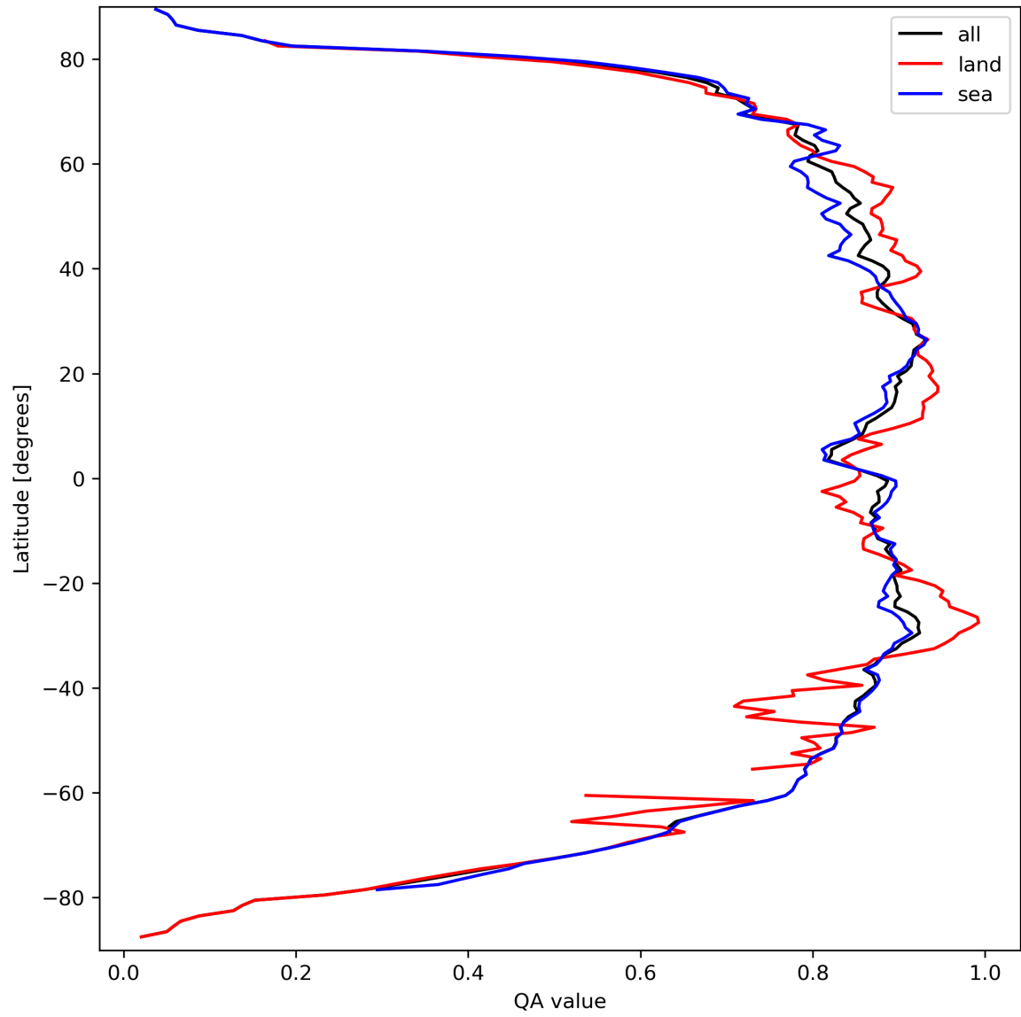
Figure 11: Zonal average of “QA value” for 2023-09-20 to 2023-09-21.
