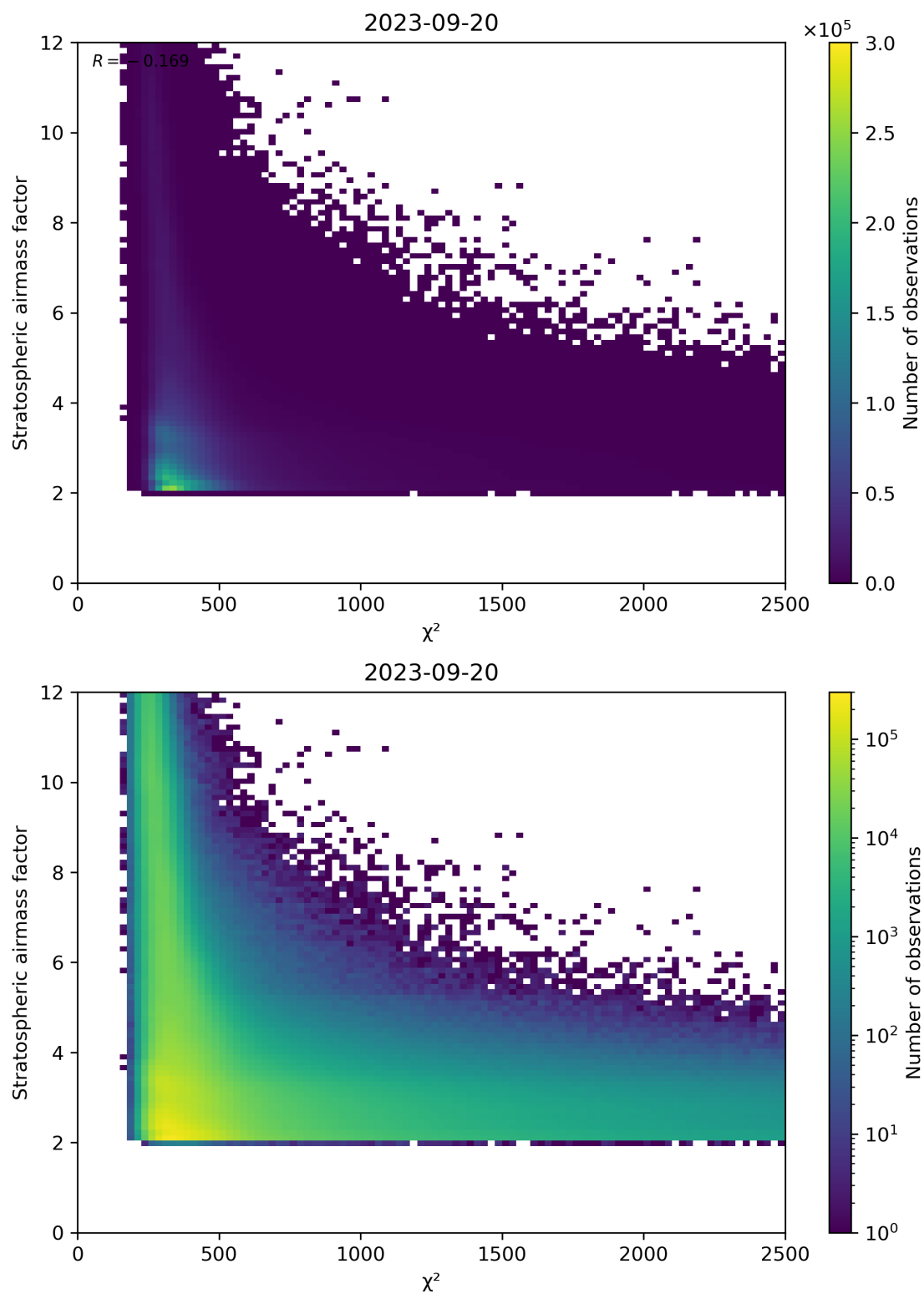
Figure 81: Scatter density plot of “ \chi^2 ” against “Stratospheric airmass factor” for 2023-09-20 to 2023-09-21.
