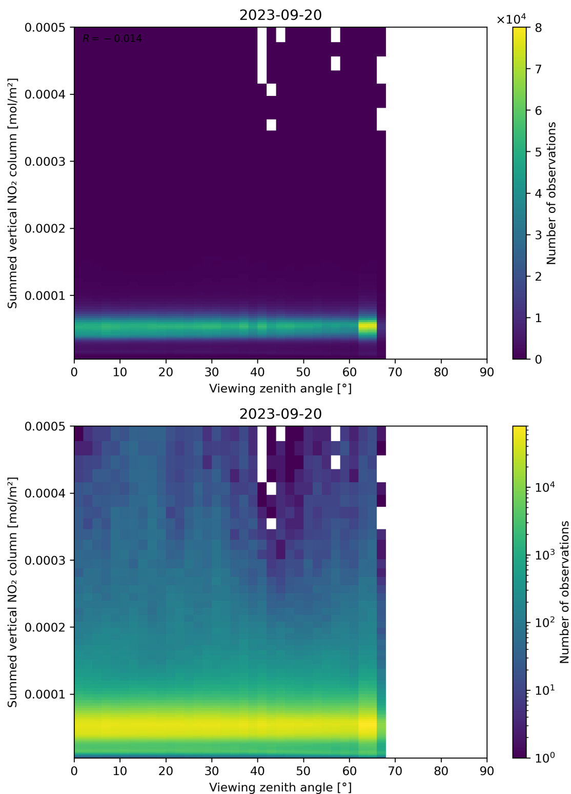
Figure 165: Scatter density plot of “Viewing zenith angle” against “Summed vertical NO 2 column” for 2023-09-20 to 2023-09-21.
