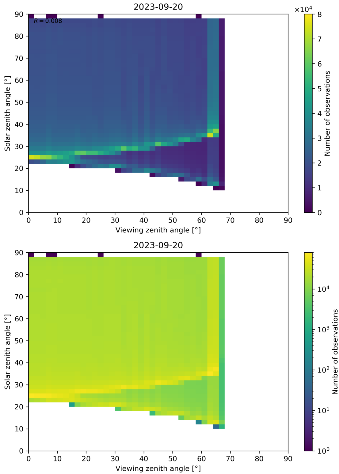
Figure 172: Scatter density plot of “Viewing zenith angle” against “Solar zenith angle” for 2023-09-20 to 2023-09-21.
