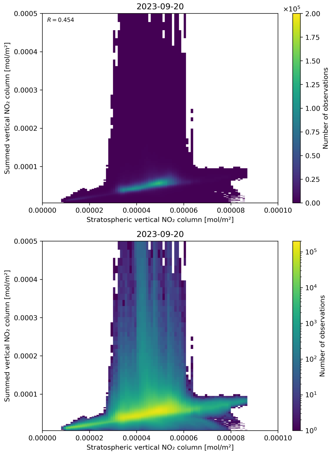
Figure 98: Scatter density plot of “Stratospheric vertical NO 2 column” against “Summed vertical NO 2 column” for 2023-09-20 to 2023-09-21.
