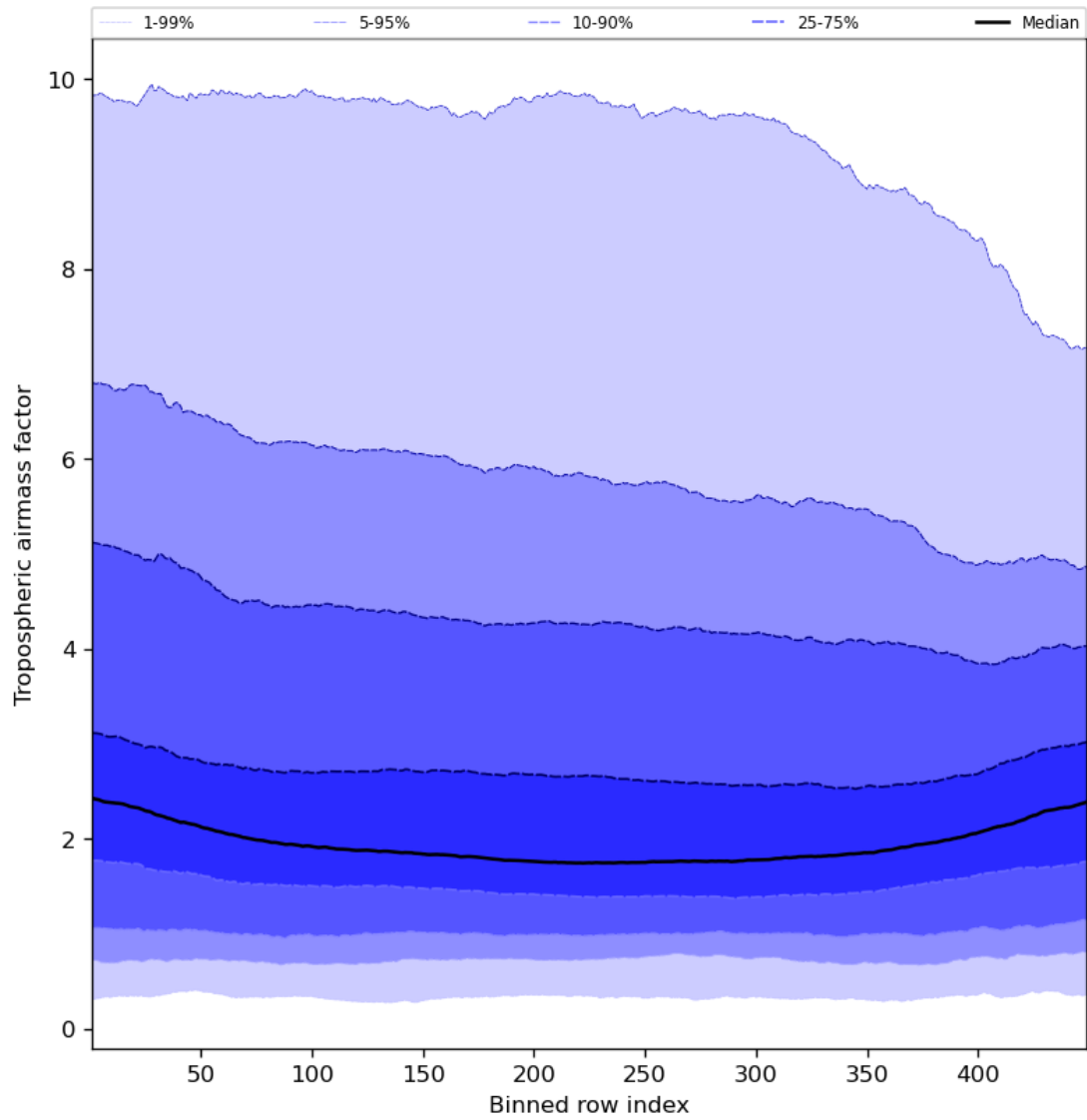
Figure 48: Along track statistics of “Tropospheric air mass factor” for 2023-09-20 to 2023-09-21
