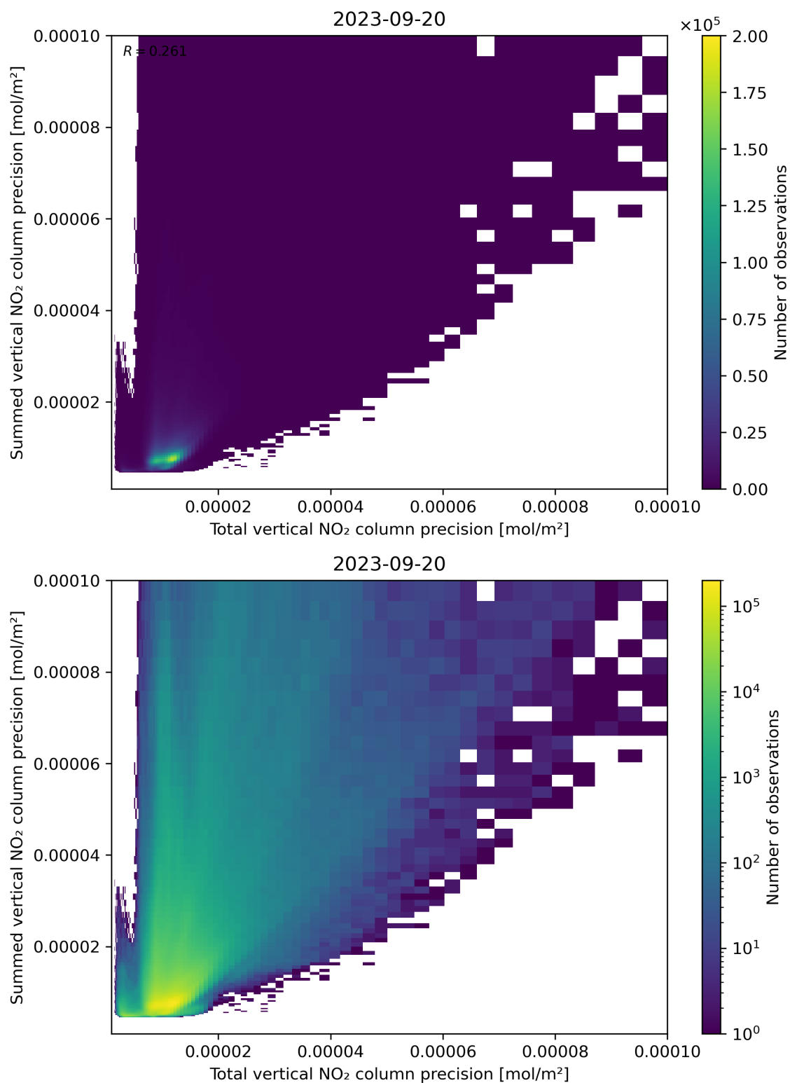
Figure 118: Scatter density plot of “Total vertical NO 2 column precision” against “Summed vertical NO 2 column precision” for 2023-09-20 to 2023-09-21.
