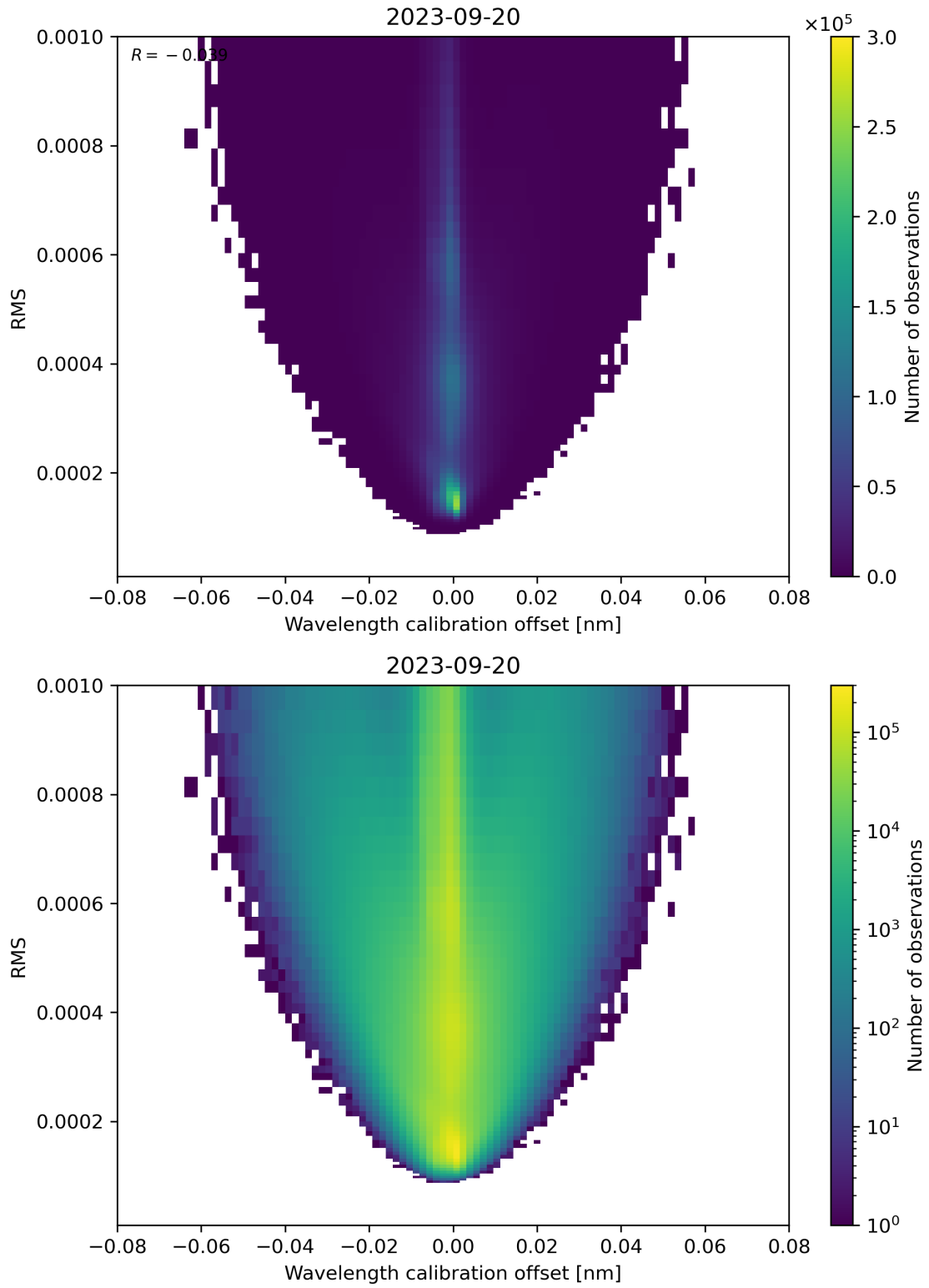
Figure 181: Scatter density plot of “Wavelength calibration offset” against “RMS” for 2023-09-20 to 2023-09-21.
