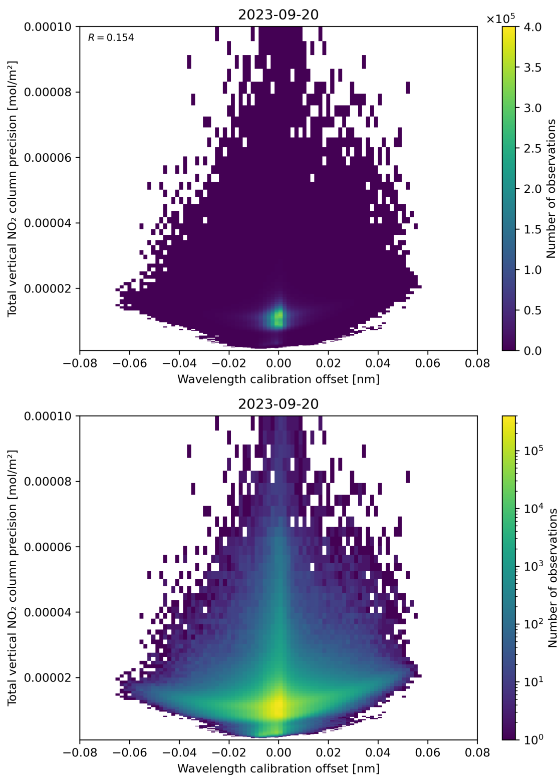
Figure 180: Scatter density plot of “Wavelength calibration offset” against “Total vertical NO 2 column precision” for 2023-09-20 to 2023-09-21.
