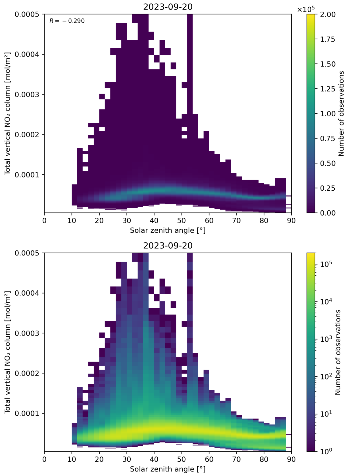
Figure 153: Scatter density plot of “Solar zenith angle” against “Total vertical NO 2 column” for 2023-09-20 to 2023-09-21.
