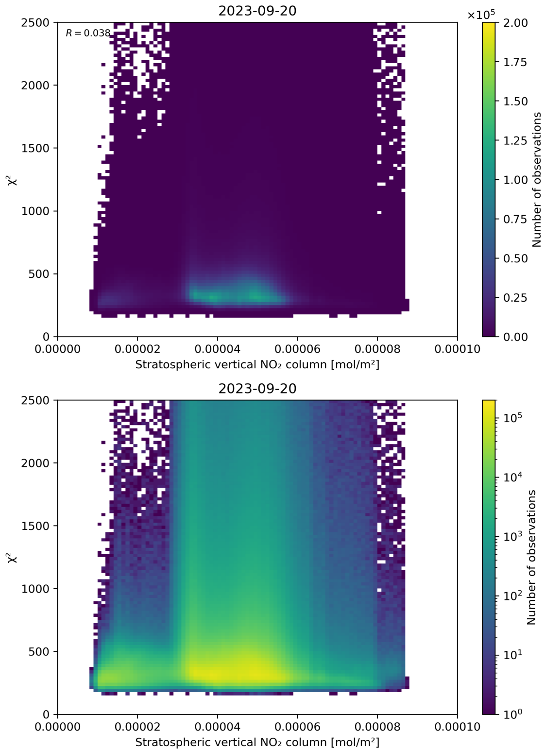
Figure 97: Scatter density plot of “Stratospheric vertical NO 2 column” against “ \chi^2 ” for 2023-09-20 to 2023-09-21.
