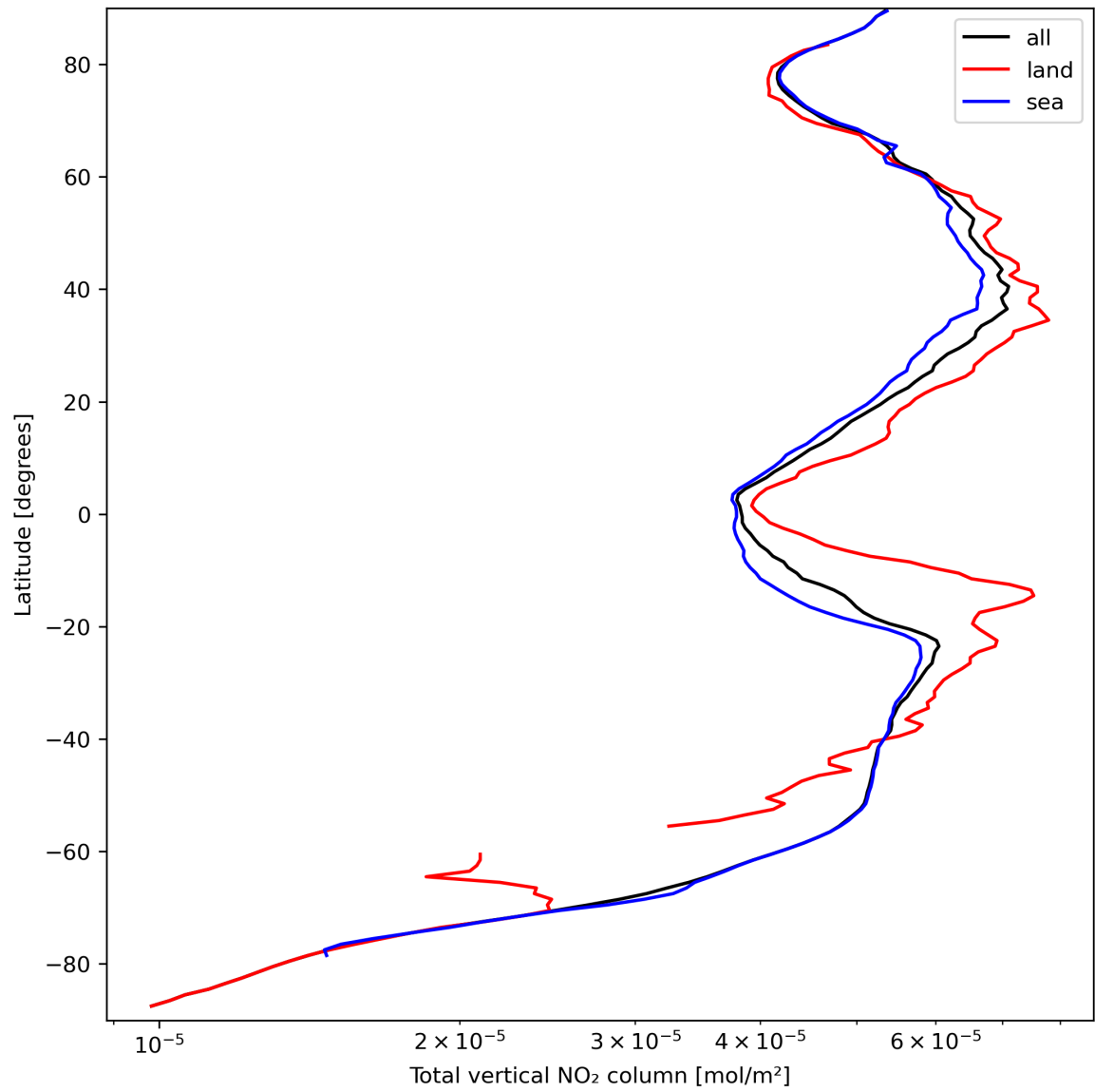
Figure 21: Zonal average of “Total vertical NO 2 column” for 2023-09-20 to 2023-09-21.
