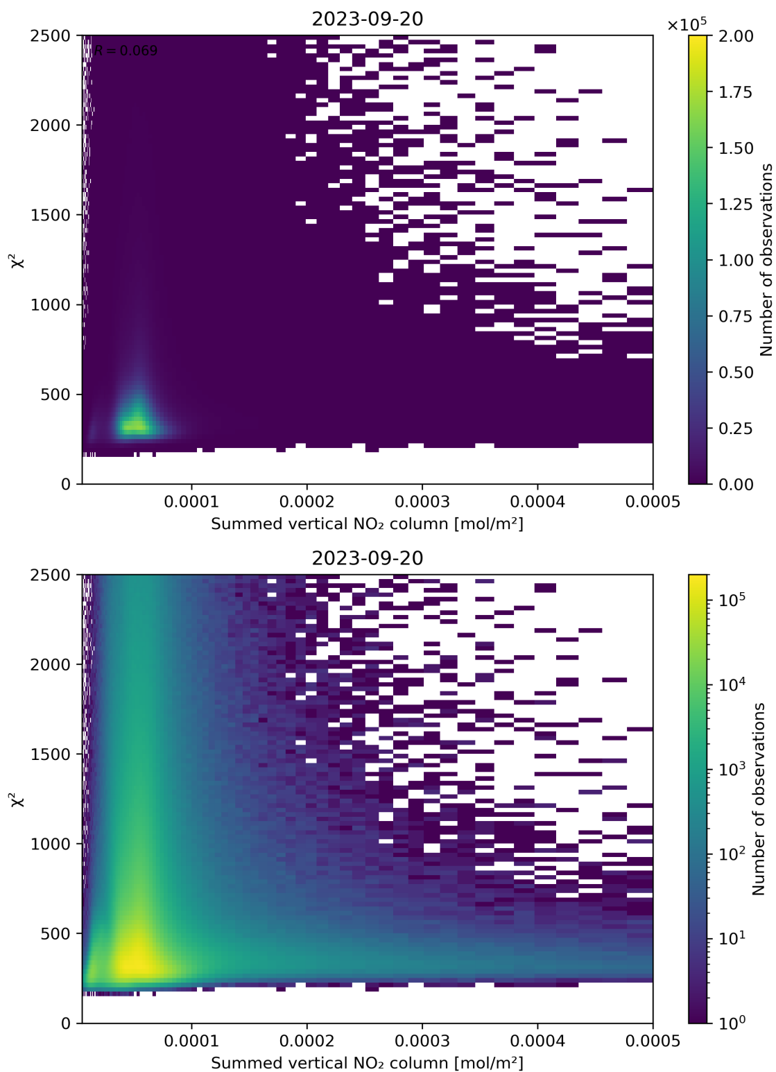
Figure 104: Scatter density plot of “Summed vertical NO 2 column” against “ \chi^2 ” for 2023-09-20 to 2023-09-21.
