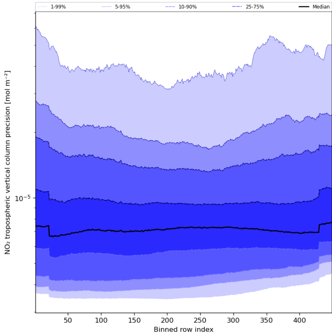
Figure 47: Along track statistics of “NO 2 tropospheric vertical column precision” for 2023-09-20 to 2023-09-21
