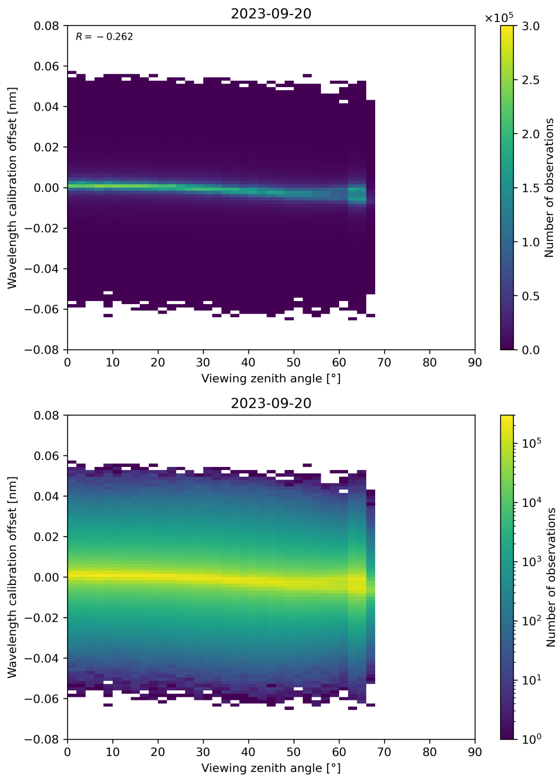
Figure 173: Scatter density plot of “Viewing zenith angle” against “Wavelength calibration offset” for 2023-09-20 to 2023-09-21.
