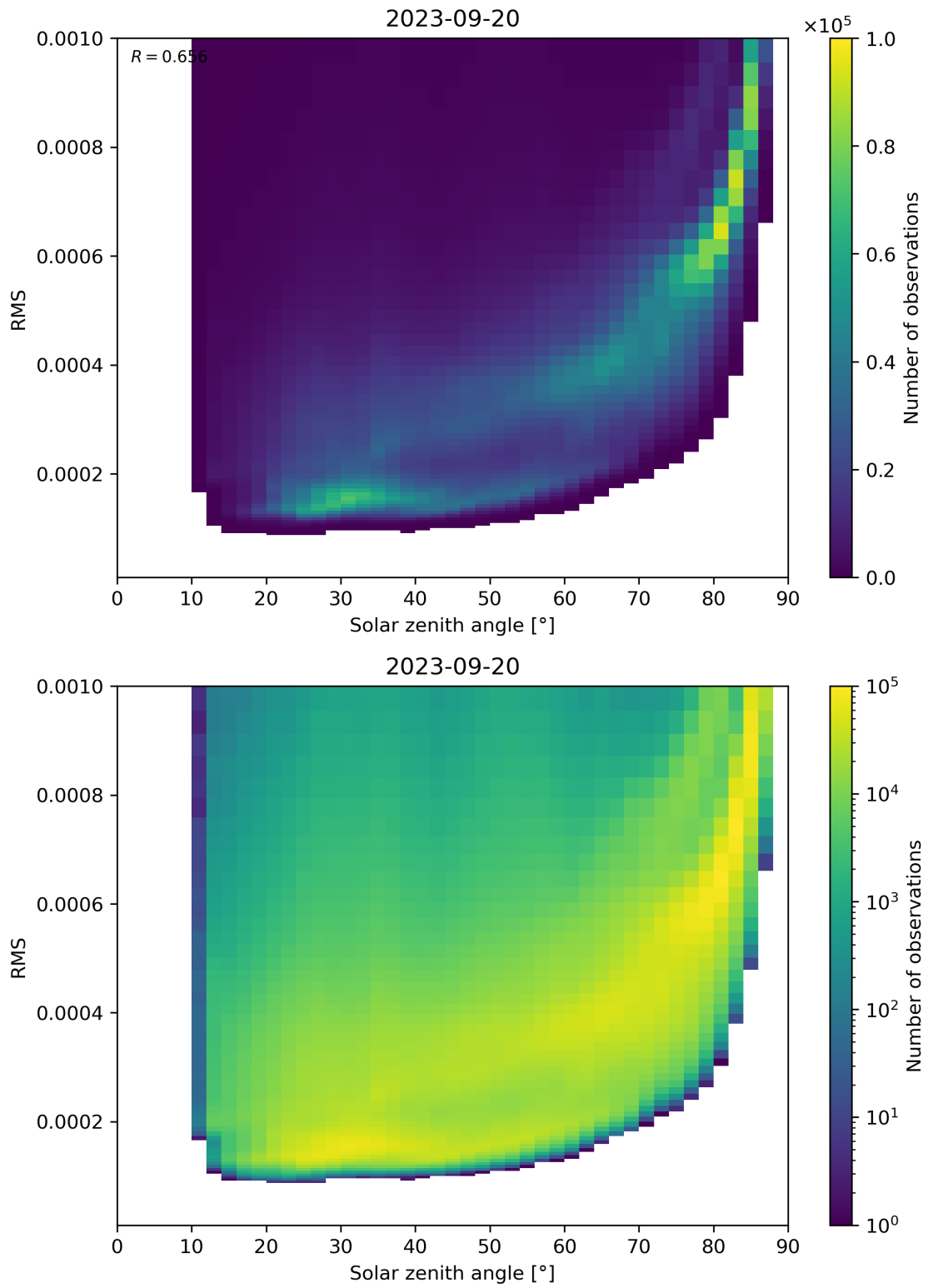
Figure 157: Scatter density plot of “Solar zenith angle” against “RMS” for 2023-09-20 to 2023-09-21.
