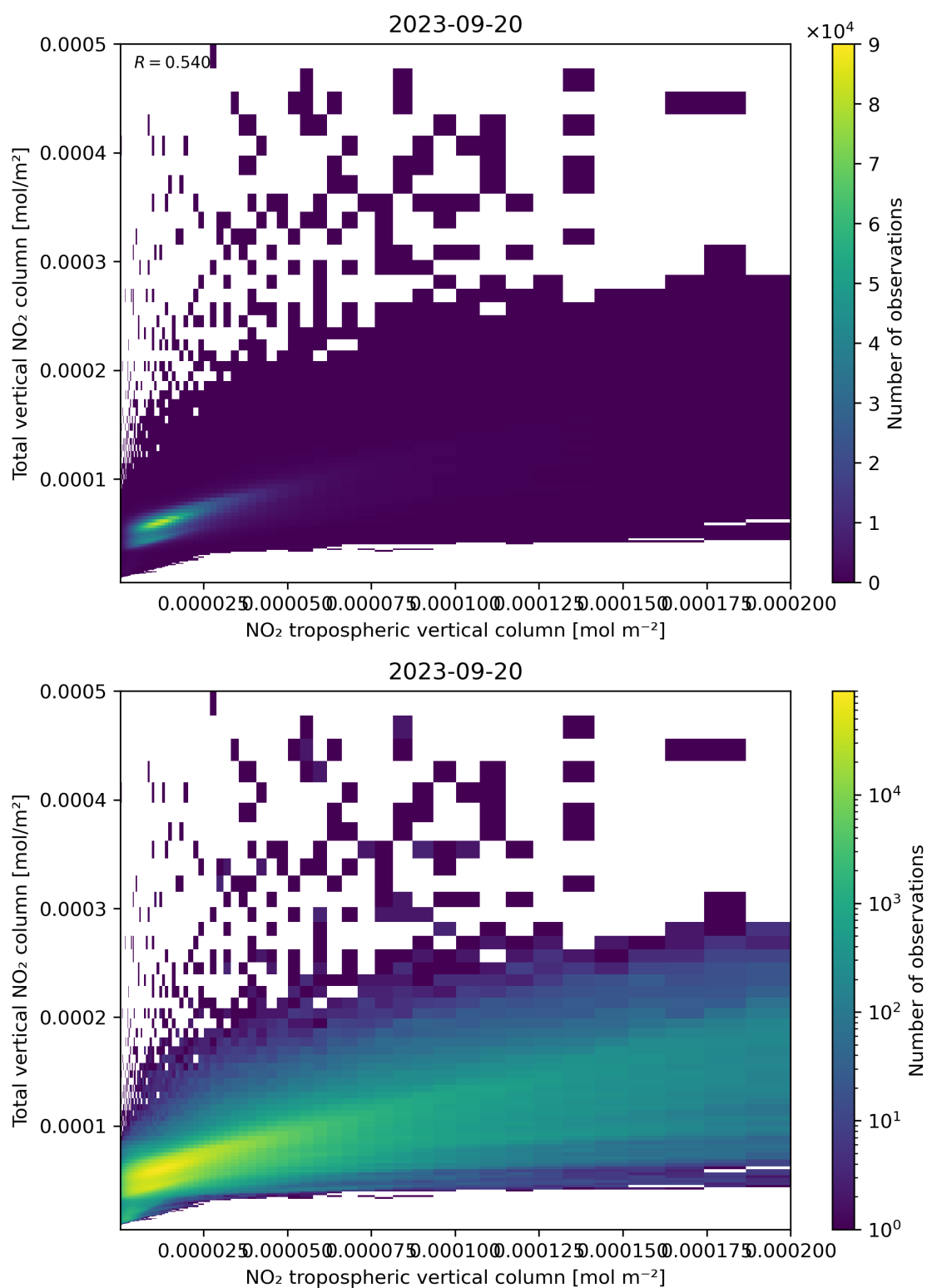
Figure 128: Scatter density plot of “NO 2 tropospheric vertical column” against “Total vertical NO 2 column” for 2023-09-20 to 2023-09-21.
