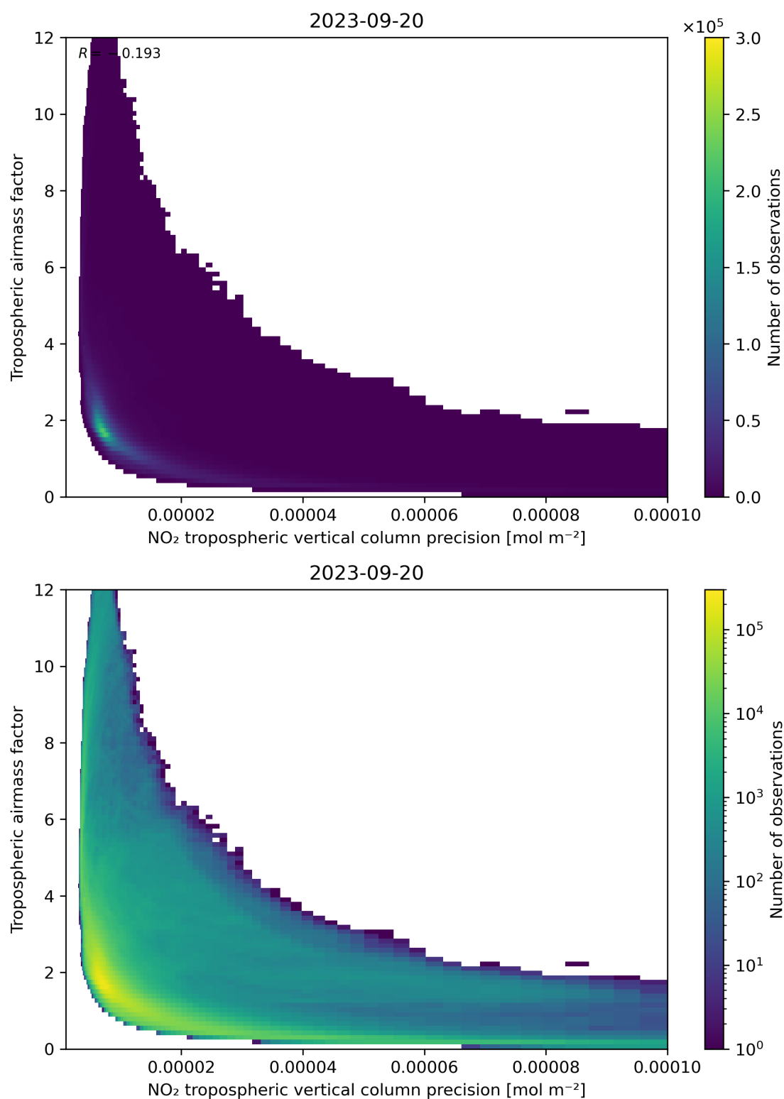
Figure 133: Scatter density plot of “NO 2 tropospheric vertical column precision” against “Tropospheric airmass factor” for 2023-09-20 to 2023-09-21.
