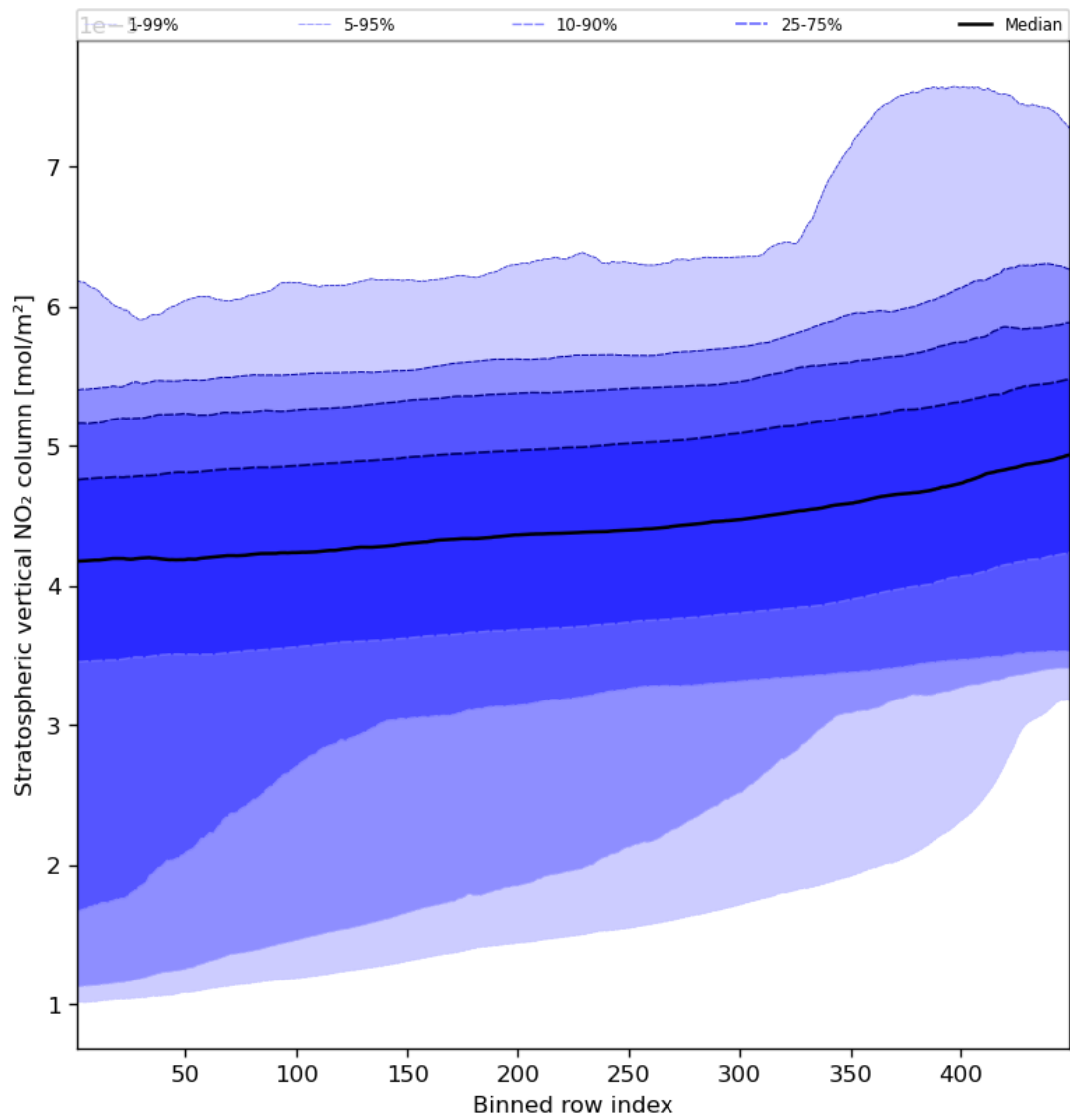
Figure 53: Along track statistics of “Stratospheric vertical NO 2 column” for 2023-09-20 to 2023-09-21
