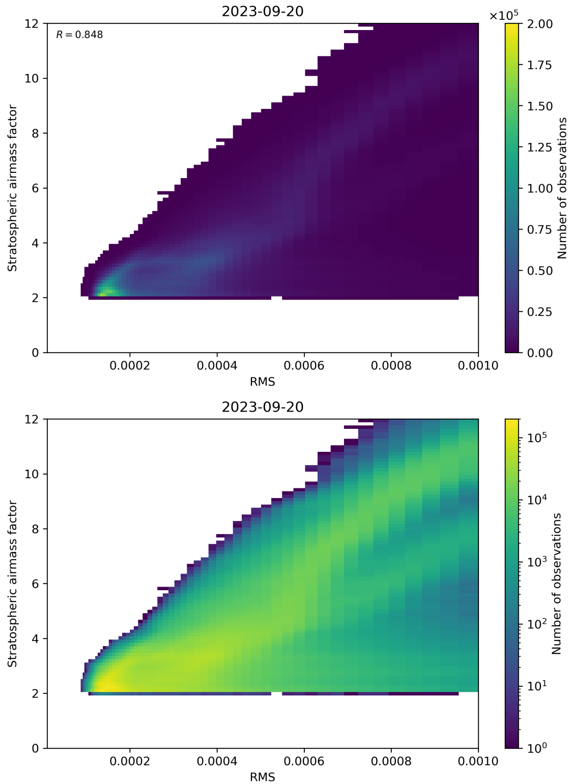
Figure 144: Scatter density plot of “RMS” against “Stratospheric airmass factor” for 2023-09-20 to 2023-09-21.
