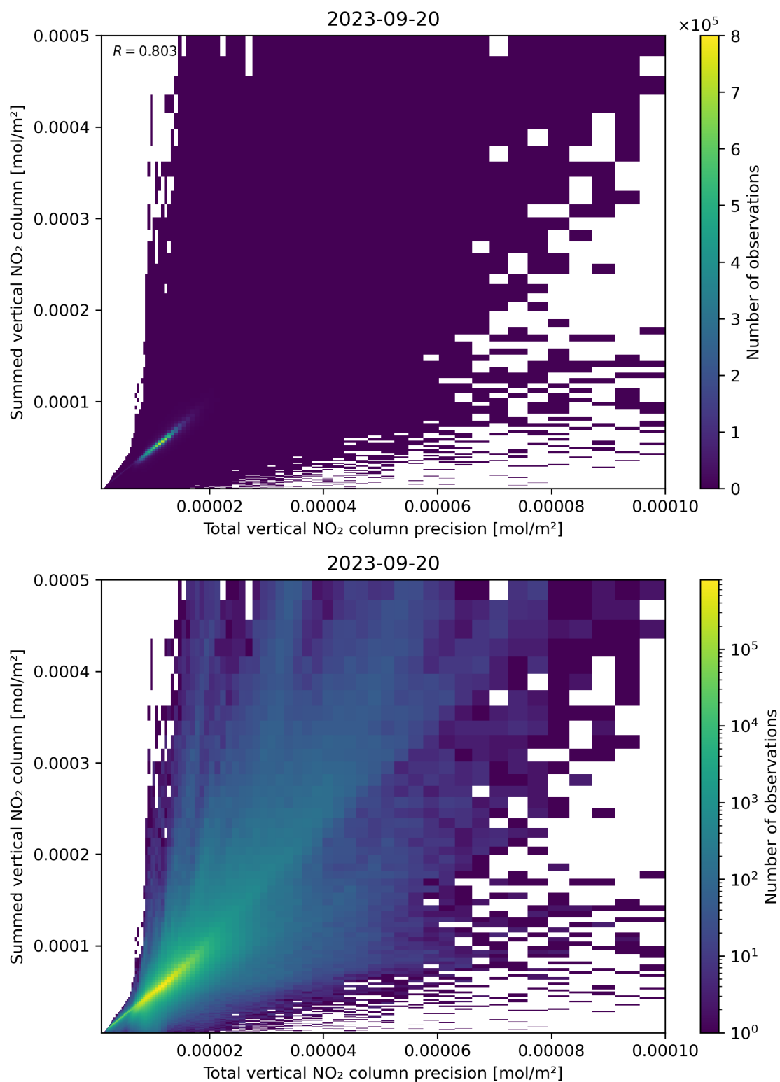
Figure 117: Scatter density plot of “Total vertical NO 2 column precision” against “Summed vertical NO 2 column” for 2023-09-20 to 2023-09-21.
