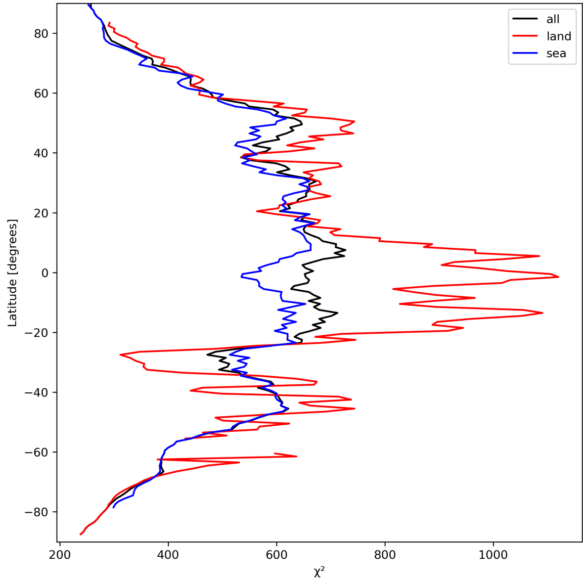
Figure 25: Zonal average of “ \chi^2 ” for 2023-09-20 to 2023-09-21.
