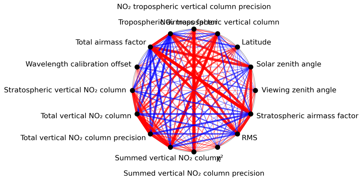
Figure 1: Map of correlation graph for 2023-09-20 to 2023-09-21.
