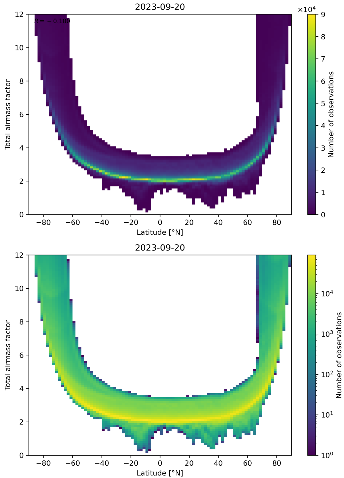
Figure 84: Scatter density plot of “Latitude” against “Total airmass factor” for 2023-09-20 to 2023-09-21.
