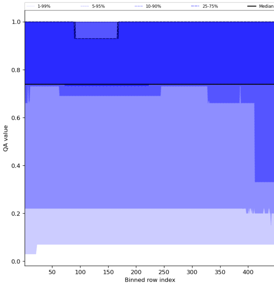
Figure 45: Along track statistics of "QA value" for 2023-09-20 to 2023-09-21
