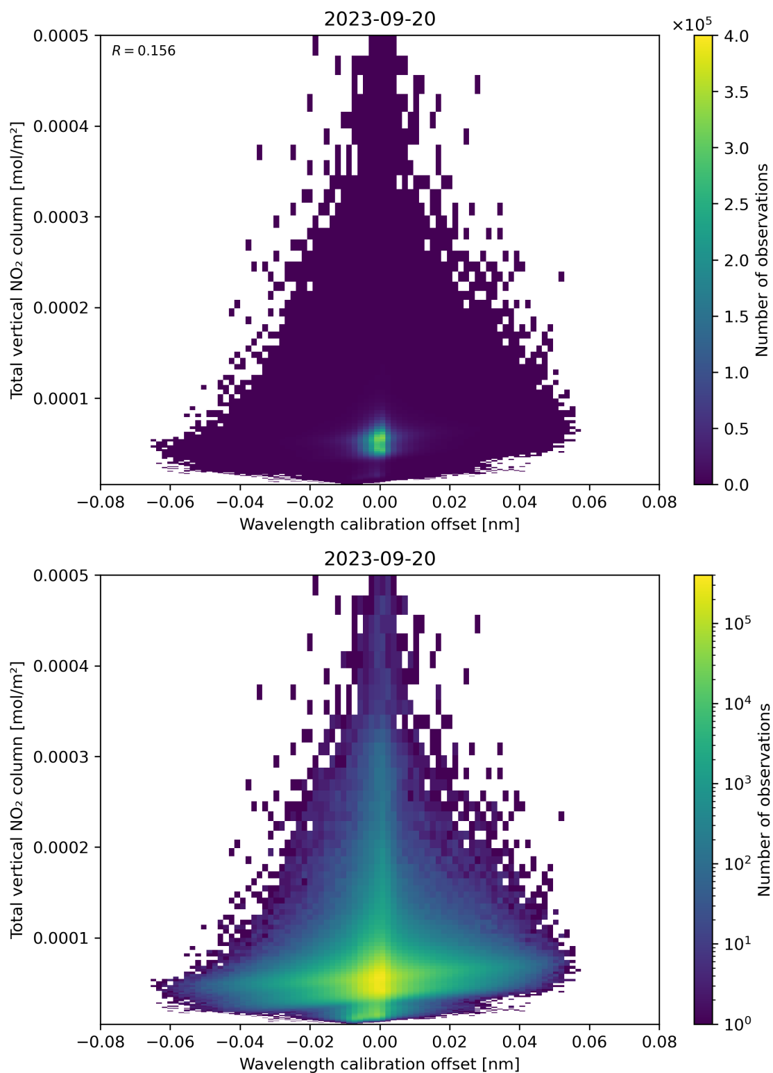
Figure 179: Scatter density plot of “Wavelength calibration offset” against “Total vertical NO 2 column” for 2023-09-20 to 2023-09-21.
