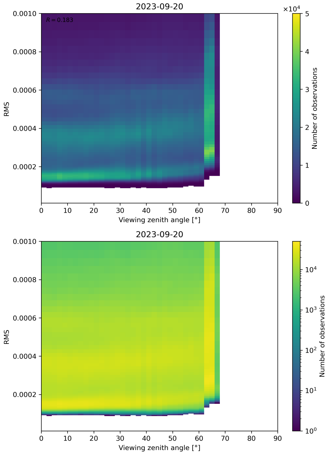
Figure 171: Scatter density plot of “Viewing zenith angle” against “RMS” for 2023-09-20 to 2023-09-21.
