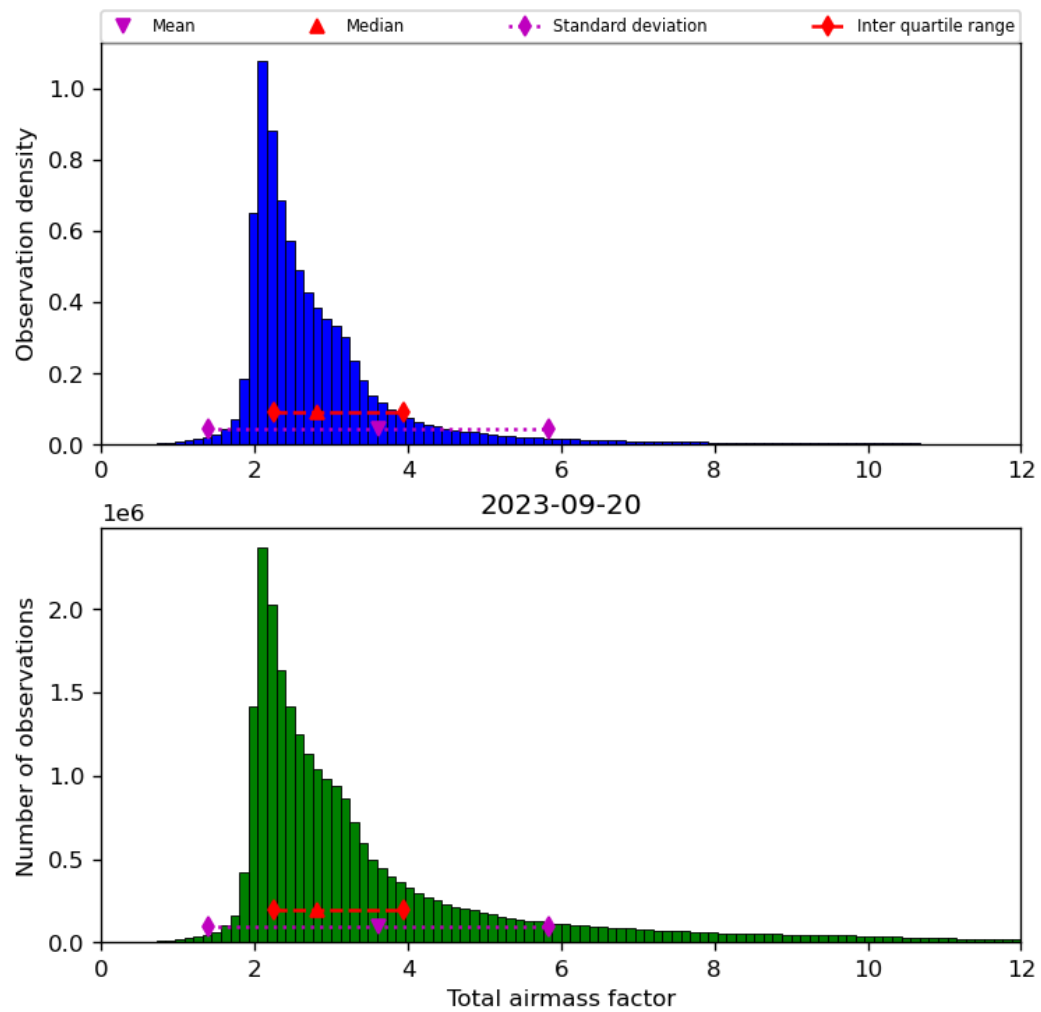
Figure 32: Histogram of “Total airmass factor” for 2023-09-20 to 2023-09-21
