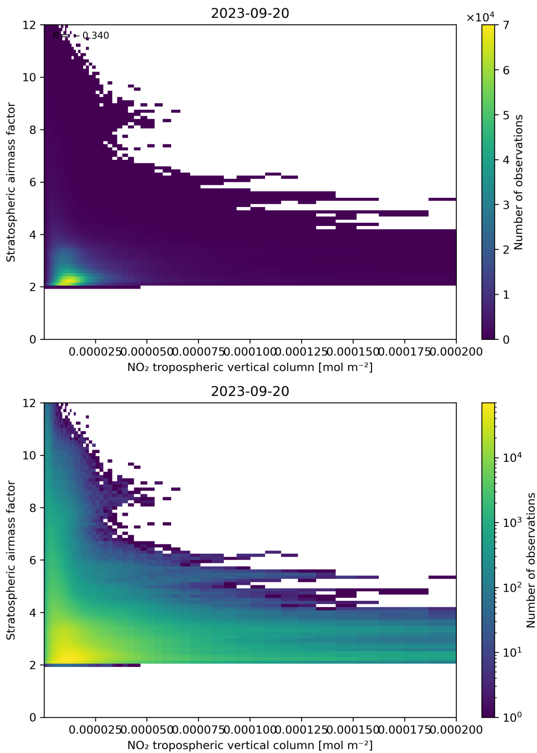
Figure 121: Scatter density plot of “NO 2 tropospheric vertical column” against “Stratospheric air mass factor” for 2023-09-20 to 2023-09-21.
