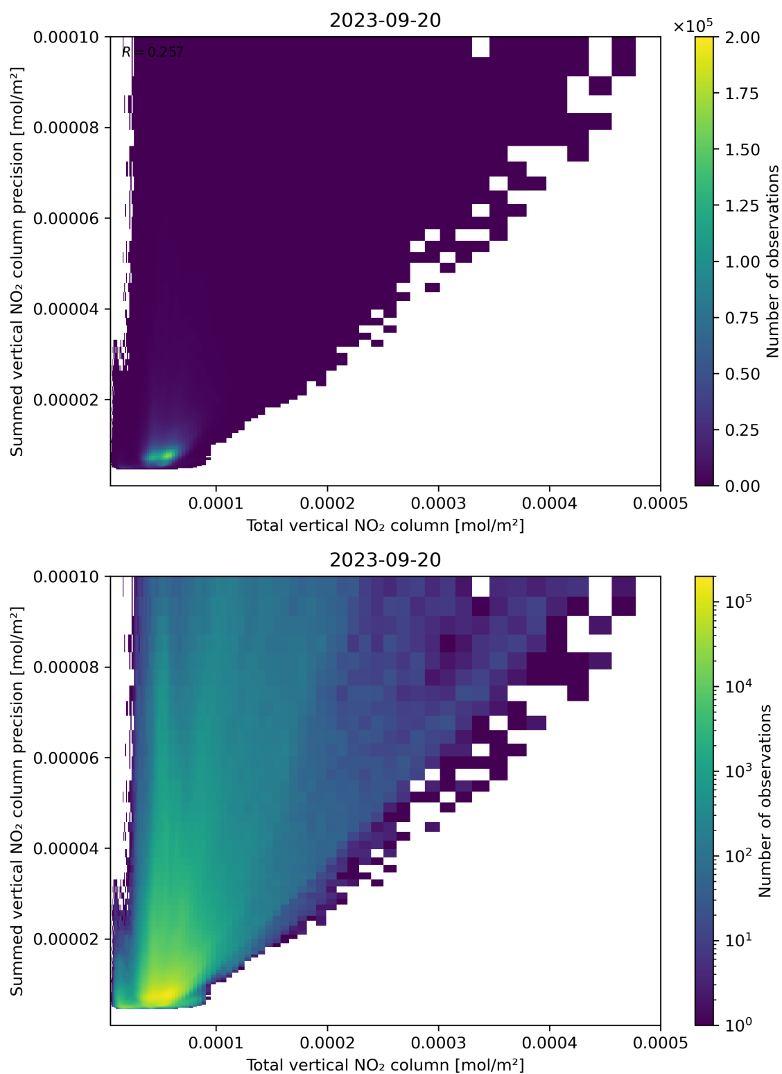
Figure 113: Scatter density plot of “Total vertical NO 2 column” against “Summed vertical NO 2 column precision” for 2023-09-20 to 2023-09-21.
