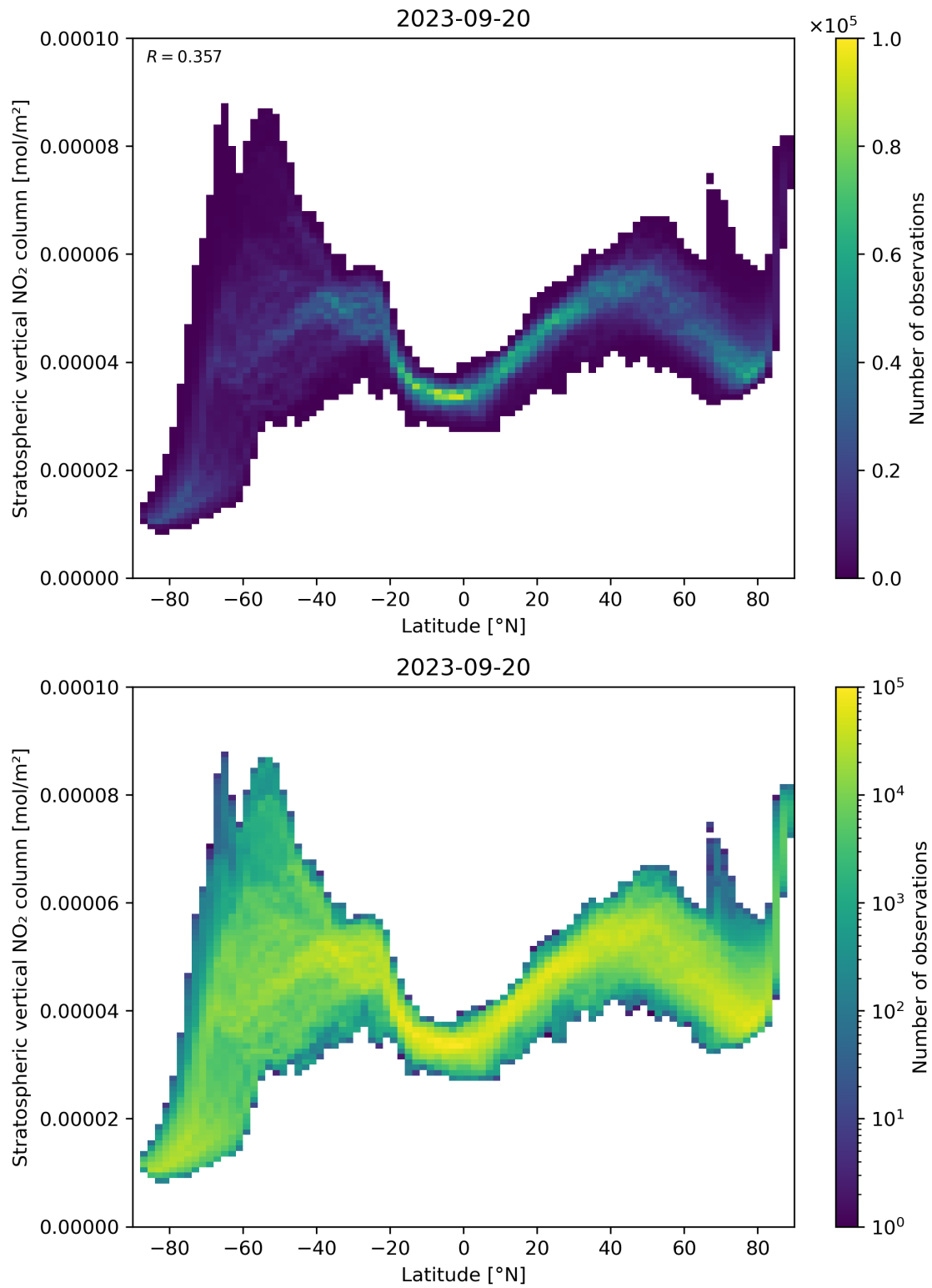
Figure 87: Scatter density plot of “Latitude” against “Stratospheric vertical NO 2 column” for 2023-09-20 to 2023-09-21.
