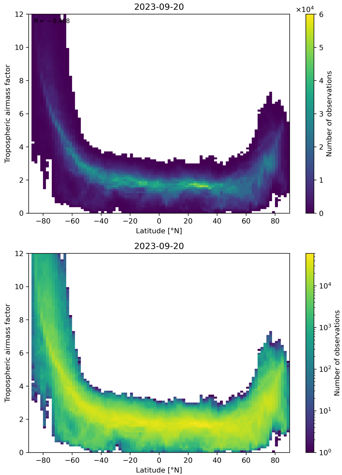
Figure 85: Scatter density plot of “Latitude” against “Tropospheric airmass factor” for 2023-09-20 to 2023-09-21.
