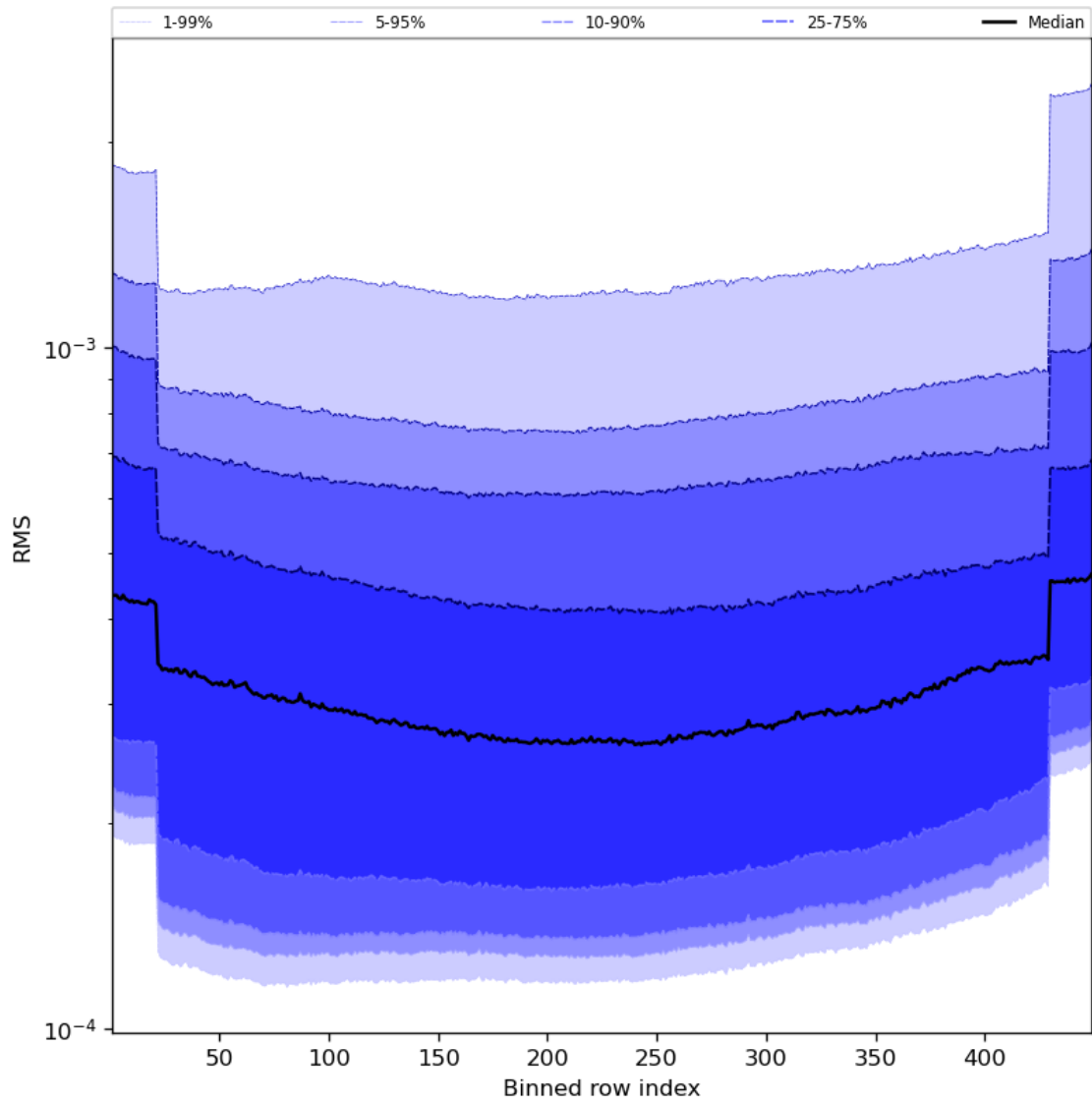
Figure 60: Along track statistics of “RMS” for 2023-09-20 to 2023-09-21
