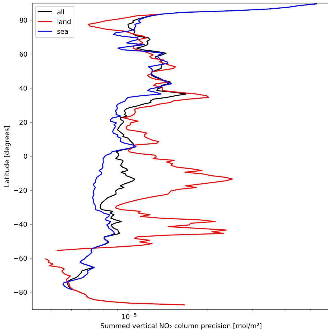
Figure 24: Zonal average of “Summed vertical NO 2 column precision” for 2023-09-20 to 2023-09-21.
