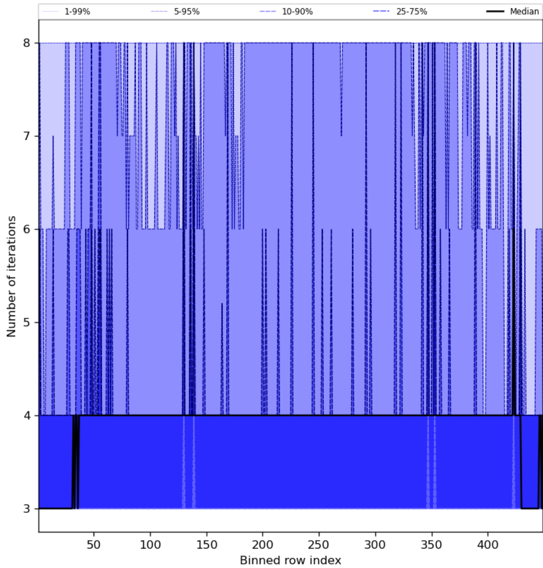
Figure 51: Along track statistics of “Number of iterations” for 2023-09-20 to 2023-09-21
