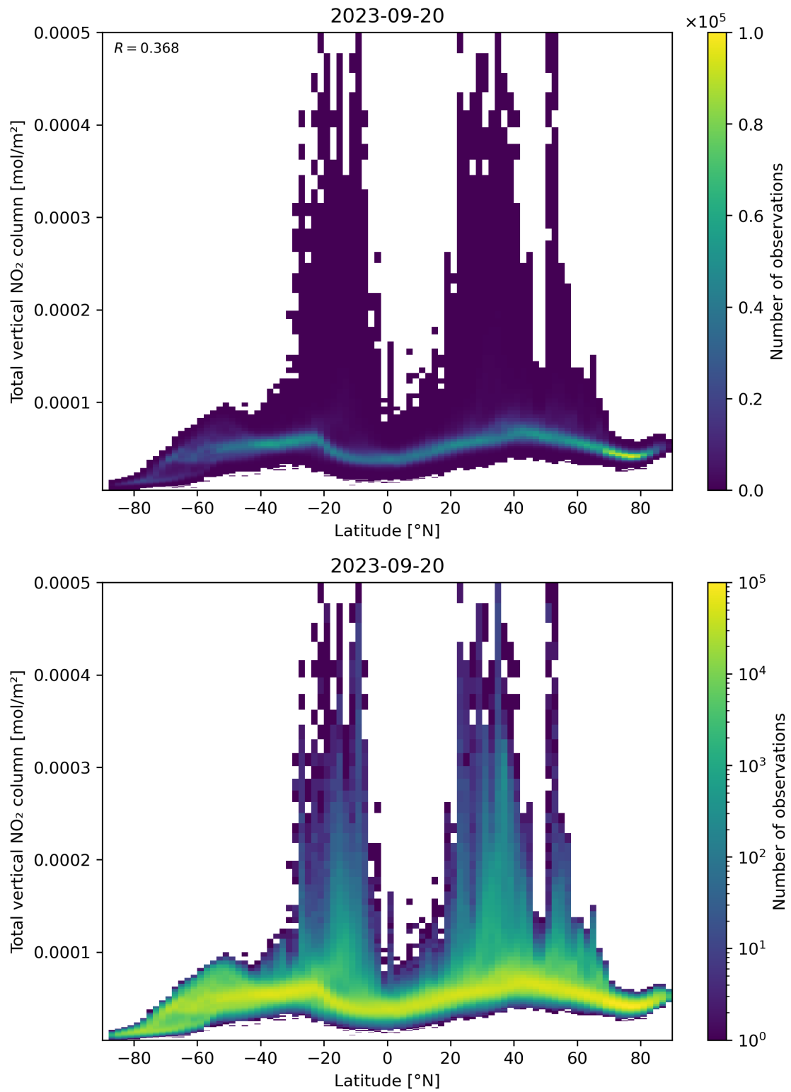
Figure 90: Scatter density plot of “Latitude” against “Total vertical NO 2 column” for 2023-09-20 to 2023-09-21.
