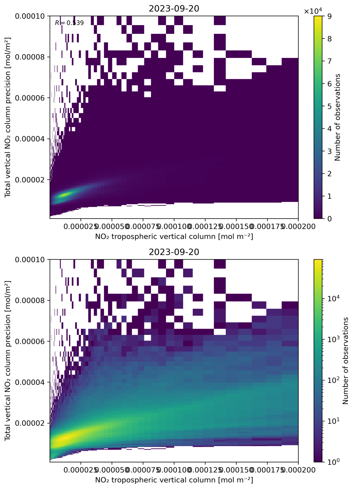
Figure 129: Scatter density plot of “NO 2 tropospheric vertical column” against “Total vertical NO 2 column precision” for 2023-09-20 to 2023-09-21.
