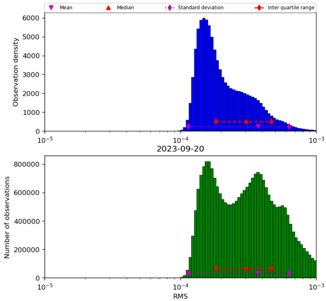
Figure 43: Histogram of “RMS” for 2023-09-20 to 2023-09-21
