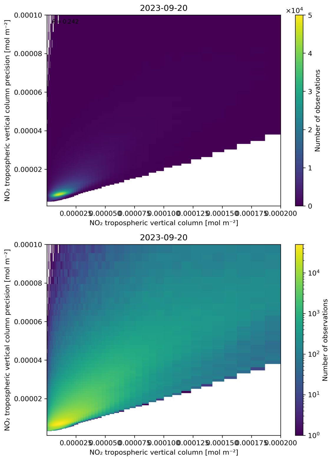
Figure 130: Scatter density plot of “NO 2 tropospheric vertical column” against “NO 2 tropospheric vertical column precision” for 2023-09-20 to 2023-09-21.
