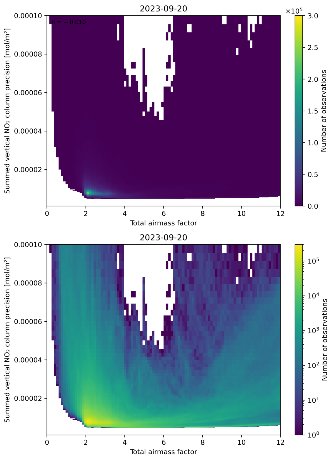
Figure 66: Scatter density plot of “Total airmass factor” against “Summed vertical NO 2 column precision” for 2023-09-20 to 2023-09-21.
