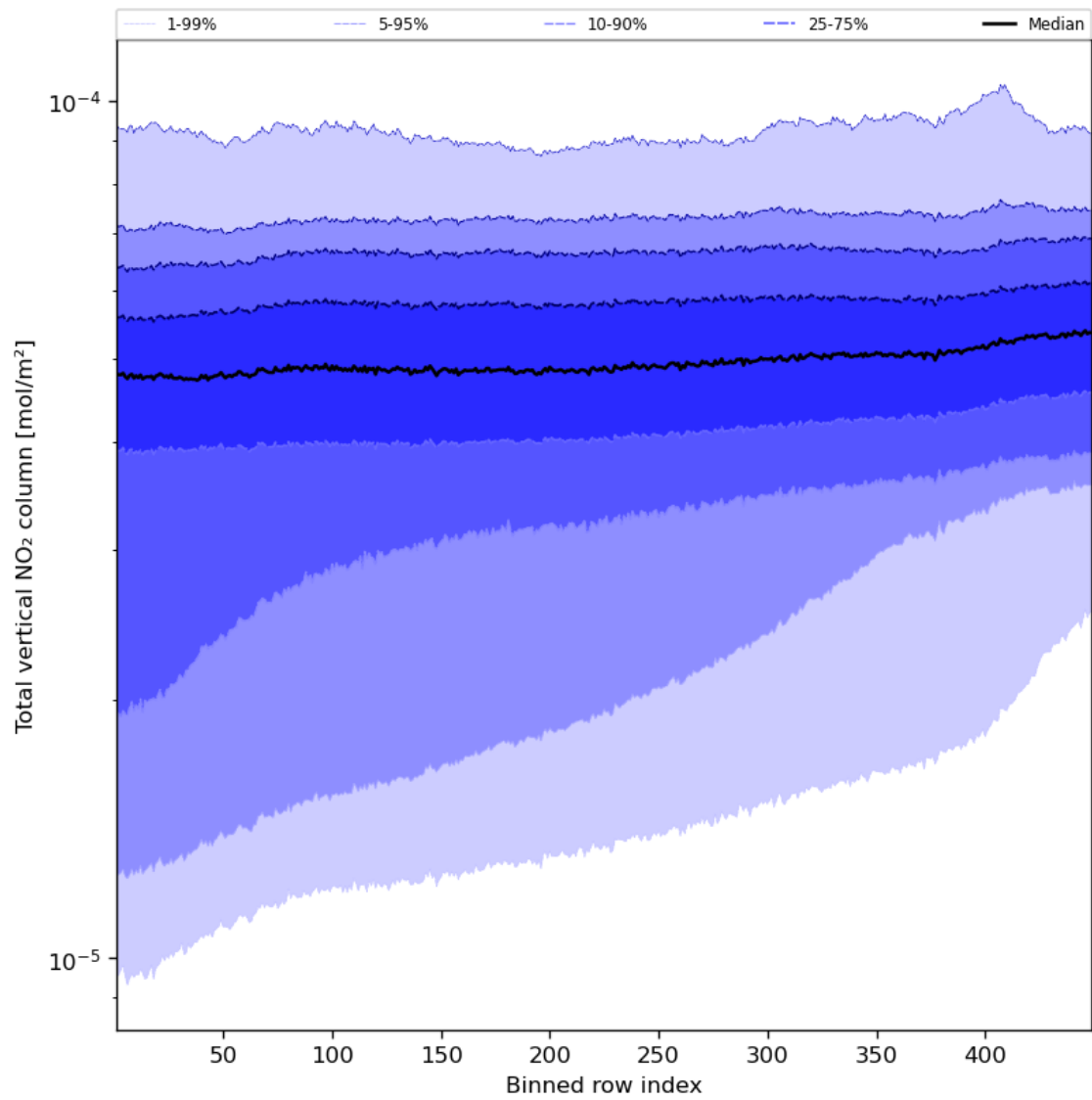
Figure 55: Along track statistics of “Total vertical NO 2 column” for 2023-09-20 to 2023-09-21
