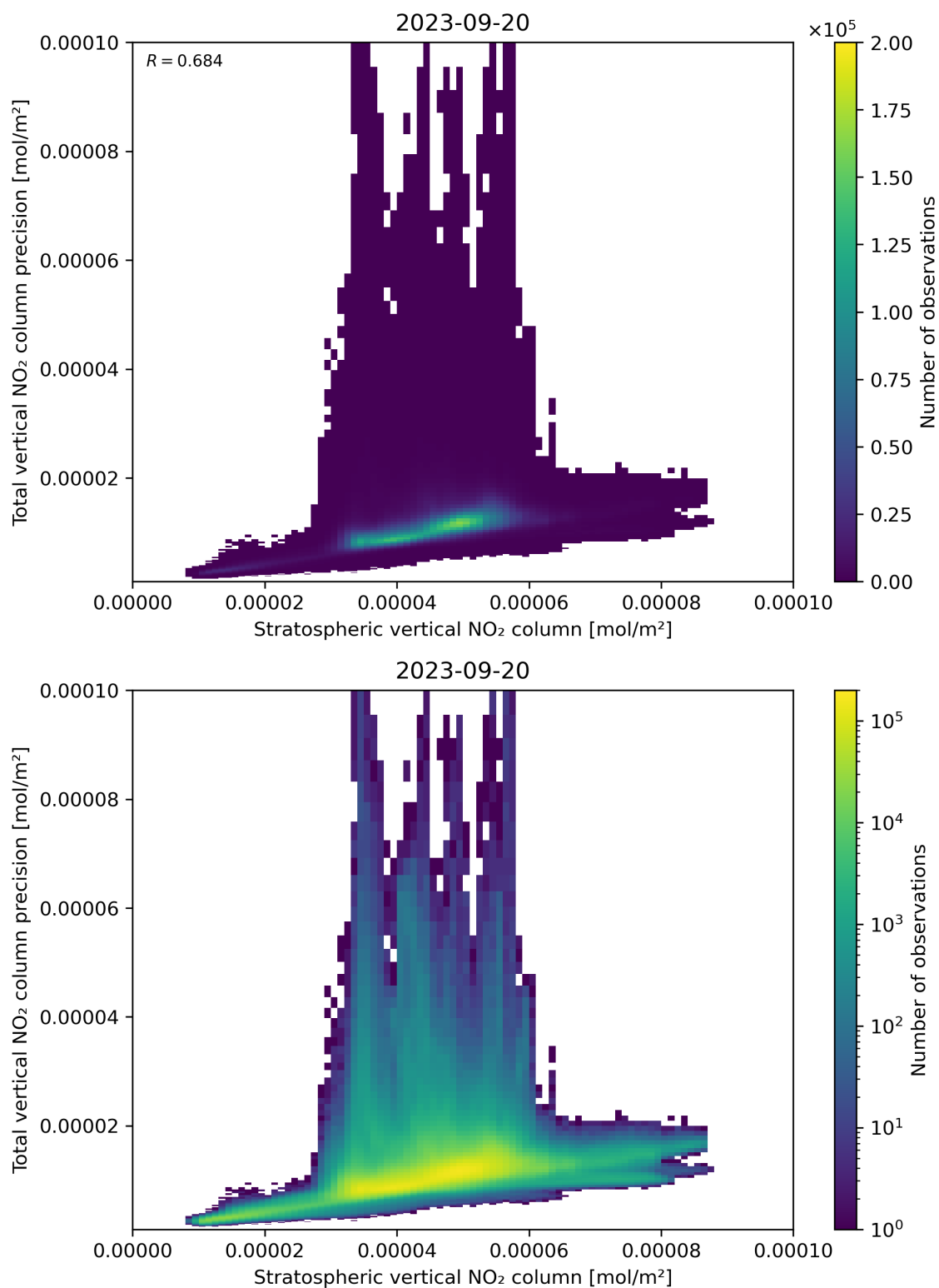
Figure 101: Scatter density plot of “Stratospheric vertical NO 2 column” against “Total vertical NO 2 column precision” for 2023-09-20 to 2023-09-21.
