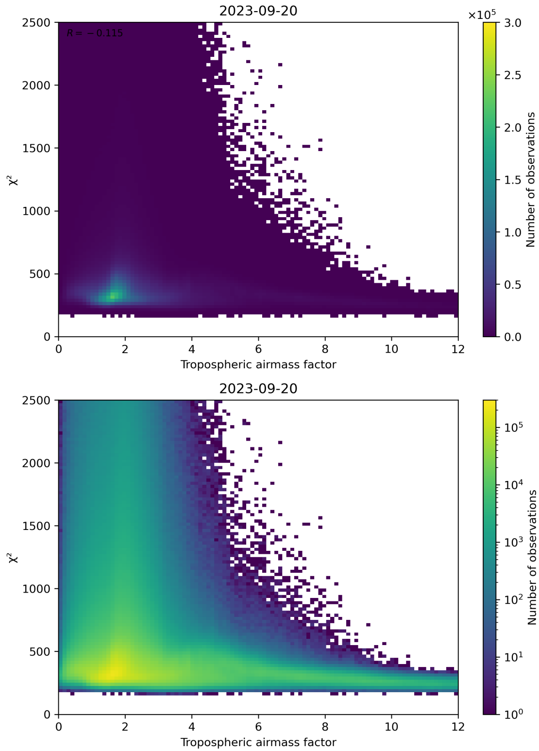
Figure 73: Scatter density plot of “Tropospheric airmass factor” against “ \chi^2 ” for 2023-09-20 to 2023-09-21.
