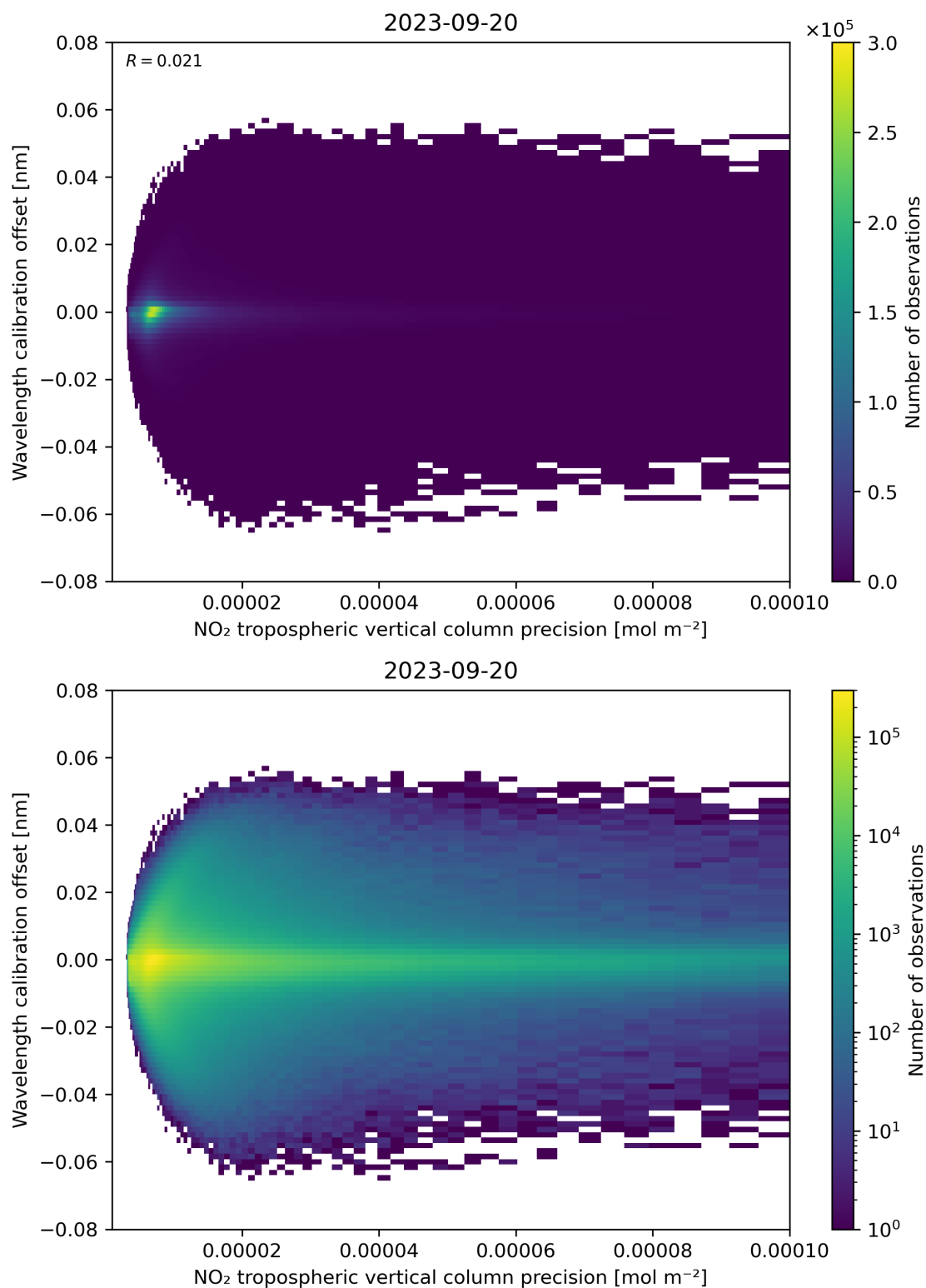
Figure 141: Scatter density plot of “NO 2 tropospheric vertical column precision” against “Wavelength calibration offset” for 2023-09-20 to 2023-09-21.
