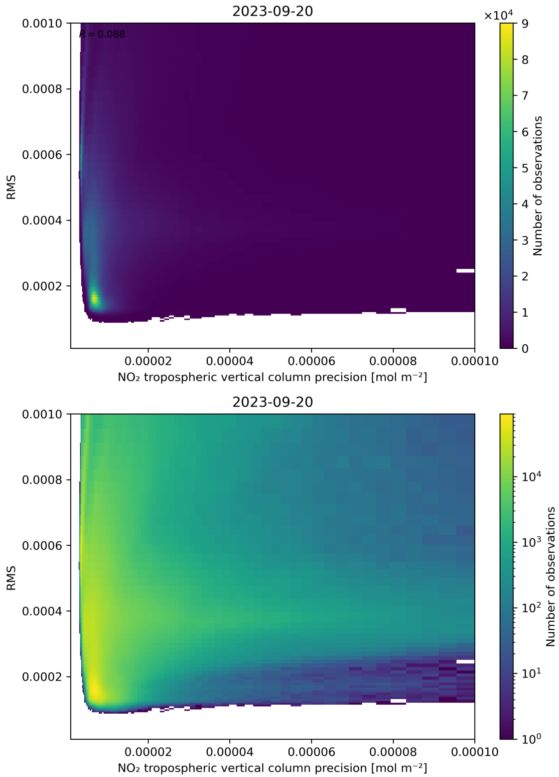
Figure 140: Scatter density plot of “NO 2 tropospheric vertical column precision” against “RMS” for 2023-09-20 to 2023-09-21.
