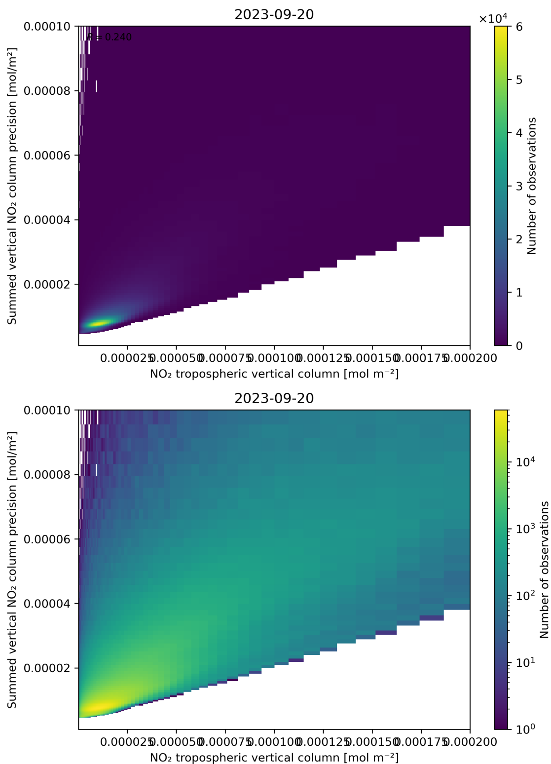
Figure 127: Scatter density plot of “NO 2 tropospheric vertical column” against “Summed vertical NO 2 column precision” for 2023-09-20 to 2023-09-21.
