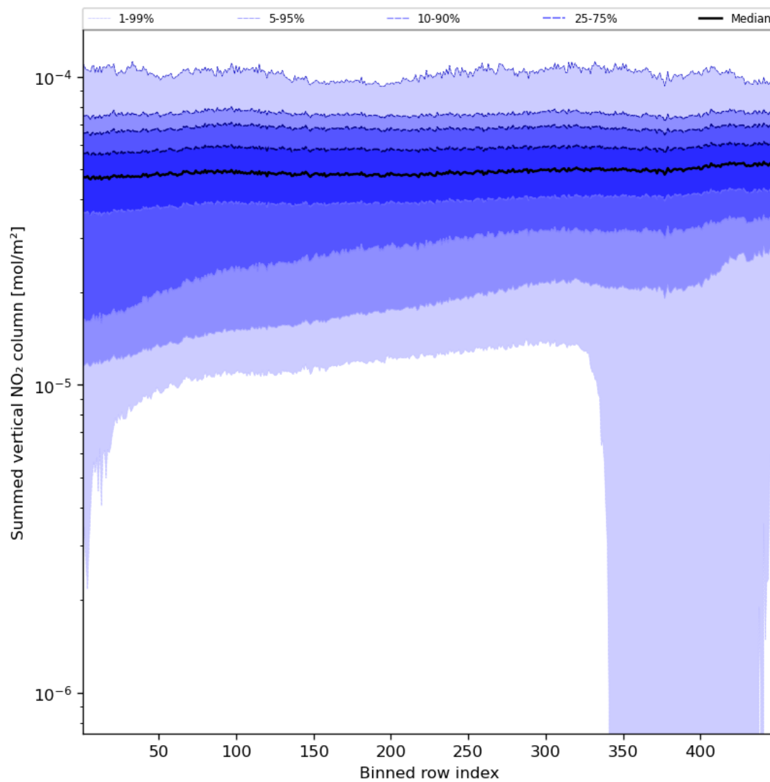
Figure 57: Along track statistics of “Summed vertical NO 2 column” for 2023-09-20 to 2023-09-21
