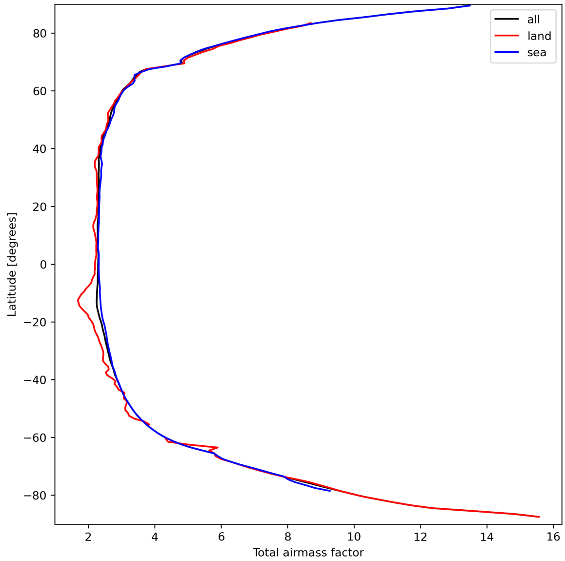
Figure 15: Zonal average of “Total airmass factor” for 2023-09-20 to 2023-09-21.
