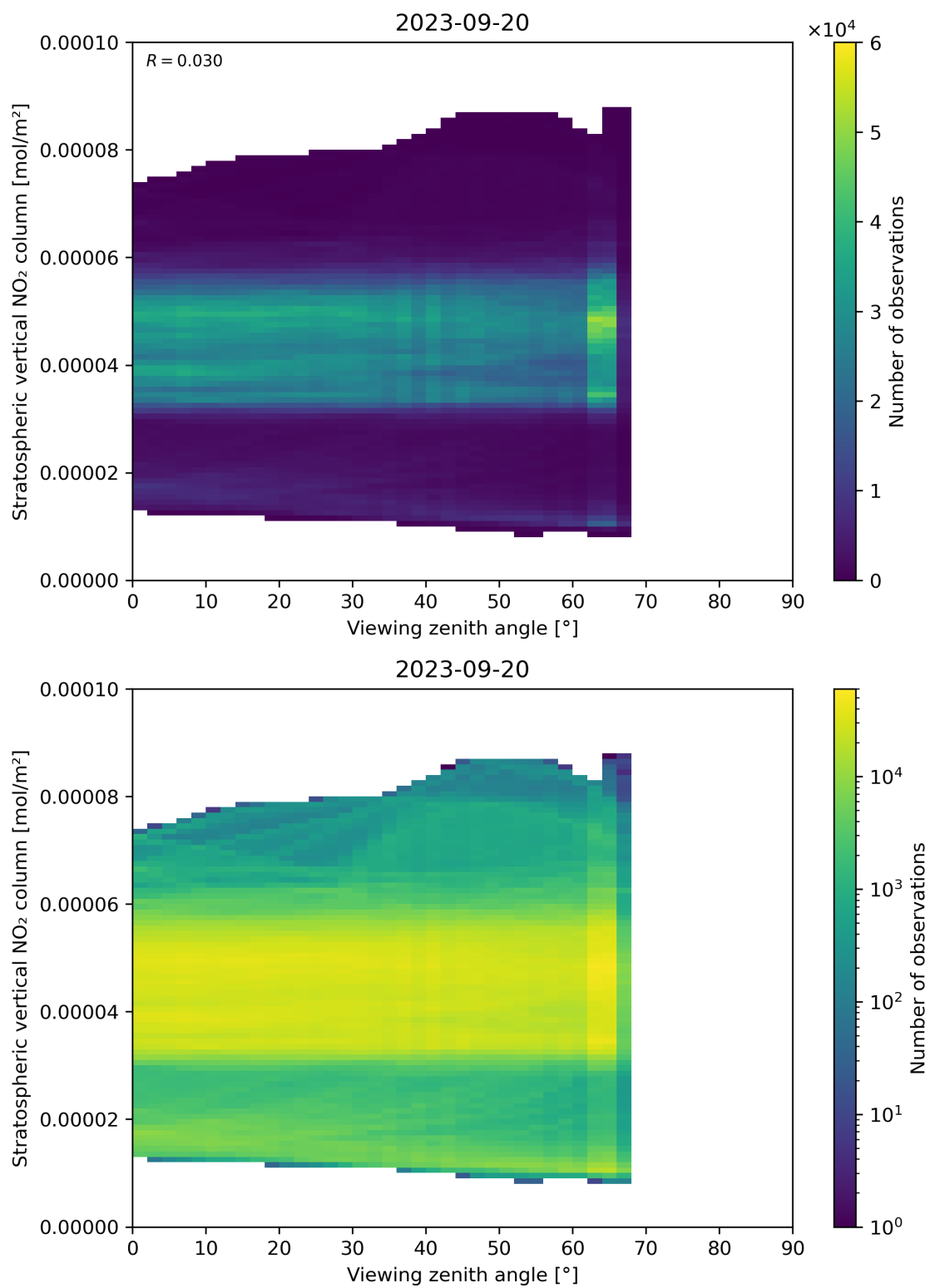
Figure 164: Scatter density plot of “Viewing zenith angle” against “Stratospheric vertical NO 2 column” for 2023-09-20 to 2023-09-21.
