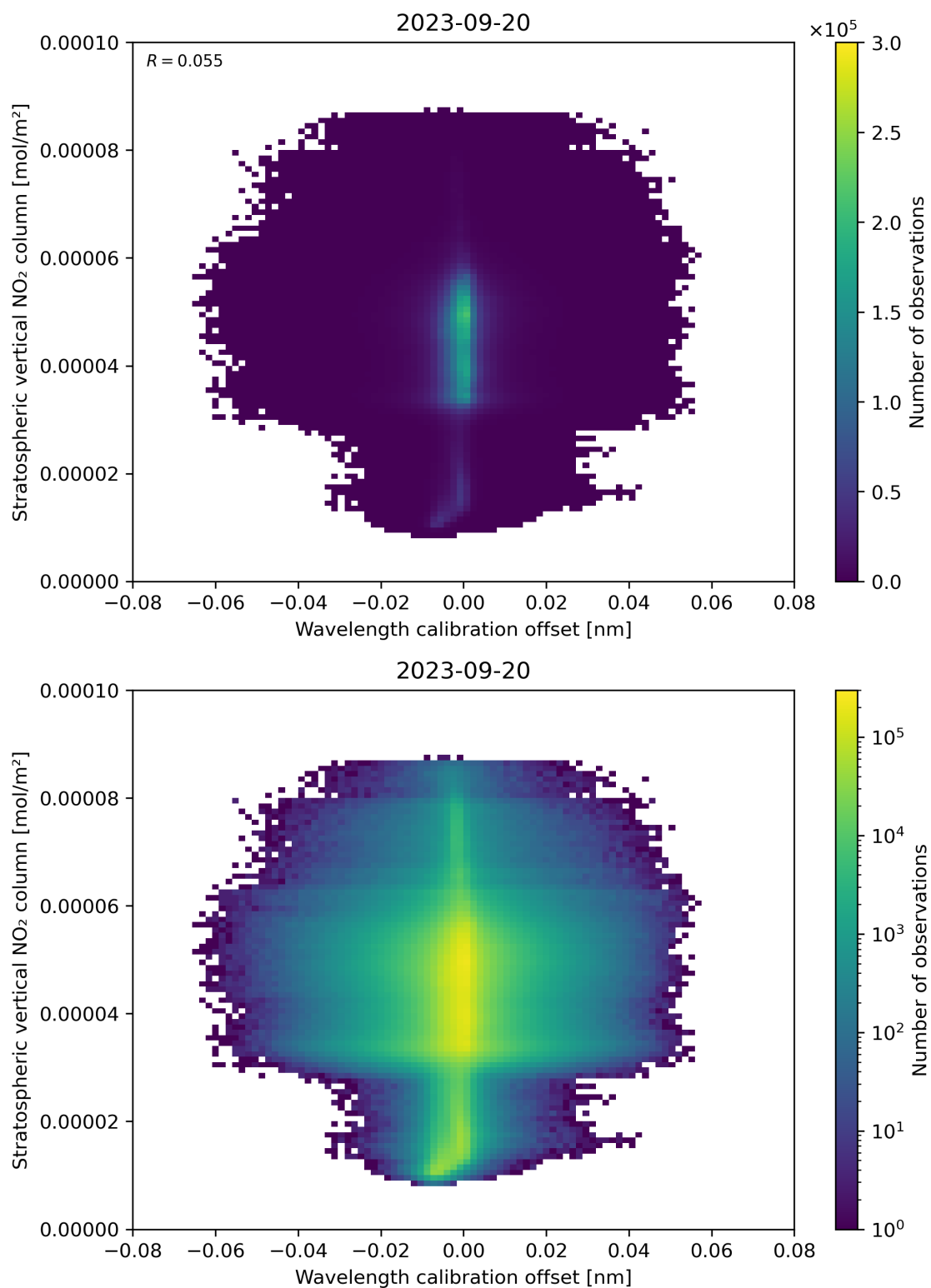
Figure 176: Scatter density plot of “Wavelength calibration offset” against “Stratospheric vertical NO 2 column” for 2023-09-20 to 2023-09-21.
