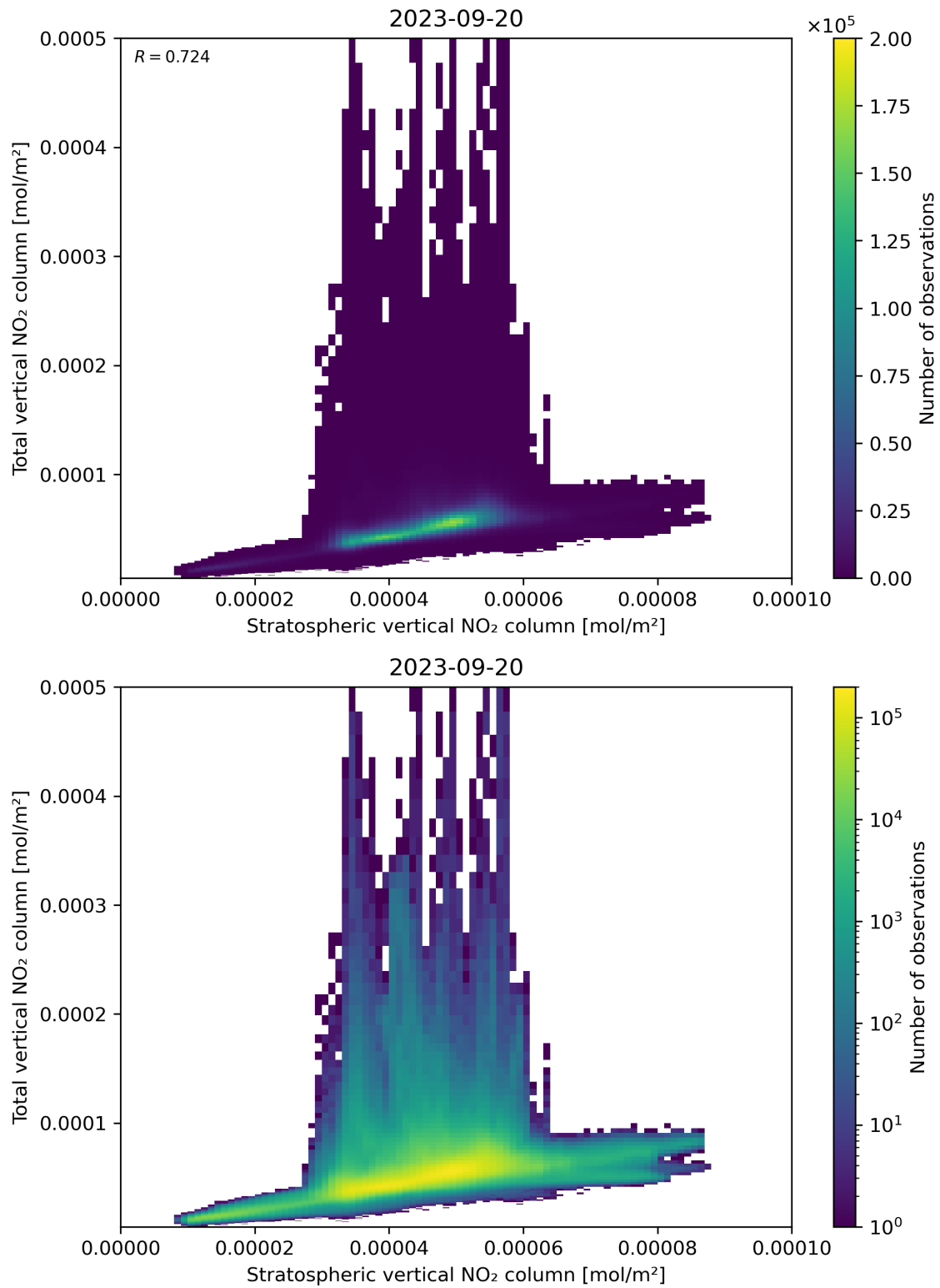
Figure 100: Scatter density plot of “Stratospheric vertical NO 2 column” against “Total vertical NO 2 column” for 2023-09-20 to 2023-09-21.
