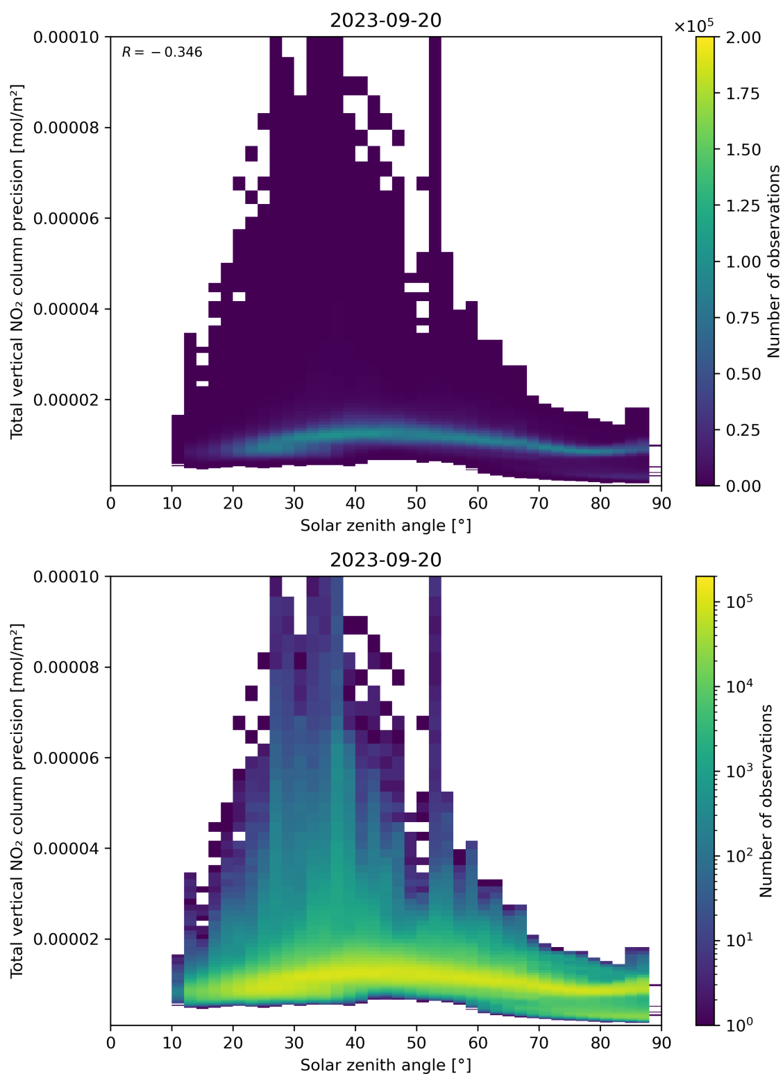
Figure 154: Scatter density plot of “Solar zenith angle” against “Total vertical NO 2 column precision” for 2023-09-20 to 2023-09-21.
