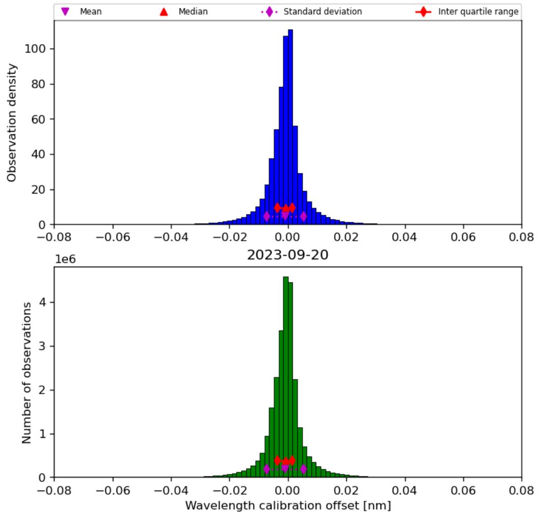
Figure 35: Histogram of “Wavelength calibration offset” for 2023-09-20 to 2023-09-21
