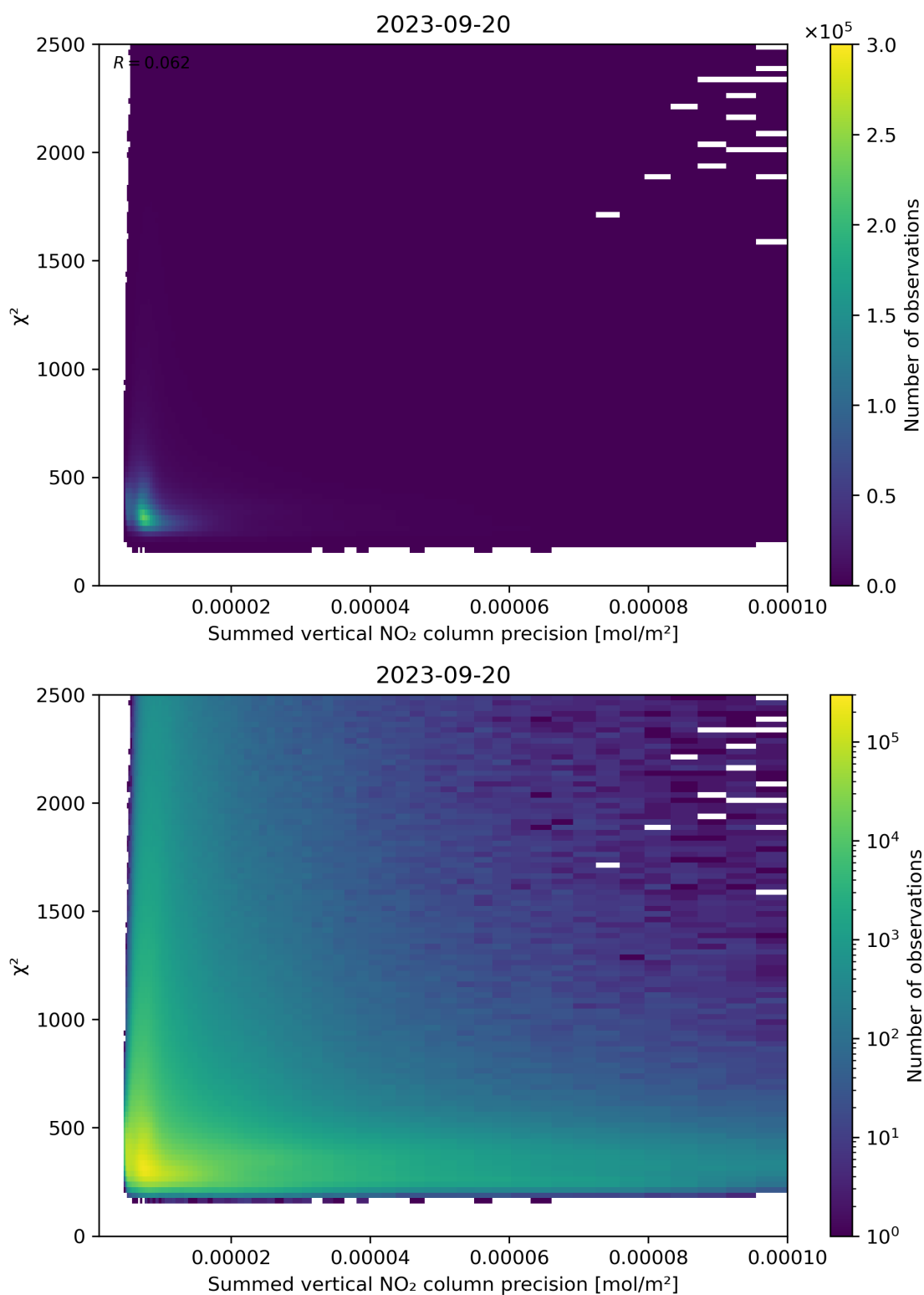
Figure 107: Scatter density plot of “Summed vertical NO 2 column precision” against “ \chi^2 ” for 2023-09-20 to 2023-09-21.
