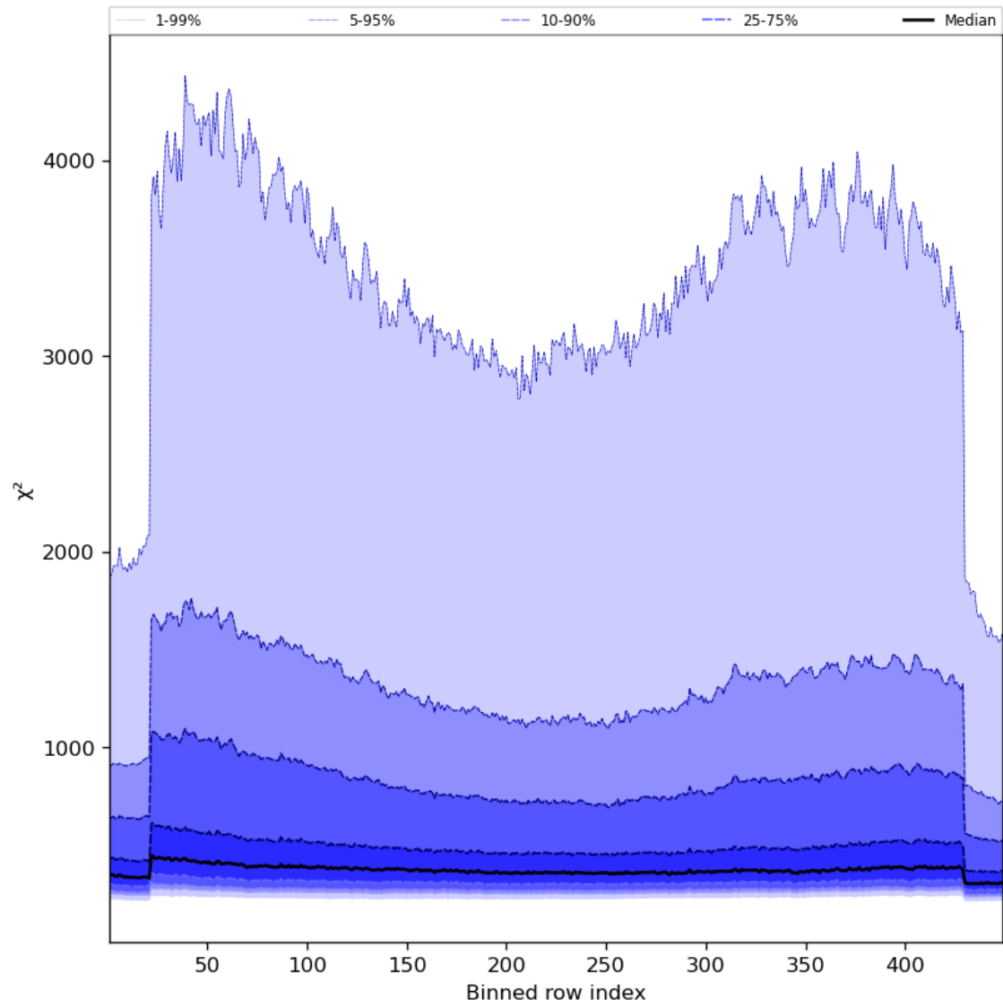
Figure 59: Along track statistics of “ \chi^2 ” for 2023-09-20 to 2023-09-21
