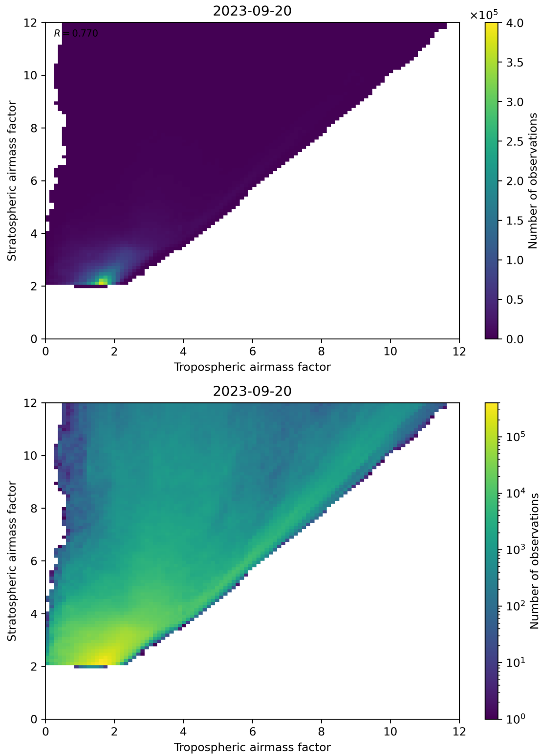
Figure 71: Scatter density plot of “Tropospheric airmass factor” against “Stratospheric airmass factor” for 2023-09-20 to 2023-09-21.
