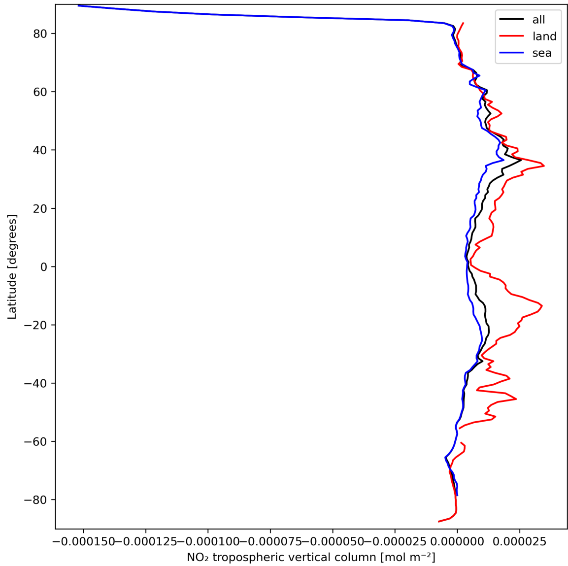
Figure 12: Zonal average of “NO 2 tropospheric vertical column” for 2023-09-20 to 2023-09-21.
