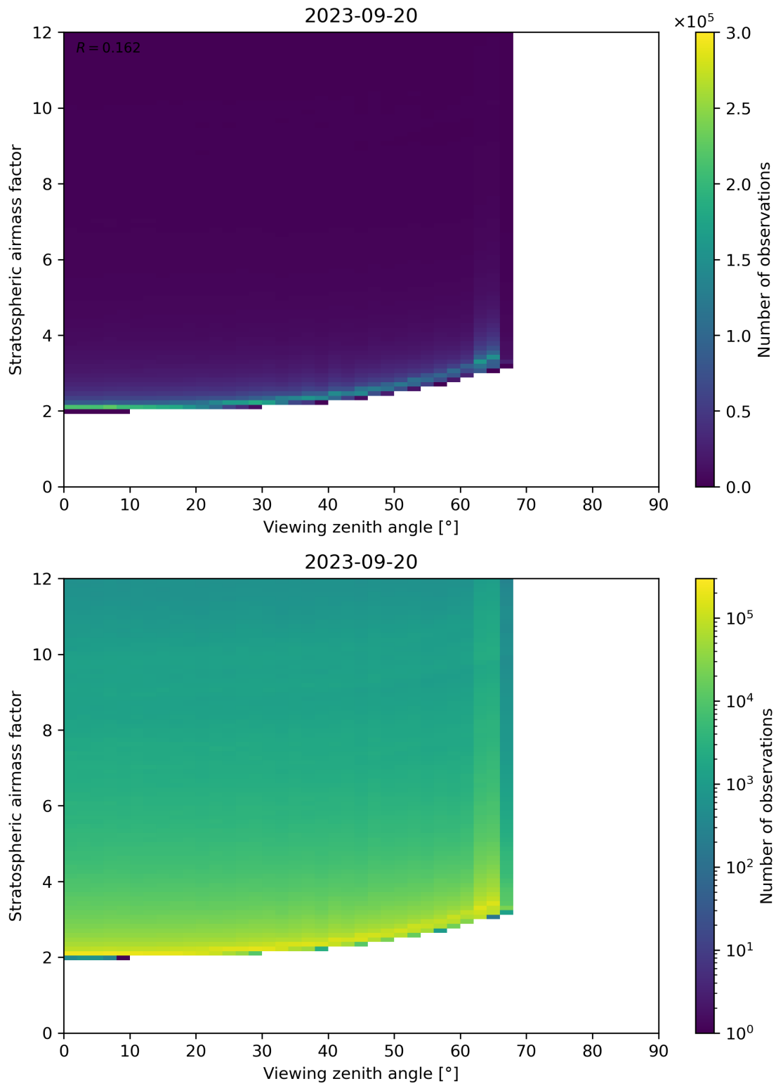
Figure 159: Scatter density plot of “Viewing zenith angle” against “Stratospheric airmass factor” for 2023-09-20 to 2023-09-21.
