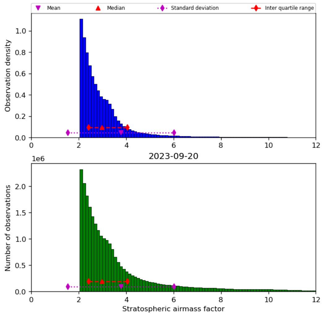
Figure 44: Histogram of “Stratospheric airmass factor” for 2023-09-20 to 2023-09-21
