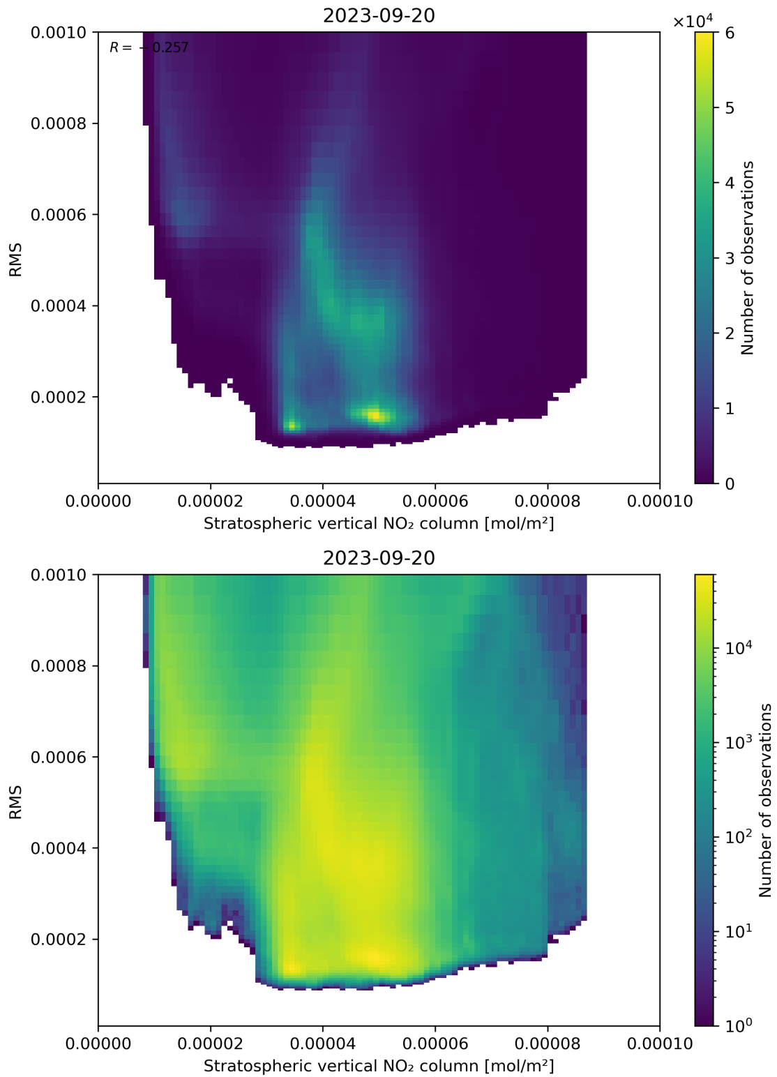
Figure 102: Scatter density plot of “Stratospheric vertical NO 2 column” against “RMS” for 2023-09-20 to 2023-09-21.
