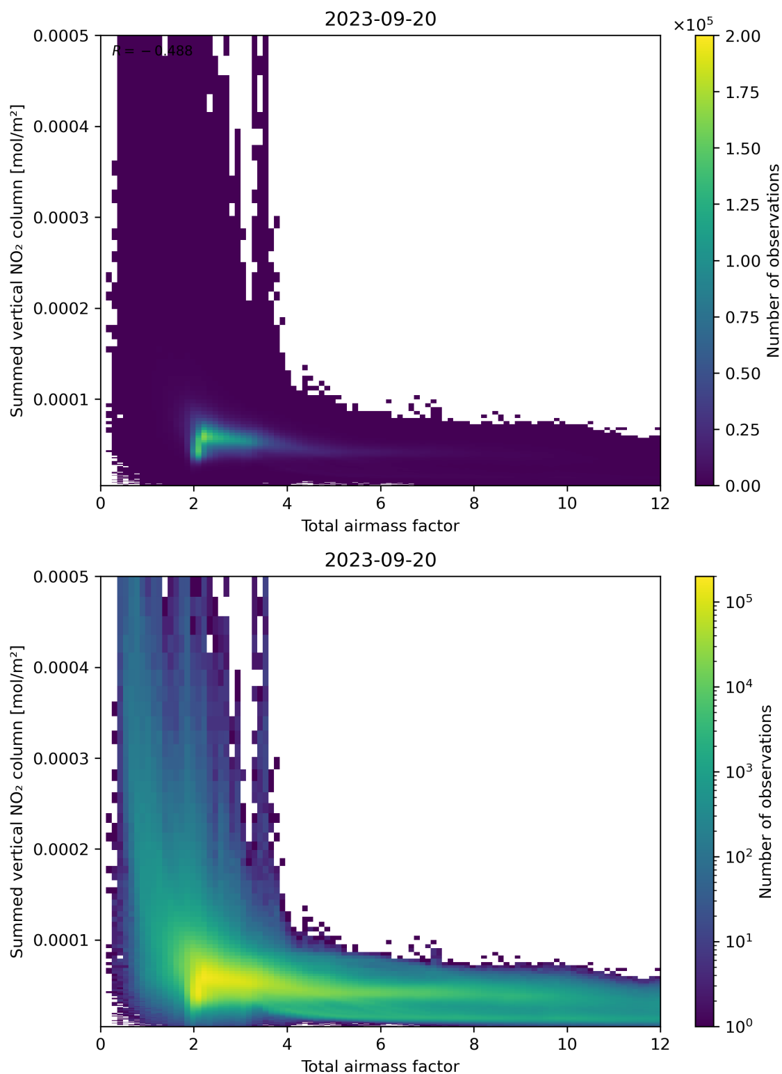
Figure 65: Scatter density plot of “Total airmass factor” against “Summed vertical NO 2 column” for 2023-09-20 to 2023-09-21.
