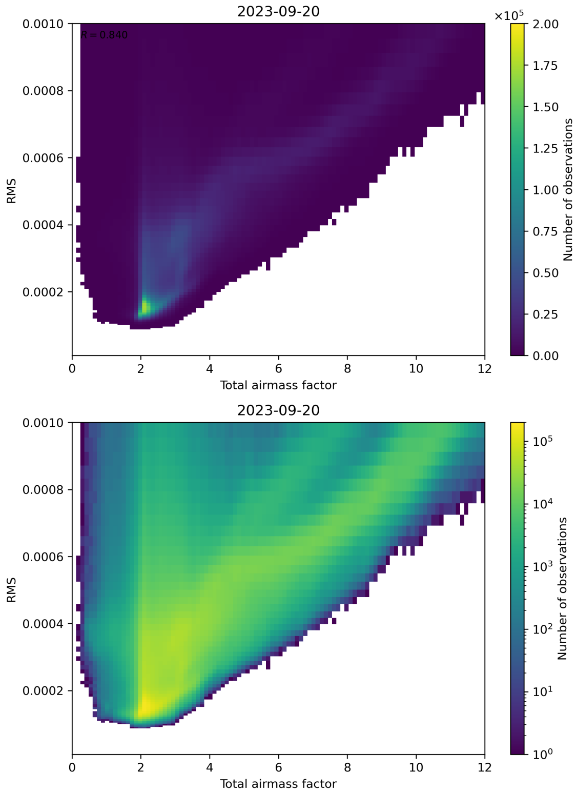
Figure 69: Scatter density plot of “Total airmass factor” against “RMS” for 2023-09-20 to 2023-09-21.
