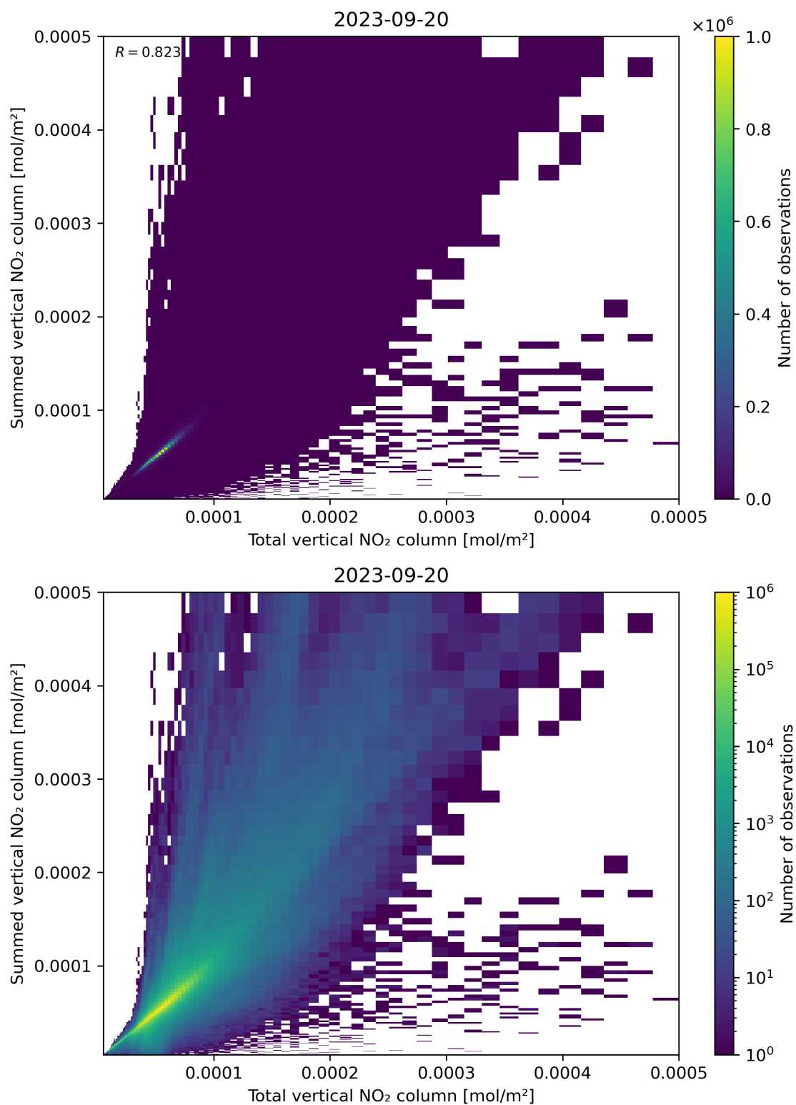
Figure 112: Scatter density plot of “Total vertical NO 2 column” against “Summed vertical NO 2 column” for 2023-09-20 to 2023-09-21.
