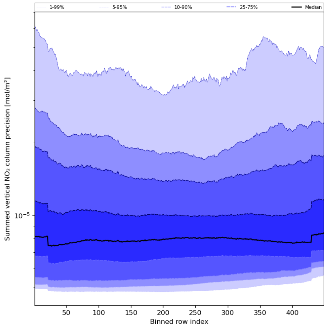
Figure 58: Along track statistics of “Summed vertical NO 2 column precision” for 2023-09-20 to 2023-09-21
