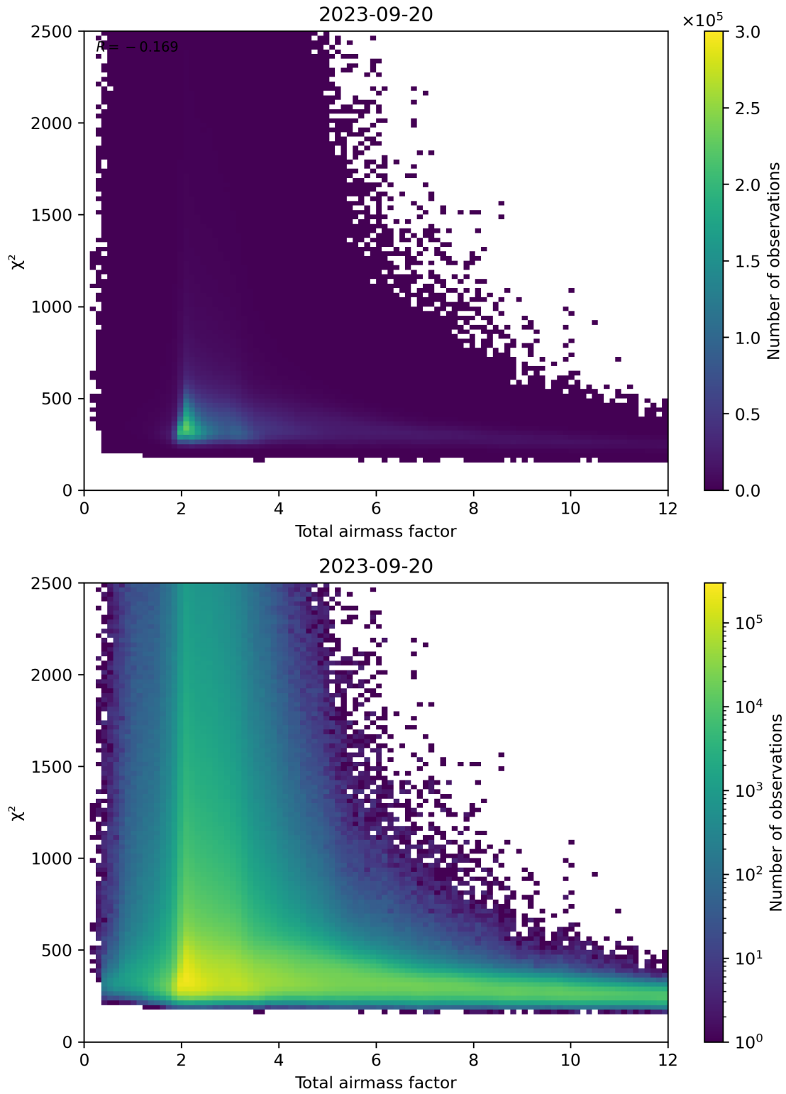
Figure 63: Scatter density plot of “Total airmass factor” against “ \chi^2 ” for 2023-09-20 to 2023-09-21.
