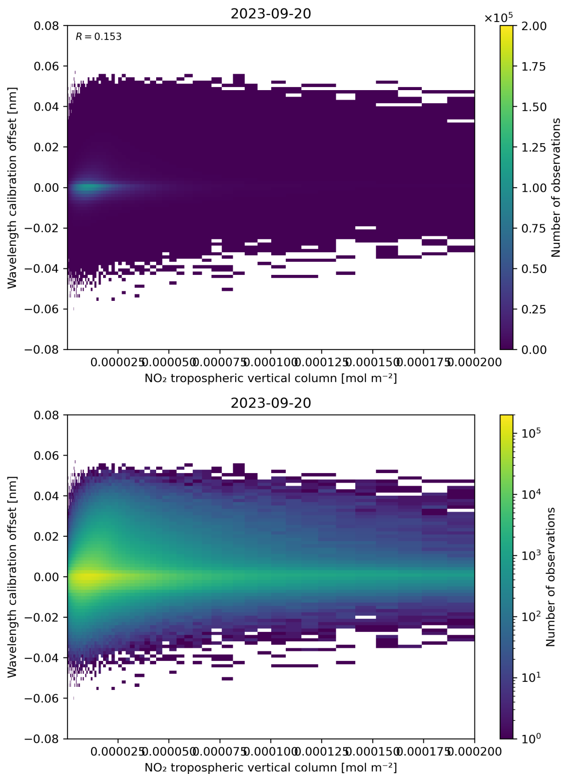
Figure 143: Scatter density plot of “NO 2 tropospheric vertical column” against “Wavelength calibration offset” for 2023-09-20 to 2023-09-21.
