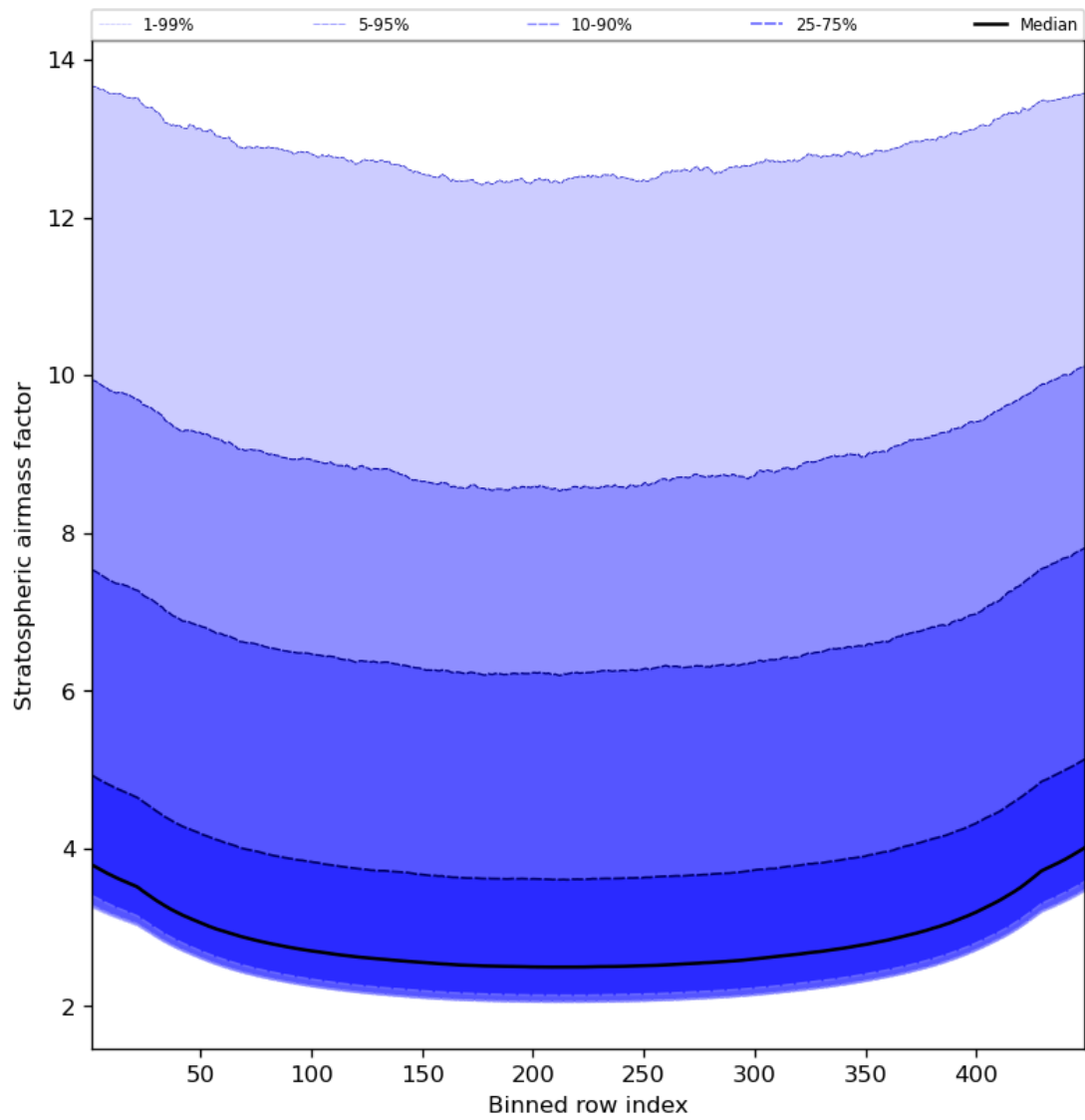
Figure 61: Along track statistics of “Stratospheric airmass factor” for 2023-09-20 to 2023-09-21
