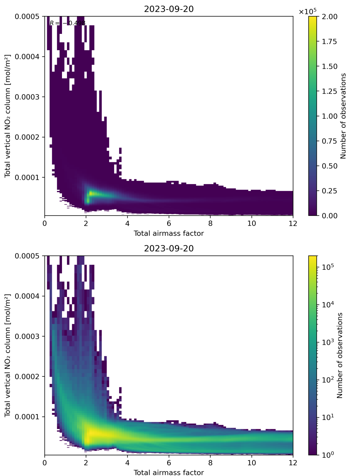
Figure 67: Scatter density plot of “Total airmass factor” against “Total vertical NO 2 column” for 2023-09-20 to 2023-09-21.
