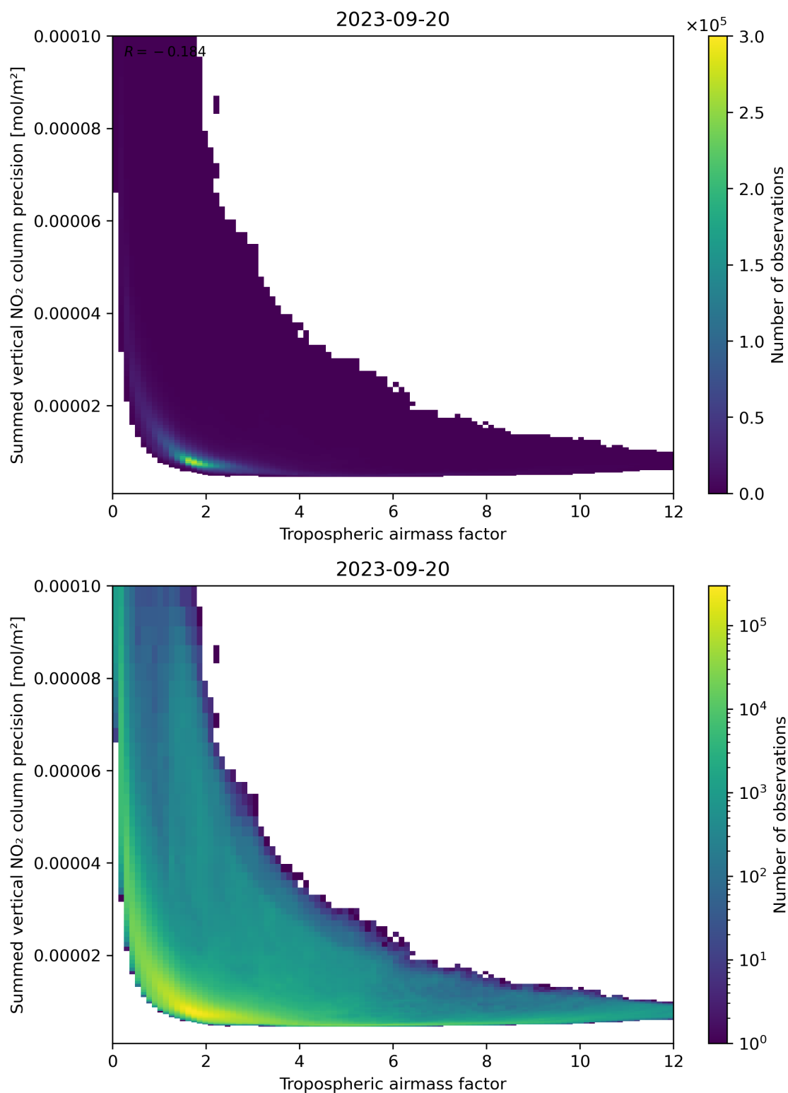
Figure 76: Scatter density plot of “Tropospheric air mass factor” against “Summed vertical NO 2 column precision” for 2023-09-20 to 2023-09-21.
