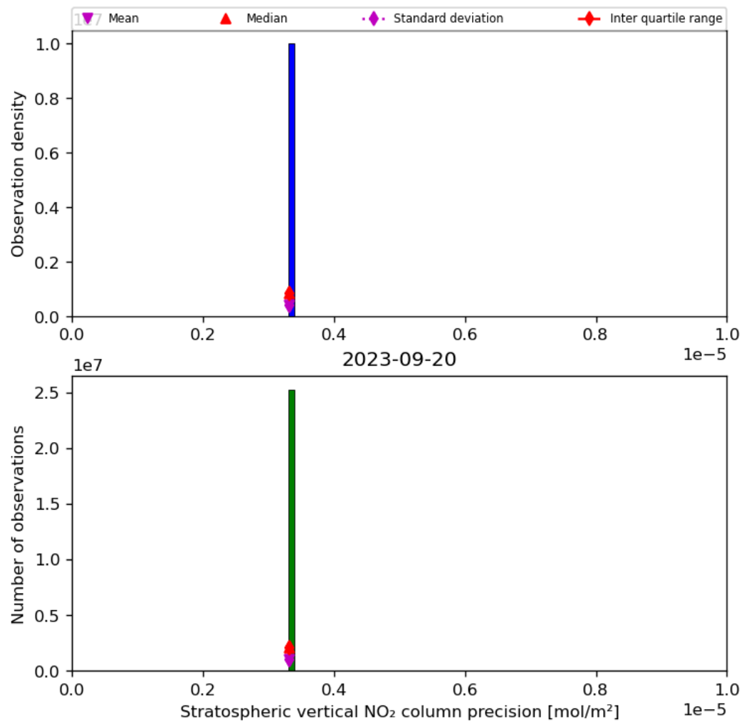
Figure 37: Histogram of “Stratospheric vertical NO 2 column precision” for 2023-09-20 to 2023-09-21
