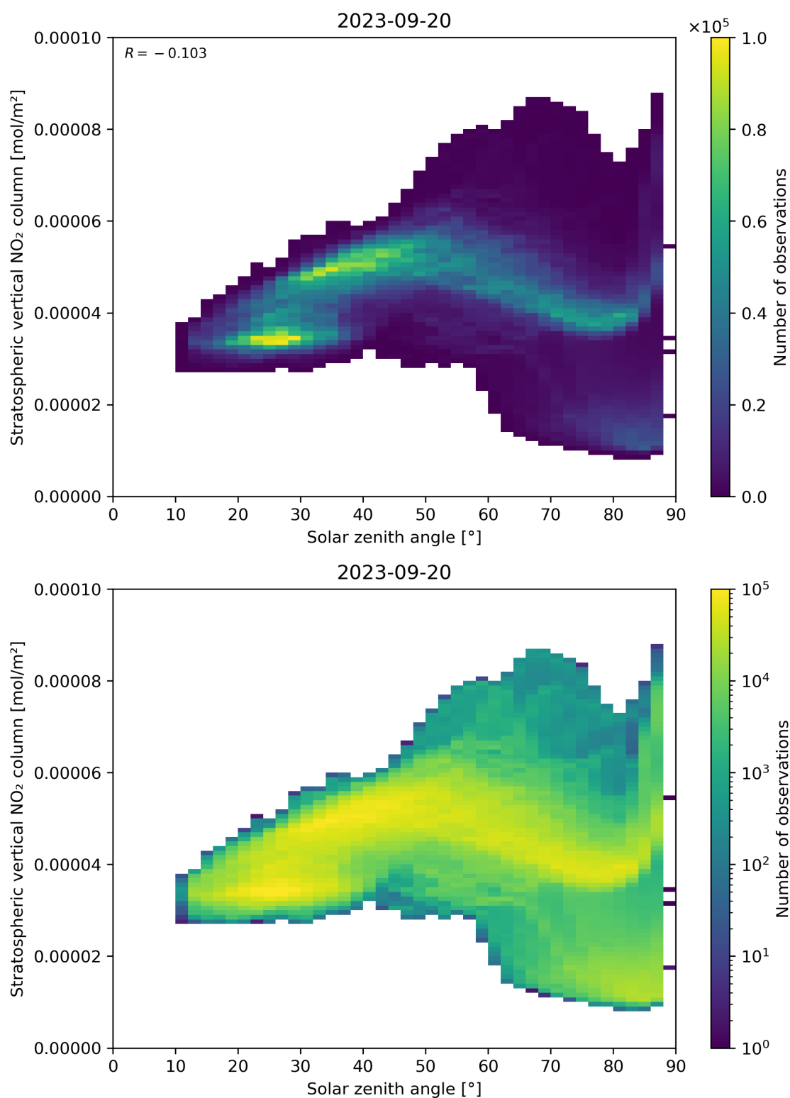
Figure 150: Scatter density plot of “Solar zenith angle” against “Stratospheric vertical NO 2 column” for 2023-09-20 to 2023-09-21.
