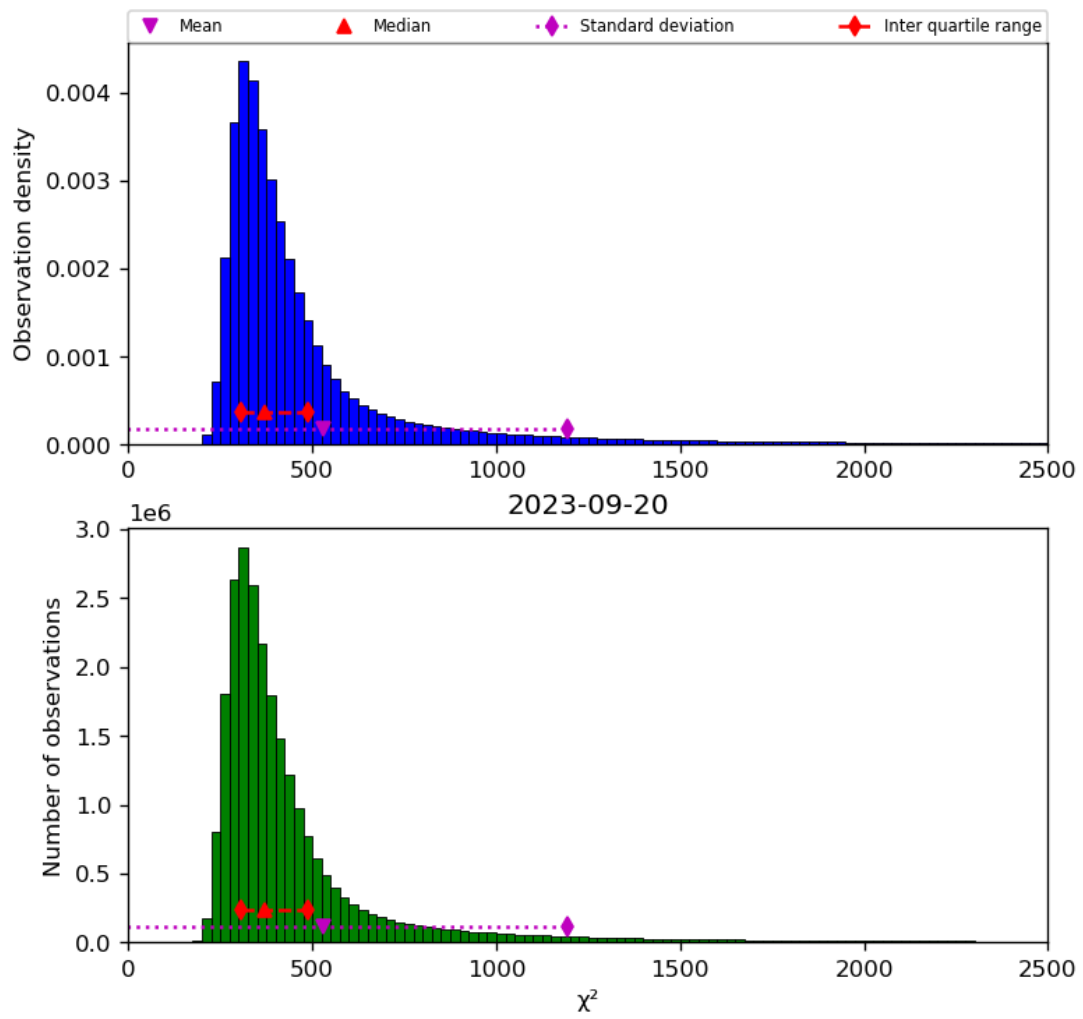
Figure 42: Histogram of “ \chi^2 ” for 2023-09-20 to 2023-09-21
