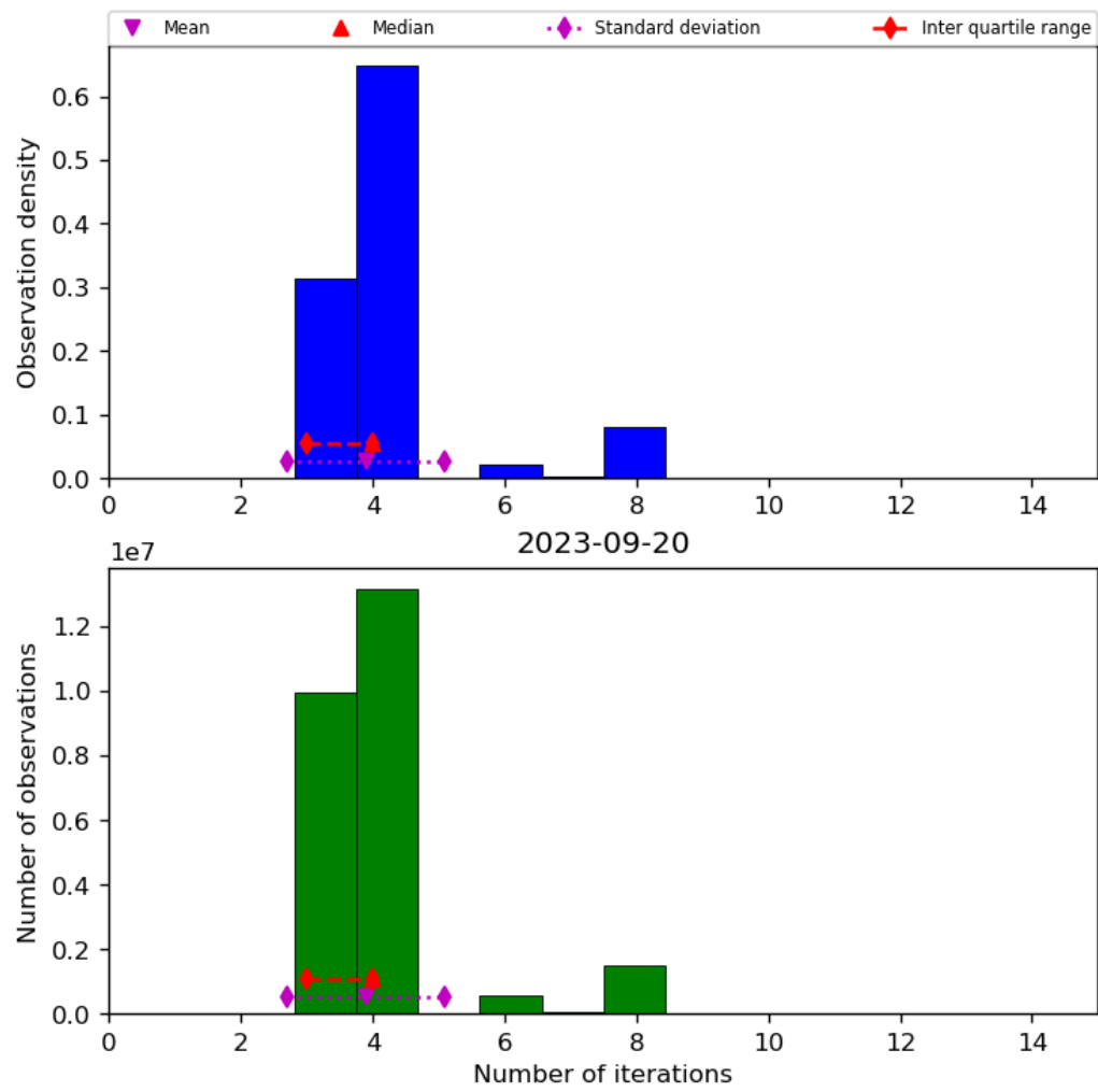
Figure 34: Histogram of “Number of iterations” for 2023-09-20 to 2023-09-21
