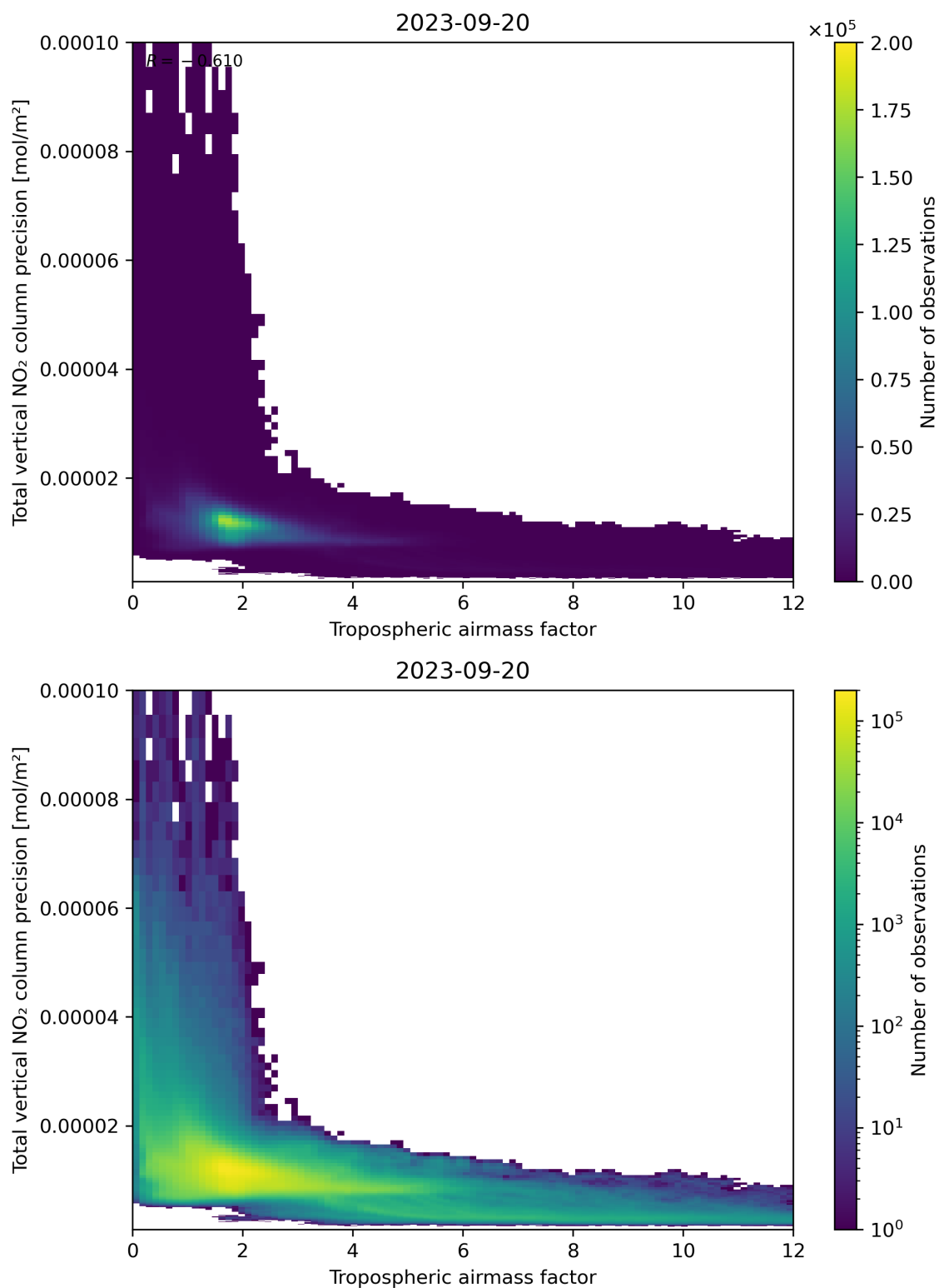
Figure 78: Scatter density plot of “Tropospheric air mass factor” against “Total vertical NO 2 column precision” for 2023-09-20 to 2023-09-21.
