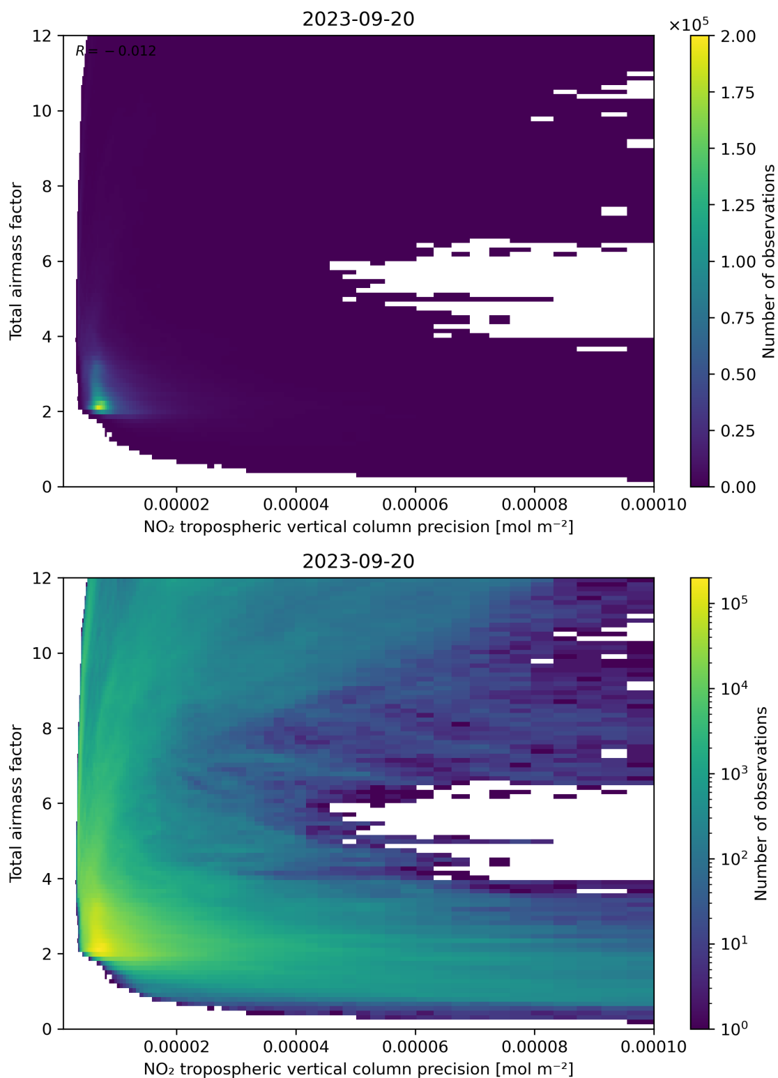
Figure 132: Scatter density plot of “NO 2 tropospheric vertical column precision” against “Total airmass factor” for 2023-09-20 to 2023-09-21.
