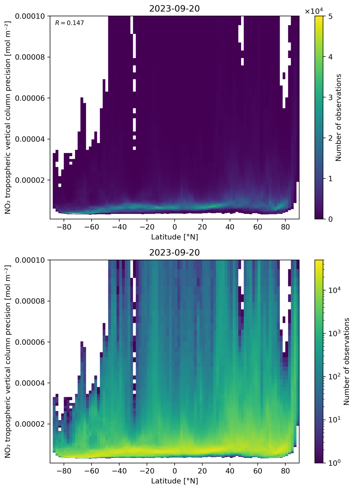
Figure 93: Scatter density plot of “Latitude” against “NO 2 tropospheric vertical column precision” for 2023-09-20 to 2023-09-21.
