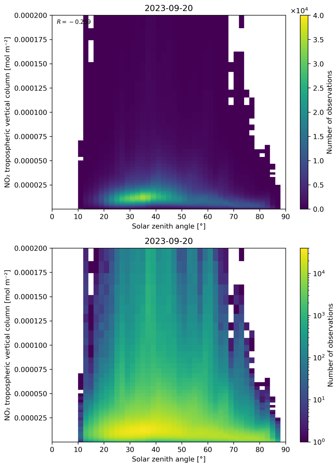
Figure 155: Scatter density plot of “Solar zenith angle” against “NO 2 tropospheric vertical column” for 2023-09-20 to 2023-09-21.
