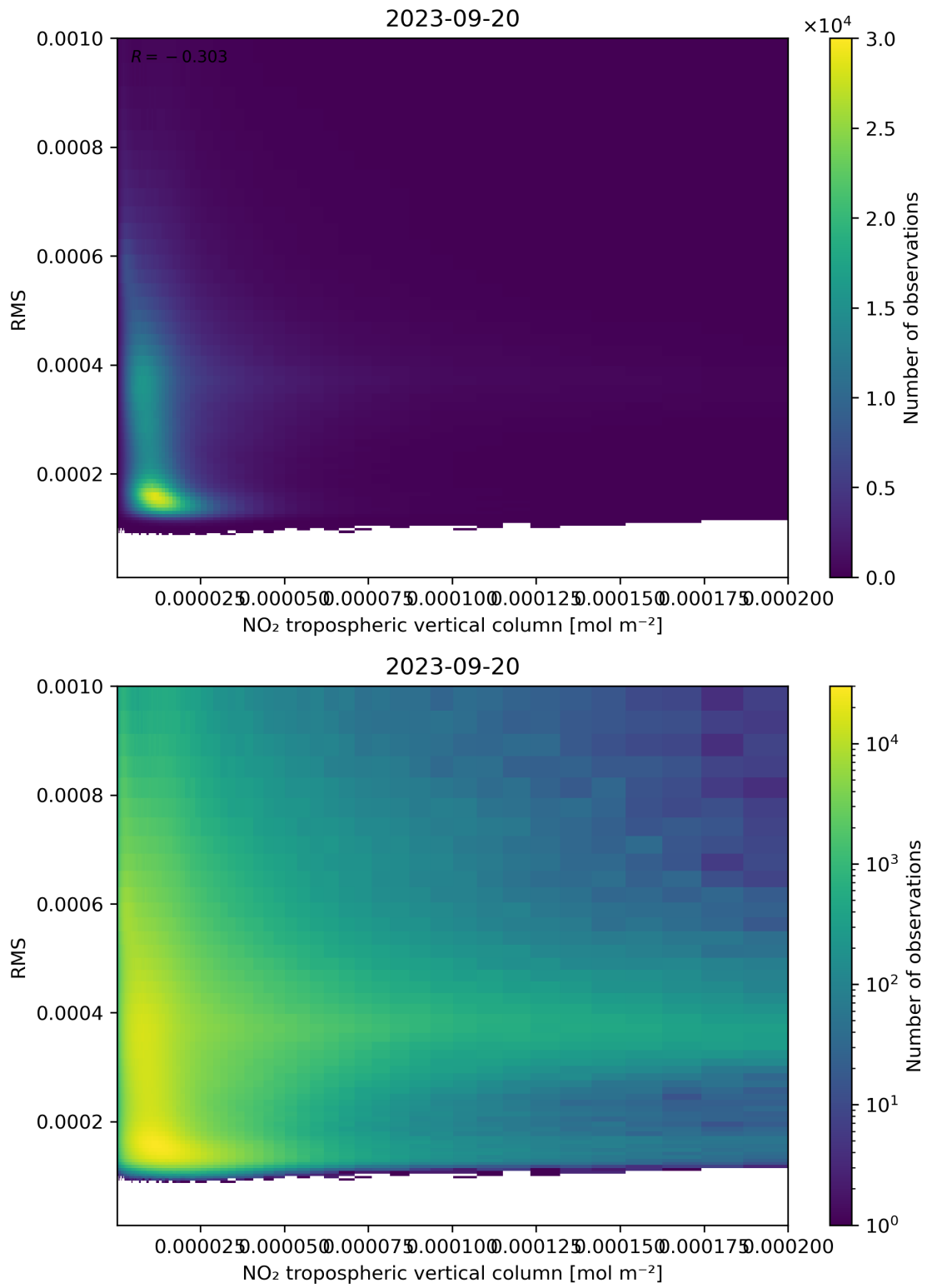
Figure 142: Scatter density plot of “NO 2 tropospheric vertical column” against “RMS” for 2023-09-20 to 2023-09-21.
