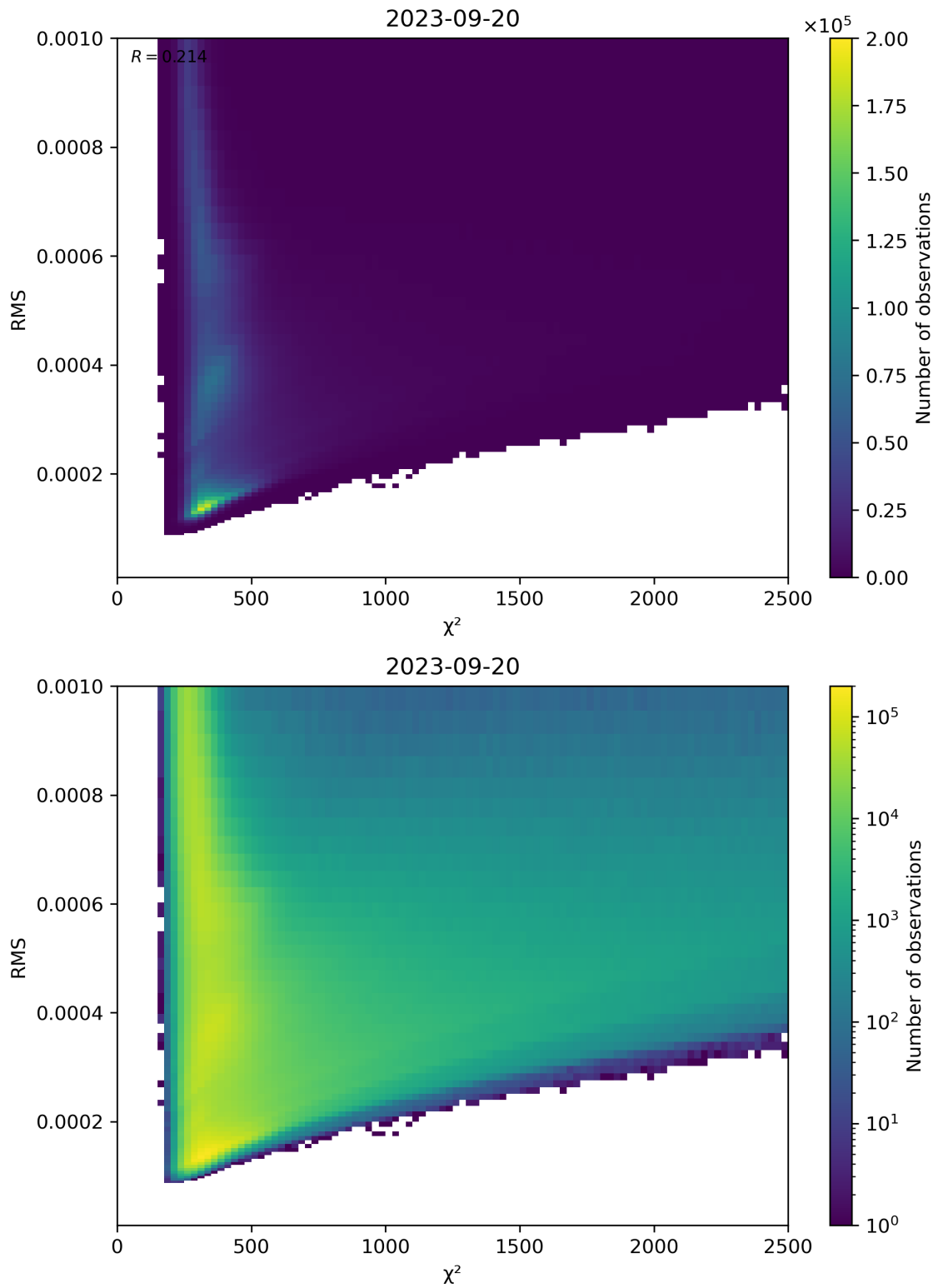
Figure 82: Scatter density plot of “ \chi^2 ” against “RMS” for 2023-09-20 to 2023-09-21.
