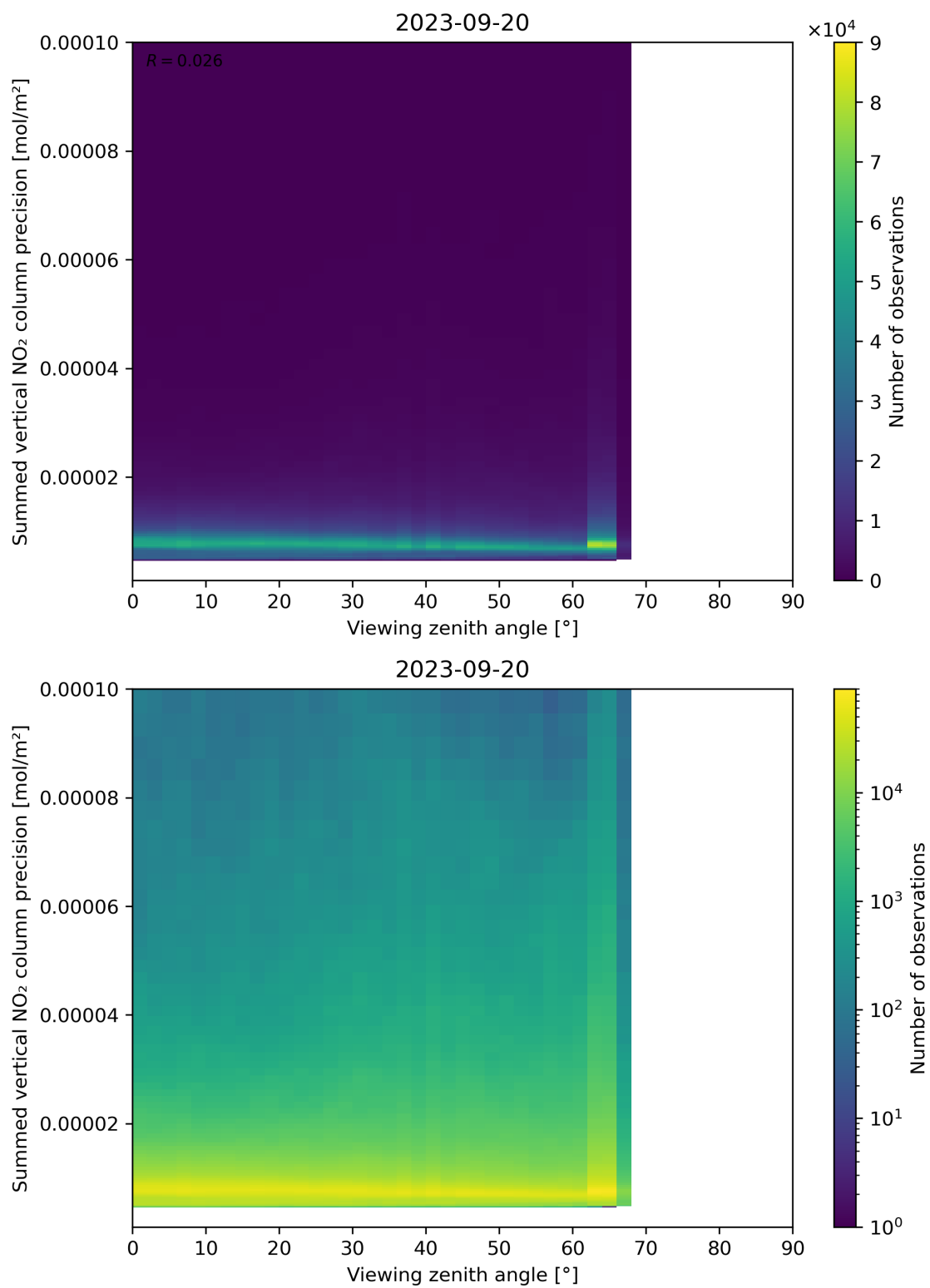
Figure 166: Scatter density plot of “Viewing zenith angle” against “Summed vertical NO 2 column precision” for 2023-09-20 to 2023-09-21.
