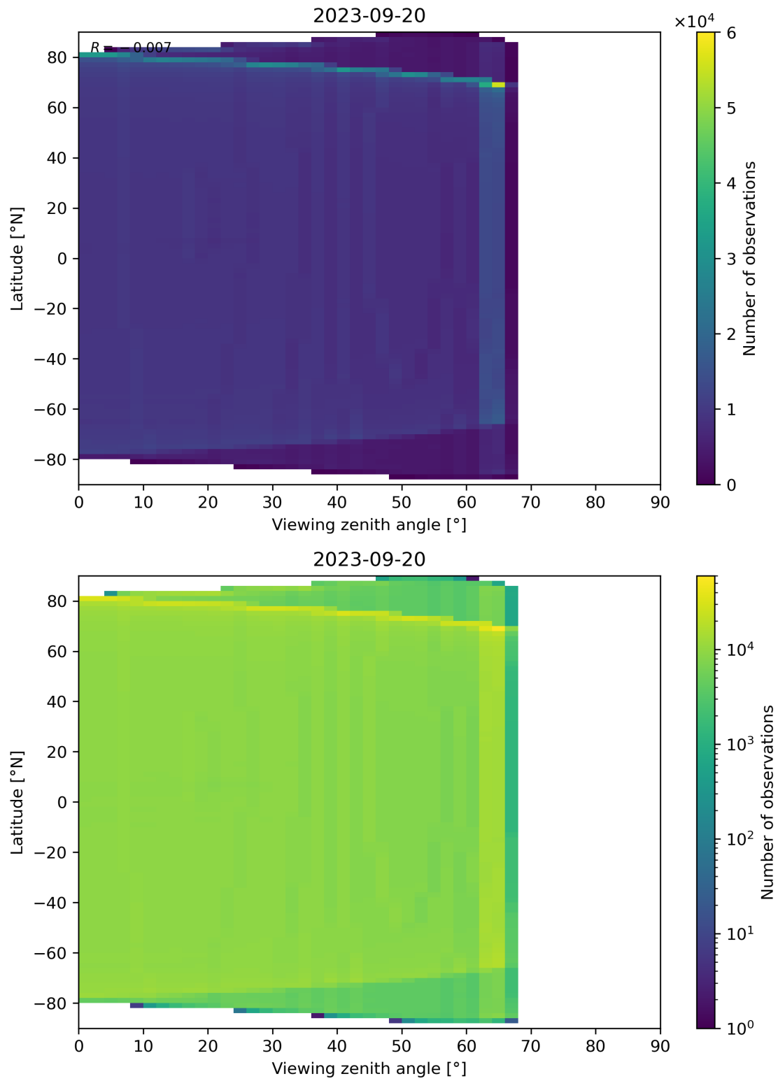
Figure 163: Scatter density plot of “Viewing zenith angle” against “Latitude” for 2023-09-20 to 2023-09-21.
