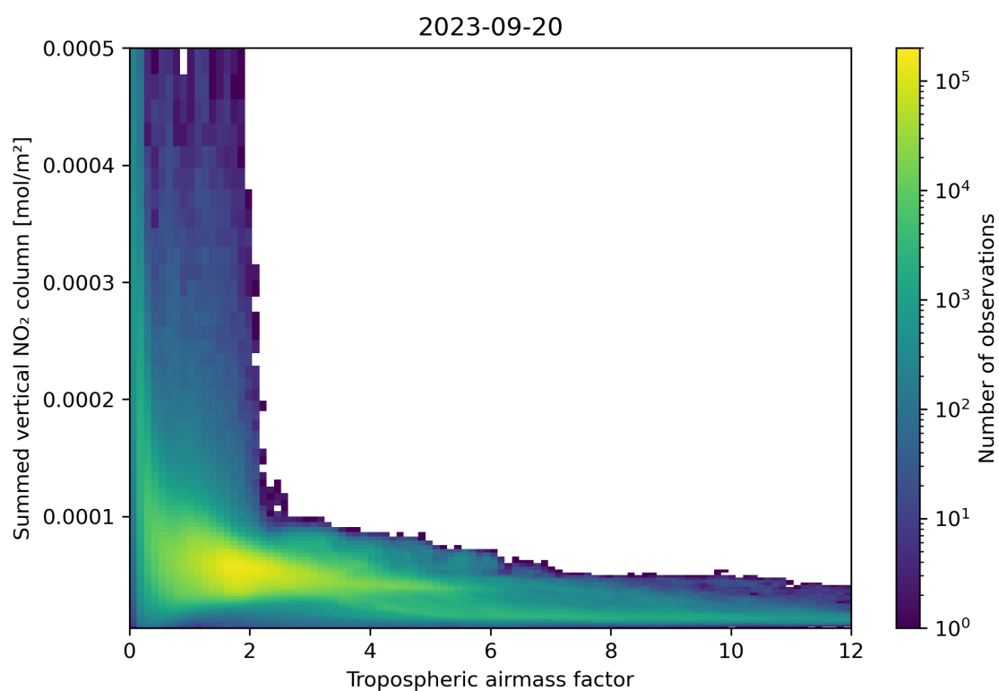
Figure 75: Scatter density plot of “Tropospheric airmass factor” against “Summed vertical NO 2 column” for 2023-09-20 to 2023-09-21.
