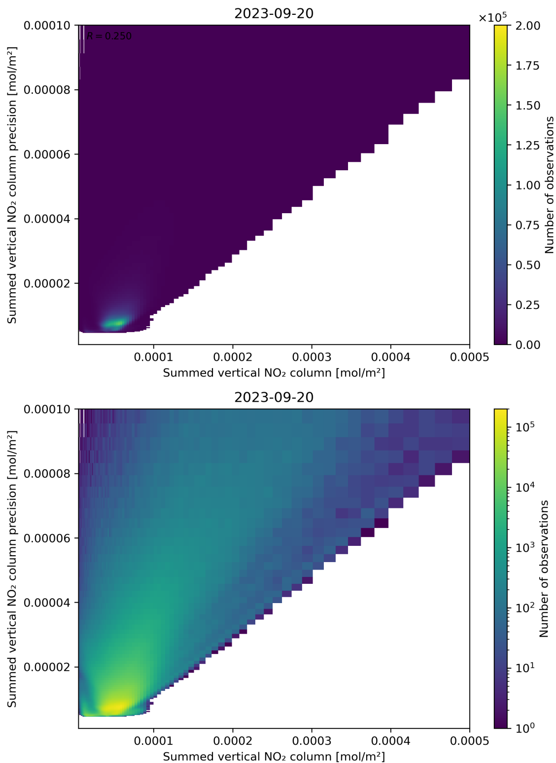
Figure 105: Scatter density plot of “Summed vertical NO 2 column” against “Summed vertical NO 2 column precision” for 2023-09-20 to 2023-09-21.
