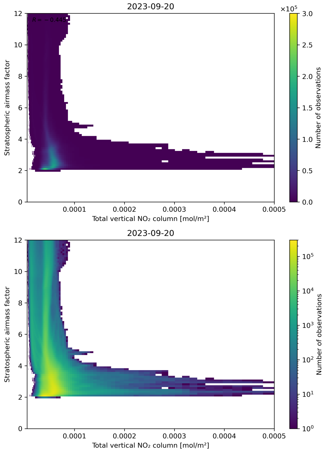
Figure 110: Scatter density plot of “Total vertical NO 2 column” against “Stratospheric airmass factor” for 2023-09-20 to 2023-09-21.
