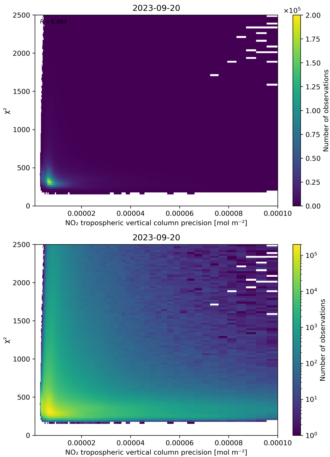
Figure 134: Scatter density plot of “NO 2 tropospheric vertical column precision” against “ \chi^2 ” for 2023-09-20 to 2023-09-21.
