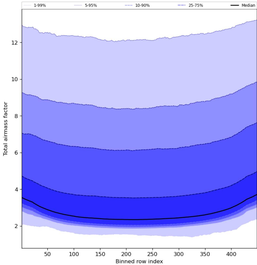
Figure 49: Along track statistics of “Total airmass factor” for 2023-09-20 to 2023-09-21
