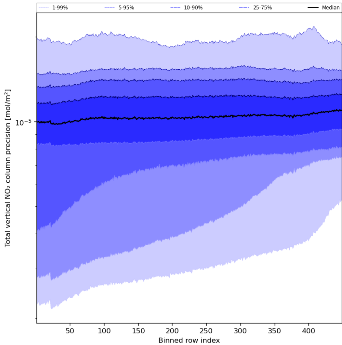
Figure 56: Along track statistics of “Total vertical NO 2 column precision” for 2023-09-20 to 2023-09-21
