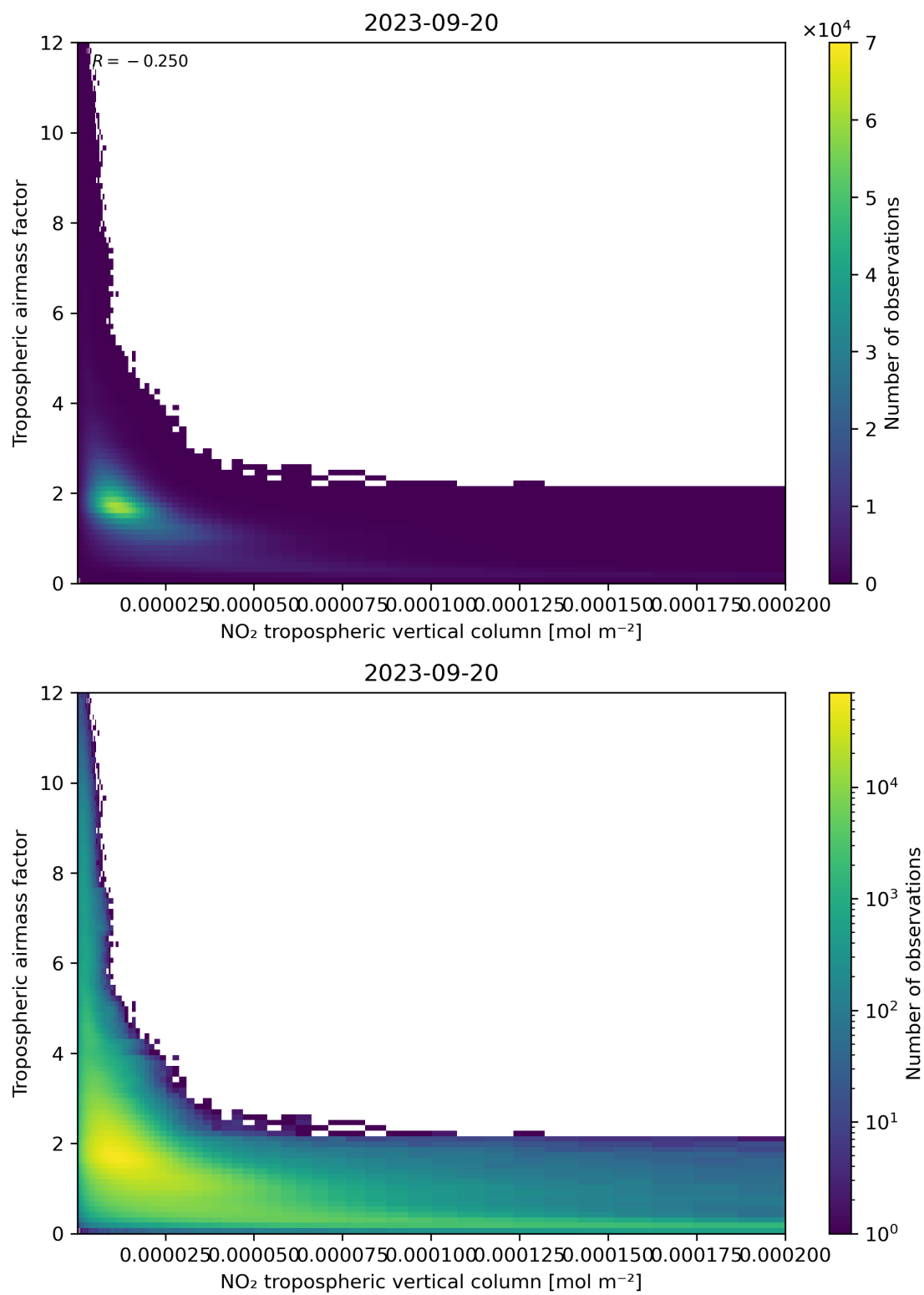
Figure 123: Scatter density plot of “NO 2 tropospheric vertical column” against “Tropospheric airmass factor” for 2023-09-20 to 2023-09-21.
