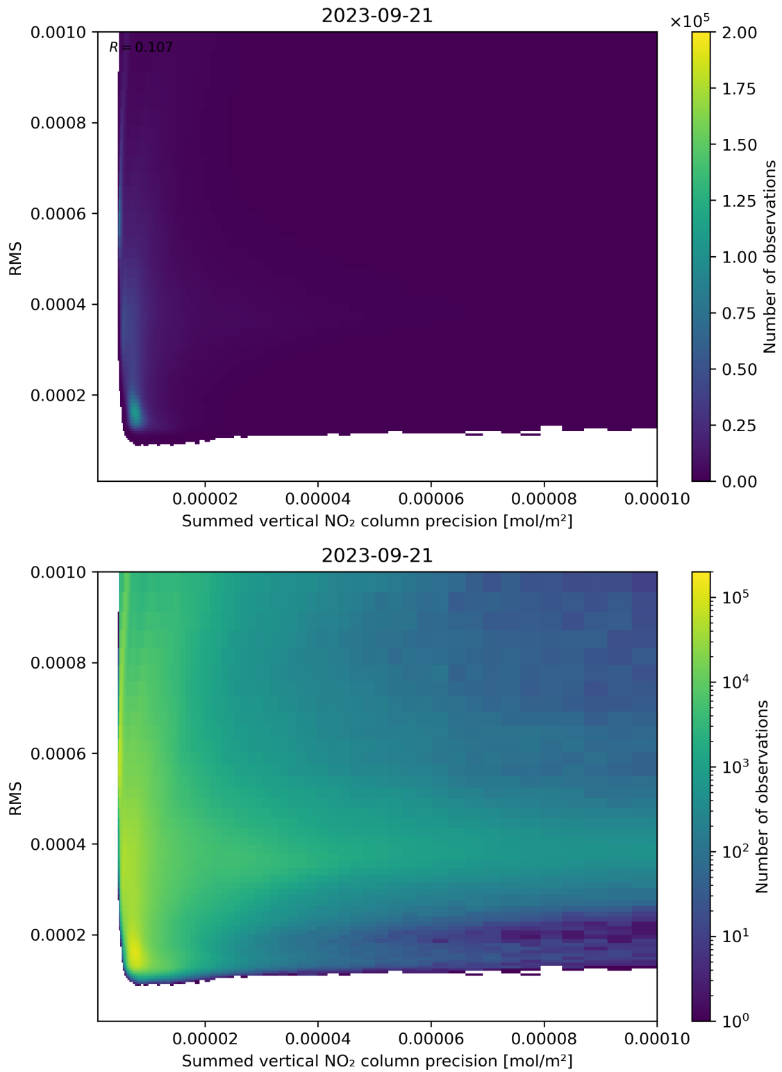
Figure 108: Scatter density plot of “Summed vertical NO 2 column precision” against “RMS” for 2023-09-20 to 2023-09-22.
