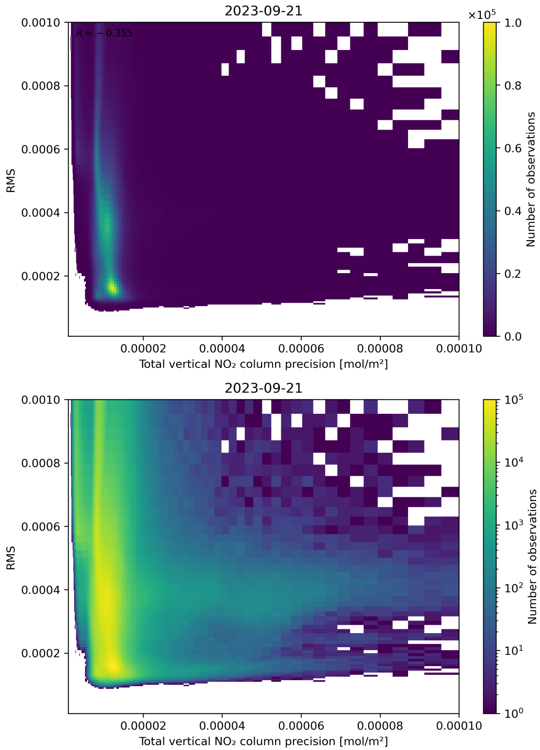
Figure 119: Scatter density plot of “Total vertical NO 2 column precision” against “RMS” for 2023-09-20 to 2023-09-22.
