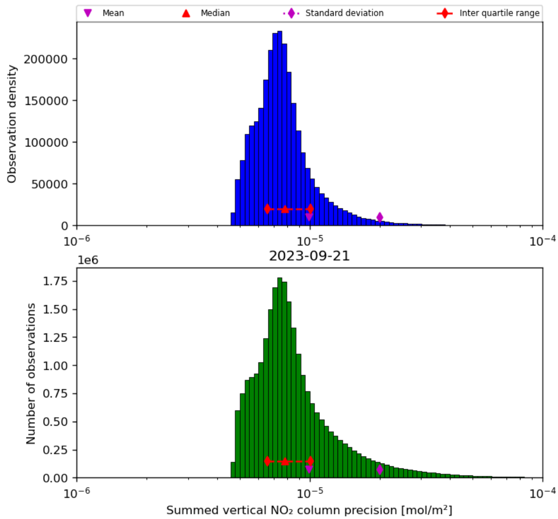
Figure 41: Histogram of "Summed vertical NO 2 column precision" for 2023-09-20 to 2023-09-22
