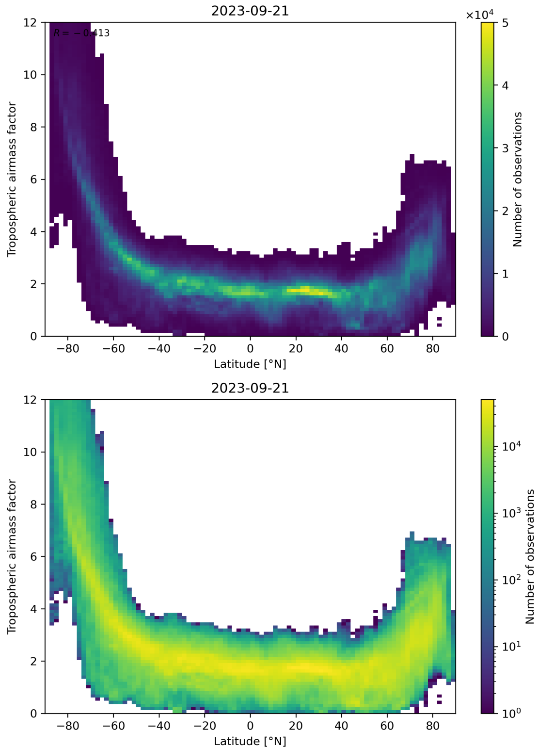
Figure 85: Scatter density plot of “Latitude” against “Tropospheric airmass factor” for 2023-09-20 to 2023-09-22.
