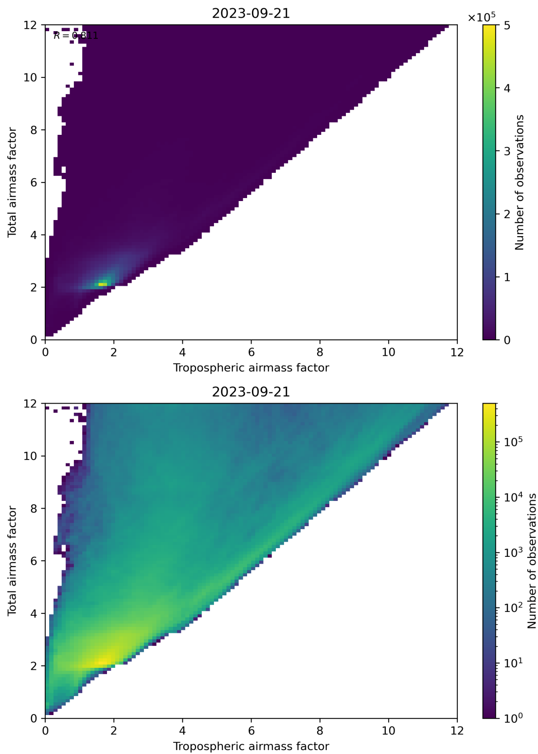
Figure 72: Scatter density plot of “Tropospheric airmass factor” against “Total airmass factor” for 2023-09-20 to 2023-09-22.
