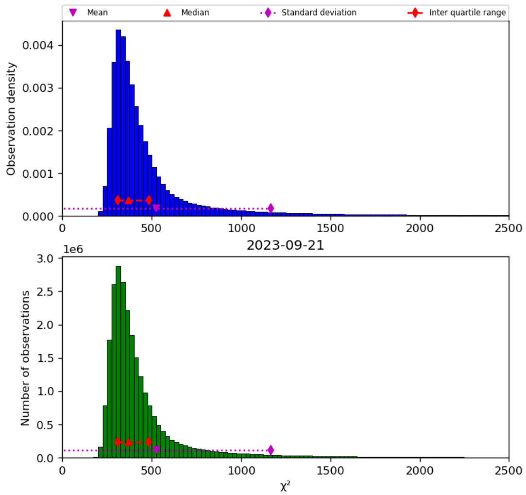
Figure 42: Histogram of “ \chi^2 ” for 2023-09-20 to 2023-09-22
