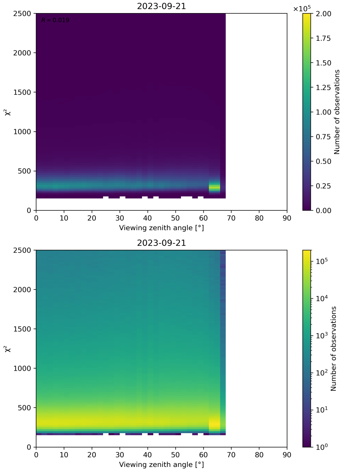
Figure 162: Scatter density plot of “Viewing zenith angle” against “ \chi^2 ” for 2023-09-20 to 2023-09-22.
