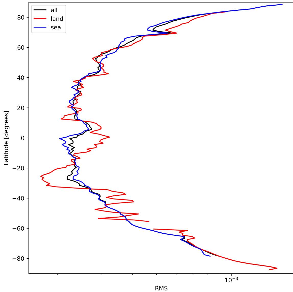
Figure 26: Zonal average of “RMS” for 2023-09-20 to 2023-09-22.
