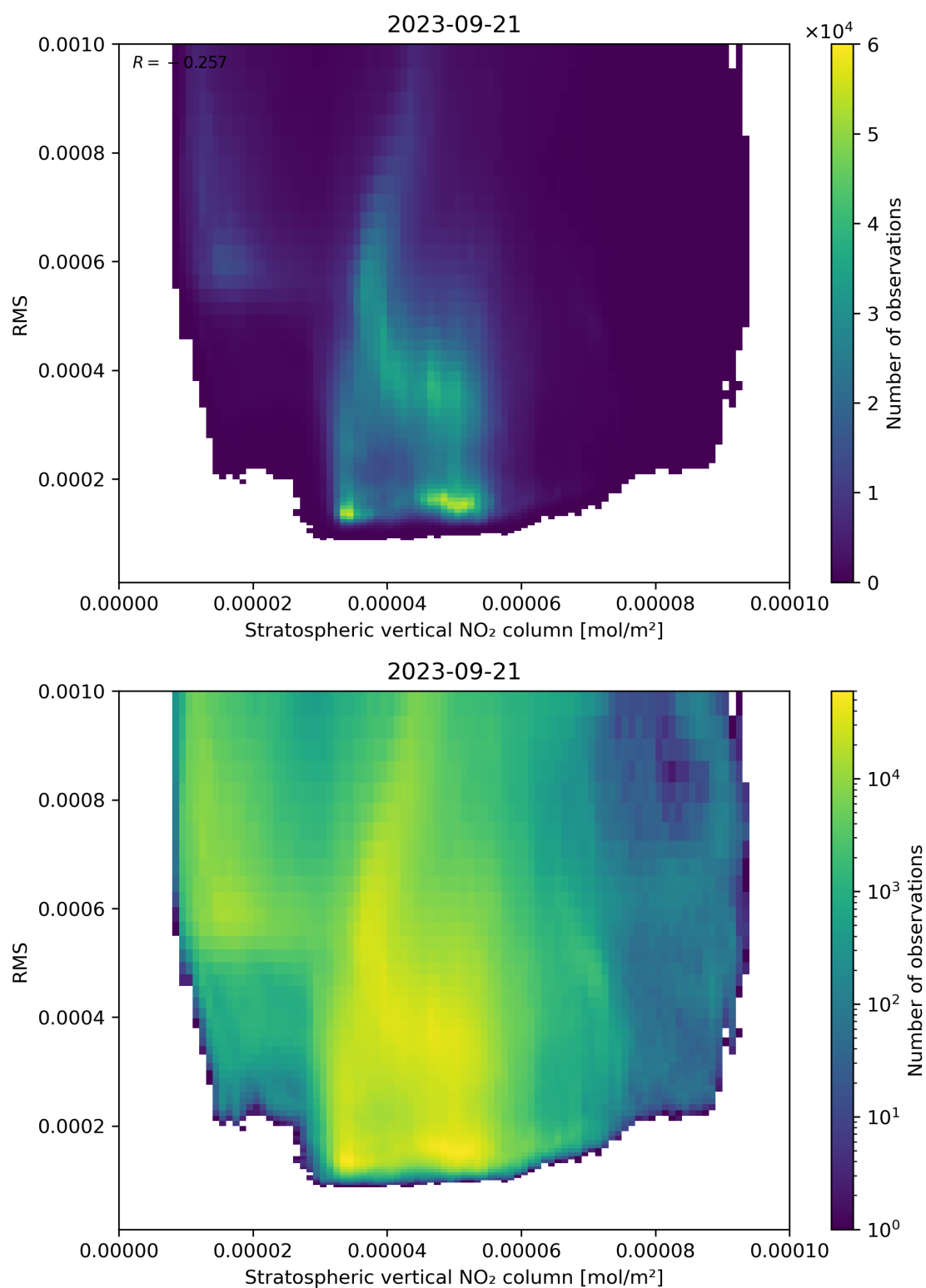
Figure 102: Scatter density plot of “Stratospheric vertical NO 2 column” against “RMS” for 2023-09-20 to 2023-09-22.
