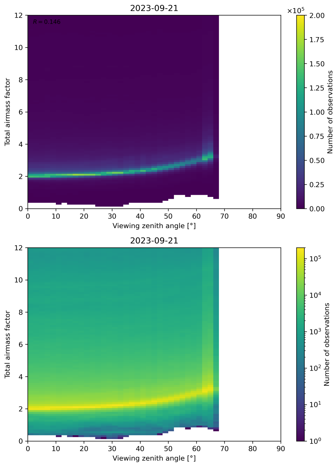
Figure 160: Scatter density plot of “Viewing zenith angle” against “Total airmass factor” for 2023-09-20 to 2023-09-22.
