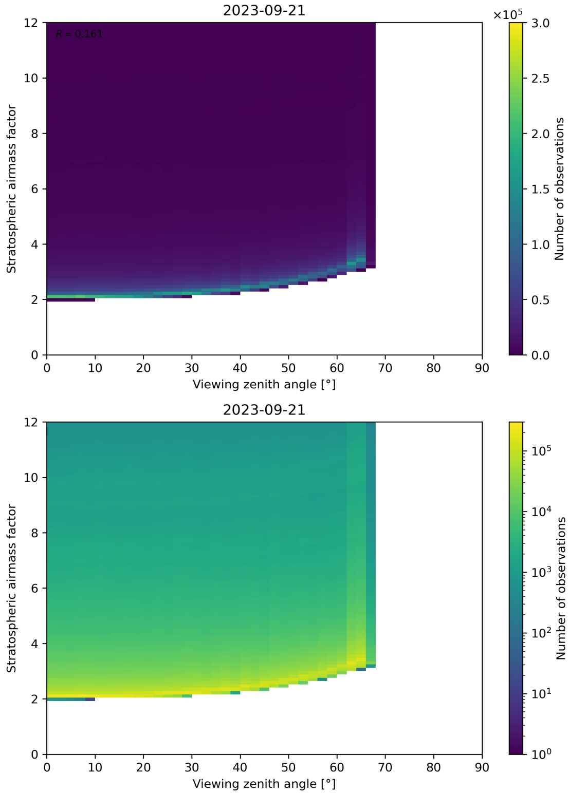
Figure 159: Scatter density plot of “Viewing zenith angle” against “Stratospheric airmass factor” for 2023-09-20 to 2023-09-22.
