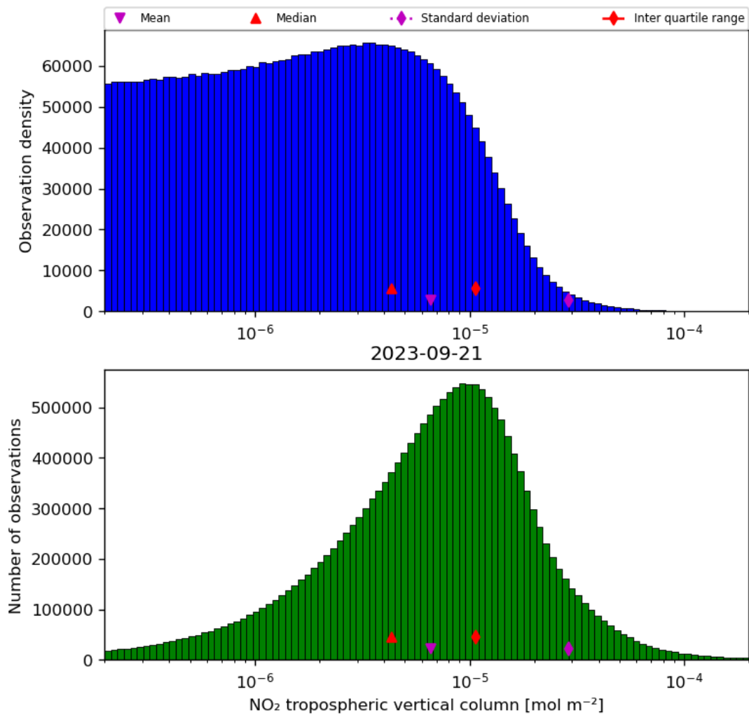
Figure 29: Histogram of “NO 2 tropospheric vertical column” for 2023-09-20 to 2023-09-22
