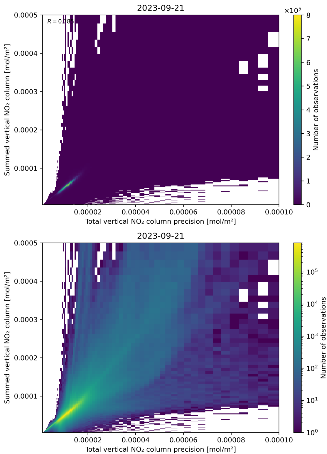
Figure 117: Scatter density plot of “Total vertical NO 2 column precision” against “Summed vertical NO 2 column” for 2023-09-20 to 2023-09-22.
