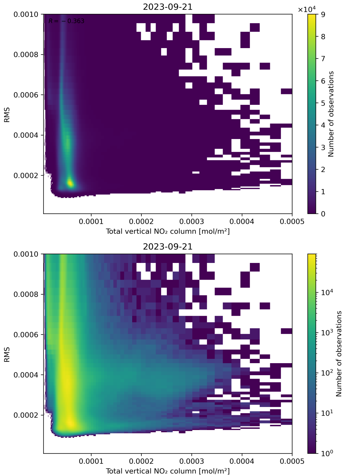
Figure 120: Scatter density plot of “Total vertical NO 2 column” against “RMS” for 2023-09-20 to 2023-09-22.
