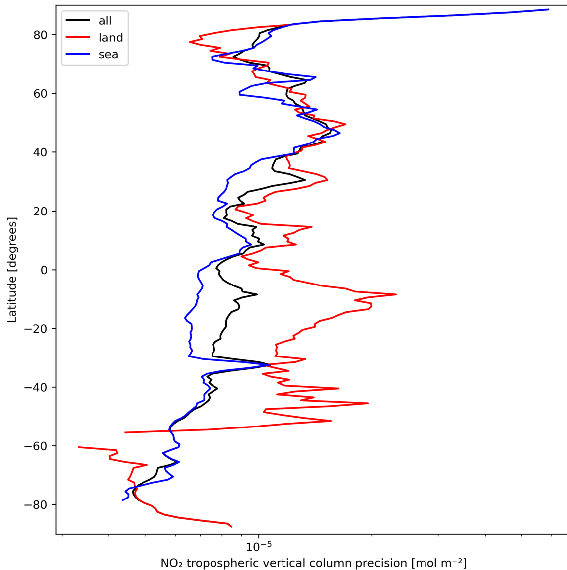
Figure 13: Zonal average of “NO 2 tropospheric vertical column precision” for 2023-09-20 to 2023-09-22.
