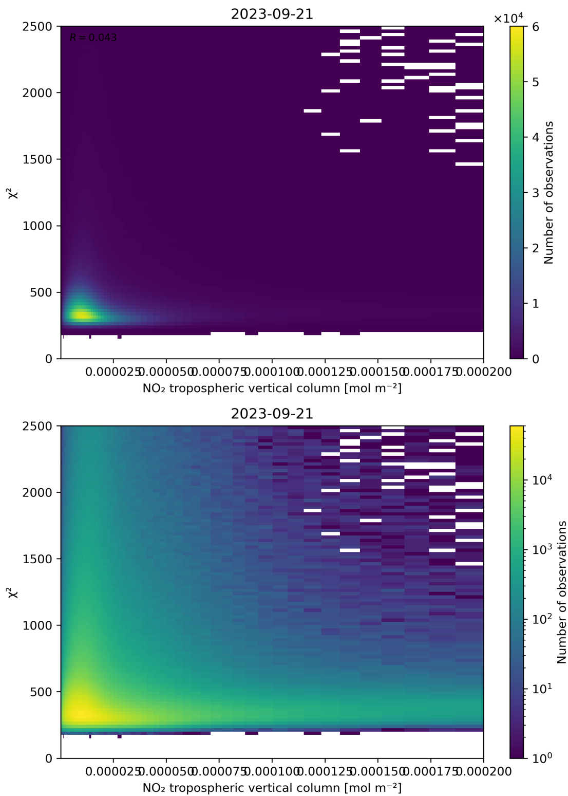
Figure 124: Scatter density plot of “NO 2 tropospheric vertical column” against “ \chi^2 ” for 2023-09-20 to 2023-09-22.
