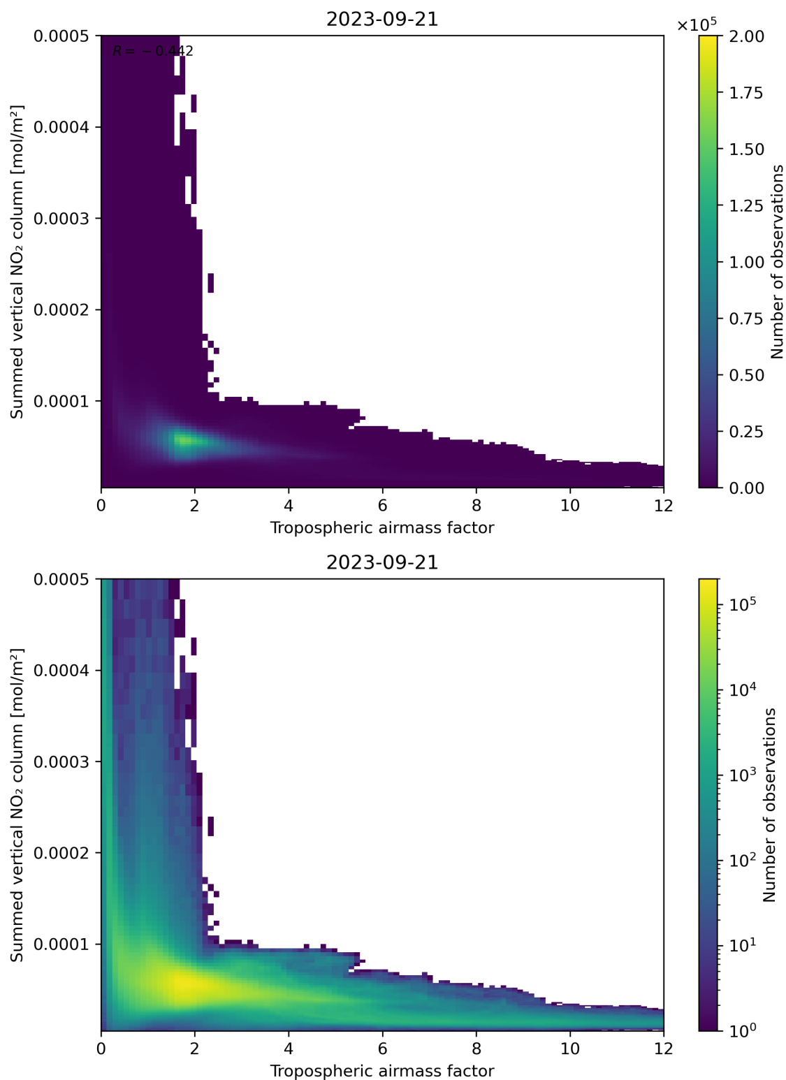
Figure 75: Scatter density plot of “Tropospheric airmass factor” against “Summed vertical NO 2 column” for 2023-09-20 to 2023-09-22.
