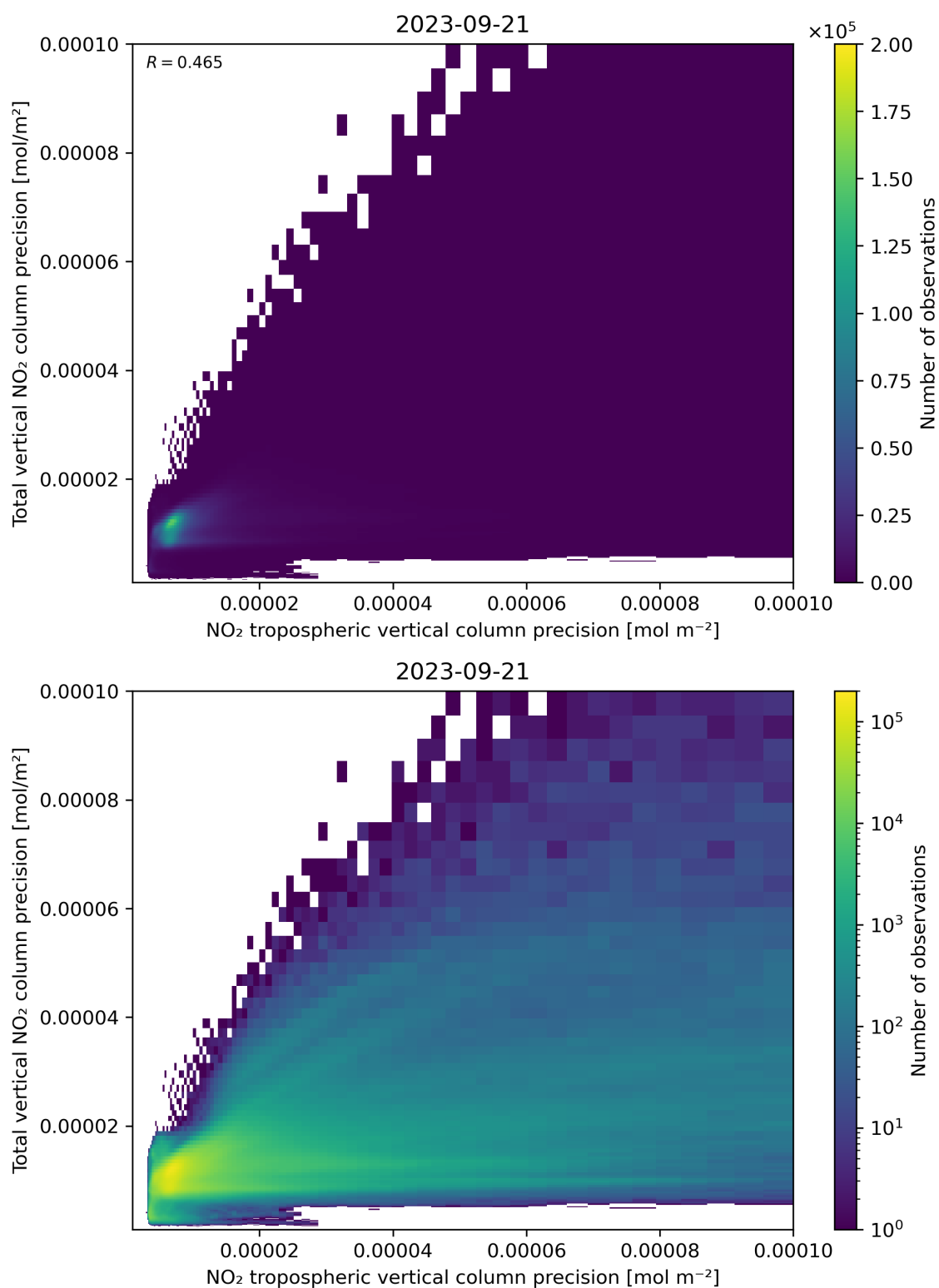
Figure 139: Scatter density plot of “NO 2 tropospheric vertical column precision” against “Total vertical NO 2 column precision” for 2023-09-20 to 2023-09-22.
