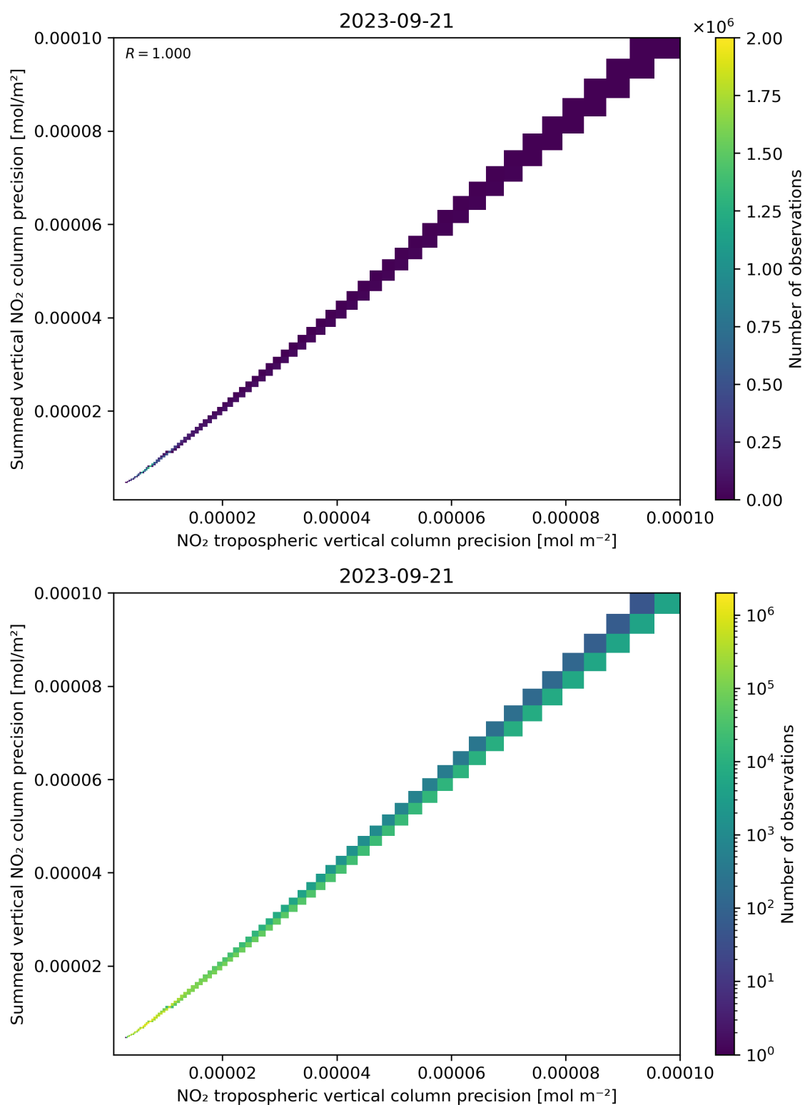
Figure 137: Scatter density plot of “NO 2 tropospheric vertical column precision” against “Summed vertical NO 2 column precision” for 2023-09-20 to 2023-09-22.
