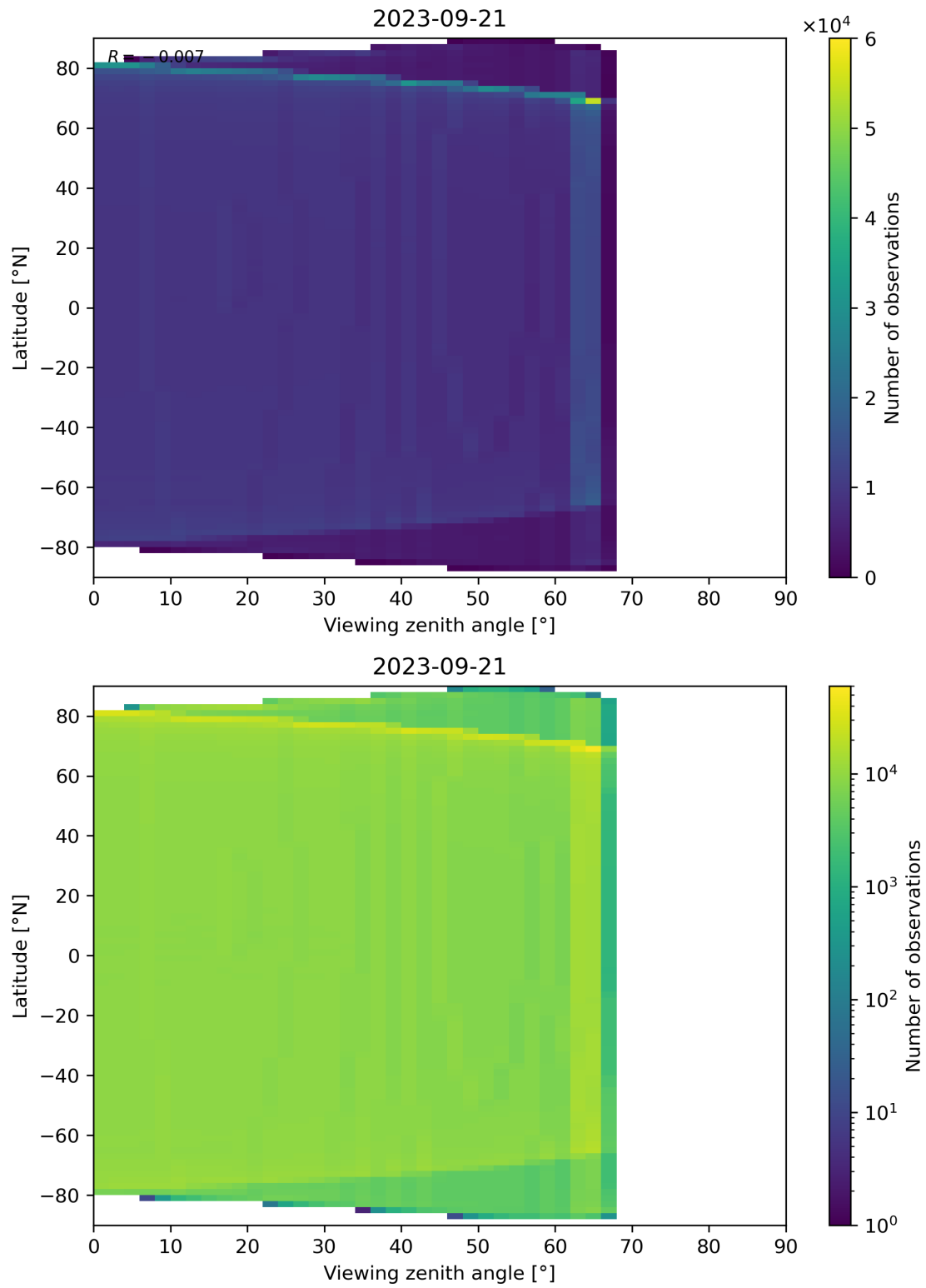
Figure 163: Scatter density plot of “Viewing zenith angle” against “Latitude” for 2023-09-20 to 2023-09-22.
