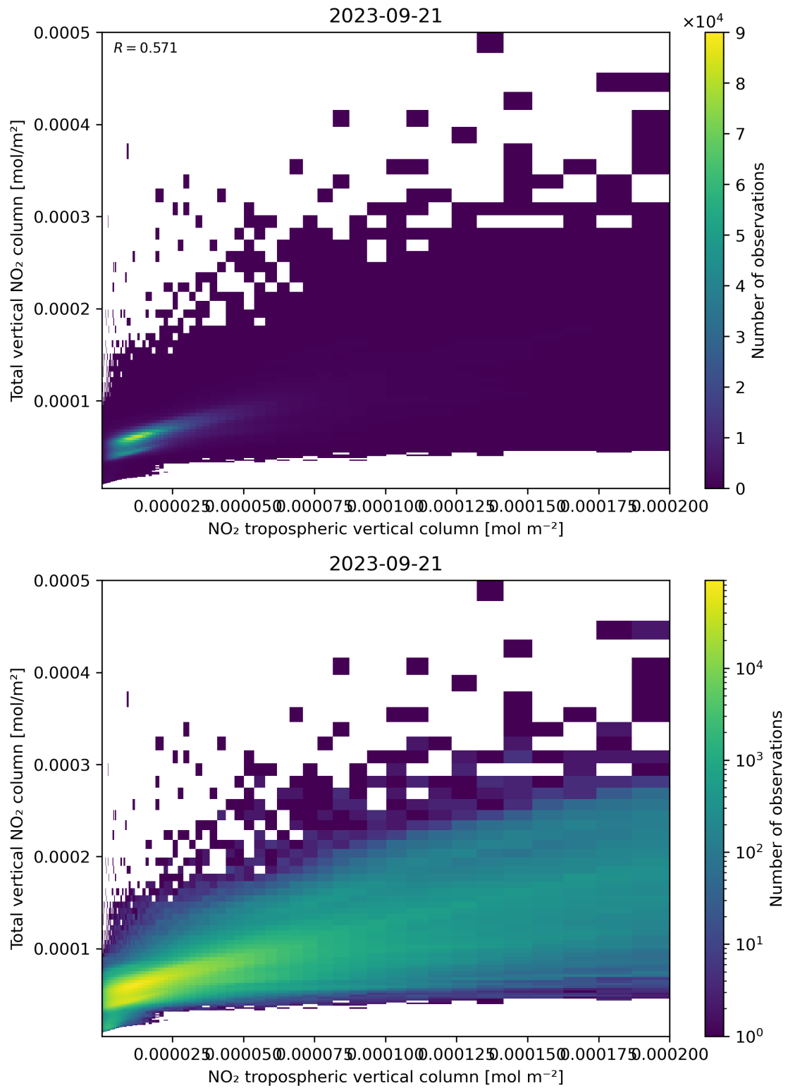
Figure 128: Scatter density plot of “NO 2 tropospheric vertical column” against “Total vertical NO 2 column” for 2023-09-20 to 2023-09-22.
