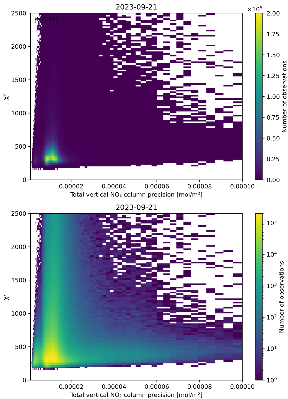
Figure 116: Scatter density plot of “Total vertical NO 2 column precision” against “ \chi^2 ” for 2023-09-20 to 2023-09-22.
