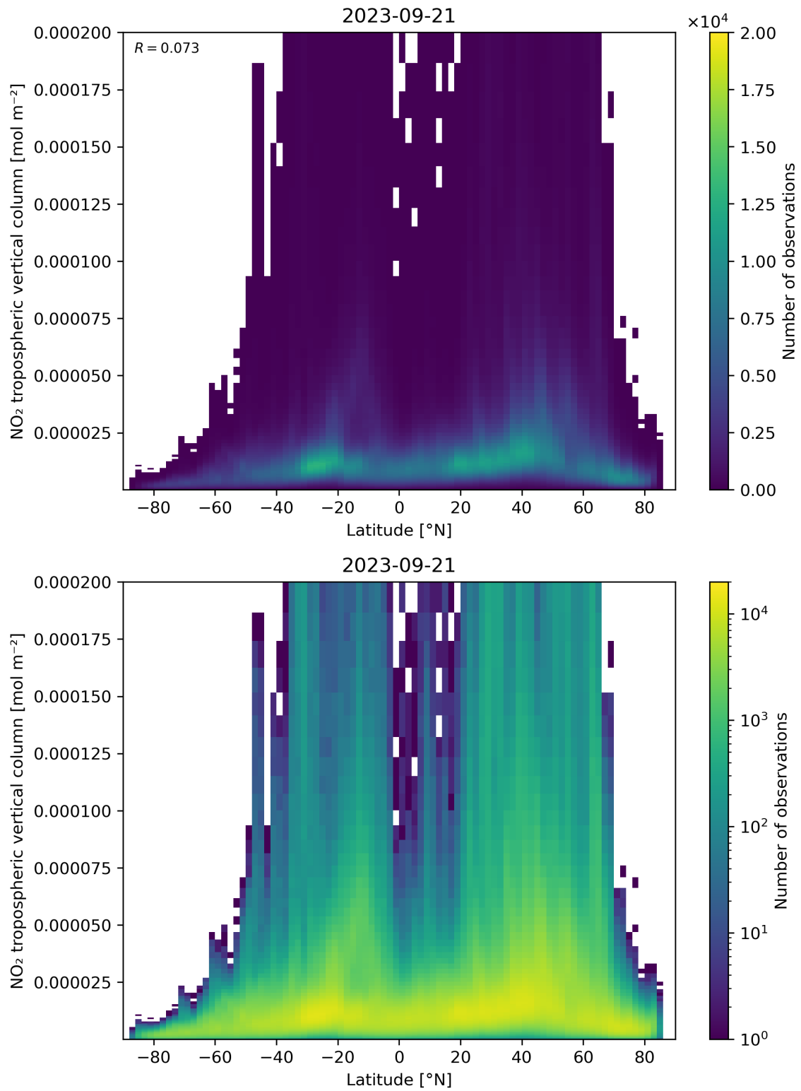
Figure 92: Scatter density plot of “Latitude” against “NO 2 tropospheric vertical column” for 2023-09-20 to 2023-09-22.
