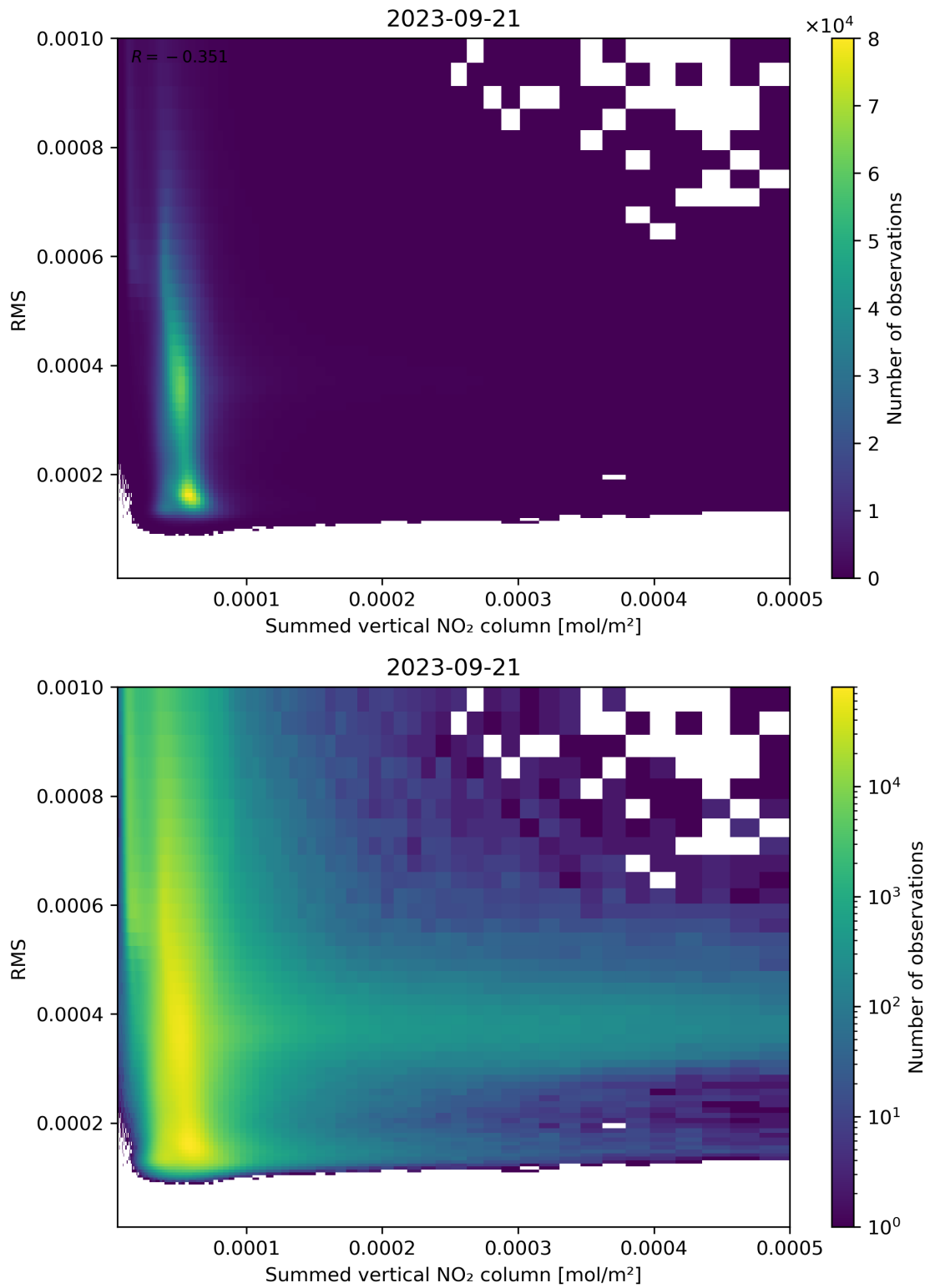
Figure 109: Scatter density plot of “Summed vertical NO 2 column” against “RMS” for 2023-09-20 to 2023-09-22.
