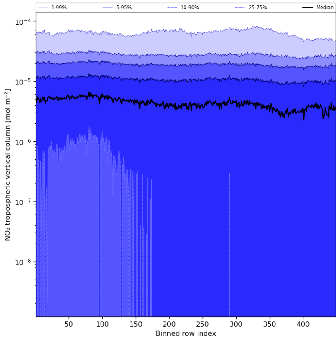
Figure 46: Along track statistics of “NO 2 tropospheric vertical column” for 2023-09-20 to 2023-09-22
