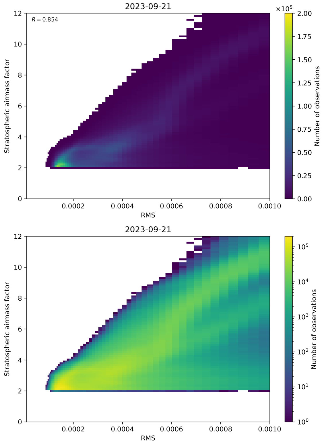
Figure 144: Scatter density plot of “RMS” against “Stratospheric airmass factor” for 2023-09-20 to 2023-09-22.
