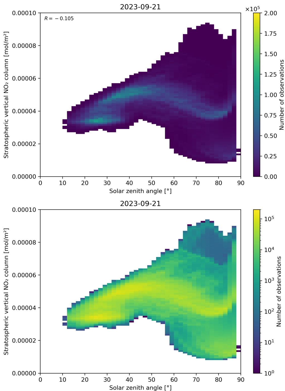
Figure 150: Scatter density plot of “Solar zenith angle” against “Stratospheric vertical NO 2 column” for 2023-09-20 to 2023-09-22.
