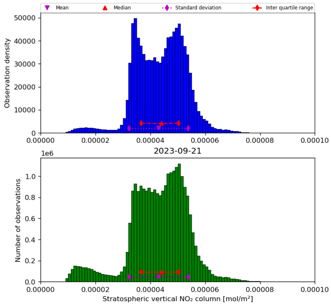
Figure 36: Histogram of “Stratospheric vertical NO 2 column” for 2023-09-20 to 2023-09-22
