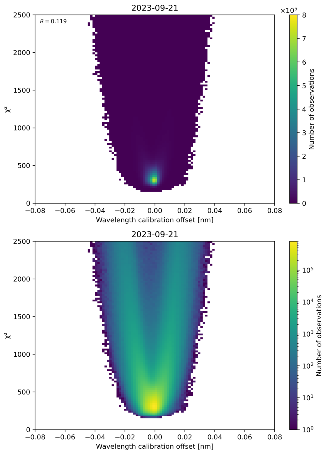
Figure 175: Scatter density plot of “Wavelength calibration offset” against “ \chi^2 ” for 2023-09-20 to 2023-09-22.
