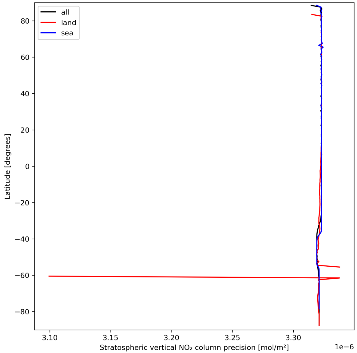
Figure 20: Zonal average of “Stratospheric vertical NO 2 column precision” for 2023-09-20 to 2023-09-22.
