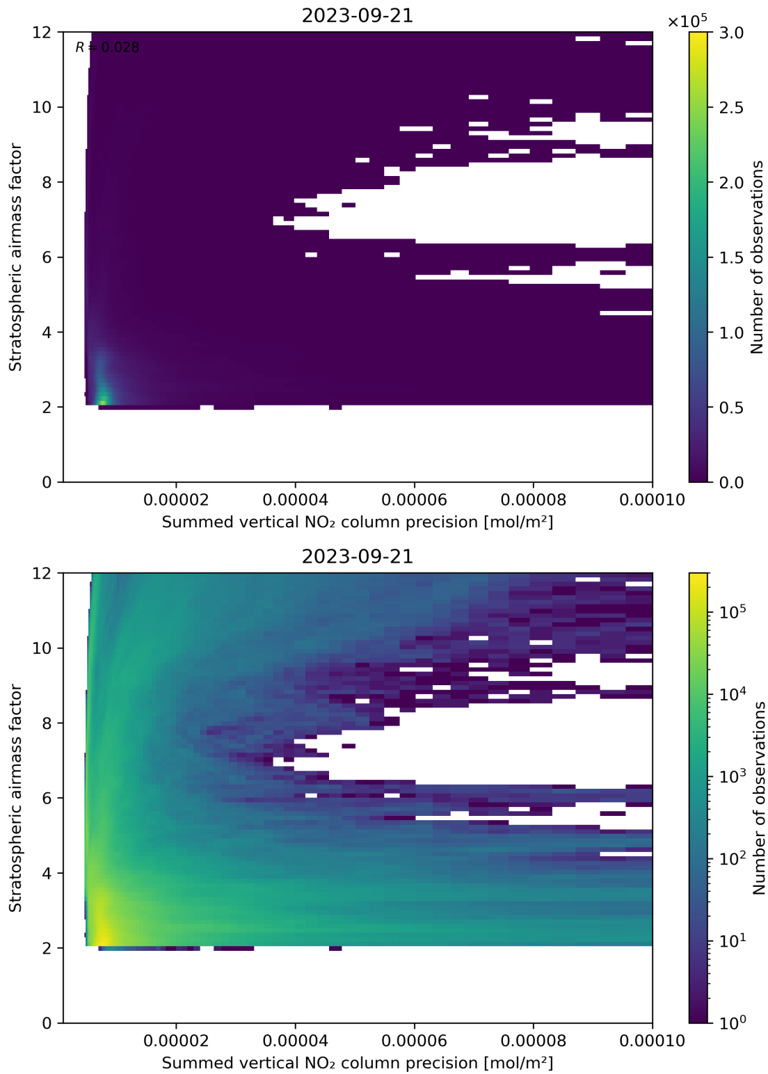
Figure 106: Scatter density plot of “Summed vertical NO 2 column precision” against “Stratospheric airmass factor” for 2023-09-20 to 2023-09-22.
