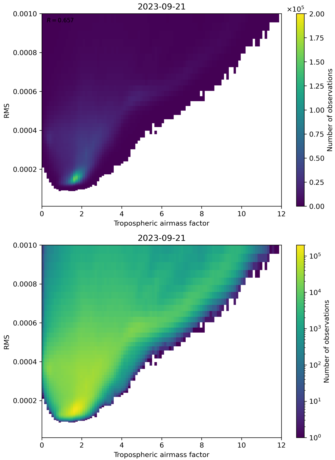
Figure 79: Scatter density plot of “Tropospheric airmass factor” against “RMS” for 2023-09-20 to 2023-09-22.
