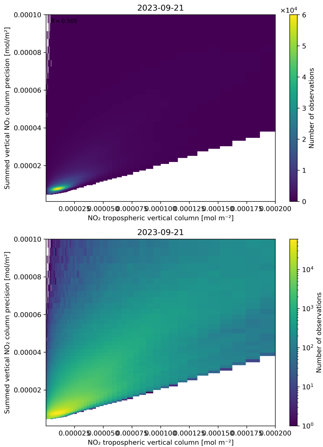
Figure 127: Scatter density plot of “NO 2 tropospheric vertical column” against “Summed vertical NO 2 column precision” for 2023-09-20 to 2023-09-22.
