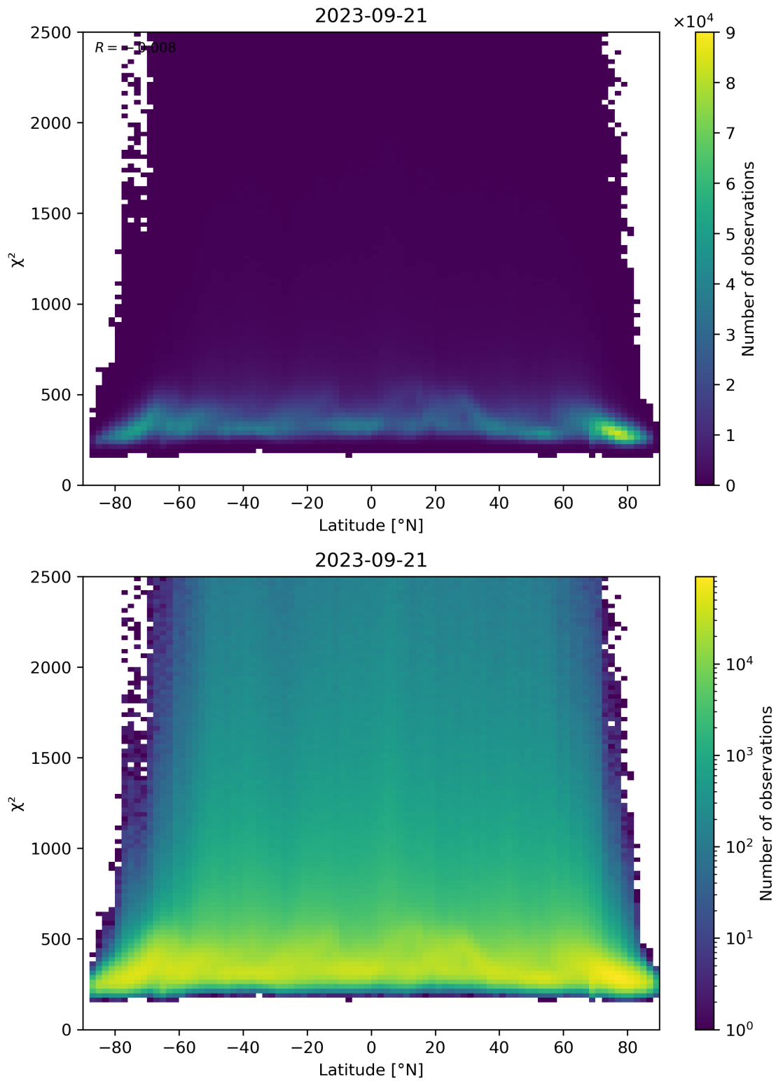
Figure 86: Scatter density plot of “Latitude” against “ \chi^2 ” for 2023-09-20 to 2023-09-22.
