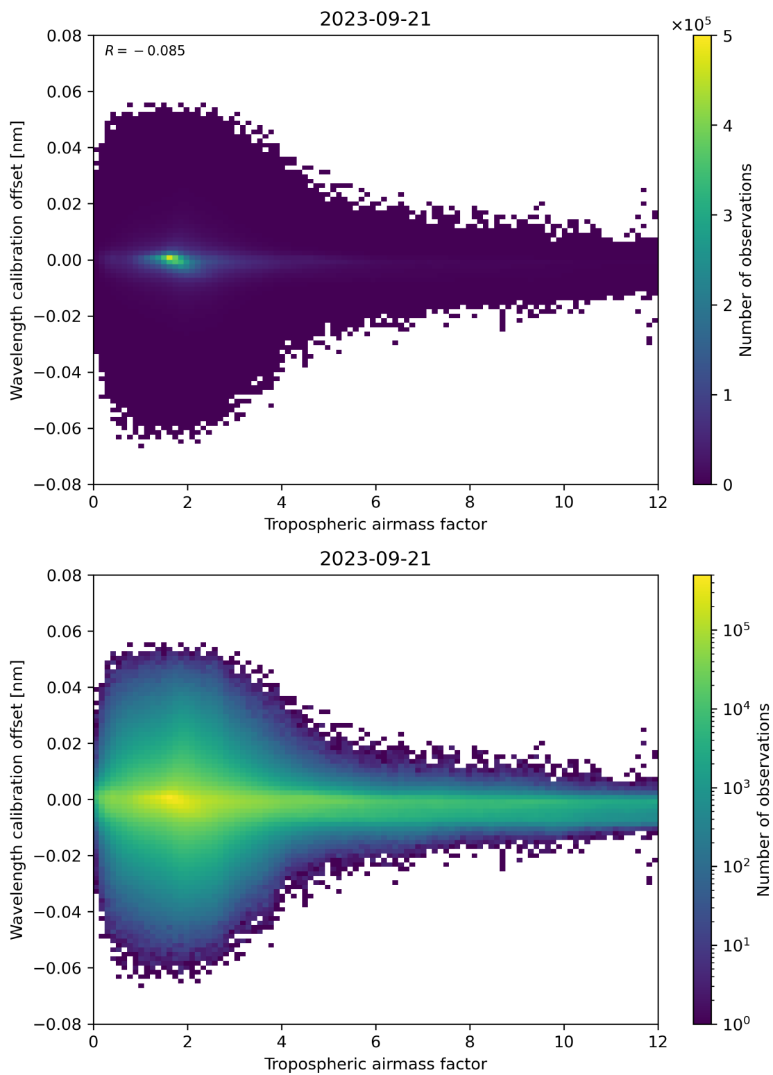
Figure 80: Scatter density plot of “Tropospheric airmass factor” against “Wavelength calibration offset” for 2023-09-20 to 2023-09-22.
