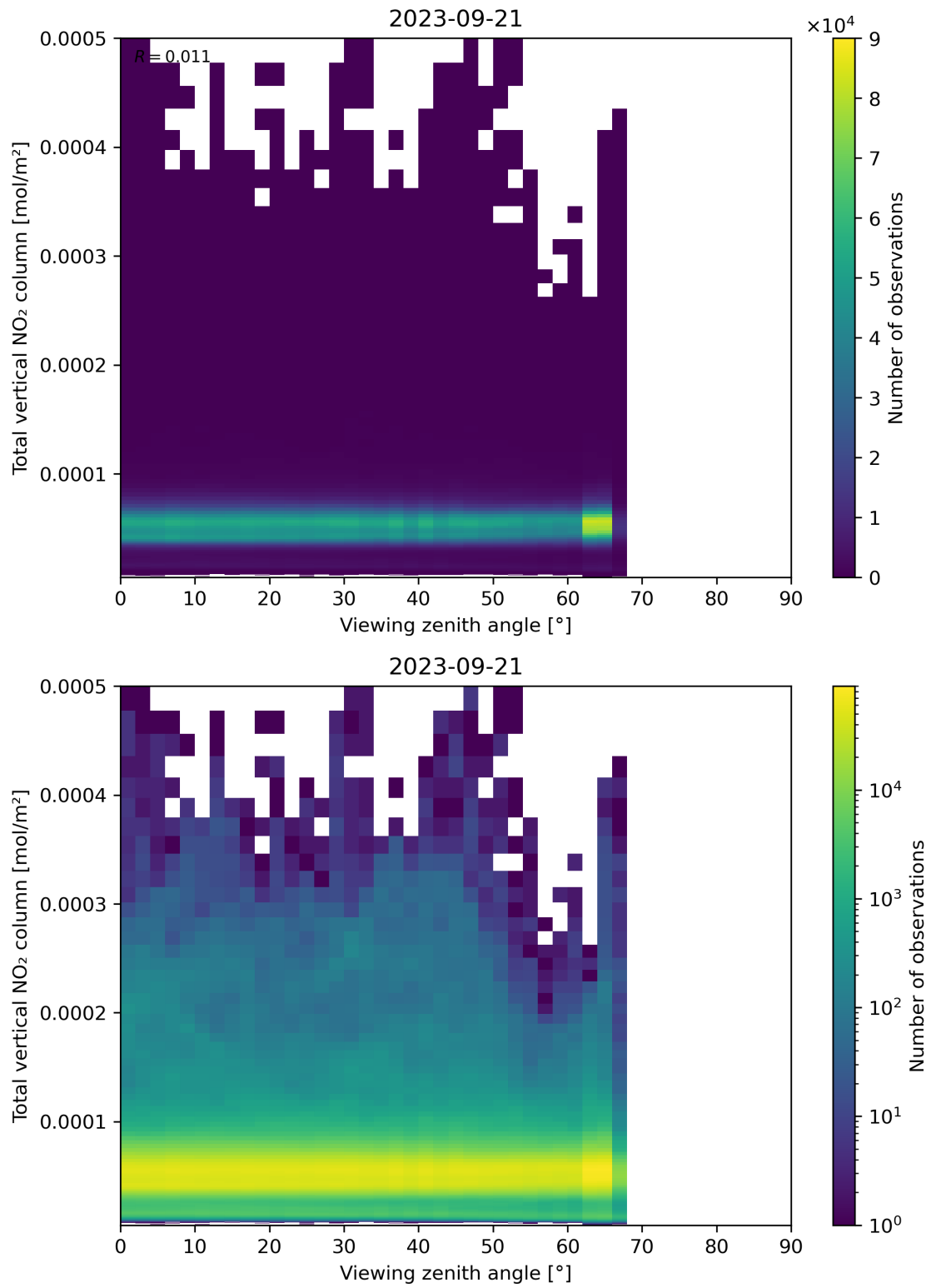
Figure 167: Scatter density plot of “Viewing zenith angle” against “Total vertical NO 2 column” for 2023-09-20 to 2023-09-22.
