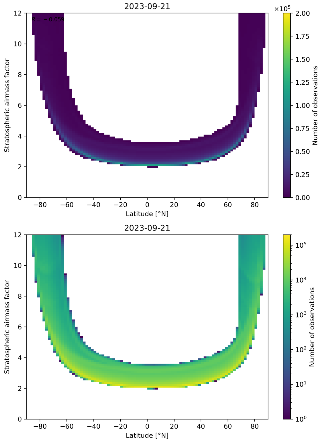
Figure 83: Scatter density plot of “Latitude” against “Stratospheric airmass factor” for 2023-09-20 to 2023-09-22.
