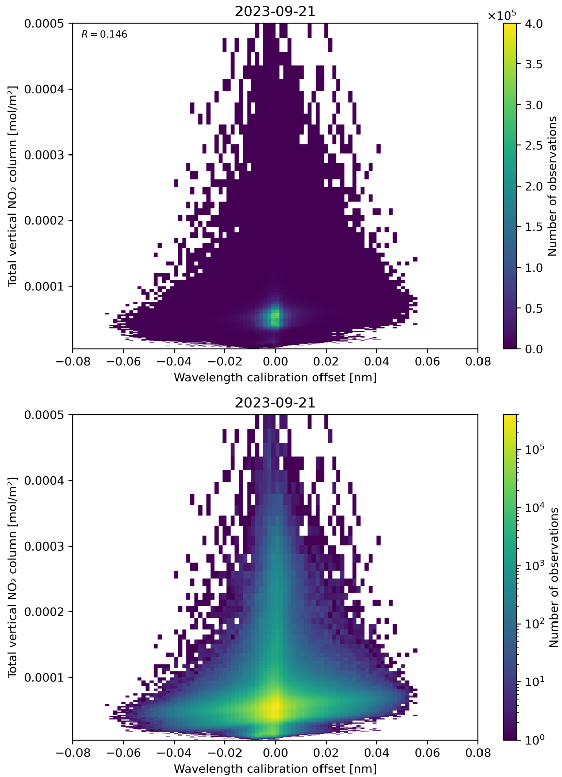
Figure 179: Scatter density plot of “Wavelength calibration offset” against “Total vertical NO 2 column” for 2023-09-20 to 2023-09-22.
