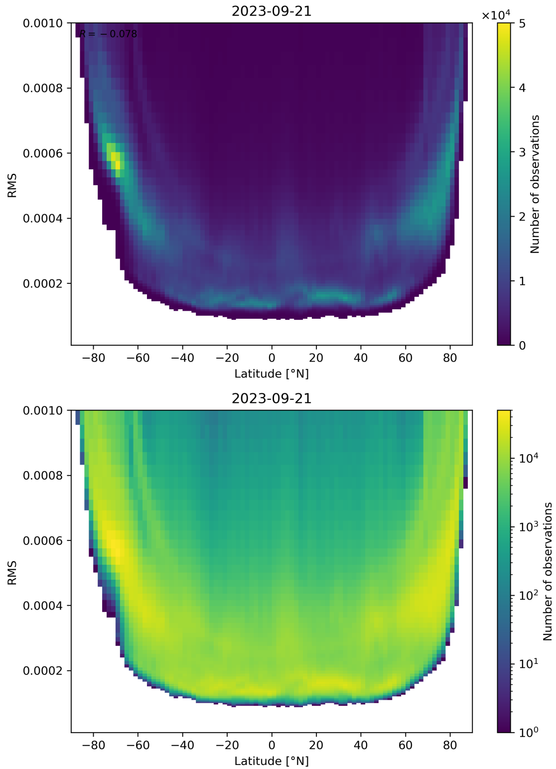
Figure 94: Scatter density plot of “Latitude” against “RMS” for 2023-09-20 to 2023-09-22.
