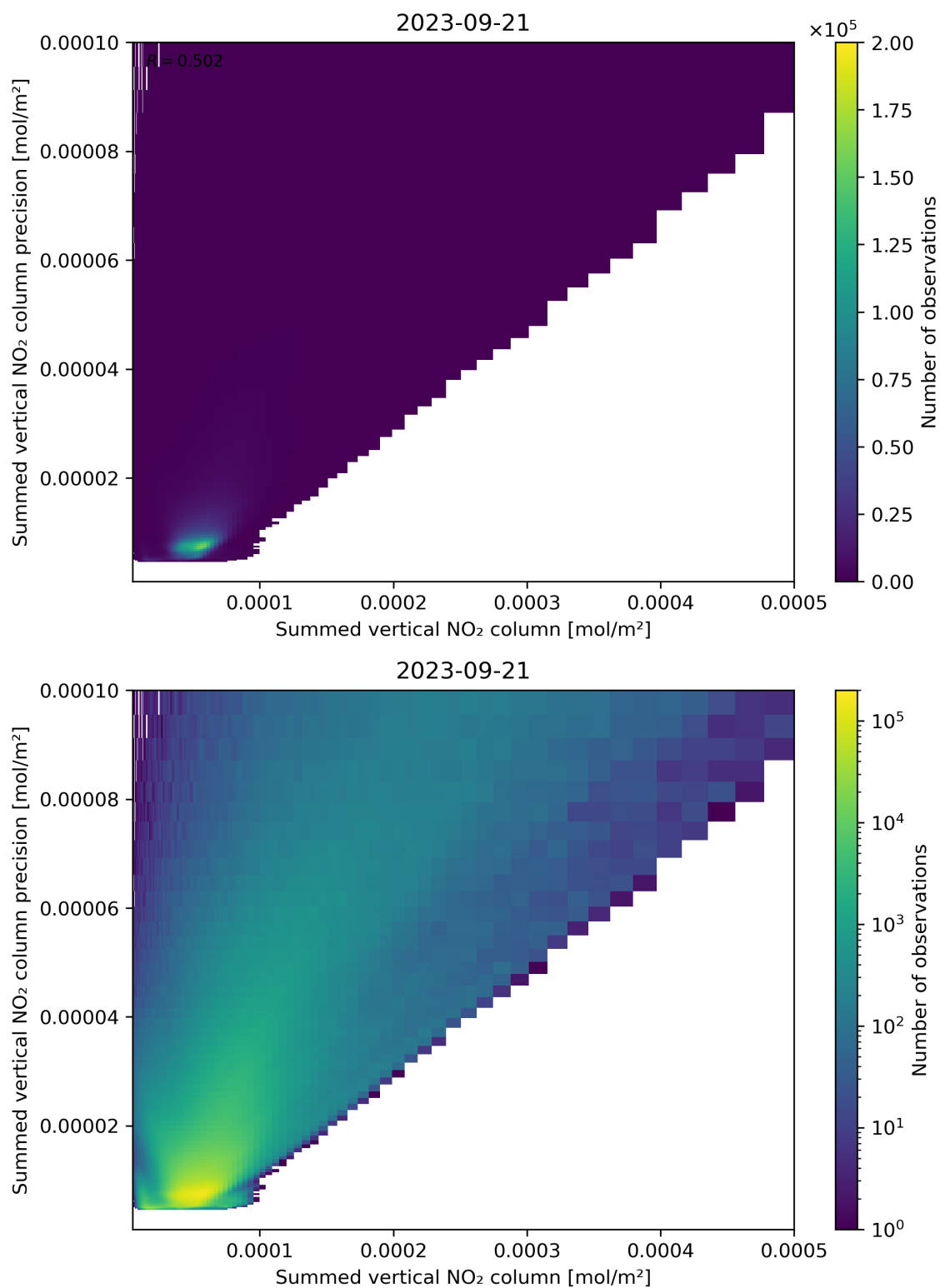
Figure 105: Scatter density plot of “Summed vertical NO 2 column” against “Summed vertical NO 2 column precision” for 2023-09-20 to 2023-09-22.
