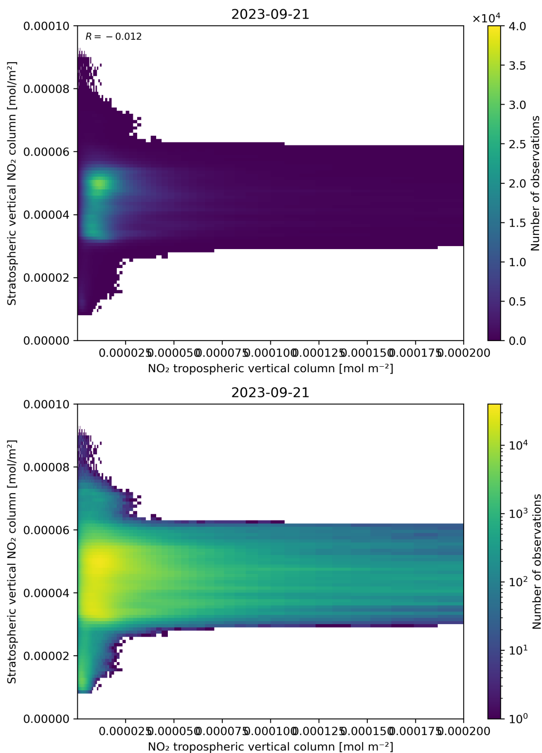
Figure 125: Scatter density plot of “NO 2 tropospheric vertical column” against “Stratospheric vertical NO 2 column” for 2023-09-20 to 2023-09-22.
