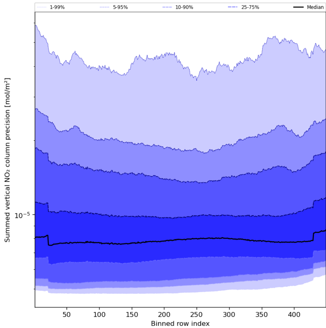
Figure 58: Along track statistics of “Summed vertical NO 2 column precision” for 2023-09-20 to 2023-09-22
