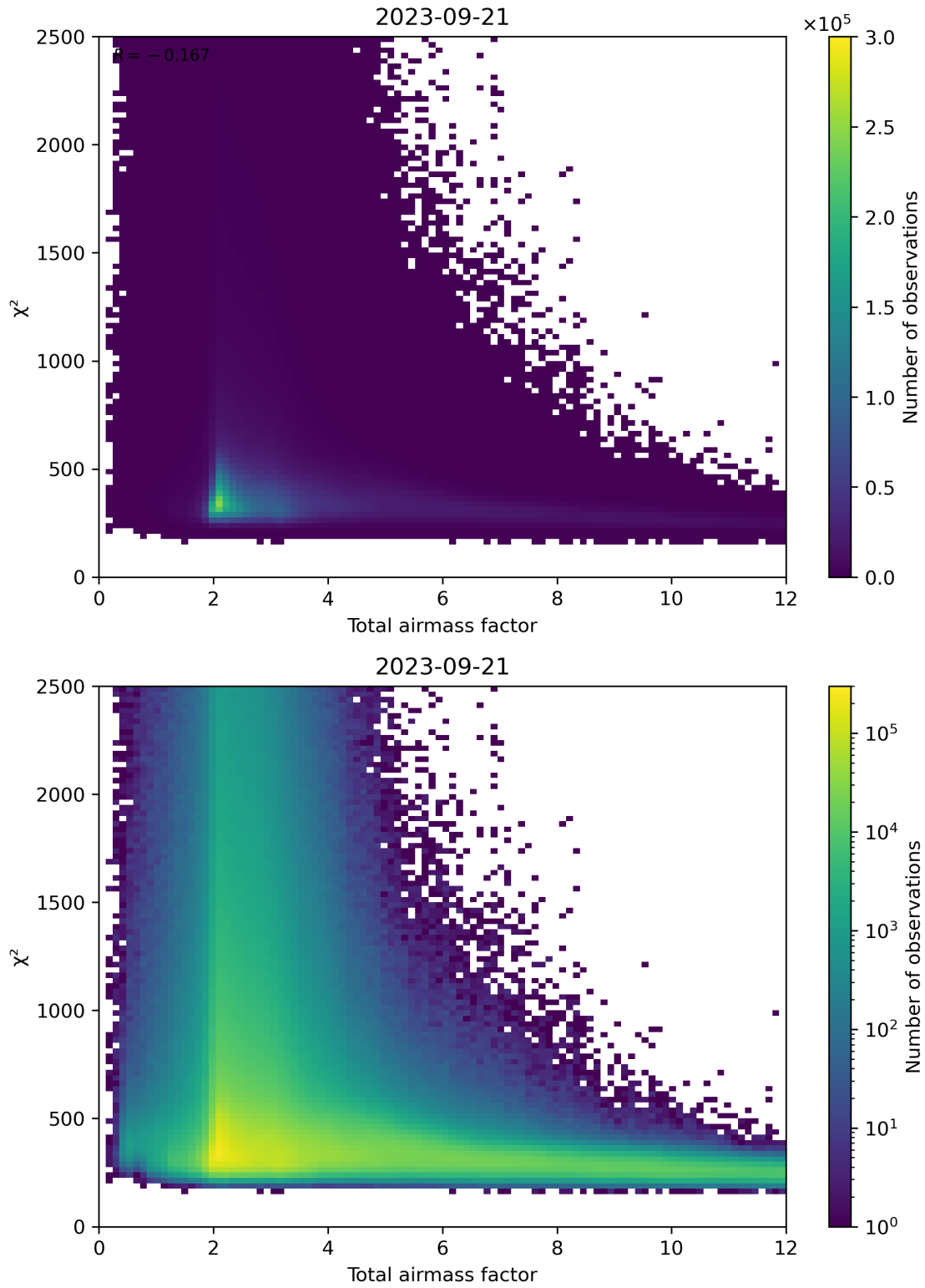
Figure 63: Scatter density plot of “Total airmass factor” against “ \chi^2 ” for 2023-09-20 to 2023-09-22.
