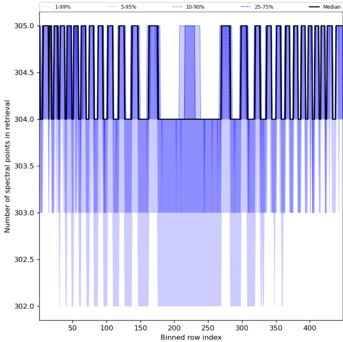
Figure 50: Along track statistics of “Number of spectral points in retrieval” for 2023-09-20 to 2023-09-22
