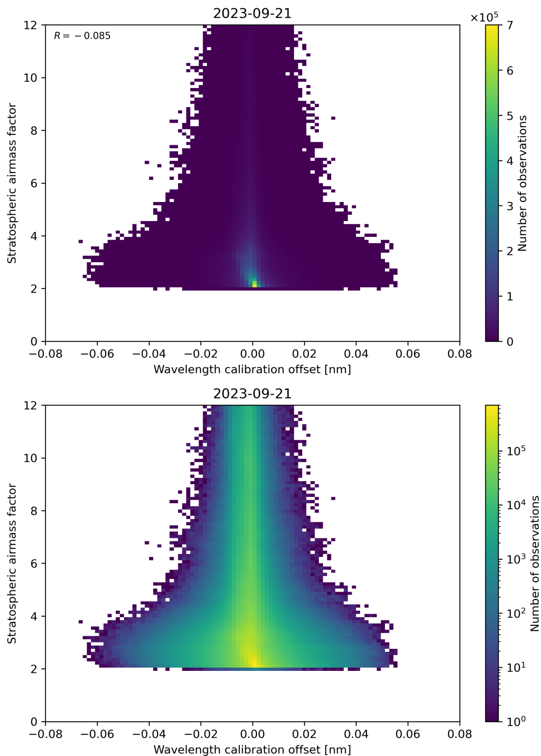
Figure 174: Scatter density plot of “Wavelength calibration offset” against “Stratospheric air mass factor” for 2023-09-20 to 2023-09-22.
