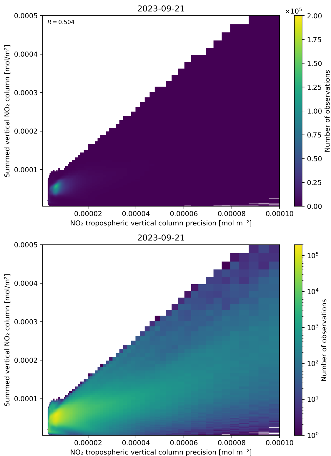
Figure 136: Scatter density plot of “NO 2 tropospheric vertical column precision” against “Summed vertical NO 2 column” for 2023-09-20 to 2023-09-22.
