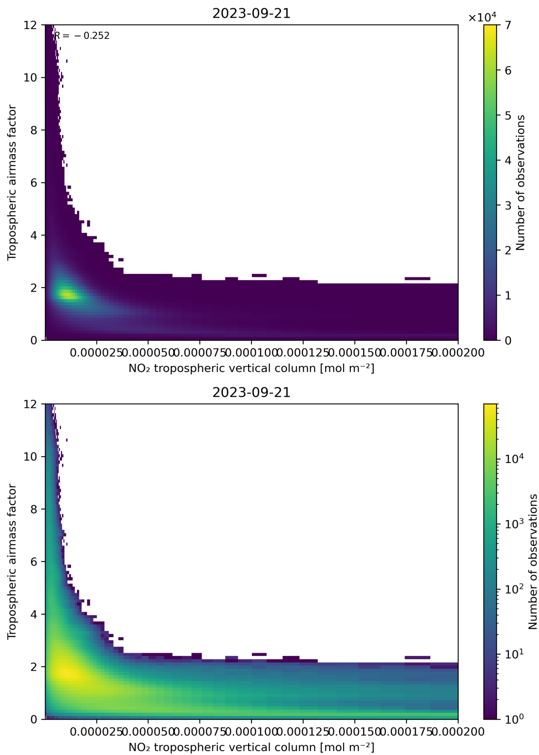
Figure 123: Scatter density plot of “NO 2 tropospheric vertical column” against “Tropospheric air mass factor” for 2023-09-20 to 2023-09-22.
