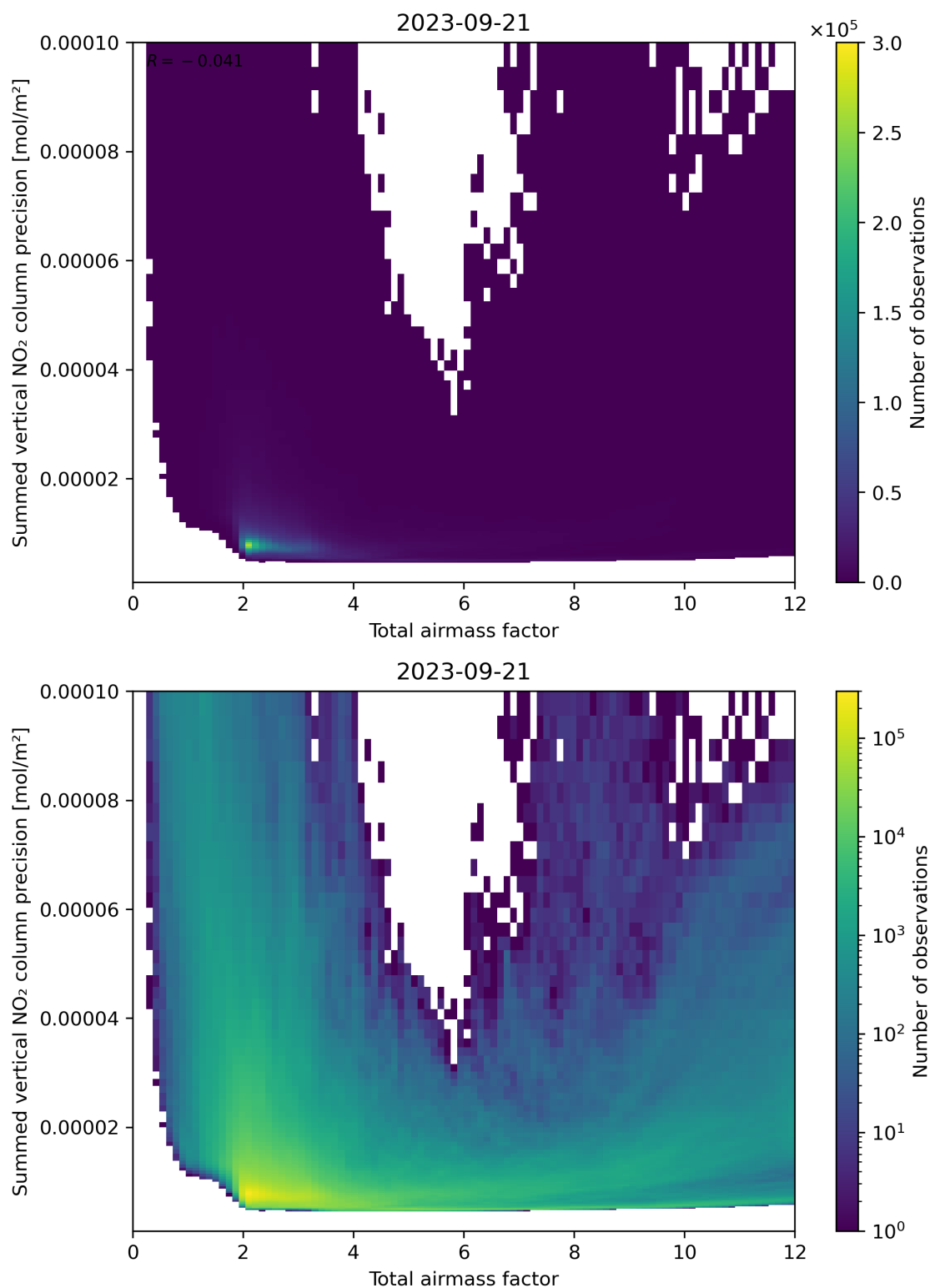
Figure 66: Scatter density plot of “Total airmass factor” against “Summed vertical NO 2 column precision” for 2023-09-20 to 2023-09-22.
