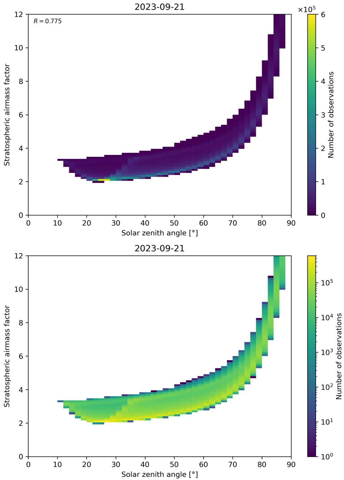
Figure 145: Scatter density plot of “Solar zenith angle” against “Stratospheric airmass factor” for 2023-09-20 to 2023-09-22.
