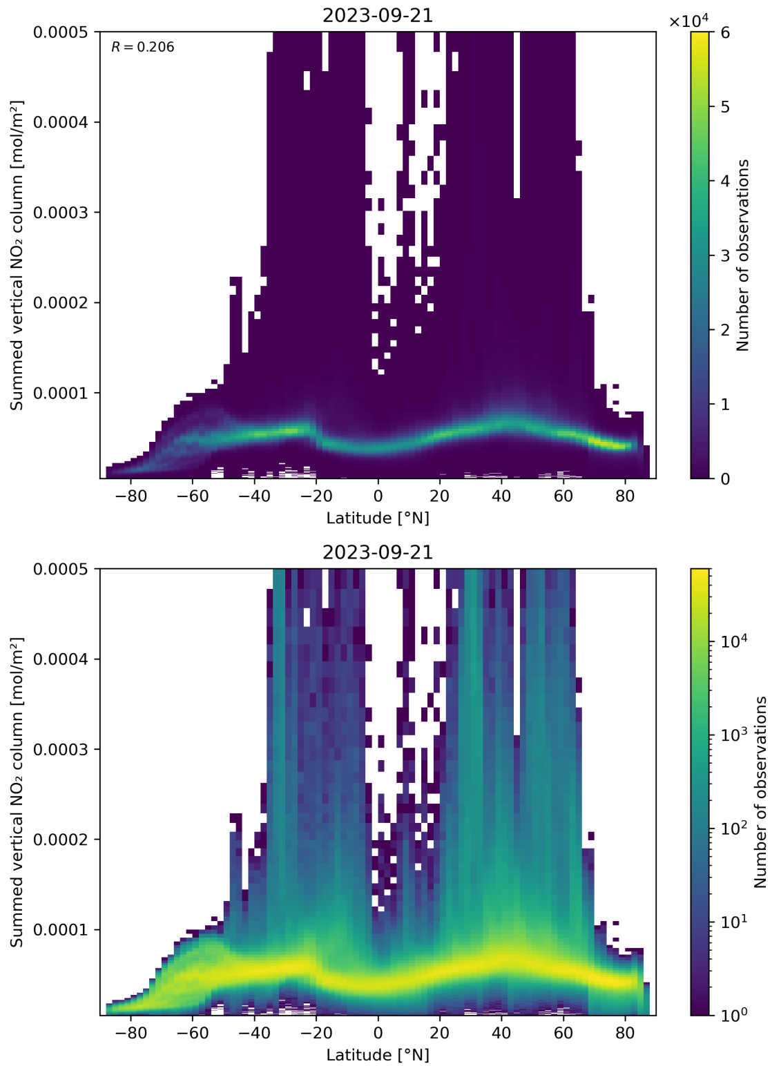
Figure 88: Scatter density plot of “Latitude” against “Summed vertical NO 2 column” for 2023-09-20 to 2023-09-22.
