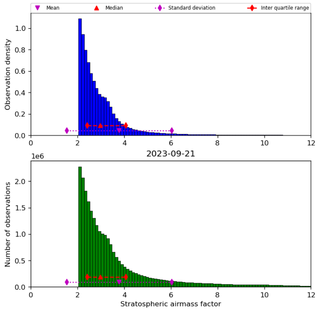
Figure 44: Histogram of “Stratospheric airmass factor” for 2023-09-20 to 2023-09-22
