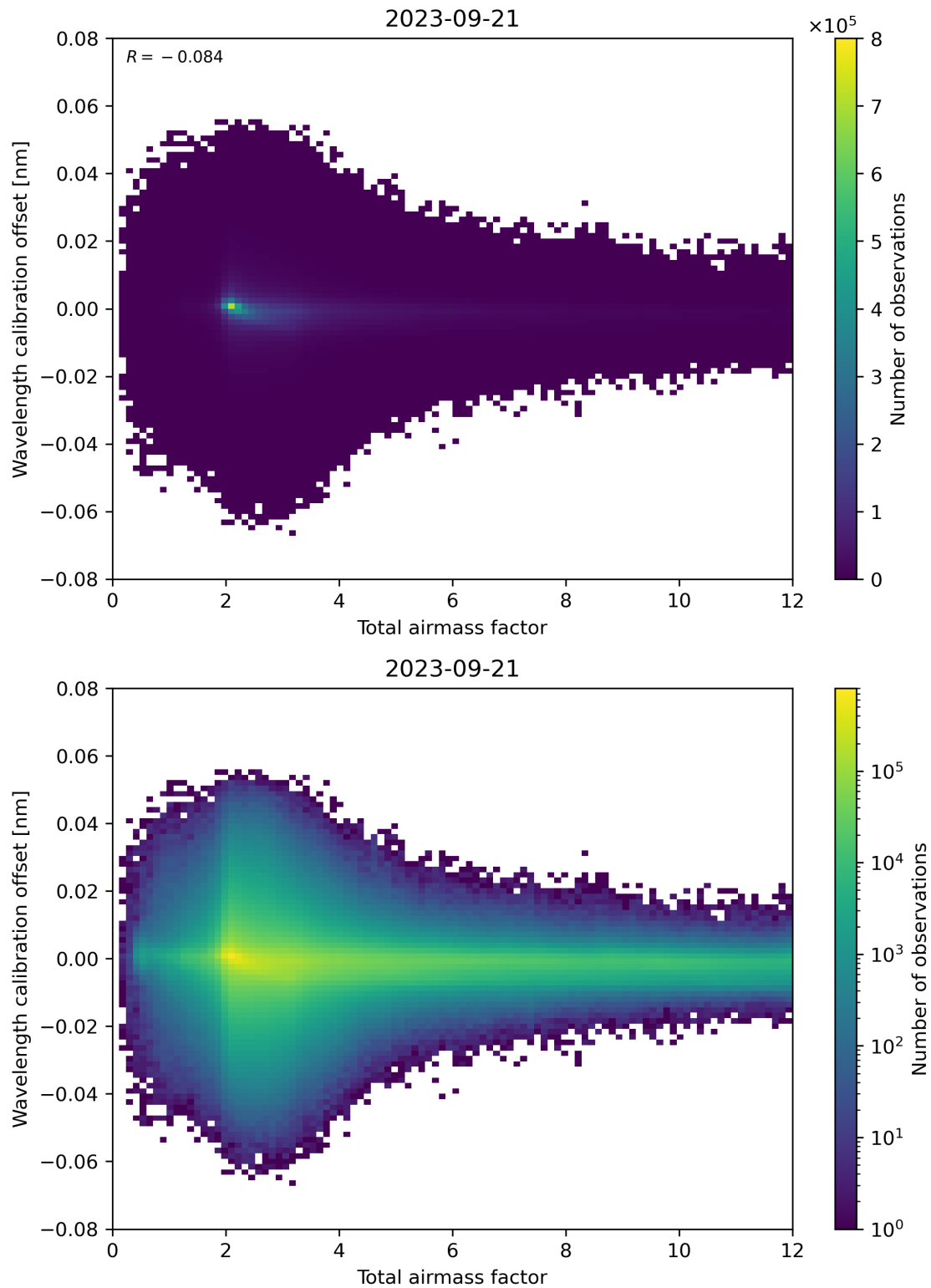
Figure 70: Scatter density plot of “Total airmass factor” against “Wavelength calibration offset” for 2023-09-20 to 2023-09-22.
