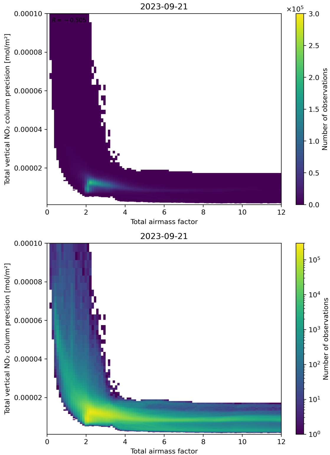
Figure 68: Scatter density plot of “Total airmass factor” against “Total vertical NO 2 column precision” for 2023-09-20 to 2023-09-22.
