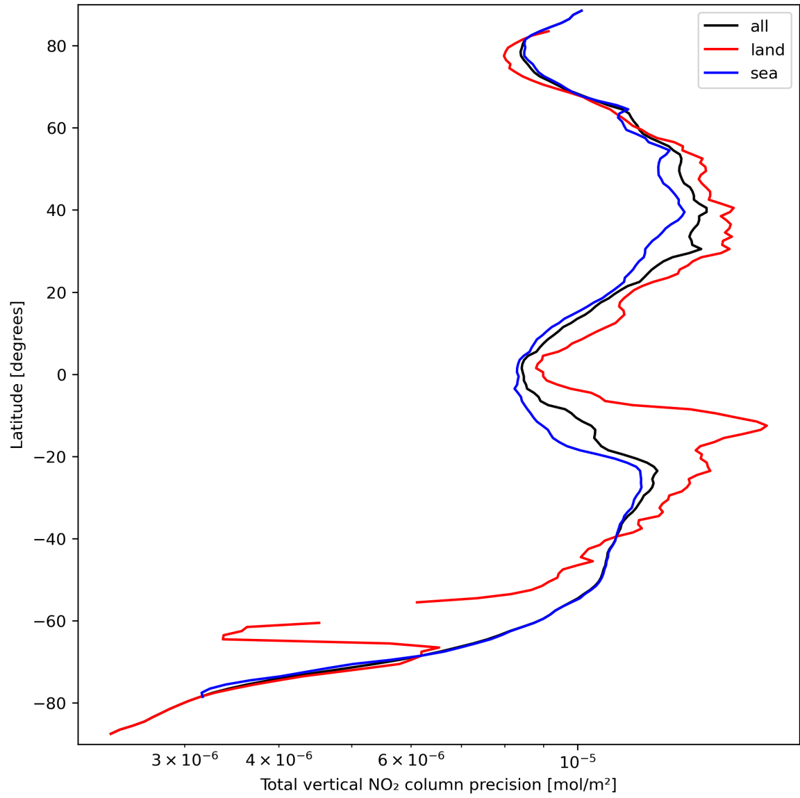
Figure 22: Zonal average of “Total vertical NO 2 column precision” for 2023-09-20 to 2023-09-22.
