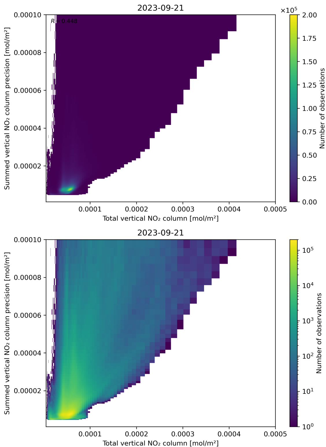
Figure 113: Scatter density plot of “Total vertical NO 2 column” against “Summed vertical NO 2 column precision” for 2023-09-20 to 2023-09-22.
