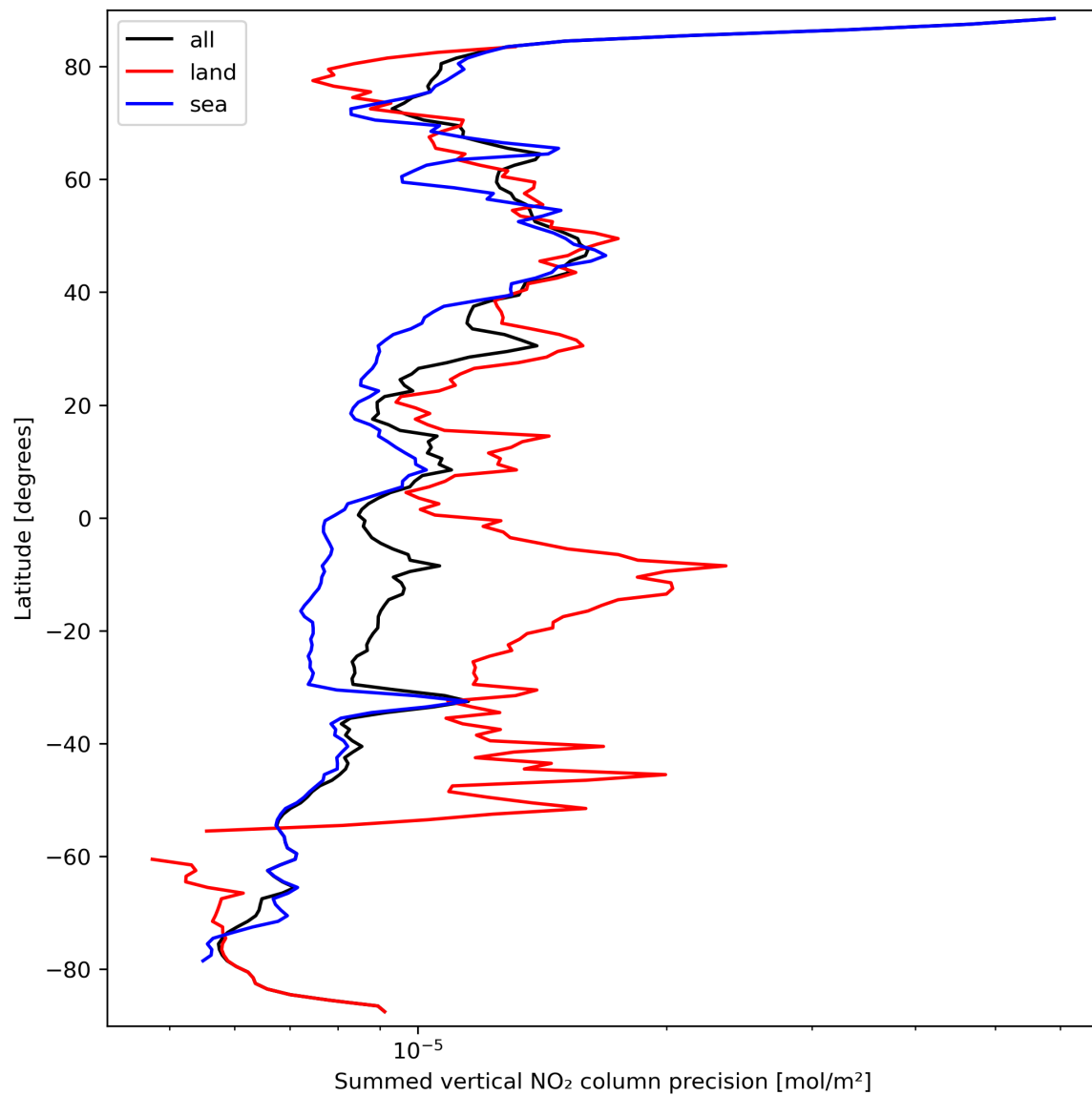
Figure 24: Zonal average of “Summed vertical NO 2 column precision” for 2023-09-20 to 2023-09-22.
