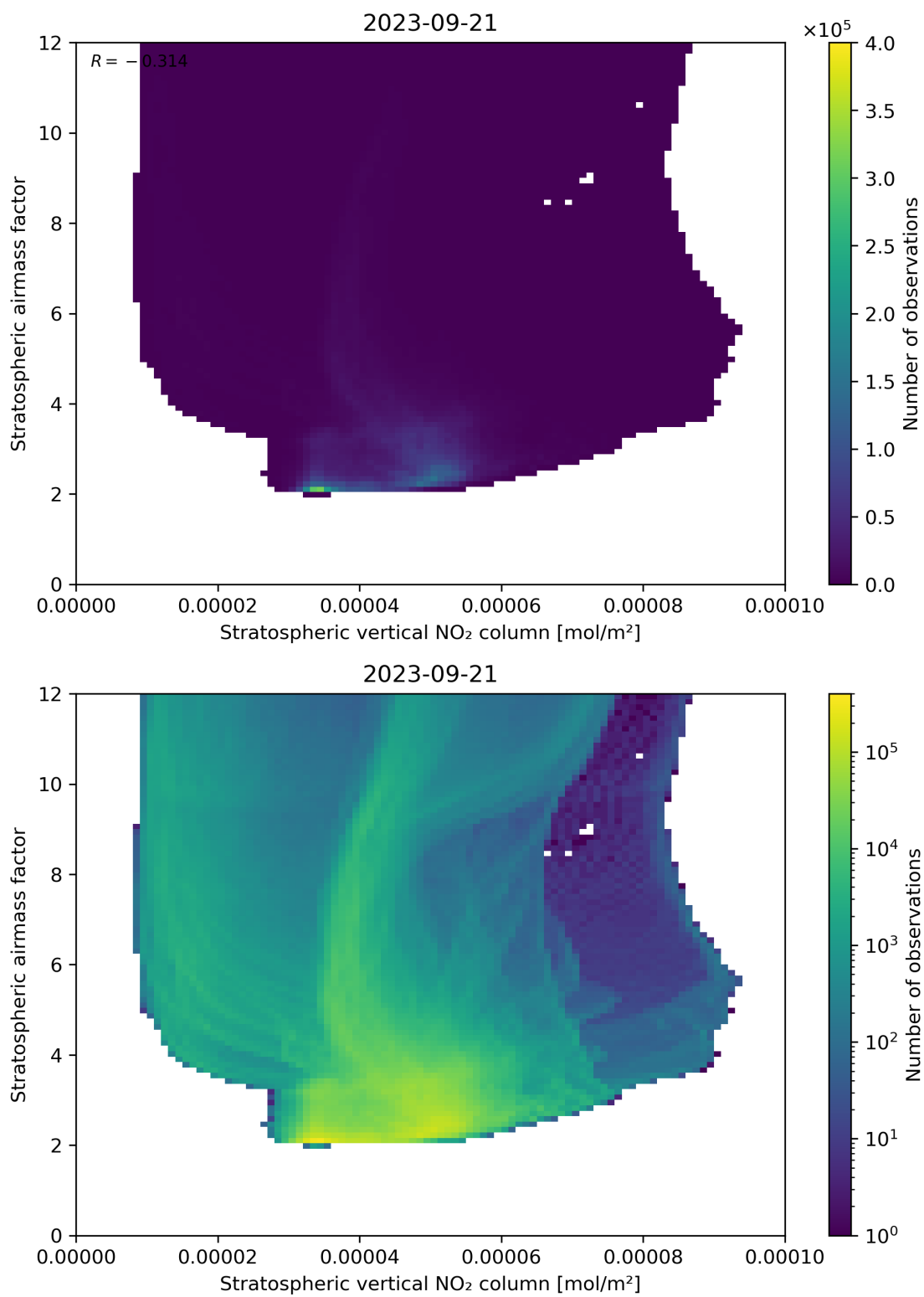
Figure 96: Scatter density plot of “Stratospheric vertical NO 2 column” against “Stratospheric airmass factor” for 2023-09-20 to 2023-09-22.
