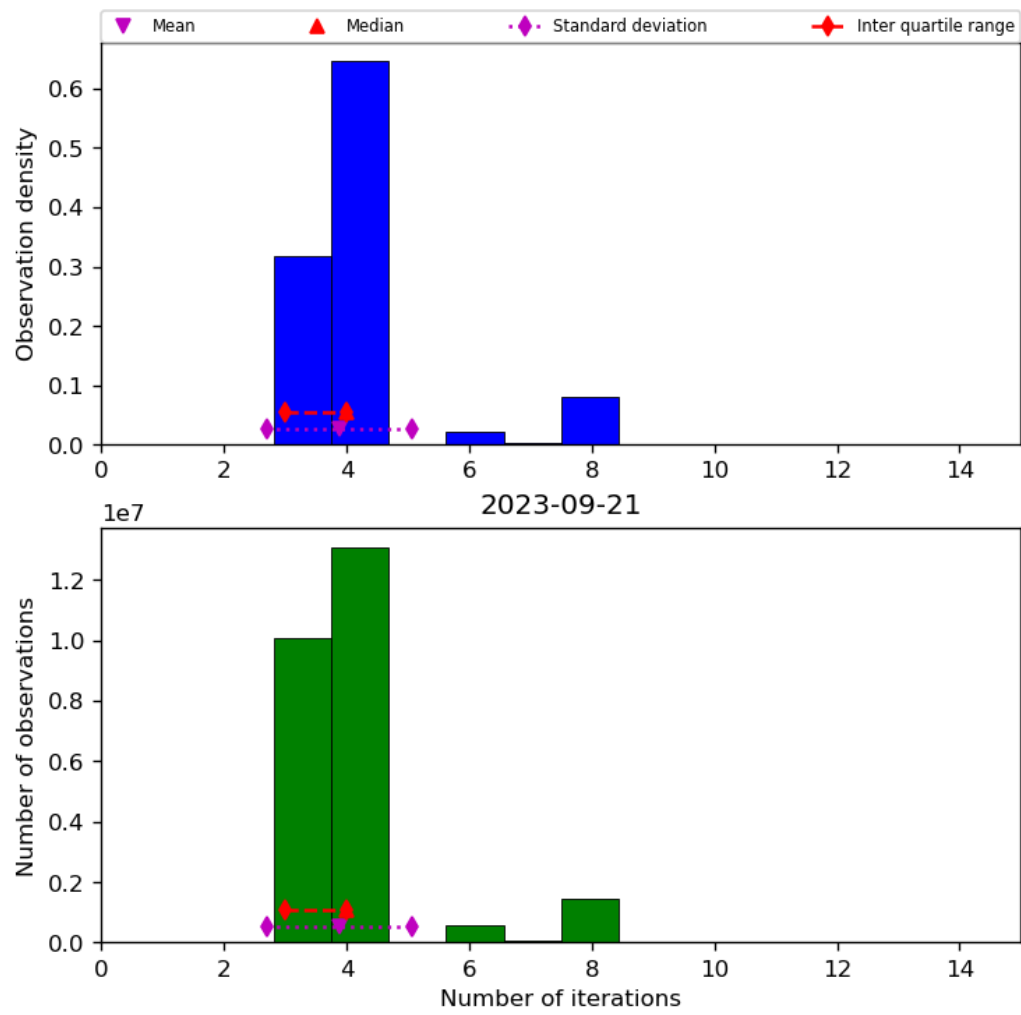
Figure 34: Histogram of “Number of iterations” for 2023-09-20 to 2023-09-22
