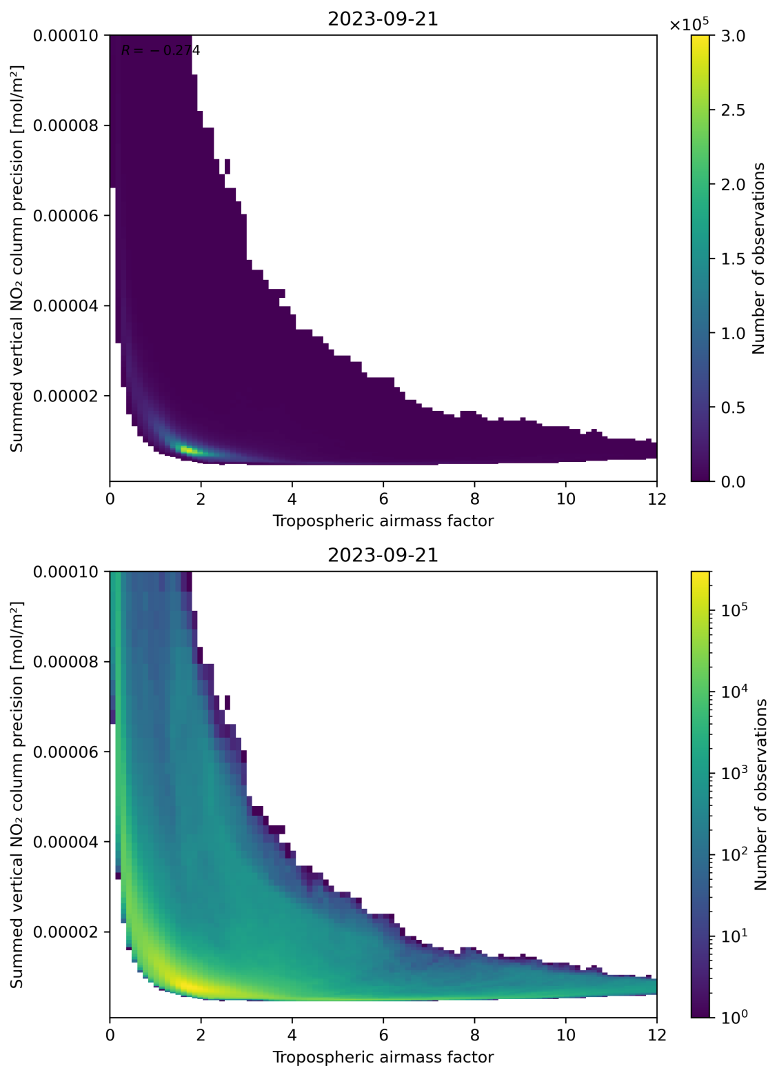
Figure 76: Scatter density plot of “Tropospheric airmass factor” against “Summed vertical NO 2 column precision” for 2023-09-20 to 2023-09-22.
