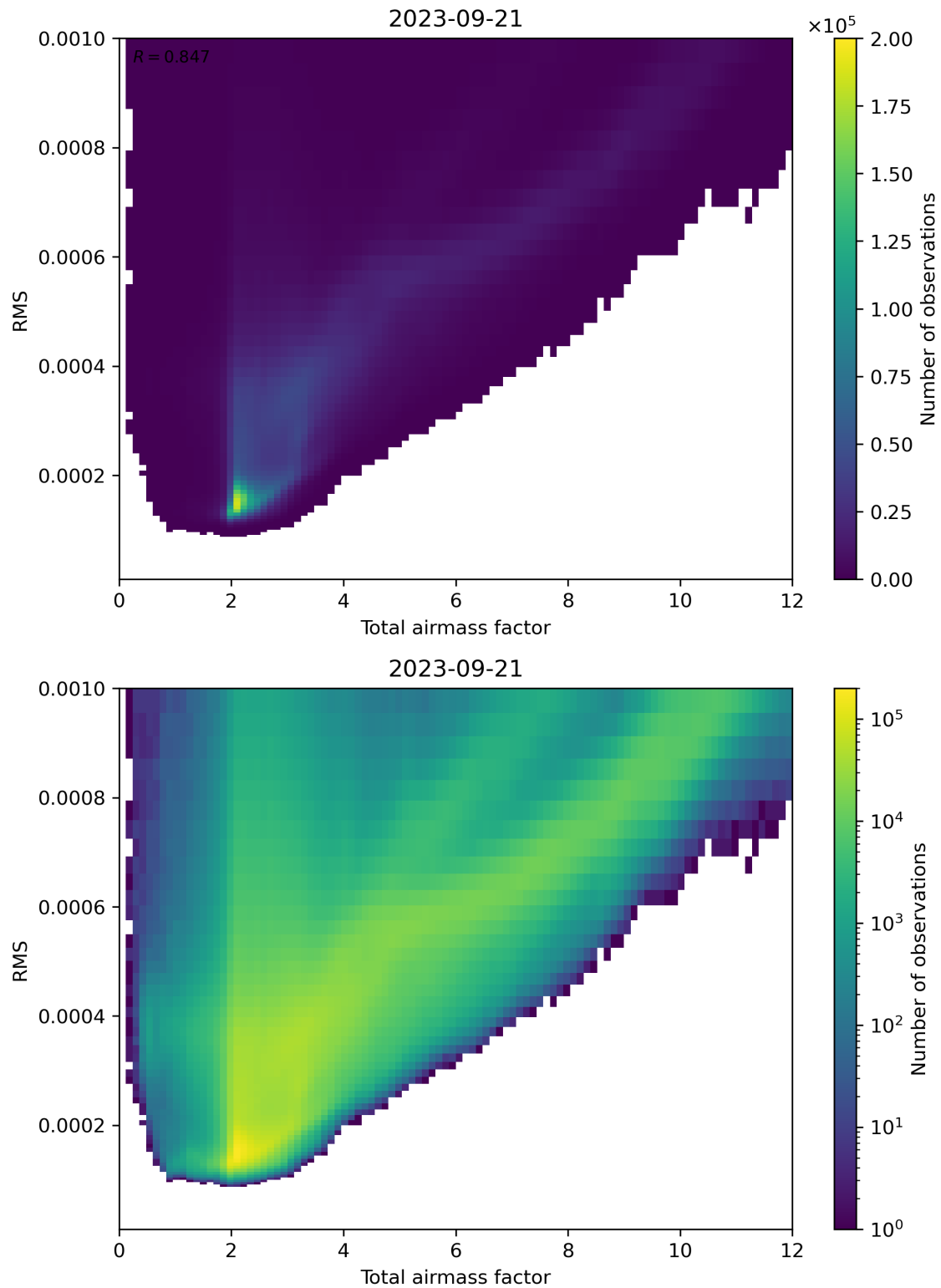
Figure 69: Scatter density plot of “Total airmass factor” against “RMS” for 2023-09-20 to 2023-09-22.
