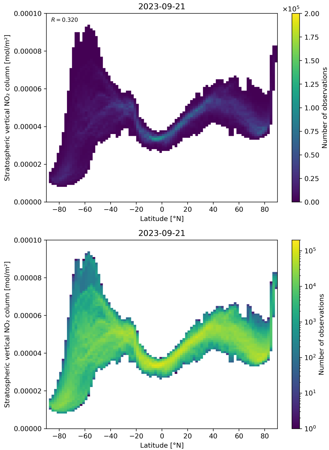
Figure 87: Scatter density plot of “Latitude” against “Stratospheric vertical NO 2 column” for 2023-09-20 to 2023-09-22.
