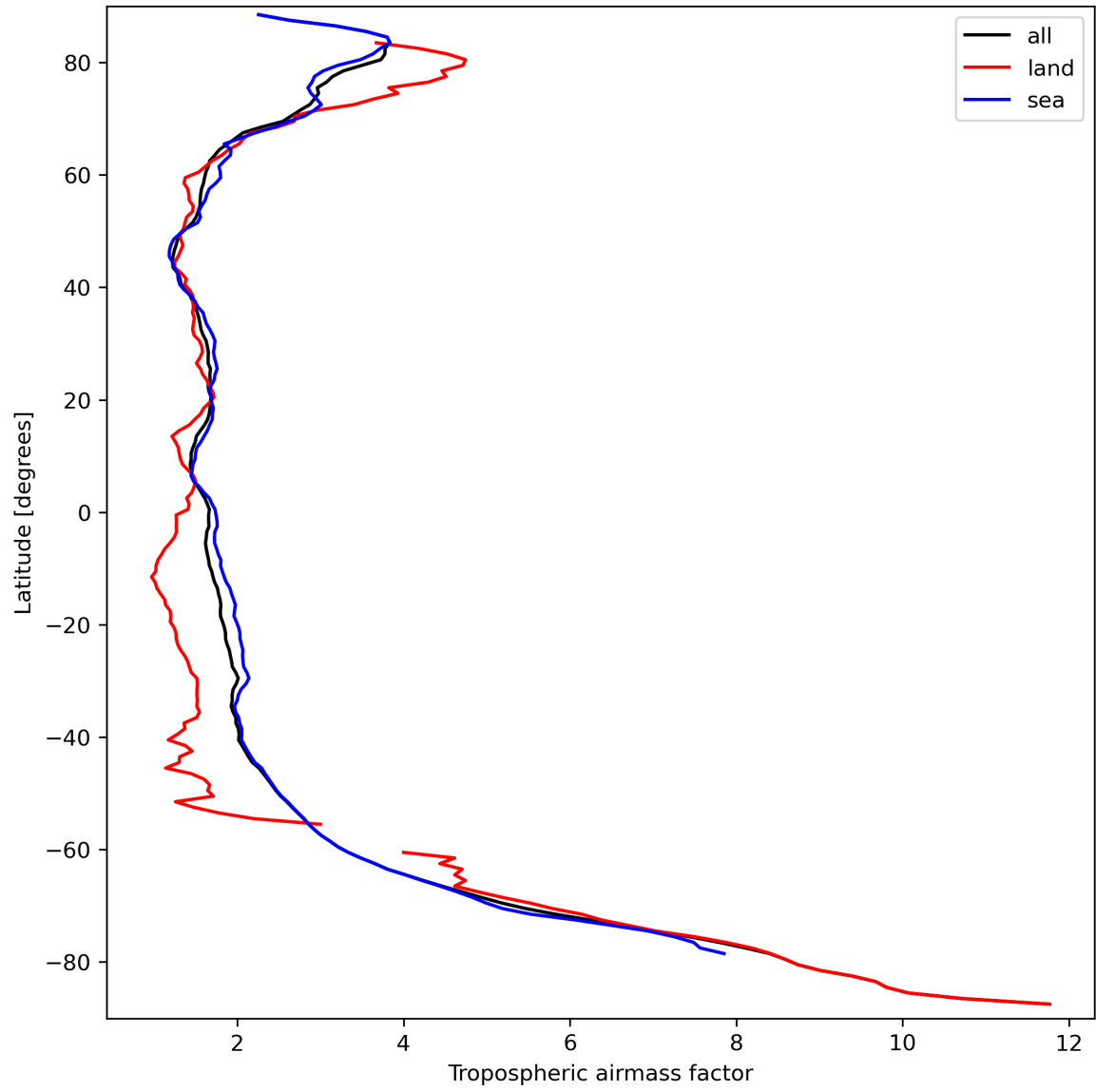
Figure 14: Zonal average of “Tropospheric airmass factor” for 2023-09-20 to 2023-09-22.
