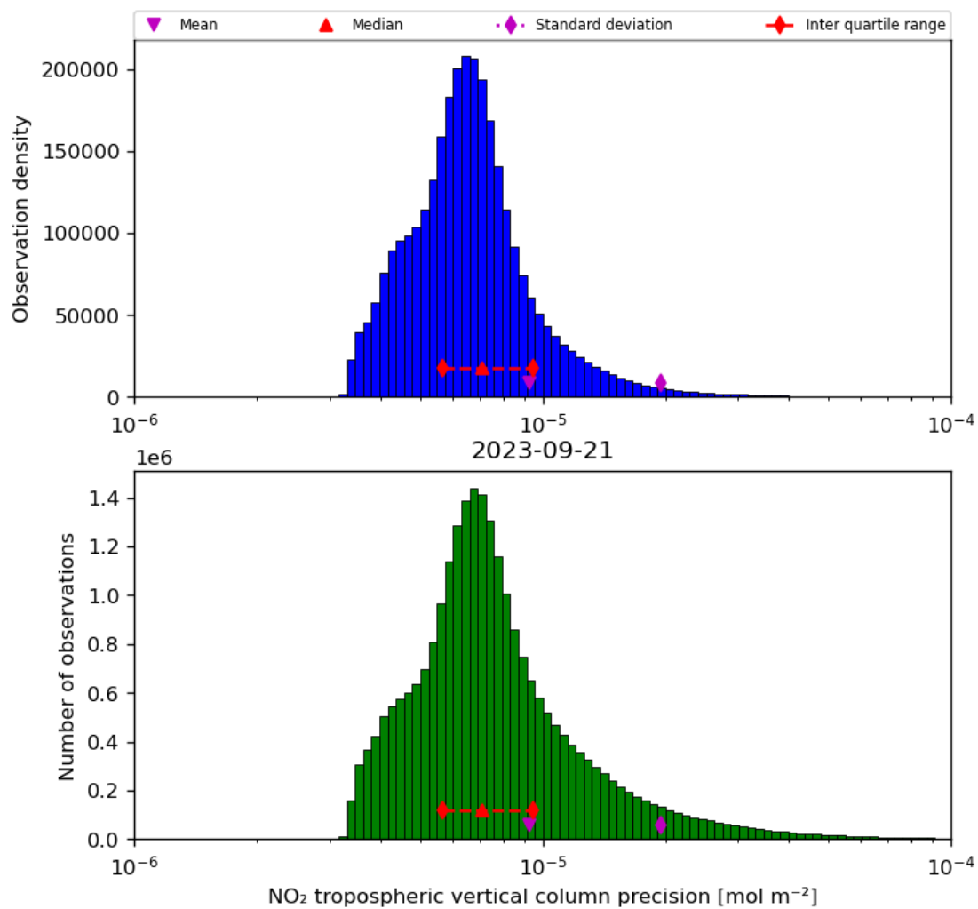
Figure 30: Histogram of “NO 2 tropospheric vertical column precision” for 2023-09-20 to 2023-09-22
