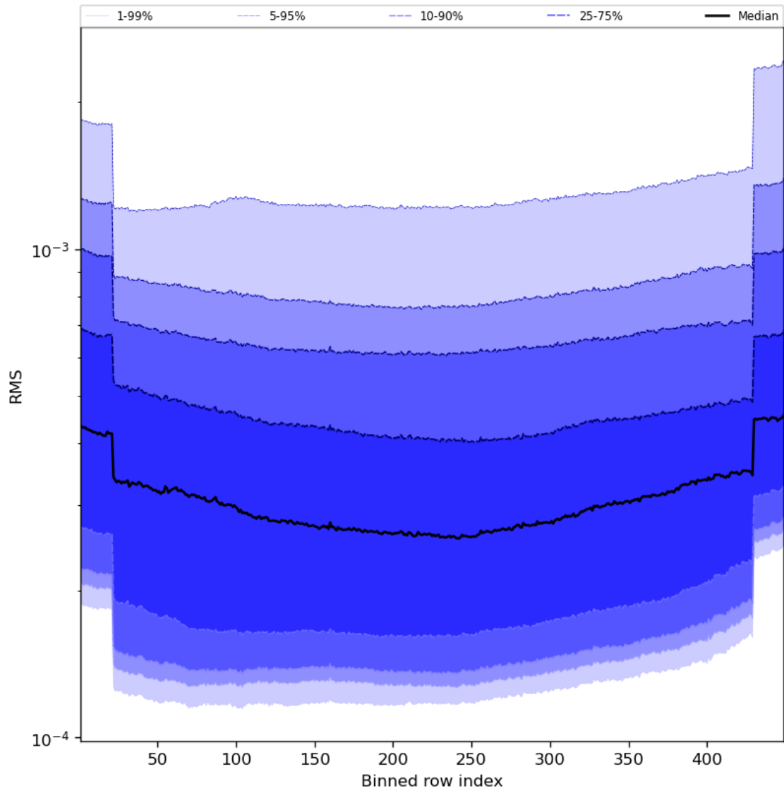
Figure 60: Along track statistics of “RMS” for 2023-09-20 to 2023-09-22
