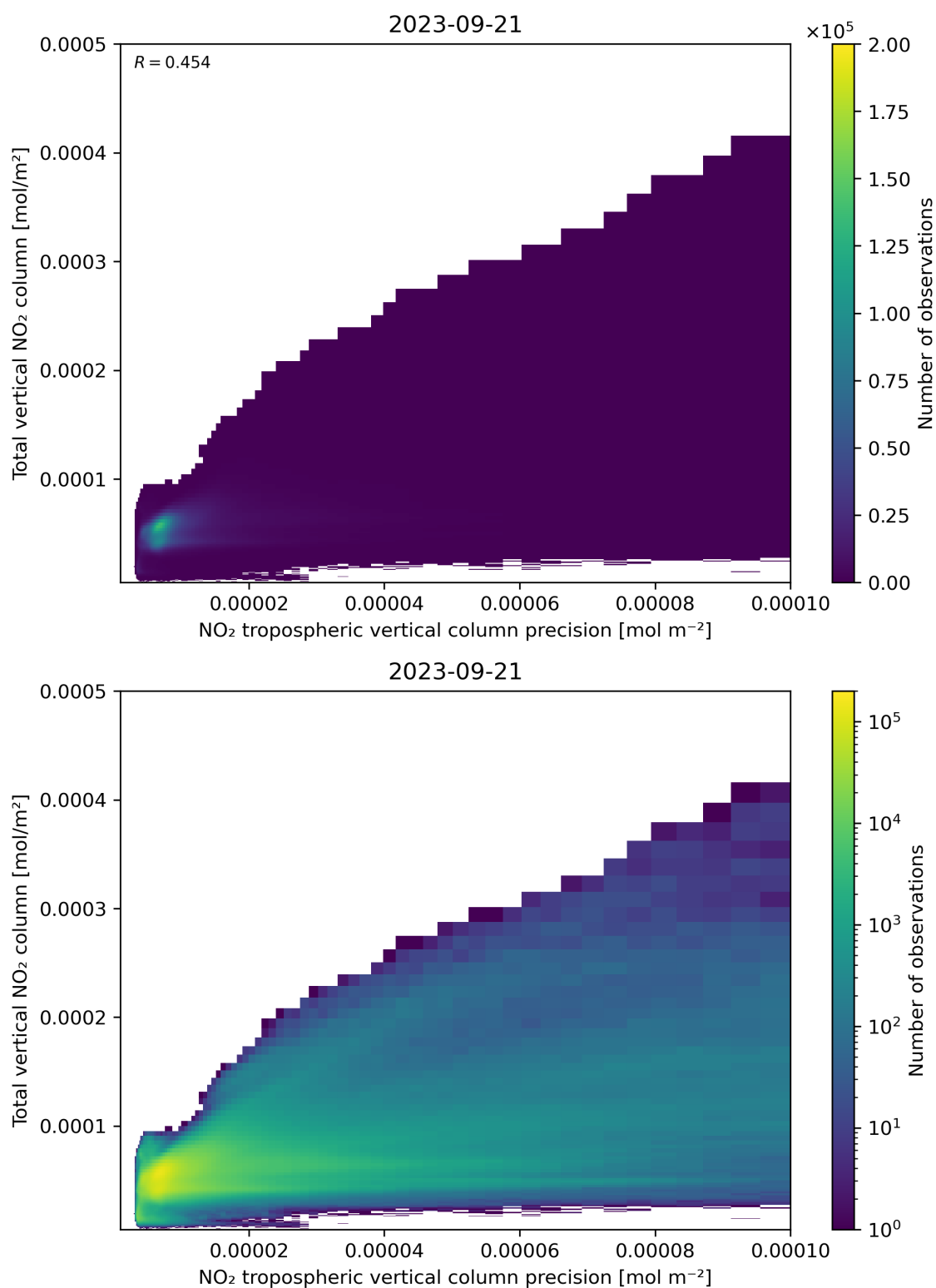
Figure 138: Scatter density plot of “NO 2 tropospheric vertical column precision” against “Total vertical NO 2 column” for 2023-09-20 to 2023-09-22.
