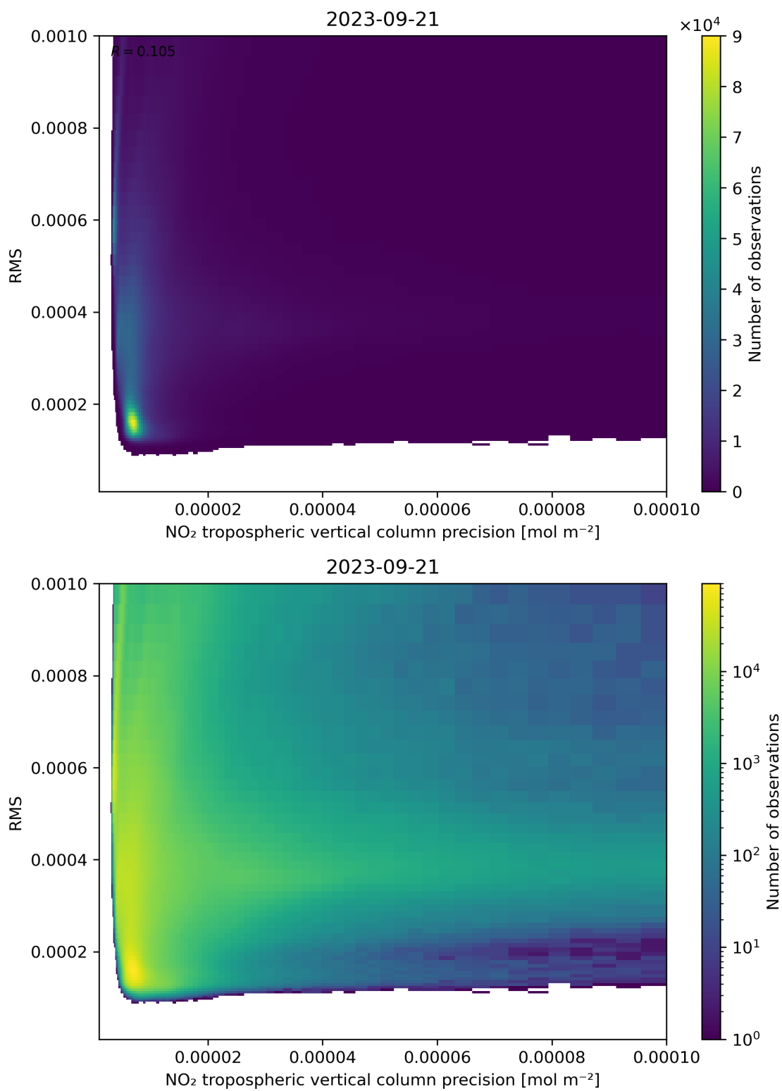
Figure 140: Scatter density plot of “NO 2 tropospheric vertical column precision” against “RMS” for 2023-09-20 to 2023-09-22.
