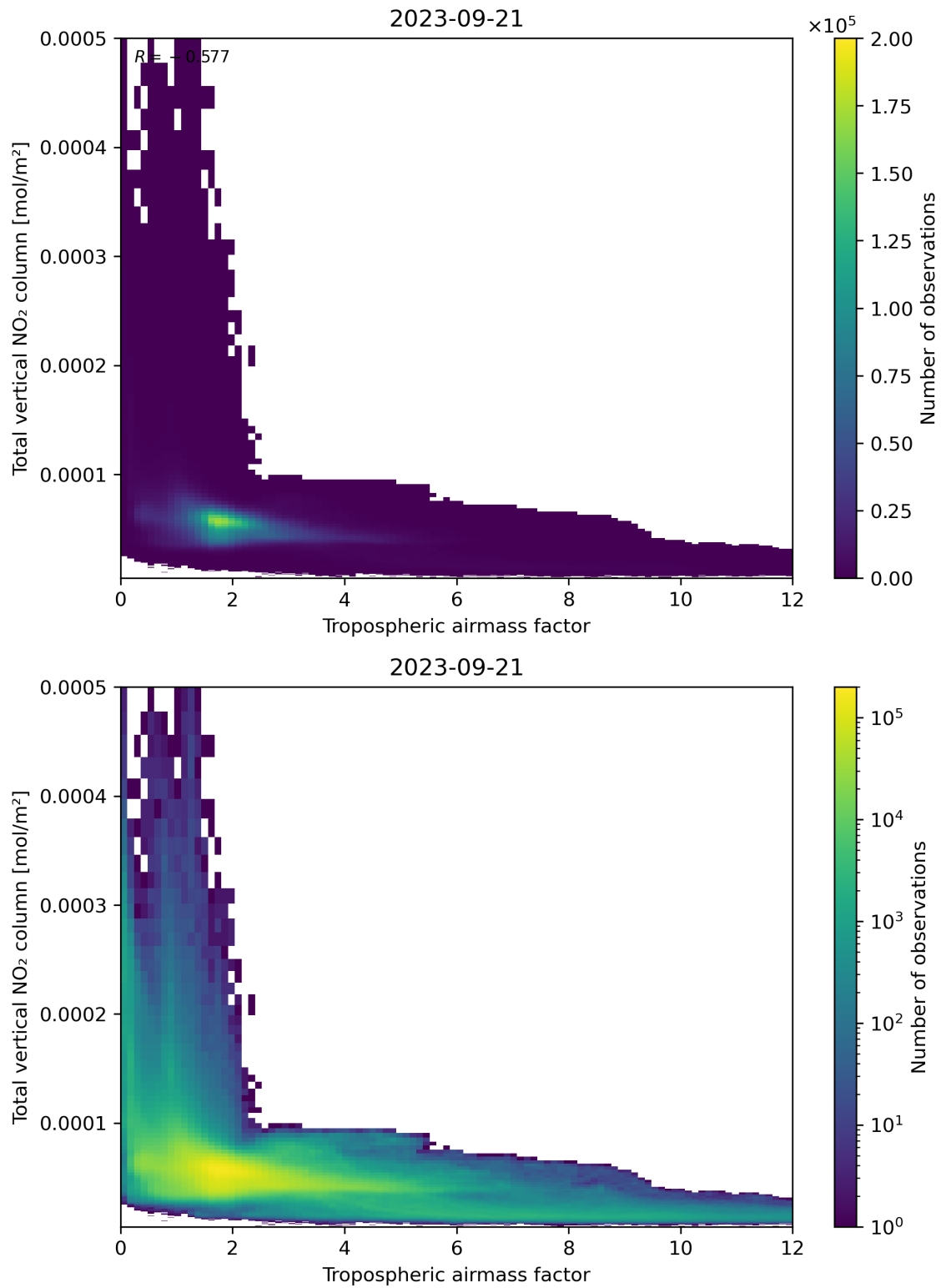
Figure 77: Scatter density plot of “Tropospheric airmass factor” against “Total vertical NO 2 column” for 2023-09-20 to 2023-09-22.
