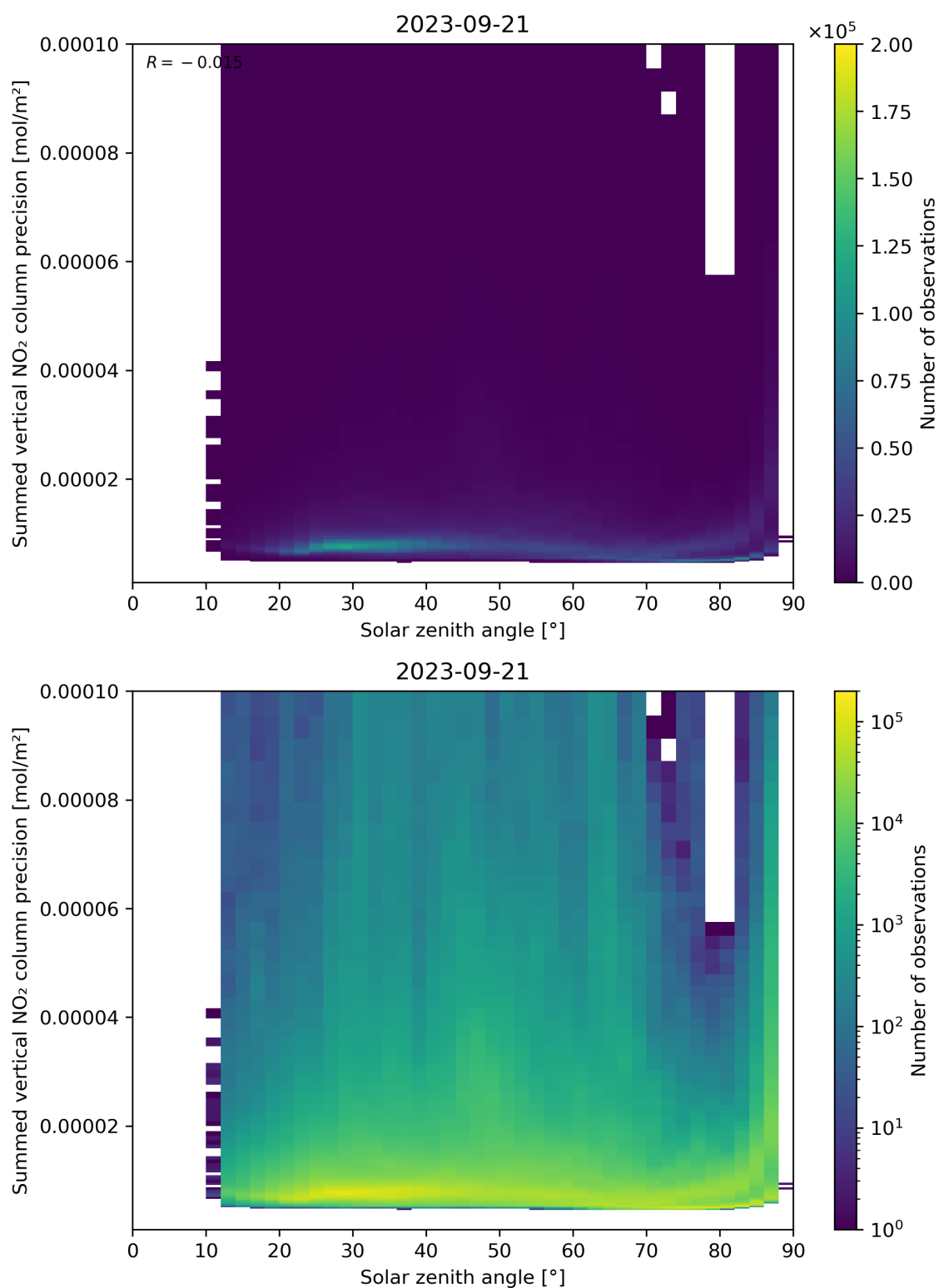
Figure 152: Scatter density plot of “Solar zenith angle” against “Summed vertical NO 2 column precision” for 2023-09-20 to 2023-09-22.
