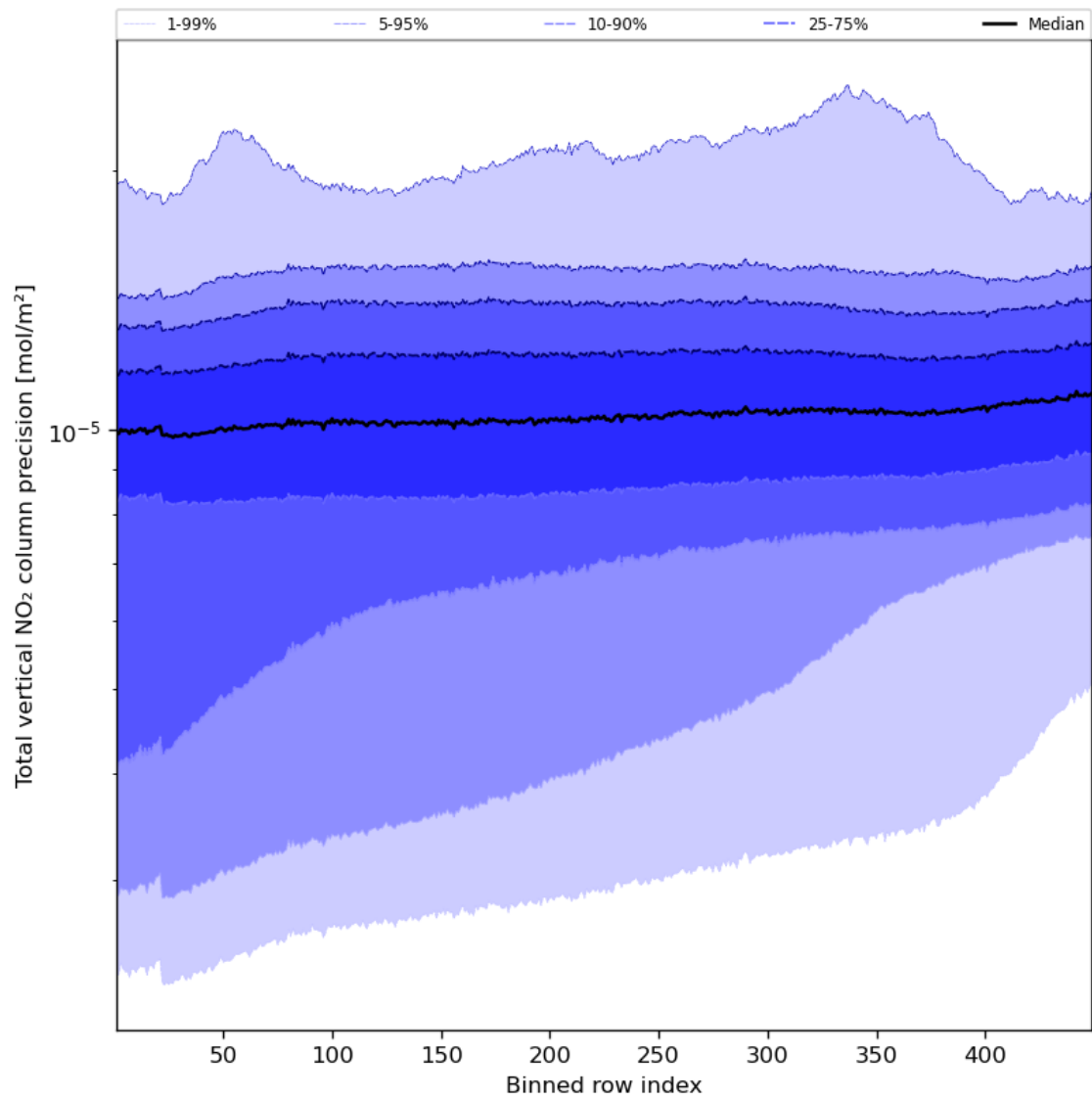
Figure 56: Along track statistics of “Total vertical NO 2 column precision” for 2023-09-20 to 2023-09-22
