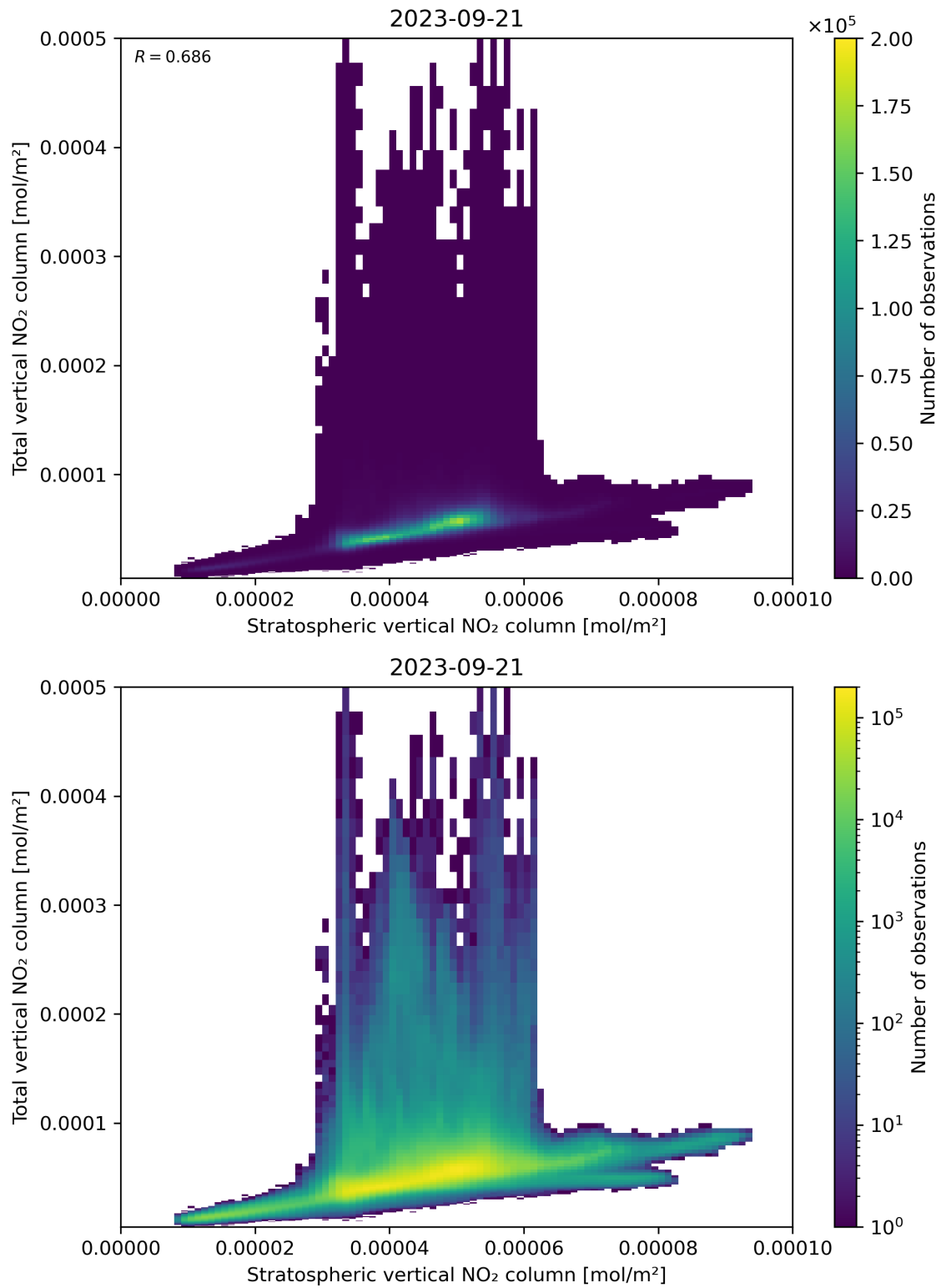
Figure 100: Scatter density plot of “Stratospheric vertical NO 2 column” against “Total vertical NO 2 column” for 2023-09-20 to 2023-09-22.
