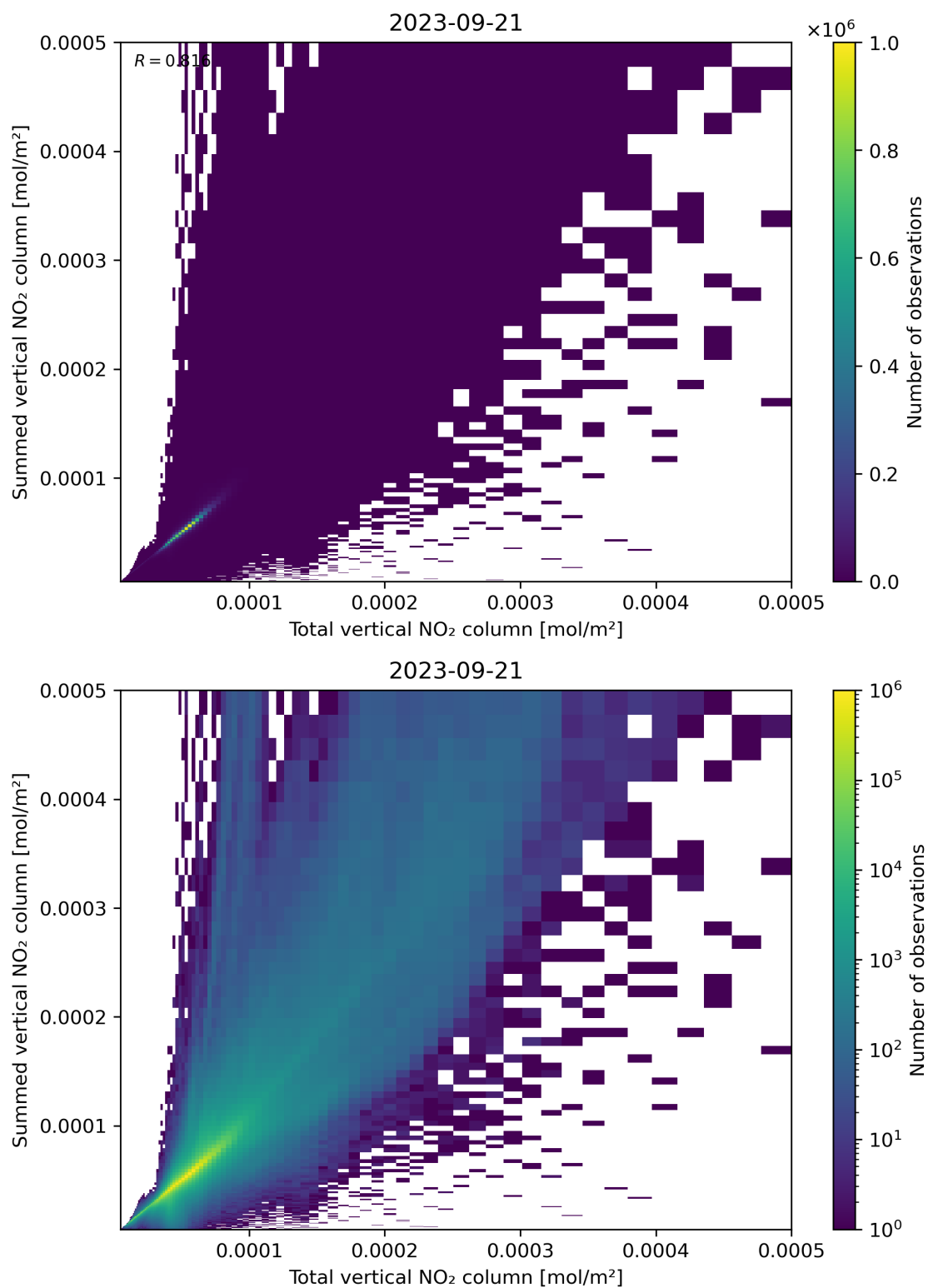
Figure 112: Scatter density plot of “Total vertical NO 2 column” against “Summed vertical NO 2 column” for 2023-09-20 to 2023-09-22.
