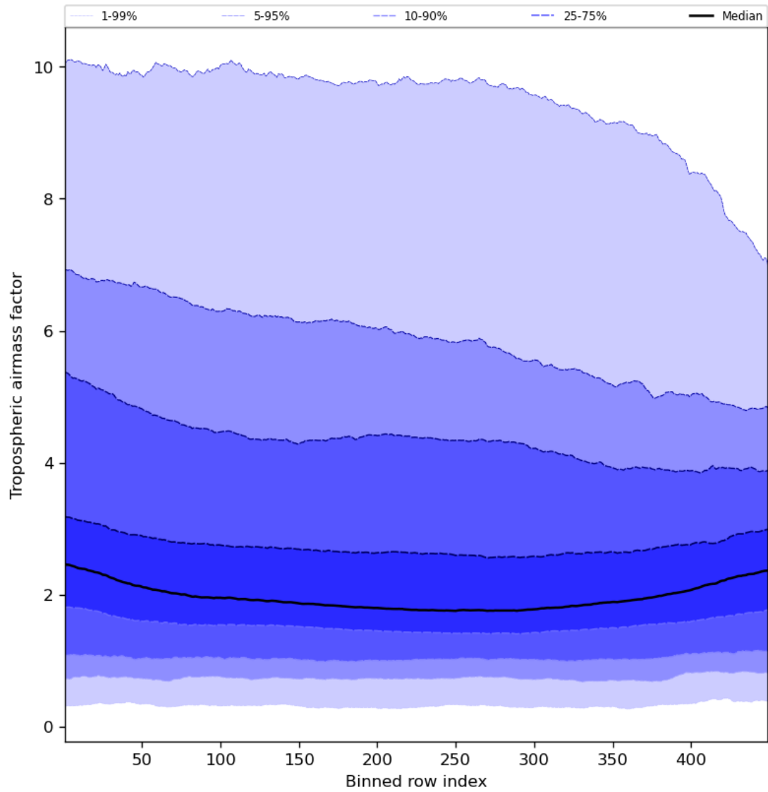
Figure 48: Along track statistics of “Tropospheric air mass factor” for 2023-09-20 to 2023-09-22
