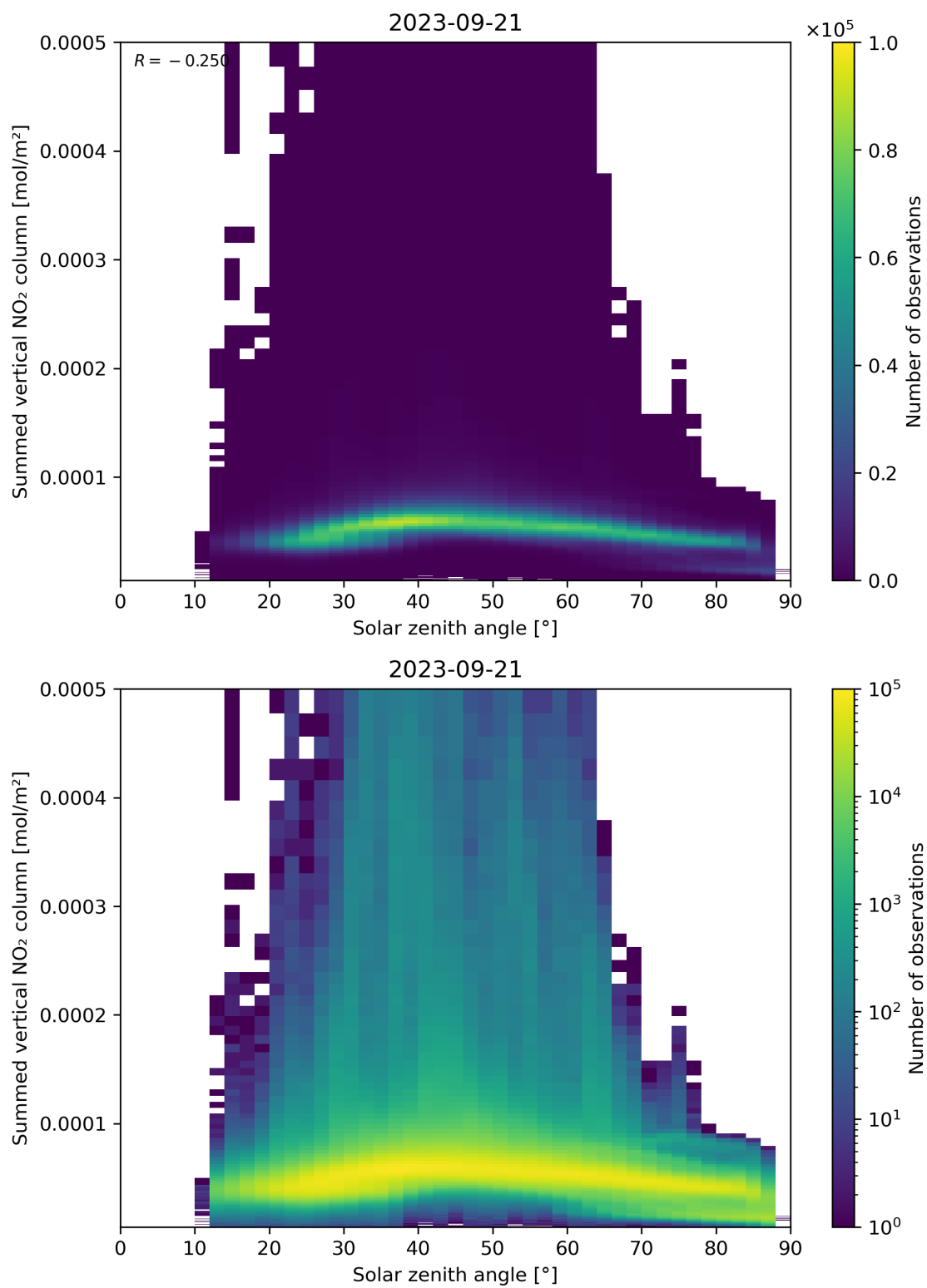
Figure 151: Scatter density plot of “Solar zenith angle” against “Summed vertical NO 2 column” for 2023-09-20 to 2023-09-22.
