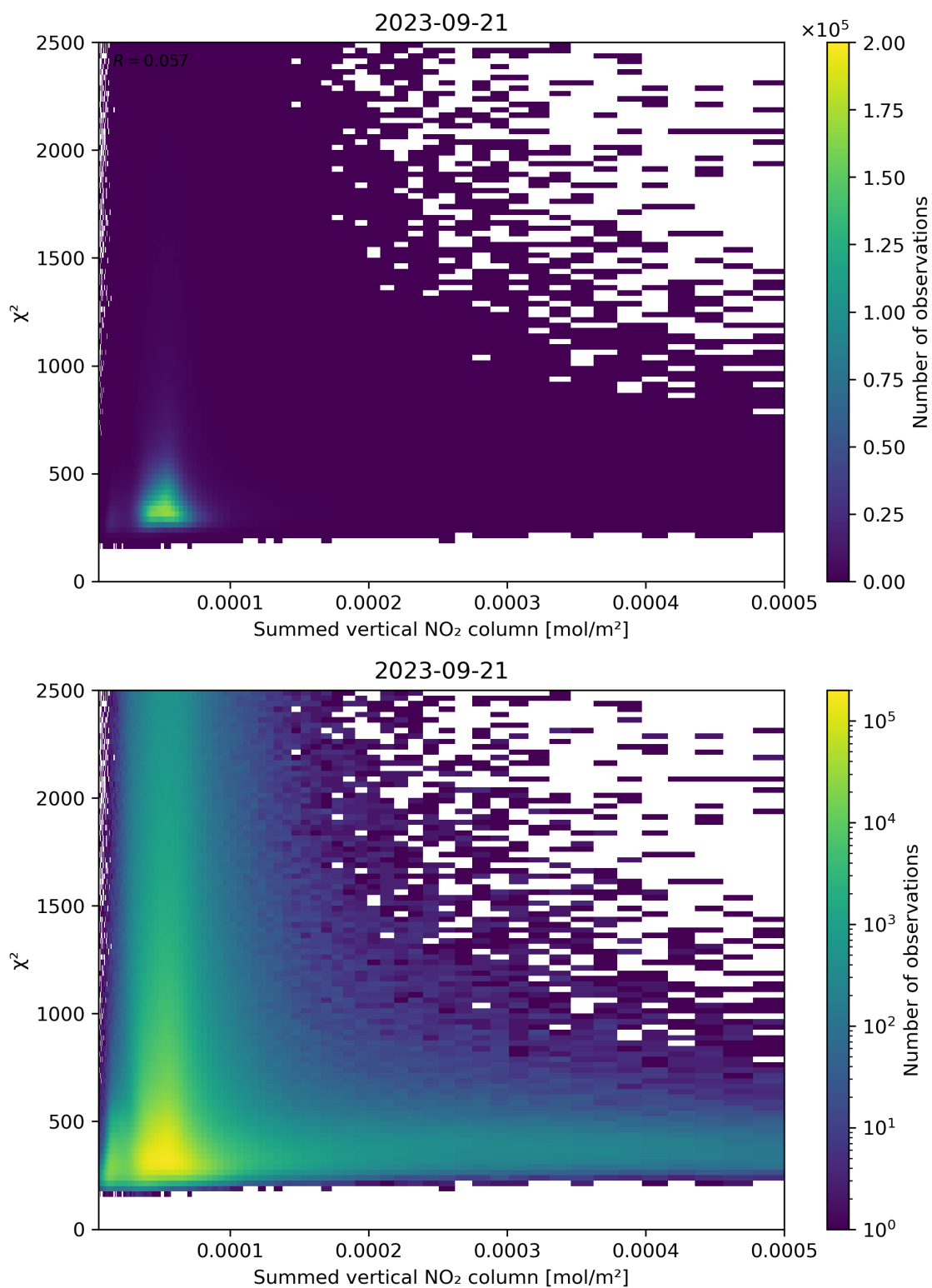
Figure 104: Scatter density plot of “Summed vertical NO 2 column” against “ \chi^2 ” for 2023-09-20 to 2023-09-22.
