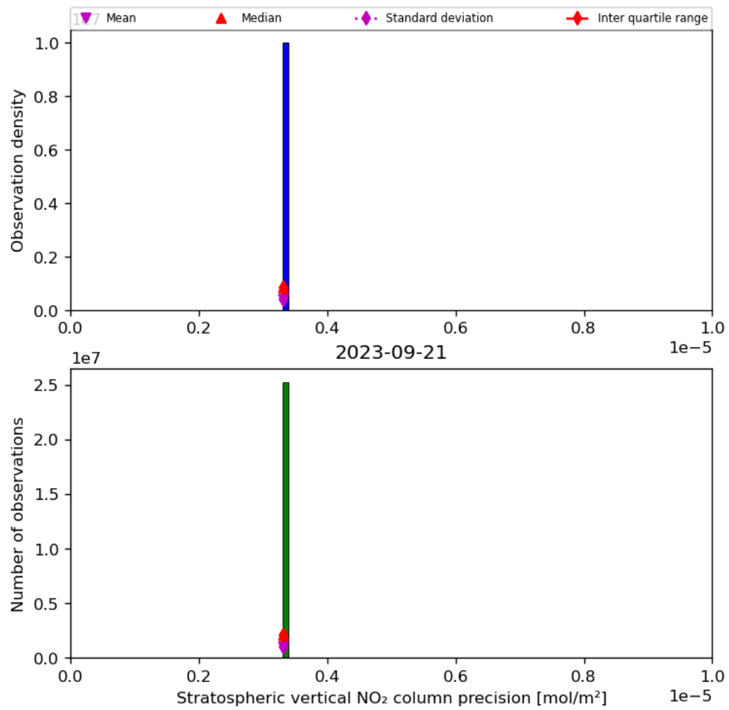
Figure 37: Histogram of “Stratospheric vertical NO 2 column precision” for 2023-09-20 to 2023-09-22
