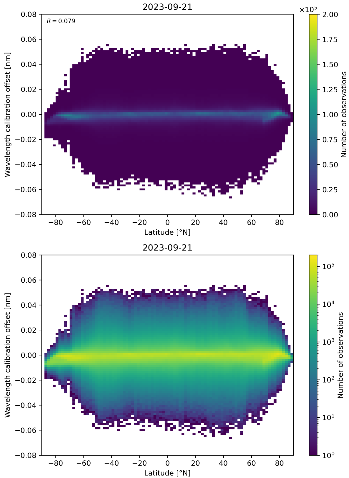
Figure 95: Scatter density plot of “Latitude” against “Wavelength calibration offset” for 2023-09-20 to 2023-09-22.
