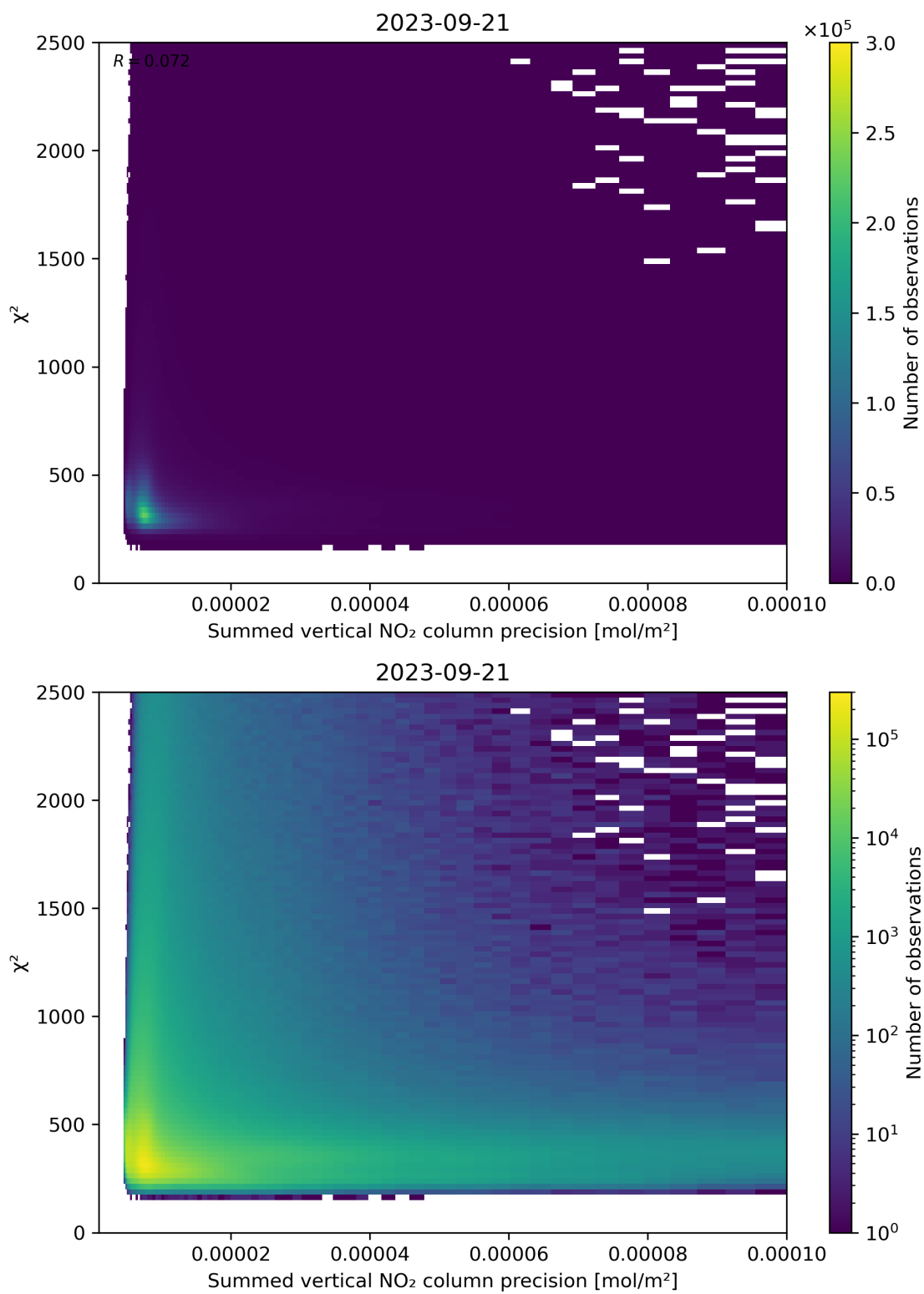
Figure 107: Scatter density plot of “Summed vertical NO 2 column precision” against “ \chi^2 ” for 2023-09-20 to 2023-09-22.
