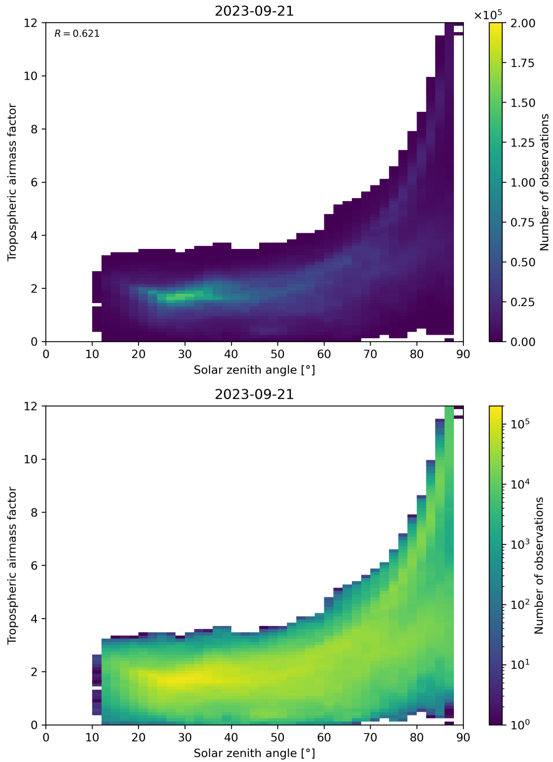
Figure 147: Scatter density plot of “Solar zenith angle” against “Tropospheric airmass factor” for 2023-09-20 to 2023-09-22.
