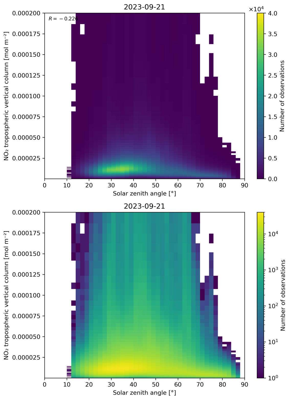
Figure 155: Scatter density plot of “Solar zenith angle” against “NO 2 tropospheric vertical column” for 2023-09-20 to 2023-09-22.
