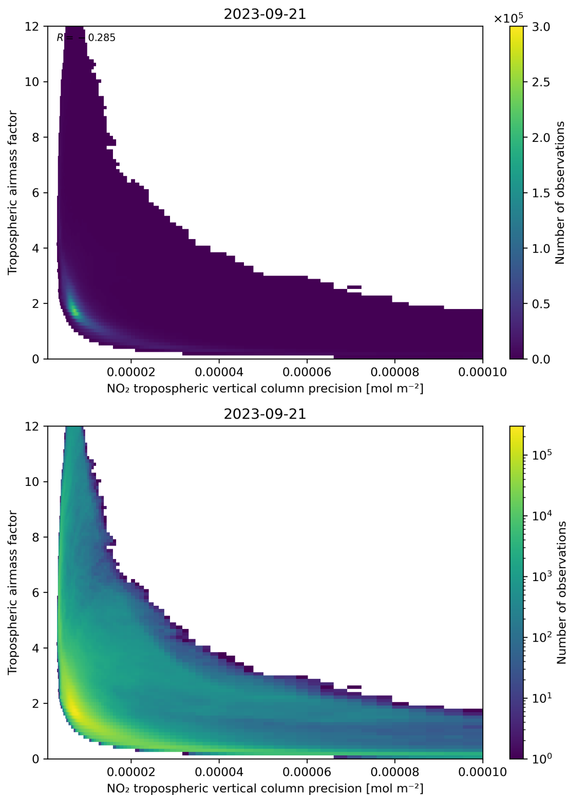
Figure 133: Scatter density plot of “NO 2 tropospheric vertical column precision” against “Tropospheric airmass factor” for 2023-09-20 to 2023-09-22.
