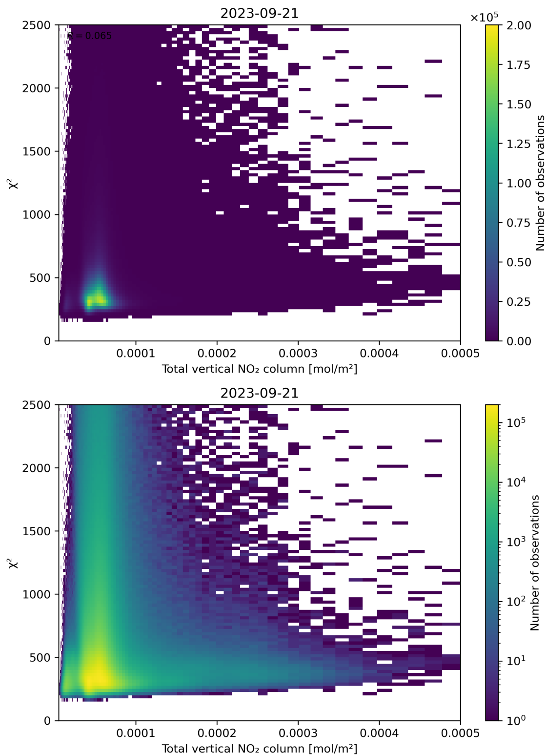
Figure 111: Scatter density plot of “Total vertical NO 2 column” against “ \chi^2 ” for 2023-09-20 to 2023-09-22.
