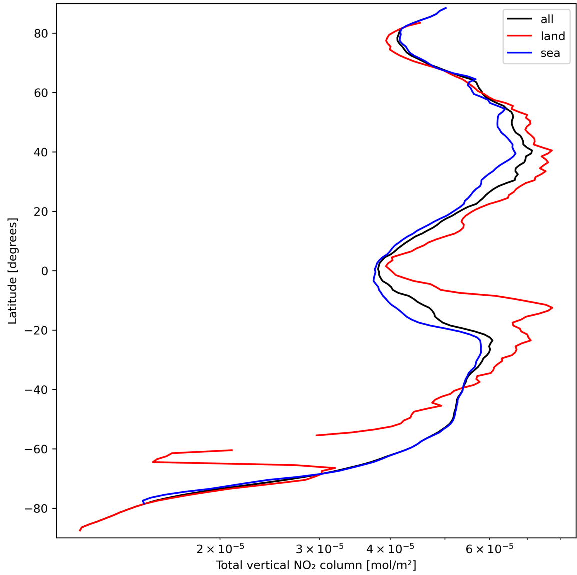
Figure 21: Zonal average of “Total vertical NO 2 column” for 2023-09-20 to 2023-09-22.
