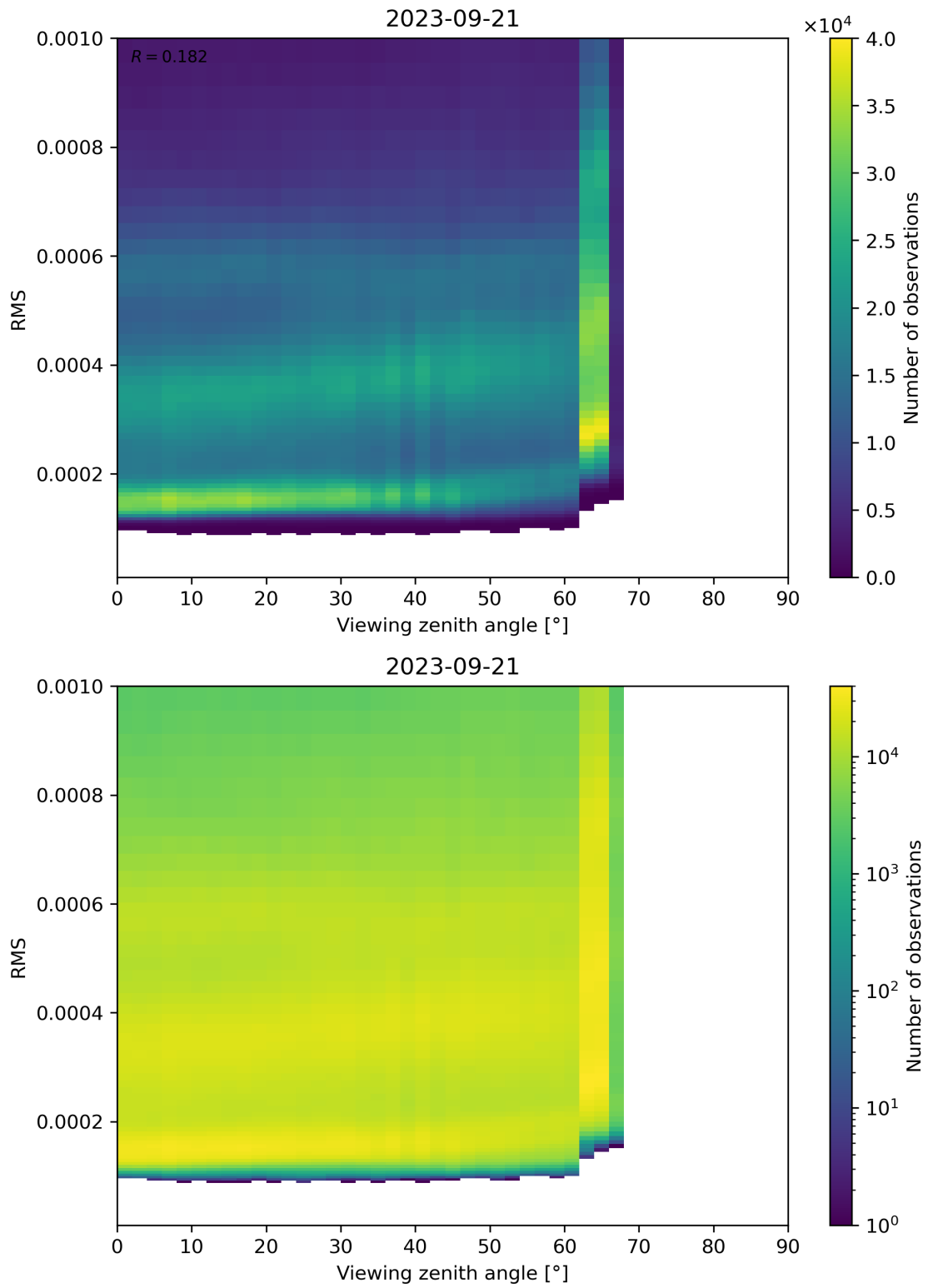
Figure 171: Scatter density plot of “Viewing zenith angle” against “RMS” for 2023-09-20 to 2023-09-22.
