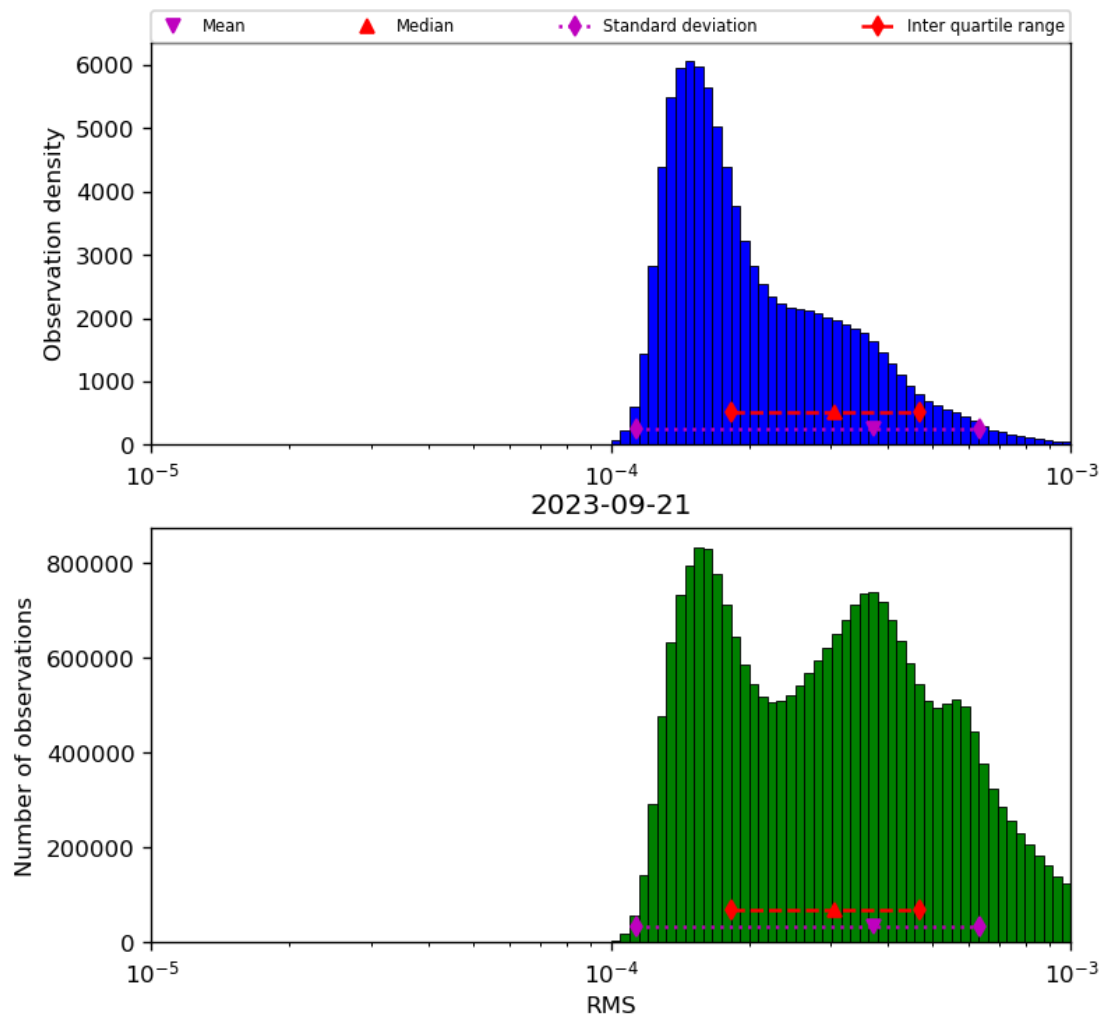
Figure 43: Histogram of “RMS” for 2023-09-20 to 2023-09-22
