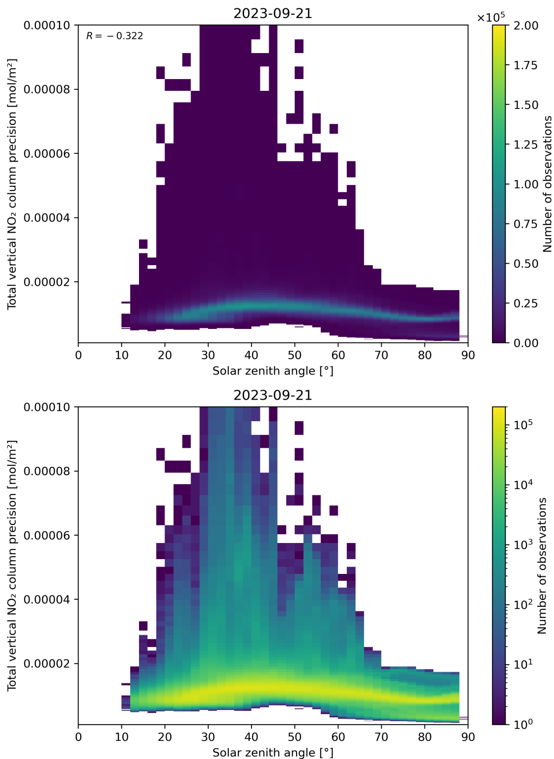
Figure 154: Scatter density plot of “Solar zenith angle” against “Total vertical NO 2 column precision” for 2023-09-20 to 2023-09-22.
