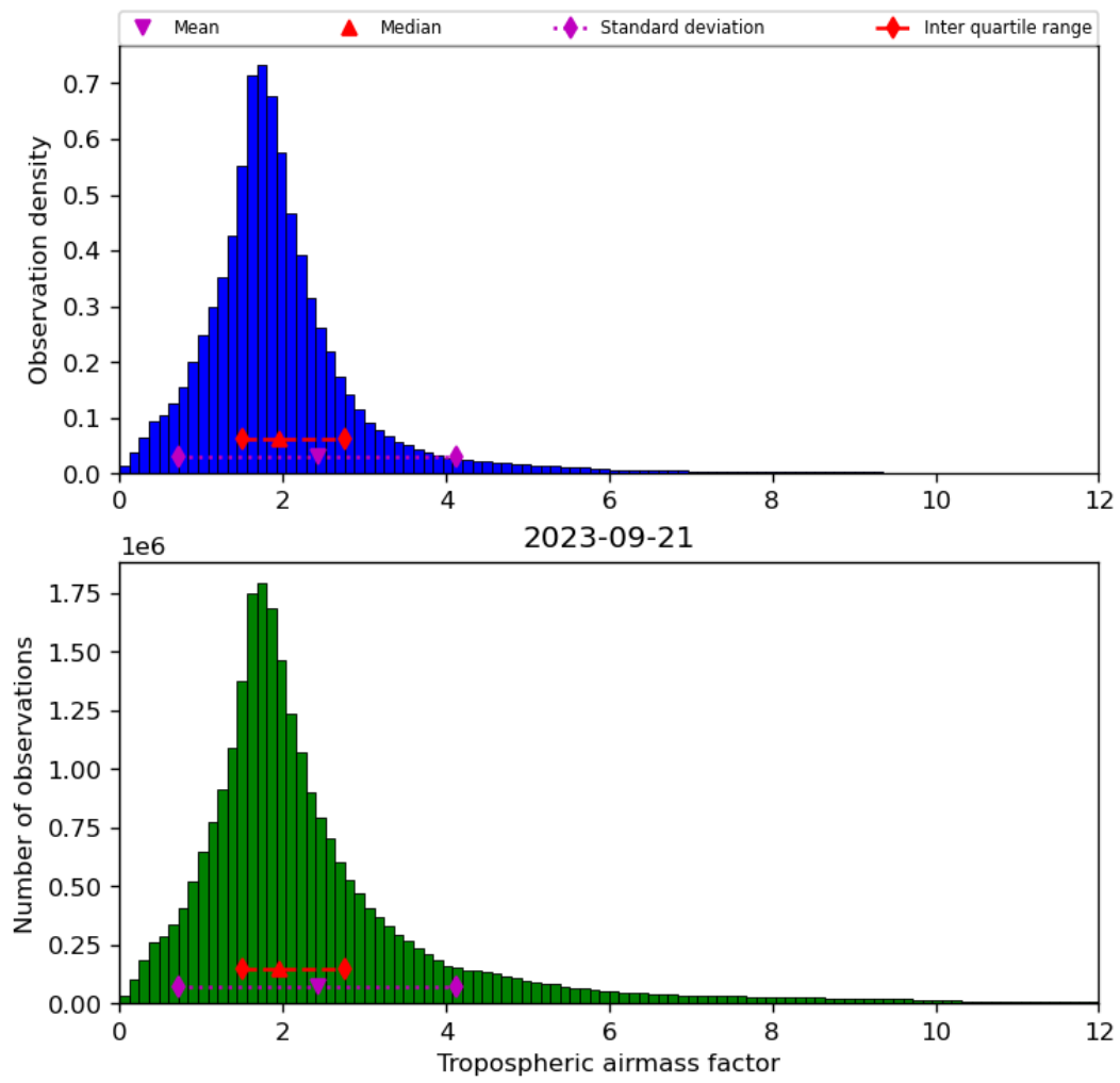
Figure 31: Histogram of “Tropospheric airmass factor” for 2023-09-20 to 2023-09-22
