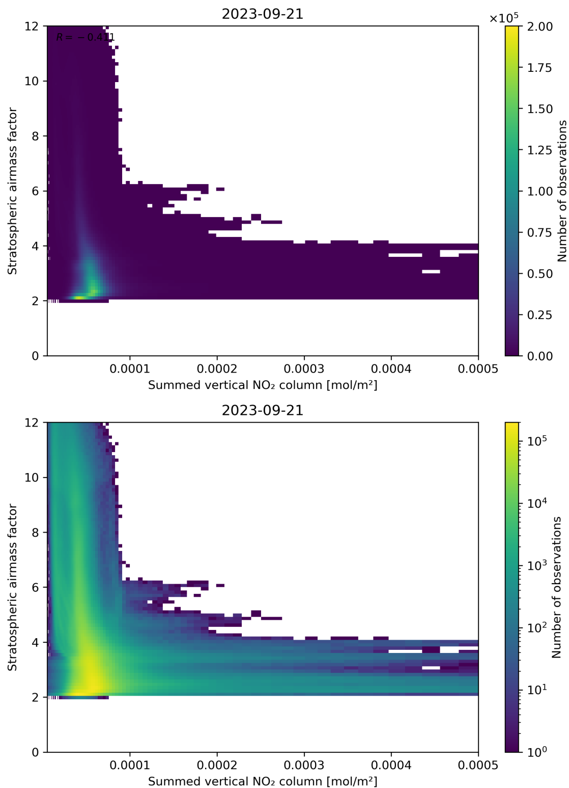
Figure 103: Scatter density plot of “Summed vertical NO 2 column” against “Stratospheric air mass factor” for 2023-09-20 to 2023-09-22.
