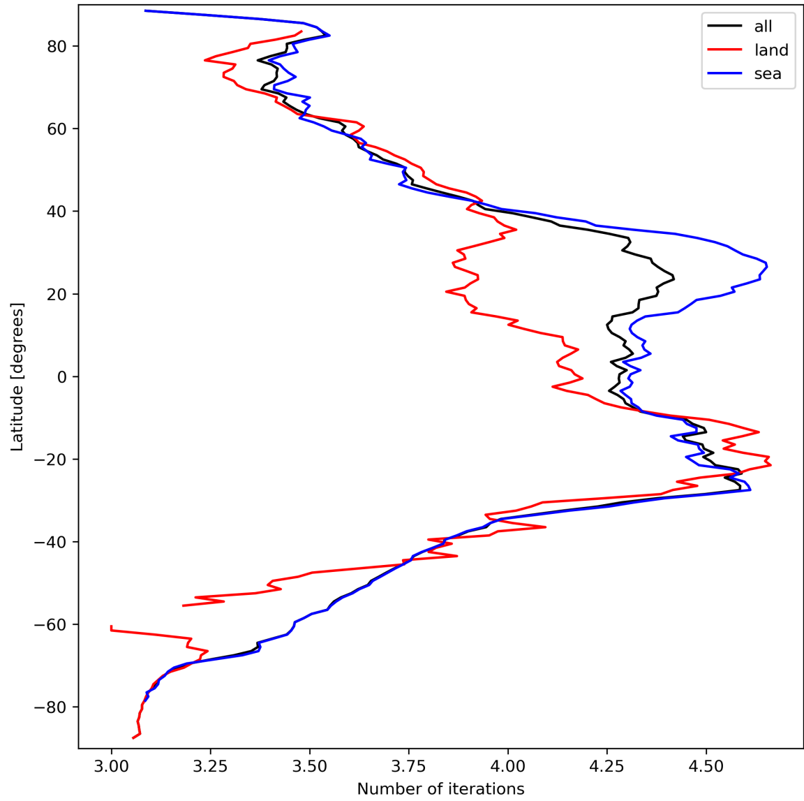
Figure 17: Zonal average of “Number of iterations” for 2023-09-20 to 2023-09-22.
