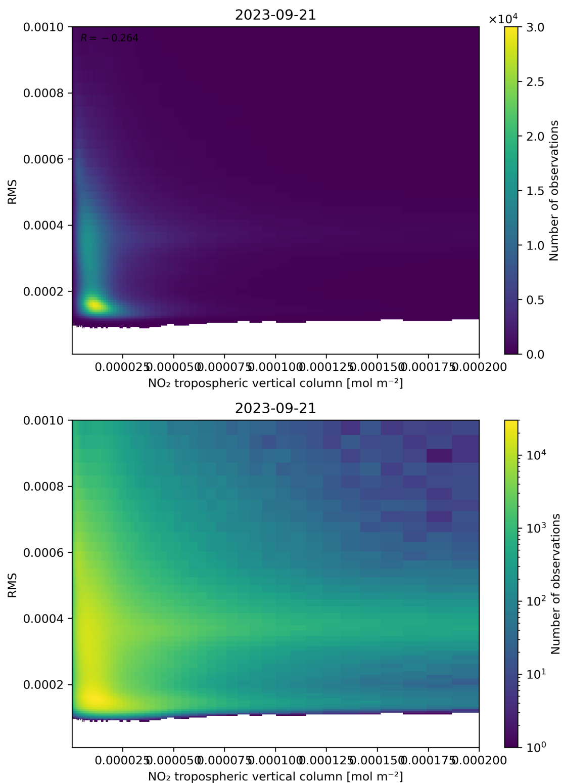
Figure 142: Scatter density plot of “NO 2 tropospheric vertical column” against “RMS” for 2023-09-20 to 2023-09-22.
