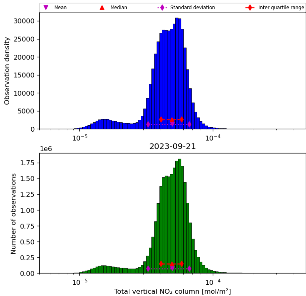
Figure 38: Histogram of “Total vertical NO 2 column” for 2023-09-20 to 2023-09-22
