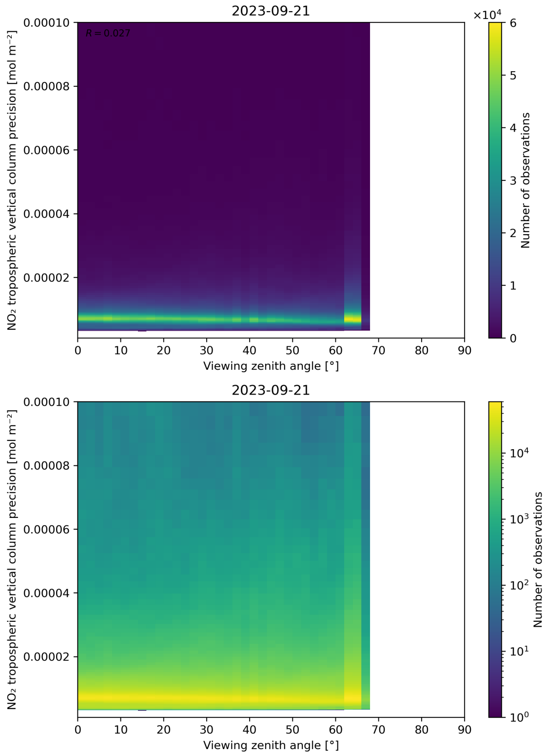
Figure 170: Scatter density plot of “Viewing zenith angle” against “NO 2 tropospheric vertical column precision” for 2023-09-20 to 2023-09-22.
