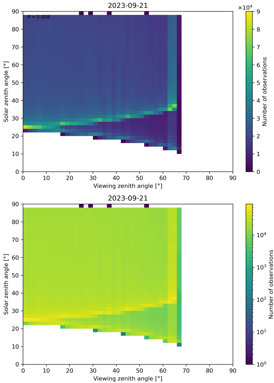
Figure 172: Scatter density plot of “Viewing zenith angle” against “Solar zenith angle” for 2023-09-20 to 2023-09-22.
