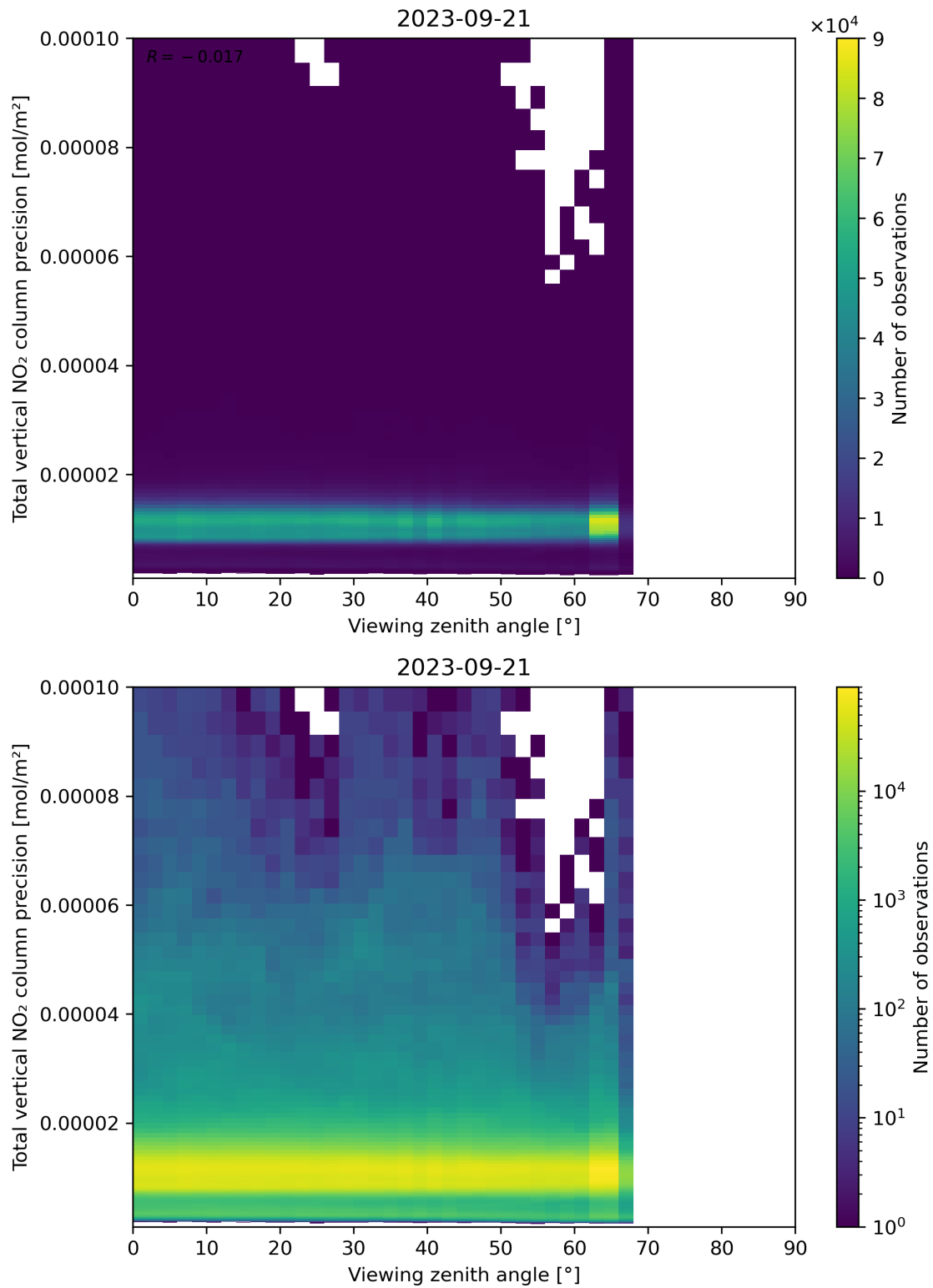
Figure 168: Scatter density plot of “Viewing zenith angle” against “Total vertical NO 2 column precision” for 2023-09-20 to 2023-09-22.
