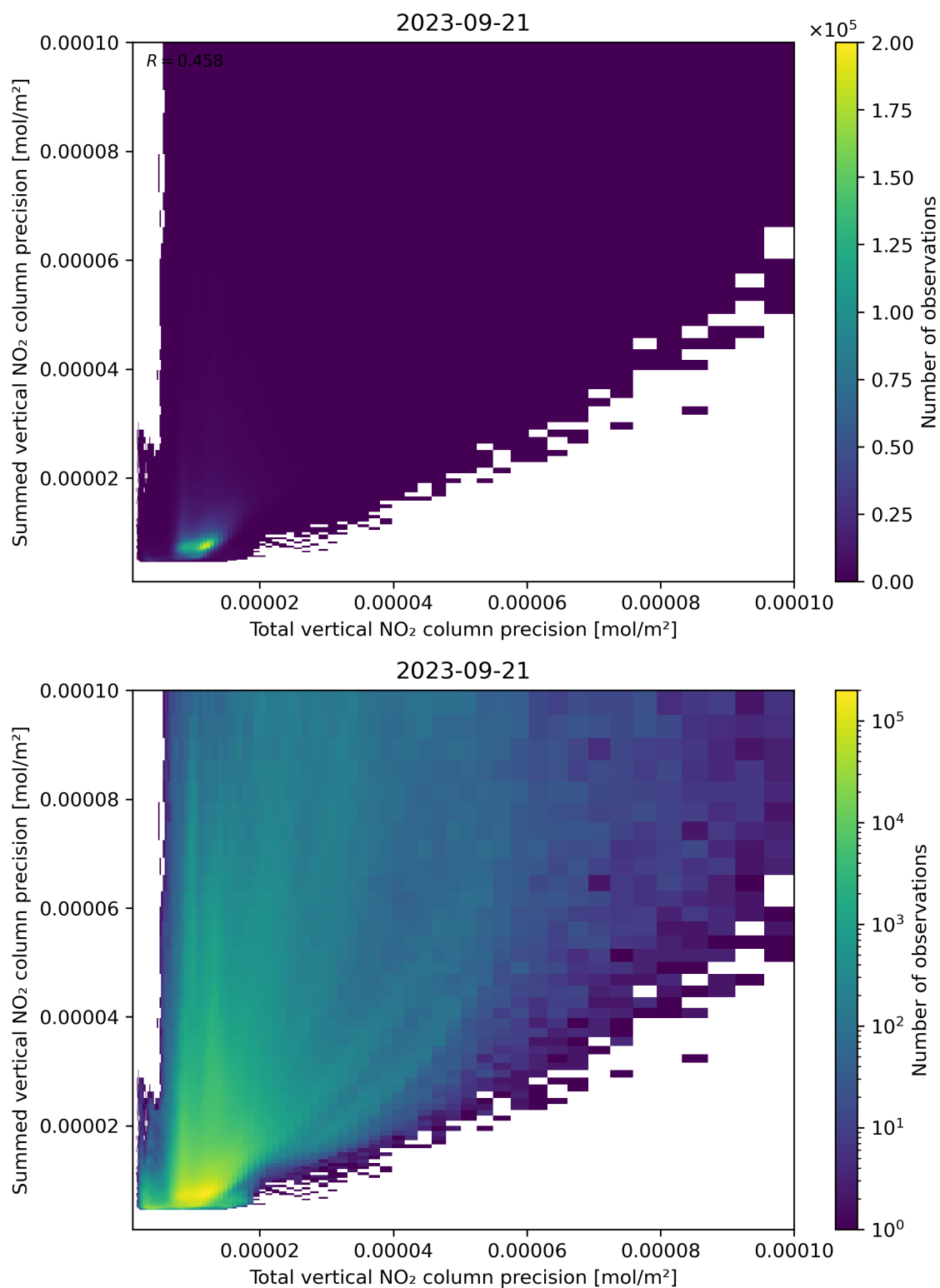
Figure 118: Scatter density plot of “Total vertical NO 2 column precision” against “Summed vertical NO 2 column precision” for 2023-09-20 to 2023-09-22.
