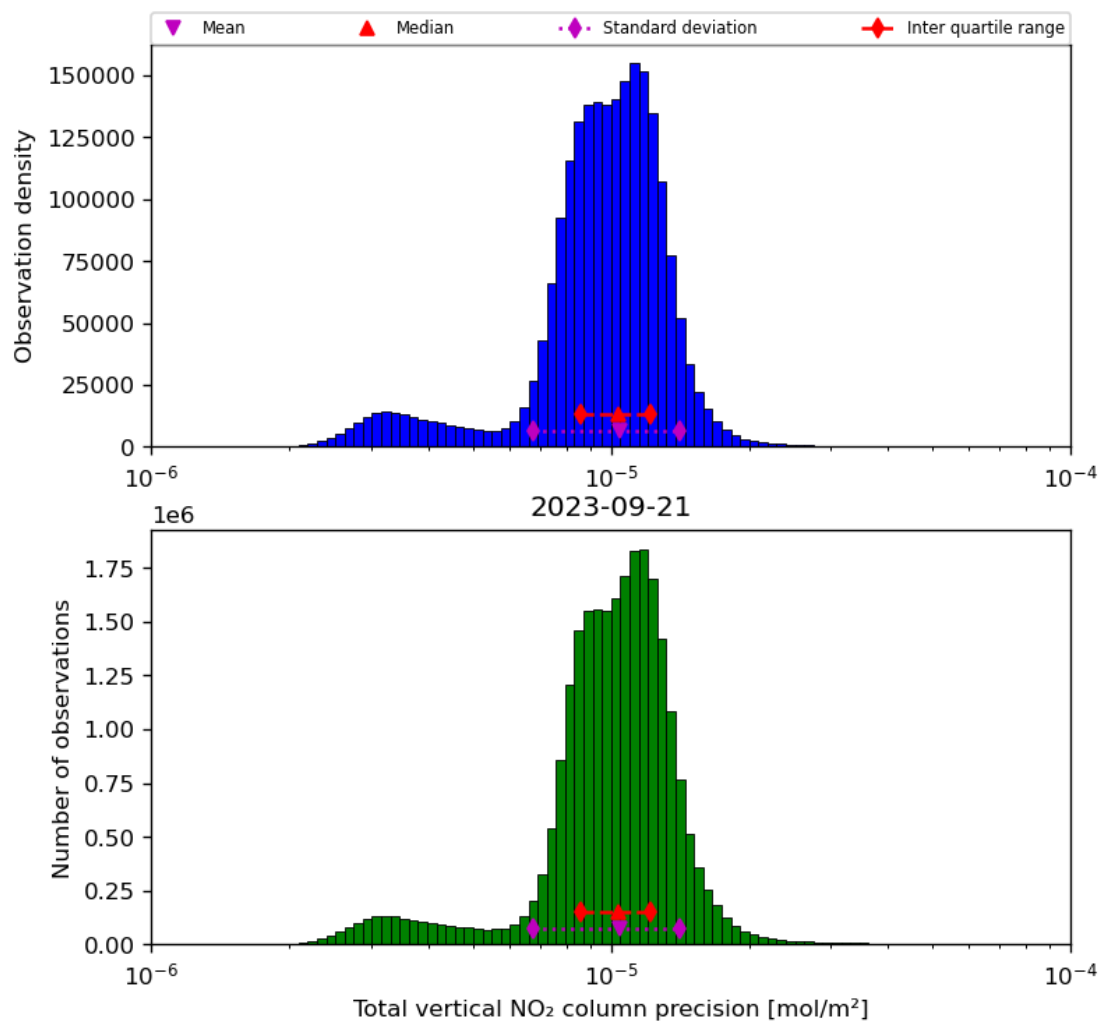
Figure 39: Histogram of “Total vertical NO 2 column precision” for 2023-09-20 to 2023-09-22
