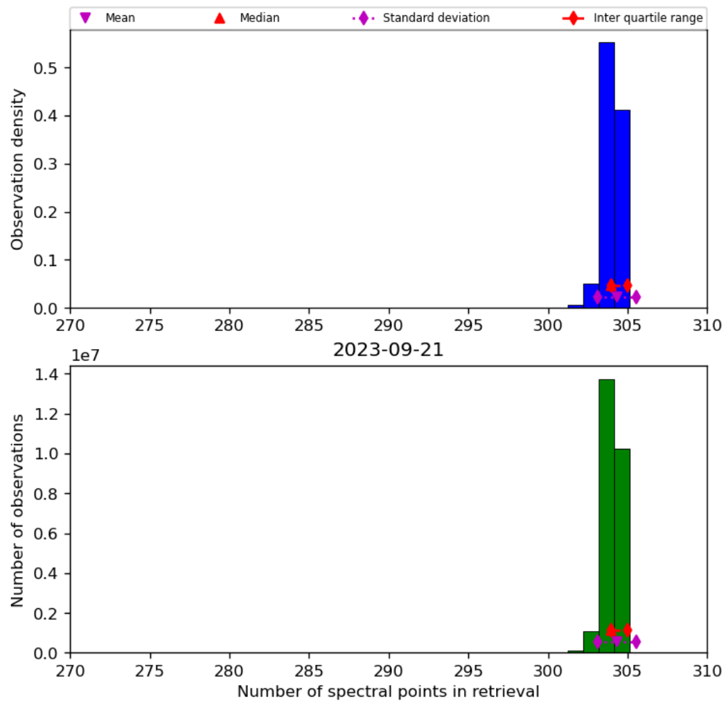
Figure 33: Histogram of “Number of spectral points in retrieval” for 2023-09-20 to 2023-09-22
