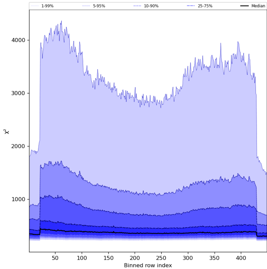
Figure 59: Along track statistics of “ \chi^2 ” for 2023-09-20 to 2023-09-22
