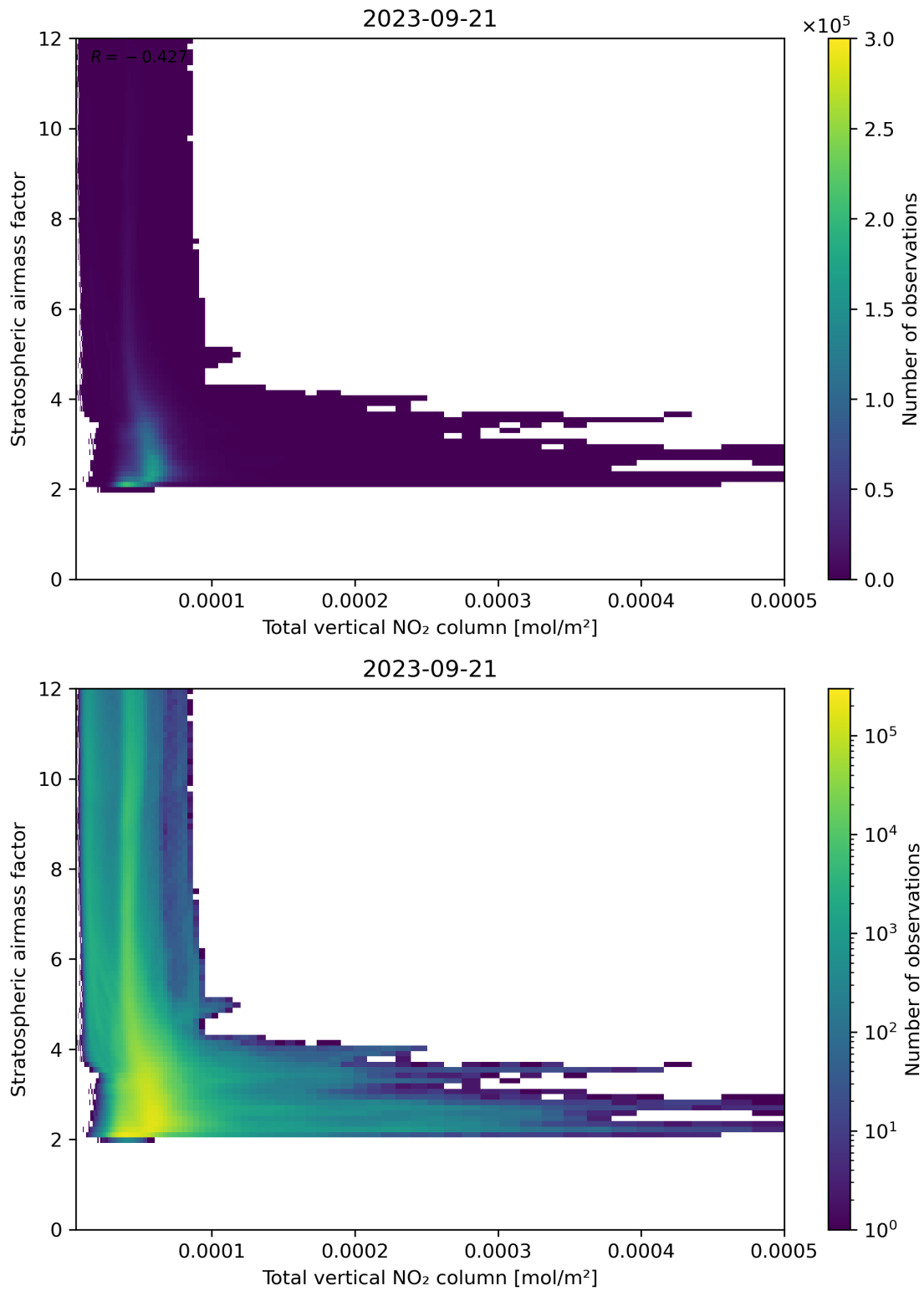
Figure 110: Scatter density plot of “Total vertical NO 2 column” against “Stratospheric airmass factor” for 2023-09-20 to 2023-09-22.
