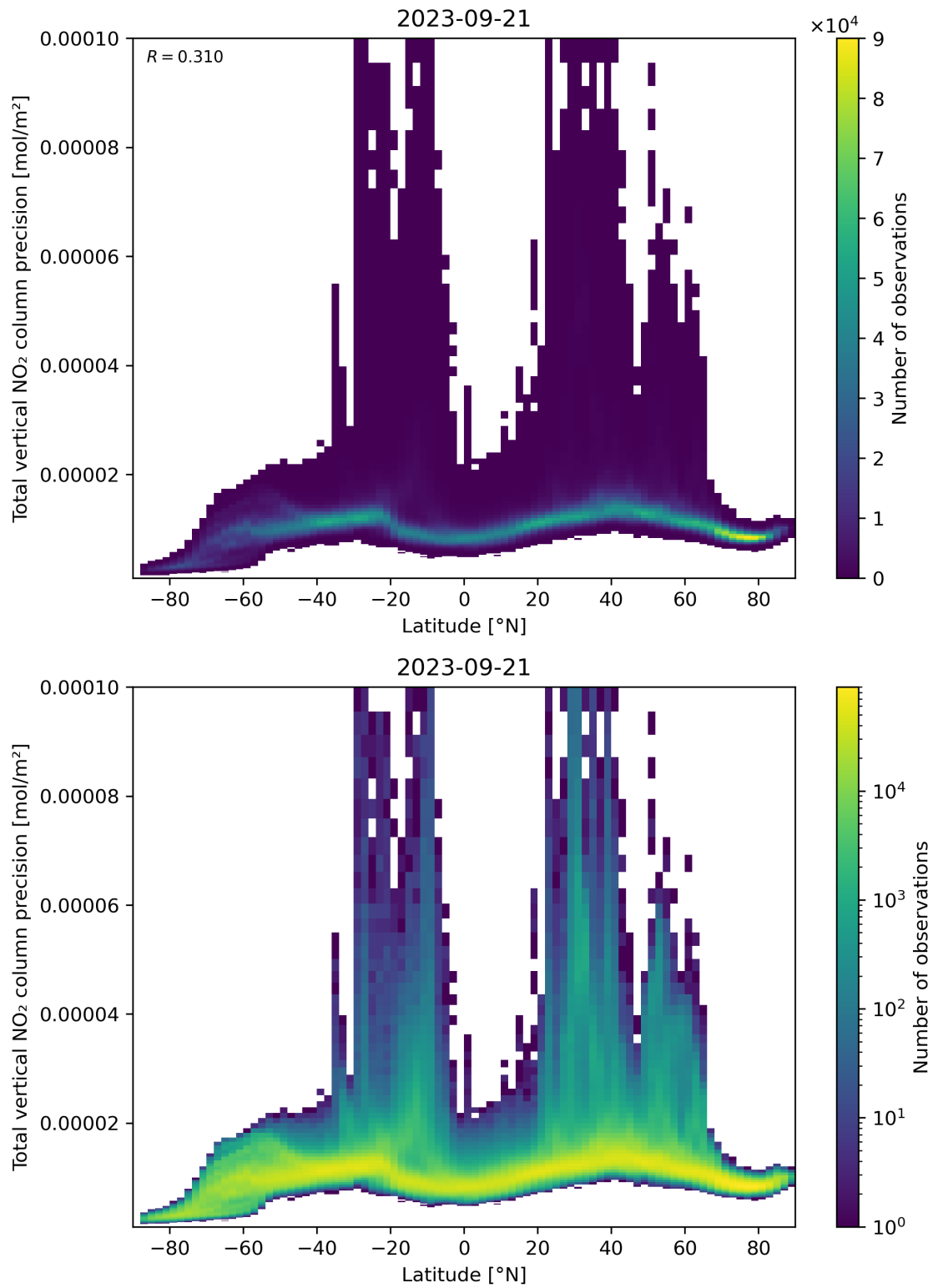
Figure 91: Scatter density plot of “Latitude” against “Total vertical NO 2 column precision” for 2023-09-20 to 2023-09-22.
