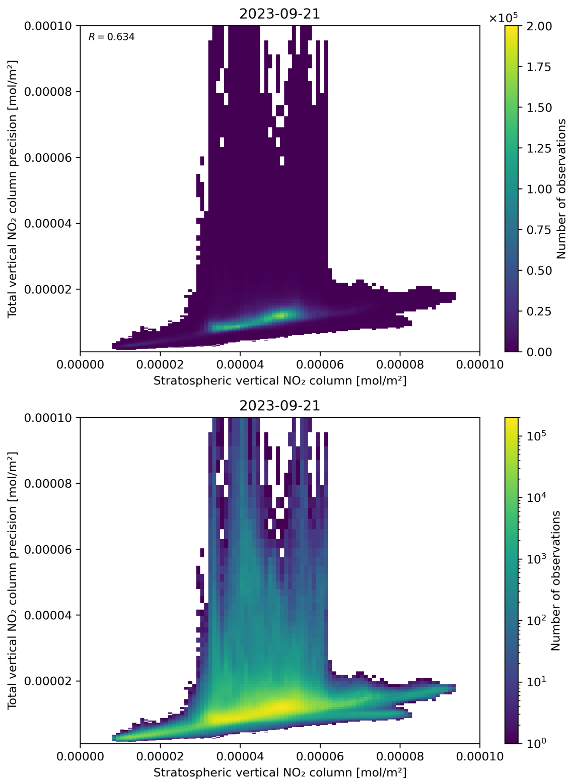
Figure 101: Scatter density plot of “Stratospheric vertical NO 2 column” against “Total vertical NO 2 column precision” for 2023-09-20 to 2023-09-22.
