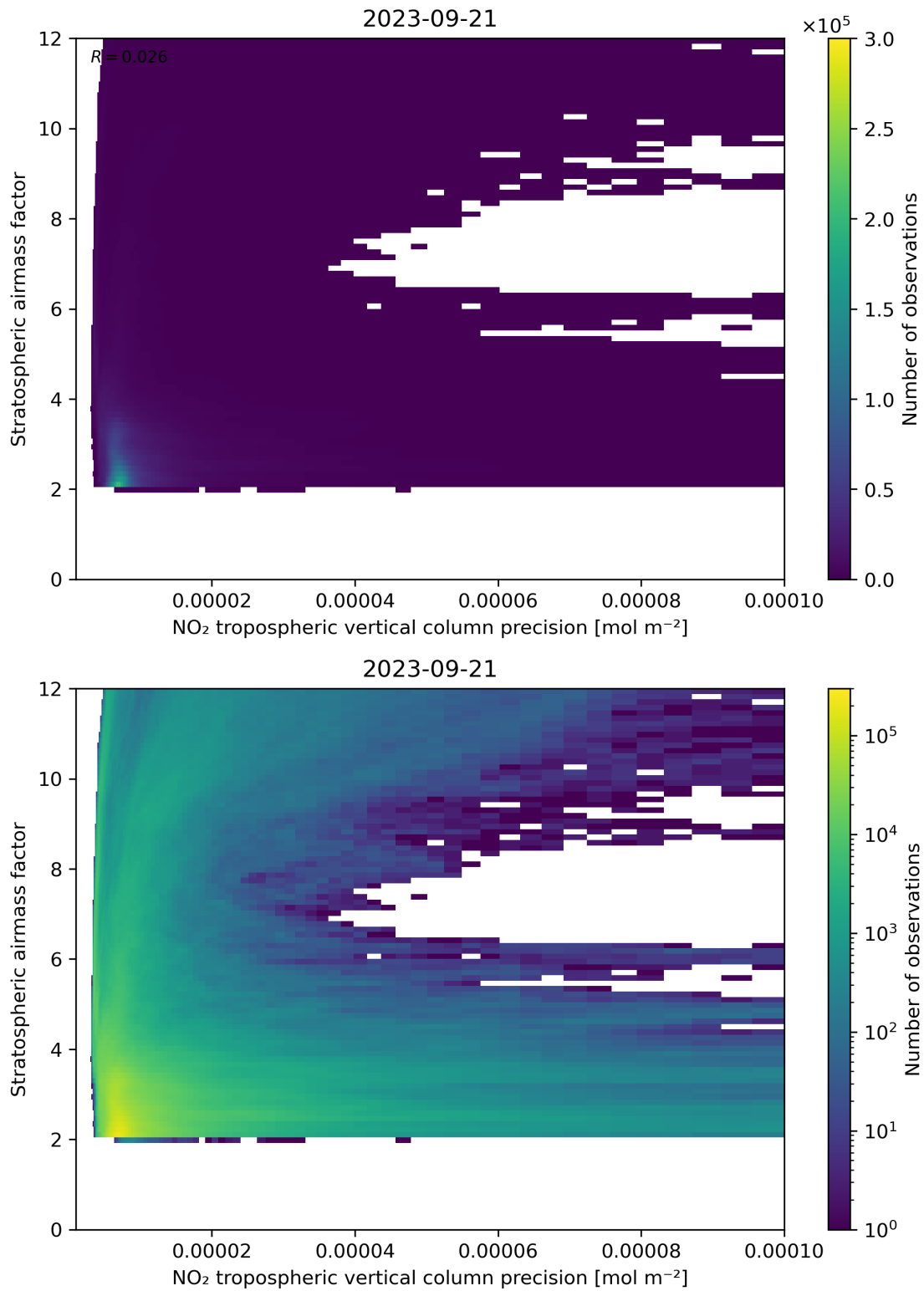
Figure 131: Scatter density plot of “NO 2 tropospheric vertical column precision” against “Stratospheric airmass factor” for 2023-09-20 to 2023-09-22.
