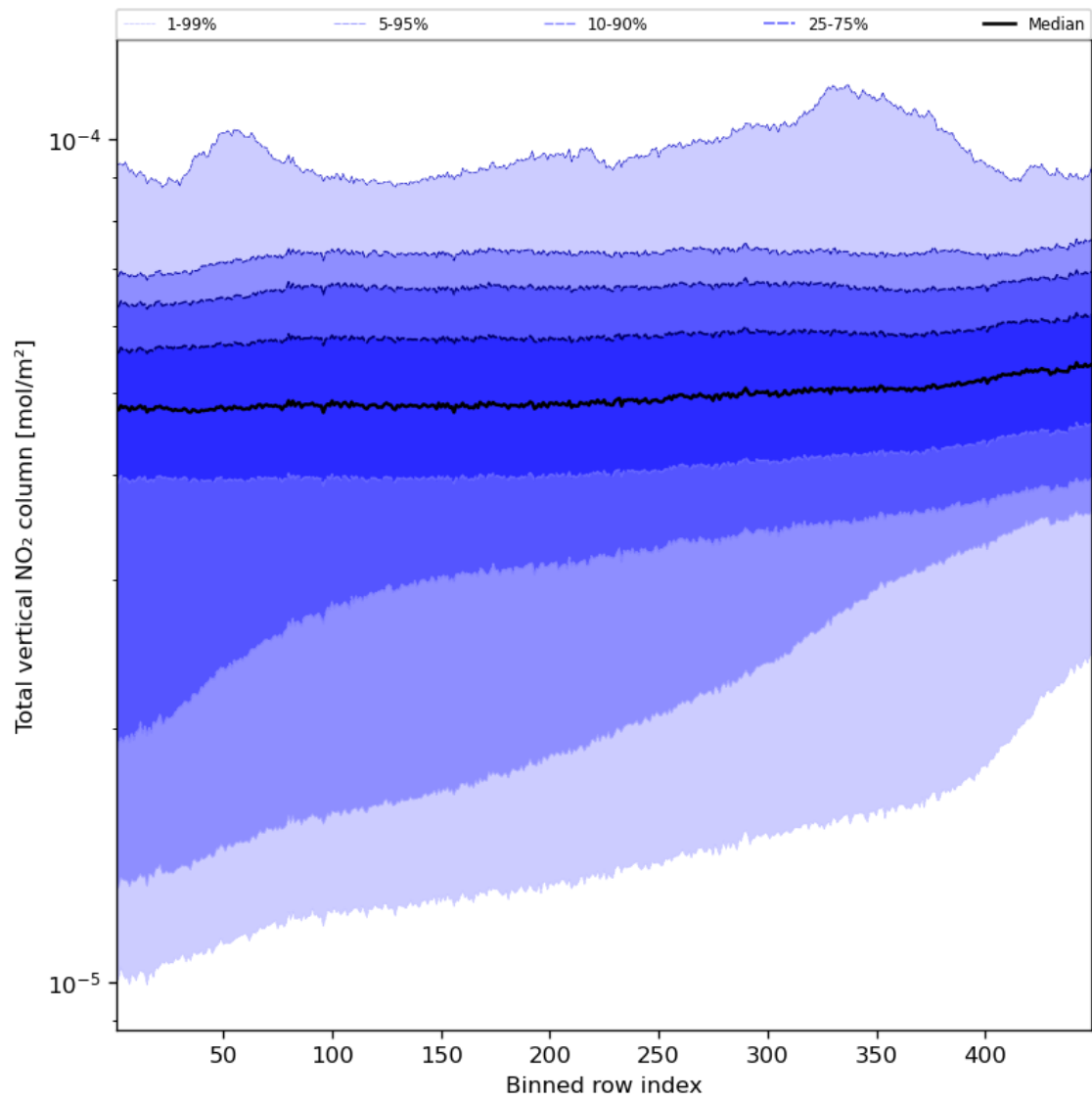
Figure 55: Along track statistics of “Total vertical NO 2 column” for 2023-09-20 to 2023-09-22
