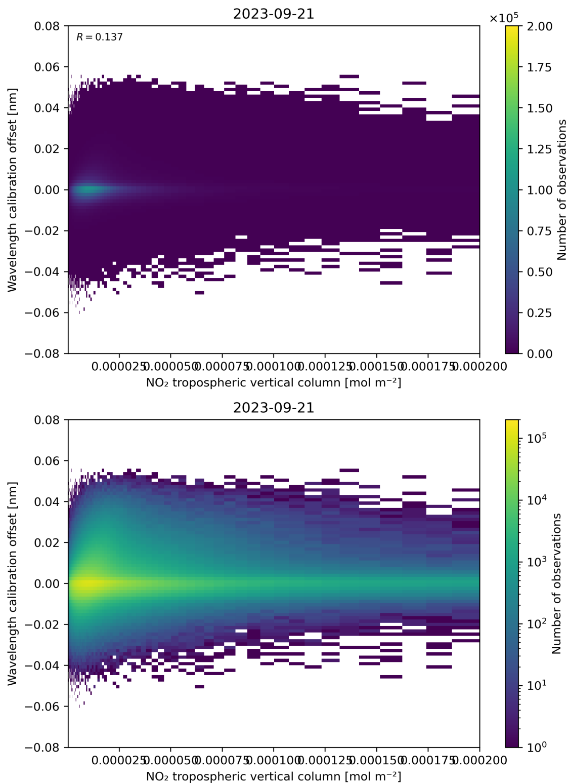
Figure 143: Scatter density plot of “NO 2 tropospheric vertical column” against “Wavelength calibration offset” for 2023-09-20 to 2023-09-22.
