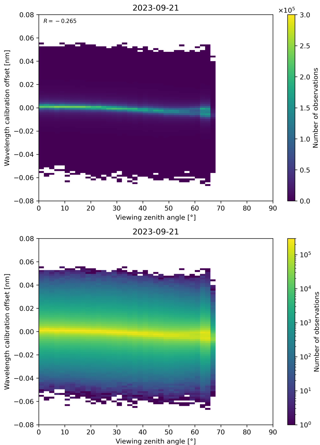
Figure 173: Scatter density plot of “Viewing zenith angle” against “Wavelength calibration offset” for 2023-09-20 to 2023-09-22.
