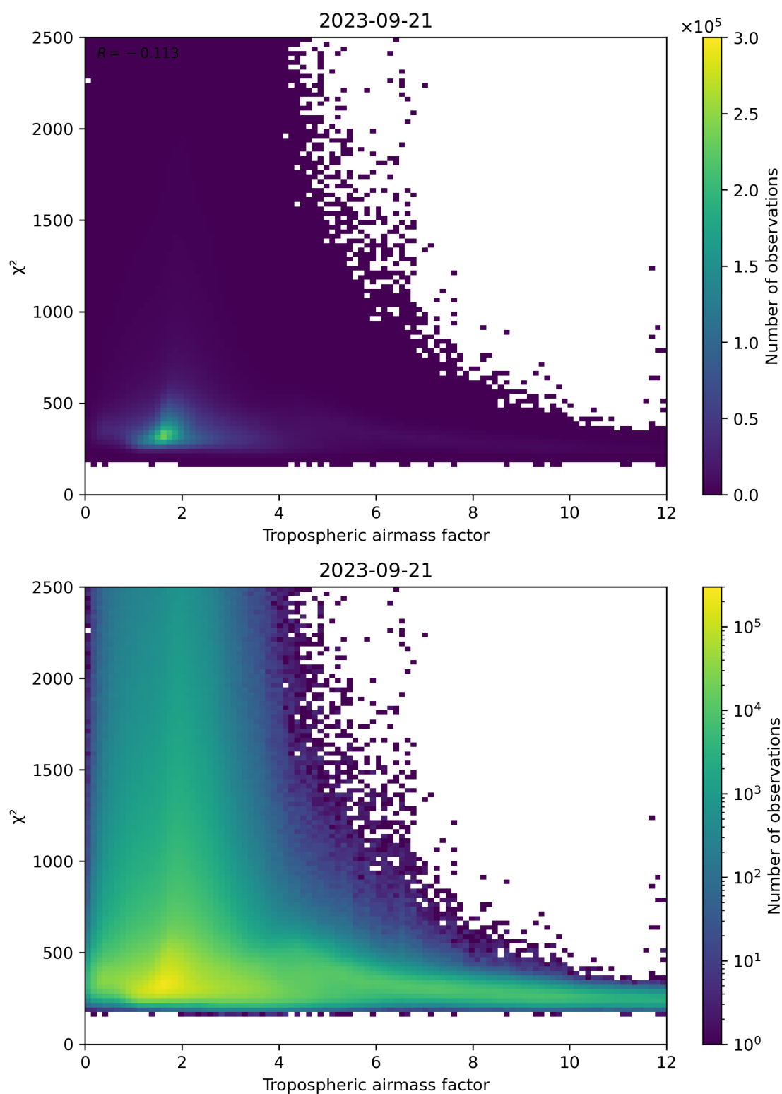
Figure 73: Scatter density plot of “Tropospheric airmass factor” against “ \chi^2 ” for 2023-09-20 to 2023-09-22.
