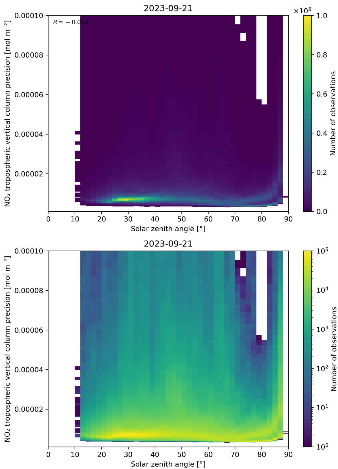
Figure 156: Scatter density plot of “Solar zenith angle” against “NO 2 tropospheric vertical column precision” for 2023-09-20 to 2023-09-22.
