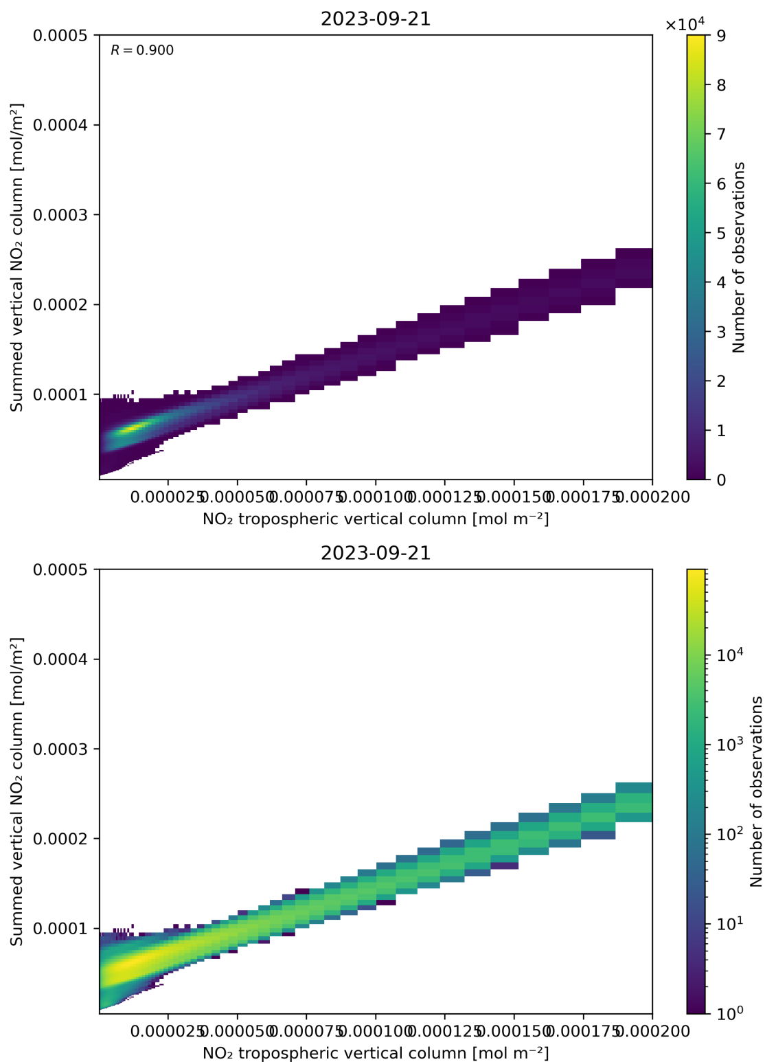
Figure 126: Scatter density plot of “NO 2 tropospheric vertical column” against “Summed vertical NO 2 column” for 2023-09-20 to 2023-09-22.
