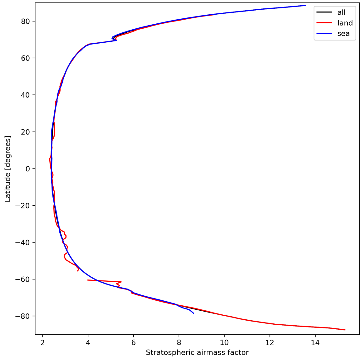
Figure 27: Zonal average of “Stratospheric airmass factor” for 2023-09-20 to 2023-09-22.
