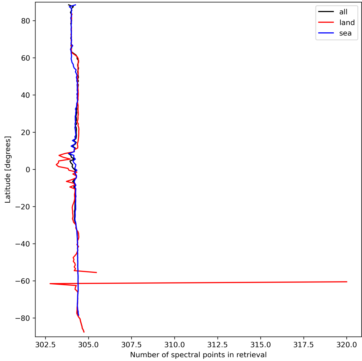
Figure 16: Zonal average of “Number of spectral points in retrieval” for 2023-09-20 to 2023-09-22.
