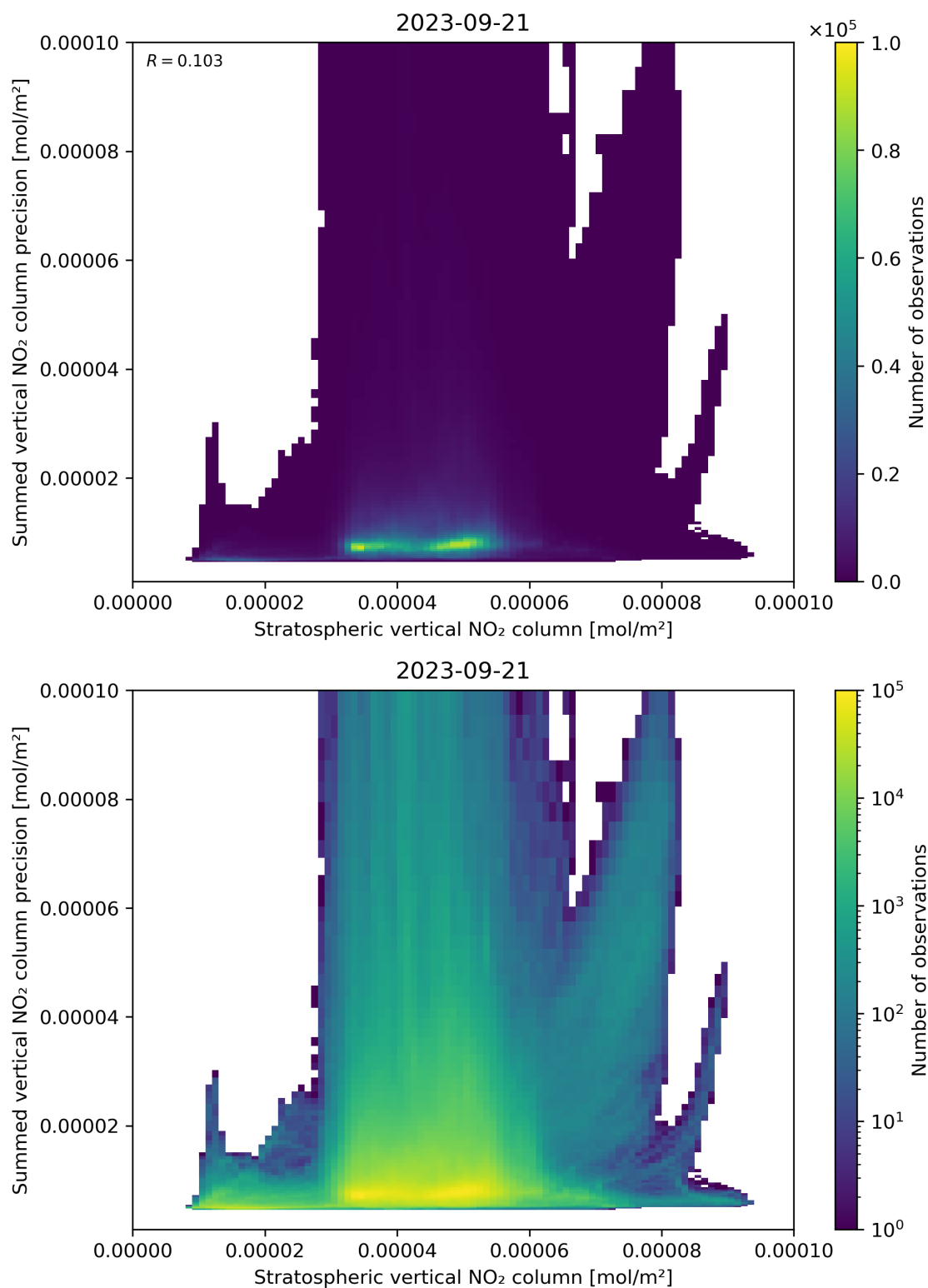
Figure 99: Scatter density plot of “Stratospheric vertical NO 2 column” against “Summed vertical NO 2 column precision” for 2023-09-20 to 2023-09-22.
