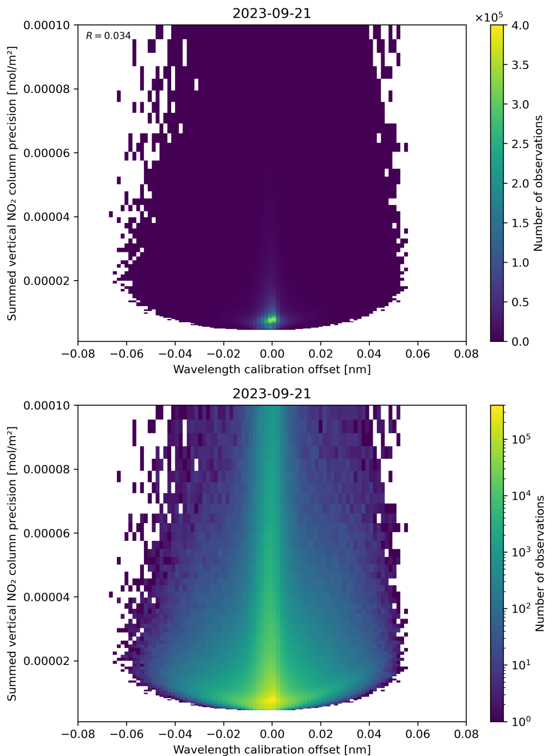
Figure 178: Scatter density plot of “Wavelength calibration offset” against “Summed vertical NO 2 column precision” for 2023-09-20 to 2023-09-22.
