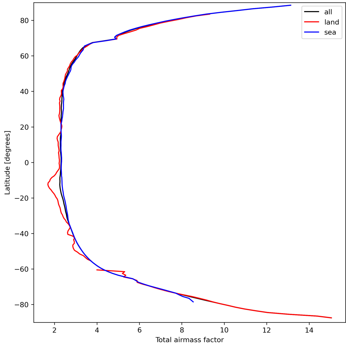
Figure 15: Zonal average of “Total airmass factor” for 2023-09-20 to 2023-09-22.
