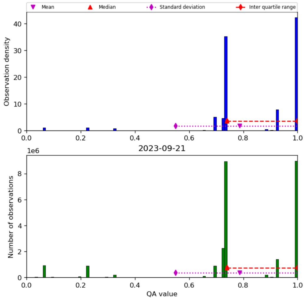
Figure 28: Histogram of “QA value” for 2023-09-20 to 2023-09-22
