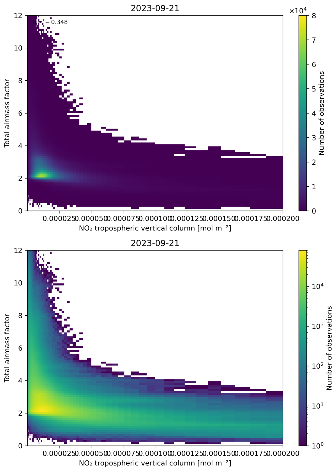
Figure 122: Scatter density plot of “NO 2 tropospheric vertical column” against “Total air mass factor” for 2023-09-20 to 2023-09-22.
