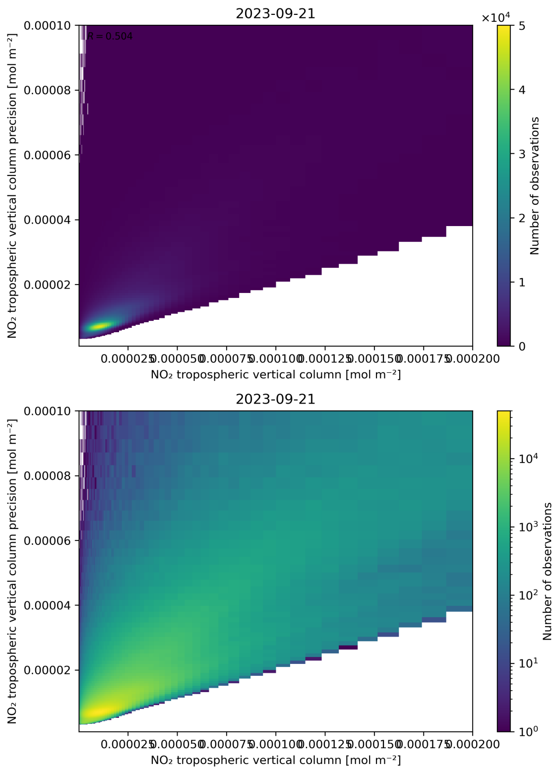
Figure 130: Scatter density plot of “NO 2 tropospheric vertical column” against “NO 2 tropospheric vertical column precision” for 2023-09-20 to 2023-09-22.
