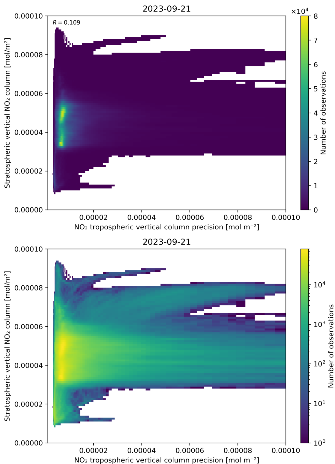
Figure 135: Scatter density plot of “NO 2 tropospheric vertical column precision” against “Stratospheric vertical NO 2 column” for 2023-09-20 to 2023-09-22.
