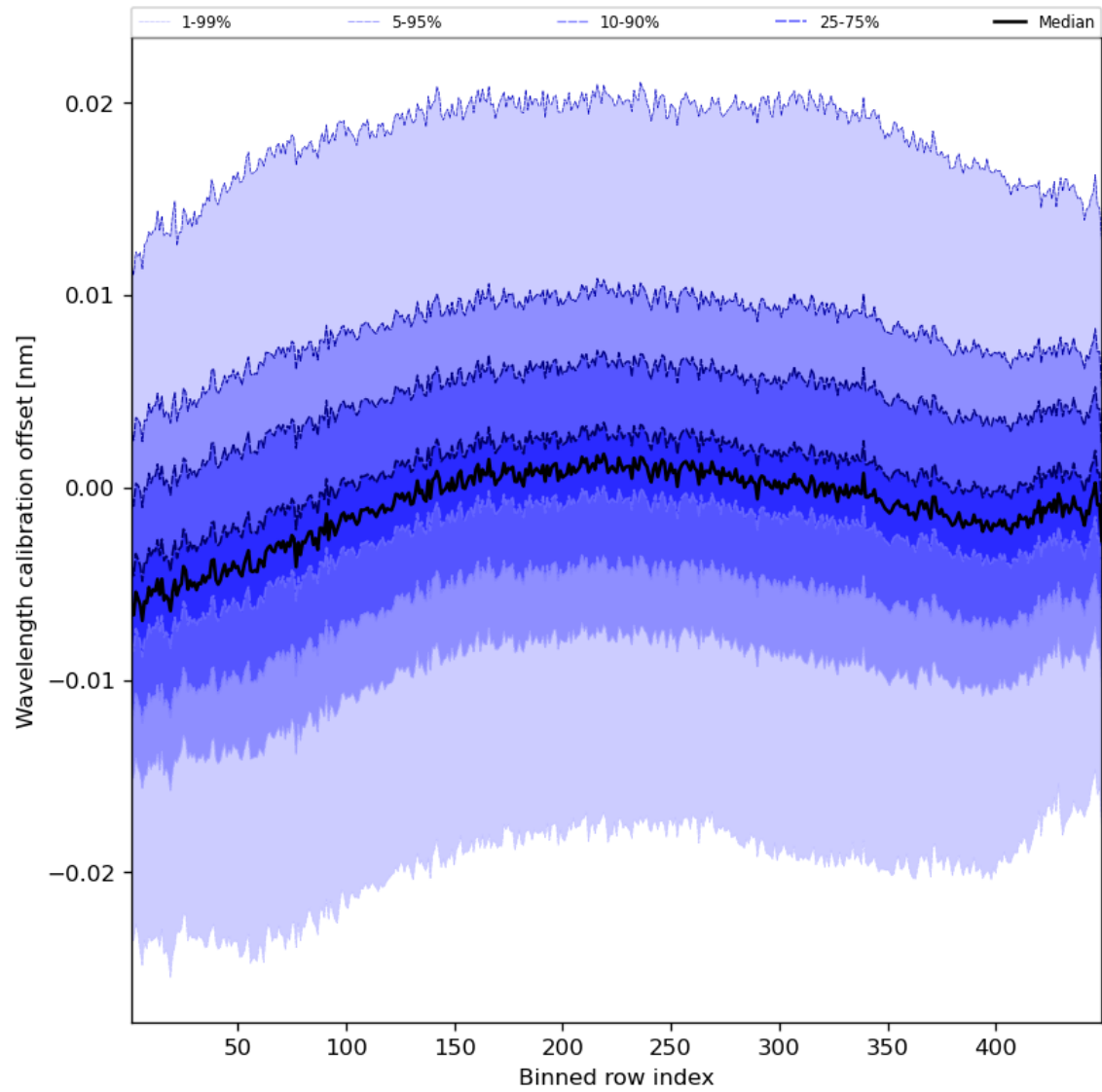
Figure 52: Along track statistics of “Wavelength calibration offset” for 2023-09-20 to 2023-09-22
