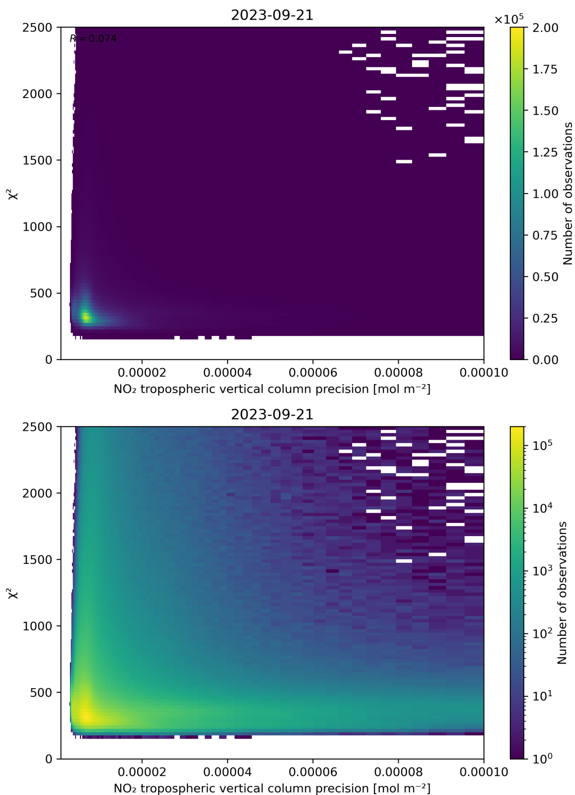
Figure 134: Scatter density plot of “NO 2 tropospheric vertical column precision” against “ \chi^2 ” for 2023-09-20 to 2023-09-22.
