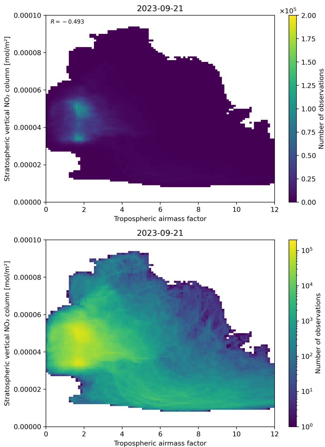
Figure 74: Scatter density plot of “Tropospheric air mass factor” against “Stratospheric vertical NO 2 column” for 2023-09-20 to 2023-09-22.
