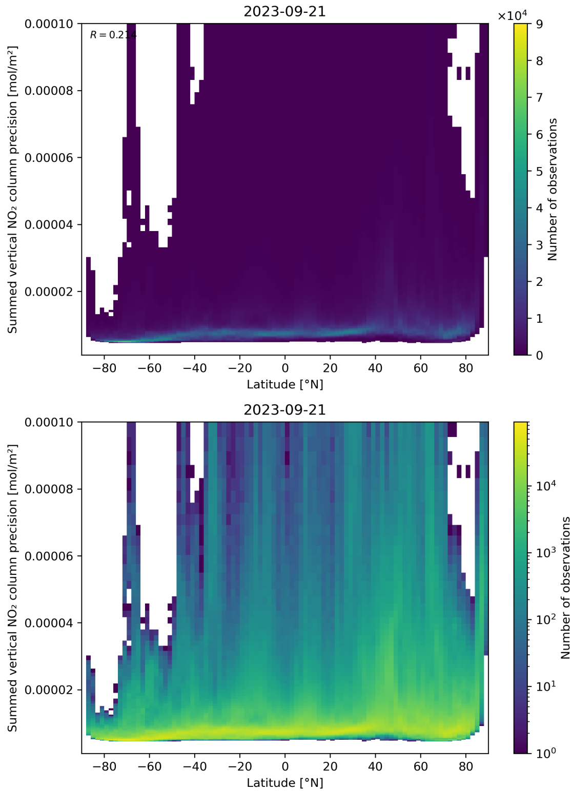
Figure 89: Scatter density plot of “Latitude” against “Summed vertical NO 2 column precision” for 2023-09-20 to 2023-09-22.
