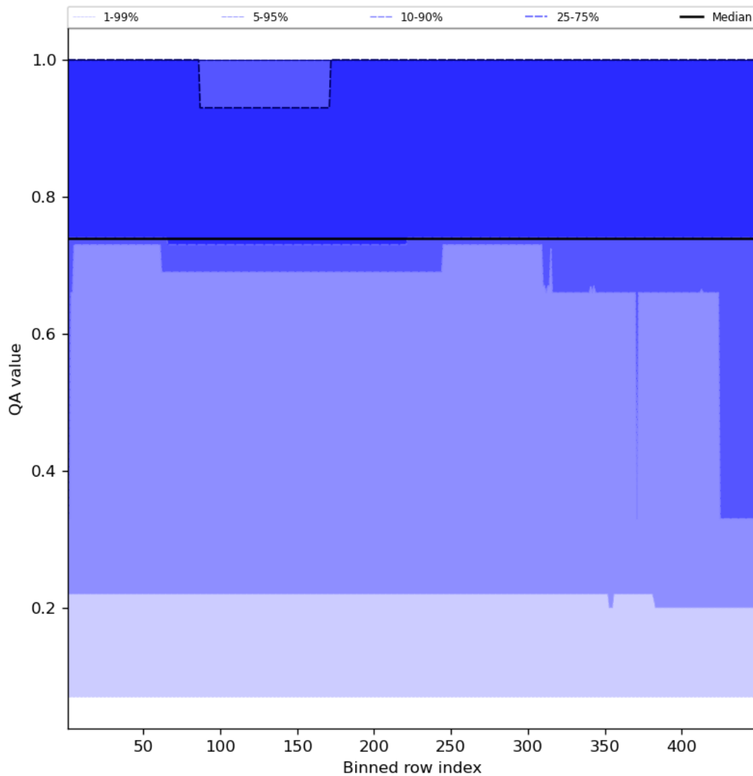
Figure 45: Along track statistics of “QA value” for 2023-09-20 to 2023-09-22
