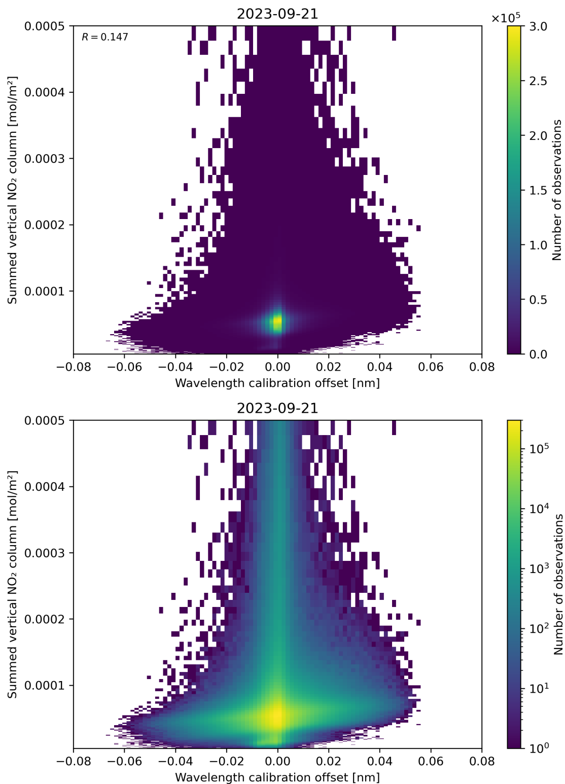
Figure 177: Scatter density plot of “Wavelength calibration offset” against “Summed vertical NO 2 column” for 2023-09-20 to 2023-09-22.
