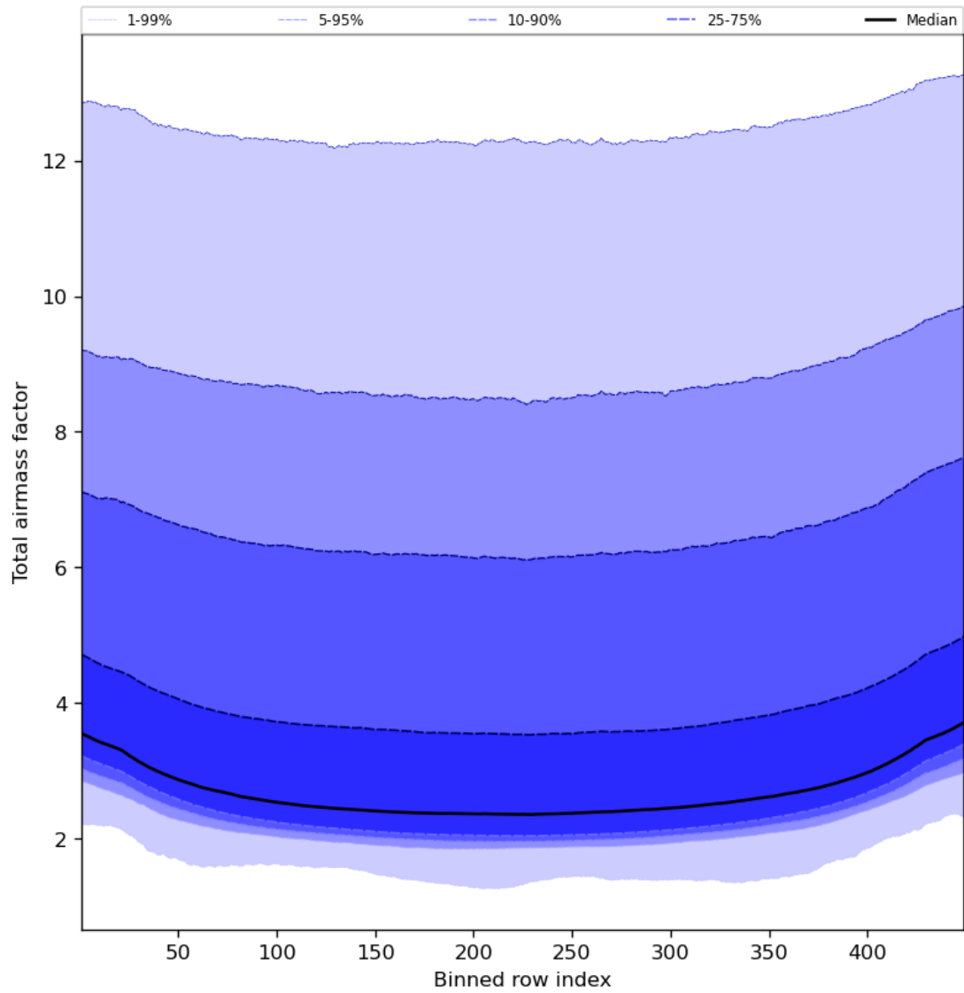
Figure 49: Along track statistics of “Total airmass factor” for 2023-09-20 to 2023-09-22
