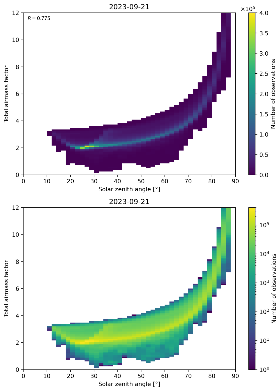
Figure 146: Scatter density plot of “Solar zenith angle” against “Total air mass factor” for 2023-09-20 to 2023-09-22.
