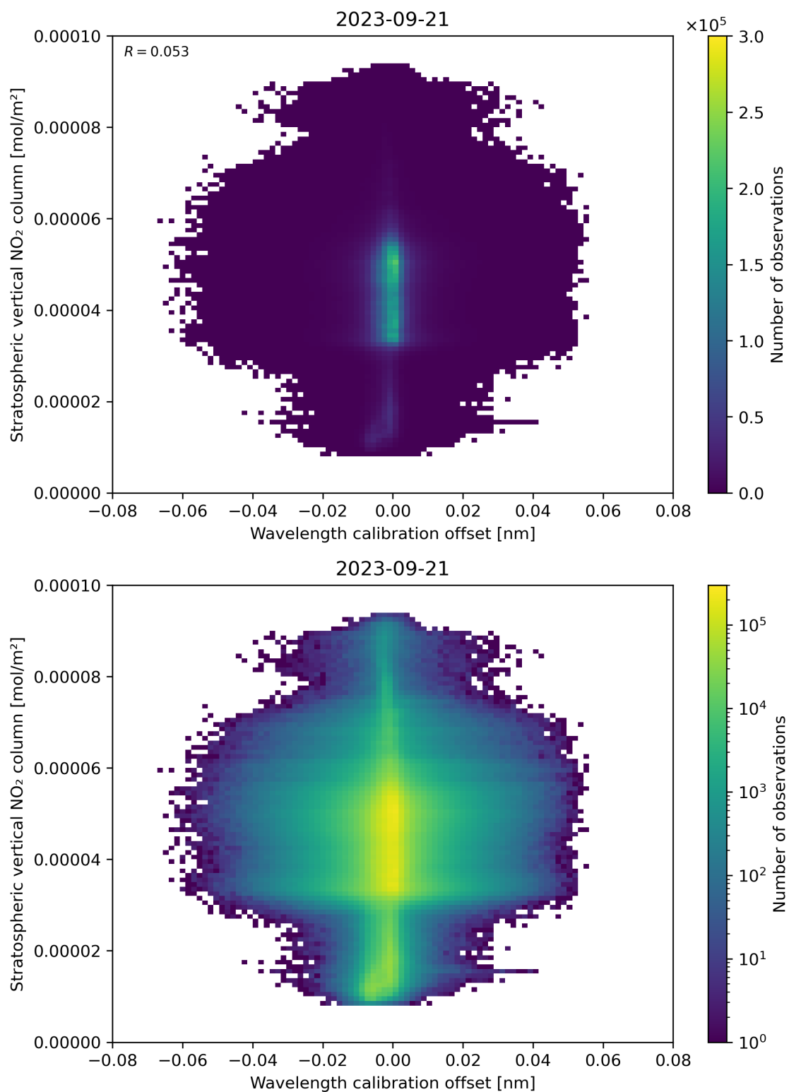
Figure 176: Scatter density plot of “Wavelength calibration offset” against “Stratospheric vertical \text{NO}_2 column” for 2023-09-20 to 2023-09-22.
