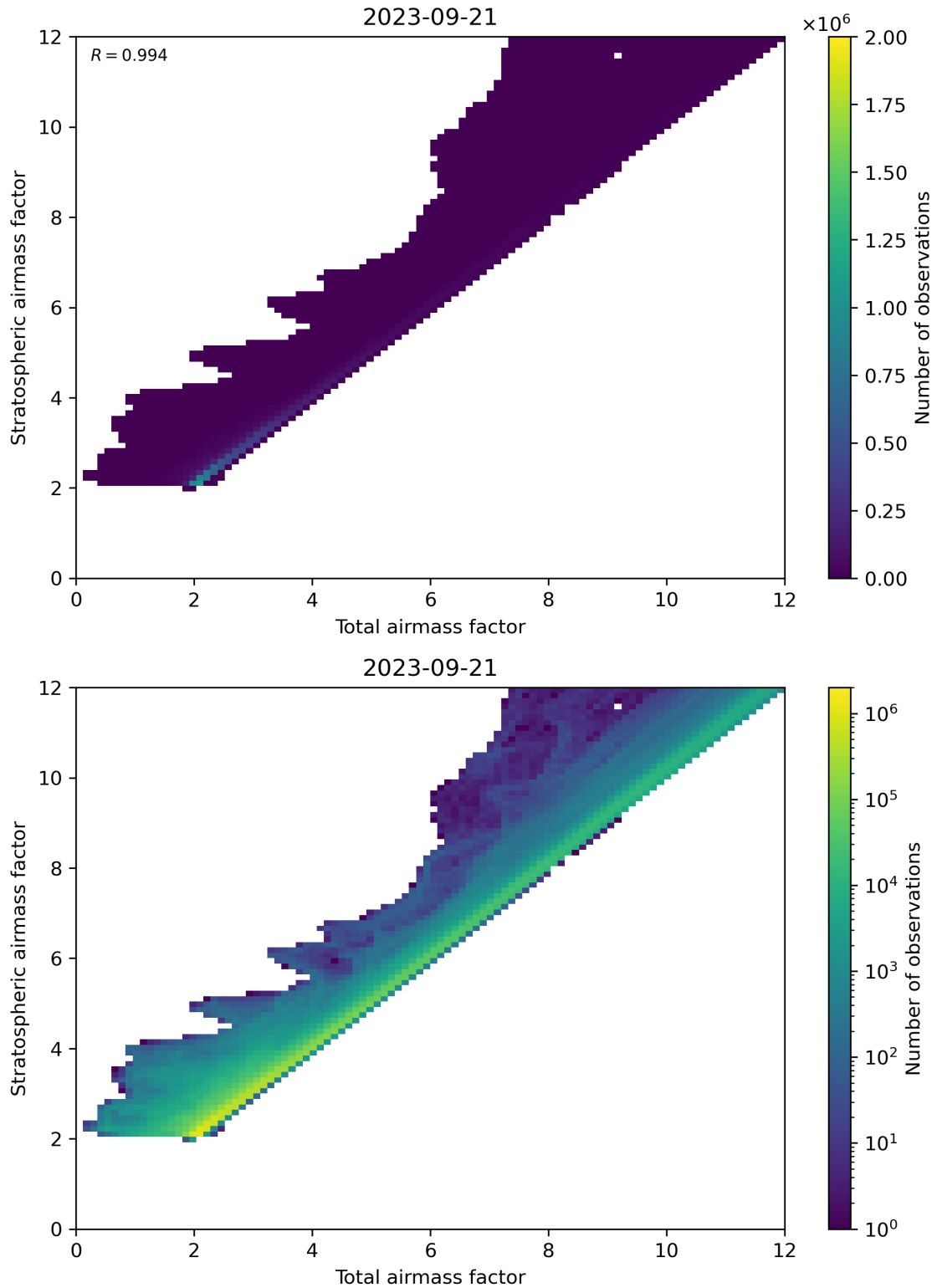
Figure 62: Scatter density plot of “Total airmass factor” against “Stratospheric airmass factor” for 2023-09-20 to 2023-09-22.
