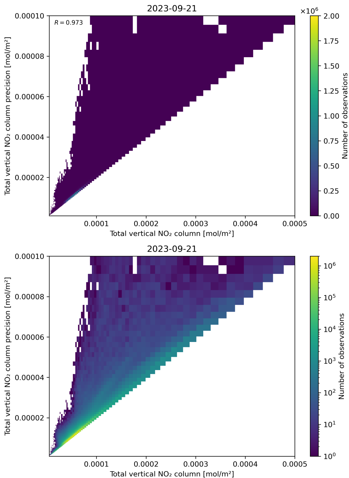
Figure 114: Scatter density plot of “Total vertical NO 2 column” against “Total vertical NO 2 column precision” for 2023-09-20 to 2023-09-22.
