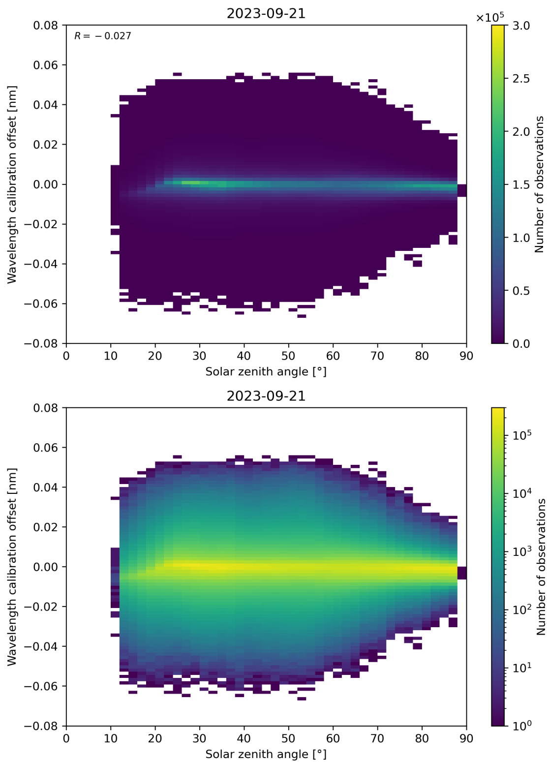
Figure 158: Scatter density plot of “Solar zenith angle” against “Wavelength calibration offset” for 2023-09-20 to 2023-09-22.
