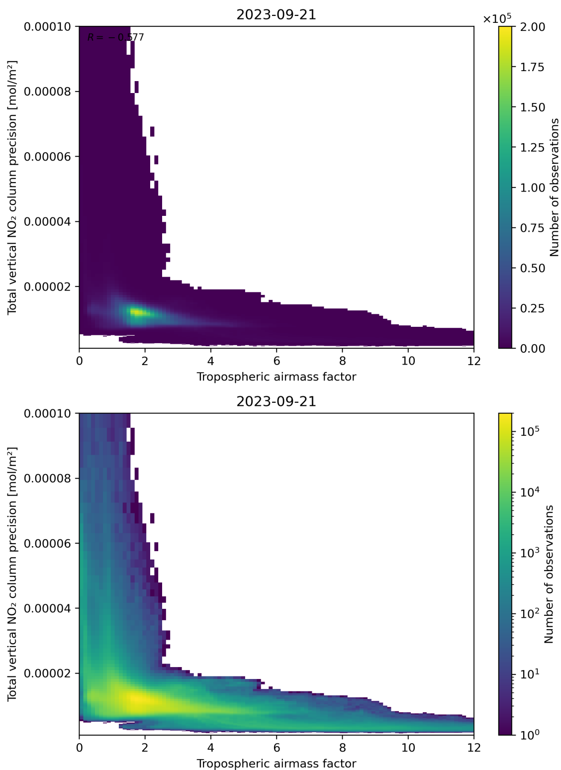
Figure 78: Scatter density plot of “Tropospheric air mass factor” against “Total vertical NO 2 column precision” for 2023-09-20 to 2023-09-22.
