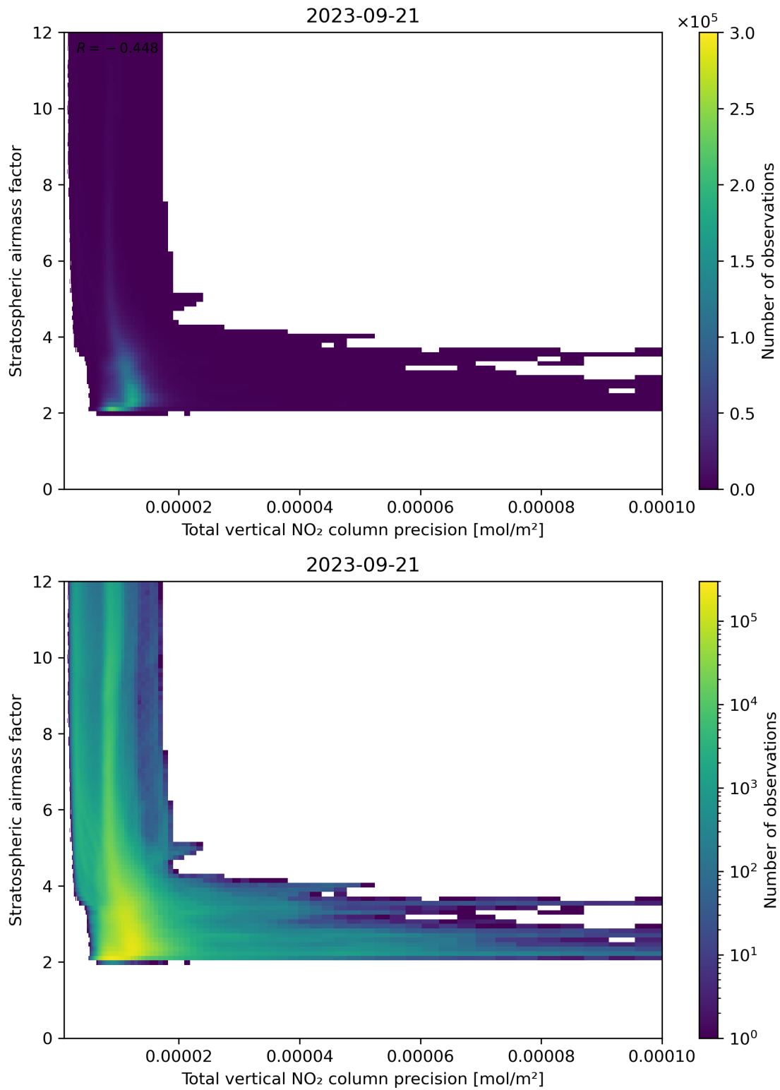
Figure 115: Scatter density plot of “Total vertical NO 2 column precision” against “Stratospheric air mass factor” for 2023-09-20 to 2023-09-22.
