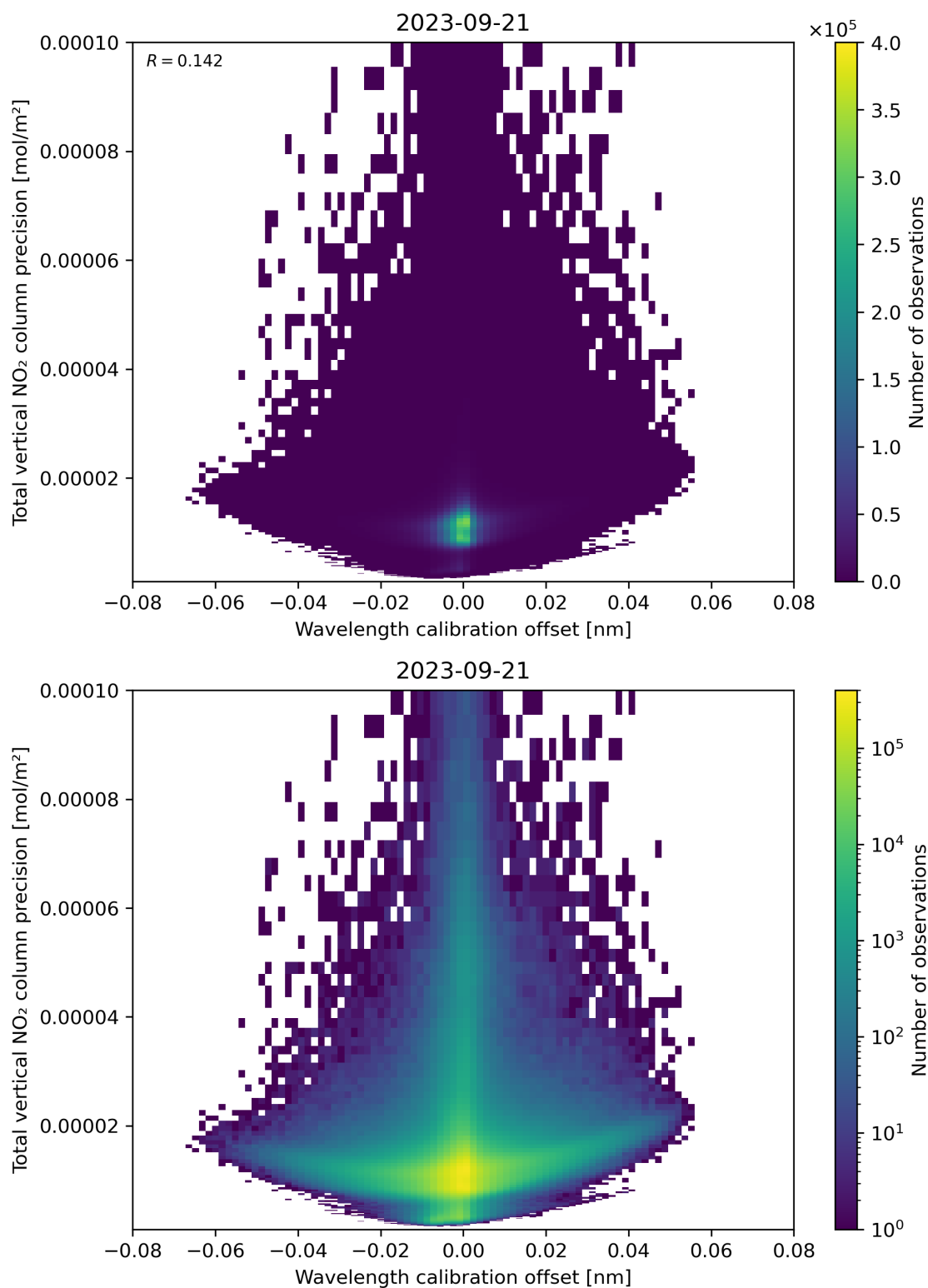
Figure 180: Scatter density plot of “Wavelength calibration offset” against “Total vertical NO 2 column precision” for 2023-09-20 to 2023-09-22.
