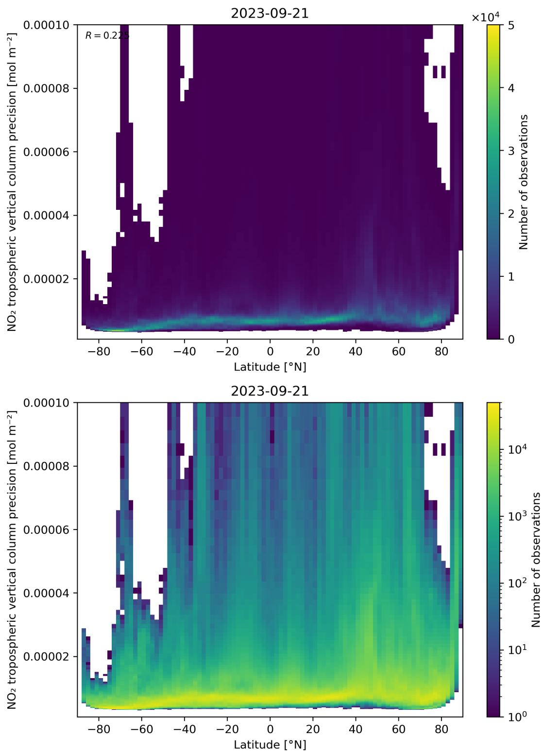
Figure 93: Scatter density plot of “Latitude” against “NO 2 tropospheric vertical column precision” for 2023-09-20 to 2023-09-22.
