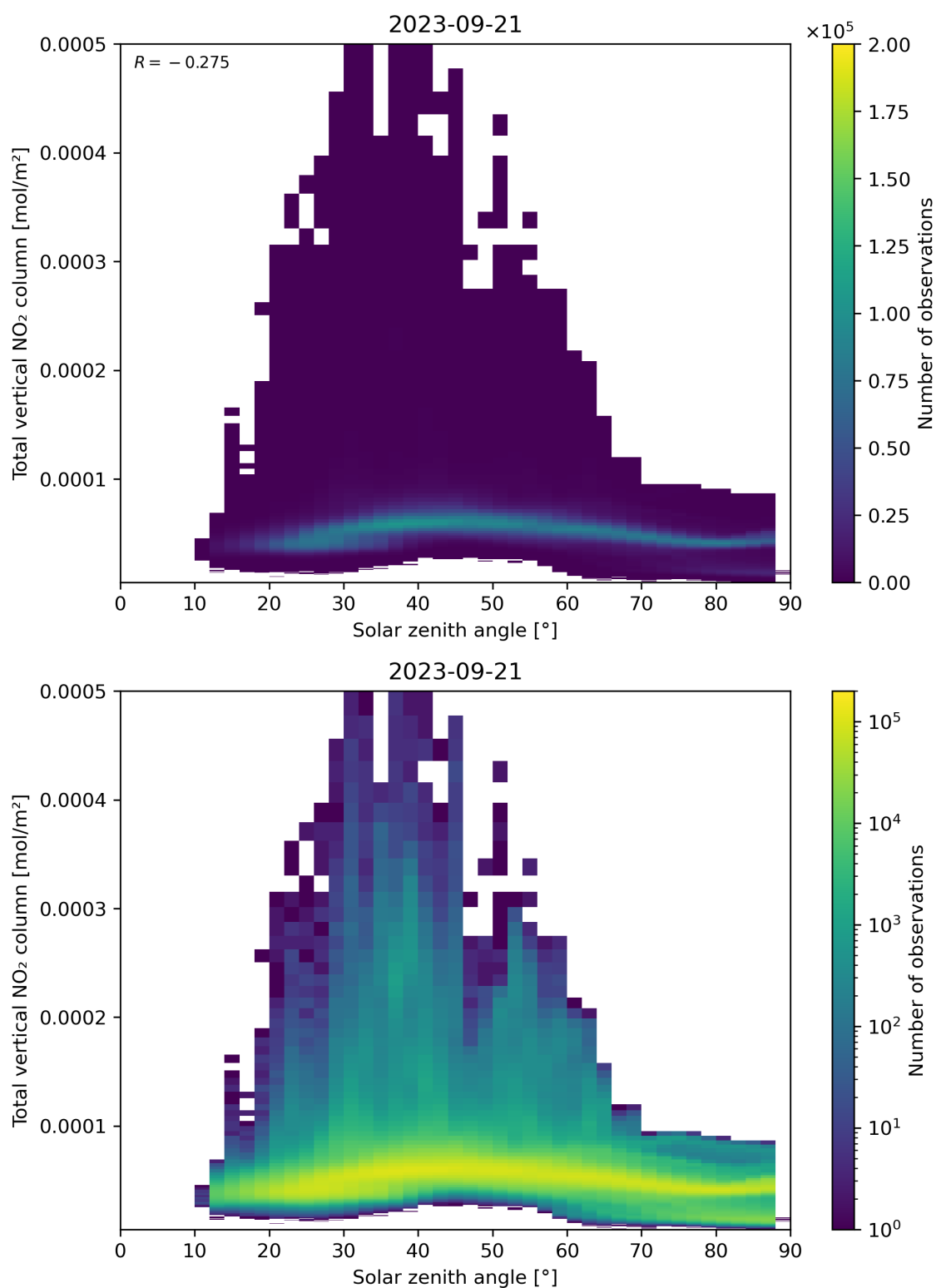
Figure 153: Scatter density plot of “Solar zenith angle” against “Total vertical NO 2 column” for 2023-09-20 to 2023-09-22.
