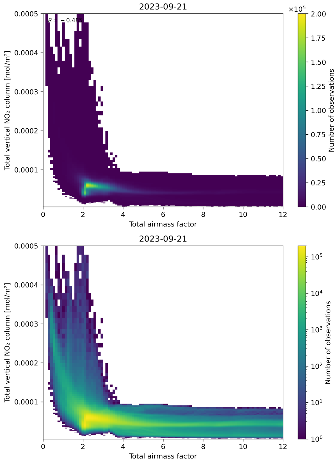
Figure 67: Scatter density plot of “Total airmass factor” against “Total vertical NO 2 column” for 2023-09-20 to 2023-09-22.
