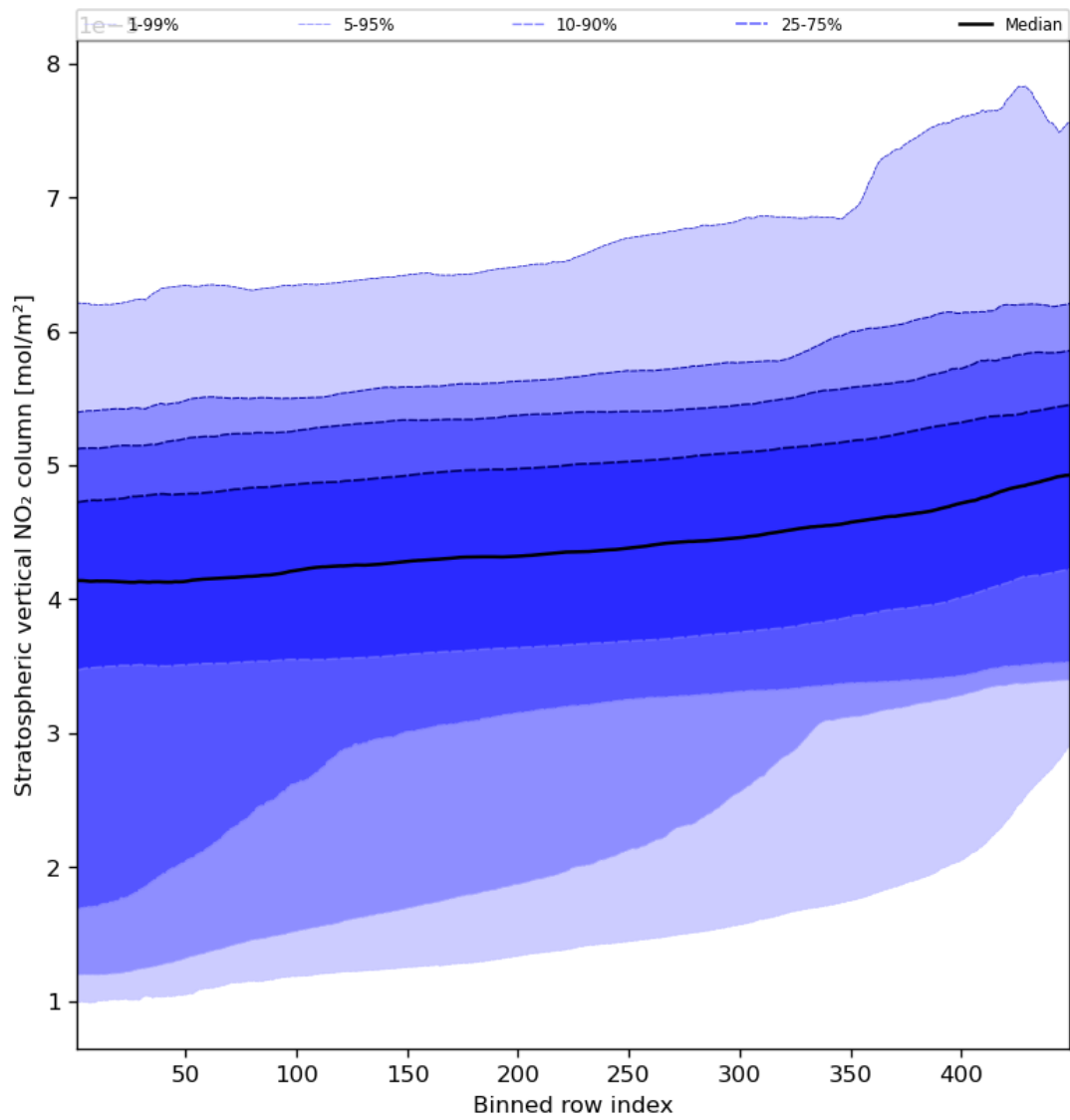
Figure 53: Along track statistics of “Stratospheric vertical NO 2 column” for 2023-09-20 to 2023-09-22
