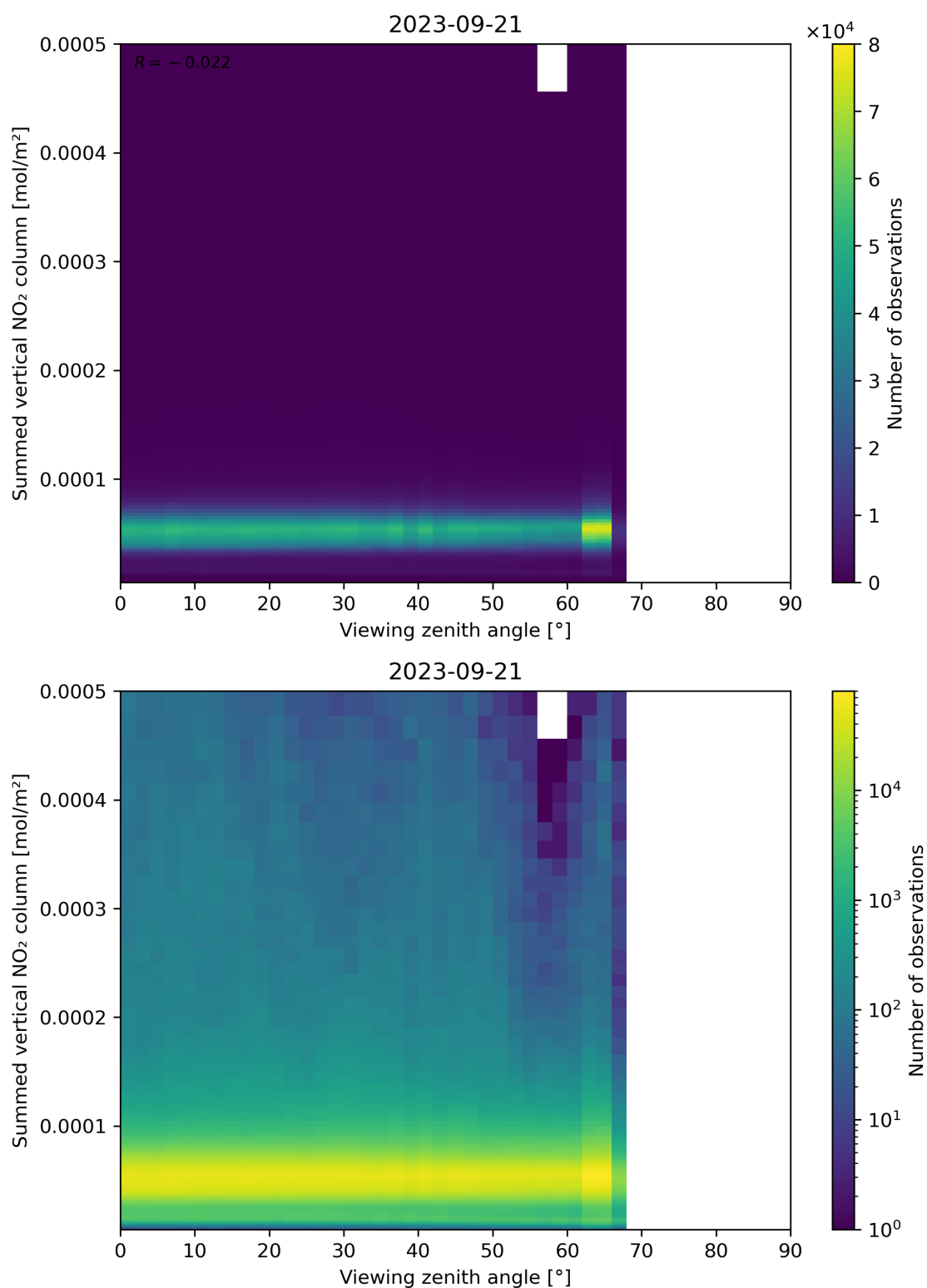
Figure 165: Scatter density plot of “Viewing zenith angle” against “Summed vertical NO 2 column” for 2023-09-20 to 2023-09-22.
