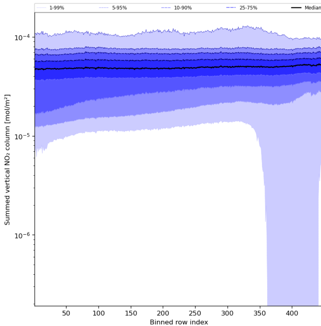
Figure 57: Along track statistics of “Summed vertical NO 2 column” for 2023-09-20 to 2023-09-22
