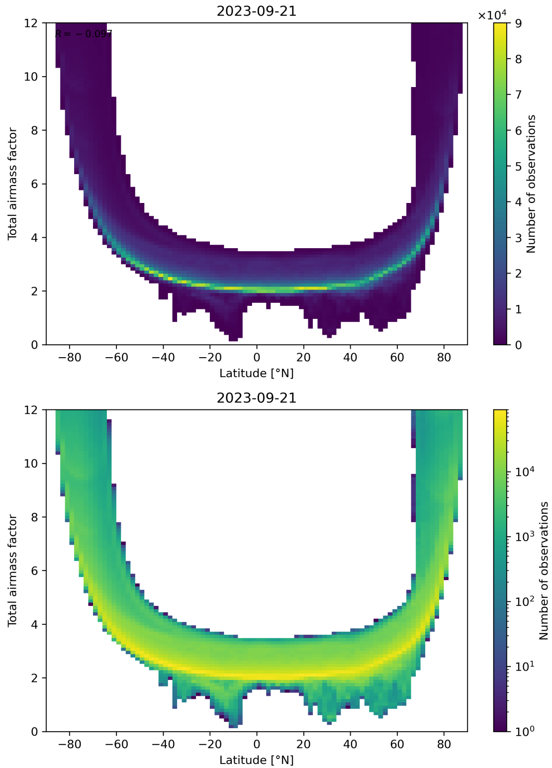
Figure 84: Scatter density plot of “Latitude” against “Total airmass factor” for 2023-09-20 to 2023-09-22.
