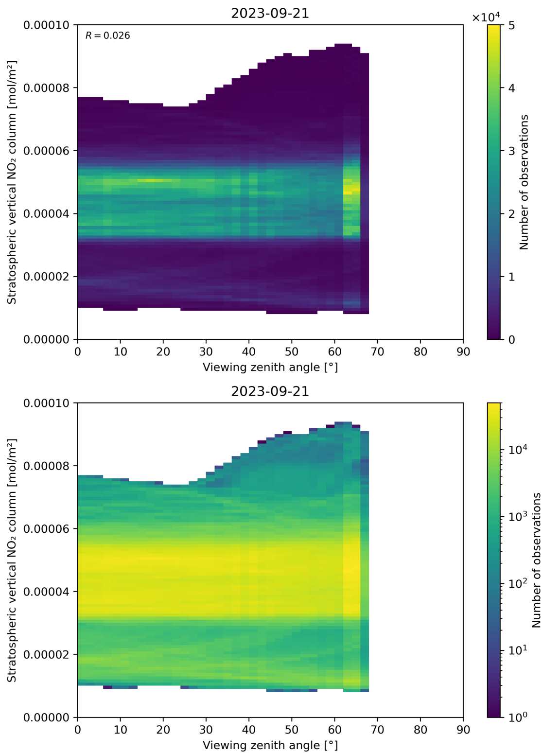
Figure 164: Scatter density plot of “Viewing zenith angle” against “Stratospheric vertical \text{NO}_2 column” for 2023-09-20 to 2023-09-22.
