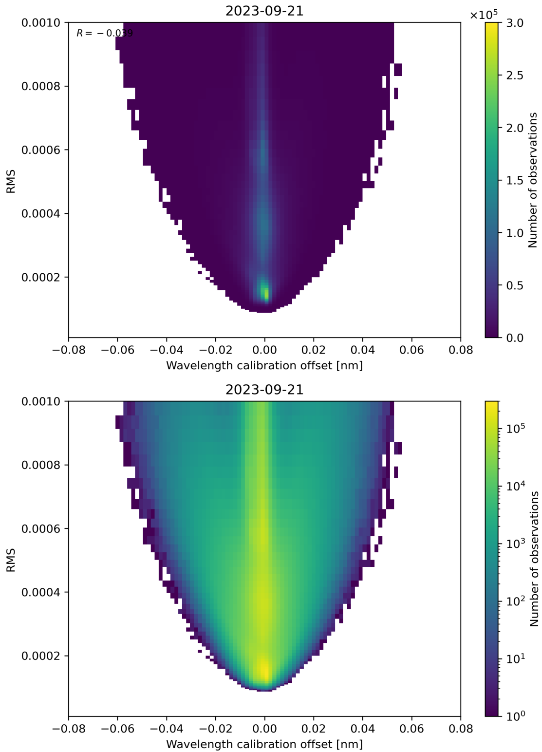
Figure 181: Scatter density plot of “Wavelength calibration offset” against “RMS” for 2023-09-20 to 2023-09-22.
