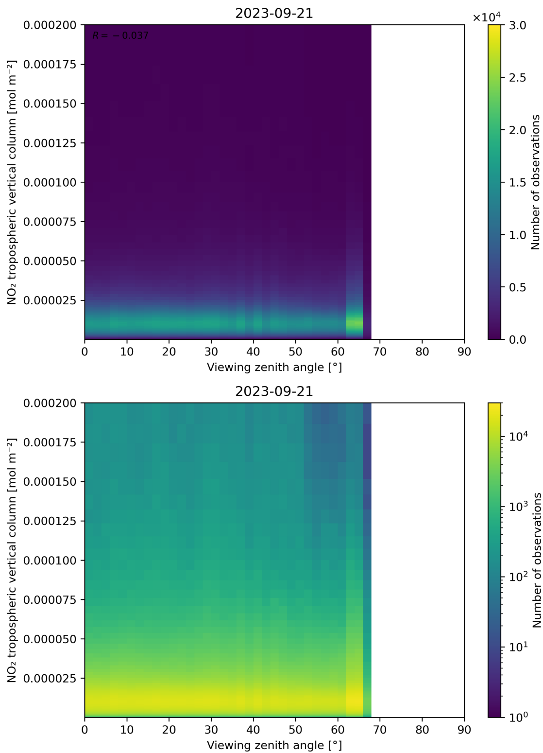
Figure 169: Scatter density plot of “Viewing zenith angle” against “NO 2 tropospheric vertical column” for 2023-09-20 to 2023-09-22.
