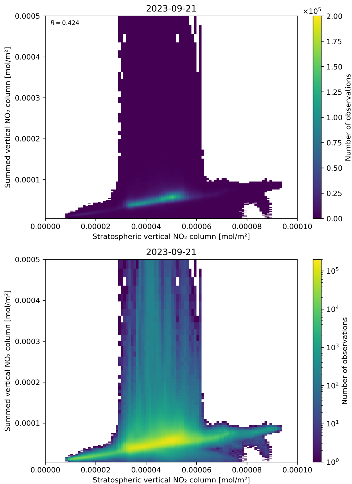
Figure 98: Scatter density plot of “Stratospheric vertical NO 2 column” against “Summed vertical NO 2 column” for 2023-09-20 to 2023-09-22.
