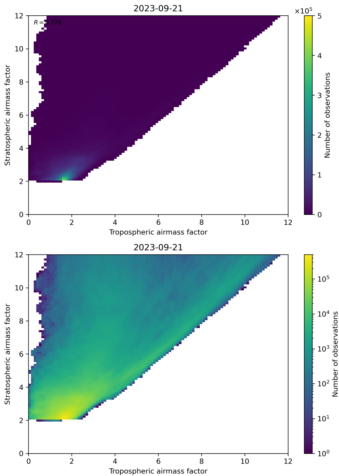
Figure 71: Scatter density plot of “Tropospheric airmass factor” against “Stratospheric airmass factor” for 2023-09-20 to 2023-09-22.
