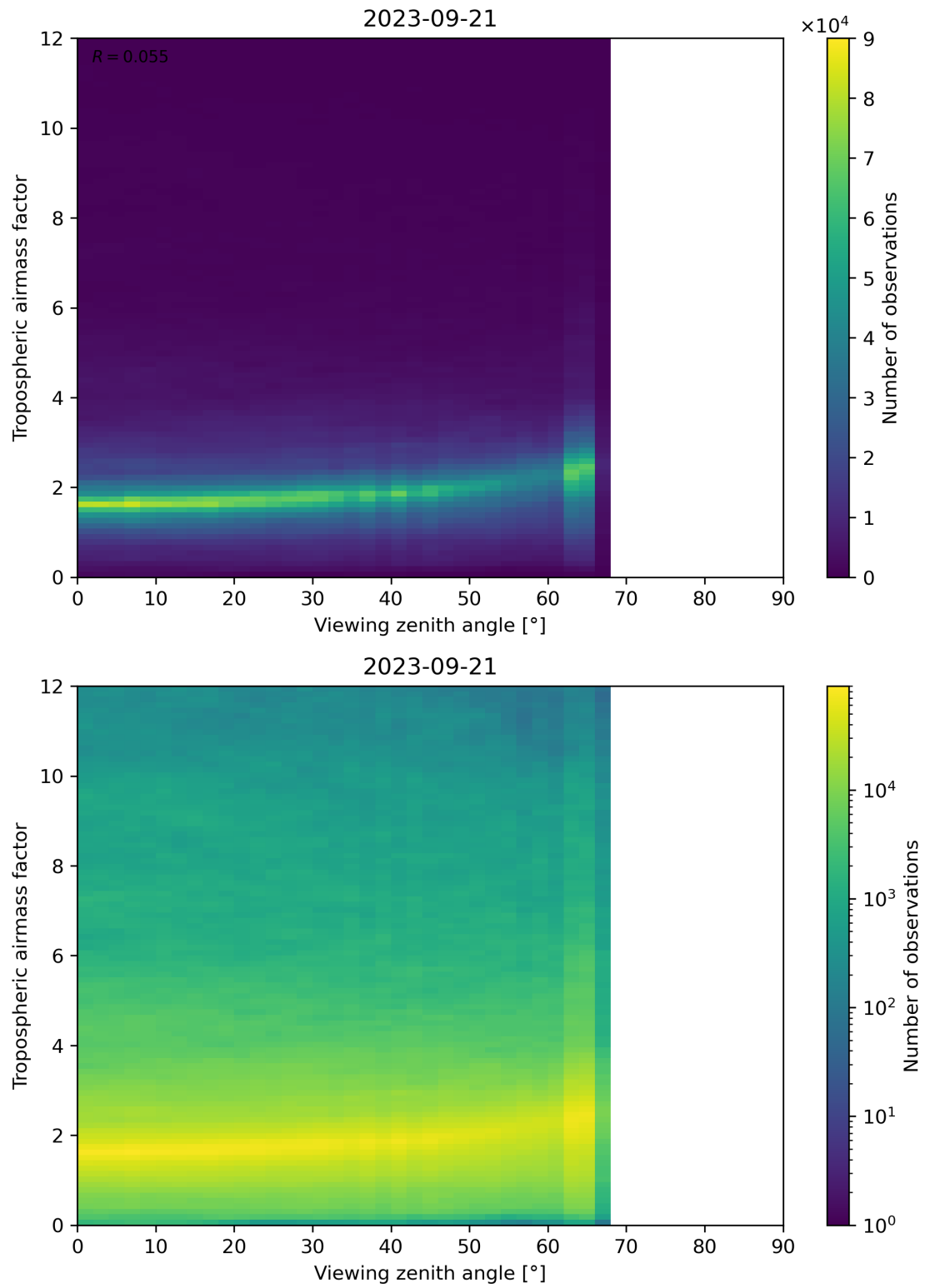
Figure 161: Scatter density plot of “Viewing zenith angle” against “Tropospheric airmass factor” for 2023-09-20 to 2023-09-22.
