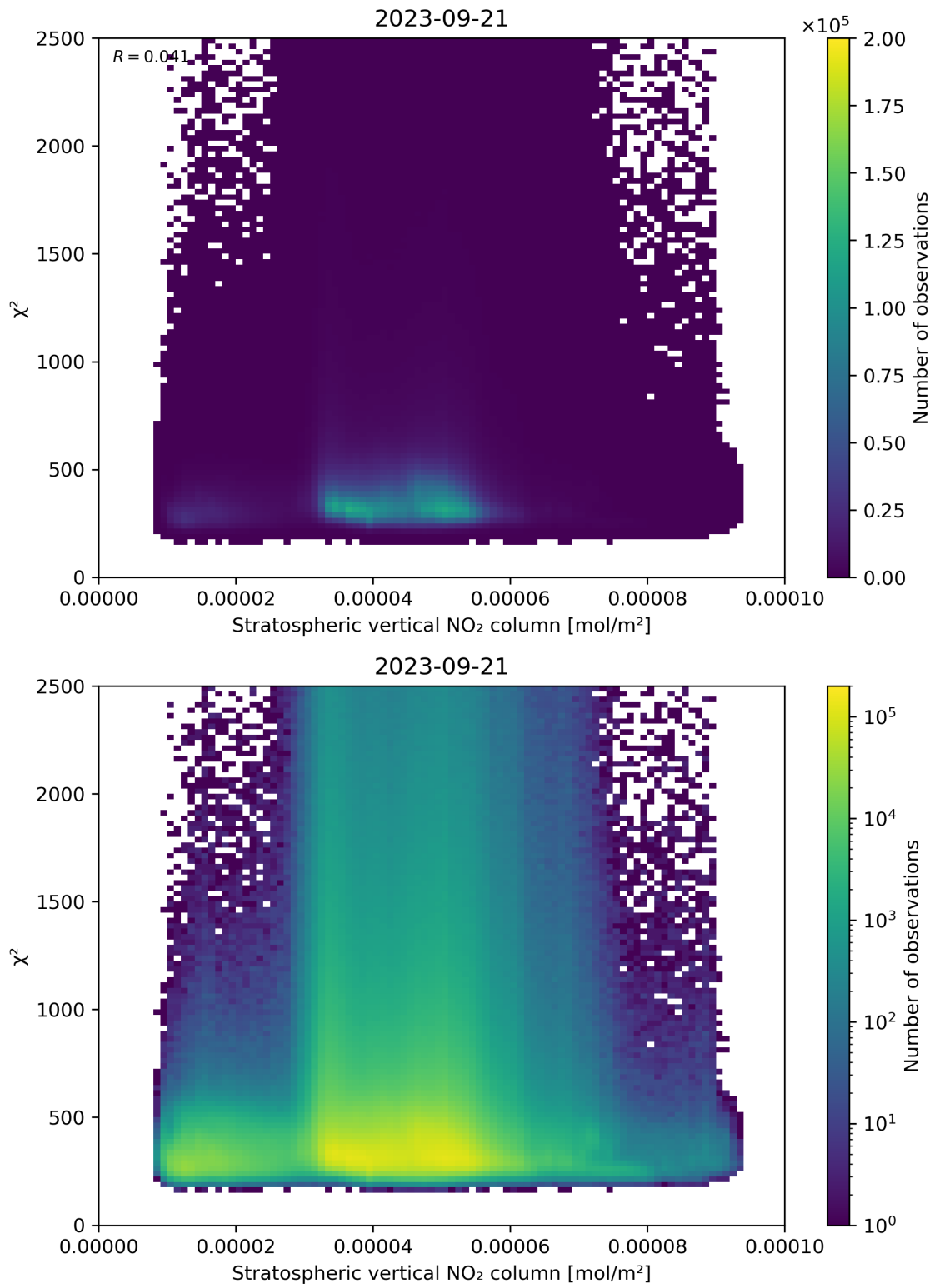
Figure 97: Scatter density plot of “Stratospheric vertical NO 2 column” against “ \chi^2 ” for 2023-09-20 to 2023-09-22.
