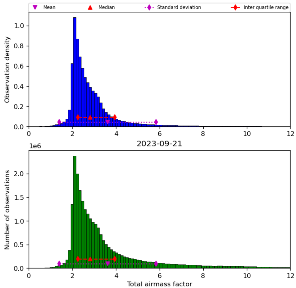
Figure 32: Histogram of “Total airmass factor” for 2023-09-20 to 2023-09-22
