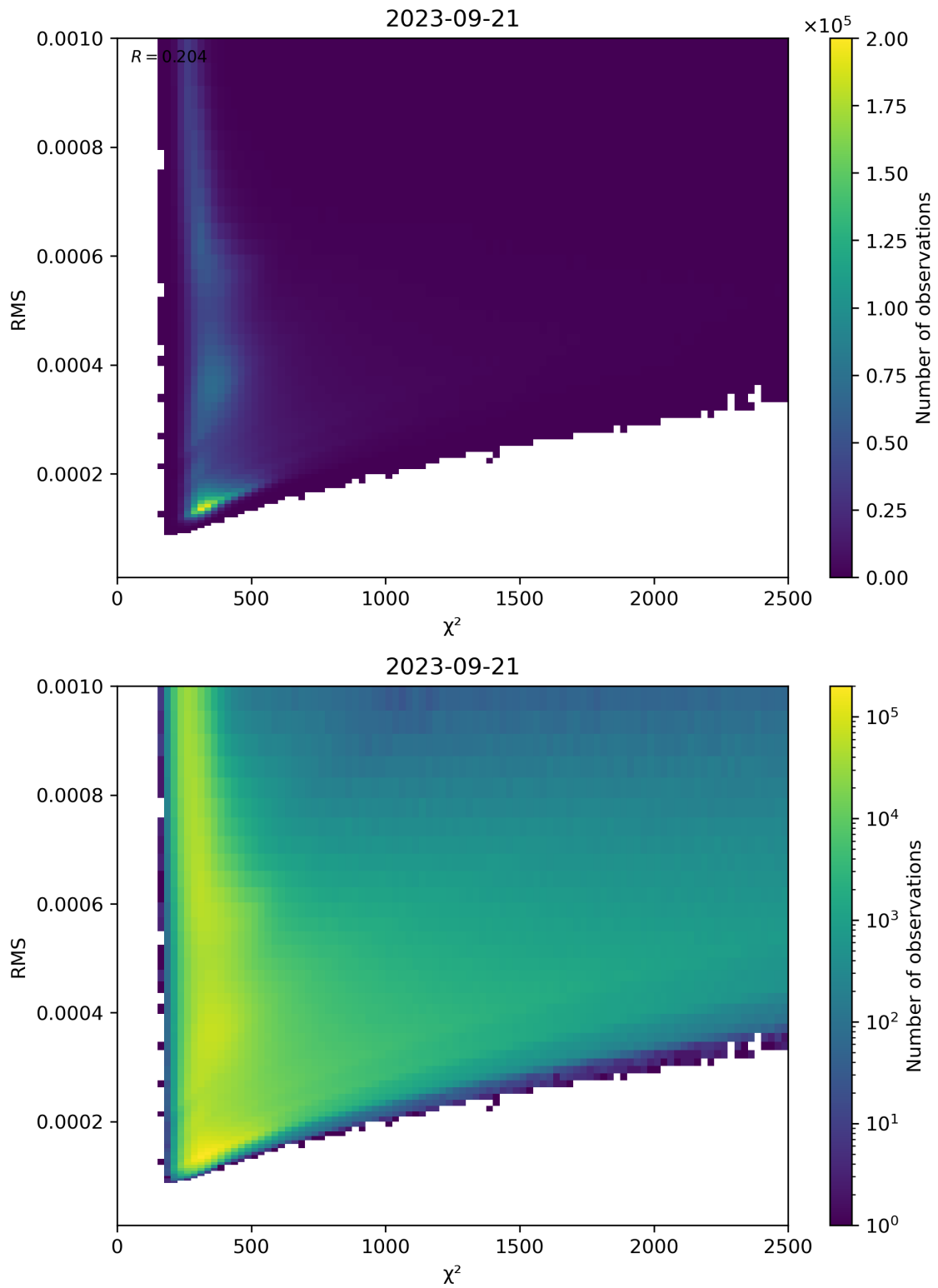
Figure 82: Scatter density plot of “ \chi^2 ” against “RMS” for 2023-09-20 to 2023-09-22.
