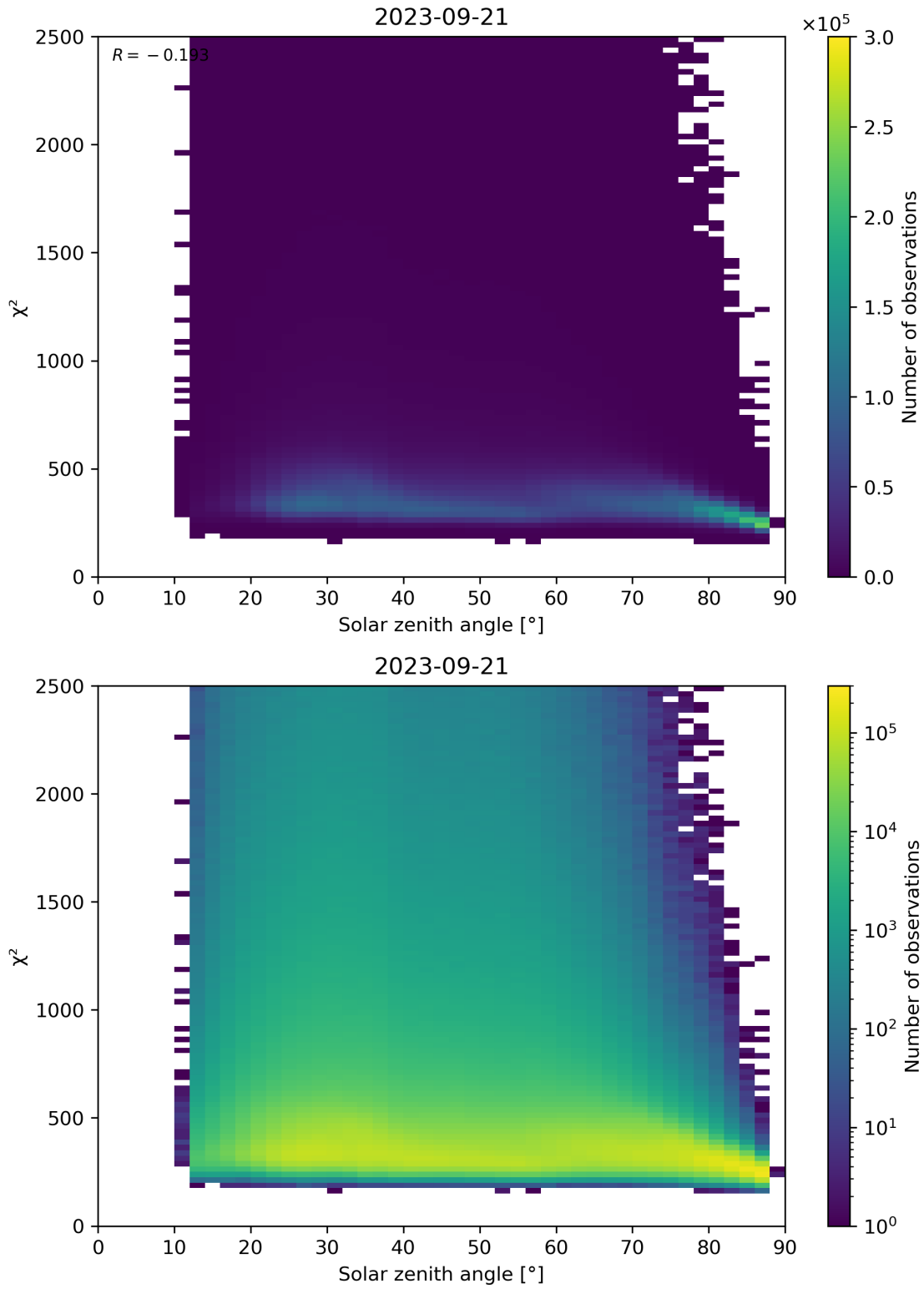
Figure 148: Scatter density plot of “Solar zenith angle” against “ \chi^2 ” for 2023-09-20 to 2023-09-22.
