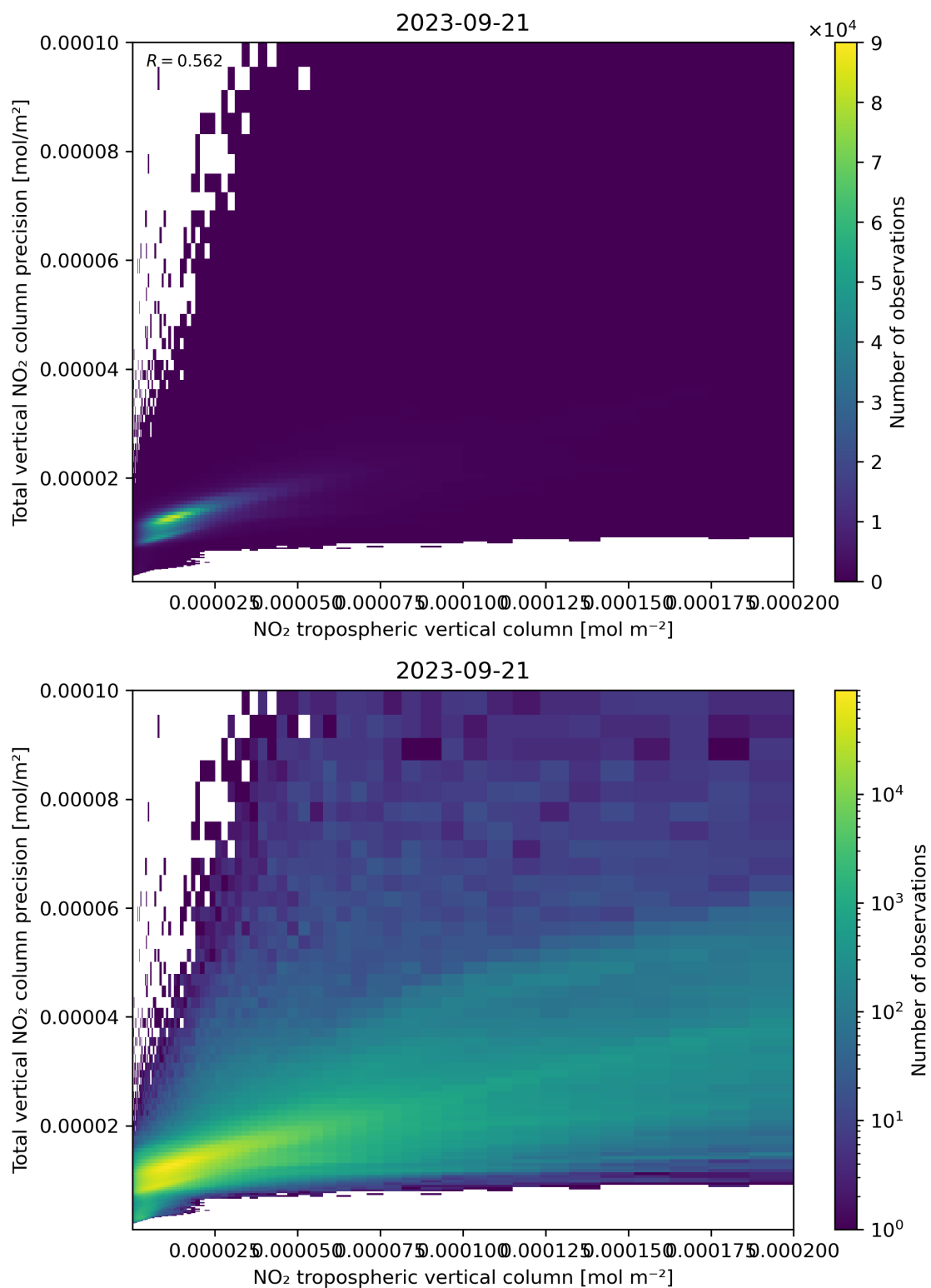
Figure 129: Scatter density plot of “NO 2 tropospheric vertical column” against “Total vertical NO 2 column precision” for 2023-09-20 to 2023-09-22.
