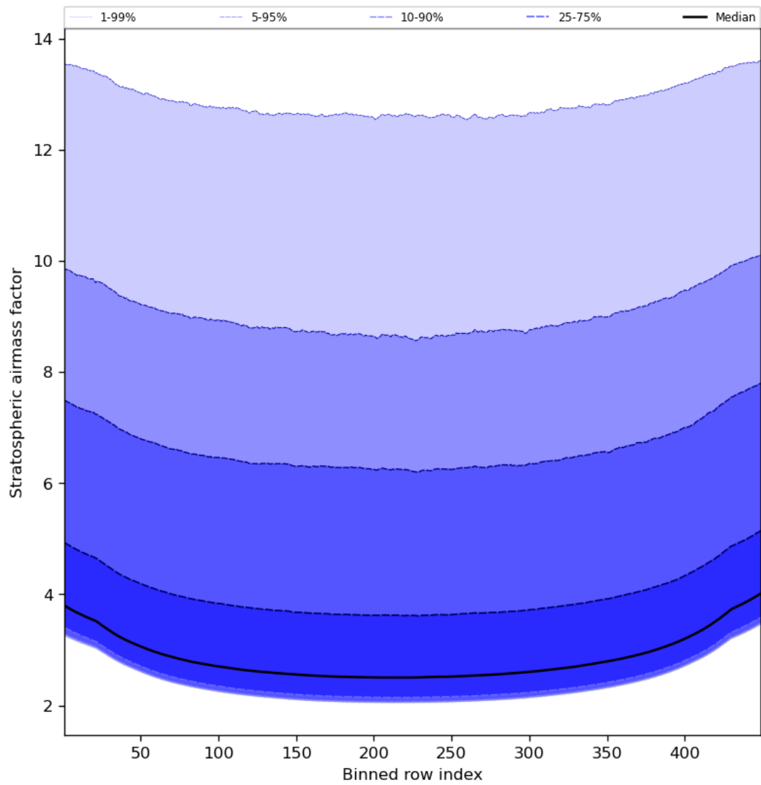
Figure 61: Along track statistics of “Stratospheric airmass factor” for 2023-09-20 to 2023-09-22
