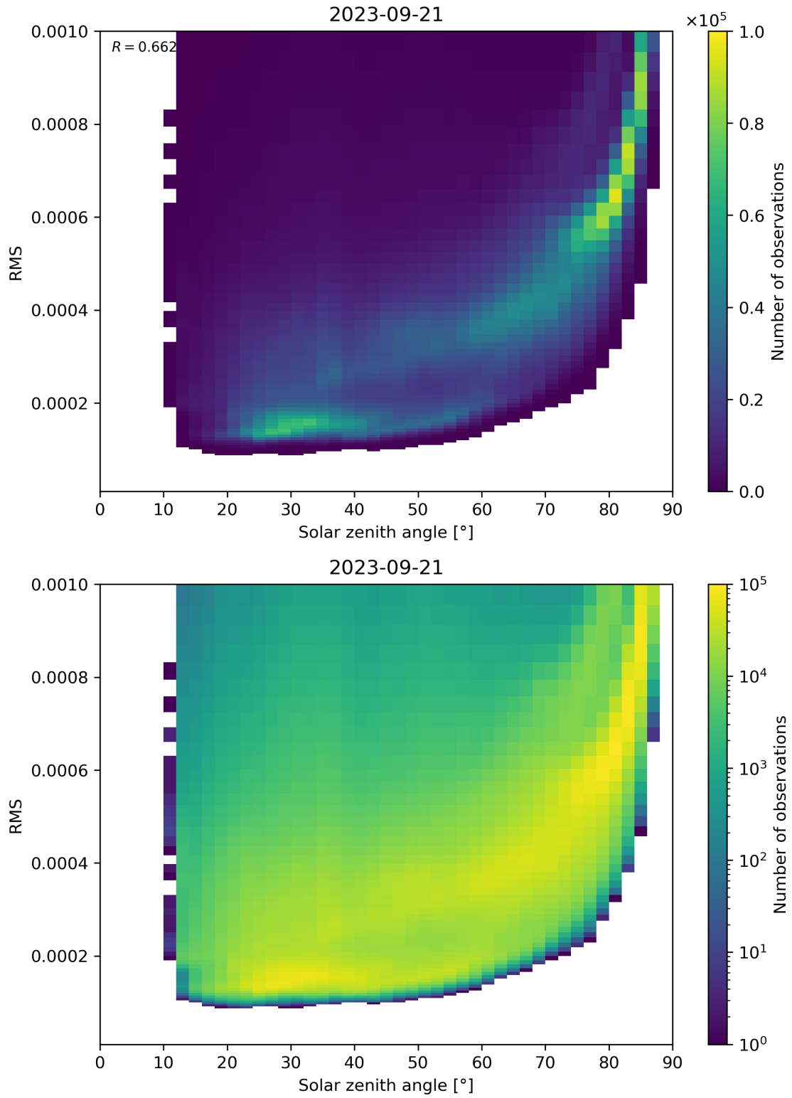
Figure 157: Scatter density plot of “Solar zenith angle” against “RMS” for 2023-09-20 to 2023-09-22.
