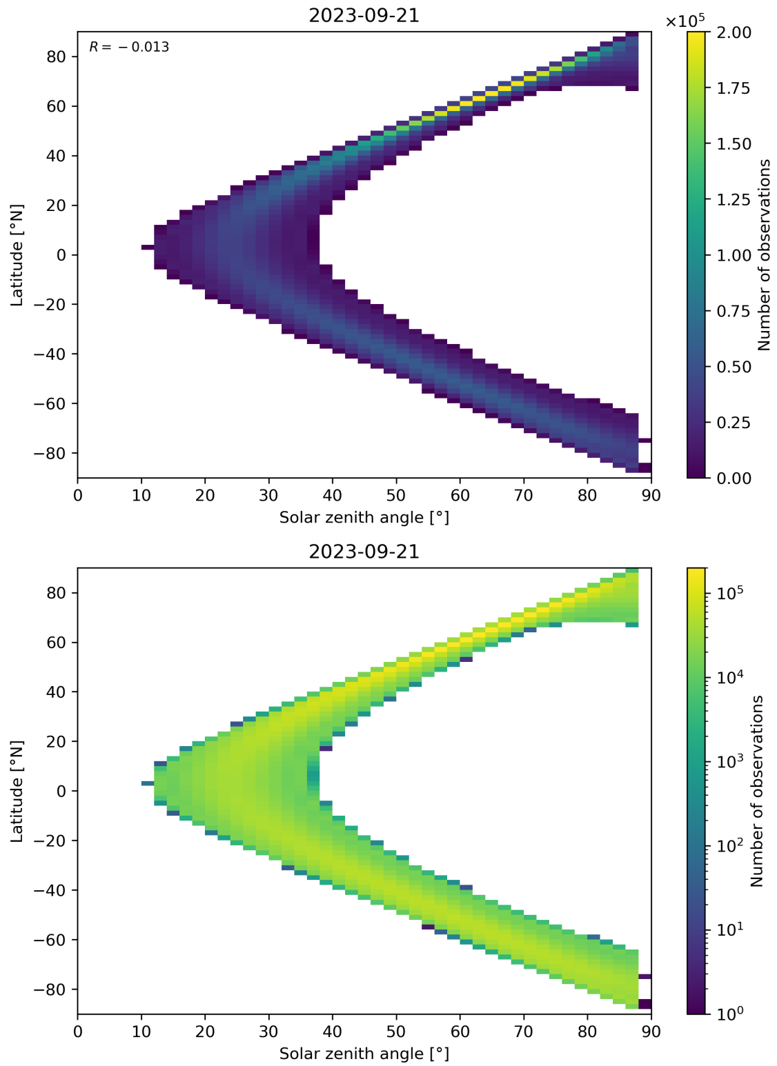
Figure 149: Scatter density plot of “Solar zenith angle” against “Latitude” for 2023-09-20 to 2023-09-22.
