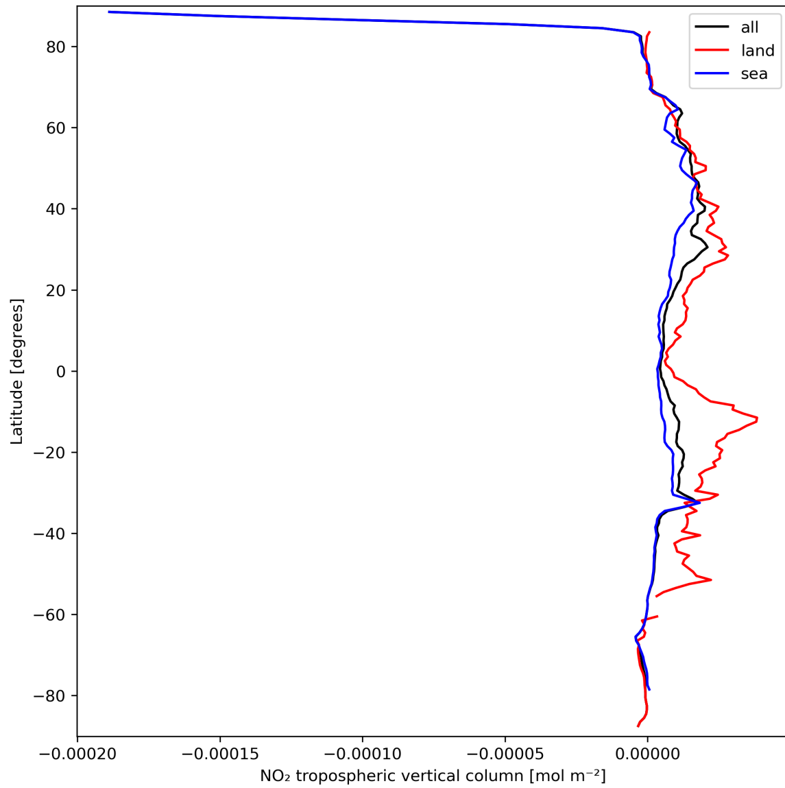
Figure 12: Zonal average of “NO 2 tropospheric vertical column” for 2023-09-20 to 2023-09-22.
