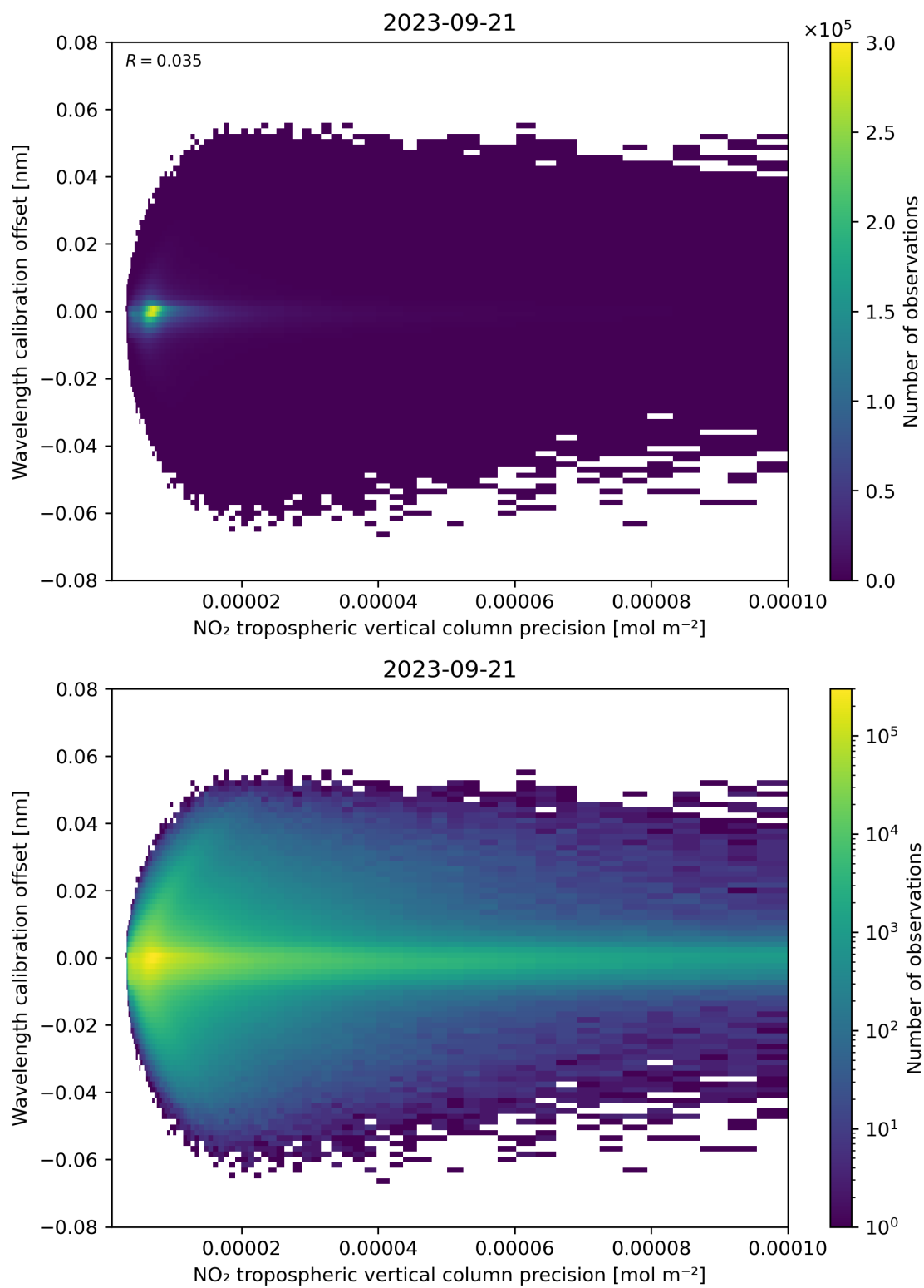
Figure 141: Scatter density plot of “NO 2 tropospheric vertical column precision” against “Wavelength calibration offset” for 2023-09-20 to 2023-09-22.
