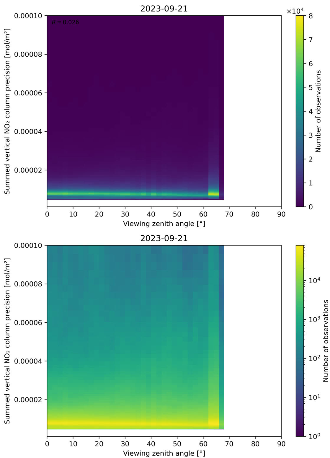
Figure 166: Scatter density plot of “Viewing zenith angle” against “Summed vertical NO 2 column precision” for 2023-09-20 to 2023-09-22.
