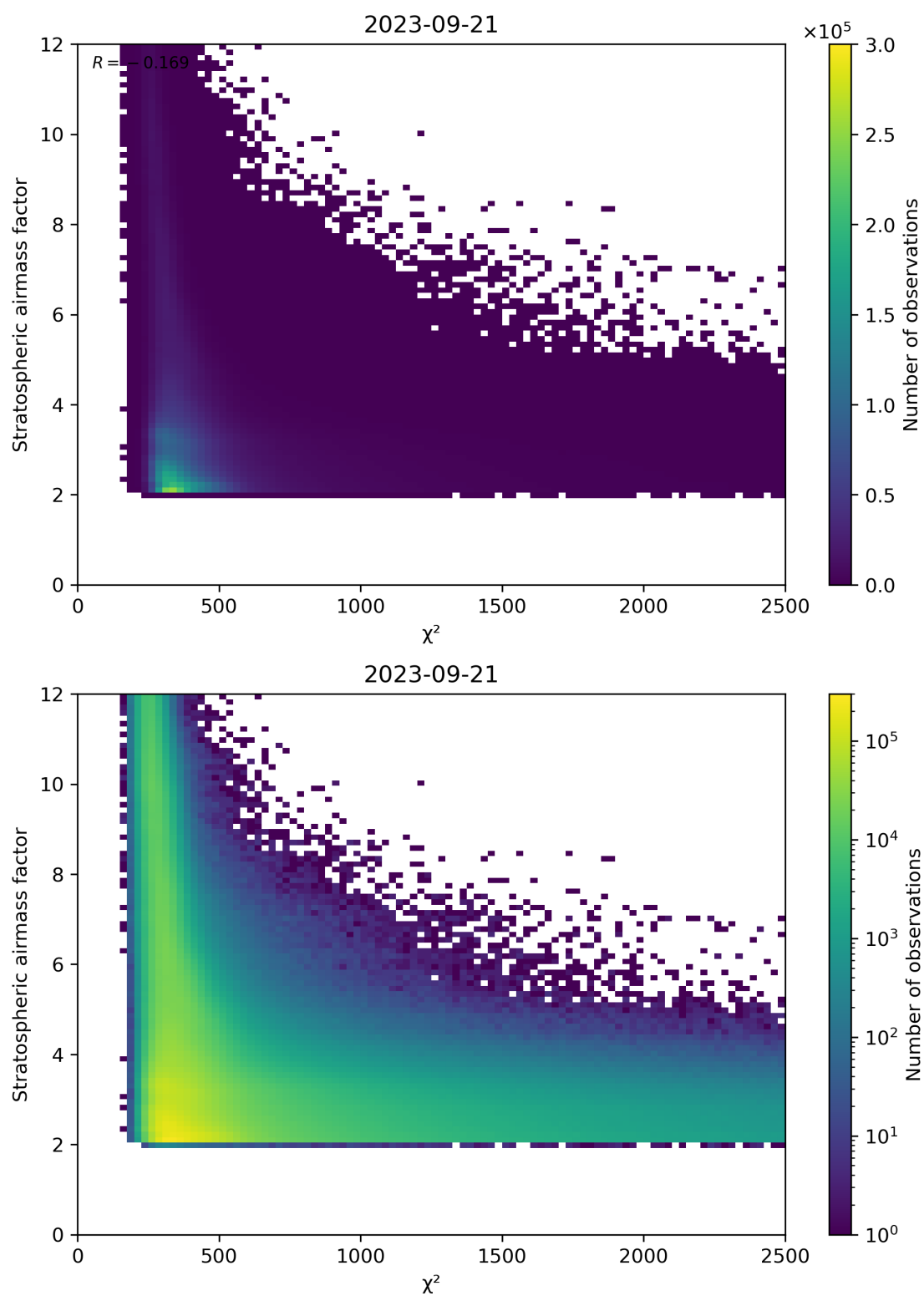
Figure 81: Scatter density plot of “ \chi^2 ” against “Stratospheric airmass factor” for 2023-09-20 to 2023-09-22.
