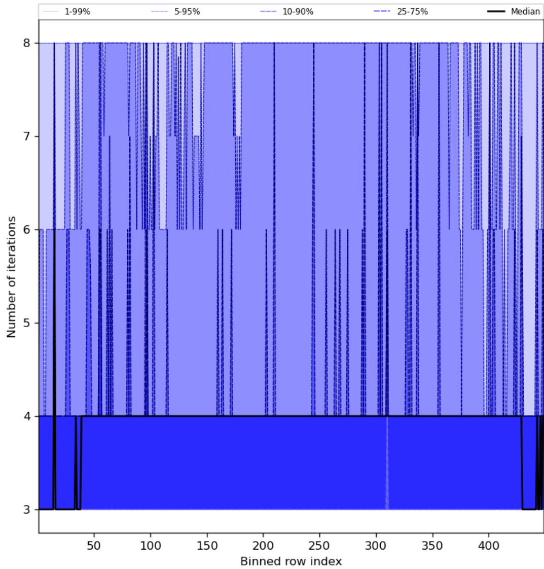
Figure 51: Along track statistics of “Number of iterations” for 2023-09-20 to 2023-09-22
