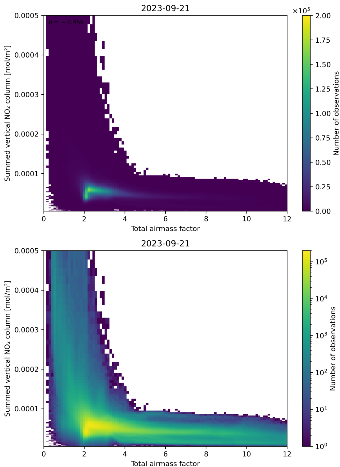
Figure 65: Scatter density plot of “Total airmass factor” against “Summed vertical NO 2 column” for 2023-09-20 to 2023-09-22.
