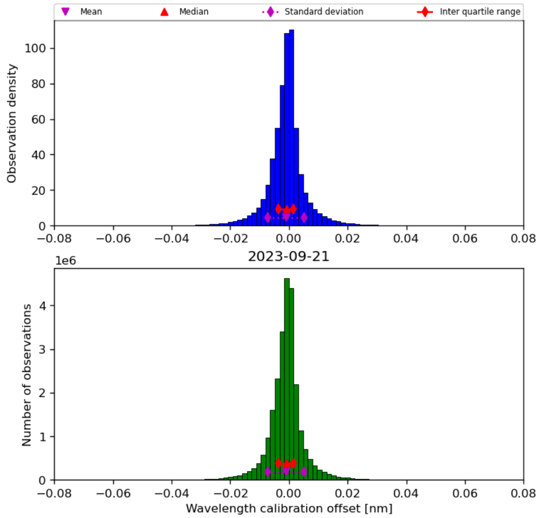
Figure 35: Histogram of “Wavelength calibration offset” for 2023-09-20 to 2023-09-22
