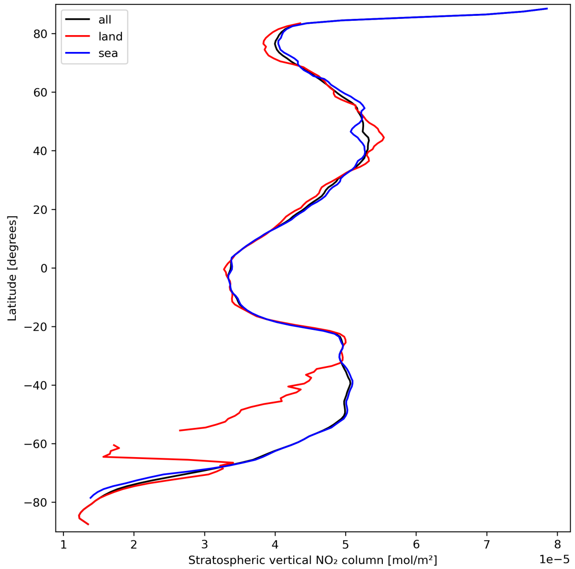
Figure 19: Zonal average of “Stratospheric vertical NO 2 column” for 2023-09-20 to 2023-09-22.
