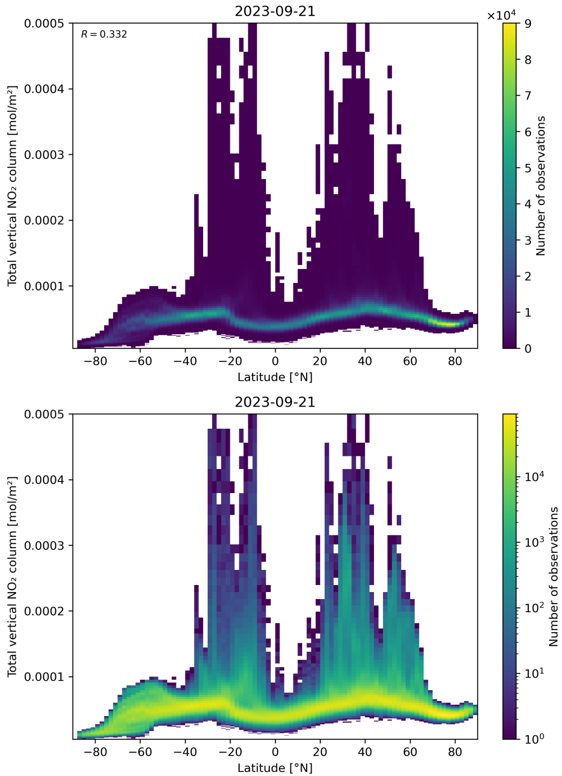
Figure 90: Scatter density plot of “Latitude” against “Total vertical NO 2 column” for 2023-09-20 to 2023-09-22.
