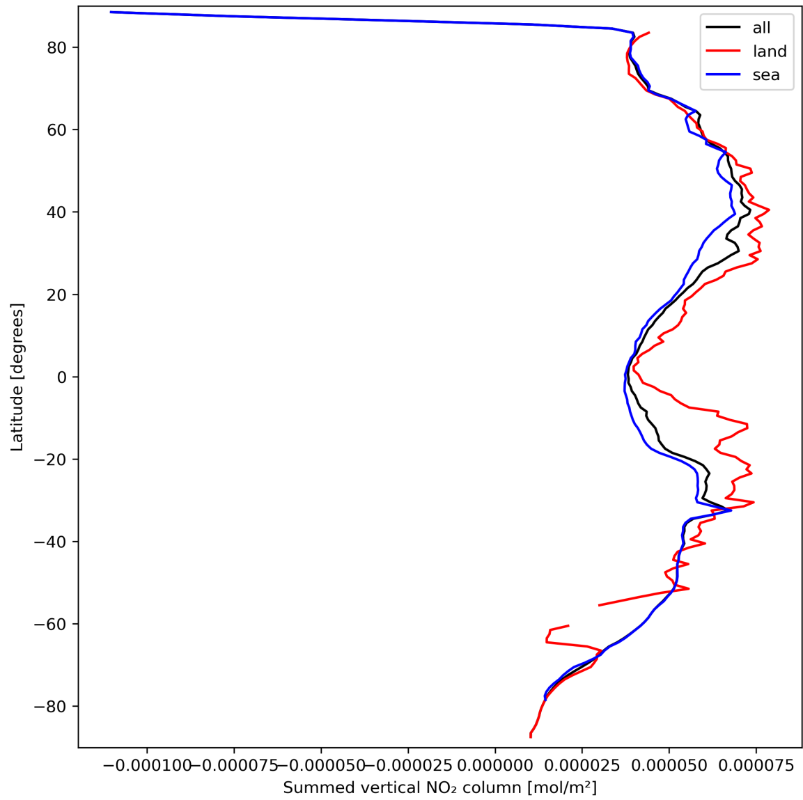
Figure 23: Zonal average of “Summed vertical NO 2 column” for 2023-09-20 to 2023-09-22.
