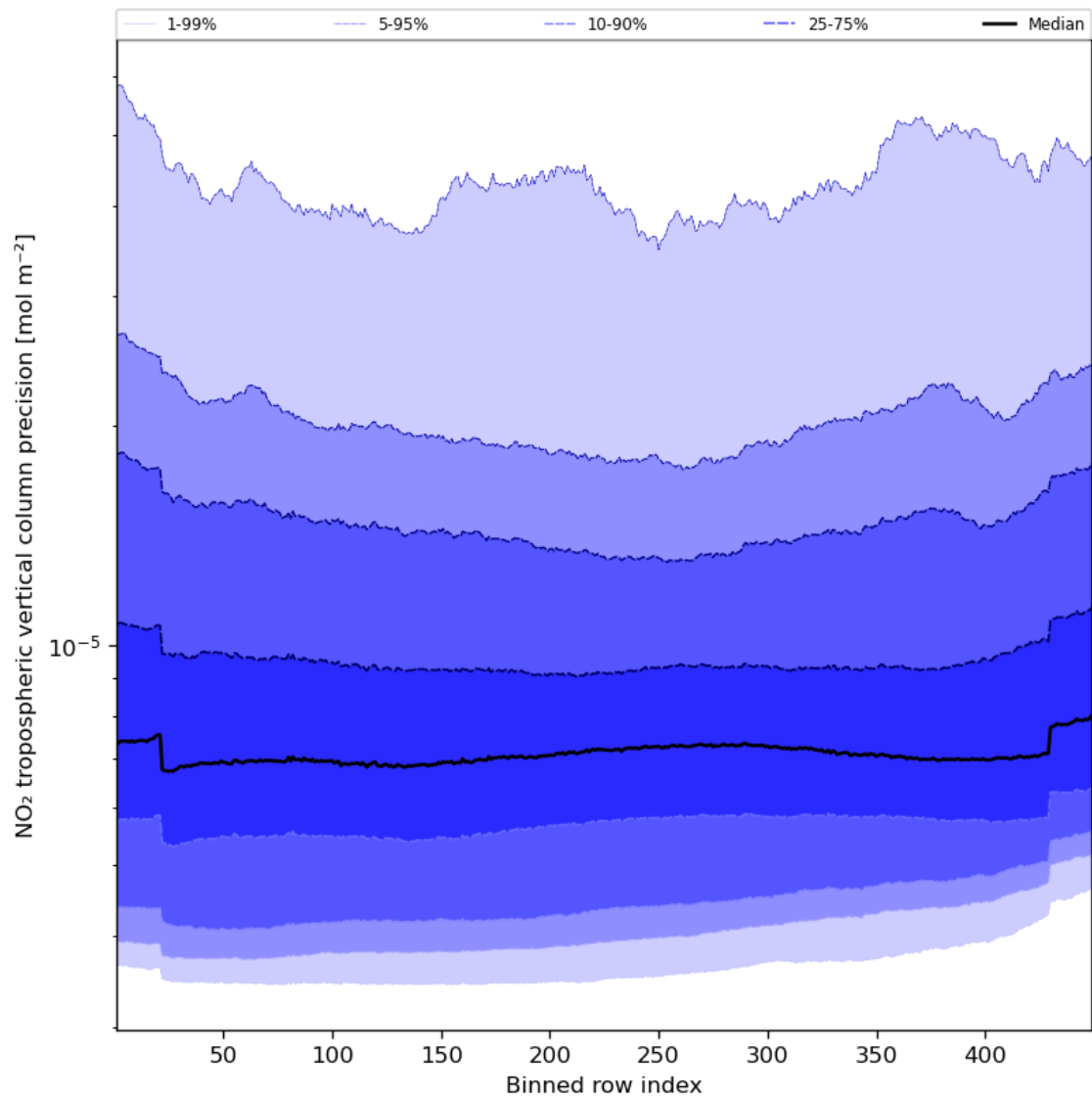
Figure 47: Along track statistics of “NO 2 tropospheric vertical column precision” for 2023-09-20 to 2023-09-22
