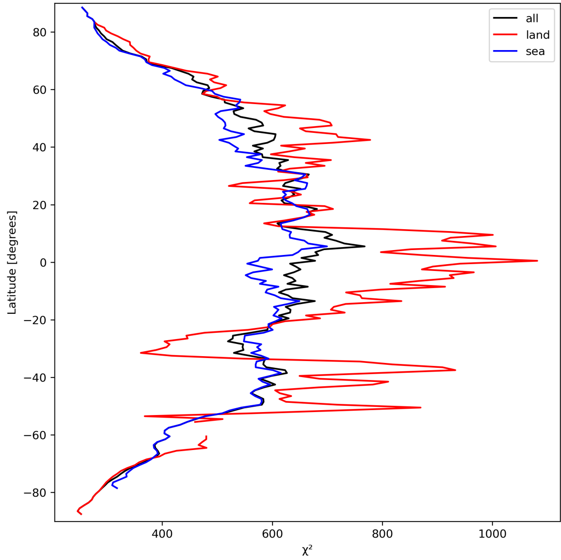
Figure 25: Zonal average of “ \chi^2 ” for 2023-09-20 to 2023-09-22.
