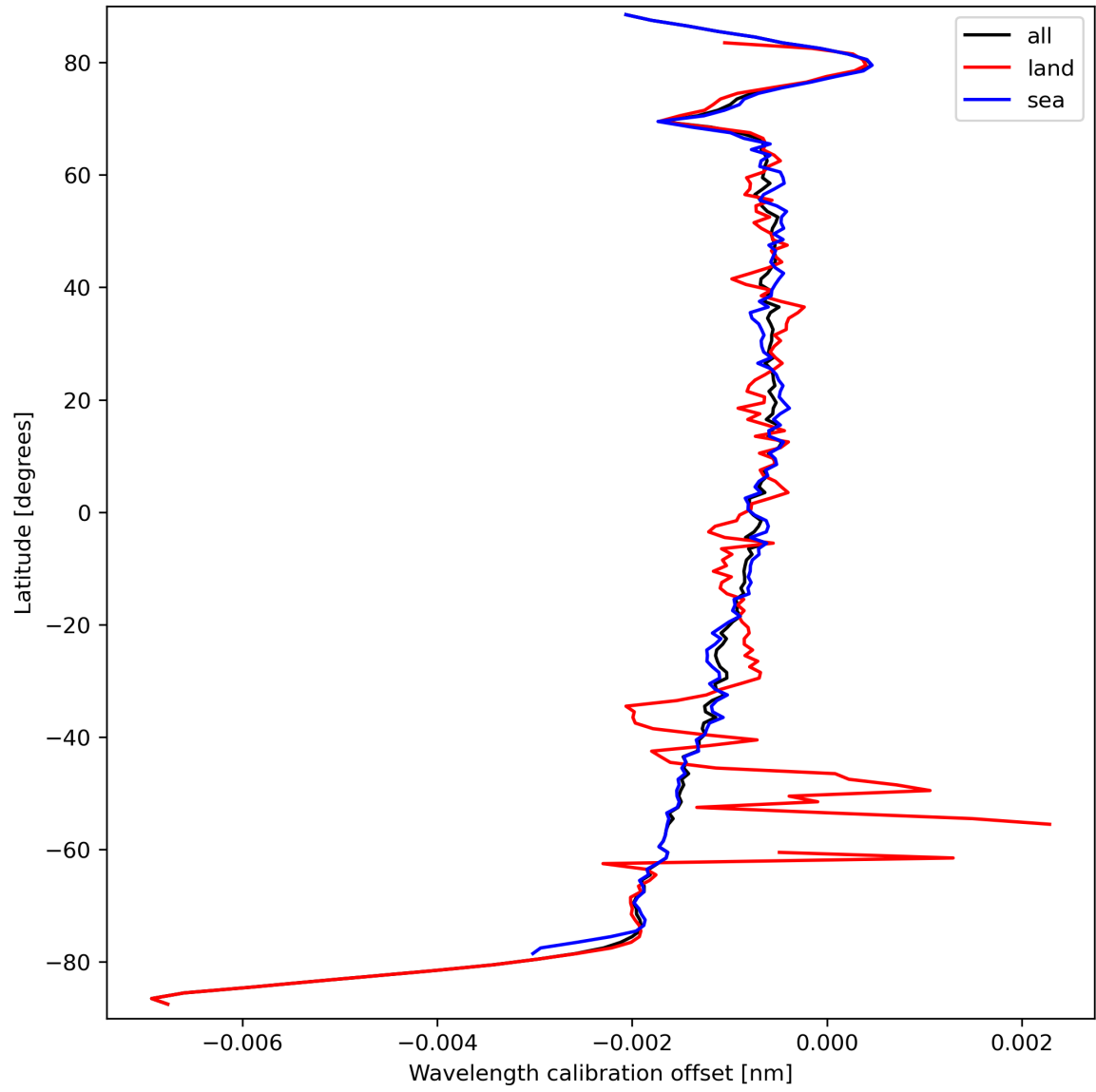
Figure 18: Zonal average of “Wavelength calibration offset” for 2023-09-20 to 2023-09-22.
