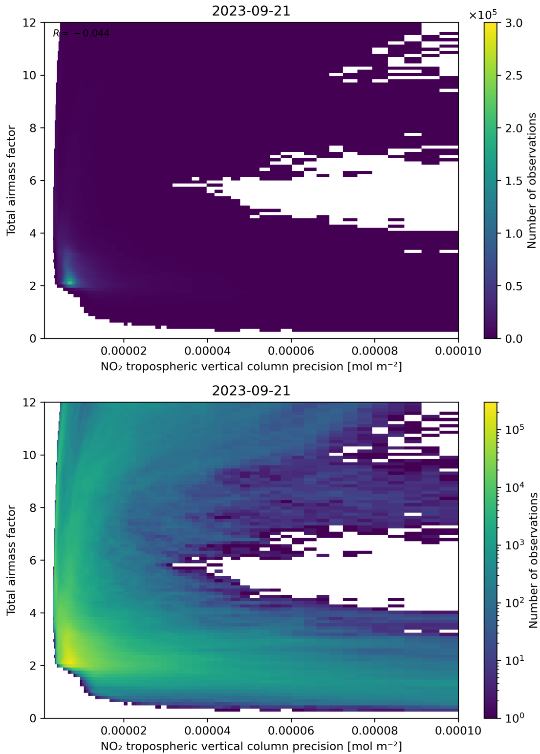
Figure 132: Scatter density plot of “NO 2 tropospheric vertical column precision” against “Total air mass factor” for 2023-09-20 to 2023-09-22.
