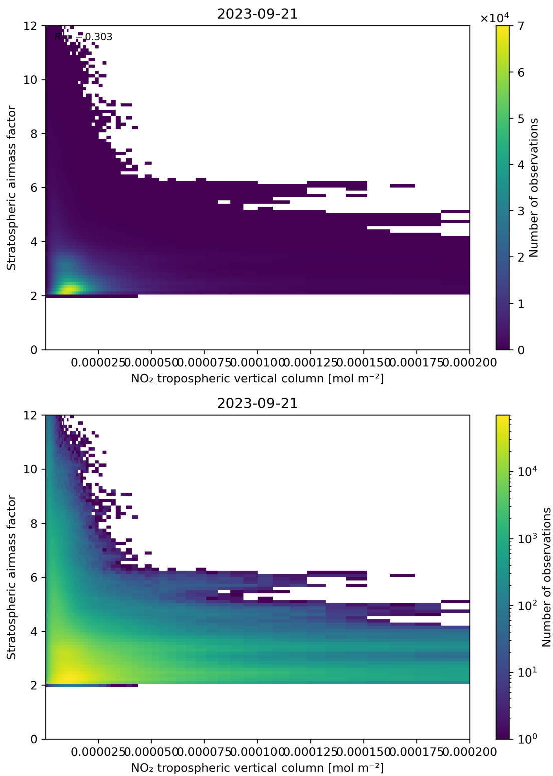
Figure 121: Scatter density plot of “NO 2 tropospheric vertical column” against “Stratospheric air mass factor” for 2023-09-20 to 2023-09-22.
