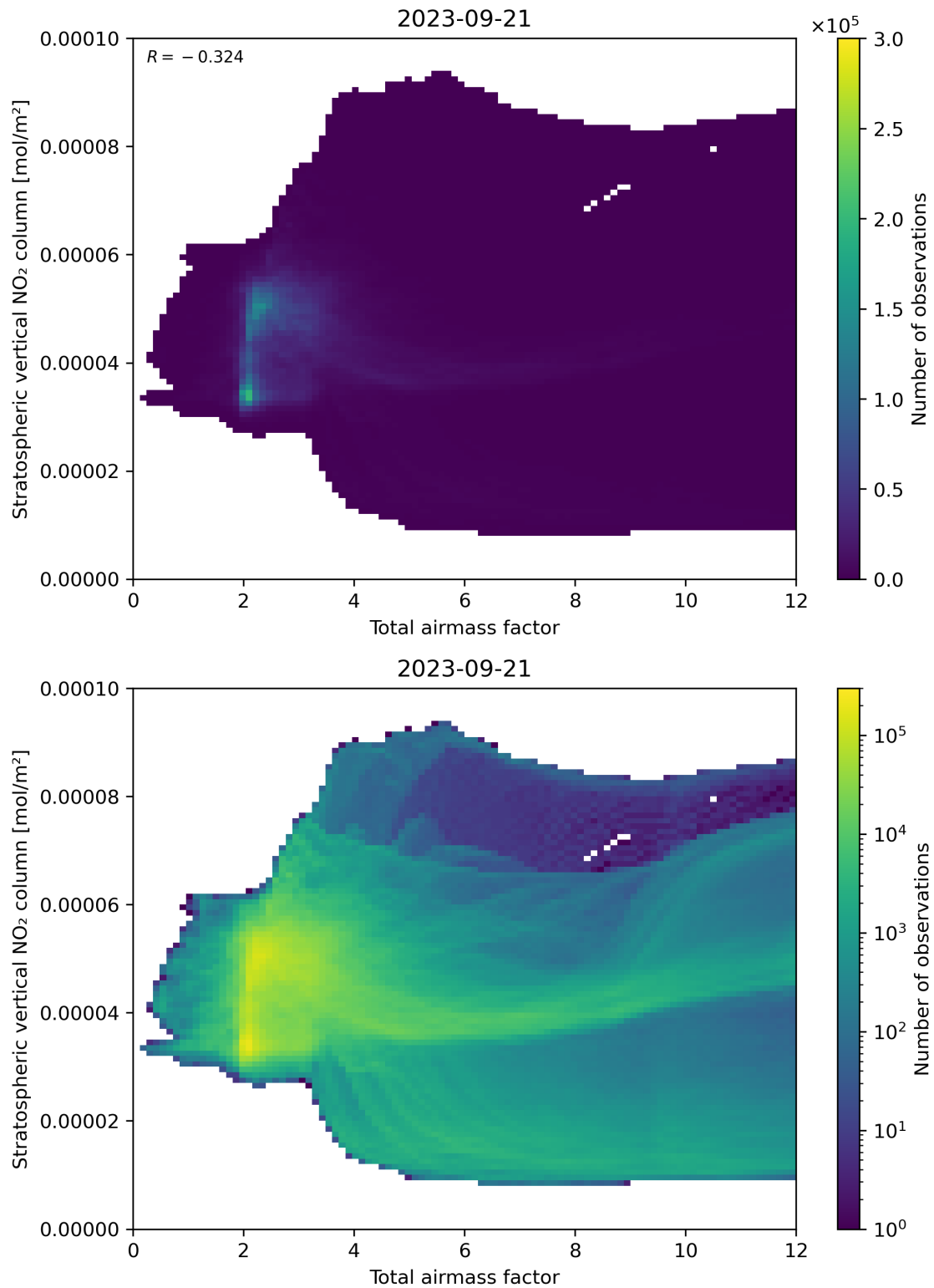
Figure 64: Scatter density plot of “Total airmass factor” against “Stratospheric vertical NO 2 column” for 2023-09-20 to 2023-09-22.
