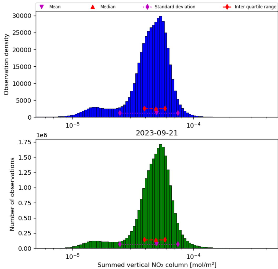
Figure 40: Histogram of “Summed vertical NO 2 column” for 2023-09-20 to 2023-09-22
