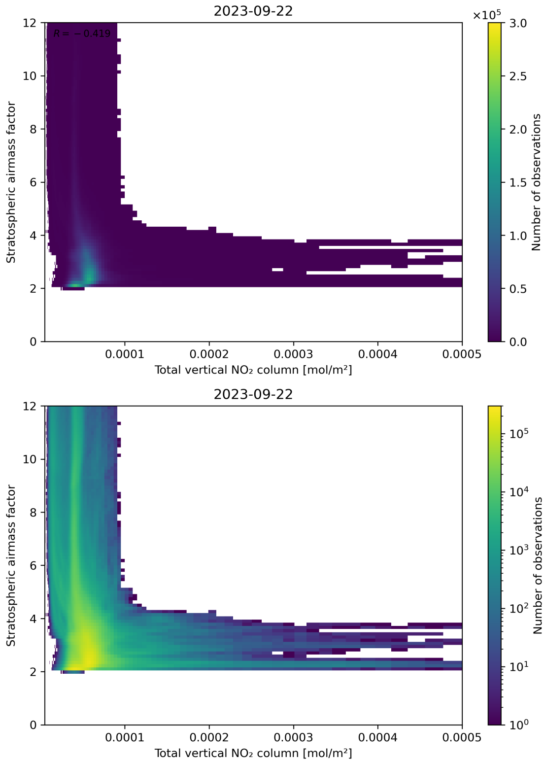
Figure 110: Scatter density plot of “Total vertical NO 2 column” against “Stratospheric airmass factor” for 2023-09-21 to 2023-09-23.
