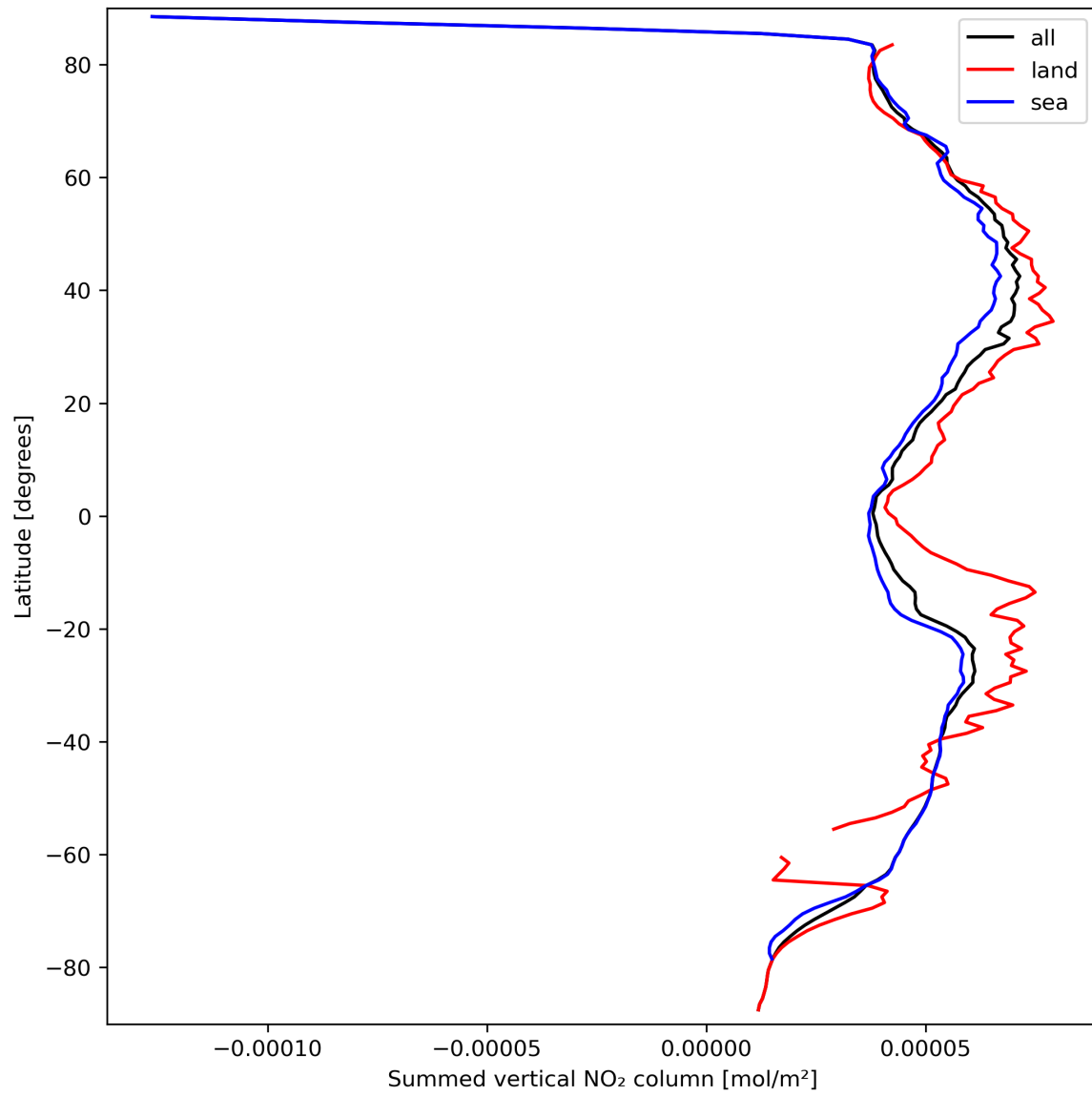
Figure 23: Zonal average of “Summed vertical NO 2 column” for 2023-09-21 to 2023-09-23.
