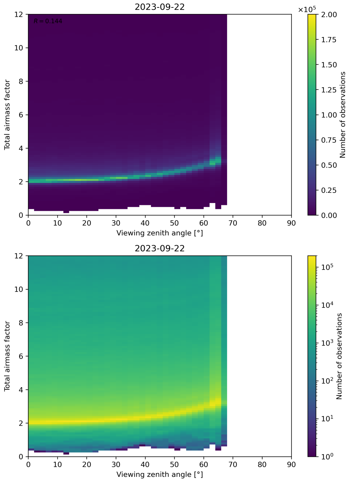
Figure 160: Scatter density plot of “Viewing zenith angle” against “Total airmass factor” for 2023-09-21 to 2023-09-23.
