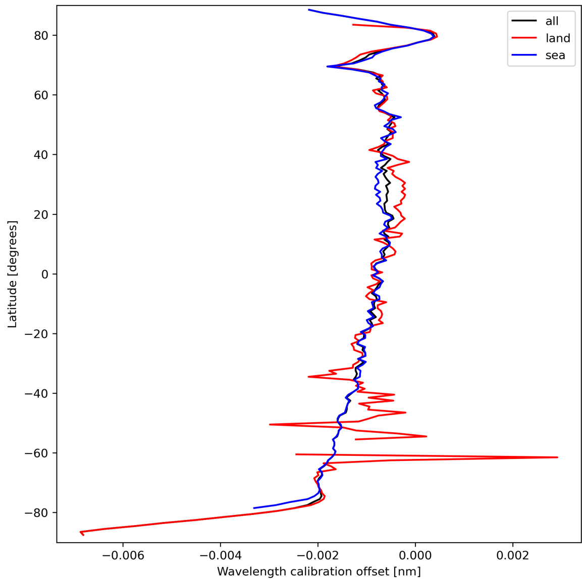
Figure 18: Zonal average of “Wavelength calibration offset” for 2023-09-21 to 2023-09-23.
