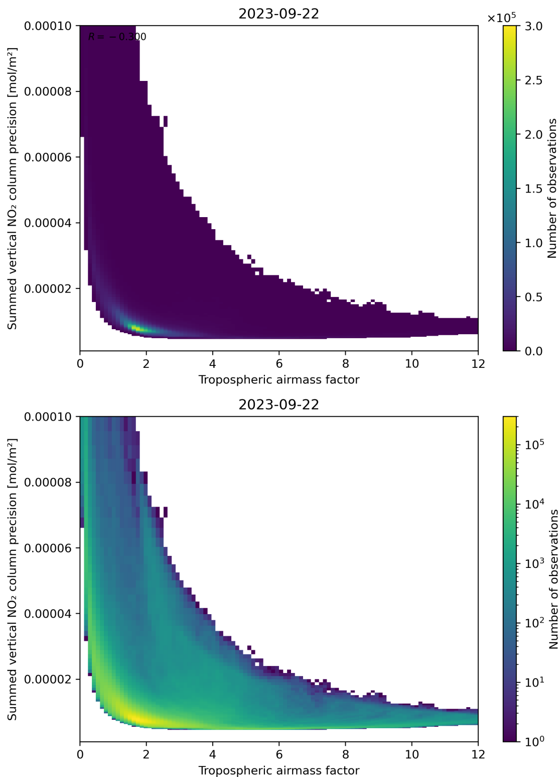
Figure 76: Scatter density plot of “Tropospheric air mass factor” against “Summed vertical NO 2 column precision” for 2023-09-21 to 2023-09-23.
