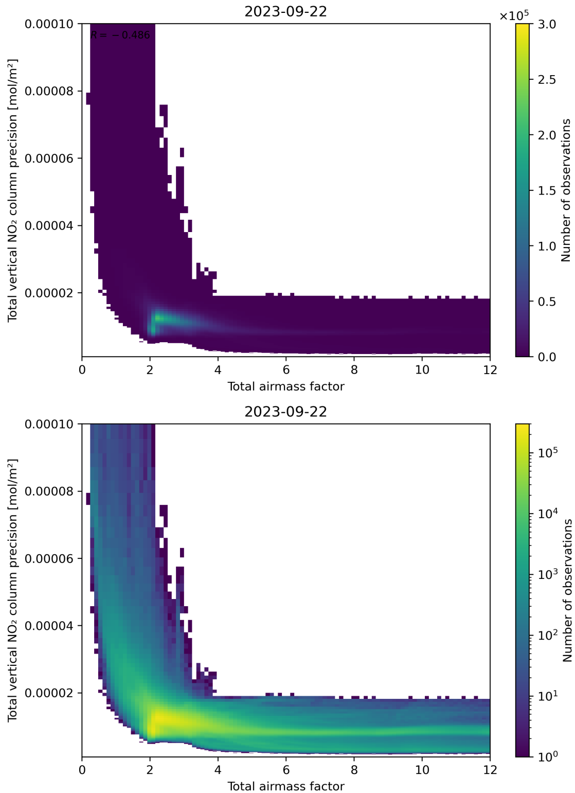
Figure 68: Scatter density plot of “Total airmass factor” against “Total vertical NO 2 column precision” for 2023-09-21 to 2023-09-23.
