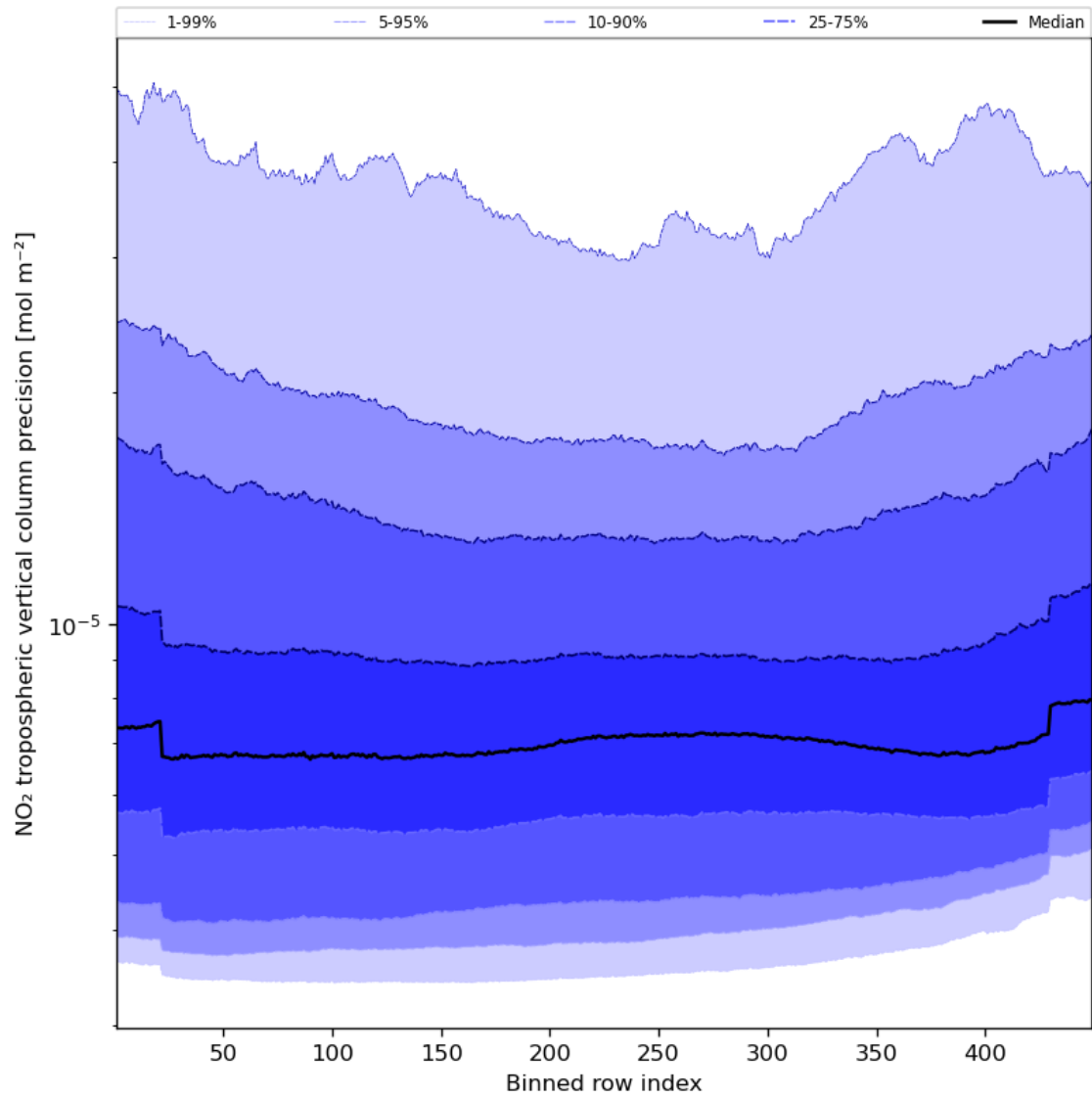
Figure 47: Along track statistics of “NO 2 tropospheric vertical column precision” for 2023-09-21 to 2023-09-23
