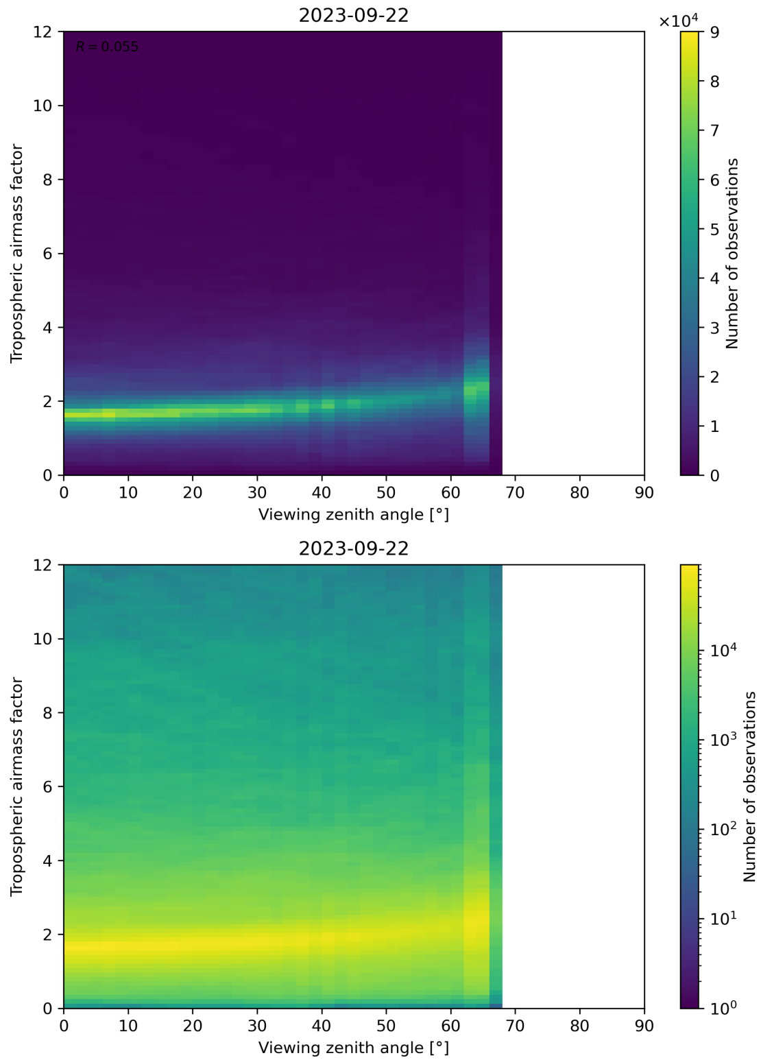
Figure 161: Scatter density plot of “Viewing zenith angle” against “Tropospheric airmass factor” for 2023-09-21 to 2023-09-23.
