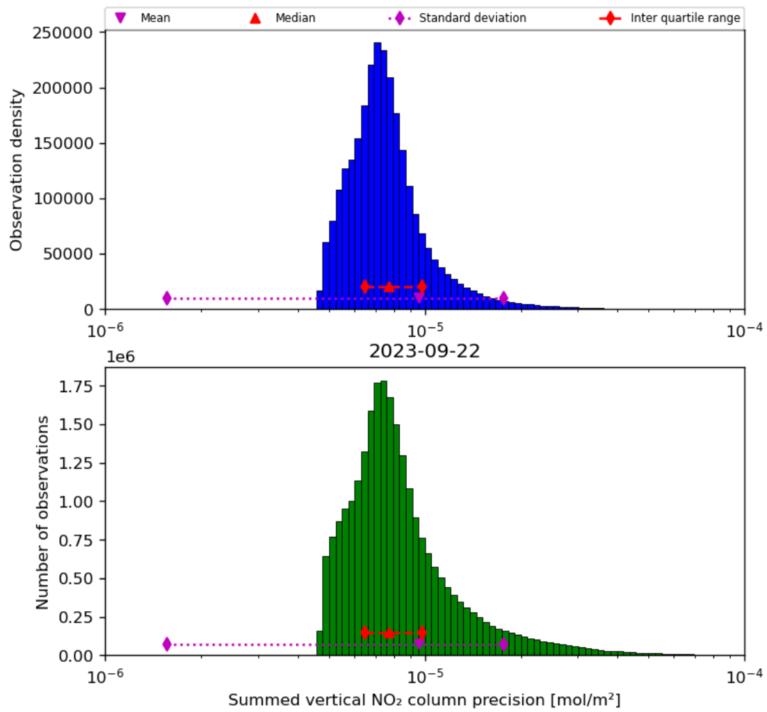
Figure 41: Histogram of "Summed vertical NO 2 column precision" for 2023-09-21 to 2023-09-23
