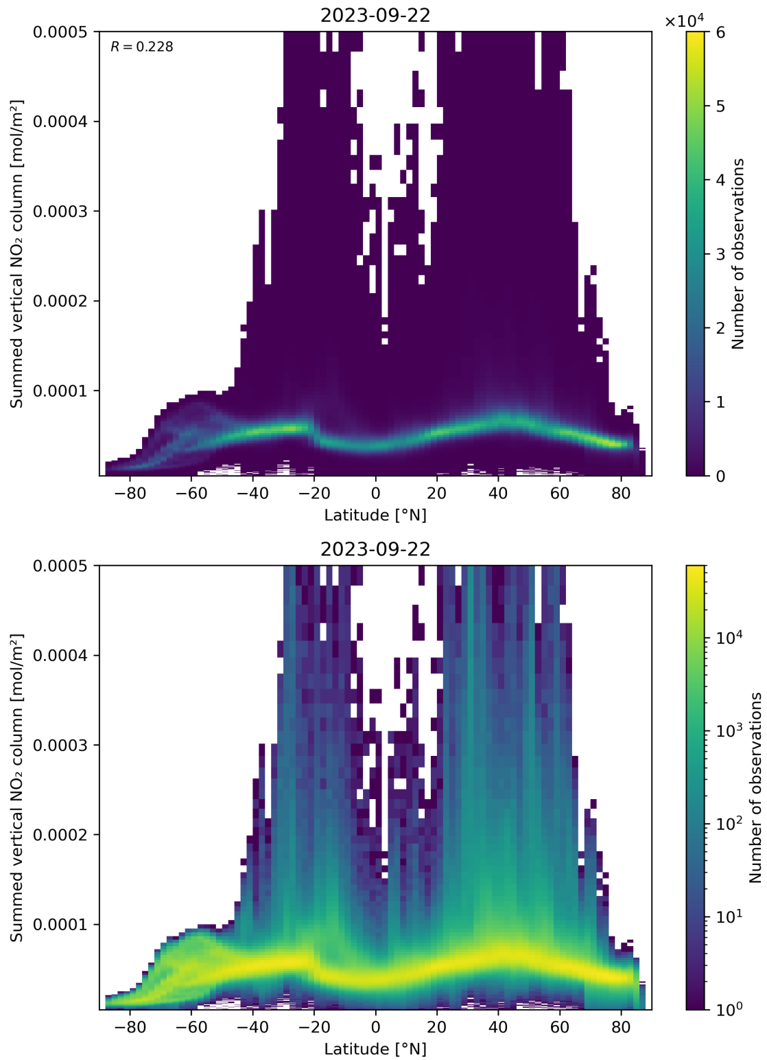
Figure 88: Scatter density plot of “Latitude” against “Summed vertical NO 2 column” for 2023-09-21 to 2023-09-23.
