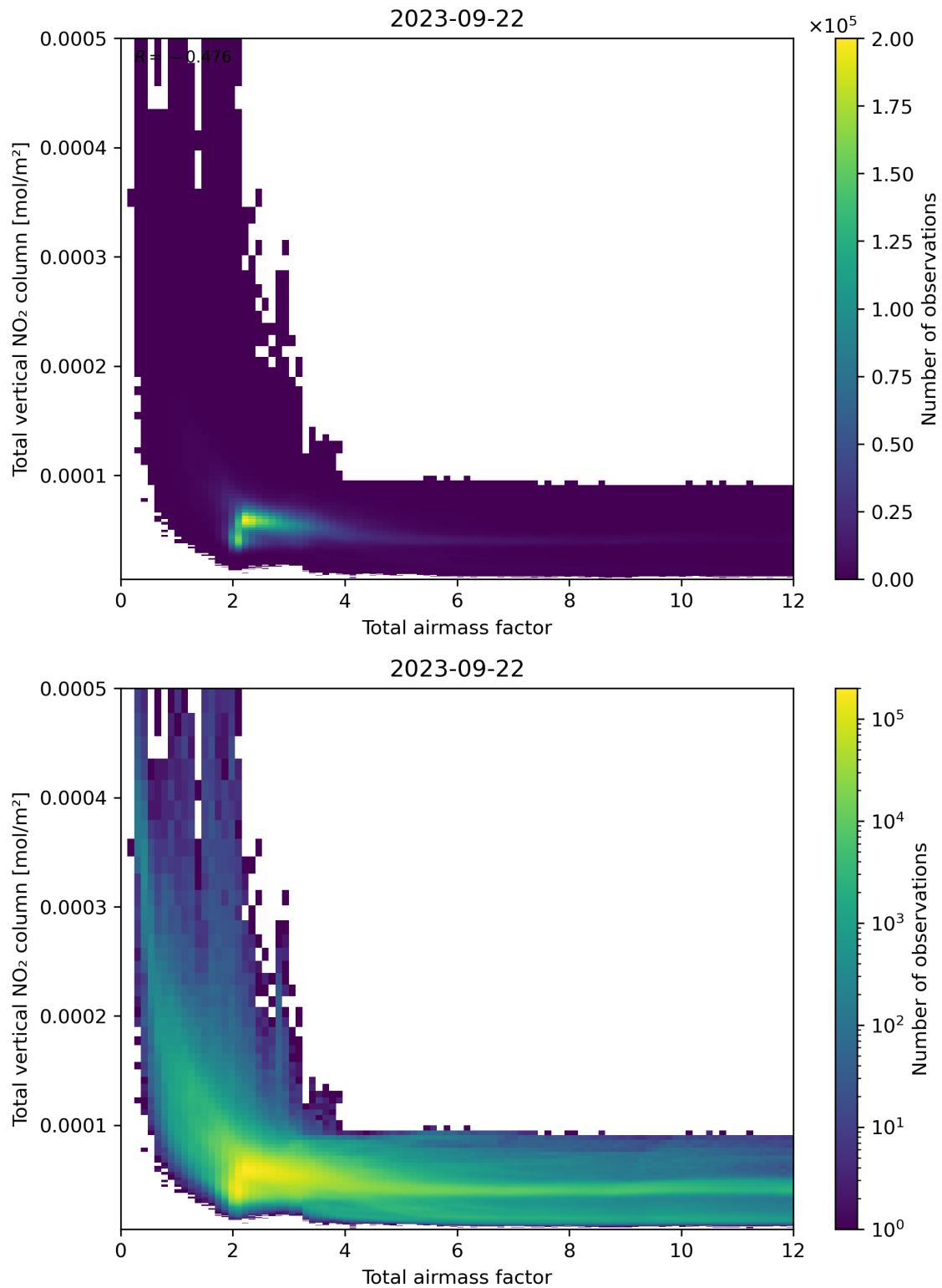
Figure 67: Scatter density plot of “Total airmass factor” against “Total vertical NO 2 column” for 2023-09-21 to 2023-09-23.
