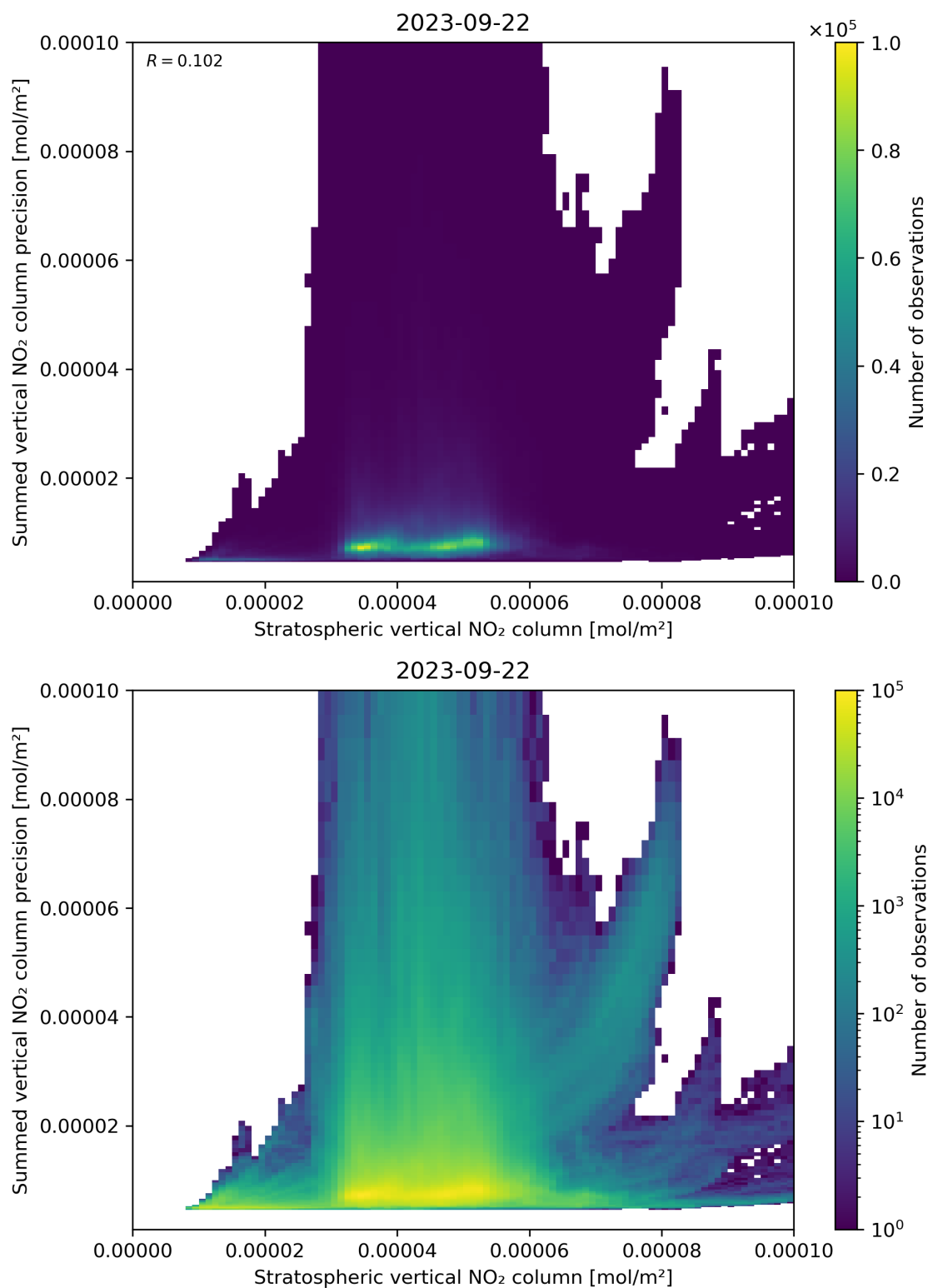
Figure 99: Scatter density plot of “Stratospheric vertical NO 2 column” against “Summed vertical NO 2 column precision” for 2023-09-21 to 2023-09-23.
