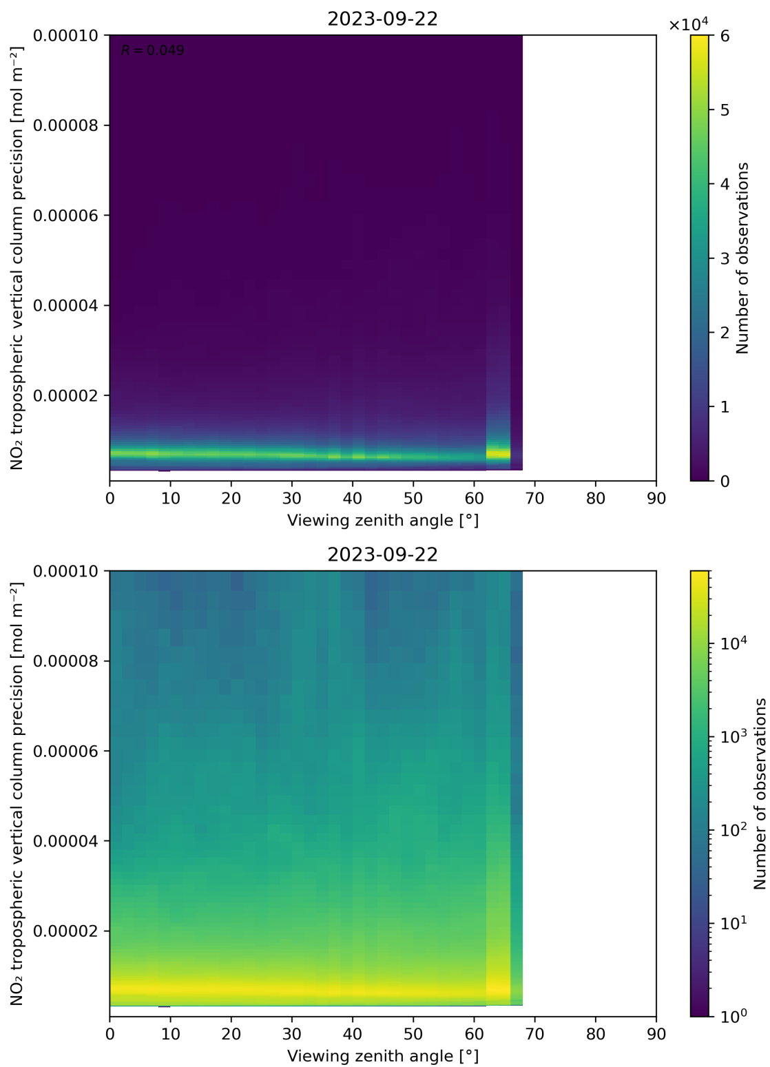
Figure 170: Scatter density plot of “Viewing zenith angle” against “NO 2 tropospheric vertical column precision” for 2023-09-21 to 2023-09-23.
