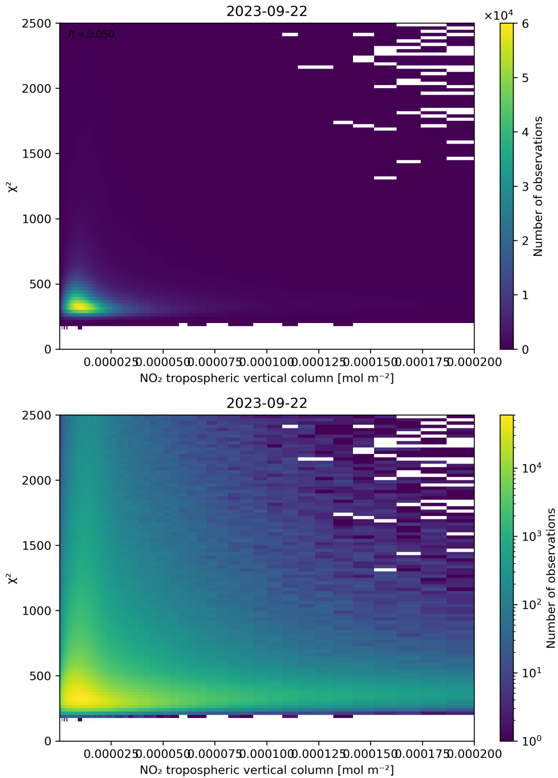
Figure 124: Scatter density plot of “NO 2 tropospheric vertical column” against “ \chi^2 ” for 2023-09-21 to 2023-09-23.
