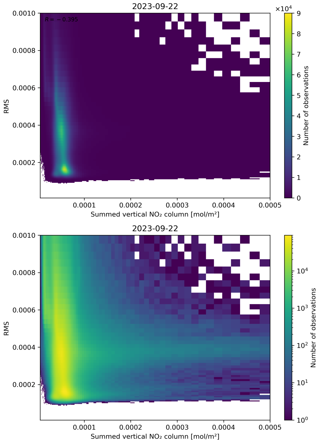
Figure 109: Scatter density plot of “Summed vertical NO 2 column” against “RMS” for 2023-09-21 to 2023-09-23.
