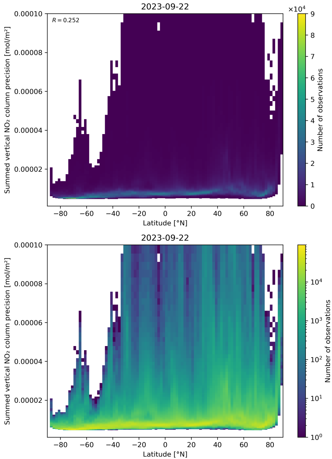
Figure 89: Scatter density plot of “Latitude” against “Summed vertical NO 2 column precision” for 2023-09-21 to 2023-09-23.
