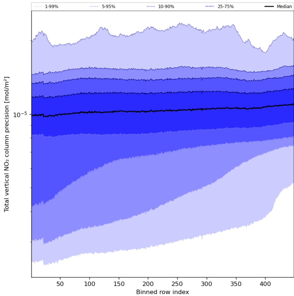
Figure 56: Along track statistics of “Total vertical NO 2 column precision” for 2023-09-21 to 2023-09-23
