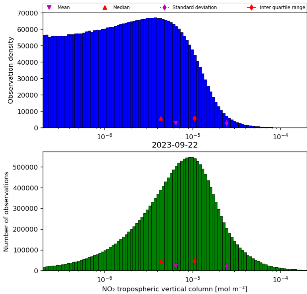
Figure 29: Histogram of “ \text{NO}_2 tropospheric vertical column” for 2023-09-21 to 2023-09-23
