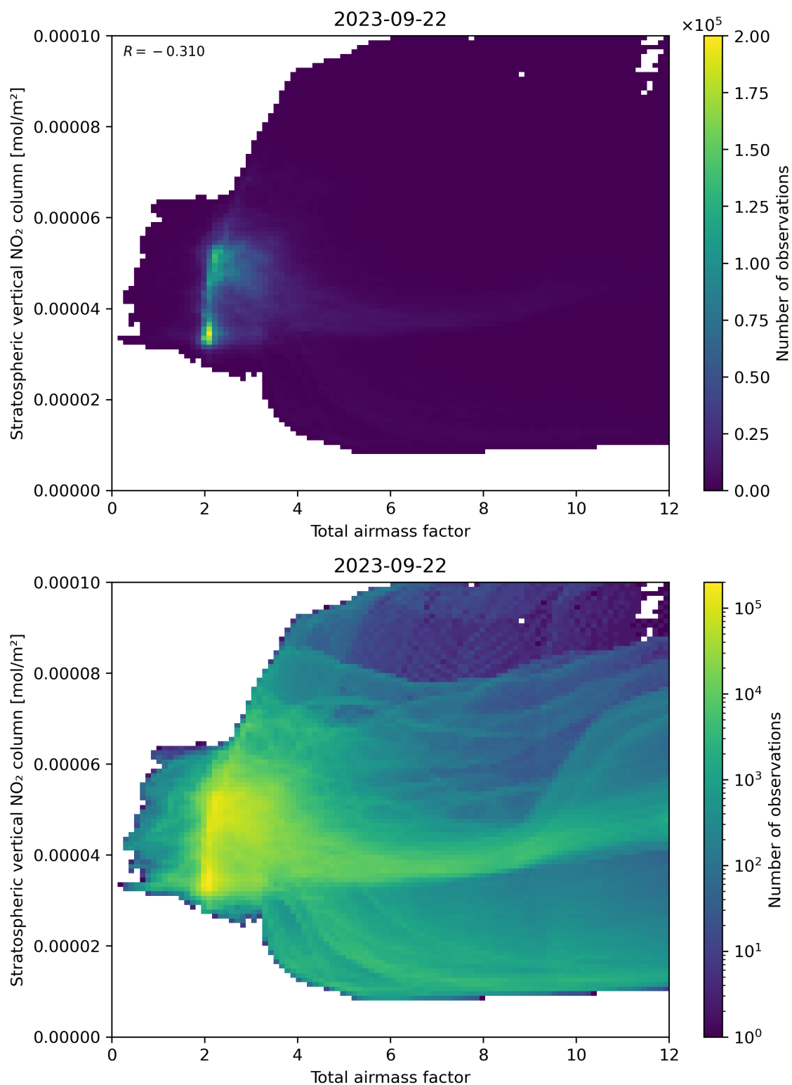
Figure 64: Scatter density plot of “Total airmass factor” against “Stratospheric vertical NO 2 column” for 2023-09-21 to 2023-09-23.
