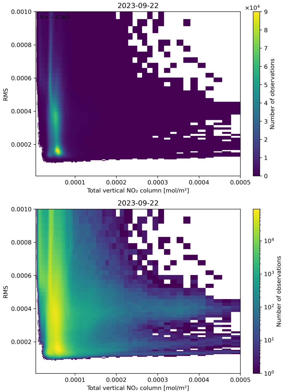
Figure 120: Scatter density plot of “Total vertical NO 2 column” against “RMS” for 2023-09-21 to 2023-09-23.
