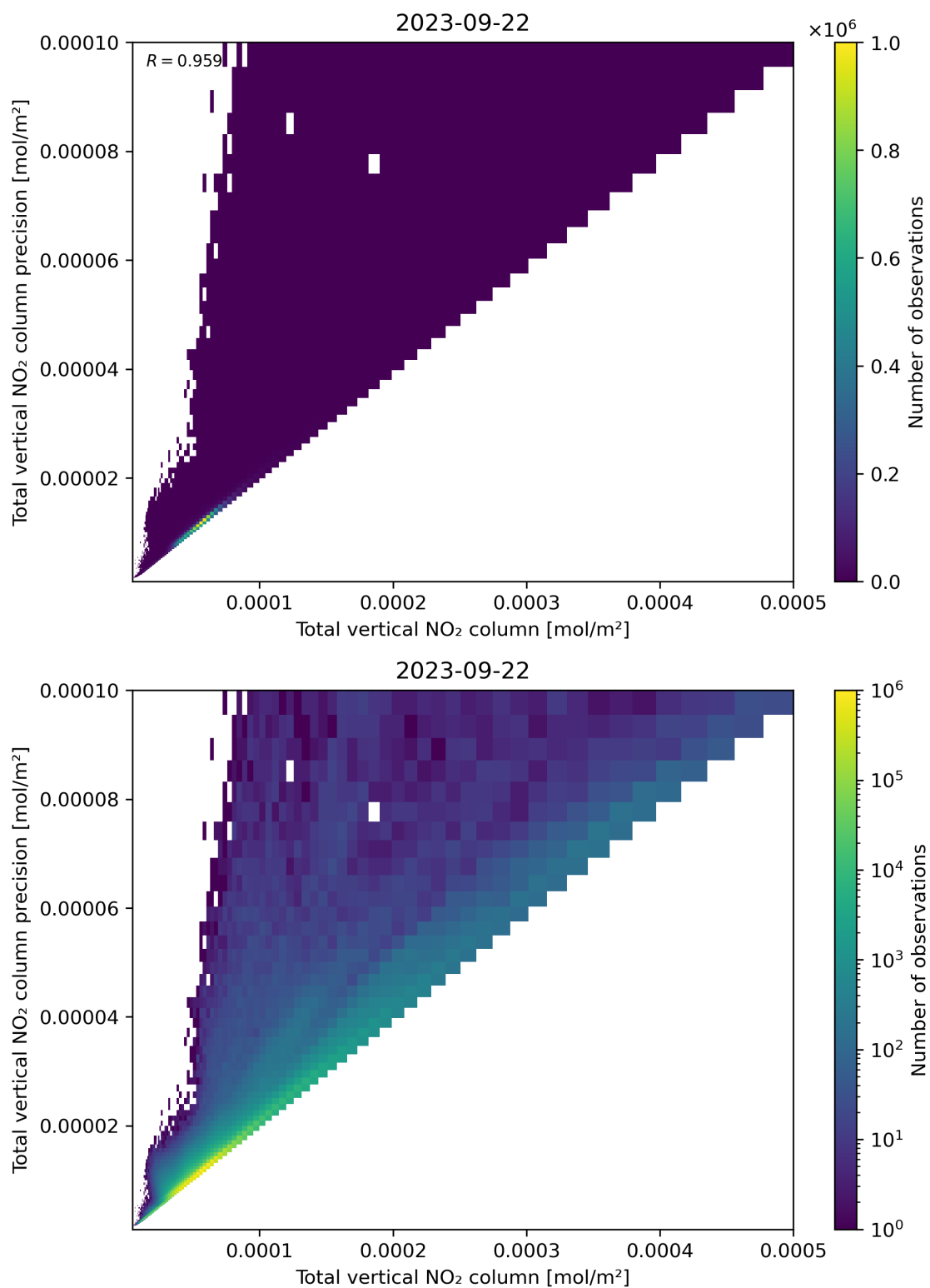
Figure 114: Scatter density plot of “Total vertical NO 2 column” against “Total vertical NO 2 column precision” for 2023-09-21 to 2023-09-23.
