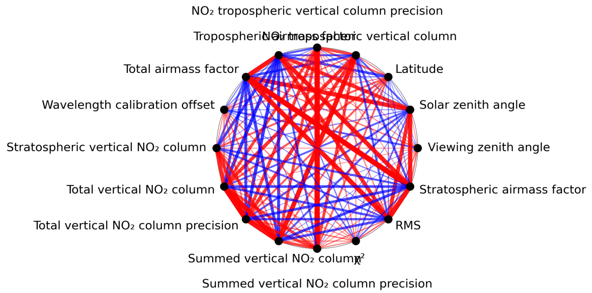
Figure 1: Map of correlation graph for 2023-09-21 to 2023-09-23.
