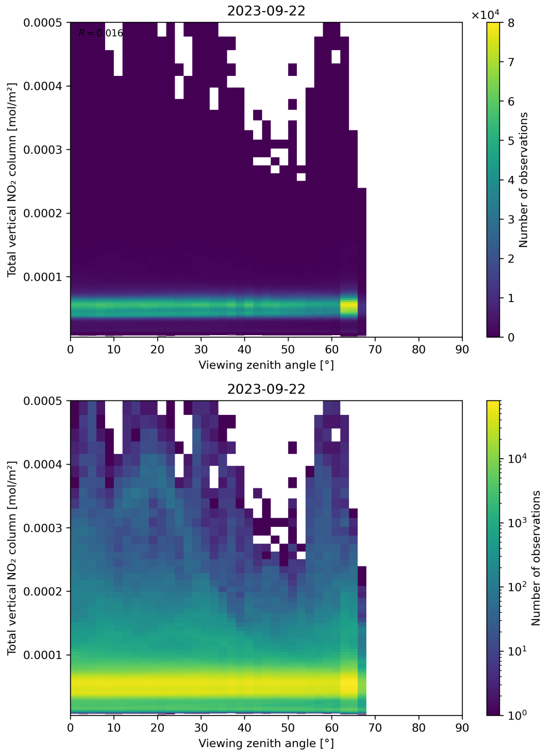
Figure 167: Scatter density plot of “Viewing zenith angle” against “Total vertical NO 2 column” for 2023-09-21 to 2023-09-23.
