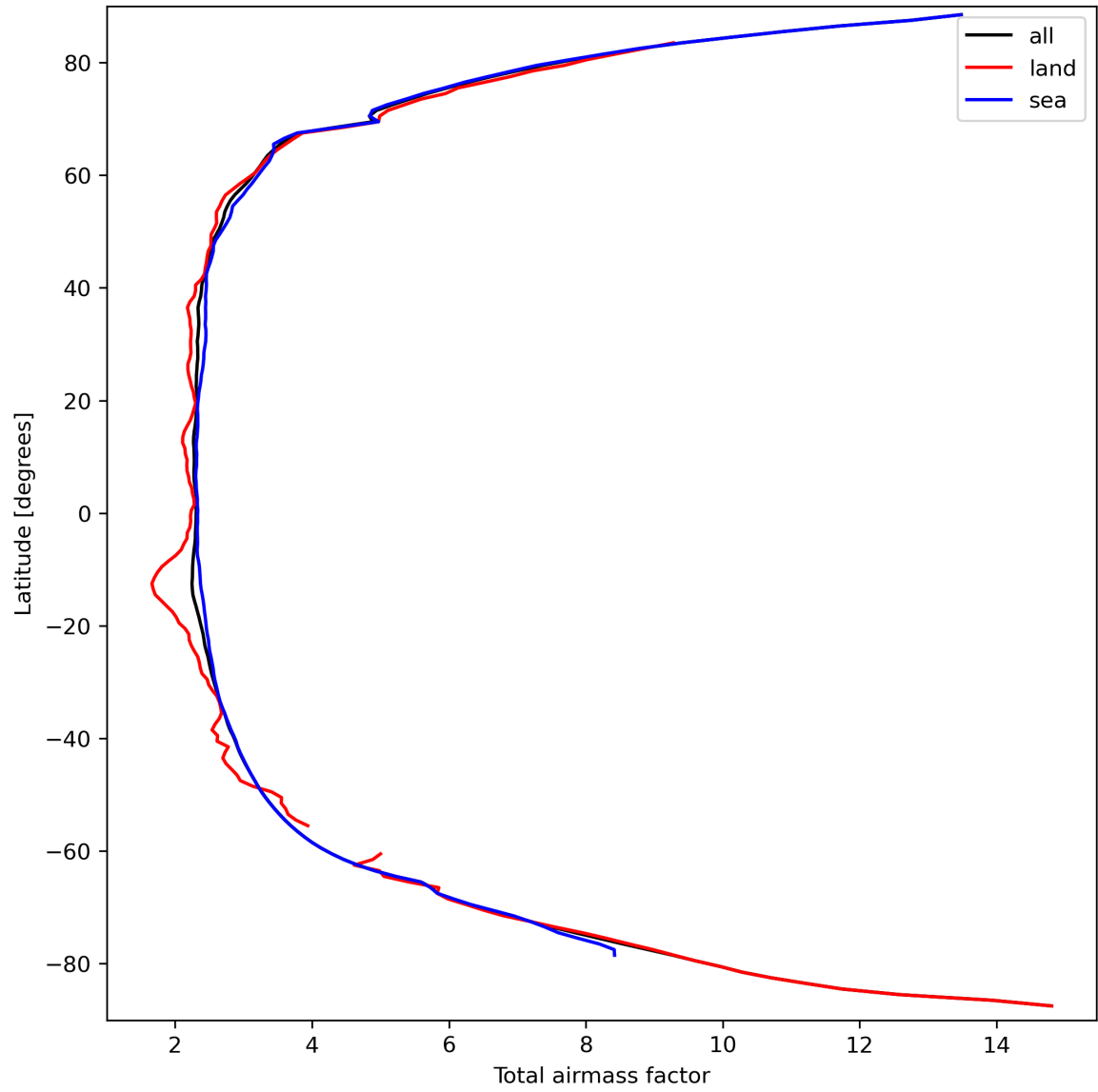
Figure 15: Zonal average of “Total airmass factor” for 2023-09-21 to 2023-09-23.
