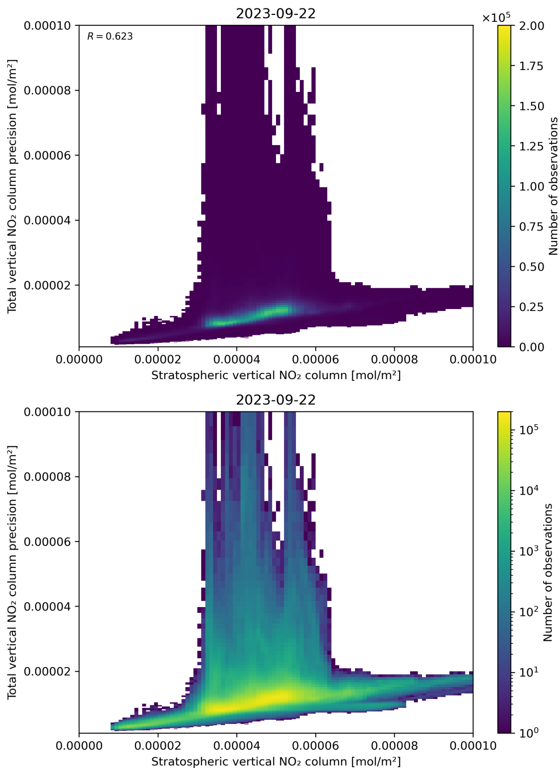
Figure 101: Scatter density plot of “Stratospheric vertical NO 2 column” against “Total vertical NO 2 column precision” for 2023-09-21 to 2023-09-23.
