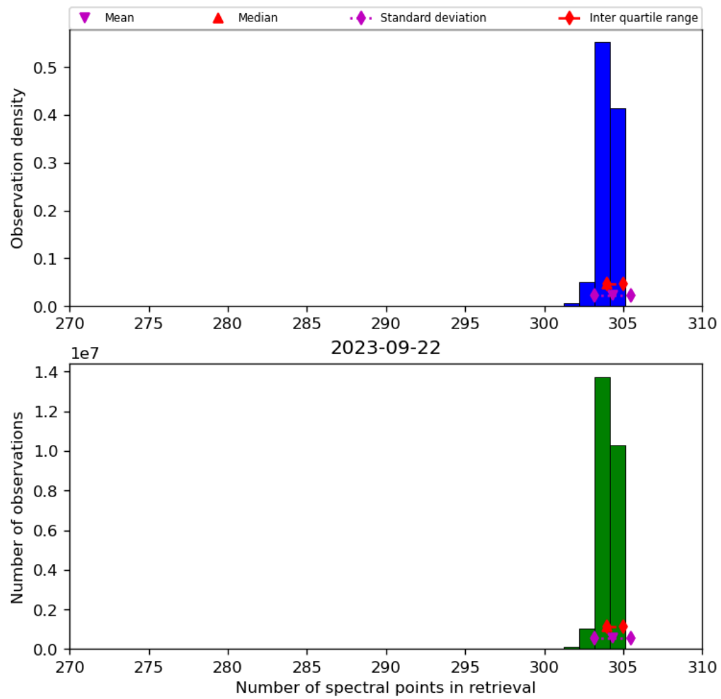
Figure 33: Histogram of “Number of spectral points in retrieval” for 2023-09-21 to 2023-09-23
