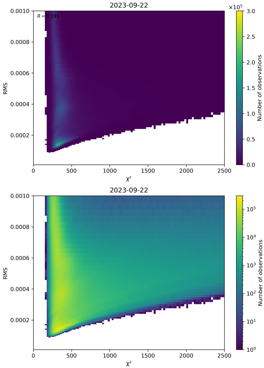
Figure 82: Scatter density plot of “ \chi^2 ” against “RMS” for 2023-09-21 to 2023-09-23.
