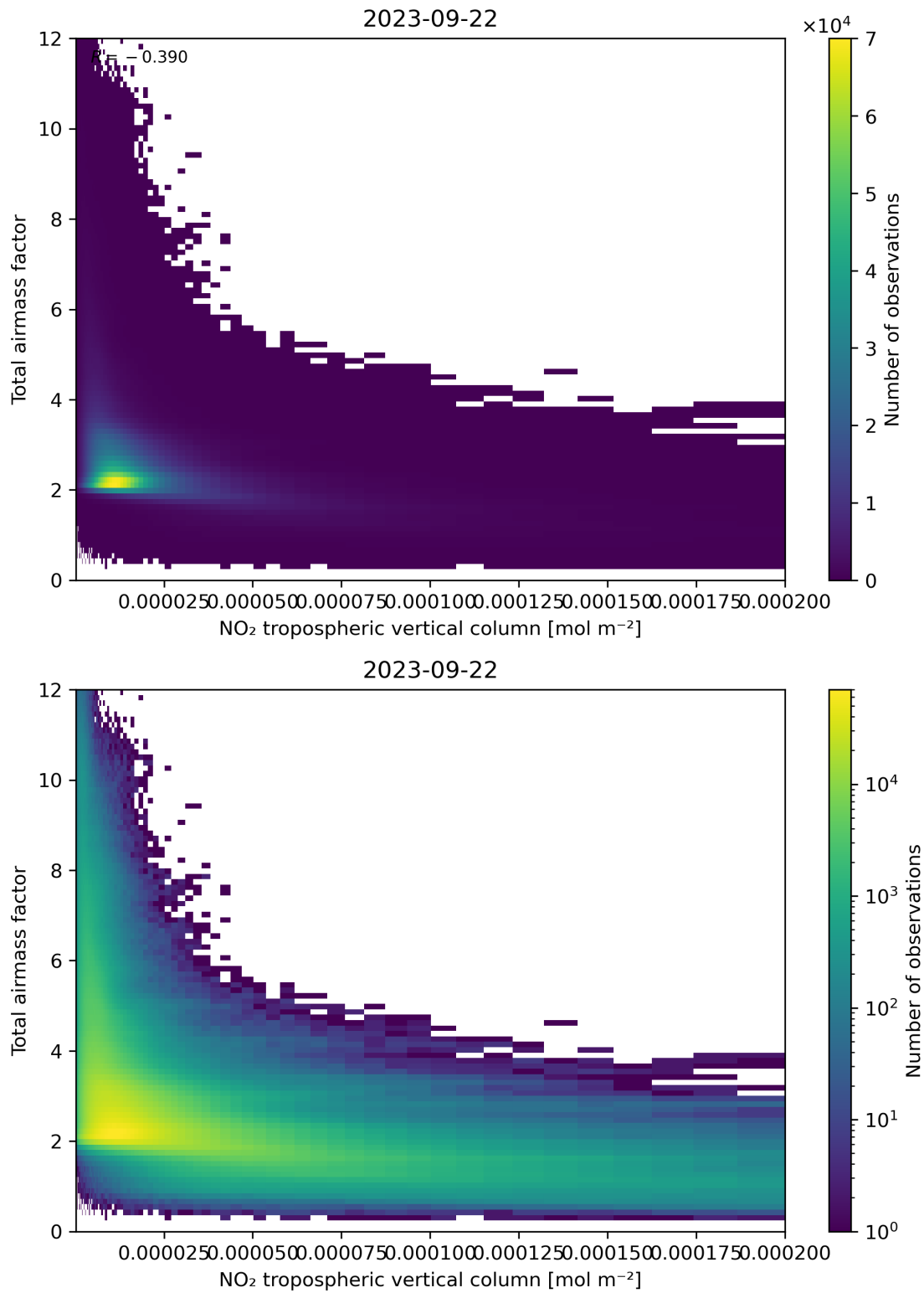
Figure 122: Scatter density plot of “NO 2 tropospheric vertical column” against “Total air mass factor” for 2023-09-21 to 2023-09-23.
