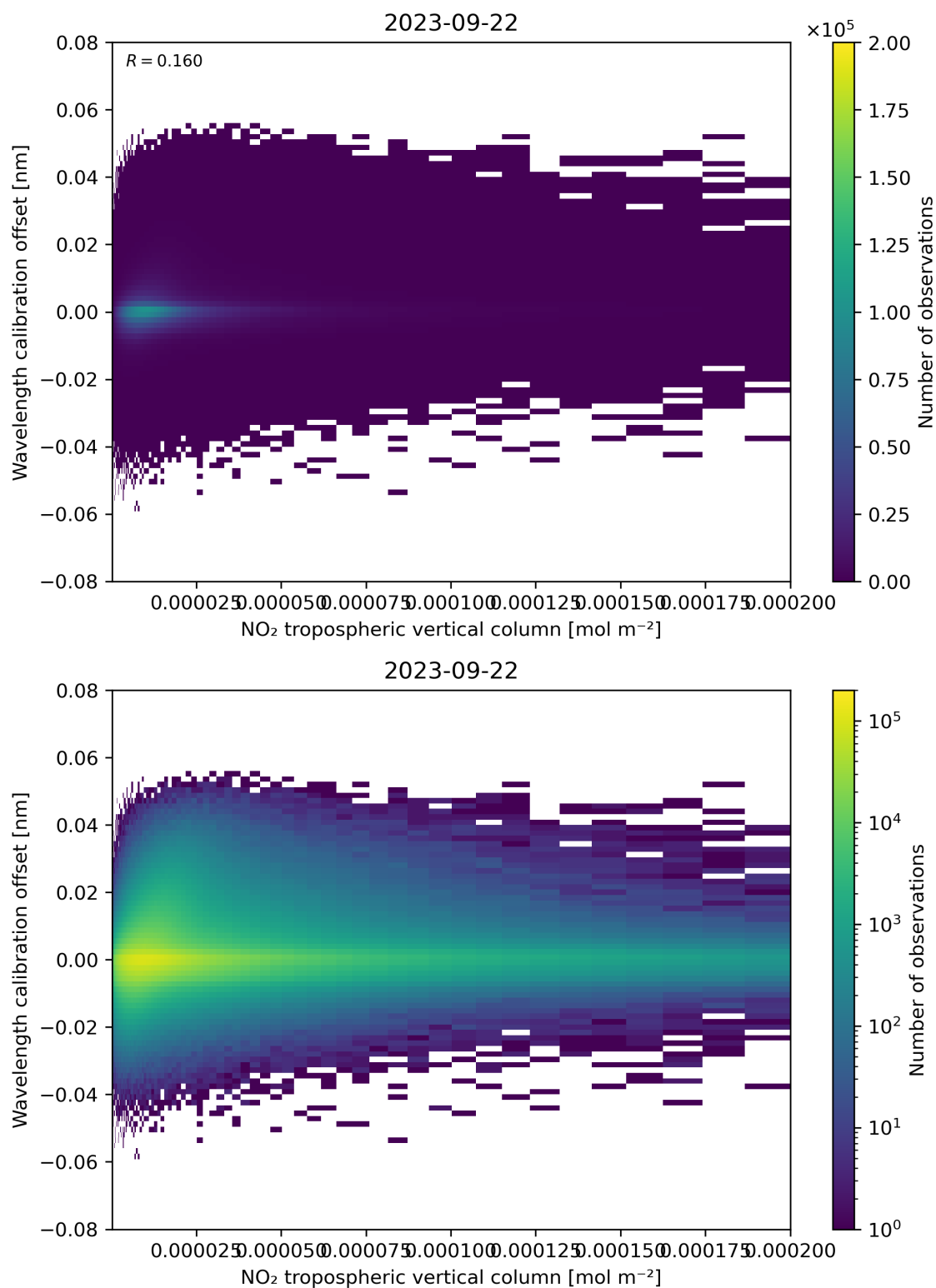
Figure 143: Scatter density plot of “NO 2 tropospheric vertical column” against “Wavelength calibration offset” for 2023-09-21 to 2023-09-23.
