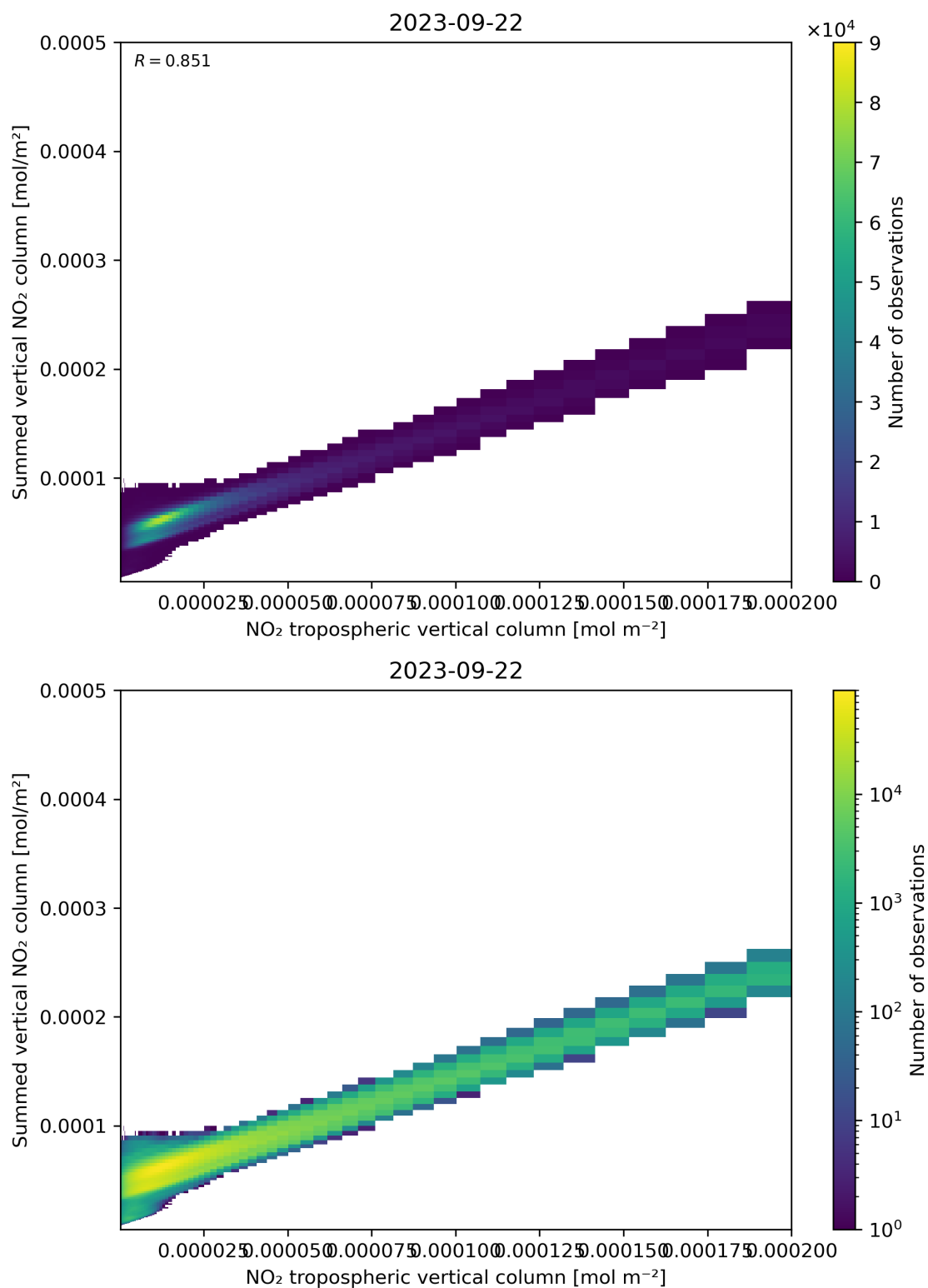
Figure 126: Scatter density plot of “NO 2 tropospheric vertical column” against “Summed vertical NO 2 column” for 2023-09-21 to 2023-09-23.
