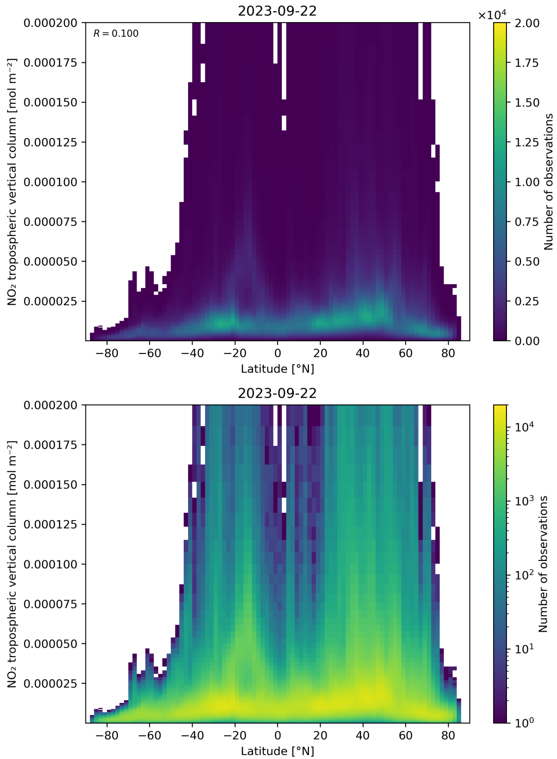
Figure 92: Scatter density plot of “Latitude” against “NO 2 tropospheric vertical column” for 2023-09-21 to 2023-09-23.
