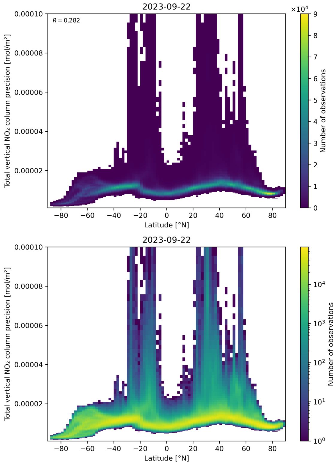
Figure 91: Scatter density plot of “Latitude” against “Total vertical NO 2 column precision” for 2023-09-21 to 2023-09-23.
