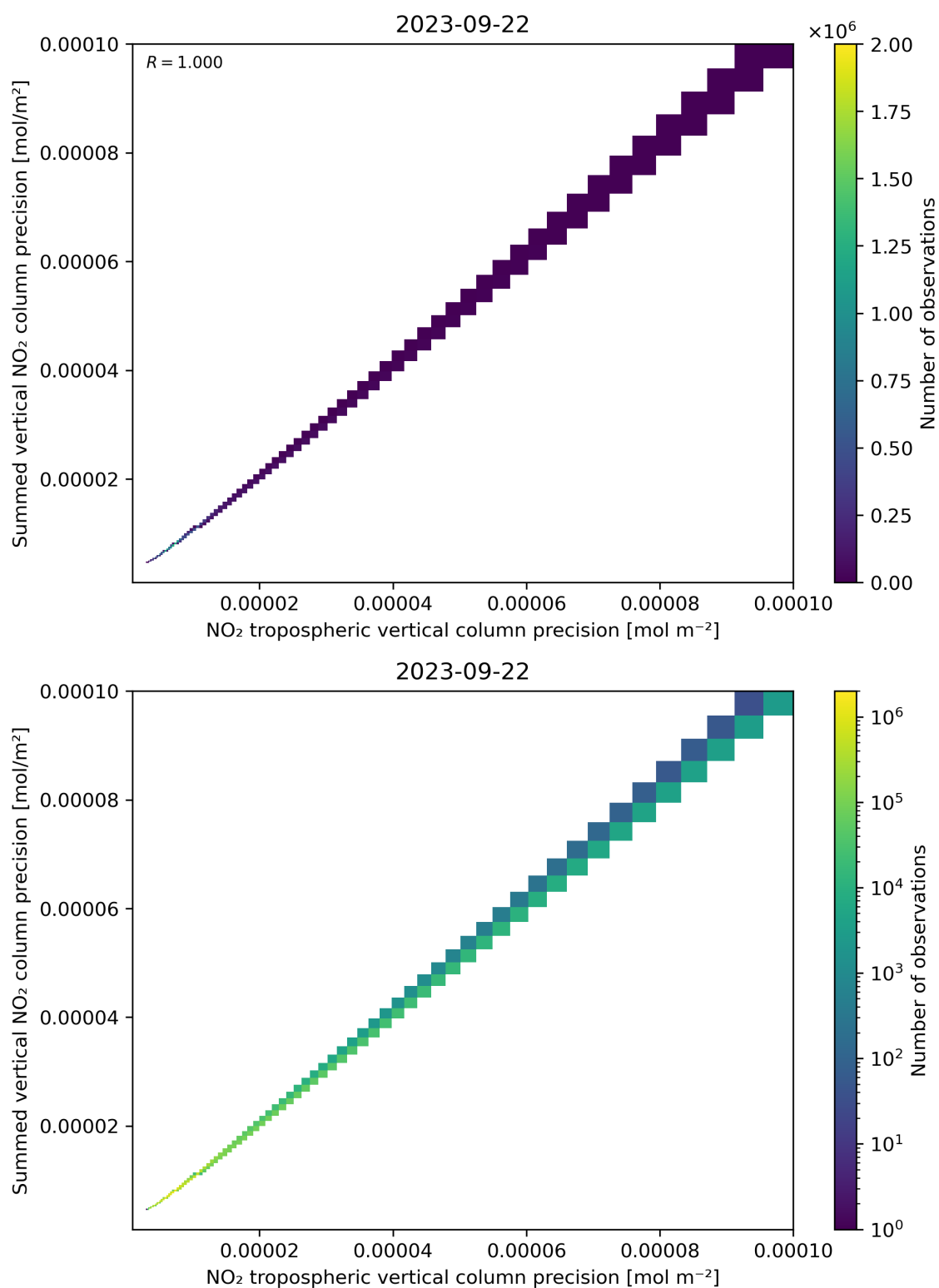
Figure 137: Scatter density plot of “NO 2 tropospheric vertical column precision” against “Summed vertical NO 2 column precision” for 2023-09-21 to 2023-09-23.
