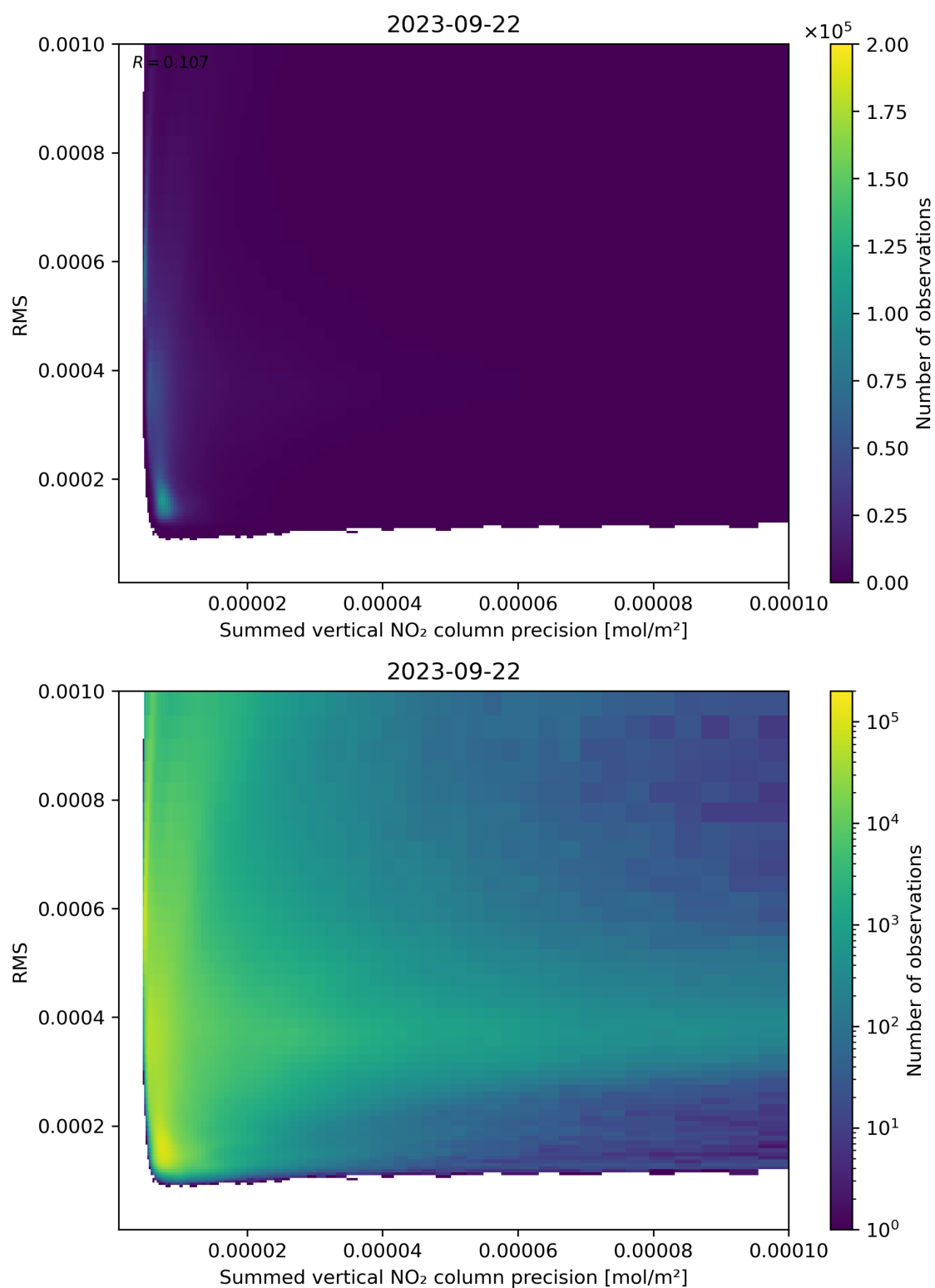
Figure 108: Scatter density plot of “Summed vertical NO 2 column precision” against “RMS” for 2023-09-21 to 2023-09-23.
