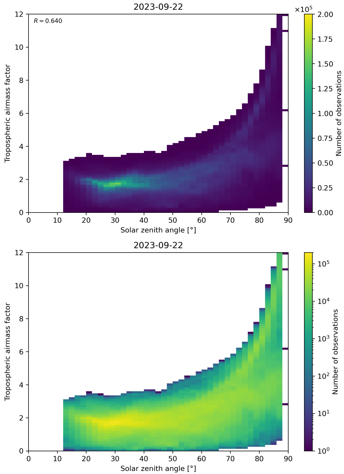
Figure 147: Scatter density plot of “Solar zenith angle” against “Tropospheric airmass factor” for 2023-09-21 to 2023-09-23.
