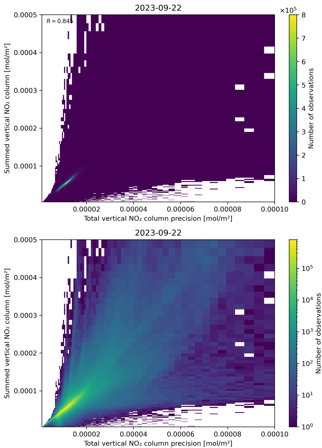
Figure 117: Scatter density plot of “Total vertical NO 2 column precision” against “Summed vertical NO 2 column” for 2023-09-21 to 2023-09-23.
