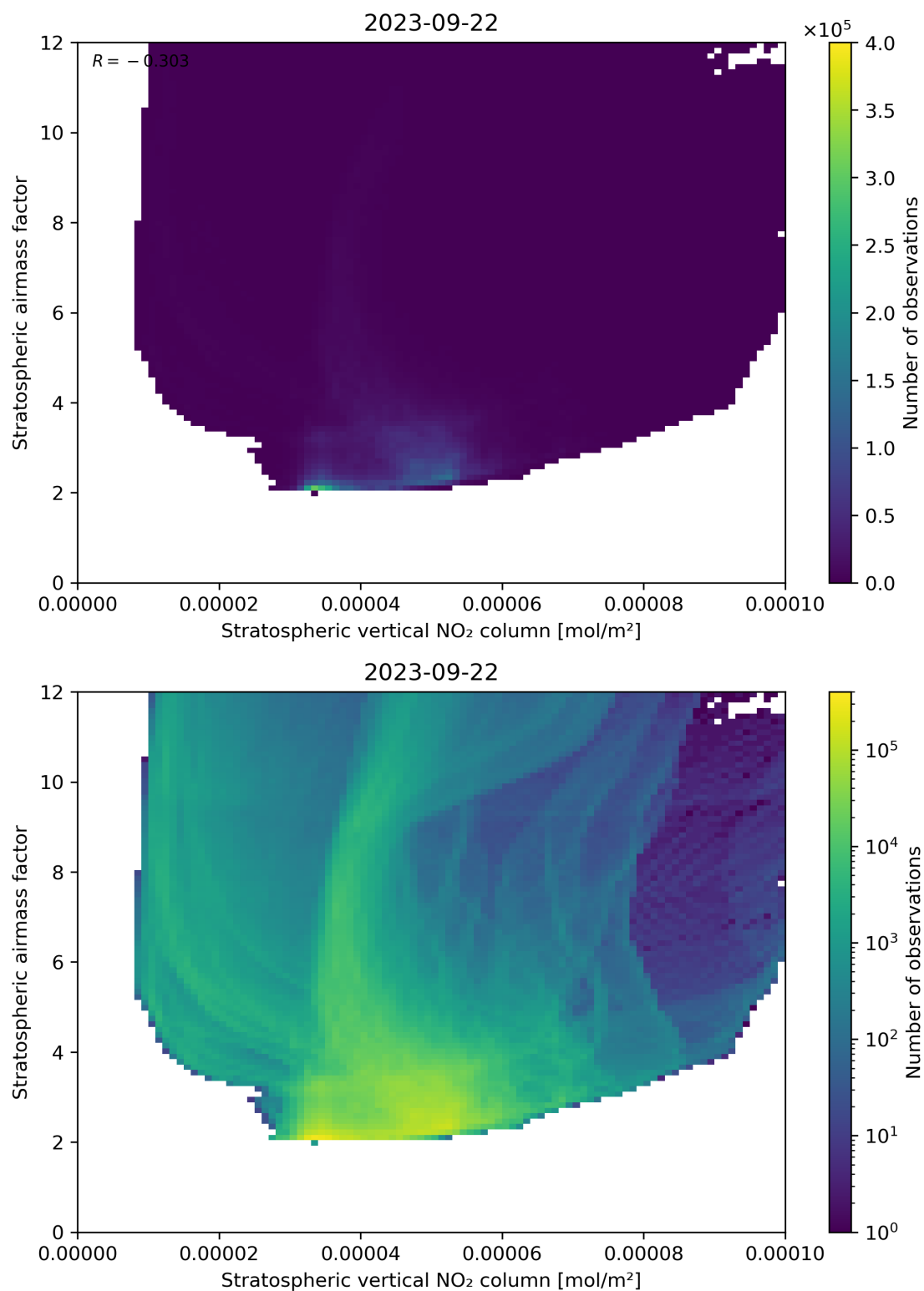
Figure 96: Scatter density plot of “Stratospheric vertical NO 2 column” against “Stratospheric airmass factor” for 2023-09-21 to 2023-09-23.
