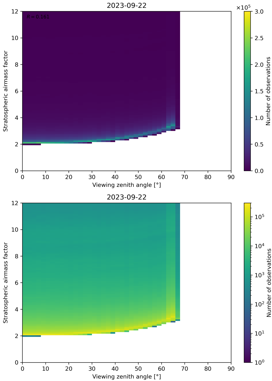
Figure 159: Scatter density plot of “Viewing zenith angle” against “Stratospheric airmass factor” for 2023-09-21 to 2023-09-23.
