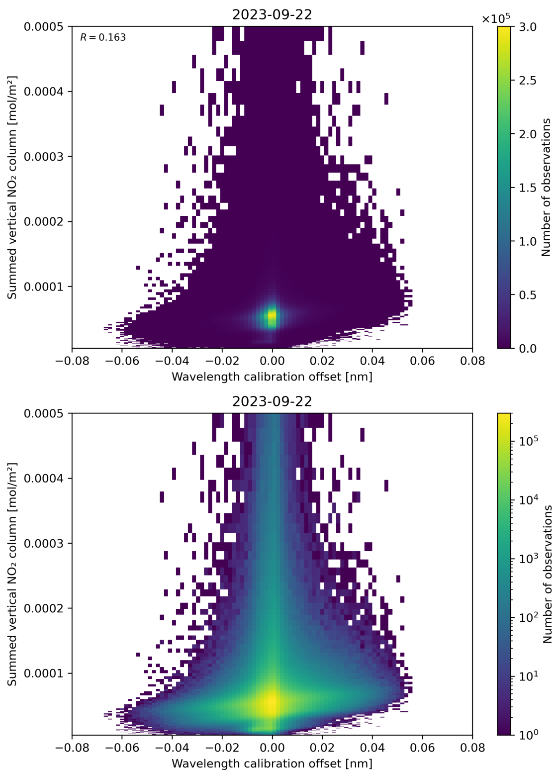
Figure 177: Scatter density plot of “Wavelength calibration offset” against “Summed vertical NO 2 column” for 2023-09-21 to 2023-09-23.
