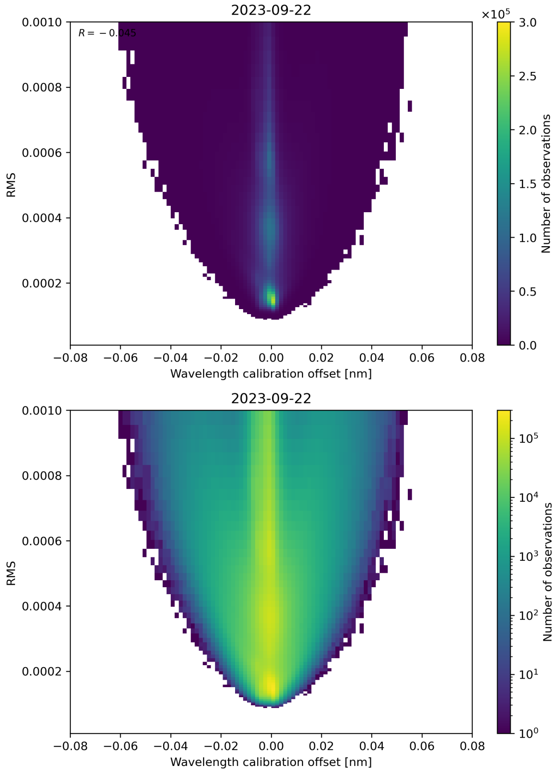
Figure 181: Scatter density plot of “Wavelength calibration offset” against “RMS” for 2023-09-21 to 2023-09-23.
