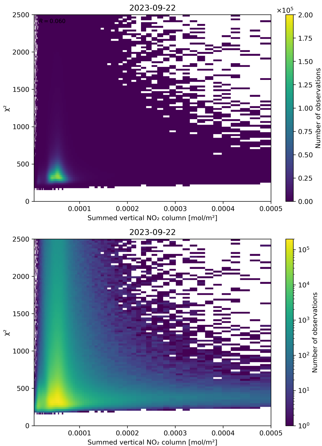
Figure 104: Scatter density plot of “Summed vertical NO 2 column” against “ \chi^2 ” for 2023-09-21 to 2023-09-23.
