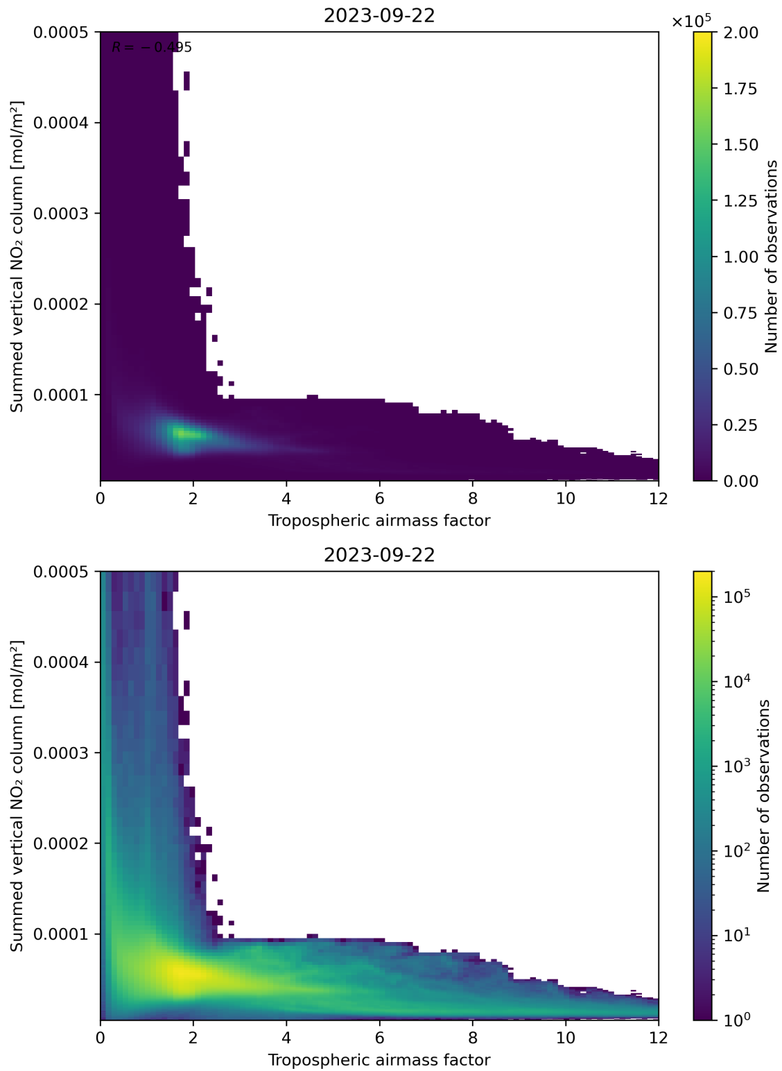
Figure 75: Scatter density plot of “Tropospheric air mass factor” against “Summed vertical NO 2 column” for 2023-09-21 to 2023-09-23.
