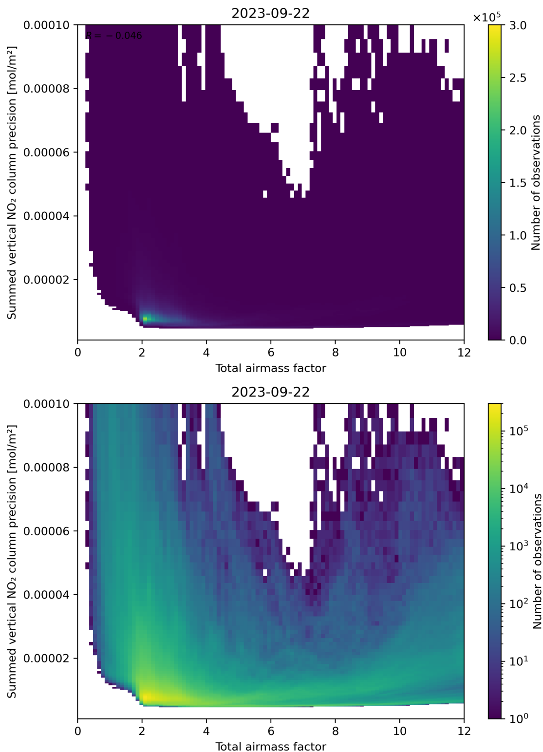
Figure 66: Scatter density plot of “Total airmass factor” against “Summed vertical NO 2 column precision” for 2023-09-21 to 2023-09-23.
