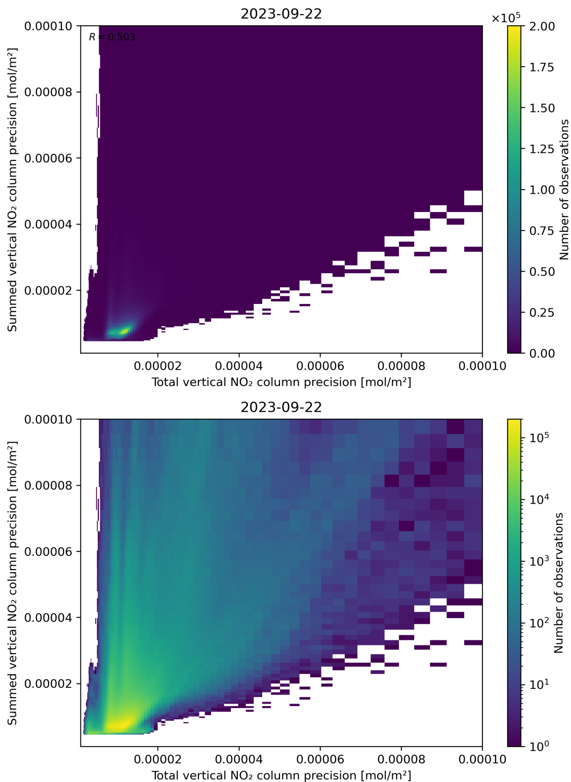
Figure 118: Scatter density plot of “Total vertical NO 2 column precision” against “Summed vertical NO 2 column precision” for 2023-09-21 to 2023-09-23.
