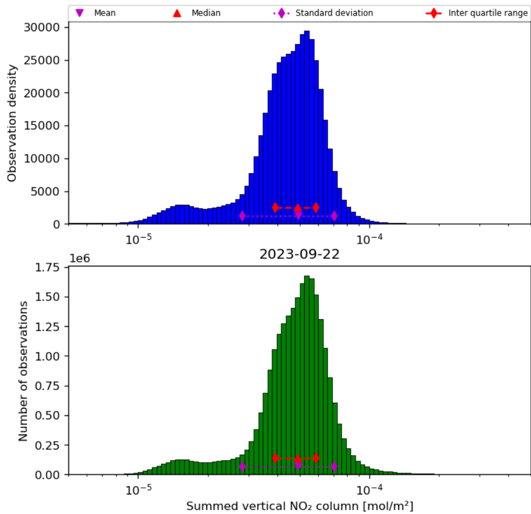
Figure 40: Histogram of “Summed vertical NO 2 column” for 2023-09-21 to 2023-09-23
