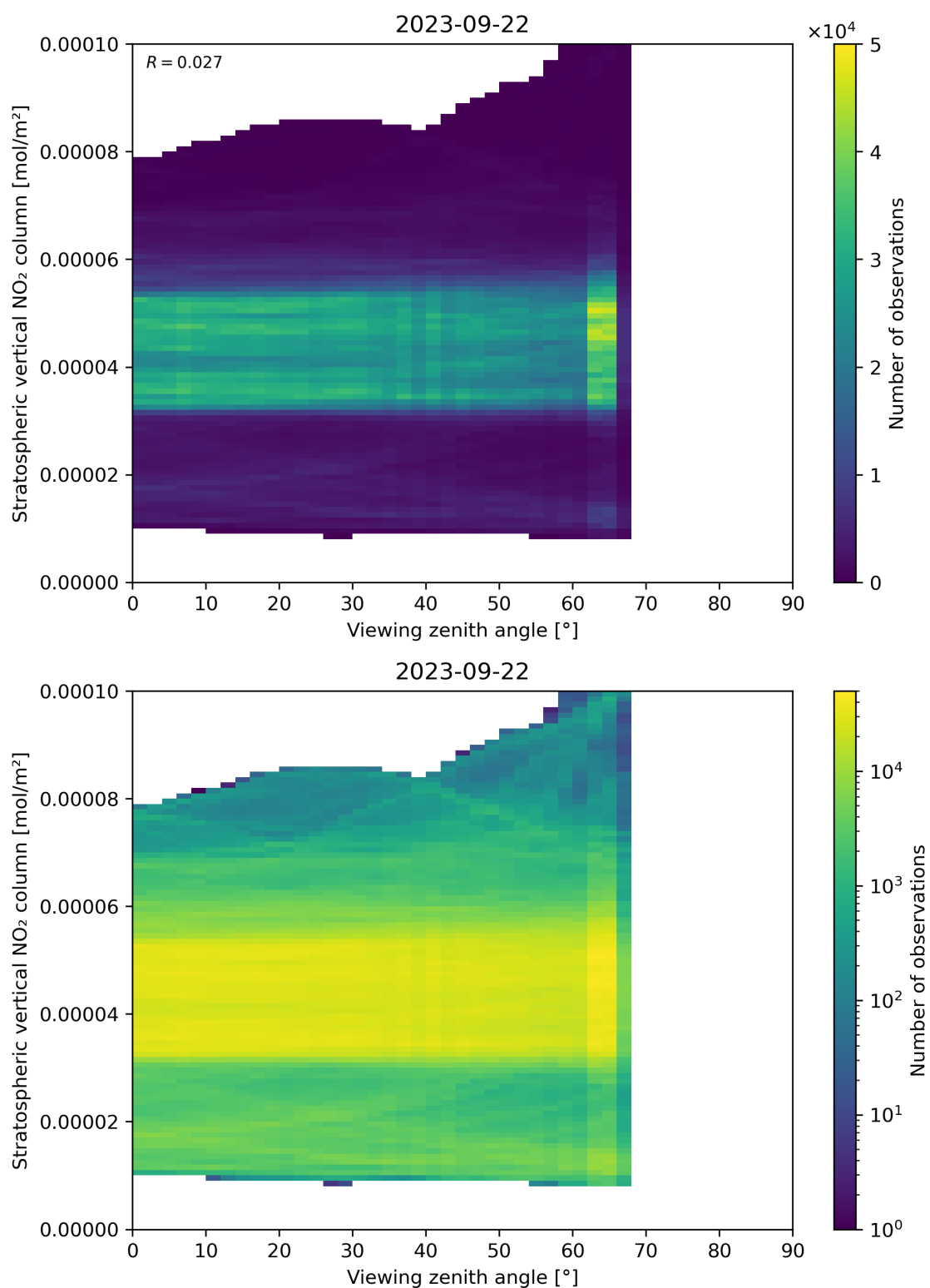
Figure 164: Scatter density plot of “Viewing zenith angle” against “Stratospheric vertical NO 2 column” for 2023-09-21 to 2023-09-23.
