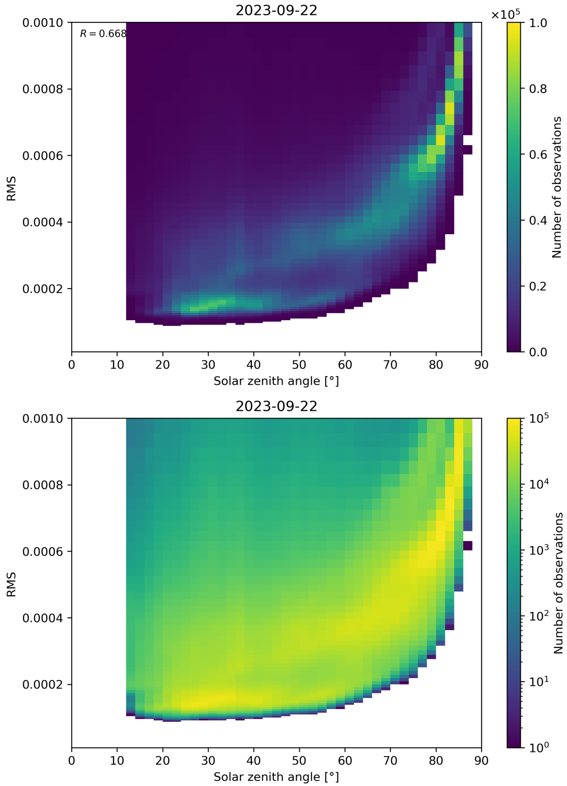
Figure 157: Scatter density plot of “Solar zenith angle” against “RMS” for 2023-09-21 to 2023-09-23.
