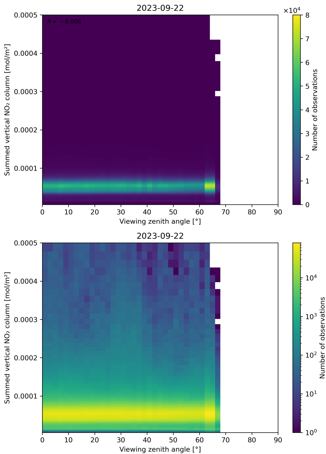
Figure 165: Scatter density plot of “Viewing zenith angle” against “Summed vertical NO 2 column” for 2023-09-21 to 2023-09-23.
