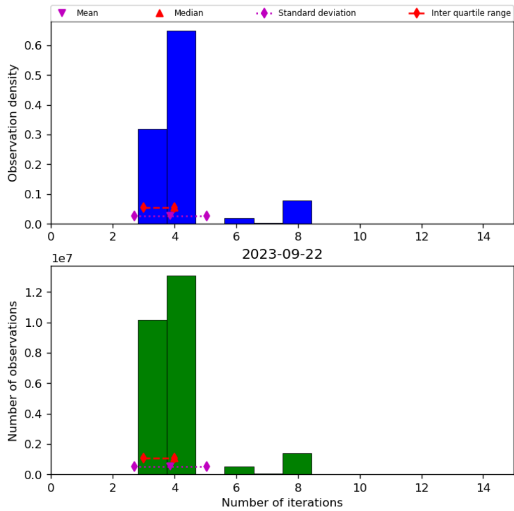
Figure 34: Histogram of “Number of iterations” for 2023-09-21 to 2023-09-23
