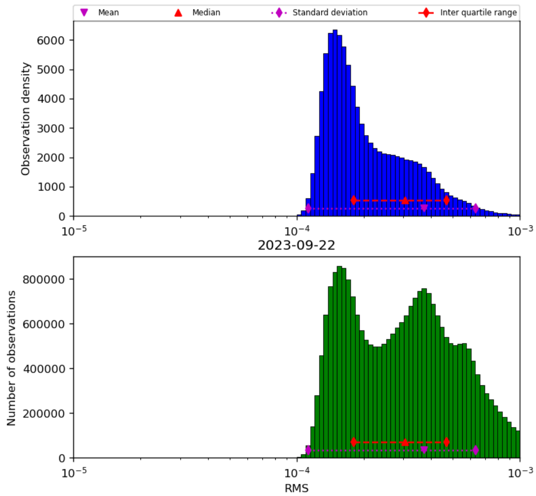
Figure 43: Histogram of “RMS” for 2023-09-21 to 2023-09-23
