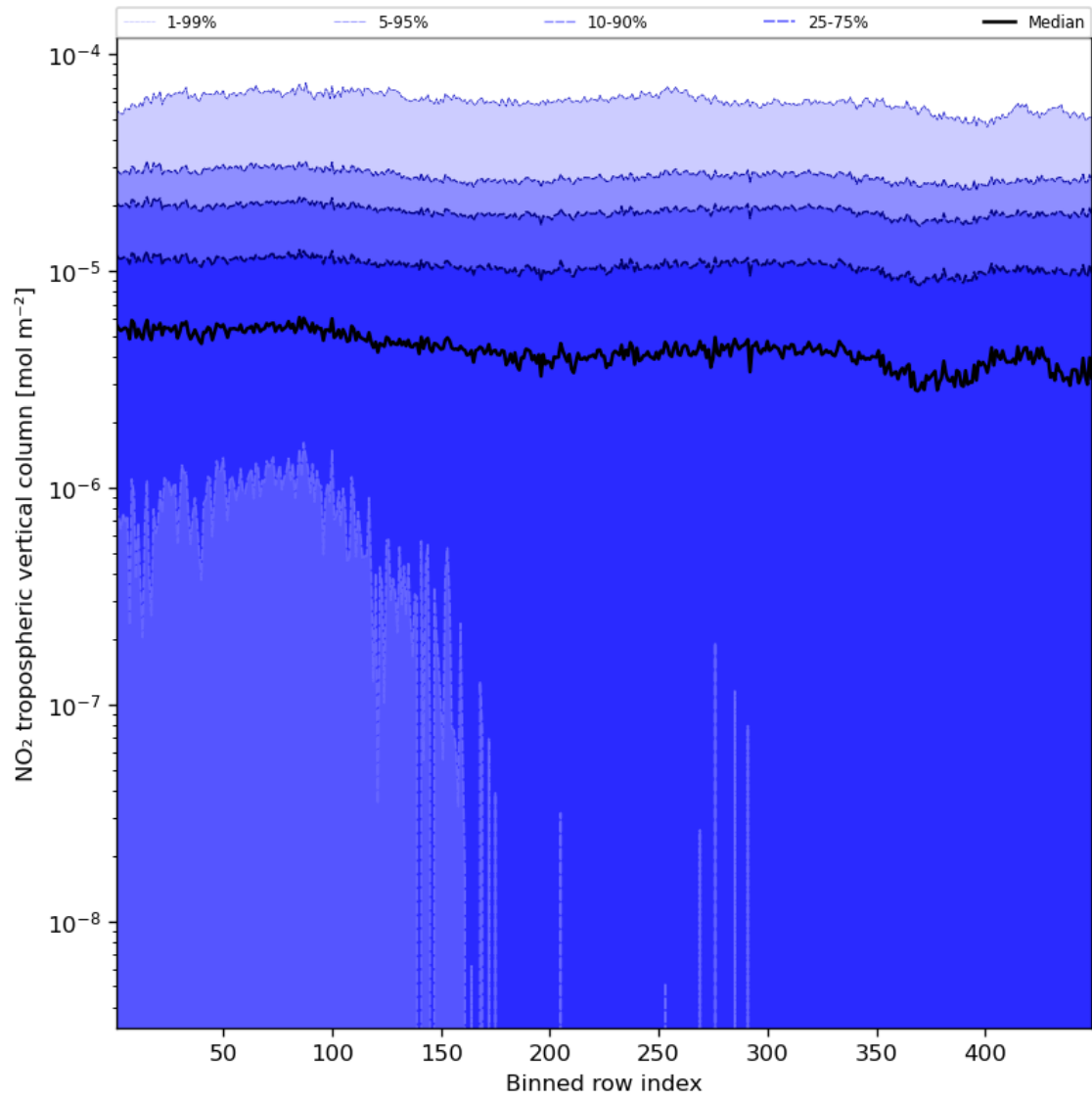
Figure 46: Along track statistics of “ \text{NO}_2 tropospheric vertical column” for 2023-09-21 to 2023-09-23
