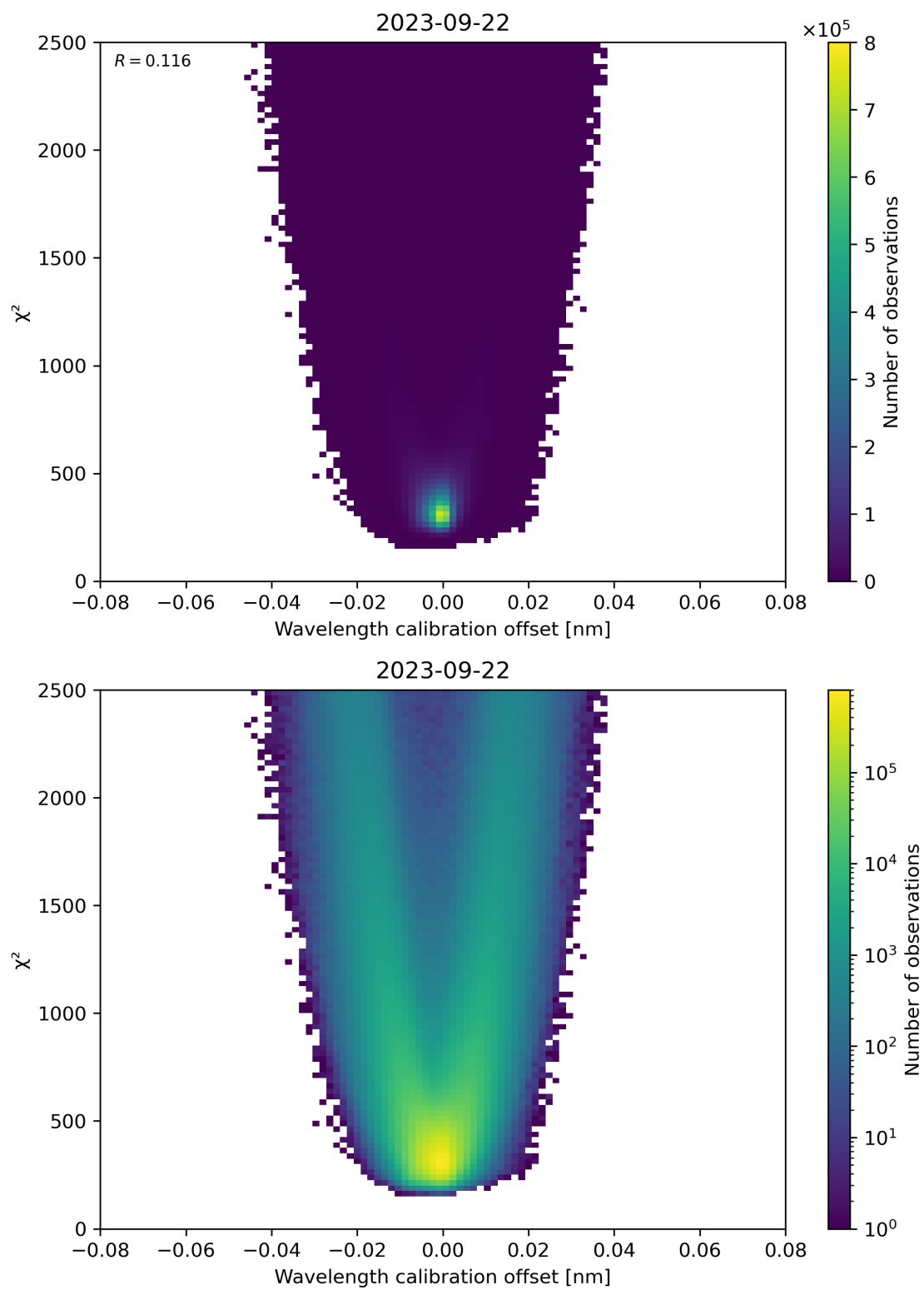
Figure 175: Scatter density plot of “Wavelength calibration offset” against “ \chi^2 ” for 2023-09-21 to 2023-09-23.
