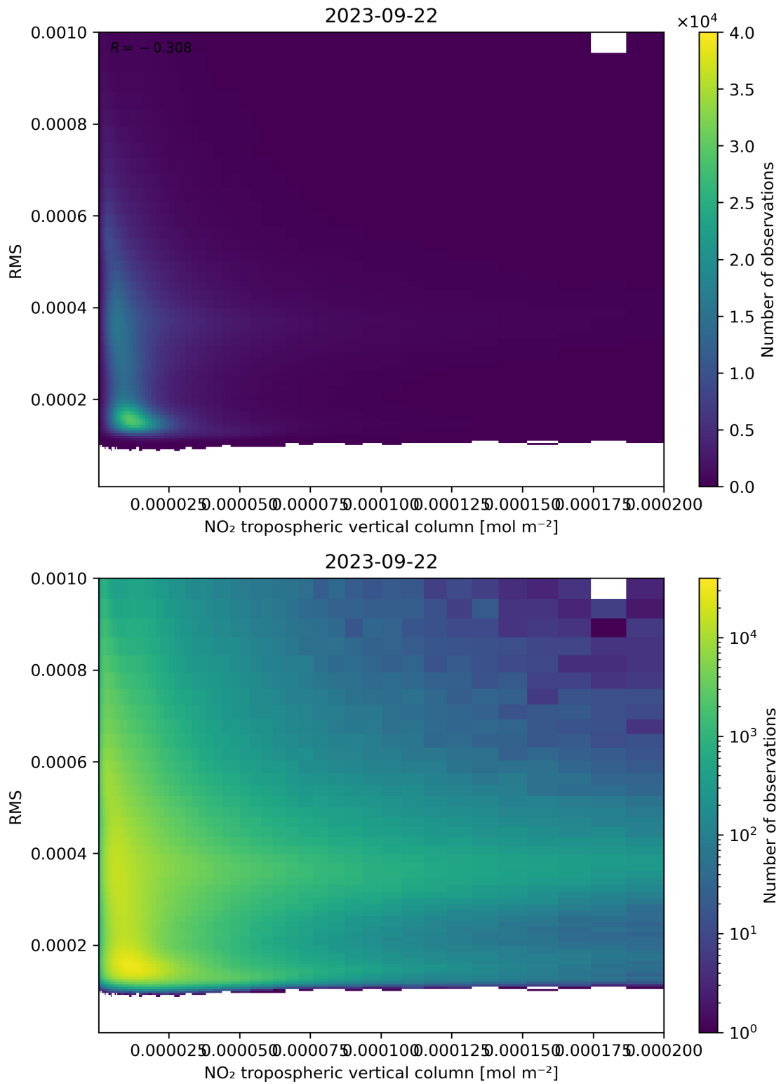
Figure 142: Scatter density plot of “NO 2 tropospheric vertical column” against “RMS” for 2023-09-21 to 2023-09-23.
