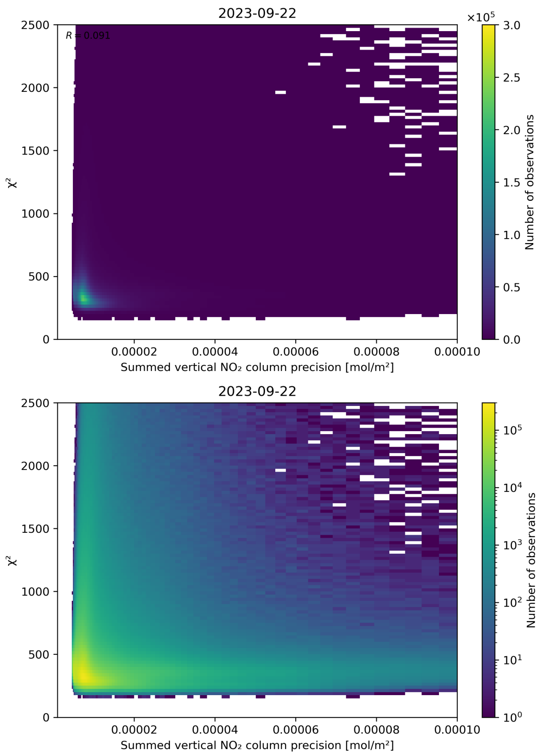
Figure 107: Scatter density plot of “Summed vertical NO 2 column precision” against “ \chi^2 ” for 2023-09-21 to 2023-09-23.
