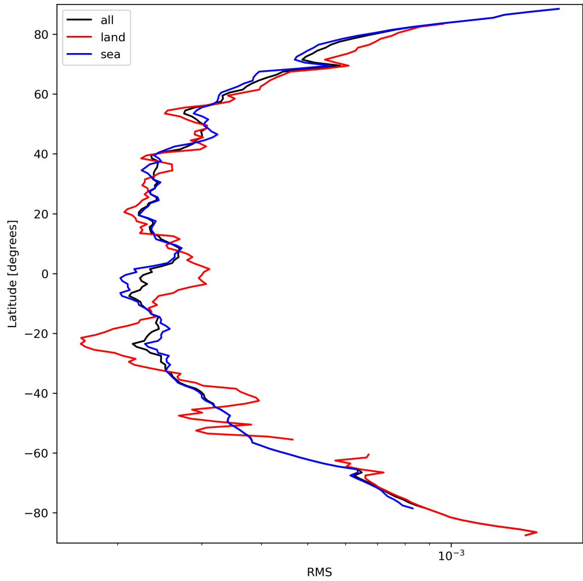
Figure 26: Zonal average of “RMS” for 2023-09-21 to 2023-09-23.
