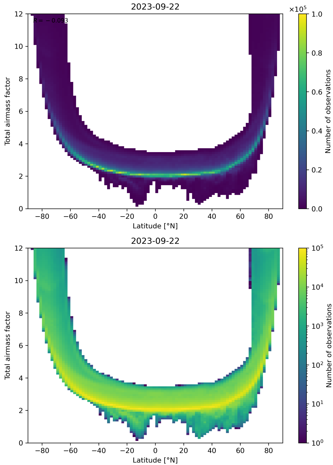
Figure 84: Scatter density plot of “Latitude” against “Total airmass factor” for 2023-09-21 to 2023-09-23.
