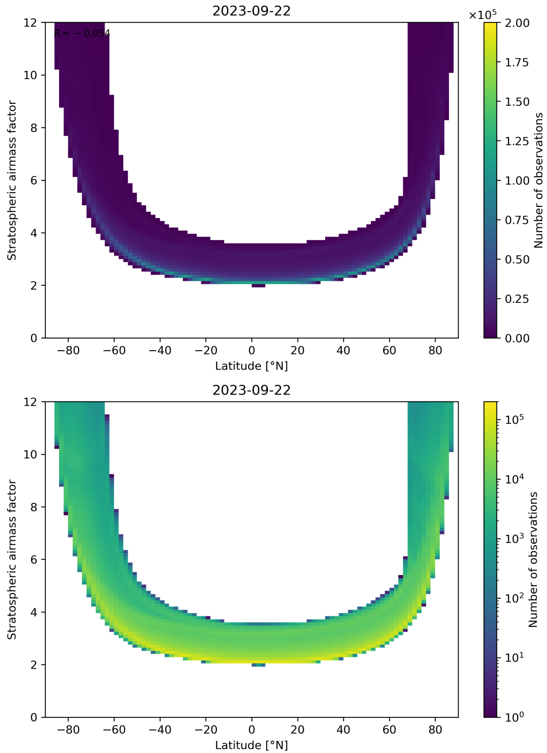
Figure 83: Scatter density plot of “Latitude” against “Stratospheric airmass factor” for 2023-09-21 to 2023-09-23.
