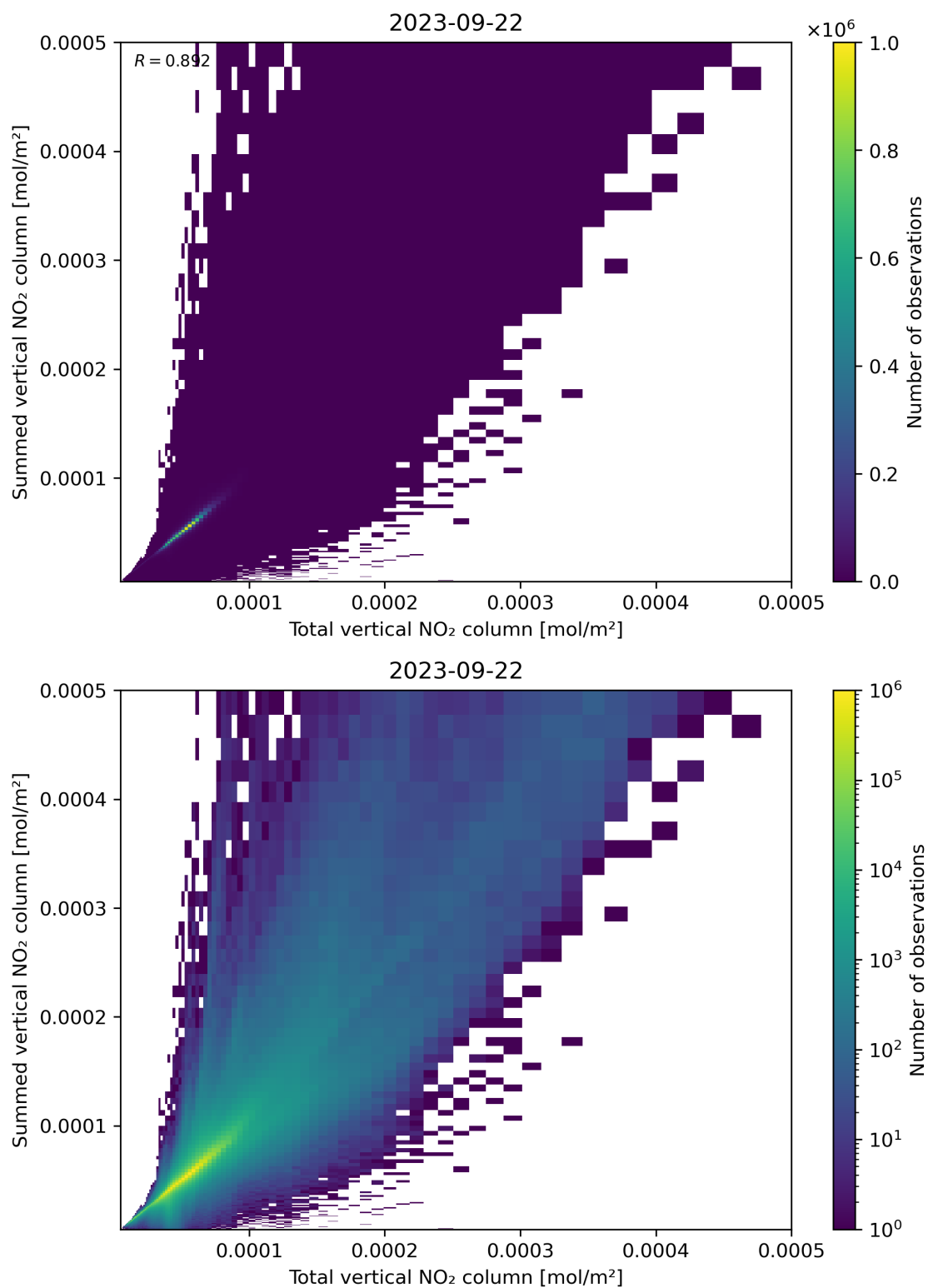
Figure 112: Scatter density plot of “Total vertical NO 2 column” against “Summed vertical NO 2 column” for 2023-09-21 to 2023-09-23.
