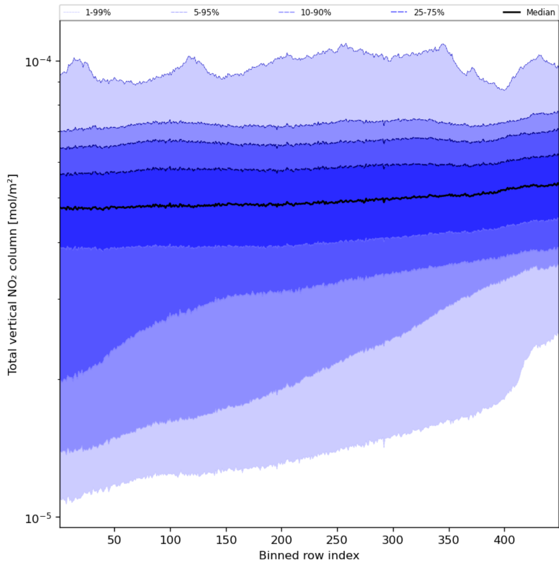
Figure 55: Along track statistics of “Total vertical NO 2 column” for 2023-09-21 to 2023-09-23
