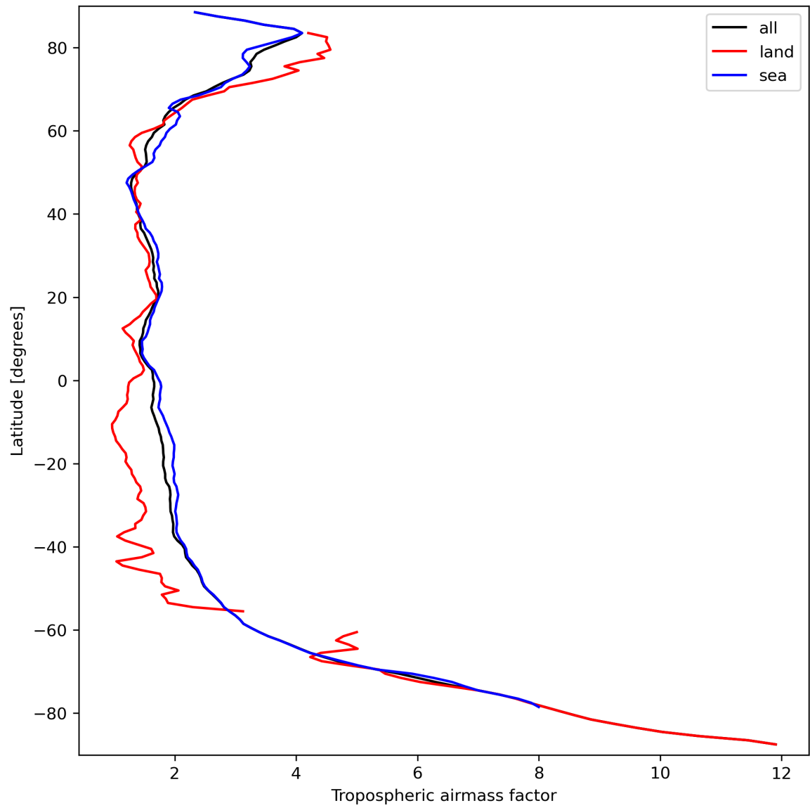
Figure 14: Zonal average of “Tropospheric airmass factor” for 2023-09-21 to 2023-09-23.
