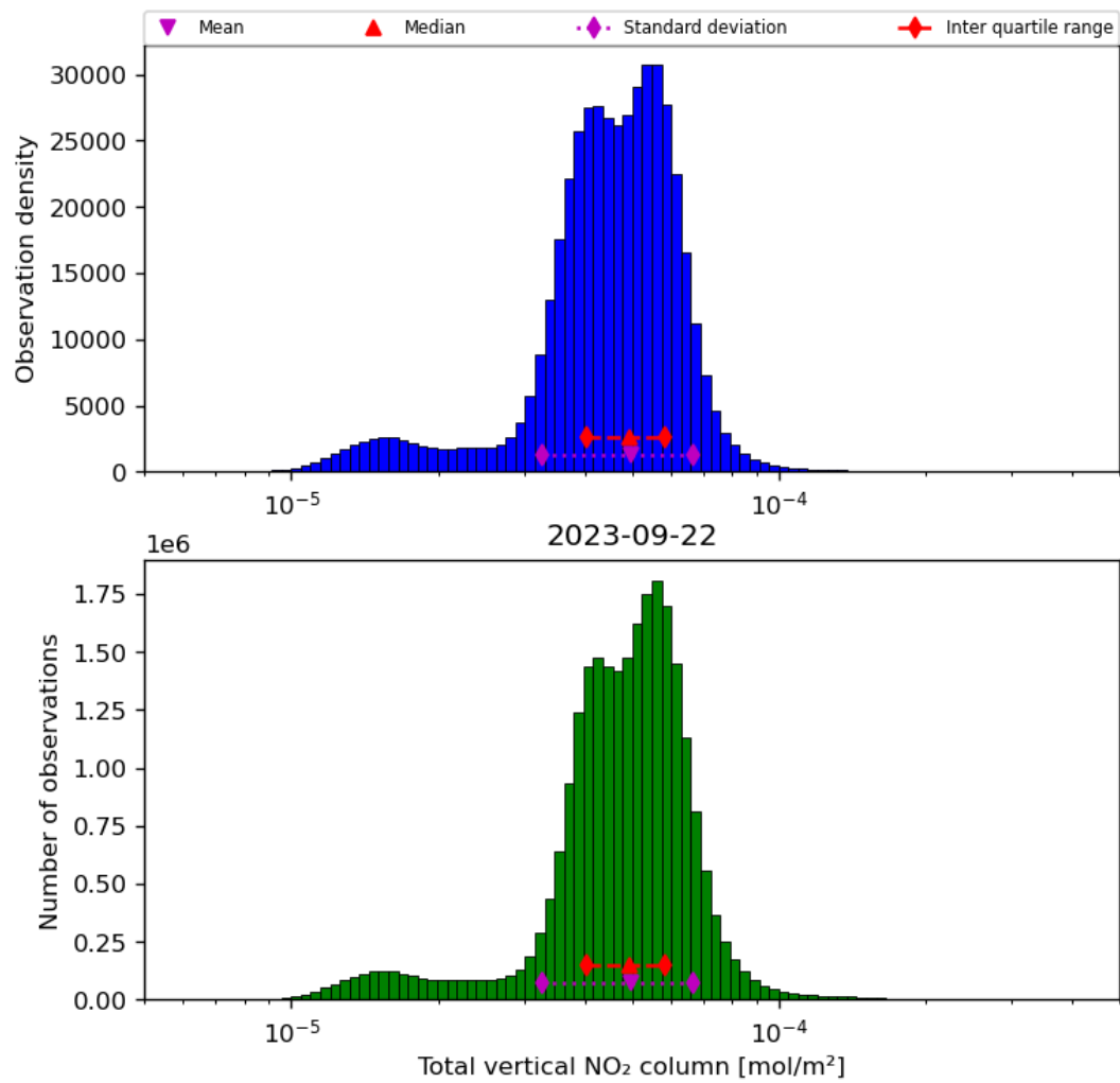
Figure 38: Histogram of “Total vertical NO 2 column” for 2023-09-21 to 2023-09-23
