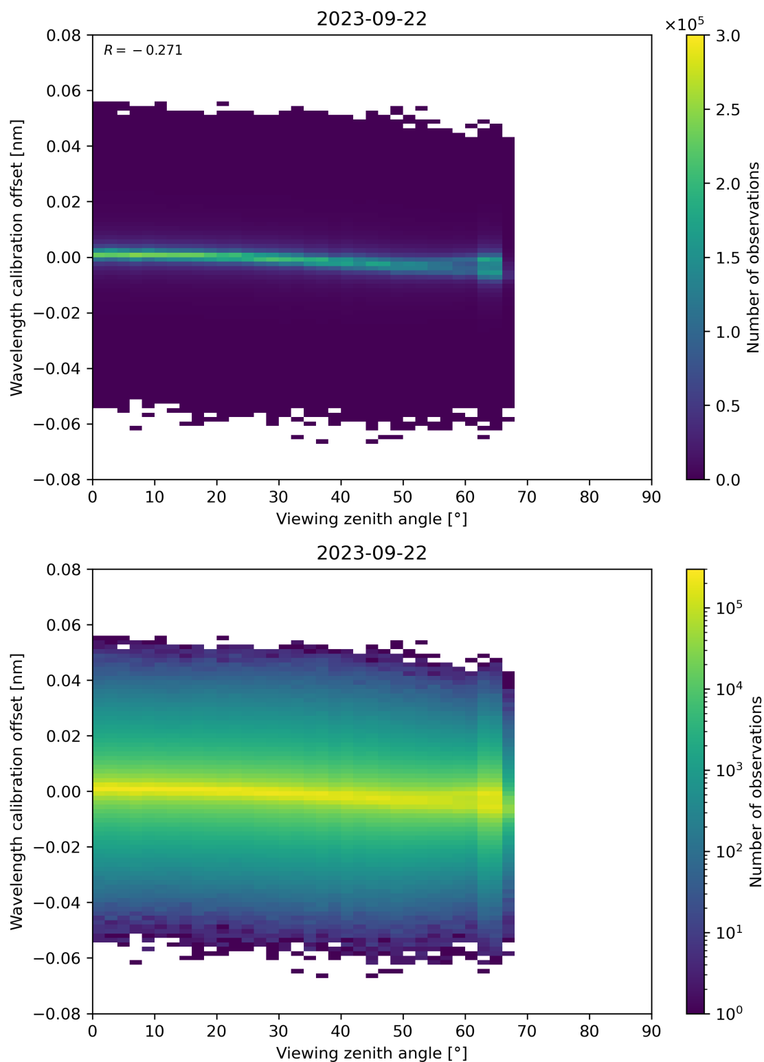
Figure 173: Scatter density plot of “Viewing zenith angle” against “Wavelength calibration offset” for 2023-09-21 to 2023-09-23.
