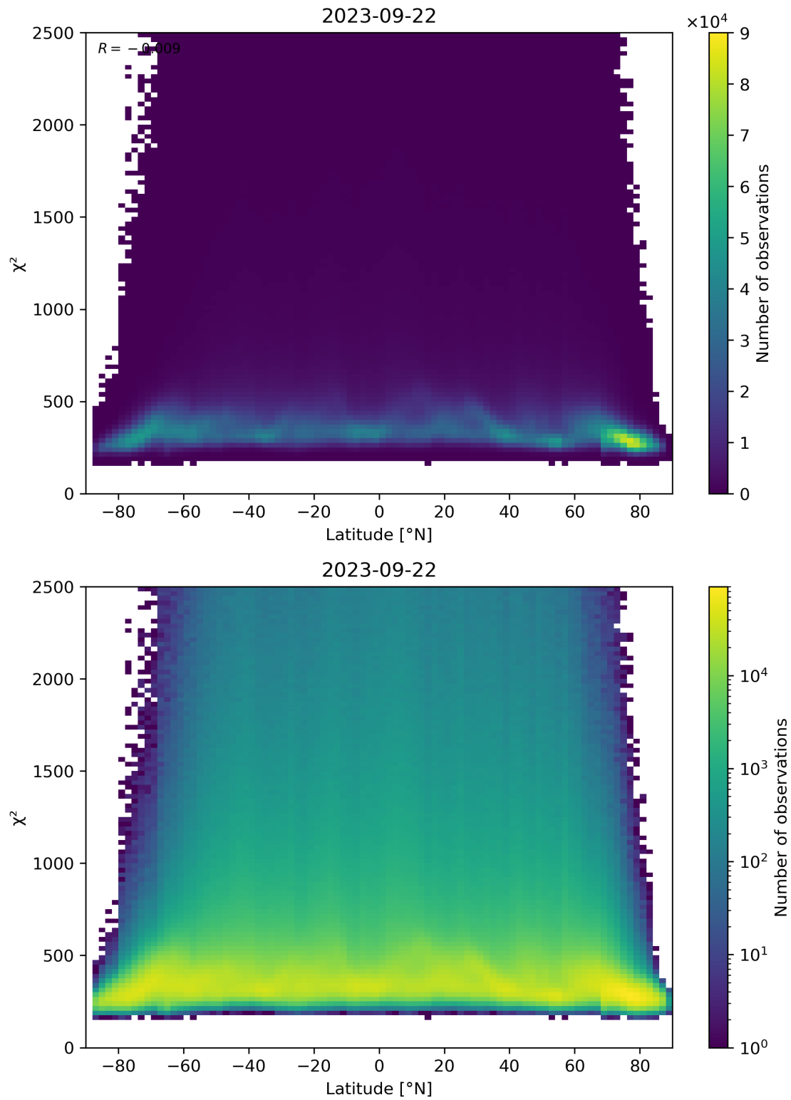
Figure 86: Scatter density plot of “Latitude” against “ \chi^2 ” for 2023-09-21 to 2023-09-23.
