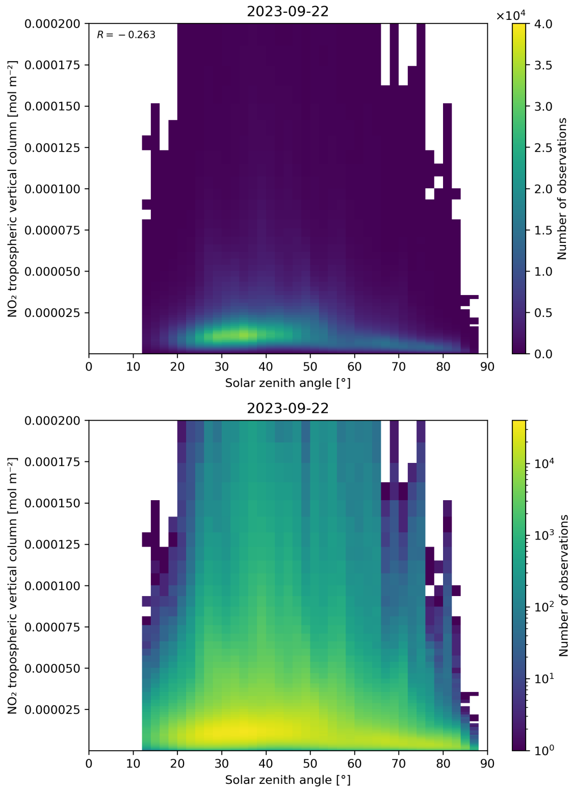
Figure 155: Scatter density plot of “Solar zenith angle” against “NO 2 tropospheric vertical column” for 2023-09-21 to 2023-09-23.
