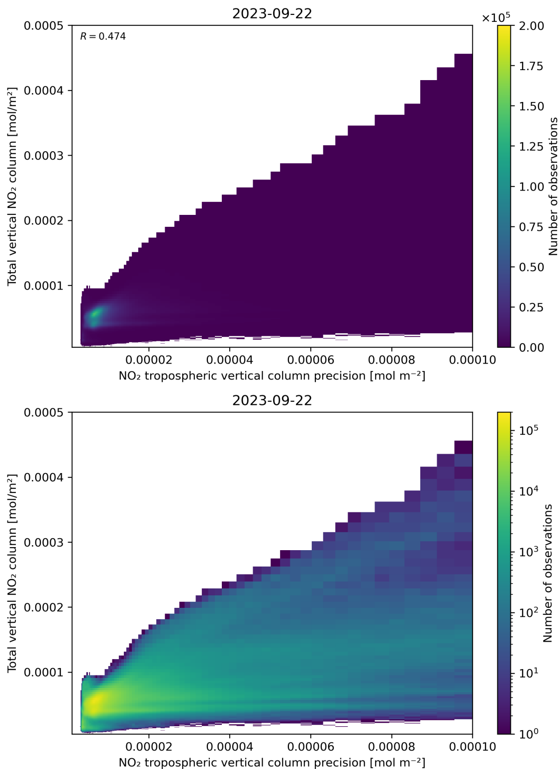
Figure 138: Scatter density plot of “NO 2 tropospheric vertical column precision” against “Total vertical NO 2 column” for 2023-09-21 to 2023-09-23.
