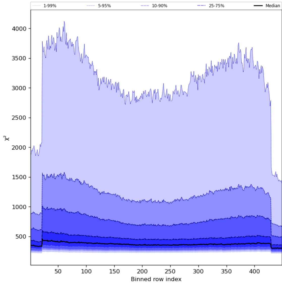
Figure 59: Along track statistics of “ \chi^2 ” for 2023-09-21 to 2023-09-23
