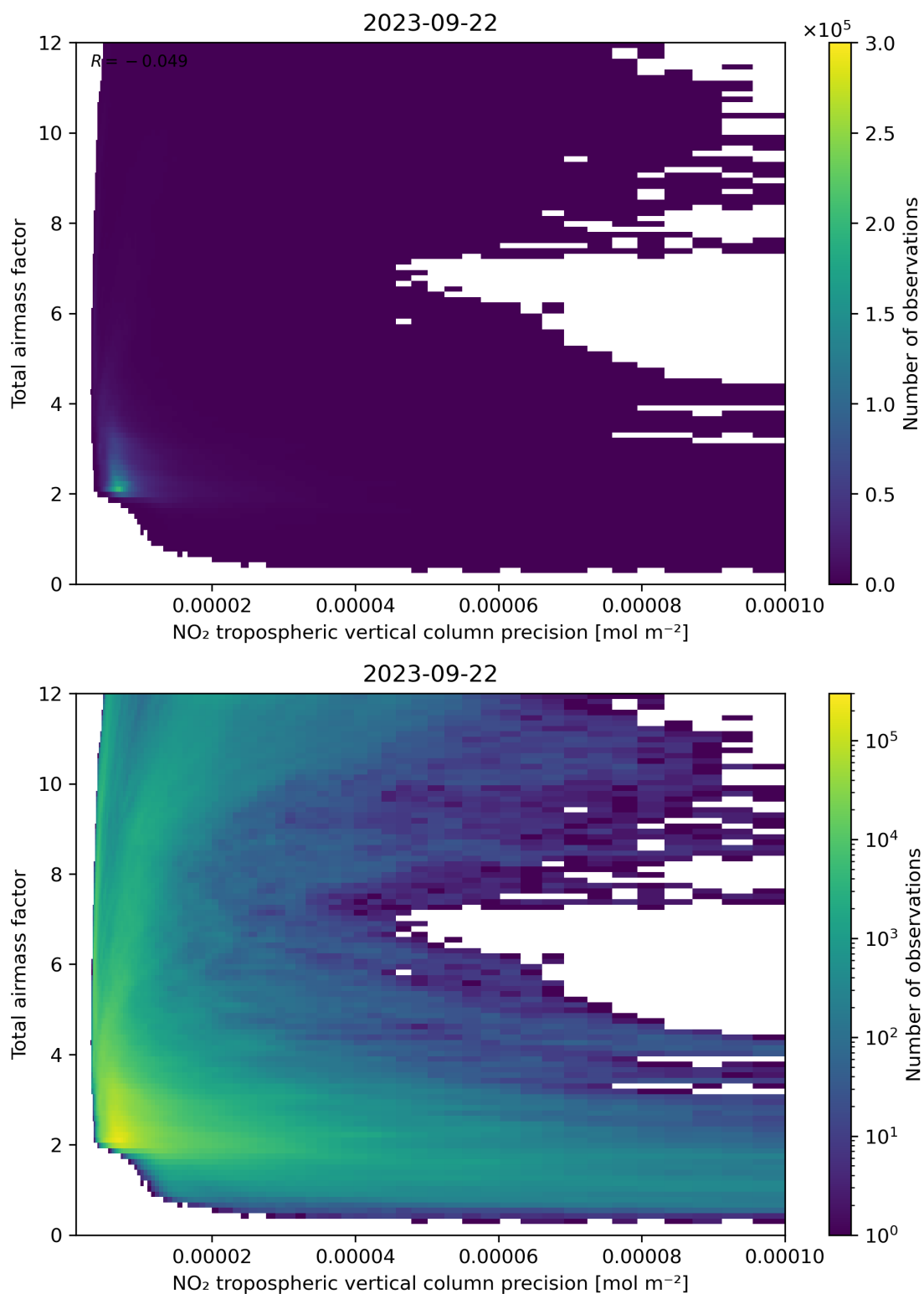
Figure 132: Scatter density plot of “NO 2 tropospheric vertical column precision” against “Total air mass factor” for 2023-09-21 to 2023-09-23.
