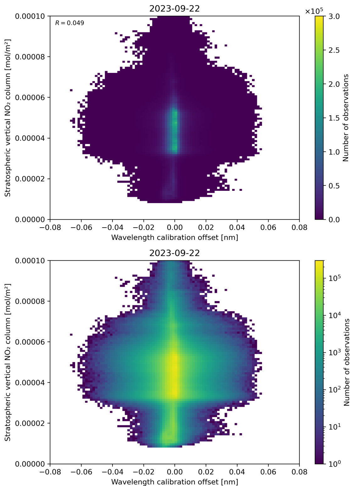
Figure 176: Scatter density plot of “Wavelength calibration offset” against “Stratospheric vertical NO 2 column” for 2023-09-21 to 2023-09-23.
