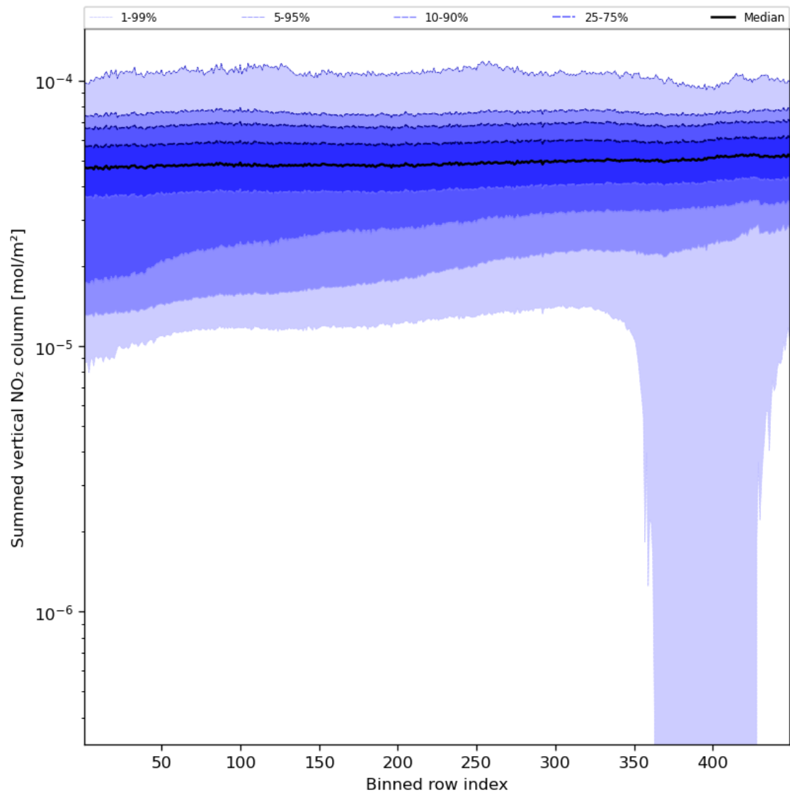
Figure 57: Along track statistics of “Summed vertical NO 2 column” for 2023-09-21 to 2023-09-23
