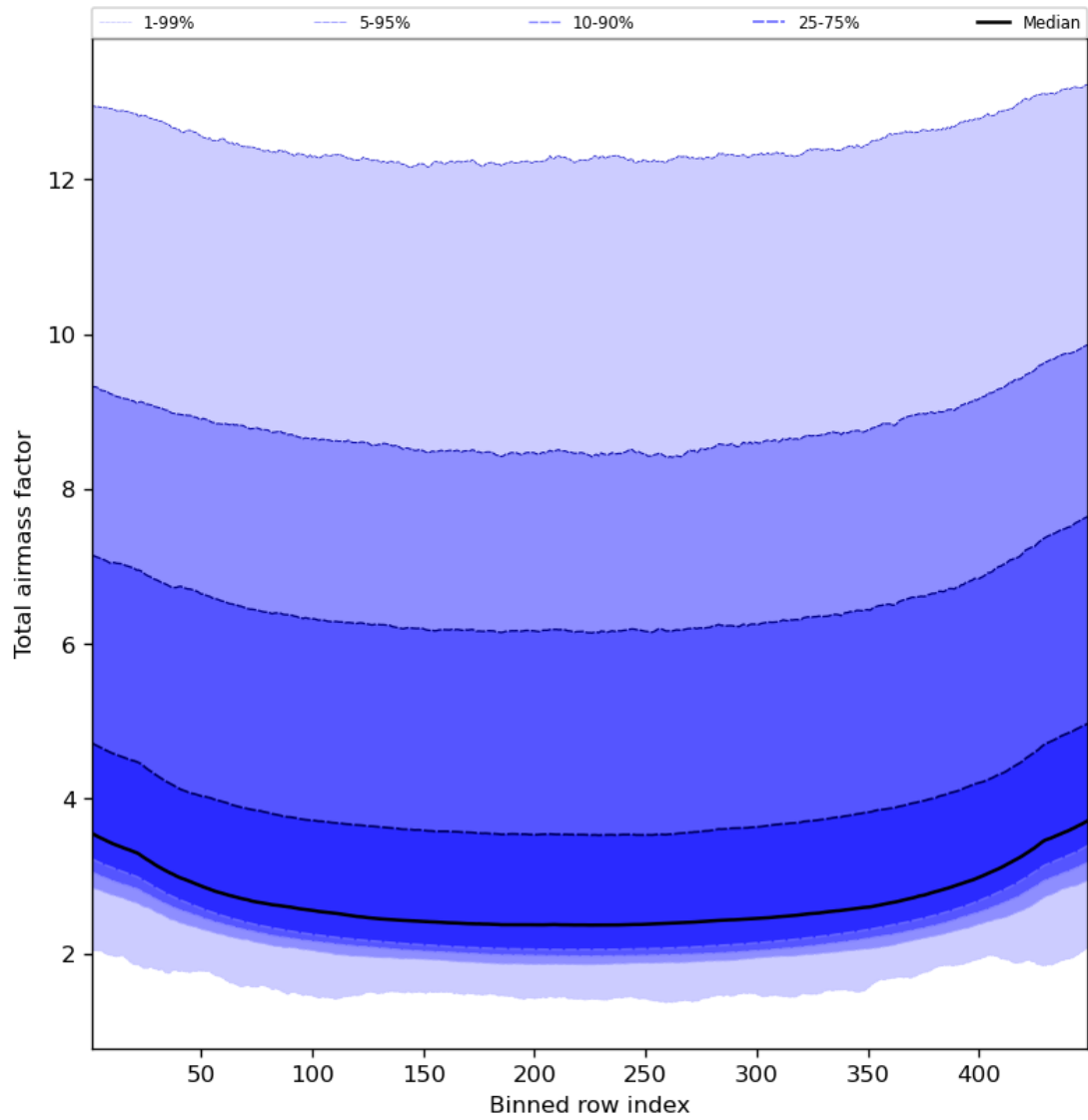
Figure 49: Along track statistics of “Total airmass factor” for 2023-09-21 to 2023-09-23
