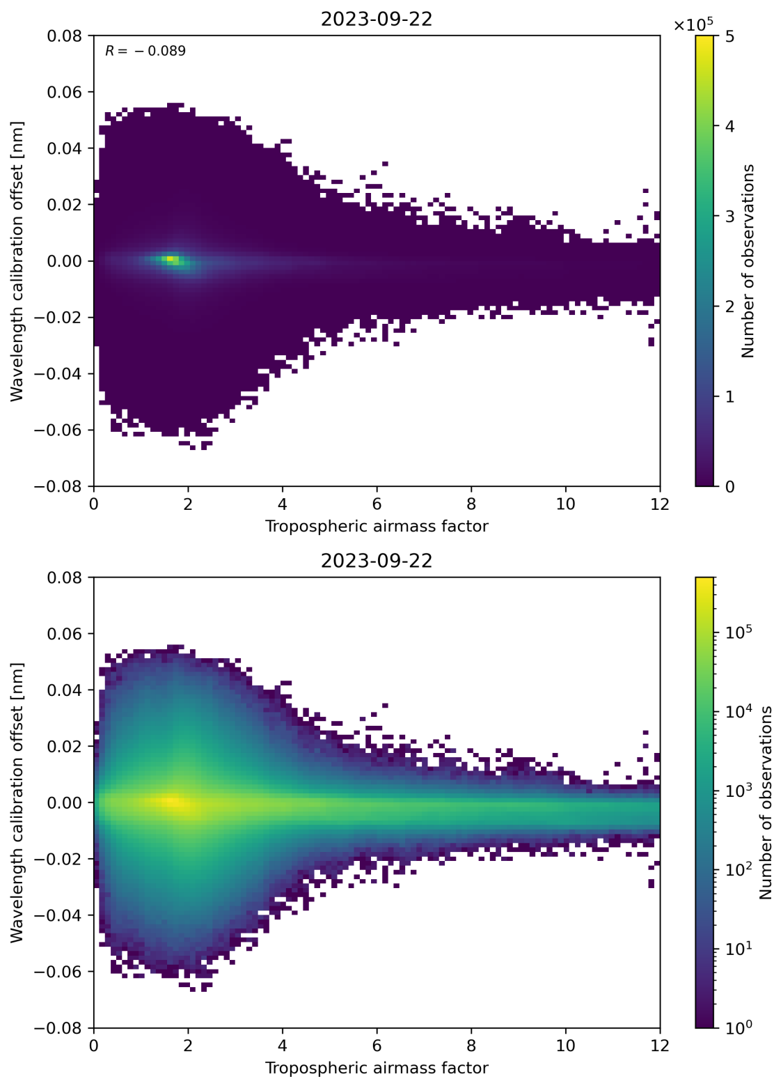
Figure 80: Scatter density plot of “Tropospheric airmass factor” against “Wavelength calibration offset” for 2023-09-21 to 2023-09-23.
