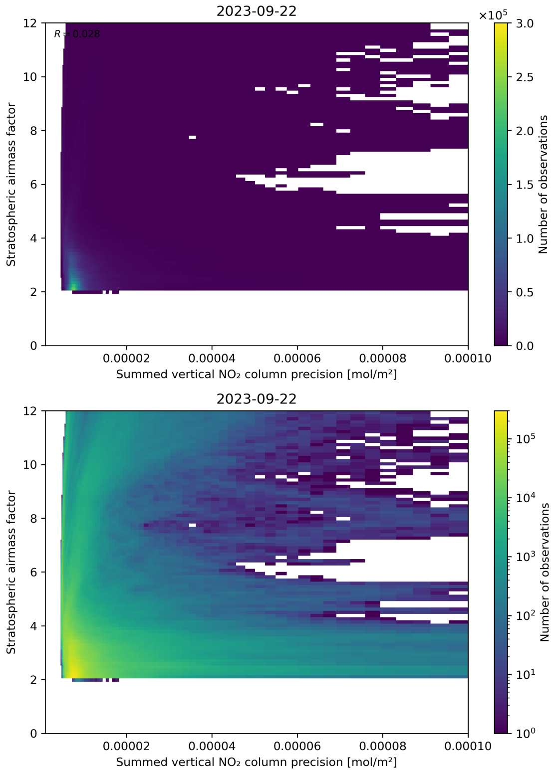
Figure 106: Scatter density plot of “Summed vertical NO 2 column precision” against “Stratospheric airmass factor” for 2023-09-21 to 2023-09-23.
