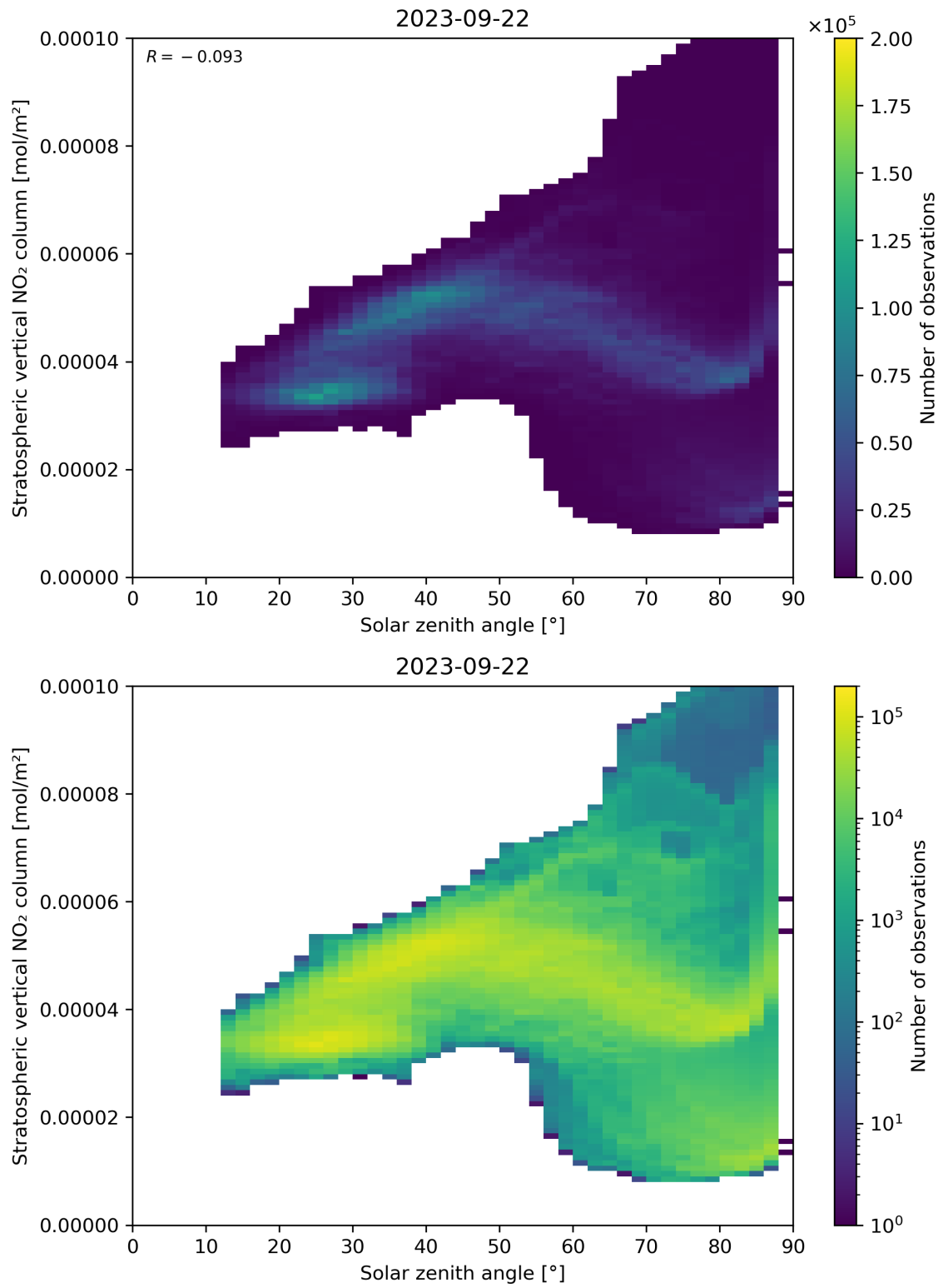
Figure 150: Scatter density plot of “Solar zenith angle” against “Stratospheric vertical NO 2 column” for 2023-09-21 to 2023-09-23.
