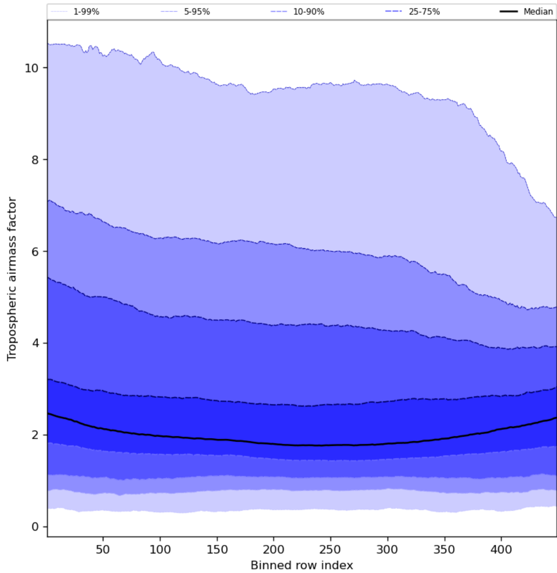
Figure 48: Along track statistics of “Tropospheric airmass factor” for 2023-09-21 to 2023-09-23
