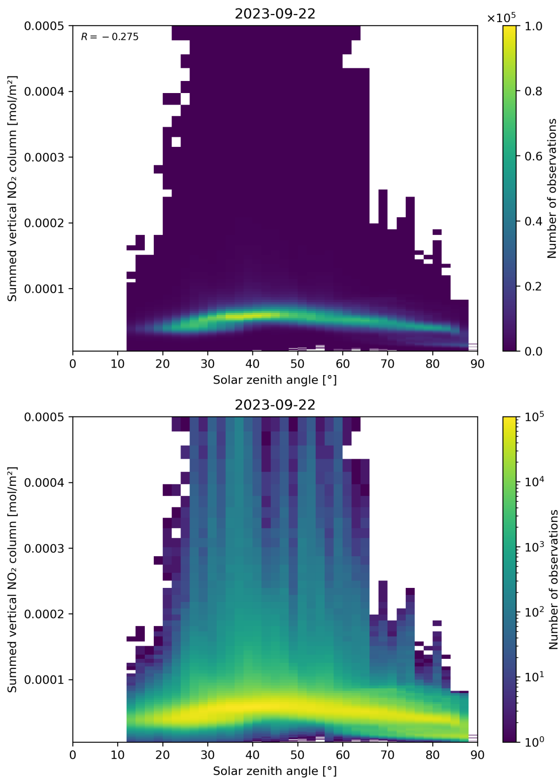
Figure 151: Scatter density plot of “Solar zenith angle” against “Summed vertical NO 2 column” for 2023-09-21 to 2023-09-23.
