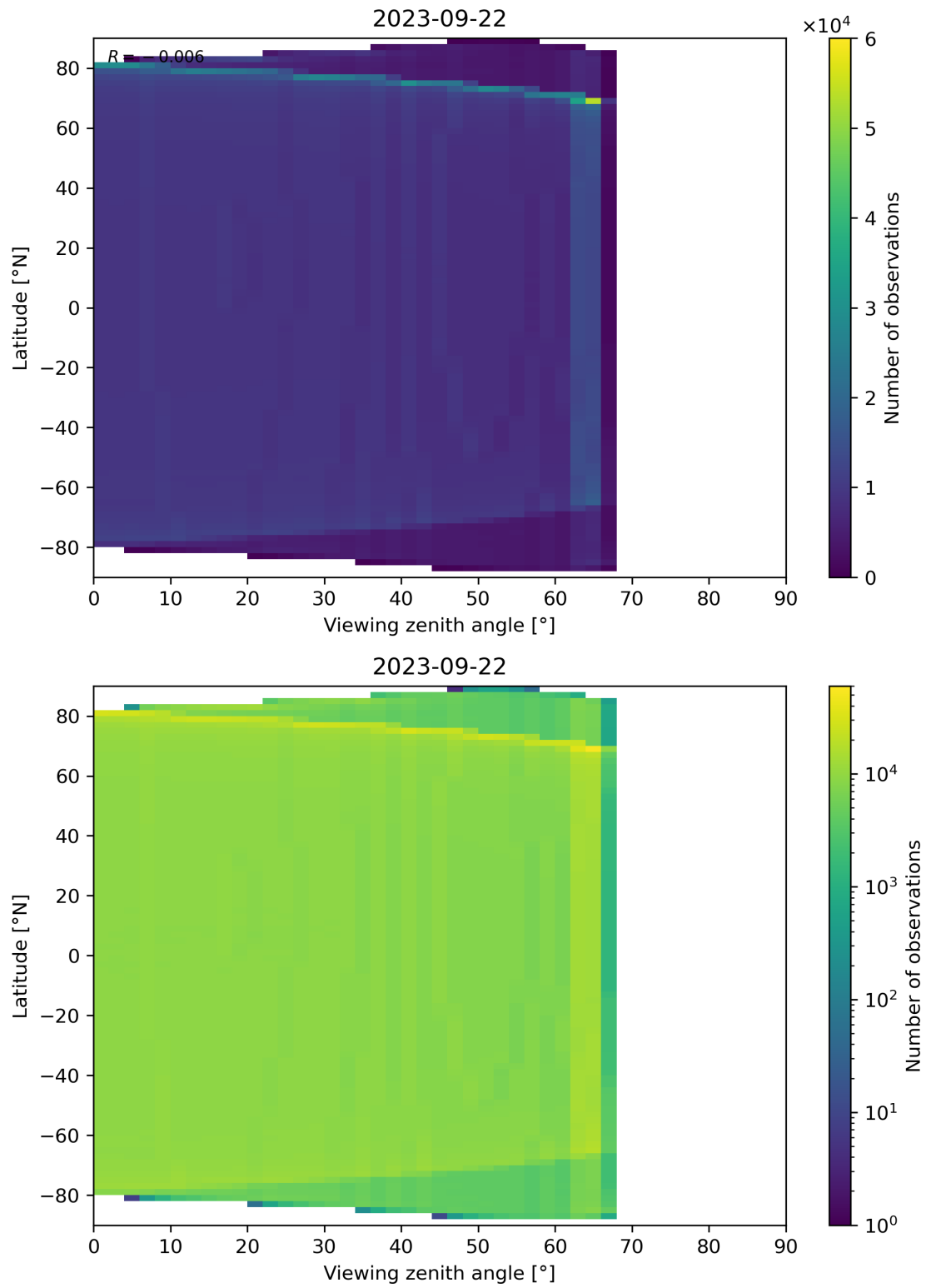
Figure 163: Scatter density plot of “Viewing zenith angle” against “Latitude” for 2023-09-21 to 2023-09-23.
