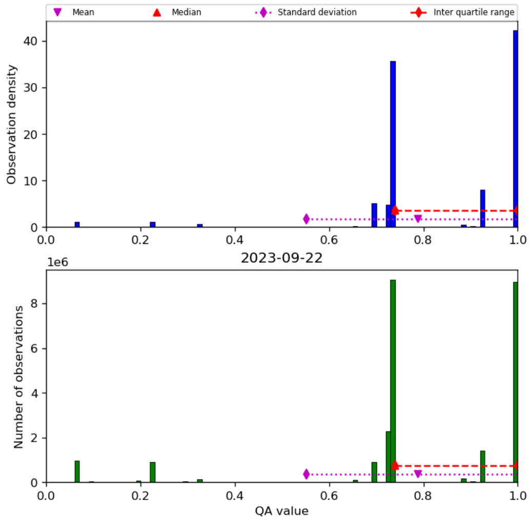
Figure 28: Histogram of “QA value” for 2023-09-21 to 2023-09-23
