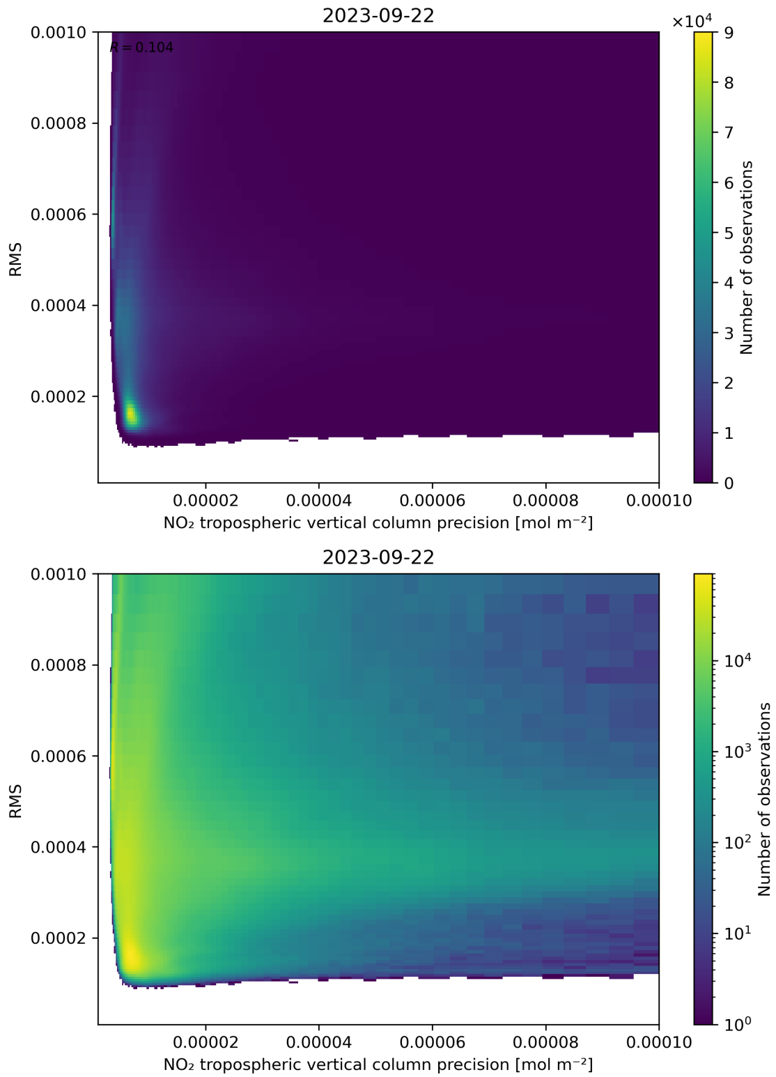
Figure 140: Scatter density plot of “NO 2 tropospheric vertical column precision” against “RMS” for 2023-09-21 to 2023-09-23.
