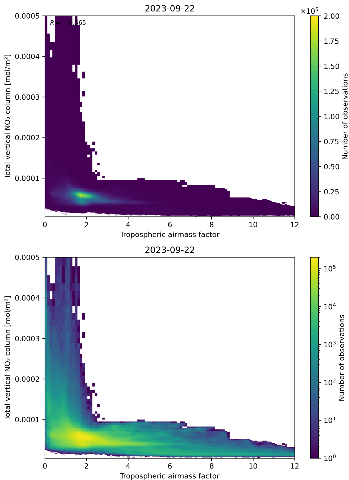
Figure 77: Scatter density plot of “Tropospheric airmass factor” against “Total vertical \text{NO}_2 column” for 2023-09-21 to 2023-09-23.
