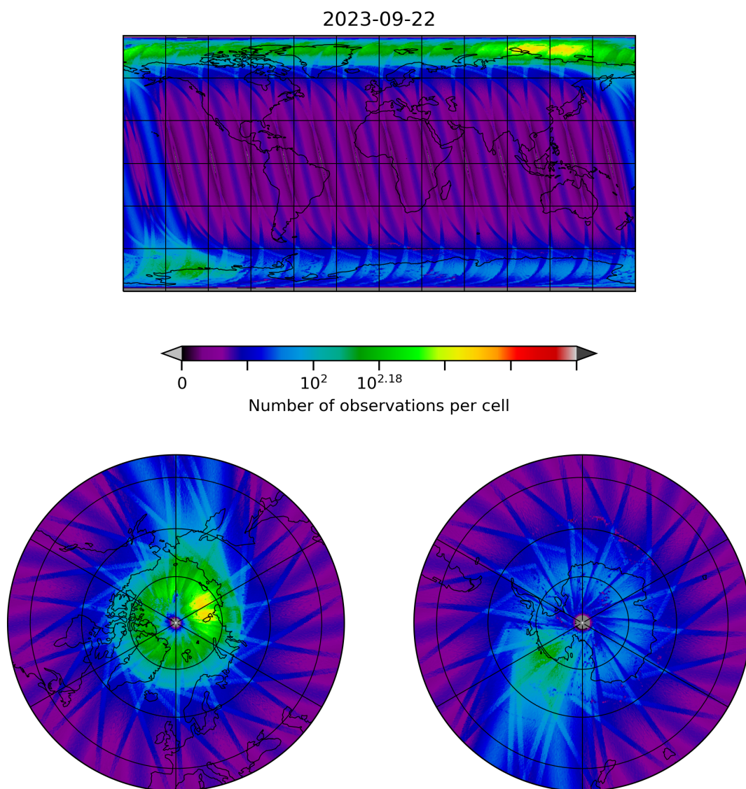
Figure 10: Map of the number of observations for 2023-09-21 to 2023-09-23
