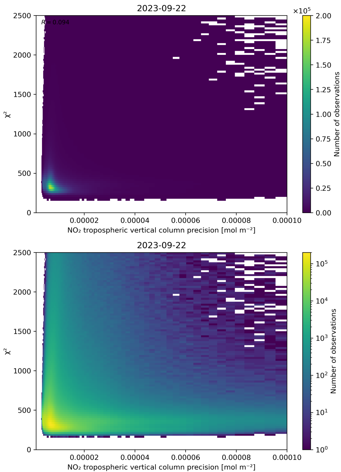
Figure 134: Scatter density plot of “NO 2 tropospheric vertical column precision” against “ \chi^2 ” for 2023-09-21 to 2023-09-23.
