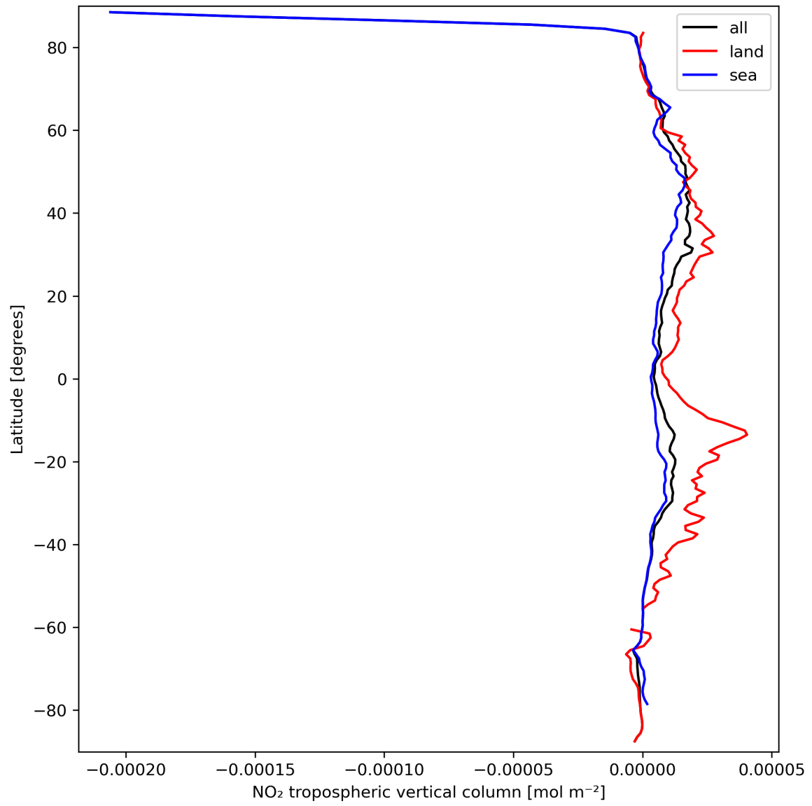
Figure 12: Zonal average of “NO 2 tropospheric vertical column” for 2023-09-21 to 2023-09-23.
