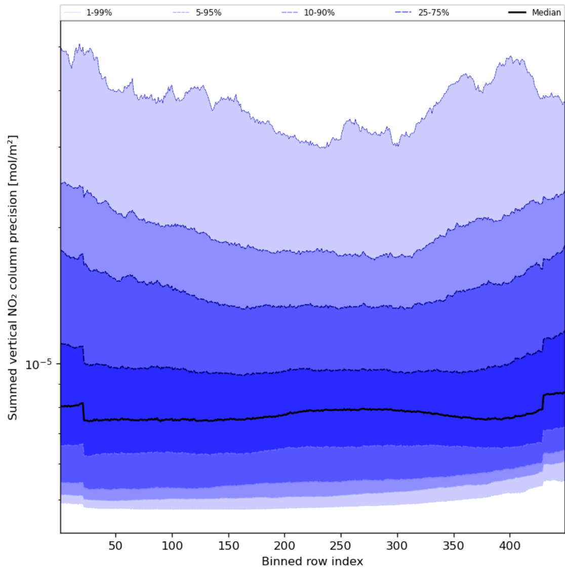
Figure 58: Along track statistics of “Summed vertical NO 2 column precision” for 2023-09-21 to 2023-09-23
