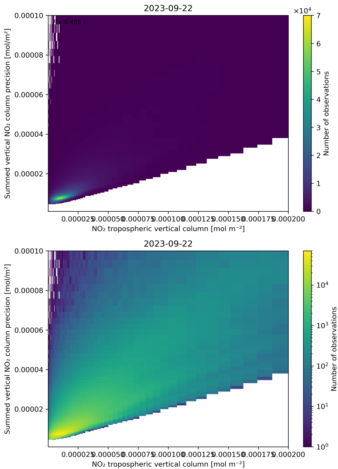
Figure 127: Scatter density plot of “NO 2 tropospheric vertical column” against “Summed vertical NO 2 column precision” for 2023-09-21 to 2023-09-23.
