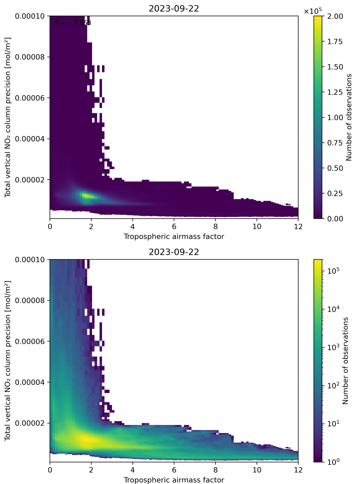
Figure 78: Scatter density plot of “Tropospheric air mass factor” against “Total vertical NO 2 column precision” for 2023-09-21 to 2023-09-23.
