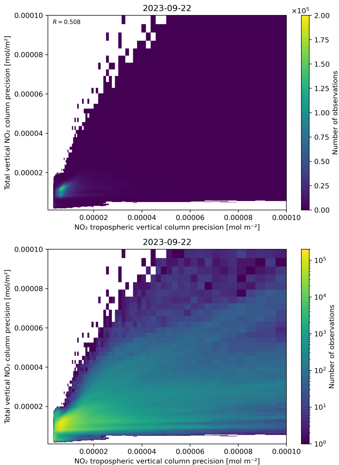
Figure 139: Scatter density plot of “NO 2 tropospheric vertical column precision” against “Total vertical NO 2 column precision” for 2023-09-21 to 2023-09-23.
