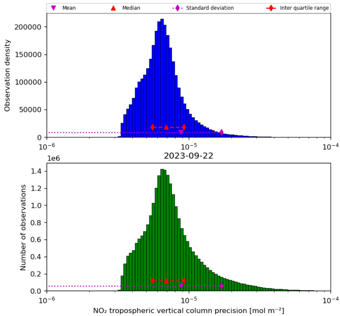
Figure 30: Histogram of “NO 2 tropospheric vertical column precision” for 2023-09-21 to 2023-09-23
