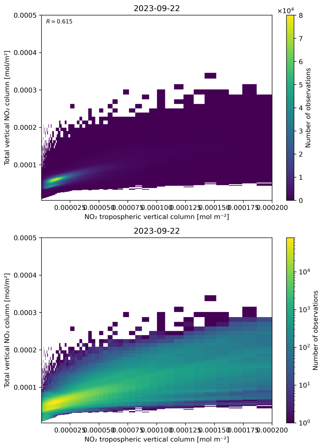
Figure 128: Scatter density plot of “NO 2 tropospheric vertical column” against “Total vertical NO 2 column” for 2023-09-21 to 2023-09-23.
