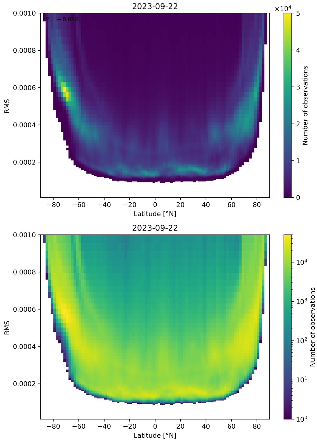
Figure 94: Scatter density plot of “Latitude” against “RMS” for 2023-09-21 to 2023-09-23.
