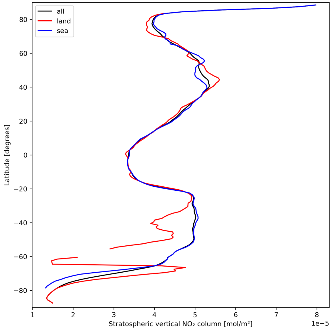
Figure 19: Zonal average of “Stratospheric vertical NO 2 column” for 2023-09-21 to 2023-09-23.
