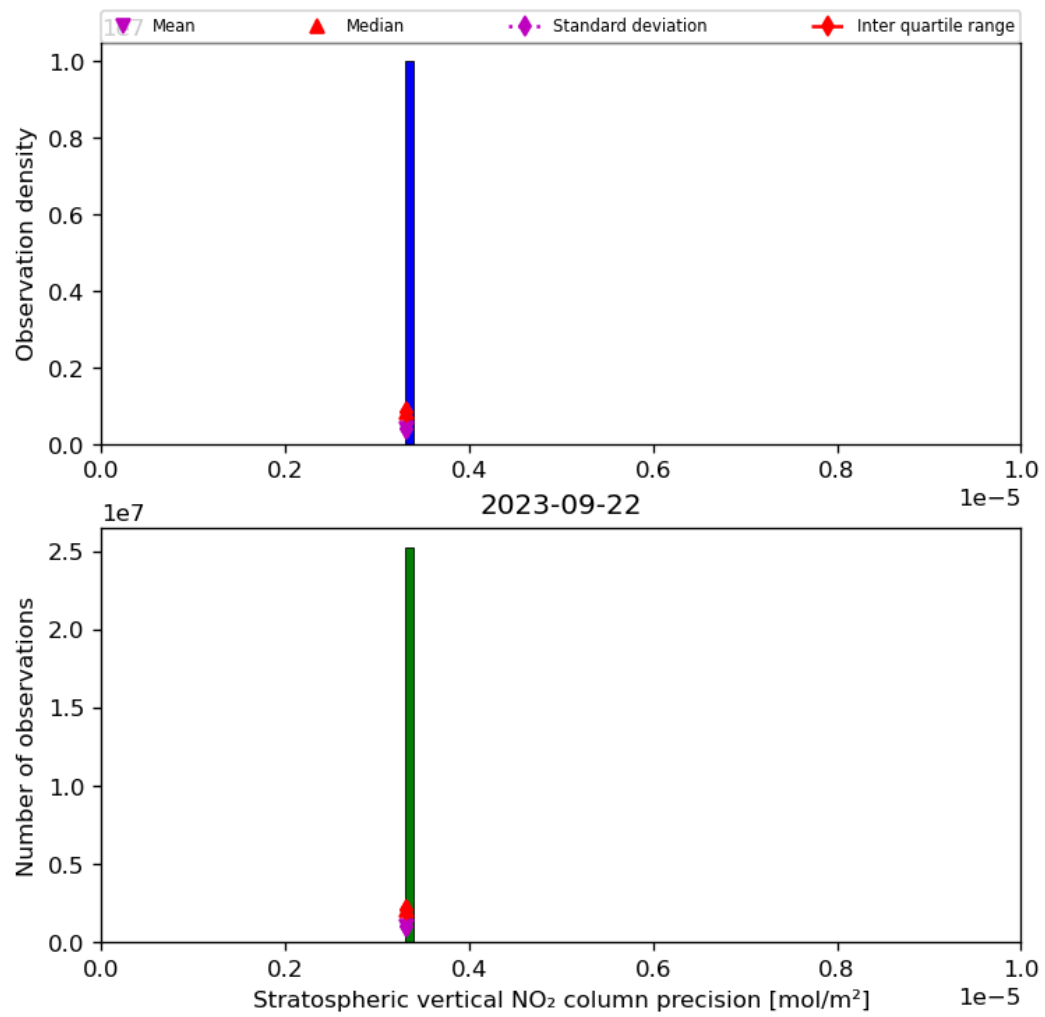
Figure 37: Histogram of “Stratospheric vertical NO 2 column precision” for 2023-09-21 to 2023-09-23
