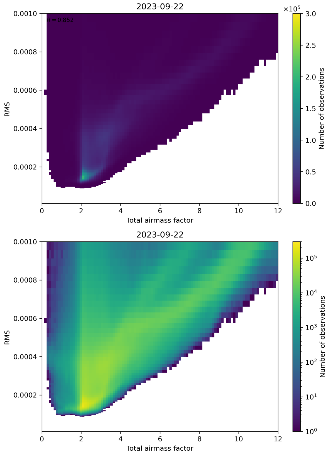
Figure 69: Scatter density plot of “Total airmass factor” against “RMS” for 2023-09-21 to 2023-09-23.
