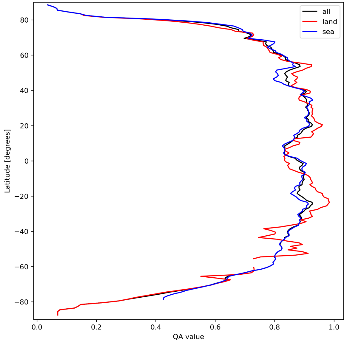
Figure 11: Zonal average of “QA value” for 2023-09-21 to 2023-09-23.
