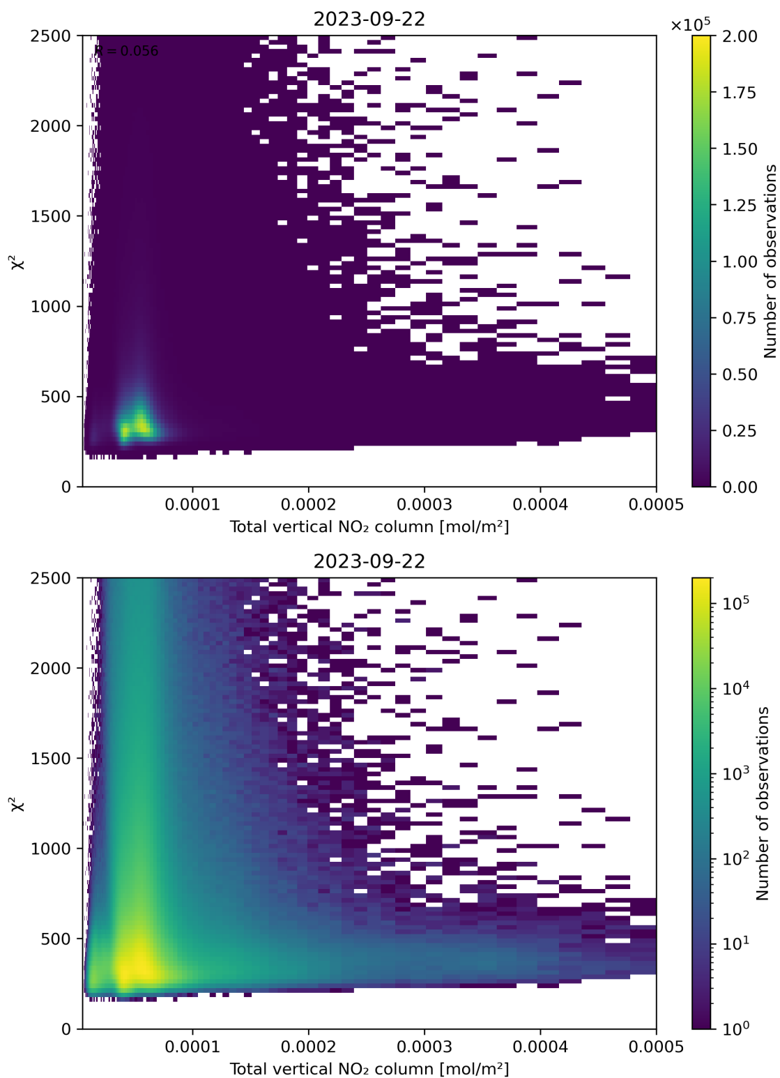
Figure 111: Scatter density plot of “Total vertical NO 2 column” against “ \chi^2 ” for 2023-09-21 to 2023-09-23.
