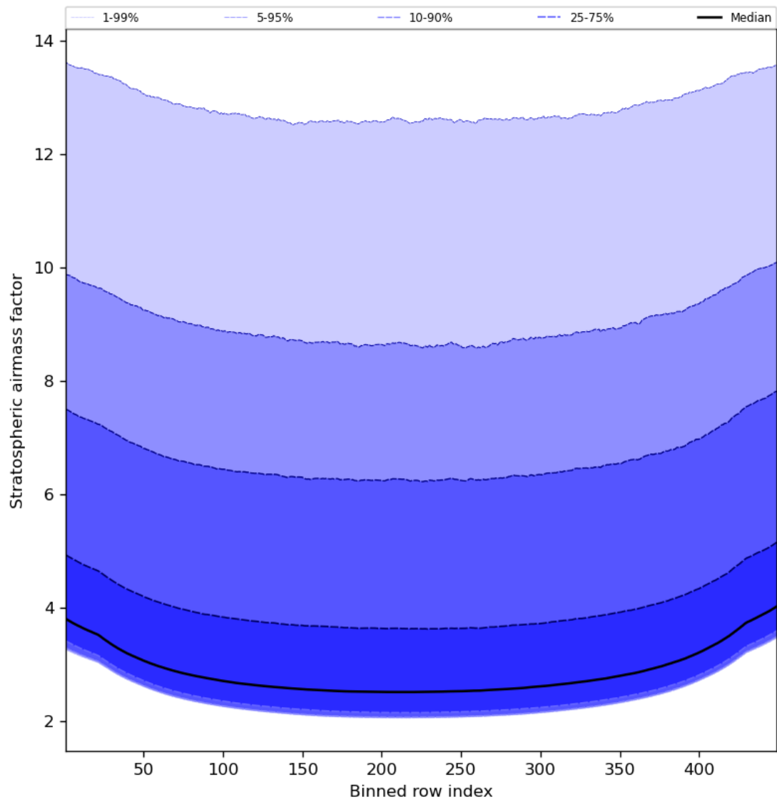
Figure 61: Along track statistics of “Stratospheric airmass factor” for 2023-09-21 to 2023-09-23
