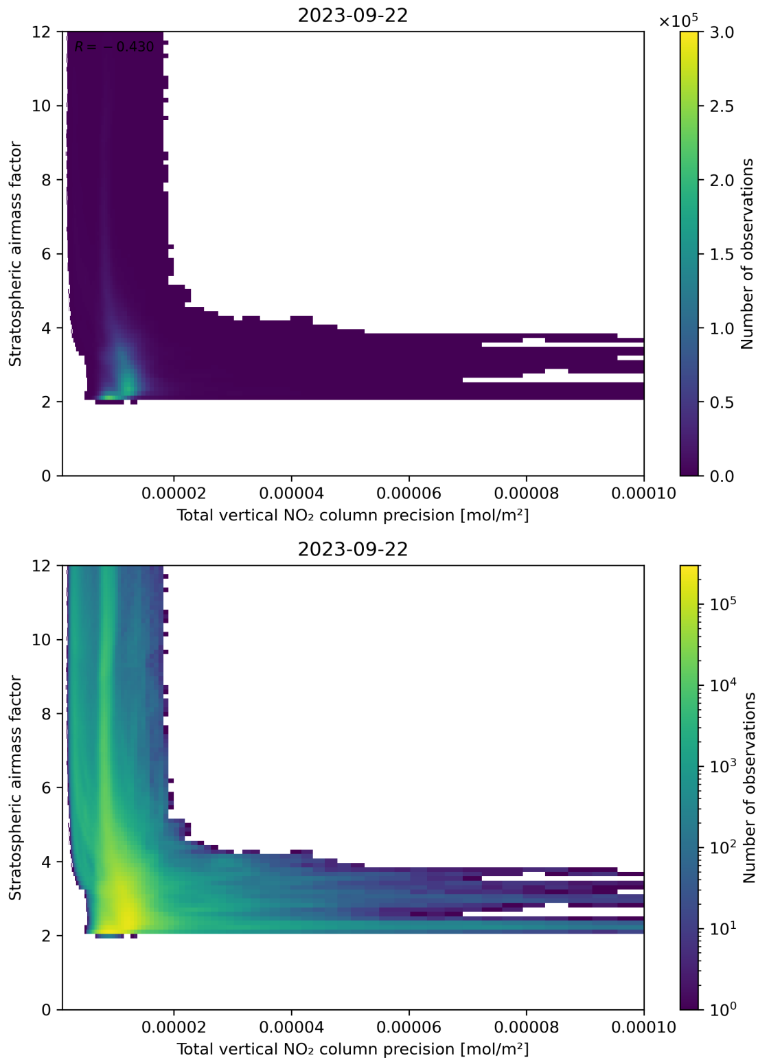
Figure 115: Scatter density plot of “Total vertical NO 2 column precision” against “Stratospheric airmass factor” for 2023-09-21 to 2023-09-23.
