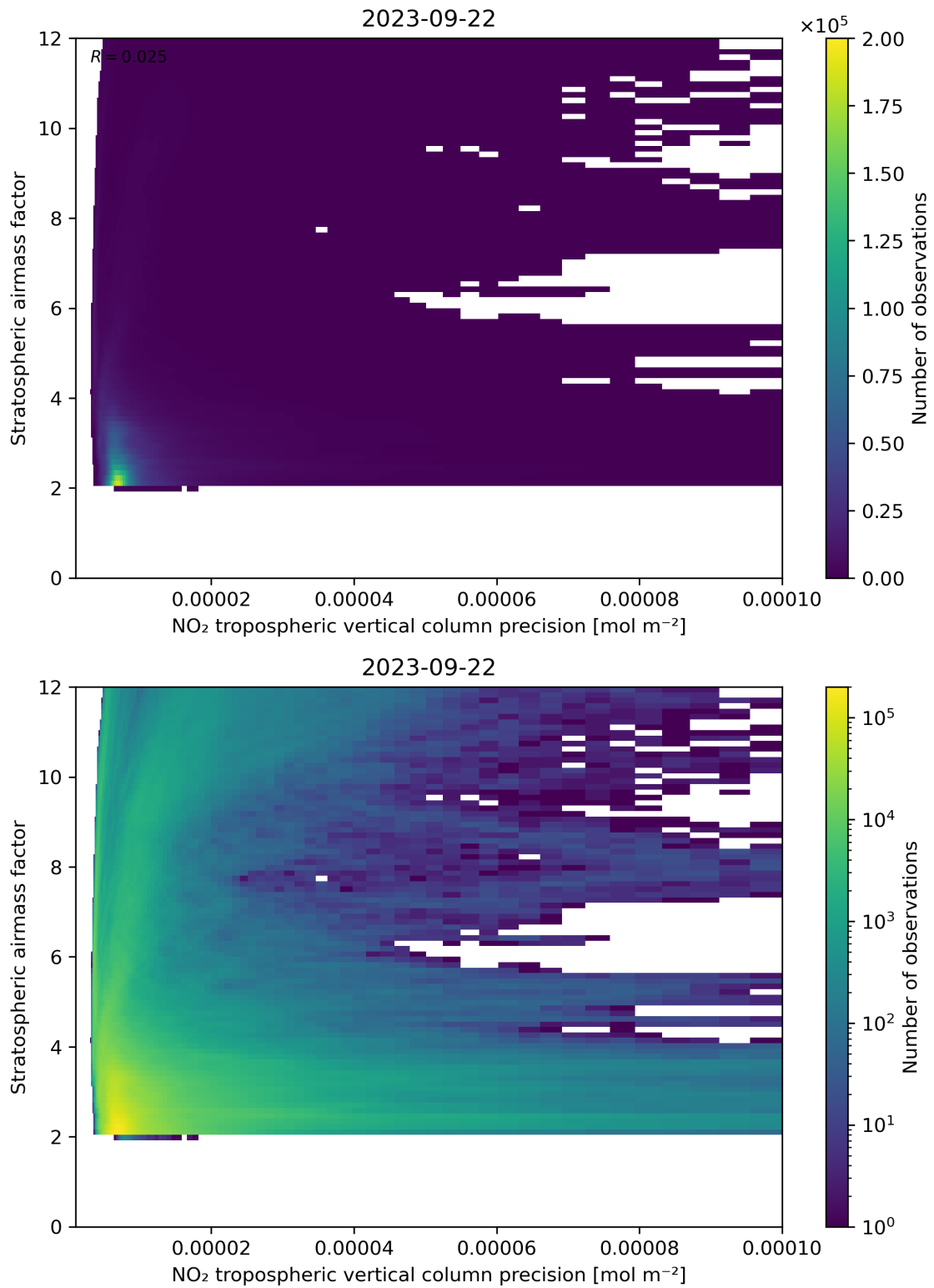
Figure 131: Scatter density plot of “NO 2 tropospheric vertical column precision” against “Stratospheric airmass factor” for 2023-09-21 to 2023-09-23.
