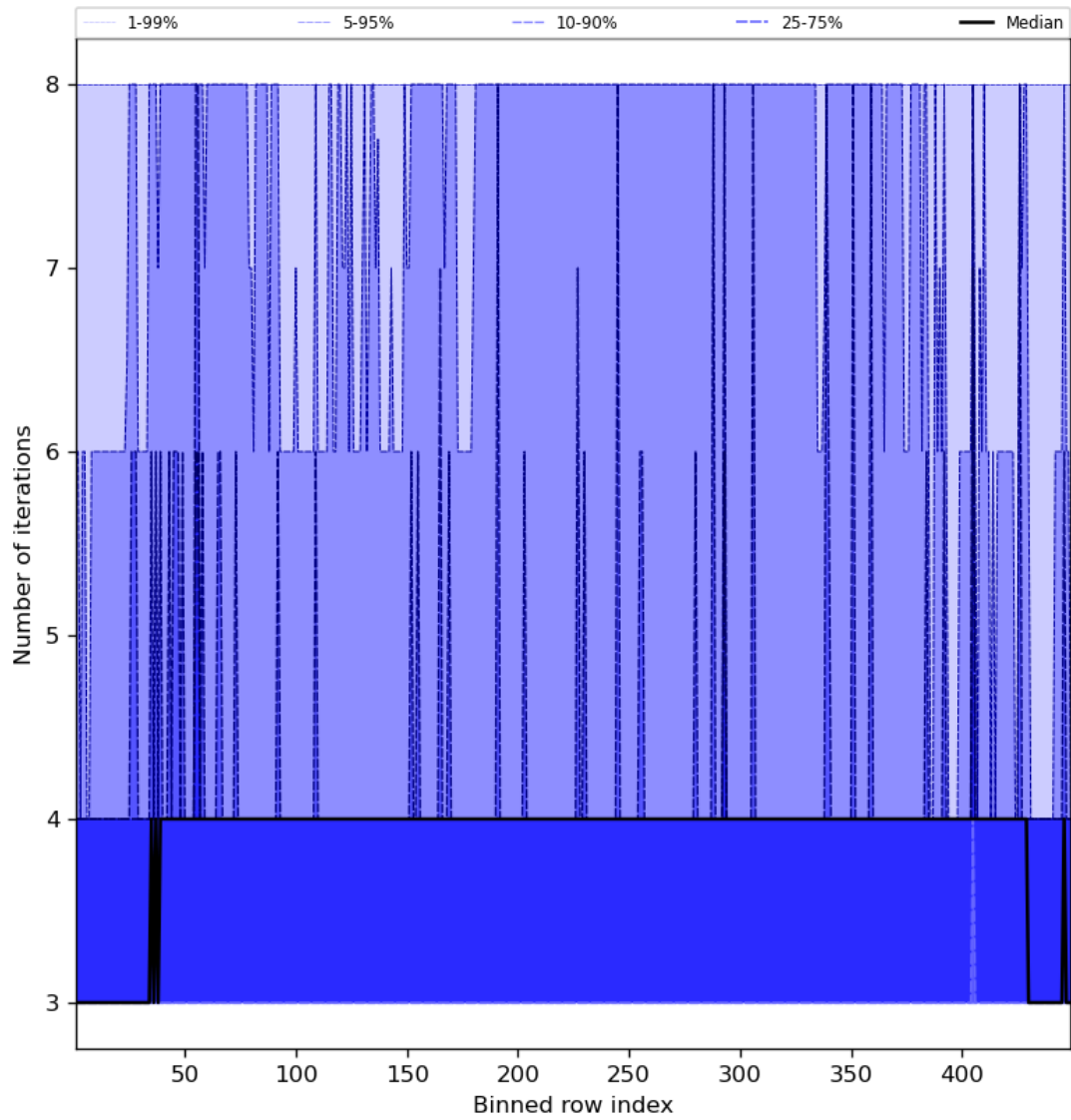
Figure 51: Along track statistics of “Number of iterations” for 2023-09-21 to 2023-09-23
