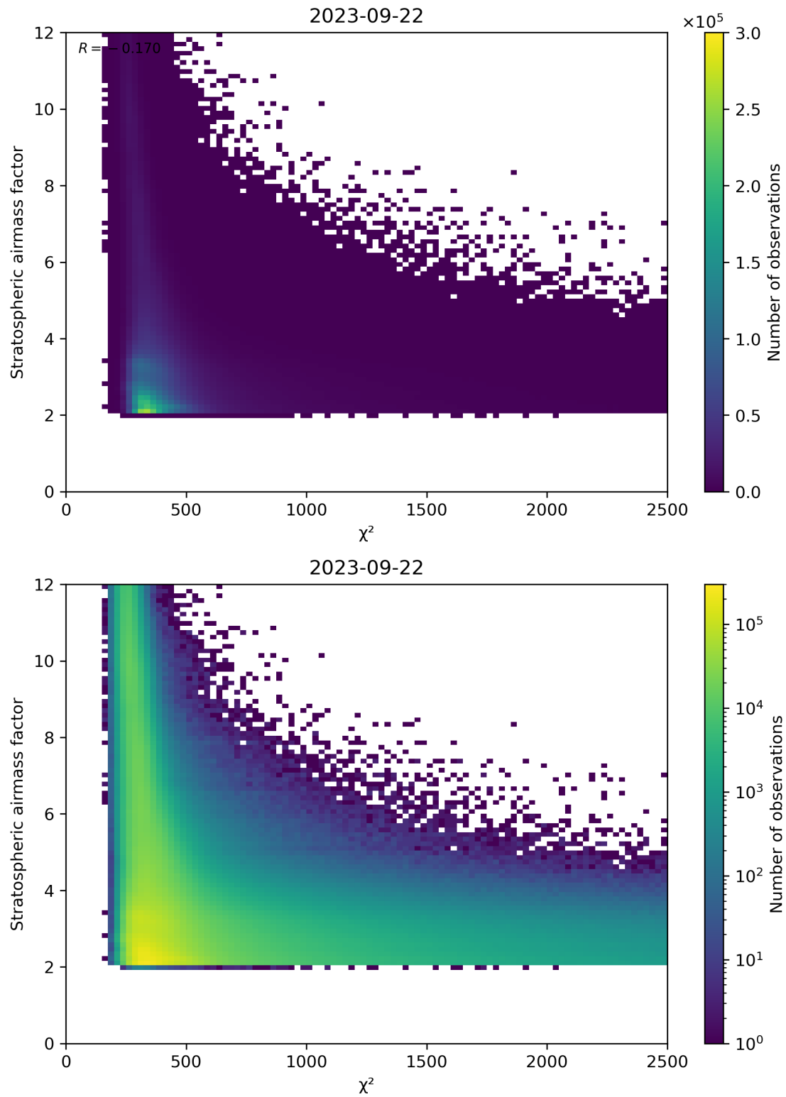
Figure 81: Scatter density plot of “ \chi^2 ” against “Stratospheric airmass factor” for 2023-09-21 to 2023-09-23.
