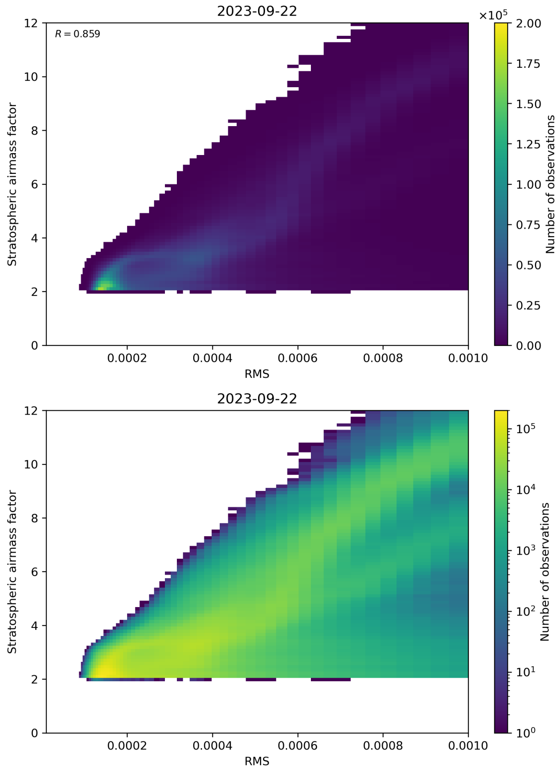
Figure 144: Scatter density plot of “RMS” against “Stratospheric airmass factor” for 2023-09-21 to 2023-09-23.
