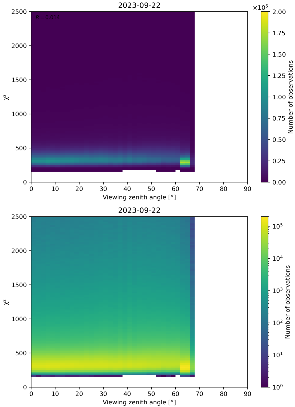
Figure 162: Scatter density plot of “Viewing zenith angle” against “ \chi^2 ” for 2023-09-21 to 2023-09-23.
