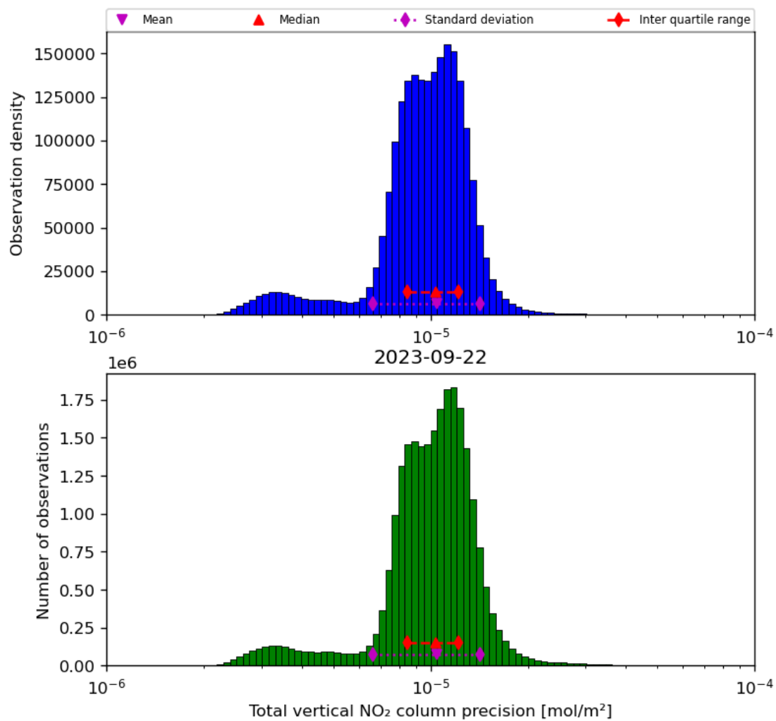
Figure 39: Histogram of “Total vertical NO 2 column precision” for 2023-09-21 to 2023-09-23
