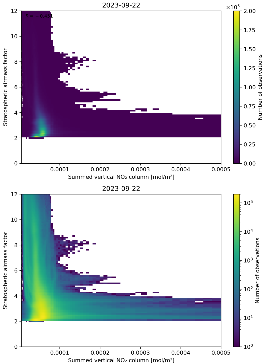
Figure 103: Scatter density plot of “Summed vertical NO 2 column” against “Stratospheric air mass factor” for 2023-09-21 to 2023-09-23.
