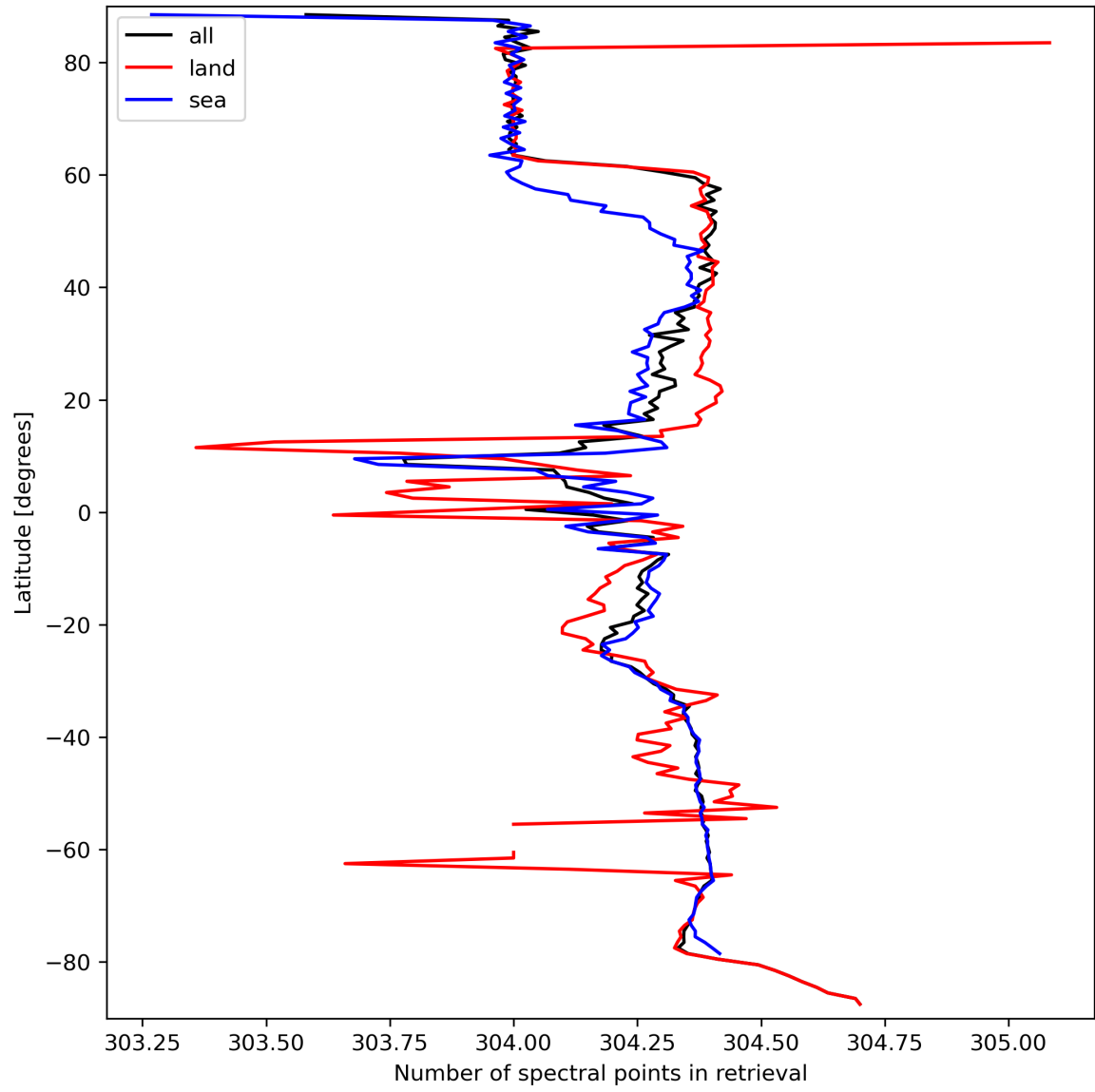
Figure 16: Zonal average of “Number of spectral points in retrieval” for 2023-09-21 to 2023-09-23.
