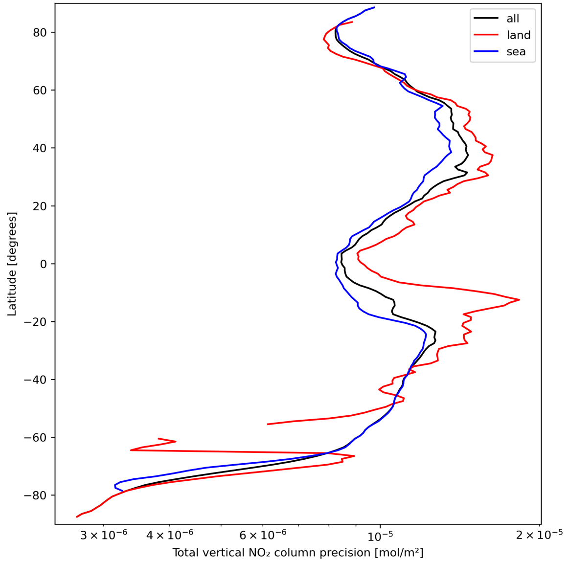
Figure 22: Zonal average of “Total vertical NO 2 column precision” for 2023-09-21 to 2023-09-23.
