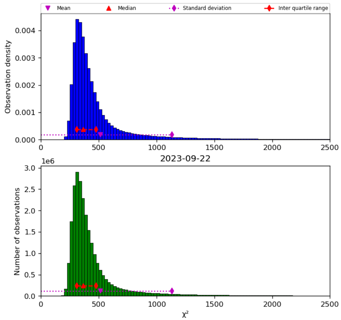
Figure 42: Histogram of “ \chi^2 ” for 2023-09-21 to 2023-09-23
