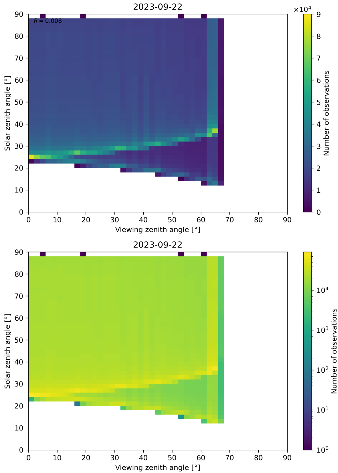
Figure 172: Scatter density plot of “Viewing zenith angle” against “Solar zenith angle” for 2023-09-21 to 2023-09-23.
