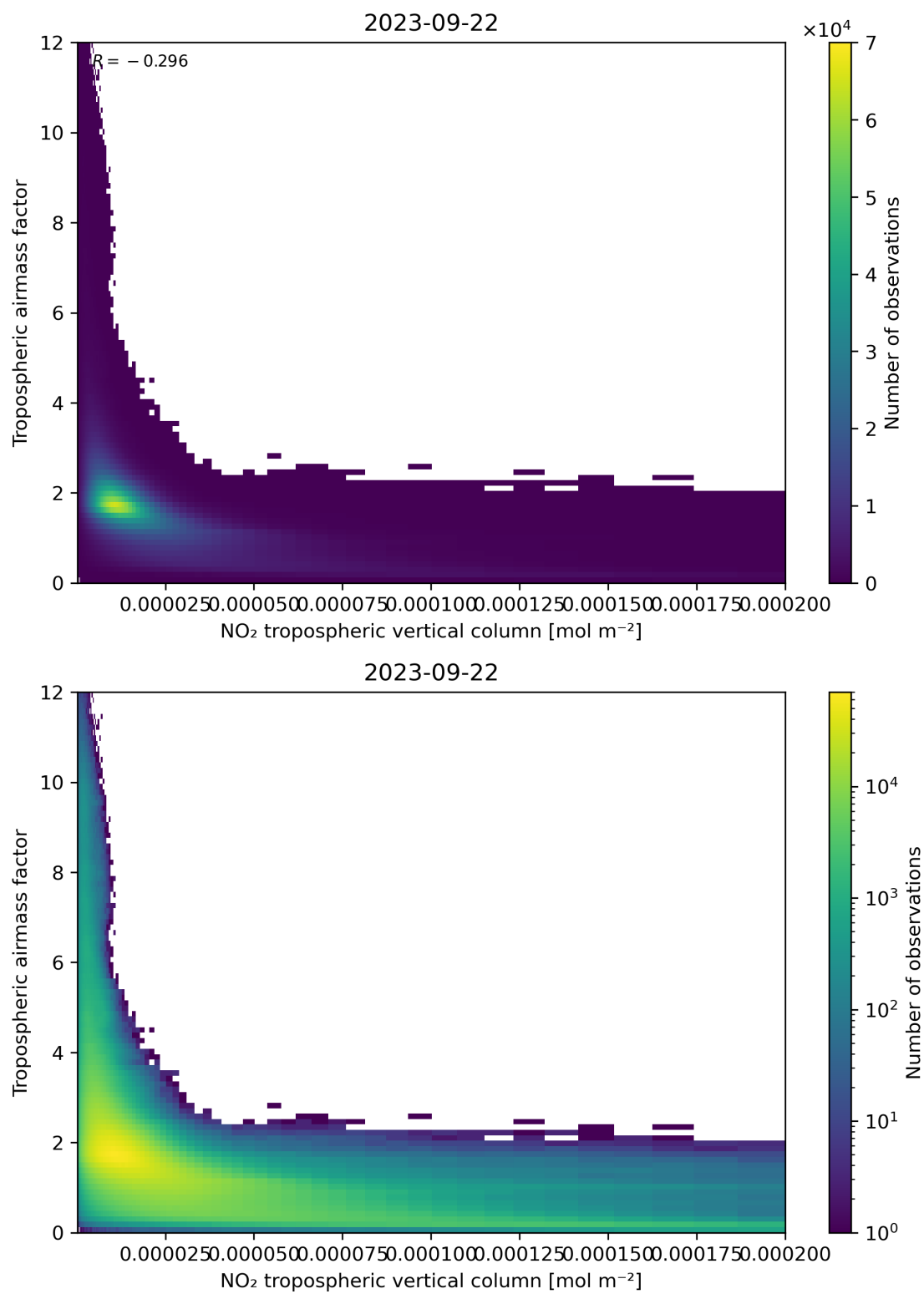
Figure 123: Scatter density plot of “NO 2 tropospheric vertical column” against “Tropospheric air mass factor” for 2023-09-21 to 2023-09-23.
