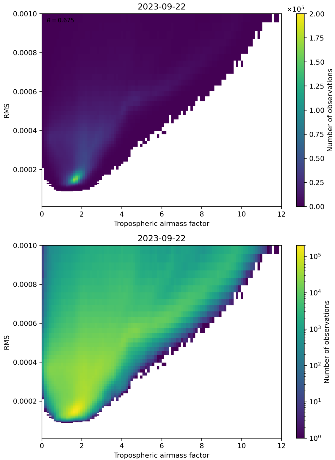
Figure 79: Scatter density plot of “Tropospheric airmass factor” against “RMS” for 2023-09-21 to 2023-09-23.
