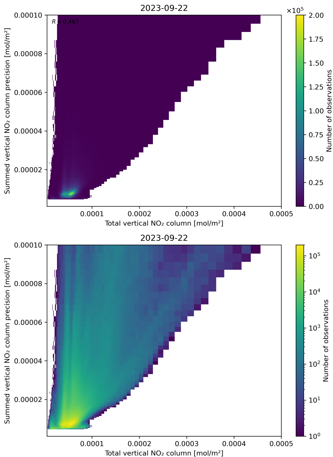
Figure 113: Scatter density plot of “Total vertical NO 2 column” against “Summed vertical NO 2 column precision” for 2023-09-21 to 2023-09-23.
