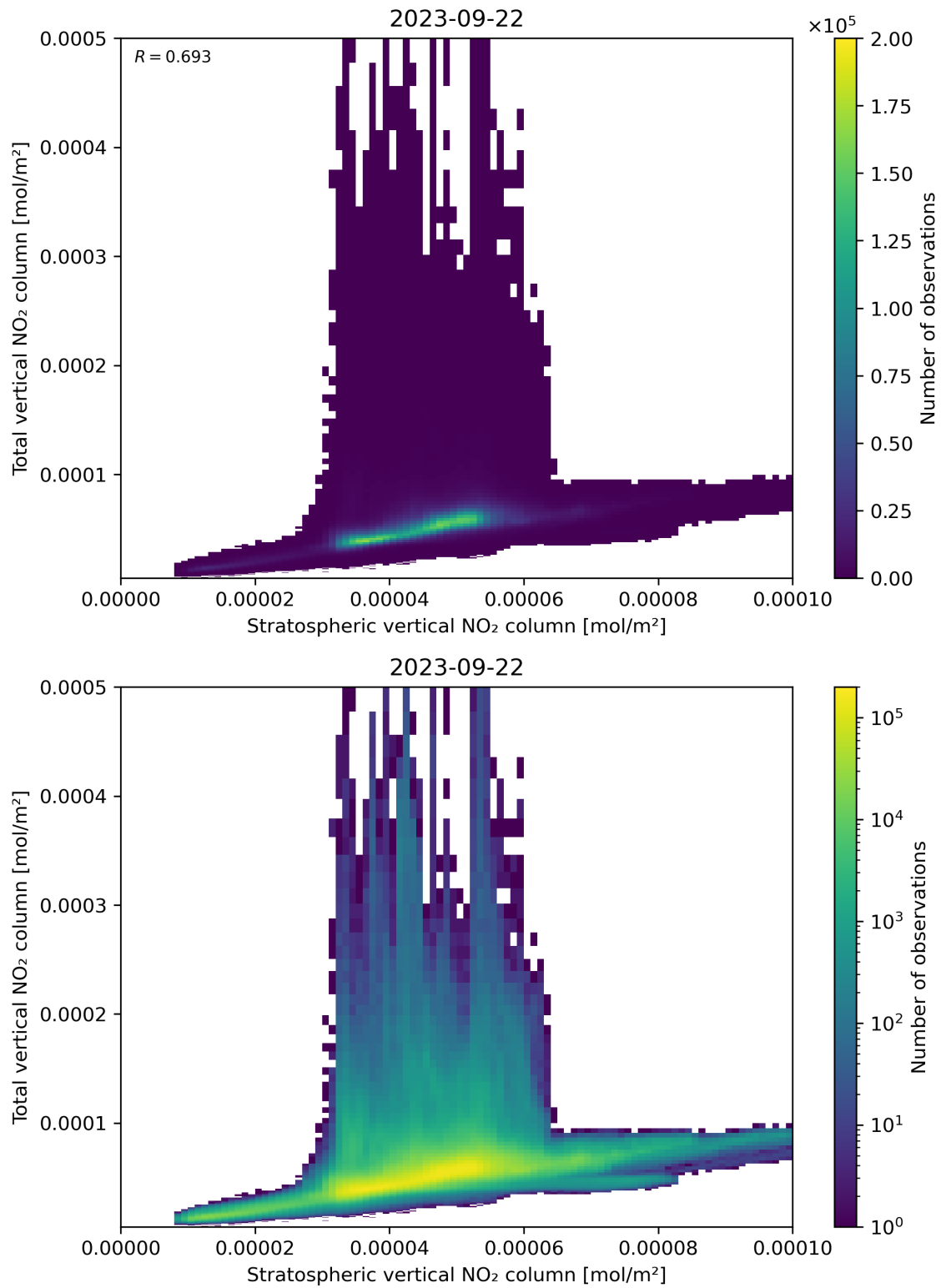
Figure 100: Scatter density plot of “Stratospheric vertical NO 2 column” against “Total vertical NO 2 column” for 2023-09-21 to 2023-09-23.
