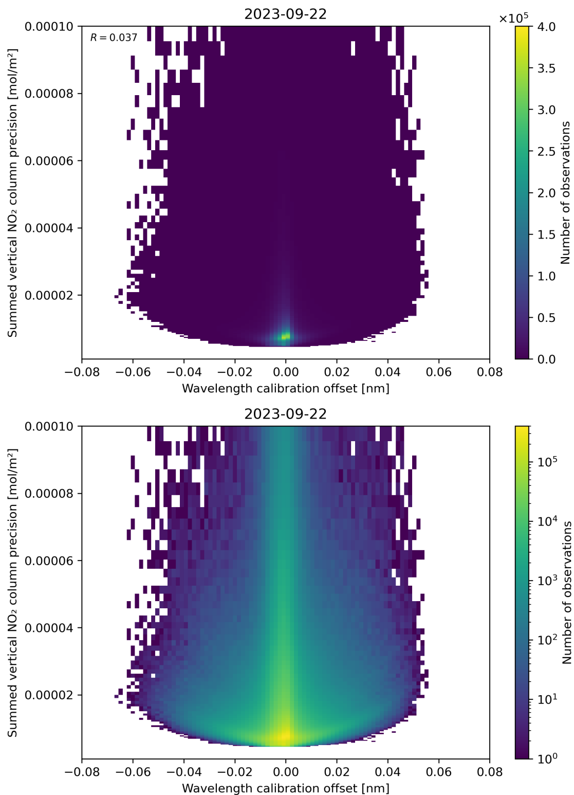
Figure 178: Scatter density plot of “Wavelength calibration offset” against “Summed vertical NO 2 column precision” for 2023-09-21 to 2023-09-23.
