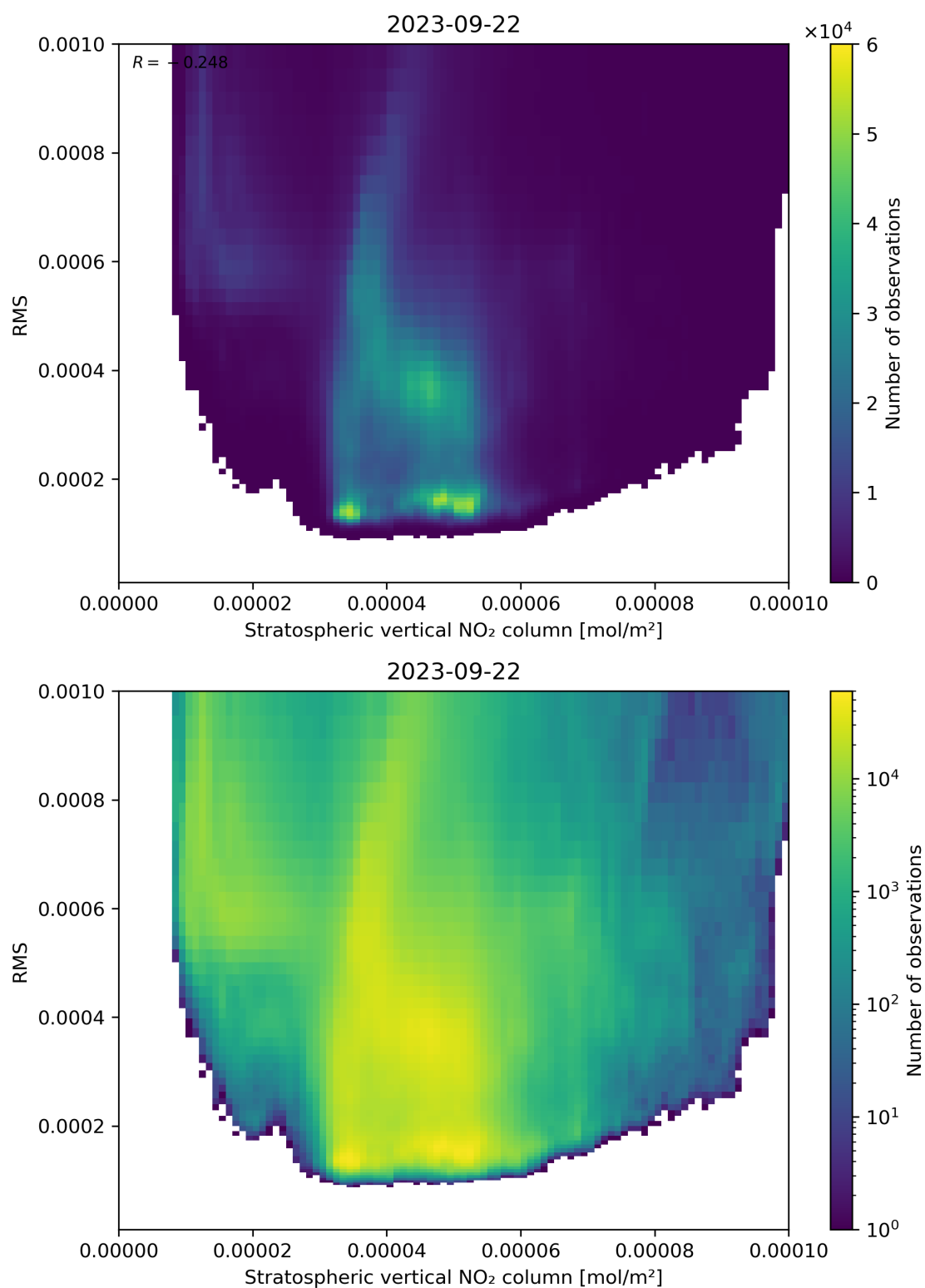
Figure 102: Scatter density plot of “Stratospheric vertical NO 2 column” against “RMS” for 2023-09-21 to 2023-09-23.
