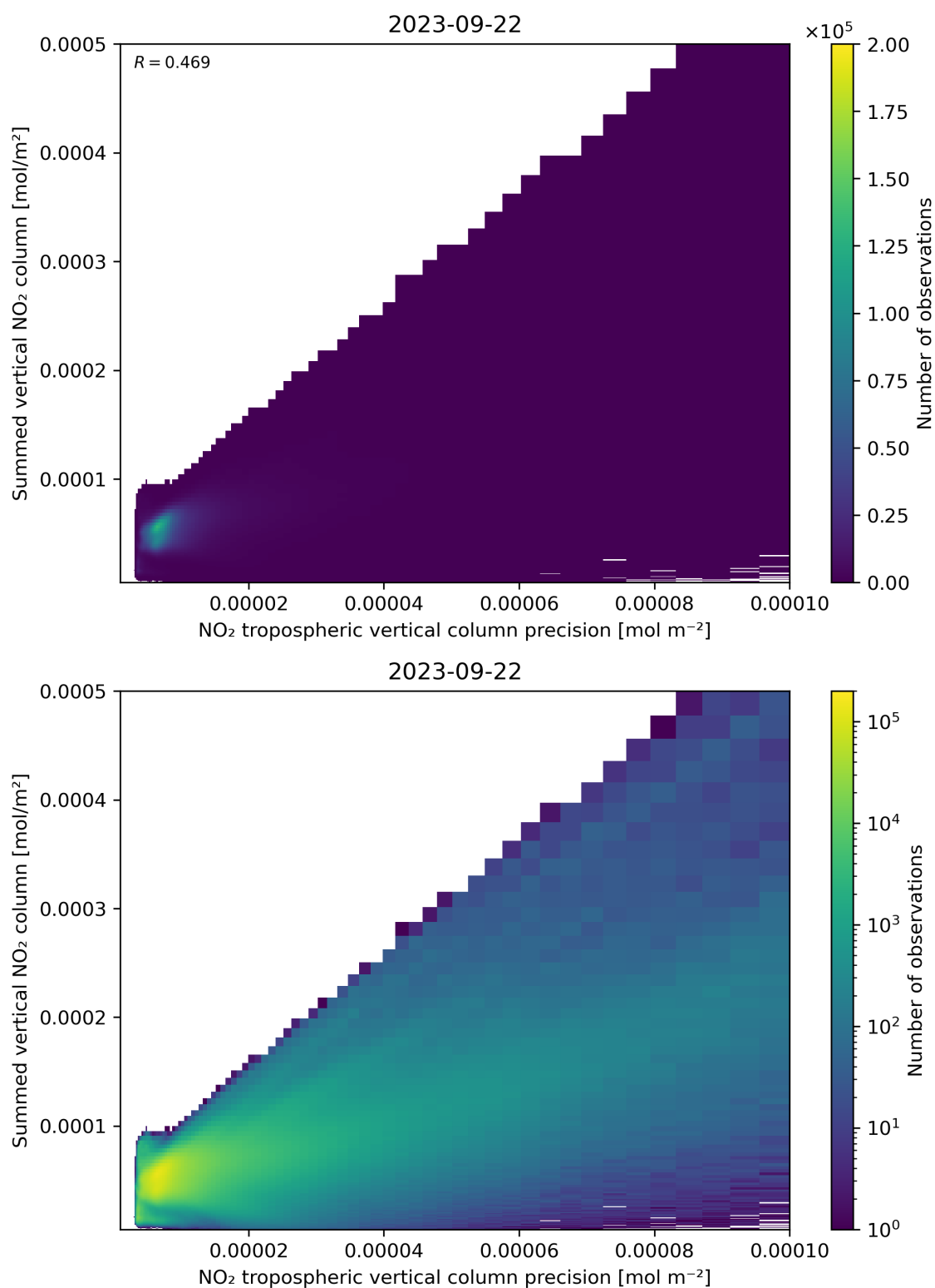
Figure 136: Scatter density plot of “NO 2 tropospheric vertical column precision” against “Summed vertical NO 2 column” for 2023-09-21 to 2023-09-23.
