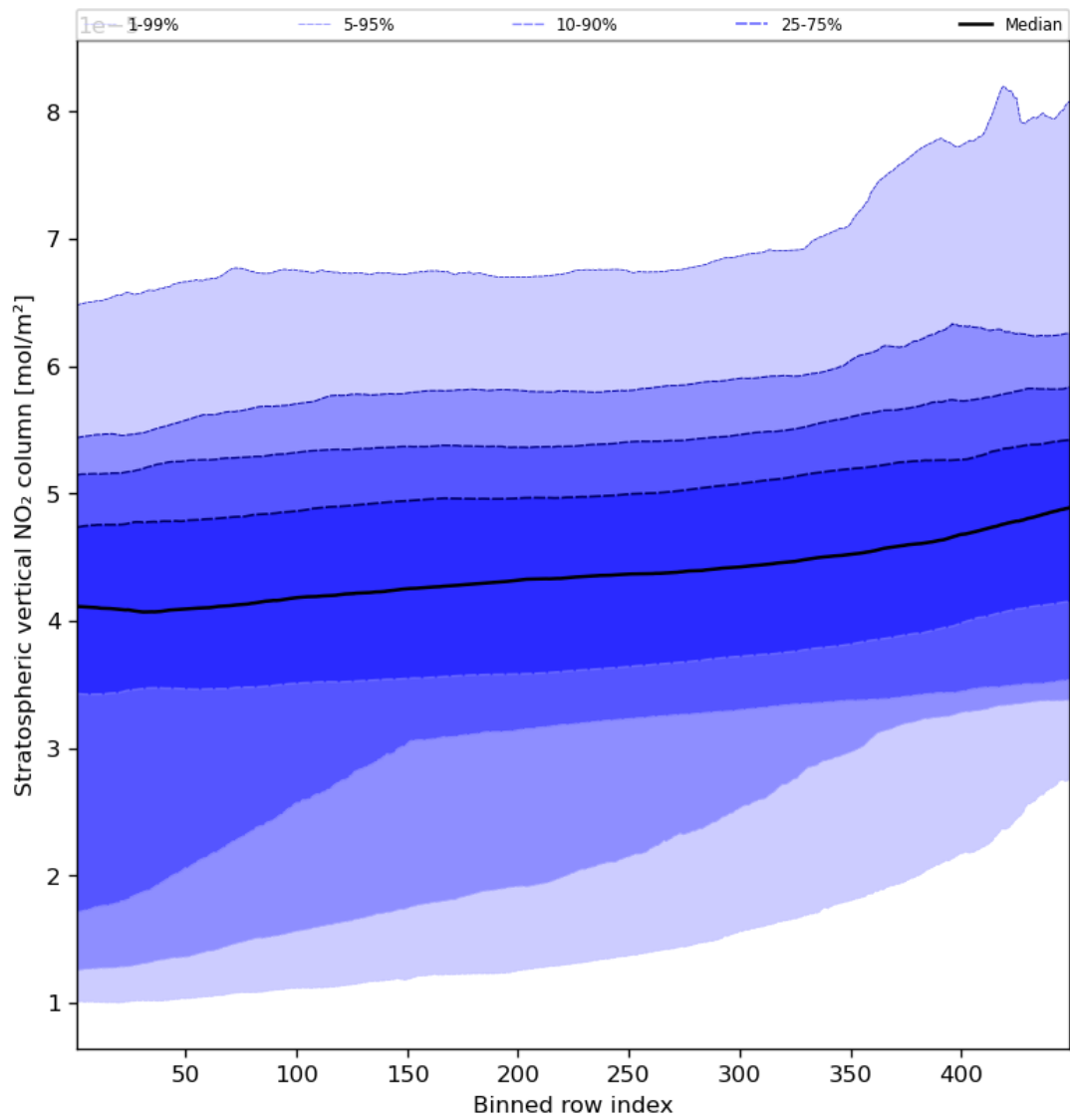
Figure 53: Along track statistics of “Stratospheric vertical NO 2 column” for 2023-09-21 to 2023-09-23
