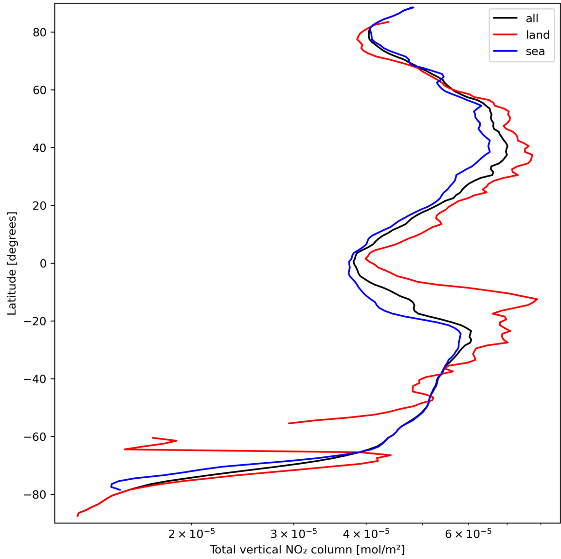
Figure 21: Zonal average of “Total vertical NO 2 column” for 2023-09-21 to 2023-09-23.
