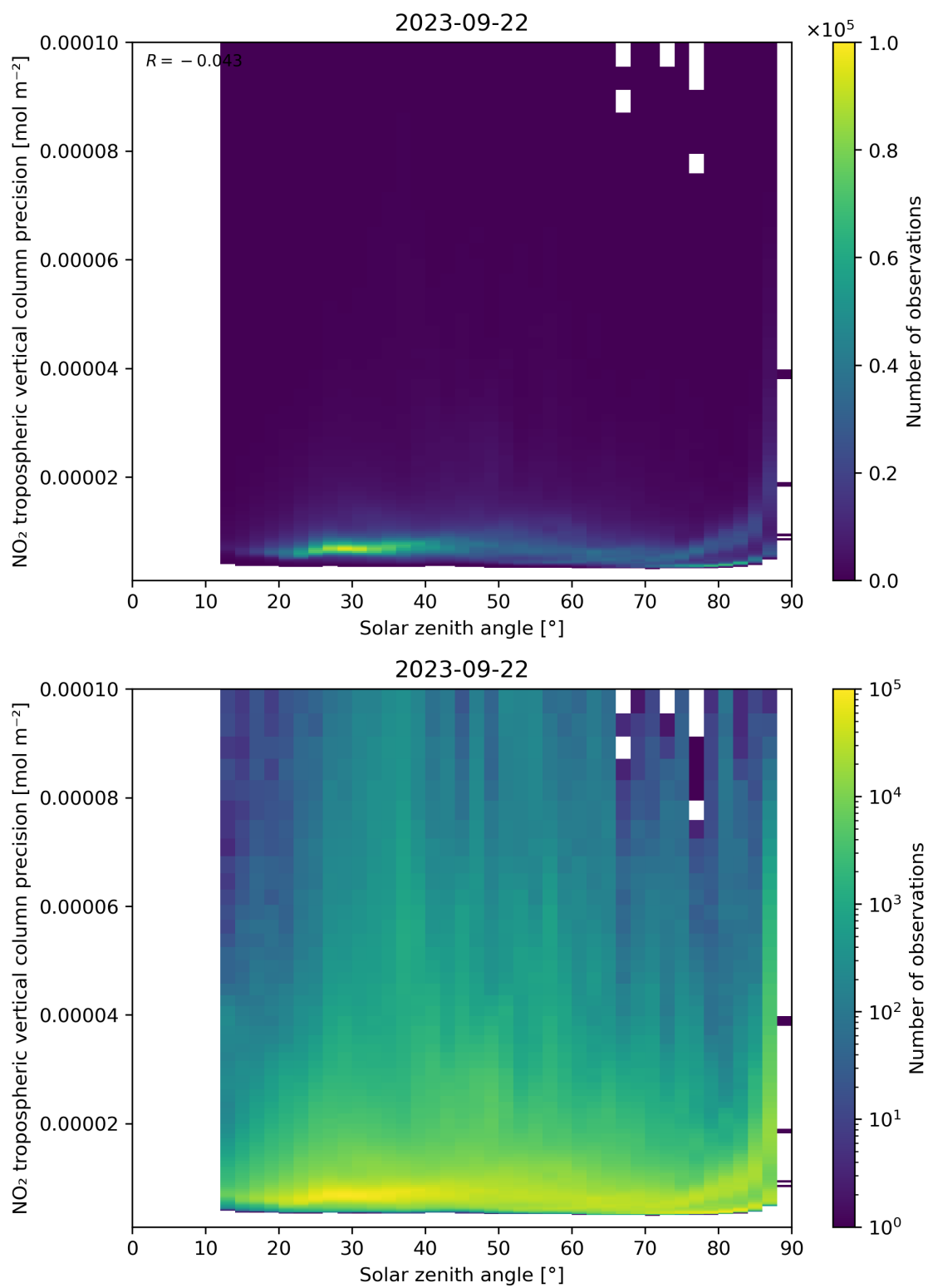
Figure 156: Scatter density plot of “Solar zenith angle” against “NO 2 tropospheric vertical column precision” for 2023-09-21 to 2023-09-23.
