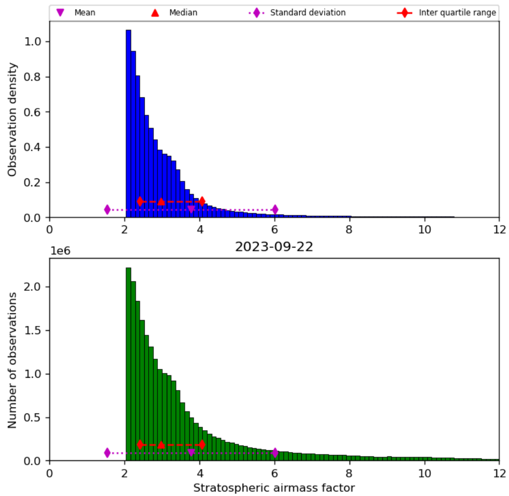
Figure 44: Histogram of “Stratospheric airmass factor” for 2023-09-21 to 2023-09-23
