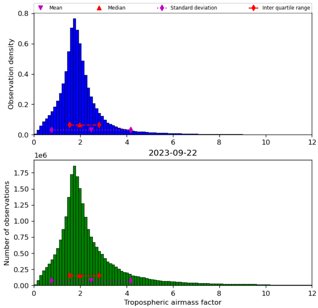
Figure 31: Histogram of “Tropospheric airmass factor” for 2023-09-21 to 2023-09-23
