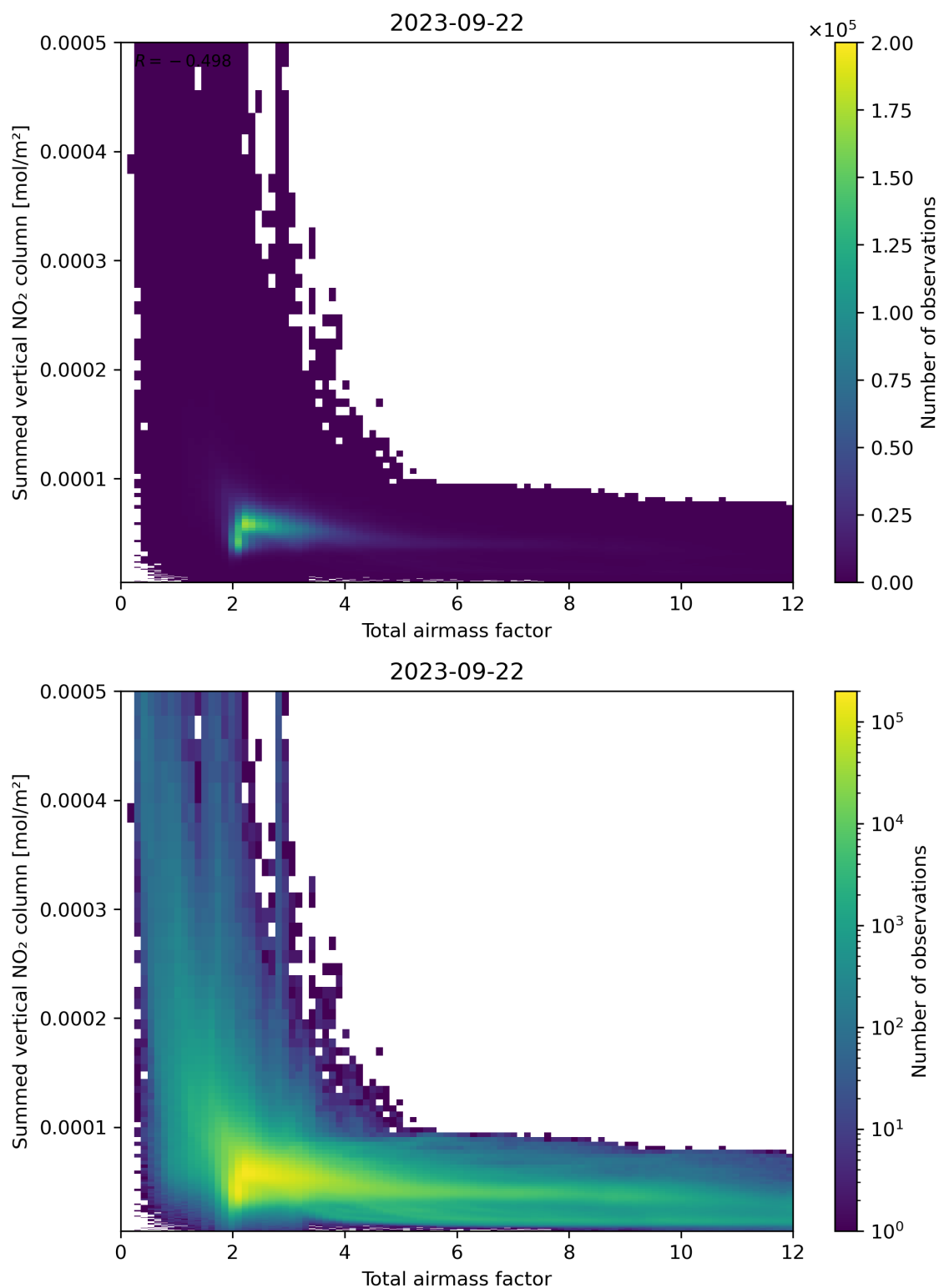
Figure 65: Scatter density plot of “Total airmass factor” against “Summed vertical NO 2 column” for 2023-09-21 to 2023-09-23.
