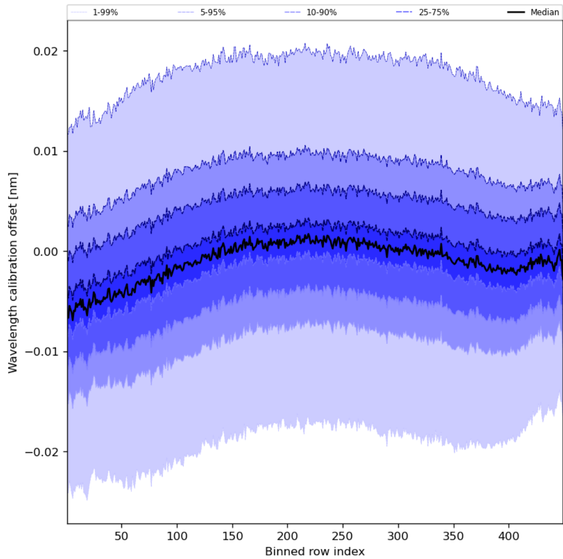
Figure 52: Along track statistics of “Wavelength calibration offset” for 2023-09-21 to 2023-09-23
