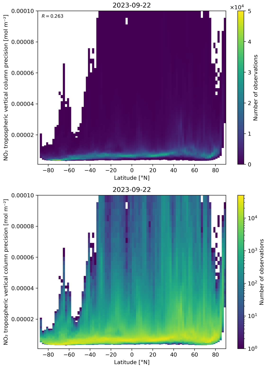
Figure 93: Scatter density plot of “Latitude” against “NO 2 tropospheric vertical column precision” for 2023-09-21 to 2023-09-23.
