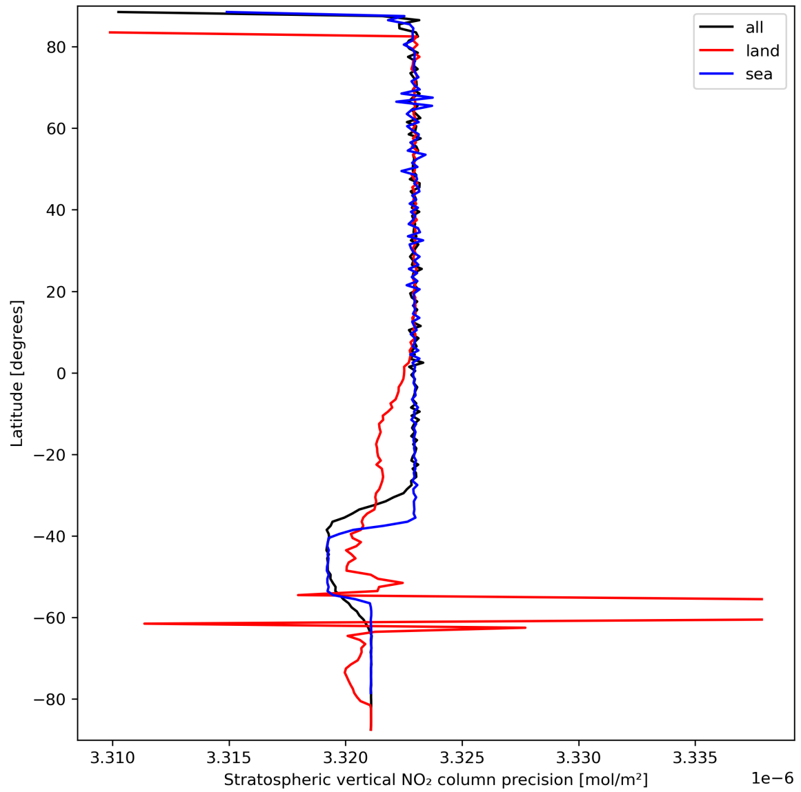
Figure 20: Zonal average of “Stratospheric vertical NO 2 column precision” for 2023-09-21 to 2023-09-23.
