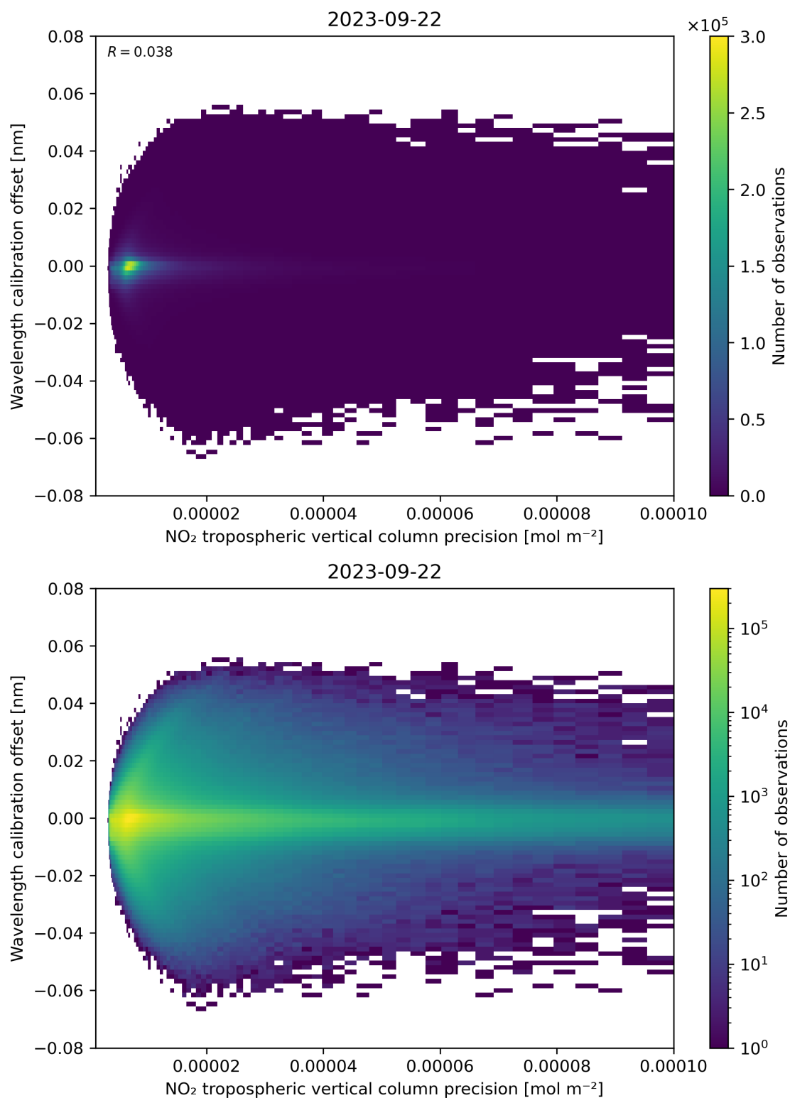
Figure 141: Scatter density plot of “NO 2 tropospheric vertical column precision” against “Wavelength calibration offset” for 2023-09-21 to 2023-09-23.
