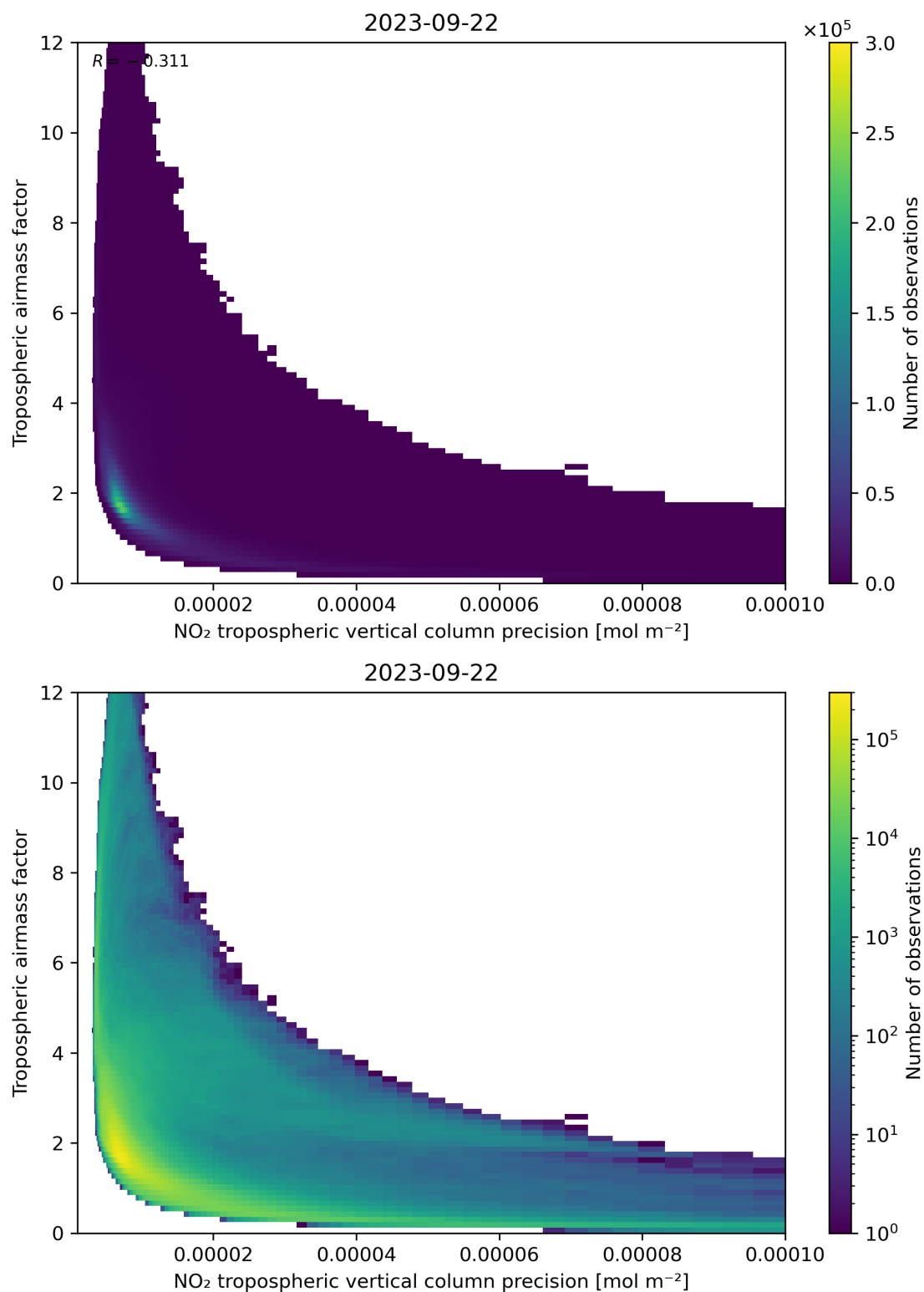
Figure 133: Scatter density plot of “NO 2 tropospheric vertical column precision” against “Tropospheric airmass factor” for 2023-09-21 to 2023-09-23.
