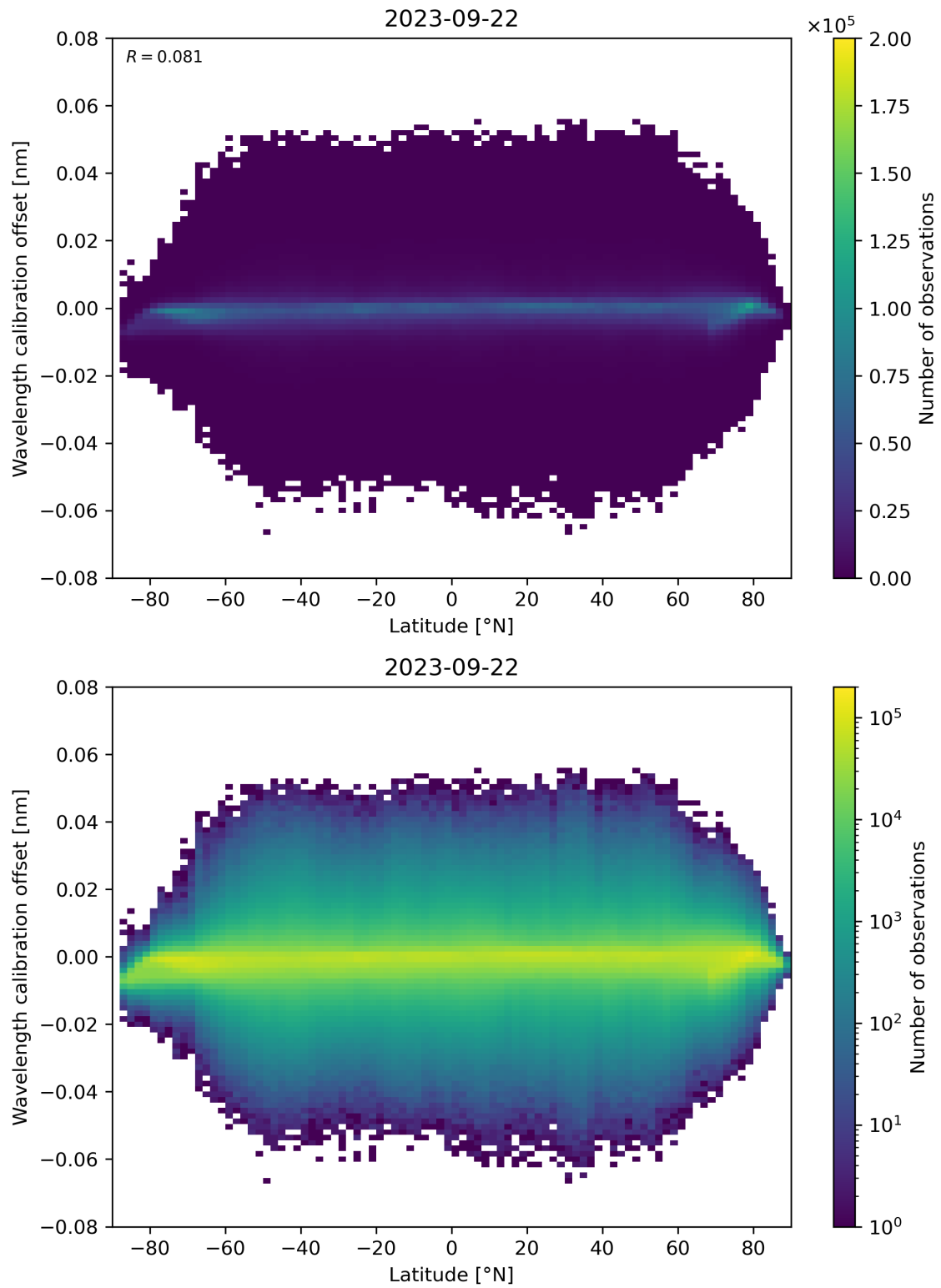
Figure 95: Scatter density plot of “Latitude” against “Wavelength calibration offset” for 2023-09-21 to 2023-09-23.
