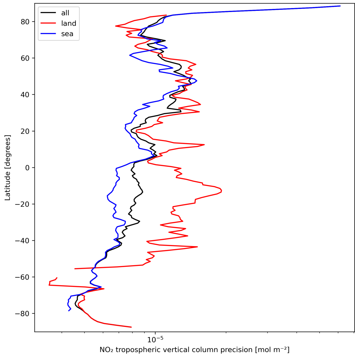
Figure 13: Zonal average of “NO 2 tropospheric vertical column precision” for 2023-09-21 to 2023-09-23.
