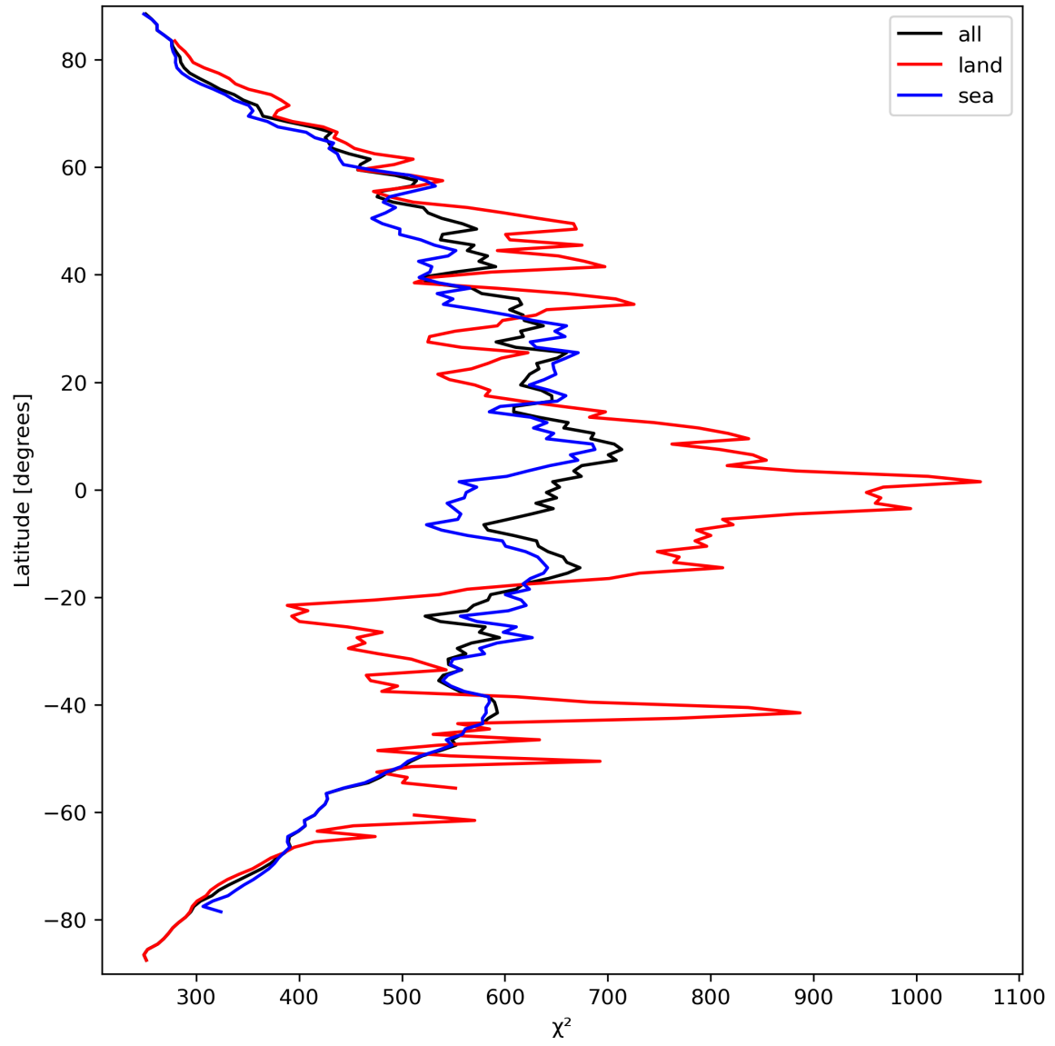
Figure 25: Zonal average of “ \chi^2 ” for 2023-09-21 to 2023-09-23.
