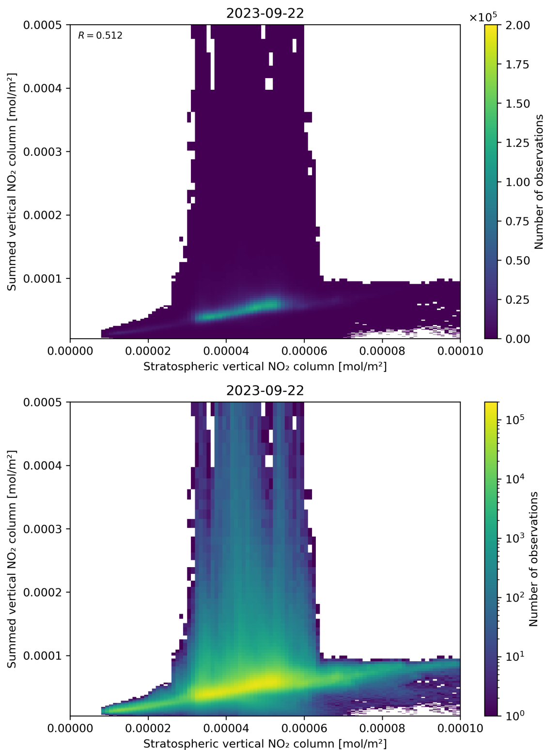
Figure 98: Scatter density plot of “Stratospheric vertical NO 2 column” against “Summed vertical NO 2 column” for 2023-09-21 to 2023-09-23.
