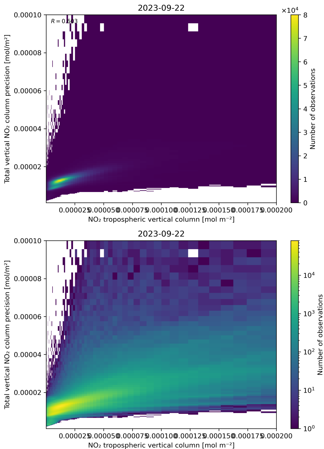
Figure 129: Scatter density plot of “NO 2 tropospheric vertical column” against “Total vertical NO 2 column precision” for 2023-09-21 to 2023-09-23.
