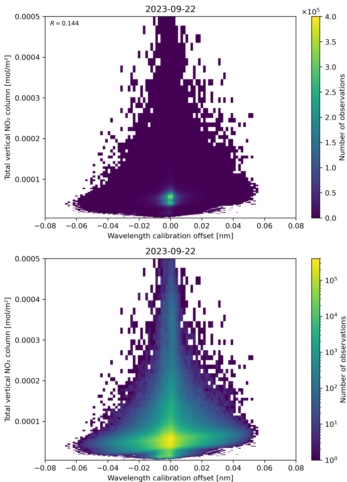
Figure 179: Scatter density plot of “Wavelength calibration offset” against “Total vertical NO 2 column” for 2023-09-21 to 2023-09-23.
