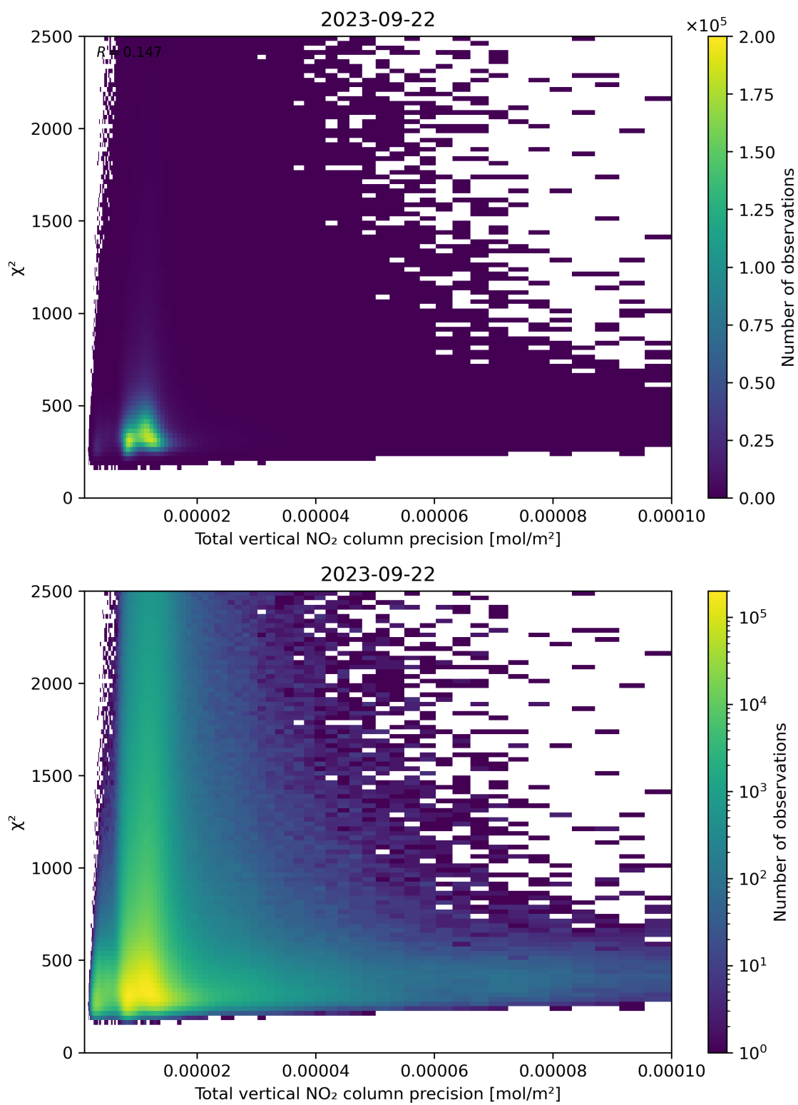
Figure 116: Scatter density plot of “Total vertical NO 2 column precision” against “ \chi^2 ” for 2023-09-21 to 2023-09-23.
