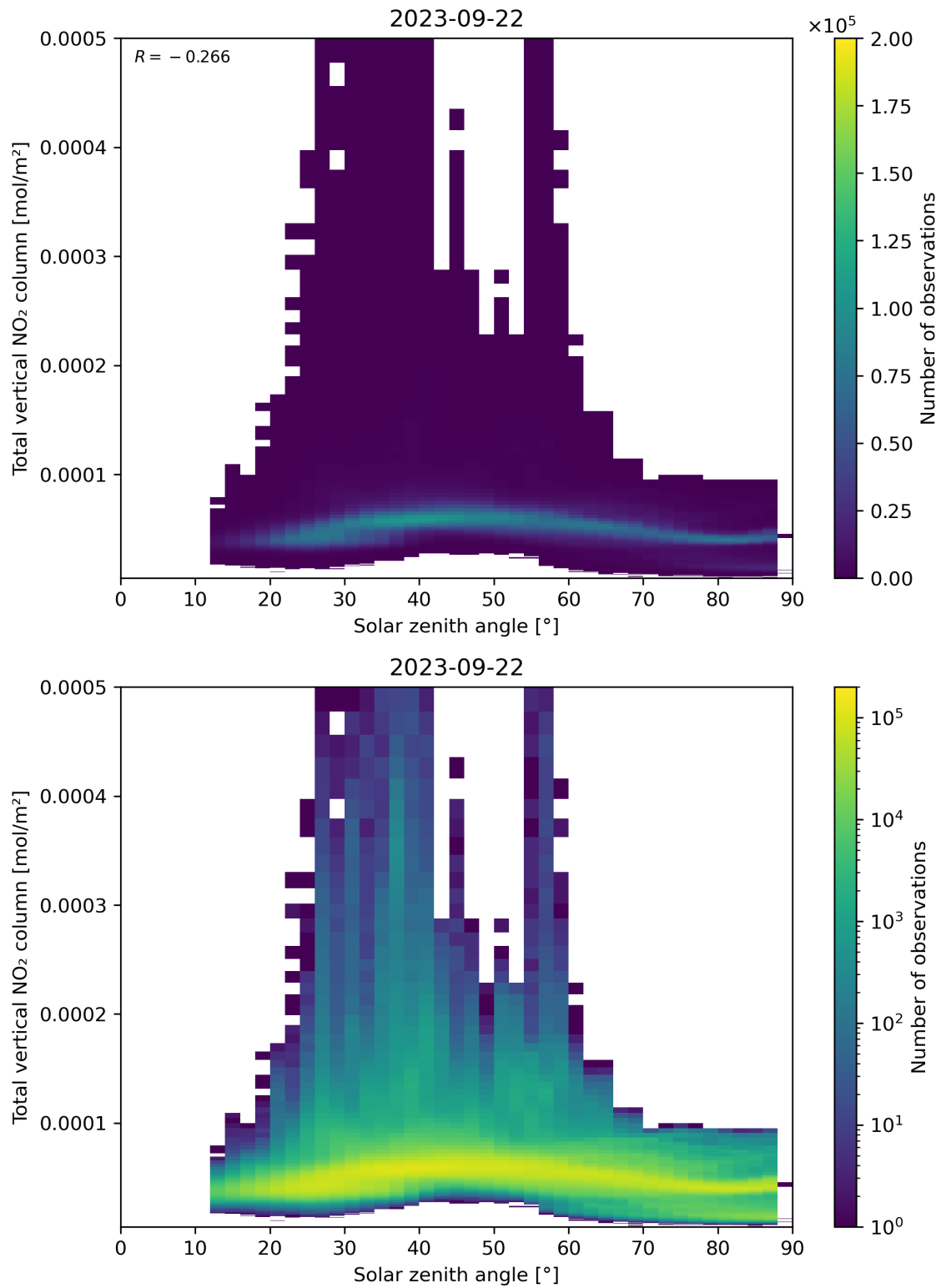
Figure 153: Scatter density plot of “Solar zenith angle” against “Total vertical NO 2 column” for 2023-09-21 to 2023-09-23.
