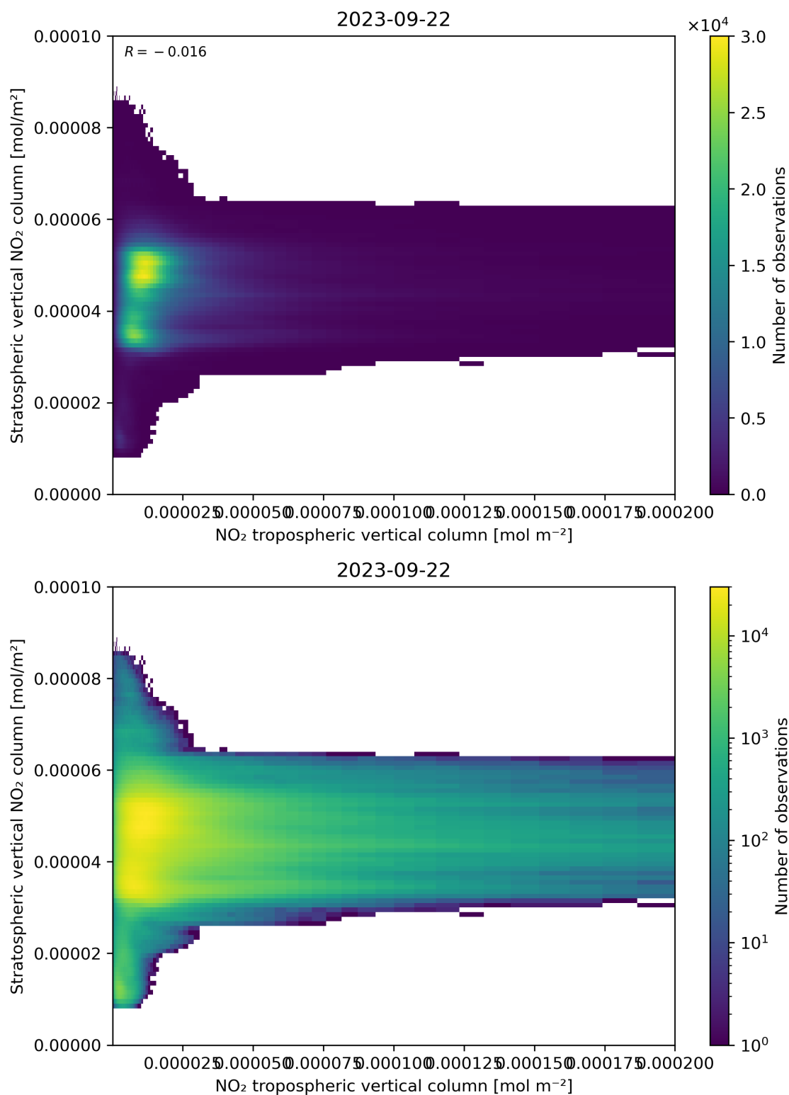
Figure 125: Scatter density plot of “NO 2 tropospheric vertical column” against “Stratospheric vertical NO 2 column” for 2023-09-21 to 2023-09-23.
