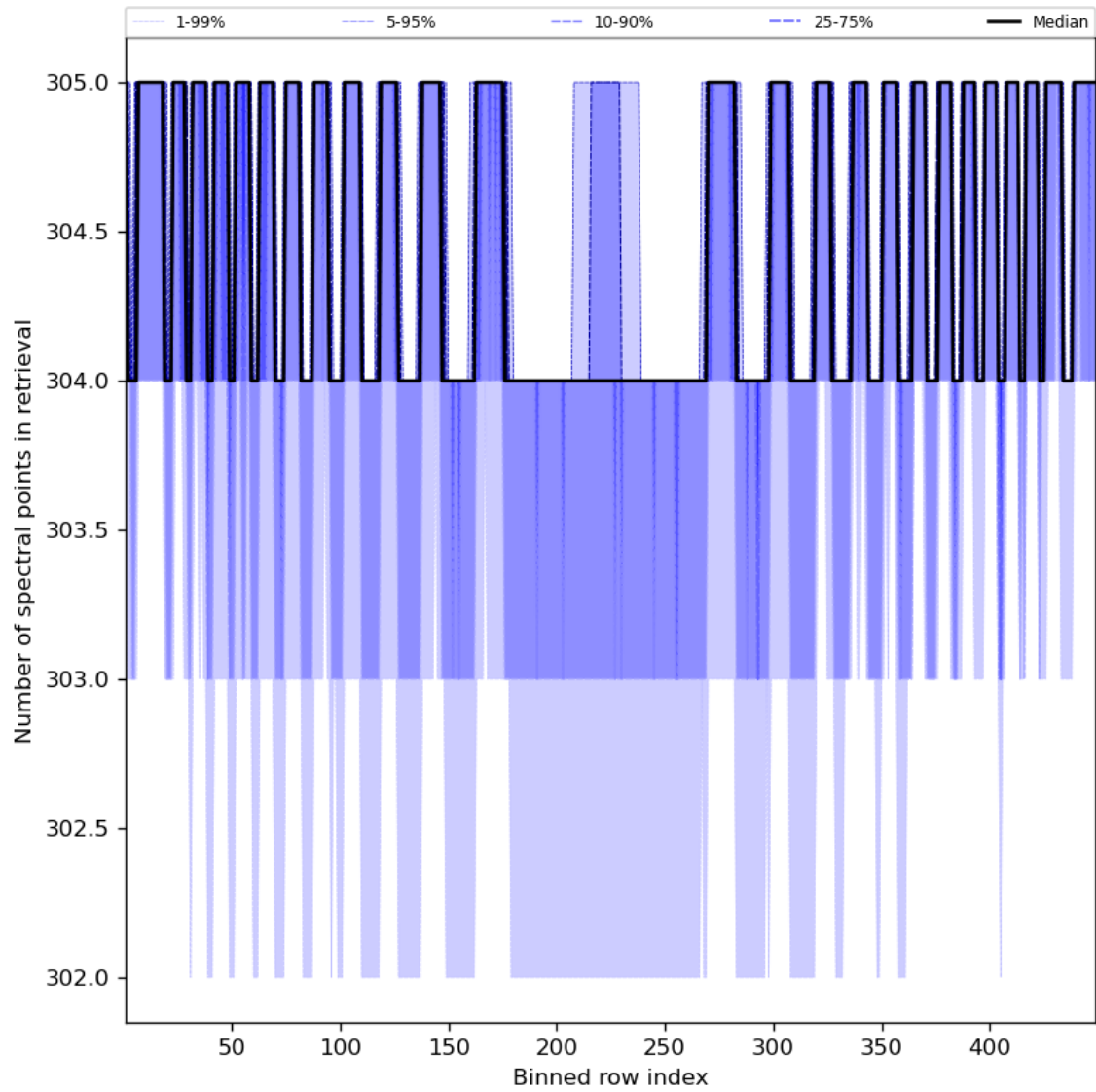
Figure 50: Along track statistics of “Number of spectral points in retrieval” for 2023-09-21 to 2023-09-23
