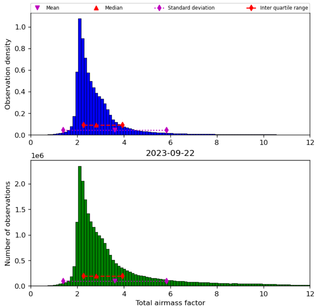
Figure 32: Histogram of “Total airmass factor” for 2023-09-21 to 2023-09-23
