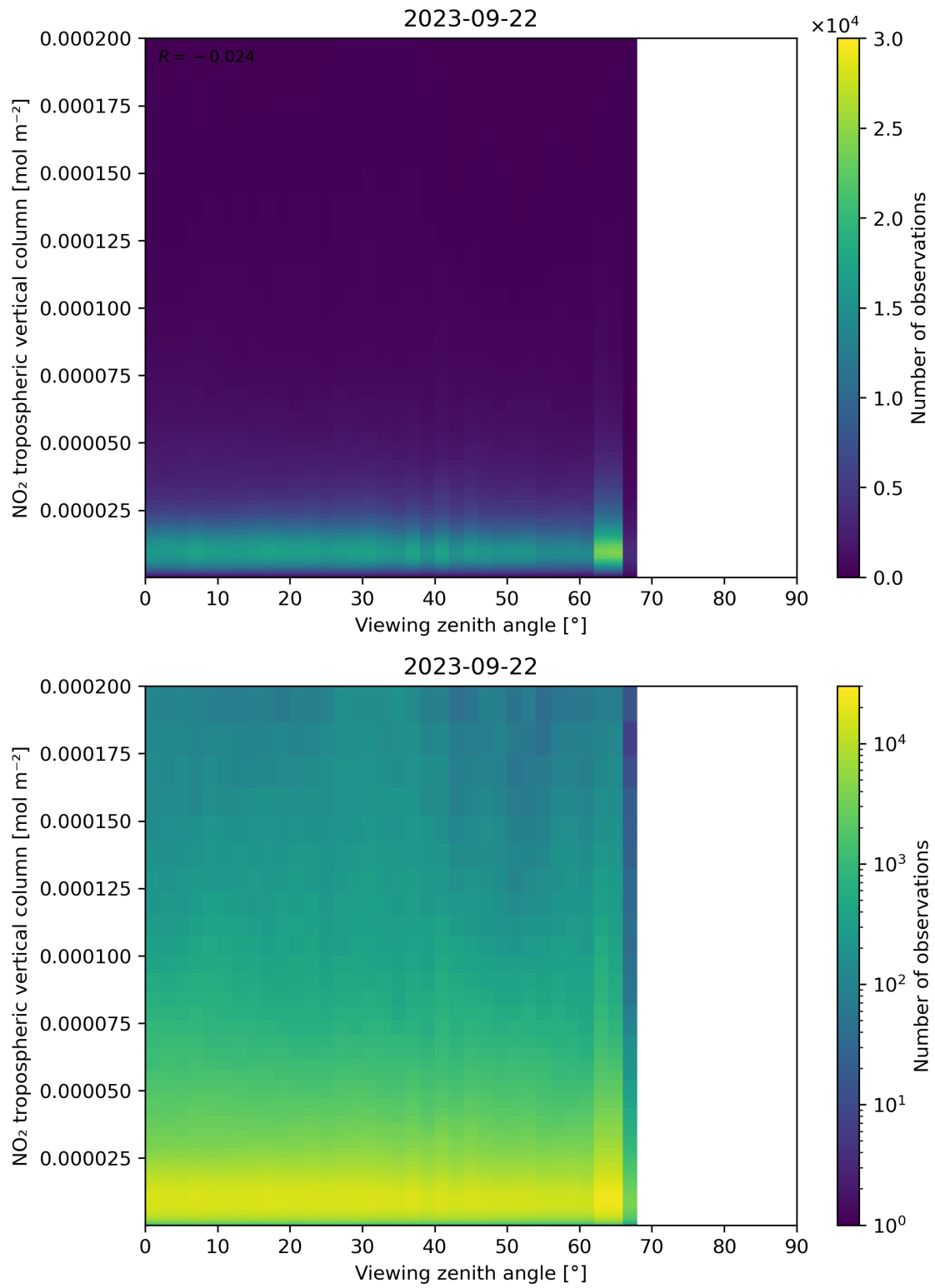
Figure 169: Scatter density plot of “Viewing zenith angle” against “NO 2 tropospheric vertical column” for 2023-09-21 to 2023-09-23.
