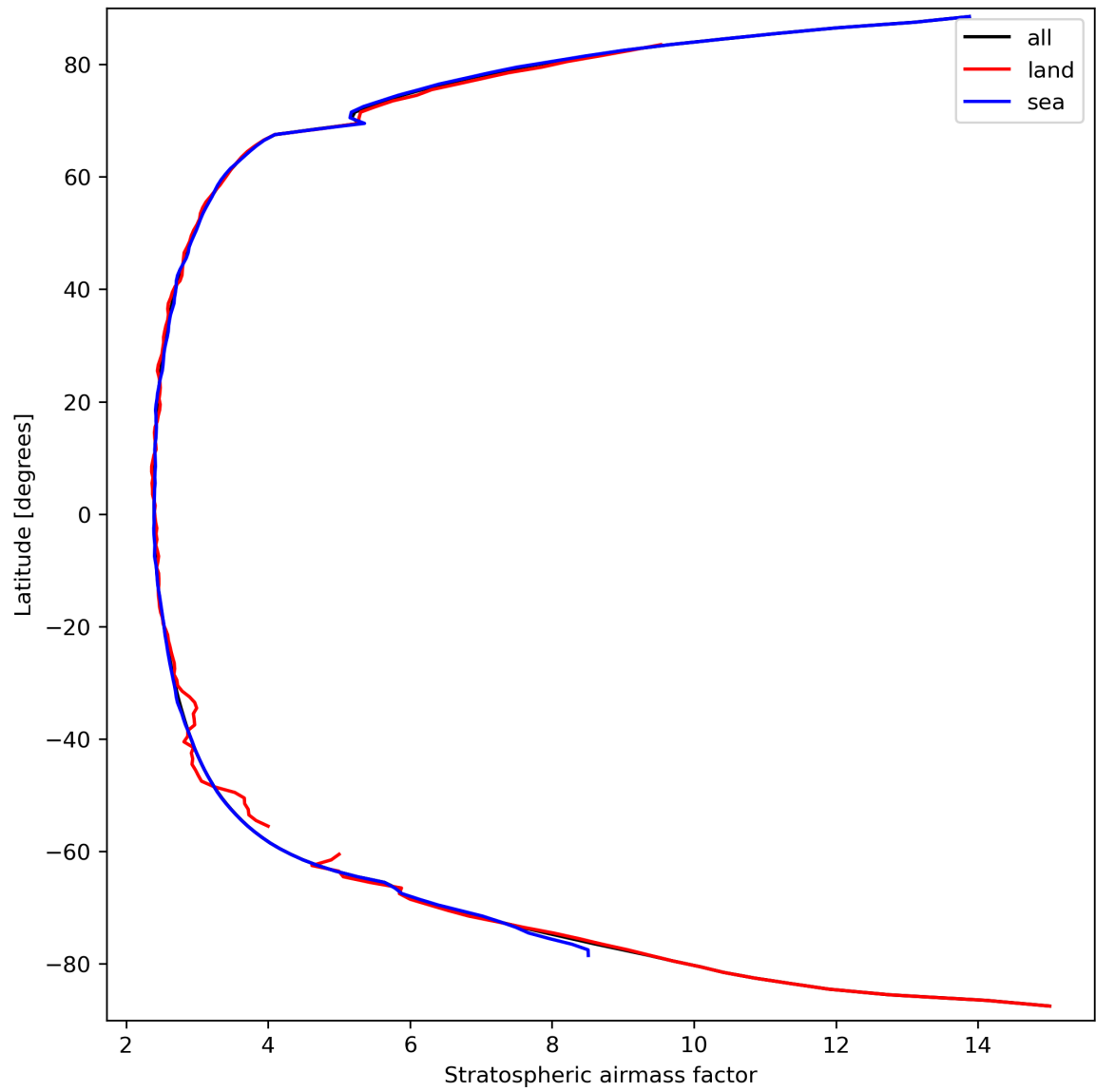
Figure 27: Zonal average of “Stratospheric airmass factor” for 2023-09-21 to 2023-09-23.
