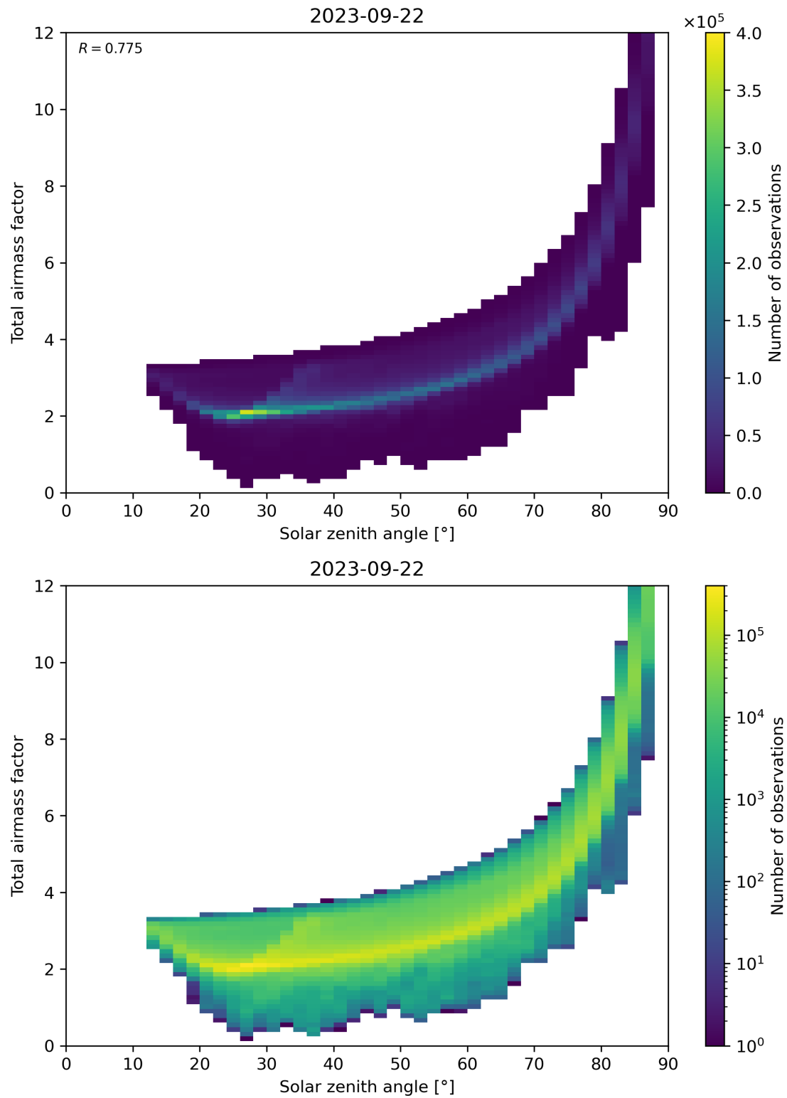
Figure 146: Scatter density plot of “Solar zenith angle” against “Total airmass factor” for 2023-09-21 to 2023-09-23.
