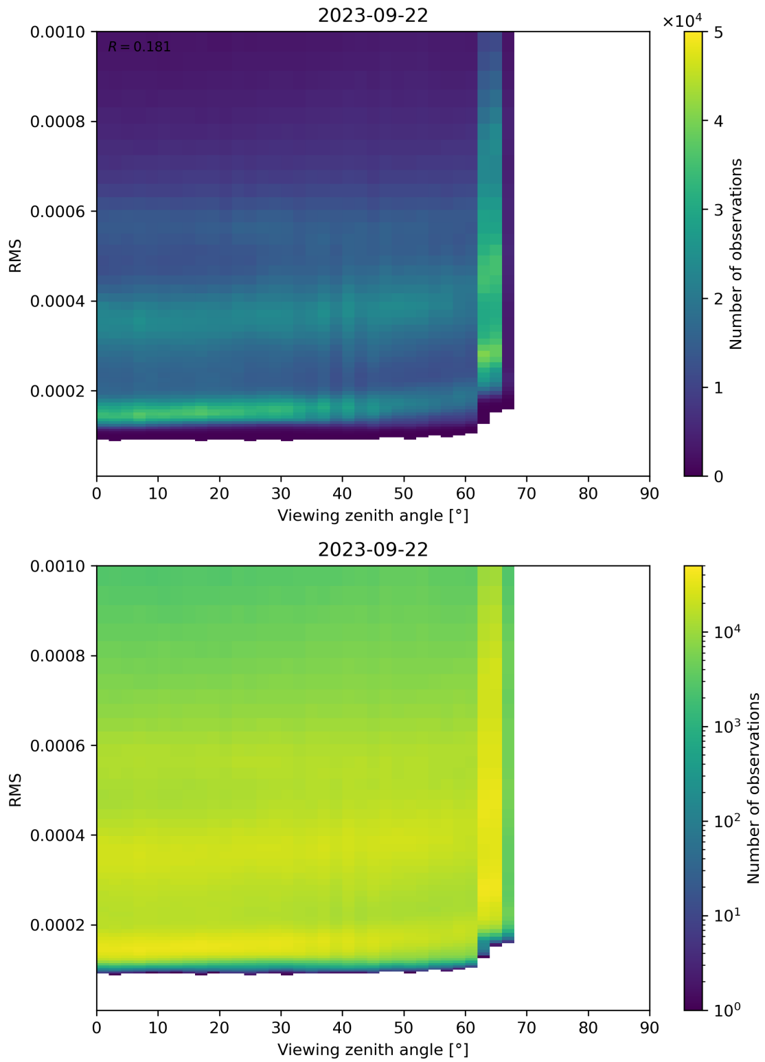
Figure 171: Scatter density plot of “Viewing zenith angle” against “RMS” for 2023-09-21 to 2023-09-23.
