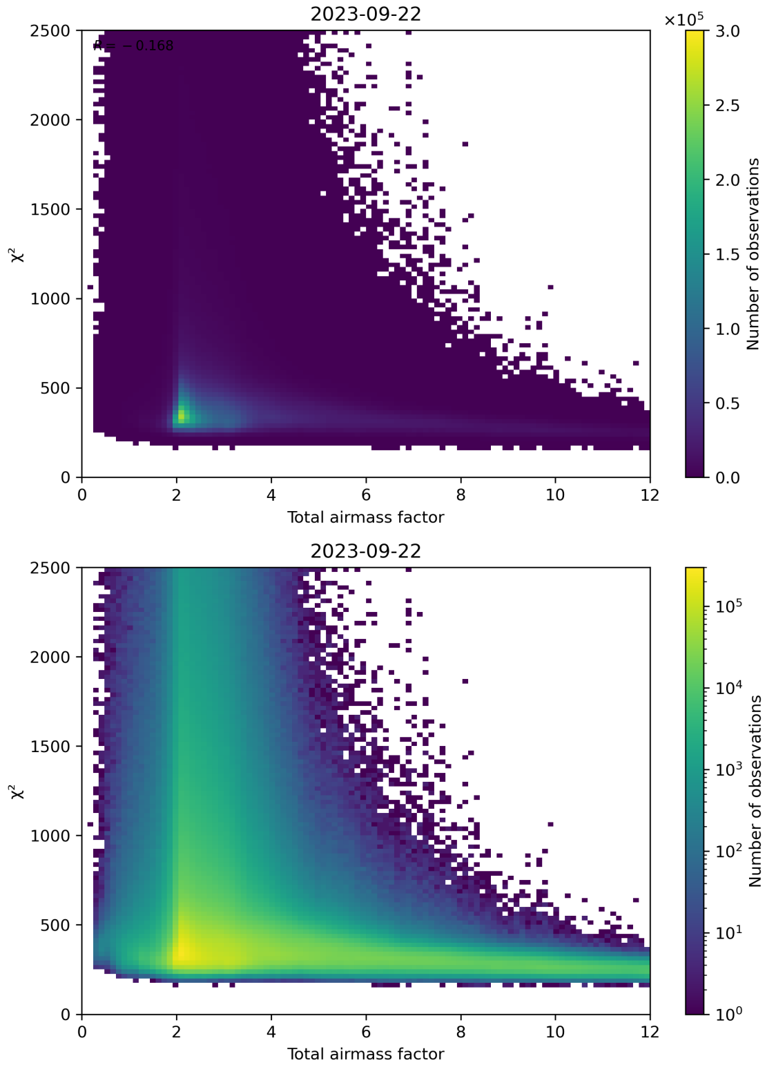
Figure 63: Scatter density plot of “Total airmass factor” against “ \chi^2 ” for 2023-09-21 to 2023-09-23.
