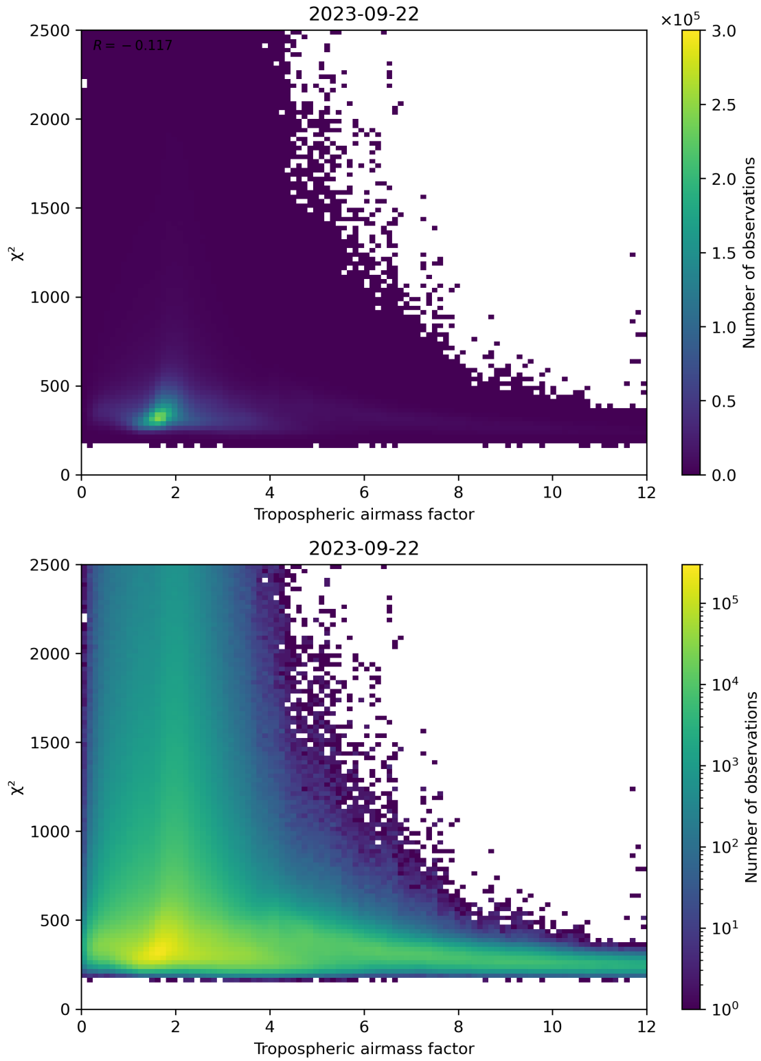
Figure 73: Scatter density plot of “Tropospheric airmass factor” against “ \chi^2 ” for 2023-09-21 to 2023-09-23.
