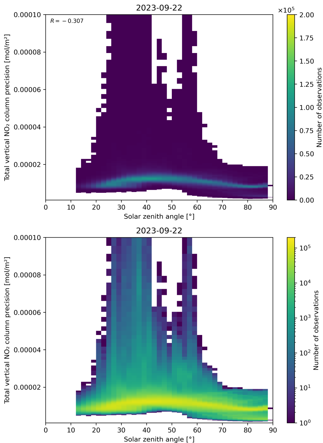
Figure 154: Scatter density plot of “Solar zenith angle” against “Total vertical NO 2 column precision” for 2023-09-21 to 2023-09-23.
