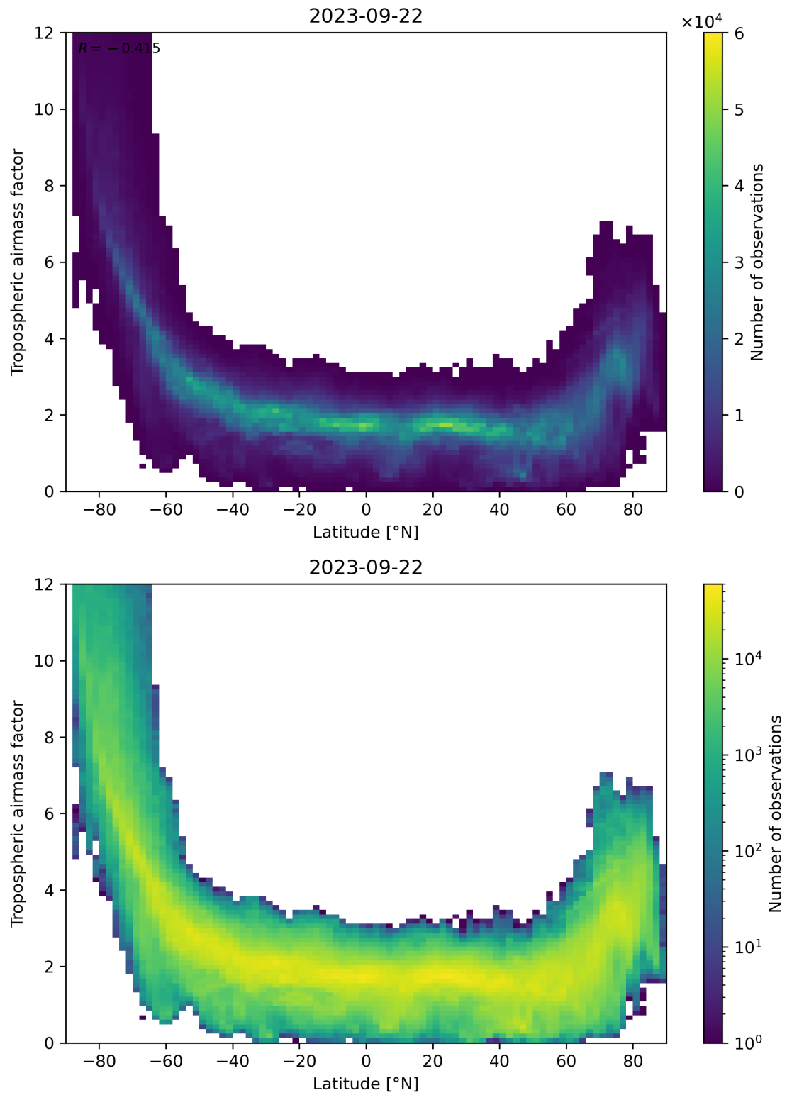
Figure 85: Scatter density plot of “Latitude” against “Tropospheric airmass factor” for 2023-09-21 to 2023-09-23.
