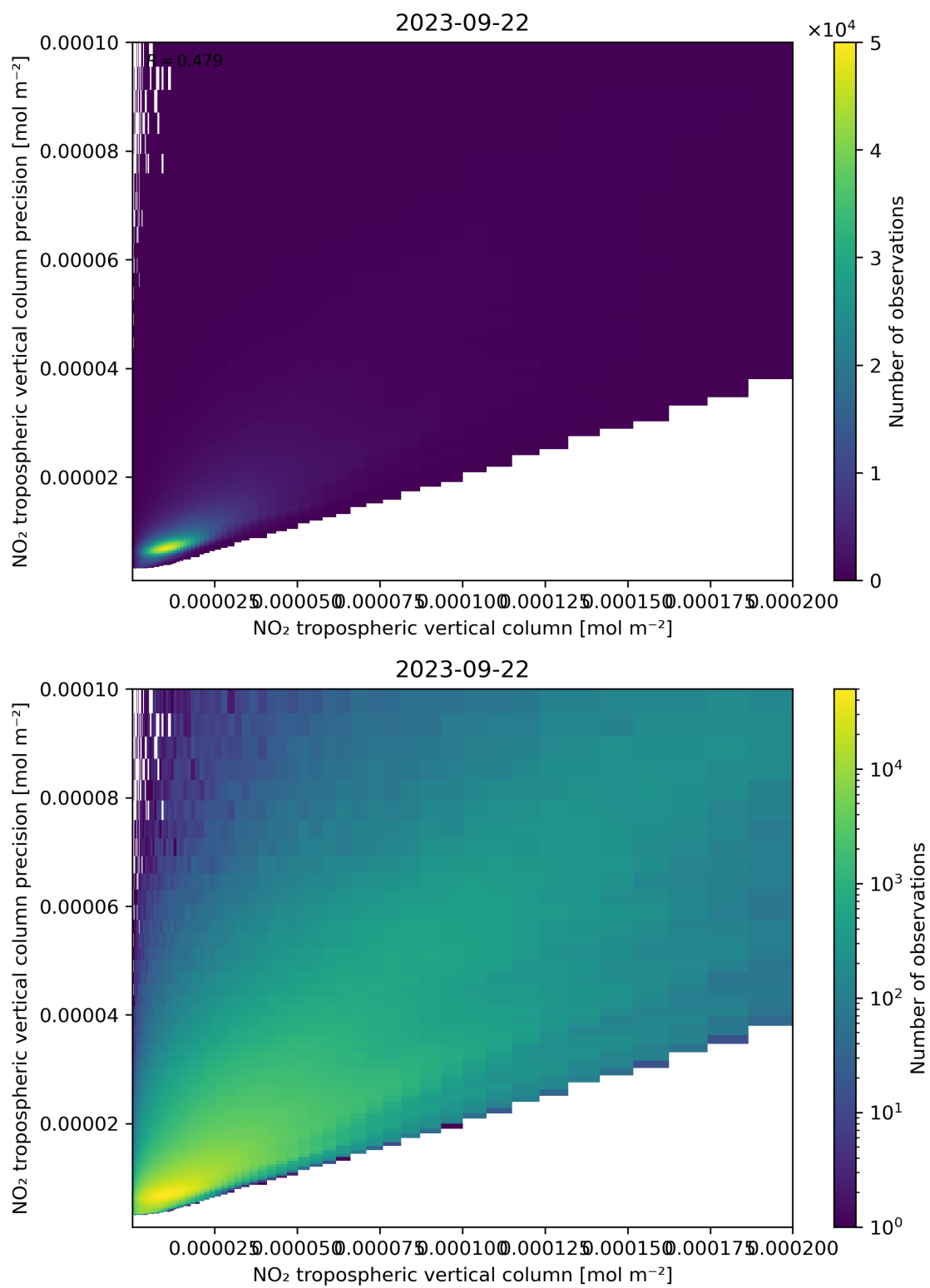
Figure 130: Scatter density plot of “NO 2 tropospheric vertical column” against “NO 2 tropospheric vertical column precision” for 2023-09-21 to 2023-09-23.
