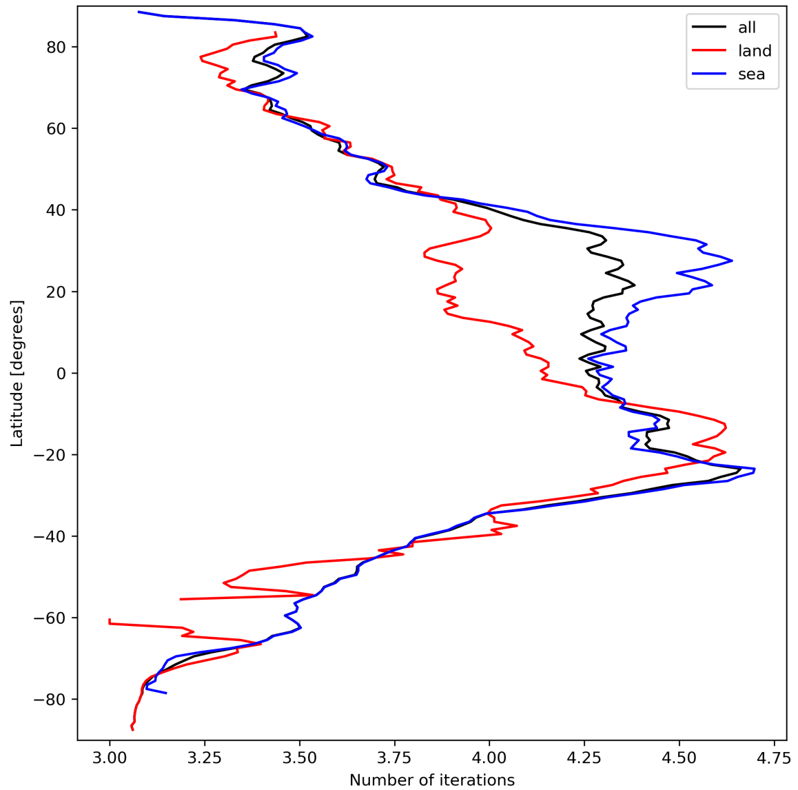
Figure 17: Zonal average of “Number of iterations” for 2023-09-21 to 2023-09-23.
