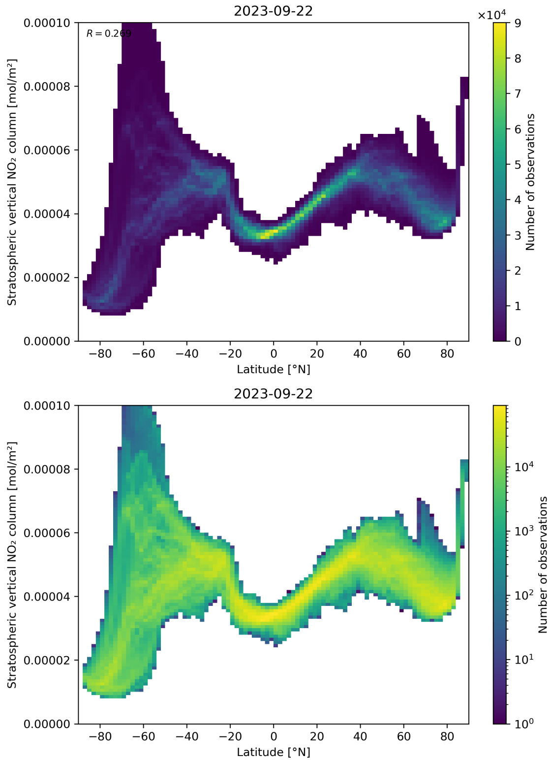
Figure 87: Scatter density plot of “Latitude” against “Stratospheric vertical NO 2 column” for 2023-09-21 to 2023-09-23.
