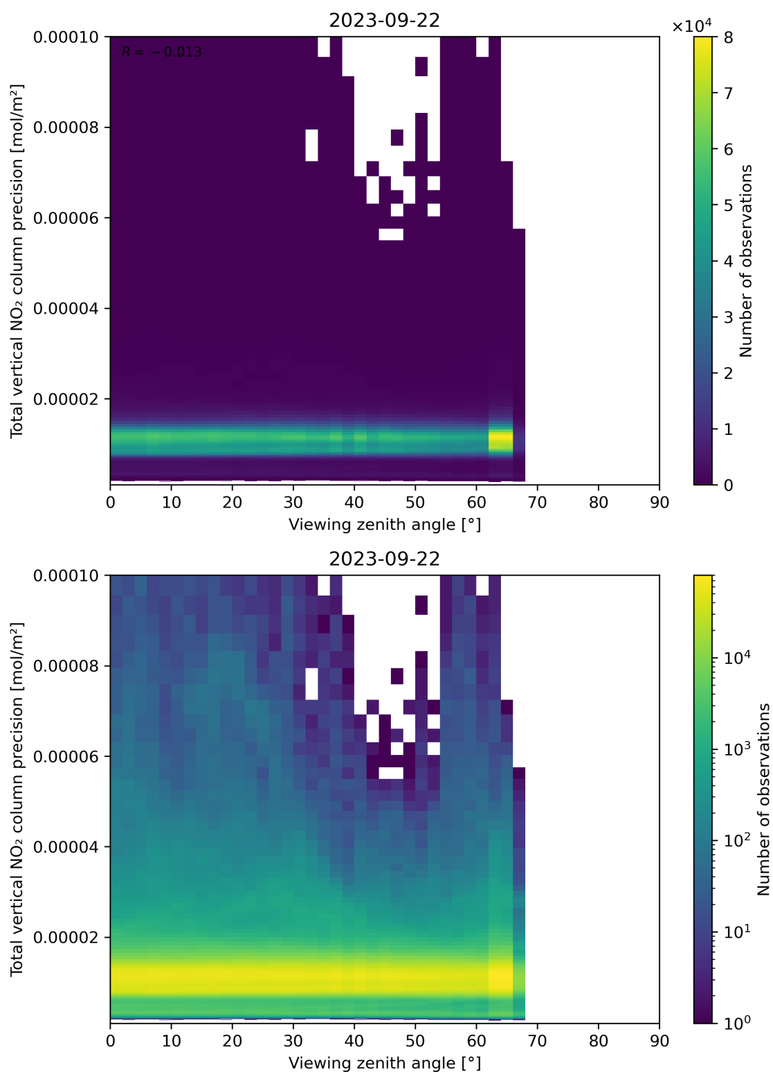
Figure 168: Scatter density plot of “Viewing zenith angle” against “Total vertical NO 2 column precision” for 2023-09-21 to 2023-09-23.
