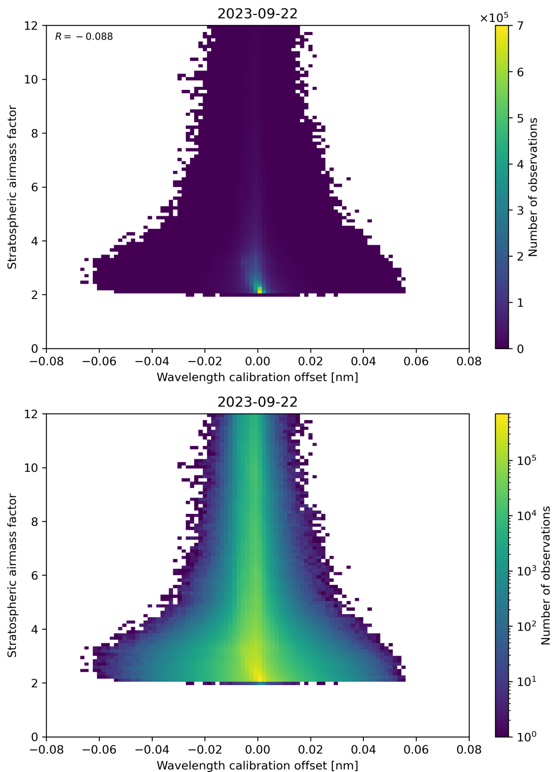
Figure 174: Scatter density plot of “Wavelength calibration offset” against “Stratospheric air mass factor” for 2023-09-21 to 2023-09-23.
