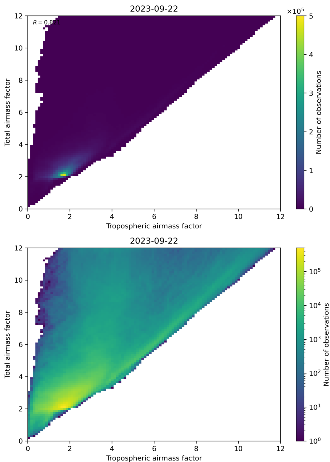
Figure 72: Scatter density plot of “Tropospheric airmass factor” against “Total airmass factor” for 2023-09-21 to 2023-09-23.
