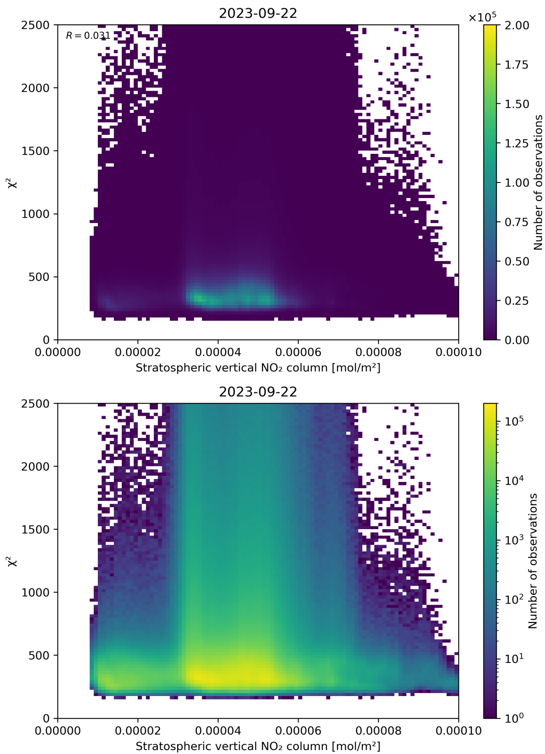
Figure 97: Scatter density plot of “Stratospheric vertical NO 2 column” against “ \chi^2 ” for 2023-09-21 to 2023-09-23.
