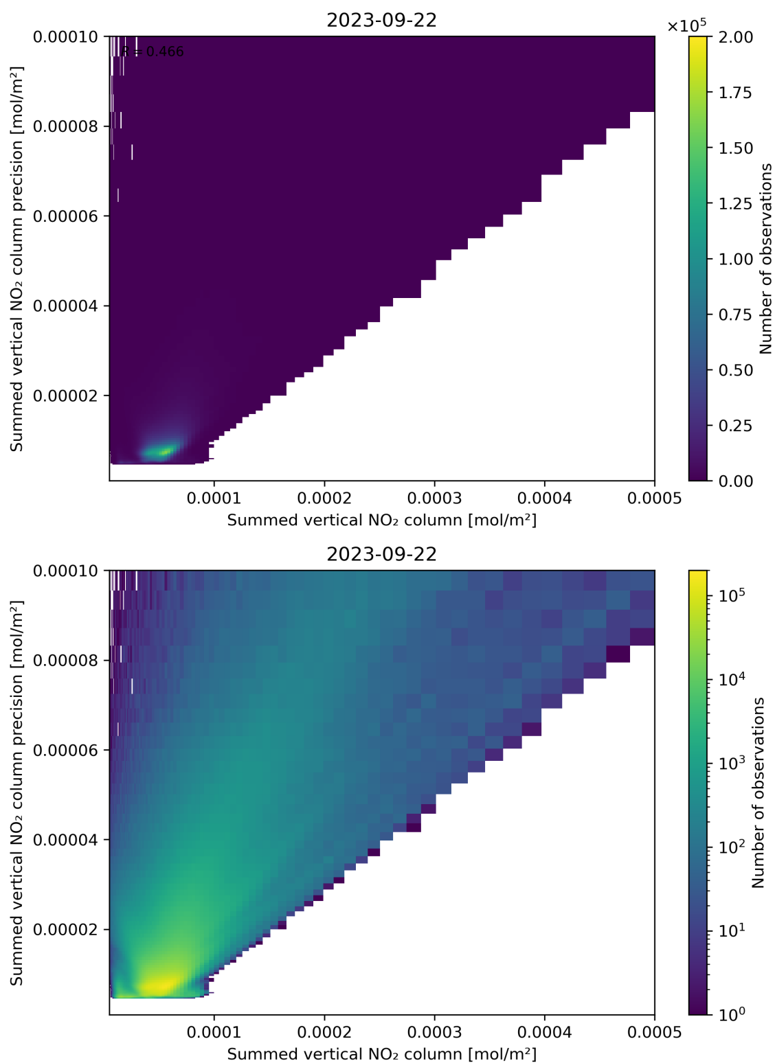
Figure 105: Scatter density plot of “Summed vertical NO 2 column” against “Summed vertical NO 2 column precision” for 2023-09-21 to 2023-09-23.
