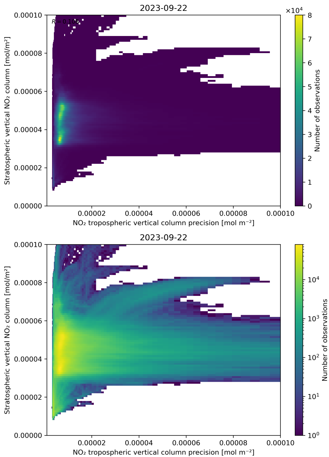
Figure 135: Scatter density plot of “NO 2 tropospheric vertical column precision” against “Stratospheric vertical NO 2 column” for 2023-09-21 to 2023-09-23.
