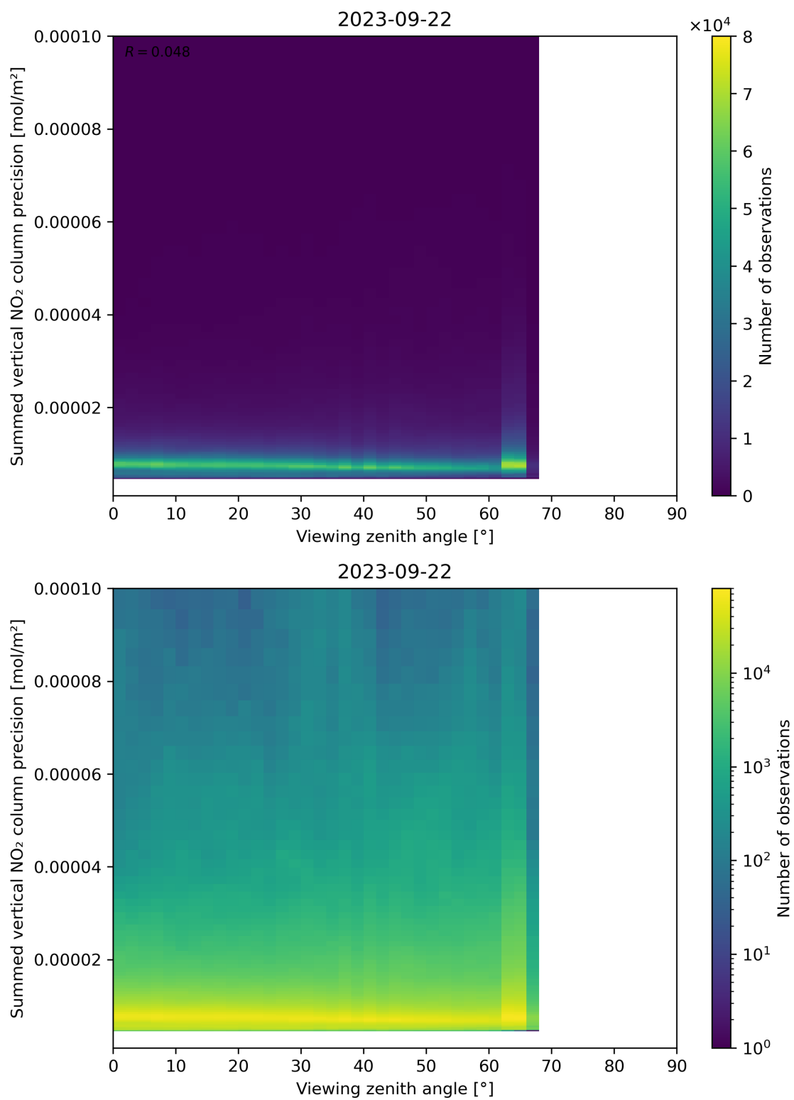
Figure 166: Scatter density plot of “Viewing zenith angle” against “Summed vertical NO 2 column precision” for 2023-09-21 to 2023-09-23.
