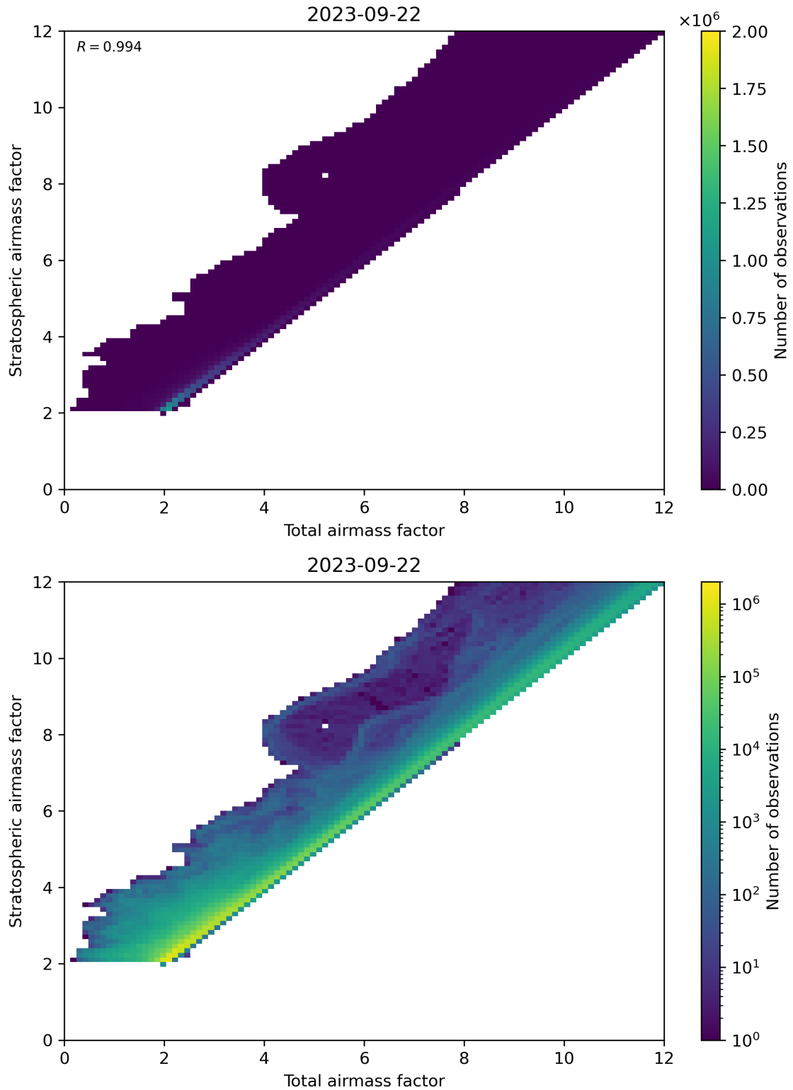
Figure 62: Scatter density plot of “Total airmass factor” against “Stratospheric airmass factor” for 2023-09-21 to 2023-09-23.
