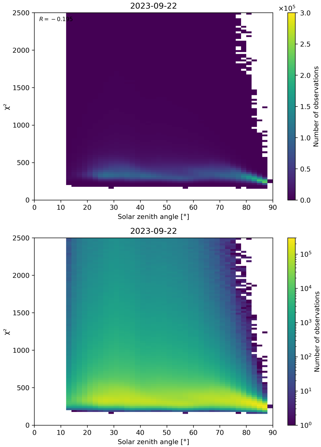
Figure 148: Scatter density plot of “Solar zenith angle” against “ \chi^2 ” for 2023-09-21 to 2023-09-23.
