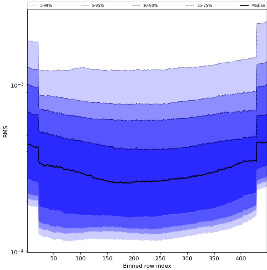
Figure 60: Along track statistics of “RMS” for 2023-09-21 to 2023-09-23
