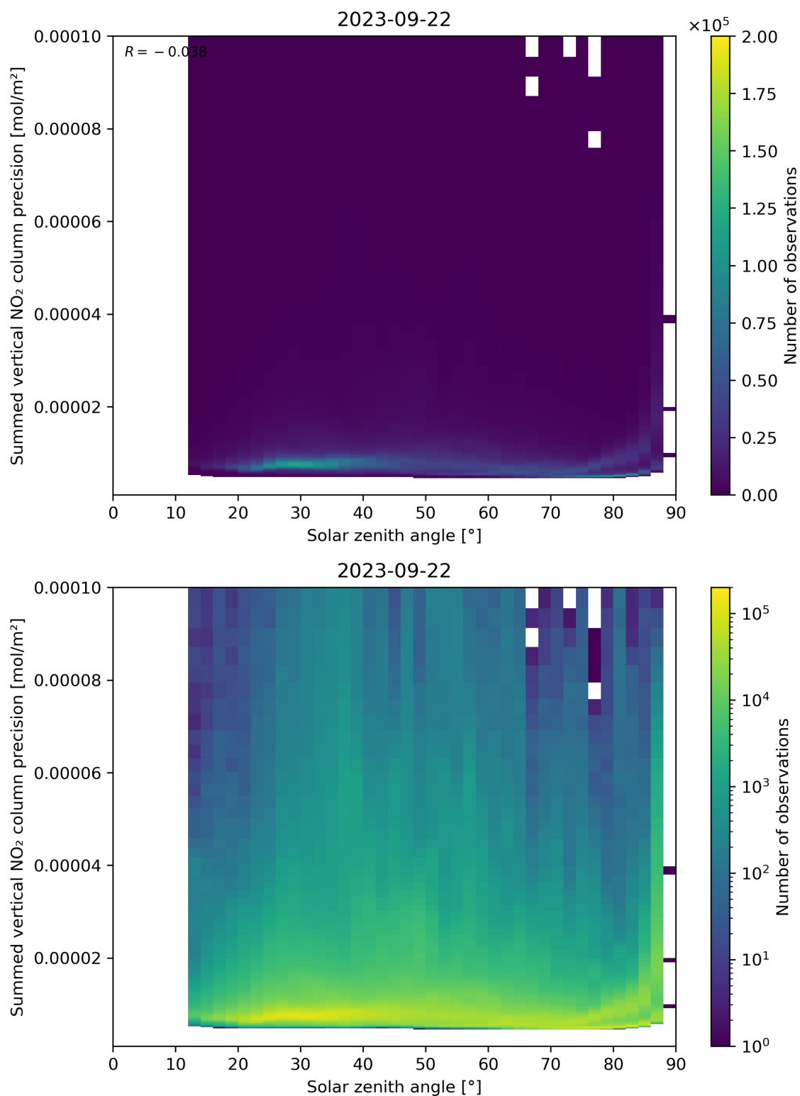
Figure 152: Scatter density plot of “Solar zenith angle” against “Summed vertical NO 2 column precision” for 2023-09-21 to 2023-09-23.
