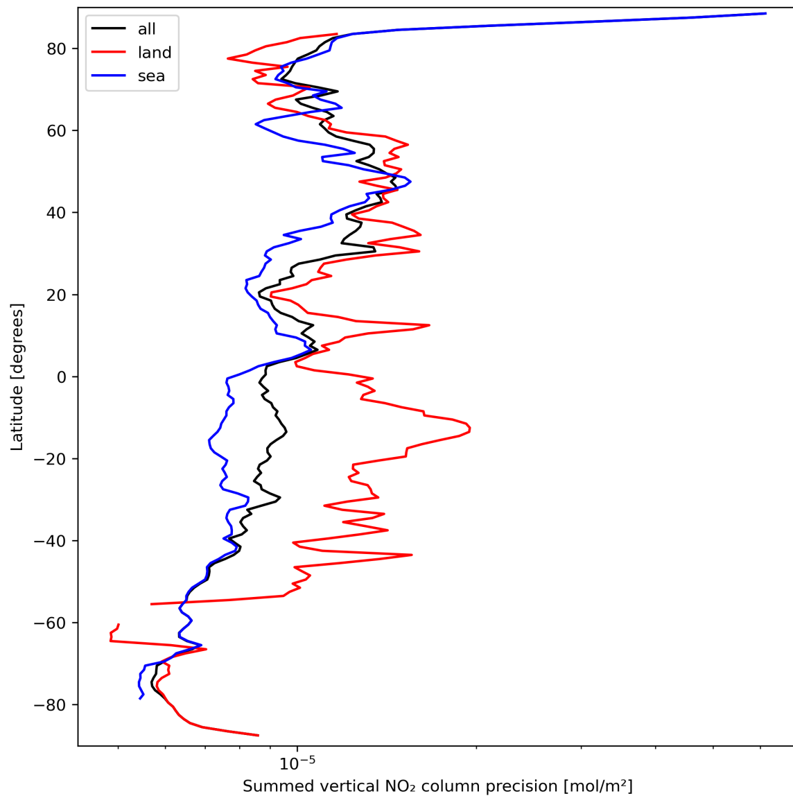
Figure 24: Zonal average of “Summed vertical NO 2 column precision” for 2023-09-21 to 2023-09-23.
