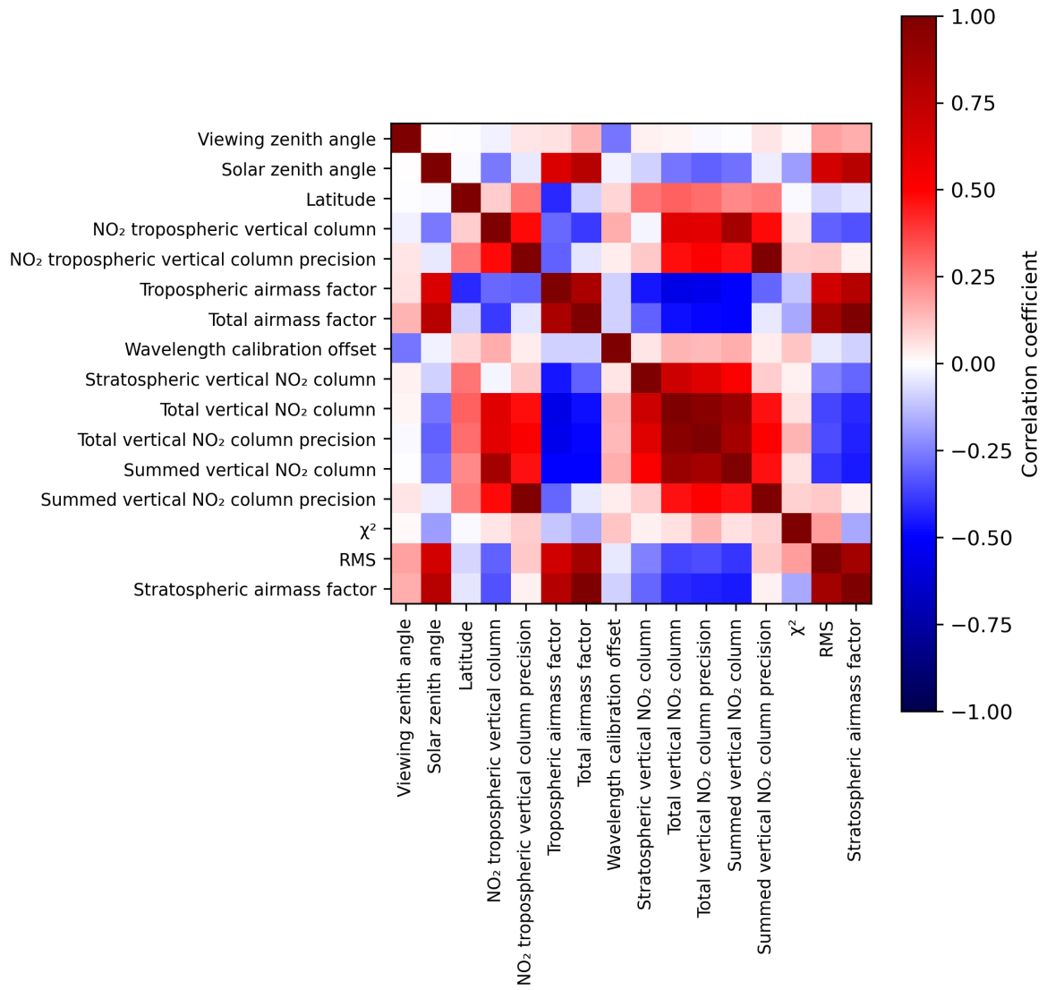
Figure 2: Map of correlation matrix for 2023-09-21 to 2023-09-23.
