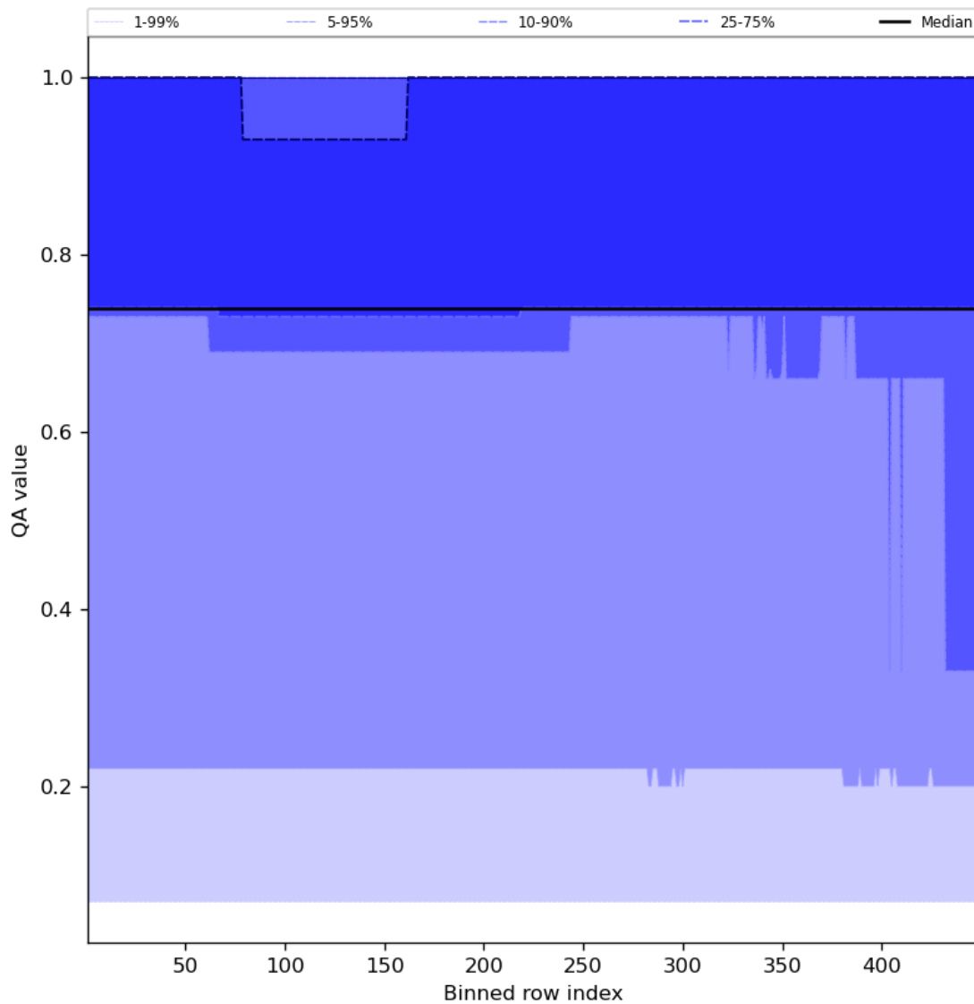
Figure 45: Along track statistics of “QA value” for 2023-09-21 to 2023-09-23
