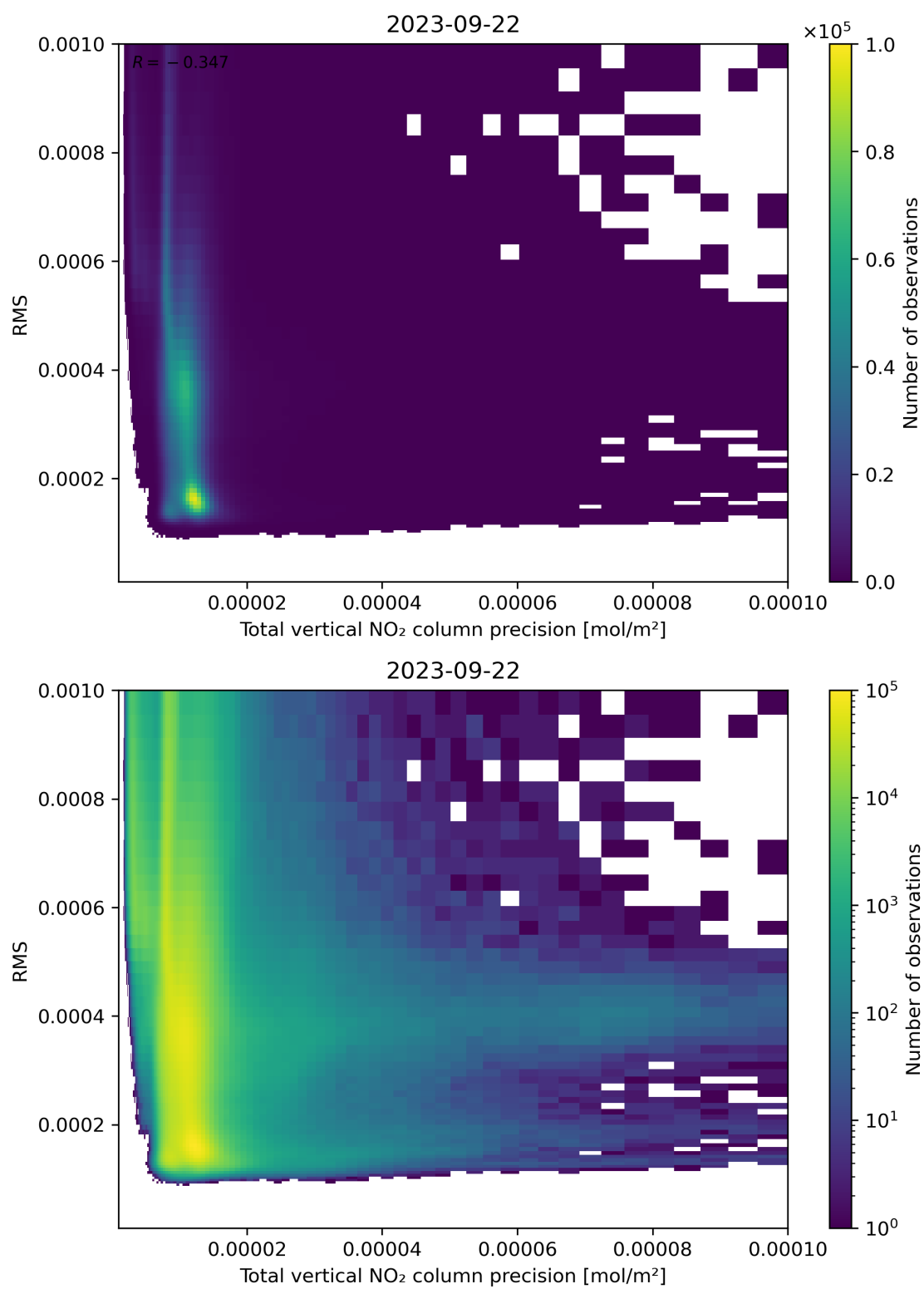
Figure 119: Scatter density plot of “Total vertical NO 2 column precision” against “RMS” for 2023-09-21 to 2023-09-23.
