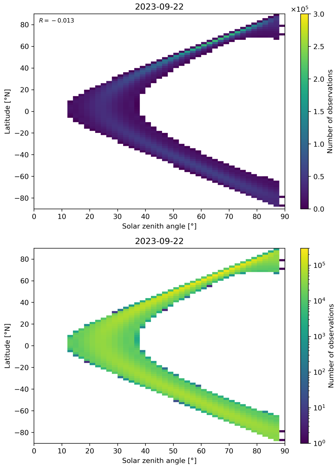
Figure 149: Scatter density plot of “Solar zenith angle” against “Latitude” for 2023-09-21 to 2023-09-23.
