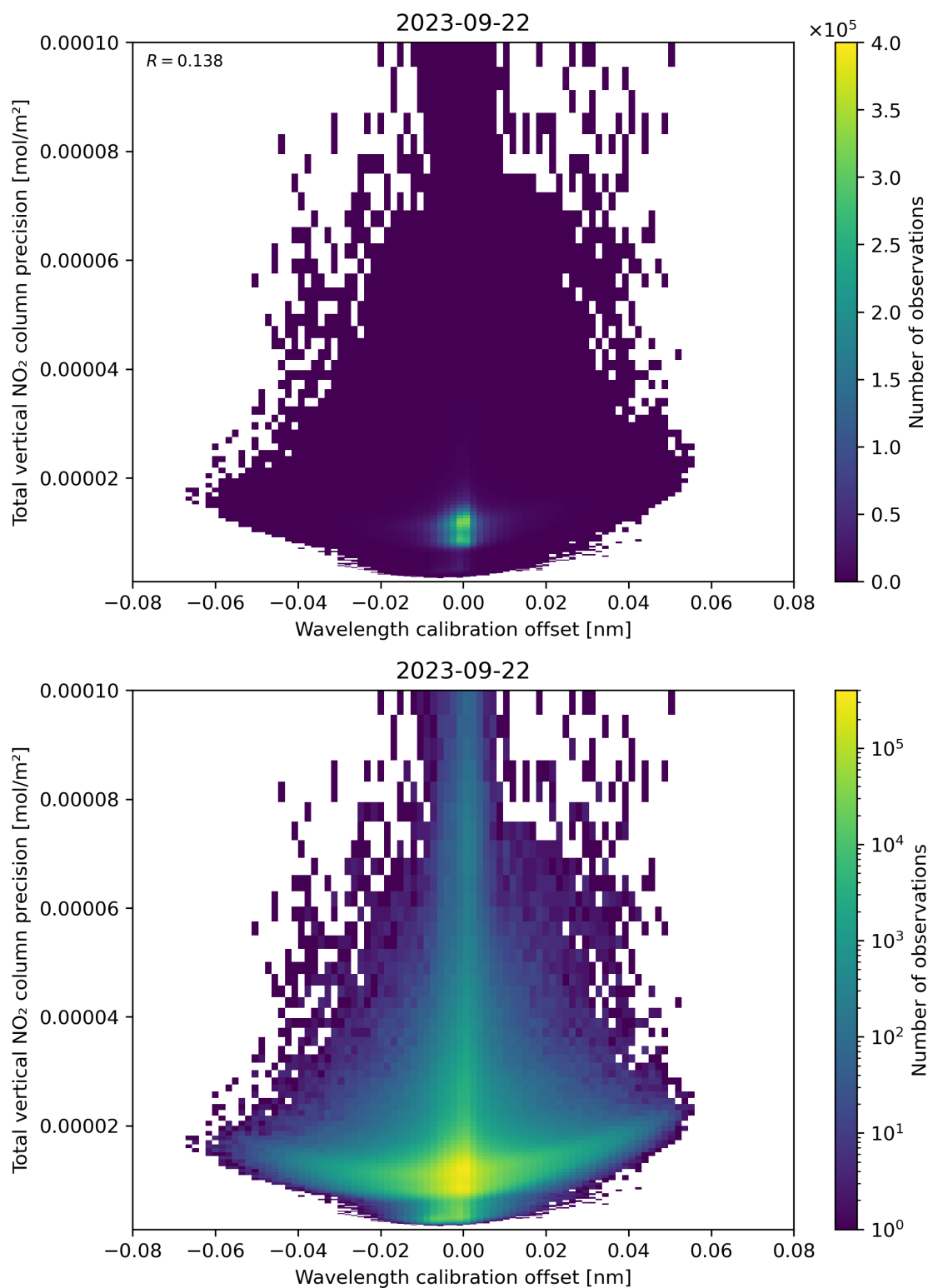
Figure 180: Scatter density plot of “Wavelength calibration offset” against “Total vertical NO 2 column precision” for 2023-09-21 to 2023-09-23.
