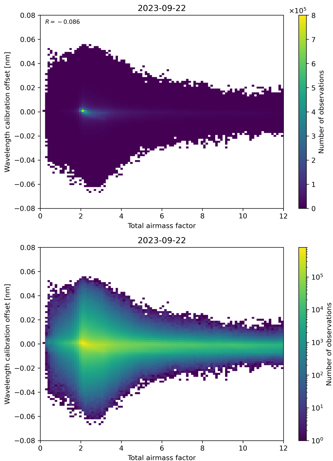
Figure 70: Scatter density plot of “Total airmass factor” against “Wavelength calibration offset” for 2023-09-21 to 2023-09-23.
