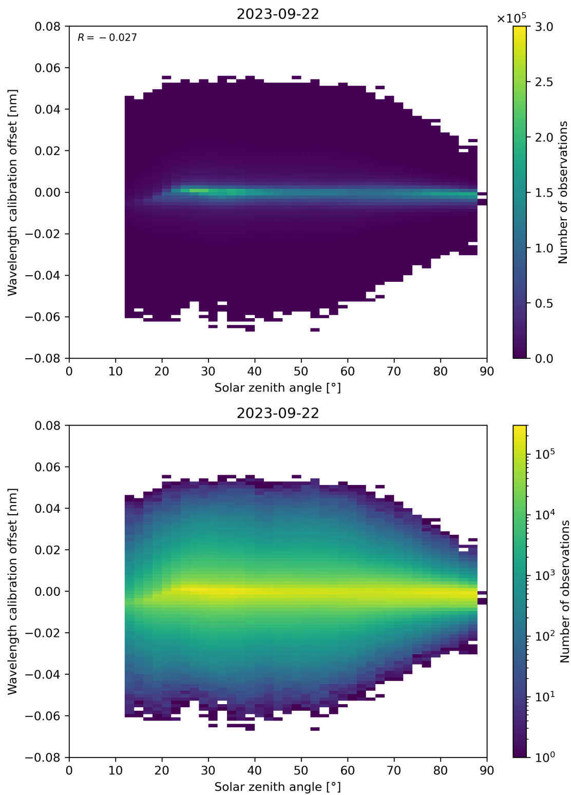
Figure 158: Scatter density plot of “Solar zenith angle” against “Wavelength calibration offset” for 2023-09-21 to 2023-09-23.
