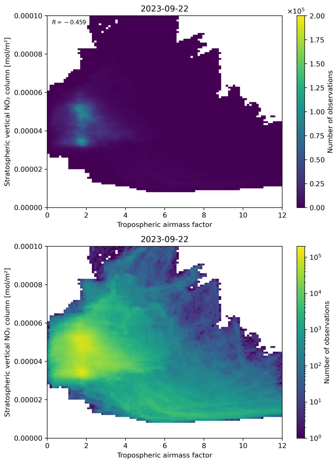
Figure 74: Scatter density plot of “Tropospheric air mass factor” against “Stratospheric vertical NO 2 column” for 2023-09-21 to 2023-09-23.
