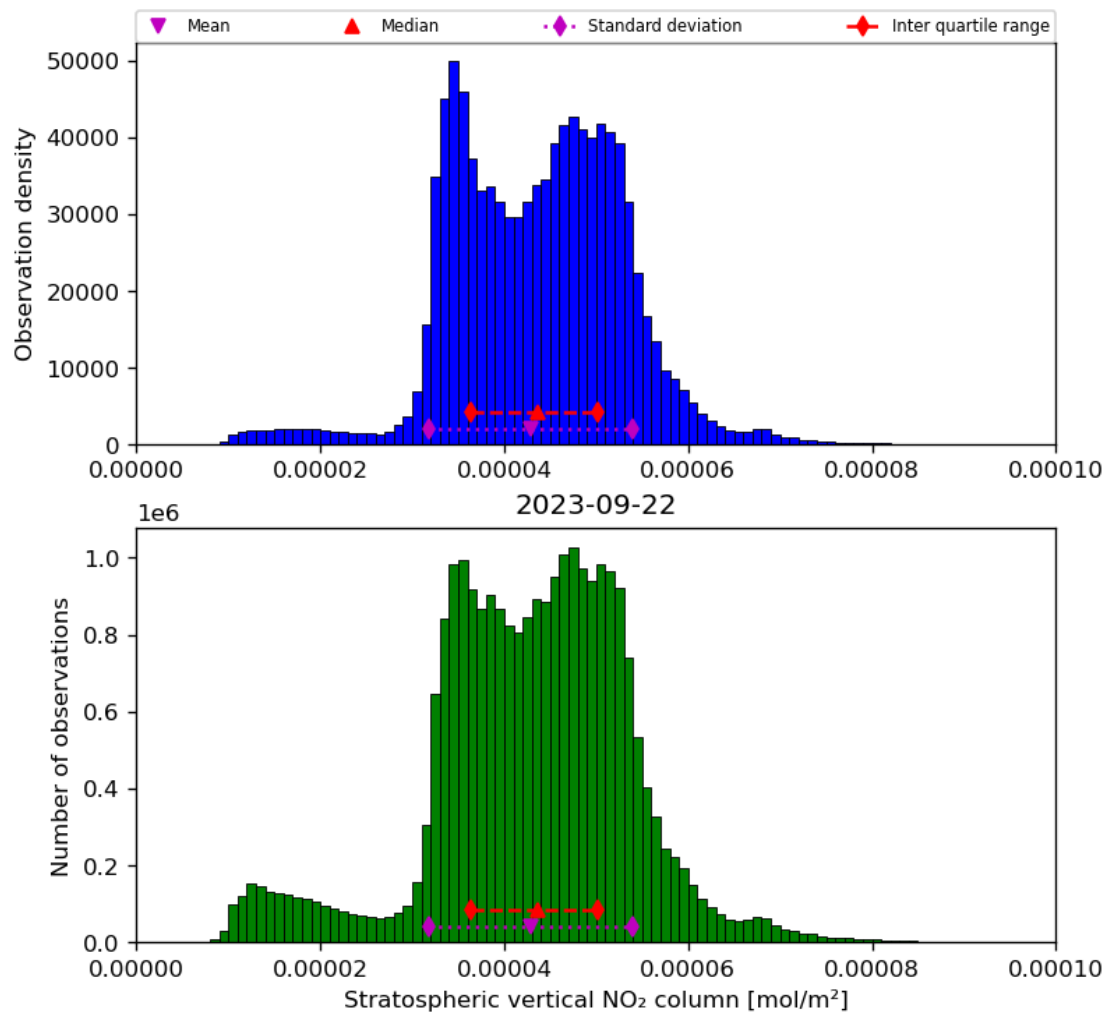
Figure 36: Histogram of “Stratospheric vertical NO 2 column” for 2023-09-21 to 2023-09-23
