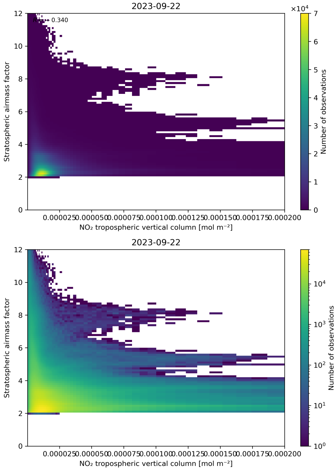
Figure 121: Scatter density plot of “NO 2 tropospheric vertical column” against “Stratospheric air mass factor” for 2023-09-21 to 2023-09-23.
