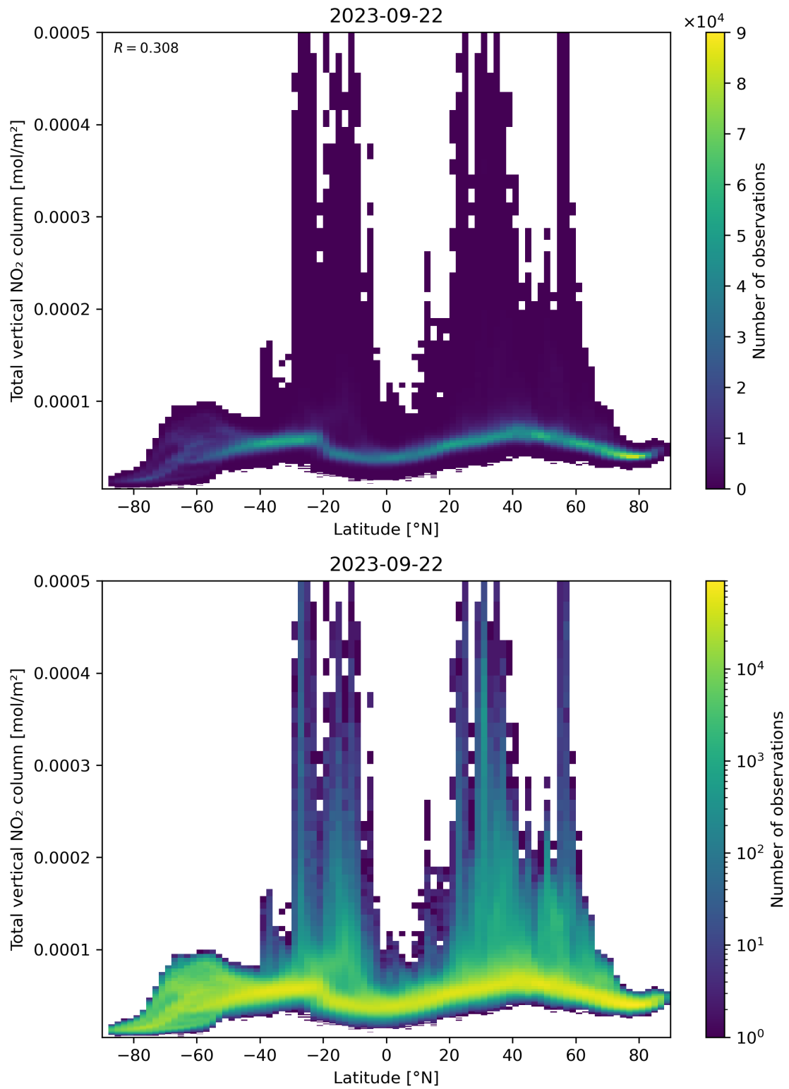
Figure 90: Scatter density plot of “Latitude” against “Total vertical NO 2 column” for 2023-09-21 to 2023-09-23.
