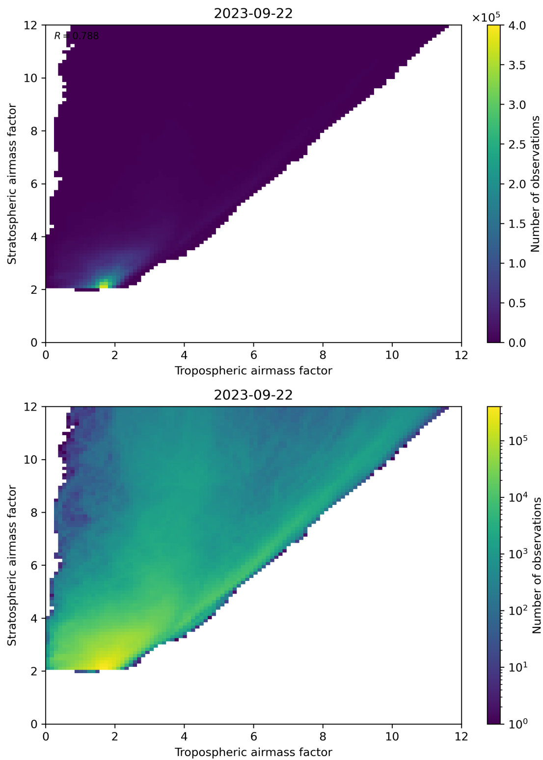
Figure 71: Scatter density plot of “Tropospheric airmass factor” against “Stratospheric airmass factor” for 2023-09-21 to 2023-09-23.
