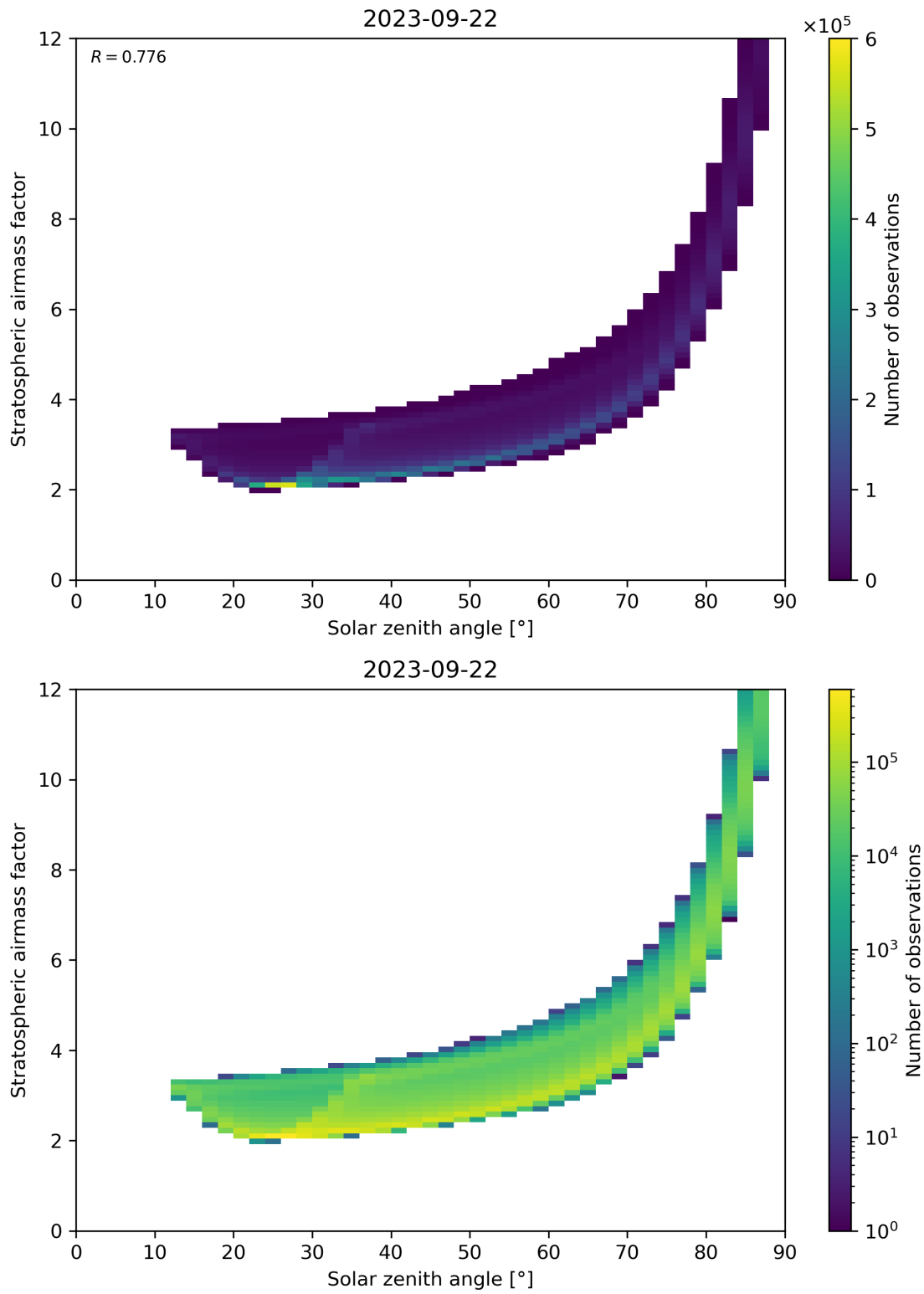
Figure 145: Scatter density plot of “Solar zenith angle” against “Stratospheric airmass factor” for 2023-09-21 to 2023-09-23.
