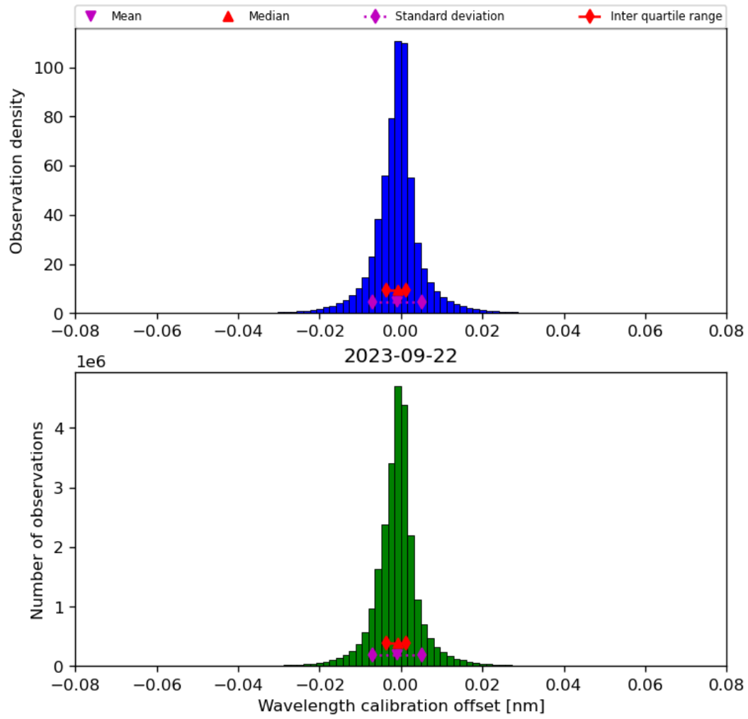
Figure 35: Histogram of “Wavelength calibration offset” for 2023-09-21 to 2023-09-23
