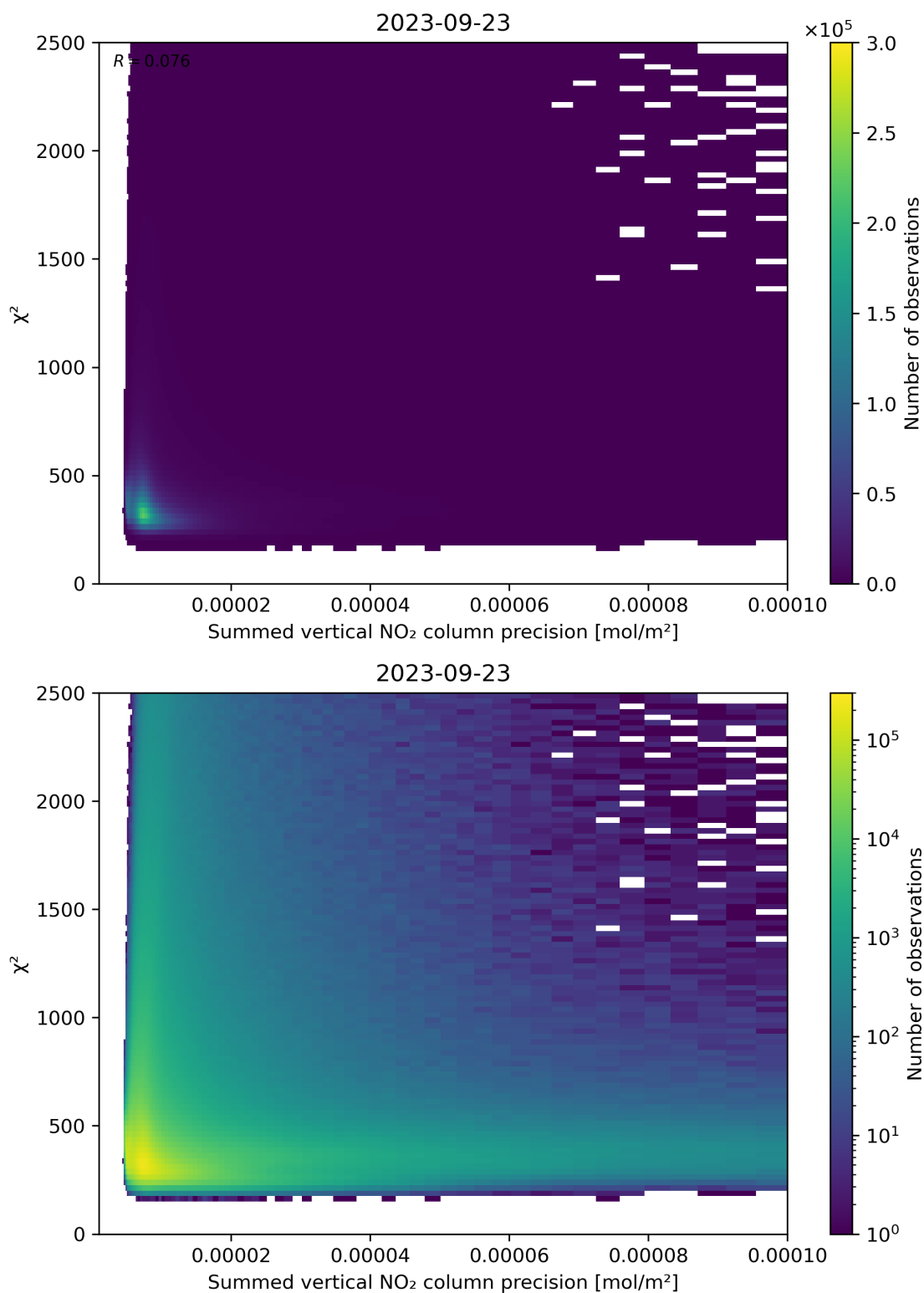
Figure 107: Scatter density plot of “Summed vertical NO 2 column precision” against “ \chi^2 ” for 2023-09-22 to 2023-09-24.
