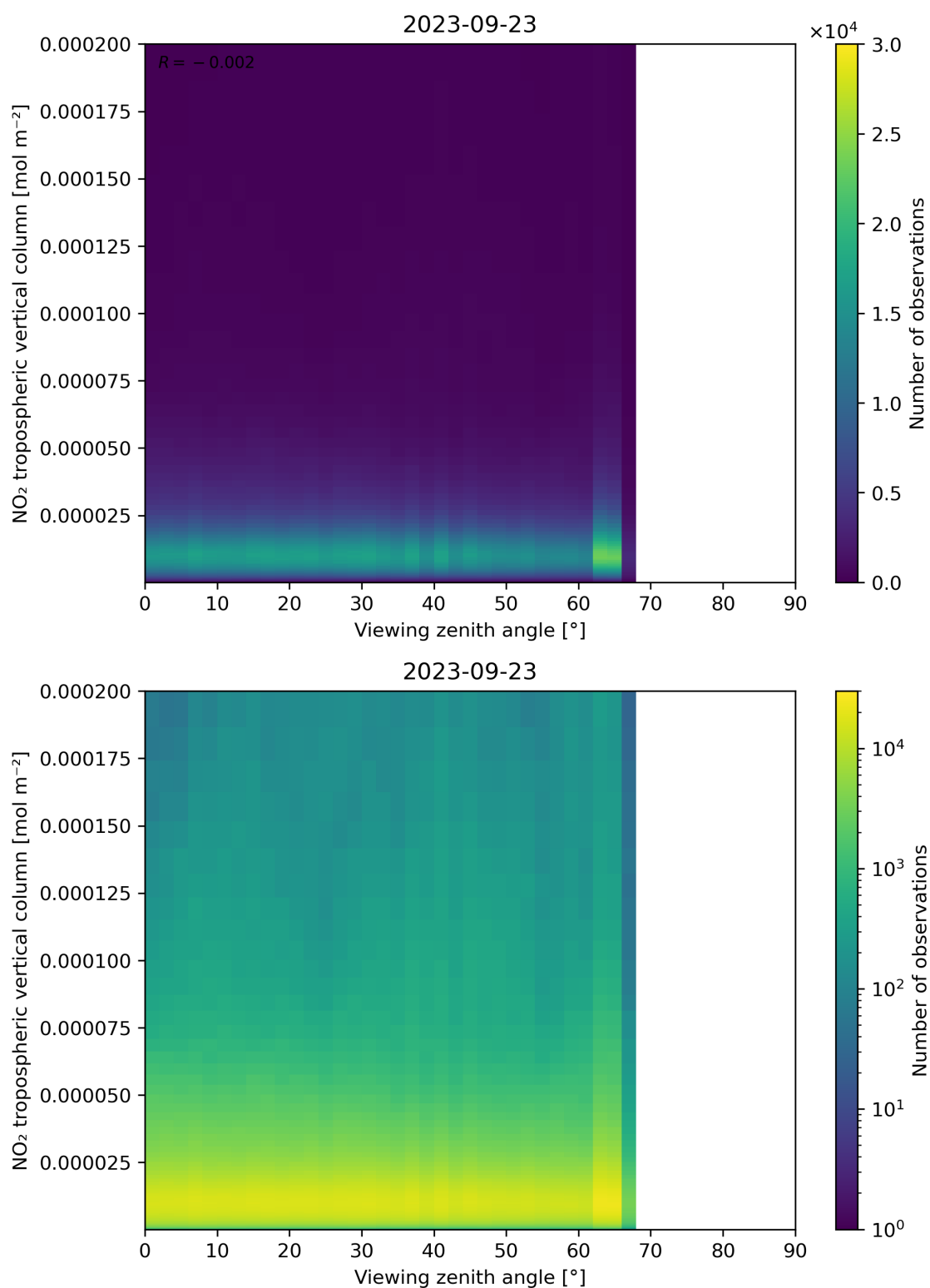
Figure 169: Scatter density plot of “Viewing zenith angle” against “NO 2 tropospheric vertical column” for 2023-09-22 to 2023-09-24.
