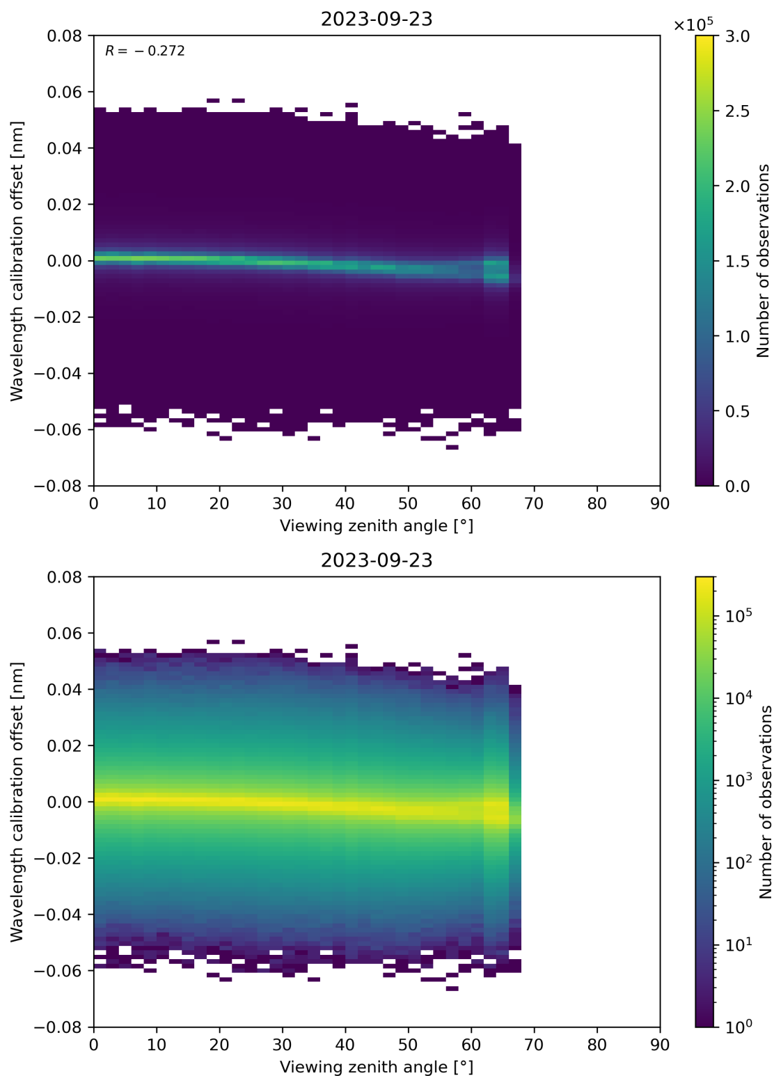
Figure 173: Scatter density plot of “Viewing zenith angle” against “Wavelength calibration offset” for 2023-09-22 to 2023-09-24.
