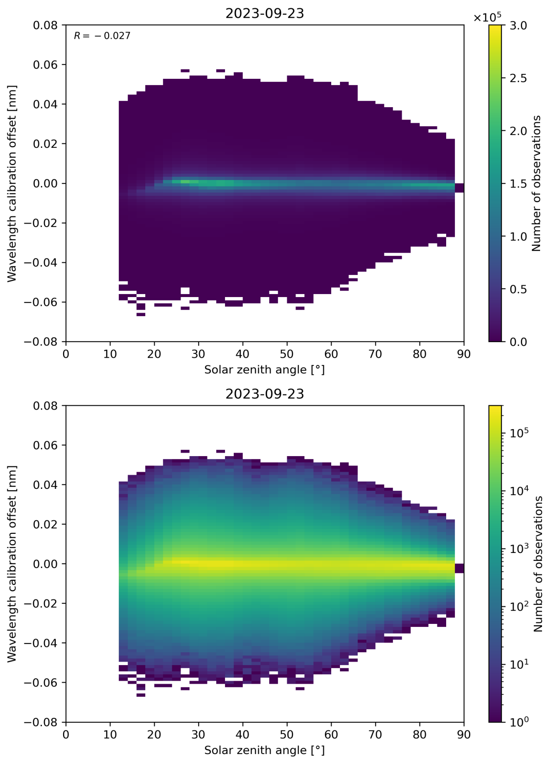
Figure 158: Scatter density plot of “Solar zenith angle” against “Wavelength calibration offset” for 2023-09-22 to 2023-09-24.
