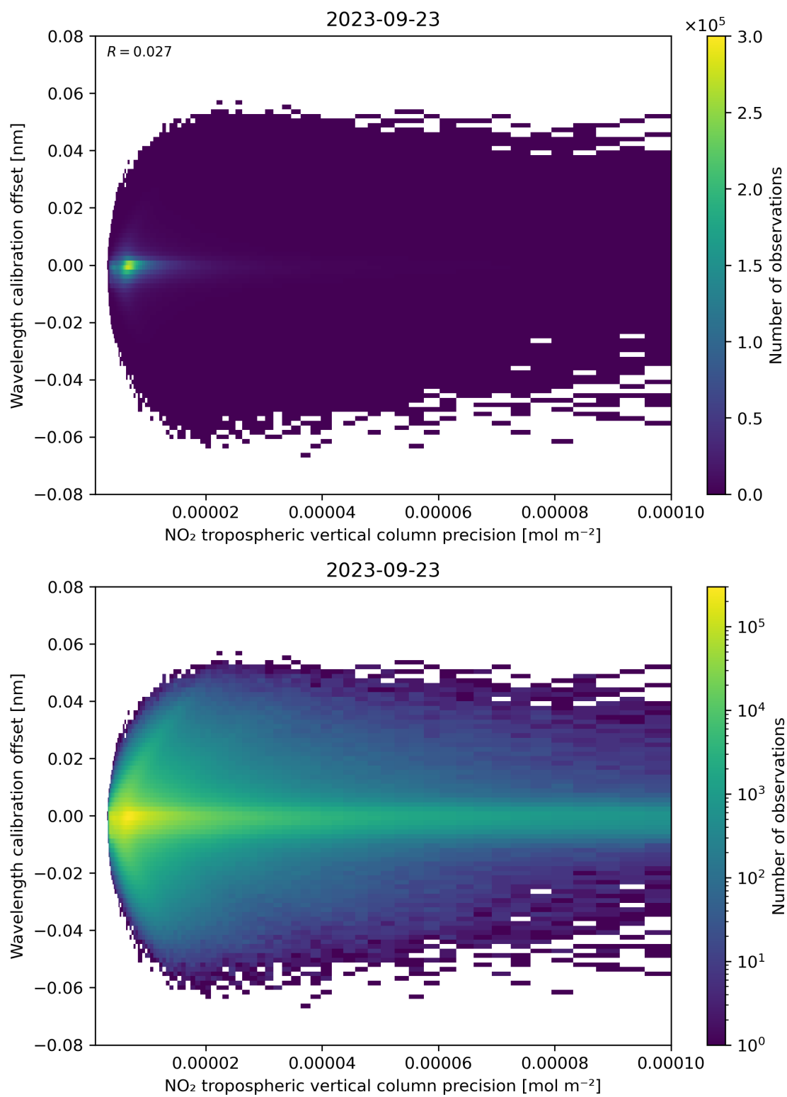
Figure 141: Scatter density plot of “NO 2 tropospheric vertical column precision” against “Wavelength calibration offset” for 2023-09-22 to 2023-09-24.
