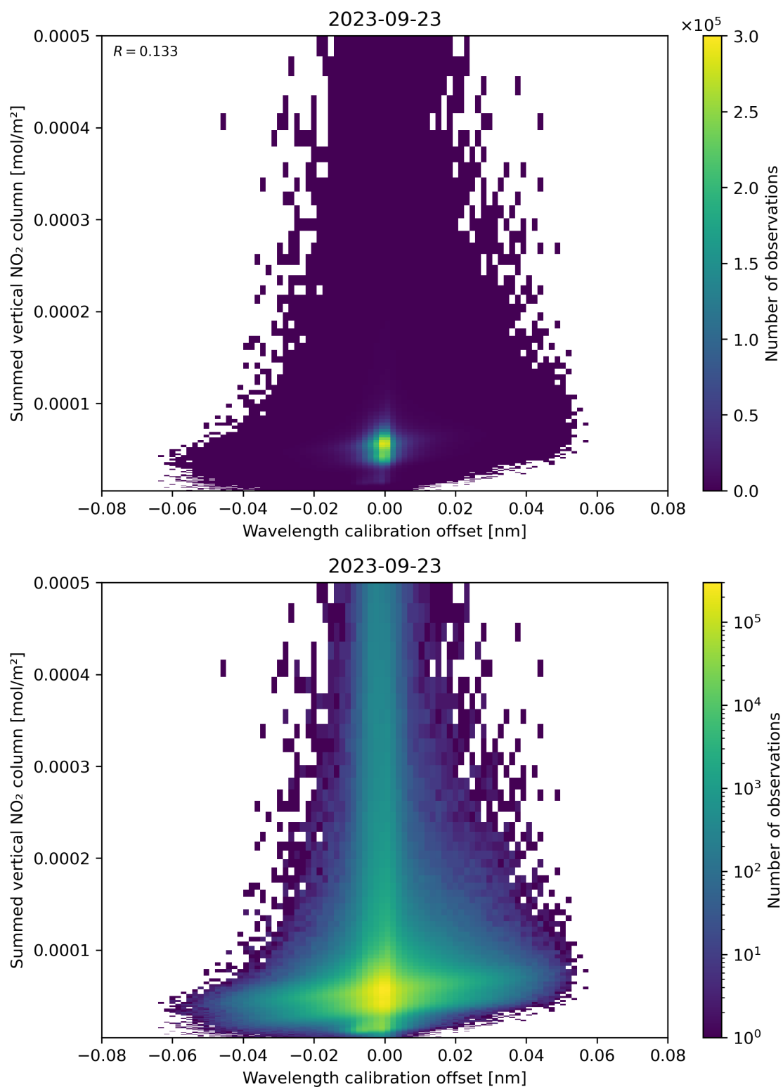
Figure 177: Scatter density plot of “Wavelength calibration offset” against “Summed vertical NO 2 column” for 2023-09-22 to 2023-09-24.
