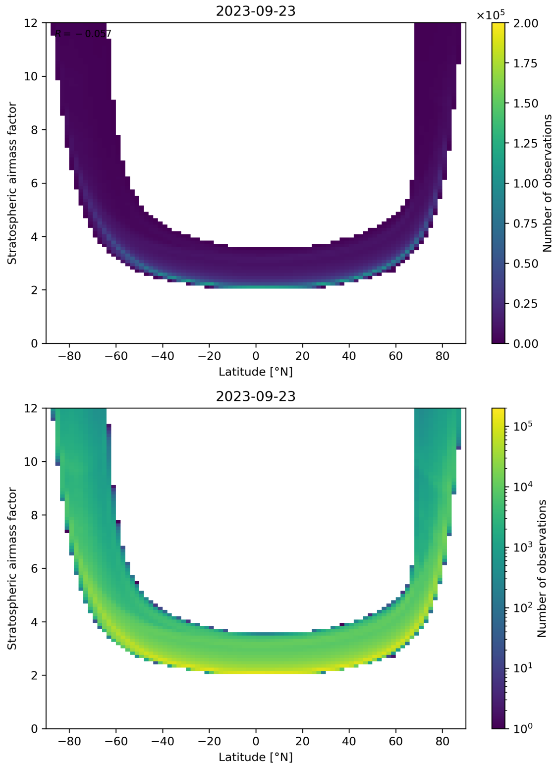
Figure 83: Scatter density plot of “Latitude” against “Stratospheric air mass factor” for 2023-09-22 to 2023-09-24.
