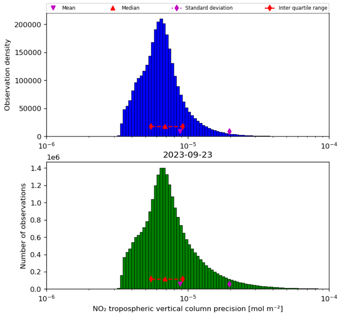
Figure 30: Histogram of “NO 2 tropospheric vertical column precision” for 2023-09-22 to 2023-09-24
