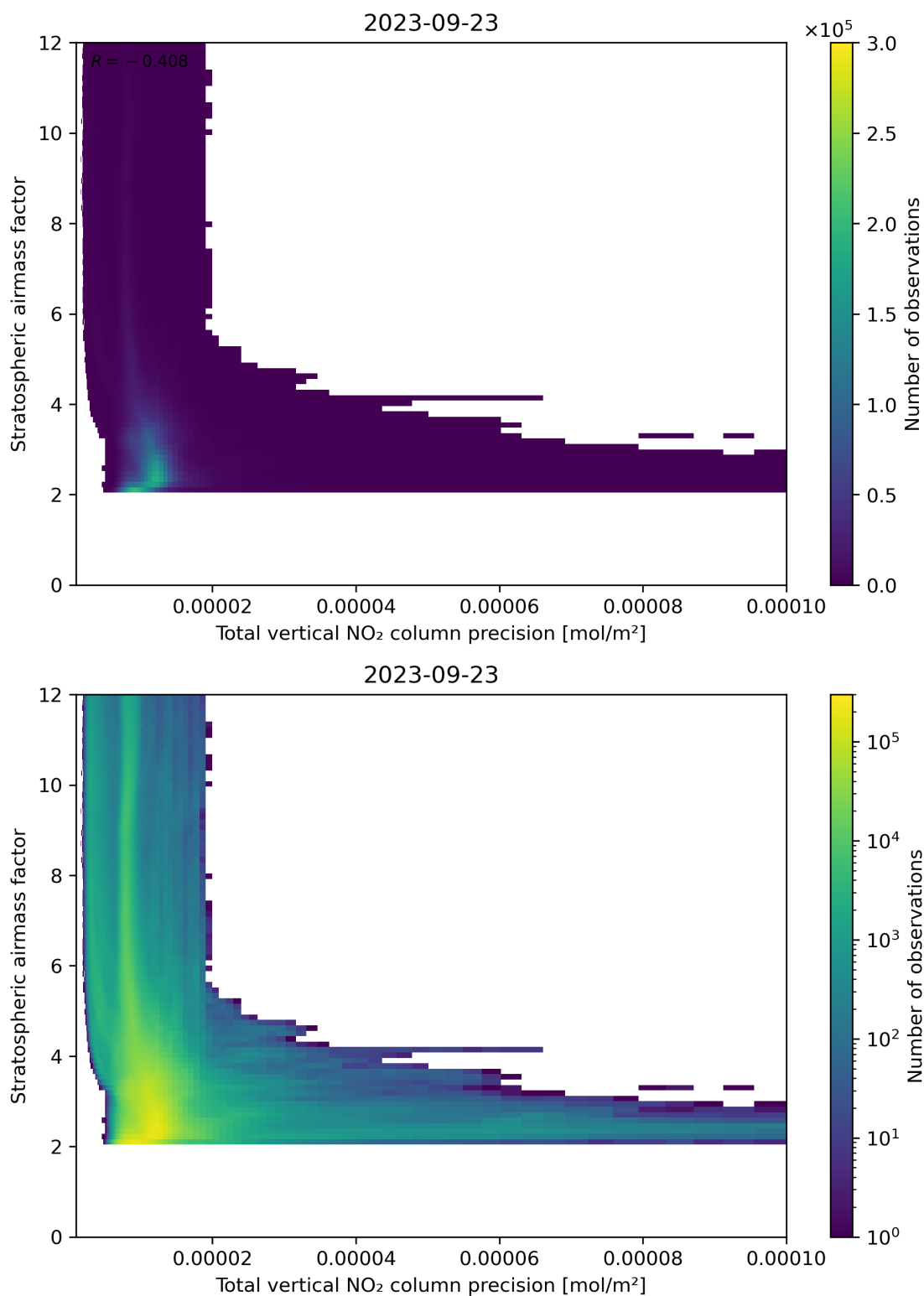
Figure 115: Scatter density plot of “Total vertical NO 2 column precision” against “Stratospheric airmass factor” for 2023-09-22 to 2023-09-24.
