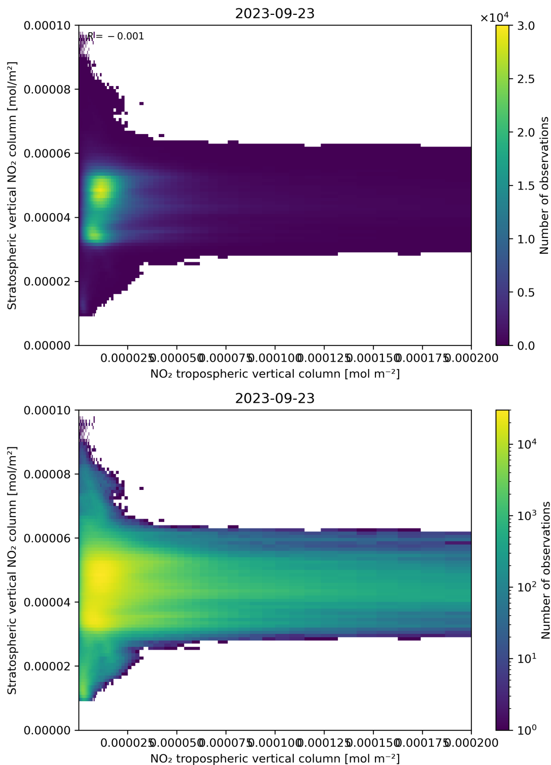
Figure 125: Scatter density plot of “NO 2 tropospheric vertical column” against “Stratospheric vertical NO 2 column” for 2023-09-22 to 2023-09-24.
