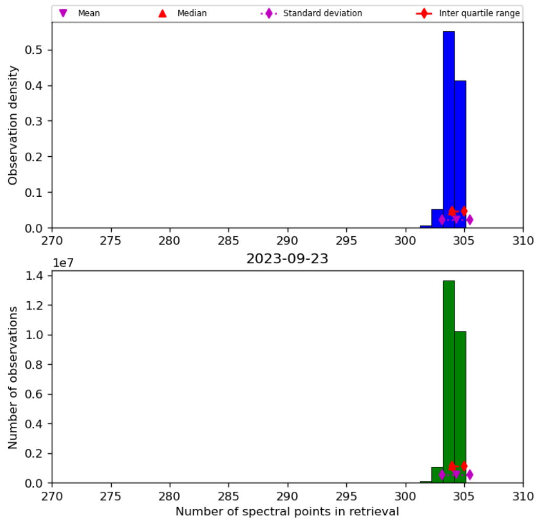
Figure 33: Histogram of “Number of spectral points in retrieval” for 2023-09-22 to 2023-09-24
