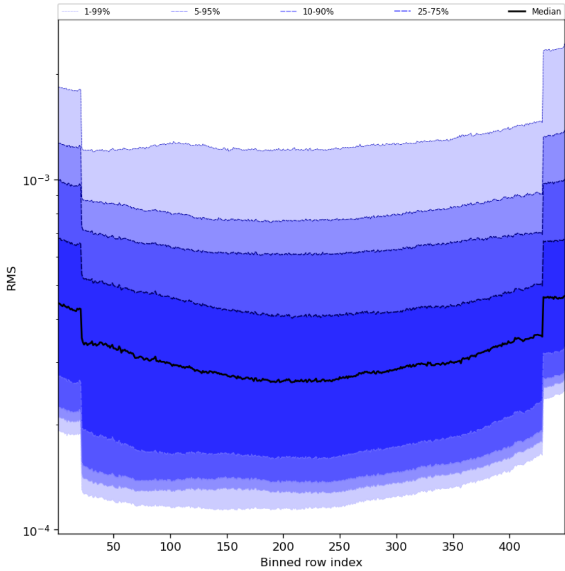
Figure 60: Along track statistics of “RMS” for 2023-09-22 to 2023-09-24
