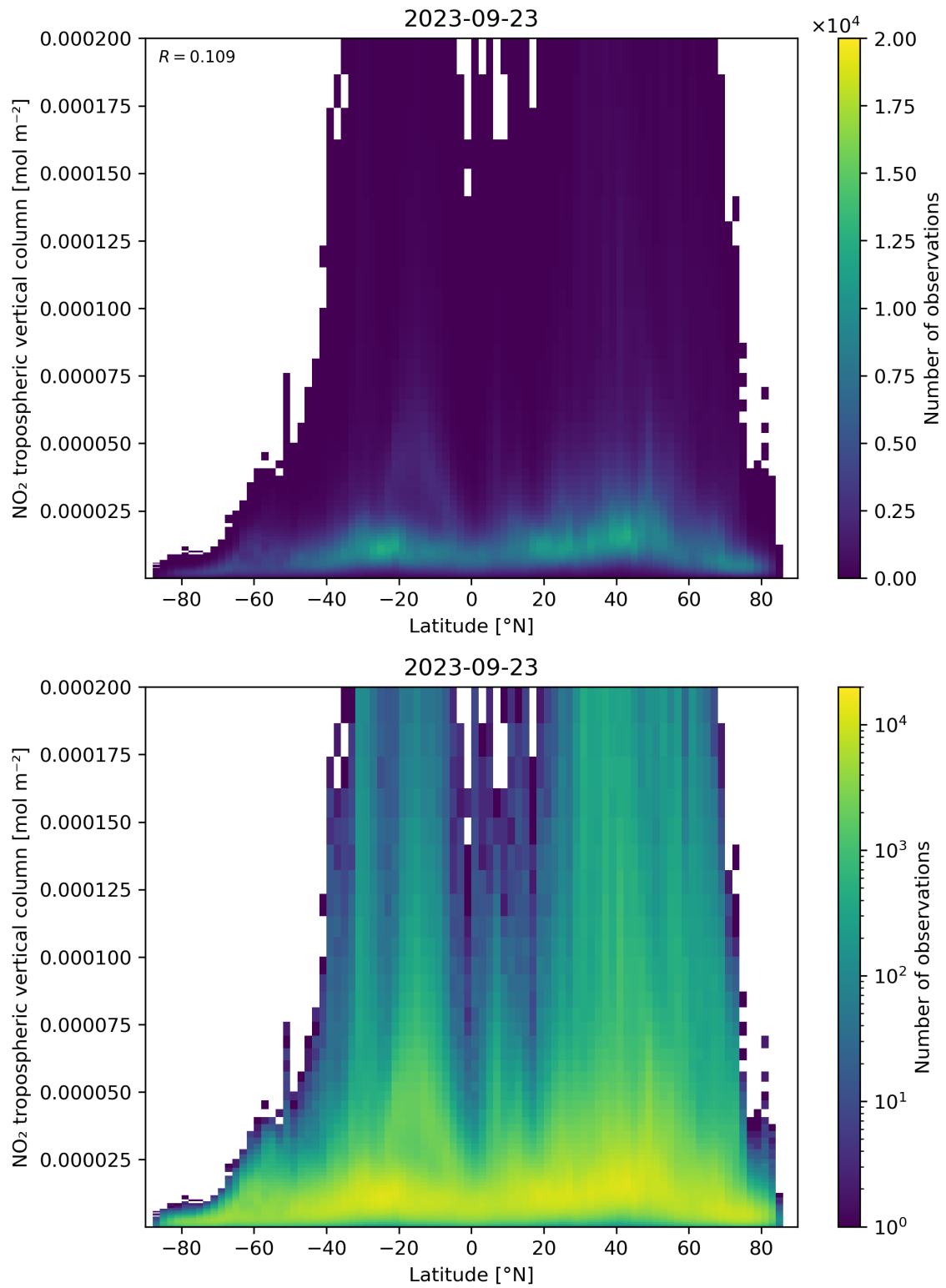
Figure 92: Scatter density plot of “Latitude” against “NO 2 tropospheric vertical column” for 2023-09-22 to 2023-09-24.
