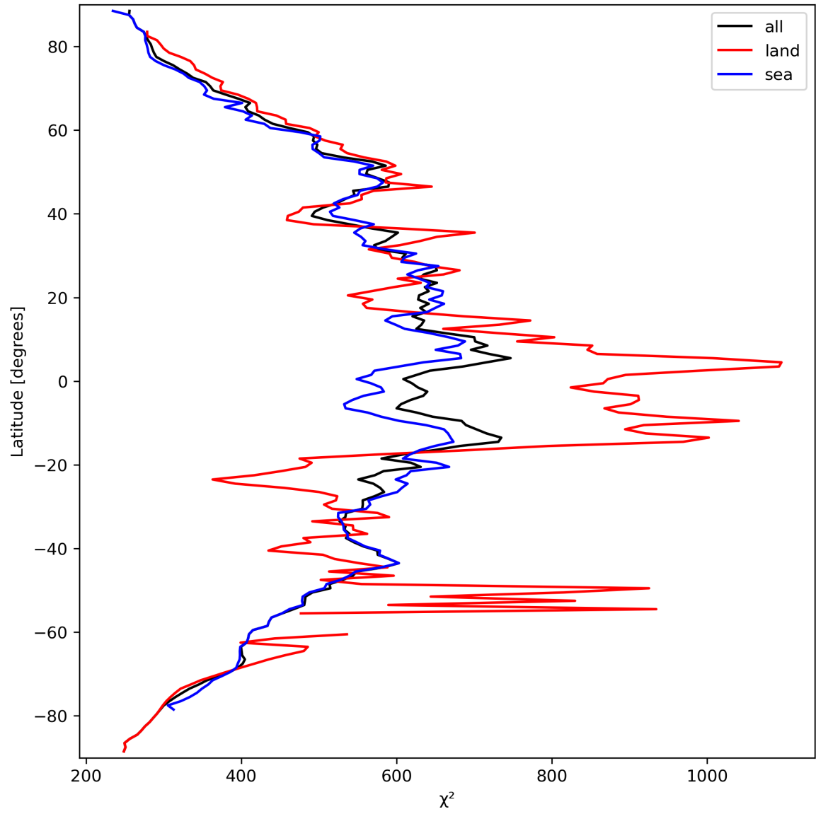
Figure 25: Zonal average of “ \chi^2 ” for 2023-09-22 to 2023-09-24.
