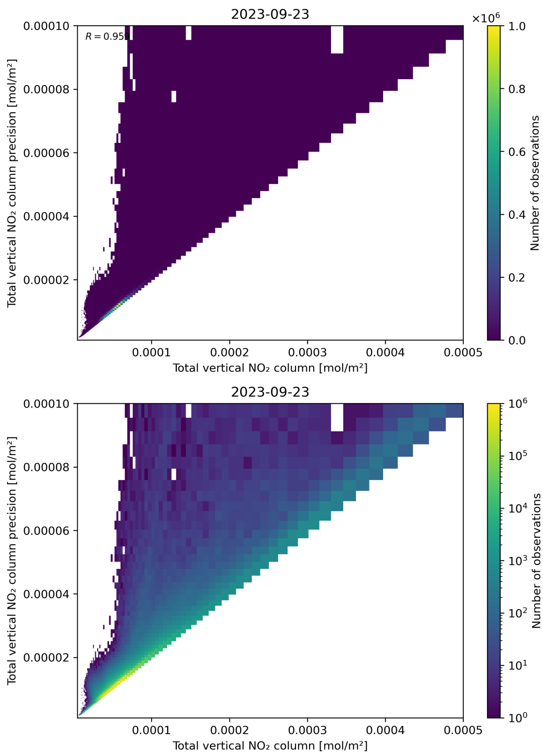
Figure 114: Scatter density plot of “Total vertical NO 2 column” against “Total vertical NO 2 column precision” for 2023-09-22 to 2023-09-24.
