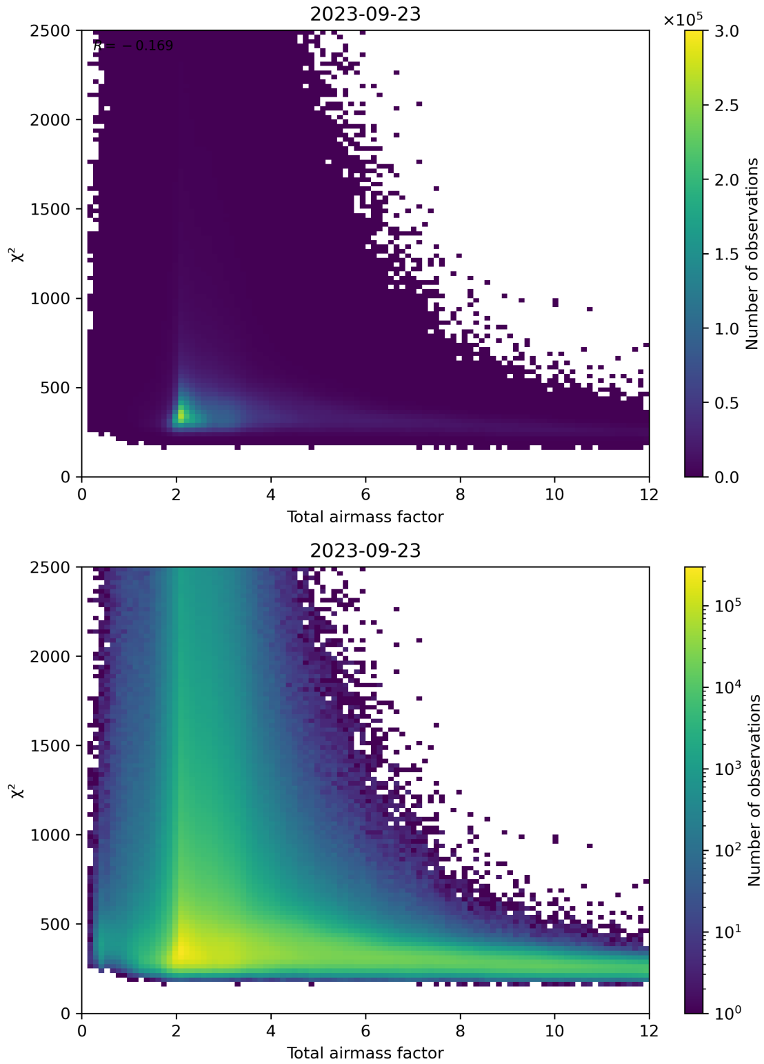
Figure 63: Scatter density plot of “Total airmass factor” against “ \chi^2 ” for 2023-09-22 to 2023-09-24.
