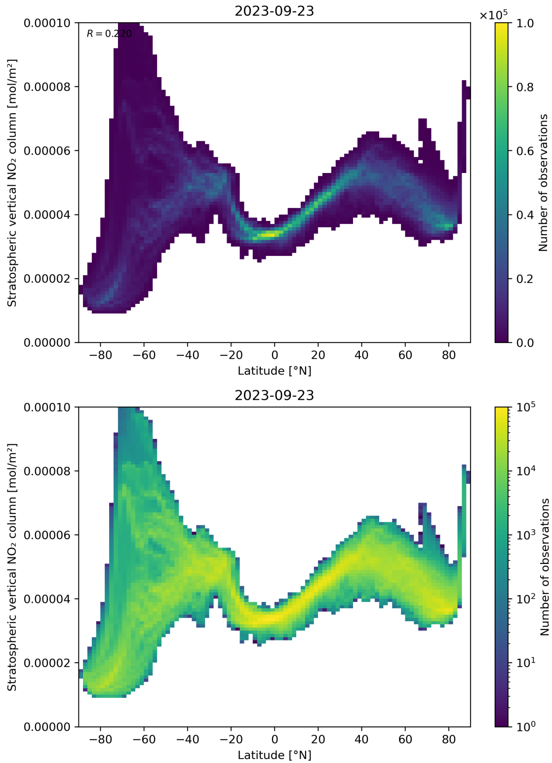
Figure 87: Scatter density plot of “Latitude” against “Stratospheric vertical NO 2 column” for 2023-09-22 to 2023-09-24.
