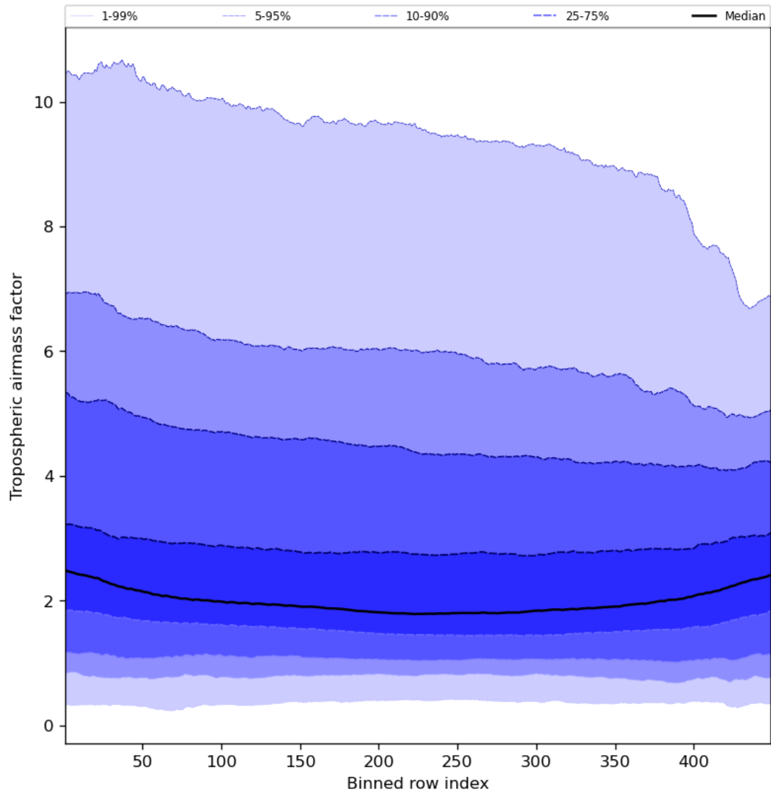
Figure 48: Along track statistics of “Tropospheric airmass factor” for 2023-09-22 to 2023-09-24
