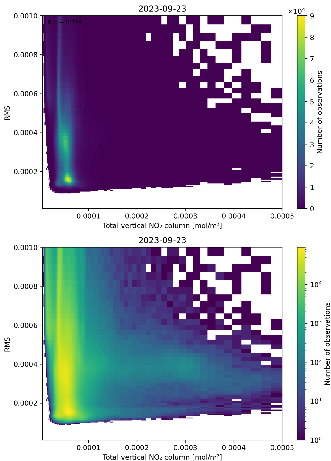
Figure 120: Scatter density plot of “Total vertical NO 2 column” against “RMS” for 2023-09-22 to 2023-09-24.
