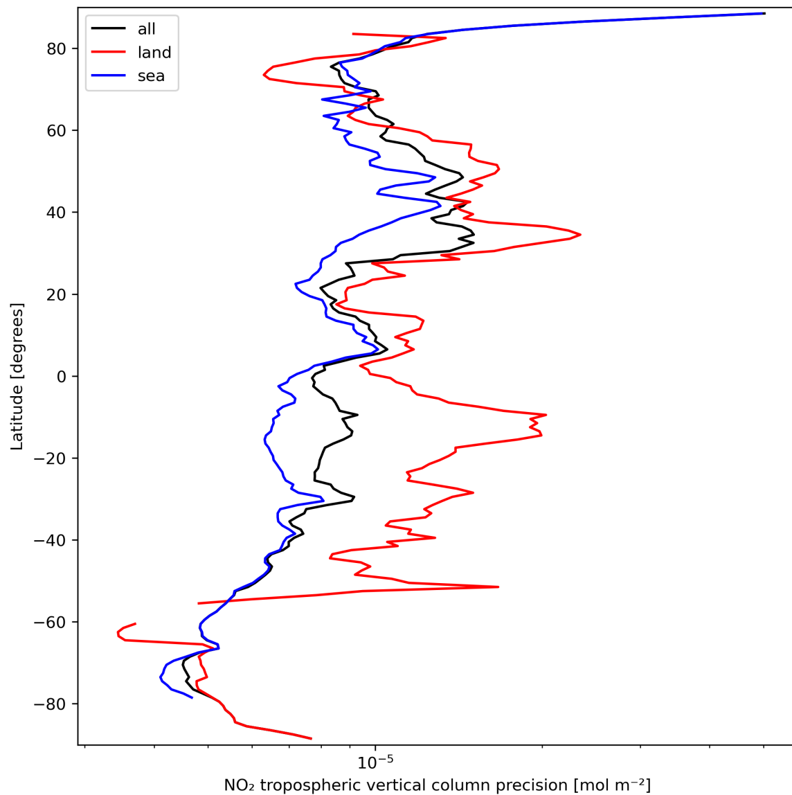
Figure 13: Zonal average of “NO 2 tropospheric vertical column precision” for 2023-09-22 to 2023-09-24.
