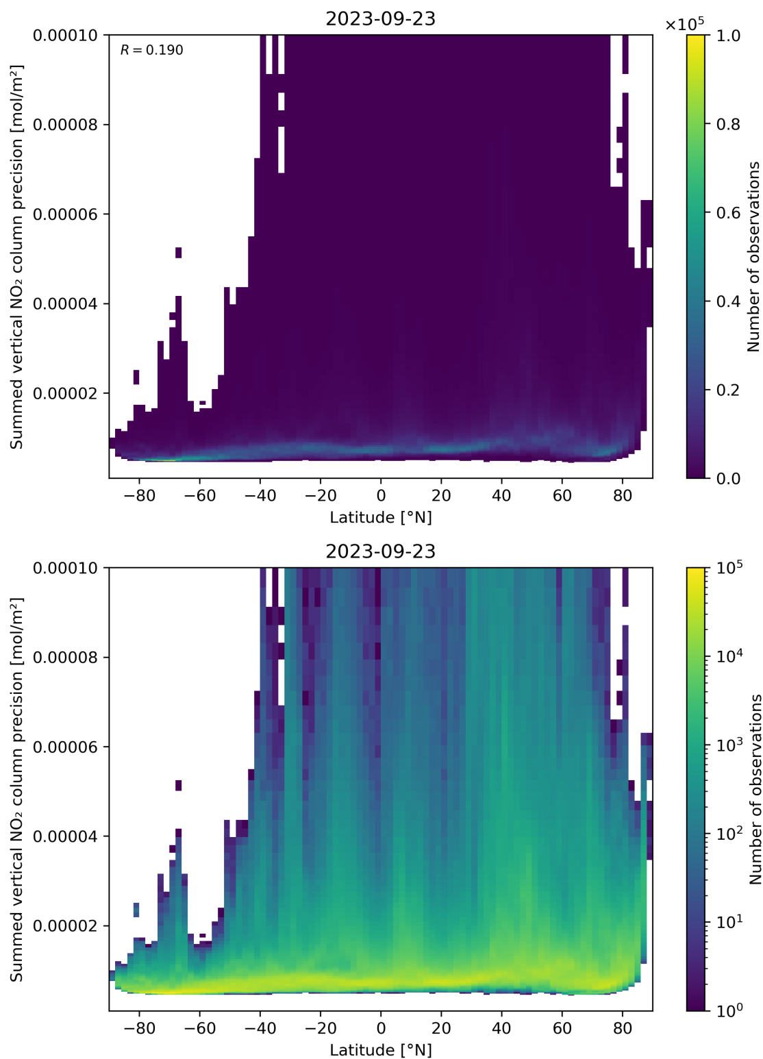
Figure 89: Scatter density plot of “Latitude” against “Summed vertical NO 2 column precision” for 2023-09-22 to 2023-09-24.
