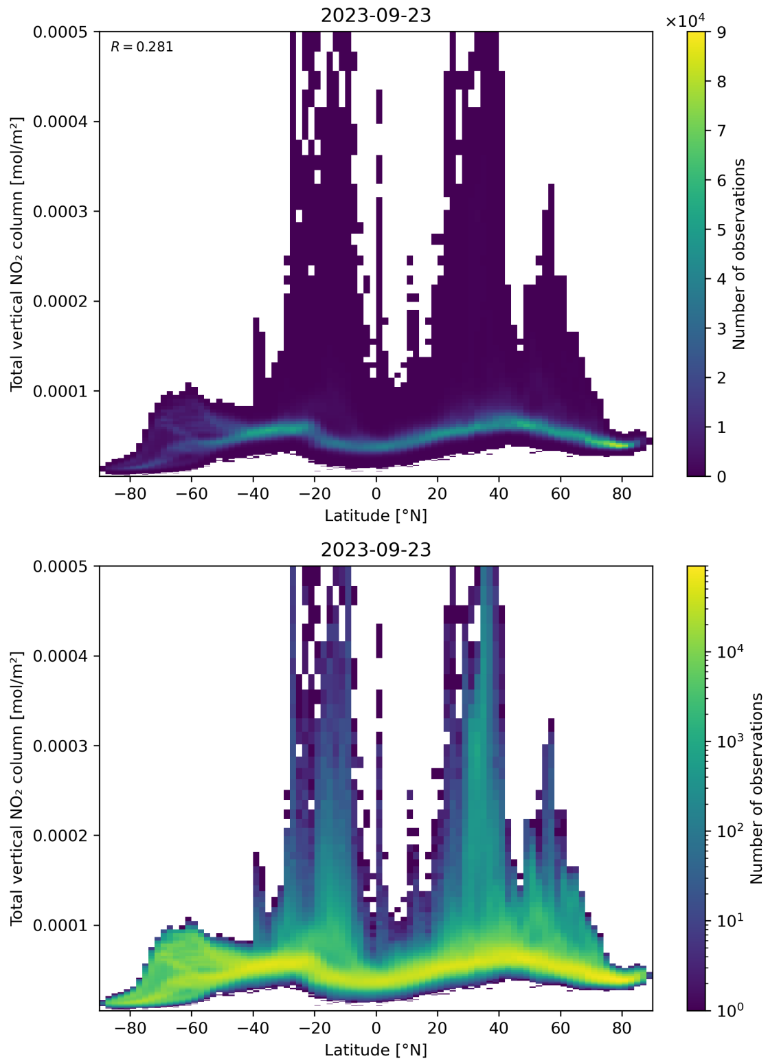
Figure 90: Scatter density plot of “Latitude” against “Total vertical NO 2 column” for 2023-09-22 to 2023-09-24.
