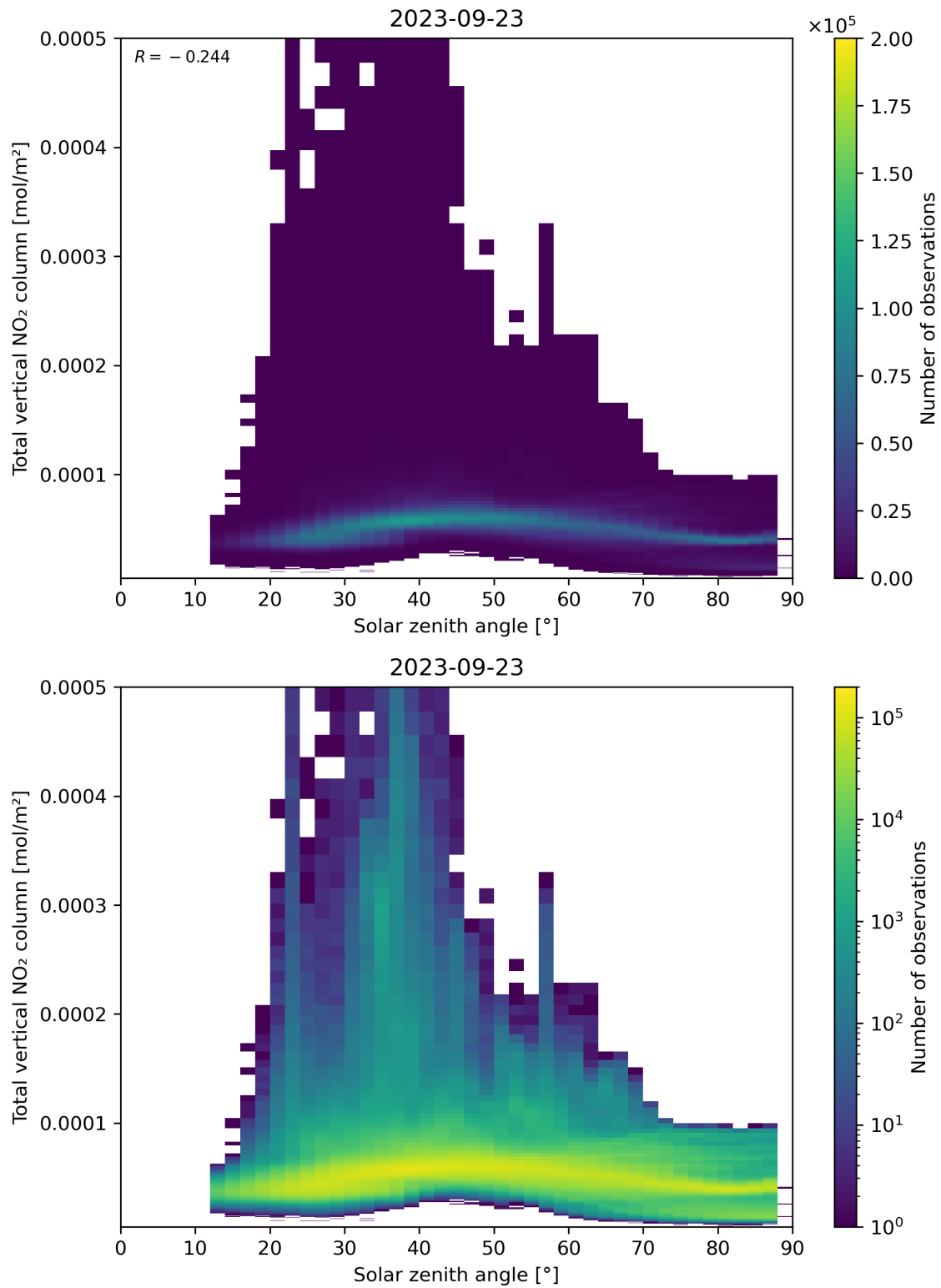
Figure 153: Scatter density plot of “Solar zenith angle” against “Total vertical NO 2 column” for 2023-09-22 to 2023-09-24.
