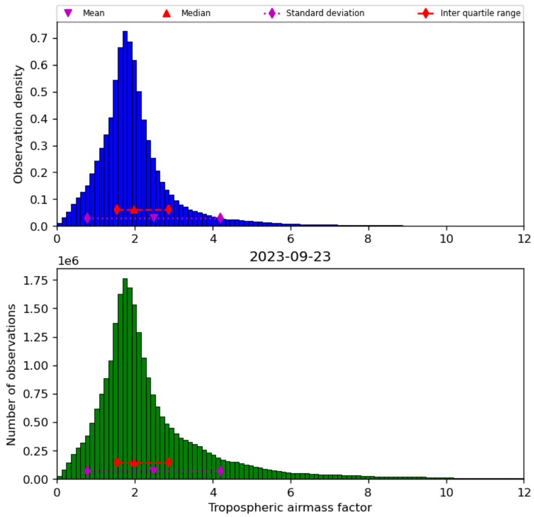
Figure 31: Histogram of “Tropospheric airmass factor” for 2023-09-22 to 2023-09-24
