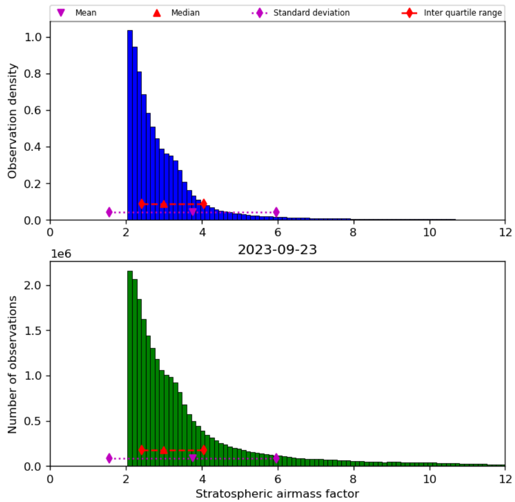
Figure 44: Histogram of “Stratospheric airmass factor” for 2023-09-22 to 2023-09-24
