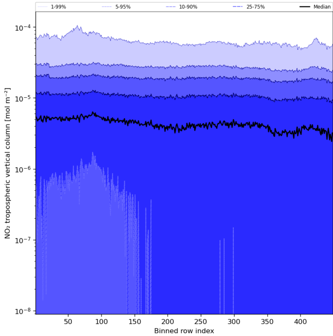
Figure 46: Along track statistics of “NO 2 tropospheric vertical column” for 2023-09-22 to 2023-09-24
