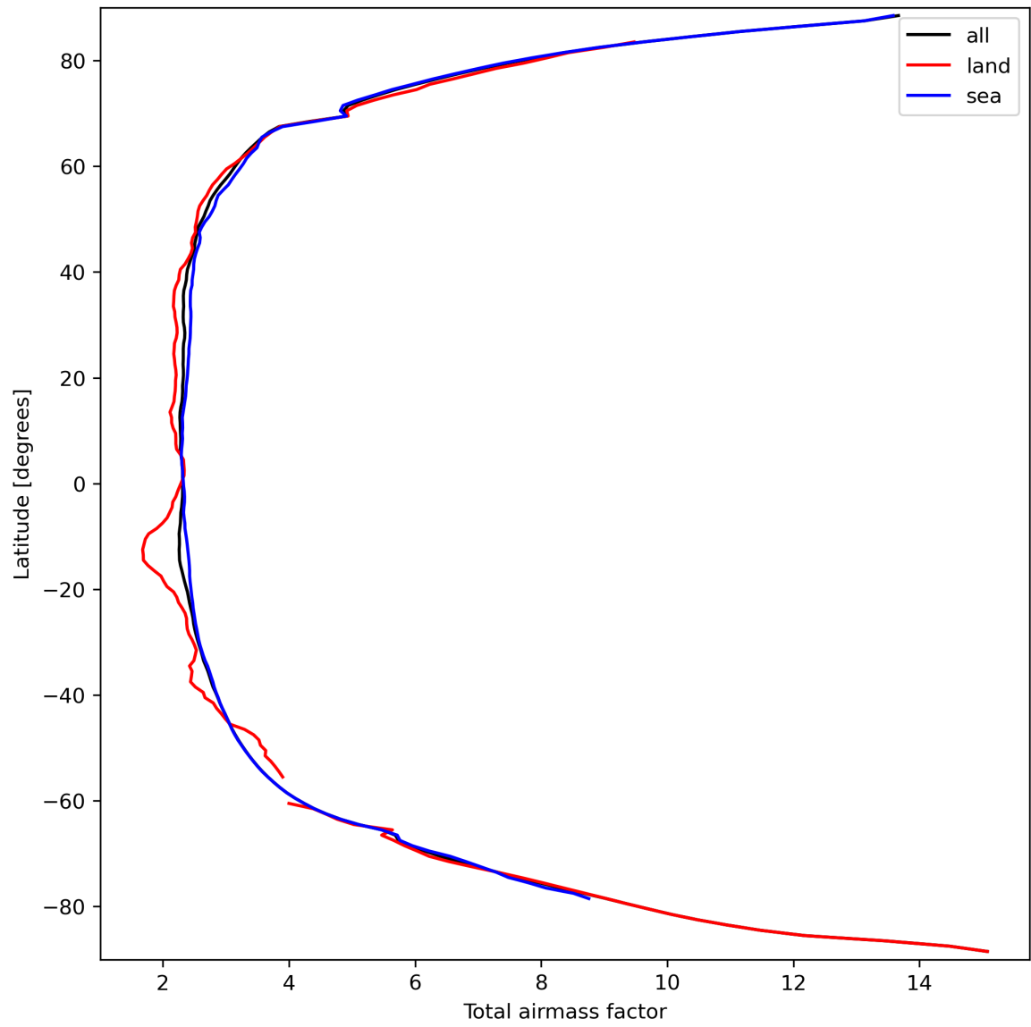
Figure 15: Zonal average of “Total airmass factor” for 2023-09-22 to 2023-09-24.
