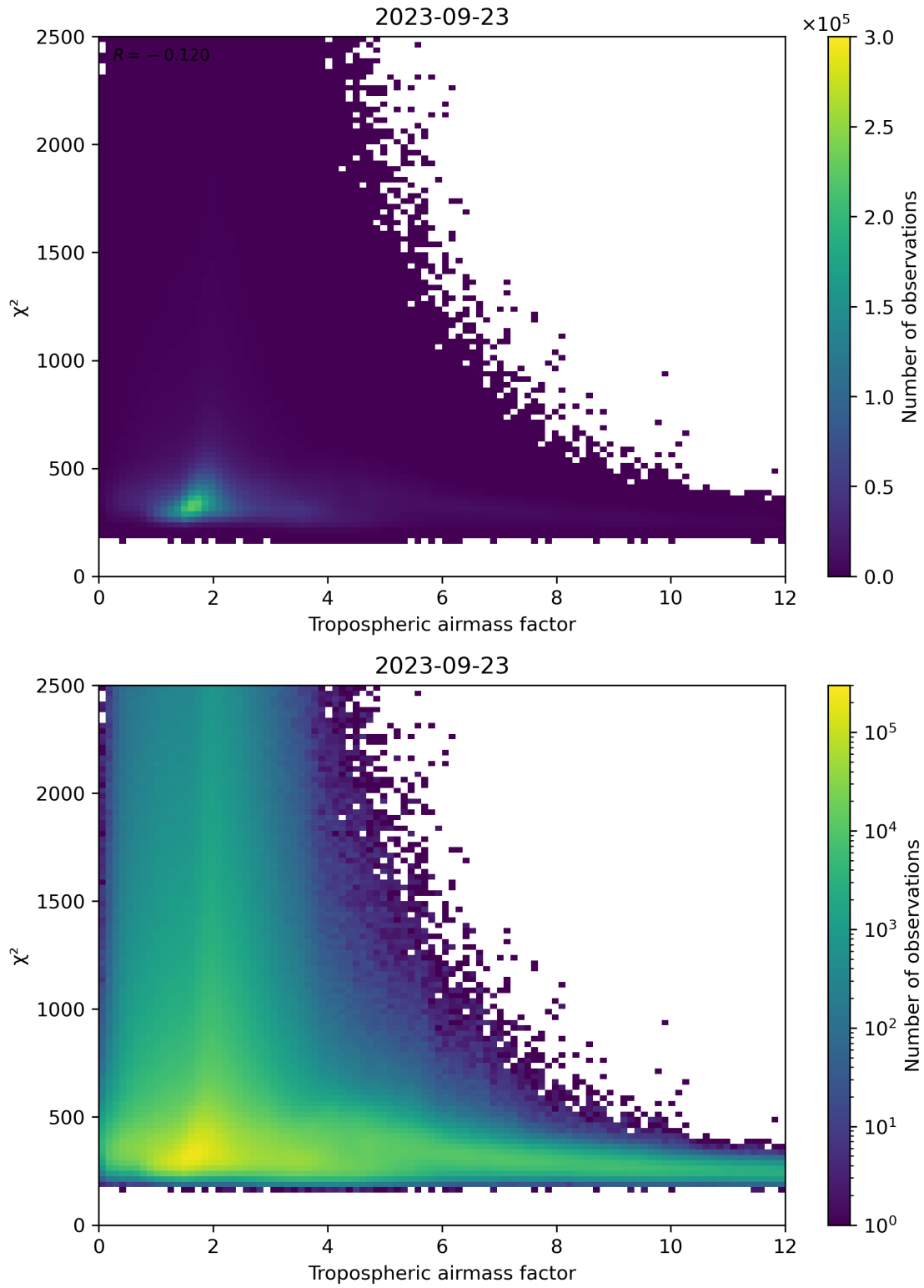
Figure 73: Scatter density plot of “Tropospheric airmass factor” against “ \chi^2 ” for 2023-09-22 to 2023-09-24.
