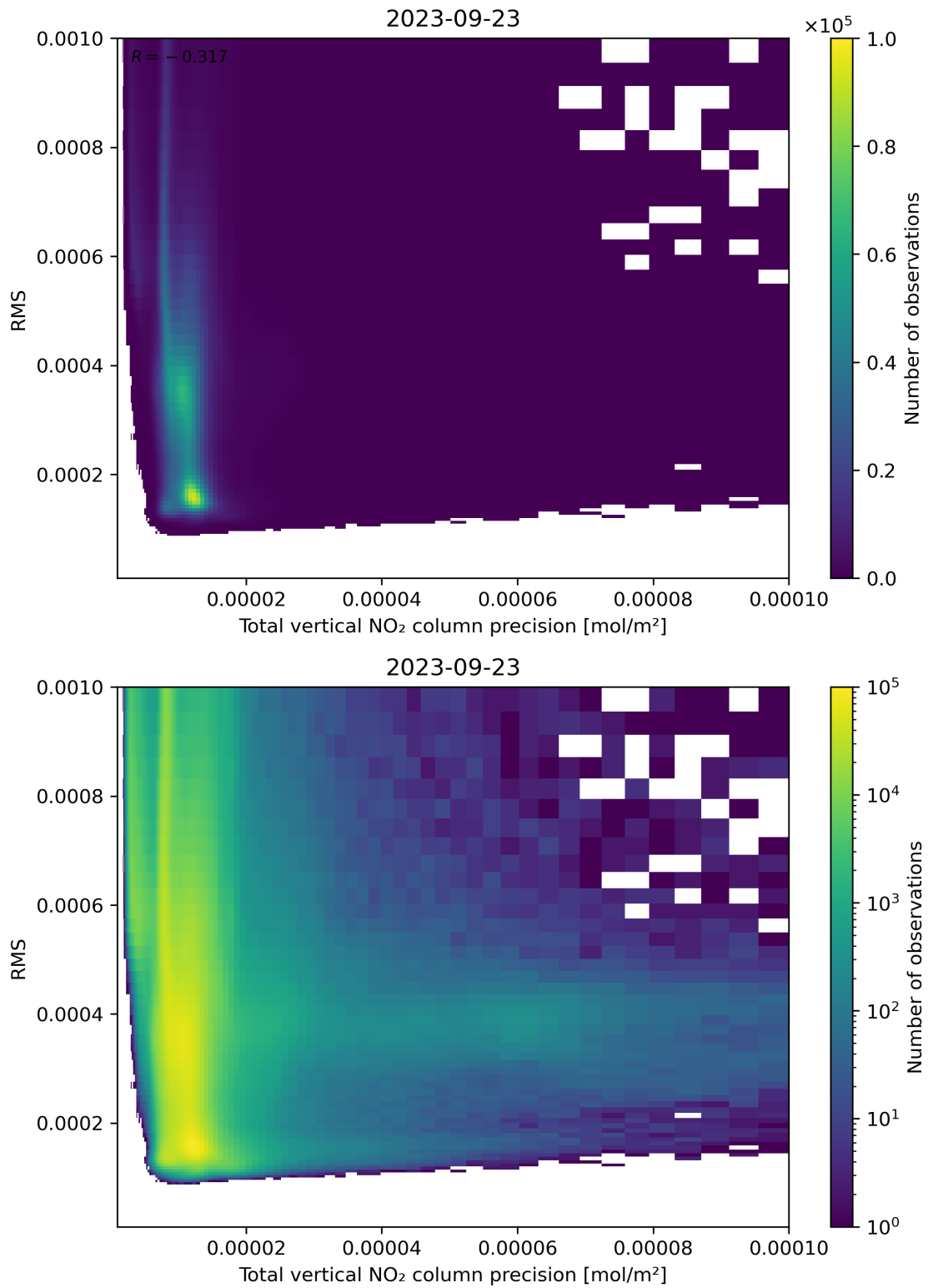
Figure 119: Scatter density plot of “Total vertical NO 2 column precision” against “RMS” for 2023-09-22 to 2023-09-24.
