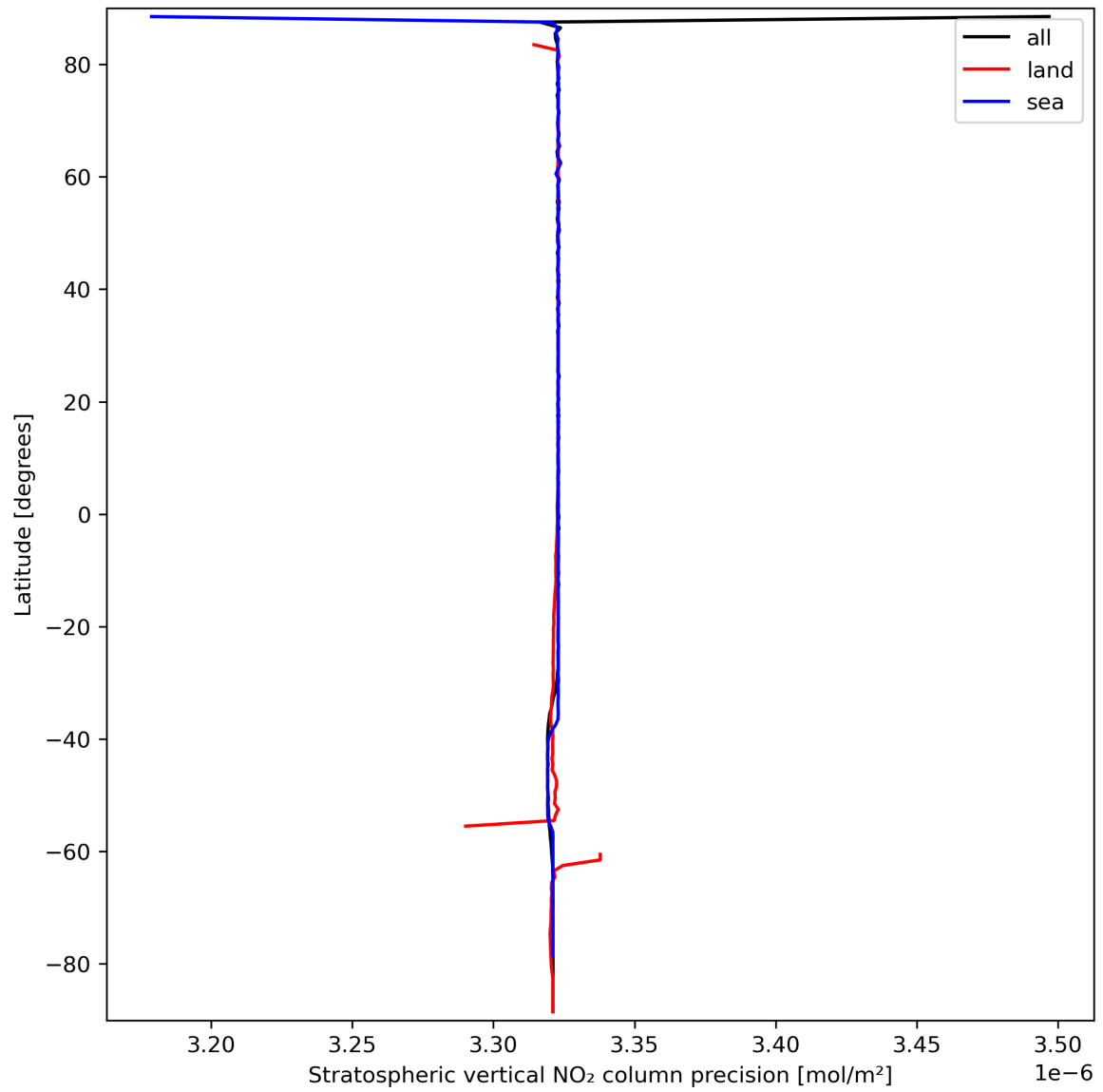
Figure 20: Zonal average of “Stratospheric vertical NO 2 column precision” for 2023-09-22 to 2023-09-24.
