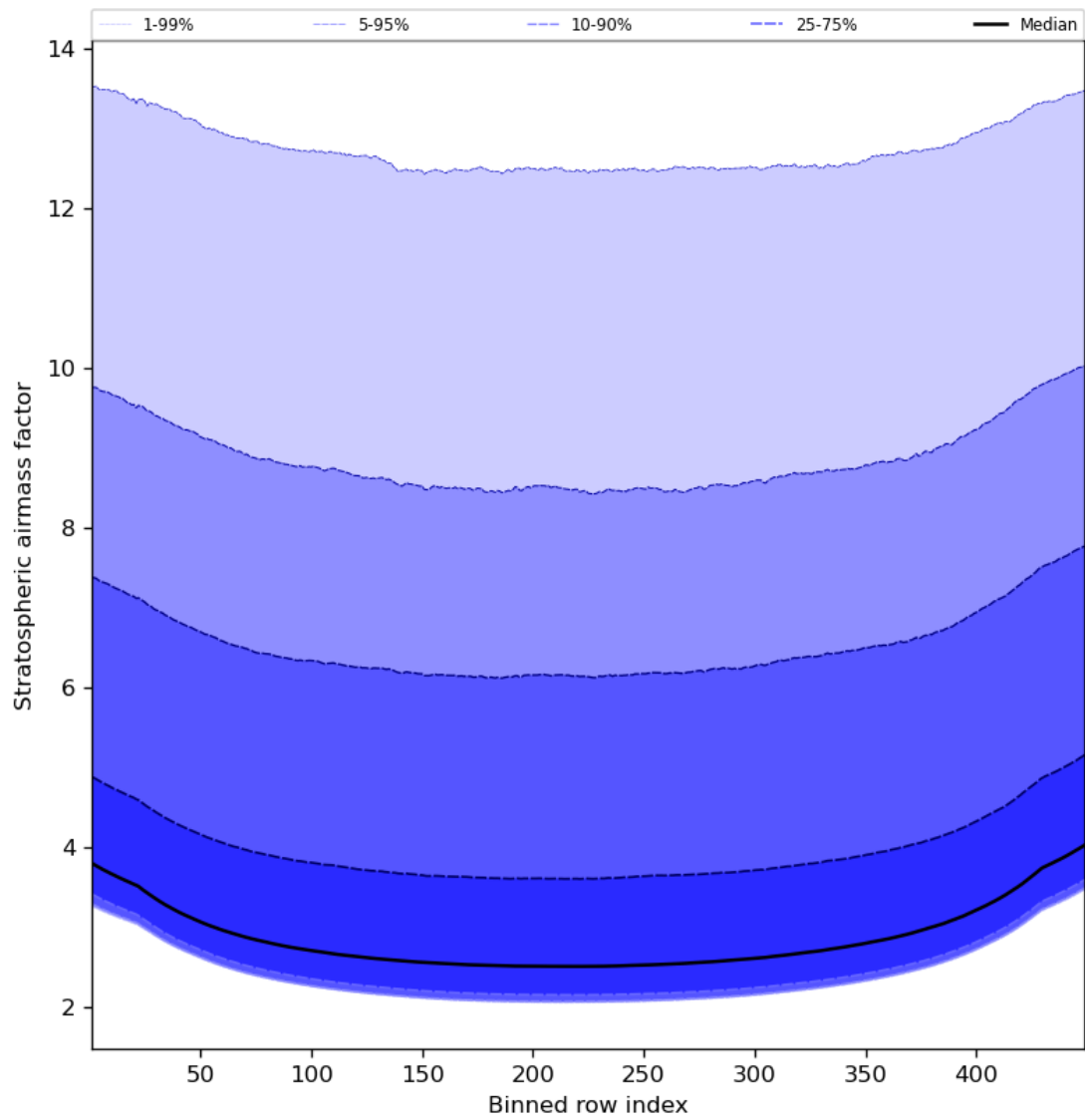
Figure 61: Along track statistics of “Stratospheric airmass factor” for 2023-09-22 to 2023-09-24
