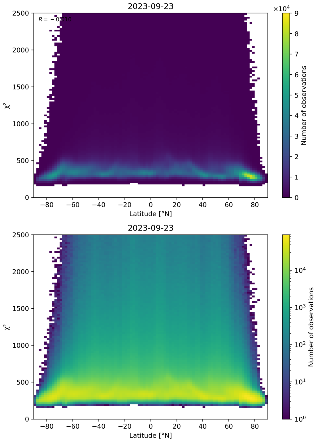
Figure 86: Scatter density plot of “Latitude” against “ \chi^2 ” for 2023-09-22 to 2023-09-24.
