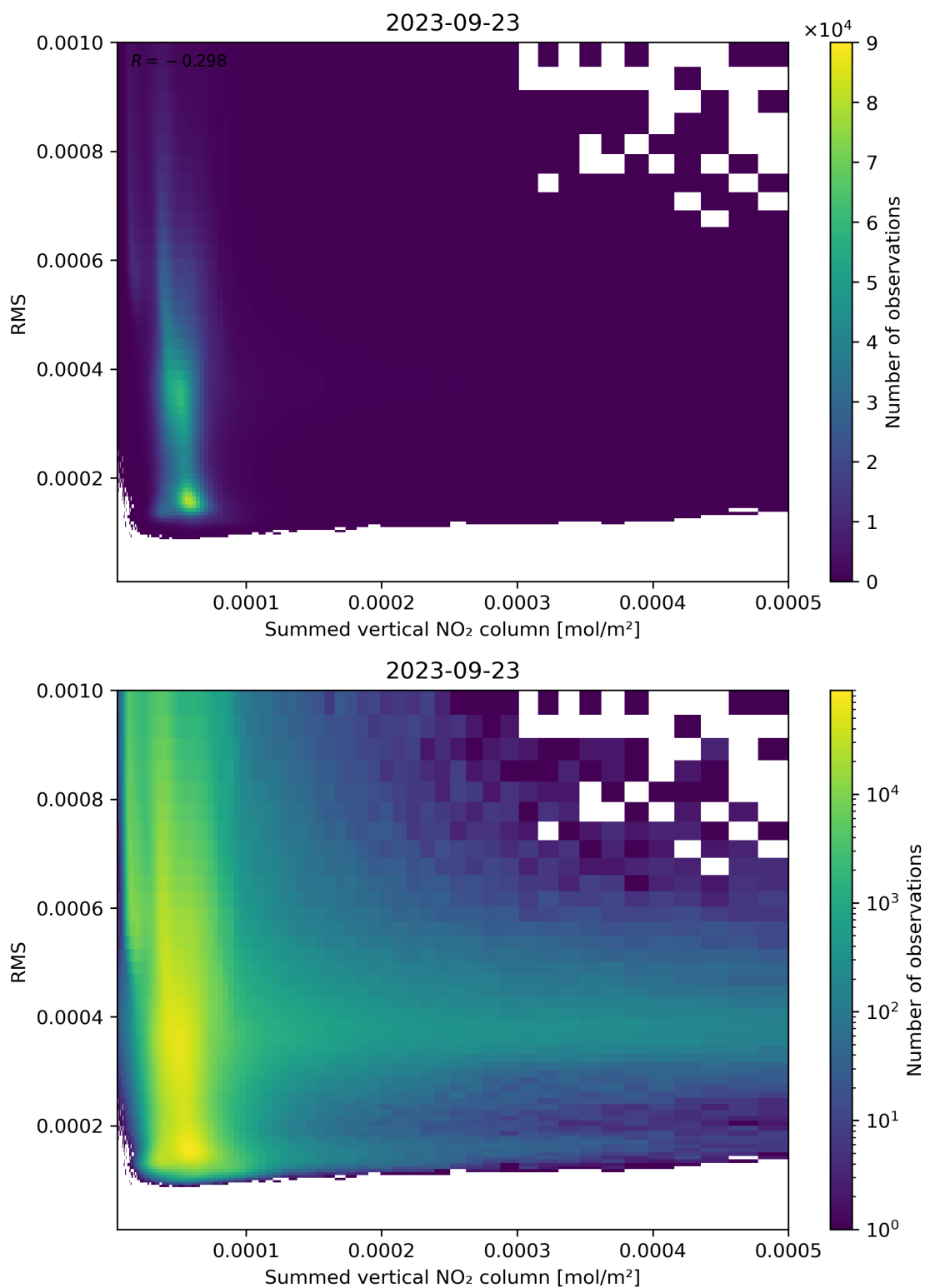
Figure 109: Scatter density plot of “Summed vertical NO 2 column” against “RMS” for 2023-09-22 to 2023-09-24.
