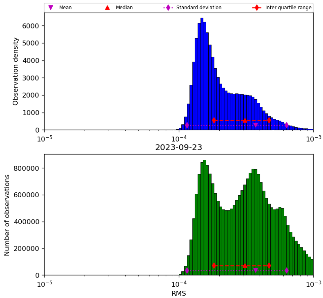
Figure 43: Histogram of “RMS” for 2023-09-22 to 2023-09-24
