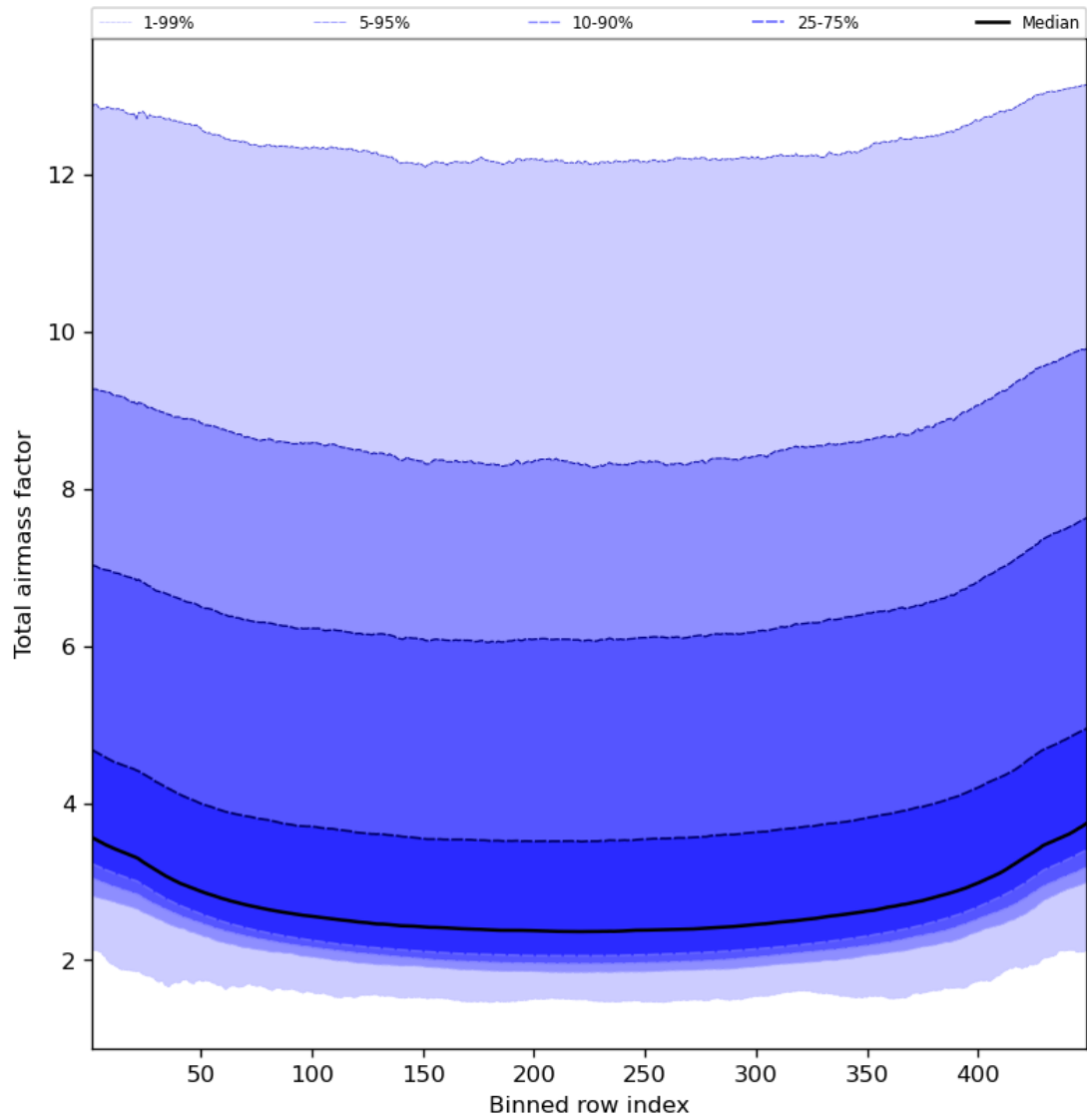
Figure 49: Along track statistics of “Total airmass factor” for 2023-09-22 to 2023-09-24
