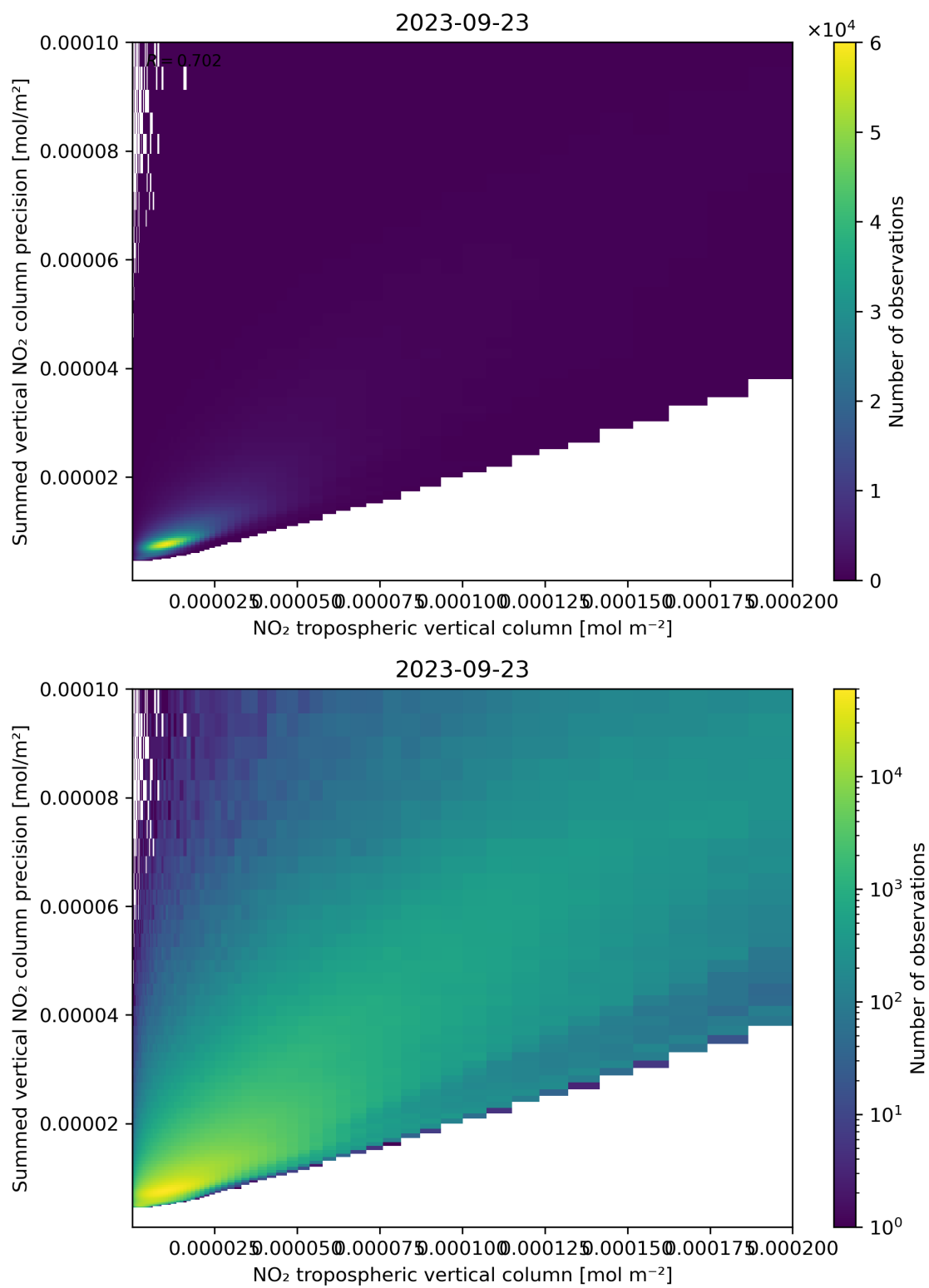
Figure 127: Scatter density plot of “NO 2 tropospheric vertical column” against “Summed vertical NO 2 column precision” for 2023-09-22 to 2023-09-24.
