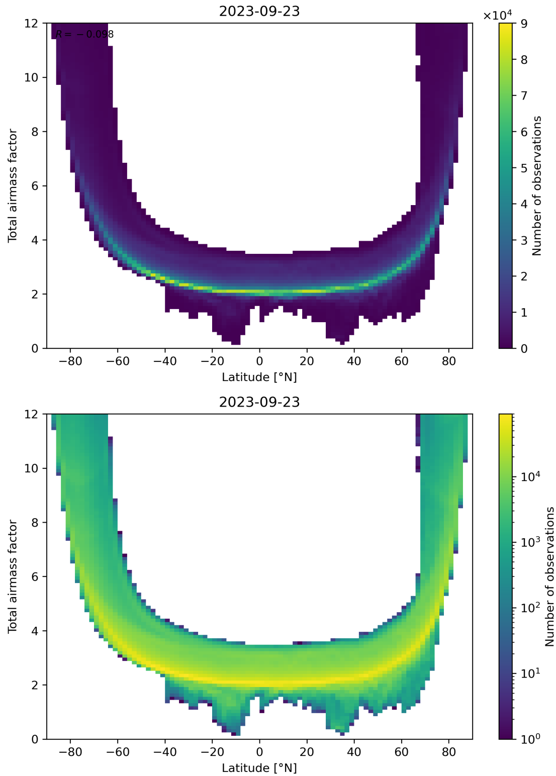
Figure 84: Scatter density plot of “Latitude” against “Total airmass factor” for 2023-09-22 to 2023-09-24.
