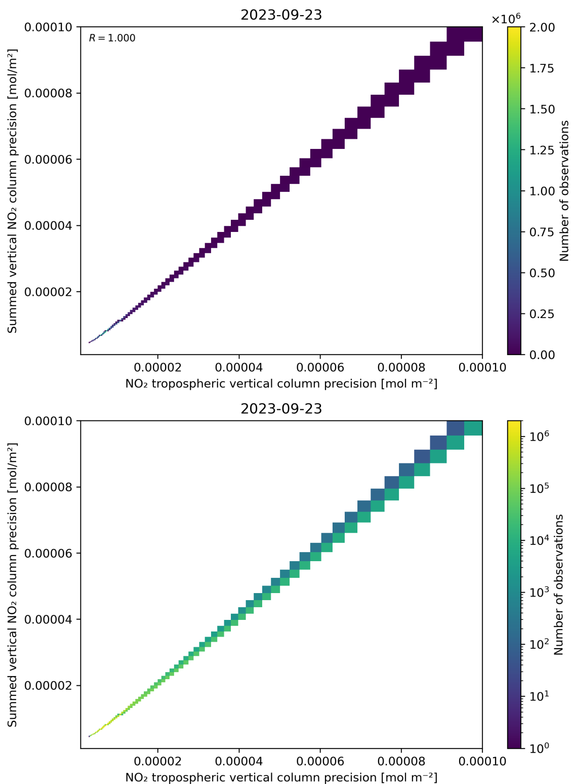
Figure 137: Scatter density plot of “NO 2 tropospheric vertical column precision” against “Summed vertical NO 2 column precision” for 2023-09-22 to 2023-09-24.
