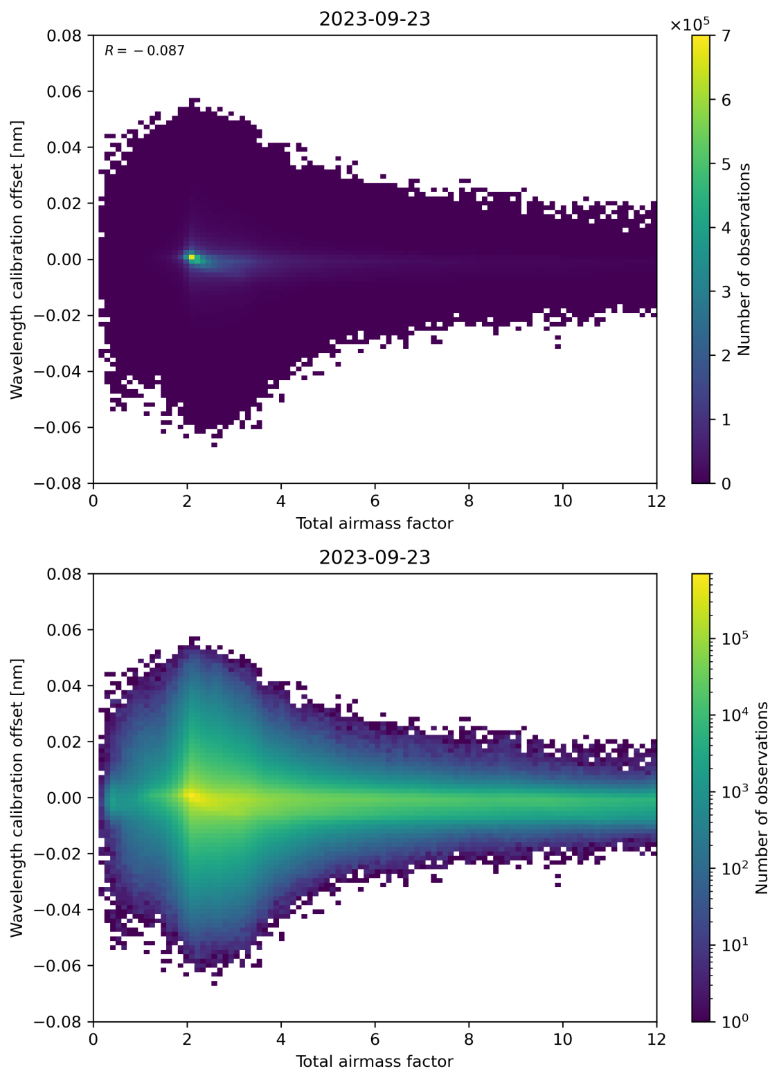
Figure 70: Scatter density plot of “Total airmass factor” against “Wavelength calibration offset” for 2023-09-22 to 2023-09-24.
