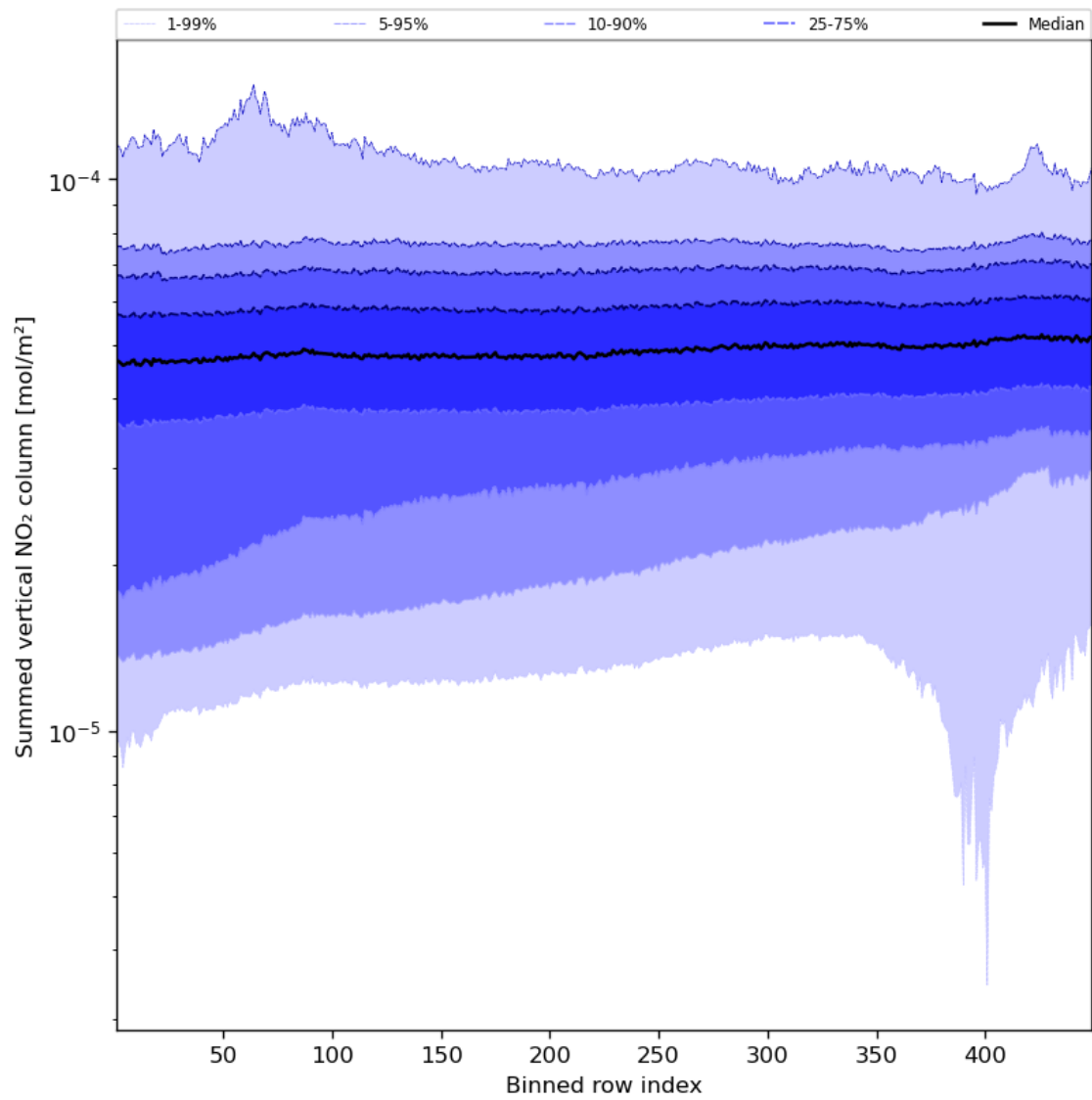
Figure 57: Along track statistics of “Summed vertical NO 2 column” for 2023-09-22 to 2023-09-24
