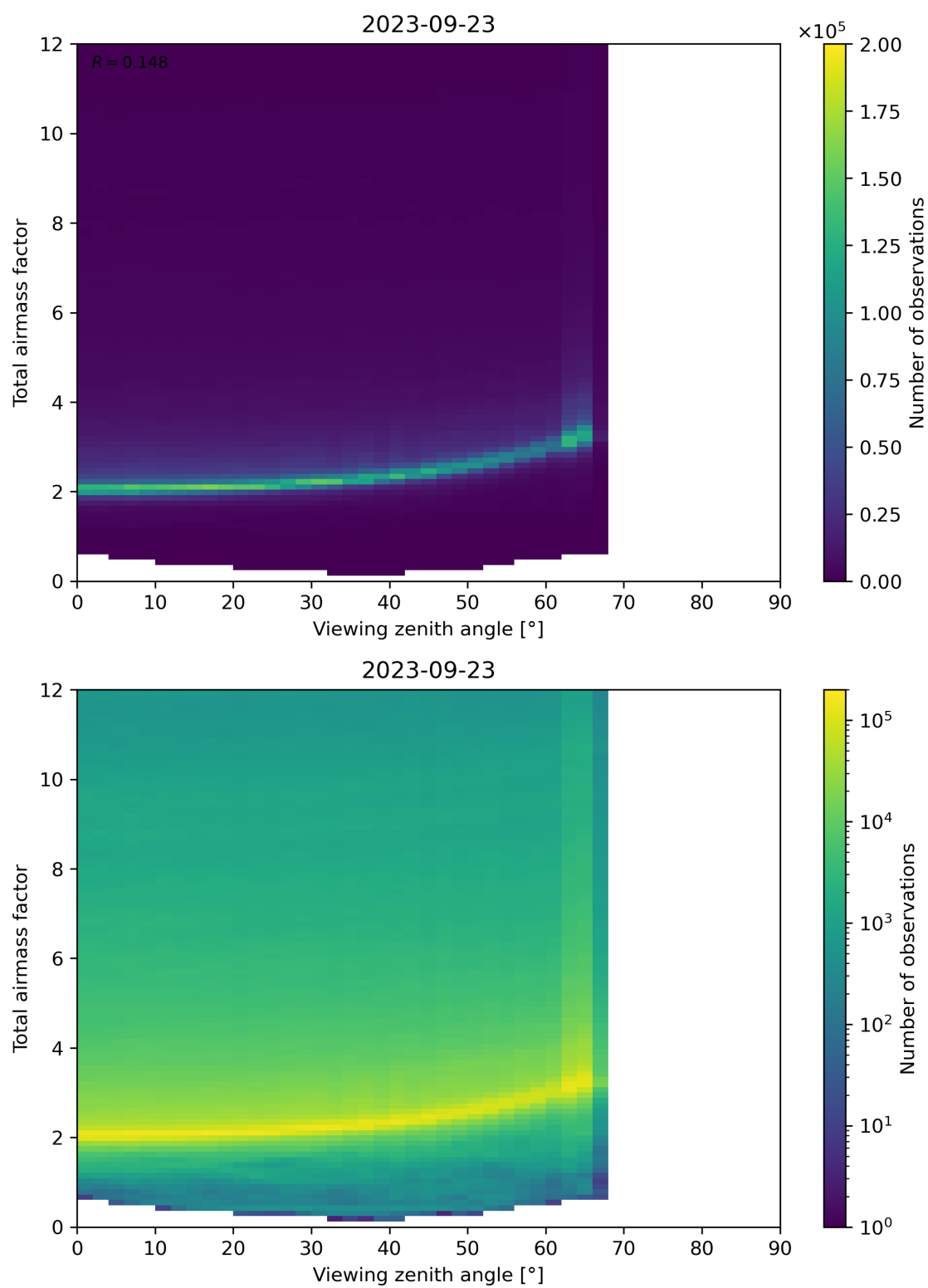
Figure 160: Scatter density plot of “Viewing zenith angle” against “Total airmass factor” for 2023-09-22 to 2023-09-24.
