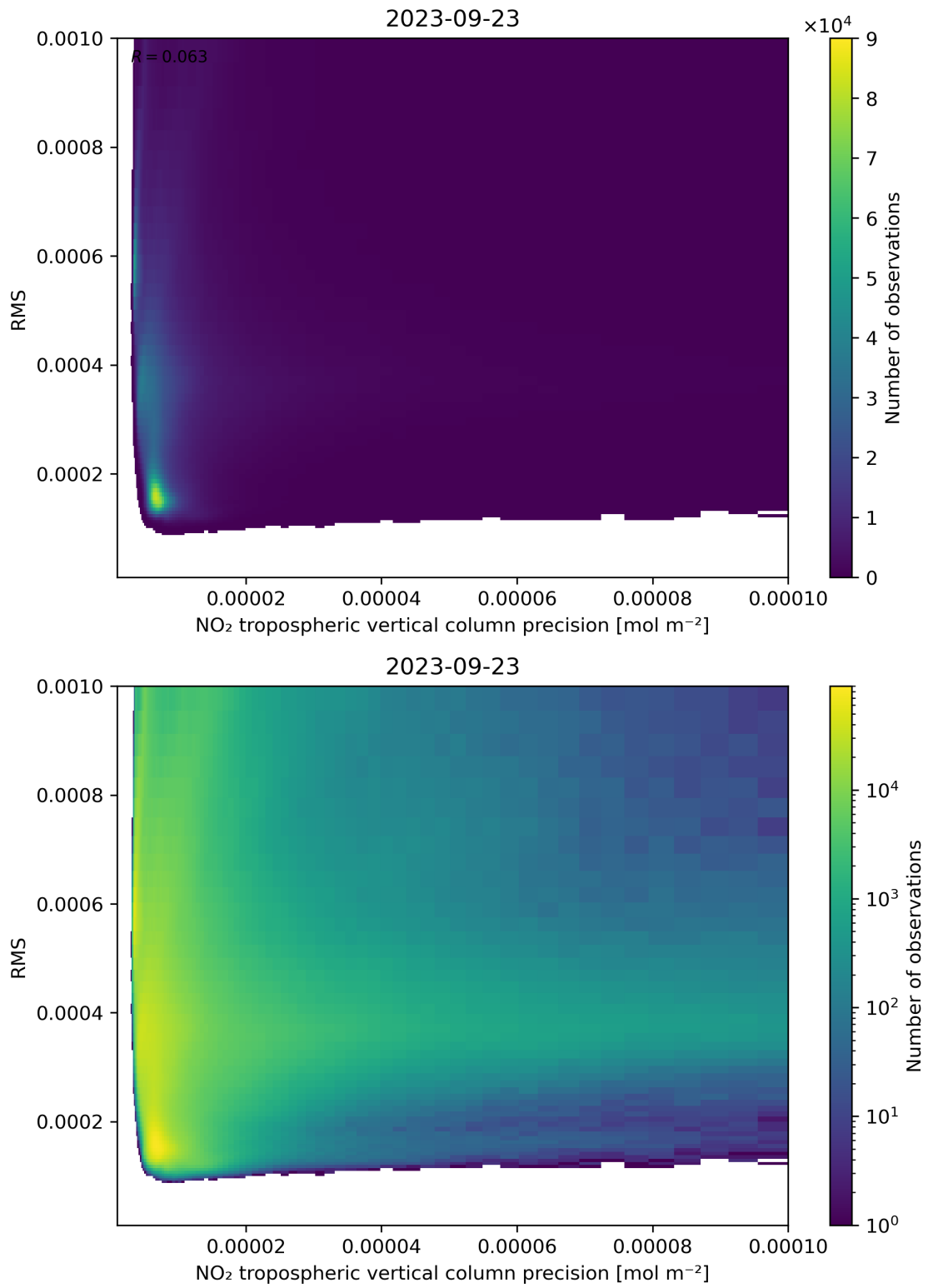
Figure 140: Scatter density plot of “NO 2 tropospheric vertical column precision” against “RMS” for 2023-09-22 to 2023-09-24.
