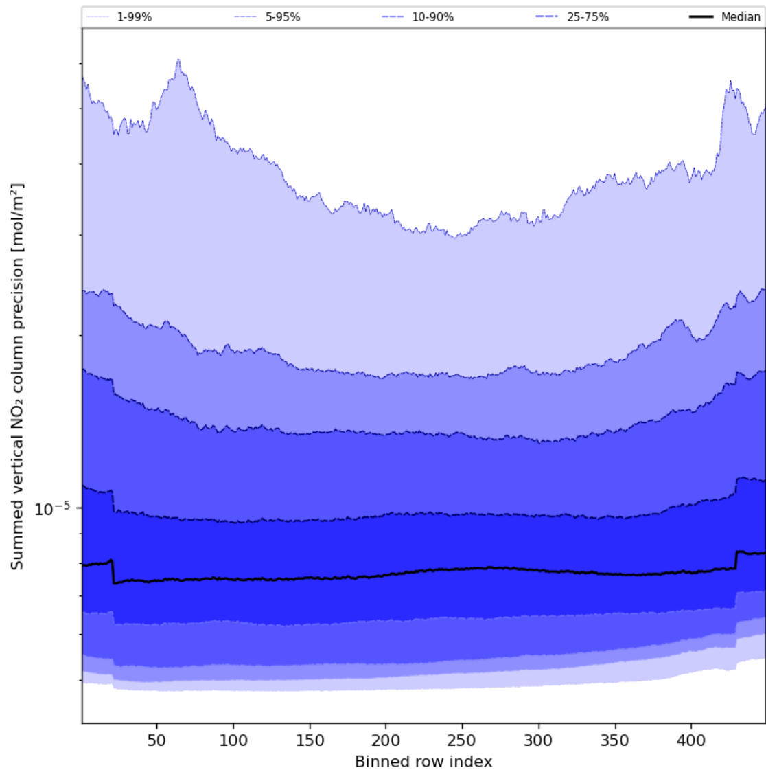
Figure 58: Along track statistics of “Summed vertical NO 2 column precision” for 2023-09-22 to 2023-09-24
