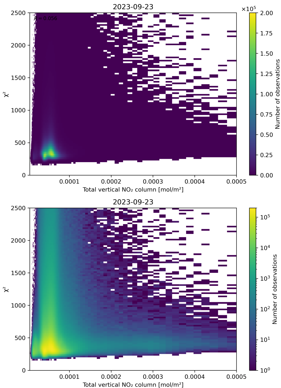
Figure 111: Scatter density plot of “Total vertical NO 2 column” against “ \chi^2 ” for 2023-09-22 to 2023-09-24.
