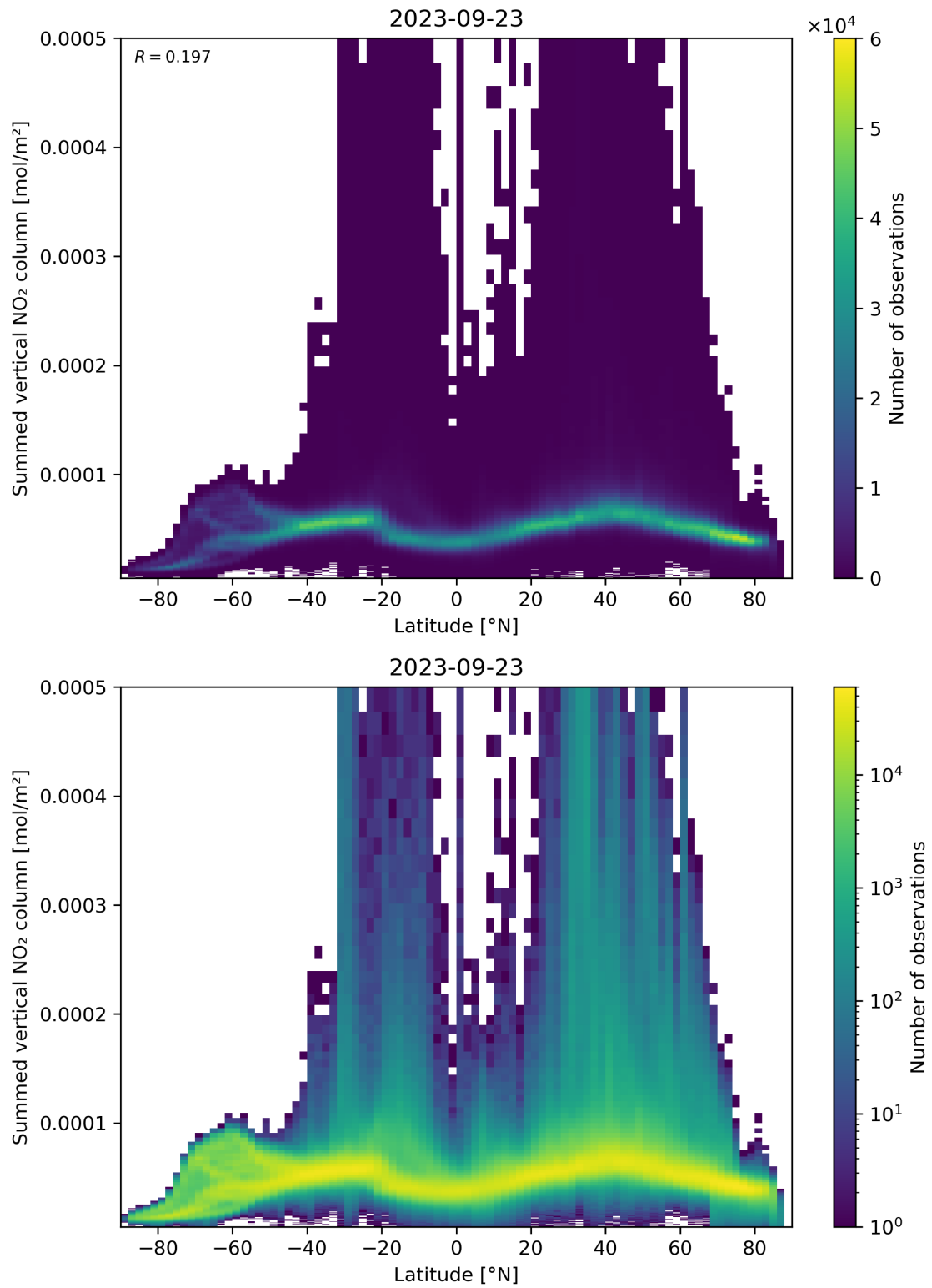
Figure 88: Scatter density plot of “Latitude” against “Summed vertical NO 2 column” for 2023-09-22 to 2023-09-24.
