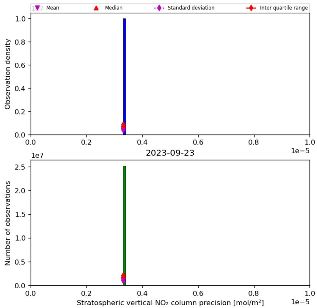
Figure 37: Histogram of “Stratospheric vertical NO 2 column precision” for 2023-09-22 to 2023-09-24
