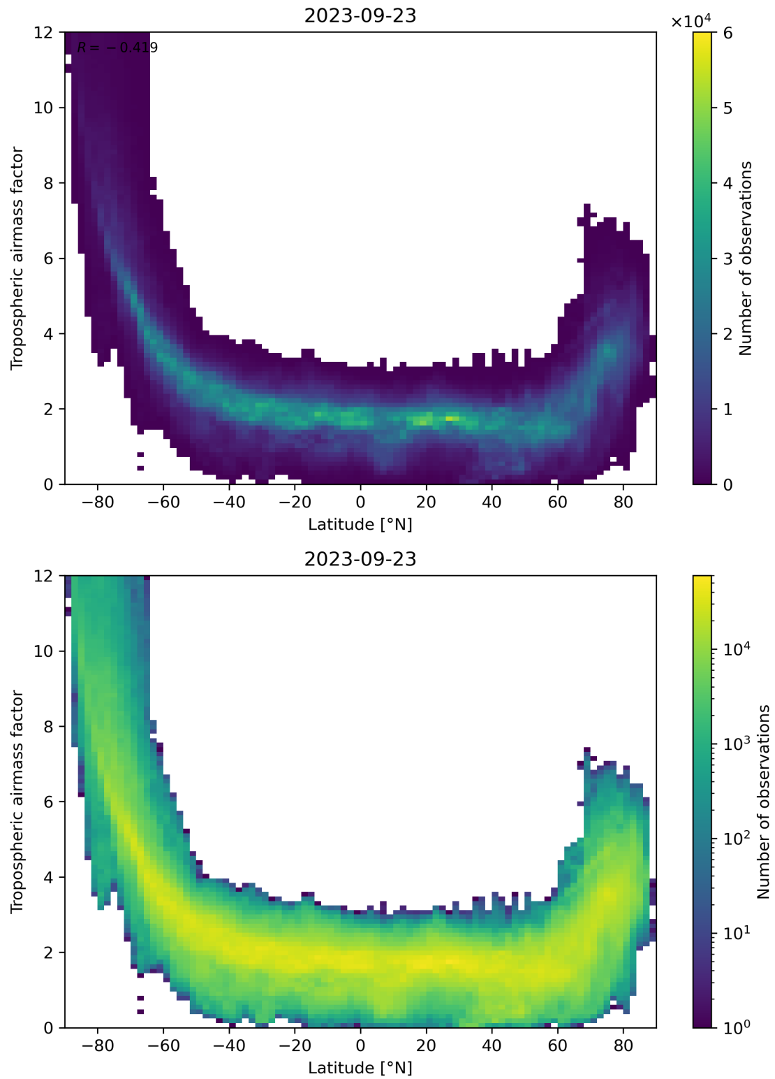
Figure 85: Scatter density plot of “Latitude” against “Tropospheric airmass factor” for 2023-09-22 to 2023-09-24.
