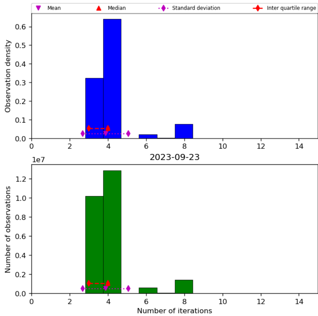
Figure 34: Histogram of “Number of iterations” for 2023-09-22 to 2023-09-24
