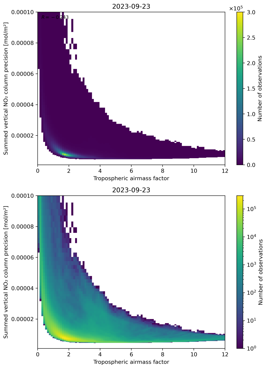
Figure 76: Scatter density plot of “Tropospheric air mass factor” against “Summed vertical NO 2 column precision” for 2023-09-22 to 2023-09-24.
