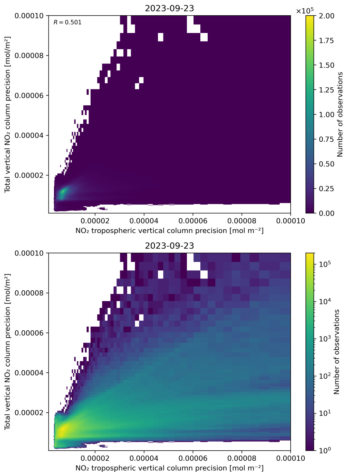
Figure 139: Scatter density plot of “NO 2 tropospheric vertical column precision” against “Total vertical NO 2 column precision” for 2023-09-22 to 2023-09-24.
