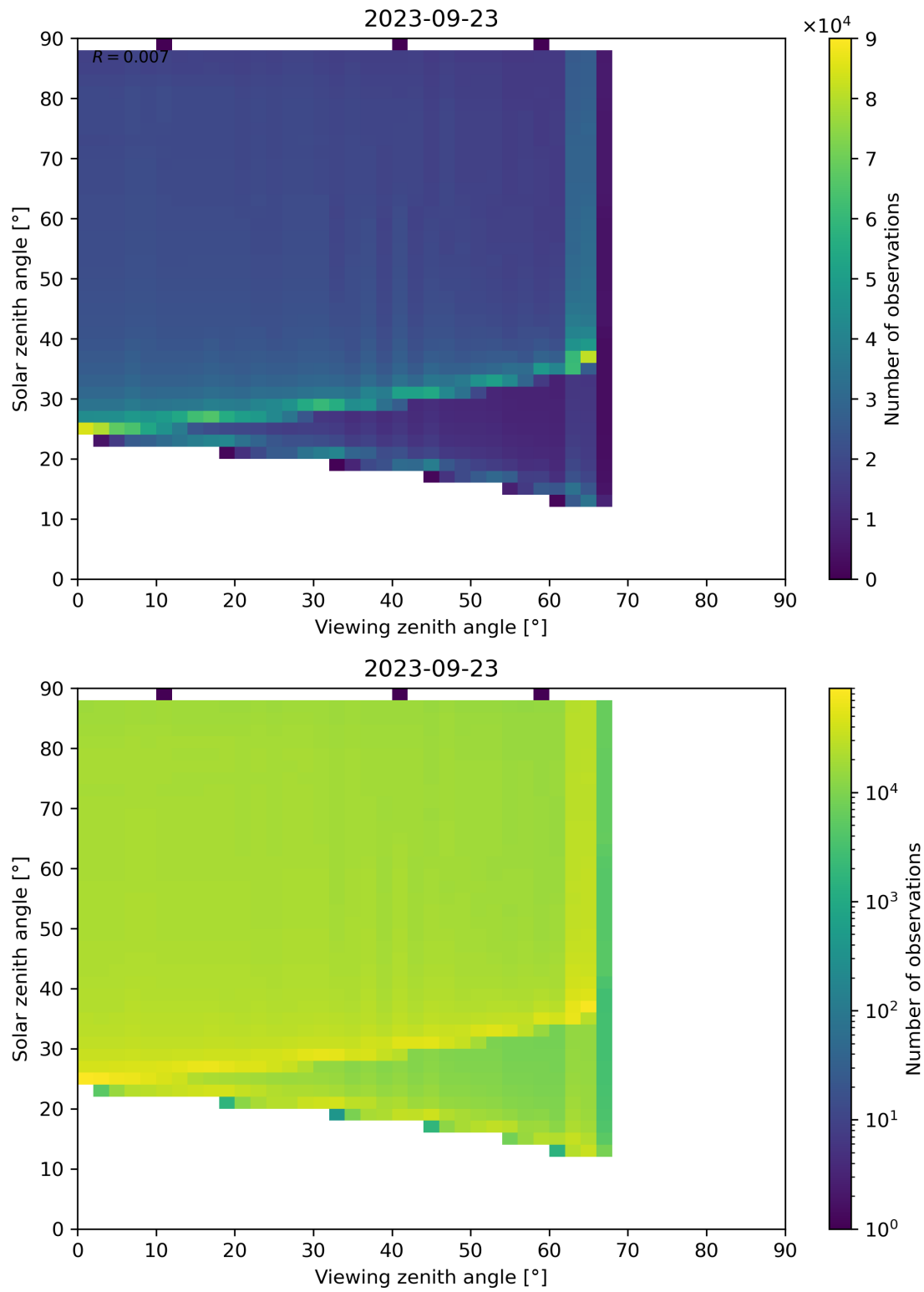
Figure 172: Scatter density plot of “Viewing zenith angle” against “Solar zenith angle” for 2023-09-22 to 2023-09-24.
