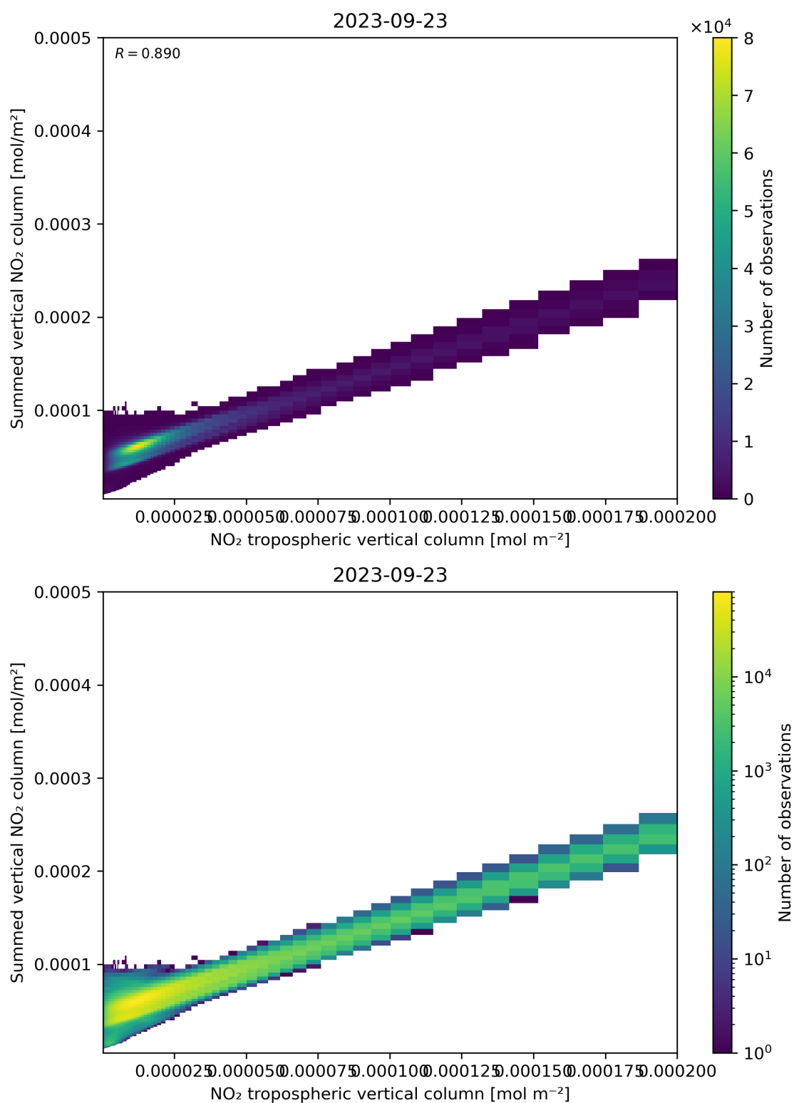
Figure 126: Scatter density plot of “NO 2 tropospheric vertical column” against “Summed vertical NO 2 column” for 2023-09-22 to 2023-09-24.
