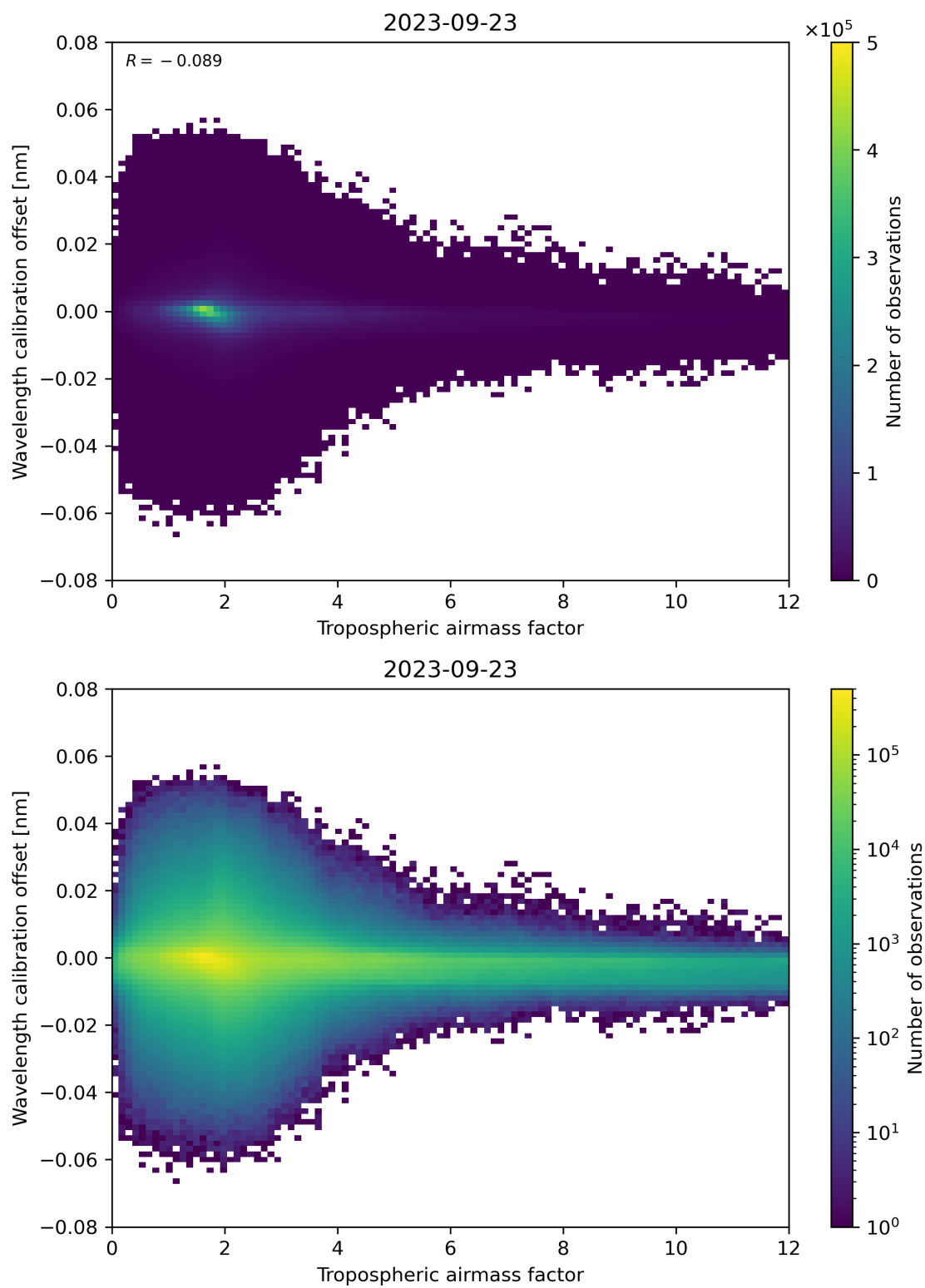
Figure 80: Scatter density plot of “Tropospheric airmass factor” against “Wavelength calibration offset” for 2023-09-22 to 2023-09-24.
