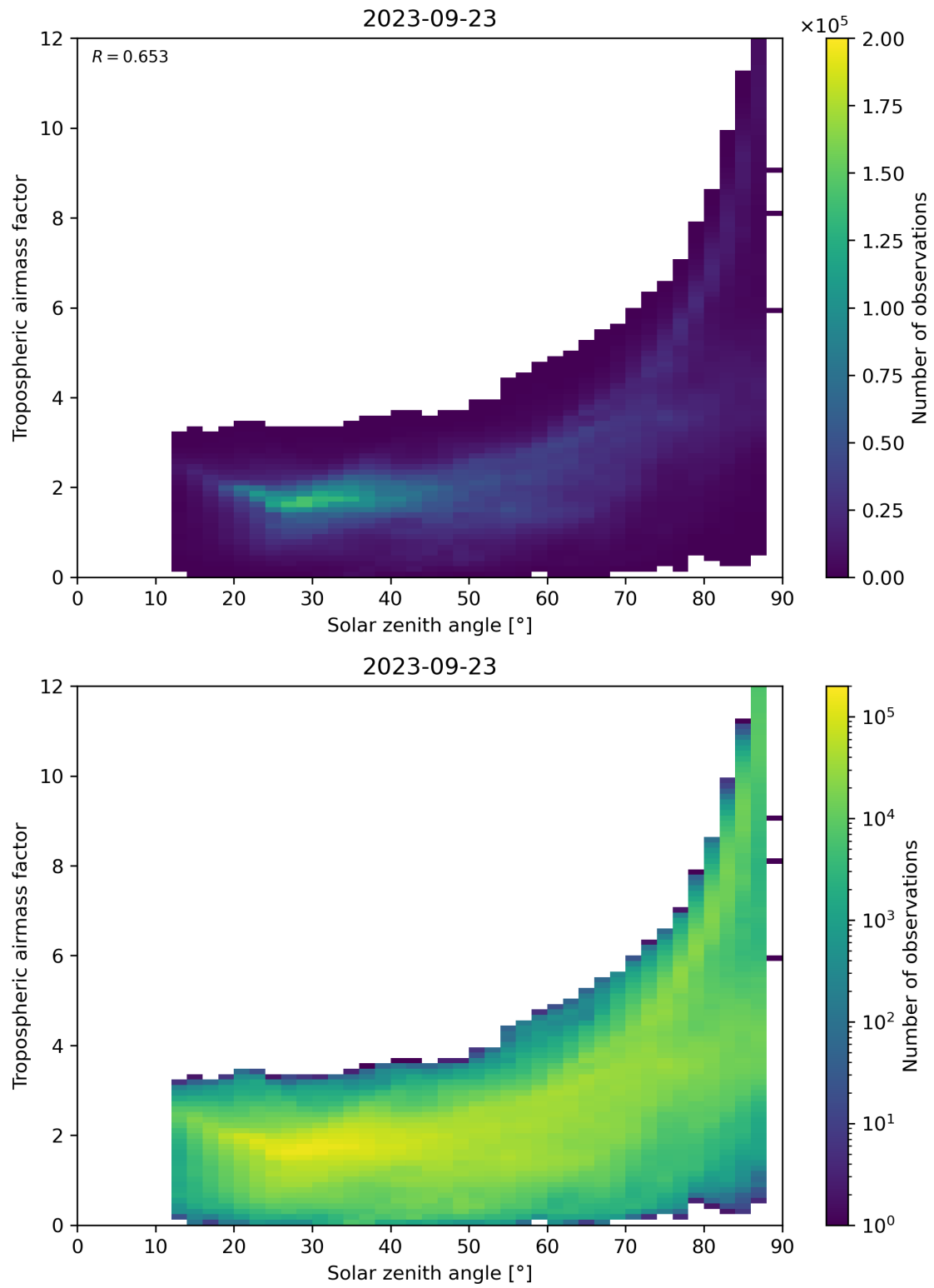
Figure 147: Scatter density plot of “Solar zenith angle” against “Tropospheric airmass factor” for 2023-09-22 to 2023-09-24.
