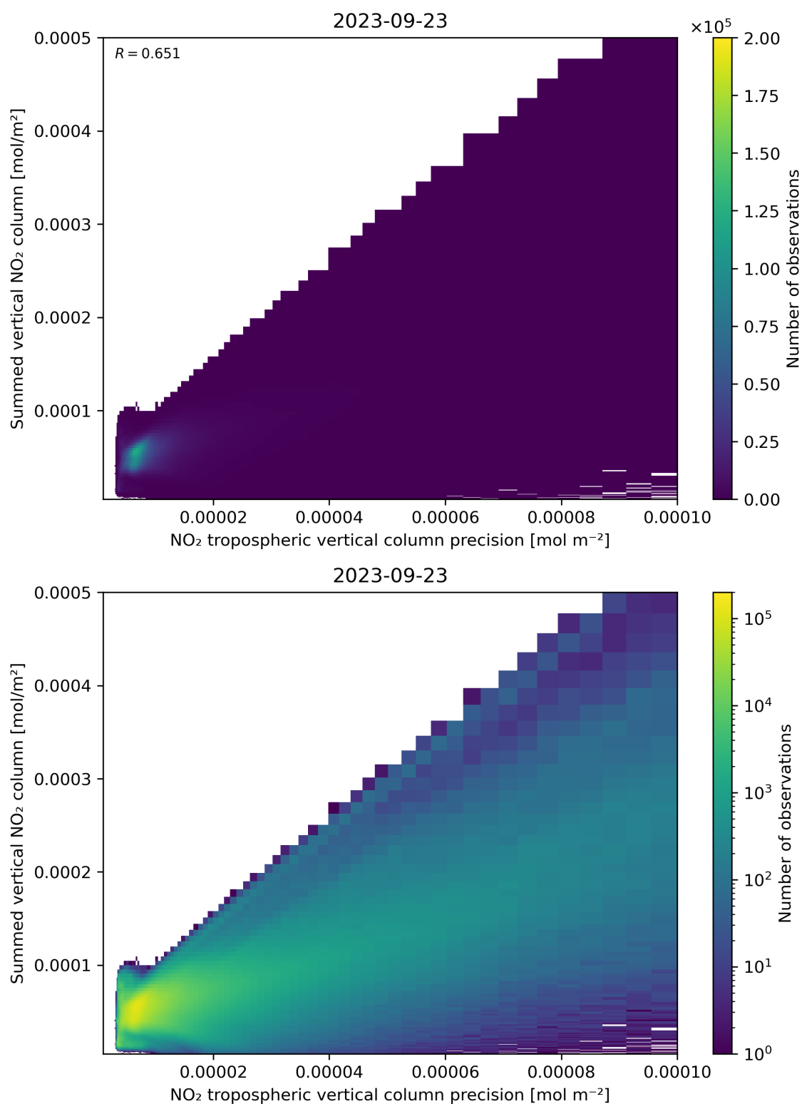
Figure 136: Scatter density plot of “NO 2 tropospheric vertical column precision” against “Summed vertical NO 2 column” for 2023-09-22 to 2023-09-24.
