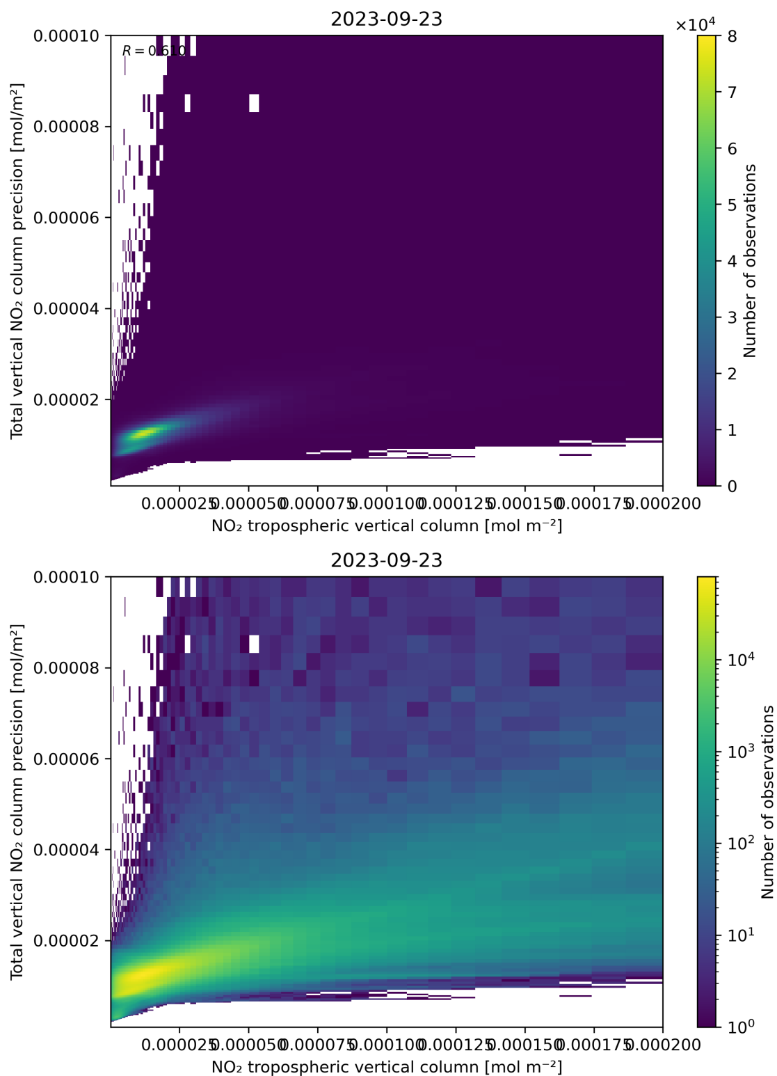
Figure 129: Scatter density plot of “NO 2 tropospheric vertical column” against “Total vertical NO 2 column precision” for 2023-09-22 to 2023-09-24.
