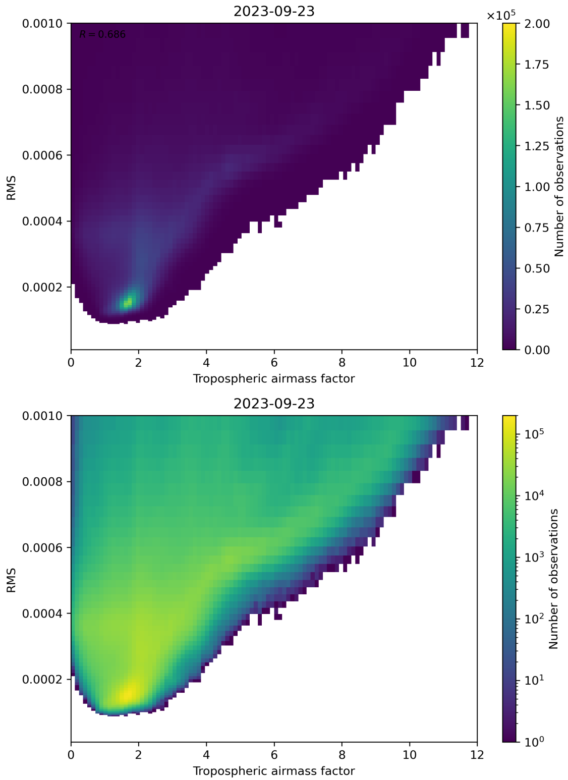
Figure 79: Scatter density plot of “Tropospheric airmass factor” against “RMS” for 2023-09-22 to 2023-09-24.
