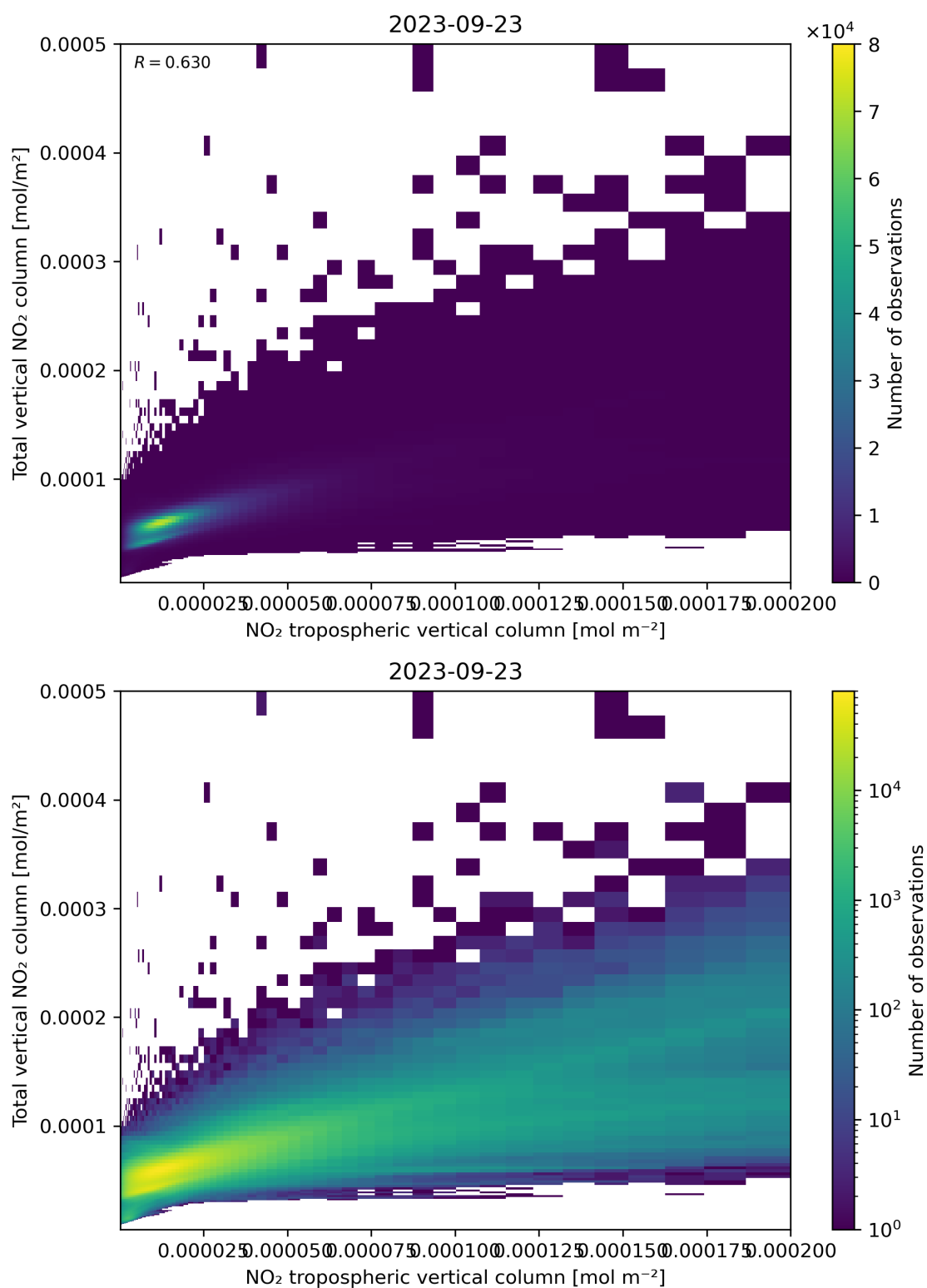
Figure 128: Scatter density plot of “NO 2 tropospheric vertical column” against “Total vertical NO 2 column” for 2023-09-22 to 2023-09-24.
