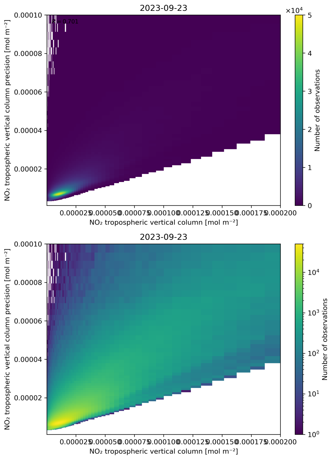
Figure 130: Scatter density plot of “NO 2 tropospheric vertical column” against “NO 2 tropospheric vertical column precision” for 2023-09-22 to 2023-09-24.
