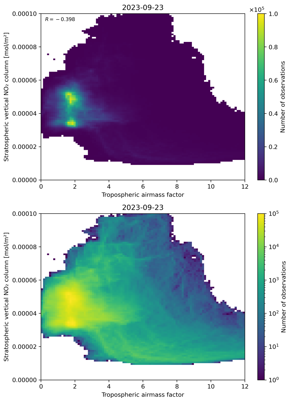
Figure 74: Scatter density plot of “Tropospheric air mass factor” against “Stratospheric vertical NO 2 column” for 2023-09-22 to 2023-09-24.
