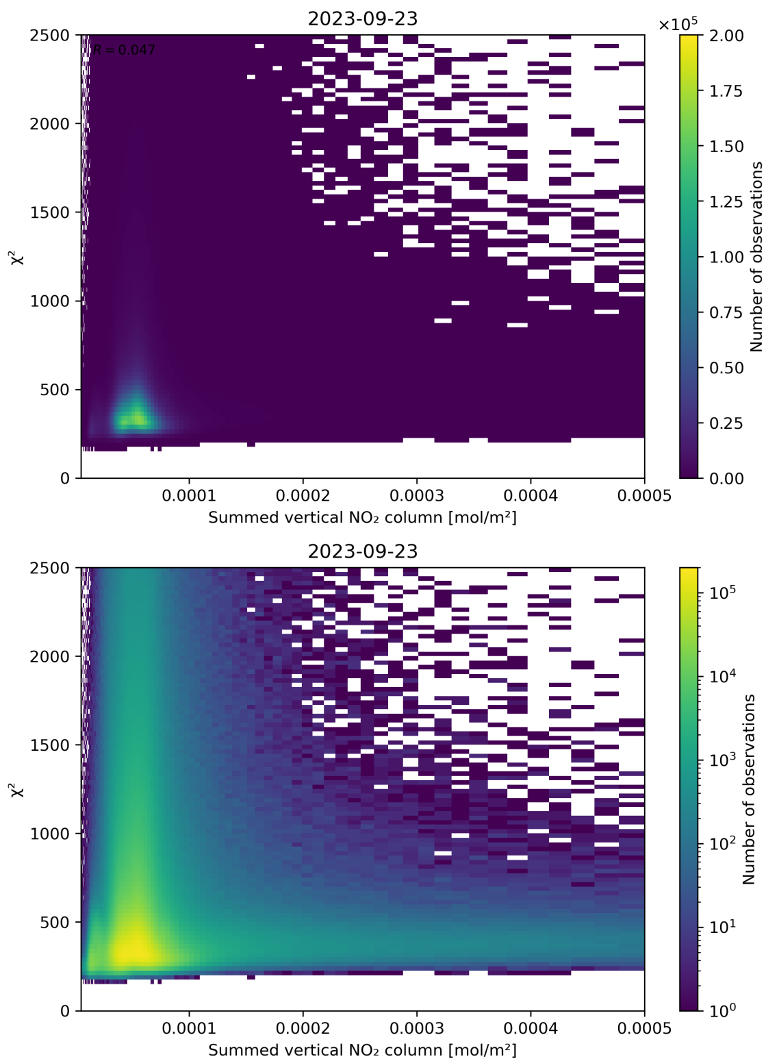
Figure 104: Scatter density plot of “Summed vertical NO 2 column” against “ \chi^2 ” for 2023-09-22 to 2023-09-24.
