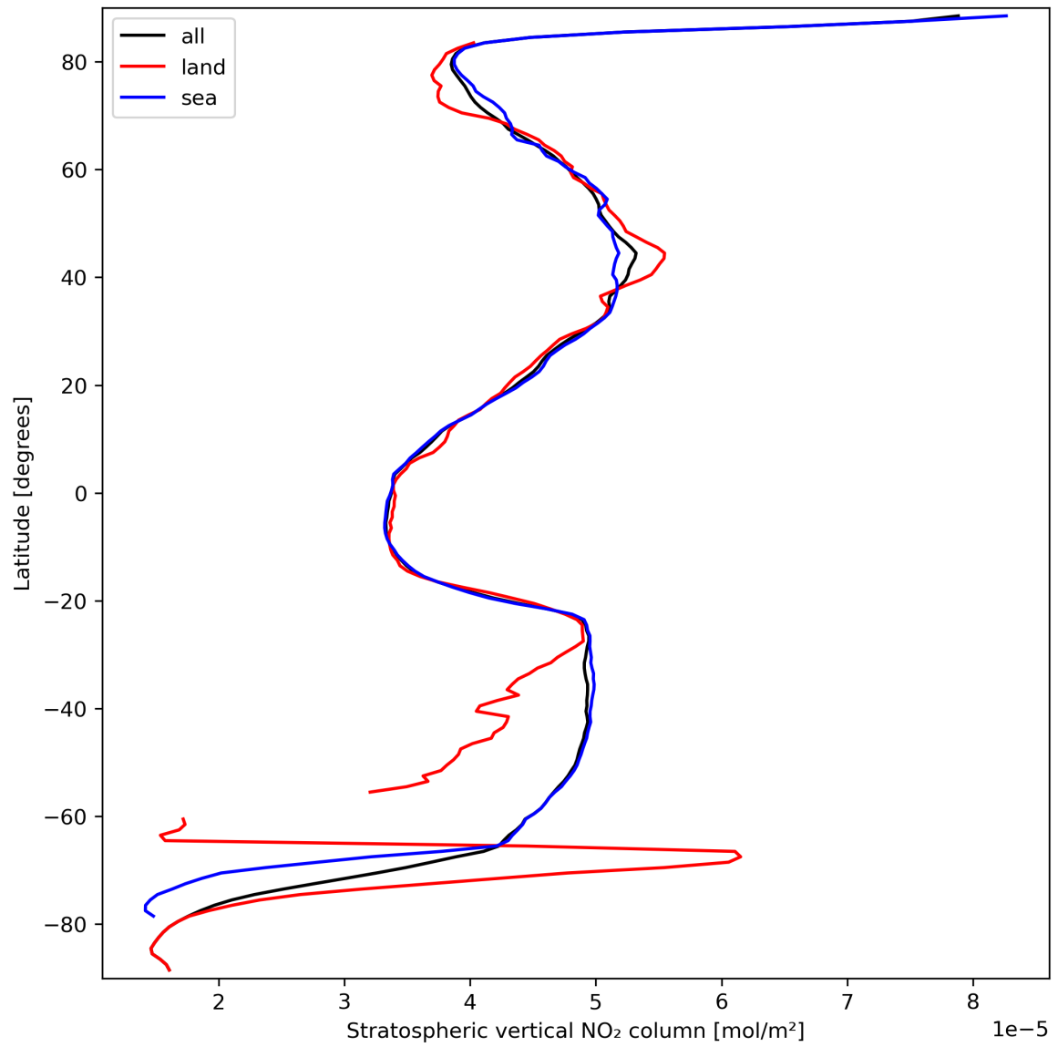
Figure 19: Zonal average of “Stratospheric vertical NO 2 column” for 2023-09-22 to 2023-09-24.
