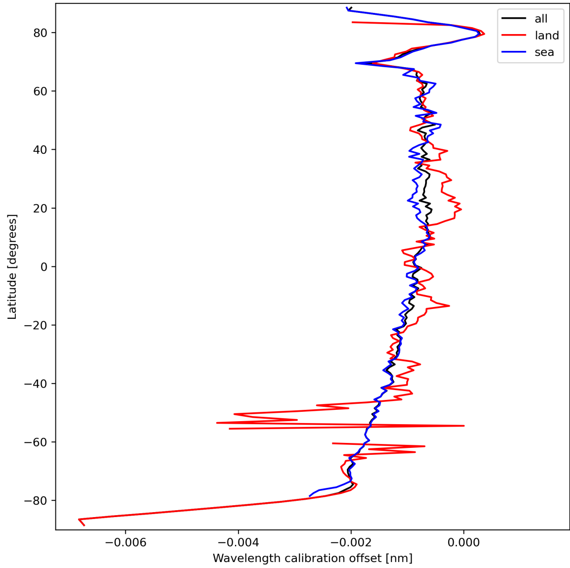
Figure 18: Zonal average of “Wavelength calibration offset” for 2023-09-22 to 2023-09-24.
