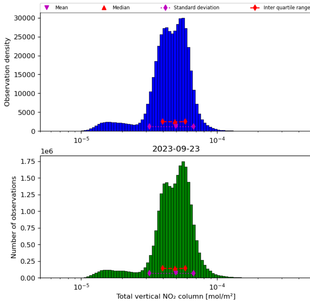
Figure 38: Histogram of “Total vertical NO 2 column” for 2023-09-22 to 2023-09-24
