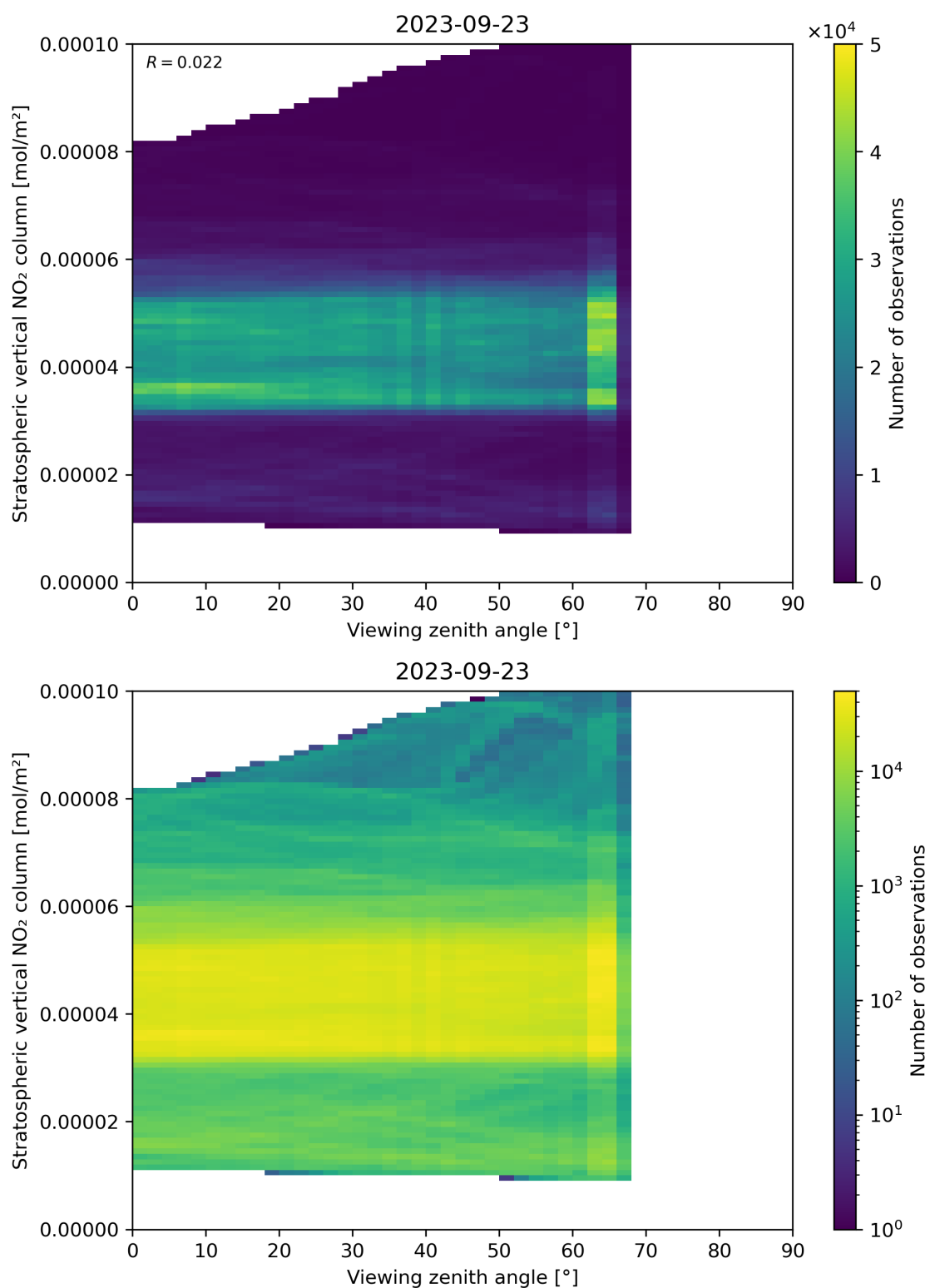
Figure 164: Scatter density plot of “Viewing zenith angle” against “Stratospheric vertical NO 2 column” for 2023-09-22 to 2023-09-24.
