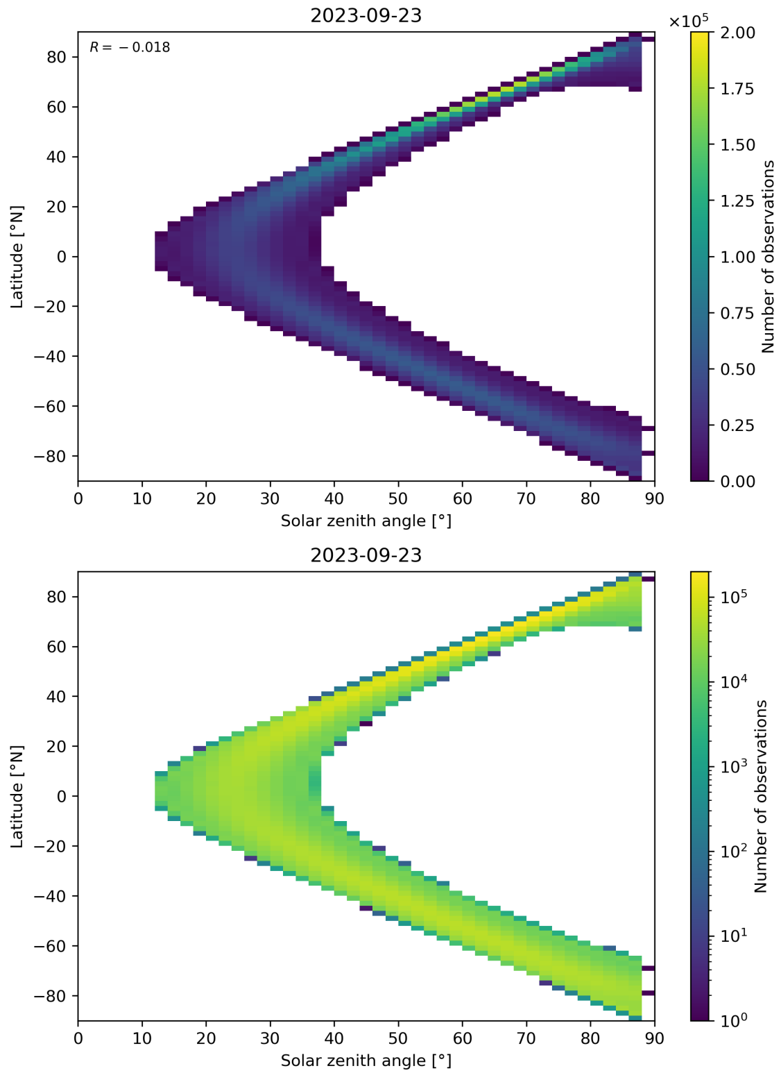
Figure 149: Scatter density plot of “Solar zenith angle” against “Latitude” for 2023-09-22 to 2023-09-24.
