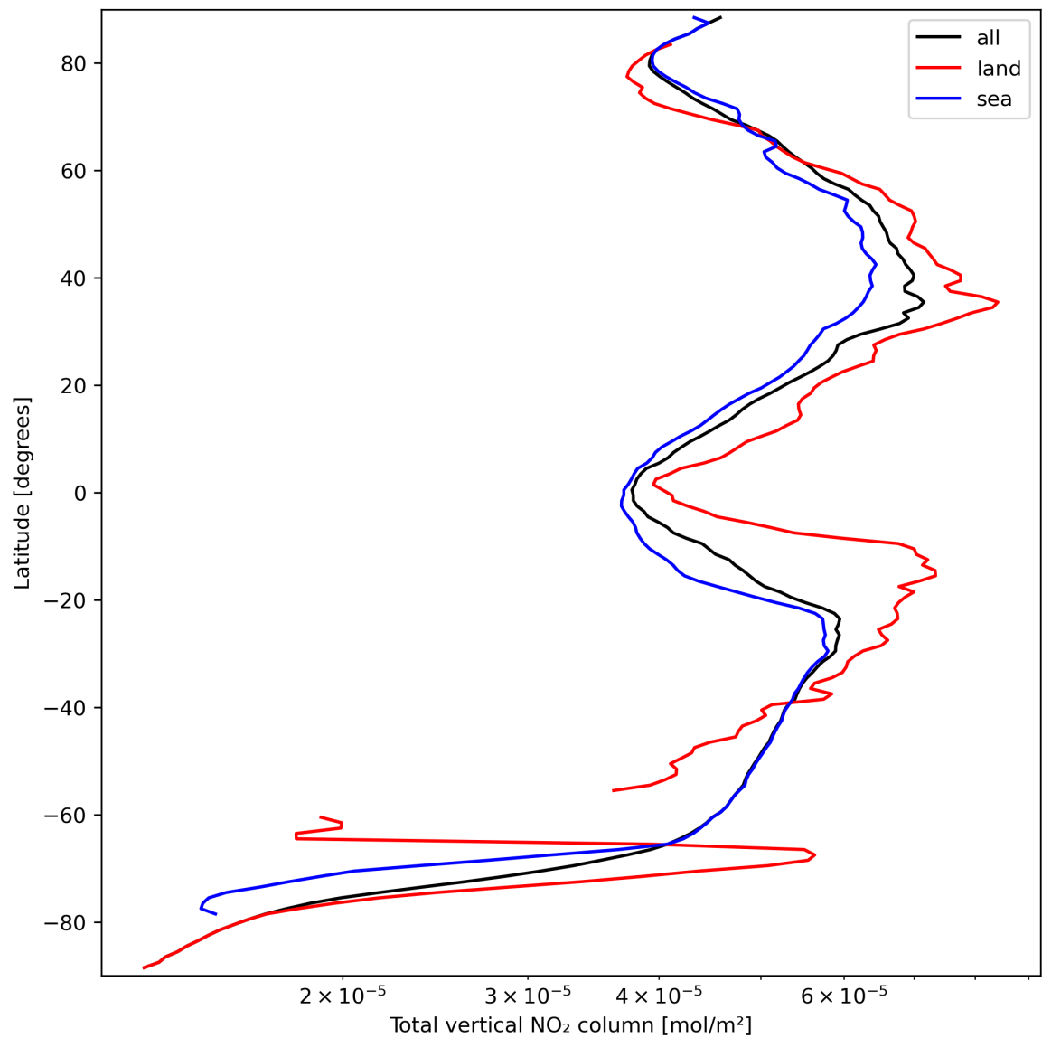
Figure 21: Zonal average of “Total vertical NO 2 column” for 2023-09-22 to 2023-09-24.
