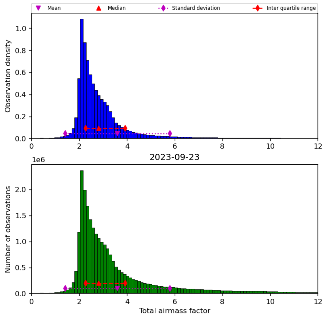
Figure 32: Histogram of “Total airmass factor” for 2023-09-22 to 2023-09-24
