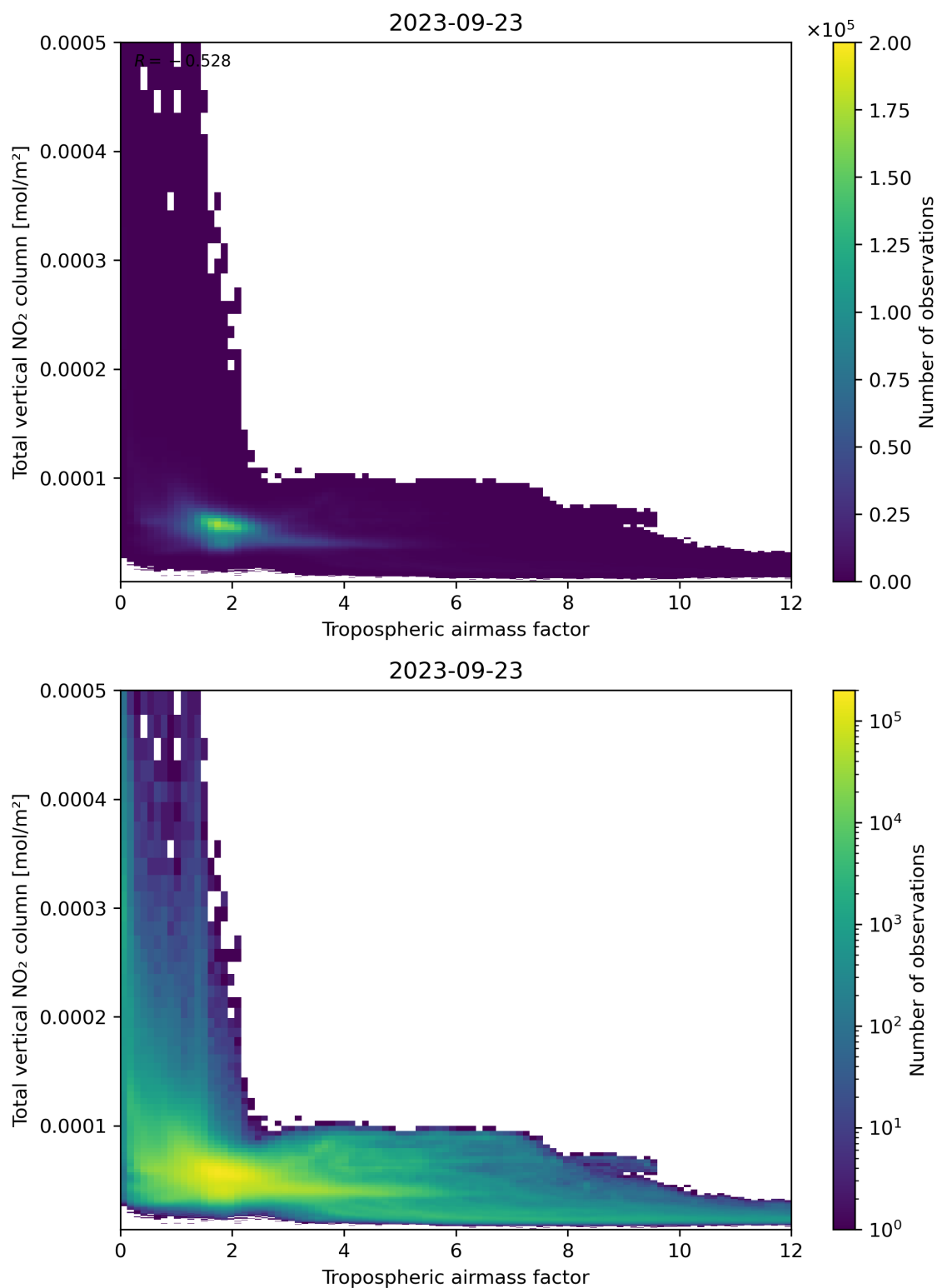
Figure 77: Scatter density plot of “Tropospheric airmass factor” against “Total vertical NO 2 column” for 2023-09-22 to 2023-09-24.
