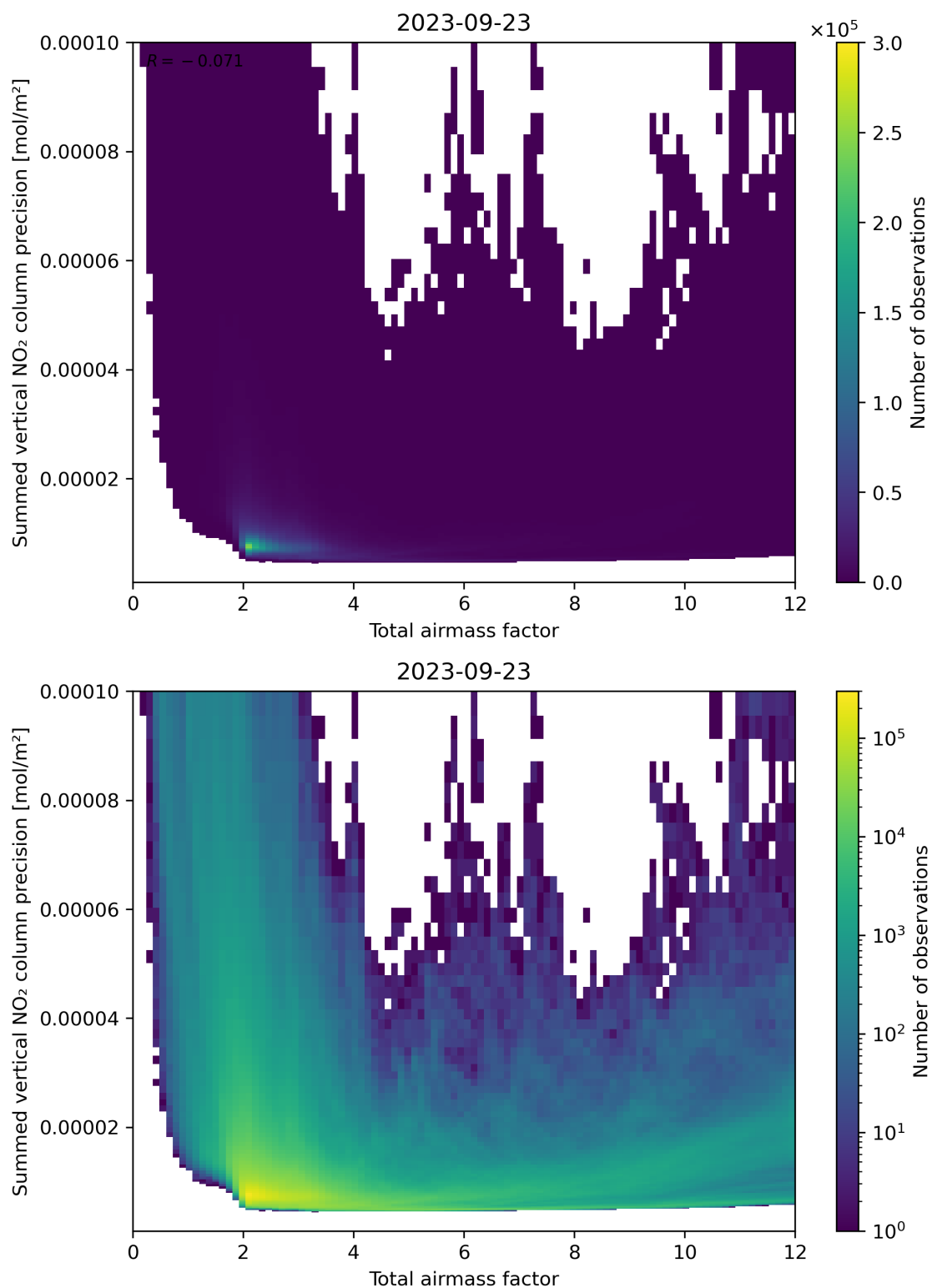
Figure 66: Scatter density plot of “Total airmass factor” against “Summed vertical NO 2 column precision” for 2023-09-22 to 2023-09-24.
