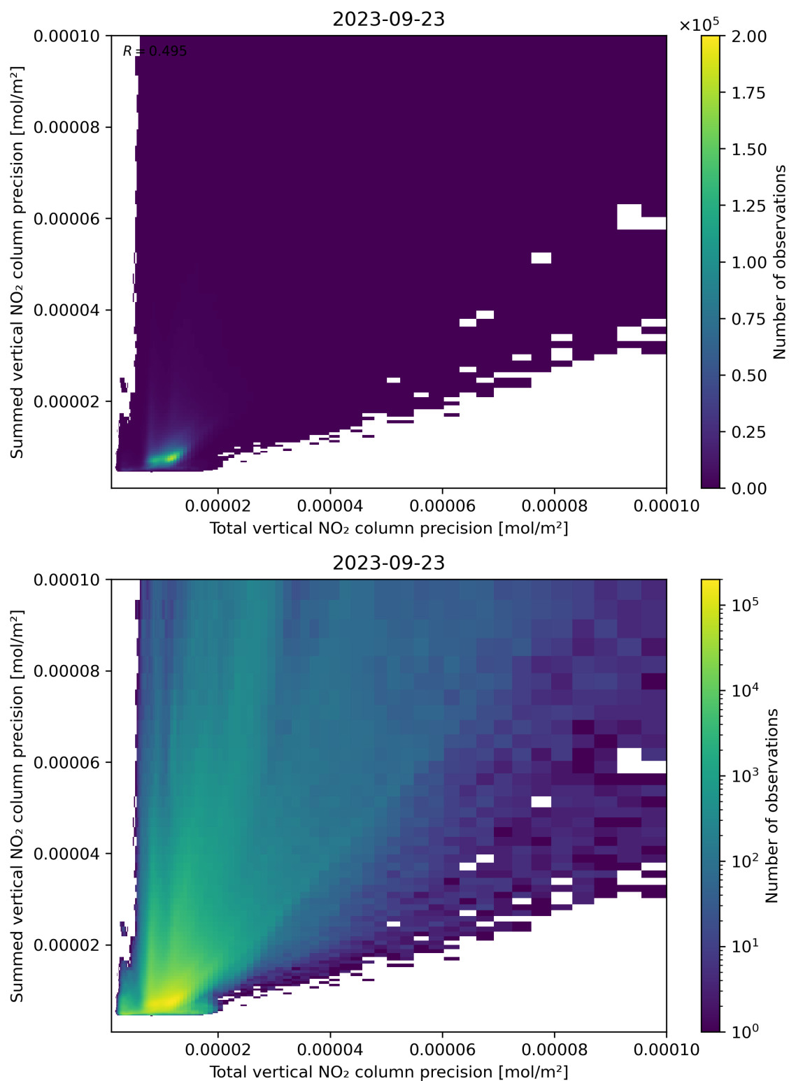
Figure 118: Scatter density plot of “Total vertical NO 2 column precision” against “Summed vertical NO 2 column precision” for 2023-09-22 to 2023-09-24.
