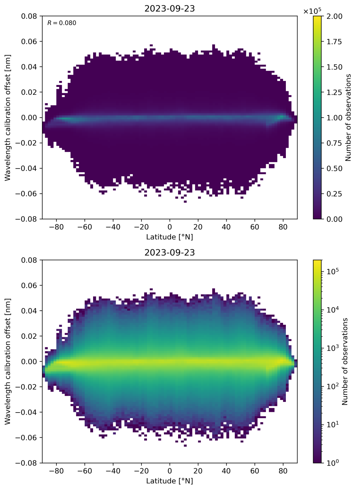
Figure 95: Scatter density plot of “Latitude” against “Wavelength calibration offset” for 2023-09-22 to 2023-09-24.
