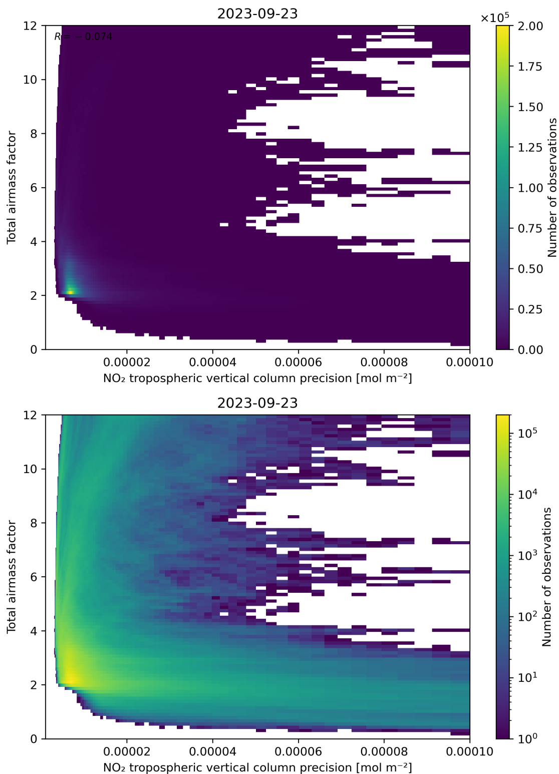
Figure 132: Scatter density plot of “NO 2 tropospheric vertical column precision” against “Total airmass factor” for 2023-09-22 to 2023-09-24.
