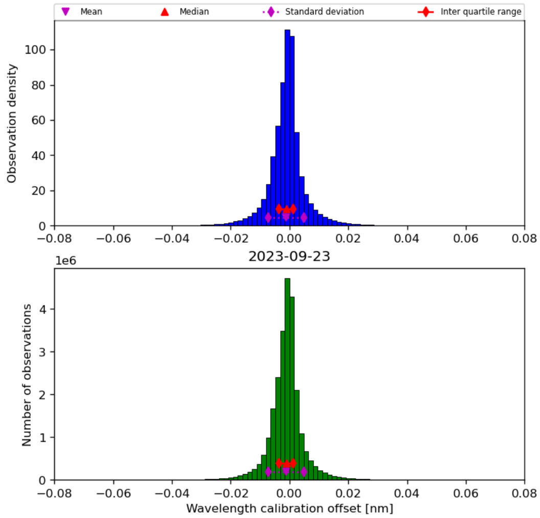
Figure 35: Histogram of “Wavelength calibration offset” for 2023-09-22 to 2023-09-24
