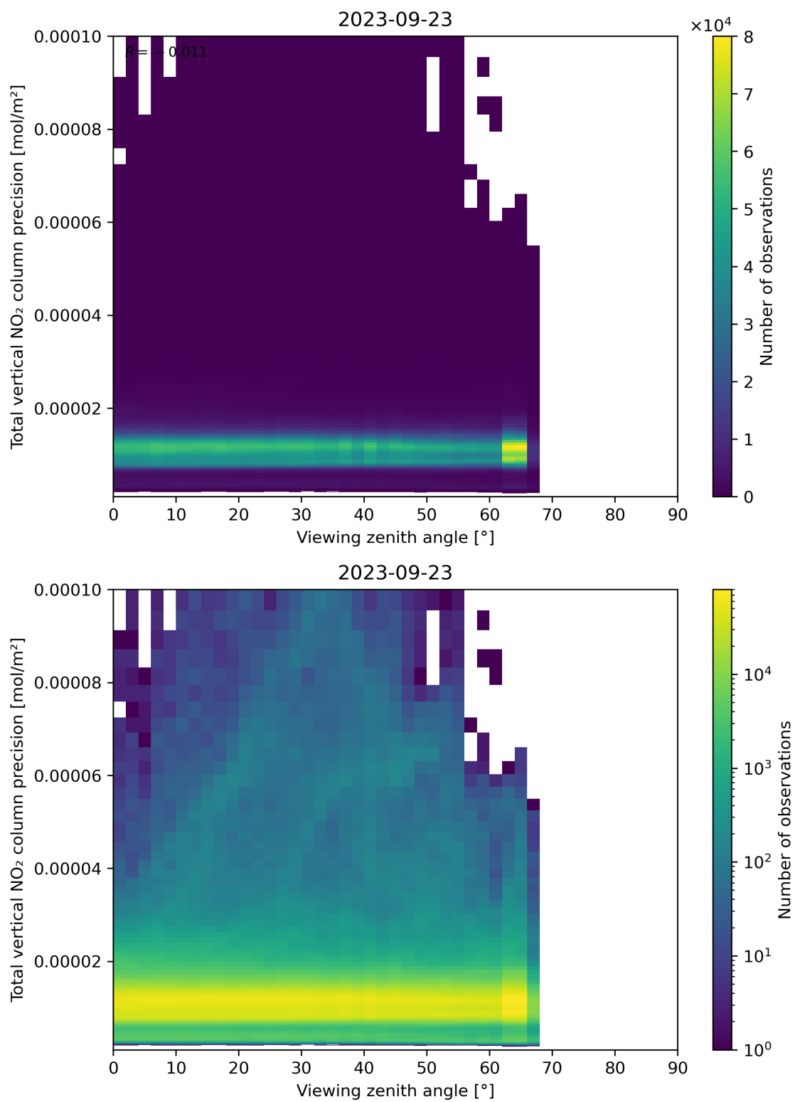
Figure 168: Scatter density plot of “Viewing zenith angle” against “Total vertical NO 2 column precision” for 2023-09-22 to 2023-09-24.
