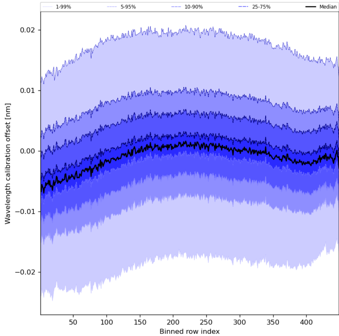
Figure 52: Along track statistics of “Wavelength calibration offset” for 2023-09-22 to 2023-09-24
