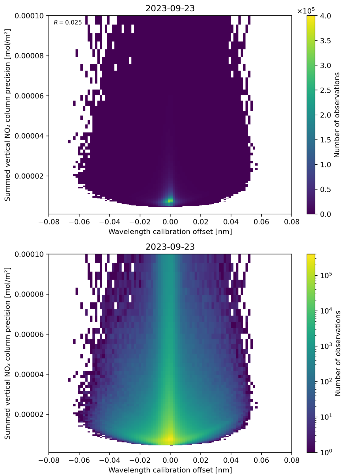
Figure 178: Scatter density plot of “Wavelength calibration offset” against “Summed vertical NO 2 column precision” for 2023-09-22 to 2023-09-24.
