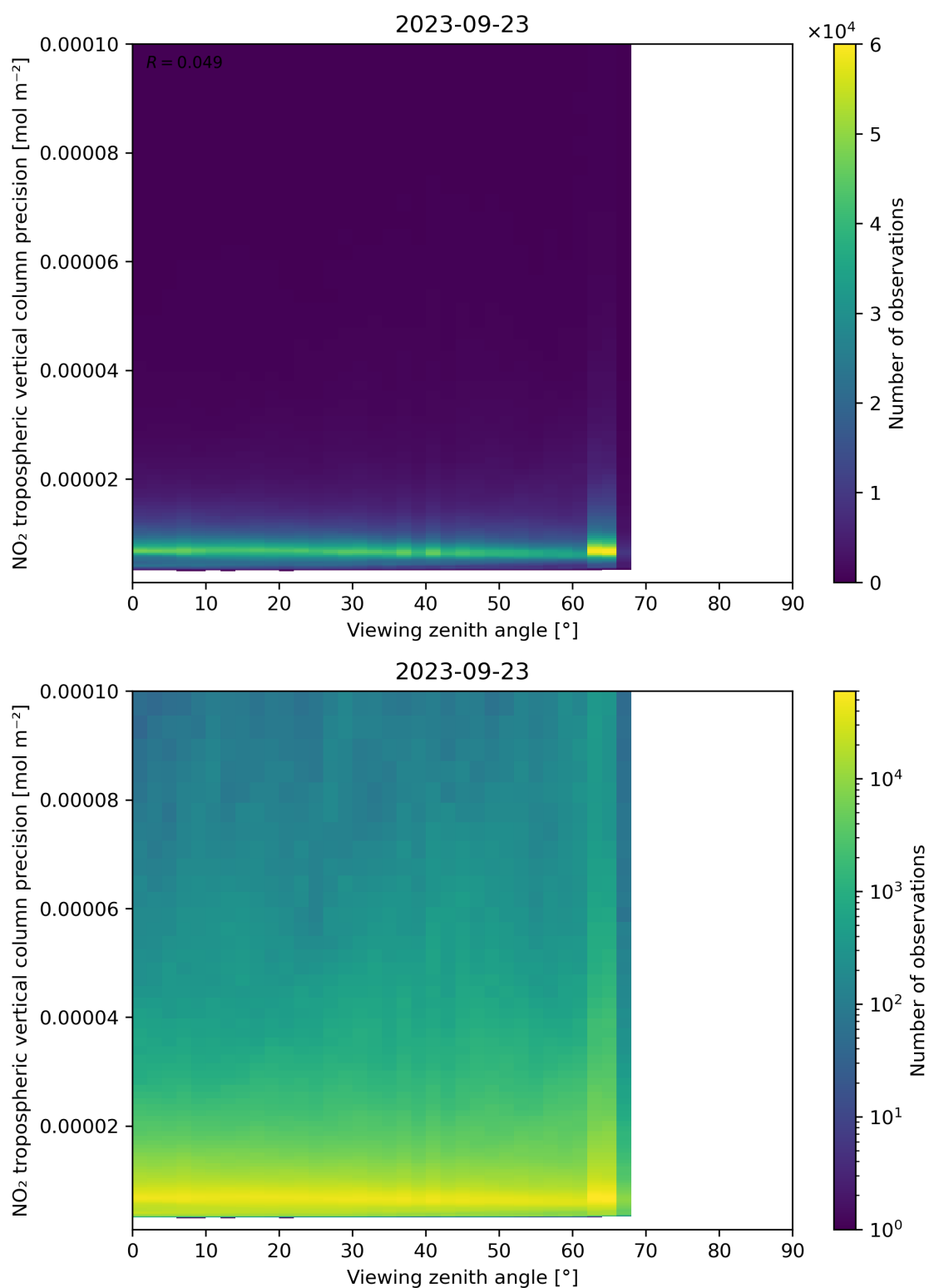
Figure 170: Scatter density plot of “Viewing zenith angle” against “NO 2 tropospheric vertical column precision” for 2023-09-22 to 2023-09-24.
