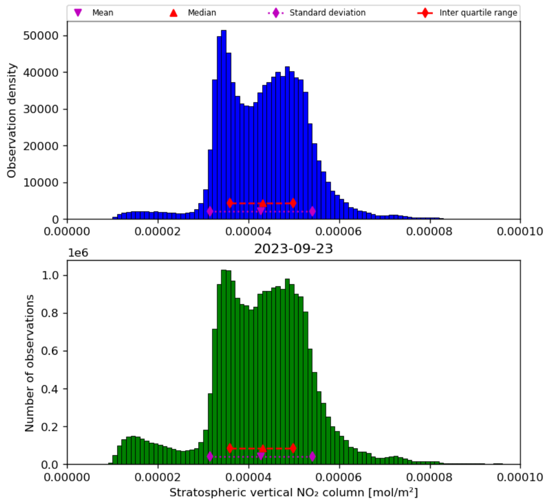
Figure 36: Histogram of “Stratospheric vertical NO 2 column” for 2023-09-22 to 2023-09-24
