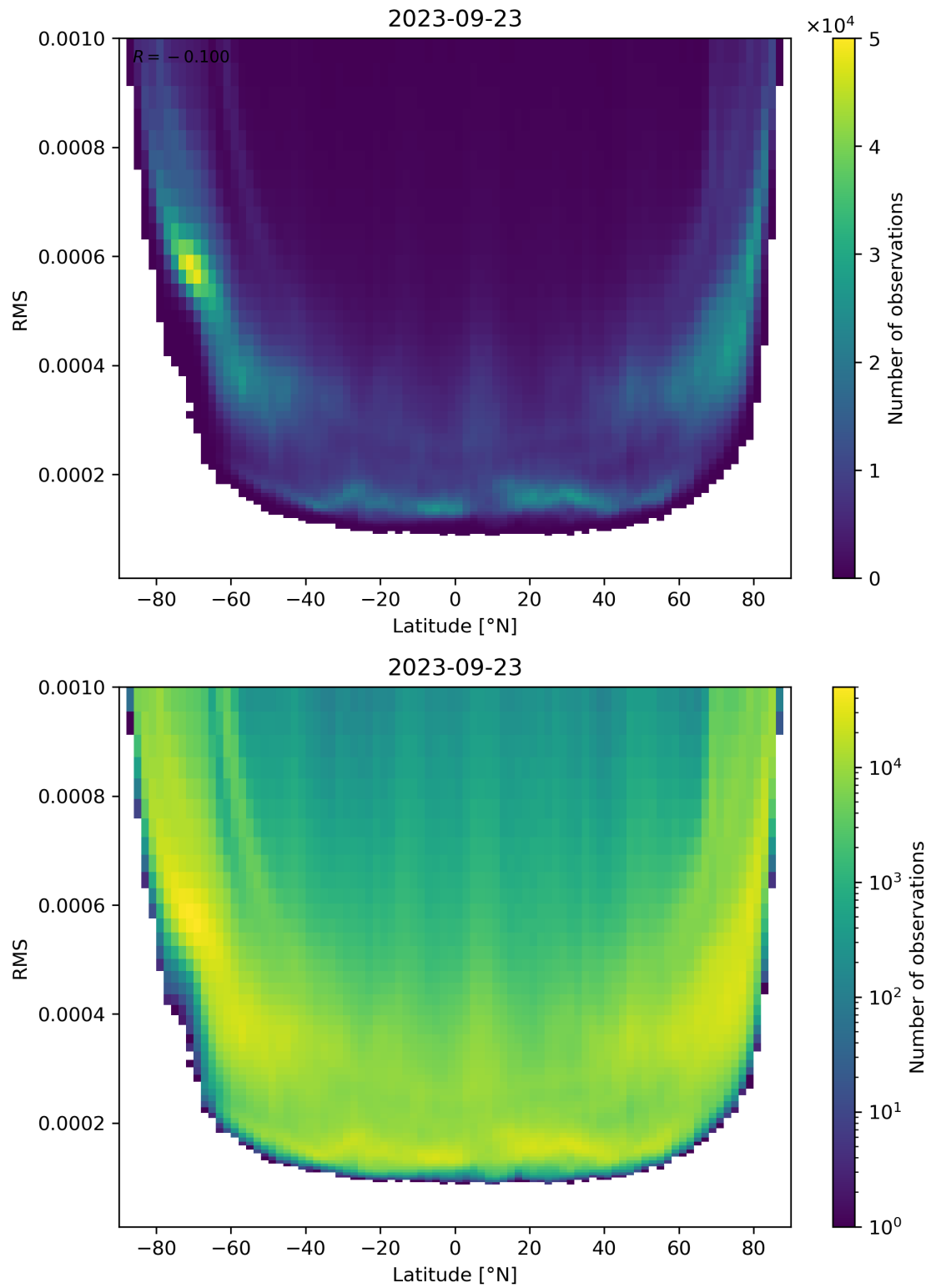
Figure 94: Scatter density plot of “Latitude” against “RMS” for 2023-09-22 to 2023-09-24.
