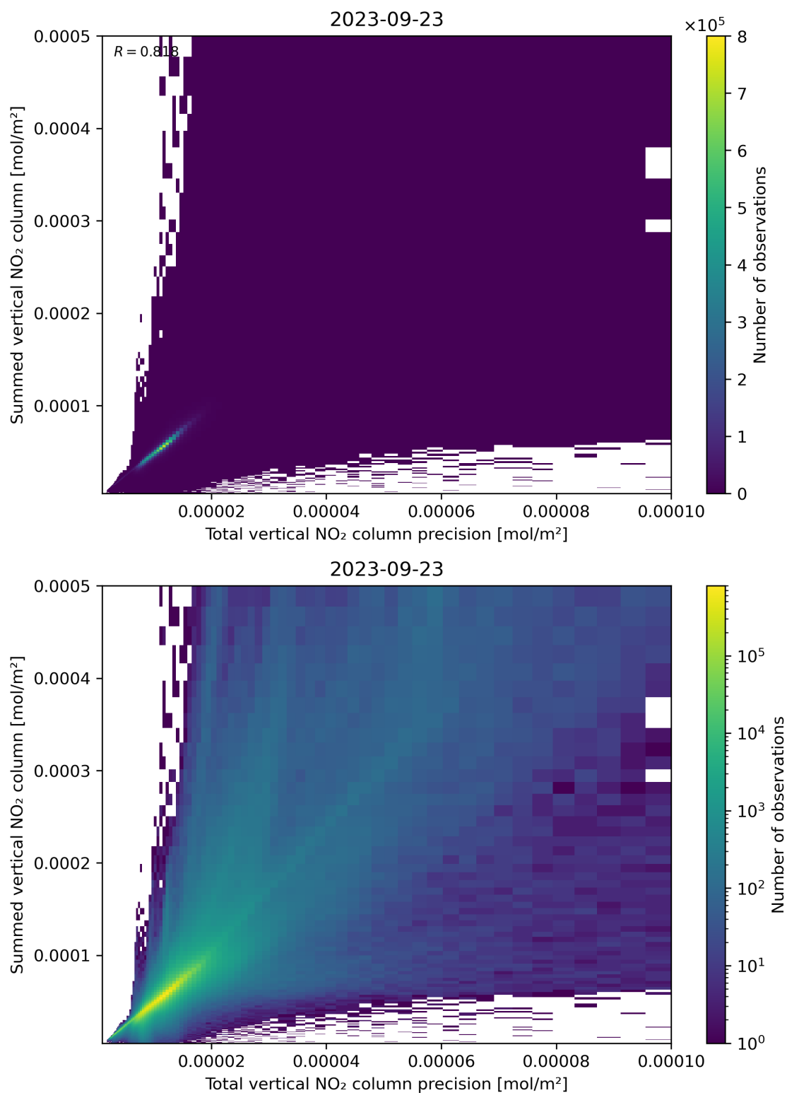
Figure 117: Scatter density plot of “Total vertical NO 2 column precision” against “Summed vertical NO 2 column” for 2023-09-22 to 2023-09-24.
