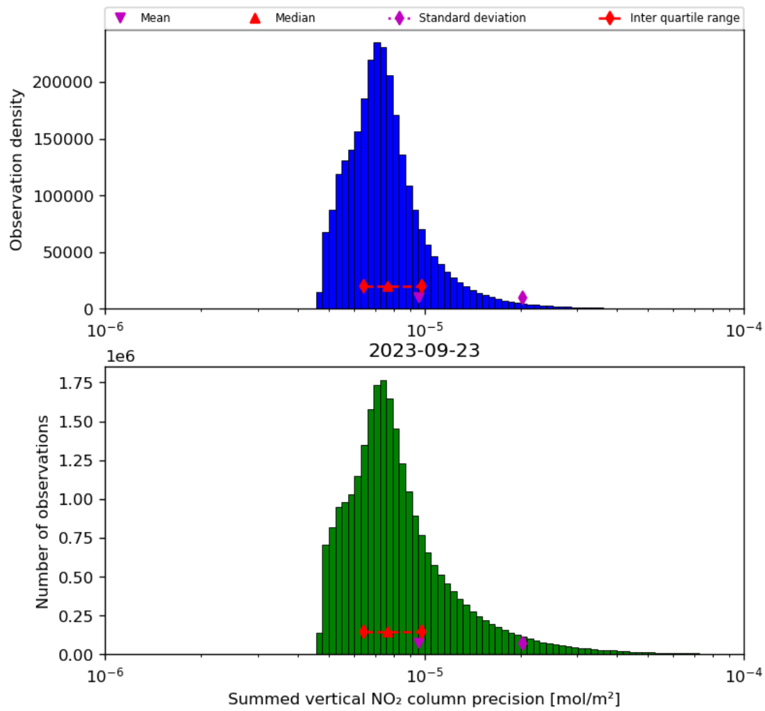
Figure 41: Histogram of “Summed vertical NO 2 column precision” for 2023-09-22 to 2023-09-24
