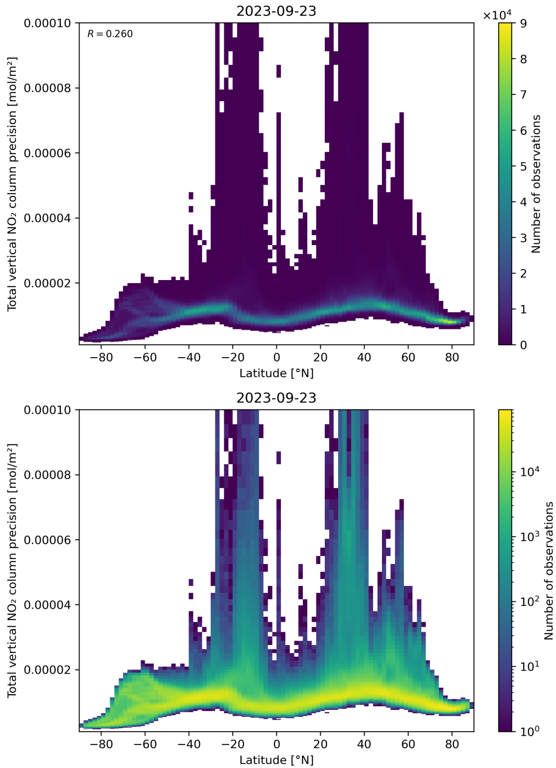
Figure 91: Scatter density plot of “Latitude” against “Total vertical NO 2 column precision” for 2023-09-22 to 2023-09-24.
