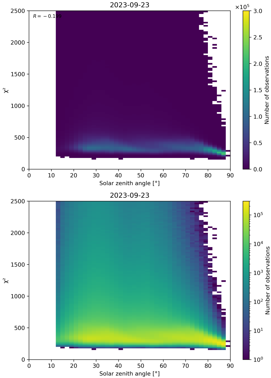
Figure 148: Scatter density plot of “Solar zenith angle” against “ \chi^2 ” for 2023-09-22 to 2023-09-24.
