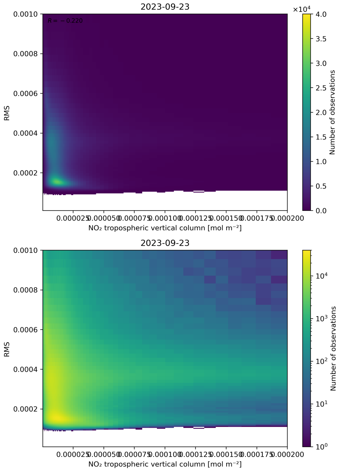
Figure 142: Scatter density plot of “NO 2 tropospheric vertical column” against “RMS” for 2023-09-22 to 2023-09-24.
