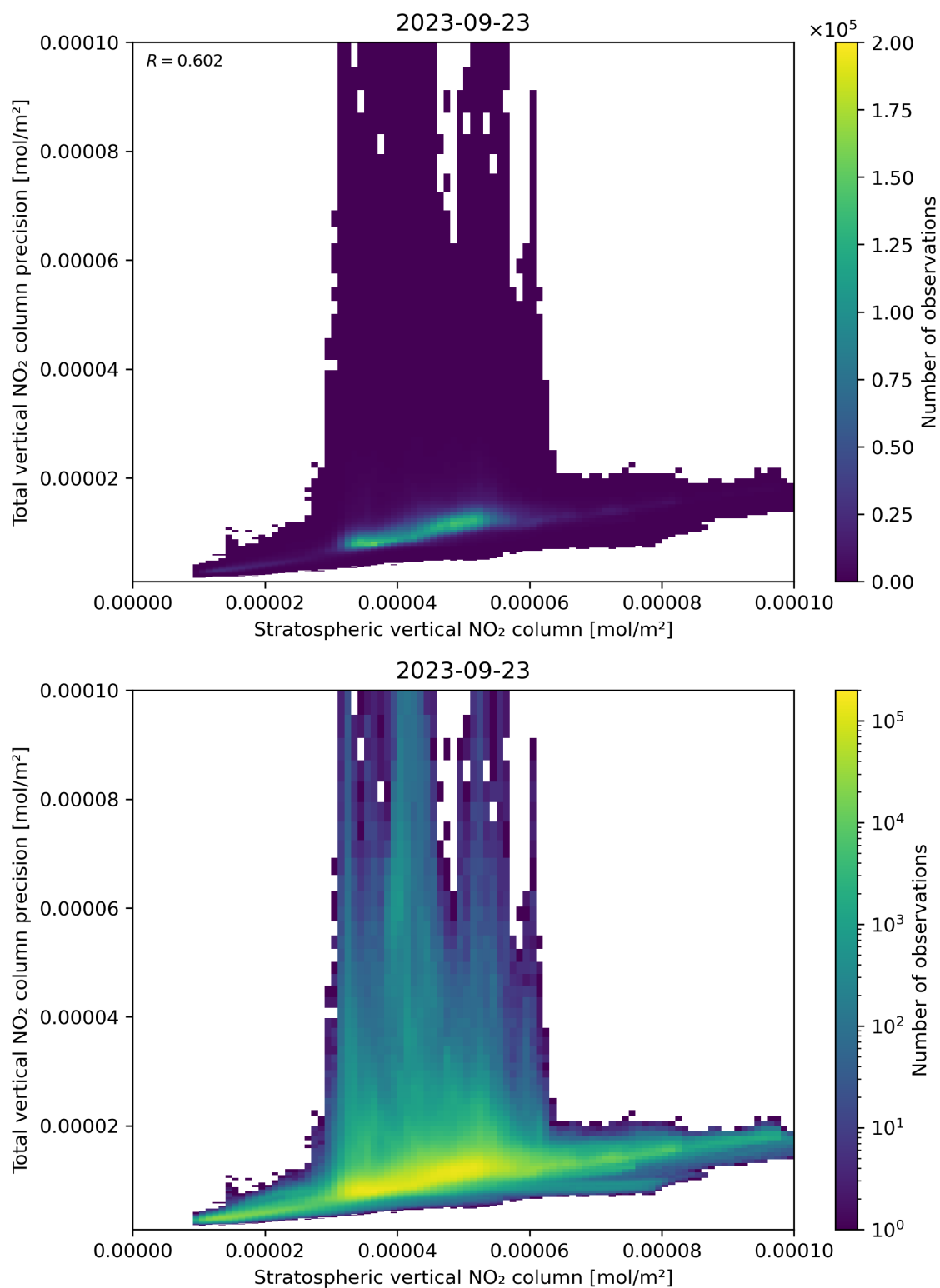
Figure 101: Scatter density plot of “Stratospheric vertical NO 2 column” against “Total vertical NO 2 column precision” for 2023-09-22 to 2023-09-24.
