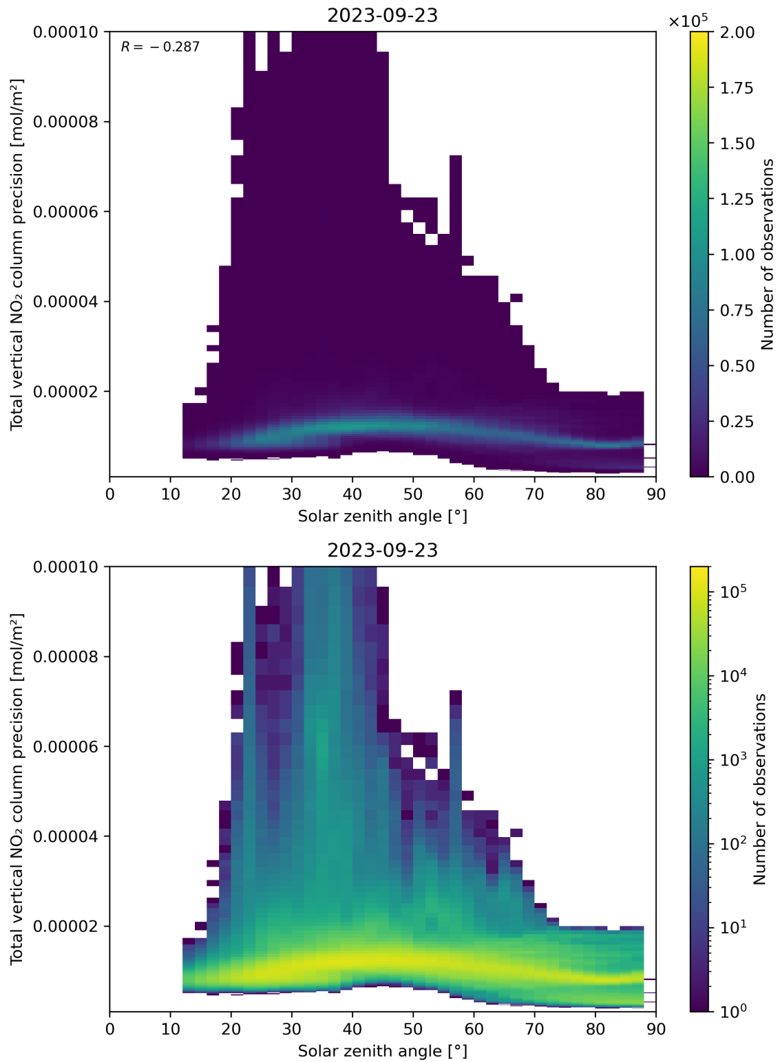
Figure 154: Scatter density plot of “Solar zenith angle” against “Total vertical NO 2 column precision” for 2023-09-22 to 2023-09-24.
