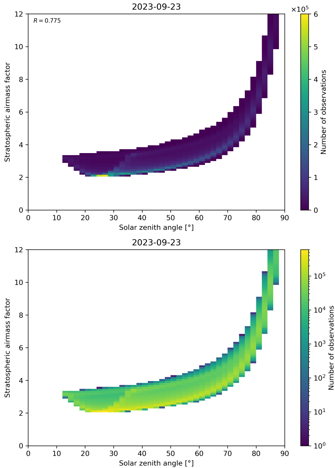
Figure 145: Scatter density plot of “Solar zenith angle” against “Stratospheric airmass factor” for 2023-09-22 to 2023-09-24.
