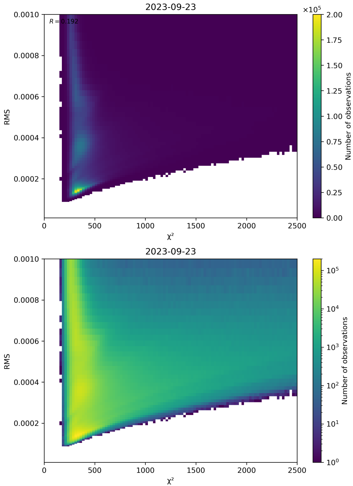
Figure 82: Scatter density plot of “ \chi^2 ” against “RMS” for 2023-09-22 to 2023-09-24.
