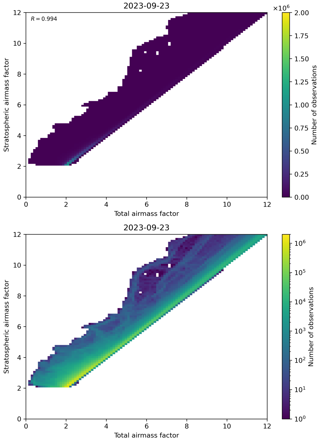
Figure 62: Scatter density plot of “Total airmass factor” against “Stratospheric airmass factor” for 2023-09-22 to 2023-09-24.
