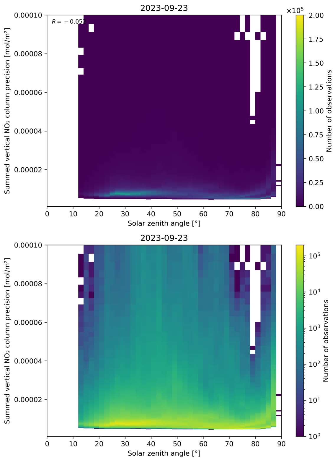
Figure 152: Scatter density plot of “Solar zenith angle” against “Summed vertical NO 2 column precision” for 2023-09-22 to 2023-09-24.
