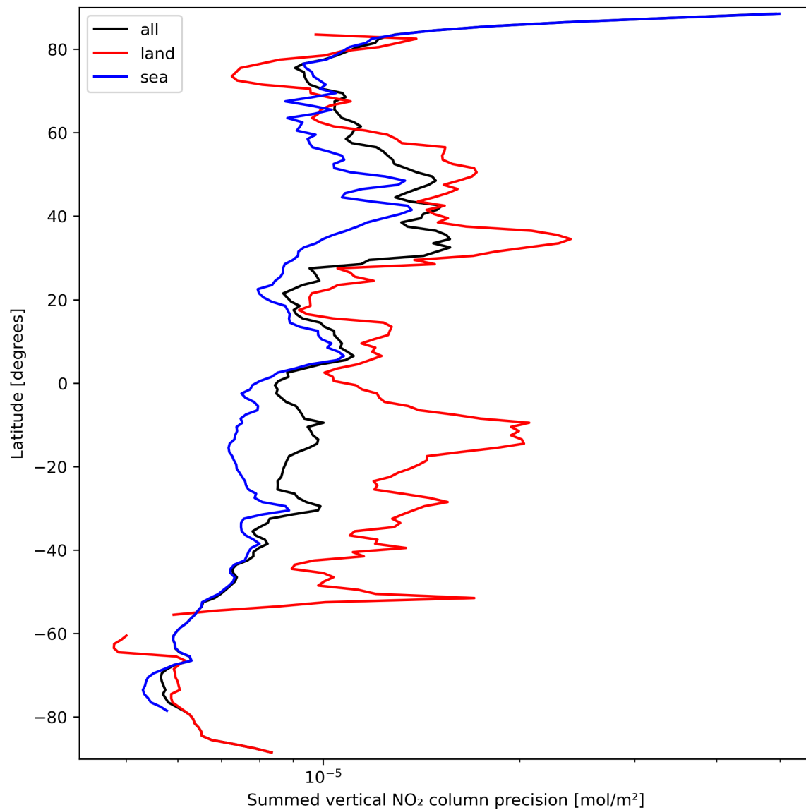
Figure 24: Zonal average of “Summed vertical NO 2 column precision” for 2023-09-22 to 2023-09-24.
