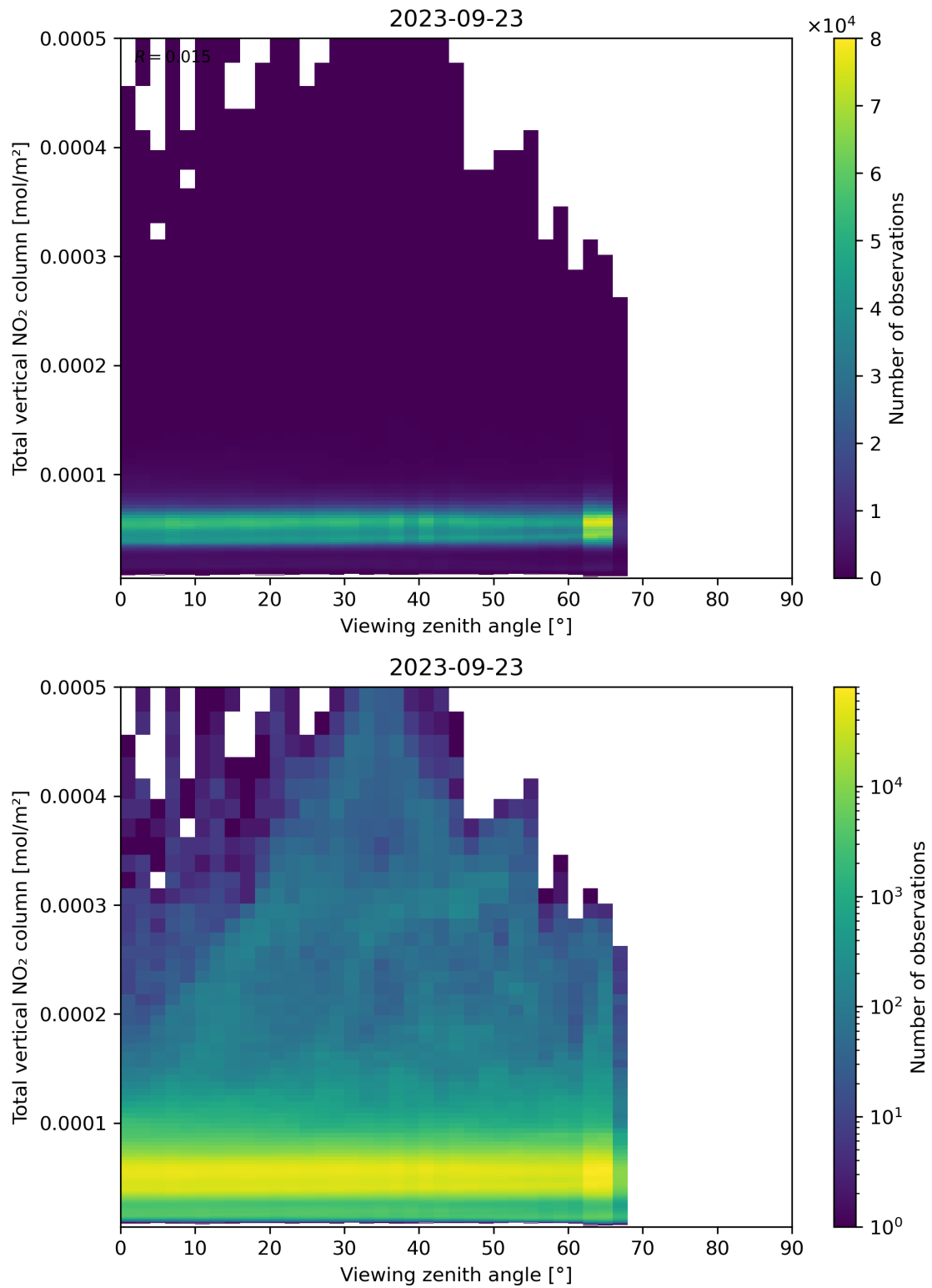
Figure 167: Scatter density plot of “Viewing zenith angle” against “Total vertical NO 2 column” for 2023-09-22 to 2023-09-24.
