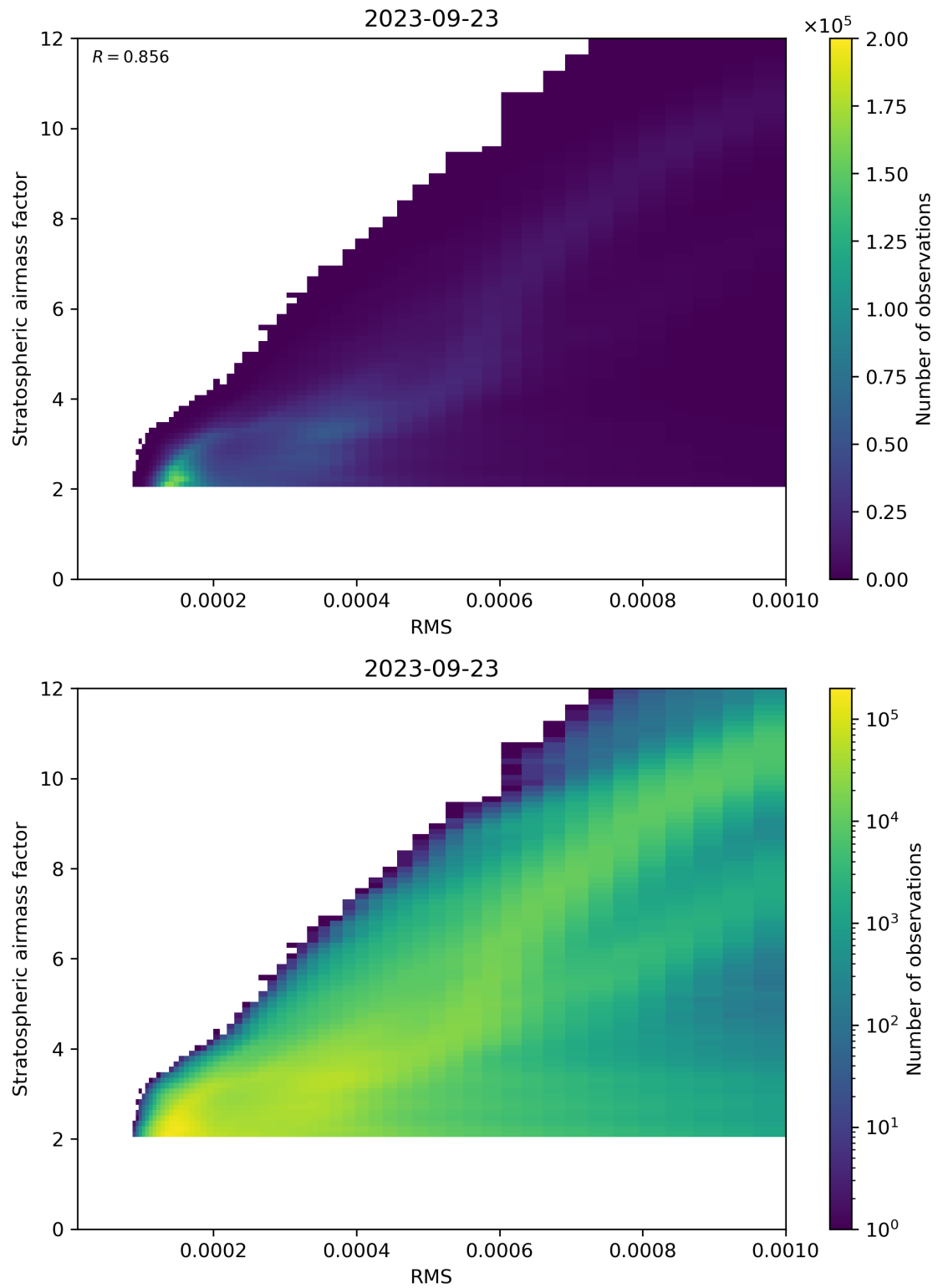
Figure 144: Scatter density plot of “RMS” against “Stratospheric airmass factor” for 2023-09-22 to 2023-09-24.
