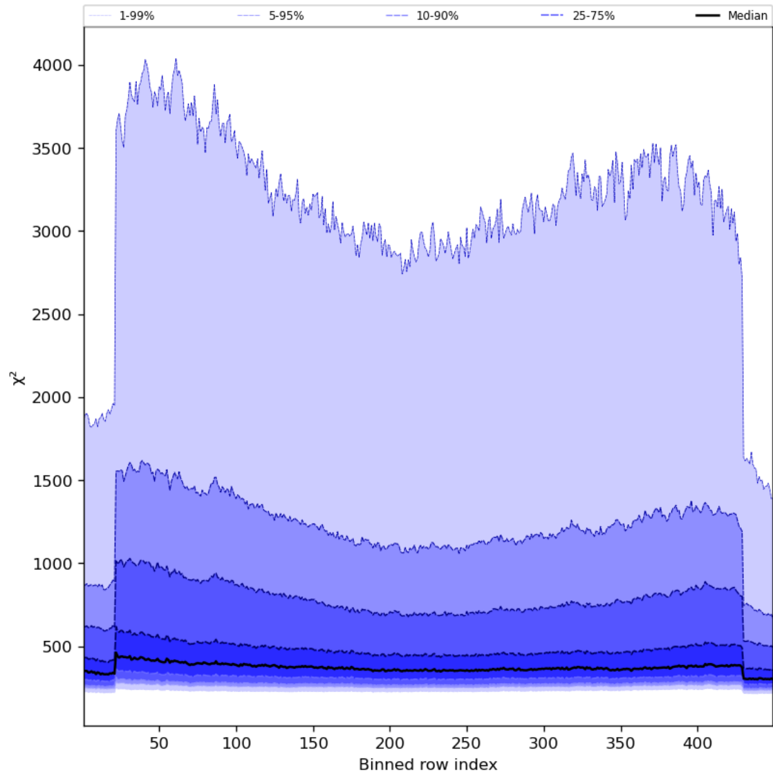
Figure 59: Along track statistics of “ \chi^2 ” for 2023-09-22 to 2023-09-24
