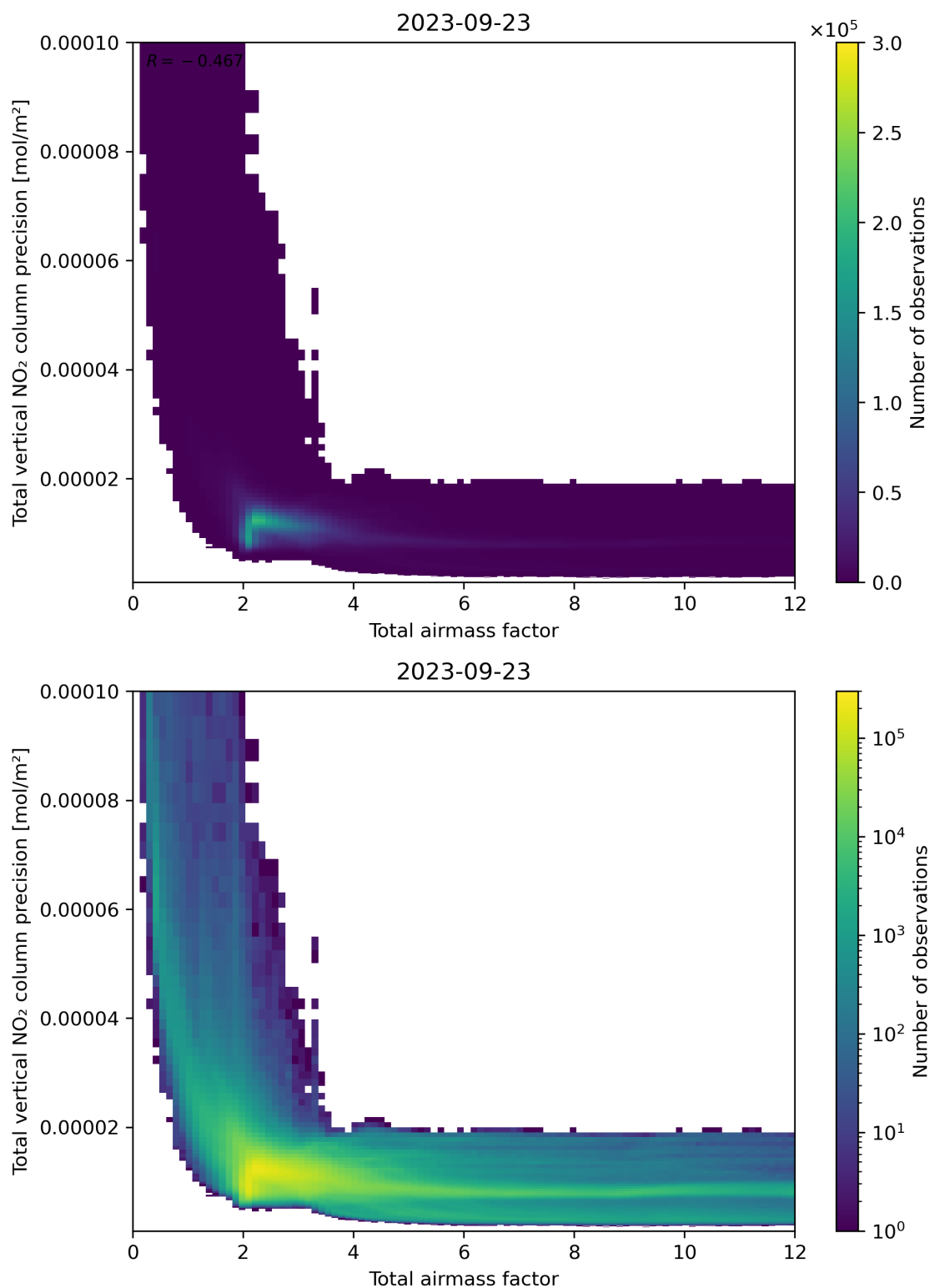
Figure 68: Scatter density plot of “Total airmass factor” against “Total vertical NO 2 column precision” for 2023-09-22 to 2023-09-24.
