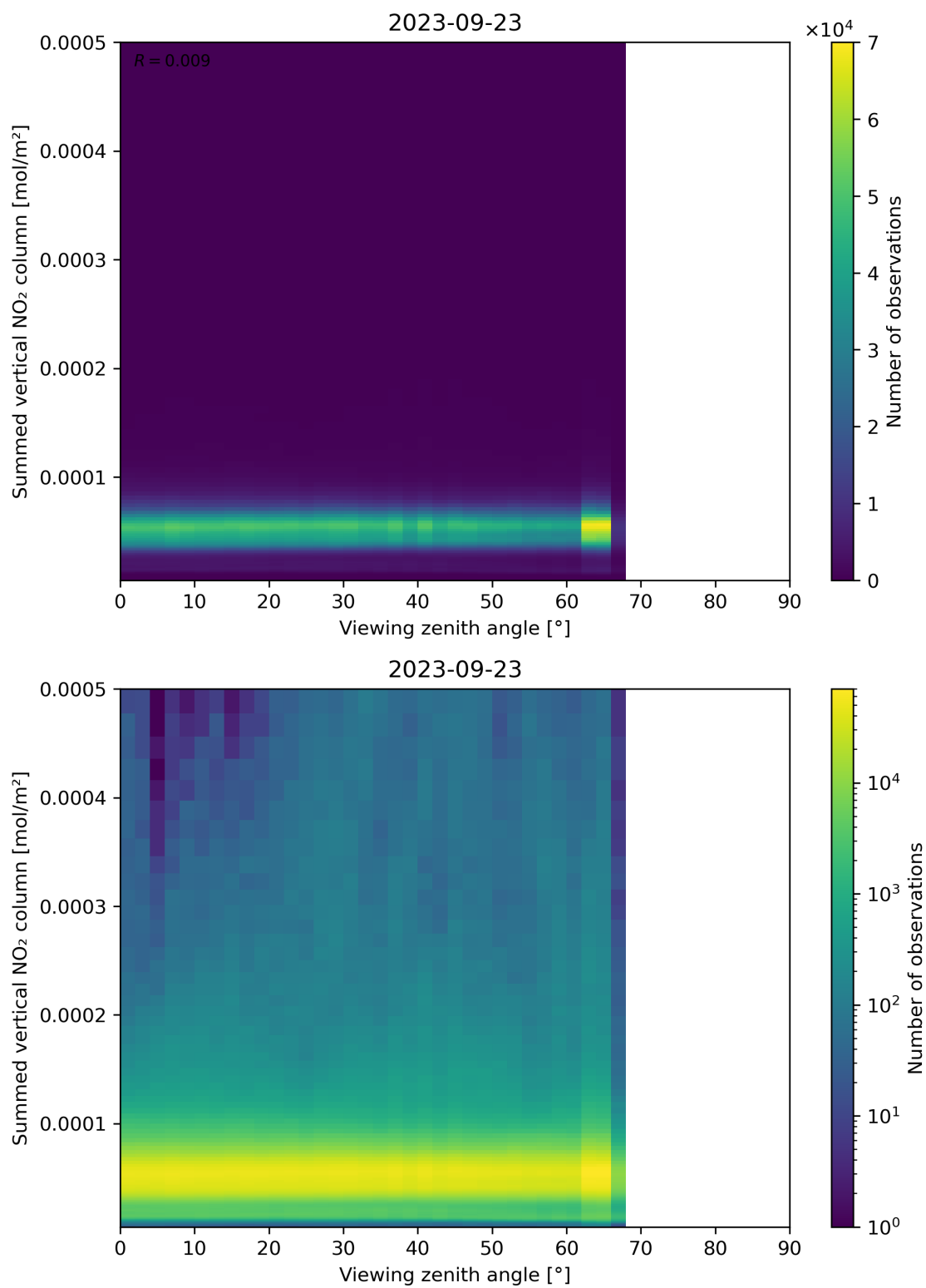
Figure 165: Scatter density plot of “Viewing zenith angle” against “Summed vertical NO 2 column” for 2023-09-22 to 2023-09-24.
