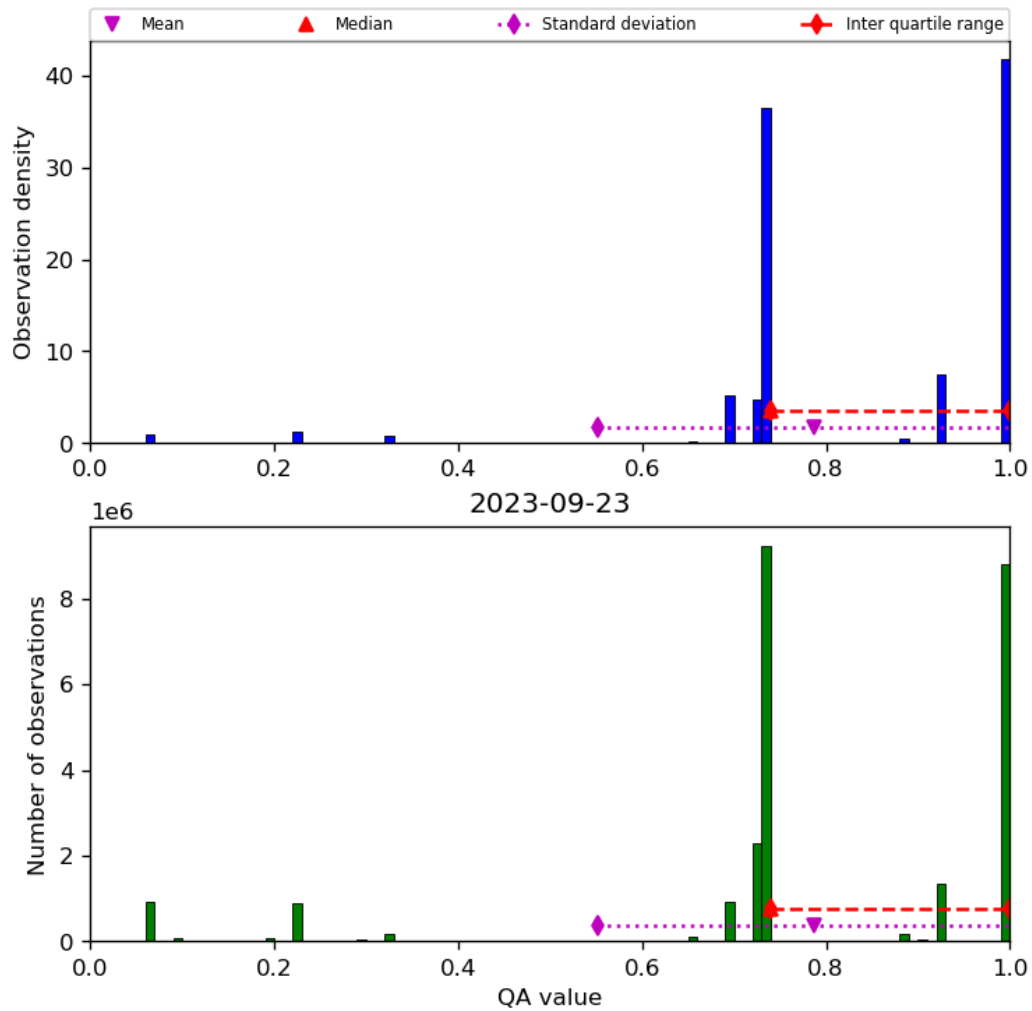
Figure 28: Histogram of “QA value” for 2023-09-22 to 2023-09-24
