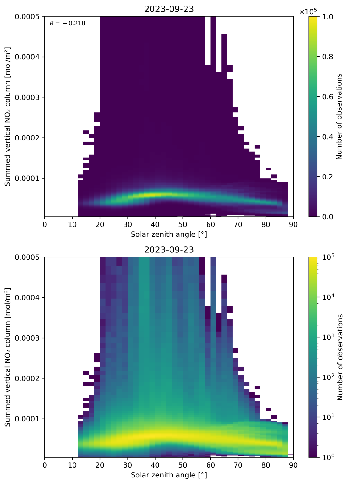
Figure 151: Scatter density plot of “Solar zenith angle” against “Summed vertical NO 2 column” for 2023-09-22 to 2023-09-24.
