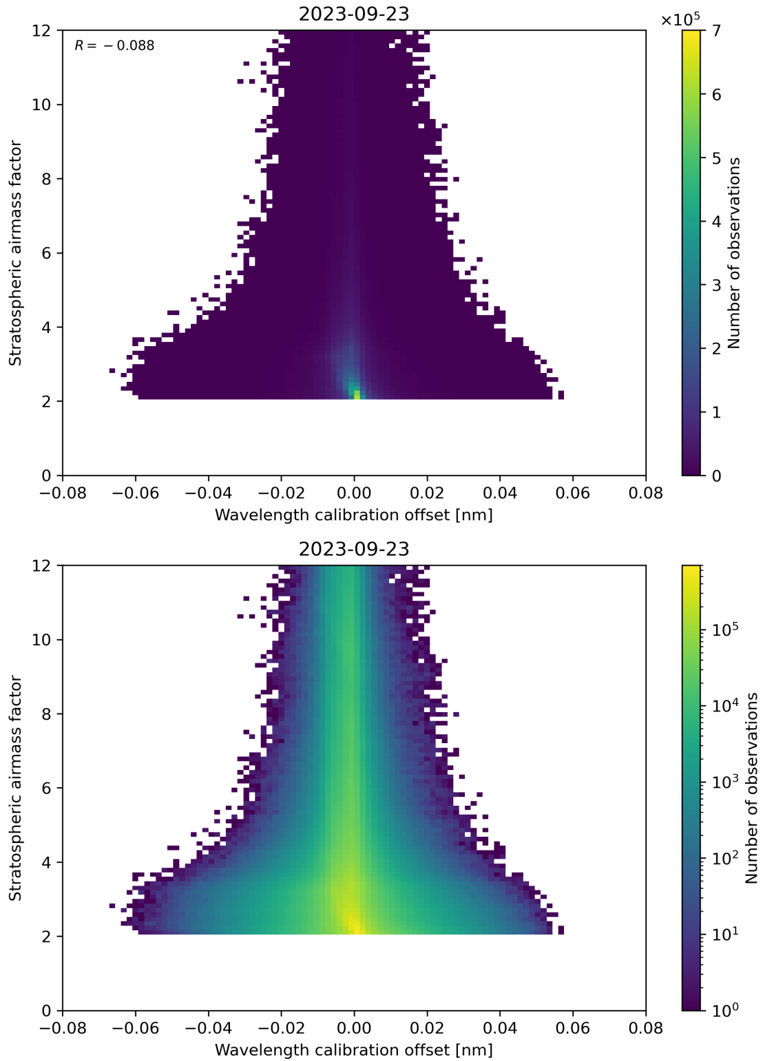
Figure 174: Scatter density plot of “Wavelength calibration offset” against “Stratospheric airmass factor” for 2023-09-22 to 2023-09-24.
