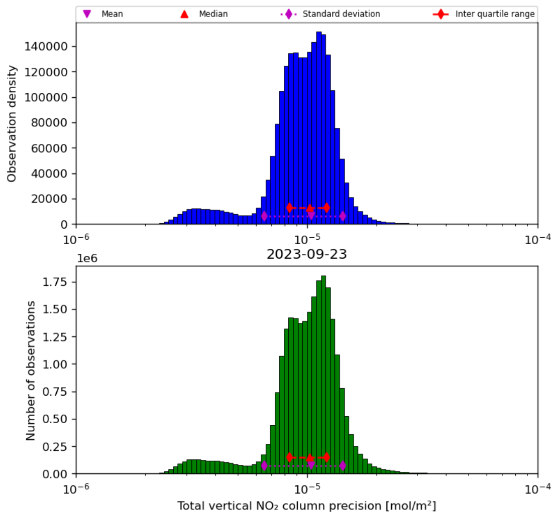
Figure 39: Histogram of “Total vertical NO 2 column precision” for 2023-09-22 to 2023-09-24
