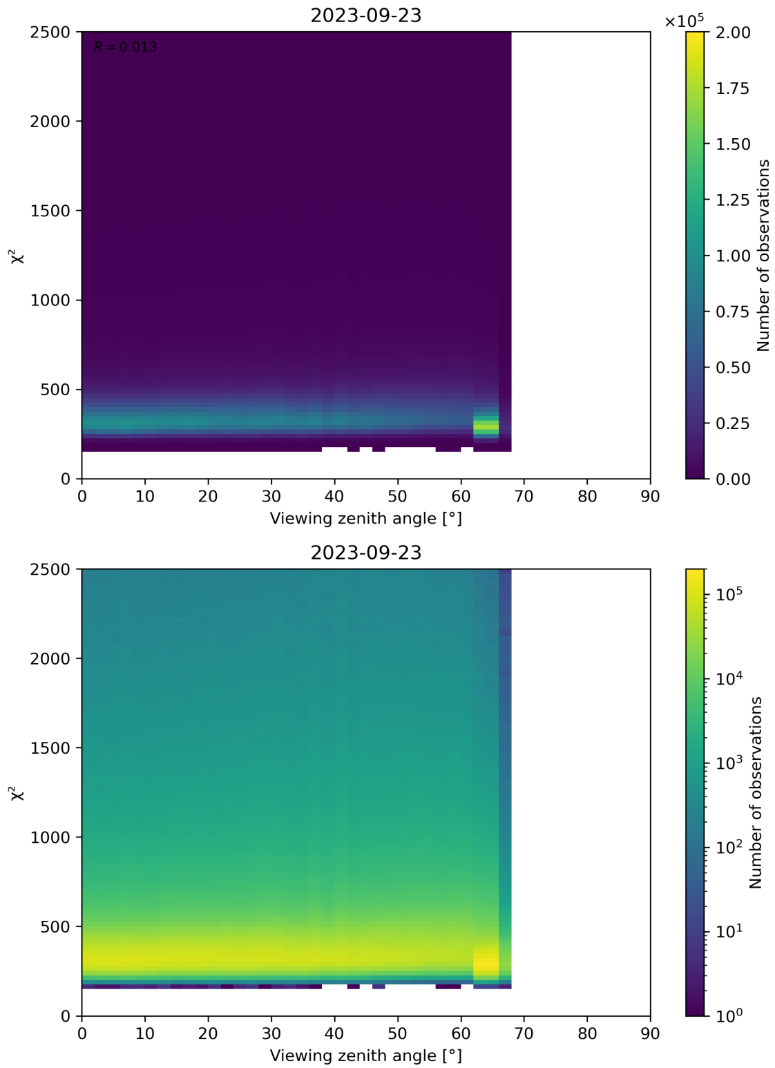
Figure 162: Scatter density plot of “Viewing zenith angle” against “ \chi^2 ” for 2023-09-22 to 2023-09-24.
