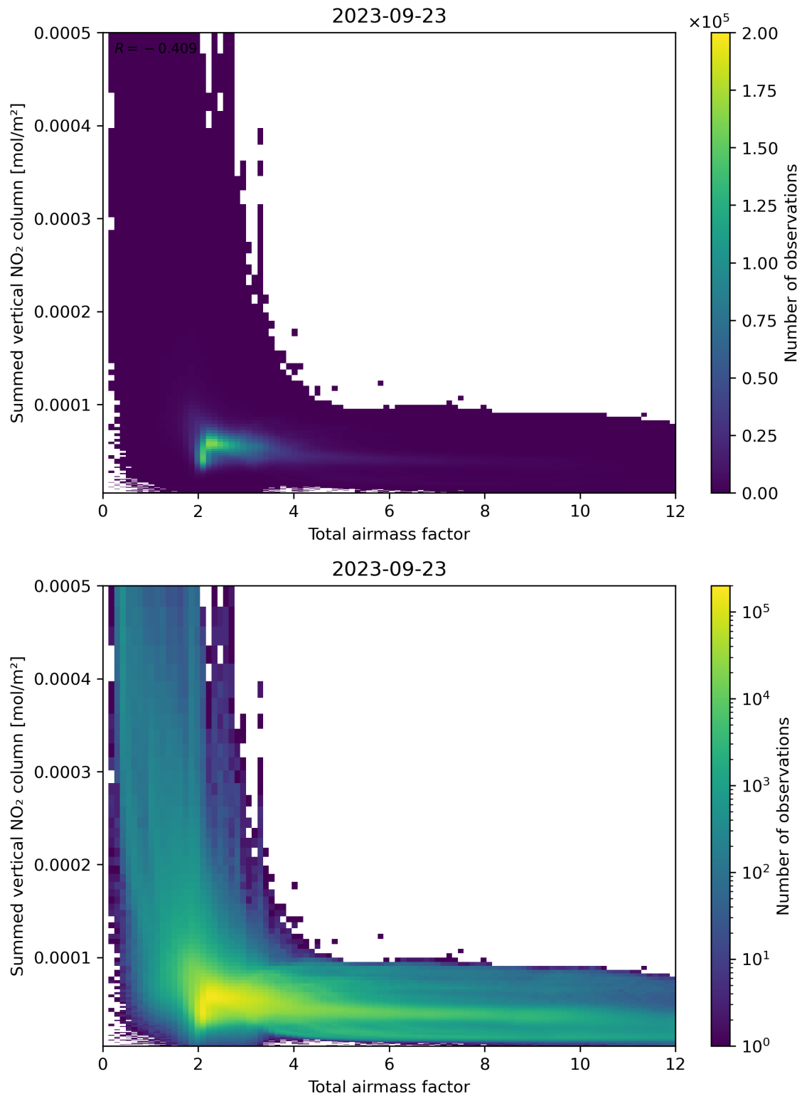
Figure 65: Scatter density plot of “Total airmass factor” against “Summed vertical NO 2 column” for 2023-09-22 to 2023-09-24.
