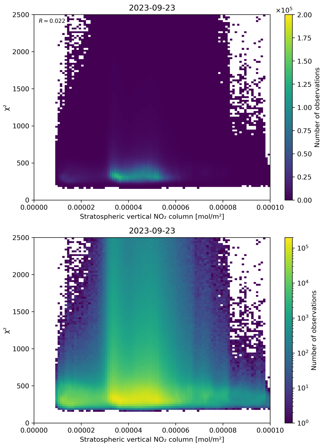
Figure 97: Scatter density plot of “Stratospheric vertical NO 2 column” against “ \chi^2 ” for 2023-09-22 to 2023-09-24.
