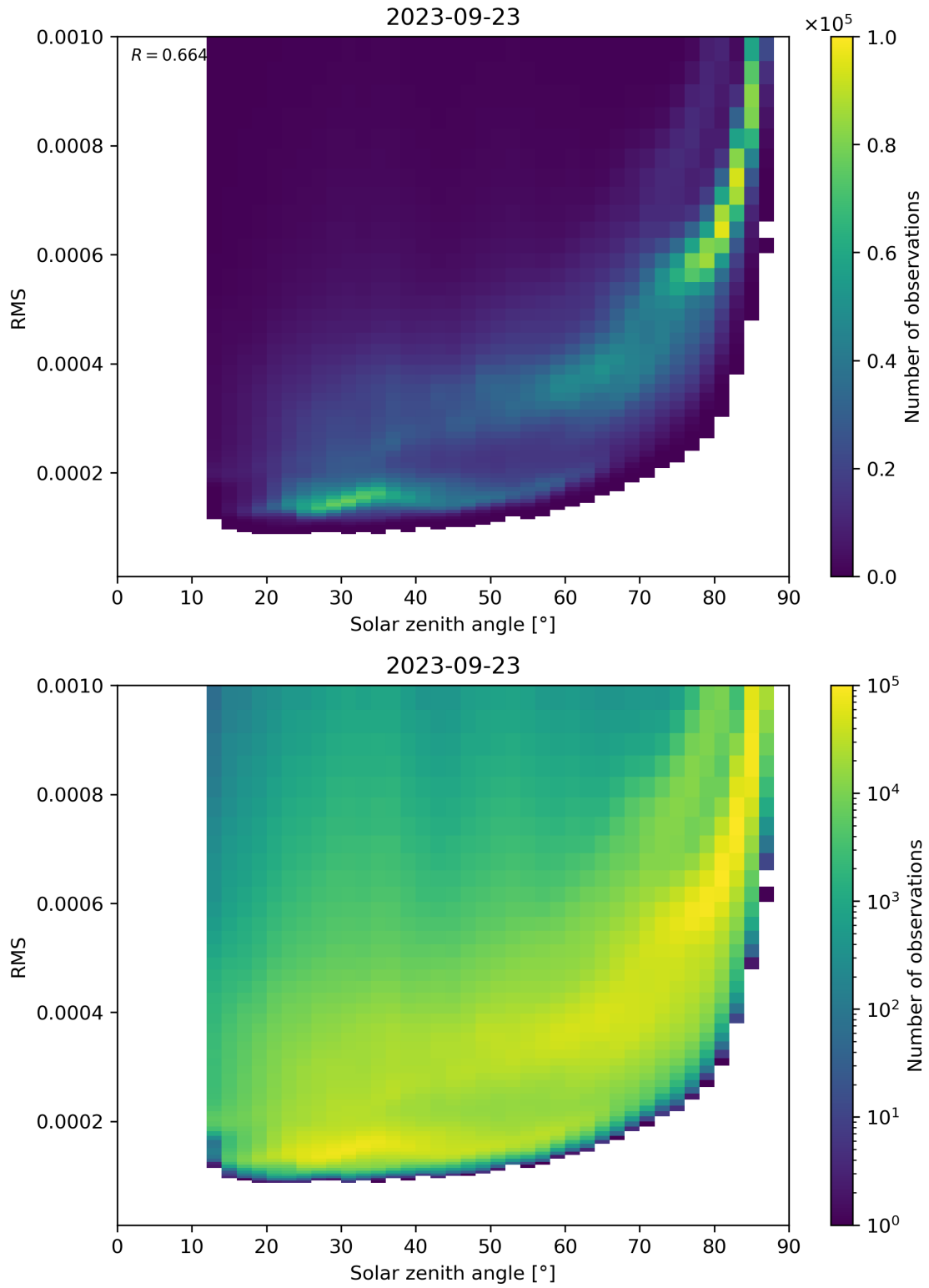
Figure 157: Scatter density plot of “Solar zenith angle” against “RMS” for 2023-09-22 to 2023-09-24.
