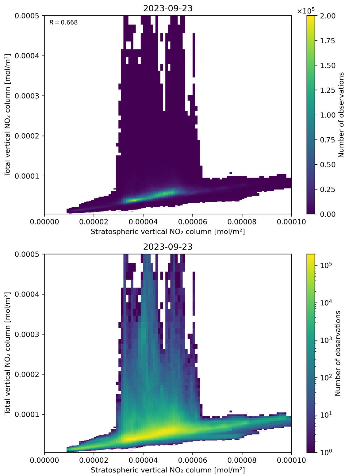
Figure 100: Scatter density plot of “Stratospheric vertical NO 2 column” against “Total vertical NO 2 column” for 2023-09-22 to 2023-09-24.
