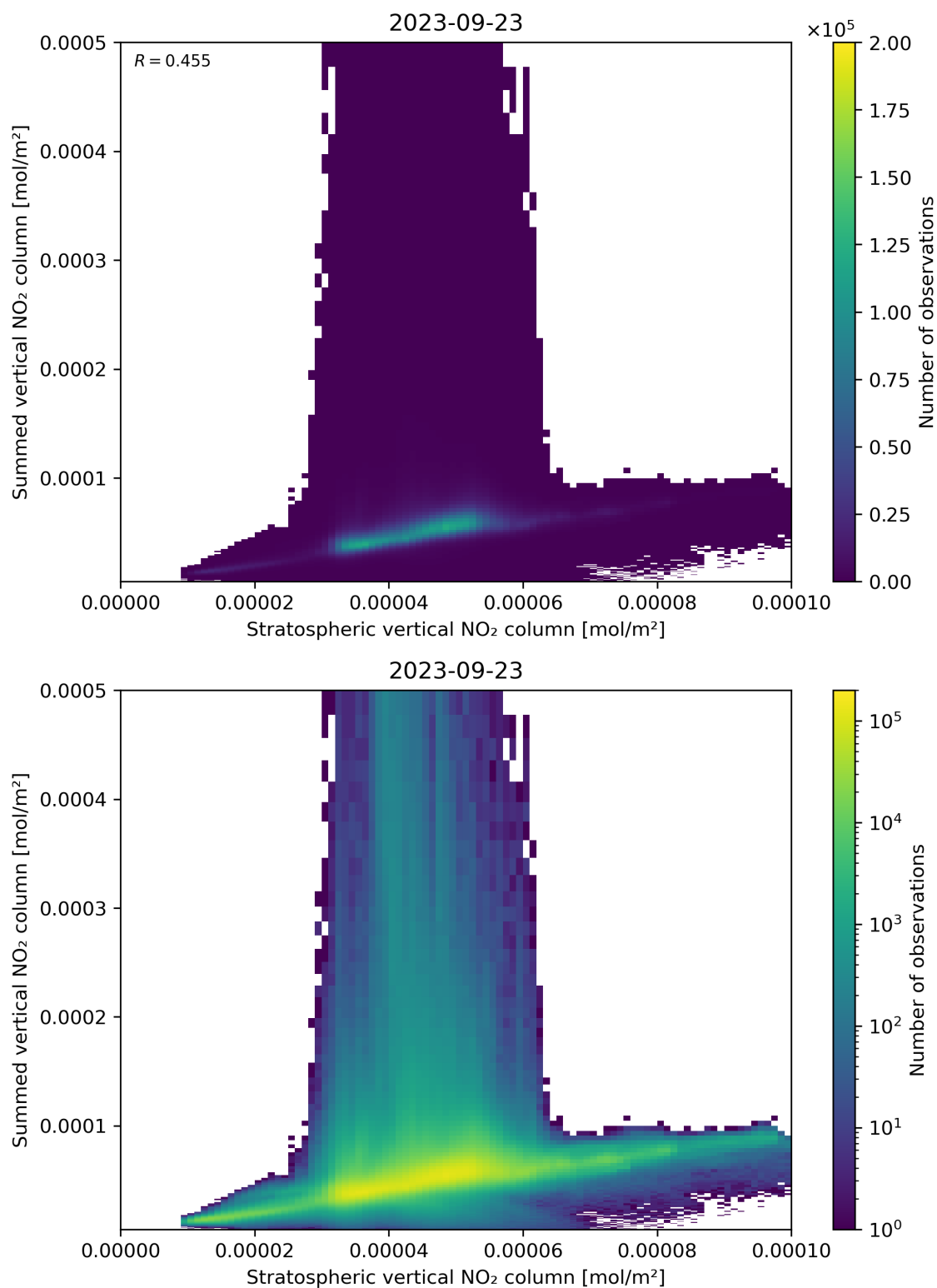
Figure 98: Scatter density plot of “Stratospheric vertical NO 2 column” against “Summed vertical NO 2 column” for 2023-09-22 to 2023-09-24.
