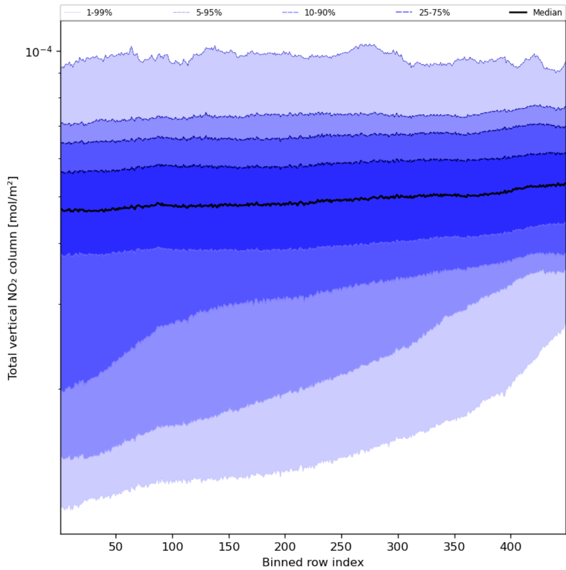
Figure 55: Along track statistics of “Total vertical NO 2 column” for 2023-09-22 to 2023-09-24
