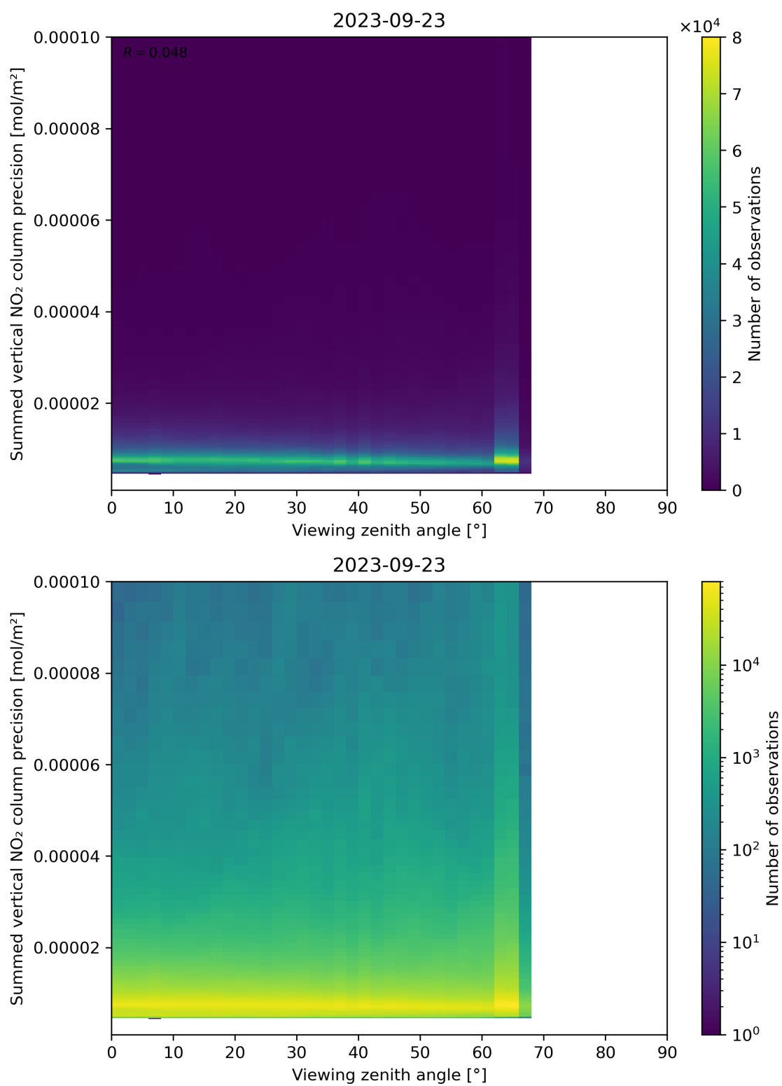
Figure 166: Scatter density plot of “Viewing zenith angle” against “Summed vertical NO 2 column precision” for 2023-09-22 to 2023-09-24.
