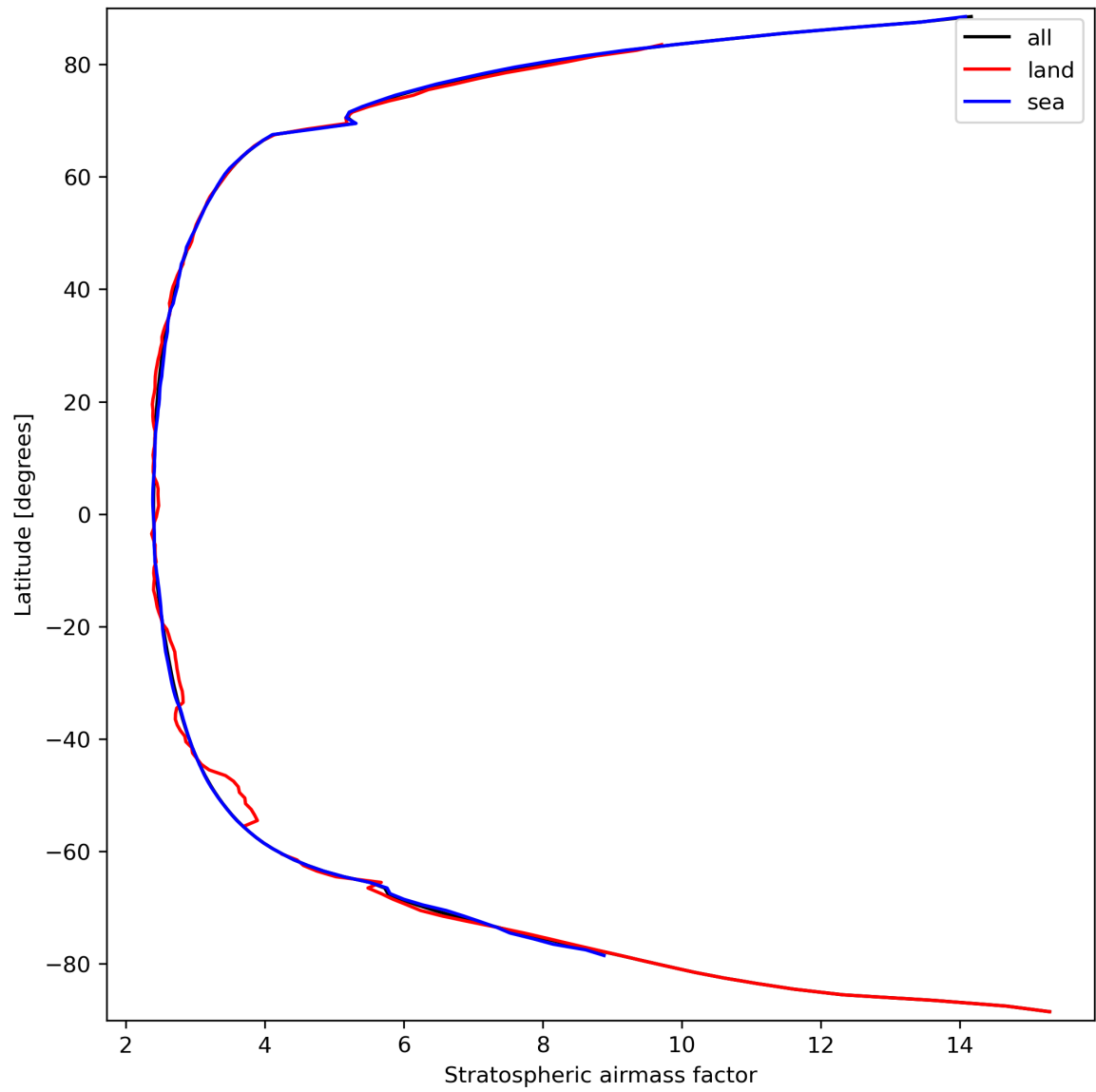
Figure 27: Zonal average of “Stratospheric airmass factor” for 2023-09-22 to 2023-09-24.
