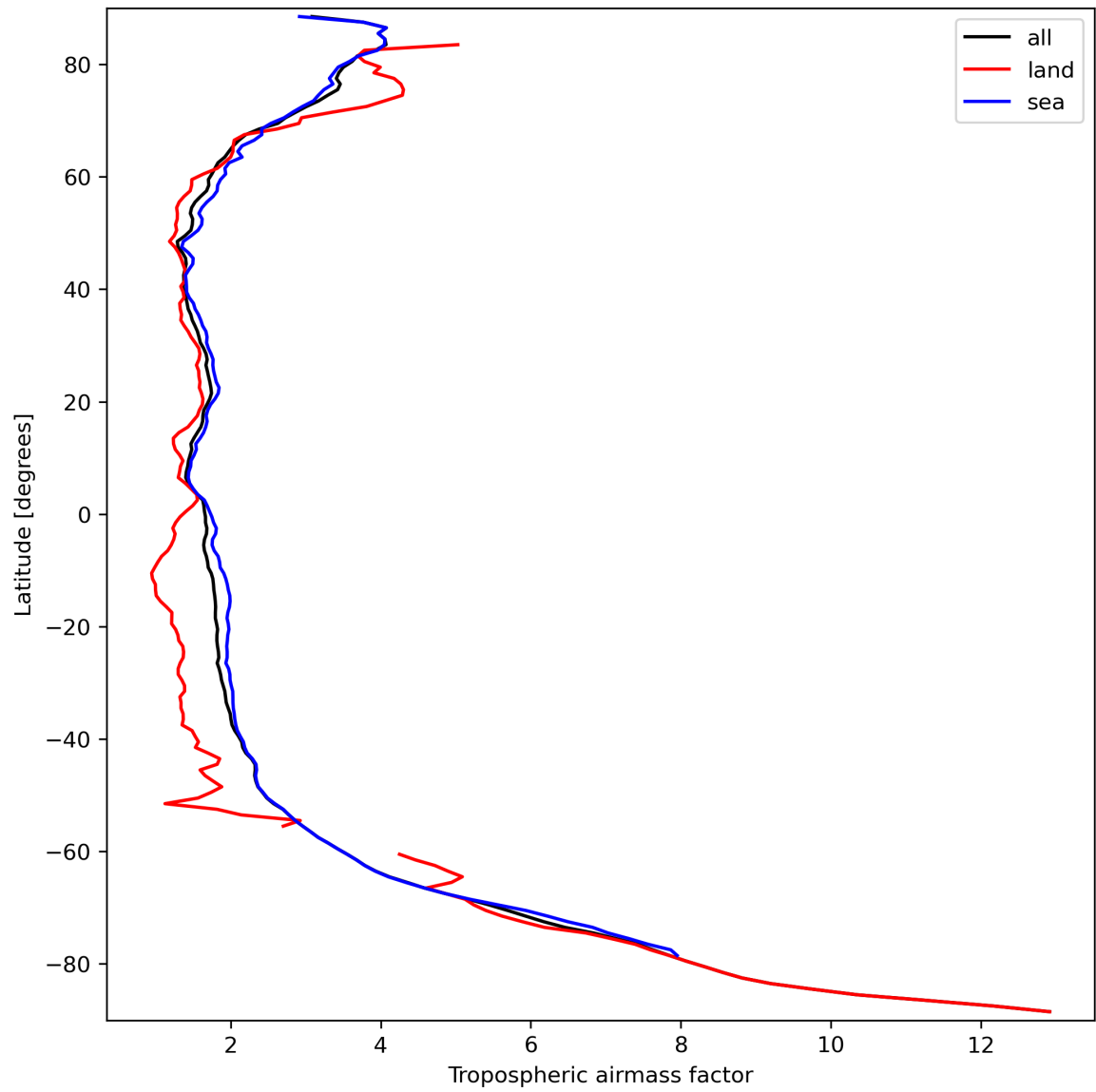
Figure 14: Zonal average of “Tropospheric airmass factor” for 2023-09-22 to 2023-09-24.
