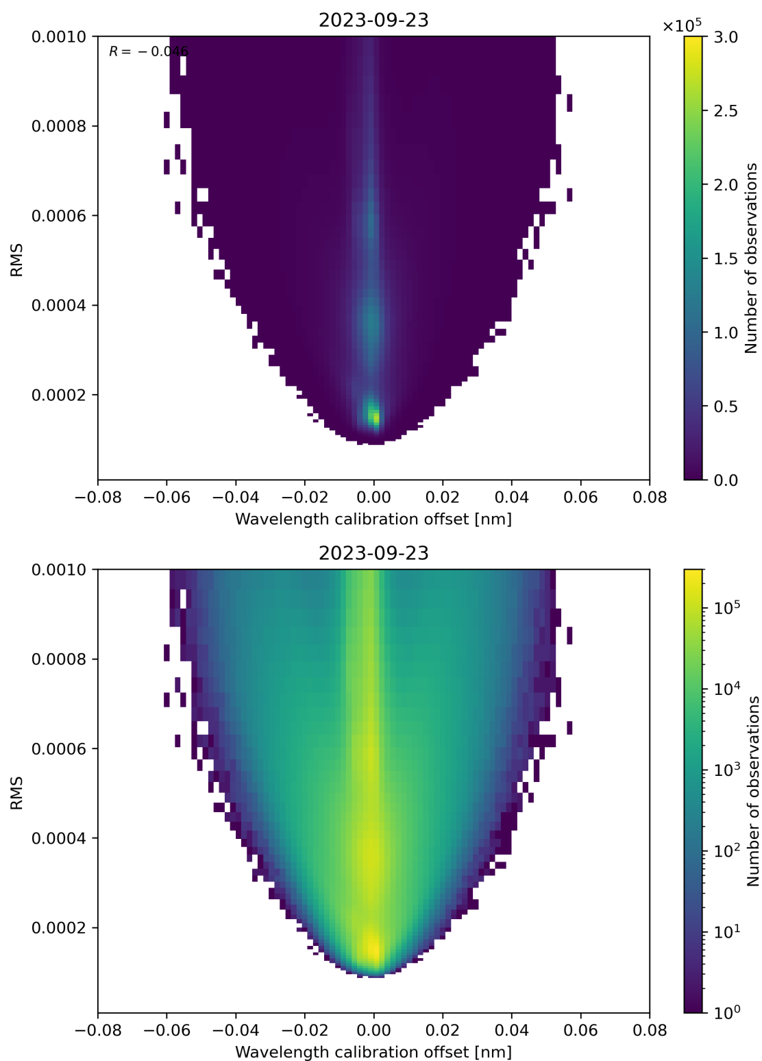
Figure 181: Scatter density plot of “Wavelength calibration offset” against “RMS” for 2023-09-22 to 2023-09-24.
