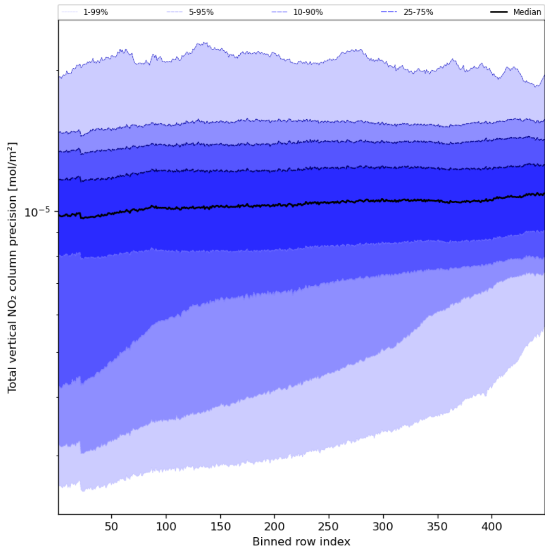
Figure 56: Along track statistics of “Total vertical NO 2 column precision” for 2023-09-22 to 2023-09-24
