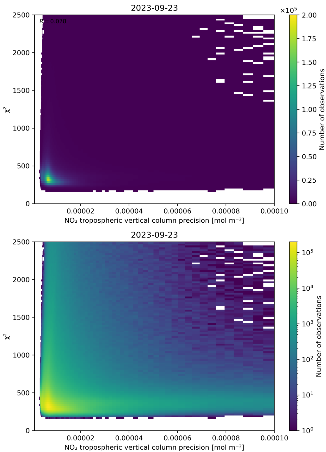
Figure 134: Scatter density plot of “NO 2 tropospheric vertical column precision” against “ \chi^2 ” for 2023-09-22 to 2023-09-24.
