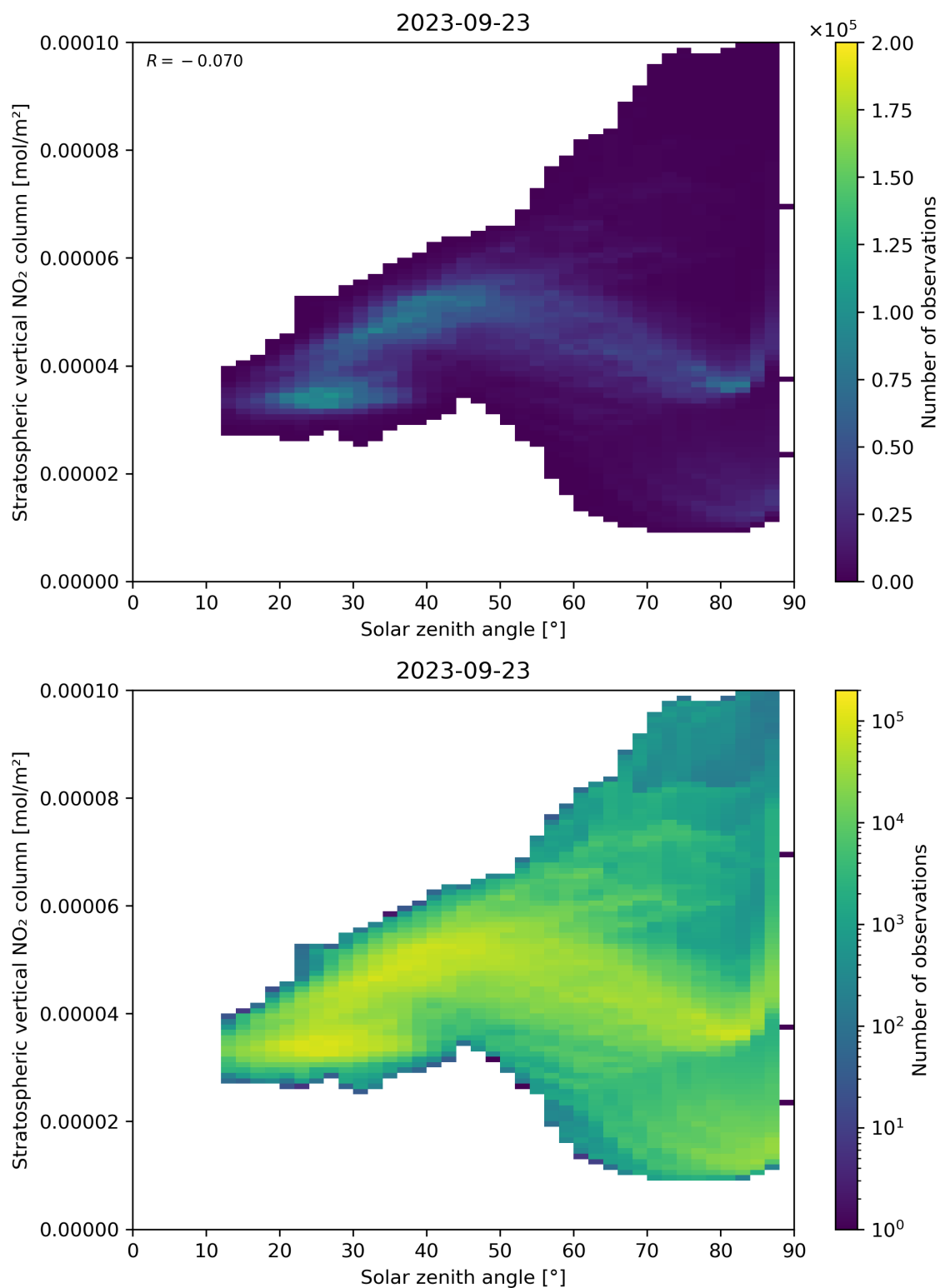
Figure 150: Scatter density plot of “Solar zenith angle” against “Stratospheric vertical NO 2 column” for 2023-09-22 to 2023-09-24.
