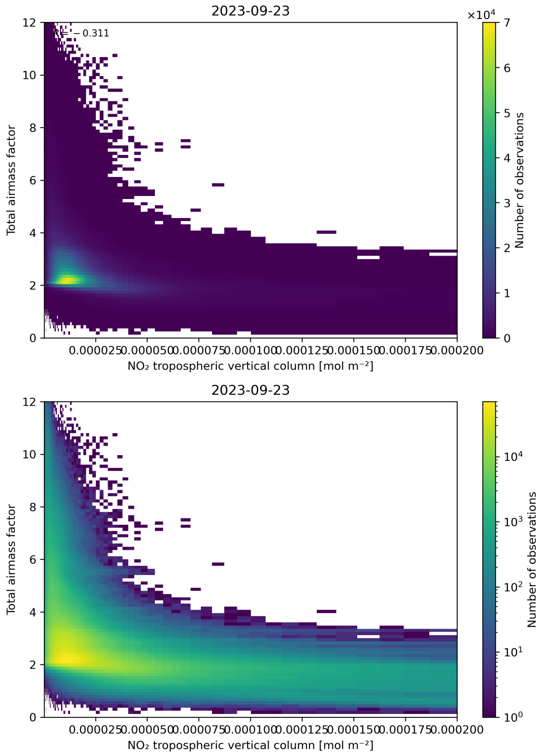
Figure 122: Scatter density plot of “NO 2 tropospheric vertical column” against “Total airmass factor” for 2023-09-22 to 2023-09-24.
