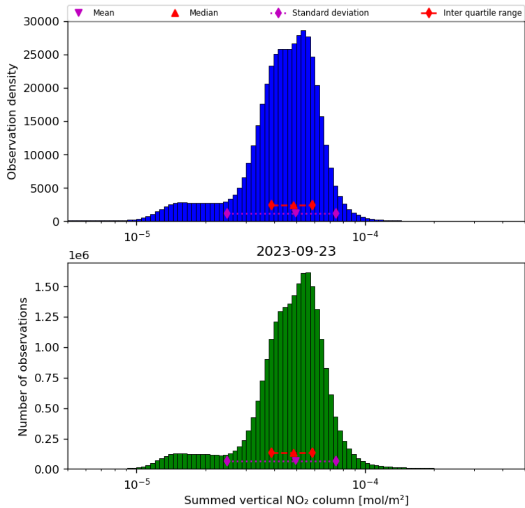
Figure 40: Histogram of “Summed vertical NO 2 column” for 2023-09-22 to 2023-09-24
