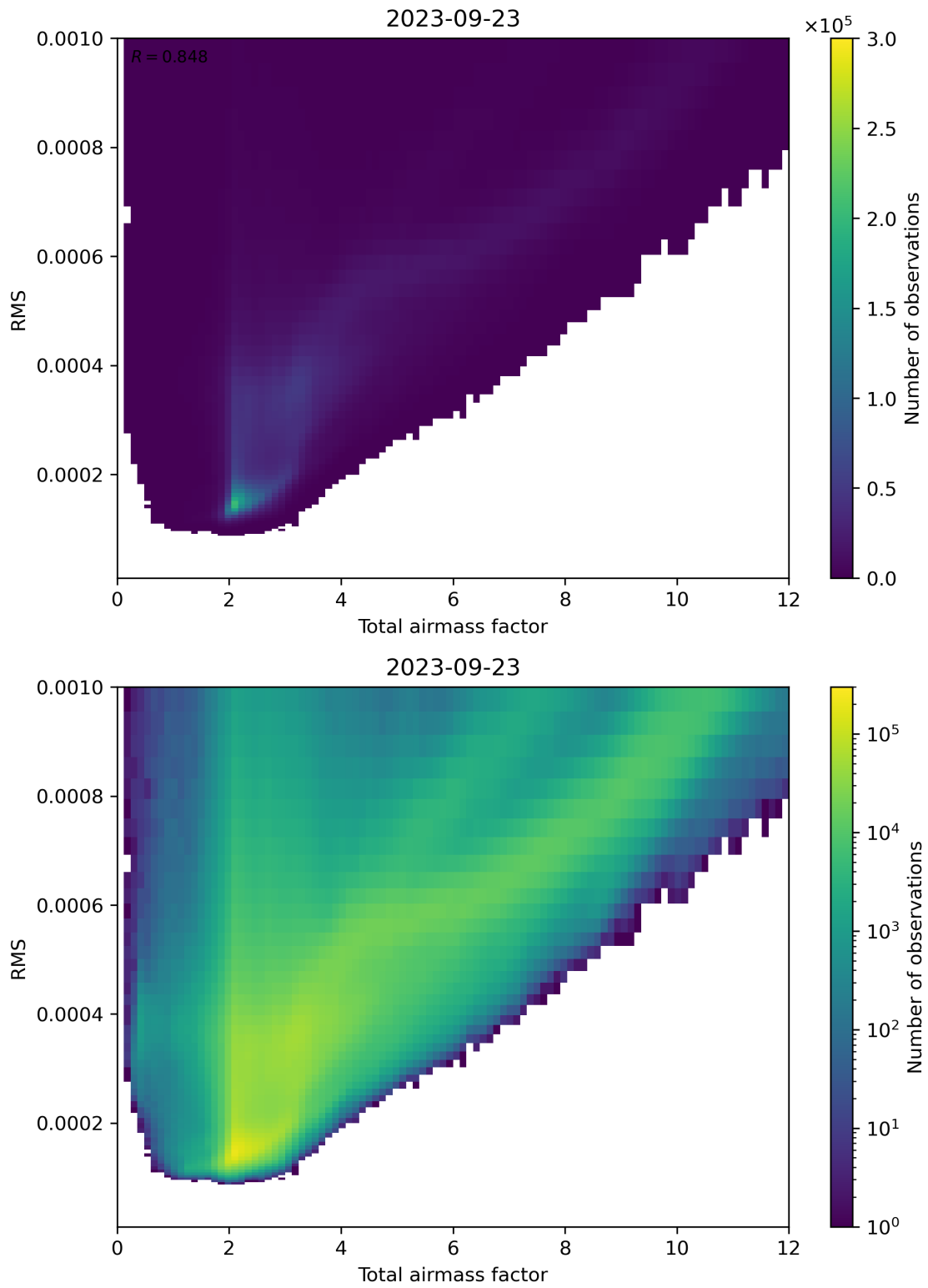
Figure 69: Scatter density plot of “Total airmass factor” against “RMS” for 2023-09-22 to 2023-09-24.
