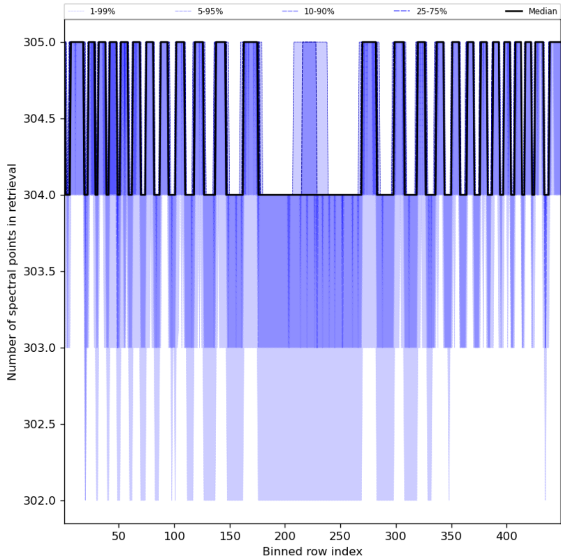
Figure 50: Along track statistics of “Number of spectral points in retrieval” for 2023-09-22 to 2023-09-24
