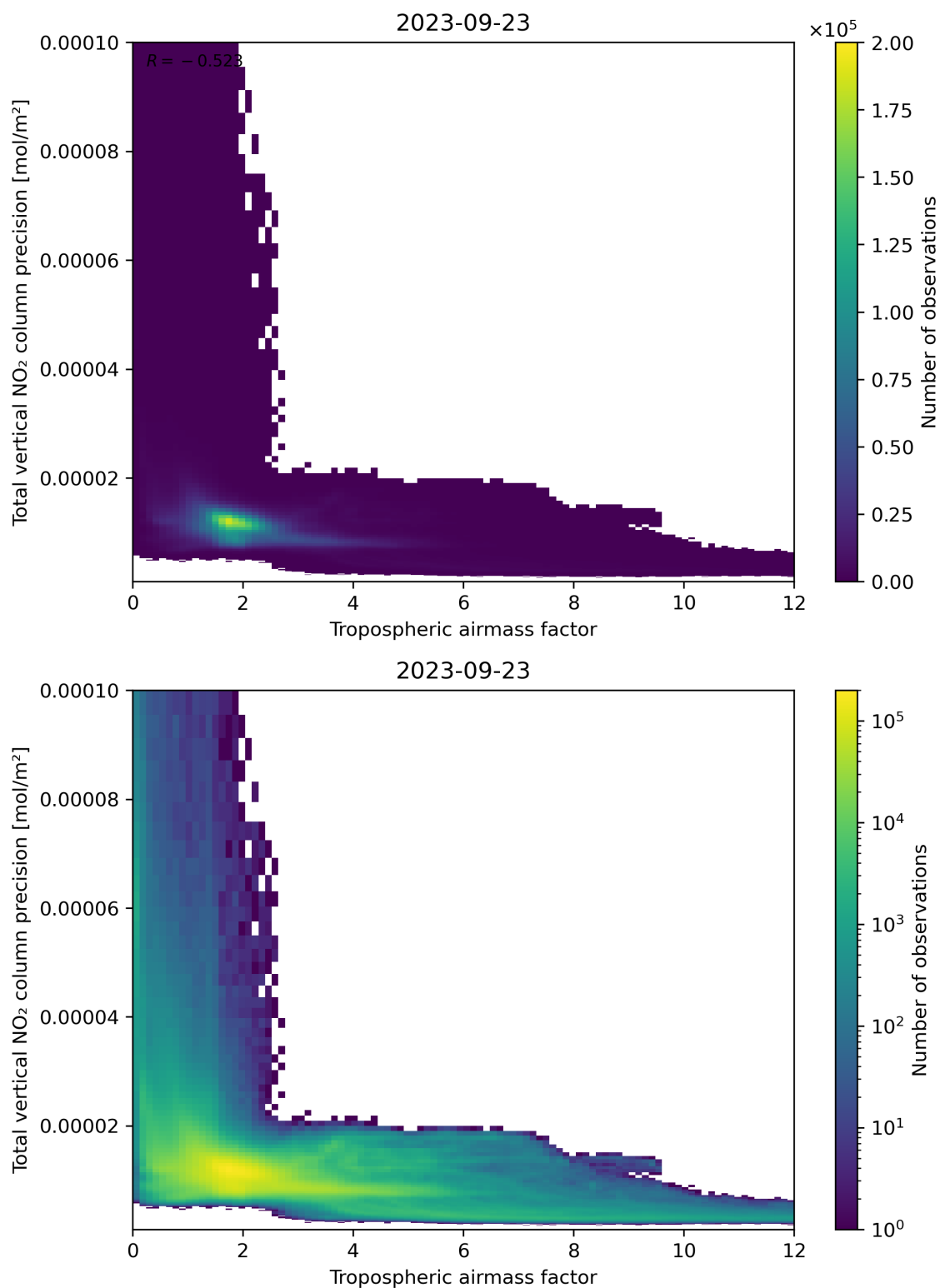
Figure 78: Scatter density plot of “Tropospheric air mass factor” against “Total vertical NO 2 column precision” for 2023-09-22 to 2023-09-24.
