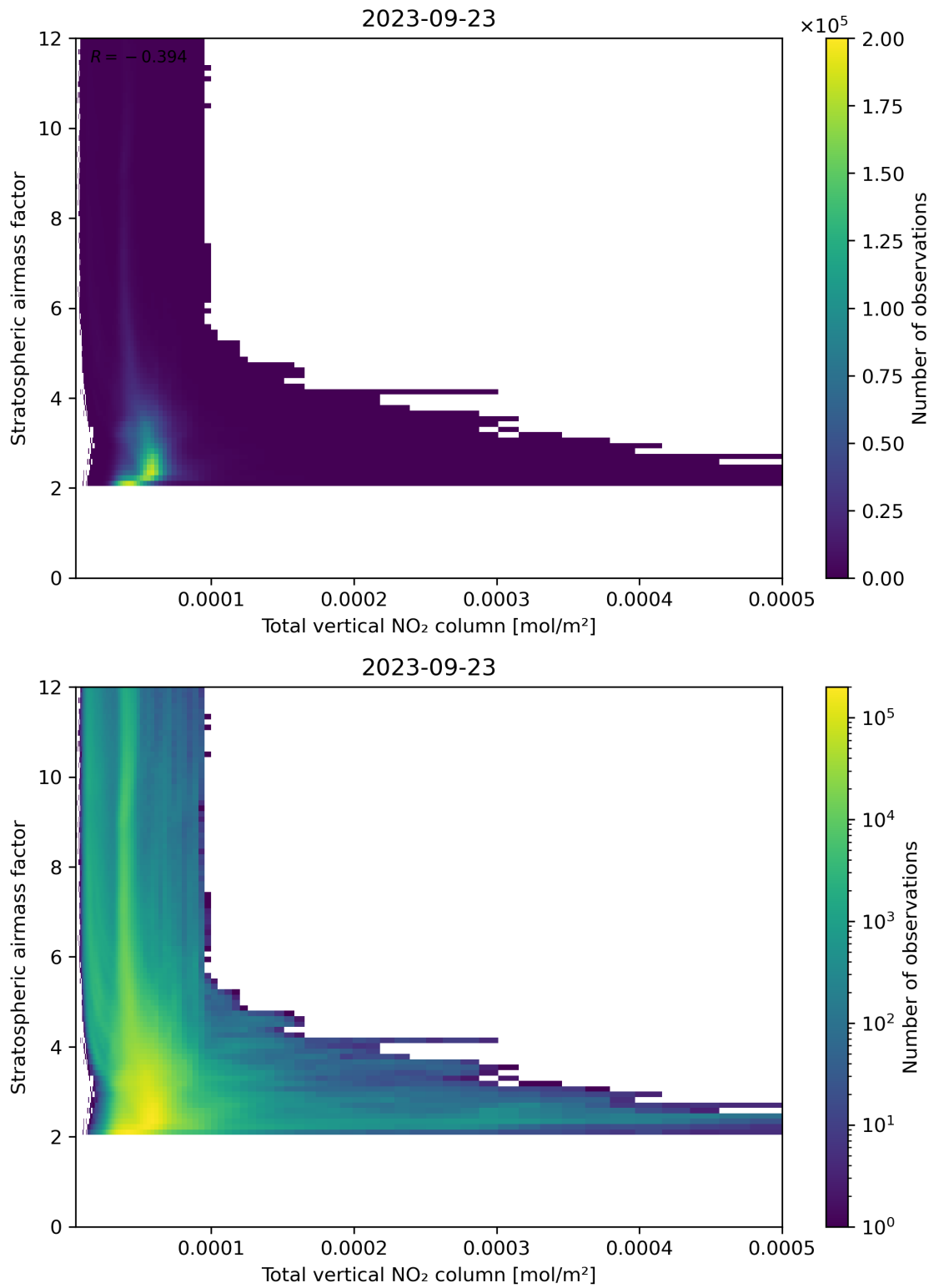
Figure 110: Scatter density plot of “Total vertical NO 2 column” against “Stratospheric airmass factor” for 2023-09-22 to 2023-09-24.
