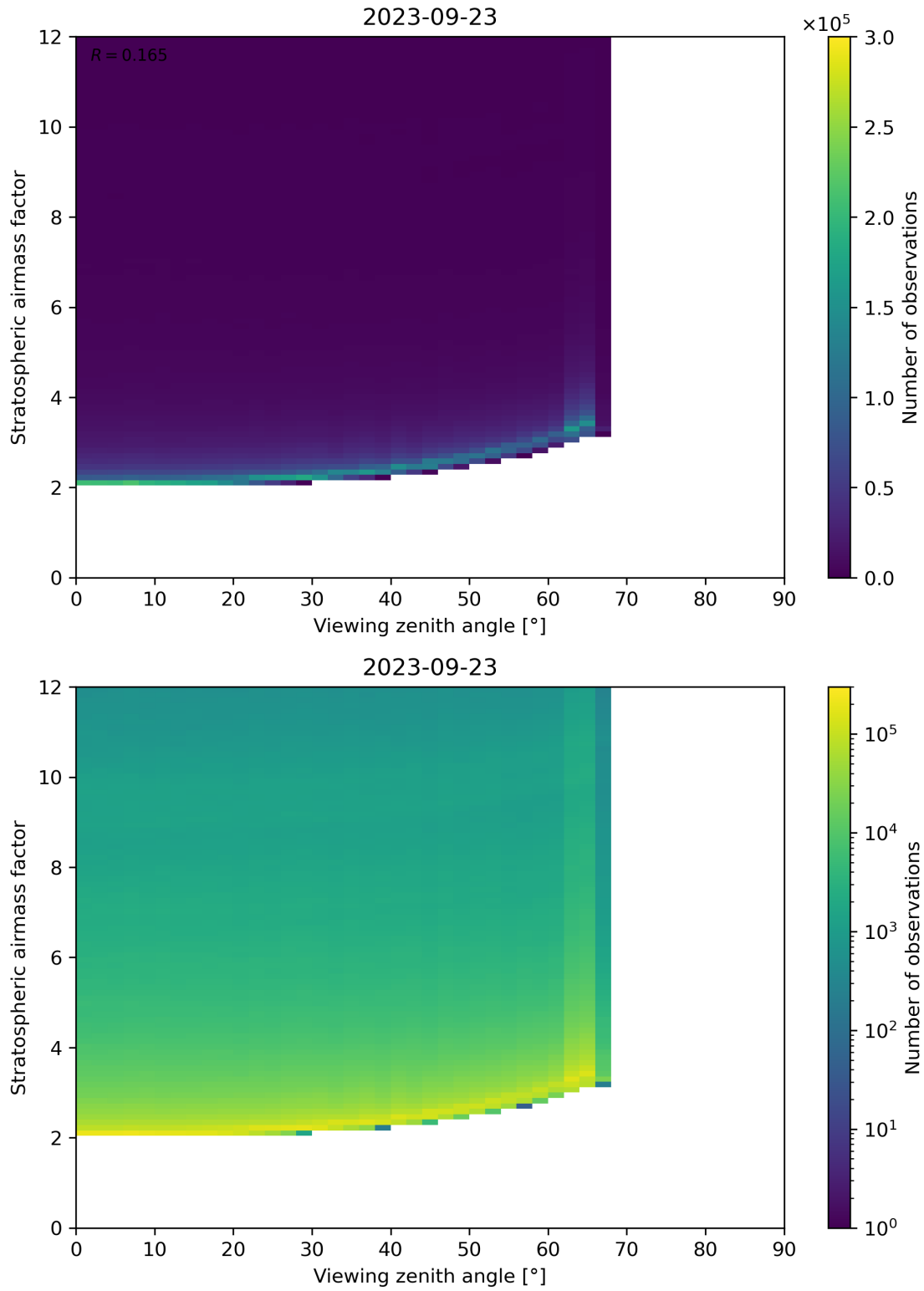
Figure 159: Scatter density plot of “Viewing zenith angle” against “Stratospheric airmass factor” for 2023-09-22 to 2023-09-24.
