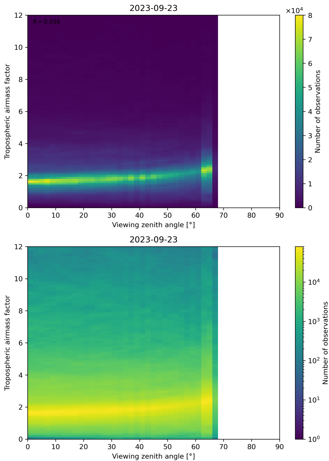
Figure 161: Scatter density plot of “Viewing zenith angle” against “Tropospheric airmass factor” for 2023-09-22 to 2023-09-24.
