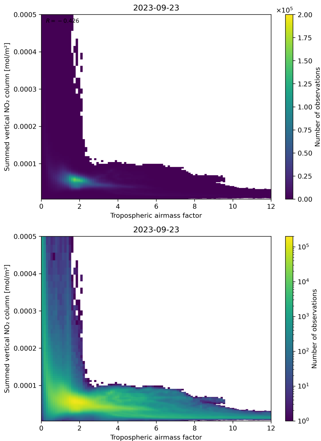
Figure 75: Scatter density plot of “Tropospheric air mass factor” against “Summed vertical NO 2 column” for 2023-09-22 to 2023-09-24.
