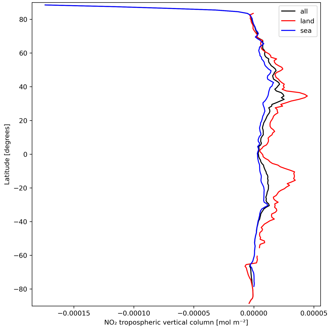
Figure 12: Zonal average of “NO 2 tropospheric vertical column” for 2023-09-22 to 2023-09-24.
