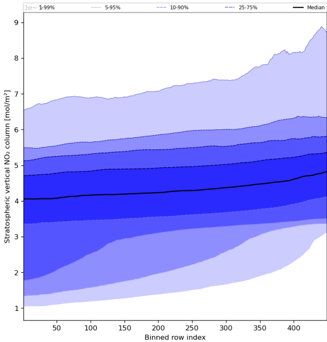
Figure 53: Along track statistics of “Stratospheric vertical NO 2 column” for 2023-09-22 to 2023-09-24
