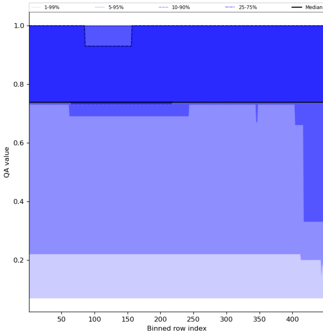
Figure 45: Along track statistics of “QA value” for 2023-09-22 to 2023-09-24
