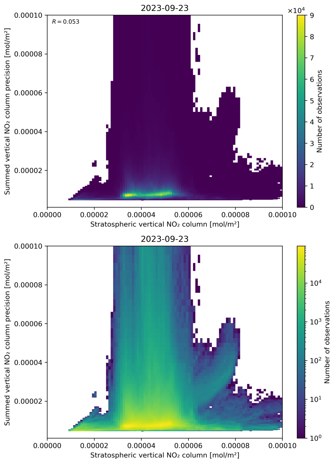
Figure 99: Scatter density plot of “Stratospheric vertical NO 2 column” against “Summed vertical NO 2 column precision” for 2023-09-22 to 2023-09-24.
