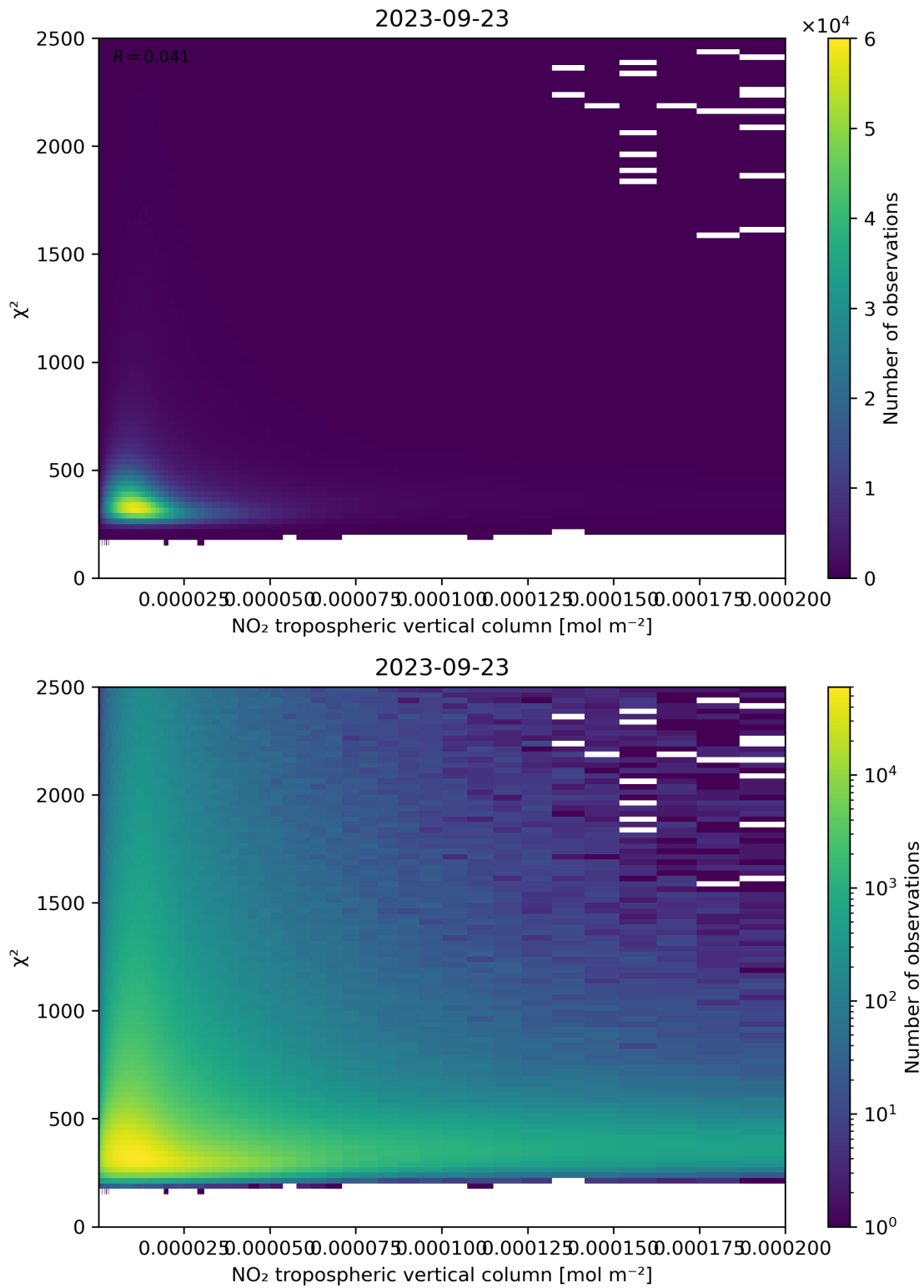
Figure 124: Scatter density plot of “NO 2 tropospheric vertical column” against “ \chi^2 ” for 2023-09-22 to 2023-09-24.
