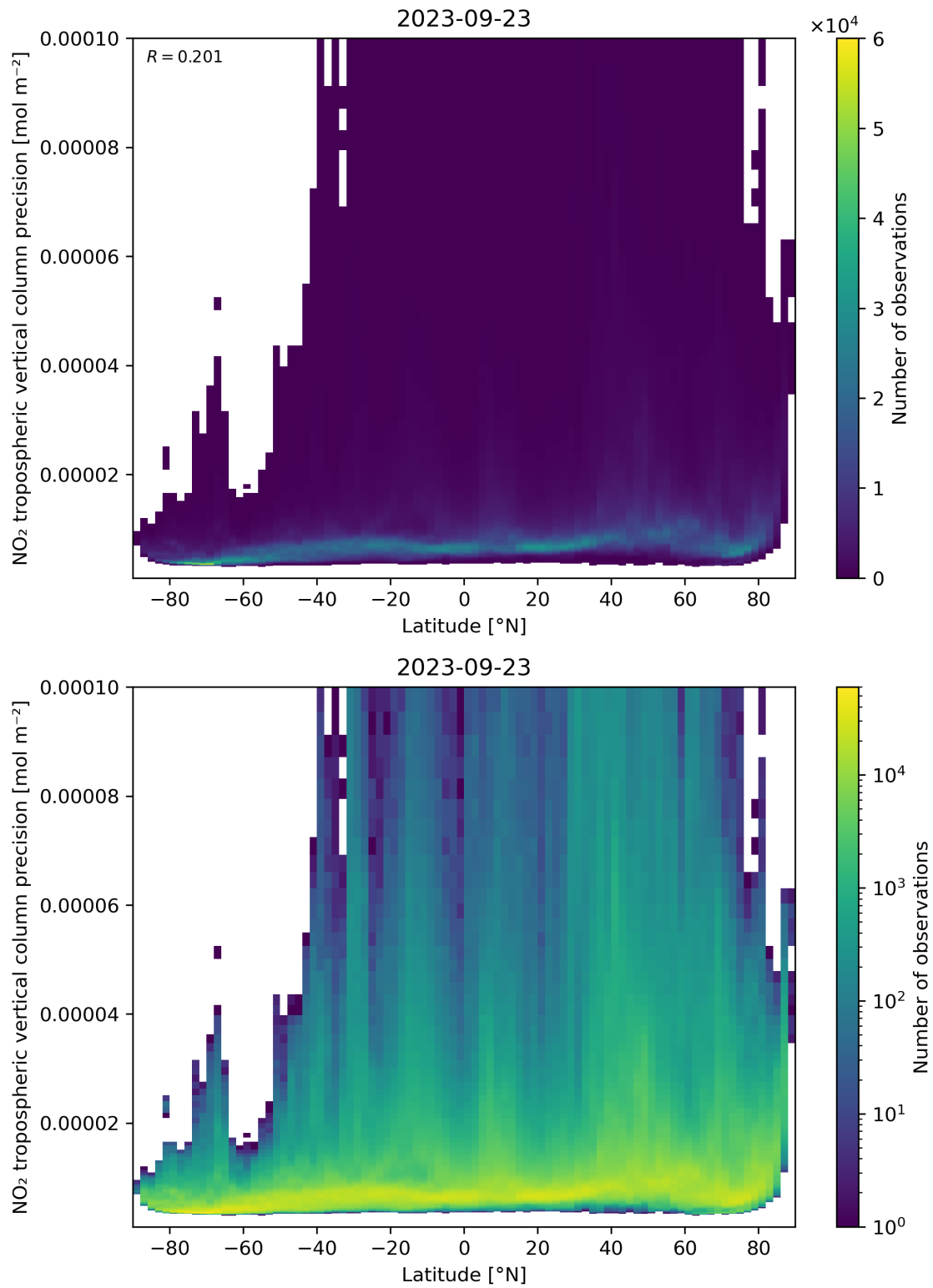
Figure 93: Scatter density plot of “Latitude” against “NO 2 tropospheric vertical column precision” for 2023-09-22 to 2023-09-24.
