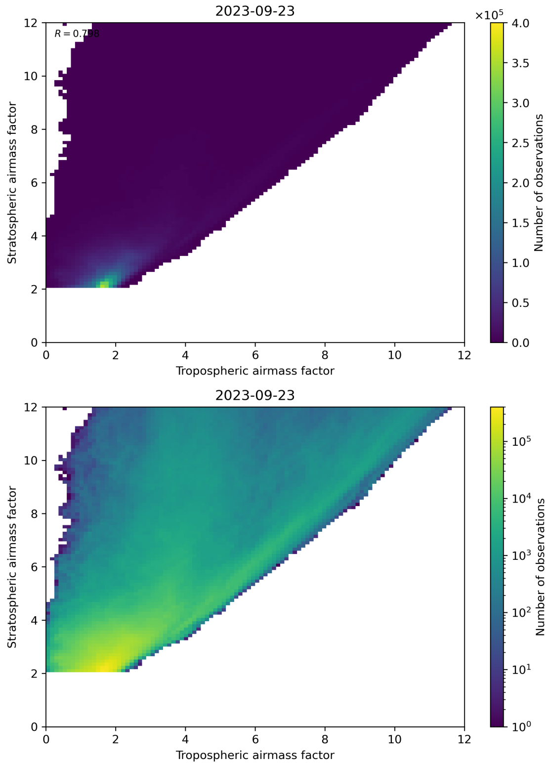
Figure 71: Scatter density plot of “Tropospheric airmass factor” against “Stratospheric airmass factor” for 2023-09-22 to 2023-09-24.
