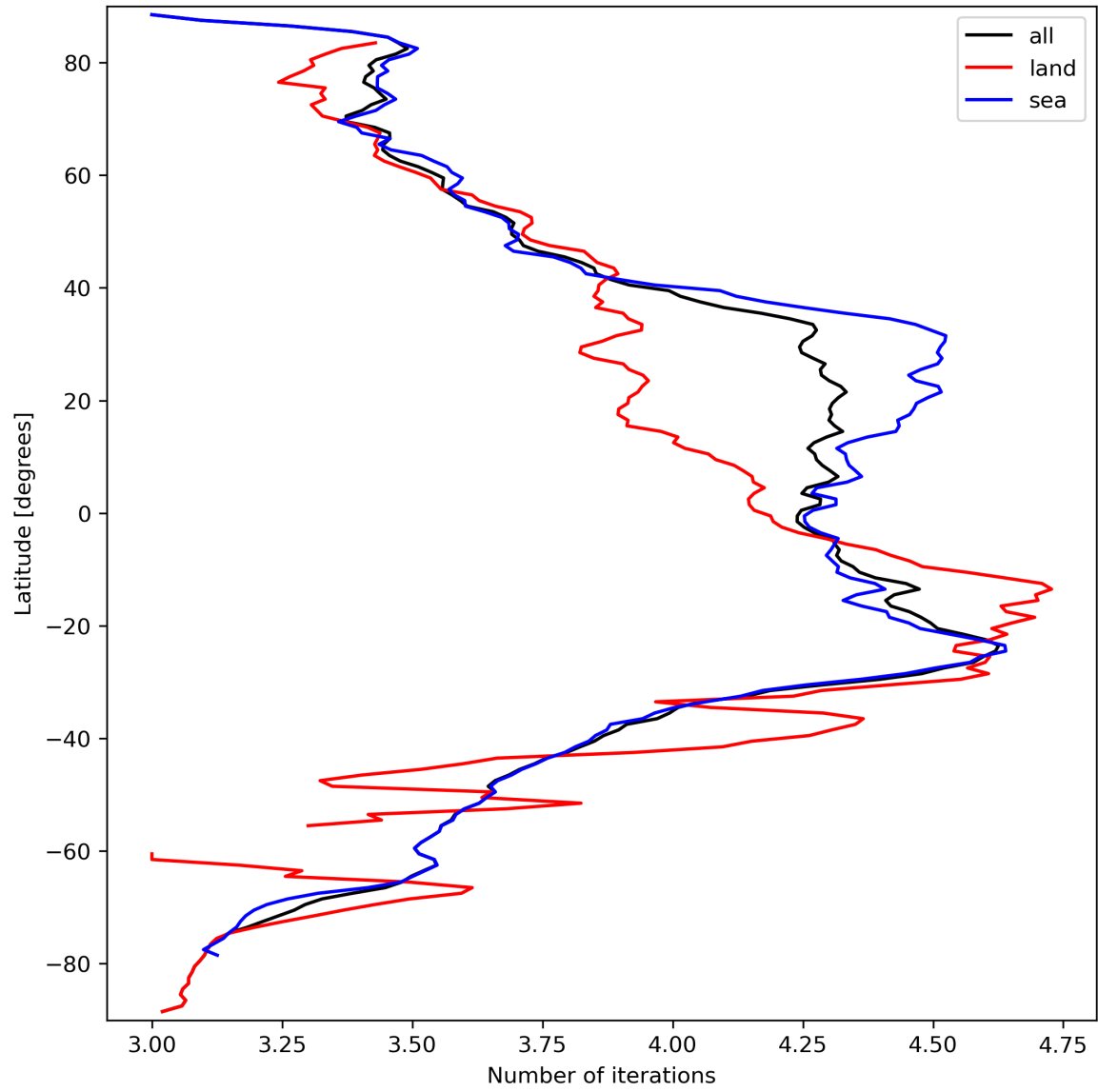
Figure 17: Zonal average of “Number of iterations” for 2023-09-22 to 2023-09-24.
