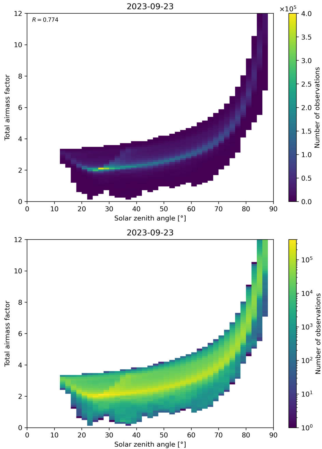
Figure 146: Scatter density plot of “Solar zenith angle” against “Total air mass factor” for 2023-09-22 to 2023-09-24.
