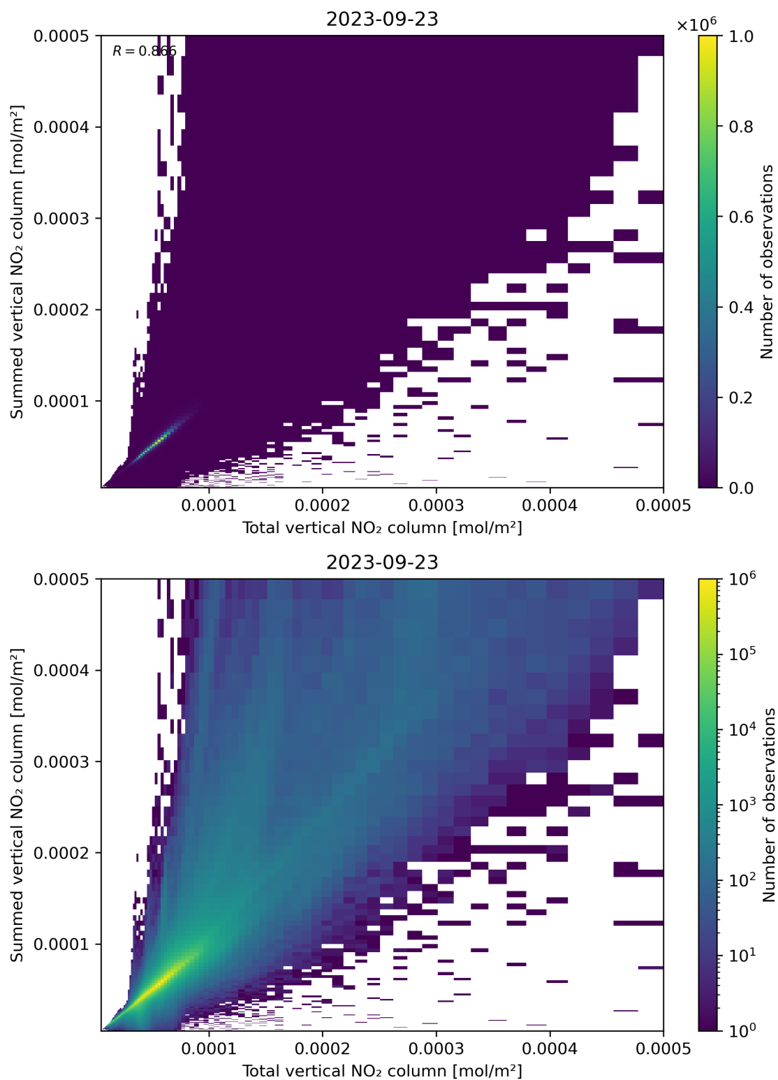
Figure 112: Scatter density plot of “Total vertical NO 2 column” against “Summed vertical NO 2 column” for 2023-09-22 to 2023-09-24.
