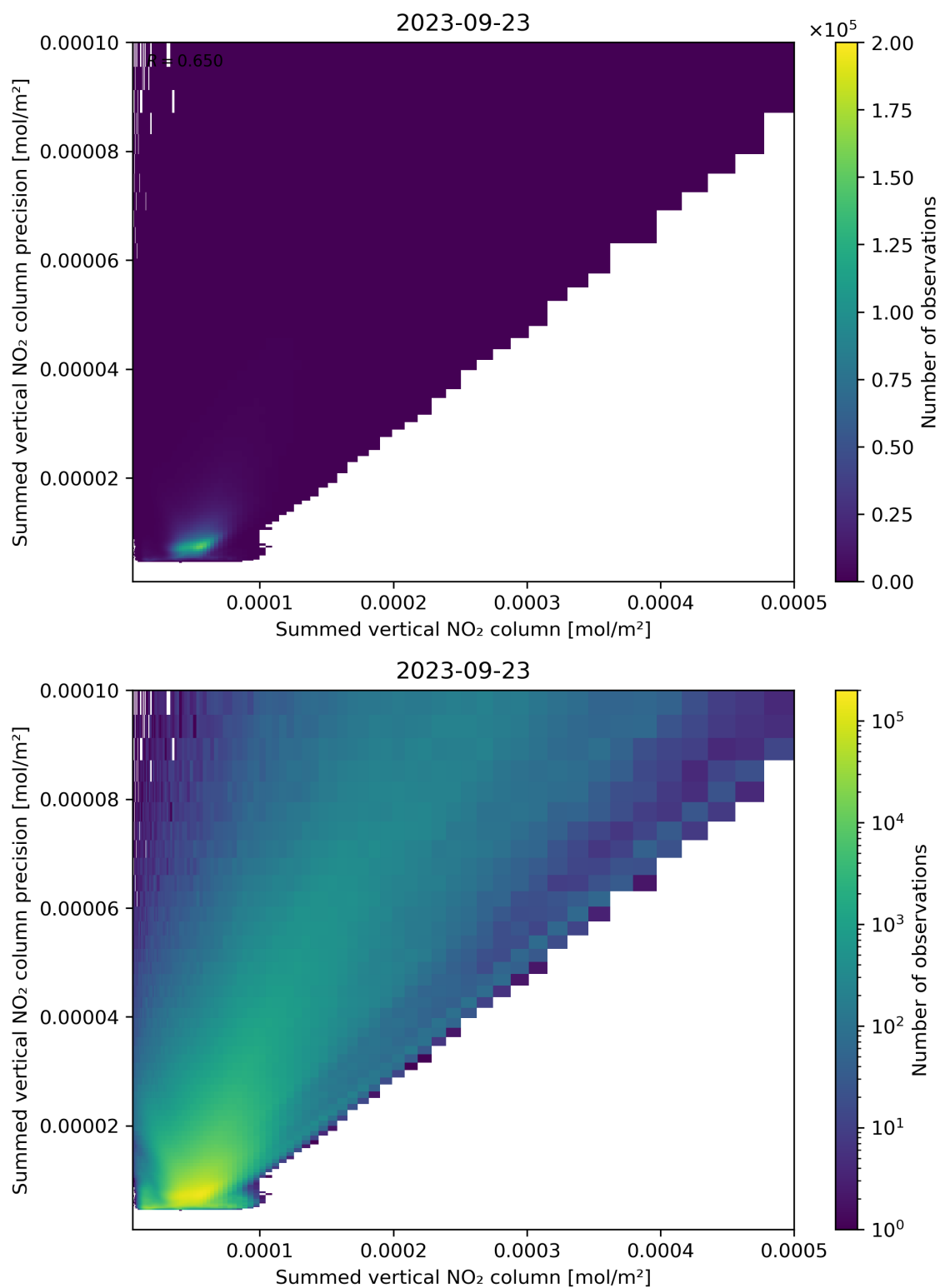
Figure 105: Scatter density plot of “Summed vertical NO 2 column” against “Summed vertical NO 2 column precision” for 2023-09-22 to 2023-09-24.
