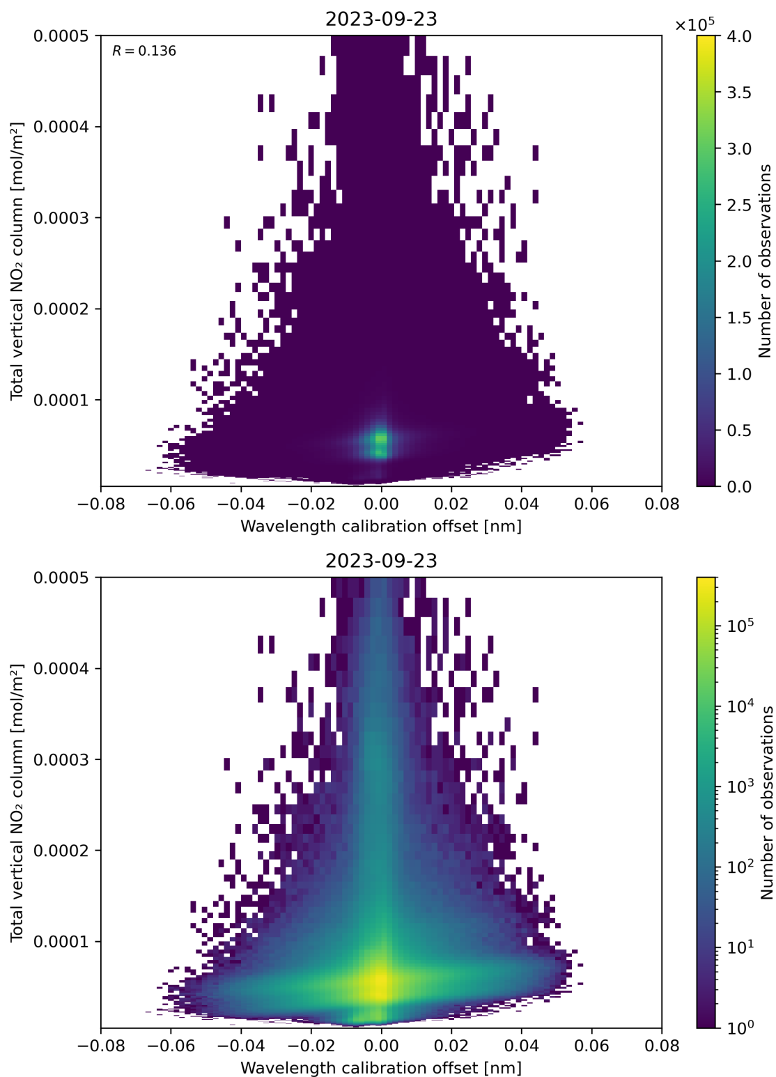
Figure 179: Scatter density plot of “Wavelength calibration offset” against “Total vertical NO 2 column” for 2023-09-22 to 2023-09-24.
