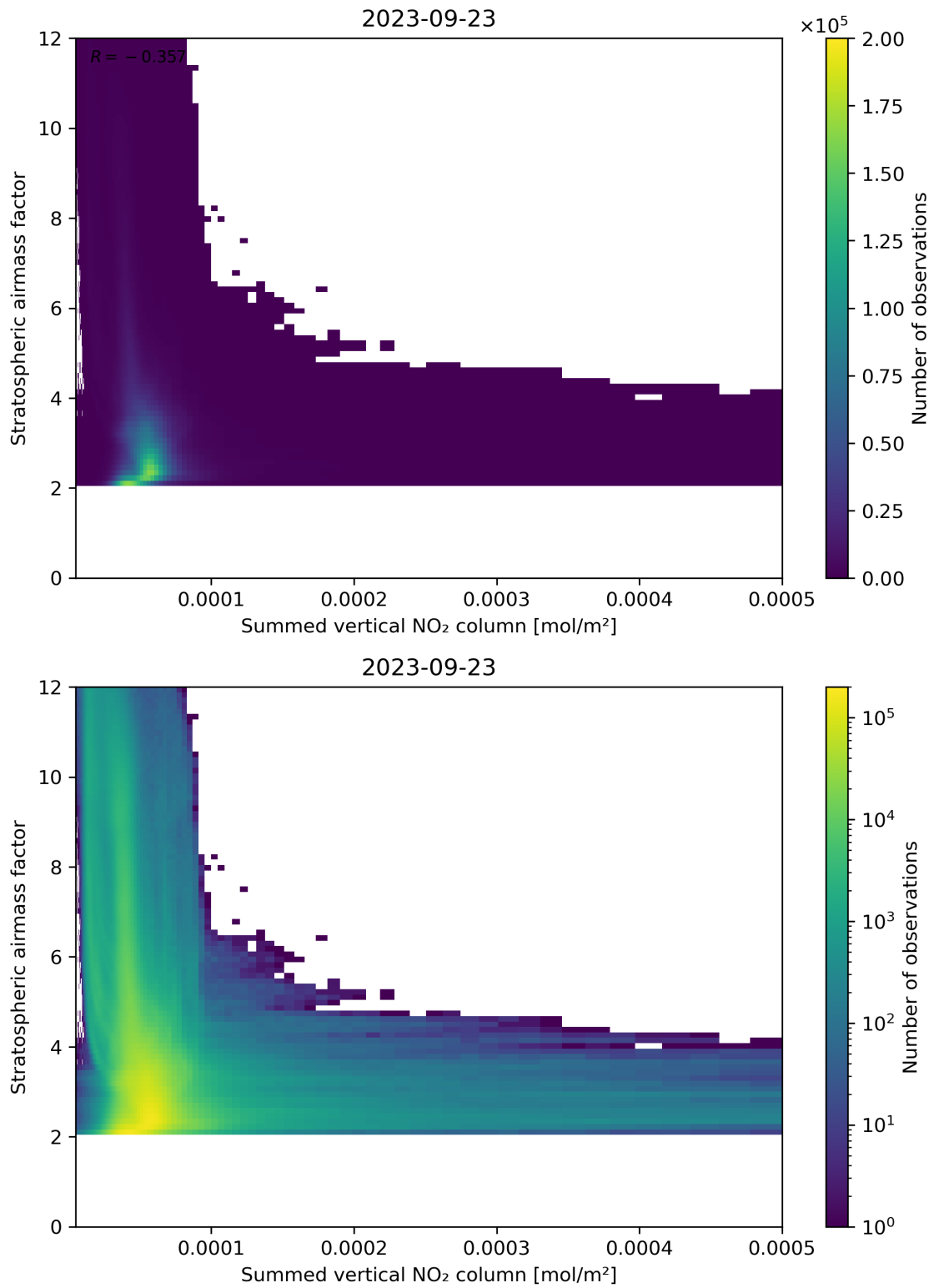
Figure 103: Scatter density plot of “Summed vertical NO 2 column” against “Stratospheric airmass factor” for 2023-09-22 to 2023-09-24.
