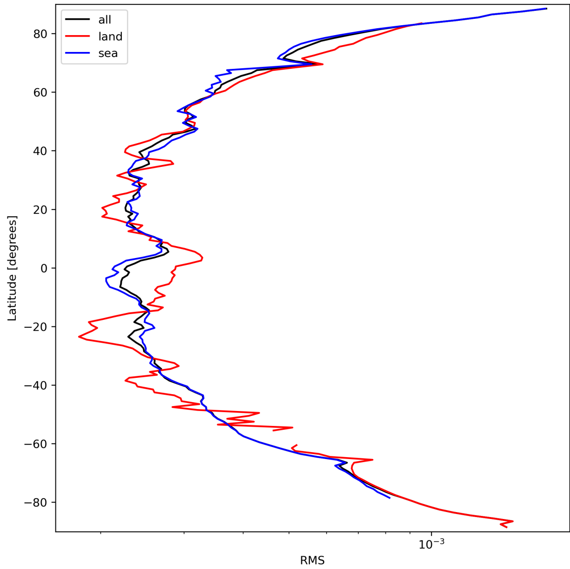
Figure 26: Zonal average of “RMS” for 2023-09-22 to 2023-09-24.
