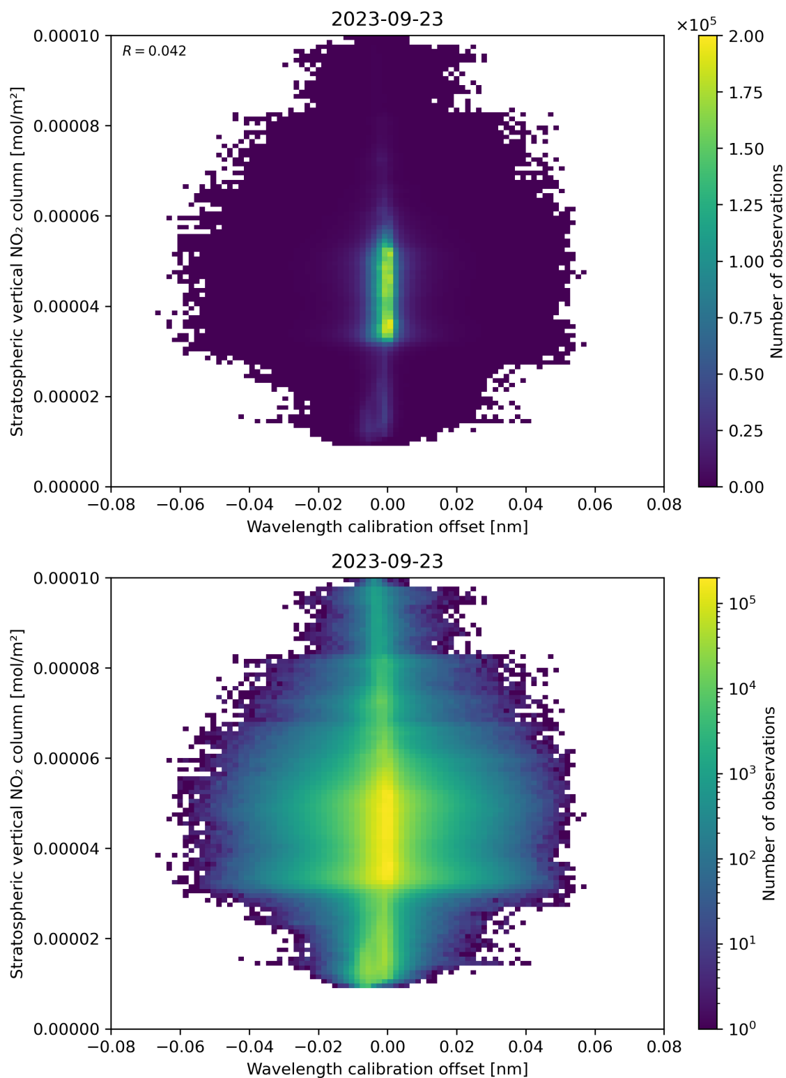
Figure 176: Scatter density plot of “Wavelength calibration offset” against “Stratospheric vertical NO 2 column” for 2023-09-22 to 2023-09-24.
