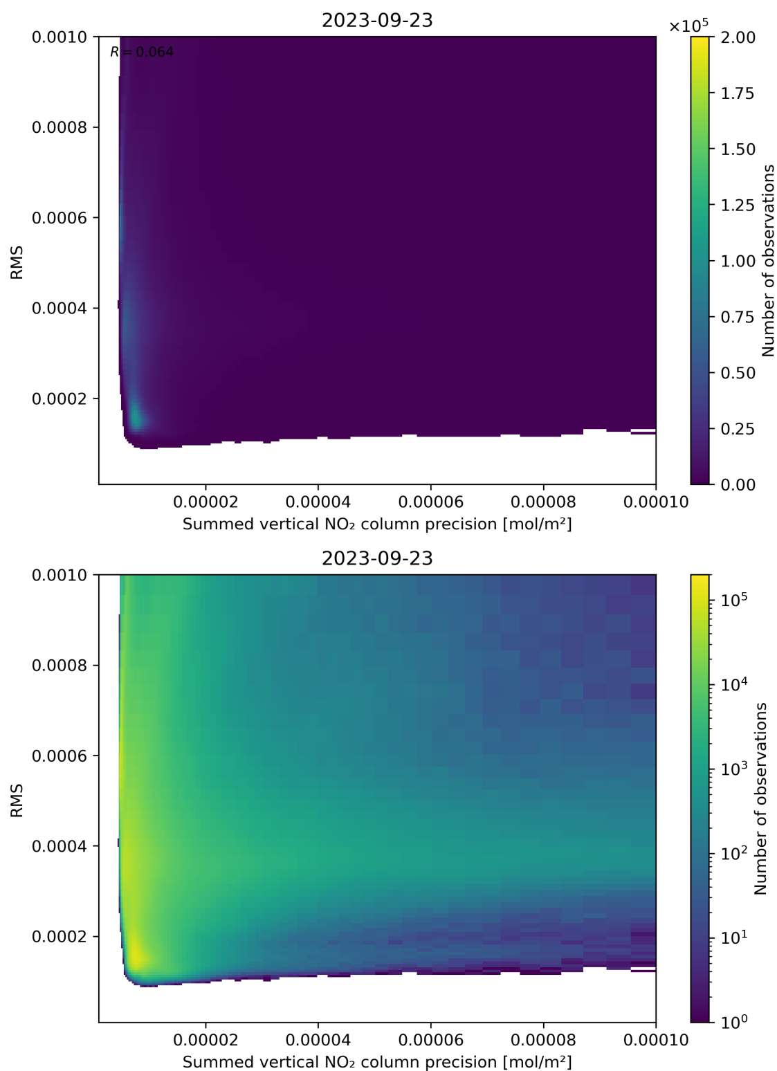
Figure 108: Scatter density plot of “Summed vertical NO 2 column precision” against “RMS” for 2023-09-22 to 2023-09-24.
