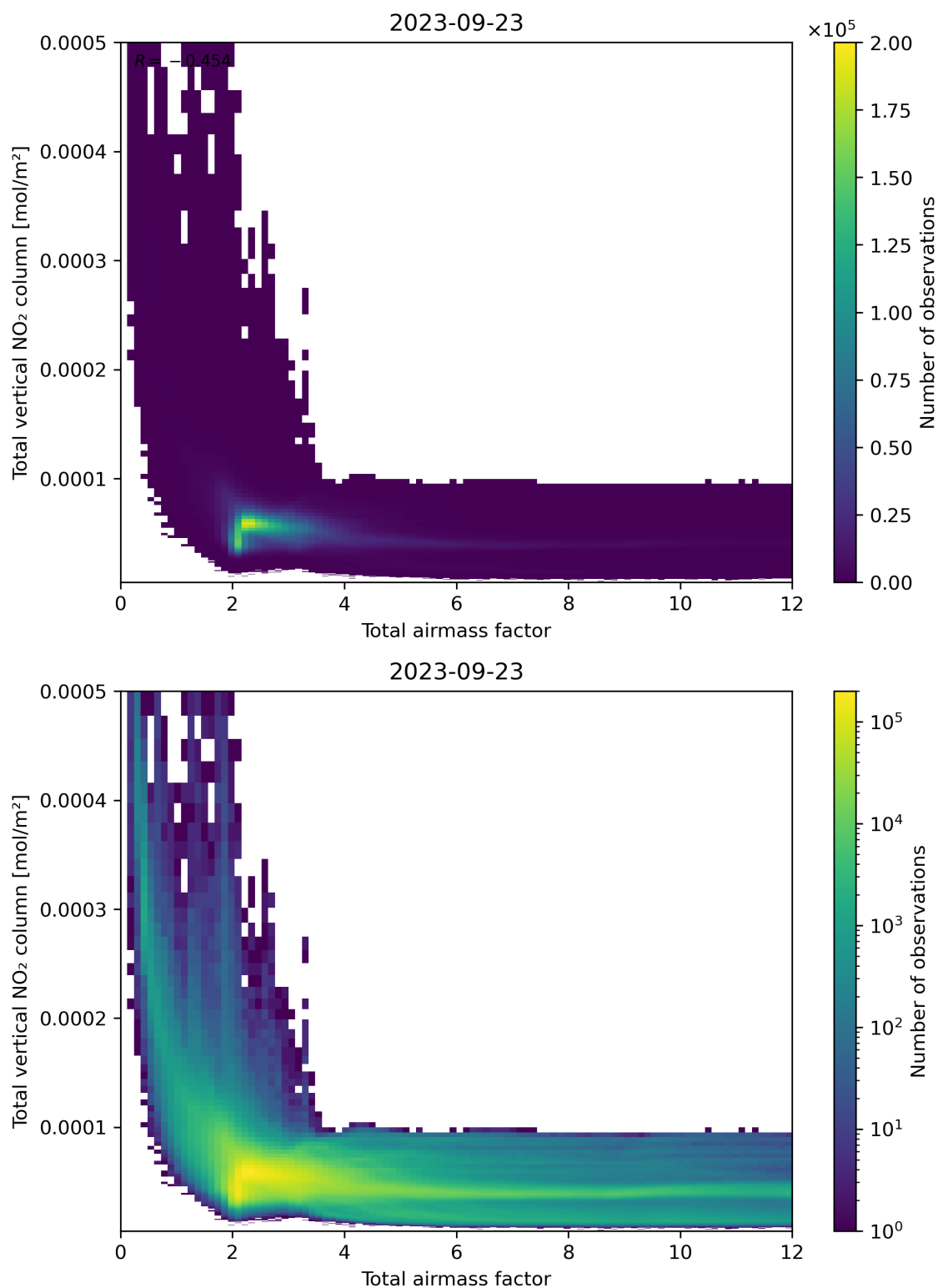
Figure 67: Scatter density plot of “Total airmass factor” against “Total vertical NO 2 column” for 2023-09-22 to 2023-09-24.
