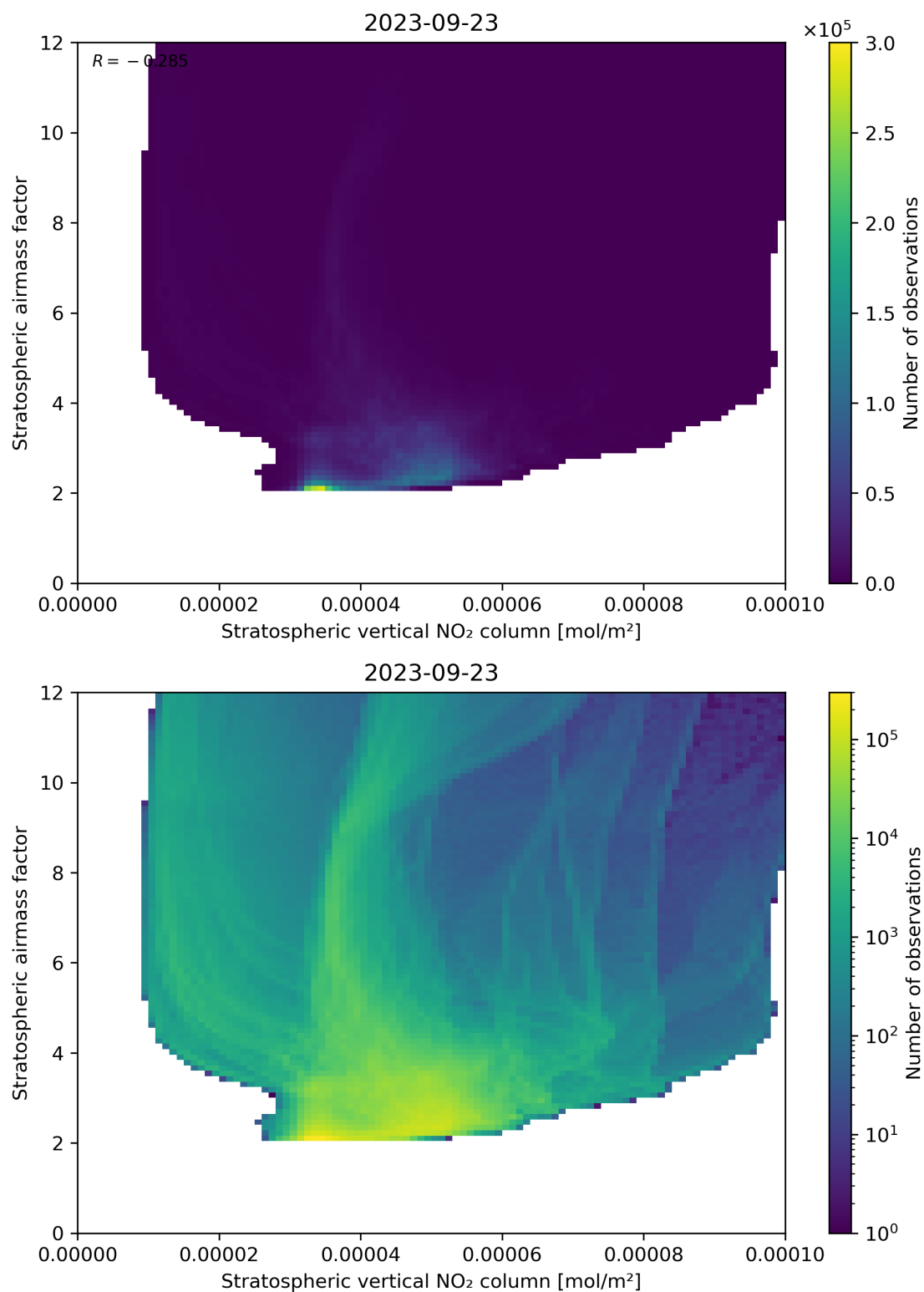
Figure 96: Scatter density plot of “Stratospheric vertical NO 2 column” against “Stratospheric airmass factor” for 2023-09-22 to 2023-09-24.
