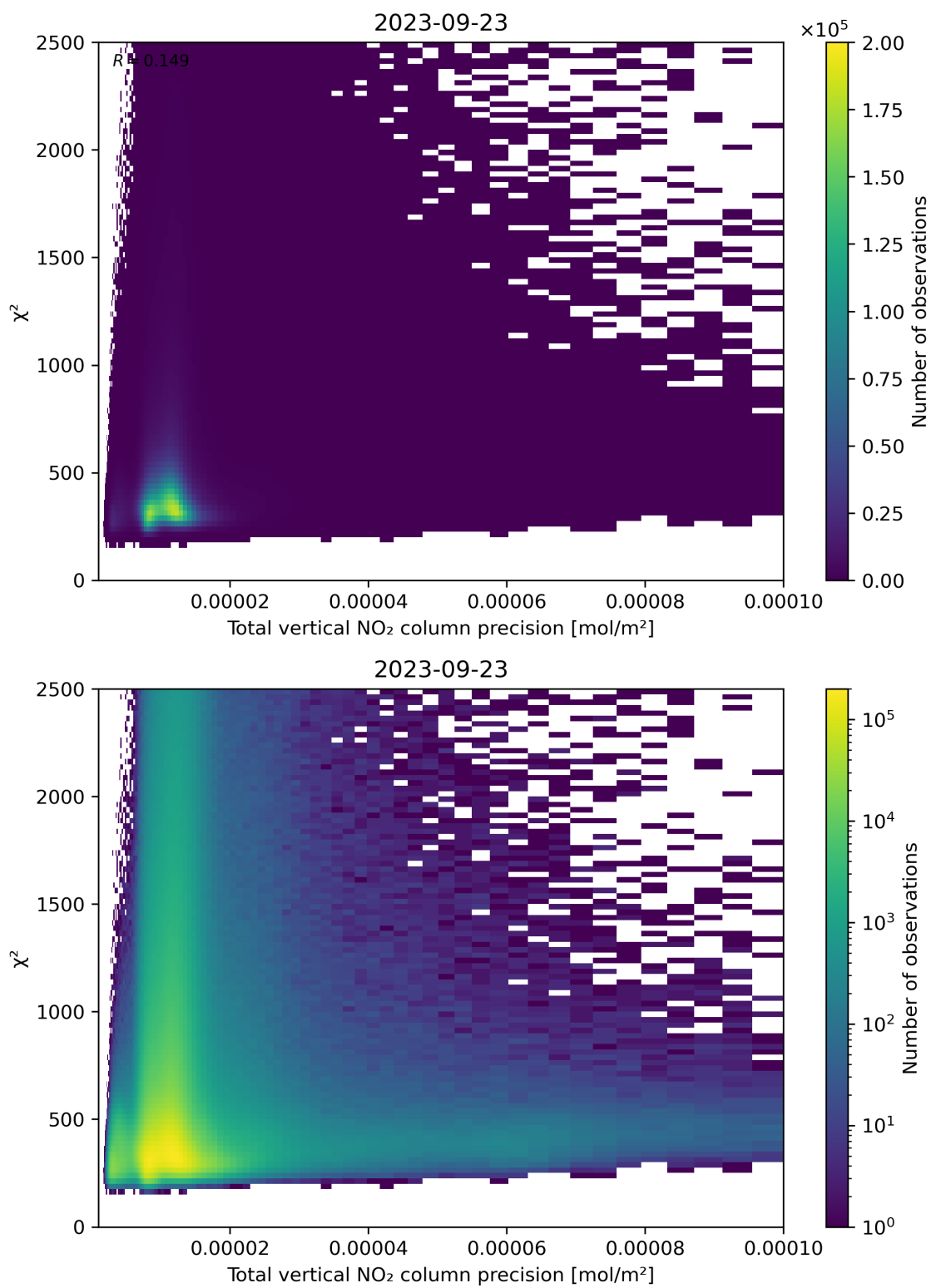
Figure 116: Scatter density plot of “Total vertical NO 2 column precision” against “ \chi^2 ” for 2023-09-22 to 2023-09-24.
