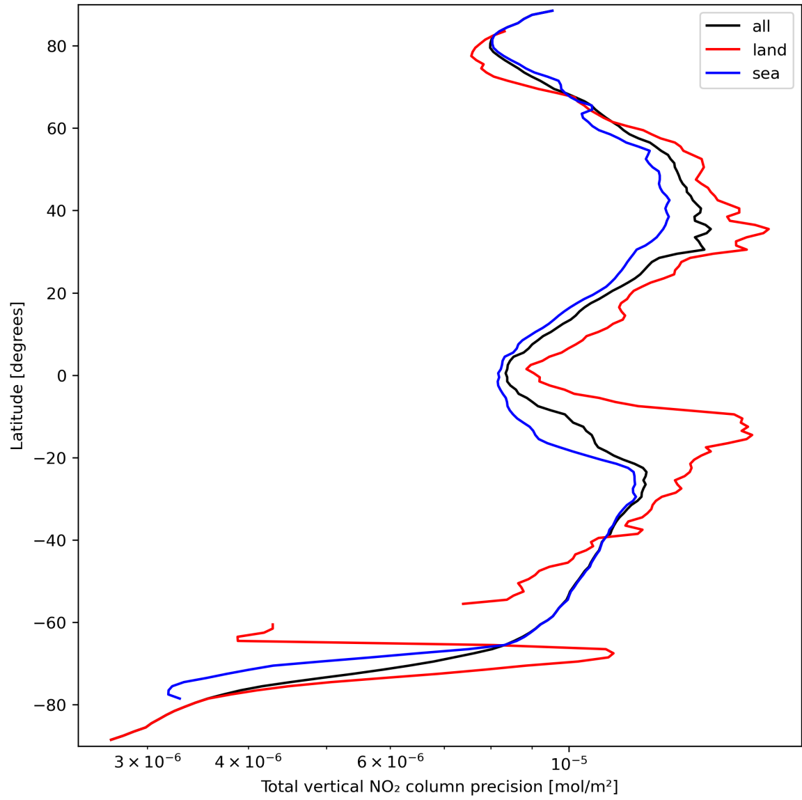
Figure 22: Zonal average of “Total vertical NO 2 column precision” for 2023-09-22 to 2023-09-24.
