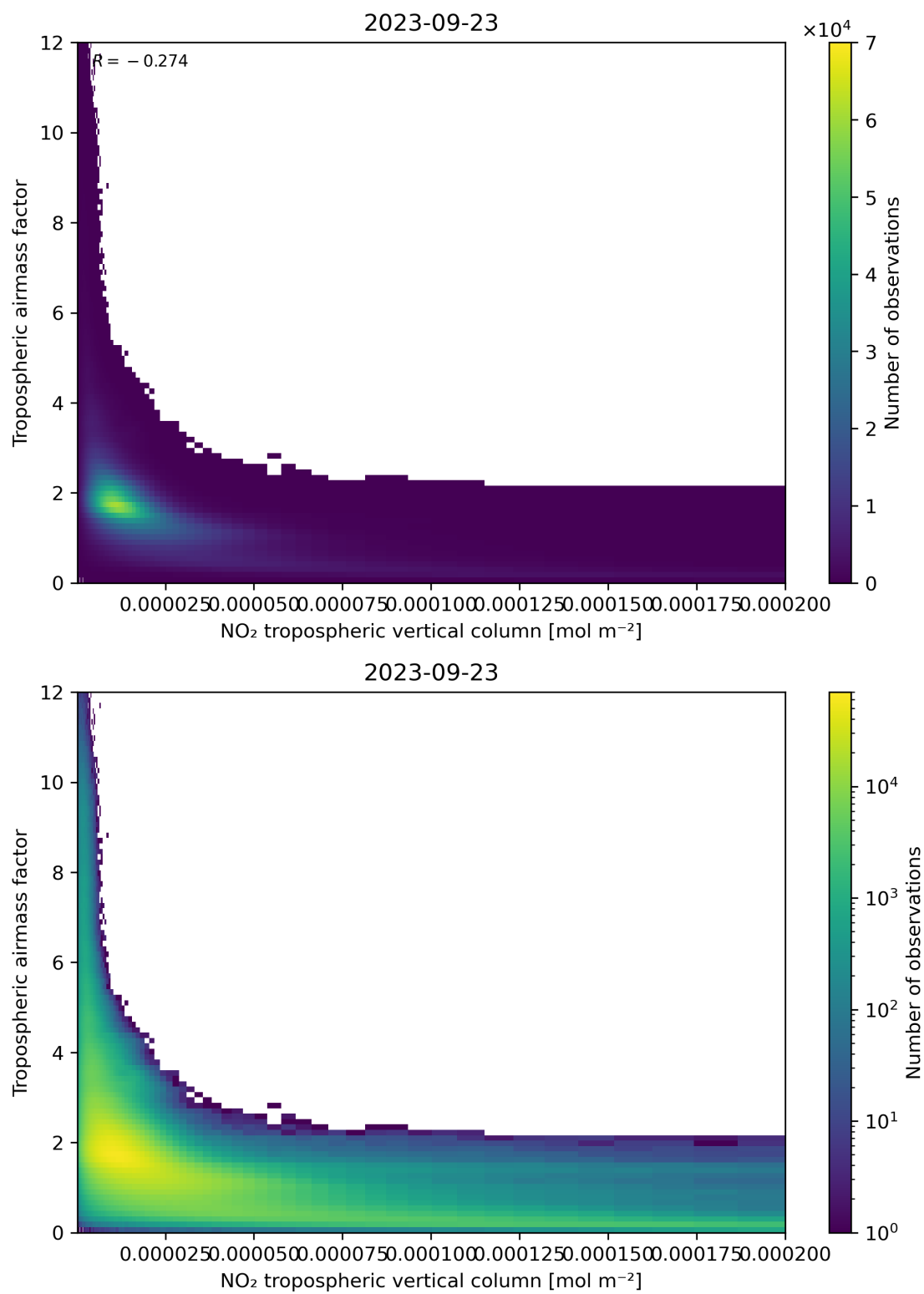
Figure 123: Scatter density plot of “NO 2 tropospheric vertical column” against “Tropospheric air mass factor” for 2023-09-22 to 2023-09-24.
