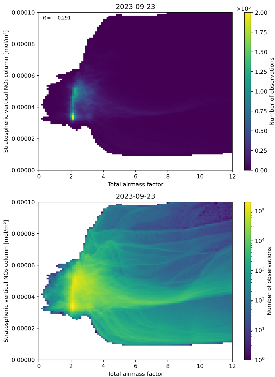
Figure 64: Scatter density plot of “Total airmass factor” against “Stratospheric vertical NO 2 column” for 2023-09-22 to 2023-09-24.
