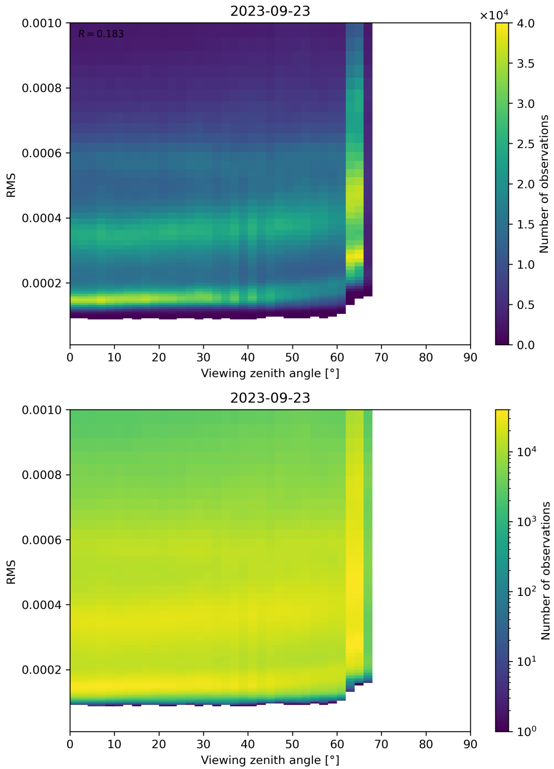
Figure 171: Scatter density plot of “Viewing zenith angle” against “RMS” for 2023-09-22 to 2023-09-24.
