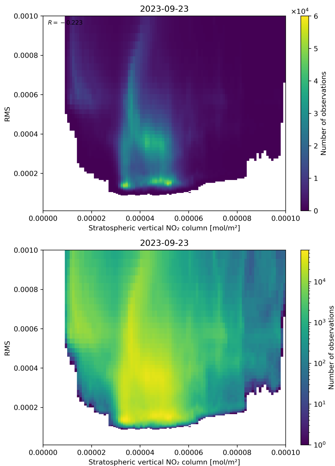
Figure 102: Scatter density plot of “Stratospheric vertical NO 2 column” against “RMS” for 2023-09-22 to 2023-09-24.
