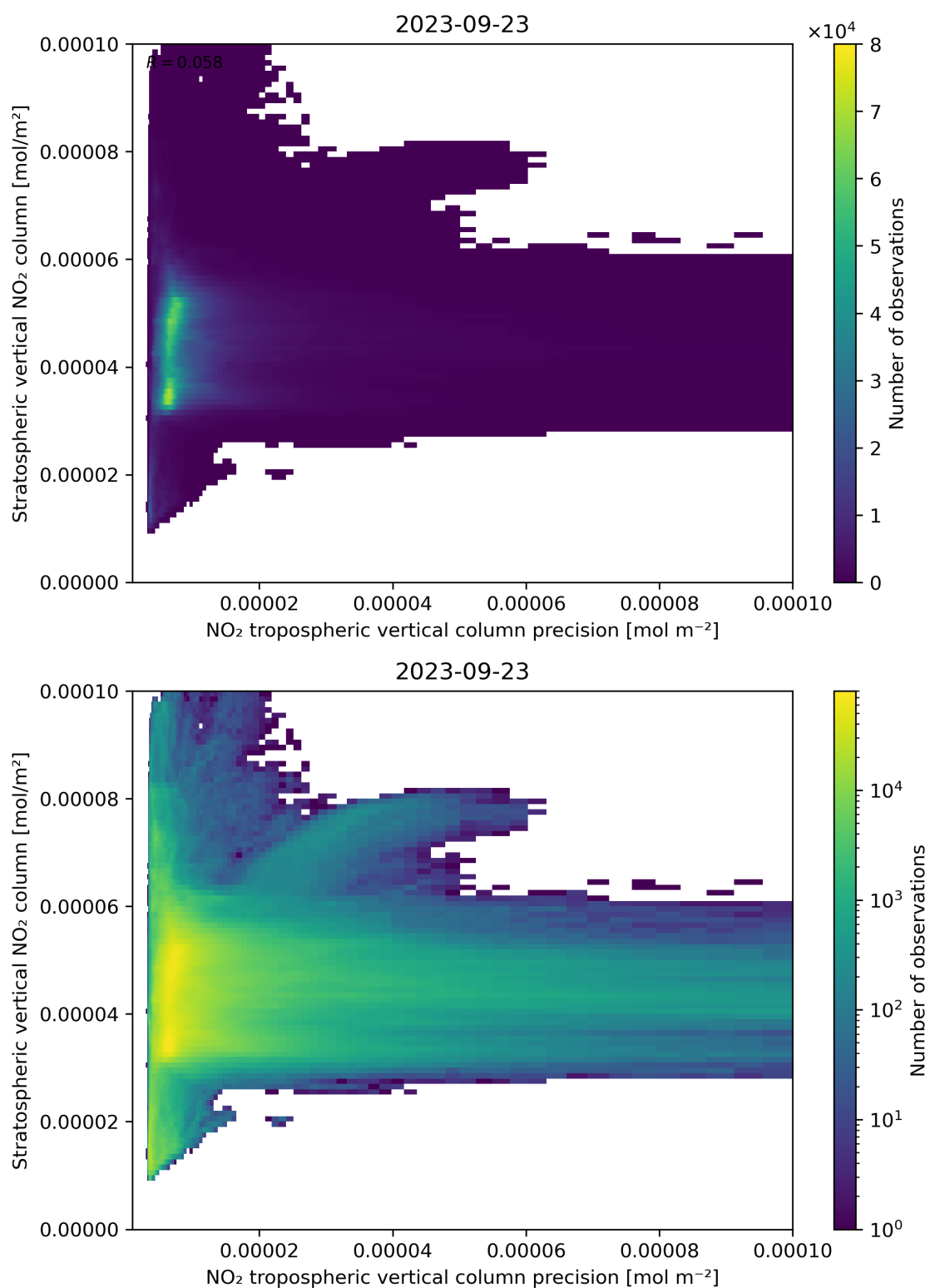
Figure 135: Scatter density plot of “NO 2 tropospheric vertical column precision” against “Stratospheric vertical NO 2 column” for 2023-09-22 to 2023-09-24.
