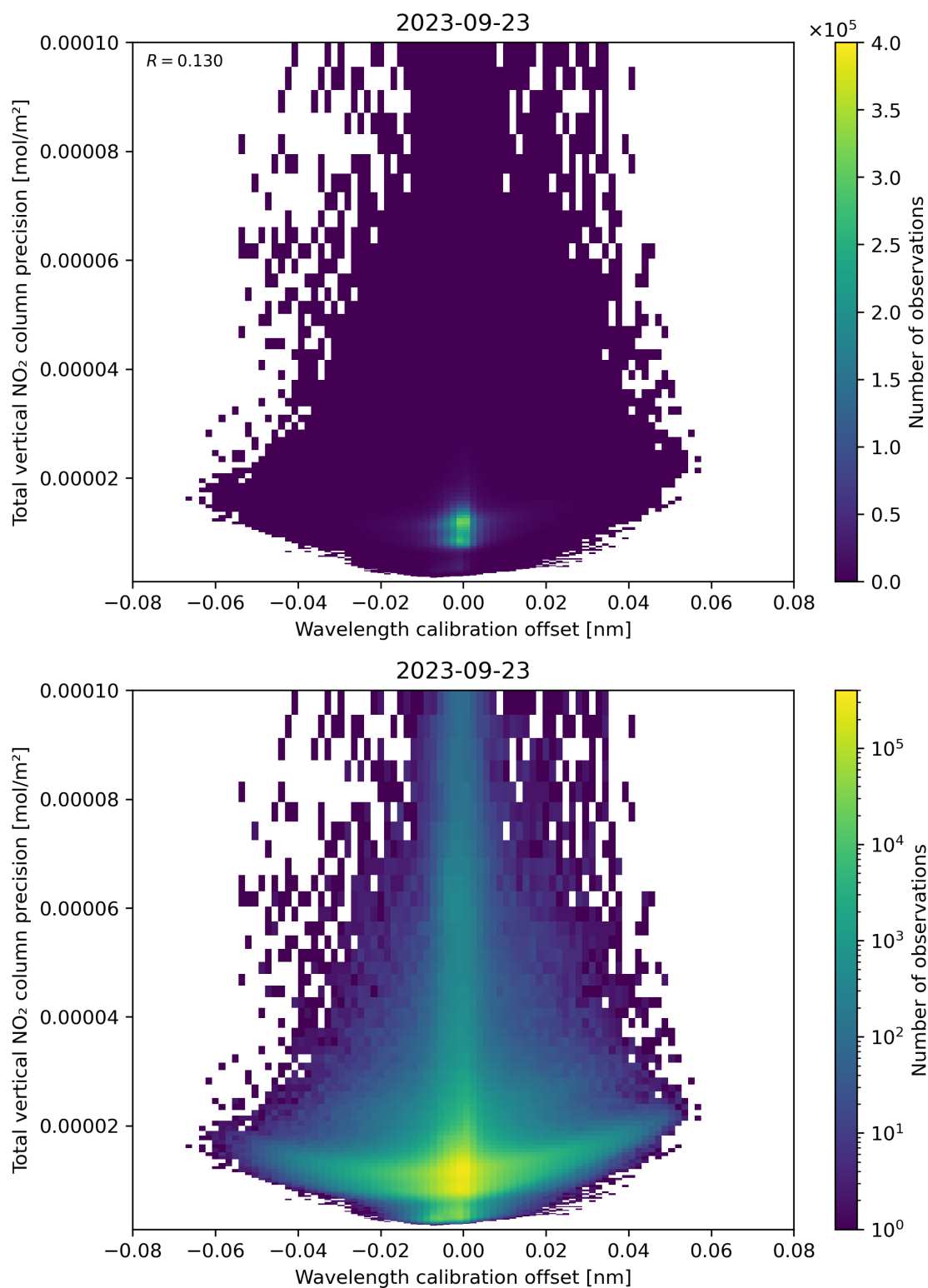
Figure 180: Scatter density plot of “Wavelength calibration offset” against “Total vertical NO 2 column precision” for 2023-09-22 to 2023-09-24.
