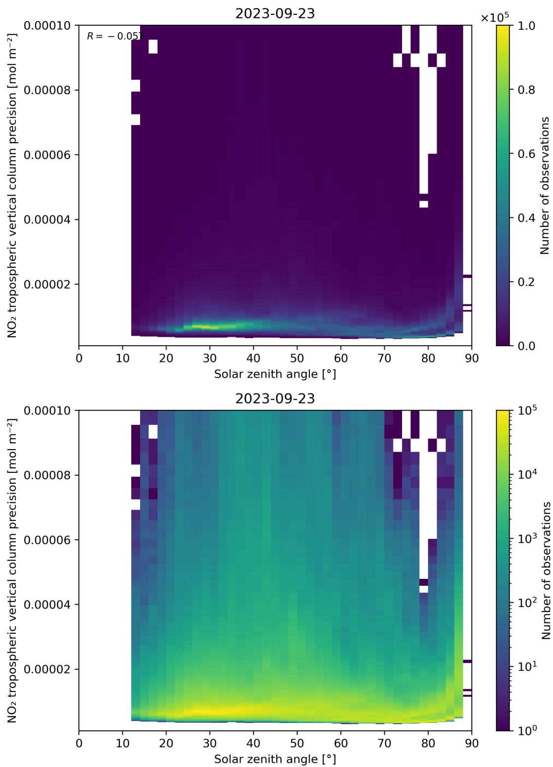
Figure 156: Scatter density plot of “Solar zenith angle” against “NO 2 tropospheric vertical column precision” for 2023-09-22 to 2023-09-24.
