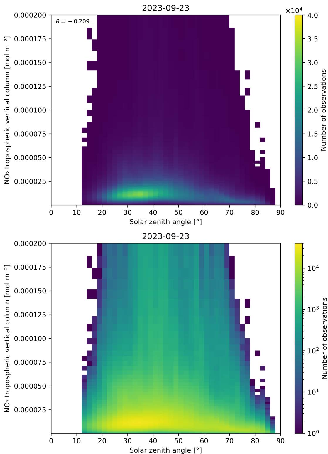
Figure 155: Scatter density plot of “Solar zenith angle” against “NO 2 tropospheric vertical column” for 2023-09-22 to 2023-09-24.
