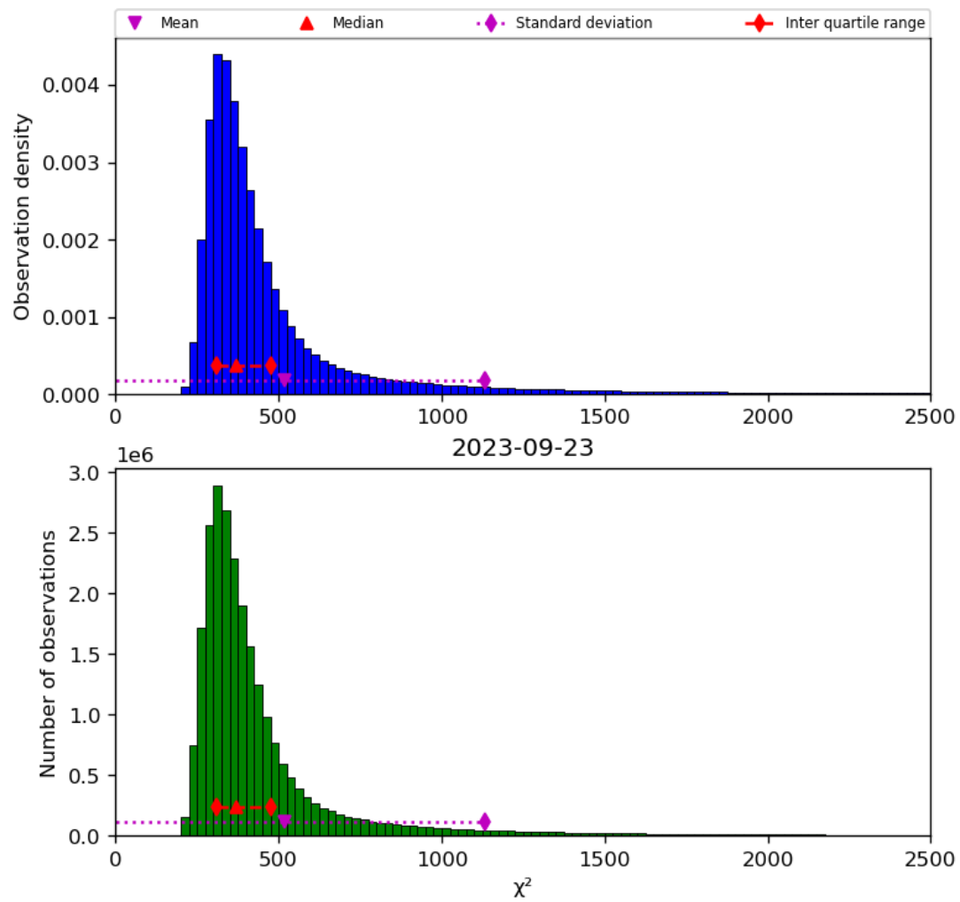
Figure 42: Histogram of “ \chi^2 ” for 2023-09-22 to 2023-09-24
