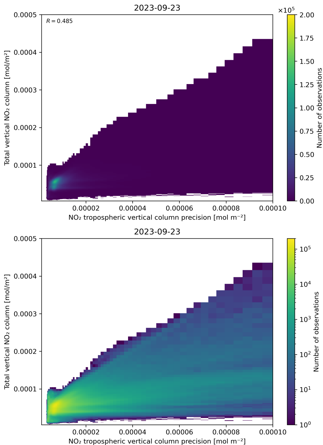
Figure 138: Scatter density plot of “NO 2 tropospheric vertical column precision” against “Total vertical NO 2 column” for 2023-09-22 to 2023-09-24.
