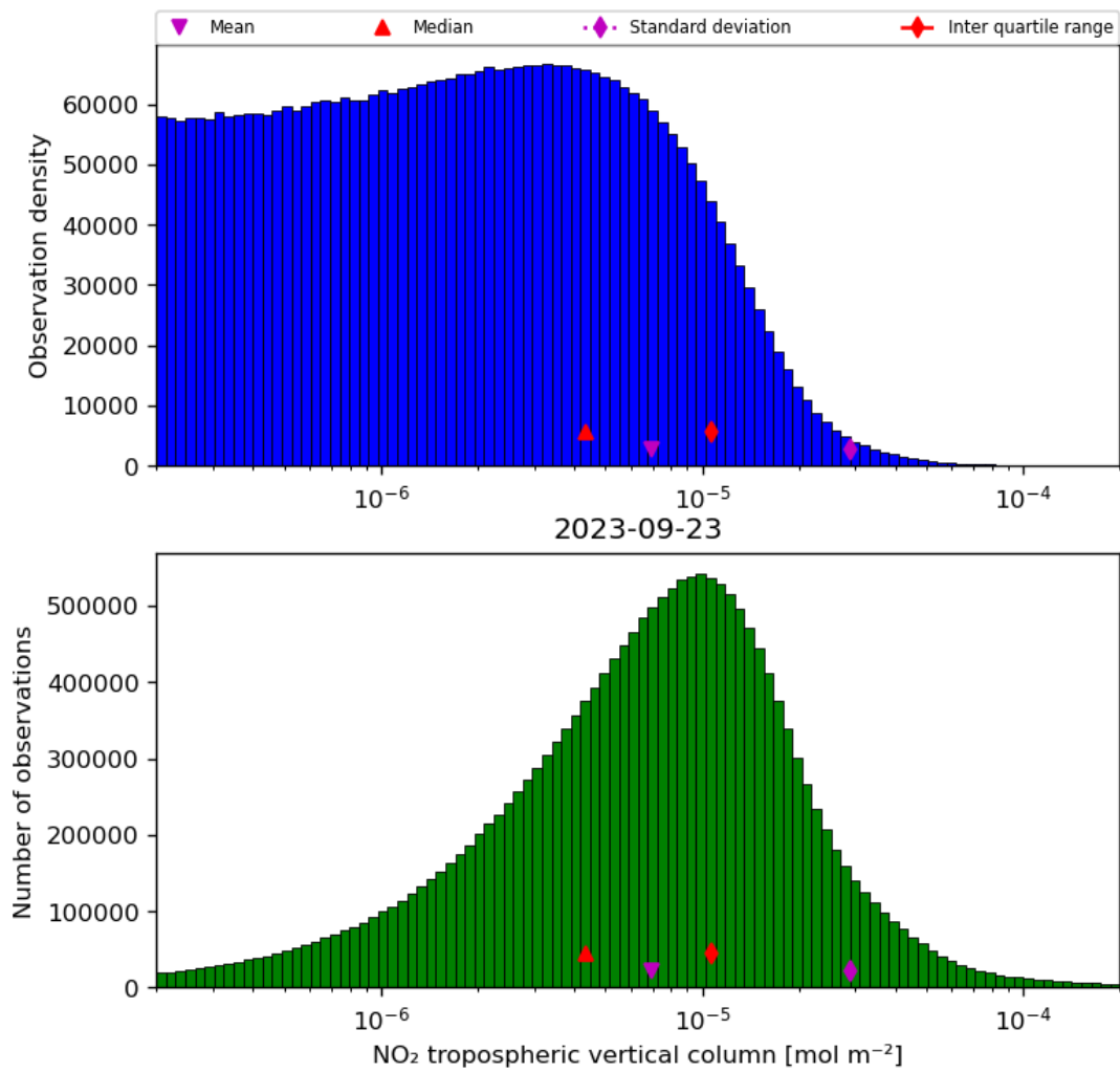
Figure 29: Histogram of “NO 2 tropospheric vertical column” for 2023-09-22 to 2023-09-24
