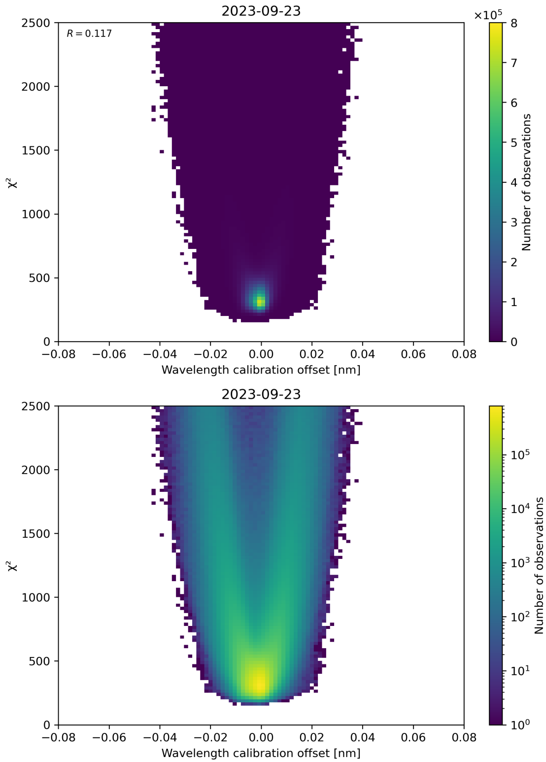
Figure 175: Scatter density plot of “Wavelength calibration offset” against “ \chi^2 ” for 2023-09-22 to 2023-09-24.
