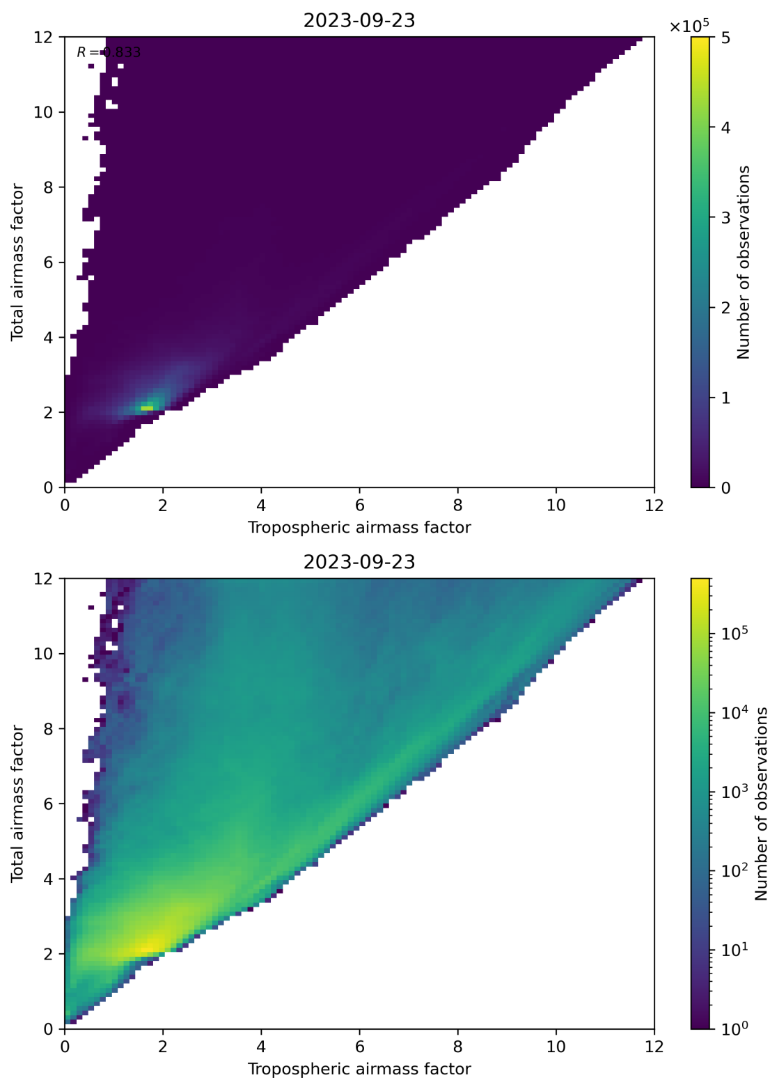
Figure 72: Scatter density plot of “Tropospheric airmass factor” against “Total airmass factor” for 2023-09-22 to 2023-09-24.
