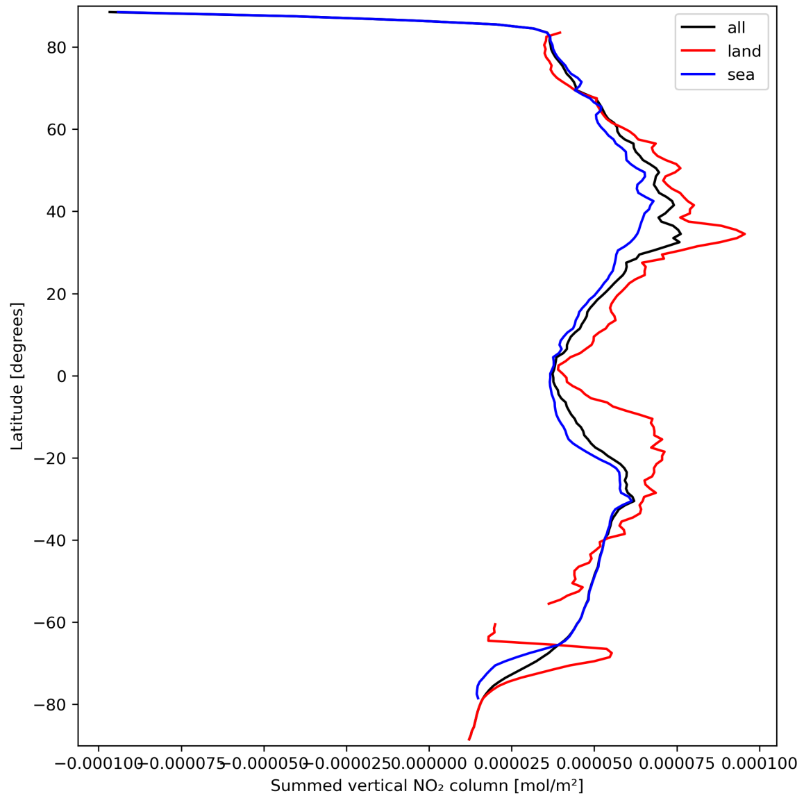
Figure 23: Zonal average of “Summed vertical NO 2 column” for 2023-09-22 to 2023-09-24.
