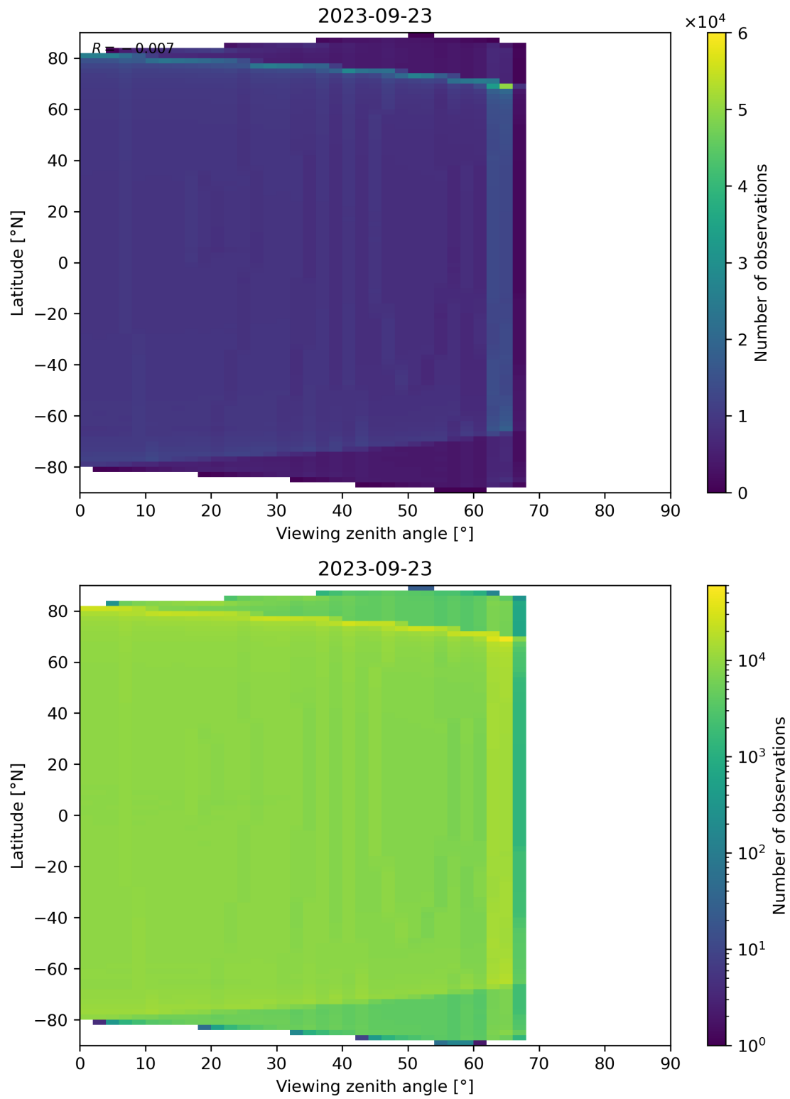
Figure 163: Scatter density plot of “Viewing zenith angle” against “Latitude” for 2023-09-22 to 2023-09-24.
