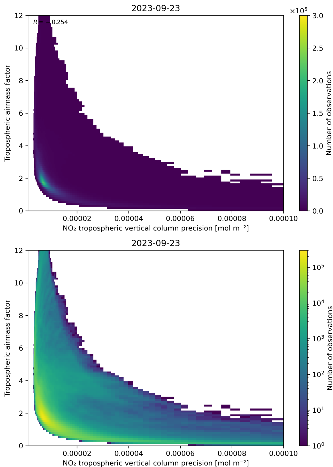
Figure 133: Scatter density plot of “NO 2 tropospheric vertical column precision” against “Tropospheric airmass factor” for 2023-09-22 to 2023-09-24.
