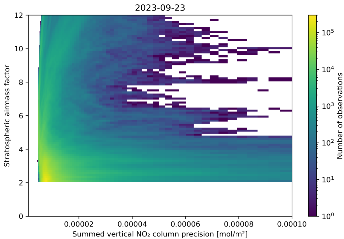
Figure 106: Scatter density plot of “Summed vertical NO 2 column precision” against “Stratospheric airmass factor” for 2023-09-22 to 2023-09-24.
