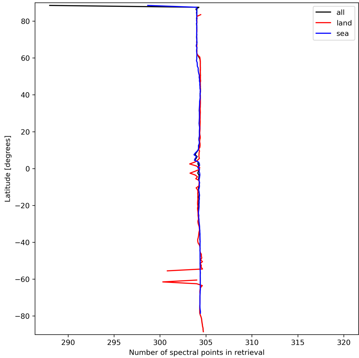
Figure 16: Zonal average of “Number of spectral points in retrieval” for 2023-09-22 to 2023-09-24.
