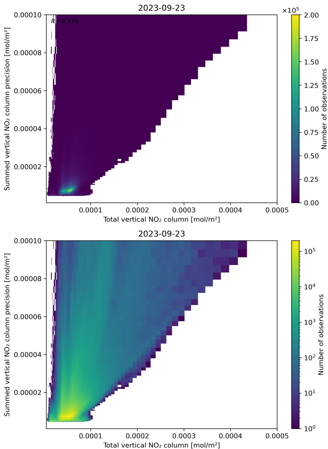
Figure 113: Scatter density plot of “Total vertical NO 2 column” against “Summed vertical NO 2 column precision” for 2023-09-22 to 2023-09-24.
