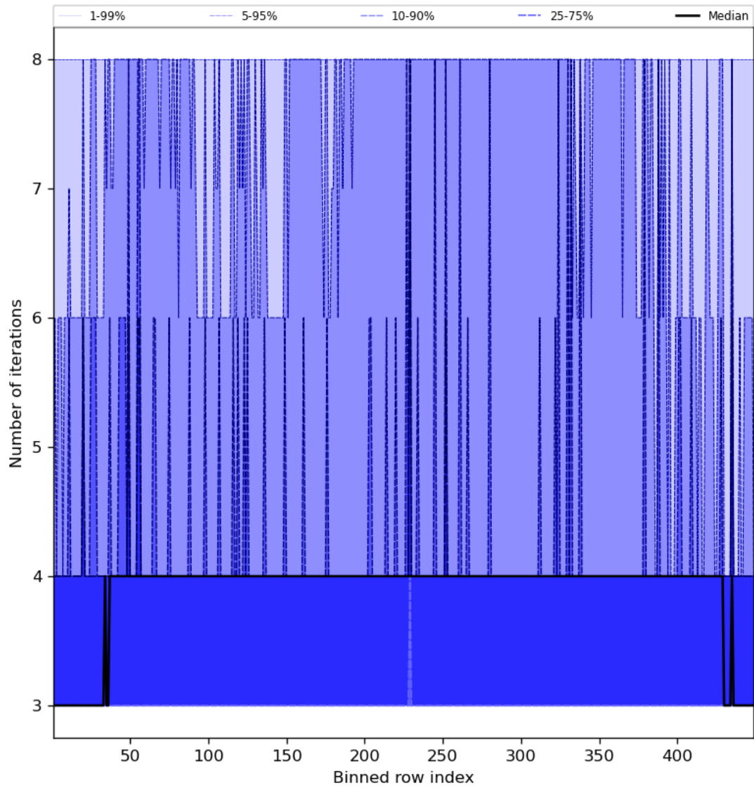
Figure 51: Along track statistics of “Number of iterations” for 2023-09-22 to 2023-09-24
