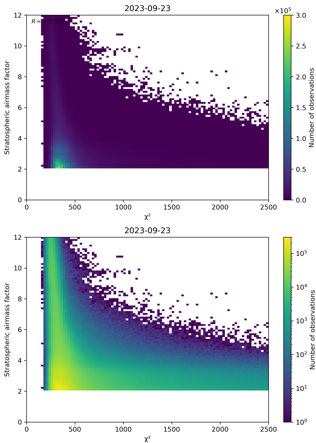
Figure 81: Scatter density plot of “ \chi^2 ” against “Stratospheric airmass factor” for 2023-09-22 to 2023-09-24.
