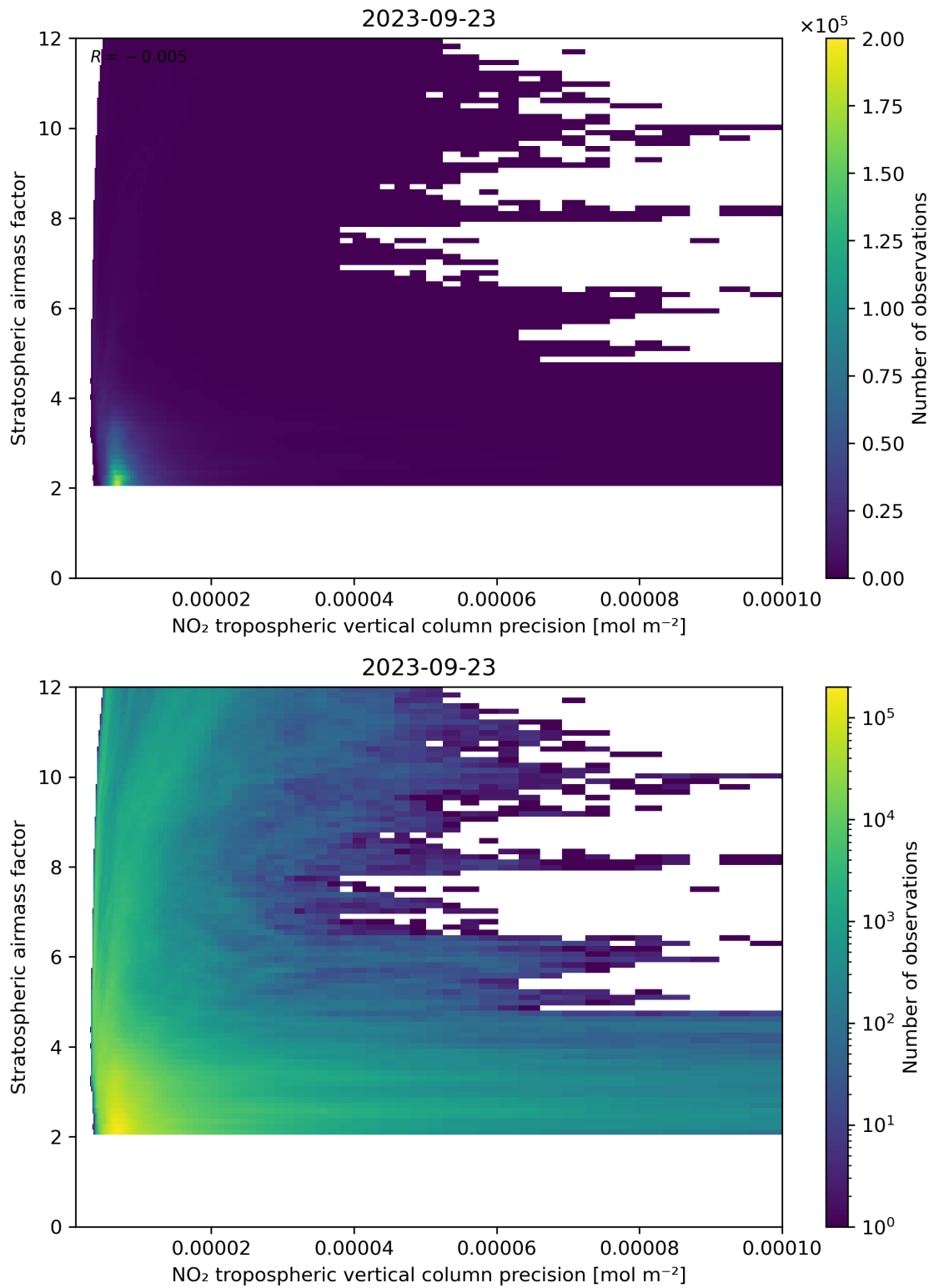
Figure 131: Scatter density plot of “NO 2 tropospheric vertical column precision” against “Stratospheric airmass factor” for 2023-09-22 to 2023-09-24.
