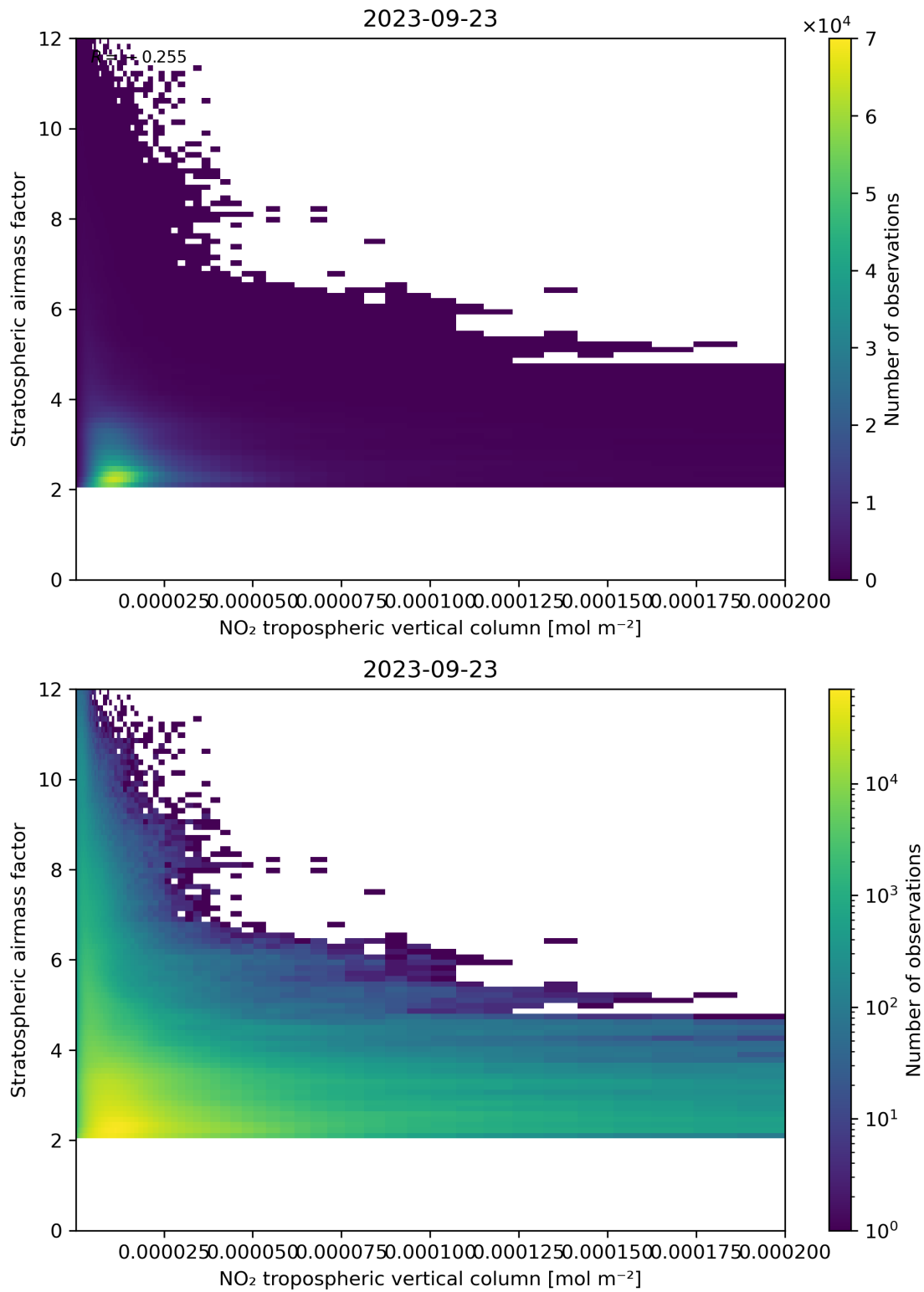
Figure 121: Scatter density plot of “NO 2 tropospheric vertical column” against “Stratospheric air mass factor” for 2023-09-22 to 2023-09-24.
