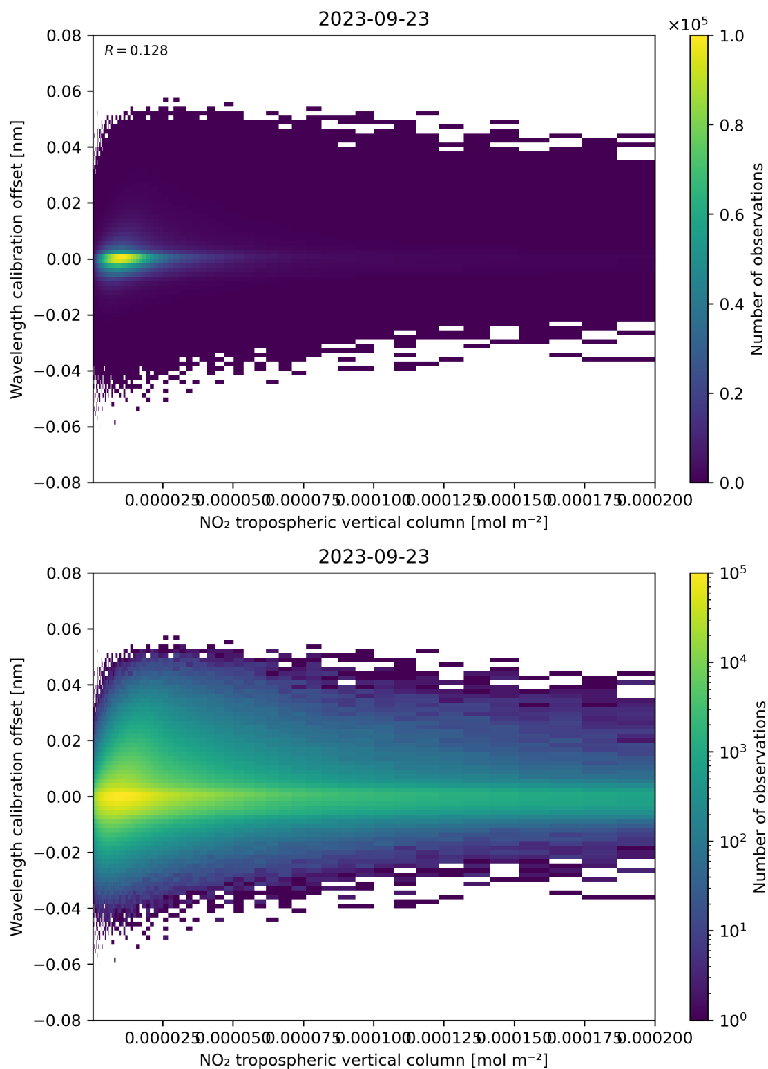
Figure 143: Scatter density plot of “NO 2 tropospheric vertical column” against “Wavelength calibration offset” for 2023-09-22 to 2023-09-24.
