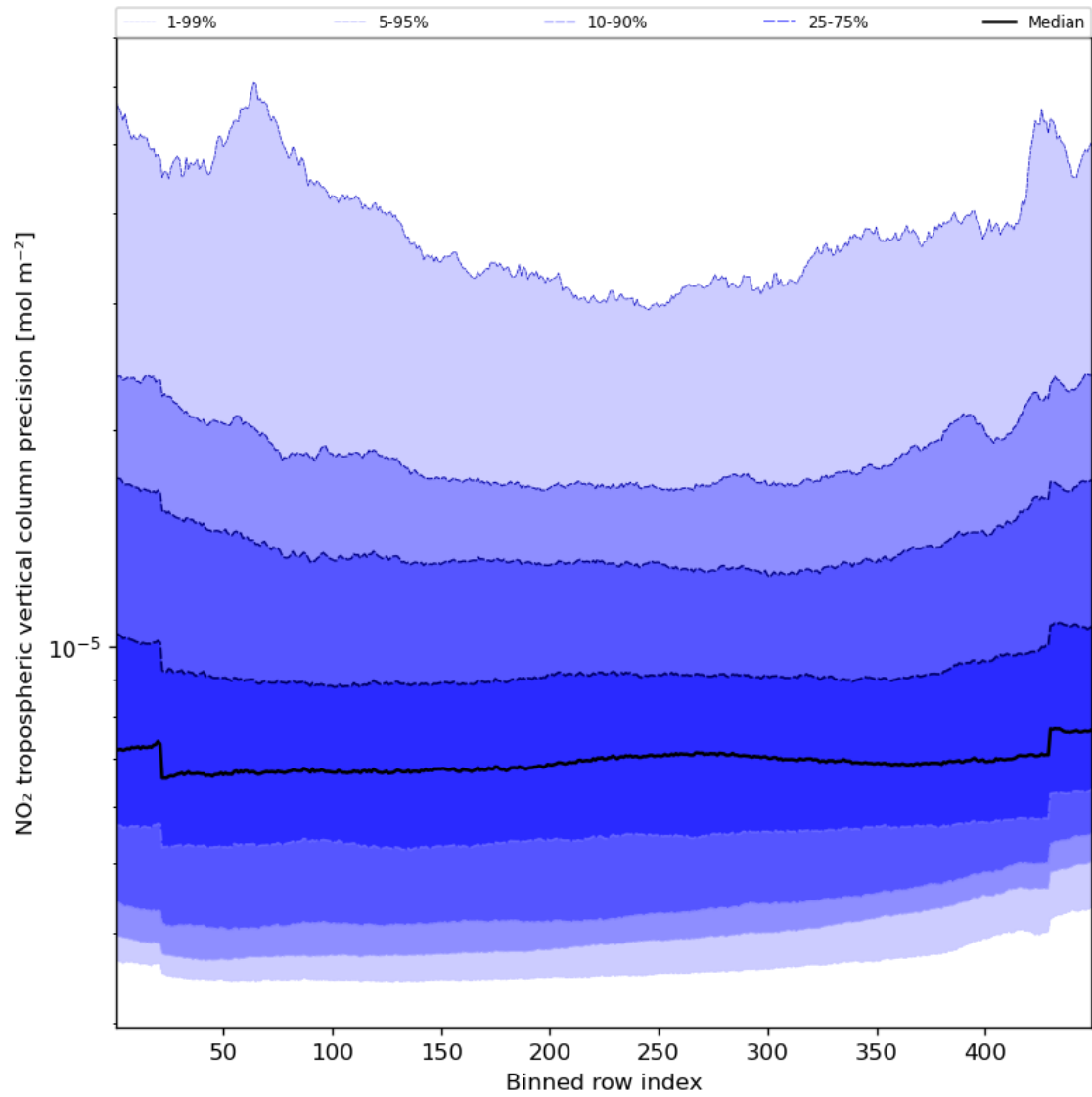
Figure 47: Along track statistics of “NO 2 tropospheric vertical column precision” for 2023-09-22 to 2023-09-24
