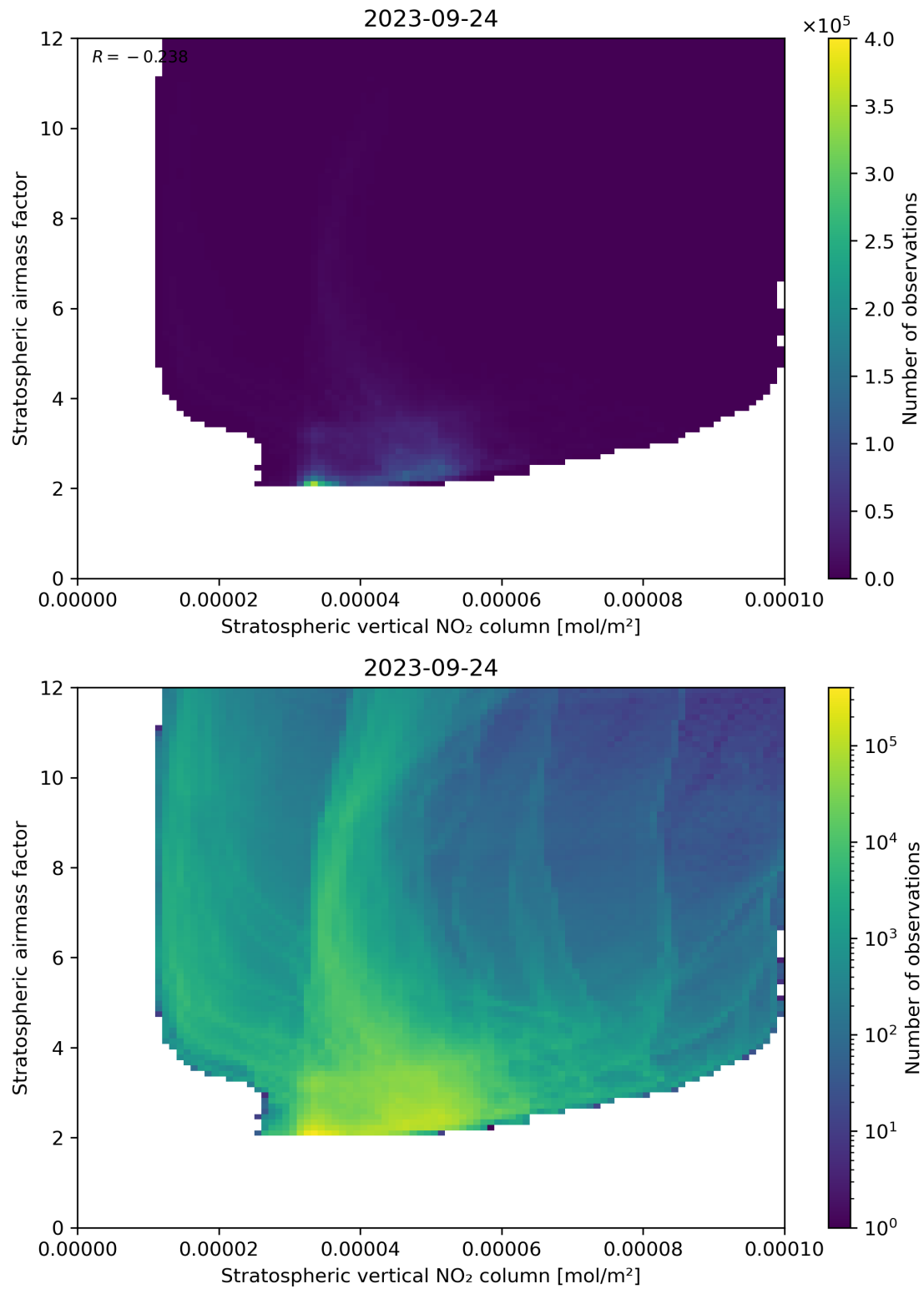
Figure 96: Scatter density plot of “Stratospheric vertical NO 2 column” against “Stratospheric airmass factor” for 2023-09-23 to 2023-09-25.
