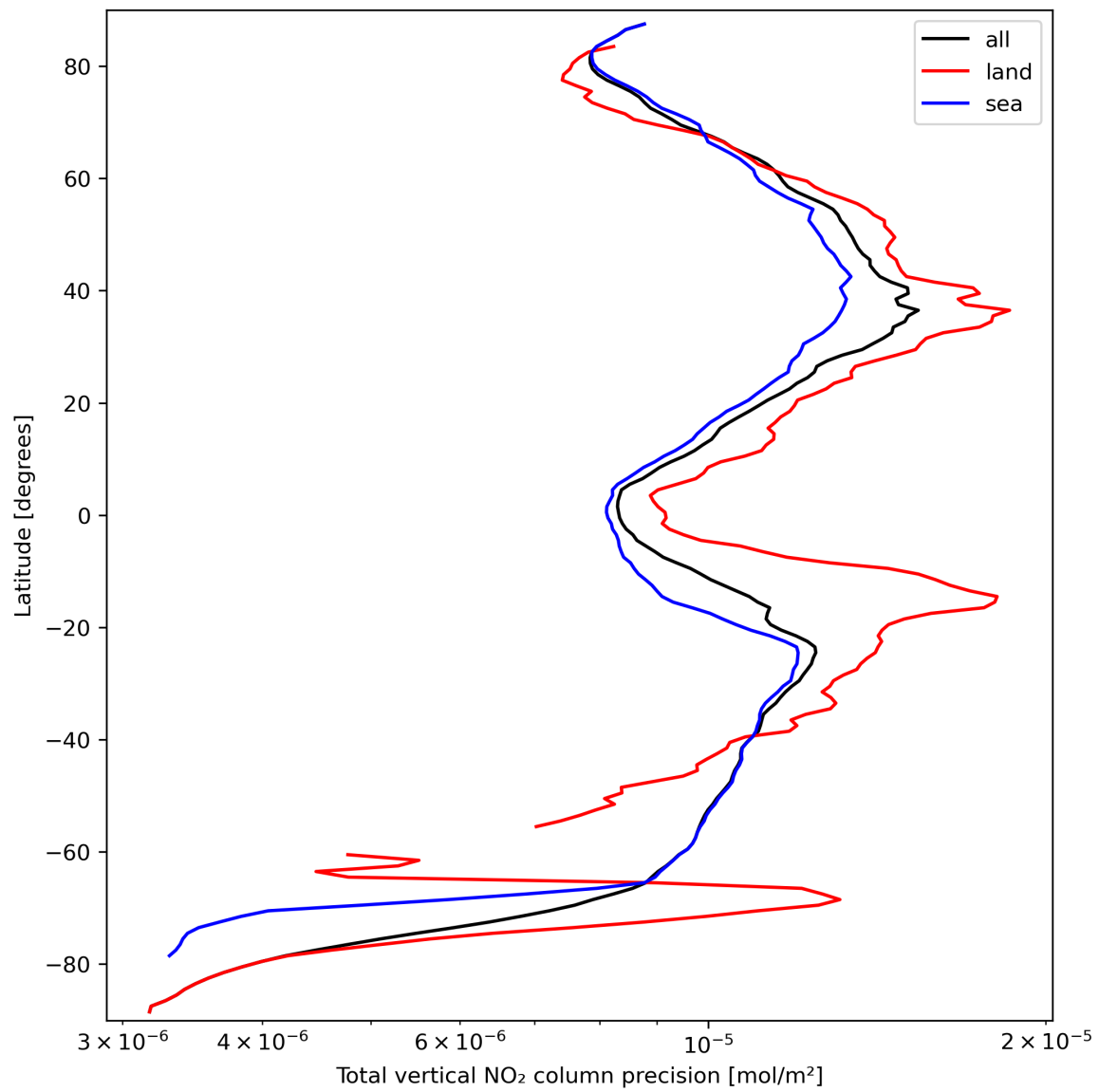
Figure 22: Zonal average of “Total vertical NO 2 column precision” for 2023-09-23 to 2023-09-25.
