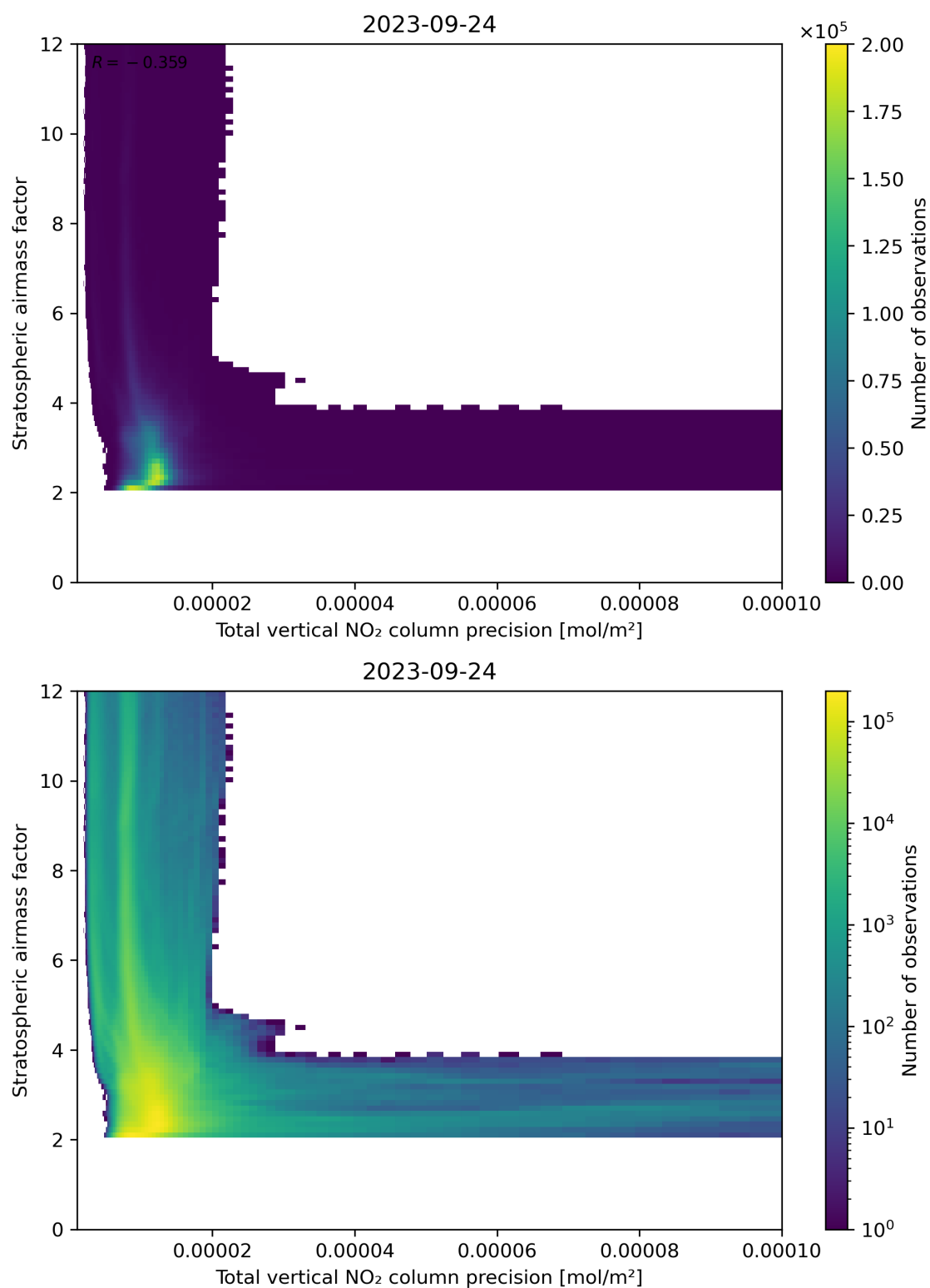
Figure 115: Scatter density plot of “Total vertical NO 2 column precision” against “Stratospheric air mass factor” for 2023-09-23 to 2023-09-25.
