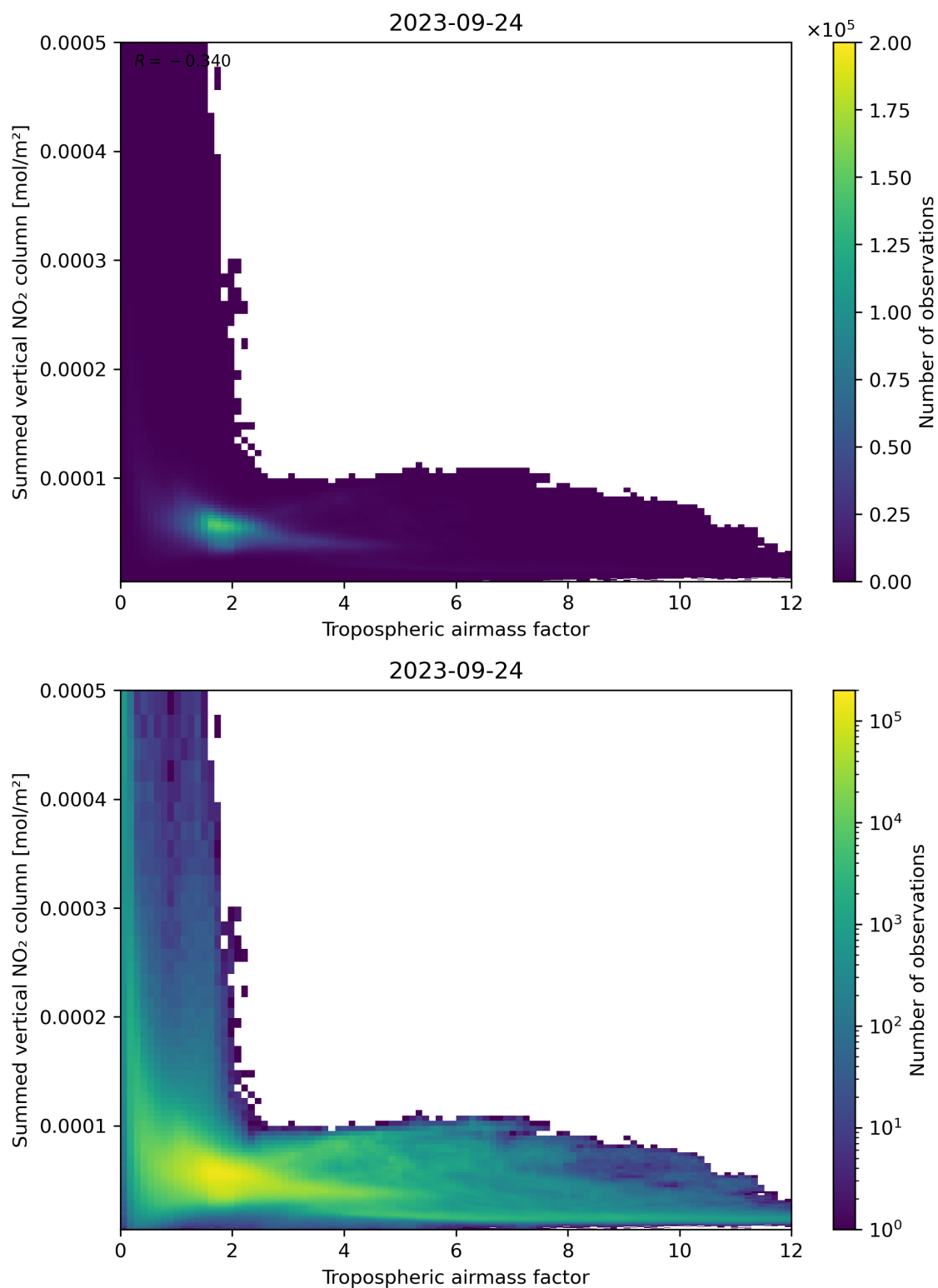
Figure 75: Scatter density plot of “Tropospheric air mass factor” against “Summed vertical NO 2 column” for 2023-09-23 to 2023-09-25.
