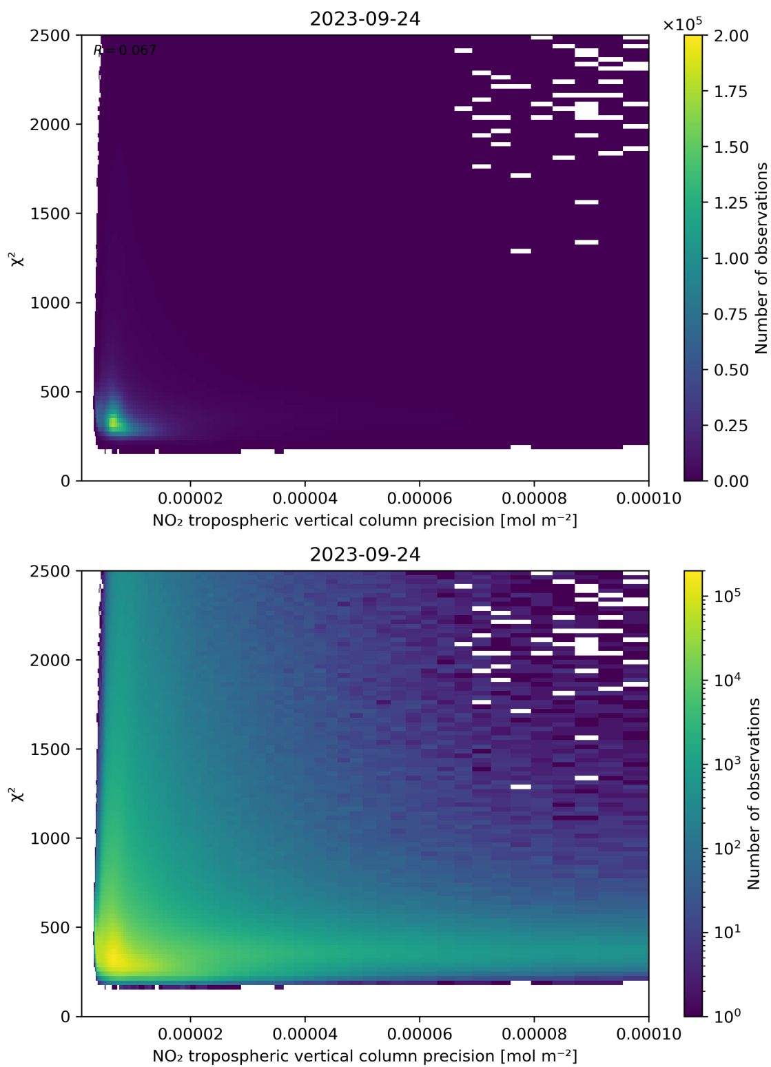
Figure 134: Scatter density plot of “NO 2 tropospheric vertical column precision” against “ \chi^2 ” for 2023-09-23 to 2023-09-25.
