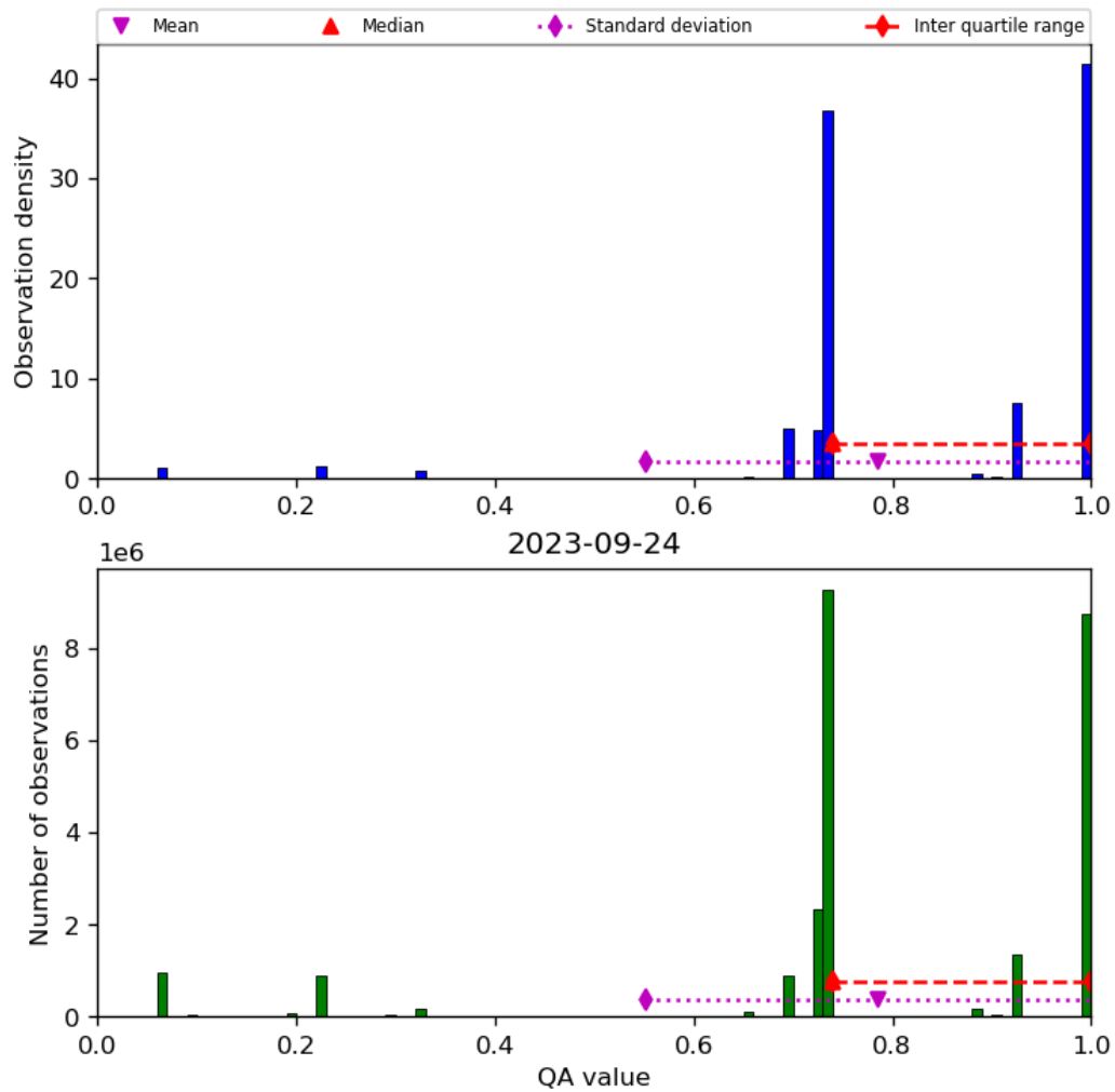
Figure 28: Histogram of “QA value” for 2023-09-23 to 2023-09-25
