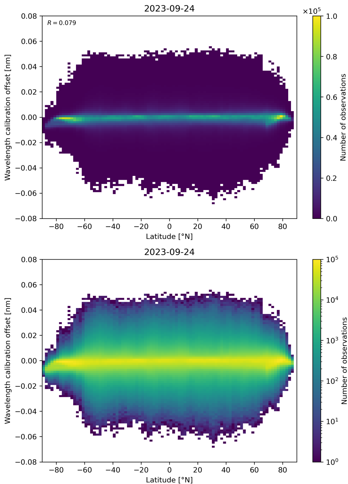
Figure 95: Scatter density plot of “Latitude” against “Wavelength calibration offset” for 2023-09-23 to 2023-09-25.
