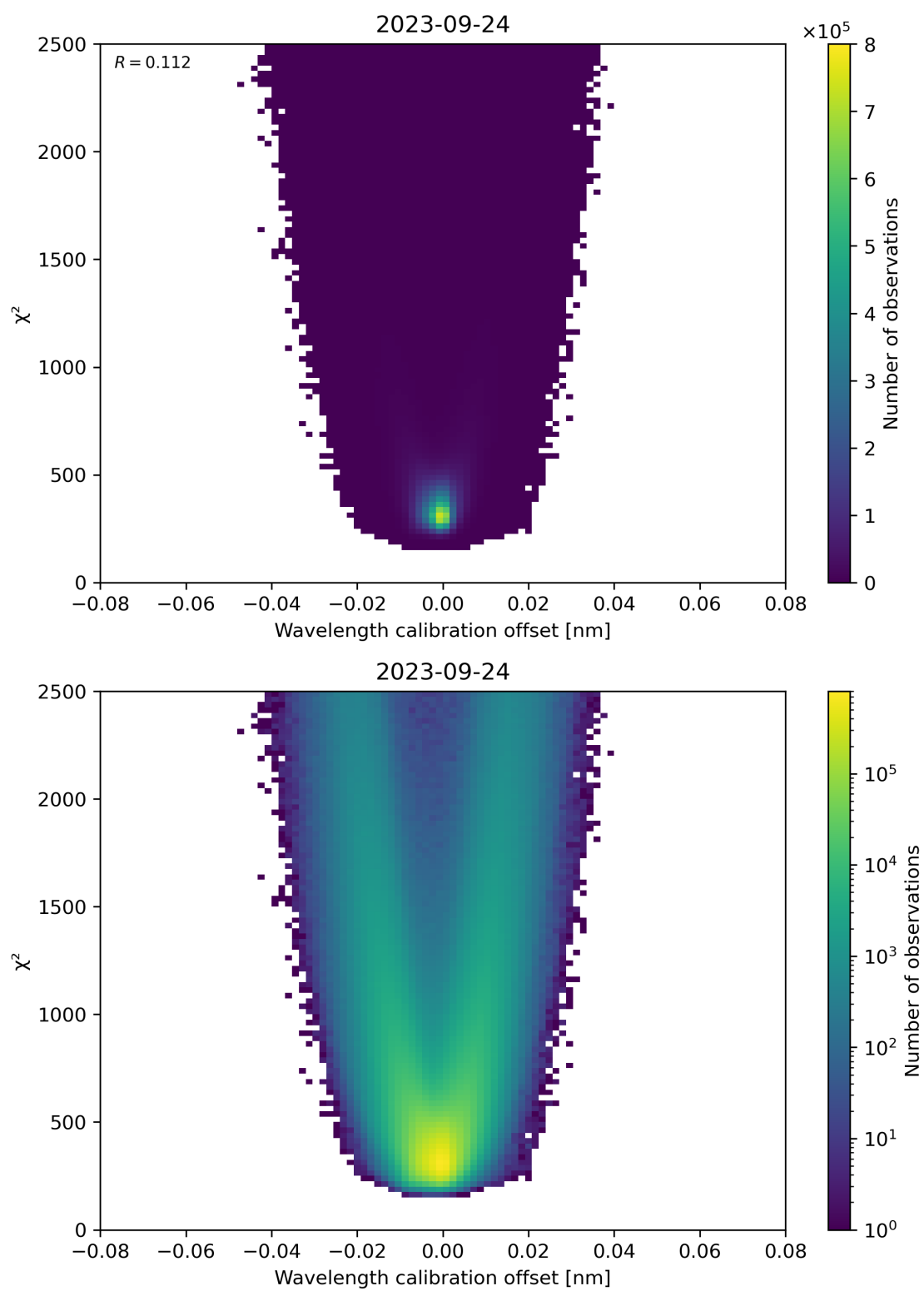
Figure 175: Scatter density plot of “Wavelength calibration offset” against “ \chi^2 ” for 2023-09-23 to 2023-09-25.
