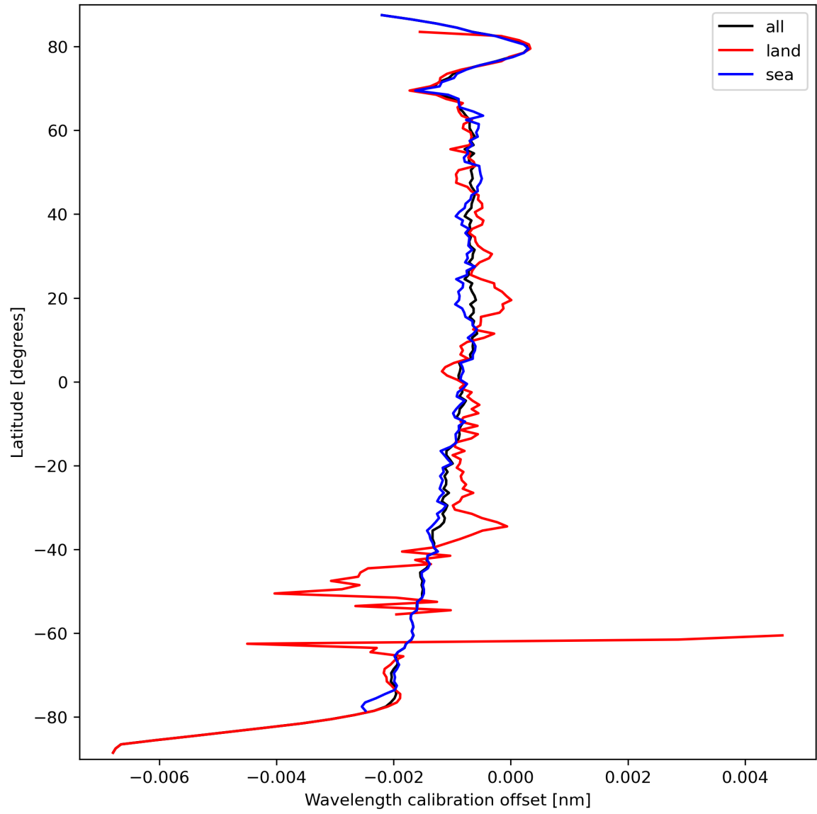
Figure 18: Zonal average of “Wavelength calibration offset” for 2023-09-23 to 2023-09-25.
