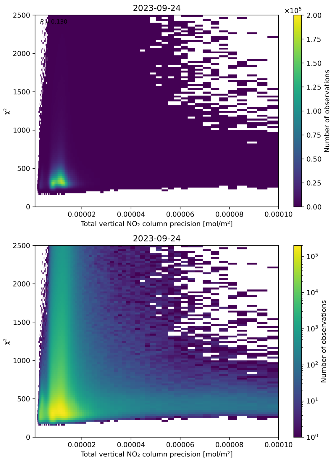
Figure 116: Scatter density plot of “Total vertical NO 2 column precision” against “ \chi^2 ” for 2023-09-23 to 2023-09-25.
