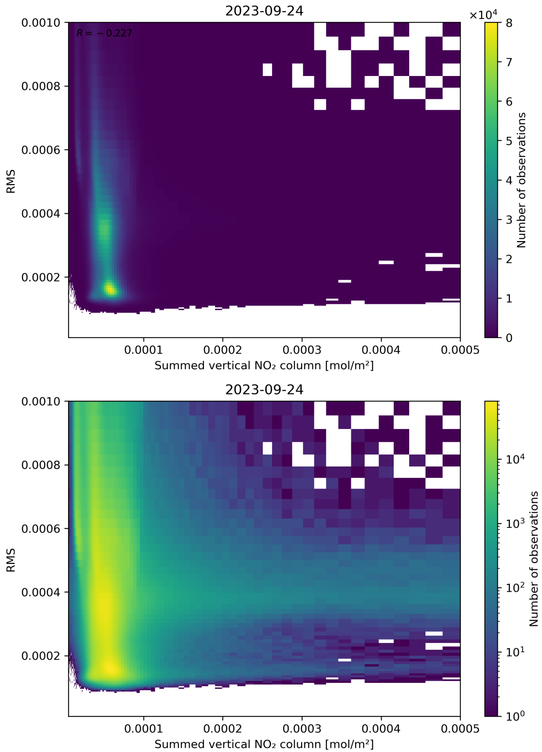
Figure 109: Scatter density plot of “Summed vertical NO 2 column” against “RMS” for 2023-09-23 to 2023-09-25.
