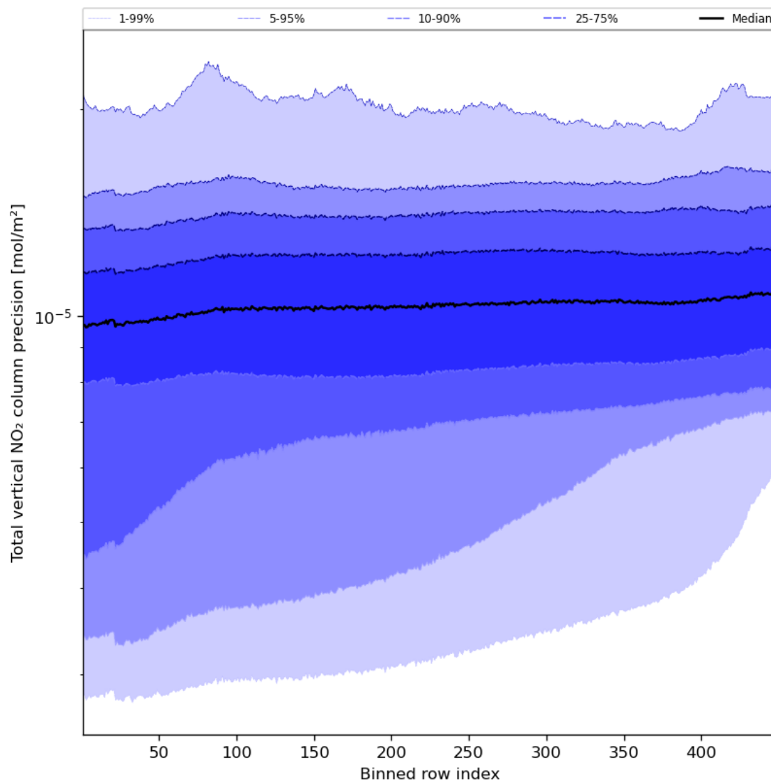
Figure 56: Along track statistics of “Total vertical NO 2 column precision” for 2023-09-23 to 2023-09-25
