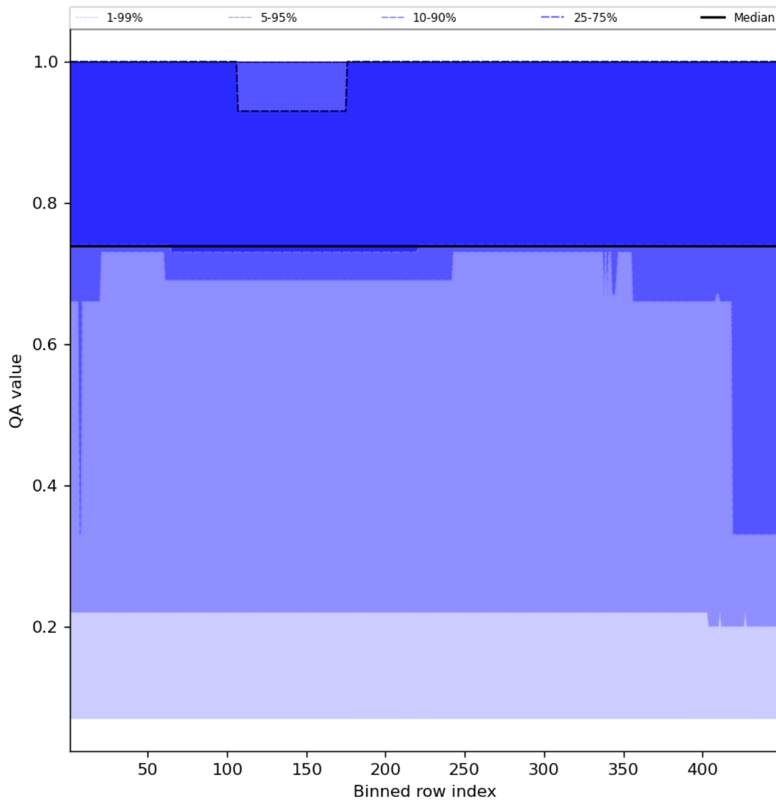
Figure 45: Along track statistics of “QA value” for 2023-09-23 to 2023-09-25
