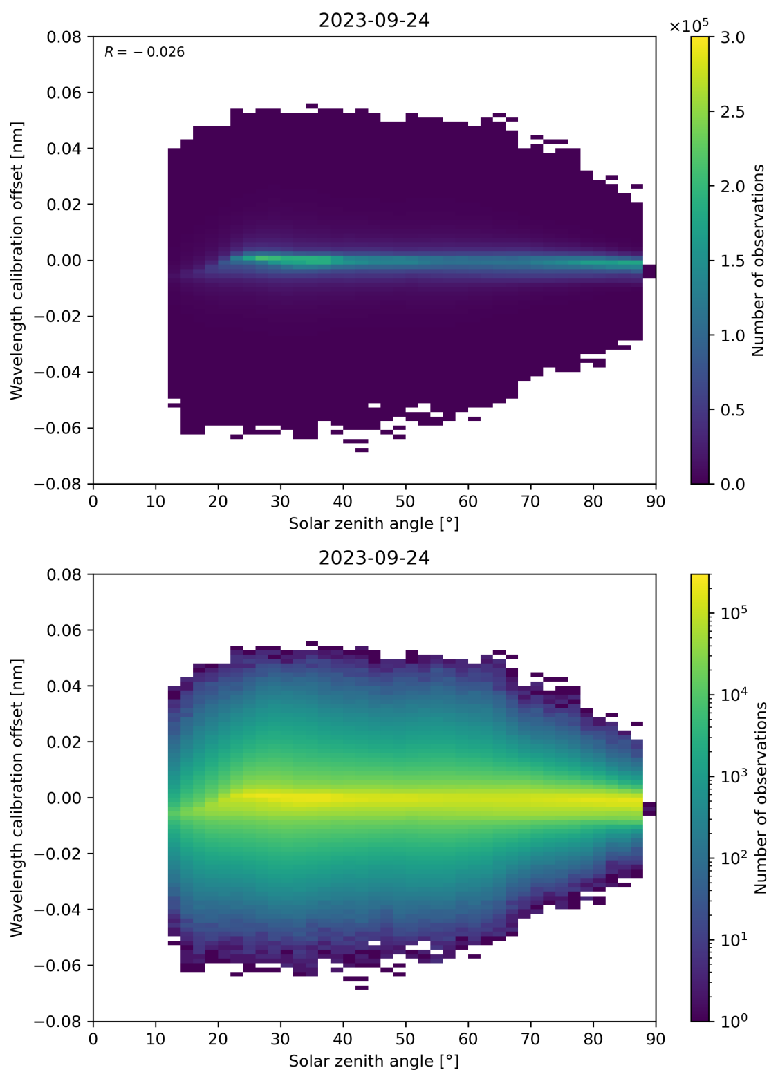
Figure 158: Scatter density plot of “Solar zenith angle” against “Wavelength calibration offset” for 2023-09-23 to 2023-09-25.
