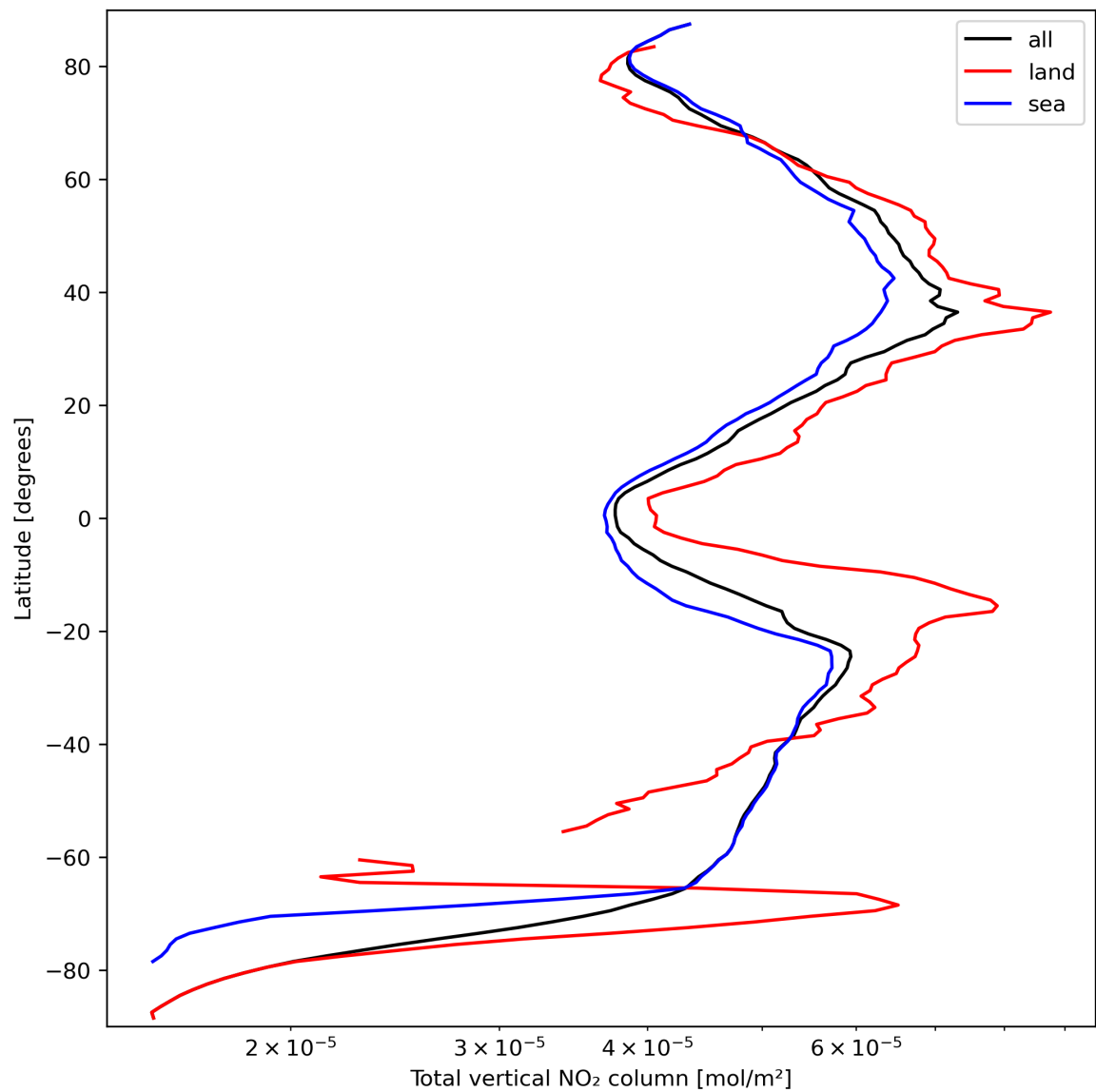
Figure 21: Zonal average of “Total vertical NO 2 column” for 2023-09-23 to 2023-09-25.
