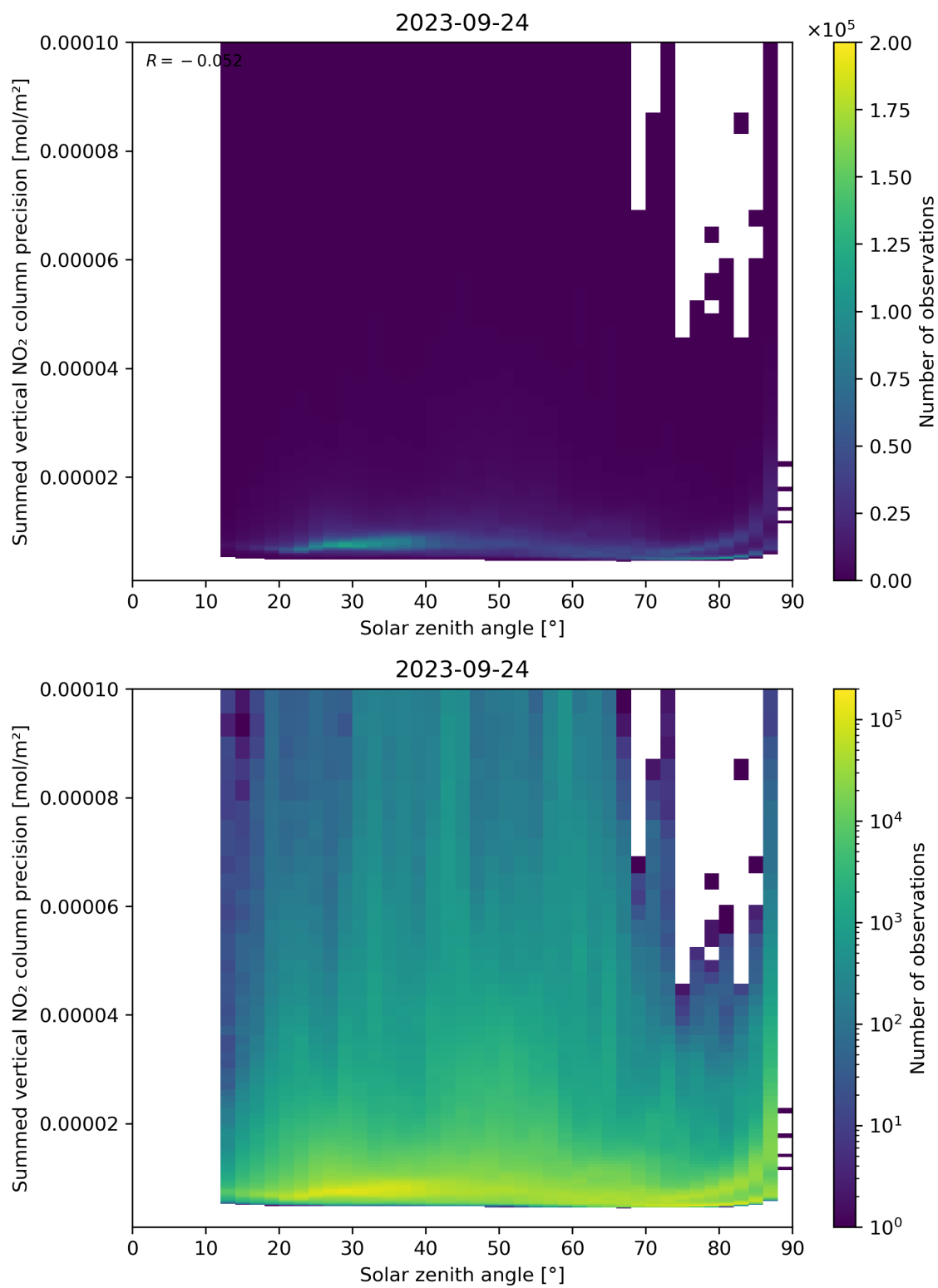
Figure 152: Scatter density plot of “Solar zenith angle” against “Summed vertical NO 2 column precision” for 2023-09-23 to 2023-09-25.
