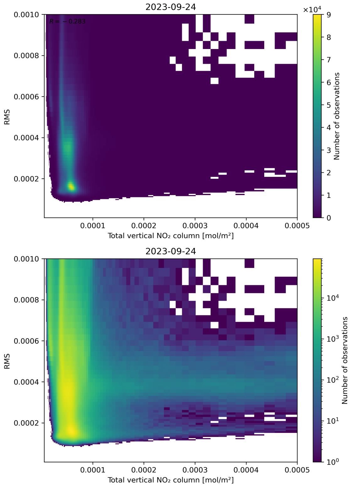
Figure 120: Scatter density plot of “Total vertical NO 2 column” against “RMS” for 2023-09-23 to 2023-09-25.
