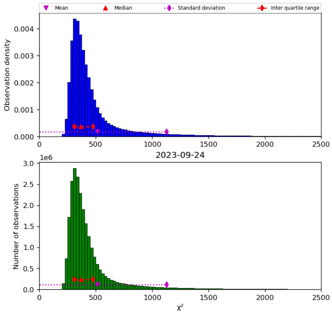
Figure 42: Histogram of “ \chi^2 ” for 2023-09-23 to 2023-09-25
