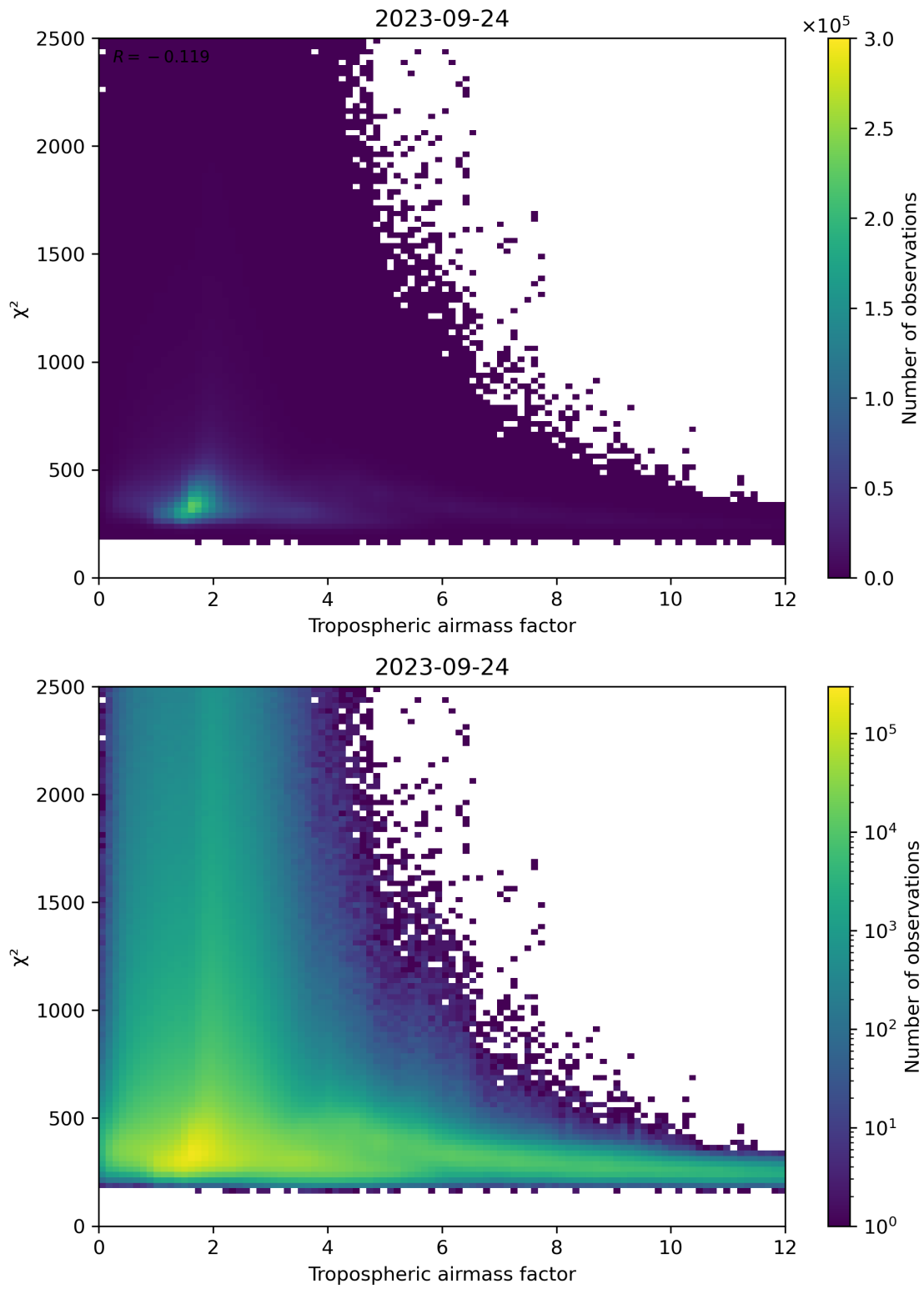
Figure 73: Scatter density plot of “Tropospheric airmass factor” against “ \chi^2 ” for 2023-09-23 to 2023-09-25.
