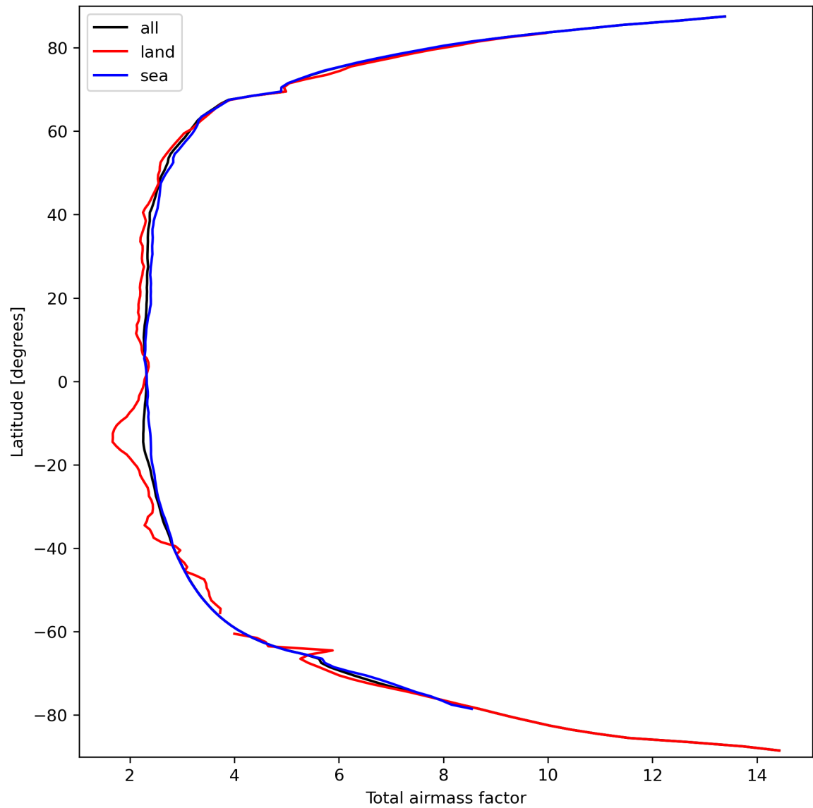
Figure 15: Zonal average of “Total airmass factor” for 2023-09-23 to 2023-09-25.
