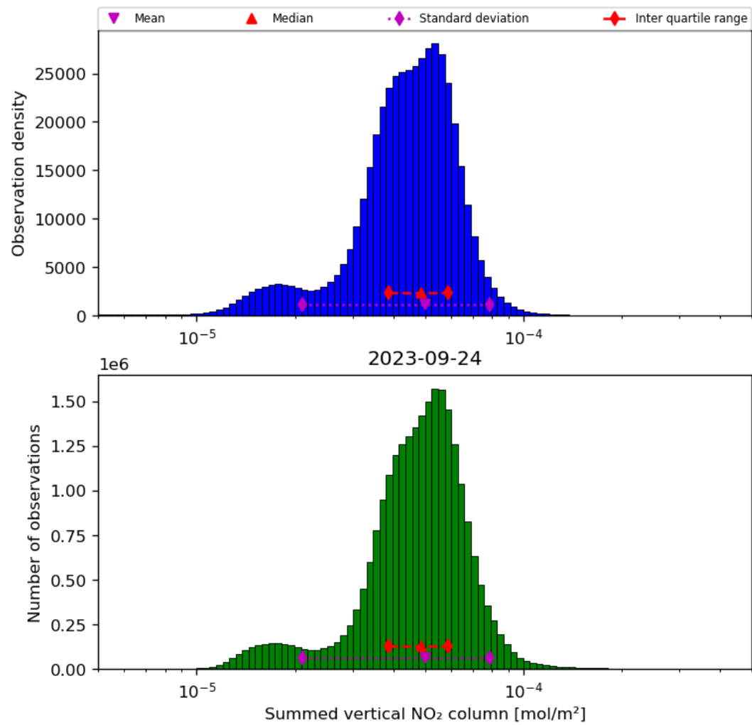
Figure 40: Histogram of “Summed vertical NO 2 column” for 2023-09-23 to 2023-09-25
