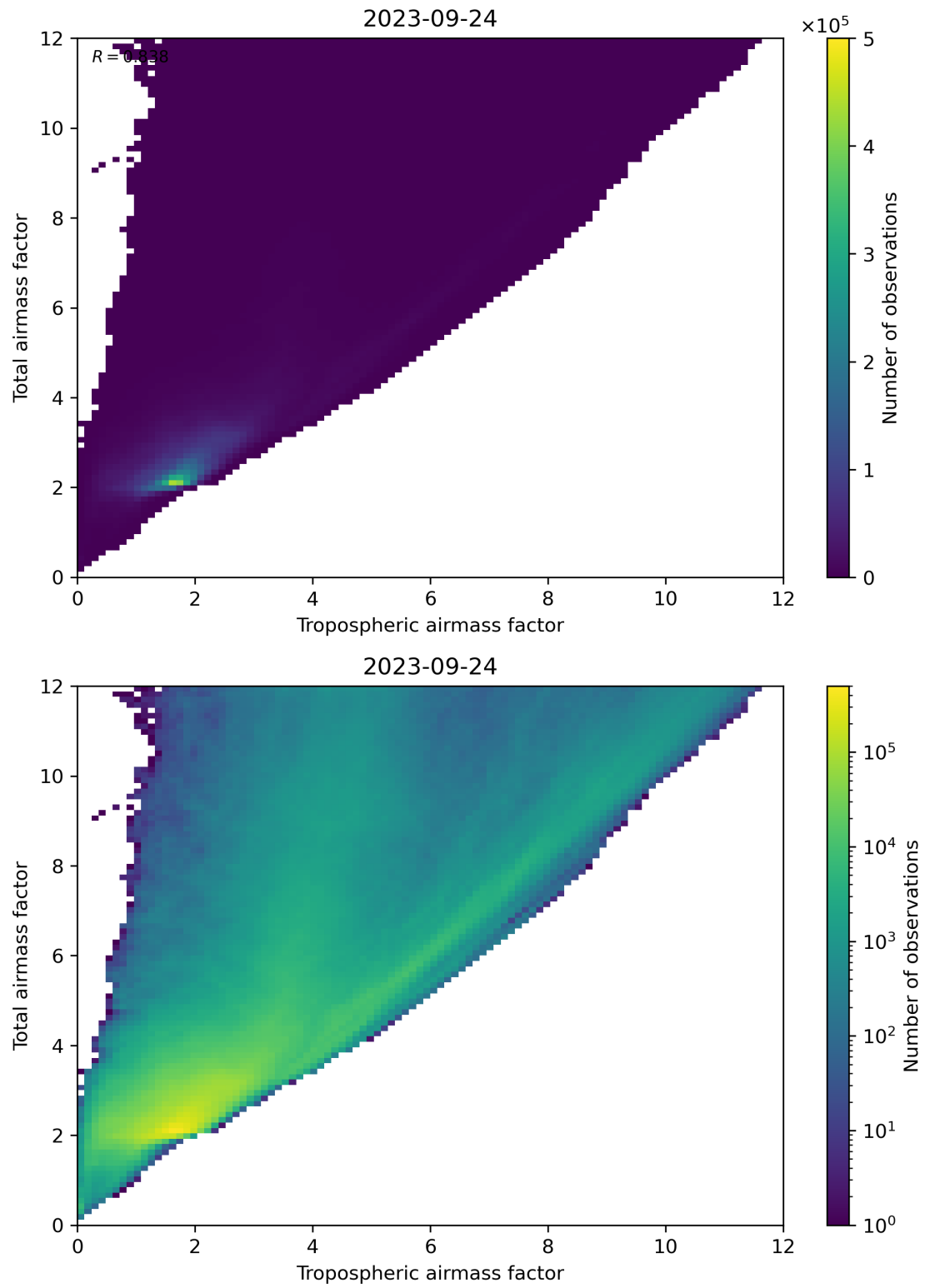
Figure 72: Scatter density plot of “Tropospheric airmass factor” against “Total airmass factor” for 2023-09-23 to 2023-09-25.
