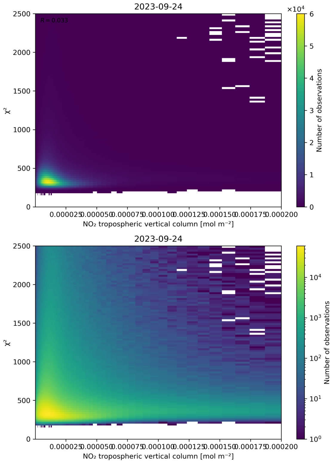
Figure 124: Scatter density plot of “NO 2 tropospheric vertical column” against “ \chi^2 ” for 2023-09-23 to 2023-09-25.
