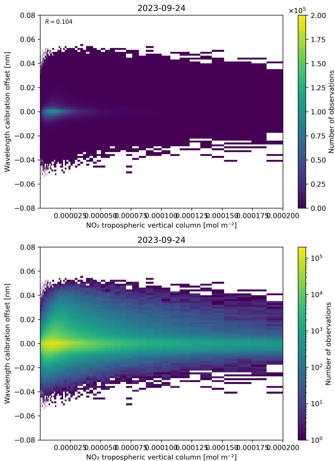
Figure 143: Scatter density plot of “NO 2 tropospheric vertical column” against “Wavelength calibration offset” for 2023-09-23 to 2023-09-25.
