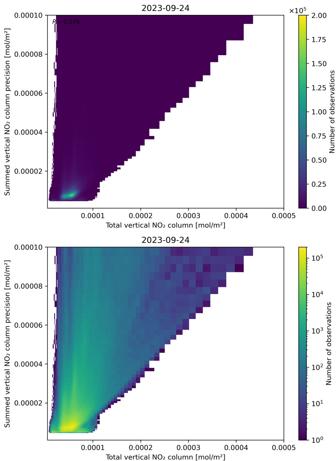
Figure 113: Scatter density plot of “Total vertical NO 2 column” against “Summed vertical NO 2 column precision” for 2023-09-23 to 2023-09-25.
