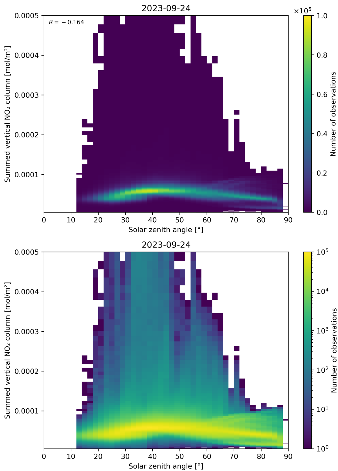
Figure 151: Scatter density plot of “Solar zenith angle” against “Summed vertical NO 2 column” for 2023-09-23 to 2023-09-25.
