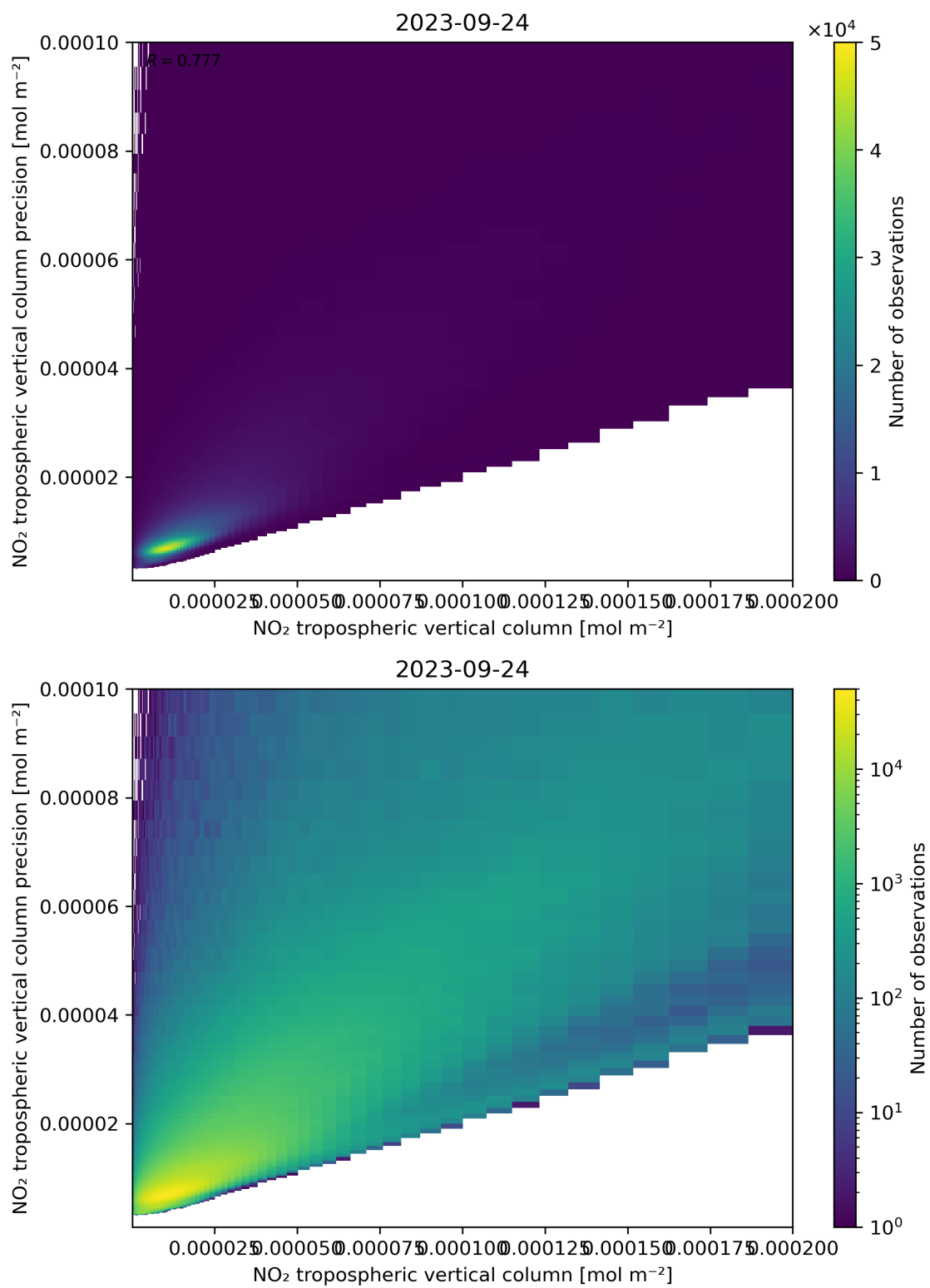
Figure 130: Scatter density plot of “NO 2 tropospheric vertical column” against “NO 2 tropospheric vertical column precision” for 2023-09-23 to 2023-09-25.
