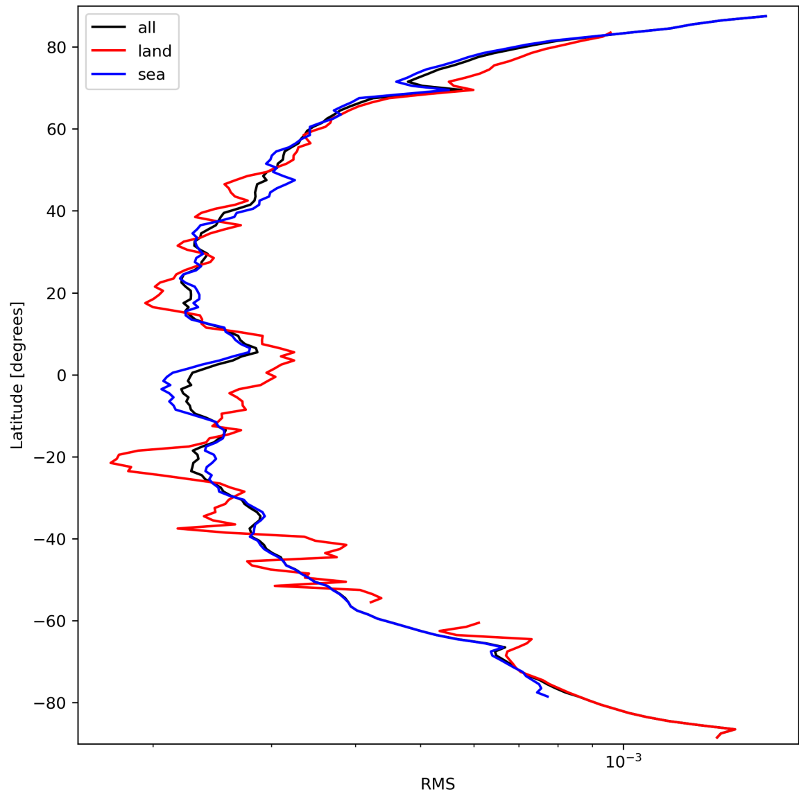
Figure 26: Zonal average of “RMS” for 2023-09-23 to 2023-09-25.
