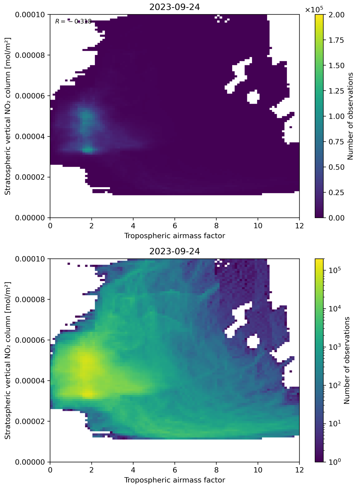
Figure 74: Scatter density plot of “Tropospheric air mass factor” against “Stratospheric vertical NO 2 column” for 2023-09-23 to 2023-09-25.
