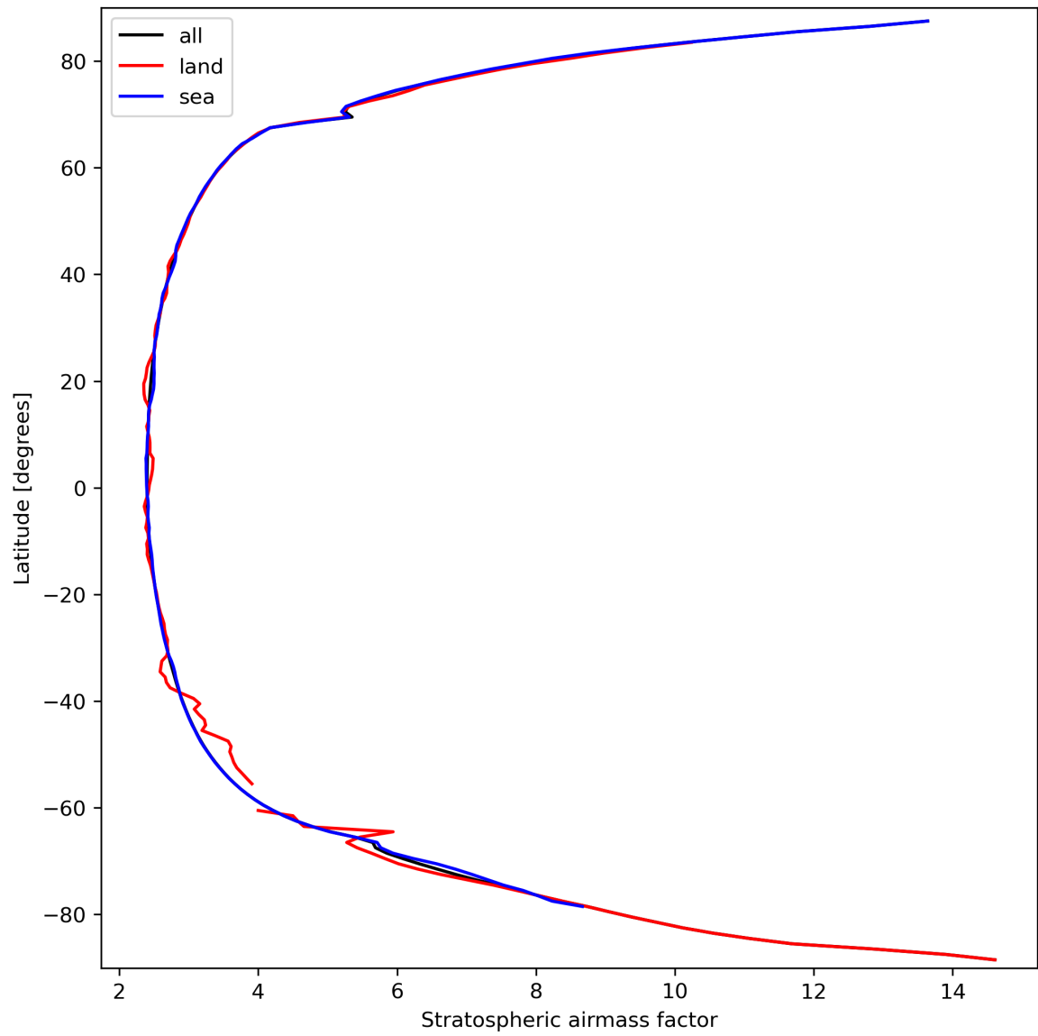
Figure 27: Zonal average of “Stratospheric air mass factor” for 2023-09-23 to 2023-09-25.
