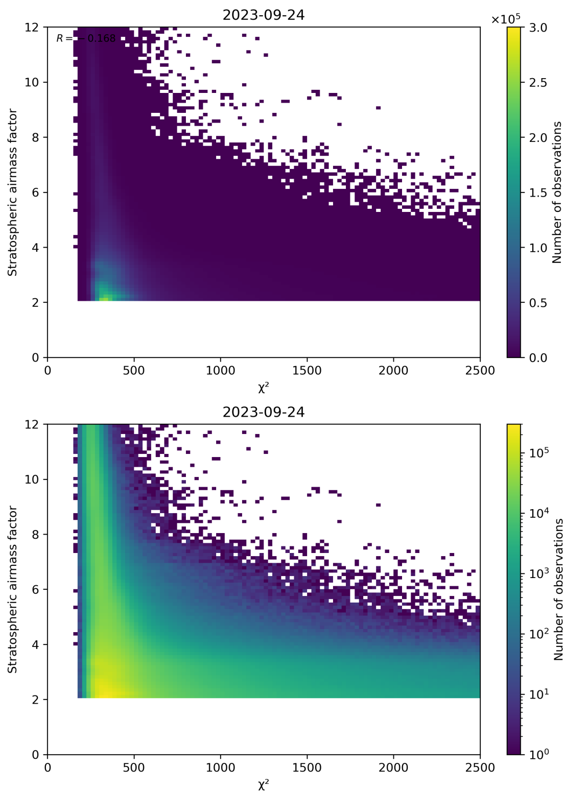
Figure 81: Scatter density plot of “ \chi^2 ” against “Stratospheric airmass factor” for 2023-09-23 to 2023-09-25.
