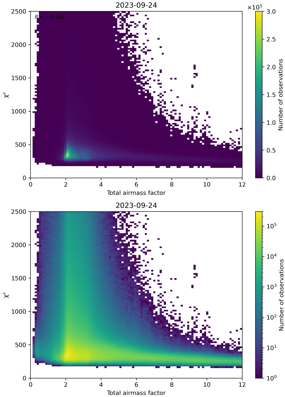
Figure 63: Scatter density plot of “Total airmass factor” against “ \chi^2 ” for 2023-09-23 to 2023-09-25.
