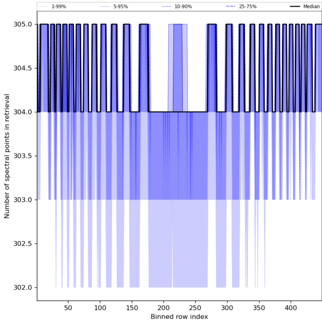
Figure 50: Along track statistics of “Number of spectral points in retrieval” for 2023-09-23 to 2023-09-25
