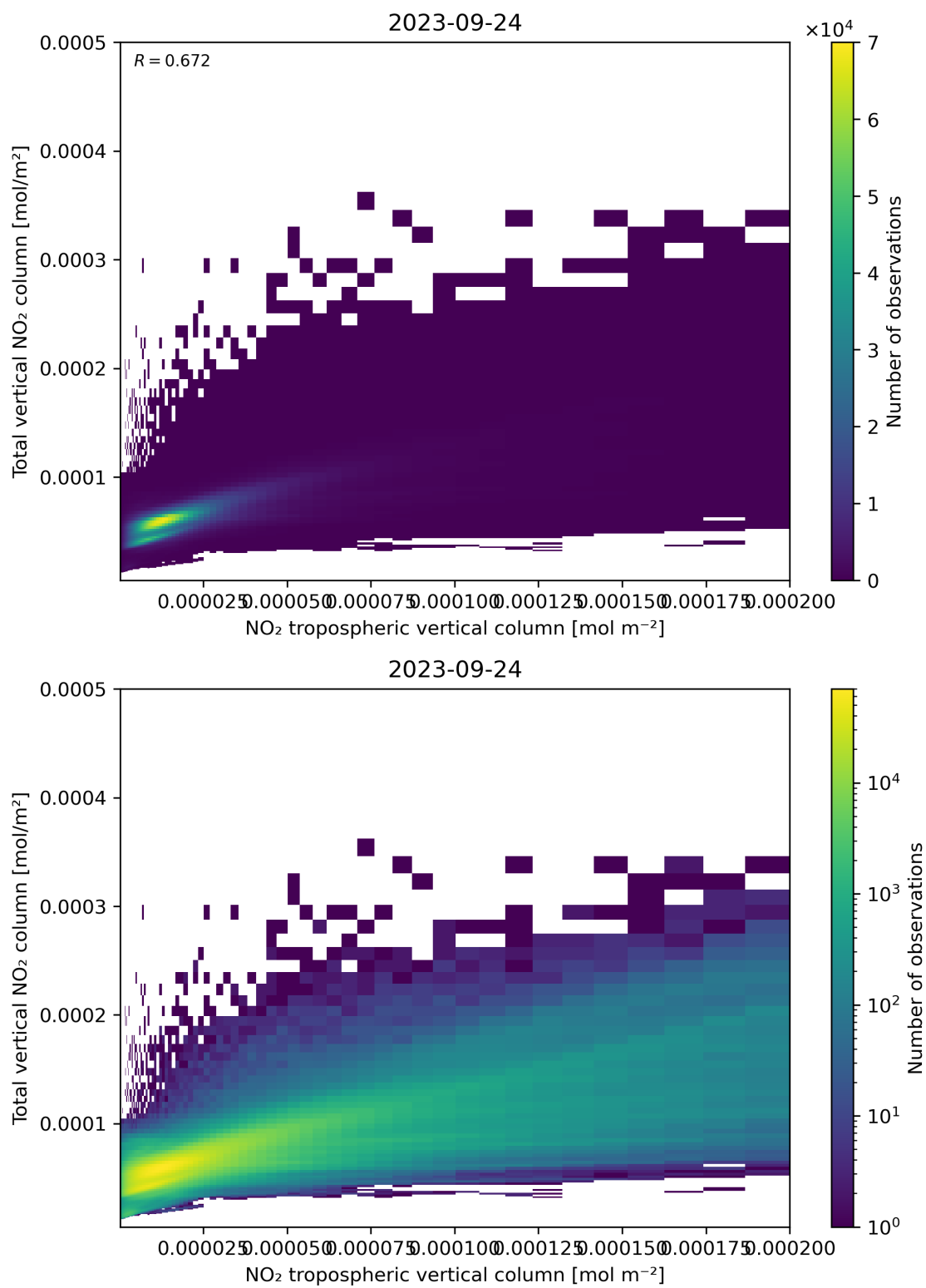
Figure 128: Scatter density plot of “NO 2 tropospheric vertical column” against “Total vertical NO 2 column” for 2023-09-23 to 2023-09-25.
