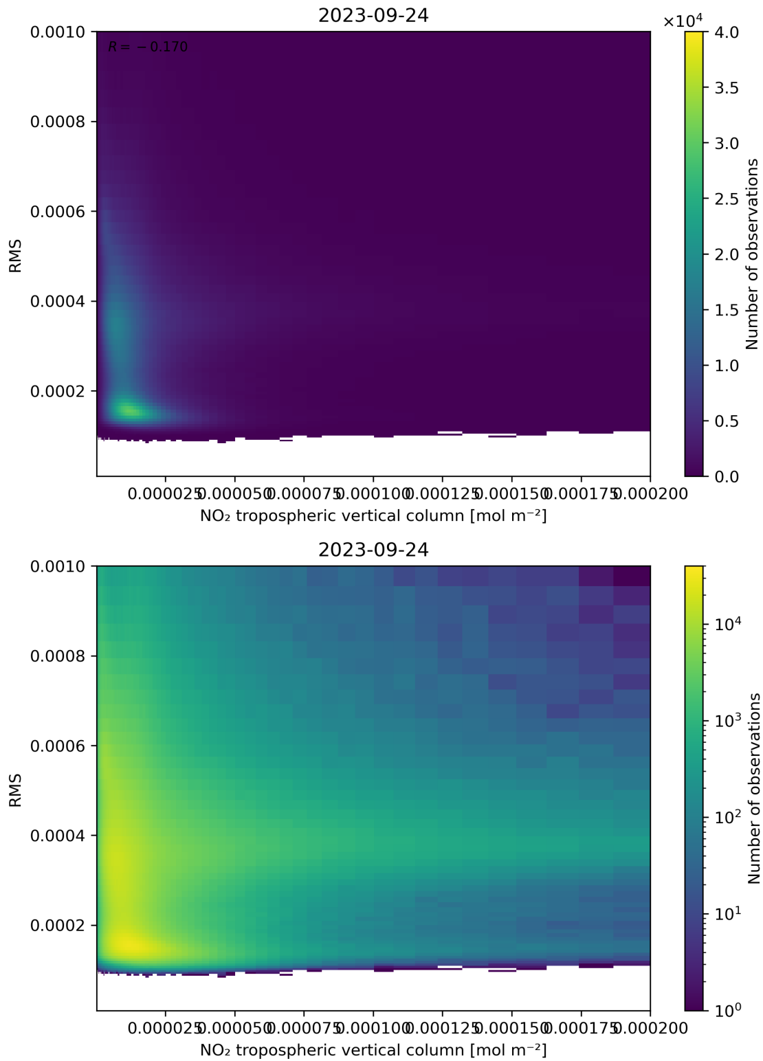
Figure 142: Scatter density plot of “NO 2 tropospheric vertical column” against “RMS” for 2023-09-23 to 2023-09-25.
