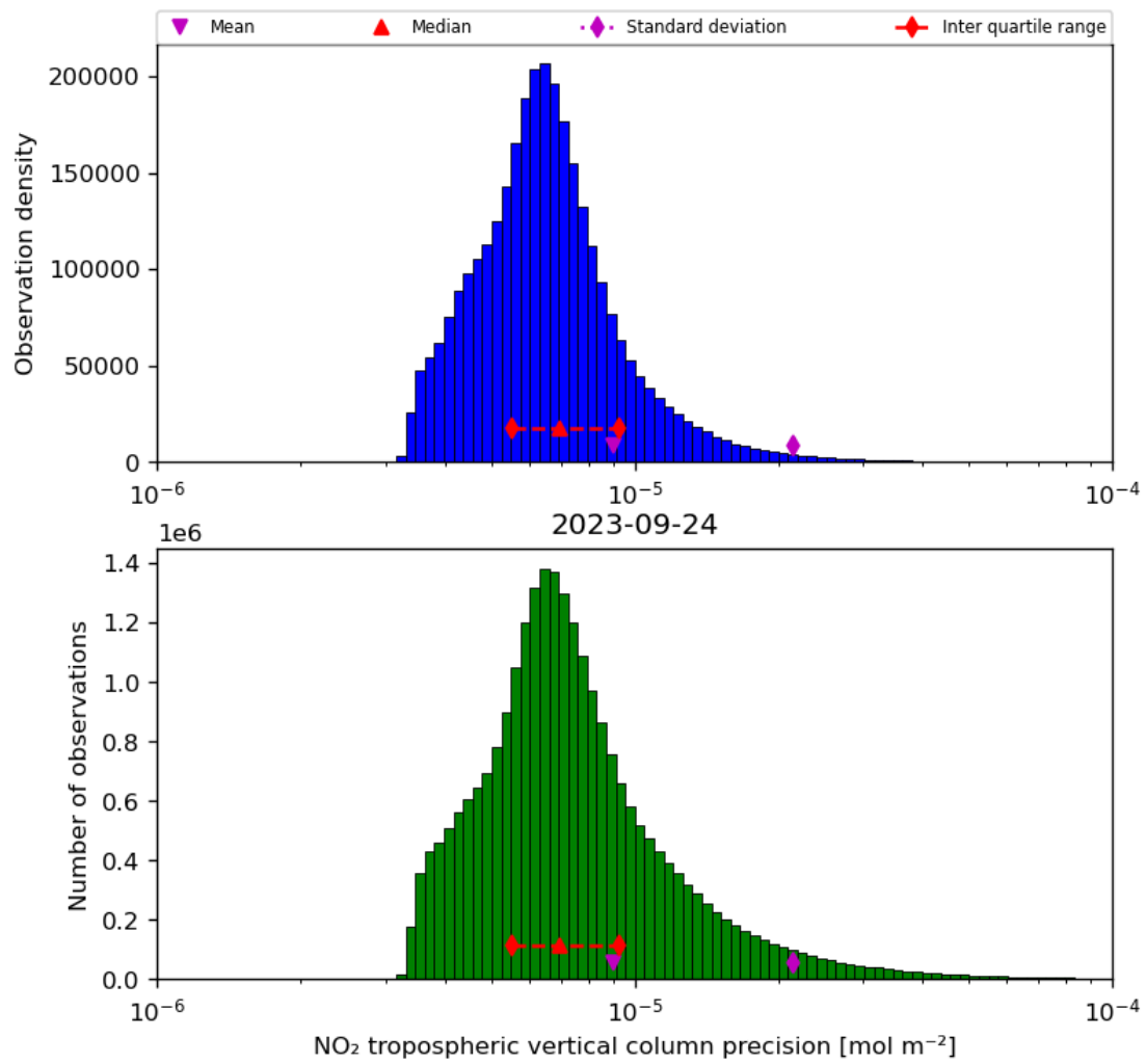
Figure 30: Histogram of “NO 2 tropospheric vertical column precision” for 2023-09-23 to 2023-09-25
