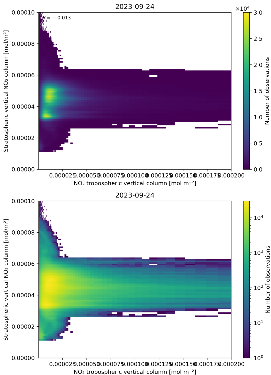
Figure 125: Scatter density plot of “NO 2 tropospheric vertical column” against “Stratospheric vertical NO 2 column” for 2023-09-23 to 2023-09-25.
