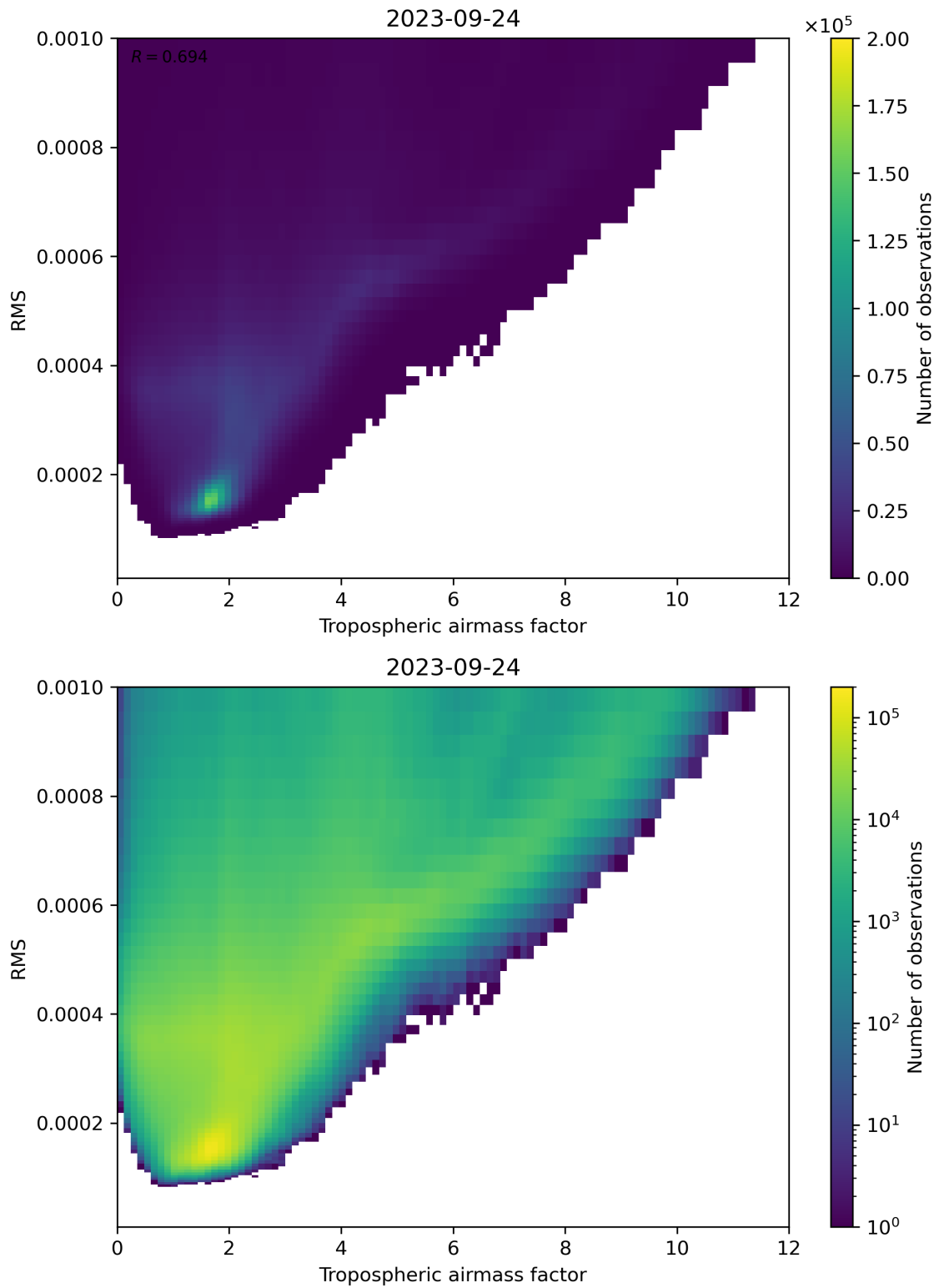
Figure 79: Scatter density plot of “Tropospheric airmass factor” against “RMS” for 2023-09-23 to 2023-09-25.
