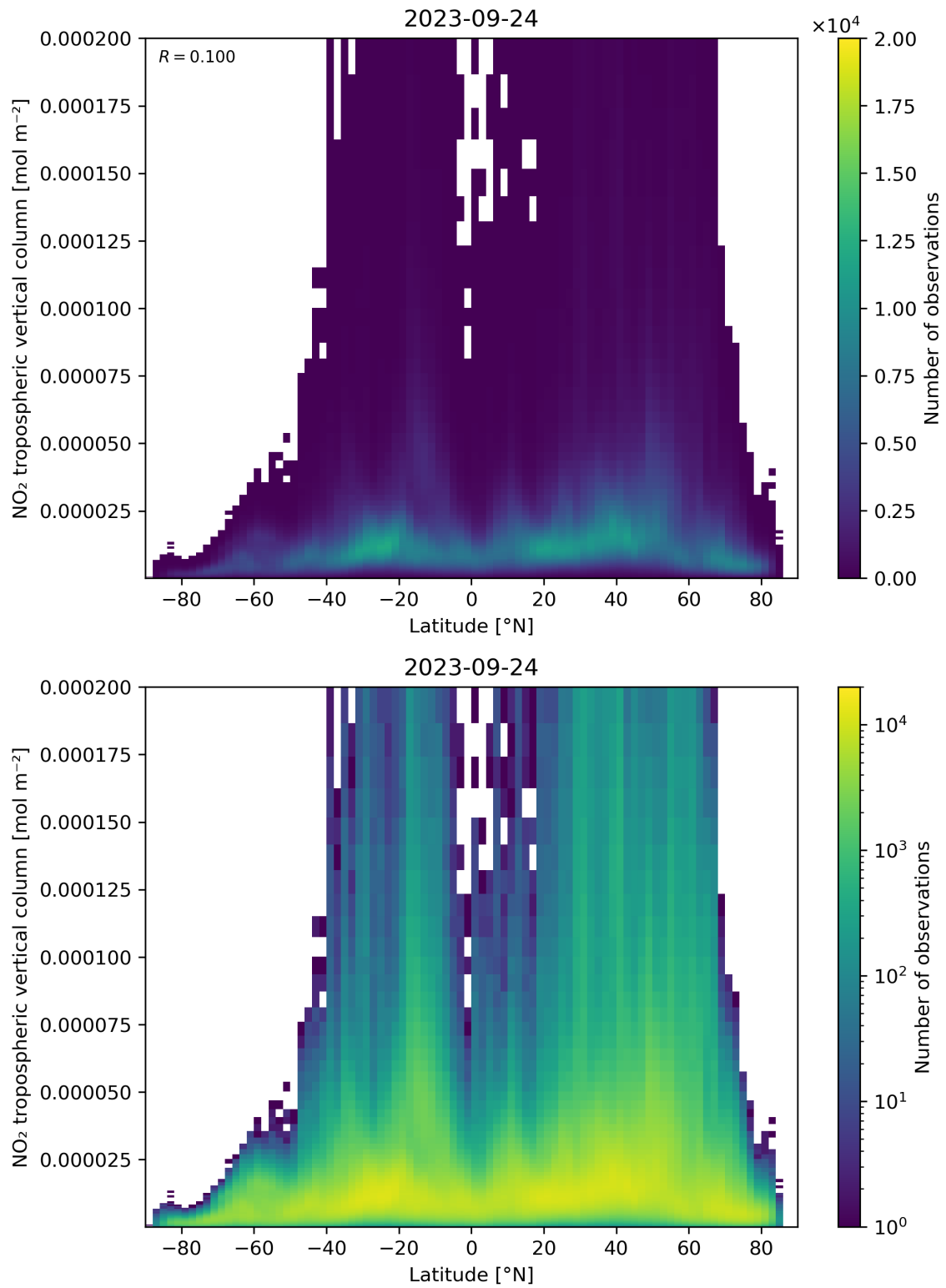
Figure 92: Scatter density plot of “Latitude” against “NO 2 tropospheric vertical column” for 2023-09-23 to 2023-09-25.
