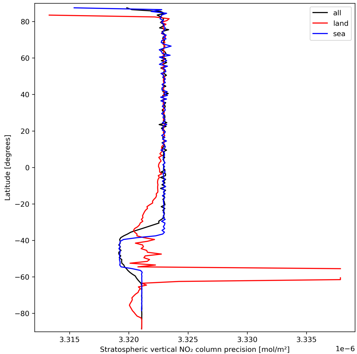
Figure 20: Zonal average of “Stratospheric vertical NO 2 column precision” for 2023-09-23 to 2023-09-25.
