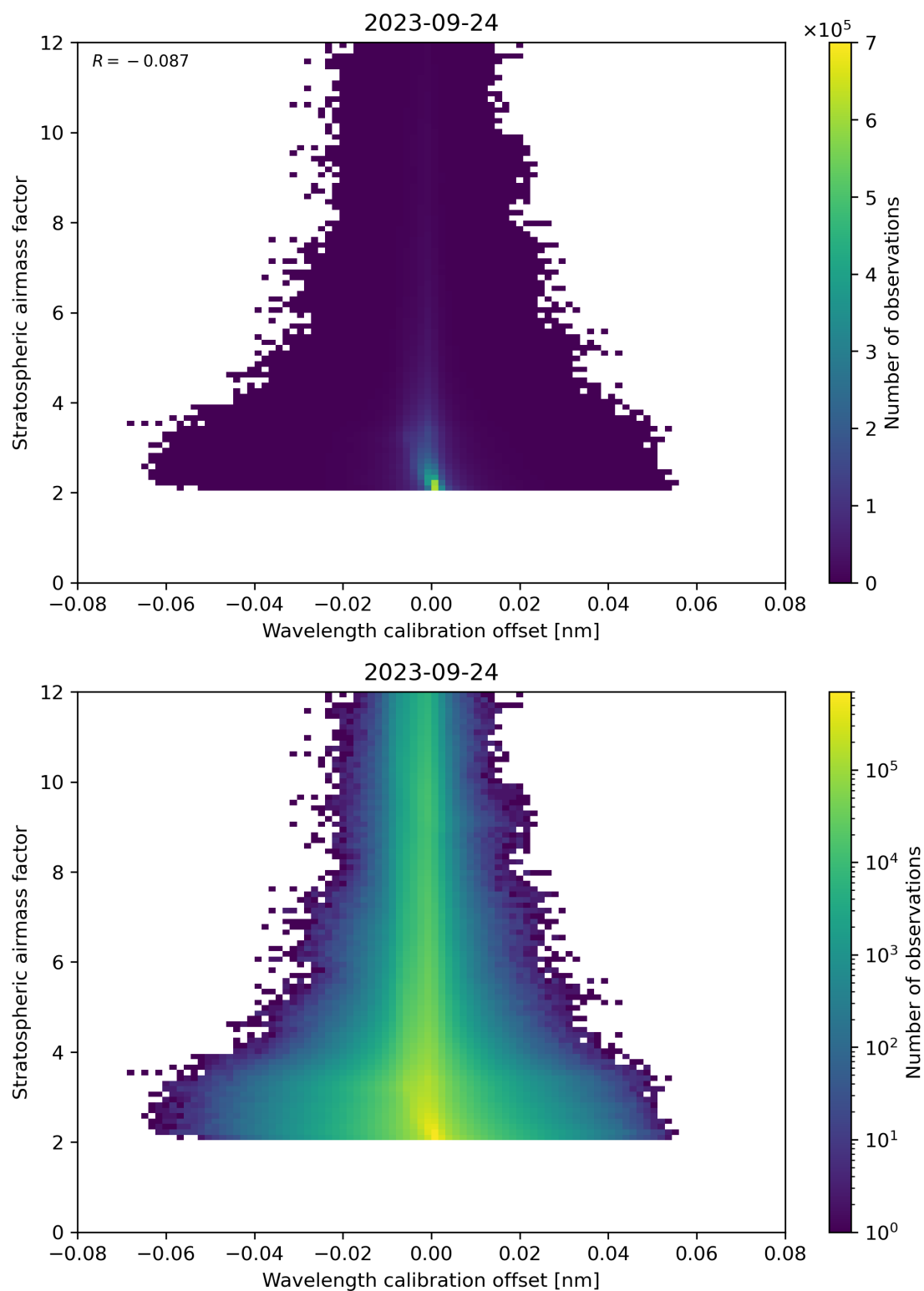
Figure 174: Scatter density plot of “Wavelength calibration offset” against “Stratospheric air mass factor” for 2023-09-23 to 2023-09-25.
