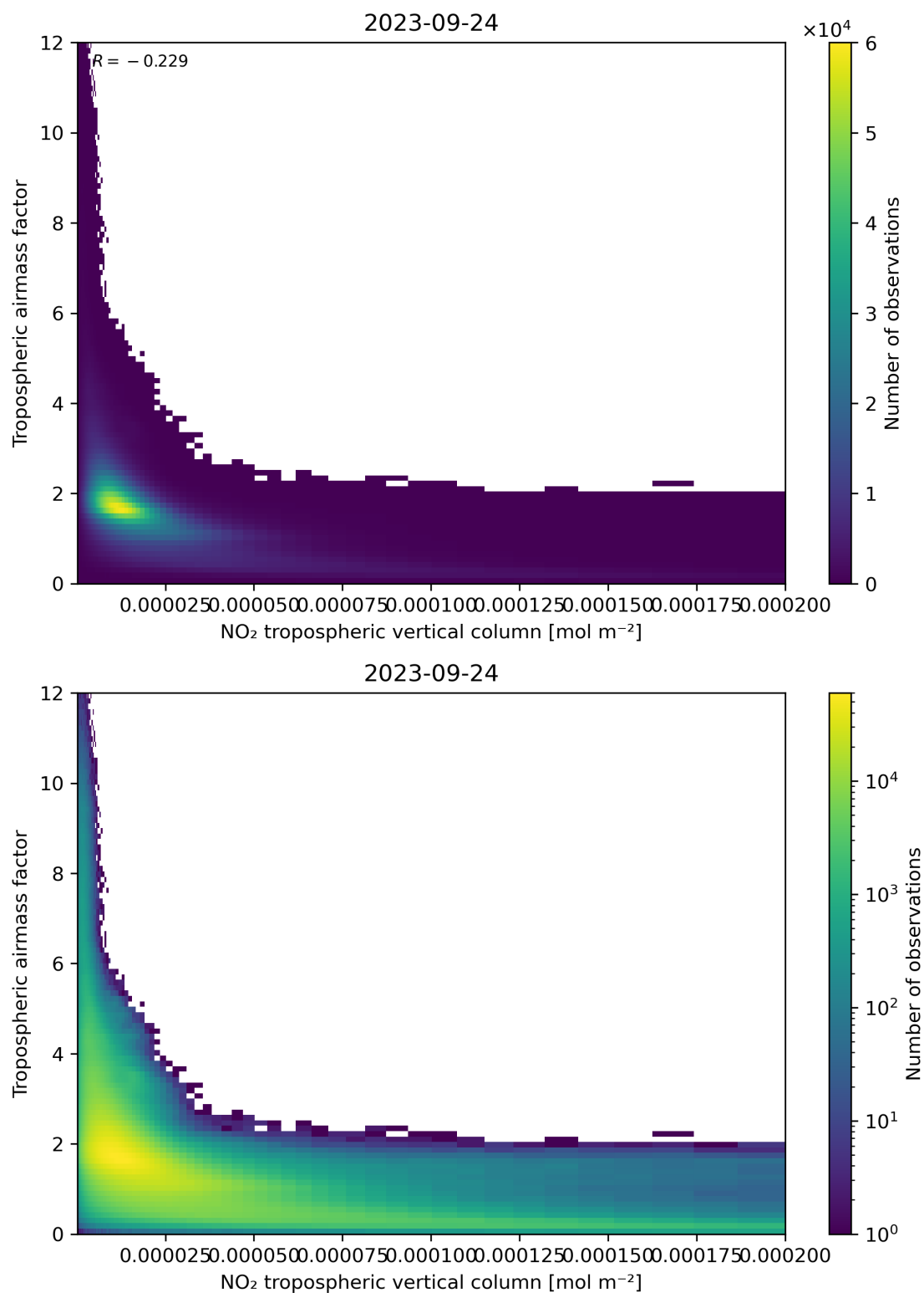
Figure 123: Scatter density plot of “NO 2 tropospheric vertical column” against “Tropospheric airmass factor” for 2023-09-23 to 2023-09-25.
