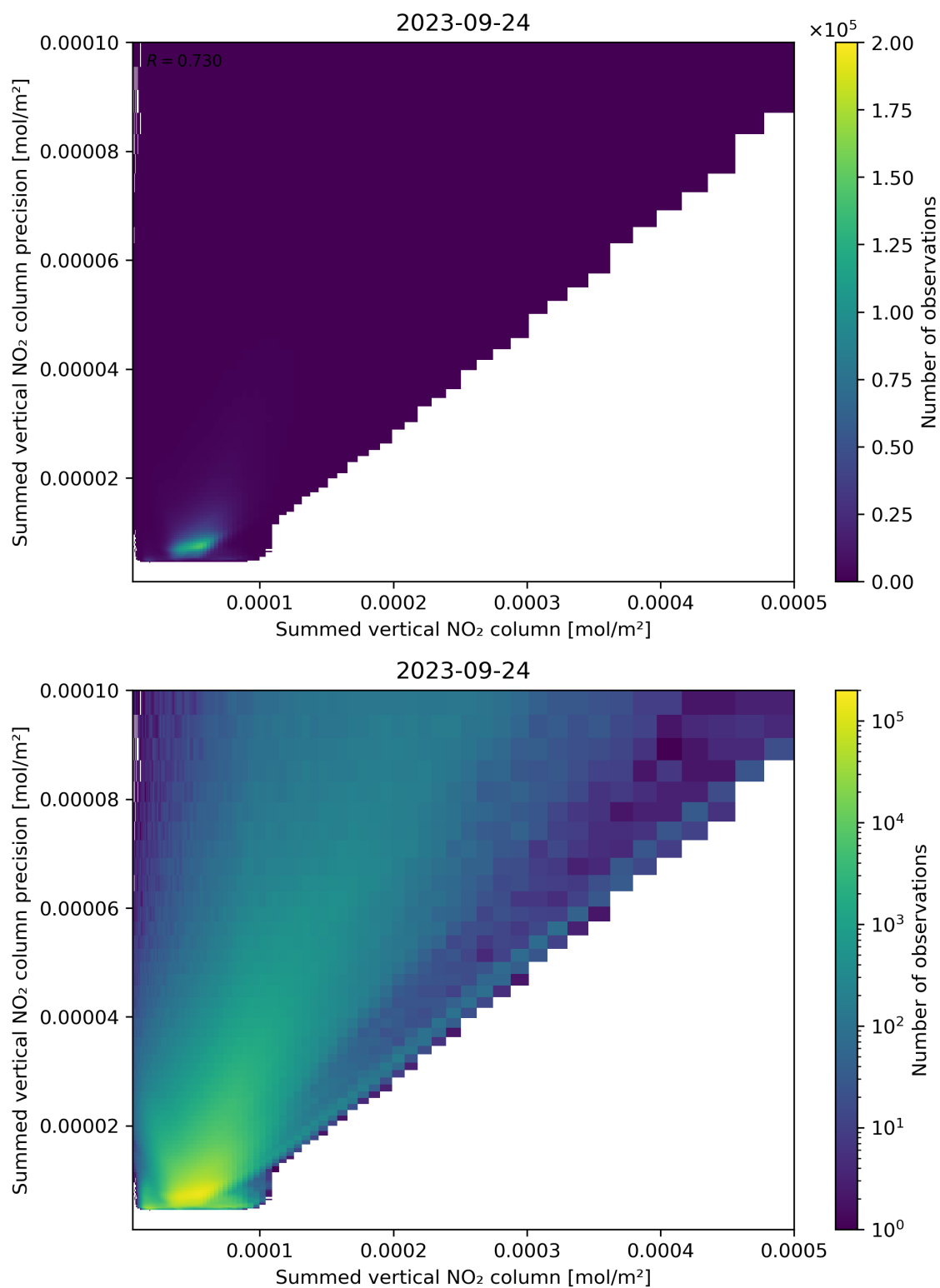
Figure 105: Scatter density plot of “Summed vertical NO 2 column” against “Summed vertical NO 2 column precision” for 2023-09-23 to 2023-09-25.
