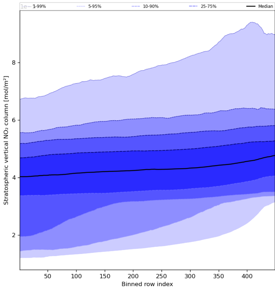
Figure 53: Along track statistics of “Stratospheric vertical NO 2 column” for 2023-09-23 to 2023-09-25
