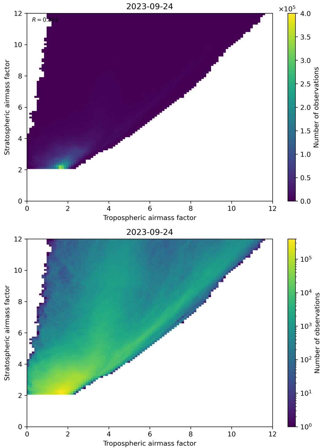
Figure 71: Scatter density plot of “Tropospheric airmass factor” against “Stratospheric airmass factor” for 2023-09-23 to 2023-09-25.
