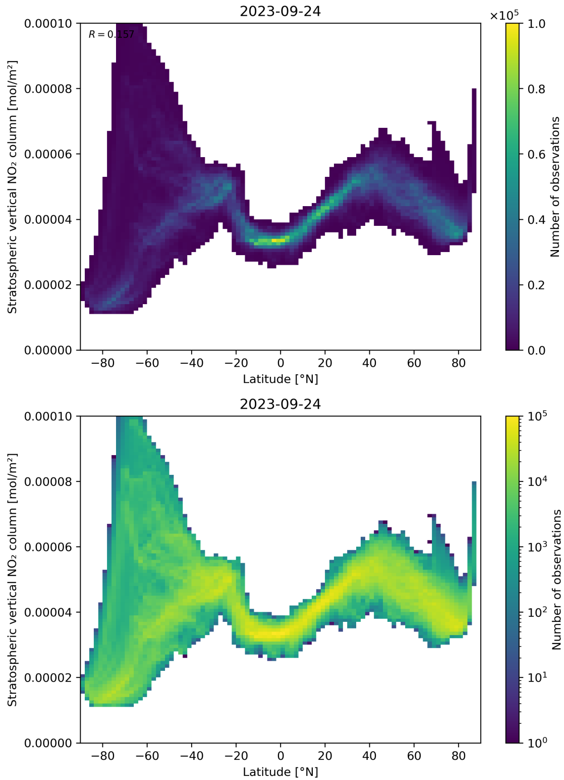
Figure 87: Scatter density plot of “Latitude” against “Stratospheric vertical NO 2 column” for 2023-09-23 to 2023-09-25.
