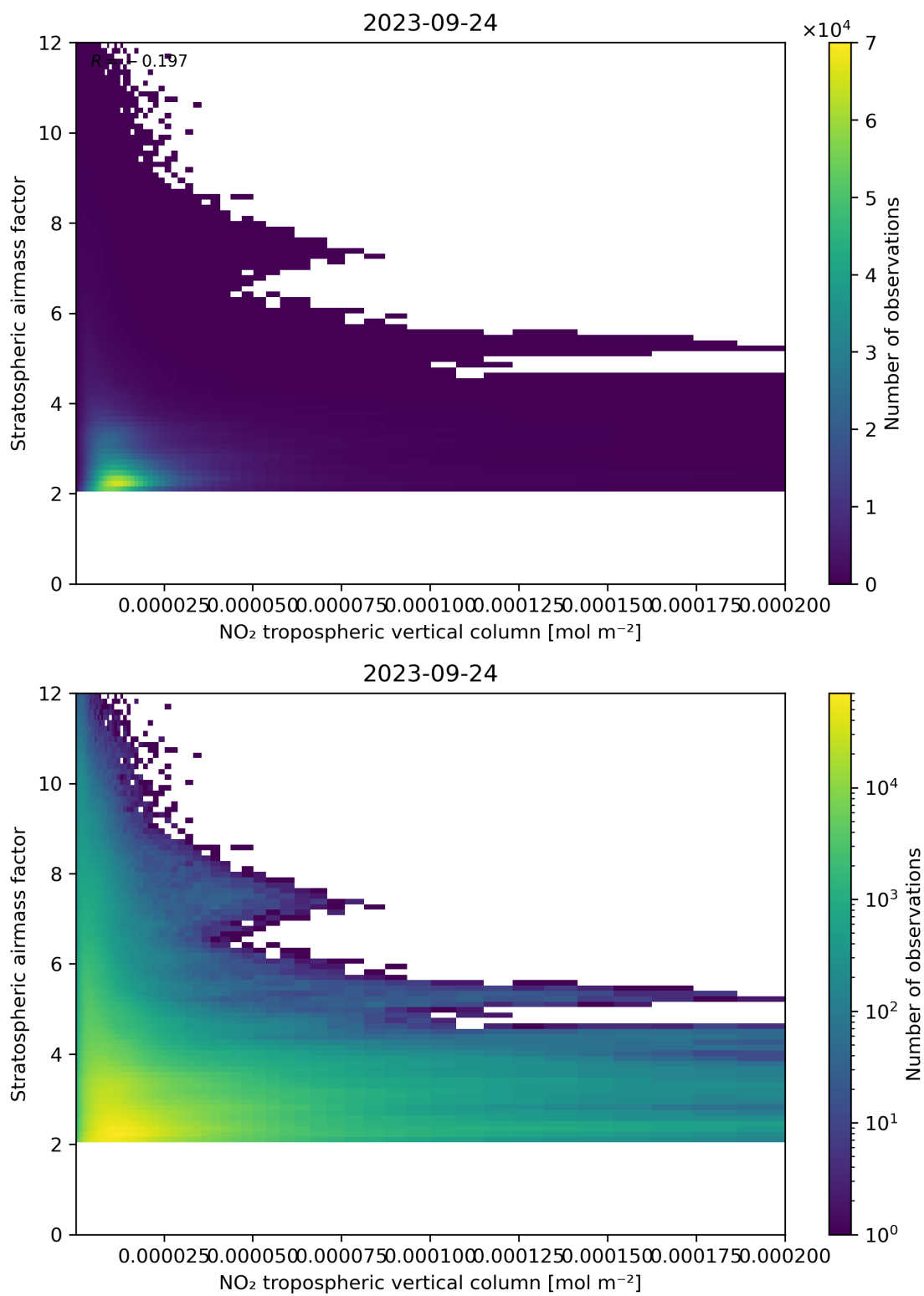
Figure 121: Scatter density plot of “NO 2 tropospheric vertical column” against “Stratospheric airmass factor” for 2023-09-23 to 2023-09-25.
