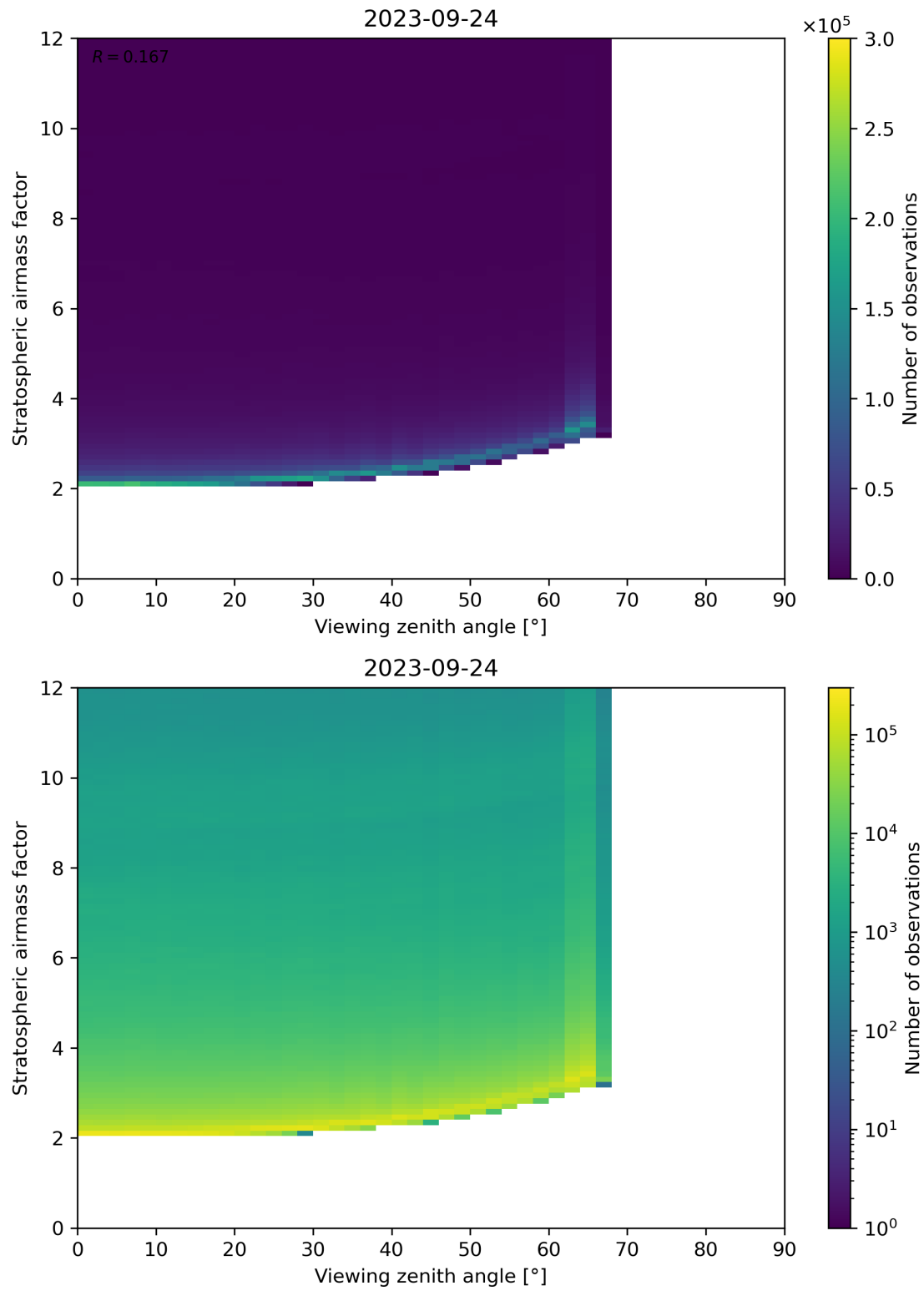
Figure 159: Scatter density plot of “Viewing zenith angle” against “Stratospheric airmass factor” for 2023-09-23 to 2023-09-25.
