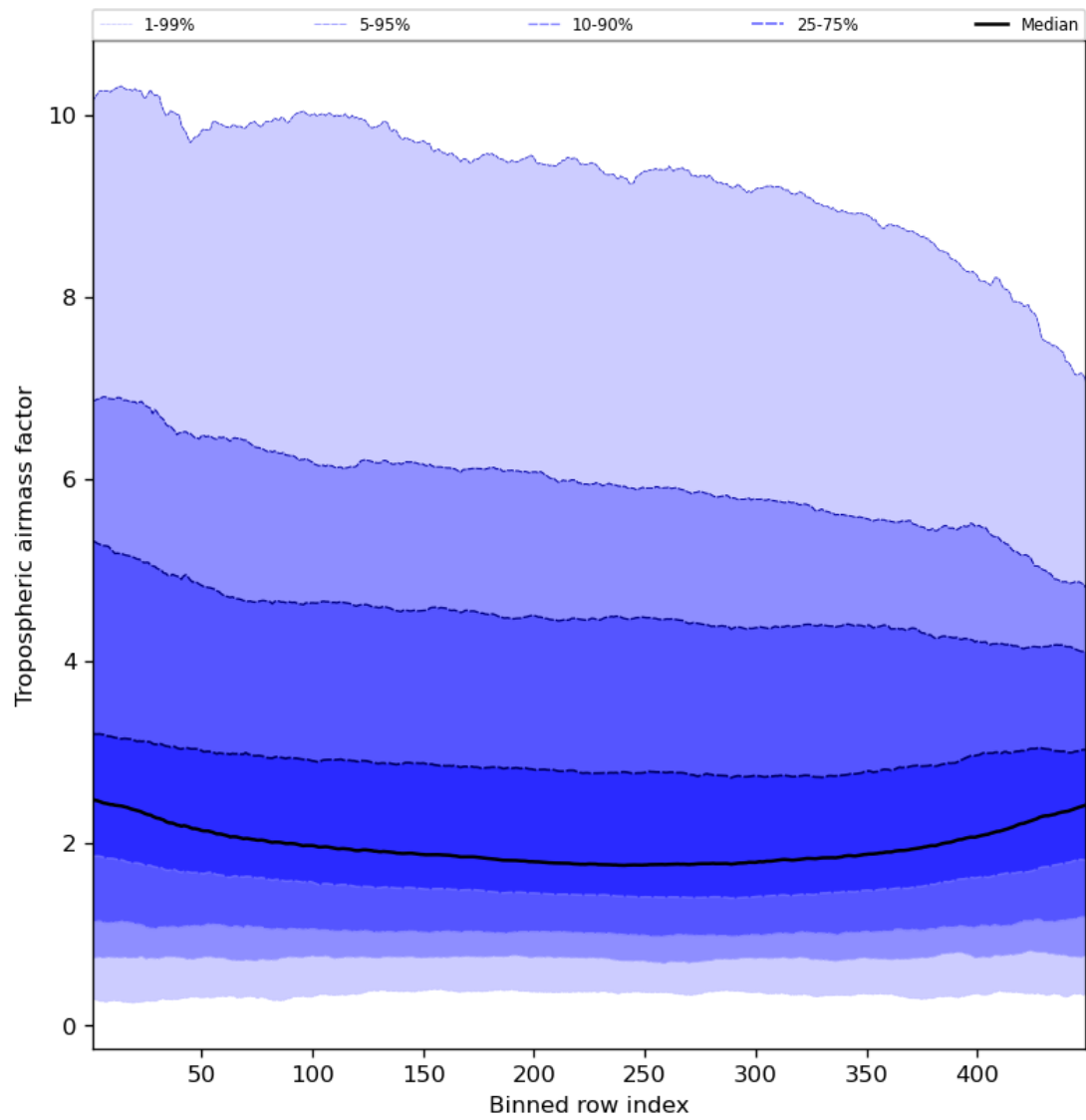
Figure 48: Along track statistics of “Tropospheric air mass factor” for 2023-09-23 to 2023-09-25
