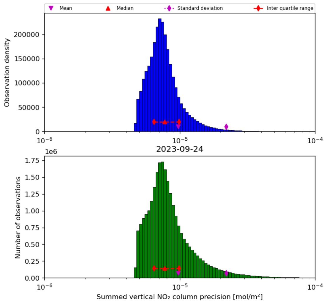
Figure 41: Histogram of “Summed vertical NO 2 column precision” for 2023-09-23 to 2023-09-25
