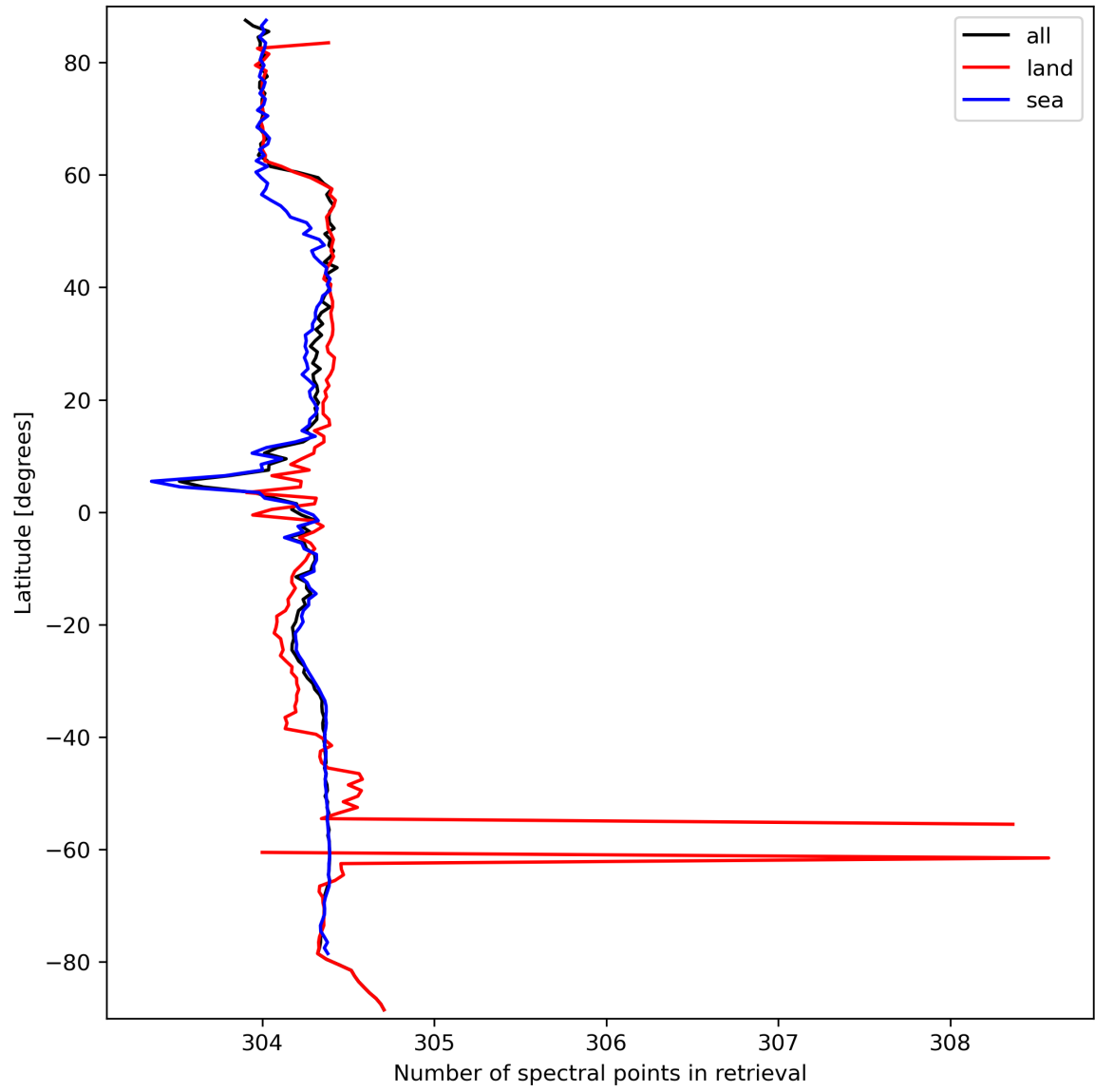
Figure 16: Zonal average of “Number of spectral points in retrieval” for 2023-09-23 to 2023-09-25.
