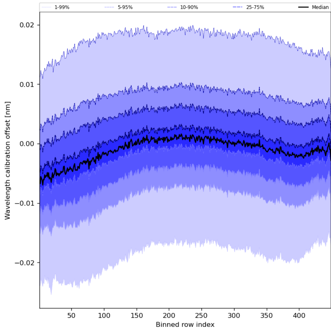
Figure 52: Along track statistics of “Wavelength calibration offset” for 2023-09-23 to 2023-09-25
