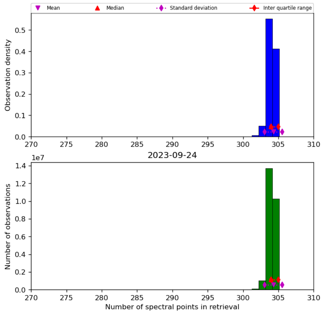
Figure 33: Histogram of “Number of spectral points in retrieval” for 2023-09-23 to 2023-09-25
