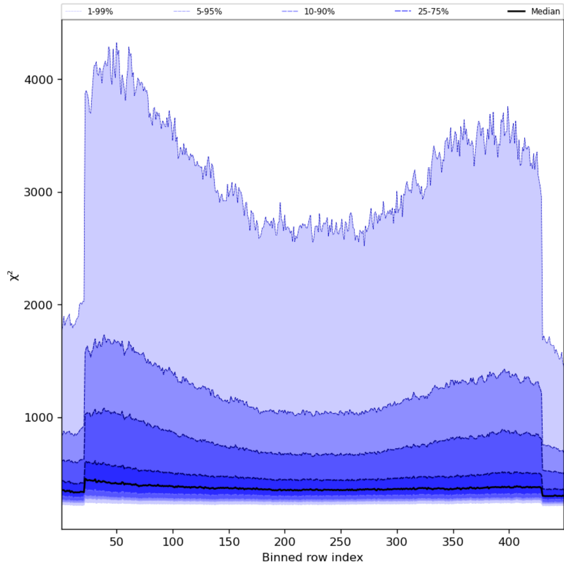
Figure 59: Along track statistics of “ \chi^2 ” for 2023-09-23 to 2023-09-25
