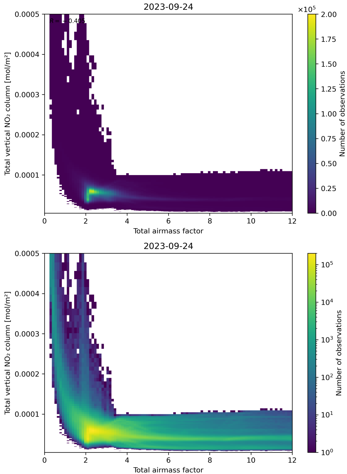
Figure 67: Scatter density plot of “Total airmass factor” against “Total vertical NO 2 column” for 2023-09-23 to 2023-09-25.
