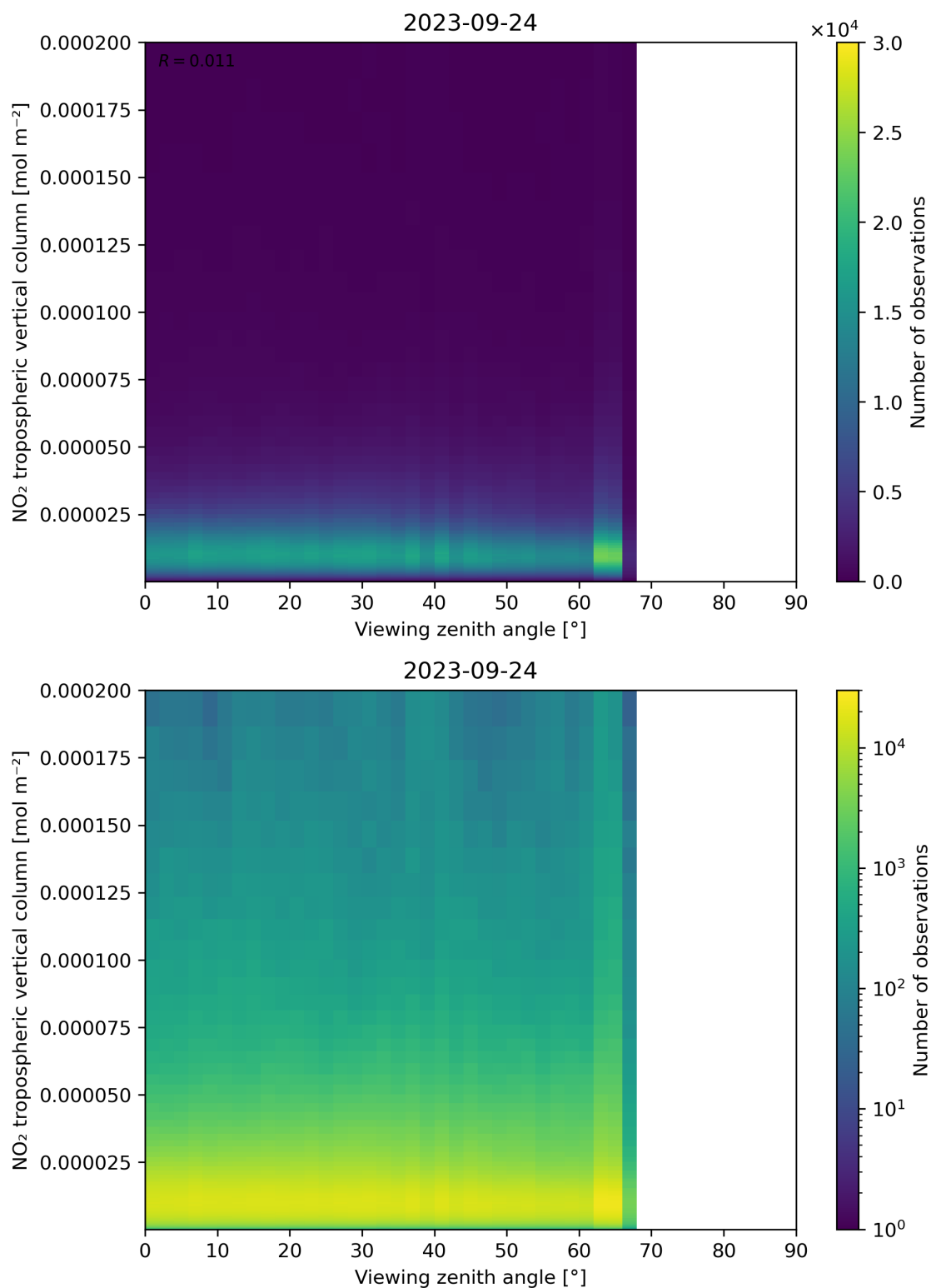
Figure 169: Scatter density plot of “Viewing zenith angle” against “NO 2 tropospheric vertical column” for 2023-09-23 to 2023-09-25.
