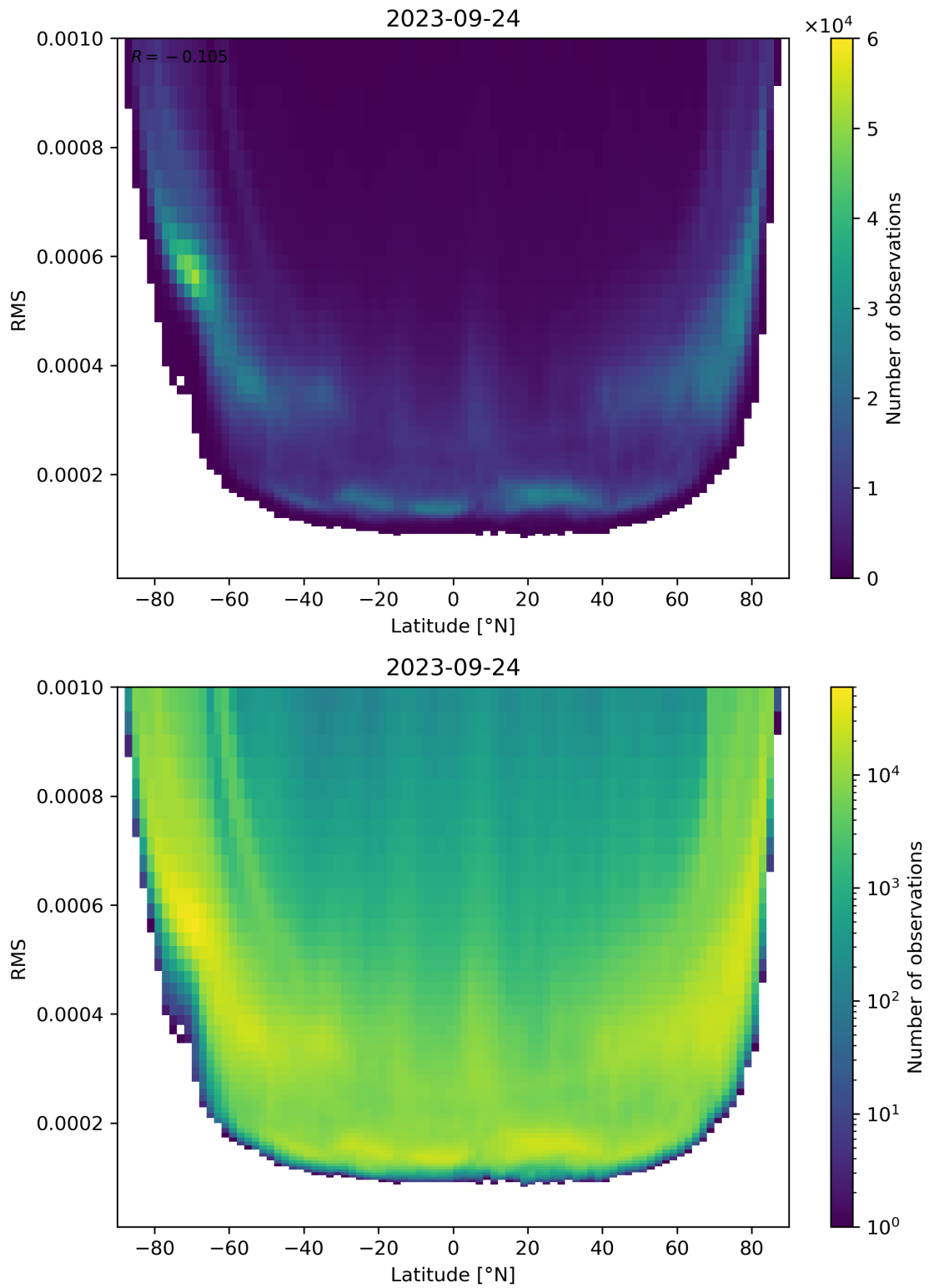
Figure 94: Scatter density plot of “Latitude” against “RMS” for 2023-09-23 to 2023-09-25.
