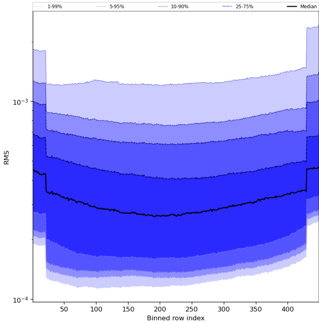
Figure 60: Along track statistics of “RMS” for 2023-09-23 to 2023-09-25
