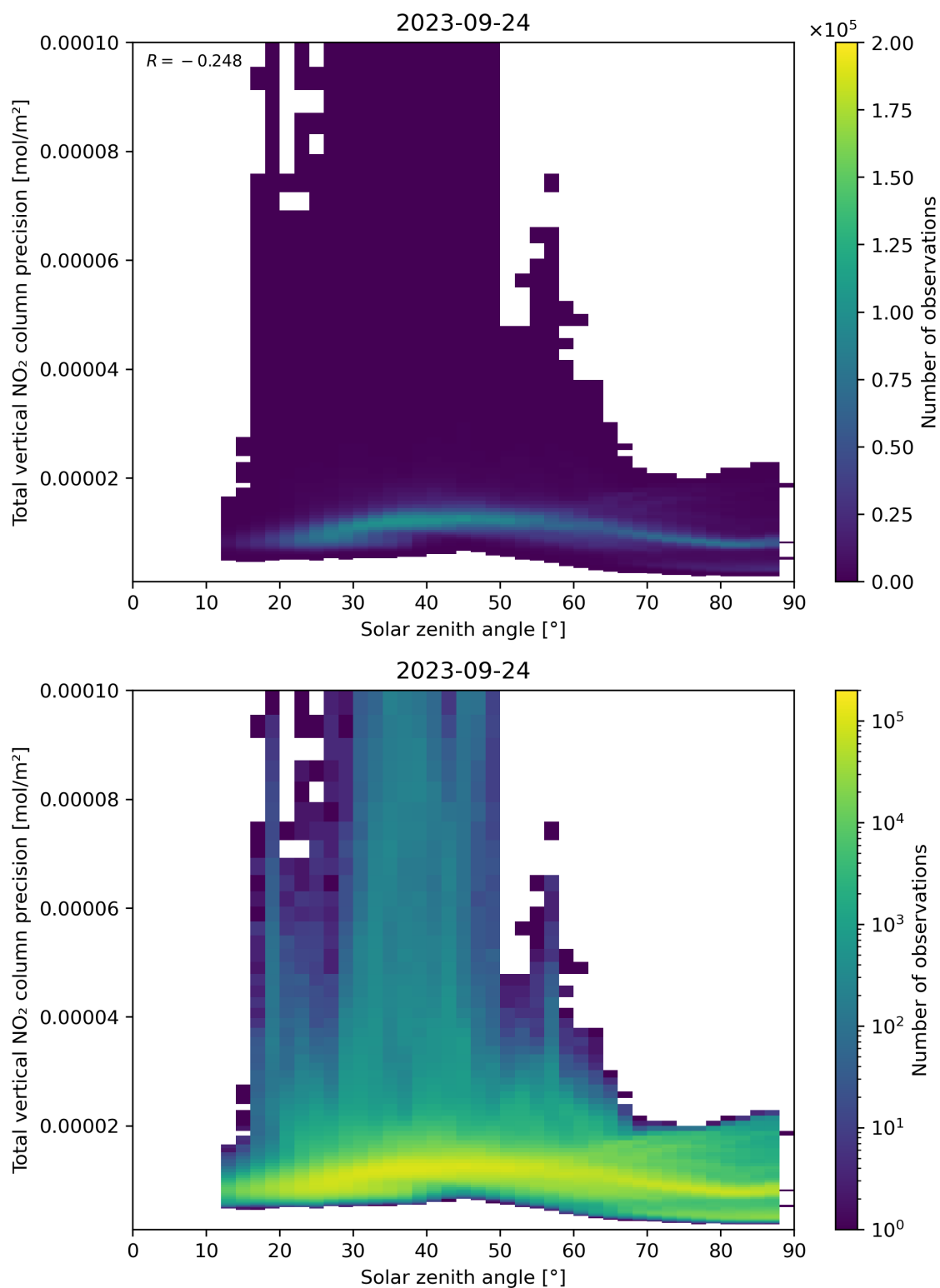
Figure 154: Scatter density plot of “Solar zenith angle” against “Total vertical NO 2 column precision” for 2023-09-23 to 2023-09-25.
