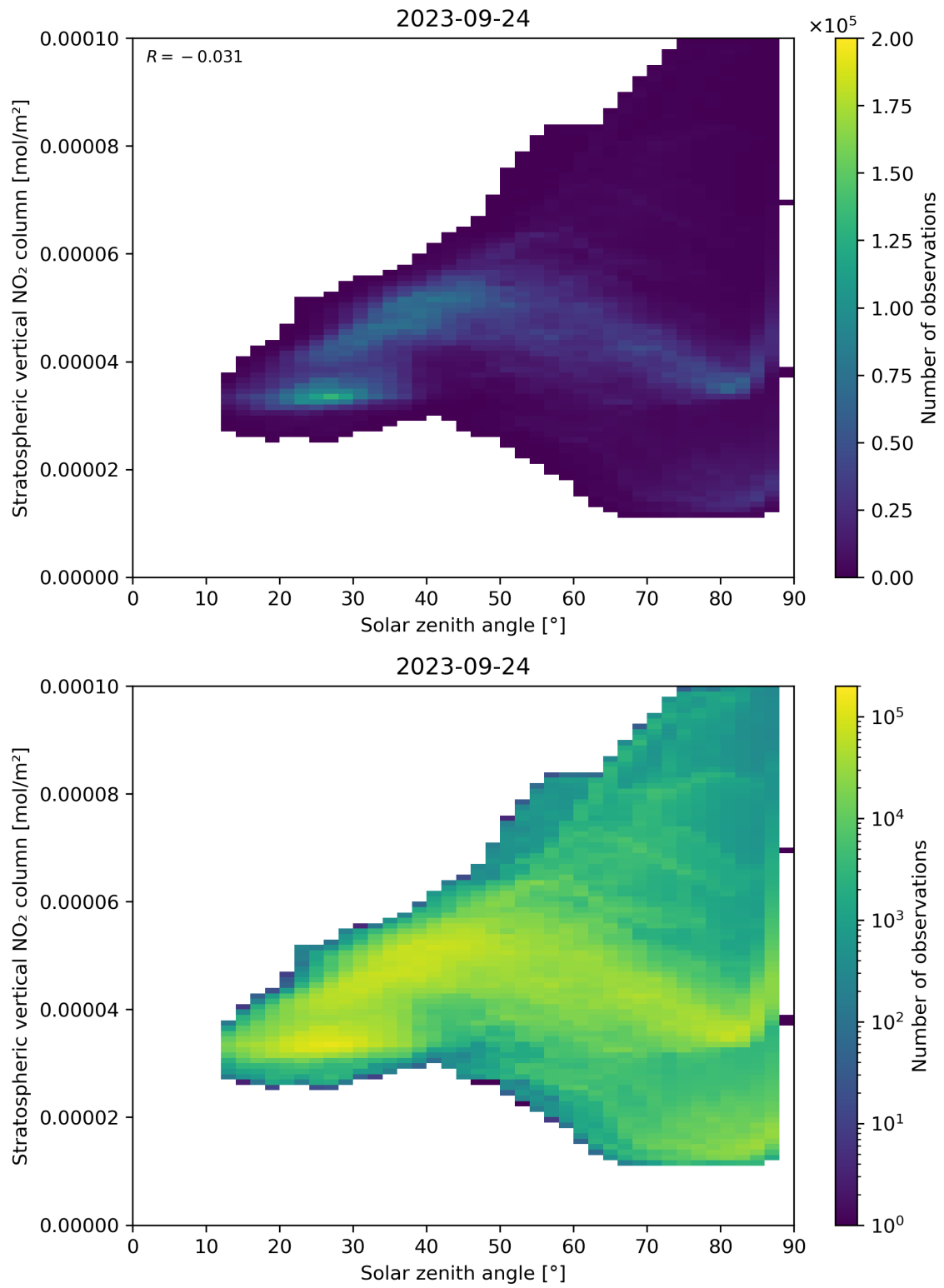
Figure 150: Scatter density plot of “Solar zenith angle” against “Stratospheric vertical NO 2 column” for 2023-09-23 to 2023-09-25.
