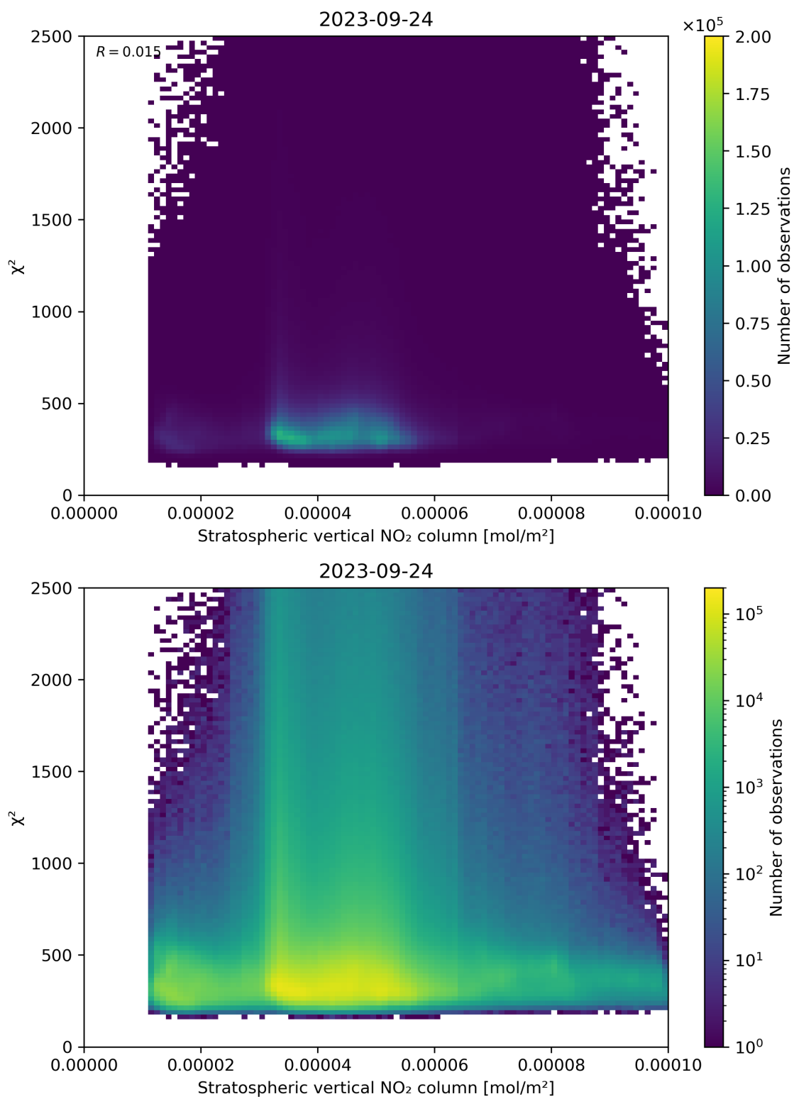
Figure 97: Scatter density plot of “Stratospheric vertical NO 2 column” against “ \chi^2 ” for 2023-09-23 to 2023-09-25.
