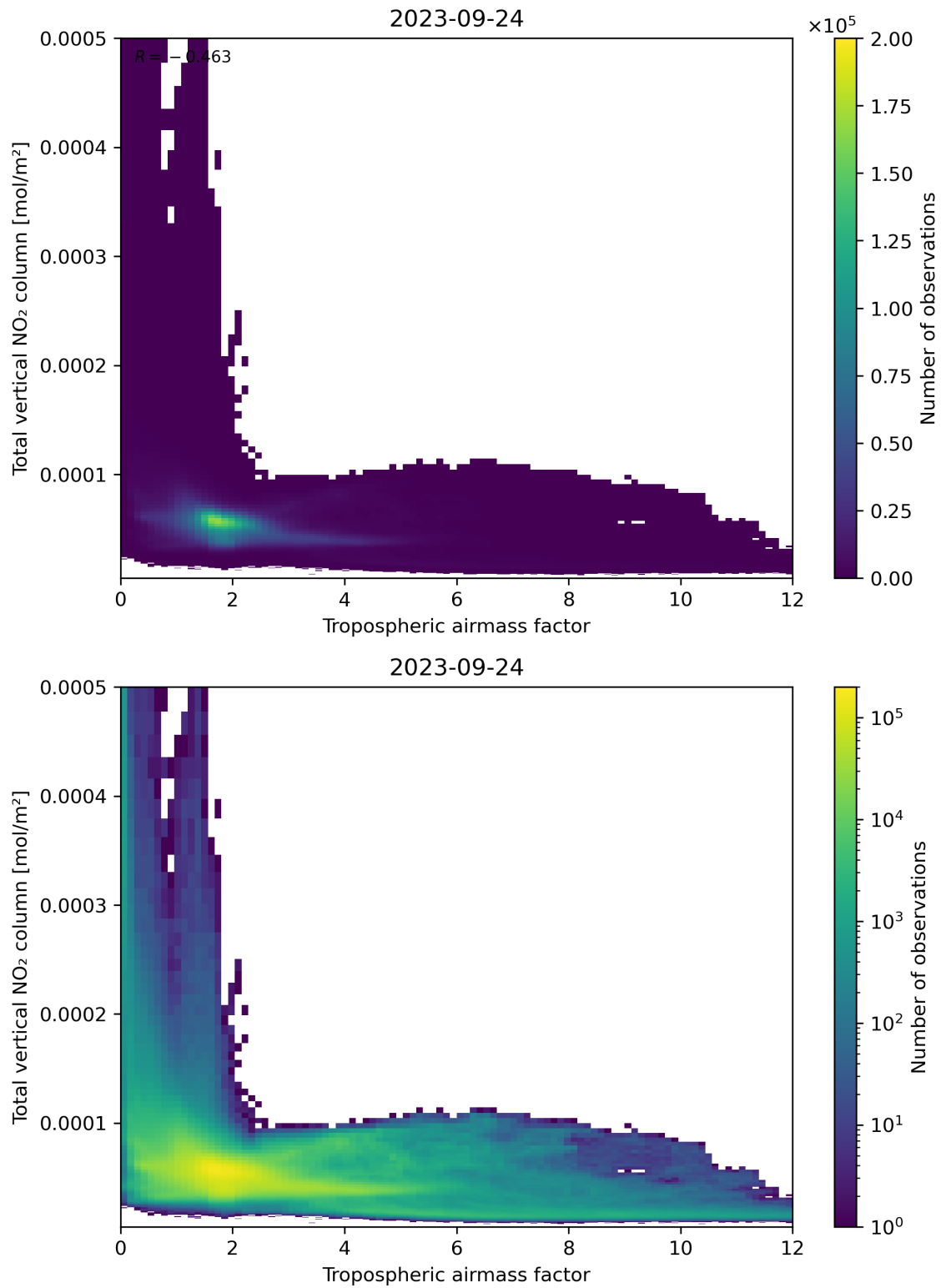
Figure 77: Scatter density plot of “Tropospheric airmass factor” against “Total vertical NO 2 column” for 2023-09-23 to 2023-09-25.
