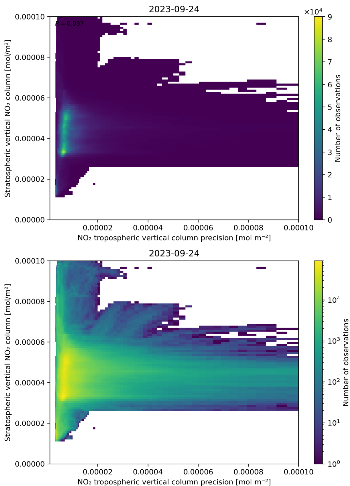
Figure 135: Scatter density plot of “NO 2 tropospheric vertical column precision” against “Stratospheric vertical NO 2 column” for 2023-09-23 to 2023-09-25.
