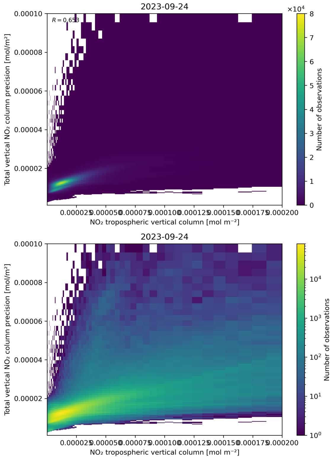
Figure 129: Scatter density plot of “NO 2 tropospheric vertical column” against “Total vertical NO 2 column precision” for 2023-09-23 to 2023-09-25.
