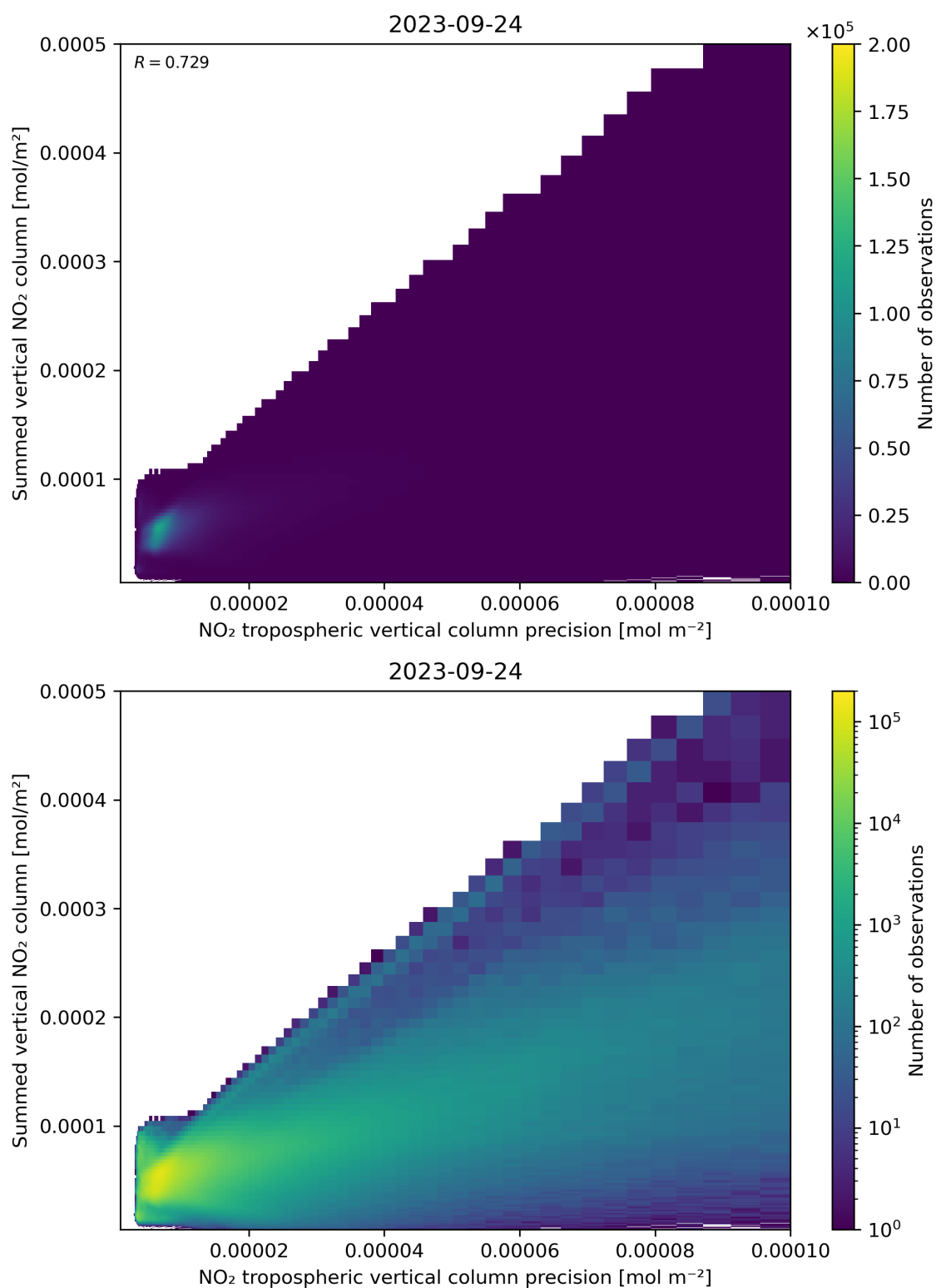
Figure 136: Scatter density plot of “NO 2 tropospheric vertical column precision” against “Summed vertical NO 2 column” for 2023-09-23 to 2023-09-25.
