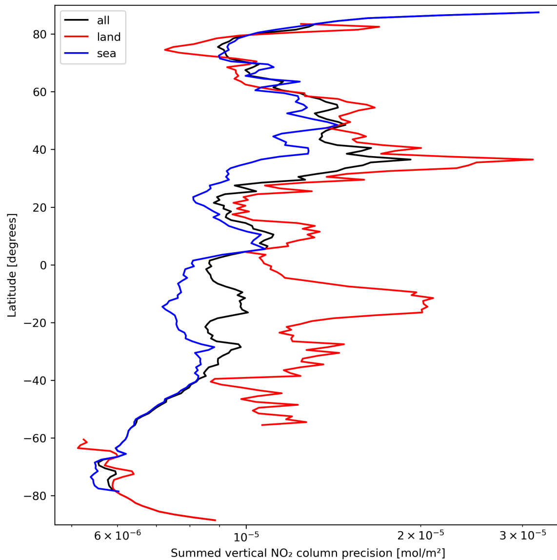
Figure 24: Zonal average of “Summed vertical NO 2 column precision” for 2023-09-23 to 2023-09-25.
