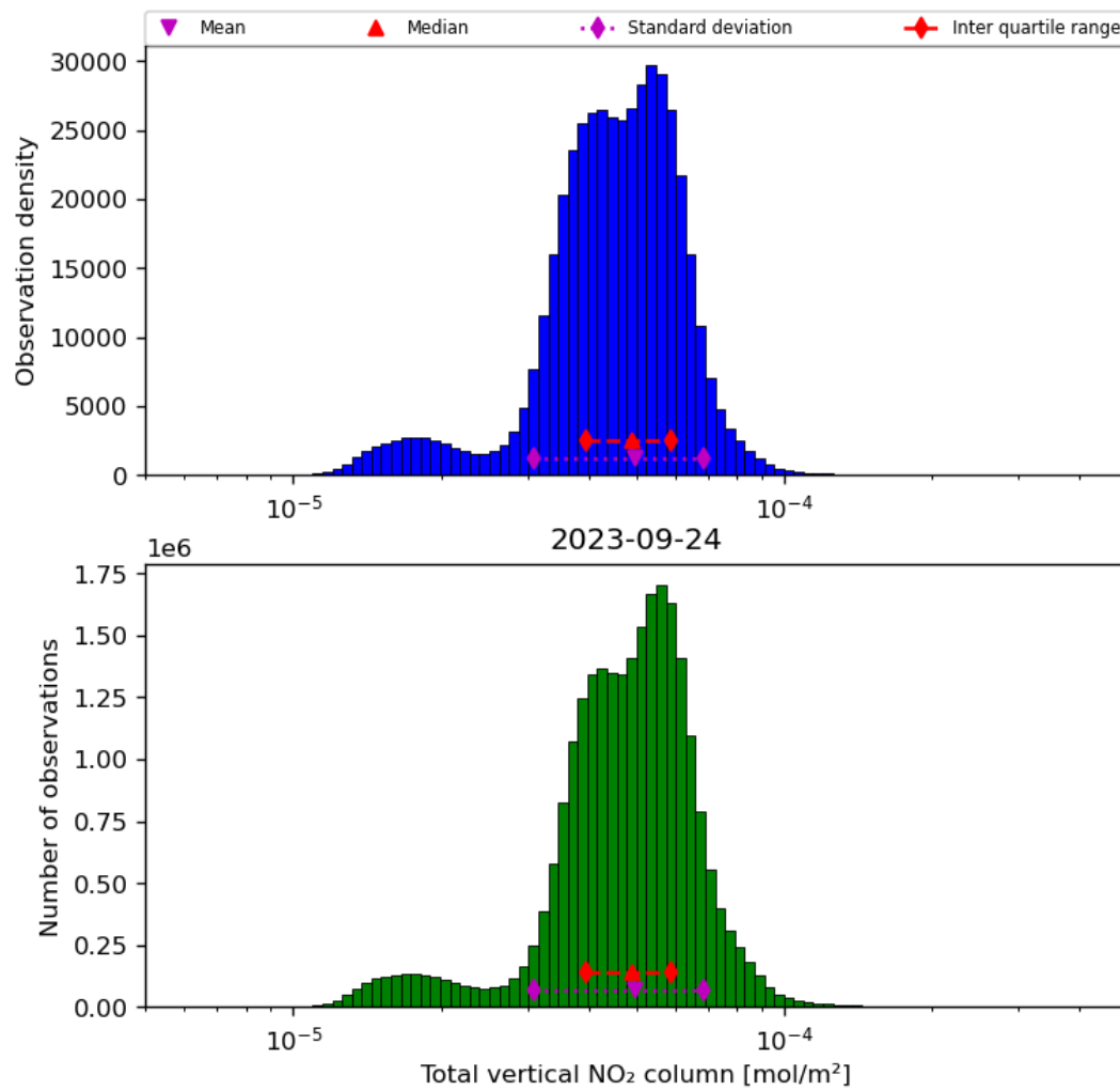
Figure 38: Histogram of “Total vertical NO 2 column” for 2023-09-23 to 2023-09-25
