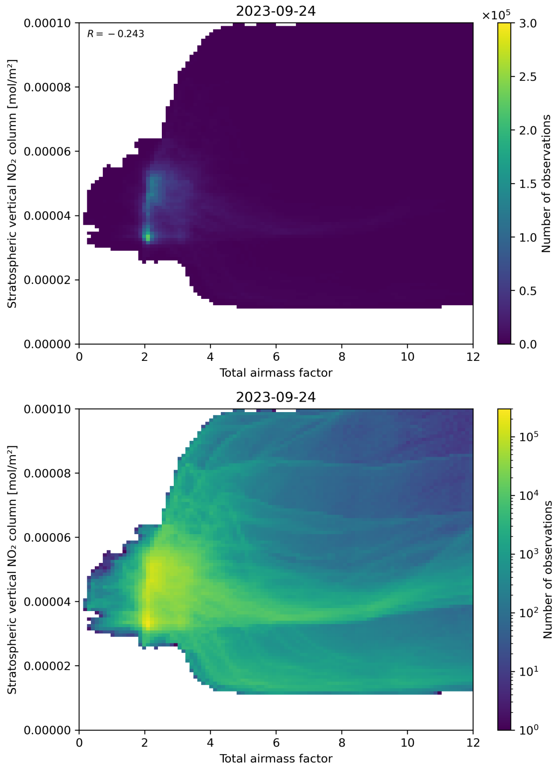
Figure 64: Scatter density plot of “Total airmass factor” against “Stratospheric vertical NO 2 column” for 2023-09-23 to 2023-09-25.
