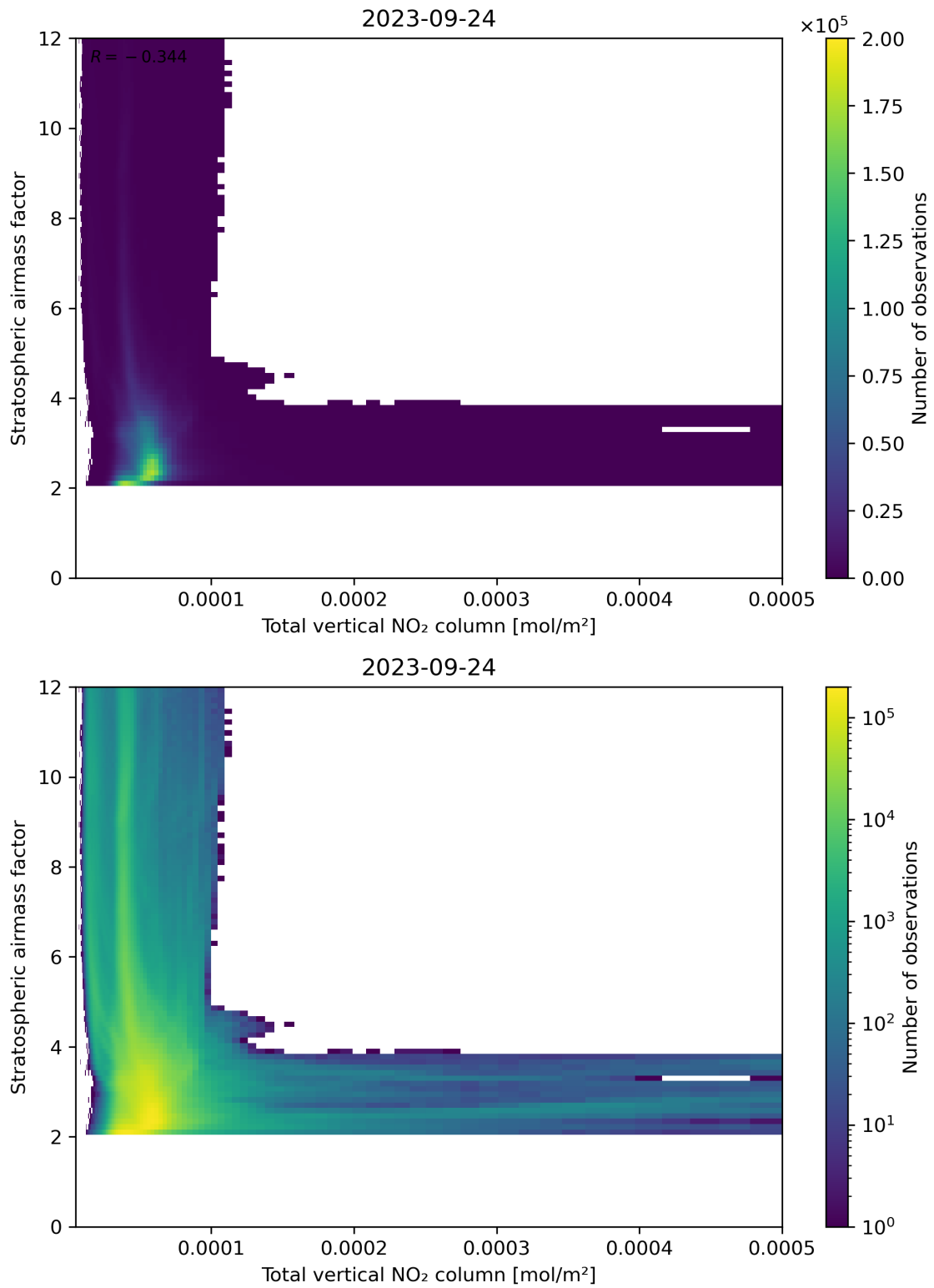
Figure 110: Scatter density plot of “Total vertical NO 2 column” against “Stratospheric airmass factor” for 2023-09-23 to 2023-09-25.
