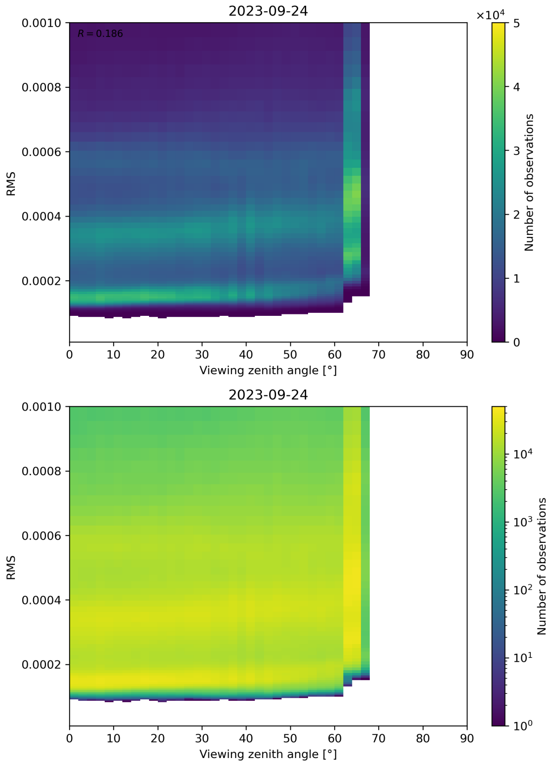
Figure 171: Scatter density plot of “Viewing zenith angle” against “RMS” for 2023-09-23 to 2023-09-25.
