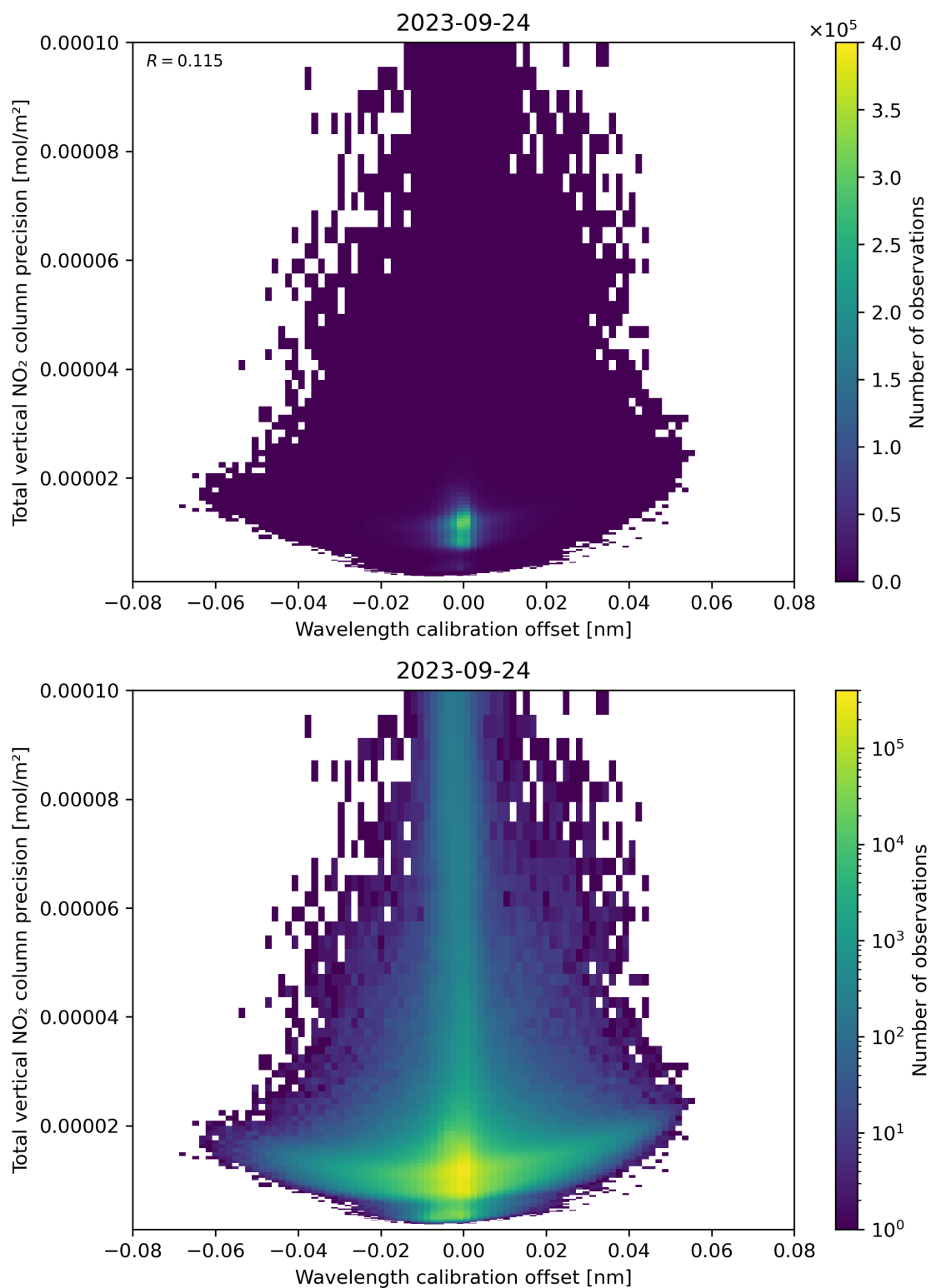
Figure 180: Scatter density plot of “Wavelength calibration offset” against “Total vertical NO 2 column precision” for 2023-09-23 to 2023-09-25.
