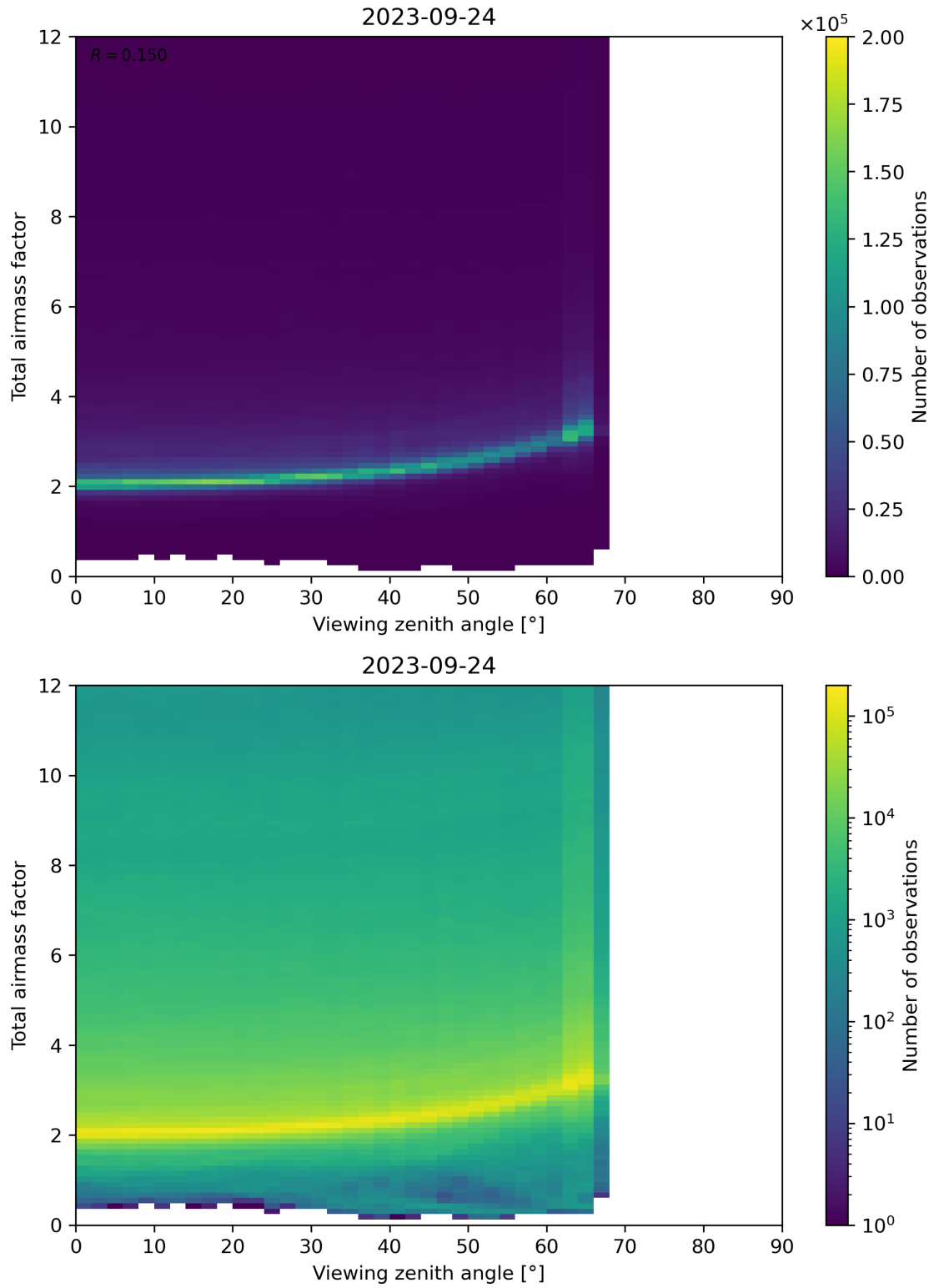
Figure 160: Scatter density plot of “Viewing zenith angle” against “Total airmass factor” for 2023-09-23 to 2023-09-25.
