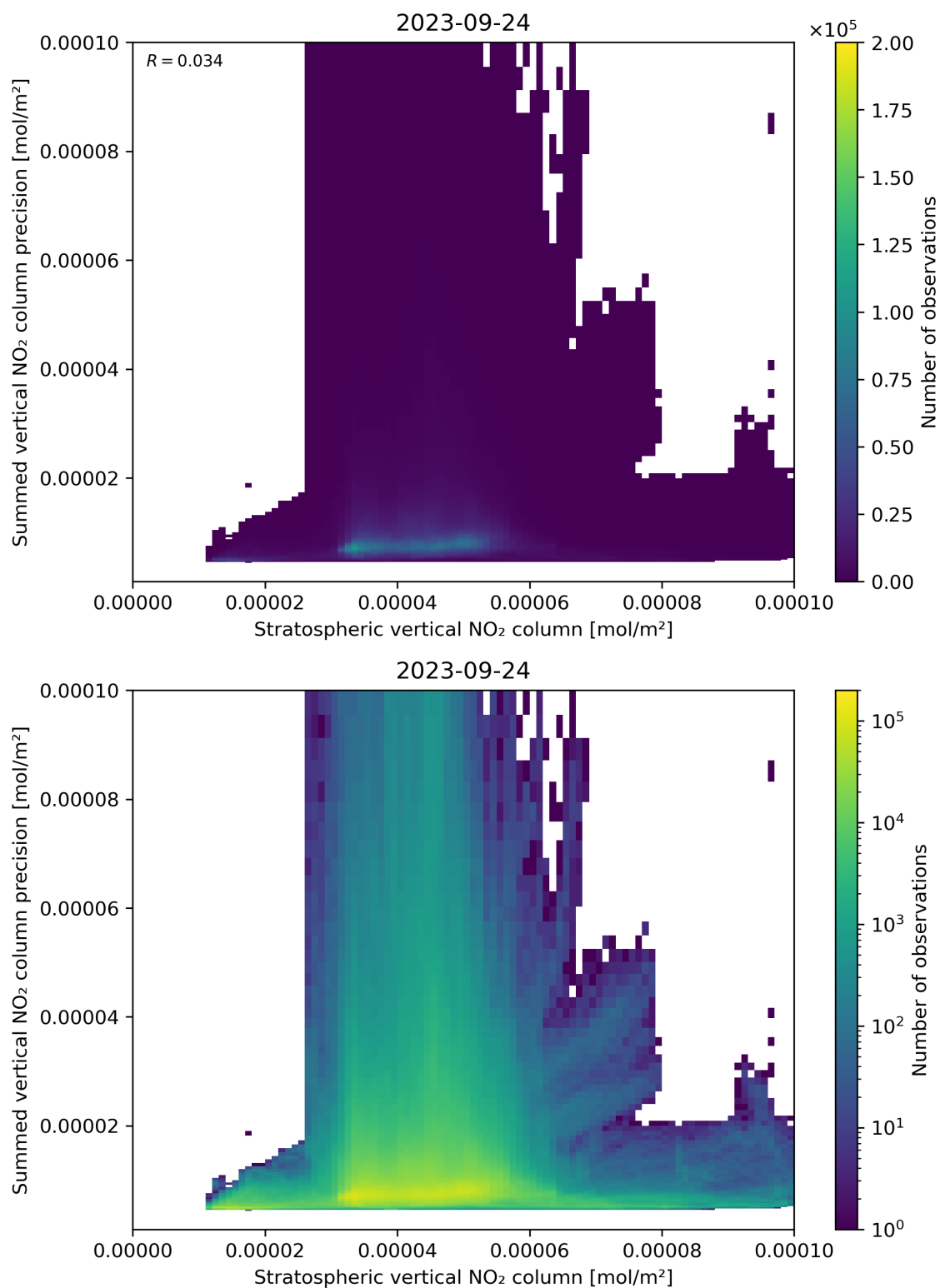
Figure 99: Scatter density plot of “Stratospheric vertical NO 2 column” against “Summed vertical NO 2 column precision” for 2023-09-23 to 2023-09-25.
