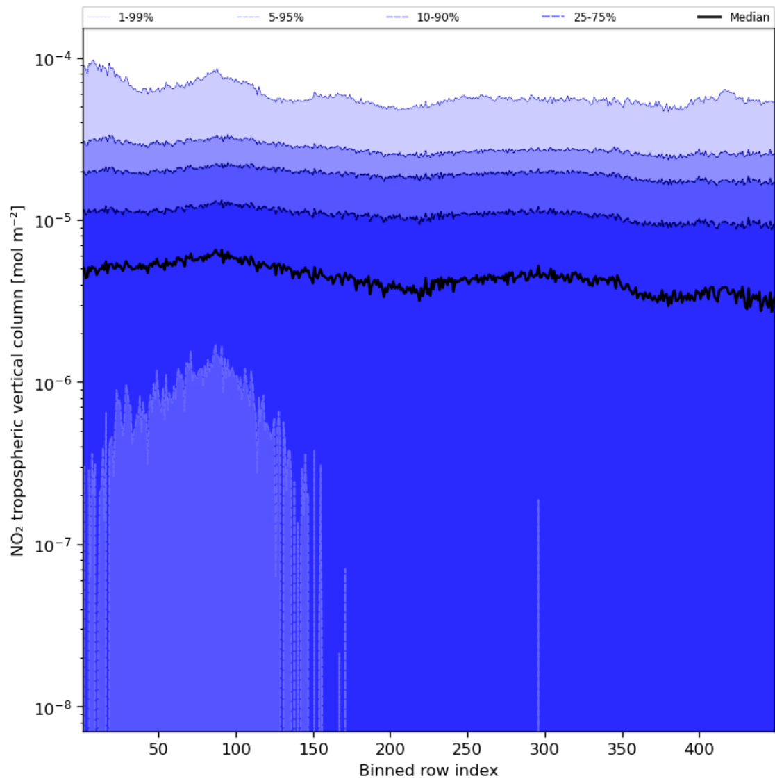
Figure 46: Along track statistics of “NO 2 tropospheric vertical column” for 2023-09-23 to 2023-09-25
