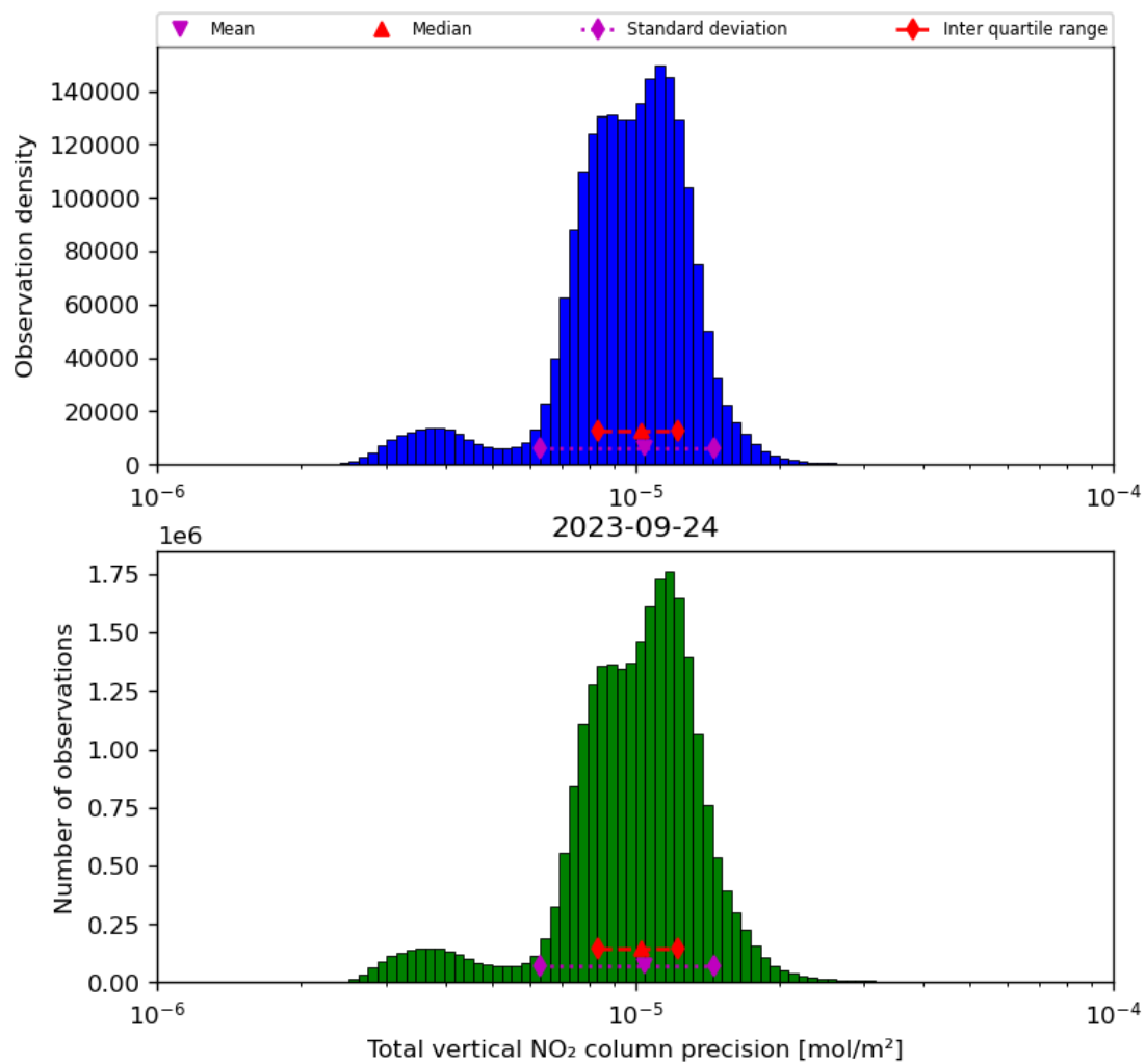
Figure 39: Histogram of “Total vertical NO 2 column precision” for 2023-09-23 to 2023-09-25
