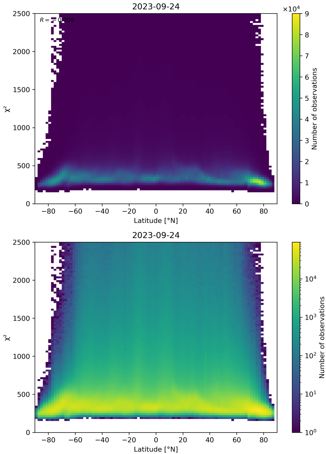
Figure 86: Scatter density plot of “Latitude” against “ \chi^2 ” for 2023-09-23 to 2023-09-25.
