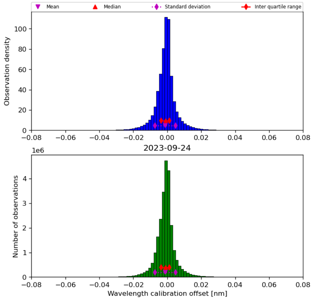
Figure 35: Histogram of “Wavelength calibration offset” for 2023-09-23 to 2023-09-25
