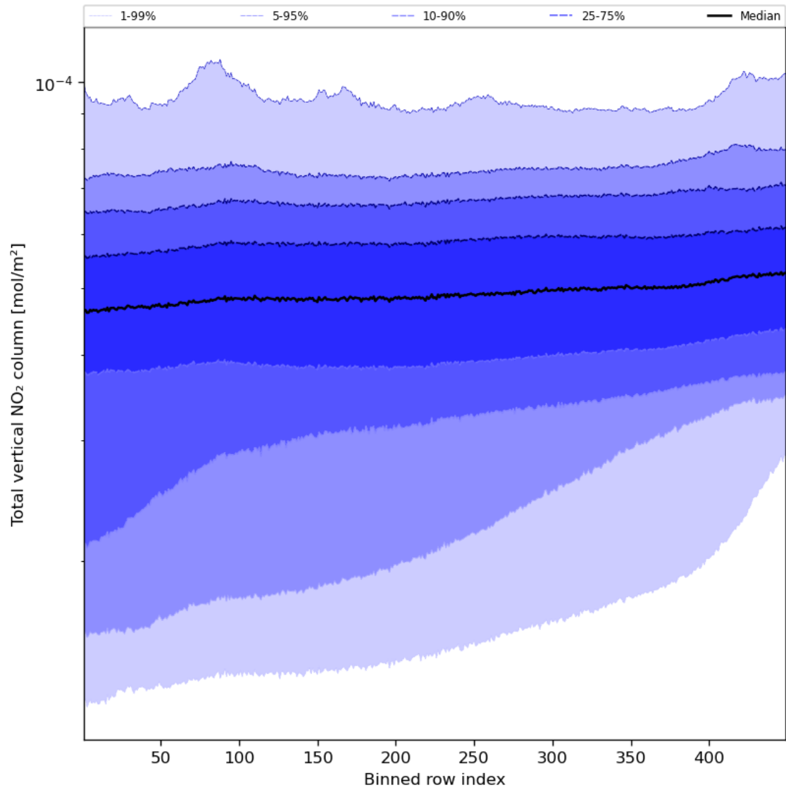
Figure 55: Along track statistics of “Total vertical NO 2 column” for 2023-09-23 to 2023-09-25
