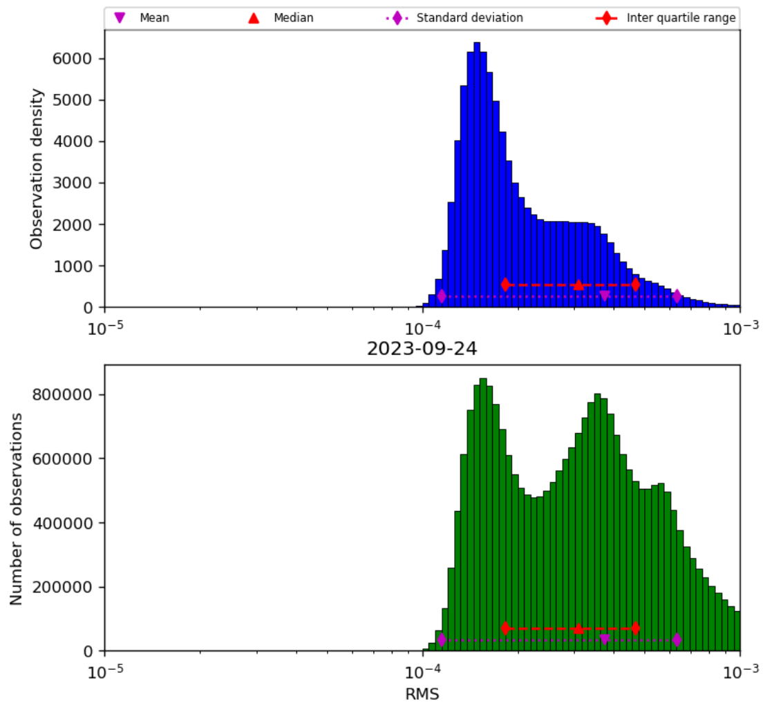
Figure 43: Histogram of “RMS” for 2023-09-23 to 2023-09-25
