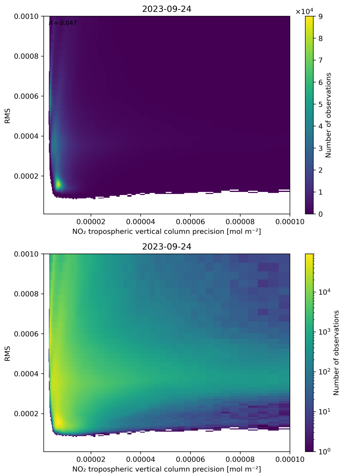
Figure 140: Scatter density plot of “NO 2 tropospheric vertical column precision” against “RMS” for 2023-09-23 to 2023-09-25.
