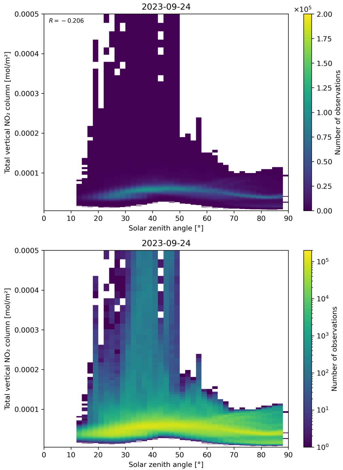
Figure 153: Scatter density plot of “Solar zenith angle” against “Total vertical NO 2 column” for 2023-09-23 to 2023-09-25.
