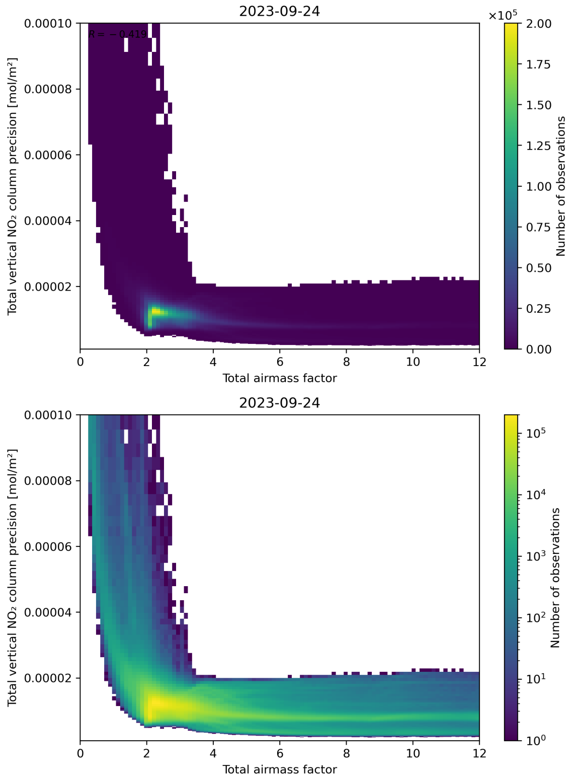
Figure 68: Scatter density plot of “Total airmass factor” against “Total vertical NO 2 column precision” for 2023-09-23 to 2023-09-25.
