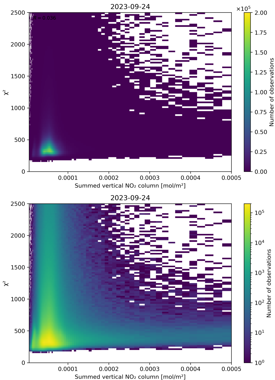
Figure 104: Scatter density plot of “Summed vertical NO 2 column” against “ \chi^2 ” for 2023-09-23 to 2023-09-25.
