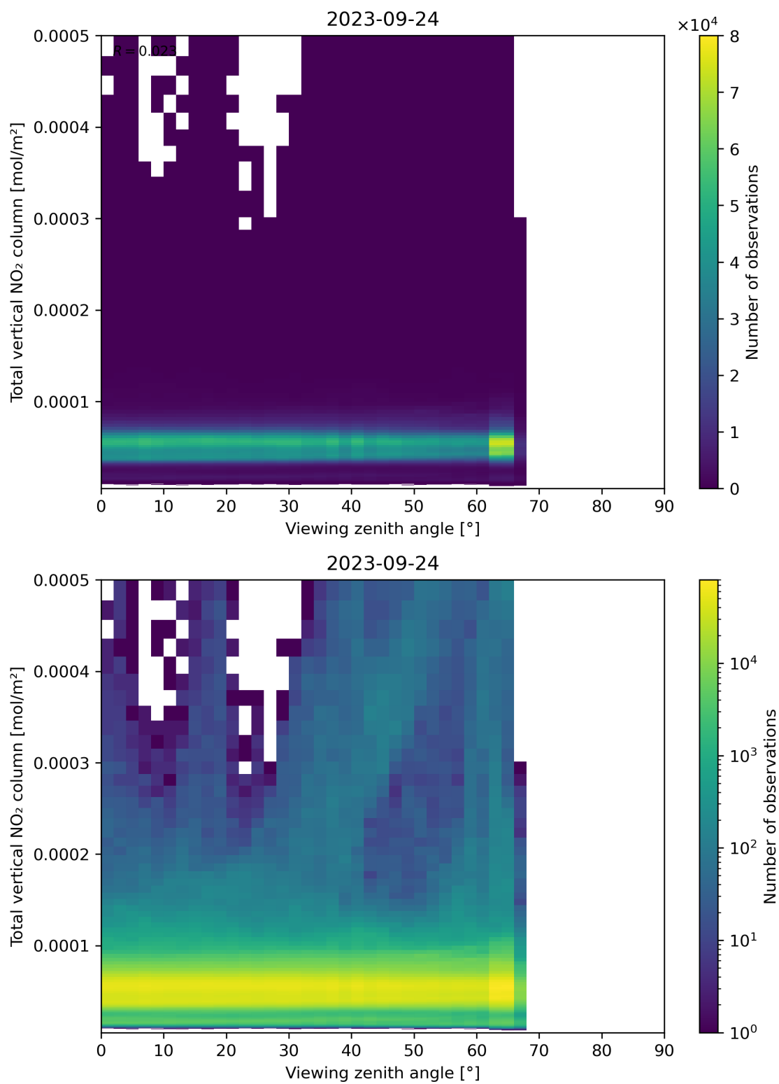
Figure 167: Scatter density plot of “Viewing zenith angle” against “Total vertical NO 2 column” for 2023-09-23 to 2023-09-25.
