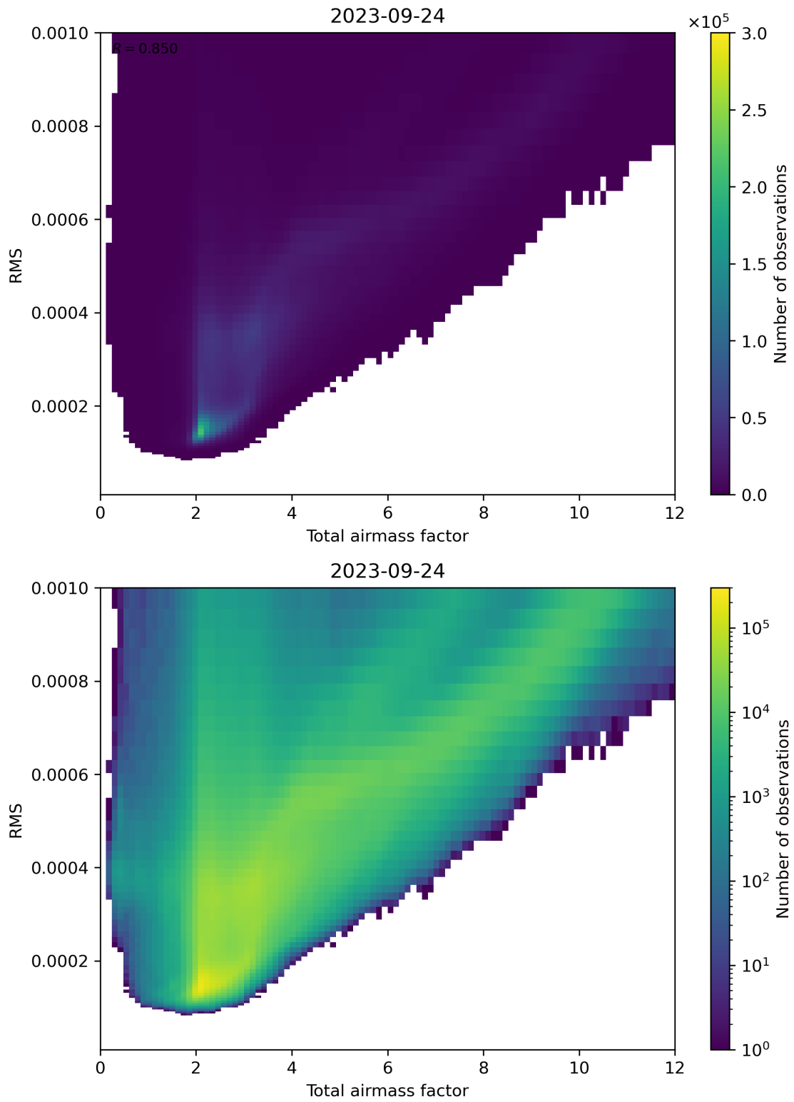
Figure 69: Scatter density plot of “Total airmass factor” against “RMS” for 2023-09-23 to 2023-09-25.
