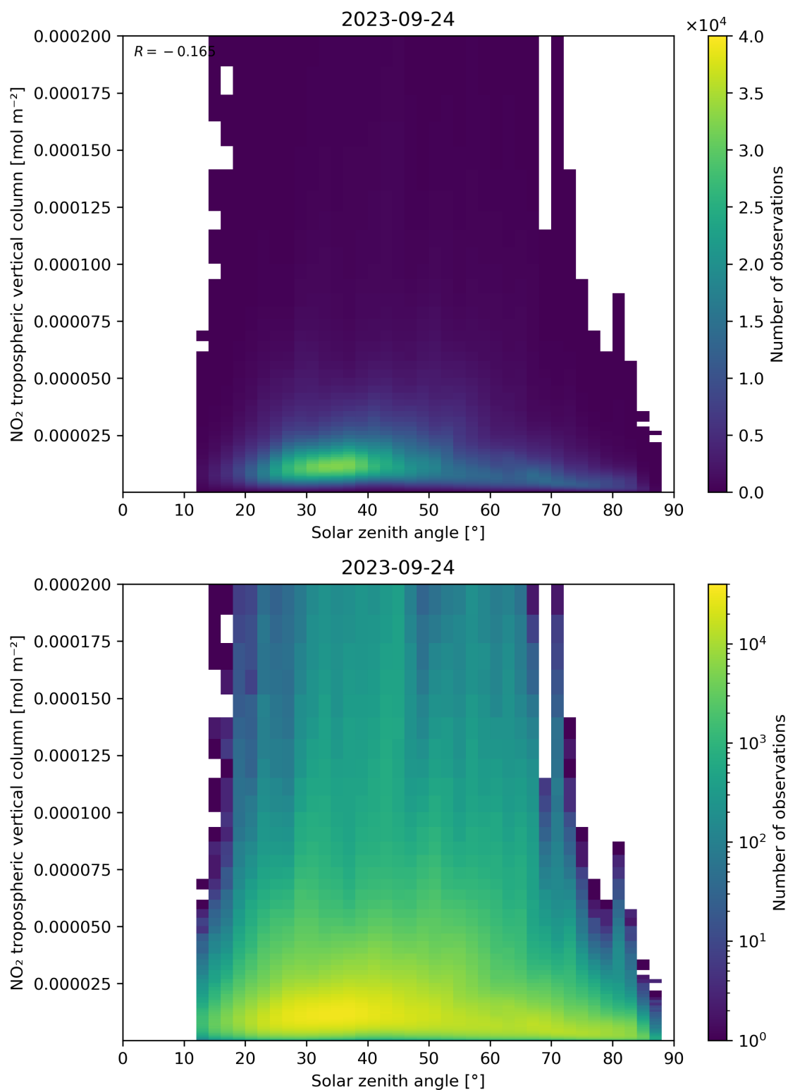
Figure 155: Scatter density plot of “Solar zenith angle” against “NO 2 tropospheric vertical column” for 2023-09-23 to 2023-09-25.
