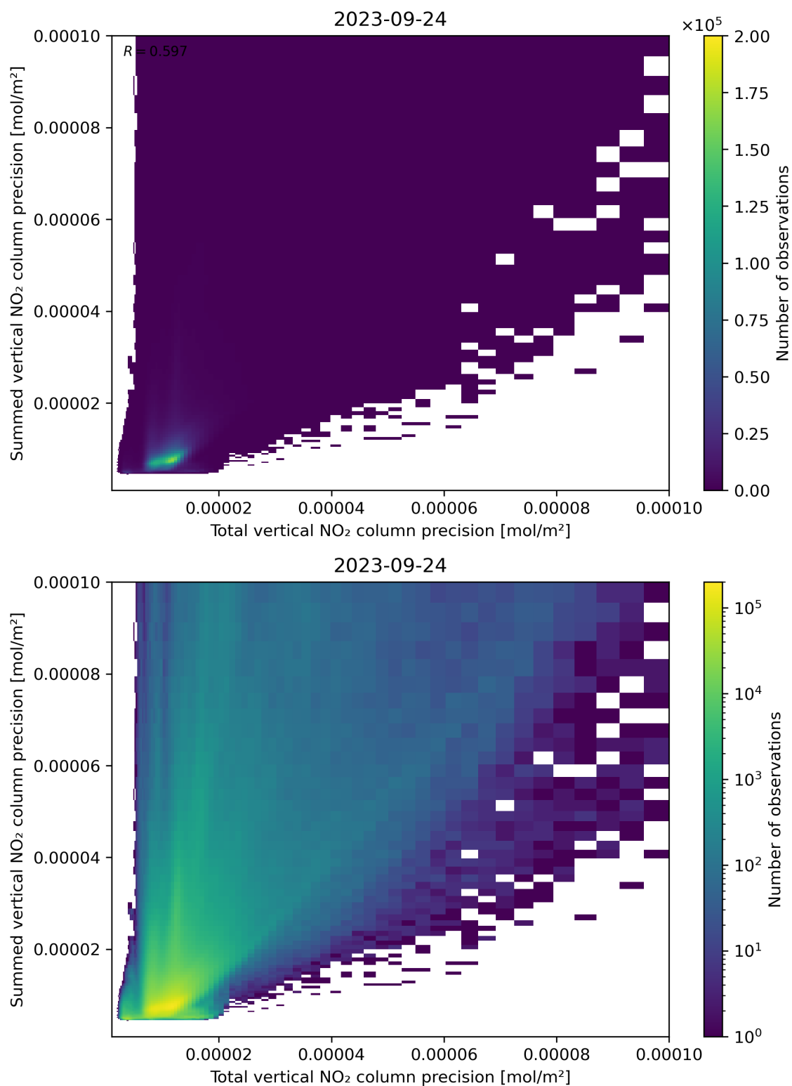
Figure 118: Scatter density plot of “Total vertical NO 2 column precision” against “Summed vertical NO 2 column precision” for 2023-09-23 to 2023-09-25.
