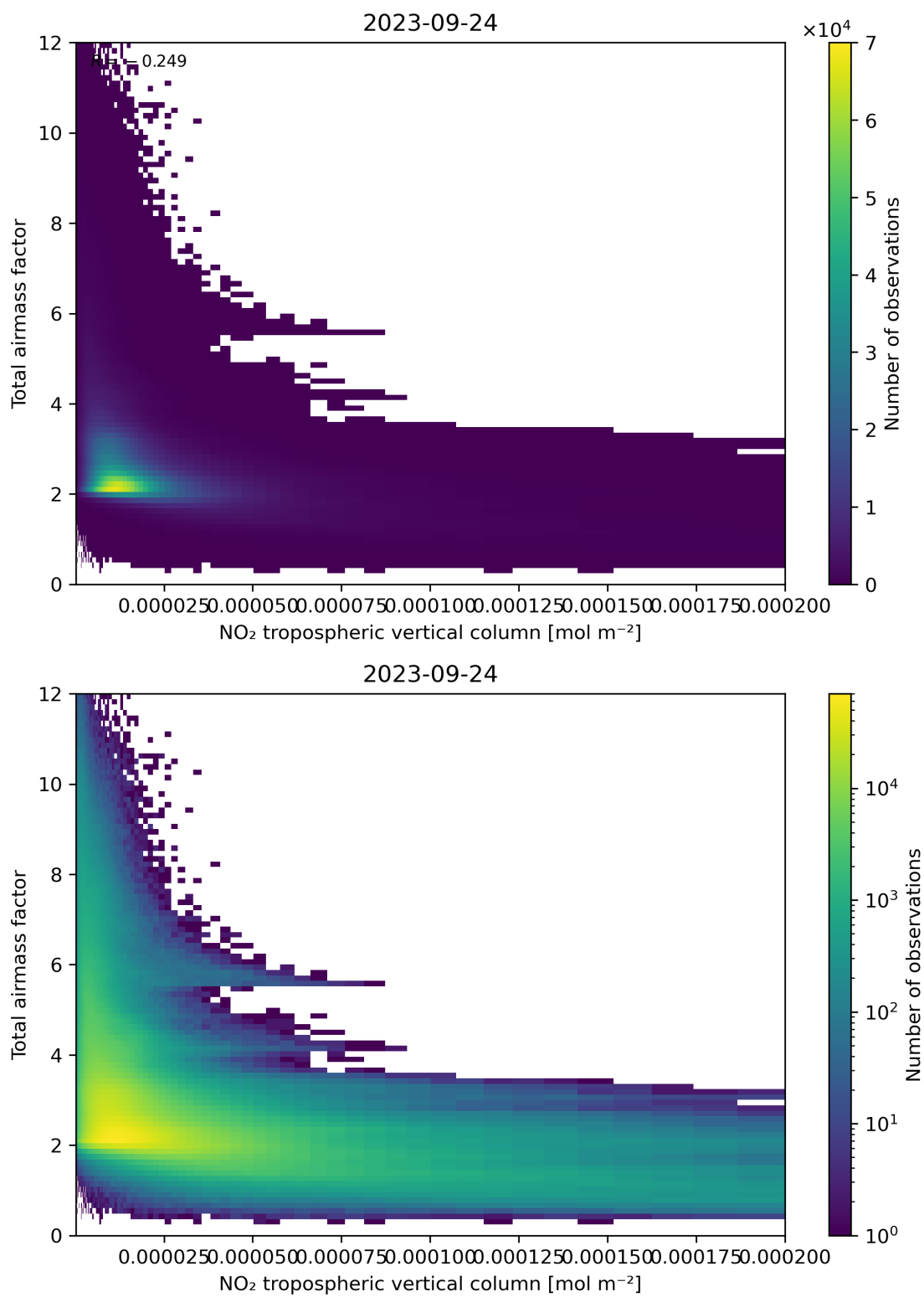
Figure 122: Scatter density plot of “NO 2 tropospheric vertical column” against “Total air mass factor” for 2023-09-23 to 2023-09-25.
