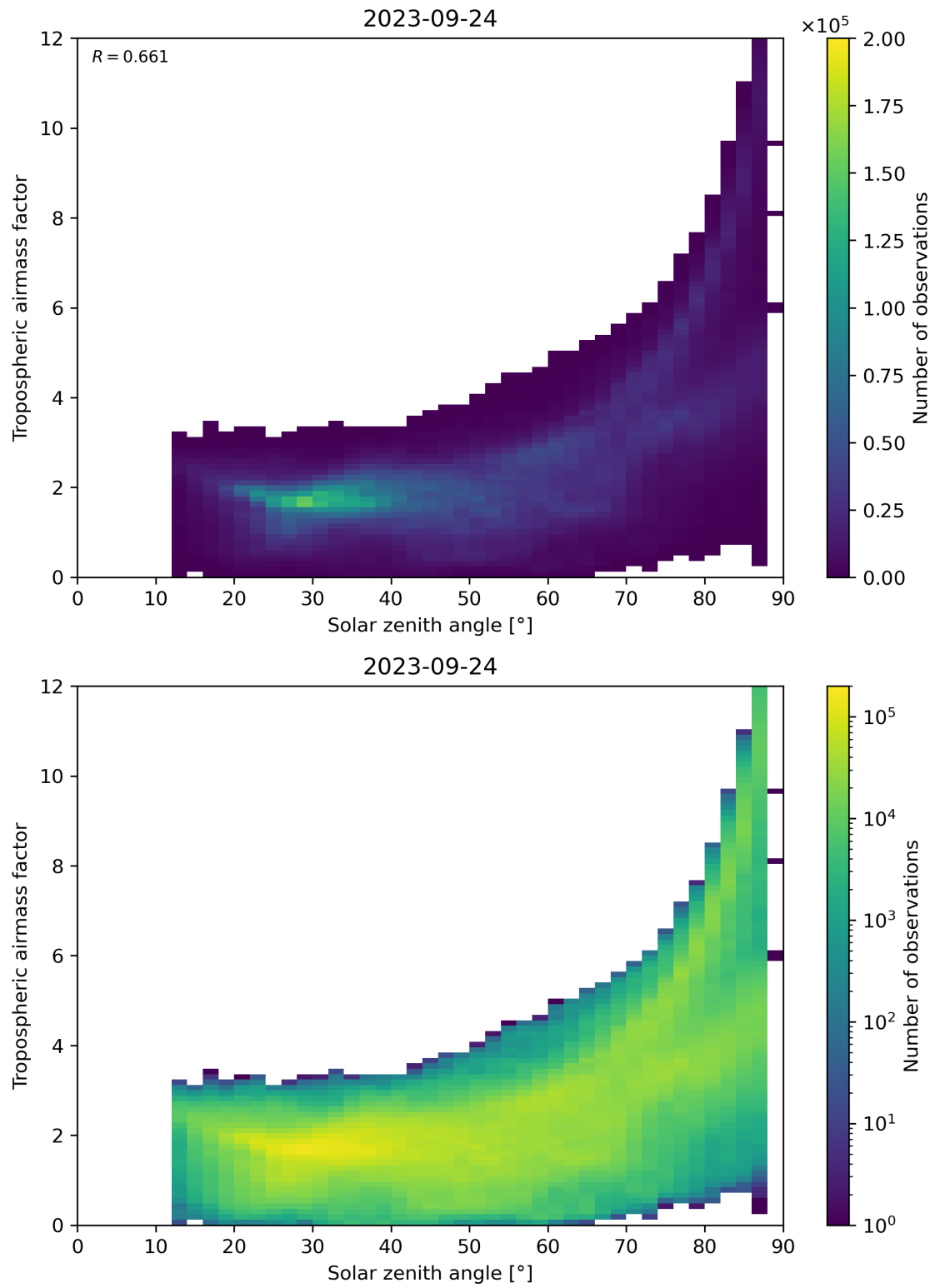
Figure 147: Scatter density plot of “Solar zenith angle” against “Tropospheric airmass factor” for 2023-09-23 to 2023-09-25.
