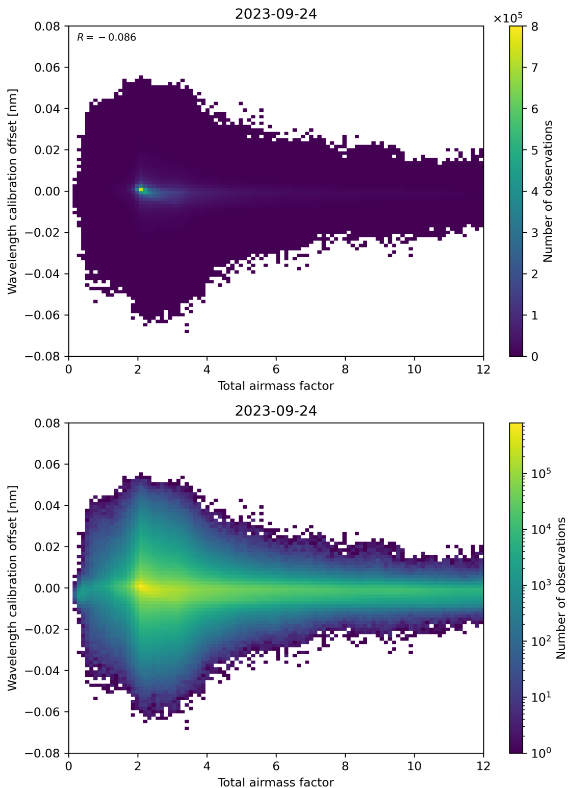
Figure 70: Scatter density plot of “Total airmass factor” against “Wavelength calibration offset” for 2023-09-23 to 2023-09-25.
