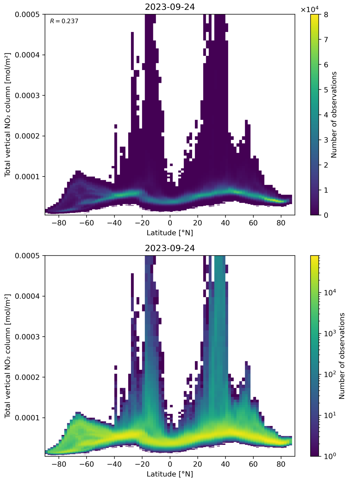
Figure 90: Scatter density plot of “Latitude” against “Total vertical NO 2 column” for 2023-09-23 to 2023-09-25.
