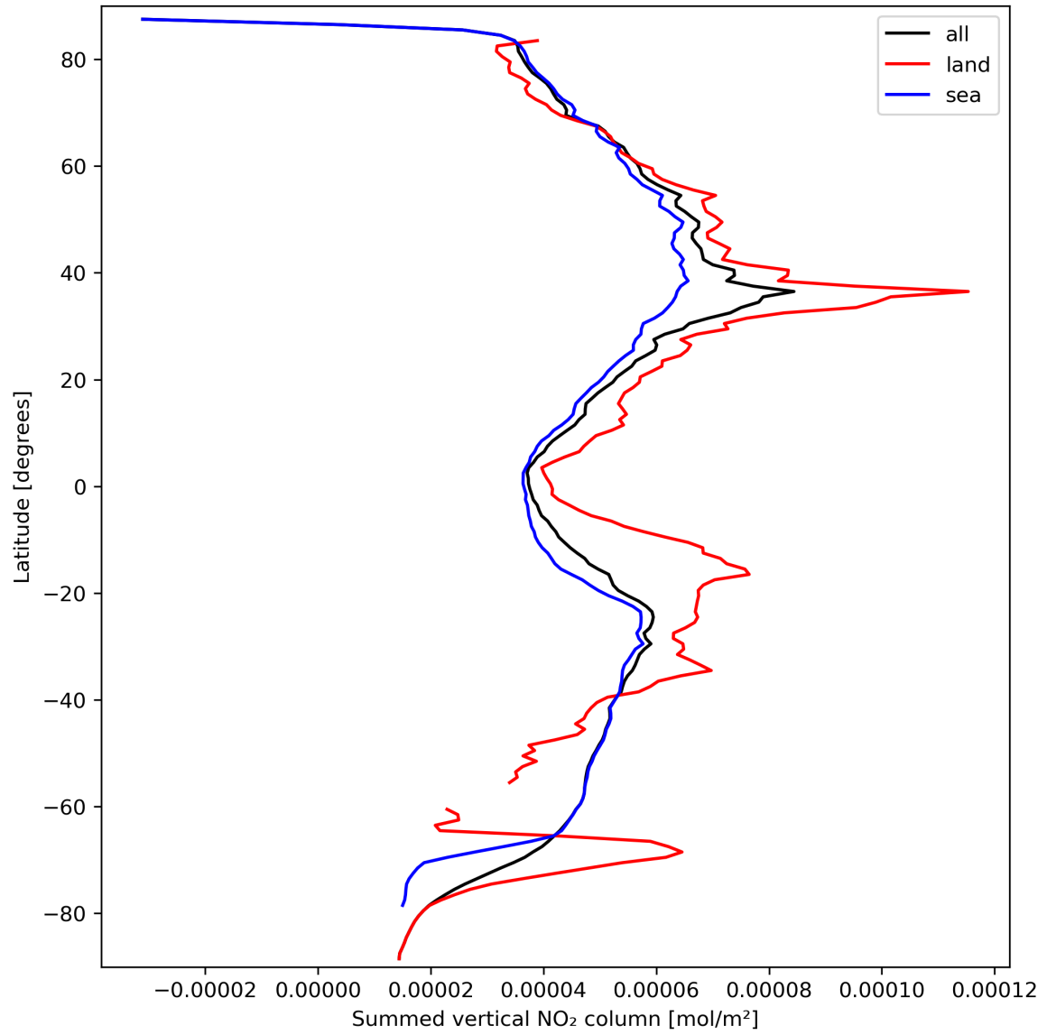
Figure 23: Zonal average of “Summed vertical NO 2 column” for 2023-09-23 to 2023-09-25.
