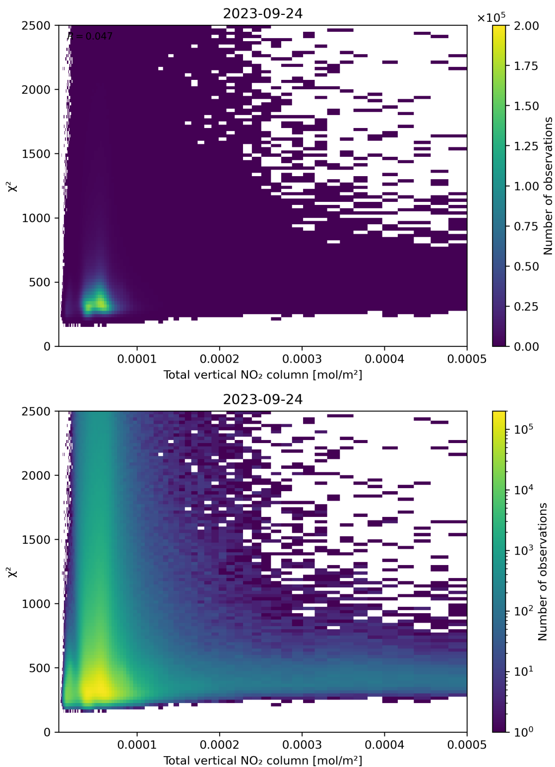
Figure 111: Scatter density plot of “Total vertical NO 2 column” against “ \chi^2 ” for 2023-09-23 to 2023-09-25.
