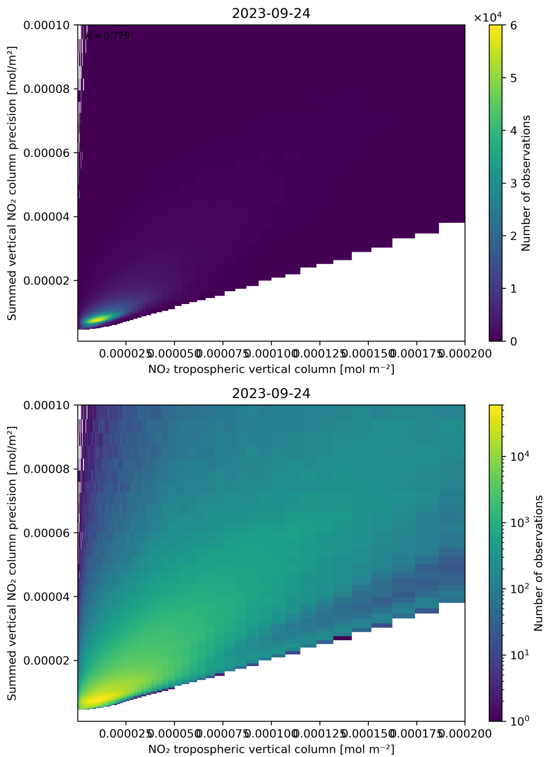
Figure 127: Scatter density plot of “NO 2 tropospheric vertical column” against “Summed vertical NO 2 column precision” for 2023-09-23 to 2023-09-25.
