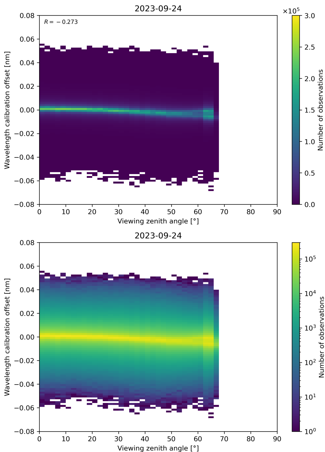
Figure 173: Scatter density plot of “Viewing zenith angle” against “Wavelength calibration offset” for 2023-09-23 to 2023-09-25.
