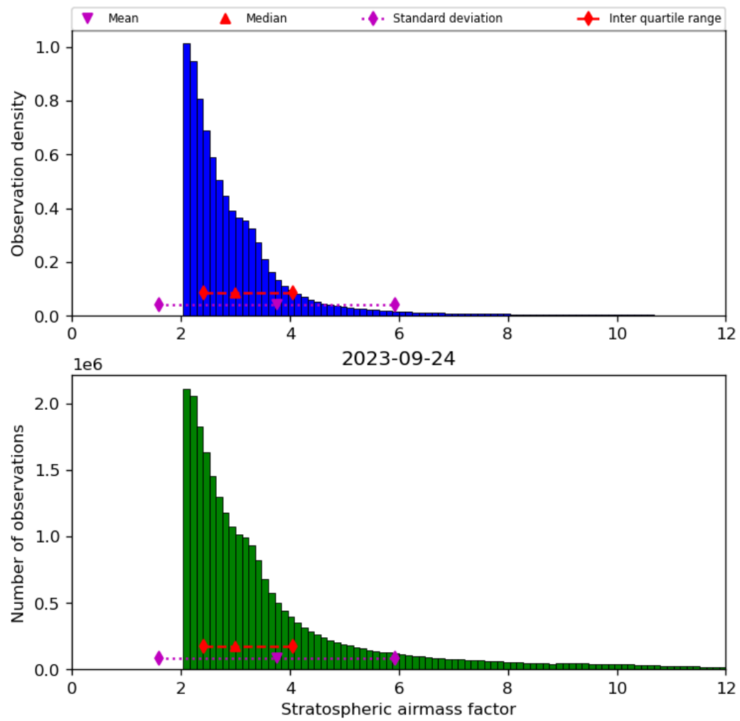
Figure 44: Histogram of “Stratospheric airmass factor” for 2023-09-23 to 2023-09-25
