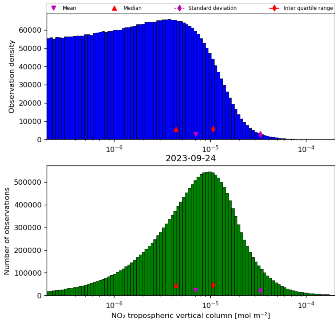
Figure 29: Histogram of “NO 2 tropospheric vertical column” for 2023-09-23 to 2023-09-25
