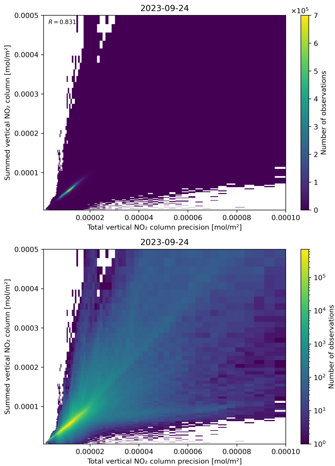
Figure 117: Scatter density plot of “Total vertical NO 2 column precision” against “Summed vertical NO 2 column” for 2023-09-23 to 2023-09-25.
