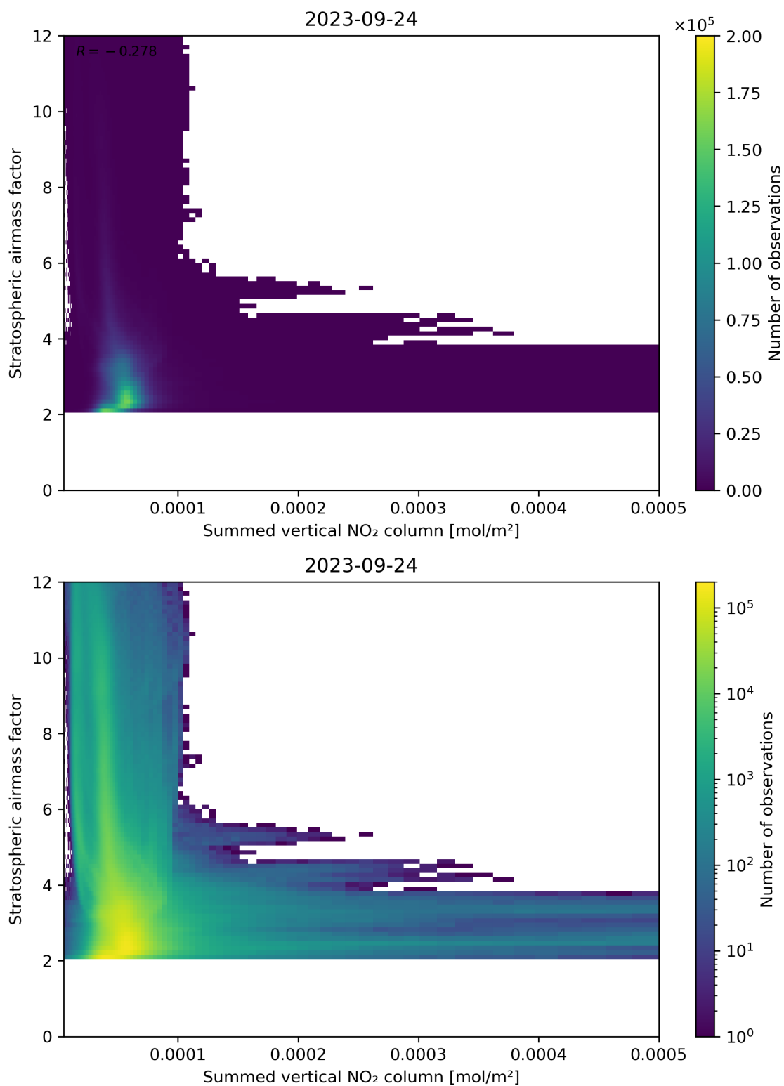
Figure 103: Scatter density plot of “Summed vertical NO 2 column” against “Stratospheric air mass factor” for 2023-09-23 to 2023-09-25.
