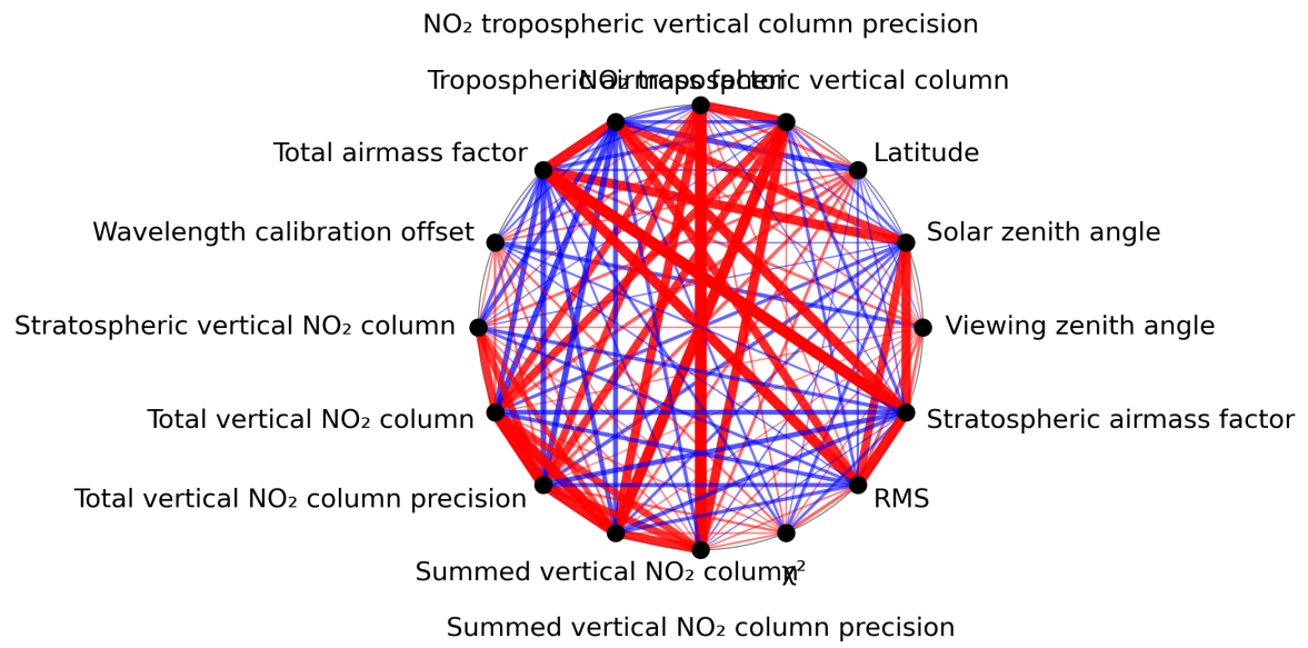
Figure 1: Map of correlation graph for 2023-09-23 to 2023-09-25.
