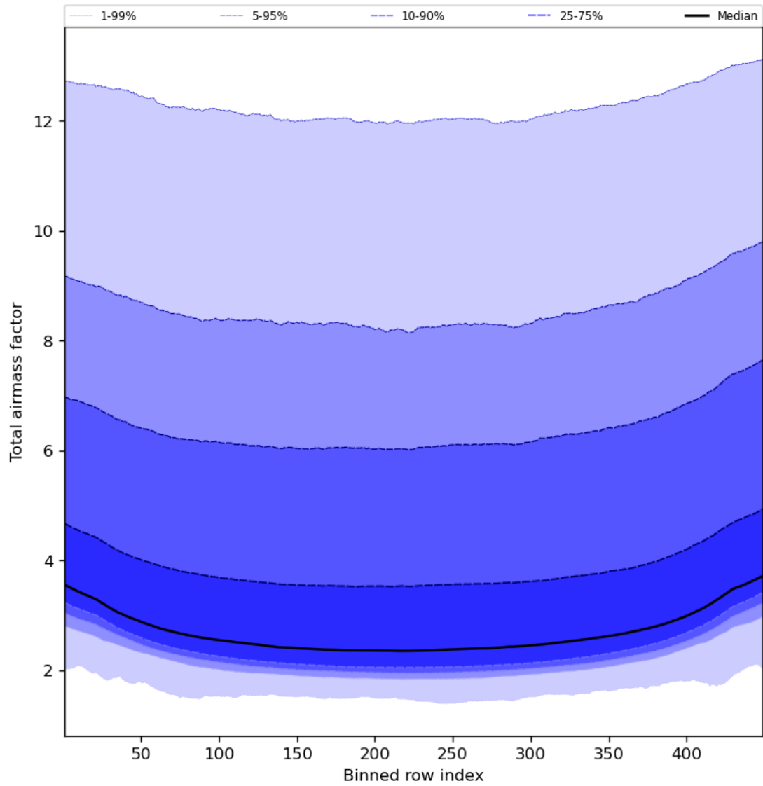
Figure 49: Along track statistics of “Total airmass factor” for 2023-09-23 to 2023-09-25
