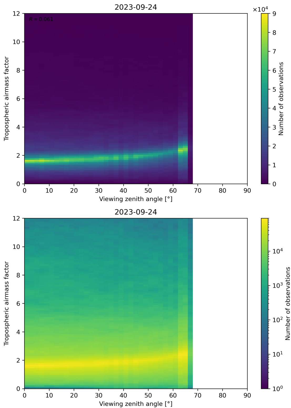
Figure 161: Scatter density plot of “Viewing zenith angle” against “Tropospheric airmass factor” for 2023-09-23 to 2023-09-25.
