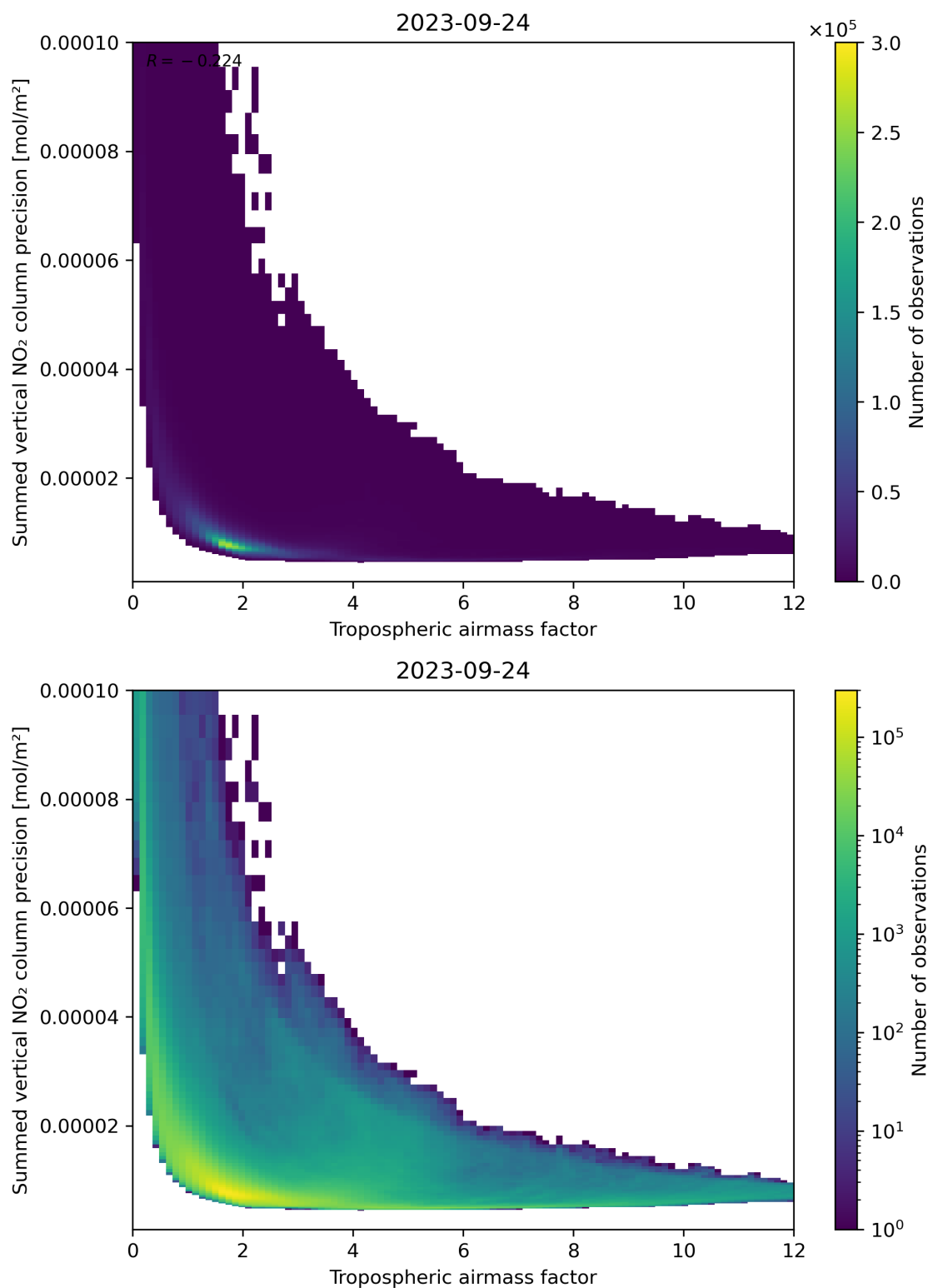
Figure 76: Scatter density plot of “Tropospheric air mass factor” against “Summed vertical NO 2 column precision” for 2023-09-23 to 2023-09-25.
