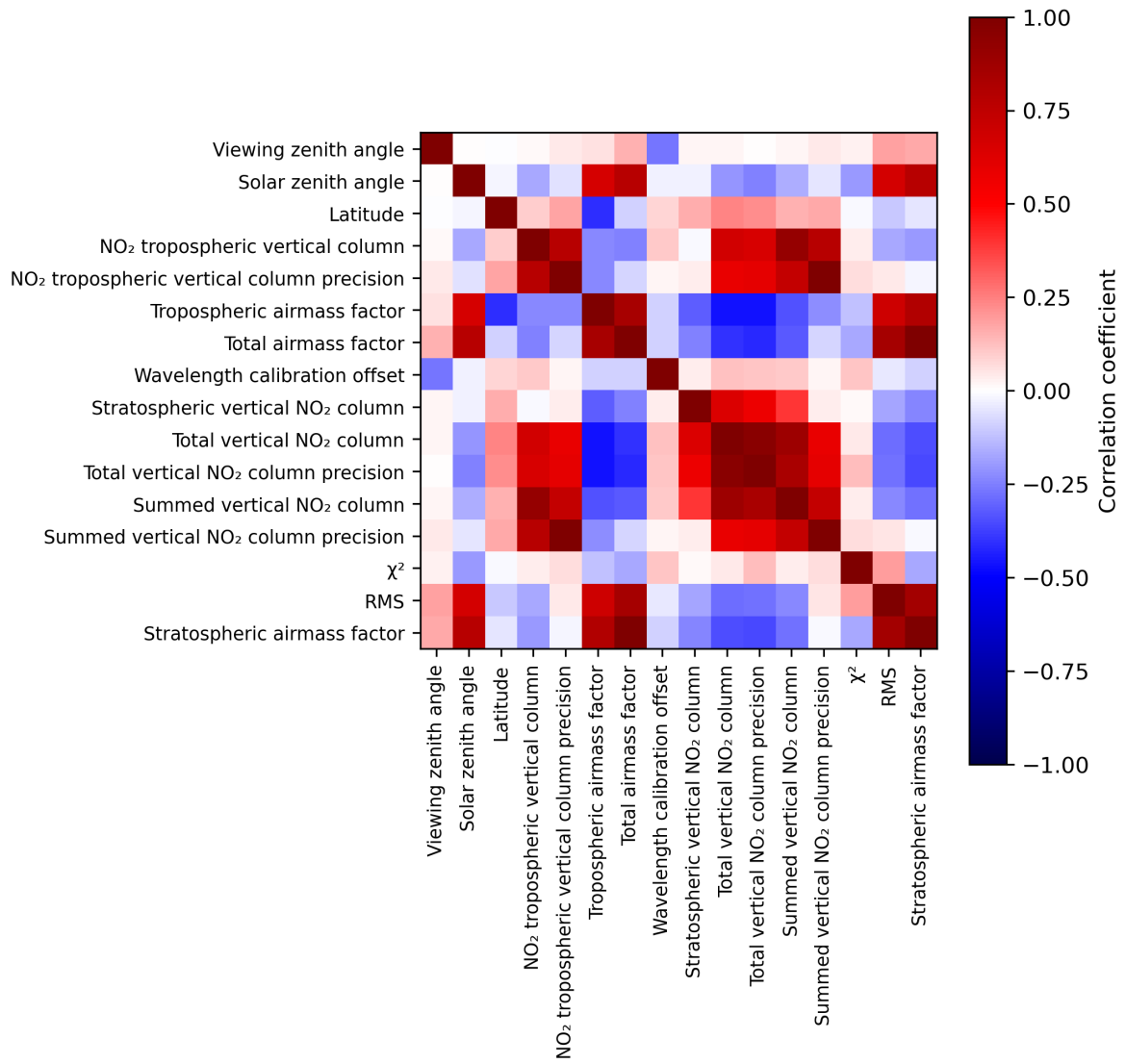
Figure 2: Map of correlation matrix for 2023-09-23 to 2023-09-25.
