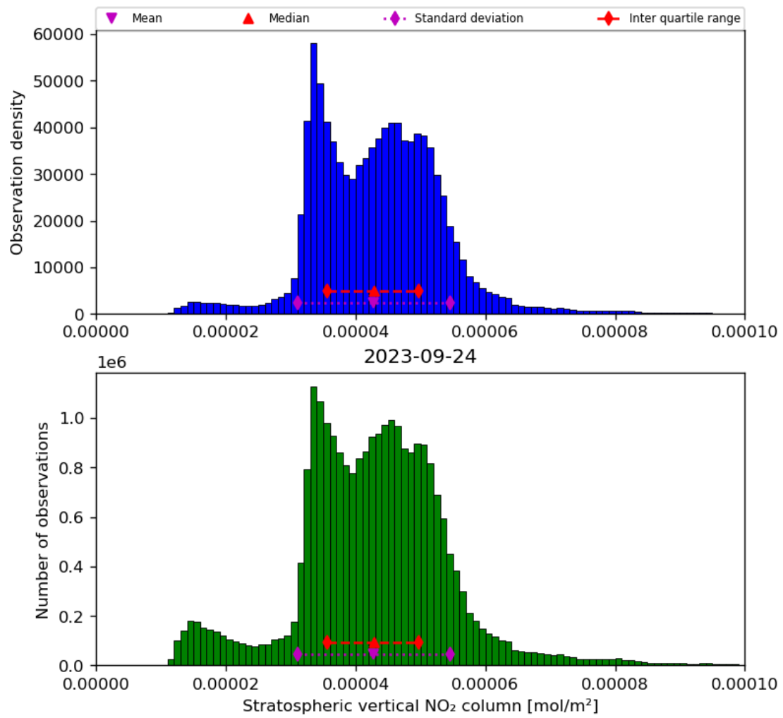
Figure 36: Histogram of “Stratospheric vertical NO 2 column” for 2023-09-23 to 2023-09-25
