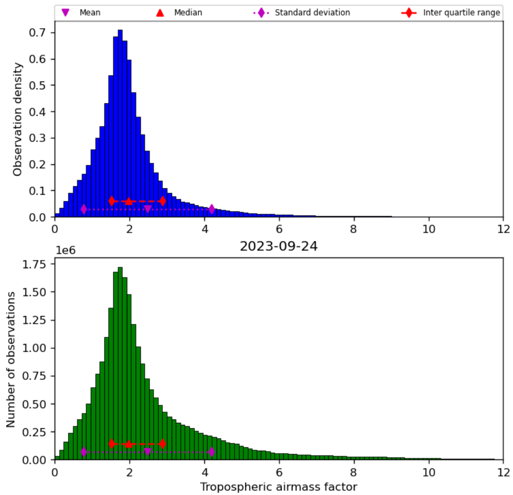
Figure 31: Histogram of “Tropospheric airmass factor” for 2023-09-23 to 2023-09-25
