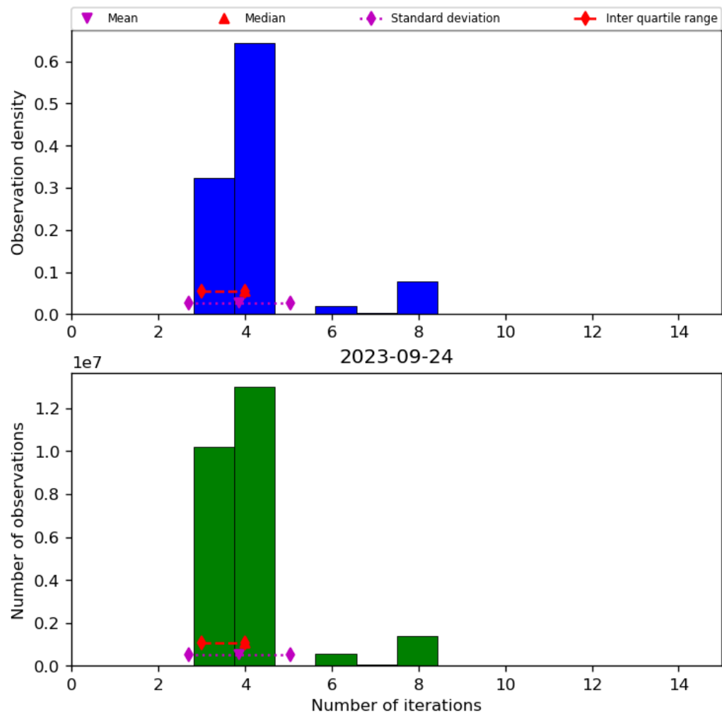
Figure 34: Histogram of “Number of iterations” for 2023-09-23 to 2023-09-25
