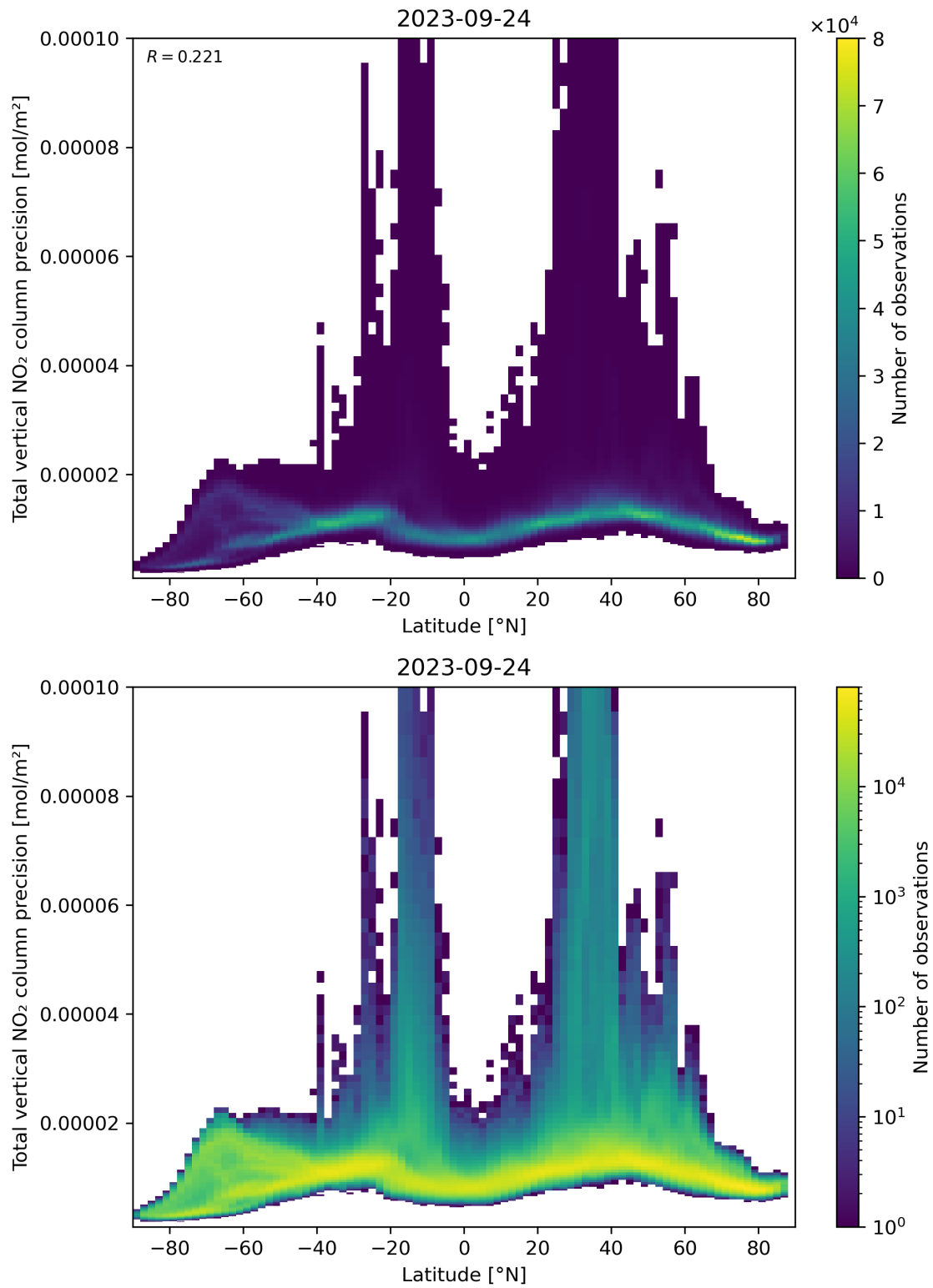
Figure 91: Scatter density plot of “Latitude” against “Total vertical NO 2 column precision” for 2023-09-23 to 2023-09-25.
