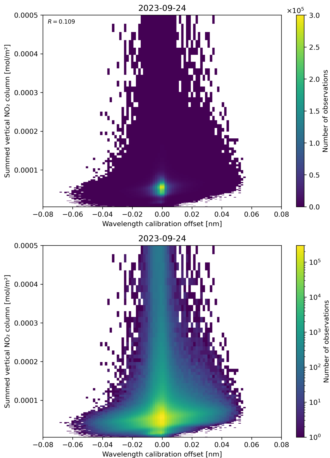
Figure 177: Scatter density plot of “Wavelength calibration offset” against “Summed vertical NO 2 column” for 2023-09-23 to 2023-09-25.
