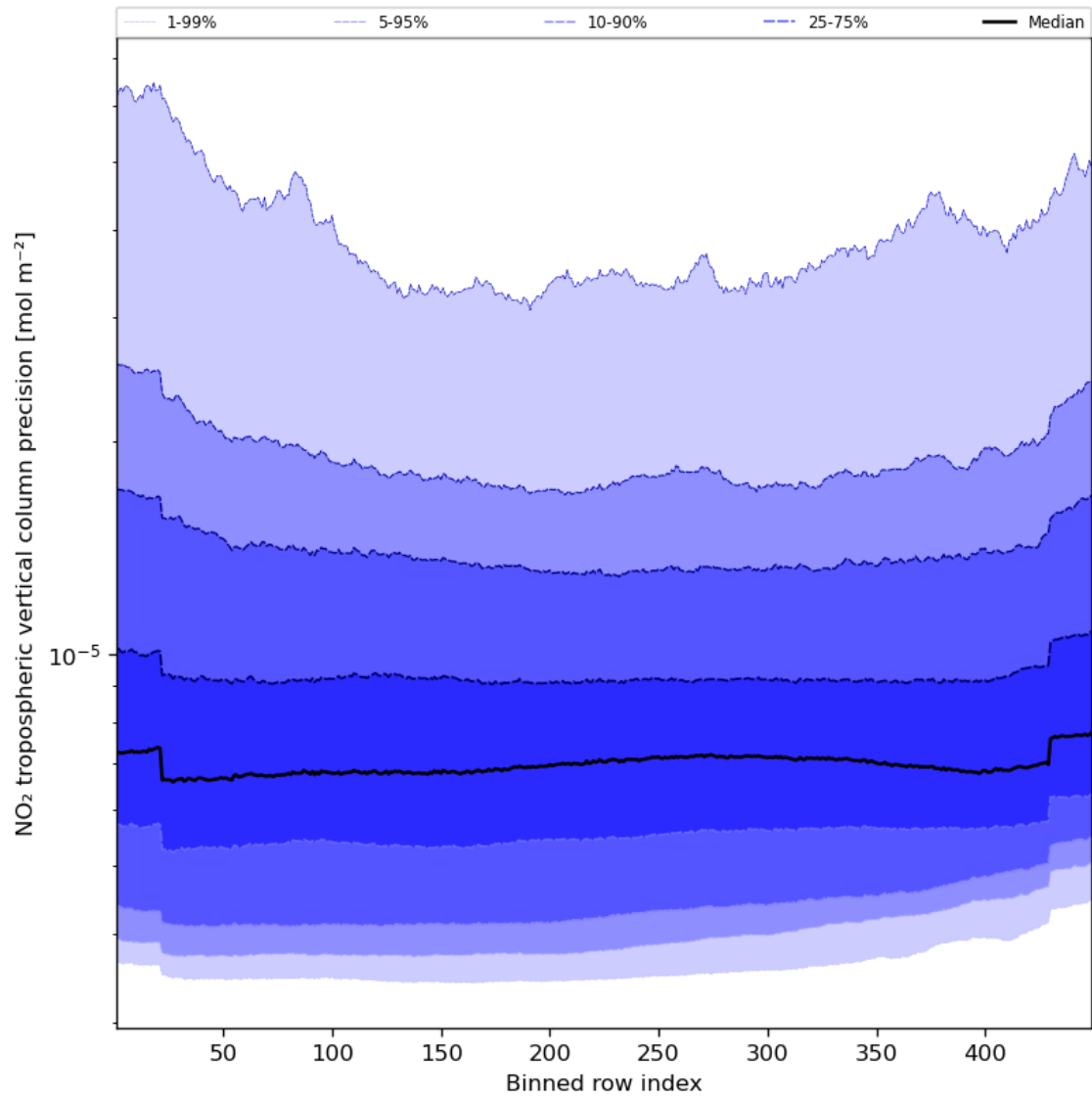
Figure 47: Along track statistics of “NO 2 tropospheric vertical column precision” for 2023-09-23 to 2023-09-25
