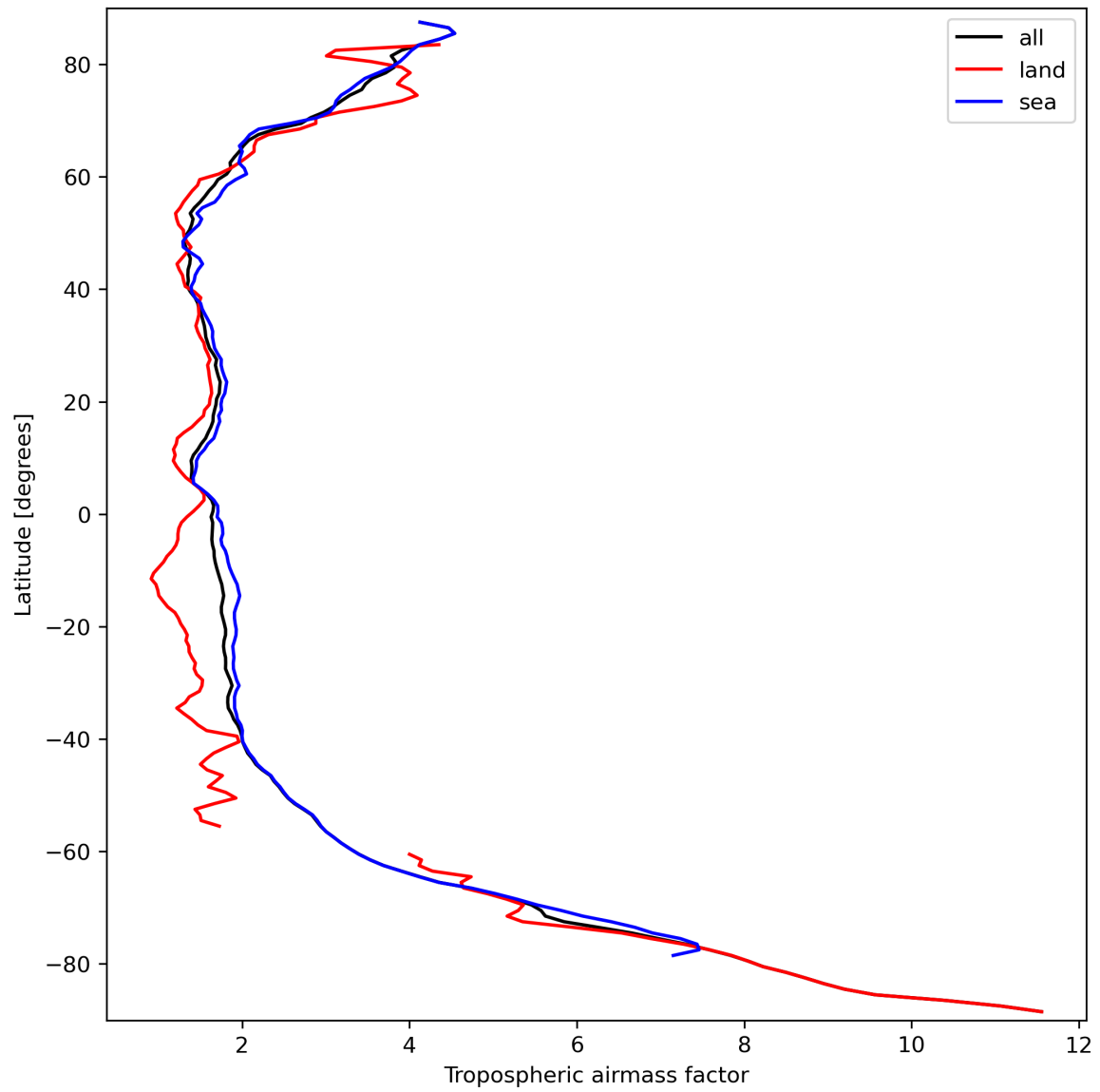
Figure 14: Zonal average of “Tropospheric airmass factor” for 2023-09-23 to 2023-09-25.
