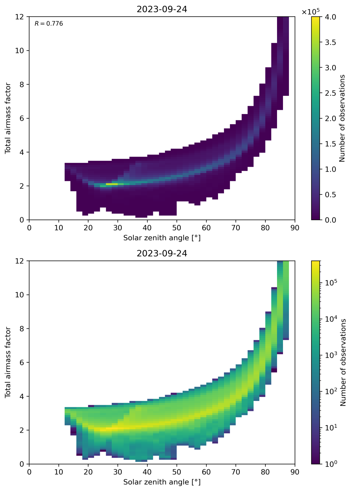
Figure 146: Scatter density plot of “Solar zenith angle” against “Total air mass factor” for 2023-09-23 to 2023-09-25.
