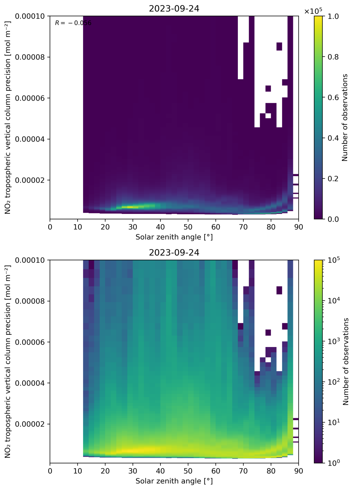
Figure 156: Scatter density plot of “Solar zenith angle” against “NO 2 tropospheric vertical column precision” for 2023-09-23 to 2023-09-25.
