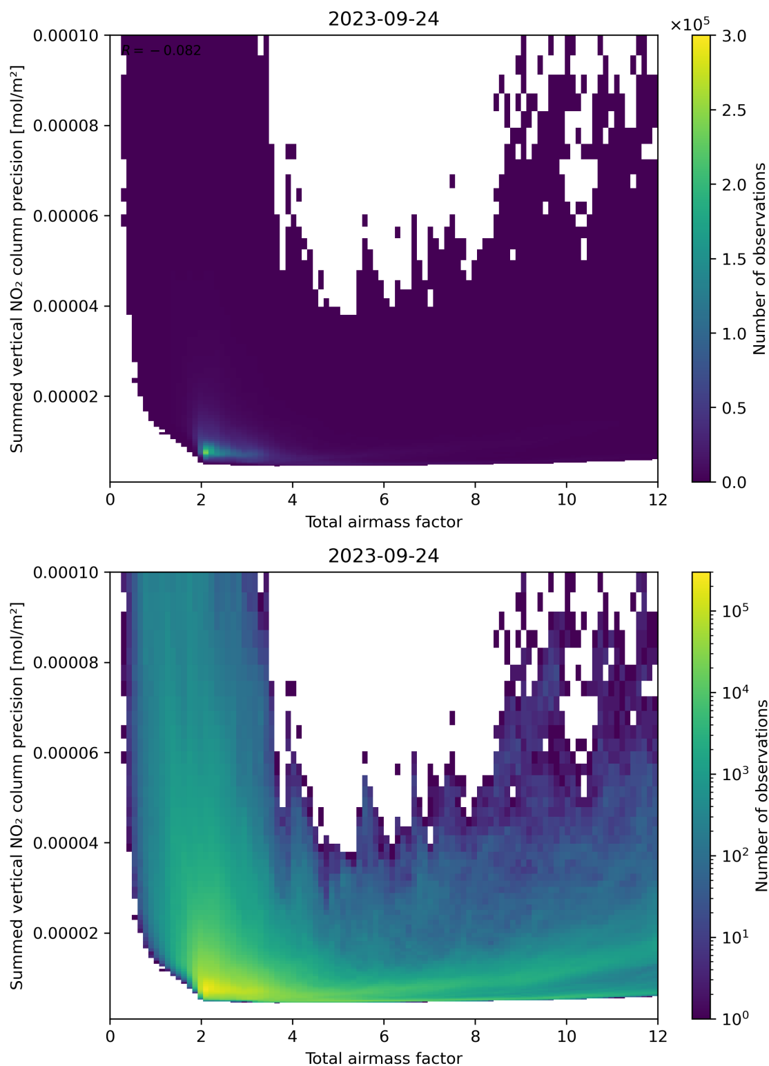
Figure 66: Scatter density plot of “Total airmass factor” against “Summed vertical NO 2 column precision” for 2023-09-23 to 2023-09-25.
