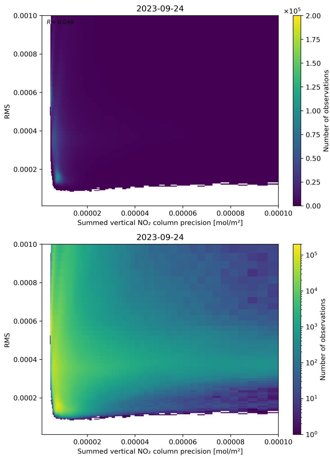
Figure 108: Scatter density plot of “Summed vertical NO 2 column precision” against “RMS” for 2023-09-23 to 2023-09-25.
