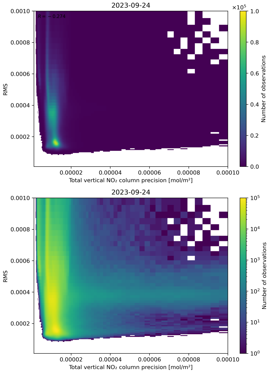
Figure 119: Scatter density plot of “Total vertical NO 2 column precision” against “RMS” for 2023-09-23 to 2023-09-25.
