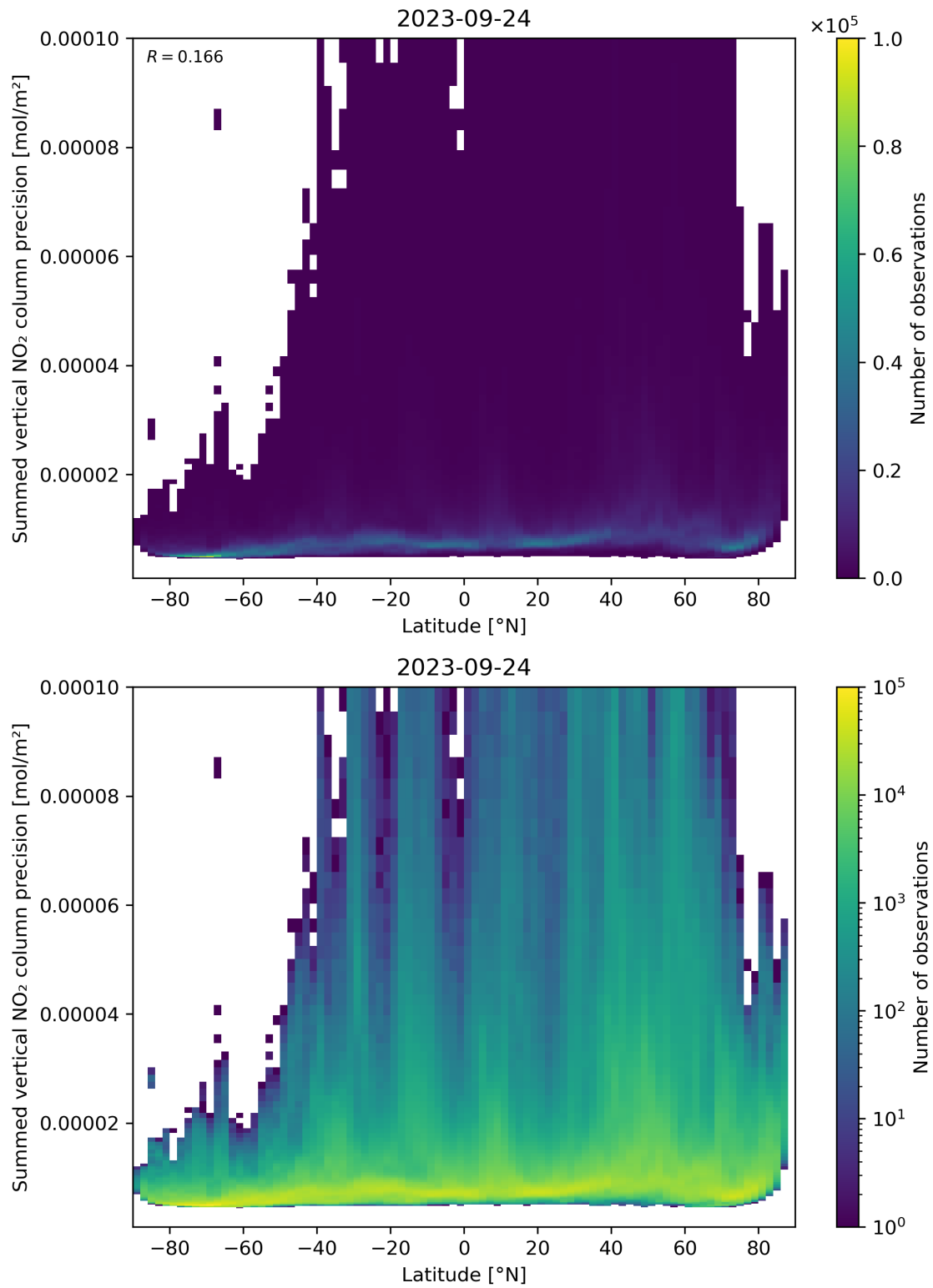
Figure 89: Scatter density plot of “Latitude” against “Summed vertical NO 2 column precision” for 2023-09-23 to 2023-09-25.
