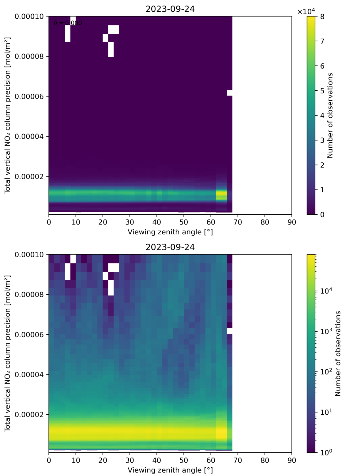
Figure 168: Scatter density plot of “Viewing zenith angle” against “Total vertical NO 2 column precision” for 2023-09-23 to 2023-09-25.
