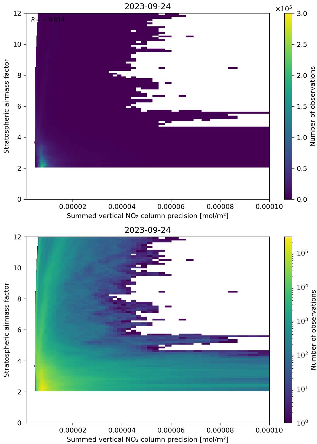
Figure 106: Scatter density plot of “Summed vertical NO 2 column precision” against “Stratospheric airmass factor” for 2023-09-23 to 2023-09-25.
