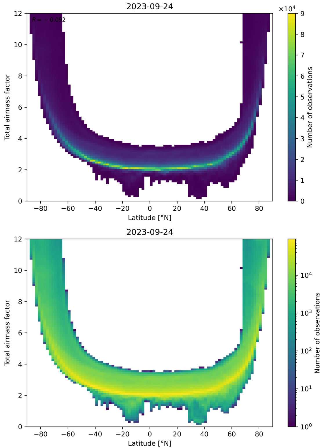
Figure 84: Scatter density plot of “Latitude” against “Total airmass factor” for 2023-09-23 to 2023-09-25.
