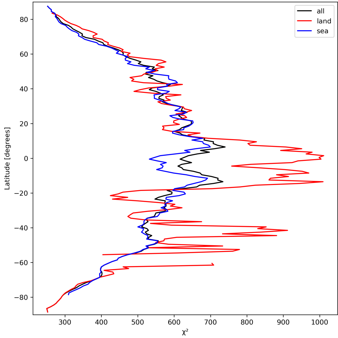
Figure 25: Zonal average of “ \chi^2 ” for 2023-09-23 to 2023-09-25.
