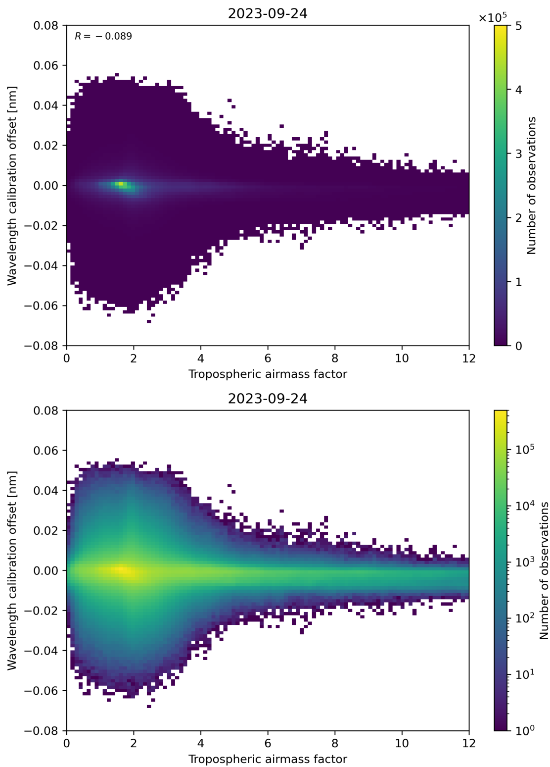
Figure 80: Scatter density plot of “Tropospheric airmass factor” against “Wavelength calibration offset” for 2023-09-23 to 2023-09-25.
