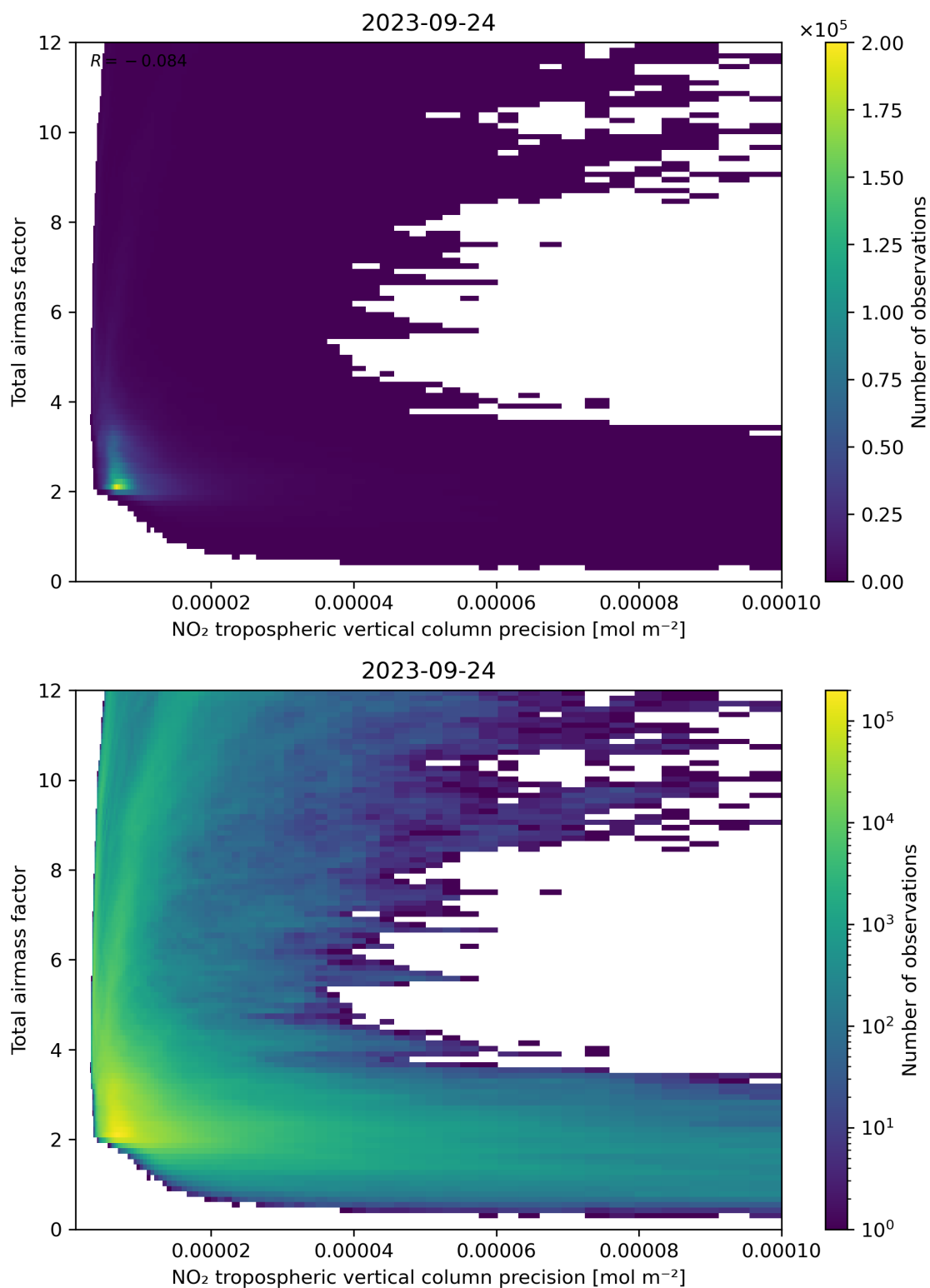
Figure 132: Scatter density plot of “NO 2 tropospheric vertical column precision” against “Total air mass factor” for 2023-09-23 to 2023-09-25.
