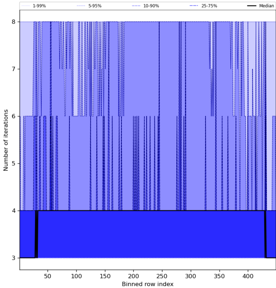
Figure 51: Along track statistics of “Number of iterations” for 2023-09-23 to 2023-09-25
