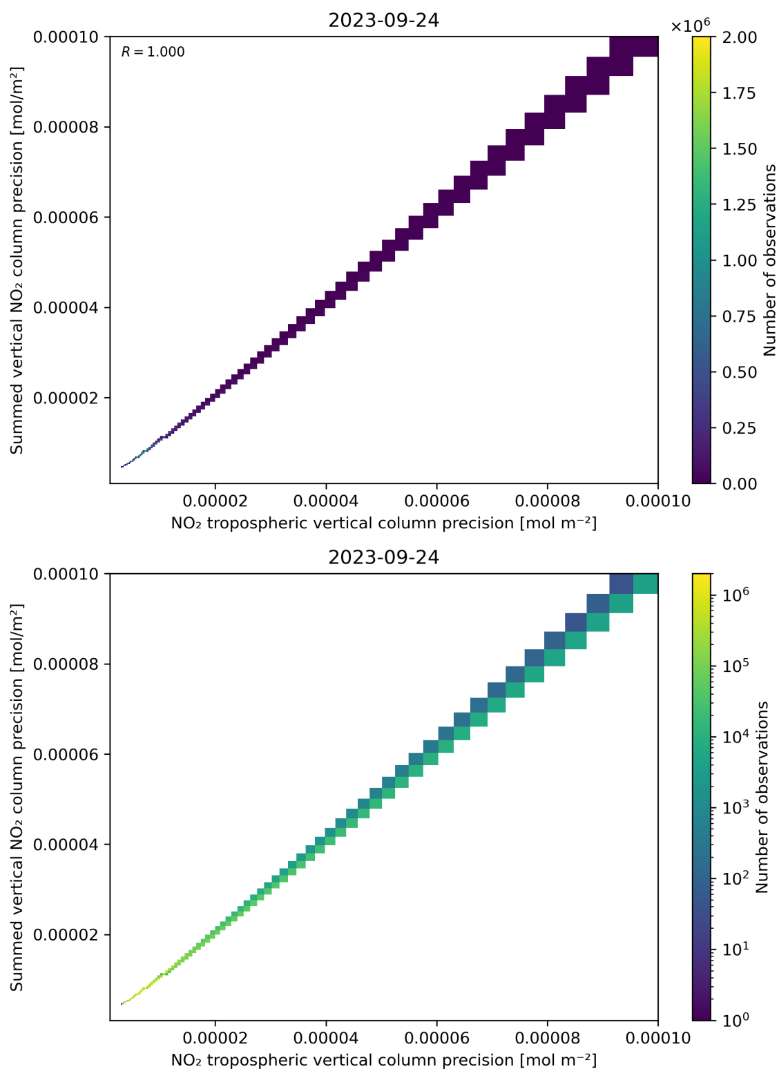
Figure 137: Scatter density plot of “NO 2 tropospheric vertical column precision” against “Summed vertical NO 2 column precision” for 2023-09-23 to 2023-09-25.
