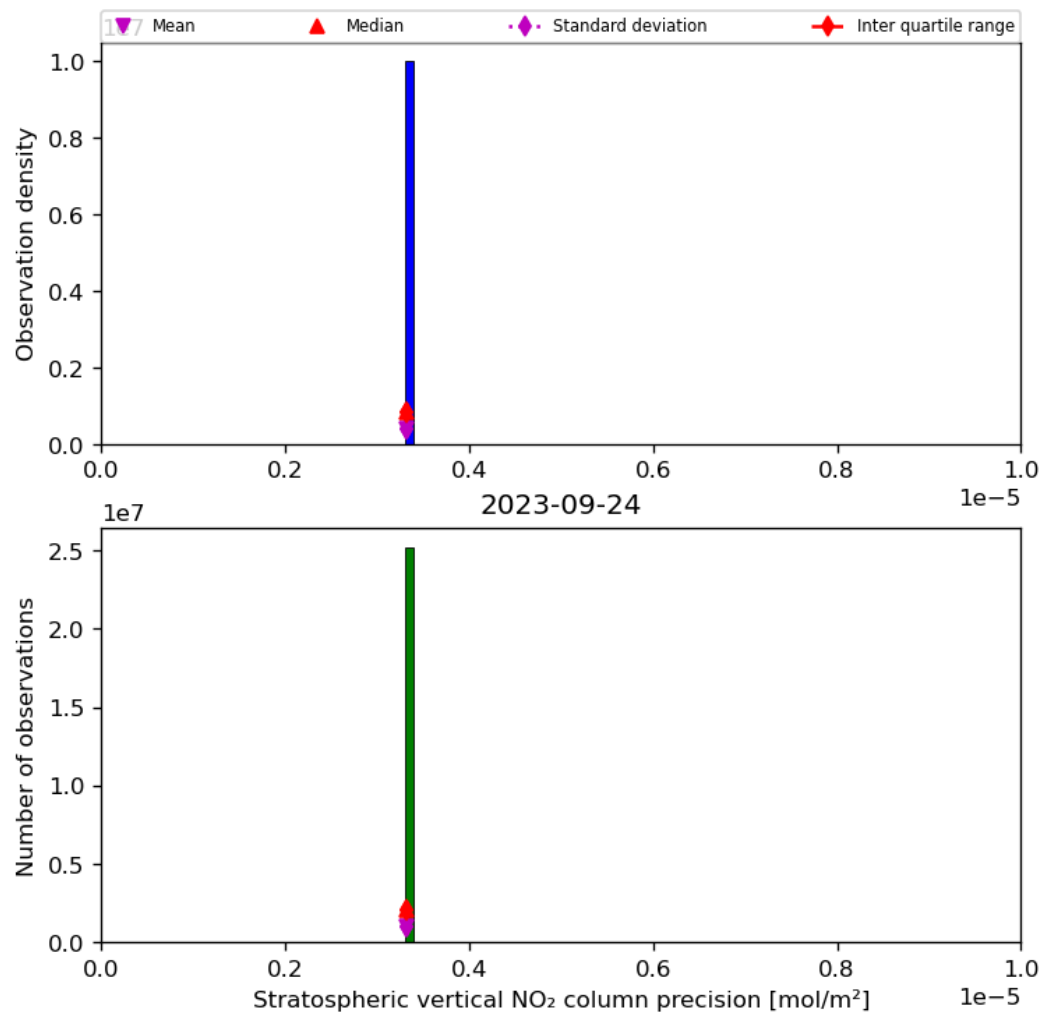
Figure 37: Histogram of “Stratospheric vertical NO 2 column precision” for 2023-09-23 to 2023-09-25
