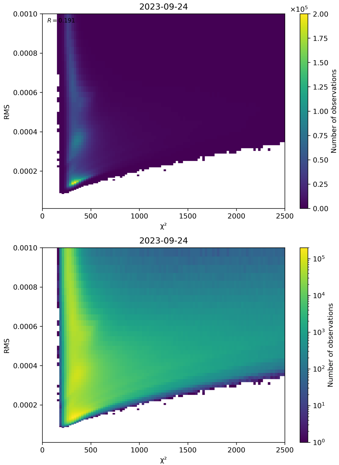
Figure 82: Scatter density plot of “ \chi^2 ” against “RMS” for 2023-09-23 to 2023-09-25.
