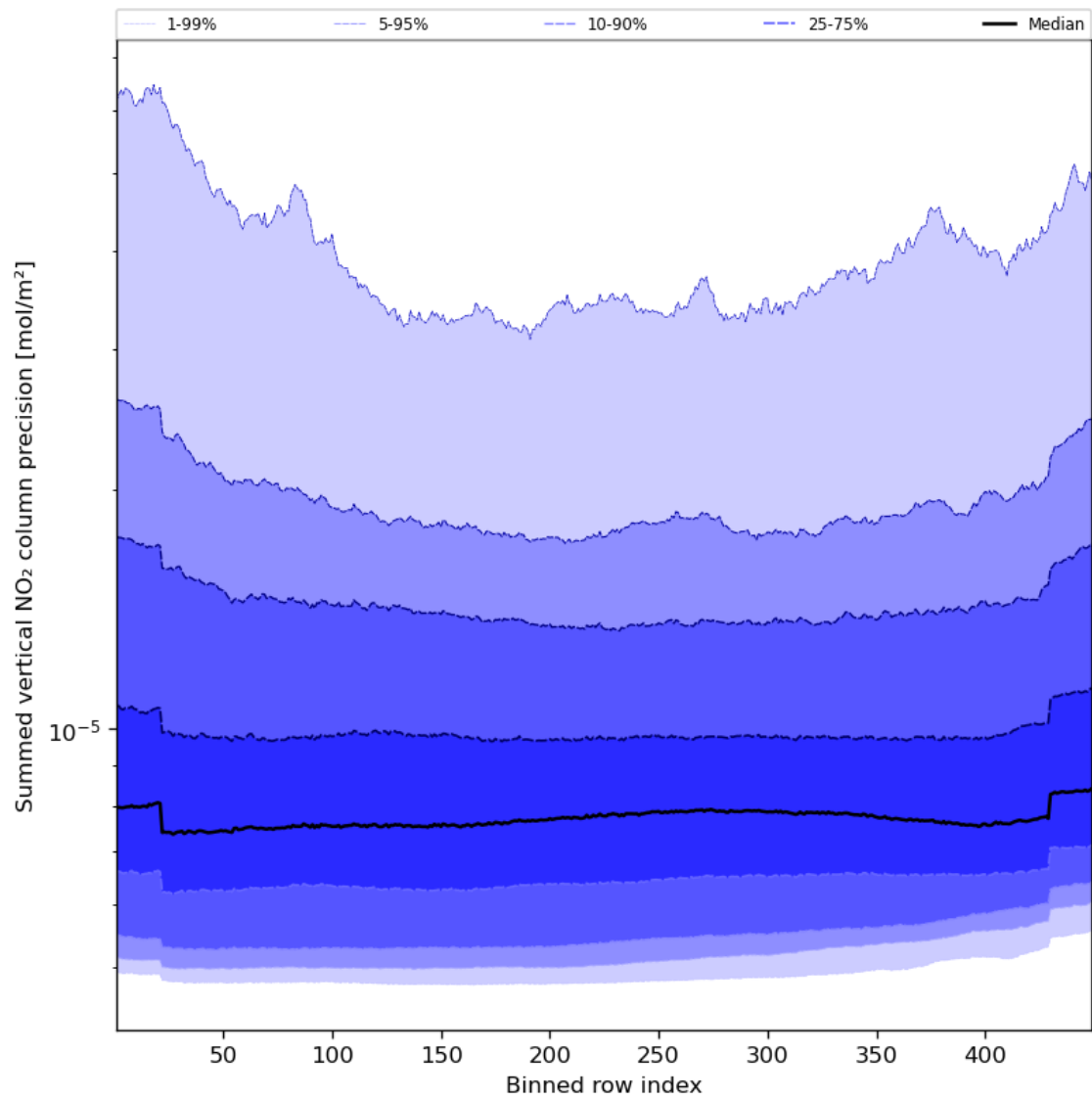
Figure 58: Along track statistics of “Summed vertical NO 2 column precision” for 2023-09-23 to 2023-09-25
