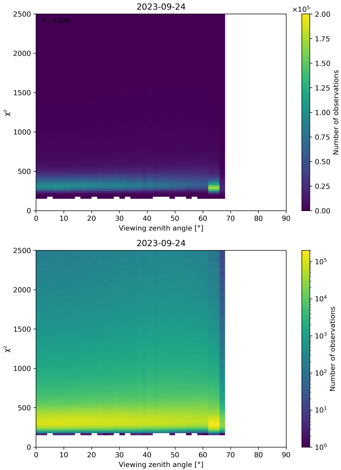
Figure 162: Scatter density plot of “Viewing zenith angle” against “ \chi^2 ” for 2023-09-23 to 2023-09-25.
