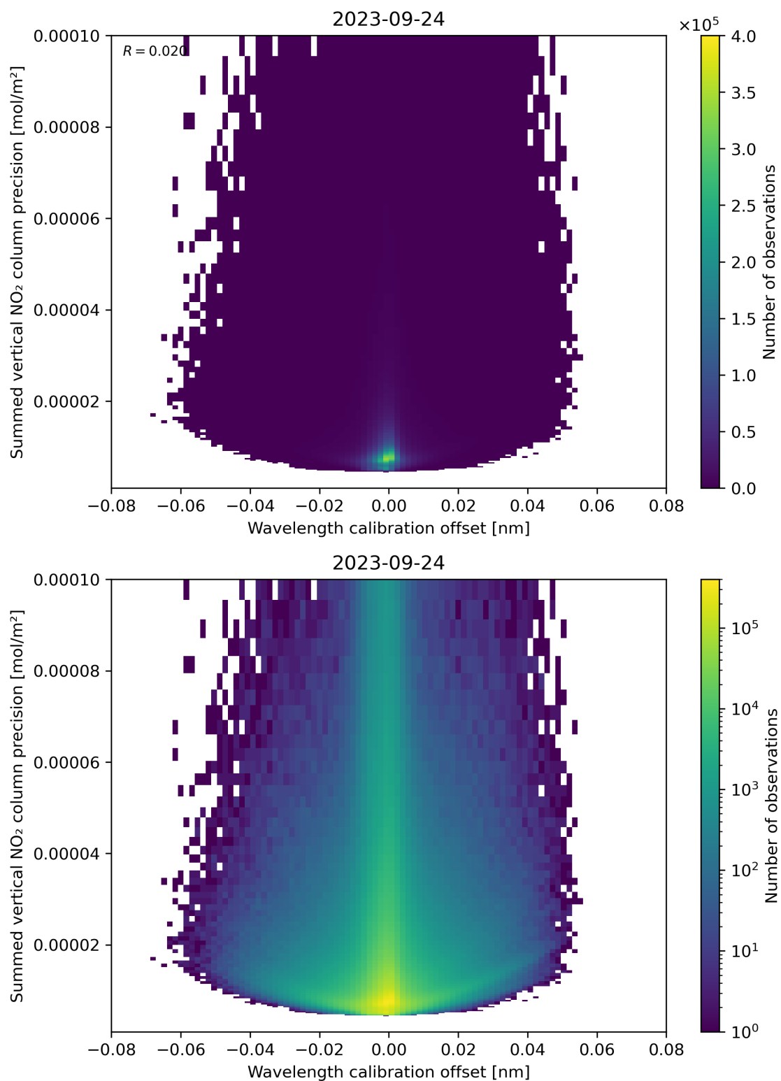
Figure 178: Scatter density plot of “Wavelength calibration offset” against “Summed vertical NO 2 column precision” for 2023-09-23 to 2023-09-25.
