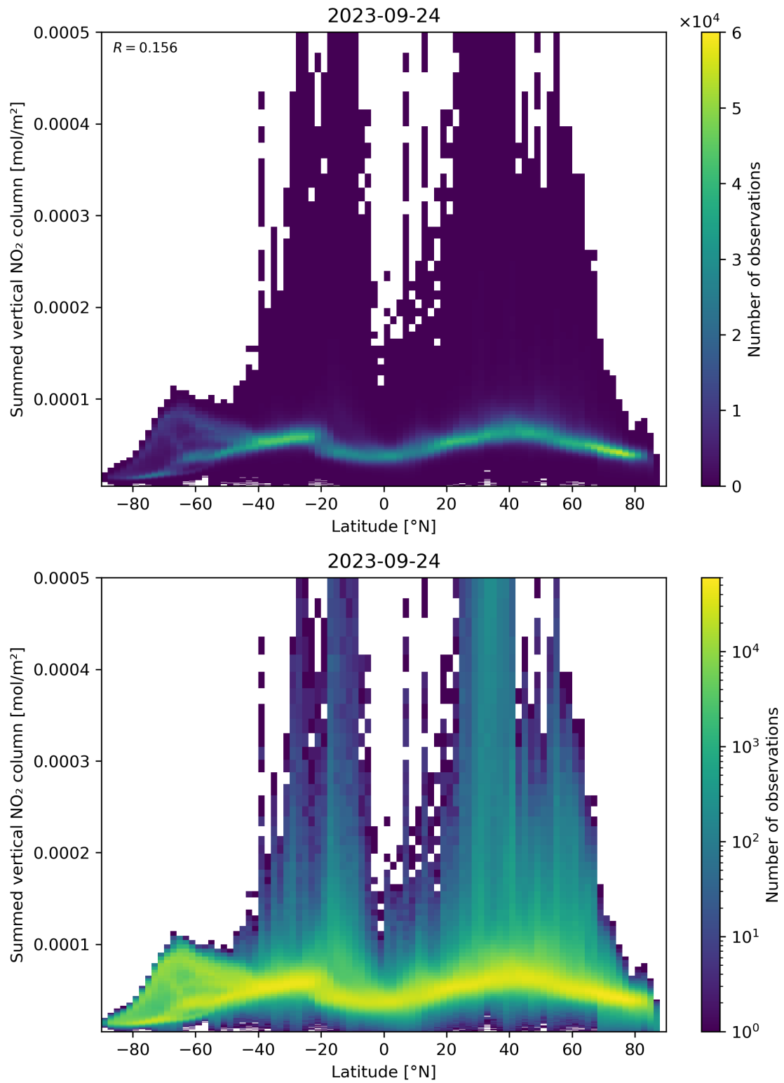
Figure 88: Scatter density plot of “Latitude” against “Summed vertical NO 2 column” for 2023-09-23 to 2023-09-25.
