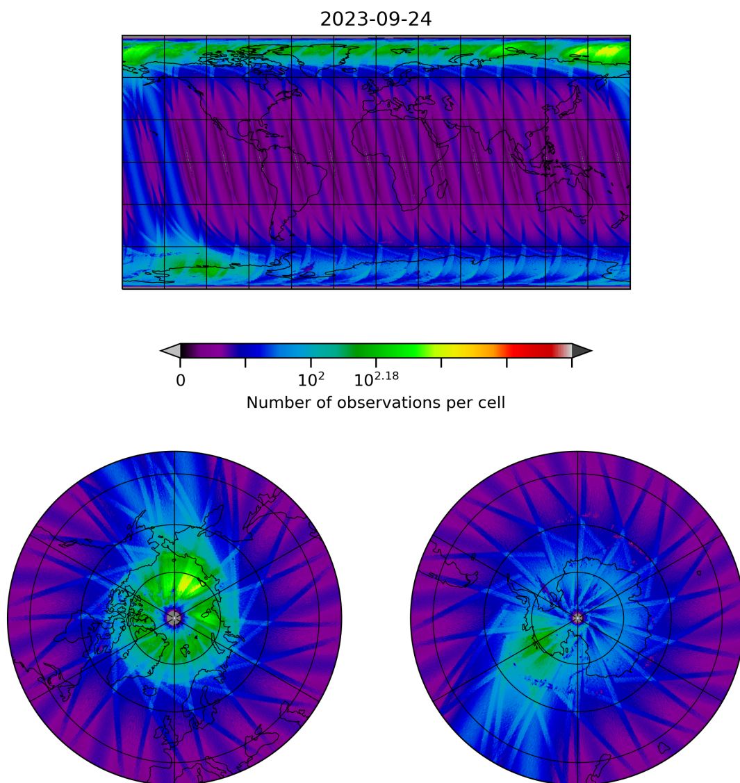
Figure 10: Map of the number of observations for 2023-09-23 to 2023-09-25
