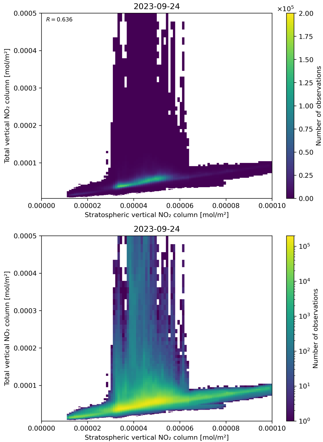
Figure 100: Scatter density plot of “Stratospheric vertical NO 2 column” against “Total vertical NO 2 column” for 2023-09-23 to 2023-09-25.
