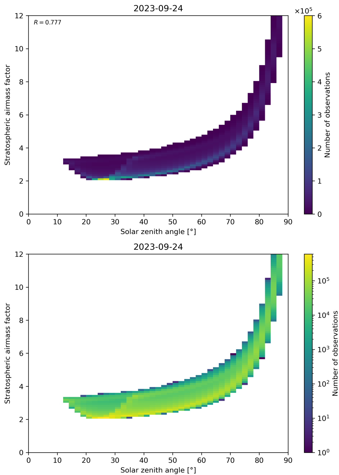
Figure 145: Scatter density plot of “Solar zenith angle” against “Stratospheric airmass factor” for 2023-09-23 to 2023-09-25.
