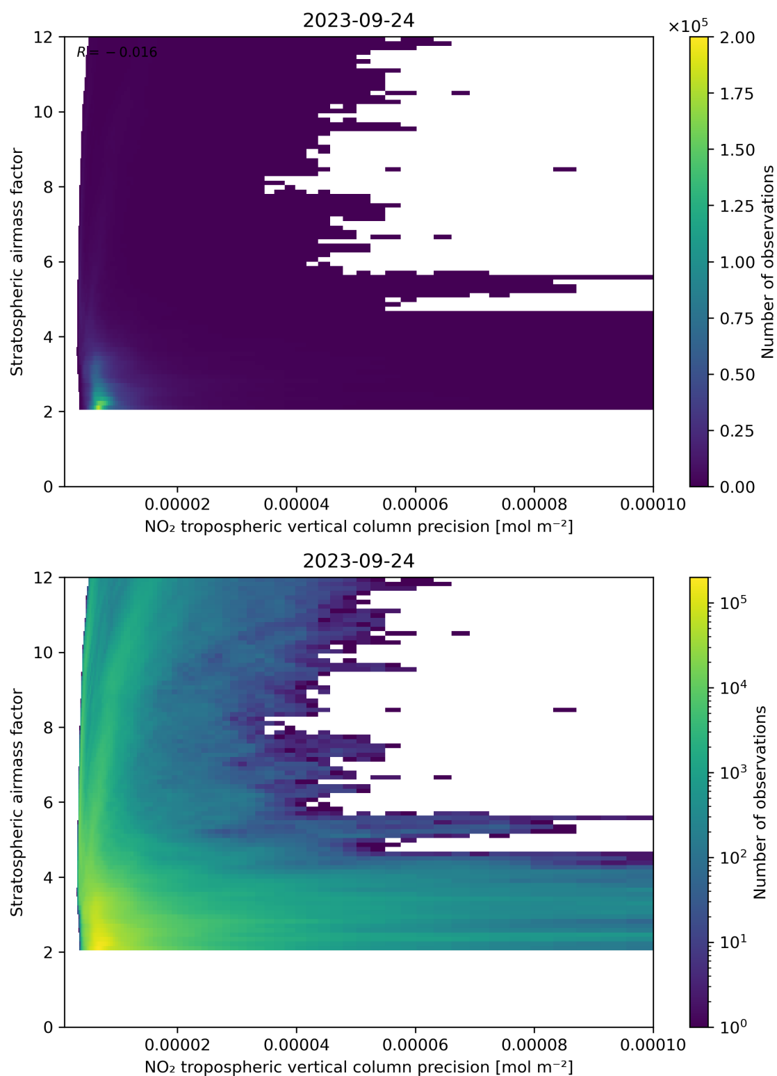
Figure 131: Scatter density plot of “NO 2 tropospheric vertical column precision” against “Stratospheric airmass factor” for 2023-09-23 to 2023-09-25.
