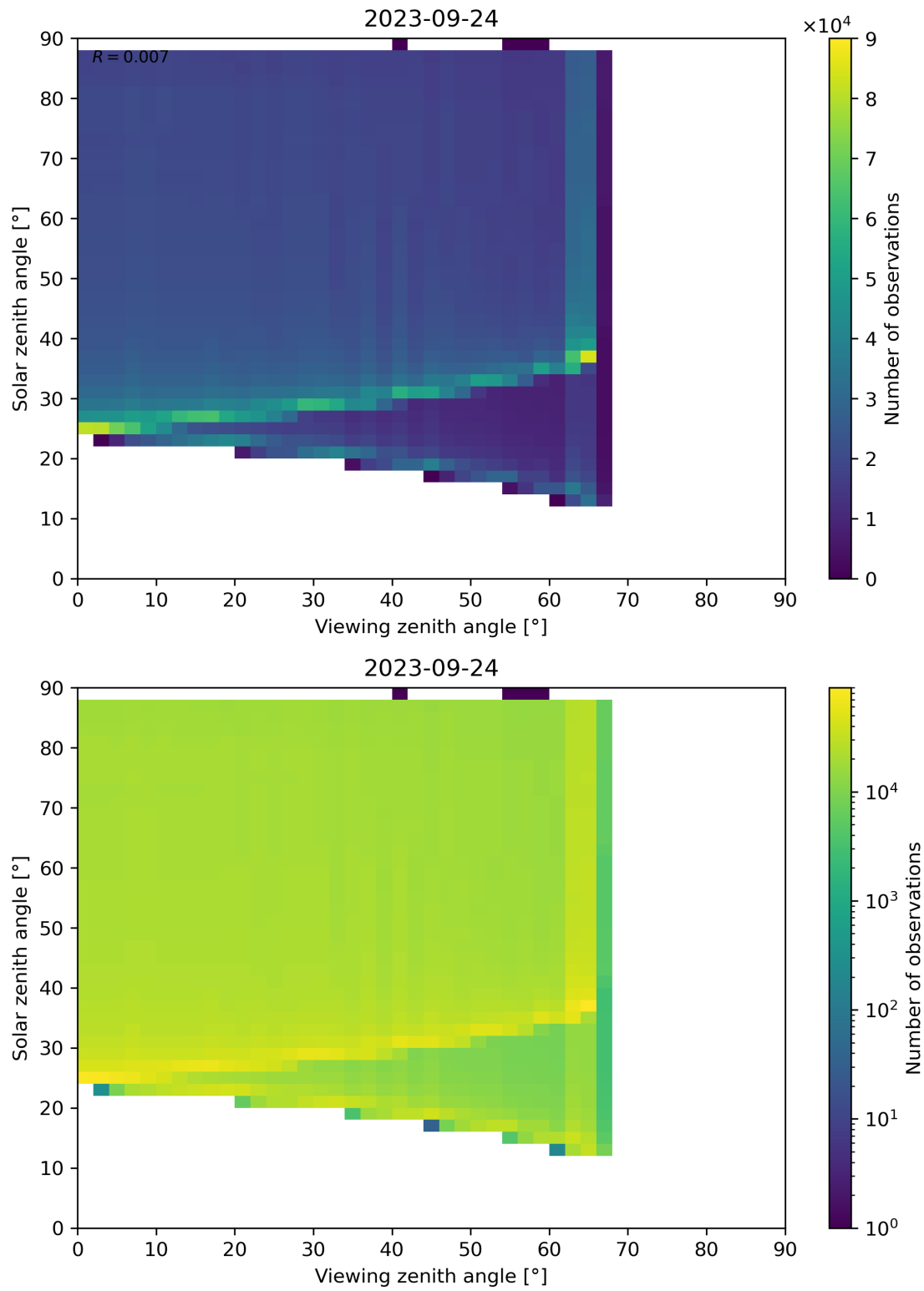
Figure 172: Scatter density plot of “Viewing zenith angle” against “Solar zenith angle” for 2023-09-23 to 2023-09-25.
