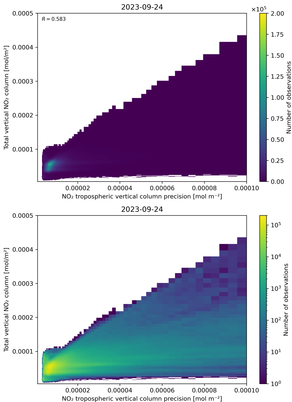
Figure 138: Scatter density plot of “NO 2 tropospheric vertical column precision” against “Total vertical NO 2 column” for 2023-09-23 to 2023-09-25.
