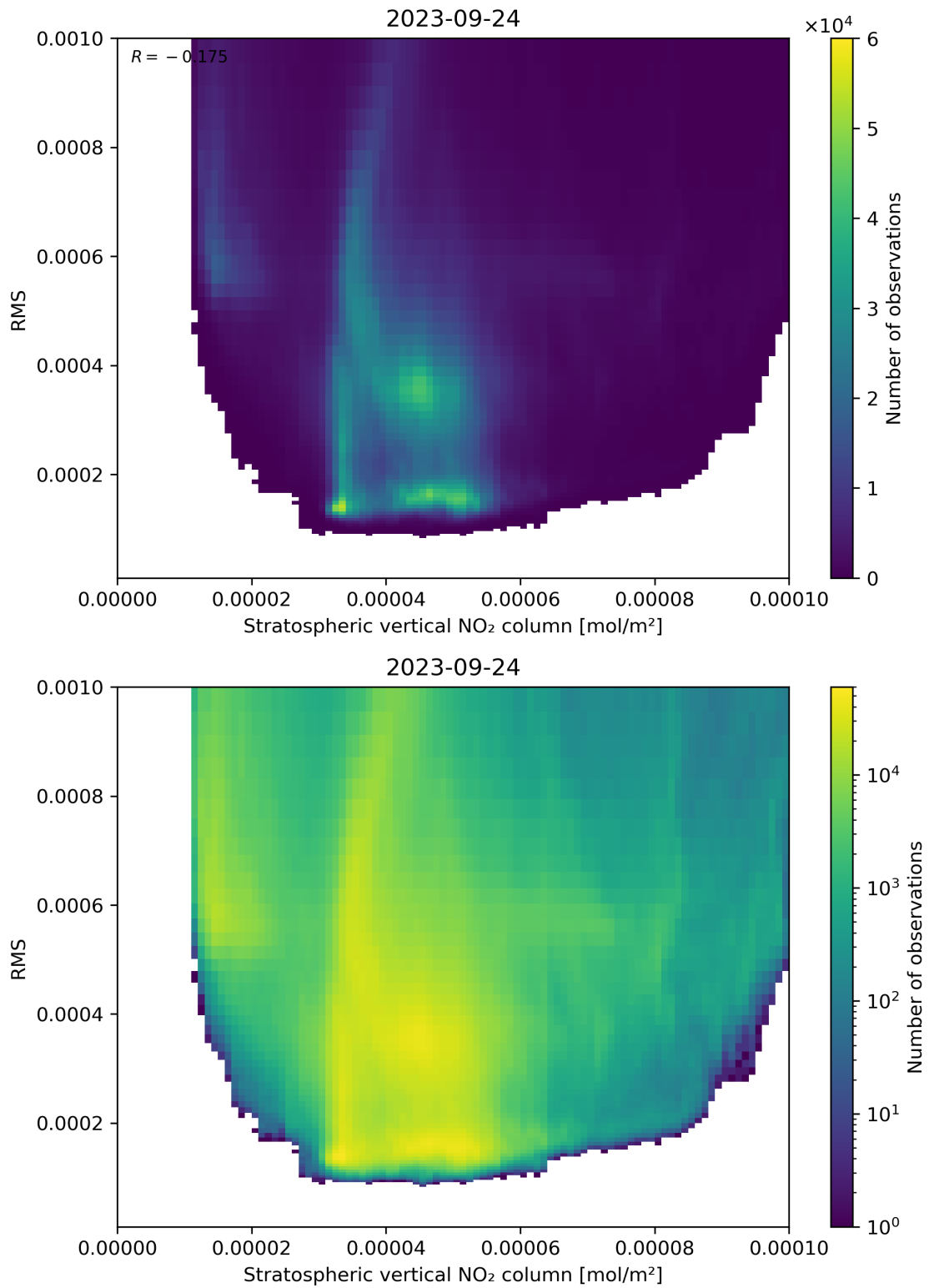
Figure 102: Scatter density plot of “Stratospheric vertical NO 2 column” against “RMS” for 2023-09-23 to 2023-09-25.
