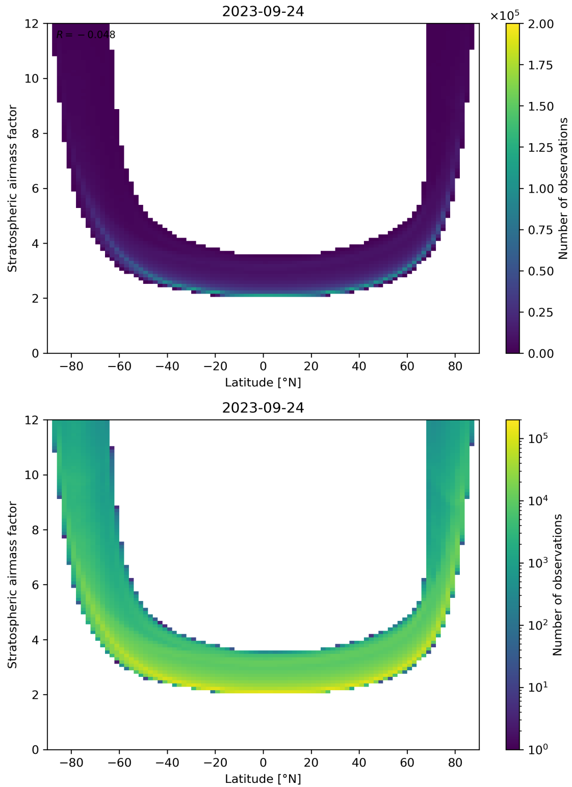
Figure 83: Scatter density plot of “Latitude” against “Stratospheric air mass factor” for 2023-09-23 to 2023-09-25.
