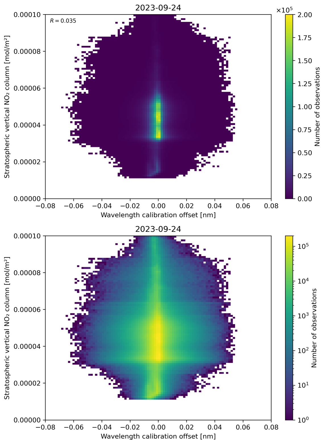
Figure 176: Scatter density plot of “Wavelength calibration offset” against “Stratospheric vertical NO 2 column” for 2023-09-23 to 2023-09-25.
