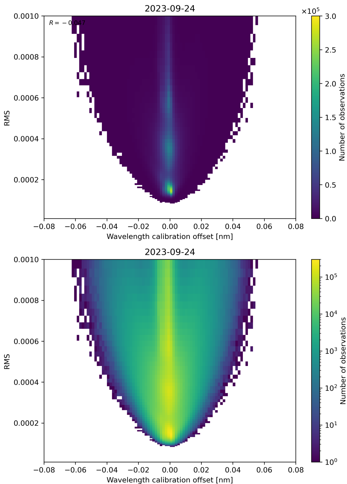
Figure 181: Scatter density plot of “Wavelength calibration offset” against “RMS” for 2023-09-23 to 2023-09-25.
