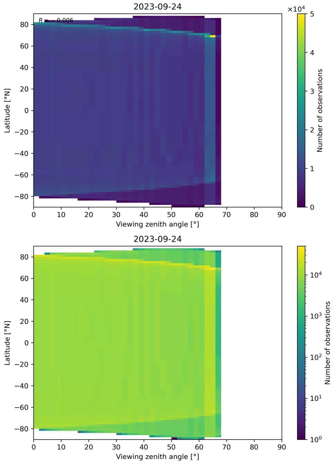
Figure 163: Scatter density plot of “Viewing zenith angle” against “Latitude” for 2023-09-23 to 2023-09-25.
