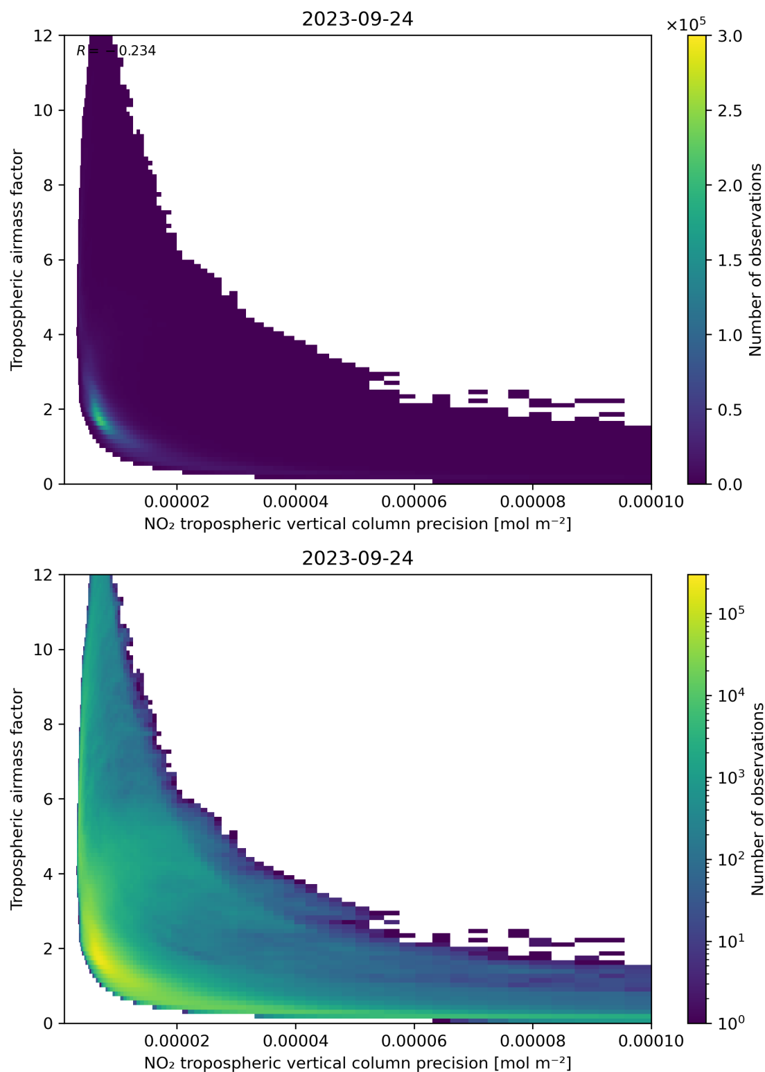
Figure 133: Scatter density plot of “NO 2 tropospheric vertical column precision” against “Tropospheric airmass factor” for 2023-09-23 to 2023-09-25.
