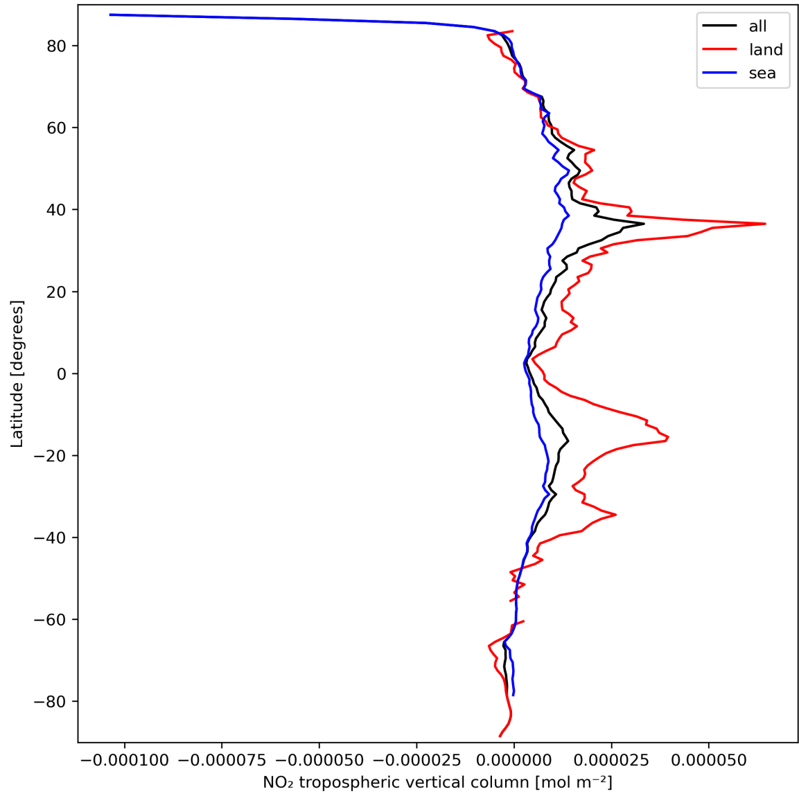
Figure 12: Zonal average of “NO 2 tropospheric vertical column” for 2023-09-23 to 2023-09-25.
