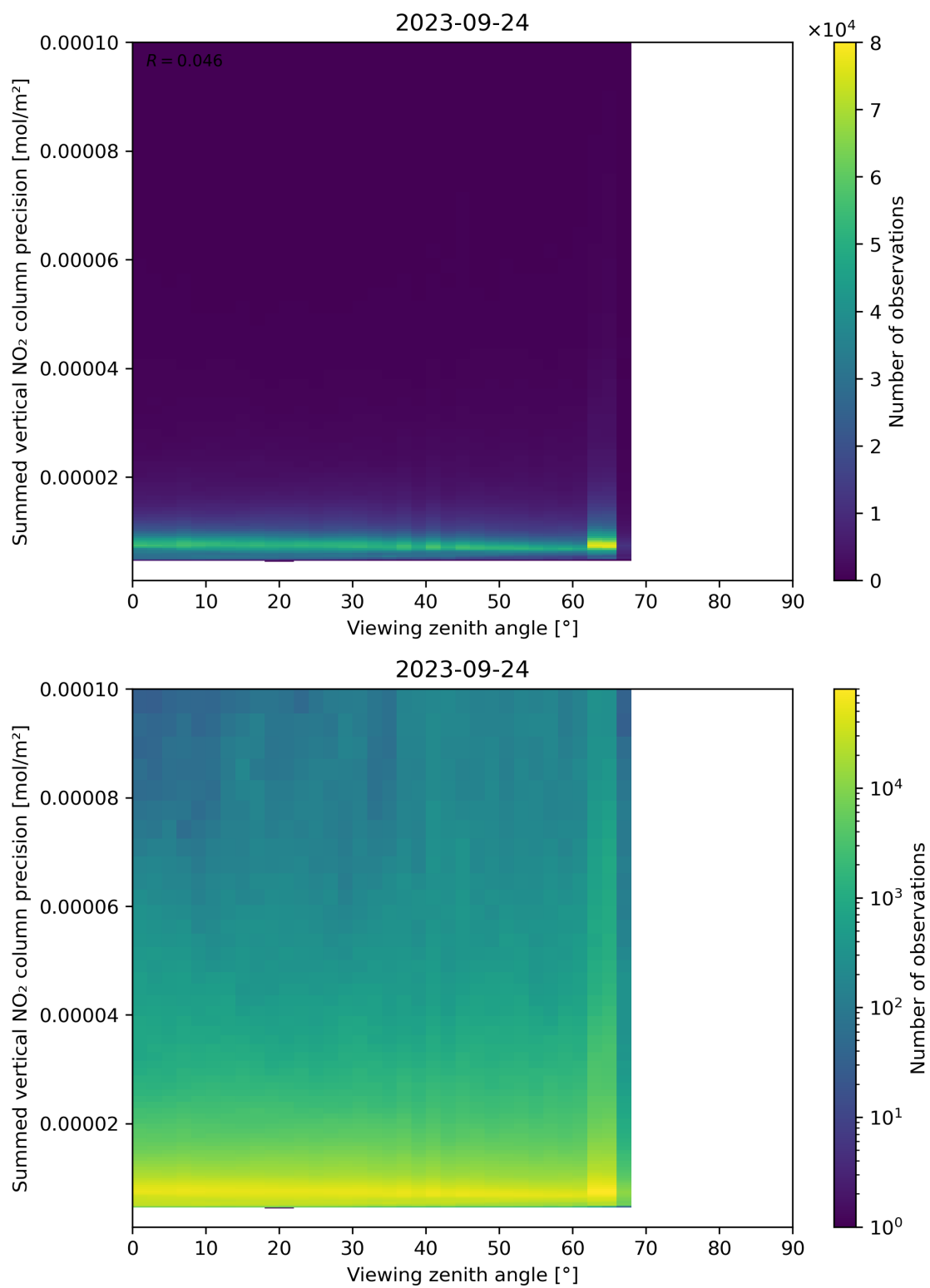
Figure 166: Scatter density plot of “Viewing zenith angle” against “Summed vertical NO 2 column precision” for 2023-09-23 to 2023-09-25.
