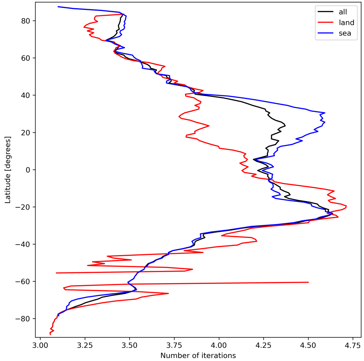
Figure 17: Zonal average of “Number of iterations” for 2023-09-23 to 2023-09-25.
