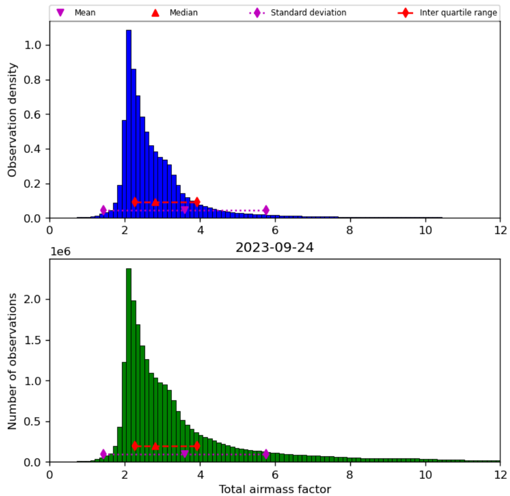
Figure 32: Histogram of “Total airmass factor” for 2023-09-23 to 2023-09-25
