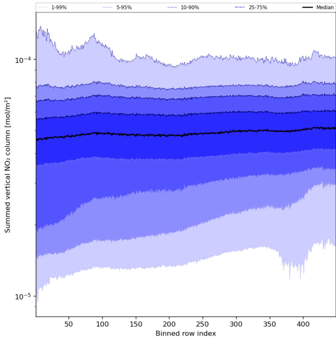
Figure 57: Along track statistics of “Summed vertical NO 2 column” for 2023-09-23 to 2023-09-25
