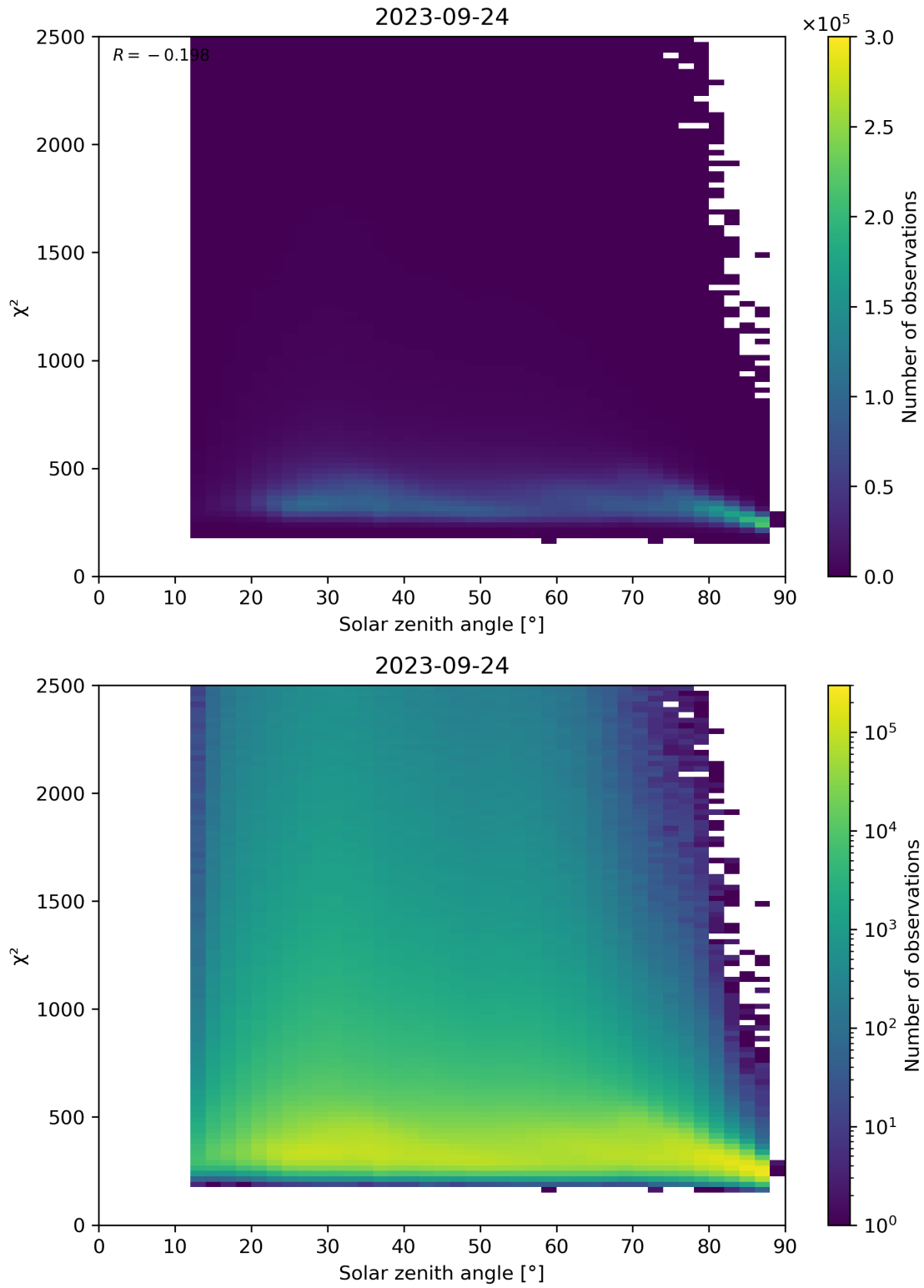
Figure 148: Scatter density plot of “Solar zenith angle” against “ \chi^2 ” for 2023-09-23 to 2023-09-25.
