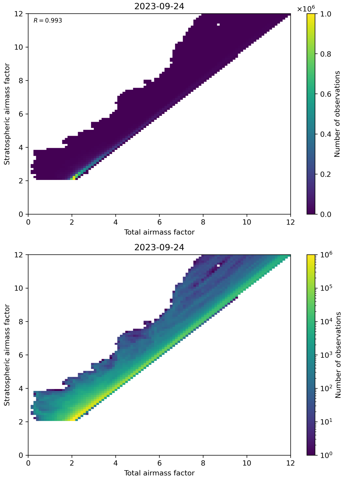
Figure 62: Scatter density plot of “Total airmass factor” against “Stratospheric airmass factor” for 2023-09-23 to 2023-09-25.
