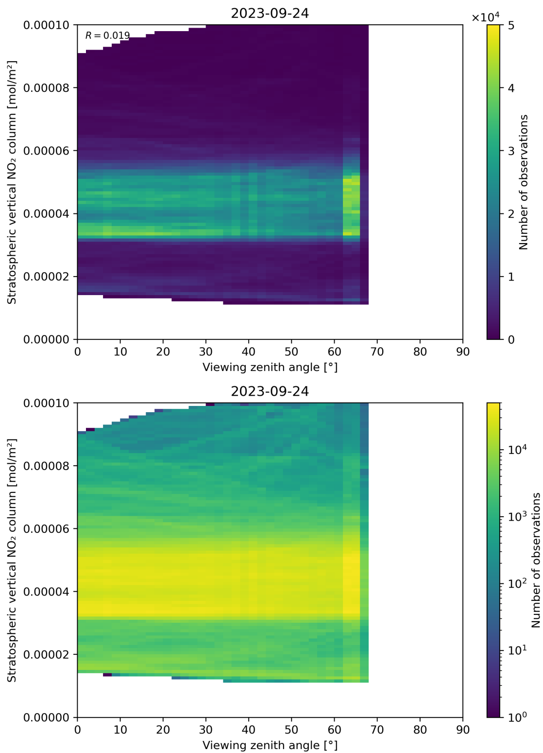
Figure 164: Scatter density plot of “Viewing zenith angle” against “Stratospheric vertical NO 2 column” for 2023-09-23 to 2023-09-25.
