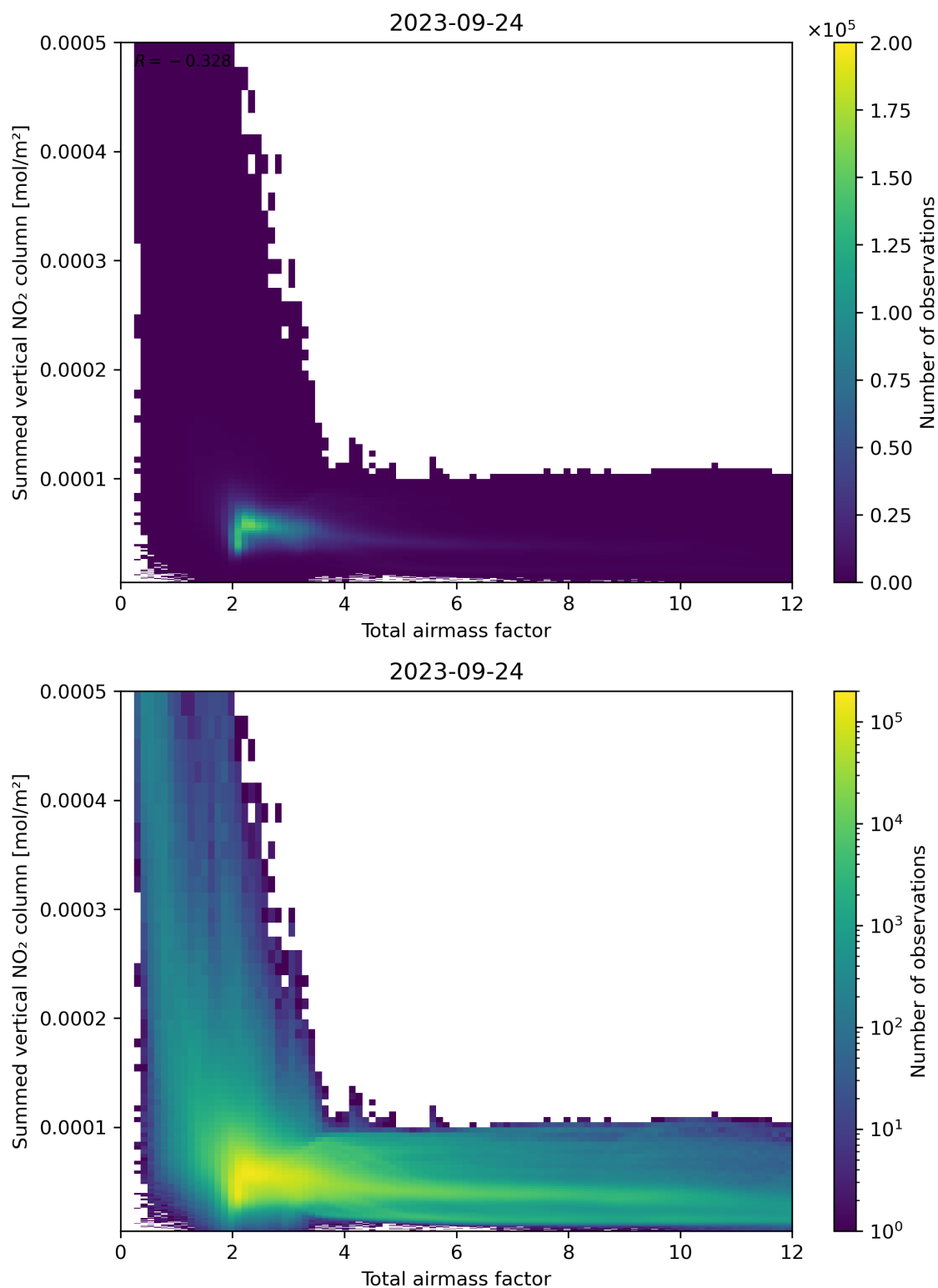
Figure 65: Scatter density plot of “Total airmass factor” against “Summed vertical NO 2 column” for 2023-09-23 to 2023-09-25.
