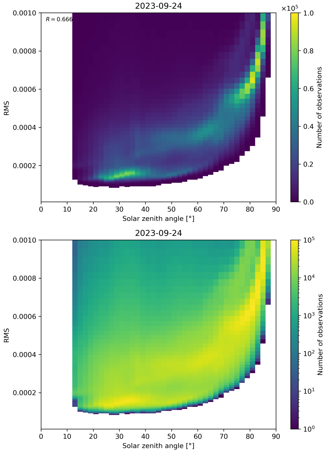
Figure 157: Scatter density plot of “Solar zenith angle” against “RMS” for 2023-09-23 to 2023-09-25.
