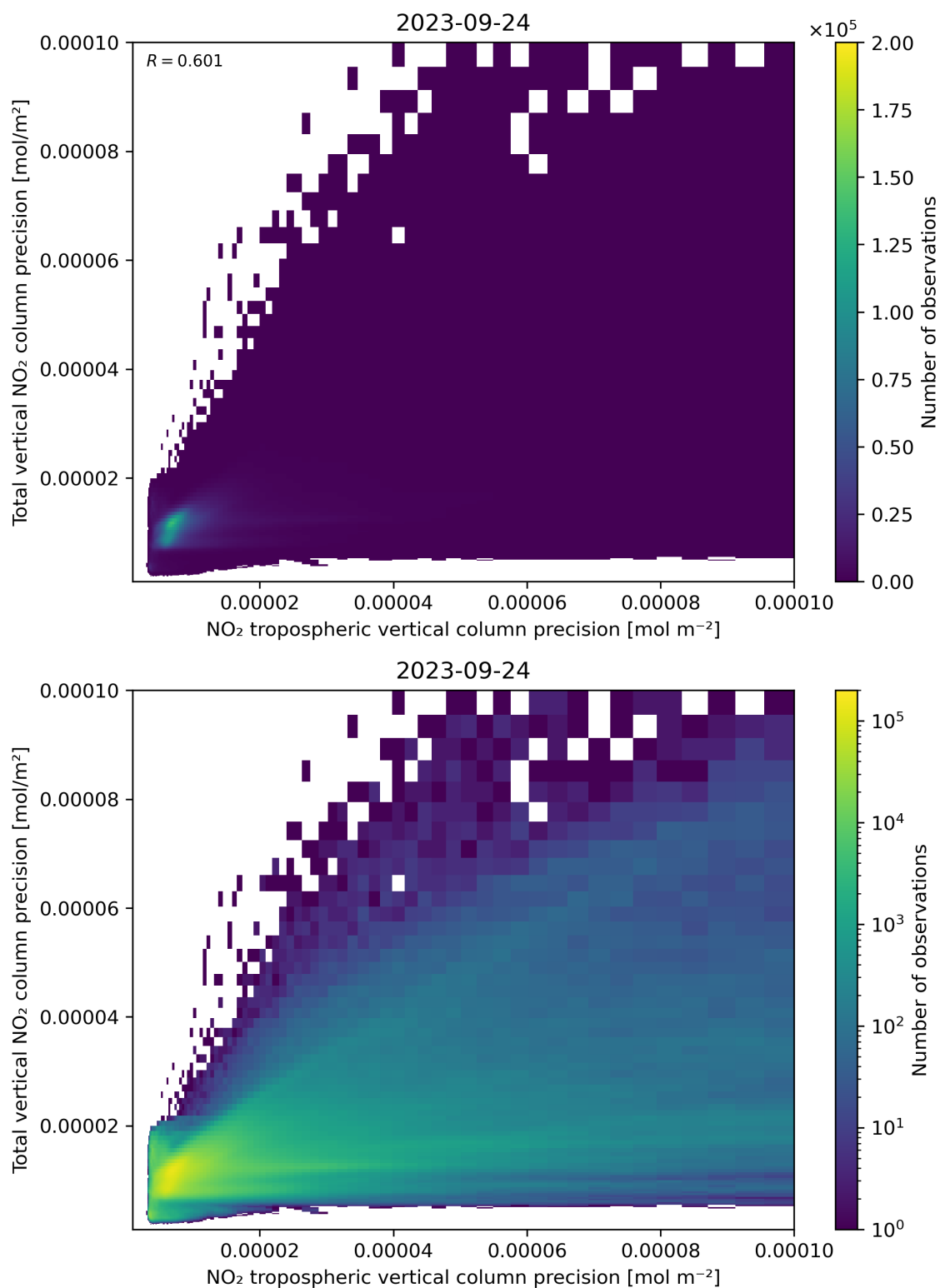
Figure 139: Scatter density plot of “NO 2 tropospheric vertical column precision” against “Total vertical NO 2 column precision” for 2023-09-23 to 2023-09-25.
