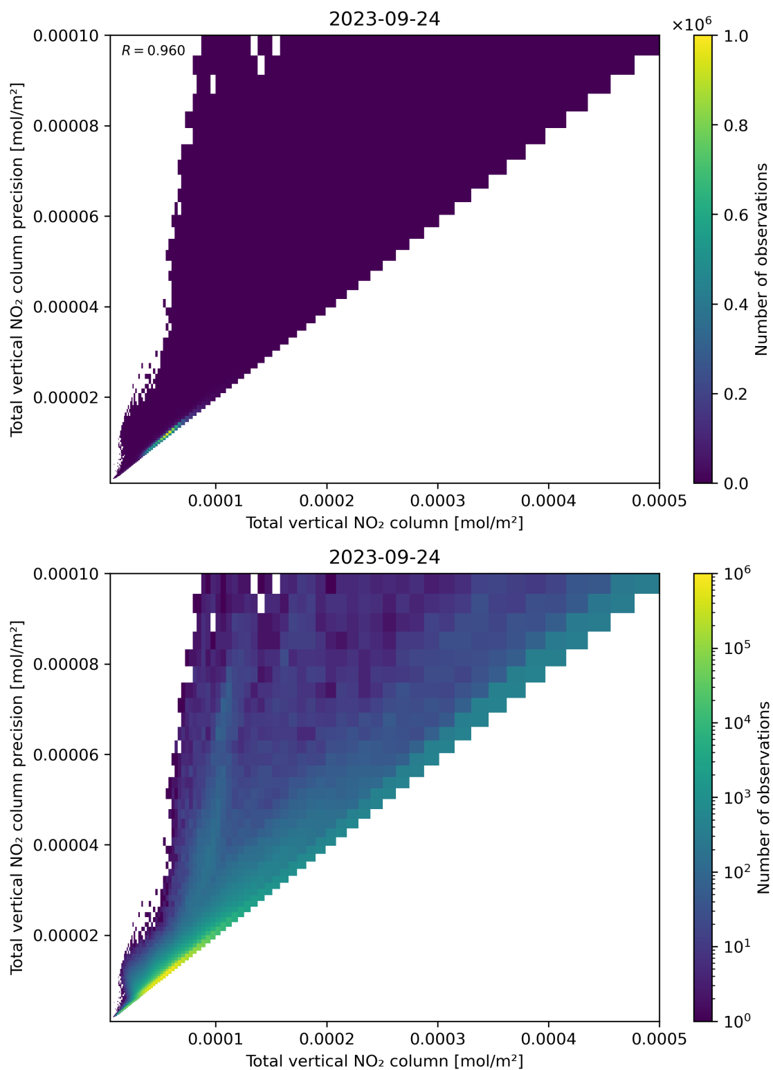
Figure 114: Scatter density plot of “Total vertical NO 2 column” against “Total vertical NO 2 column precision” for 2023-09-23 to 2023-09-25.
