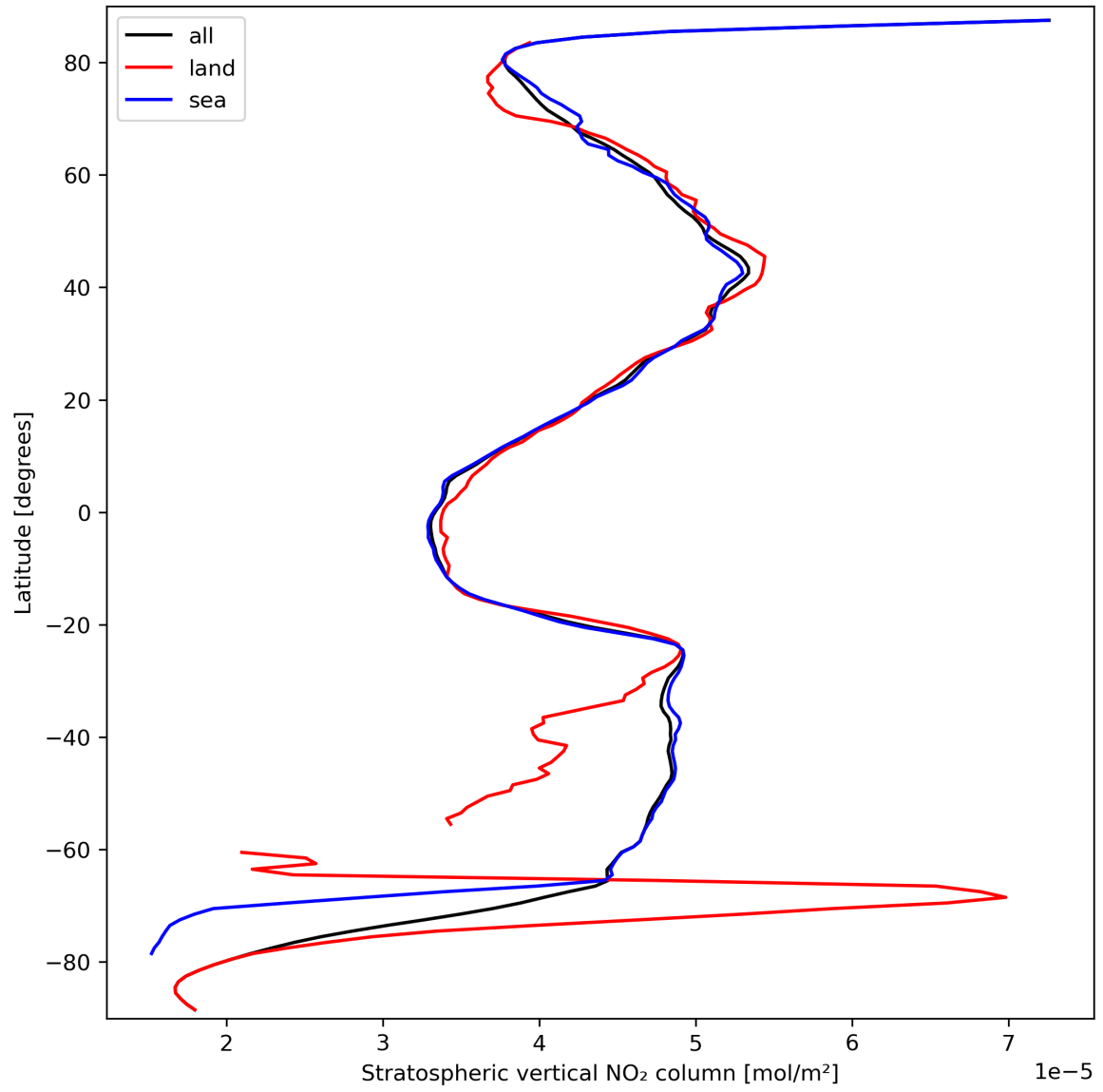
Figure 19: Zonal average of “Stratospheric vertical NO 2 column” for 2023-09-23 to 2023-09-25.
