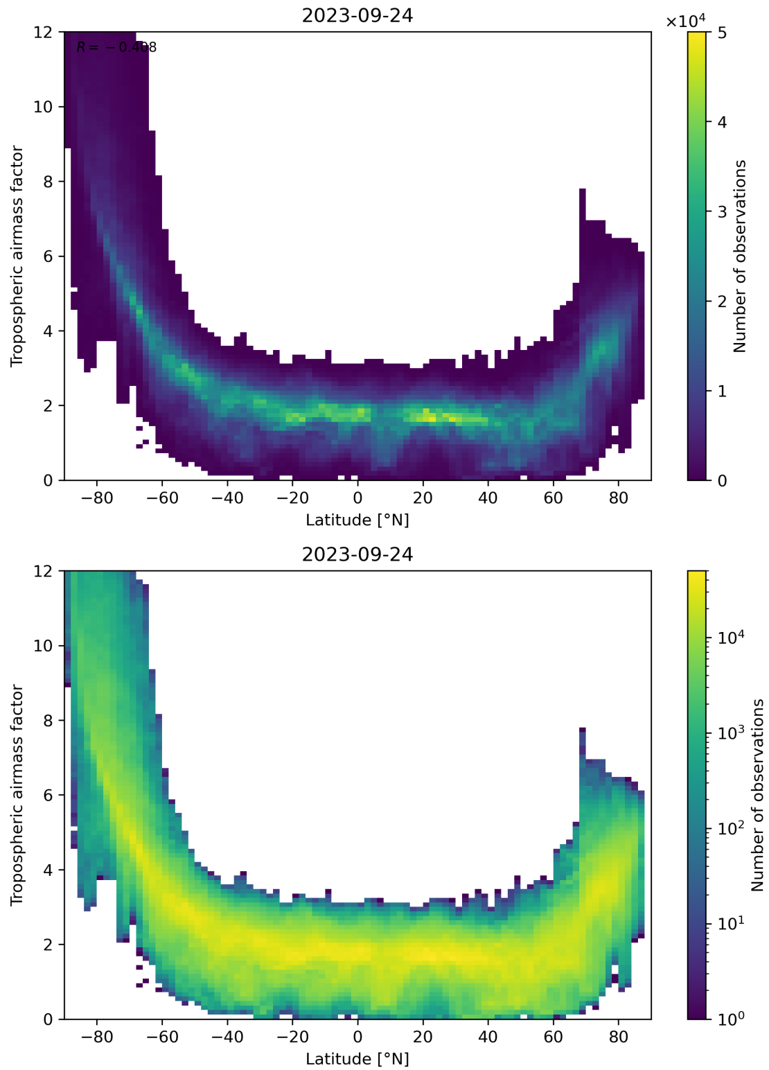
Figure 85: Scatter density plot of “Latitude” against “Tropospheric airmass factor” for 2023-09-23 to 2023-09-25.
