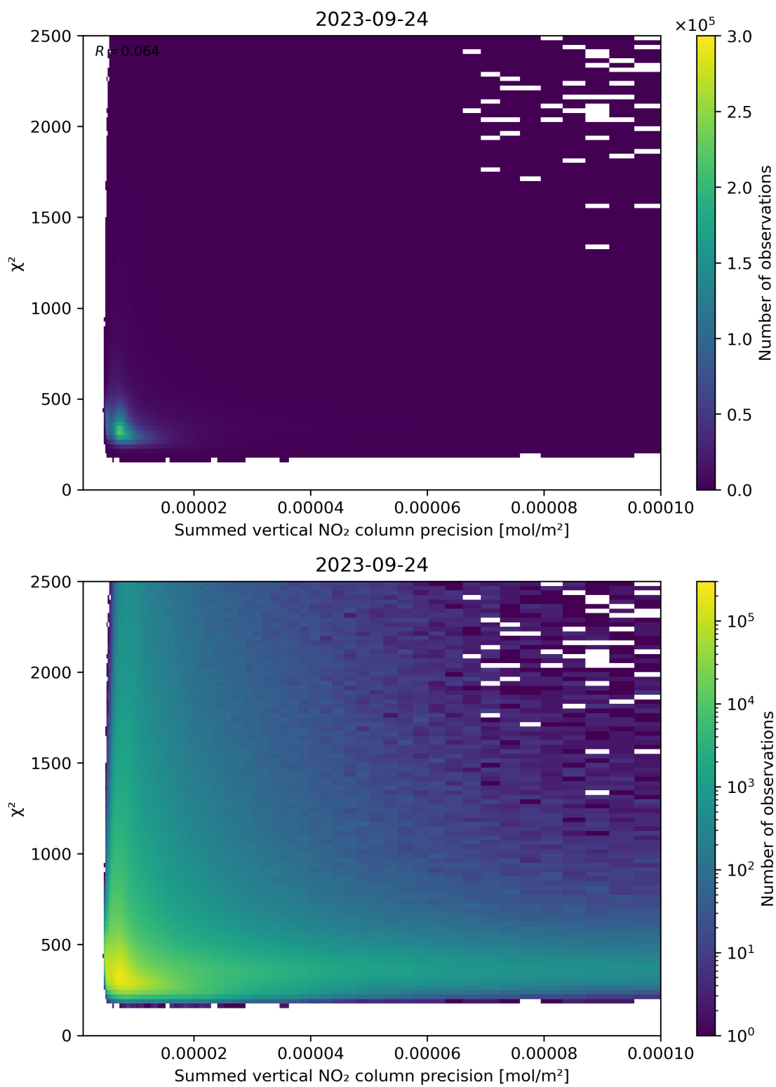
Figure 107: Scatter density plot of “Summed vertical NO 2 column precision” against “ \chi^2 ” for 2023-09-23 to 2023-09-25.
