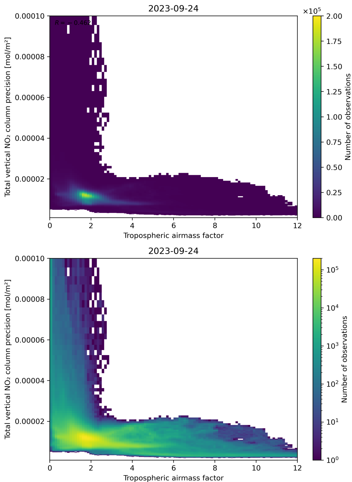
Figure 78: Scatter density plot of “Tropospheric air mass factor” against “Total vertical NO 2 column precision” for 2023-09-23 to 2023-09-25.
