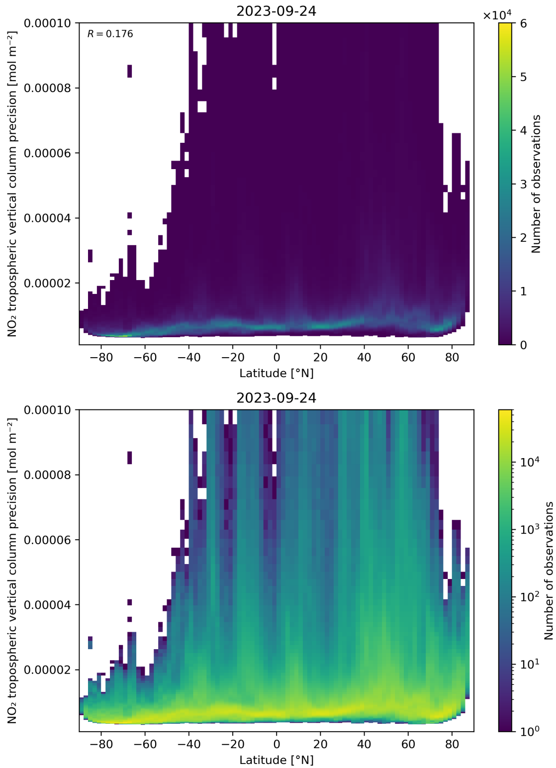
Figure 93: Scatter density plot of “Latitude” against “NO 2 tropospheric vertical column precision” for 2023-09-23 to 2023-09-25.
