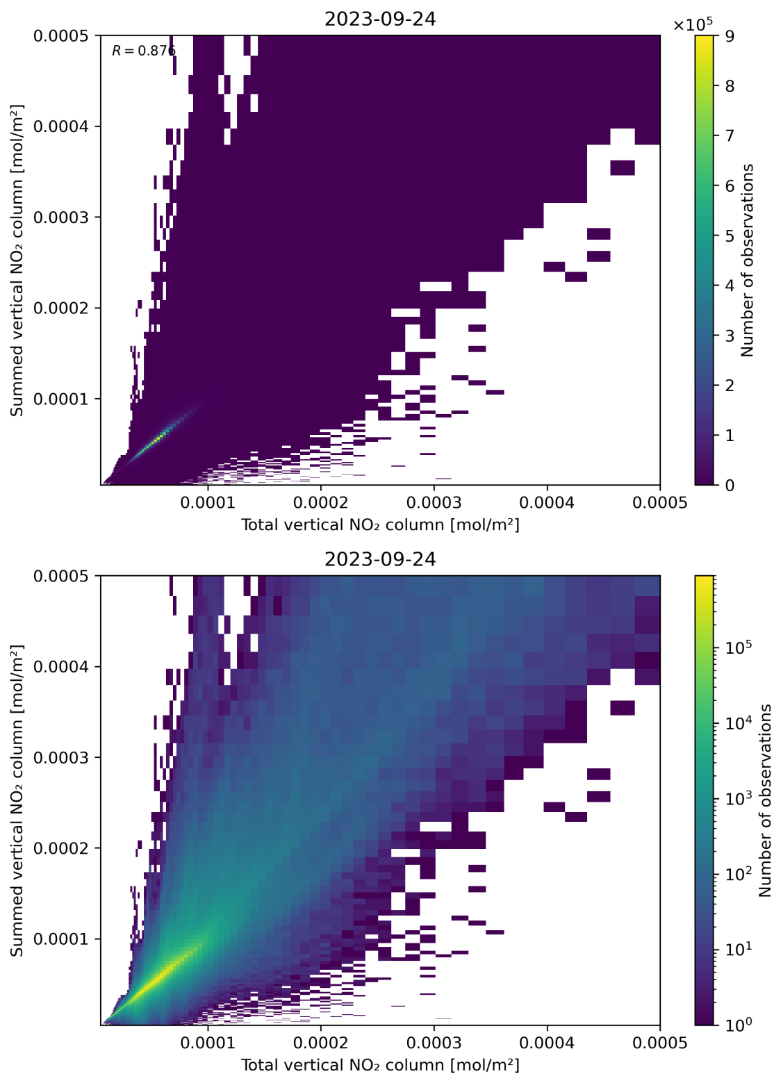
Figure 112: Scatter density plot of “Total vertical NO 2 column” against “Summed vertical NO 2 column” for 2023-09-23 to 2023-09-25.
