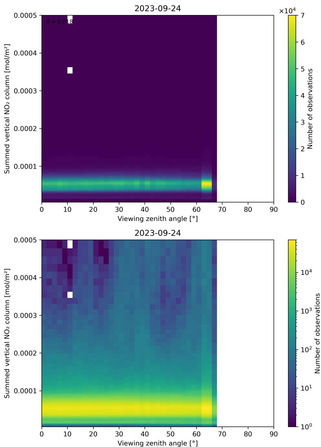
Figure 165: Scatter density plot of “Viewing zenith angle” against “Summed vertical NO 2 column” for 2023-09-23 to 2023-09-25.
