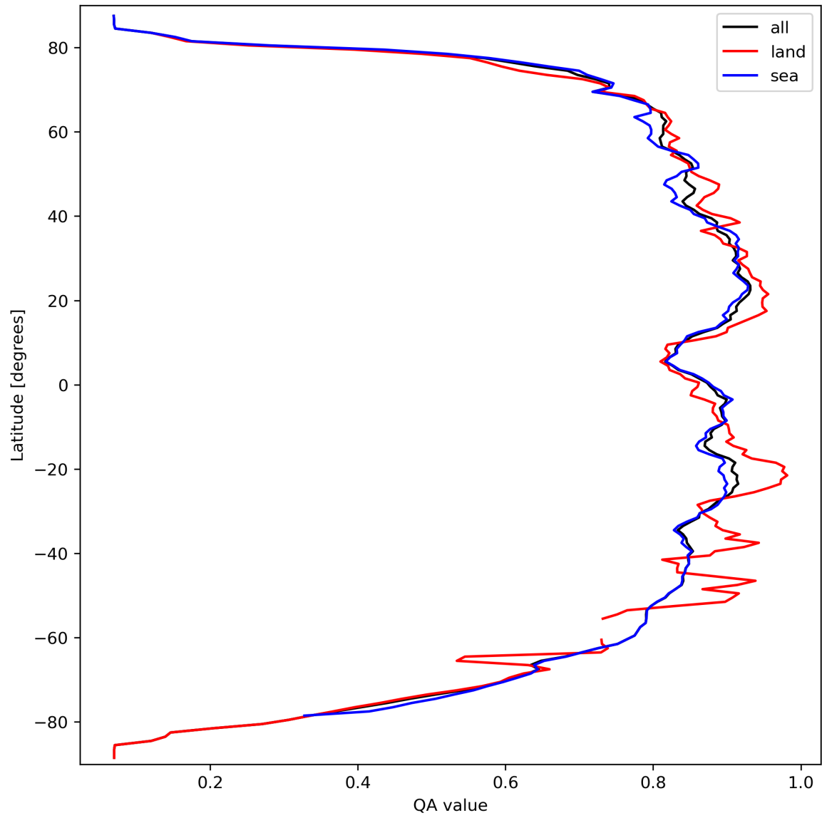
Figure 11: Zonal average of “QA value” for 2023-09-23 to 2023-09-25.
