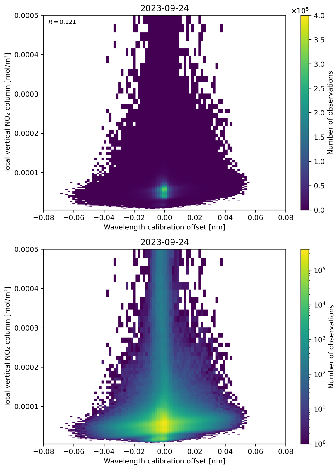
Figure 179: Scatter density plot of “Wavelength calibration offset” against “Total vertical NO 2 column” for 2023-09-23 to 2023-09-25.
