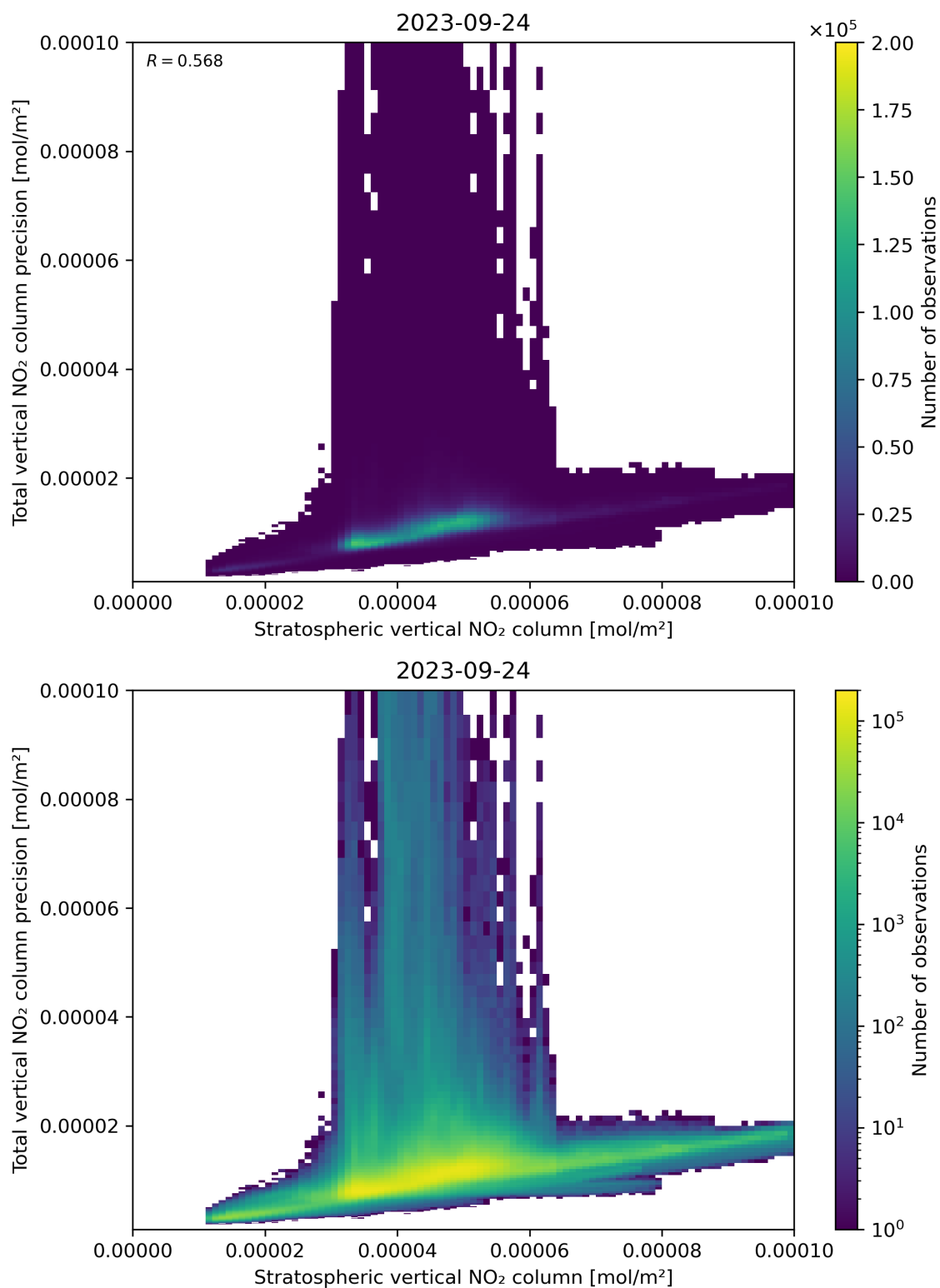
Figure 101: Scatter density plot of “Stratospheric vertical NO 2 column” against “Total vertical NO 2 column precision” for 2023-09-23 to 2023-09-25.
