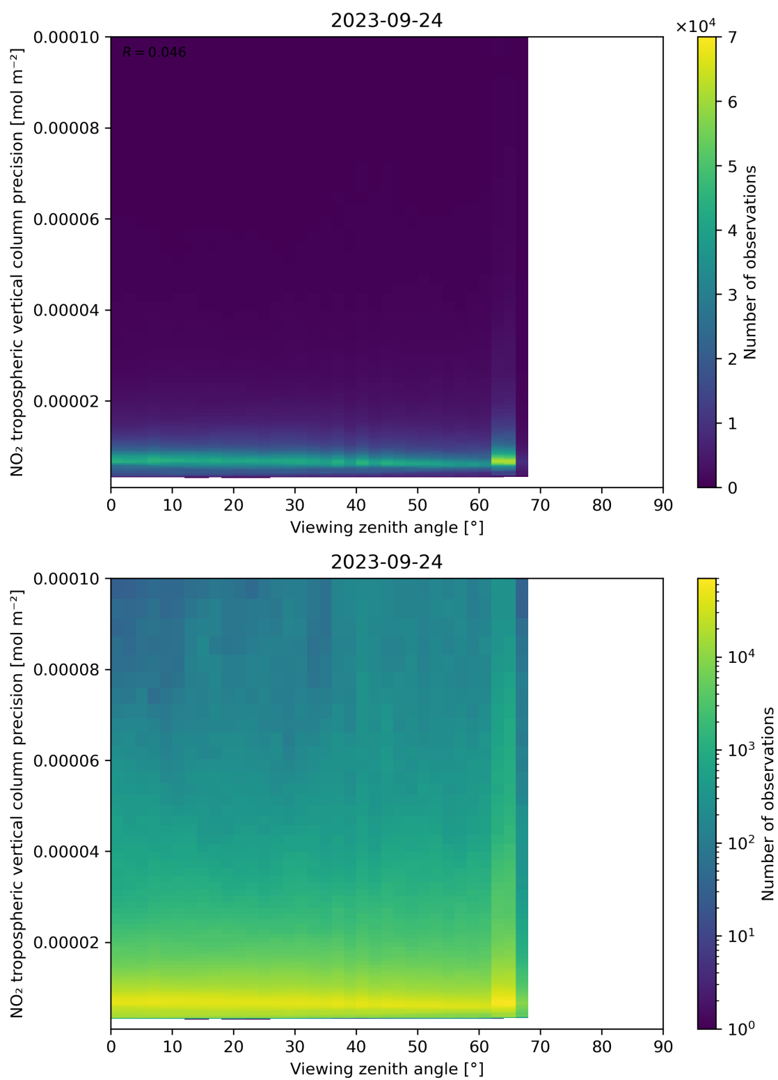
Figure 170: Scatter density plot of “Viewing zenith angle” against “NO 2 tropospheric vertical column precision” for 2023-09-23 to 2023-09-25.
