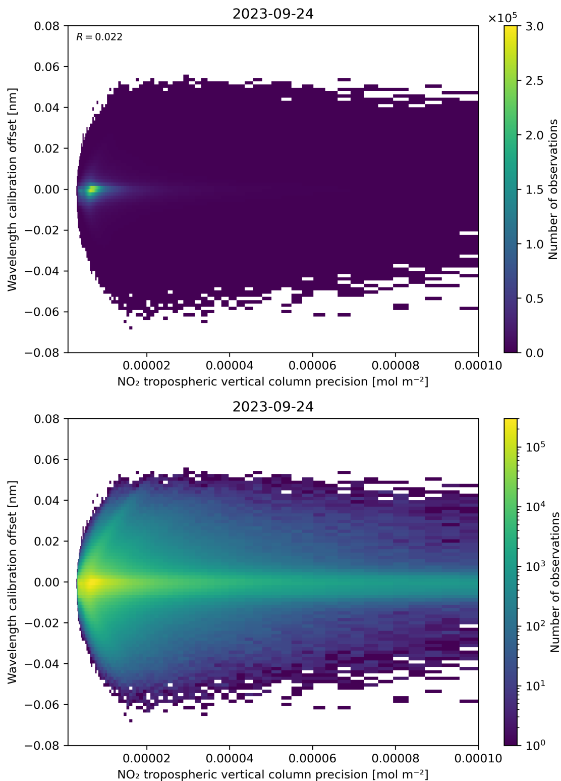
Figure 141: Scatter density plot of “NO 2 tropospheric vertical column precision” against “Wavelength calibration offset” for 2023-09-23 to 2023-09-25.
