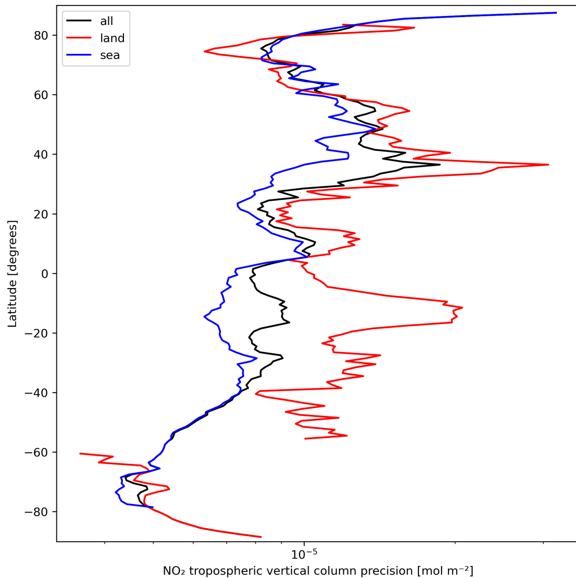
Figure 13: Zonal average of “NO 2 tropospheric vertical column precision” for 2023-09-23 to 2023-09-25.
