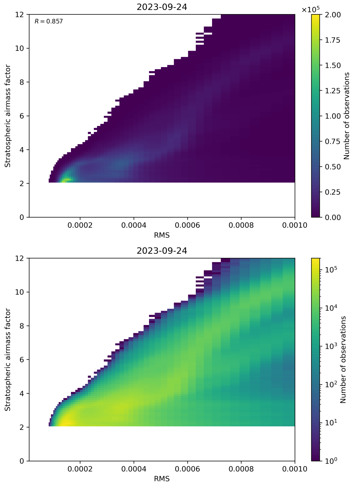
Figure 144: Scatter density plot of “RMS” against “Stratospheric airmass factor” for 2023-09-23 to 2023-09-25.
