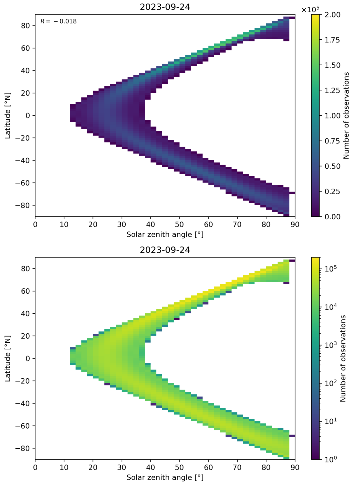
Figure 149: Scatter density plot of “Solar zenith angle” against “Latitude” for 2023-09-23 to 2023-09-25.
