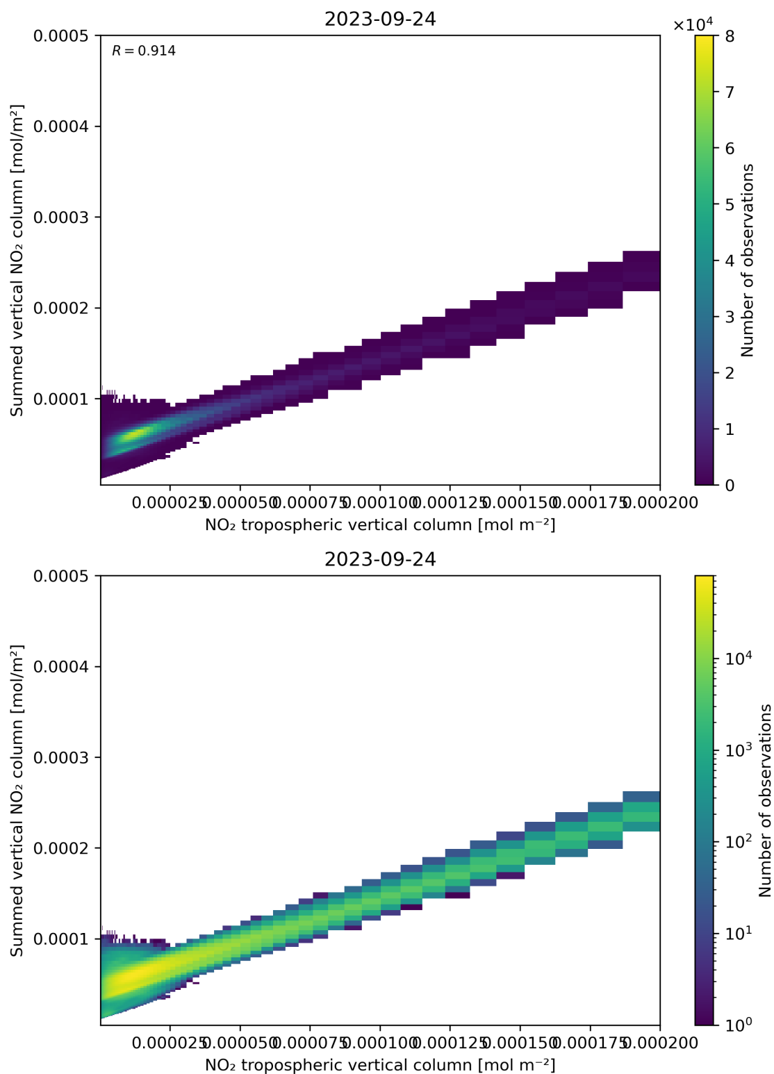
Figure 126: Scatter density plot of “NO 2 tropospheric vertical column” against “Summed vertical NO 2 column” for 2023-09-23 to 2023-09-25.
