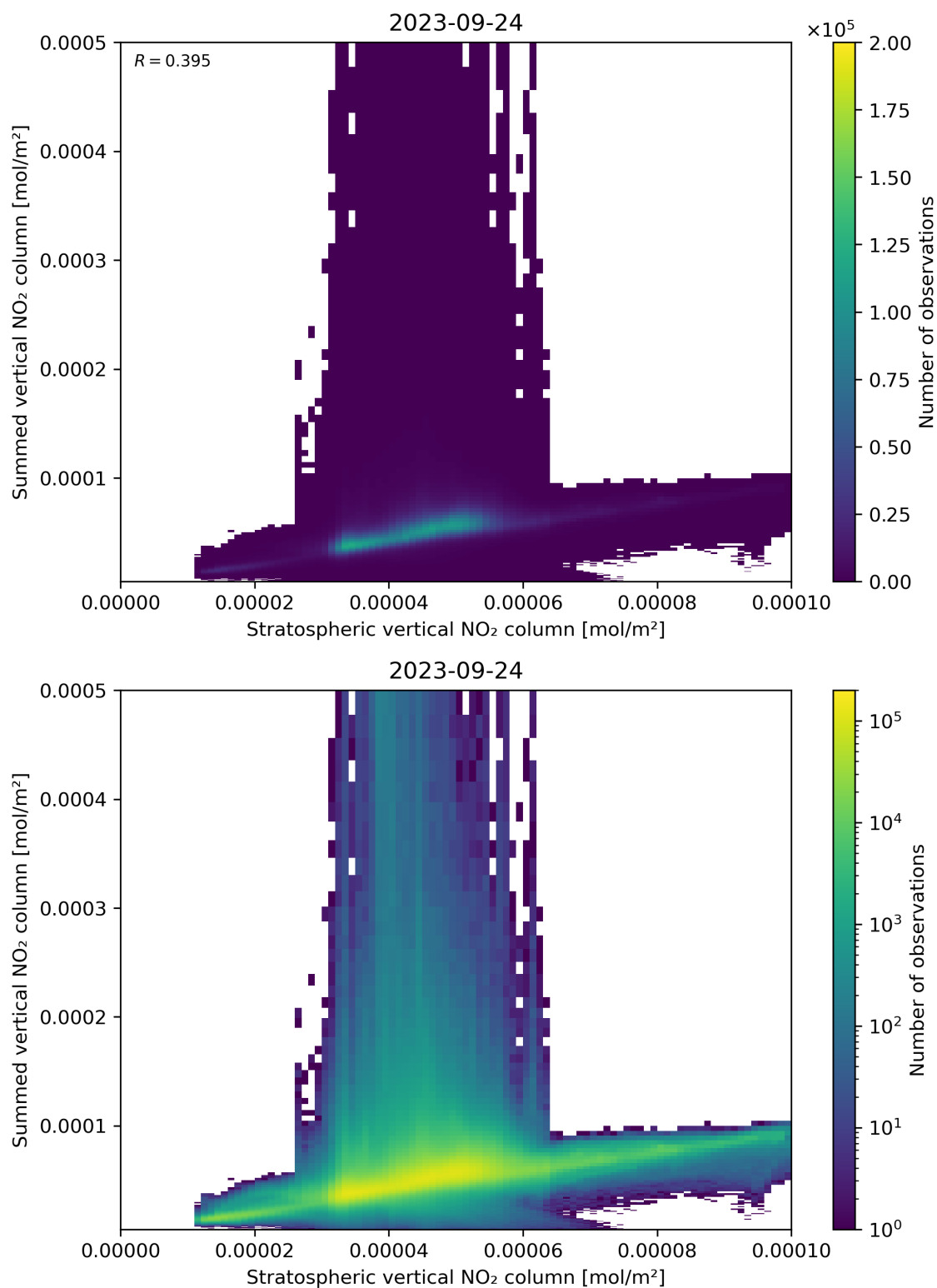
Figure 98: Scatter density plot of “Stratospheric vertical NO 2 column” against “Summed vertical NO 2 column” for 2023-09-23 to 2023-09-25.
