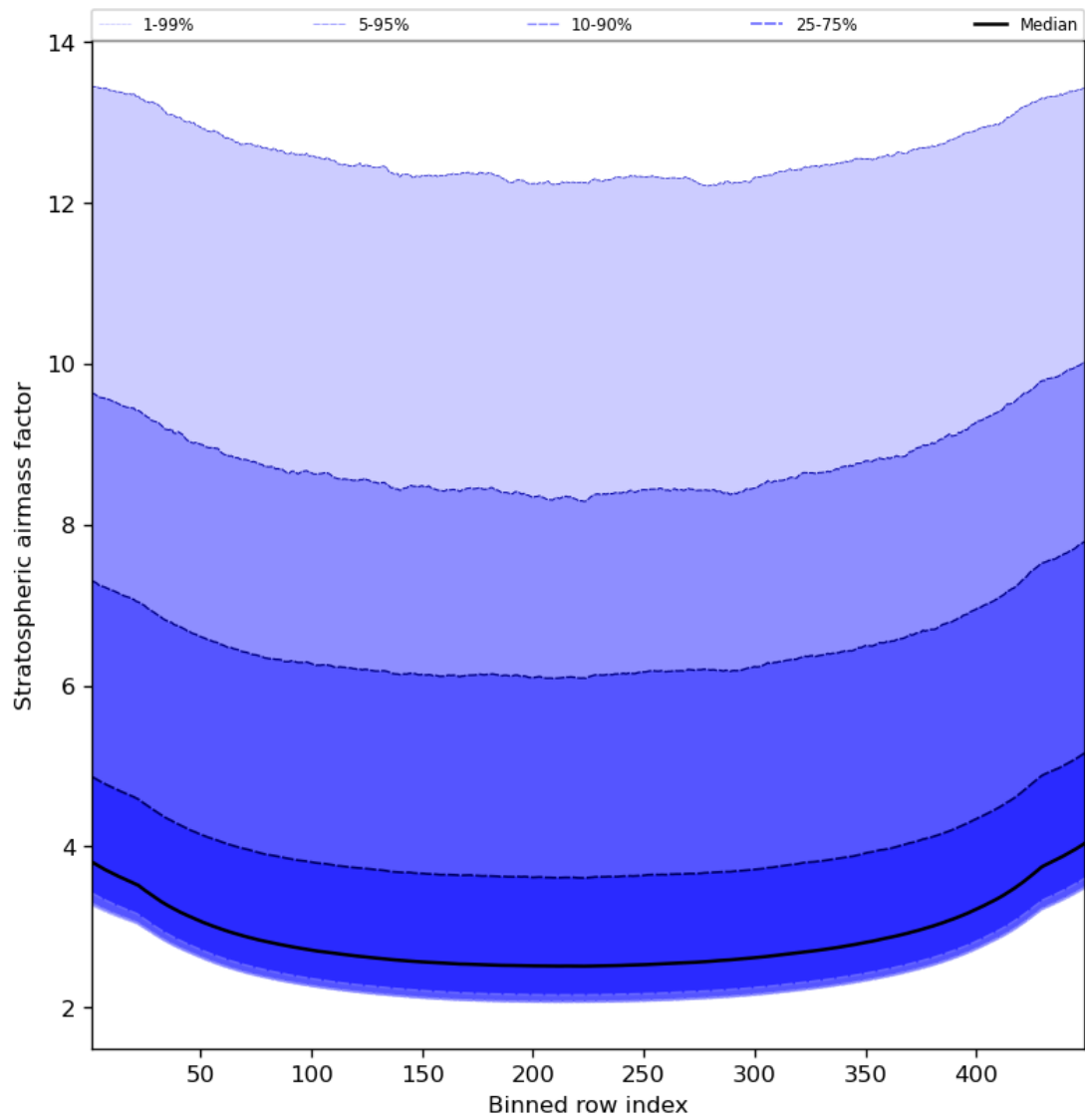
Figure 61: Along track statistics of “Stratospheric airmass factor” for 2023-09-23 to 2023-09-25
