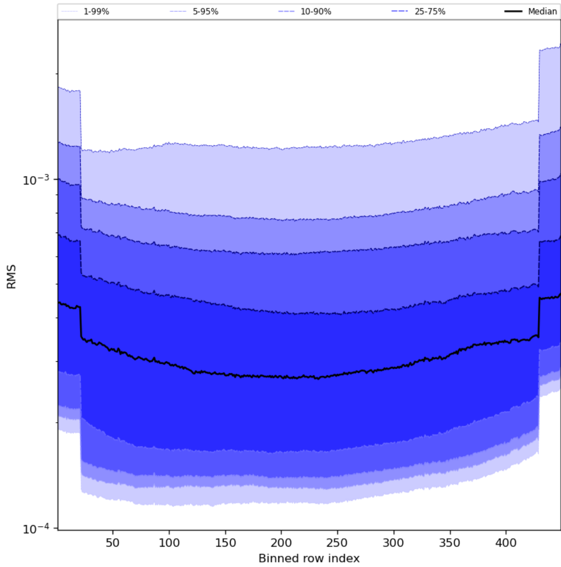
Figure 60: Along track statistics of “RMS” for 2023-09-24 to 2023-09-26
