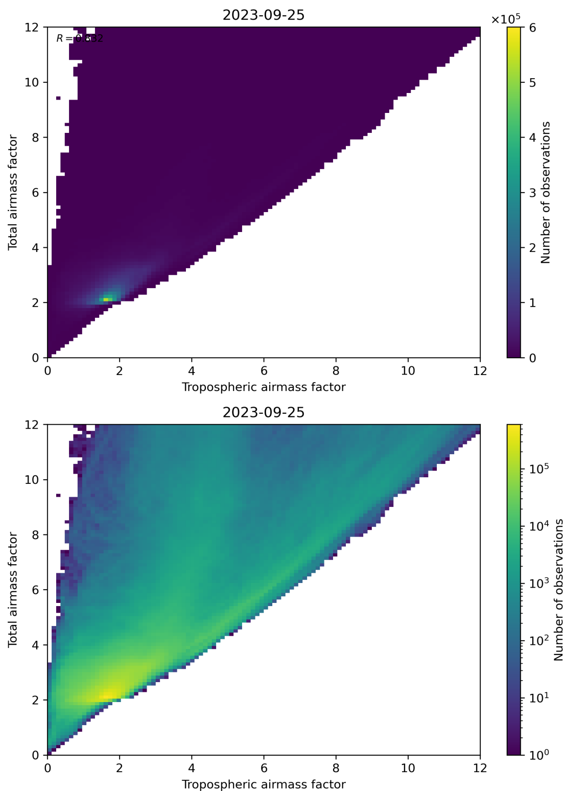
Figure 72: Scatter density plot of “Tropospheric airmass factor” against “Total airmass factor” for 2023-09-24 to 2023-09-26.
