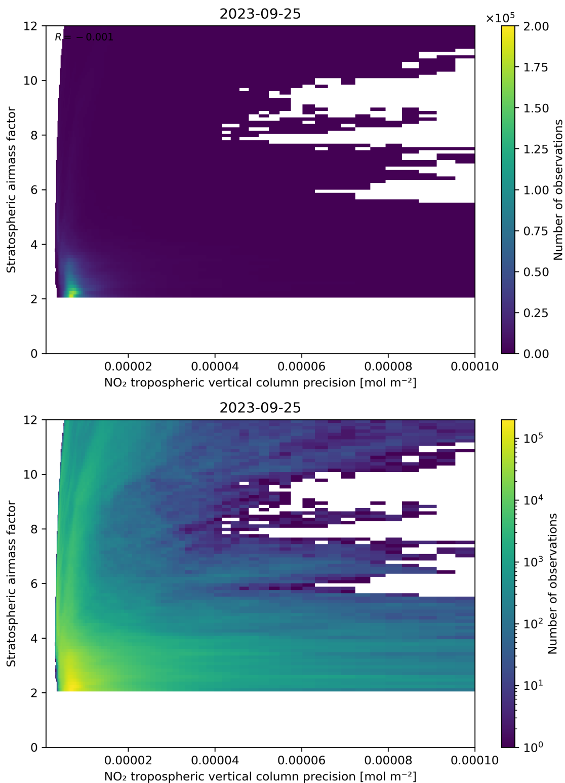
Figure 131: Scatter density plot of “NO 2 tropospheric vertical column precision” against “Stratospheric airmass factor” for 2023-09-24 to 2023-09-26.
