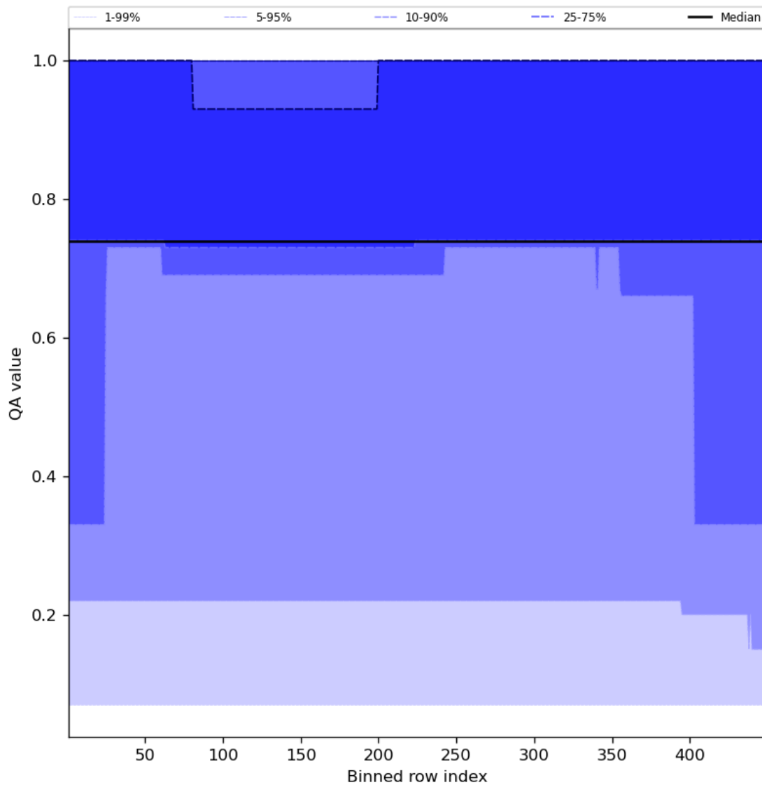
Figure 45: Along track statistics of "QA value" for 2023-09-24 to 2023-09-26
