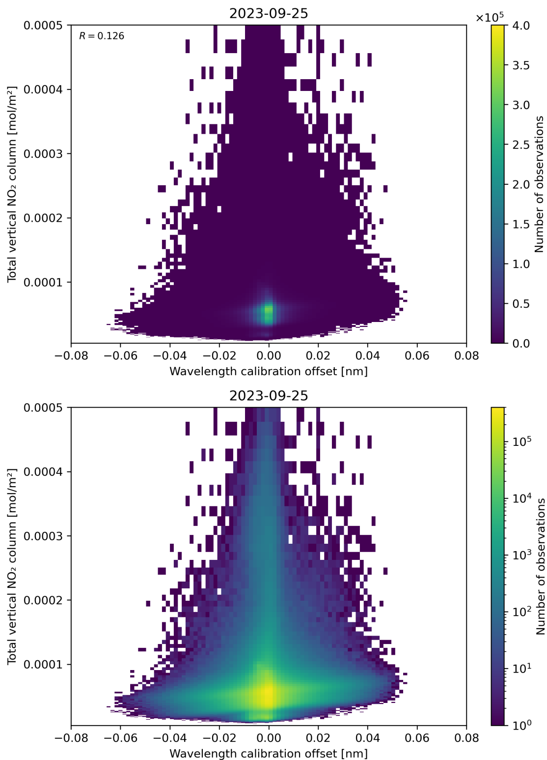
Figure 179: Scatter density plot of “Wavelength calibration offset” against “Total vertical NO 2 column” for 2023-09-24 to 2023-09-26.
