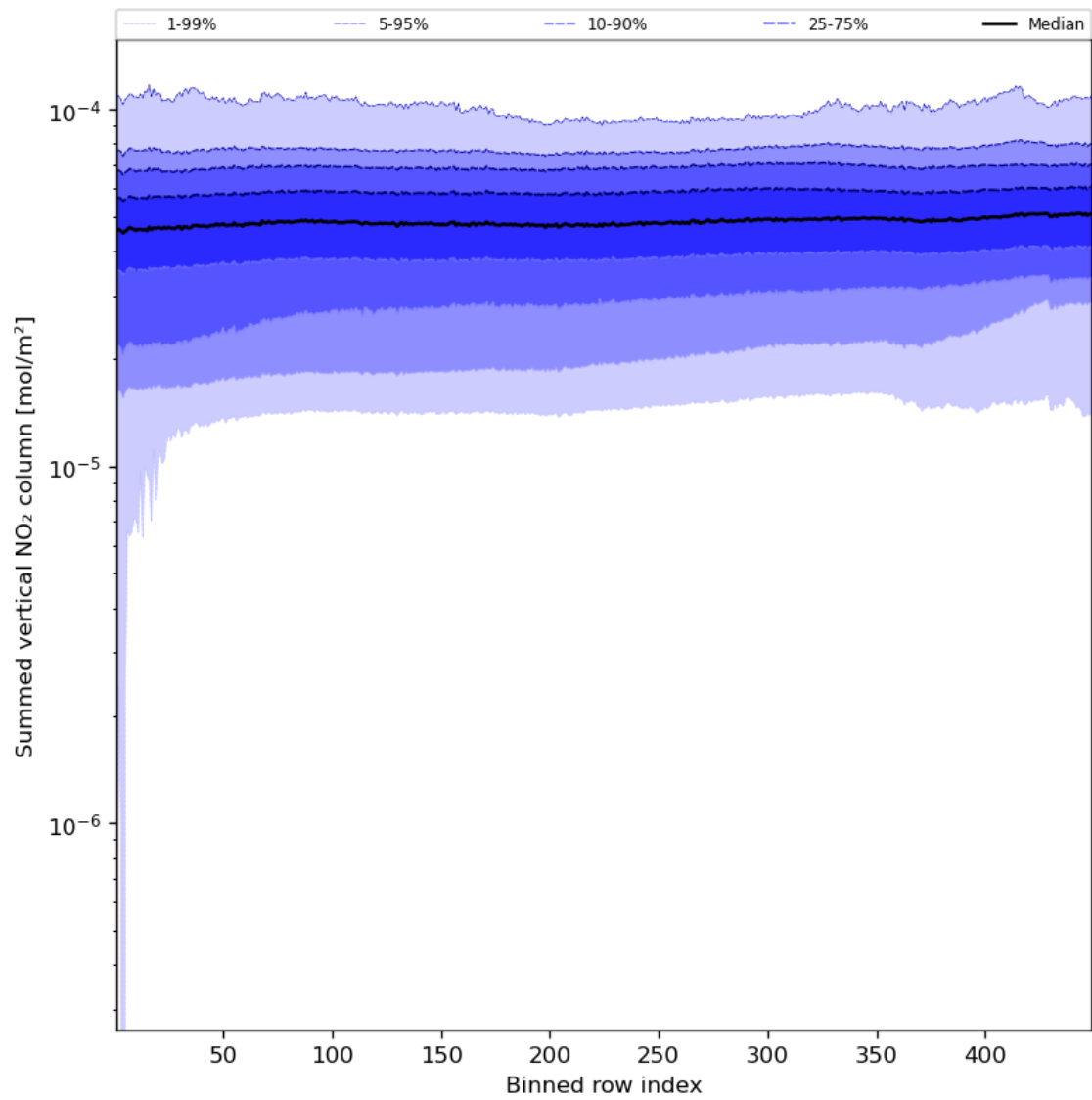
Figure 57: Along track statistics of “Summed vertical NO 2 column” for 2023-09-24 to 2023-09-26
