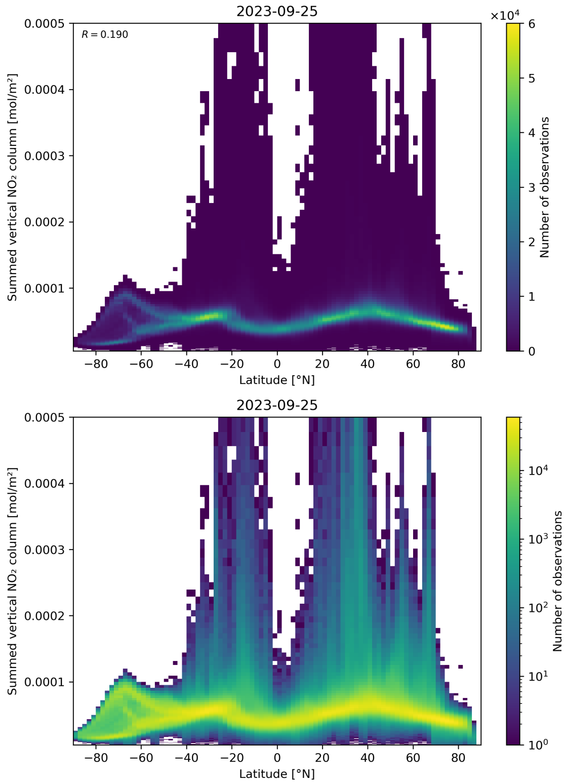
Figure 88: Scatter density plot of “Latitude” against “Summed vertical NO 2 column” for 2023-09-24 to 2023-09-26.
