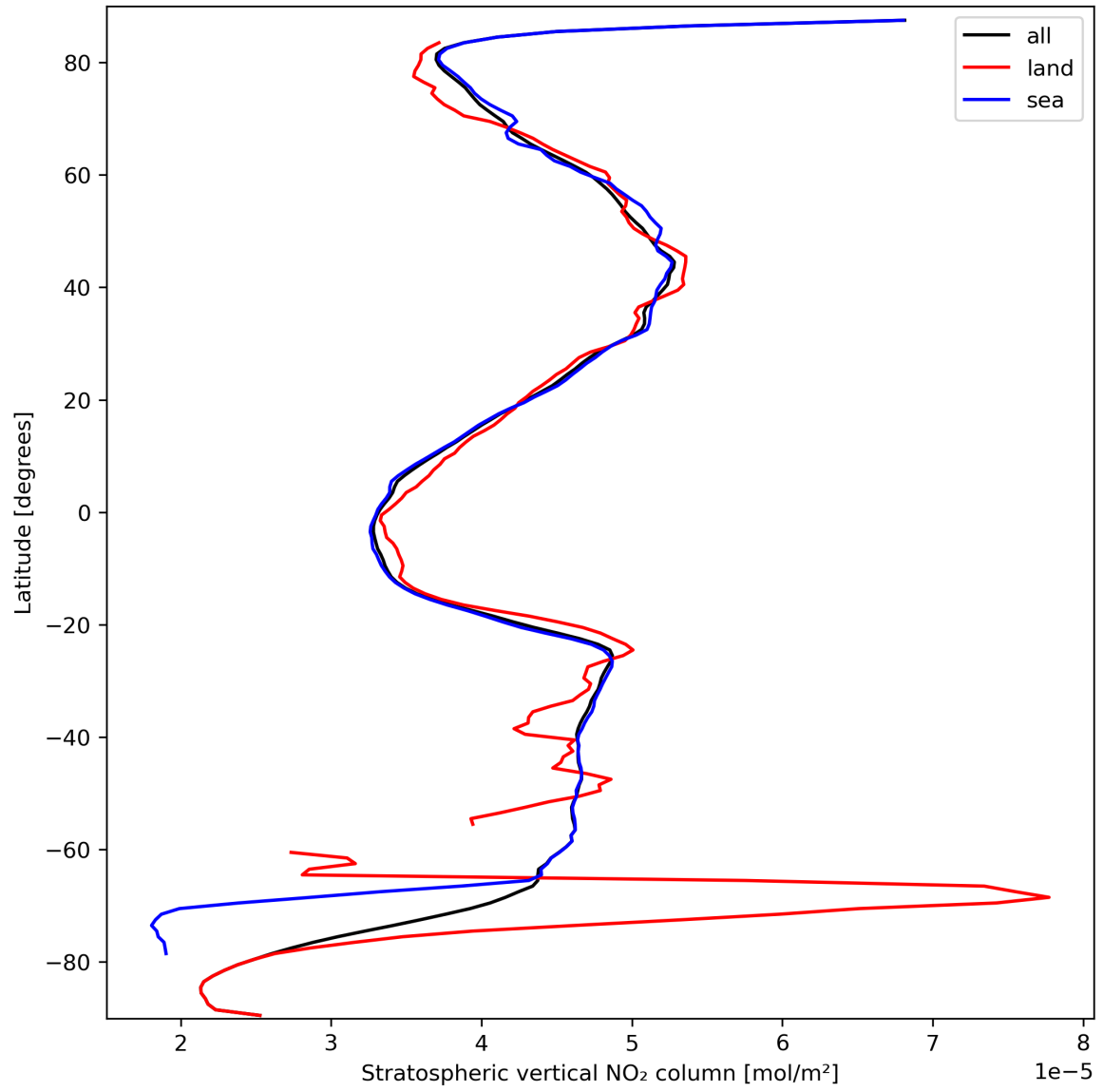
Figure 19: Zonal average of “Stratospheric vertical NO 2 column” for 2023-09-24 to 2023-09-26.
