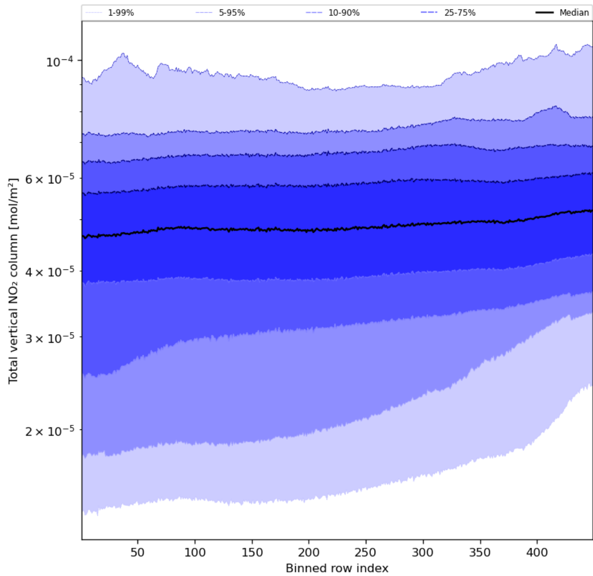
Figure 55: Along track statistics of “Total vertical NO 2 column” for 2023-09-24 to 2023-09-26
