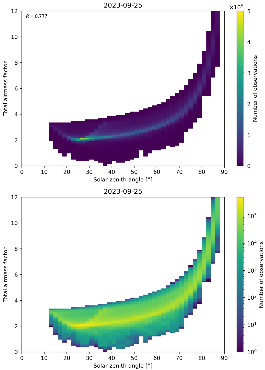
Figure 146: Scatter density plot of “Solar zenith angle” against “Total air mass factor” for 2023-09-24 to 2023-09-26.
