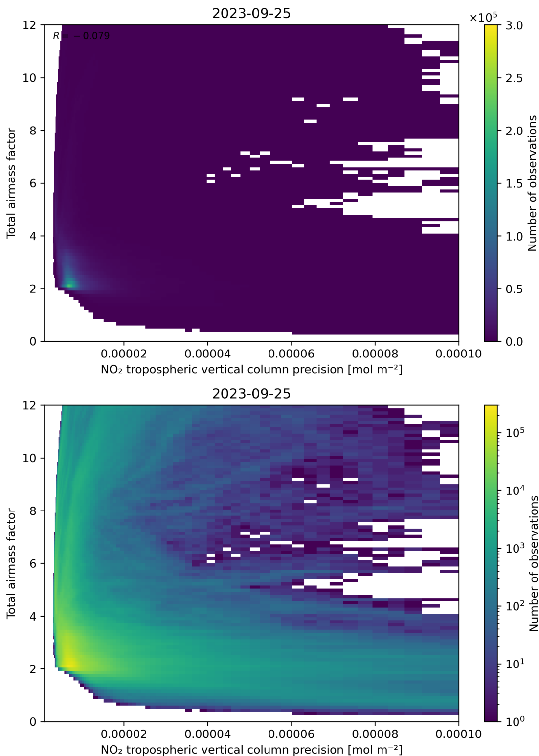
Figure 132: Scatter density plot of “NO 2 tropospheric vertical column precision” against “Total air mass factor” for 2023-09-24 to 2023-09-26.
