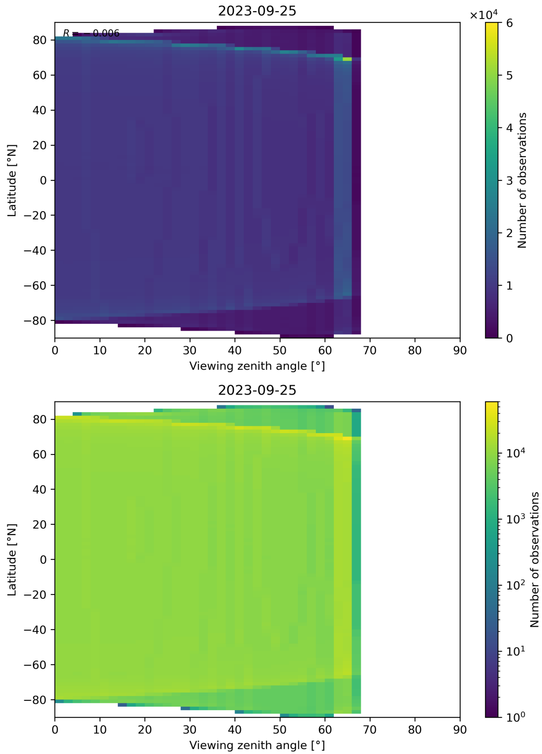
Figure 163: Scatter density plot of “Viewing zenith angle” against “Latitude” for 2023-09-24 to 2023-09-26.
