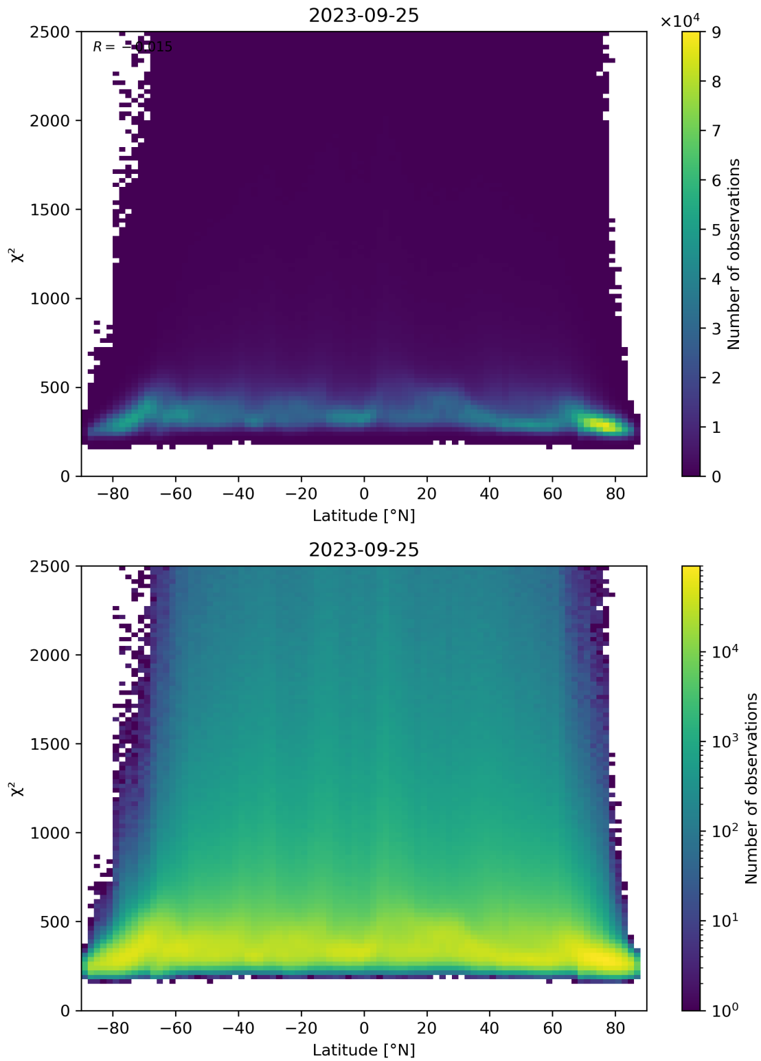
Figure 86: Scatter density plot of “Latitude” against “ \chi^2 ” for 2023-09-24 to 2023-09-26.
