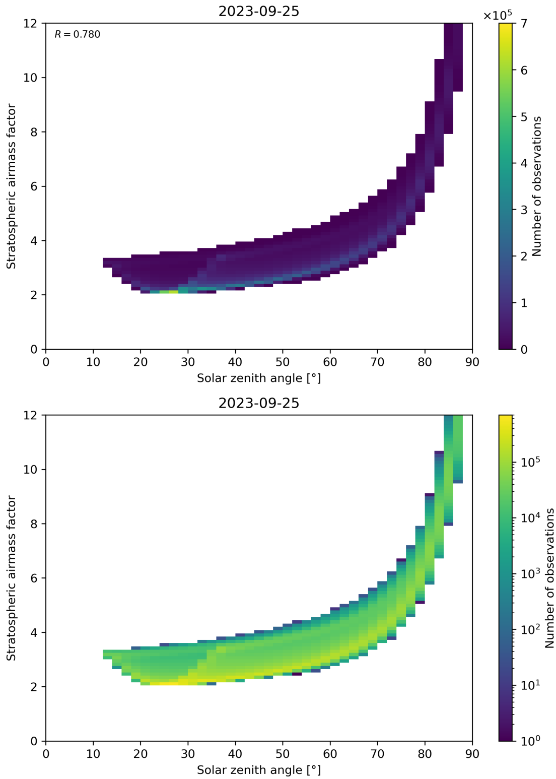
Figure 145: Scatter density plot of “Solar zenith angle” against “Stratospheric airmass factor” for 2023-09-24 to 2023-09-26.
