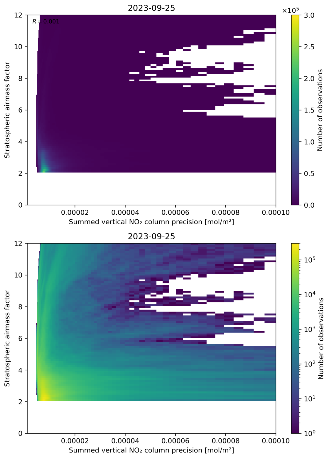
Figure 106: Scatter density plot of “Summed vertical NO 2 column precision” against “Stratospheric airmass factor” for 2023-09-24 to 2023-09-26.
