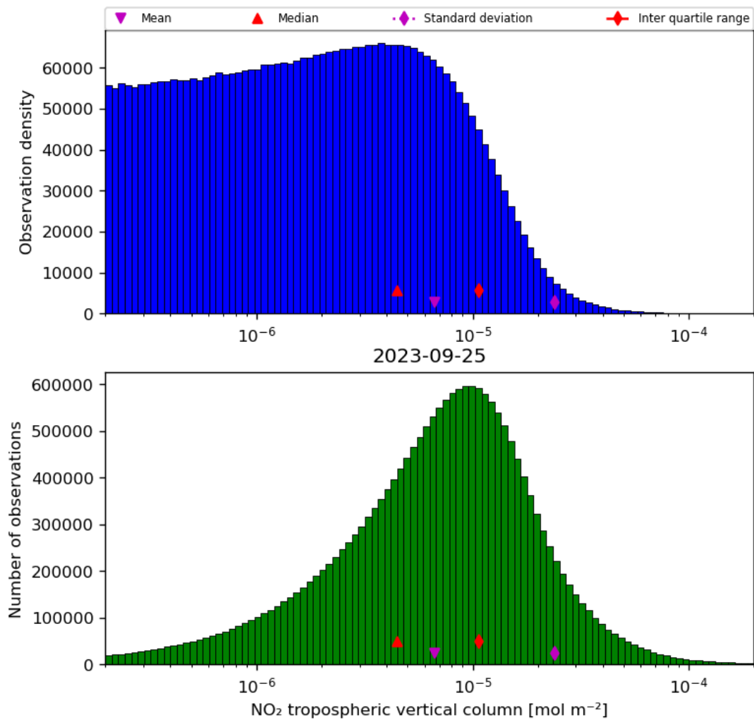
Figure 29: Histogram of “NO 2 tropospheric vertical column” for 2023-09-24 to 2023-09-26
