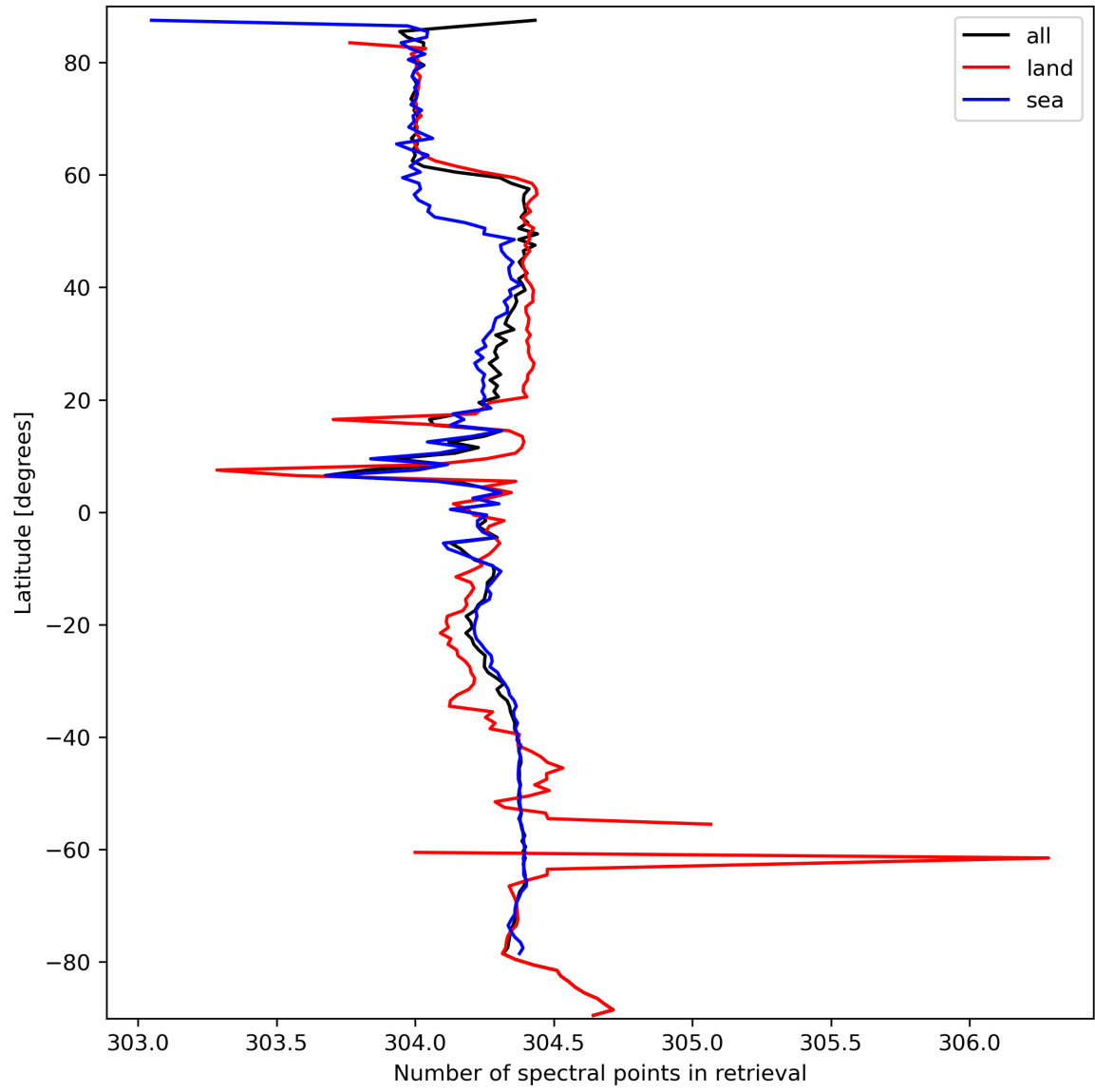
Figure 16: Zonal average of “Number of spectral points in retrieval” for 2023-09-24 to 2023-09-26.
