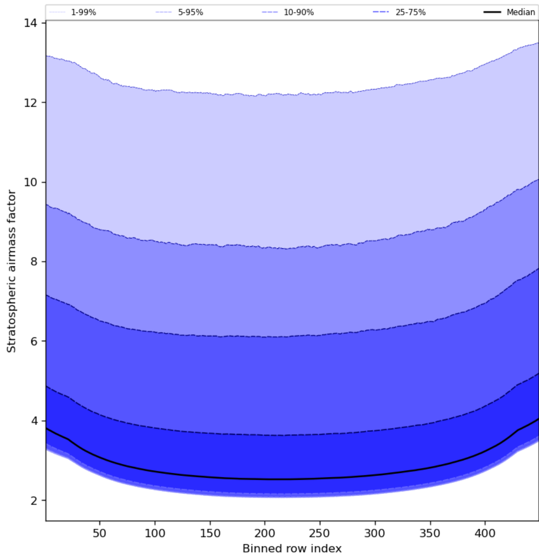
Figure 61: Along track statistics of “Stratospheric airmass factor” for 2023-09-24 to 2023-09-26
