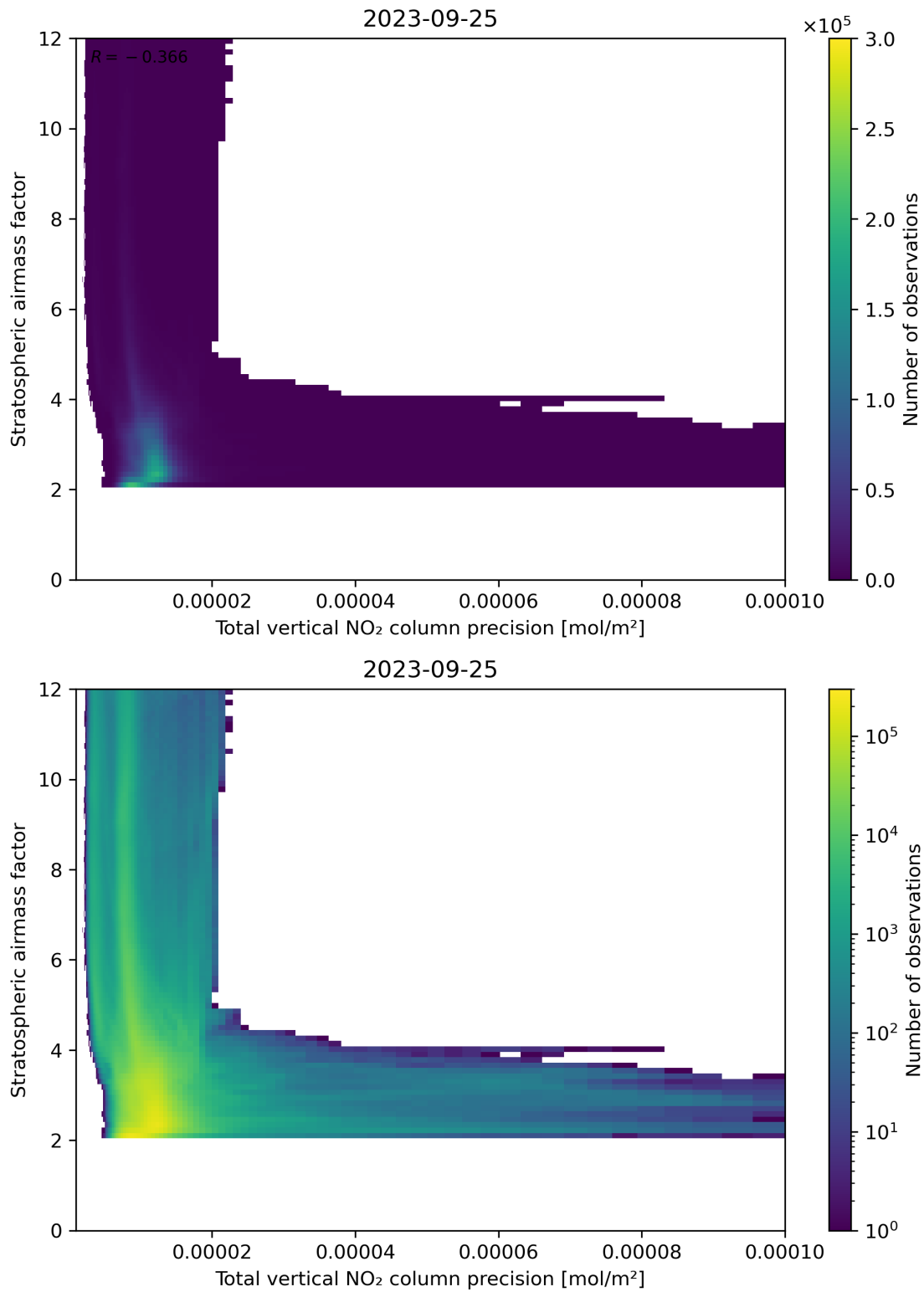
Figure 115: Scatter density plot of “Total vertical NO 2 column precision” against “Stratospheric airmass factor” for 2023-09-24 to 2023-09-26.
