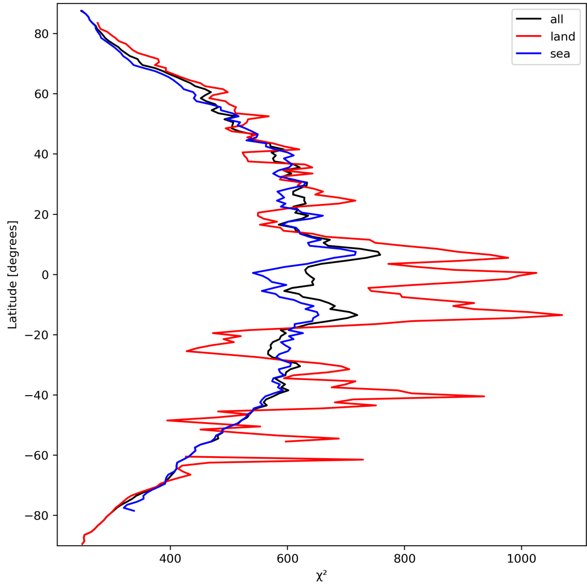
Figure 25: Zonal average of “ \chi^2 ” for 2023-09-24 to 2023-09-26.
