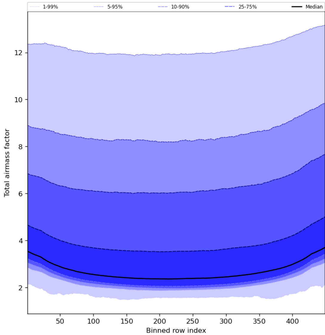
Figure 49: Along track statistics of “Total airmass factor” for 2023-09-24 to 2023-09-26
