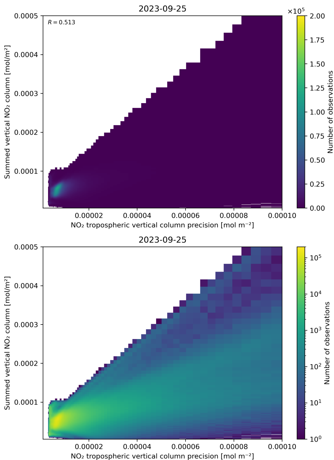
Figure 136: Scatter density plot of “NO 2 tropospheric vertical column precision” against “Summed vertical NO 2 column” for 2023-09-24 to 2023-09-26.
