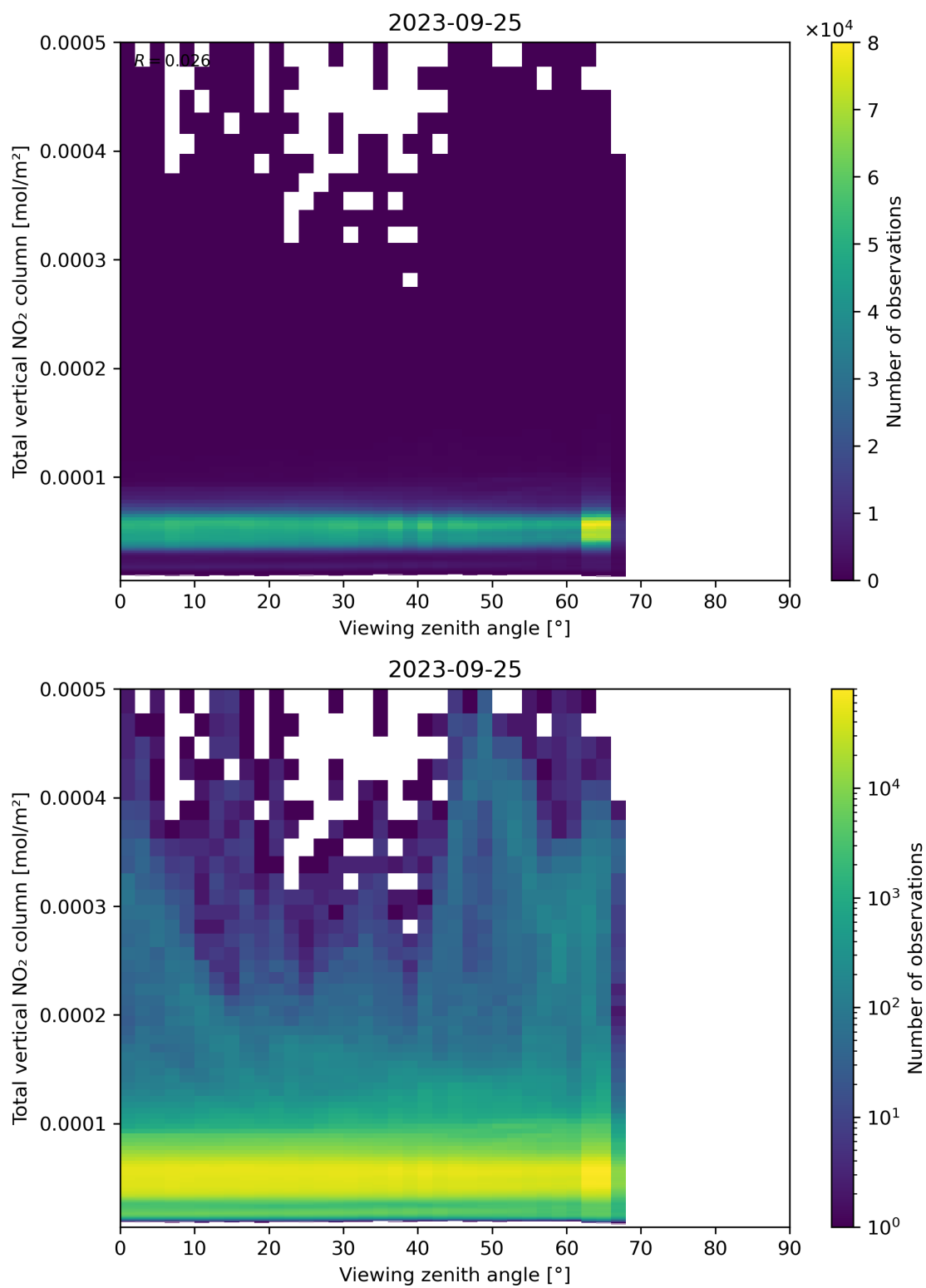
Figure 167: Scatter density plot of “Viewing zenith angle” against “Total vertical NO 2 column” for 2023-09-24 to 2023-09-26.
