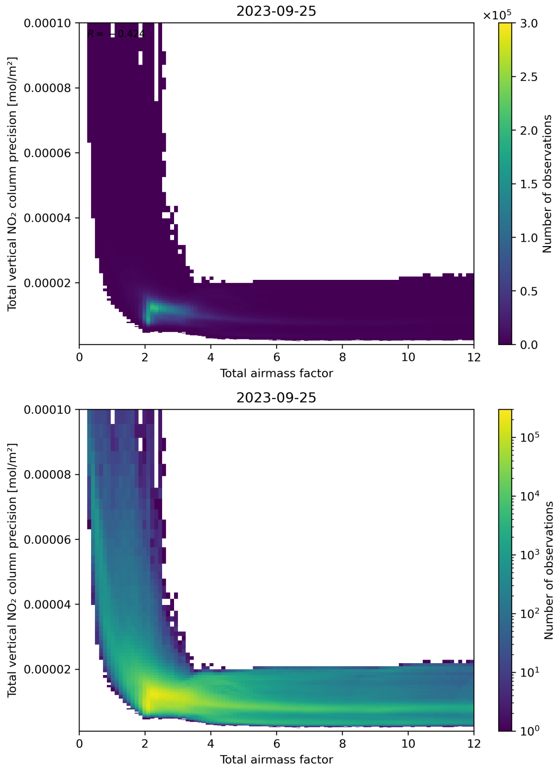
Figure 68: Scatter density plot of “Total airmass factor” against “Total vertical NO 2 column precision” for 2023-09-24 to 2023-09-26.
