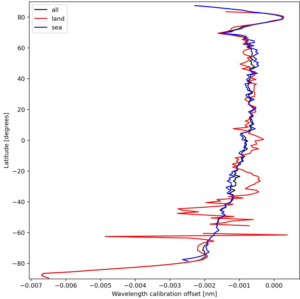
Figure 18: Zonal average of “Wavelength calibration offset” for 2023-09-24 to 2023-09-26.
