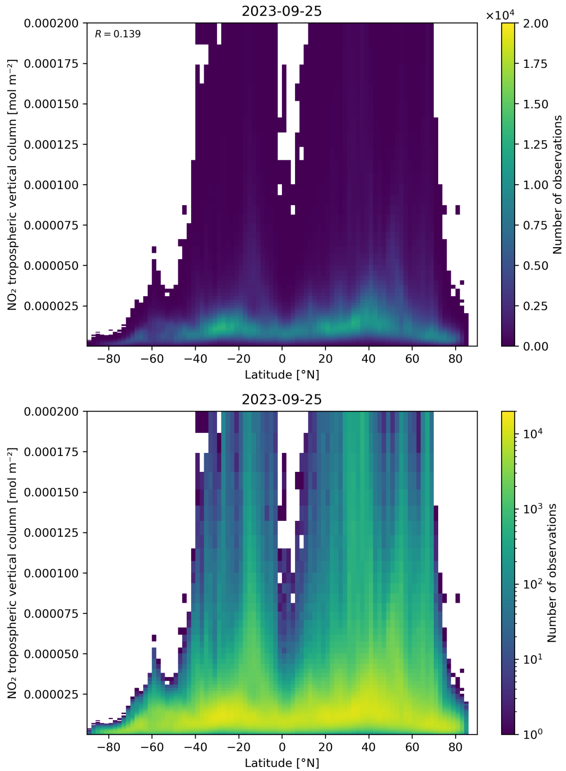
Figure 92: Scatter density plot of “Latitude” against “NO 2 tropospheric vertical column” for 2023-09-24 to 2023-09-26.
