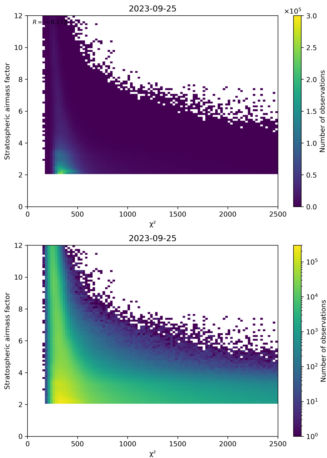
Figure 81: Scatter density plot of “ \chi^2 ” against “Stratospheric airmass factor” for 2023-09-24 to 2023-09-26.
