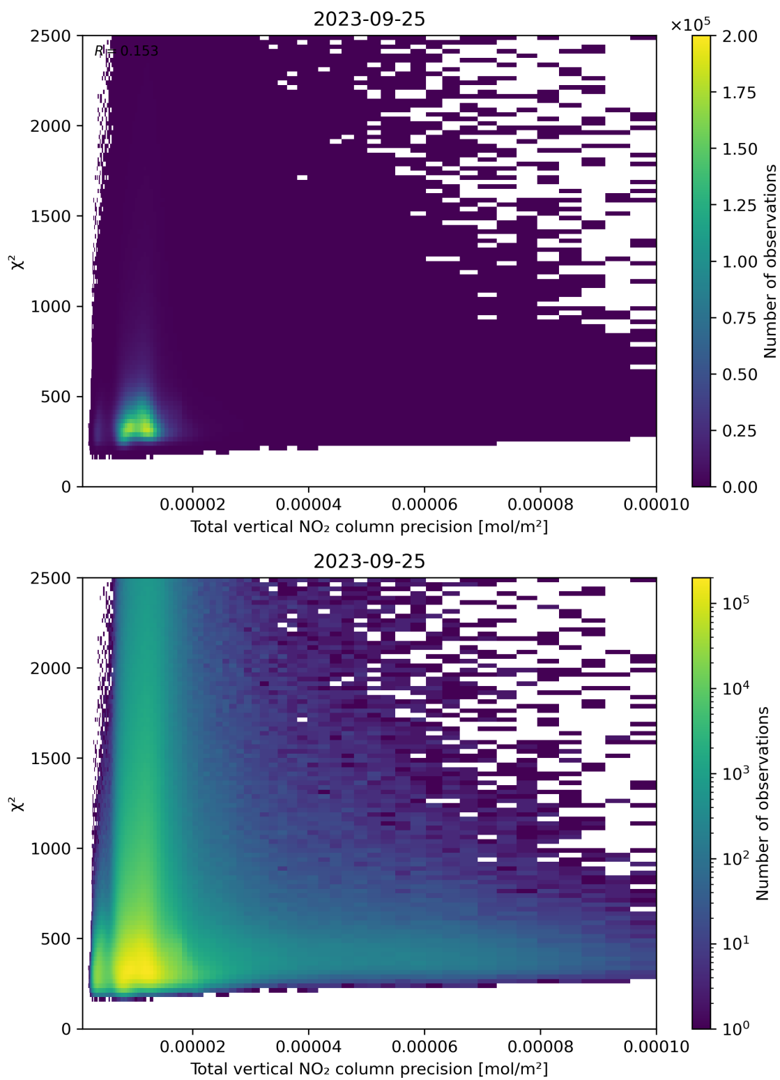
Figure 116: Scatter density plot of “Total vertical NO 2 column precision” against “ \chi^2 ” for 2023-09-24 to 2023-09-26.
