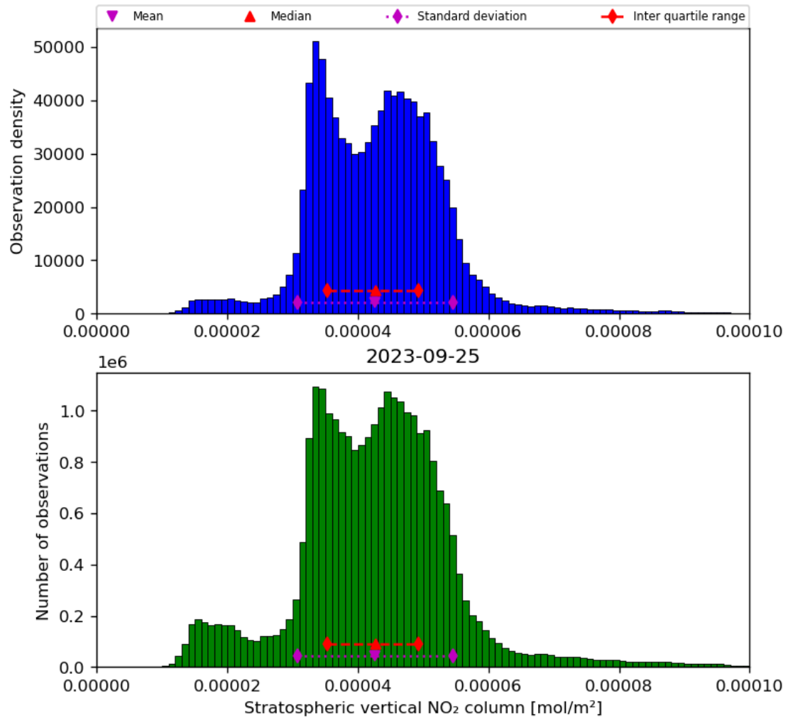
Figure 36: Histogram of “Stratospheric vertical NO 2 column” for 2023-09-24 to 2023-09-26
