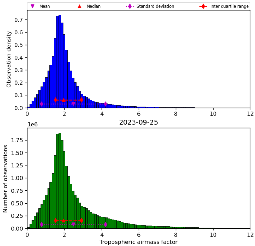
Figure 31: Histogram of “Tropospheric airmass factor” for 2023-09-24 to 2023-09-26
