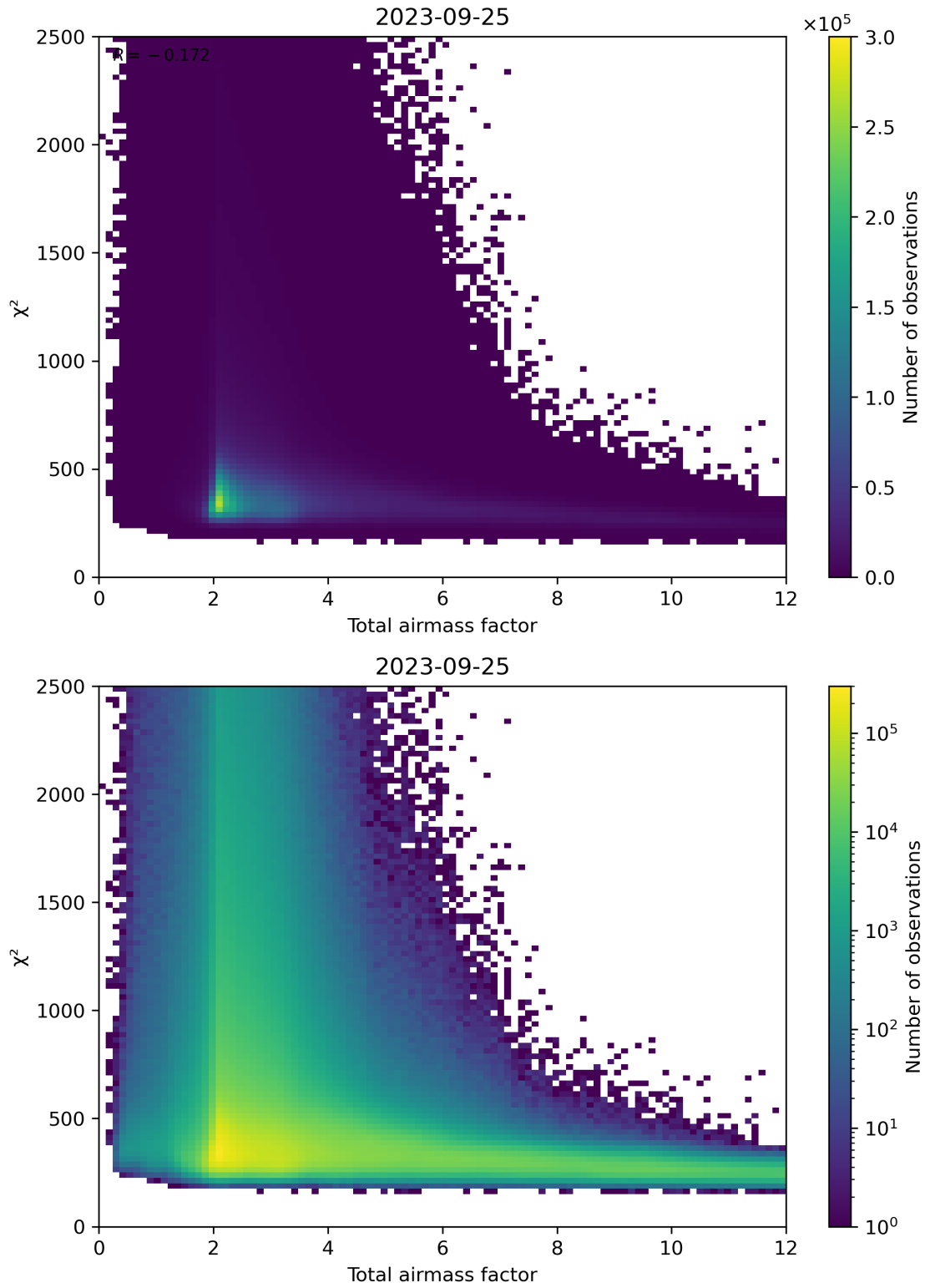
Figure 63: Scatter density plot of “Total airmass factor” against “ \chi^2 ” for 2023-09-24 to 2023-09-26.
