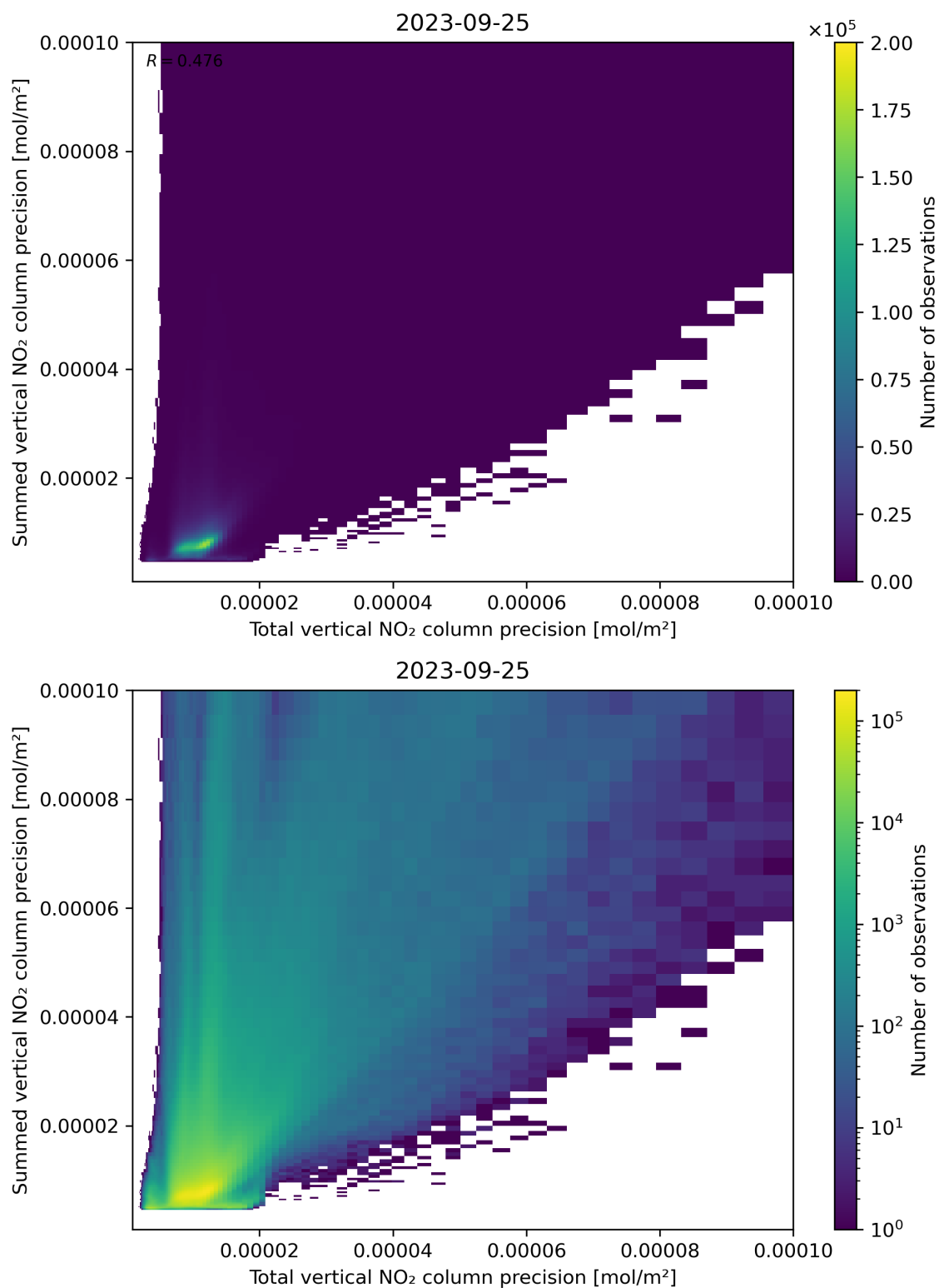
Figure 118: Scatter density plot of “Total vertical NO 2 column precision” against “Summed vertical NO 2 column precision” for 2023-09-24 to 2023-09-26.
