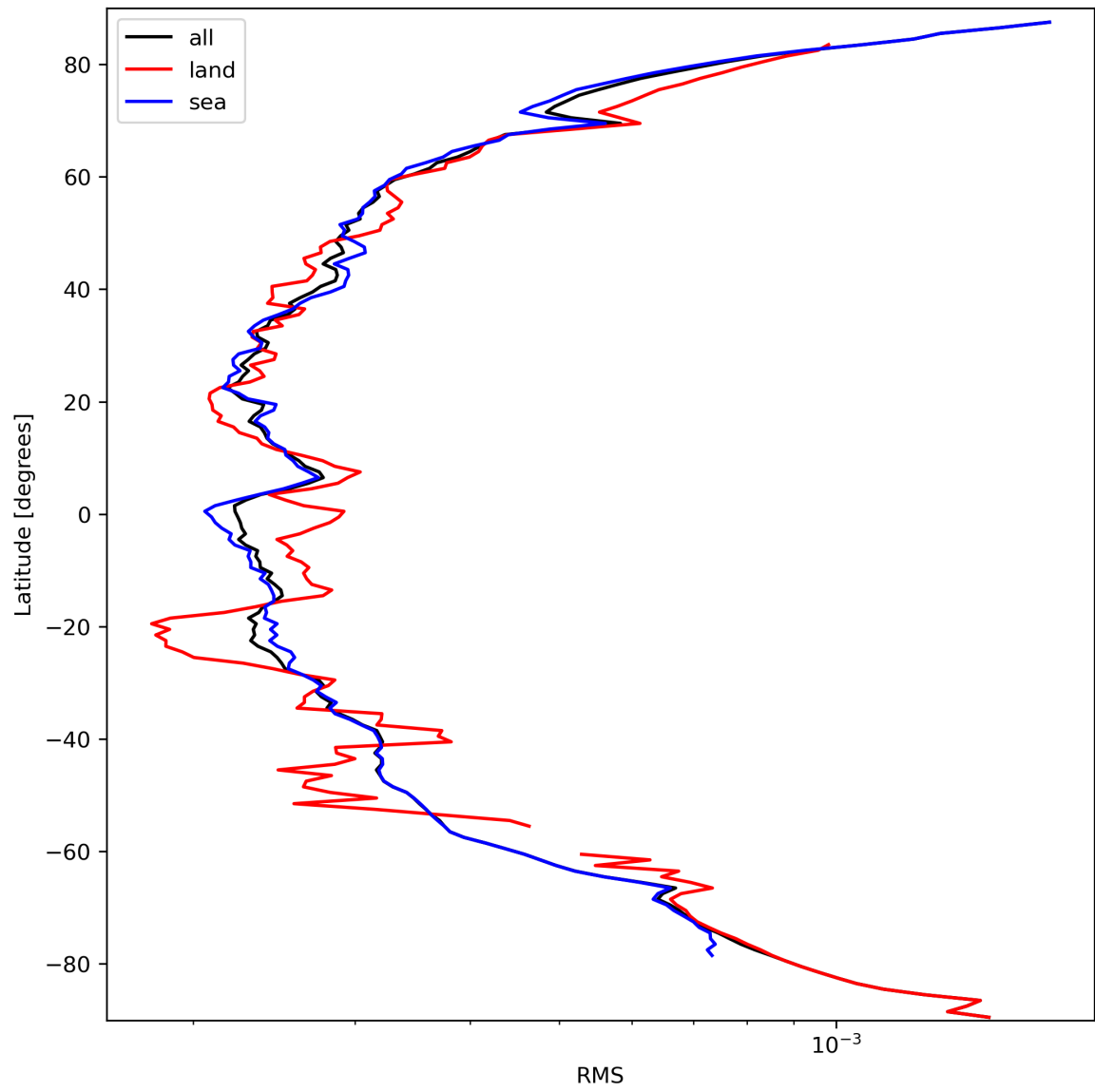
Figure 26: Zonal average of “RMS” for 2023-09-24 to 2023-09-26.
