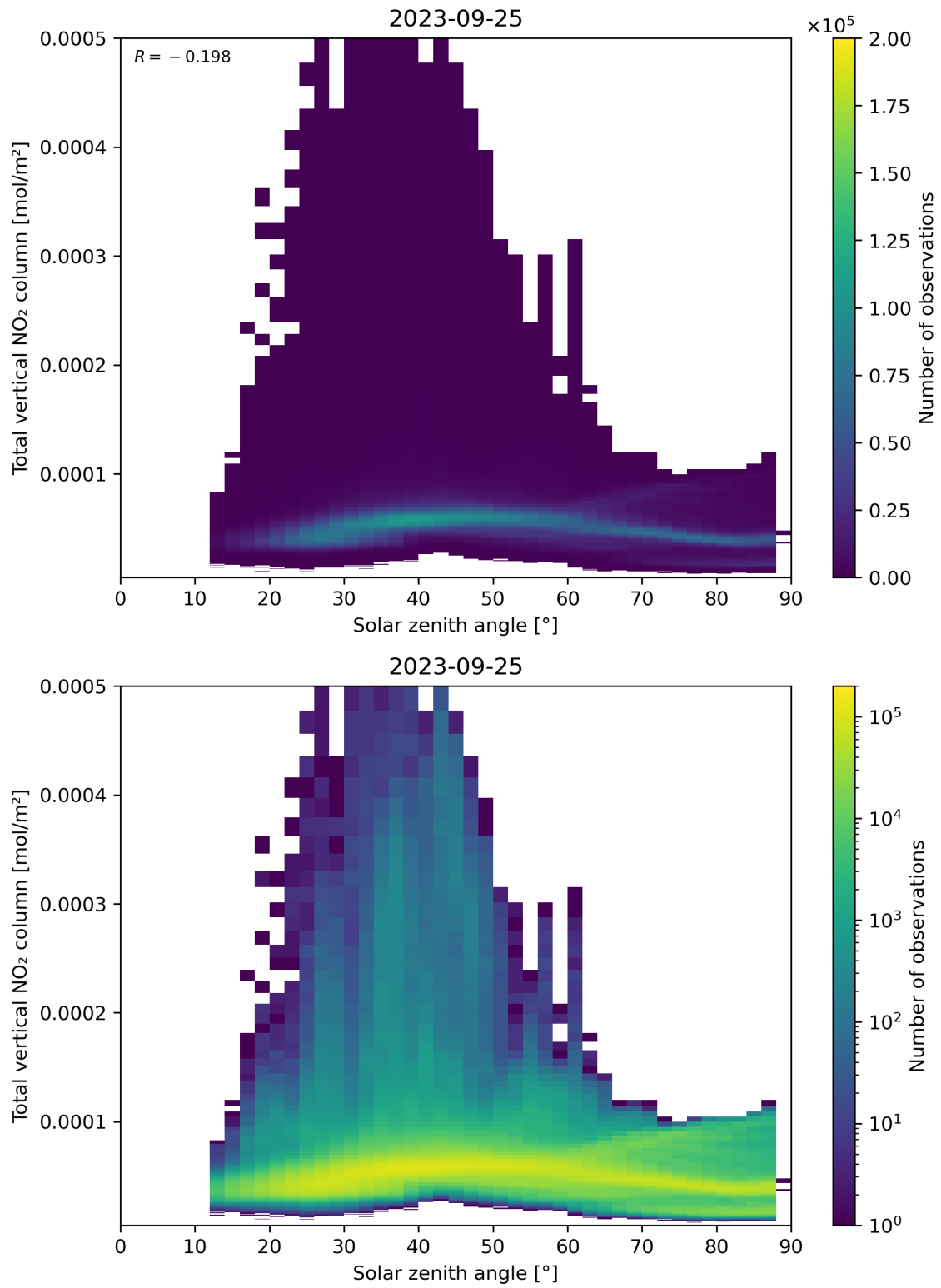
Figure 153: Scatter density plot of “Solar zenith angle” against “Total vertical NO 2 column” for 2023-09-24 to 2023-09-26.
