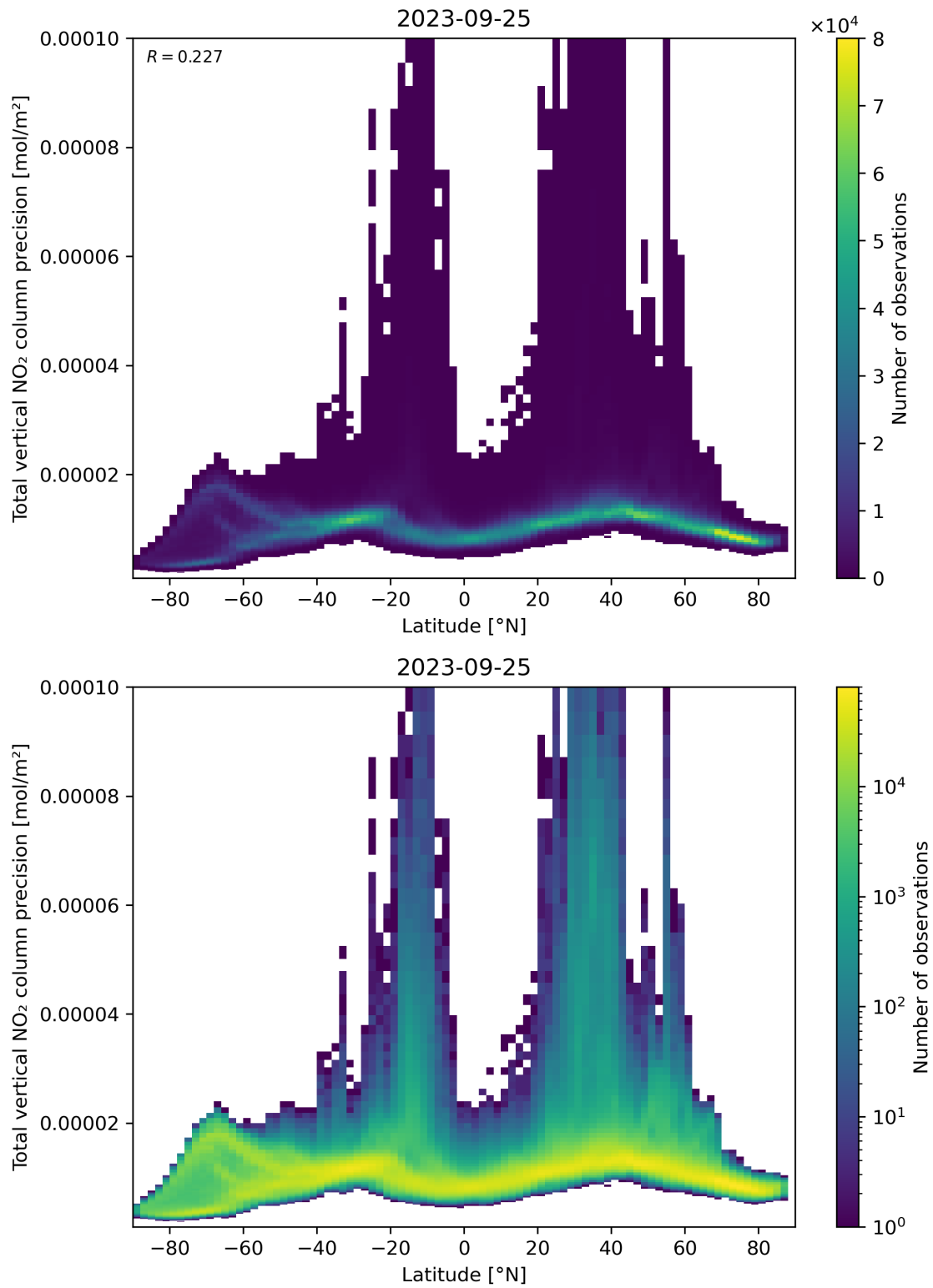
Figure 91: Scatter density plot of “Latitude” against “Total vertical NO 2 column precision” for 2023-09-24 to 2023-09-26.
