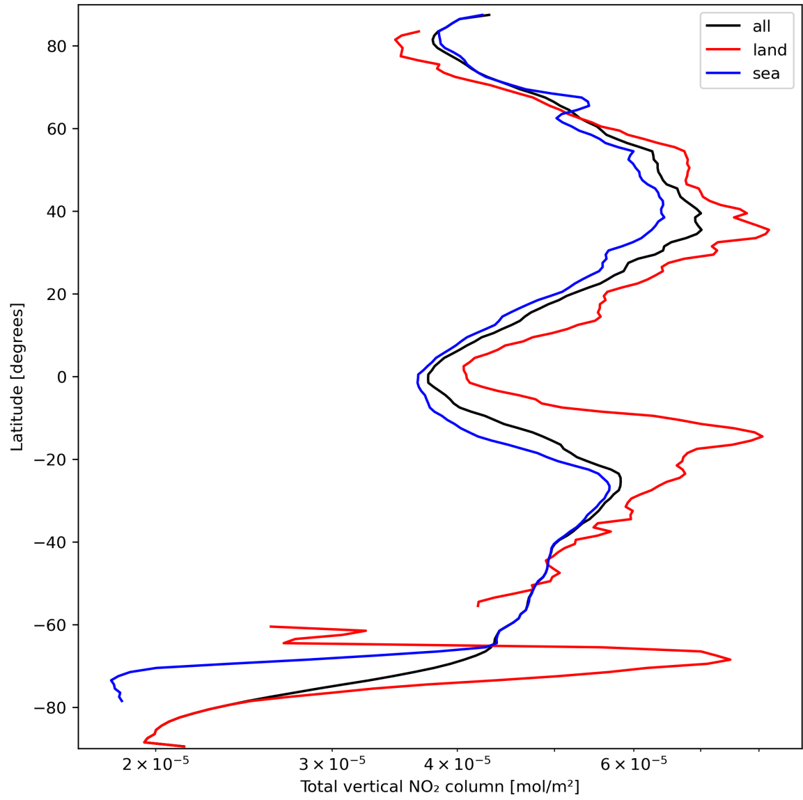
Figure 21: Zonal average of “Total vertical NO 2 column” for 2023-09-24 to 2023-09-26.
