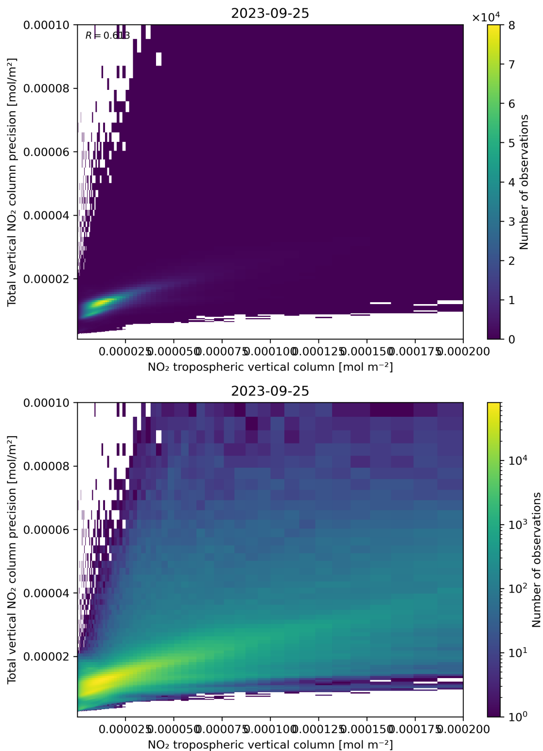
Figure 129: Scatter density plot of “NO 2 tropospheric vertical column” against “Total vertical NO 2 column precision” for 2023-09-24 to 2023-09-26.
