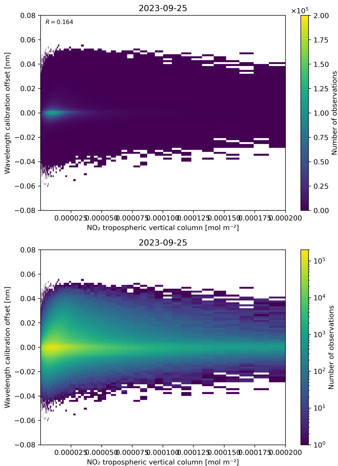
Figure 143: Scatter density plot of “NO 2 tropospheric vertical column” against “Wavelength calibration offset” for 2023-09-24 to 2023-09-26.
