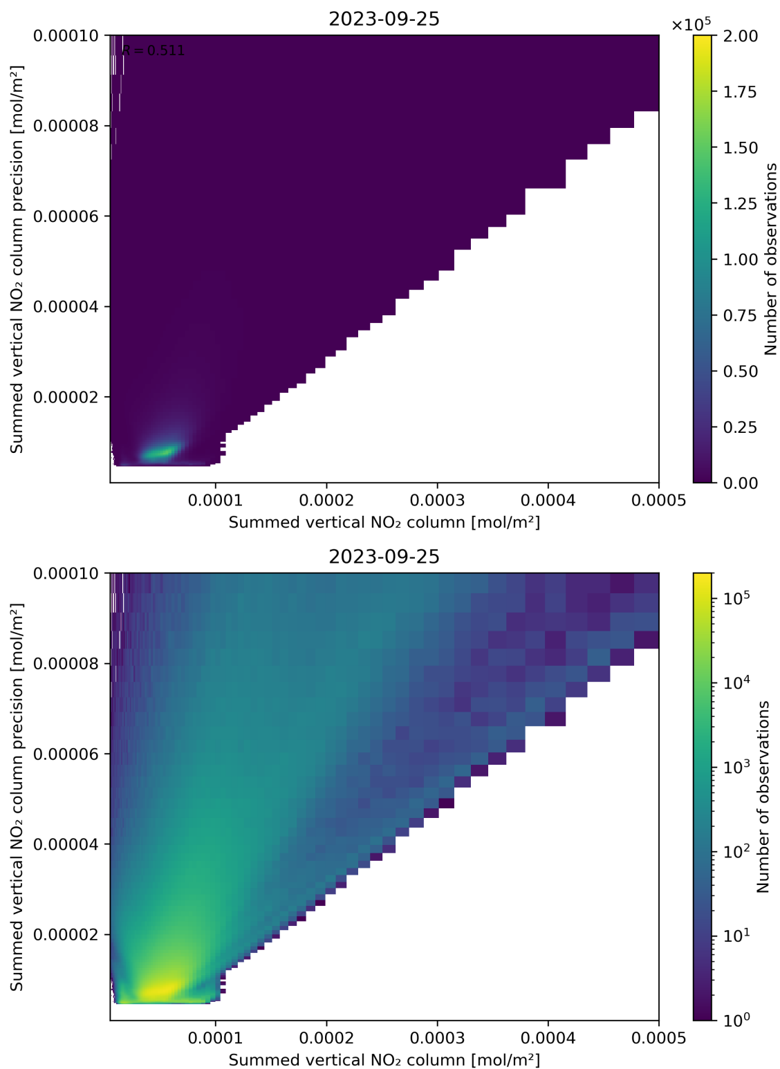
Figure 105: Scatter density plot of “Summed vertical NO 2 column” against “Summed vertical NO 2 column precision” for 2023-09-24 to 2023-09-26.
