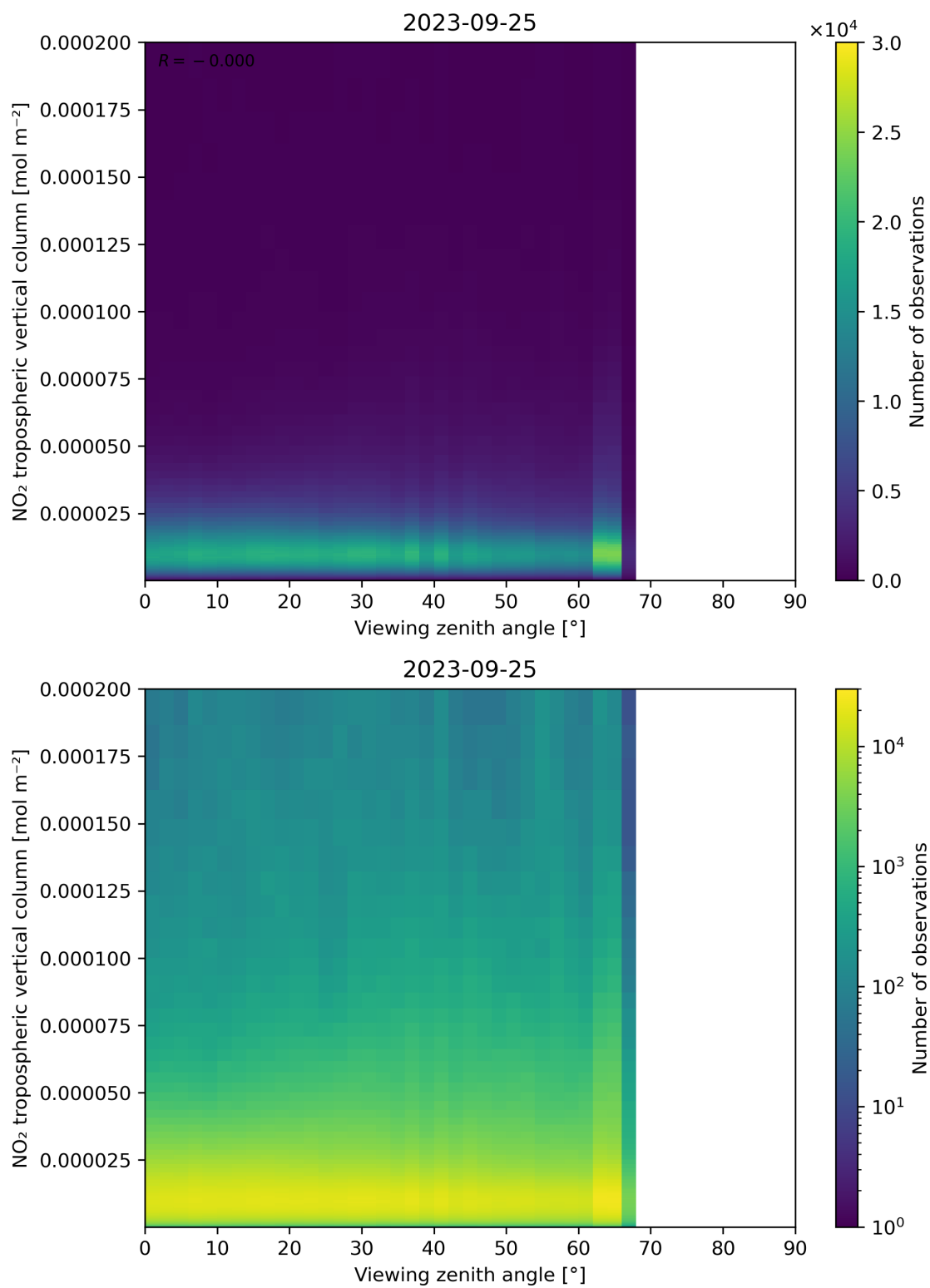
Figure 169: Scatter density plot of “Viewing zenith angle” against “NO 2 tropospheric vertical column” for 2023-09-24 to 2023-09-26.
