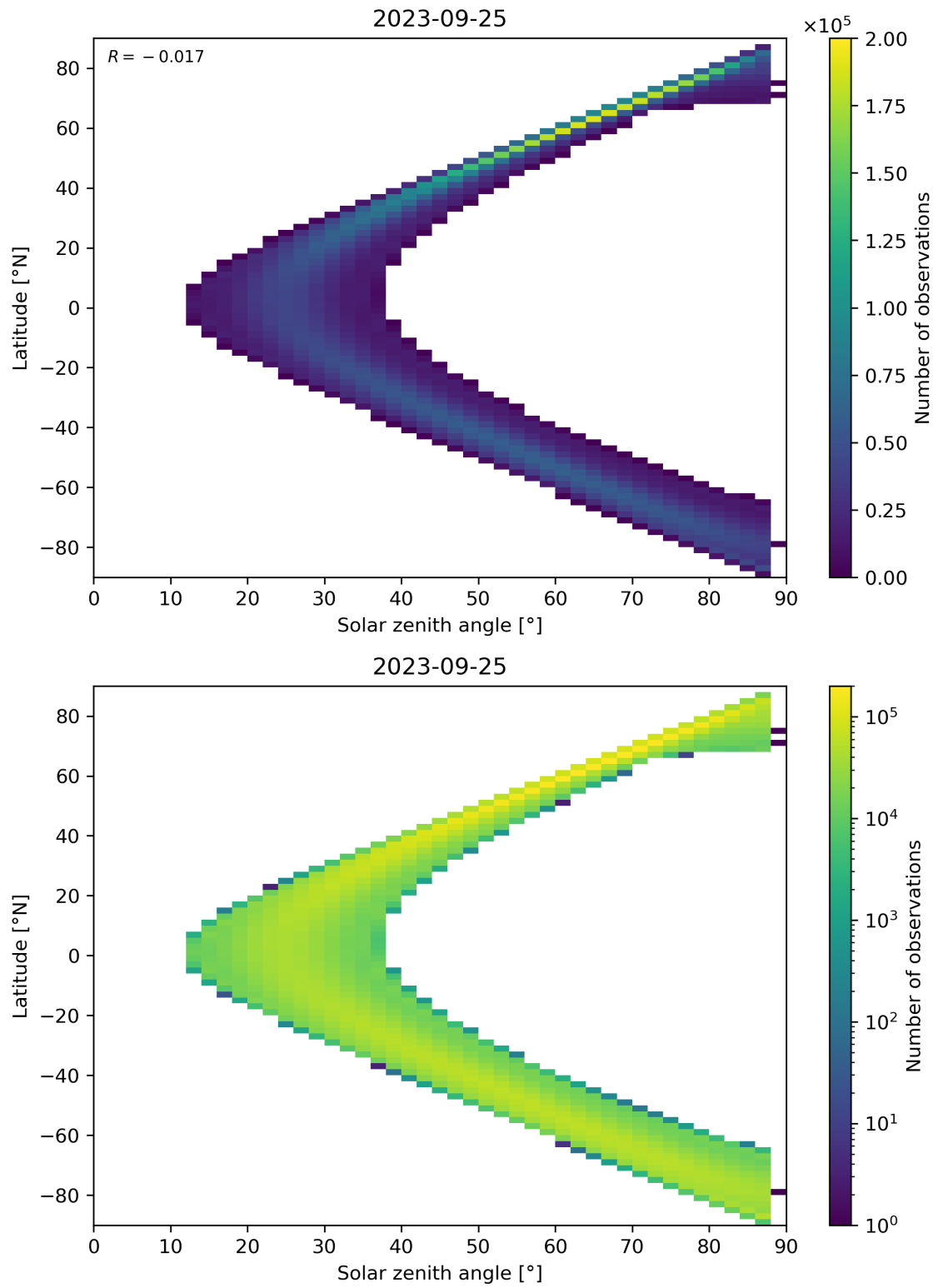
Figure 149: Scatter density plot of “Solar zenith angle” against “Latitude” for 2023-09-24 to 2023-09-26.
