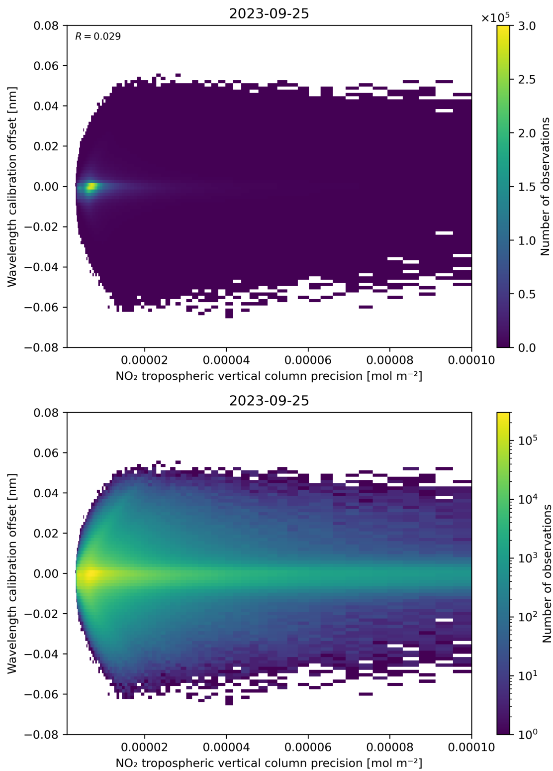
Figure 141: Scatter density plot of “NO 2 tropospheric vertical column precision” against “Wavelength calibration offset” for 2023-09-24 to 2023-09-26.
