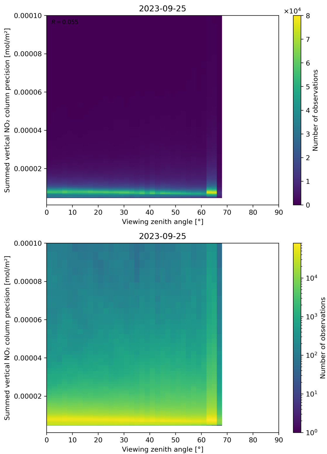
Figure 166: Scatter density plot of “Viewing zenith angle” against “Summed vertical NO 2 column precision” for 2023-09-24 to 2023-09-26.
