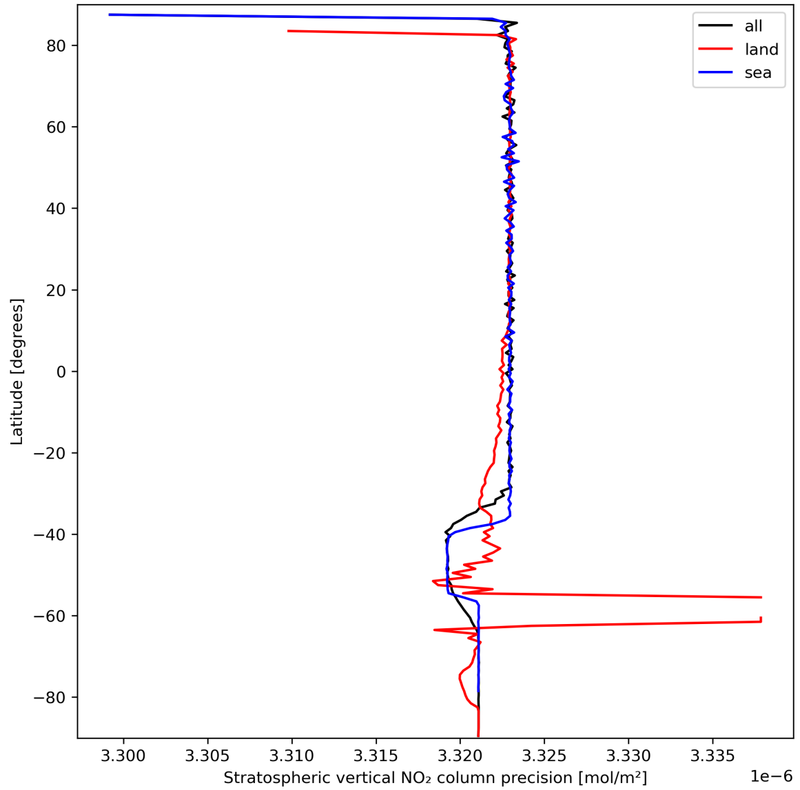
Figure 20: Zonal average of “Stratospheric vertical NO 2 column precision” for 2023-09-24 to 2023-09-26.
