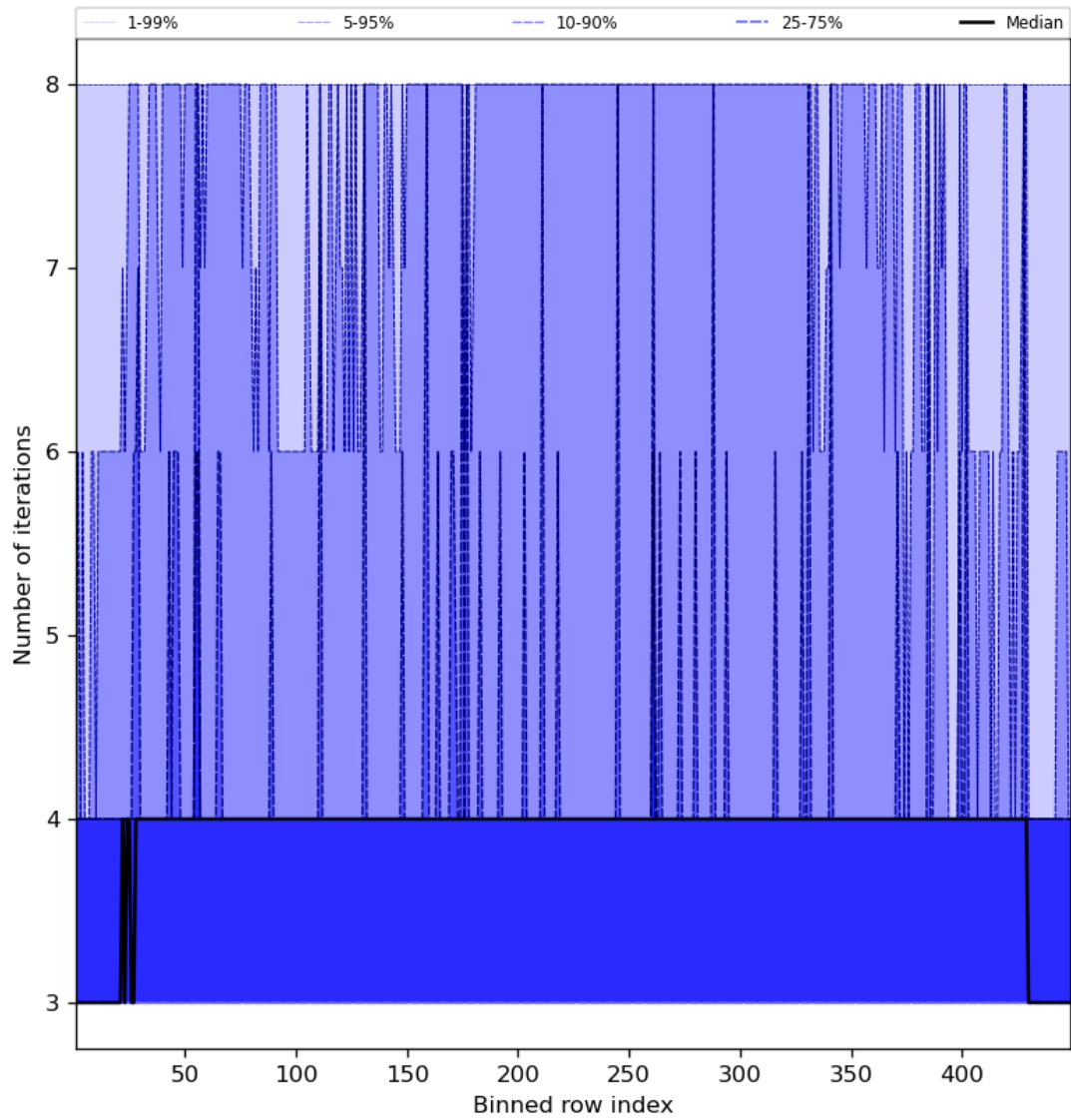
Figure 51: Along track statistics of “Number of iterations” for 2023-09-24 to 2023-09-26
