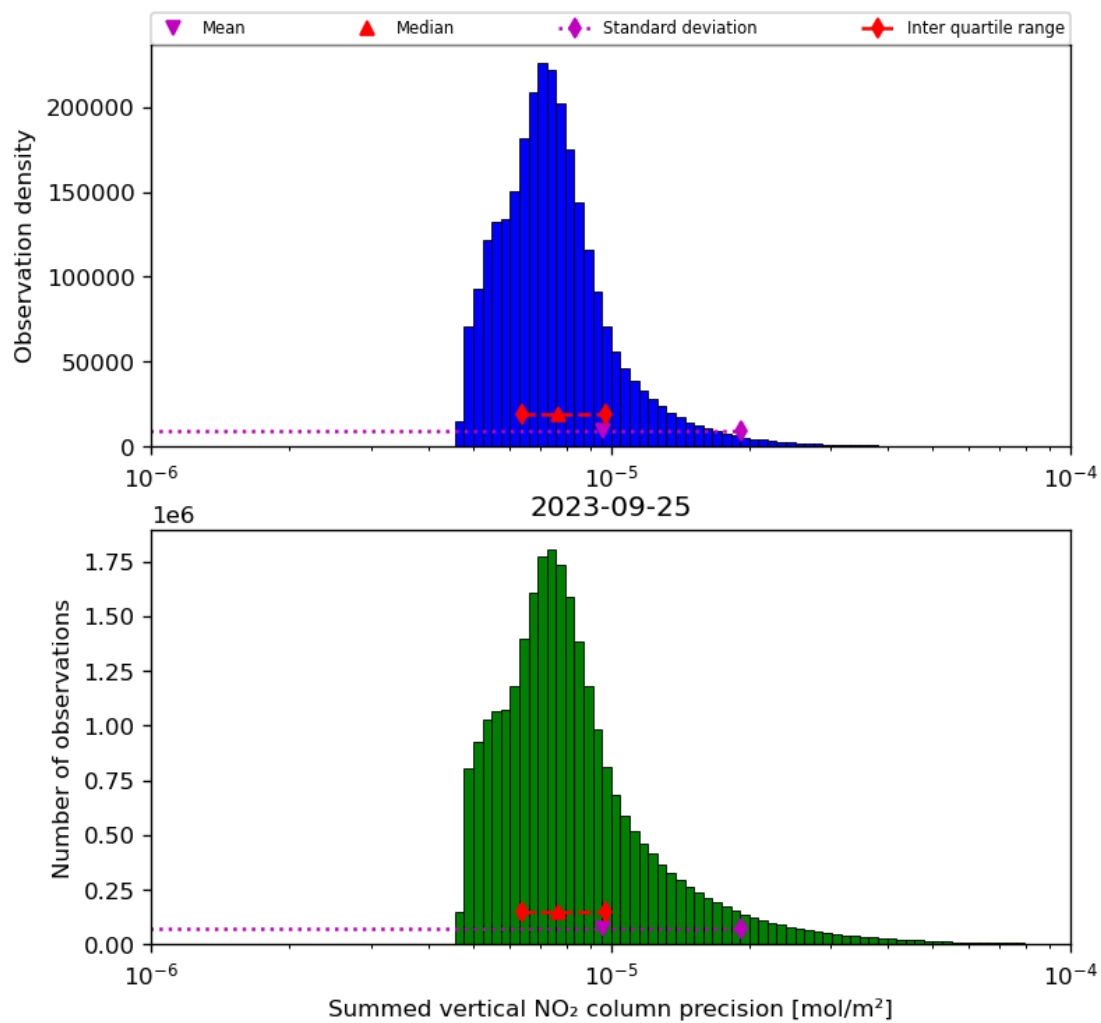
Figure 41: Histogram of “Summed vertical NO 2 column precision” for 2023-09-24 to 2023-09-26
