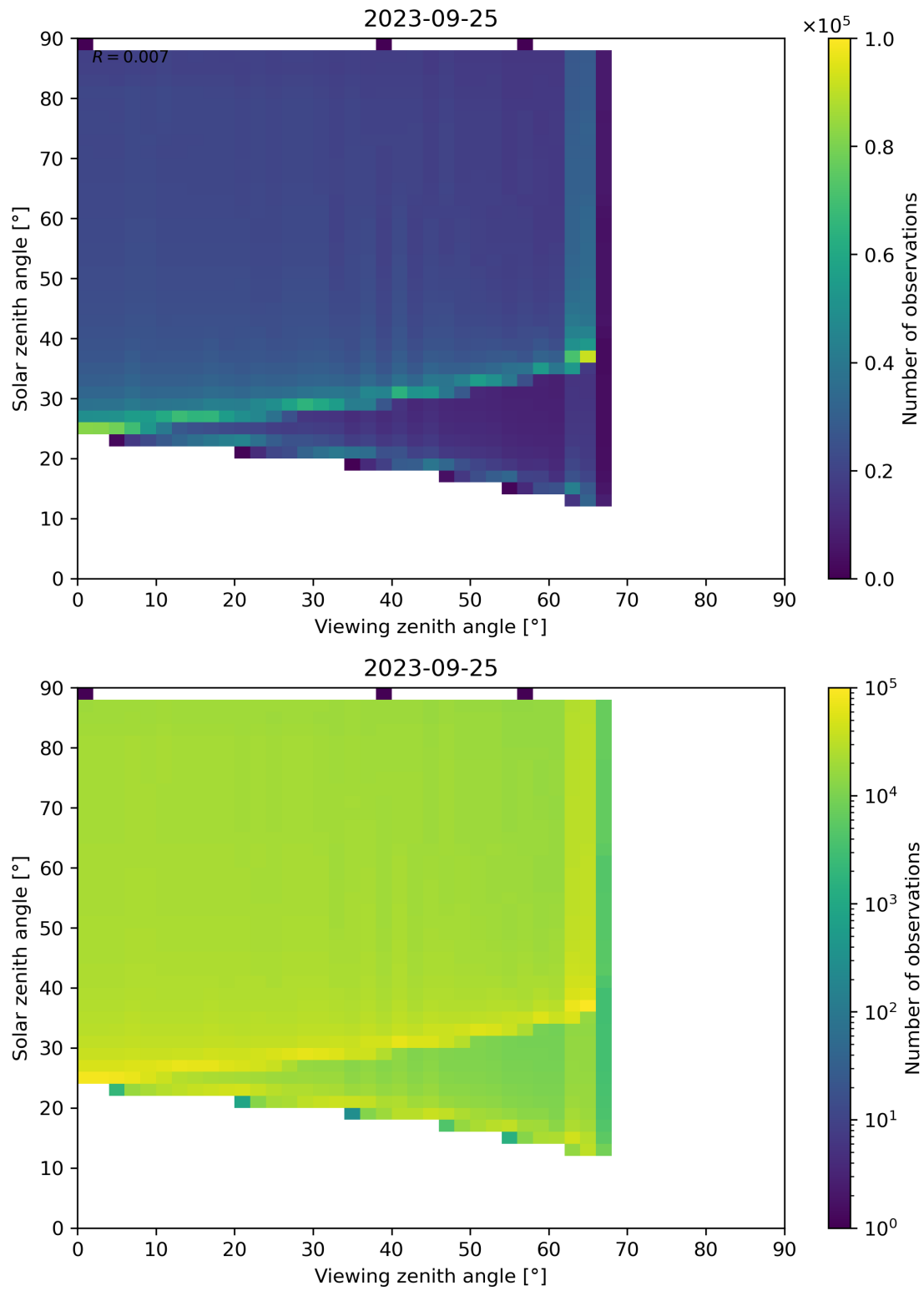
Figure 172: Scatter density plot of “Viewing zenith angle” against “Solar zenith angle” for 2023-09-24 to 2023-09-26.
