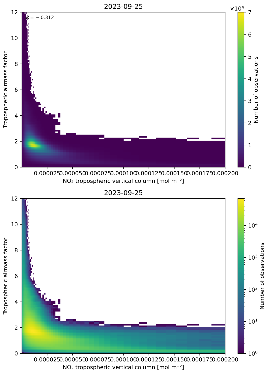
Figure 123: Scatter density plot of “NO 2 tropospheric vertical column” against “Tropospheric air mass factor” for 2023-09-24 to 2023-09-26.
