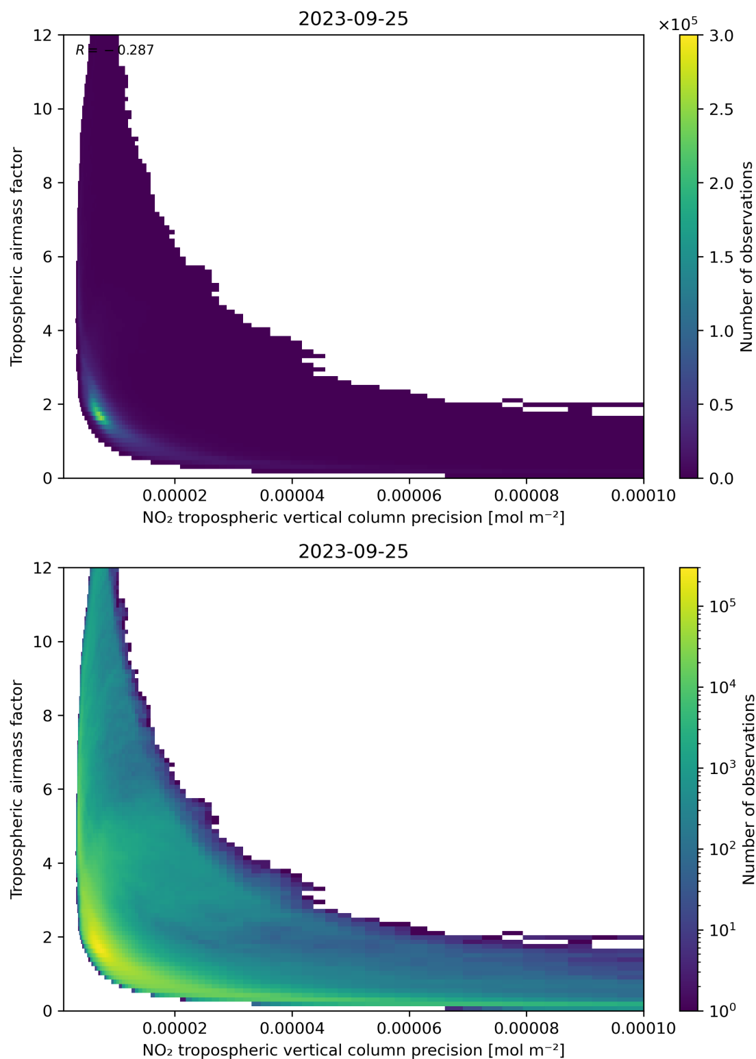
Figure 133: Scatter density plot of “NO 2 tropospheric vertical column precision” against “Tropospheric air mass factor” for 2023-09-24 to 2023-09-26.
