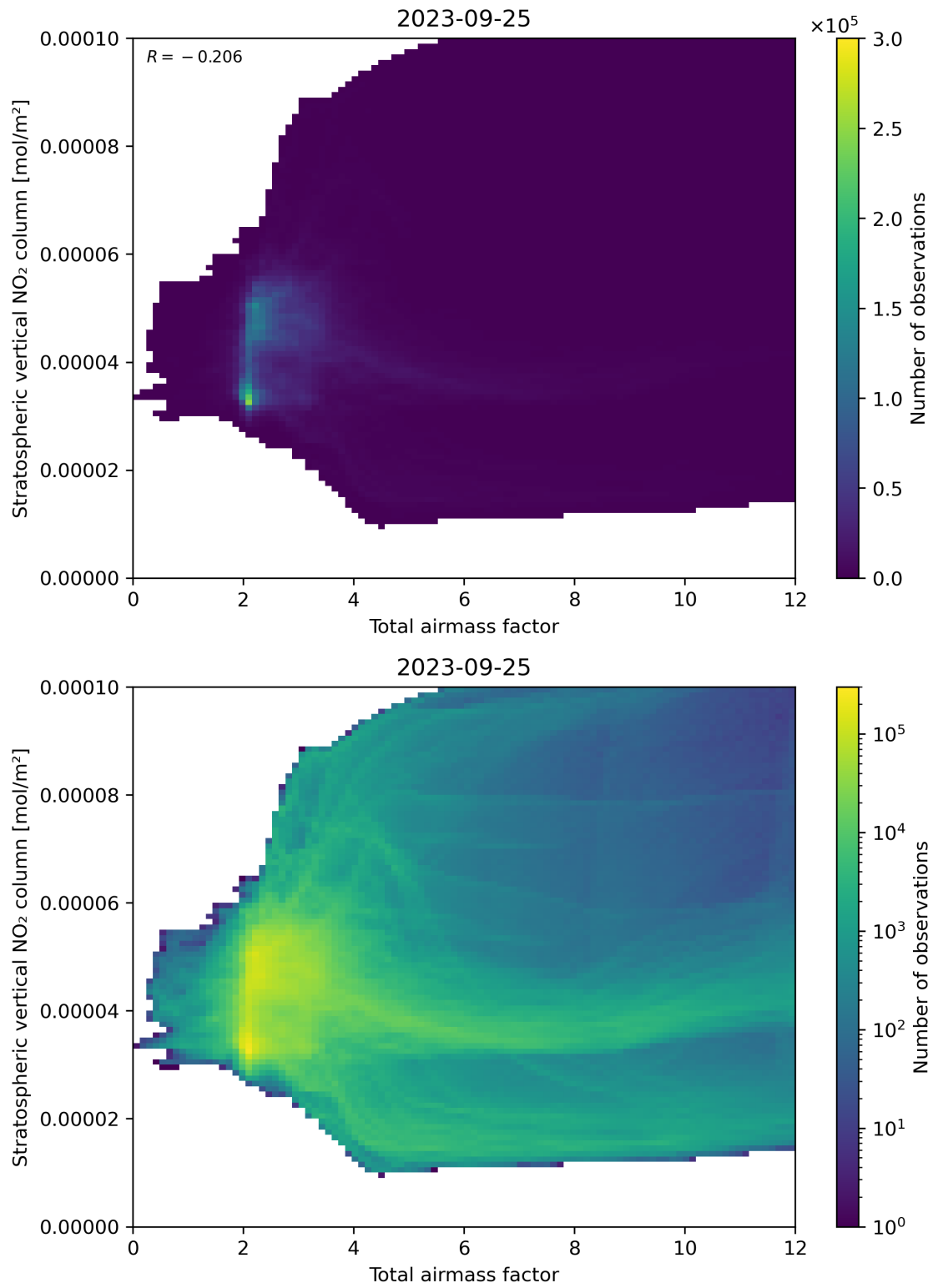
Figure 64: Scatter density plot of “Total airmass factor” against “Stratospheric vertical NO 2 column” for 2023-09-24 to 2023-09-26.
