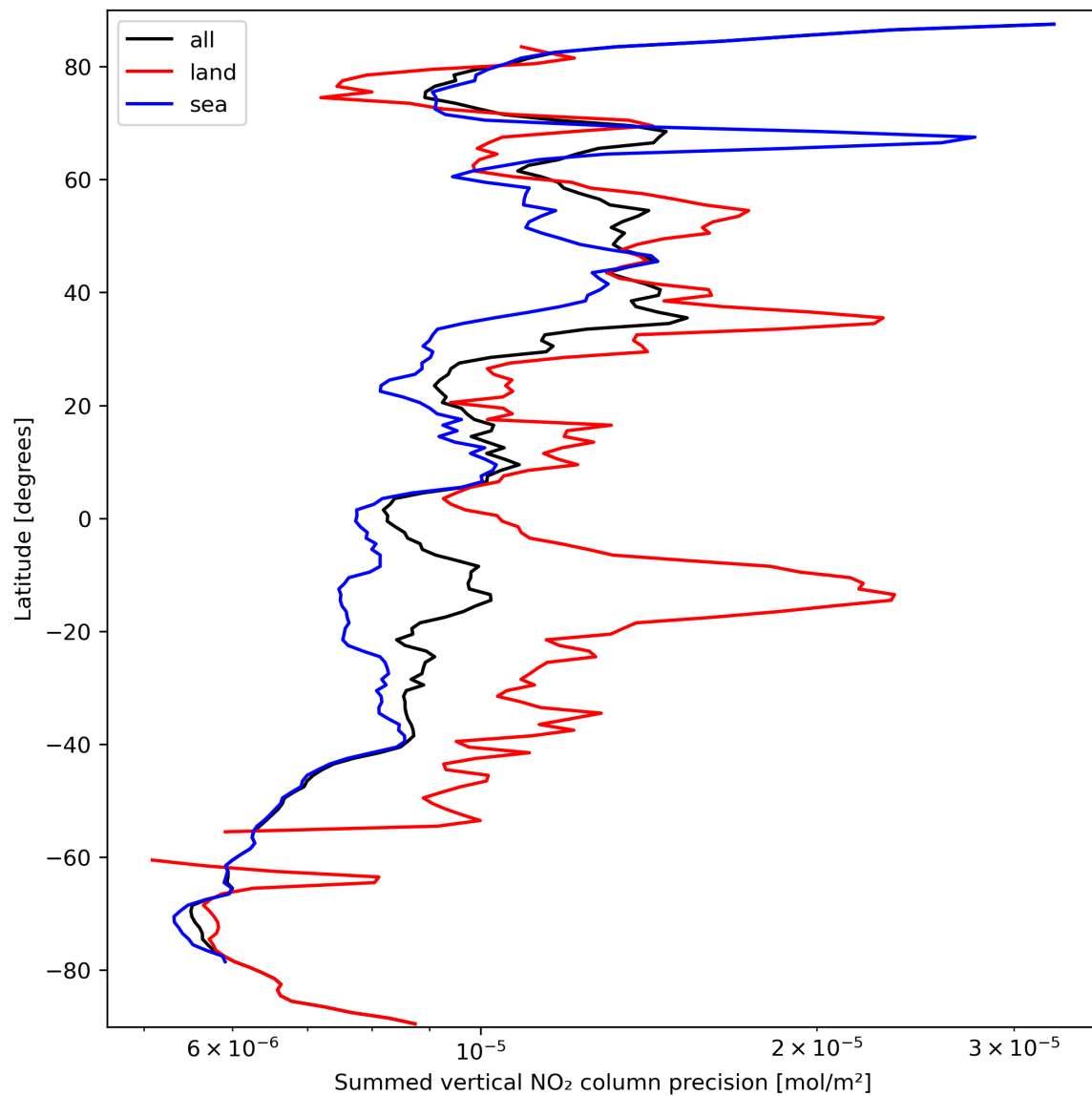
Figure 24: Zonal average of “Summed vertical NO 2 column precision” for 2023-09-24 to 2023-09-26.
