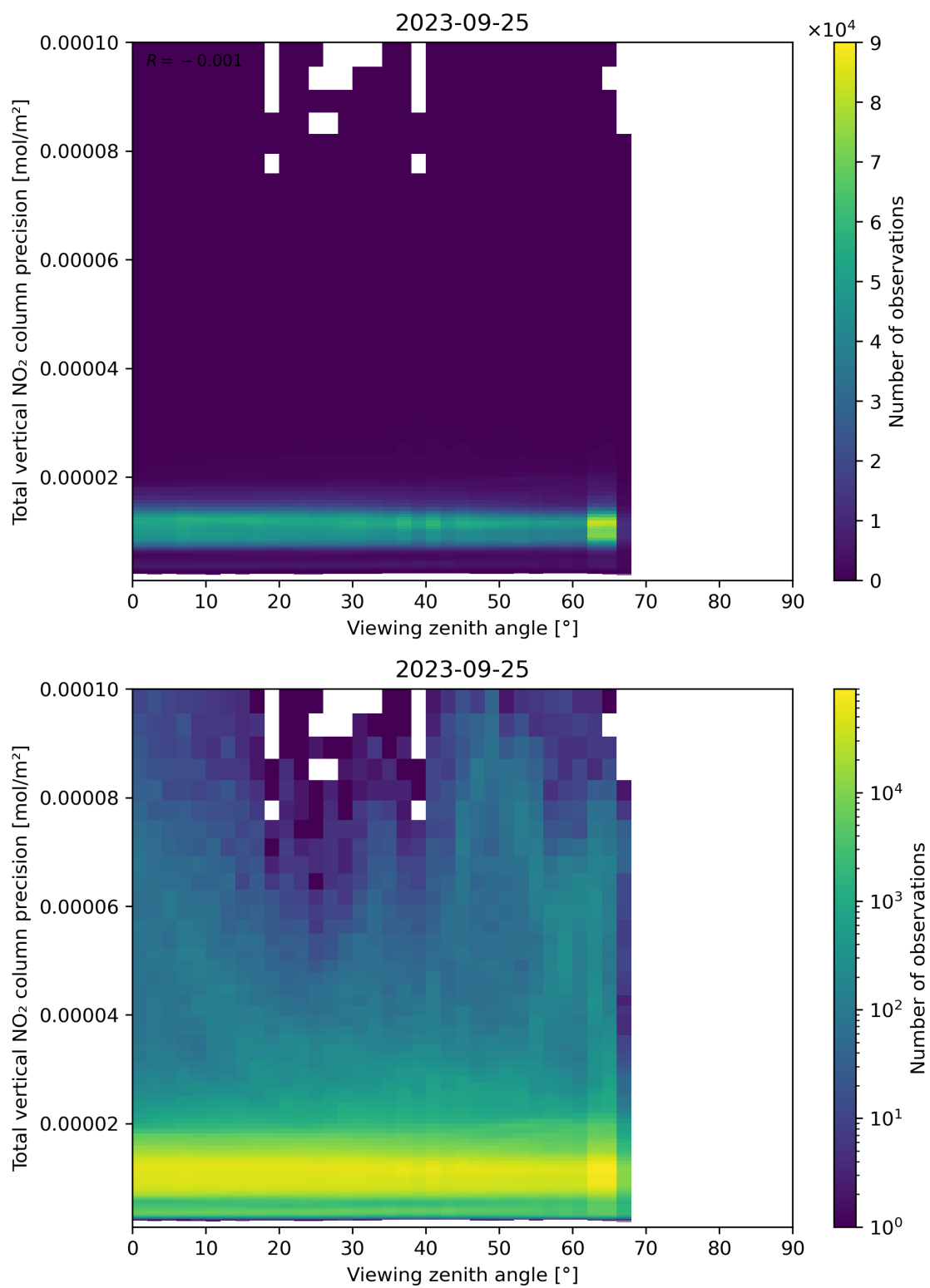
Figure 168: Scatter density plot of “Viewing zenith angle” against “Total vertical NO 2 column precision” for 2023-09-24 to 2023-09-26.
