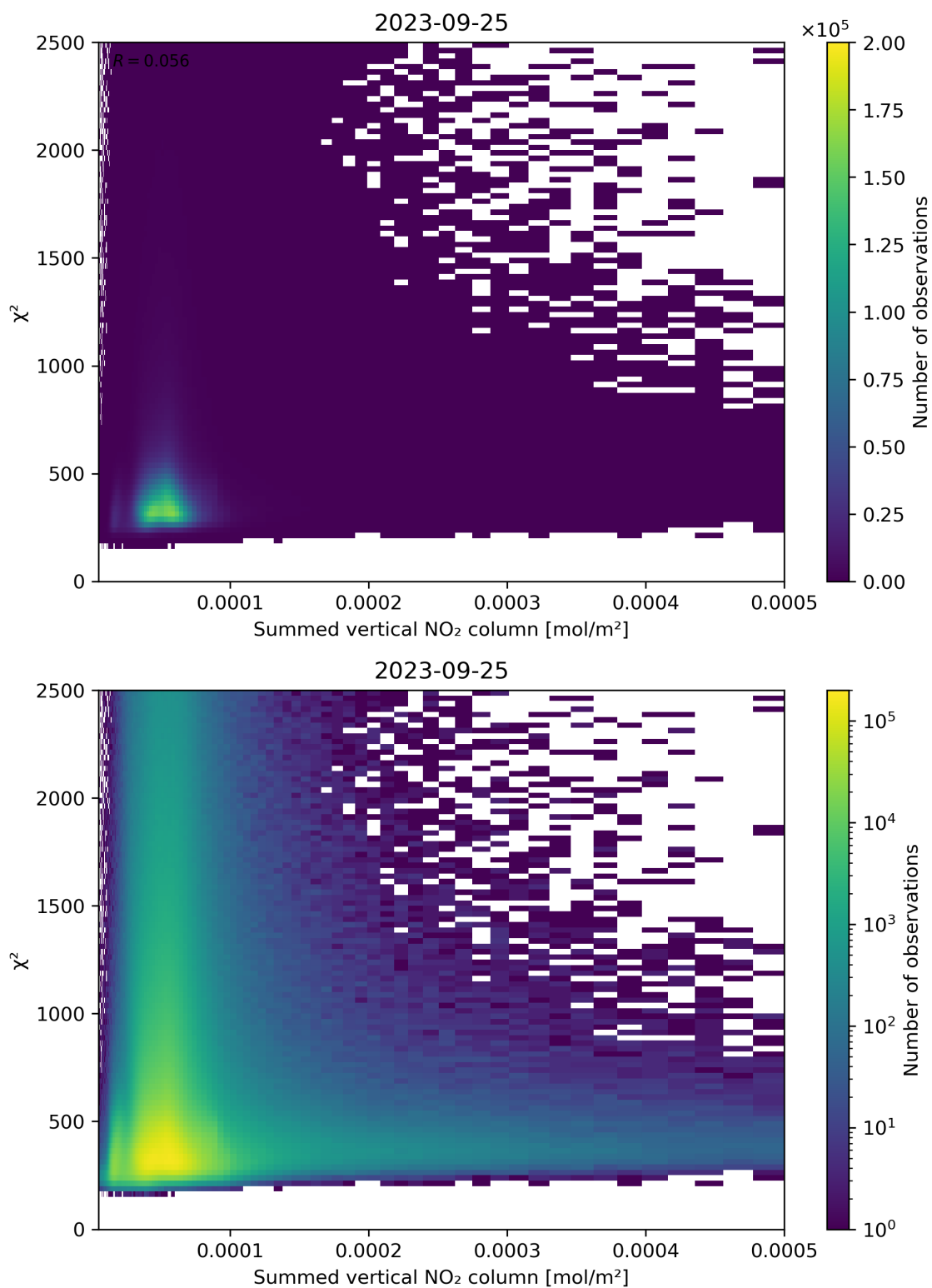
Figure 104: Scatter density plot of “Summed vertical NO 2 column” against “ \chi^2 ” for 2023-09-24 to 2023-09-26.
