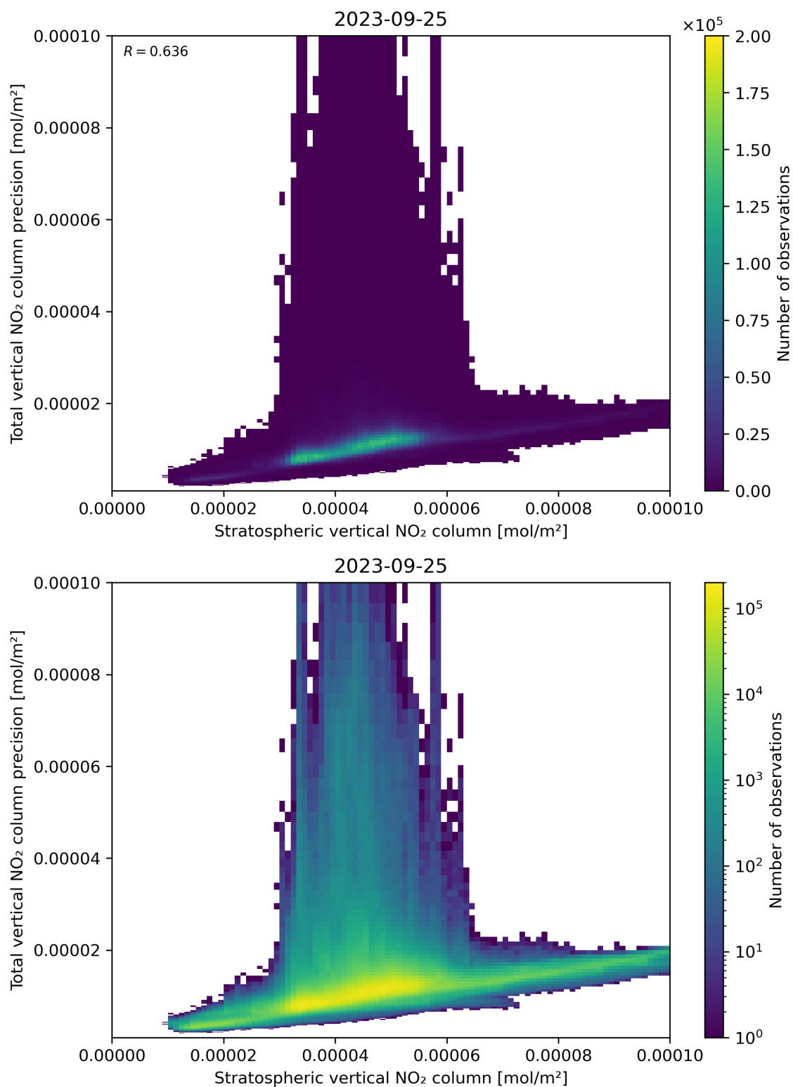
Figure 101: Scatter density plot of “Stratospheric vertical NO 2 column” against “Total vertical NO 2 column precision” for 2023-09-24 to 2023-09-26.
