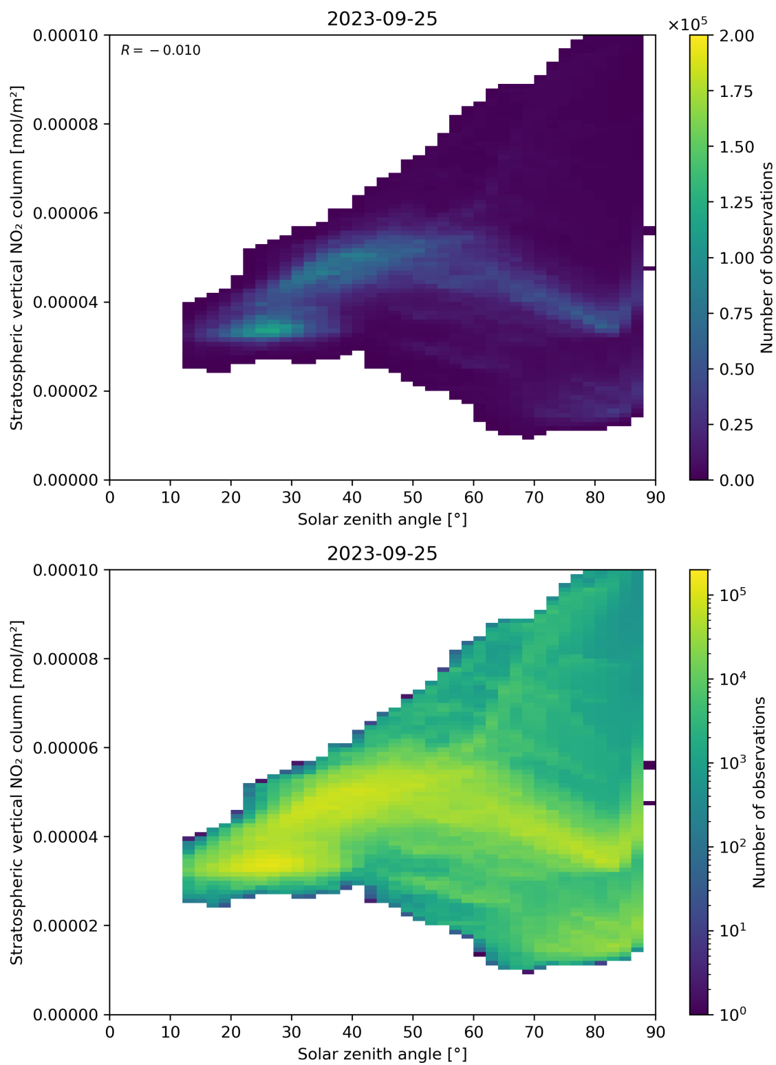
Figure 150: Scatter density plot of “Solar zenith angle” against “Stratospheric vertical NO 2 column” for 2023-09-24 to 2023-09-26.
