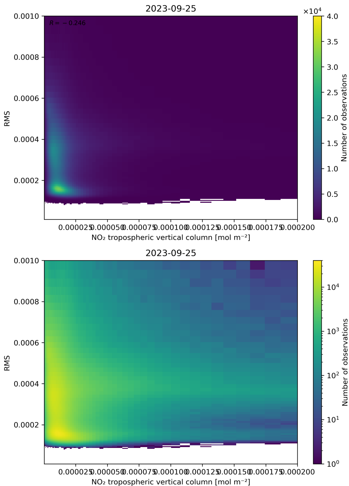
Figure 142: Scatter density plot of “NO 2 tropospheric vertical column” against “RMS” for 2023-09-24 to 2023-09-26.
