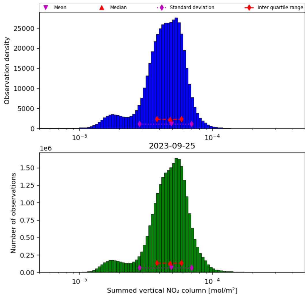
Figure 40: Histogram of “Summed vertical NO 2 column” for 2023-09-24 to 2023-09-26
