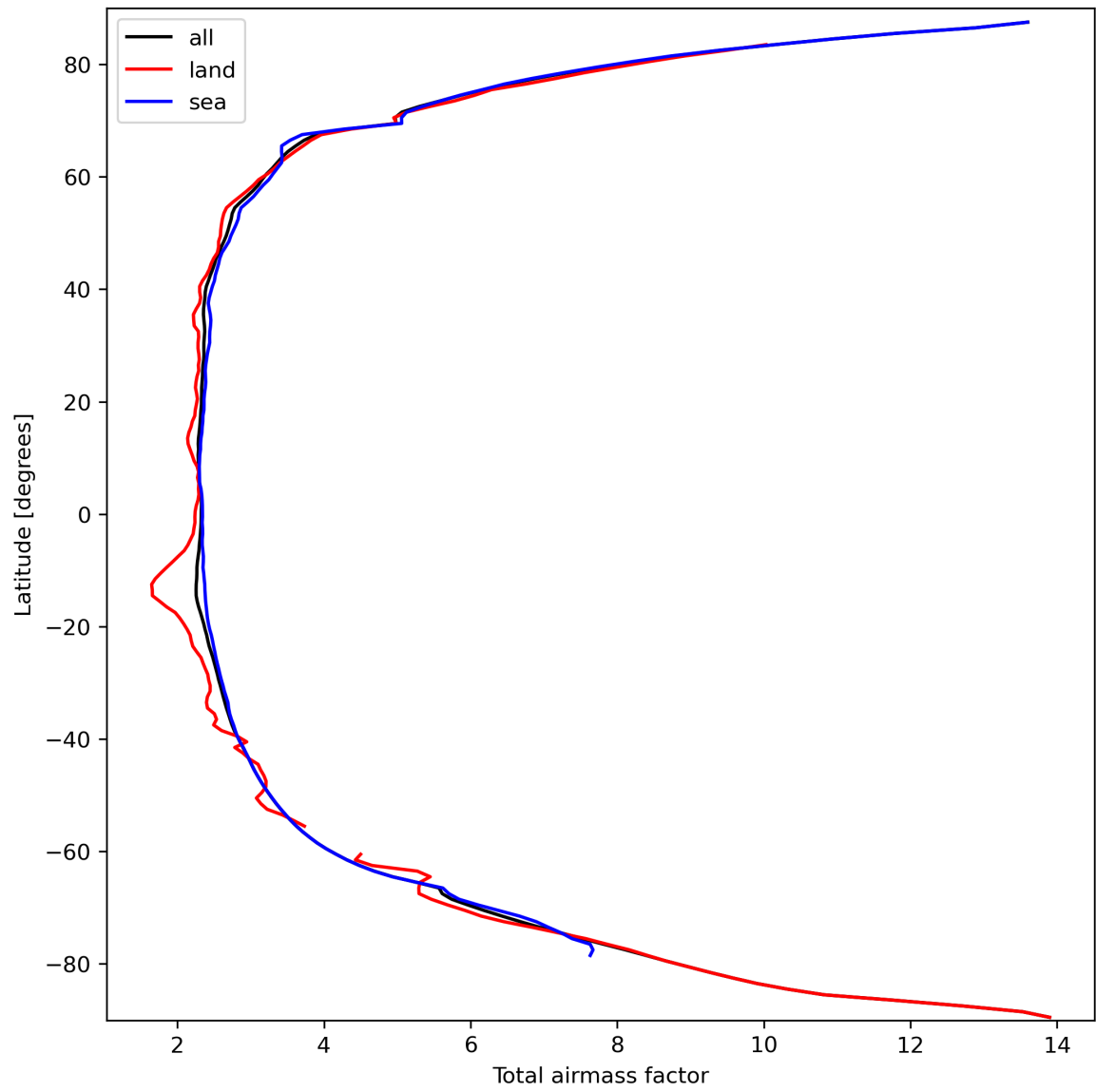
Figure 15: Zonal average of “Total airmass factor” for 2023-09-24 to 2023-09-26.
