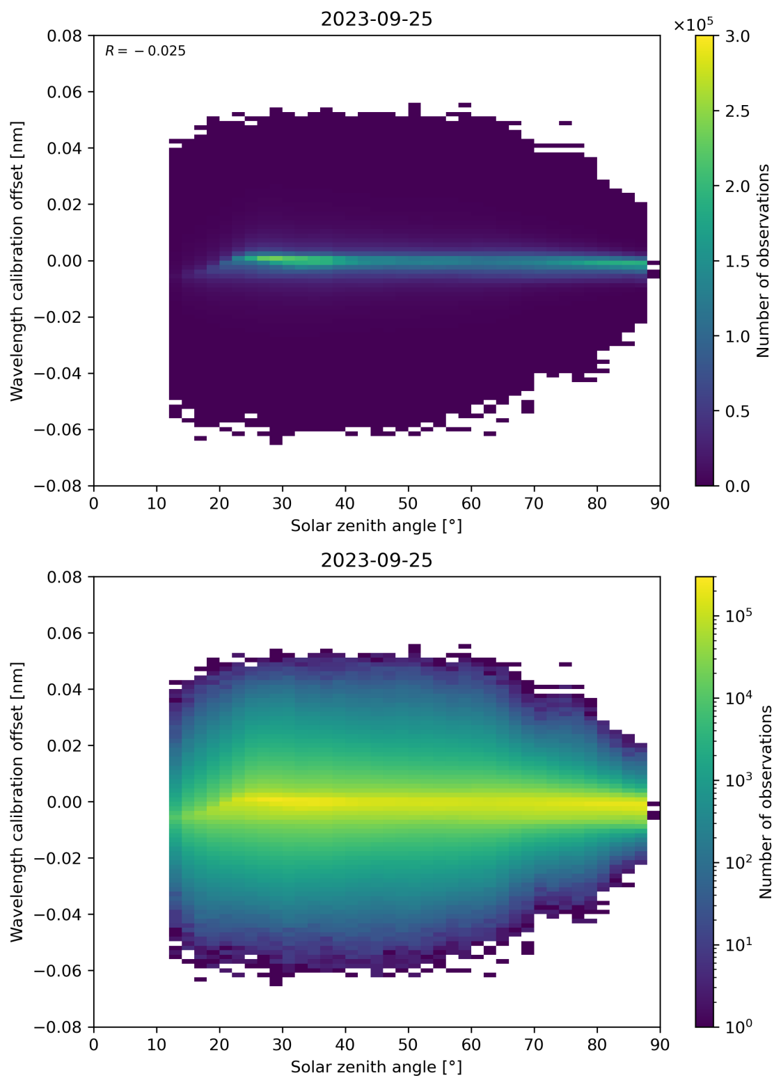
Figure 158: Scatter density plot of “Solar zenith angle” against “Wavelength calibration offset” for 2023-09-24 to 2023-09-26.
