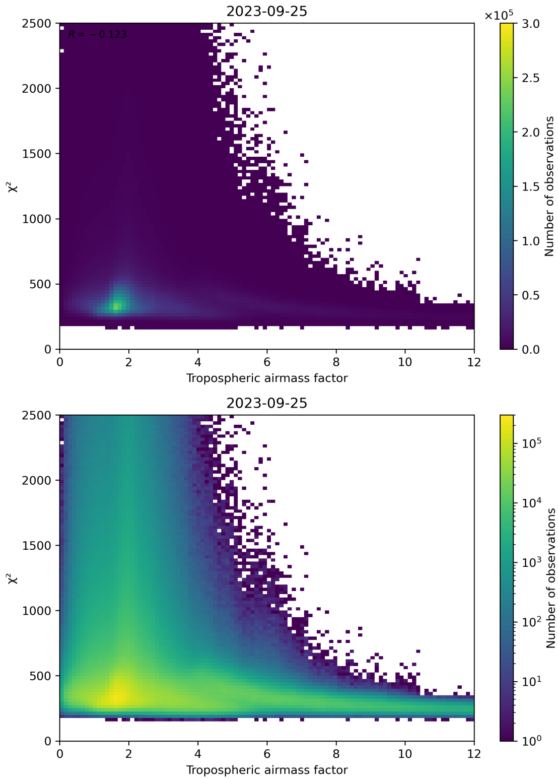
Figure 73: Scatter density plot of “Tropospheric airmass factor” against “ \chi^2 ” for 2023-09-24 to 2023-09-26.
