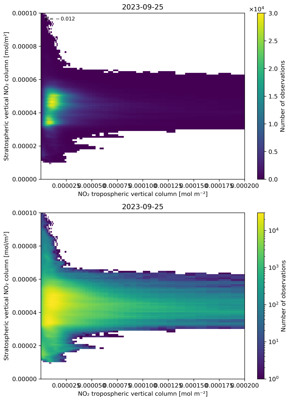
Figure 125: Scatter density plot of “NO 2 tropospheric vertical column” against “Stratospheric vertical NO 2 column” for 2023-09-24 to 2023-09-26.
