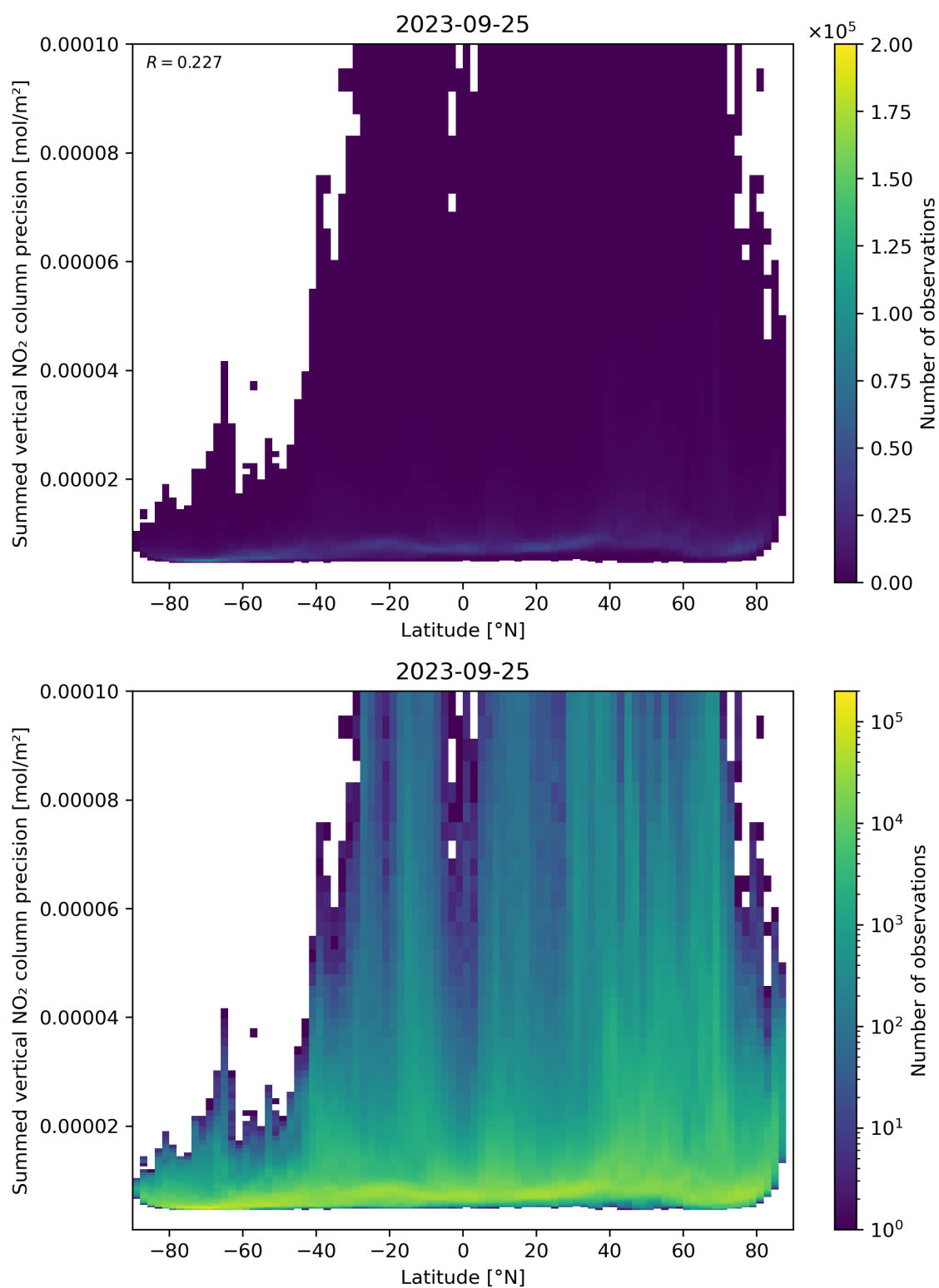
Figure 89: Scatter density plot of “Latitude” against “Summed vertical NO 2 column precision” for 2023-09-24 to 2023-09-26.
