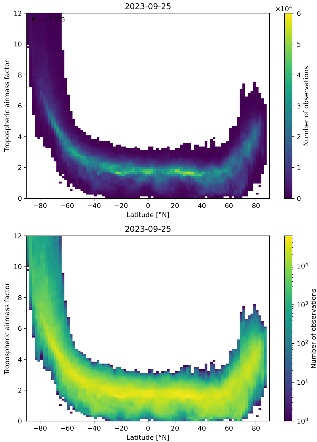
Figure 85: Scatter density plot of “Latitude” against “Tropospheric airmass factor” for 2023-09-24 to 2023-09-26.
