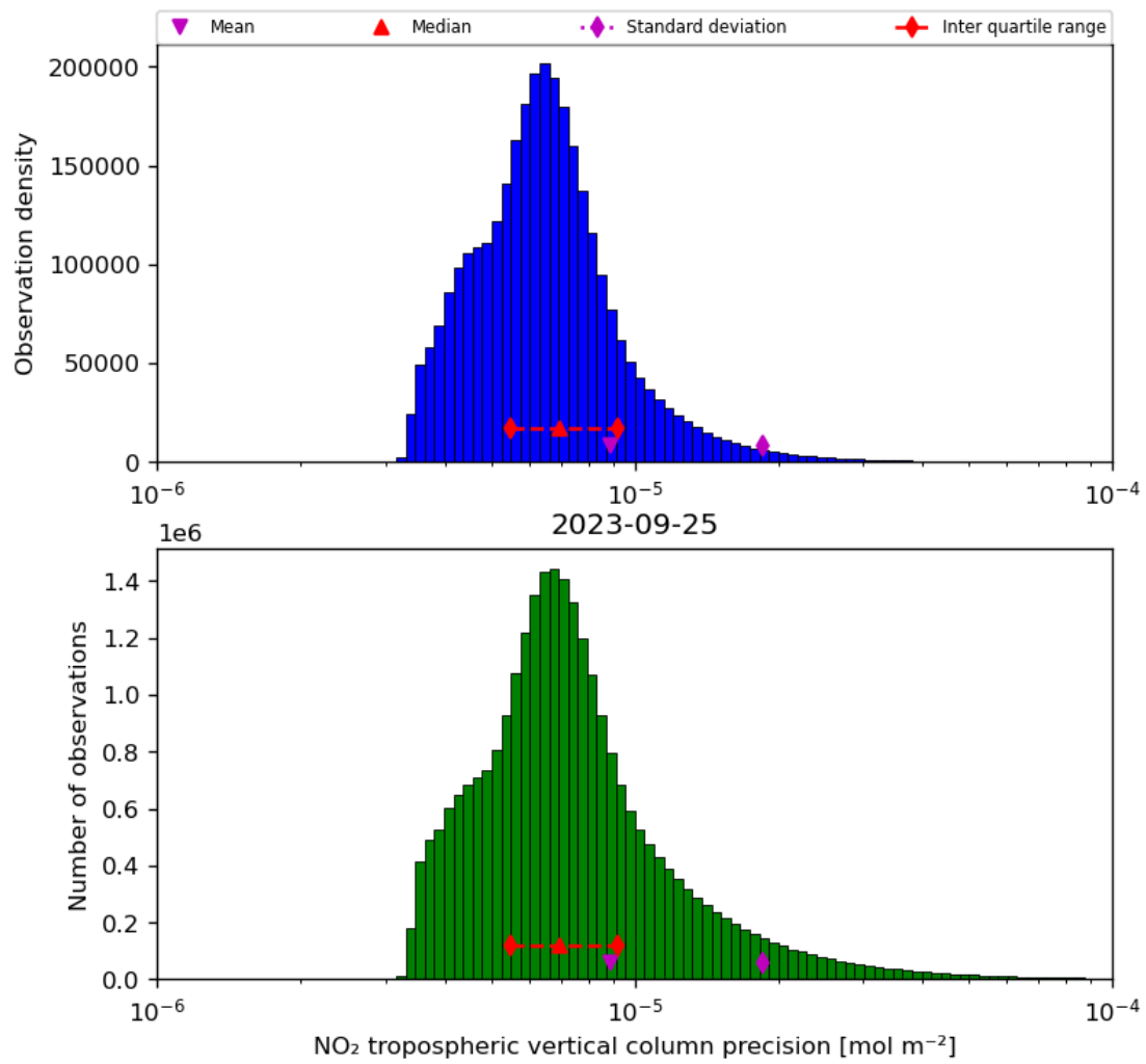
Figure 30: Histogram of “NO 2 tropospheric vertical column precision” for 2023-09-24 to 2023-09-26
