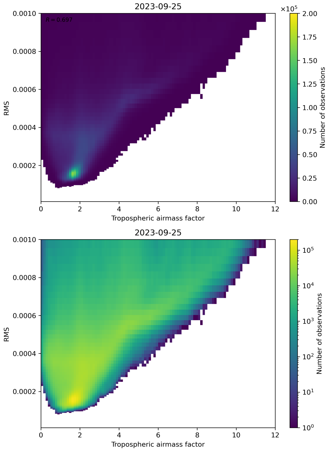
Figure 79: Scatter density plot of “Tropospheric airmass factor” against “RMS” for 2023-09-24 to 2023-09-26.
