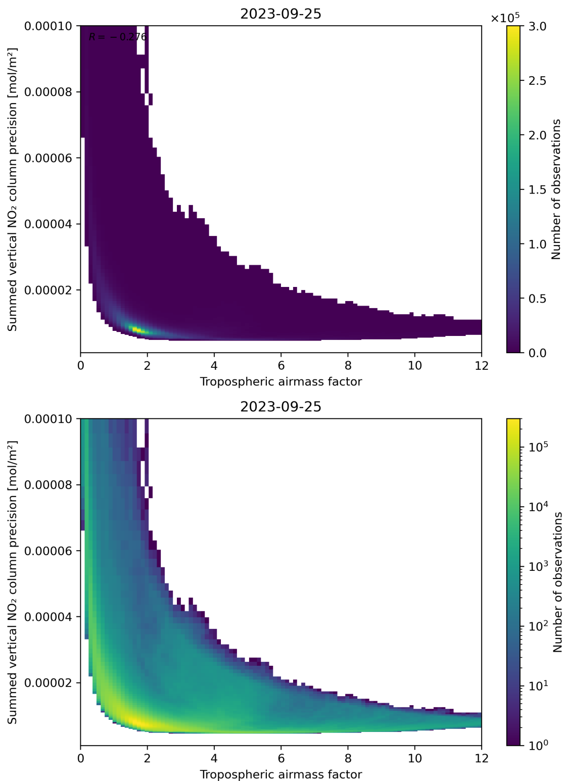
Figure 76: Scatter density plot of “Tropospheric air mass factor” against “Summed vertical NO 2 column precision” for 2023-09-24 to 2023-09-26.
