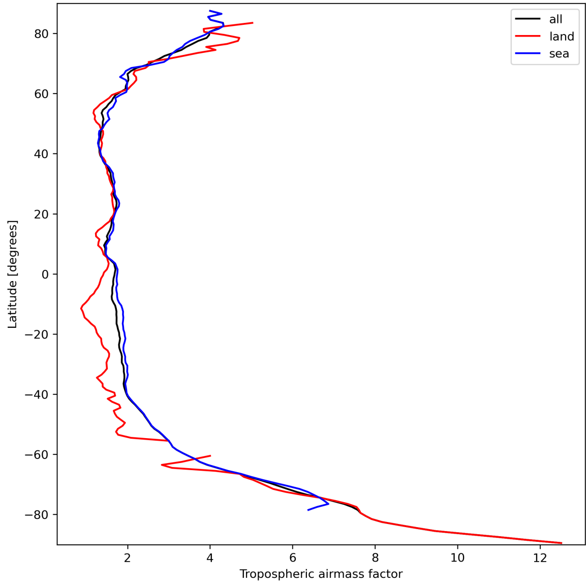
Figure 14: Zonal average of “Tropospheric airmass factor” for 2023-09-24 to 2023-09-26.
