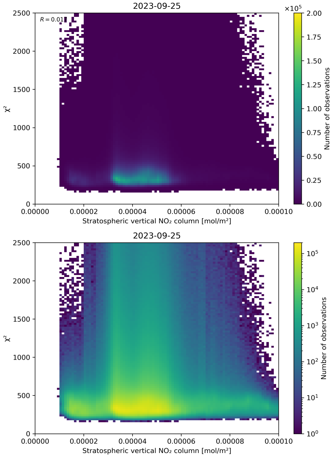
Figure 97: Scatter density plot of “Stratospheric vertical NO 2 column” against “ \chi^2 ” for 2023-09-24 to 2023-09-26.
