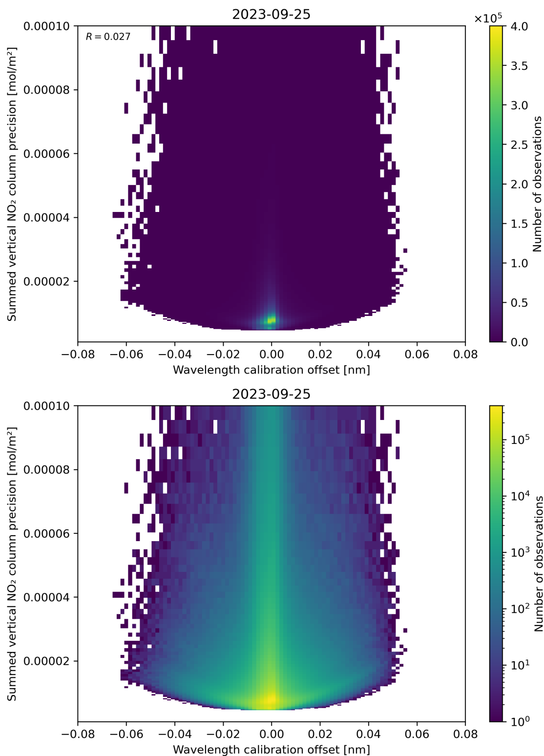
Figure 178: Scatter density plot of “Wavelength calibration offset” against “Summed vertical NO 2 column precision” for 2023-09-24 to 2023-09-26.
