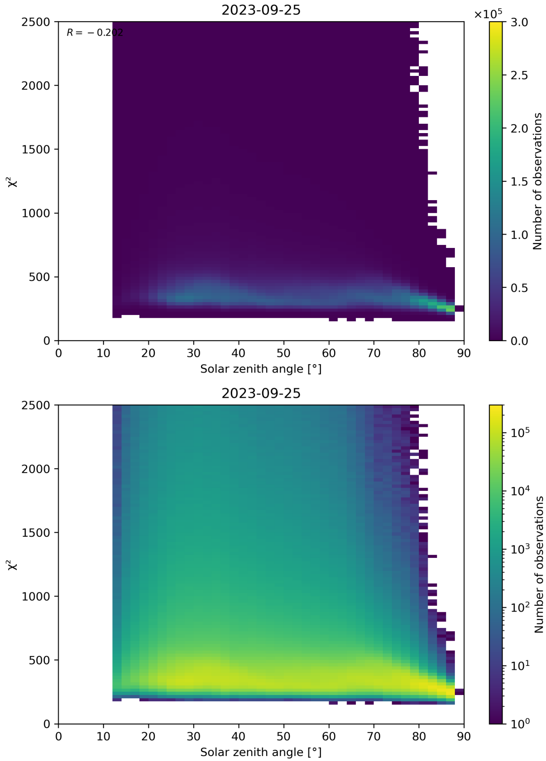
Figure 148: Scatter density plot of “Solar zenith angle” against “ \chi^2 ” for 2023-09-24 to 2023-09-26.
