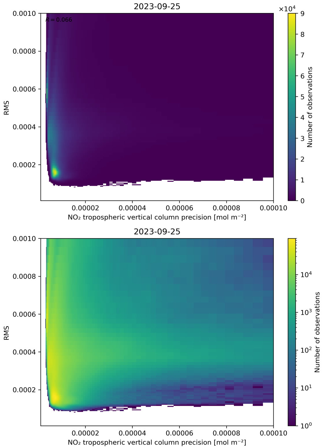
Figure 140: Scatter density plot of “NO 2 tropospheric vertical column precision” against “RMS” for 2023-09-24 to 2023-09-26.
