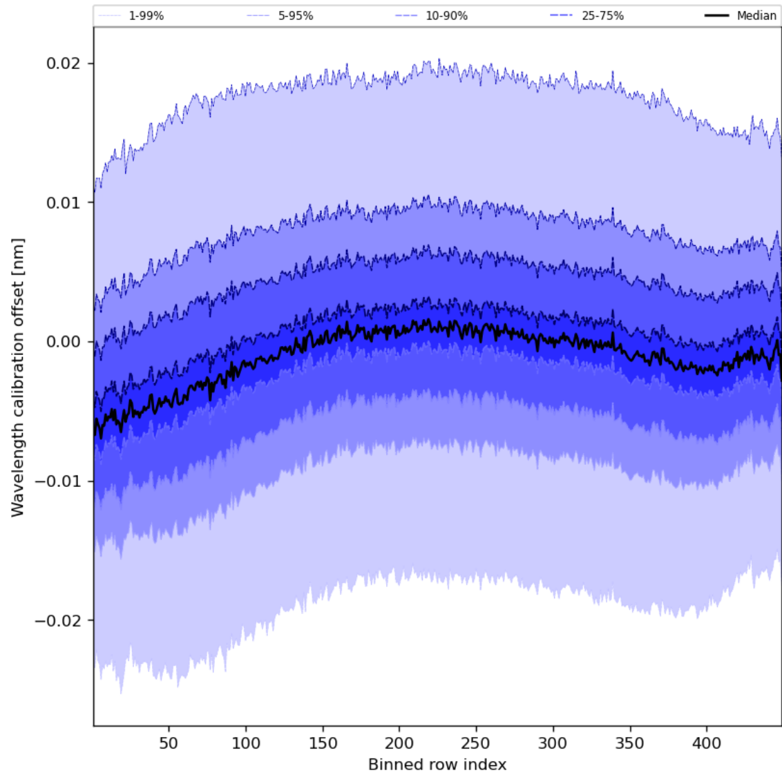
Figure 52: Along track statistics of “Wavelength calibration offset” for 2023-09-24 to 2023-09-26
