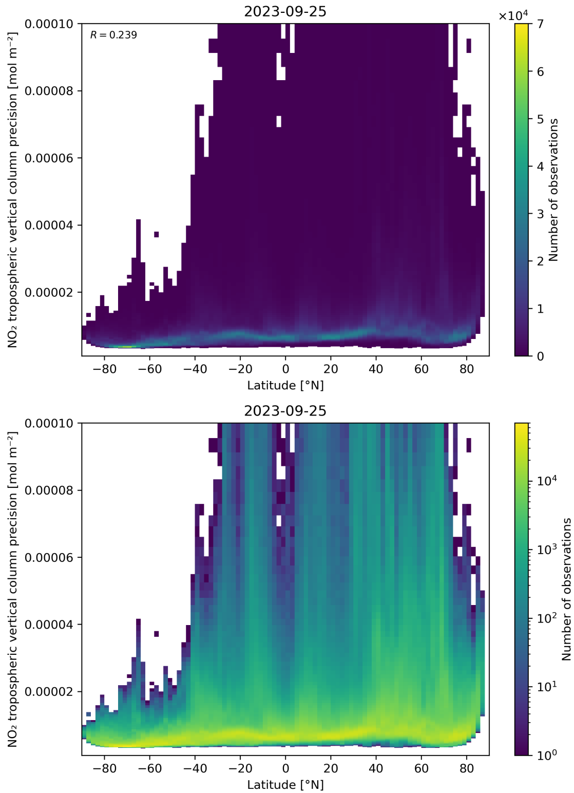
Figure 93: Scatter density plot of “Latitude” against “NO 2 tropospheric vertical column precision” for 2023-09-24 to 2023-09-26.
