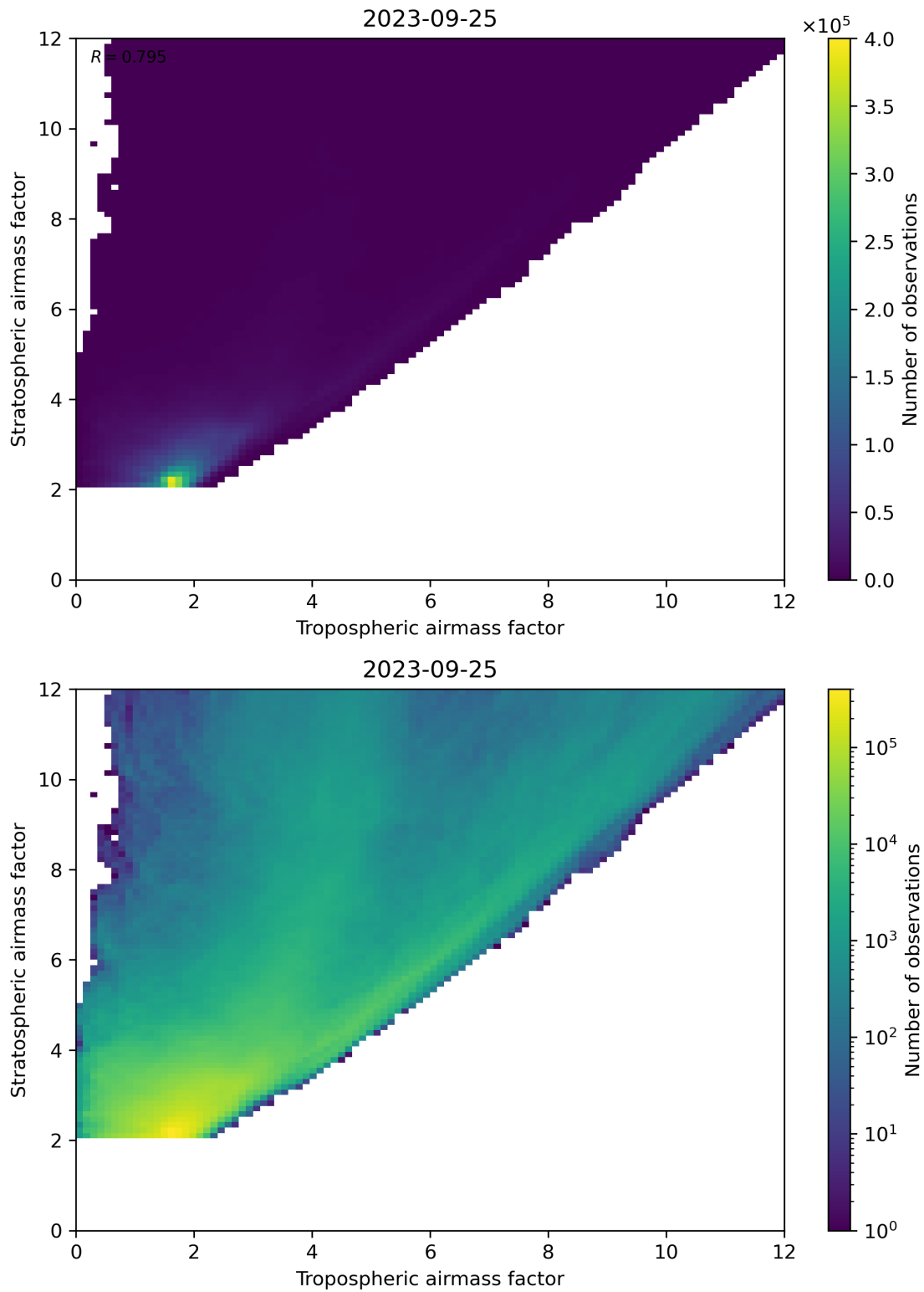
Figure 71: Scatter density plot of “Tropospheric airmass factor” against “Stratospheric airmass factor” for 2023-09-24 to 2023-09-26.
