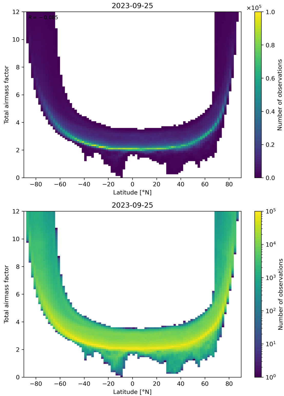
Figure 84: Scatter density plot of “Latitude” against “Total airmass factor” for 2023-09-24 to 2023-09-26.
