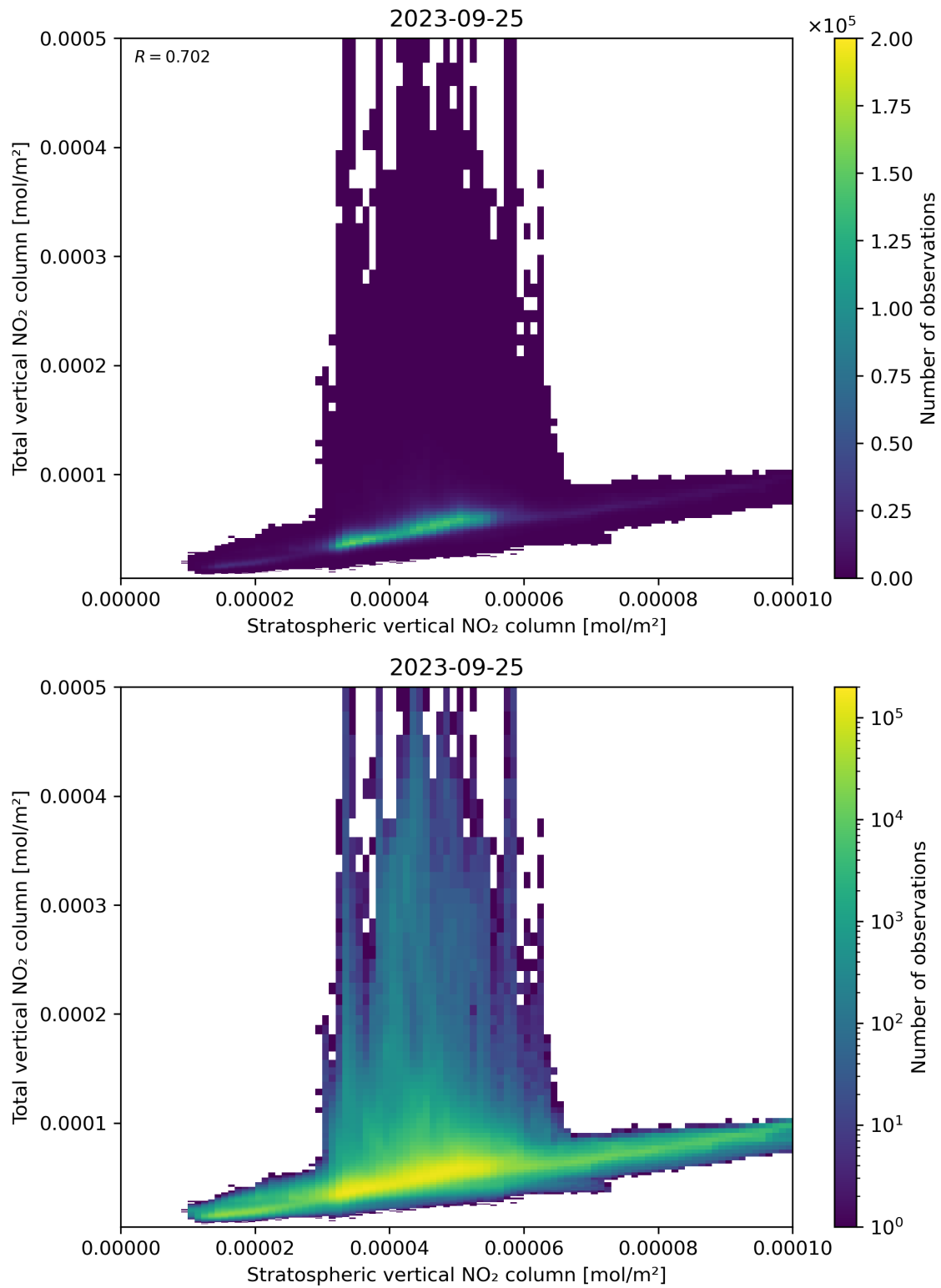
Figure 100: Scatter density plot of “Stratospheric vertical NO 2 column” against “Total vertical NO 2 column” for 2023-09-24 to 2023-09-26.
