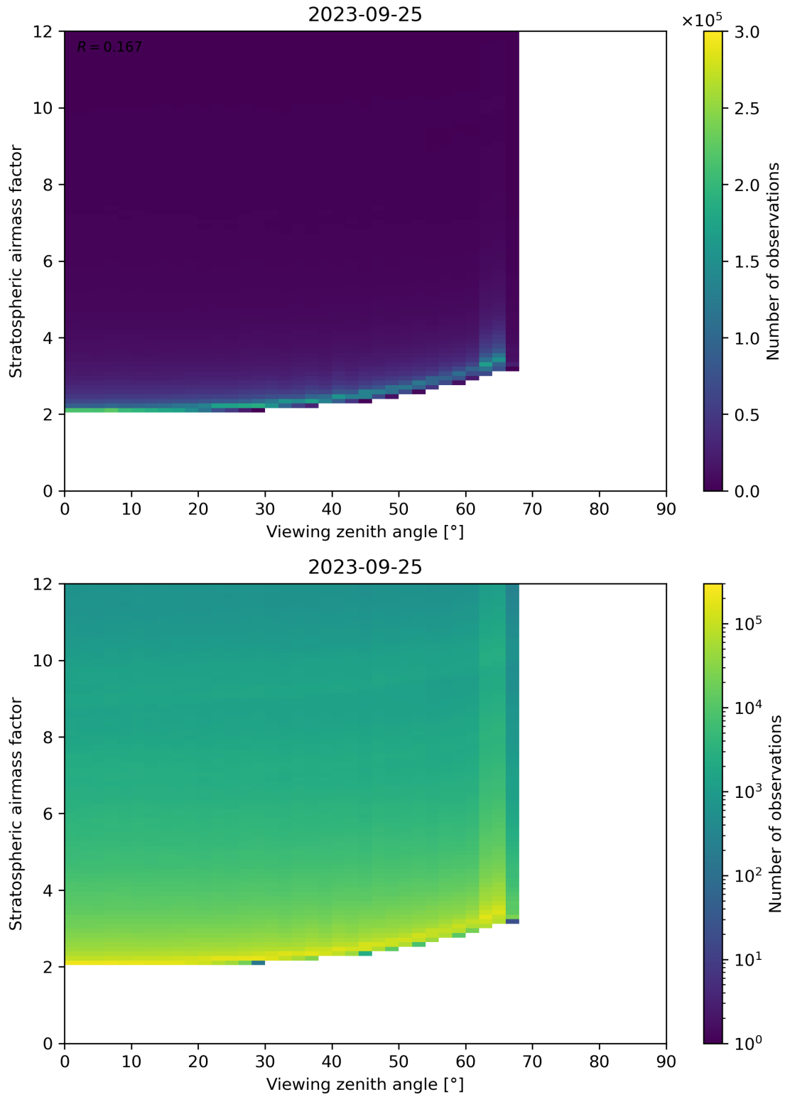
Figure 159: Scatter density plot of “Viewing zenith angle” against “Stratospheric airmass factor” for 2023-09-24 to 2023-09-26.
