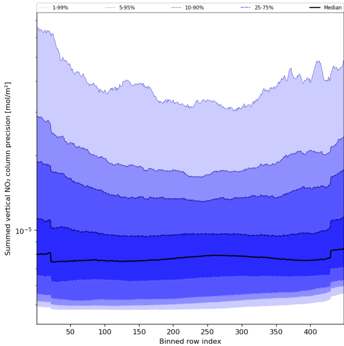
Figure 58: Along track statistics of “Summed vertical NO 2 column precision” for 2023-09-24 to 2023-09-26
