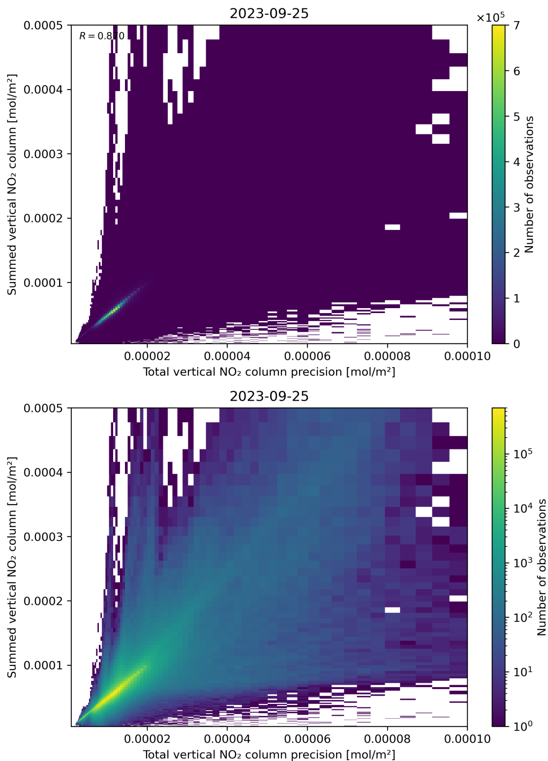
Figure 117: Scatter density plot of “Total vertical NO 2 column precision” against “Summed vertical NO 2 column” for 2023-09-24 to 2023-09-26.
