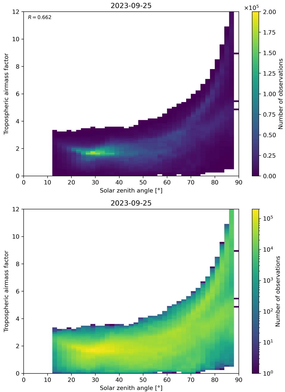
Figure 147: Scatter density plot of “Solar zenith angle” against “Tropospheric airmass factor” for 2023-09-24 to 2023-09-26.
