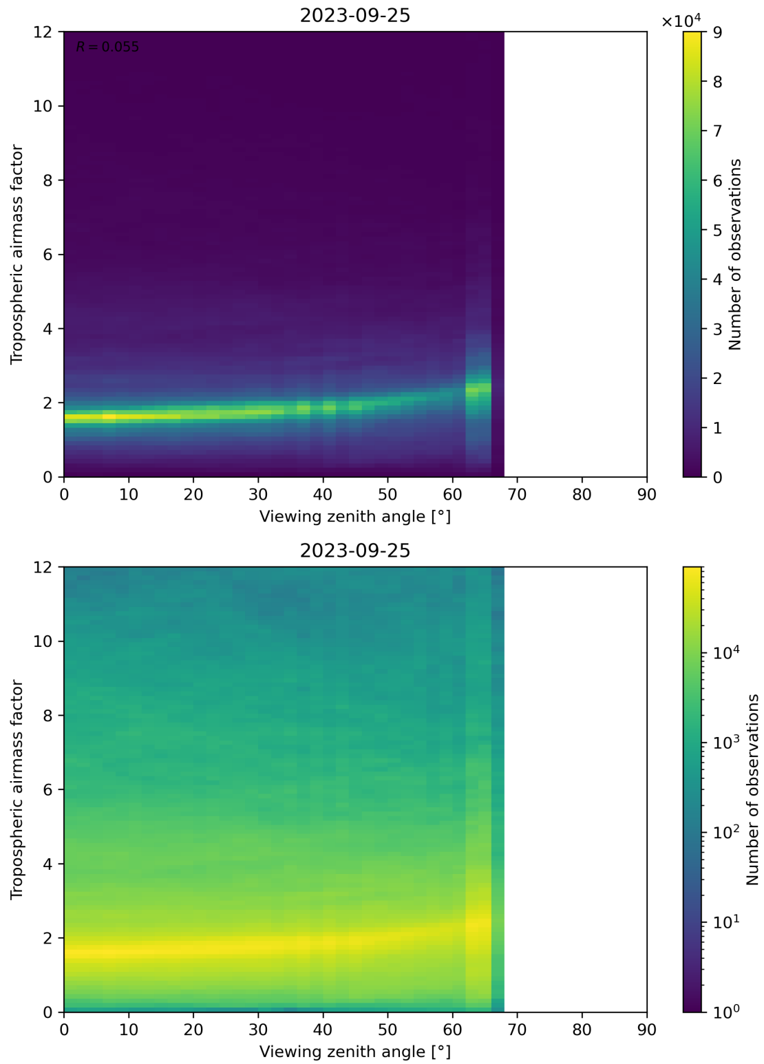
Figure 161: Scatter density plot of “Viewing zenith angle” against “Tropospheric airmass factor” for 2023-09-24 to 2023-09-26.
