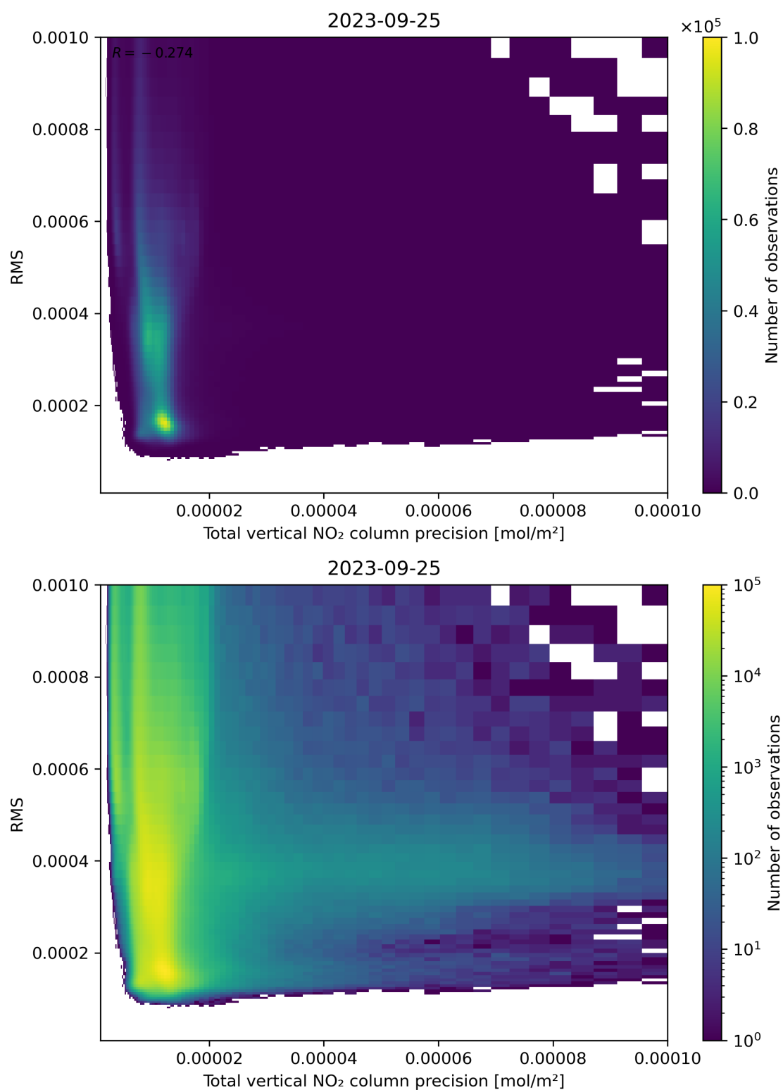
Figure 119: Scatter density plot of “Total vertical NO 2 column precision” against “RMS” for 2023-09-24 to 2023-09-26.
