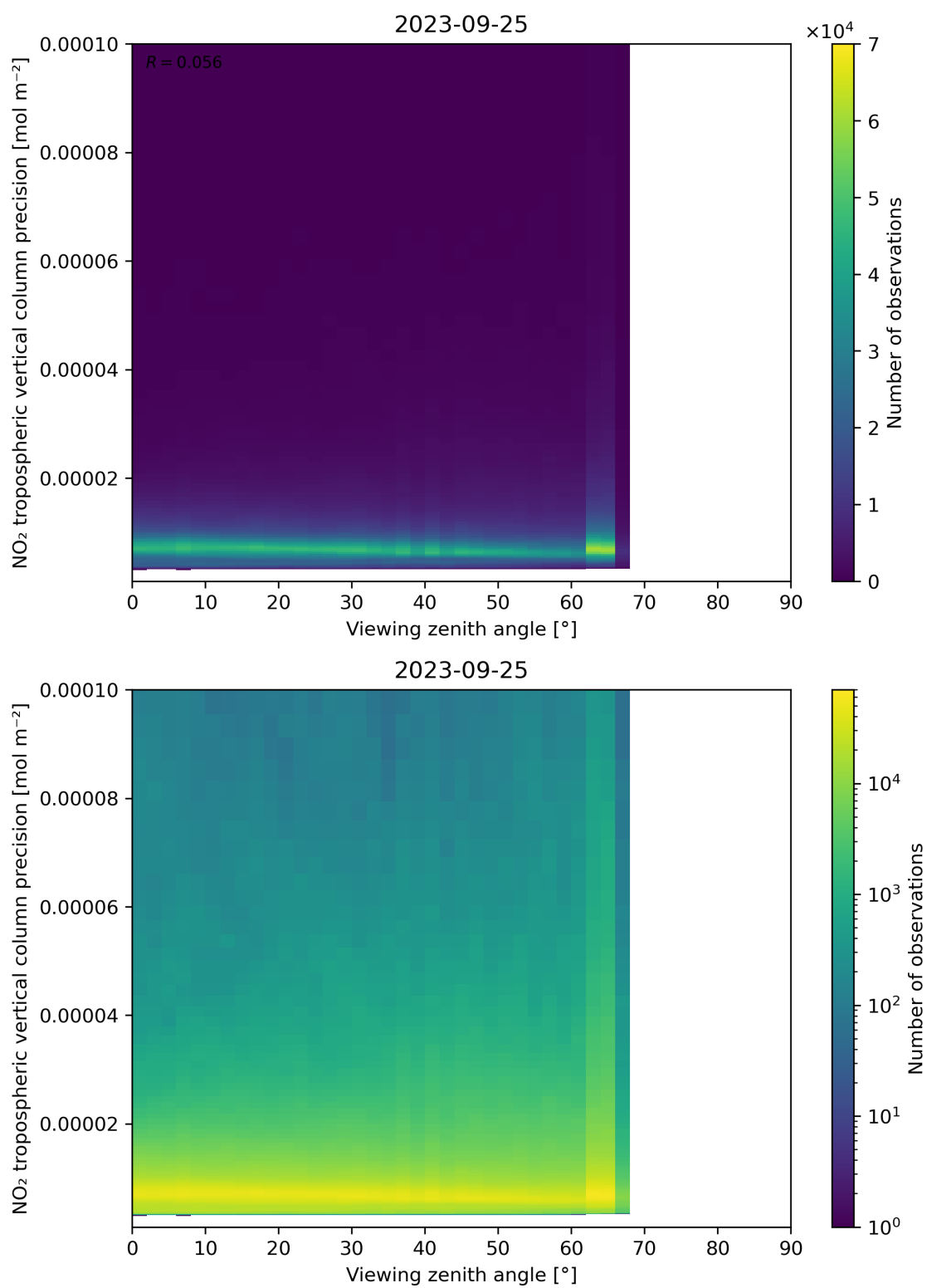
Figure 170: Scatter density plot of “Viewing zenith angle” against “NO 2 tropospheric vertical column precision” for 2023-09-24 to 2023-09-26.
