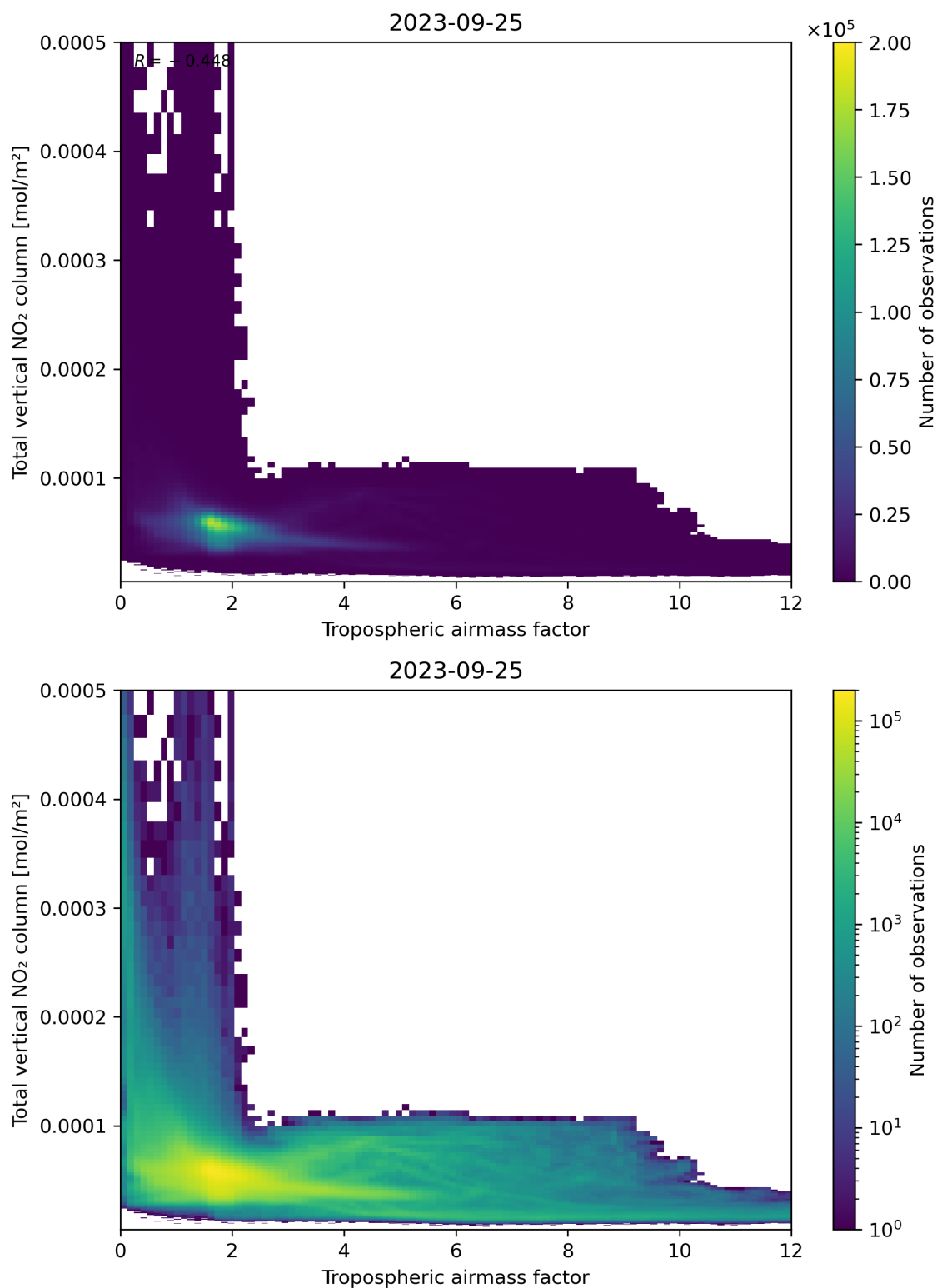
Figure 77: Scatter density plot of “Tropospheric airmass factor” against “Total vertical NO 2 column” for 2023-09-24 to 2023-09-26.
