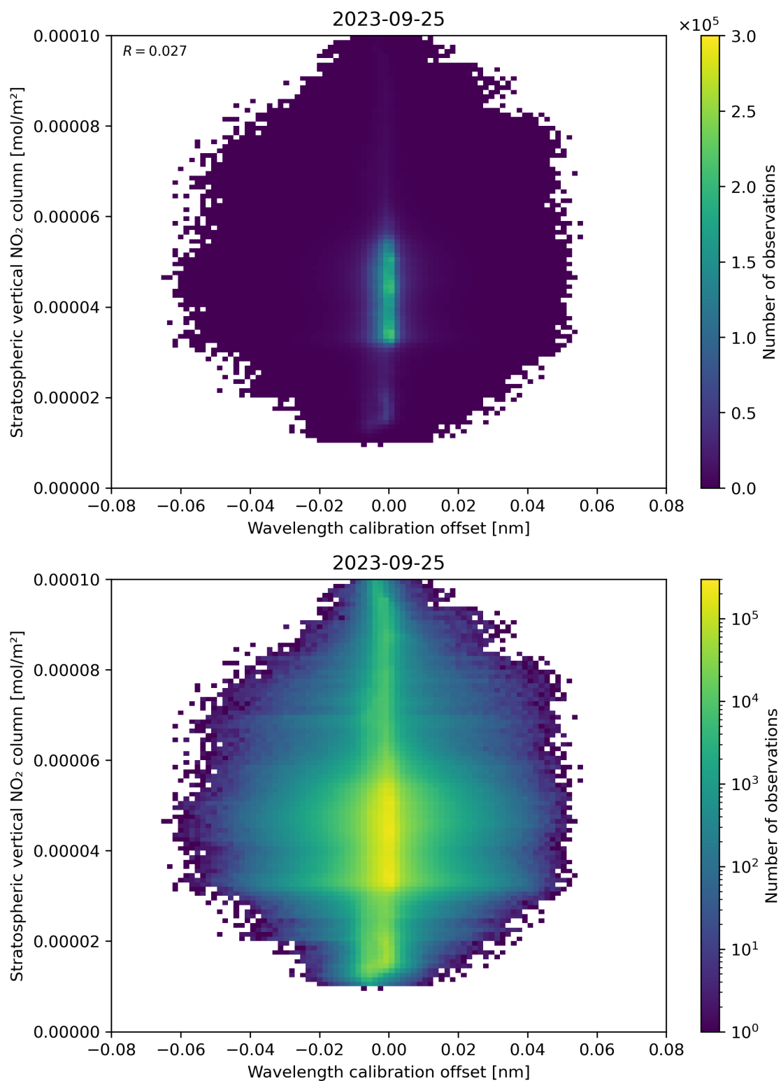
Figure 176: Scatter density plot of “Wavelength calibration offset” against “Stratospheric vertical NO 2 column” for 2023-09-24 to 2023-09-26.
