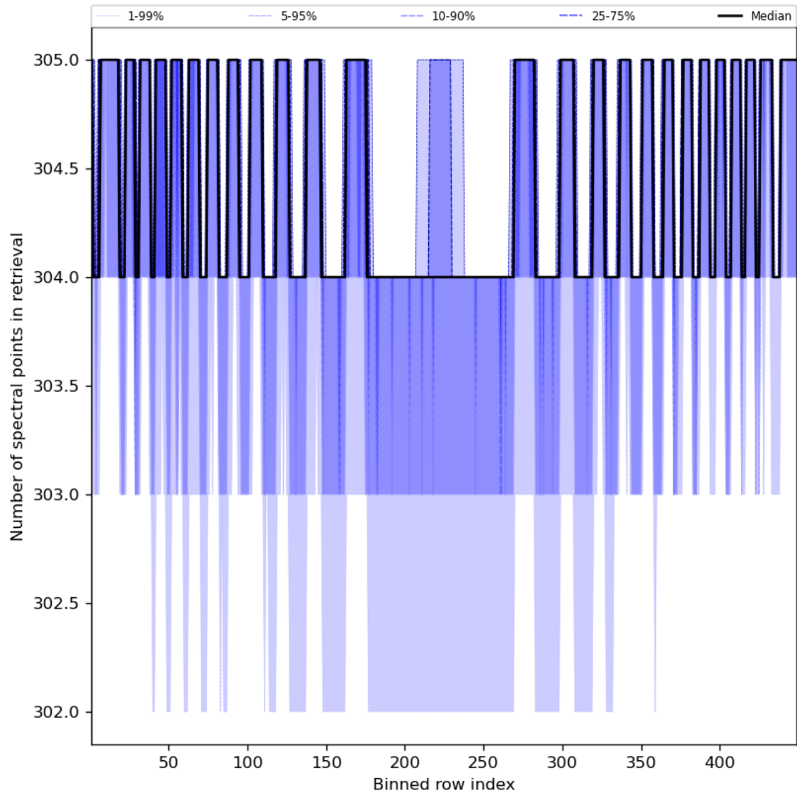
Figure 50: Along track statistics of “Number of spectral points in retrieval” for 2023-09-24 to 2023-09-26
