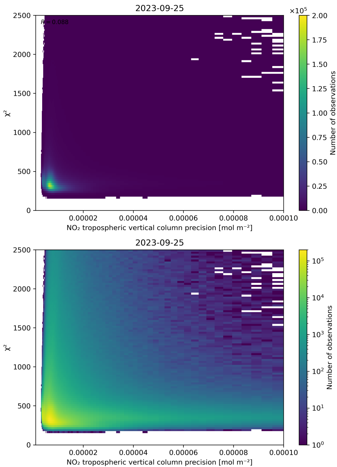
Figure 134: Scatter density plot of “NO 2 tropospheric vertical column precision” against “ \chi^2 ” for 2023-09-24 to 2023-09-26.
