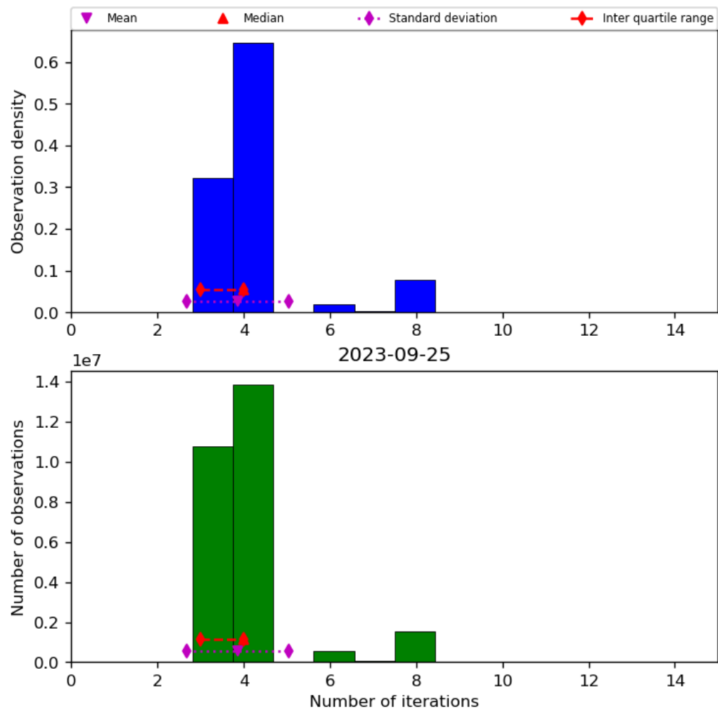
Figure 34: Histogram of “Number of iterations” for 2023-09-24 to 2023-09-26
