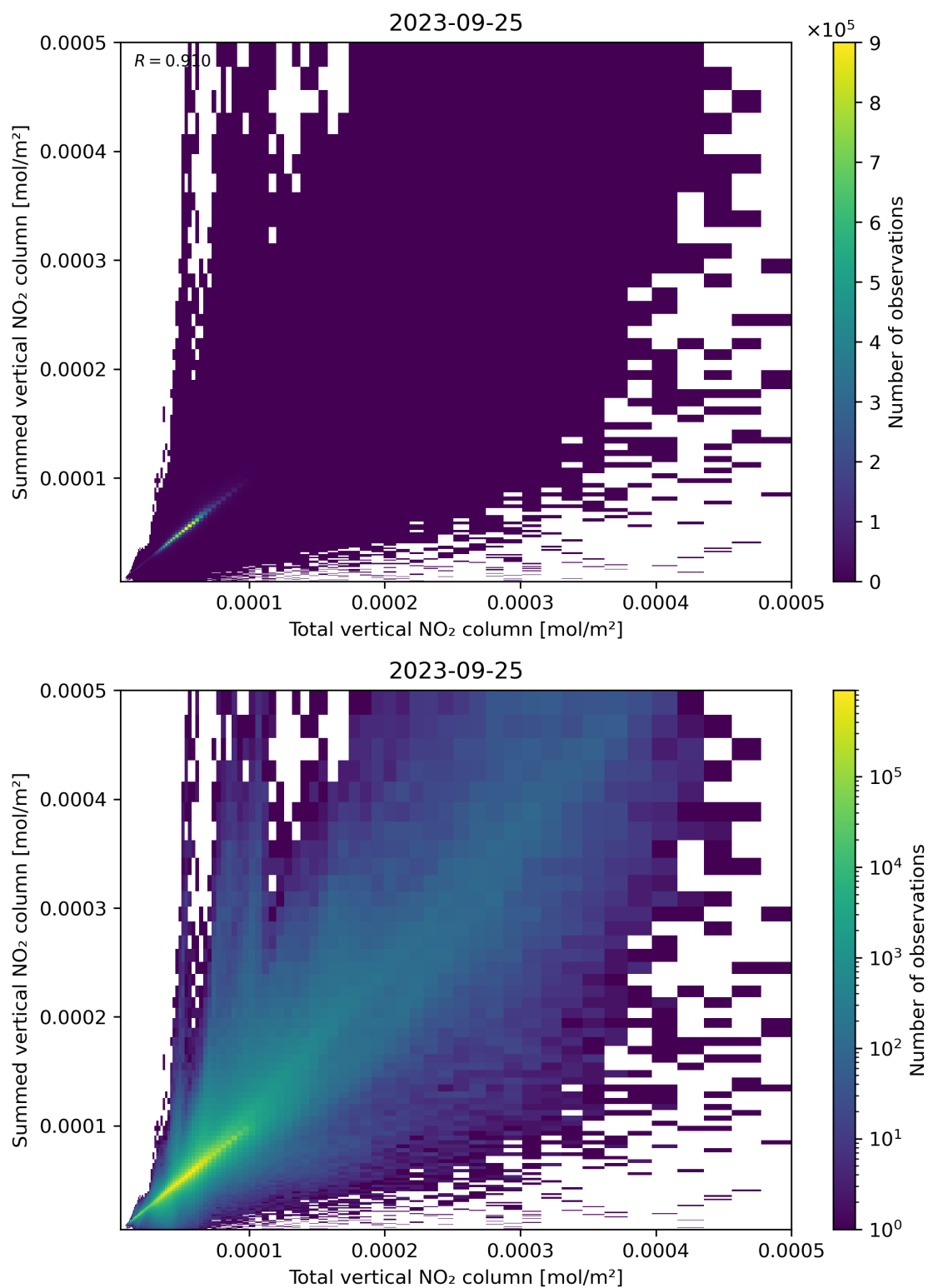
Figure 112: Scatter density plot of “Total vertical NO 2 column” against “Summed vertical NO 2 column” for 2023-09-24 to 2023-09-26.
