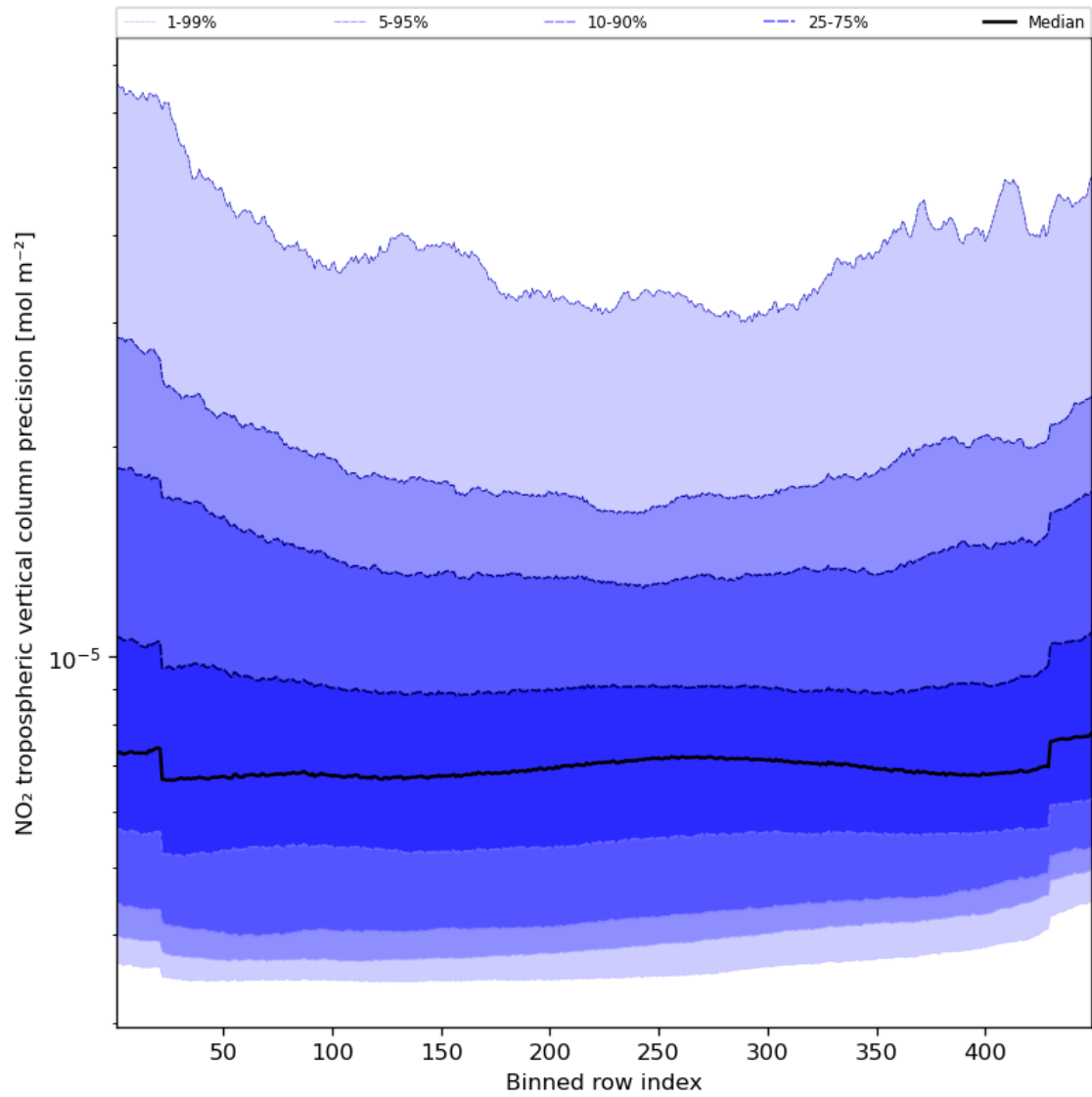
Figure 47: Along track statistics of “NO 2 tropospheric vertical column precision” for 2023-09-24 to 2023-09-26
