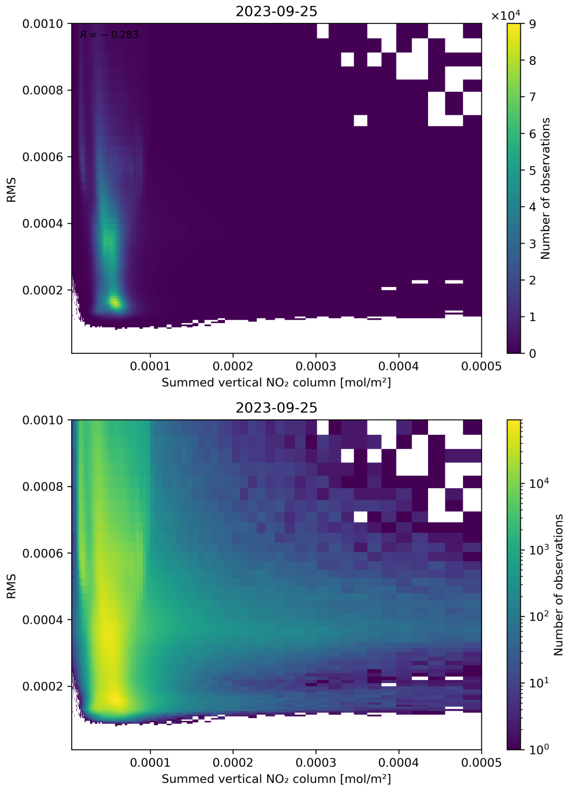
Figure 109: Scatter density plot of “Summed vertical NO 2 column” against “RMS” for 2023-09-24 to 2023-09-26.
