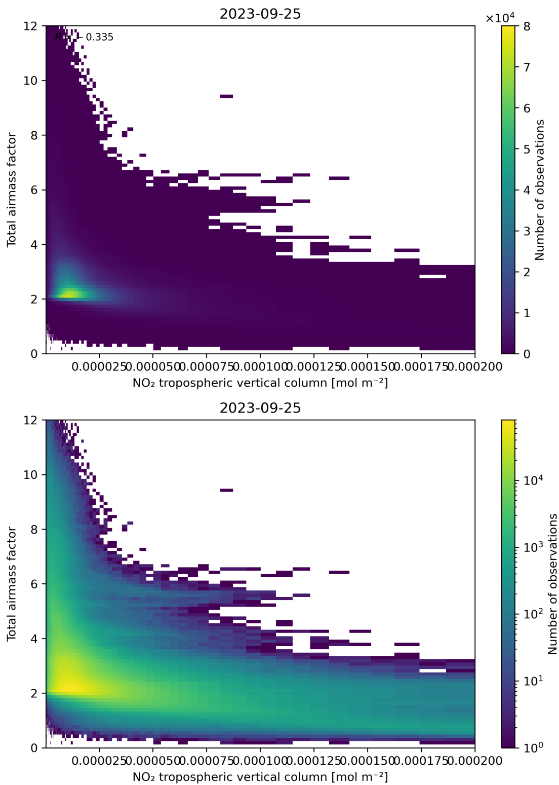
Figure 122: Scatter density plot of “NO 2 tropospheric vertical column” against “Total air mass factor” for 2023-09-24 to 2023-09-26.
