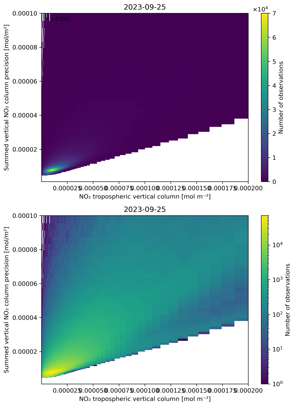
Figure 127: Scatter density plot of “NO 2 tropospheric vertical column” against “Summed vertical NO 2 column precision” for 2023-09-24 to 2023-09-26.
