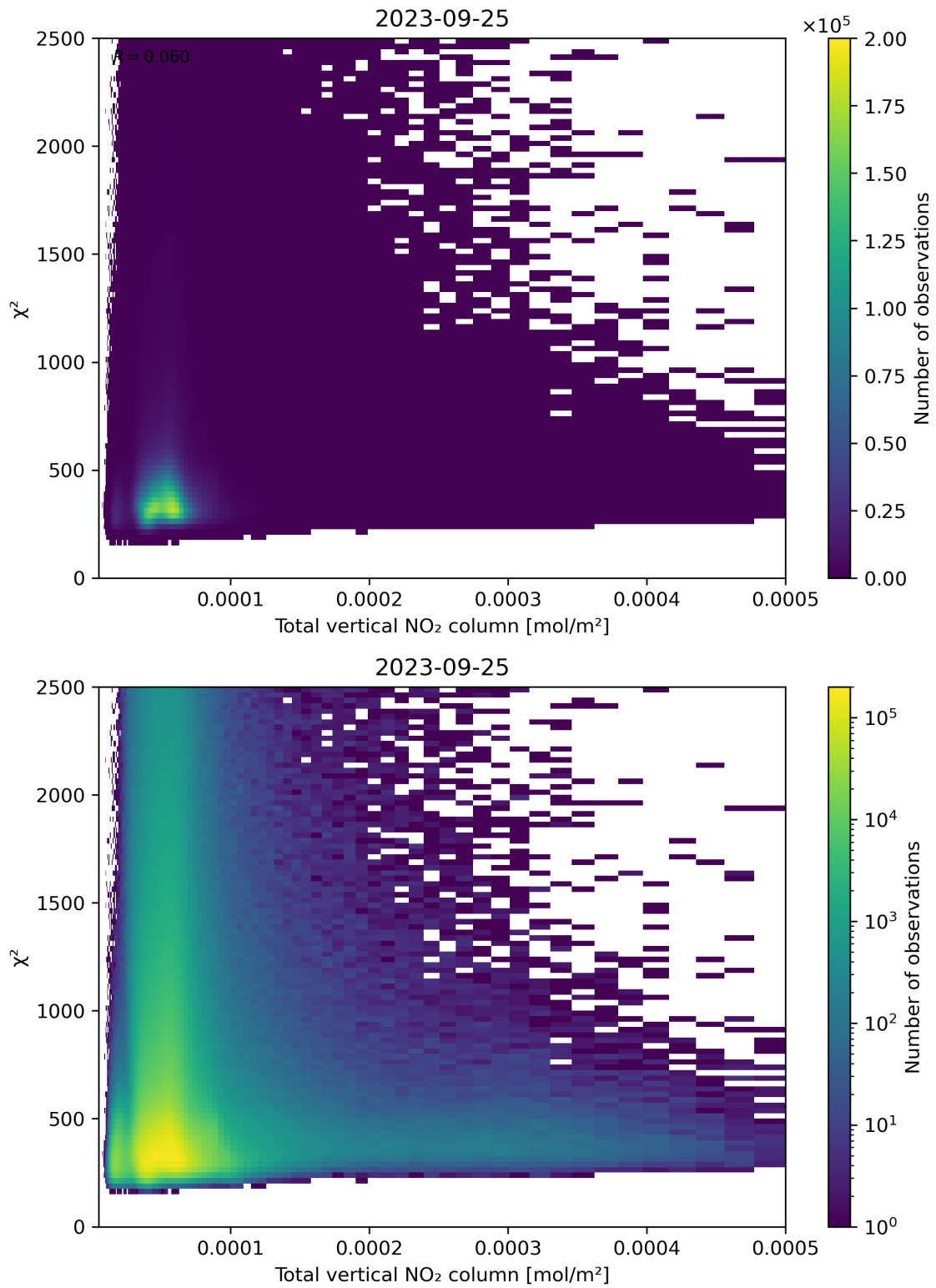
Figure 111: Scatter density plot of “Total vertical NO 2 column” against “ \chi^2 ” for 2023-09-24 to 2023-09-26.
