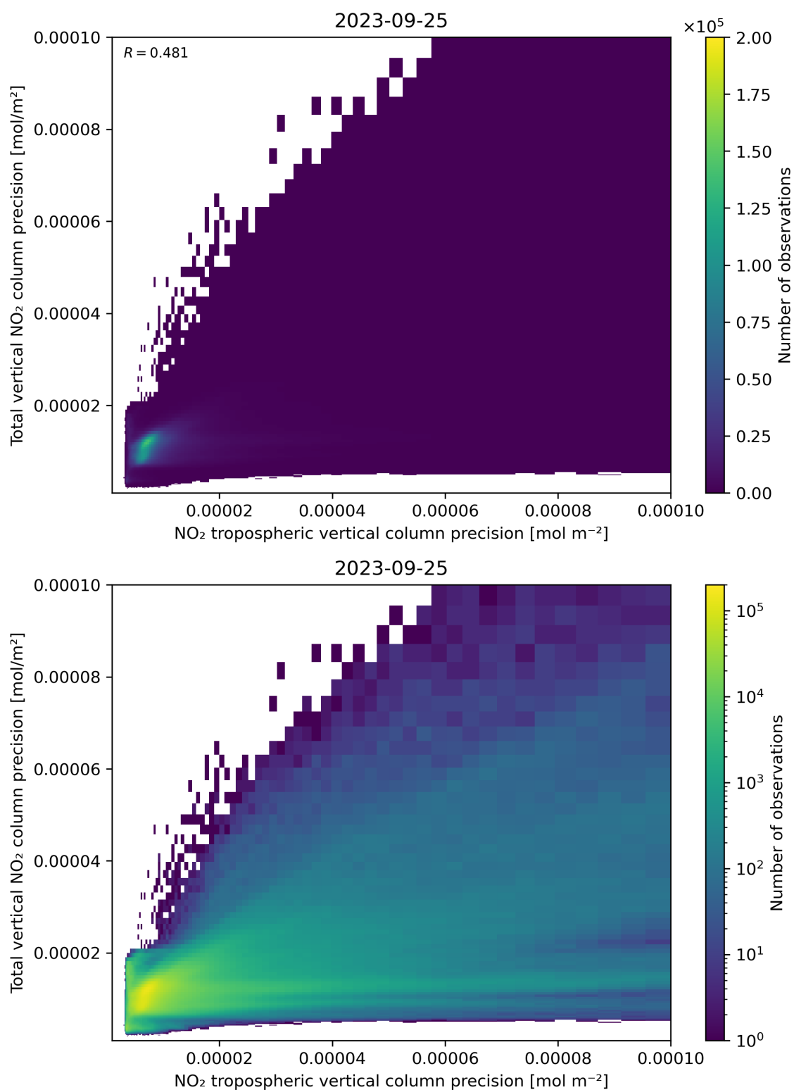
Figure 139: Scatter density plot of “NO 2 tropospheric vertical column precision” against “Total vertical NO 2 column precision” for 2023-09-24 to 2023-09-26.
