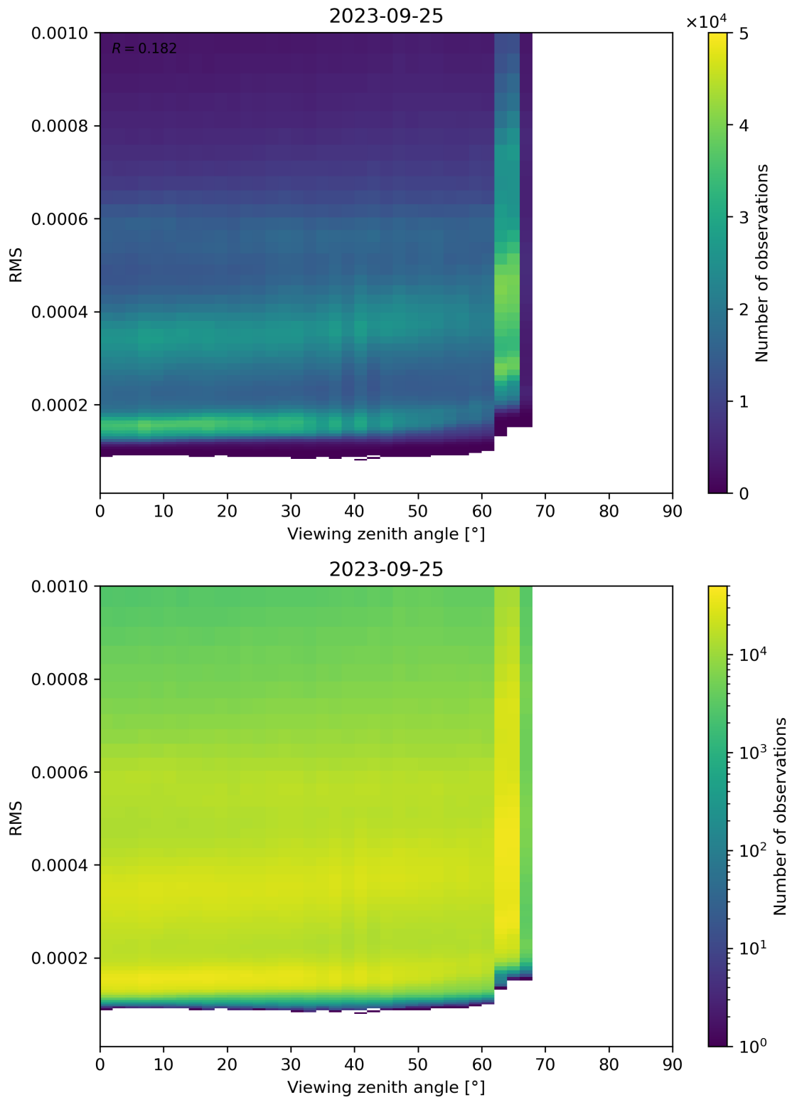
Figure 171: Scatter density plot of “Viewing zenith angle” against “RMS” for 2023-09-24 to 2023-09-26.
