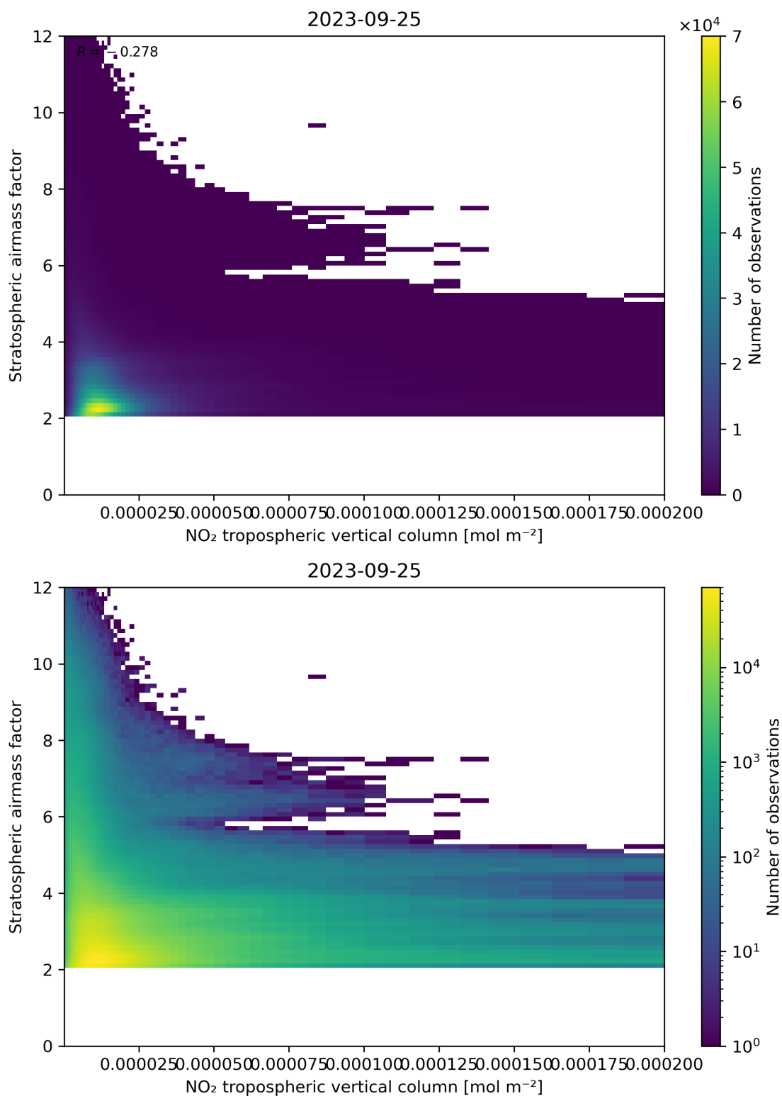
Figure 121: Scatter density plot of “NO 2 tropospheric vertical column” against “Stratospheric air mass factor” for 2023-09-24 to 2023-09-26.
