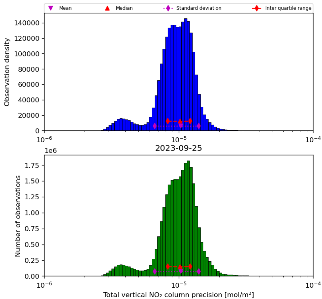
Figure 39: Histogram of “Total vertical NO 2 column precision” for 2023-09-24 to 2023-09-26
