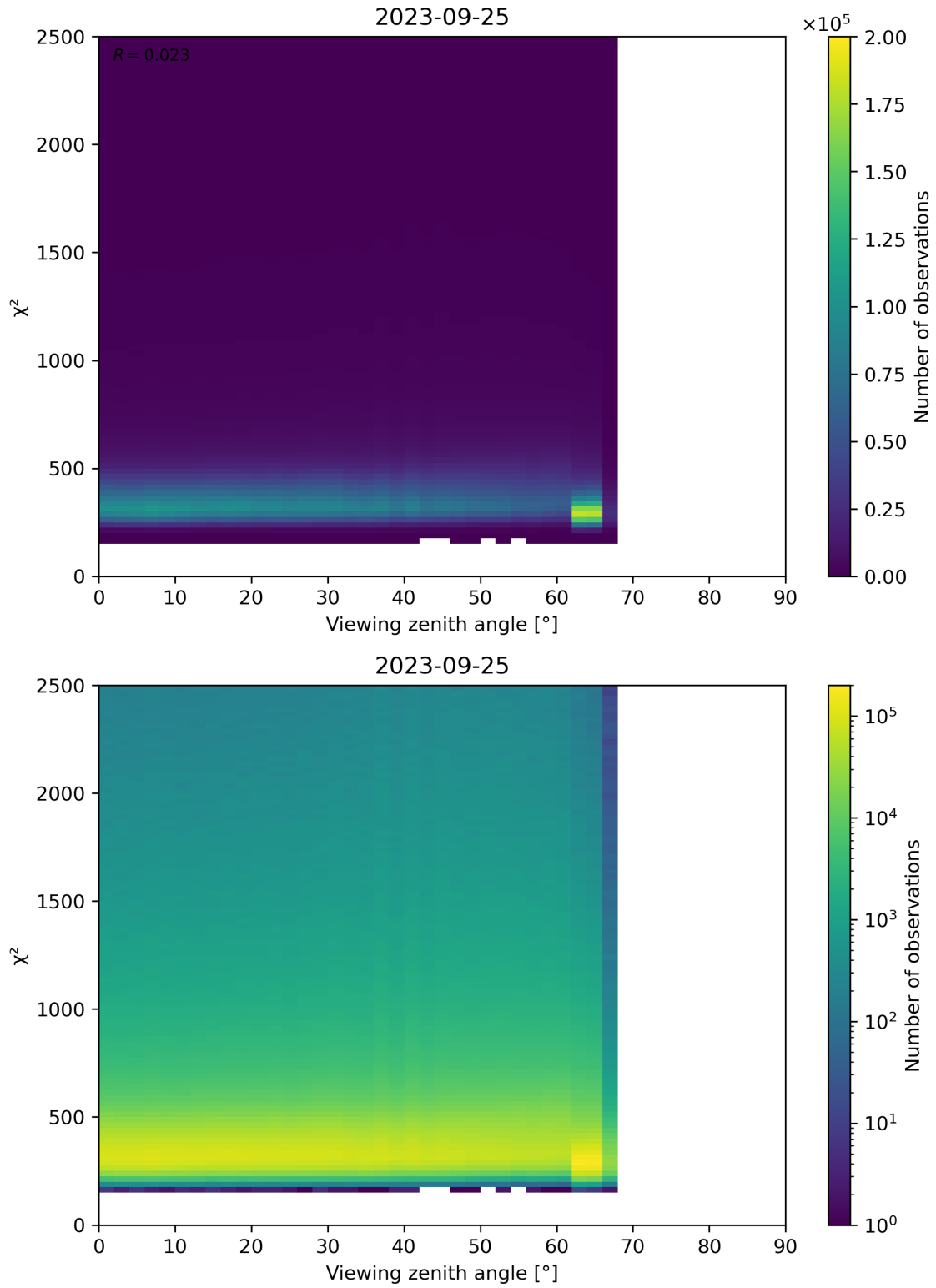
Figure 162: Scatter density plot of “Viewing zenith angle” against “ \chi^2 ” for 2023-09-24 to 2023-09-26.
