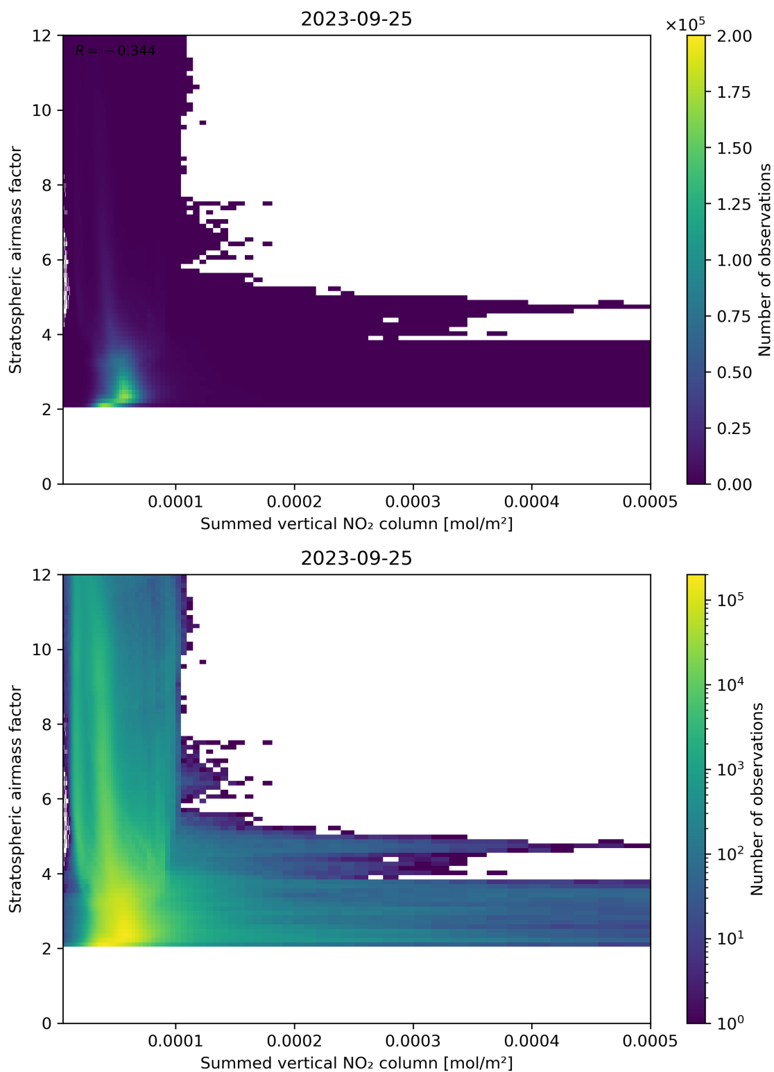
Figure 103: Scatter density plot of “Summed vertical NO 2 column” against “Stratospheric airmass factor” for 2023-09-24 to 2023-09-26.
