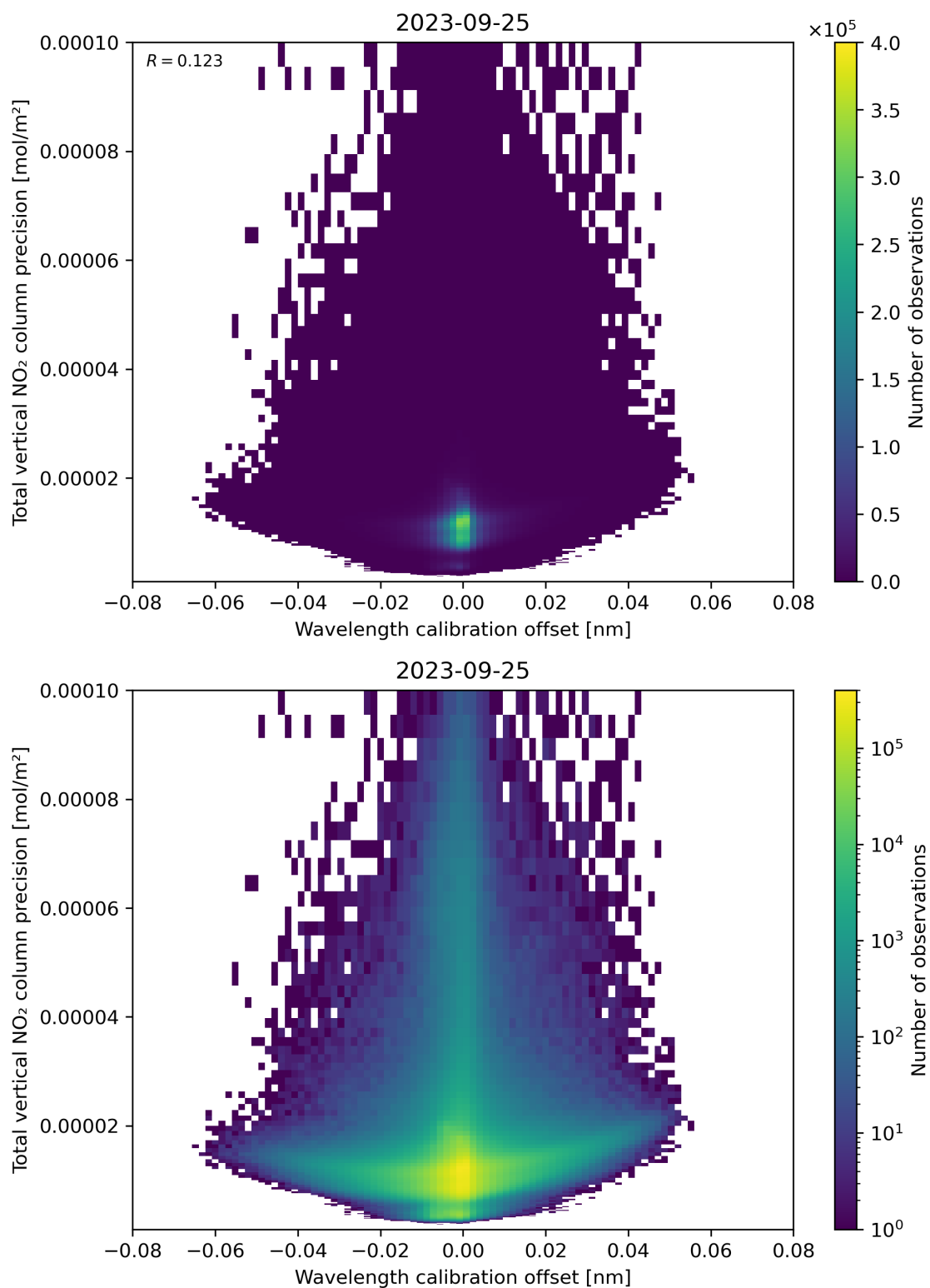
Figure 180: Scatter density plot of “Wavelength calibration offset” against “Total vertical NO 2 column precision” for 2023-09-24 to 2023-09-26.
