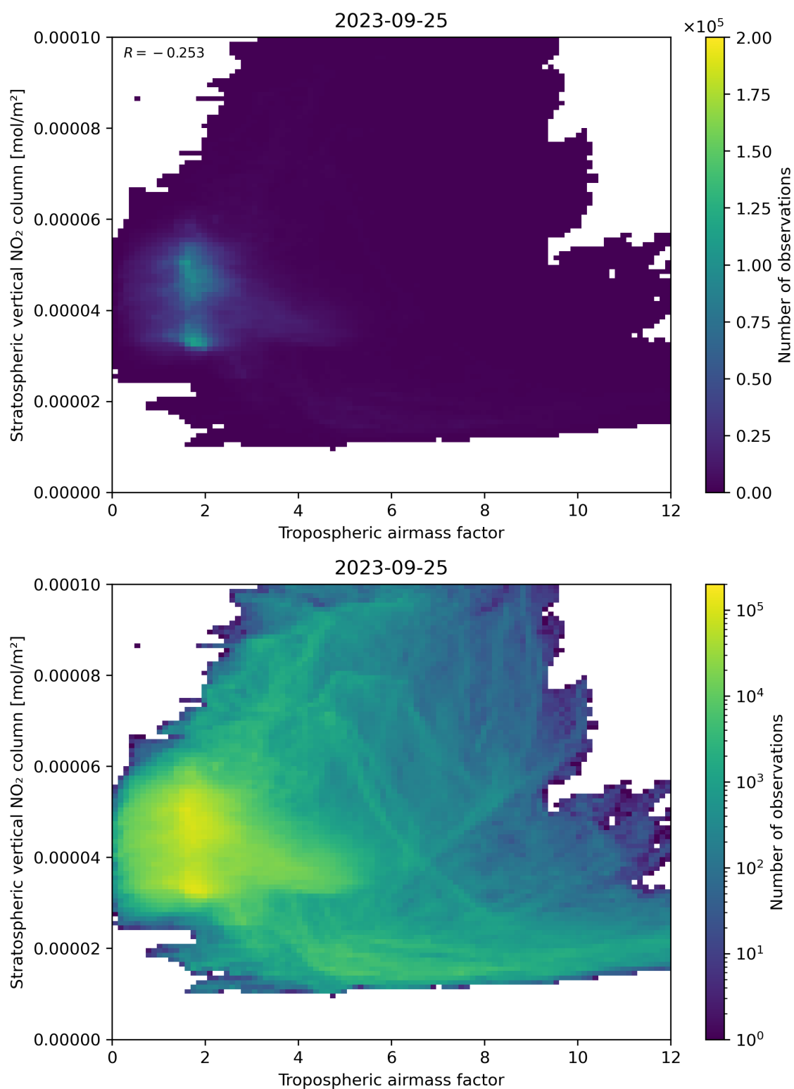
Figure 74: Scatter density plot of “Tropospheric air mass factor” against “Stratospheric vertical NO 2 column” for 2023-09-24 to 2023-09-26.
