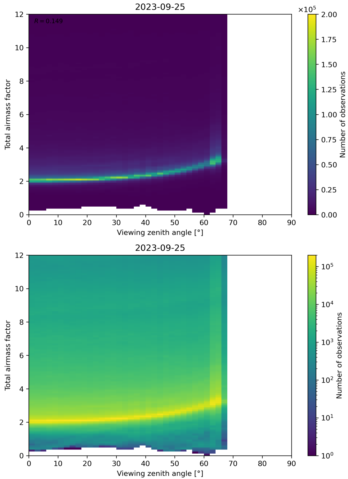
Figure 160: Scatter density plot of “Viewing zenith angle” against “Total airmass factor” for 2023-09-24 to 2023-09-26.
