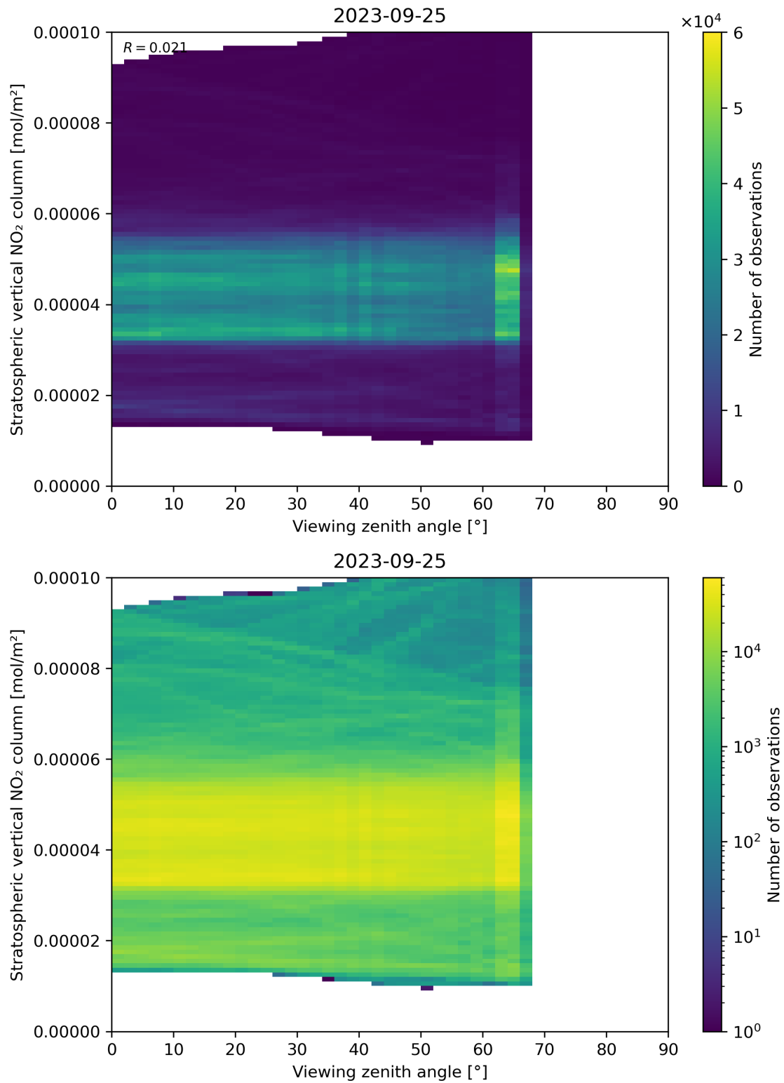
Figure 164: Scatter density plot of “Viewing zenith angle” against “Stratospheric vertical NO 2 column” for 2023-09-24 to 2023-09-26.
