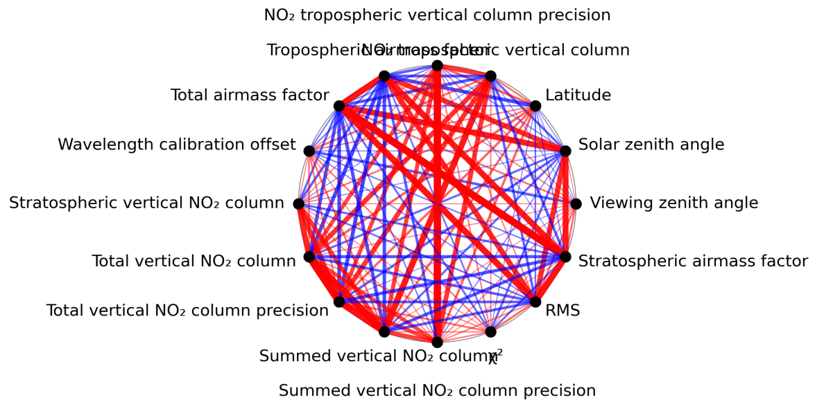
Figure 1: Map of correlation graph for 2023-09-24 to 2023-09-26.
