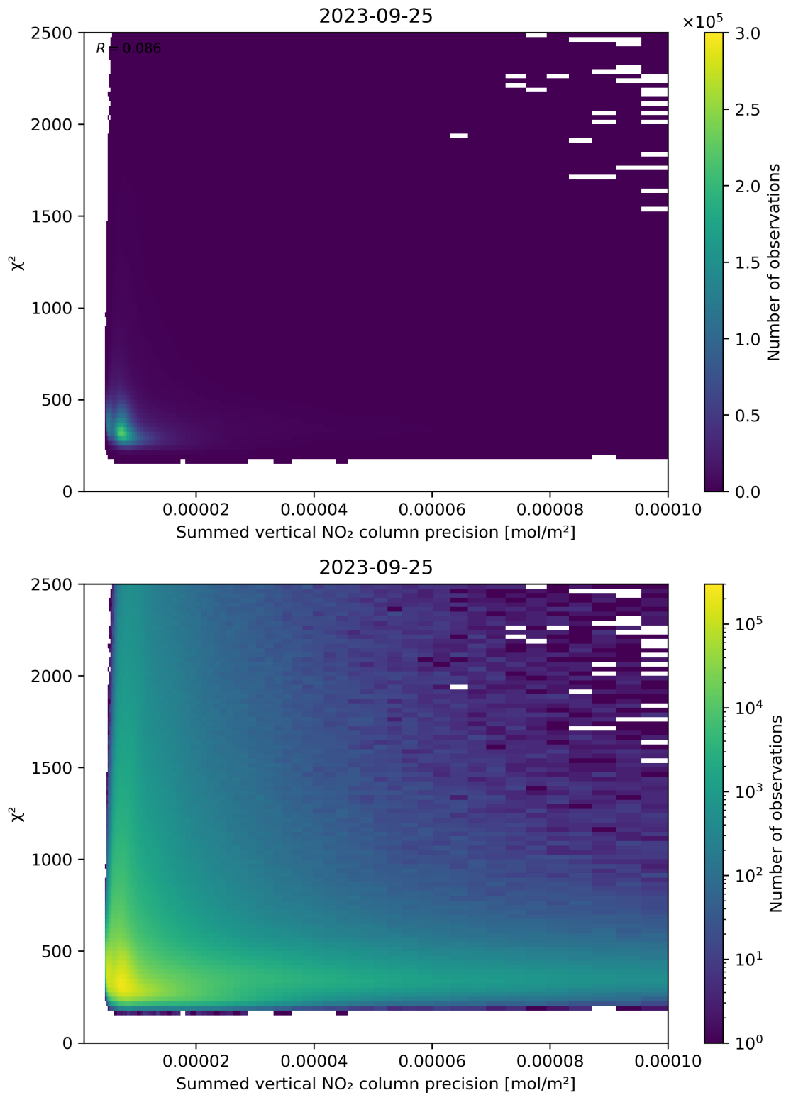
Figure 107: Scatter density plot of “Summed vertical NO 2 column precision” against “ \chi^2 ” for 2023-09-24 to 2023-09-26.
