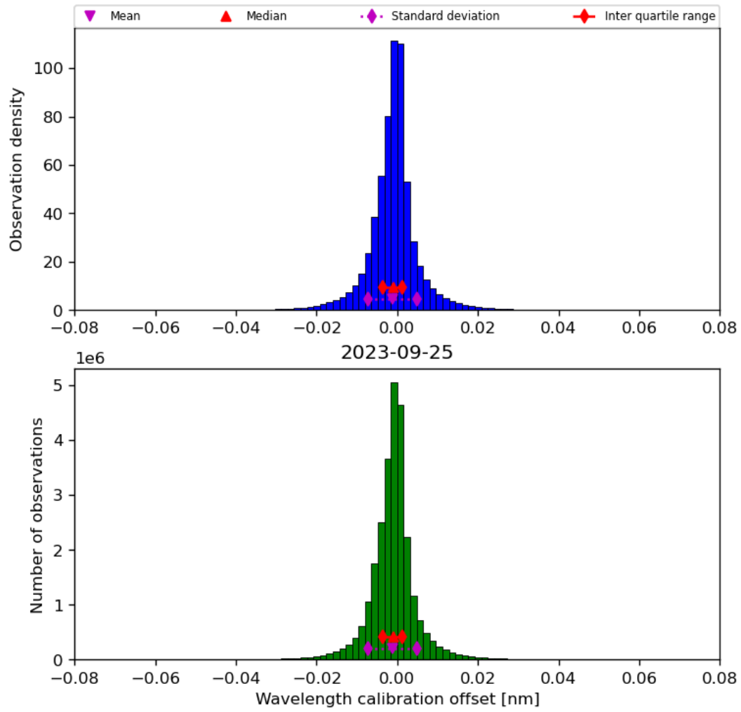
Figure 35: Histogram of “Wavelength calibration offset” for 2023-09-24 to 2023-09-26
