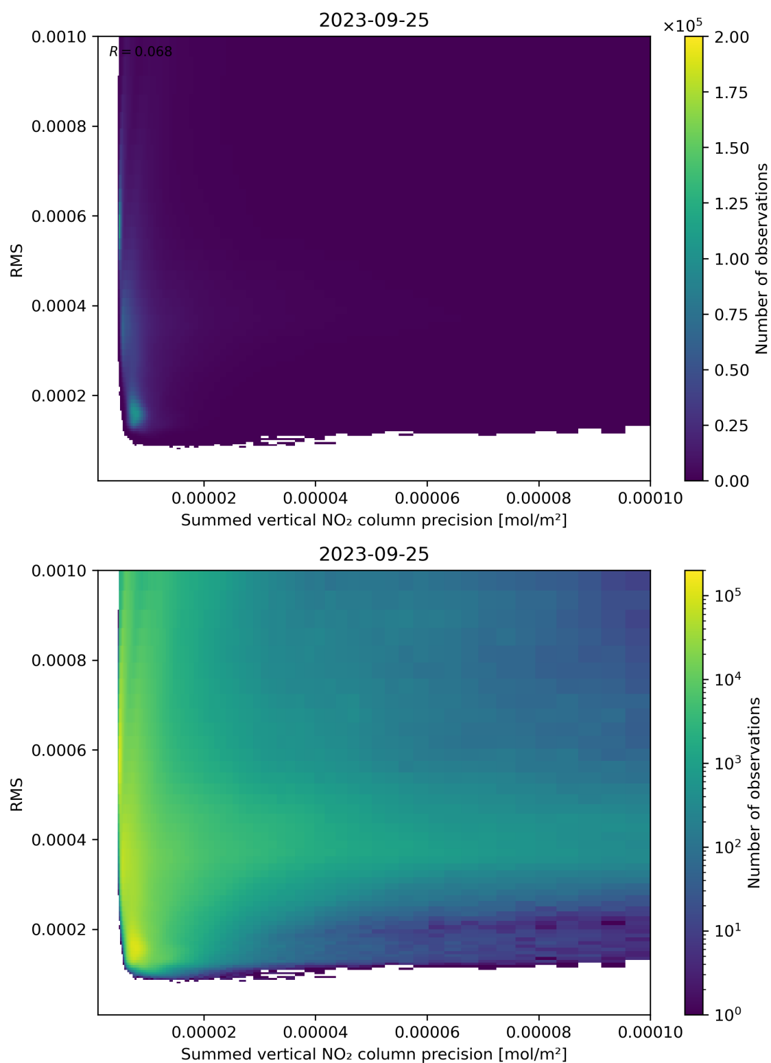
Figure 108: Scatter density plot of “Summed vertical NO 2 column precision” against “RMS” for 2023-09-24 to 2023-09-26.
