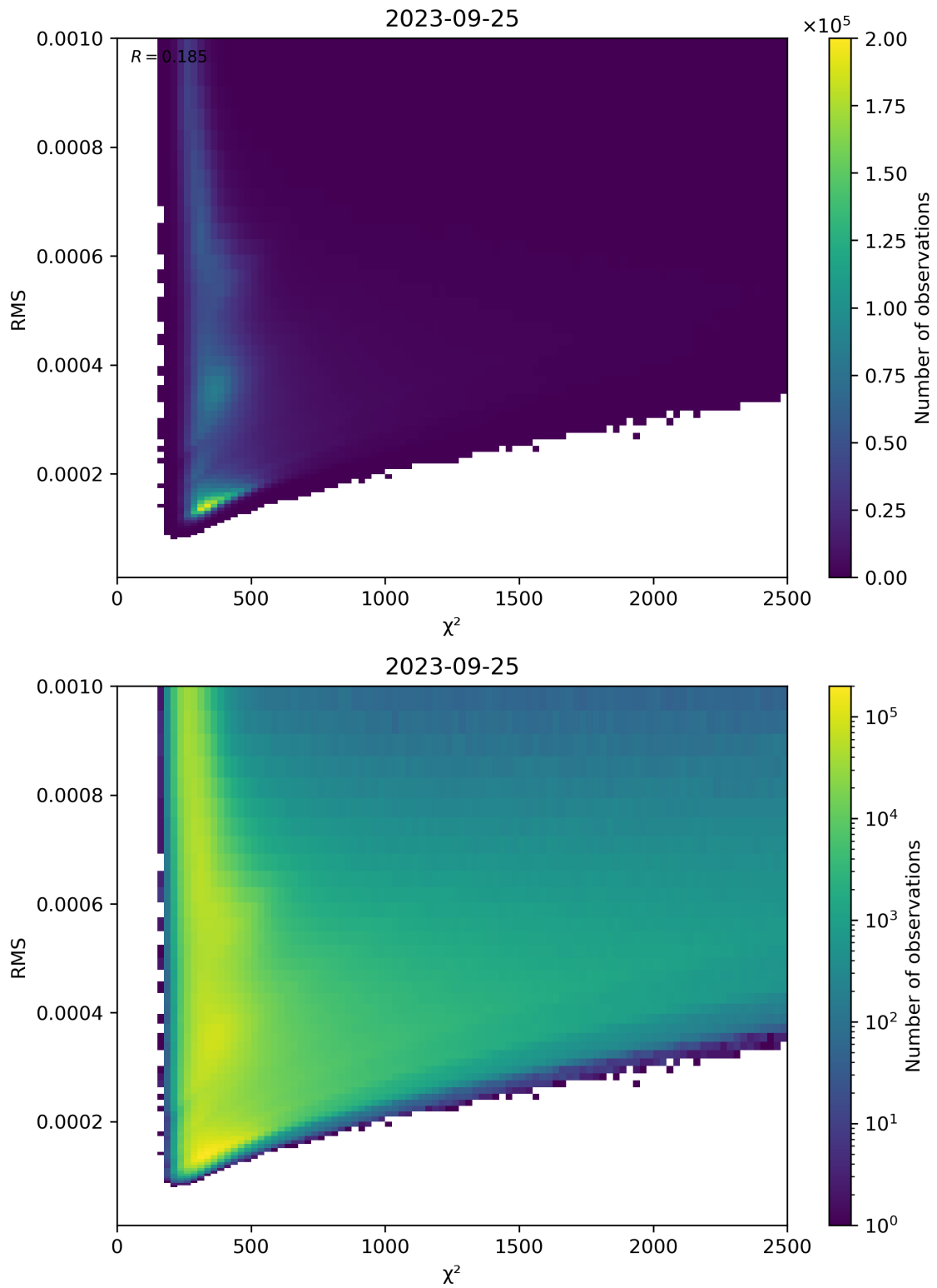
Figure 82: Scatter density plot of “ \chi^2 ” against “RMS” for 2023-09-24 to 2023-09-26.
