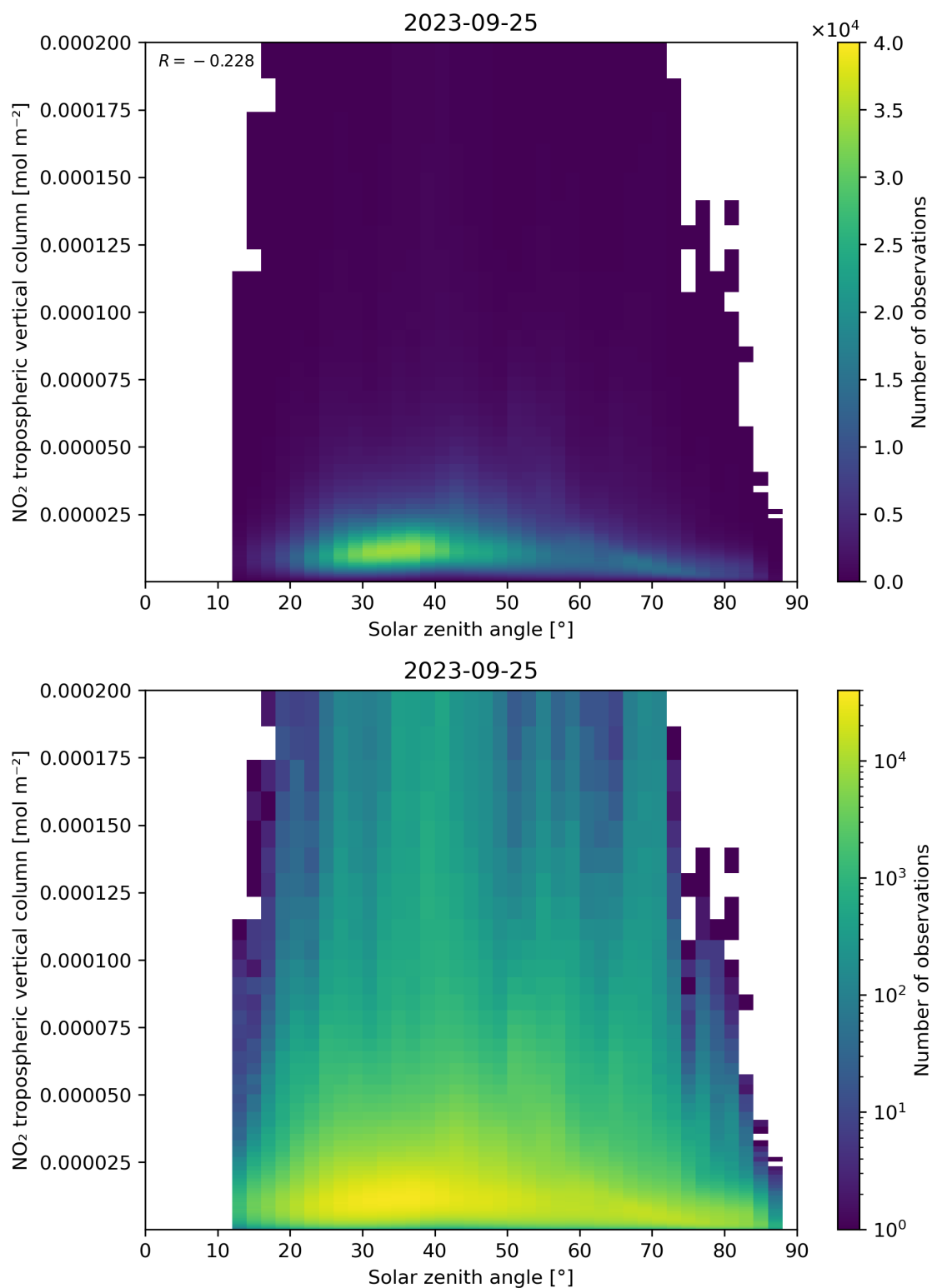
Figure 155: Scatter density plot of “Solar zenith angle” against “NO 2 tropospheric vertical column” for 2023-09-24 to 2023-09-26.
