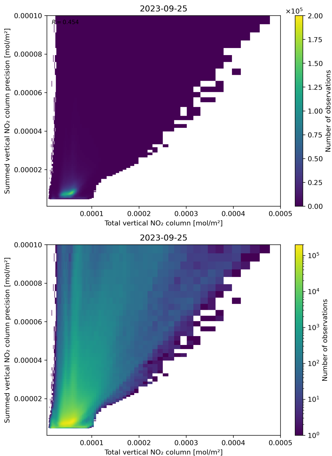
Figure 113: Scatter density plot of “Total vertical NO 2 column” against “Summed vertical NO 2 column precision” for 2023-09-24 to 2023-09-26.
