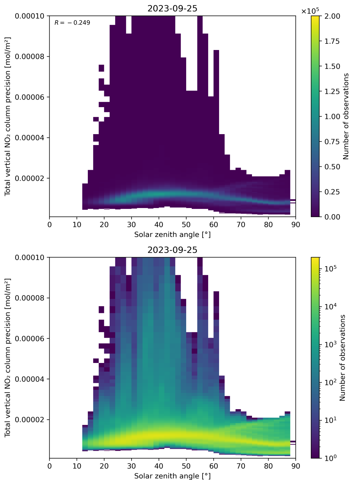
Figure 154: Scatter density plot of “Solar zenith angle” against “Total vertical NO 2 column precision” for 2023-09-24 to 2023-09-26.
