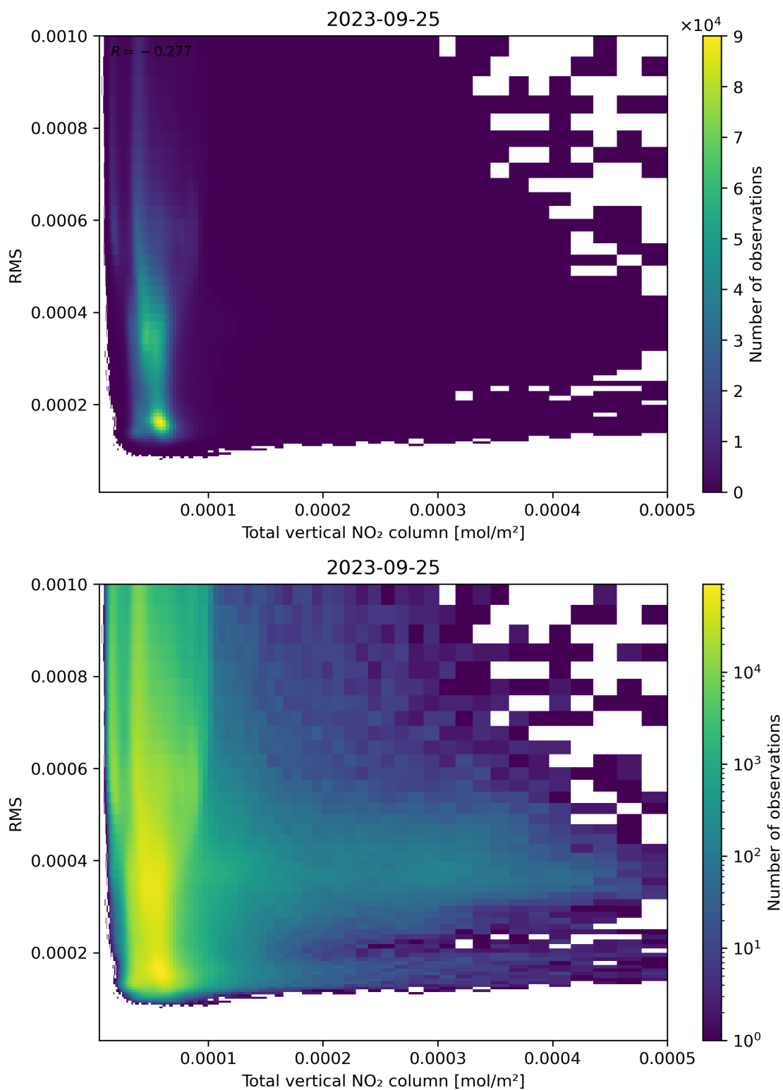
Figure 120: Scatter density plot of “Total vertical NO 2 column” against “RMS” for 2023-09-24 to 2023-09-26.
