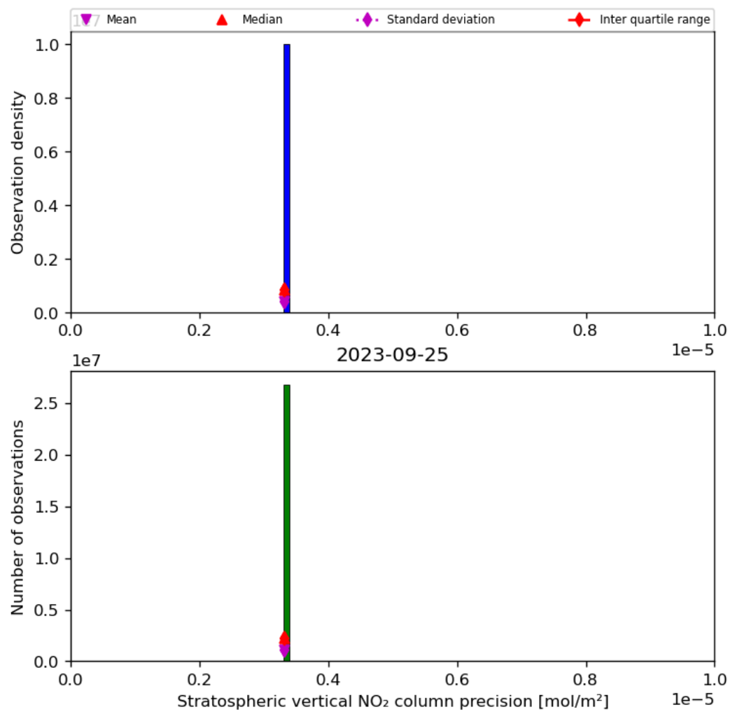
Figure 37: Histogram of “Stratospheric vertical NO 2 column precision” for 2023-09-24 to 2023-09-26
