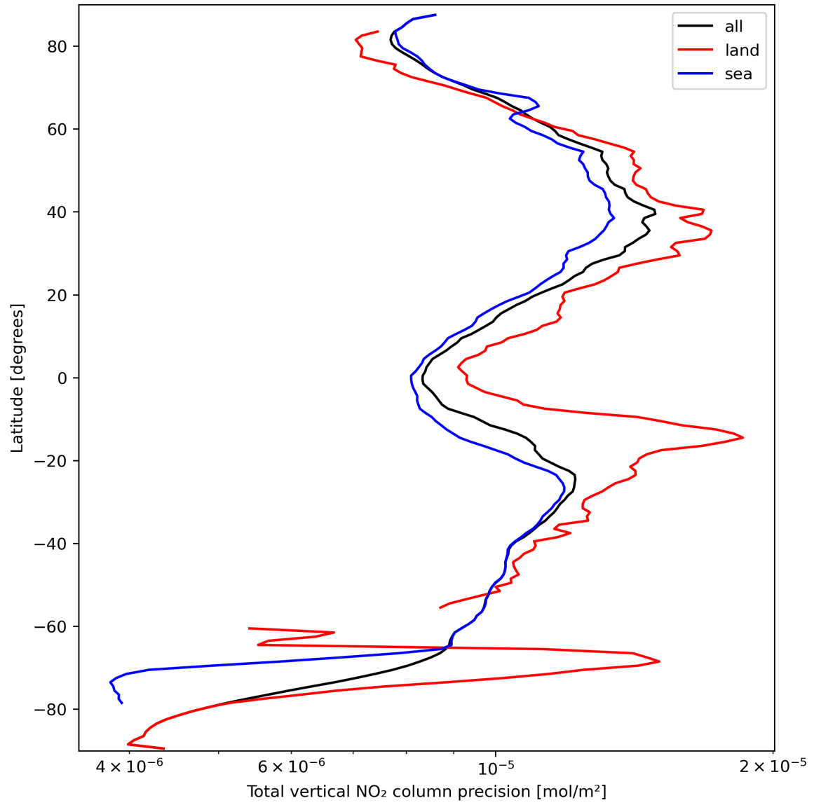
Figure 22: Zonal average of “Total vertical NO 2 column precision” for 2023-09-24 to 2023-09-26.
