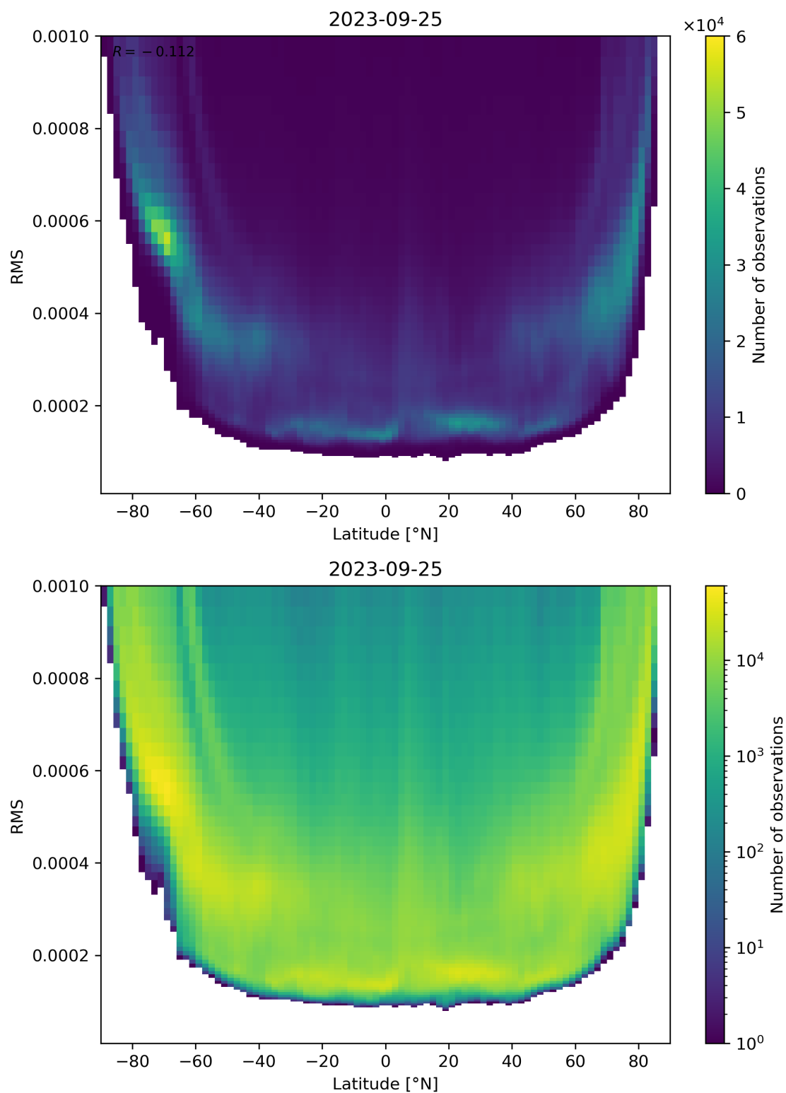
Figure 94: Scatter density plot of “Latitude” against “RMS” for 2023-09-24 to 2023-09-26.
