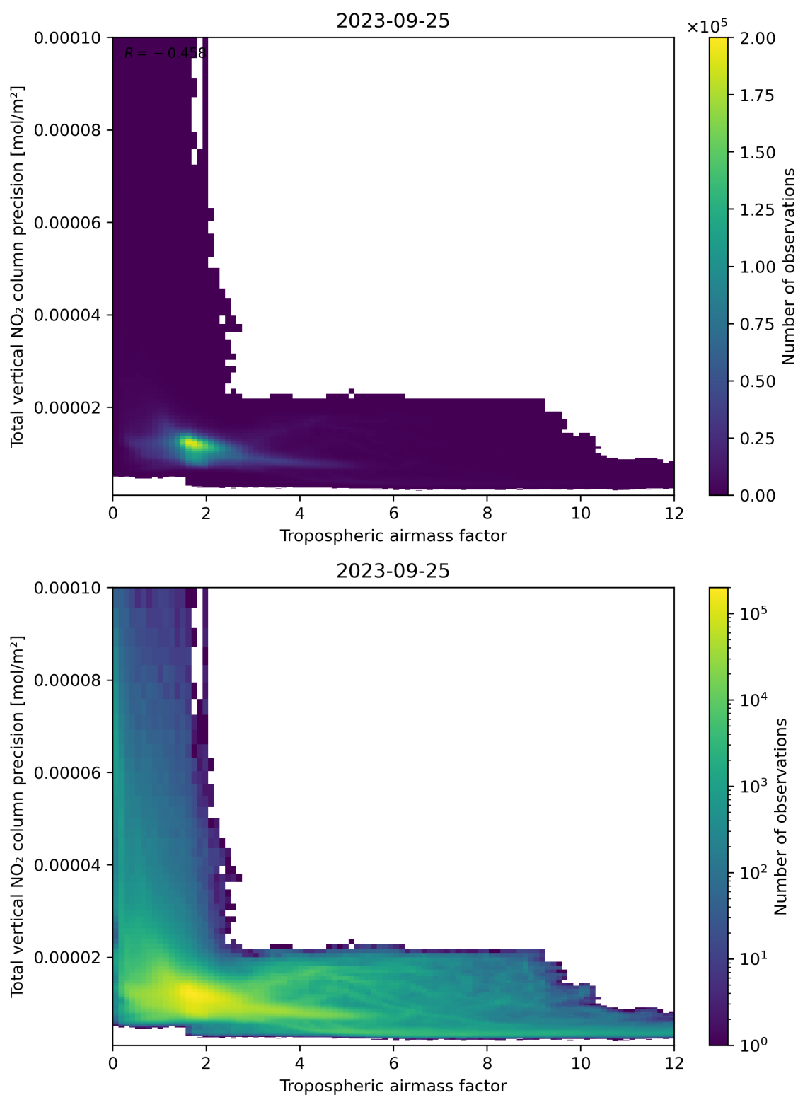
Figure 78: Scatter density plot of “Tropospheric air mass factor” against “Total vertical NO 2 column precision” for 2023-09-24 to 2023-09-26.
