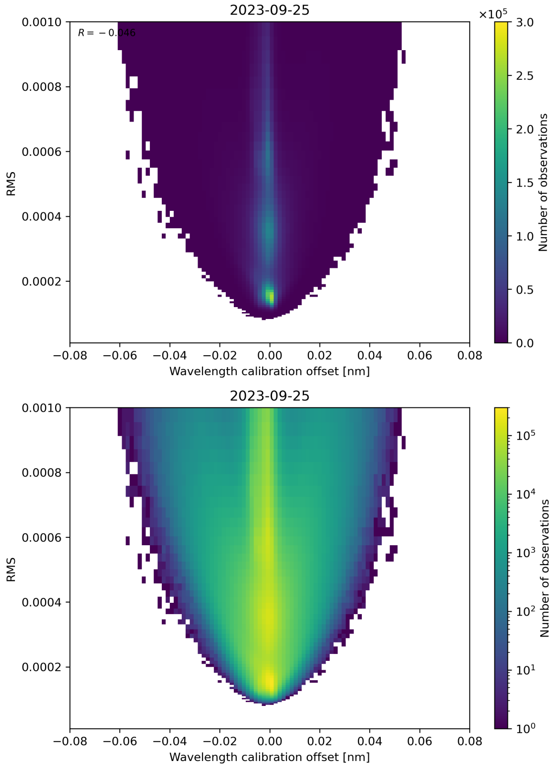
Figure 181: Scatter density plot of “Wavelength calibration offset” against “RMS” for 2023-09-24 to 2023-09-26.
