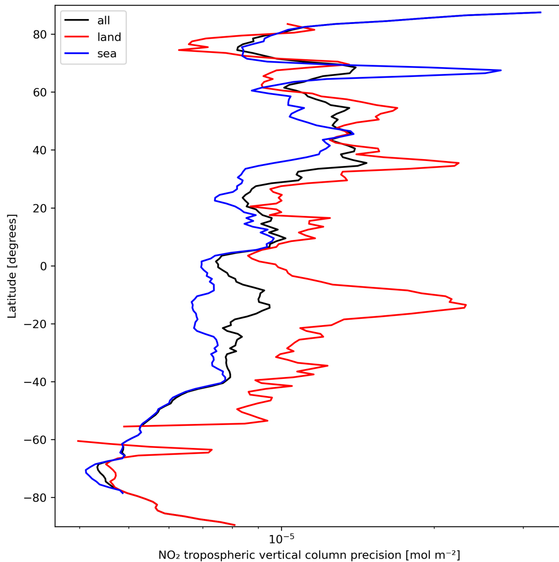
Figure 13: Zonal average of “NO 2 tropospheric vertical column precision” for 2023-09-24 to 2023-09-26.
