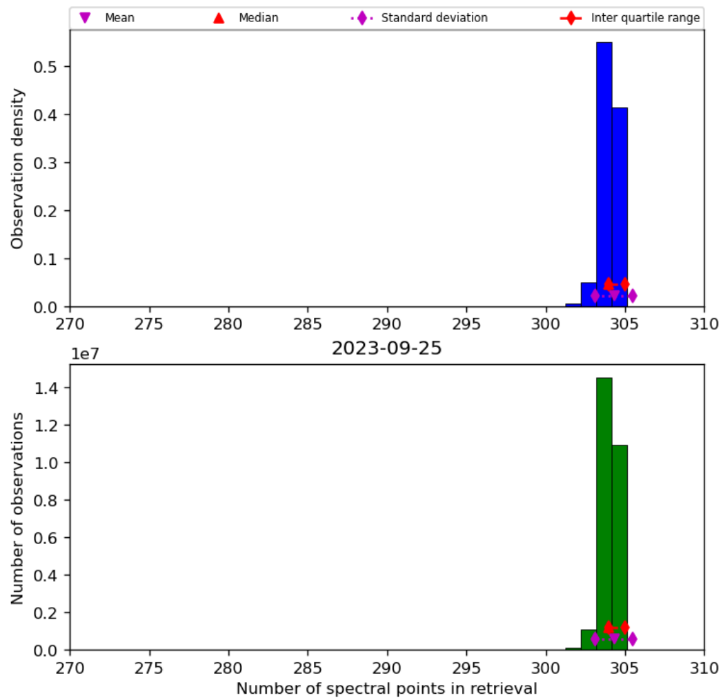
Figure 33: Histogram of “Number of spectral points in retrieval” for 2023-09-24 to 2023-09-26
