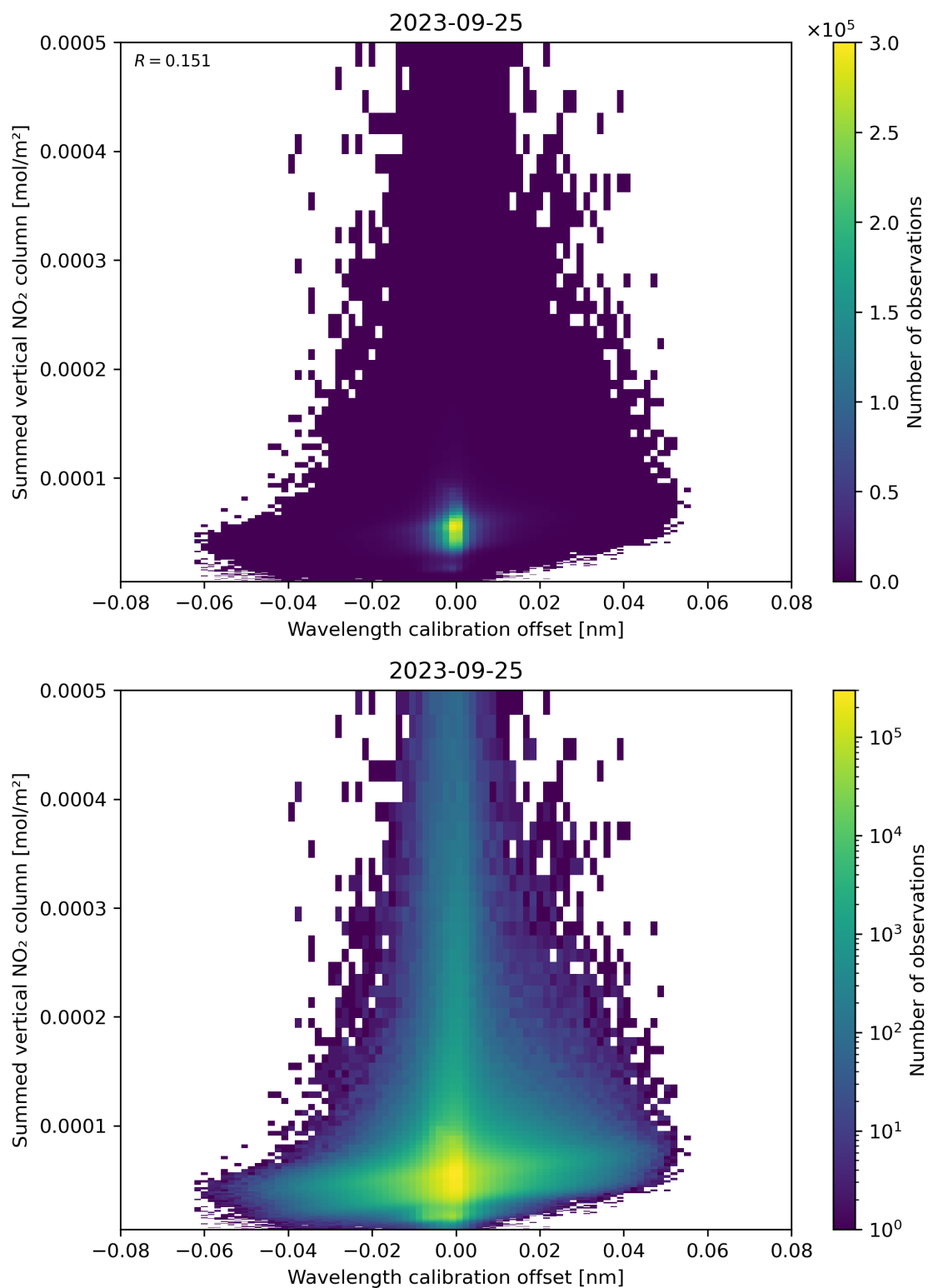
Figure 177: Scatter density plot of “Wavelength calibration offset” against “Summed vertical NO 2 column” for 2023-09-24 to 2023-09-26.
