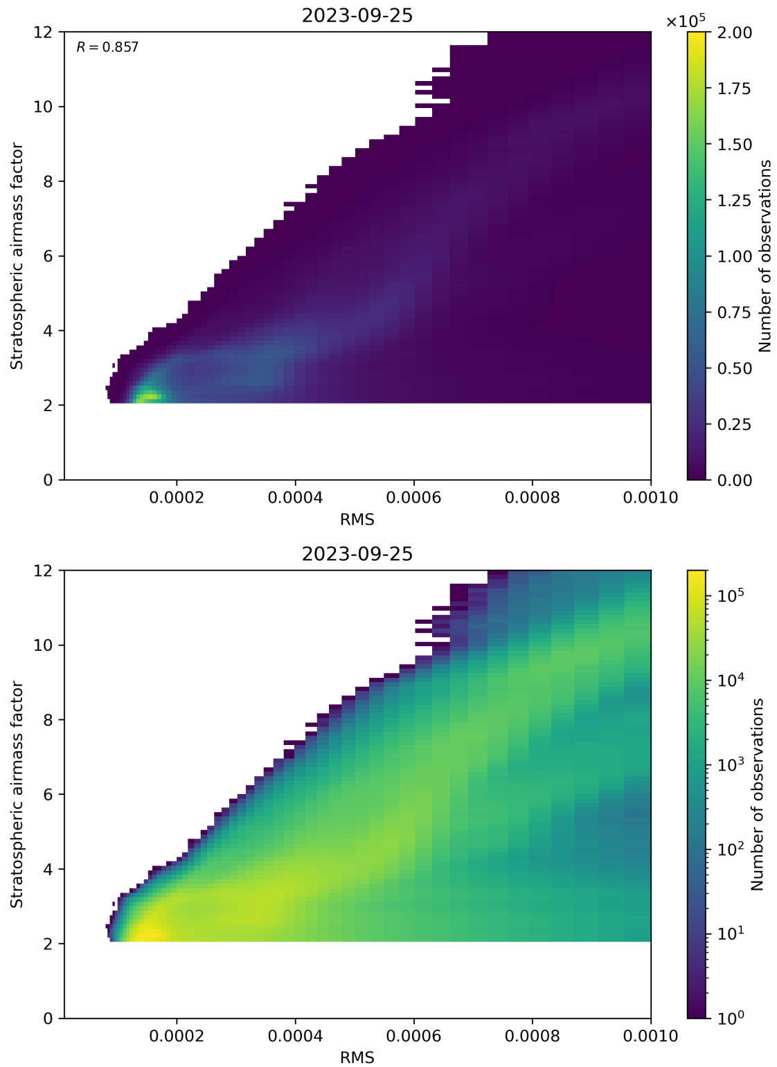
Figure 144: Scatter density plot of “RMS” against “Stratospheric airmass factor” for 2023-09-24 to 2023-09-26.
