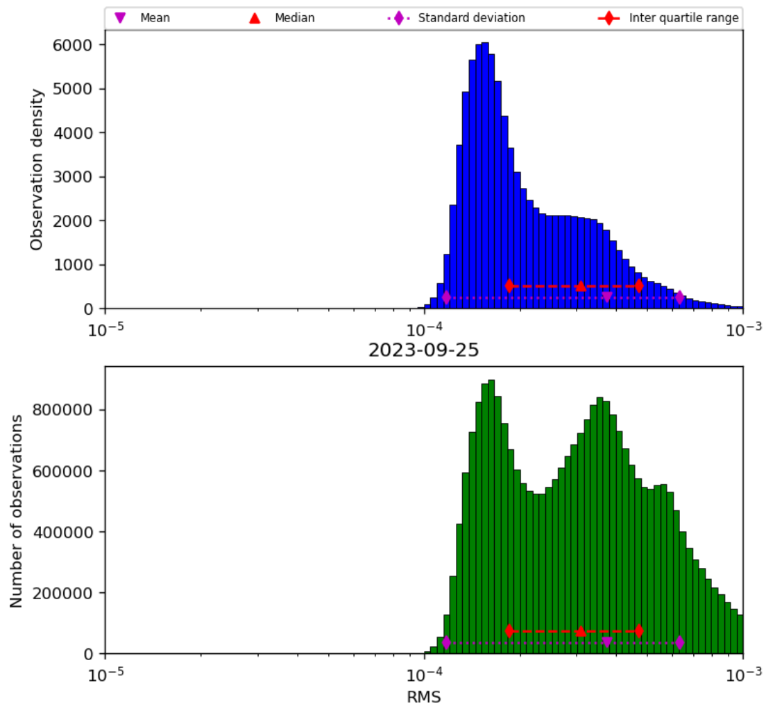
Figure 43: Histogram of “RMS” for 2023-09-24 to 2023-09-26
