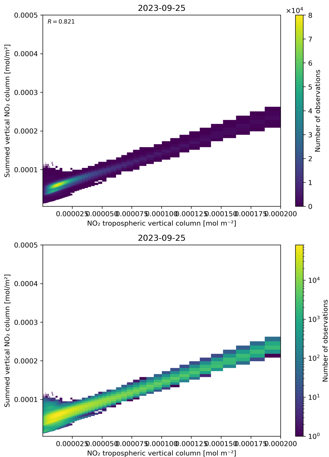
Figure 126: Scatter density plot of “NO 2 tropospheric vertical column” against “Summed vertical NO 2 column” for 2023-09-24 to 2023-09-26.
