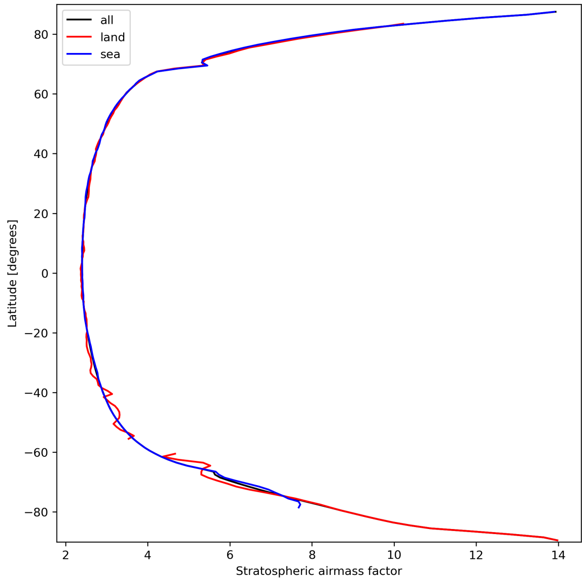
Figure 27: Zonal average of “Stratospheric air mass factor” for 2023-09-24 to 2023-09-26.
