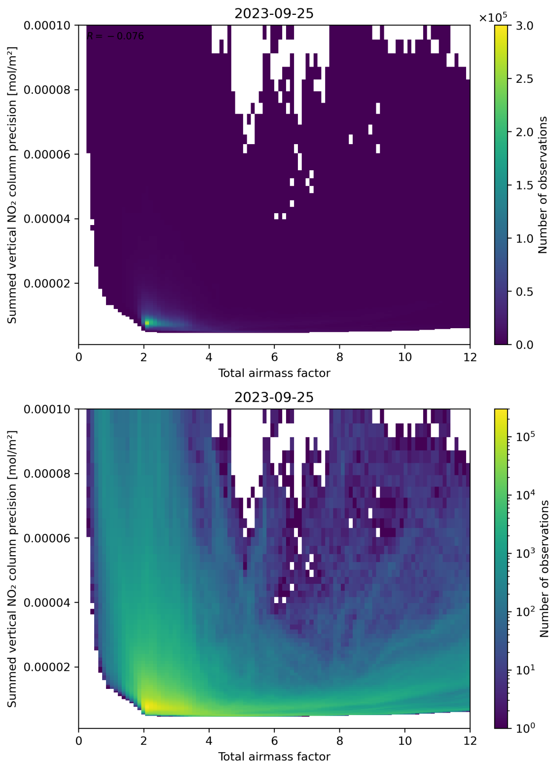
Figure 66: Scatter density plot of “Total airmass factor” against “Summed vertical NO 2 column precision” for 2023-09-24 to 2023-09-26.
