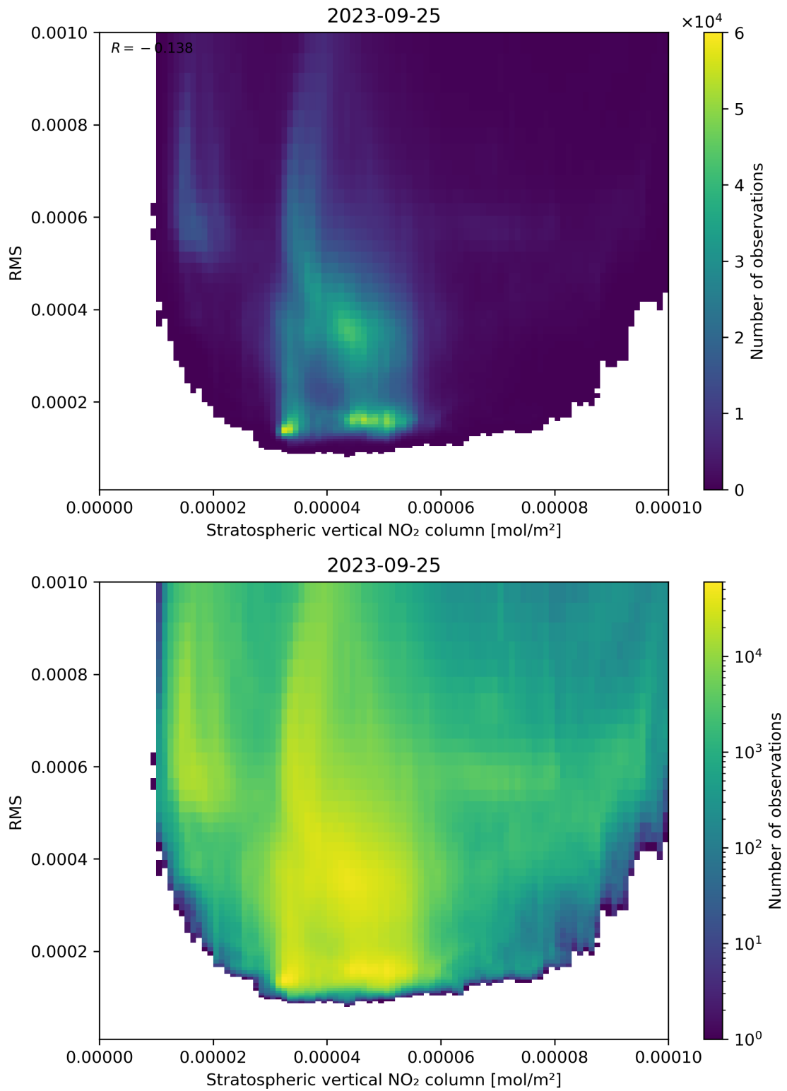
Figure 102: Scatter density plot of “Stratospheric vertical NO 2 column” against “RMS” for 2023-09-24 to 2023-09-26.
