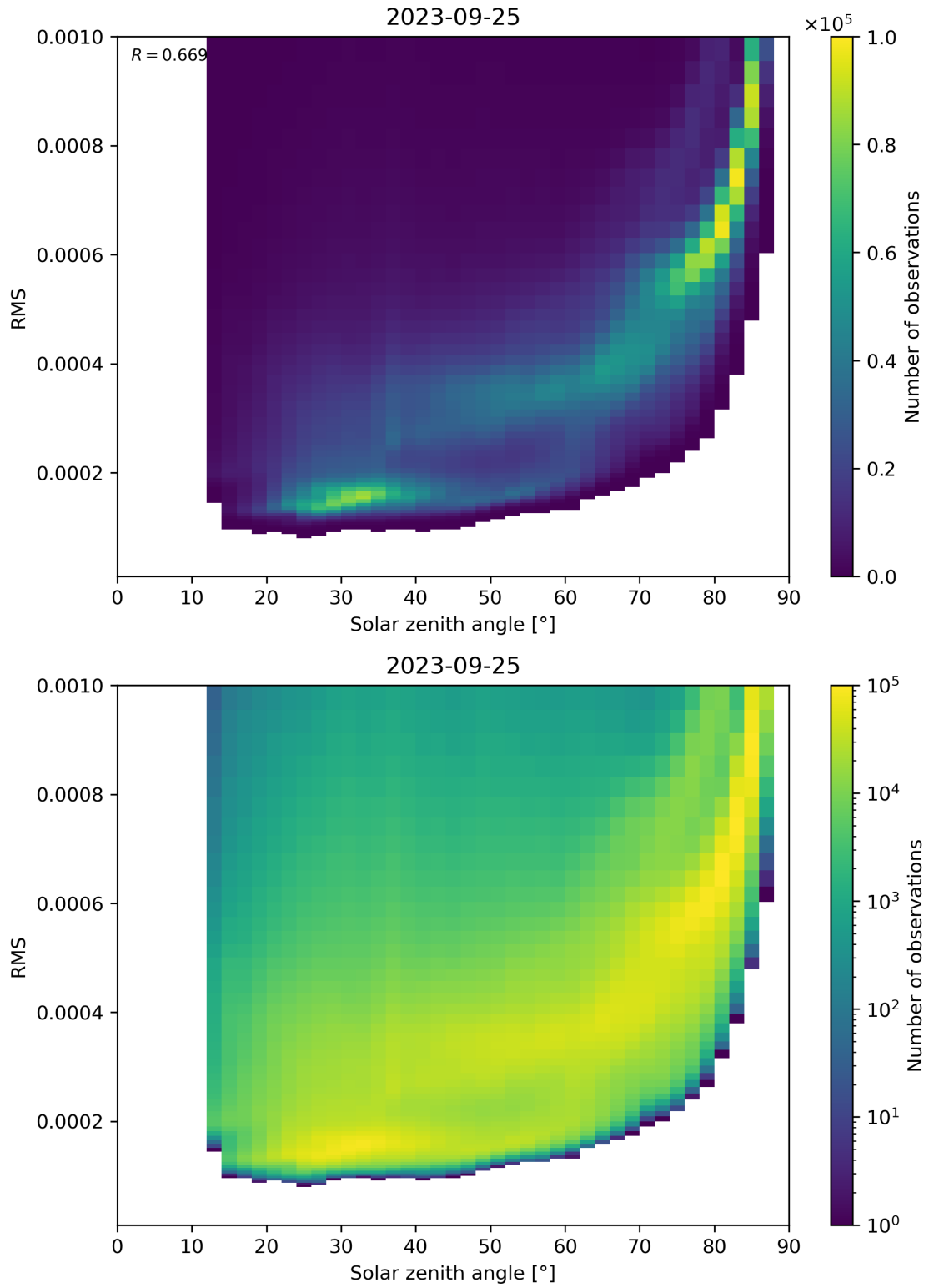
Figure 157: Scatter density plot of “Solar zenith angle” against “RMS” for 2023-09-24 to 2023-09-26.
