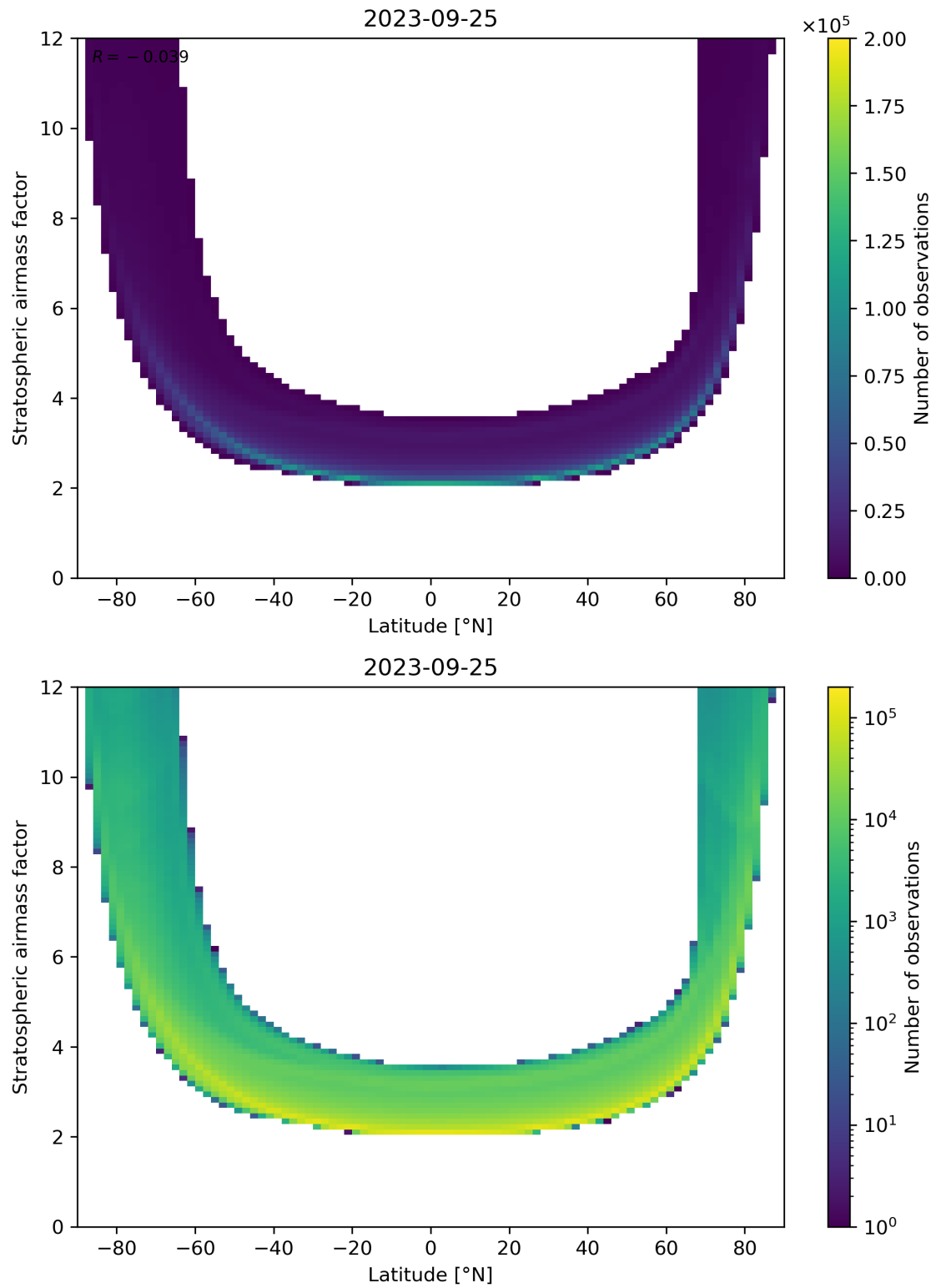
Figure 83: Scatter density plot of “Latitude” against “Stratospheric air mass factor” for 2023-09-24 to 2023-09-26.
