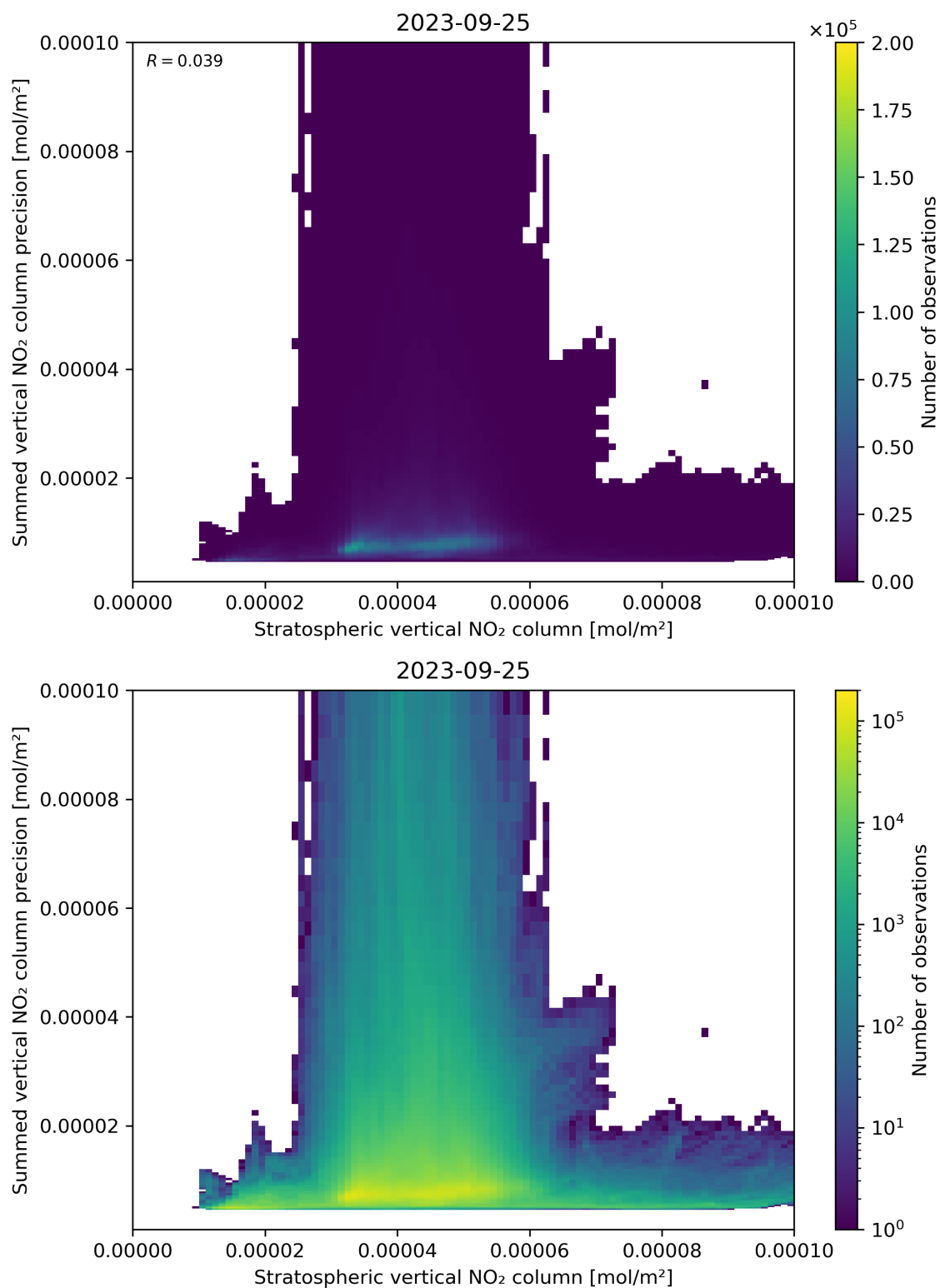
Figure 99: Scatter density plot of “Stratospheric vertical NO 2 column” against “Summed vertical NO 2 column precision” for 2023-09-24 to 2023-09-26.
