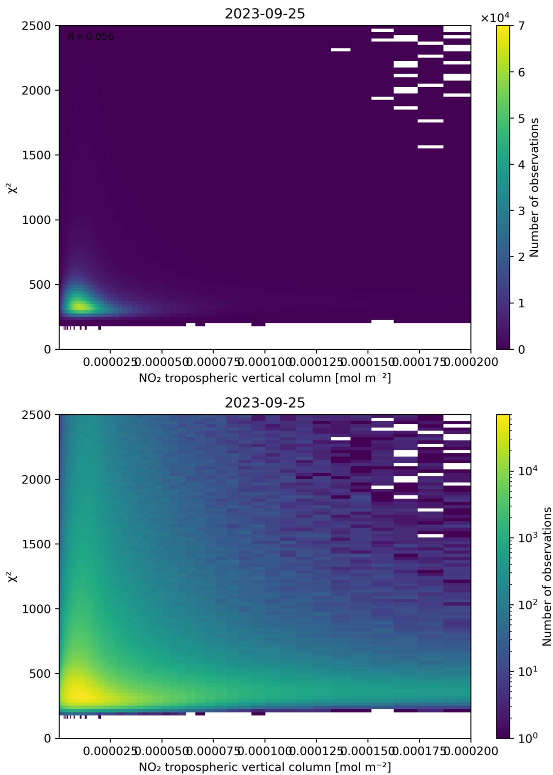
Figure 124: Scatter density plot of “NO 2 tropospheric vertical column” against “ \chi^2 ” for 2023-09-24 to 2023-09-26.
