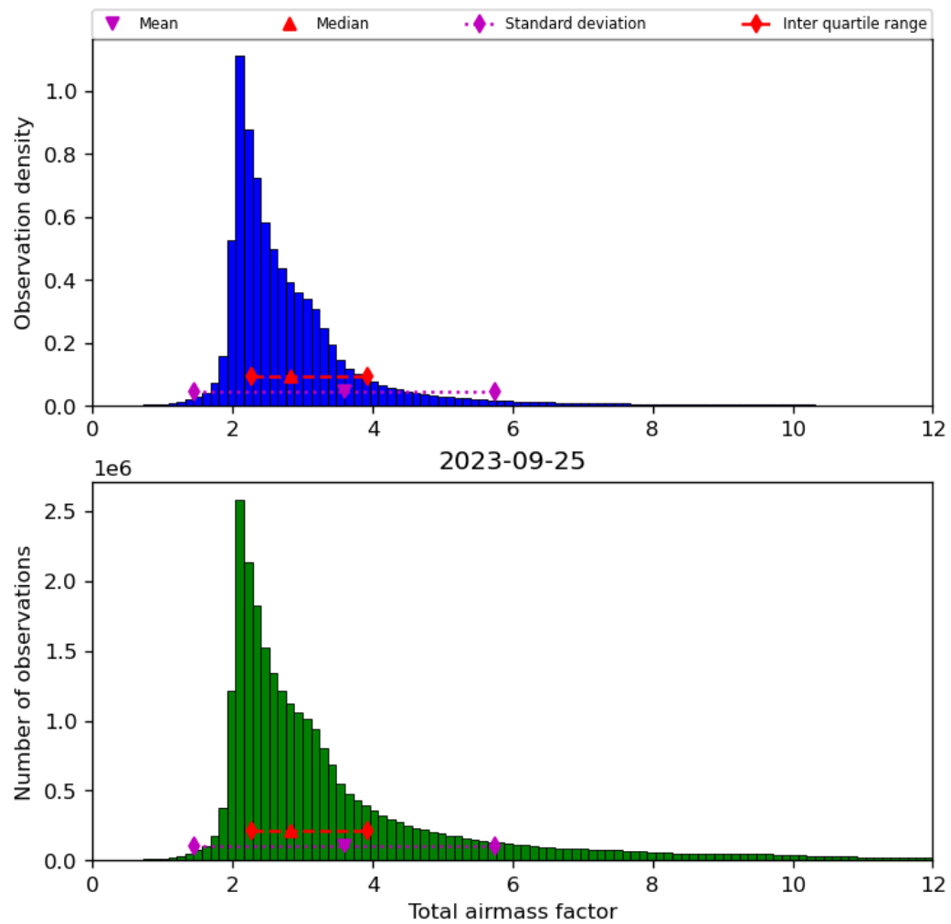
Figure 32: Histogram of “Total airmass factor” for 2023-09-24 to 2023-09-26
