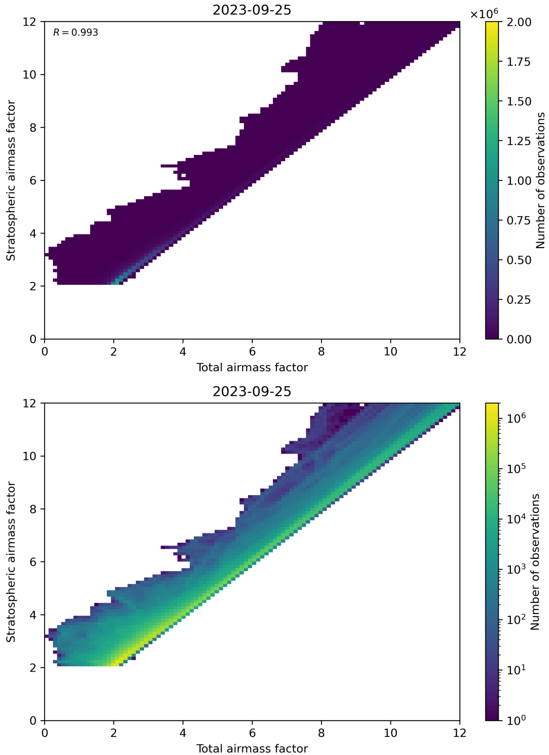
Figure 62: Scatter density plot of “Total airmass factor” against “Stratospheric airmass factor” for 2023-09-24 to 2023-09-26.
