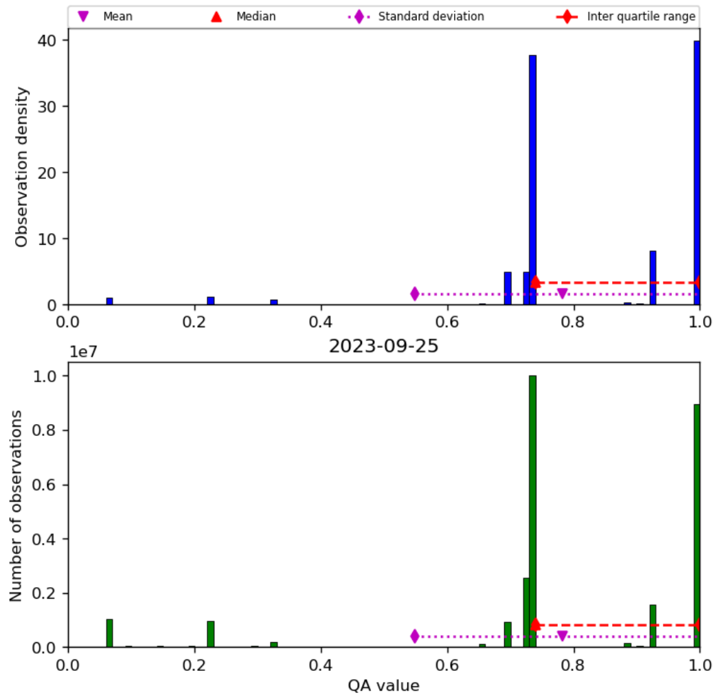
Figure 28: Histogram of “QA value” for 2023-09-24 to 2023-09-26
