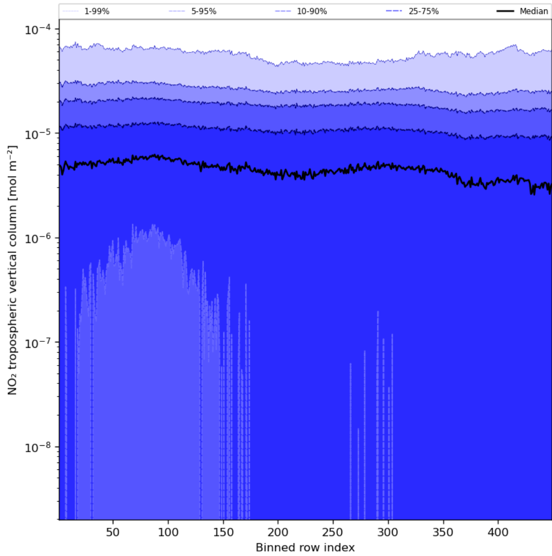
Figure 46: Along track statistics of “NO 2 tropospheric vertical column” for 2023-09-24 to 2023-09-26
