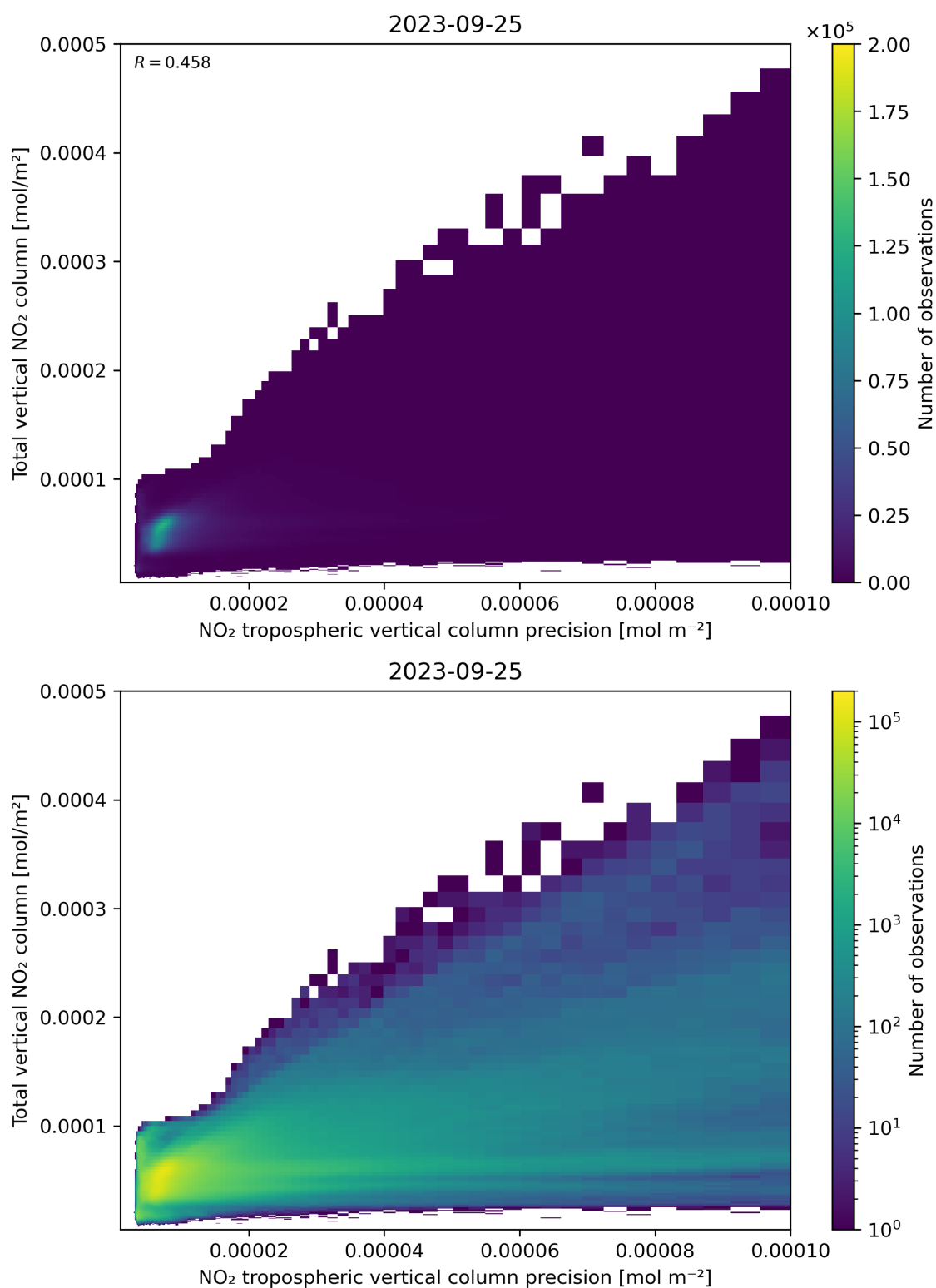
Figure 138: Scatter density plot of “NO 2 tropospheric vertical column precision” against “Total vertical NO 2 column” for 2023-09-24 to 2023-09-26.
