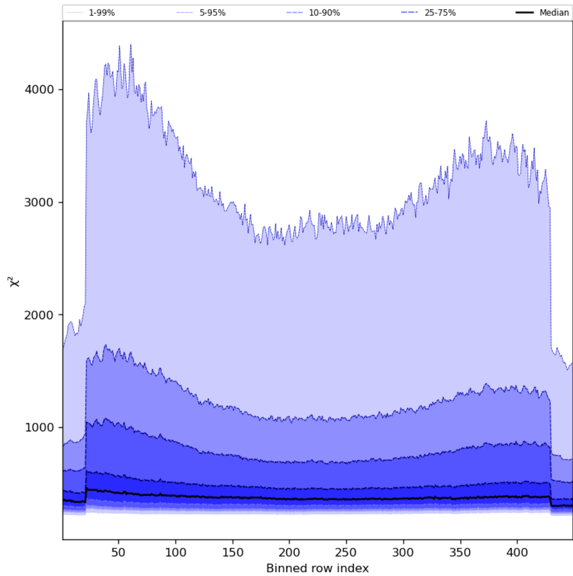
Figure 59: Along track statistics of “ \chi^2 ” for 2023-09-24 to 2023-09-26
