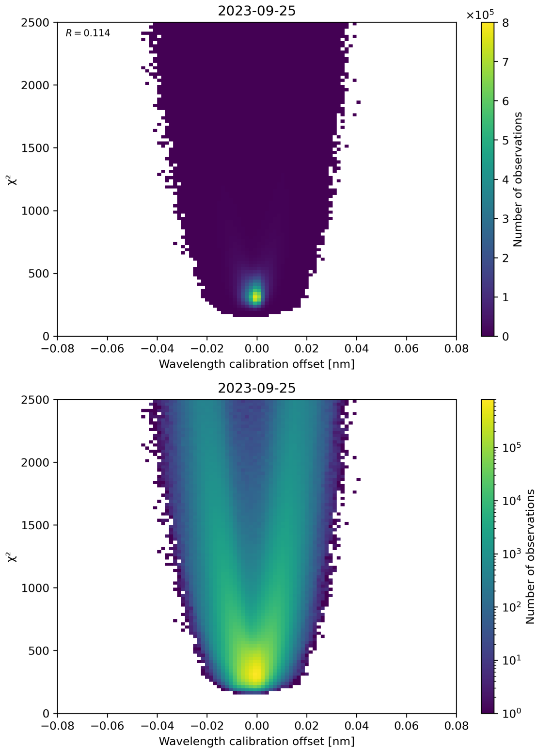
Figure 175: Scatter density plot of “Wavelength calibration offset” against “ \chi^2 ” for 2023-09-24 to 2023-09-26.
