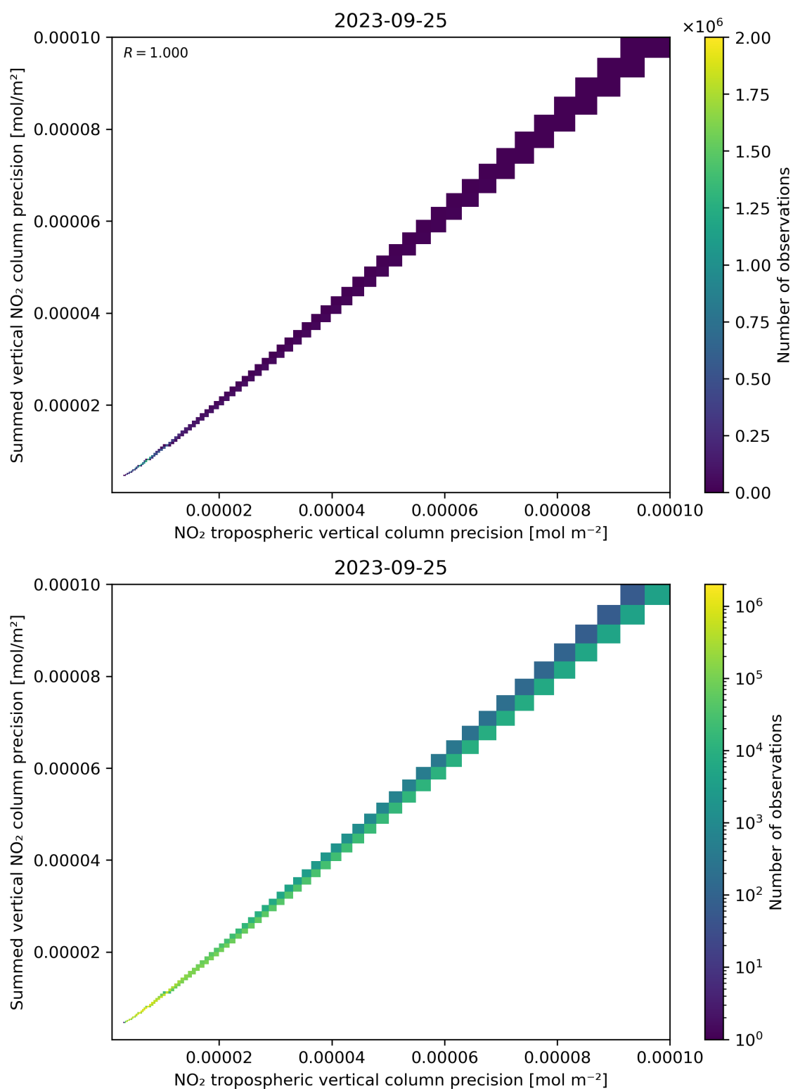
Figure 137: Scatter density plot of “NO 2 tropospheric vertical column precision” against “Summed vertical NO 2 column precision” for 2023-09-24 to 2023-09-26.
