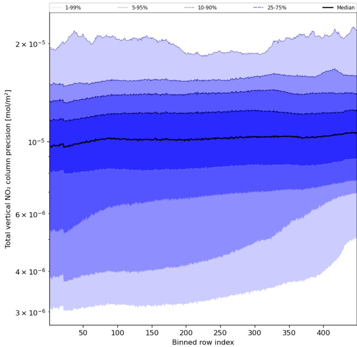
Figure 56: Along track statistics of "Total vertical NO 2 column precision" for 2023-09-24 to 2023-09-26
