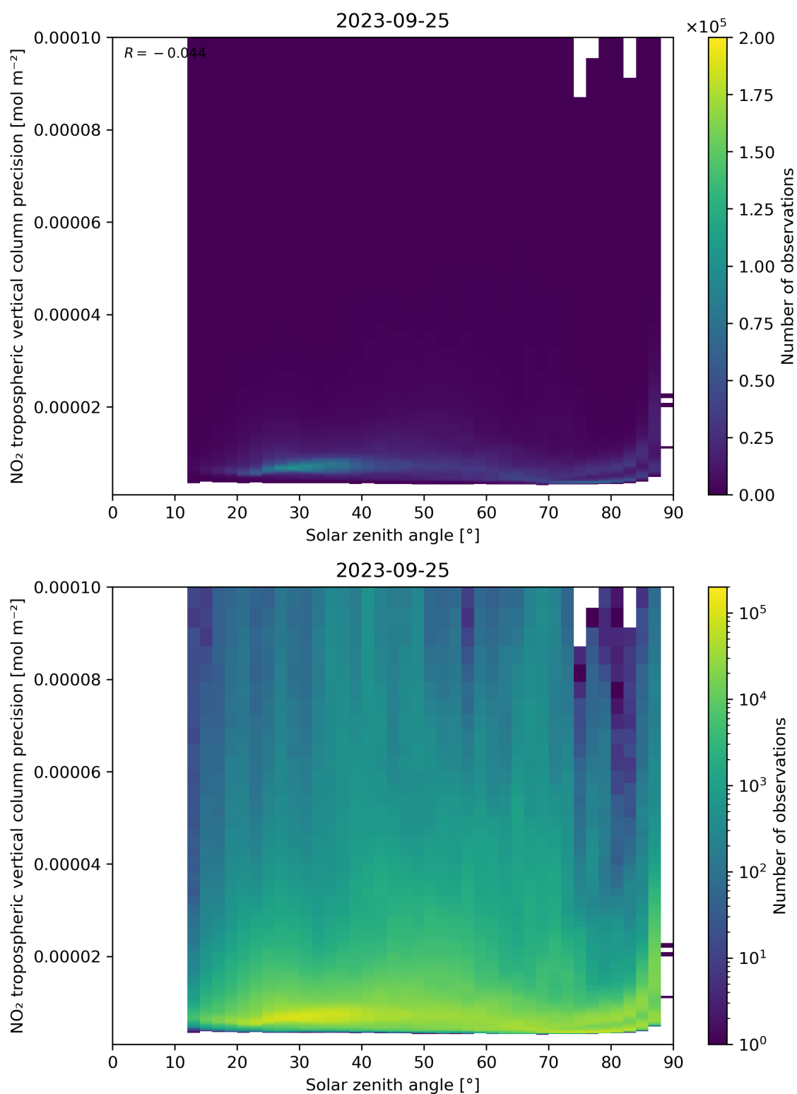
Figure 156: Scatter density plot of “Solar zenith angle” against “NO 2 tropospheric vertical column precision” for 2023-09-24 to 2023-09-26.
