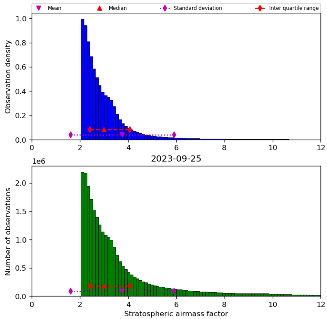
Figure 44: Histogram of “Stratospheric airmass factor” for 2023-09-24 to 2023-09-26
