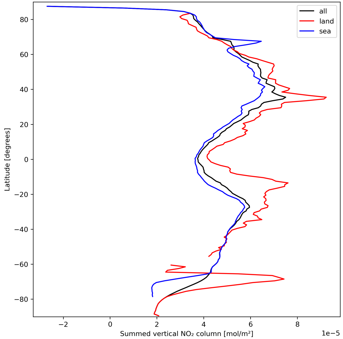
Figure 23: Zonal average of “Summed vertical NO 2 column” for 2023-09-24 to 2023-09-26.
