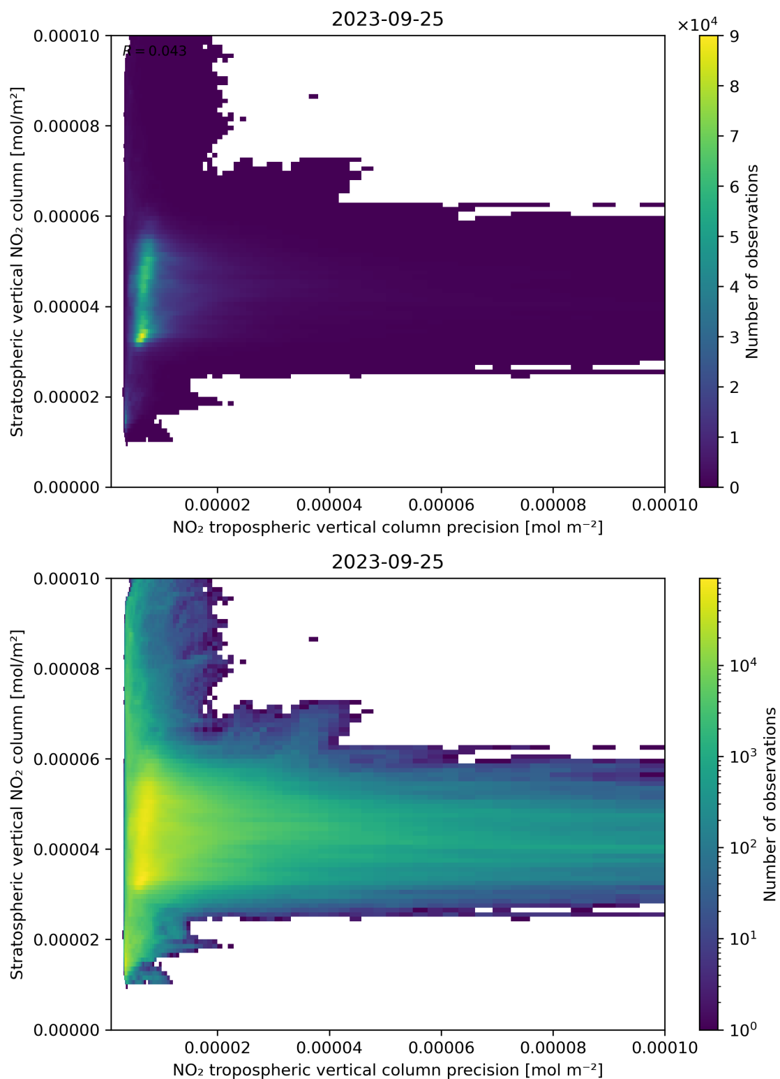
Figure 135: Scatter density plot of “NO 2 tropospheric vertical column precision” against “Stratospheric vertical NO 2 column” for 2023-09-24 to 2023-09-26.
