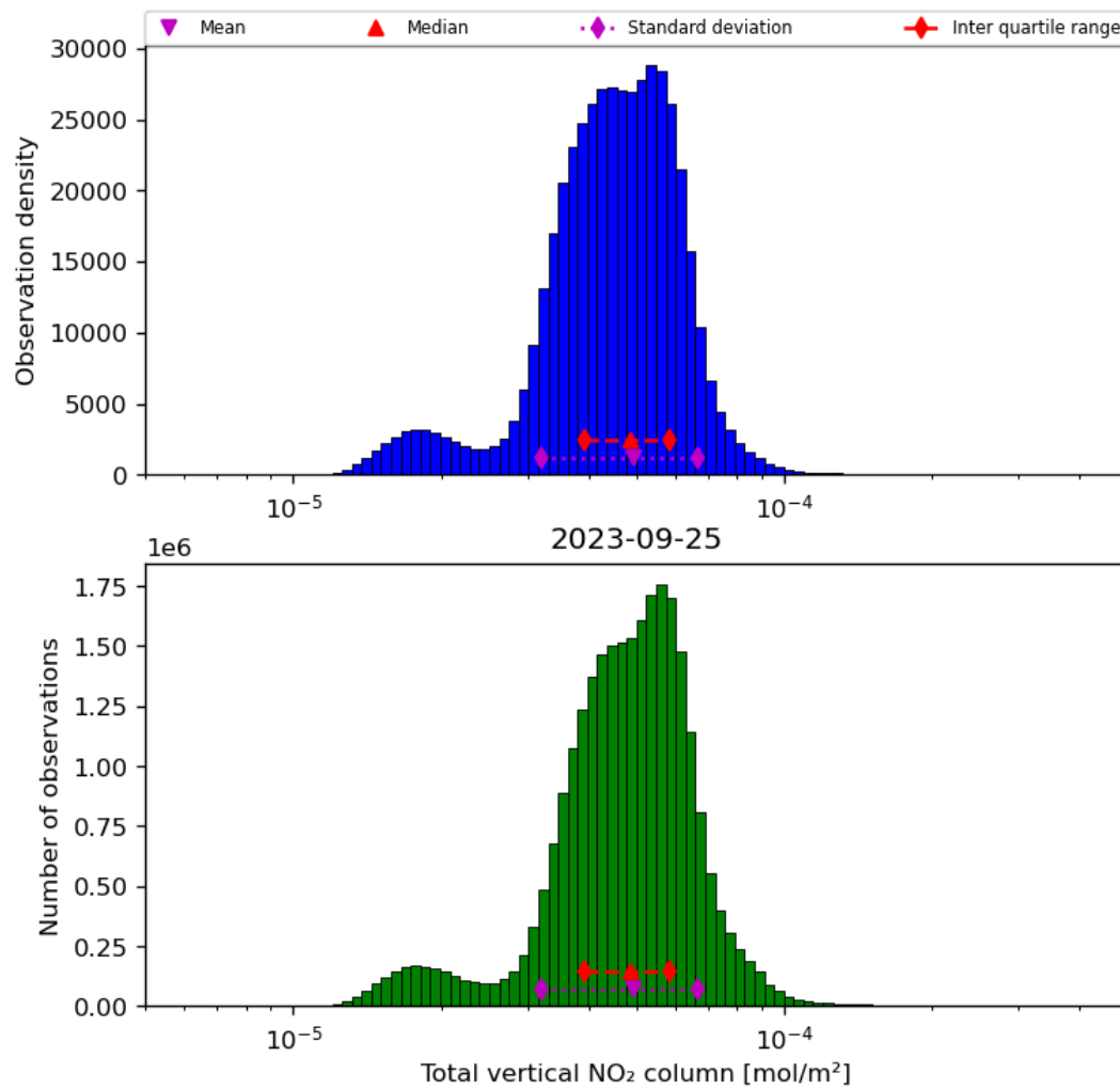
Figure 38: Histogram of “Total vertical NO 2 column” for 2023-09-24 to 2023-09-26
