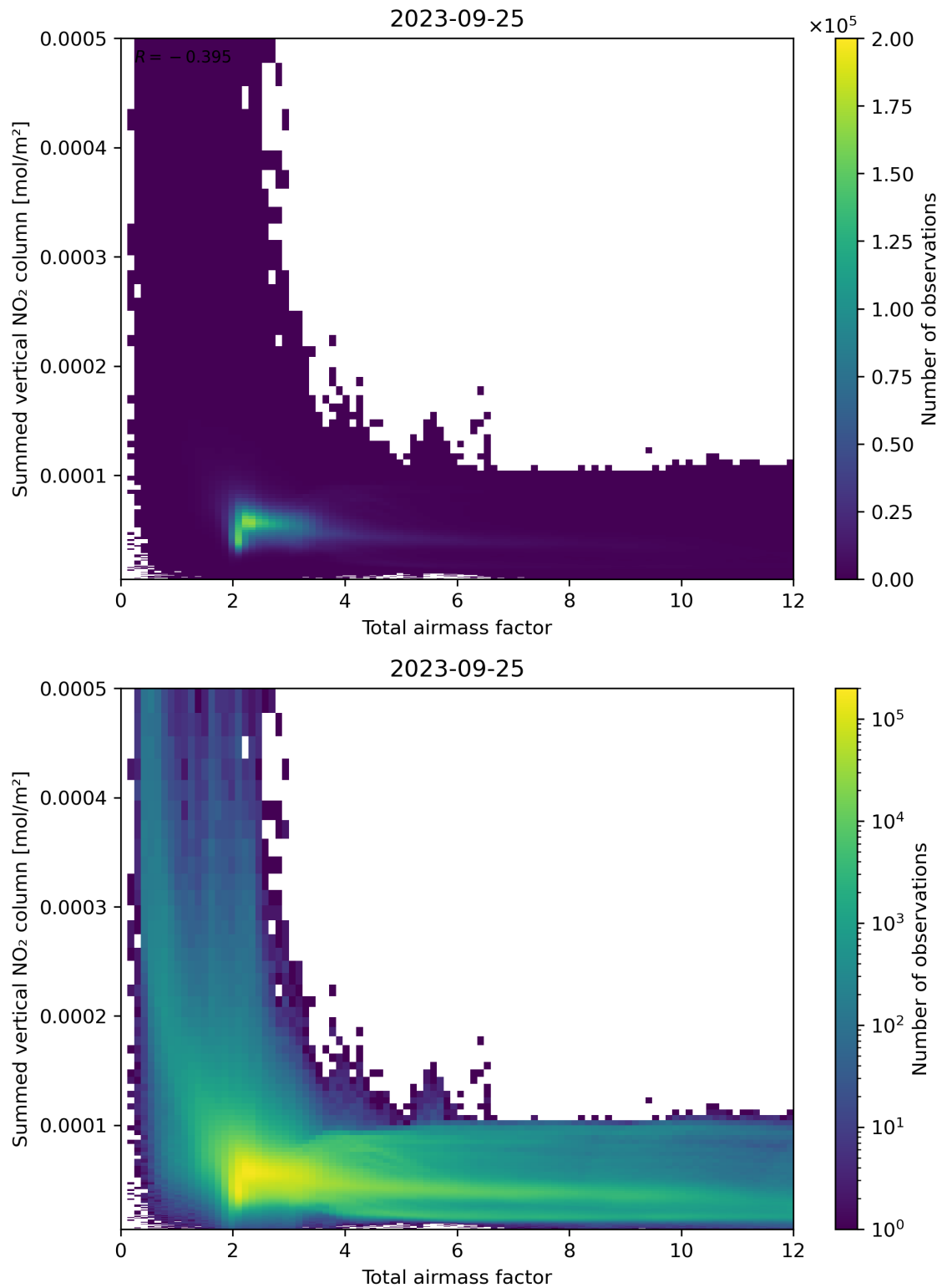
Figure 65: Scatter density plot of “Total airmass factor” against “Summed vertical NO 2 column” for 2023-09-24 to 2023-09-26.
