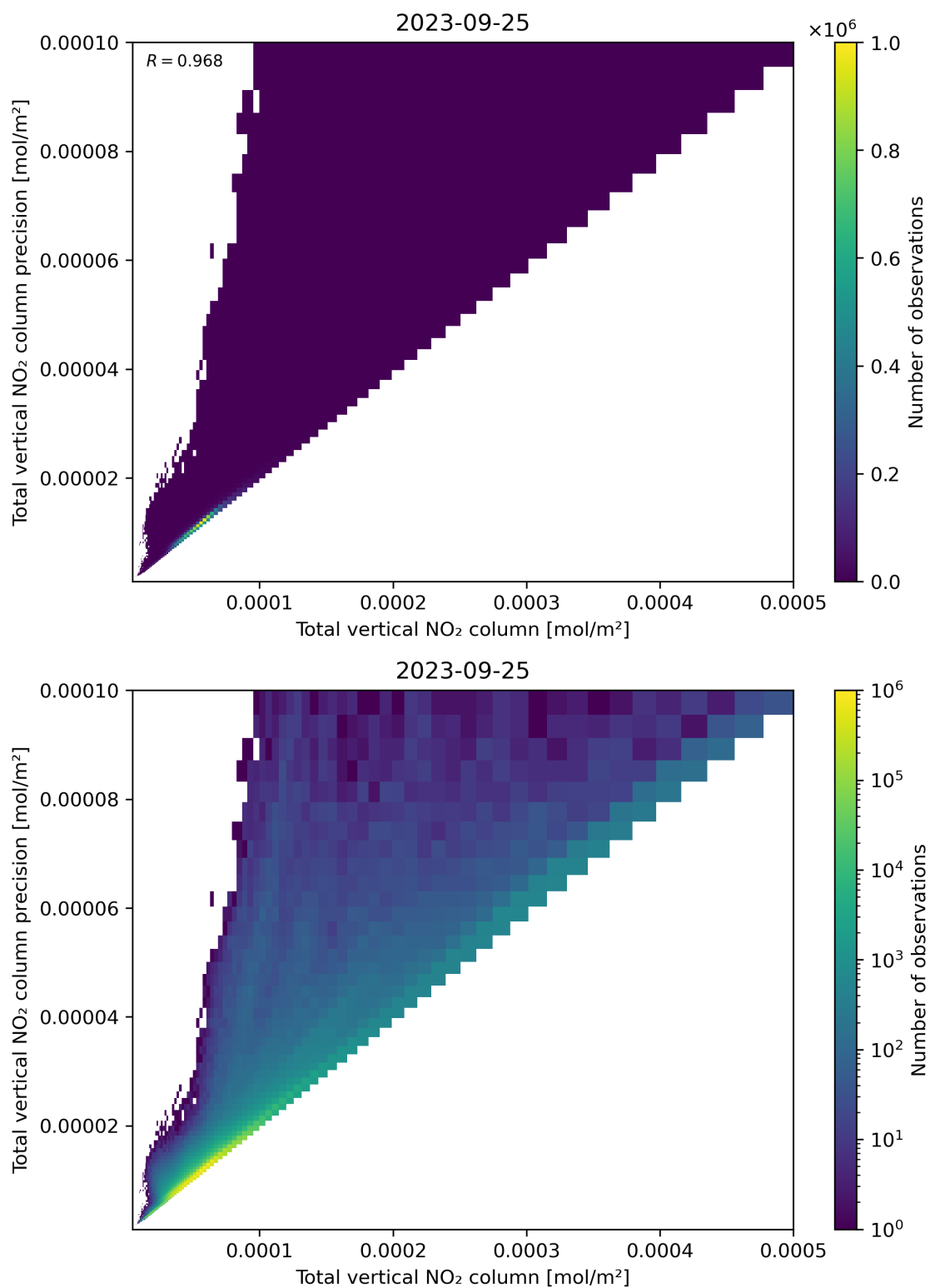
Figure 114: Scatter density plot of “Total vertical NO 2 column” against “Total vertical NO 2 column precision” for 2023-09-24 to 2023-09-26.
