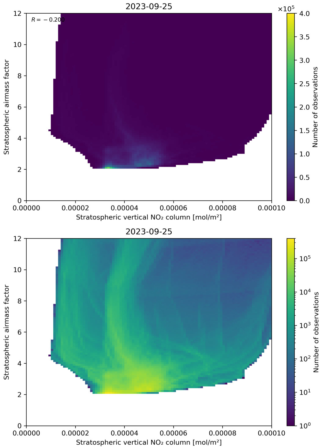
Figure 96: Scatter density plot of “Stratospheric vertical NO 2 column” against “Stratospheric airmass factor” for 2023-09-24 to 2023-09-26.
