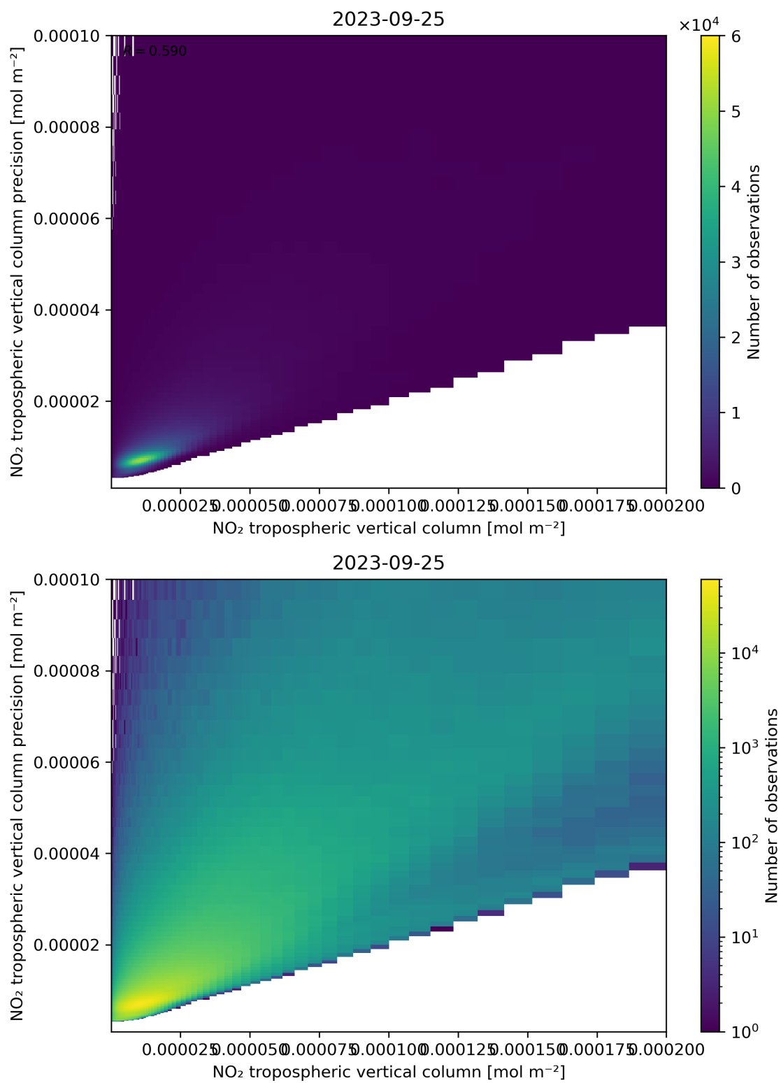
Figure 130: Scatter density plot of “NO 2 tropospheric vertical column” against “NO 2 tropospheric vertical column precision” for 2023-09-24 to 2023-09-26.
