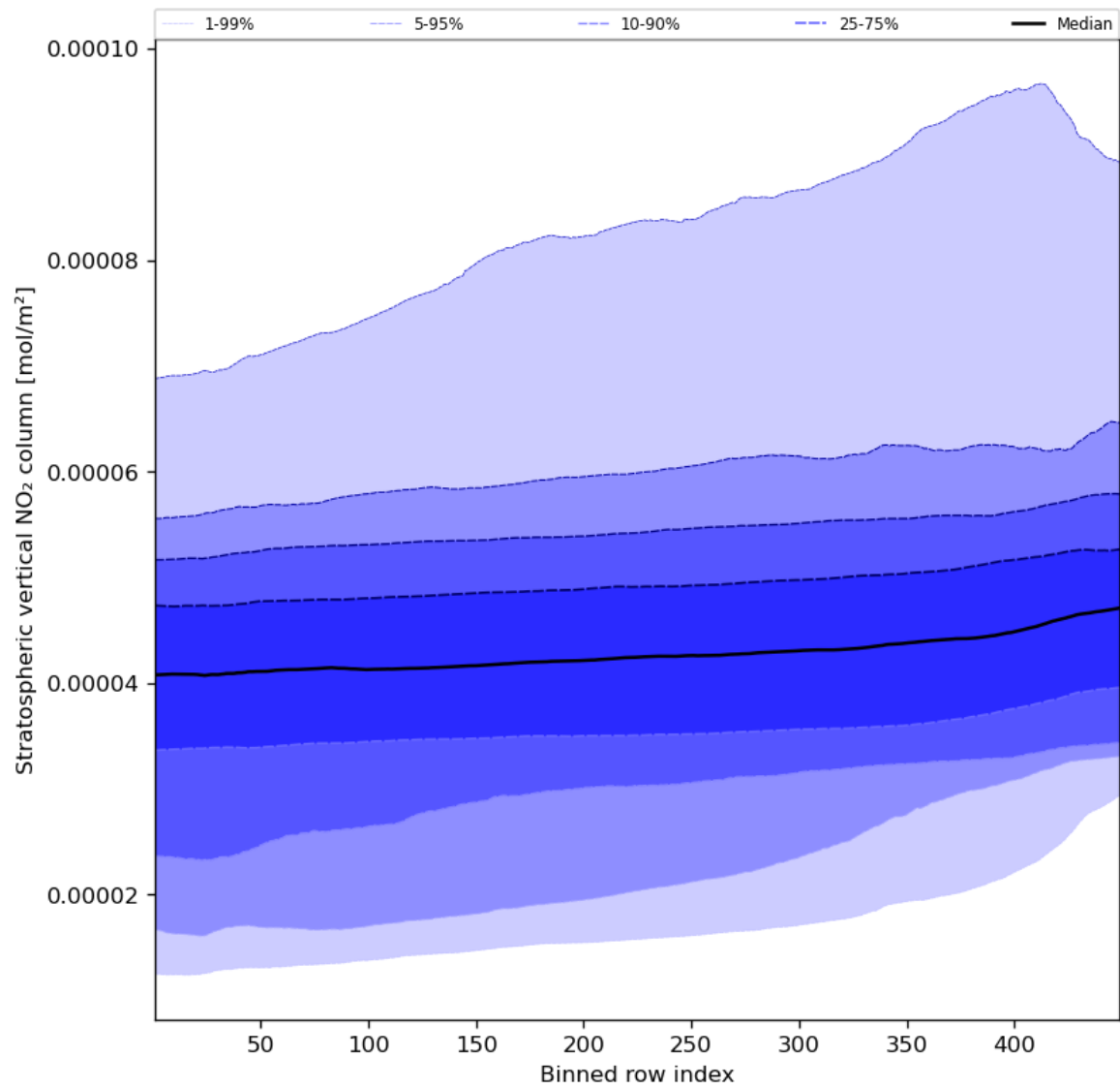
Figure 53: Along track statistics of “Stratospheric vertical NO 2 column” for 2023-09-24 to 2023-09-26
