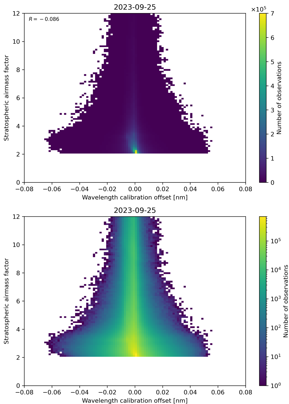
Figure 174: Scatter density plot of “Wavelength calibration offset” against “Stratospheric airmass factor” for 2023-09-24 to 2023-09-26.
