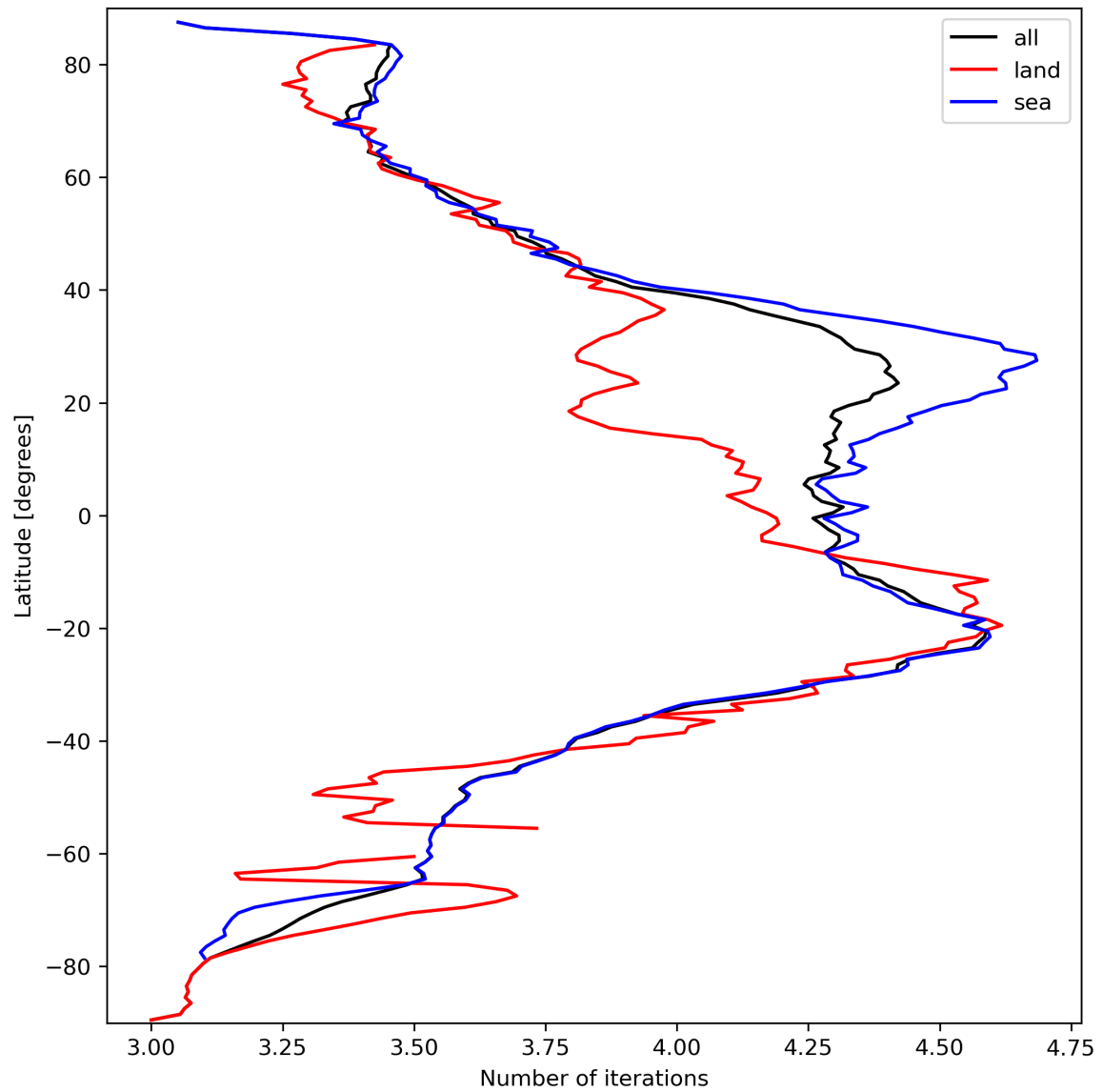
Figure 17: Zonal average of “Number of iterations” for 2023-09-24 to 2023-09-26.
