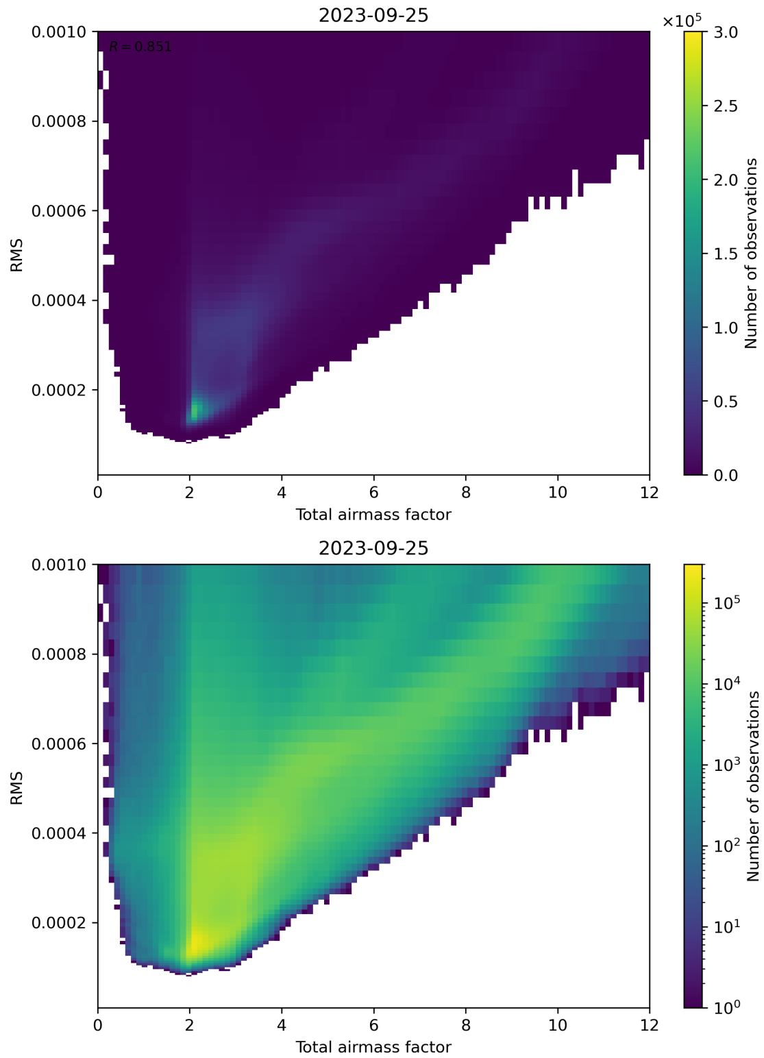
Figure 69: Scatter density plot of “Total airmass factor” against “RMS” for 2023-09-24 to 2023-09-26.
