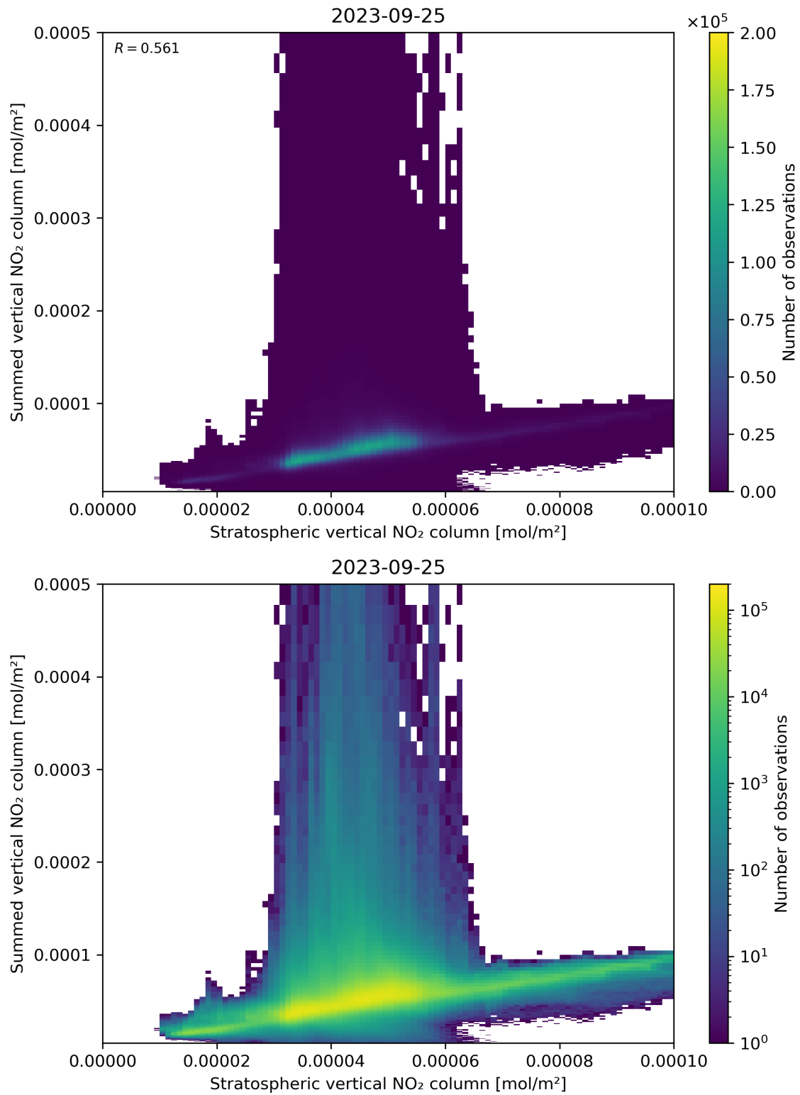
Figure 98: Scatter density plot of “Stratospheric vertical NO 2 column” against “Summed vertical NO 2 column” for 2023-09-24 to 2023-09-26.
