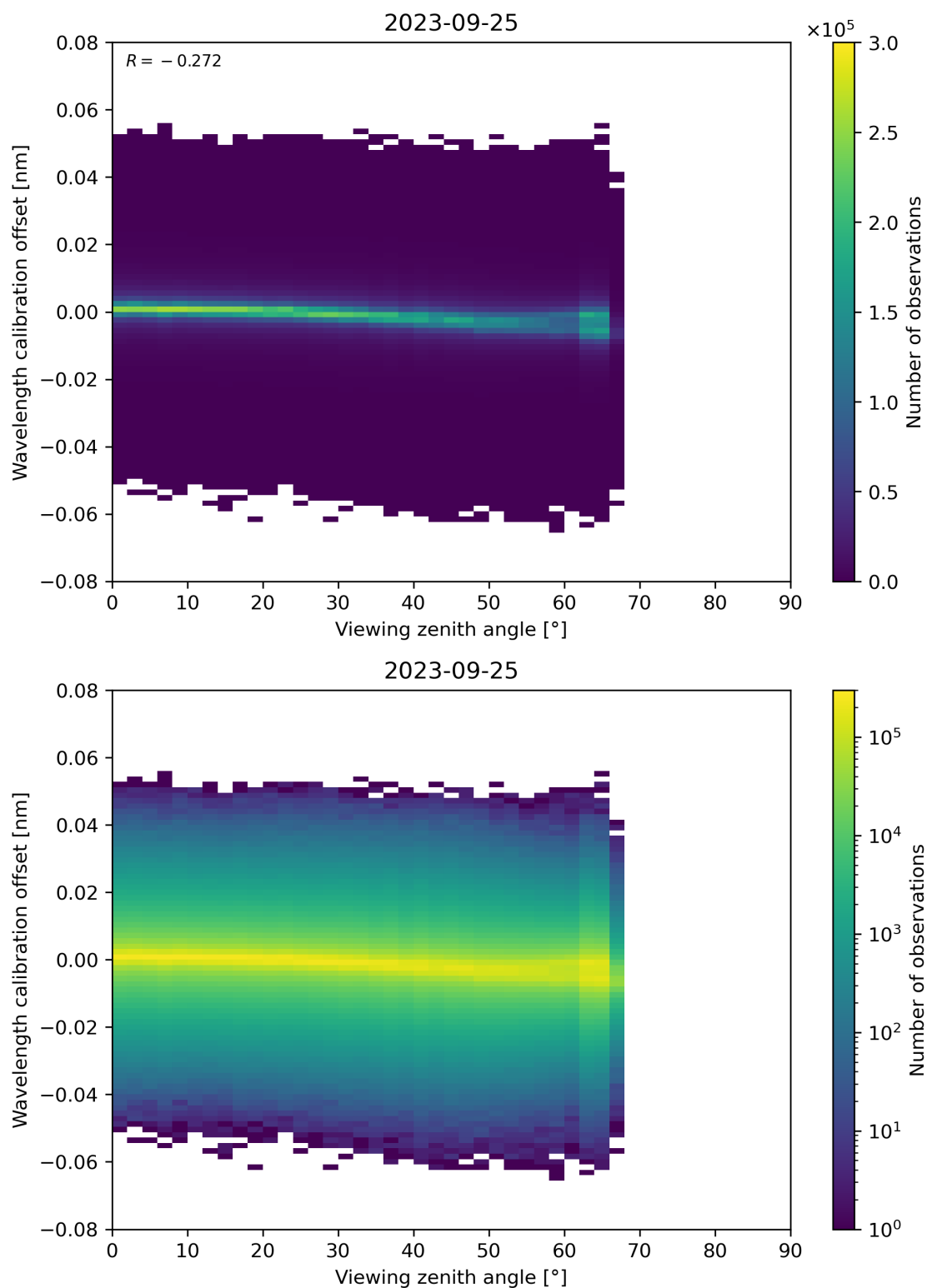
Figure 173: Scatter density plot of “Viewing zenith angle” against “Wavelength calibration offset” for 2023-09-24 to 2023-09-26.
