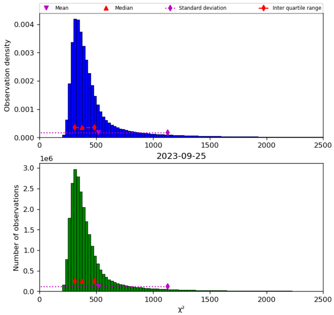
Figure 42: Histogram of “ \chi^2 ” for 2023-09-24 to 2023-09-26
