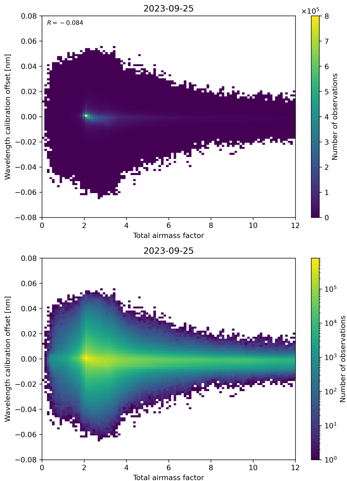
Figure 70: Scatter density plot of “Total airmass factor” against “Wavelength calibration offset” for 2023-09-24 to 2023-09-26.
