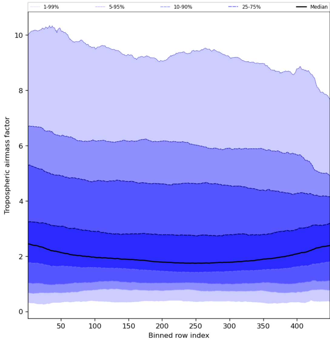
Figure 48: Along track statistics of “Tropospheric air mass factor” for 2023-09-24 to 2023-09-26
