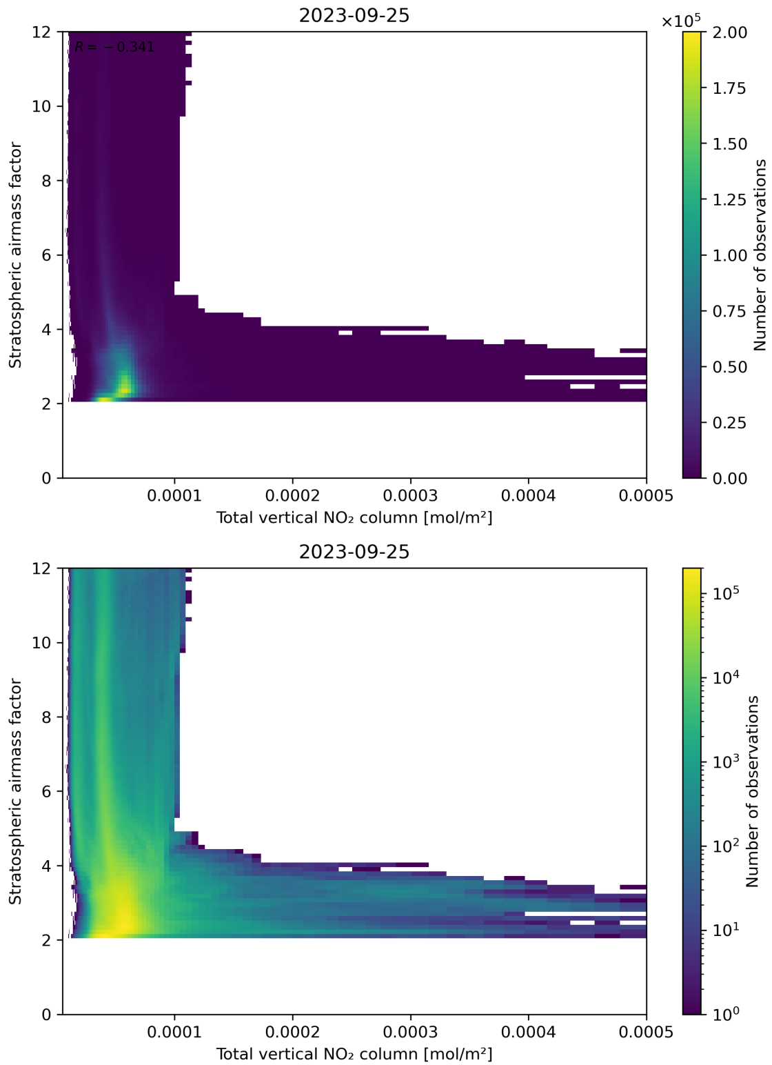
Figure 110: Scatter density plot of “Total vertical NO 2 column” against “Stratospheric airmass factor” for 2023-09-24 to 2023-09-26.
