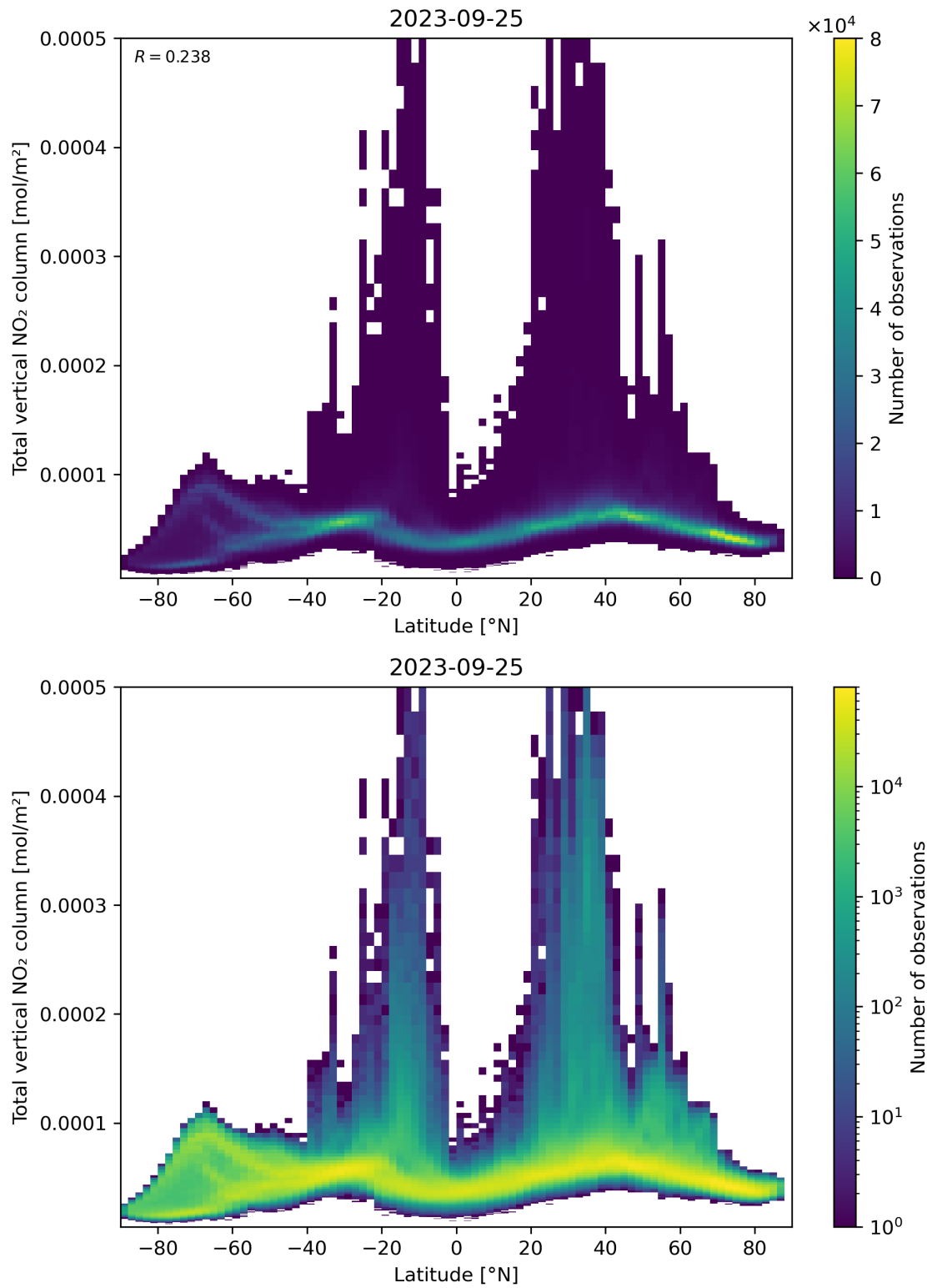
Figure 90: Scatter density plot of “Latitude” against “Total vertical NO 2 column” for 2023-09-24 to 2023-09-26.
