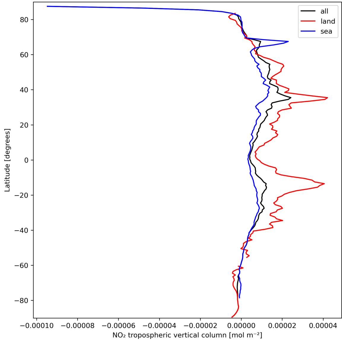
Figure 12: Zonal average of “NO 2 tropospheric vertical column” for 2023-09-24 to 2023-09-26.
