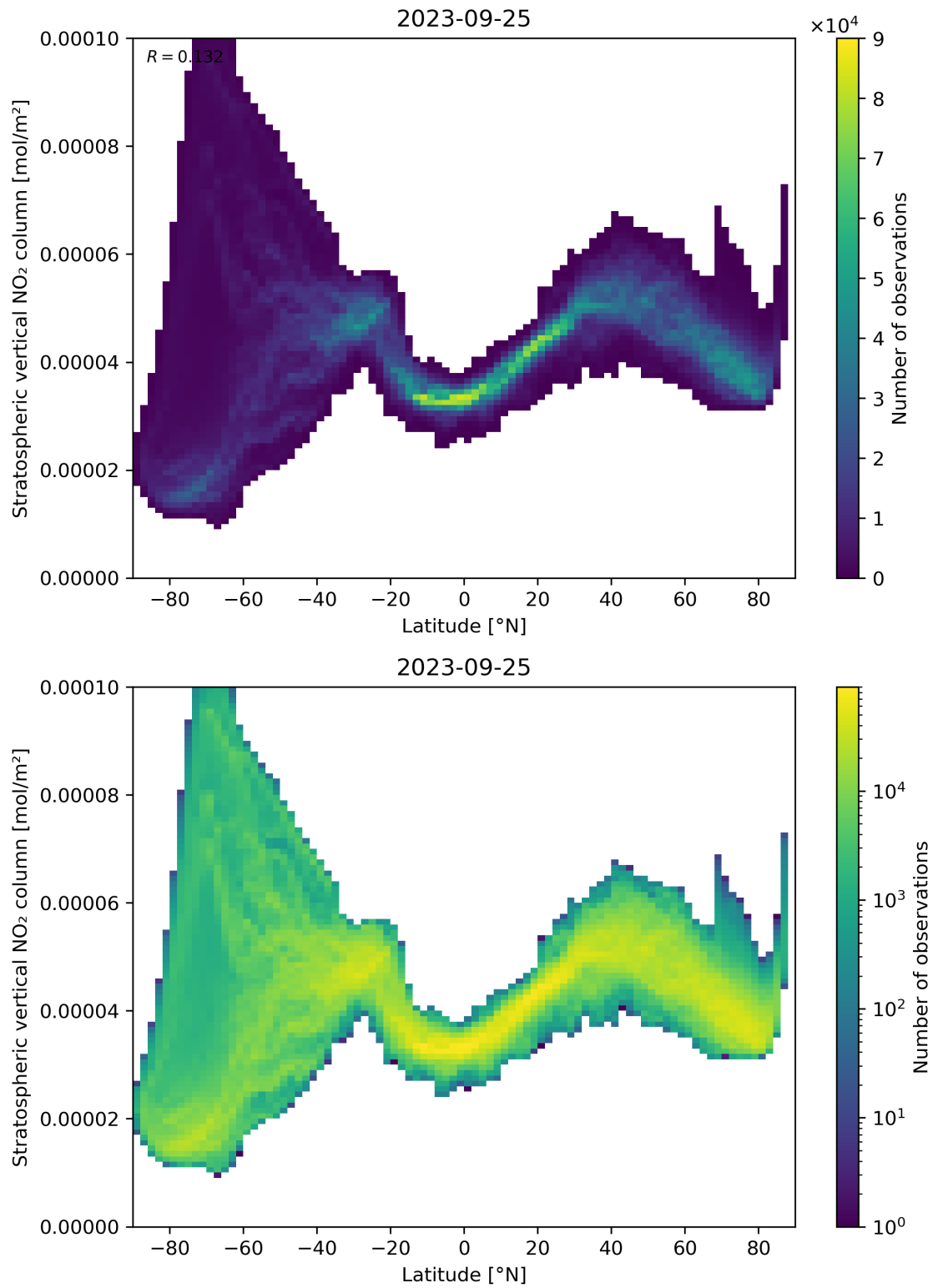
Figure 87: Scatter density plot of “Latitude” against “Stratospheric vertical NO 2 column” for 2023-09-24 to 2023-09-26.
