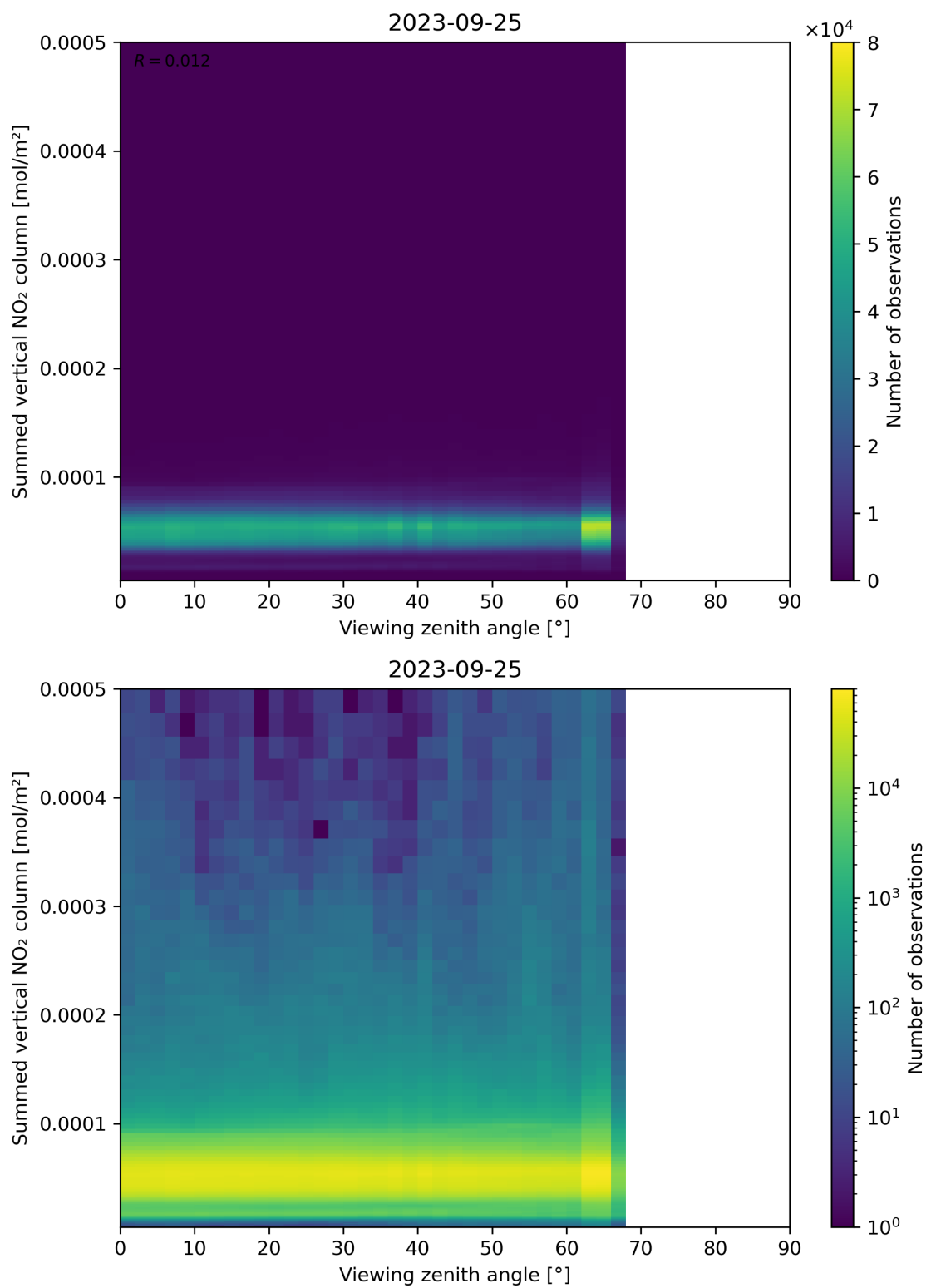
Figure 165: Scatter density plot of “Viewing zenith angle” against “Summed vertical NO 2 column” for 2023-09-24 to 2023-09-26.
