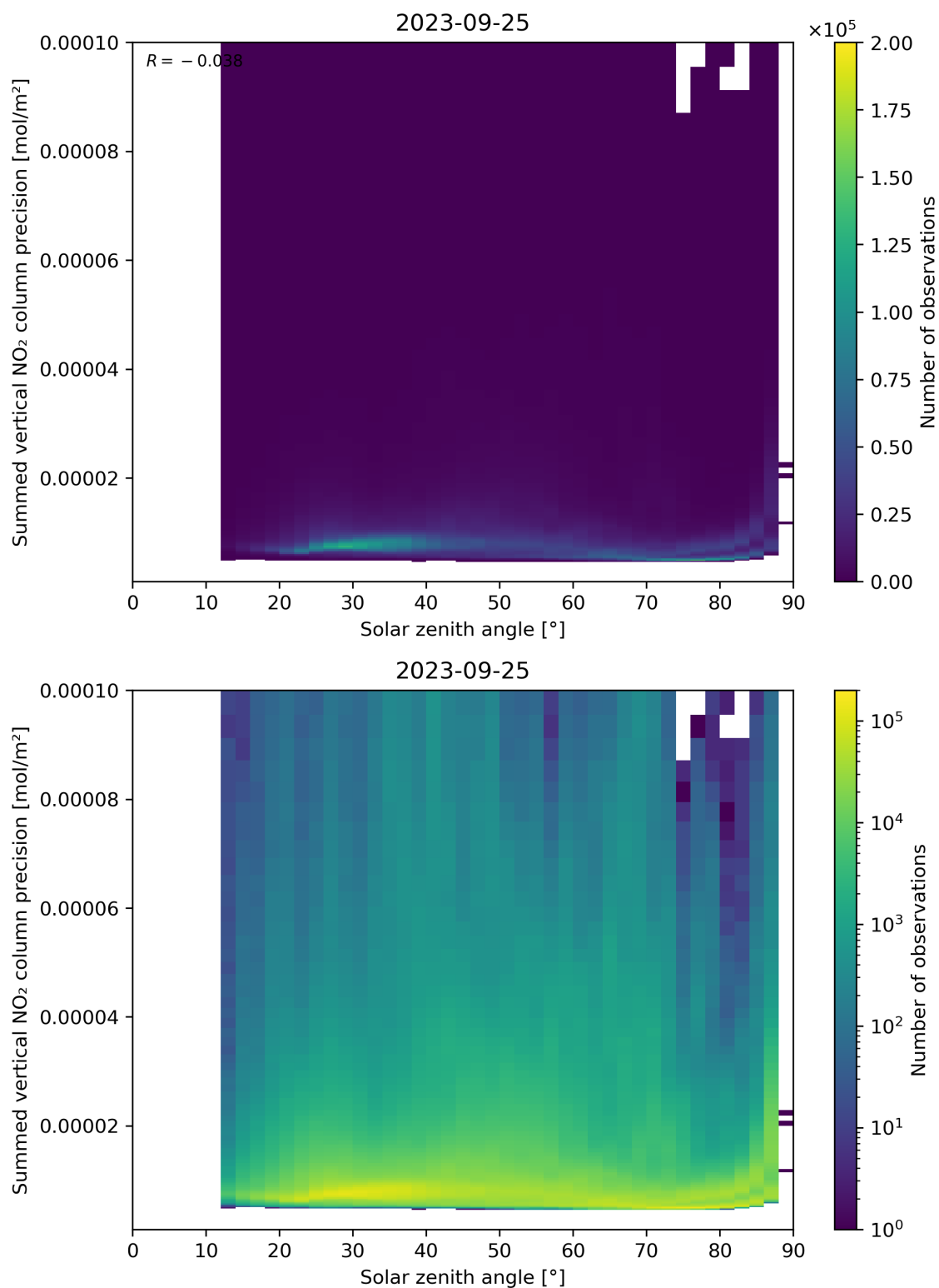
Figure 152: Scatter density plot of “Solar zenith angle” against “Summed vertical NO 2 column precision” for 2023-09-24 to 2023-09-26.
