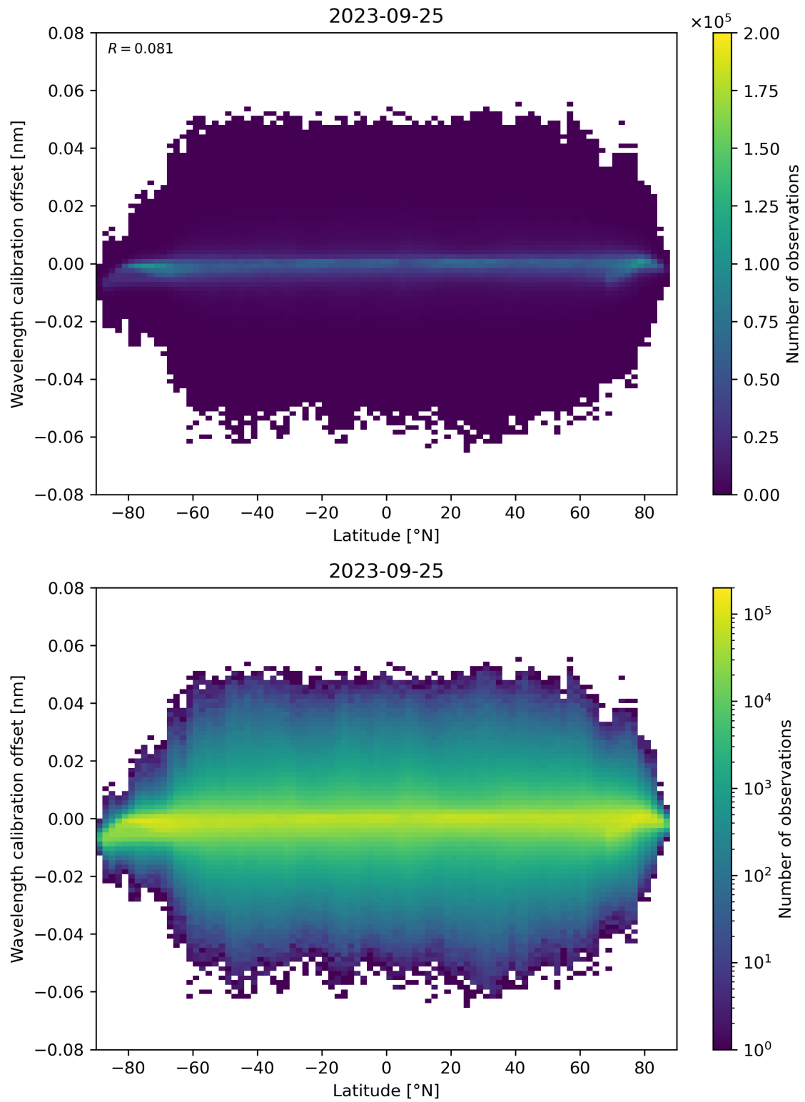
Figure 95: Scatter density plot of “Latitude” against “Wavelength calibration offset” for 2023-09-24 to 2023-09-26.
