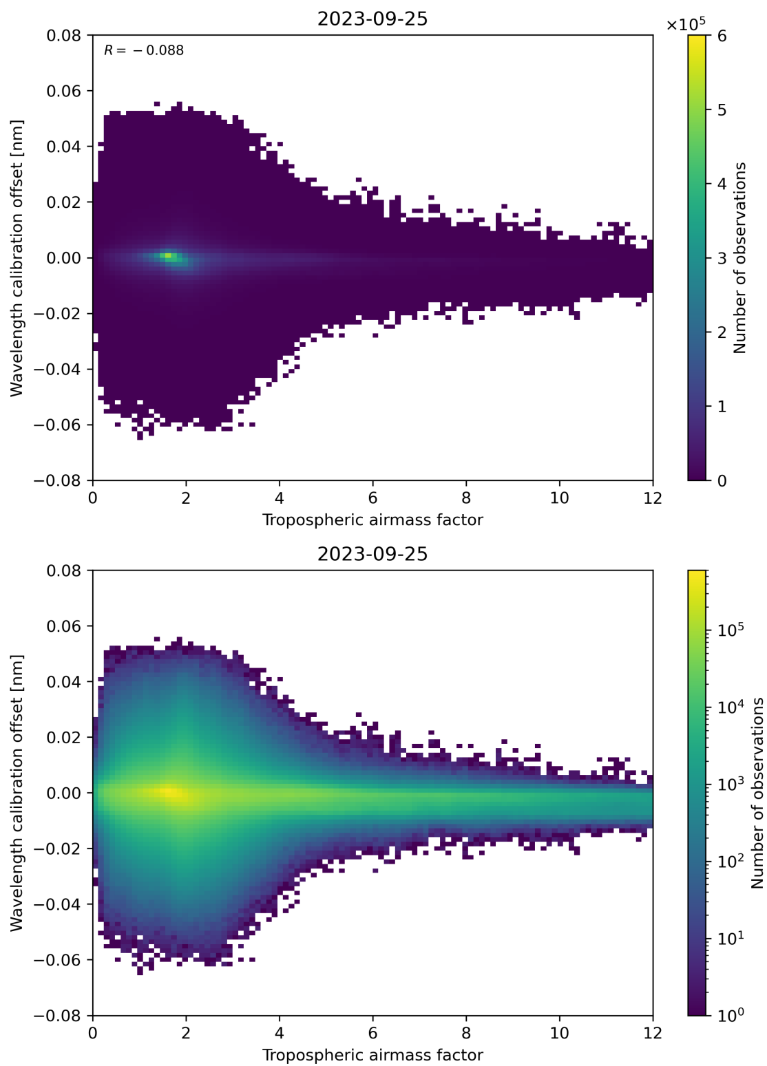
Figure 80: Scatter density plot of “Tropospheric airmass factor” against “Wavelength calibration offset” for 2023-09-24 to 2023-09-26.
