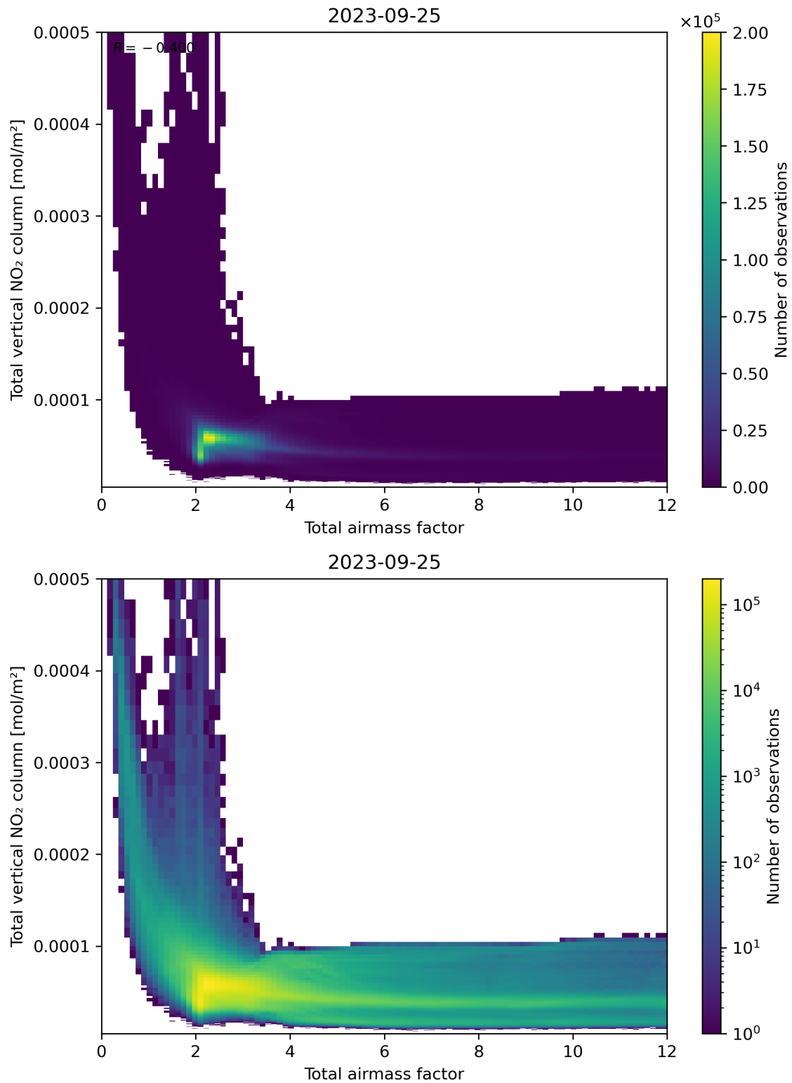
Figure 67: Scatter density plot of “Total airmass factor” against “Total vertical NO 2 column” for 2023-09-24 to 2023-09-26.
