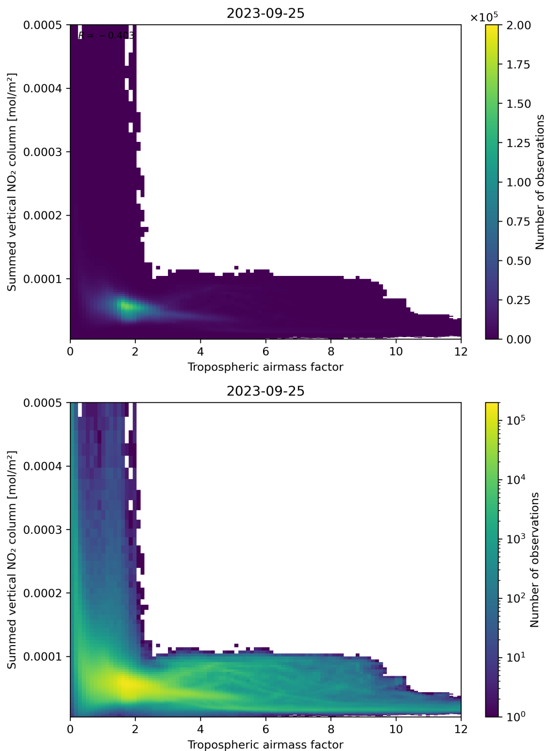
Figure 75: Scatter density plot of “Tropospheric airmass factor” against “Summed vertical NO 2 column” for 2023-09-24 to 2023-09-26.
