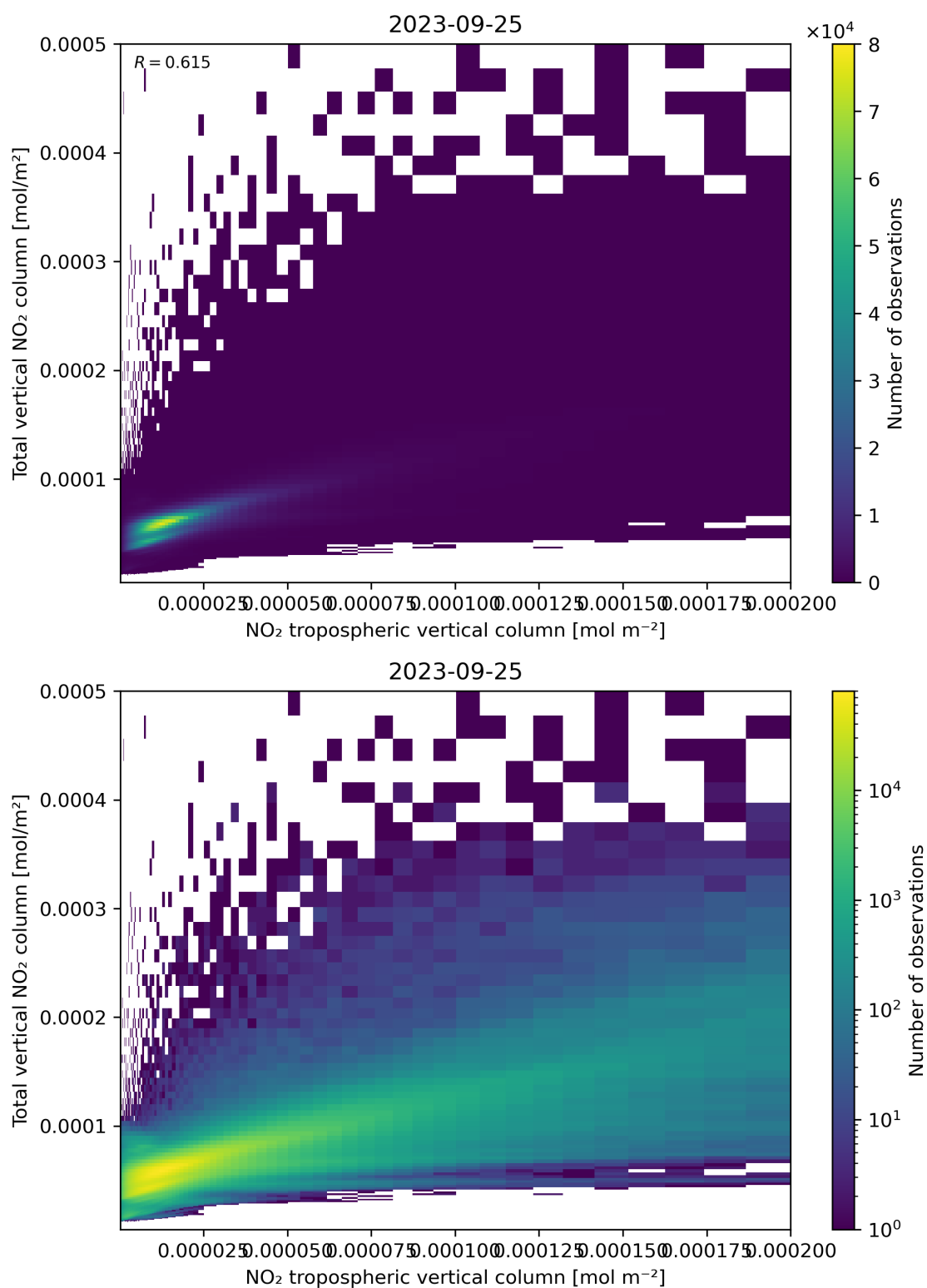
Figure 128: Scatter density plot of “NO 2 tropospheric vertical column” against “Total vertical NO 2 column” for 2023-09-24 to 2023-09-26.
