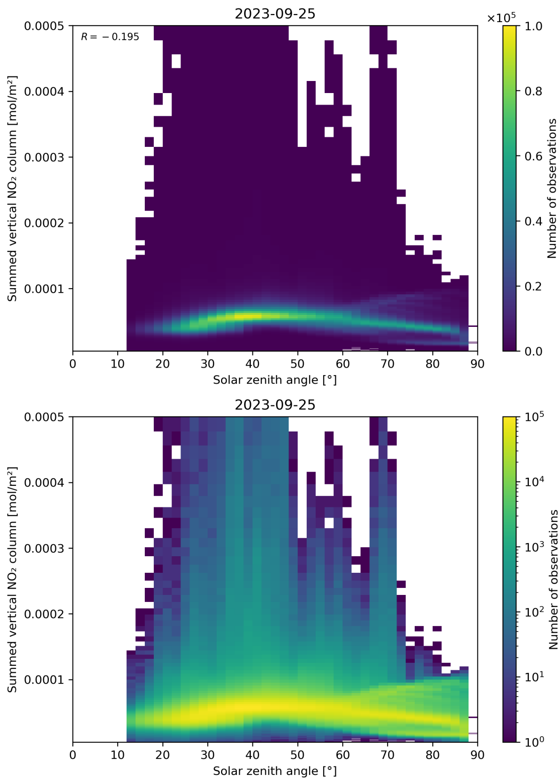
Figure 151: Scatter density plot of “Solar zenith angle” against “Summed vertical NO 2 column” for 2023-09-24 to 2023-09-26.
