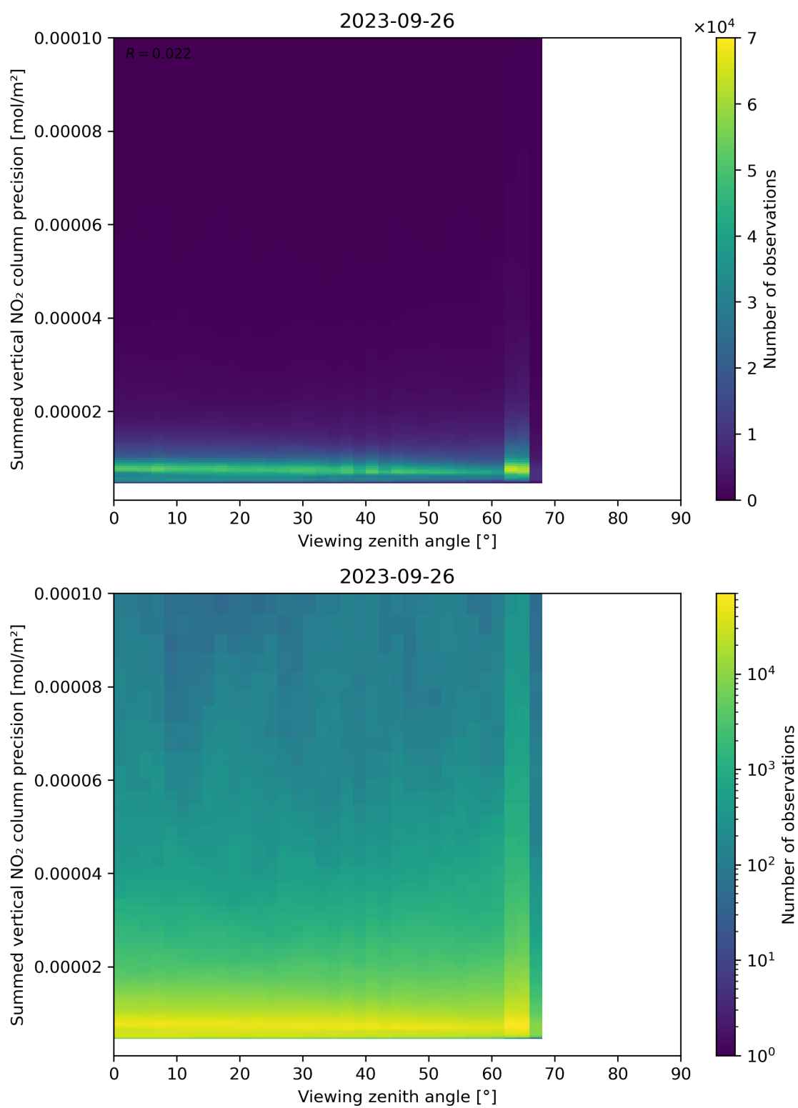
Figure 166: Scatter density plot of “Viewing zenith angle” against “Summed vertical NO 2 column precision” for 2023-09-26 to 2023-09-27.
