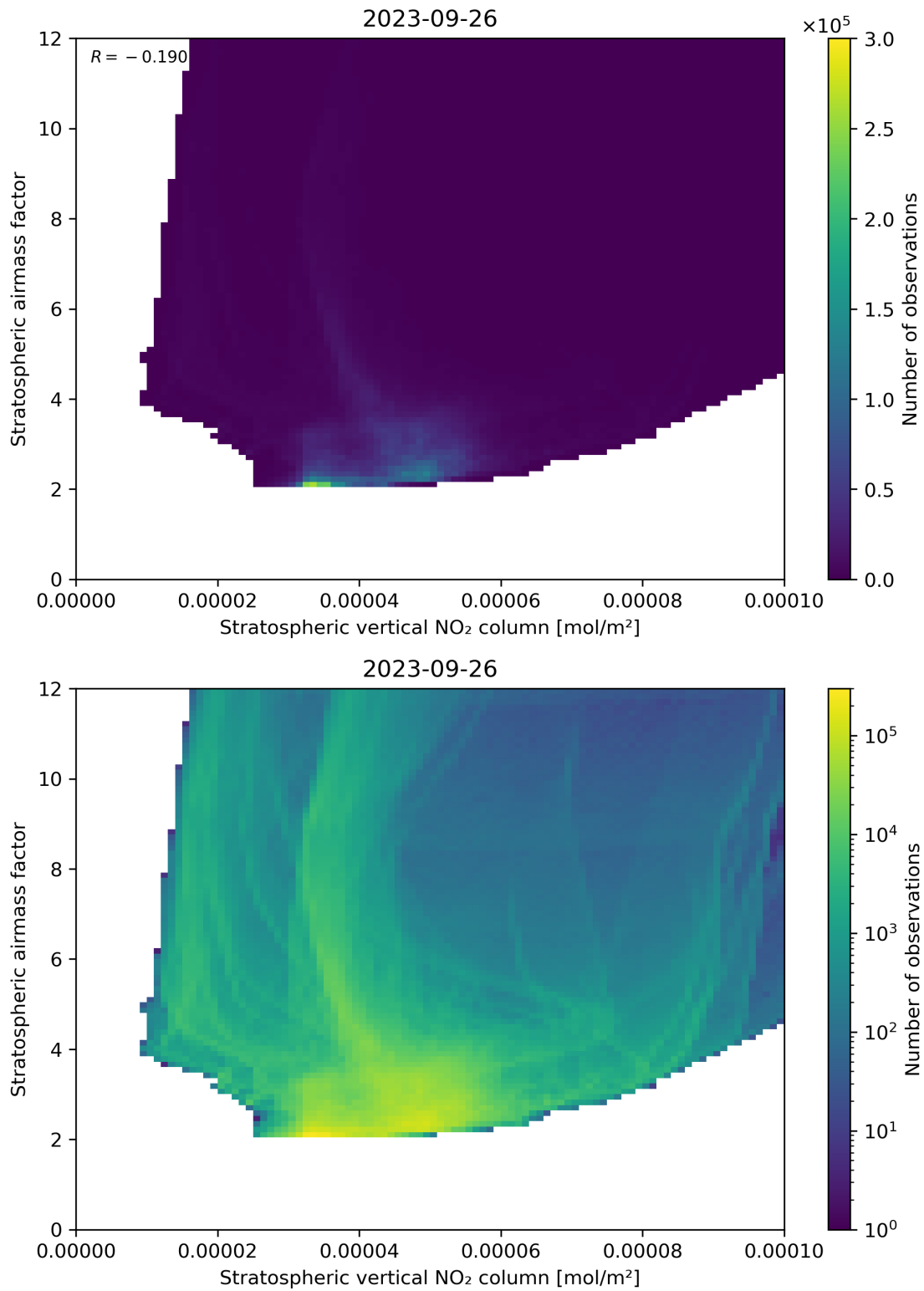
Figure 96: Scatter density plot of “Stratospheric vertical NO 2 column” against “Stratospheric airmass factor” for 2023-09-26 to 2023-09-27.
