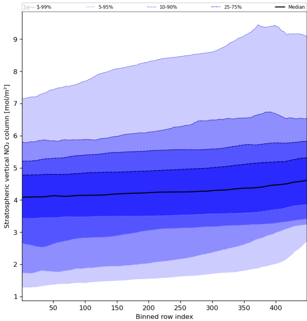
Figure 53: Along track statistics of “Stratospheric vertical NO 2 column” for 2023-09-26 to 2023-09-27
