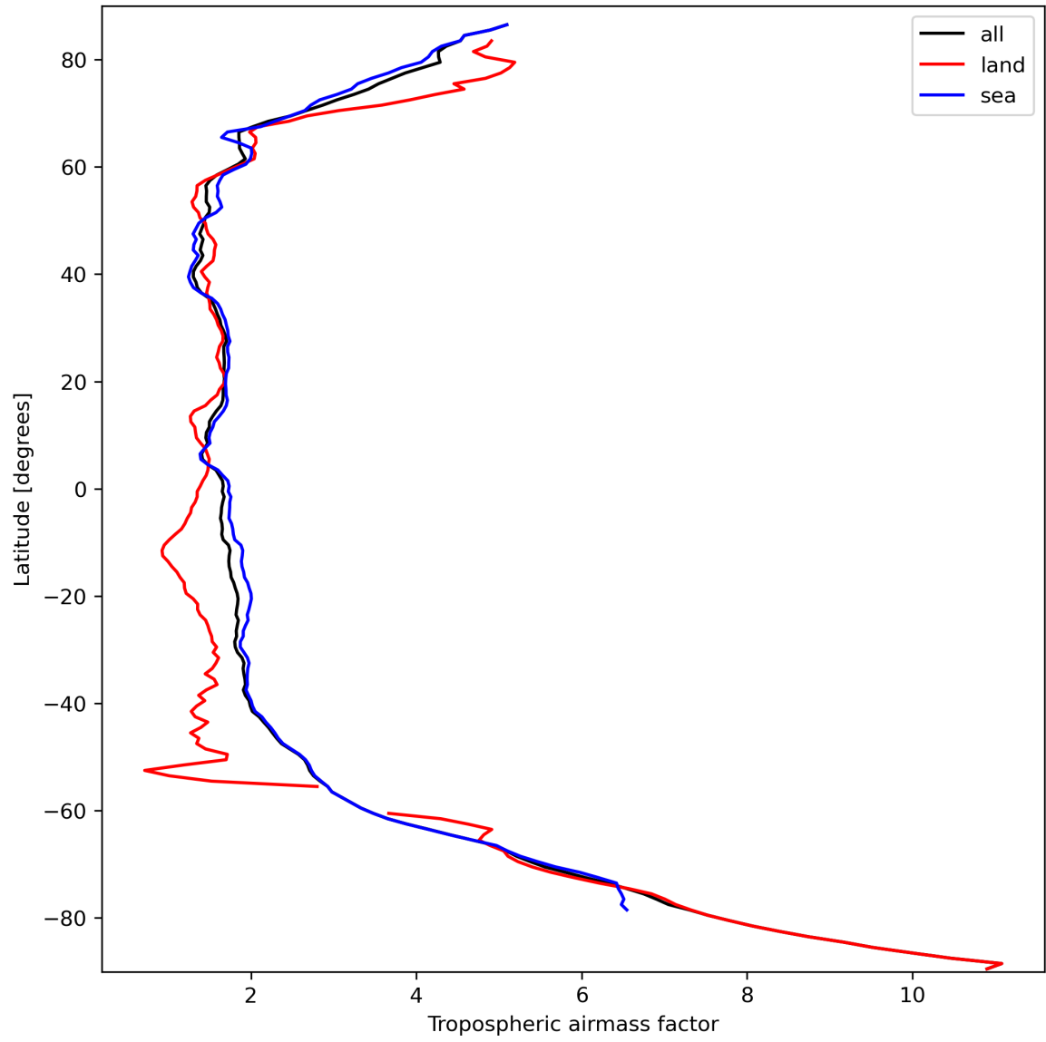
Figure 14: Zonal average of “Tropospheric airmass factor” for 2023-09-26 to 2023-09-27.
