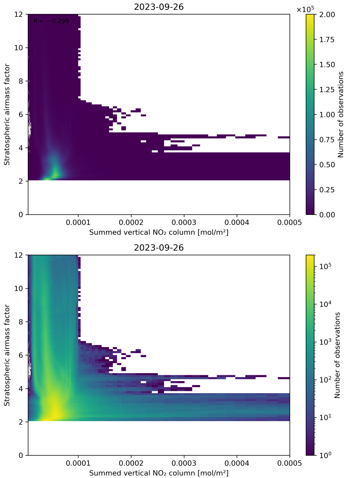
Figure 103: Scatter density plot of “Summed vertical NO 2 column” against “Stratospheric air mass factor” for 2023-09-26 to 2023-09-27.
