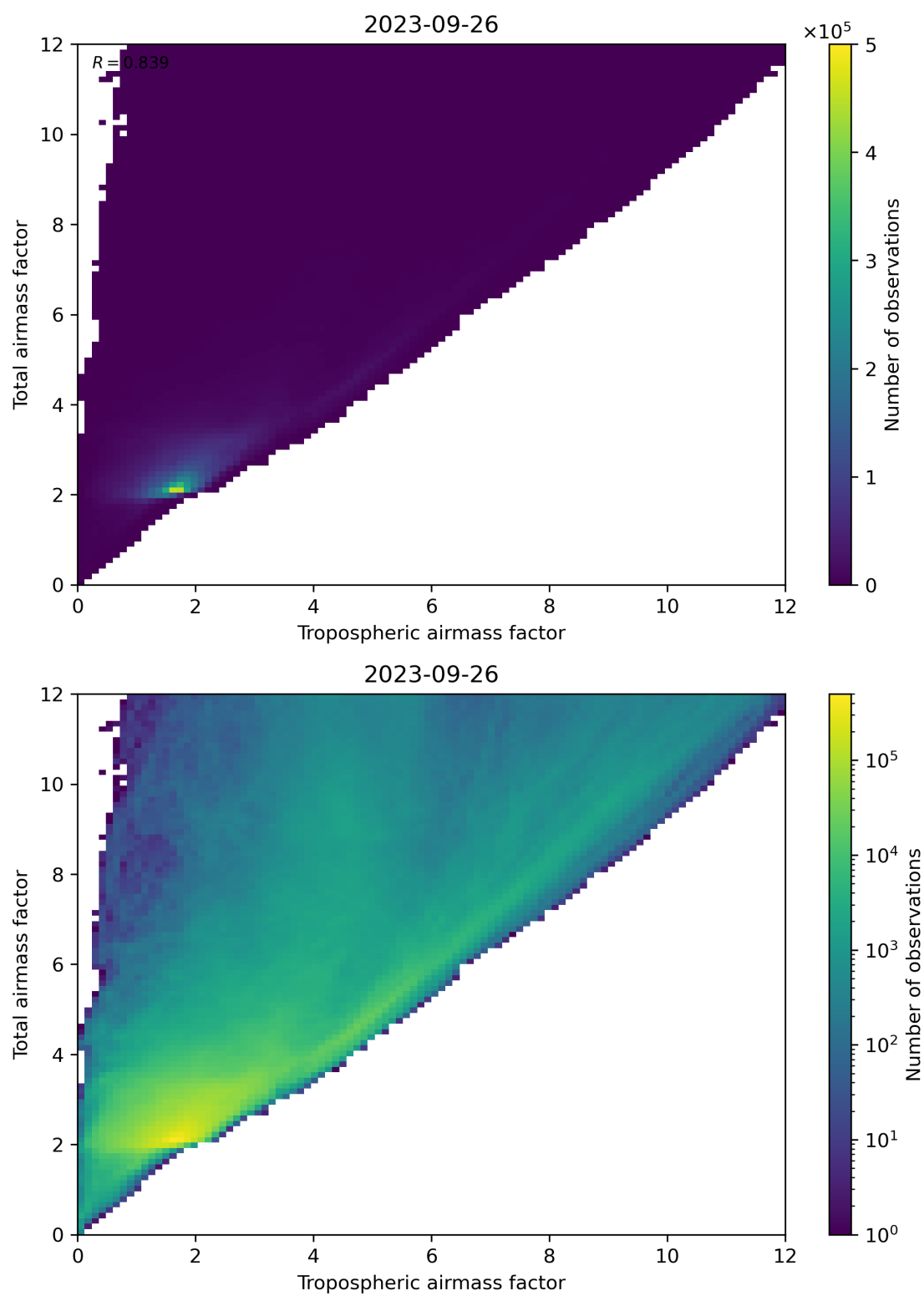
Figure 72: Scatter density plot of “Tropospheric airmass factor” against “Total airmass factor” for 2023-09-26 to 2023-09-27.
