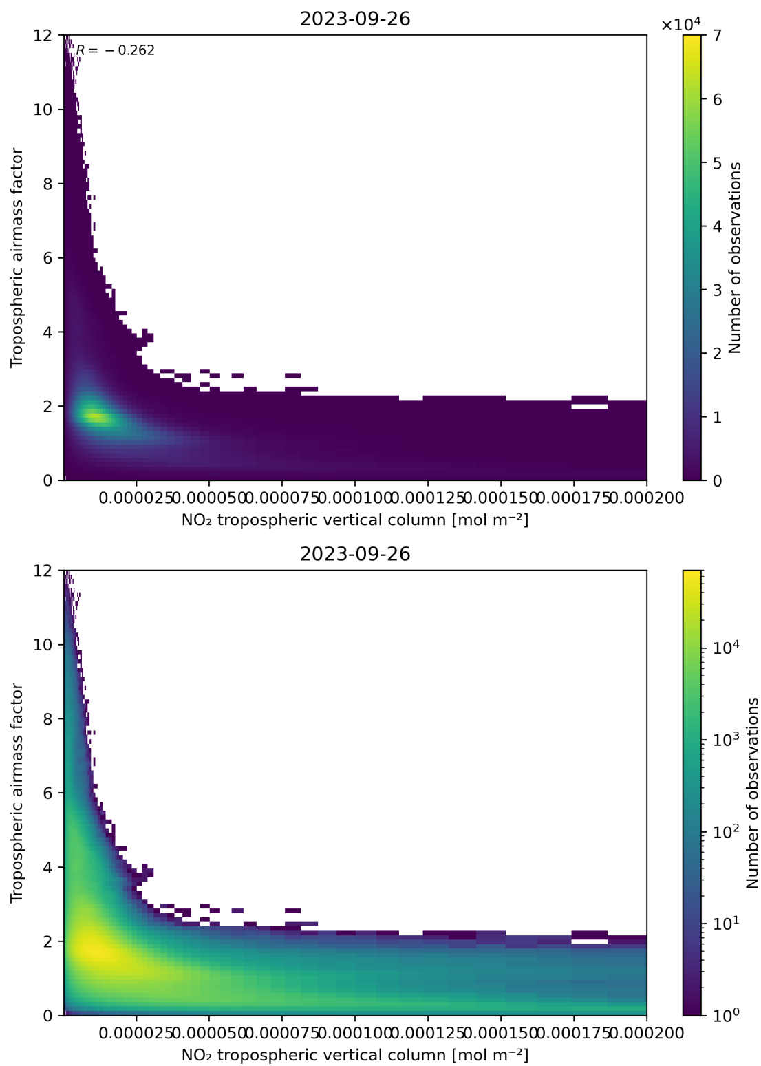
Figure 123: Scatter density plot of “NO 2 tropospheric vertical column” against “Tropospheric air mass factor” for 2023-09-26 to 2023-09-27.
