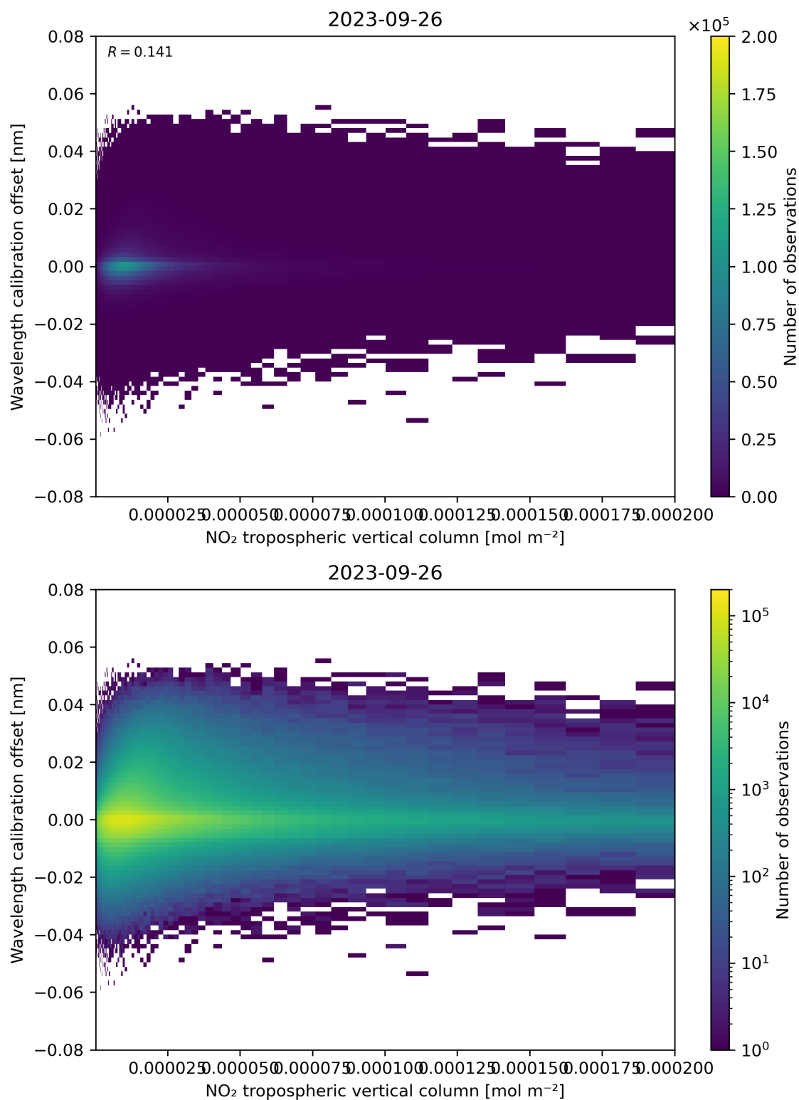
Figure 143: Scatter density plot of “NO 2 tropospheric vertical column” against “Wavelength calibration offset” for 2023-09-26 to 2023-09-27.
