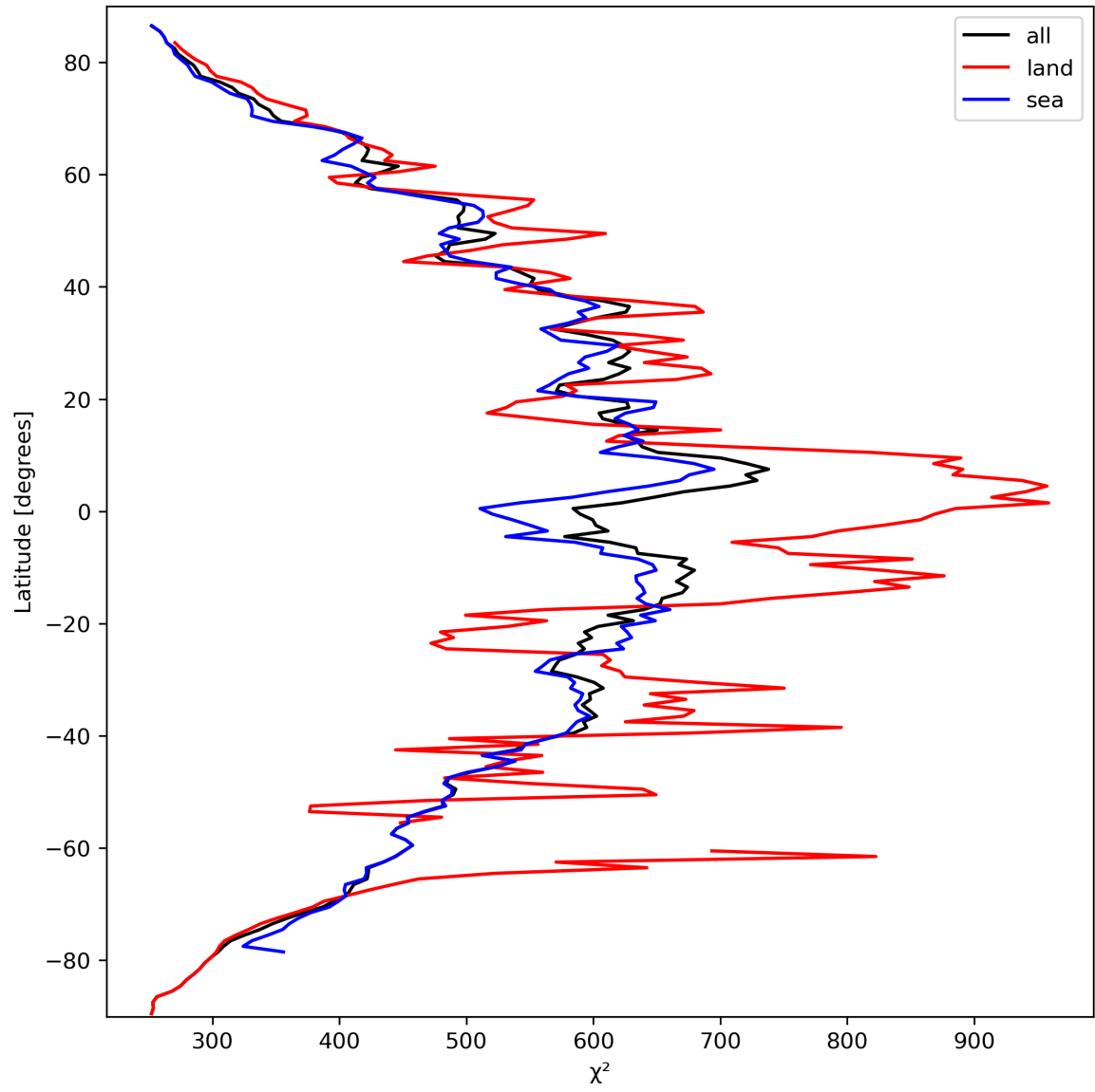
Figure 25: Zonal average of “ \chi^2 ” for 2023-09-26 to 2023-09-27.
