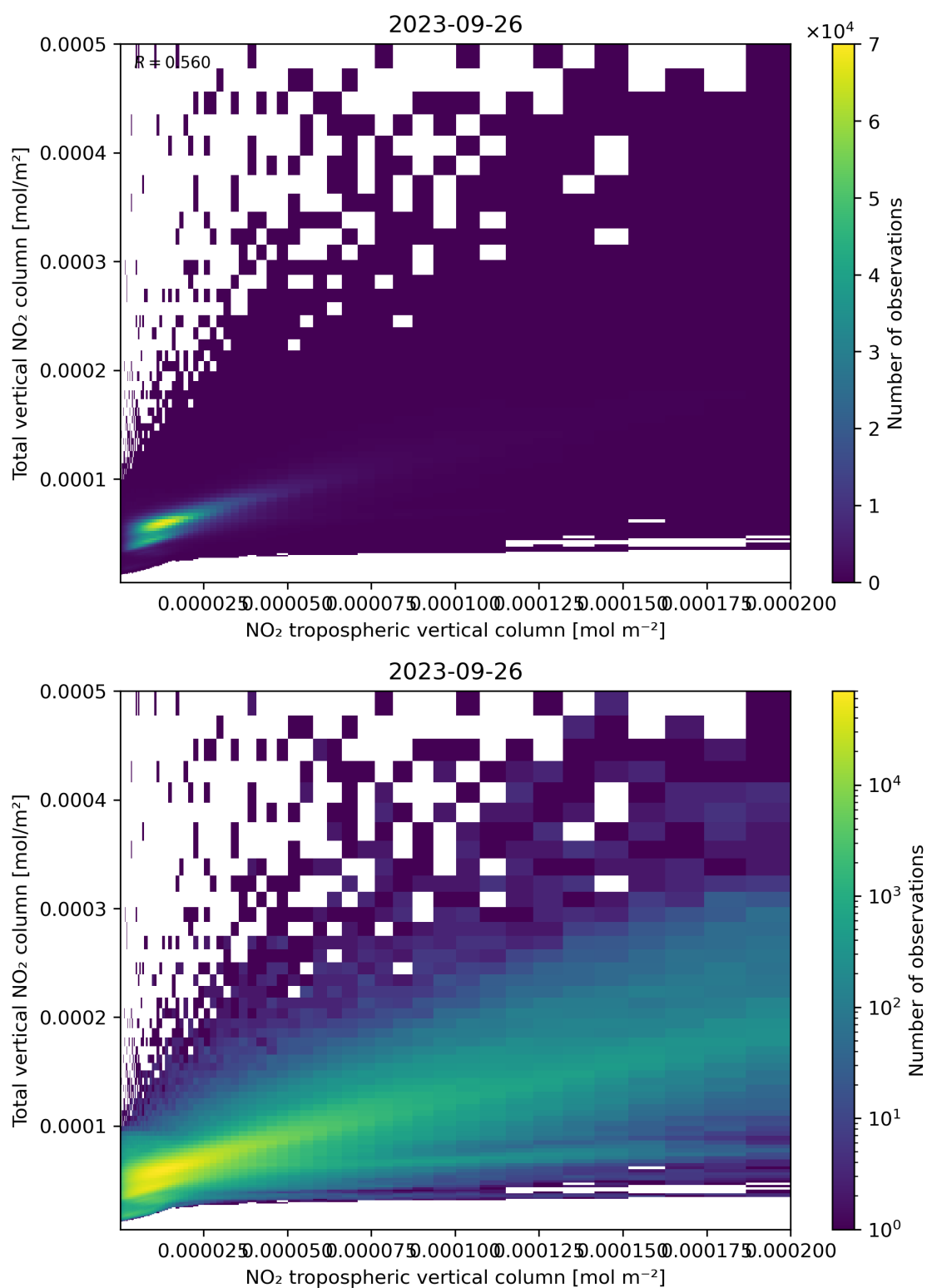
Figure 128: Scatter density plot of “NO 2 tropospheric vertical column” against “Total vertical NO 2 column” for 2023-09-26 to 2023-09-27.
