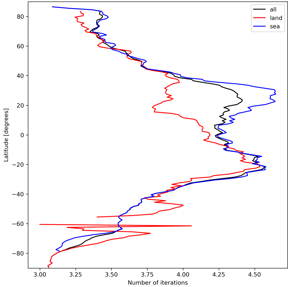
Figure 17: Zonal average of “Number of iterations” for 2023-09-26 to 2023-09-27.
