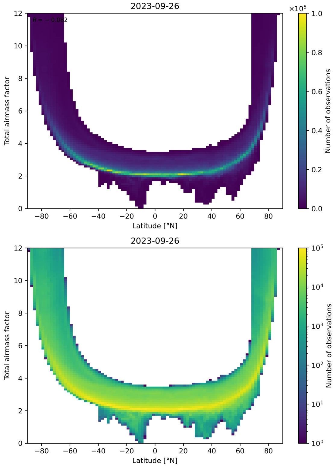
Figure 84: Scatter density plot of “Latitude” against “Total airmass factor” for 2023-09-26 to 2023-09-27.
