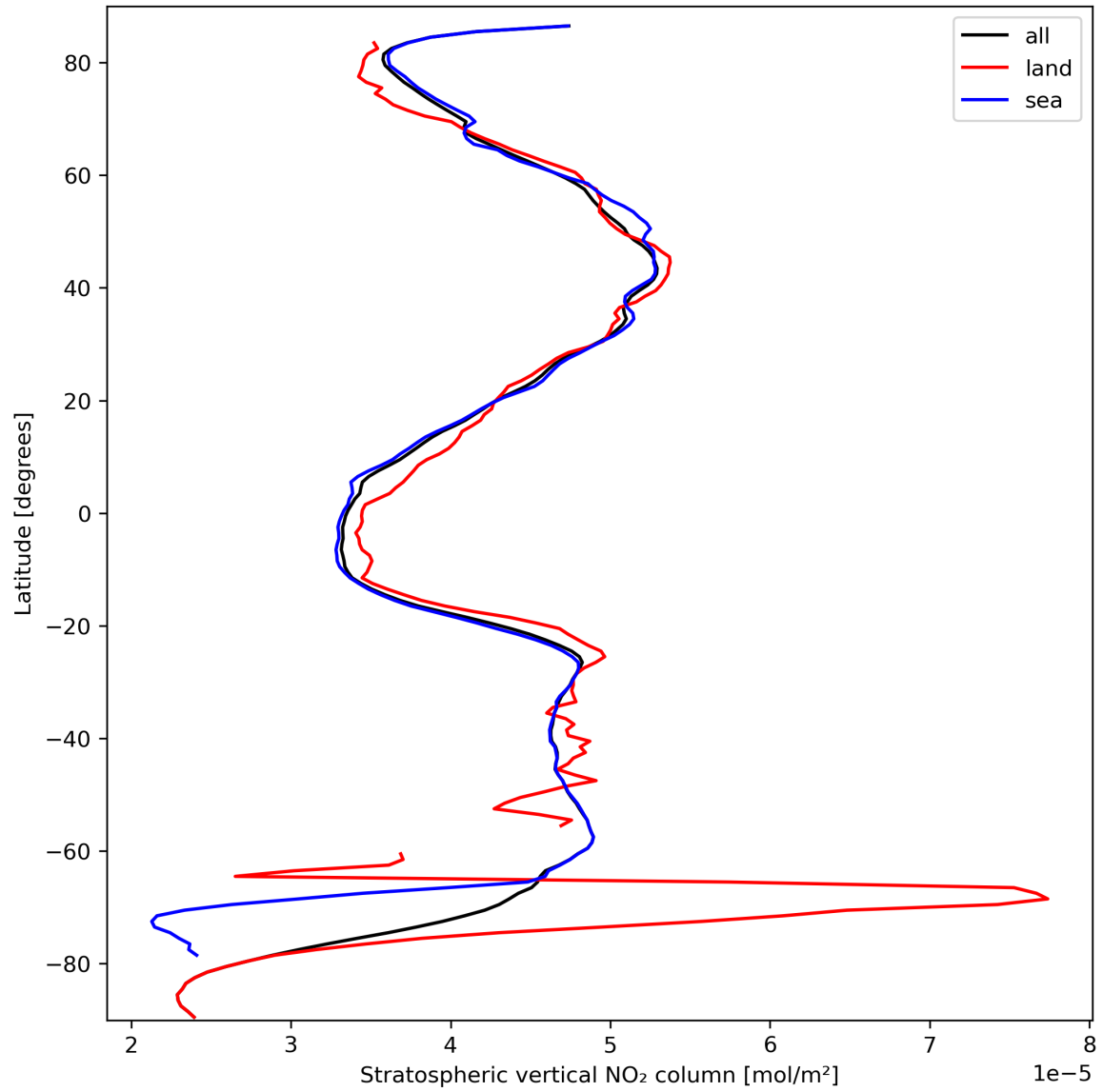
Figure 19: Zonal average of “Stratospheric vertical NO 2 column” for 2023-09-26 to 2023-09-27.
