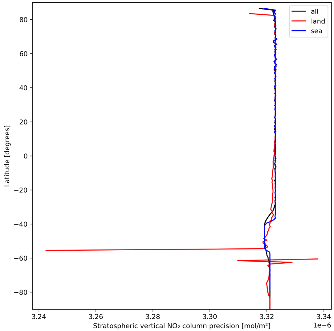
Figure 20: Zonal average of “Stratospheric vertical NO 2 column precision” for 2023-09-26 to 2023-09-27.
