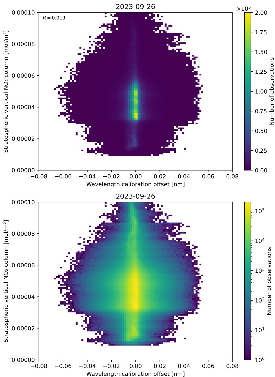
Figure 176: Scatter density plot of “Wavelength calibration offset” against “Stratospheric vertical NO 2 column” for 2023-09-26 to 2023-09-27.
