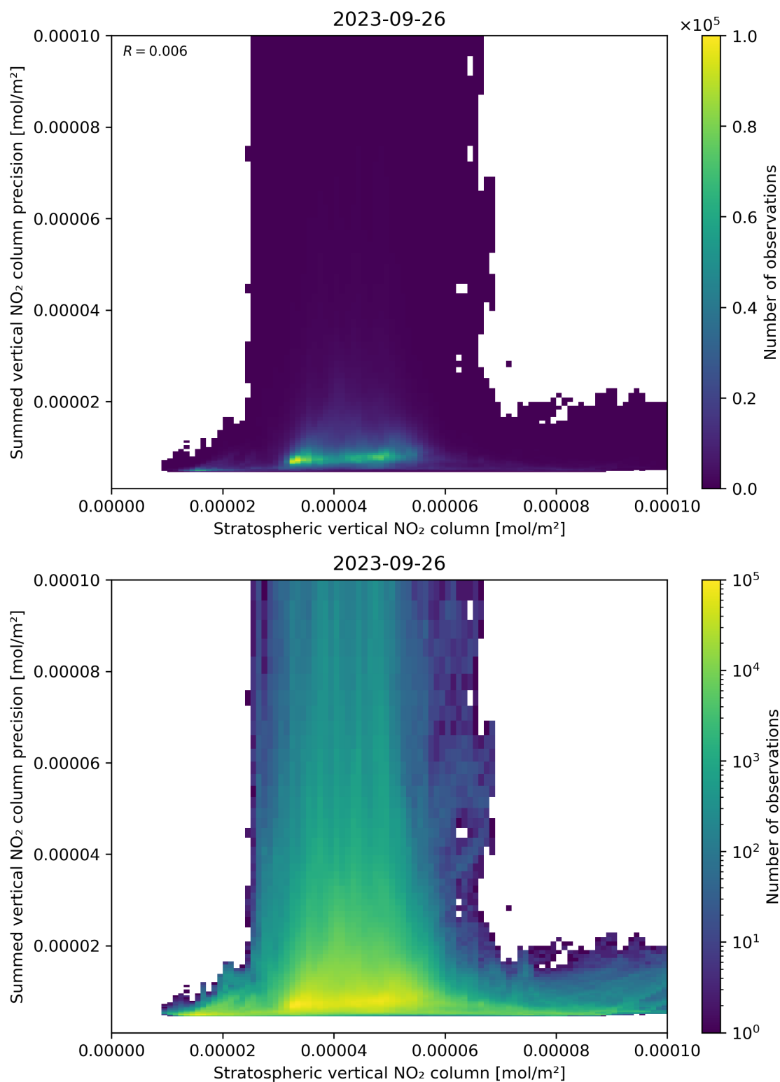
Figure 99: Scatter density plot of “Stratospheric vertical NO 2 column” against “Summed vertical NO 2 column precision” for 2023-09-26 to 2023-09-27.
