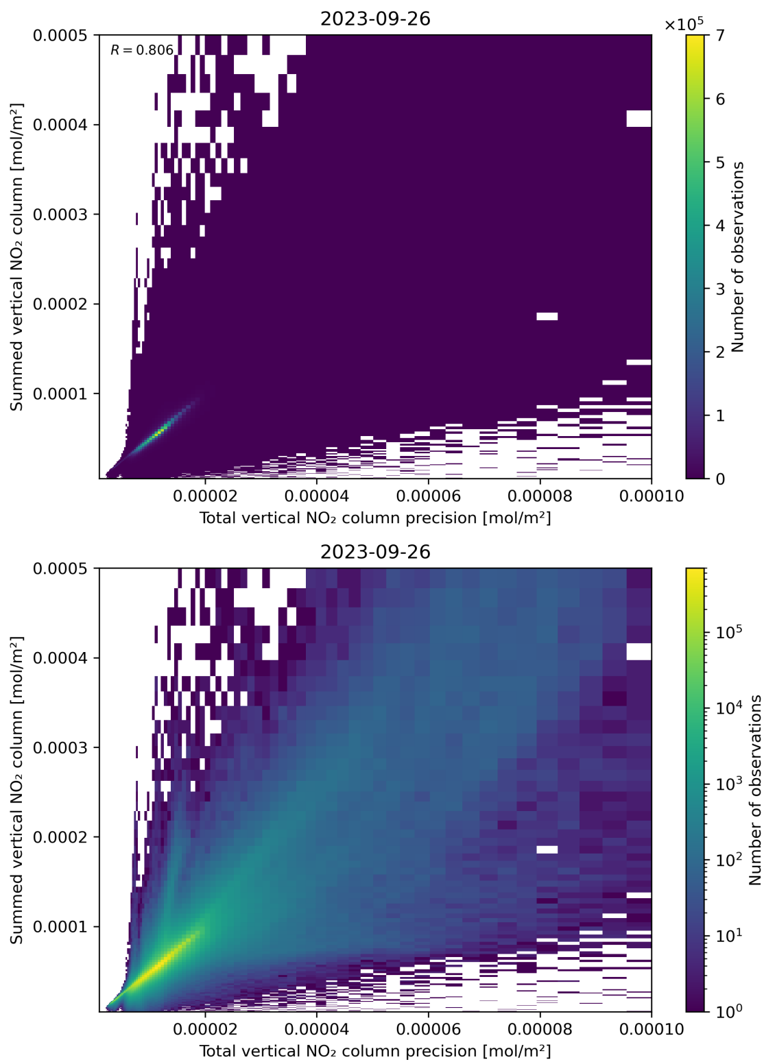
Figure 117: Scatter density plot of “Total vertical NO 2 column precision” against “Summed vertical NO 2 column” for 2023-09-26 to 2023-09-27.
