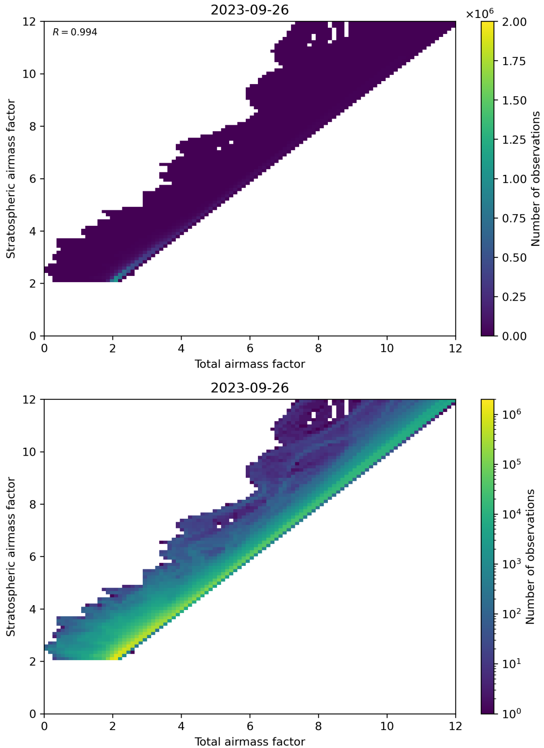
Figure 62: Scatter density plot of “Total airmass factor” against “Stratospheric airmass factor” for 2023-09-26 to 2023-09-27.
