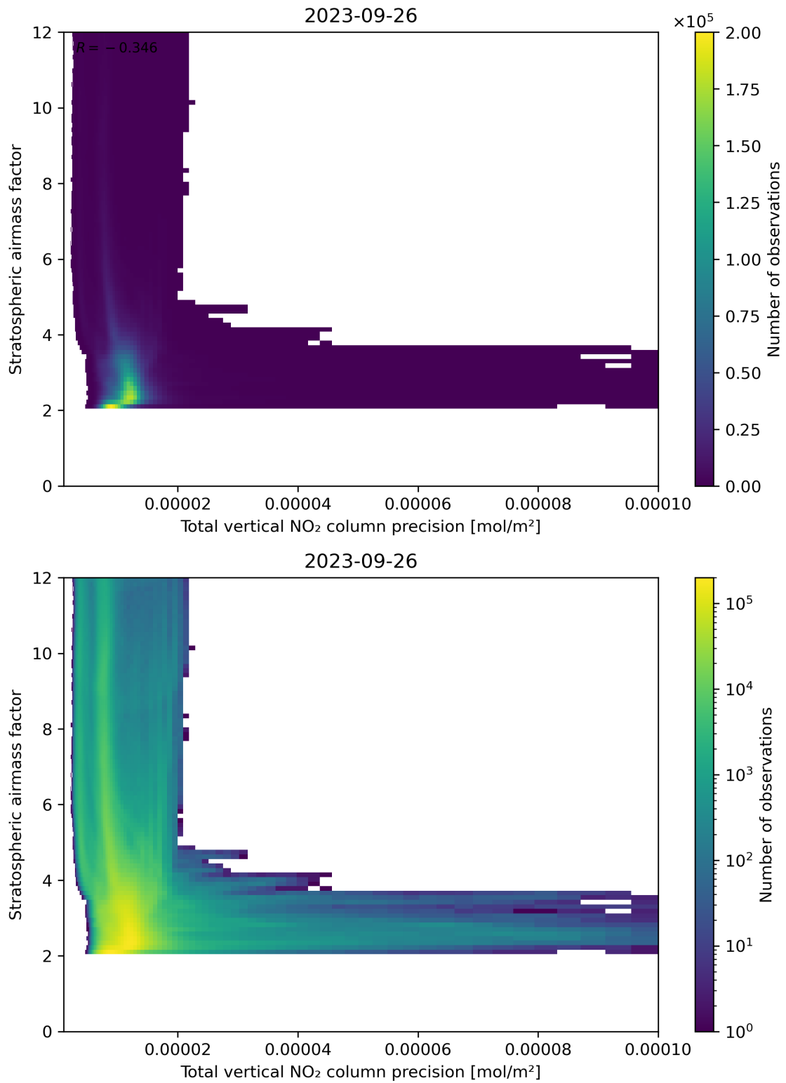
Figure 115: Scatter density plot of “Total vertical NO 2 column precision” against “Stratospheric air mass factor” for 2023-09-26 to 2023-09-27.
