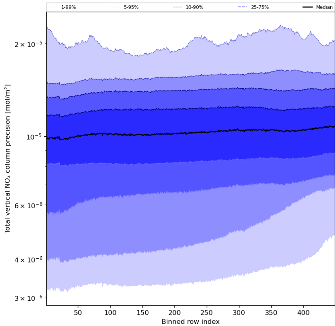
Figure 56: Along track statistics of “Total vertical NO 2 column precision” for 2023-09-26 to 2023-09-27
