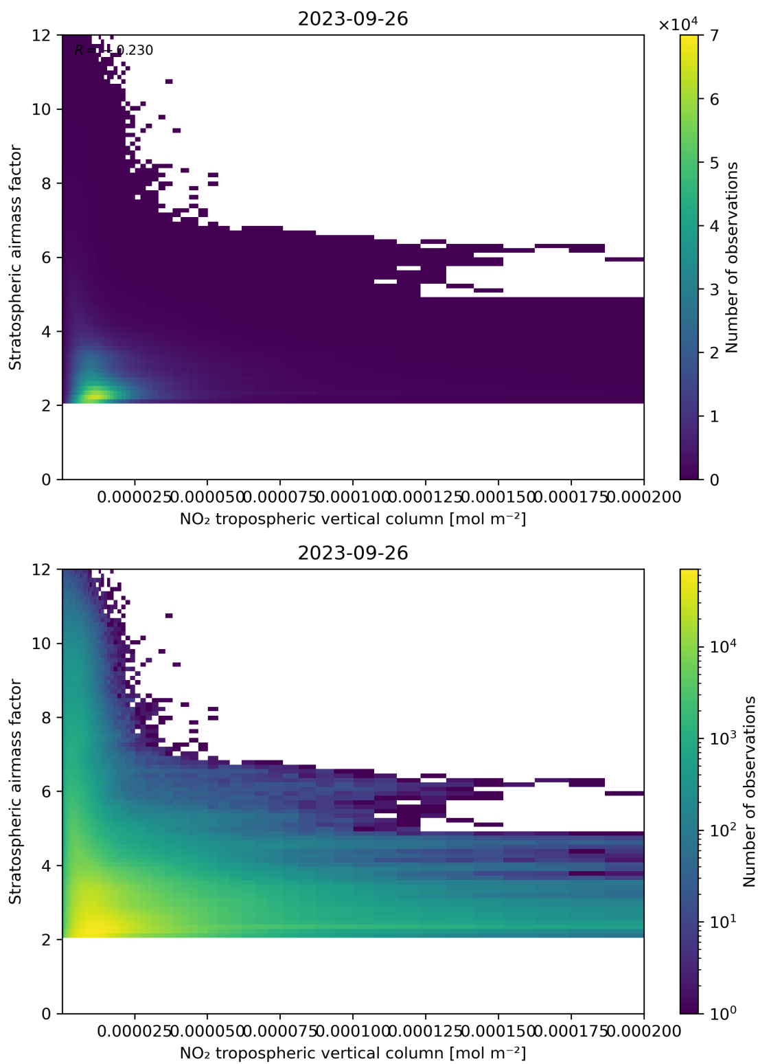
Figure 121: Scatter density plot of “NO 2 tropospheric vertical column” against “Stratospheric air mass factor” for 2023-09-26 to 2023-09-27.
