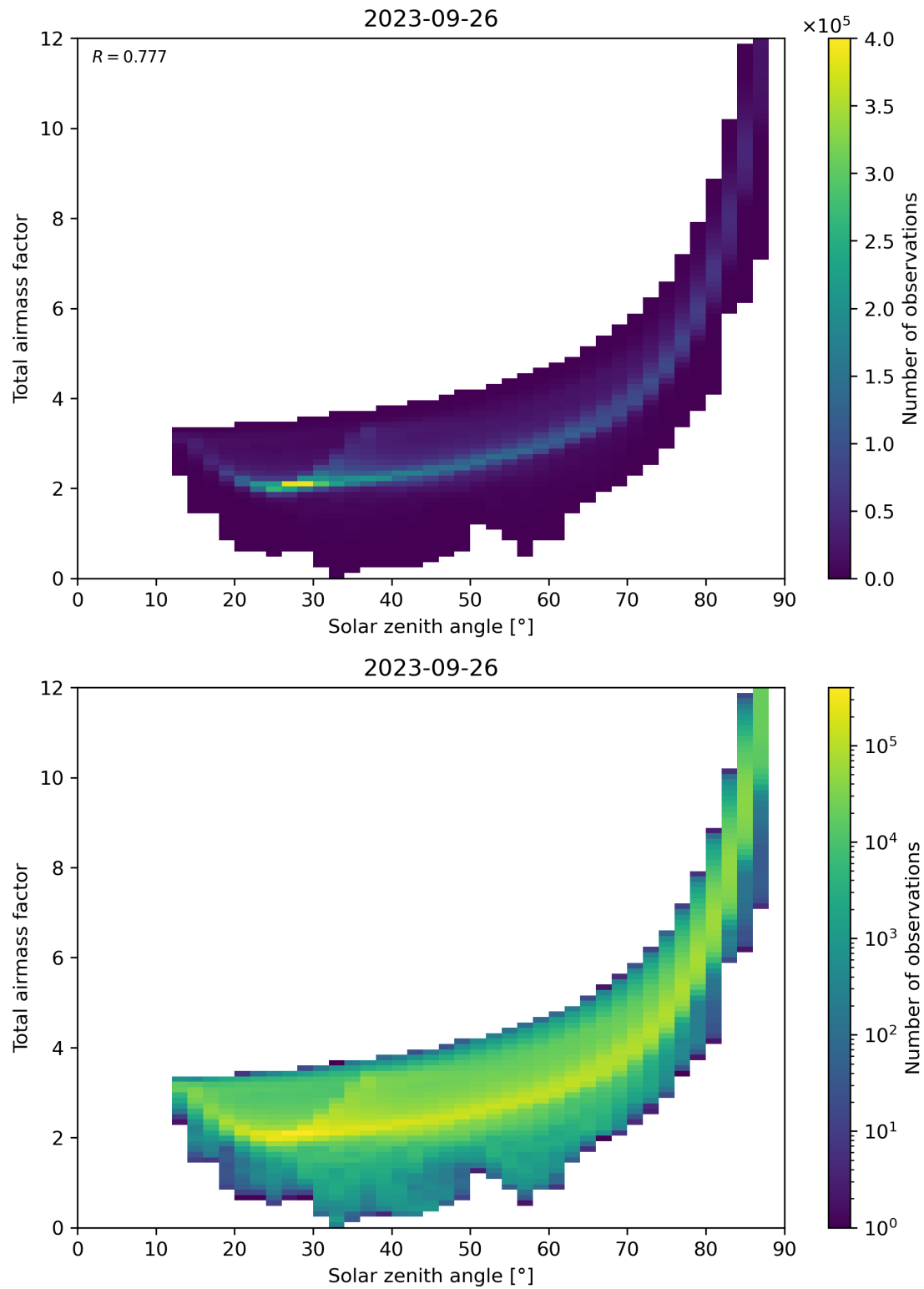
Figure 146: Scatter density plot of “Solar zenith angle” against “Total airmass factor” for 2023-09-26 to 2023-09-27.
