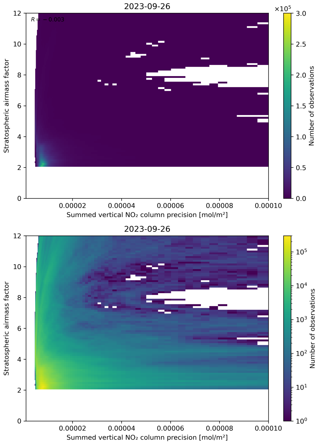
Figure 106: Scatter density plot of “Summed vertical NO 2 column precision” against “Stratospheric airmass factor” for 2023-09-26 to 2023-09-27.
