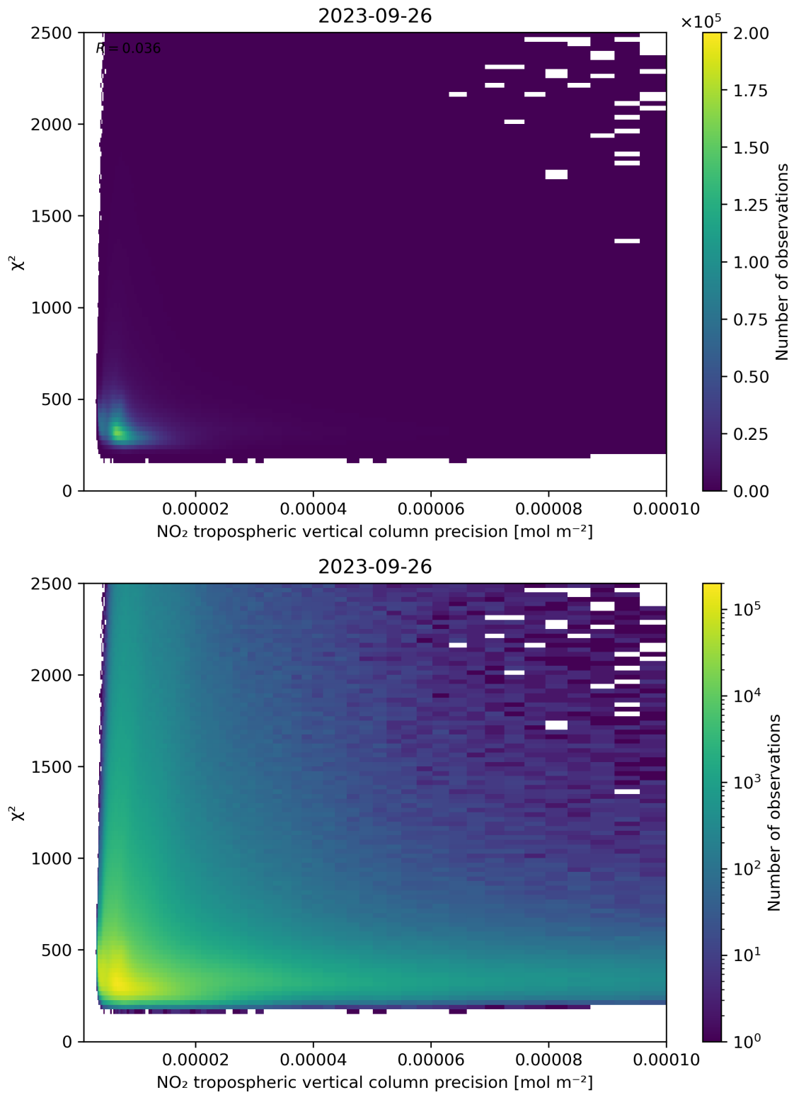
Figure 134: Scatter density plot of “NO 2 tropospheric vertical column precision” against “ \chi^2 ” for 2023-09-26 to 2023-09-27.
