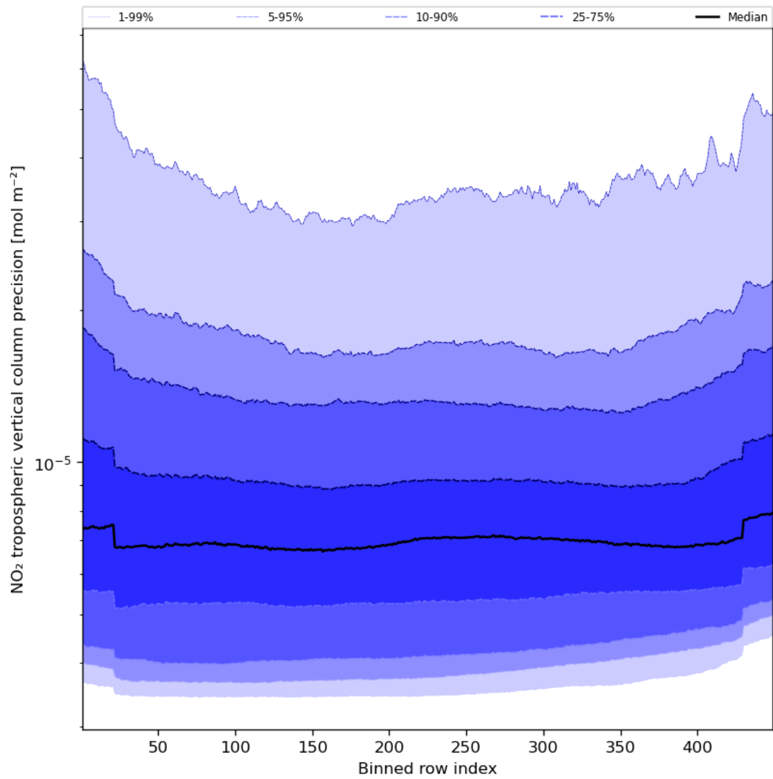
Figure 47: Along track statistics of “NO 2 tropospheric vertical column precision” for 2023-09-26 to 2023-09-27
