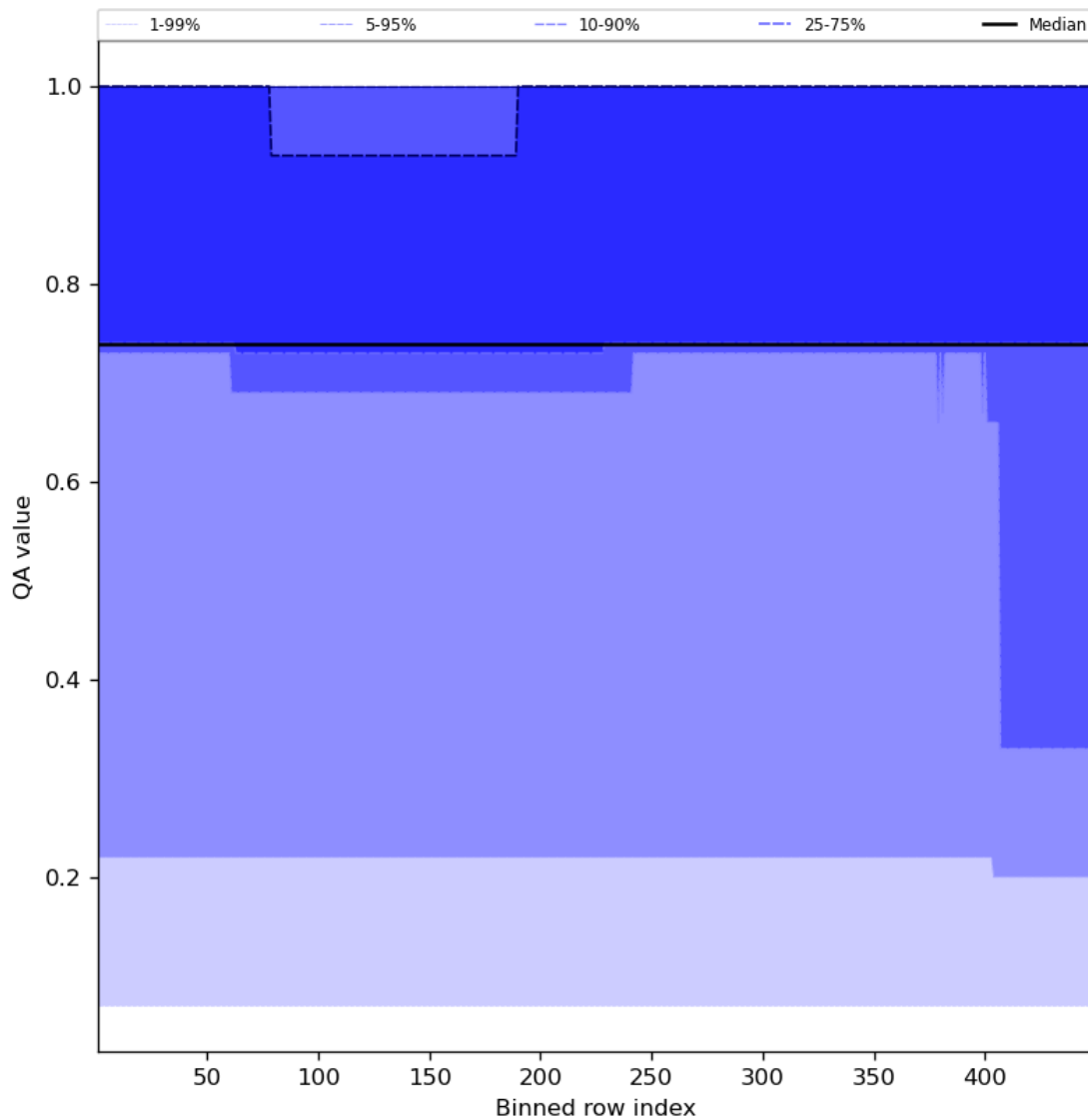
Figure 45: Along track statistics of “QA value” for 2023-09-26 to 2023-09-27
