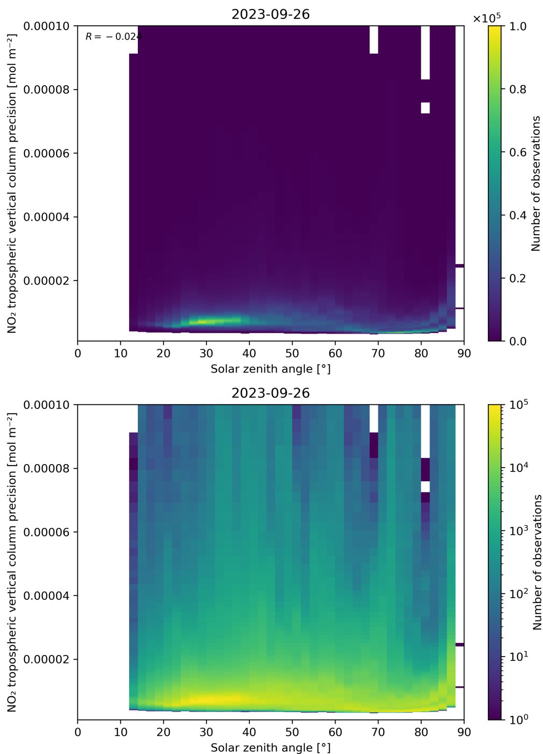
Figure 156: Scatter density plot of “Solar zenith angle” against “NO 2 tropospheric vertical column precision” for 2023-09-26 to 2023-09-27.
