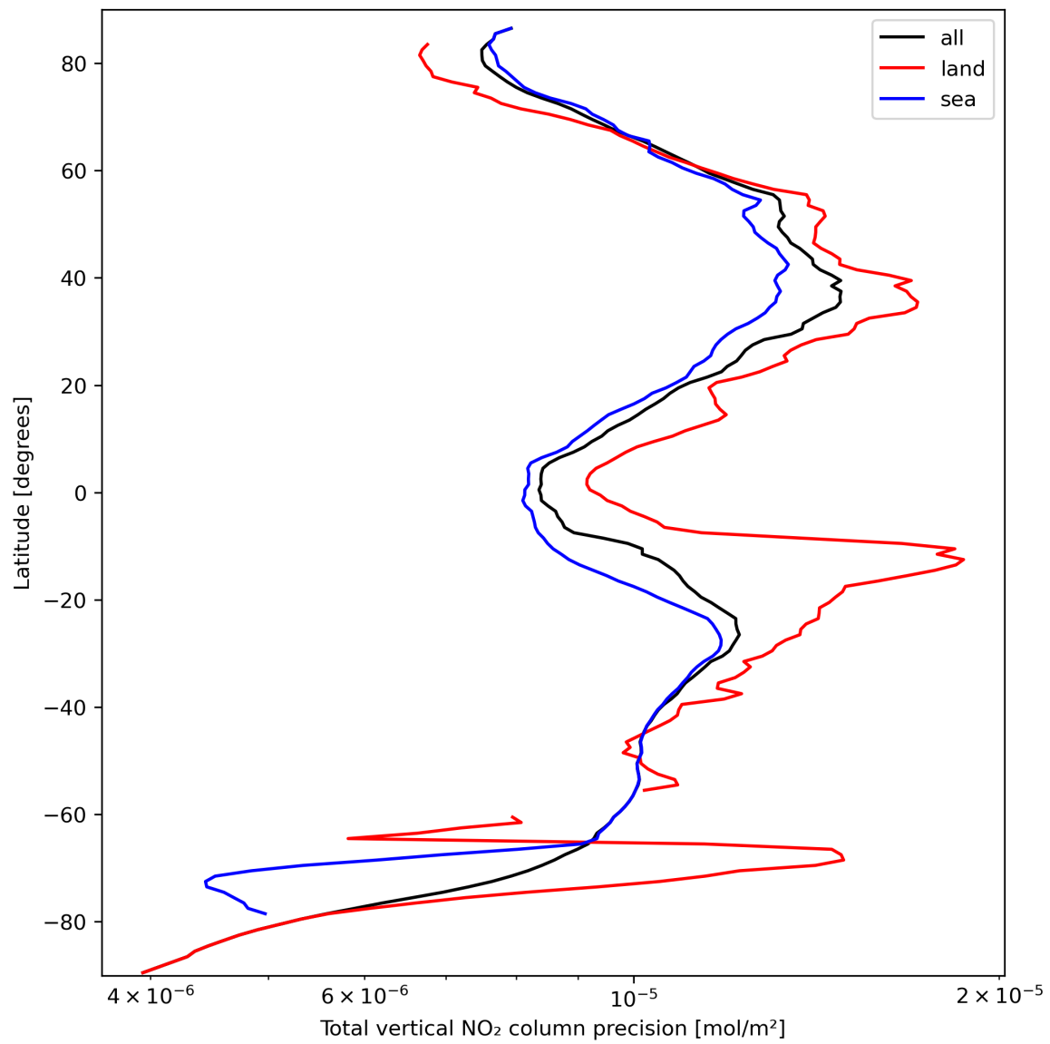
Figure 22: Zonal average of “Total vertical NO 2 column precision” for 2023-09-26 to 2023-09-27.
