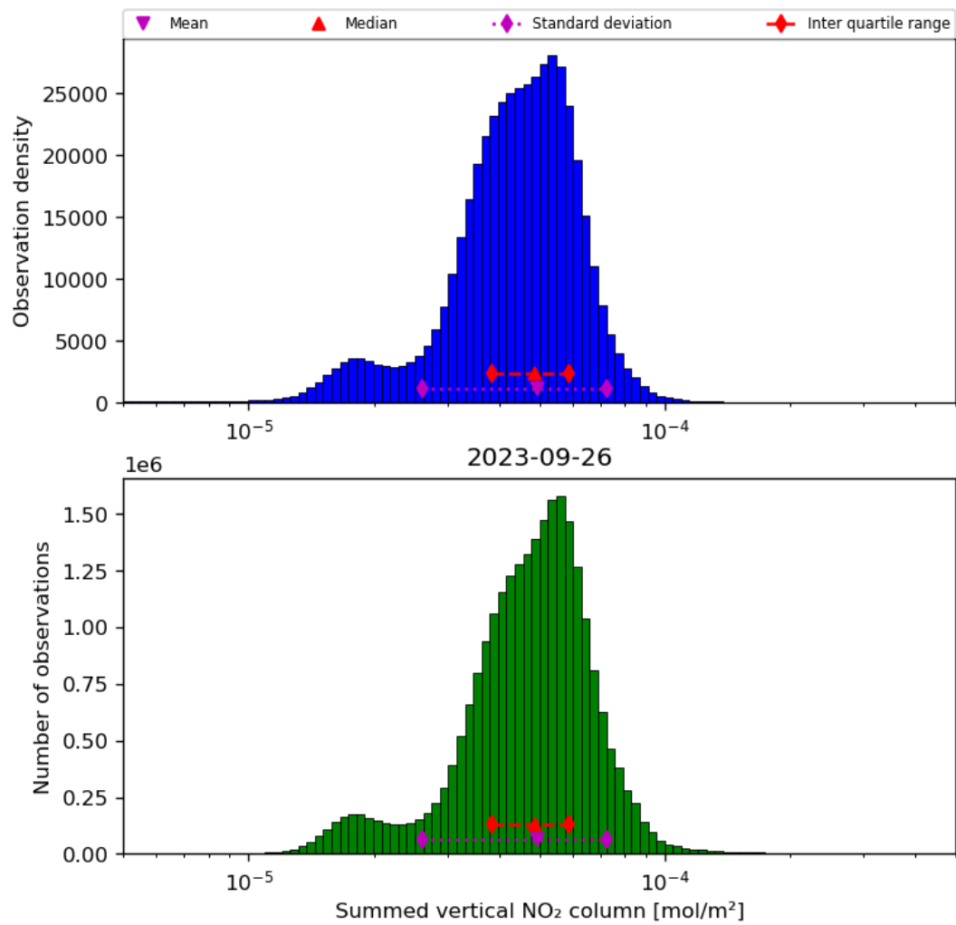
Figure 40: Histogram of “Summed vertical NO 2 column” for 2023-09-26 to 2023-09-27
