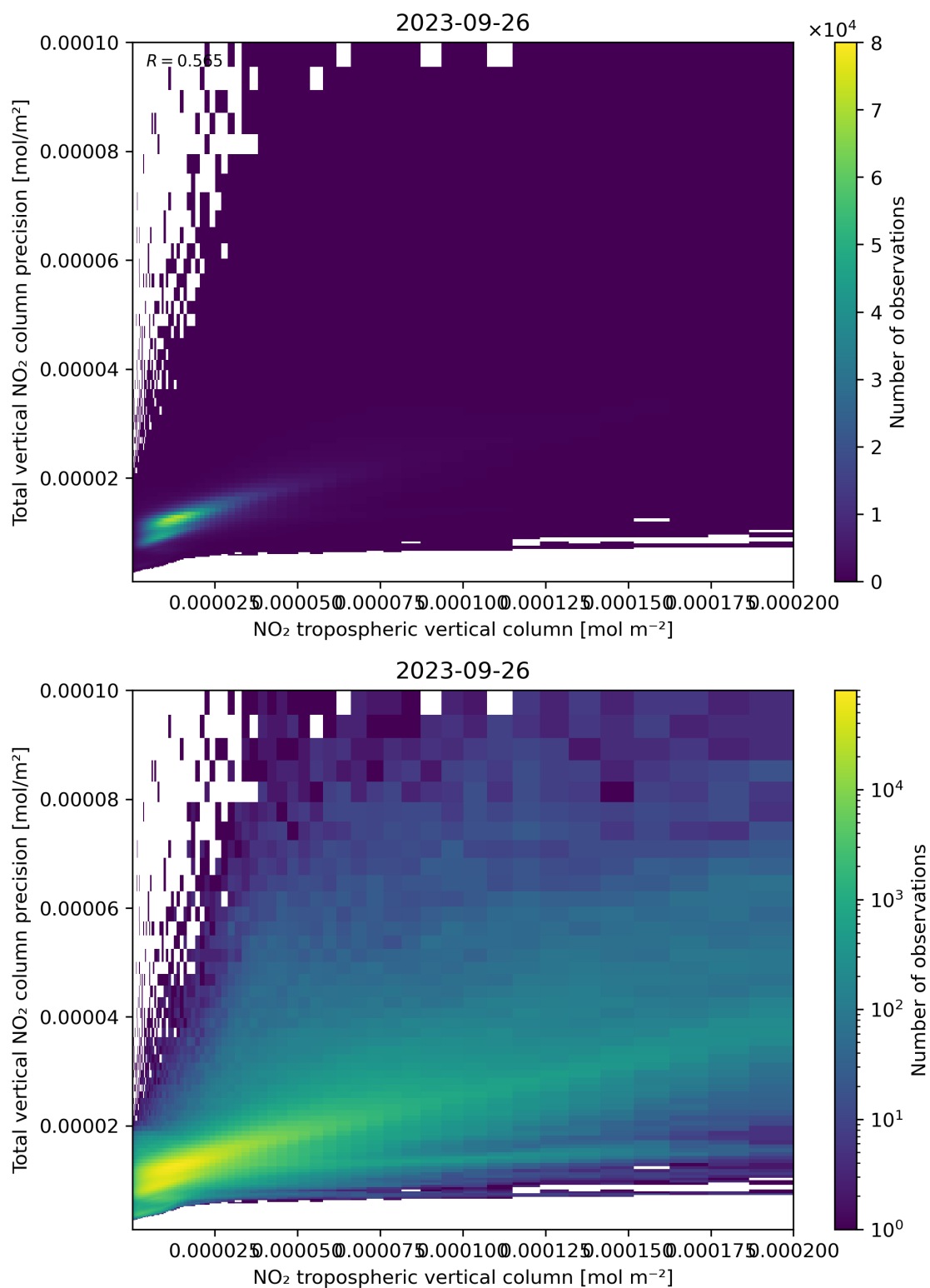
Figure 129: Scatter density plot of “NO 2 tropospheric vertical column” against “Total vertical NO 2 column precision” for 2023-09-26 to 2023-09-27.
