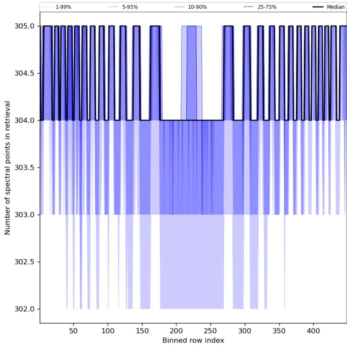
Figure 50: Along track statistics of “Number of spectral points in retrieval” for 2023-09-26 to 2023-09-27
