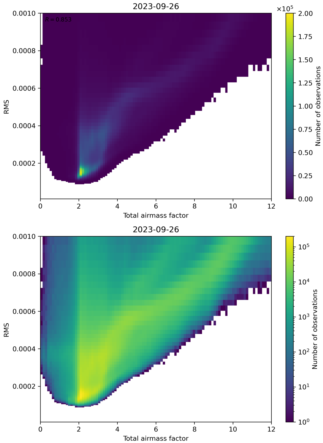
Figure 69: Scatter density plot of “Total airmass factor” against “RMS” for 2023-09-26 to 2023-09-27.
