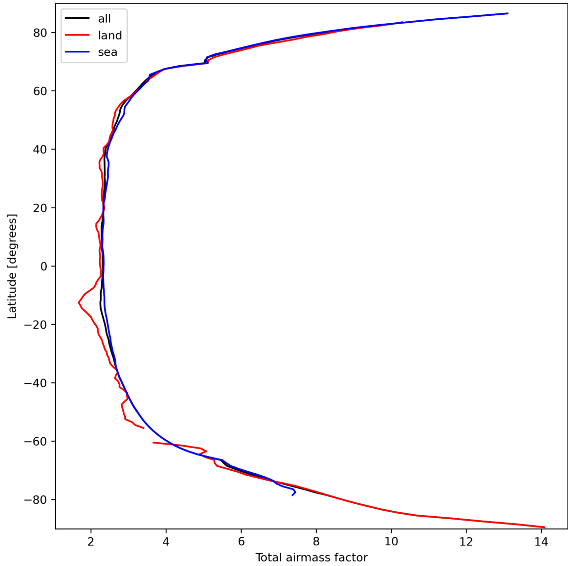
Figure 15: Zonal average of “Total airmass factor” for 2023-09-26 to 2023-09-27.
