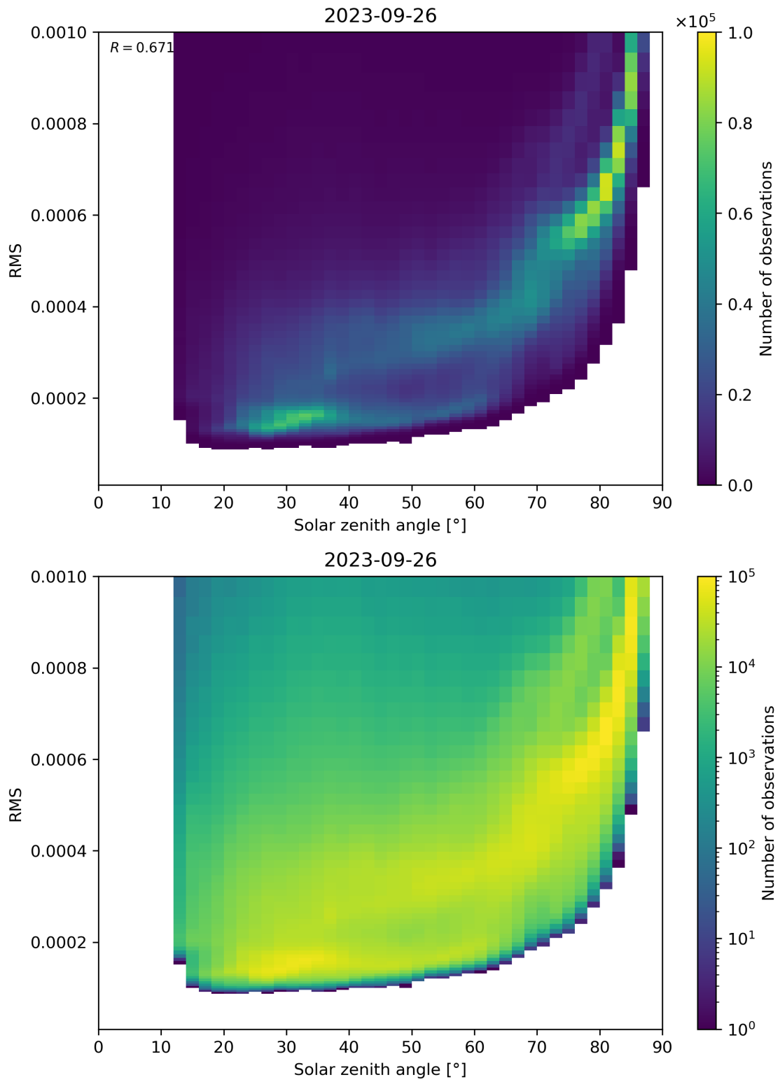
Figure 157: Scatter density plot of “Solar zenith angle” against “RMS” for 2023-09-26 to 2023-09-27.
