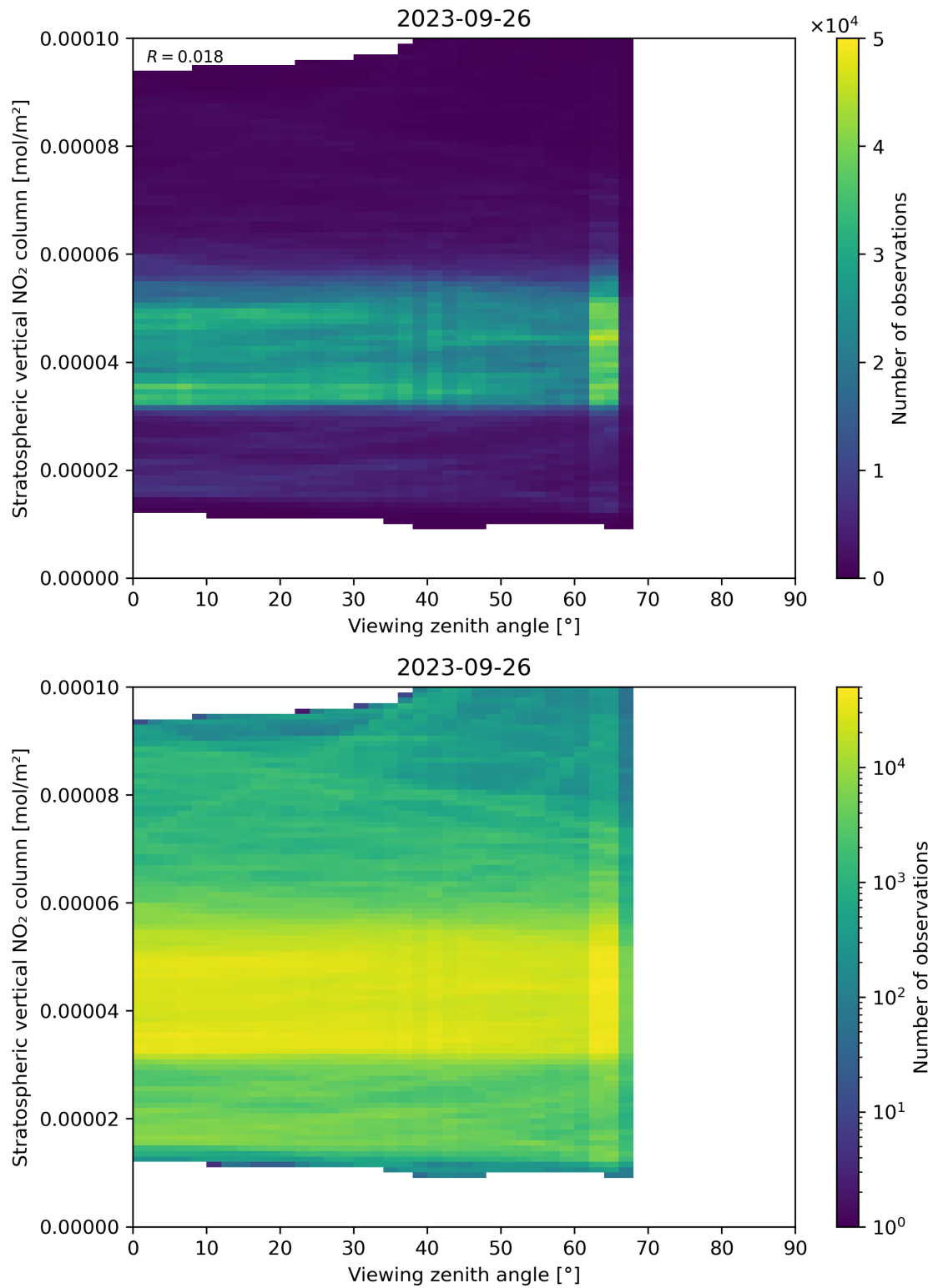
Figure 164: Scatter density plot of “Viewing zenith angle” against “Stratospheric vertical NO 2 column” for 2023-09-26 to 2023-09-27.
