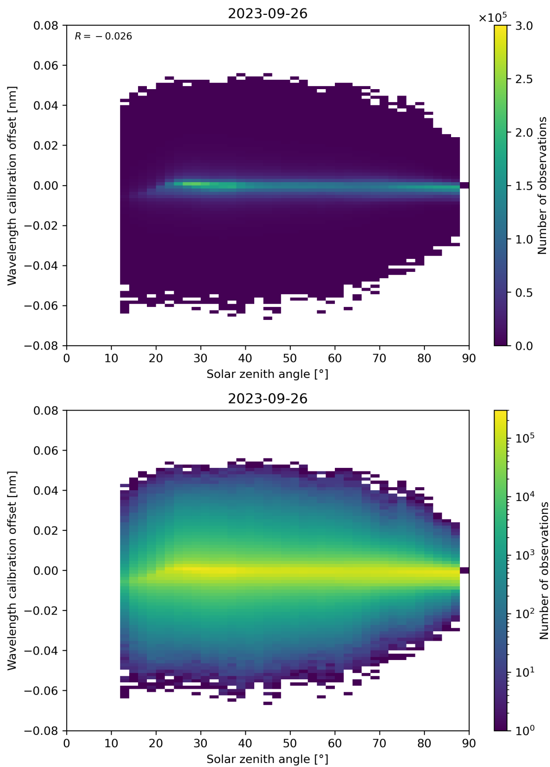
Figure 158: Scatter density plot of “Solar zenith angle” against “Wavelength calibration offset” for 2023-09-26 to 2023-09-27.
