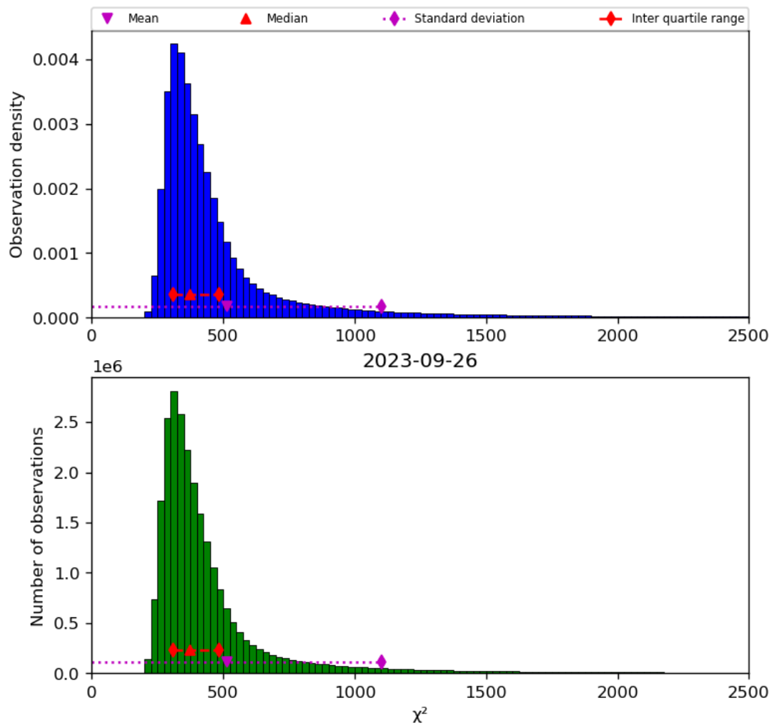
Figure 42: Histogram of “ \chi^2 ” for 2023-09-26 to 2023-09-27
