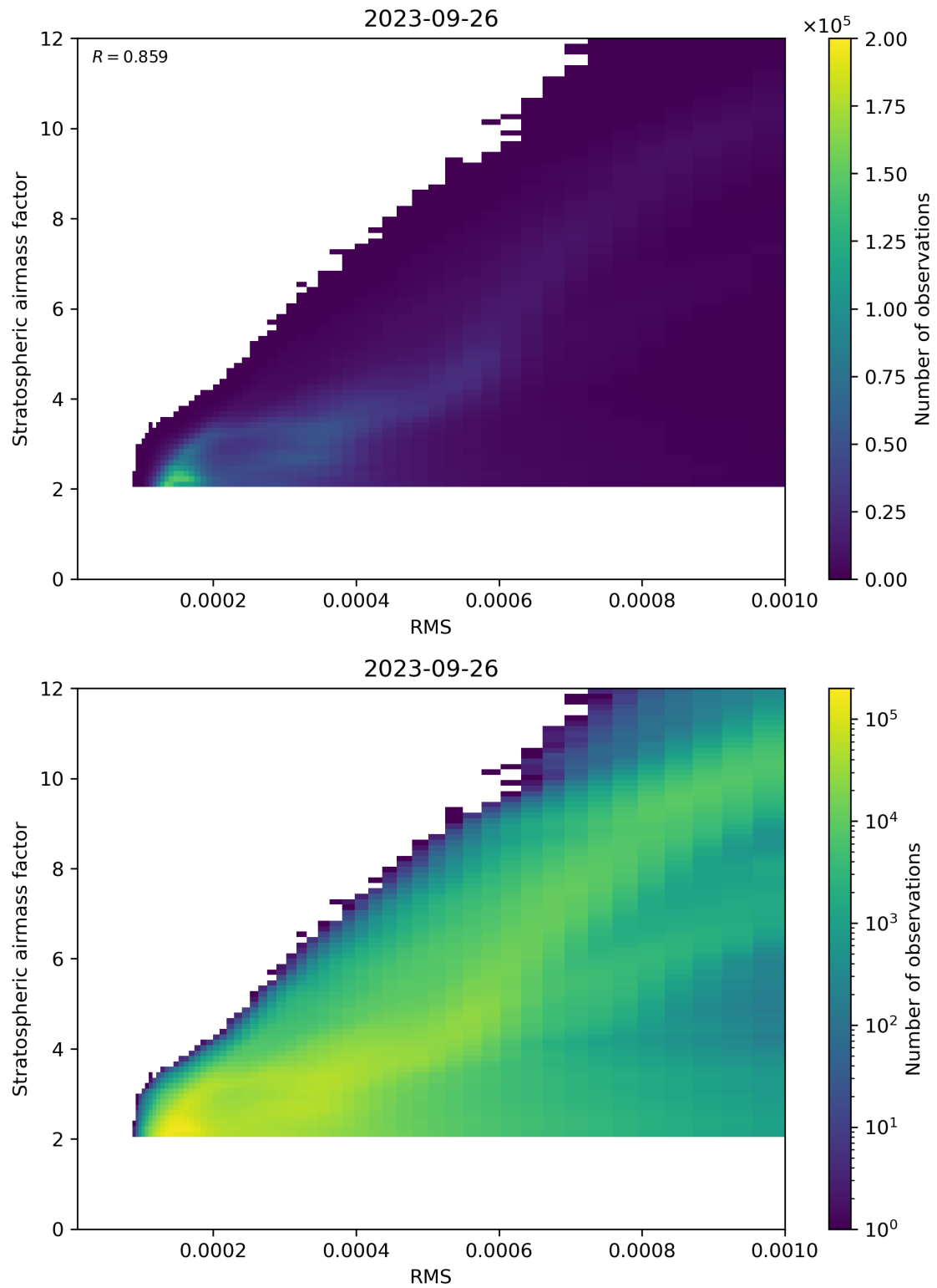
Figure 144: Scatter density plot of “RMS” against “Stratospheric airmass factor” for 2023-09-26 to 2023-09-27.
