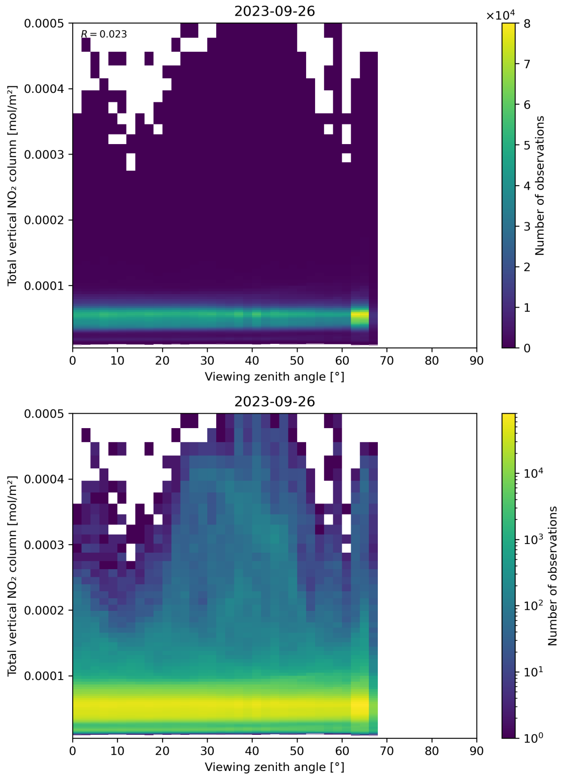
Figure 167: Scatter density plot of “Viewing zenith angle” against “Total vertical NO 2 column” for 2023-09-26 to 2023-09-27.
