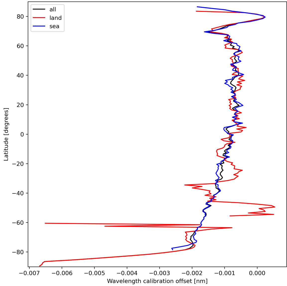
Figure 18: Zonal average of “Wavelength calibration offset” for 2023-09-26 to 2023-09-27.
