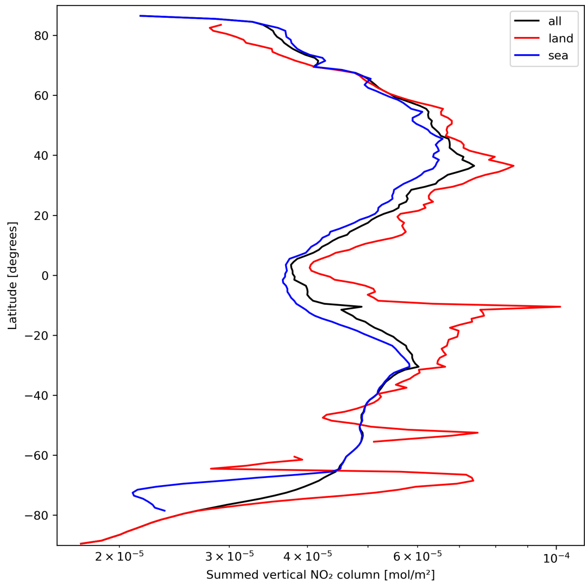
Figure 23: Zonal average of “Summed vertical NO 2 column” for 2023-09-26 to 2023-09-27.
