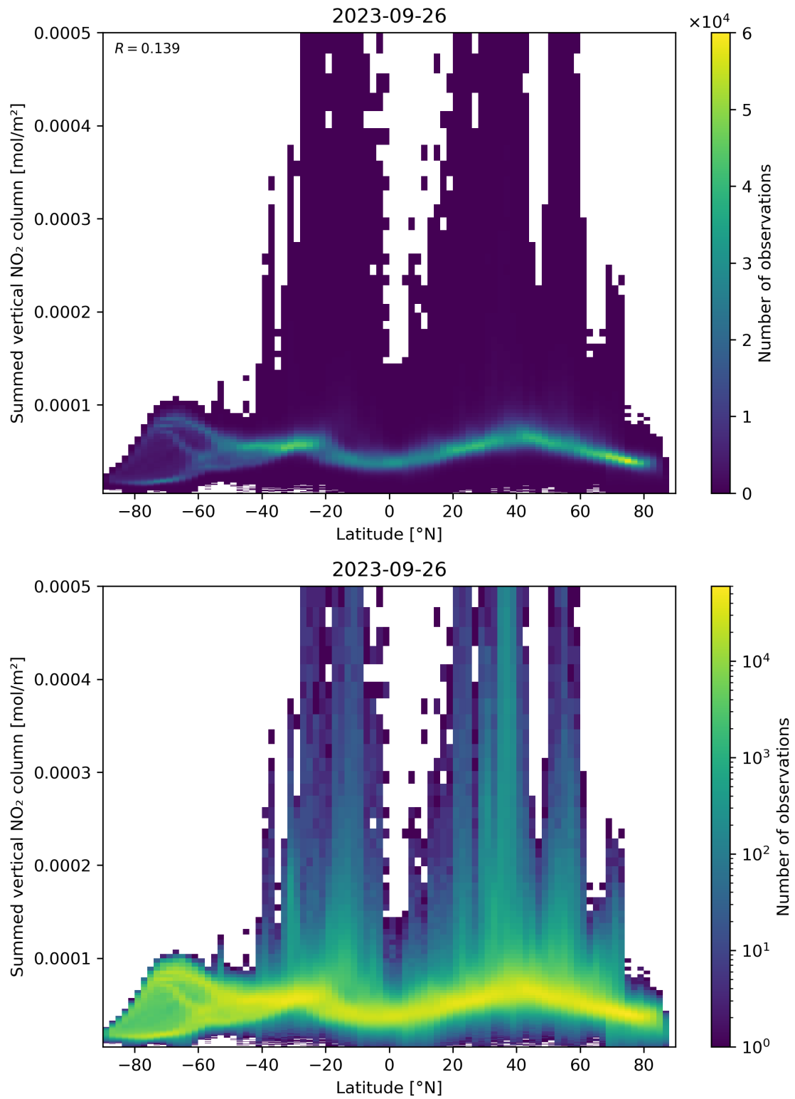
Figure 88: Scatter density plot of “Latitude” against “Summed vertical NO 2 column” for 2023-09-26 to 2023-09-27.
