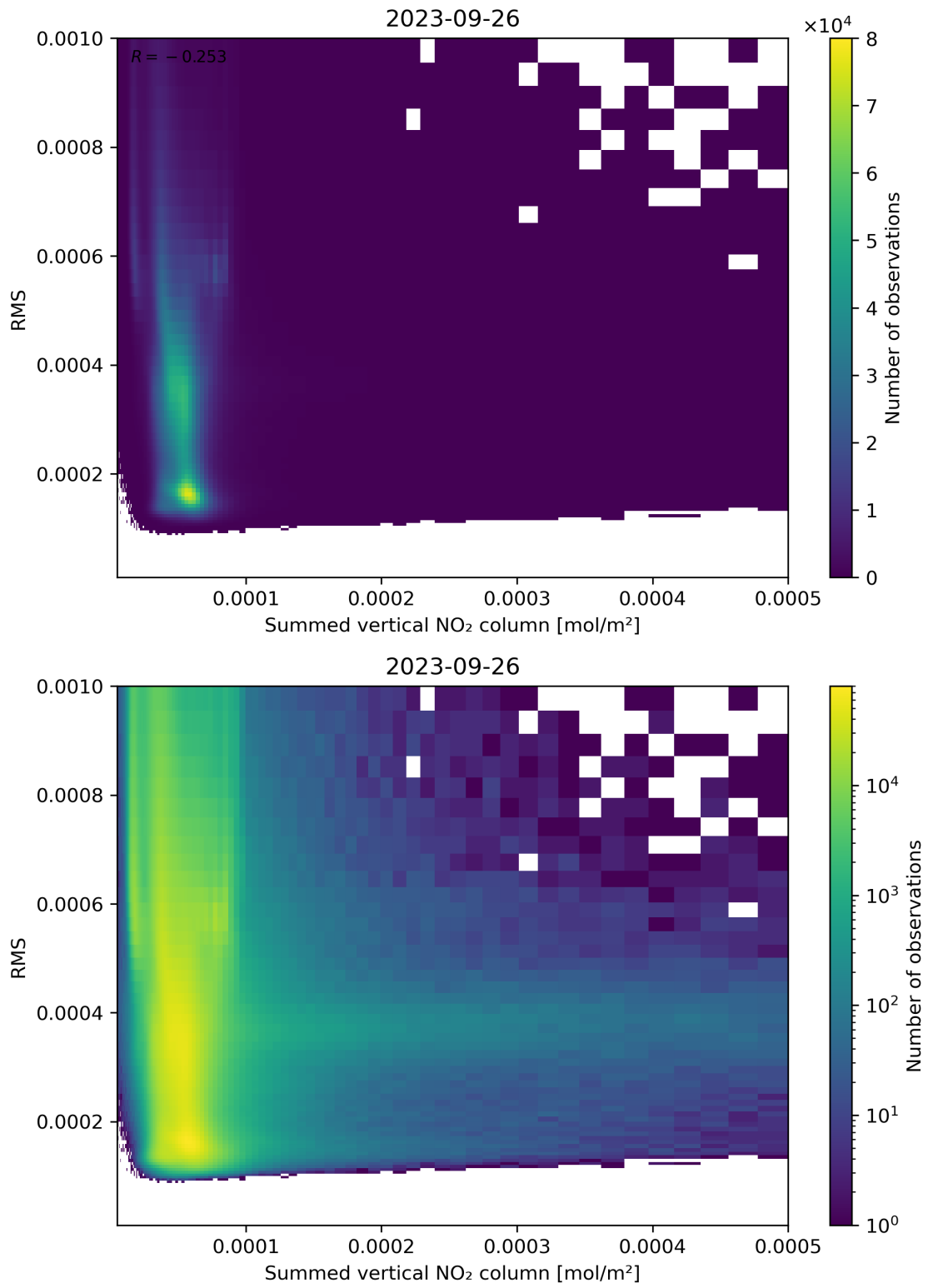
Figure 109: Scatter density plot of “Summed vertical NO 2 column” against “RMS” for 2023-09-26 to 2023-09-27.
