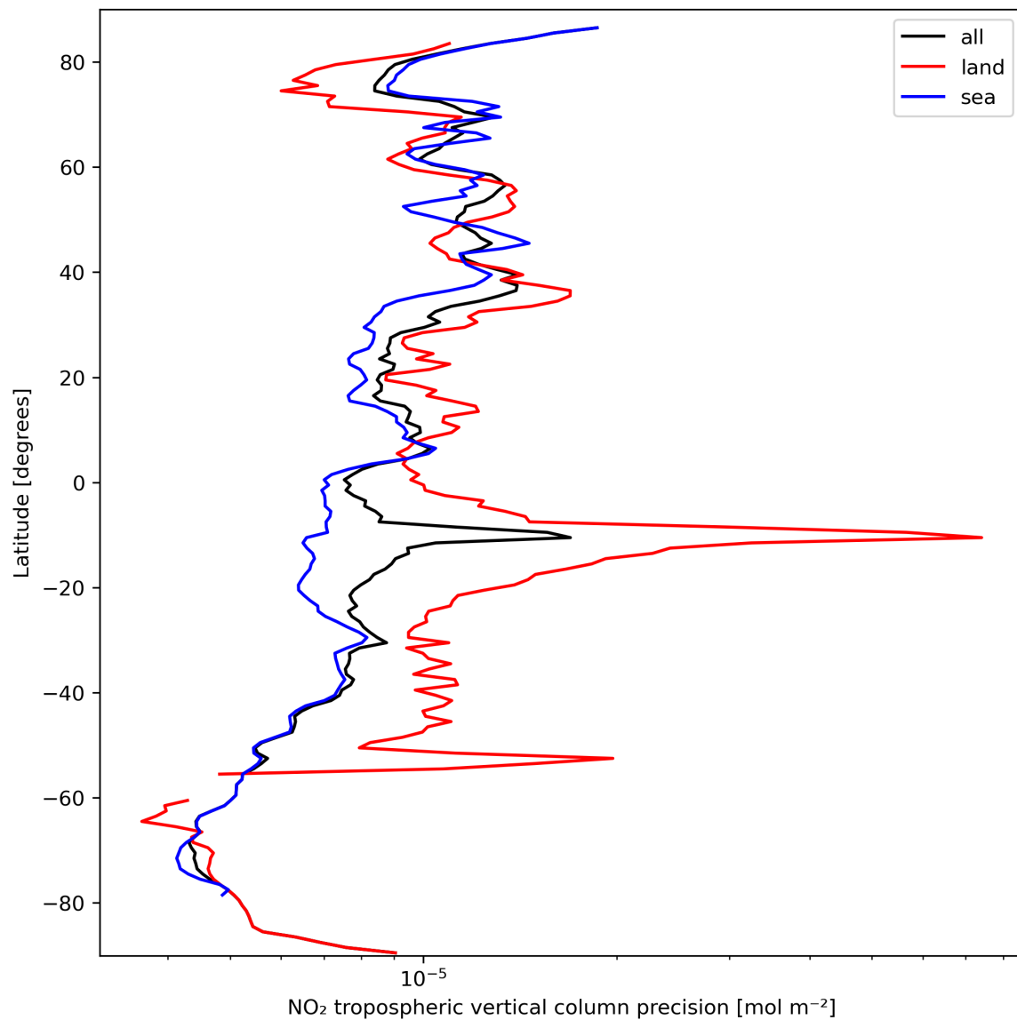
Figure 13: Zonal average of “NO 2 tropospheric vertical column precision” for 2023-09-26 to 2023-09-27.
