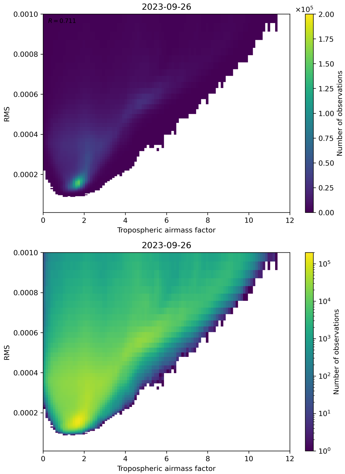
Figure 79: Scatter density plot of “Tropospheric airmass factor” against “RMS” for 2023-09-26 to 2023-09-27.
