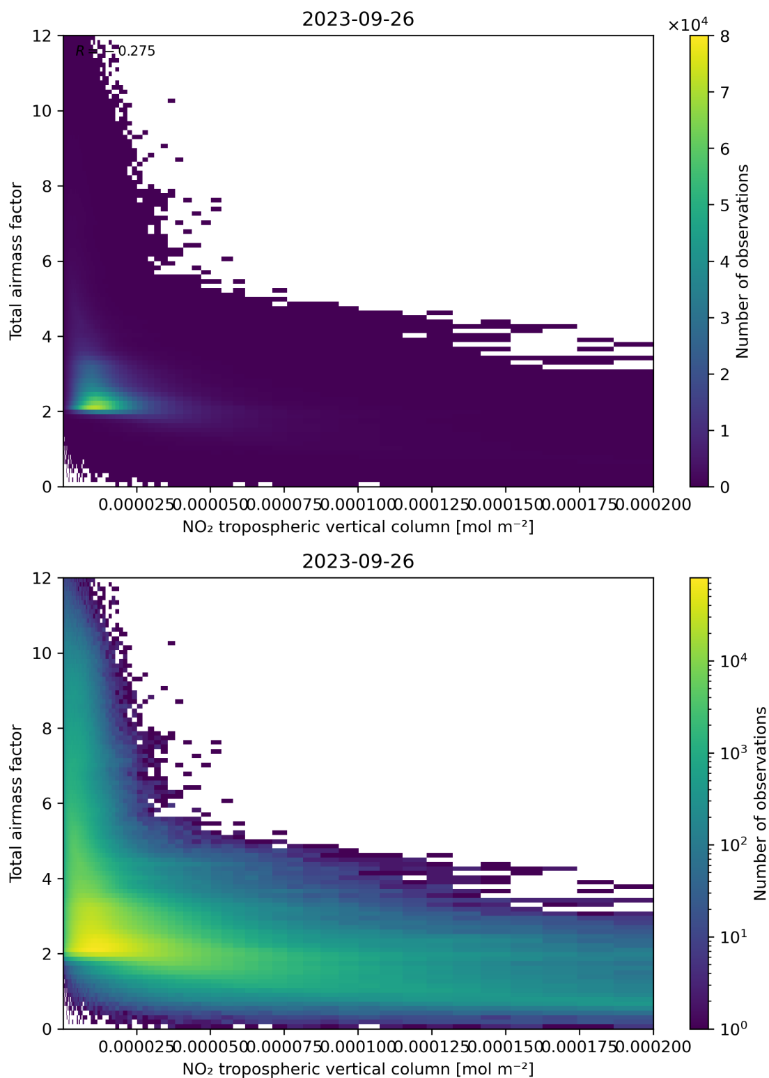
Figure 122: Scatter density plot of “NO 2 tropospheric vertical column” against “Total air mass factor” for 2023-09-26 to 2023-09-27.
