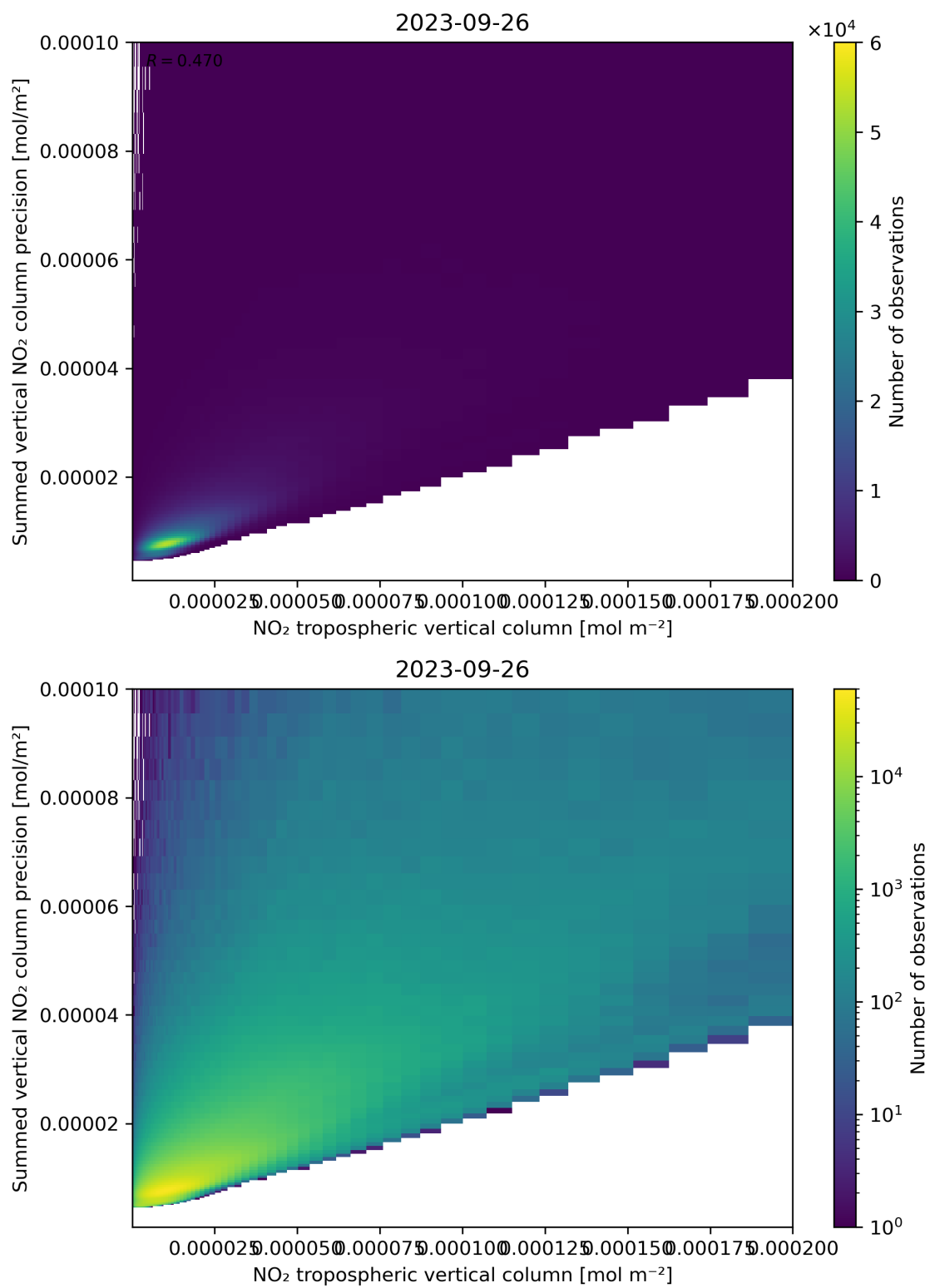
Figure 127: Scatter density plot of “NO 2 tropospheric vertical column” against “Summed vertical NO 2 column precision” for 2023-09-26 to 2023-09-27.
