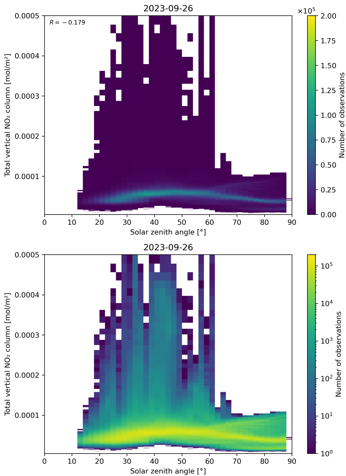
Figure 153: Scatter density plot of “Solar zenith angle” against “Total vertical NO 2 column” for 2023-09-26 to 2023-09-27.
