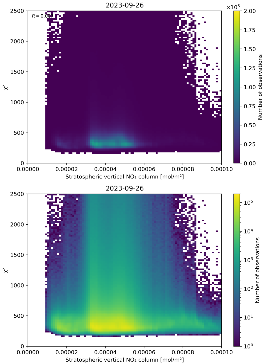
Figure 97: Scatter density plot of “Stratospheric vertical NO 2 column” against “ \chi^2 ” for 2023-09-26 to 2023-09-27.
