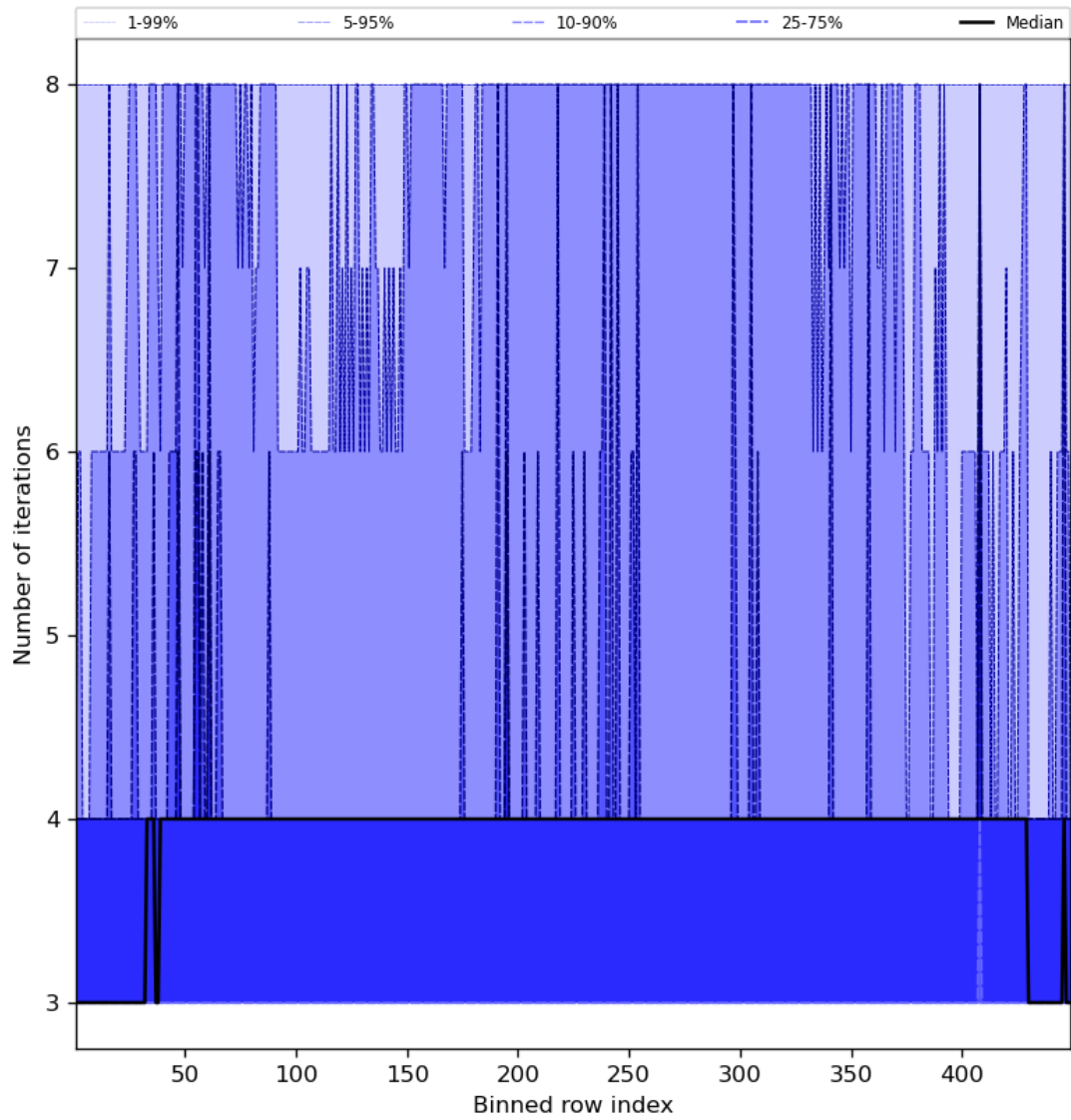
Figure 51: Along track statistics of “Number of iterations” for 2023-09-26 to 2023-09-27
