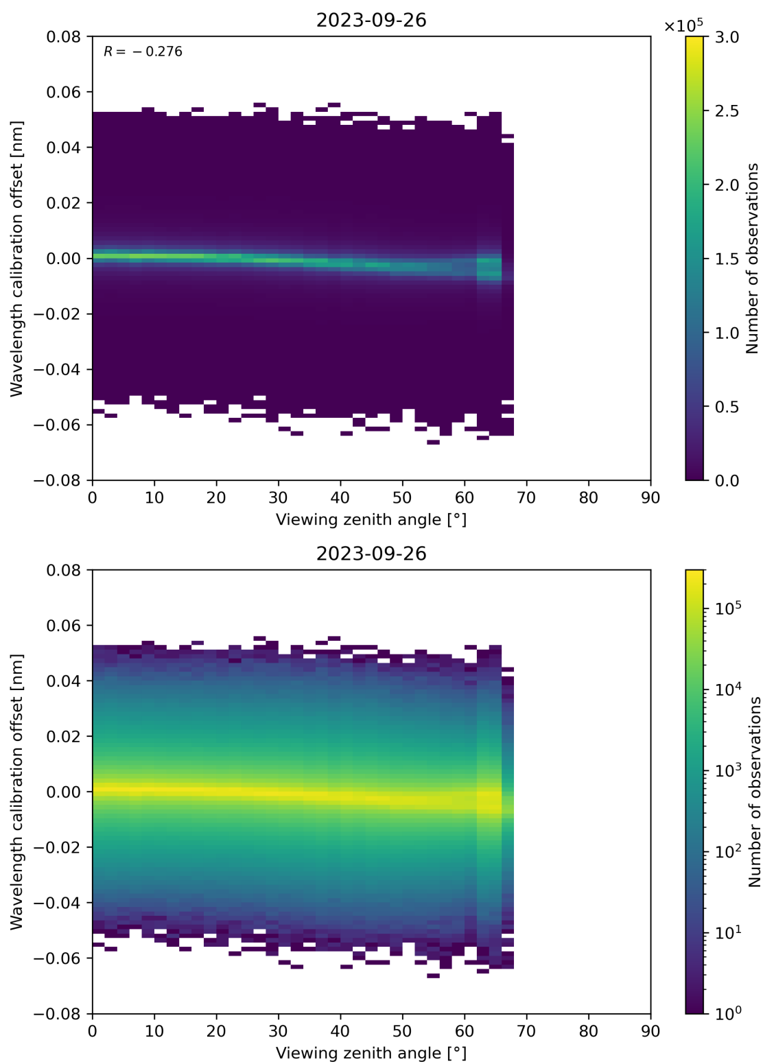
Figure 173: Scatter density plot of “Viewing zenith angle” against “Wavelength calibration offset” for 2023-09-26 to 2023-09-27.
