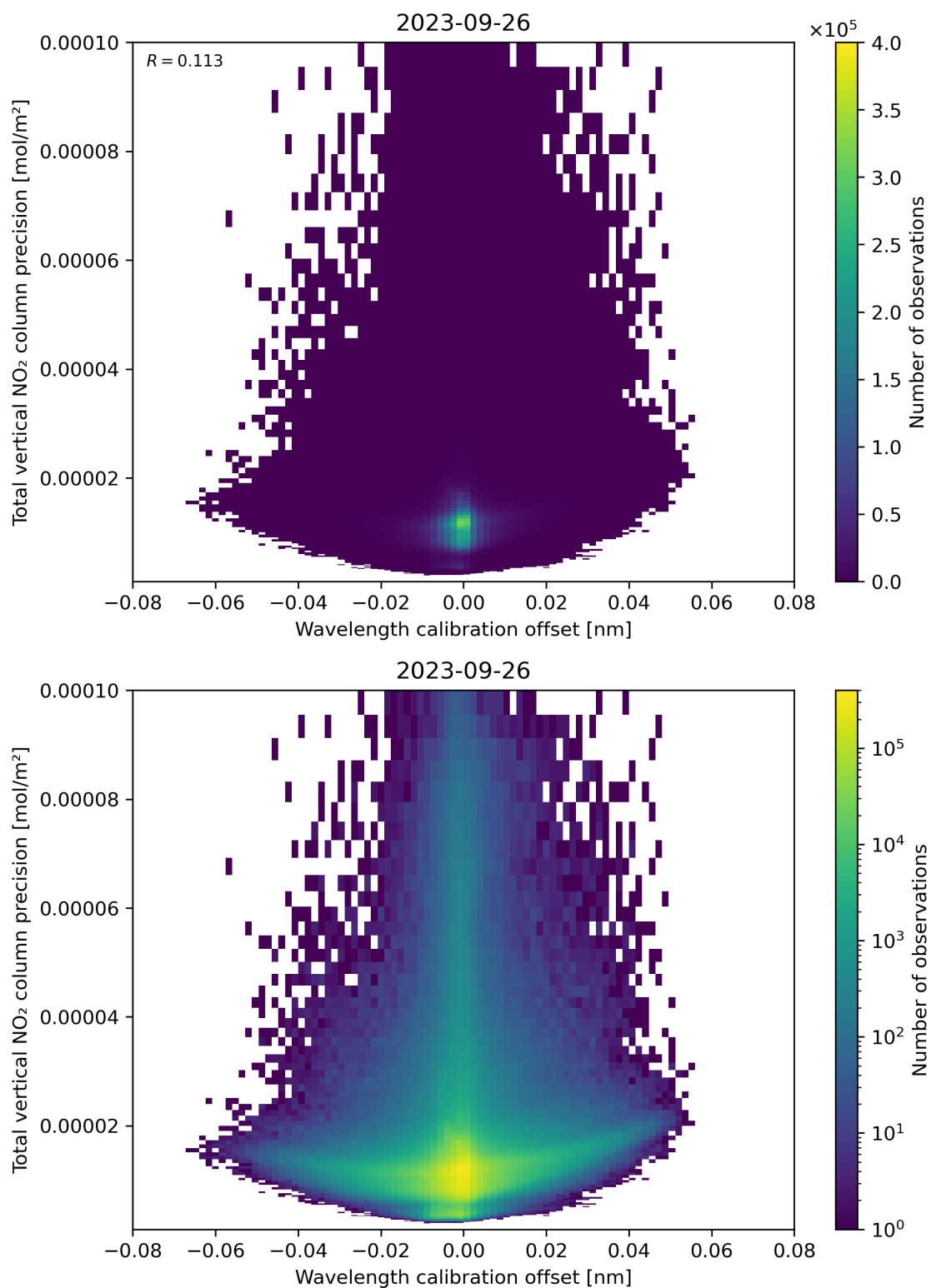
Figure 180: Scatter density plot of “Wavelength calibration offset” against “Total vertical NO 2 column precision” for 2023-09-26 to 2023-09-27.
