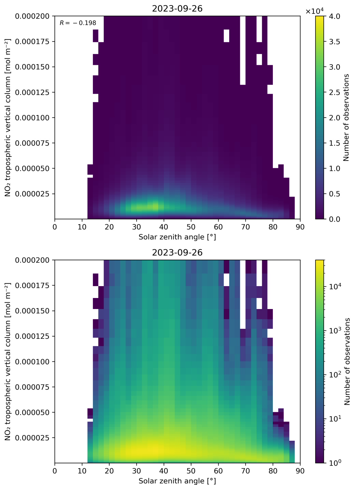
Figure 155: Scatter density plot of “Solar zenith angle” against “NO 2 tropospheric vertical column” for 2023-09-26 to 2023-09-27.
