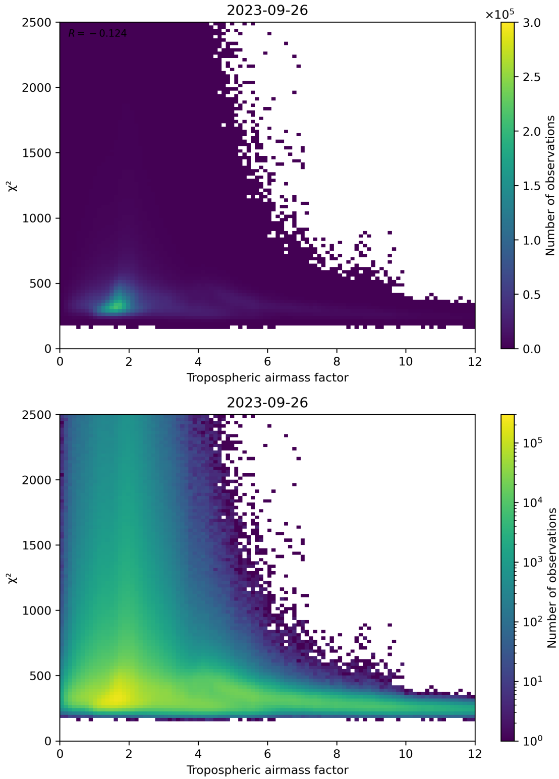
Figure 73: Scatter density plot of “Tropospheric airmass factor” against “ \chi^2 ” for 2023-09-26 to 2023-09-27.
