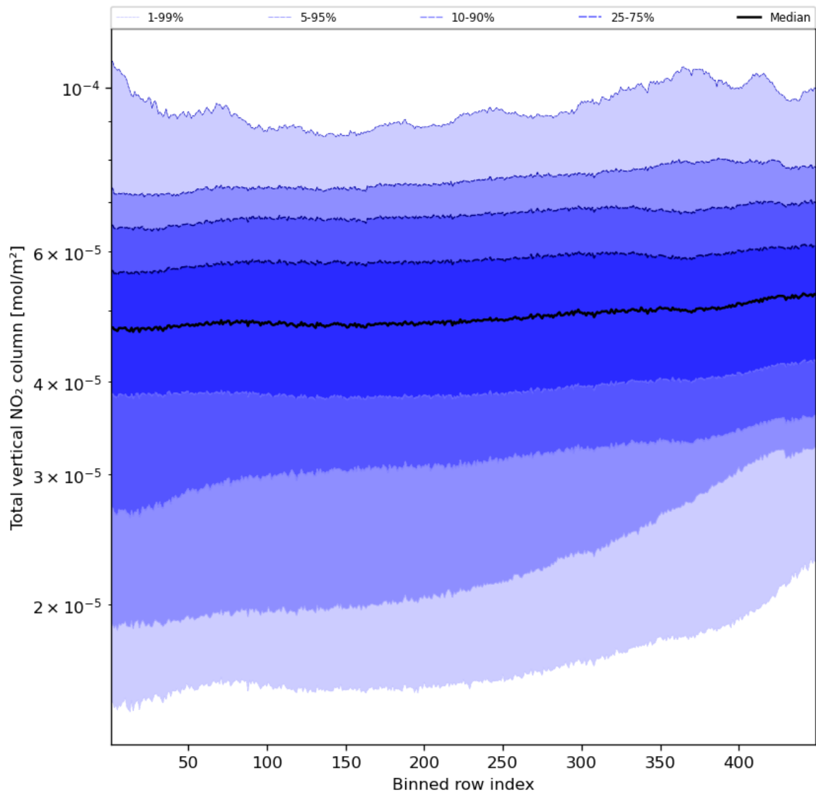
Figure 55: Along track statistics of “Total vertical NO 2 column” for 2023-09-26 to 2023-09-27
