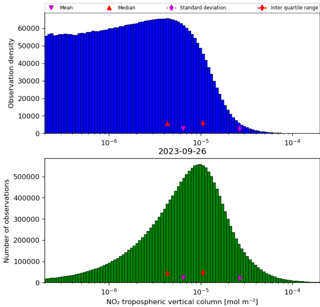
Figure 29: Histogram of “NO 2 tropospheric vertical column” for 2023-09-26 to 2023-09-27
