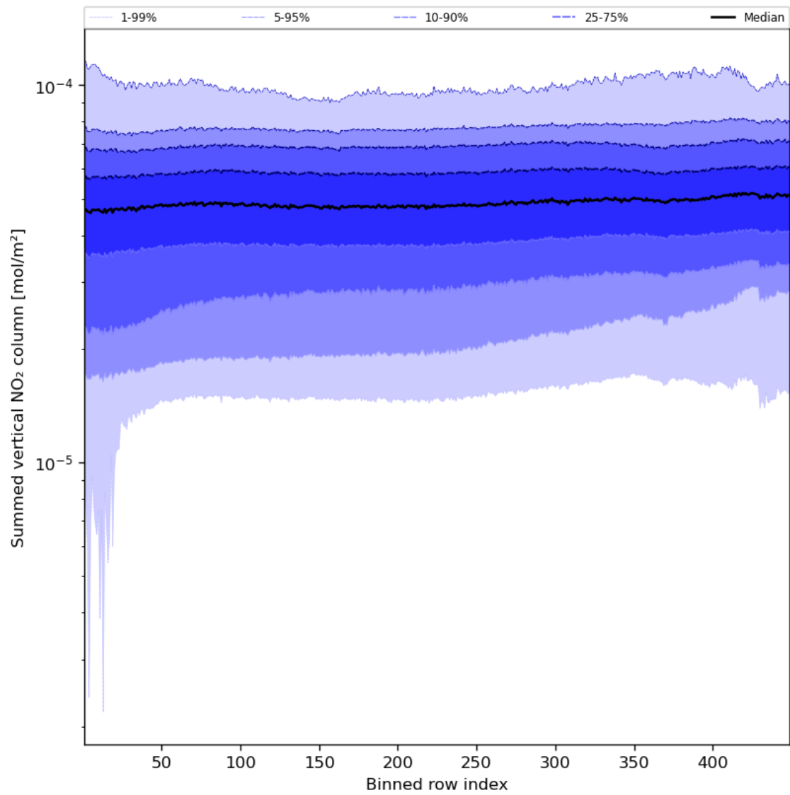
Figure 57: Along track statistics of “Summed vertical NO 2 column” for 2023-09-26 to 2023-09-27
