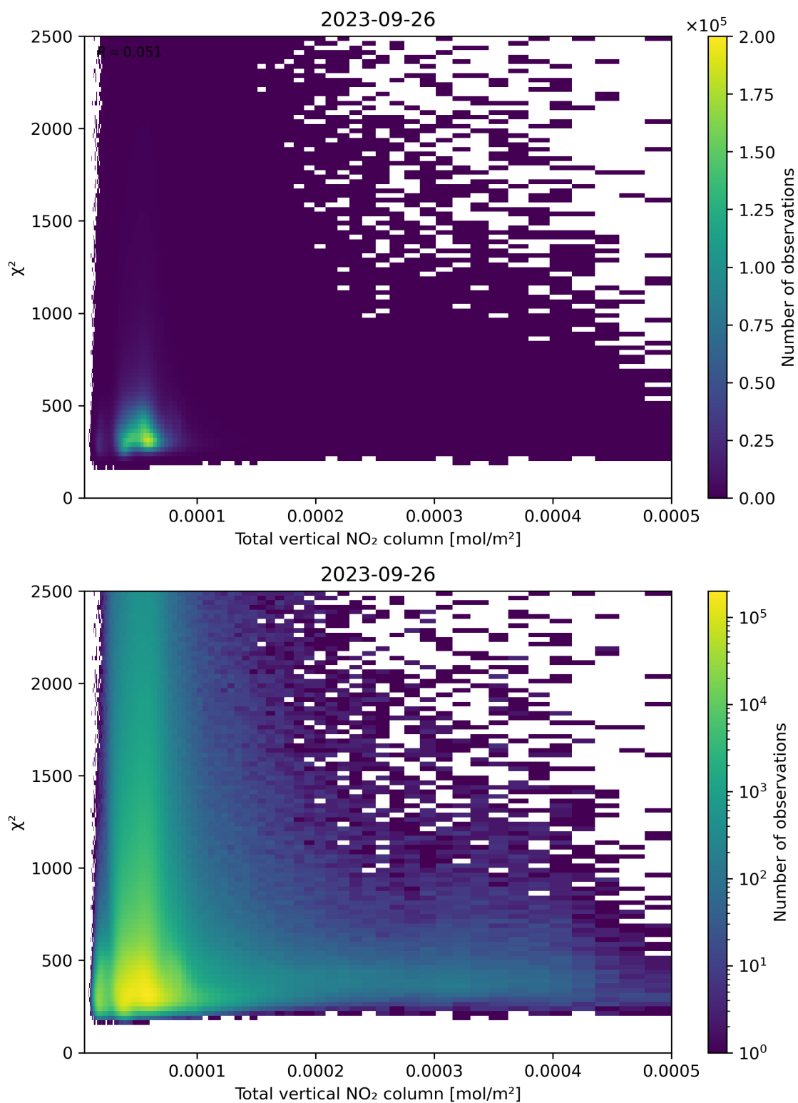
Figure 111: Scatter density plot of “Total vertical NO 2 column” against “ \chi^2 ” for 2023-09-26 to 2023-09-27.
