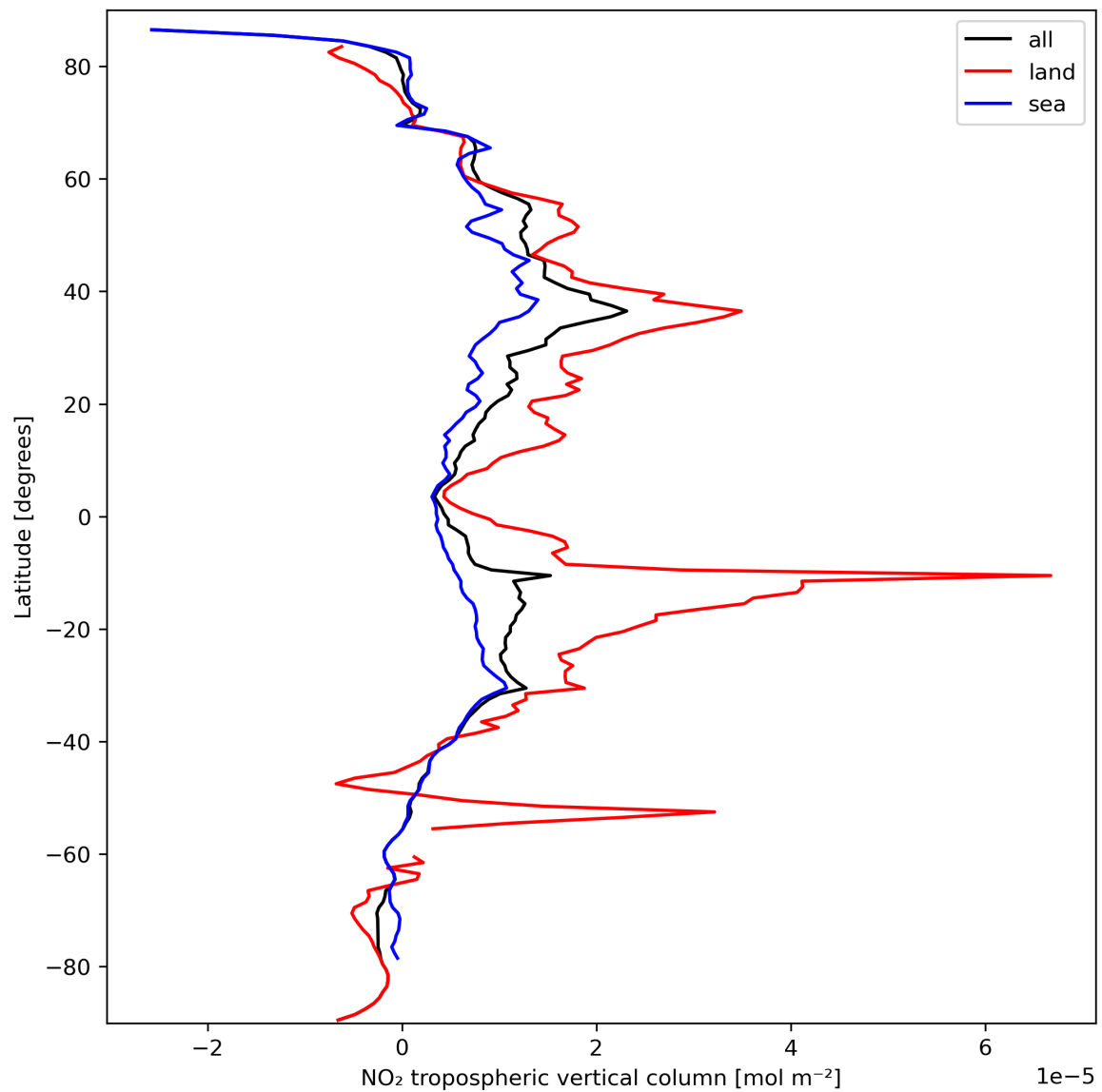
Figure 12: Zonal average of “NO 2 tropospheric vertical column” for 2023-09-26 to 2023-09-27.
