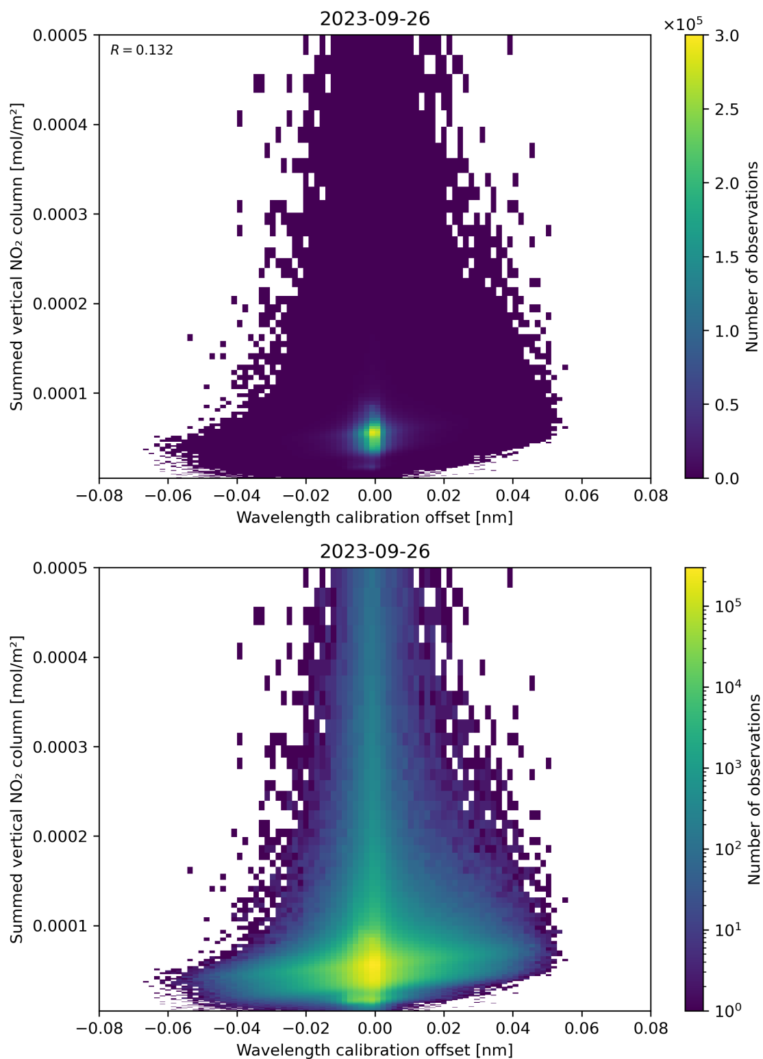
Figure 177: Scatter density plot of “Wavelength calibration offset” against “Summed vertical NO 2 column” for 2023-09-26 to 2023-09-27.
