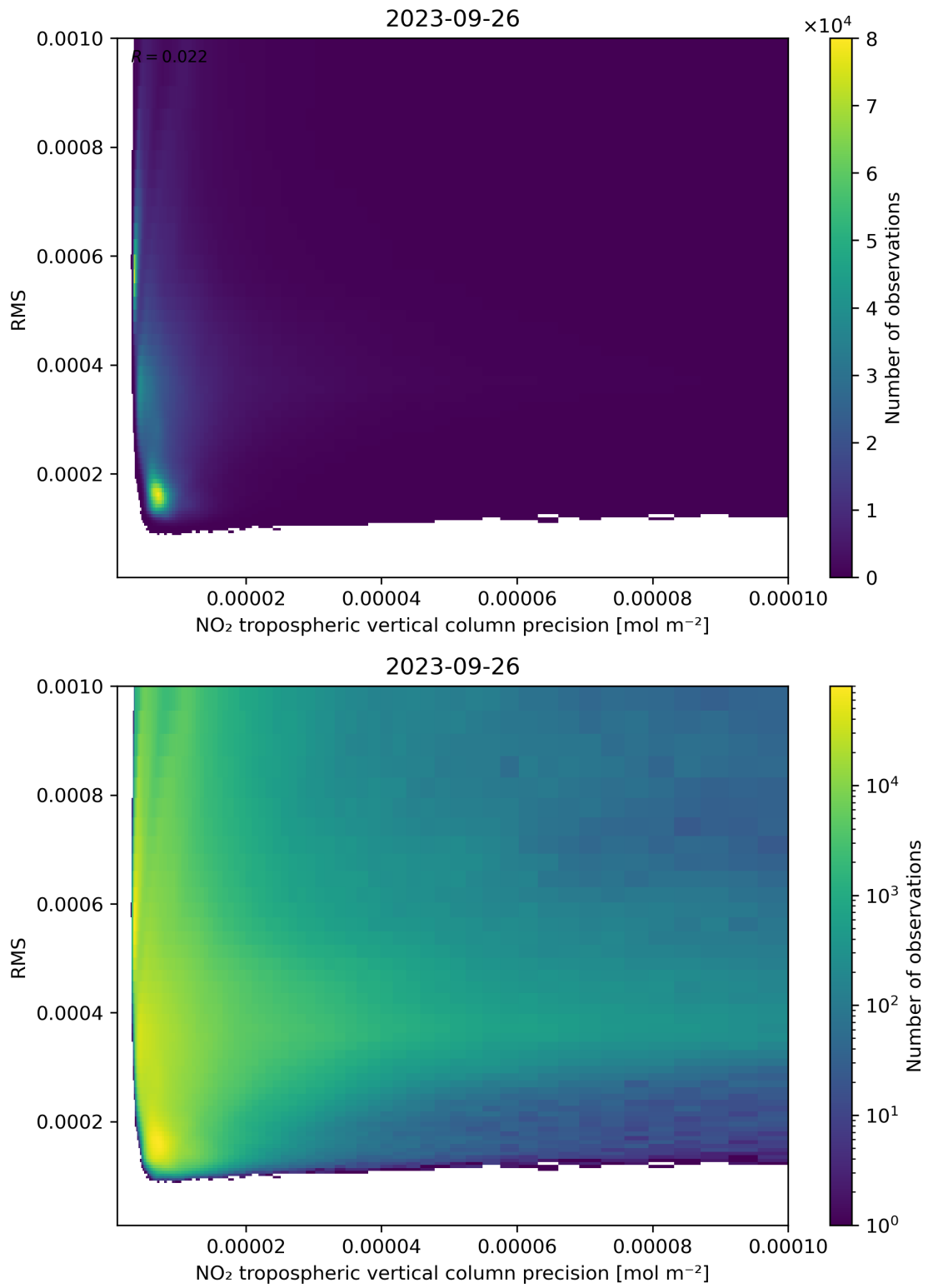
Figure 140: Scatter density plot of “NO 2 tropospheric vertical column precision” against “RMS” for 2023-09-26 to 2023-09-27.
