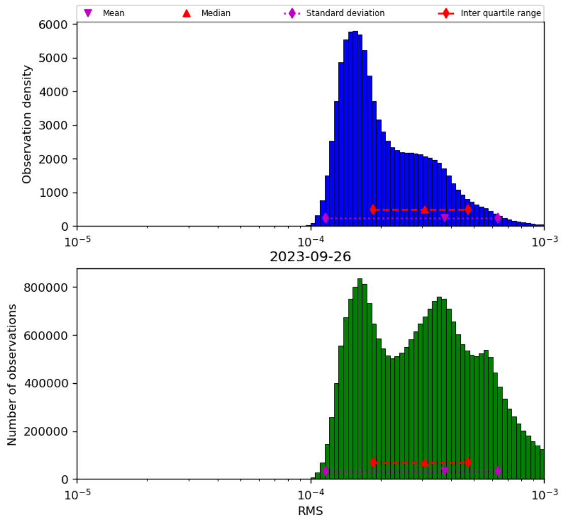
Figure 43: Histogram of “RMS” for 2023-09-26 to 2023-09-27
