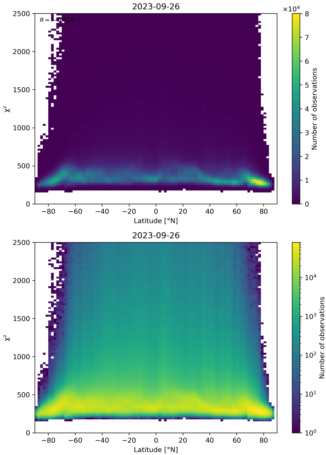
Figure 86: Scatter density plot of “Latitude” against “ \chi^2 ” for 2023-09-26 to 2023-09-27.
