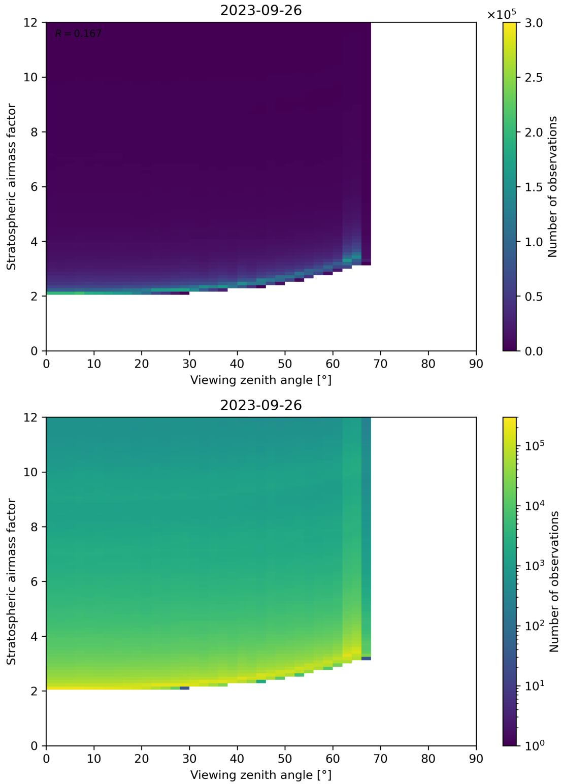
Figure 159: Scatter density plot of “Viewing zenith angle” against “Stratospheric airmass factor” for 2023-09-26 to 2023-09-27.
