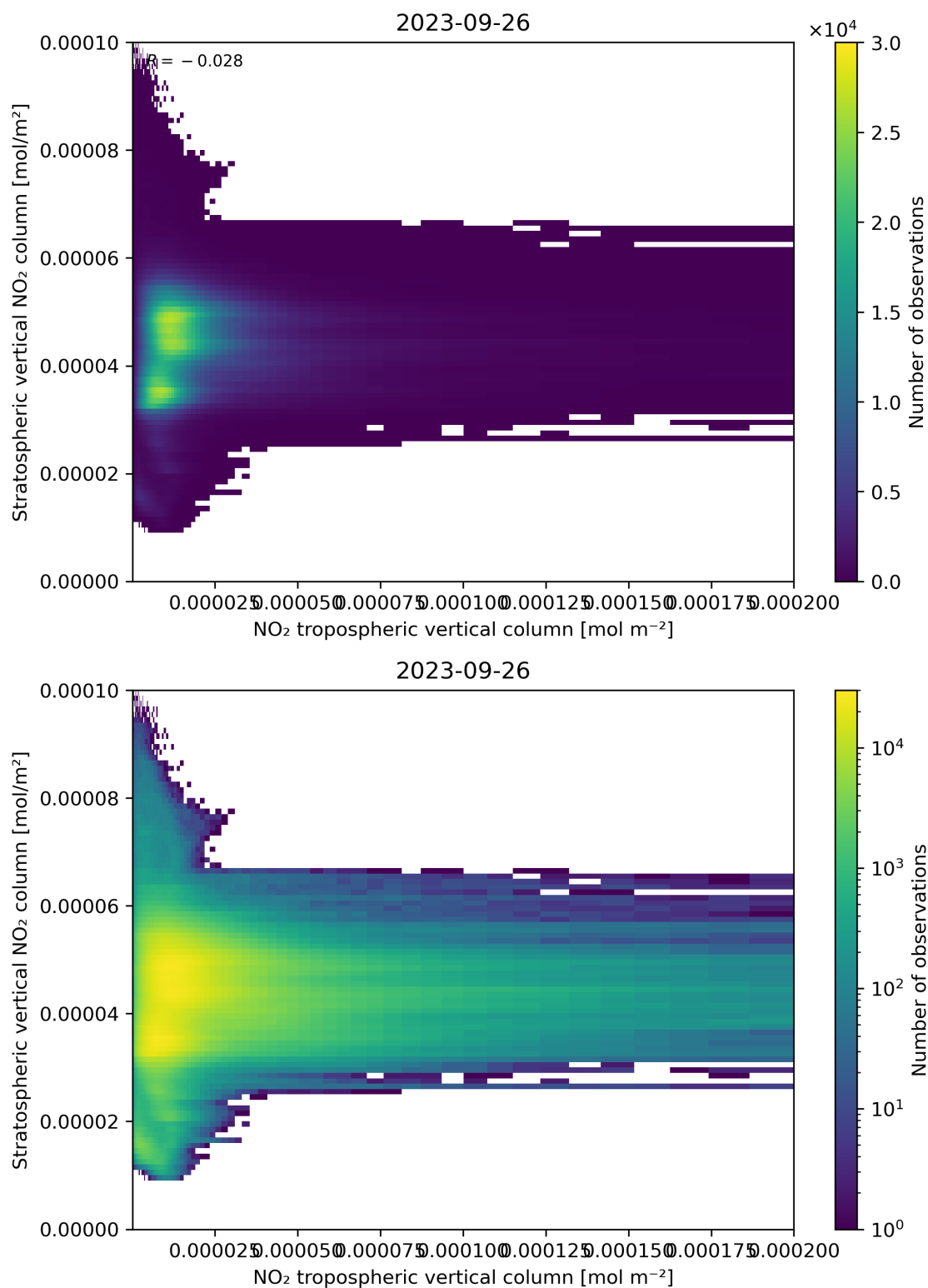
Figure 125: Scatter density plot of “NO 2 tropospheric vertical column” against “Stratospheric vertical NO 2 column” for 2023-09-26 to 2023-09-27.
