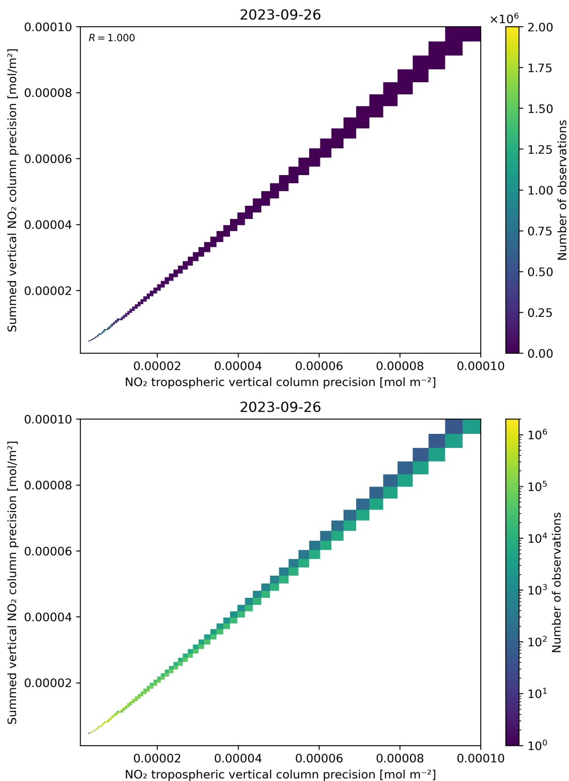
Figure 137: Scatter density plot of “NO 2 tropospheric vertical column precision” against “Summed vertical NO 2 column precision” for 2023-09-26 to 2023-09-27.
