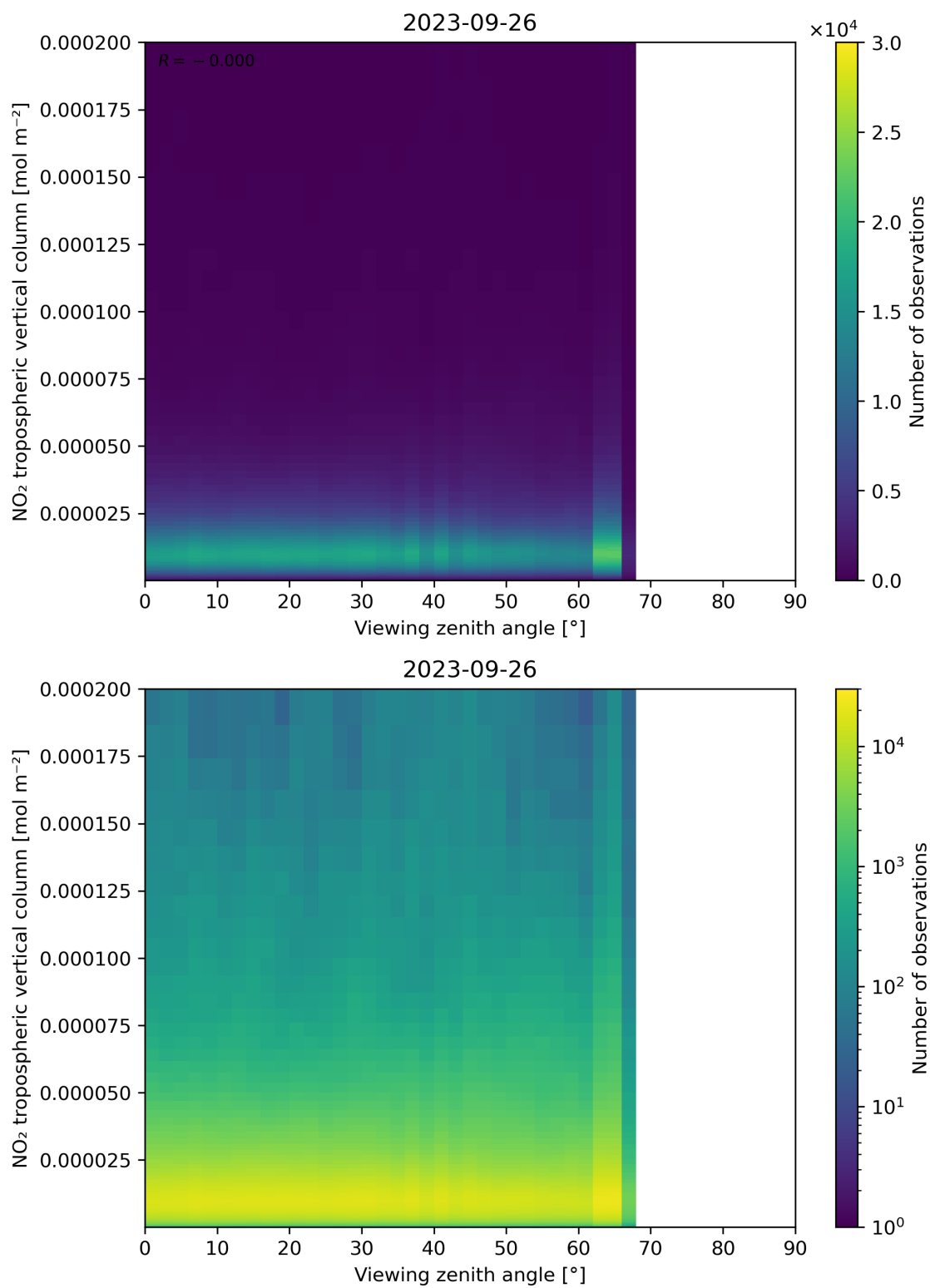
Figure 169: Scatter density plot of “Viewing zenith angle” against “NO 2 tropospheric vertical column” for 2023-09-26 to 2023-09-27.
