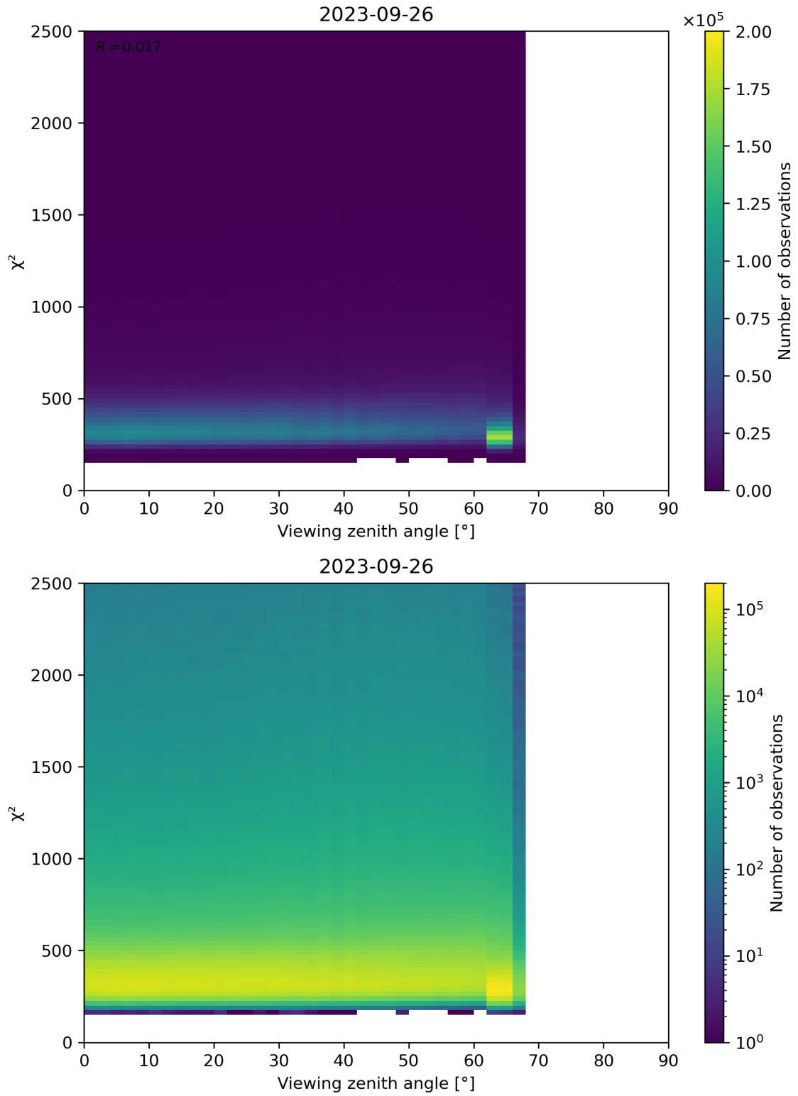
Figure 162: Scatter density plot of “Viewing zenith angle” against “ \chi^2 ” for 2023-09-26 to 2023-09-27.
