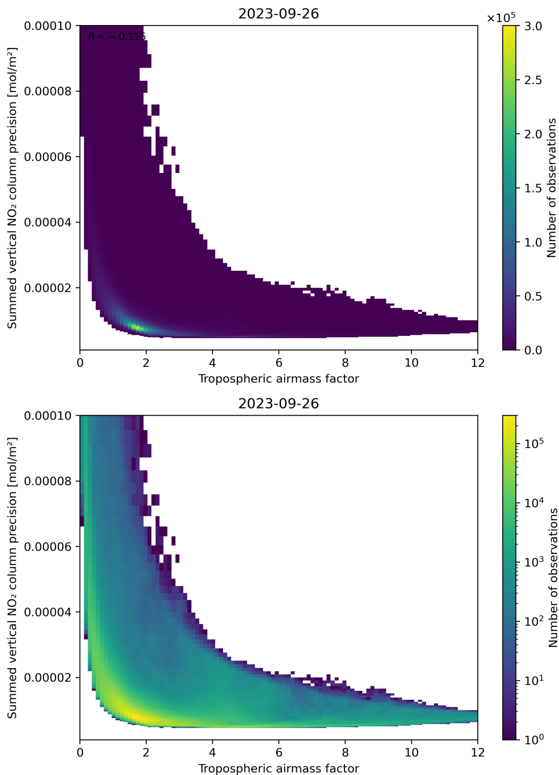
Figure 76: Scatter density plot of “Tropospheric air mass factor” against “Summed vertical NO 2 column precision” for 2023-09-26 to 2023-09-27.
