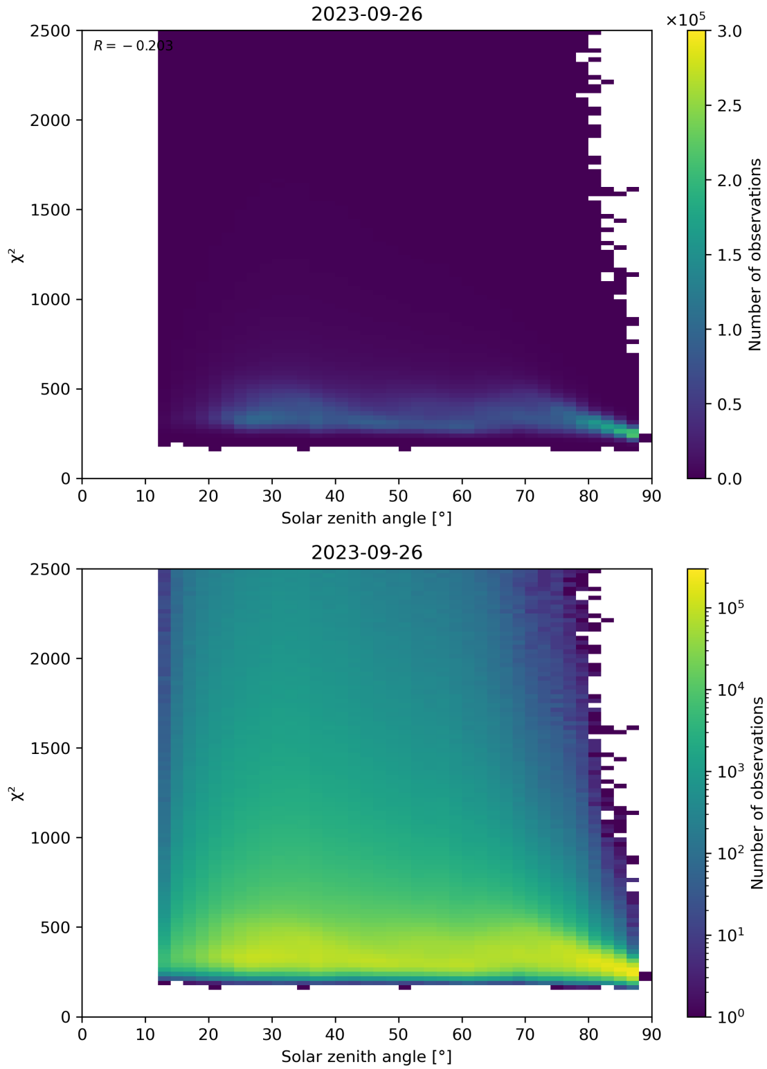
Figure 148: Scatter density plot of “Solar zenith angle” against “ \chi^2 ” for 2023-09-26 to 2023-09-27.
