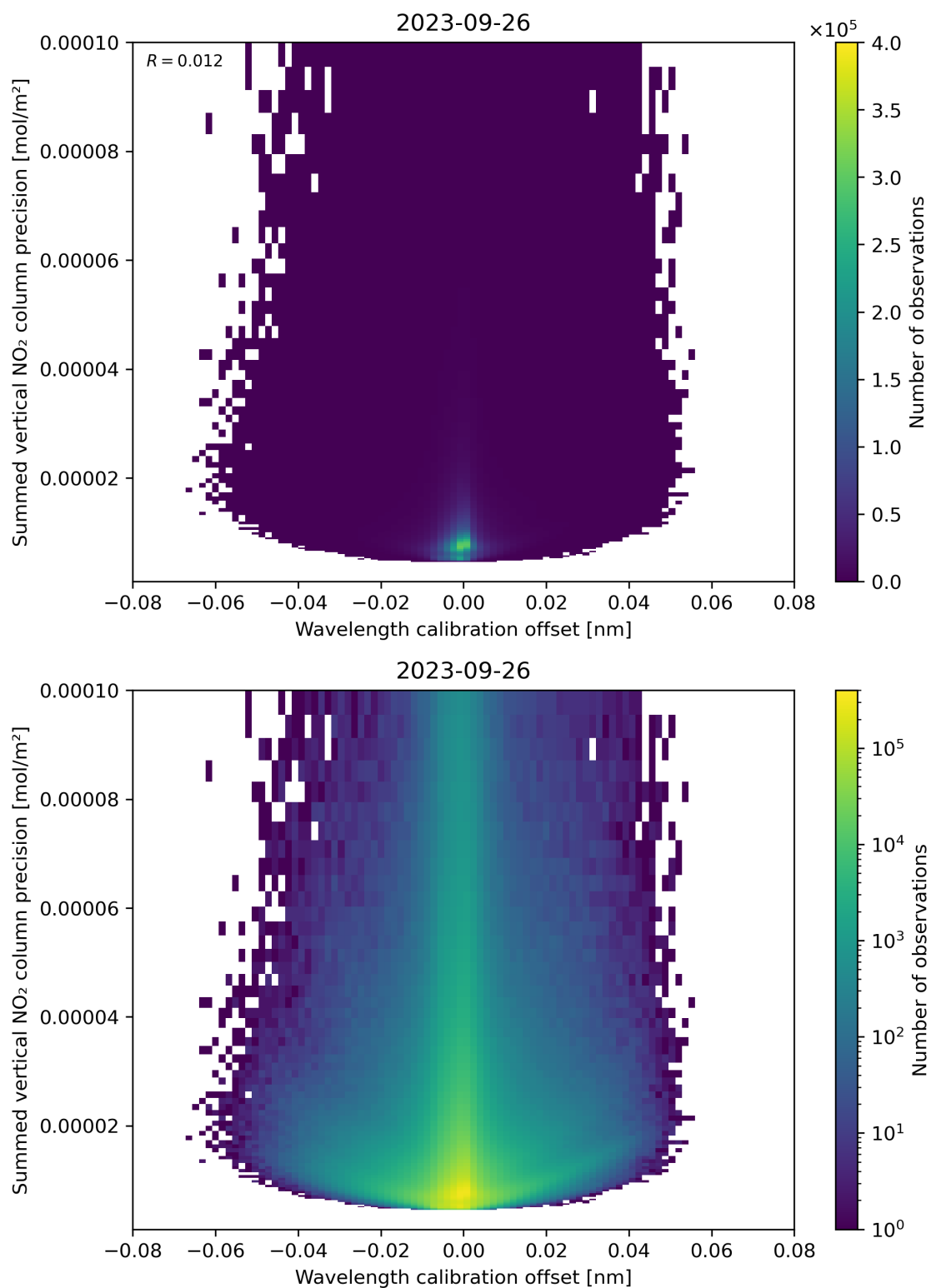
Figure 178: Scatter density plot of “Wavelength calibration offset” against “Summed vertical NO 2 column precision” for 2023-09-26 to 2023-09-27.
