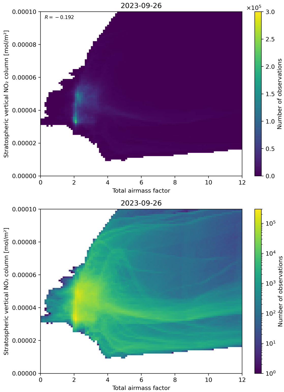
Figure 64: Scatter density plot of “Total airmass factor” against “Stratospheric vertical \text{NO}_2 column” for 2023-09-26 to 2023-09-27.
