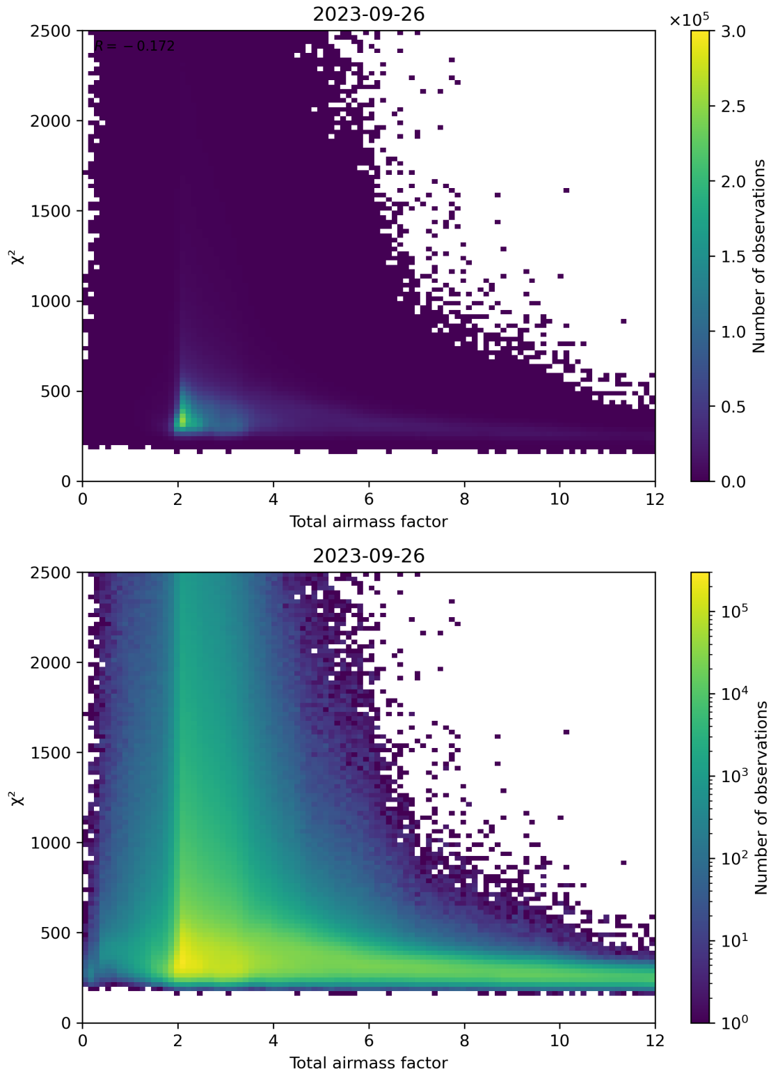
Figure 63: Scatter density plot of “Total airmass factor” against “ \chi^2 ” for 2023-09-26 to 2023-09-27.
