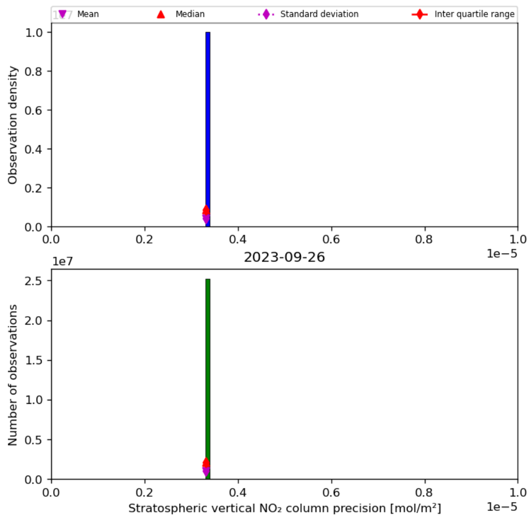
Figure 37: Histogram of “Stratospheric vertical NO 2 column precision” for 2023-09-26 to 2023-09-27
