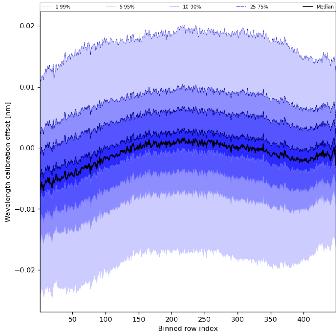
Figure 52: Along track statistics of “Wavelength calibration offset” for 2023-09-26 to 2023-09-27
