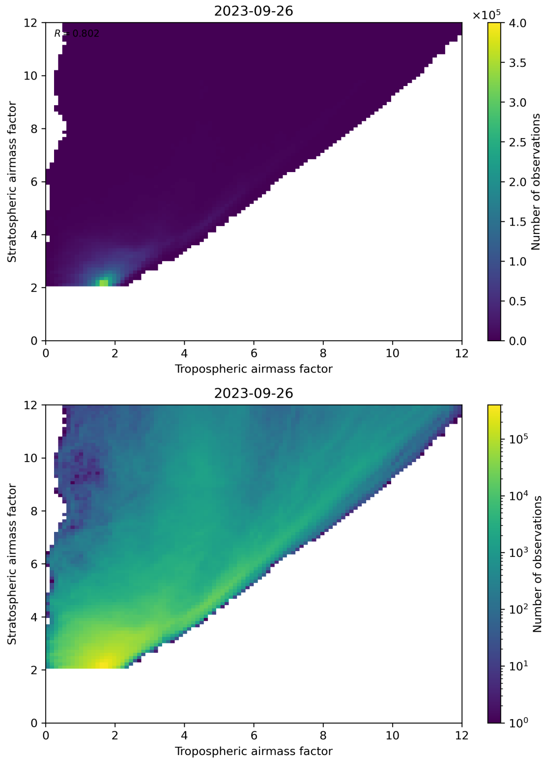
Figure 71: Scatter density plot of “Tropospheric airmass factor” against “Stratospheric airmass factor” for 2023-09-26 to 2023-09-27.
