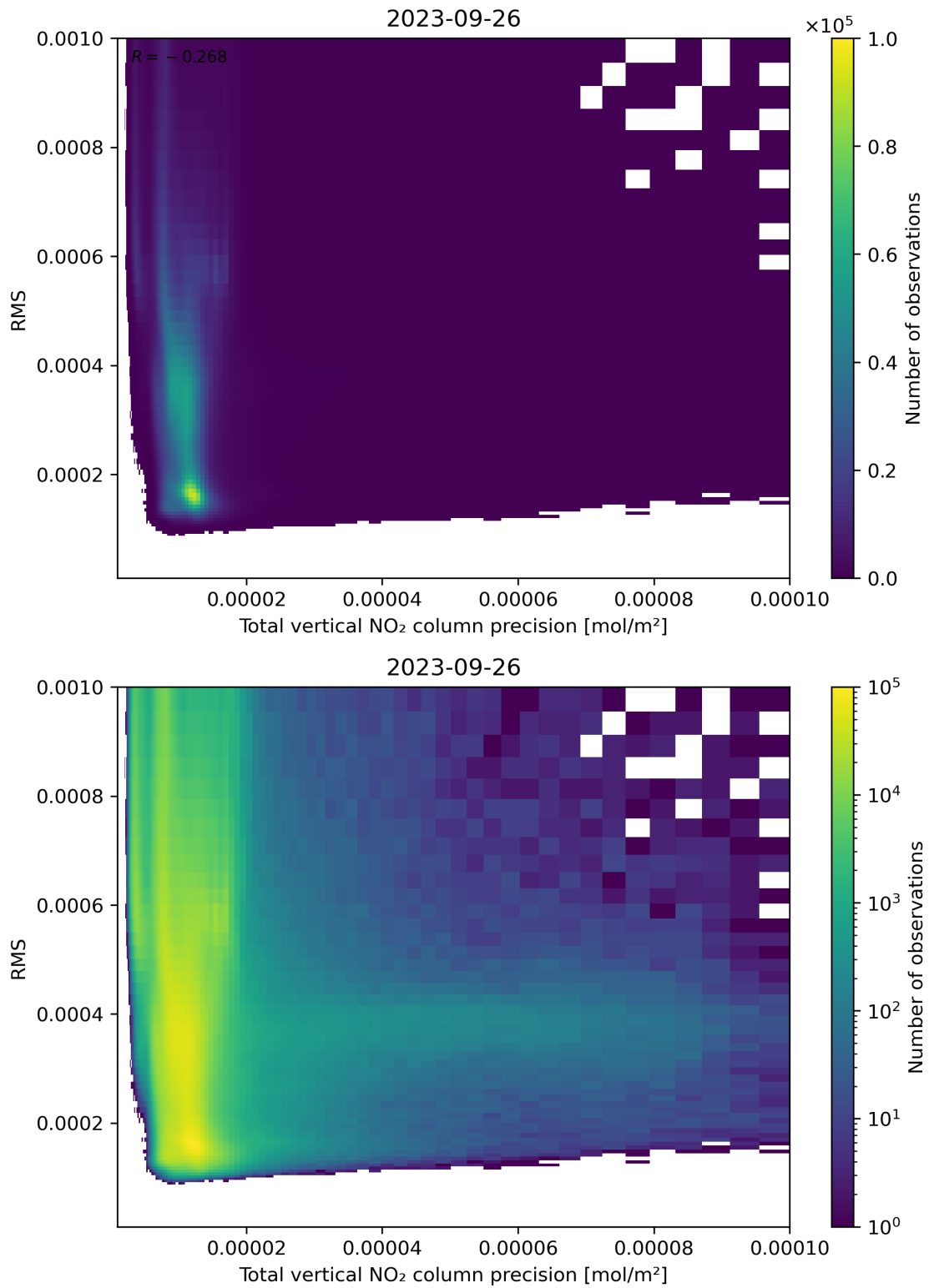
Figure 119: Scatter density plot of “Total vertical NO 2 column precision” against “RMS” for 2023-09-26 to 2023-09-27.
