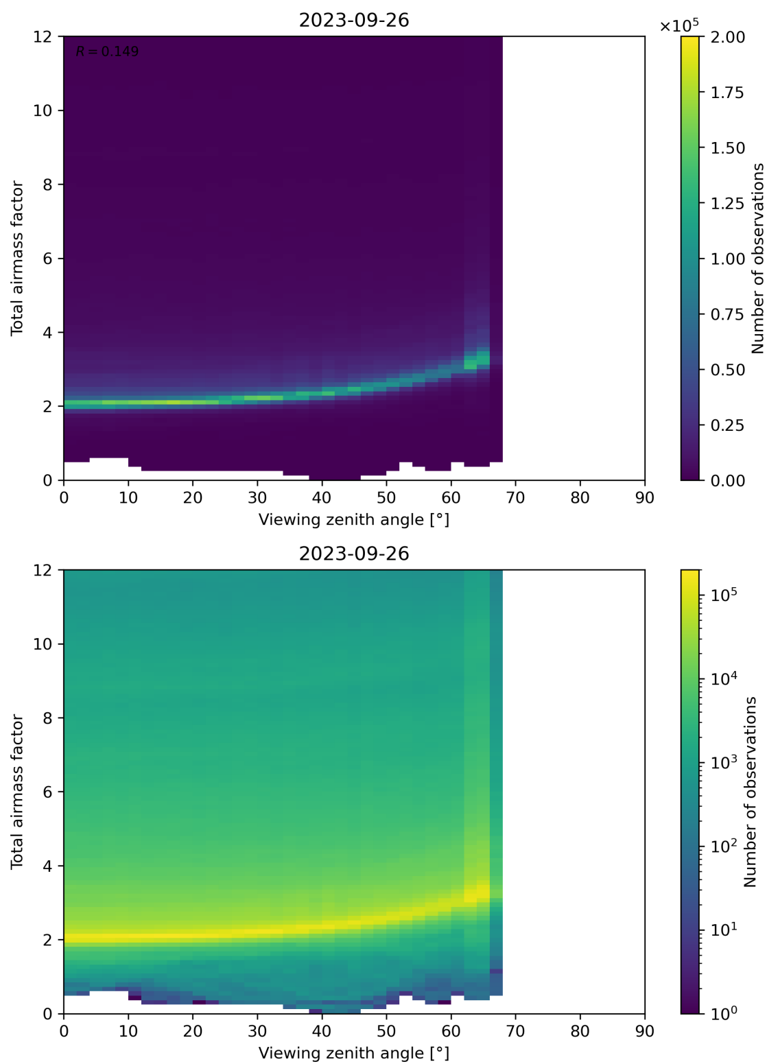
Figure 160: Scatter density plot of “Viewing zenith angle” against “Total airmass factor” for 2023-09-26 to 2023-09-27.
