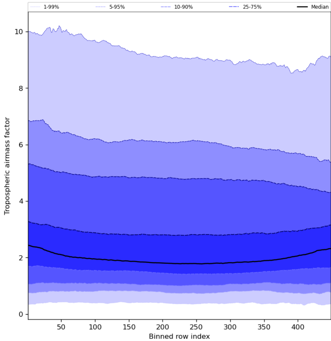
Figure 48: Along track statistics of “Tropospheric airmass factor” for 2023-09-26 to 2023-09-27
