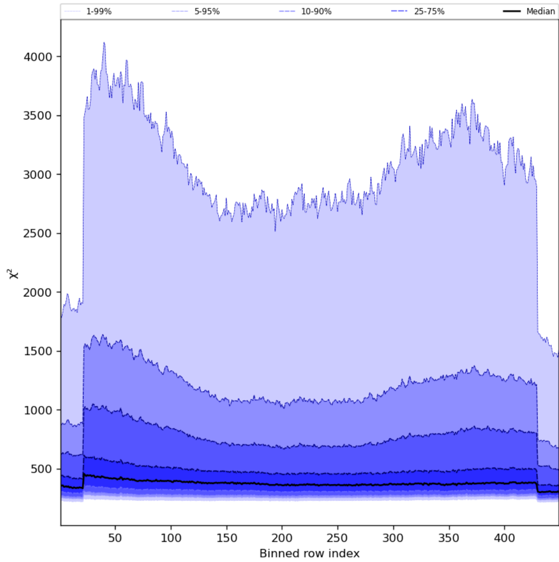
Figure 59: Along track statistics of “ \chi^2 ” for 2023-09-26 to 2023-09-27
