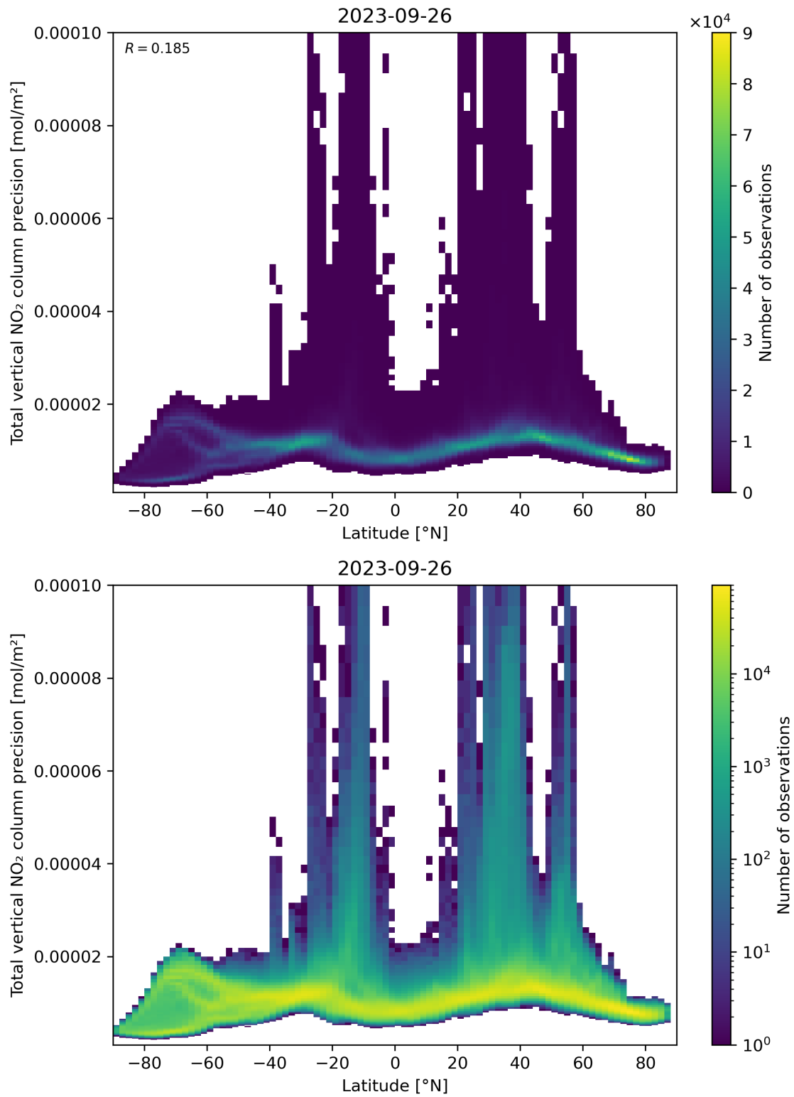
Figure 91: Scatter density plot of “Latitude” against “Total vertical NO 2 column precision” for 2023-09-26 to 2023-09-27.
