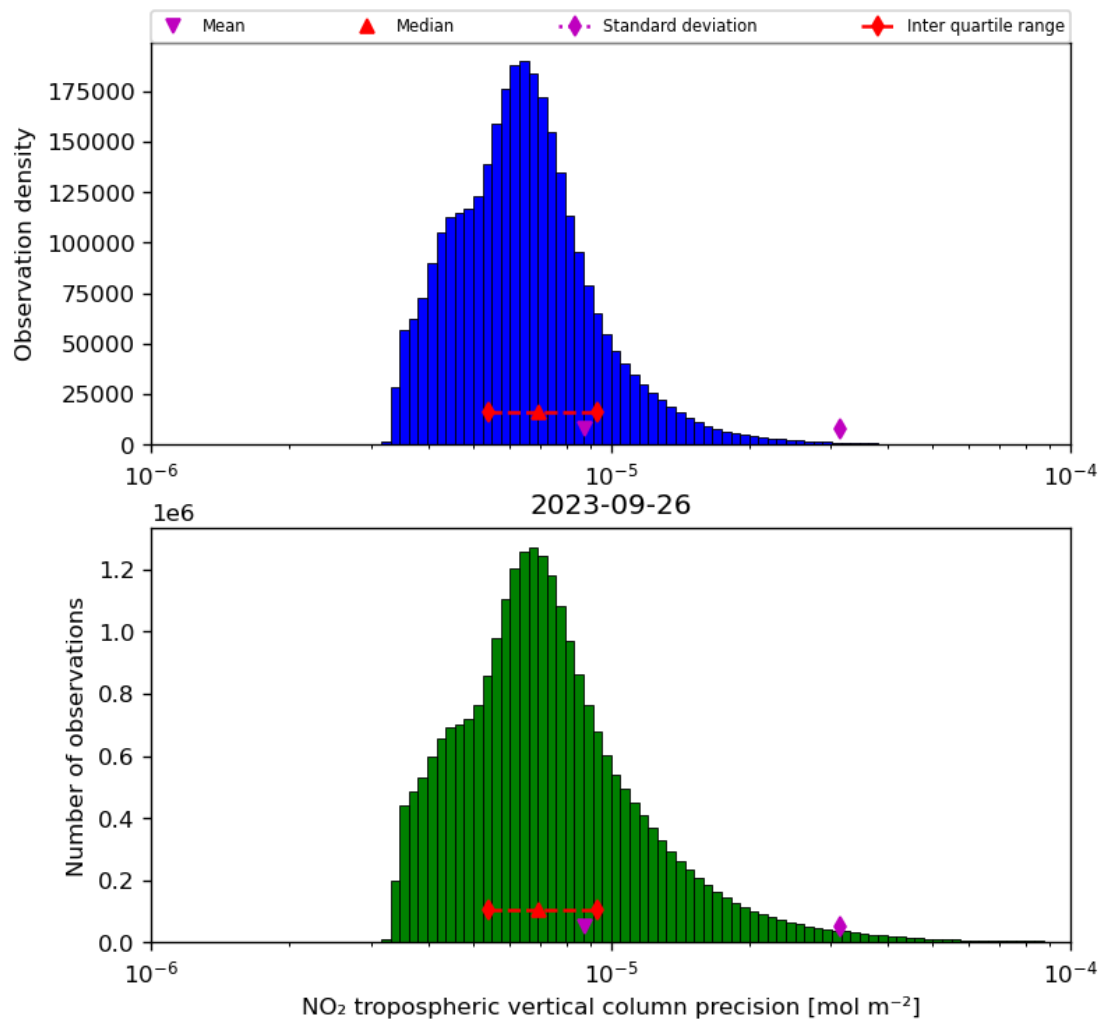
Figure 30: Histogram of “NO 2 tropospheric vertical column precision” for 2023-09-26 to 2023-09-27
