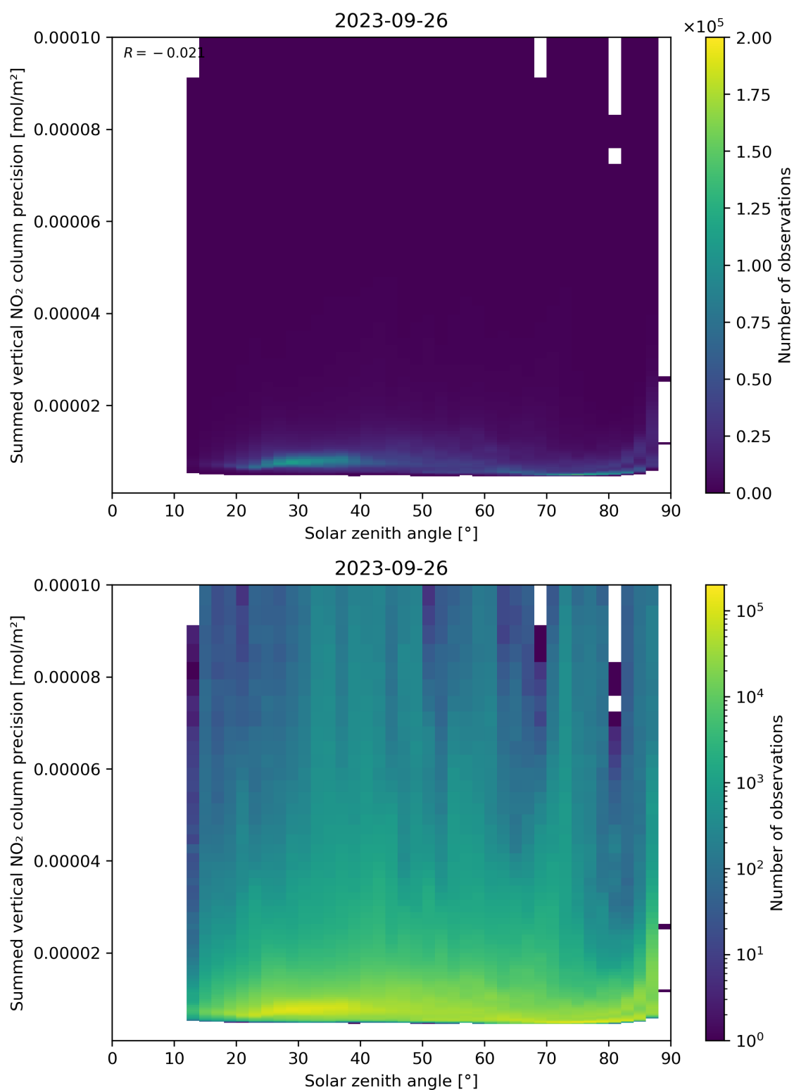
Figure 152: Scatter density plot of “Solar zenith angle” against “Summed vertical NO 2 column precision” for 2023-09-26 to 2023-09-27.
