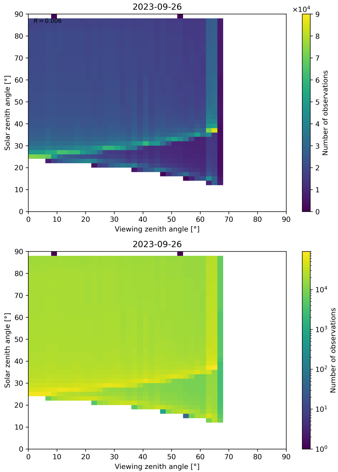
Figure 172: Scatter density plot of “Viewing zenith angle” against “Solar zenith angle” for 2023-09-26 to 2023-09-27.
