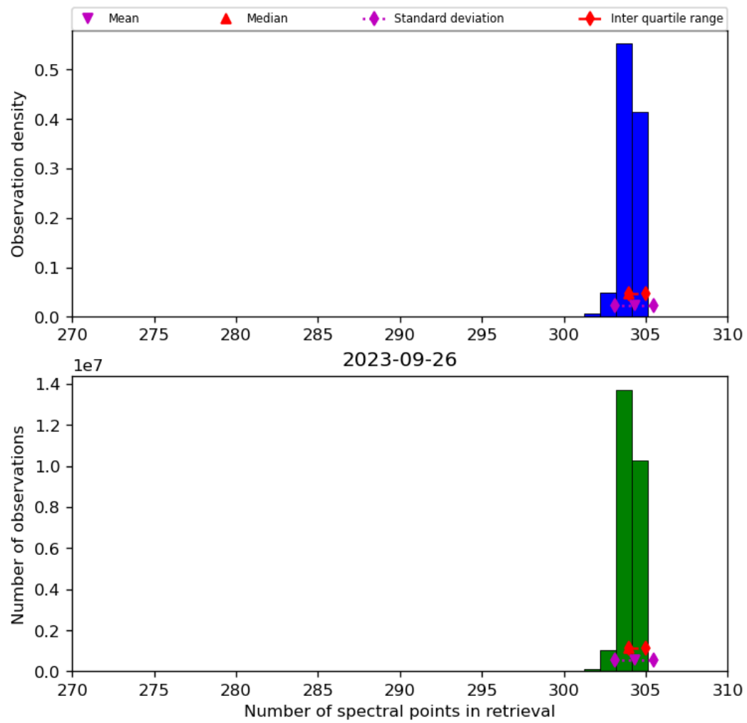
Figure 33: Histogram of “Number of spectral points in retrieval” for 2023-09-26 to 2023-09-27
