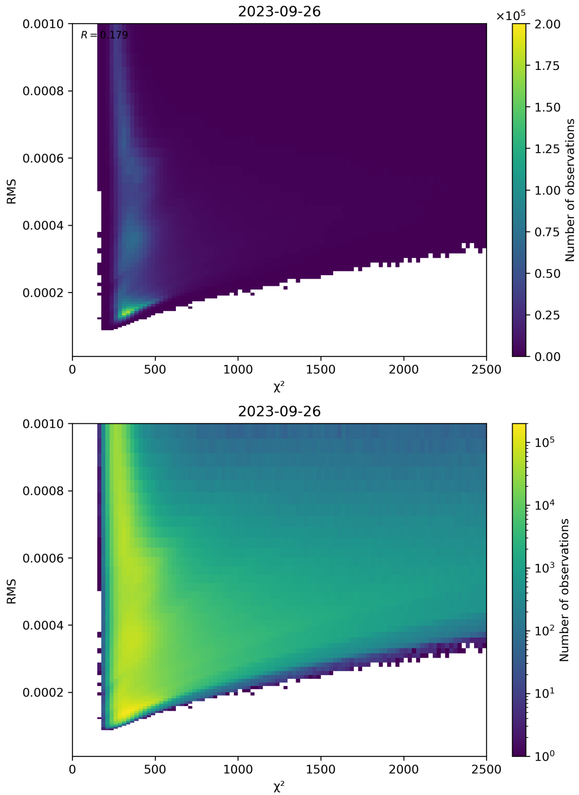
Figure 82: Scatter density plot of “ \chi^2 ” against “RMS” for 2023-09-26 to 2023-09-27.
