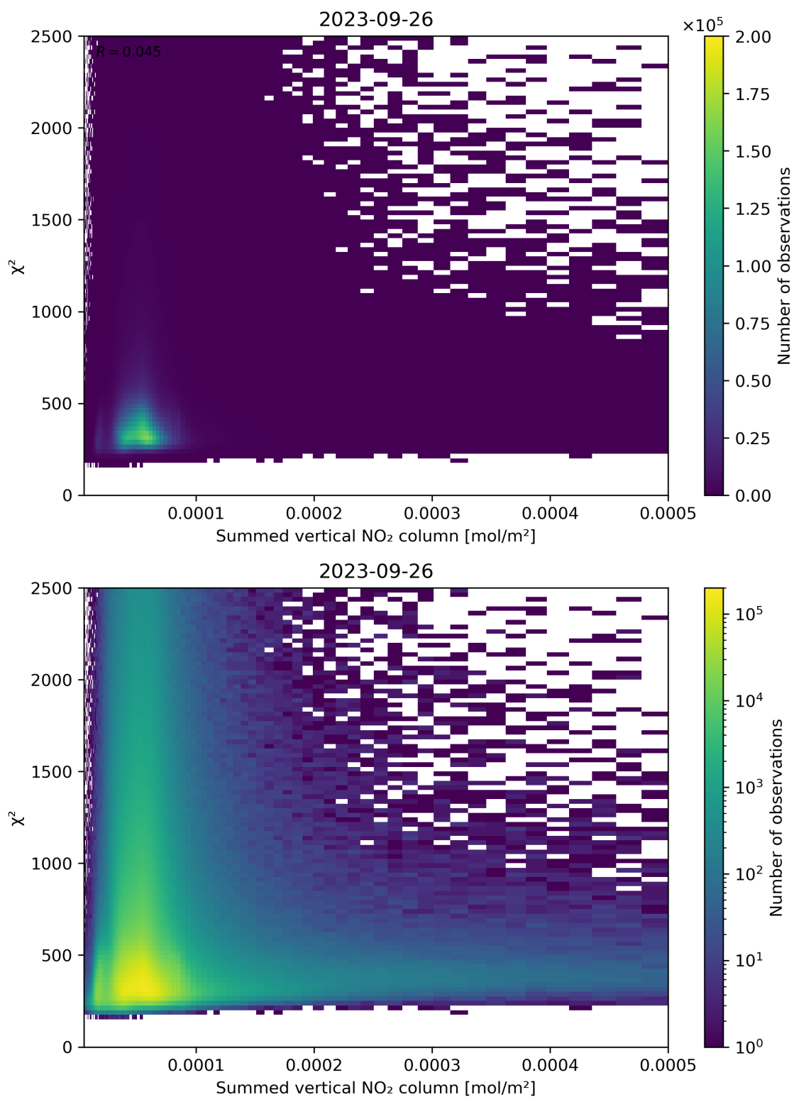
Figure 104: Scatter density plot of “Summed vertical NO 2 column” against “ \chi^2 ” for 2023-09-26 to 2023-09-27.
