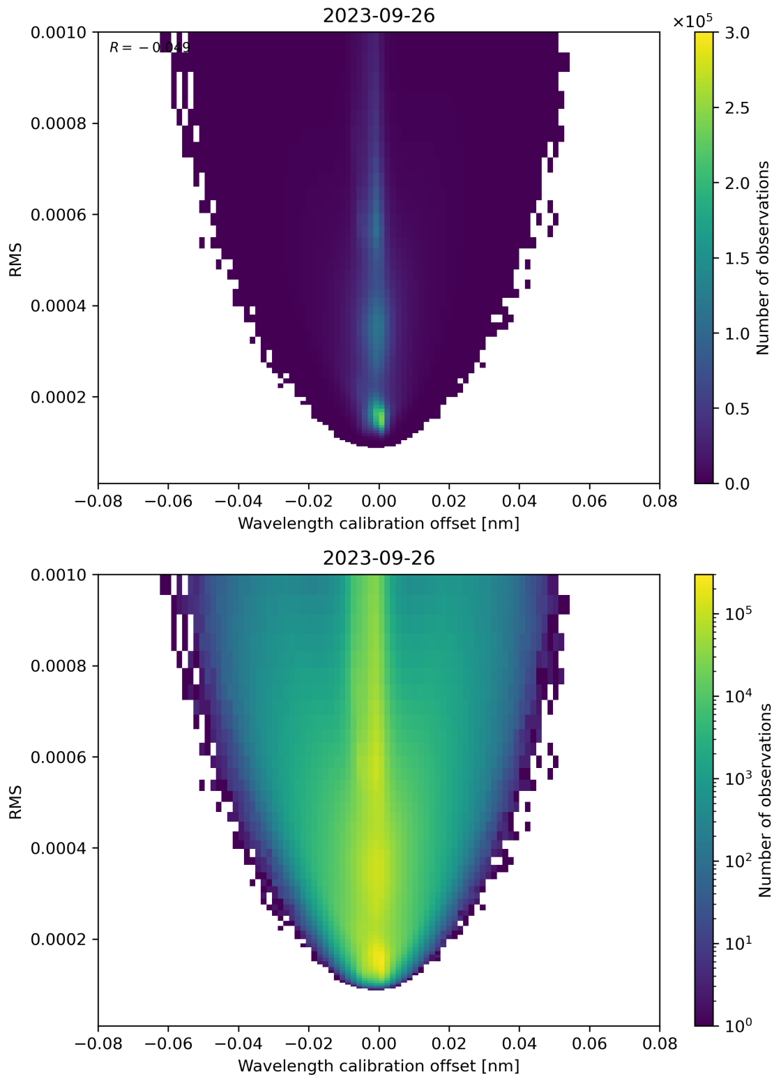
Figure 181: Scatter density plot of “Wavelength calibration offset” against “RMS” for 2023-09-26 to 2023-09-27.
