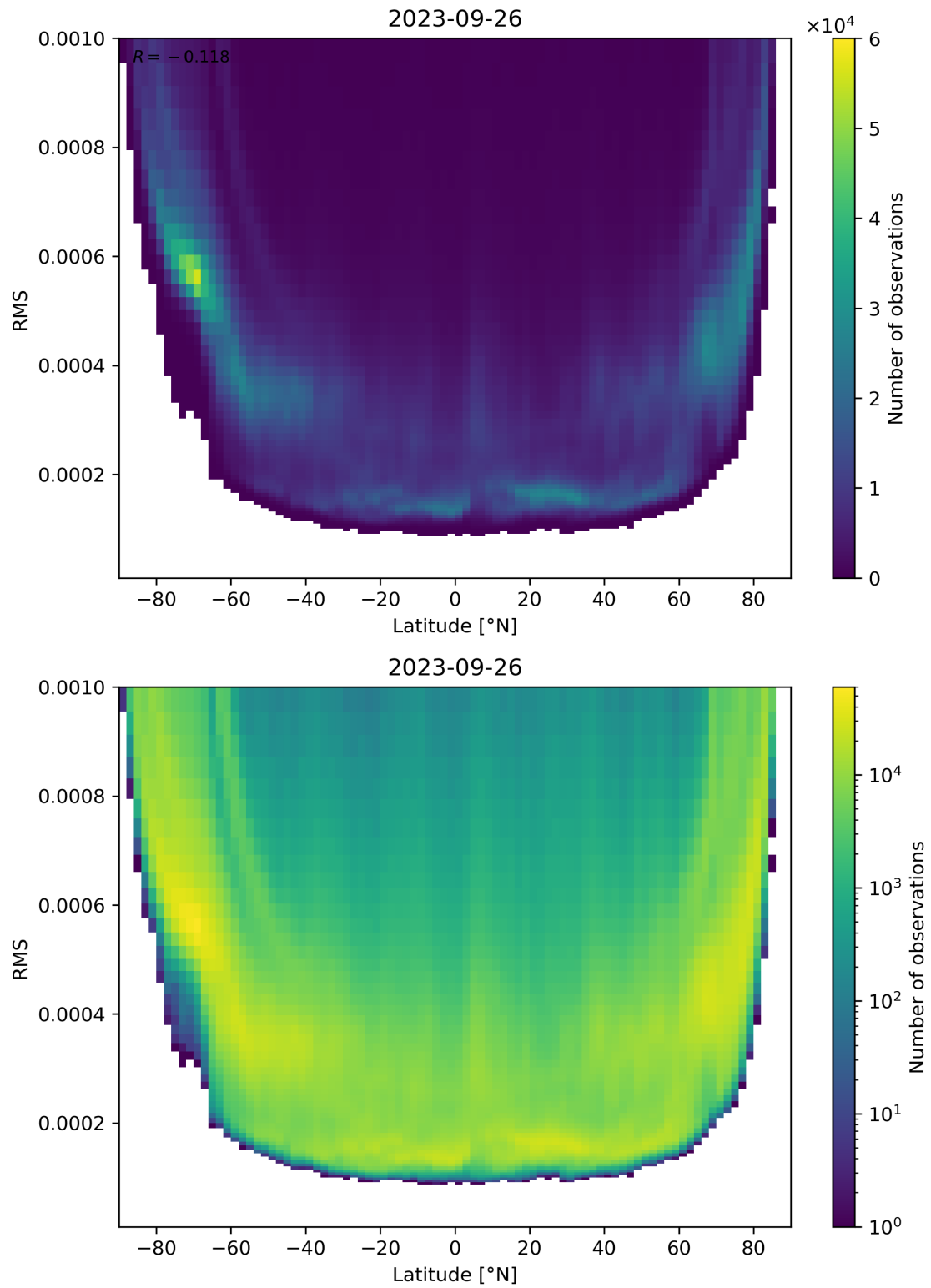
Figure 94: Scatter density plot of “Latitude” against “RMS” for 2023-09-26 to 2023-09-27.
