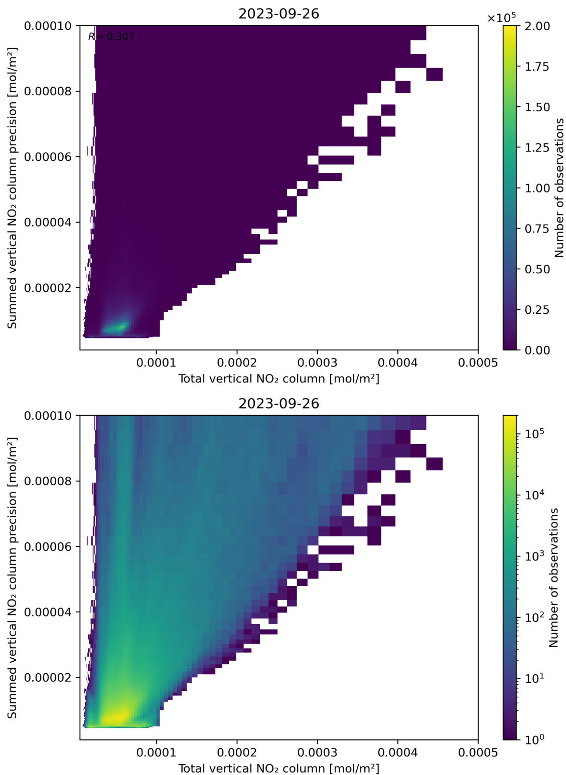
Figure 113: Scatter density plot of “Total vertical NO 2 column” against “Summed vertical NO 2 column precision” for 2023-09-26 to 2023-09-27.
