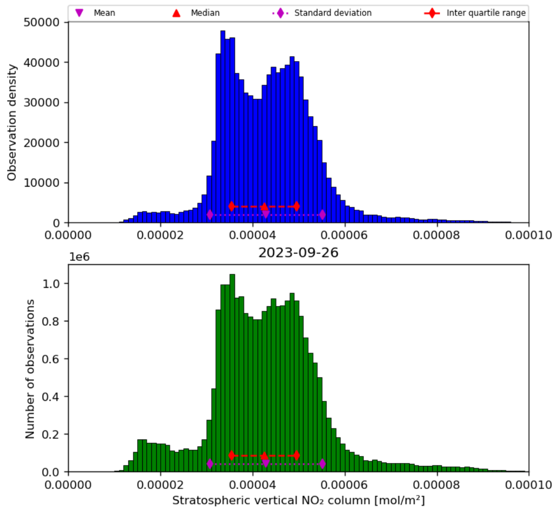
Figure 36: Histogram of “Stratospheric vertical NO 2 column” for 2023-09-26 to 2023-09-27
