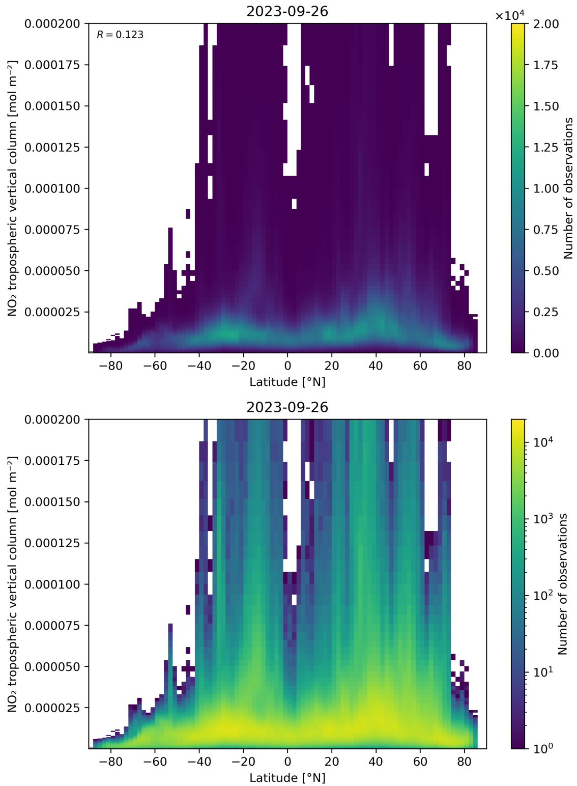
Figure 92: Scatter density plot of “Latitude” against “NO 2 tropospheric vertical column” for 2023-09-26 to 2023-09-27.
