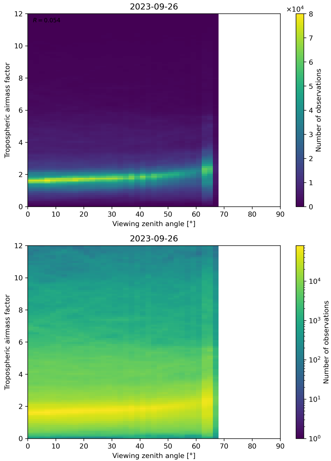
Figure 161: Scatter density plot of “Viewing zenith angle” against “Tropospheric airmass factor” for 2023-09-26 to 2023-09-27.
