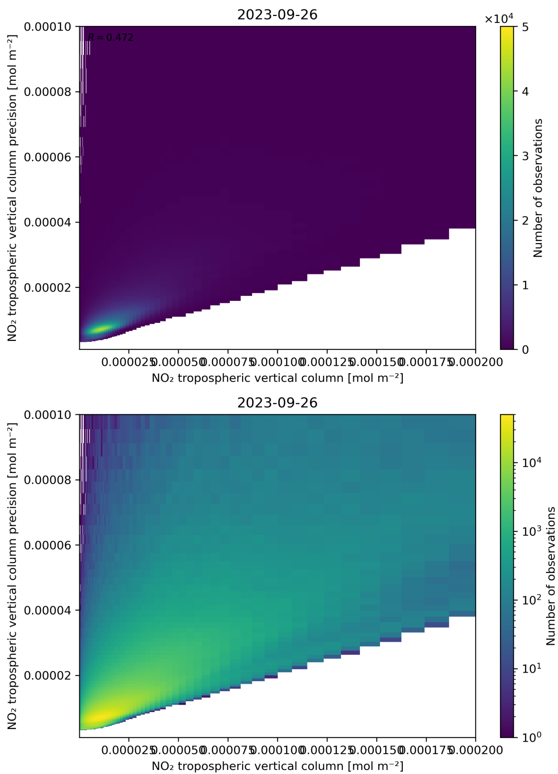
Figure 130: Scatter density plot of “NO 2 tropospheric vertical column” against “NO 2 tropospheric vertical column precision” for 2023-09-26 to 2023-09-27.
