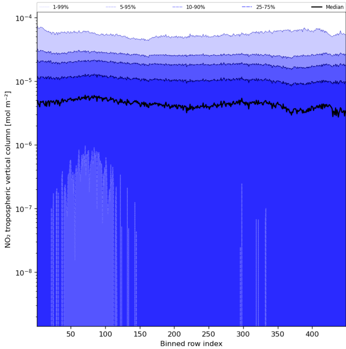
Figure 46: Along track statistics of “NO 2 tropospheric vertical column” for 2023-09-26 to 2023-09-27
