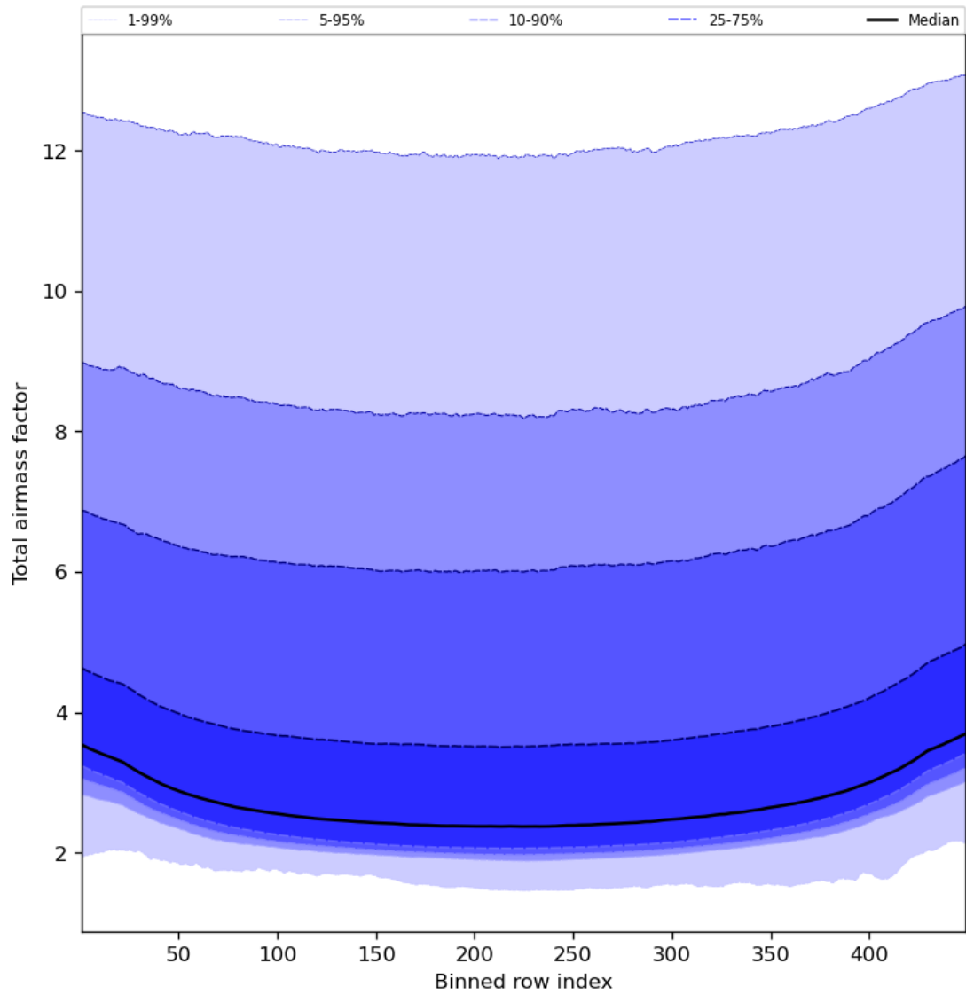
Figure 49: Along track statistics of “Total airmass factor” for 2023-09-26 to 2023-09-27
