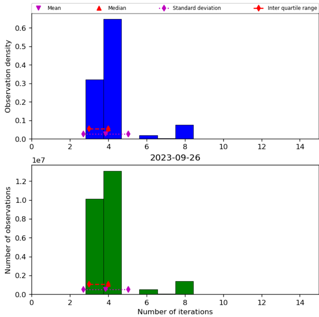
Figure 34: Histogram of “Number of iterations” for 2023-09-26 to 2023-09-27
