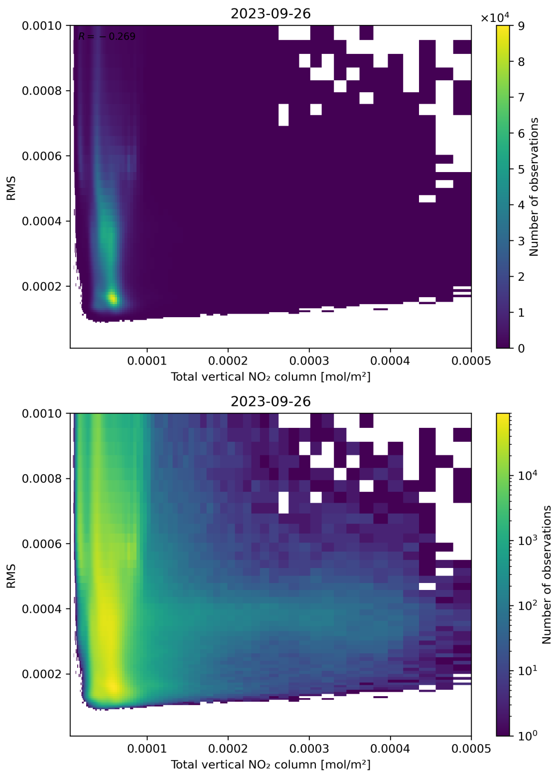
Figure 120: Scatter density plot of “Total vertical NO 2 column” against “RMS” for 2023-09-26 to 2023-09-27.
