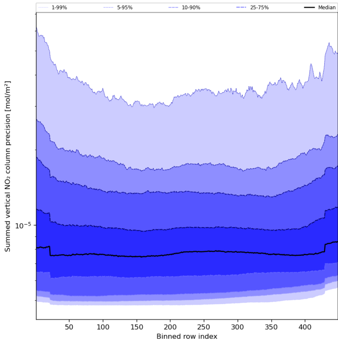
Figure 58: Along track statistics of “Summed vertical NO 2 column precision” for 2023-09-26 to 2023-09-27
