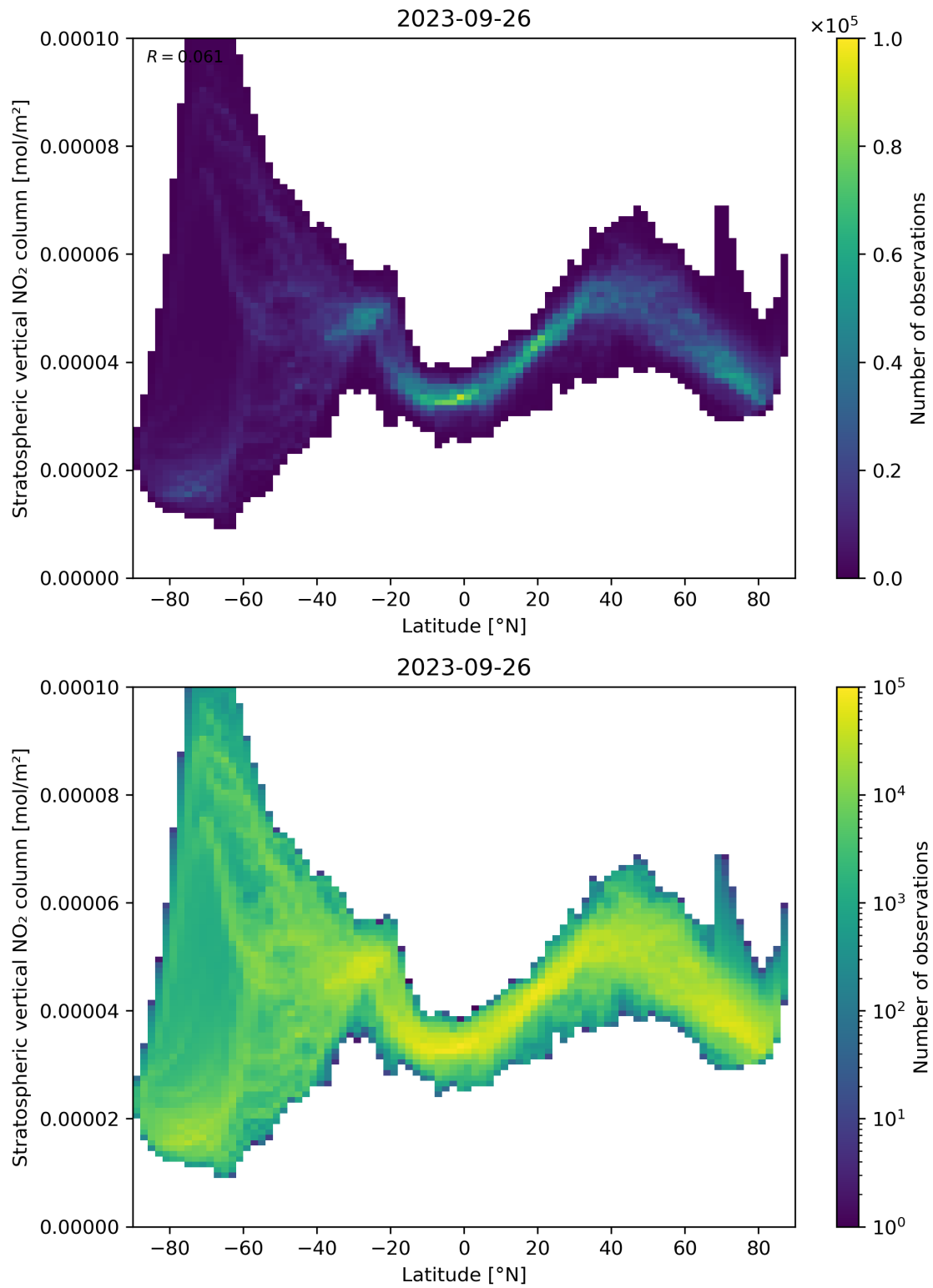
Figure 87: Scatter density plot of “Latitude” against “Stratospheric vertical NO 2 column” for 2023-09-26 to 2023-09-27.
