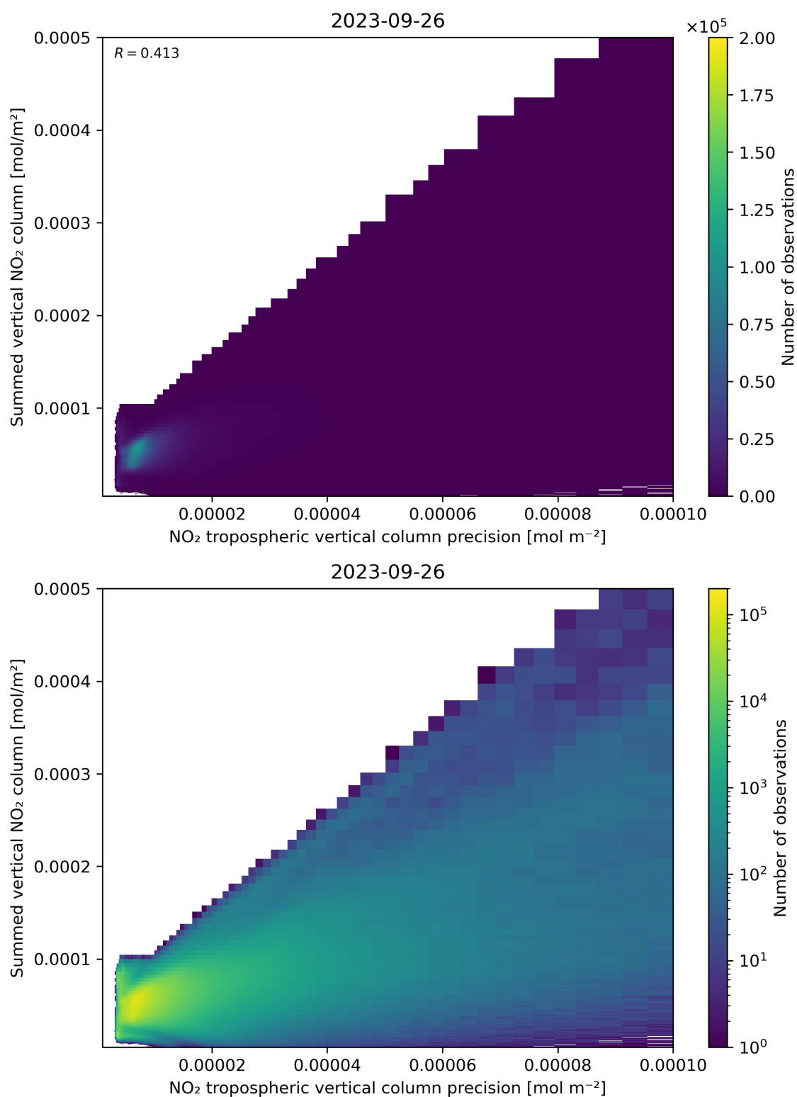
Figure 136: Scatter density plot of “NO 2 tropospheric vertical column precision” against “Summed vertical NO 2 column” for 2023-09-26 to 2023-09-27.
