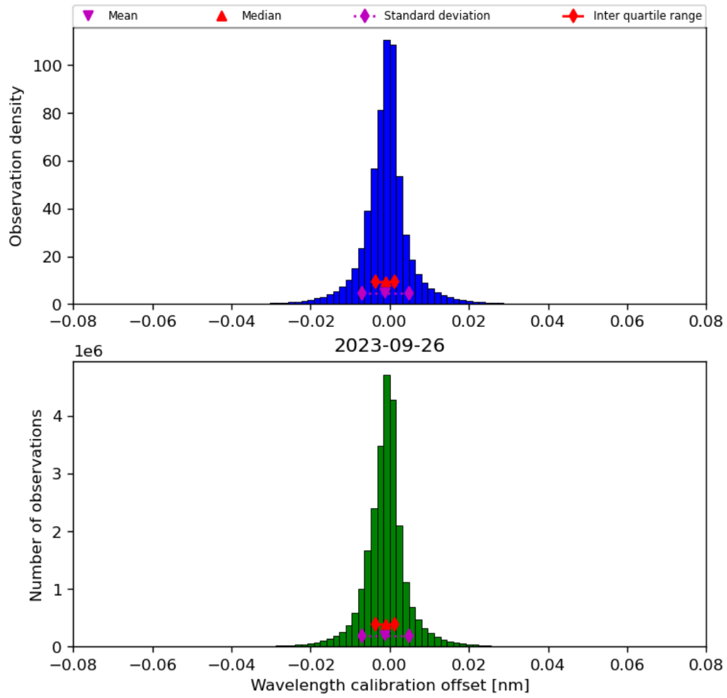
Figure 35: Histogram of “Wavelength calibration offset” for 2023-09-26 to 2023-09-27
