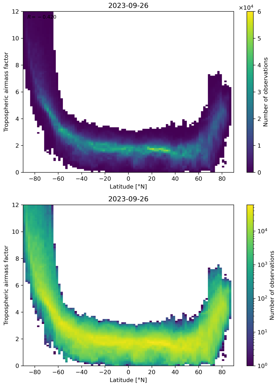
Figure 85: Scatter density plot of “Latitude” against “Tropospheric air mass factor” for 2023-09-26 to 2023-09-27.
