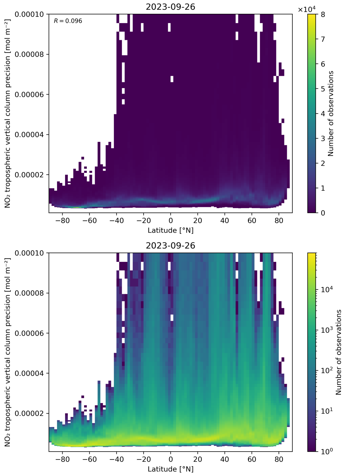
Figure 93: Scatter density plot of “Latitude” against “NO 2 tropospheric vertical column precision” for 2023-09-26 to 2023-09-27.
