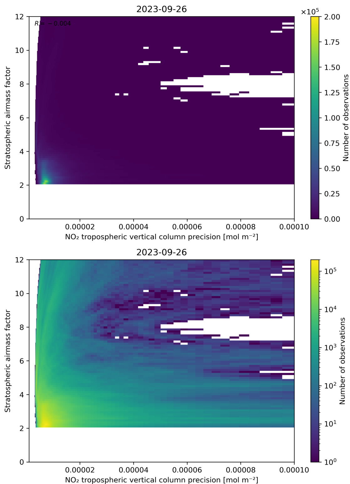
Figure 131: Scatter density plot of “NO 2 tropospheric vertical column precision” against “Stratospheric airmass factor” for 2023-09-26 to 2023-09-27.
