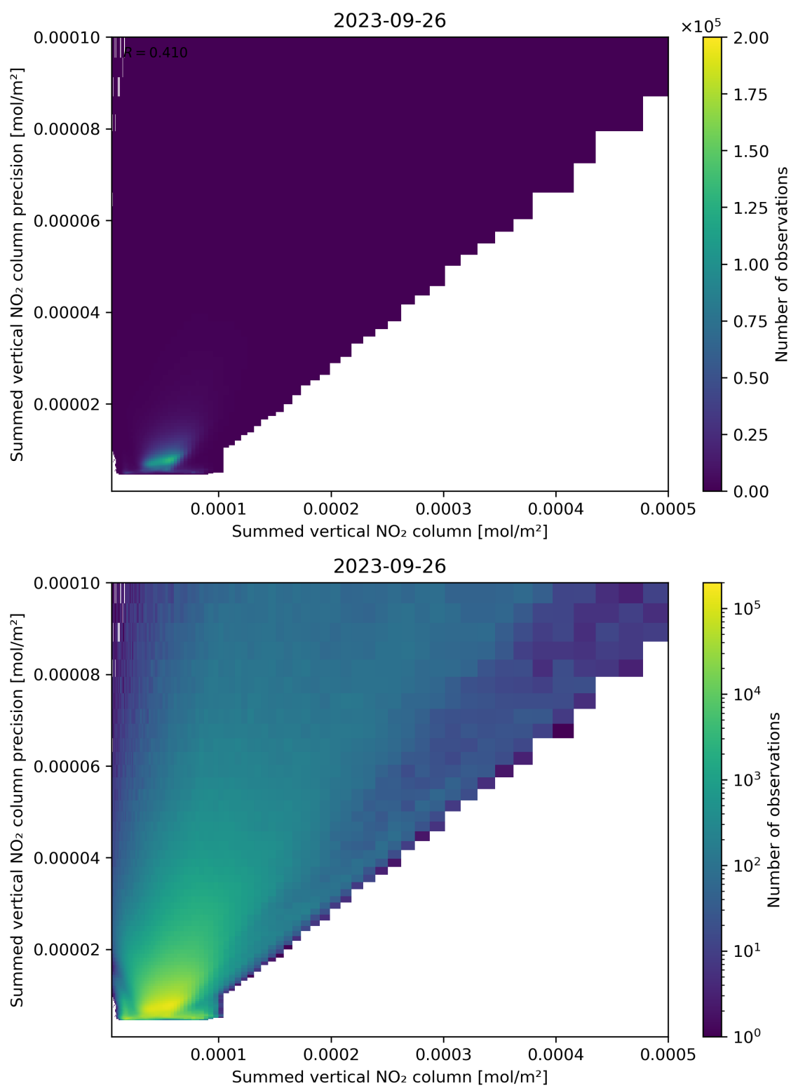
Figure 105: Scatter density plot of “Summed vertical NO 2 column” against “Summed vertical NO 2 column precision” for 2023-09-26 to 2023-09-27.
