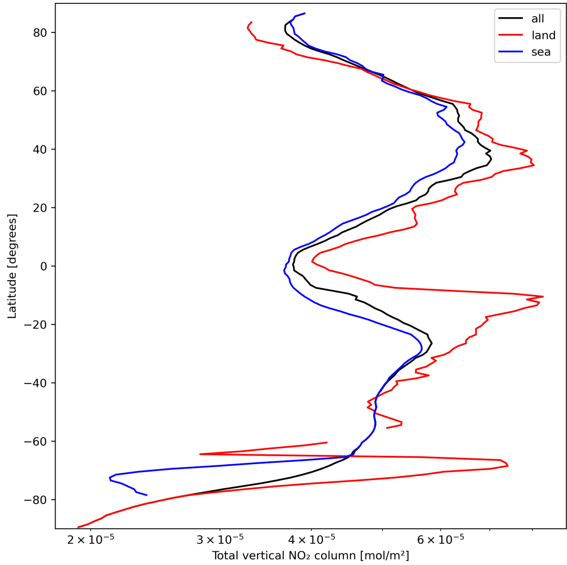
Figure 21: Zonal average of “Total vertical NO 2 column” for 2023-09-26 to 2023-09-27.
