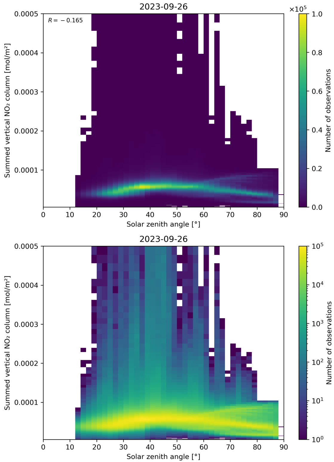
Figure 151: Scatter density plot of “Solar zenith angle” against “Summed vertical NO 2 column” for 2023-09-26 to 2023-09-27.
