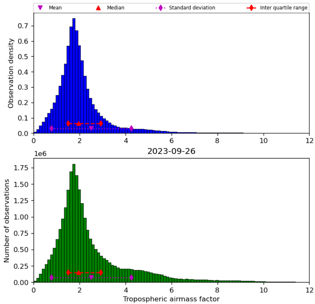
Figure 31: Histogram of “Tropospheric airmass factor” for 2023-09-26 to 2023-09-27
