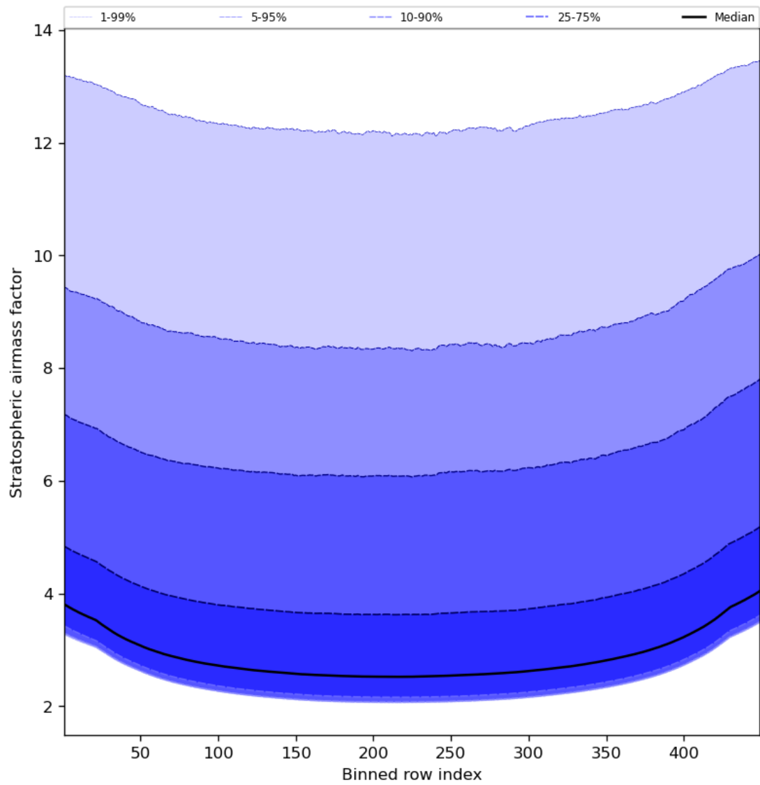
Figure 61: Along track statistics of “Stratospheric airmass factor” for 2023-09-26 to 2023-09-27
