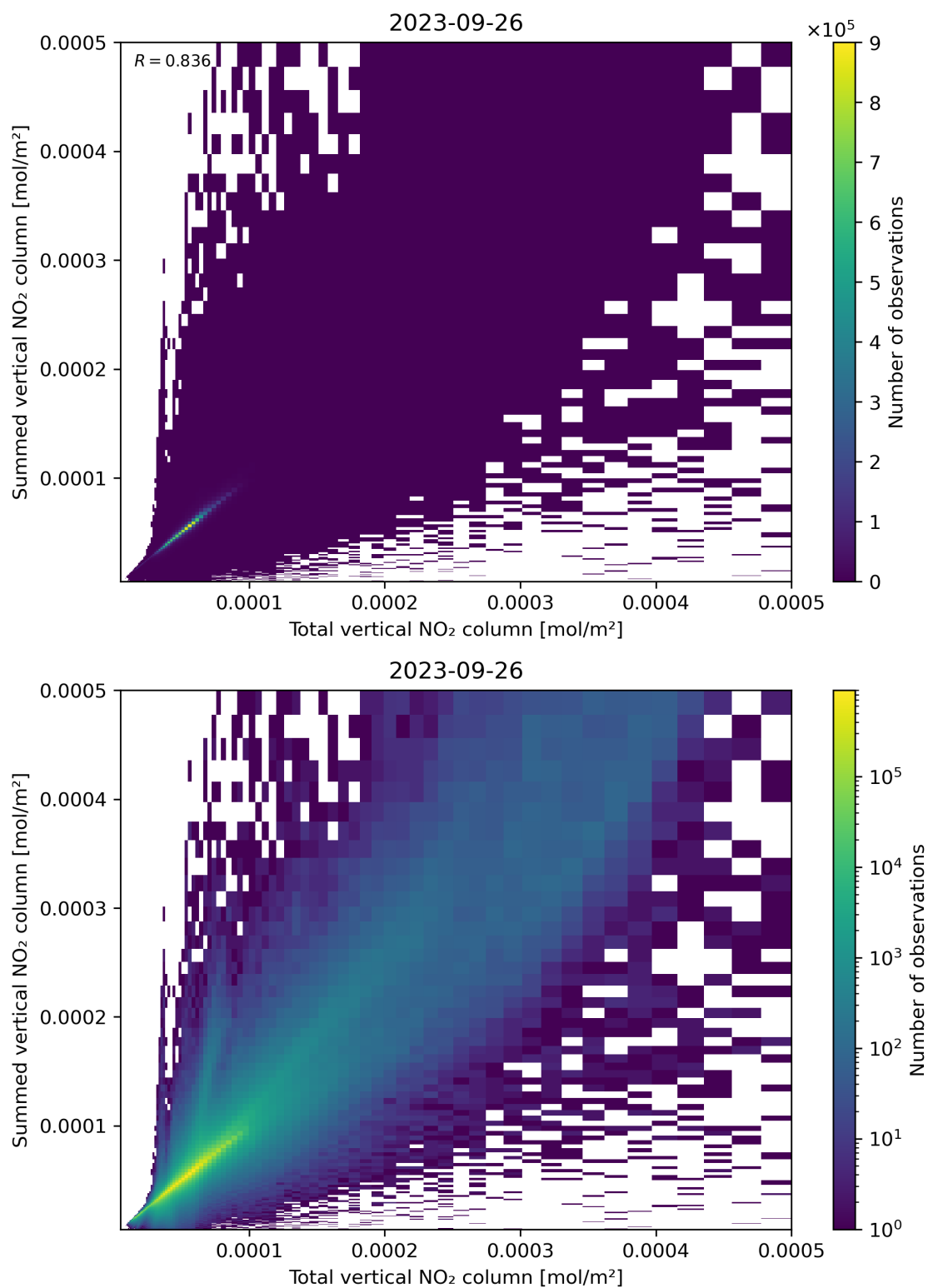
Figure 112: Scatter density plot of “Total vertical NO 2 column” against “Summed vertical NO 2 column” for 2023-09-26 to 2023-09-27.
