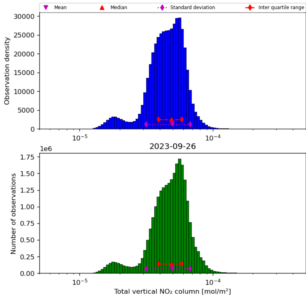
Figure 38: Histogram of “Total vertical NO 2 column” for 2023-09-26 to 2023-09-27
