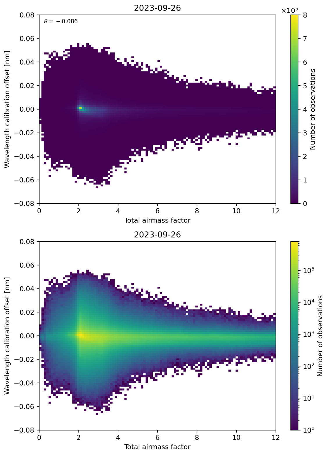
Figure 70: Scatter density plot of “Total airmass factor” against “Wavelength calibration offset” for 2023-09-26 to 2023-09-27.
