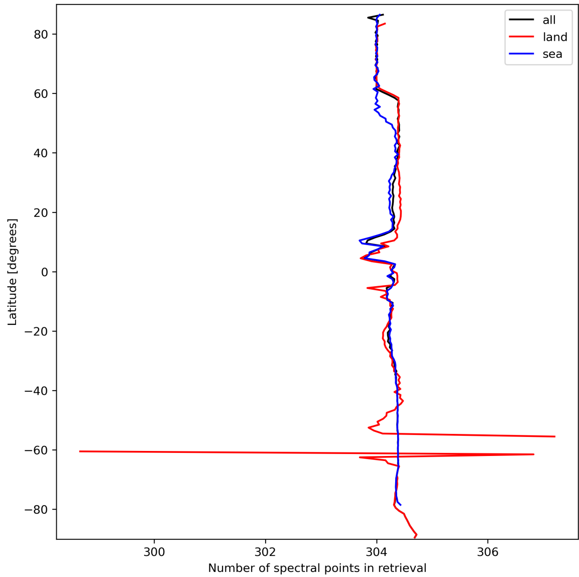
Figure 16: Zonal average of “Number of spectral points in retrieval” for 2023-09-26 to 2023-09-27.
