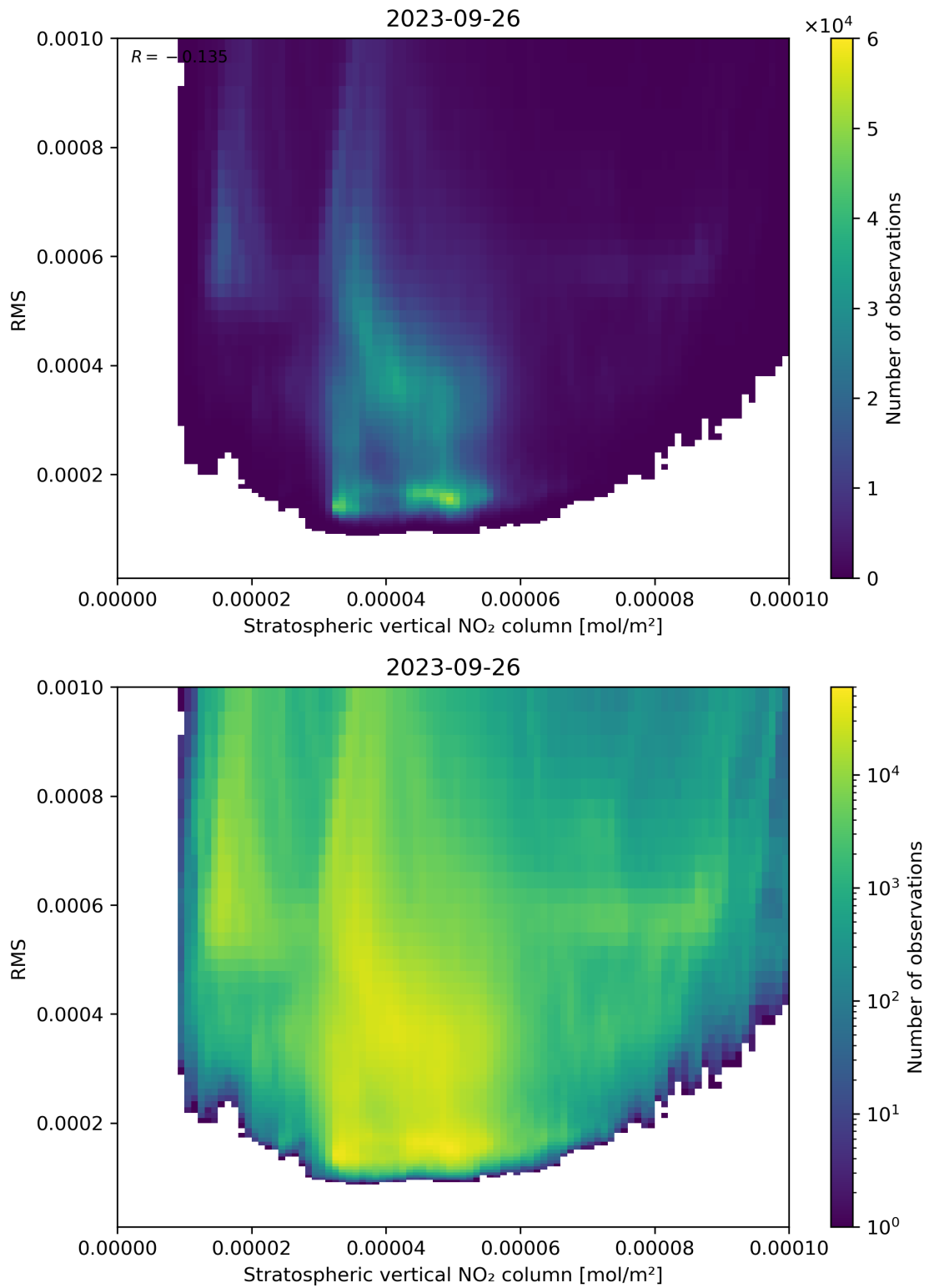
Figure 102: Scatter density plot of “Stratospheric vertical NO 2 column” against “RMS” for 2023-09-26 to 2023-09-27.
