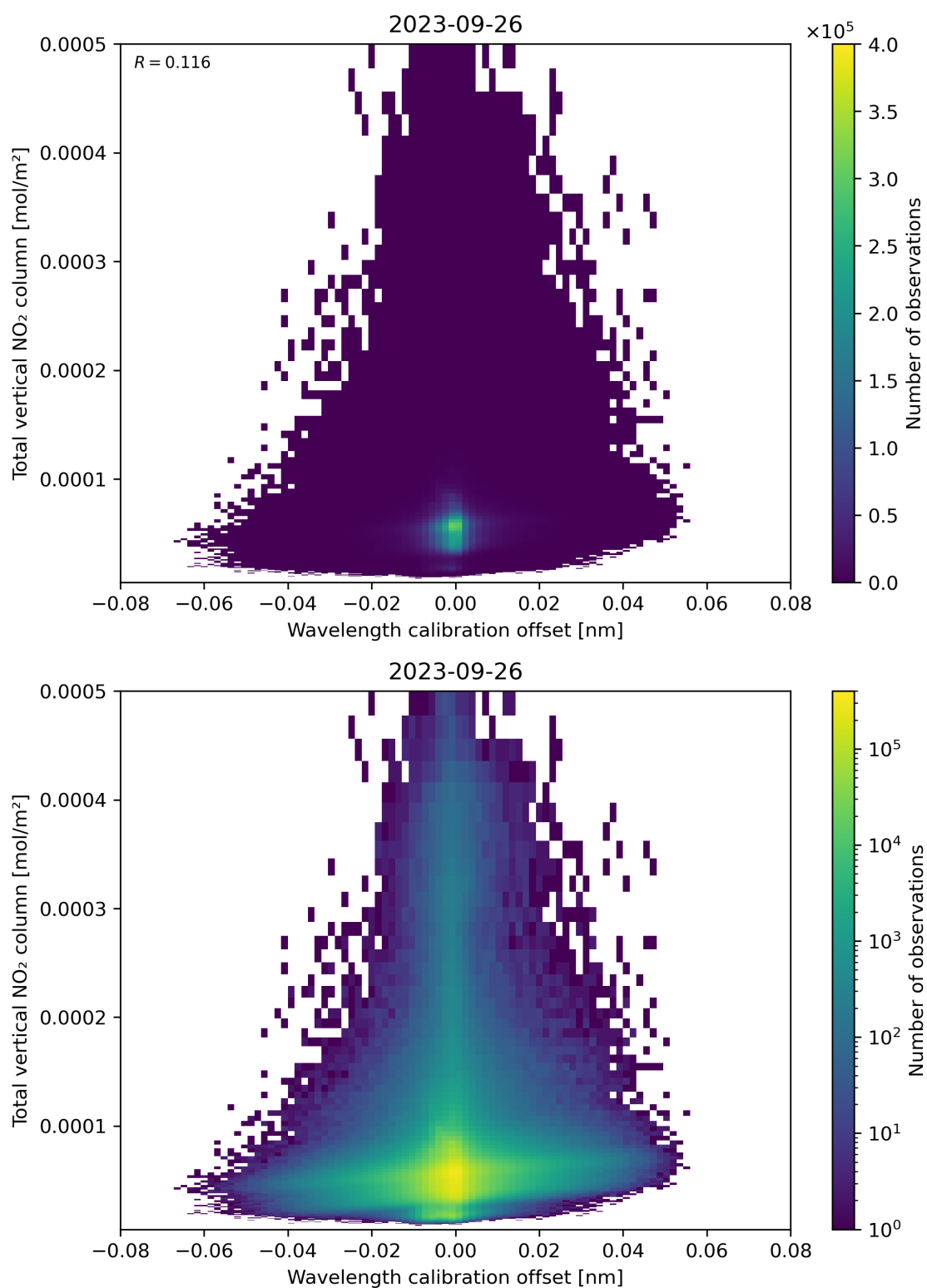
Figure 179: Scatter density plot of “Wavelength calibration offset” against “Total vertical NO 2 column” for 2023-09-26 to 2023-09-27.
