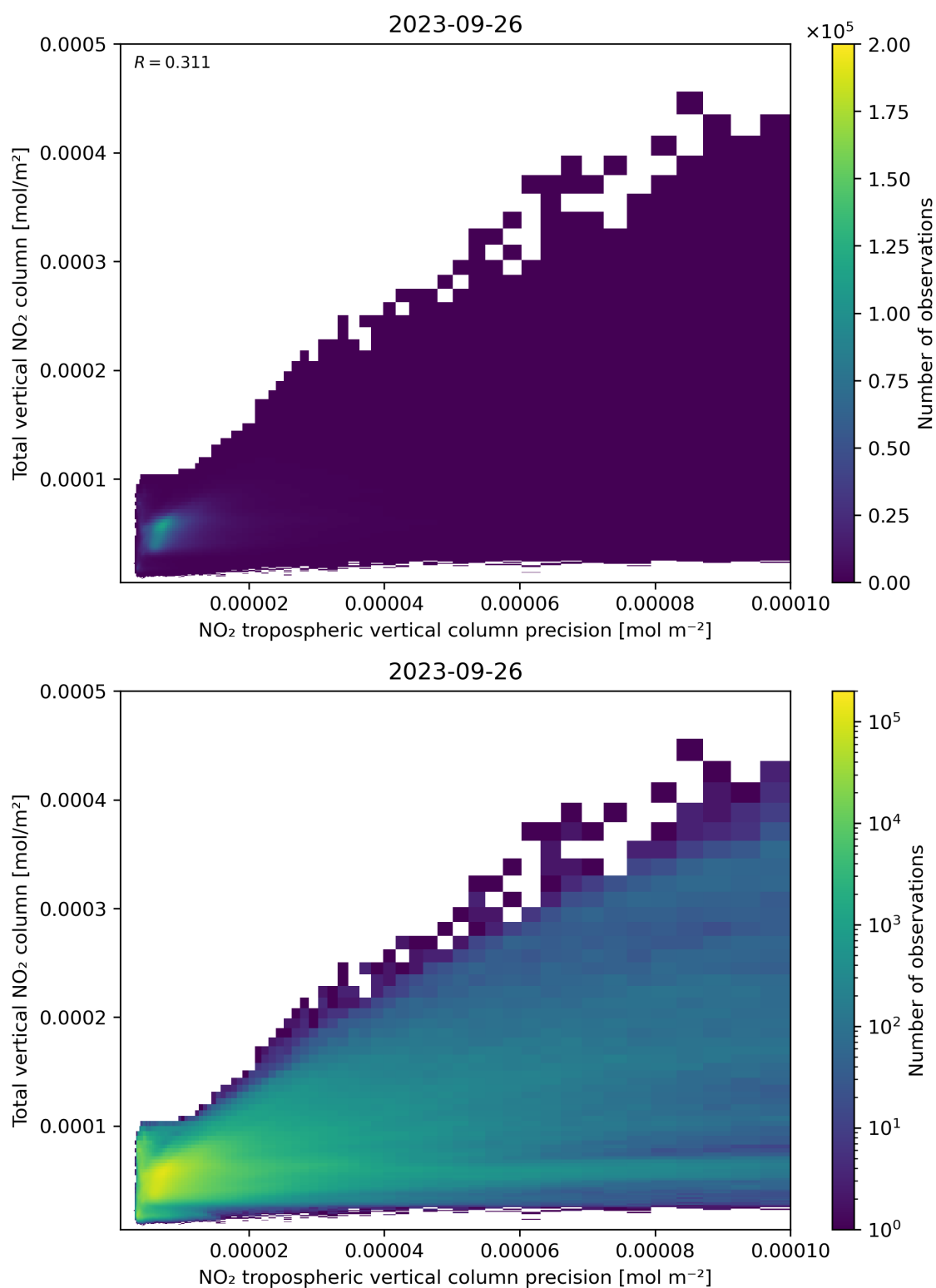
Figure 138: Scatter density plot of “NO 2 tropospheric vertical column precision” against “Total vertical NO 2 column” for 2023-09-26 to 2023-09-27.
