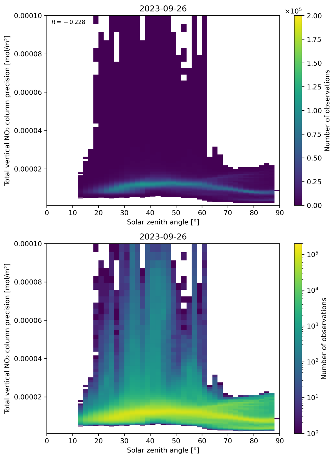
Figure 154: Scatter density plot of “Solar zenith angle” against “Total vertical NO 2 column precision” for 2023-09-26 to 2023-09-27.
