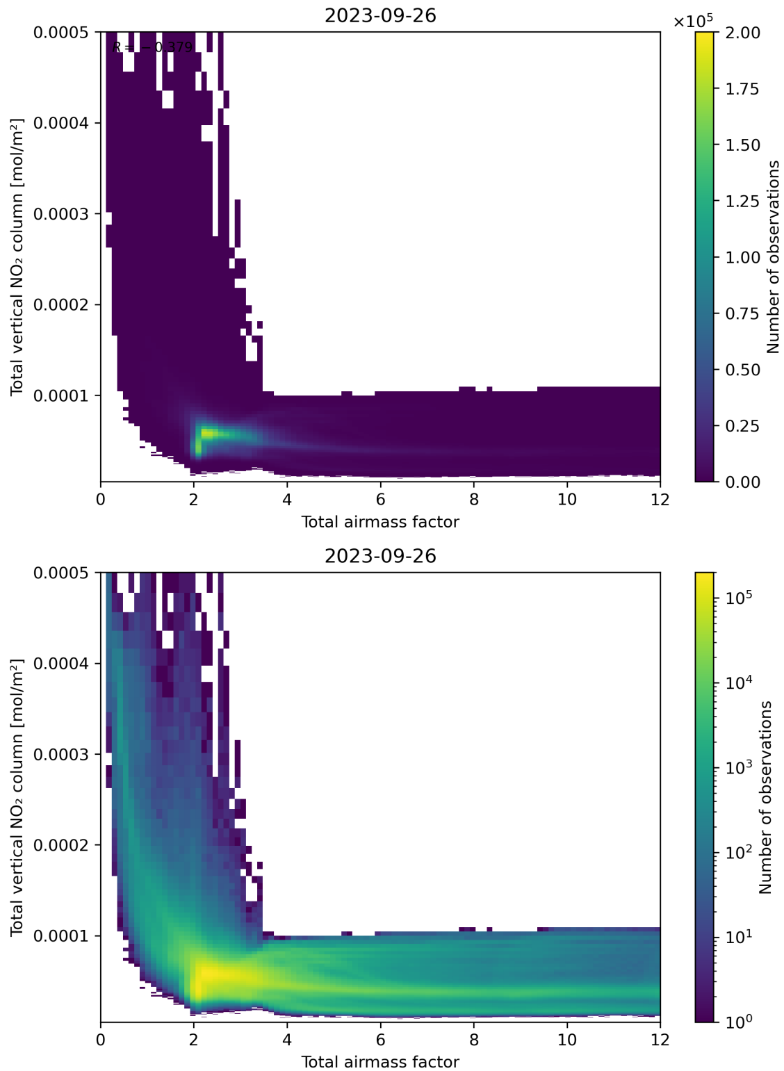
Figure 67: Scatter density plot of “Total airmass factor” against “Total vertical NO 2 column” for 2023-09-26 to 2023-09-27.
