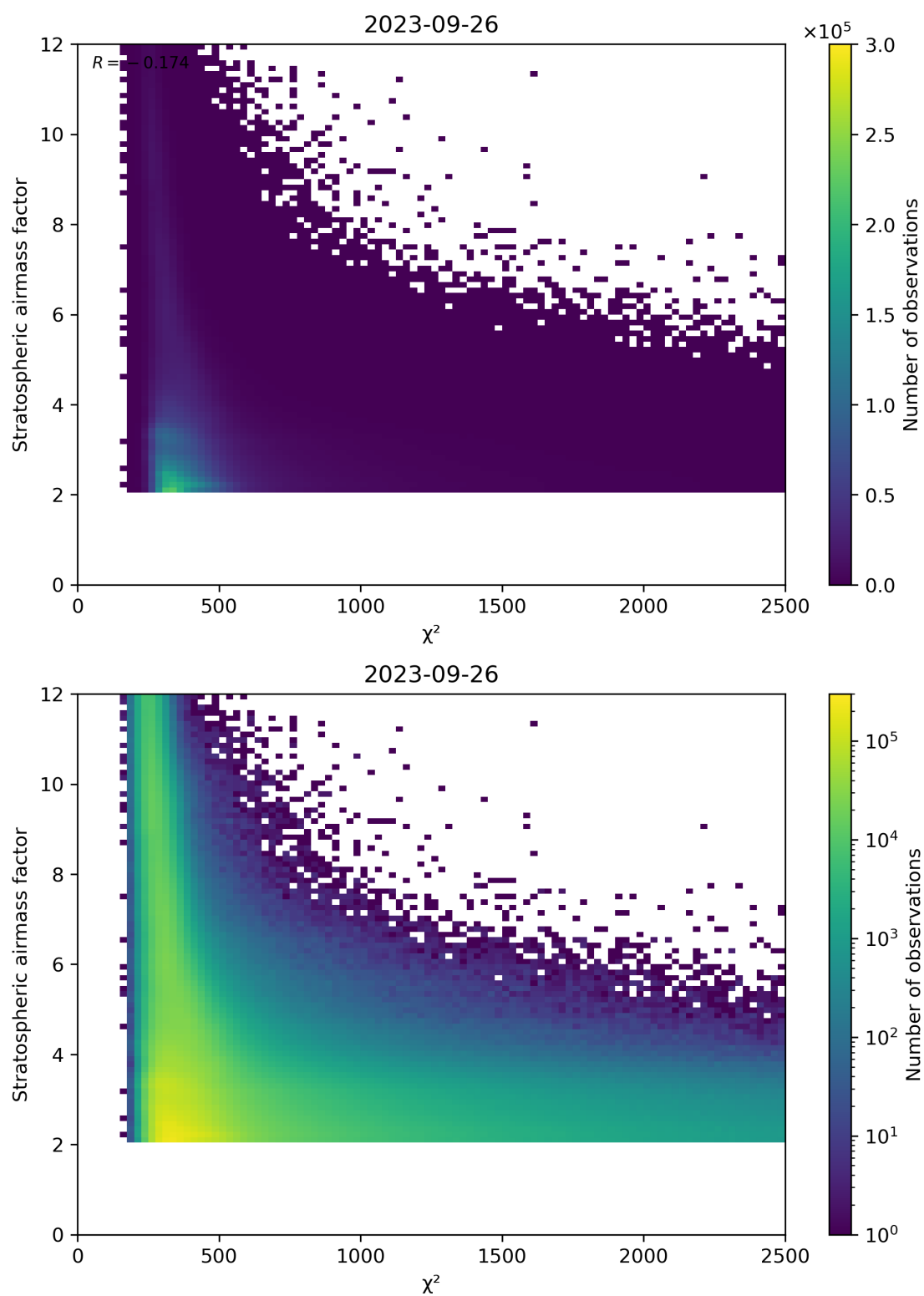
Figure 81: Scatter density plot of “ \chi^2 ” against “Stratospheric airmass factor” for 2023-09-26 to 2023-09-27.
