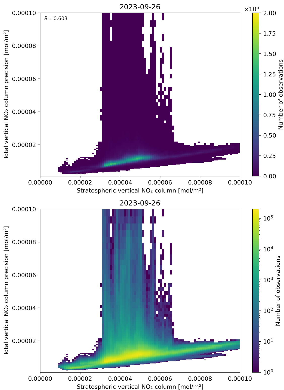
Figure 101: Scatter density plot of “Stratospheric vertical NO 2 column” against “Total vertical NO 2 column precision” for 2023-09-26 to 2023-09-27.
