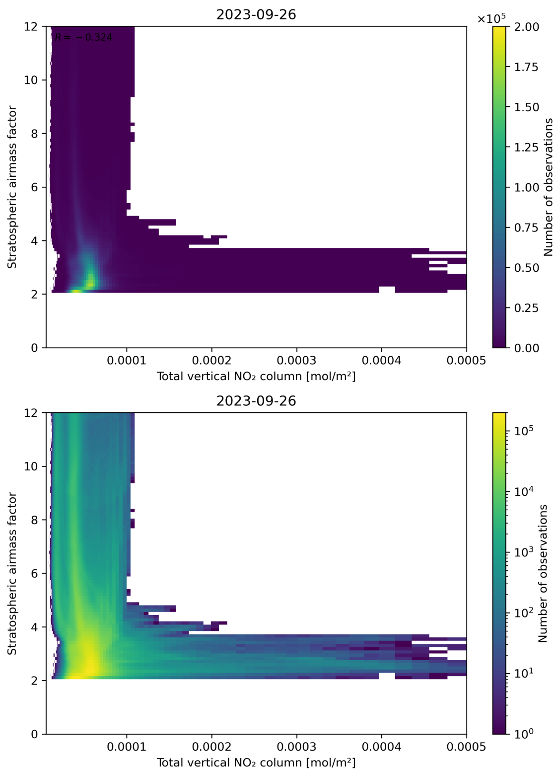
Figure 110: Scatter density plot of “Total vertical NO 2 column” against “Stratospheric airmass factor” for 2023-09-26 to 2023-09-27.
