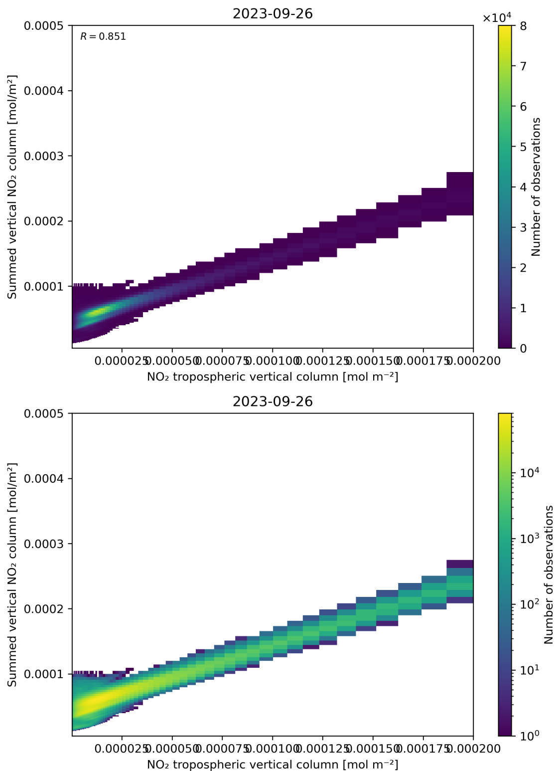
Figure 126: Scatter density plot of “NO 2 tropospheric vertical column” against “Summed vertical NO 2 column” for 2023-09-26 to 2023-09-27.
