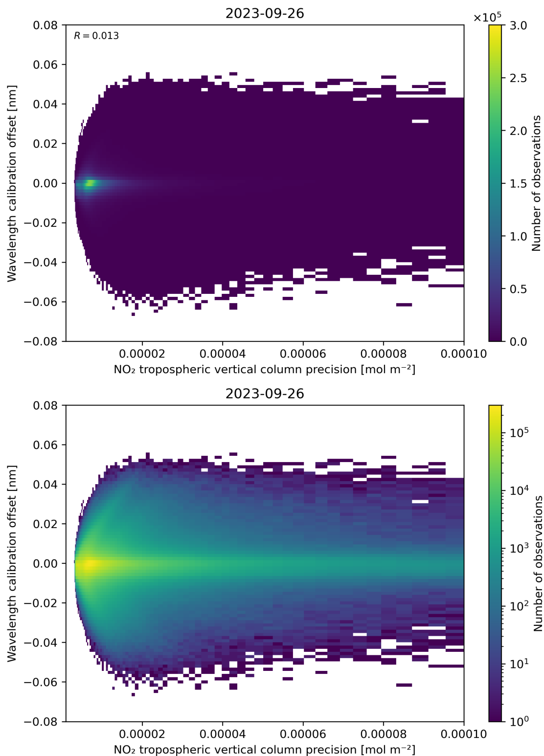
Figure 141: Scatter density plot of “NO 2 tropospheric vertical column precision” against “Wavelength calibration offset” for 2023-09-26 to 2023-09-27.
