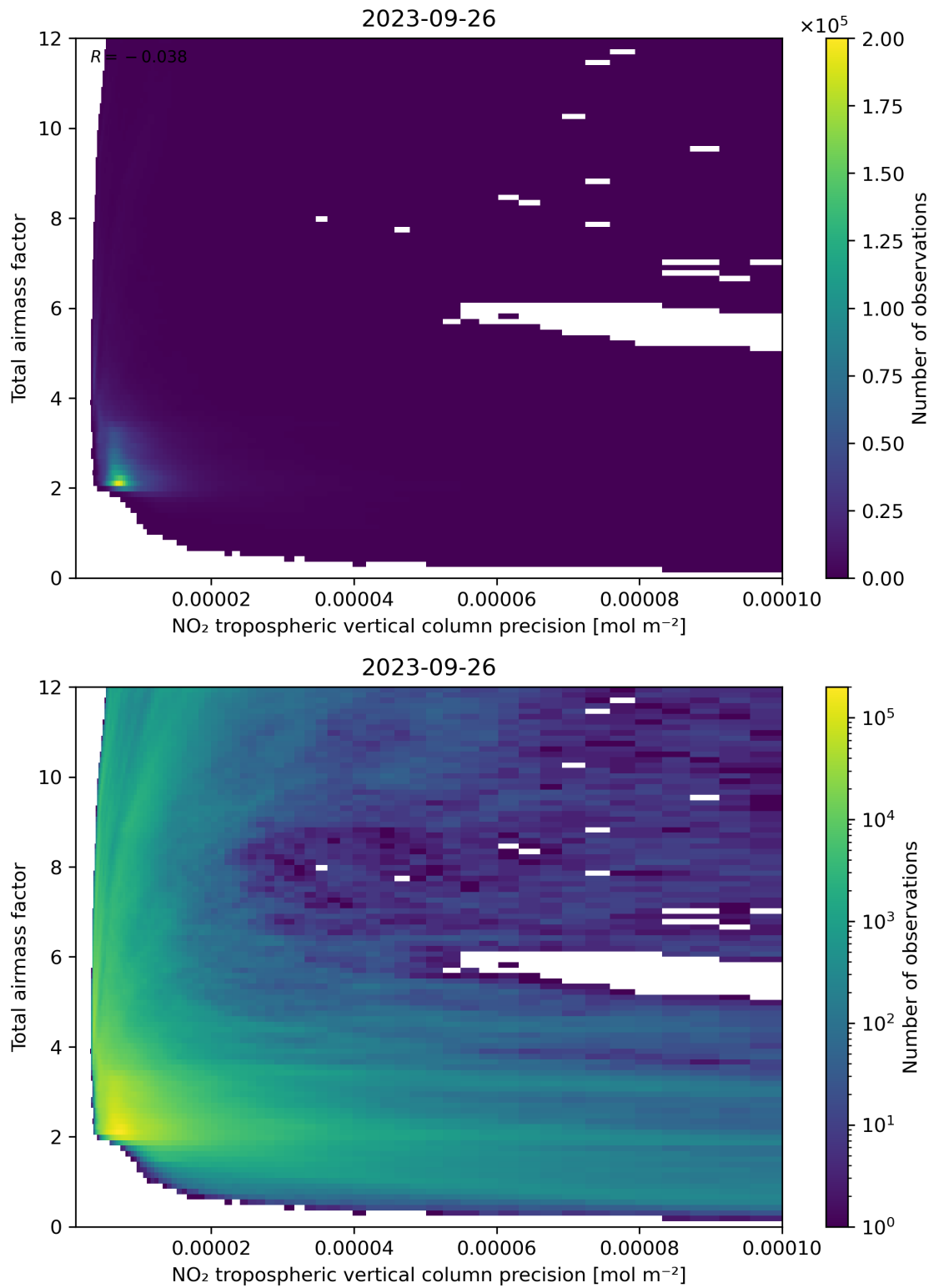
Figure 132: Scatter density plot of “NO 2 tropospheric vertical column precision” against “Total air mass factor” for 2023-09-26 to 2023-09-27.
