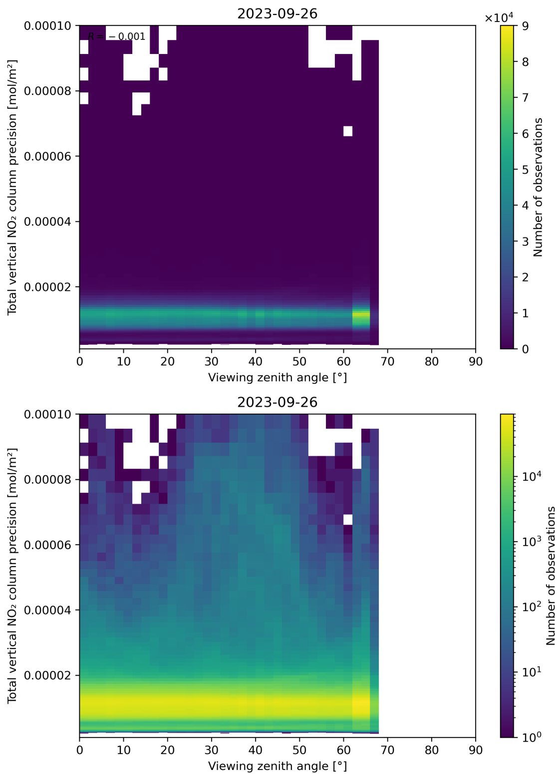
Figure 168: Scatter density plot of “Viewing zenith angle” against “Total vertical NO 2 column precision” for 2023-09-26 to 2023-09-27.
