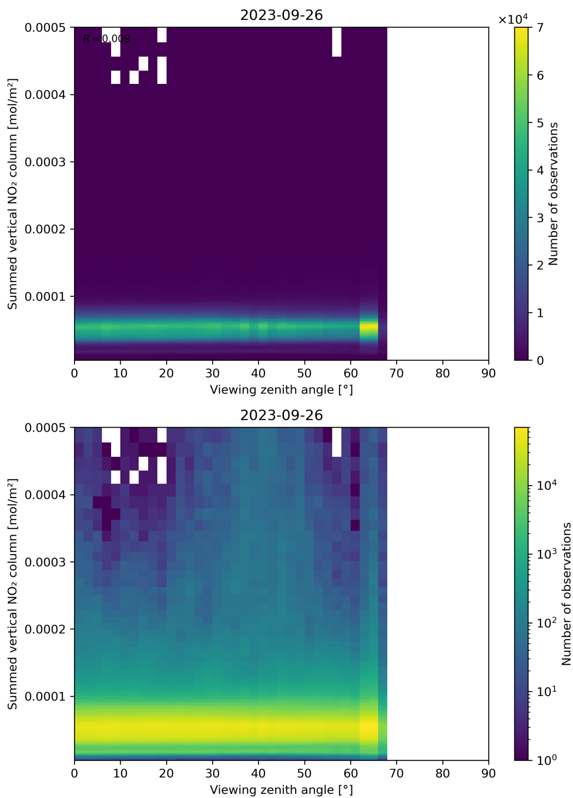
Figure 165: Scatter density plot of “Viewing zenith angle” against “Summed vertical NO 2 column” for 2023-09-26 to 2023-09-27.
