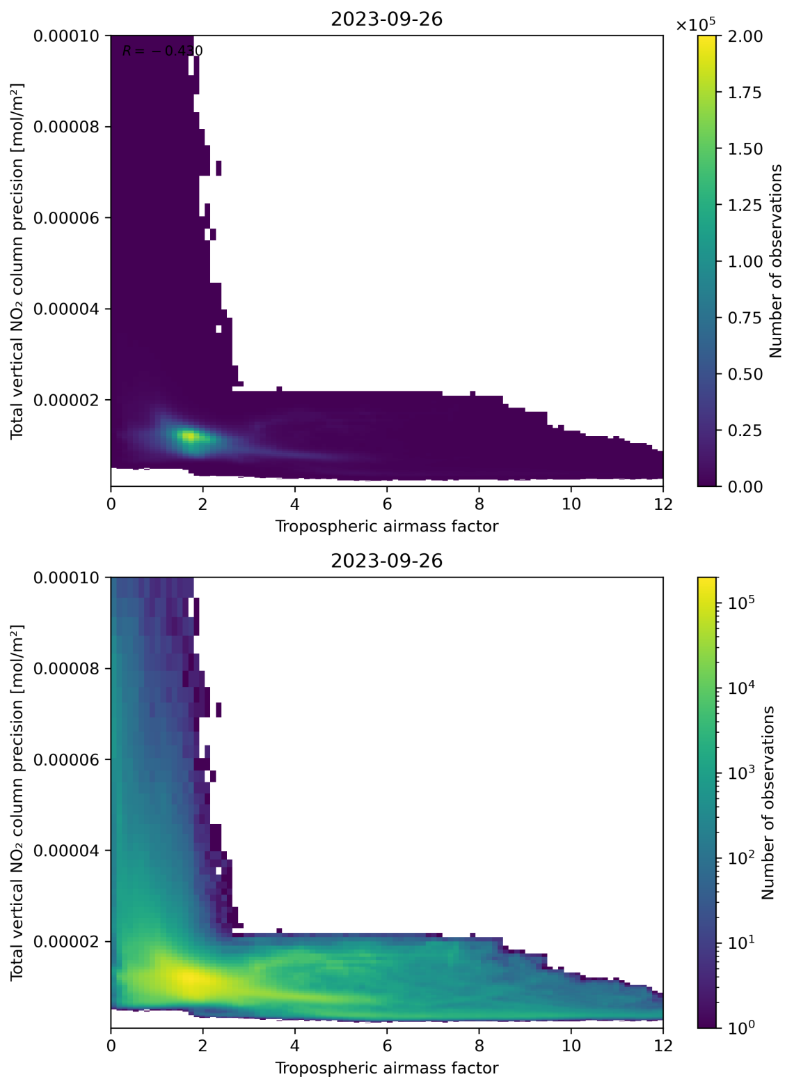
Figure 78: Scatter density plot of “Tropospheric air mass factor” against “Total vertical NO 2 column precision” for 2023-09-26 to 2023-09-27.
