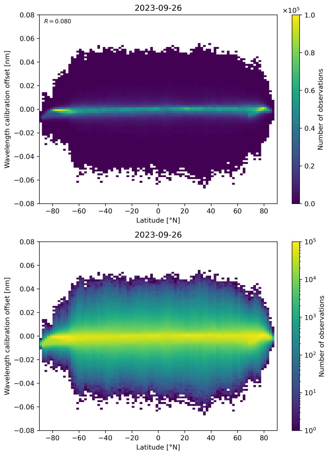
Figure 95: Scatter density plot of “Latitude” against “Wavelength calibration offset” for 2023-09-26 to 2023-09-27.
