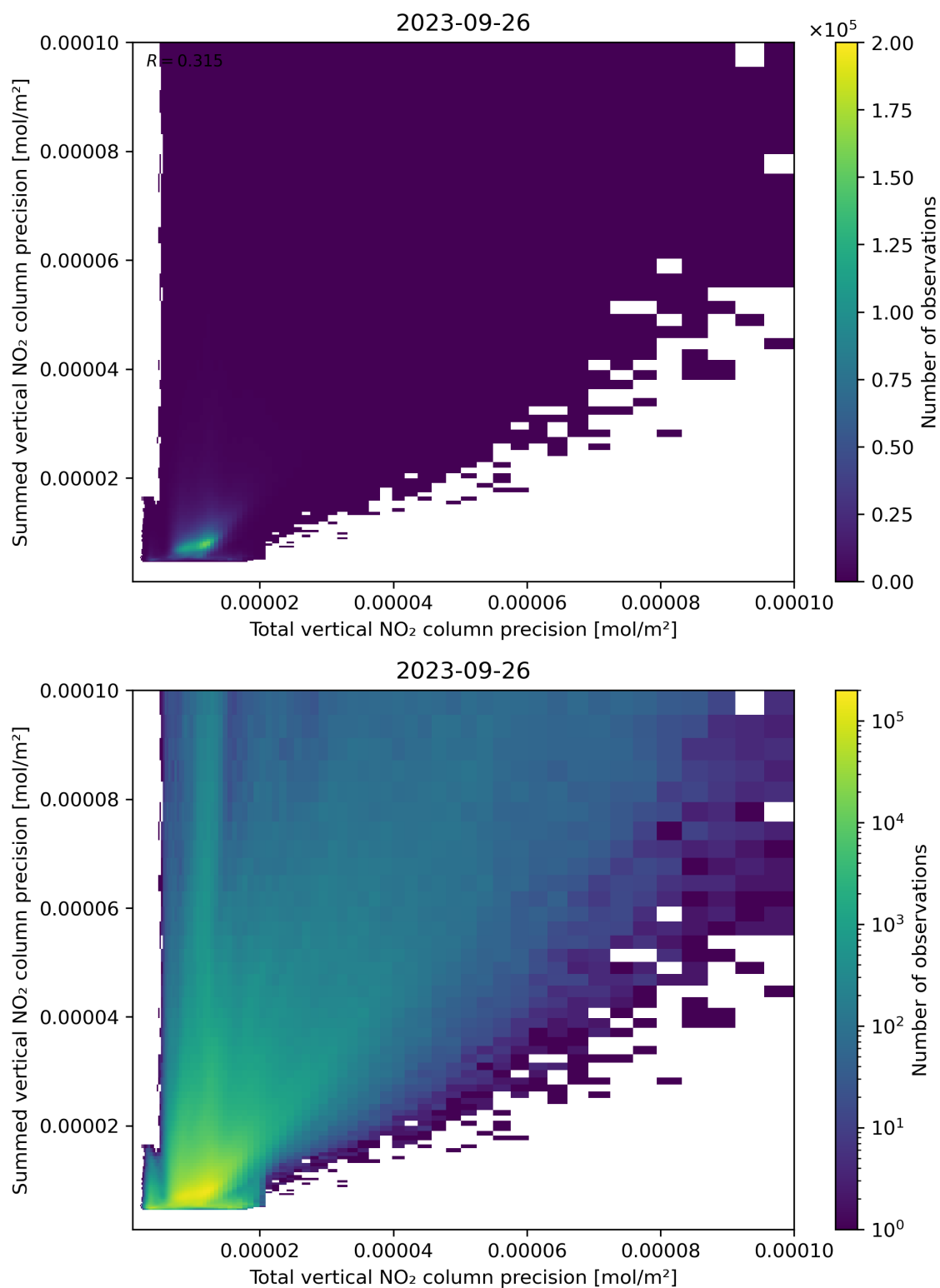
Figure 118: Scatter density plot of “Total vertical NO 2 column precision” against “Summed vertical NO 2 column precision” for 2023-09-26 to 2023-09-27.
