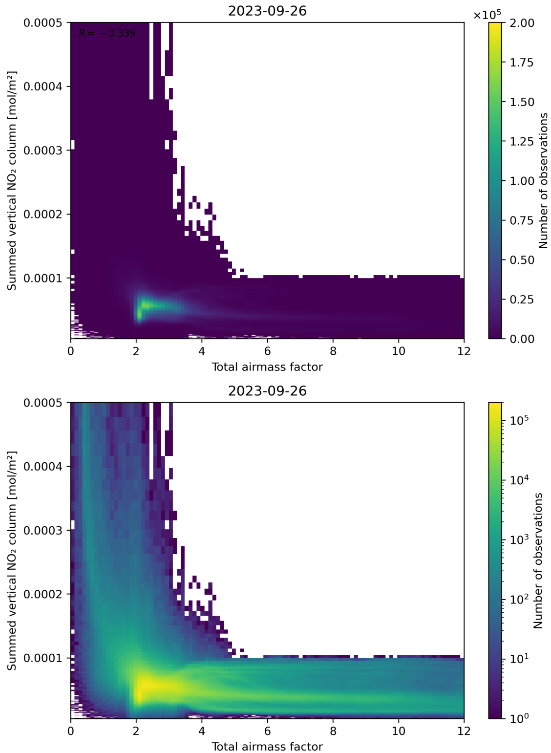
Figure 65: Scatter density plot of “Total airmass factor” against “Summed vertical NO 2 column” for 2023-09-26 to 2023-09-27.
