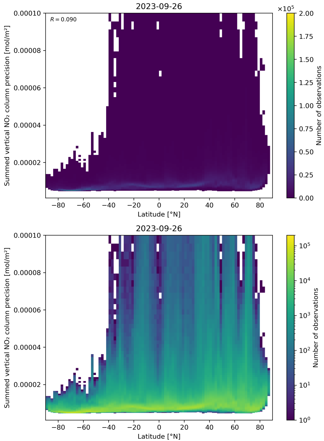
Figure 89: Scatter density plot of “Latitude” against “Summed vertical NO 2 column precision” for 2023-09-26 to 2023-09-27.
