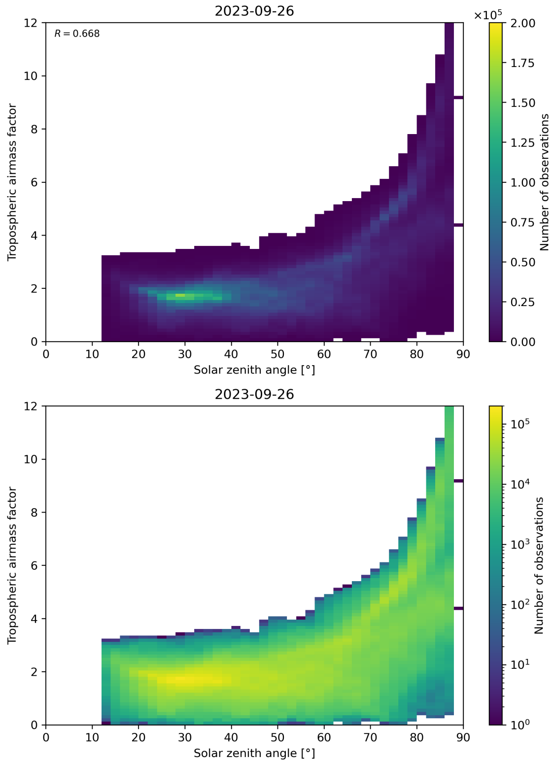
Figure 147: Scatter density plot of “Solar zenith angle” against “Tropospheric airmass factor” for 2023-09-26 to 2023-09-27.
