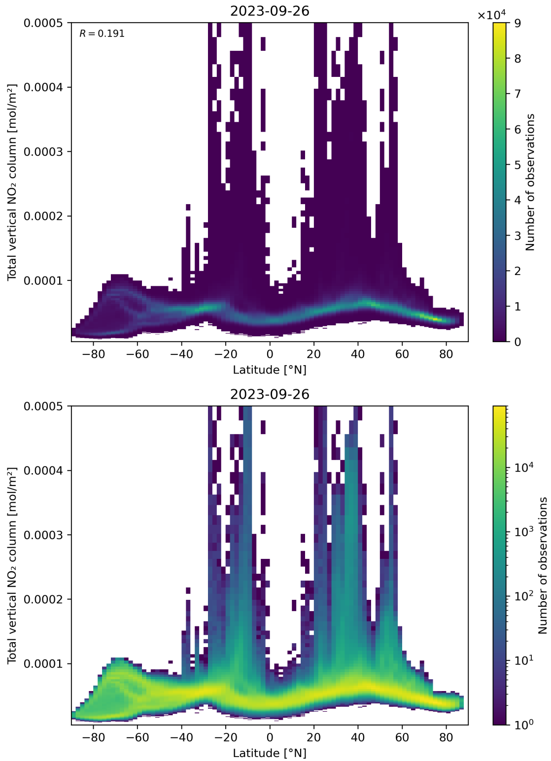
Figure 90: Scatter density plot of “Latitude” against “Total vertical NO 2 column” for 2023-09-26 to 2023-09-27.
