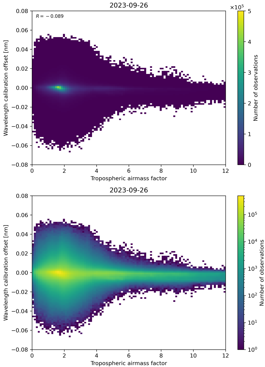
Figure 80: Scatter density plot of “Tropospheric airmass factor” against “Wavelength calibration offset” for 2023-09-26 to 2023-09-27.
