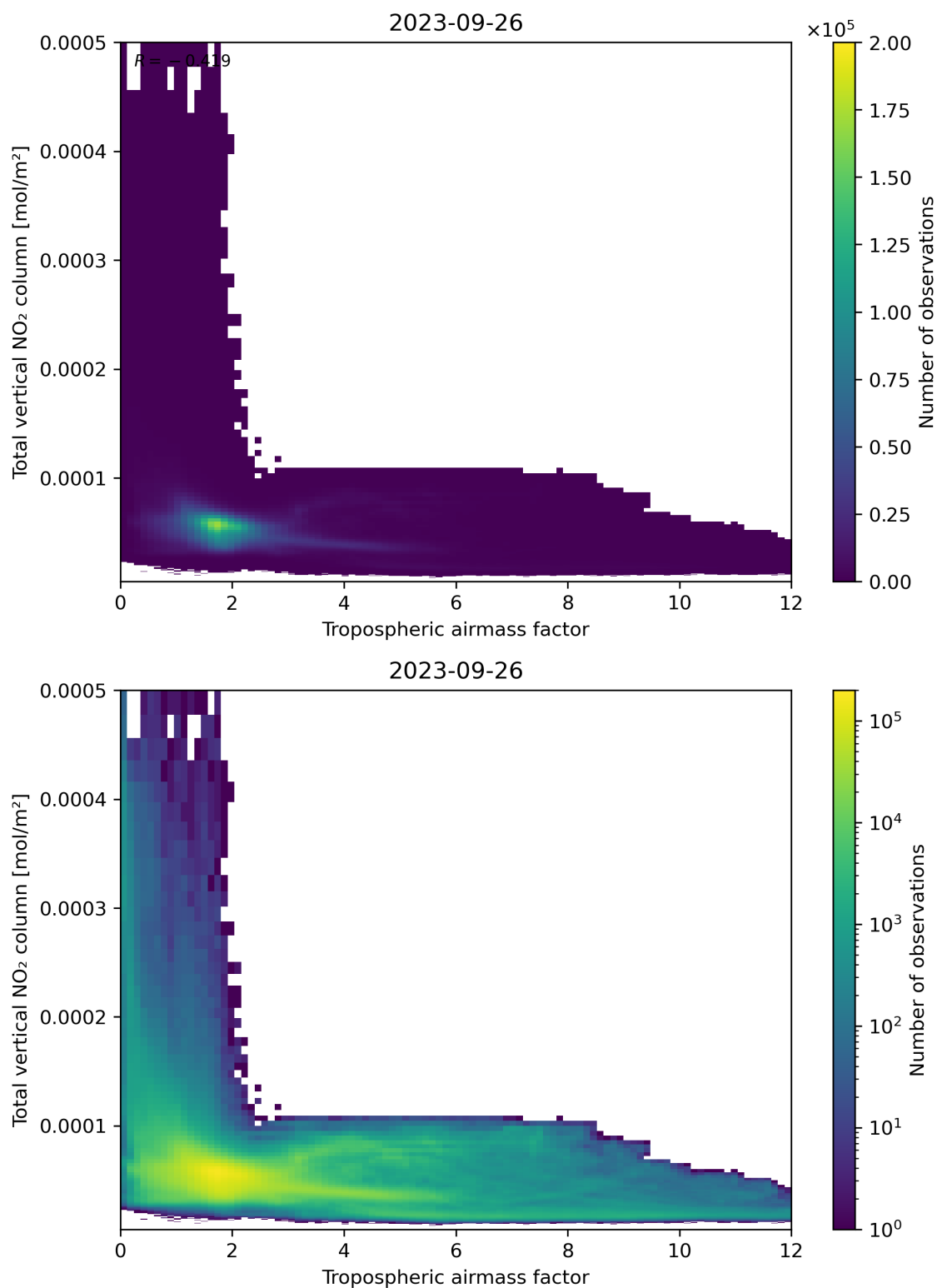
Figure 77: Scatter density plot of “Tropospheric airmass factor” against “Total vertical NO 2 column” for 2023-09-26 to 2023-09-27.
