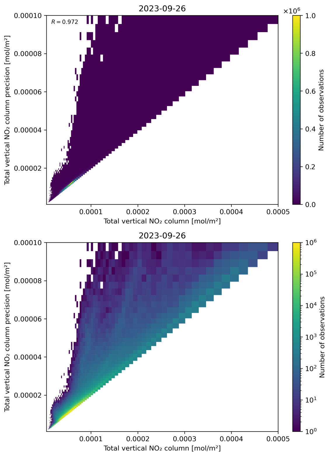
Figure 114: Scatter density plot of “Total vertical NO 2 column” against “Total vertical NO 2 column precision” for 2023-09-26 to 2023-09-27.
