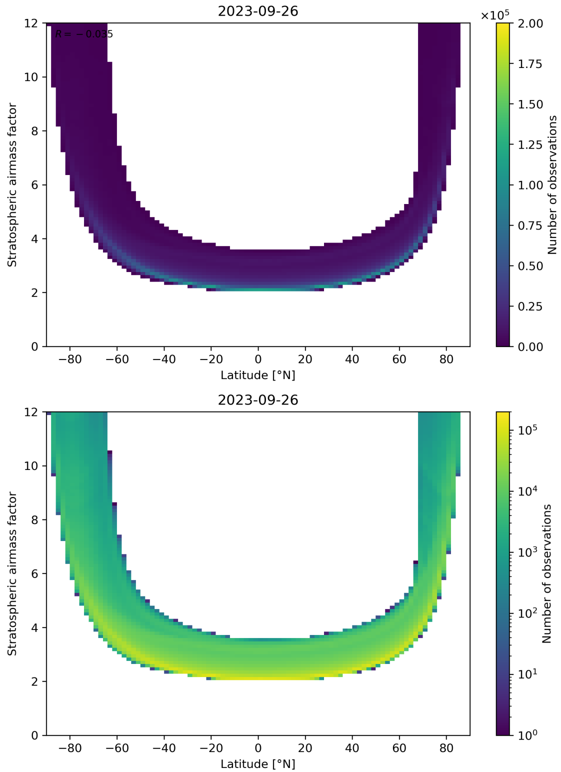
Figure 83: Scatter density plot of “Latitude” against “Stratospheric air mass factor” for 2023-09-26 to 2023-09-27.
