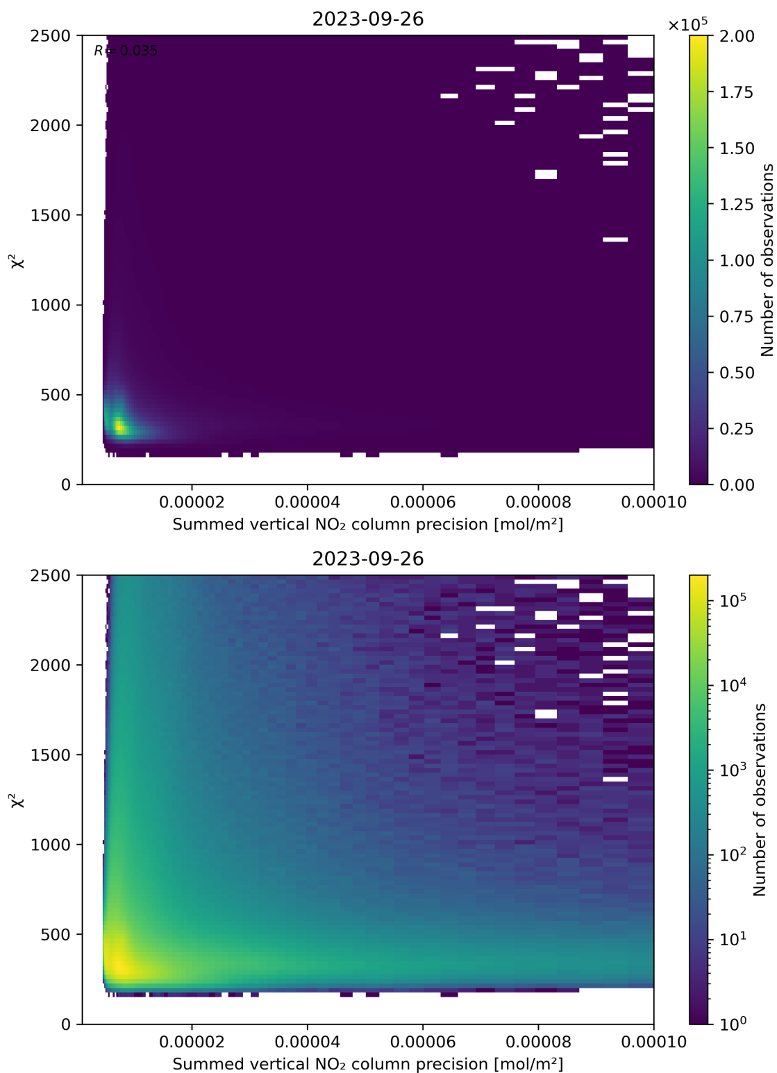
Figure 107: Scatter density plot of “Summed vertical NO 2 column precision” against “ \chi^2 ” for 2023-09-26 to 2023-09-27.
