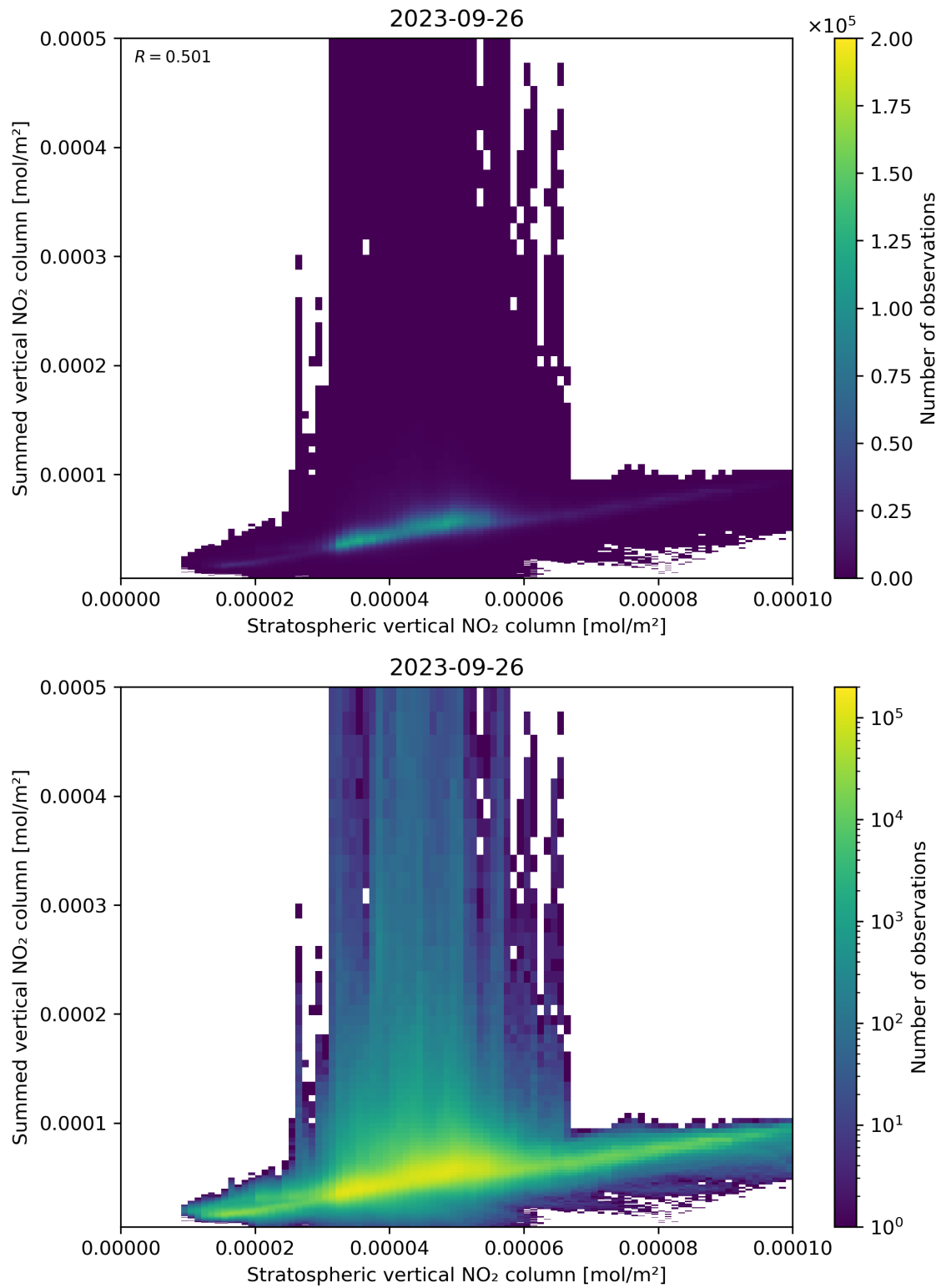
Figure 98: Scatter density plot of “Stratospheric vertical NO 2 column” against “Summed vertical NO 2 column” for 2023-09-26 to 2023-09-27.
