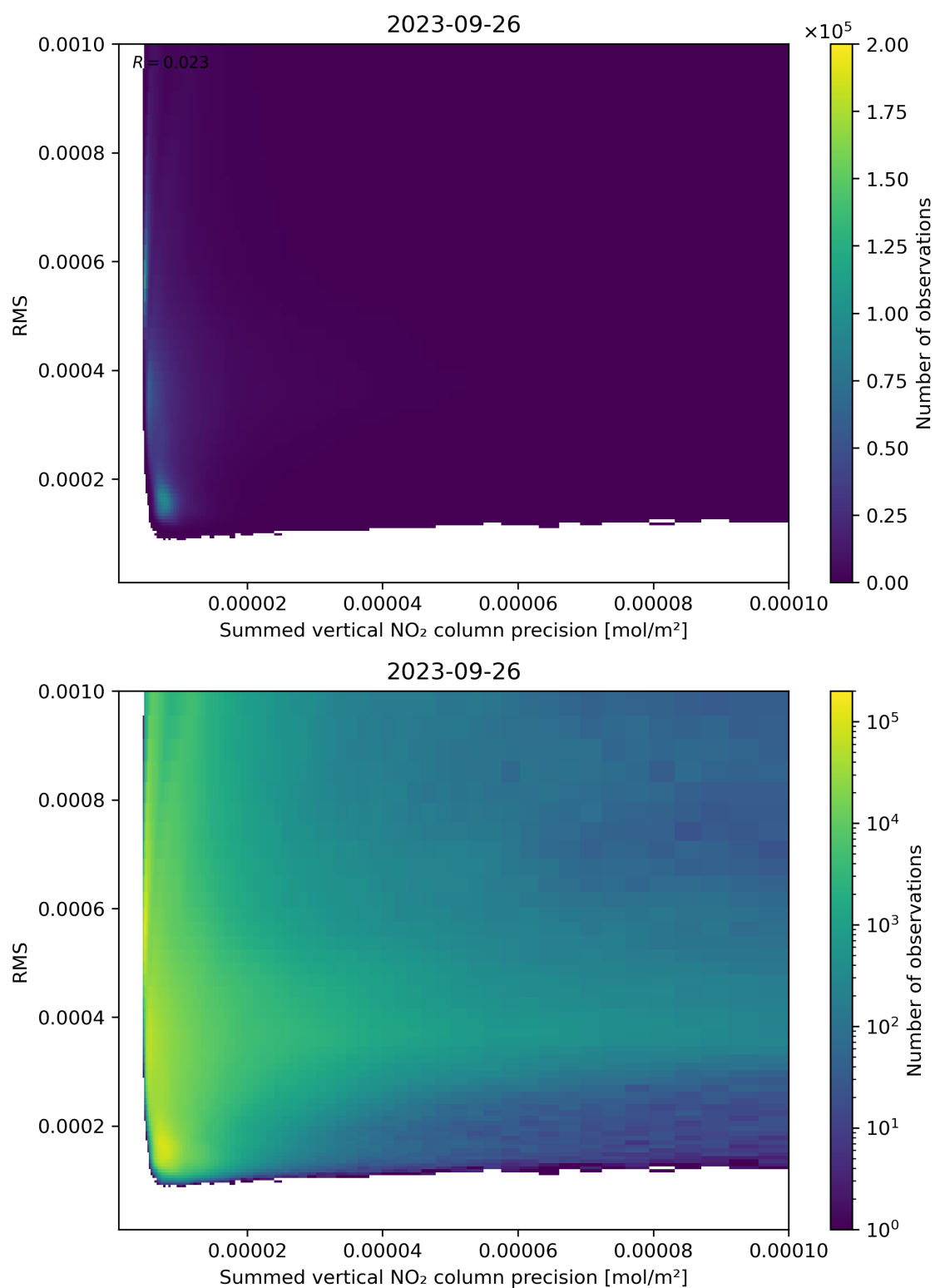
Figure 108: Scatter density plot of “Summed vertical NO 2 column precision” against “RMS” for 2023-09-26 to 2023-09-27.
