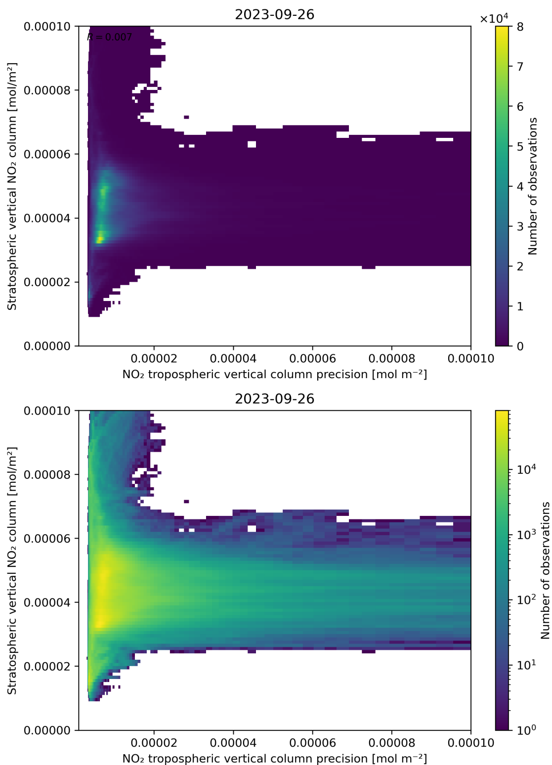
Figure 135: Scatter density plot of “NO 2 tropospheric vertical column precision” against “Stratospheric vertical NO 2 column” for 2023-09-26 to 2023-09-27.
