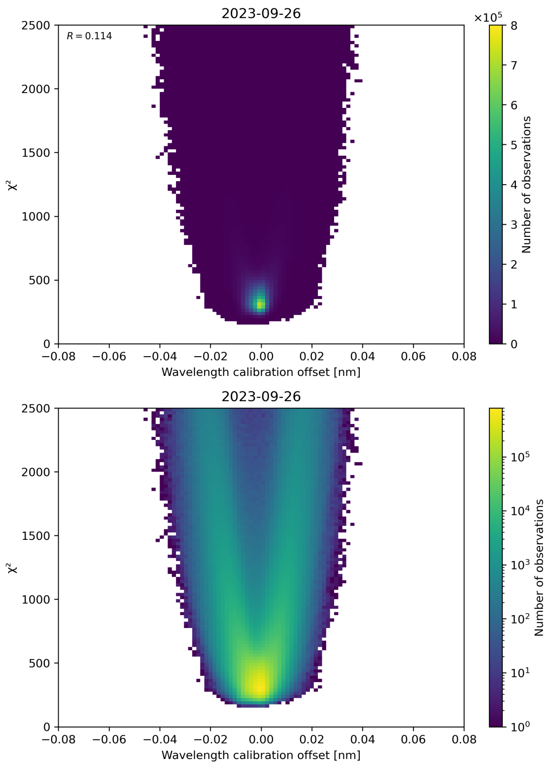
Figure 175: Scatter density plot of “Wavelength calibration offset” against “ \chi^2 ” for 2023-09-26 to 2023-09-27.
