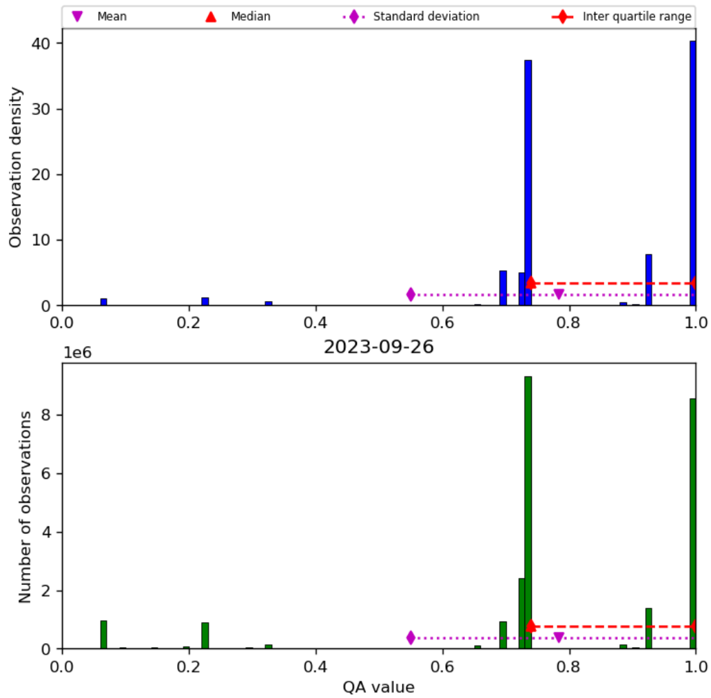
Figure 28: Histogram of “QA value” for 2023-09-26 to 2023-09-27
