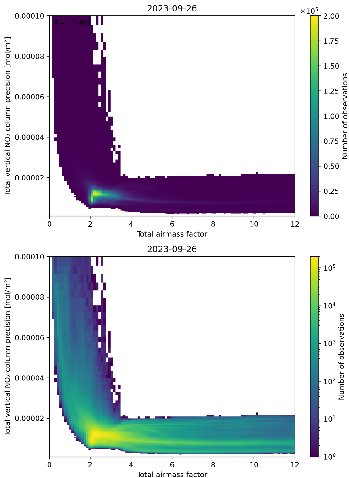
Figure 68: Scatter density plot of “Total airmass factor” against “Total vertical NO 2 column precision” for 2023-09-26 to 2023-09-27.
