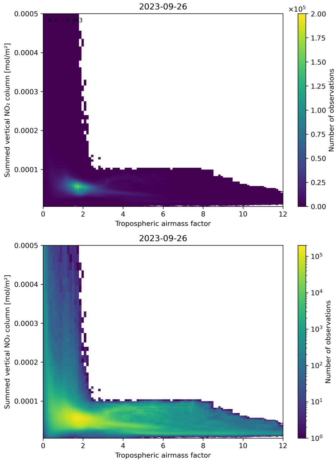
Figure 75: Scatter density plot of “Tropospheric air mass factor” against “Summed vertical NO 2 column” for 2023-09-26 to 2023-09-27.
