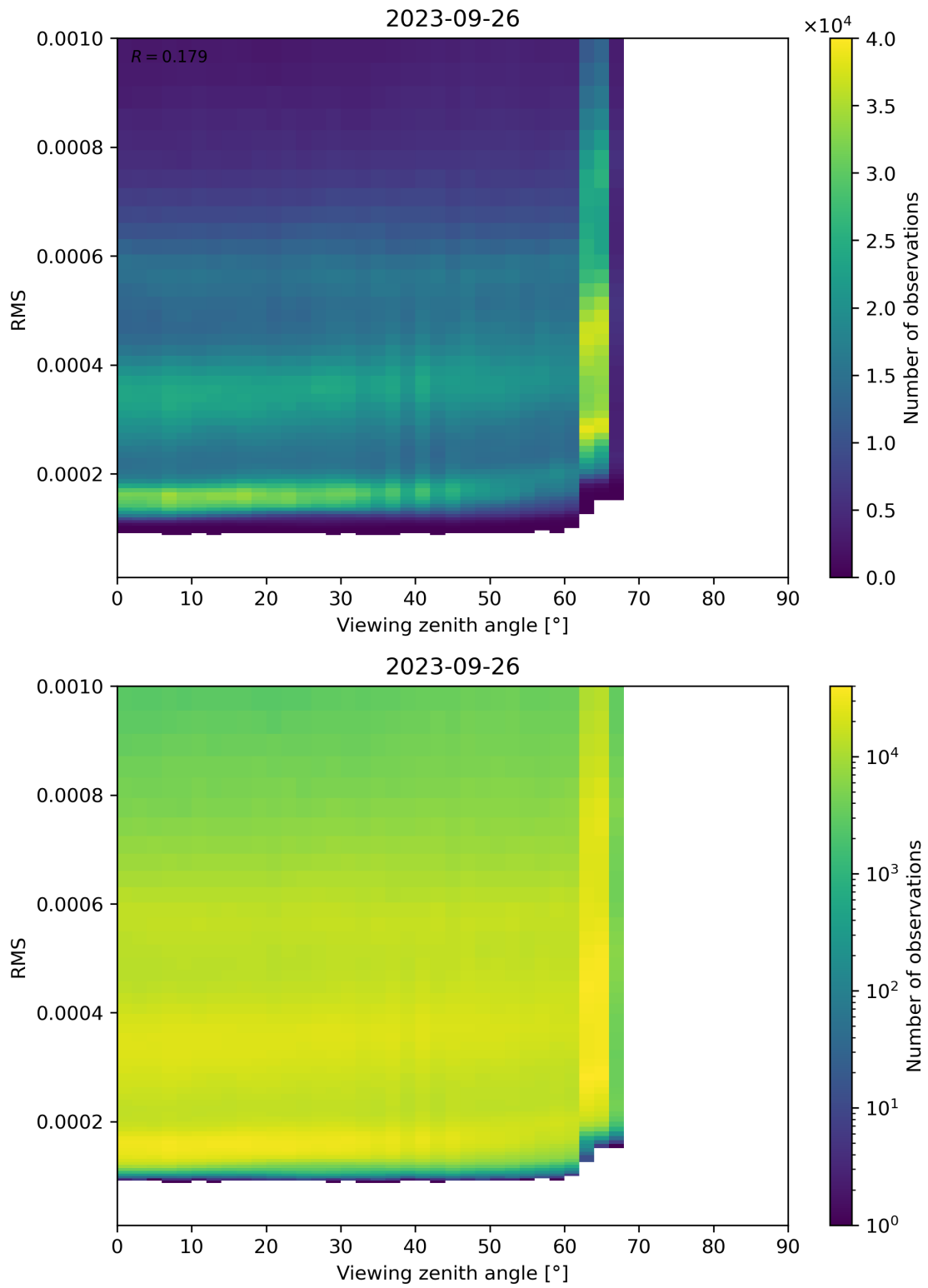
Figure 171: Scatter density plot of “Viewing zenith angle” against “RMS” for 2023-09-26 to 2023-09-27.
