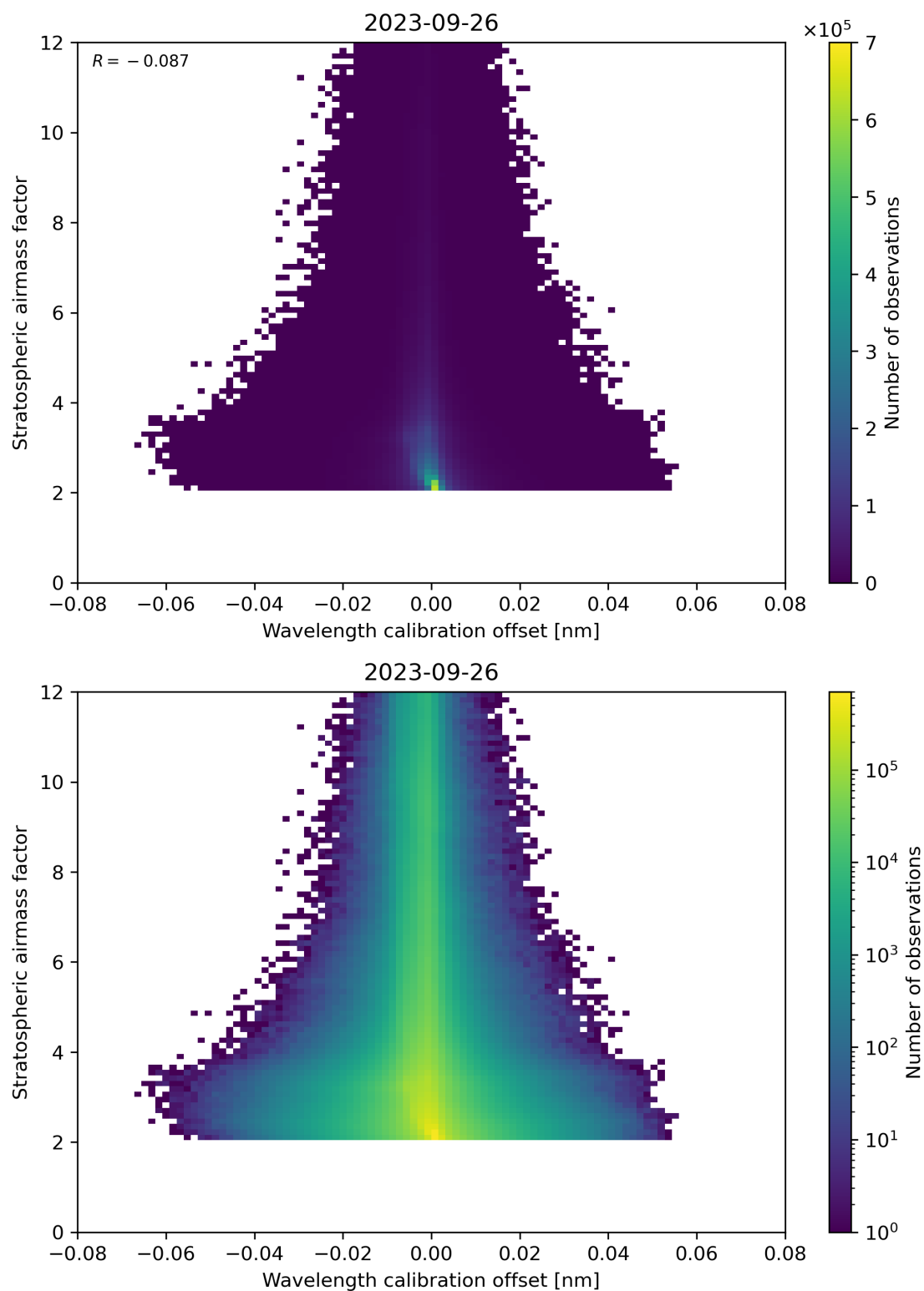
Figure 174: Scatter density plot of “Wavelength calibration offset” against “Stratospheric airmass factor” for 2023-09-26 to 2023-09-27.
