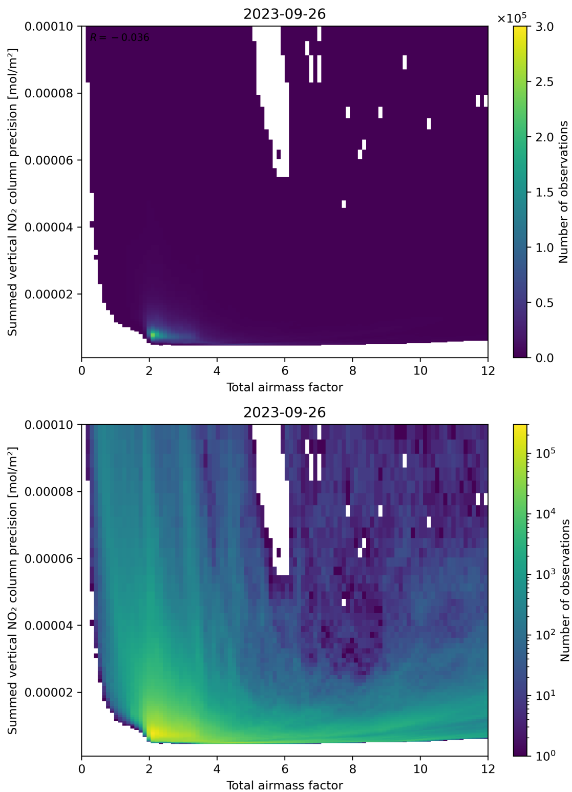
Figure 66: Scatter density plot of “Total airmass factor” against “Summed vertical NO 2 column precision” for 2023-09-26 to 2023-09-27.
