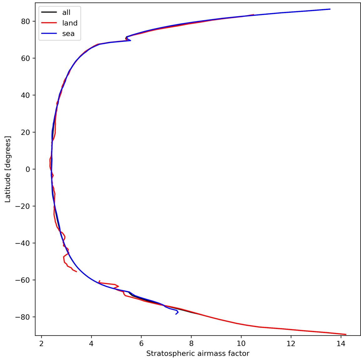
Figure 27: Zonal average of “Stratospheric air mass factor” for 2023-09-26 to 2023-09-27.
