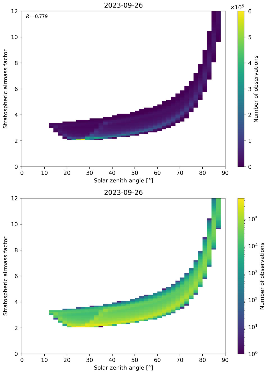
Figure 145: Scatter density plot of “Solar zenith angle” against “Stratospheric airmass factor” for 2023-09-26 to 2023-09-27.
