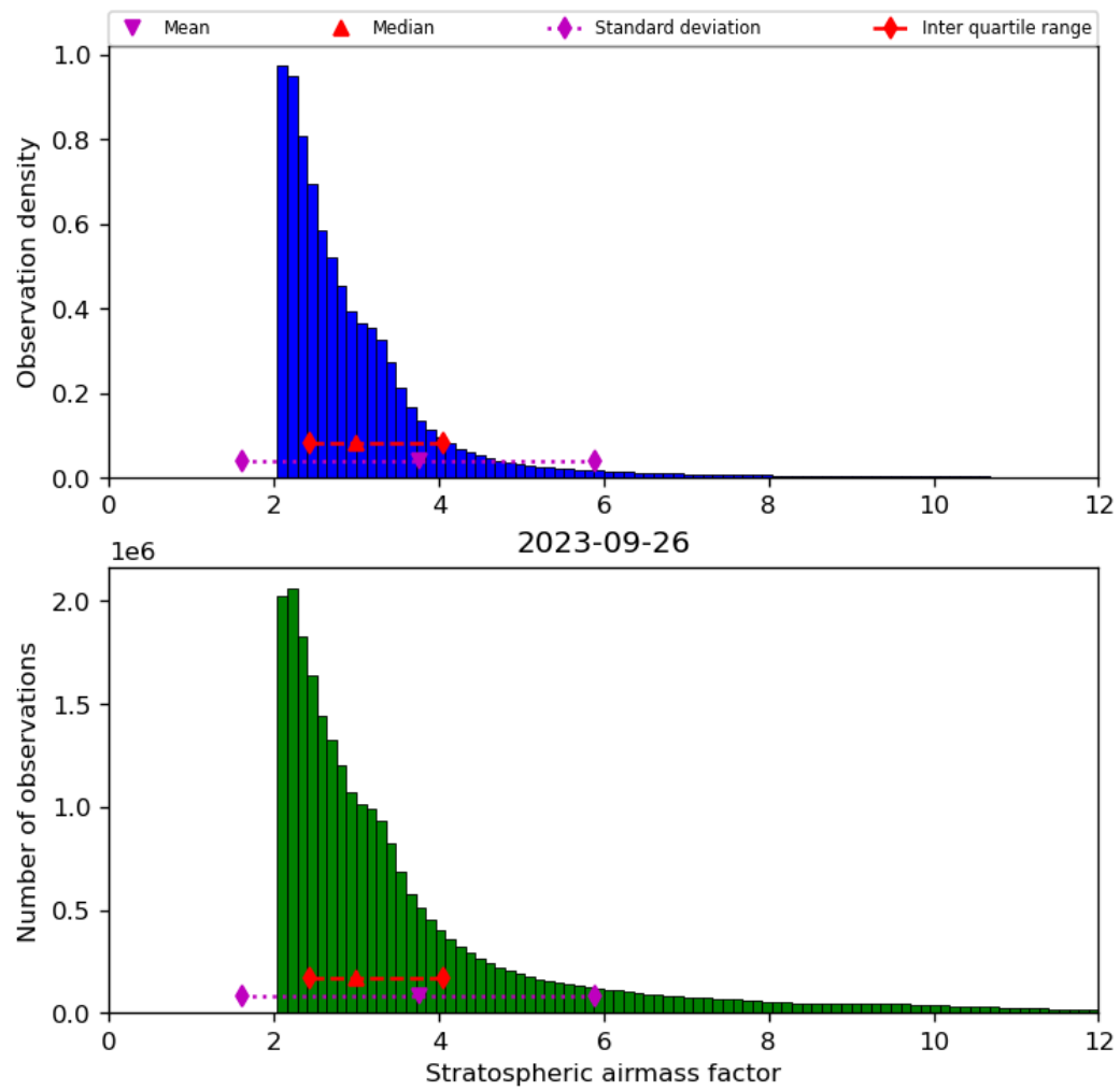
Figure 44: Histogram of “Stratospheric airmass factor” for 2023-09-26 to 2023-09-27
