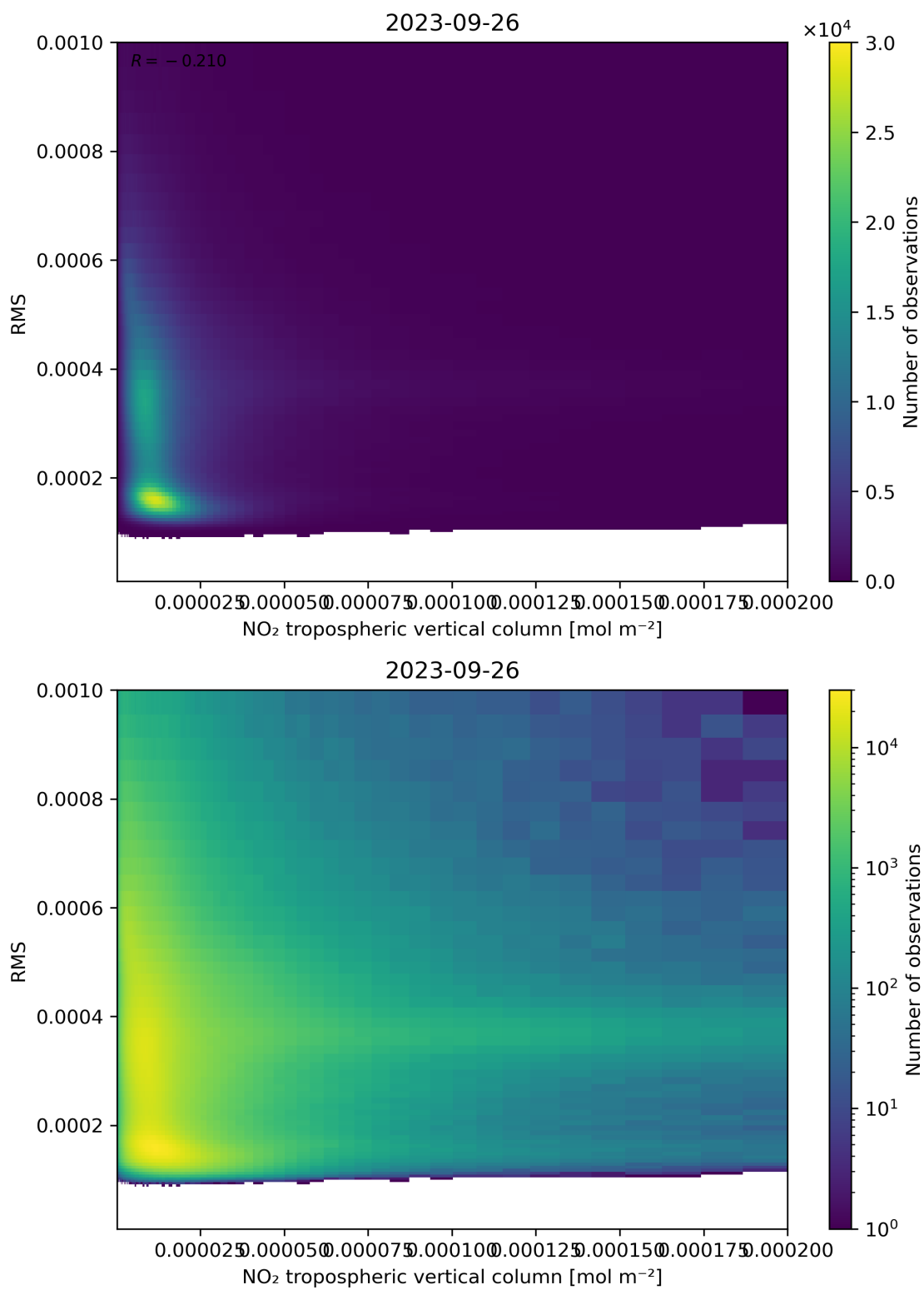
Figure 142: Scatter density plot of “NO 2 tropospheric vertical column” against “RMS” for 2023-09-26 to 2023-09-27.
