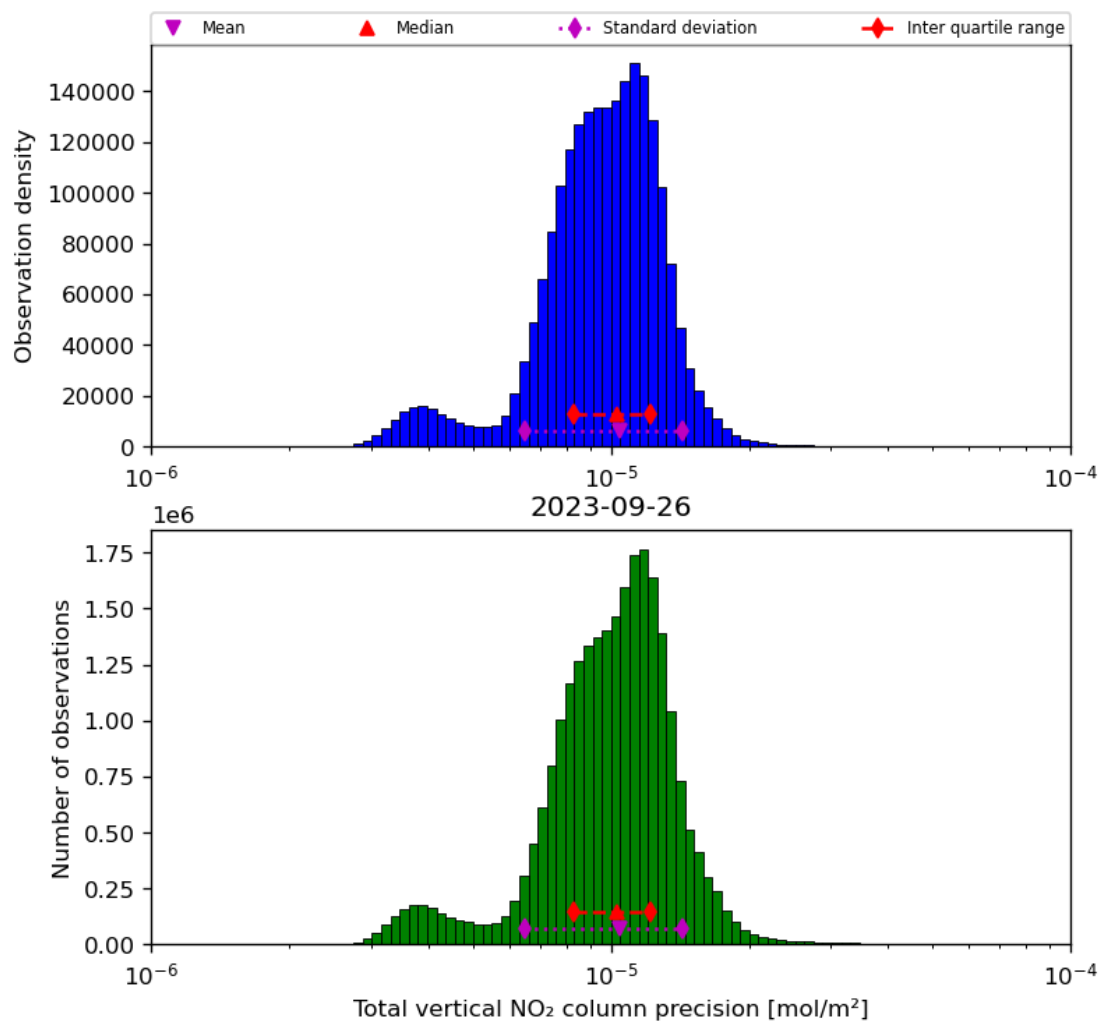
Figure 39: Histogram of “Total vertical NO 2 column precision” for 2023-09-26 to 2023-09-27
