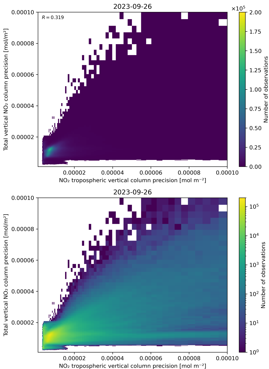
Figure 139: Scatter density plot of “NO 2 tropospheric vertical column precision” against “Total vertical NO 2 column precision” for 2023-09-26 to 2023-09-27.
