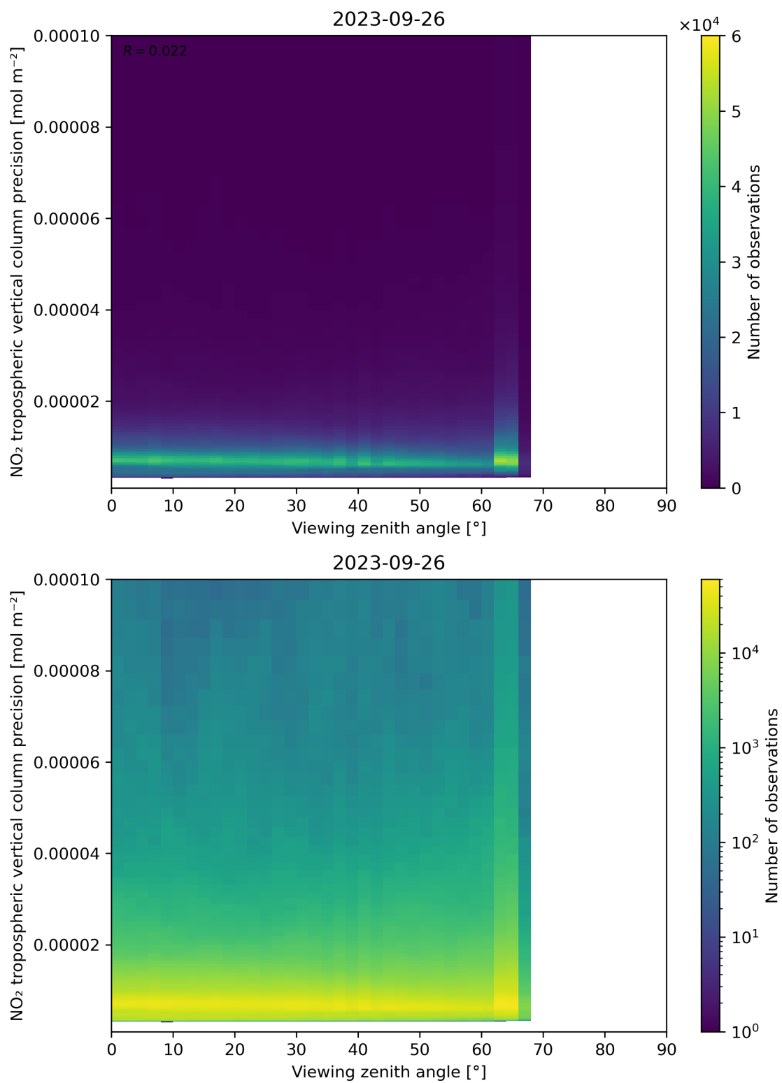
Figure 170: Scatter density plot of “Viewing zenith angle” against “NO 2 tropospheric vertical column precision” for 2023-09-26 to 2023-09-27.
