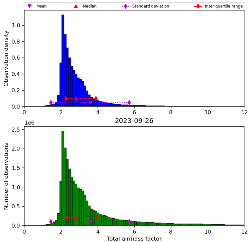
Figure 32: Histogram of “Total airmass factor” for 2023-09-26 to 2023-09-27
