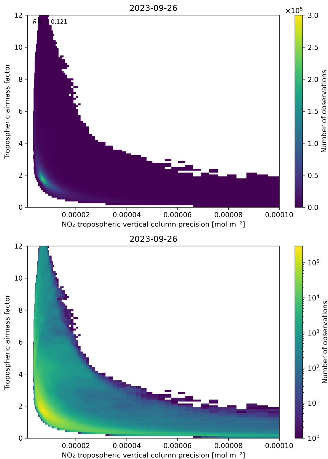
Figure 133: Scatter density plot of “NO 2 tropospheric vertical column precision” against “Tropospheric airmass factor” for 2023-09-26 to 2023-09-27.
