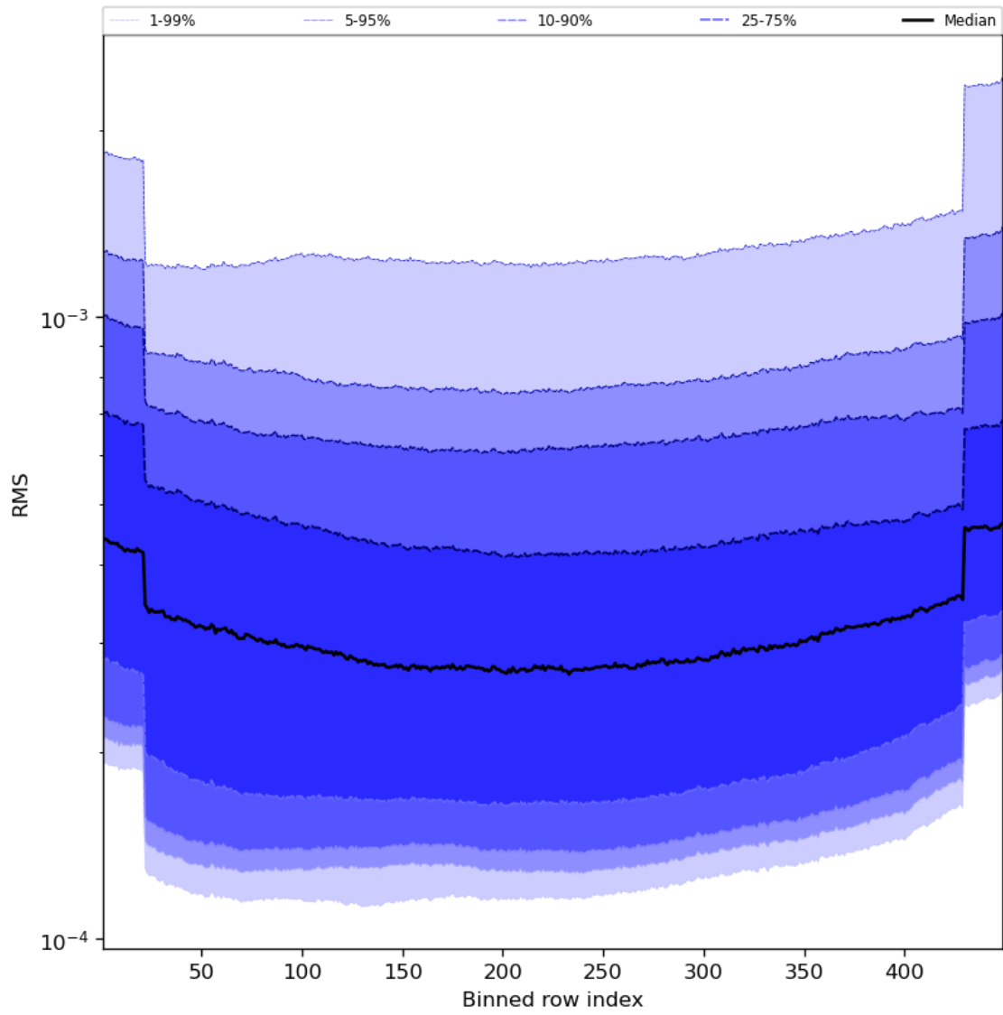
Figure 60: Along track statistics of “RMS” for 2023-09-26 to 2023-09-27
