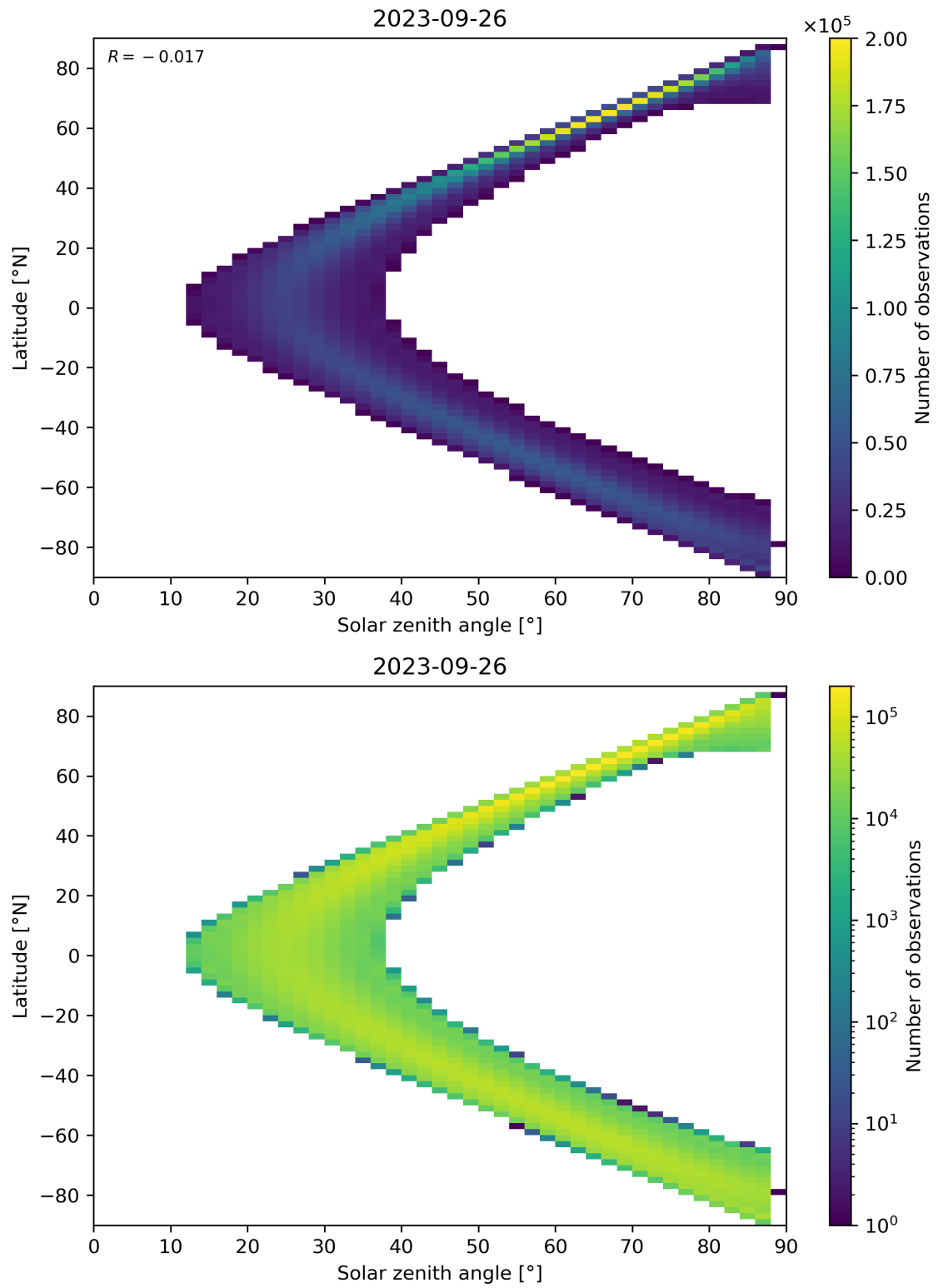
Figure 149: Scatter density plot of “Solar zenith angle” against “Latitude” for 2023-09-26 to 2023-09-27.
