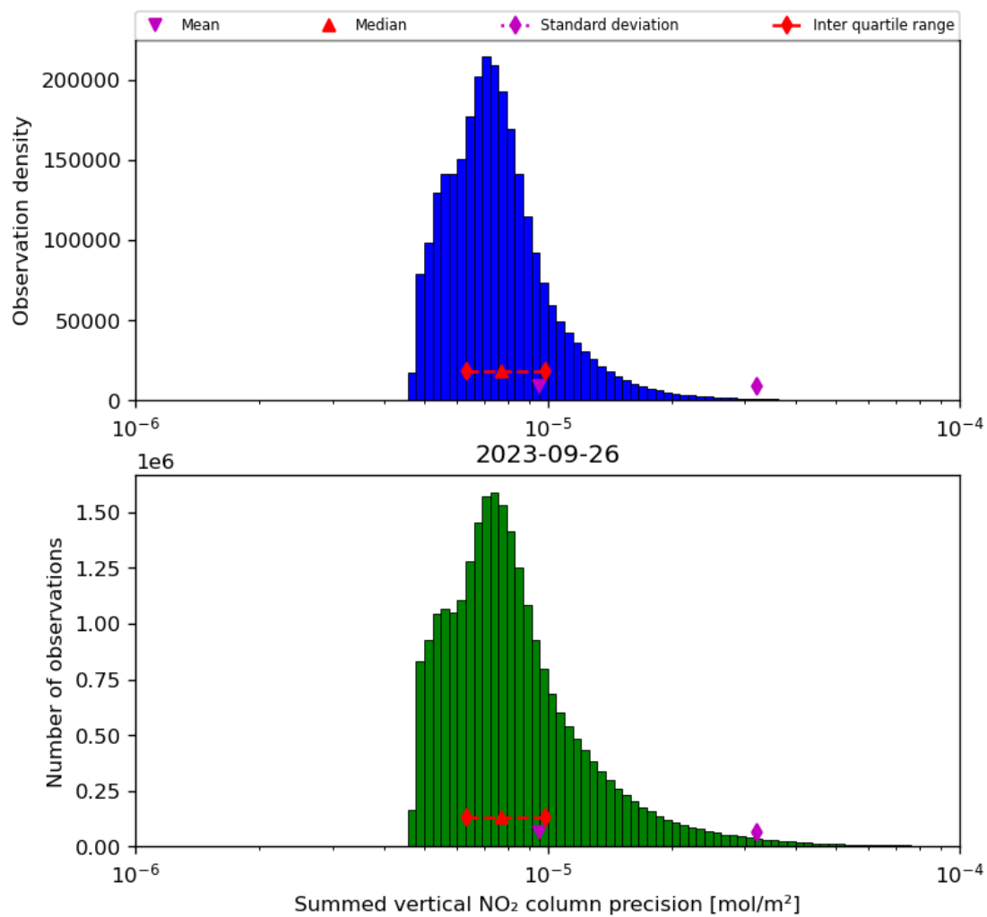
Figure 41: Histogram of “Summed vertical NO 2 column precision” for 2023-09-26 to 2023-09-27
