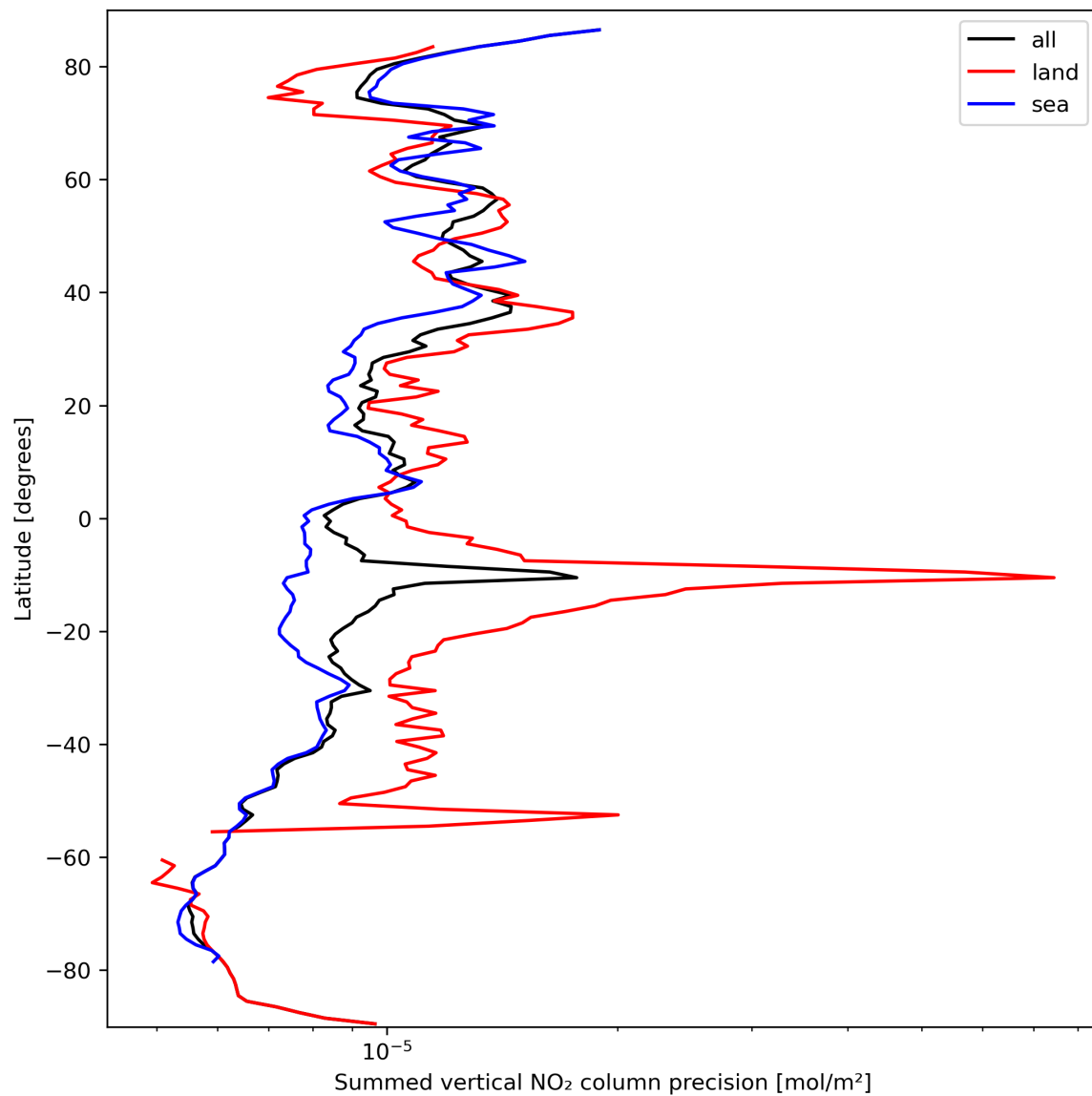
Figure 24: Zonal average of “Summed vertical NO 2 column precision” for 2023-09-26 to 2023-09-27.
