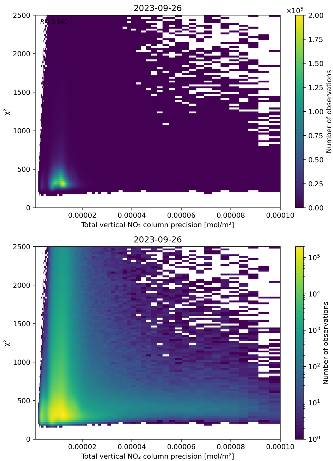
Figure 116: Scatter density plot of “Total vertical NO 2 column precision” against “ \chi^2 ” for 2023-09-26 to 2023-09-27.
