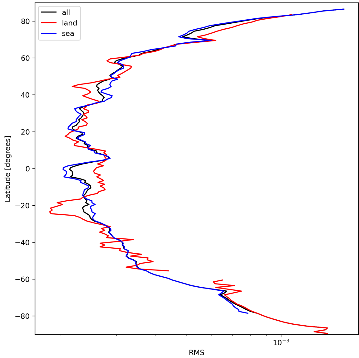
Figure 26: Zonal average of “RMS” for 2023-09-26 to 2023-09-27.
