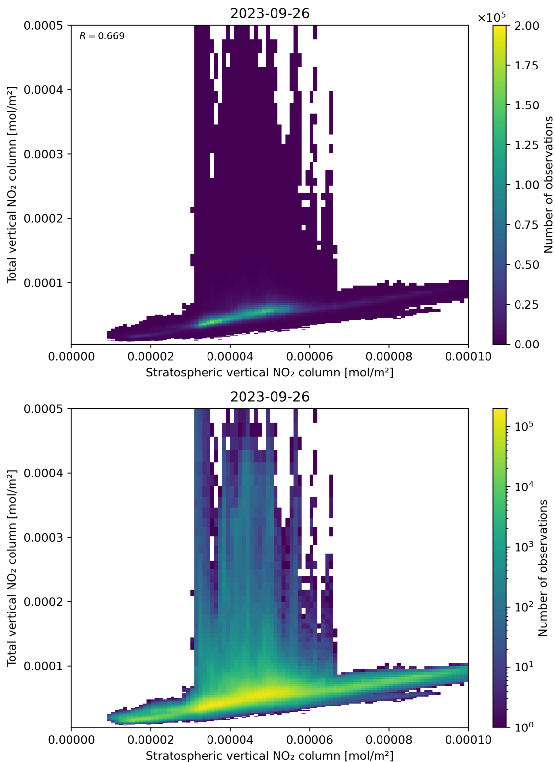
Figure 100: Scatter density plot of “Stratospheric vertical NO 2 column” against “Total vertical NO 2 column” for 2023-09-26 to 2023-09-27.
