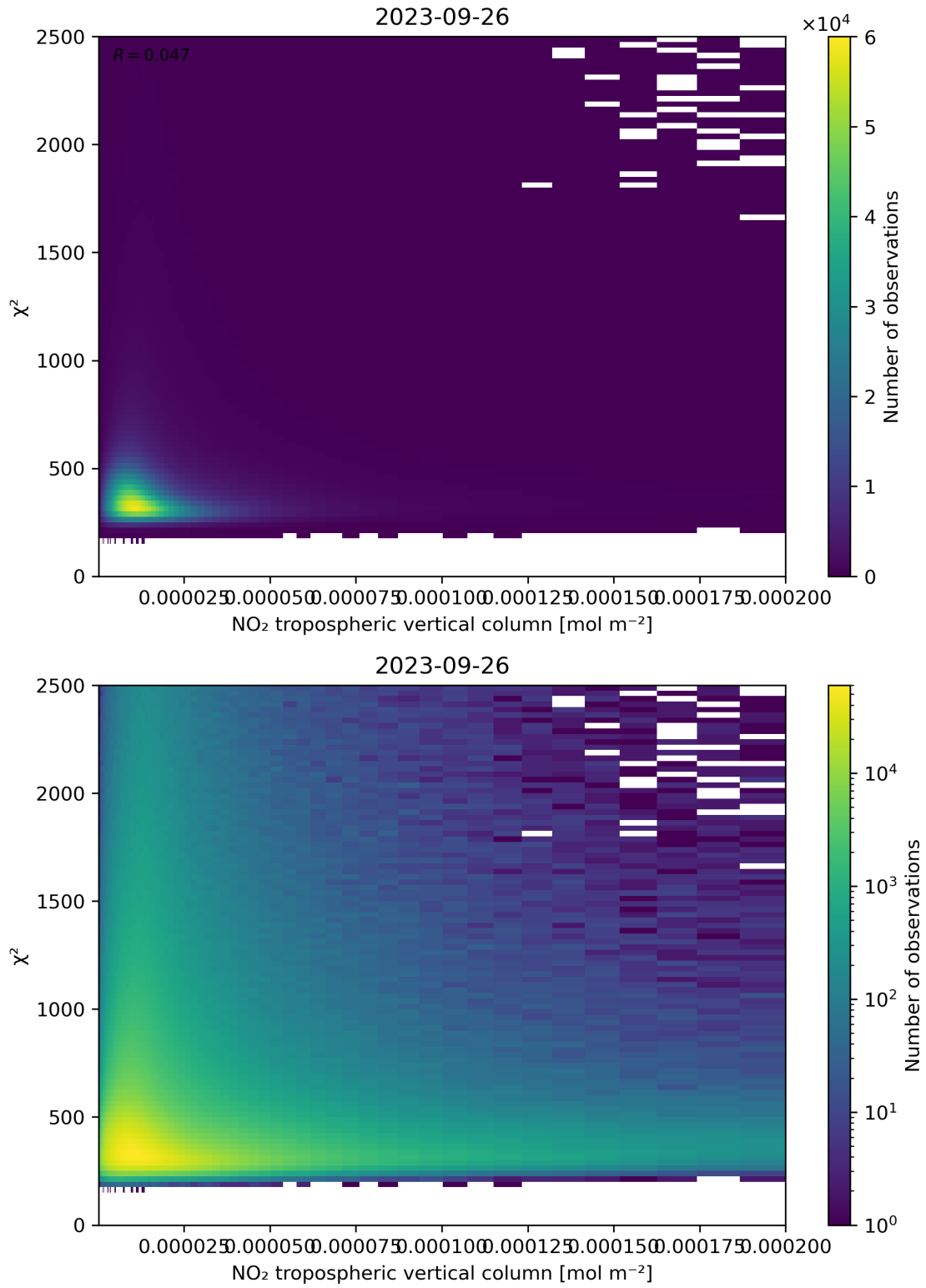
Figure 124: Scatter density plot of “NO 2 tropospheric vertical column” against “ \chi^2 ” for 2023-09-26 to 2023-09-27.
