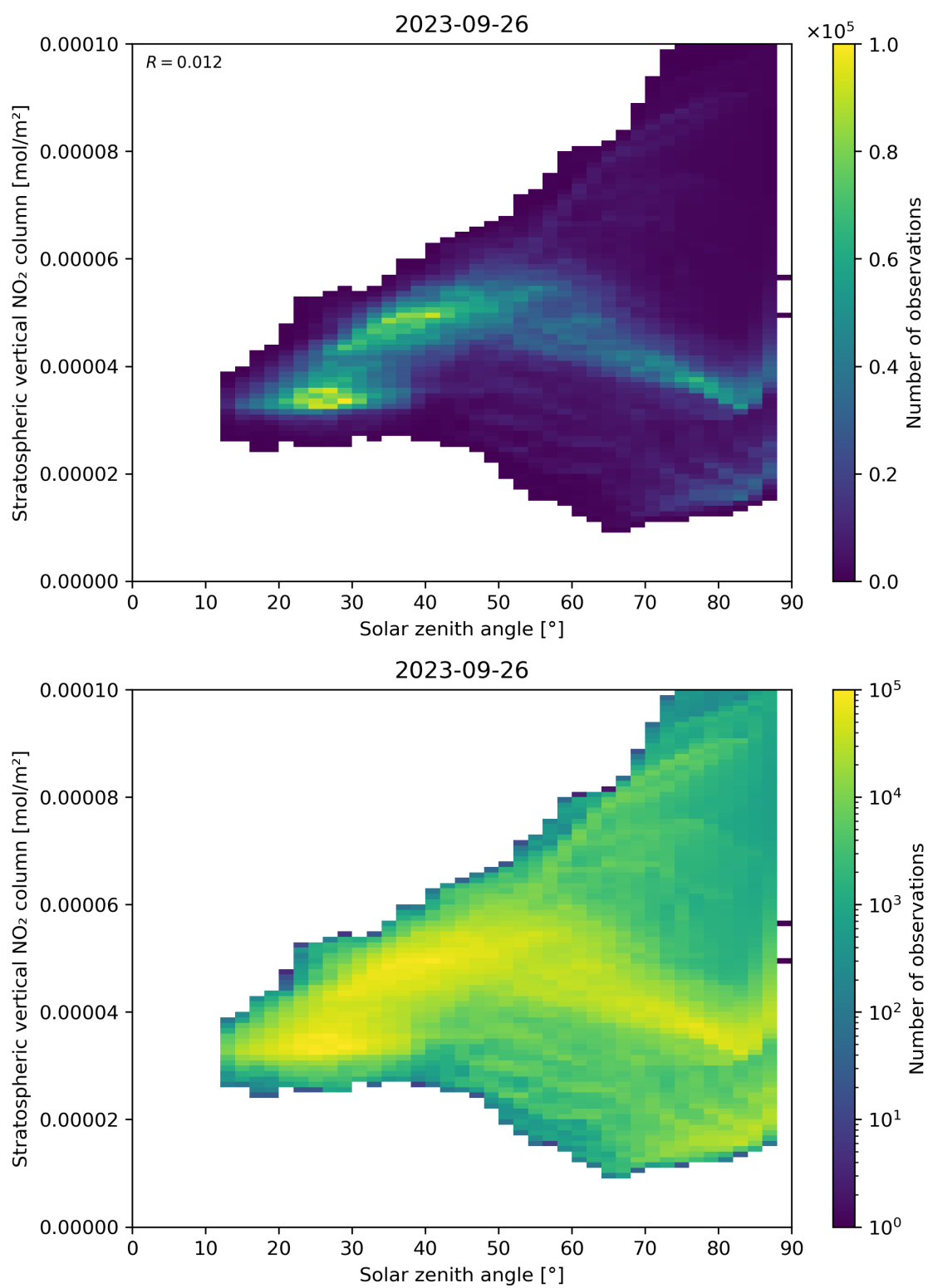
Figure 150: Scatter density plot of “Solar zenith angle” against “Stratospheric vertical NO 2 column” for 2023-09-26 to 2023-09-27.
