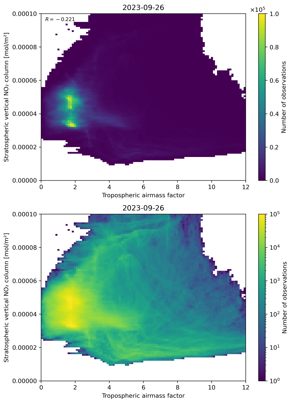
Figure 74: Scatter density plot of “Tropospheric air mass factor” against “Stratospheric vertical NO 2 column” for 2023-09-26 to 2023-09-27.
