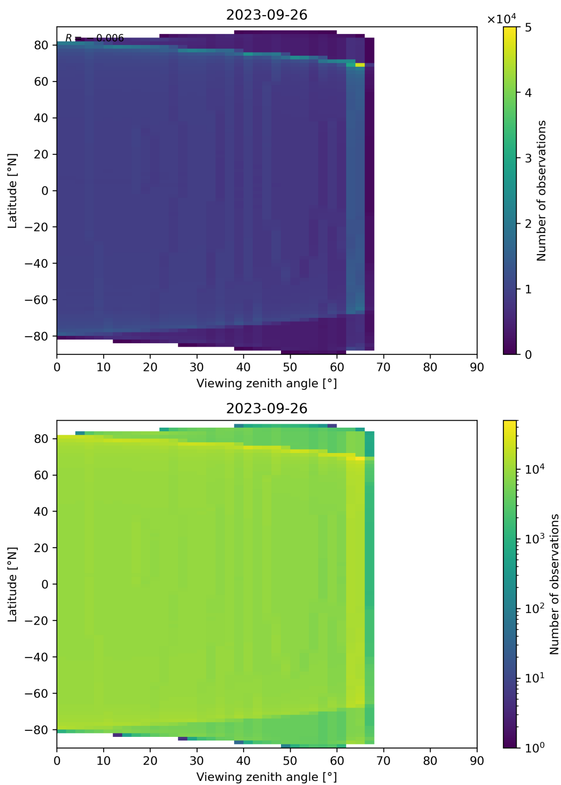
Figure 163: Scatter density plot of “Viewing zenith angle” against “Latitude” for 2023-09-26 to 2023-09-27.
