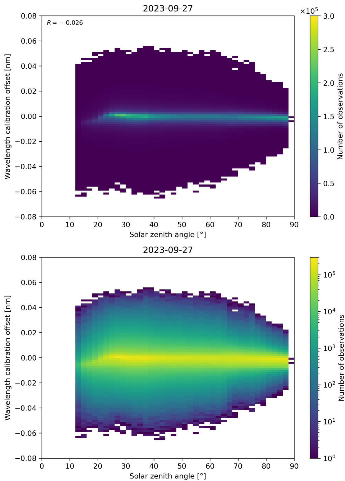
Figure 158: Scatter density plot of “Solar zenith angle” against “Wavelength calibration offset” for 2023-09-26 to 2023-09-28.
