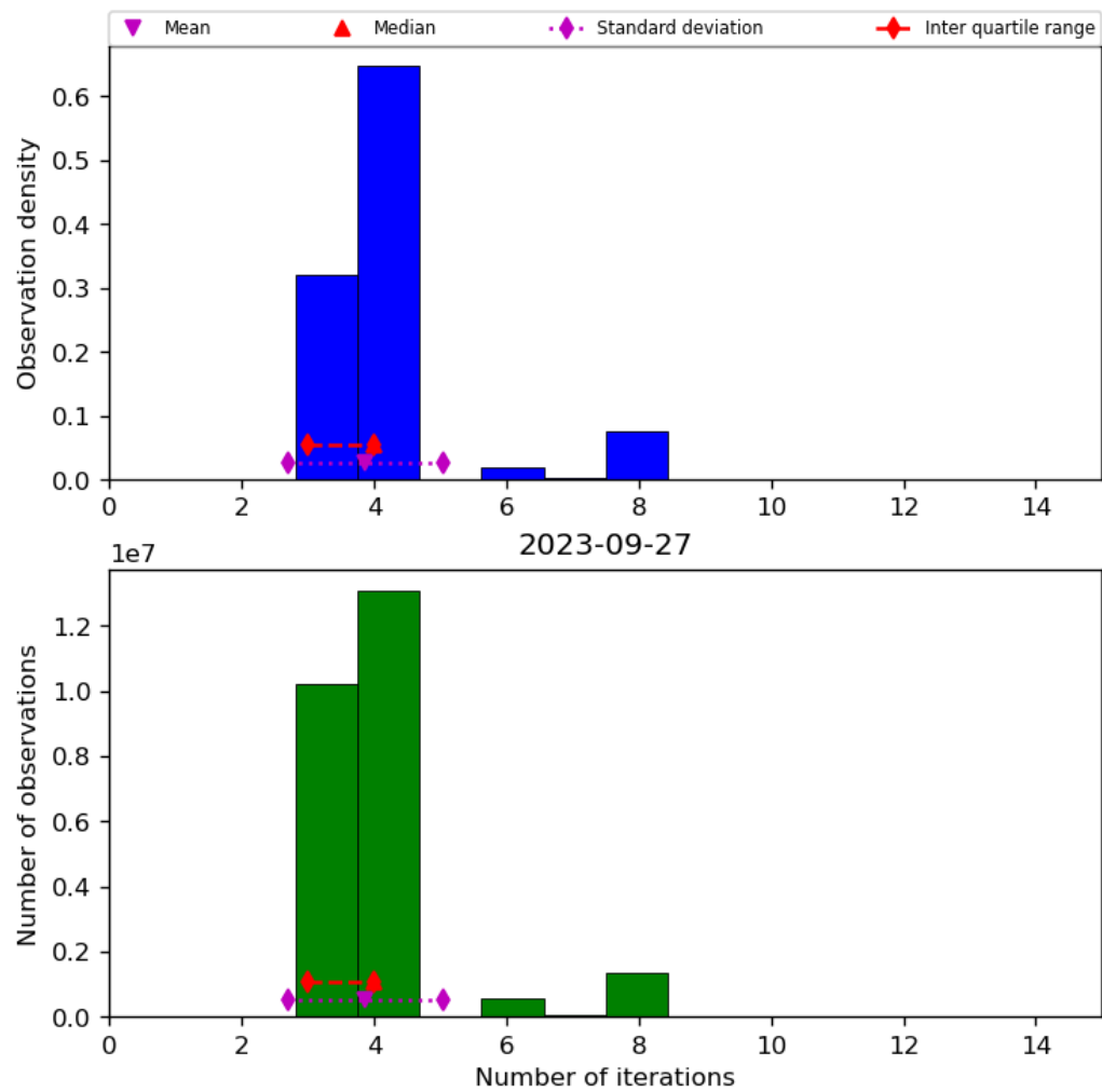
Figure 34: Histogram of “Number of iterations” for 2023-09-26 to 2023-09-28
