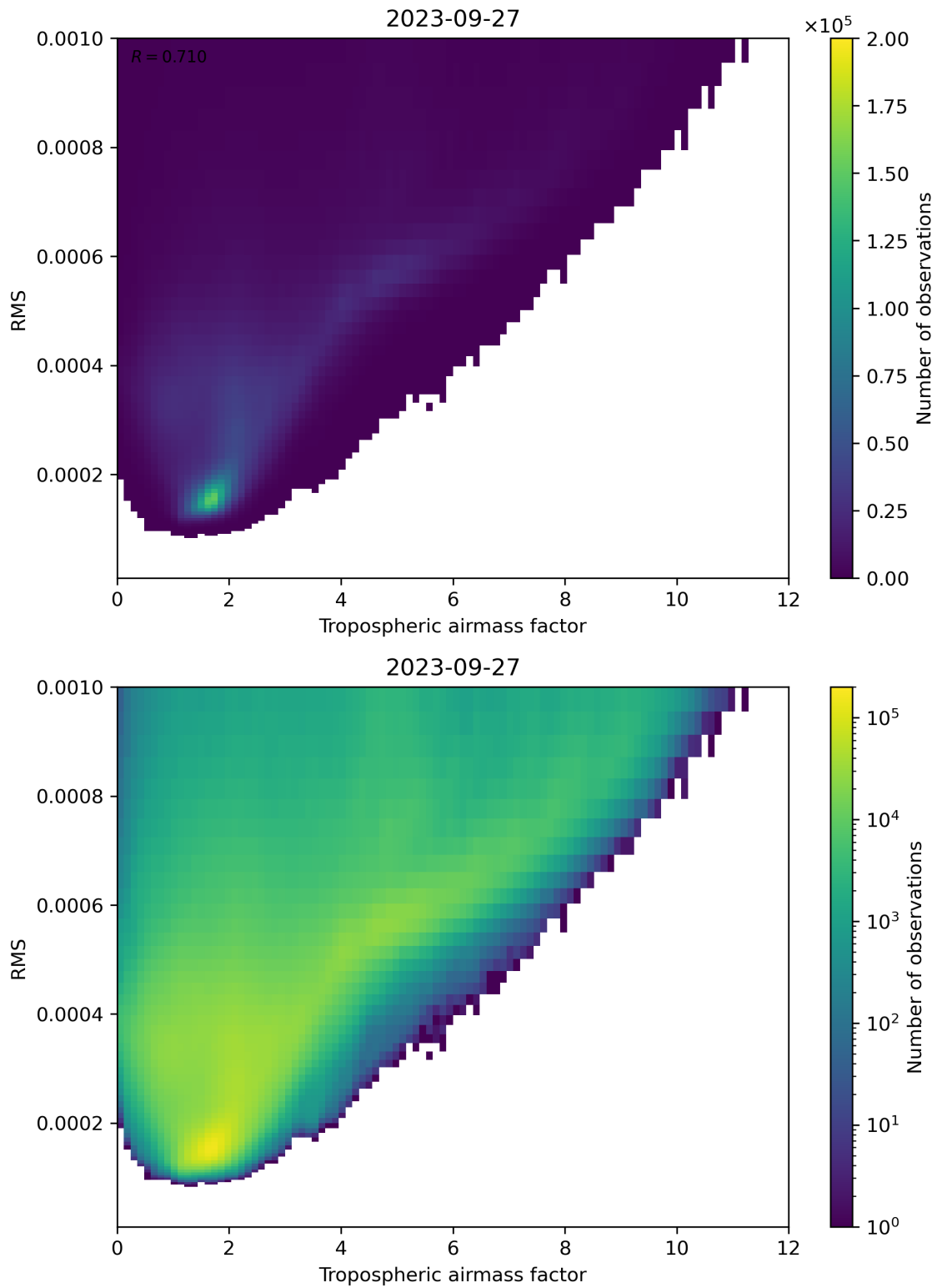
Figure 79: Scatter density plot of “Tropospheric airmass factor” against “RMS” for 2023-09-26 to 2023-09-28.
