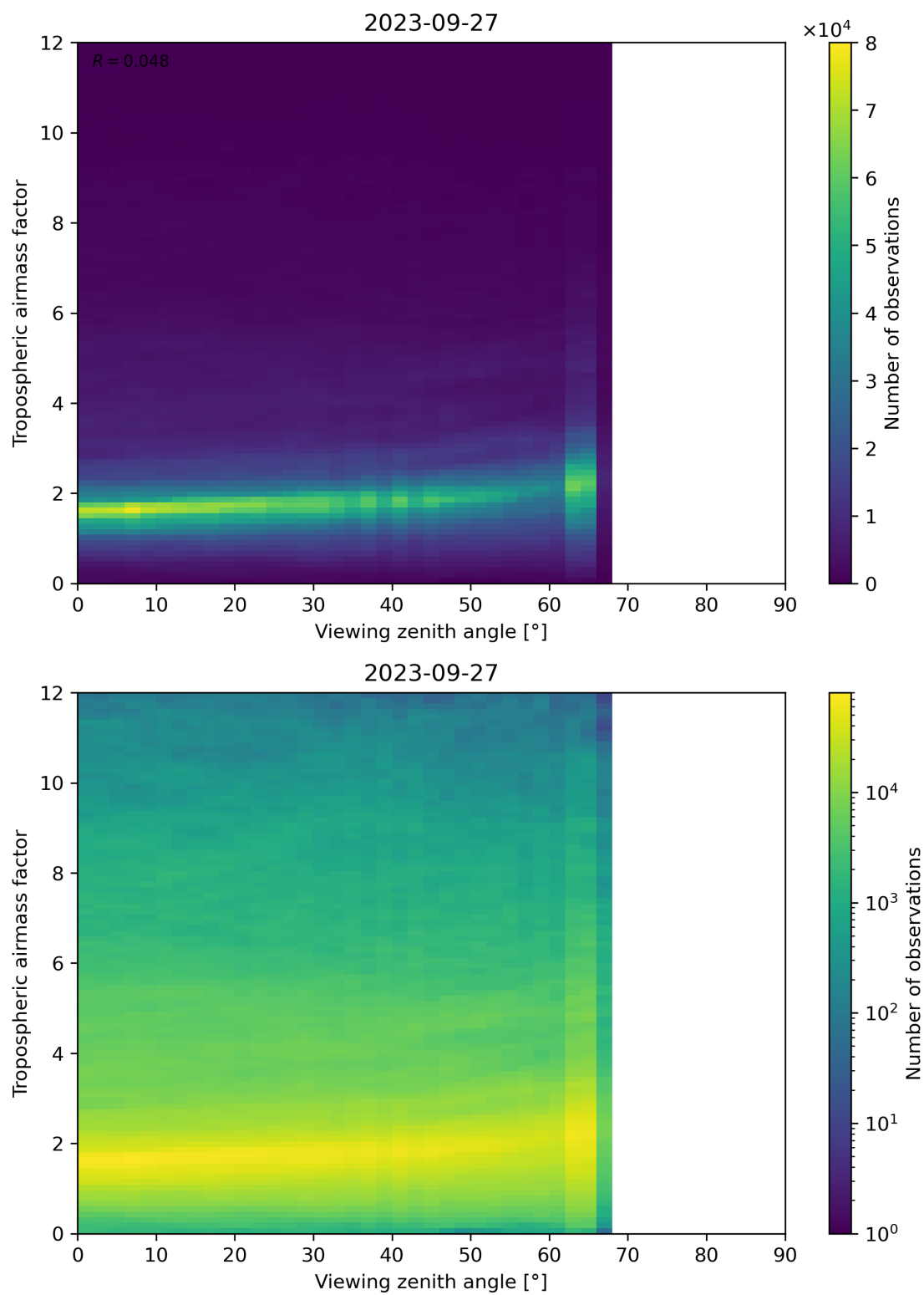
Figure 161: Scatter density plot of “Viewing zenith angle” against “Tropospheric airmass factor” for 2023-09-26 to 2023-09-28.
