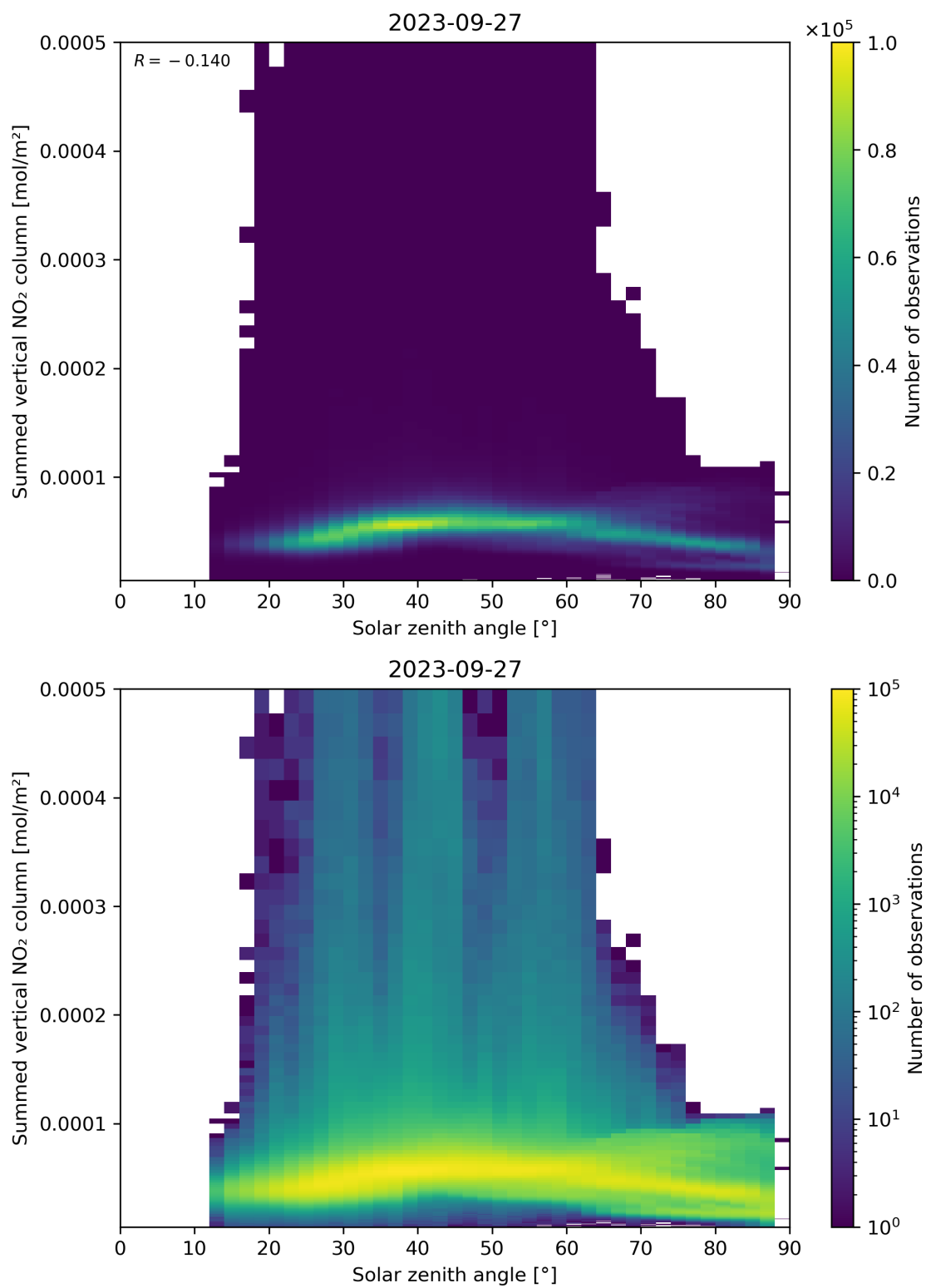
Figure 151: Scatter density plot of “Solar zenith angle” against “Summed vertical NO 2 column” for 2023-09-26 to 2023-09-28.
