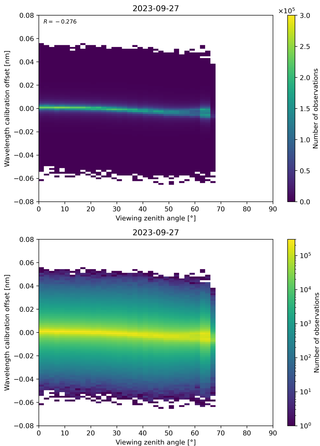
Figure 173: Scatter density plot of “Viewing zenith angle” against “Wavelength calibration offset” for 2023-09-26 to 2023-09-28.
