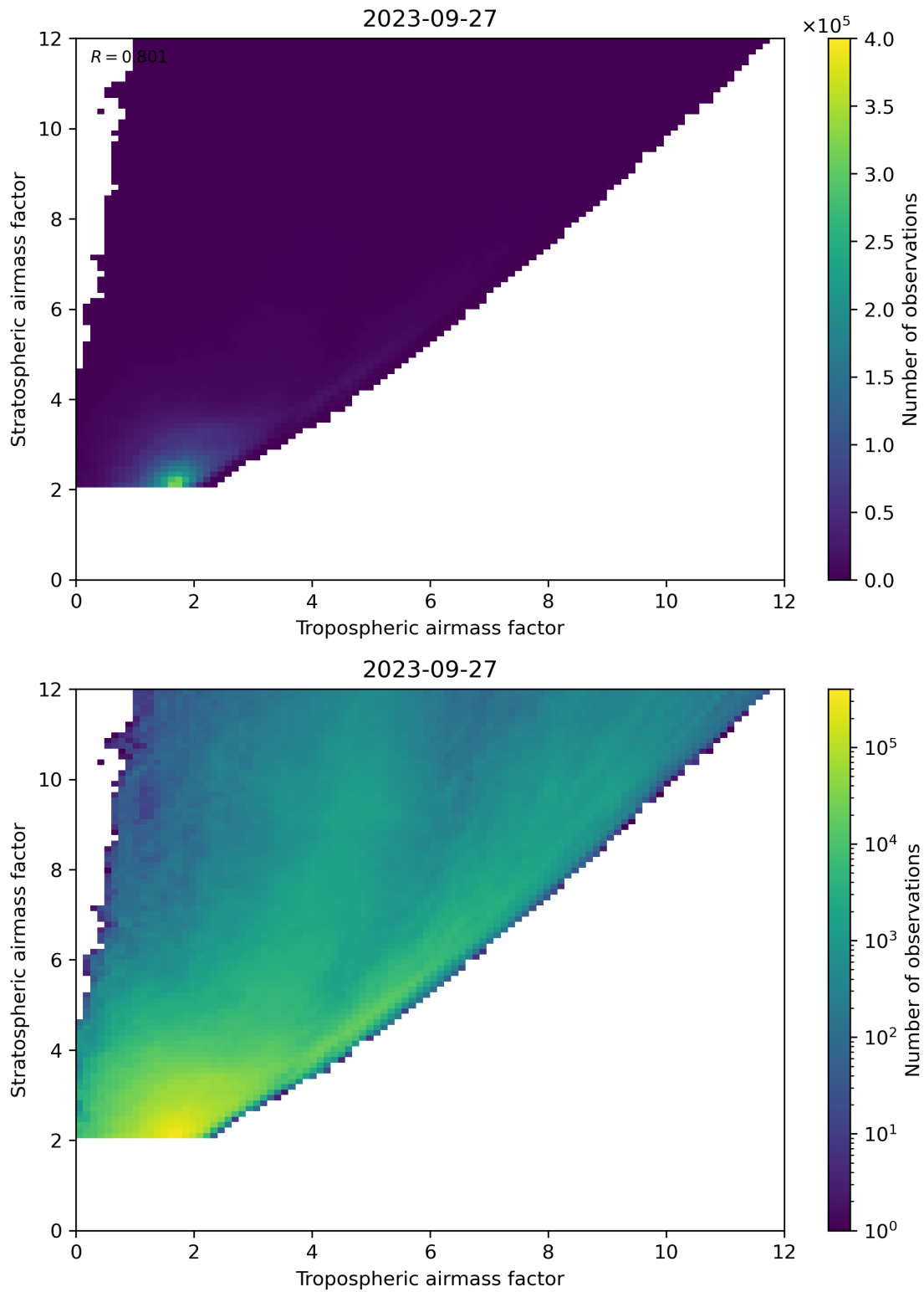
Figure 71: Scatter density plot of “Tropospheric airmass factor” against “Stratospheric airmass factor” for 2023-09-26 to 2023-09-28.
