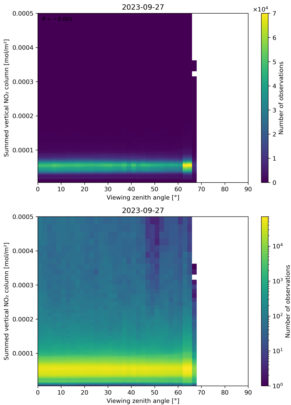
Figure 165: Scatter density plot of “Viewing zenith angle” against “Summed vertical NO 2 column” for 2023-09-26 to 2023-09-28.
