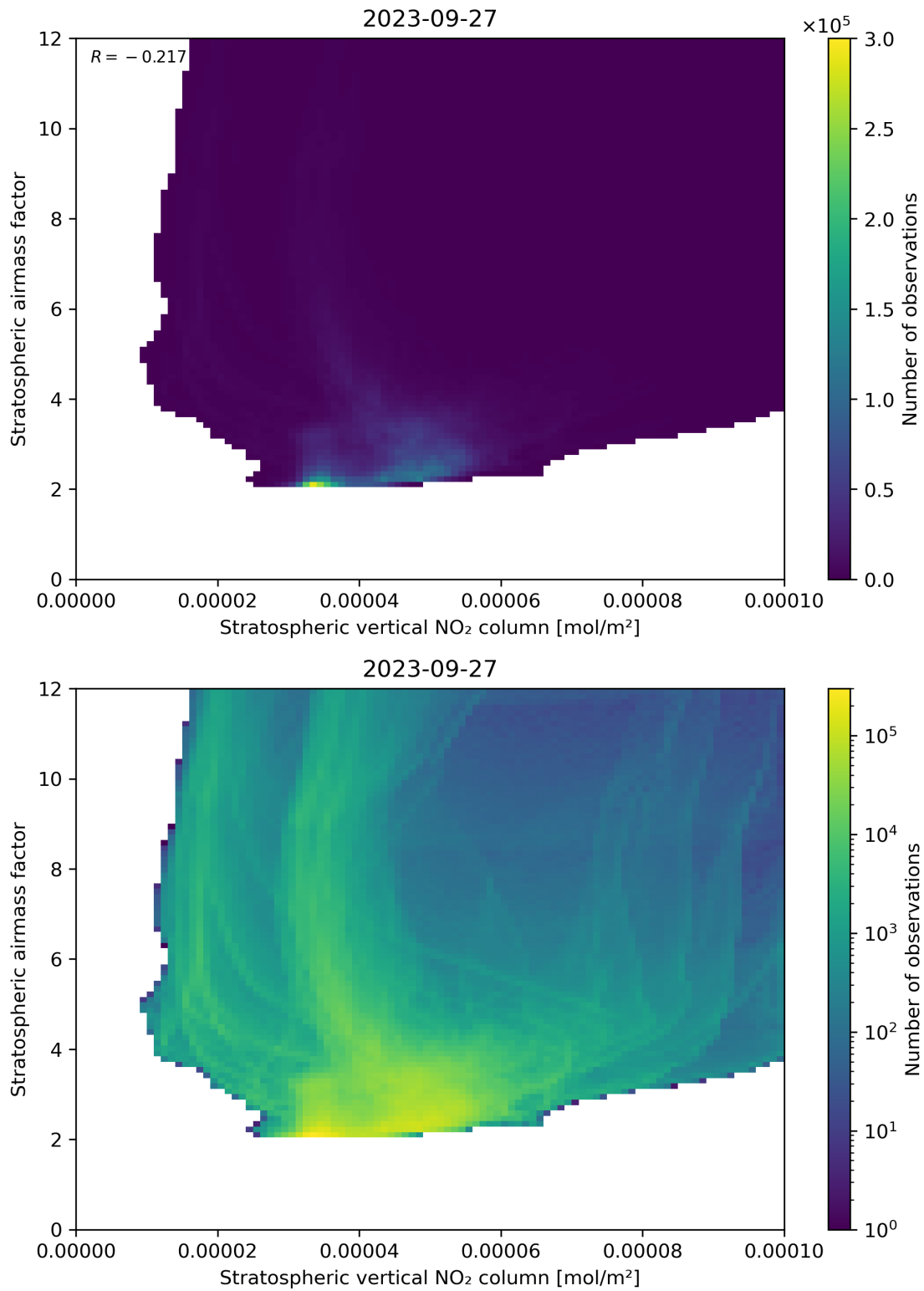
Figure 96: Scatter density plot of “Stratospheric vertical NO 2 column” against “Stratospheric airmass factor” for 2023-09-26 to 2023-09-28.
