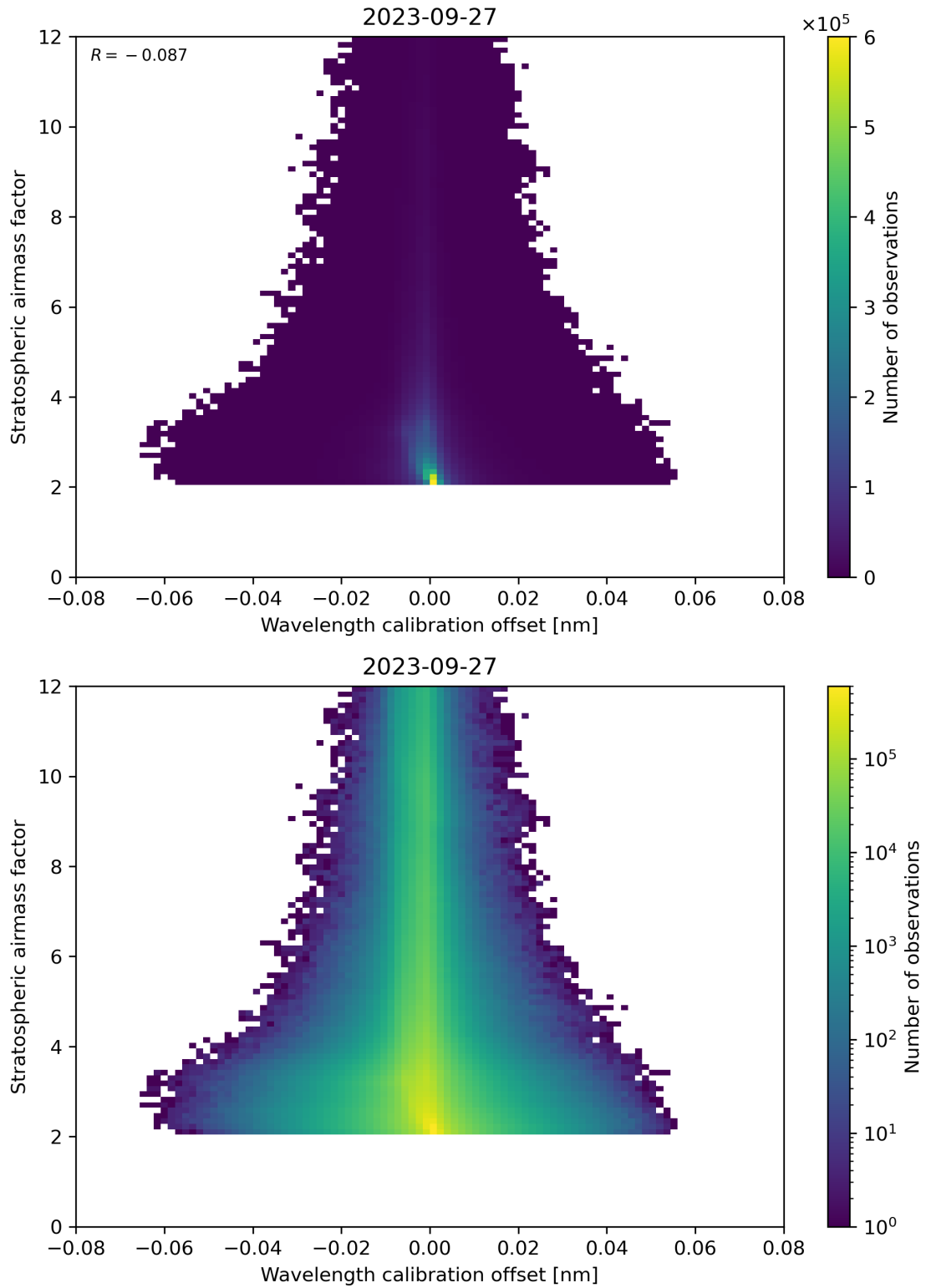
Figure 174: Scatter density plot of “Wavelength calibration offset” against “Stratospheric air mass factor” for 2023-09-26 to 2023-09-28.
