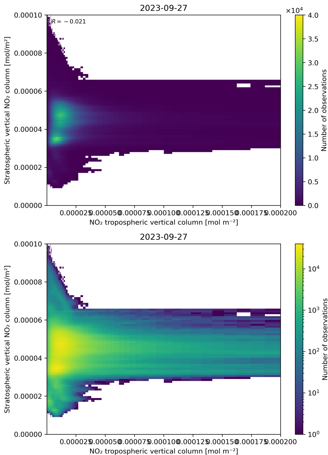
Figure 125: Scatter density plot of “NO 2 tropospheric vertical column” against “Stratospheric vertical NO 2 column” for 2023-09-26 to 2023-09-28.
