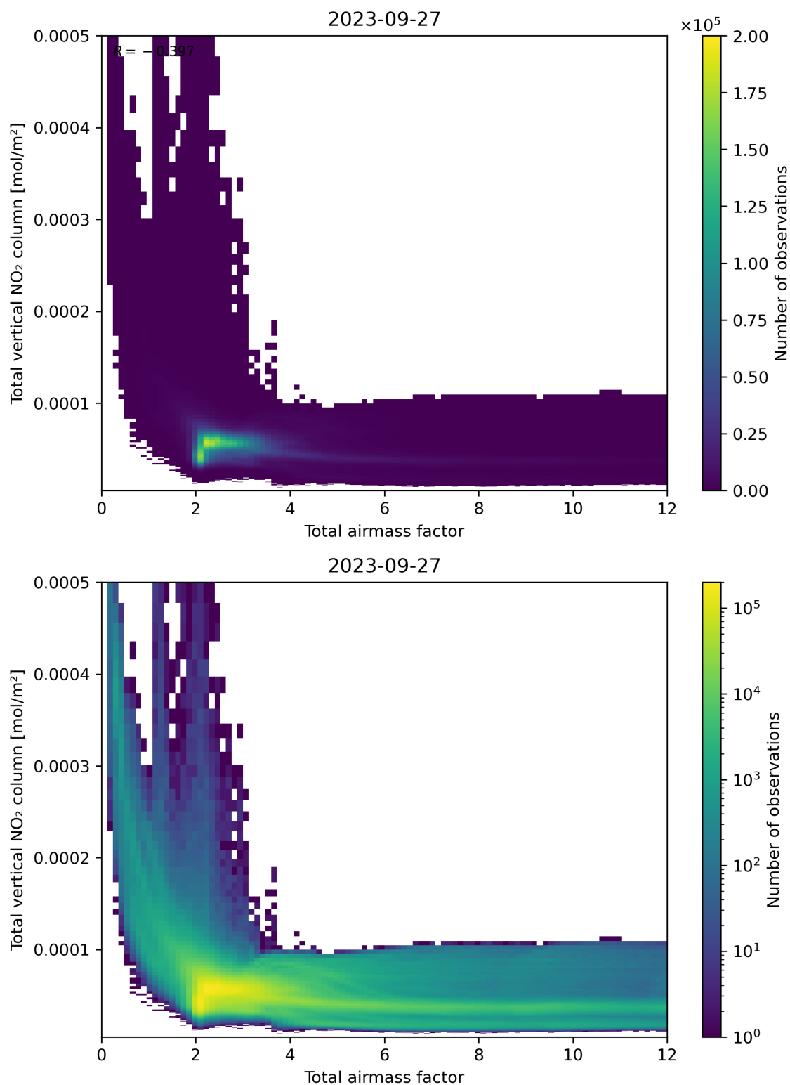
Figure 67: Scatter density plot of “Total airmass factor” against “Total vertical NO 2 column” for 2023-09-26 to 2023-09-28.
