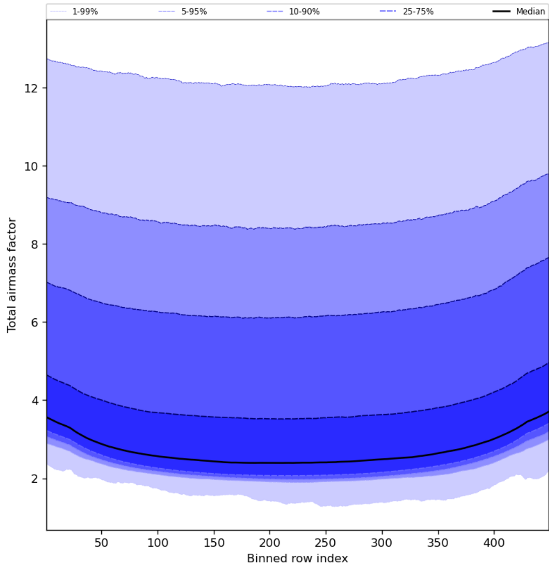
Figure 49: Along track statistics of “Total airmass factor” for 2023-09-26 to 2023-09-28
