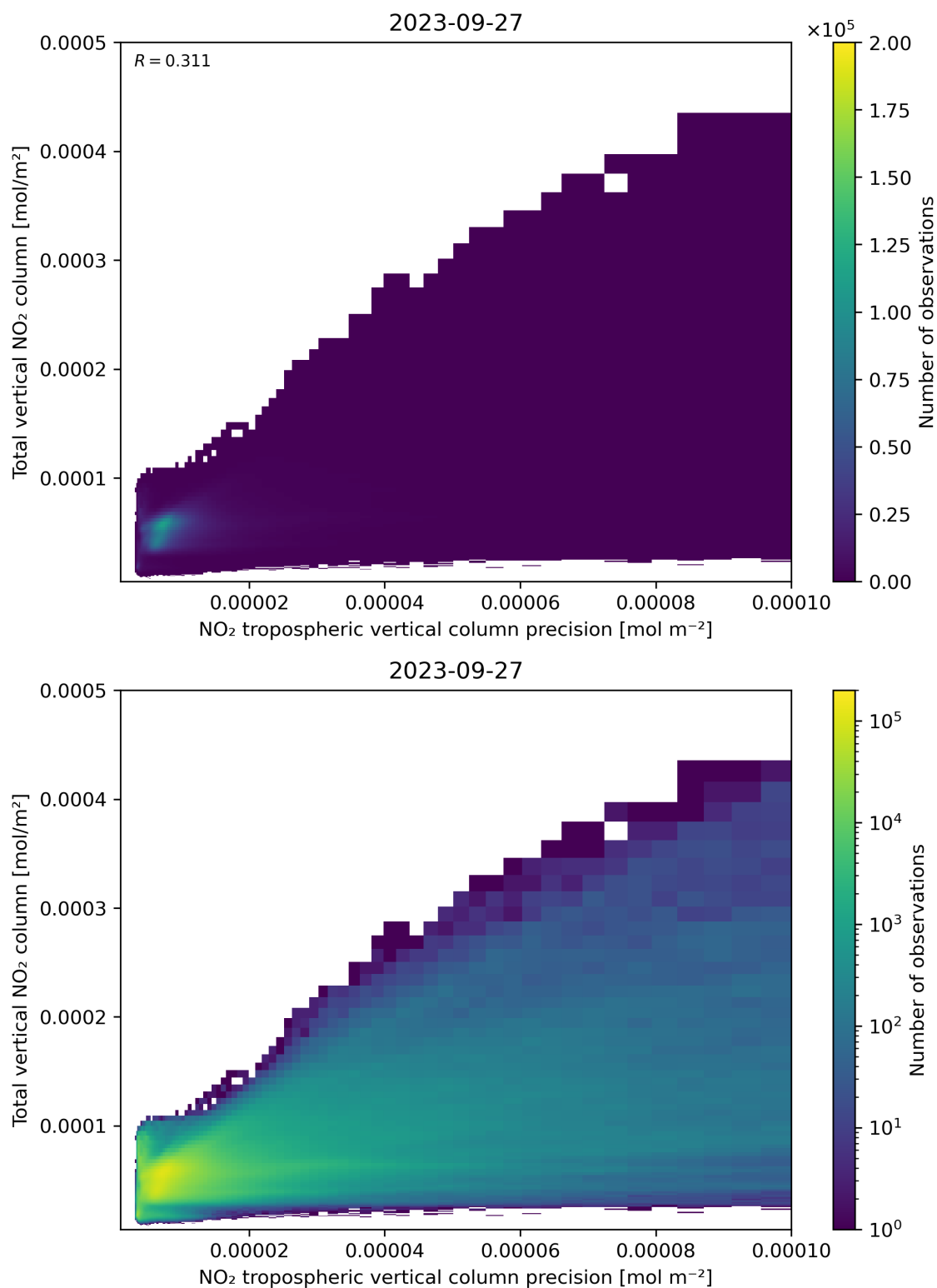
Figure 138: Scatter density plot of “NO 2 tropospheric vertical column precision” against “Total vertical NO 2 column” for 2023-09-26 to 2023-09-28.
