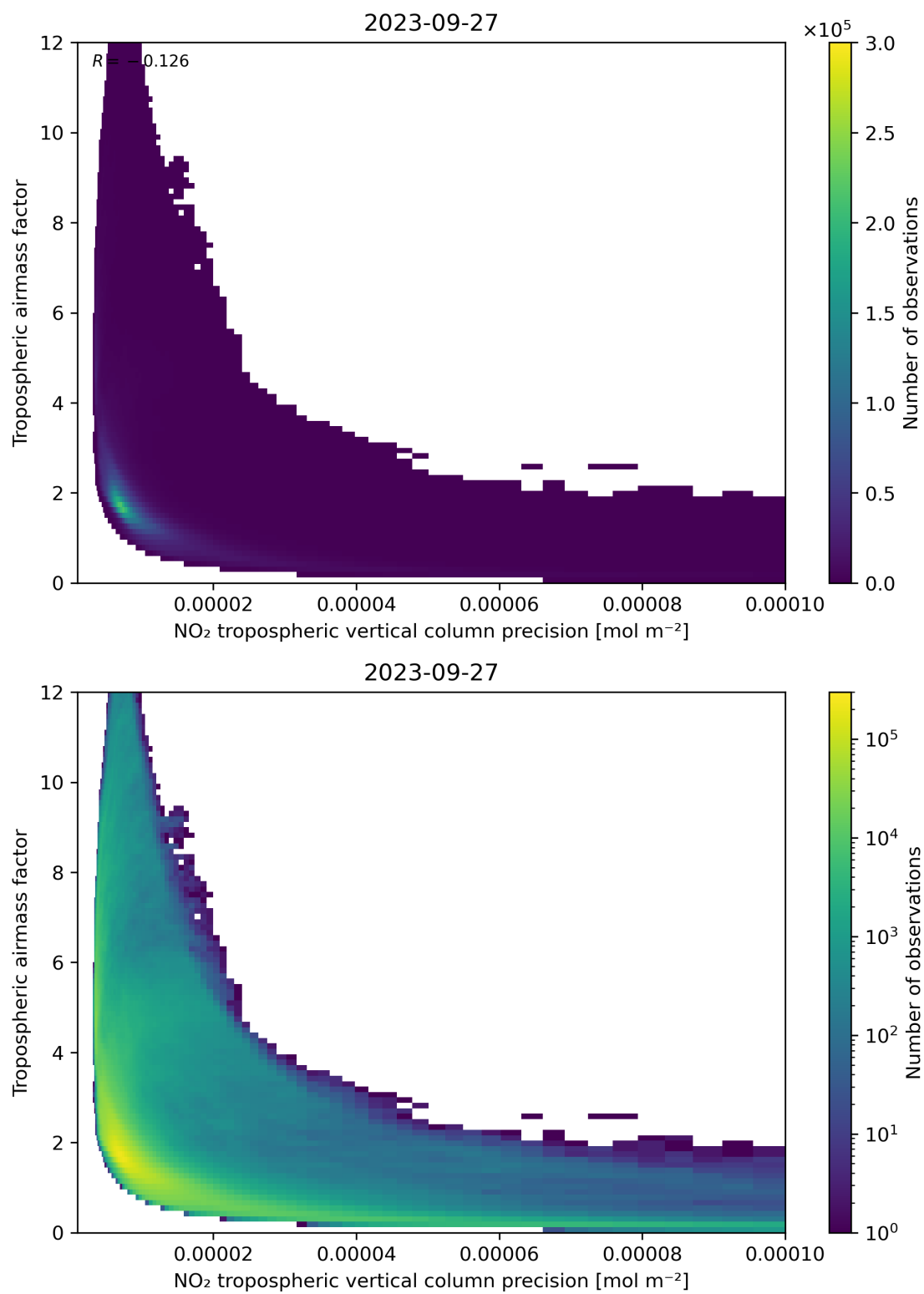
Figure 133: Scatter density plot of “NO 2 tropospheric vertical column precision” against “Tropospheric airmass factor” for 2023-09-26 to 2023-09-28.
