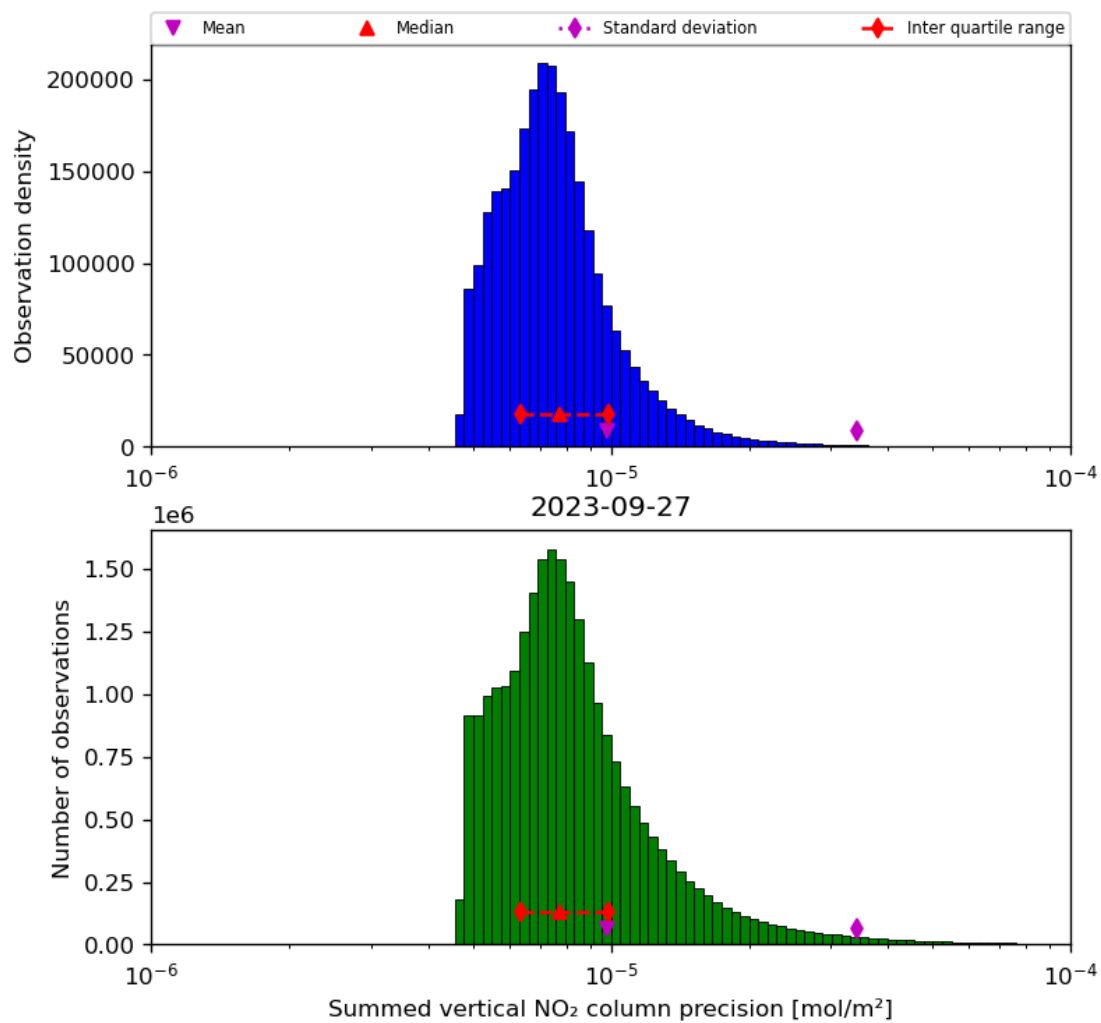
Figure 41: Histogram of "Summed vertical NO 2 column precision" for 2023-09-26 to 2023-09-28
