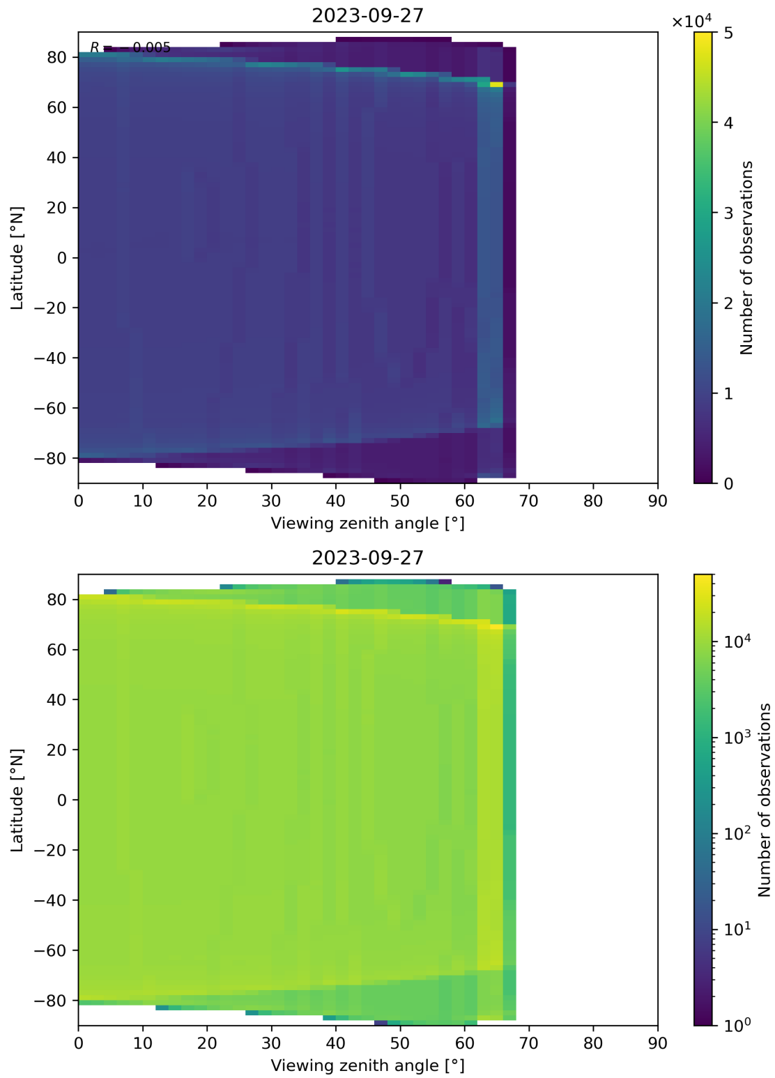
Figure 163: Scatter density plot of “Viewing zenith angle” against “Latitude” for 2023-09-26 to 2023-09-28.
