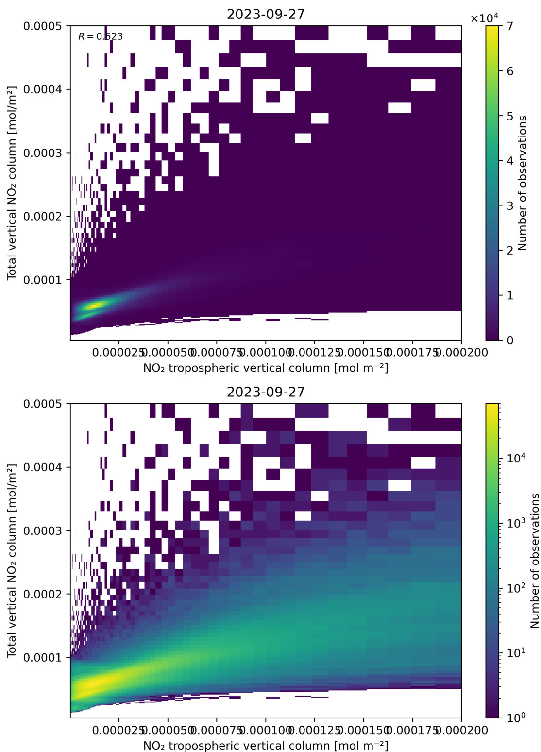
Figure 128: Scatter density plot of “NO 2 tropospheric vertical column” against “Total vertical NO 2 column” for 2023-09-26 to 2023-09-28.
