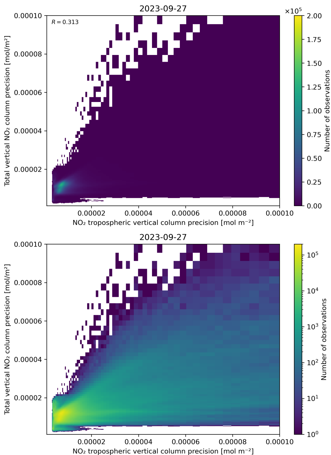
Figure 139: Scatter density plot of “NO 2 tropospheric vertical column precision” against “Total vertical NO 2 column precision” for 2023-09-26 to 2023-09-28.
