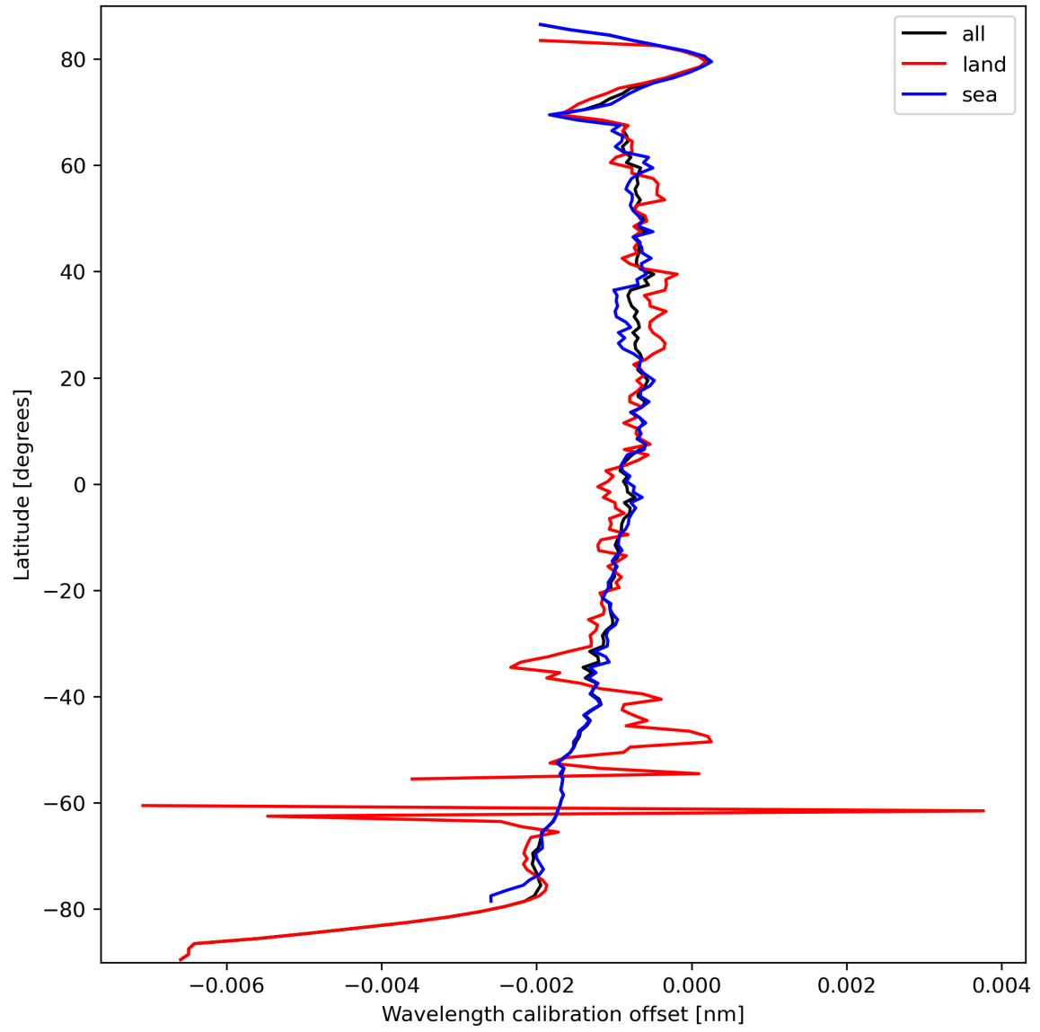
Figure 18: Zonal average of “Wavelength calibration offset” for 2023-09-26 to 2023-09-28.
