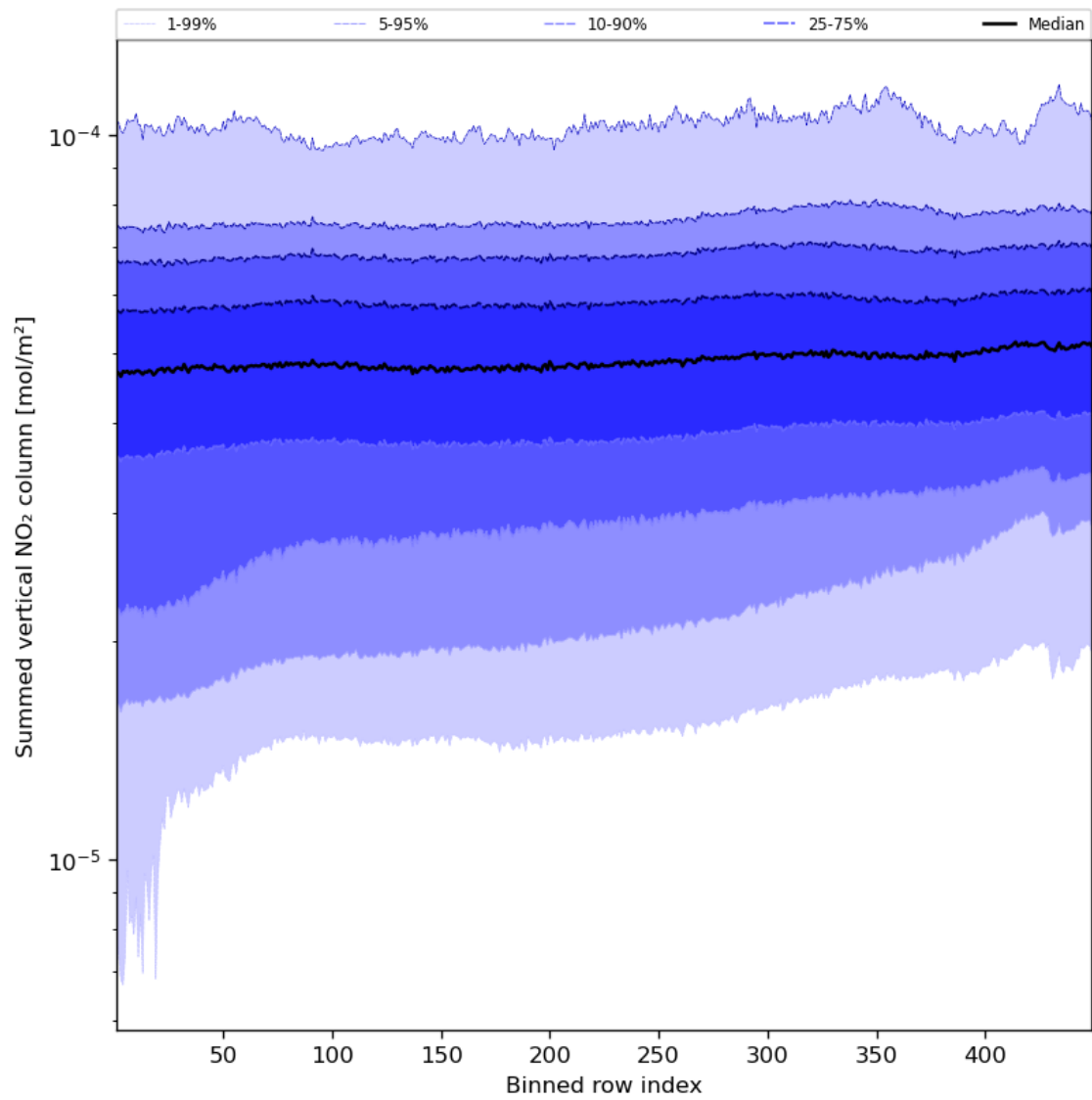
Figure 57: Along track statistics of “Summed vertical NO 2 column” for 2023-09-26 to 2023-09-28
