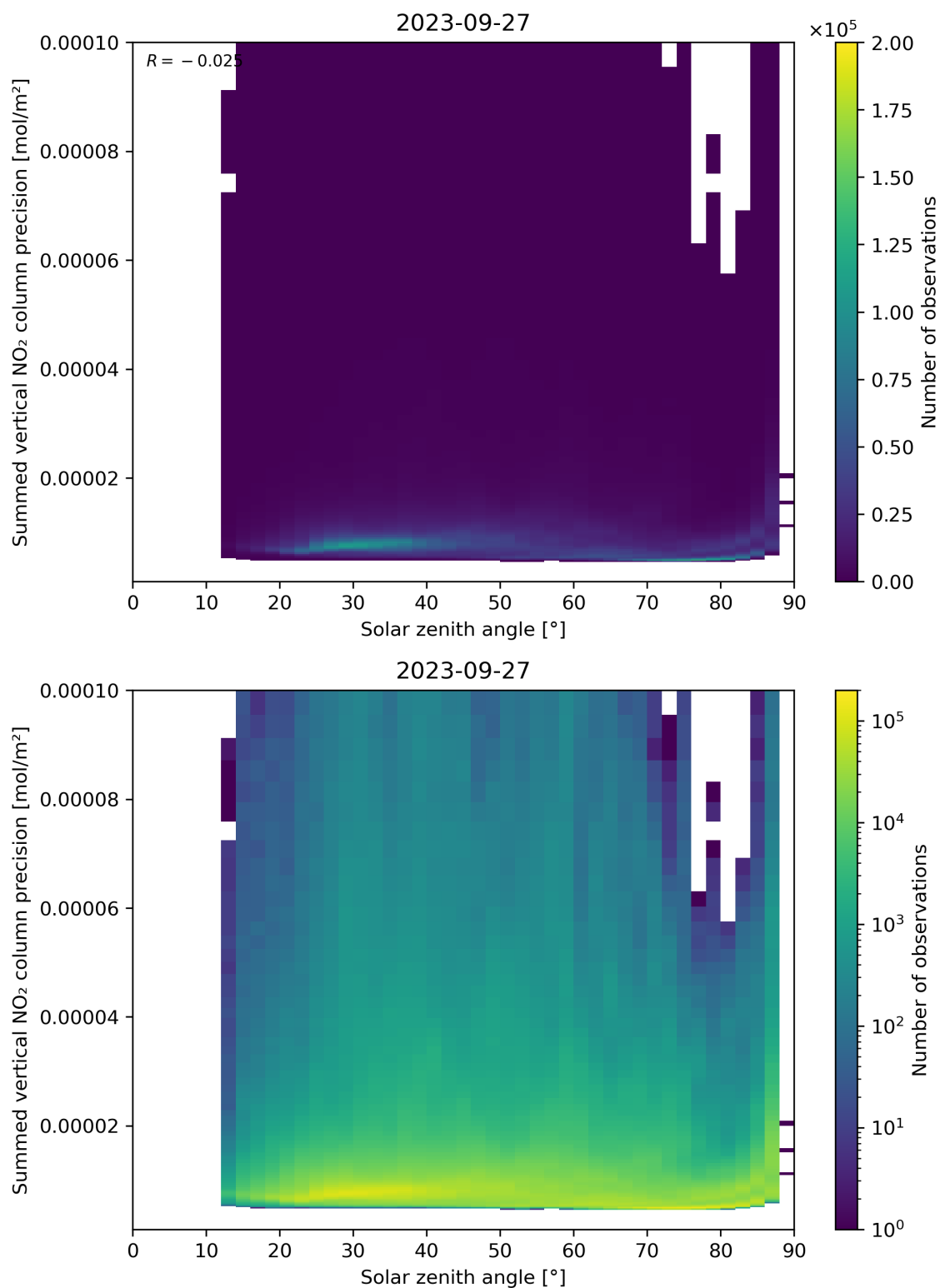
Figure 152: Scatter density plot of “Solar zenith angle” against “Summed vertical NO 2 column precision” for 2023-09-26 to 2023-09-28.
