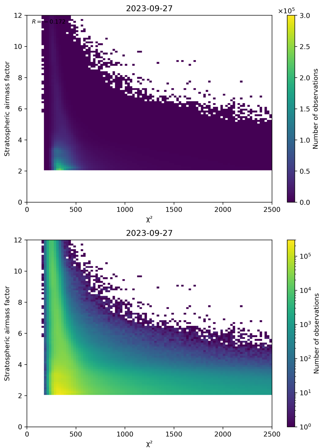
Figure 81: Scatter density plot of “ \chi^2 ” against “Stratospheric airmass factor” for 2023-09-26 to 2023-09-28.
