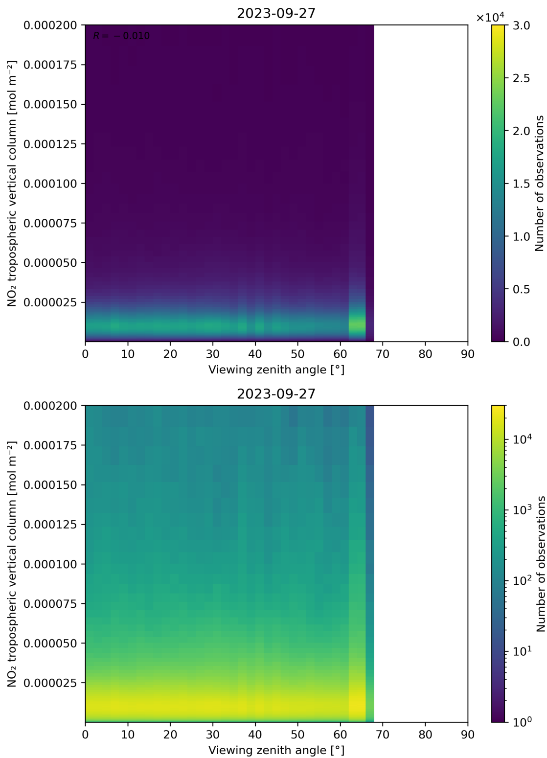
Figure 169: Scatter density plot of “Viewing zenith angle” against “NO 2 tropospheric vertical column” for 2023-09-26 to 2023-09-28.
