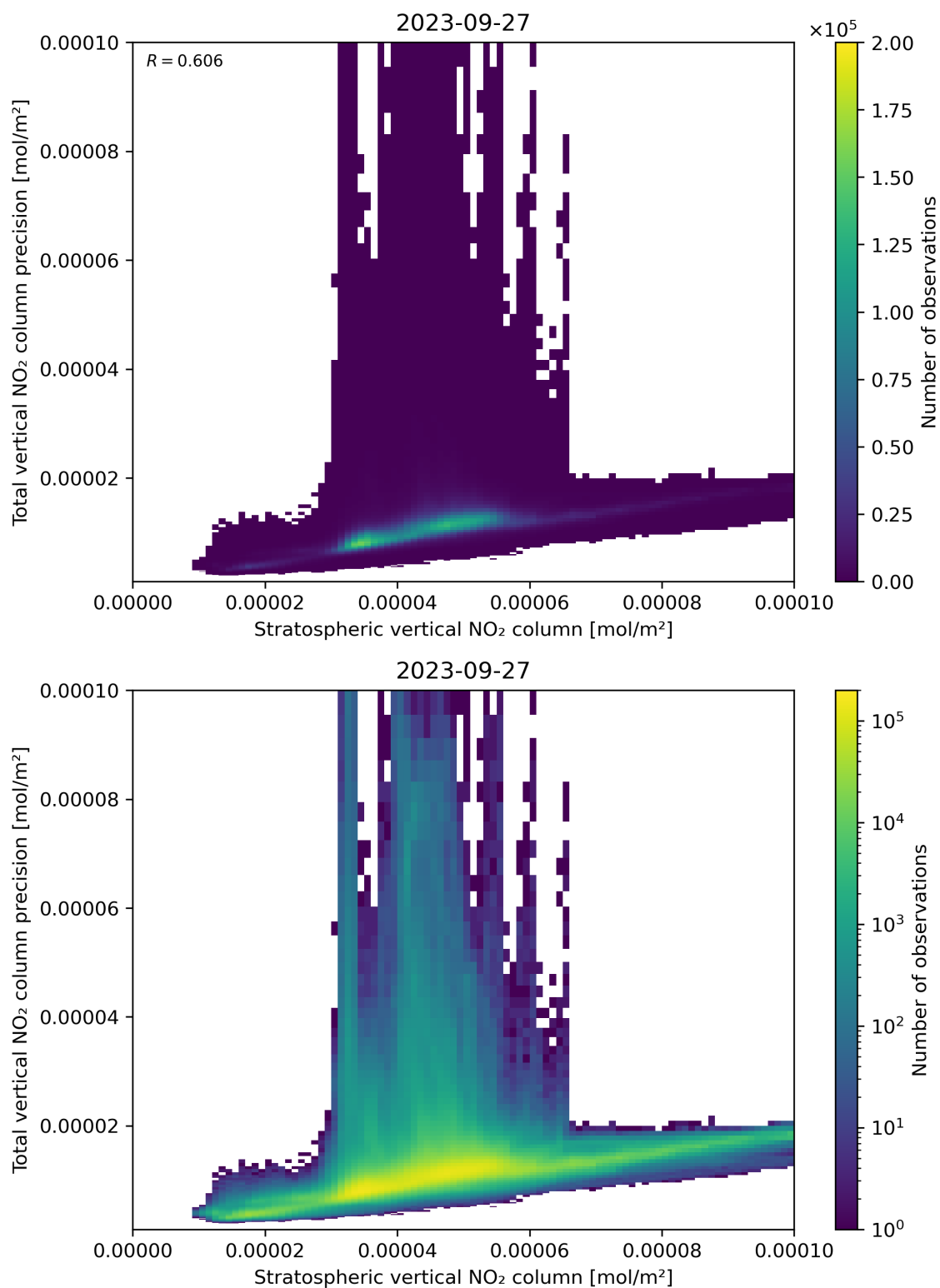
Figure 101: Scatter density plot of “Stratospheric vertical NO 2 column” against “Total vertical NO 2 column precision” for 2023-09-26 to 2023-09-28.
