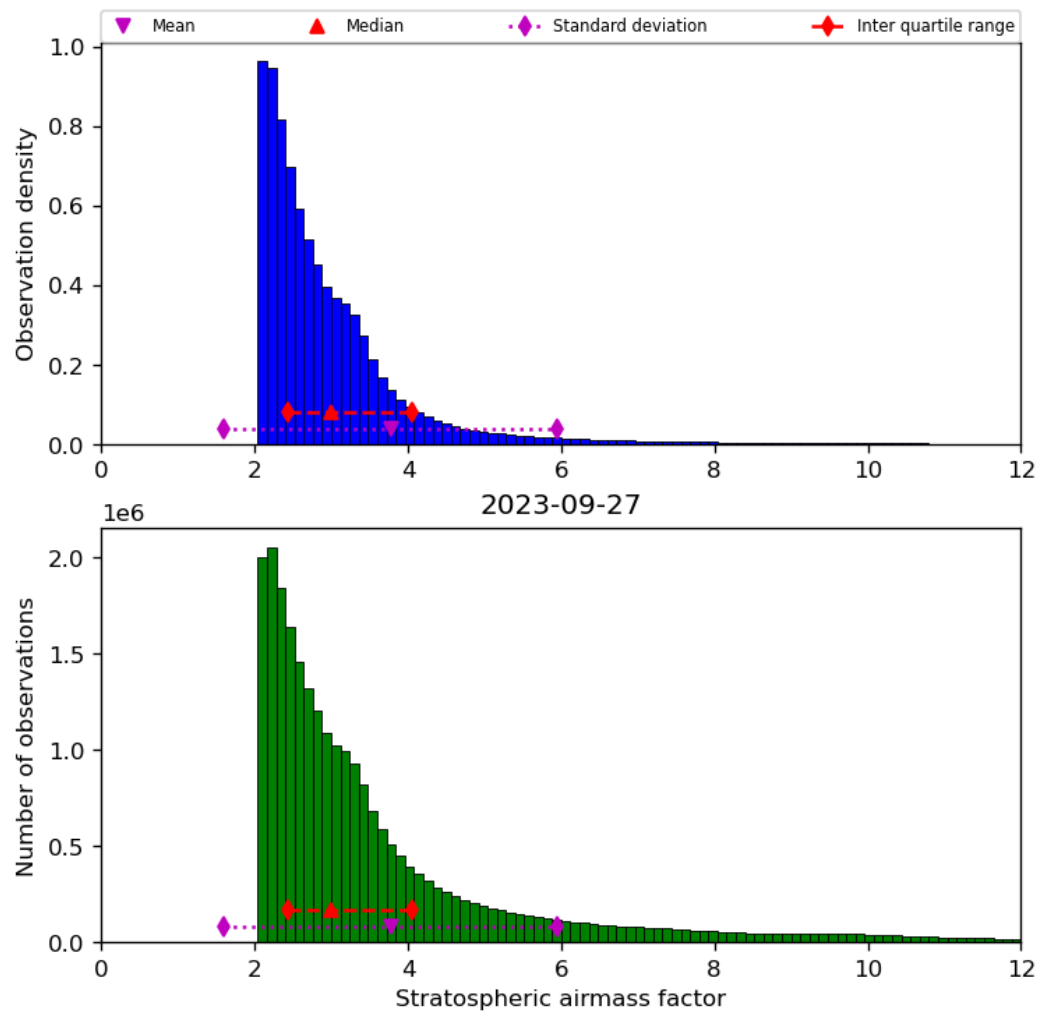
Figure 44: Histogram of “Stratospheric airmass factor” for 2023-09-26 to 2023-09-28
