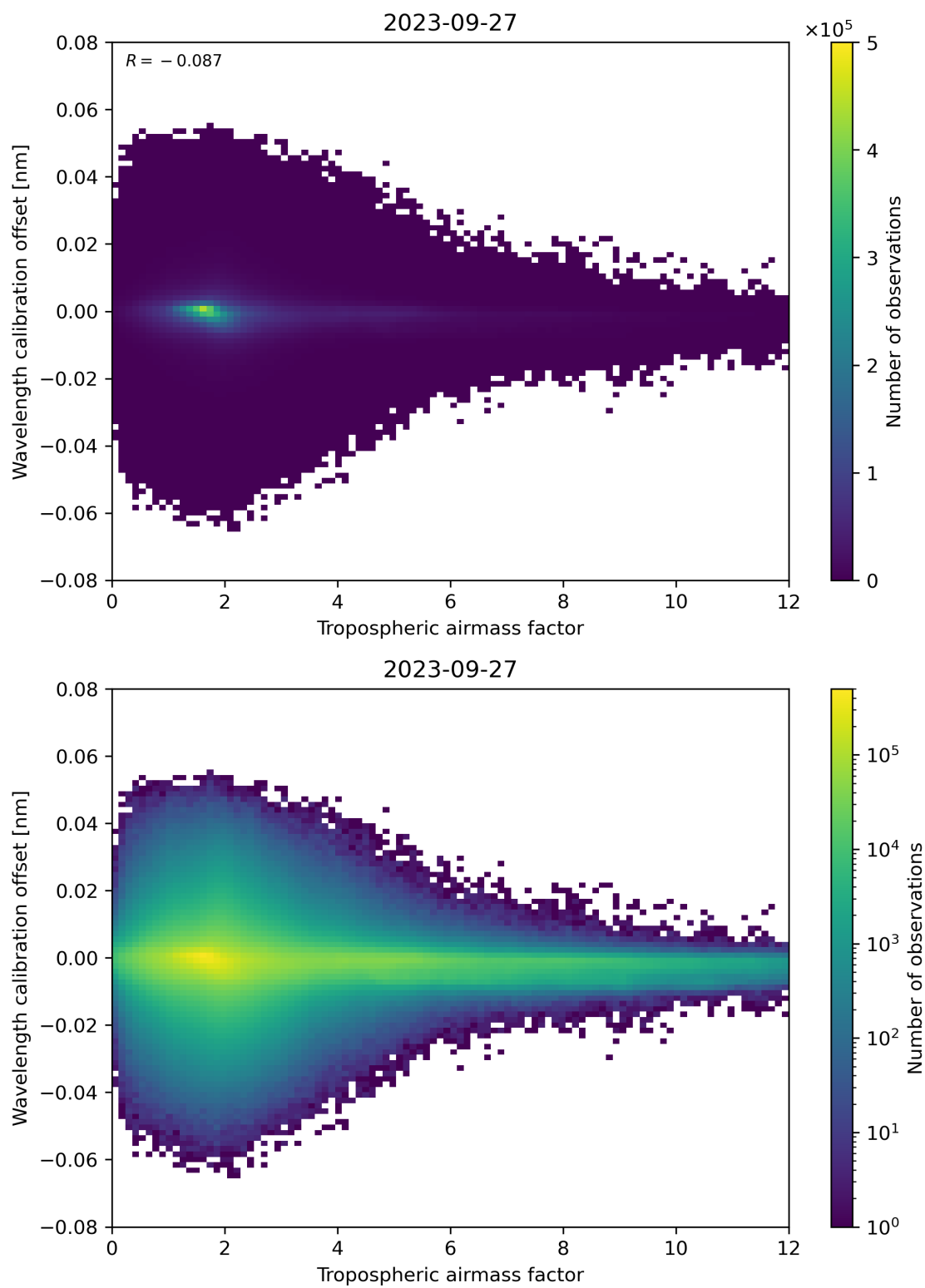
Figure 80: Scatter density plot of “Tropospheric air mass factor” against “Wavelength calibration offset” for 2023-09-26 to 2023-09-28.
