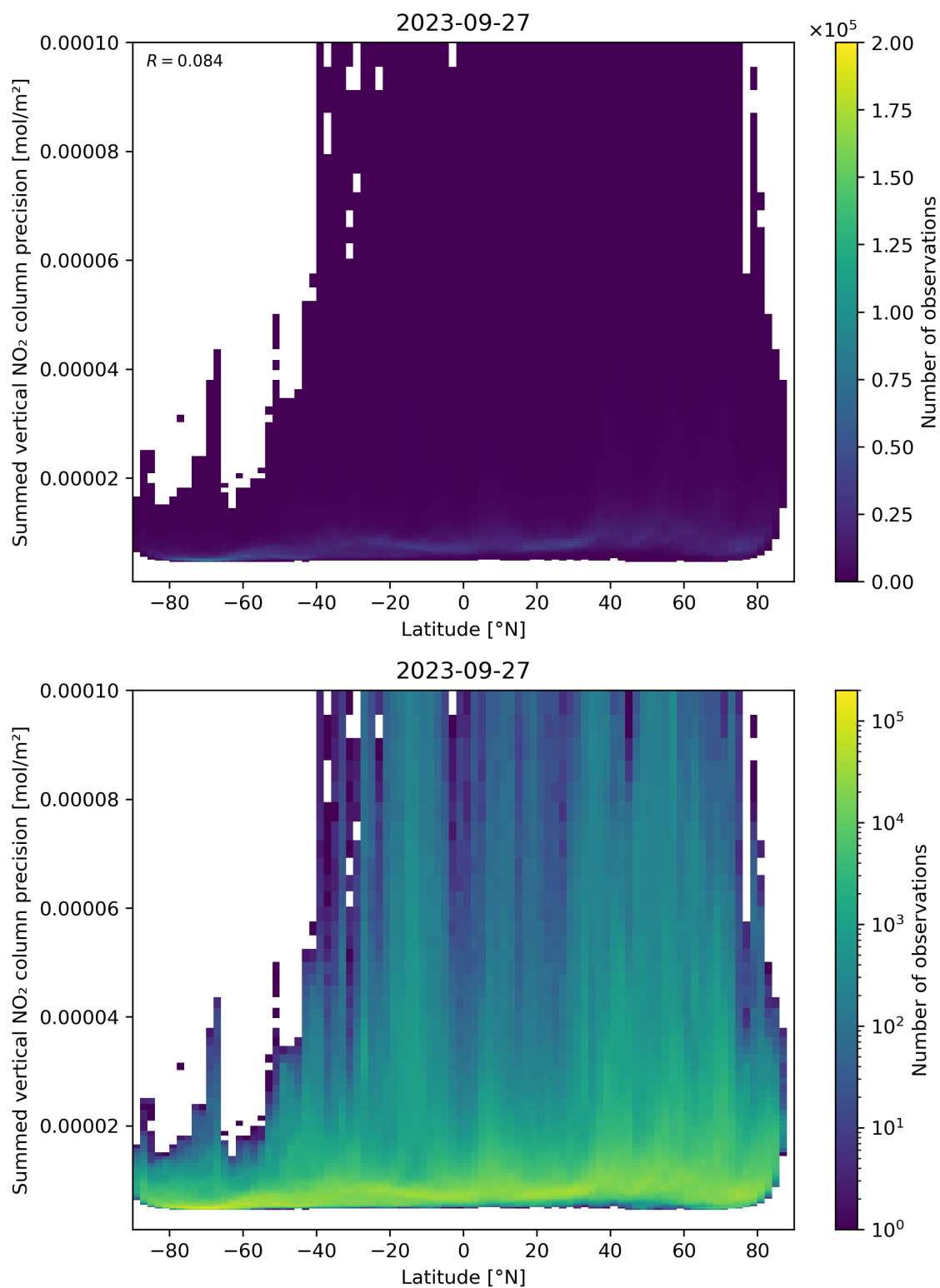
Figure 89: Scatter density plot of “Latitude” against “Summed vertical NO 2 column precision” for 2023-09-26 to 2023-09-28.
