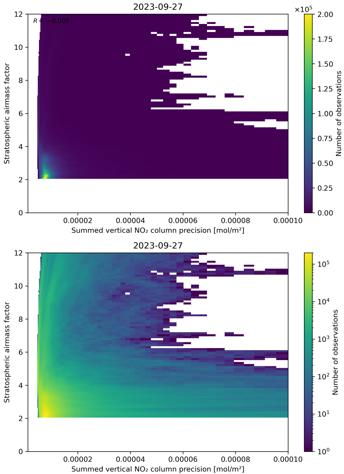
Figure 106: Scatter density plot of “Summed vertical NO 2 column precision” against “Stratospheric airmass factor” for 2023-09-26 to 2023-09-28.
