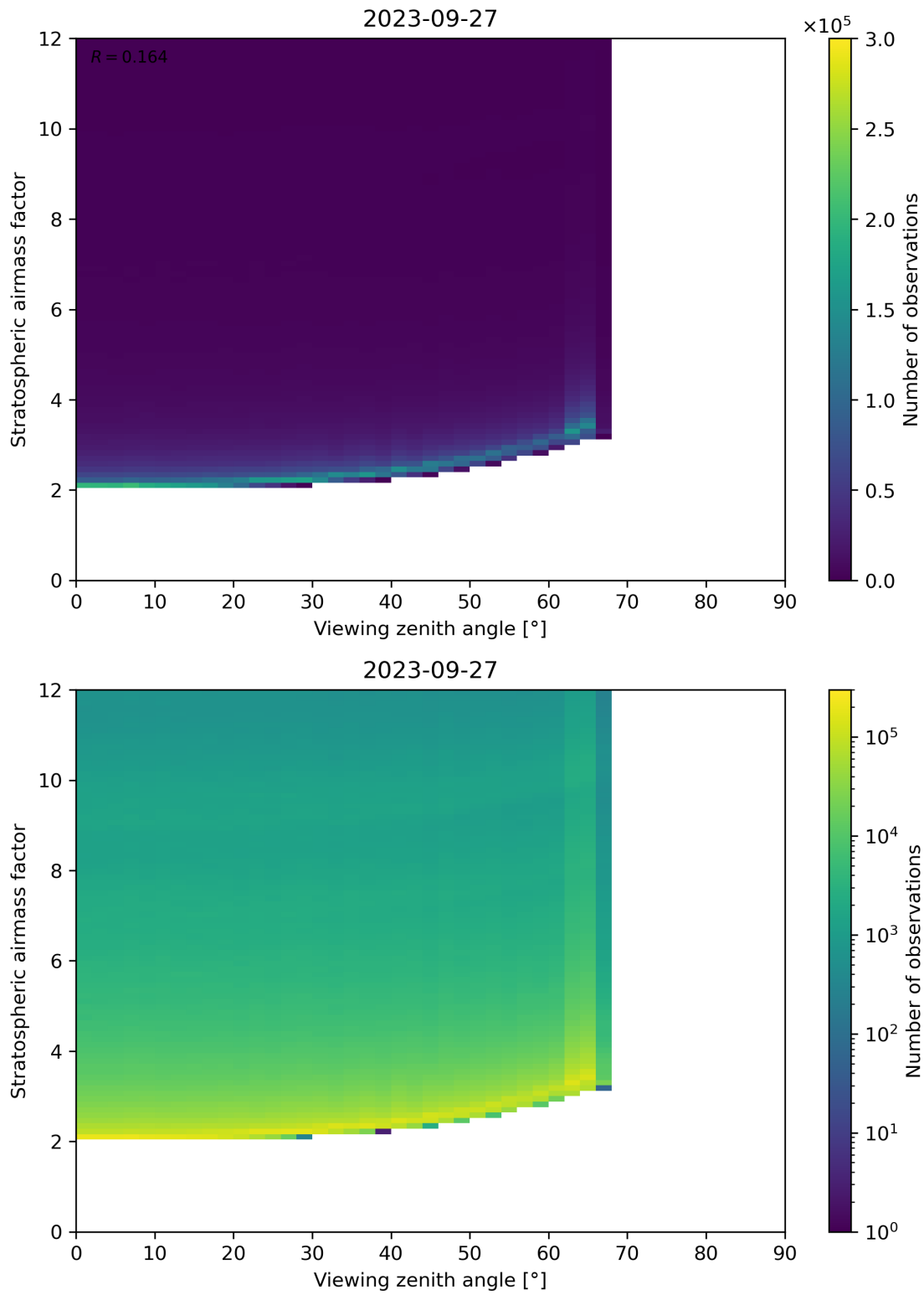
Figure 159: Scatter density plot of “Viewing zenith angle” against “Stratospheric airmass factor” for 2023-09-26 to 2023-09-28.
