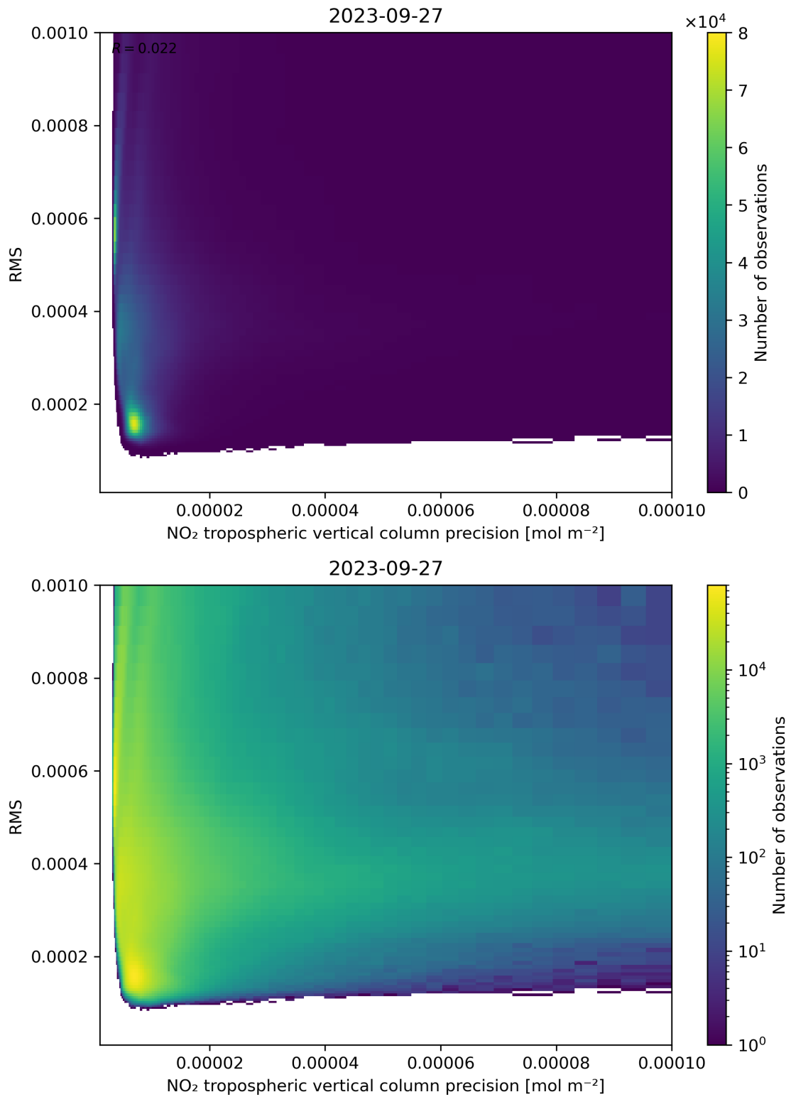
Figure 140: Scatter density plot of “NO 2 tropospheric vertical column precision” against “RMS” for 2023-09-26 to 2023-09-28.
