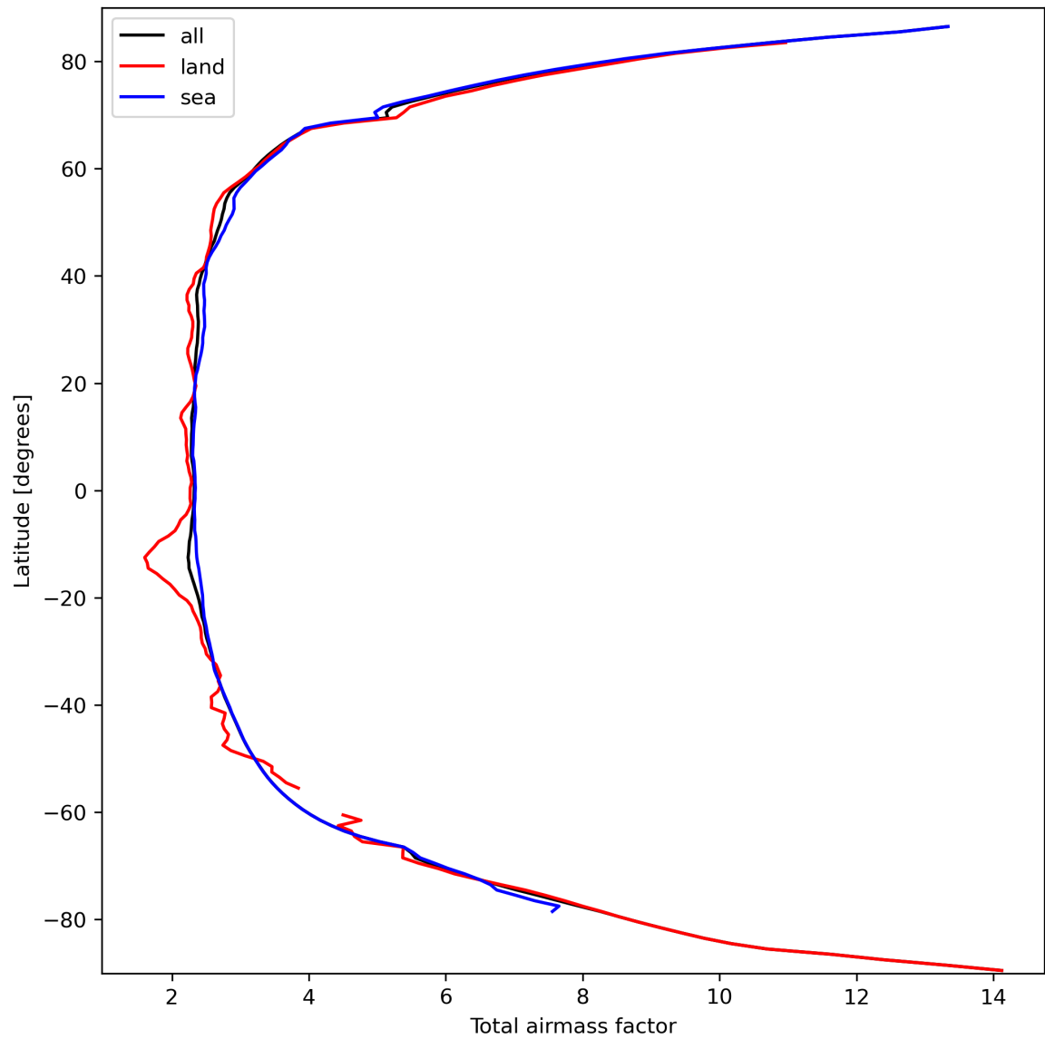
Figure 15: Zonal average of “Total airmass factor” for 2023-09-26 to 2023-09-28.
