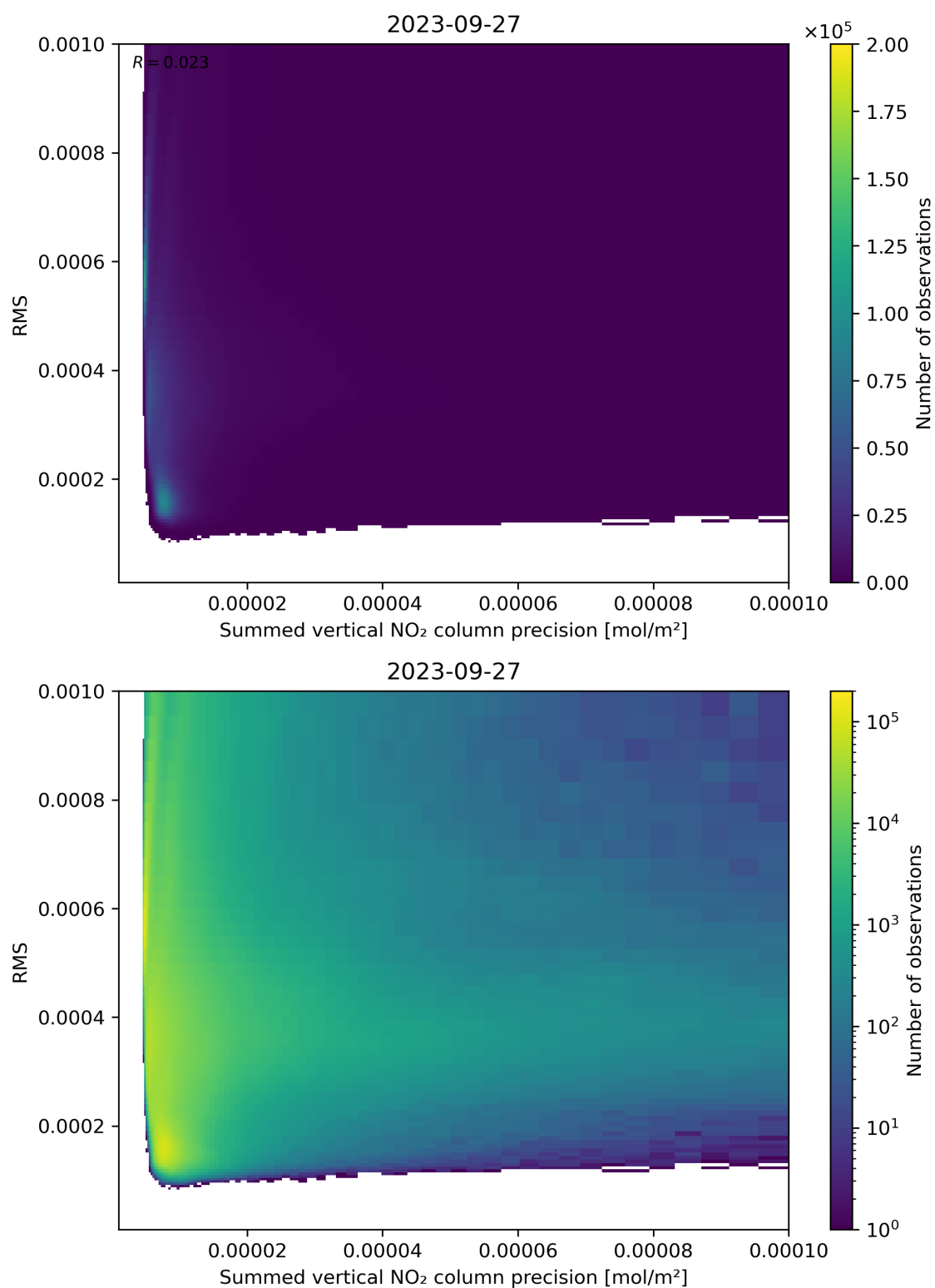
Figure 108: Scatter density plot of “Summed vertical NO 2 column precision” against “RMS” for 2023-09-26 to 2023-09-28.
