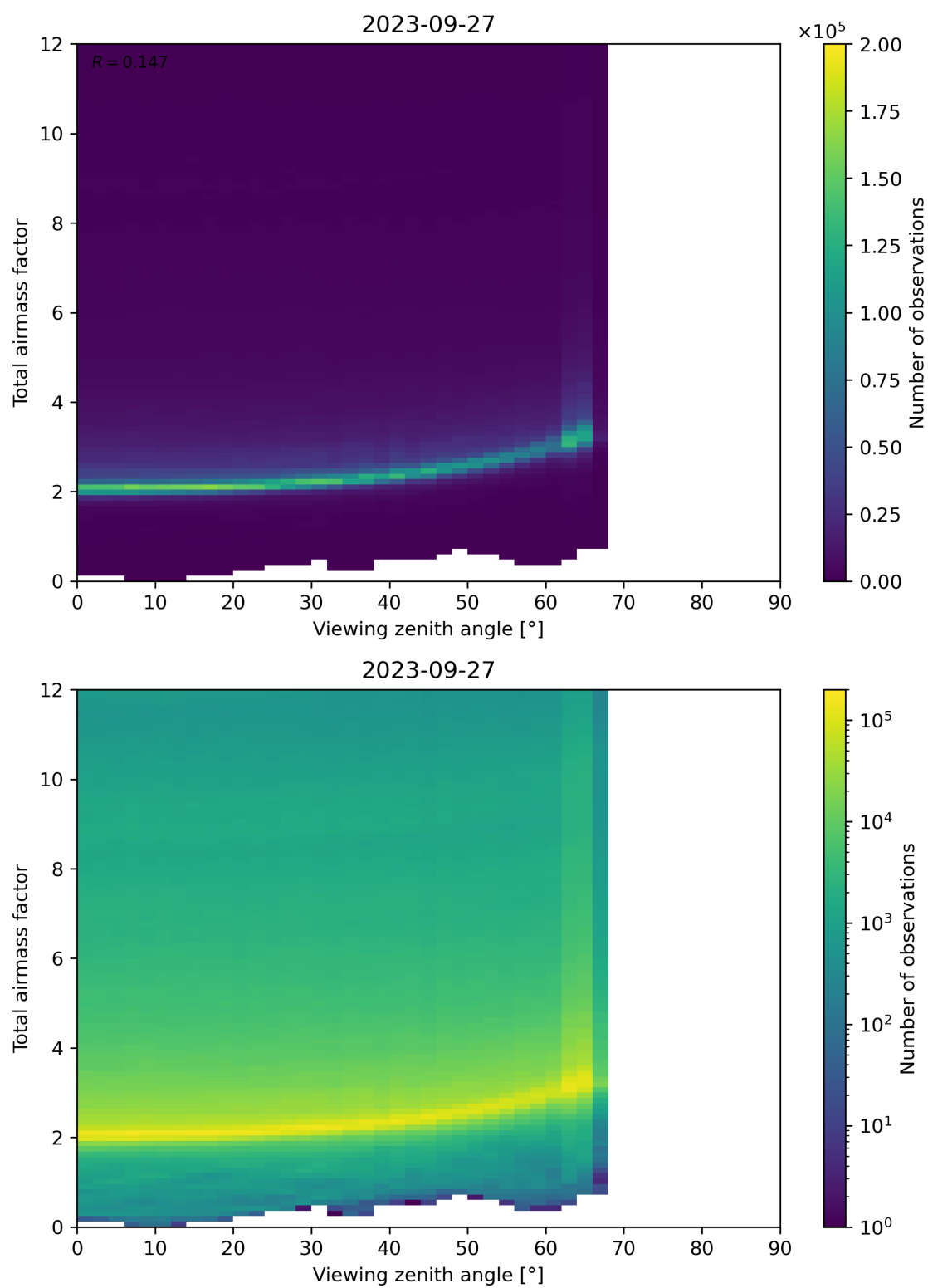
Figure 160: Scatter density plot of “Viewing zenith angle” against “Total airmass factor” for 2023-09-26 to 2023-09-28.
