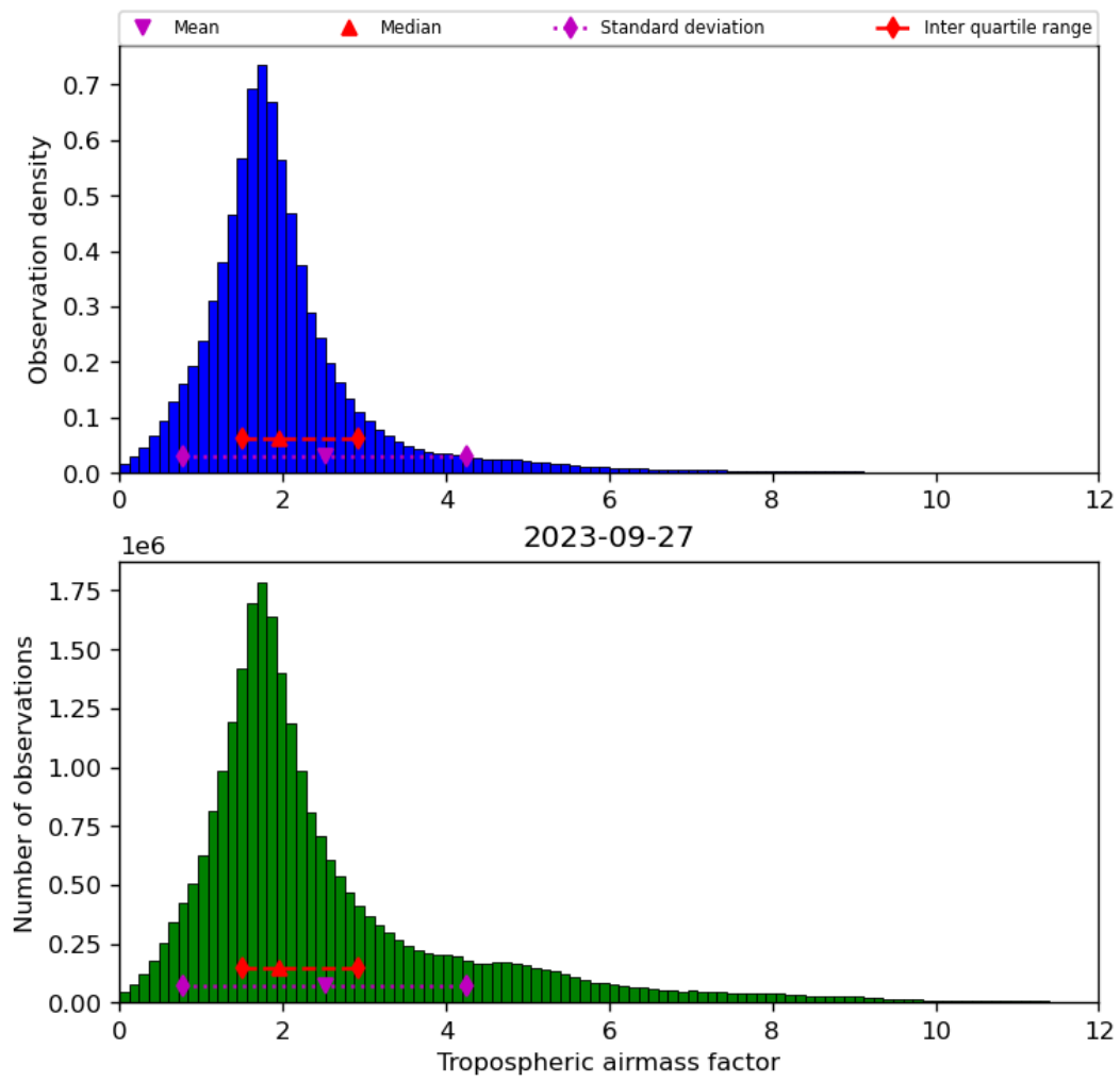
Figure 31: Histogram of “Tropospheric airmass factor” for 2023-09-26 to 2023-09-28
