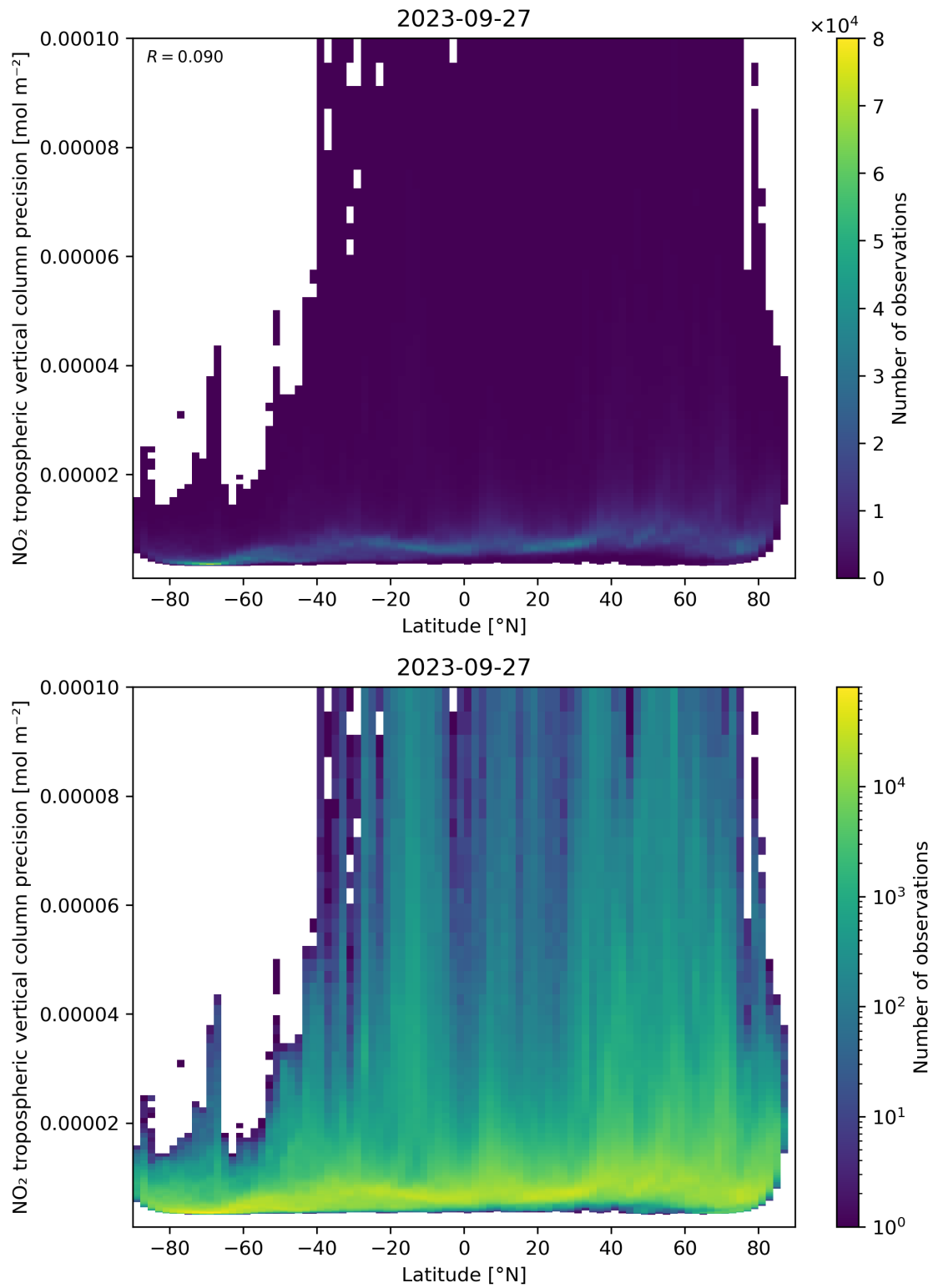
Figure 93: Scatter density plot of “Latitude” against “NO 2 tropospheric vertical column precision” for 2023-09-26 to 2023-09-28.
