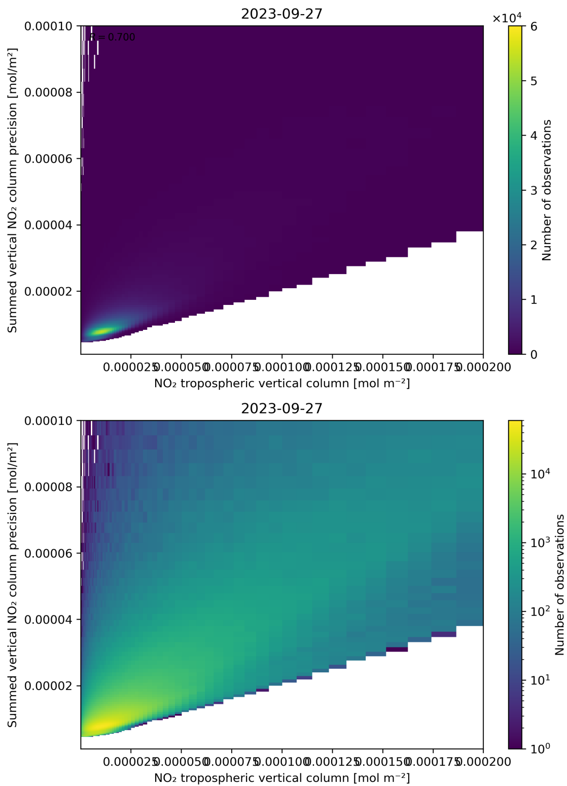
Figure 127: Scatter density plot of “NO 2 tropospheric vertical column” against “Summed vertical NO 2 column precision” for 2023-09-26 to 2023-09-28.
