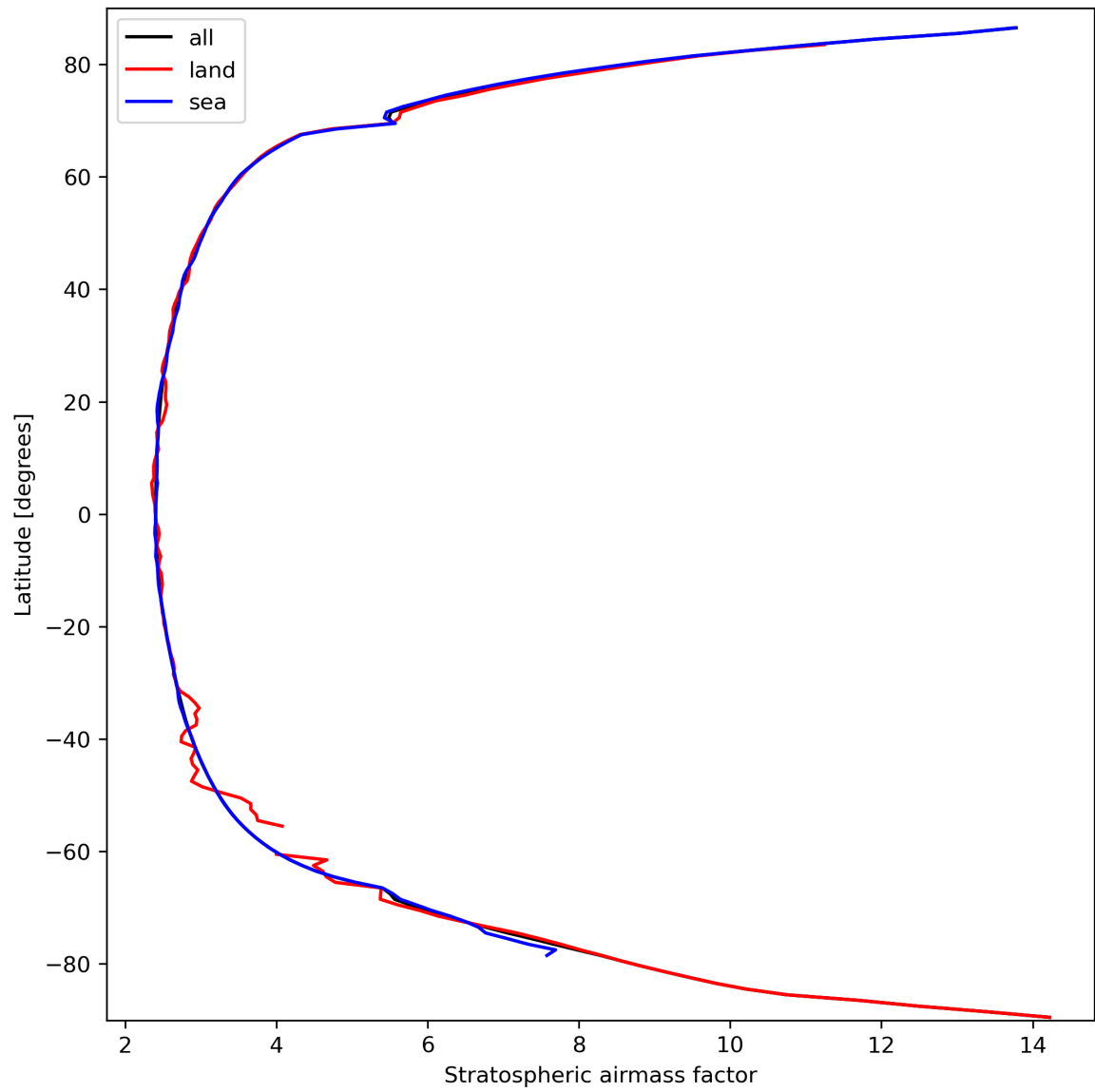
Figure 27: Zonal average of “Stratospheric airmass factor” for 2023-09-26 to 2023-09-28.
