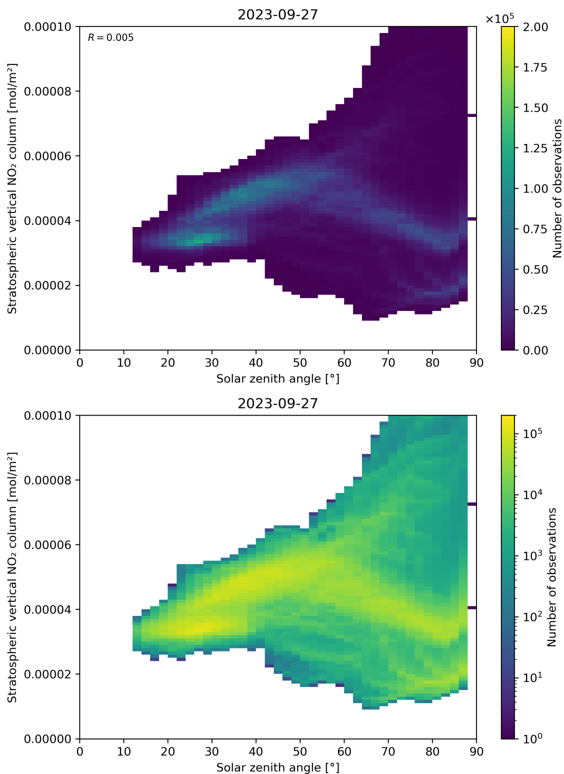
Figure 150: Scatter density plot of “Solar zenith angle” against “Stratospheric vertical NO 2 column” for 2023-09-26 to 2023-09-28.
