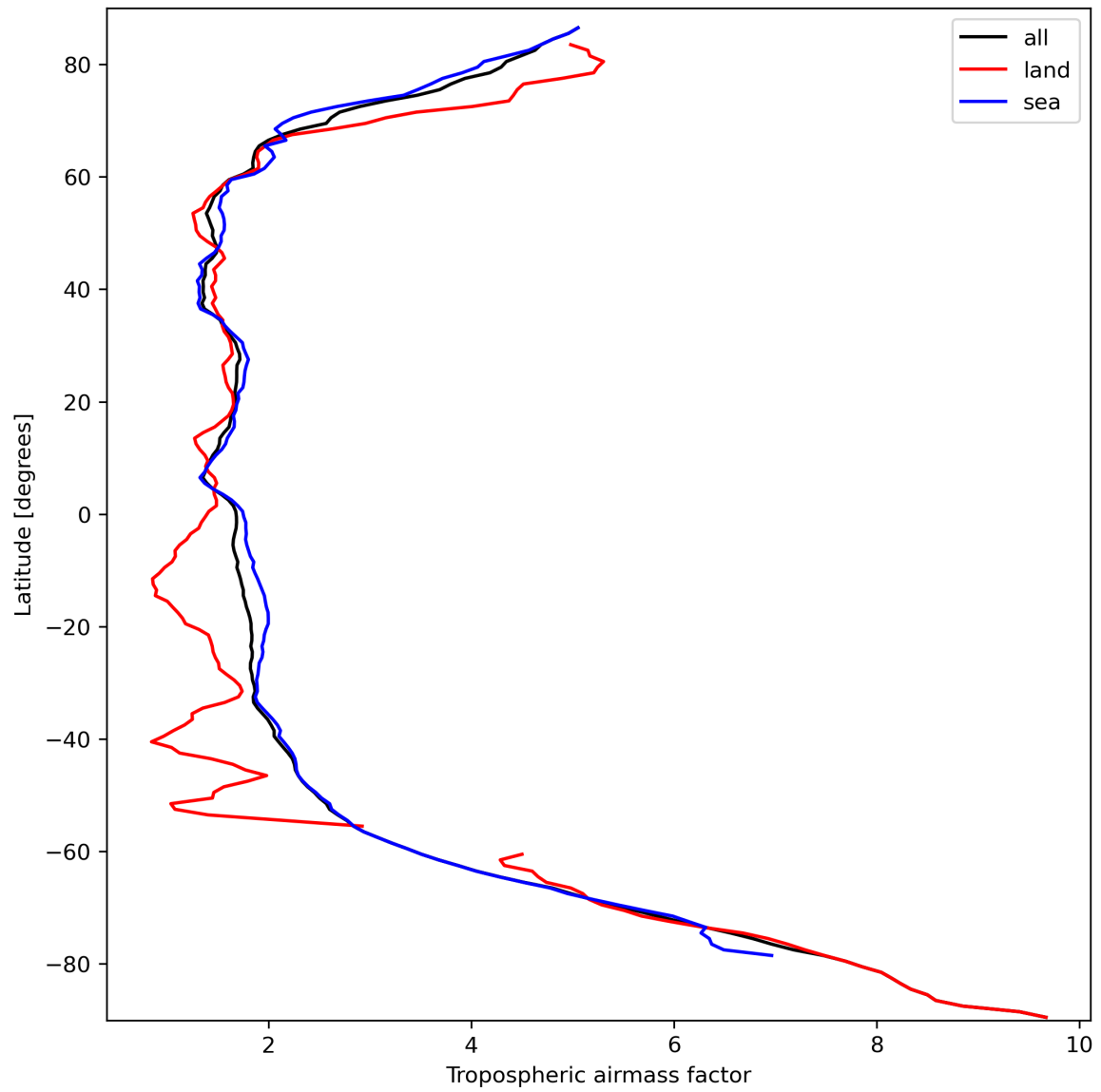
Figure 14: Zonal average of “Tropospheric airmass factor” for 2023-09-26 to 2023-09-28.
