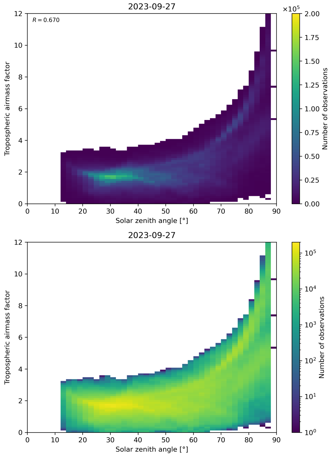
Figure 147: Scatter density plot of “Solar zenith angle” against “Tropospheric airmass factor” for 2023-09-26 to 2023-09-28.
