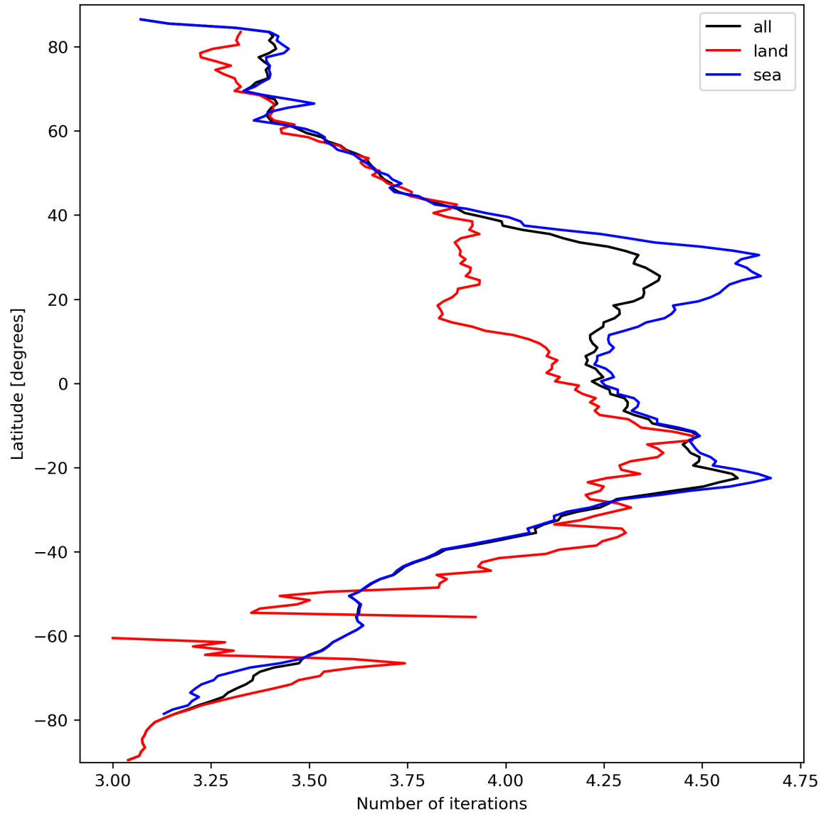
Figure 17: Zonal average of “Number of iterations” for 2023-09-26 to 2023-09-28.
