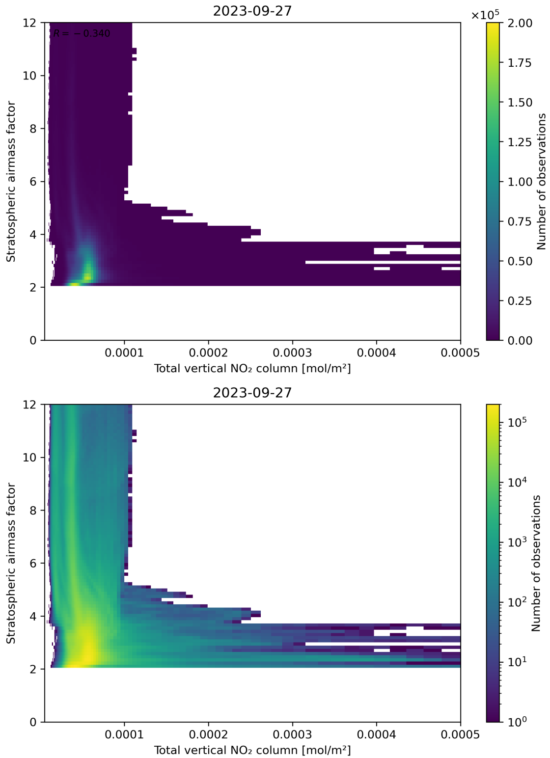
Figure 110: Scatter density plot of “Total vertical NO 2 column” against “Stratospheric airmass factor” for 2023-09-26 to 2023-09-28.
