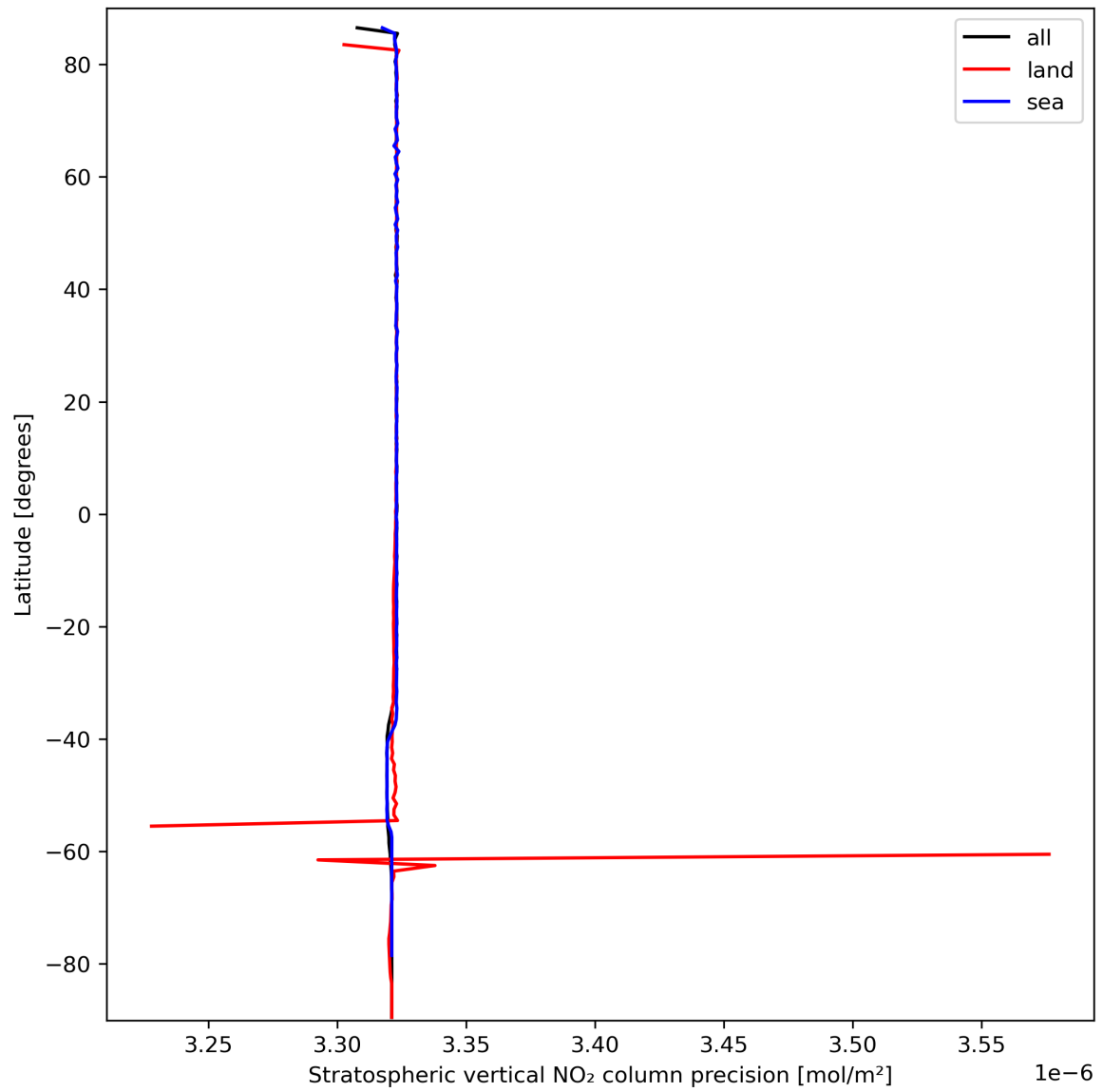
Figure 20: Zonal average of “Stratospheric vertical NO 2 column precision” for 2023-09-26 to 2023-09-28.
