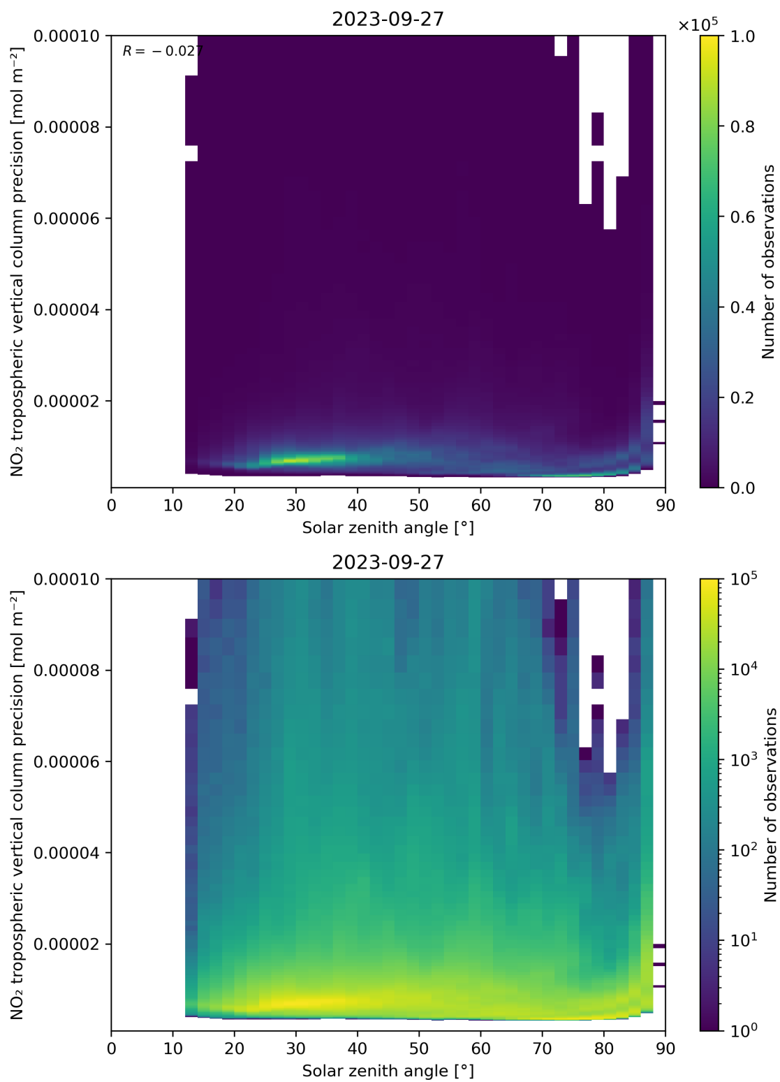
Figure 156: Scatter density plot of “Solar zenith angle” against “NO 2 tropospheric vertical column precision” for 2023-09-26 to 2023-09-28.
