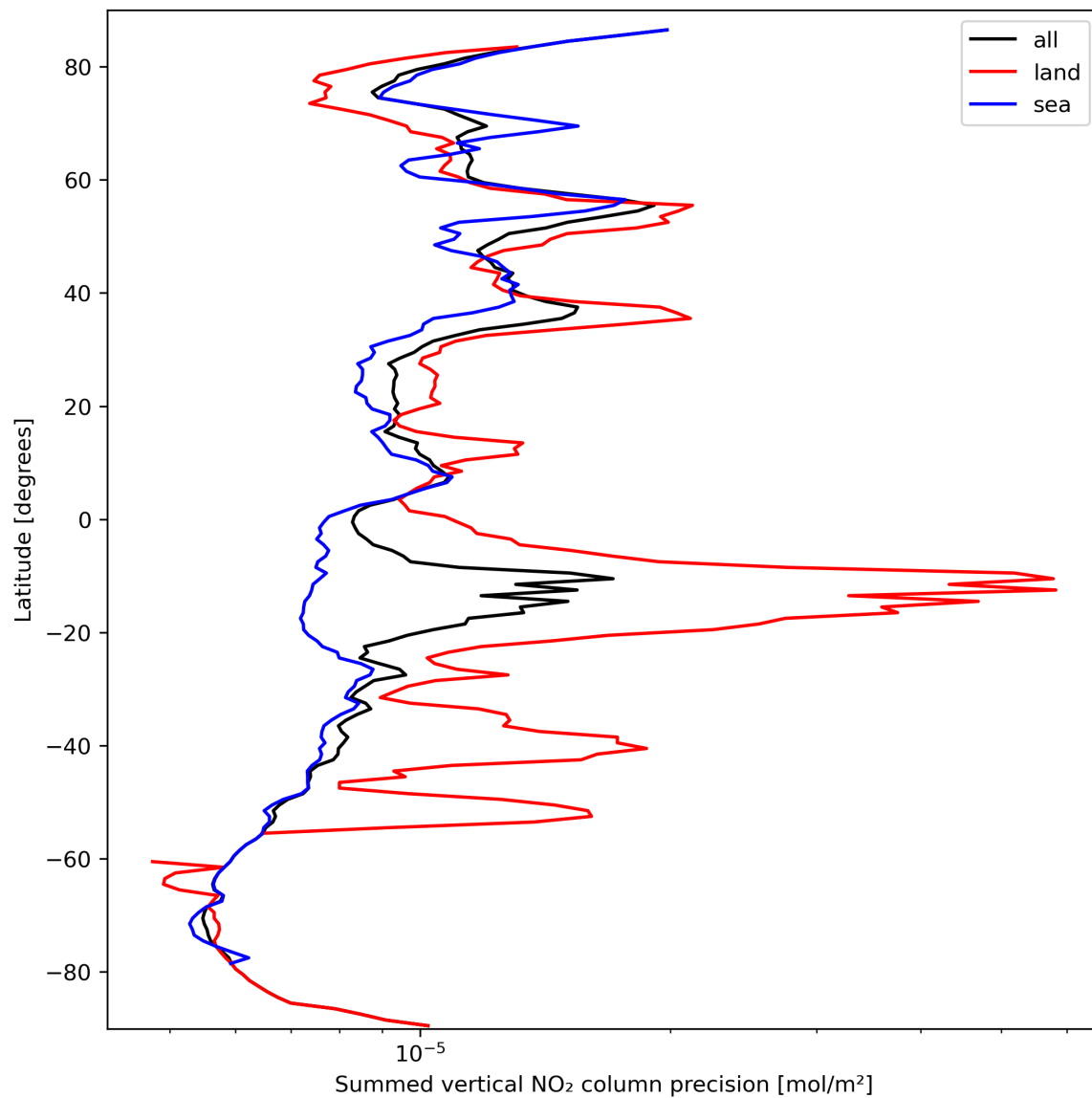
Figure 24: Zonal average of “Summed vertical NO 2 column precision” for 2023-09-26 to 2023-09-28.
