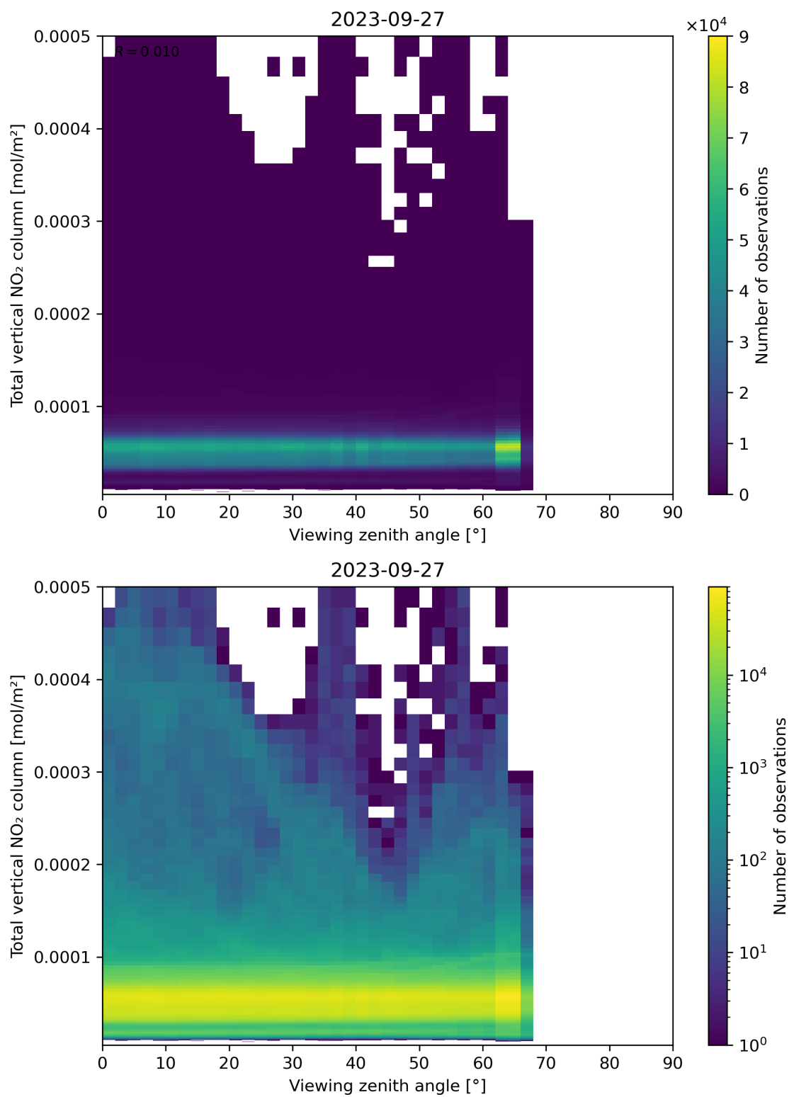
Figure 167: Scatter density plot of “Viewing zenith angle” against “Total vertical NO 2 column” for 2023-09-26 to 2023-09-28.
