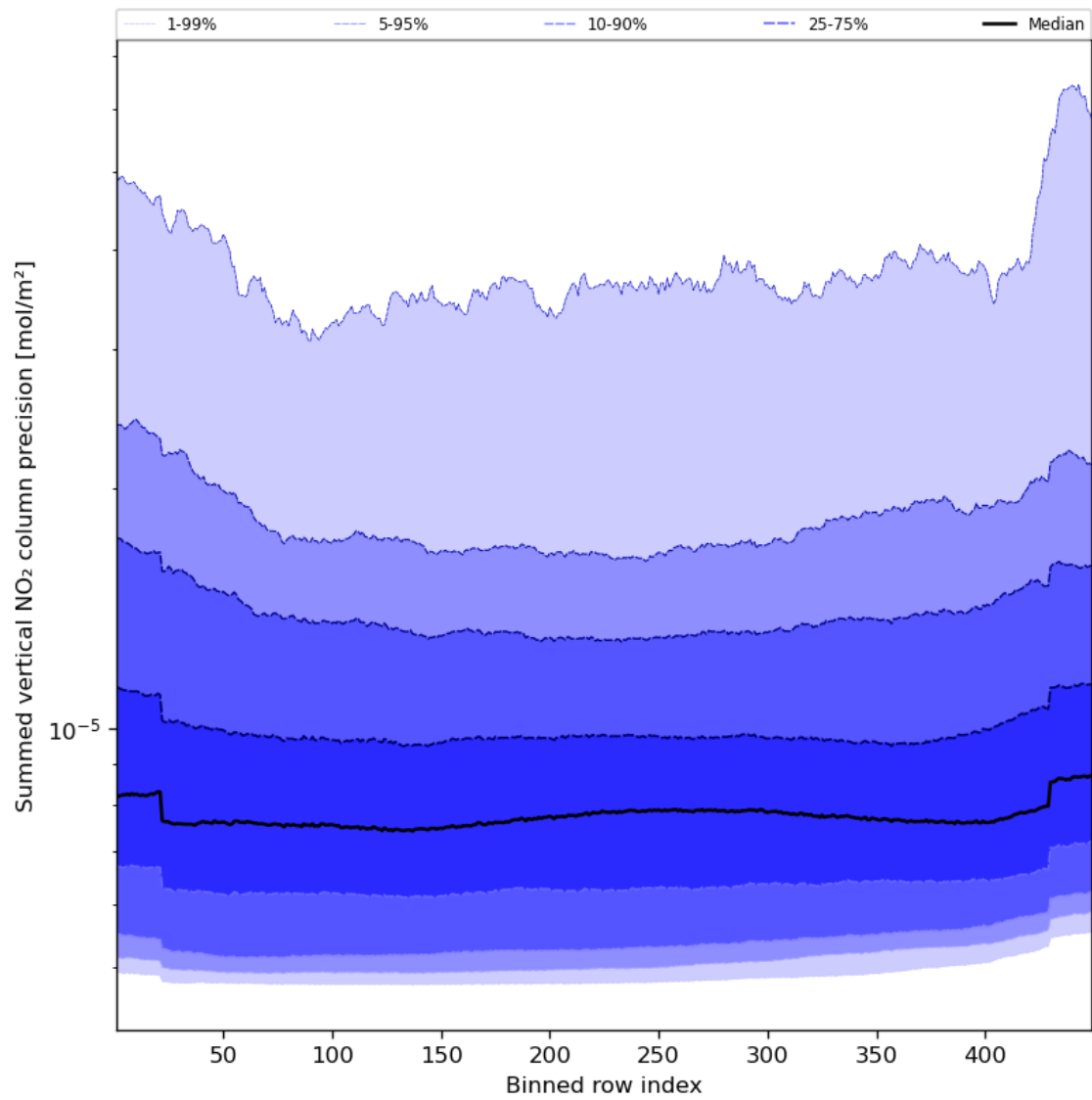
Figure 58: Along track statistics of “Summed vertical NO 2 column precision” for 2023-09-26 to 2023-09-28
