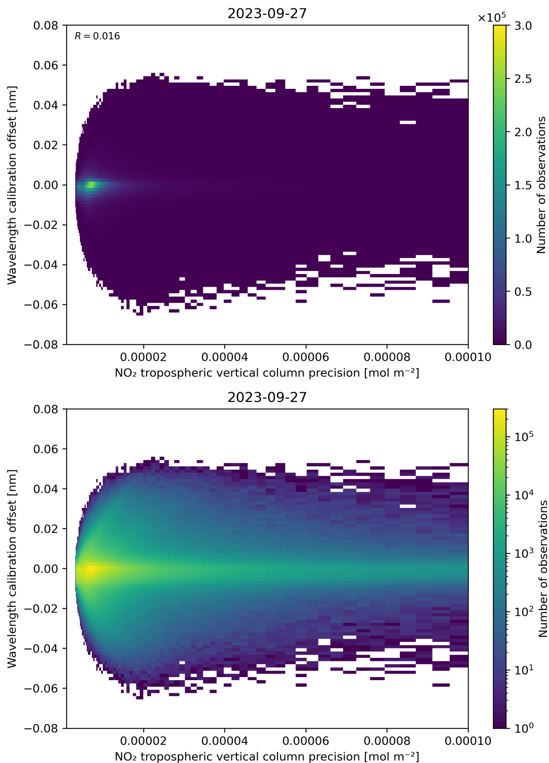
Figure 141: Scatter density plot of “NO 2 tropospheric vertical column precision” against “Wavelength calibration offset” for 2023-09-26 to 2023-09-28.
