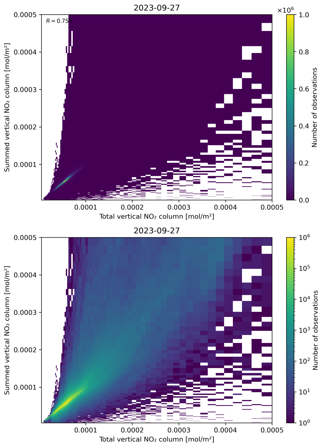
Figure 112: Scatter density plot of “Total vertical NO 2 column” against “Summed vertical NO 2 column” for 2023-09-26 to 2023-09-28.
