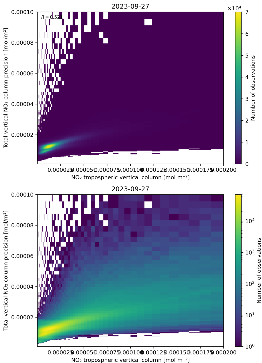
Figure 129: Scatter density plot of “NO 2 tropospheric vertical column” against “Total vertical NO 2 column precision” for 2023-09-26 to 2023-09-28.
