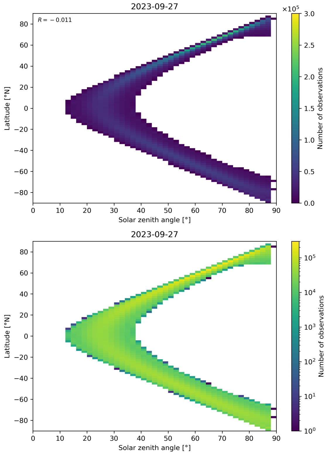
Figure 149: Scatter density plot of “Solar zenith angle” against “Latitude” for 2023-09-26 to 2023-09-28.
