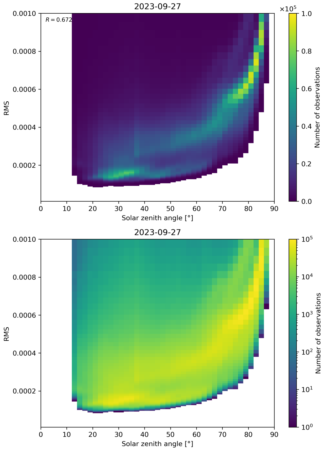
Figure 157: Scatter density plot of “Solar zenith angle” against “RMS” for 2023-09-26 to 2023-09-28.
