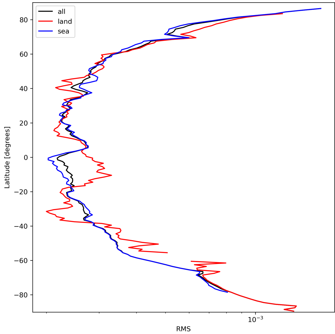
Figure 26: Zonal average of “RMS” for 2023-09-26 to 2023-09-28.
