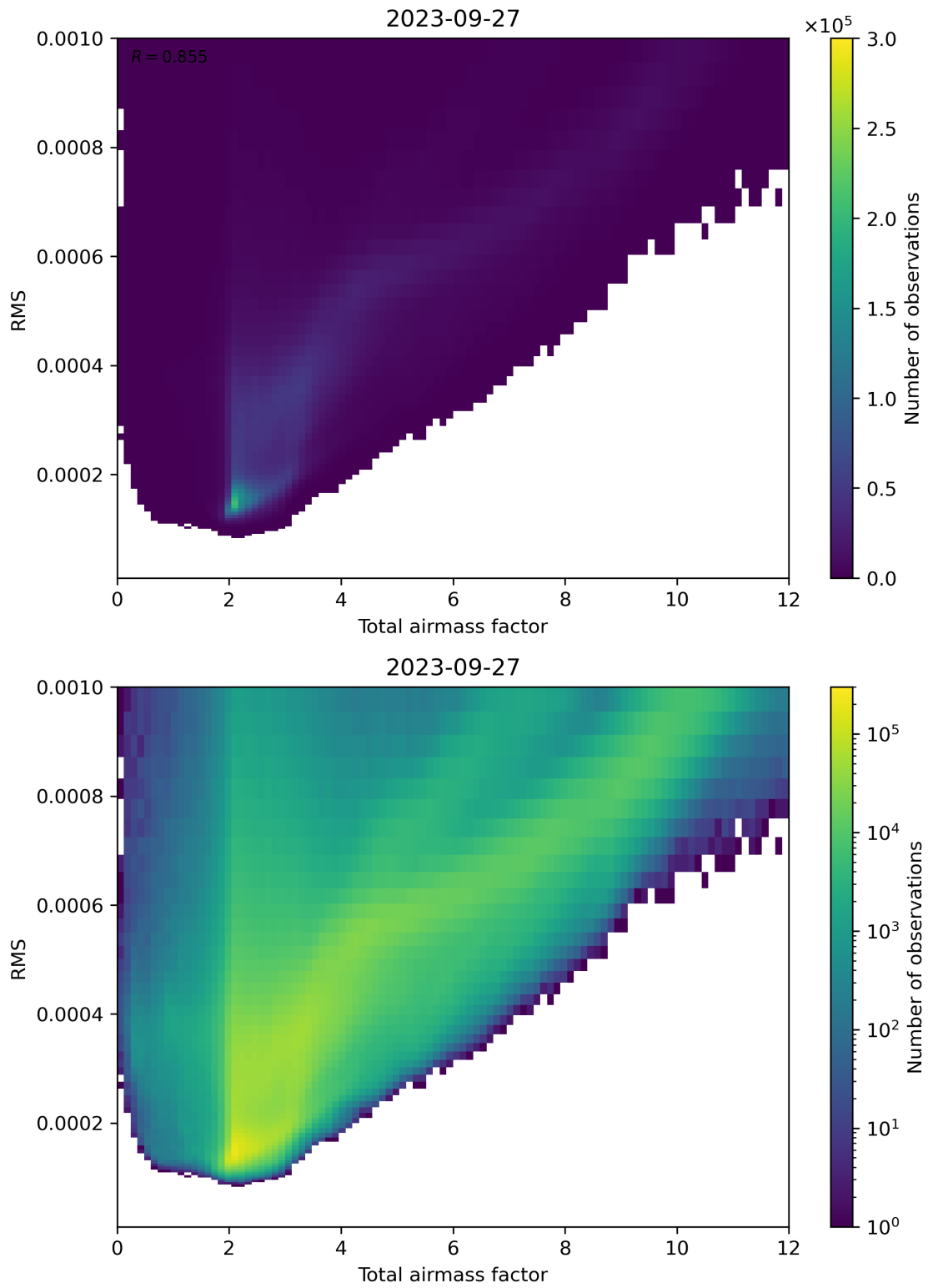
Figure 69: Scatter density plot of “Total airmass factor” against “RMS” for 2023-09-26 to 2023-09-28.
