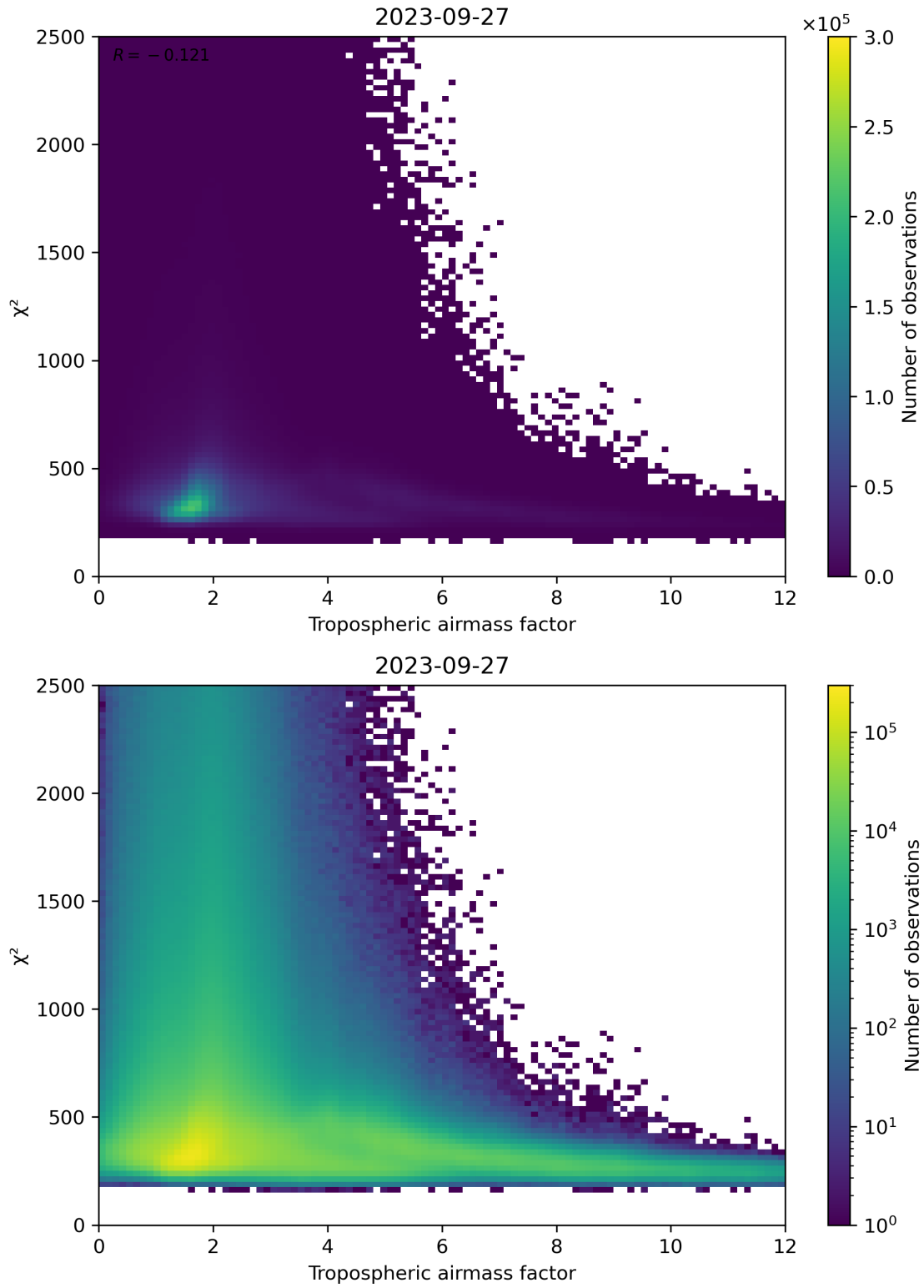
Figure 73: Scatter density plot of “Tropospheric airmass factor” against “ \chi^2 ” for 2023-09-26 to 2023-09-28.
