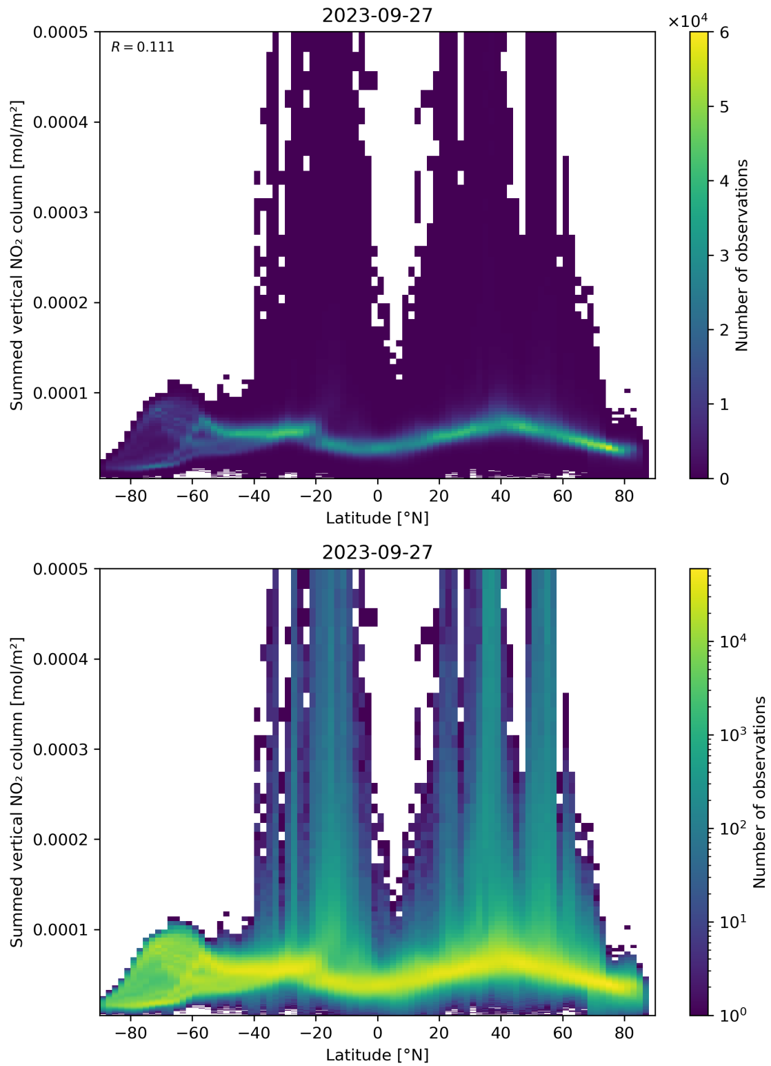
Figure 88: Scatter density plot of “Latitude” against “Summed vertical NO 2 column” for 2023-09-26 to 2023-09-28.
