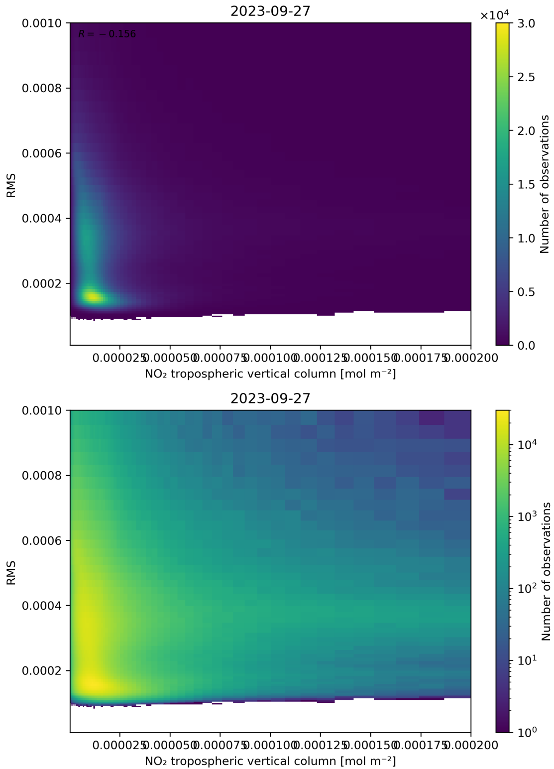
Figure 142: Scatter density plot of “NO 2 tropospheric vertical column” against “RMS” for 2023-09-26 to 2023-09-28.
