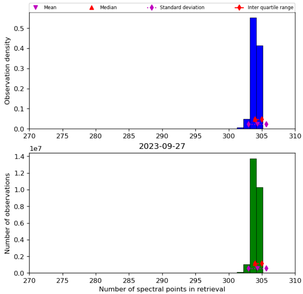
Figure 33: Histogram of “Number of spectral points in retrieval” for 2023-09-26 to 2023-09-28
