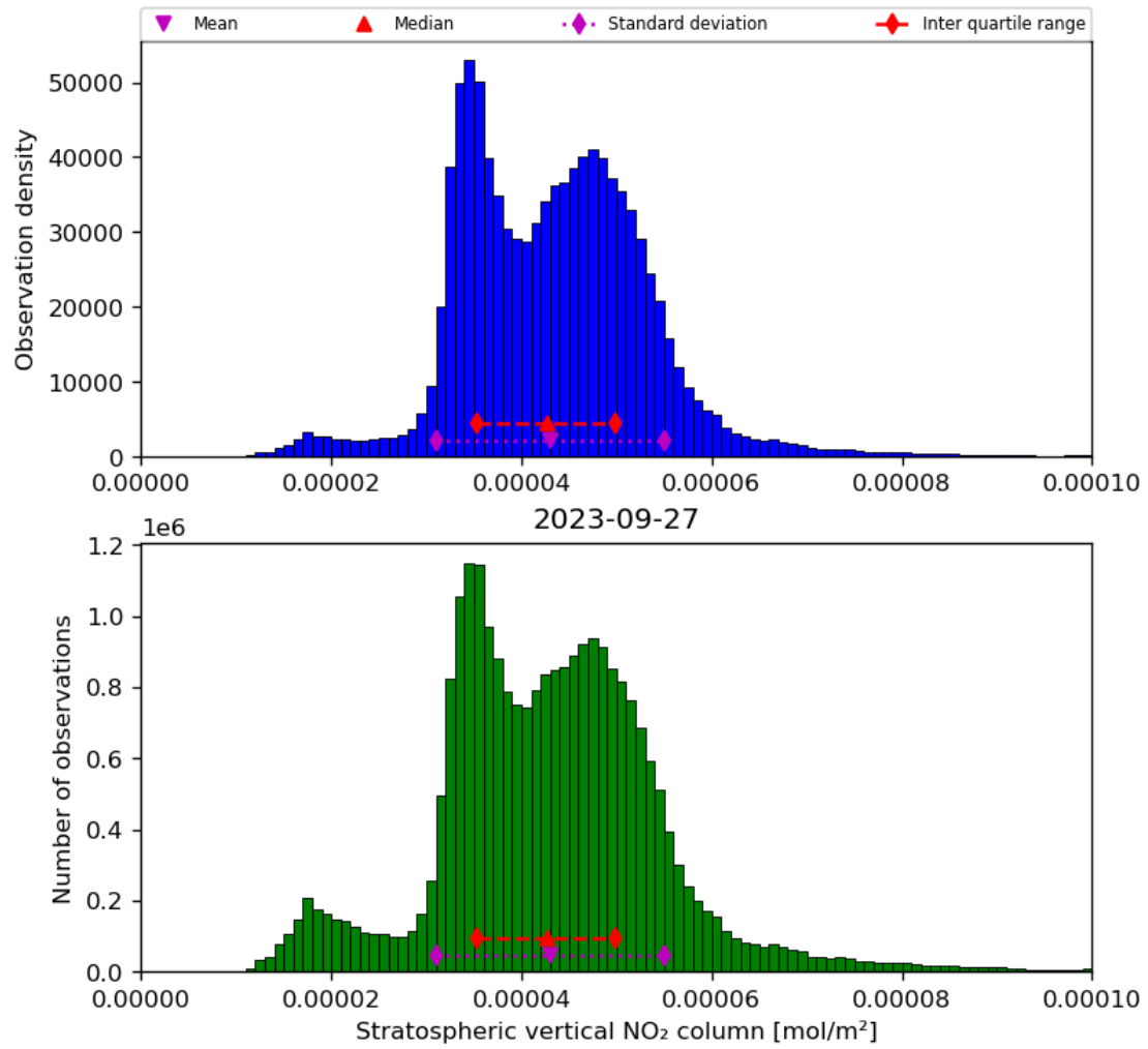
Figure 36: Histogram of “Stratospheric vertical NO 2 column” for 2023-09-26 to 2023-09-28
