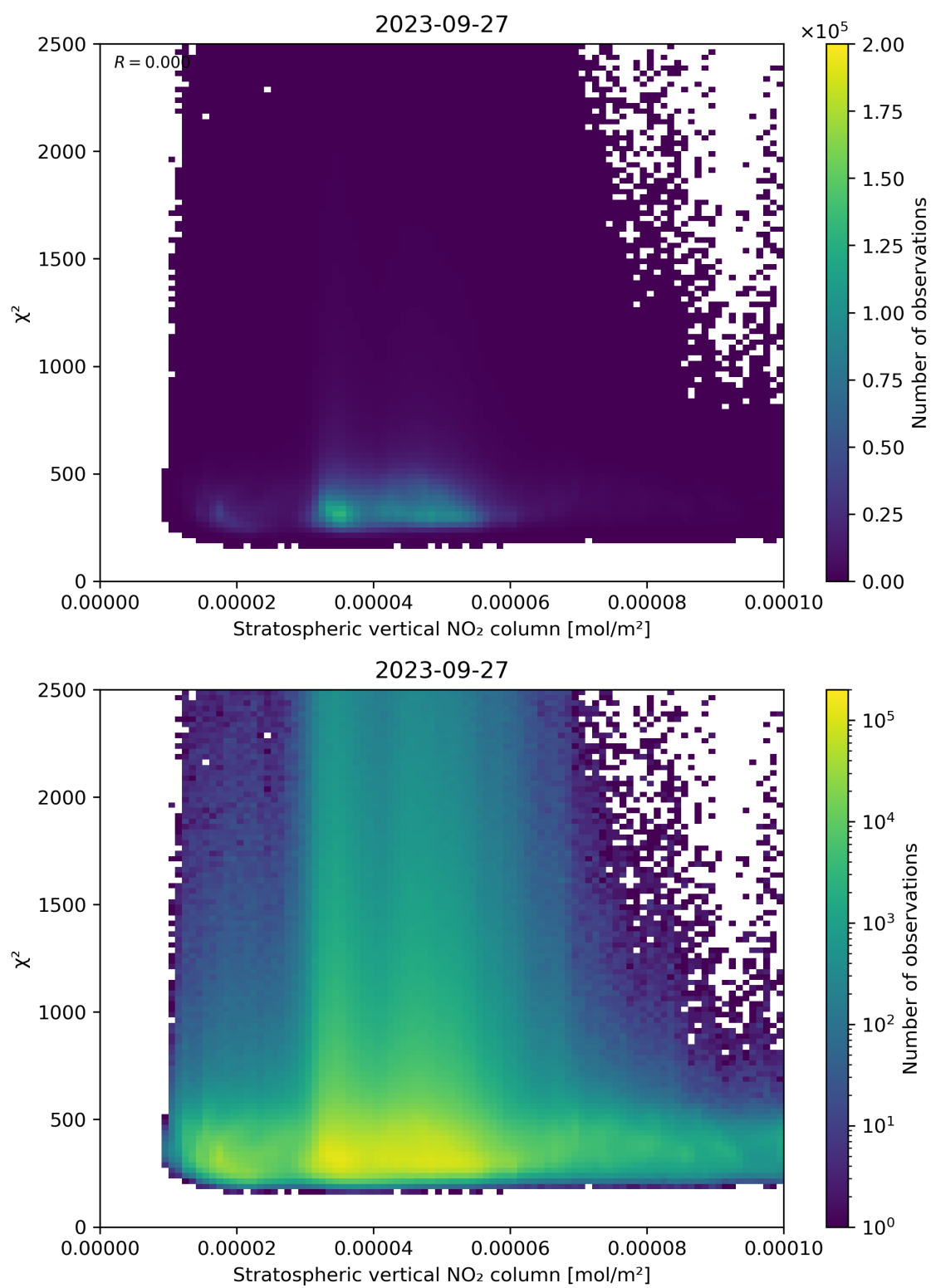
Figure 97: Scatter density plot of “Stratospheric vertical NO 2 column” against “ \chi^2 ” for 2023-09-26 to 2023-09-28.
