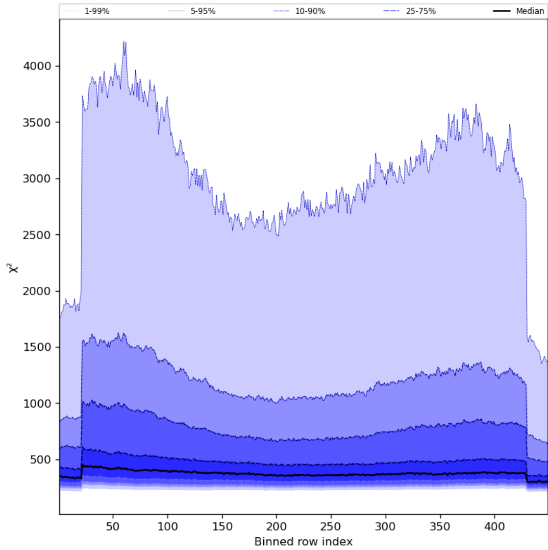
Figure 59: Along track statistics of “ \chi^2 ” for 2023-09-26 to 2023-09-28
