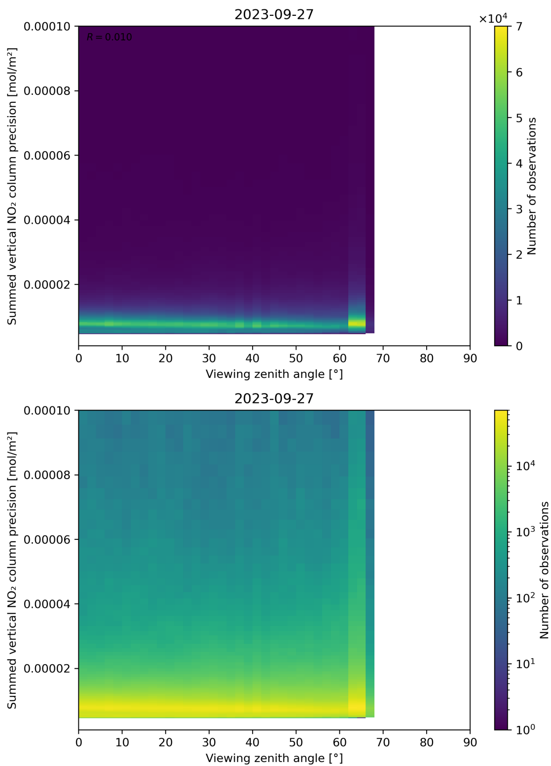
Figure 166: Scatter density plot of “Viewing zenith angle” against “Summed vertical NO 2 column precision” for 2023-09-26 to 2023-09-28.
