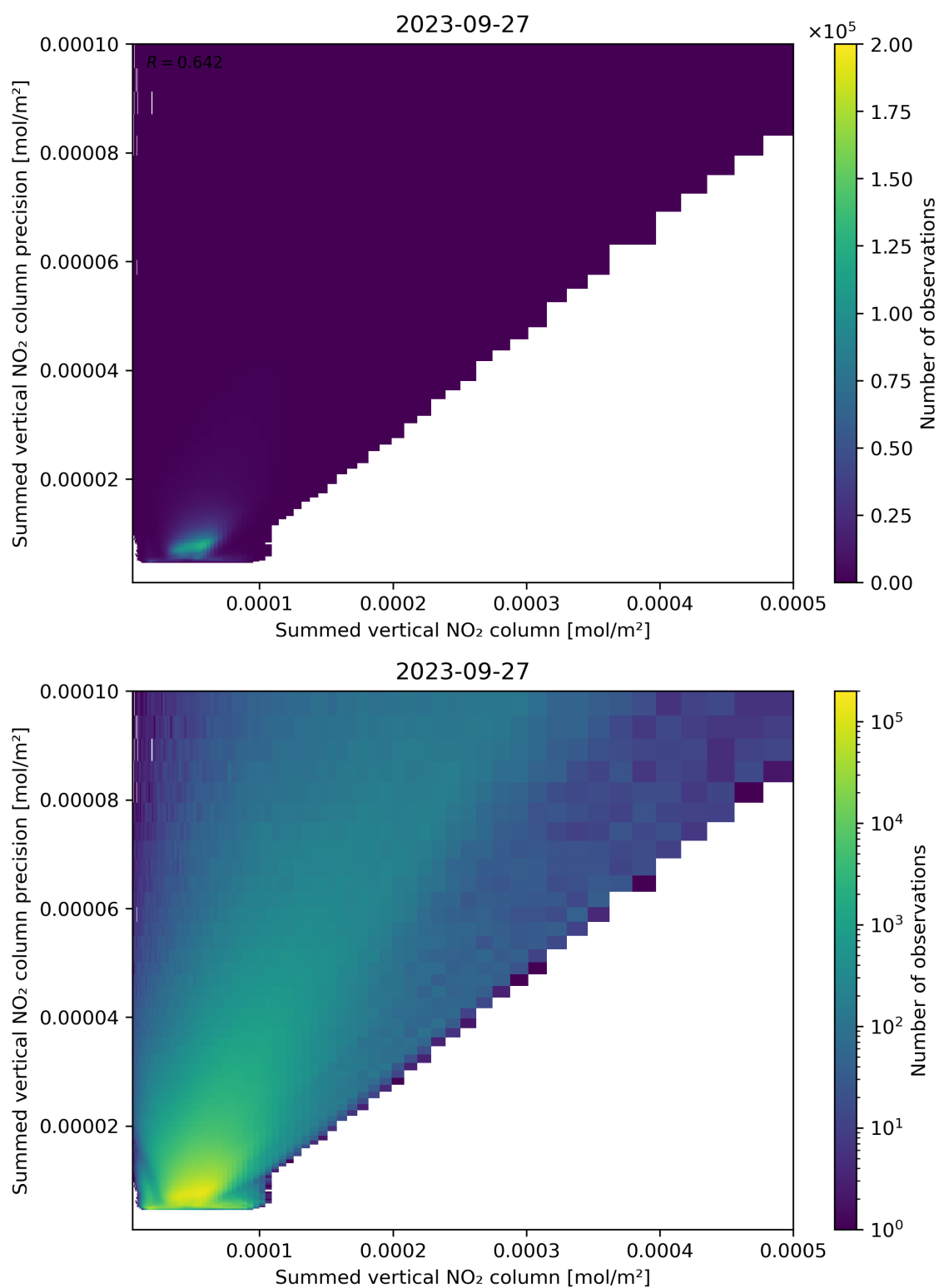
Figure 105: Scatter density plot of “Summed vertical NO 2 column” against “Summed vertical NO 2 column precision” for 2023-09-26 to 2023-09-28.
