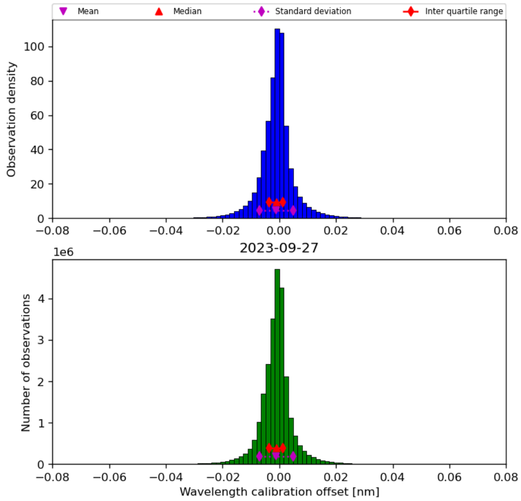
Figure 35: Histogram of “Wavelength calibration offset” for 2023-09-26 to 2023-09-28
