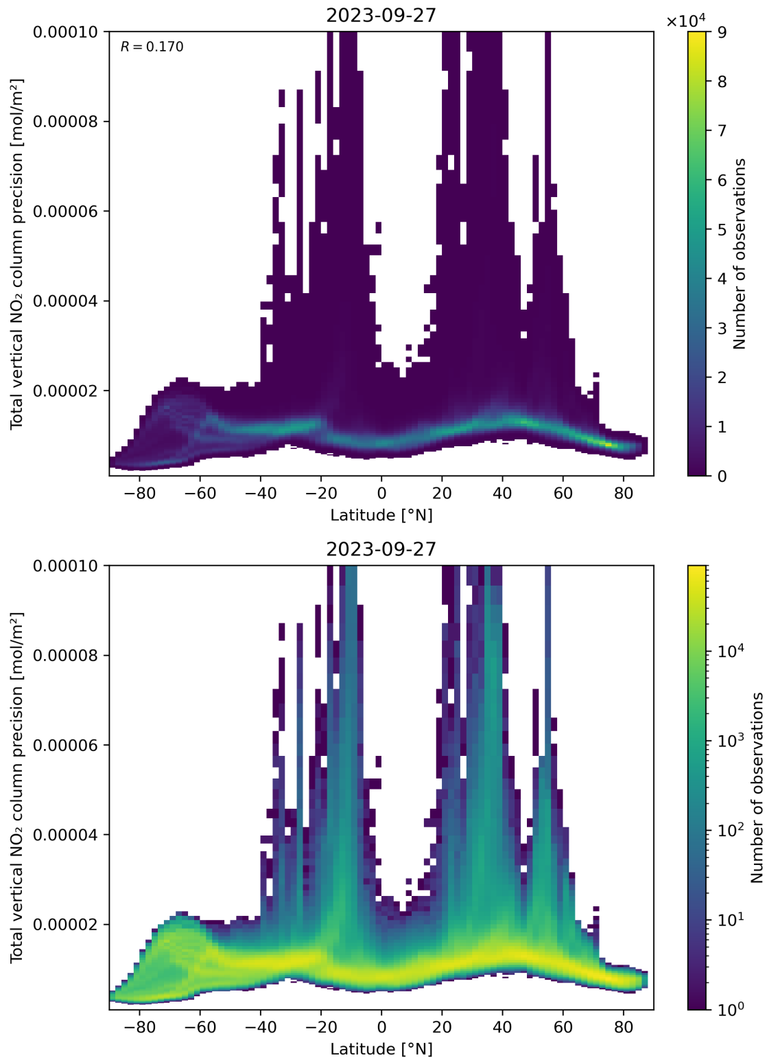
Figure 91: Scatter density plot of “Latitude” against “Total vertical NO 2 column precision” for 2023-09-26 to 2023-09-28.
