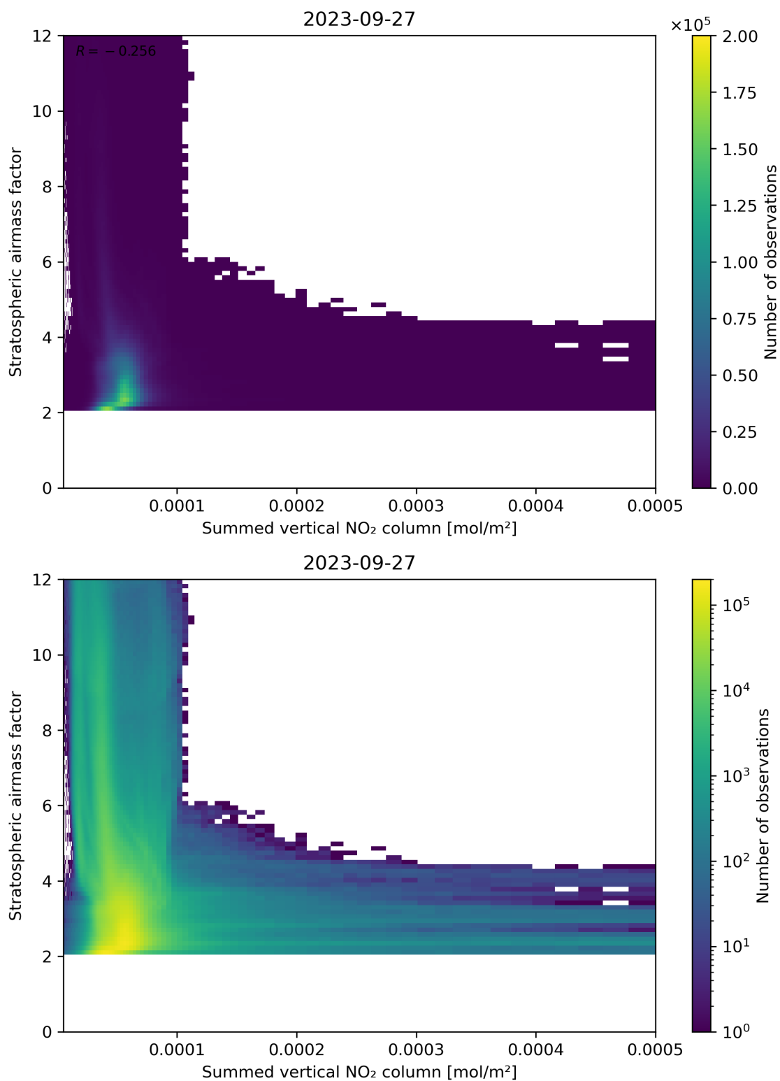
Figure 103: Scatter density plot of “Summed vertical NO 2 column” against “Stratospheric airmass factor” for 2023-09-26 to 2023-09-28.
