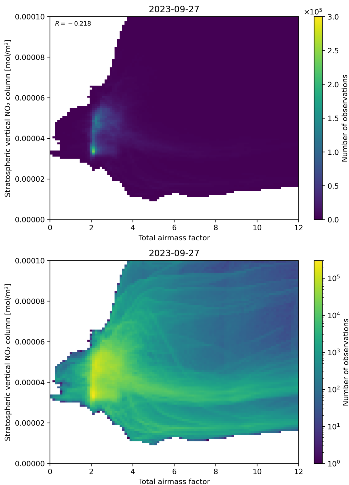
Figure 64: Scatter density plot of “Total airmass factor” against “Stratospheric vertical NO 2 column” for 2023-09-26 to 2023-09-28.
