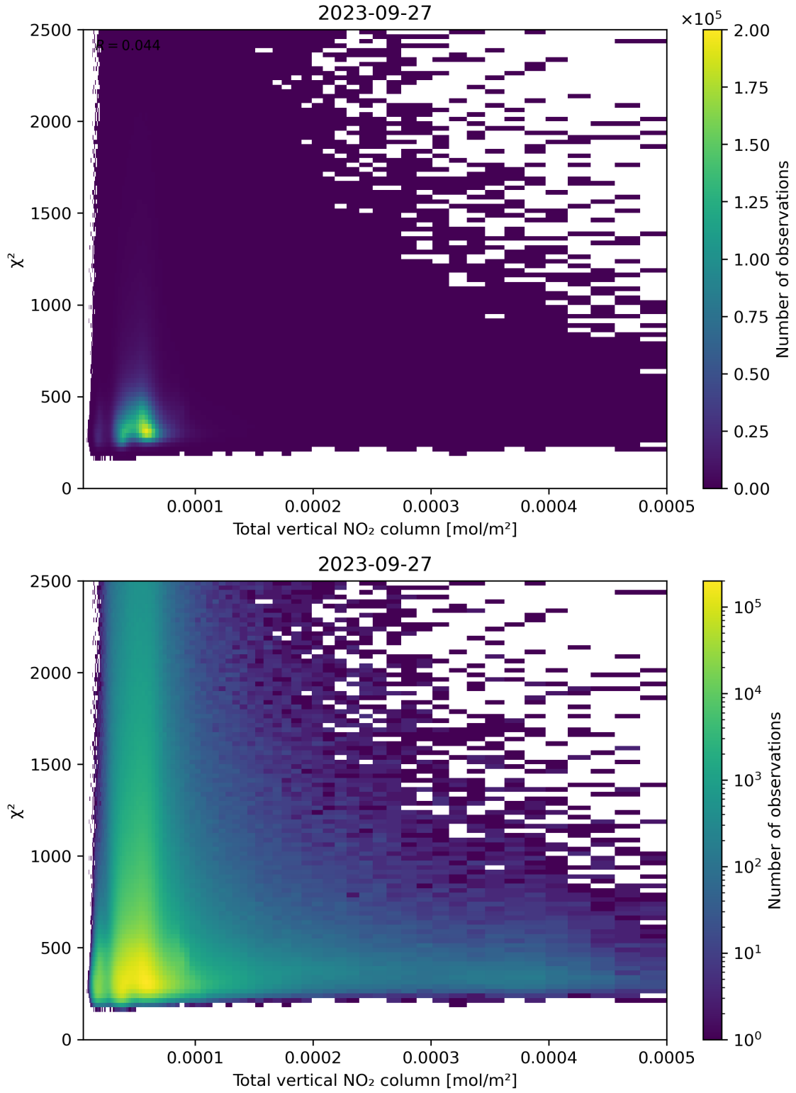
Figure 111: Scatter density plot of “Total vertical NO 2 column” against “ \chi^2 ” for 2023-09-26 to 2023-09-28.
