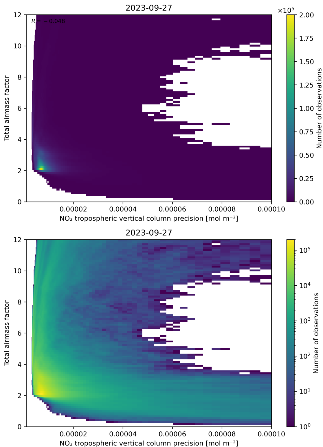
Figure 132: Scatter density plot of “NO 2 tropospheric vertical column precision” against “Total air mass factor” for 2023-09-26 to 2023-09-28.
