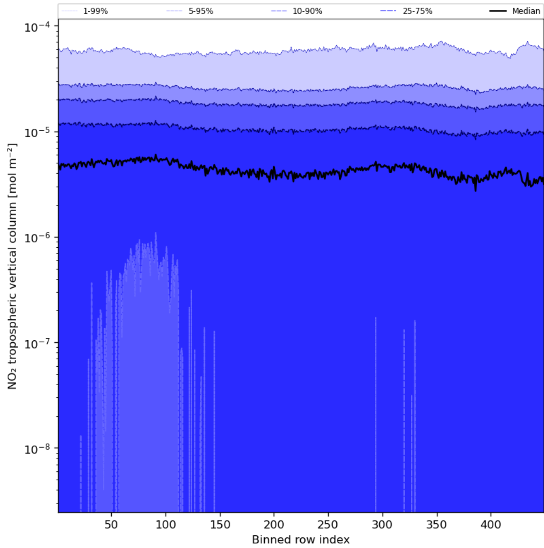
Figure 46: Along track statistics of “NO 2 tropospheric vertical column” for 2023-09-26 to 2023-09-28
