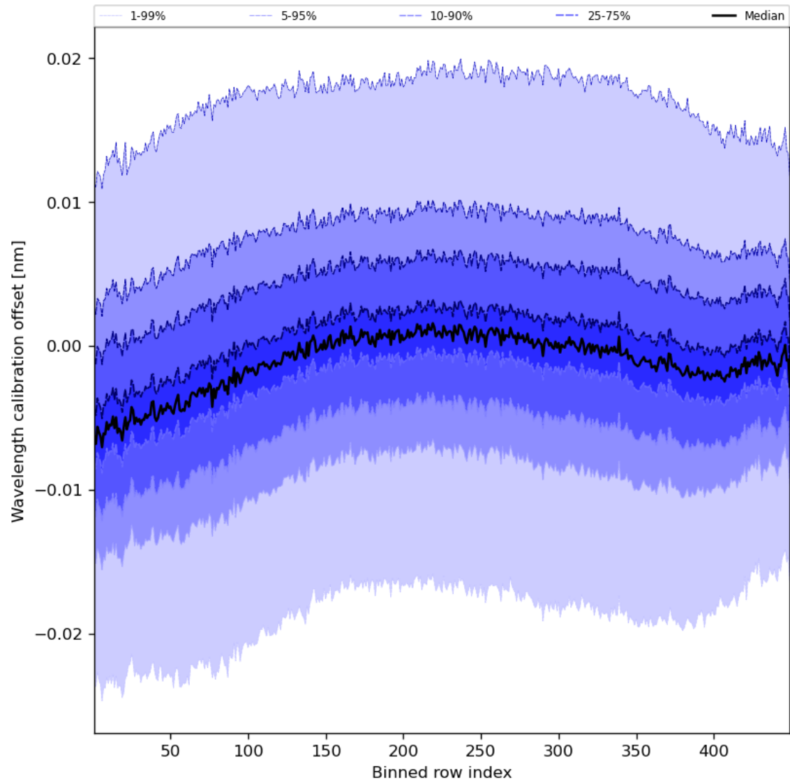
Figure 52: Along track statistics of “Wavelength calibration offset” for 2023-09-26 to 2023-09-28
