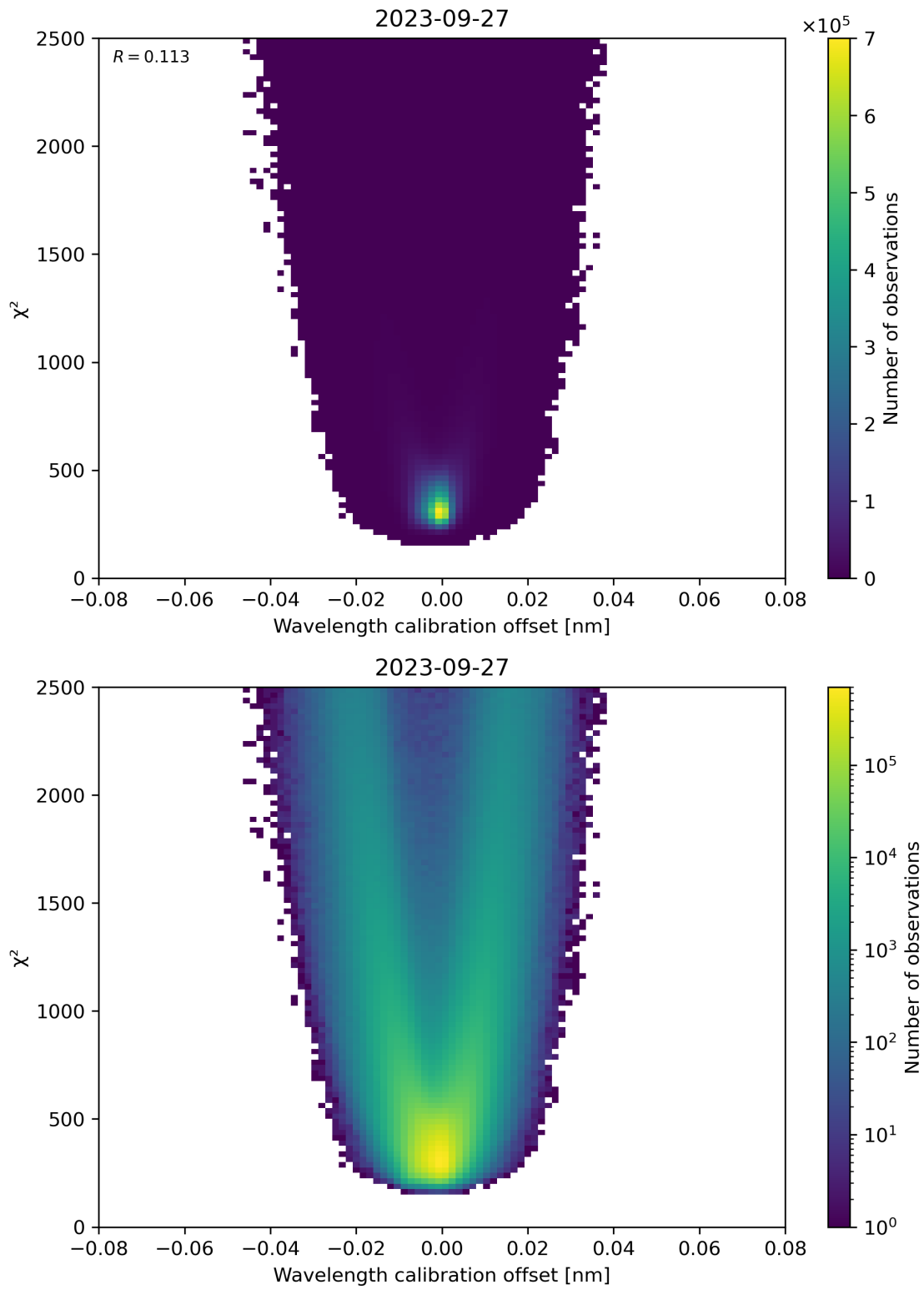
Figure 175: Scatter density plot of “Wavelength calibration offset” against “ \chi^2 ” for 2023-09-26 to 2023-09-28.
