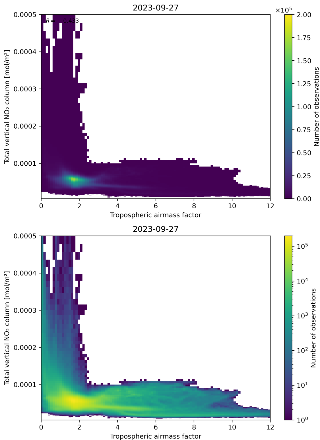
Figure 77: Scatter density plot of “Tropospheric airmass factor” against “Total vertical NO 2 column” for 2023-09-26 to 2023-09-28.
