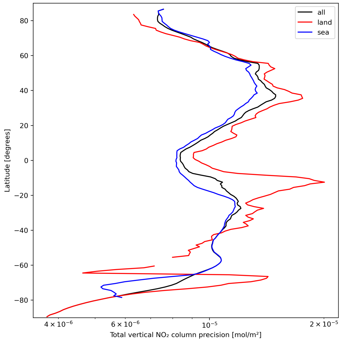
Figure 22: Zonal average of “Total vertical NO 2 column precision” for 2023-09-26 to 2023-09-28.
