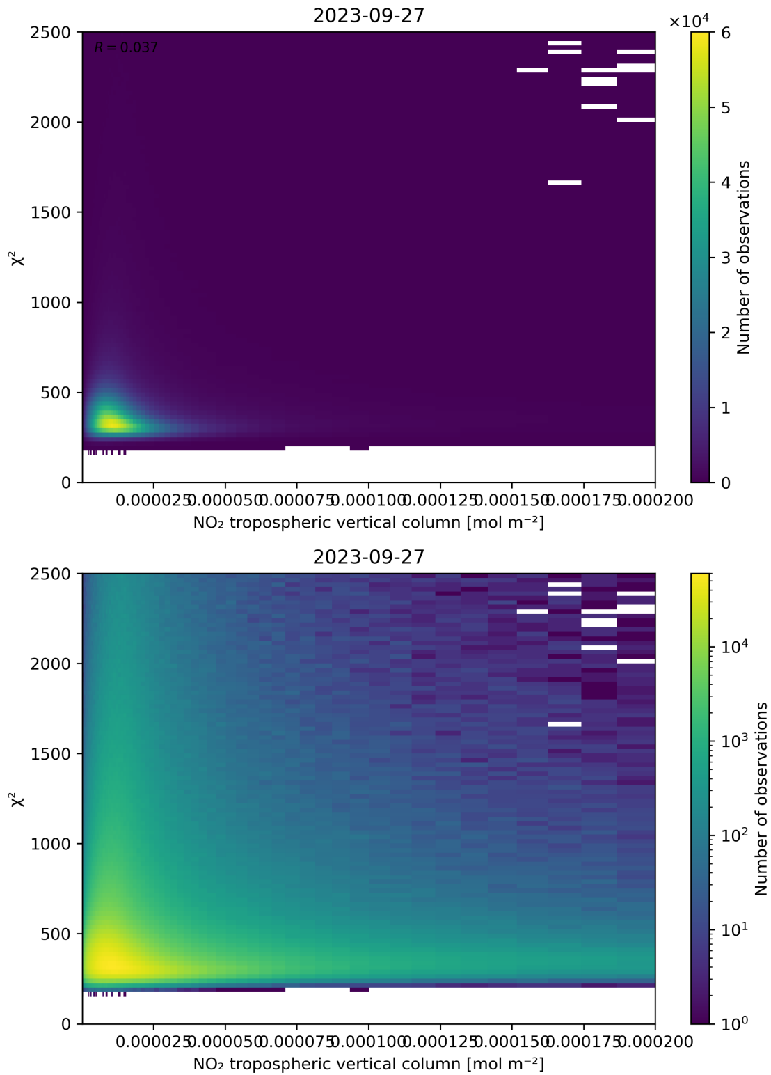
Figure 124: Scatter density plot of “NO 2 tropospheric vertical column” against “ \chi^2 ” for 2023-09-26 to 2023-09-28.
