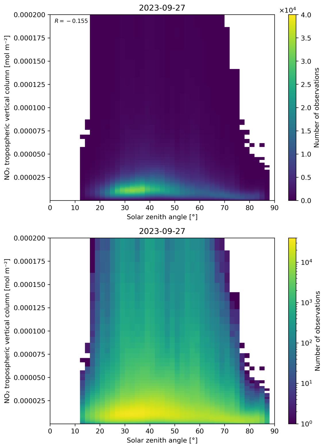
Figure 155: Scatter density plot of “Solar zenith angle” against “NO 2 tropospheric vertical column” for 2023-09-26 to 2023-09-28.
