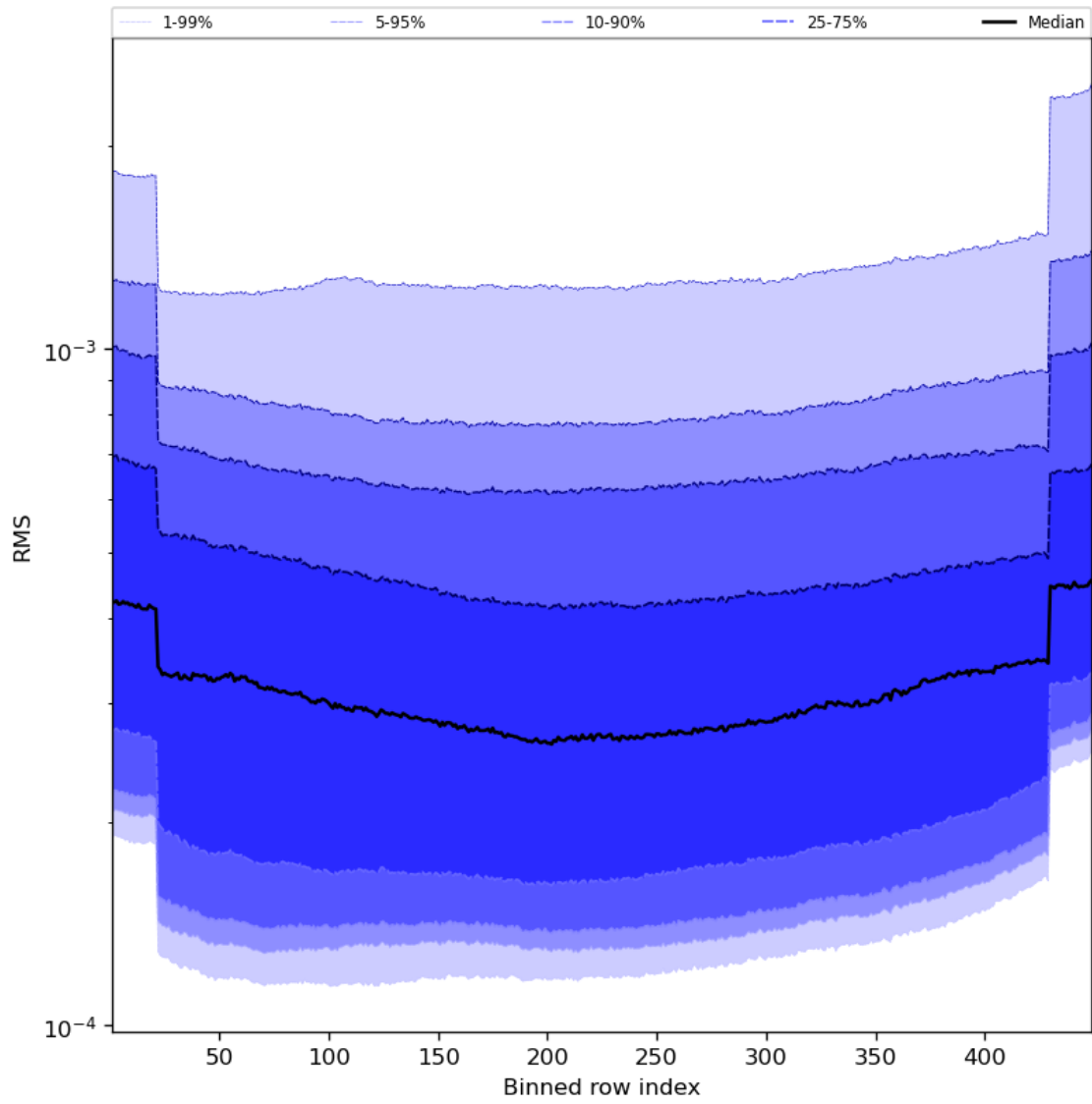
Figure 60: Along track statistics of “RMS” for 2023-09-26 to 2023-09-28
