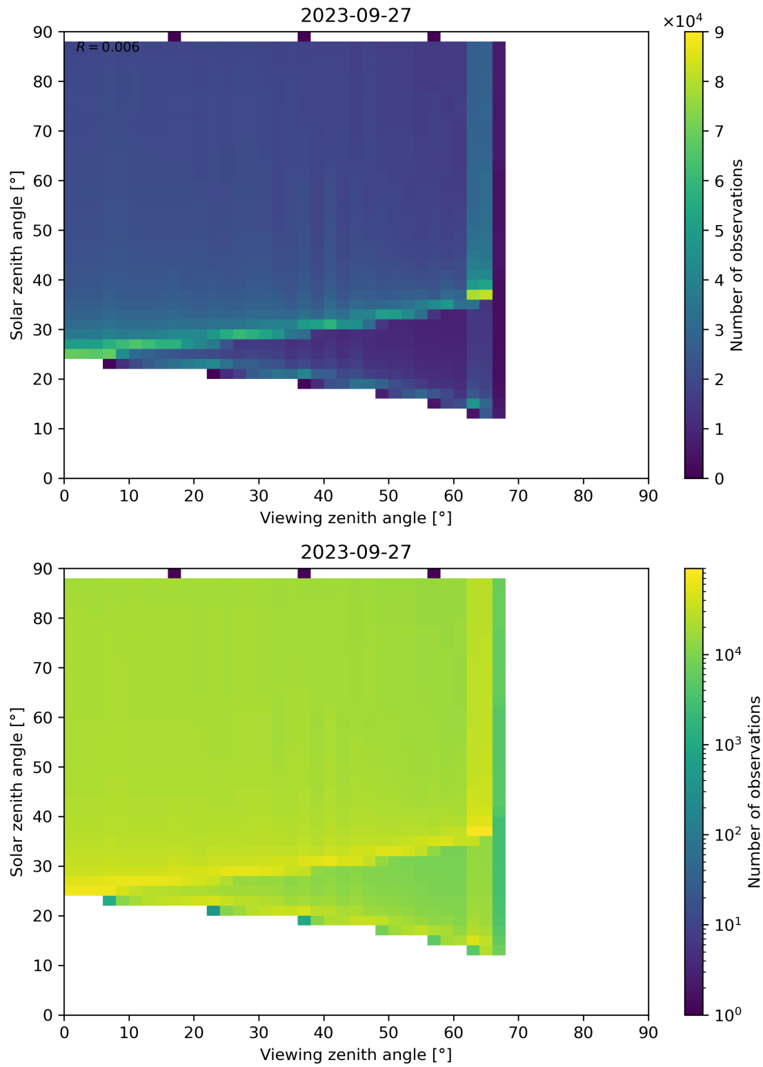
Figure 172: Scatter density plot of “Viewing zenith angle” against “Solar zenith angle” for 2023-09-26 to 2023-09-28.
