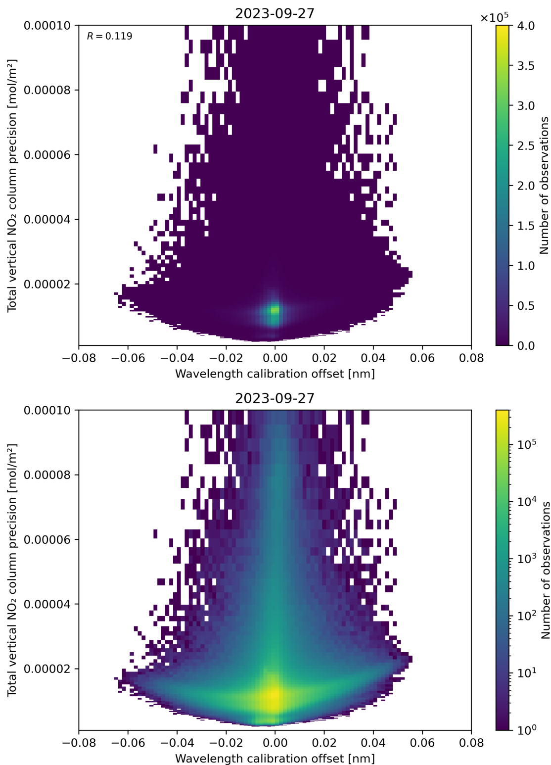
Figure 180: Scatter density plot of “Wavelength calibration offset” against “Total vertical NO 2 column precision” for 2023-09-26 to 2023-09-28.
