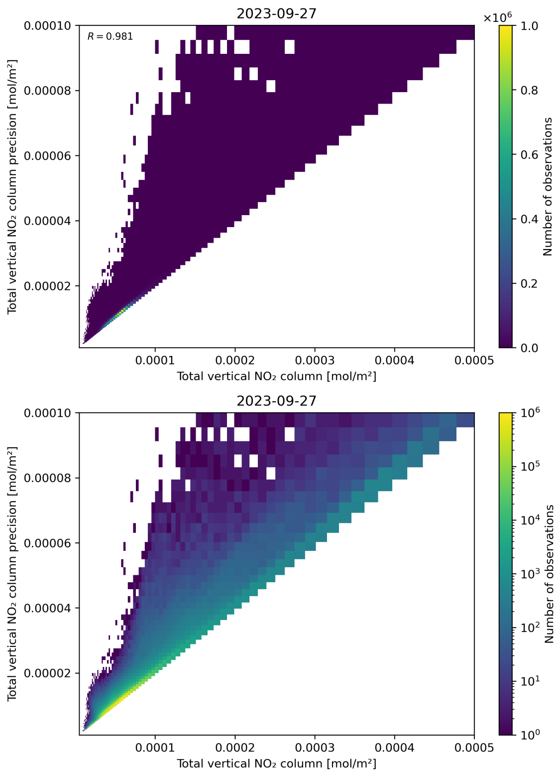
Figure 114: Scatter density plot of “Total vertical NO 2 column” against “Total vertical NO 2 column precision” for 2023-09-26 to 2023-09-28.
