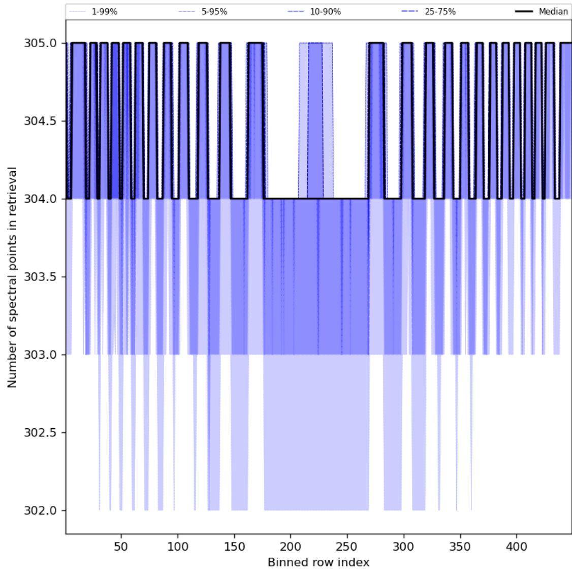
Figure 50: Along track statistics of “Number of spectral points in retrieval” for 2023-09-26 to 2023-09-28
