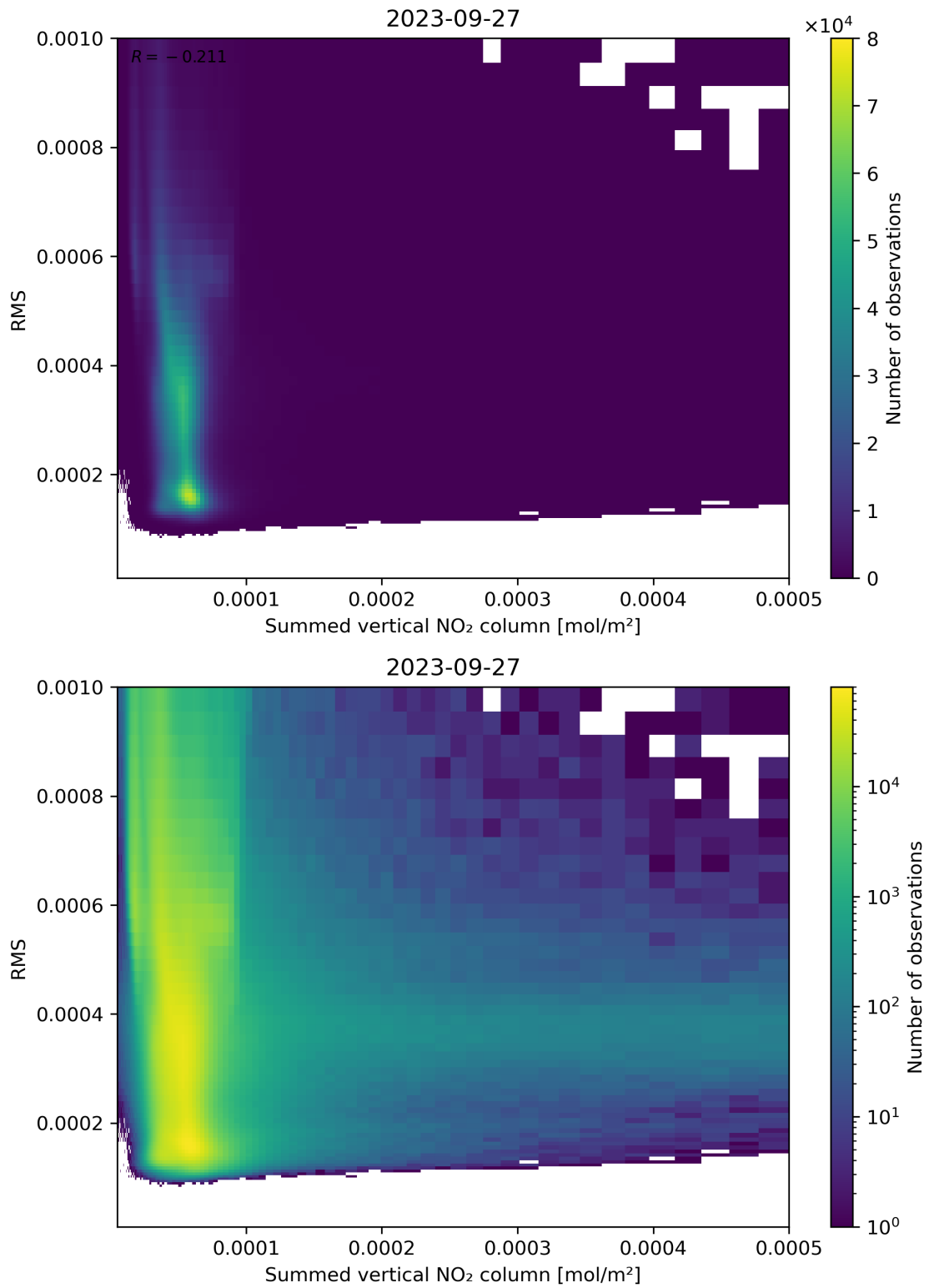
Figure 109: Scatter density plot of “Summed vertical NO 2 column” against “RMS” for 2023-09-26 to 2023-09-28.
