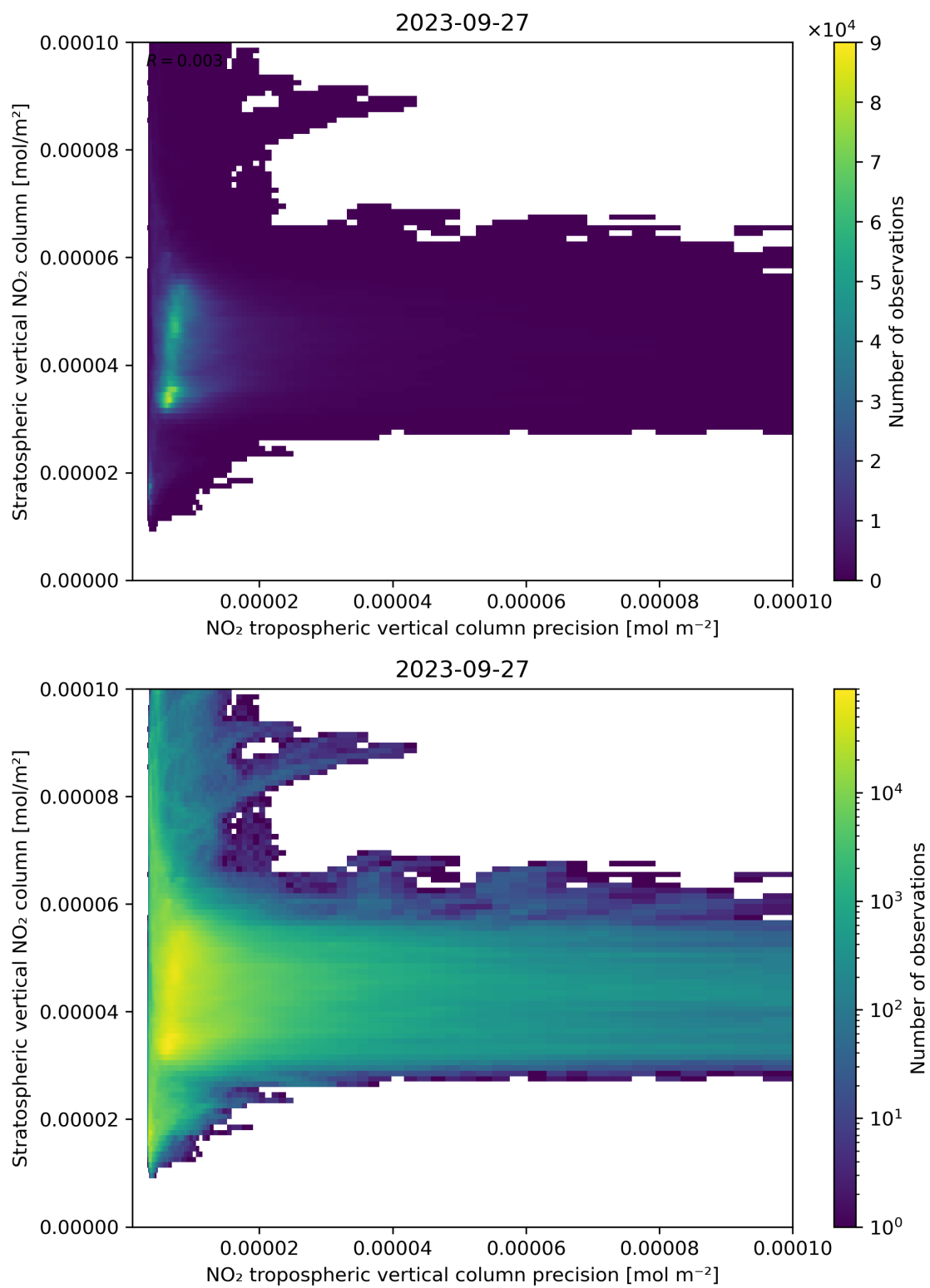
Figure 135: Scatter density plot of “NO 2 tropospheric vertical column precision” against “Stratospheric vertical NO 2 column” for 2023-09-26 to 2023-09-28.
