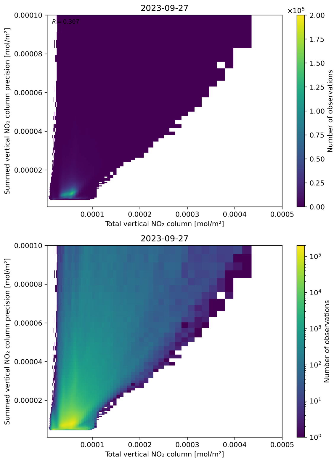
Figure 113: Scatter density plot of “Total vertical NO 2 column” against “Summed vertical NO 2 column precision” for 2023-09-26 to 2023-09-28.
