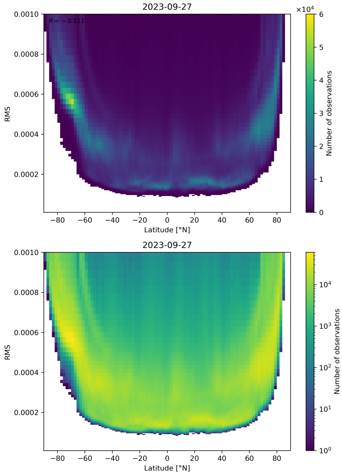
Figure 94: Scatter density plot of “Latitude” against “RMS” for 2023-09-26 to 2023-09-28.
