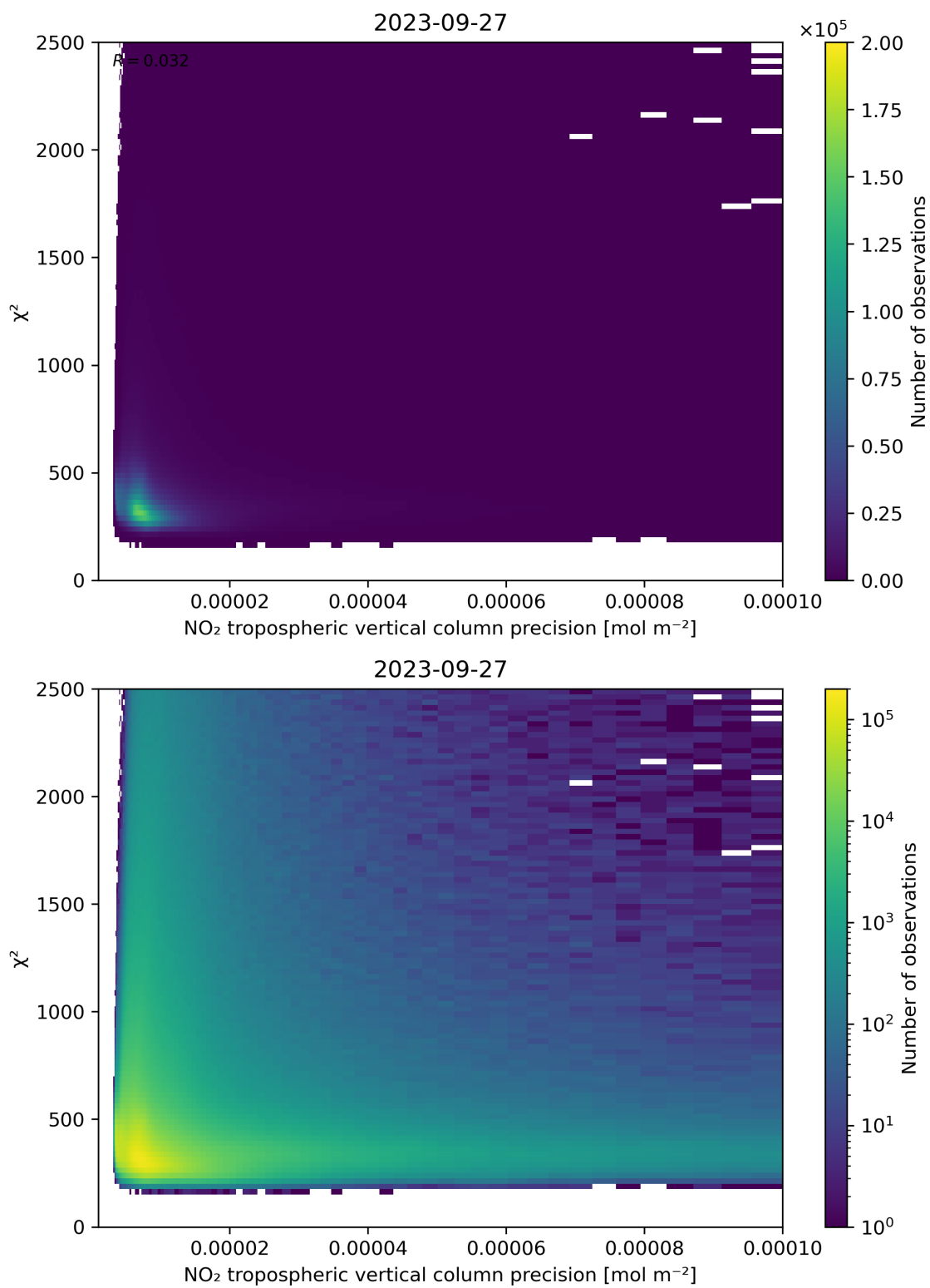
Figure 134: Scatter density plot of “NO 2 tropospheric vertical column precision” against “ \chi^2 ” for 2023-09-26 to 2023-09-28.
