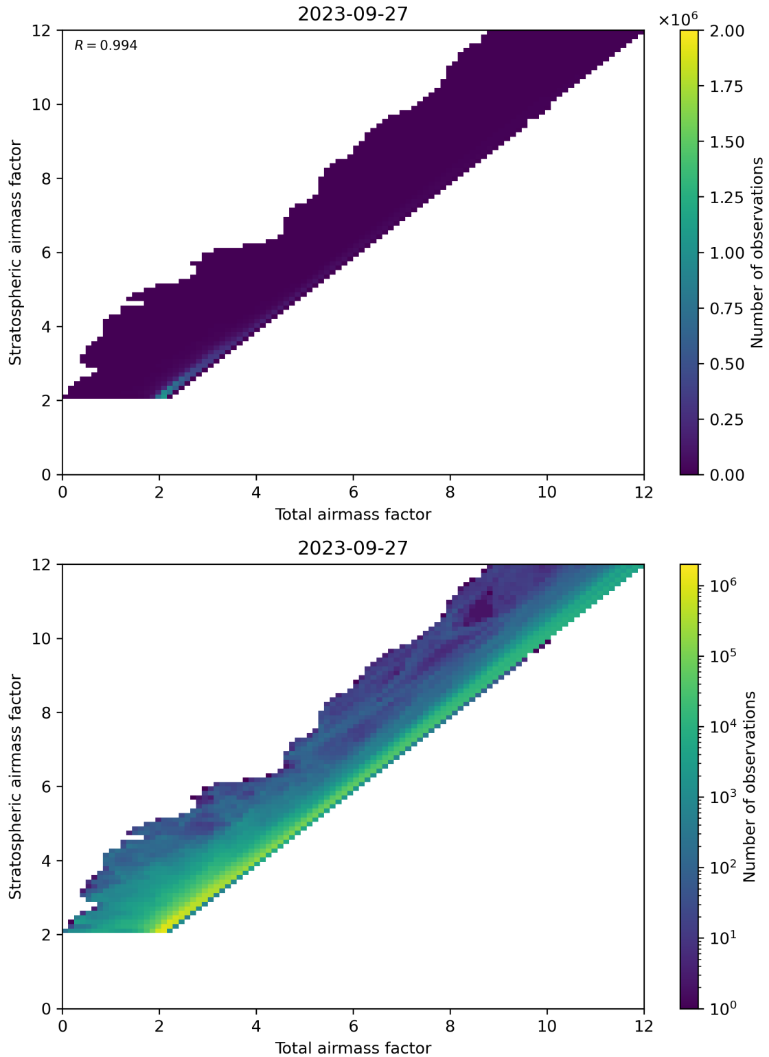
Figure 62: Scatter density plot of “Total airmass factor” against “Stratospheric airmass factor” for 2023-09-26 to 2023-09-28.
