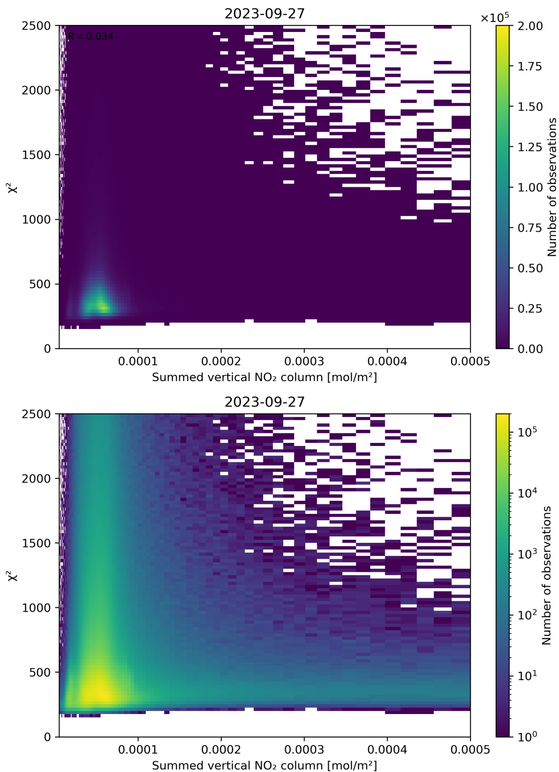
Figure 104: Scatter density plot of “Summed vertical NO 2 column” against “ \chi^2 ” for 2023-09-26 to 2023-09-28.
