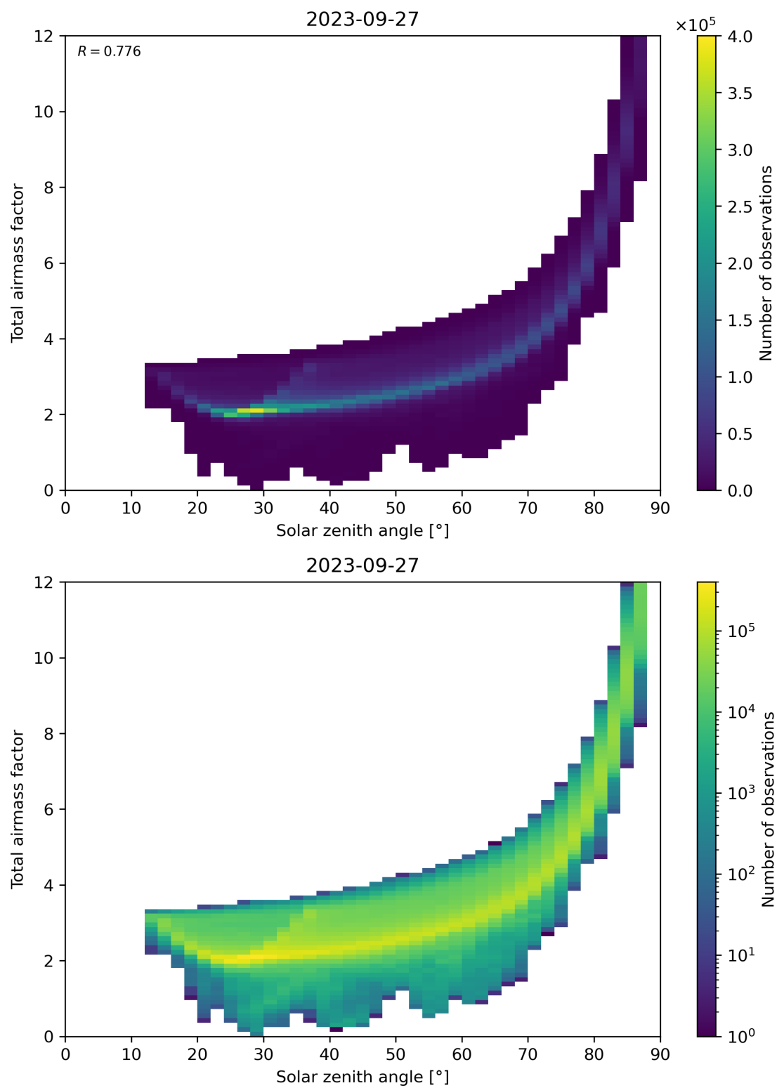
Figure 146: Scatter density plot of “Solar zenith angle” against “Total airmass factor” for 2023-09-26 to 2023-09-28.
