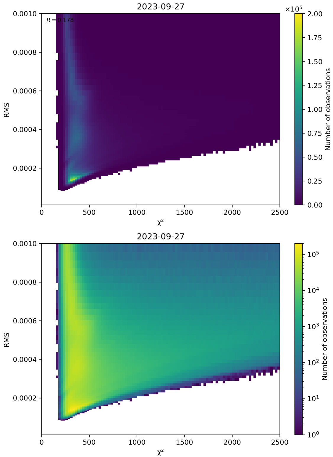
Figure 82: Scatter density plot of “ \chi^2 ” against “RMS” for 2023-09-26 to 2023-09-28.
