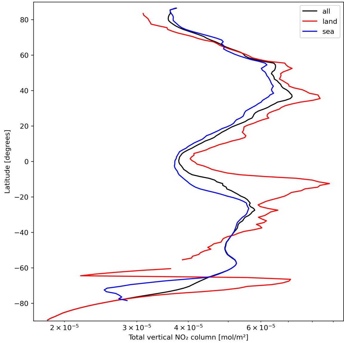
Figure 21: Zonal average of “Total vertical NO 2 column” for 2023-09-26 to 2023-09-28.
