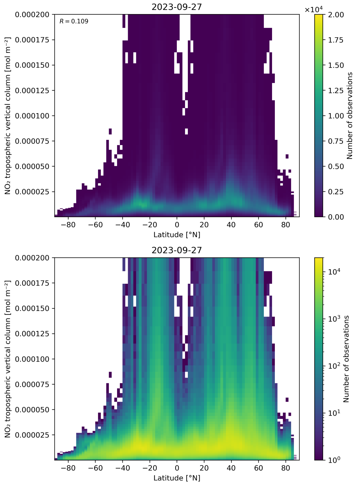
Figure 92: Scatter density plot of “Latitude” against “NO 2 tropospheric vertical column” for 2023-09-26 to 2023-09-28.
