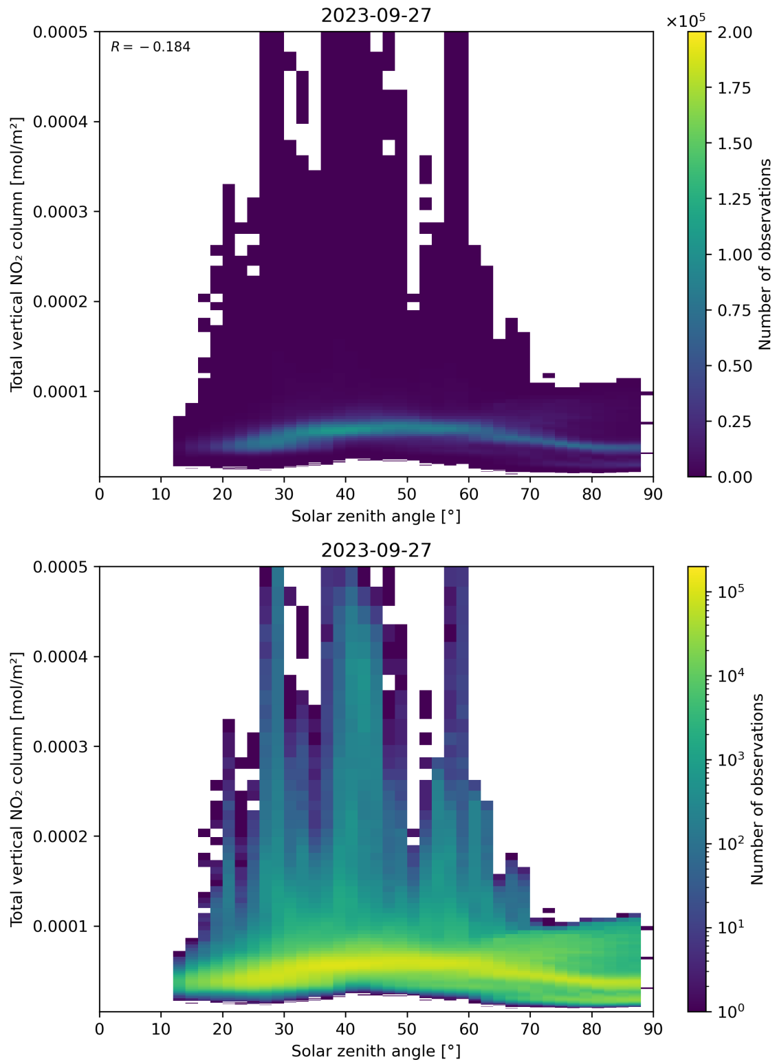
Figure 153: Scatter density plot of “Solar zenith angle” against “Total vertical NO 2 column” for 2023-09-26 to 2023-09-28.
