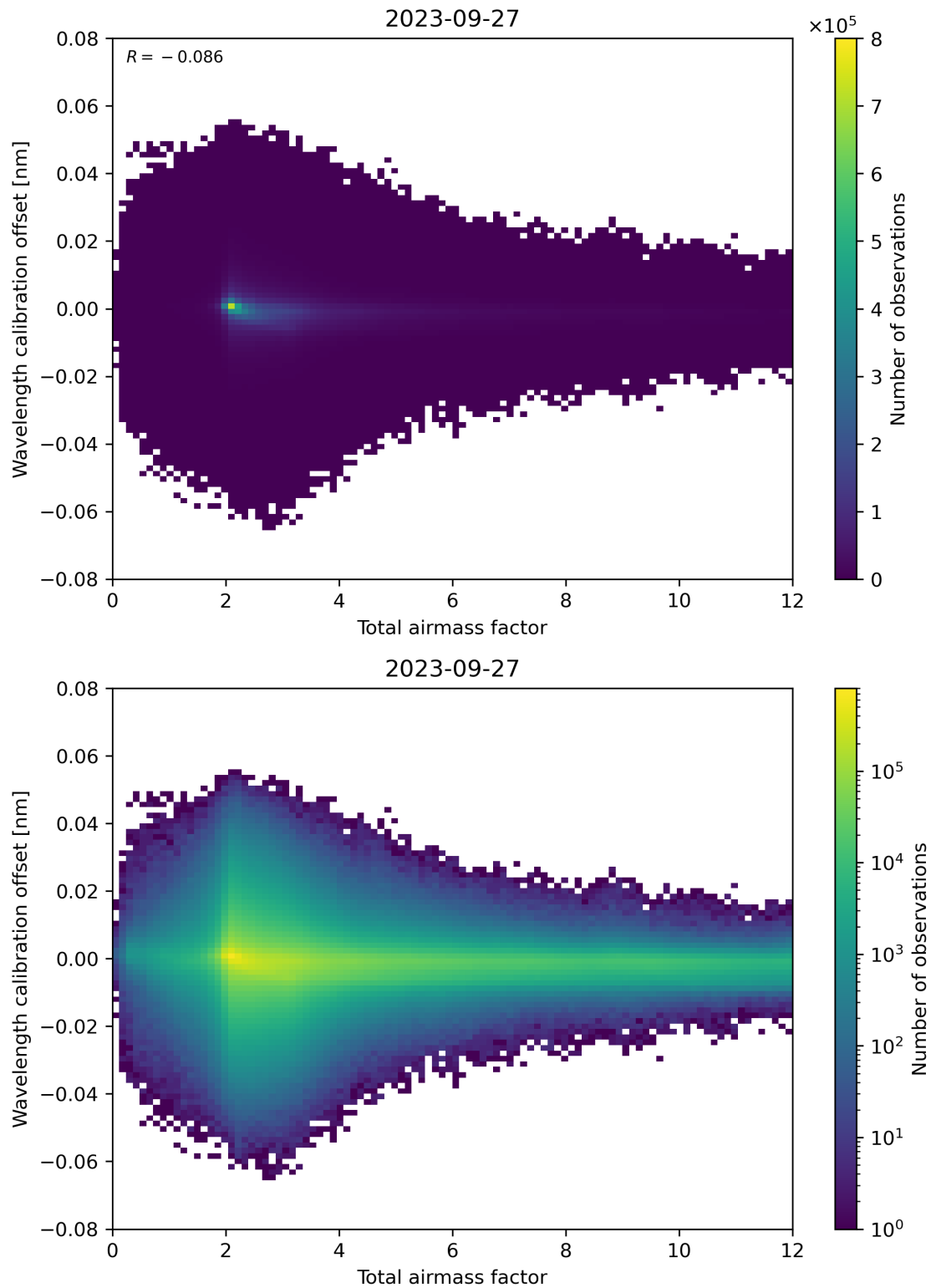
Figure 70: Scatter density plot of “Total airmass factor” against “Wavelength calibration offset” for 2023-09-26 to 2023-09-28.
