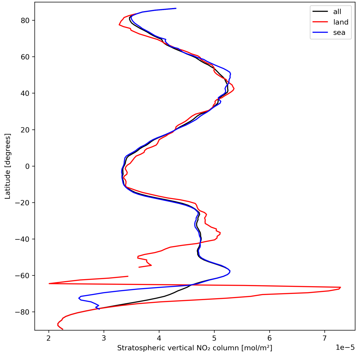
Figure 19: Zonal average of “Stratospheric vertical NO 2 column” for 2023-09-26 to 2023-09-28.
