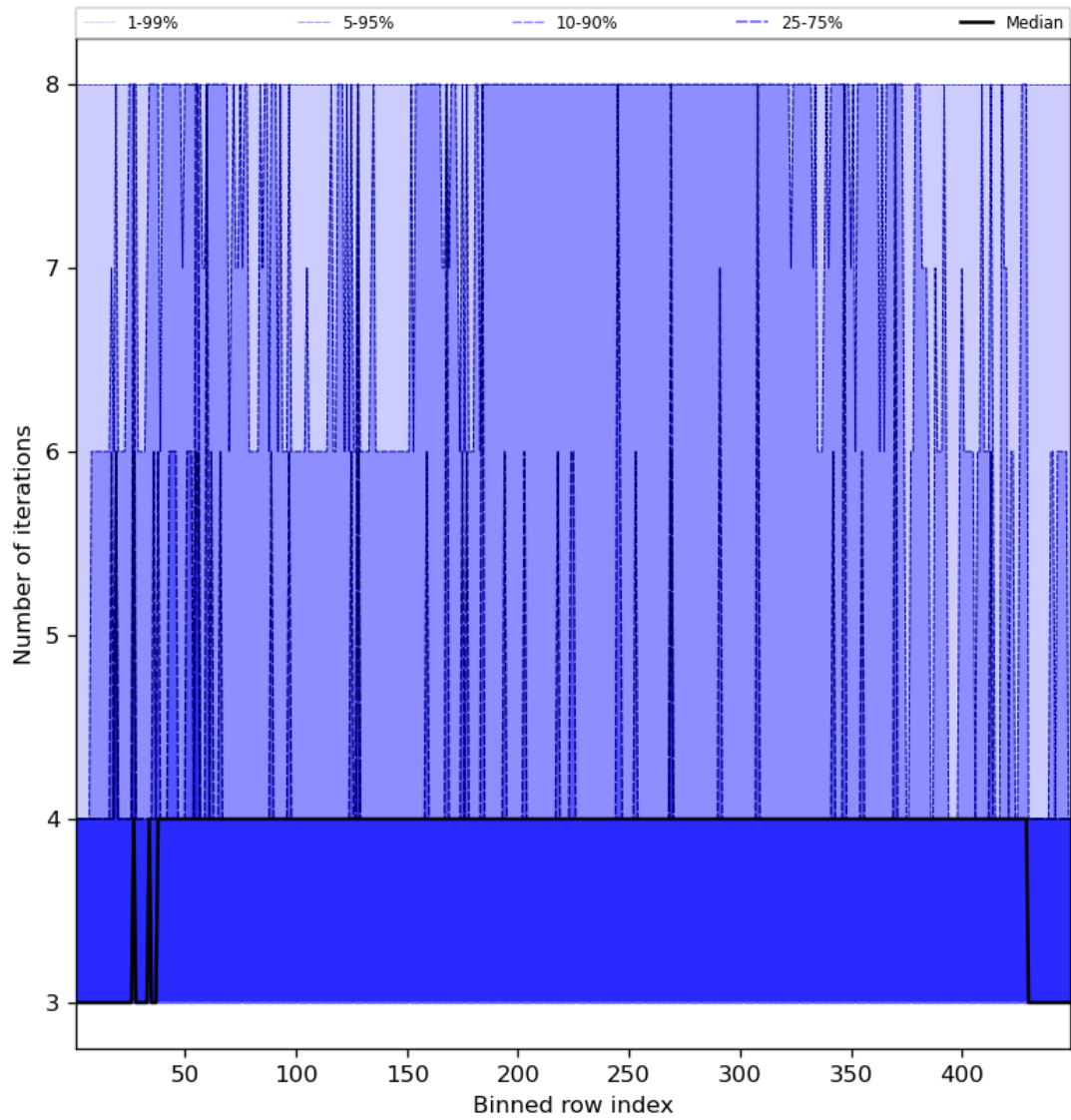
Figure 51: Along track statistics of “Number of iterations” for 2023-09-26 to 2023-09-28
