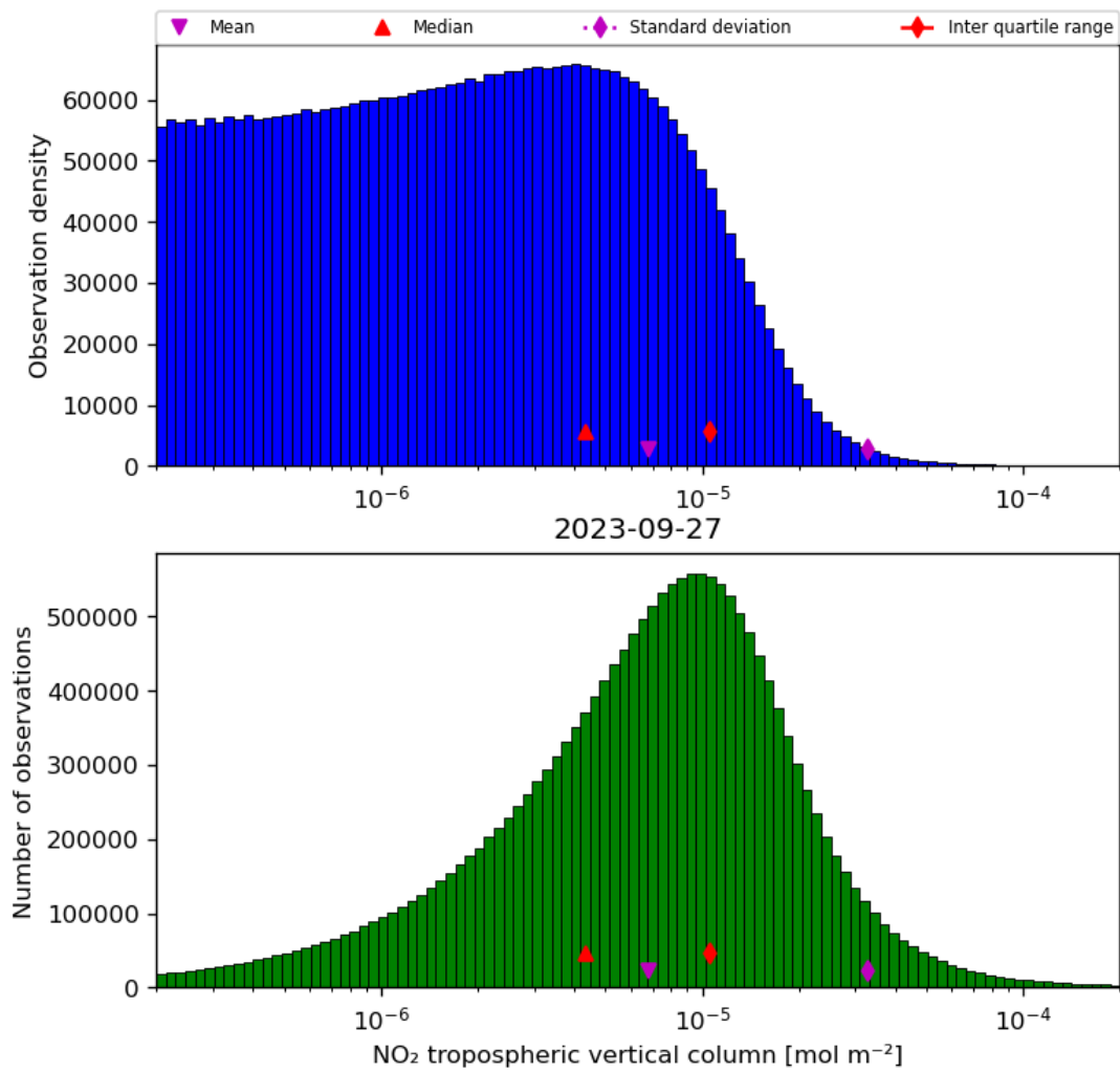
Figure 29: Histogram of “NO 2 tropospheric vertical column” for 2023-09-26 to 2023-09-28
