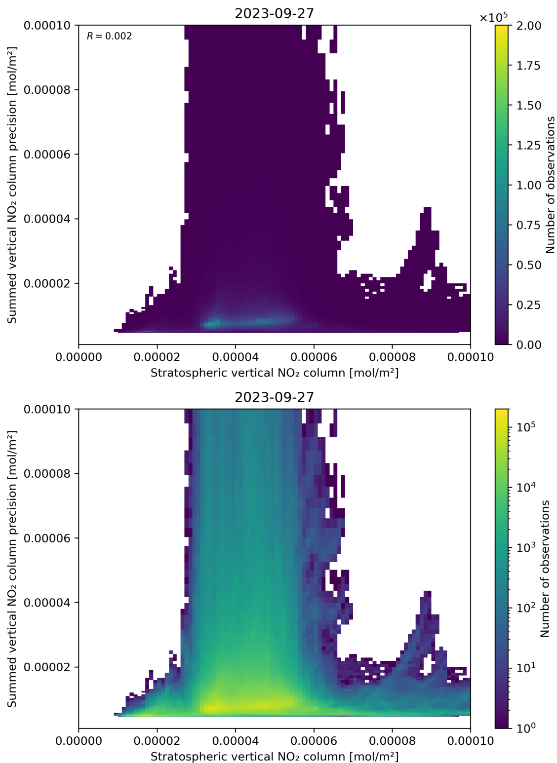
Figure 99: Scatter density plot of “Stratospheric vertical NO 2 column” against “Summed vertical NO 2 column precision” for 2023-09-26 to 2023-09-28.
