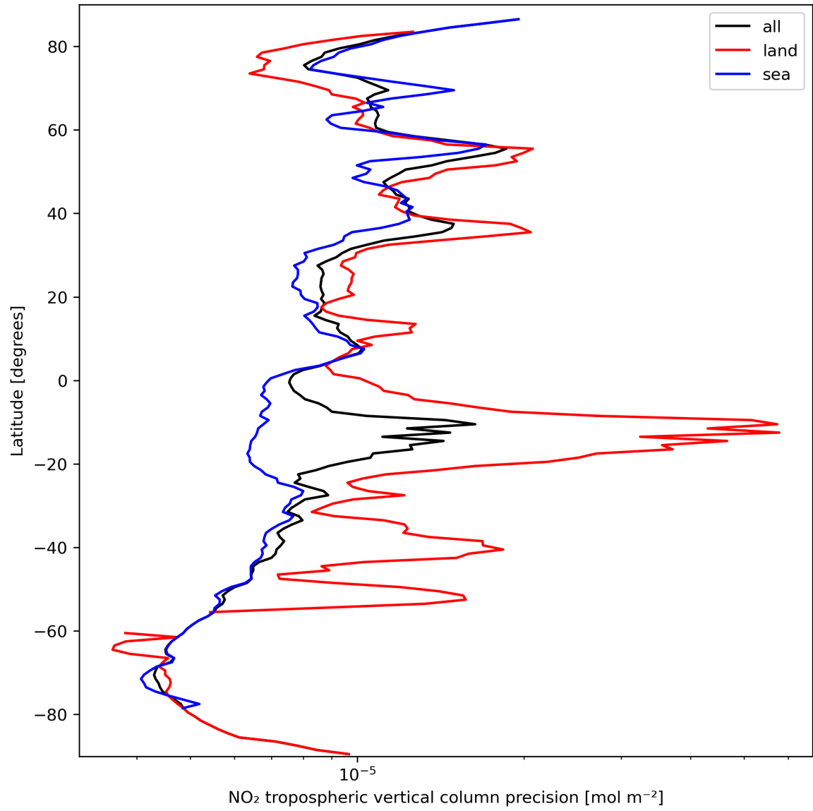
Figure 13: Zonal average of “NO 2 tropospheric vertical column precision” for 2023-09-26 to 2023-09-28.
