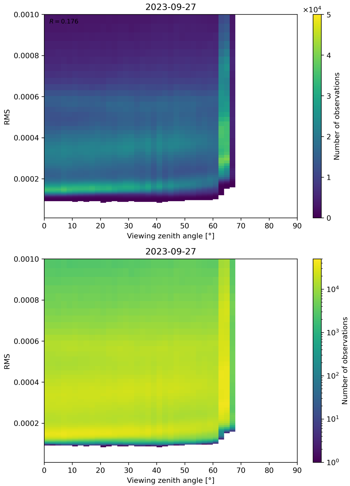
Figure 171: Scatter density plot of “Viewing zenith angle” against “RMS” for 2023-09-26 to 2023-09-28.
