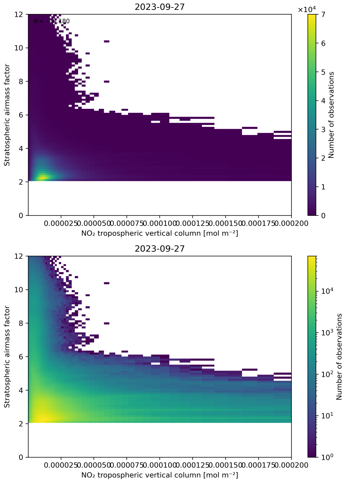
Figure 121: Scatter density plot of “NO 2 tropospheric vertical column” against “Stratospheric air mass factor” for 2023-09-26 to 2023-09-28.
