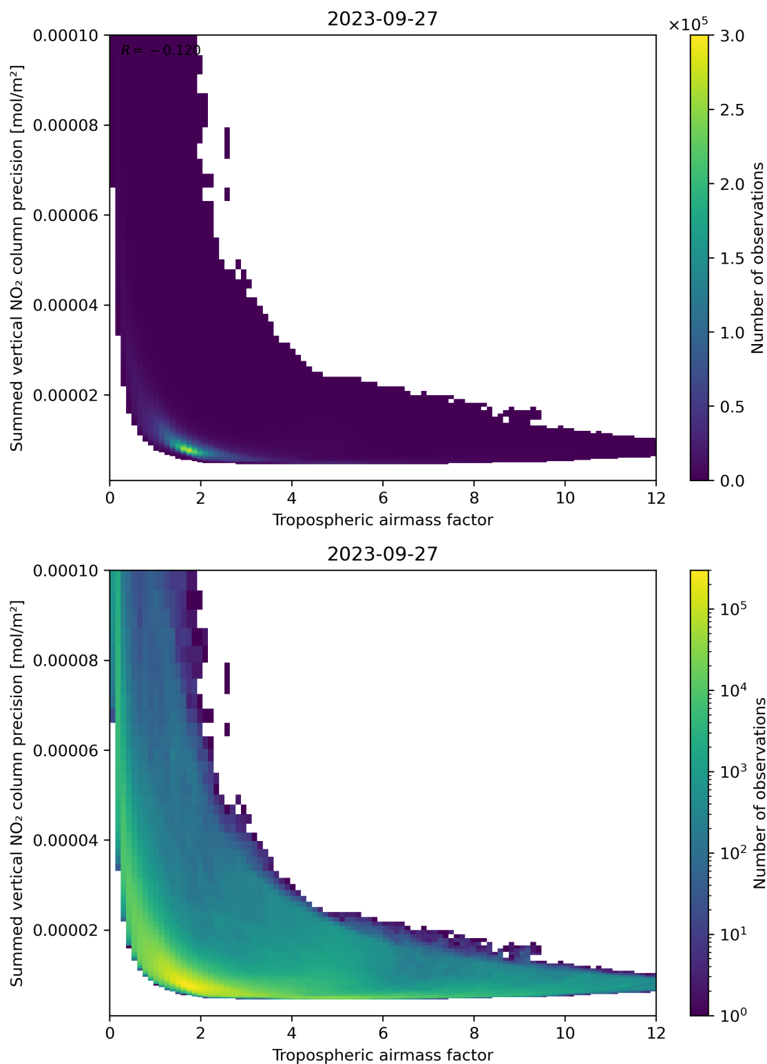
Figure 76: Scatter density plot of “Tropospheric air mass factor” against “Summed vertical NO 2 column precision” for 2023-09-26 to 2023-09-28.
