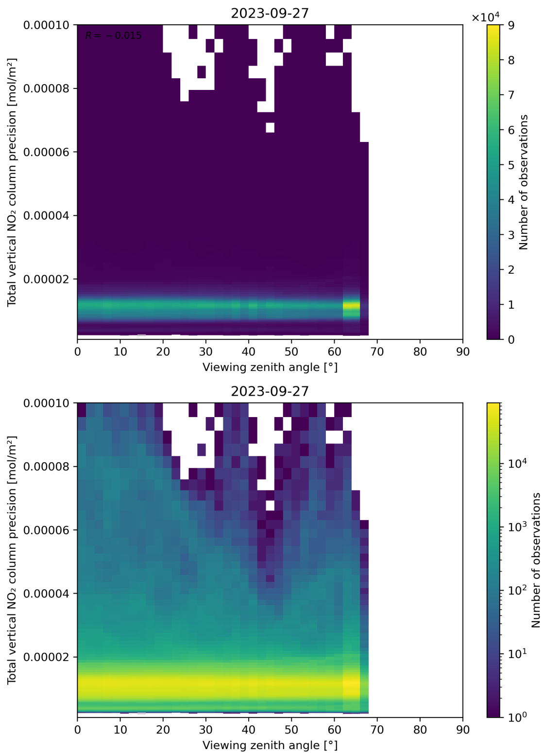
Figure 168: Scatter density plot of “Viewing zenith angle” against “Total vertical NO 2 column precision” for 2023-09-26 to 2023-09-28.
