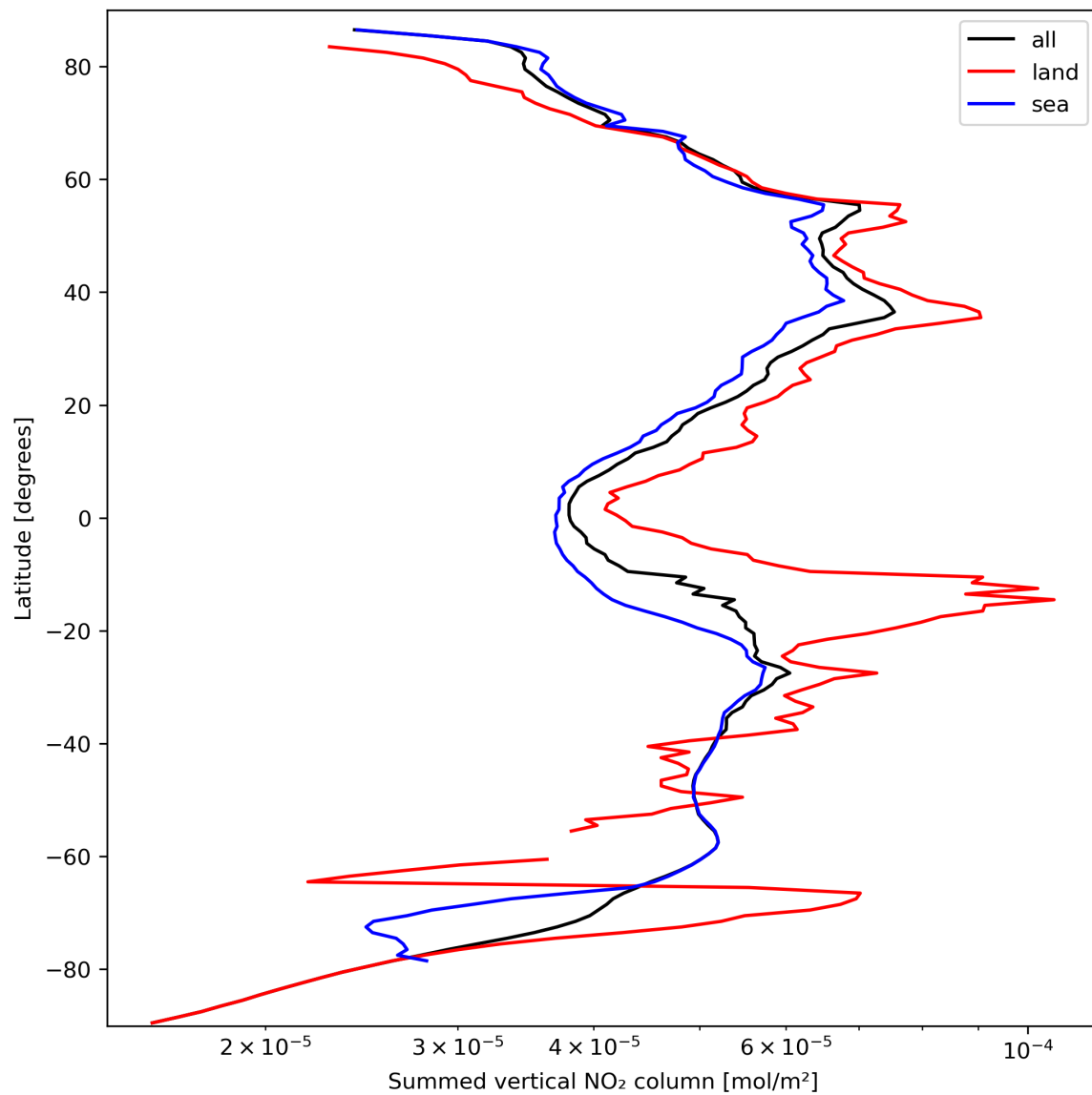
Figure 23: Zonal average of “Summed vertical NO 2 column” for 2023-09-26 to 2023-09-28.
