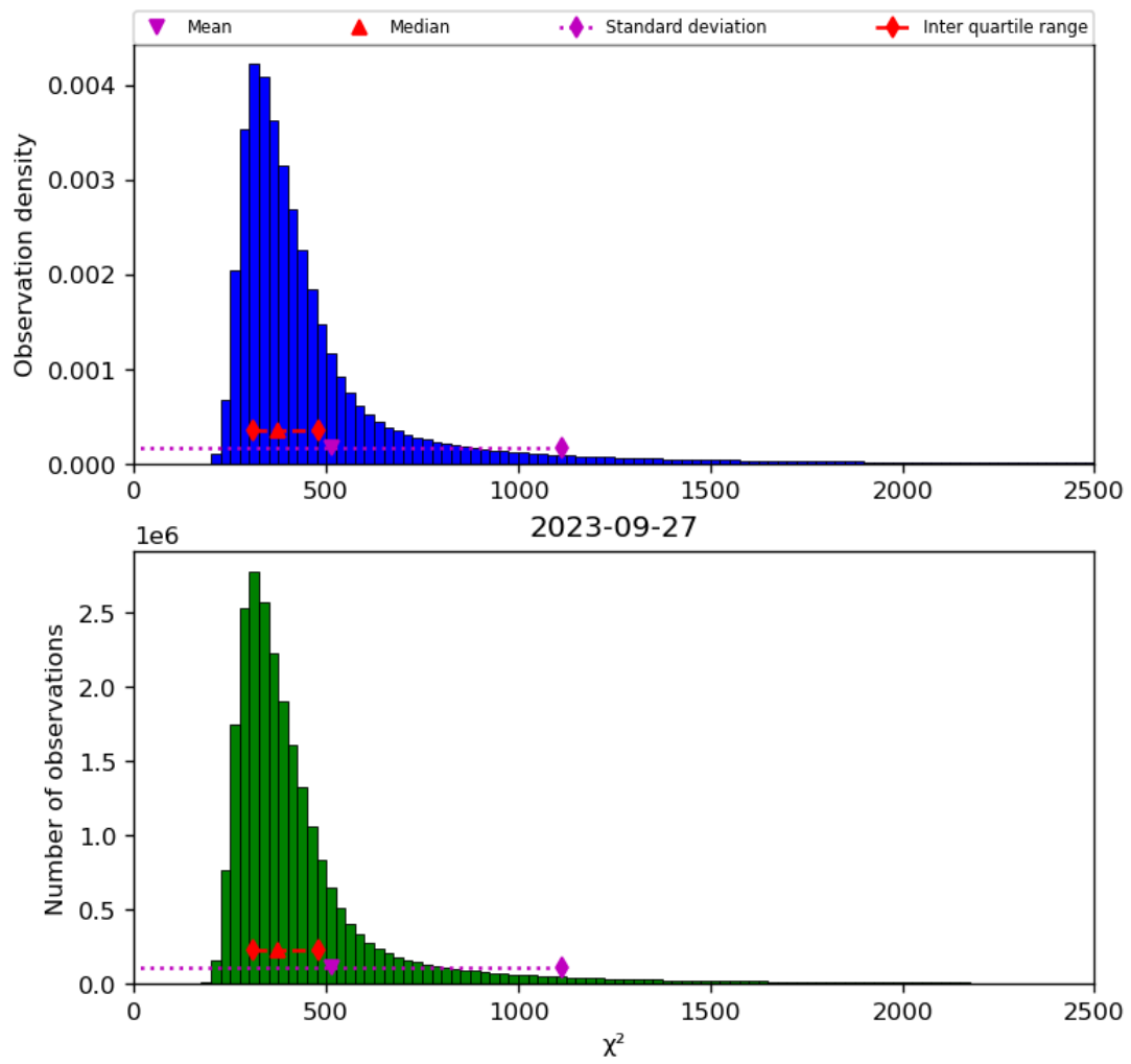
Figure 42: Histogram of “ \chi^2 ” for 2023-09-26 to 2023-09-28
