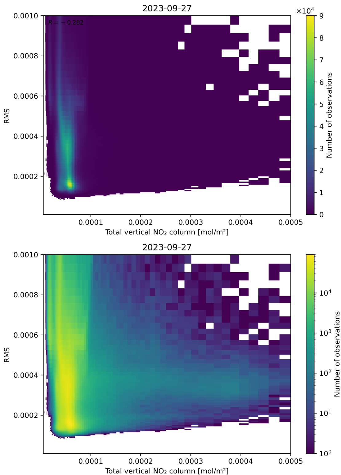
Figure 120: Scatter density plot of “Total vertical NO 2 column” against “RMS” for 2023-09-26 to 2023-09-28.
