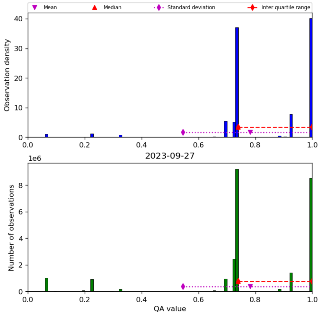
Figure 28: Histogram of “QA value” for 2023-09-26 to 2023-09-28
