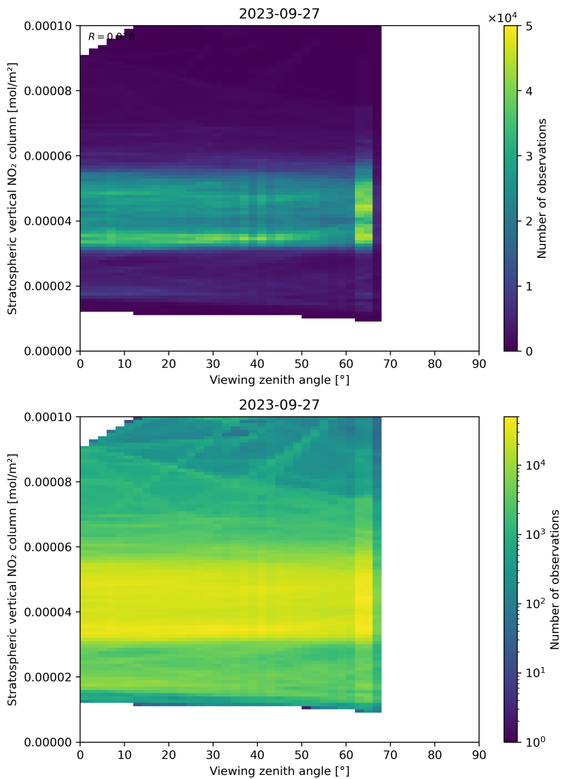
Figure 164: Scatter density plot of “Viewing zenith angle” against “Stratospheric vertical NO 2 column” for 2023-09-26 to 2023-09-28.
