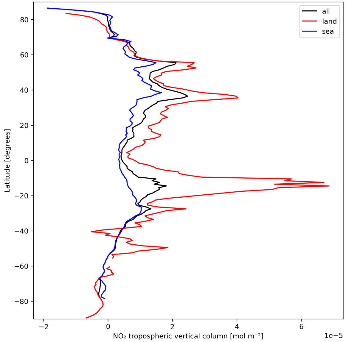
Figure 12: Zonal average of “NO 2 tropospheric vertical column” for 2023-09-26 to 2023-09-28.
