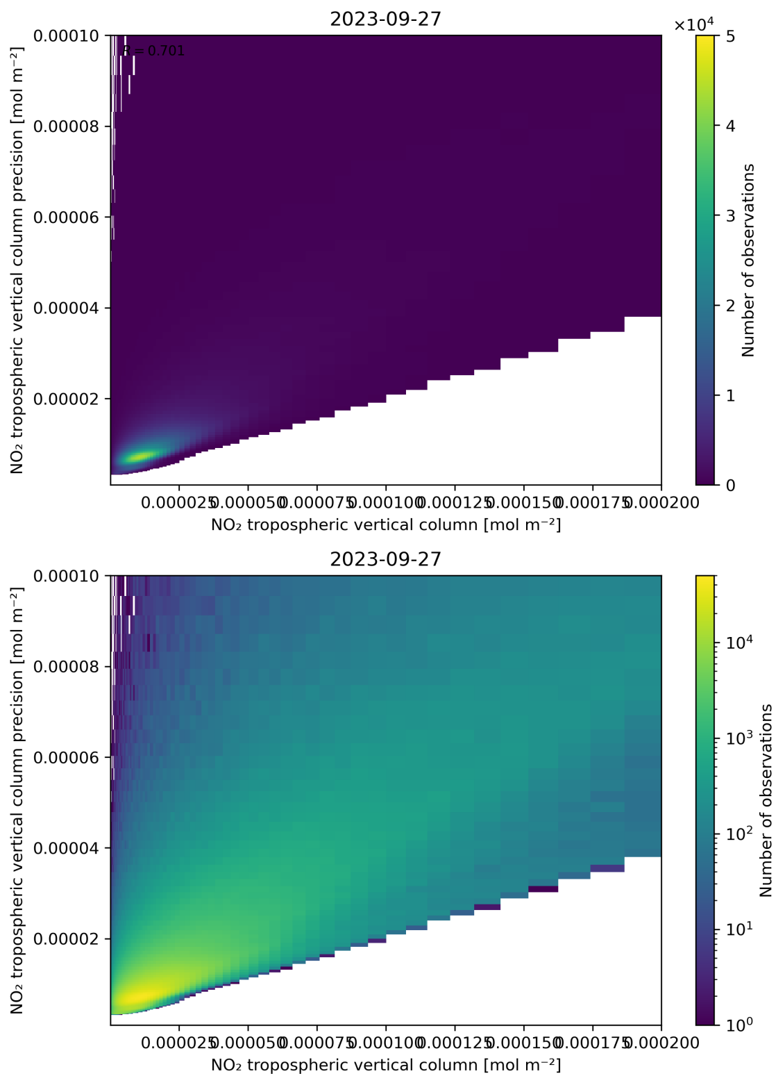
Figure 130: Scatter density plot of “NO 2 tropospheric vertical column” against “NO 2 tropospheric vertical column precision” for 2023-09-26 to 2023-09-28.
