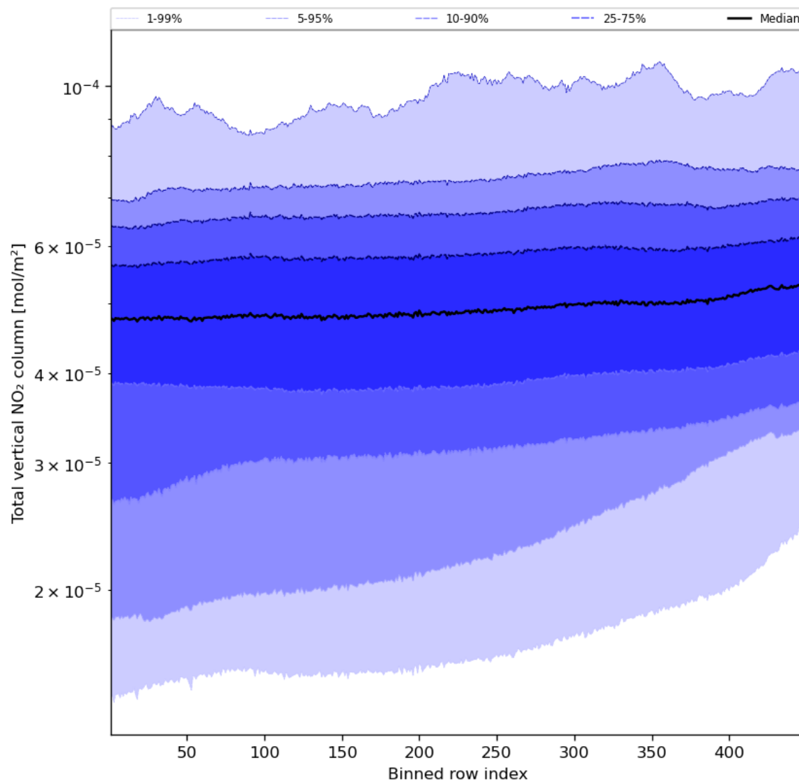
Figure 55: Along track statistics of “Total vertical NO 2 column” for 2023-09-26 to 2023-09-28
