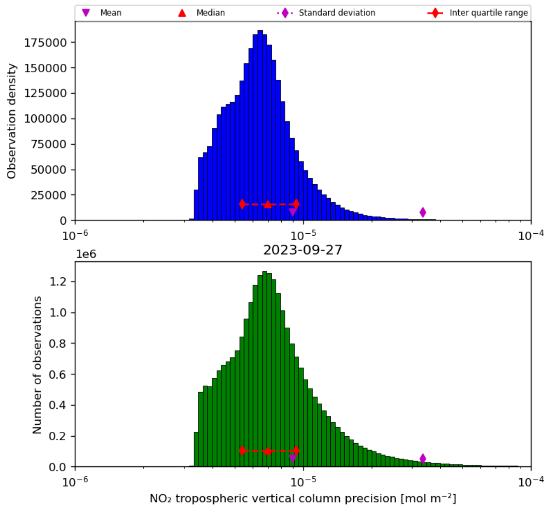
Figure 30: Histogram of “NO 2 tropospheric vertical column precision” for 2023-09-26 to 2023-09-28
