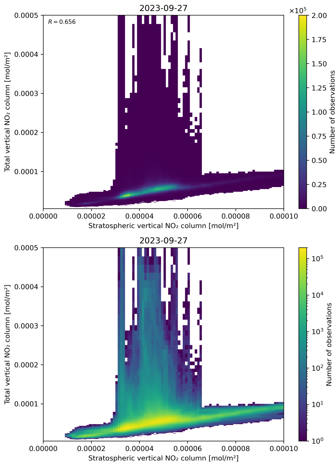
Figure 100: Scatter density plot of “Stratospheric vertical NO 2 column” against “Total vertical NO 2 column” for 2023-09-26 to 2023-09-28.
