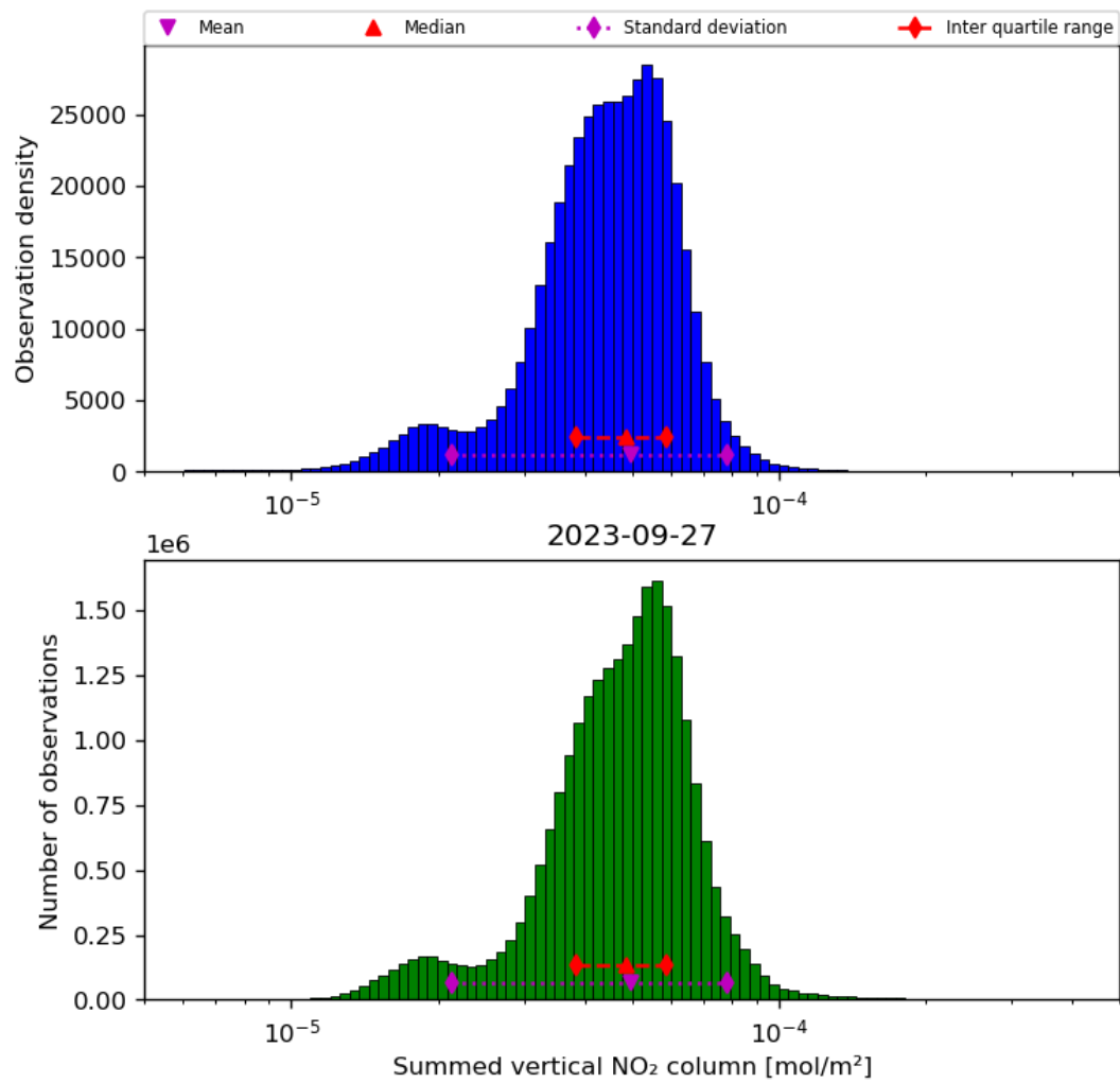
Figure 40: Histogram of “Summed vertical NO 2 column” for 2023-09-26 to 2023-09-28
