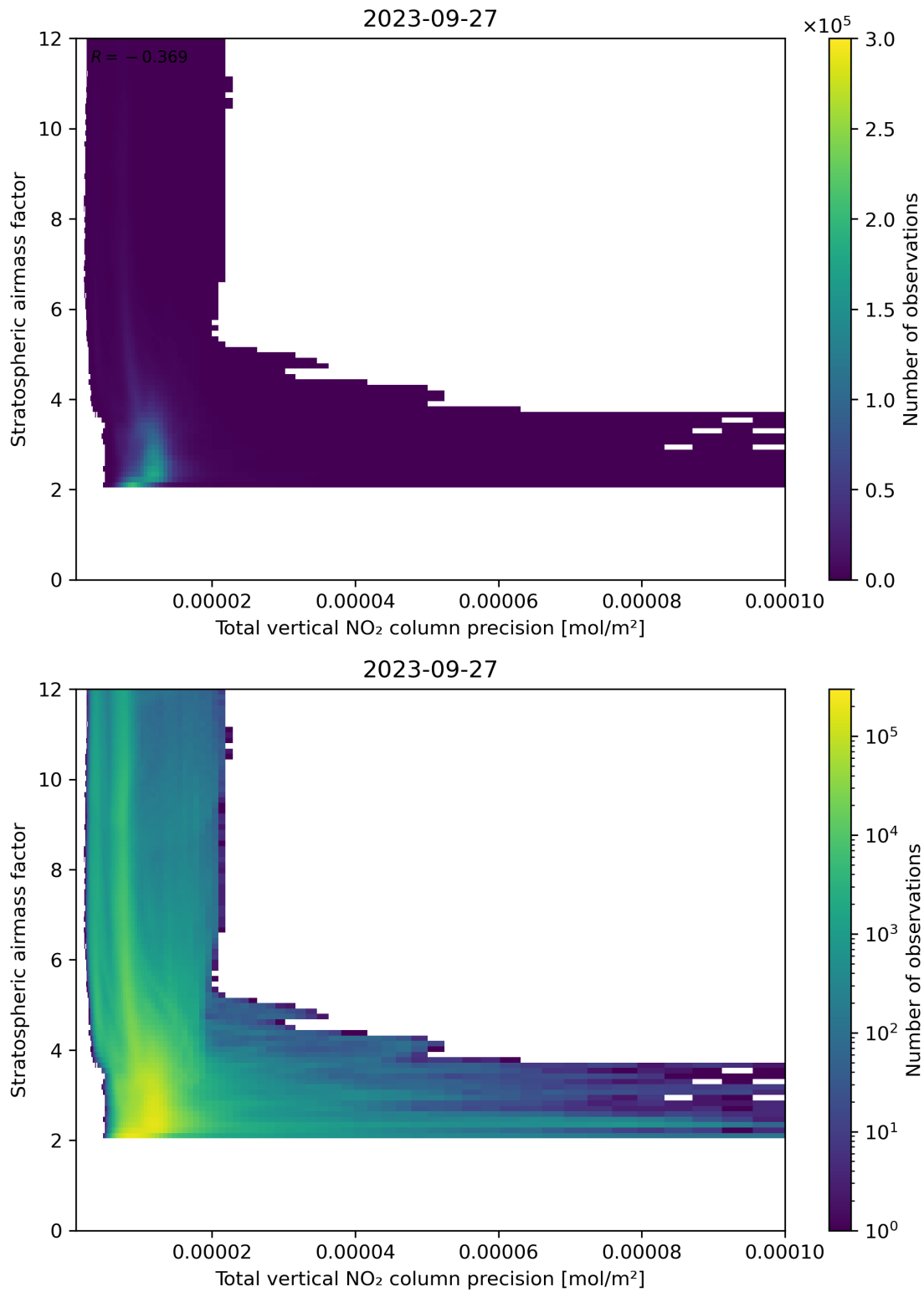
Figure 115: Scatter density plot of “Total vertical NO 2 column precision” against “Stratospheric air mass factor” for 2023-09-26 to 2023-09-28.
