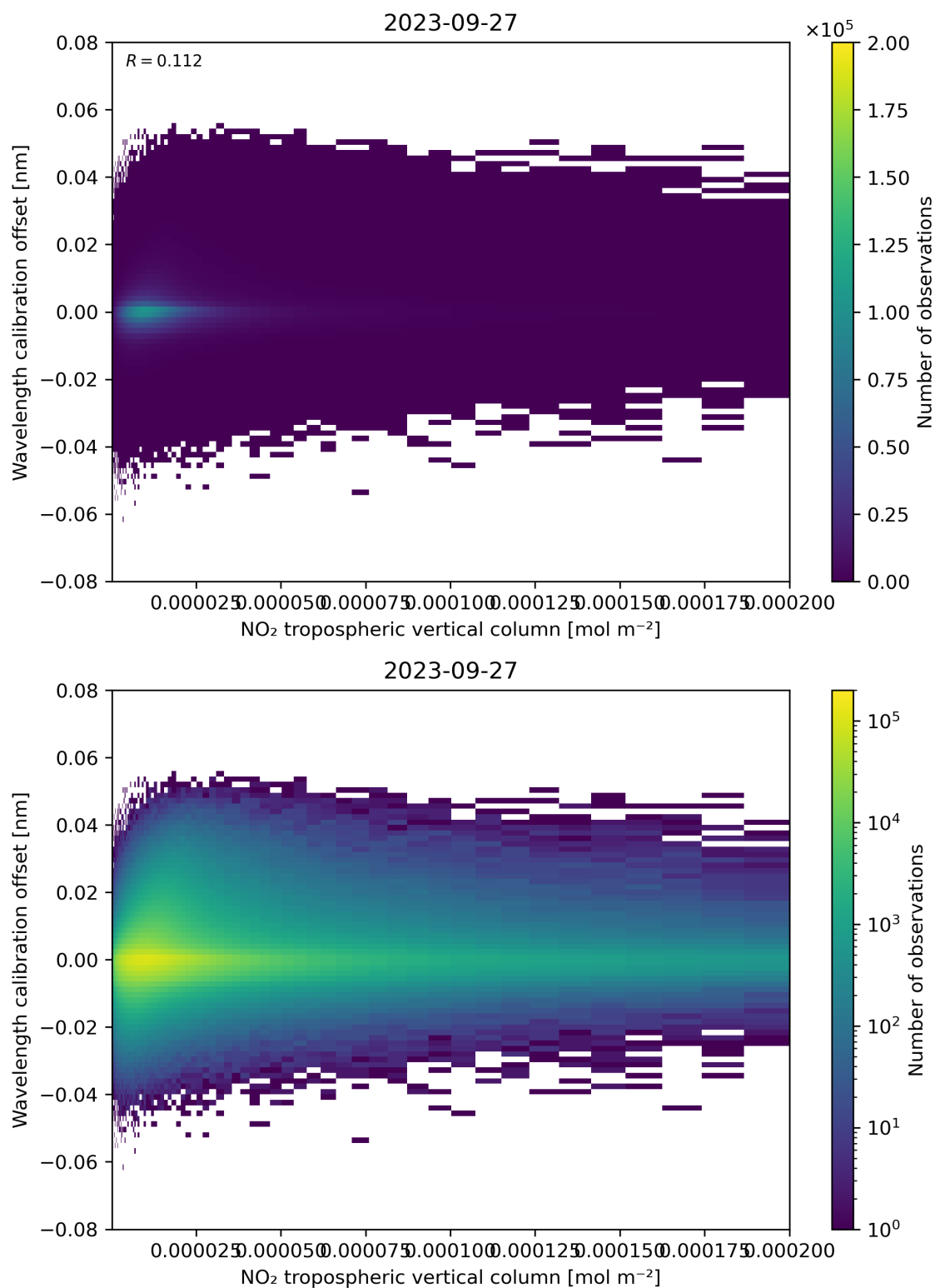
Figure 143: Scatter density plot of “NO 2 tropospheric vertical column” against “Wavelength calibration offset” for 2023-09-26 to 2023-09-28.
