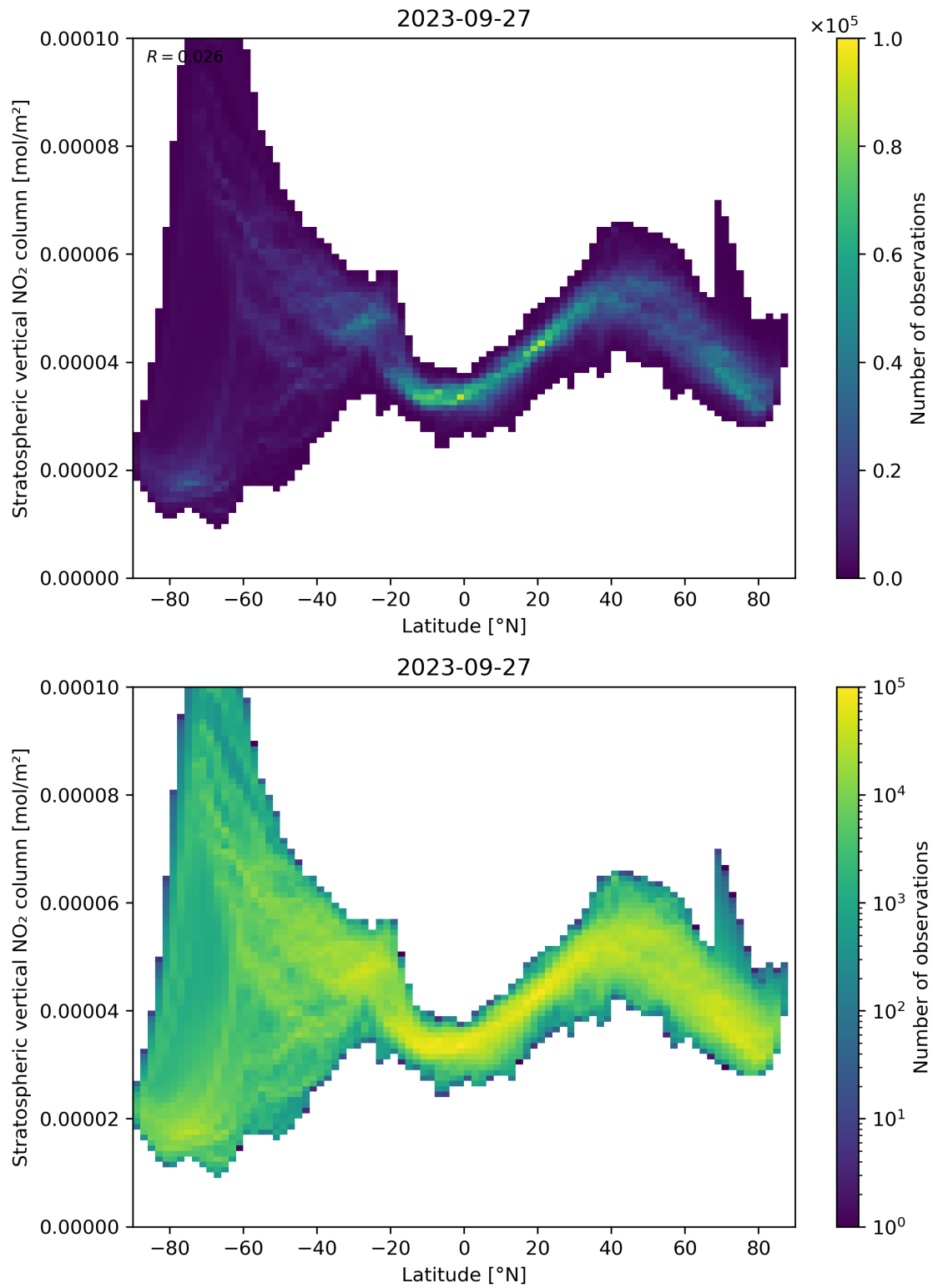
Figure 87: Scatter density plot of “Latitude” against “Stratospheric vertical NO 2 column” for 2023-09-26 to 2023-09-28.
