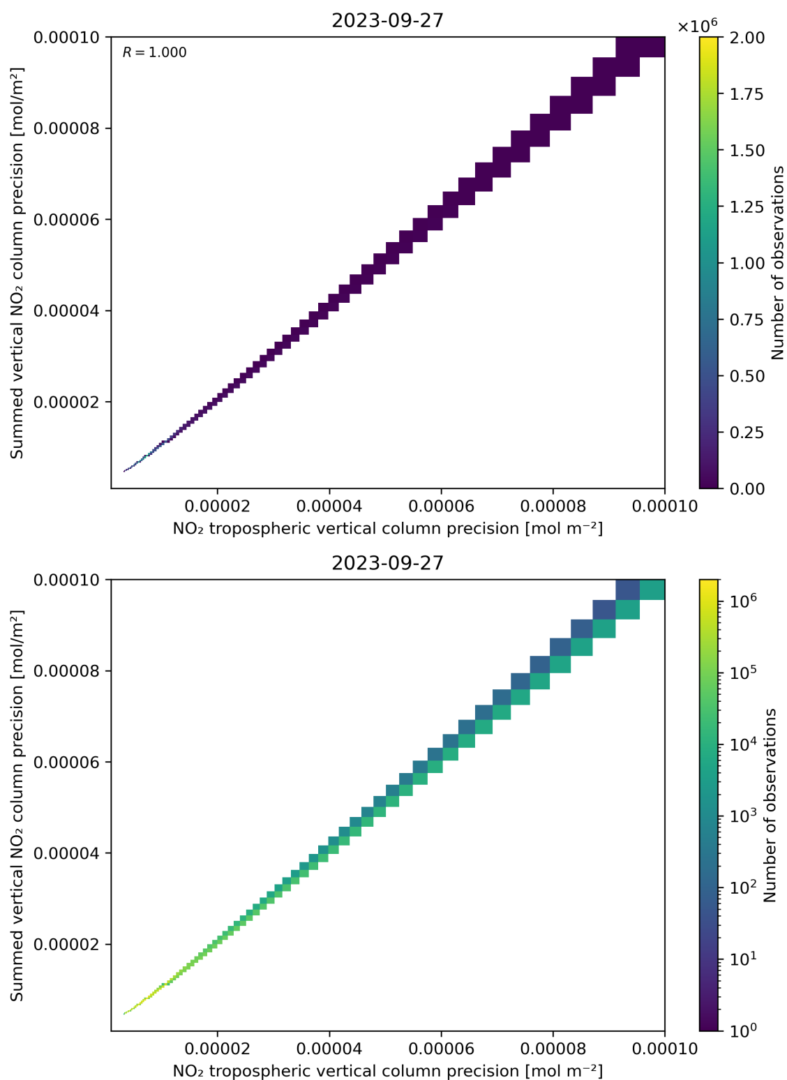
Figure 137: Scatter density plot of “NO 2 tropospheric vertical column precision” against “Summed vertical NO 2 column precision” for 2023-09-26 to 2023-09-28.
