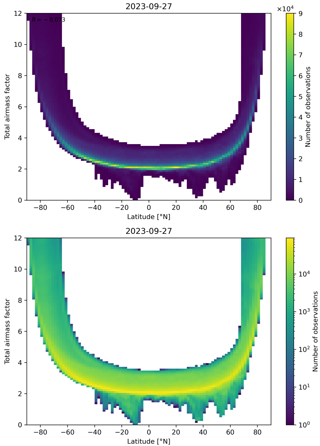
Figure 84: Scatter density plot of “Latitude” against “Total airmass factor” for 2023-09-26 to 2023-09-28.
