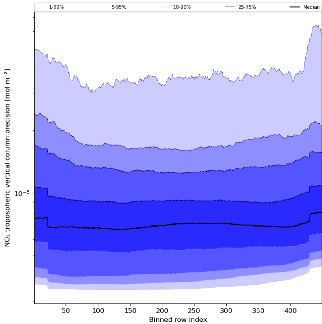
Figure 47: Along track statistics of “NO 2 tropospheric vertical column precision” for 2023-09-26 to 2023-09-28
