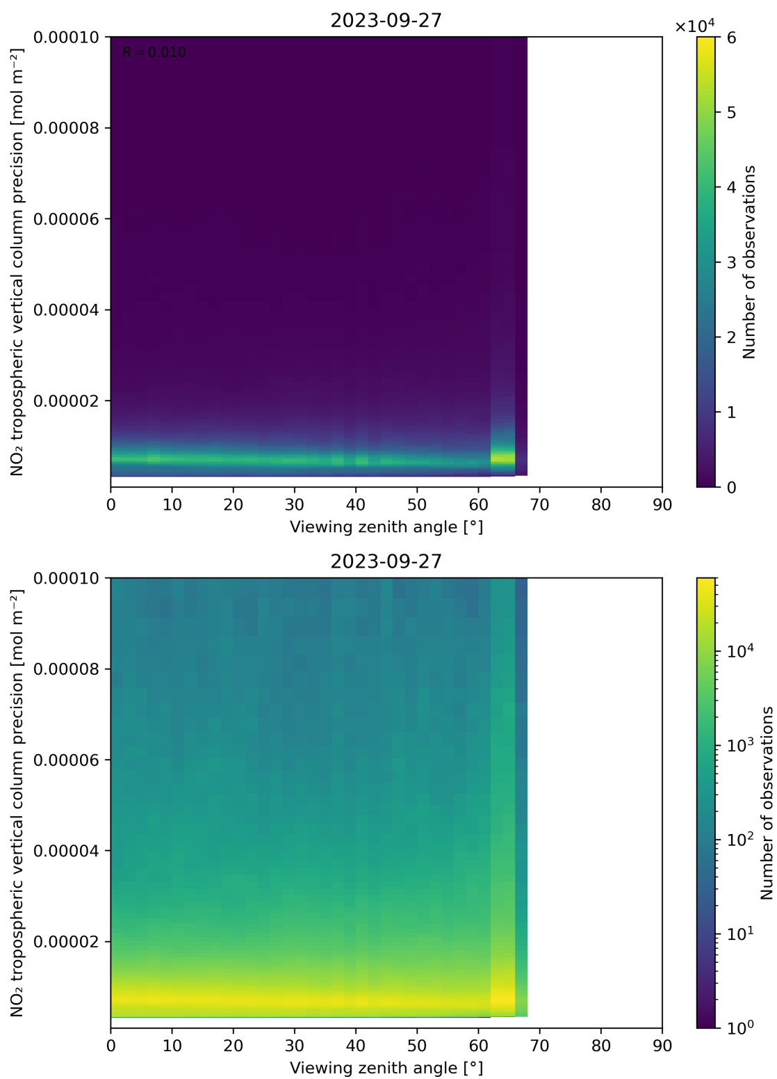
Figure 170: Scatter density plot of “Viewing zenith angle” against “NO 2 tropospheric vertical column precision” for 2023-09-26 to 2023-09-28.
