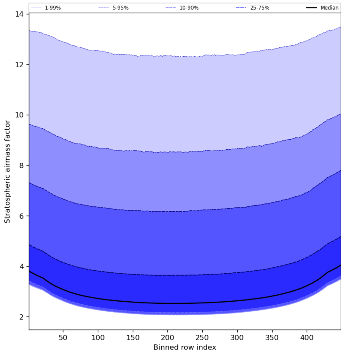
Figure 61: Along track statistics of “Stratospheric airmass factor” for 2023-09-26 to 2023-09-28
