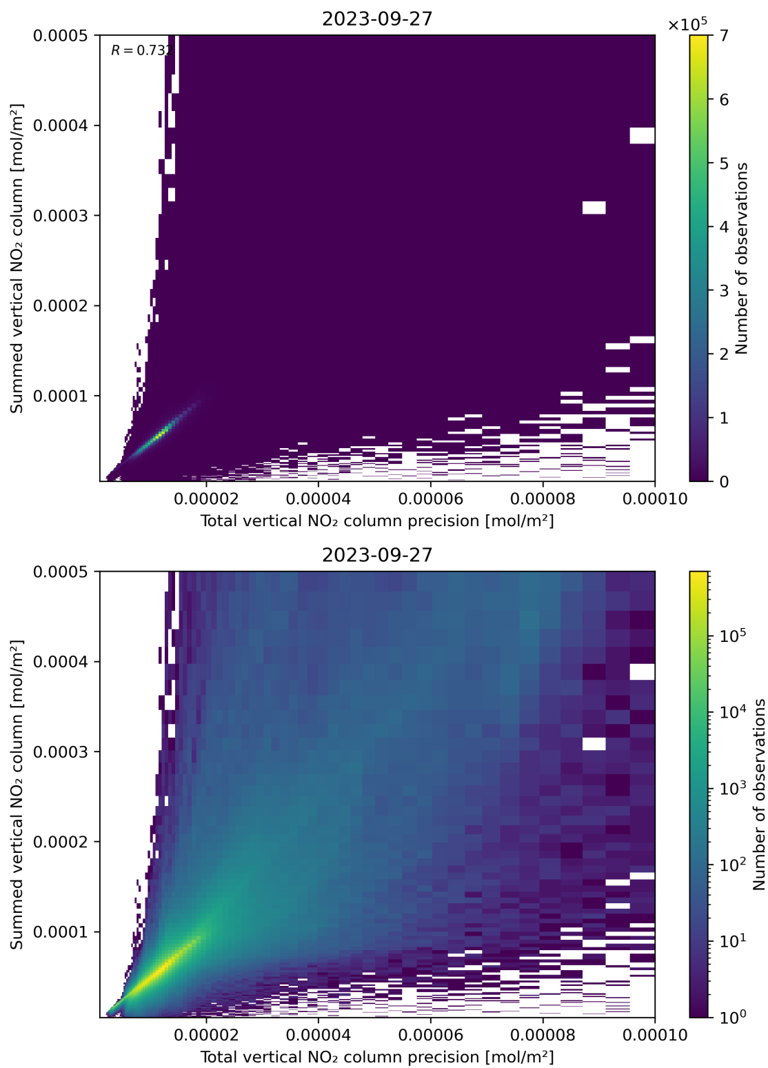
Figure 117: Scatter density plot of “Total vertical NO 2 column precision” against “Summed vertical NO 2 column” for 2023-09-26 to 2023-09-28.
