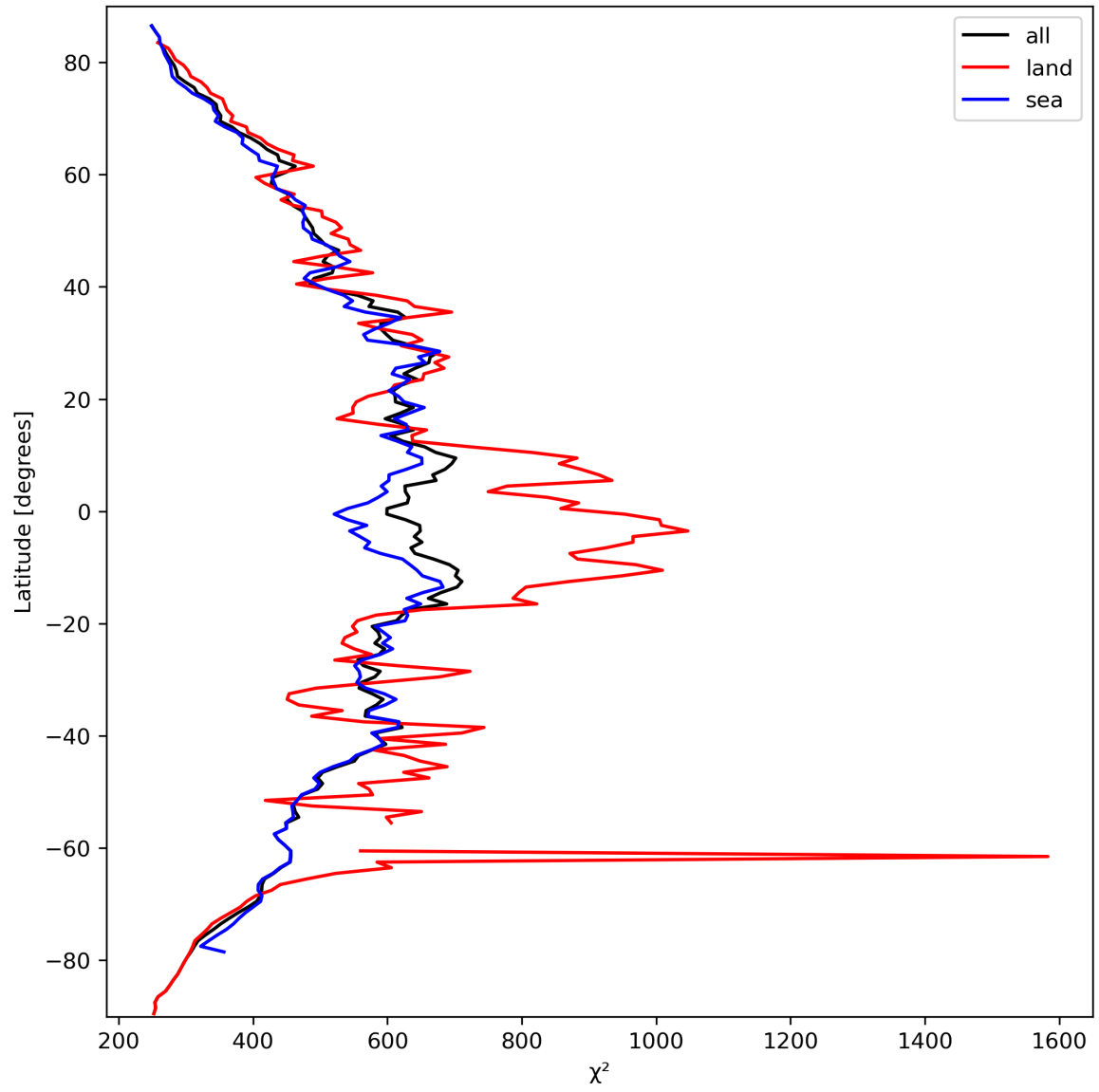
Figure 25: Zonal average of “ \chi^2 ” for 2023-09-26 to 2023-09-28.
