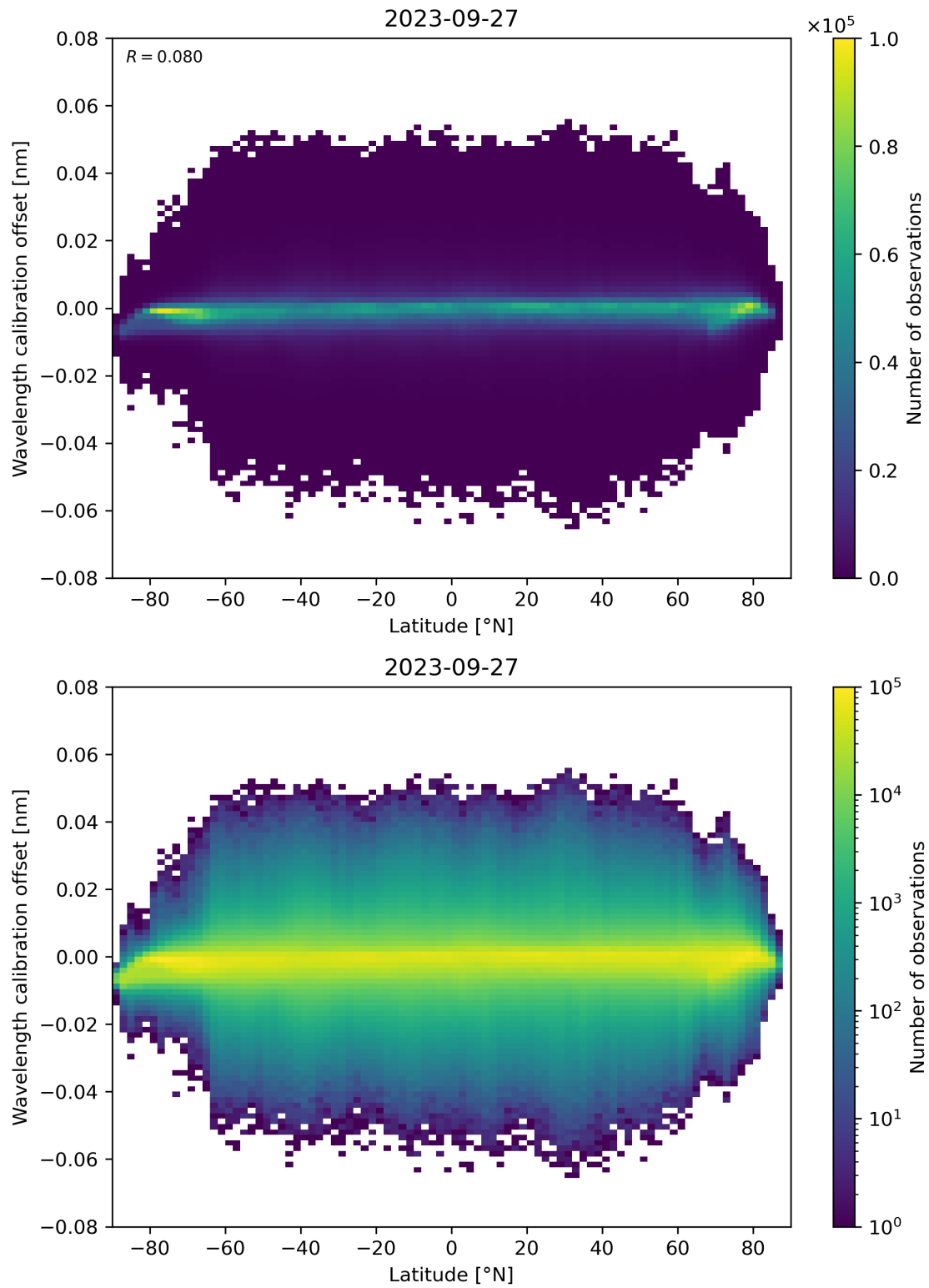
Figure 95: Scatter density plot of “Latitude” against “Wavelength calibration offset” for 2023-09-26 to 2023-09-28.
