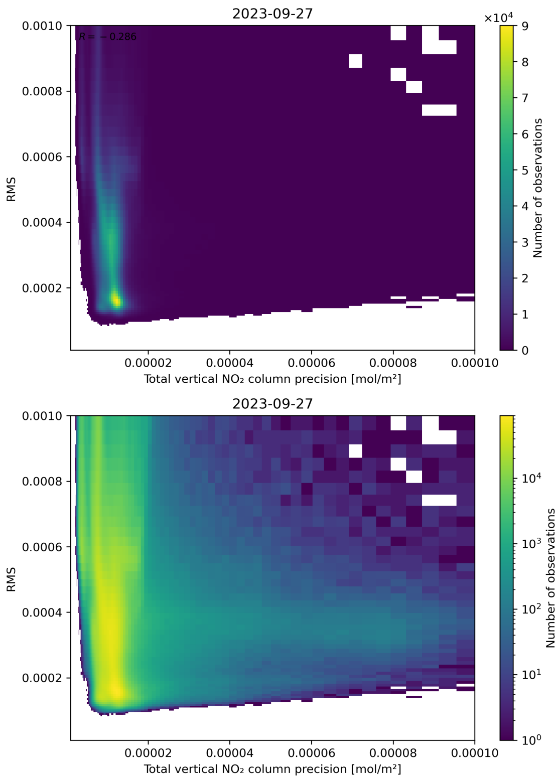
Figure 119: Scatter density plot of “Total vertical NO 2 column precision” against “RMS” for 2023-09-26 to 2023-09-28.
