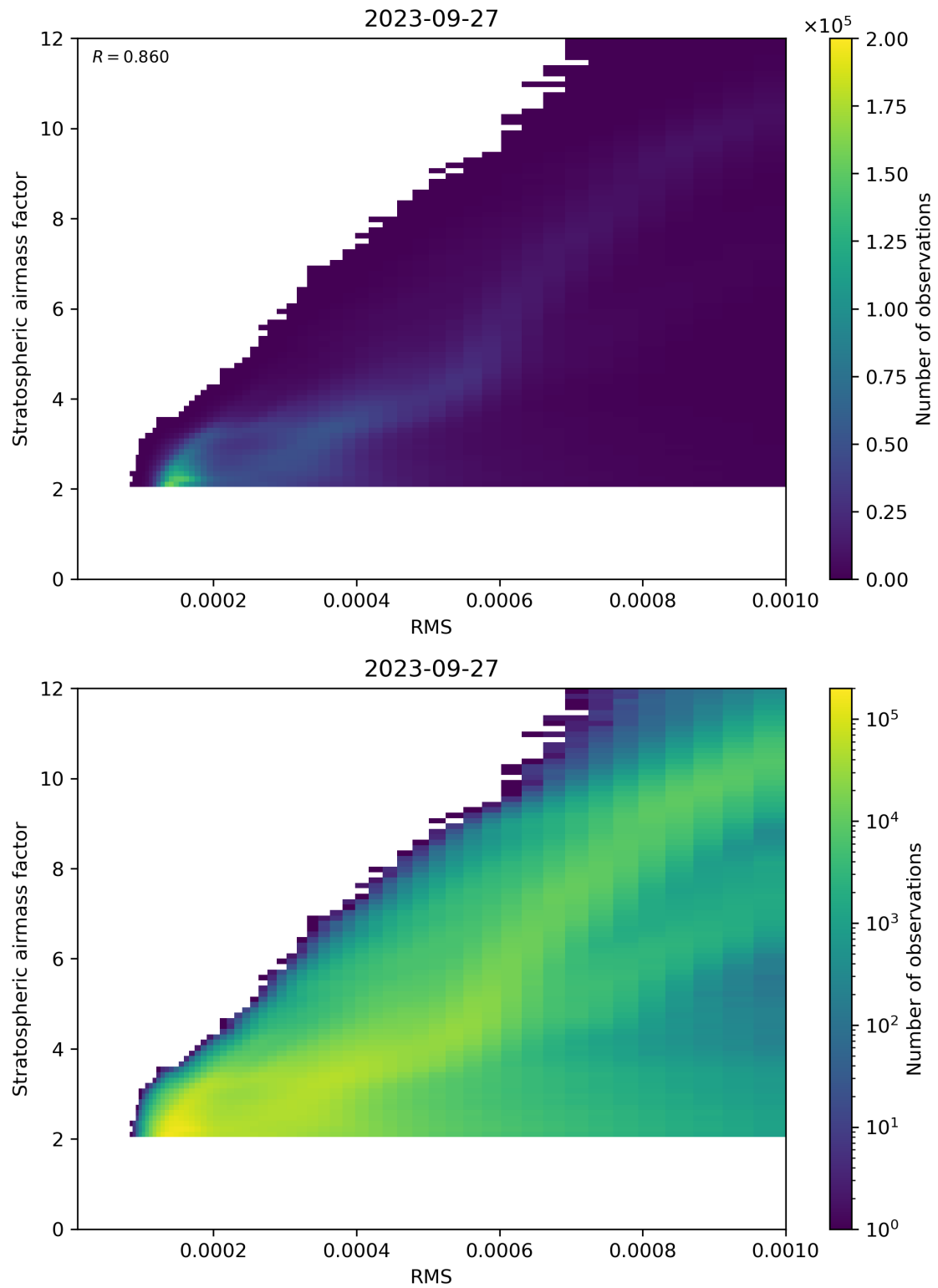
Figure 144: Scatter density plot of “RMS” against “Stratospheric airmass factor” for 2023-09-26 to 2023-09-28.
