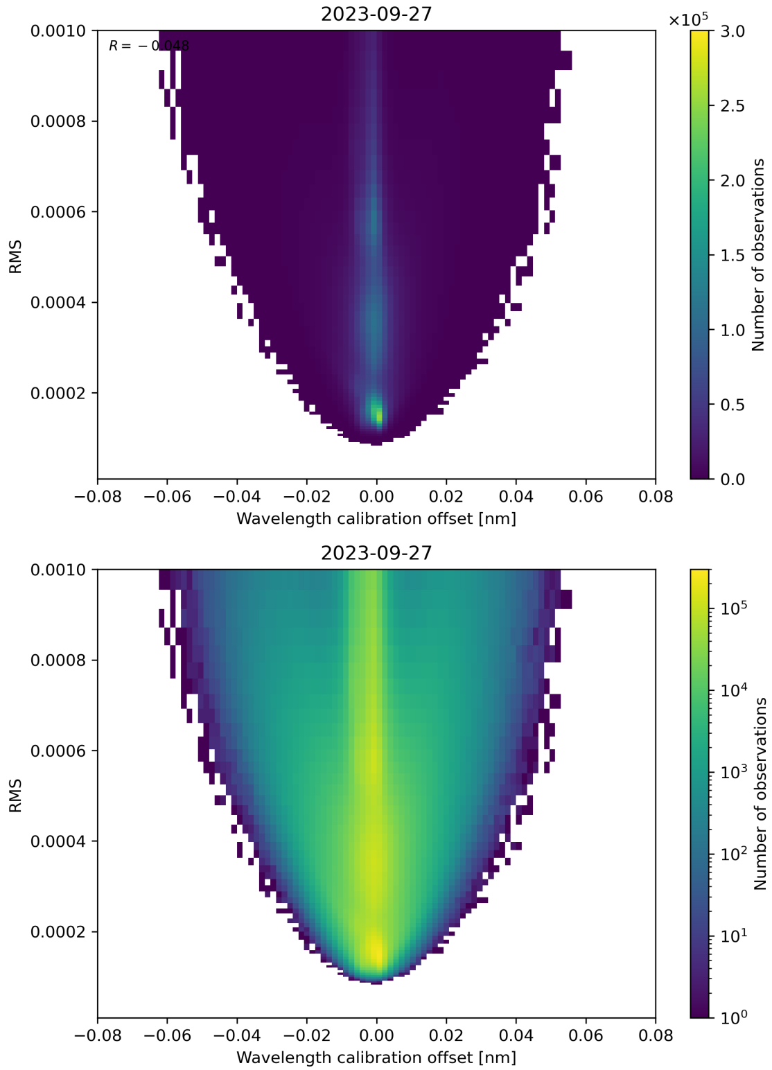
Figure 181: Scatter density plot of “Wavelength calibration offset” against “RMS” for 2023-09-26 to 2023-09-28.
