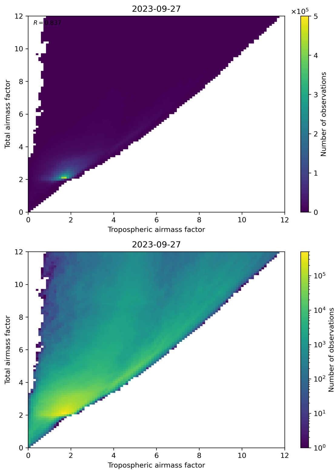
Figure 72: Scatter density plot of “Tropospheric airmass factor” against “Total airmass factor” for 2023-09-26 to 2023-09-28.
