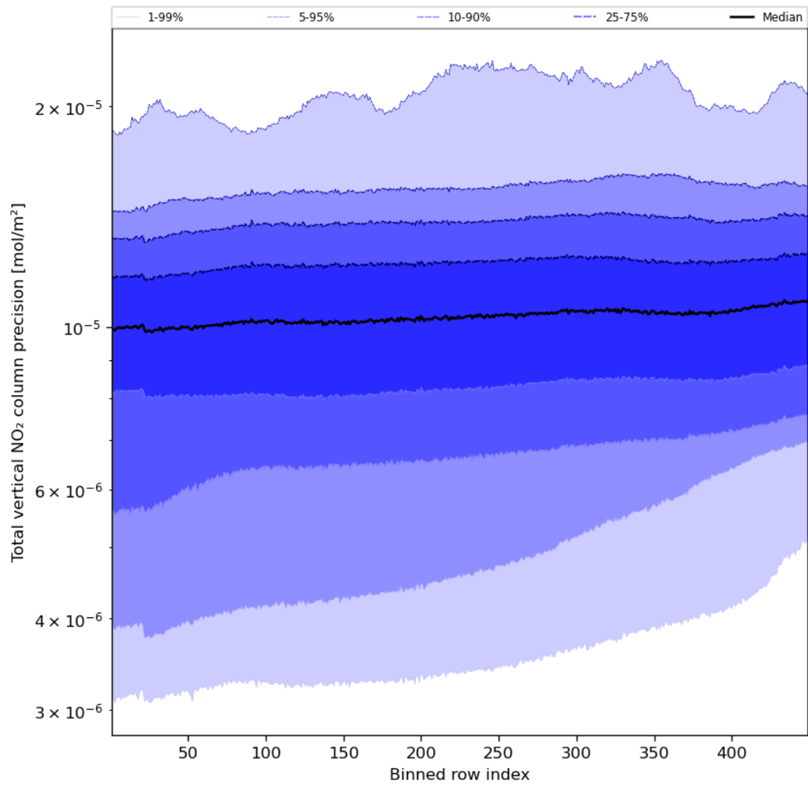
Figure 56: Along track statistics of “Total vertical NO 2 column precision” for 2023-09-26 to 2023-09-28
