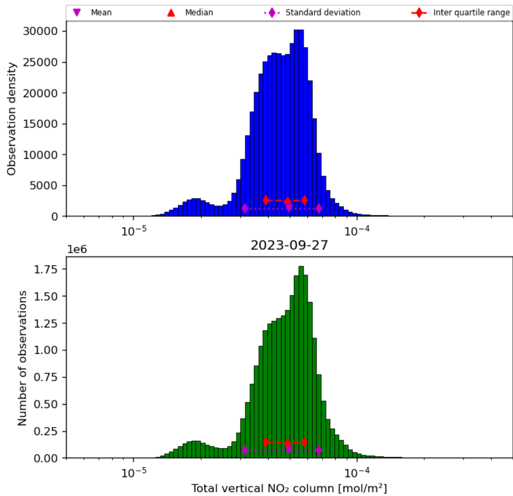
Figure 38: Histogram of “Total vertical NO 2 column” for 2023-09-26 to 2023-09-28
