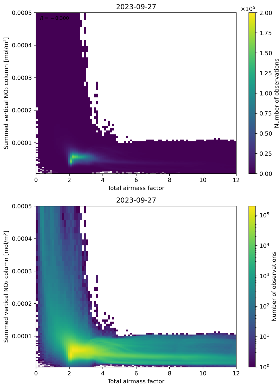
Figure 65: Scatter density plot of “Total airmass factor” against “Summed vertical NO 2 column” for 2023-09-26 to 2023-09-28.
