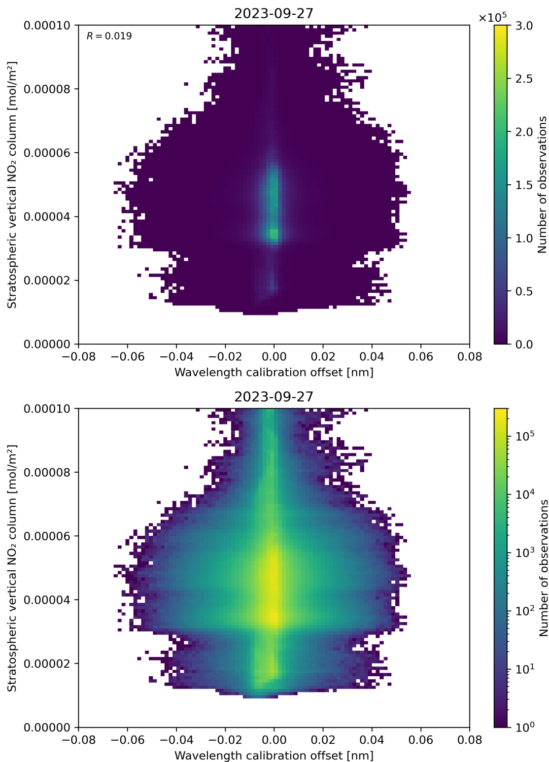
Figure 176: Scatter density plot of “Wavelength calibration offset” against “Stratospheric vertical NO 2 column” for 2023-09-26 to 2023-09-28.
