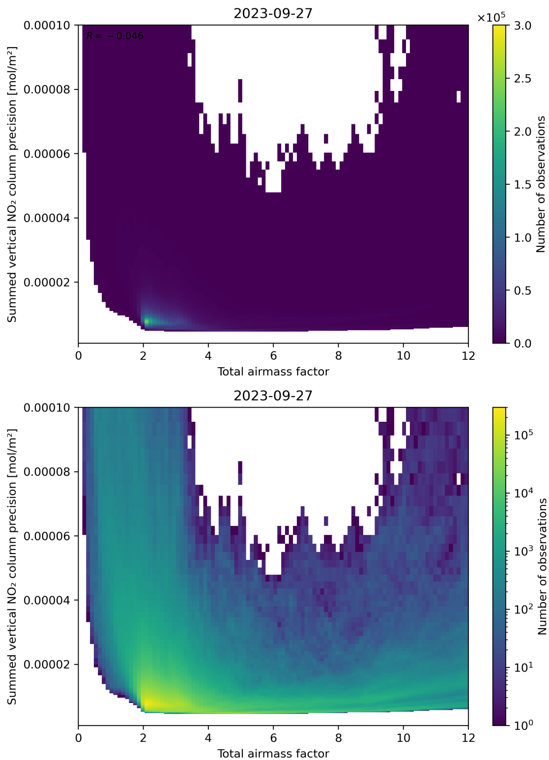
Figure 66: Scatter density plot of “Total airmass factor” against “Summed vertical NO 2 column precision” for 2023-09-26 to 2023-09-28.
