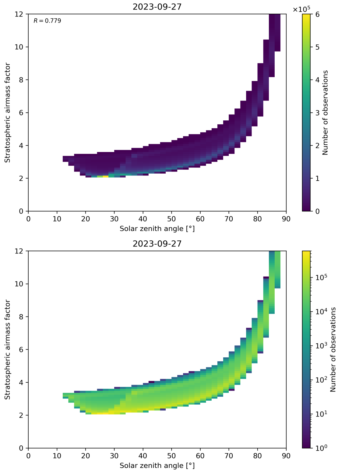
Figure 145: Scatter density plot of “Solar zenith angle” against “Stratospheric airmass factor” for 2023-09-26 to 2023-09-28.
