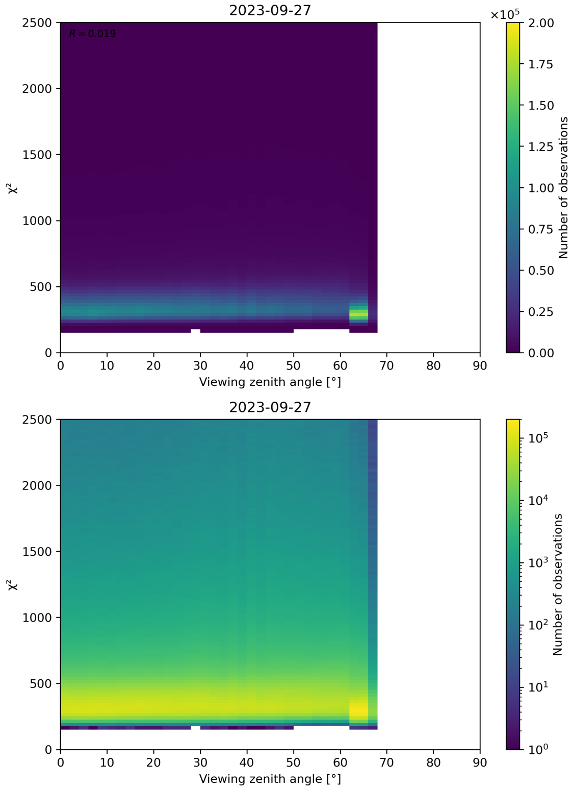
Figure 162: Scatter density plot of “Viewing zenith angle” against “ \chi^2 ” for 2023-09-26 to 2023-09-28.
