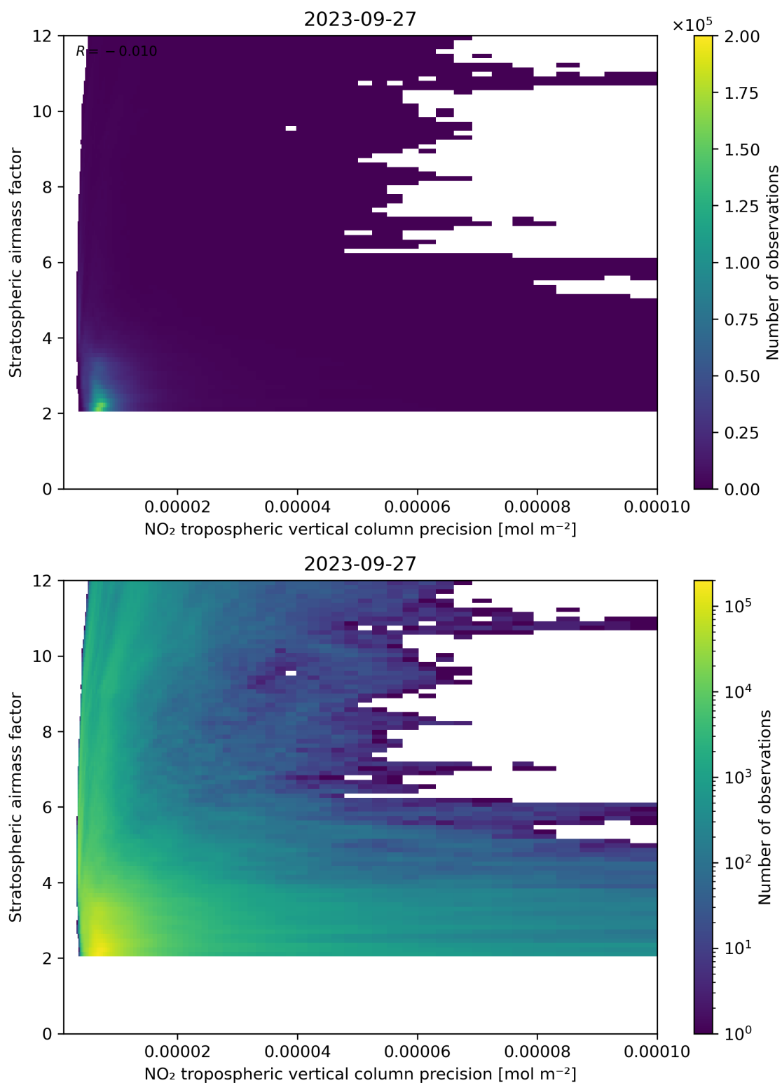
Figure 131: Scatter density plot of “NO 2 tropospheric vertical column precision” against “Stratospheric airmass factor” for 2023-09-26 to 2023-09-28.
