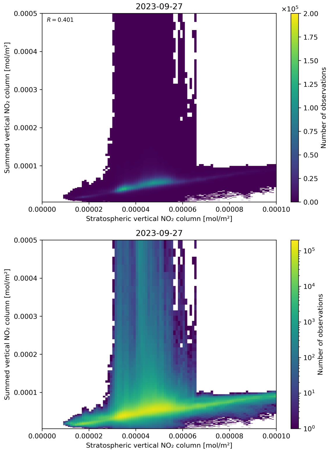
Figure 98: Scatter density plot of “Stratospheric vertical NO 2 column” against “Summed vertical NO 2 column” for 2023-09-26 to 2023-09-28.
