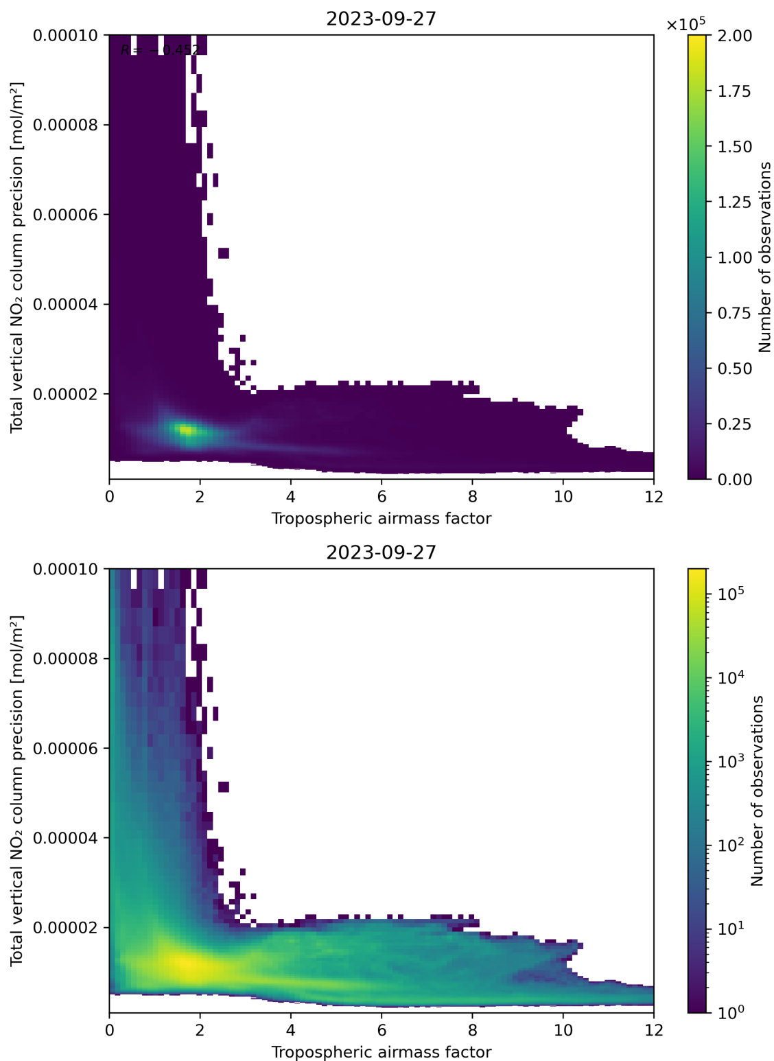
Figure 78: Scatter density plot of “Tropospheric air mass factor” against “Total vertical NO 2 column precision” for 2023-09-26 to 2023-09-28.
