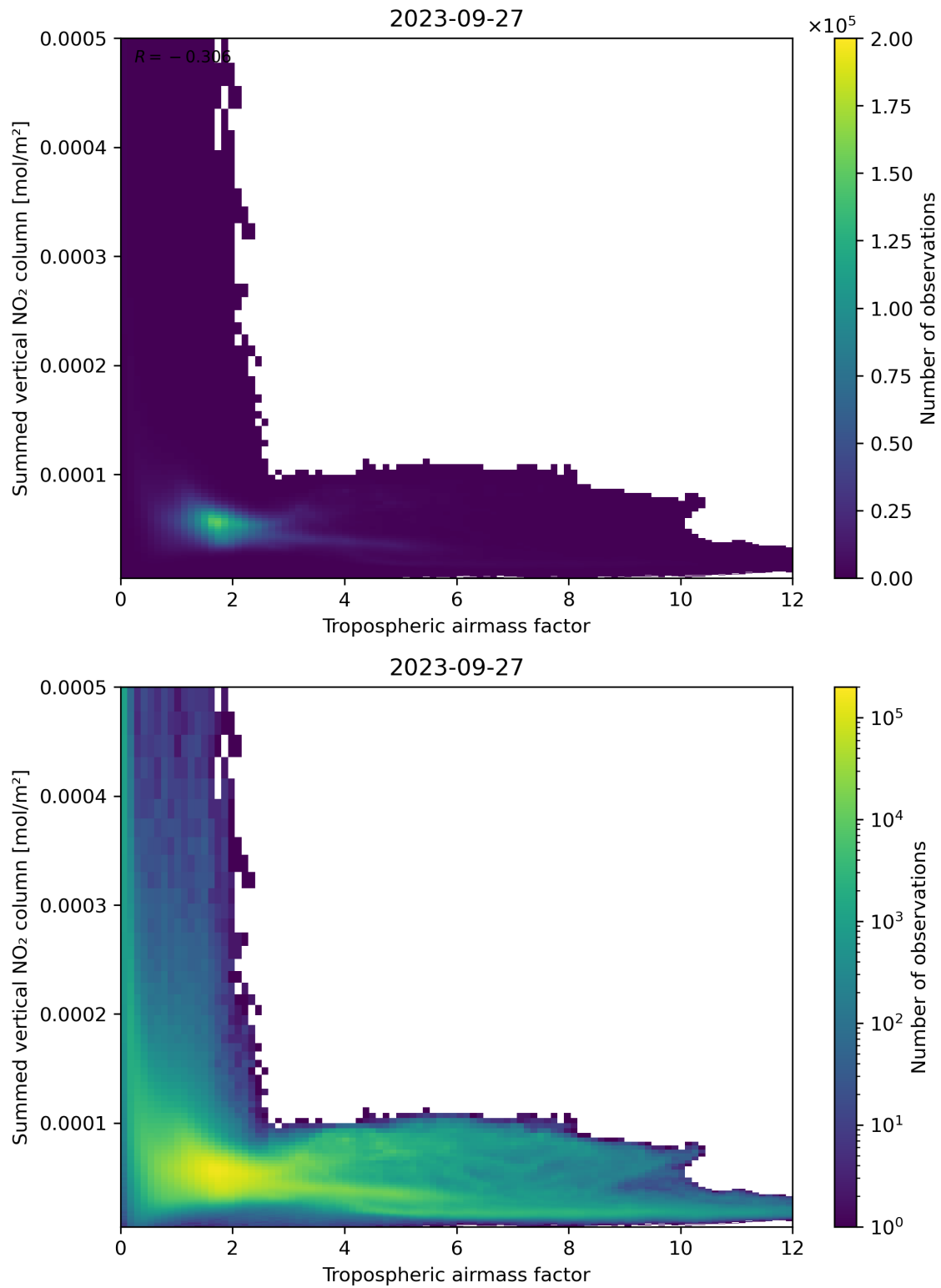
Figure 75: Scatter density plot of “Tropospheric airmass factor” against “Summed vertical NO 2 column” for 2023-09-26 to 2023-09-28.
