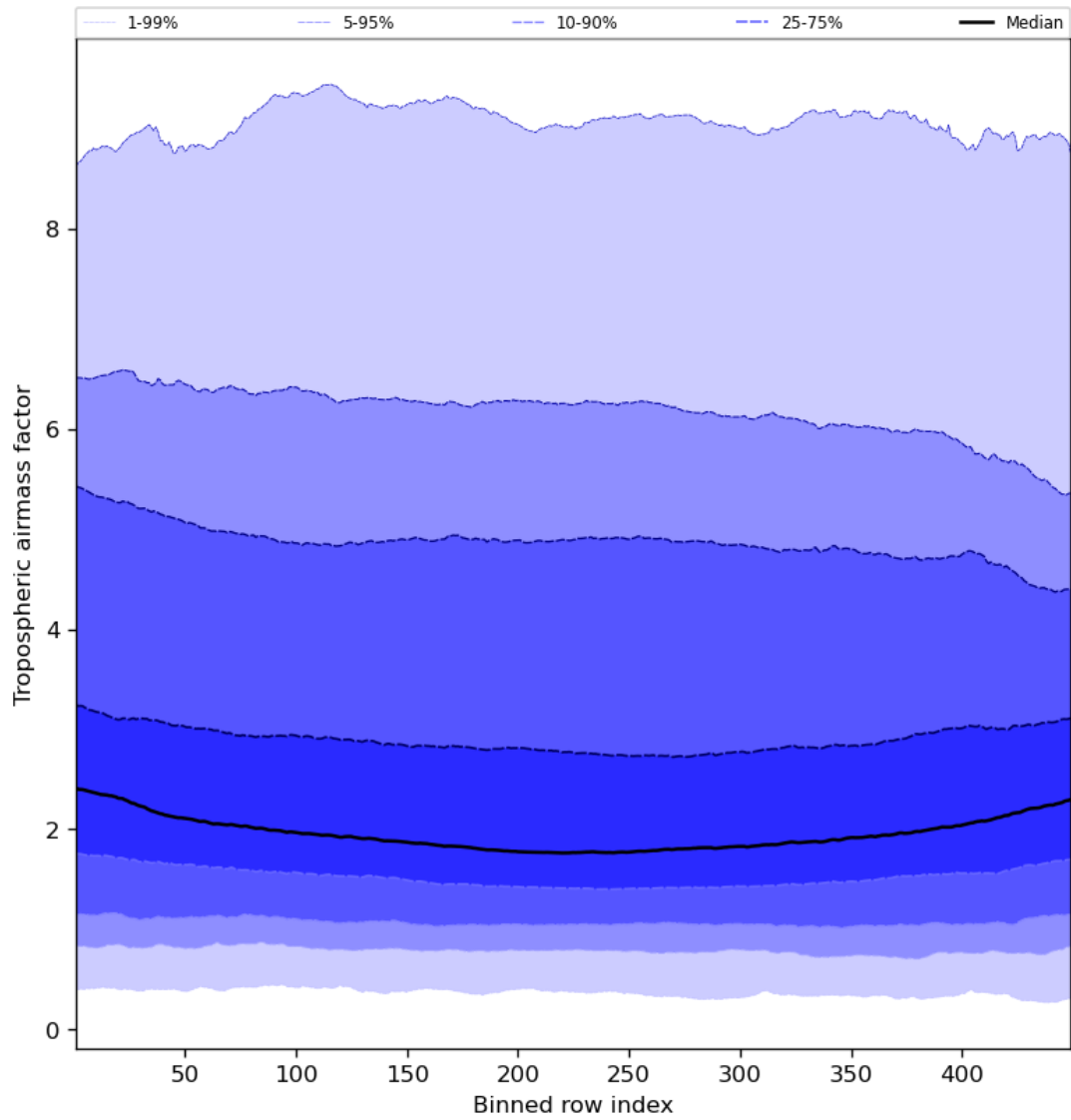
Figure 48: Along track statistics of “Tropospheric air mass factor” for 2023-09-26 to 2023-09-28
