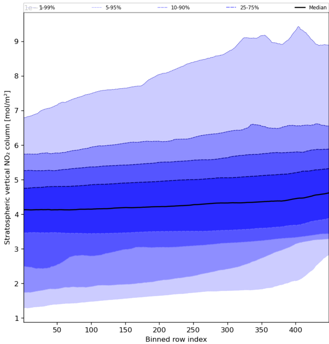
Figure 53: Along track statistics of “Stratospheric vertical NO 2 column” for 2023-09-26 to 2023-09-28
