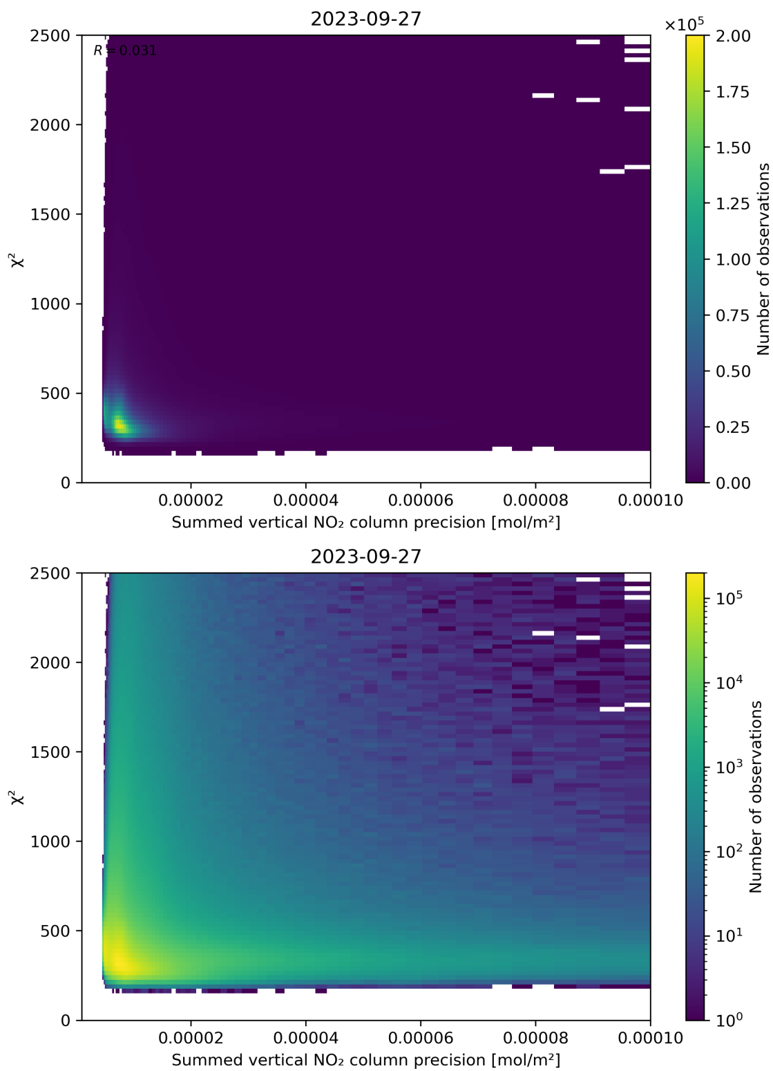
Figure 107: Scatter density plot of “Summed vertical NO 2 column precision” against “ \chi^2 ” for 2023-09-26 to 2023-09-28.
