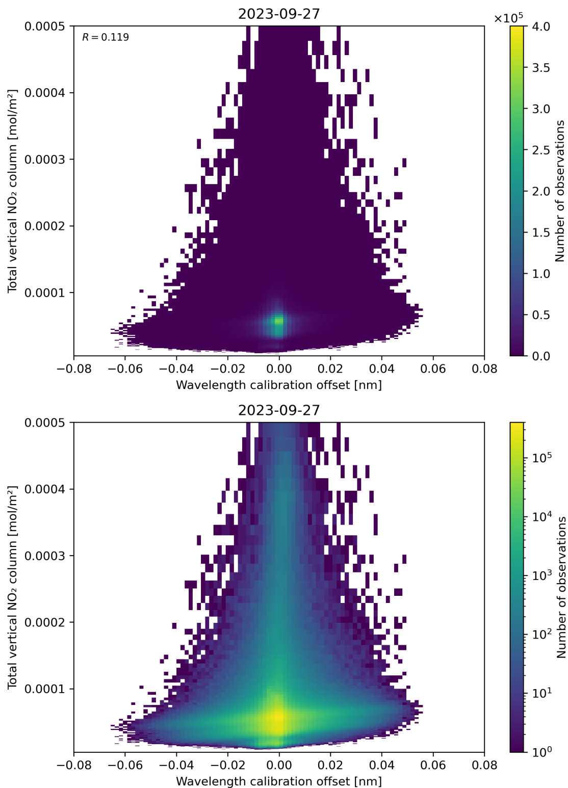
Figure 179: Scatter density plot of “Wavelength calibration offset” against “Total vertical NO 2 column” for 2023-09-26 to 2023-09-28.
