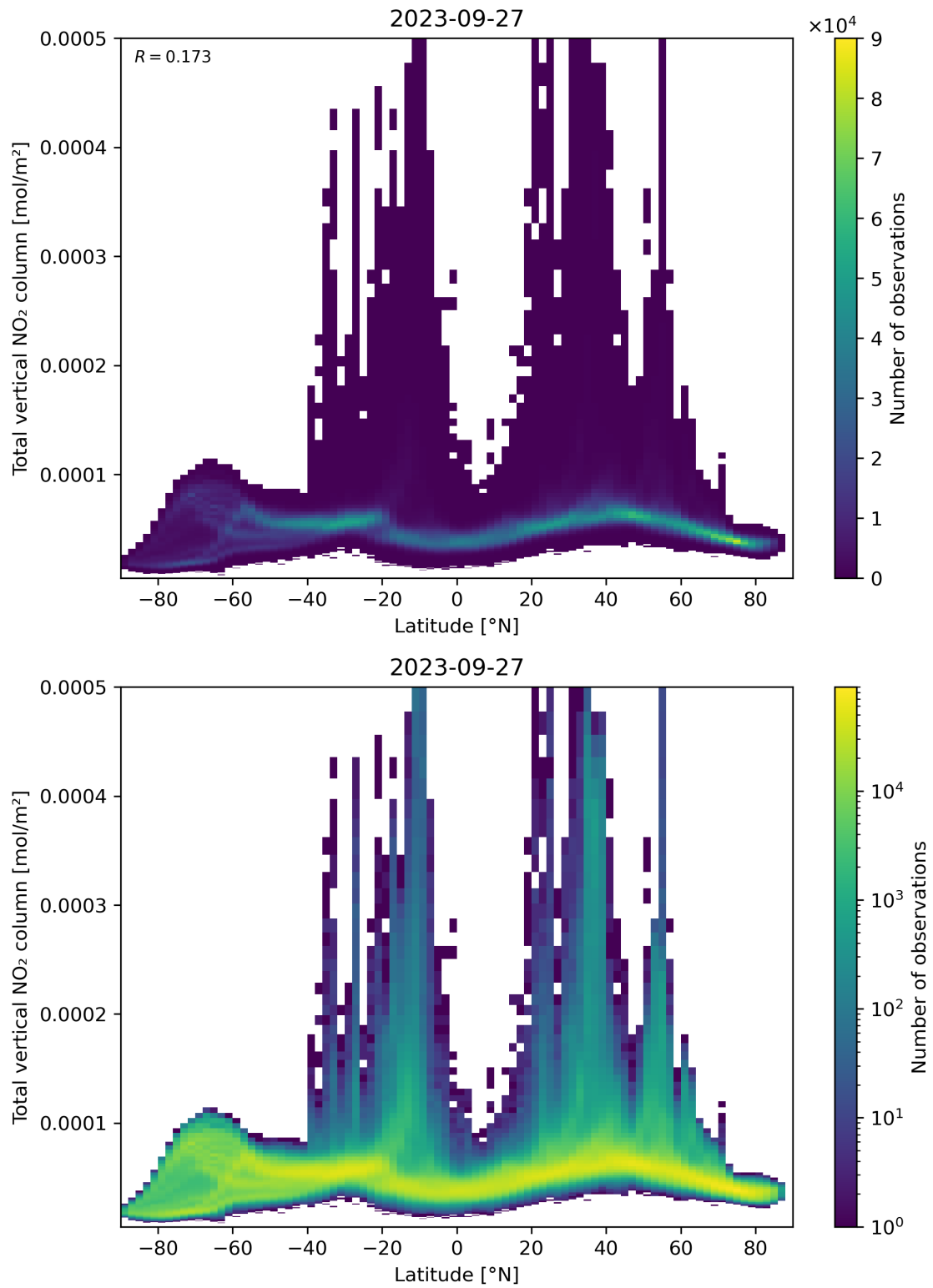
Figure 90: Scatter density plot of “Latitude” against “Total vertical NO 2 column” for 2023-09-26 to 2023-09-28.
