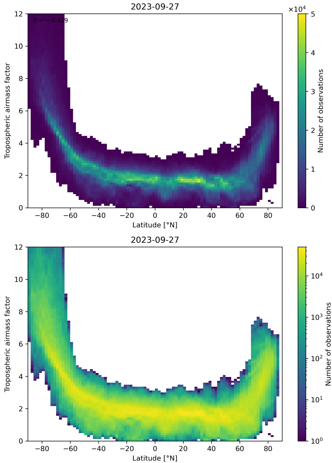
Figure 85: Scatter density plot of “Latitude” against “Tropospheric airmass factor” for 2023-09-26 to 2023-09-28.
