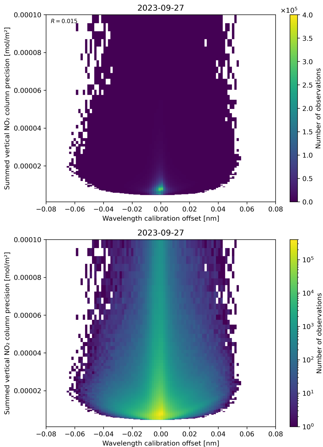
Figure 178: Scatter density plot of “Wavelength calibration offset” against “Summed vertical NO 2 column precision” for 2023-09-26 to 2023-09-28.
