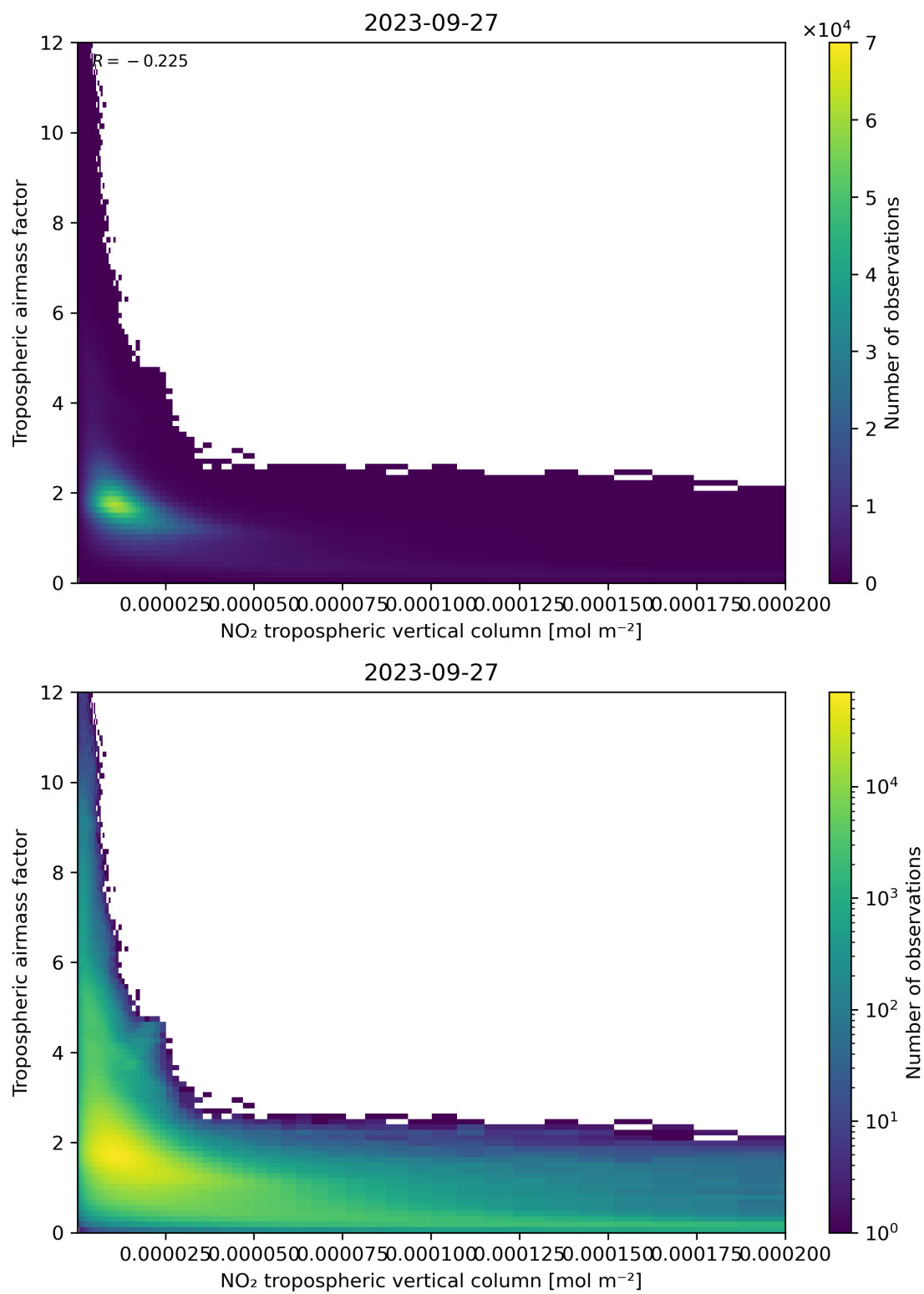
Figure 123: Scatter density plot of “NO 2 tropospheric vertical column” against “Tropospheric air mass factor” for 2023-09-26 to 2023-09-28.
