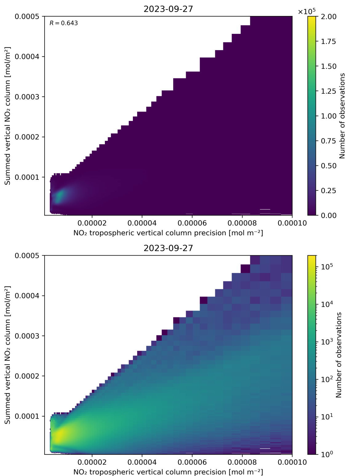
Figure 136: Scatter density plot of “NO 2 tropospheric vertical column precision” against “Summed vertical NO 2 column” for 2023-09-26 to 2023-09-28.
