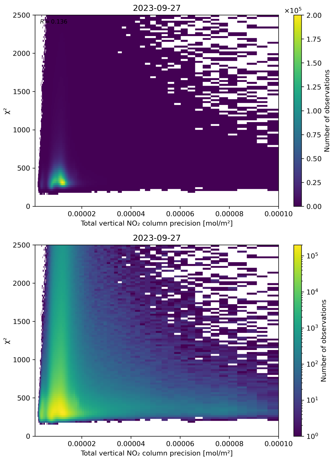
Figure 116: Scatter density plot of “Total vertical NO 2 column precision” against “ \chi^2 ” for 2023-09-26 to 2023-09-28.
