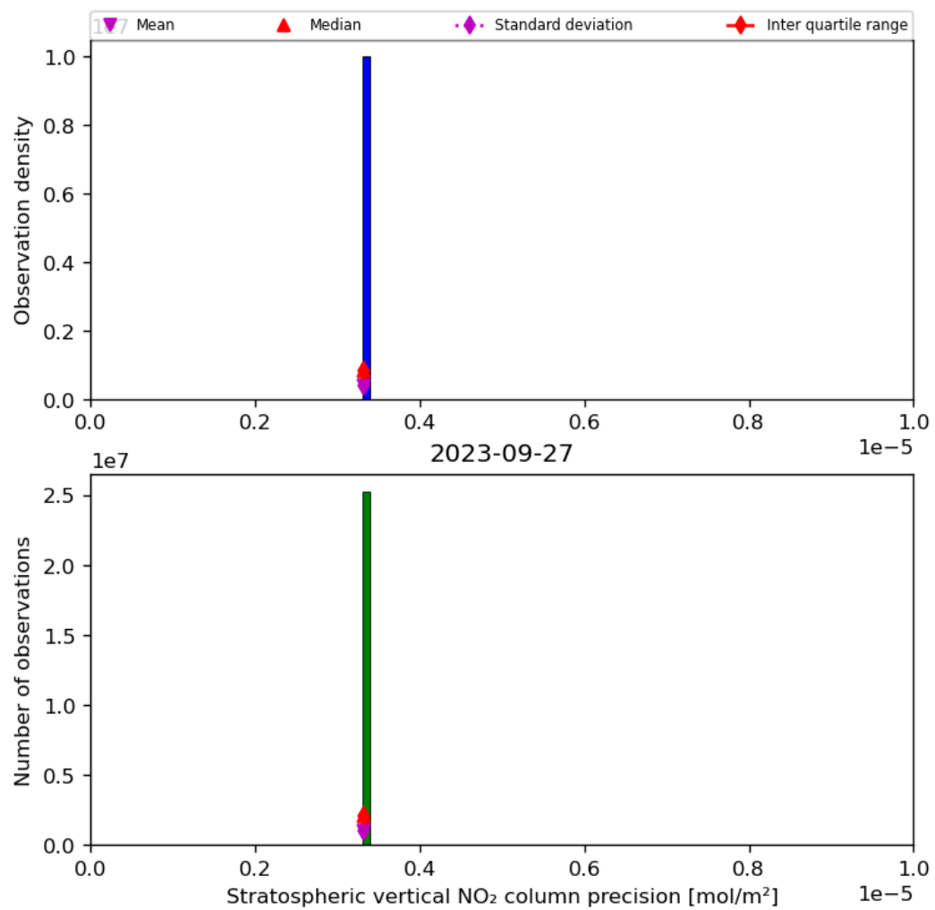
Figure 37: Histogram of “Stratospheric vertical NO 2 column precision” for 2023-09-26 to 2023-09-28
