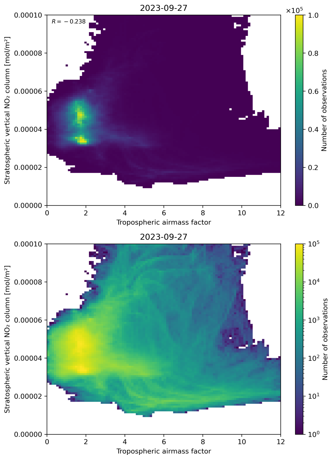
Figure 74: Scatter density plot of “Tropospheric air mass factor” against “Stratospheric vertical NO 2 column” for 2023-09-26 to 2023-09-28.
