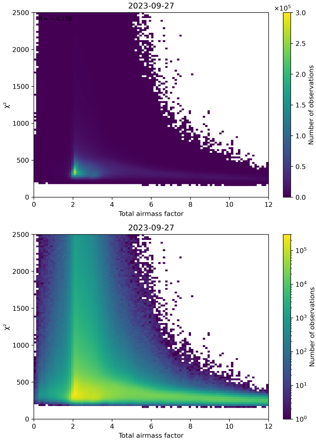
Figure 63: Scatter density plot of “Total airmass factor” against “ \chi^2 ” for 2023-09-26 to 2023-09-28.
