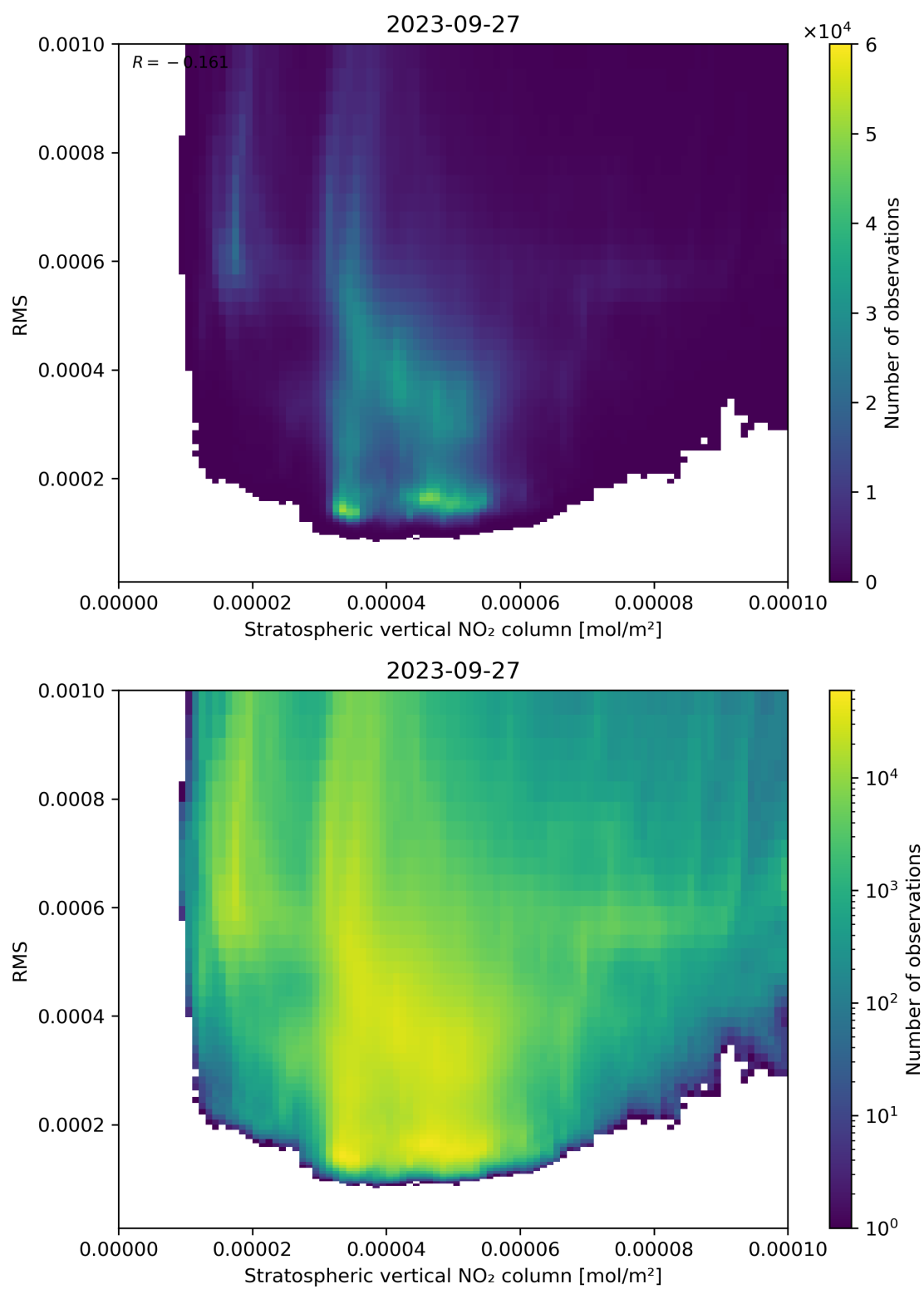
Figure 102: Scatter density plot of “Stratospheric vertical NO 2 column” against “RMS” for 2023-09-26 to 2023-09-28.
