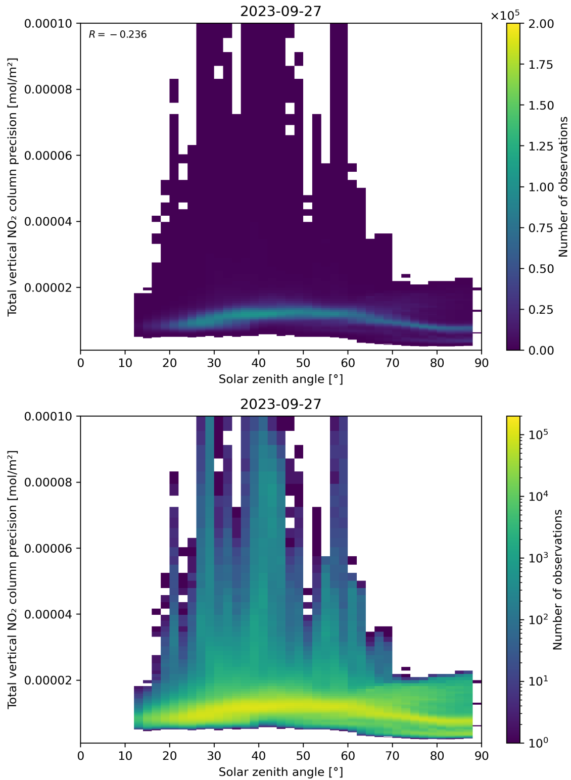
Figure 154: Scatter density plot of “Solar zenith angle” against “Total vertical NO 2 column precision” for 2023-09-26 to 2023-09-28.
