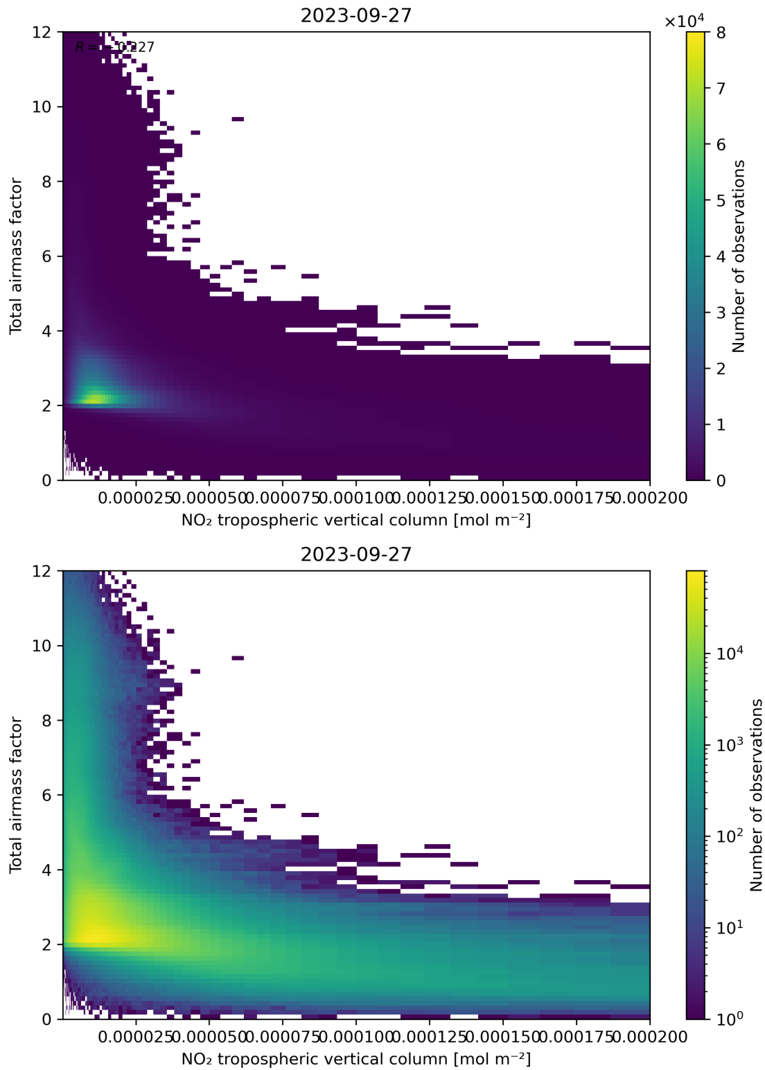
Figure 122: Scatter density plot of “NO 2 tropospheric vertical column” against “Total airmass factor” for 2023-09-26 to 2023-09-28.
