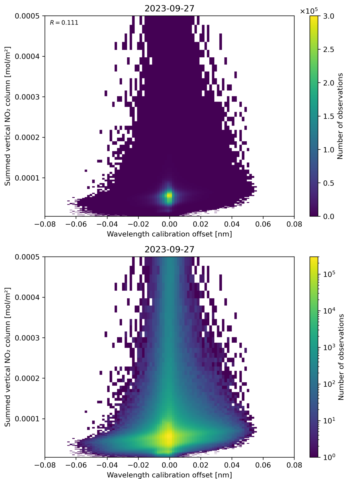
Figure 177: Scatter density plot of “Wavelength calibration offset” against “Summed vertical NO 2 column” for 2023-09-26 to 2023-09-28.
