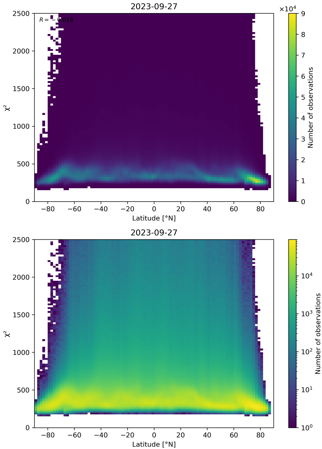
Figure 86: Scatter density plot of “Latitude” against “ \chi^2 ” for 2023-09-26 to 2023-09-28.
