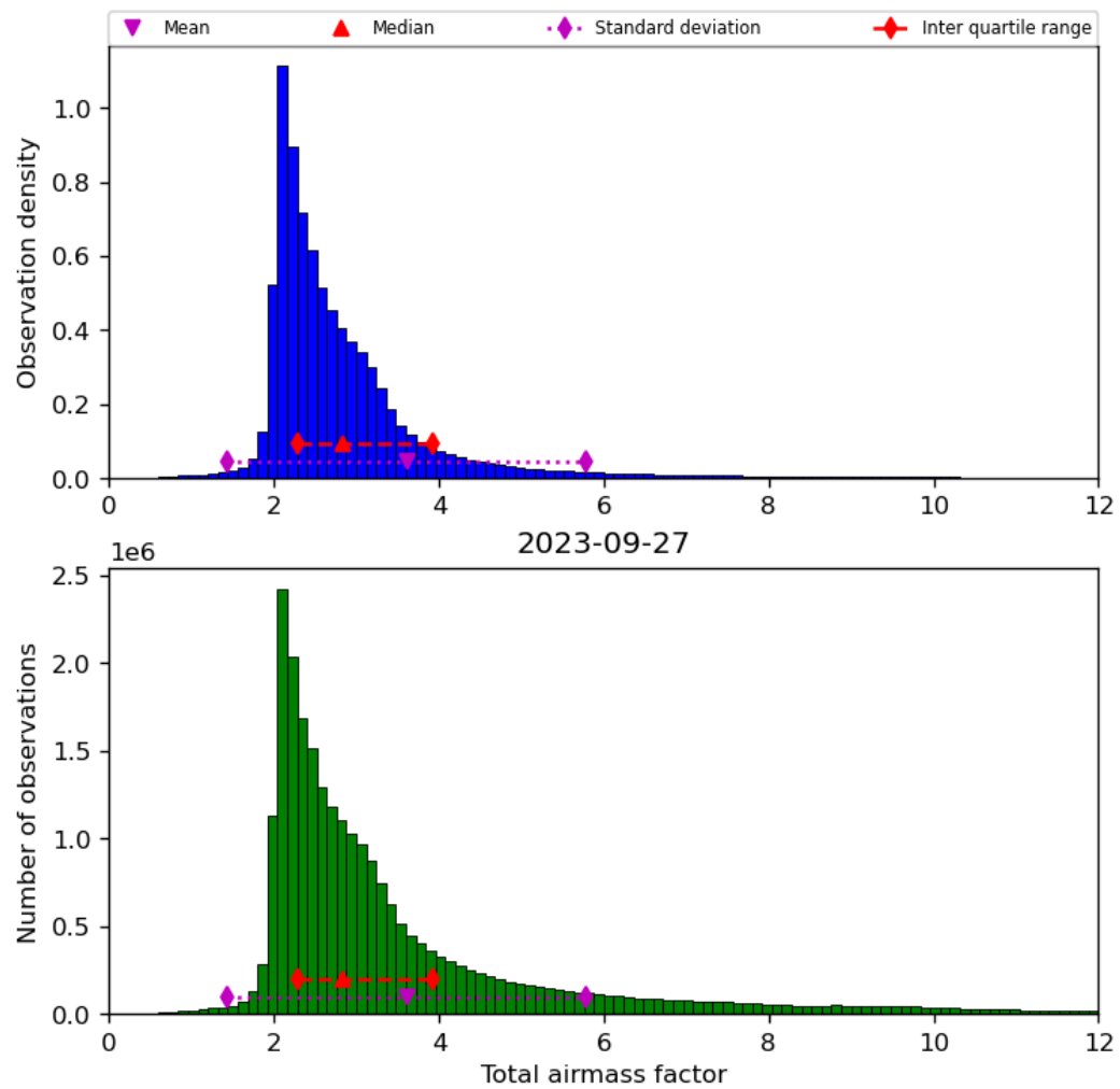
Figure 32: Histogram of “Total airmass factor” for 2023-09-26 to 2023-09-28
