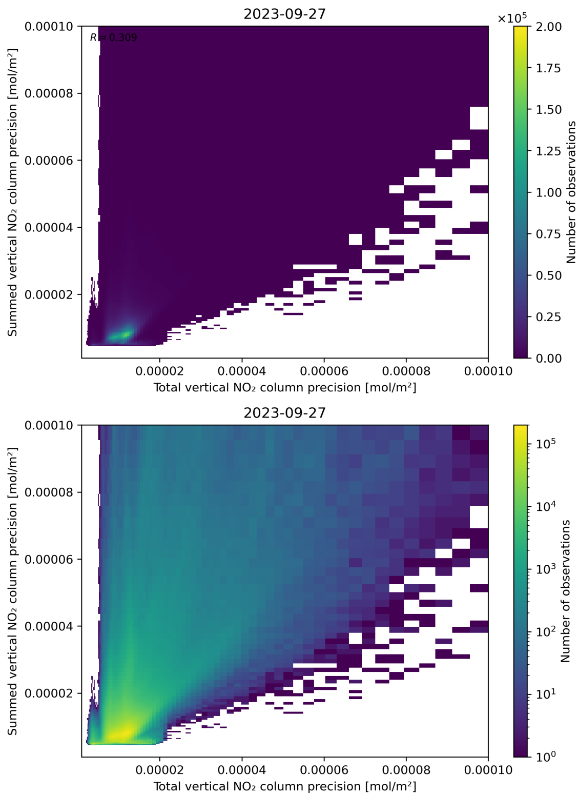
Figure 118: Scatter density plot of “Total vertical NO 2 column precision” against “Summed vertical NO 2 column precision” for 2023-09-26 to 2023-09-28.
