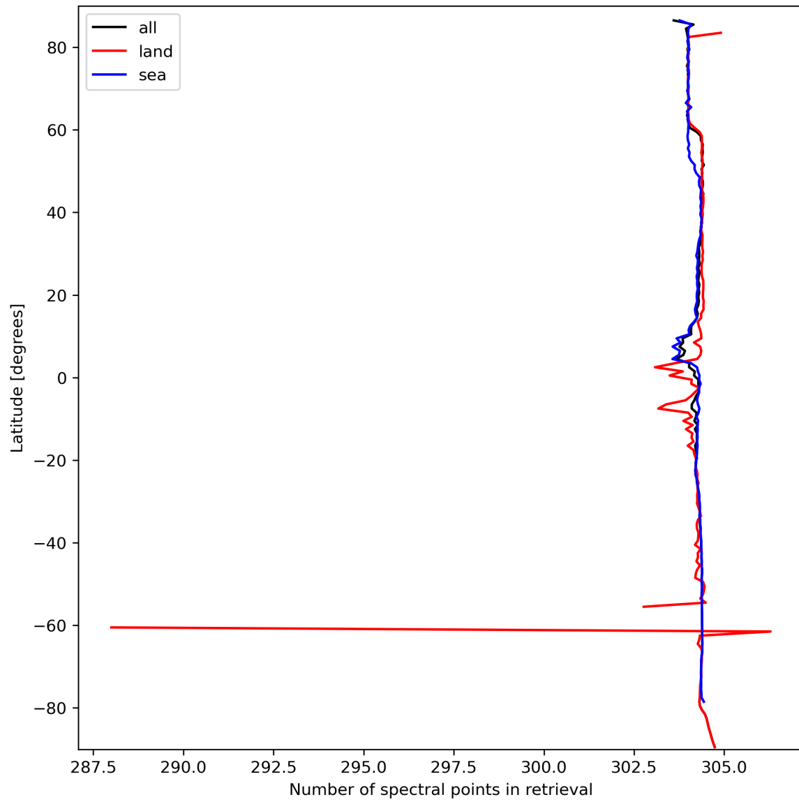
Figure 16: Zonal average of “Number of spectral points in retrieval” for 2023-09-26 to 2023-09-28.
