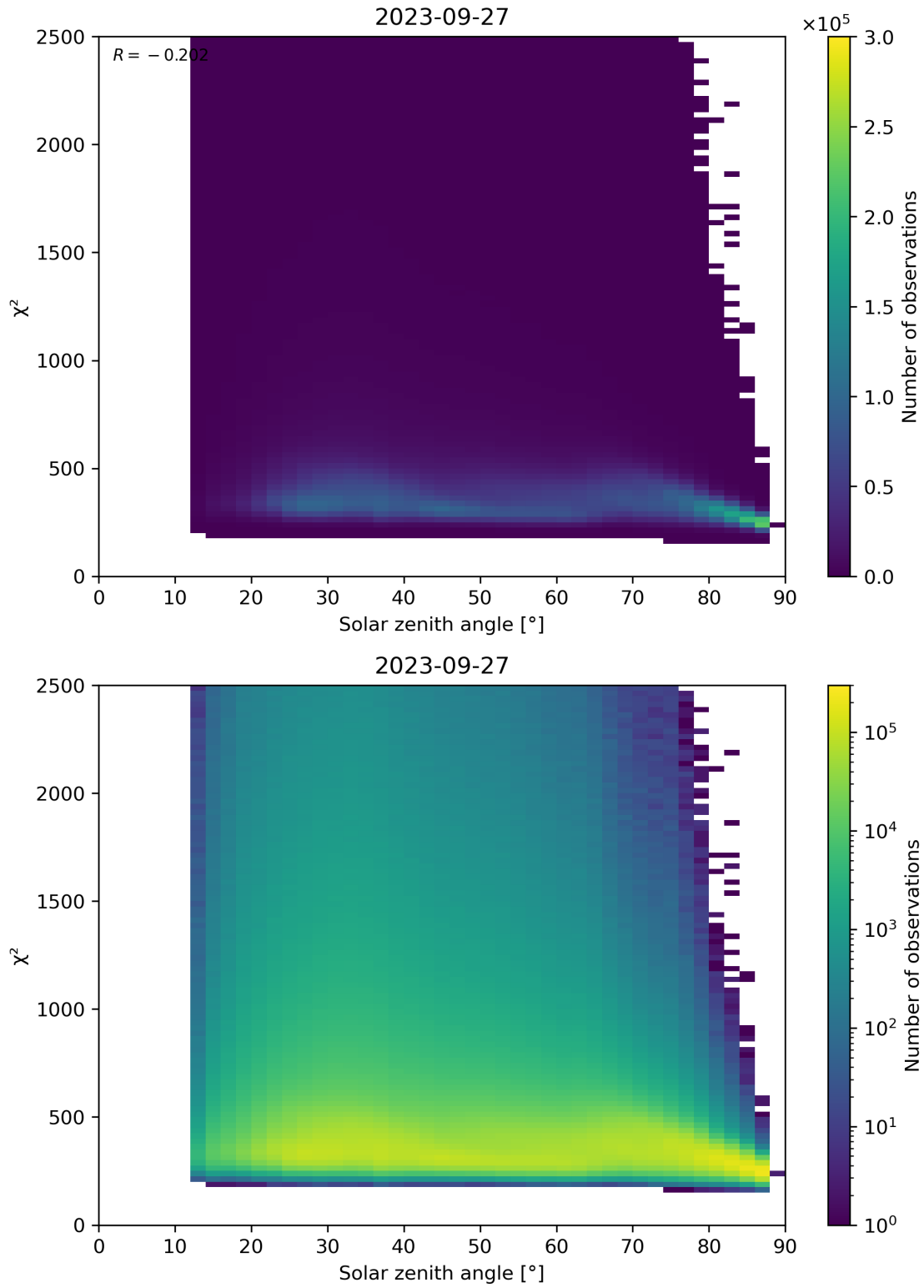
Figure 148: Scatter density plot of “Solar zenith angle” against “ \chi^2 ” for 2023-09-26 to 2023-09-28.
