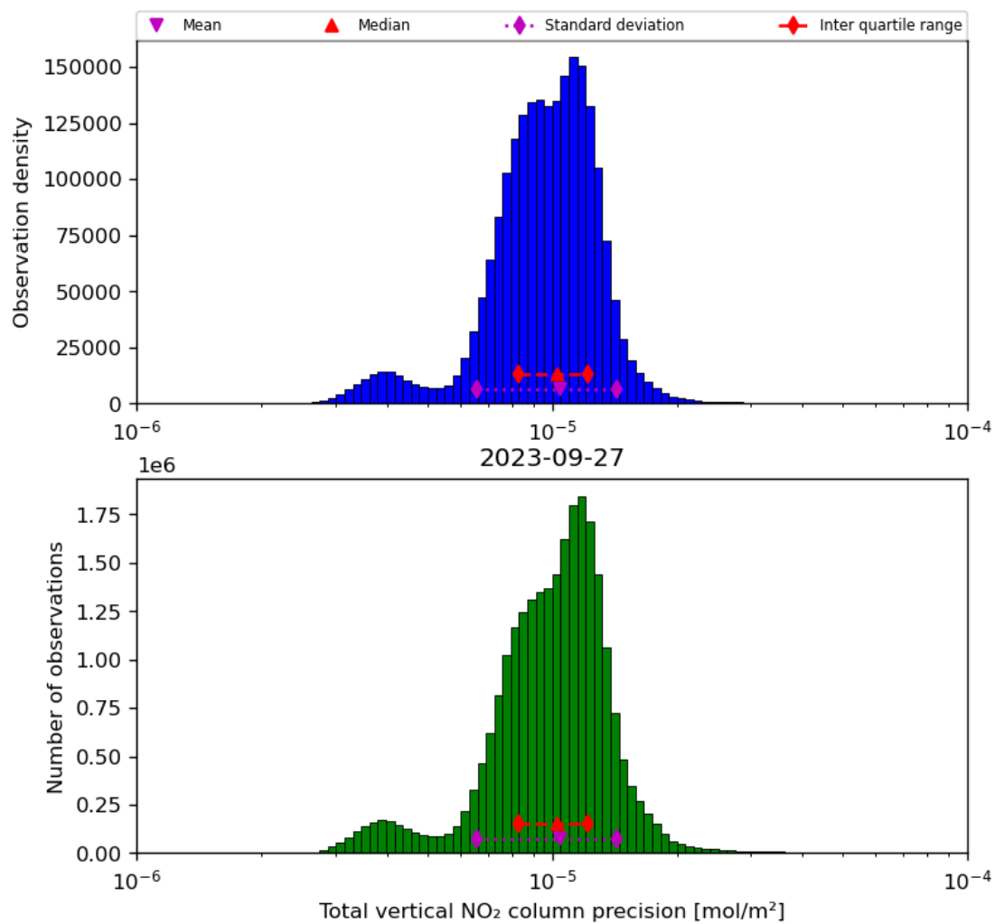
Figure 39: Histogram of “Total vertical NO 2 column precision” for 2023-09-26 to 2023-09-28
