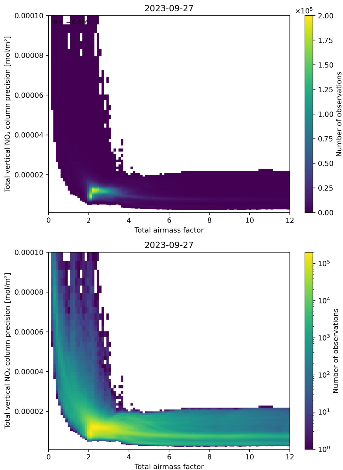
Figure 68: Scatter density plot of “Total airmass factor” against “Total vertical NO 2 column precision” for 2023-09-26 to 2023-09-28.
