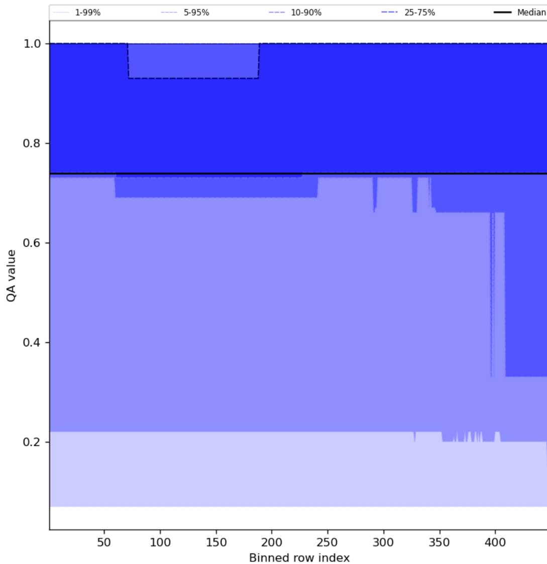
Figure 45: Along track statistics of “QA value” for 2023-09-26 to 2023-09-28
