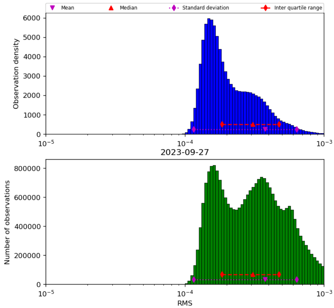
Figure 43: Histogram of “RMS” for 2023-09-26 to 2023-09-28
