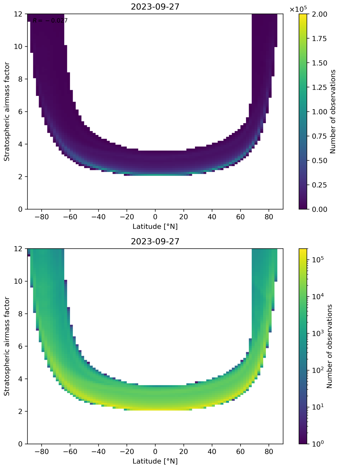
Figure 83: Scatter density plot of “Latitude” against “Stratospheric air mass factor” for 2023-09-26 to 2023-09-28.
