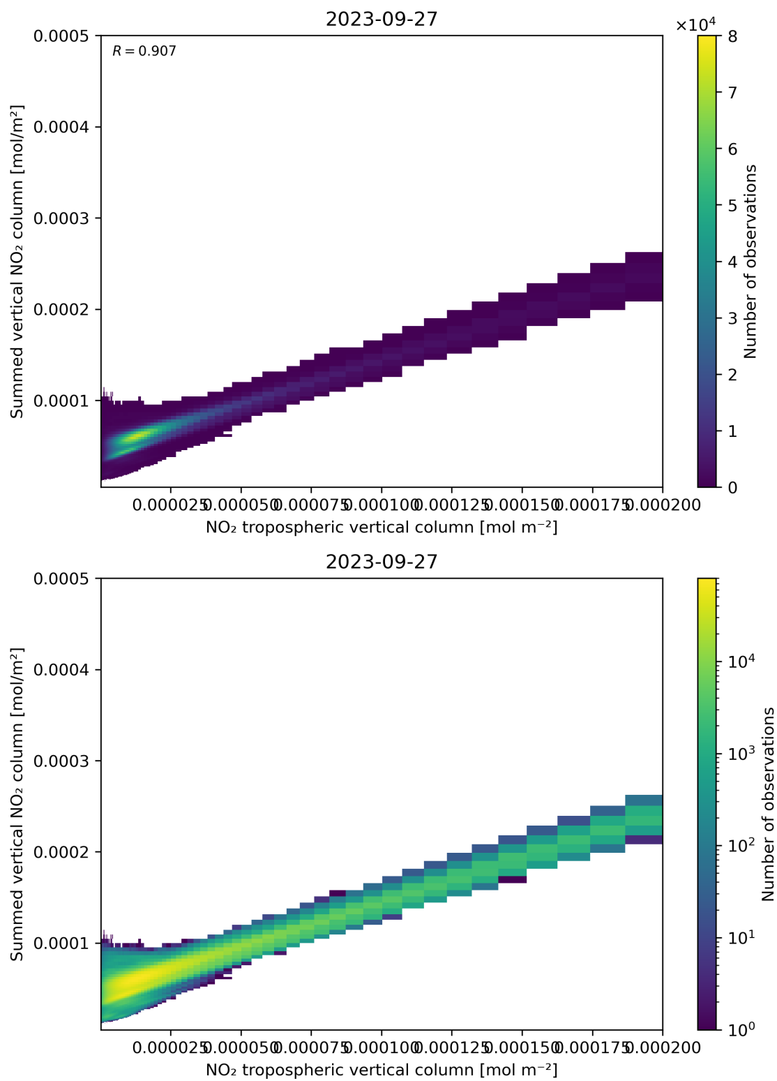
Figure 126: Scatter density plot of “NO 2 tropospheric vertical column” against “Summed vertical NO 2 column” for 2023-09-26 to 2023-09-28.
