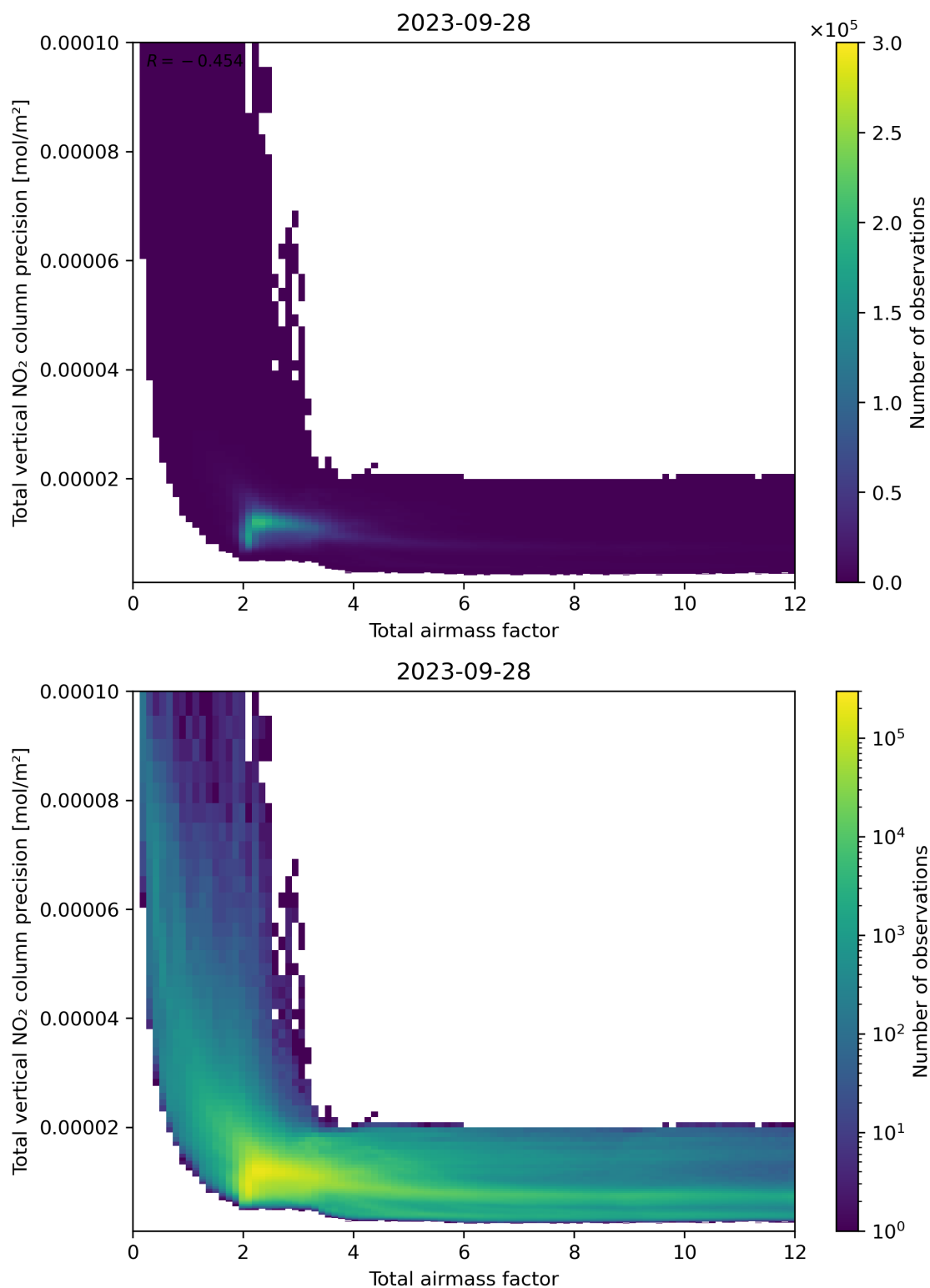
Figure 68: Scatter density plot of “Total airmass factor” against “Total vertical NO 2 column precision” for 2023-09-27 to 2023-09-29.
