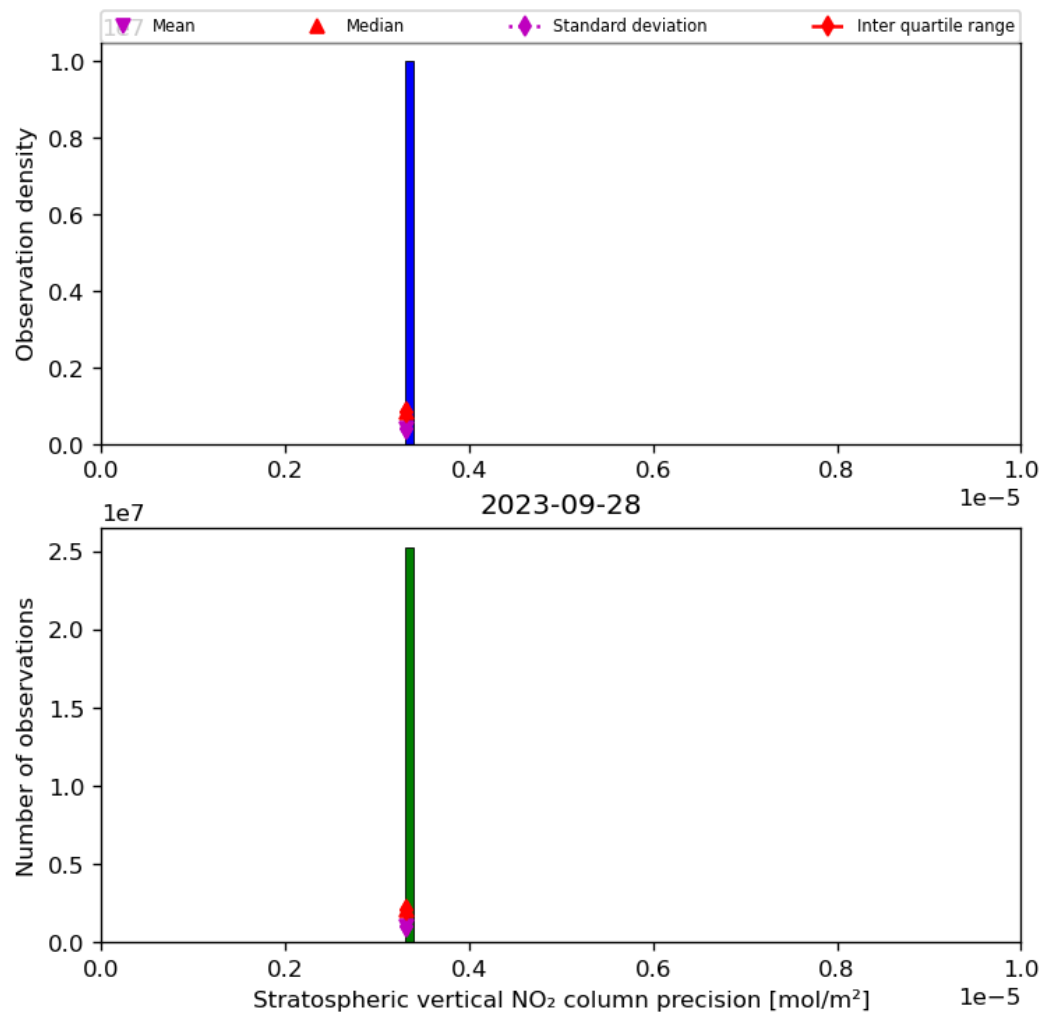
Figure 37: Histogram of “Stratospheric vertical NO 2 column precision” for 2023-09-27 to 2023-09-29
