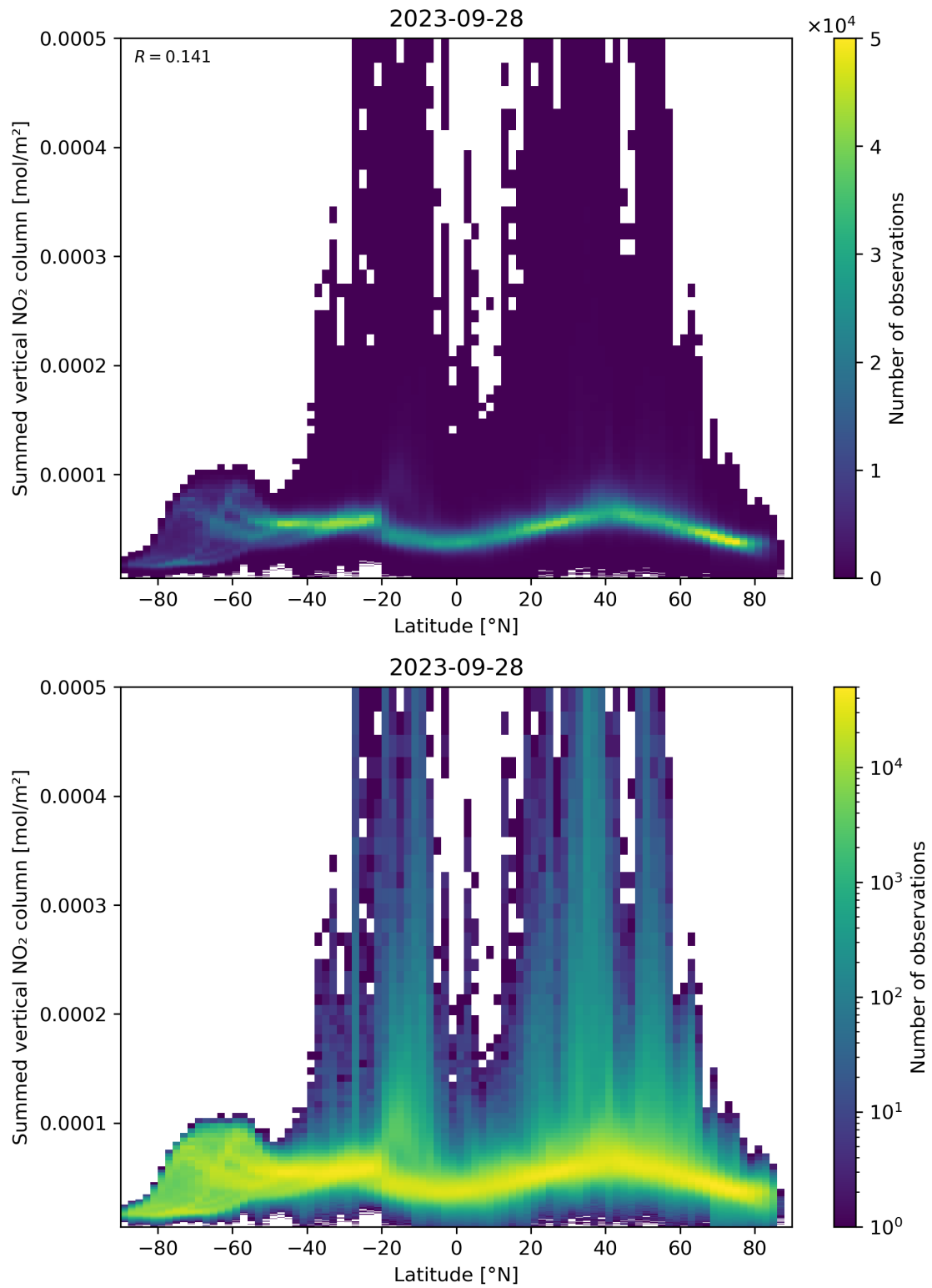
Figure 88: Scatter density plot of “Latitude” against “Summed vertical NO 2 column” for 2023-09-27 to 2023-09-29.
