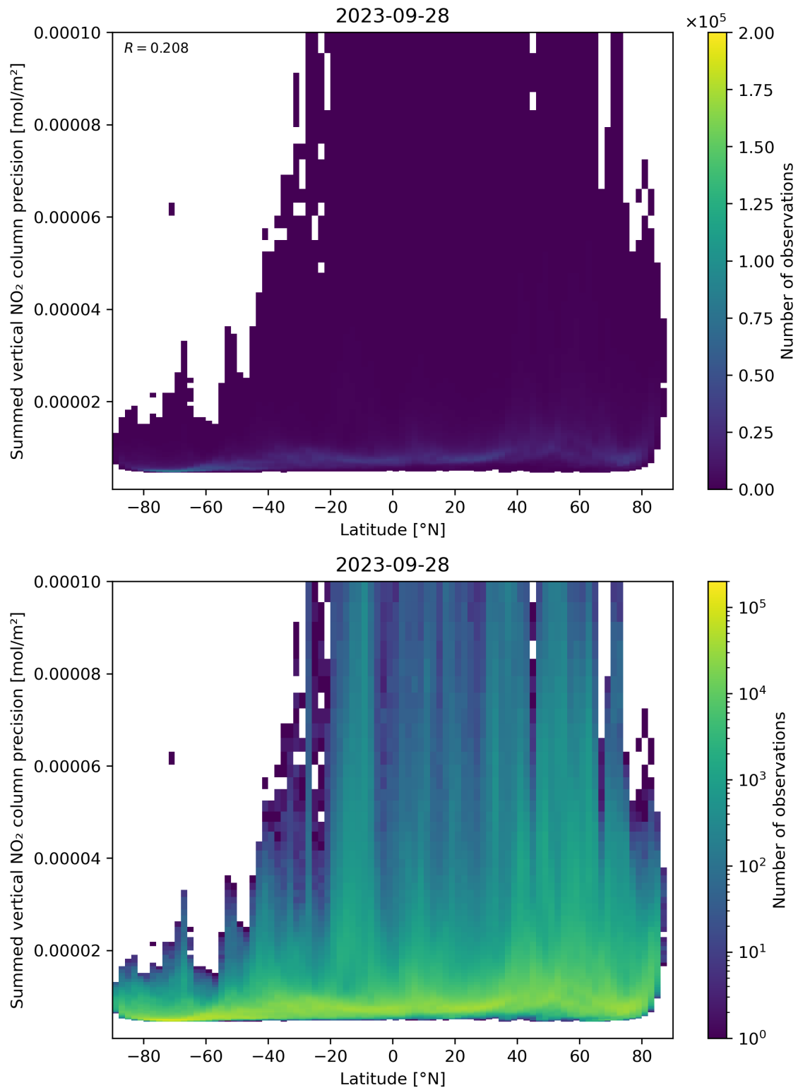
Figure 89: Scatter density plot of “Latitude” against “Summed vertical NO 2 column precision” for 2023-09-27 to 2023-09-29.
