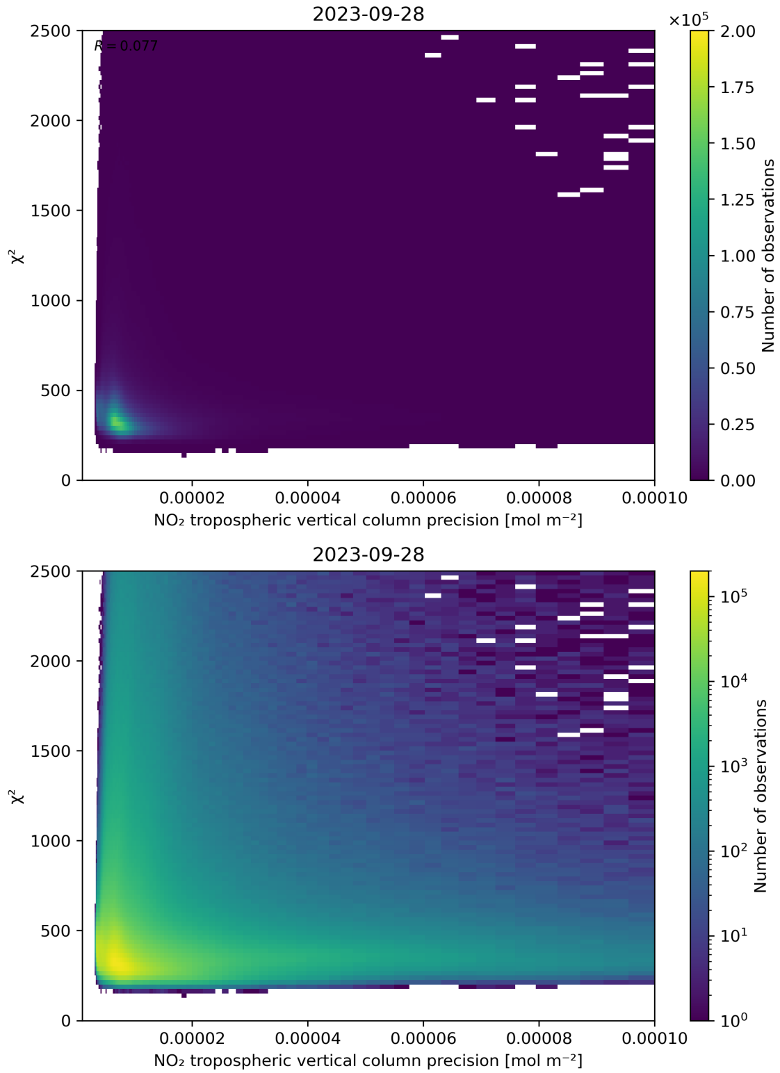
Figure 134: Scatter density plot of “NO 2 tropospheric vertical column precision” against “ \chi^2 ” for 2023-09-27 to 2023-09-29.
