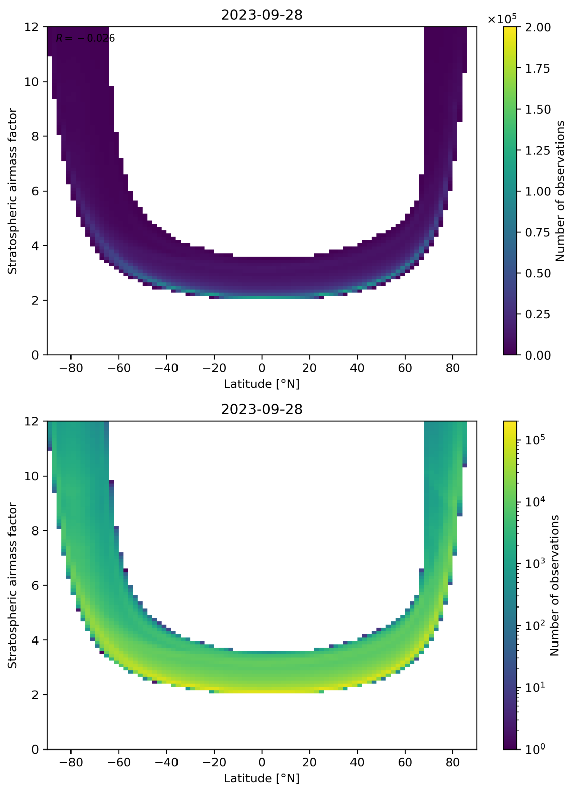
Figure 83: Scatter density plot of “Latitude” against “Stratospheric air mass factor” for 2023-09-27 to 2023-09-29.
