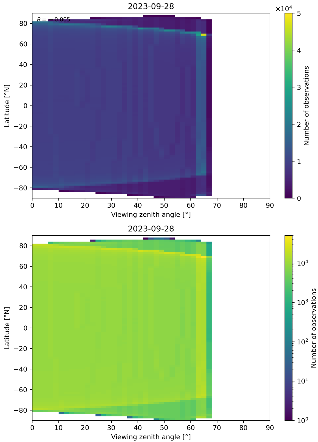
Figure 163: Scatter density plot of “Viewing zenith angle” against “Latitude” for 2023-09-27 to 2023-09-29.
