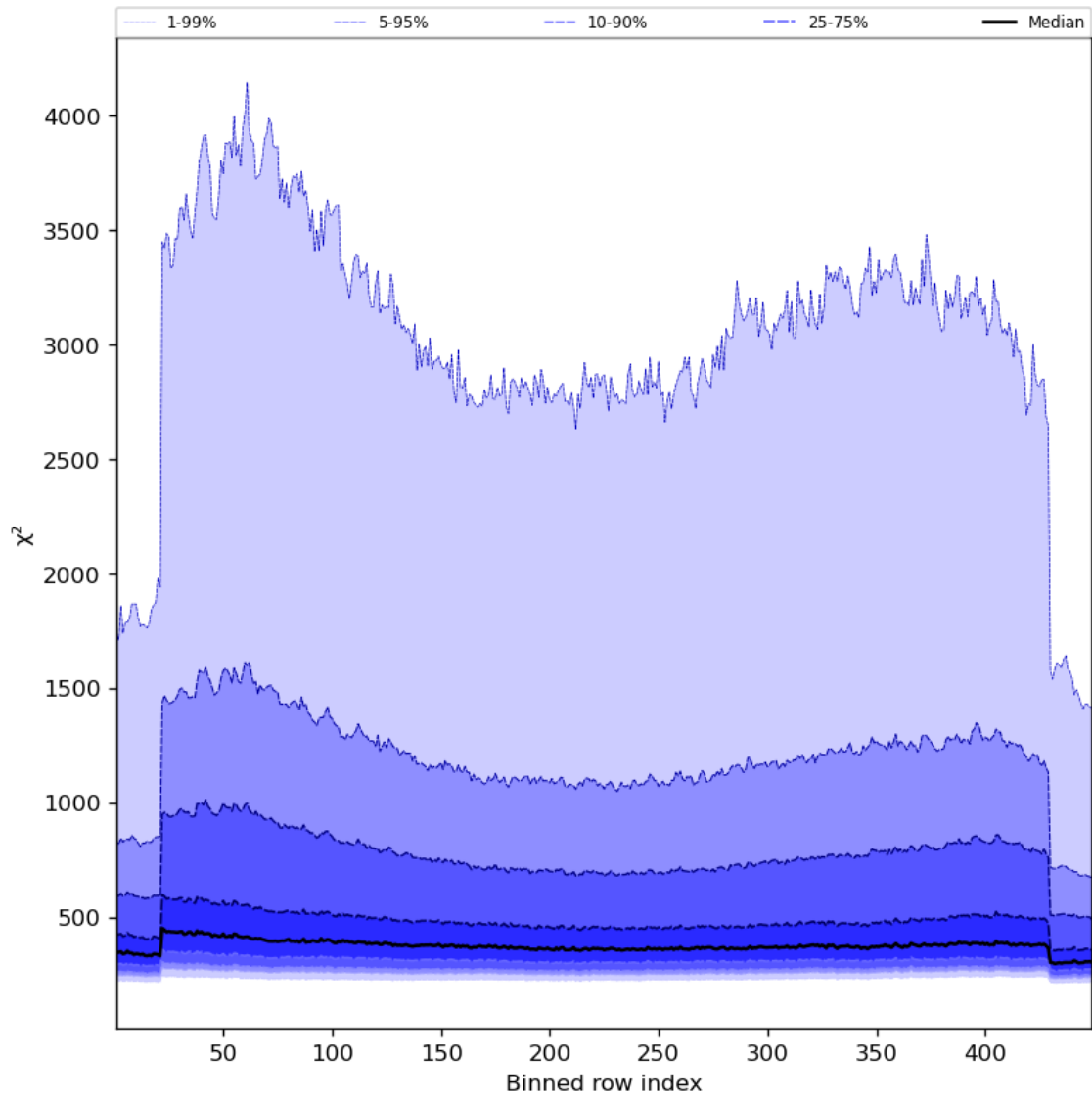
Figure 59: Along track statistics of “ \chi^2 ” for 2023-09-27 to 2023-09-29
