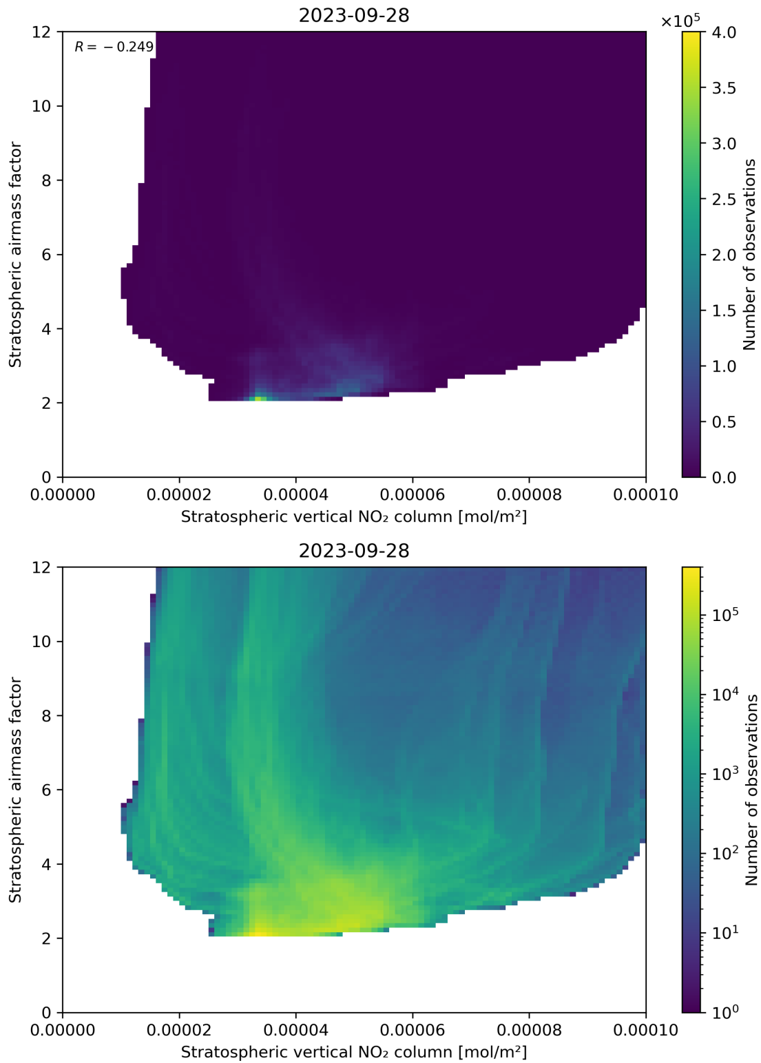
Figure 96: Scatter density plot of “Stratospheric vertical NO 2 column” against “Stratospheric airmass factor” for 2023-09-27 to 2023-09-29.
