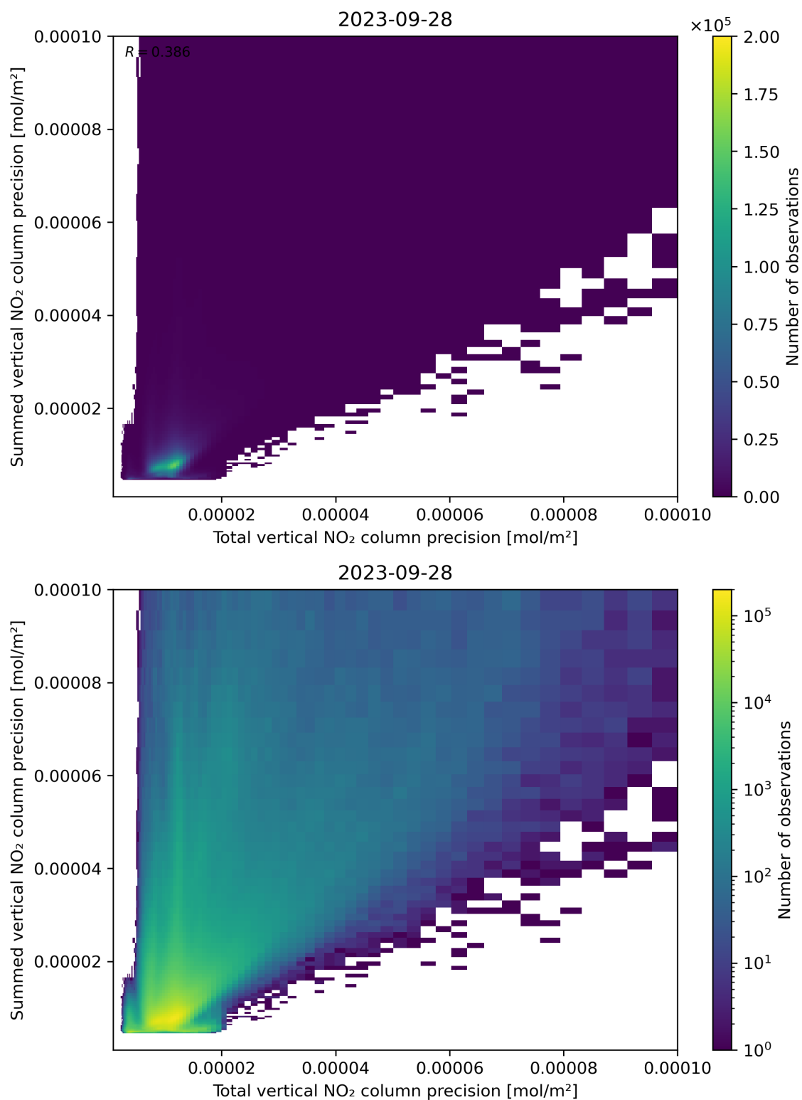
Figure 118: Scatter density plot of “Total vertical NO 2 column precision” against “Summed vertical NO 2 column precision” for 2023-09-27 to 2023-09-29.
