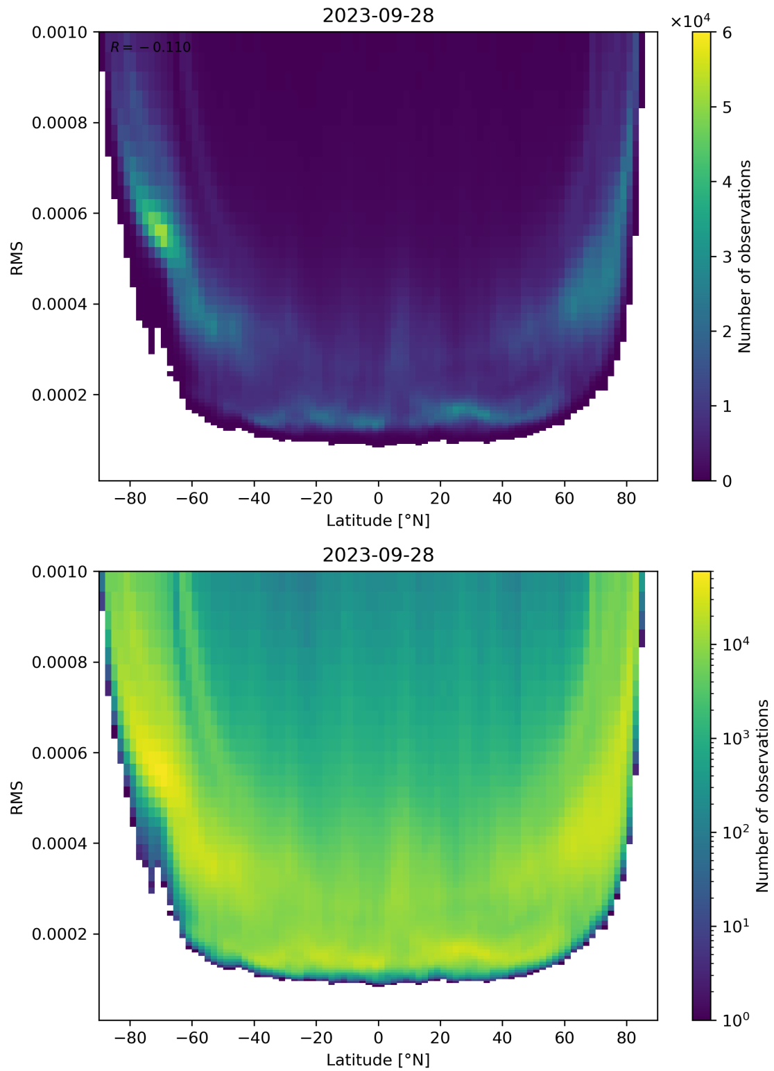
Figure 94: Scatter density plot of “Latitude” against “RMS” for 2023-09-27 to 2023-09-29.
