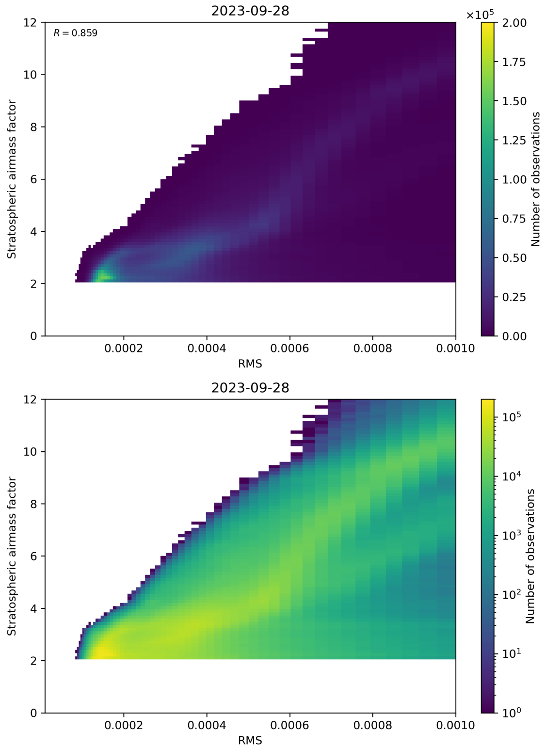
Figure 144: Scatter density plot of “RMS” against “Stratospheric airmass factor” for 2023-09-27 to 2023-09-29.
