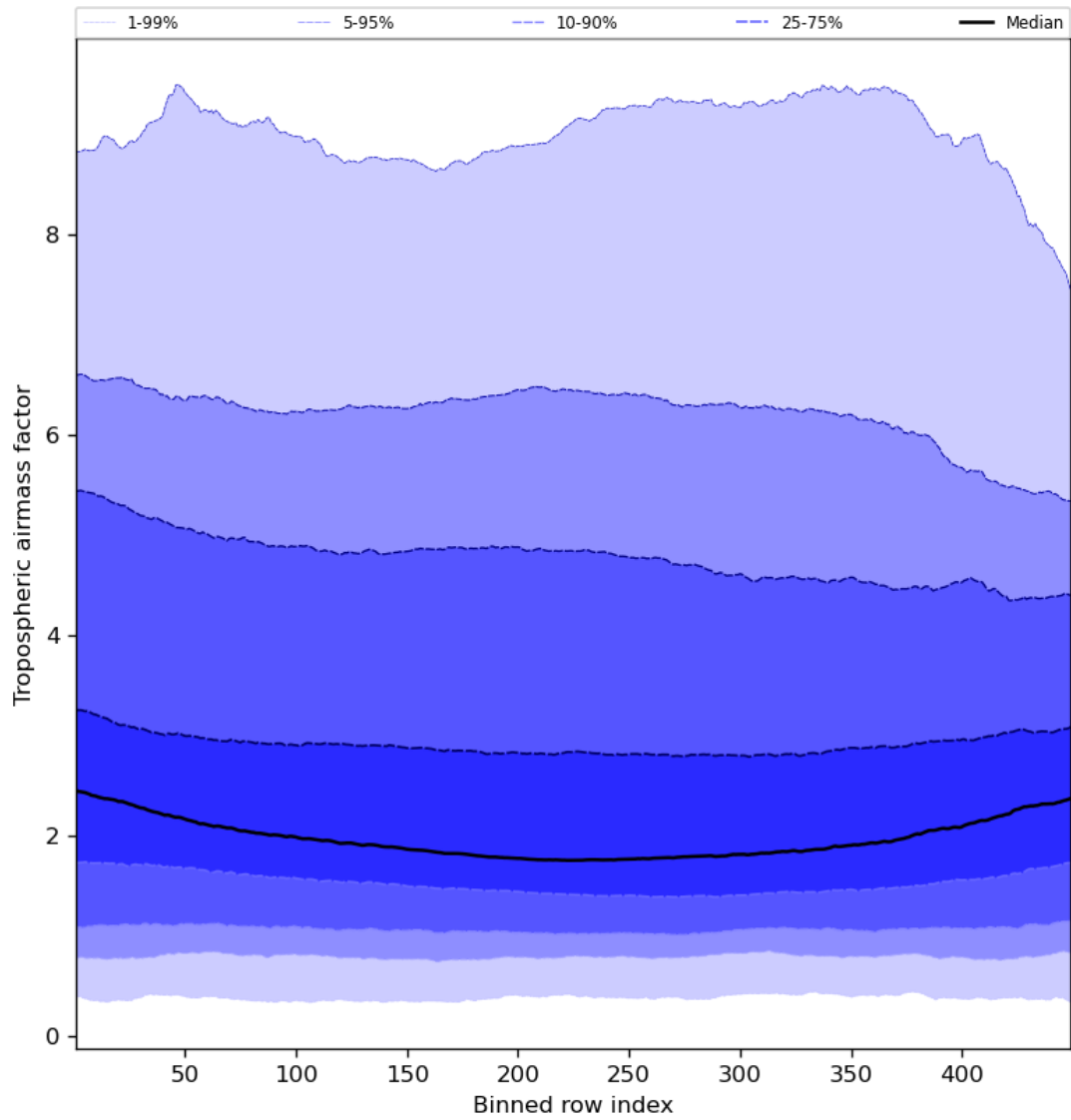
Figure 48: Along track statistics of “Tropospheric airmass factor” for 2023-09-27 to 2023-09-29
