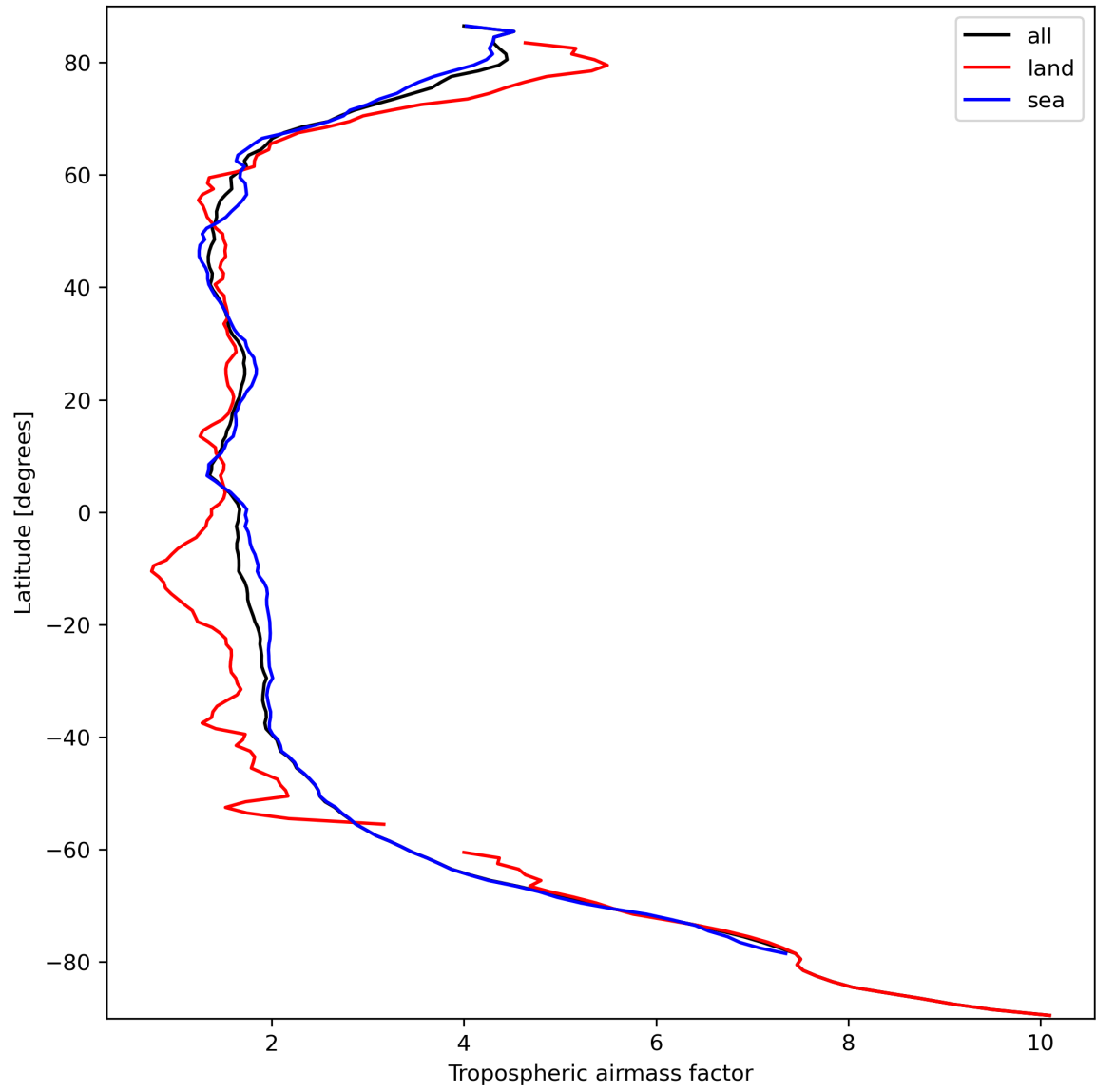
Figure 14: Zonal average of “Tropospheric airmass factor” for 2023-09-27 to 2023-09-29.
