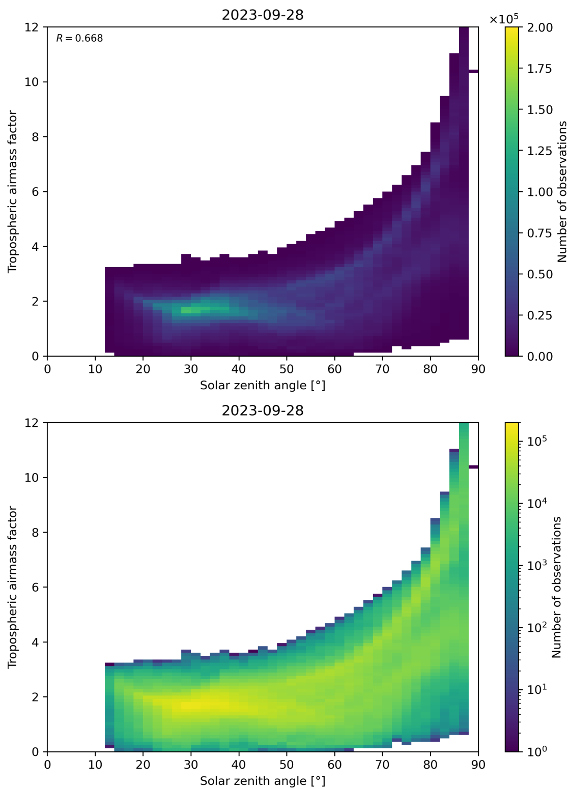
Figure 147: Scatter density plot of “Solar zenith angle” against “Tropospheric airmass factor” for 2023-09-27 to 2023-09-29.
