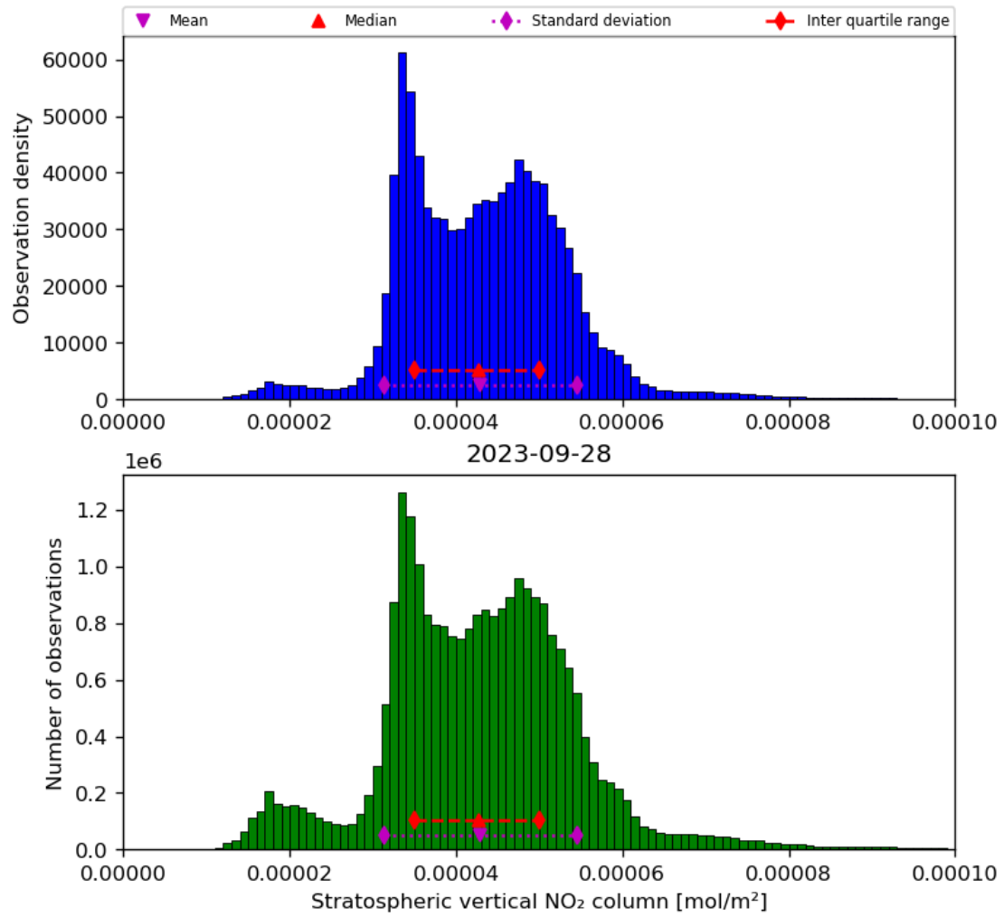
Figure 36: Histogram of “Stratospheric vertical NO 2 column” for 2023-09-27 to 2023-09-29
