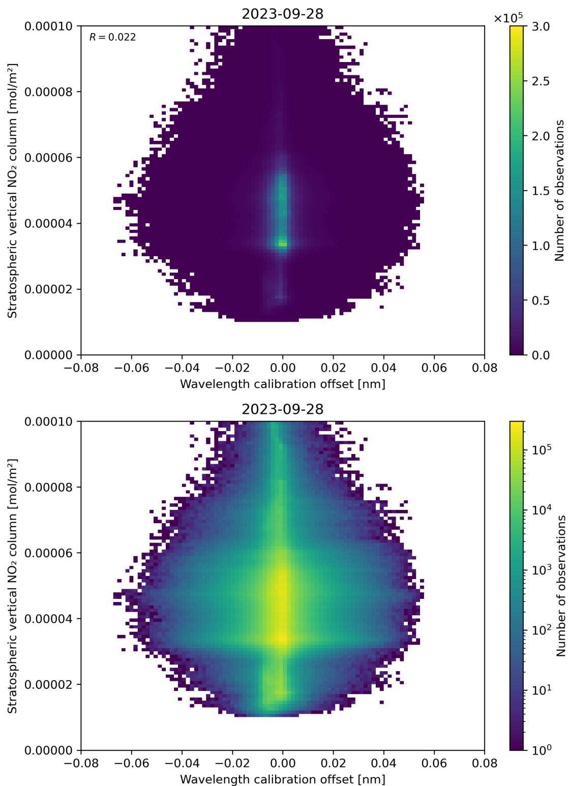
Figure 176: Scatter density plot of “Wavelength calibration offset” against “Stratospheric vertical NO 2 column” for 2023-09-27 to 2023-09-29.
