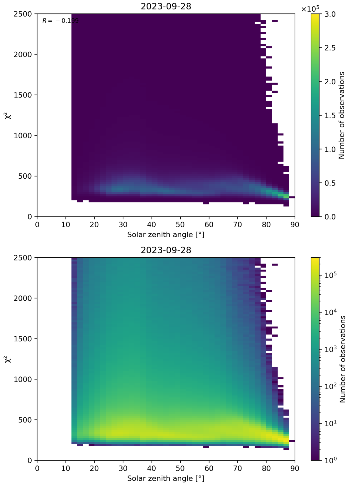
Figure 148: Scatter density plot of “Solar zenith angle” against “ \chi^2 ” for 2023-09-27 to 2023-09-29.
