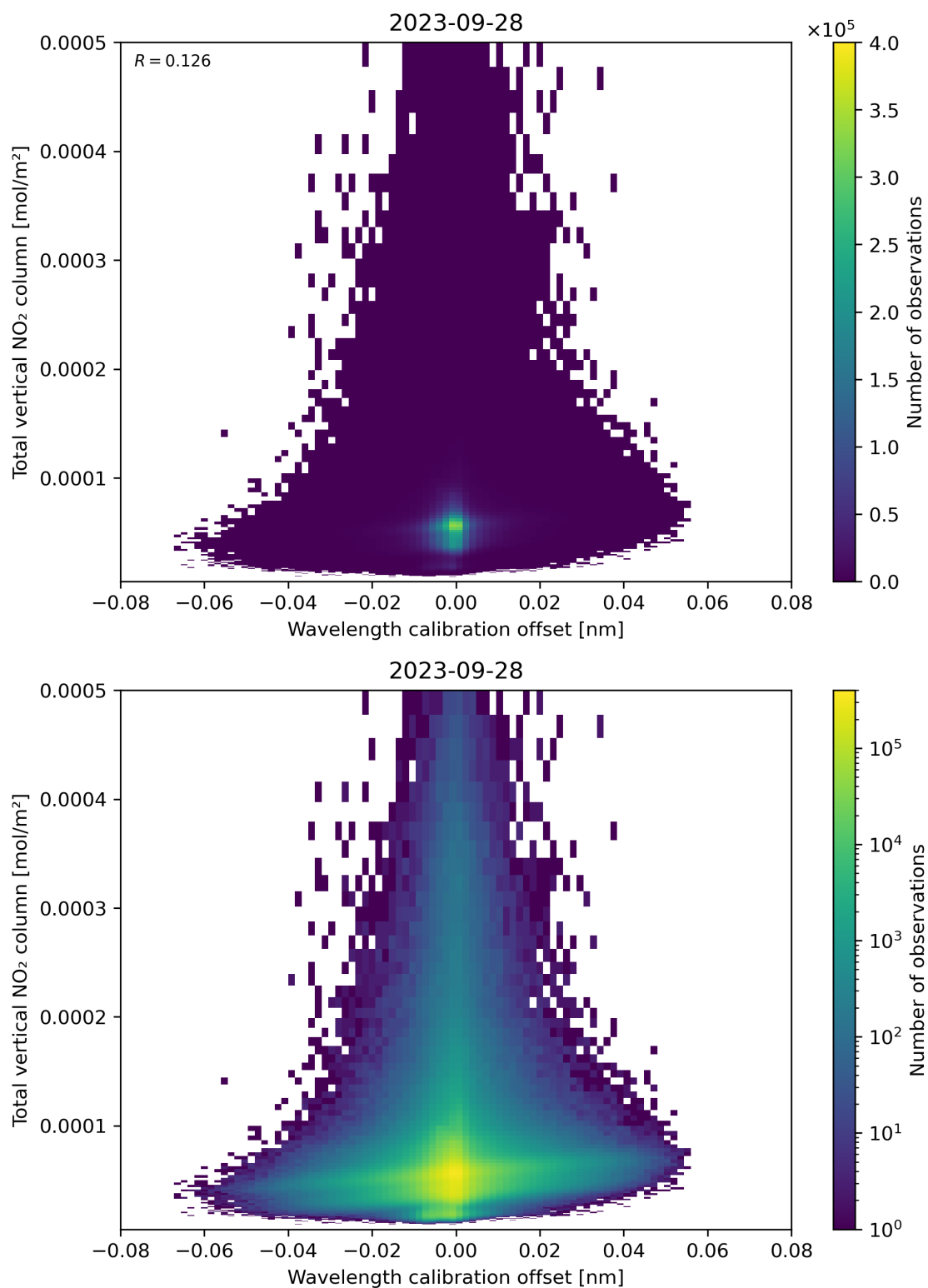
Figure 179: Scatter density plot of “Wavelength calibration offset” against “Total vertical NO 2 column” for 2023-09-27 to 2023-09-29.
