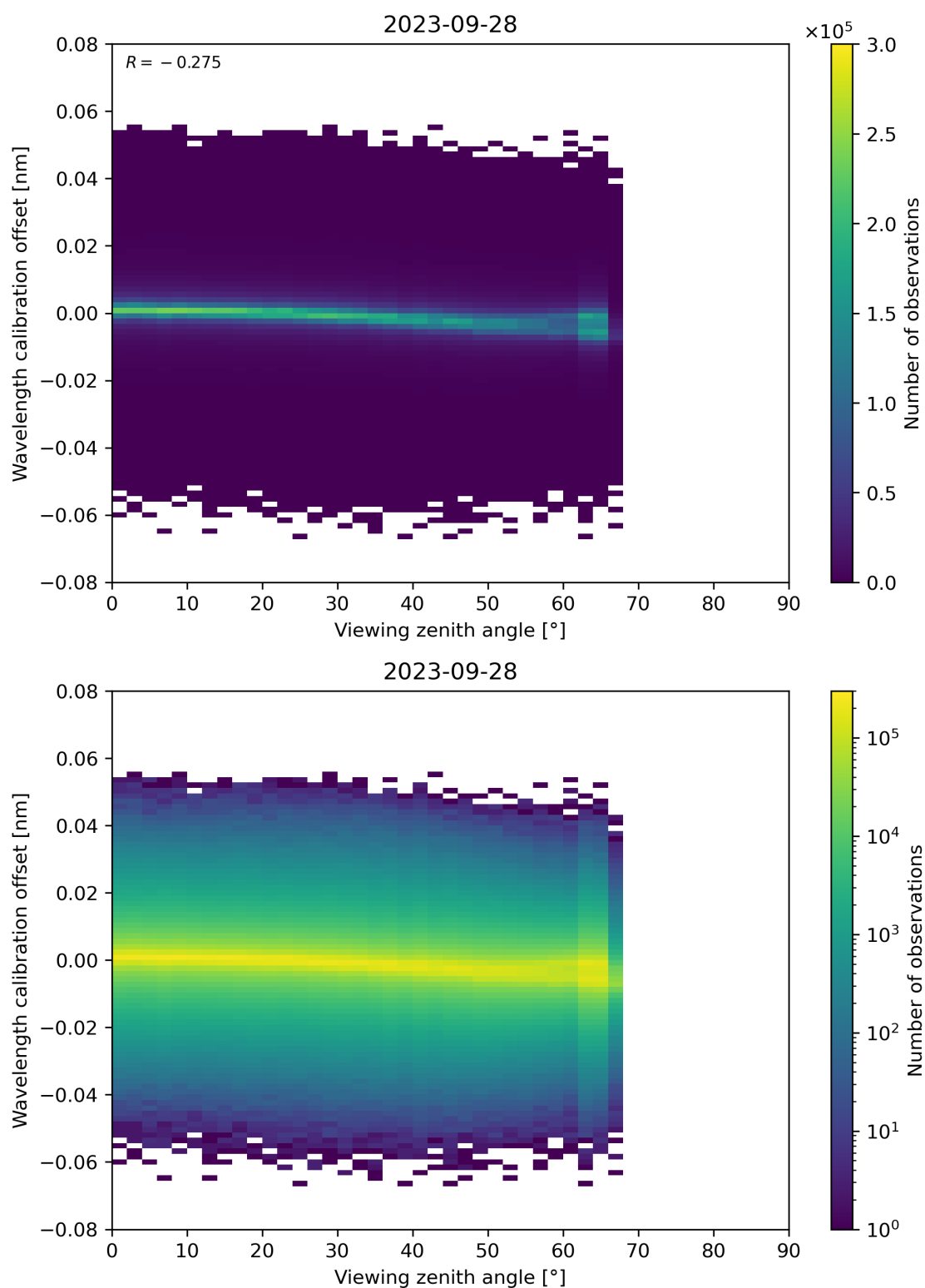
Figure 173: Scatter density plot of “Viewing zenith angle” against “Wavelength calibration offset” for 2023-09-27 to 2023-09-29.
