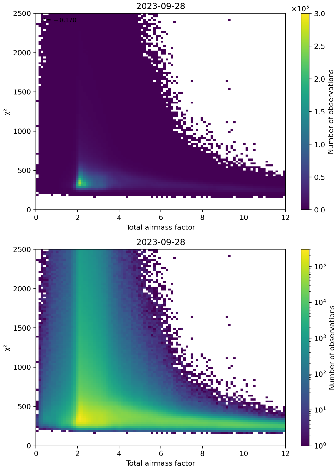
Figure 63: Scatter density plot of “Total airmass factor” against “ \chi^2 ” for 2023-09-27 to 2023-09-29.
