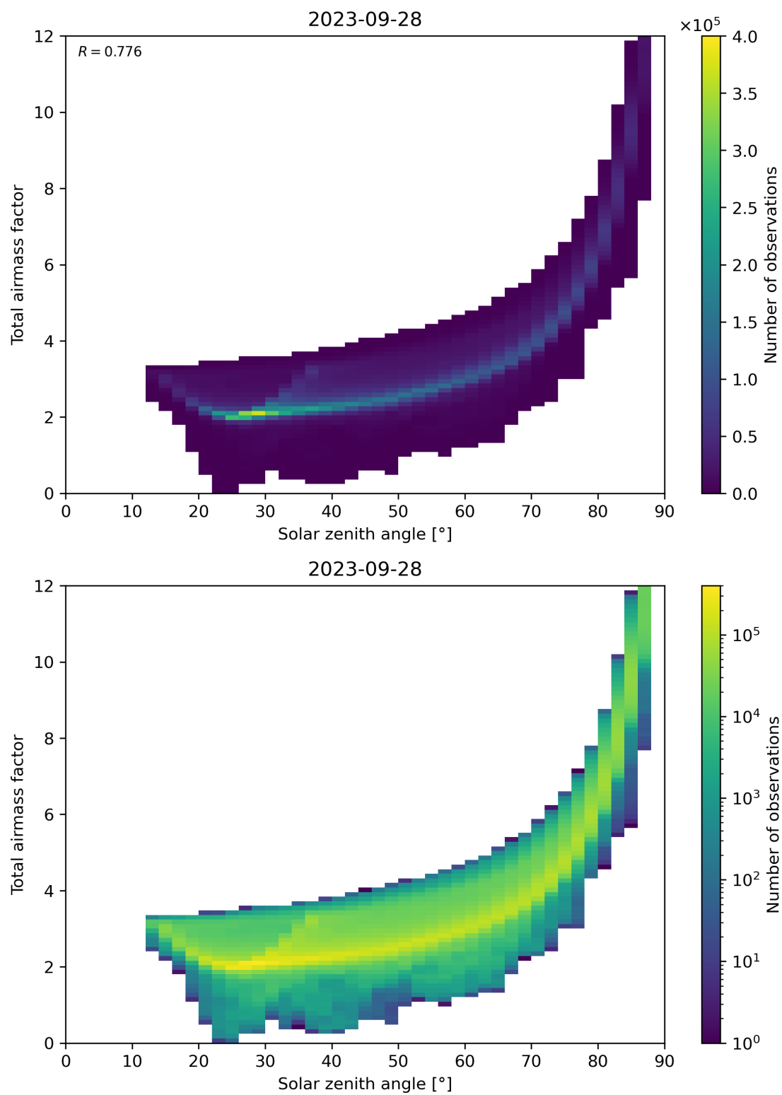
Figure 146: Scatter density plot of “Solar zenith angle” against “Total airmass factor” for 2023-09-27 to 2023-09-29.
