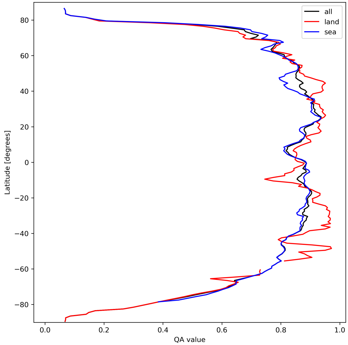
Figure 11: Zonal average of “QA value” for 2023-09-27 to 2023-09-29.
