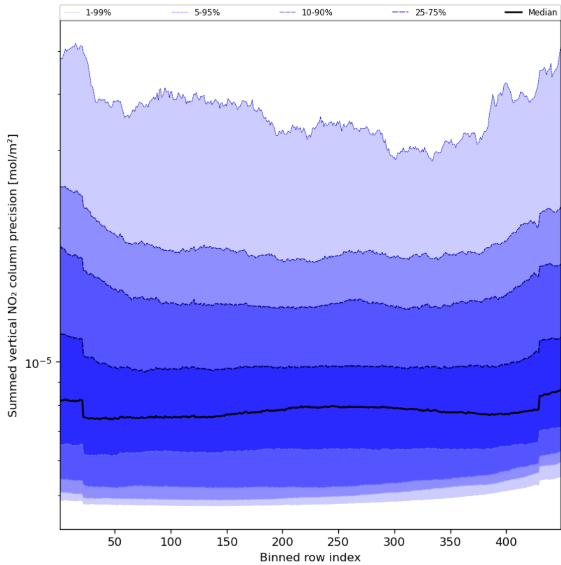
Figure 58: Along track statistics of “Summed vertical NO 2 column precision” for 2023-09-27 to 2023-09-29
