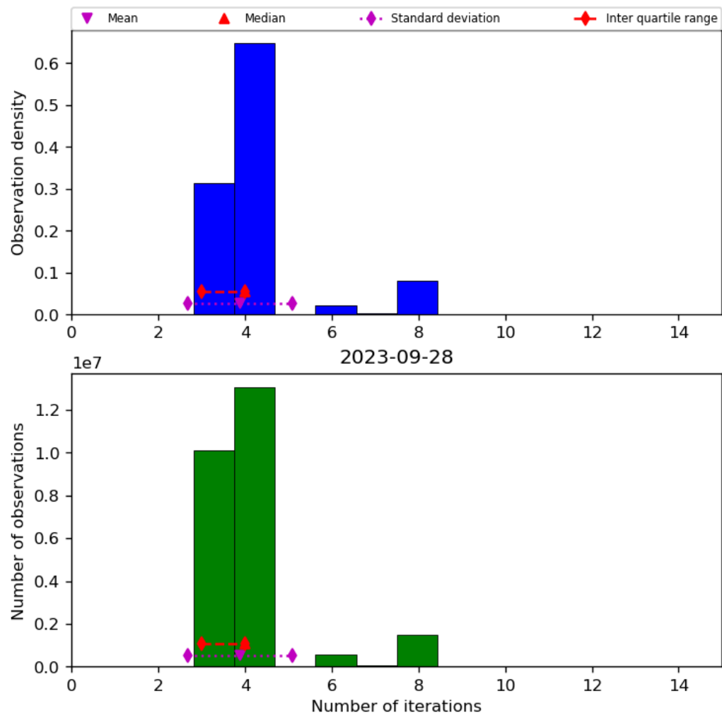
Figure 34: Histogram of “Number of iterations” for 2023-09-27 to 2023-09-29
