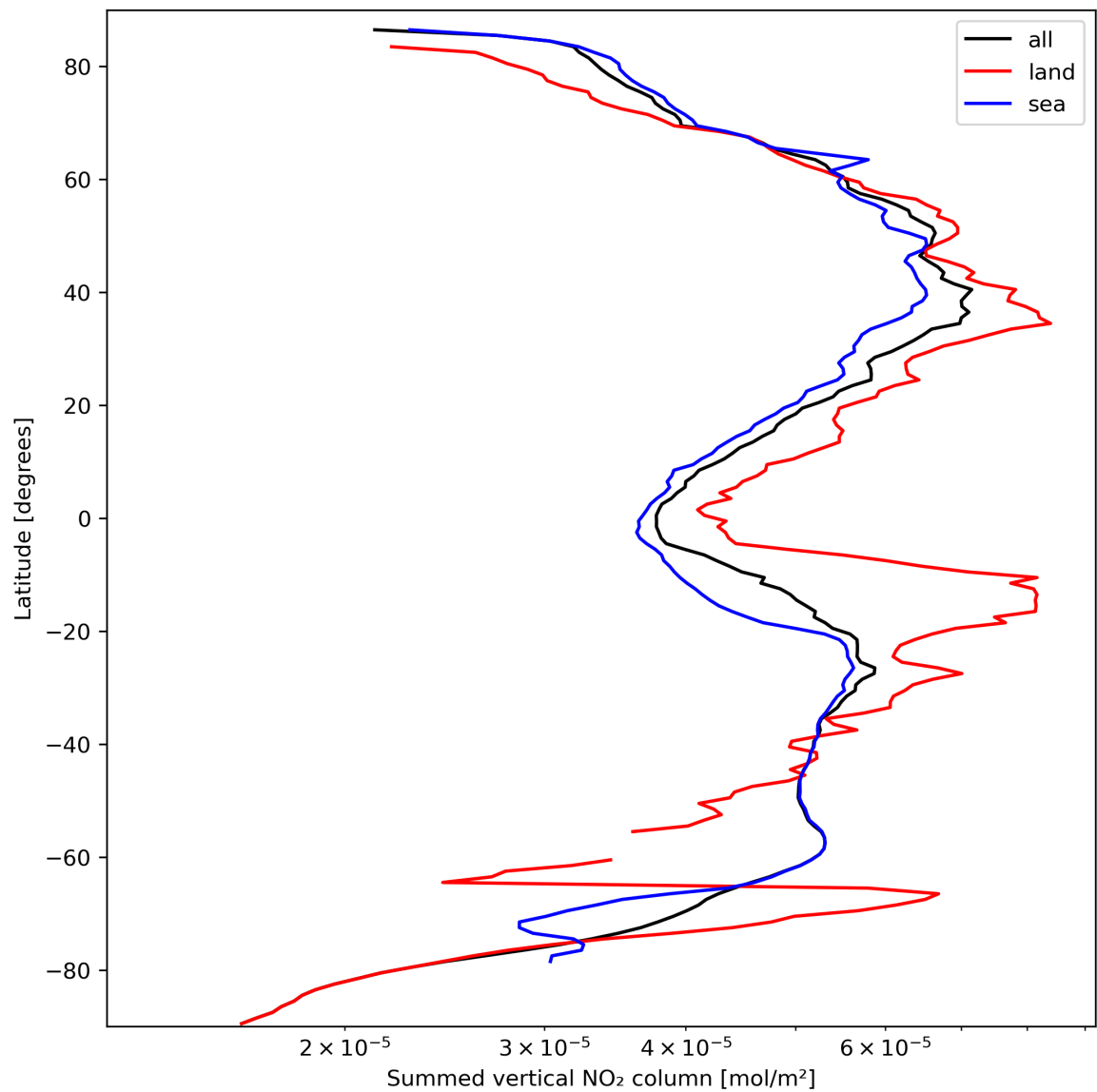
Figure 23: Zonal average of “Summed vertical NO 2 column” for 2023-09-27 to 2023-09-29.
