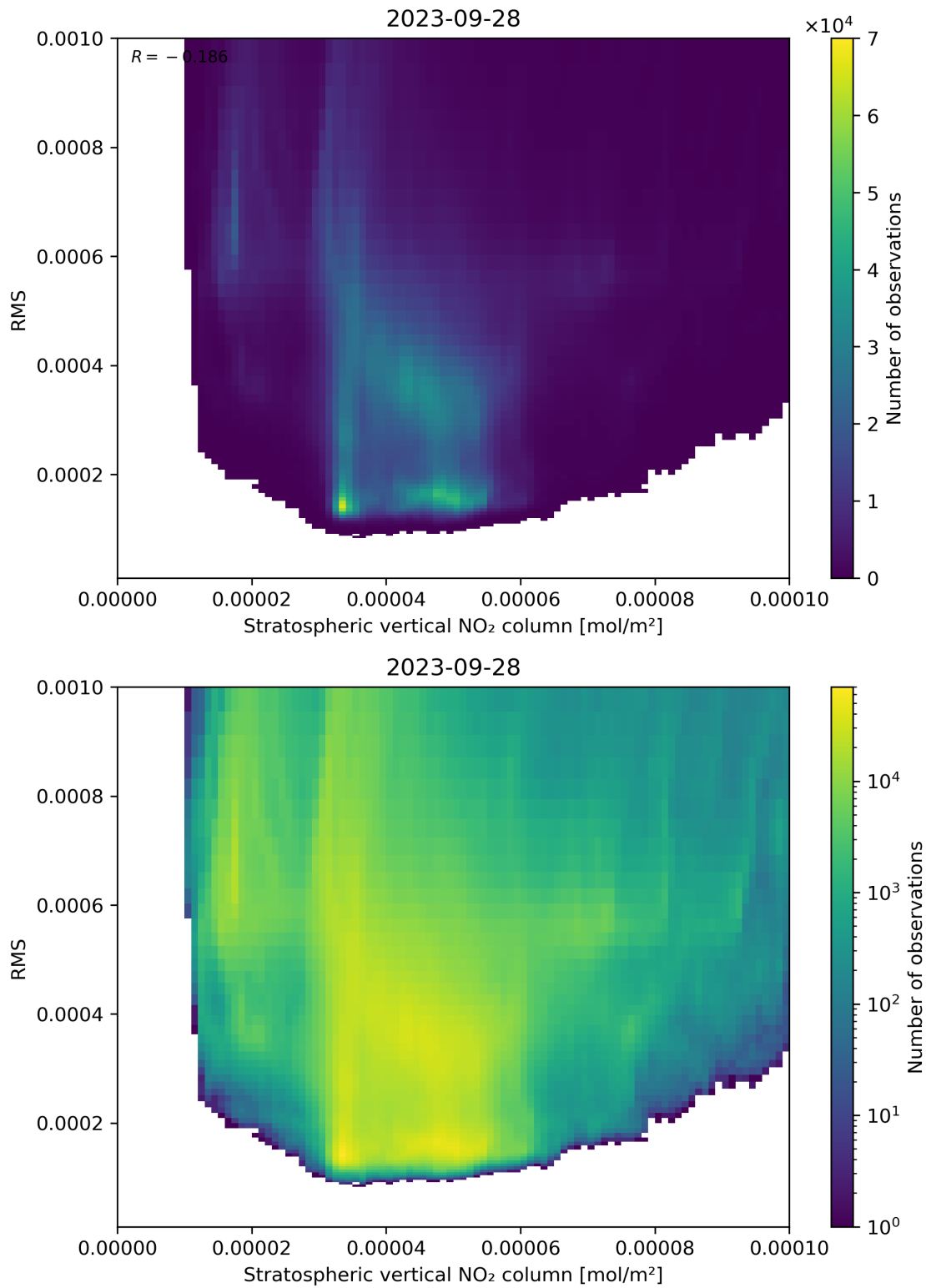
Figure 102: Scatter density plot of “Stratospheric vertical NO 2 column” against “RMS” for 2023-09-27 to 2023-09-29.
