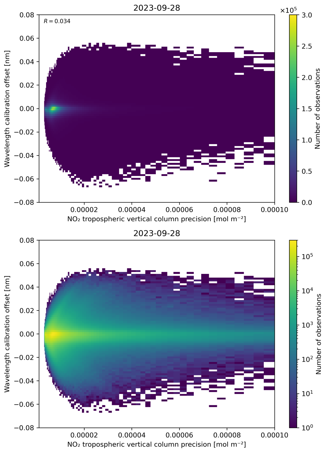
Figure 141: Scatter density plot of “NO 2 tropospheric vertical column precision” against “Wavelength calibration offset” for 2023-09-27 to 2023-09-29.
