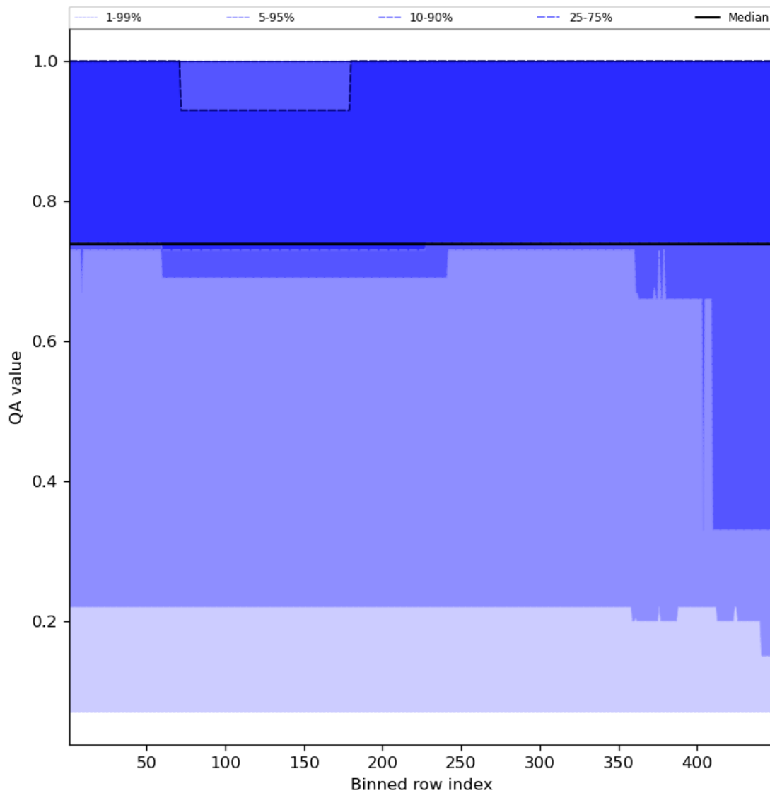
Figure 45: Along track statistics of “QA value” for 2023-09-27 to 2023-09-29
