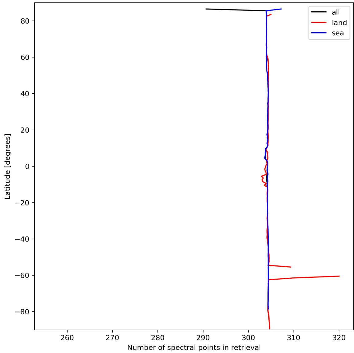
Figure 16: Zonal average of “Number of spectral points in retrieval” for 2023-09-27 to 2023-09-29.
