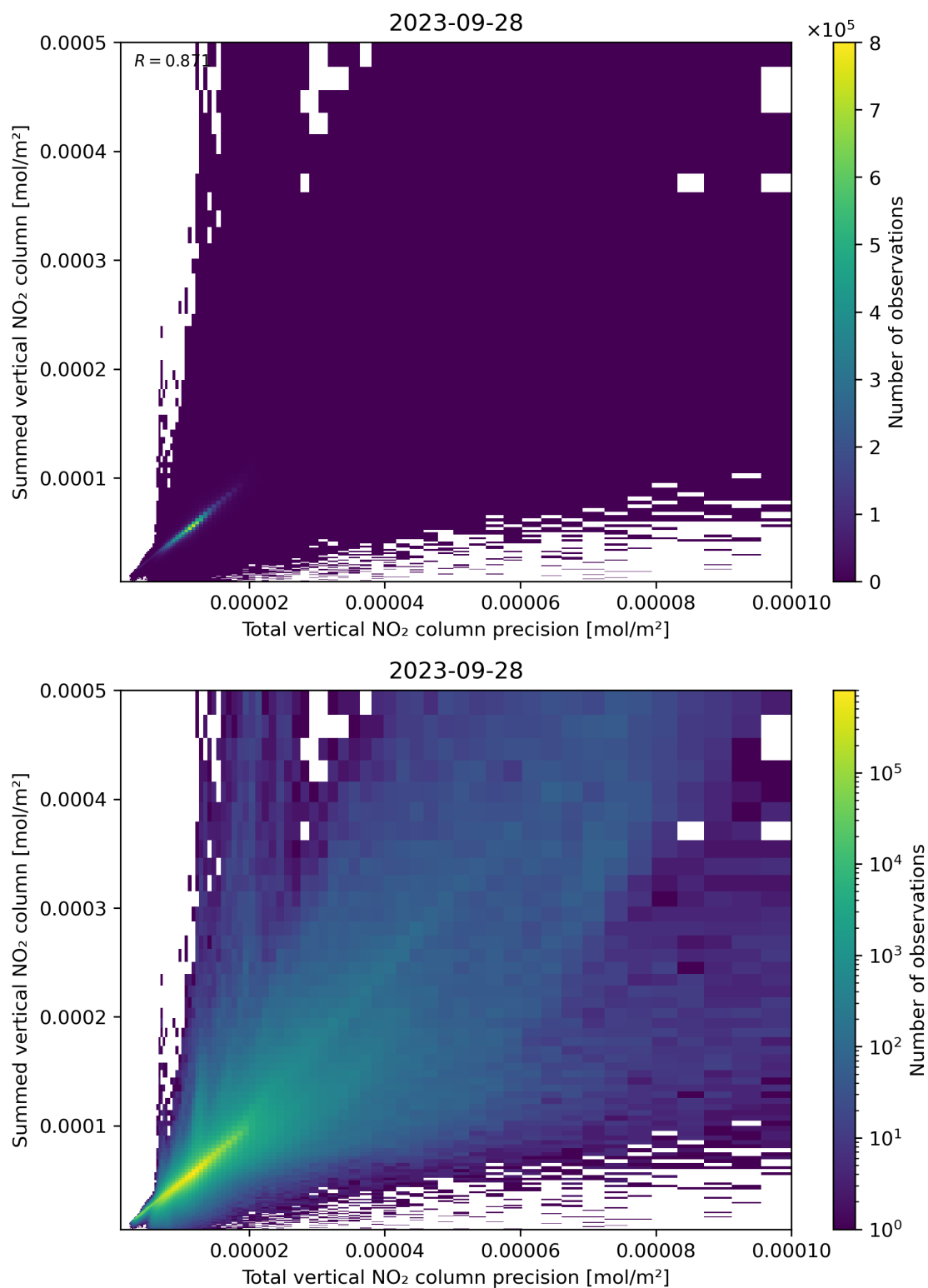
Figure 117: Scatter density plot of “Total vertical NO 2 column precision” against “Summed vertical NO 2 column” for 2023-09-27 to 2023-09-29.
