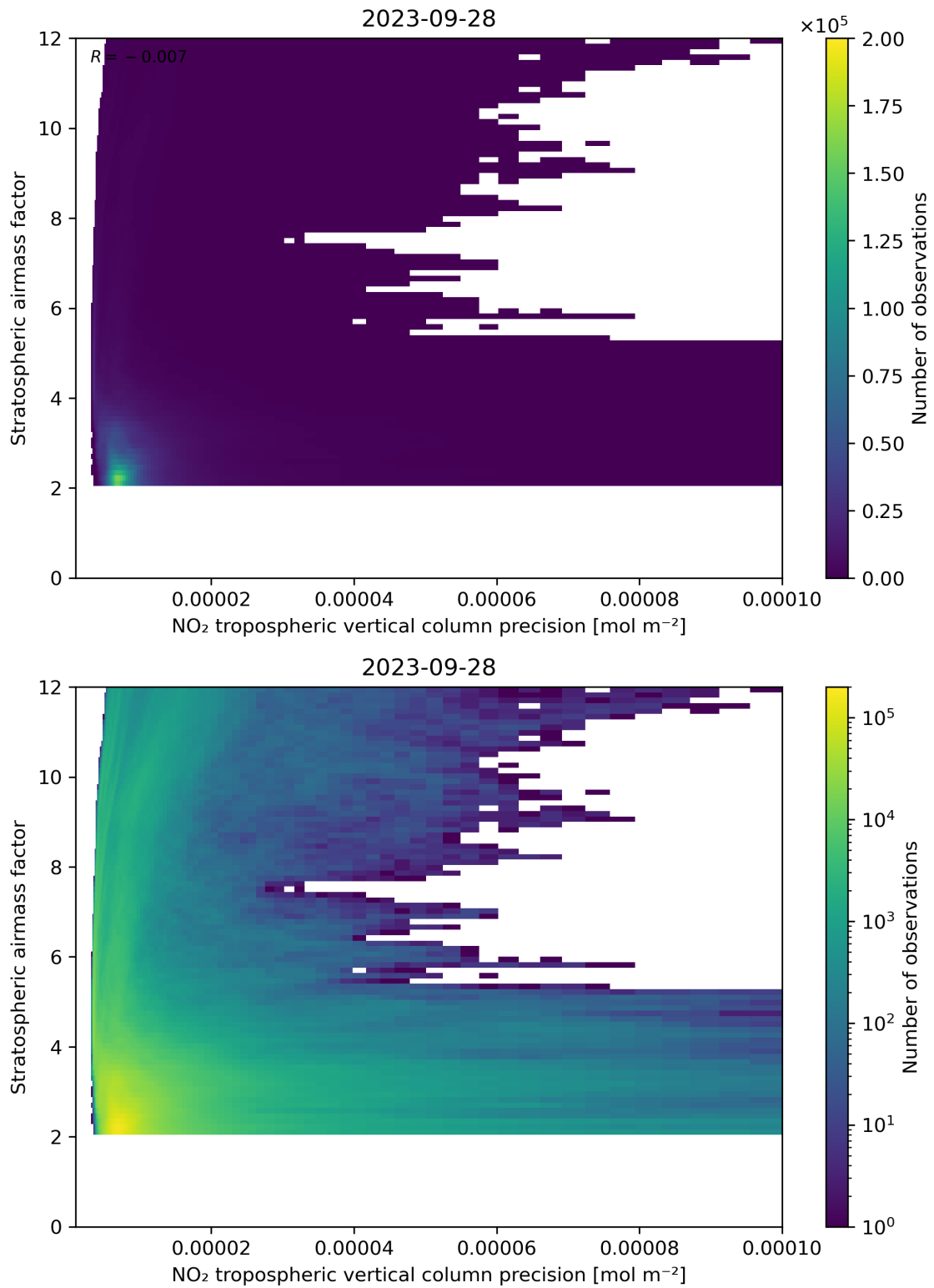
Figure 131: Scatter density plot of “NO 2 tropospheric vertical column precision” against “Stratospheric airmass factor” for 2023-09-27 to 2023-09-29.
