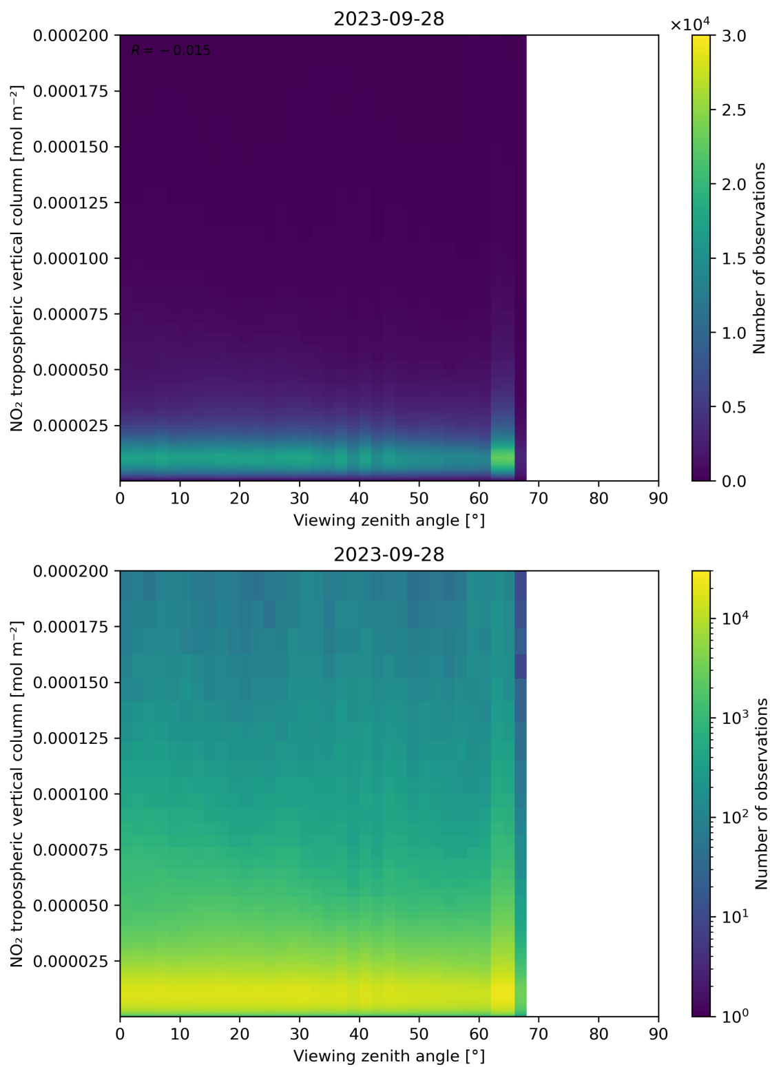
Figure 169: Scatter density plot of “Viewing zenith angle” against “NO 2 tropospheric vertical column” for 2023-09-27 to 2023-09-29.
