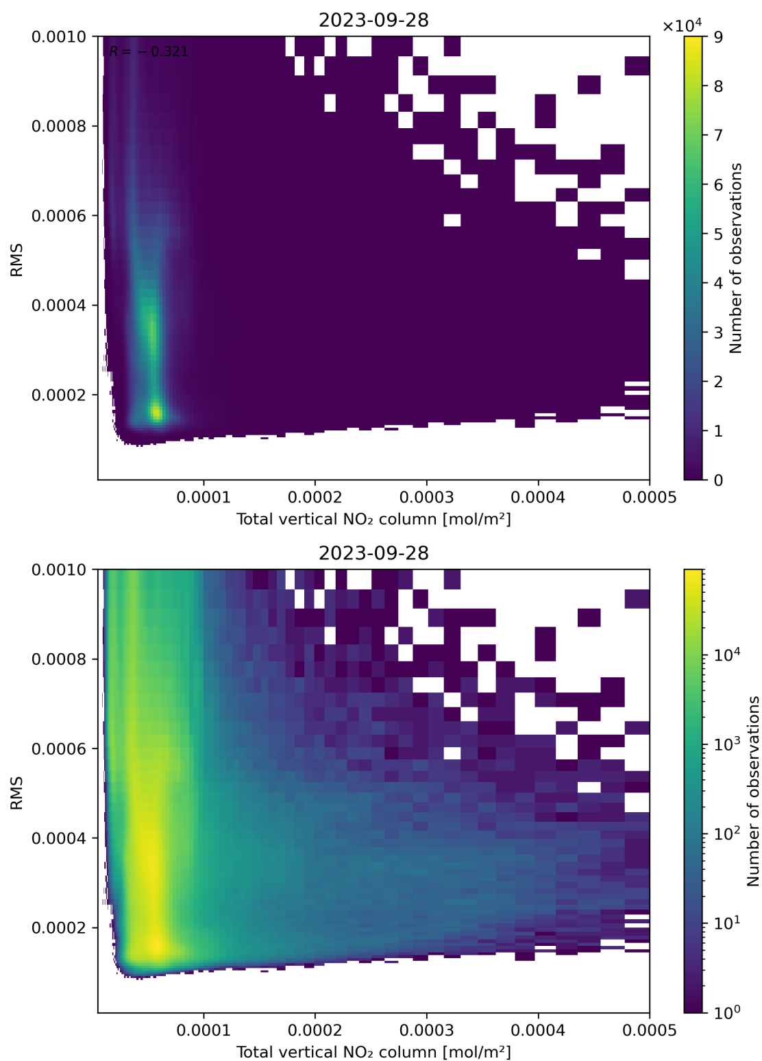
Figure 120: Scatter density plot of “Total vertical NO 2 column” against “RMS” for 2023-09-27 to 2023-09-29.
