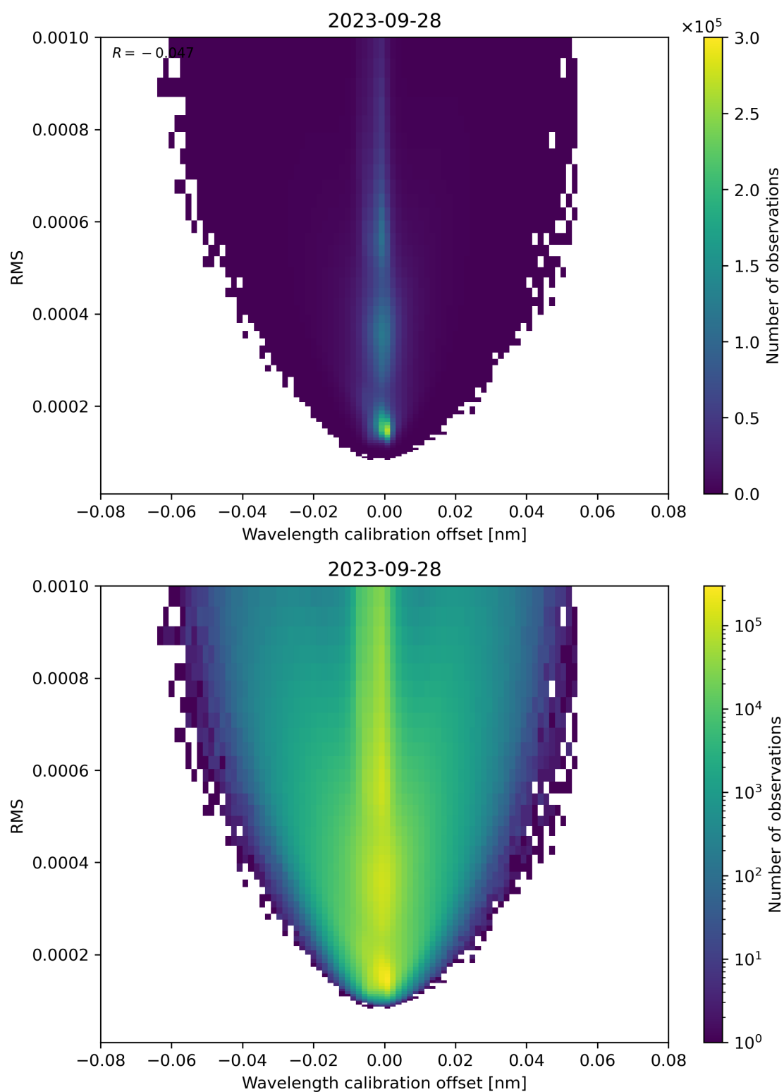
Figure 181: Scatter density plot of “Wavelength calibration offset” against “RMS” for 2023-09-27 to 2023-09-29.
