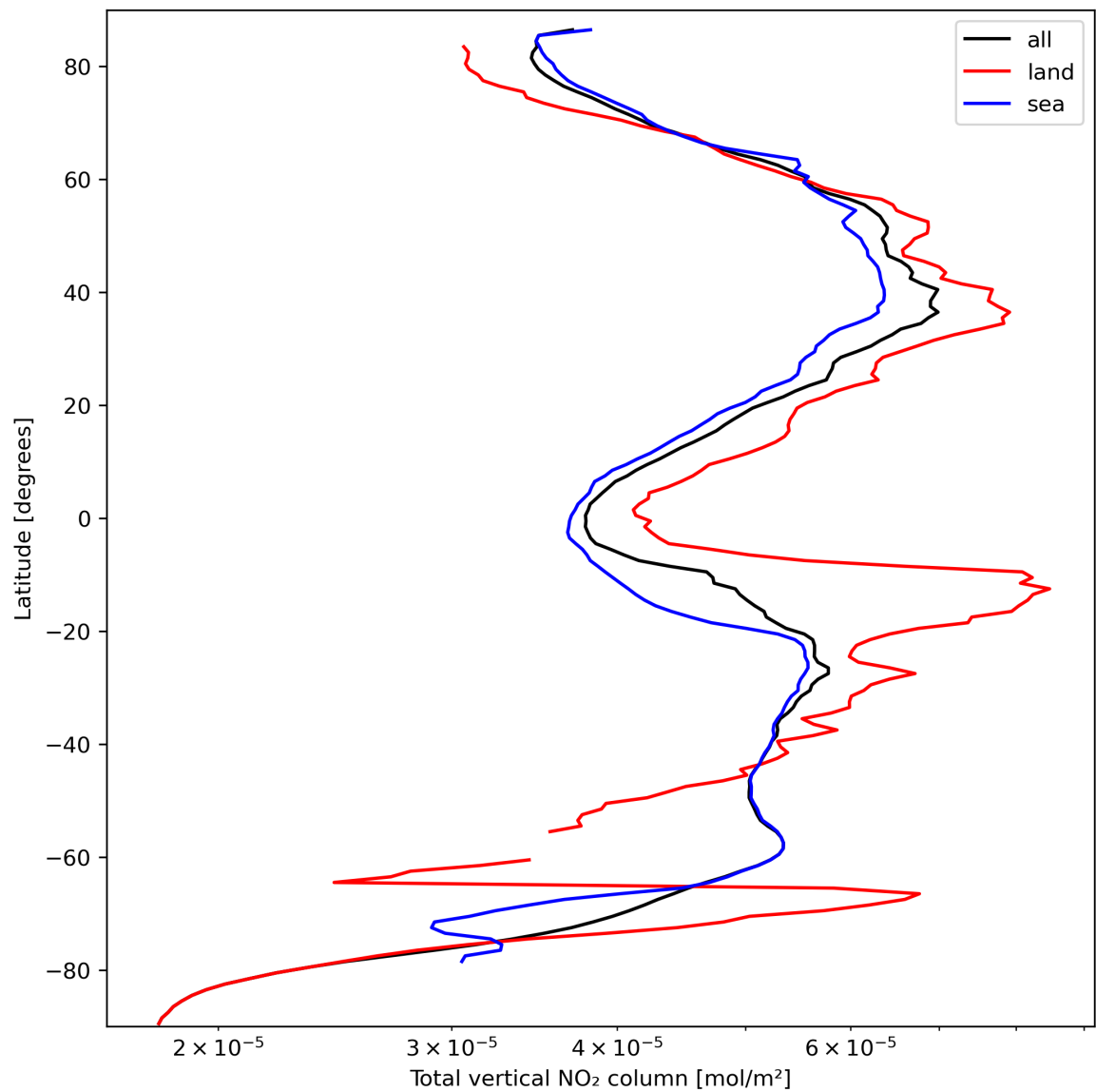
Figure 21: Zonal average of “Total vertical NO 2 column” for 2023-09-27 to 2023-09-29.
