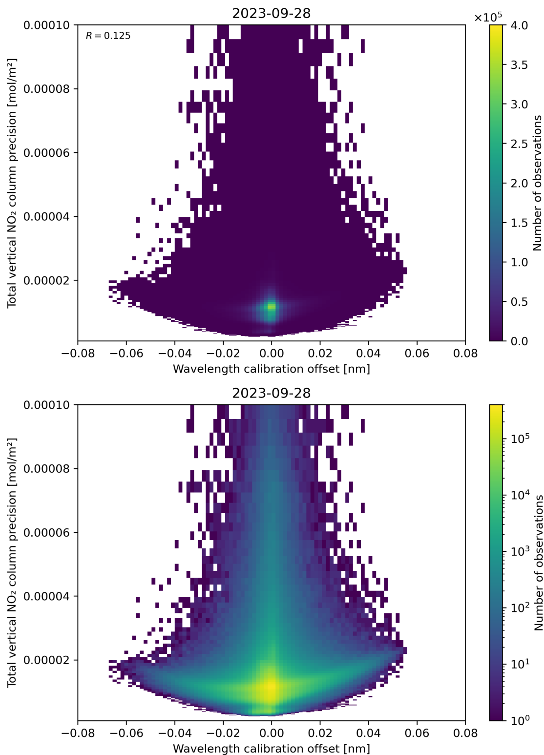
Figure 180: Scatter density plot of “Wavelength calibration offset” against “Total vertical NO 2 column precision” for 2023-09-27 to 2023-09-29.
