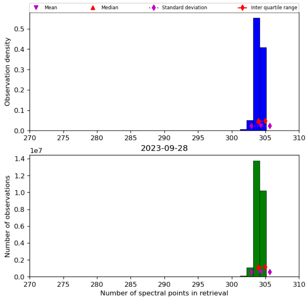
Figure 33: Histogram of “Number of spectral points in retrieval” for 2023-09-27 to 2023-09-29
