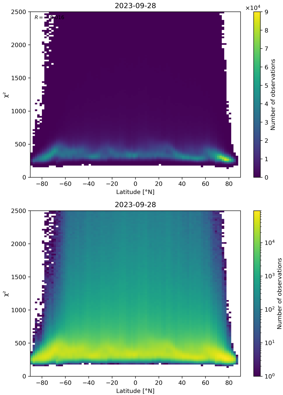
Figure 86: Scatter density plot of “Latitude” against “ \chi^2 ” for 2023-09-27 to 2023-09-29.
