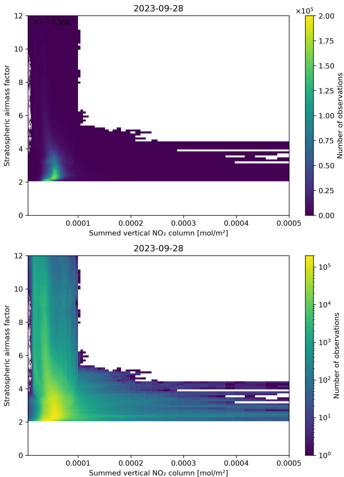
Figure 103: Scatter density plot of “Summed vertical NO 2 column” against “Stratospheric airmass factor” for 2023-09-27 to 2023-09-29.
