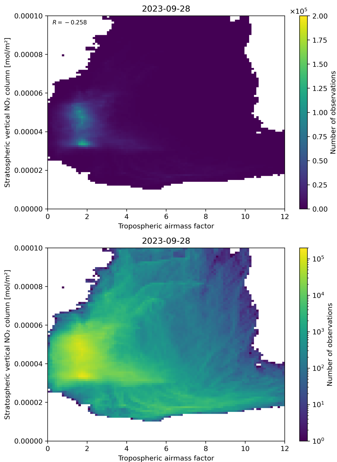
Figure 74: Scatter density plot of “Tropospheric air mass factor” against “Stratospheric vertical NO 2 column” for 2023-09-27 to 2023-09-29.
