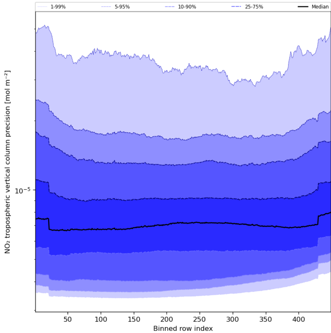
Figure 47: Along track statistics of “NO 2 tropospheric vertical column precision” for 2023-09-27 to 2023-09-29
