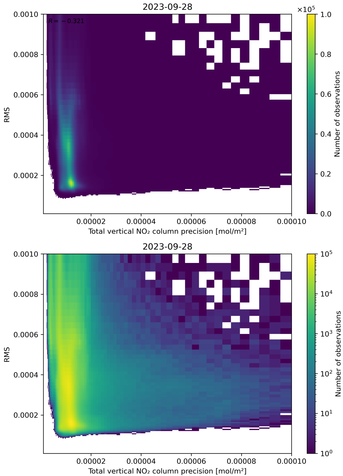
Figure 119: Scatter density plot of “Total vertical NO 2 column precision” against “RMS” for 2023-09-27 to 2023-09-29.
