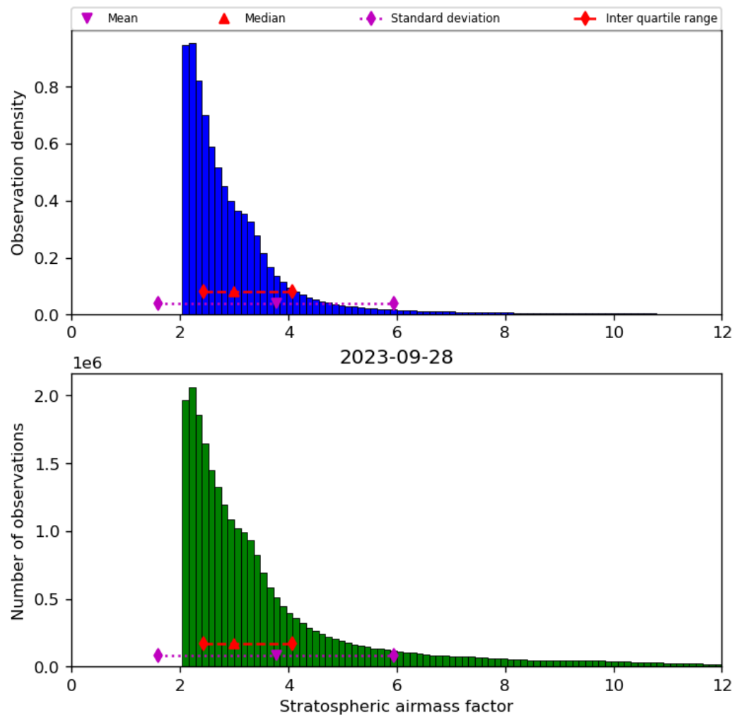
Figure 44: Histogram of “Stratospheric airmass factor” for 2023-09-27 to 2023-09-29
