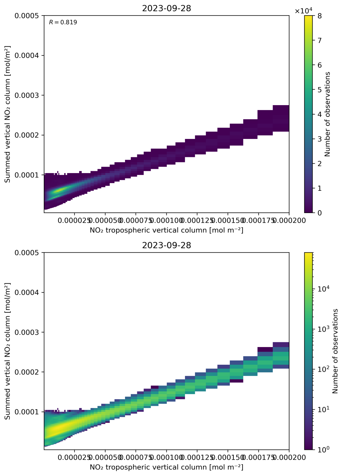
Figure 126: Scatter density plot of “NO 2 tropospheric vertical column” against “Summed vertical NO 2 column” for 2023-09-27 to 2023-09-29.
