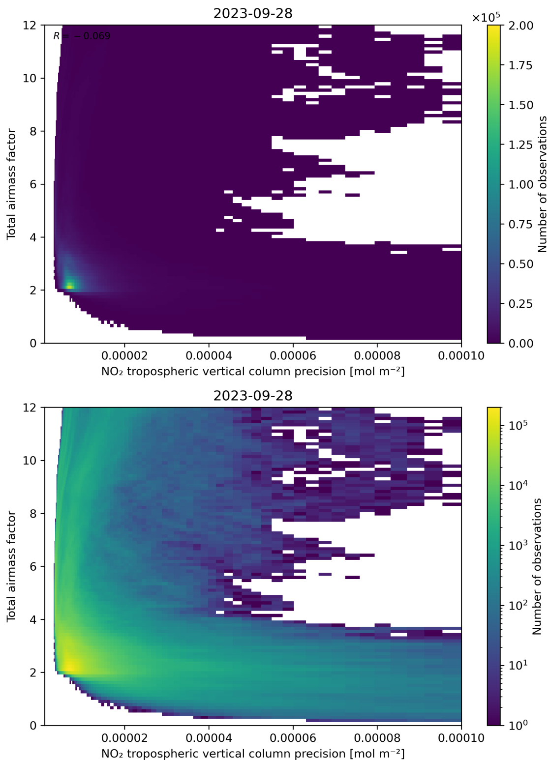
Figure 132: Scatter density plot of “NO 2 tropospheric vertical column precision” against “Total air mass factor” for 2023-09-27 to 2023-09-29.
