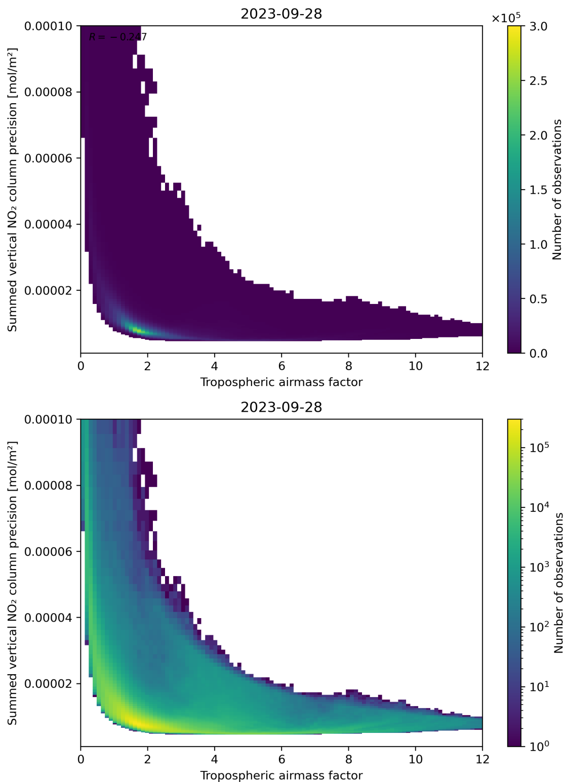
Figure 76: Scatter density plot of “Tropospheric air mass factor” against “Summed vertical NO 2 column precision” for 2023-09-27 to 2023-09-29.
