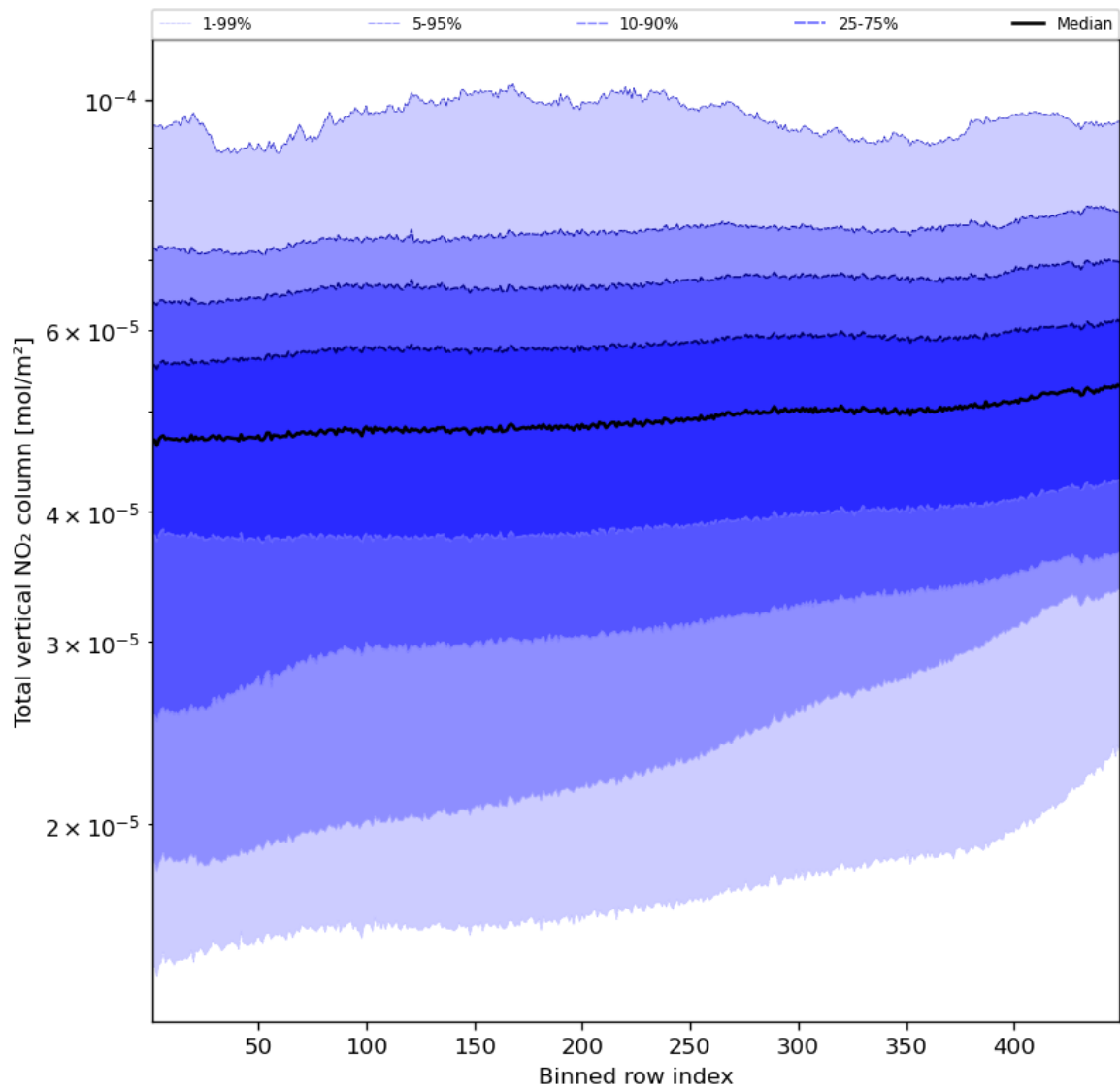
Figure 55: Along track statistics of “Total vertical NO 2 column” for 2023-09-27 to 2023-09-29
