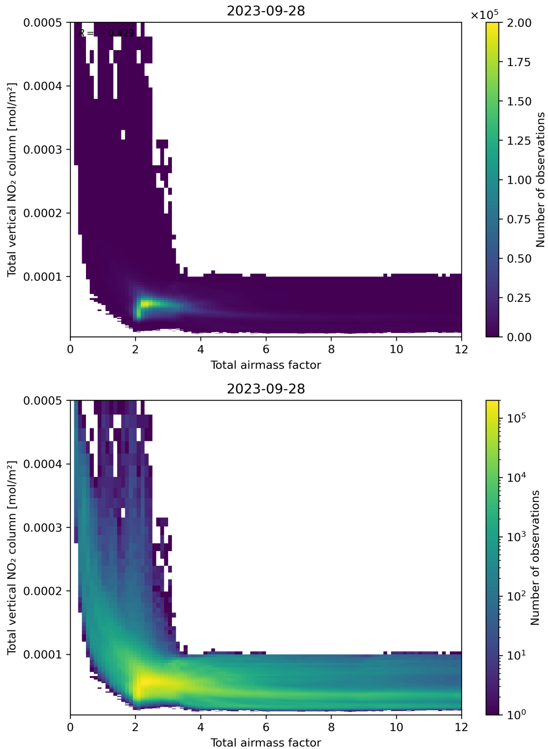
Figure 67: Scatter density plot of “Total airmass factor” against “Total vertical NO 2 column” for 2023-09-27 to 2023-09-29.
