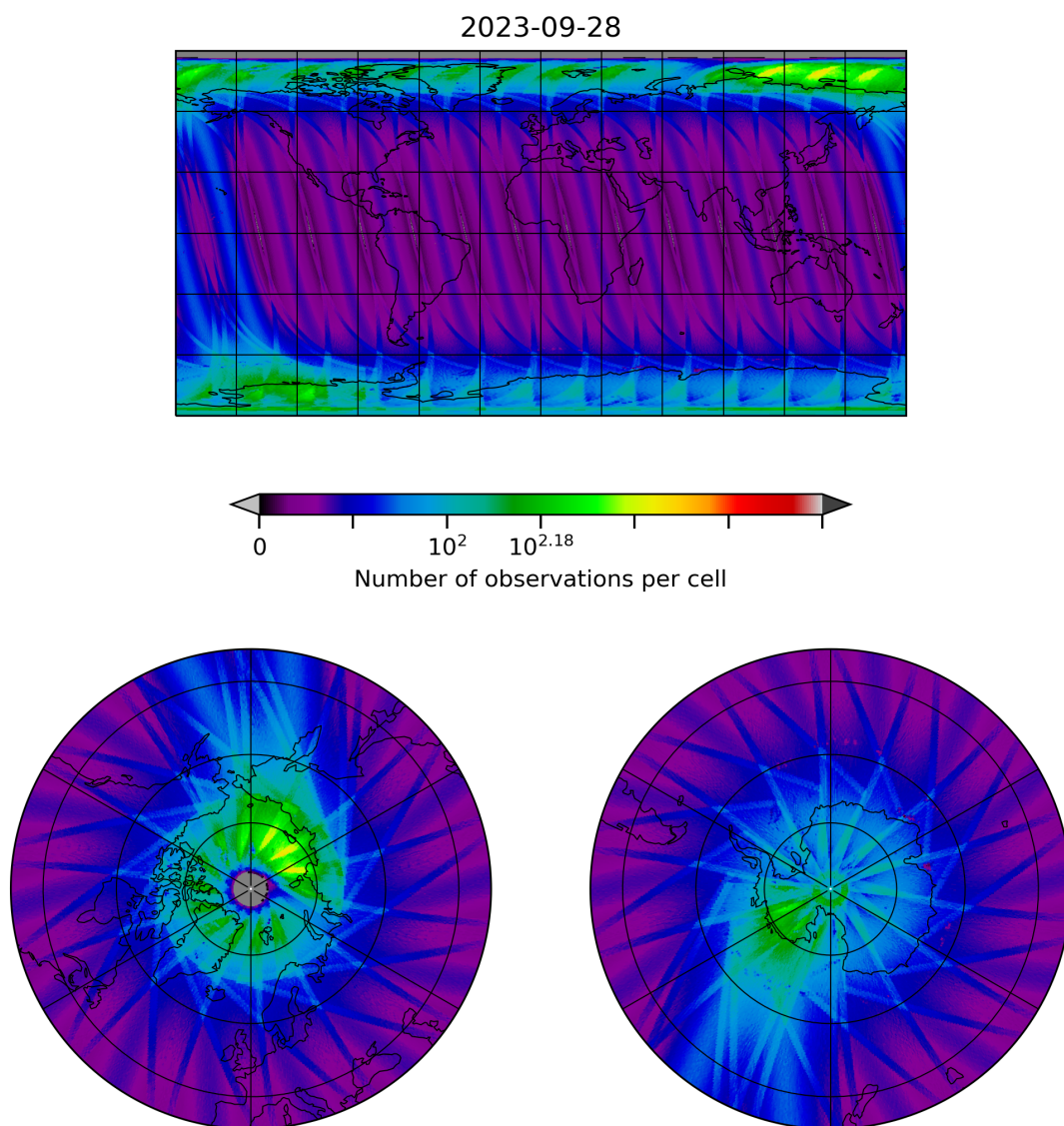
Figure 10: Map of the number of observations for 2023-09-27 to 2023-09-29
