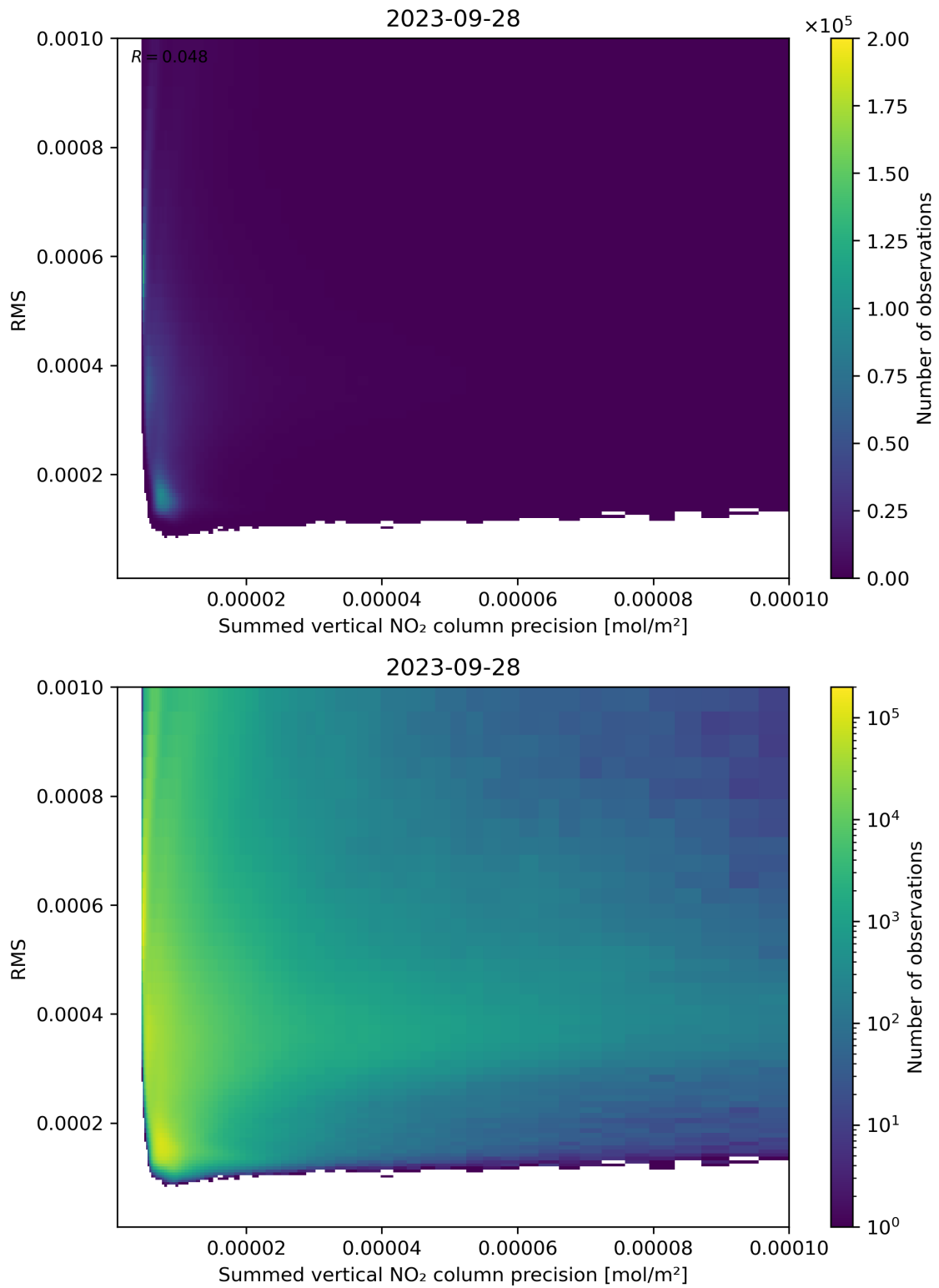
Figure 108: Scatter density plot of “Summed vertical NO 2 column precision” against “RMS” for 2023-09-27 to 2023-09-29.
