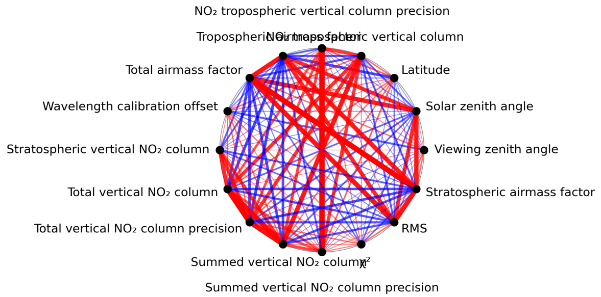
Figure 1: Map of correlation graph for 2023-09-27 to 2023-09-29.
