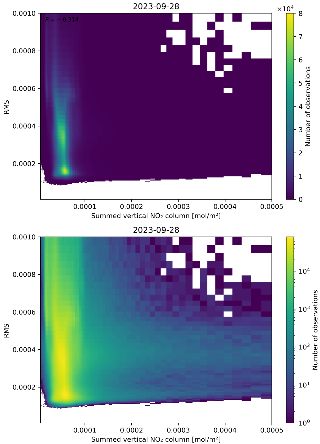
Figure 109: Scatter density plot of “Summed vertical NO 2 column” against “RMS” for 2023-09-27 to 2023-09-29.
