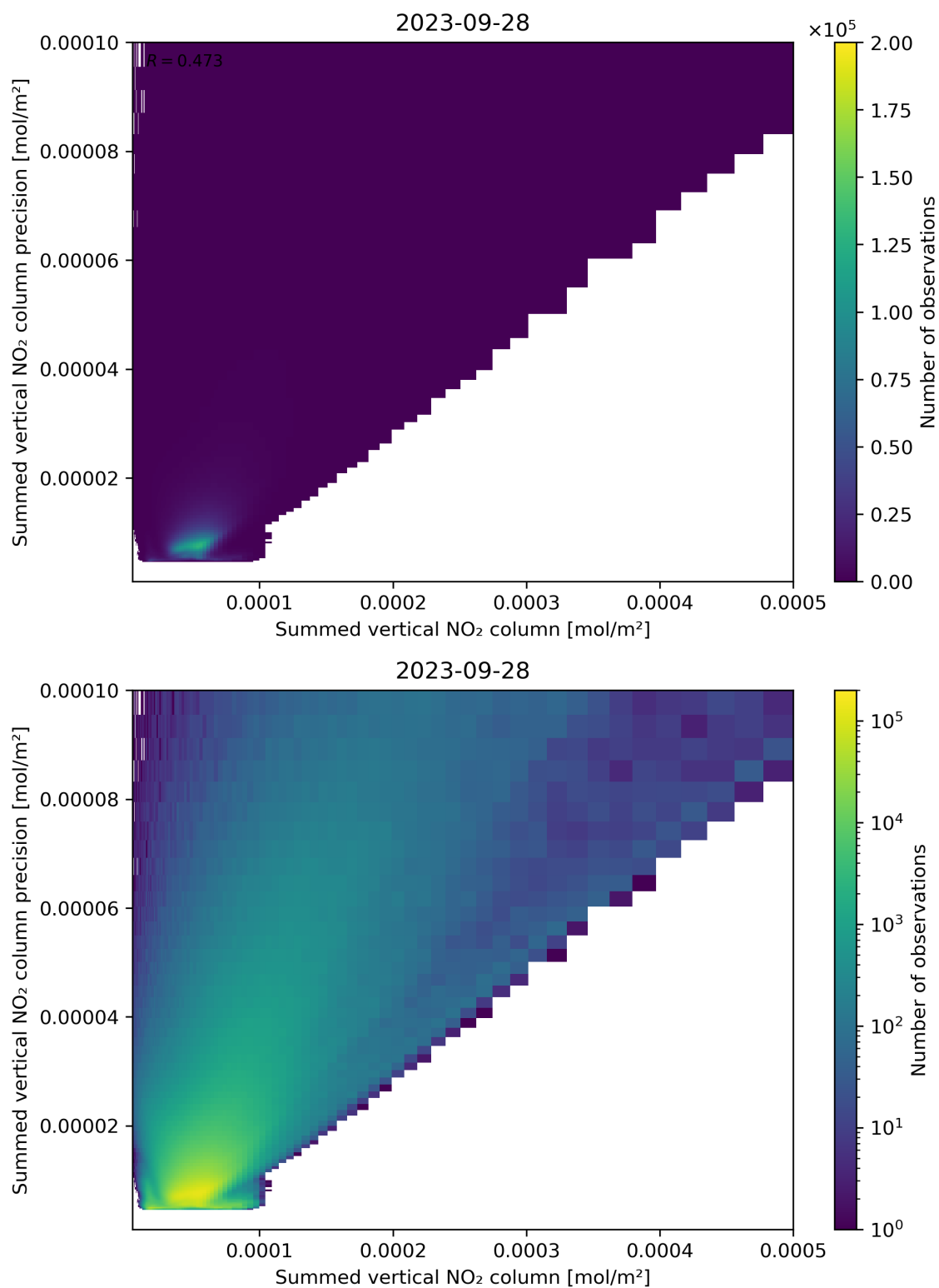
Figure 105: Scatter density plot of “Summed vertical NO 2 column” against “Summed vertical NO 2 column precision” for 2023-09-27 to 2023-09-29.
