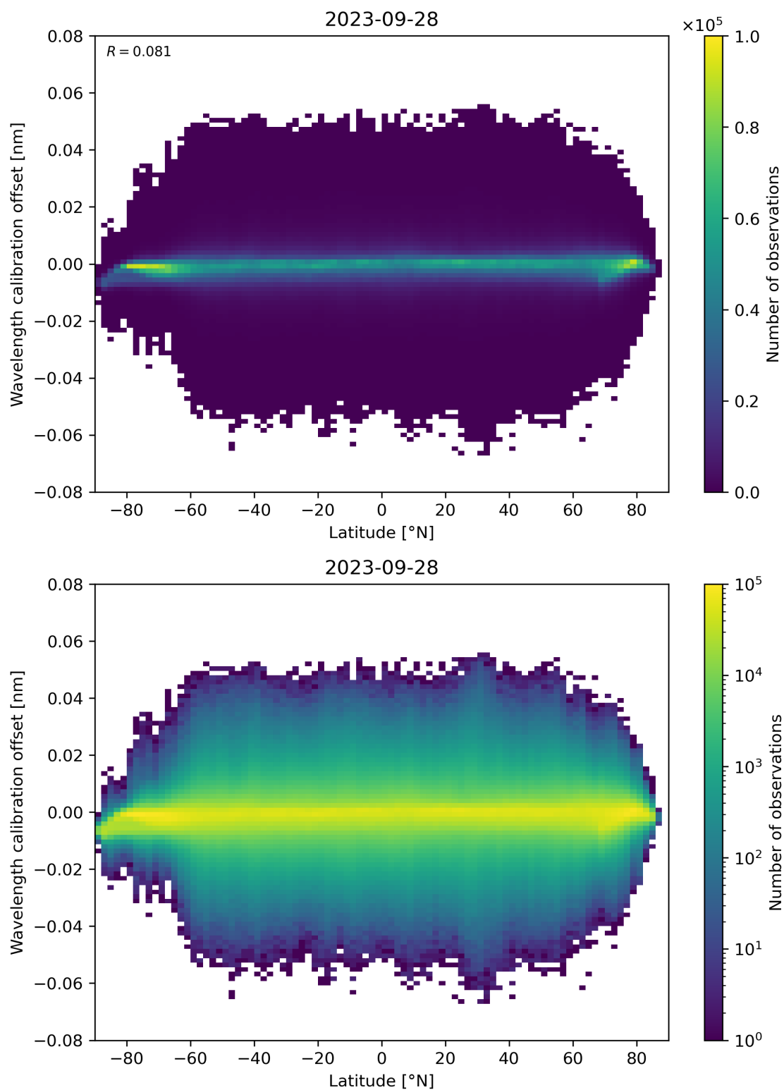
Figure 95: Scatter density plot of “Latitude” against “Wavelength calibration offset” for 2023-09-27 to 2023-09-29.
