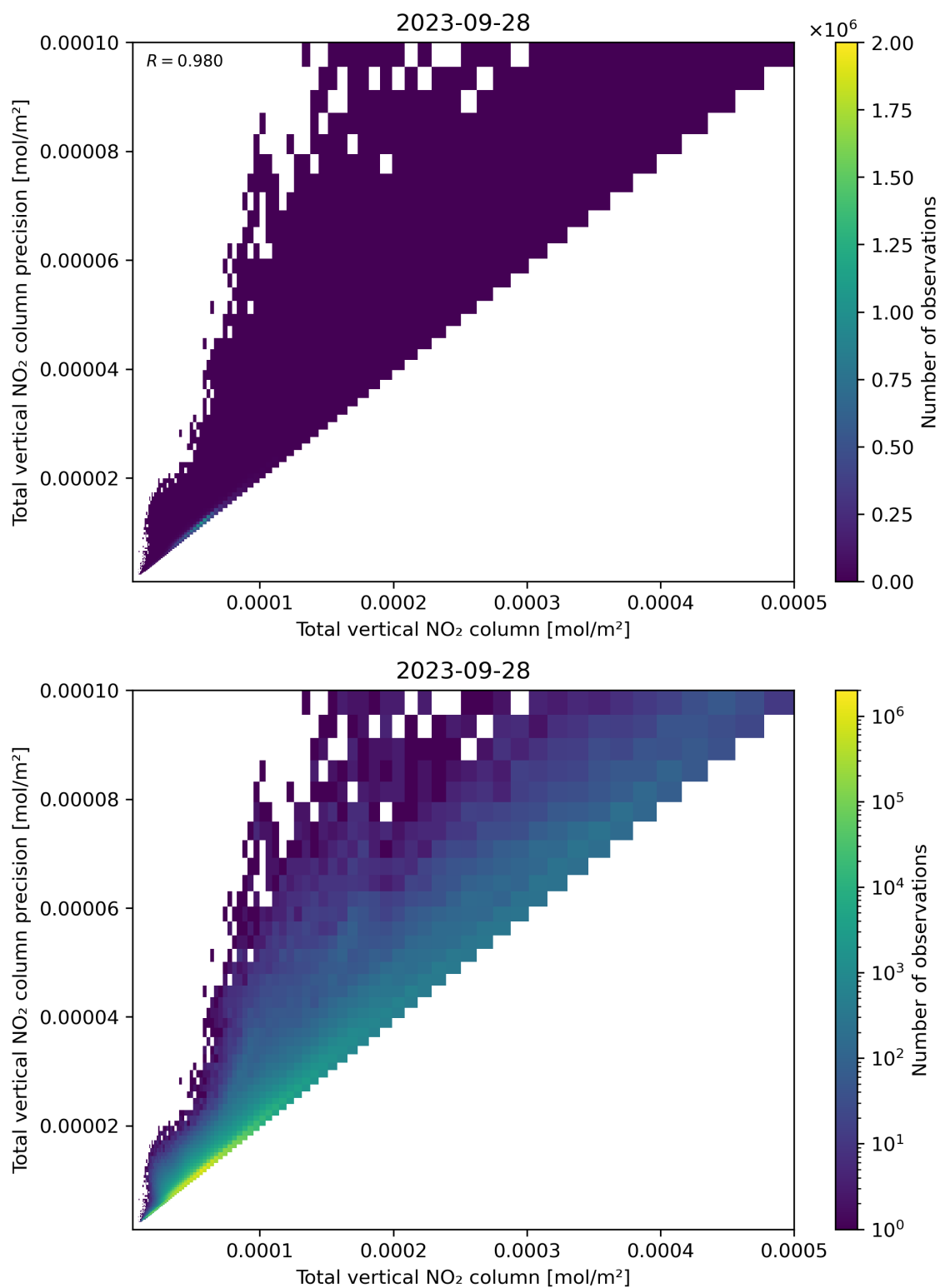
Figure 114: Scatter density plot of “Total vertical NO 2 column” against “Total vertical NO 2 column precision” for 2023-09-27 to 2023-09-29.
