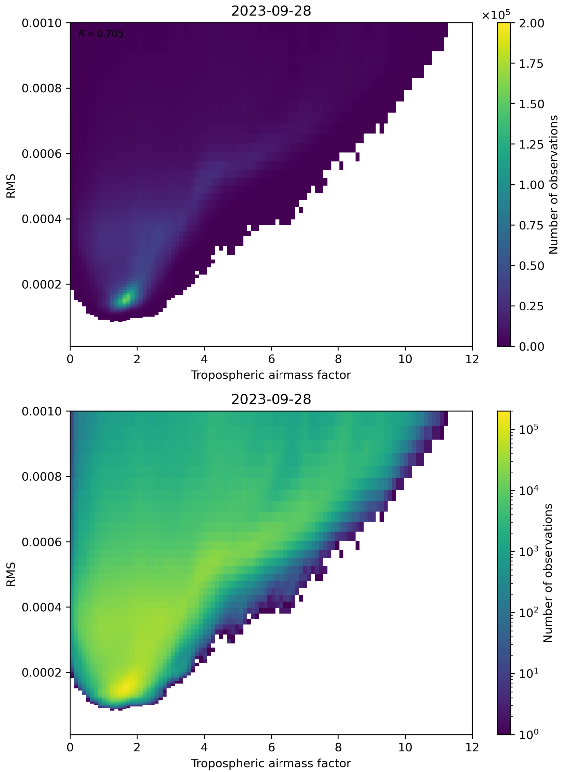
Figure 79: Scatter density plot of “Tropospheric airmass factor” against “RMS” for 2023-09-27 to 2023-09-29.
