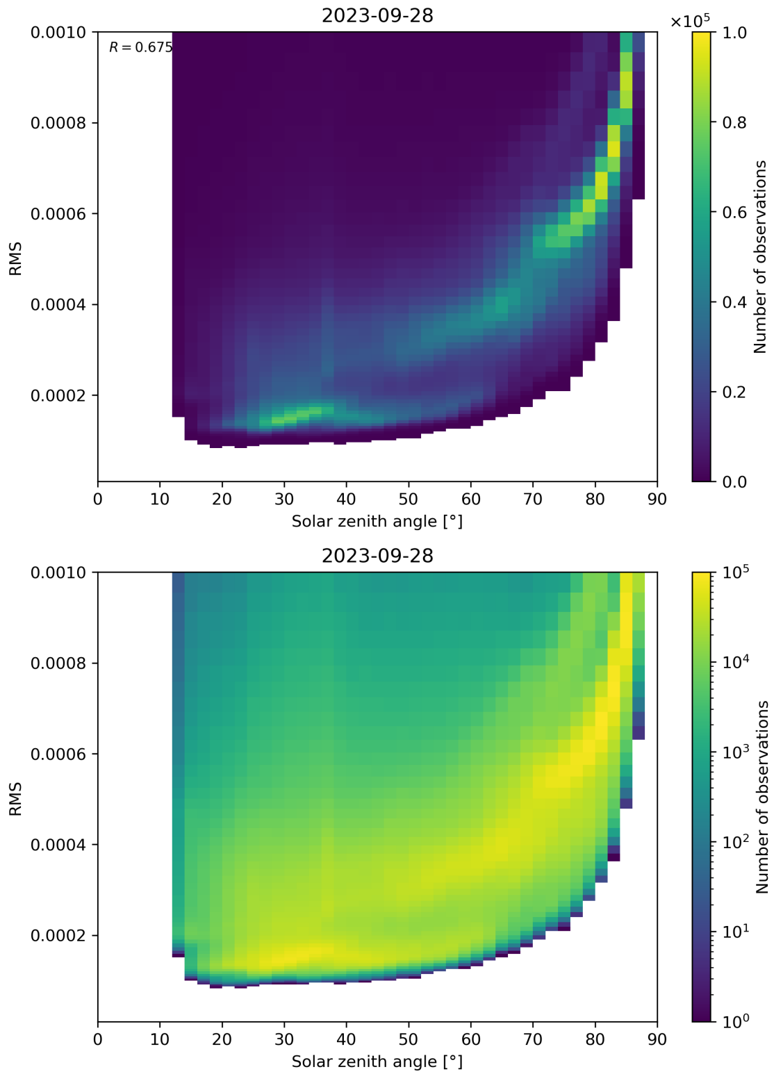
Figure 157: Scatter density plot of “Solar zenith angle” against “RMS” for 2023-09-27 to 2023-09-29.
