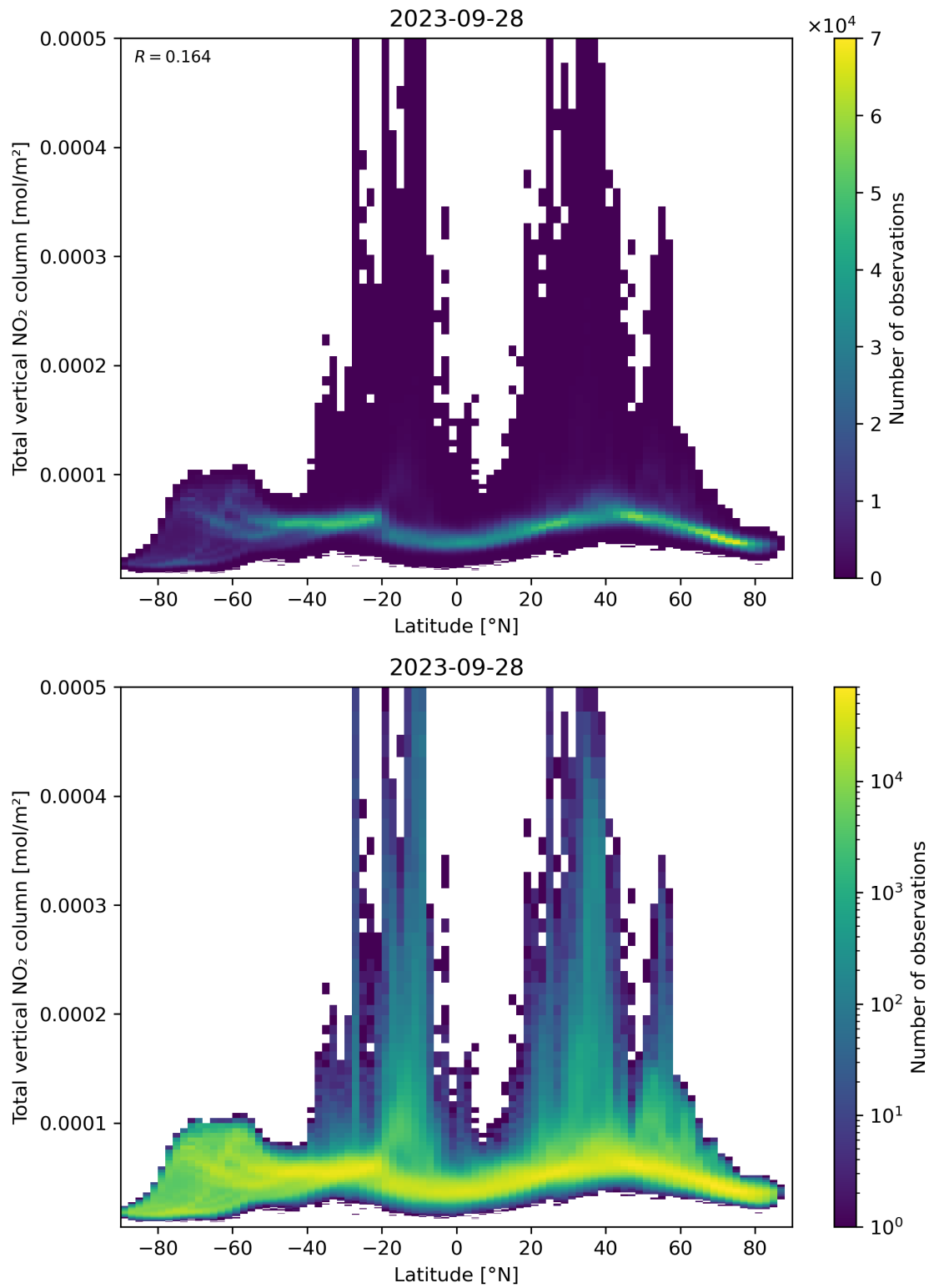
Figure 90: Scatter density plot of “Latitude” against “Total vertical NO 2 column” for 2023-09-27 to 2023-09-29.
