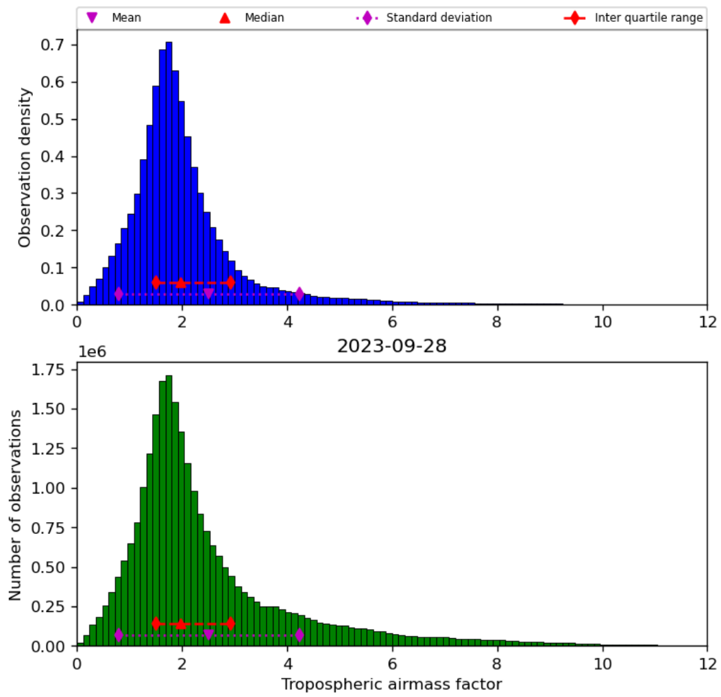
Figure 31: Histogram of “Tropospheric airmass factor” for 2023-09-27 to 2023-09-29
