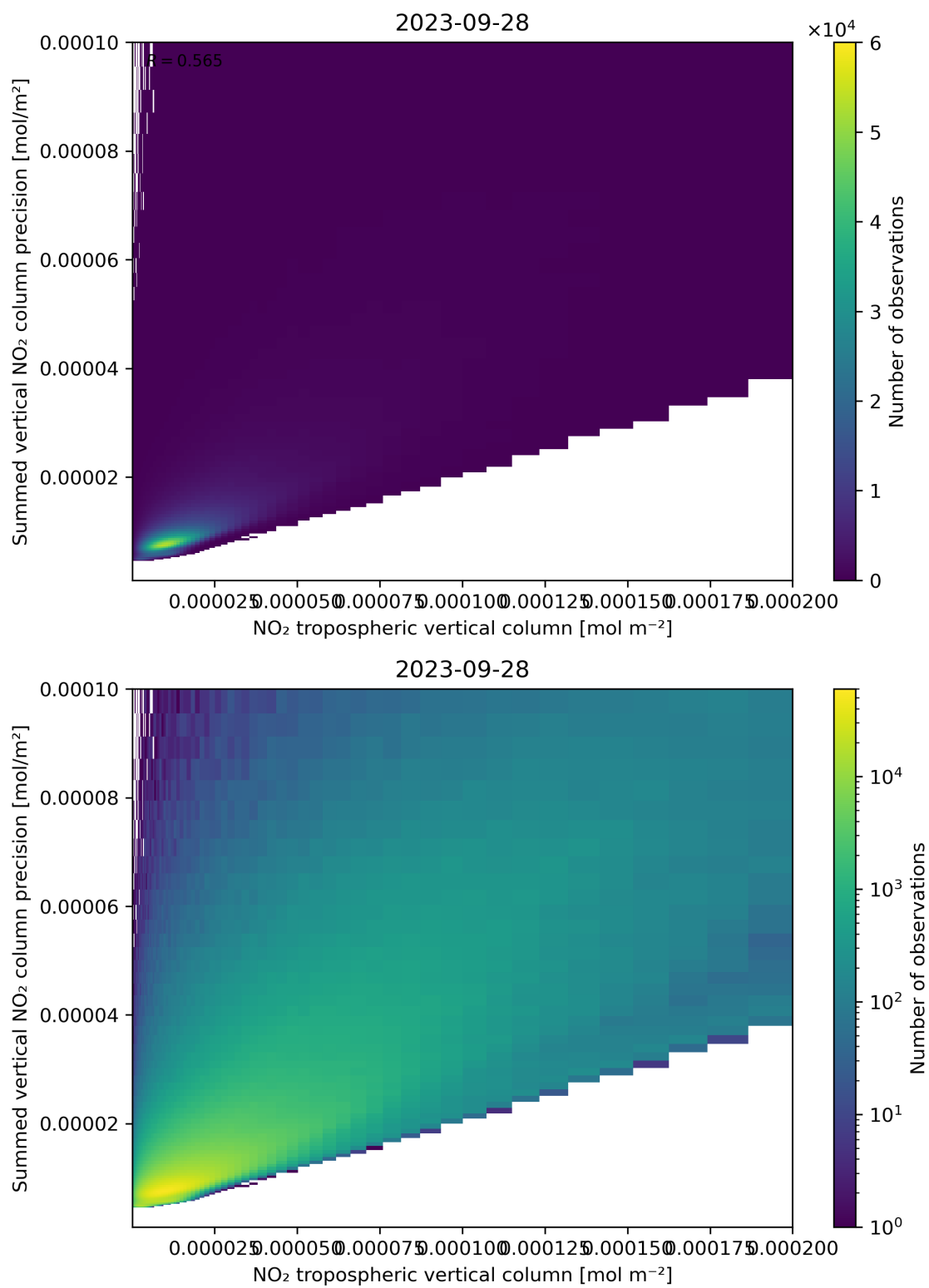
Figure 127: Scatter density plot of “NO 2 tropospheric vertical column” against “Summed vertical NO 2 column precision” for 2023-09-27 to 2023-09-29.
