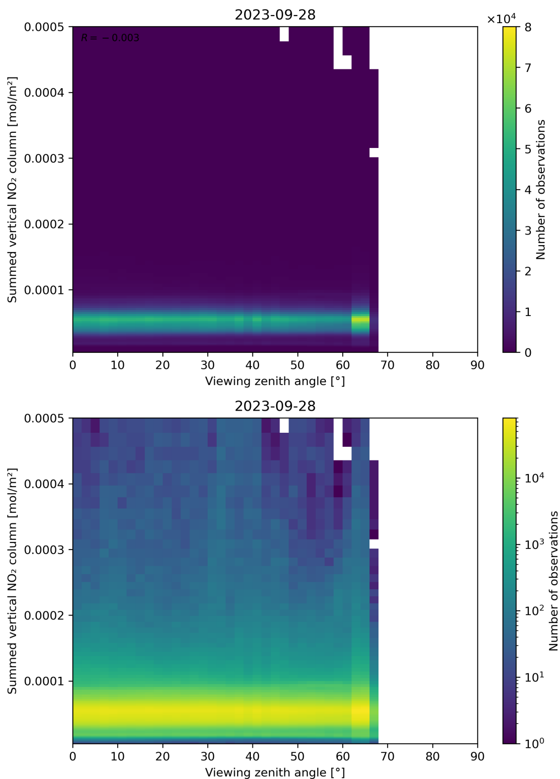
Figure 165: Scatter density plot of “Viewing zenith angle” against “Summed vertical NO 2 column” for 2023-09-27 to 2023-09-29.
