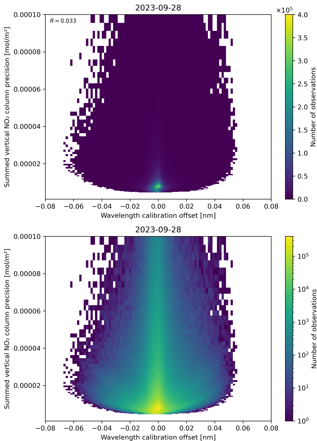
Figure 178: Scatter density plot of “Wavelength calibration offset” against “Summed vertical NO 2 column precision” for 2023-09-27 to 2023-09-29.
