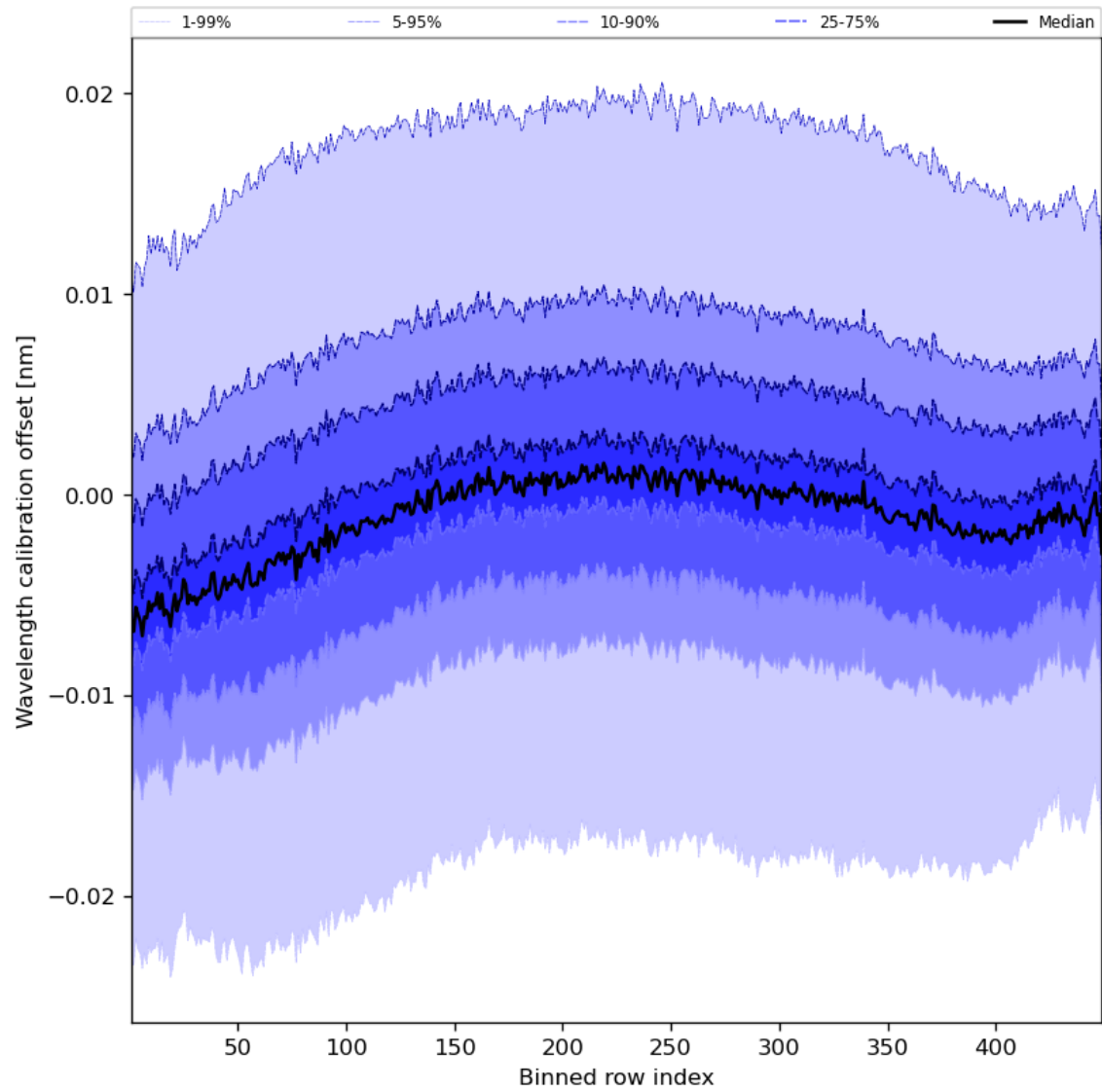
Figure 52: Along track statistics of “Wavelength calibration offset” for 2023-09-27 to 2023-09-29
