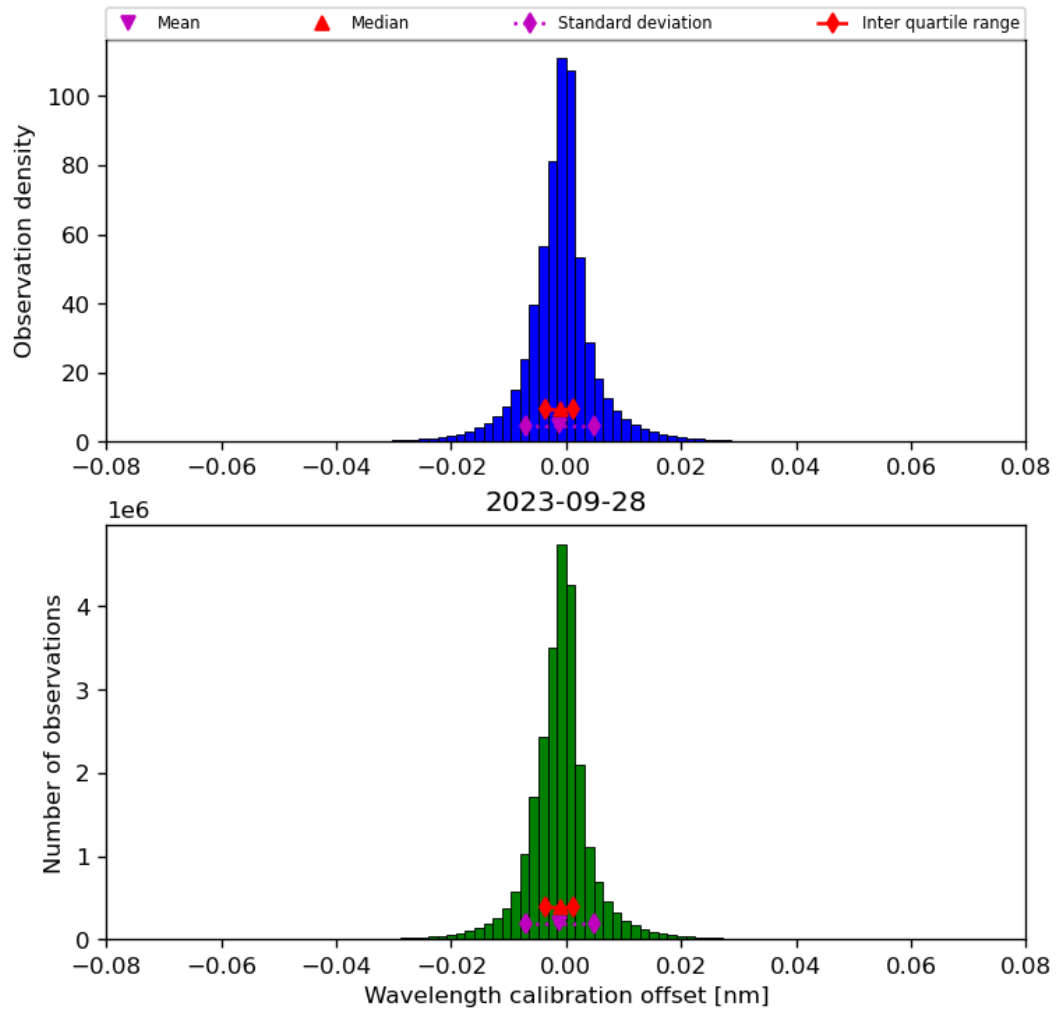
Figure 35: Histogram of “Wavelength calibration offset” for 2023-09-27 to 2023-09-29
