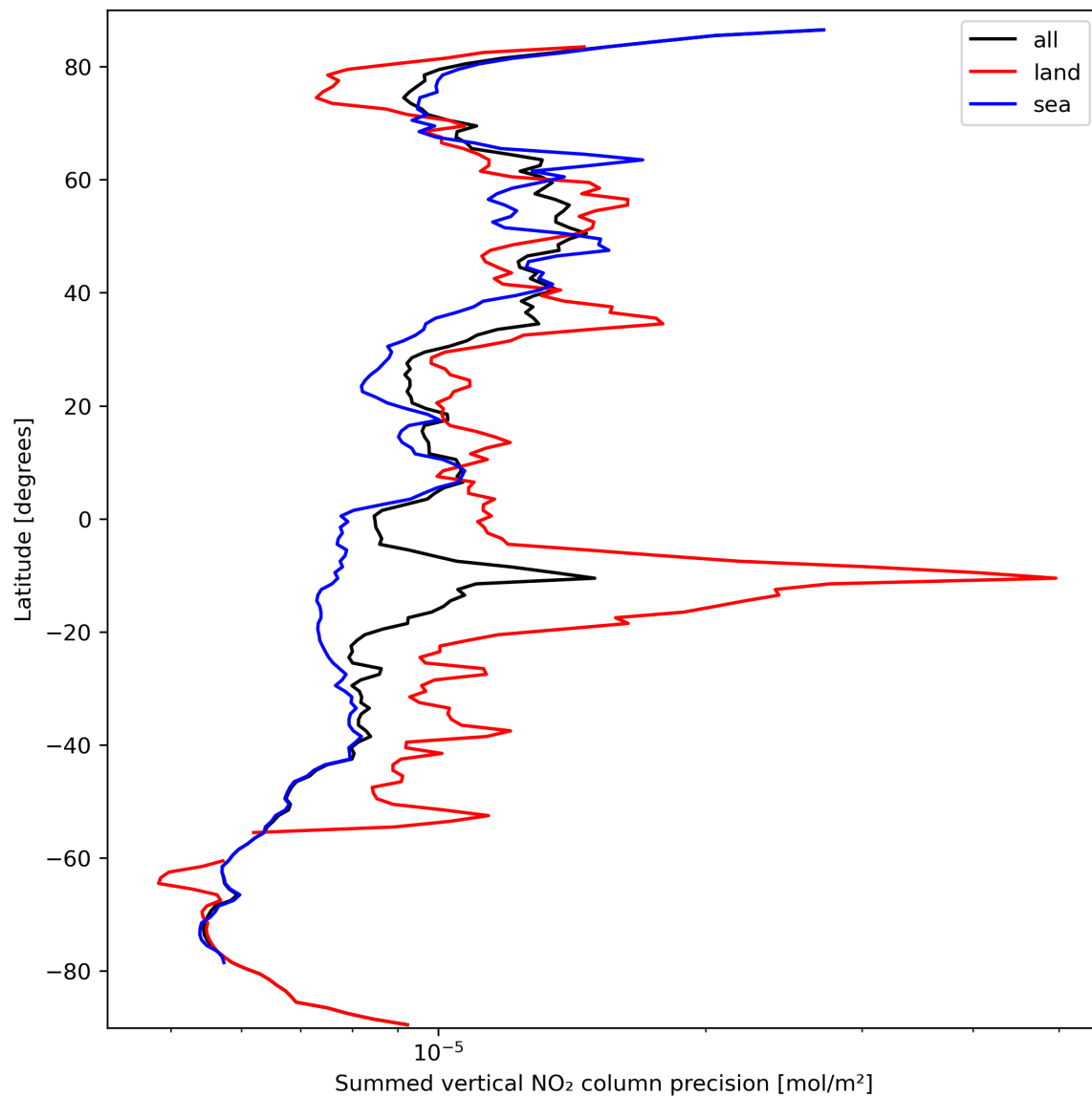
Figure 24: Zonal average of “Summed vertical NO 2 column precision” for 2023-09-27 to 2023-09-29.
