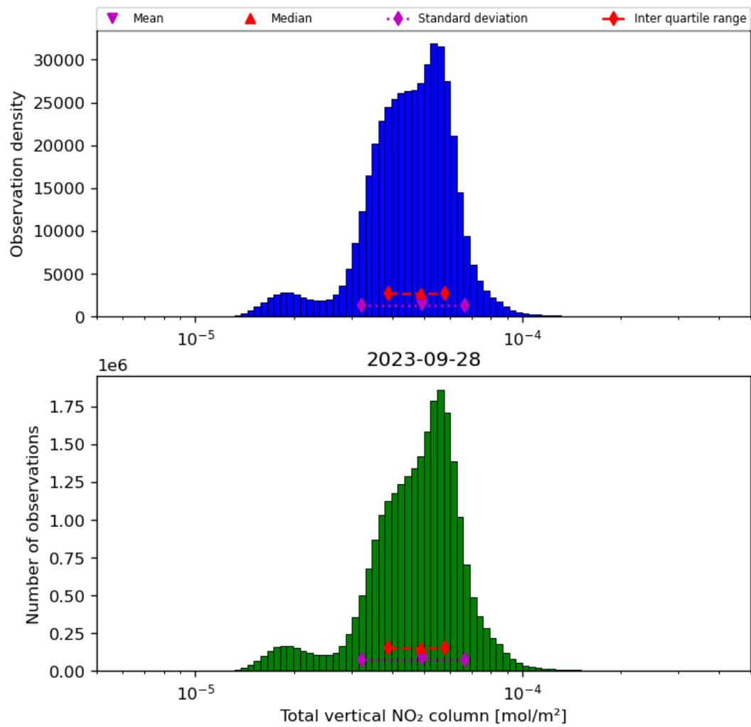
Figure 38: Histogram of "Total vertical NO 2 column" for 2023-09-27 to 2023-09-29
