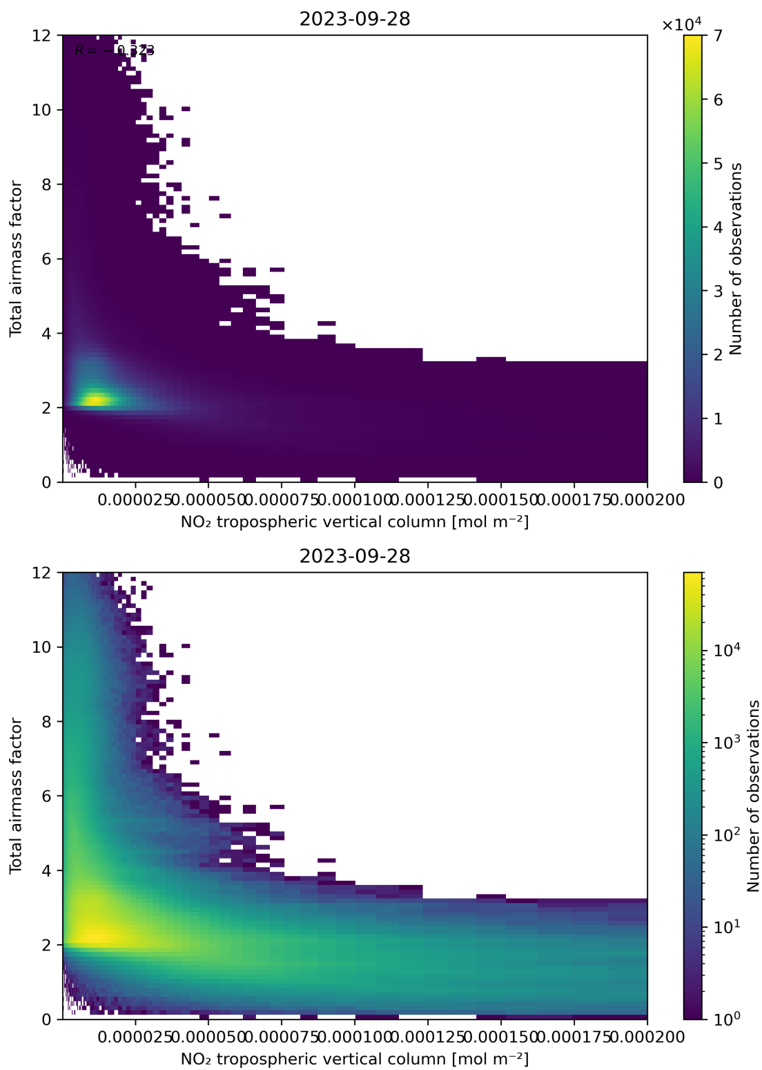
Figure 122: Scatter density plot of “NO 2 tropospheric vertical column” against “Total air mass factor” for 2023-09-27 to 2023-09-29.
