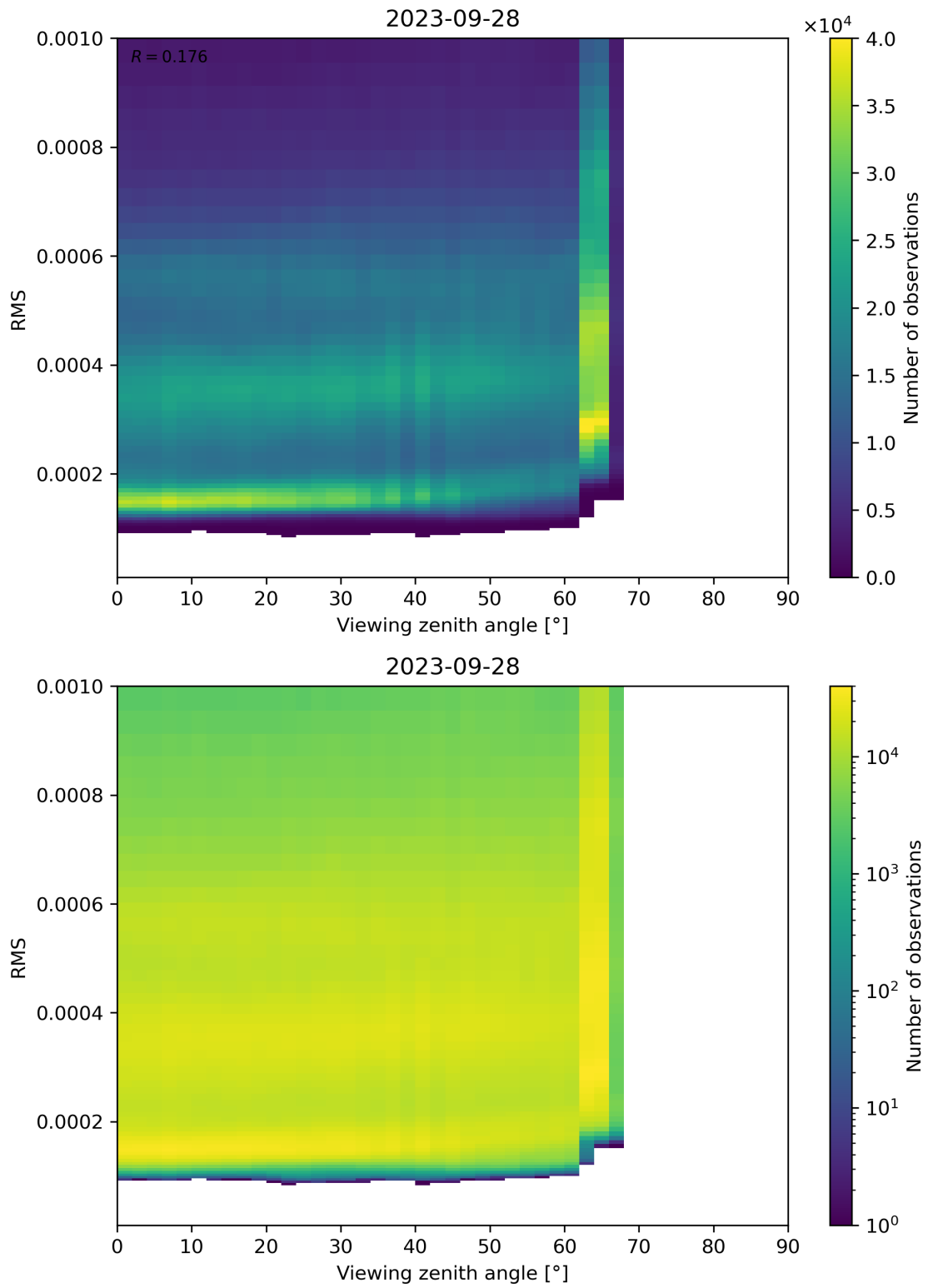
Figure 171: Scatter density plot of “Viewing zenith angle” against “RMS” for 2023-09-27 to 2023-09-29.
