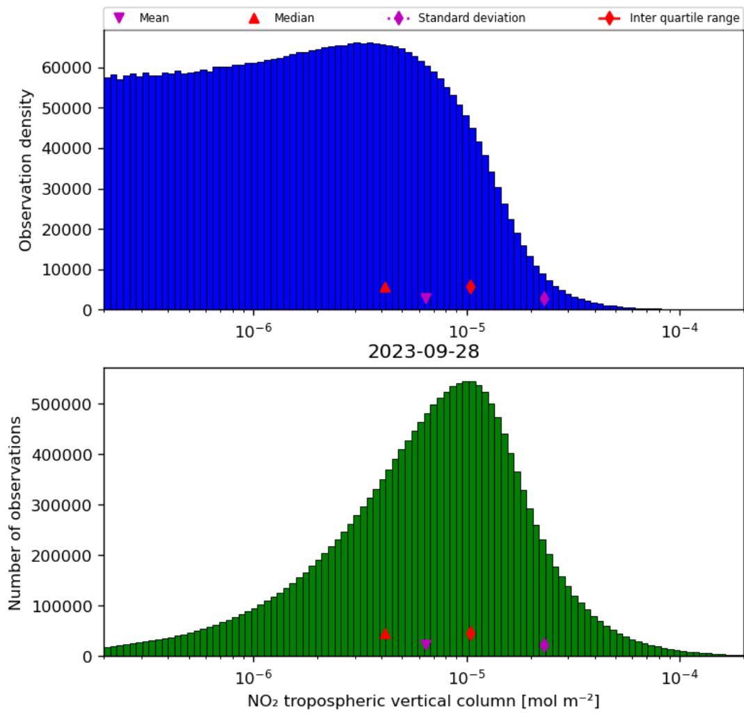
Figure 29: Histogram of “NO 2 tropospheric vertical column” for 2023-09-27 to 2023-09-29
