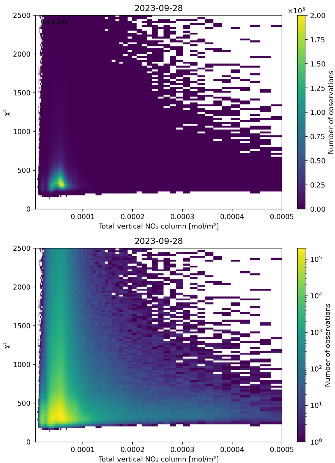
Figure 111: Scatter density plot of “Total vertical NO 2 column” against “ \chi^2 ” for 2023-09-27 to 2023-09-29.
