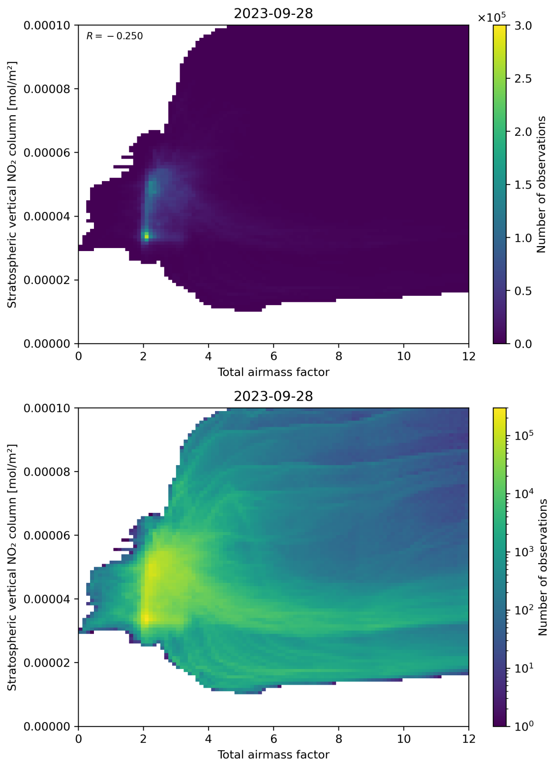
Figure 64: Scatter density plot of “Total airmass factor” against “Stratospheric vertical NO 2 column” for 2023-09-27 to 2023-09-29.
