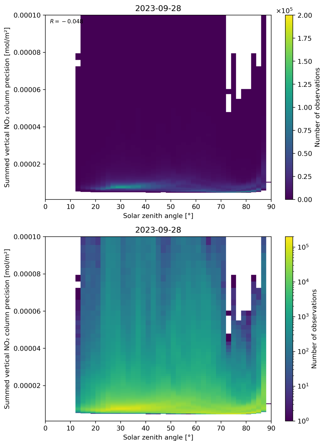
Figure 152: Scatter density plot of “Solar zenith angle” against “Summed vertical NO 2 column precision” for 2023-09-27 to 2023-09-29.
