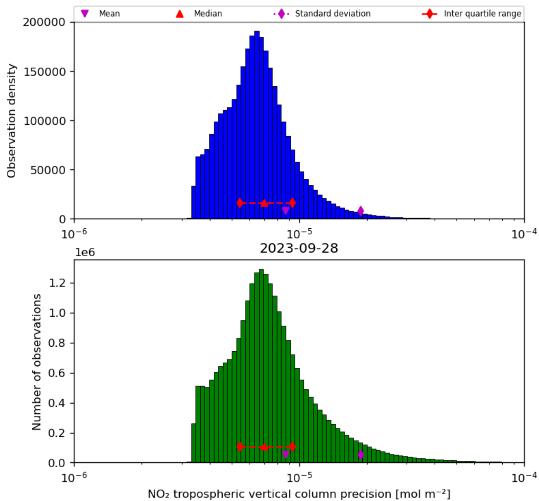
Figure 30: Histogram of “NO 2 tropospheric vertical column precision” for 2023-09-27 to 2023-09-29
