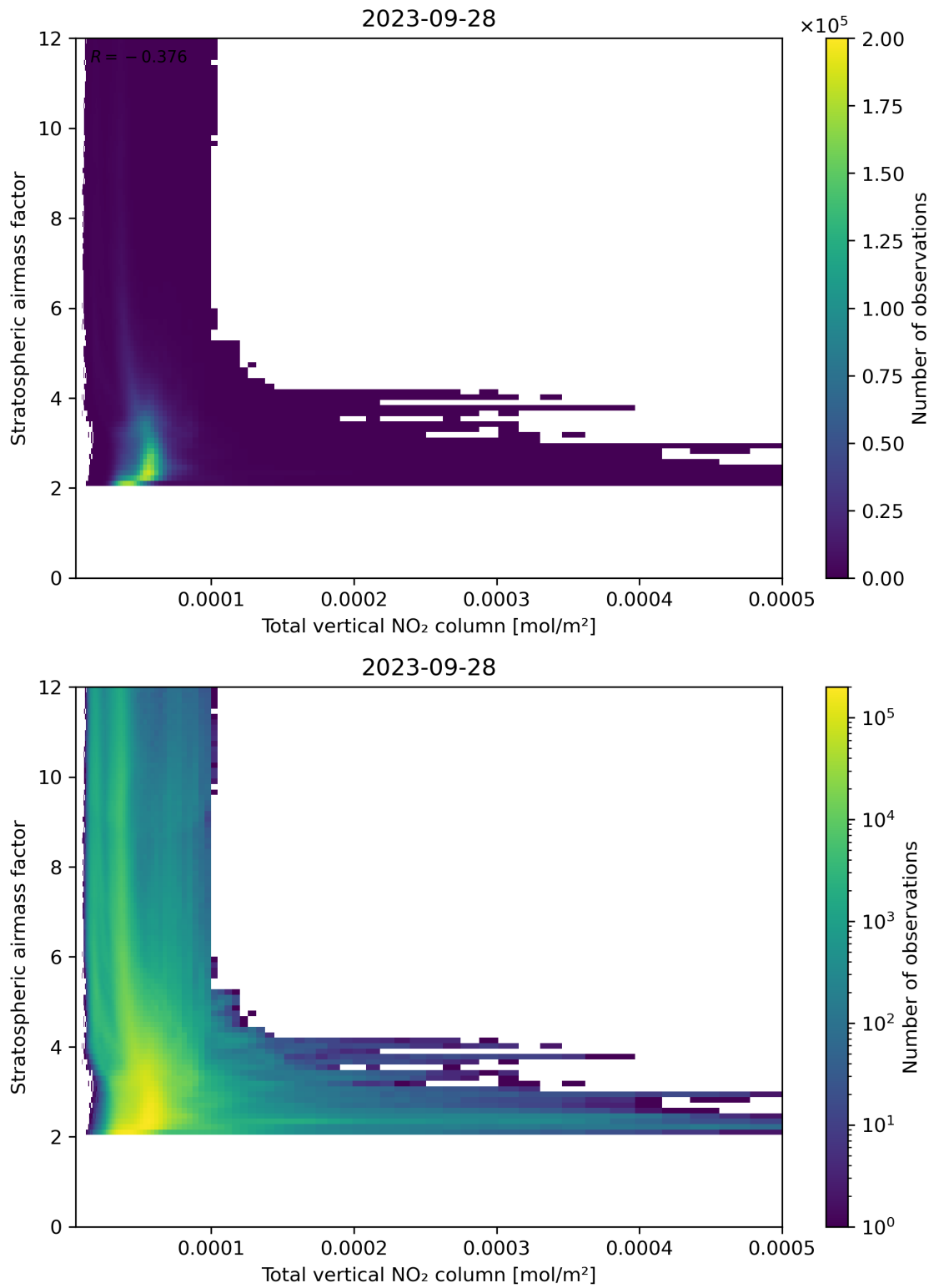
Figure 110: Scatter density plot of “Total vertical NO 2 column” against “Stratospheric airmass factor” for 2023-09-27 to 2023-09-29.
