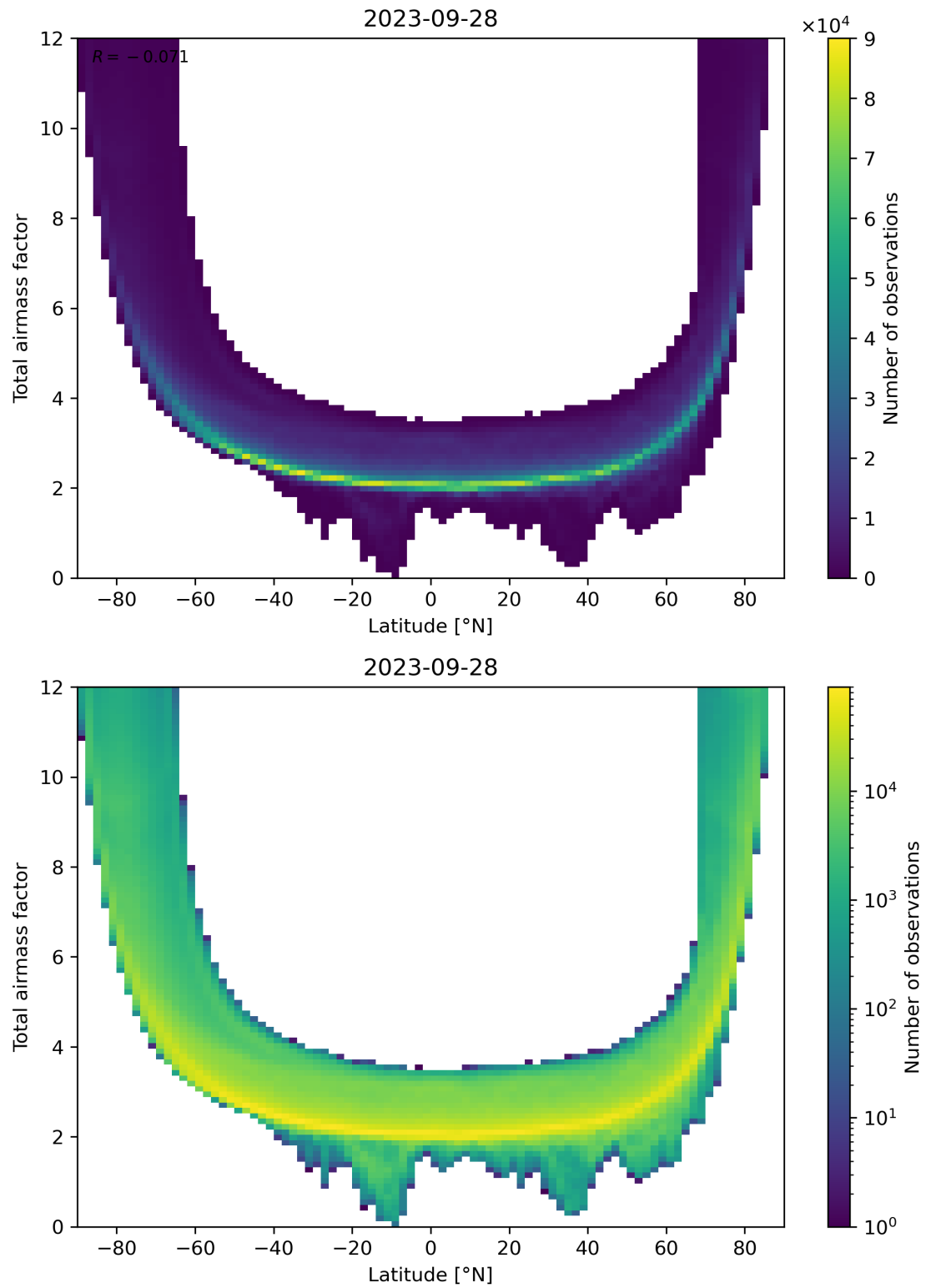
Figure 84: Scatter density plot of “Latitude” against “Total airmass factor” for 2023-09-27 to 2023-09-29.
