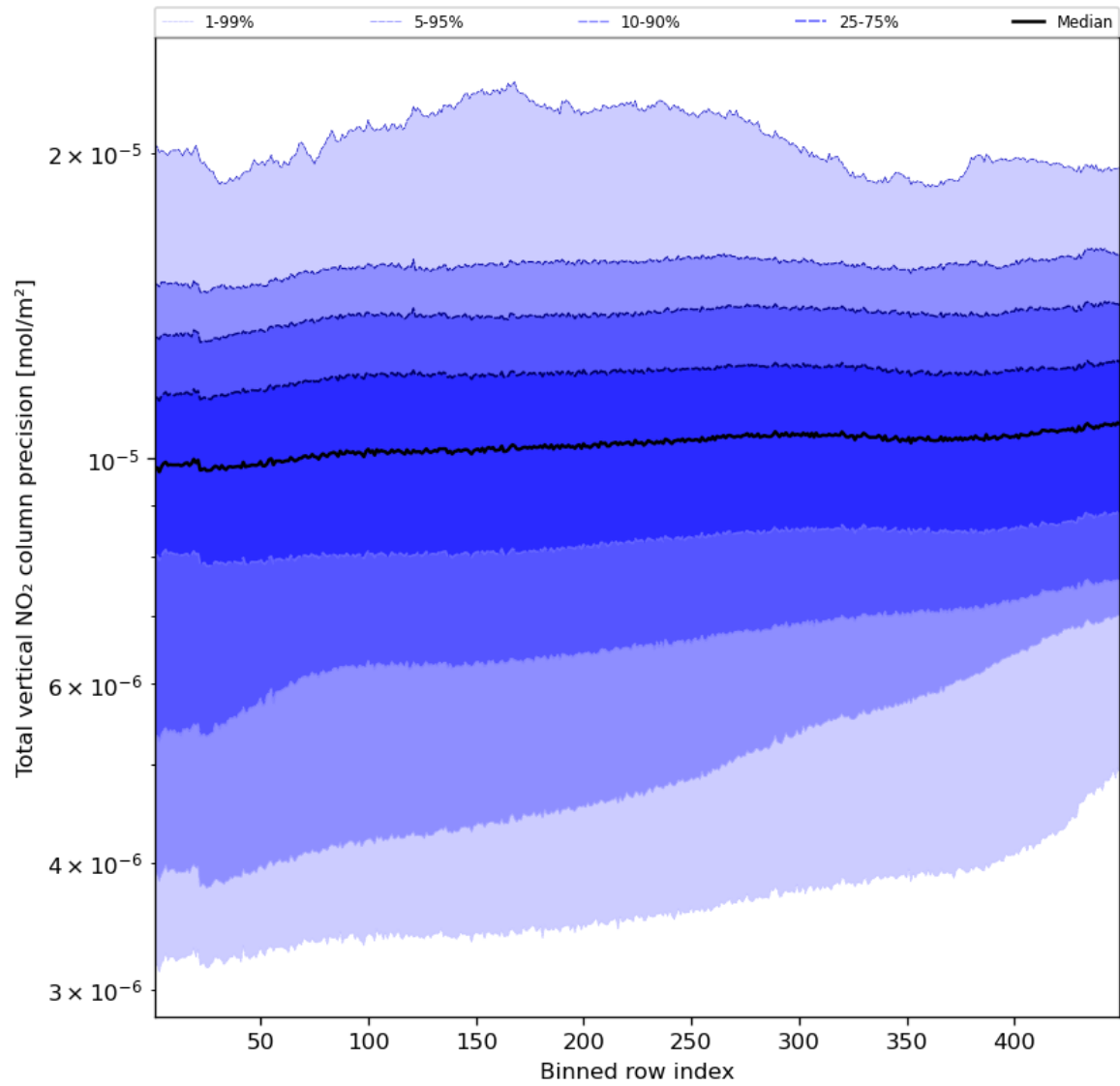
Figure 56: Along track statistics of “Total vertical NO 2 column precision” for 2023-09-27 to 2023-09-29
