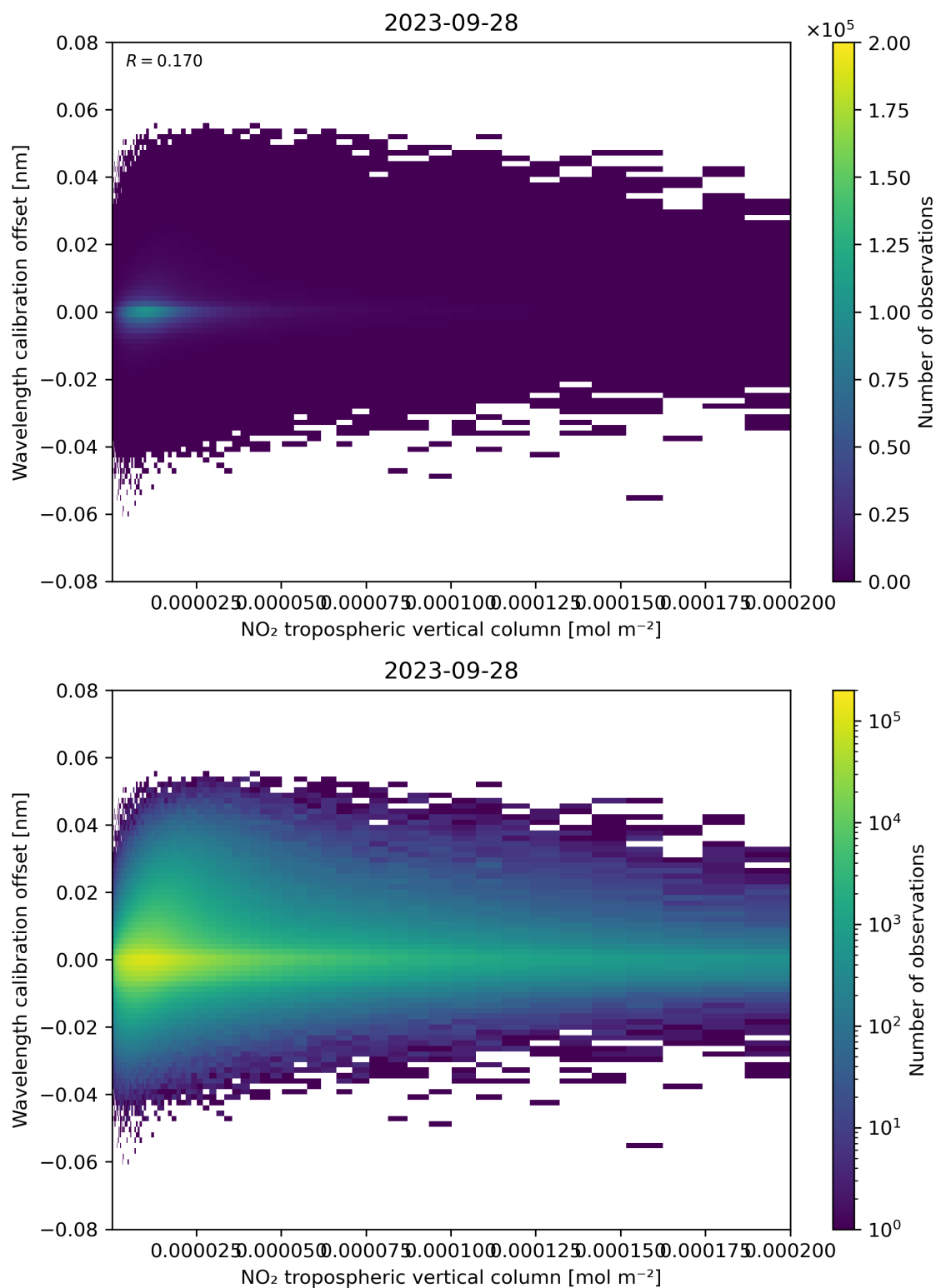
Figure 143: Scatter density plot of “NO 2 tropospheric vertical column” against “Wavelength calibration offset” for 2023-09-27 to 2023-09-29.
