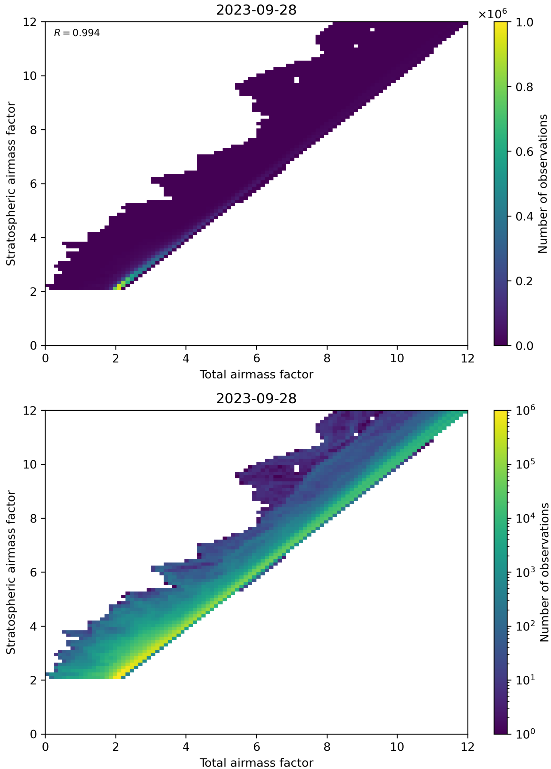
Figure 62: Scatter density plot of “Total airmass factor” against “Stratospheric airmass factor” for 2023-09-27 to 2023-09-29.
