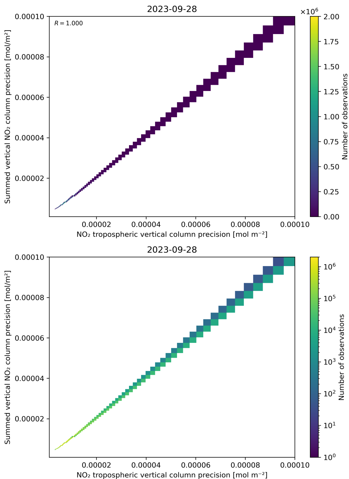
Figure 137: Scatter density plot of “NO 2 tropospheric vertical column precision” against “Summed vertical NO 2 column precision” for 2023-09-27 to 2023-09-29.
