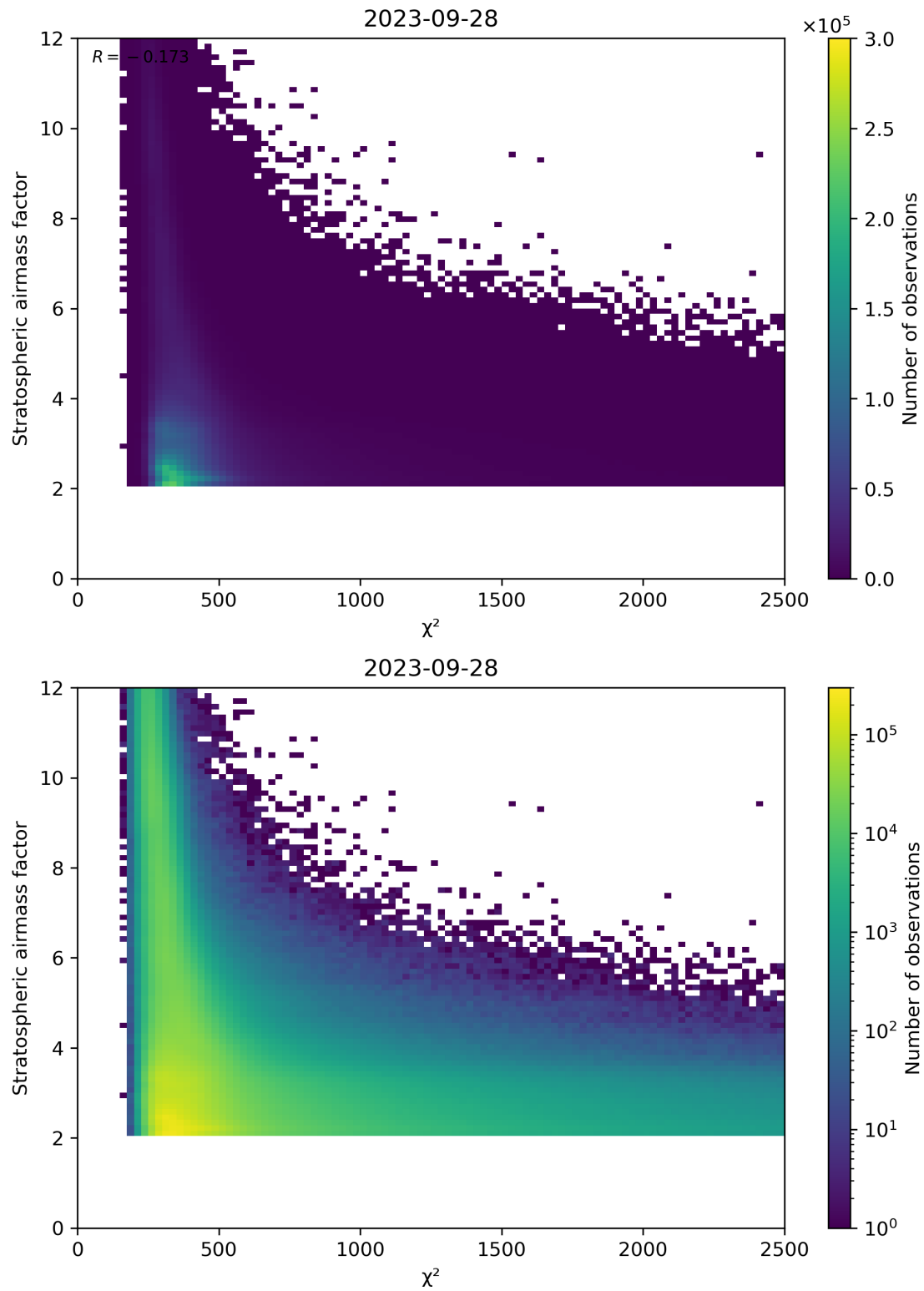
Figure 81: Scatter density plot of “ \chi^2 ” against “Stratospheric airmass factor” for 2023-09-27 to 2023-09-29.
