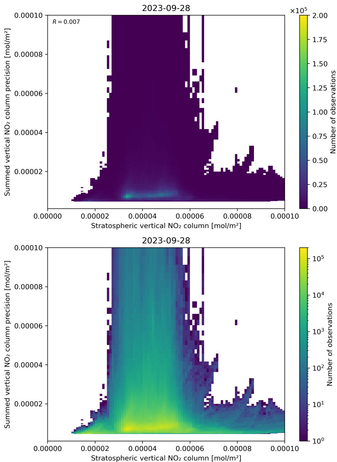
Figure 99: Scatter density plot of “Stratospheric vertical NO 2 column” against “Summed vertical NO 2 column precision” for 2023-09-27 to 2023-09-29.
