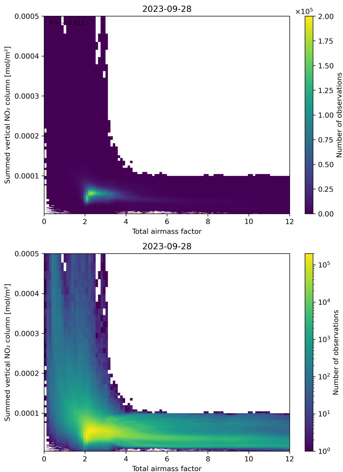
Figure 65: Scatter density plot of “Total airmass factor” against “Summed vertical NO 2 column” for 2023-09-27 to 2023-09-29.
