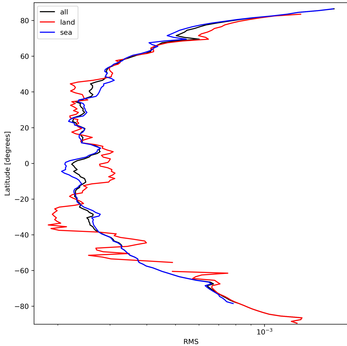
Figure 26: Zonal average of “RMS” for 2023-09-27 to 2023-09-29.
