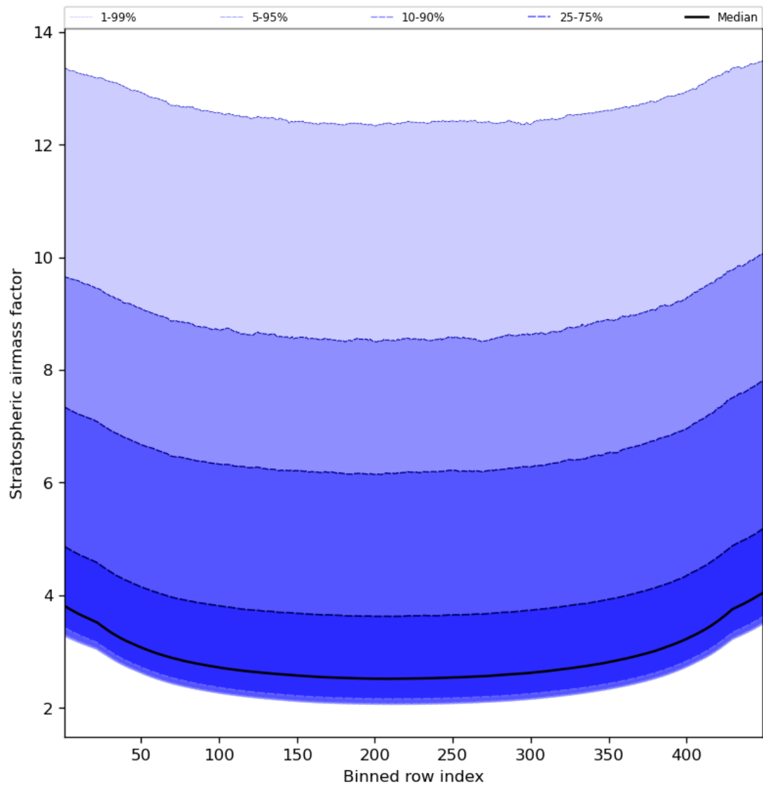
Figure 61: Along track statistics of “Stratospheric air mass factor” for 2023-09-27 to 2023-09-29
