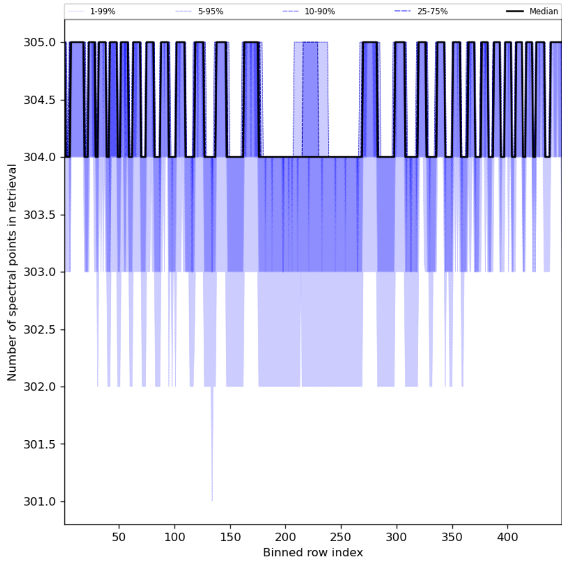
Figure 50: Along track statistics of “Number of spectral points in retrieval” for 2023-09-27 to 2023-09-29
