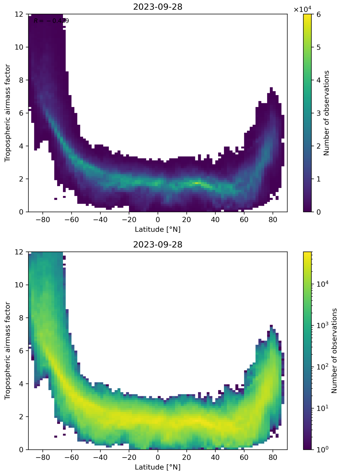
Figure 85: Scatter density plot of “Latitude” against “Tropospheric airmass factor” for 2023-09-27 to 2023-09-29.
