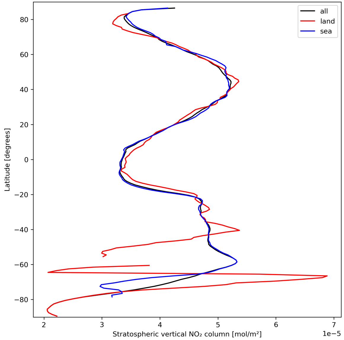
Figure 19: Zonal average of “Stratospheric vertical NO 2 column” for 2023-09-27 to 2023-09-29.
