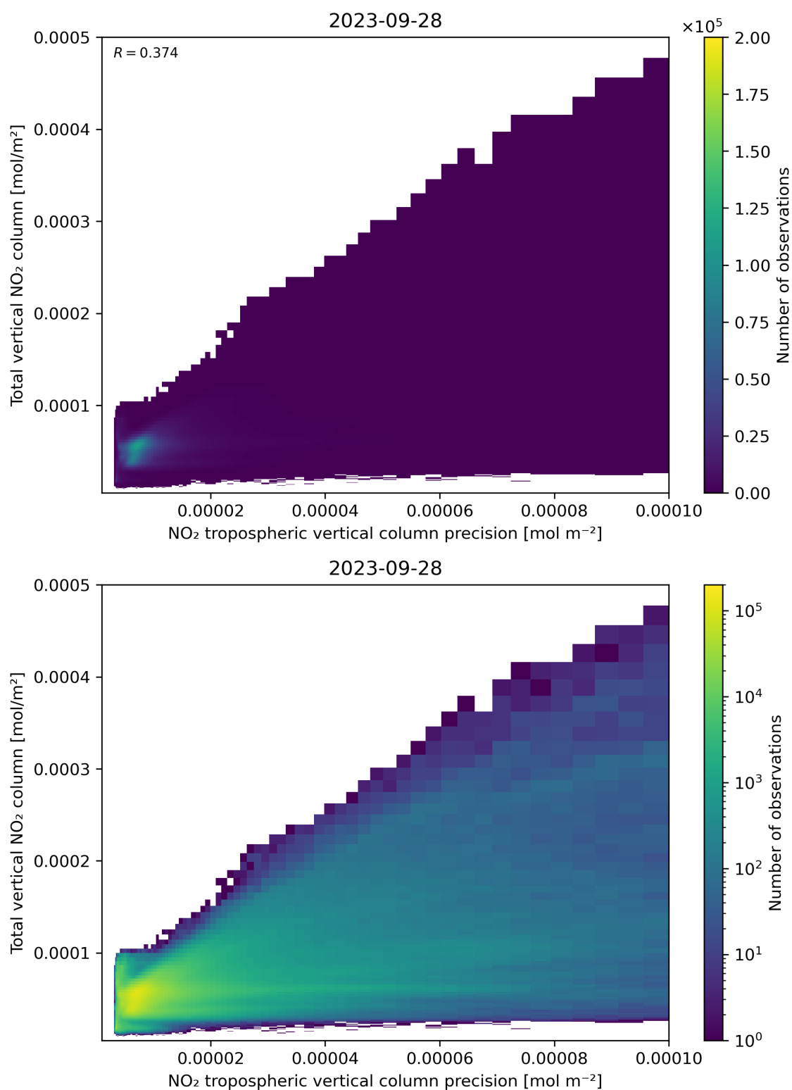
Figure 138: Scatter density plot of “NO 2 tropospheric vertical column precision” against “Total vertical NO 2 column” for 2023-09-27 to 2023-09-29.
