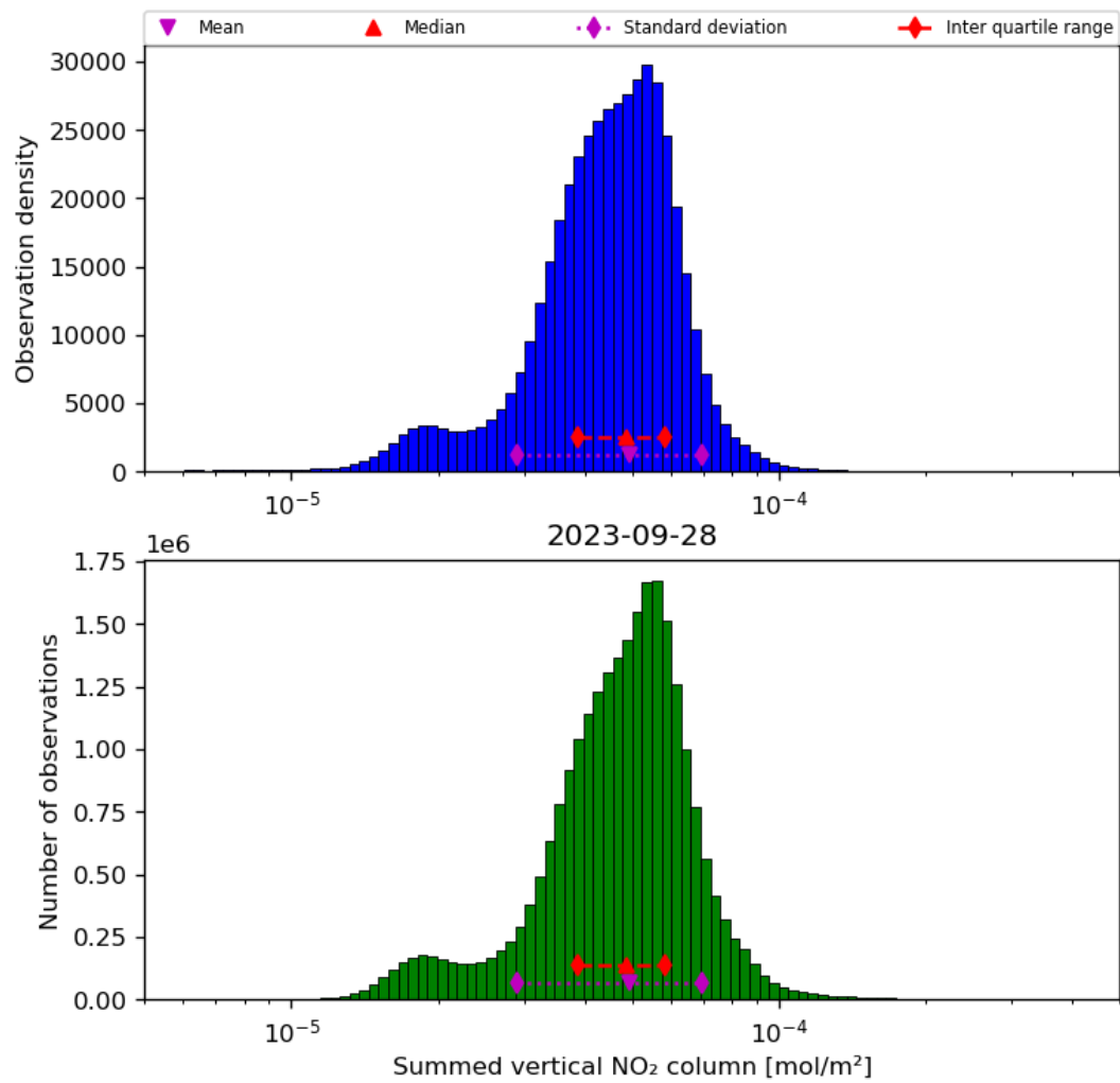
Figure 40: Histogram of “Summed vertical NO 2 column” for 2023-09-27 to 2023-09-29
