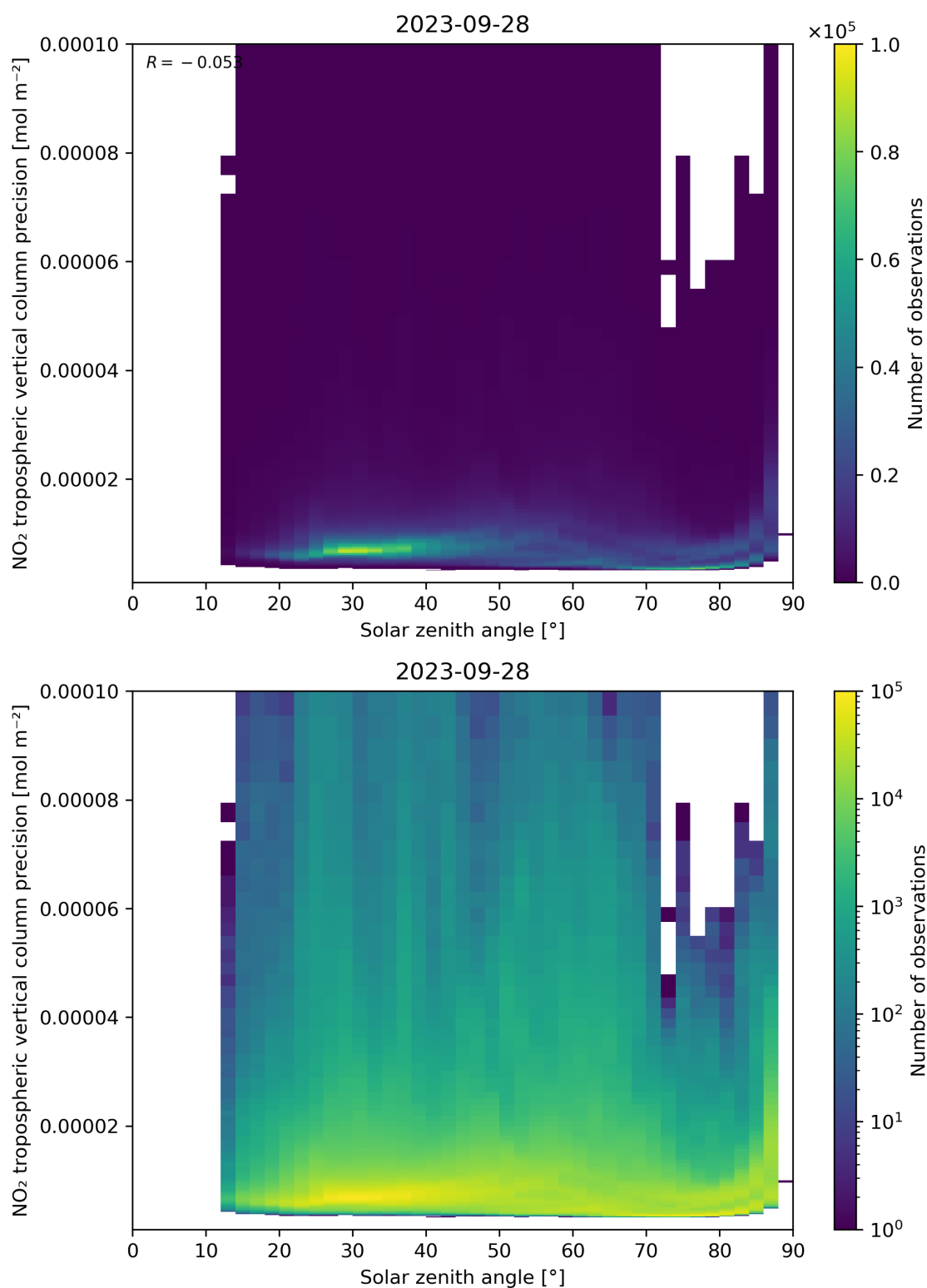
Figure 156: Scatter density plot of “Solar zenith angle” against “NO 2 tropospheric vertical column precision” for 2023-09-27 to 2023-09-29.
