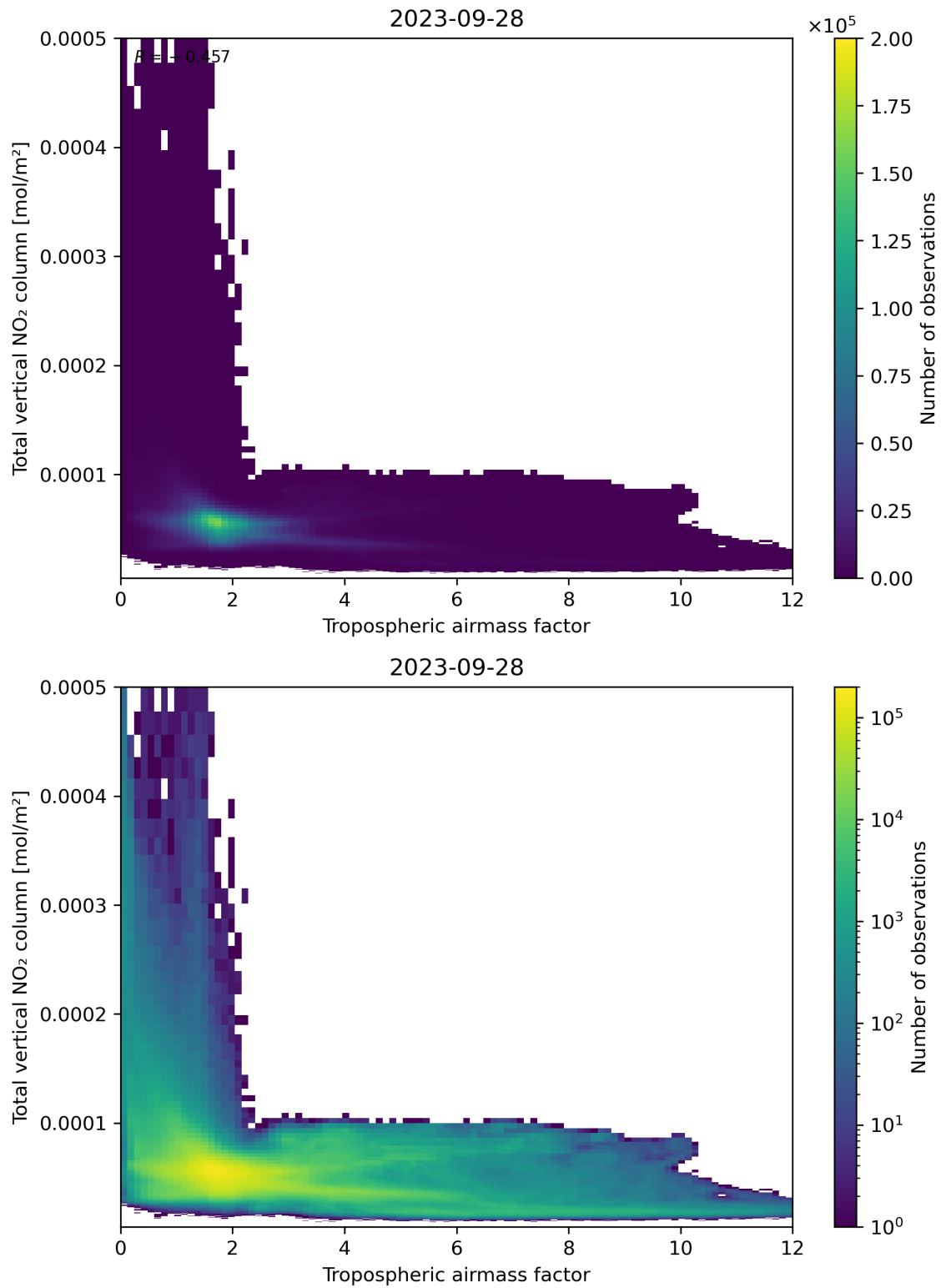
Figure 77: Scatter density plot of “Tropospheric airmass factor” against “Total vertical NO 2 column” for 2023-09-27 to 2023-09-29.
