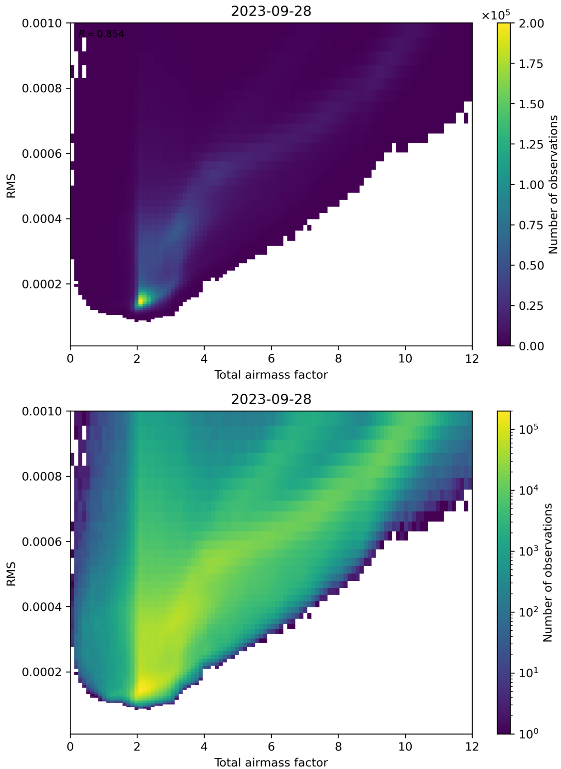
Figure 69: Scatter density plot of “Total airmass factor” against “RMS” for 2023-09-27 to 2023-09-29.
