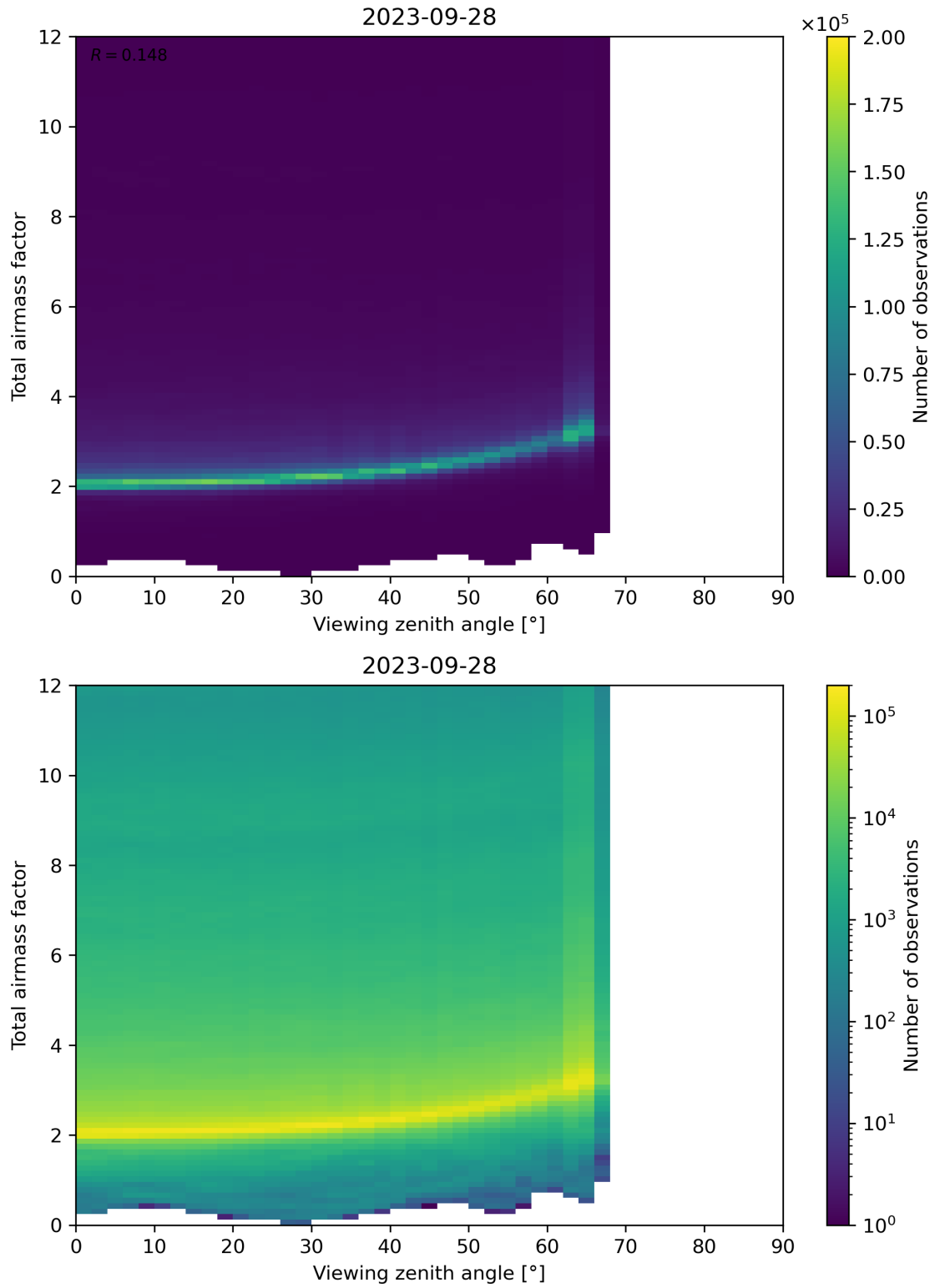
Figure 160: Scatter density plot of “Viewing zenith angle” against “Total airmass factor” for 2023-09-27 to 2023-09-29.
