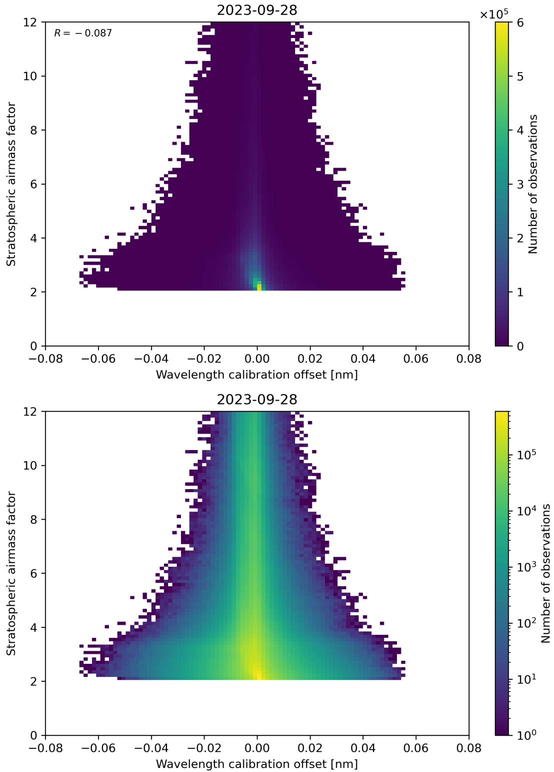
Figure 174: Scatter density plot of “Wavelength calibration offset” against “Stratospheric air mass factor” for 2023-09-27 to 2023-09-29.
