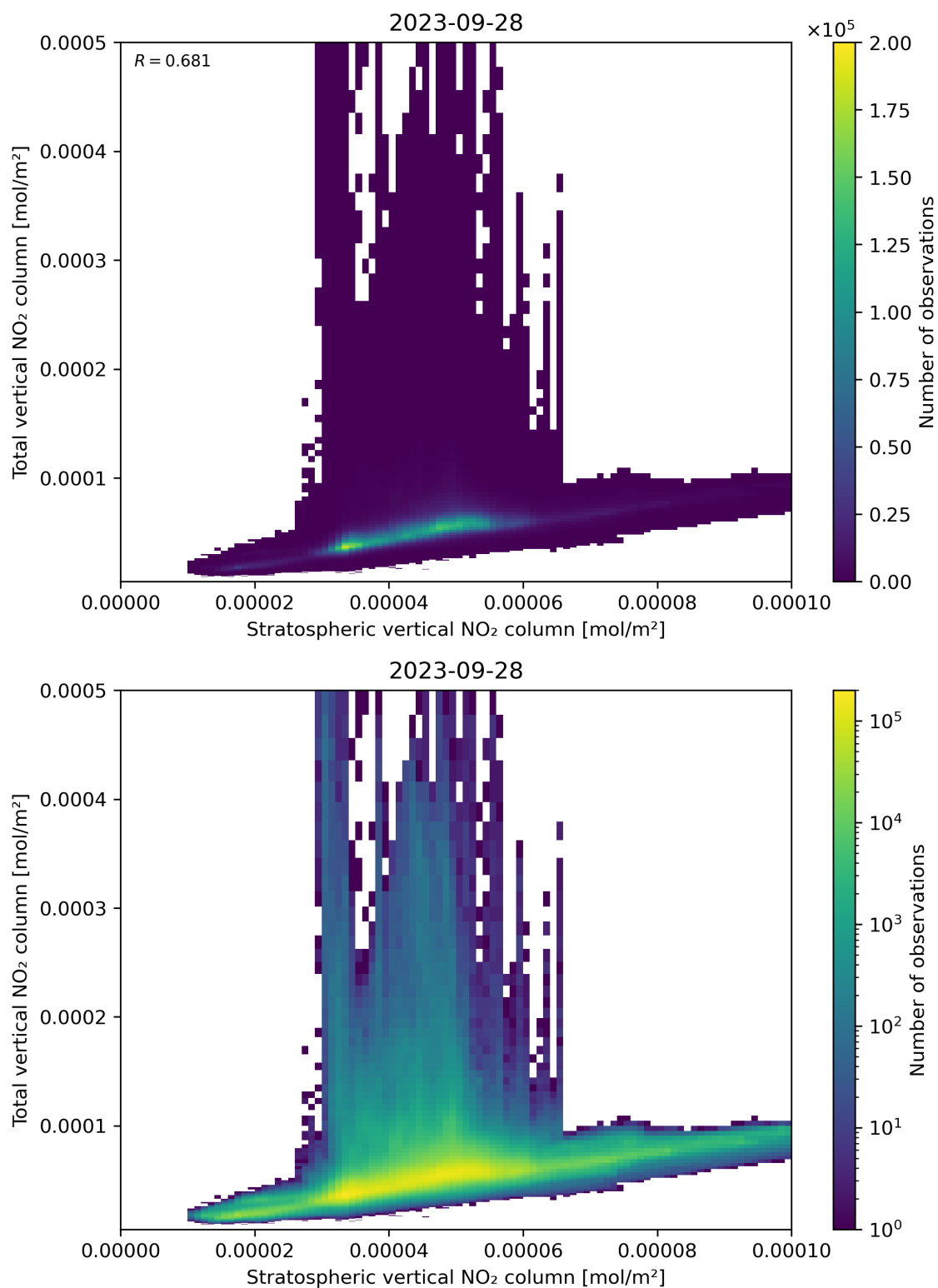
Figure 100: Scatter density plot of “Stratospheric vertical NO 2 column” against “Total vertical NO 2 column” for 2023-09-27 to 2023-09-29.
