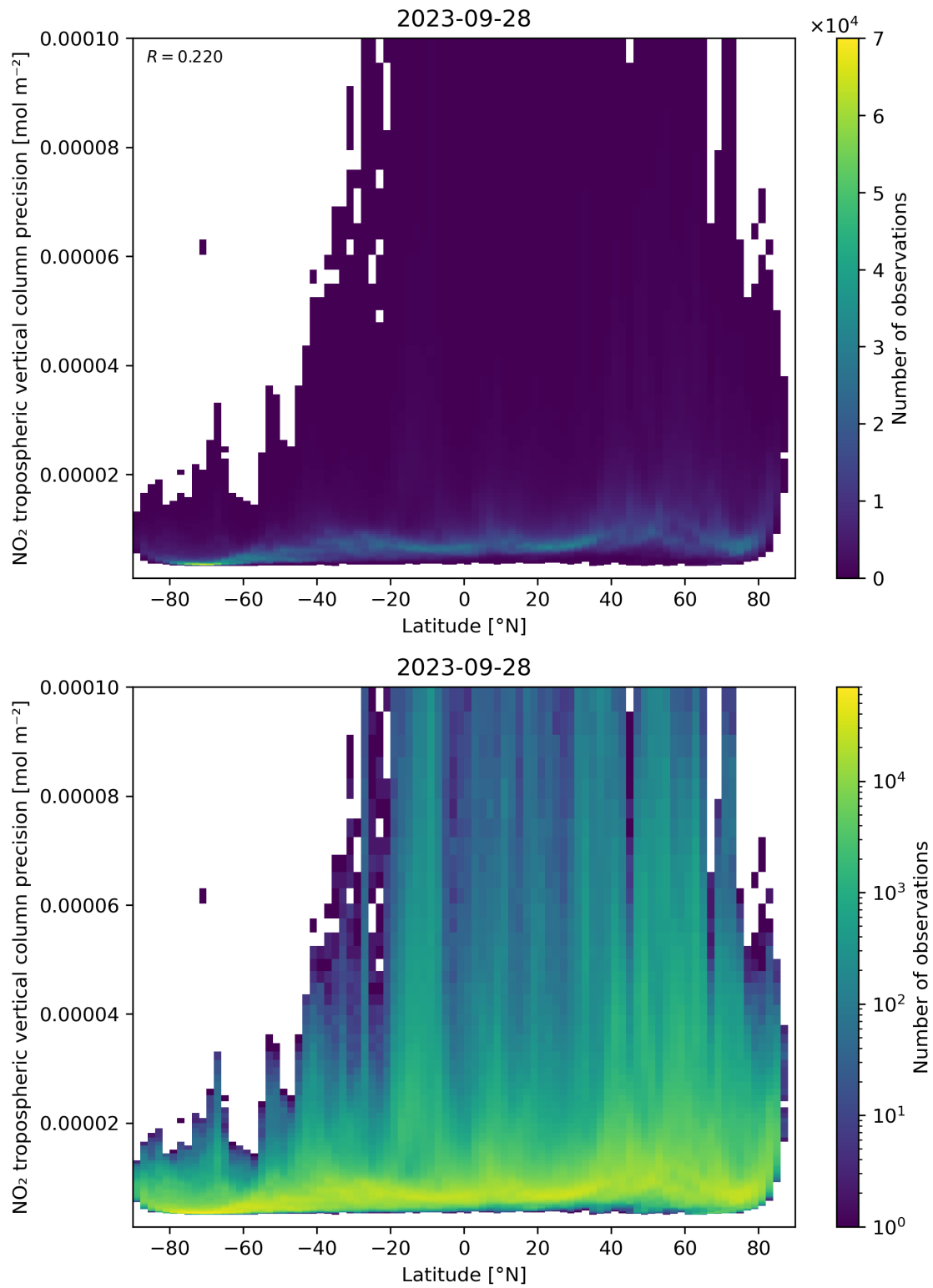
Figure 93: Scatter density plot of “Latitude” against “NO 2 tropospheric vertical column precision” for 2023-09-27 to 2023-09-29.
