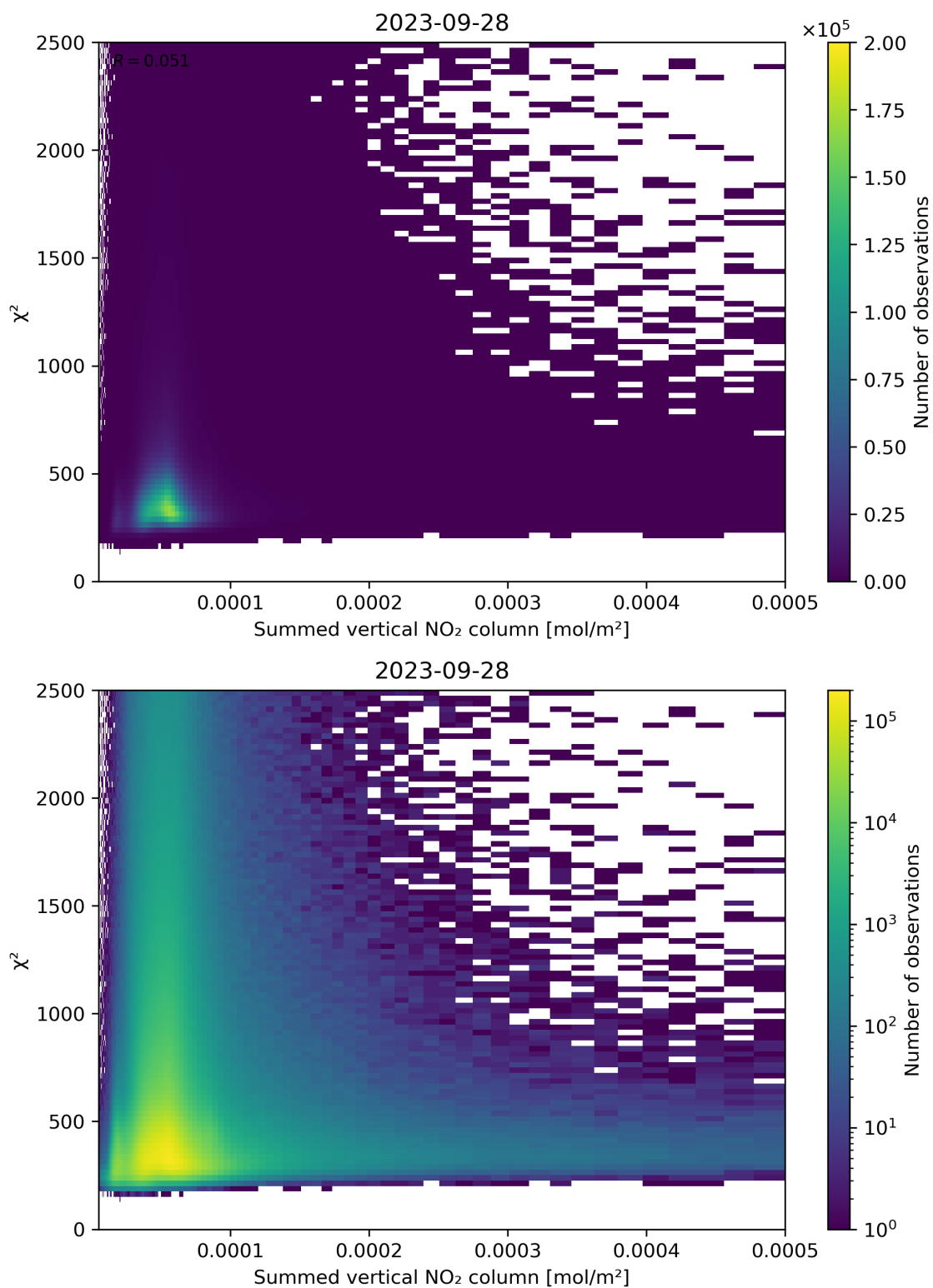
Figure 104: Scatter density plot of “Summed vertical NO 2 column” against “ \chi^2 ” for 2023-09-27 to 2023-09-29.
