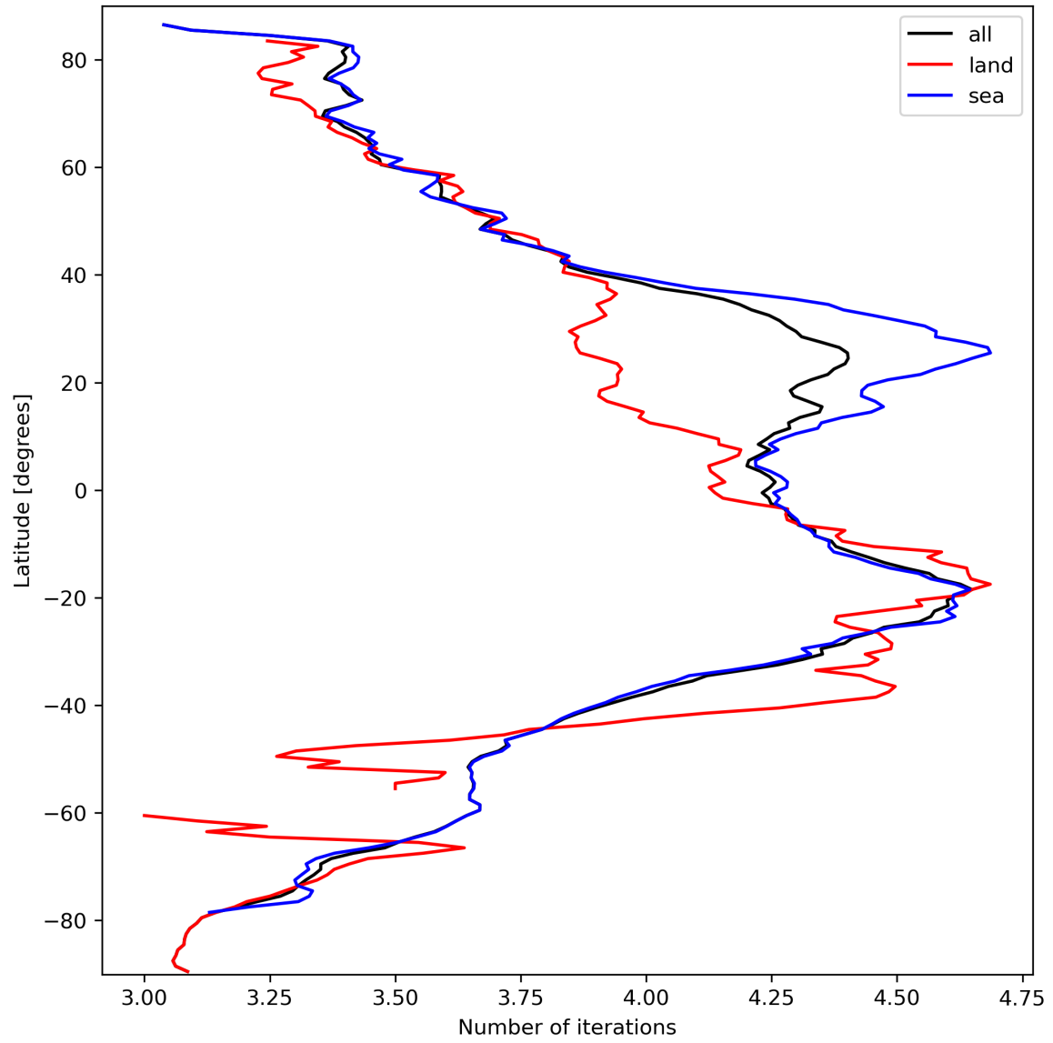
Figure 17: Zonal average of “Number of iterations” for 2023-09-27 to 2023-09-29.
