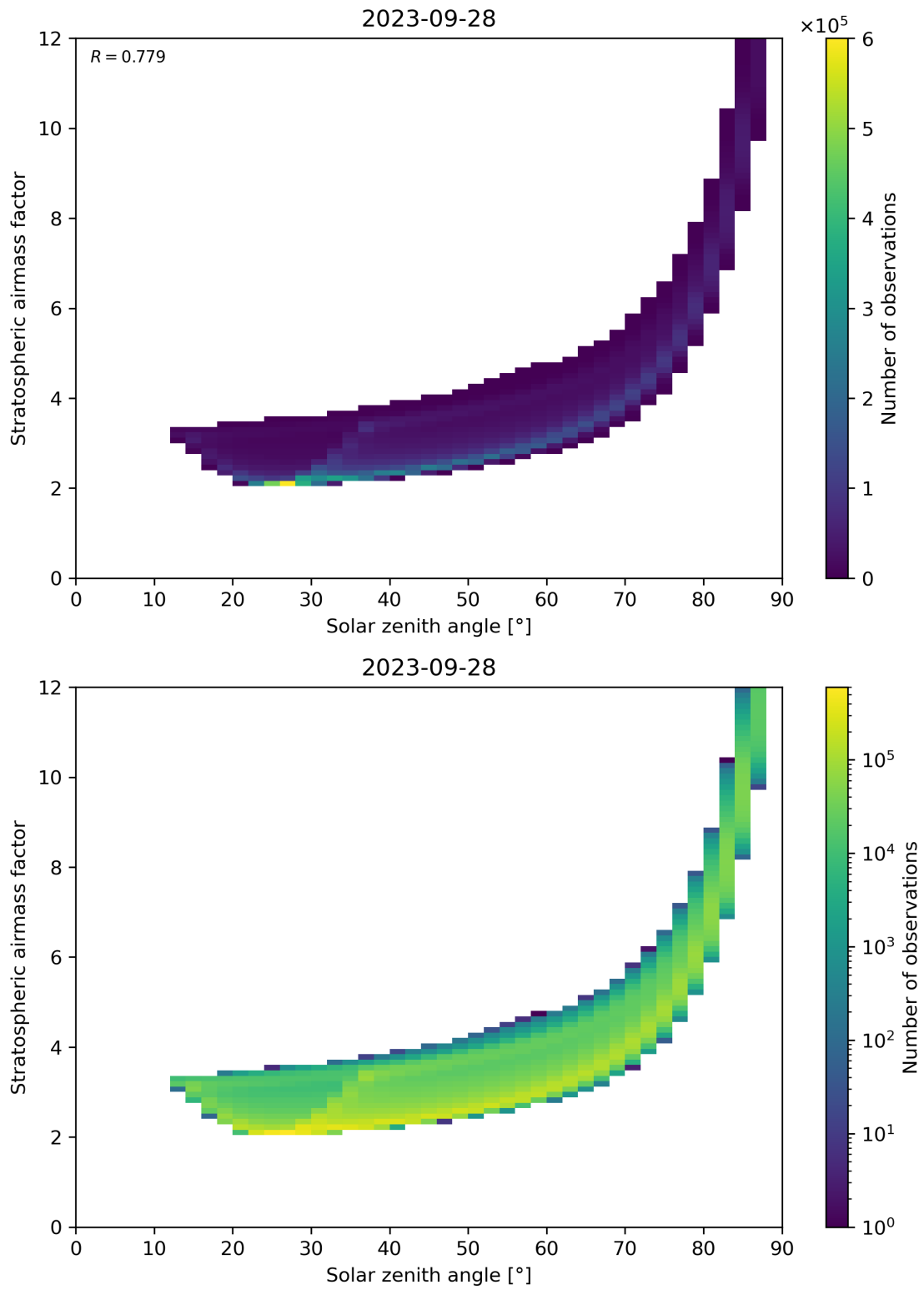
Figure 145: Scatter density plot of “Solar zenith angle” against “Stratospheric airmass factor” for 2023-09-27 to 2023-09-29.
