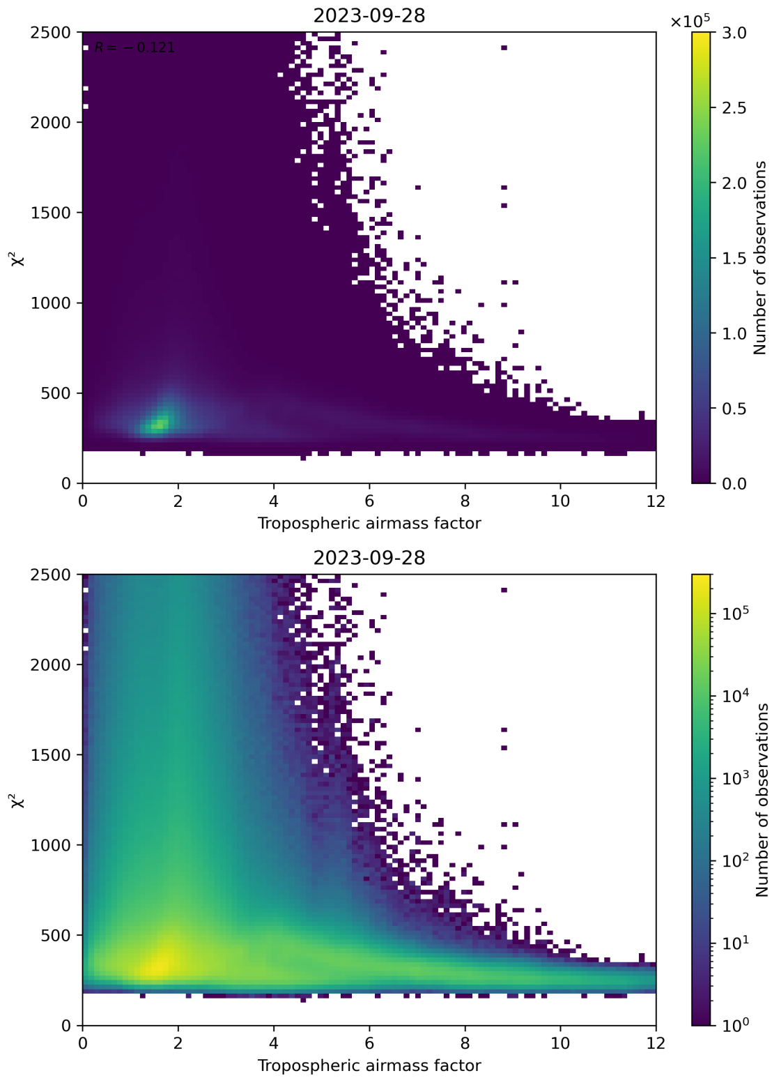
Figure 73: Scatter density plot of “Tropospheric airmass factor” against “ \chi^2 ” for 2023-09-27 to 2023-09-29.
