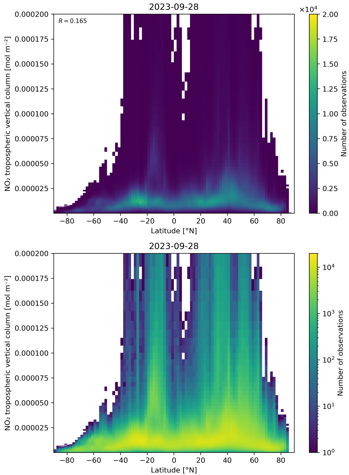
Figure 92: Scatter density plot of “Latitude” against “NO 2 tropospheric vertical column” for 2023-09-27 to 2023-09-29.
