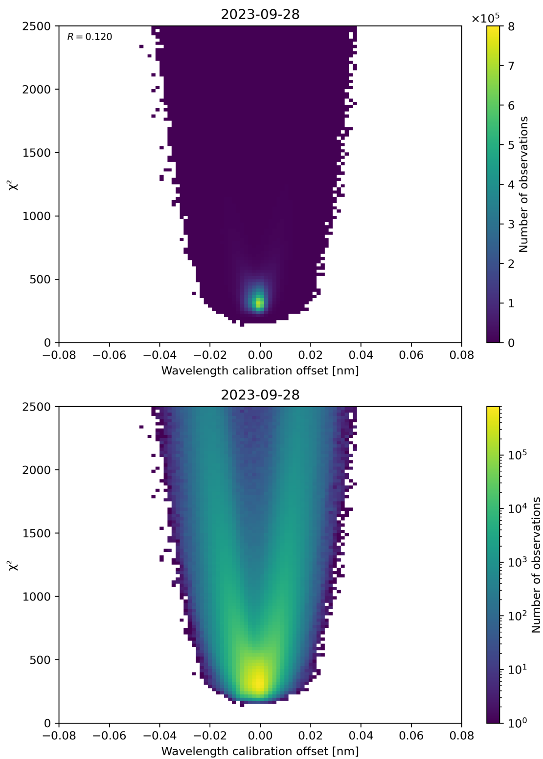
Figure 175: Scatter density plot of “Wavelength calibration offset” against “ \chi^2 ” for 2023-09-27 to 2023-09-29.
