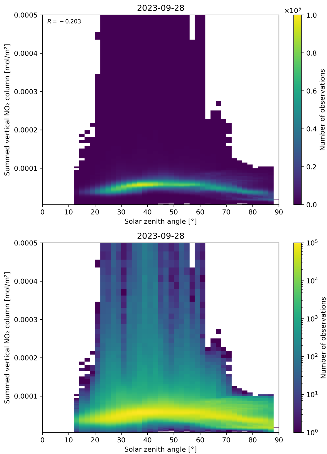
Figure 151: Scatter density plot of “Solar zenith angle” against “Summed vertical NO 2 column” for 2023-09-27 to 2023-09-29.
