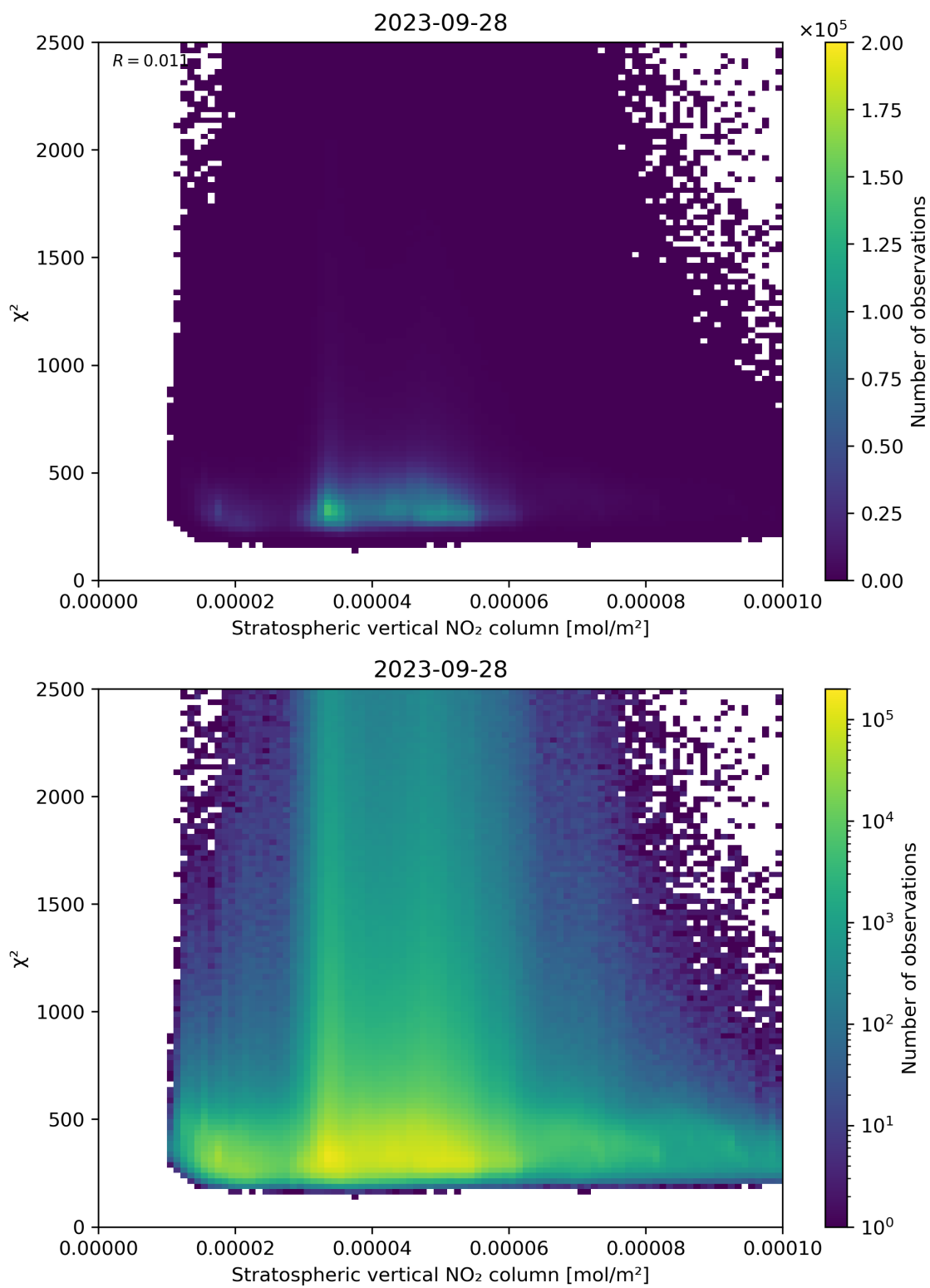
Figure 97: Scatter density plot of “Stratospheric vertical NO 2 column” against “ \chi^2 ” for 2023-09-27 to 2023-09-29.
