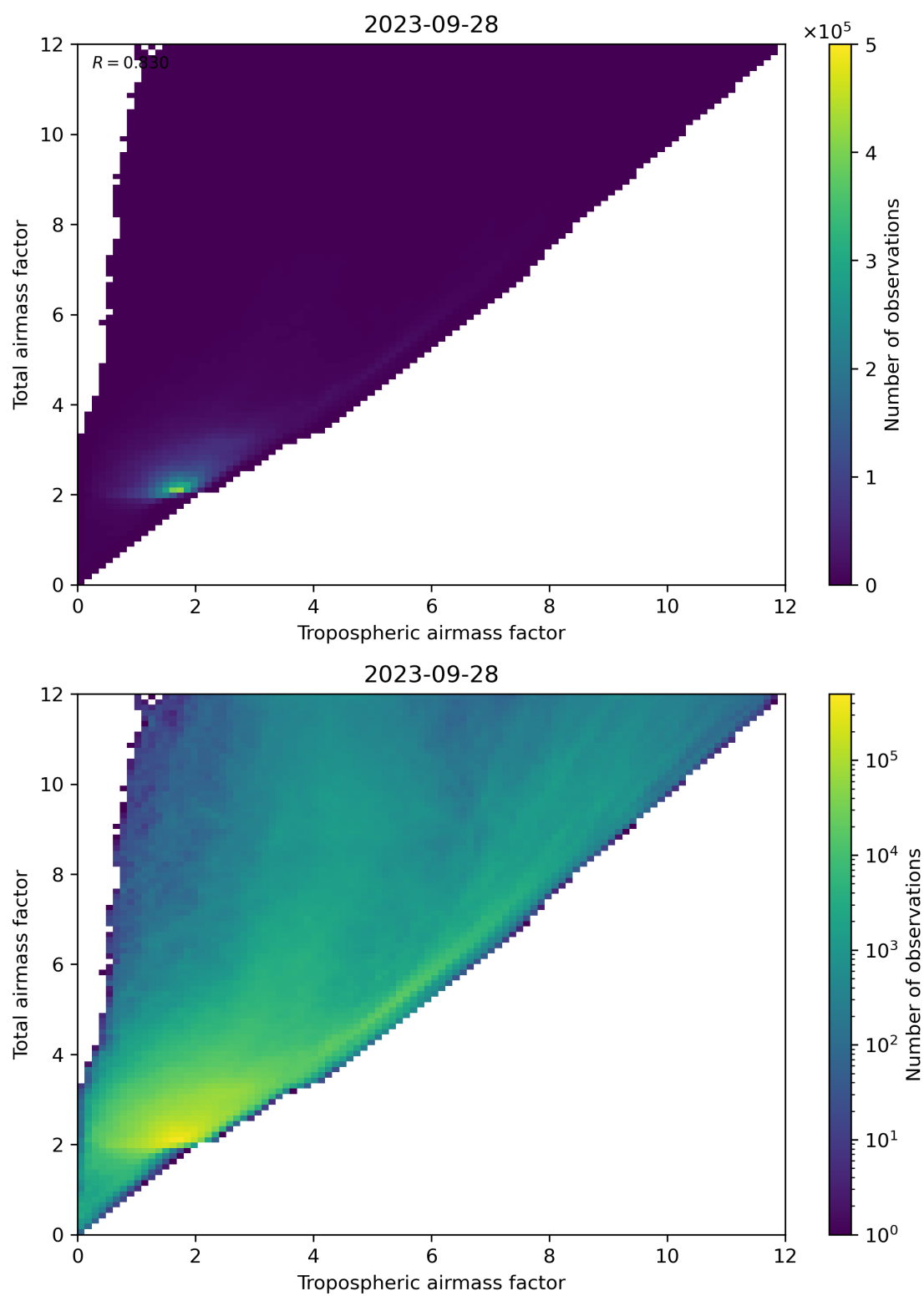
Figure 72: Scatter density plot of “Tropospheric airmass factor” against “Total airmass factor” for 2023-09-27 to 2023-09-29.
