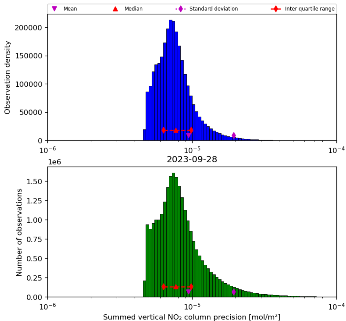
Figure 41: Histogram of “Summed vertical NO 2 column precision” for 2023-09-27 to 2023-09-29
