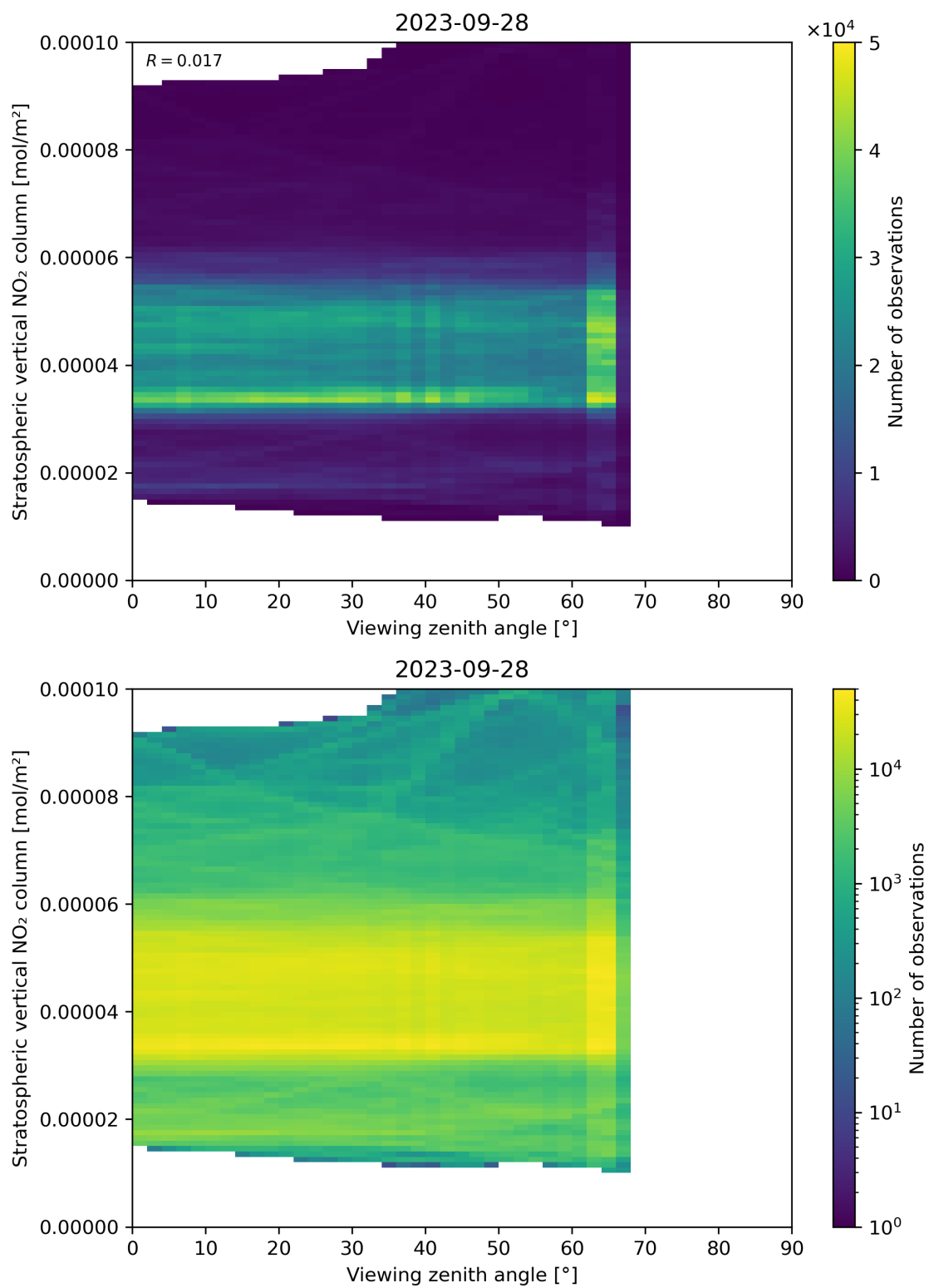
Figure 164: Scatter density plot of “Viewing zenith angle” against “Stratospheric vertical NO 2 column” for 2023-09-27 to 2023-09-29.
