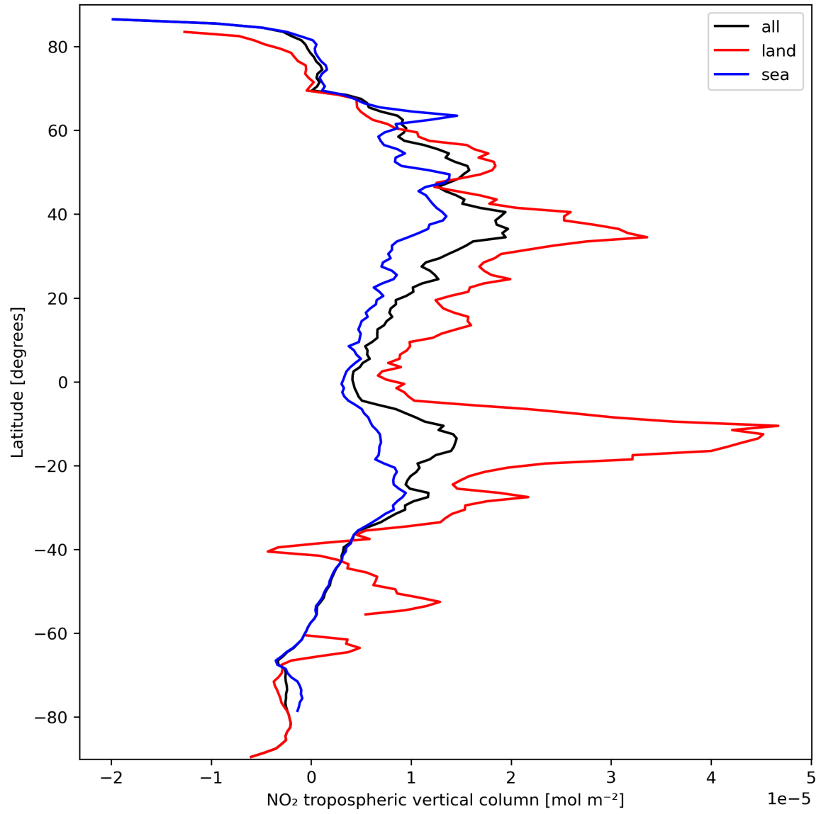
Figure 12: Zonal average of “NO 2 tropospheric vertical column” for 2023-09-27 to 2023-09-29.
