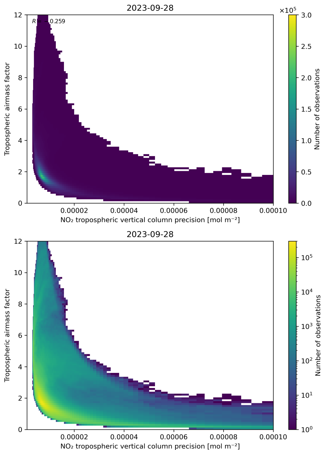
Figure 133: Scatter density plot of “NO 2 tropospheric vertical column precision” against “Tropospheric air mass factor” for 2023-09-27 to 2023-09-29.
