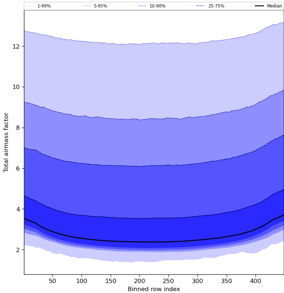
Figure 49: Along track statistics of “Total airmass factor” for 2023-09-27 to 2023-09-29
