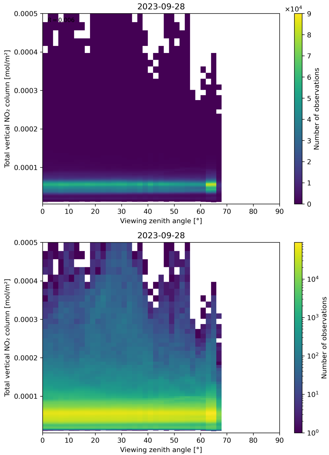
Figure 167: Scatter density plot of “Viewing zenith angle” against “Total vertical NO 2 column” for 2023-09-27 to 2023-09-29.
