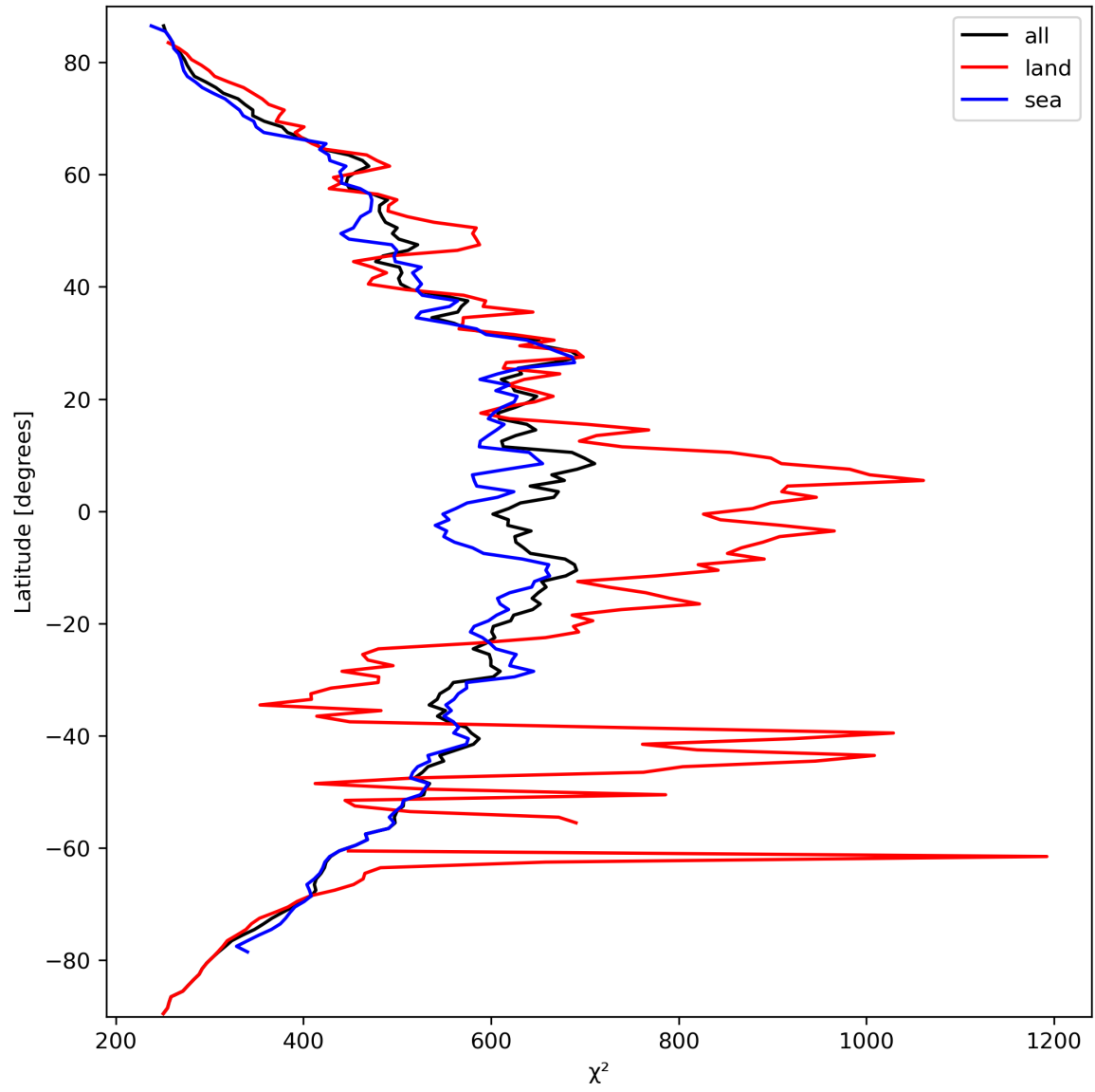
Figure 25: Zonal average of “ \chi^2 ” for 2023-09-27 to 2023-09-29.
