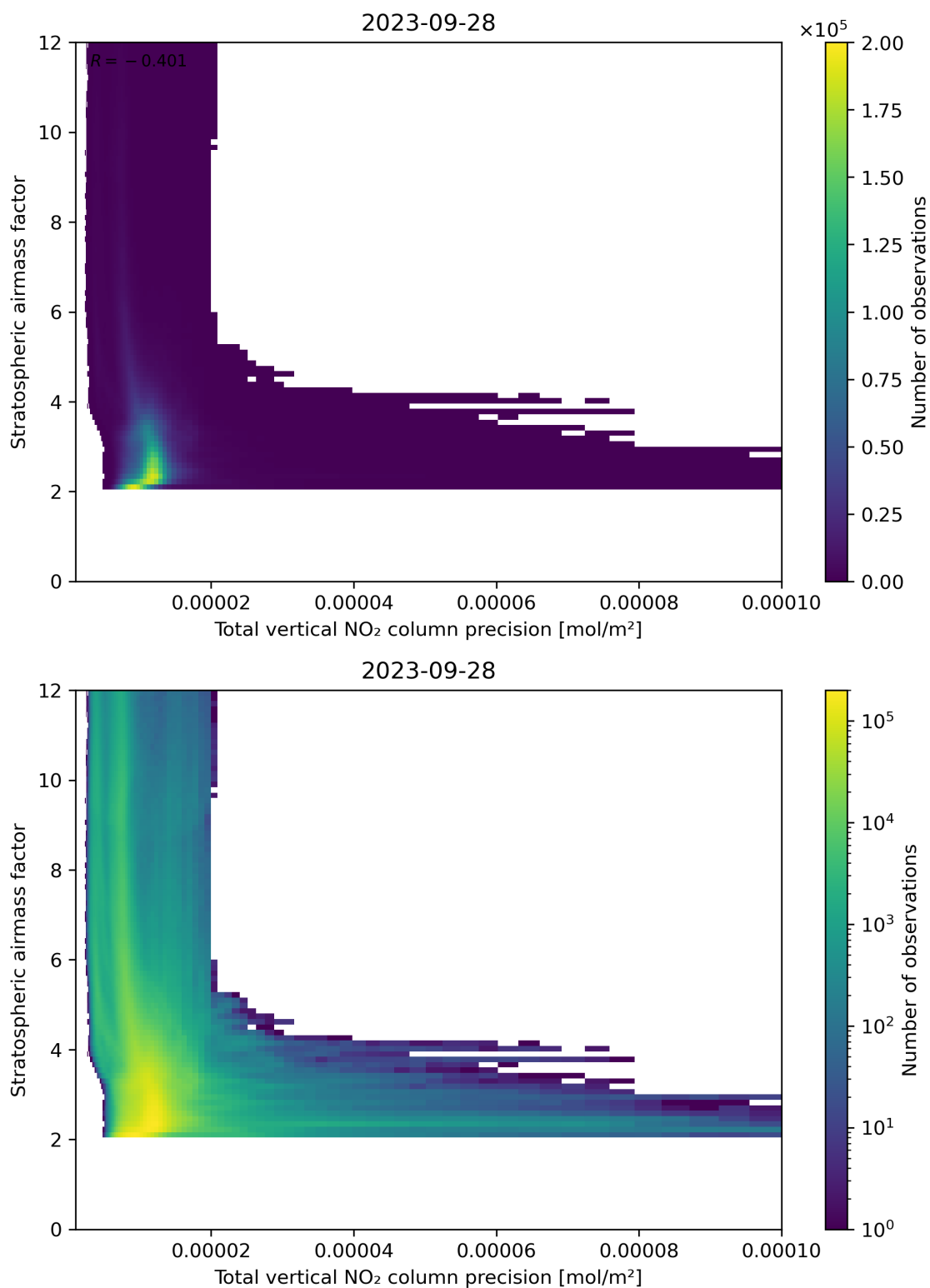
Figure 115: Scatter density plot of “Total vertical NO 2 column precision” against “Stratospheric airmass factor” for 2023-09-27 to 2023-09-29.
