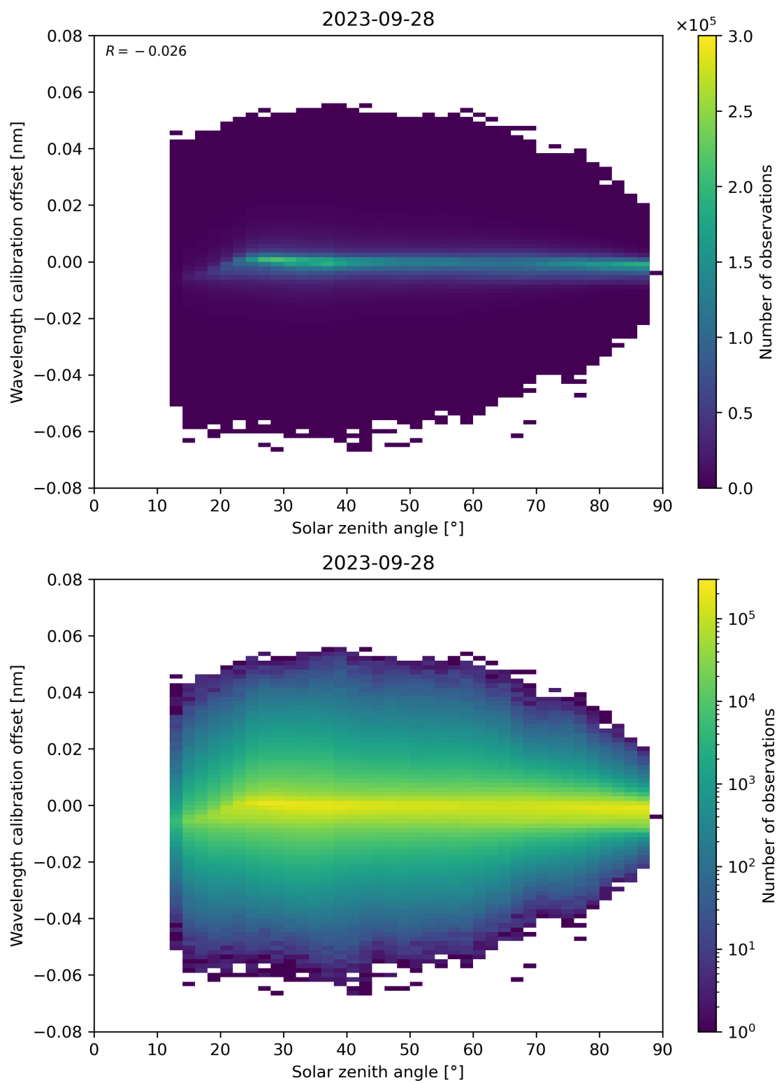
Figure 158: Scatter density plot of “Solar zenith angle” against “Wavelength calibration offset” for 2023-09-27 to 2023-09-29.
