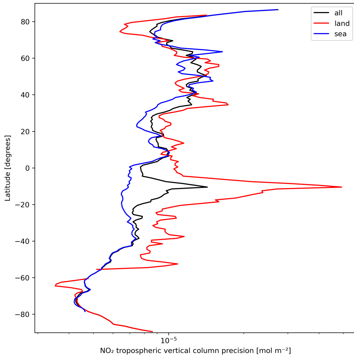
Figure 13: Zonal average of “NO 2 tropospheric vertical column precision” for 2023-09-27 to 2023-09-29.
