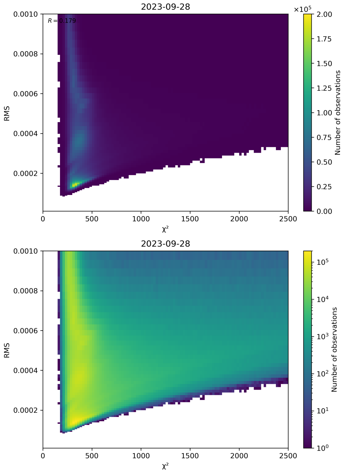
Figure 82: Scatter density plot of “ \chi^2 ” against “RMS” for 2023-09-27 to 2023-09-29.
