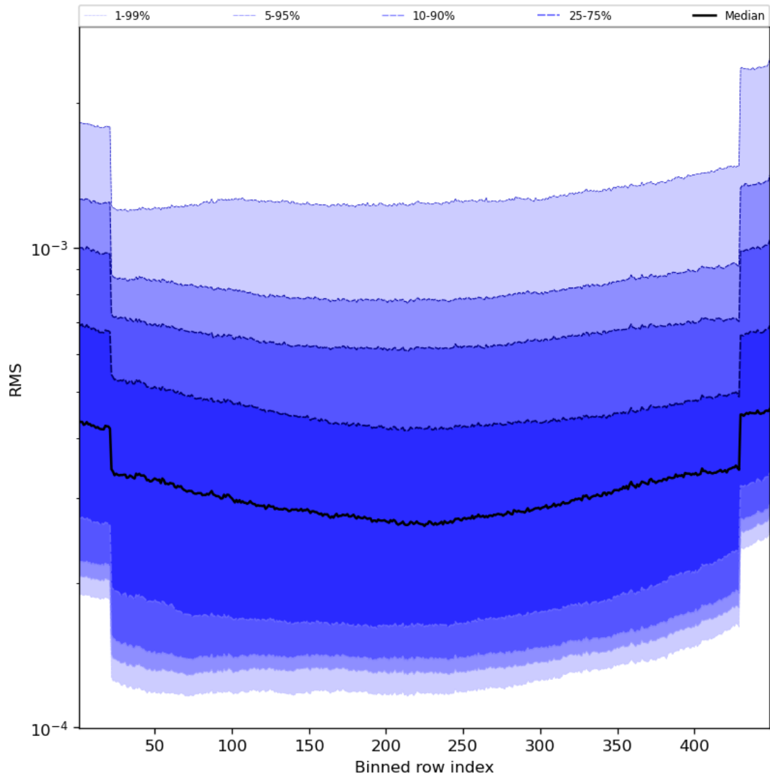
Figure 60: Along track statistics of “RMS” for 2023-09-27 to 2023-09-29
