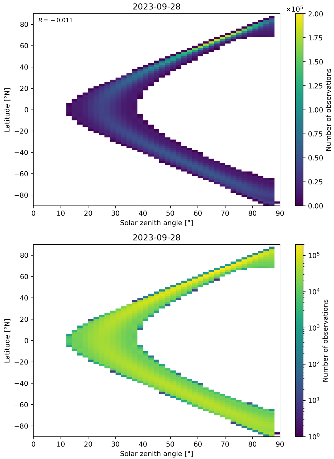
Figure 149: Scatter density plot of “Solar zenith angle” against “Latitude” for 2023-09-27 to 2023-09-29.
