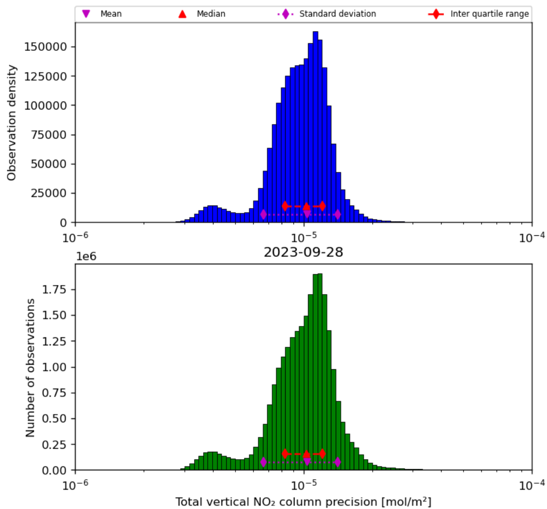
Figure 39: Histogram of "Total vertical NO 2 column precision" for 2023-09-27 to 2023-09-29
