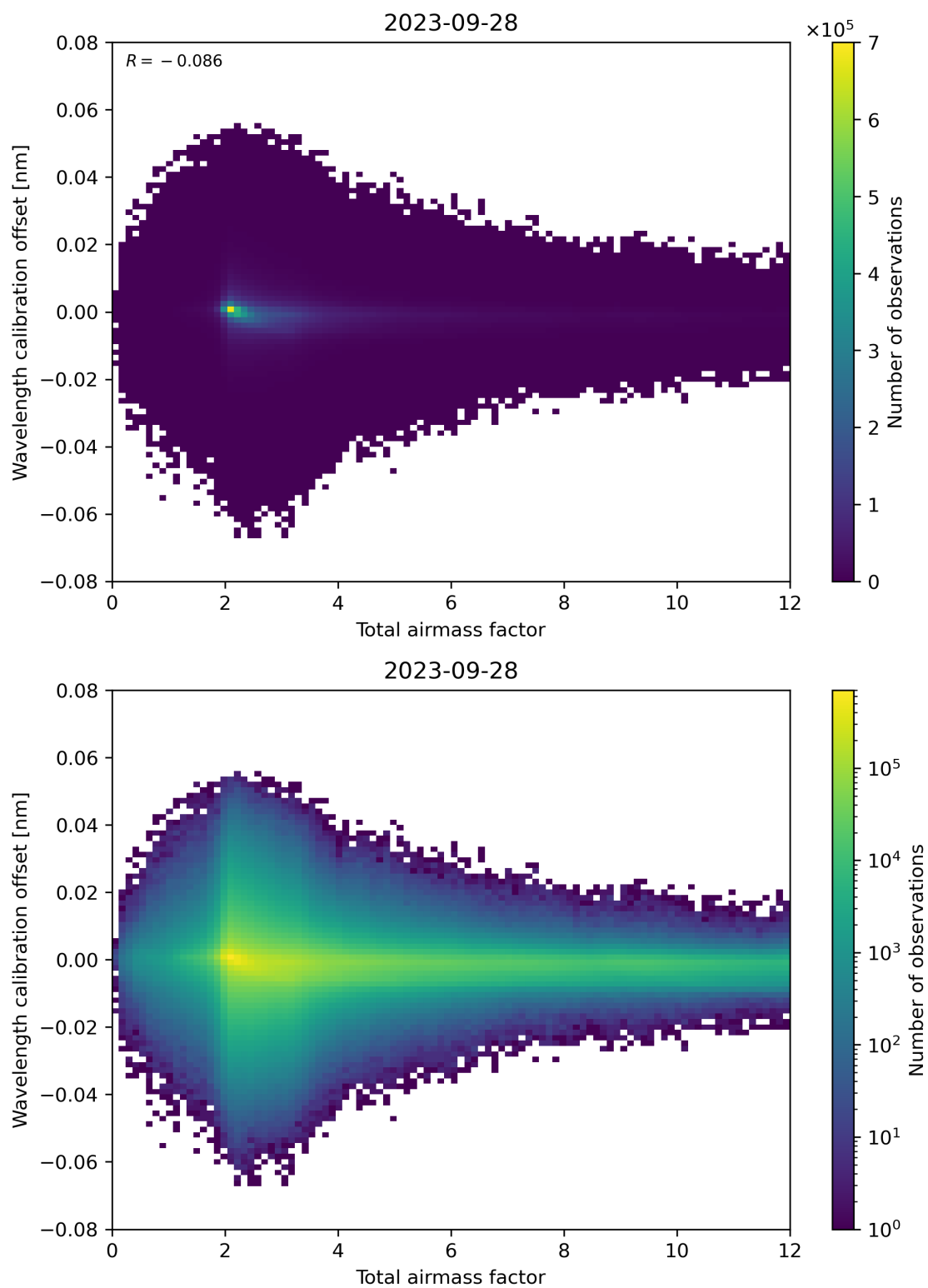
Figure 70: Scatter density plot of “Total airmass factor” against “Wavelength calibration offset” for 2023-09-27 to 2023-09-29.
