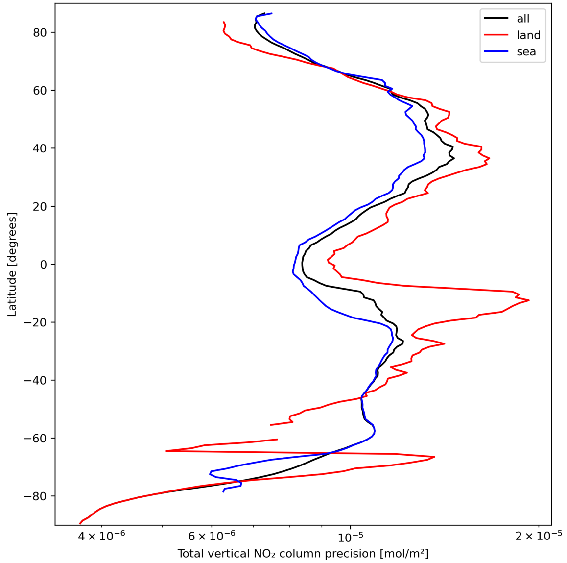
Figure 22: Zonal average of "Total vertical NO 2 column precision" for 2023-09-27 to 2023-09-29.
