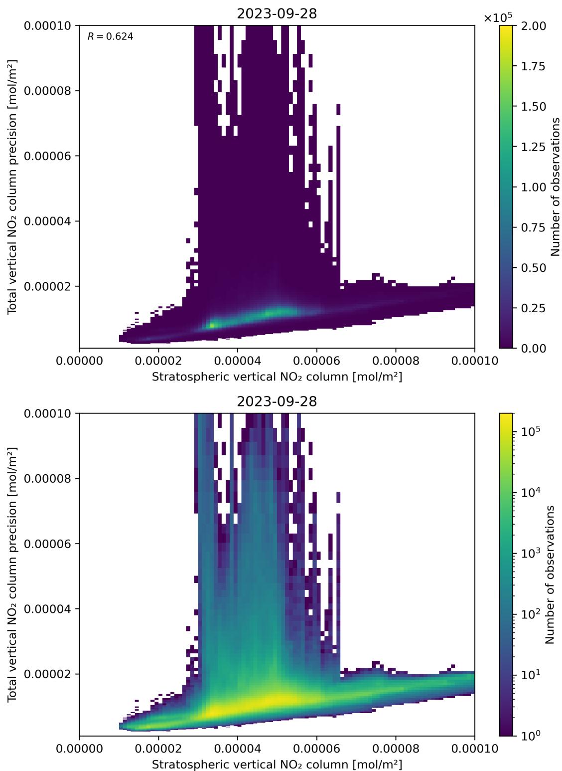
Figure 101: Scatter density plot of “Stratospheric vertical NO 2 column” against “Total vertical NO 2 column precision” for 2023-09-27 to 2023-09-29.
