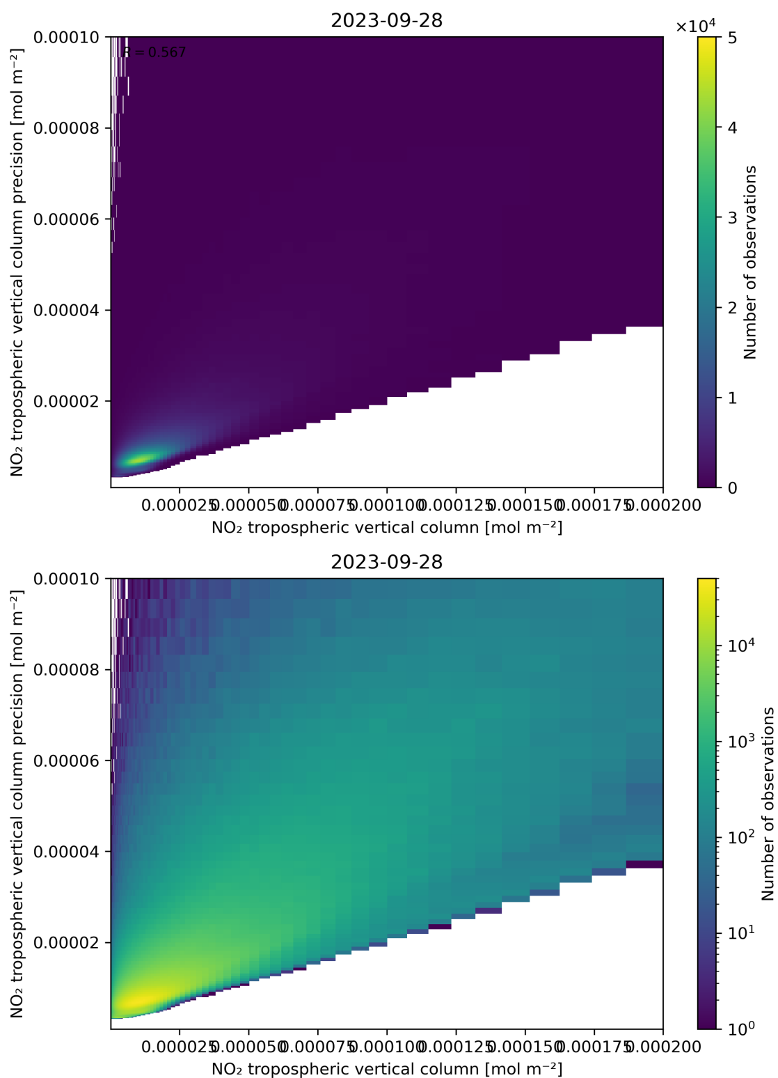
Figure 130: Scatter density plot of “NO 2 tropospheric vertical column” against “NO 2 tropospheric vertical column precision” for 2023-09-27 to 2023-09-29.
