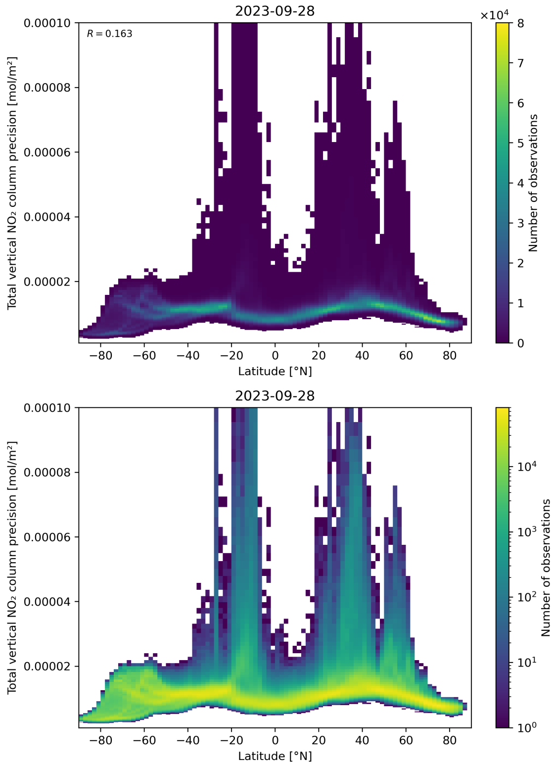
Figure 91: Scatter density plot of “Latitude” against “Total vertical NO 2 column precision” for 2023-09-27 to 2023-09-29.
