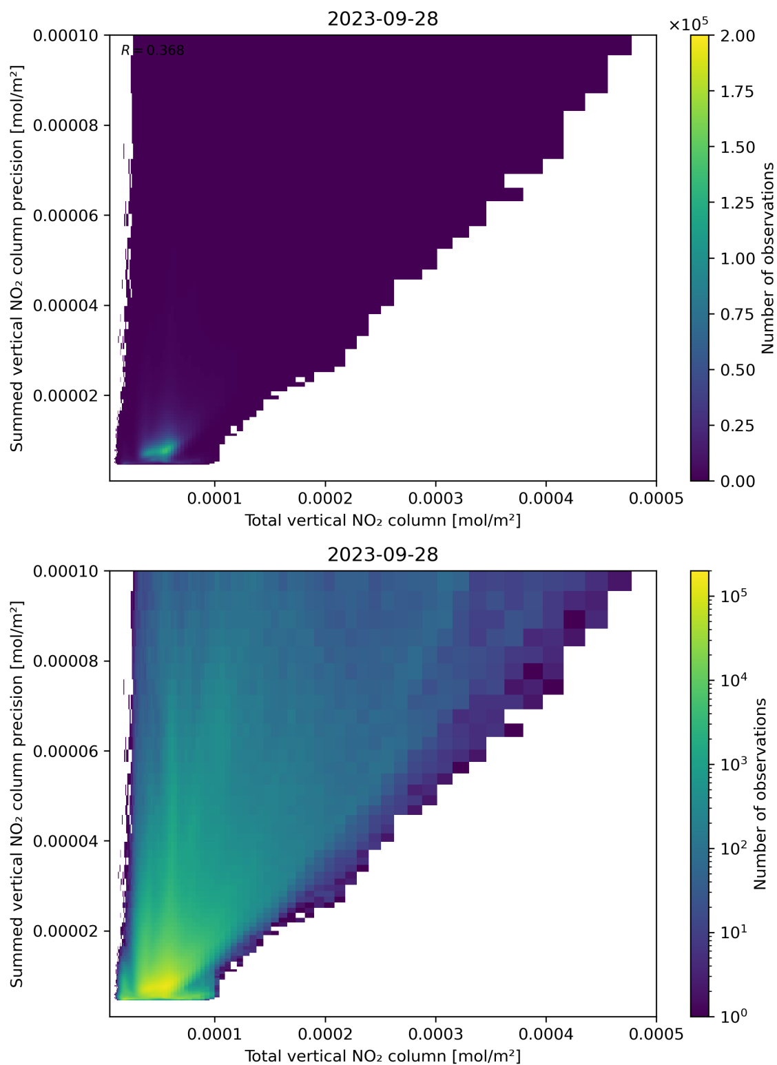
Figure 113: Scatter density plot of “Total vertical NO 2 column” against “Summed vertical NO 2 column precision” for 2023-09-27 to 2023-09-29.
