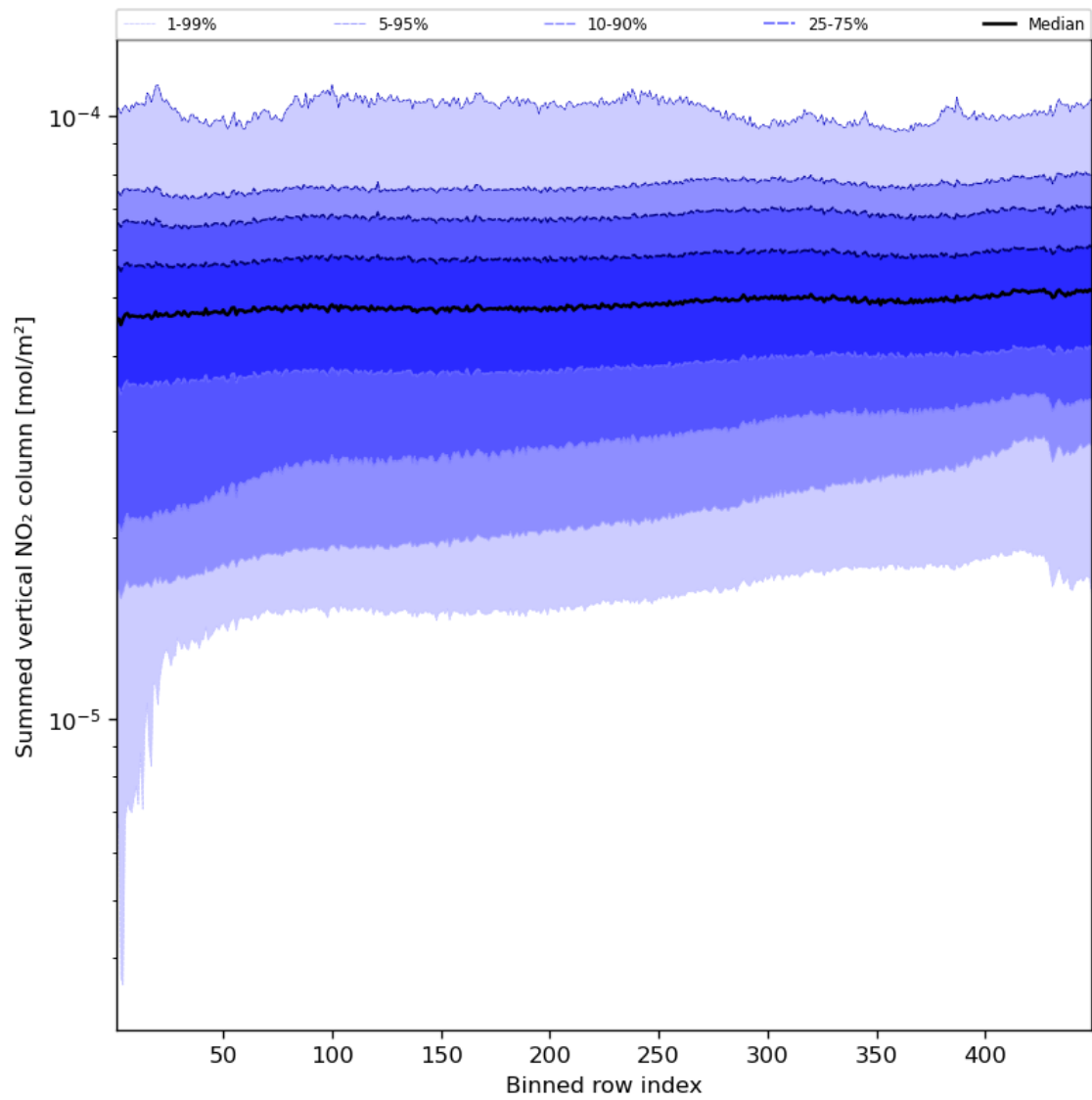
Figure 57: Along track statistics of “Summed vertical NO 2 column” for 2023-09-27 to 2023-09-29
