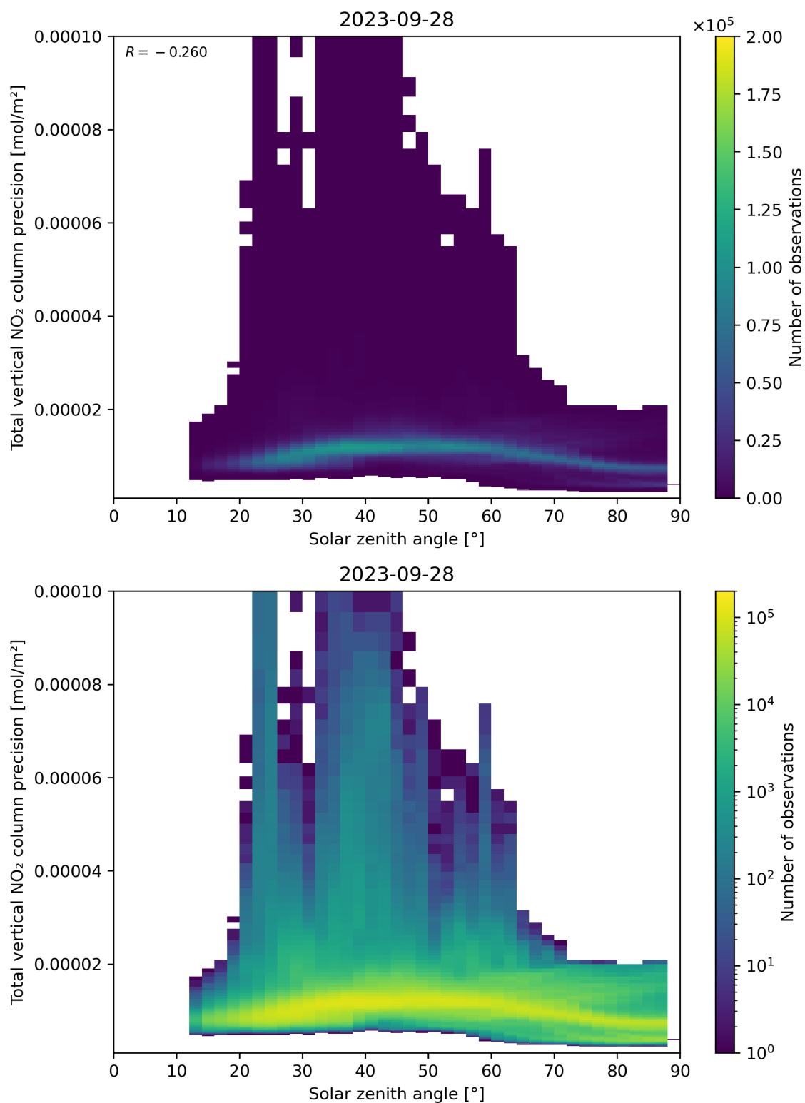
Figure 154: Scatter density plot of “Solar zenith angle” against “Total vertical NO 2 column precision” for 2023-09-27 to 2023-09-29.
