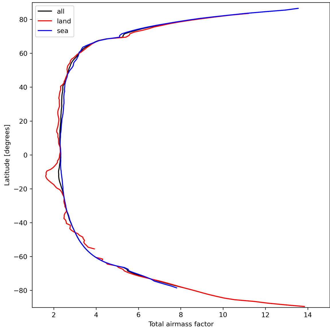
Figure 15: Zonal average of “Total airmass factor” for 2023-09-27 to 2023-09-29.
