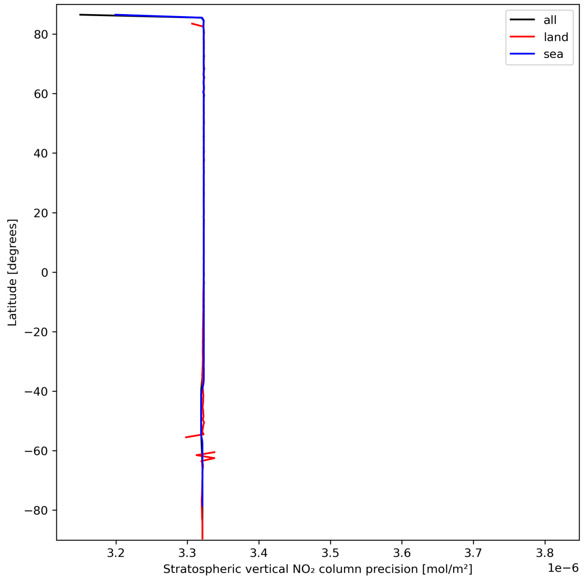
Figure 20: Zonal average of “Stratospheric vertical NO 2 column precision” for 2023-09-27 to 2023-09-29.
