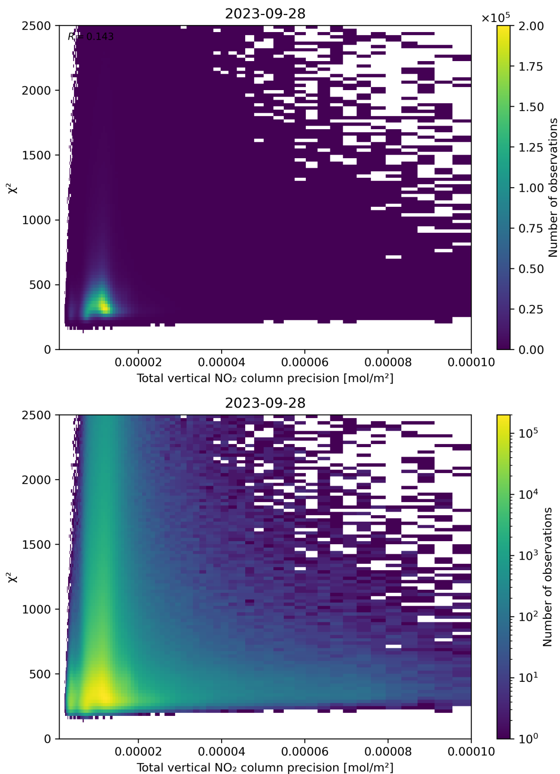
Figure 116: Scatter density plot of “Total vertical NO 2 column precision” against “ \chi^2 ” for 2023-09-27 to 2023-09-29.
