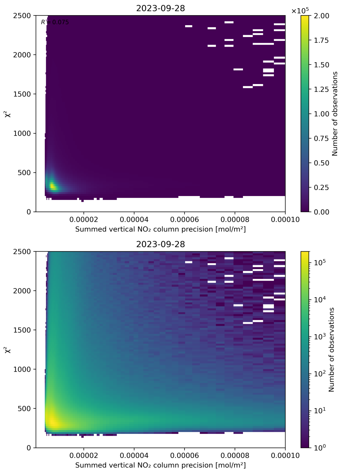
Figure 107: Scatter density plot of “Summed vertical NO 2 column precision” against “ \chi^2 ” for 2023-09-27 to 2023-09-29.
