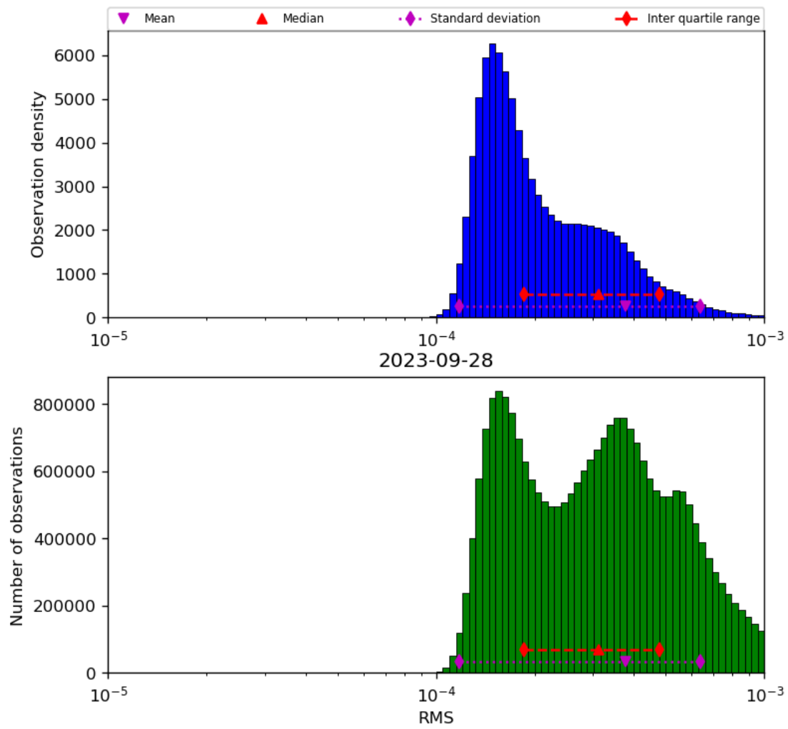
Figure 43: Histogram of “RMS” for 2023-09-27 to 2023-09-29
