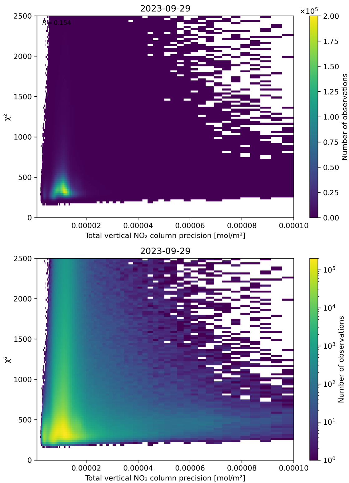
Figure 116: Scatter density plot of “Total vertical NO 2 column precision” against “ \chi^2 ” for 2023-09-28 to 2023-09-30.
