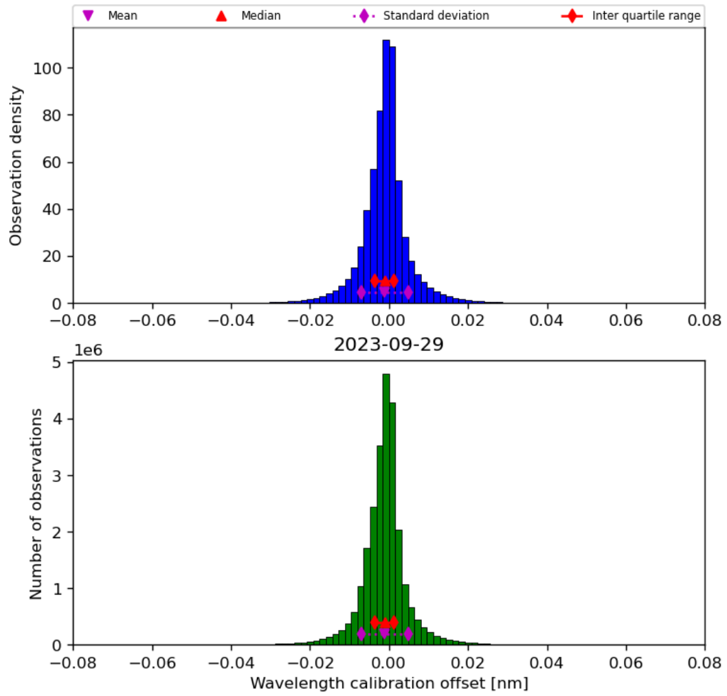
Figure 35: Histogram of “Wavelength calibration offset” for 2023-09-28 to 2023-09-30
