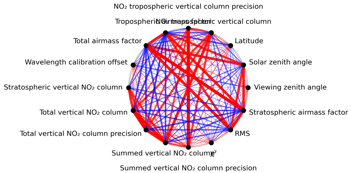
Figure 1: Map of correlation graph for 2023-09-28 to 2023-09-30.
