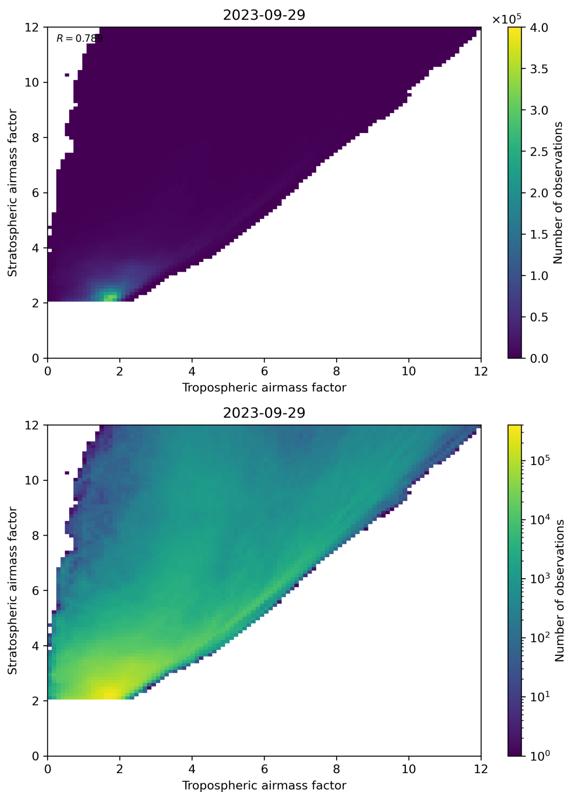
Figure 71: Scatter density plot of “Tropospheric airmass factor” against “Stratospheric airmass factor” for 2023-09-28 to 2023-09-30.
