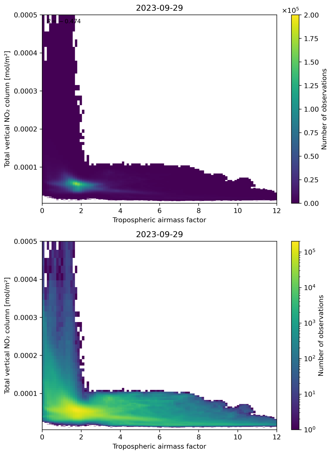
Figure 77: Scatter density plot of “Tropospheric airmass factor” against “Total vertical NO 2 column” for 2023-09-28 to 2023-09-30.
