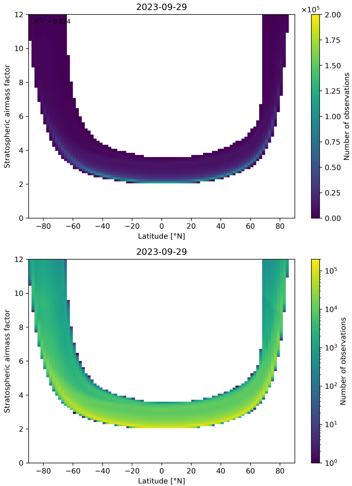
Figure 83: Scatter density plot of “Latitude” against “Stratospheric airmass factor” for 2023-09-28 to 2023-09-30.
