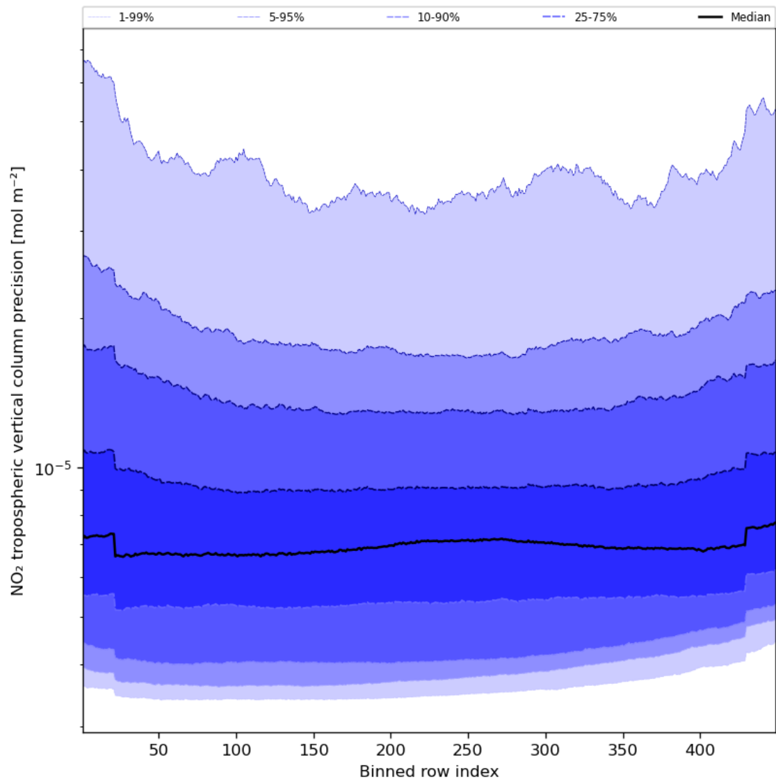
Figure 47: Along track statistics of “NO 2 tropospheric vertical column precision” for 2023-09-28 to 2023-09-30
