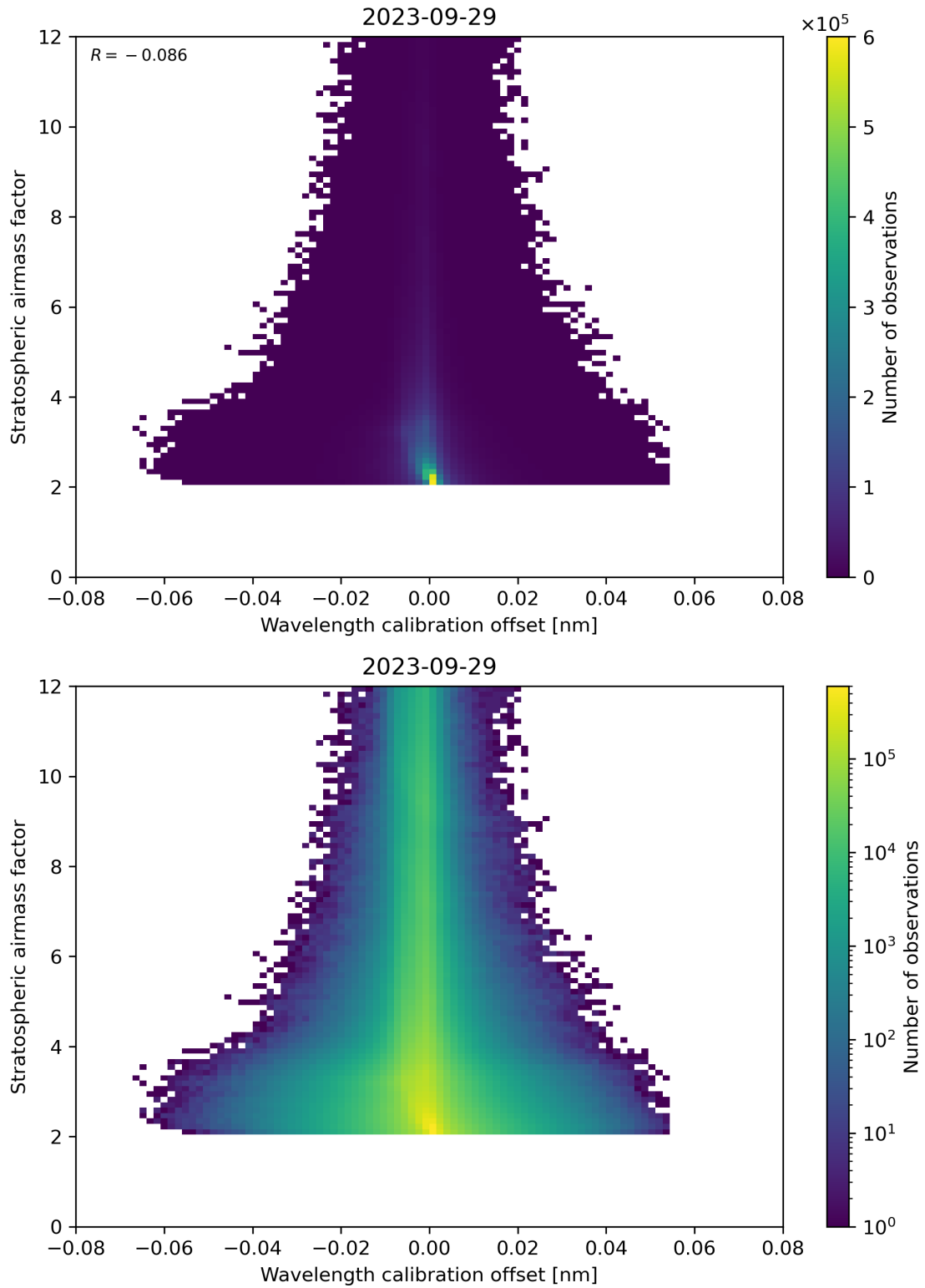
Figure 174: Scatter density plot of “Wavelength calibration offset” against “Stratospheric airmass factor” for 2023-09-28 to 2023-09-30.
