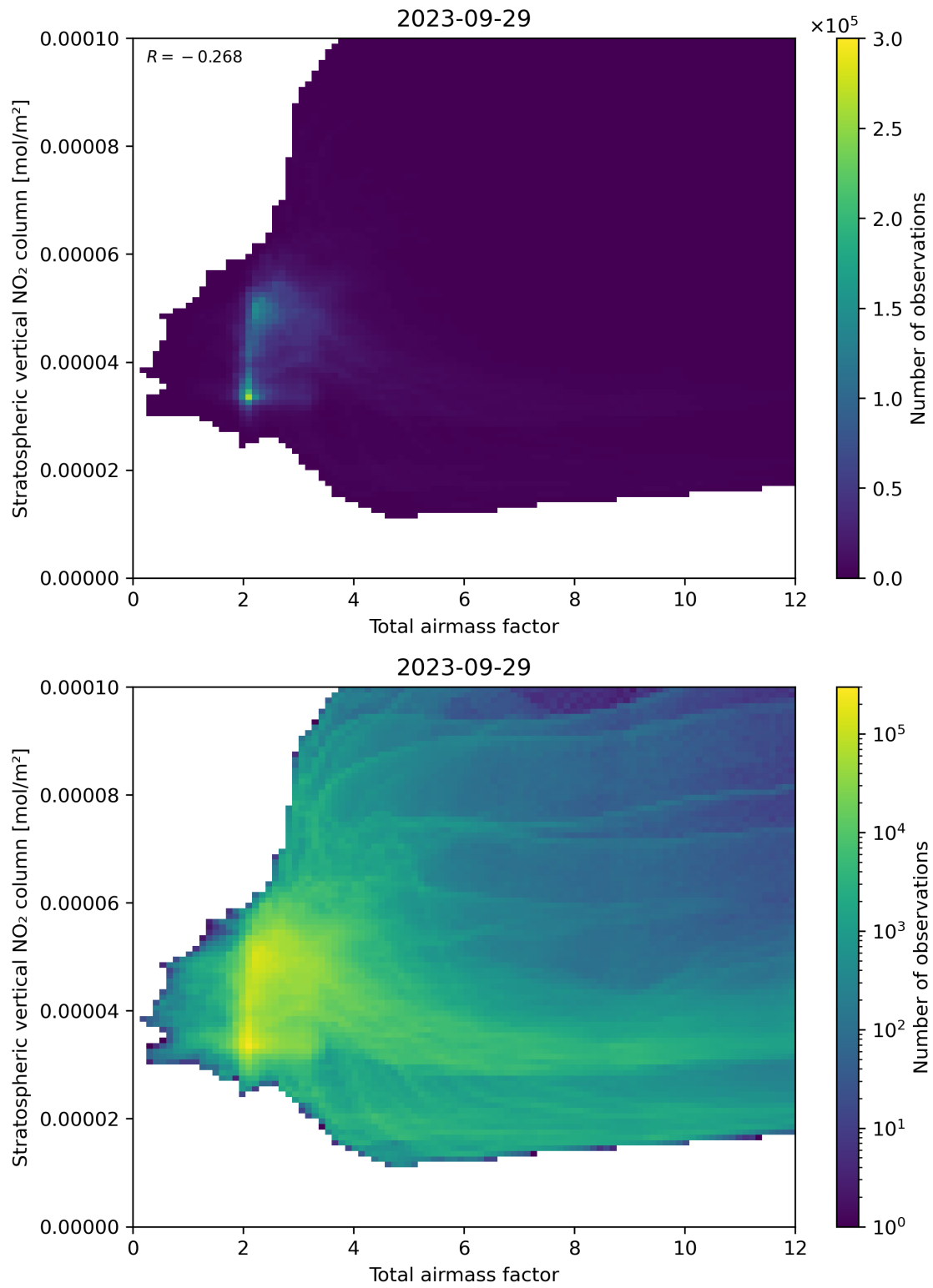
Figure 64: Scatter density plot of “Total airmass factor” against “Stratospheric vertical NO 2 column” for 2023-09-28 to 2023-09-30.
