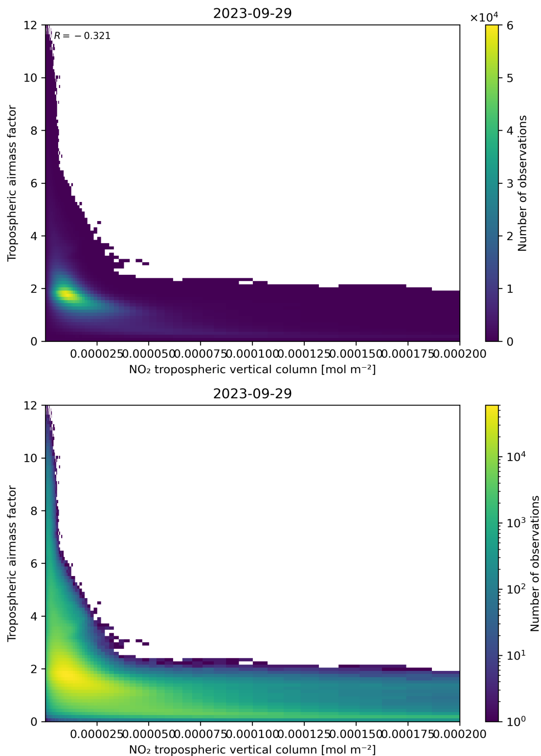
Figure 123: Scatter density plot of “NO 2 tropospheric vertical column” against “Tropospheric airmass factor” for 2023-09-28 to 2023-09-30.
