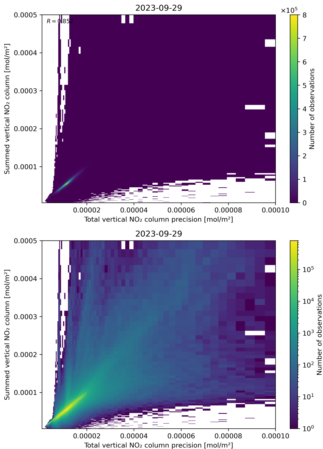
Figure 117: Scatter density plot of “Total vertical NO 2 column precision” against “Summed vertical NO 2 column” for 2023-09-28 to 2023-09-30.
