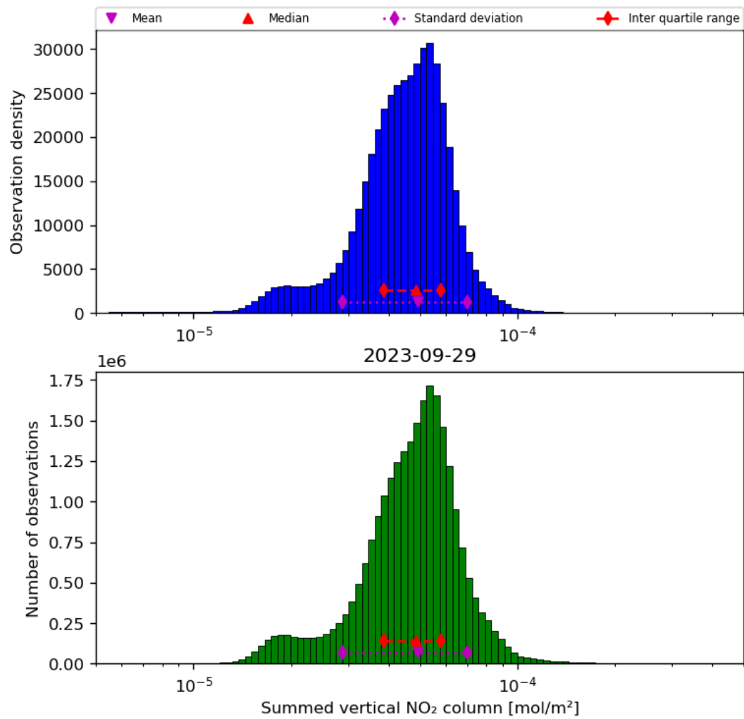
Figure 40: Histogram of “Summed vertical NO 2 column” for 2023-09-28 to 2023-09-30
