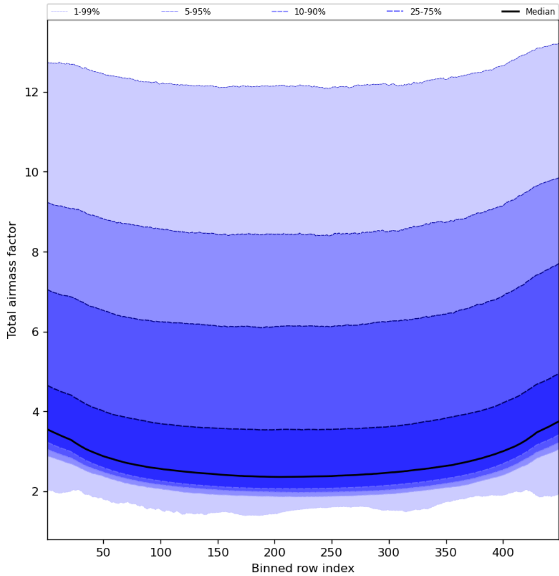
Figure 49: Along track statistics of “Total airmass factor” for 2023-09-28 to 2023-09-30
