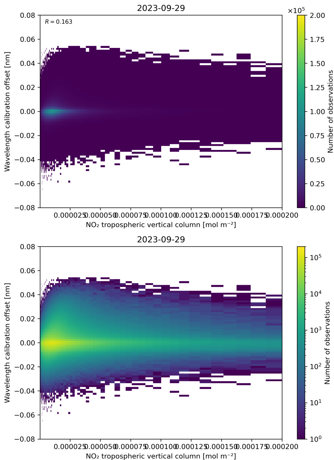
Figure 143: Scatter density plot of “NO 2 tropospheric vertical column” against “Wavelength calibration offset” for 2023-09-28 to 2023-09-30.
