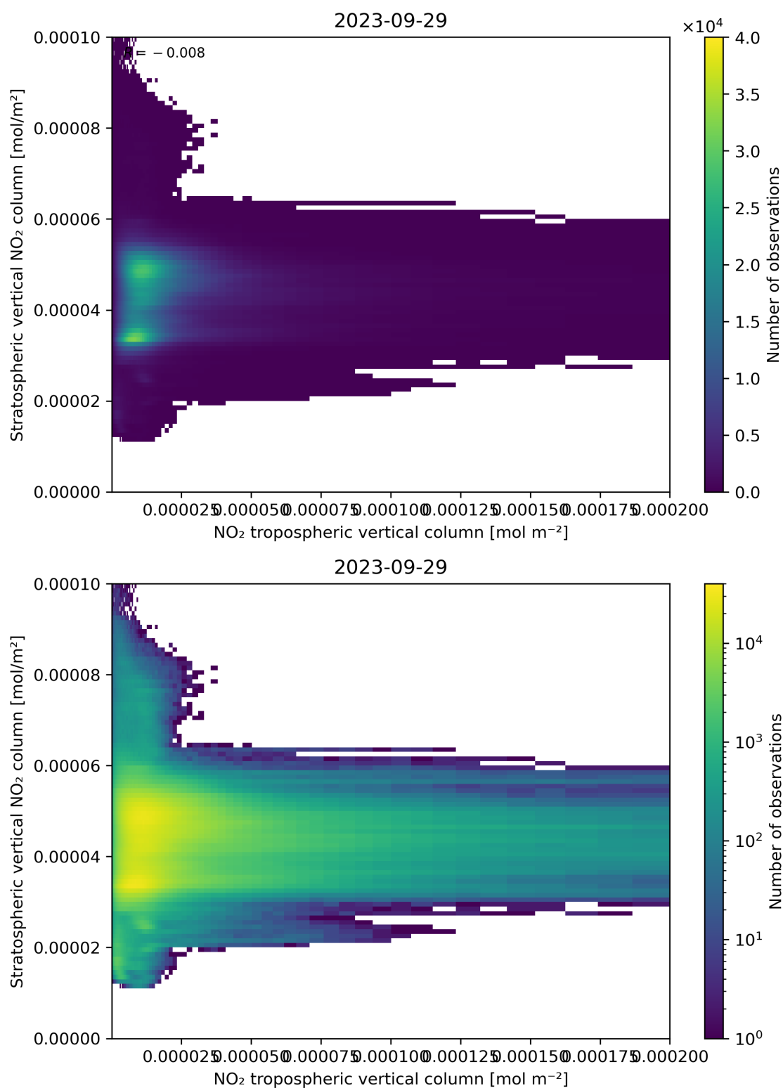
Figure 125: Scatter density plot of “NO 2 tropospheric vertical column” against “Stratospheric vertical NO 2 column” for 2023-09-28 to 2023-09-30.
