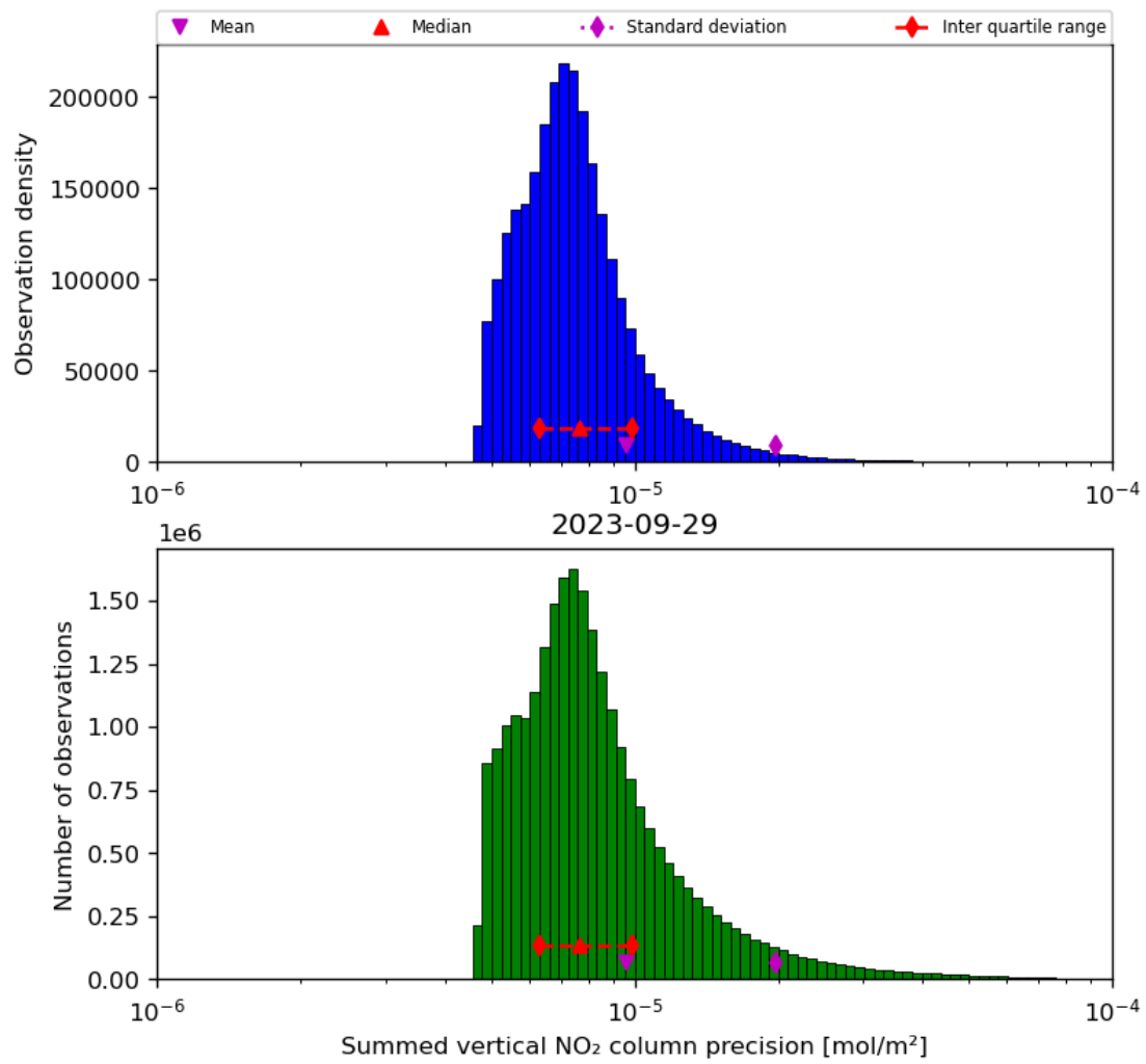
Figure 41: Histogram of “Summed vertical NO 2 column precision” for 2023-09-28 to 2023-09-30
