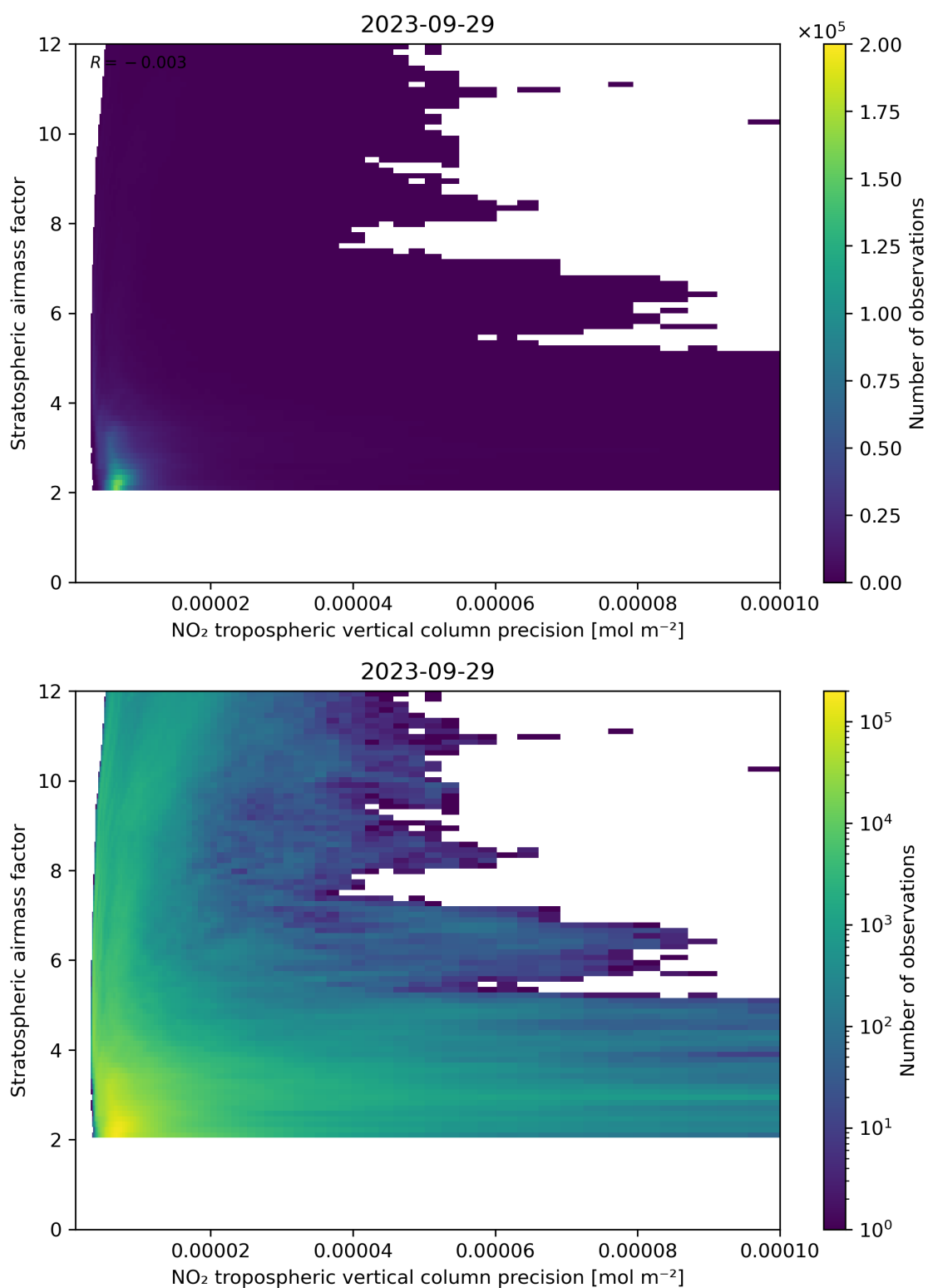
Figure 131: Scatter density plot of “NO 2 tropospheric vertical column precision” against “Stratospheric airmass factor” for 2023-09-28 to 2023-09-30.
