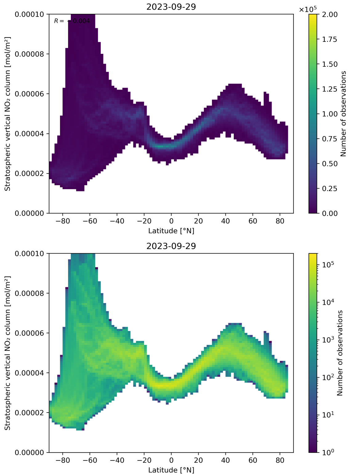
Figure 87: Scatter density plot of “Latitude” against “Stratospheric vertical NO 2 column” for 2023-09-28 to 2023-09-30.
