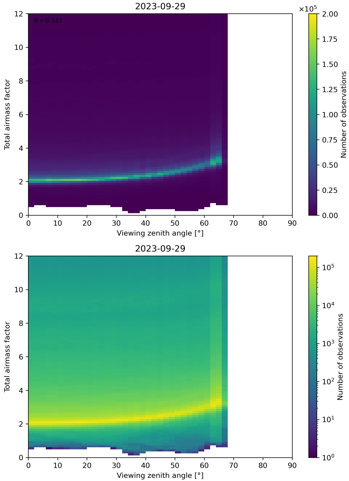
Figure 160: Scatter density plot of “Viewing zenith angle” against “Total airmass factor” for 2023-09-28 to 2023-09-30.
