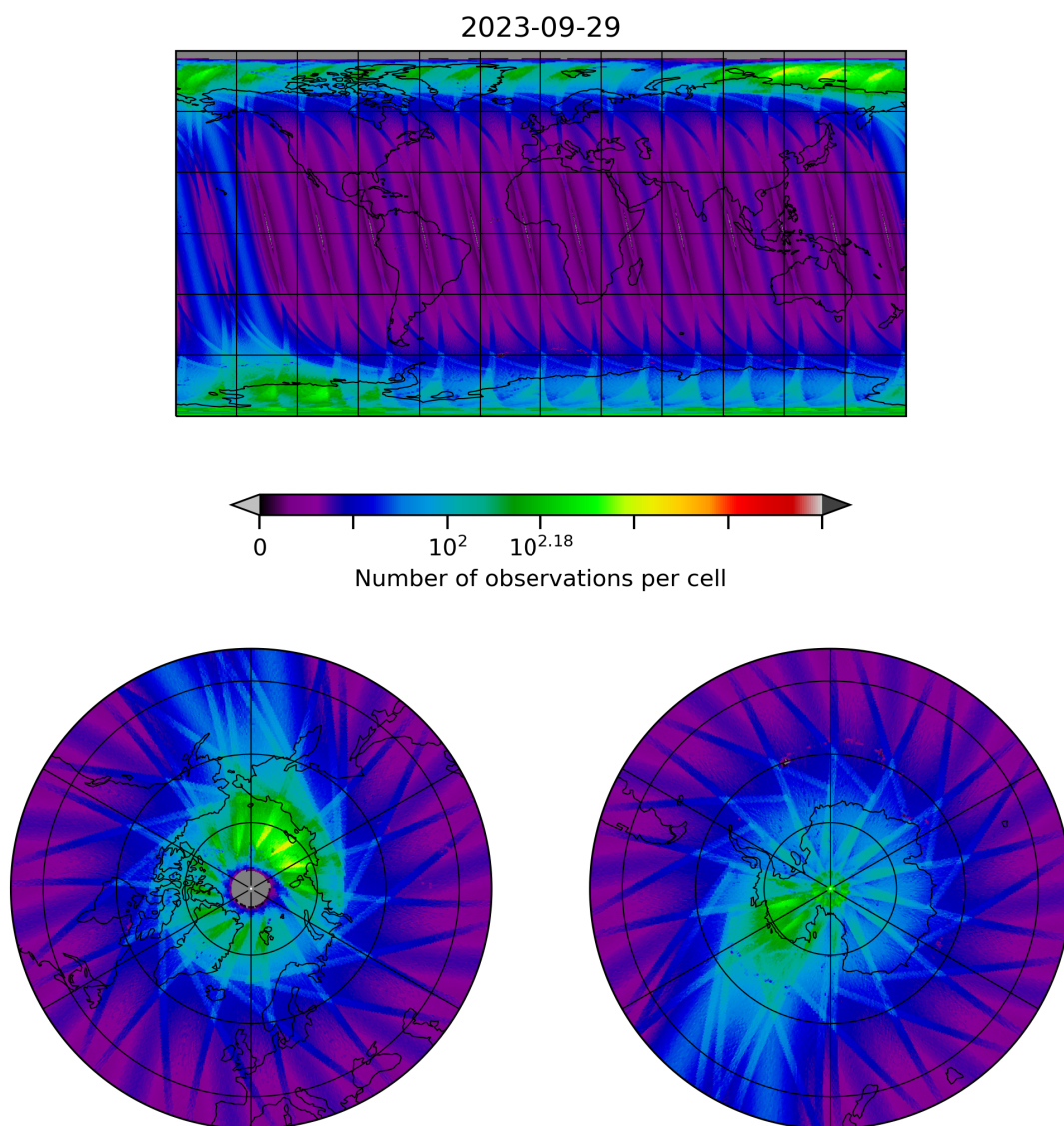
Figure 10: Map of the number of observations for 2023-09-28 to 2023-09-30
