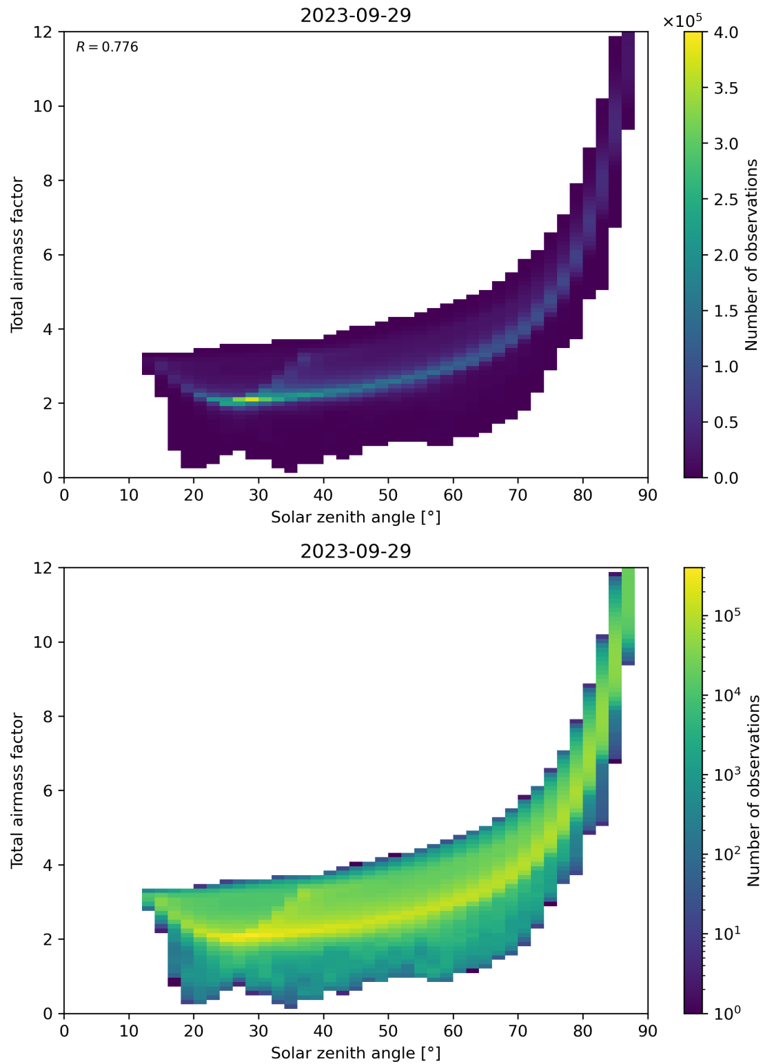
Figure 146: Scatter density plot of “Solar zenith angle” against “Total airmass factor” for 2023-09-28 to 2023-09-30.
