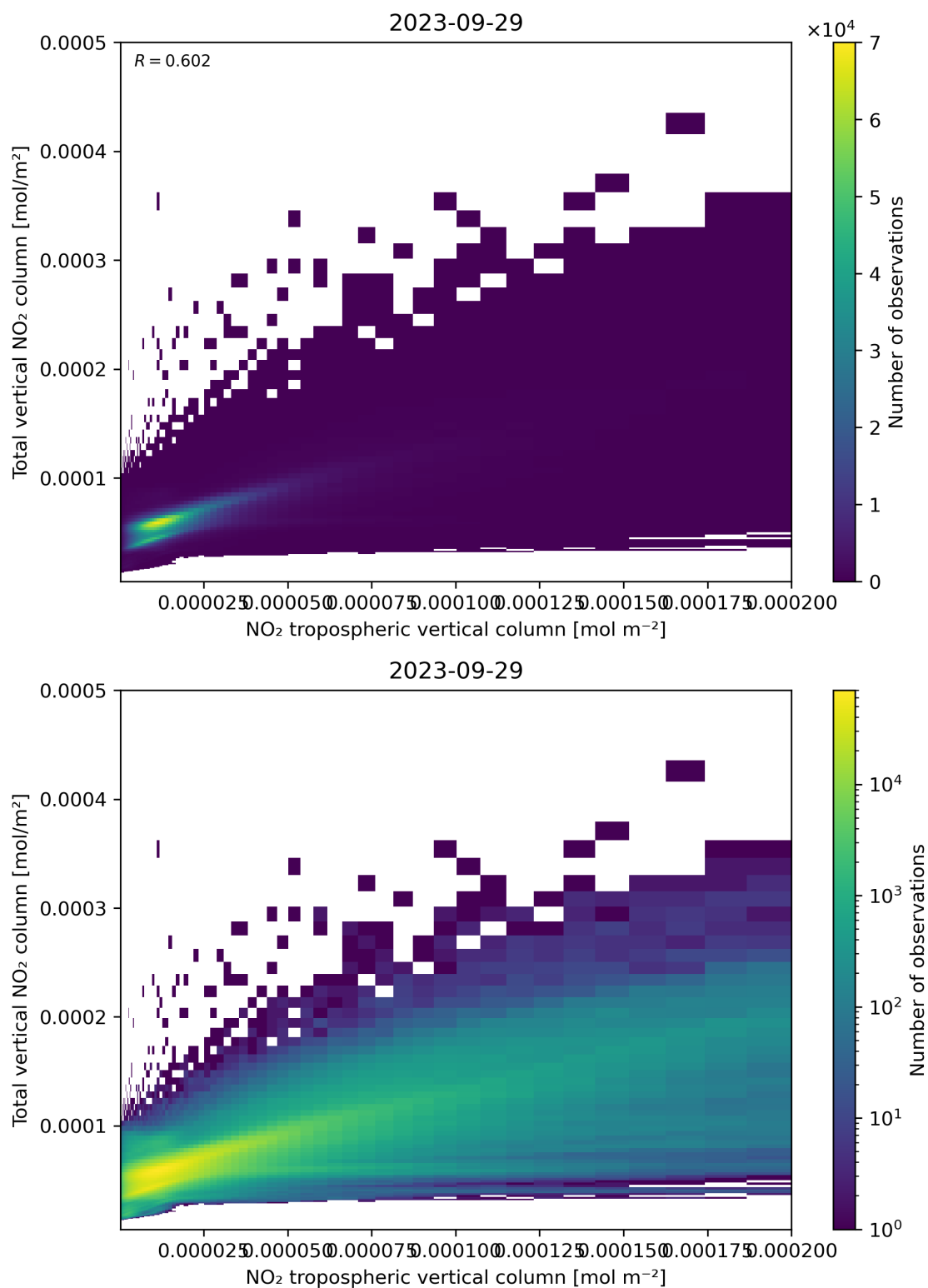
Figure 128: Scatter density plot of “NO 2 tropospheric vertical column” against “Total vertical NO 2 column” for 2023-09-28 to 2023-09-30.
