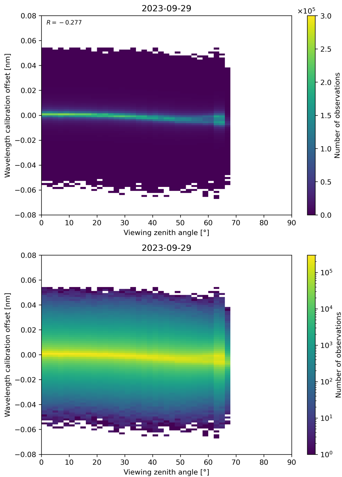
Figure 173: Scatter density plot of “Viewing zenith angle” against “Wavelength calibration offset” for 2023-09-28 to 2023-09-30.
