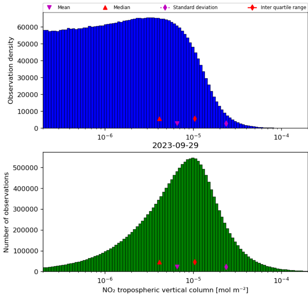
Figure 29: Histogram of “NO 2 tropospheric vertical column” for 2023-09-28 to 2023-09-30
