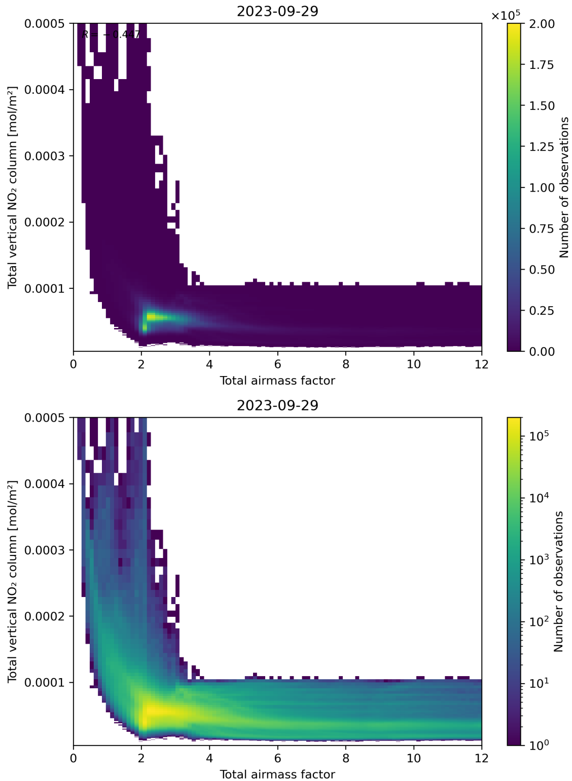
Figure 67: Scatter density plot of “Total airmass factor” against “Total vertical NO 2 column” for 2023-09-28 to 2023-09-30.
