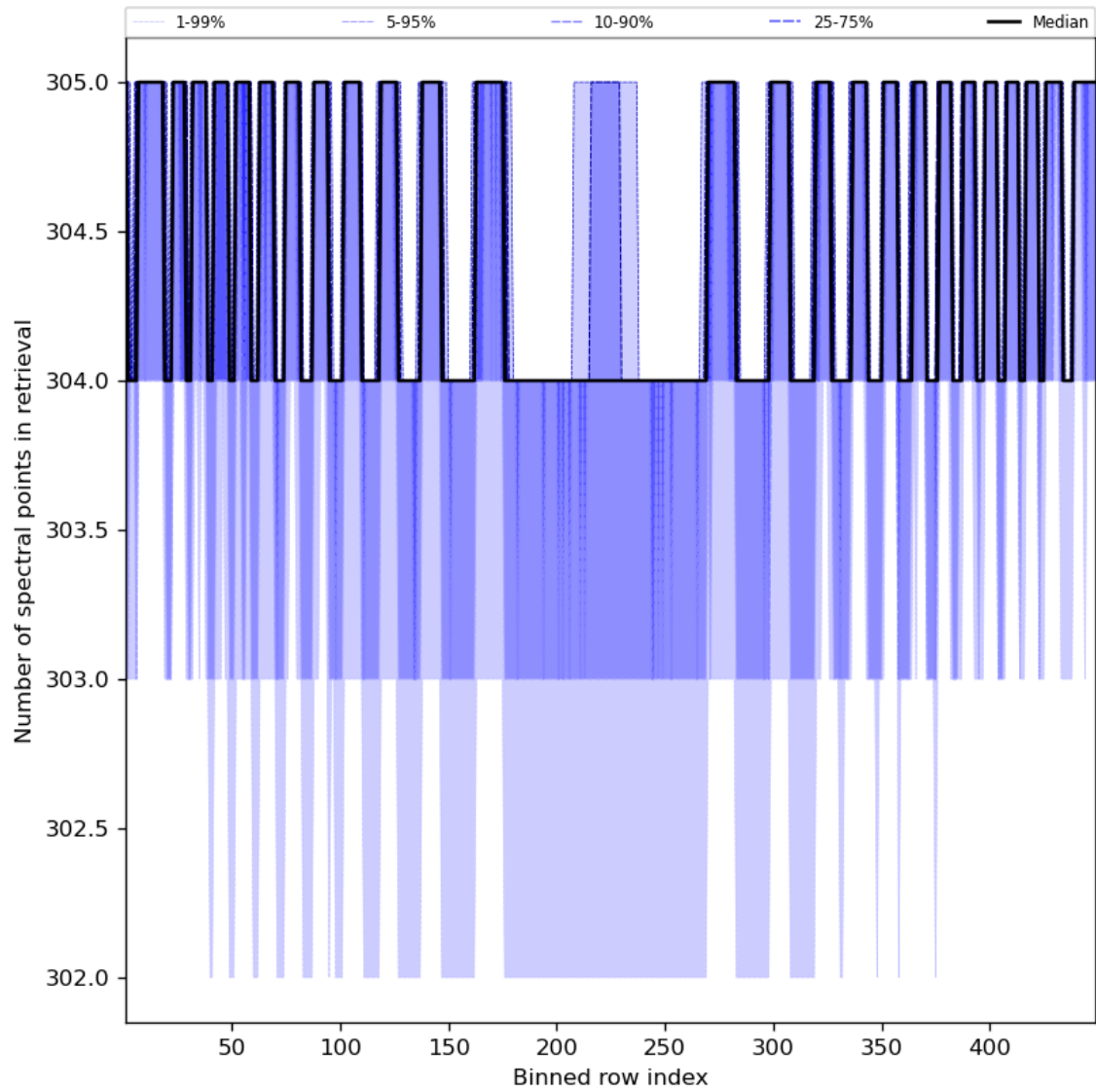
Figure 50: Along track statistics of “Number of spectral points in retrieval” for 2023-09-28 to 2023-09-30
