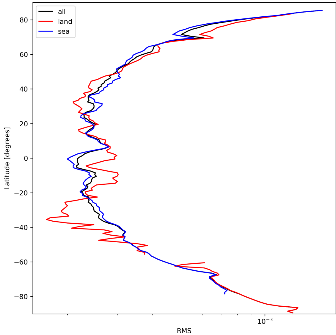
Figure 26: Zonal average of “RMS” for 2023-09-28 to 2023-09-30.
