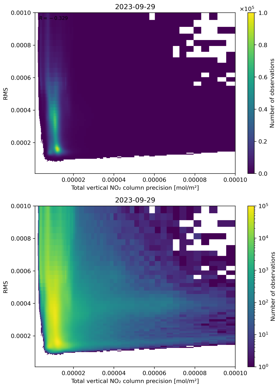
Figure 119: Scatter density plot of “Total vertical NO 2 column precision” against “RMS” for 2023-09-28 to 2023-09-30.
