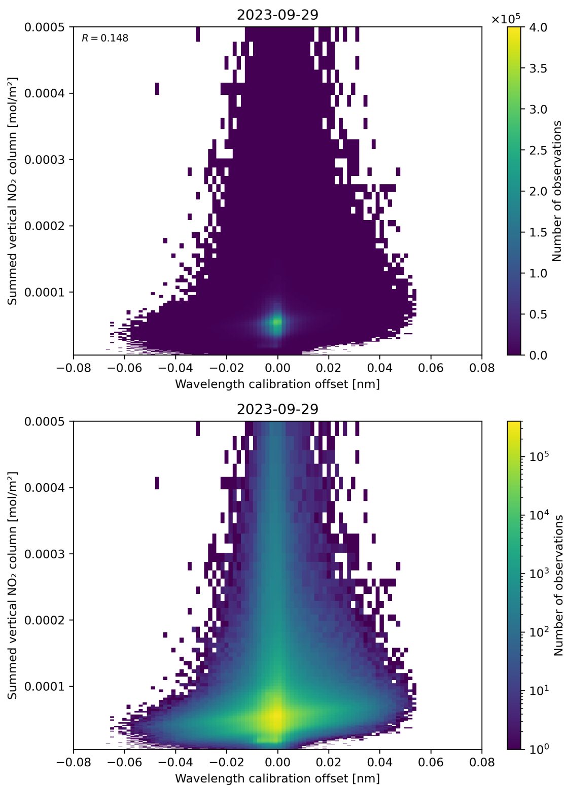
Figure 177: Scatter density plot of “Wavelength calibration offset” against “Summed vertical NO 2 column” for 2023-09-28 to 2023-09-30.
