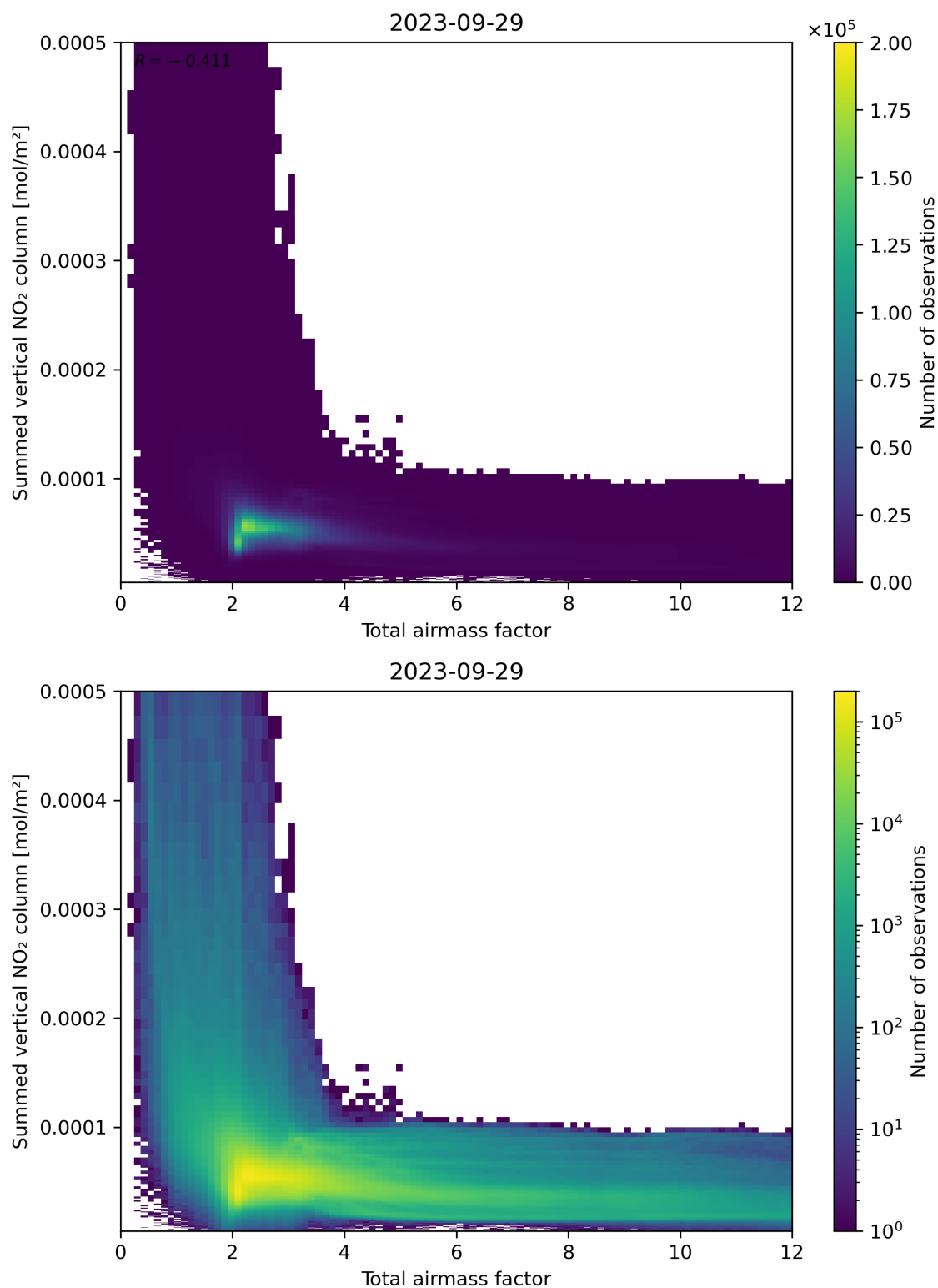
Figure 65: Scatter density plot of “Total airmass factor” against “Summed vertical NO 2 column” for 2023-09-28 to 2023-09-30.
