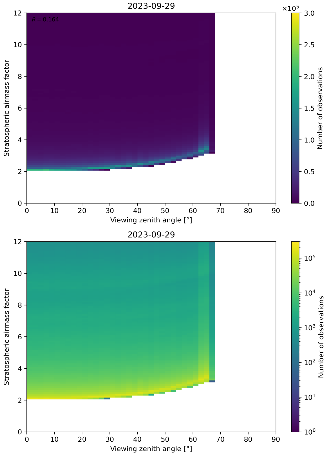
Figure 159: Scatter density plot of “Viewing zenith angle” against “Stratospheric airmass factor” for 2023-09-28 to 2023-09-30.
