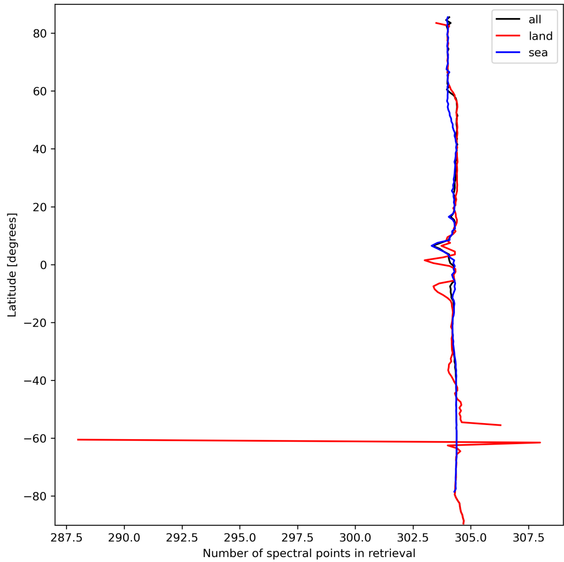
Figure 16: Zonal average of “Number of spectral points in retrieval” for 2023-09-28 to 2023-09-30.
