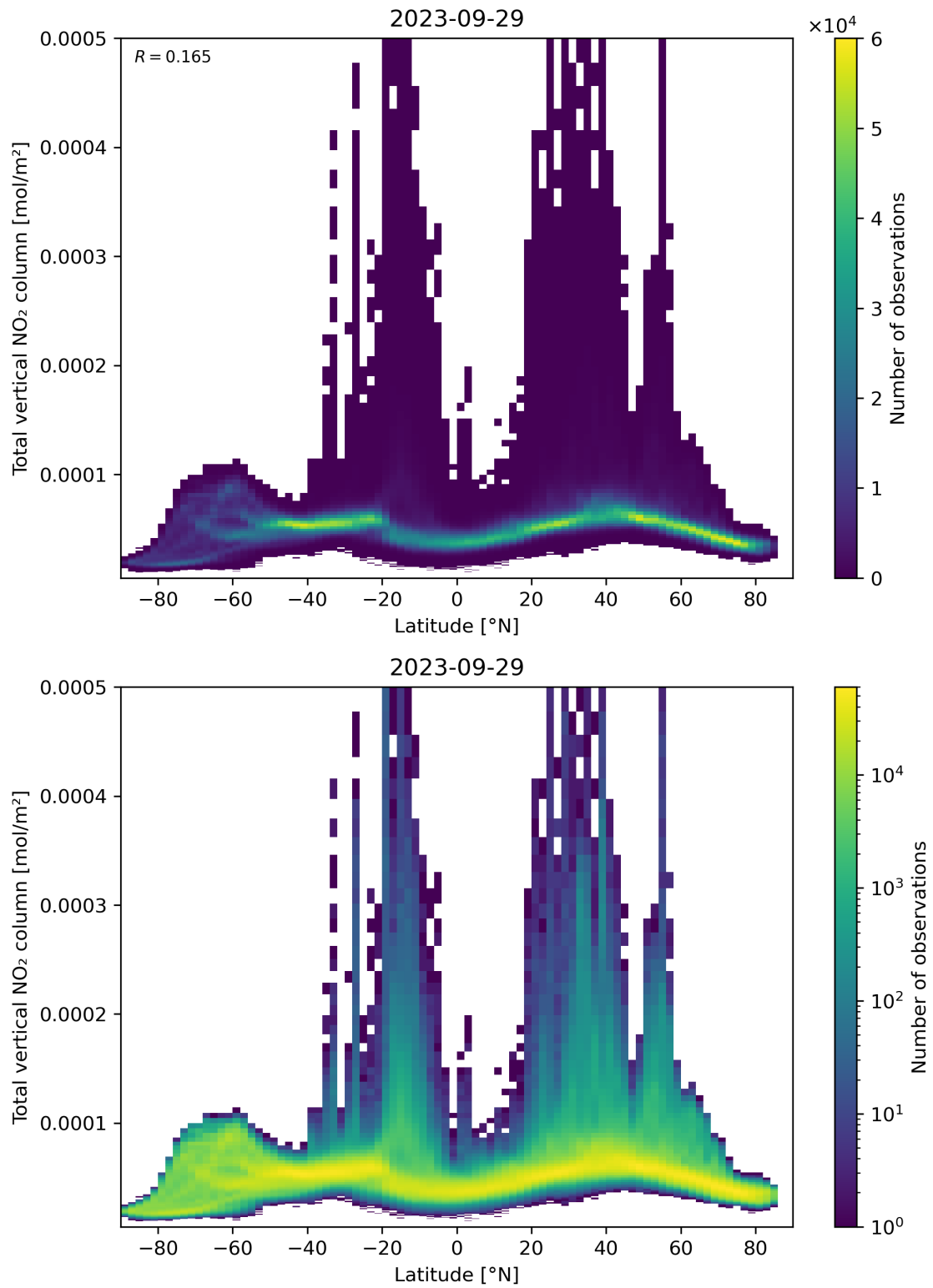
Figure 90: Scatter density plot of “Latitude” against “Total vertical NO 2 column” for 2023-09-28 to 2023-09-30.
