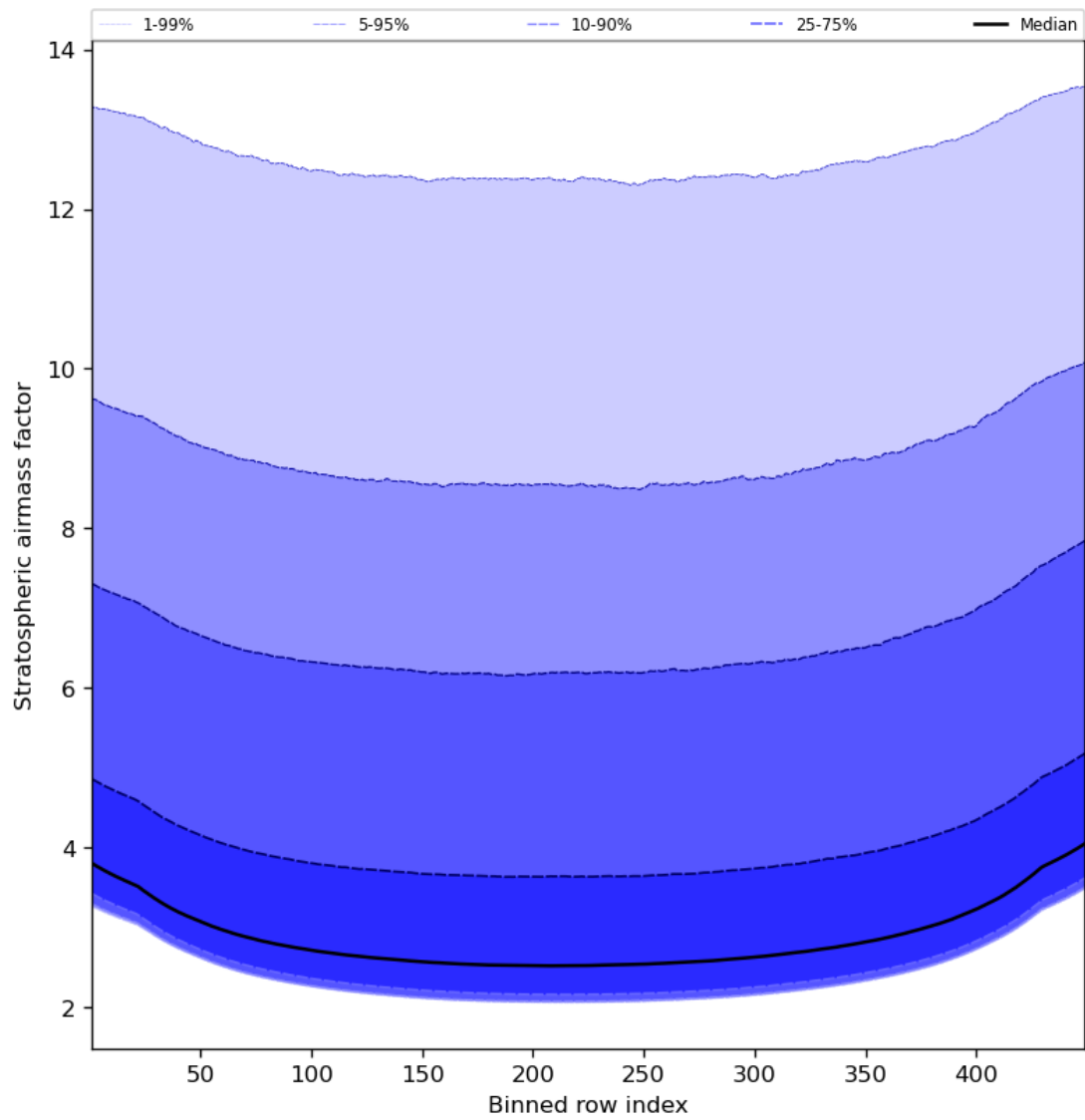
Figure 61: Along track statistics of “Stratospheric air mass factor” for 2023-09-28 to 2023-09-30
