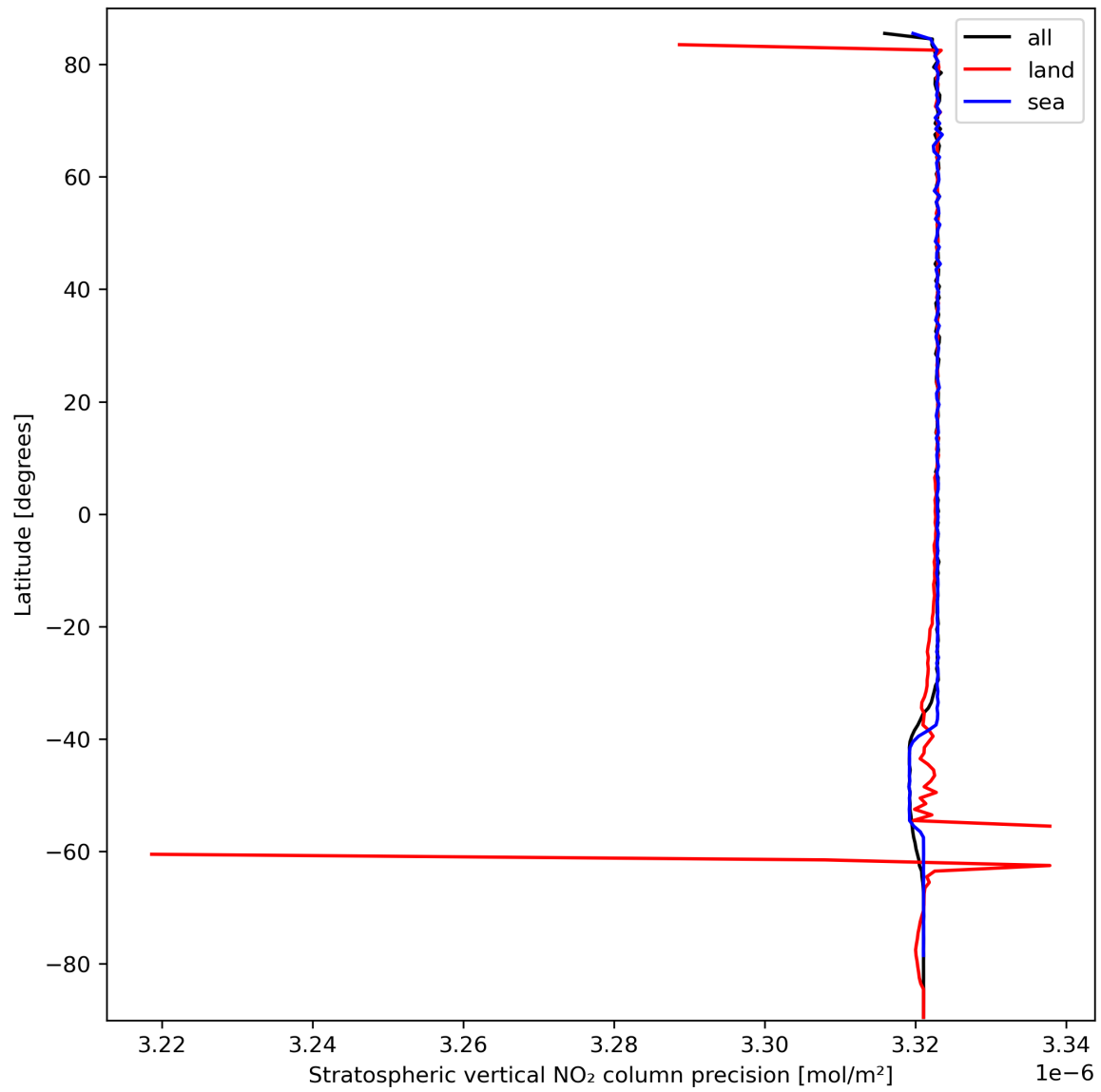
Figure 20: Zonal average of “Stratospheric vertical NO 2 column precision” for 2023-09-28 to 2023-09-30.
