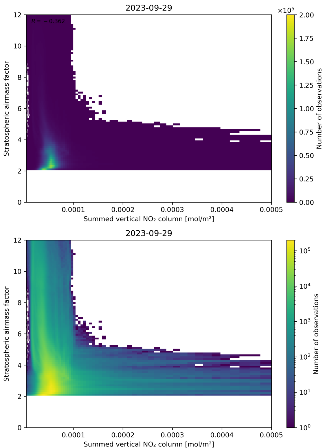
Figure 103: Scatter density plot of “Summed vertical NO 2 column” against “Stratospheric airmass factor” for 2023-09-28 to 2023-09-30.
