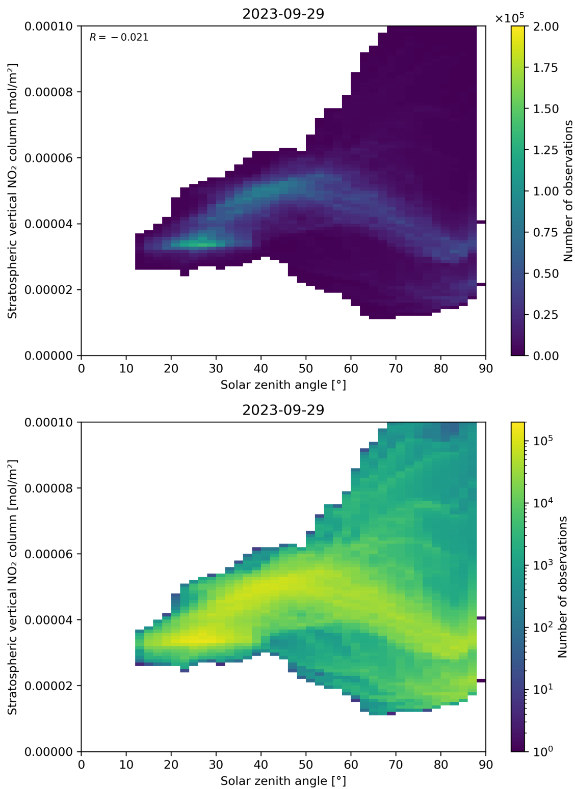
Figure 150: Scatter density plot of “Solar zenith angle” against “Stratospheric vertical NO 2 column” for 2023-09-28 to 2023-09-30.
