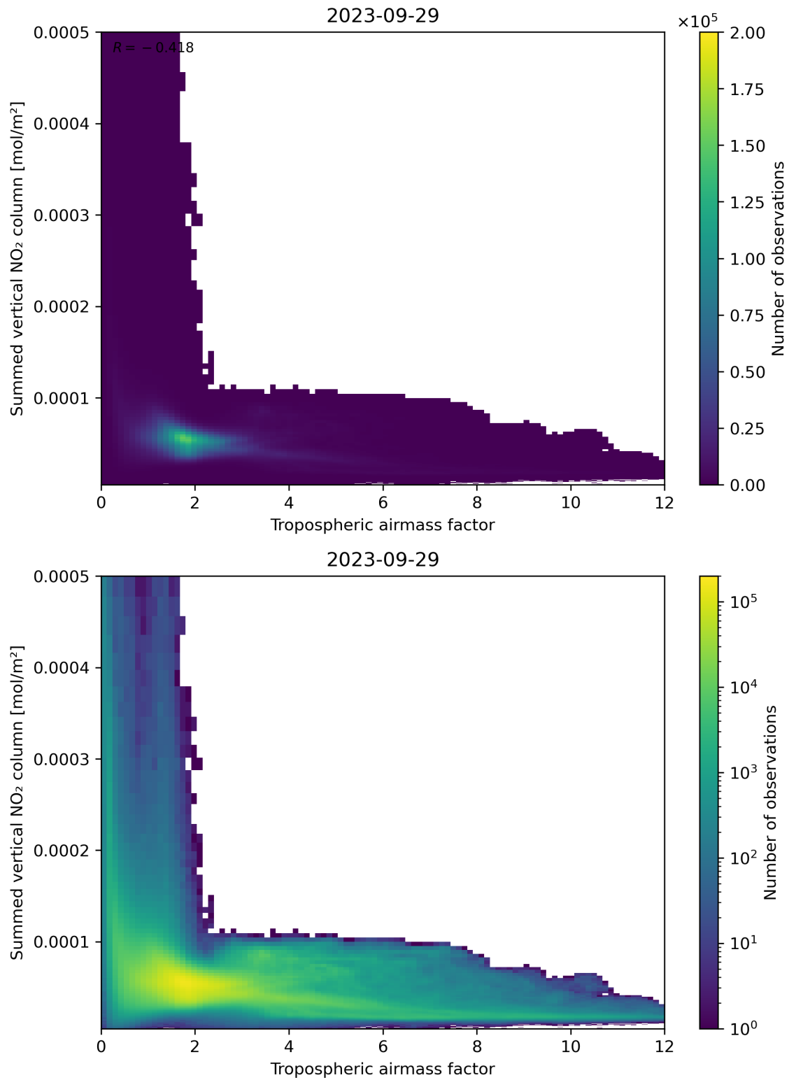
Figure 75: Scatter density plot of “Tropospheric air mass factor” against “Summed vertical NO 2 column” for 2023-09-28 to 2023-09-30.
