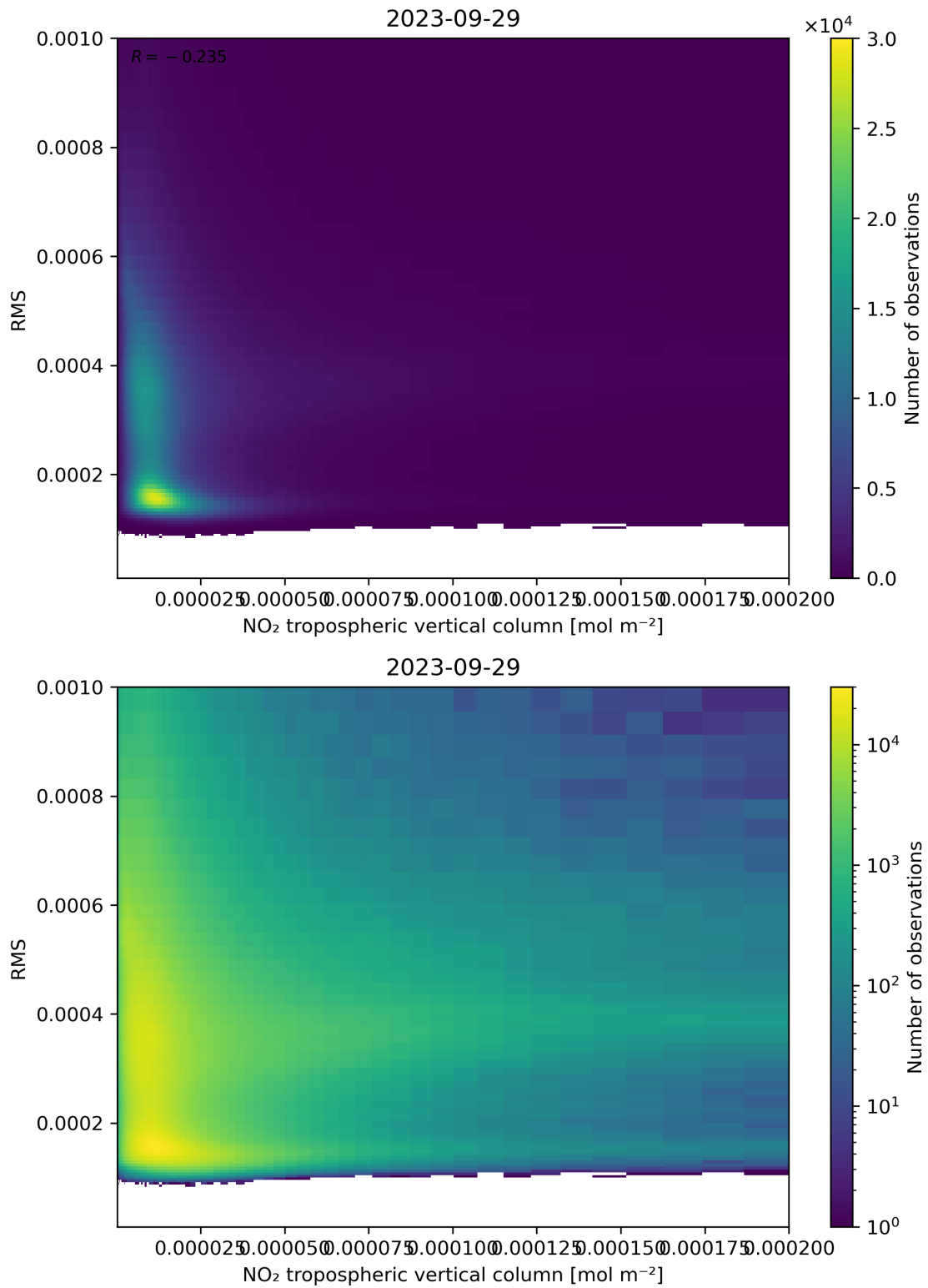
Figure 142: Scatter density plot of “NO 2 tropospheric vertical column” against “RMS” for 2023-09-28 to 2023-09-30.
