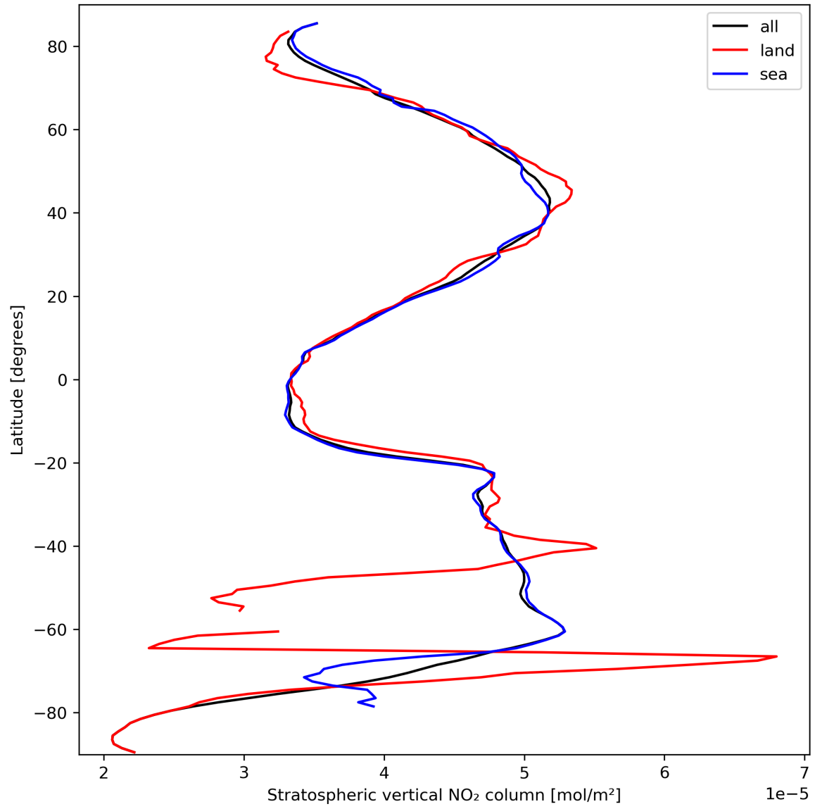
Figure 19: Zonal average of “Stratospheric vertical NO 2 column” for 2023-09-28 to 2023-09-30.
