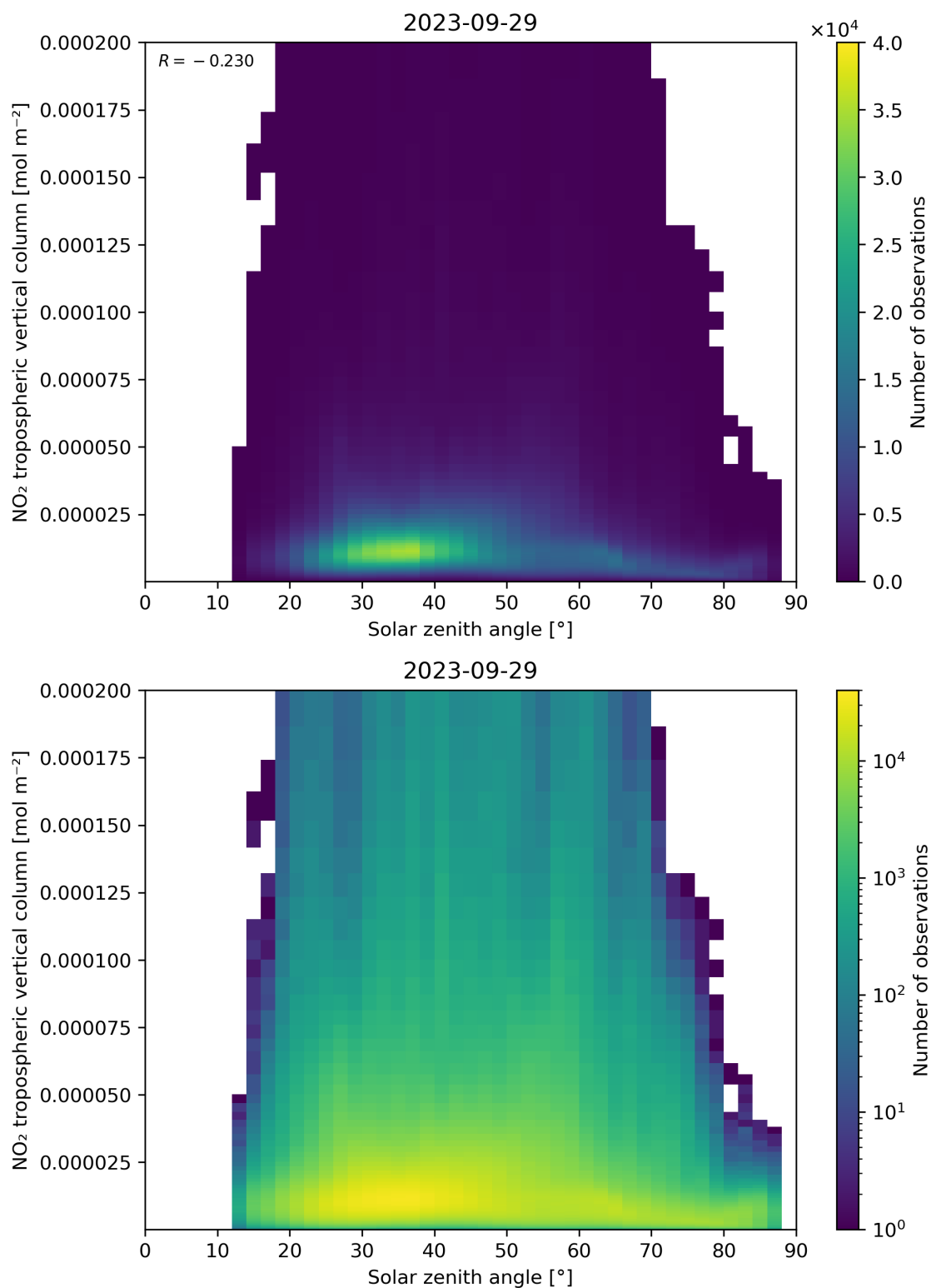
Figure 155: Scatter density plot of “Solar zenith angle” against “NO 2 tropospheric vertical column” for 2023-09-28 to 2023-09-30.
