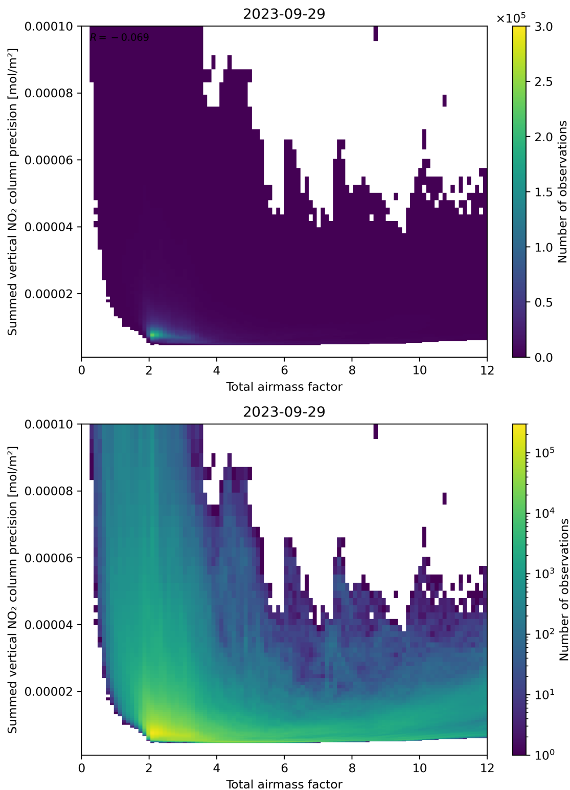
Figure 66: Scatter density plot of “Total airmass factor” against “Summed vertical NO 2 column precision” for 2023-09-28 to 2023-09-30.
