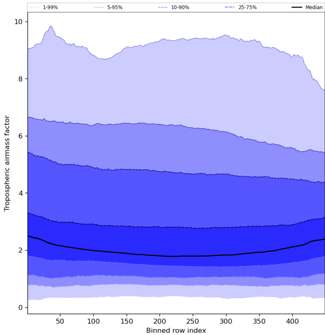
Figure 48: Along track statistics of “Tropospheric airmass factor” for 2023-09-28 to 2023-09-30
