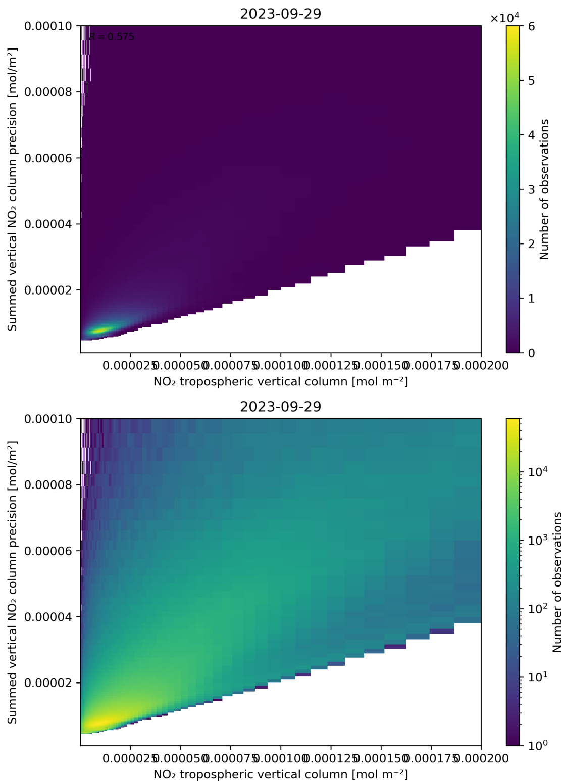
Figure 127: Scatter density plot of “NO 2 tropospheric vertical column” against “Summed vertical NO 2 column precision” for 2023-09-28 to 2023-09-30.
