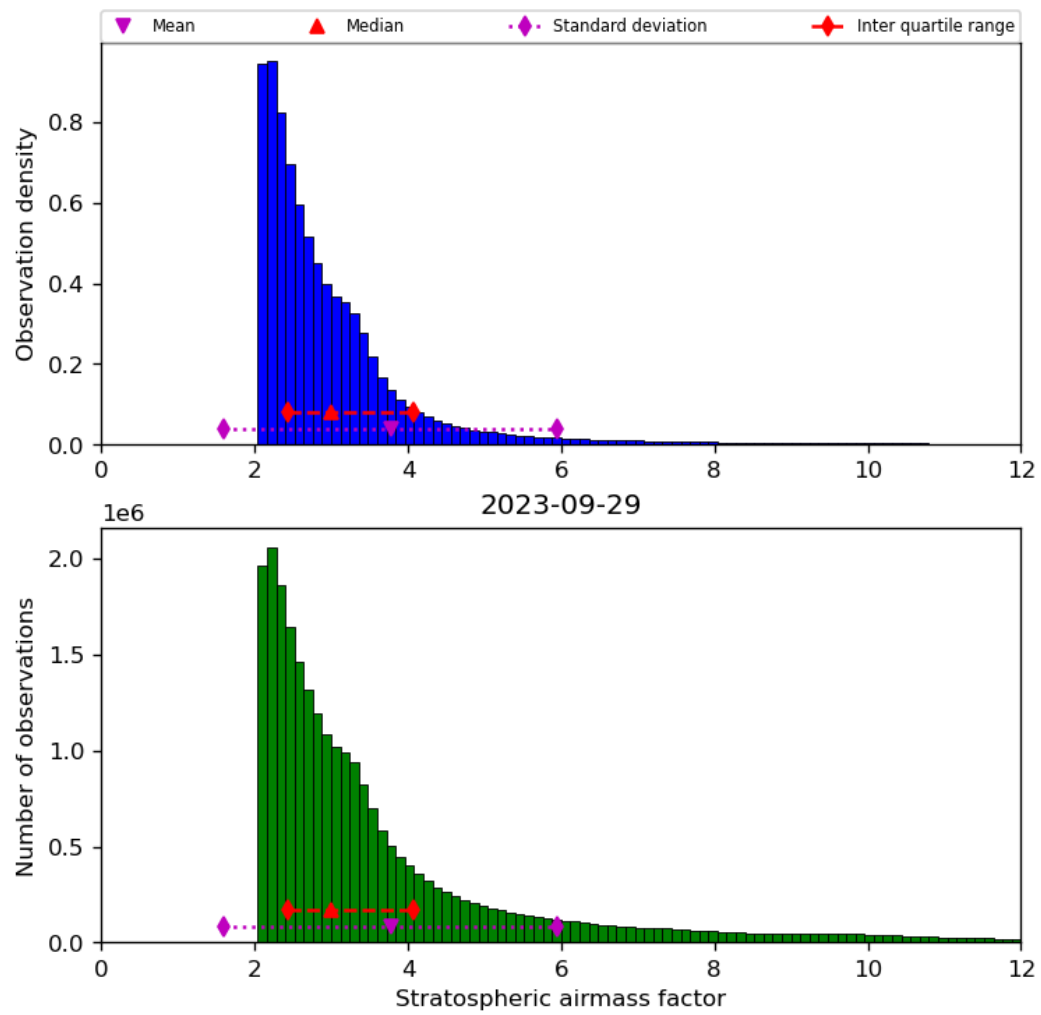
Figure 44: Histogram of “Stratospheric airmass factor” for 2023-09-28 to 2023-09-30
