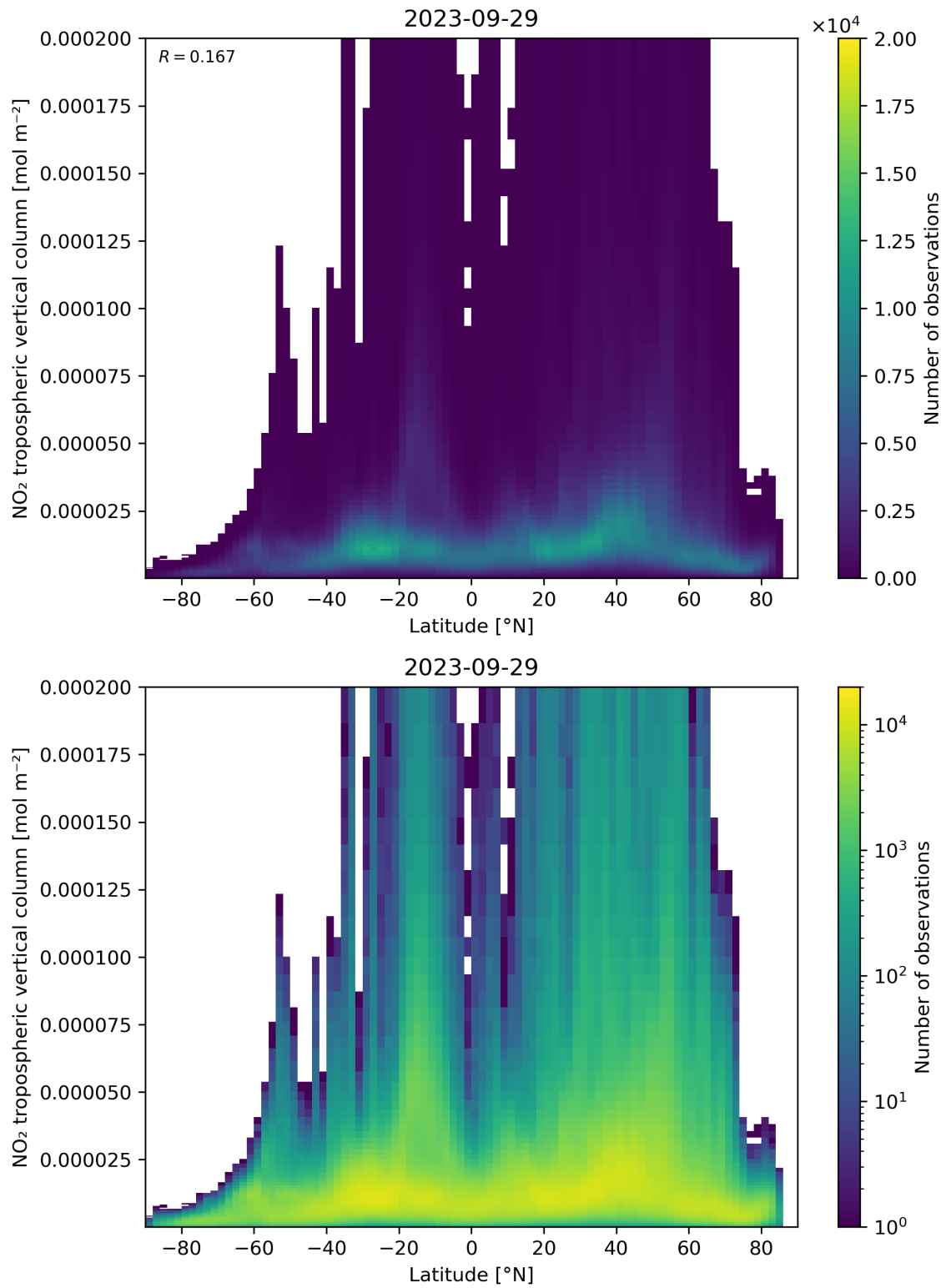
Figure 92: Scatter density plot of “Latitude” against “NO 2 tropospheric vertical column” for 2023-09-28 to 2023-09-30.
