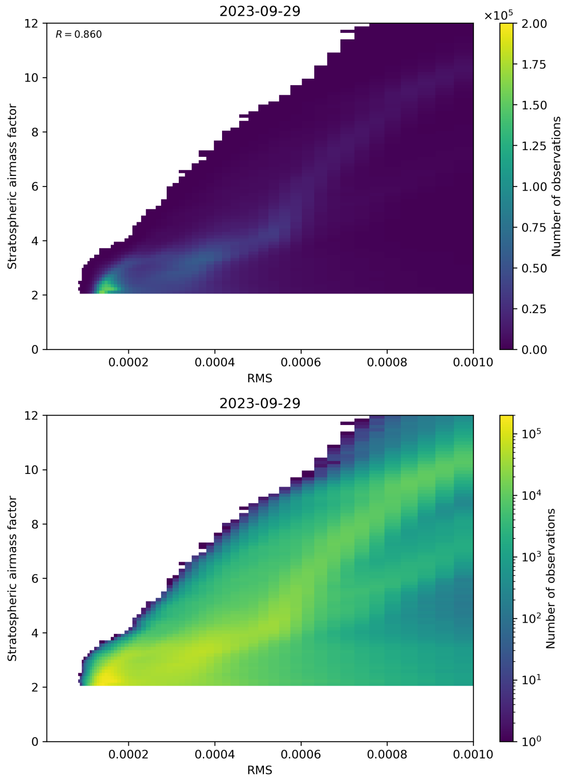
Figure 144: Scatter density plot of “RMS” against “Stratospheric airmass factor” for 2023-09-28 to 2023-09-30.
