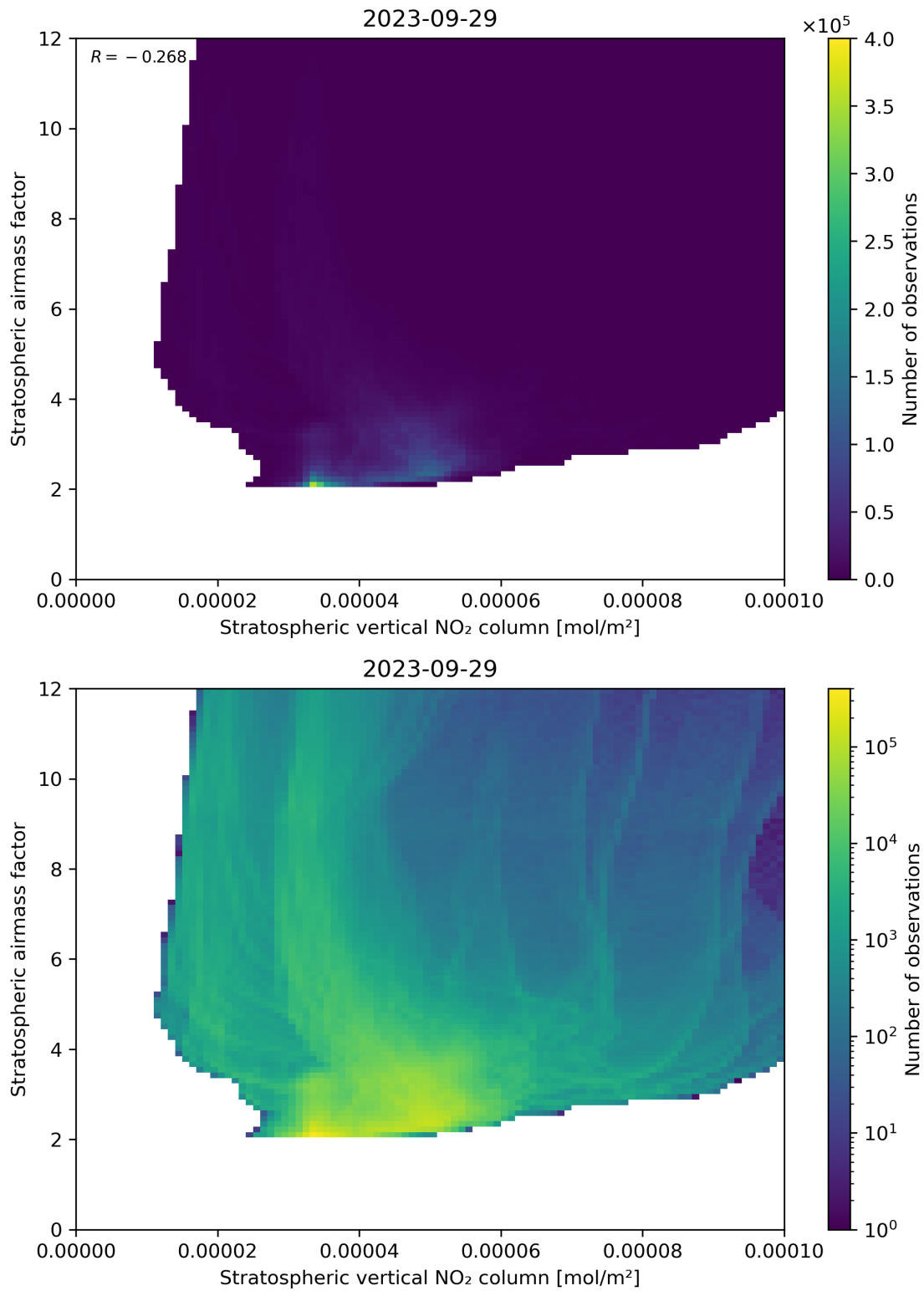
Figure 96: Scatter density plot of “Stratospheric vertical NO 2 column” against “Stratospheric airmass factor” for 2023-09-28 to 2023-09-30.
