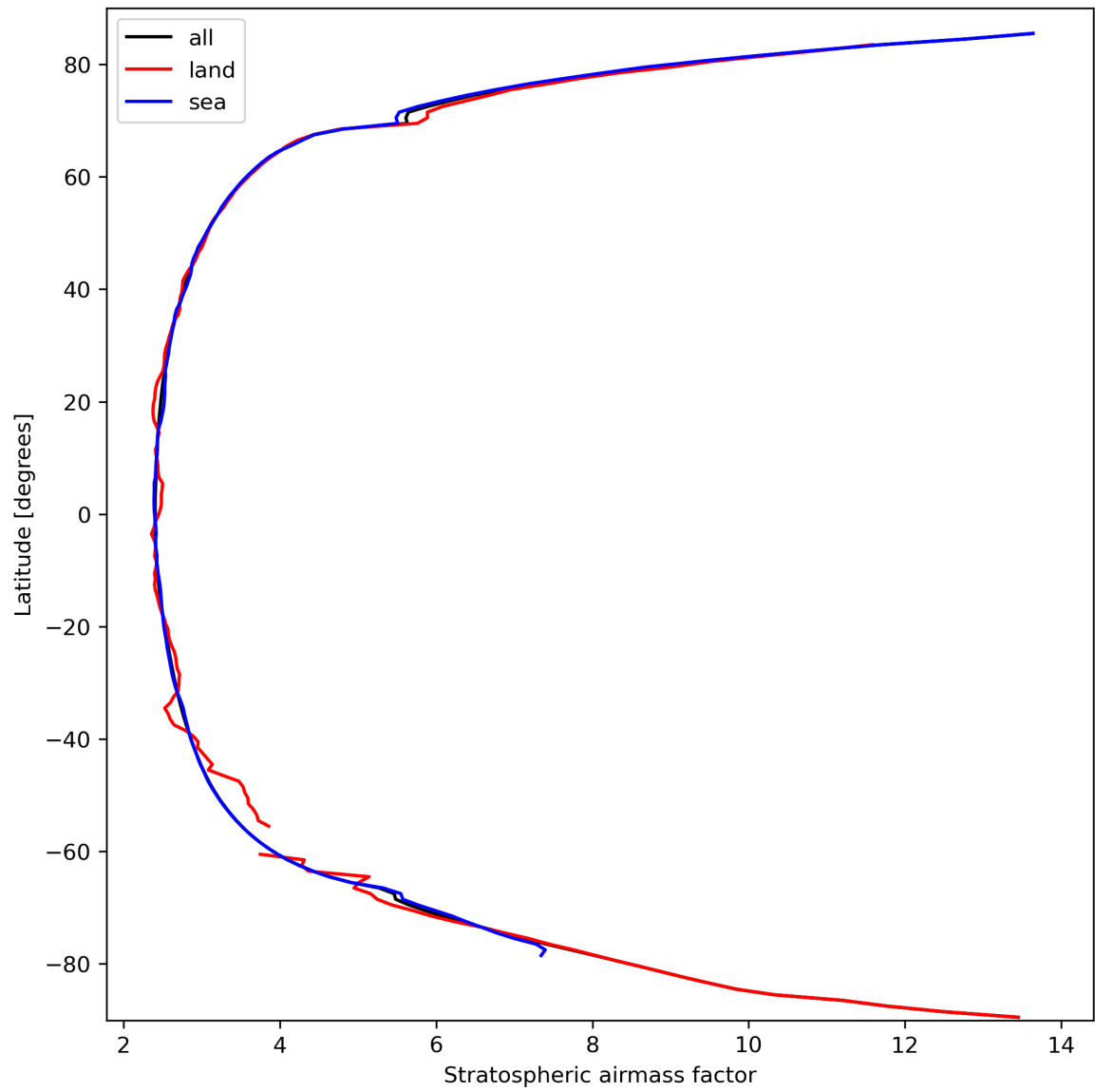
Figure 27: Zonal average of “Stratospheric air mass factor” for 2023-09-28 to 2023-09-30.
