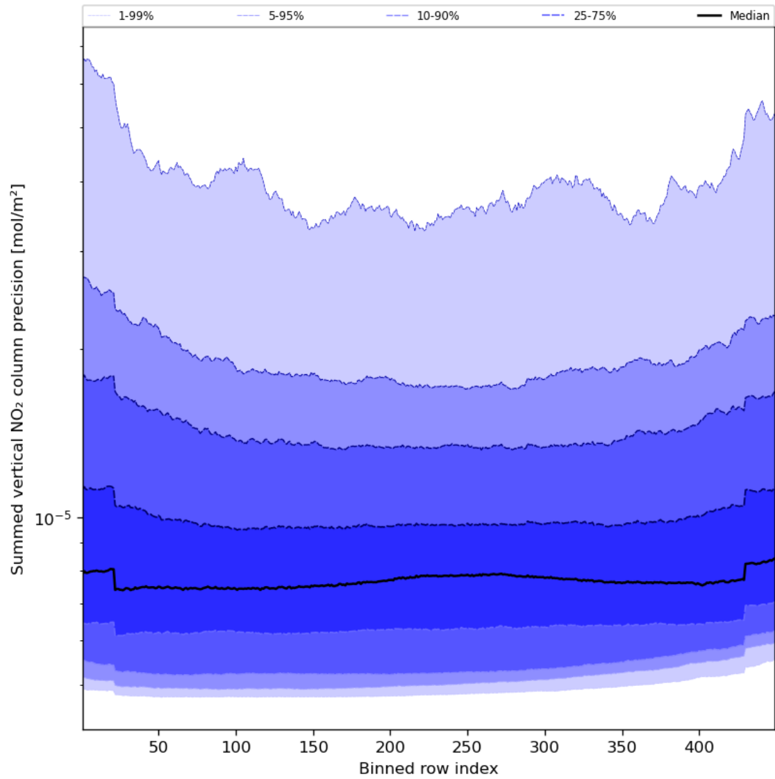
Figure 58: Along track statistics of “Summed vertical NO 2 column precision” for 2023-09-28 to 2023-09-30
