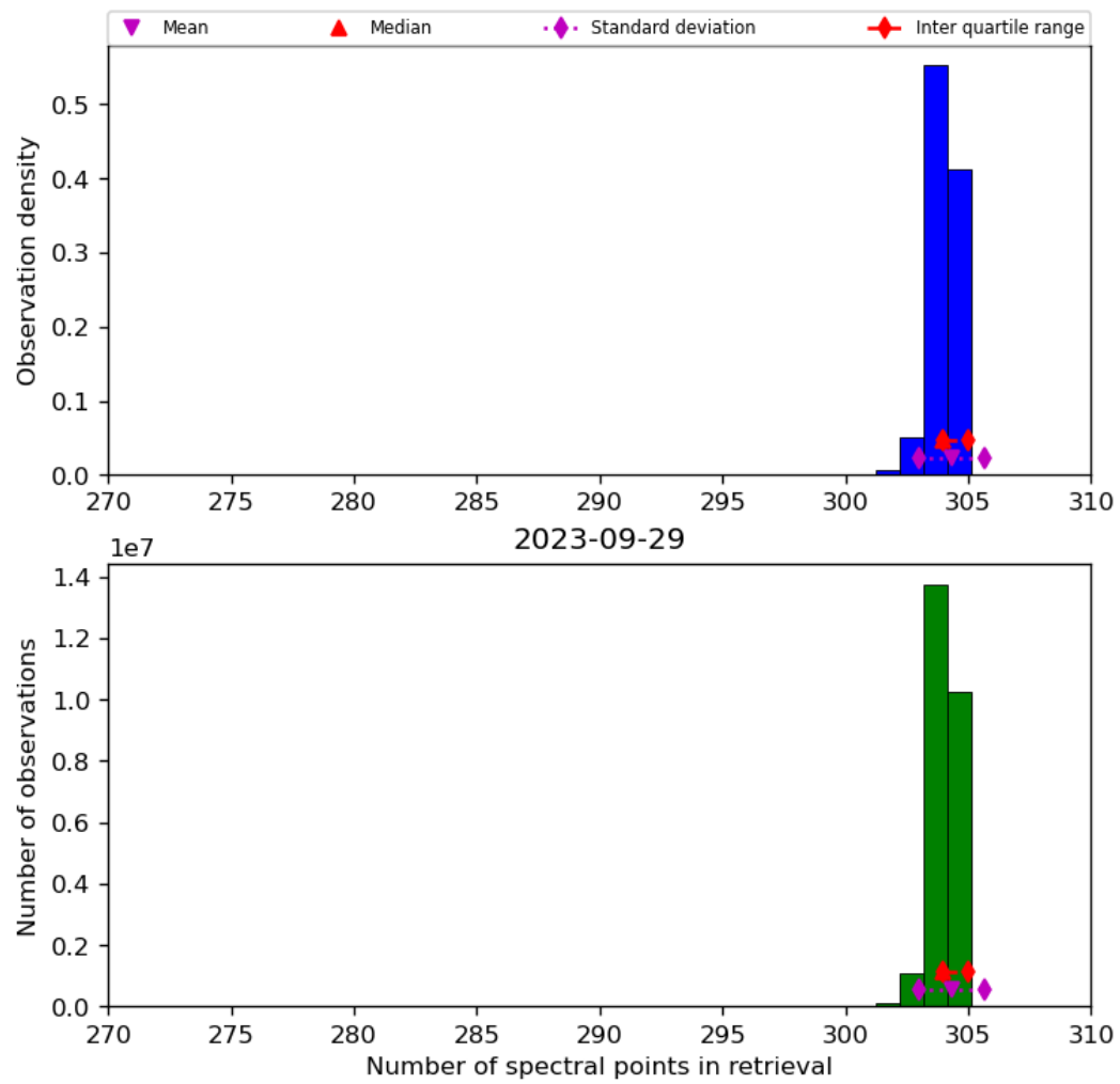
Figure 33: Histogram of “Number of spectral points in retrieval” for 2023-09-28 to 2023-09-30
