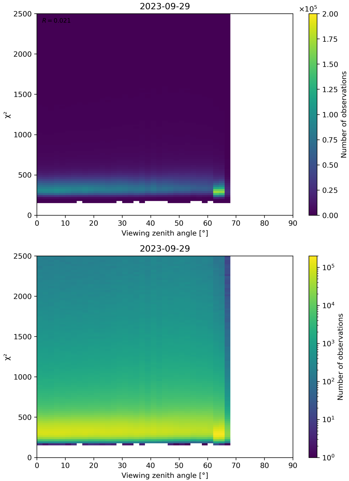
Figure 162: Scatter density plot of “Viewing zenith angle” against “ \chi^2 ” for 2023-09-28 to 2023-09-30.
