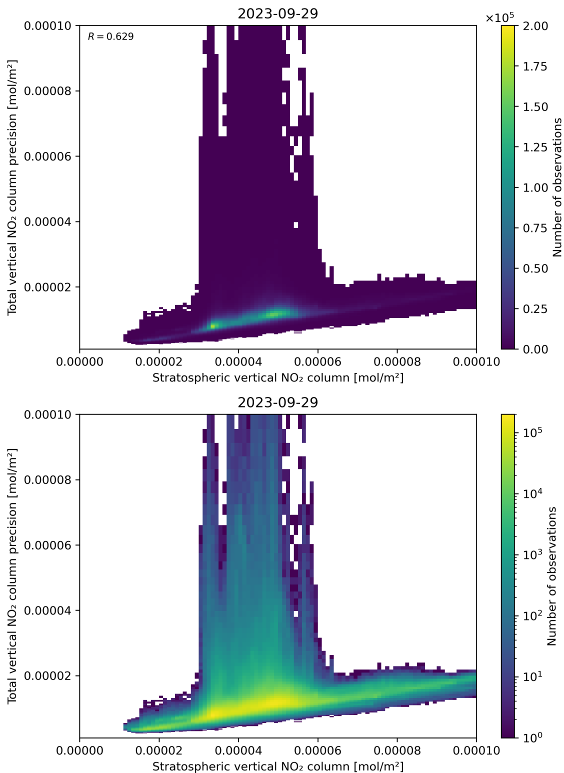
Figure 101: Scatter density plot of “Stratospheric vertical NO 2 column” against “Total vertical NO 2 column precision” for 2023-09-28 to 2023-09-30.
