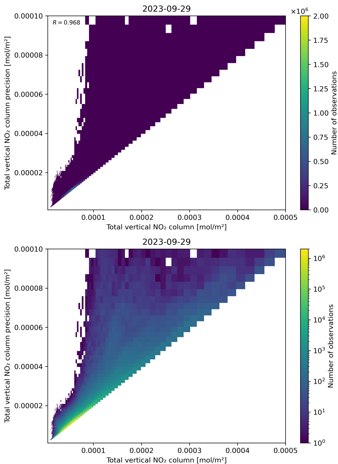
Figure 114: Scatter density plot of “Total vertical NO 2 column” against “Total vertical NO 2 column precision” for 2023-09-28 to 2023-09-30.
