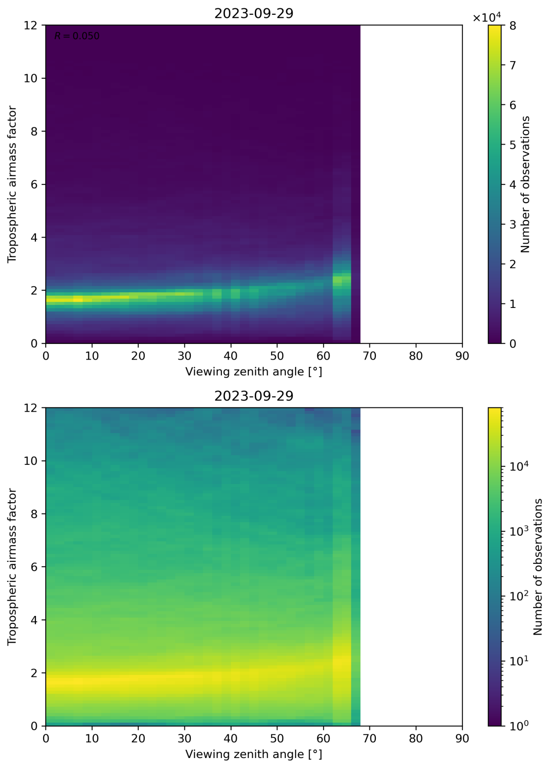
Figure 161: Scatter density plot of “Viewing zenith angle” against “Tropospheric airmass factor” for 2023-09-28 to 2023-09-30.
