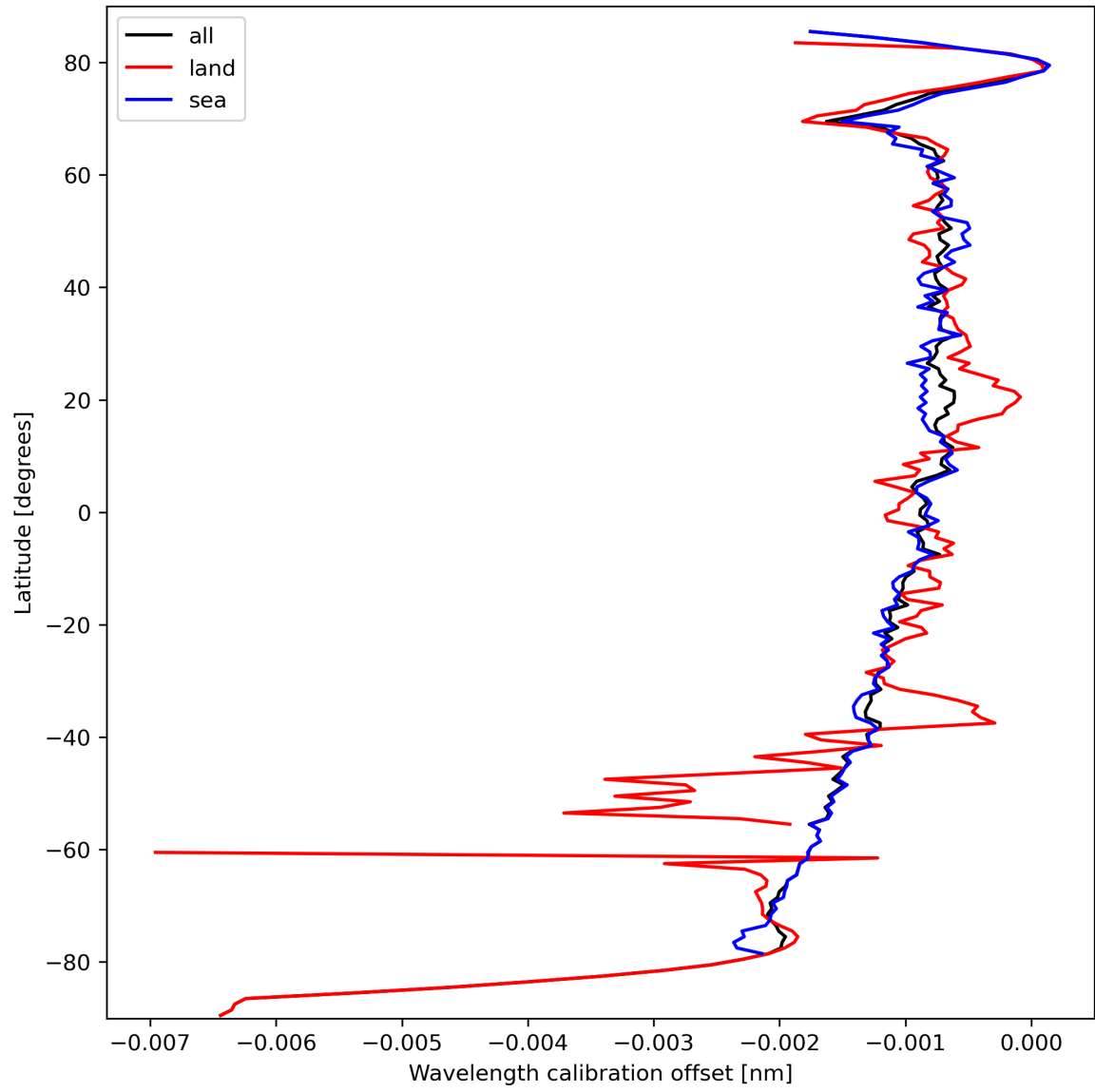
Figure 18: Zonal average of “Wavelength calibration offset” for 2023-09-28 to 2023-09-30.
