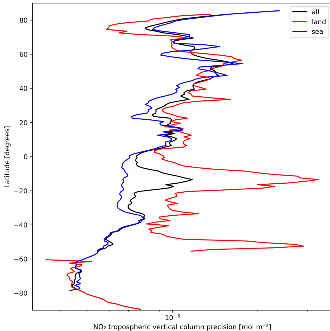
Figure 13: Zonal average of “NO 2 tropospheric vertical column precision” for 2023-09-28 to 2023-09-30.
