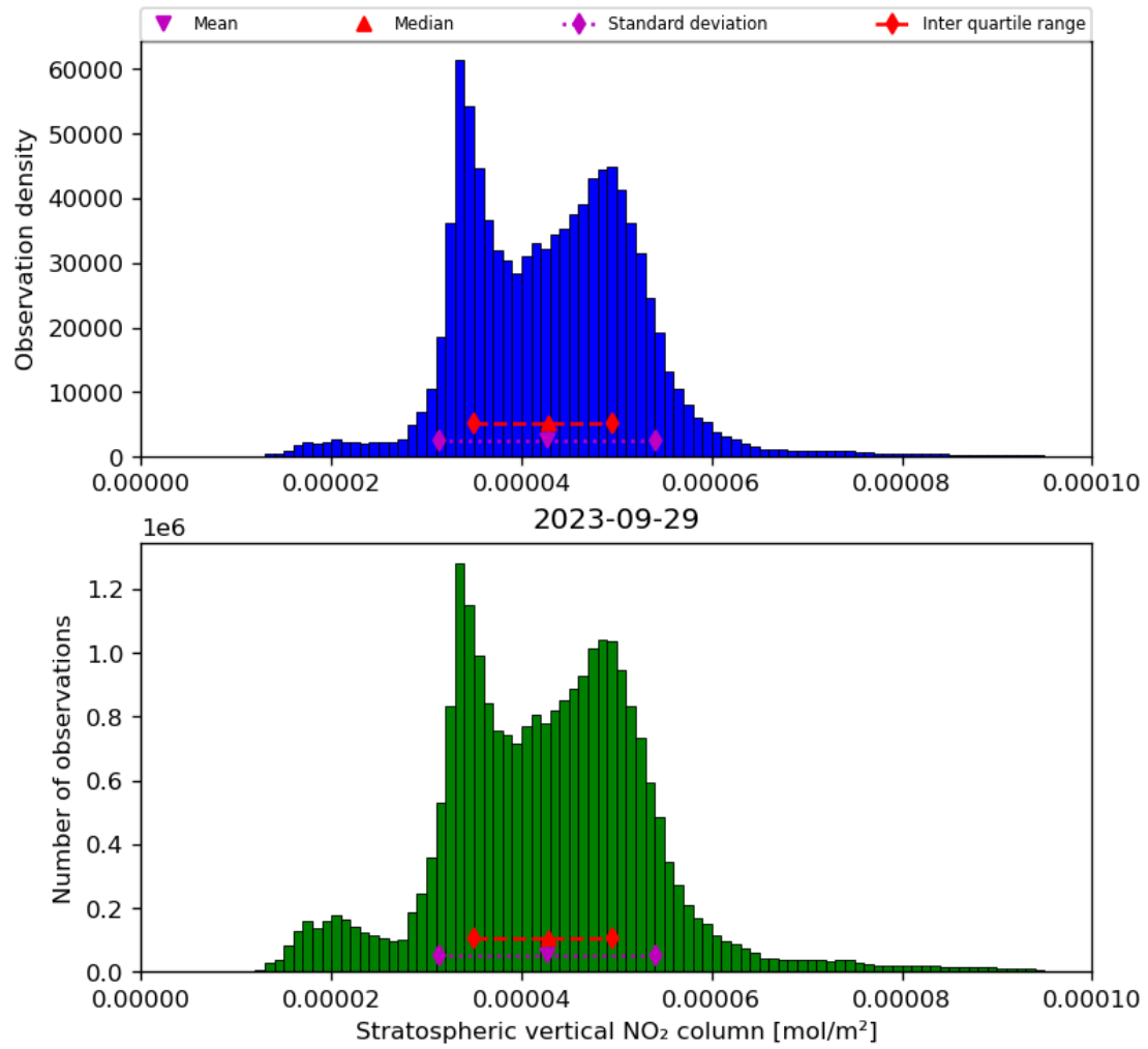
Figure 36: Histogram of “Stratospheric vertical NO 2 column” for 2023-09-28 to 2023-09-30
