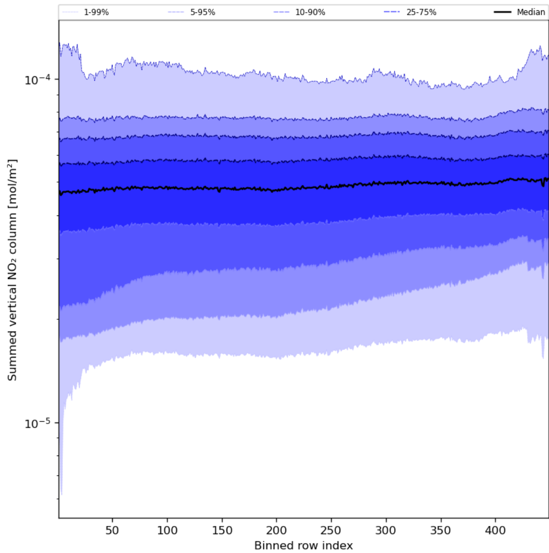
Figure 57: Along track statistics of “Summed vertical NO 2 column” for 2023-09-28 to 2023-09-30
