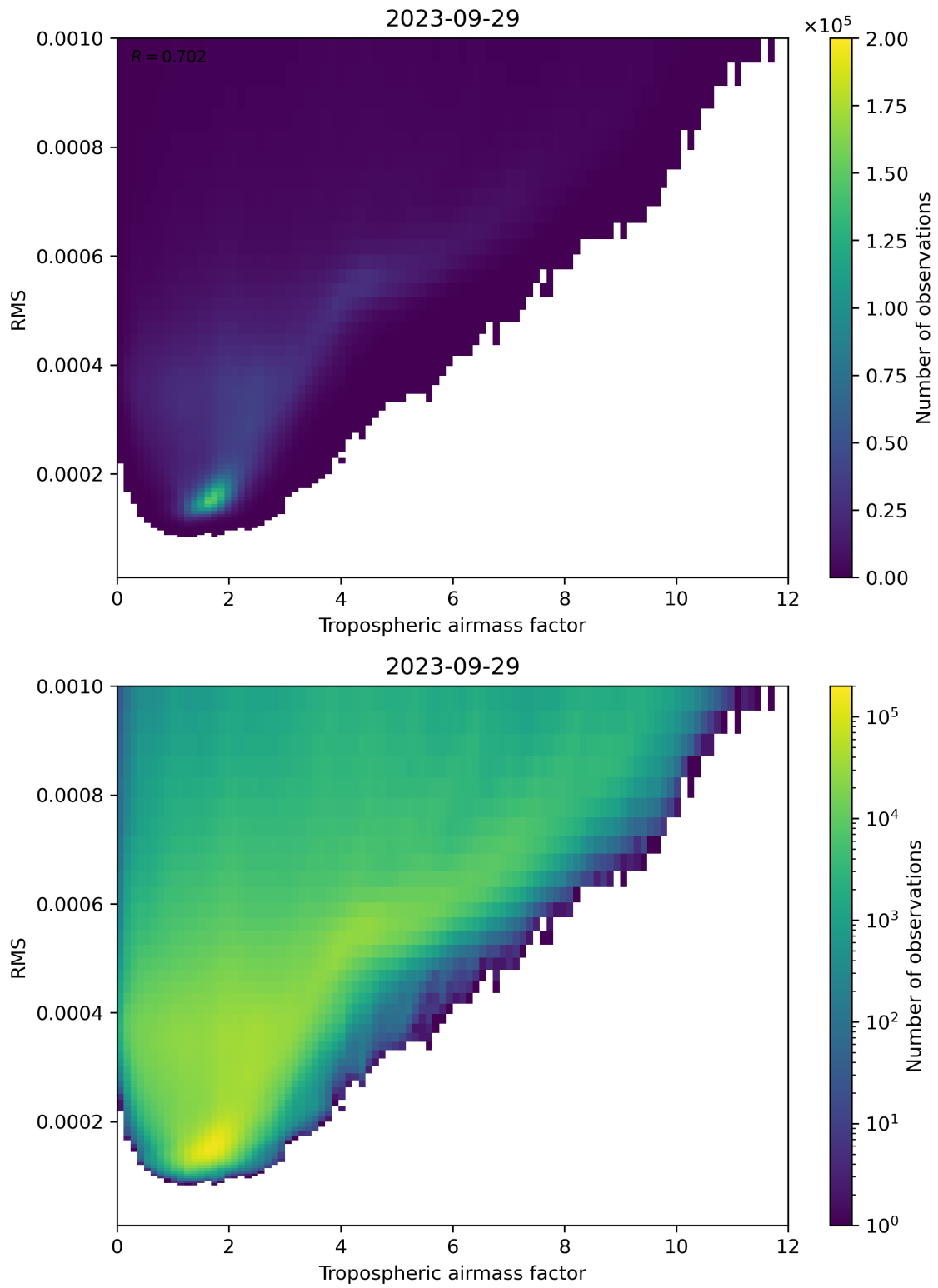
Figure 79: Scatter density plot of “Tropospheric airmass factor” against “RMS” for 2023-09-28 to 2023-09-30.
