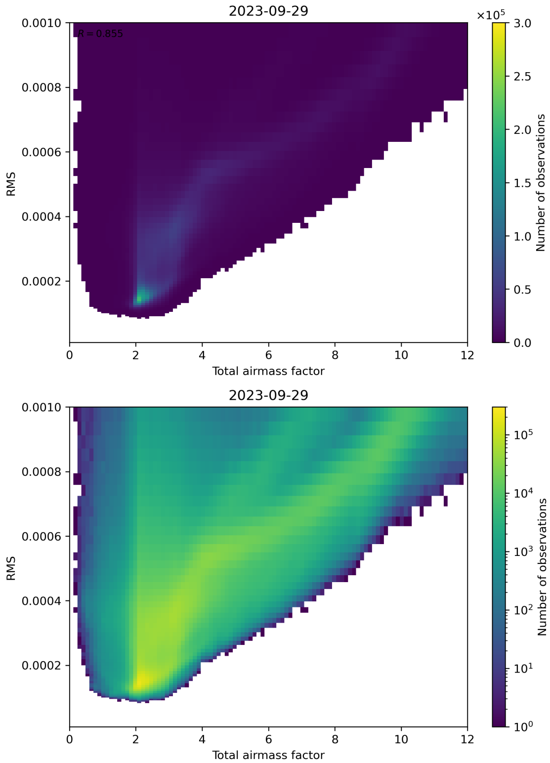
Figure 69: Scatter density plot of “Total airmass factor” against “RMS” for 2023-09-28 to 2023-09-30.
