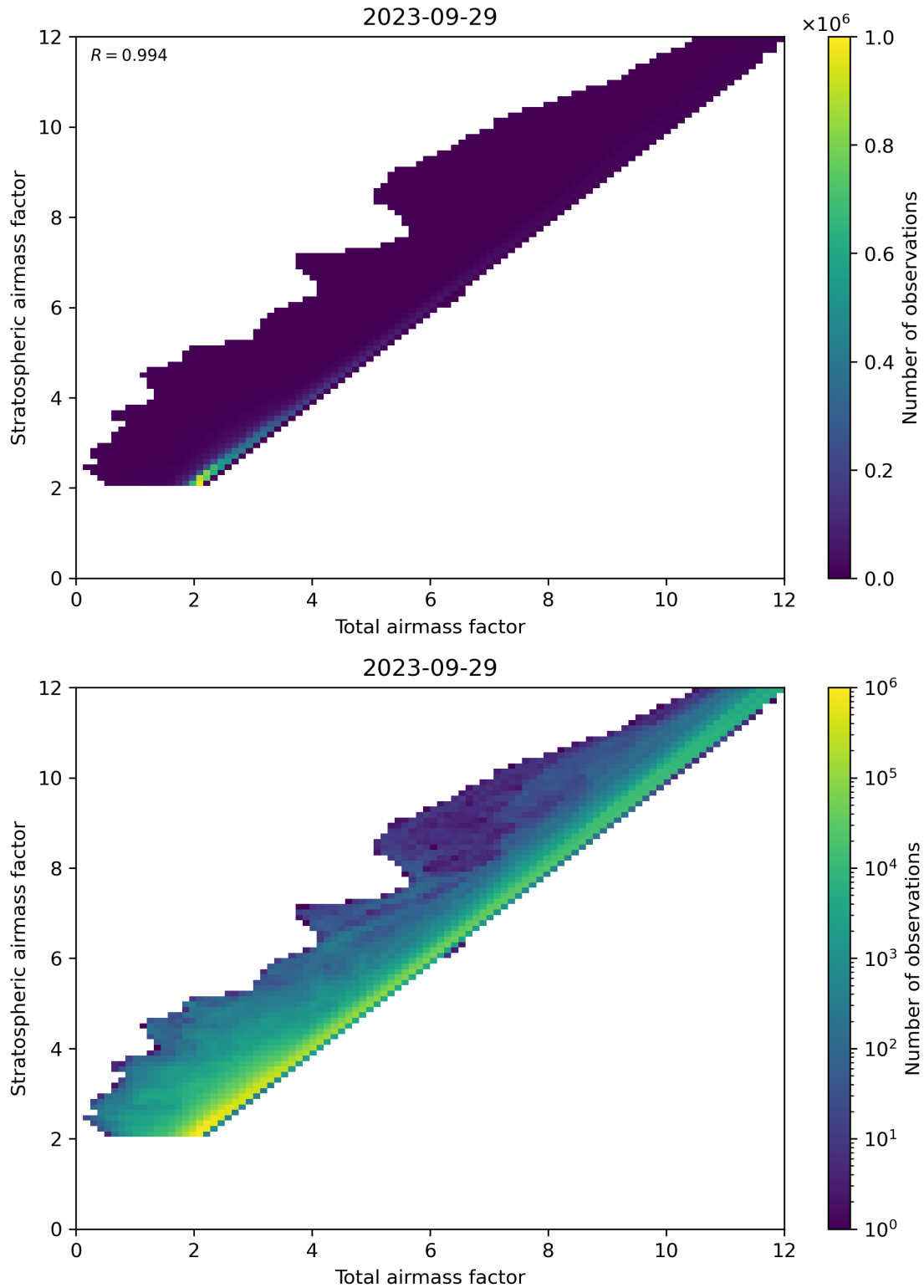
Figure 62: Scatter density plot of “Total airmass factor” against “Stratospheric airmass factor” for 2023-09-28 to 2023-09-30.
