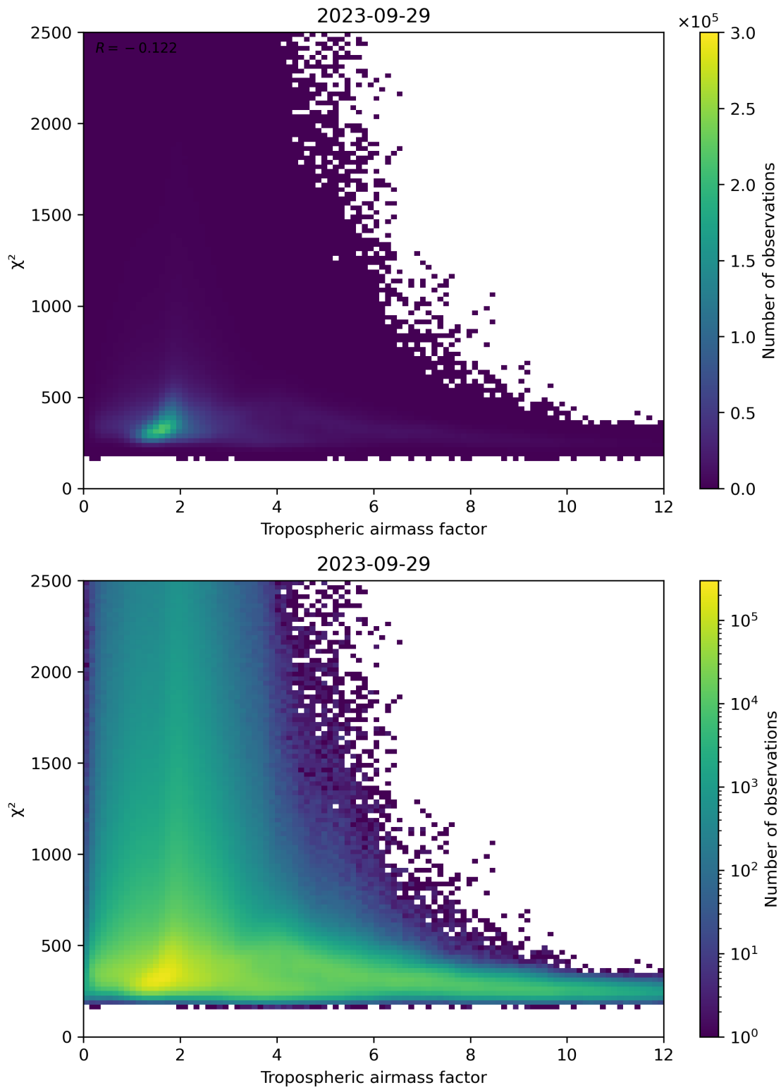
Figure 73: Scatter density plot of “Tropospheric airmass factor” against “ \chi^2 ” for 2023-09-28 to 2023-09-30.
