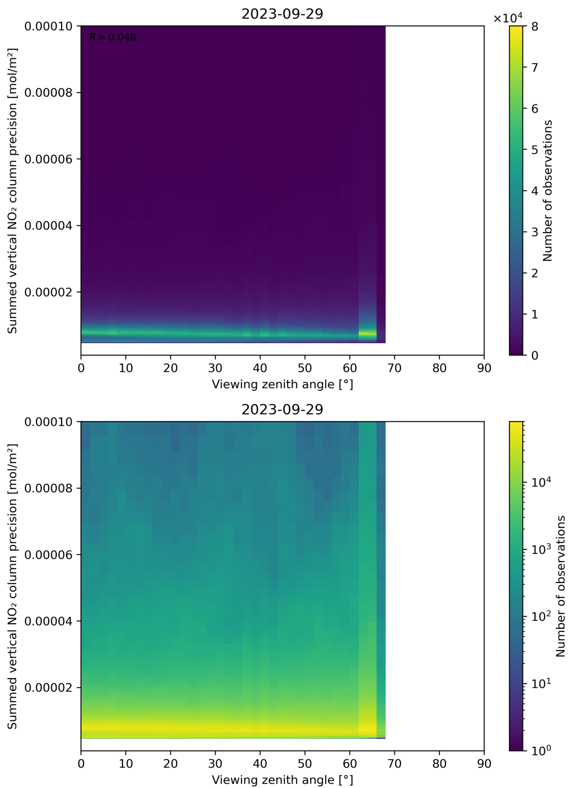
Figure 166: Scatter density plot of “Viewing zenith angle” against “Summed vertical NO 2 column precision” for 2023-09-28 to 2023-09-30.
