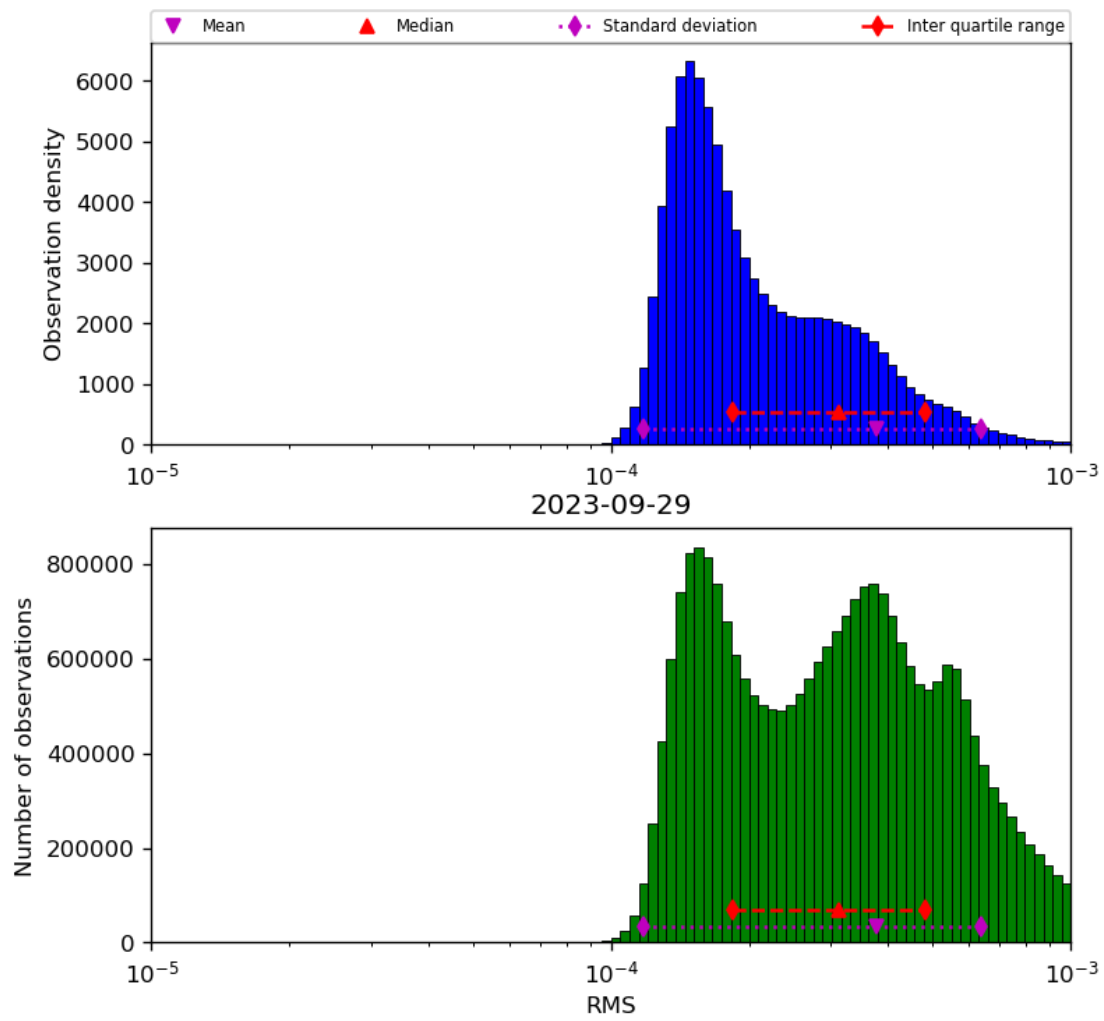
Figure 43: Histogram of “RMS” for 2023-09-28 to 2023-09-30
