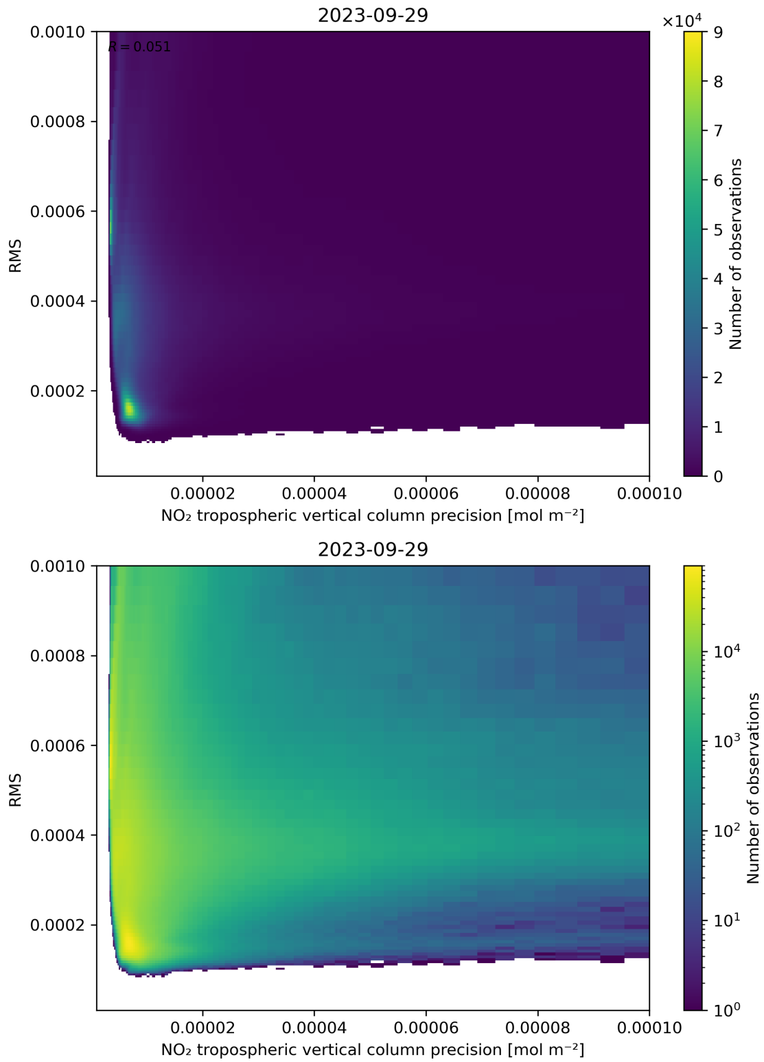
Figure 140: Scatter density plot of “NO 2 tropospheric vertical column precision” against “RMS” for 2023-09-28 to 2023-09-30.
