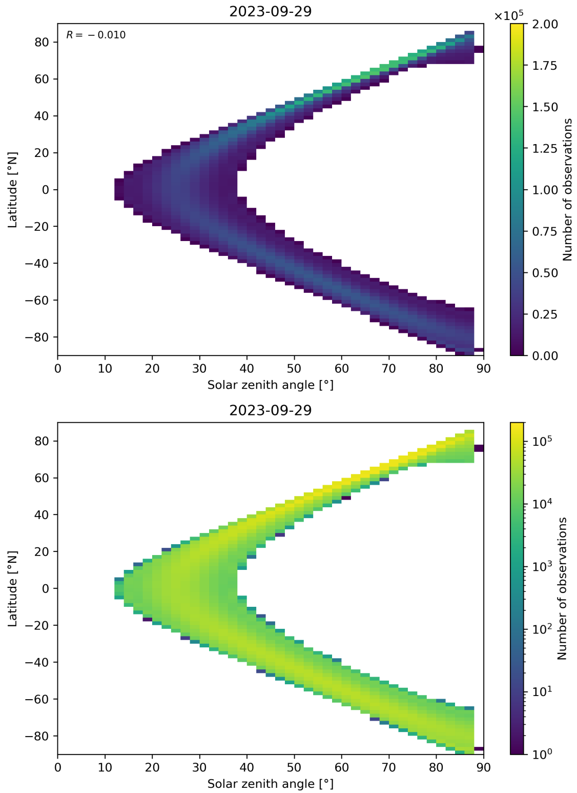
Figure 149: Scatter density plot of “Solar zenith angle” against “Latitude” for 2023-09-28 to 2023-09-30.
