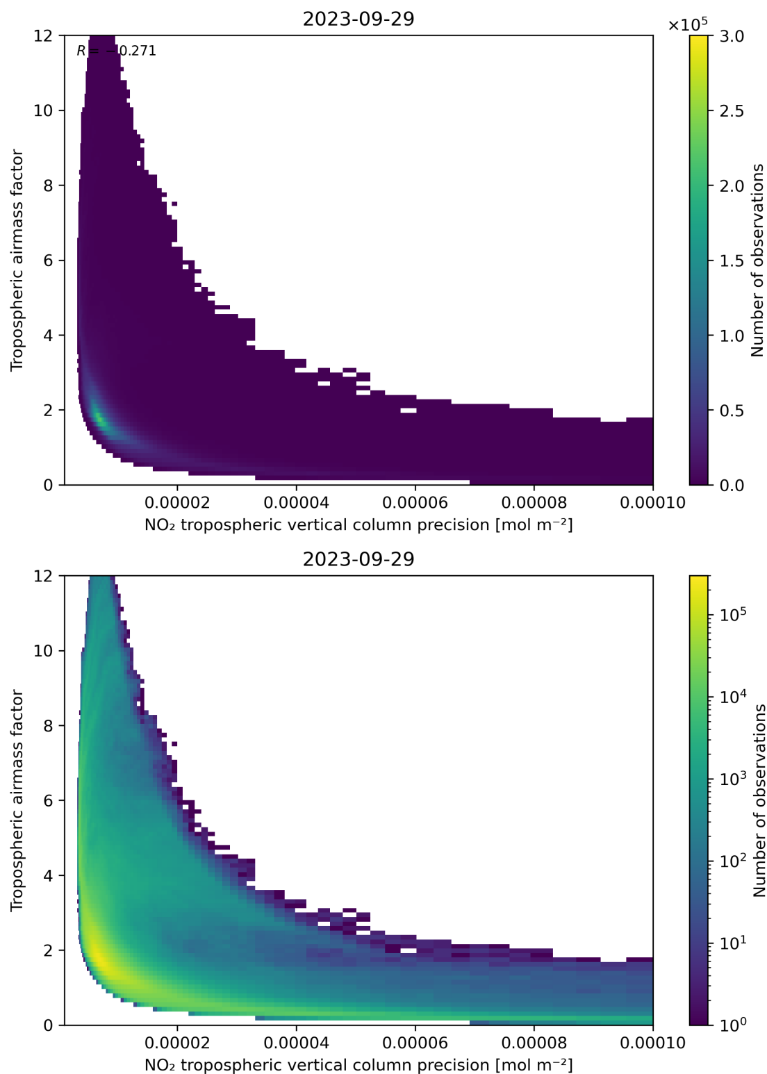
Figure 133: Scatter density plot of “NO 2 tropospheric vertical column precision” against “Tropospheric airmass factor” for 2023-09-28 to 2023-09-30.
