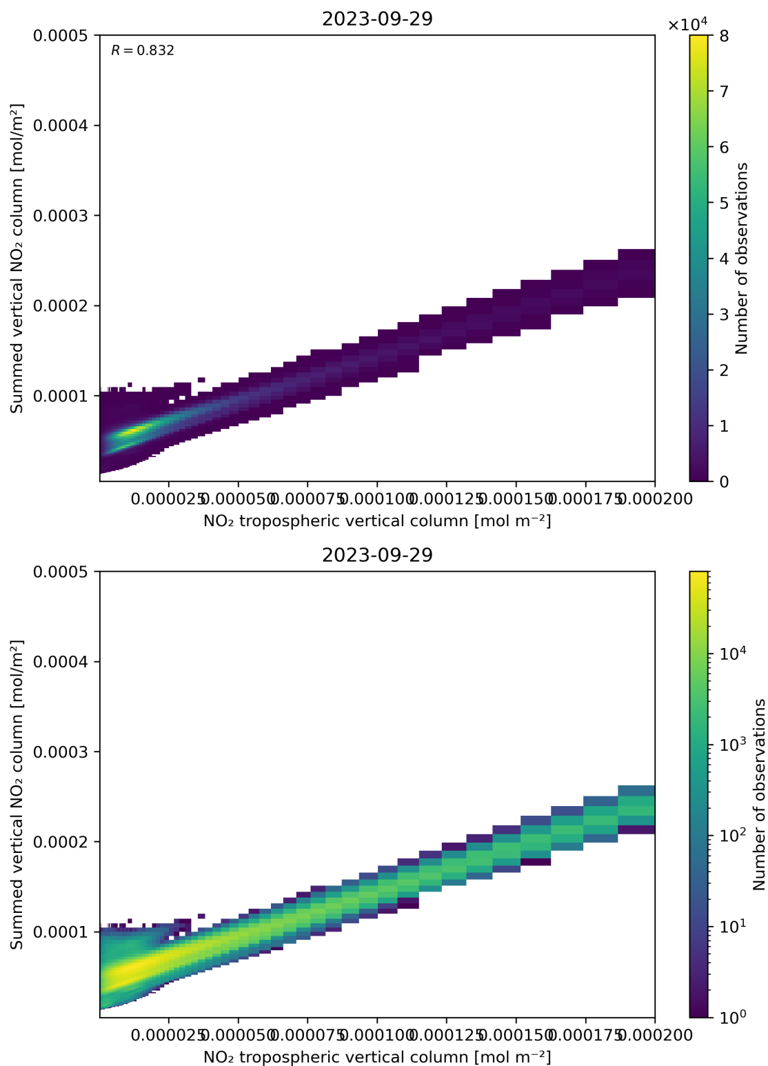
Figure 126: Scatter density plot of “NO 2 tropospheric vertical column” against “Summed vertical NO 2 column” for 2023-09-28 to 2023-09-30.
