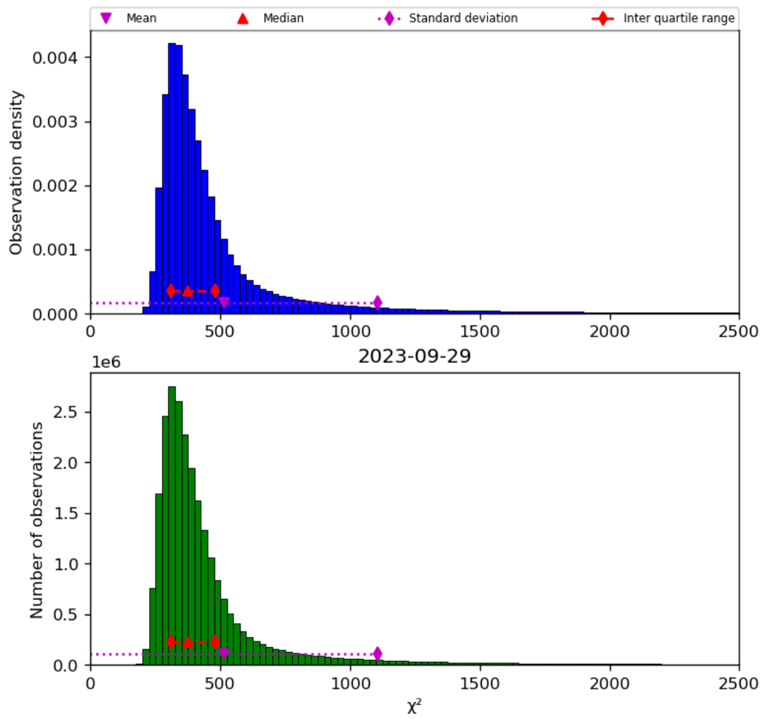
Figure 42: Histogram of “ \chi^2 ” for 2023-09-28 to 2023-09-30
