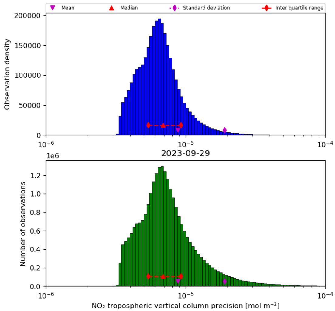
Figure 30: Histogram of “NO 2 tropospheric vertical column precision” for 2023-09-28 to 2023-09-30
