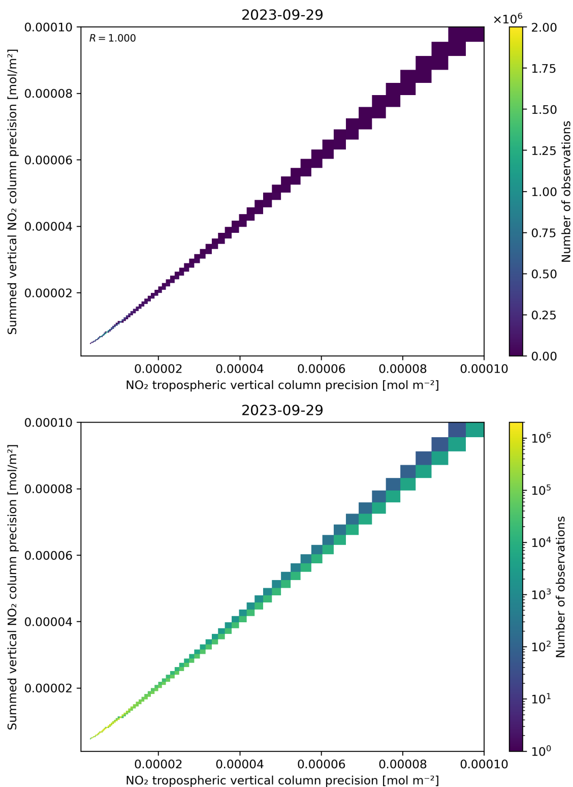
Figure 137: Scatter density plot of “NO 2 tropospheric vertical column precision” against “Summed vertical NO 2 column precision” for 2023-09-28 to 2023-09-30.
