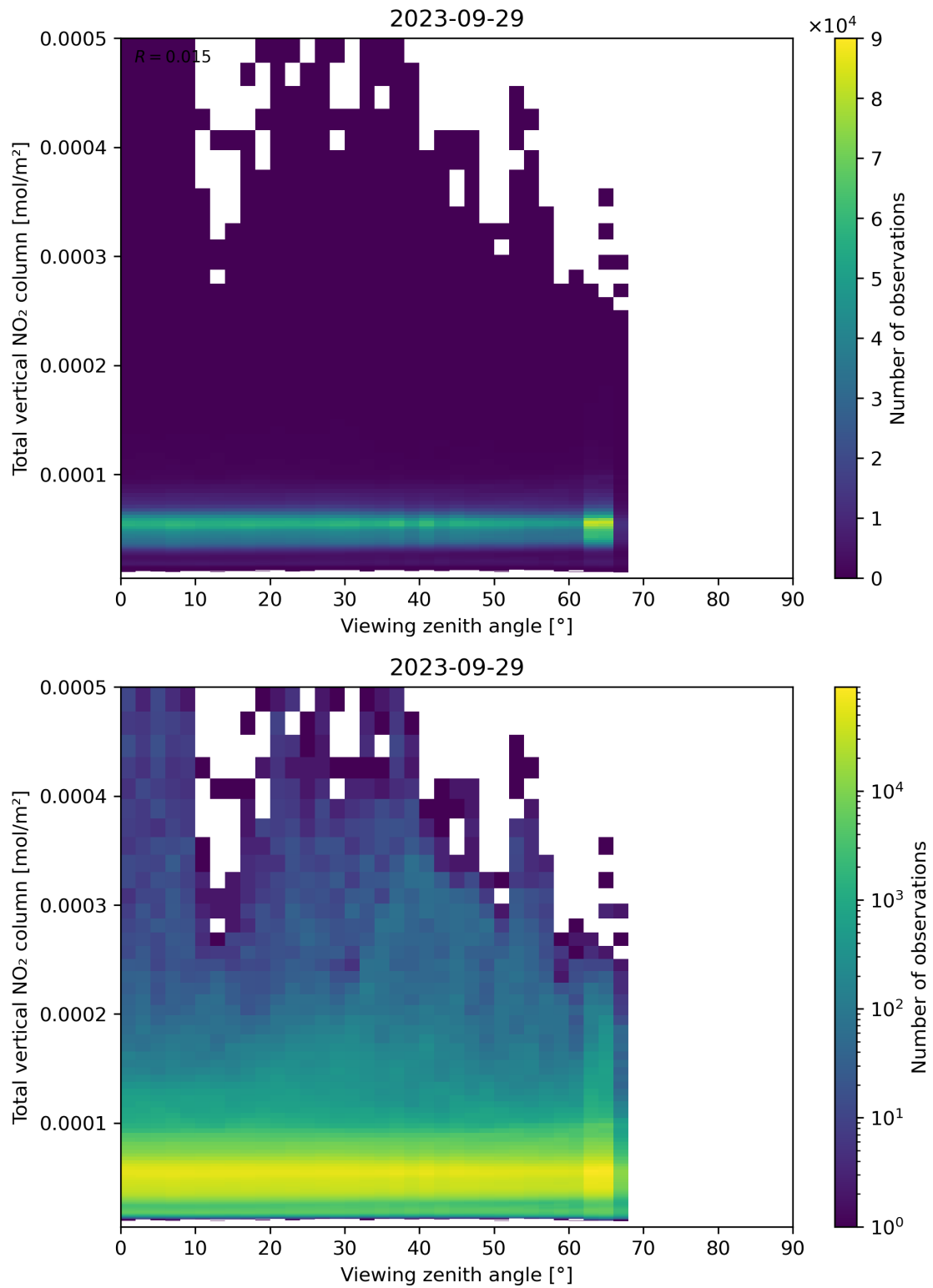
Figure 167: Scatter density plot of “Viewing zenith angle” against “Total vertical NO 2 column” for 2023-09-28 to 2023-09-30.
