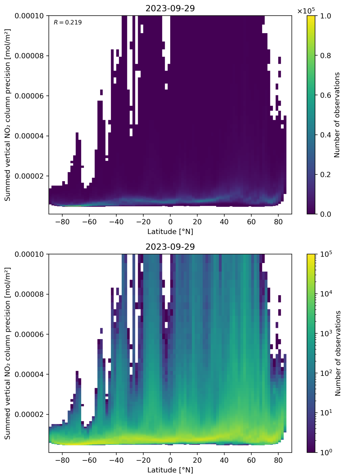
Figure 89: Scatter density plot of “Latitude” against “Summed vertical NO 2 column precision” for 2023-09-28 to 2023-09-30.
