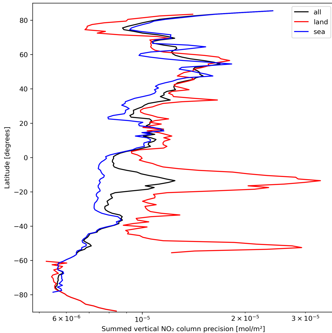
Figure 24: Zonal average of “Summed vertical NO 2 column precision” for 2023-09-28 to 2023-09-30.
