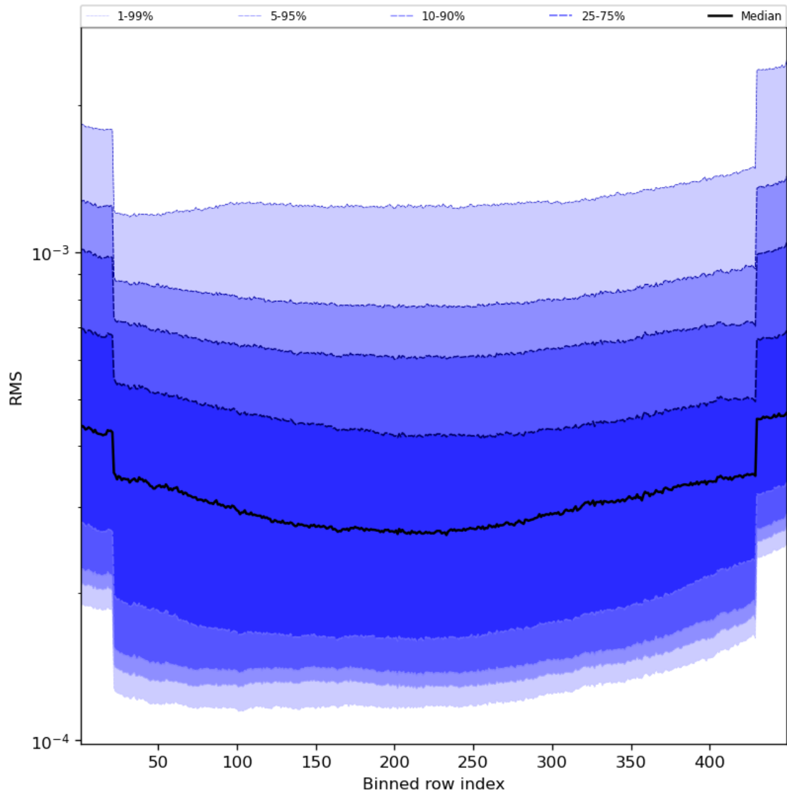
Figure 60: Along track statistics of “RMS” for 2023-09-28 to 2023-09-30
