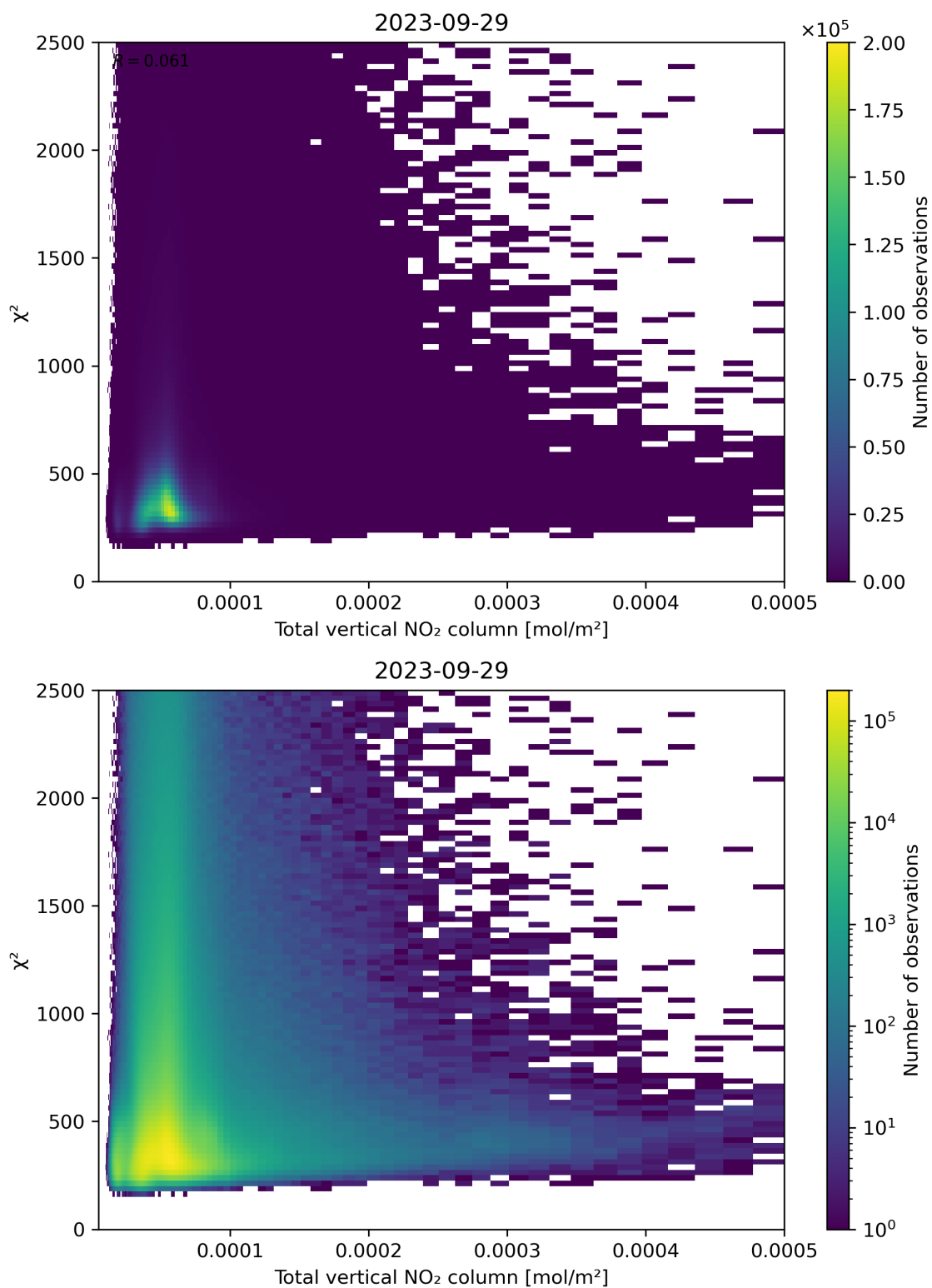
Figure 111: Scatter density plot of “Total vertical NO 2 column” against “ \chi^2 ” for 2023-09-28 to 2023-09-30.
