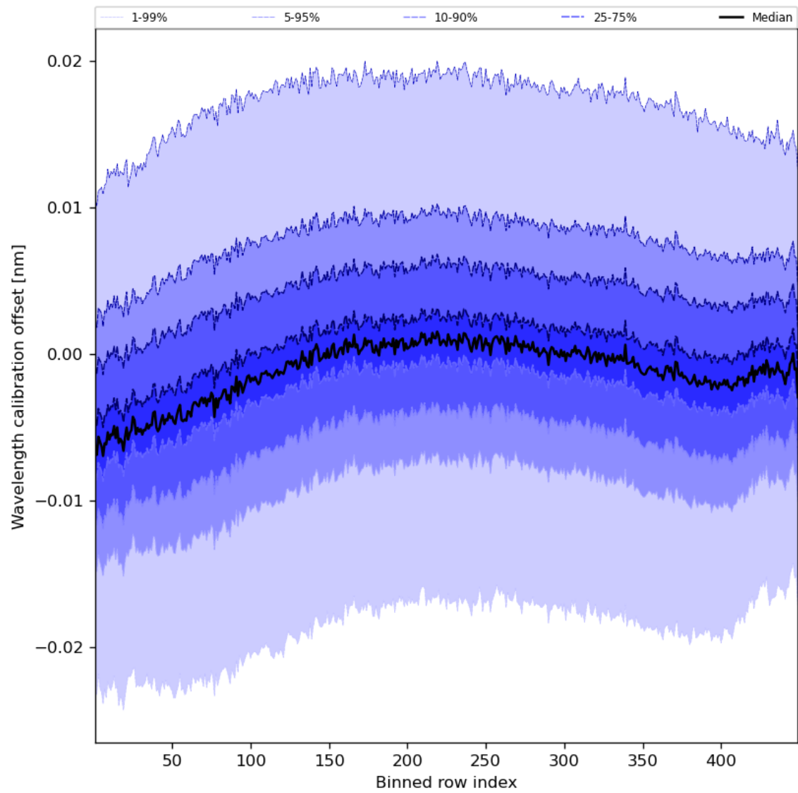
Figure 52: Along track statistics of “Wavelength calibration offset” for 2023-09-28 to 2023-09-30
