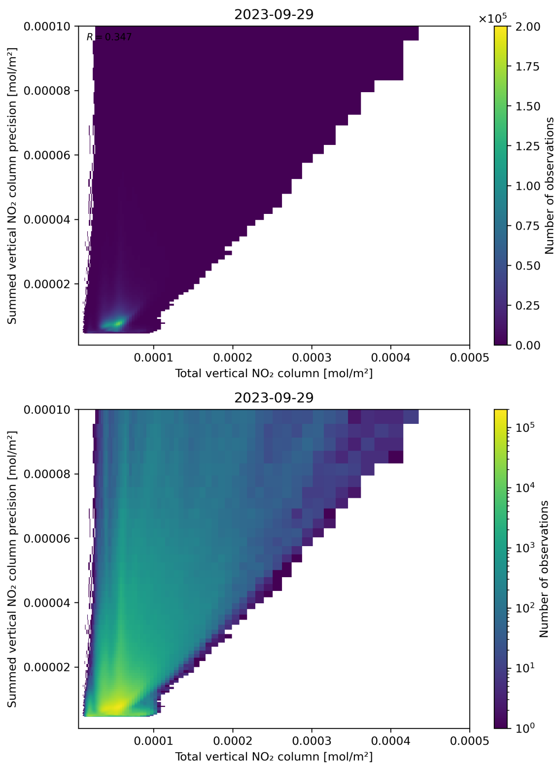
Figure 113: Scatter density plot of “Total vertical NO 2 column” against “Summed vertical NO 2 column precision” for 2023-09-28 to 2023-09-30.
