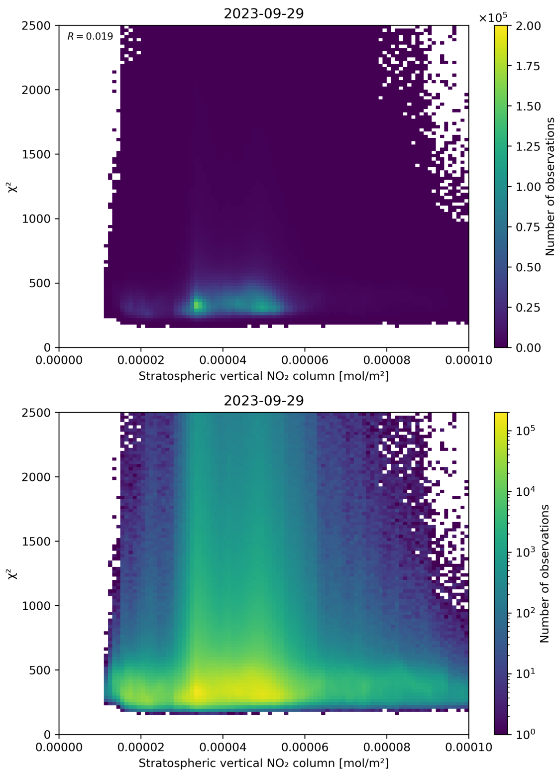
Figure 97: Scatter density plot of “Stratospheric vertical NO 2 column” against “ \chi^2 ” for 2023-09-28 to 2023-09-30.
