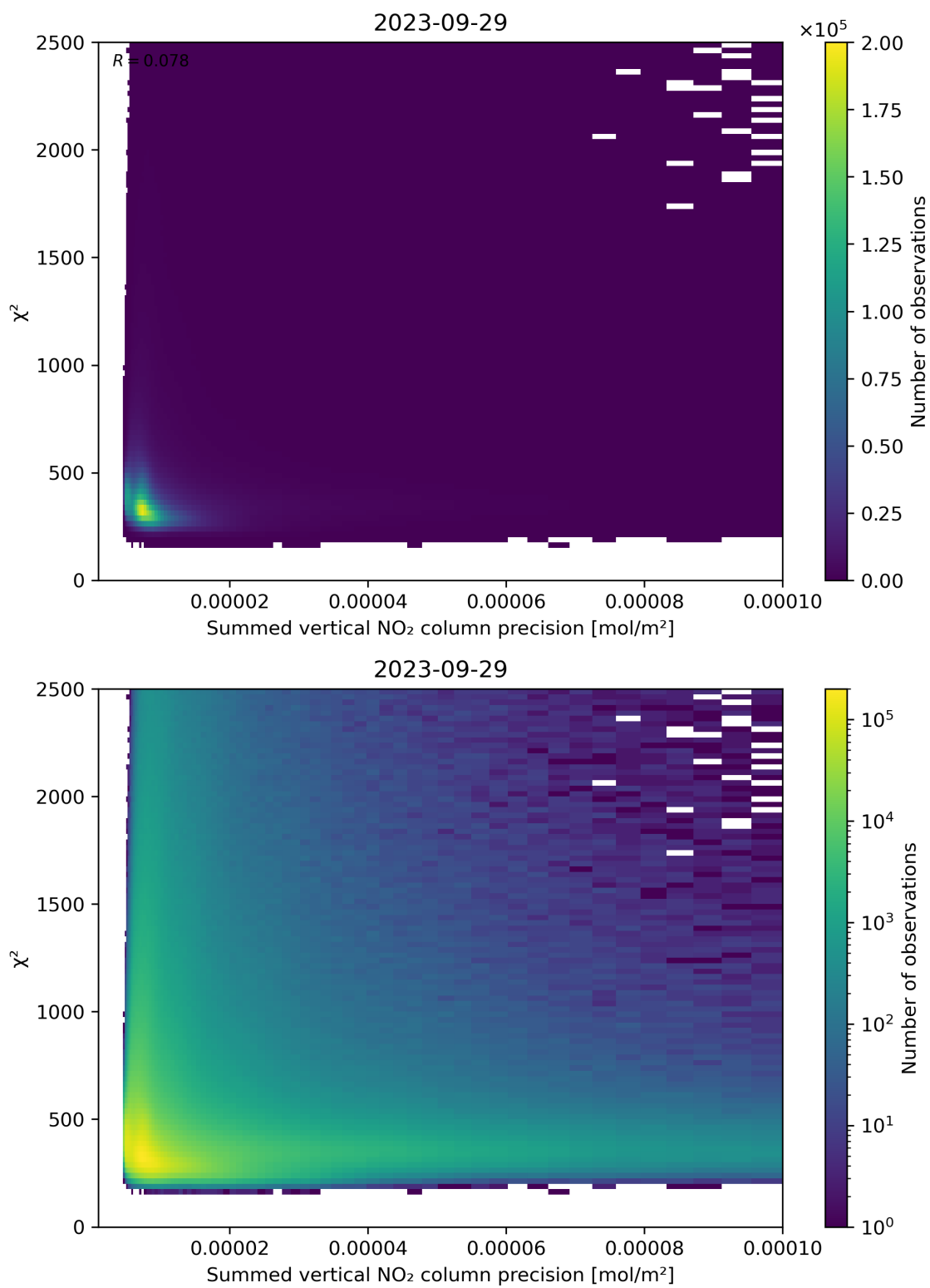
Figure 107: Scatter density plot of “Summed vertical NO 2 column precision” against “ \chi^2 ” for 2023-09-28 to 2023-09-30.
