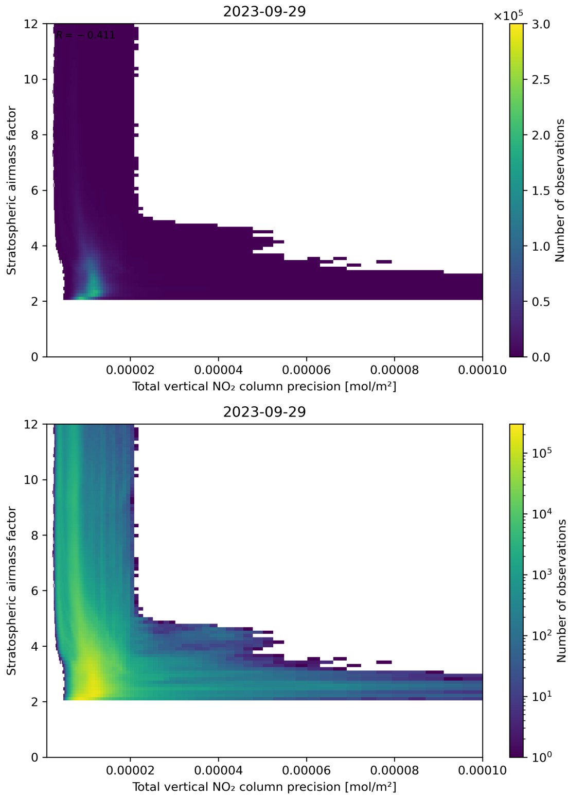
Figure 115: Scatter density plot of “Total vertical NO 2 column precision” against “Stratospheric air mass factor” for 2023-09-28 to 2023-09-30.
