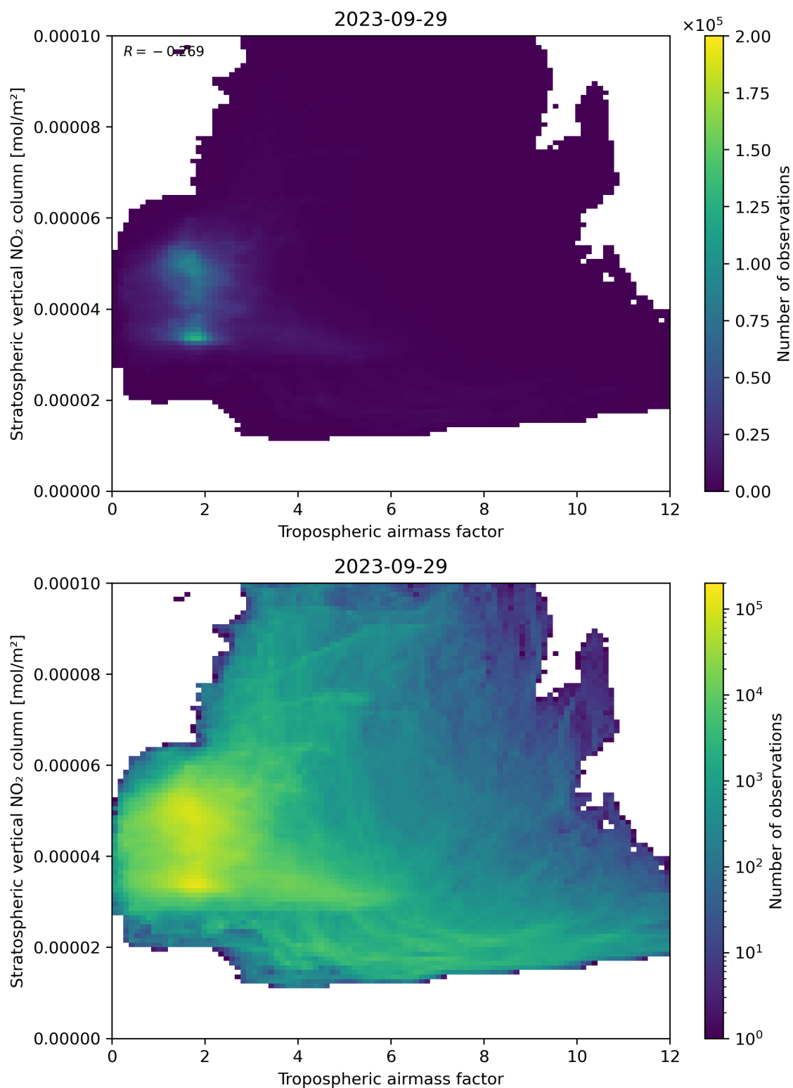
Figure 74: Scatter density plot of “Tropospheric air mass factor” against “Stratospheric vertical NO 2 column” for 2023-09-28 to 2023-09-30.
