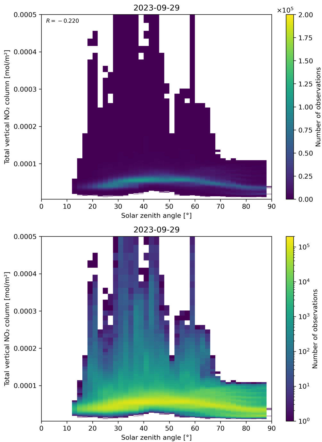
Figure 153: Scatter density plot of “Solar zenith angle” against “Total vertical NO 2 column” for 2023-09-28 to 2023-09-30.
