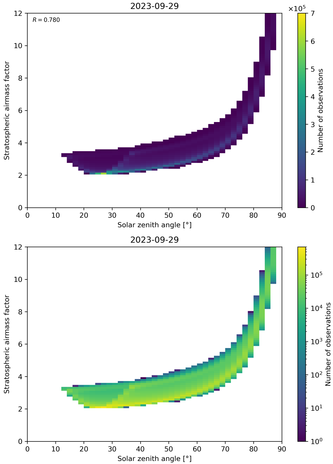
Figure 145: Scatter density plot of “Solar zenith angle” against “Stratospheric airmass factor” for 2023-09-28 to 2023-09-30.
