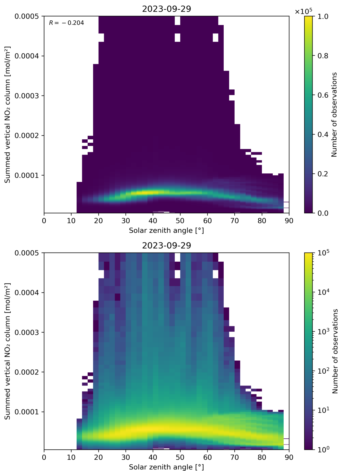
Figure 151: Scatter density plot of “Solar zenith angle” against “Summed vertical NO 2 column” for 2023-09-28 to 2023-09-30.
