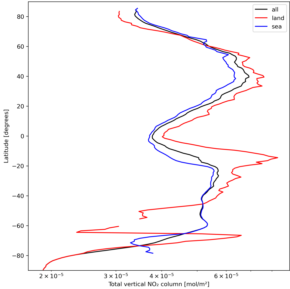
Figure 21: Zonal average of “Total vertical NO 2 column” for 2023-09-28 to 2023-09-30.
