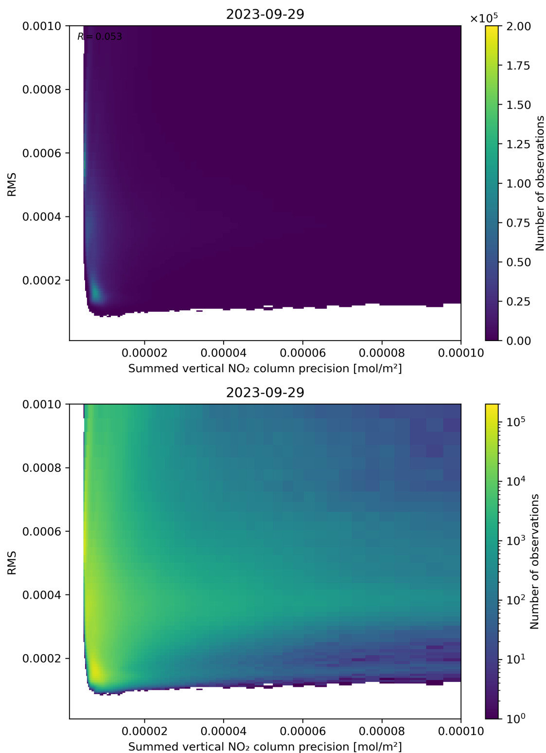
Figure 108: Scatter density plot of “Summed vertical NO 2 column precision” against “RMS” for 2023-09-28 to 2023-09-30.
