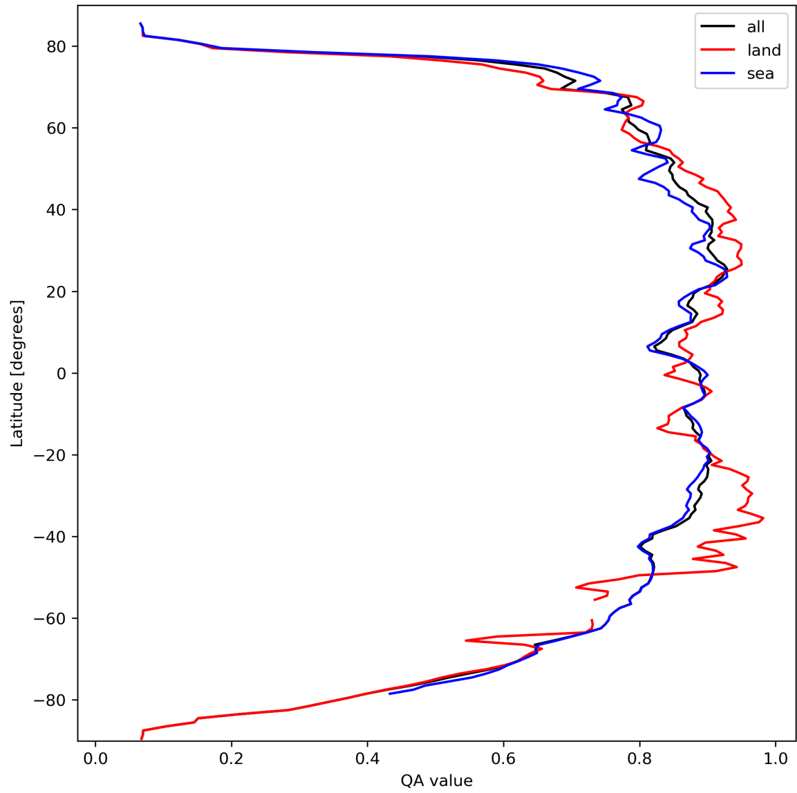
Figure 11: Zonal average of “QA value” for 2023-09-28 to 2023-09-30.
