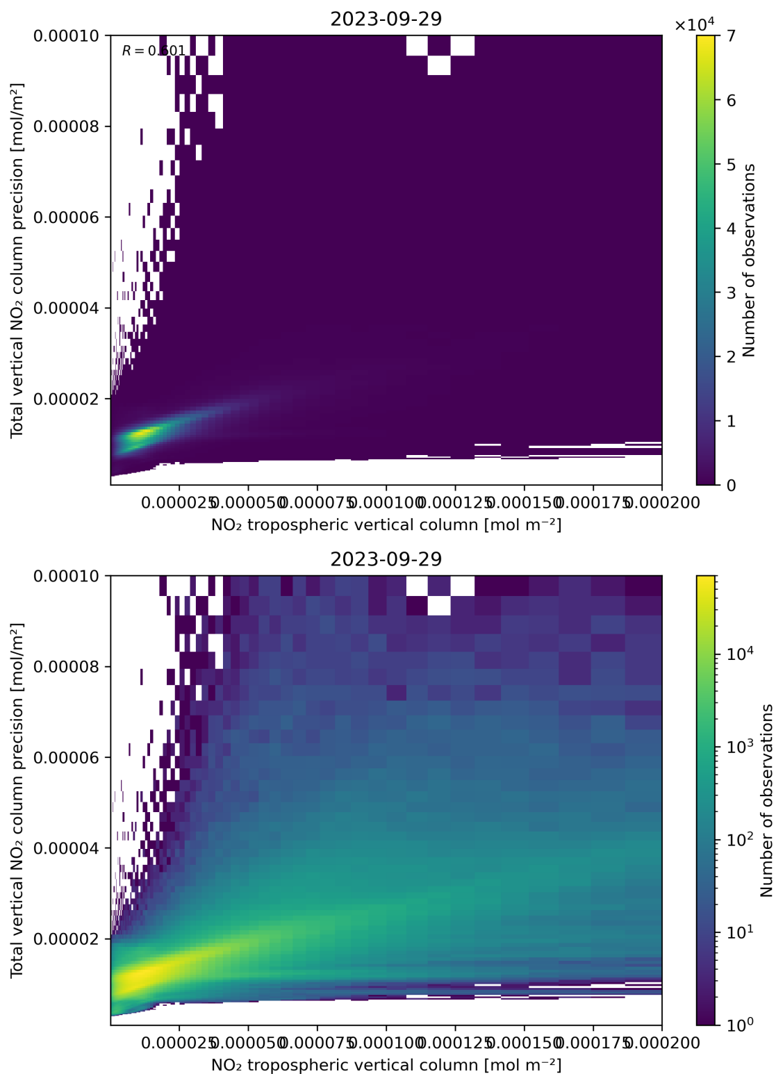
Figure 129: Scatter density plot of “NO 2 tropospheric vertical column” against “Total vertical NO 2 column precision” for 2023-09-28 to 2023-09-30.
