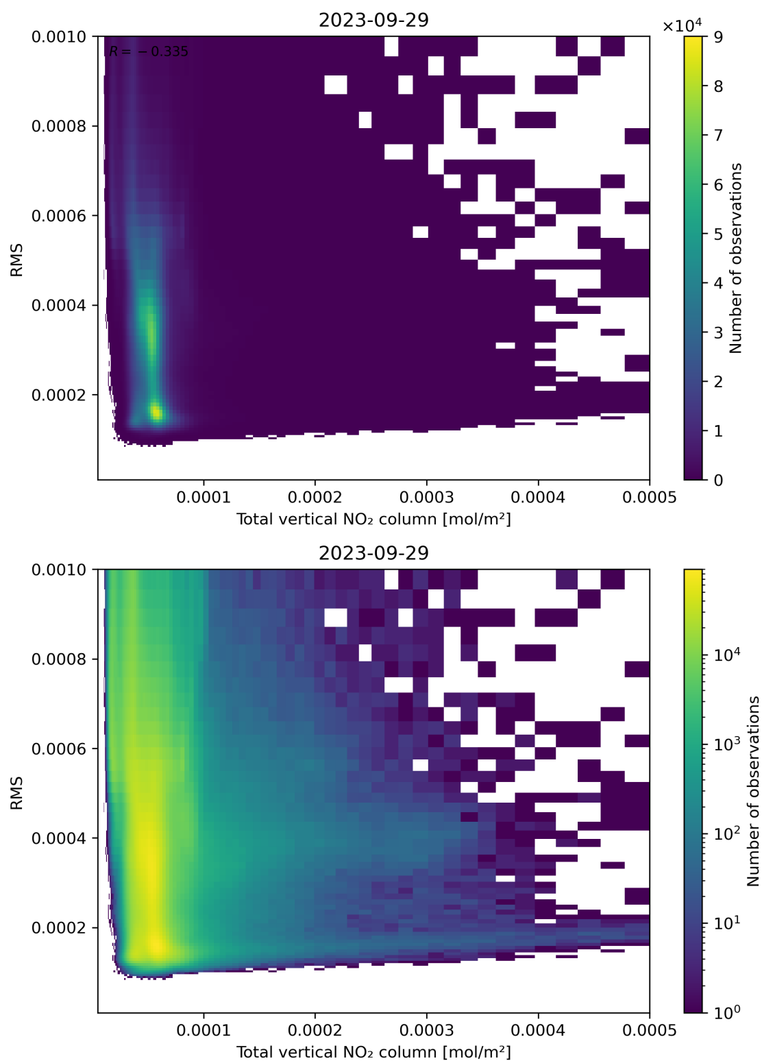
Figure 120: Scatter density plot of “Total vertical NO 2 column” against “RMS” for 2023-09-28 to 2023-09-30.
