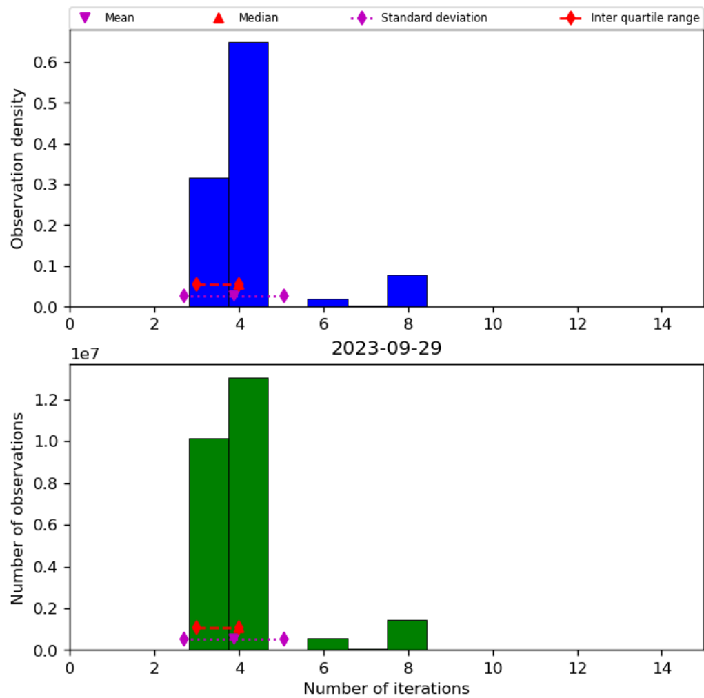
Figure 34: Histogram of “Number of iterations” for 2023-09-28 to 2023-09-30
