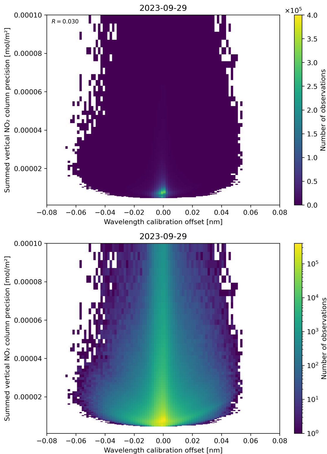
Figure 178: Scatter density plot of “Wavelength calibration offset” against “Summed vertical NO 2 column precision” for 2023-09-28 to 2023-09-30.
