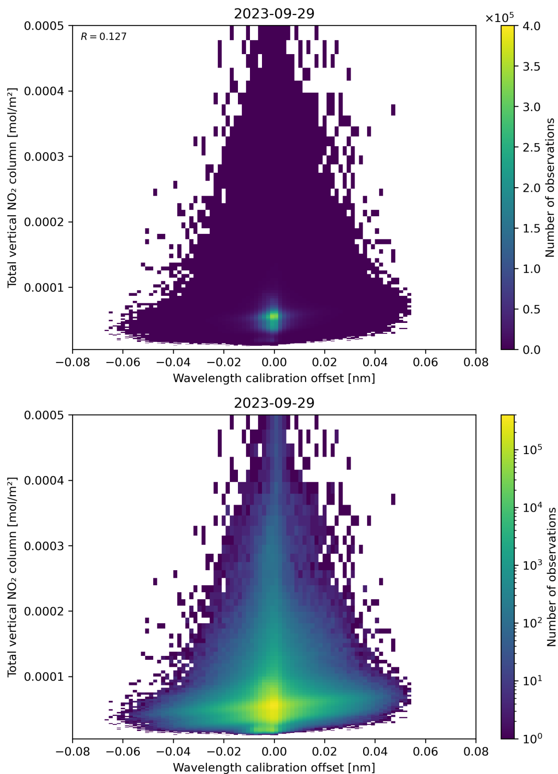
Figure 179: Scatter density plot of “Wavelength calibration offset” against “Total vertical NO 2 column” for 2023-09-28 to 2023-09-30.
