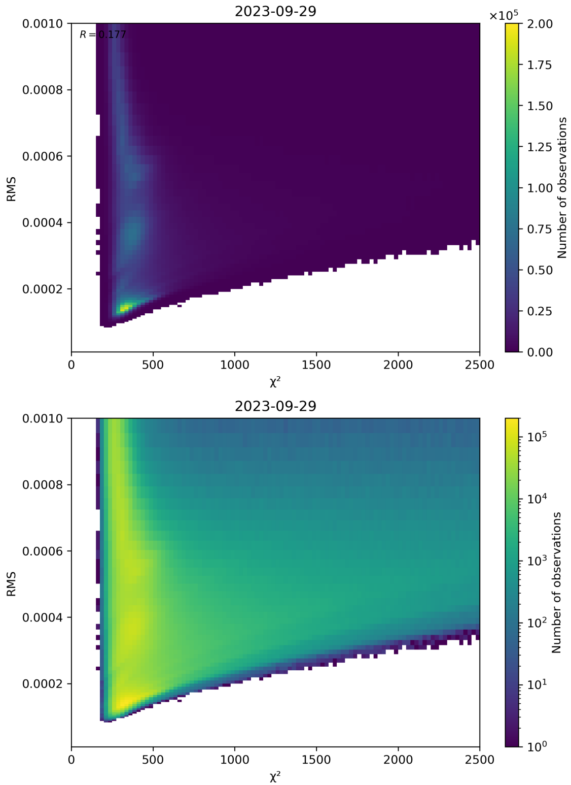
Figure 82: Scatter density plot of “ \chi^2 ” against “RMS” for 2023-09-28 to 2023-09-30.
