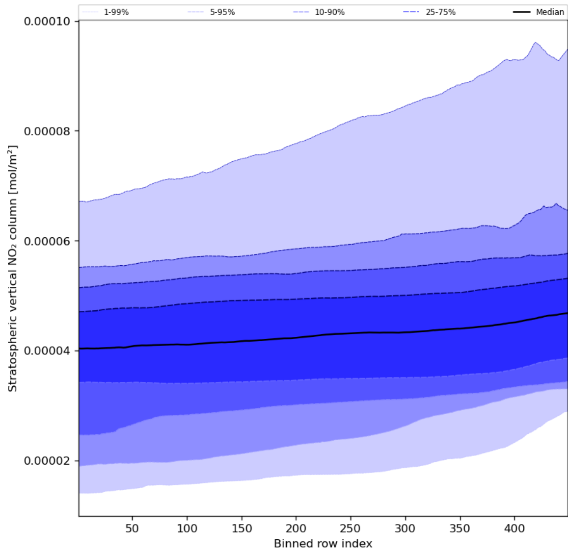
Figure 53: Along track statistics of “Stratospheric vertical NO 2 column” for 2023-09-28 to 2023-09-30
