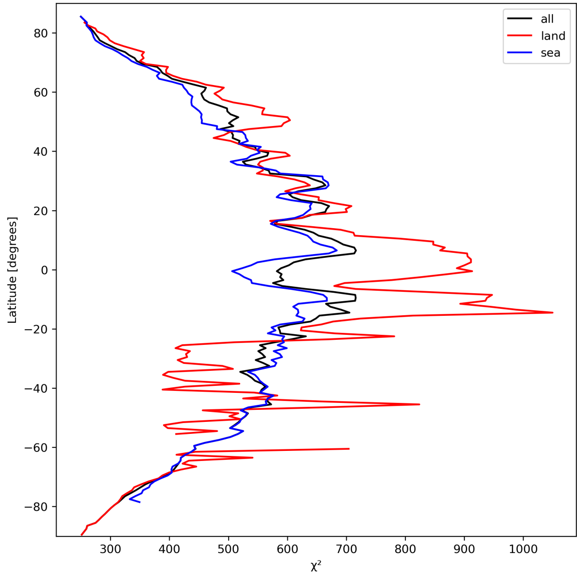
Figure 25: Zonal average of “ \chi^2 ” for 2023-09-28 to 2023-09-30.
