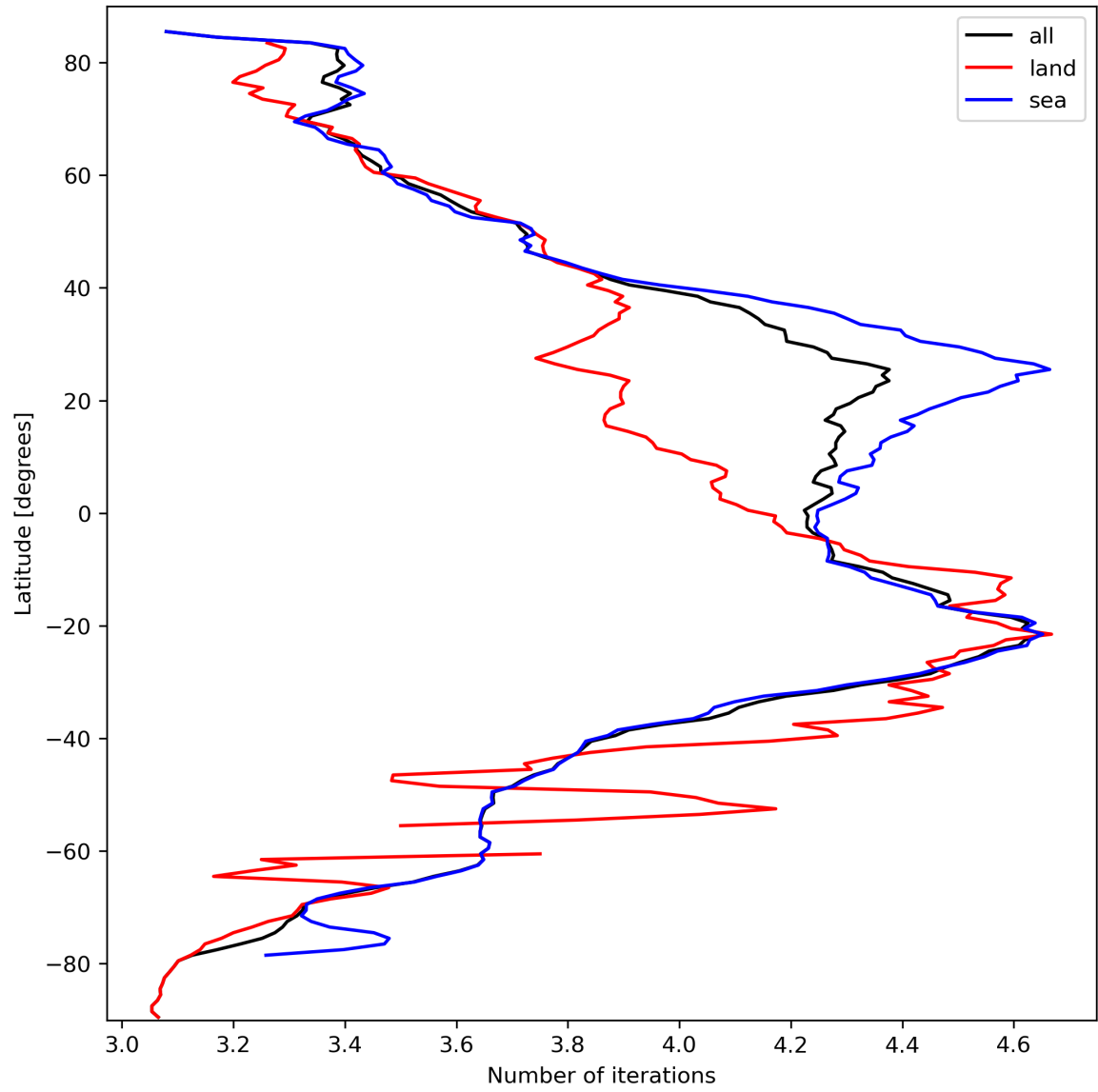
Figure 17: Zonal average of “Number of iterations” for 2023-09-28 to 2023-09-30.
