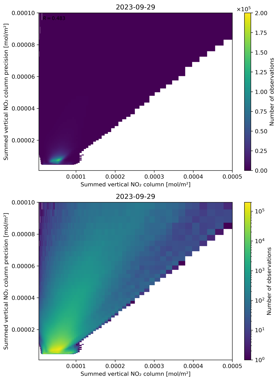
Figure 105: Scatter density plot of “Summed vertical NO 2 column” against “Summed vertical NO 2 column precision” for 2023-09-28 to 2023-09-30.
