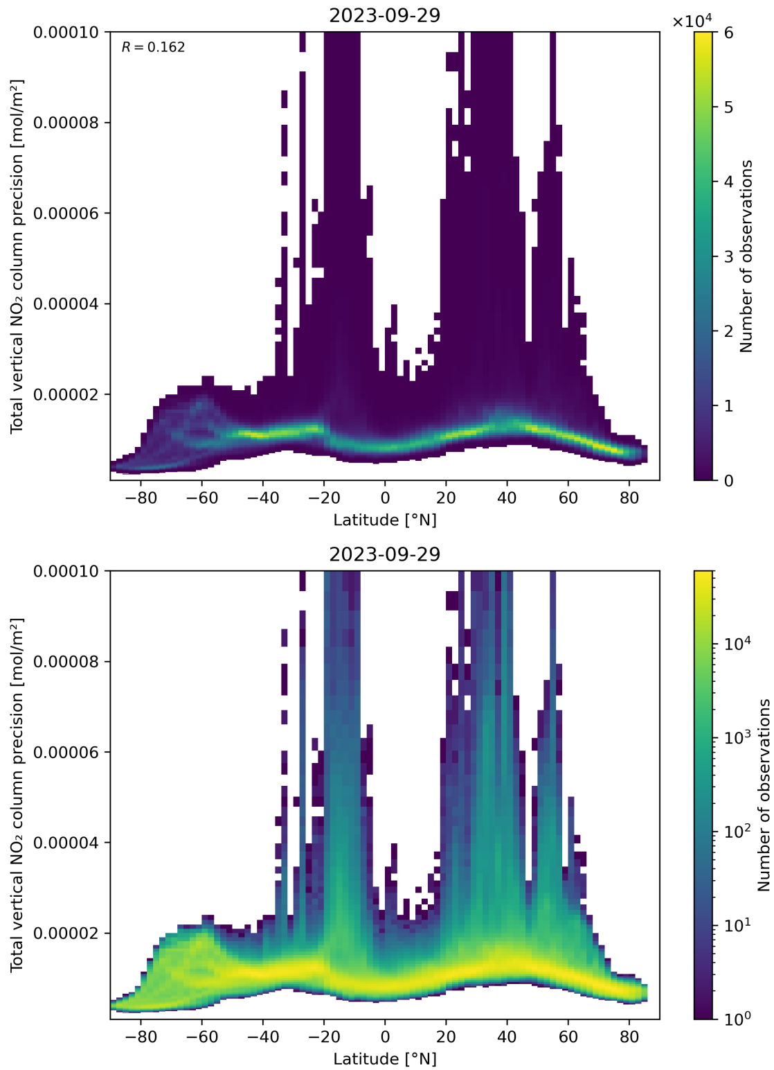
Figure 91: Scatter density plot of “Latitude” against “Total vertical NO 2 column precision” for 2023-09-28 to 2023-09-30.
