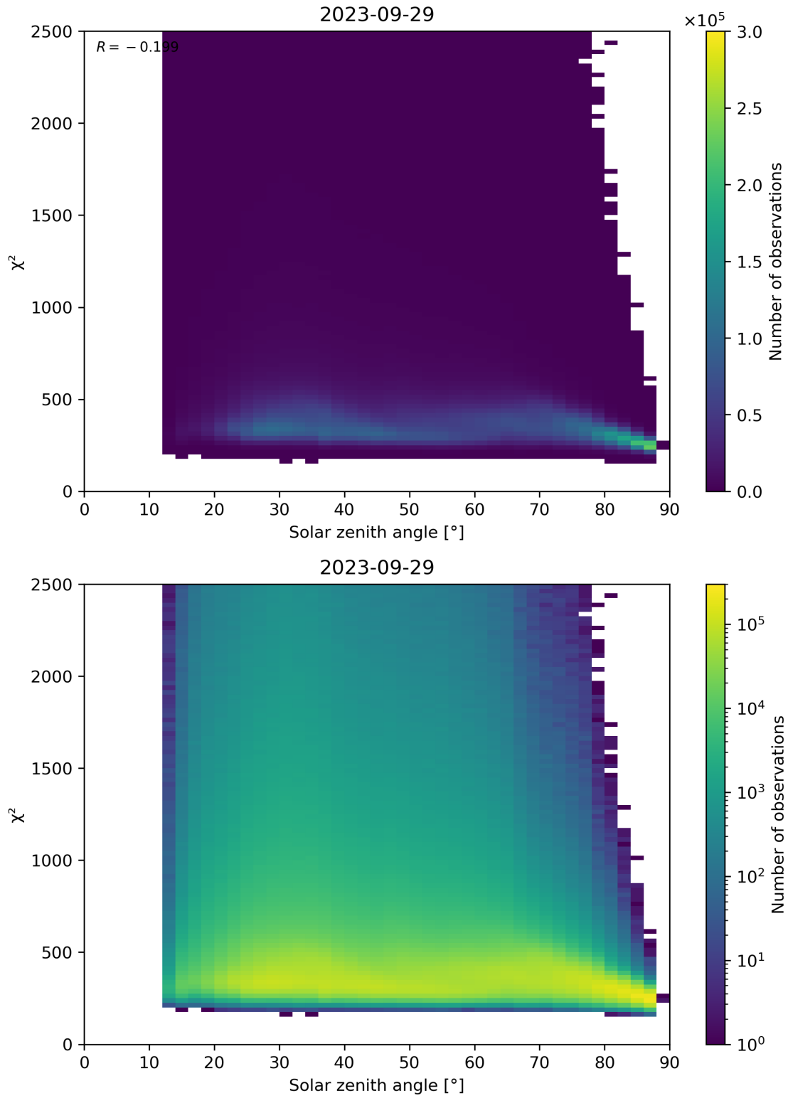
Figure 148: Scatter density plot of “Solar zenith angle” against “ \chi^2 ” for 2023-09-28 to 2023-09-30.
