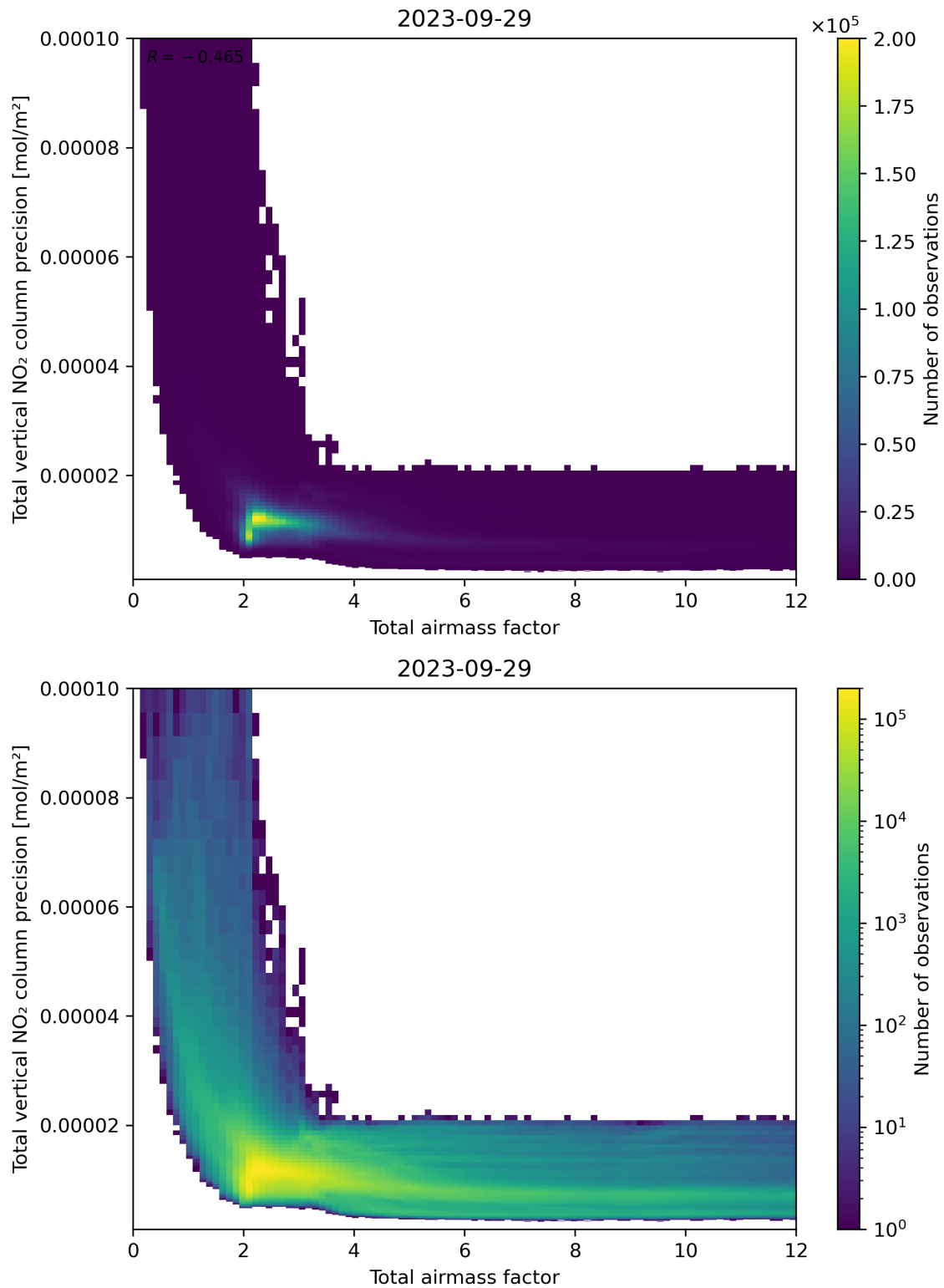
Figure 68: Scatter density plot of “Total airmass factor” against “Total vertical NO 2 column precision” for 2023-09-28 to 2023-09-30.
