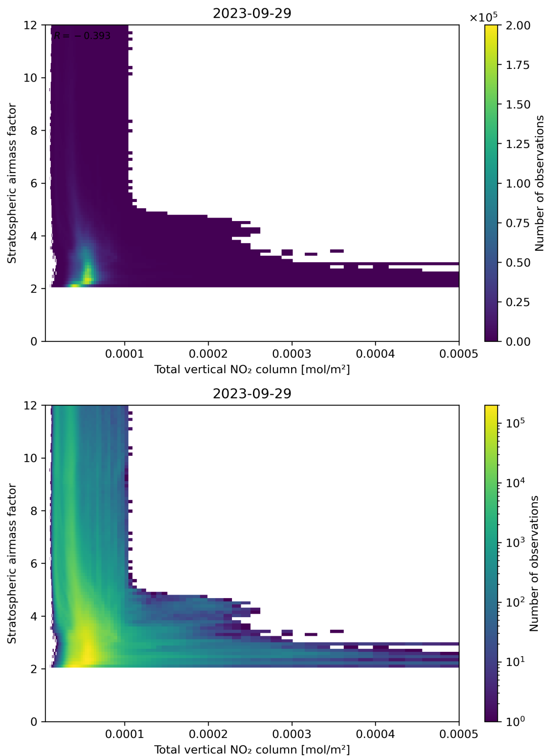
Figure 110: Scatter density plot of “Total vertical NO 2 column” against “Stratospheric airmass factor” for 2023-09-28 to 2023-09-30.
