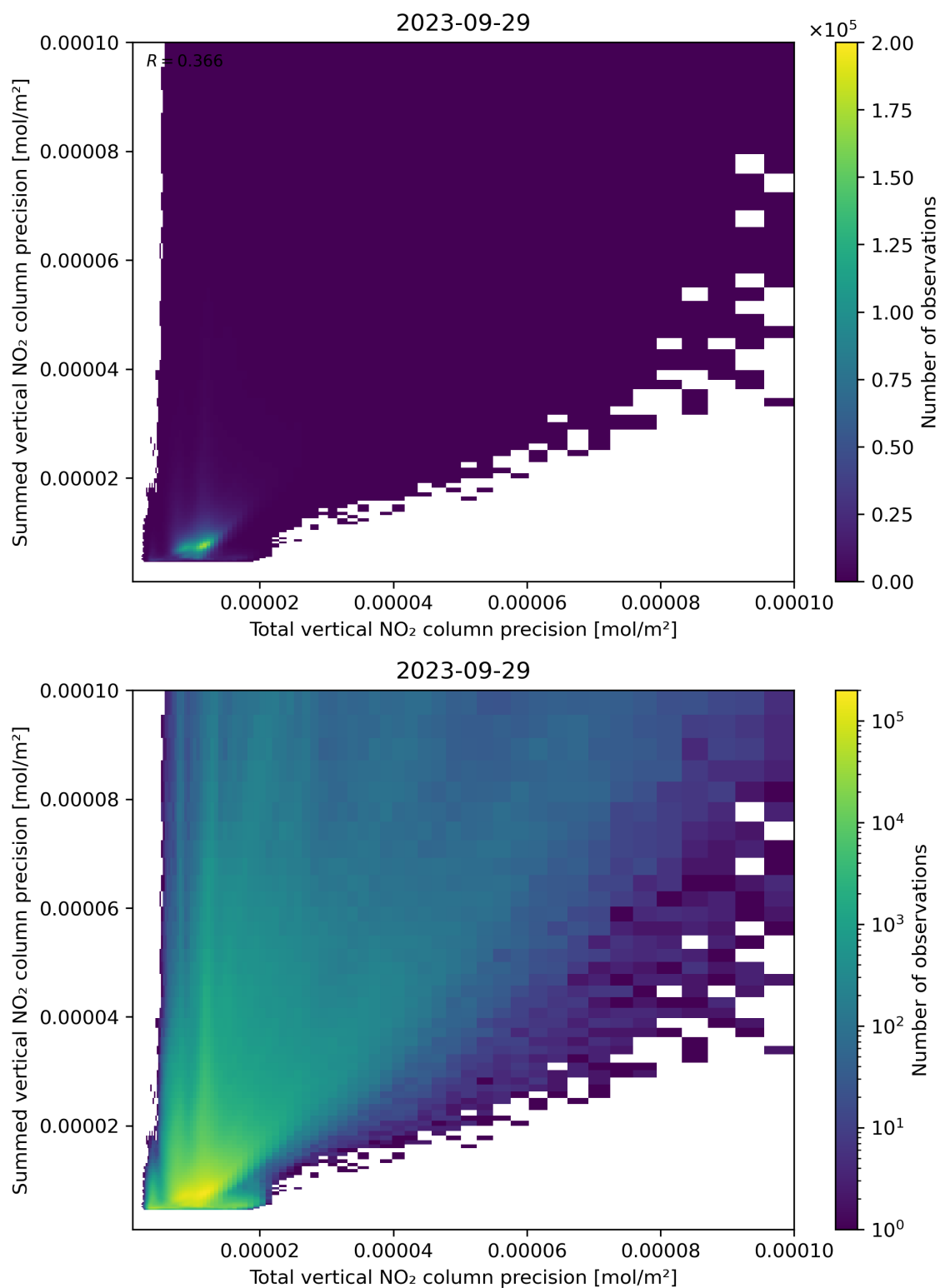
Figure 118: Scatter density plot of “Total vertical NO 2 column precision” against “Summed vertical NO 2 column precision” for 2023-09-28 to 2023-09-30.
