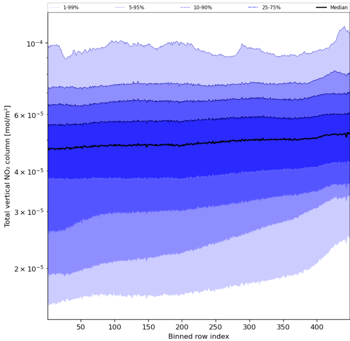
Figure 55: Along track statistics of “Total vertical NO 2 column” for 2023-09-28 to 2023-09-30
