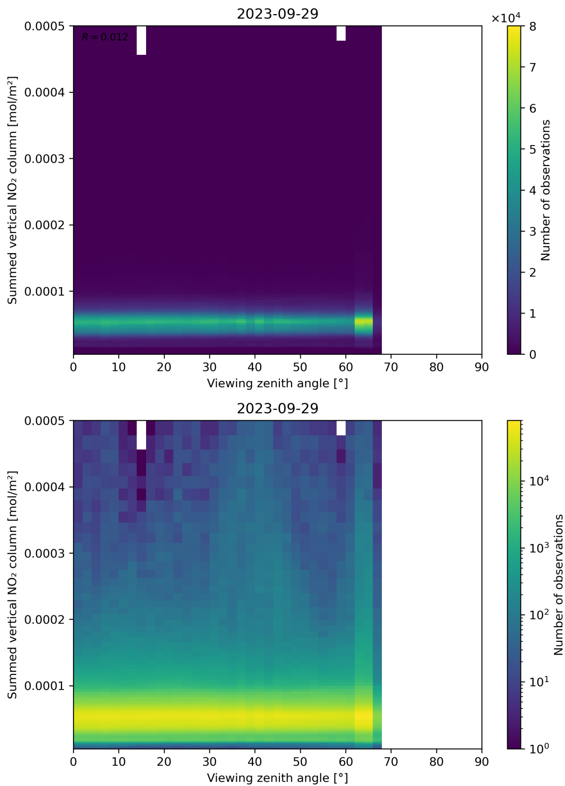
Figure 165: Scatter density plot of “Viewing zenith angle” against “Summed vertical NO 2 column” for 2023-09-28 to 2023-09-30.
