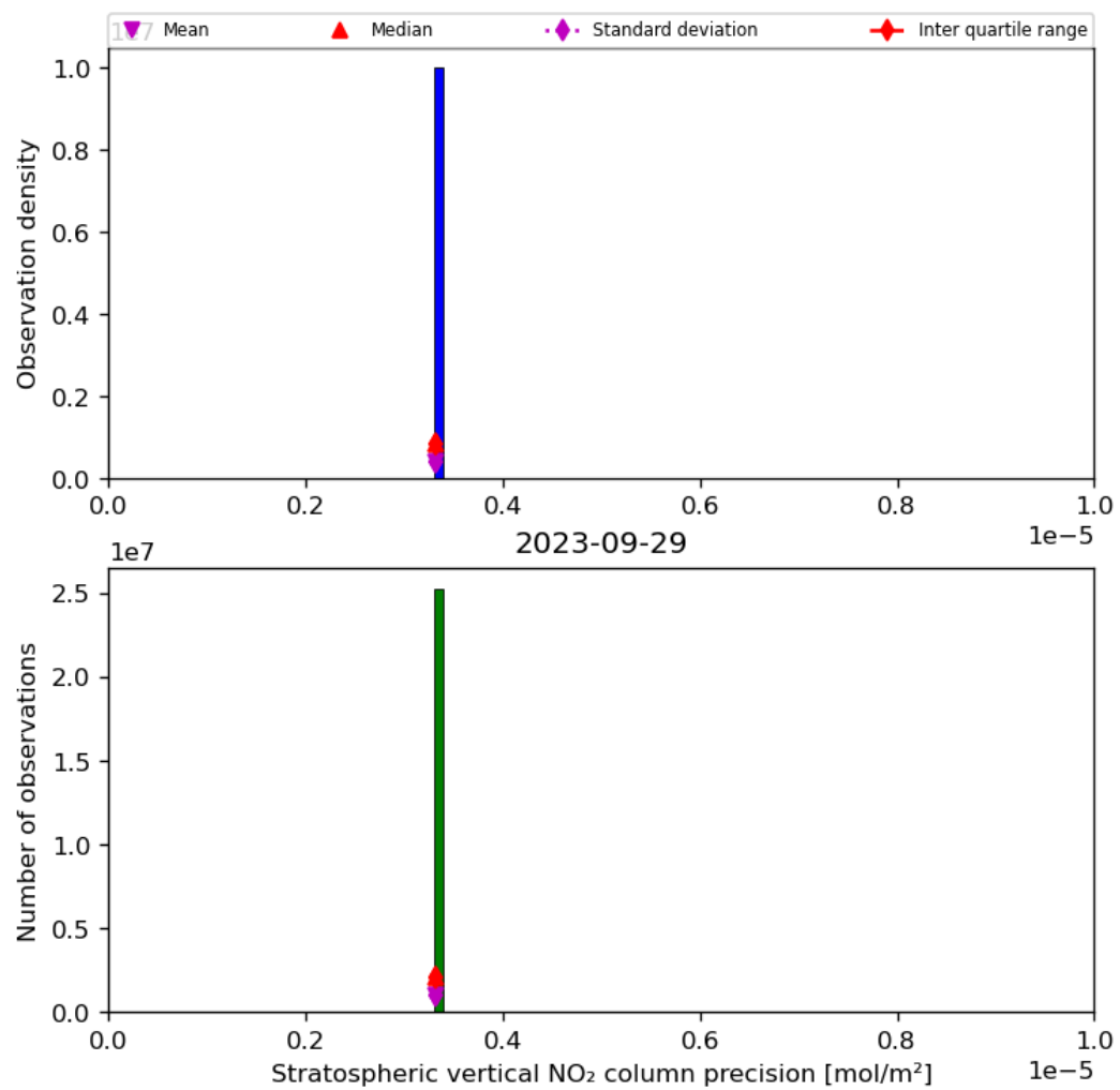
Figure 37: Histogram of “Stratospheric vertical NO 2 column precision” for 2023-09-28 to 2023-09-30
