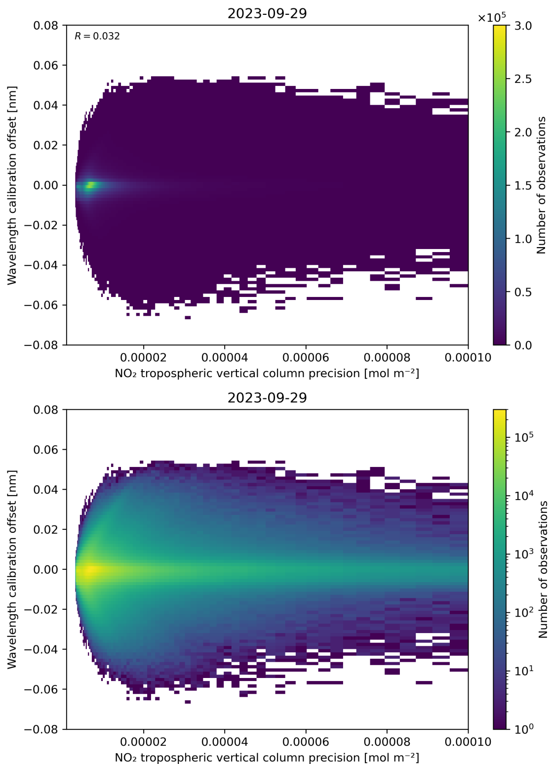
Figure 141: Scatter density plot of “NO 2 tropospheric vertical column precision” against “Wavelength calibration offset” for 2023-09-28 to 2023-09-30.
