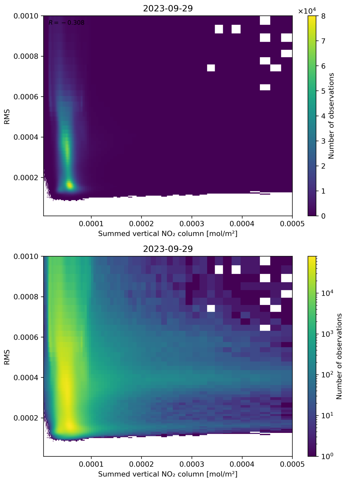
Figure 109: Scatter density plot of “Summed vertical NO 2 column” against “RMS” for 2023-09-28 to 2023-09-30.
