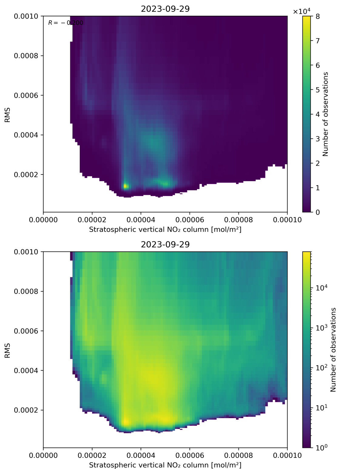
Figure 102: Scatter density plot of “Stratospheric vertical NO 2 column” against “RMS” for 2023-09-28 to 2023-09-30.
