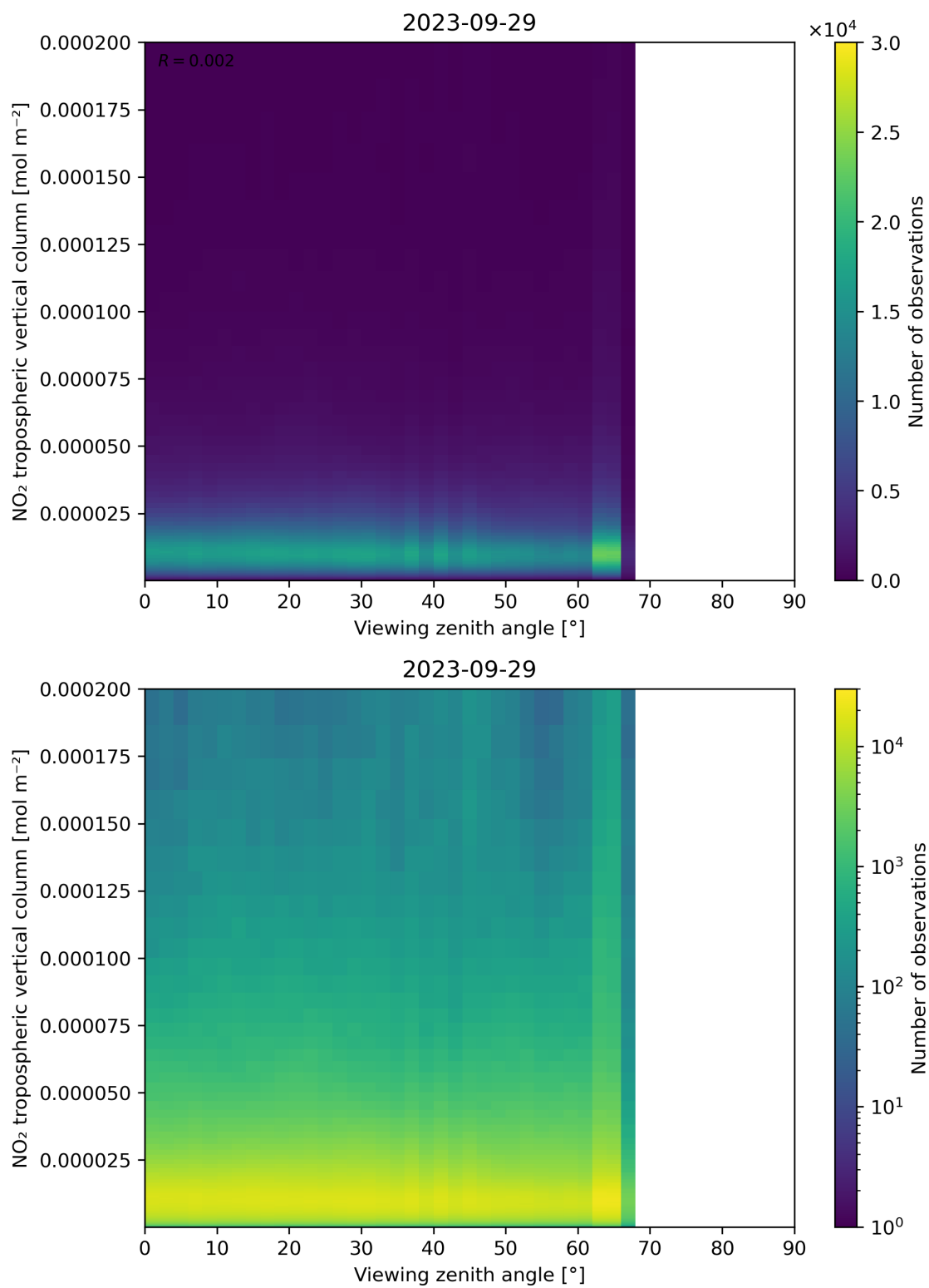
Figure 169: Scatter density plot of “Viewing zenith angle” against “NO 2 tropospheric vertical column” for 2023-09-28 to 2023-09-30.
