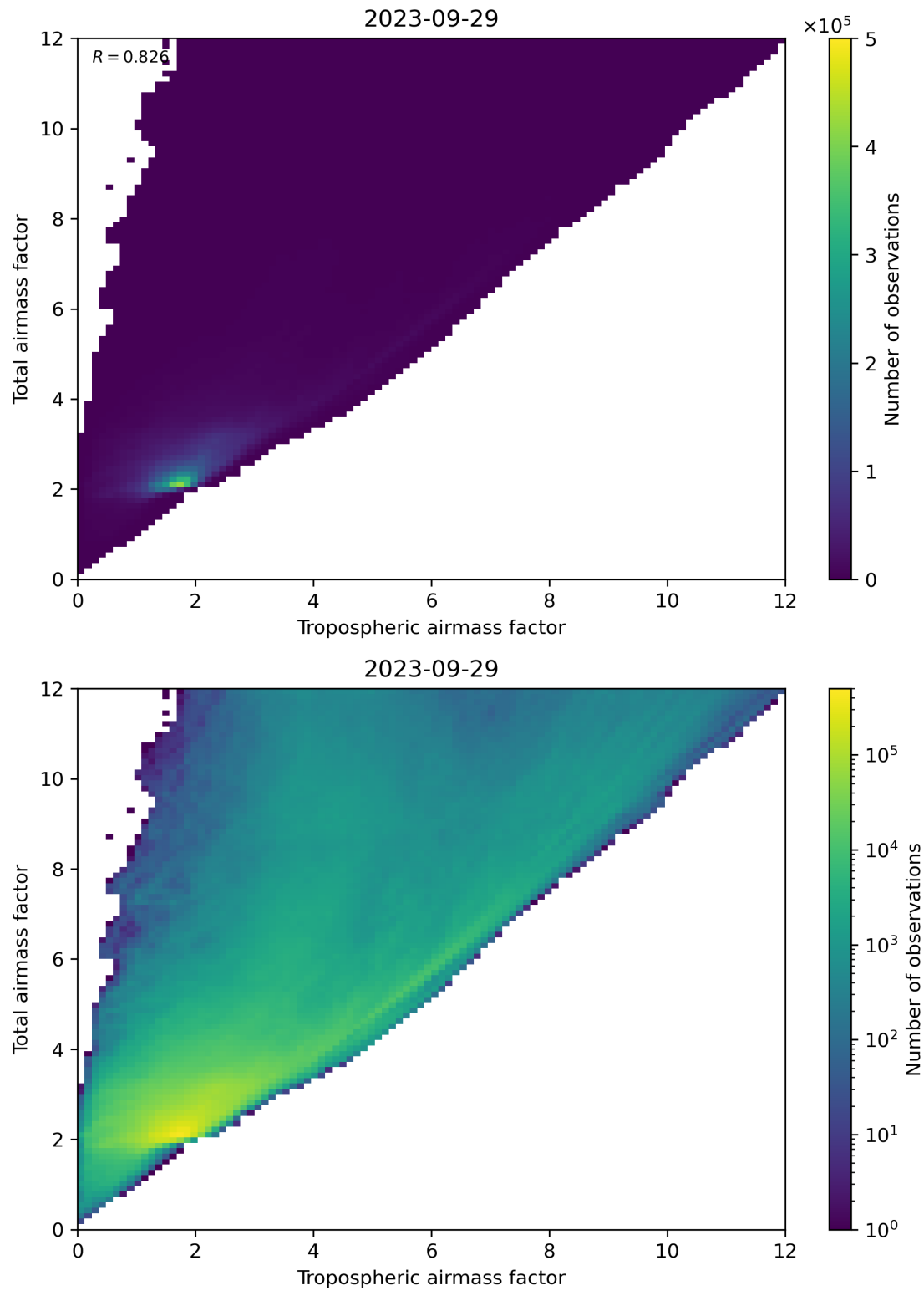
Figure 72: Scatter density plot of “Tropospheric airmass factor” against “Total airmass factor” for 2023-09-28 to 2023-09-30.
