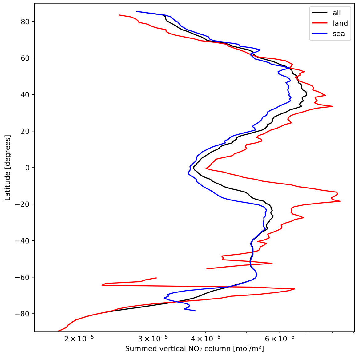
Figure 23: Zonal average of “Summed vertical NO 2 column” for 2023-09-28 to 2023-09-30.
