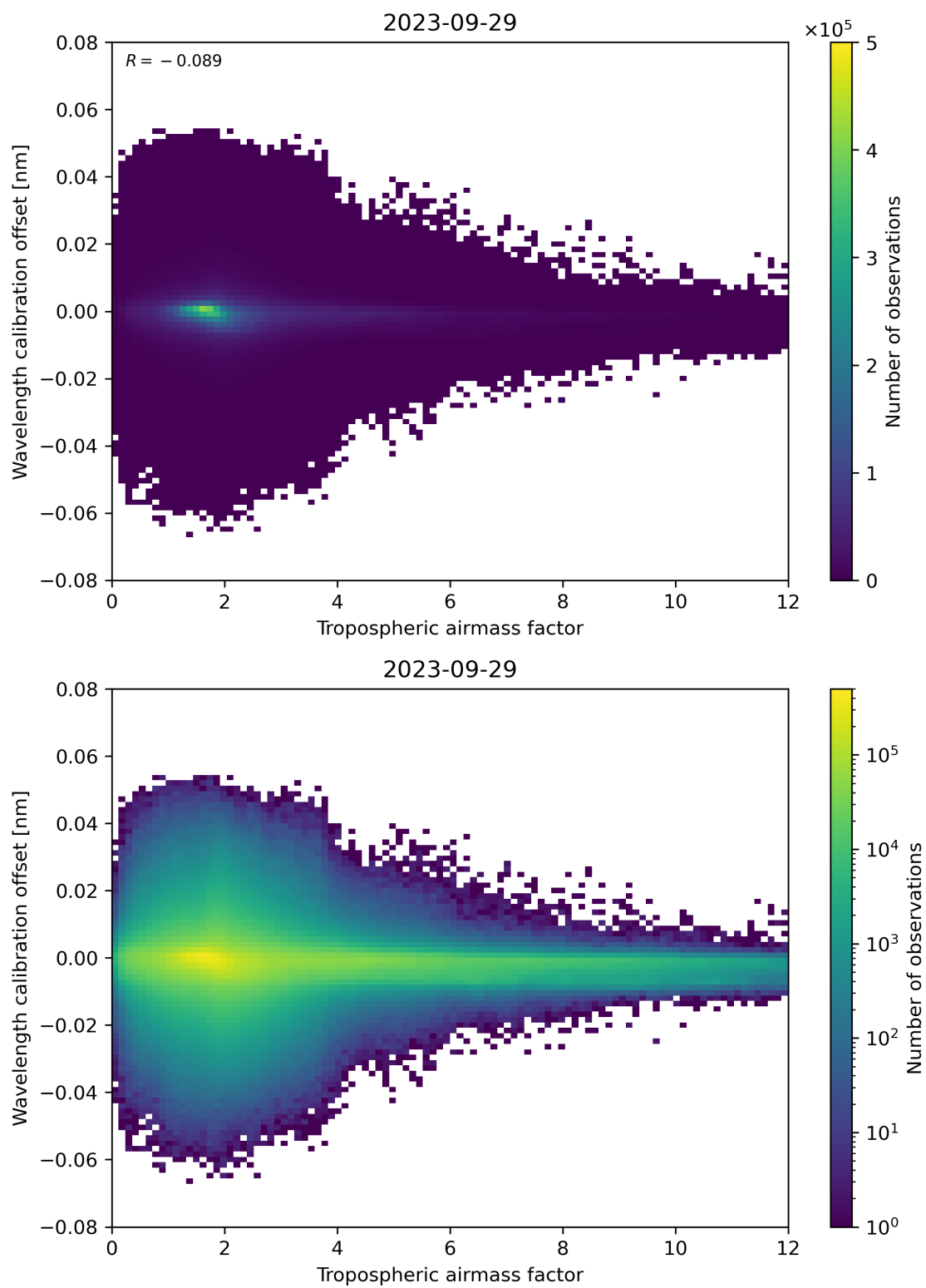
Figure 80: Scatter density plot of “Tropospheric airmass factor” against “Wavelength calibration offset” for 2023-09-28 to 2023-09-30.
