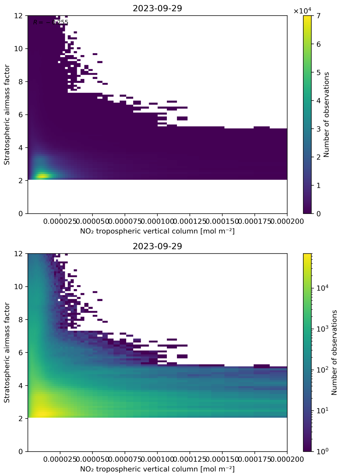
Figure 121: Scatter density plot of “NO 2 tropospheric vertical column” against “Stratospheric airmass factor” for 2023-09-28 to 2023-09-30.
