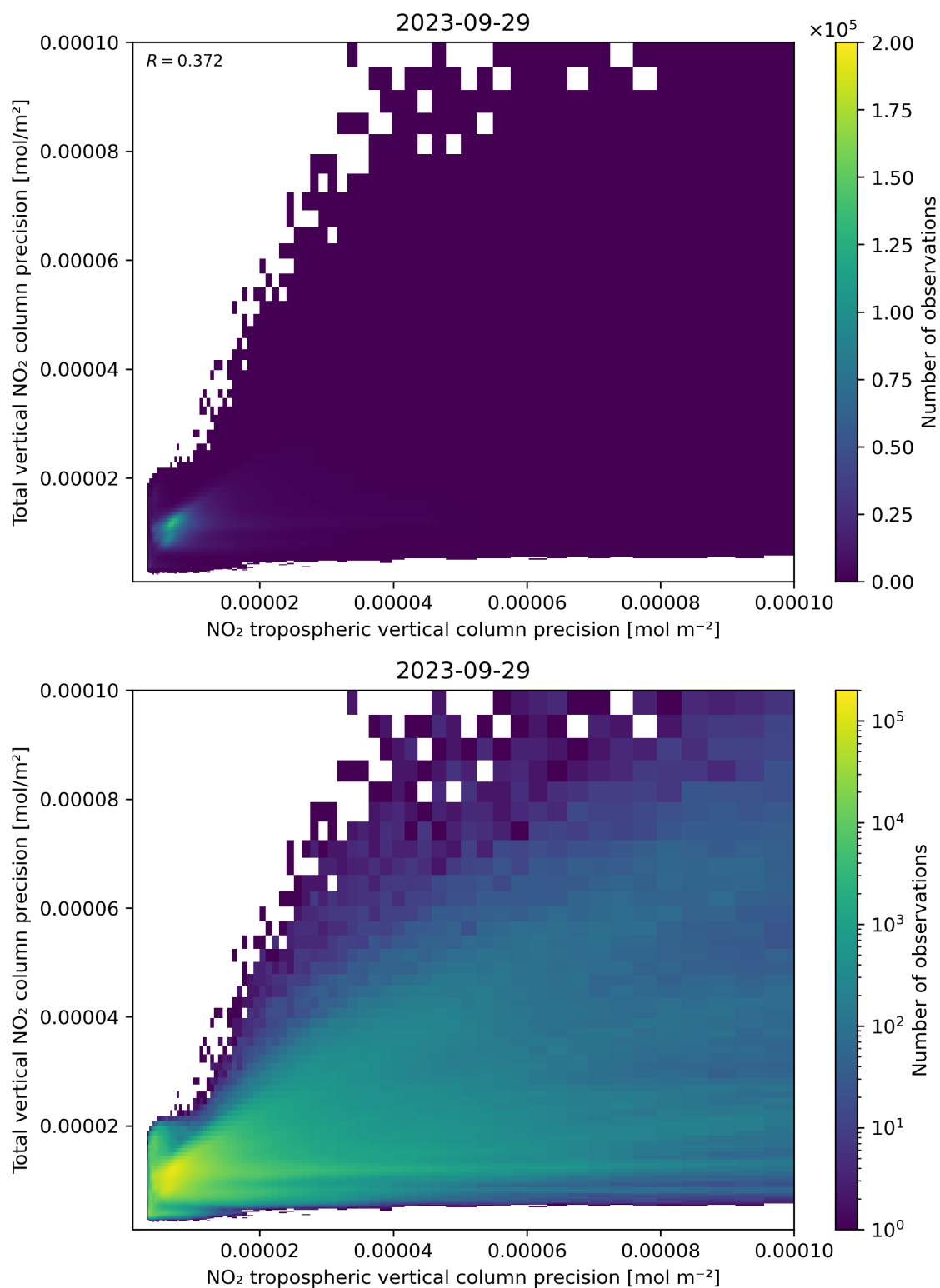
Figure 139: Scatter density plot of “NO 2 tropospheric vertical column precision” against “Total vertical NO 2 column precision” for 2023-09-28 to 2023-09-30.
