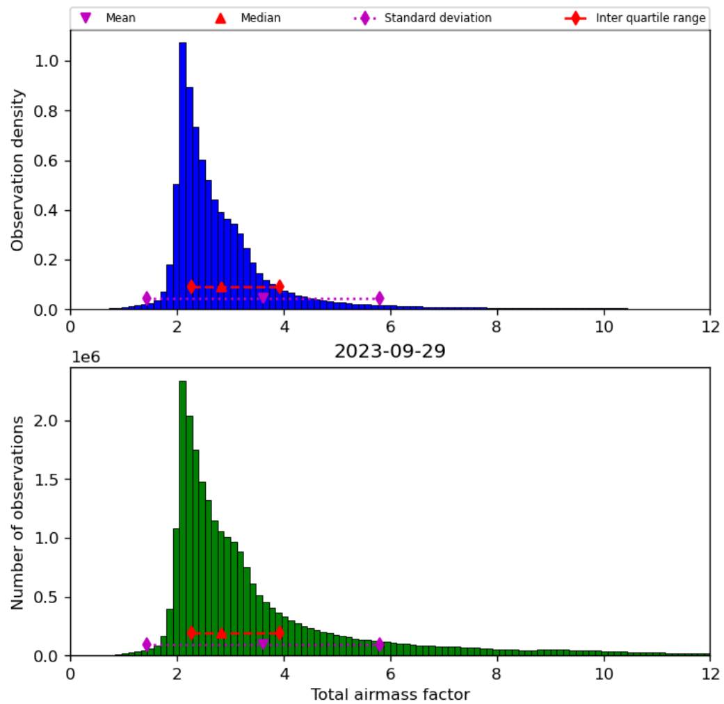
Figure 32: Histogram of “Total airmass factor” for 2023-09-28 to 2023-09-30
