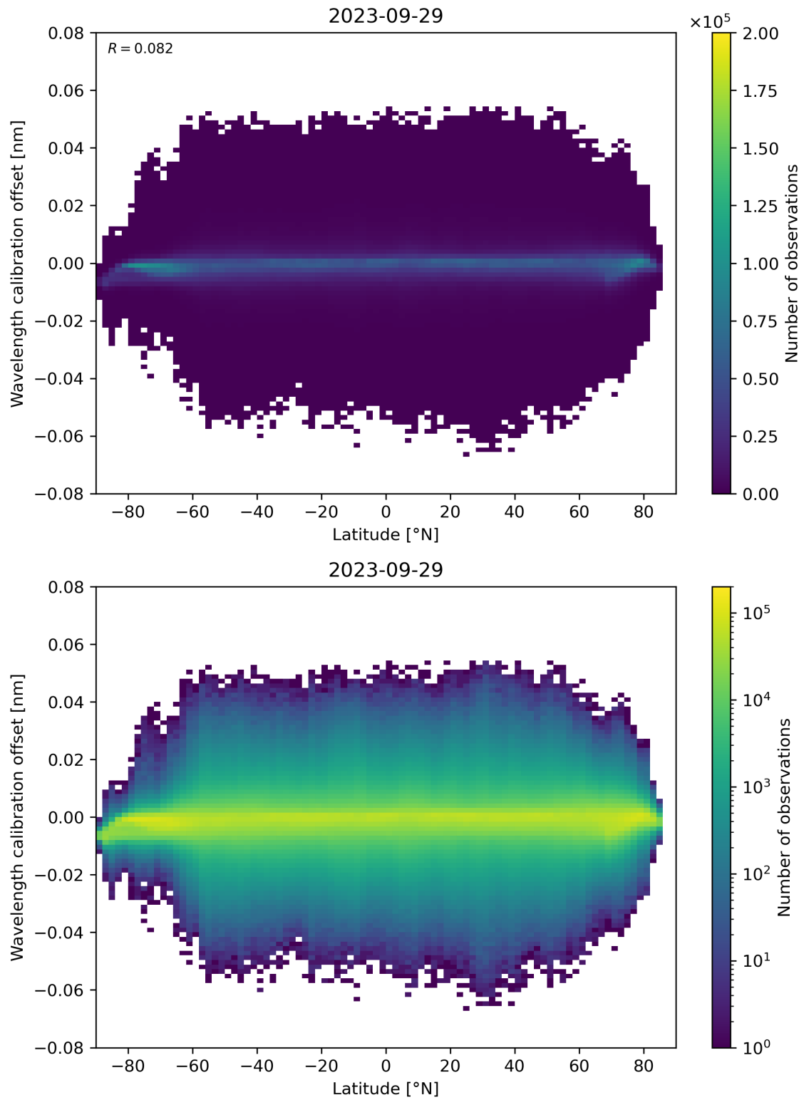
Figure 95: Scatter density plot of “Latitude” against “Wavelength calibration offset” for 2023-09-28 to 2023-09-30.
