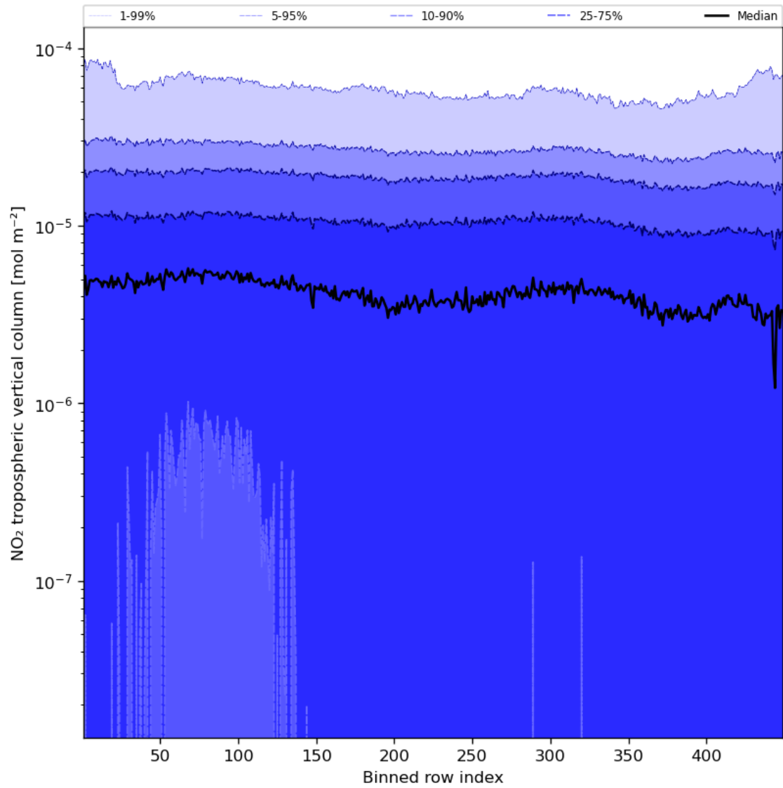
Figure 46: Along track statistics of “NO 2 tropospheric vertical column” for 2023-09-28 to 2023-09-30
