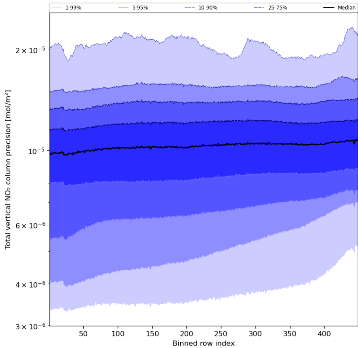
Figure 56: Along track statistics of “Total vertical NO 2 column precision” for 2023-09-28 to 2023-09-30
