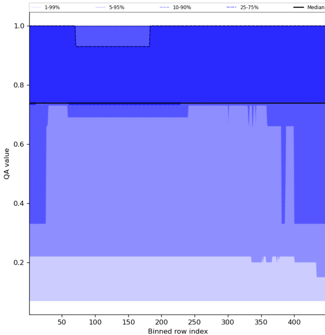
Figure 45: Along track statistics of “QA value” for 2023-09-28 to 2023-09-30
