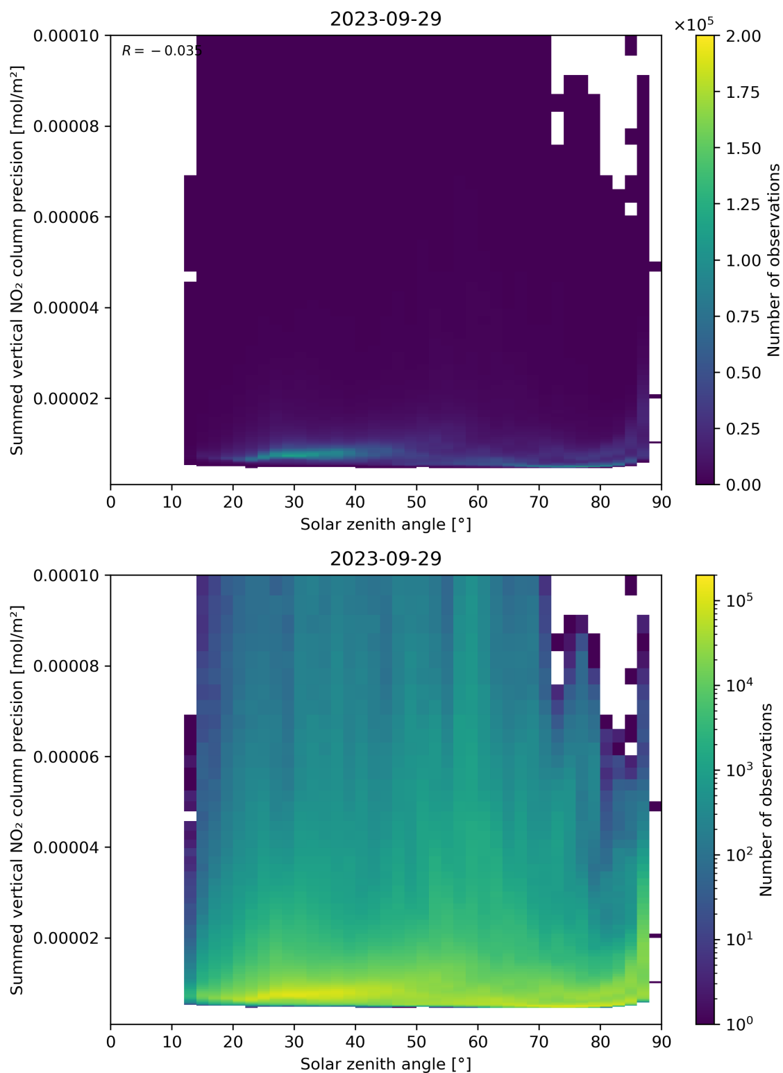
Figure 152: Scatter density plot of “Solar zenith angle” against “Summed vertical NO 2 column precision” for 2023-09-28 to 2023-09-30.
