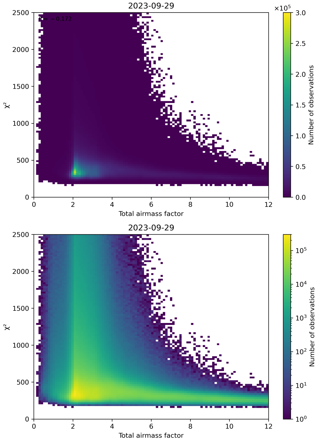
Figure 63: Scatter density plot of “Total airmass factor” against “ \chi^2 ” for 2023-09-28 to 2023-09-30.
