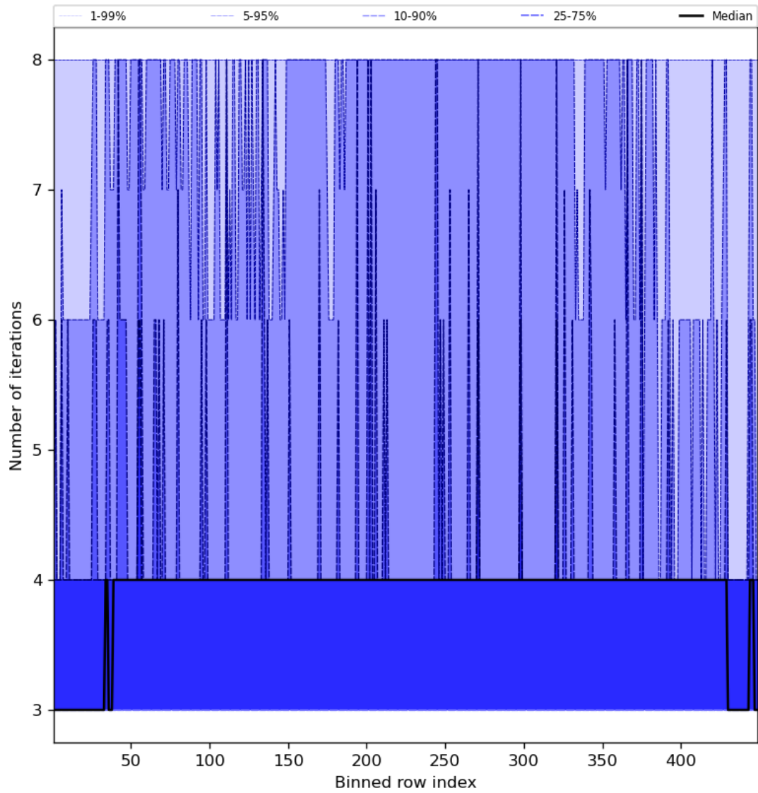
Figure 51: Along track statistics of “Number of iterations” for 2023-09-28 to 2023-09-30
