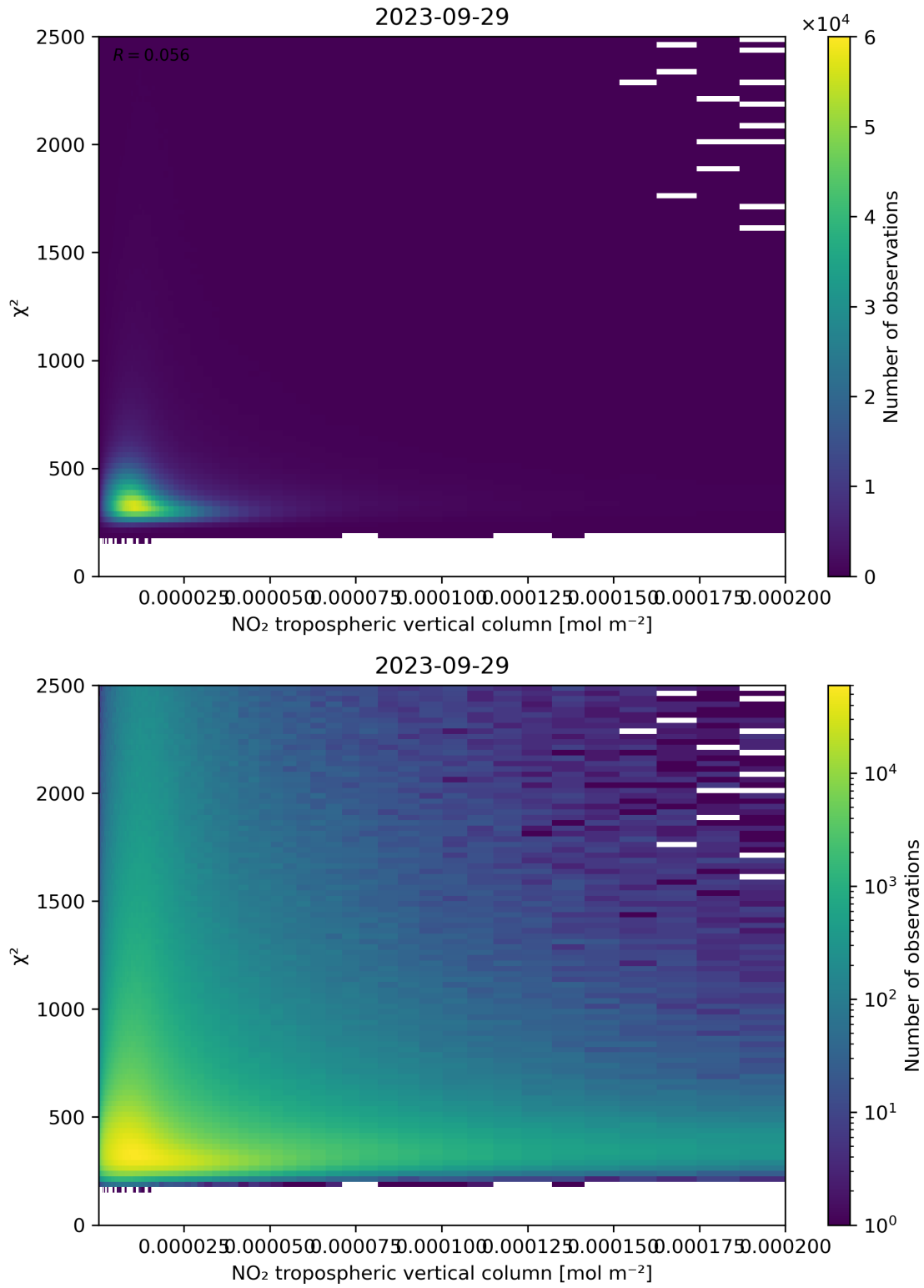
Figure 124: Scatter density plot of “NO 2 tropospheric vertical column” against “ \chi^2 ” for 2023-09-28 to 2023-09-30.
