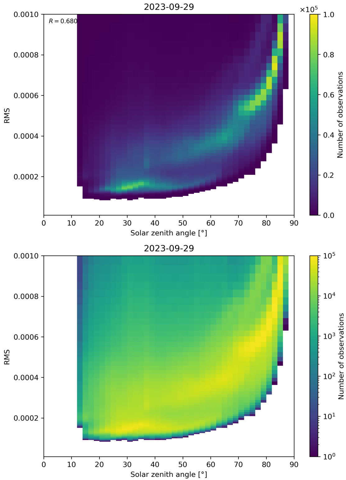
Figure 157: Scatter density plot of “Solar zenith angle” against “RMS” for 2023-09-28 to 2023-09-30.
