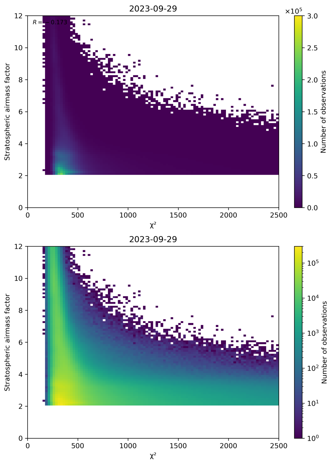
Figure 81: Scatter density plot of “ \chi^2 ” against “Stratospheric airmass factor” for 2023-09-28 to 2023-09-30.
