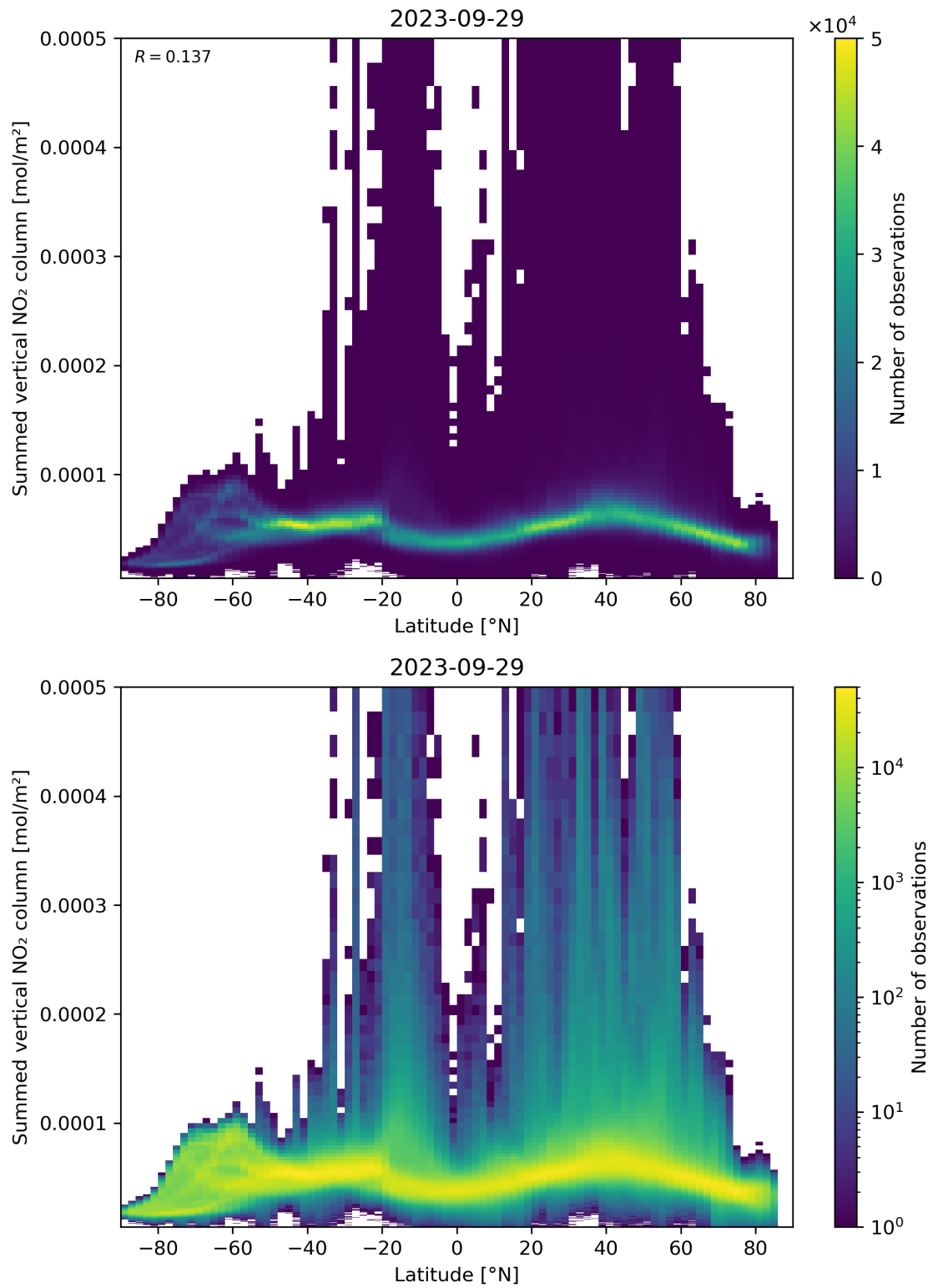
Figure 88: Scatter density plot of “Latitude” against “Summed vertical NO 2 column” for 2023-09-28 to 2023-09-30.
