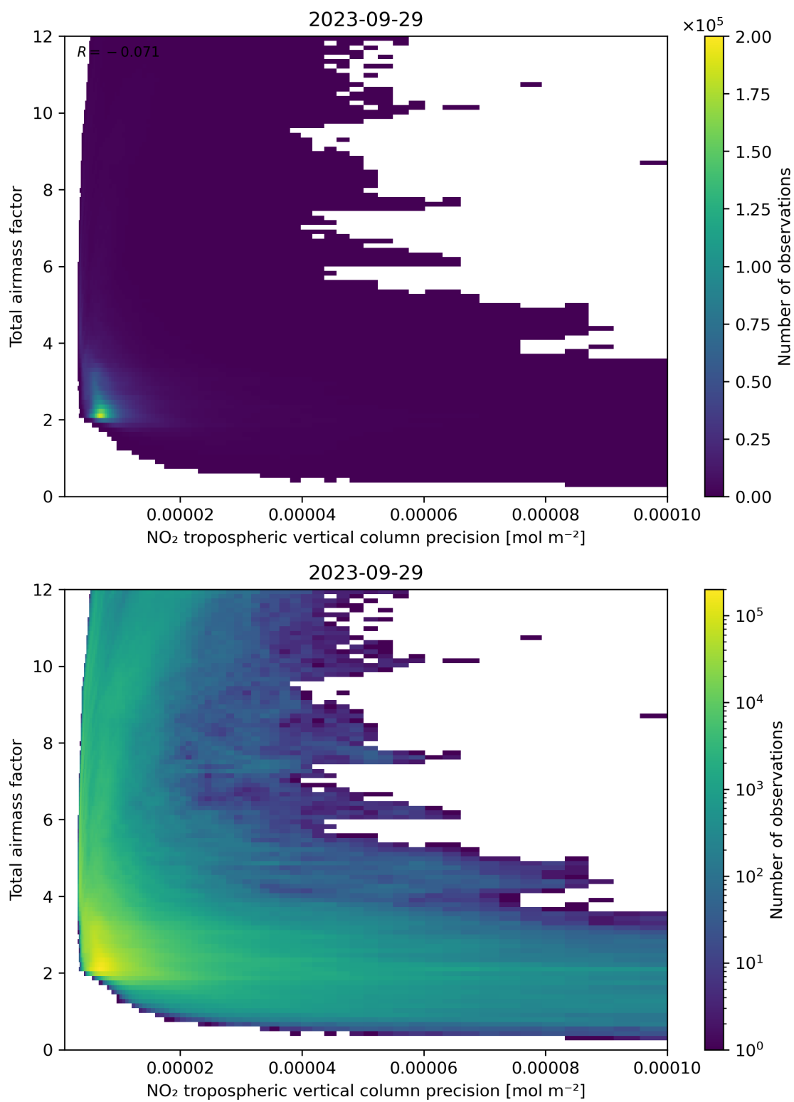
Figure 132: Scatter density plot of “NO 2 tropospheric vertical column precision” against “Total air mass factor” for 2023-09-28 to 2023-09-30.
