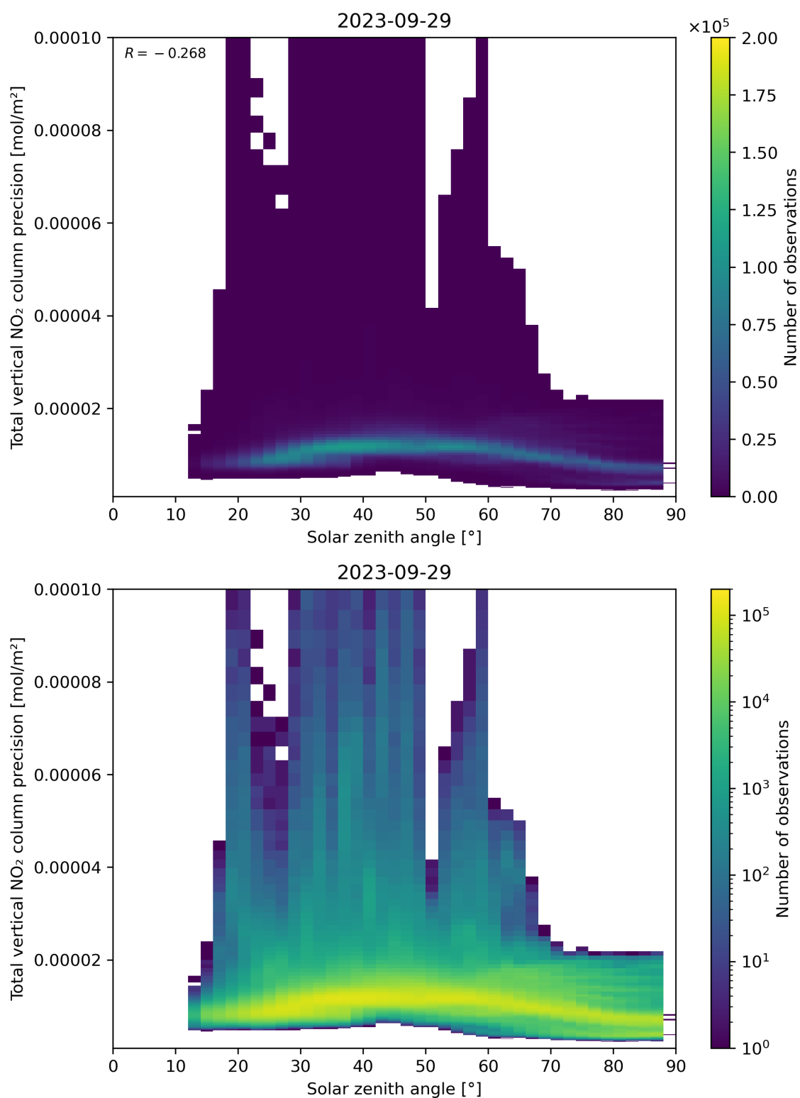
Figure 154: Scatter density plot of “Solar zenith angle” against “Total vertical NO 2 column precision” for 2023-09-28 to 2023-09-30.
