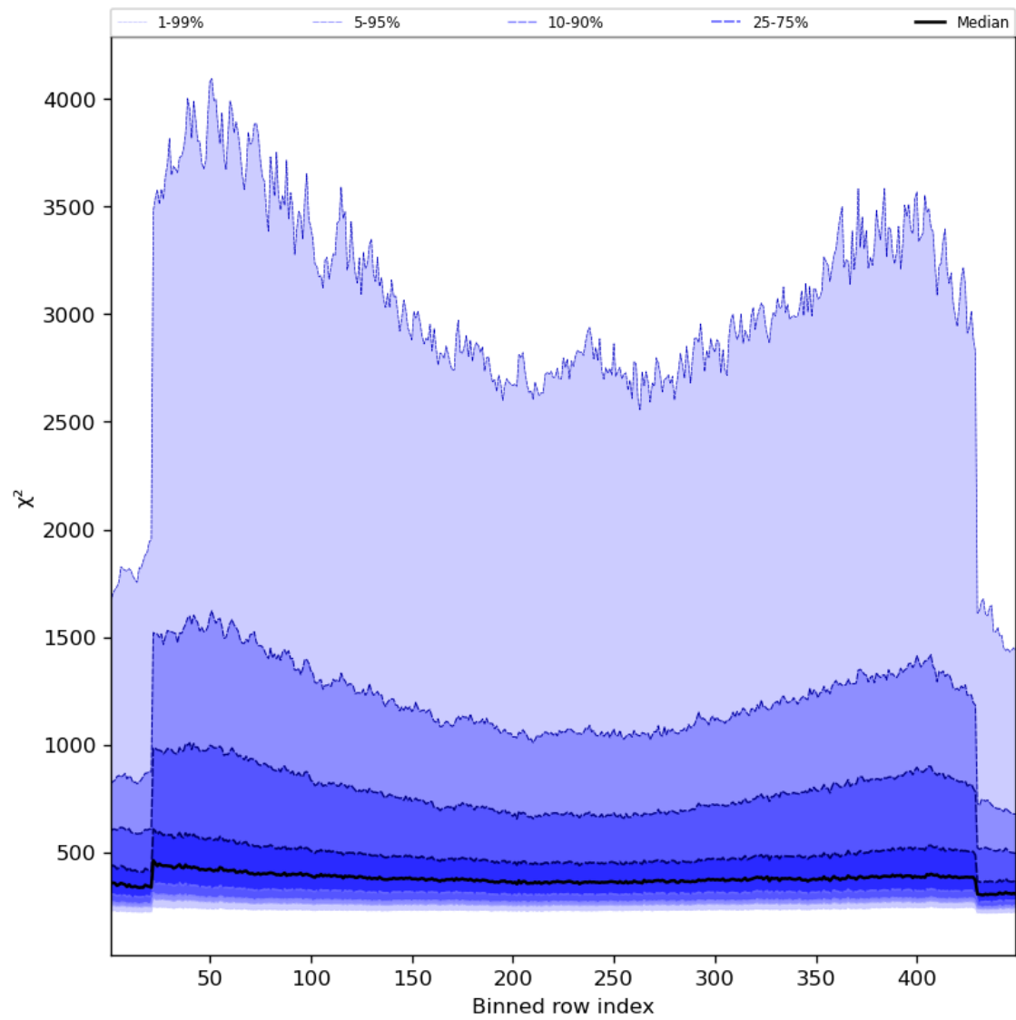
Figure 59: Along track statistics of “ \chi^2 ” for 2023-09-28 to 2023-09-30
