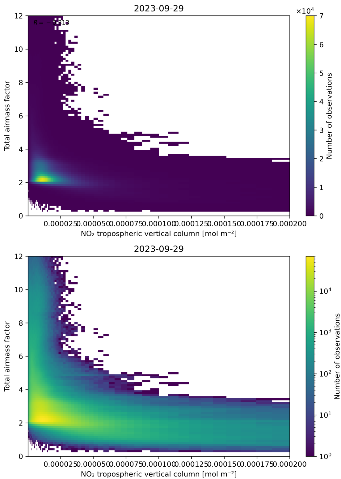
Figure 122: Scatter density plot of “NO 2 tropospheric vertical column” against “Total air mass factor” for 2023-09-28 to 2023-09-30.
