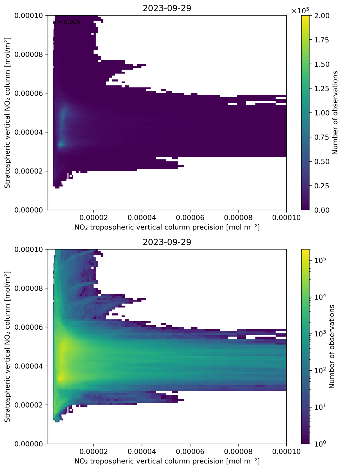
Figure 135: Scatter density plot of “NO 2 tropospheric vertical column precision” against “Stratospheric vertical NO 2 column” for 2023-09-28 to 2023-09-30.
