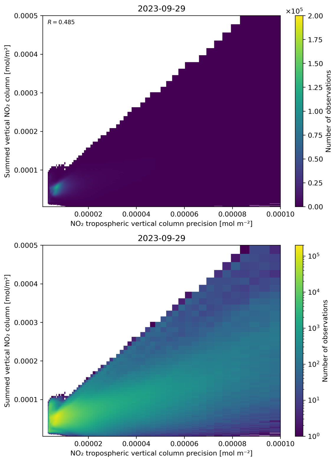
Figure 136: Scatter density plot of “NO 2 tropospheric vertical column precision” against “Summed vertical NO 2 column” for 2023-09-28 to 2023-09-30.
