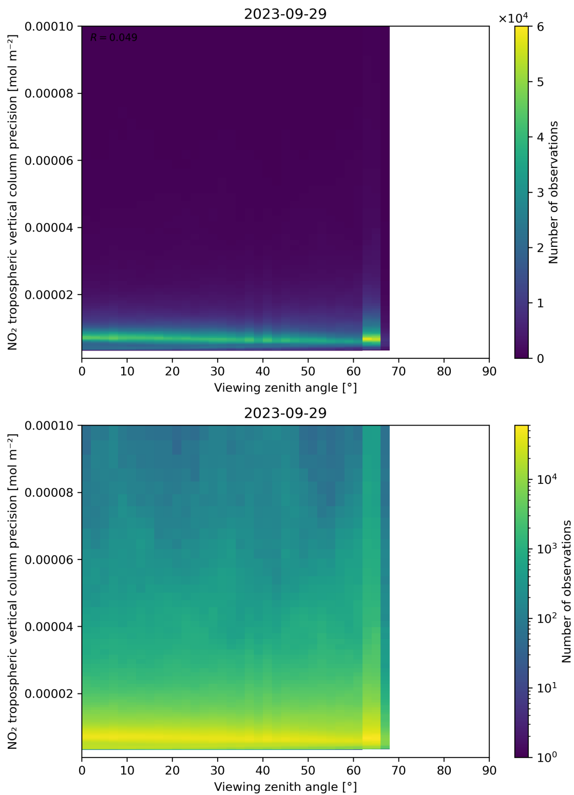
Figure 170: Scatter density plot of “Viewing zenith angle” against “NO 2 tropospheric vertical column precision” for 2023-09-28 to 2023-09-30.
