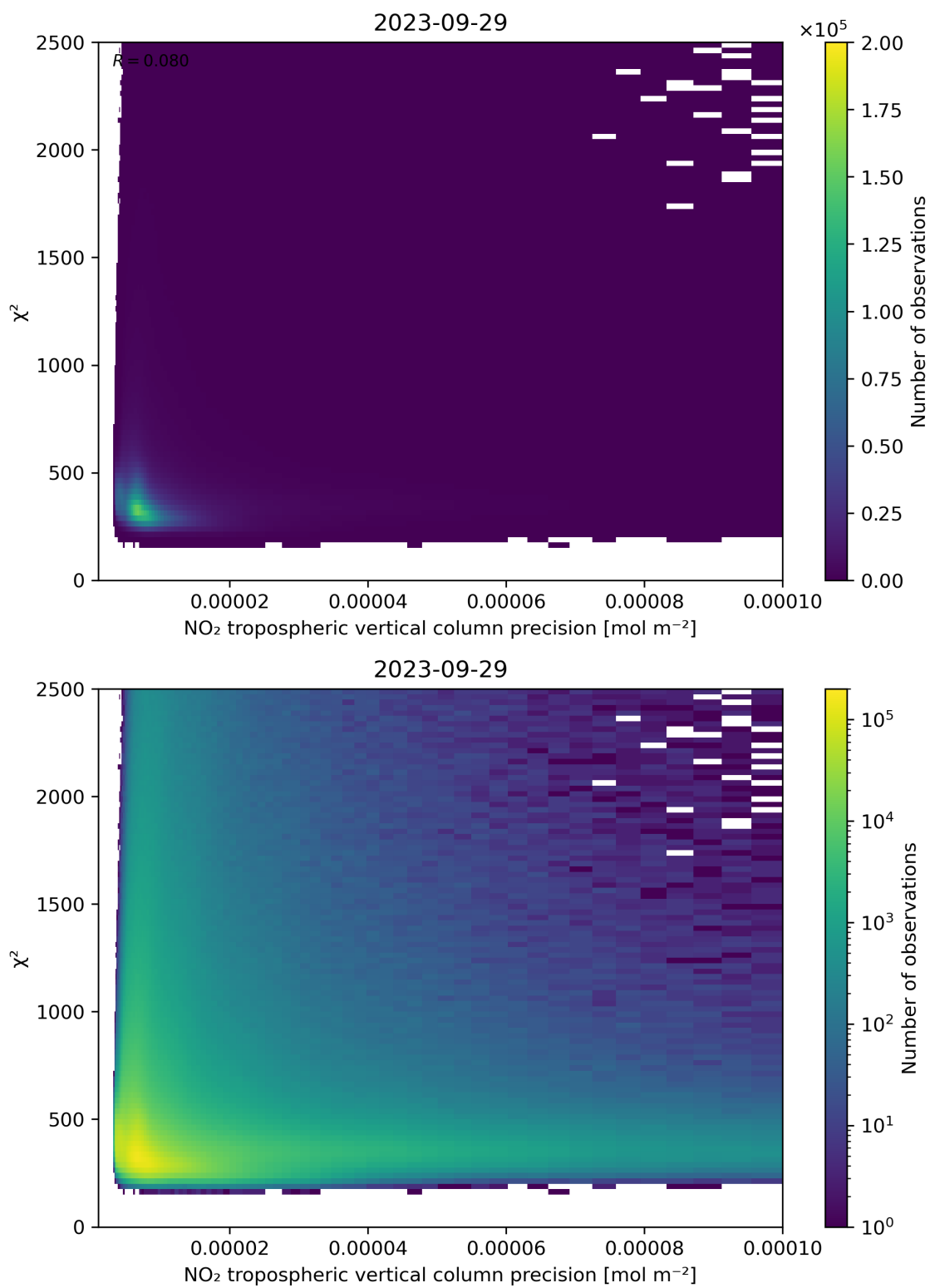
Figure 134: Scatter density plot of “NO 2 tropospheric vertical column precision” against “ \chi^2 ” for 2023-09-28 to 2023-09-30.
