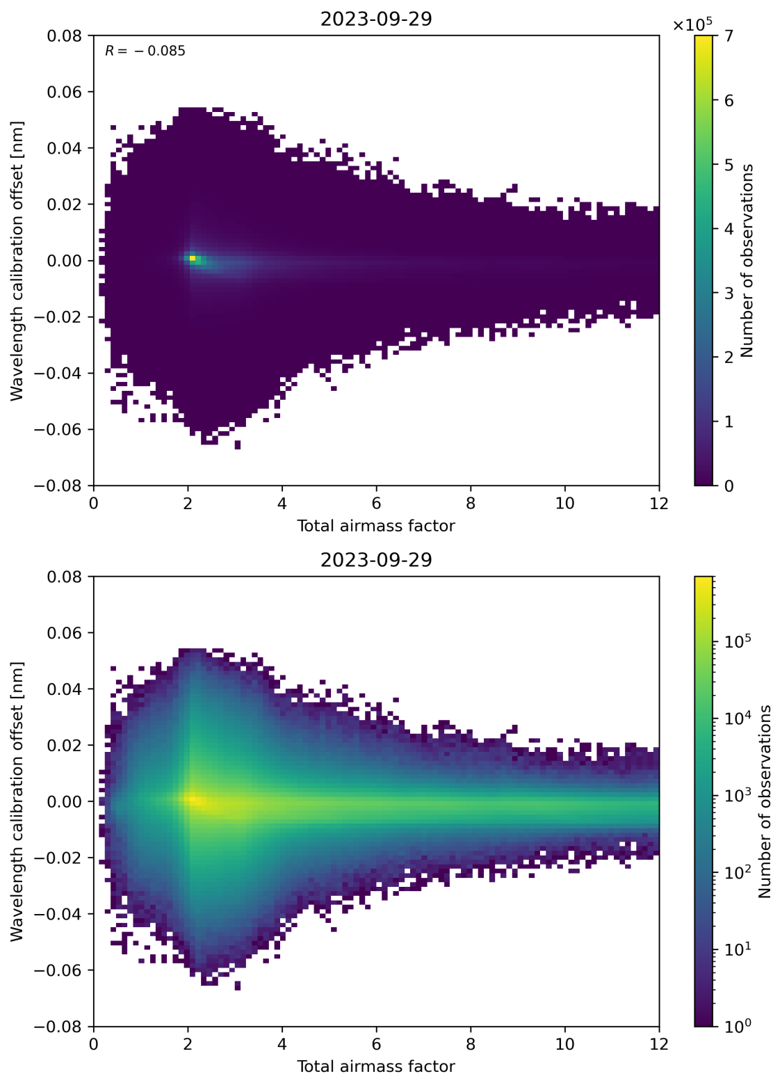
Figure 70: Scatter density plot of “Total airmass factor” against “Wavelength calibration offset” for 2023-09-28 to 2023-09-30.
