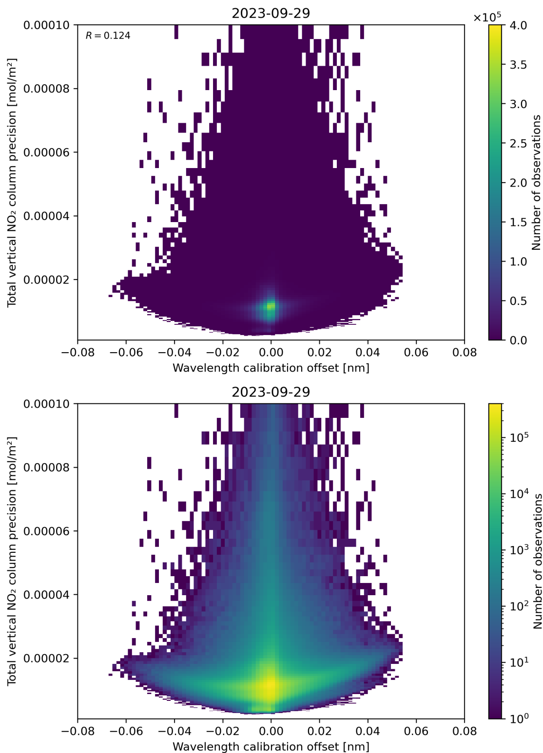
Figure 180: Scatter density plot of “Wavelength calibration offset” against “Total vertical NO 2 column precision” for 2023-09-28 to 2023-09-30.
