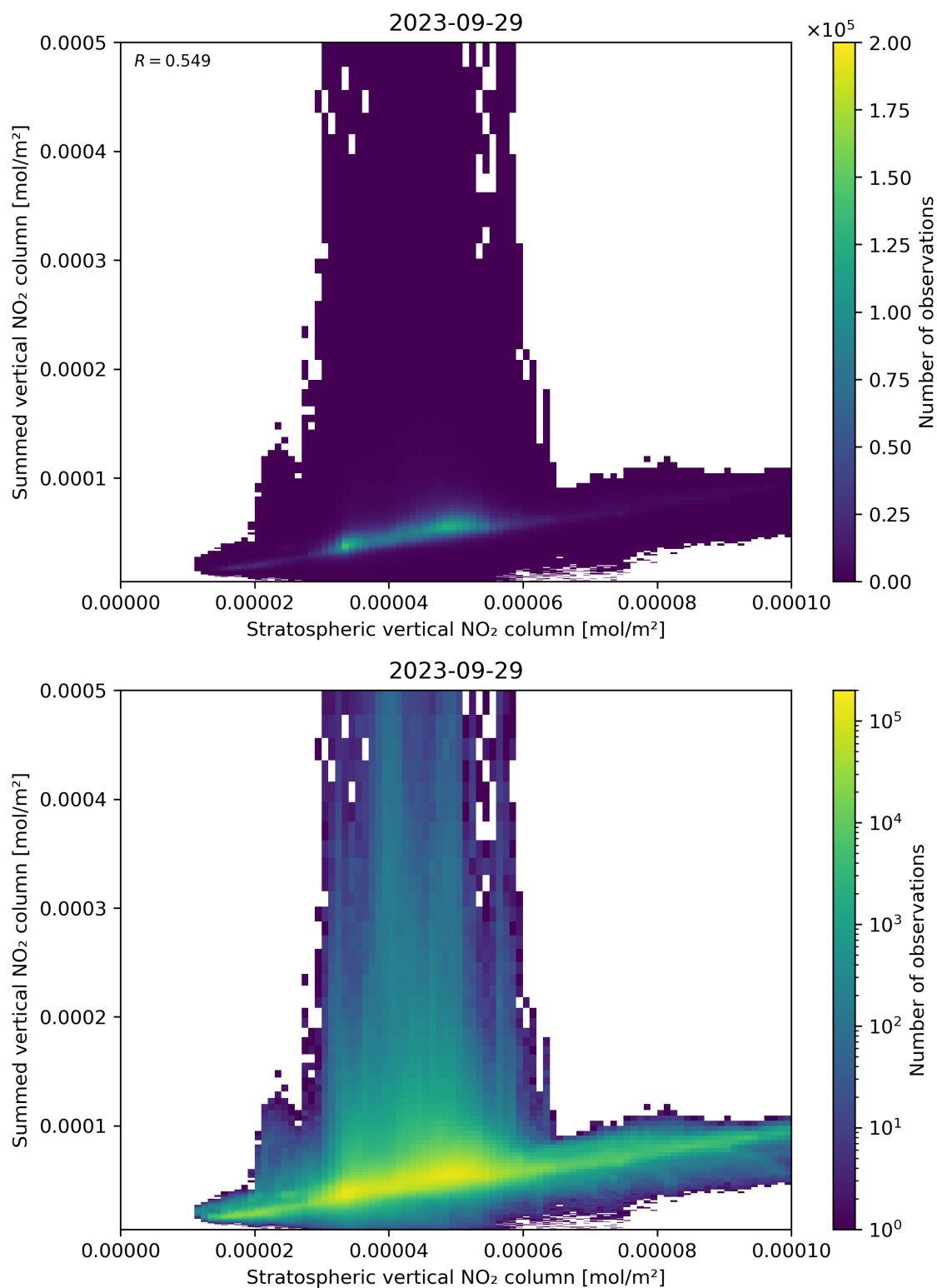
Figure 98: Scatter density plot of “Stratospheric vertical NO 2 column” against “Summed vertical NO 2 column” for 2023-09-28 to 2023-09-30.
