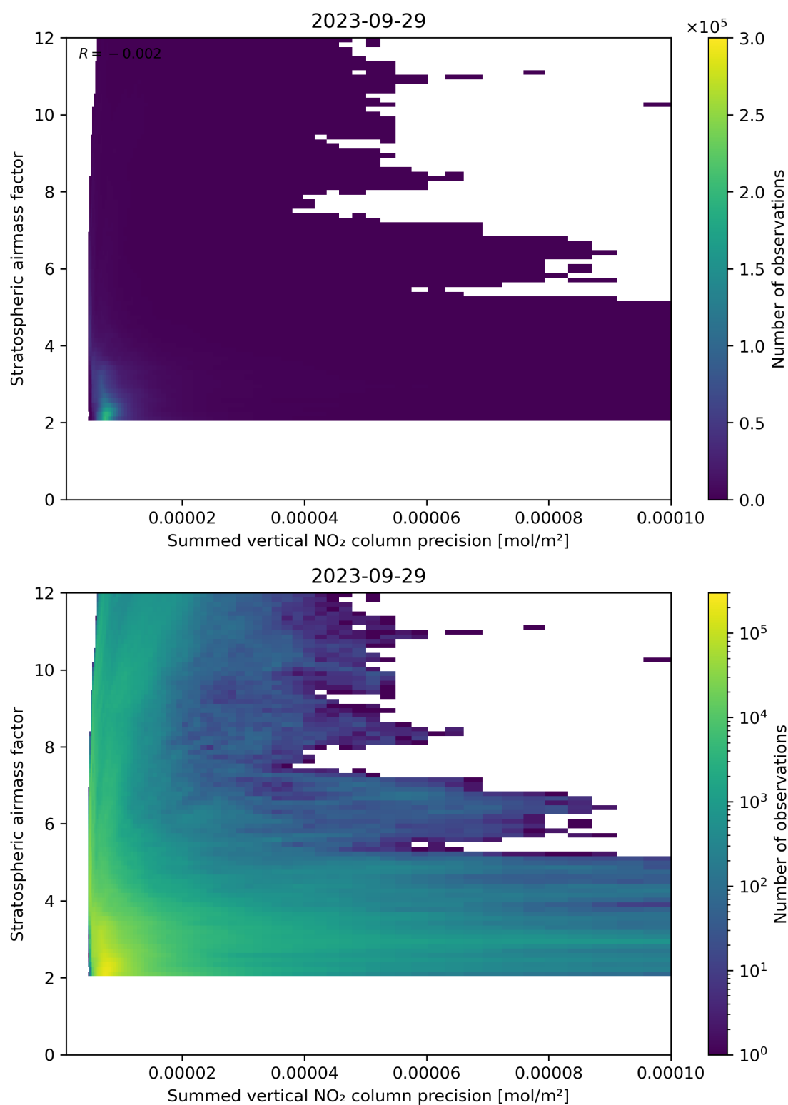
Figure 106: Scatter density plot of “Summed vertical NO 2 column precision” against “Stratospheric airmass factor” for 2023-09-28 to 2023-09-30.
