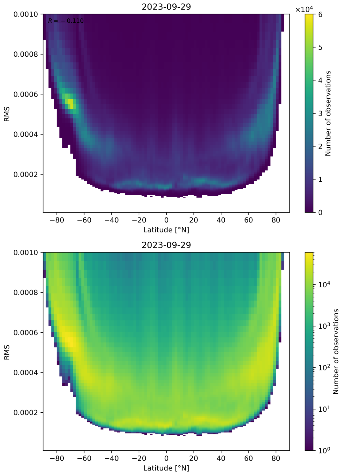
Figure 94: Scatter density plot of “Latitude” against “RMS” for 2023-09-28 to 2023-09-30.
