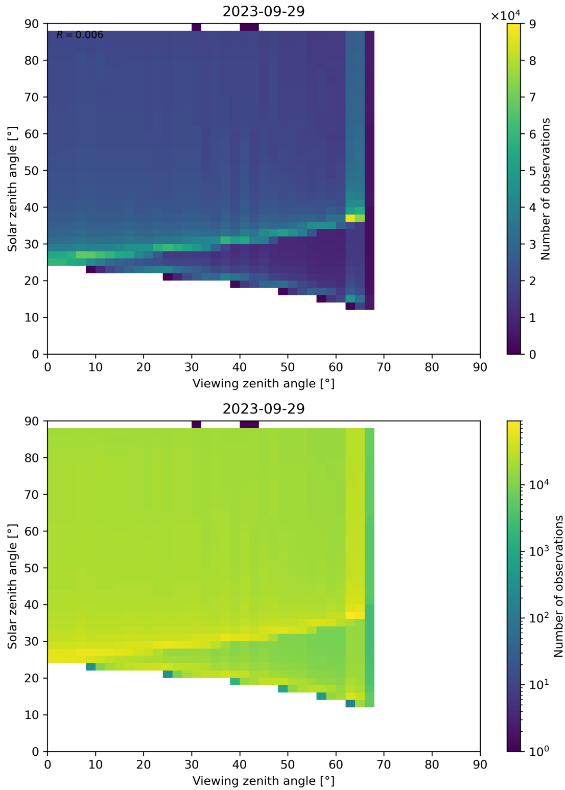
Figure 172: Scatter density plot of “Viewing zenith angle” against “Solar zenith angle” for 2023-09-28 to 2023-09-30.
