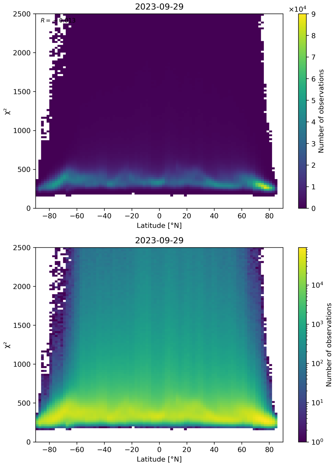
Figure 86: Scatter density plot of “Latitude” against “ \chi^2 ” for 2023-09-28 to 2023-09-30.
