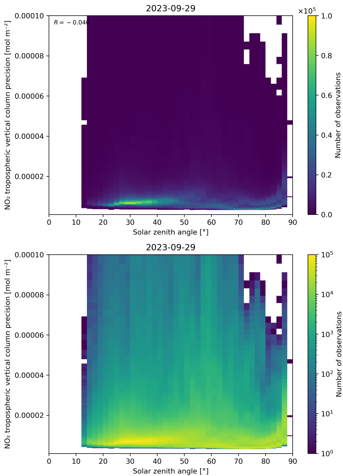
Figure 156: Scatter density plot of “Solar zenith angle” against “NO 2 tropospheric vertical column precision” for 2023-09-28 to 2023-09-30.
