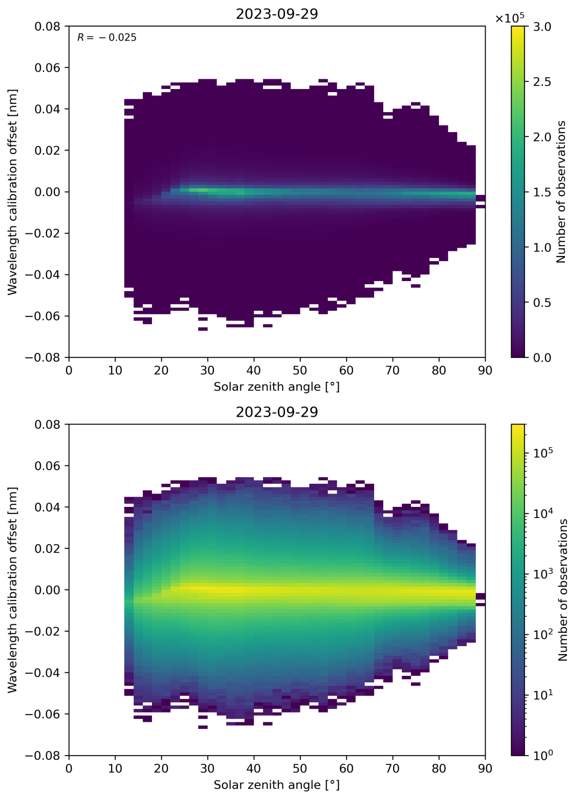
Figure 158: Scatter density plot of “Solar zenith angle” against “Wavelength calibration offset” for 2023-09-28 to 2023-09-30.
