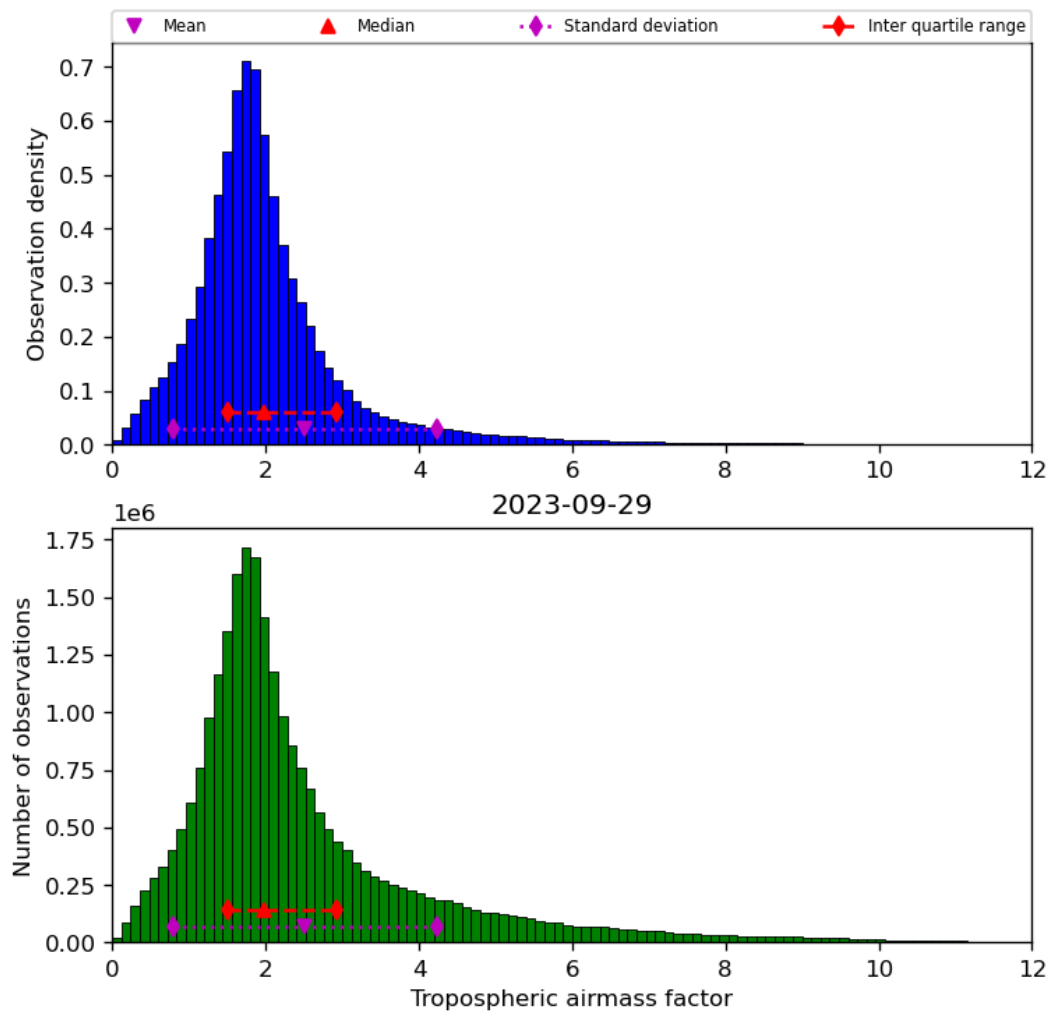
Figure 31: Histogram of “Tropospheric airmass factor” for 2023-09-28 to 2023-09-30
