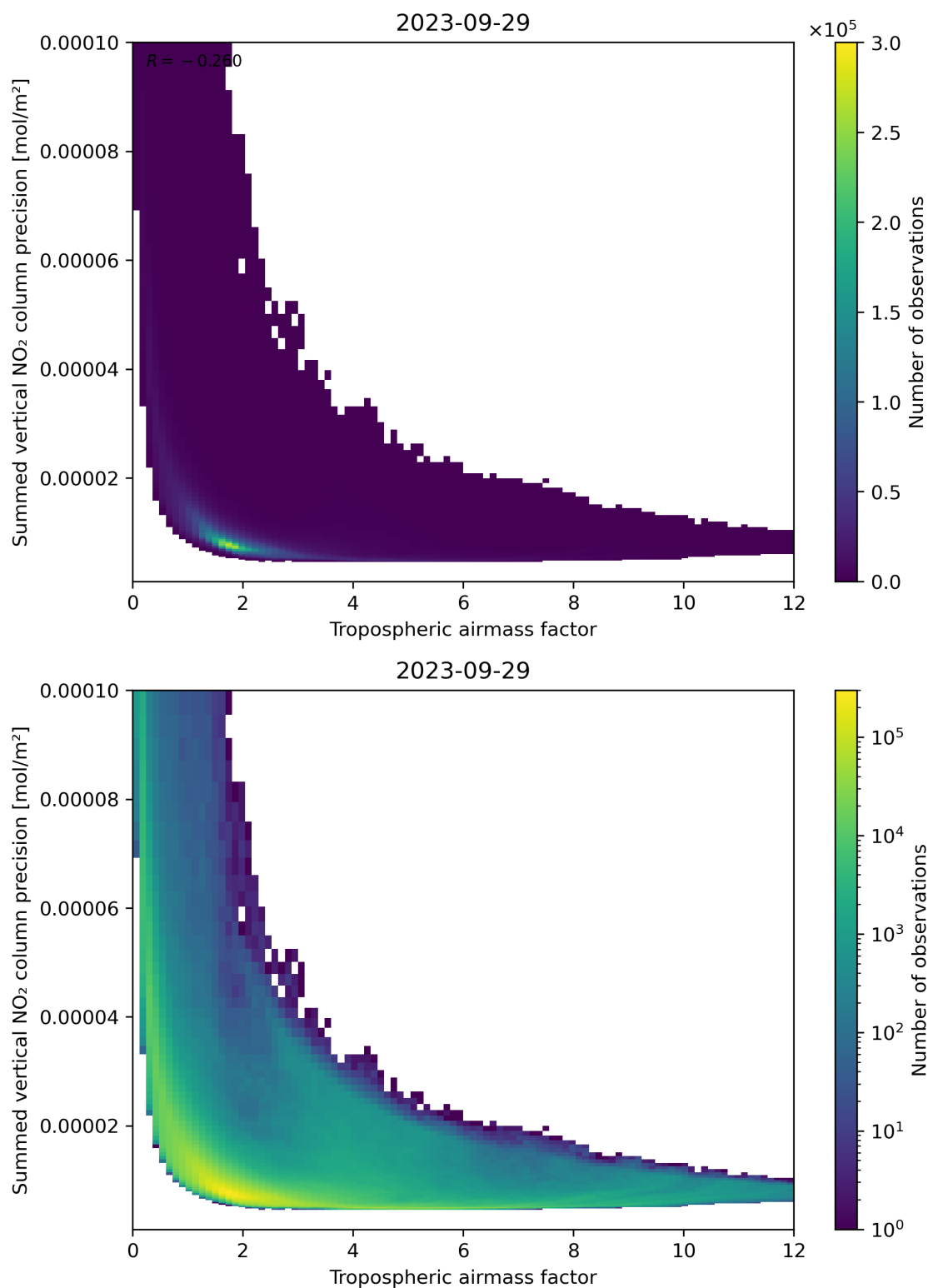
Figure 76: Scatter density plot of “Tropospheric air mass factor” against “Summed vertical NO 2 column precision” for 2023-09-28 to 2023-09-30.
