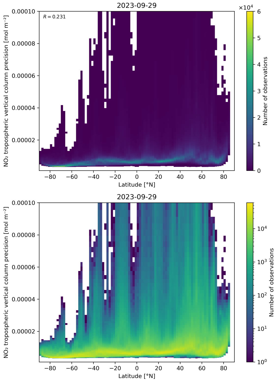
Figure 93: Scatter density plot of “Latitude” against “NO 2 tropospheric vertical column precision” for 2023-09-28 to 2023-09-30.
