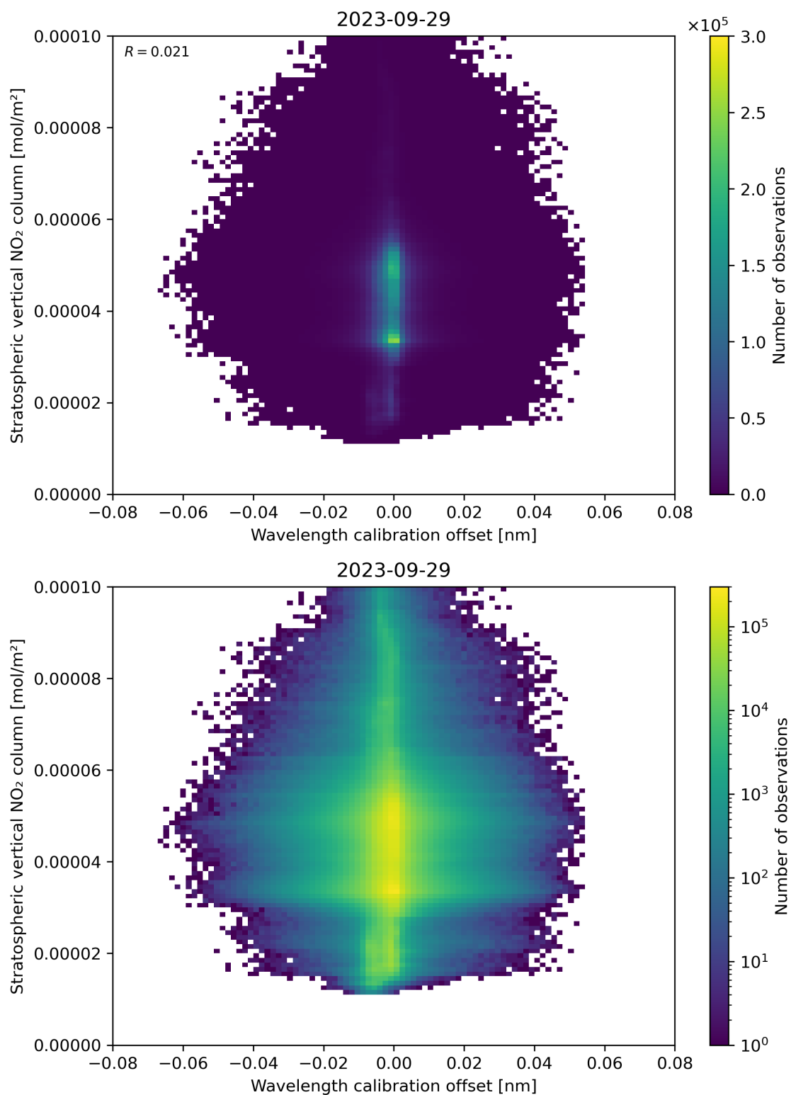
Figure 176: Scatter density plot of “Wavelength calibration offset” against “Stratospheric vertical NO 2 column” for 2023-09-28 to 2023-09-30.
