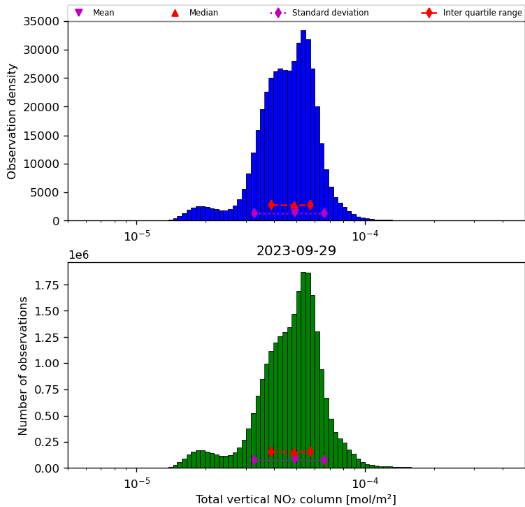
Figure 38: Histogram of “Total vertical NO 2 column” for 2023-09-28 to 2023-09-30
