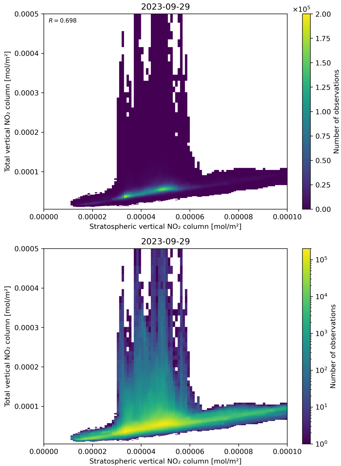
Figure 100: Scatter density plot of “Stratospheric vertical NO 2 column” against “Total vertical NO 2 column” for 2023-09-28 to 2023-09-30.
