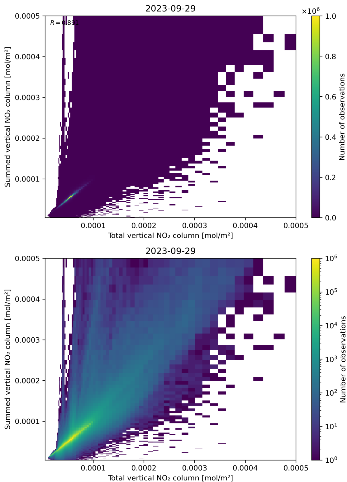
Figure 112: Scatter density plot of “Total vertical NO 2 column” against “Summed vertical NO 2 column” for 2023-09-28 to 2023-09-30.
