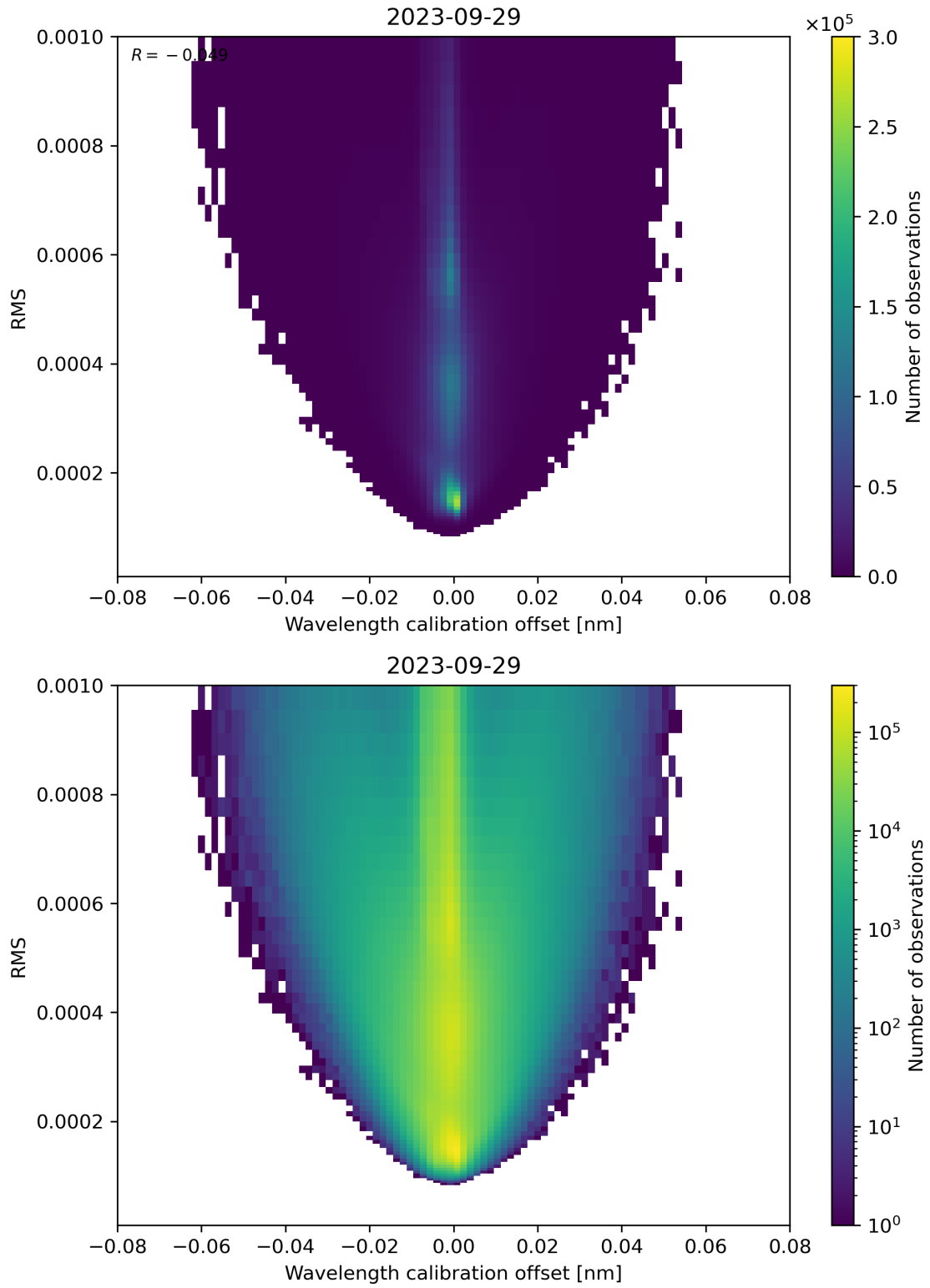
Figure 181: Scatter density plot of “Wavelength calibration offset” against “RMS” for 2023-09-28 to 2023-09-30.
