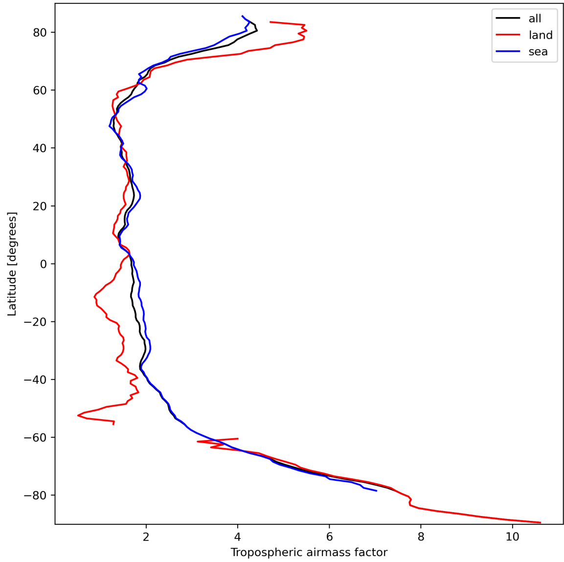
Figure 14: Zonal average of “Tropospheric airmass factor” for 2023-09-28 to 2023-09-30.
