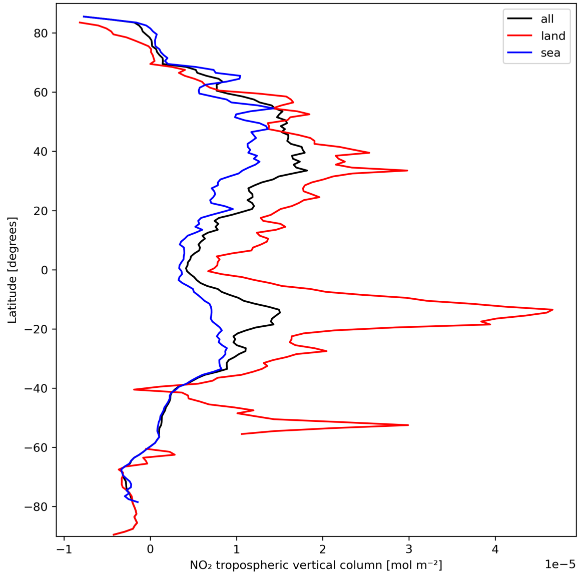
Figure 12: Zonal average of “NO 2 tropospheric vertical column” for 2023-09-28 to 2023-09-30.
