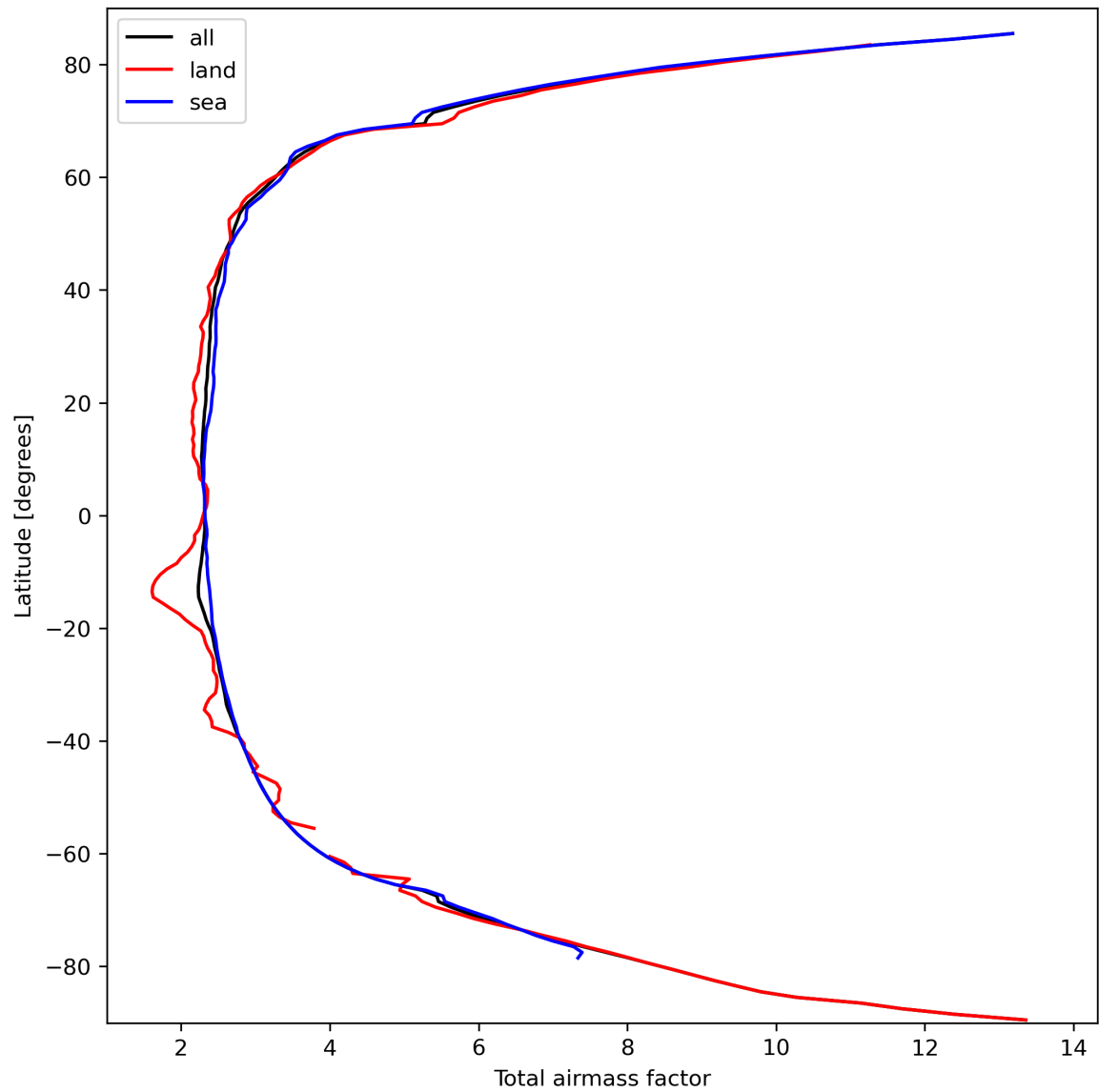
Figure 15: Zonal average of “Total airmass factor” for 2023-09-28 to 2023-09-30.
