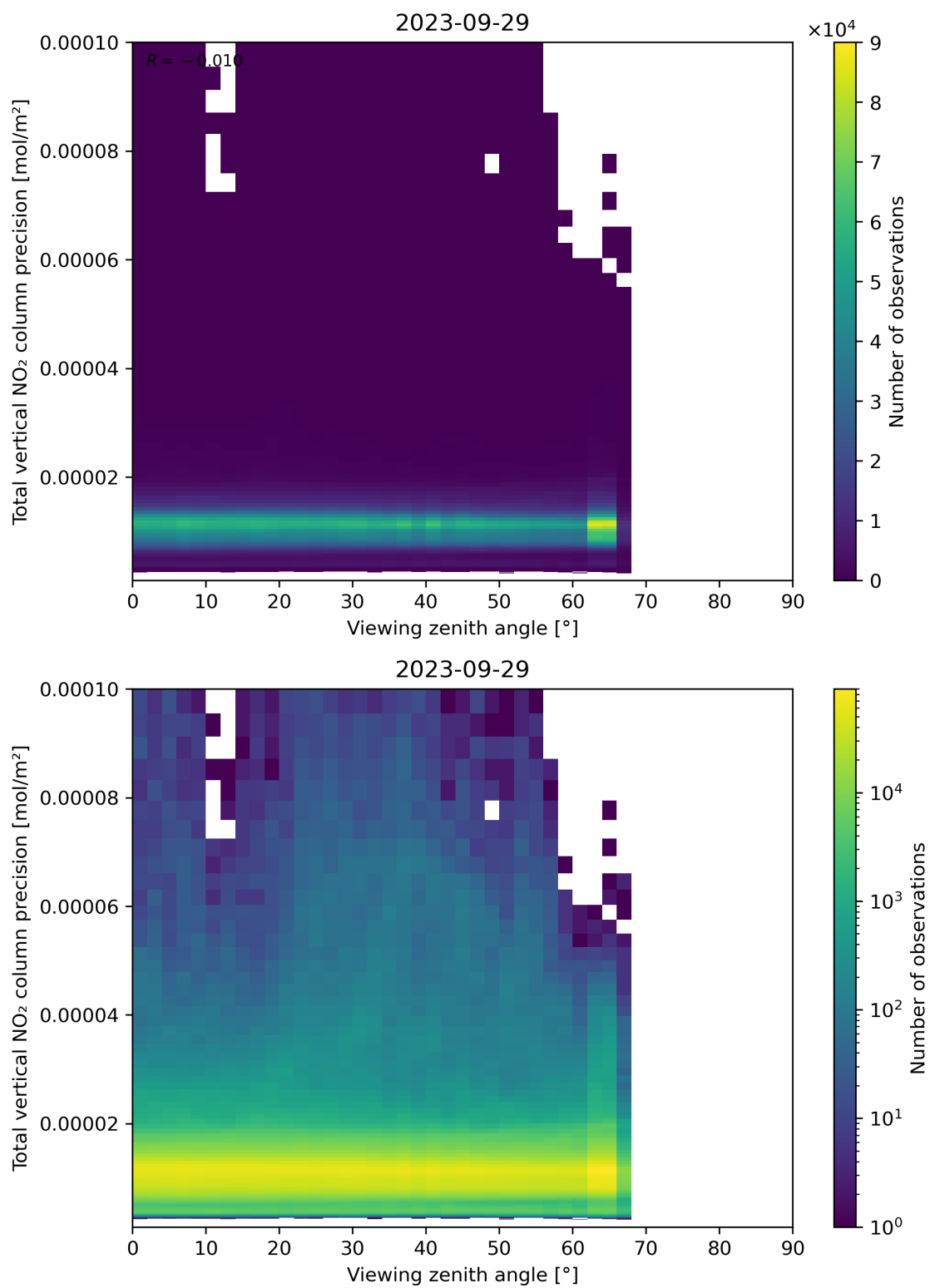
Figure 168: Scatter density plot of “Viewing zenith angle” against “Total vertical NO 2 column precision” for 2023-09-28 to 2023-09-30.
