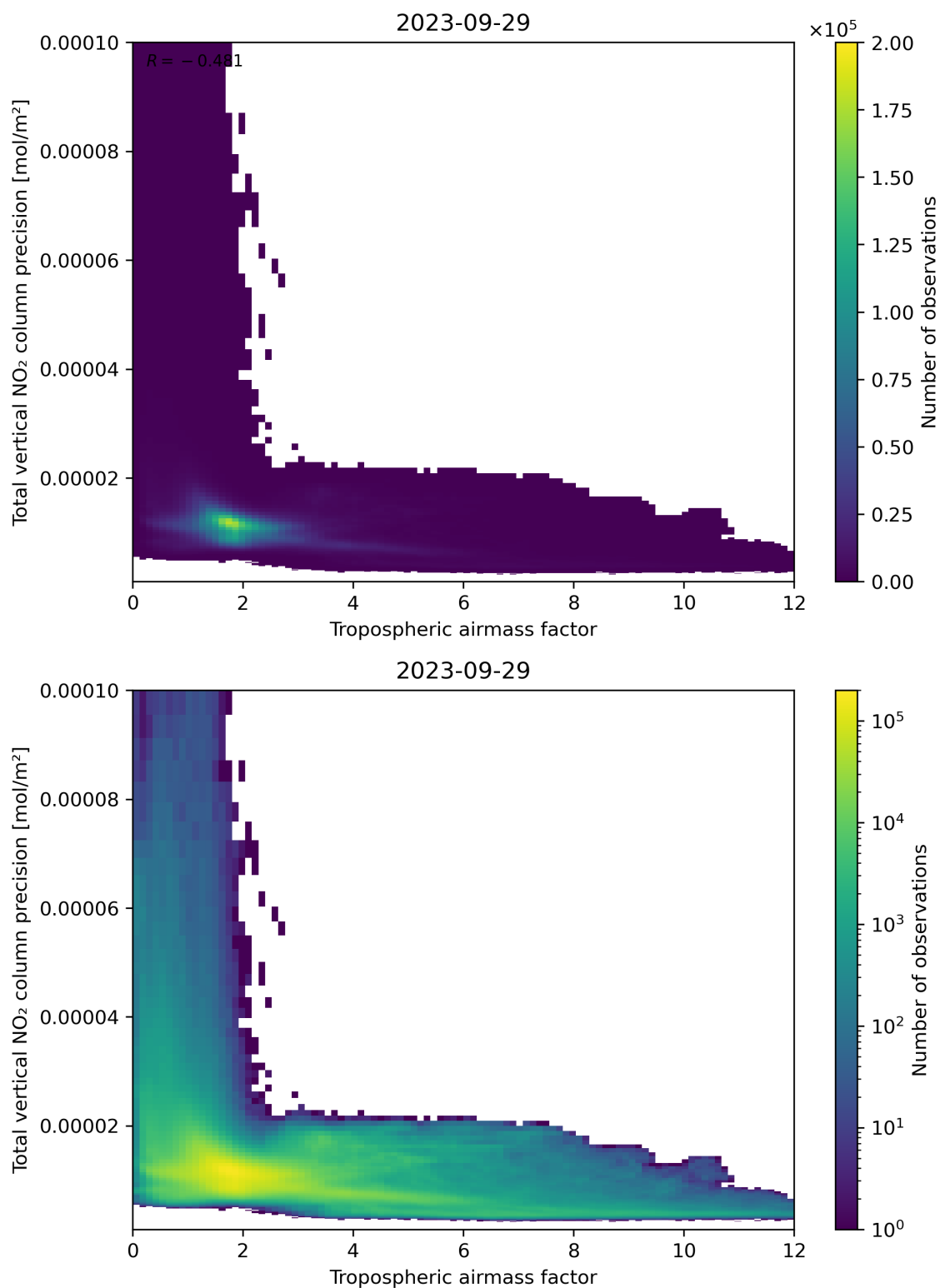
Figure 78: Scatter density plot of “Tropospheric air mass factor” against “Total vertical NO 2 column precision” for 2023-09-28 to 2023-09-30.
