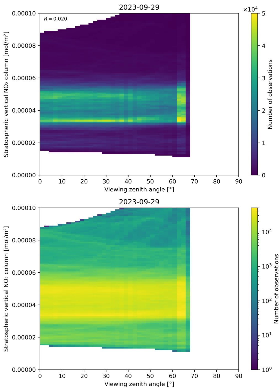
Figure 164: Scatter density plot of “Viewing zenith angle” against “Stratospheric vertical NO 2 column” for 2023-09-28 to 2023-09-30.
