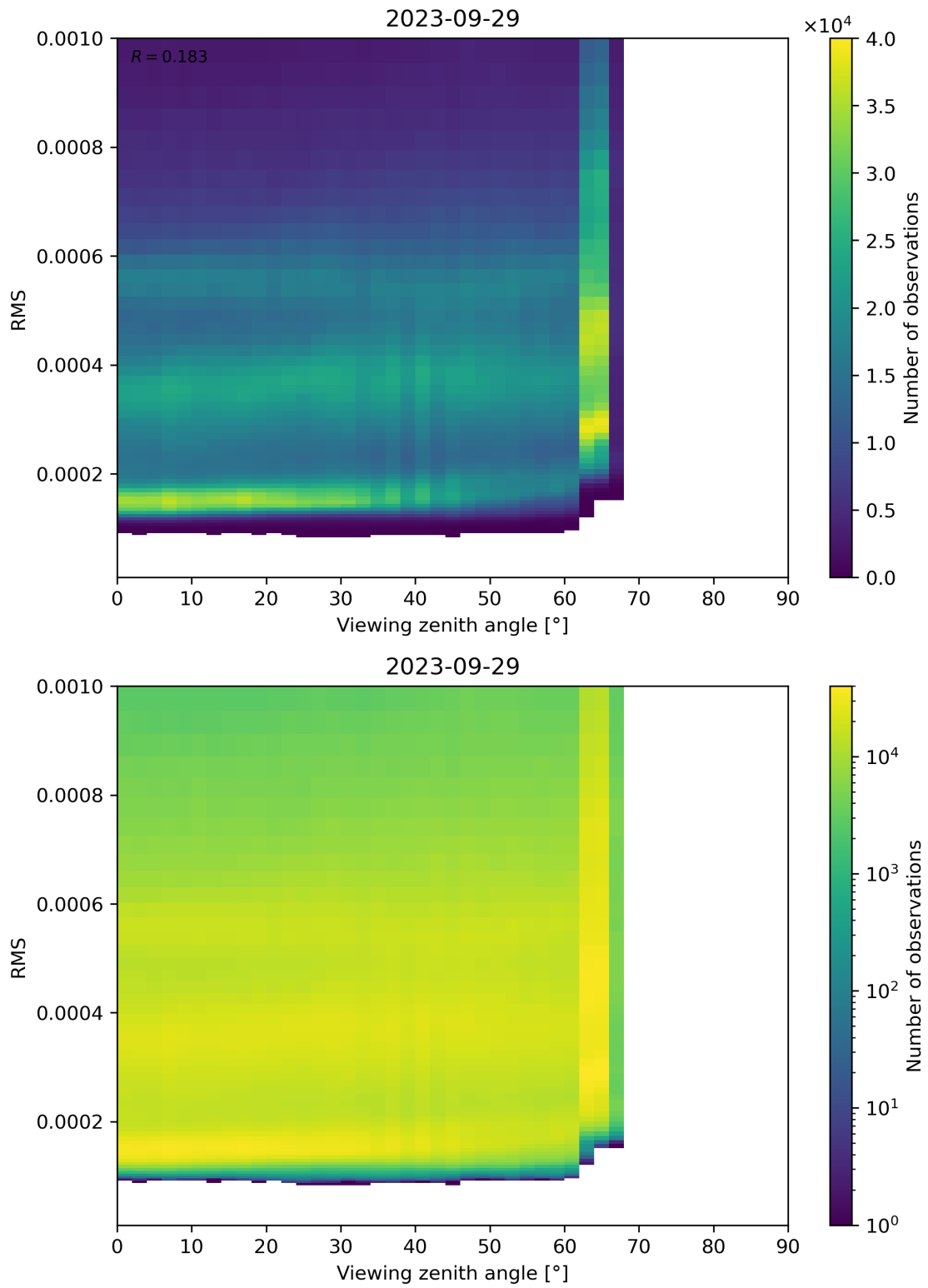
Figure 171: Scatter density plot of “Viewing zenith angle” against “RMS” for 2023-09-28 to 2023-09-30.
