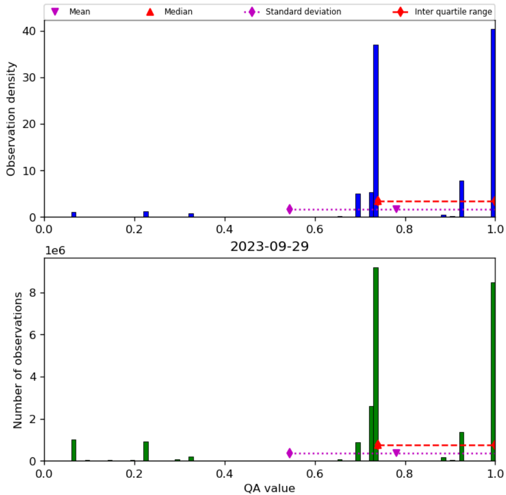
Figure 28: Histogram of “QA value” for 2023-09-28 to 2023-09-30
