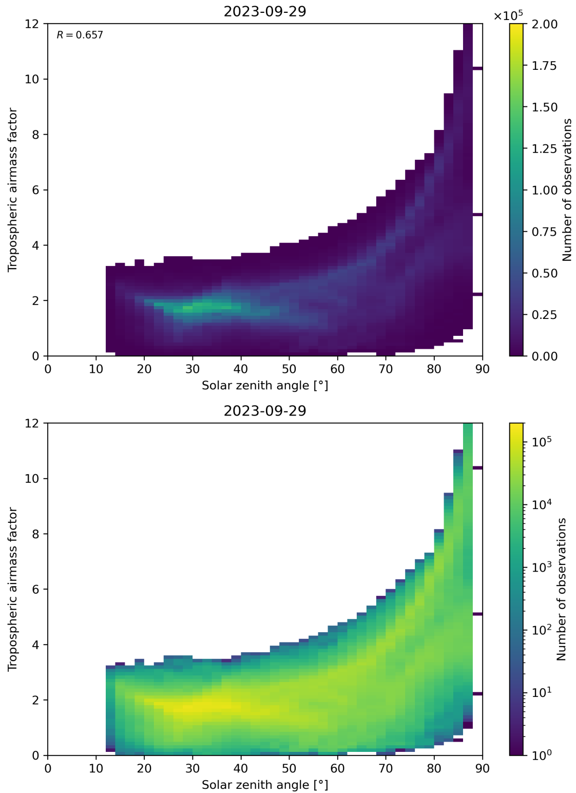
Figure 147: Scatter density plot of “Solar zenith angle” against “Tropospheric airmass factor” for 2023-09-28 to 2023-09-30.
