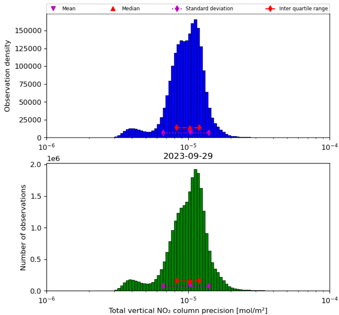
Figure 39: Histogram of "Total vertical NO 2 column precision" for 2023-09-28 to 2023-09-30
