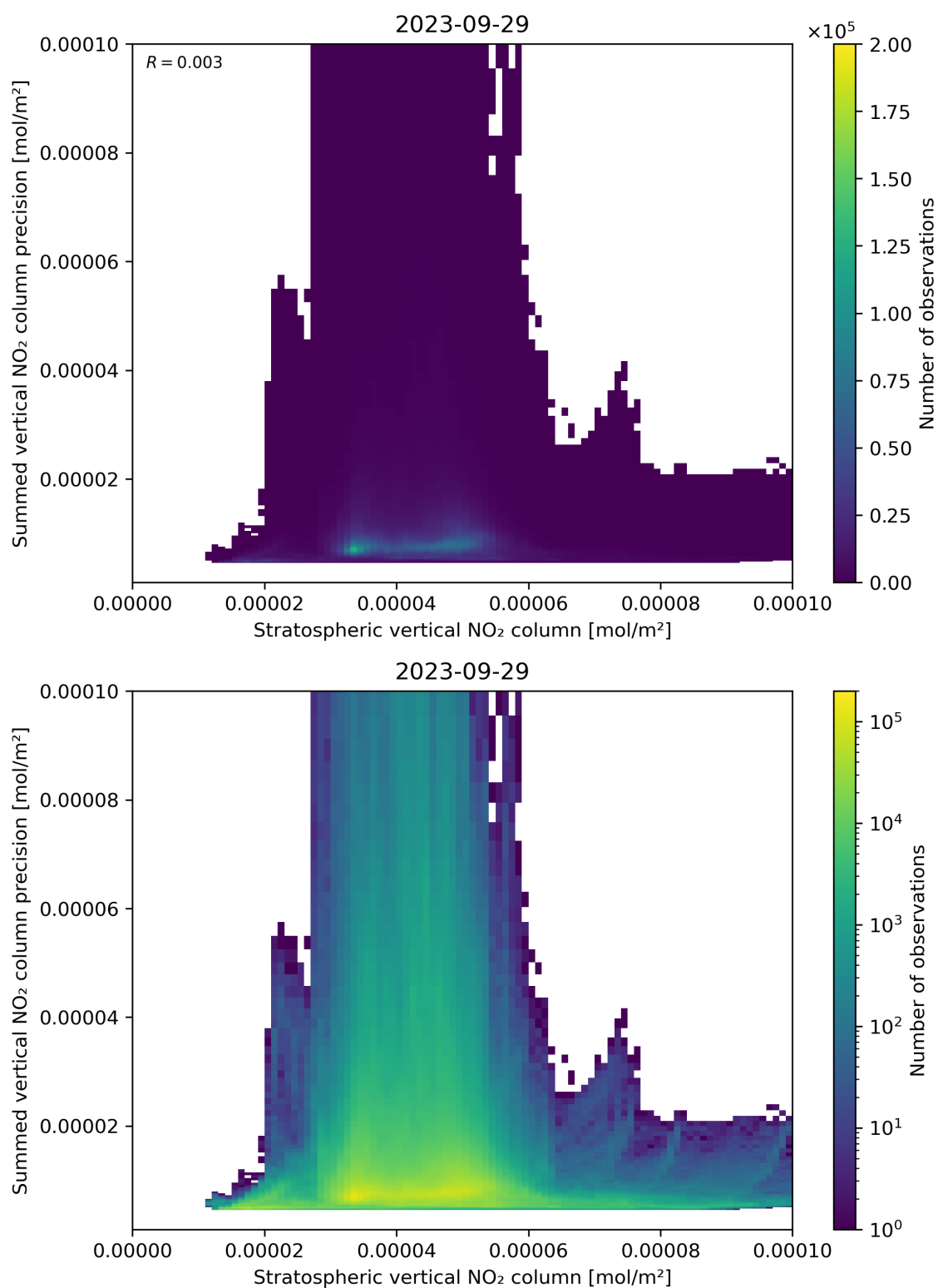
Figure 99: Scatter density plot of “Stratospheric vertical NO 2 column” against “Summed vertical NO 2 column precision” for 2023-09-28 to 2023-09-30.
