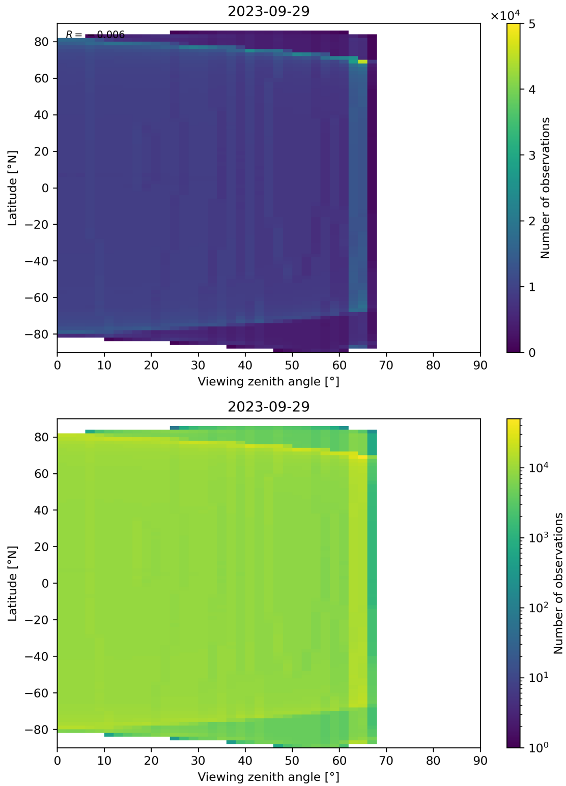
Figure 163: Scatter density plot of “Viewing zenith angle” against “Latitude” for 2023-09-28 to 2023-09-30.
