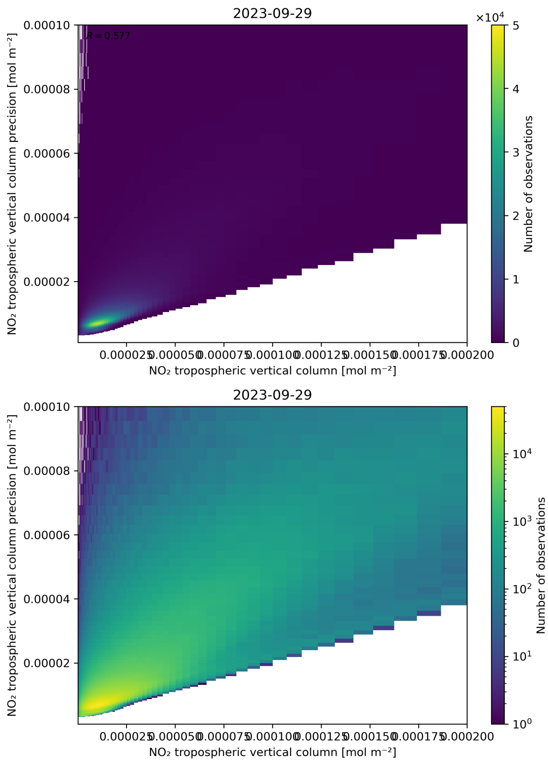
Figure 130: Scatter density plot of “NO 2 tropospheric vertical column” against “NO 2 tropospheric vertical column precision” for 2023-09-28 to 2023-09-30.
