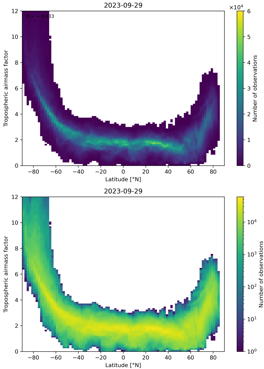
Figure 85: Scatter density plot of “Latitude” against “Tropospheric airmass factor” for 2023-09-28 to 2023-09-30.
