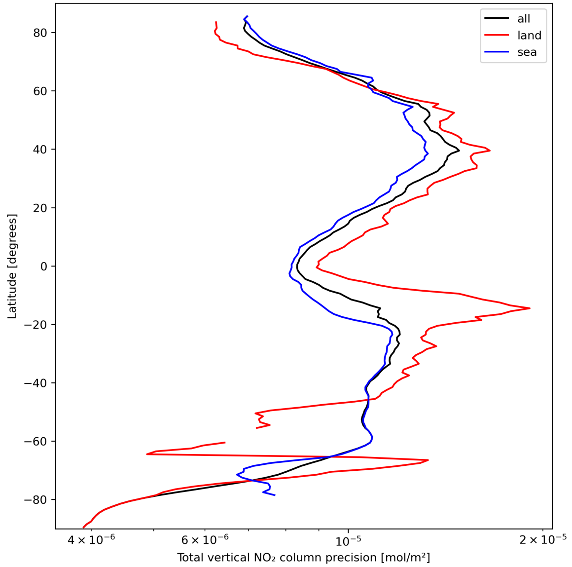
Figure 22: Zonal average of “Total vertical NO 2 column precision” for 2023-09-28 to 2023-09-30.
