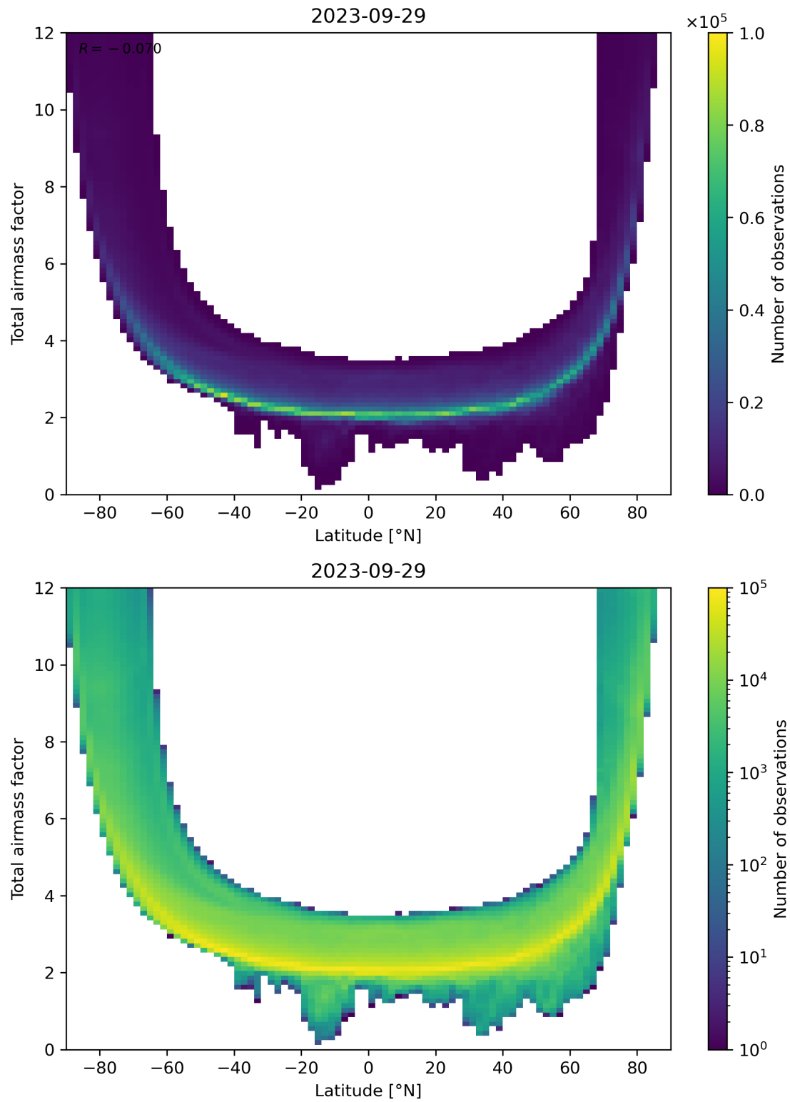
Figure 84: Scatter density plot of “Latitude” against “Total airmass factor” for 2023-09-28 to 2023-09-30.
