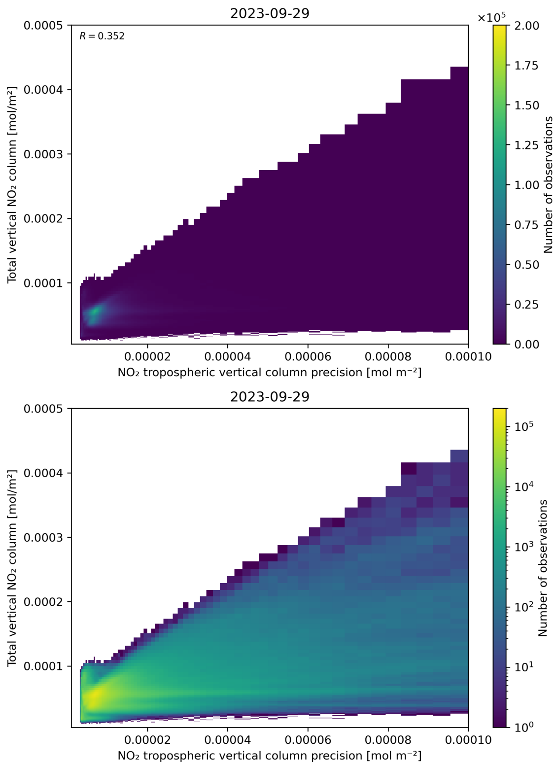
Figure 138: Scatter density plot of “NO 2 tropospheric vertical column precision” against “Total vertical NO 2 column” for 2023-09-28 to 2023-09-30.
