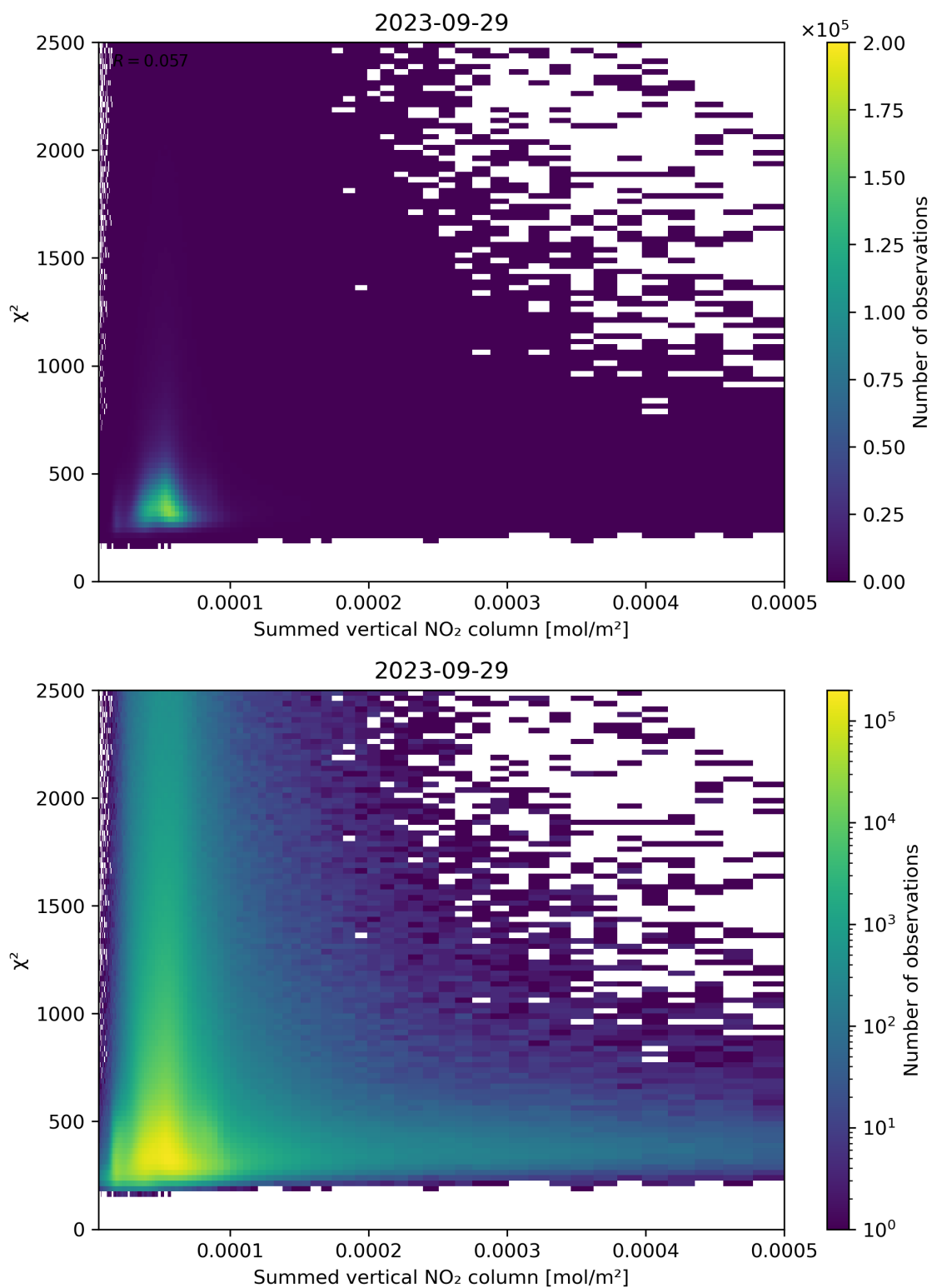
Figure 104: Scatter density plot of “Summed vertical NO 2 column” against “ \chi^2 ” for 2023-09-28 to 2023-09-30.
