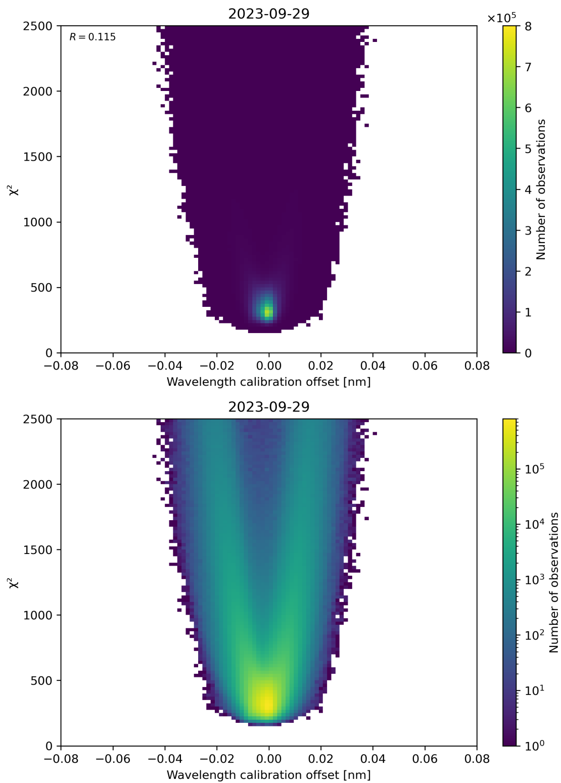
Figure 175: Scatter density plot of “Wavelength calibration offset” against “ \chi^2 ” for 2023-09-28 to 2023-09-30.
