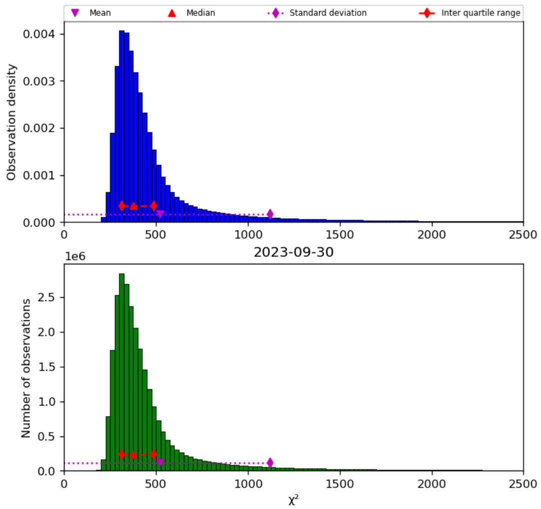
Figure 42: Histogram of “ \chi^2 ” for 2023-09-29 to 2023-10-01
