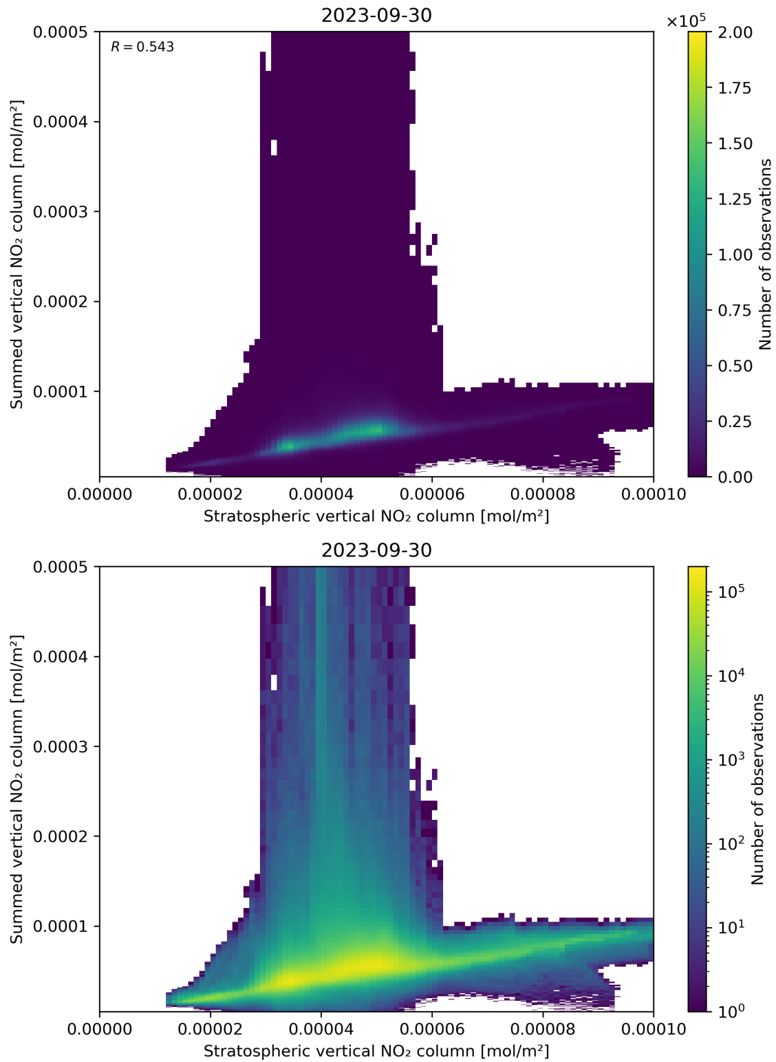
Figure 98: Scatter density plot of “Stratospheric vertical NO 2 column” against “Summed vertical NO 2 column” for 2023-09-29 to 2023-10-01.
