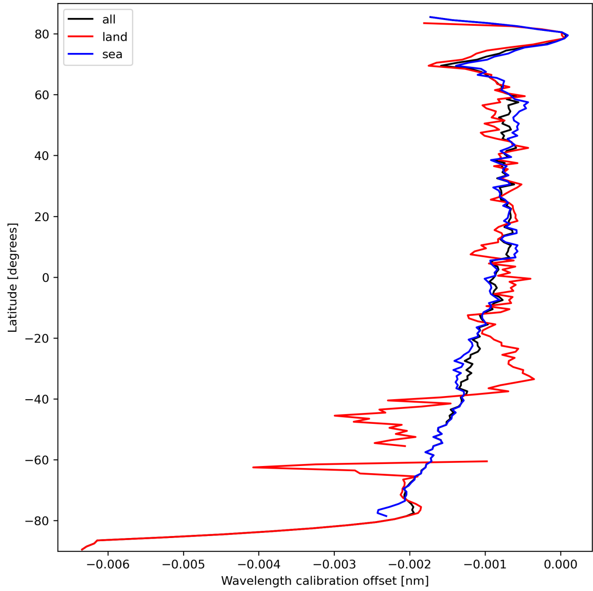
Figure 18: Zonal average of “Wavelength calibration offset” for 2023-09-29 to 2023-10-01.
