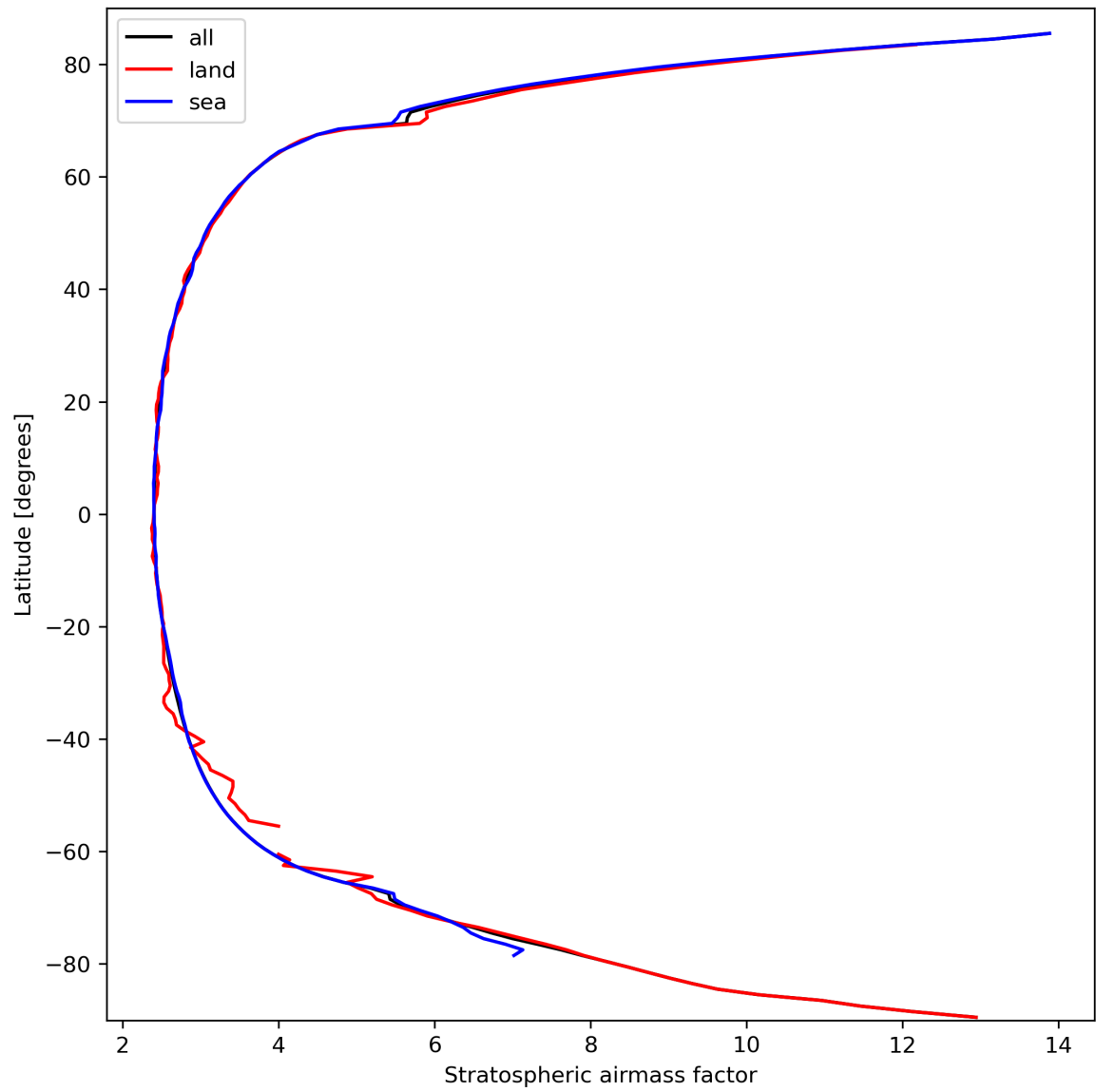
Figure 27: Zonal average of “Stratospheric airmass factor” for 2023-09-29 to 2023-10-01.
