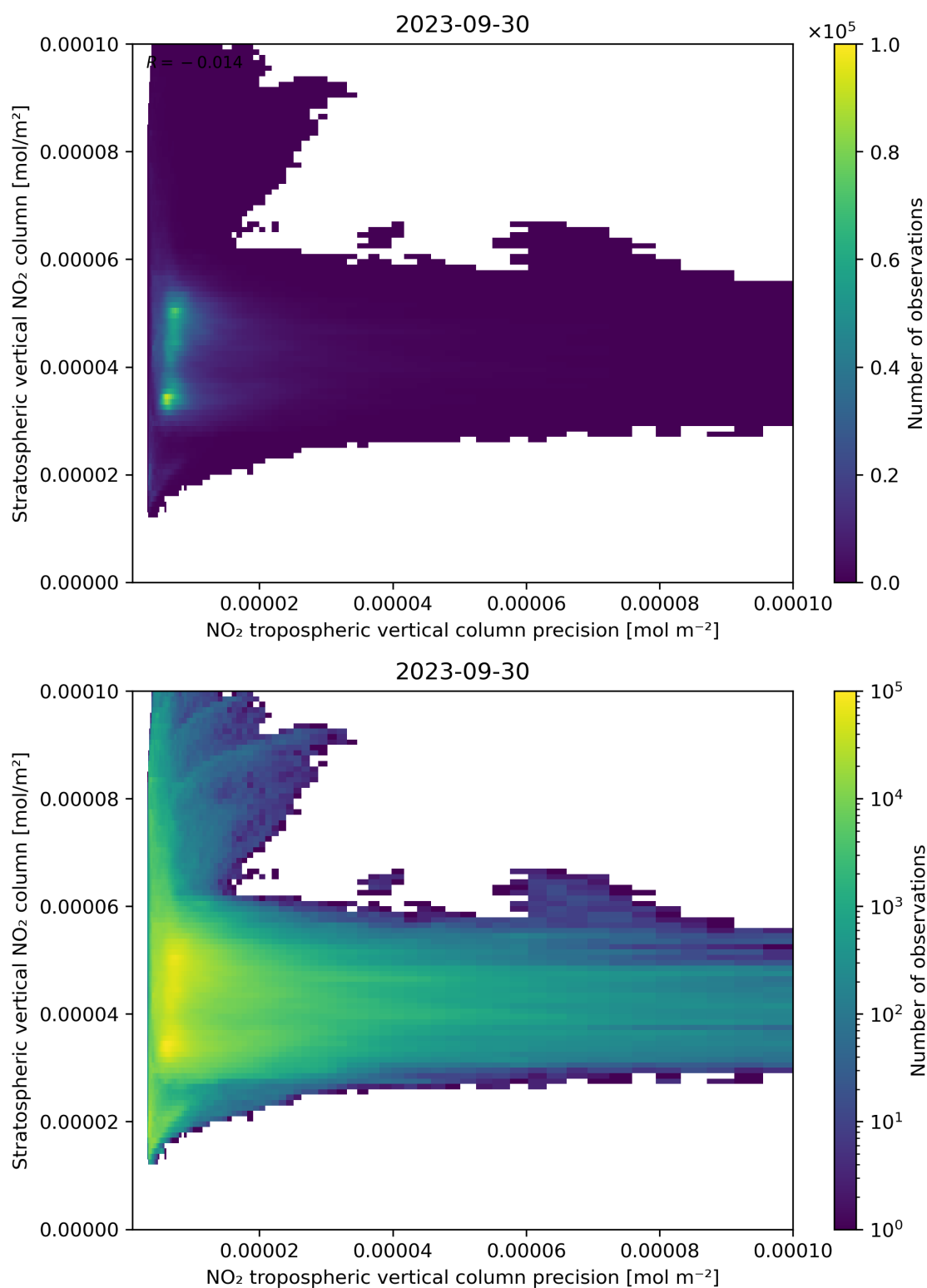
Figure 135: Scatter density plot of “NO 2 tropospheric vertical column precision” against “Stratospheric vertical NO 2 column” for 2023-09-29 to 2023-10-01.
