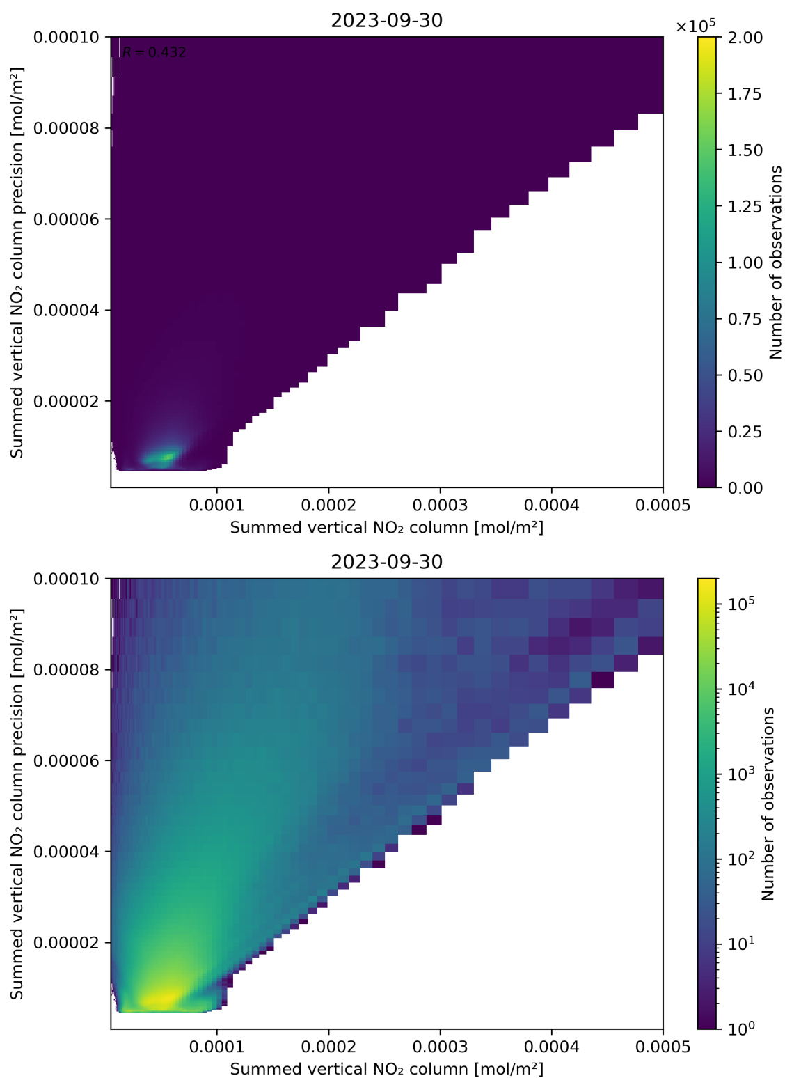
Figure 105: Scatter density plot of “Summed vertical NO 2 column” against “Summed vertical NO 2 column precision” for 2023-09-29 to 2023-10-01.
