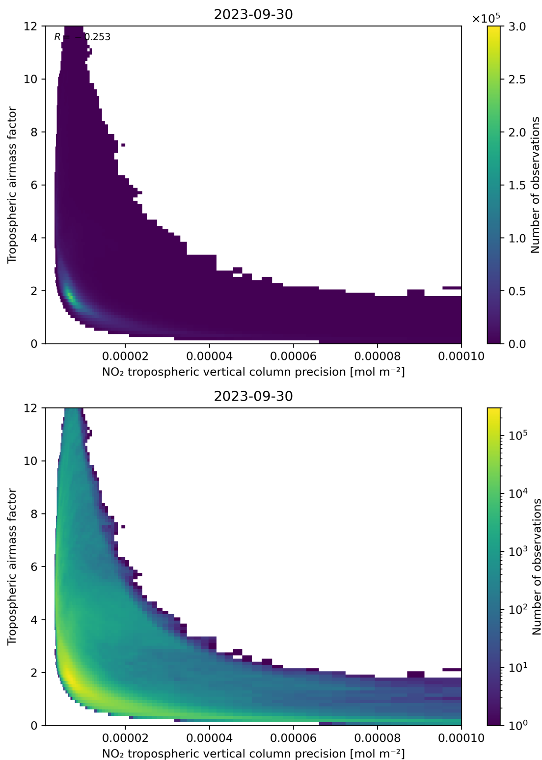
Figure 133: Scatter density plot of “NO 2 tropospheric vertical column precision” against “Tropospheric air mass factor” for 2023-09-29 to 2023-10-01.
