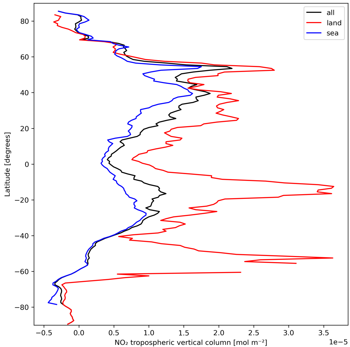
Figure 12: Zonal average of “NO 2 tropospheric vertical column” for 2023-09-29 to 2023-10-01.
