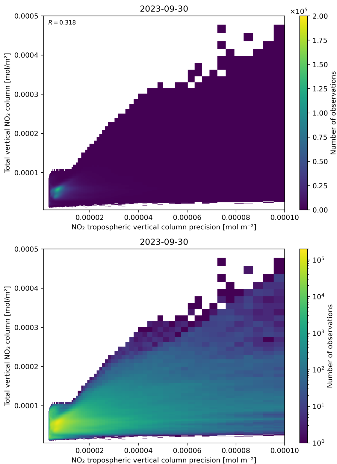
Figure 138: Scatter density plot of “NO 2 tropospheric vertical column precision” against “Total vertical NO 2 column” for 2023-09-29 to 2023-10-01.
