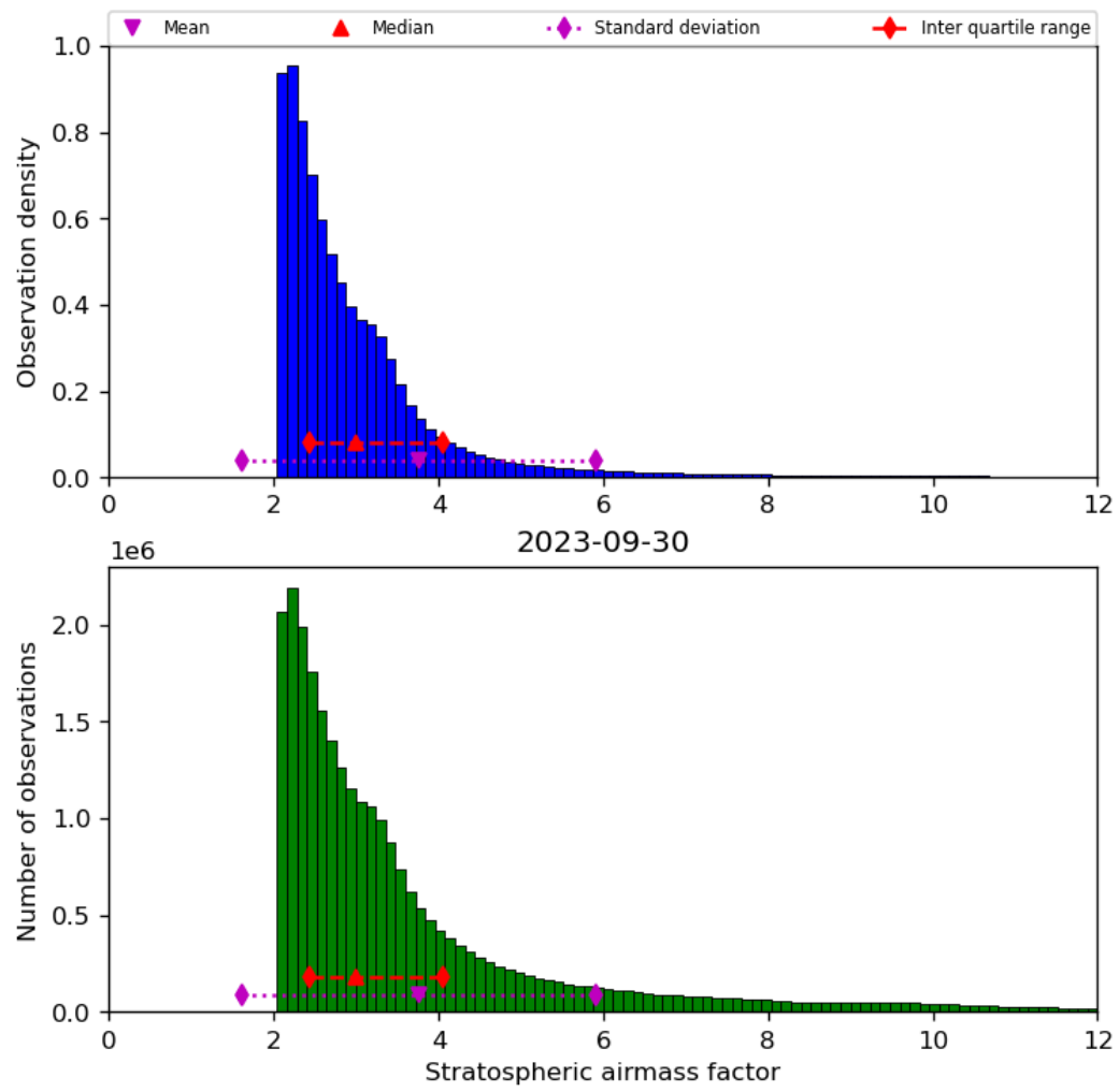
Figure 44: Histogram of “Stratospheric airmass factor” for 2023-09-29 to 2023-10-01
