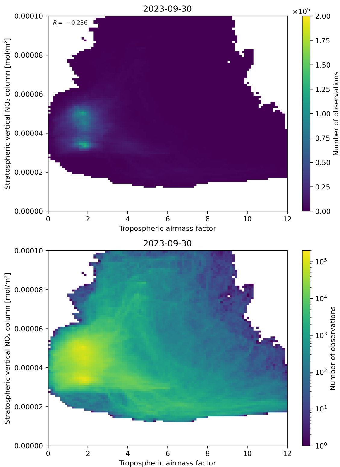
Figure 74: Scatter density plot of “Tropospheric air mass factor” against “Stratospheric vertical NO 2 column” for 2023-09-29 to 2023-10-01.
