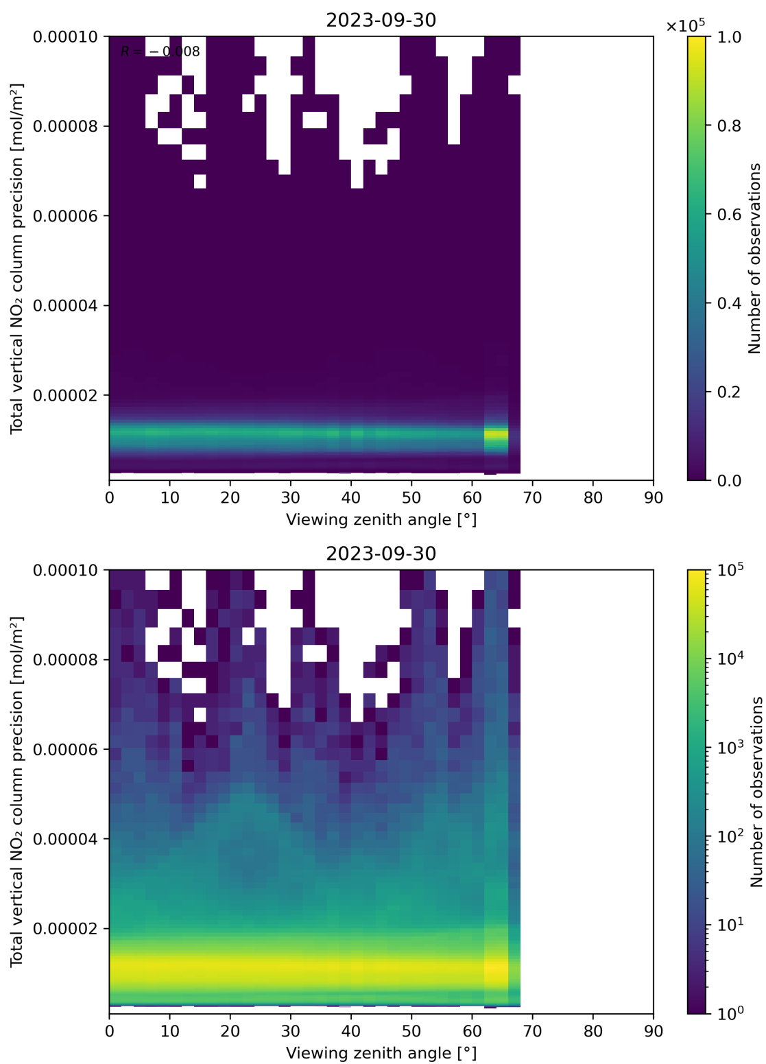
Figure 168: Scatter density plot of “Viewing zenith angle” against “Total vertical NO 2 column precision” for 2023-09-29 to 2023-10-01.
