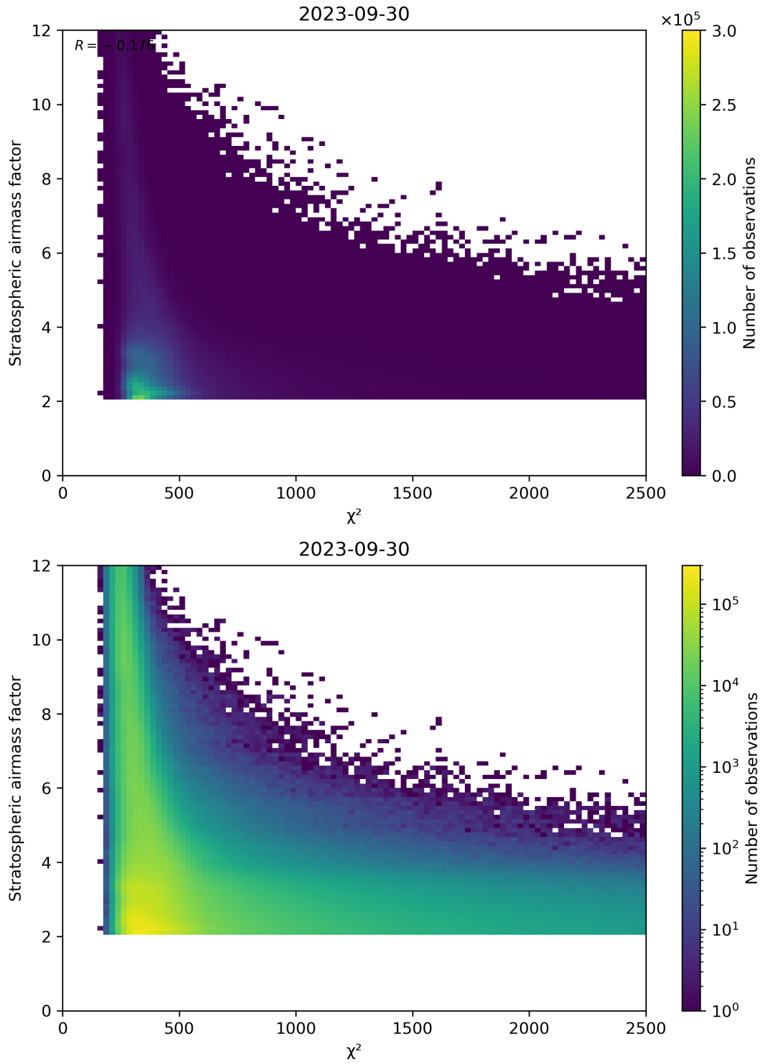
Figure 81: Scatter density plot of “ \chi^2 ” against “Stratospheric airmass factor” for 2023-09-29 to 2023-10-01.
