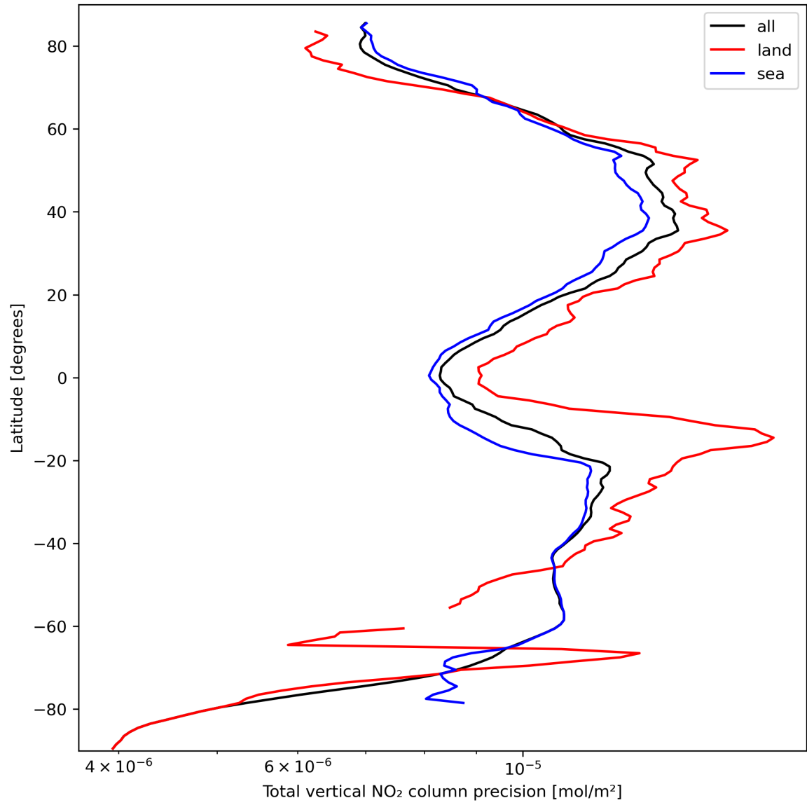
Figure 22: Zonal average of “Total vertical NO 2 column precision” for 2023-09-29 to 2023-10-01.
