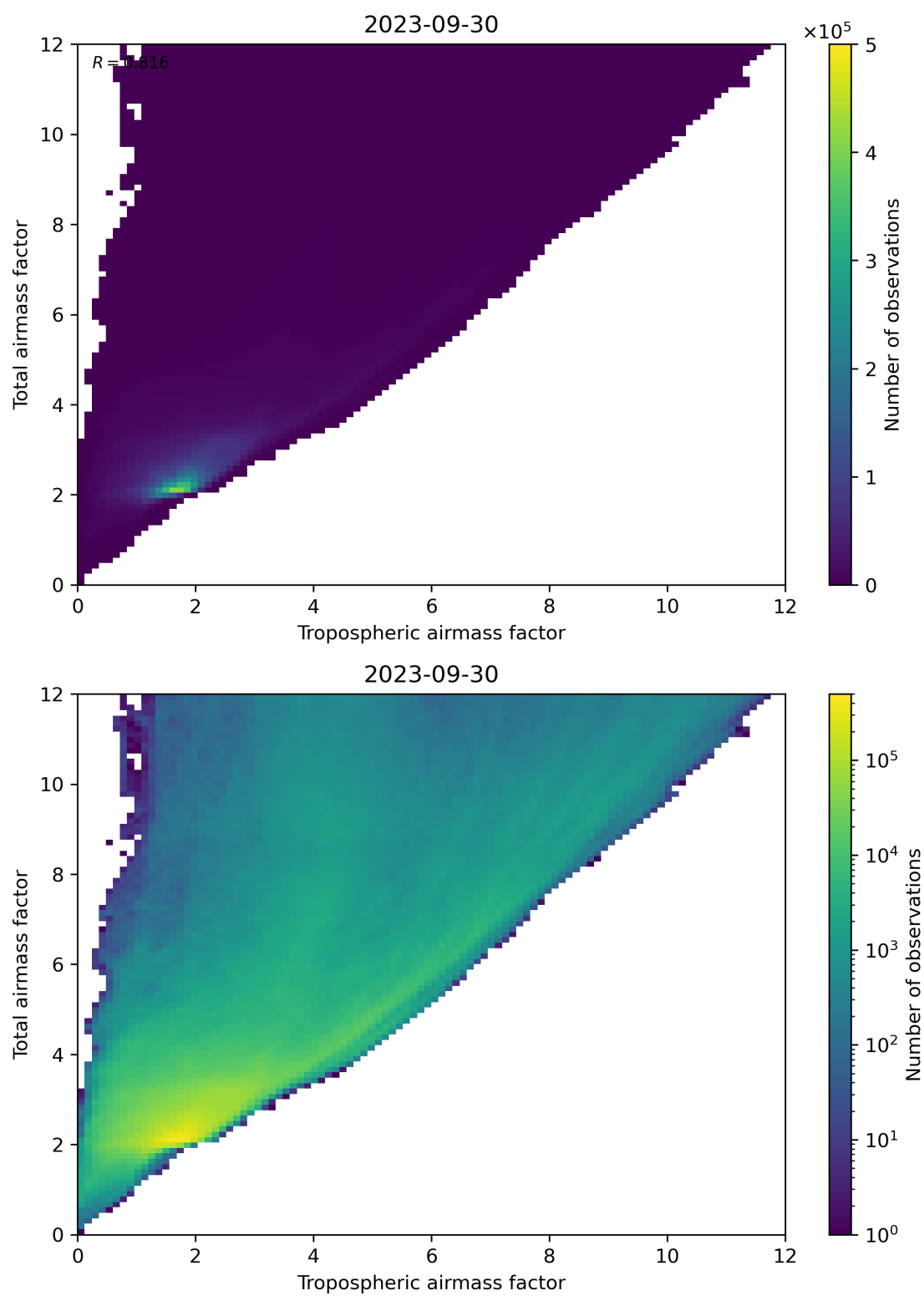
Figure 72: Scatter density plot of “Tropospheric airmass factor” against “Total airmass factor” for 2023-09-29 to 2023-10-01.
