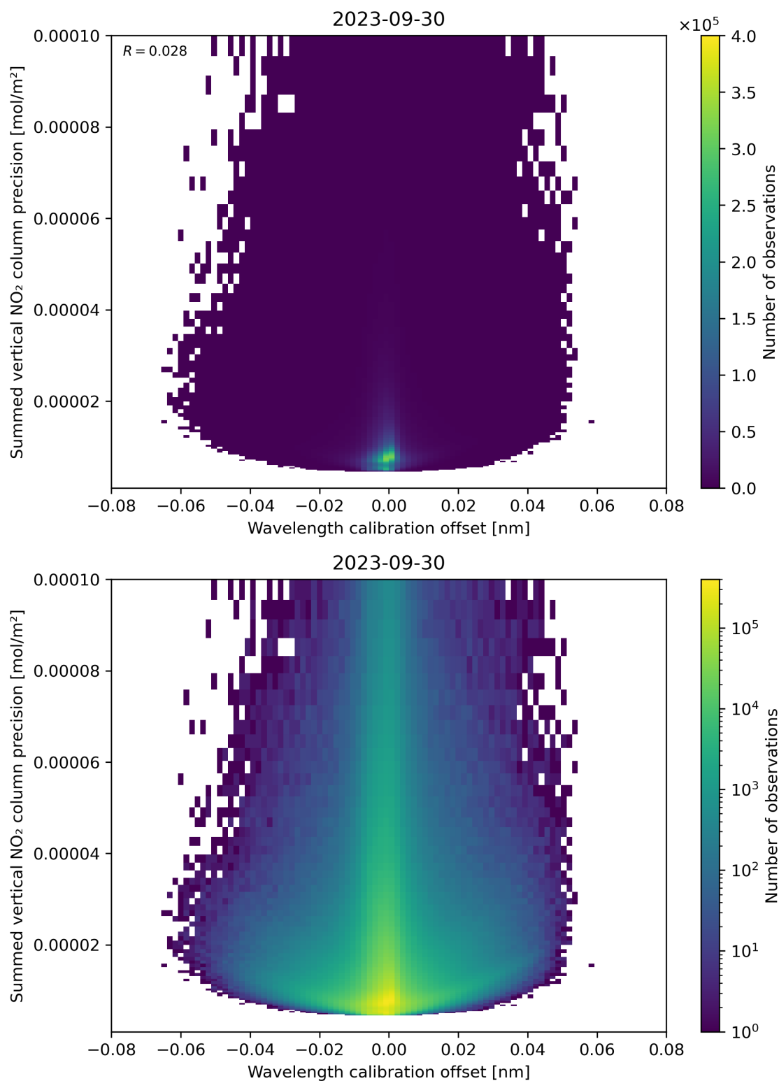
Figure 178: Scatter density plot of “Wavelength calibration offset” against “Summed vertical NO 2 column precision” for 2023-09-29 to 2023-10-01.
