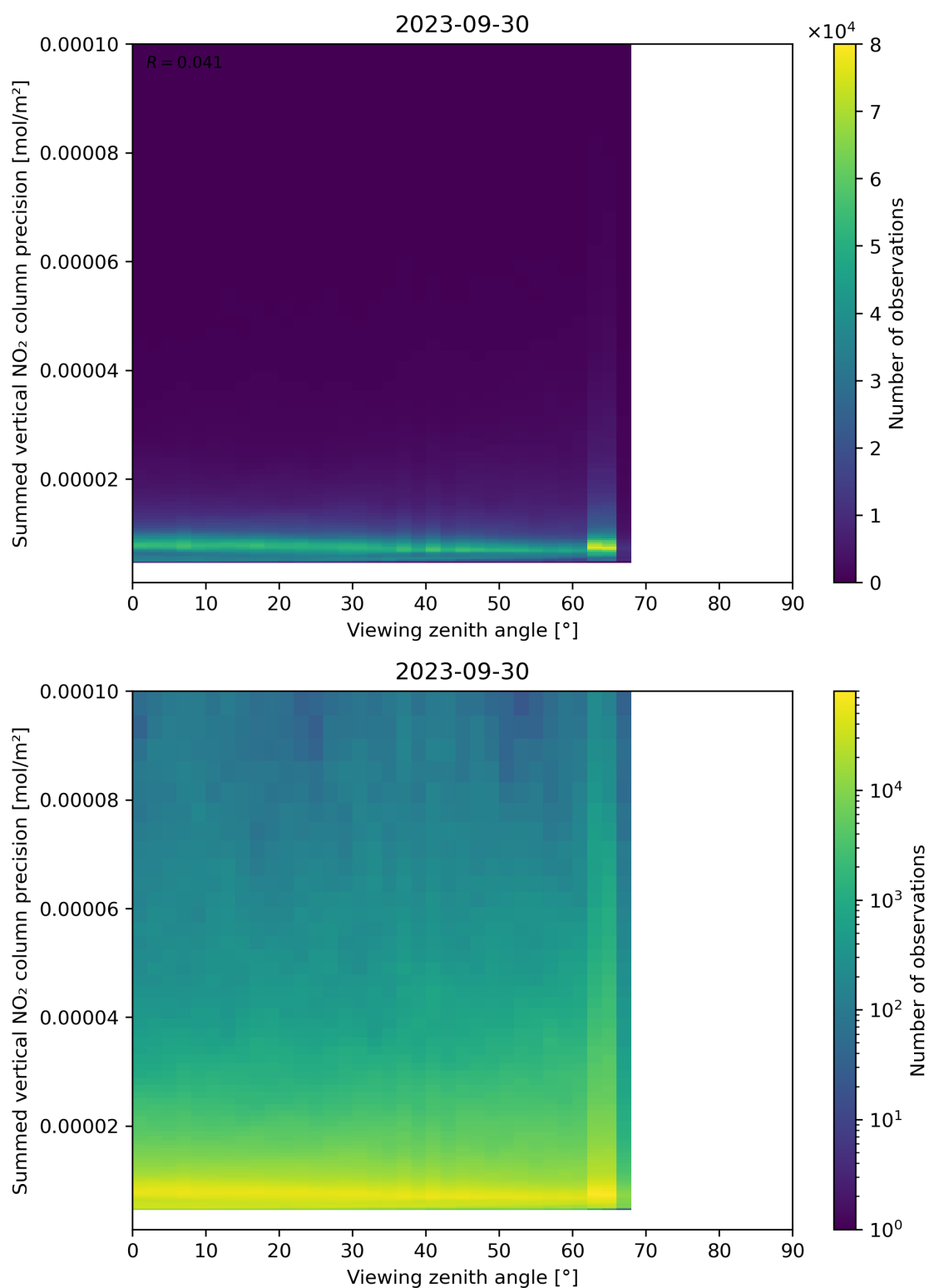
Figure 166: Scatter density plot of “Viewing zenith angle” against “Summed vertical NO 2 column precision” for 2023-09-29 to 2023-10-01.
