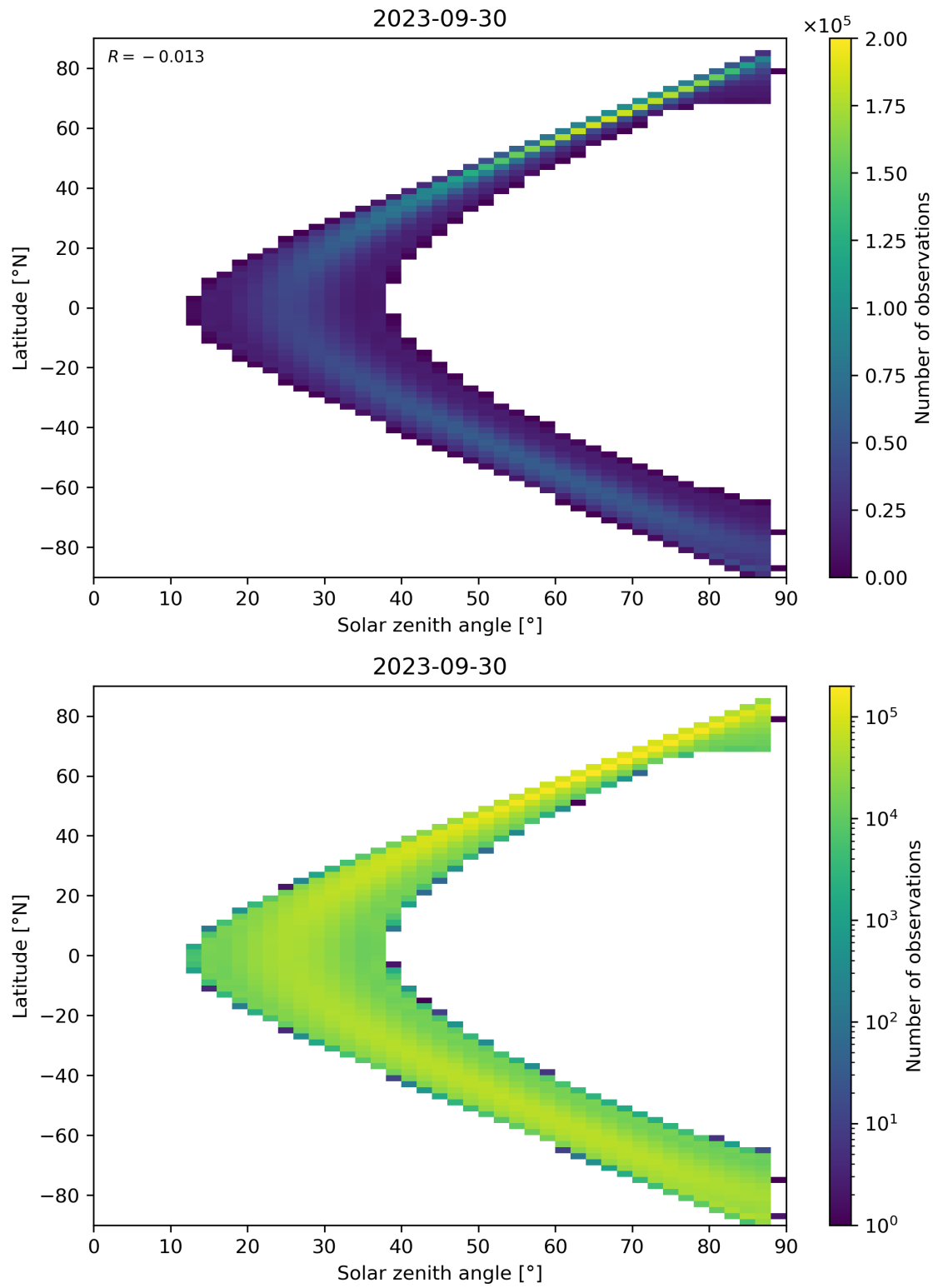
Figure 149: Scatter density plot of “Solar zenith angle” against “Latitude” for 2023-09-29 to 2023-10-01.
