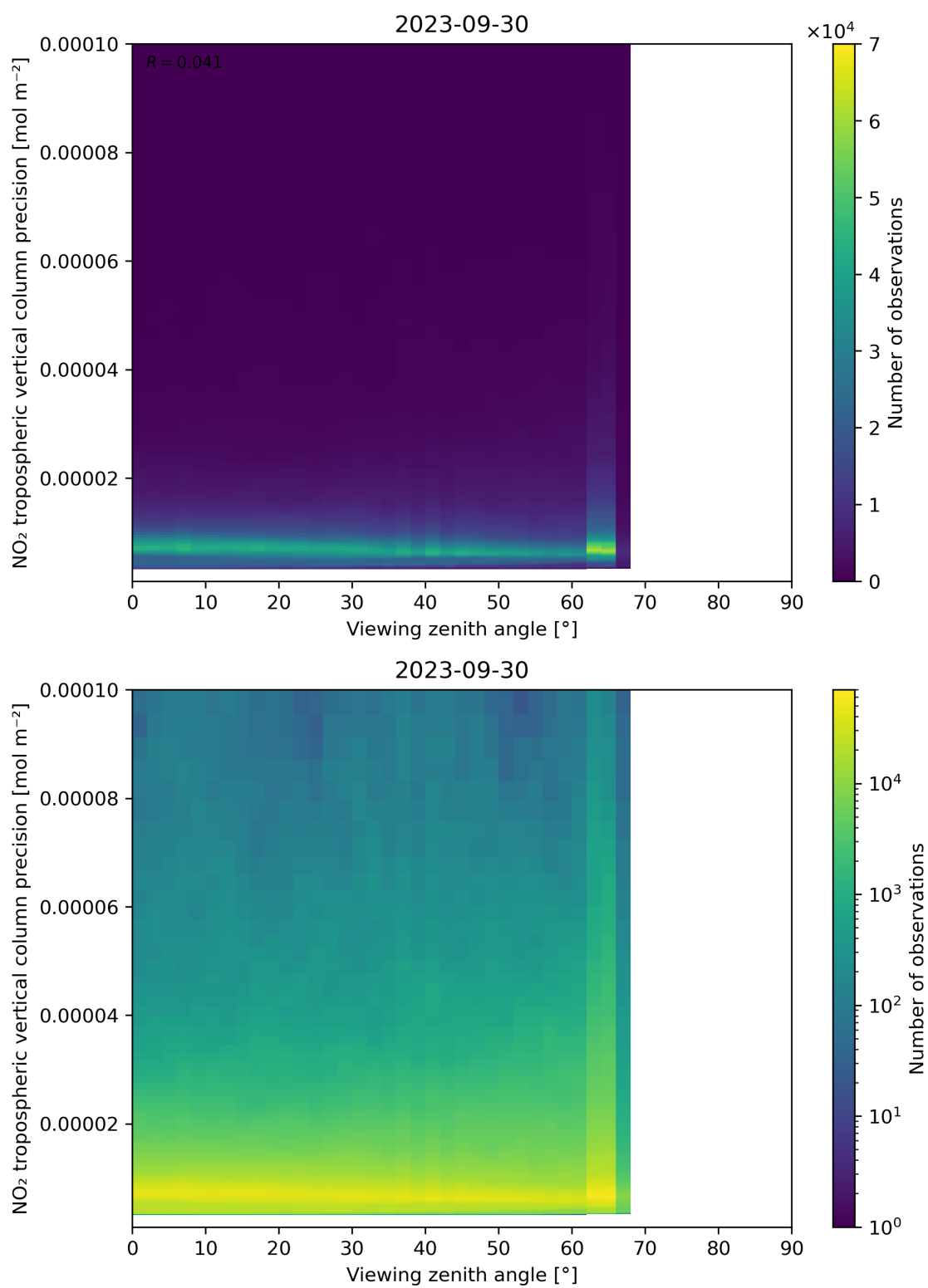
Figure 170: Scatter density plot of “Viewing zenith angle” against “NO 2 tropospheric vertical column precision” for 2023-09-29 to 2023-10-01.
