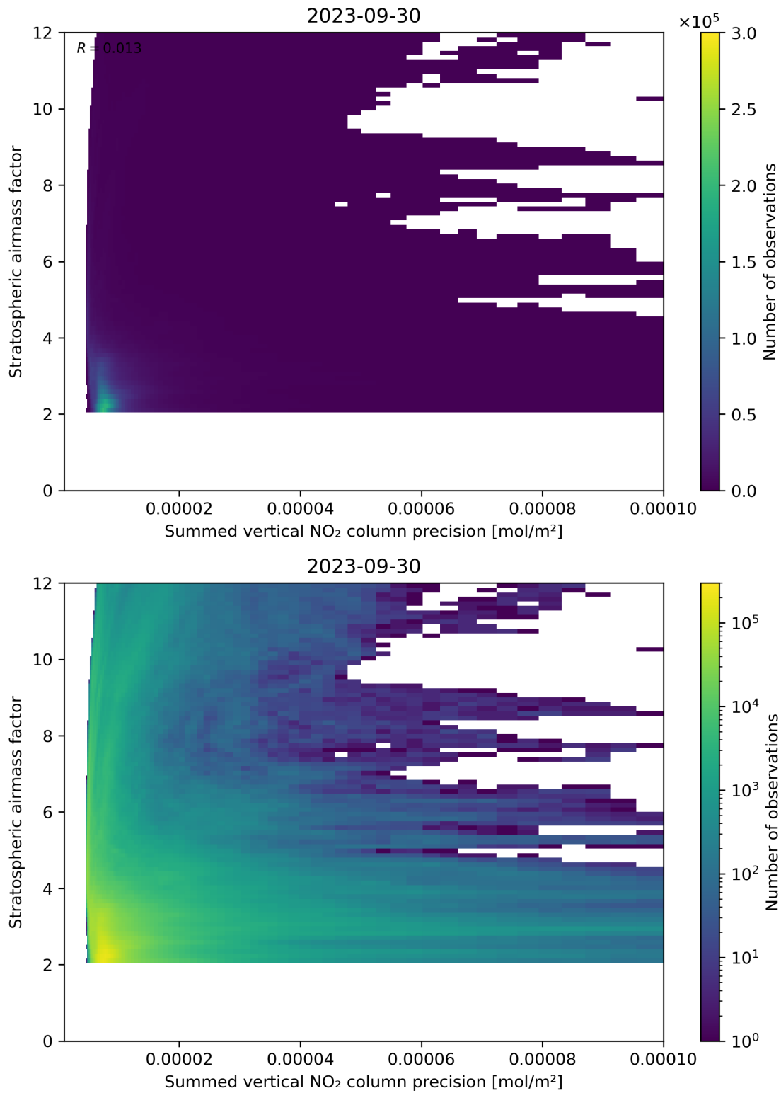
Figure 106: Scatter density plot of “Summed vertical NO 2 column precision” against “Stratospheric airmass factor” for 2023-09-29 to 2023-10-01.
