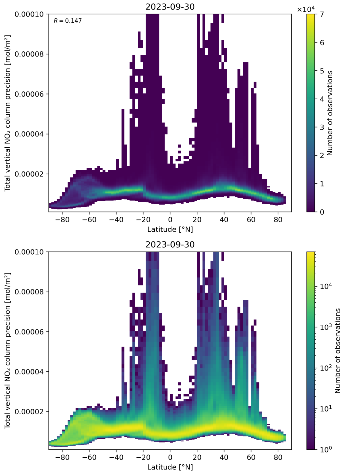
Figure 91: Scatter density plot of “Latitude” against “Total vertical NO 2 column precision” for 2023-09-29 to 2023-10-01.
