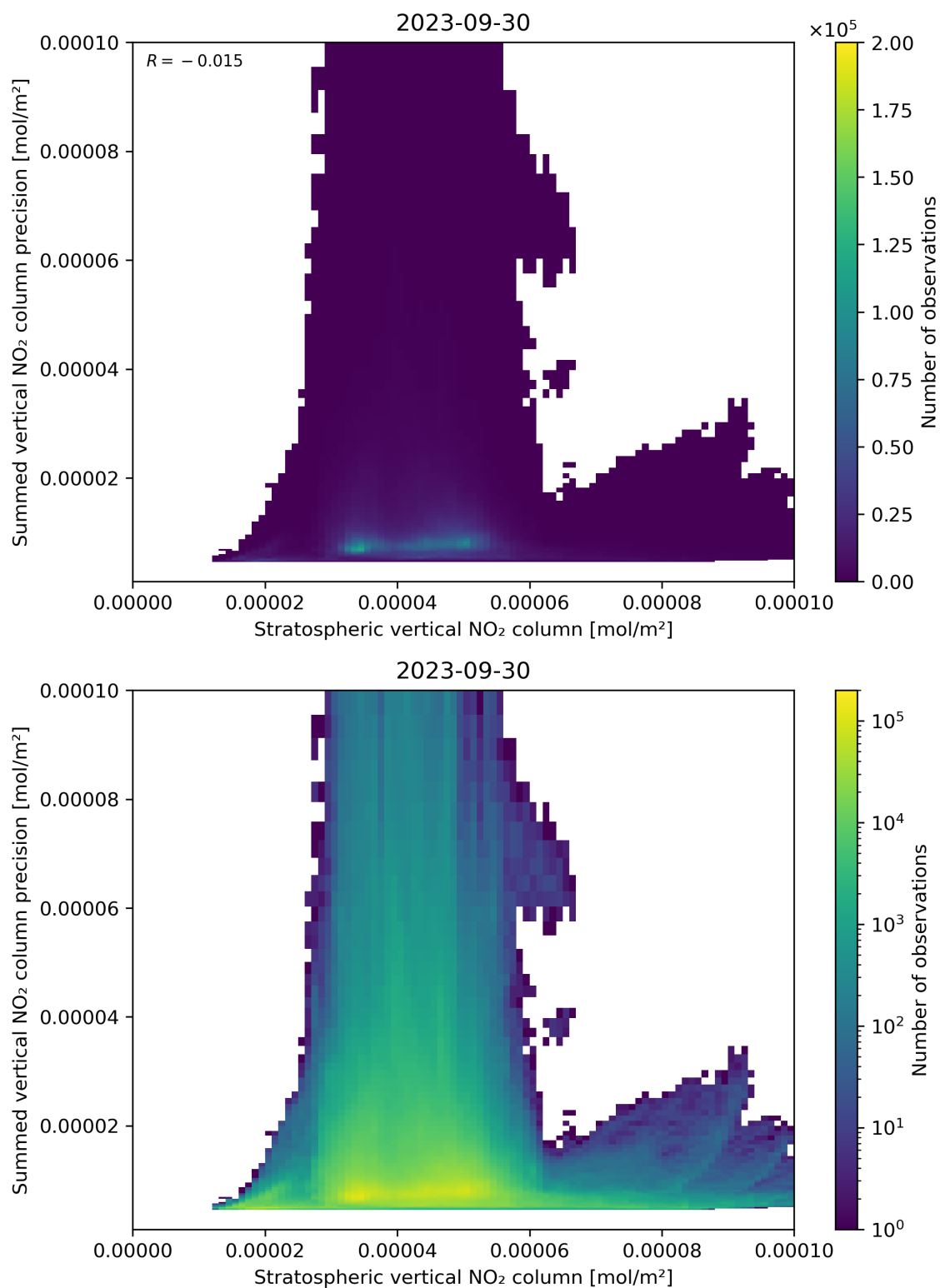
Figure 99: Scatter density plot of “Stratospheric vertical NO 2 column” against “Summed vertical NO 2 column precision” for 2023-09-29 to 2023-10-01.
