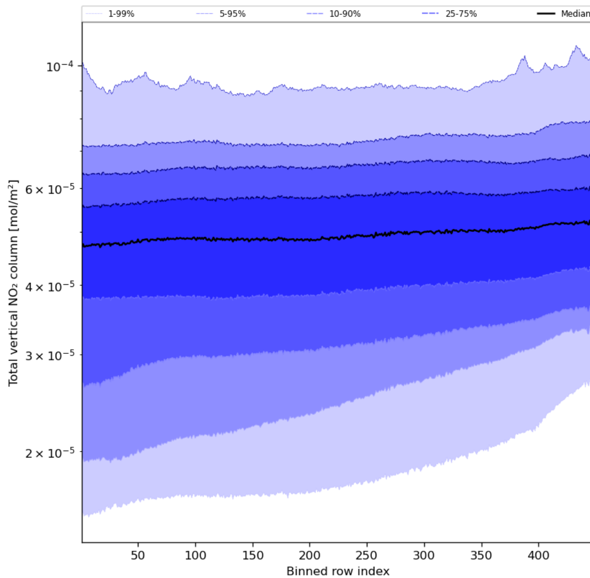
Figure 55: Along track statistics of “Total vertical NO 2 column” for 2023-09-29 to 2023-10-01
