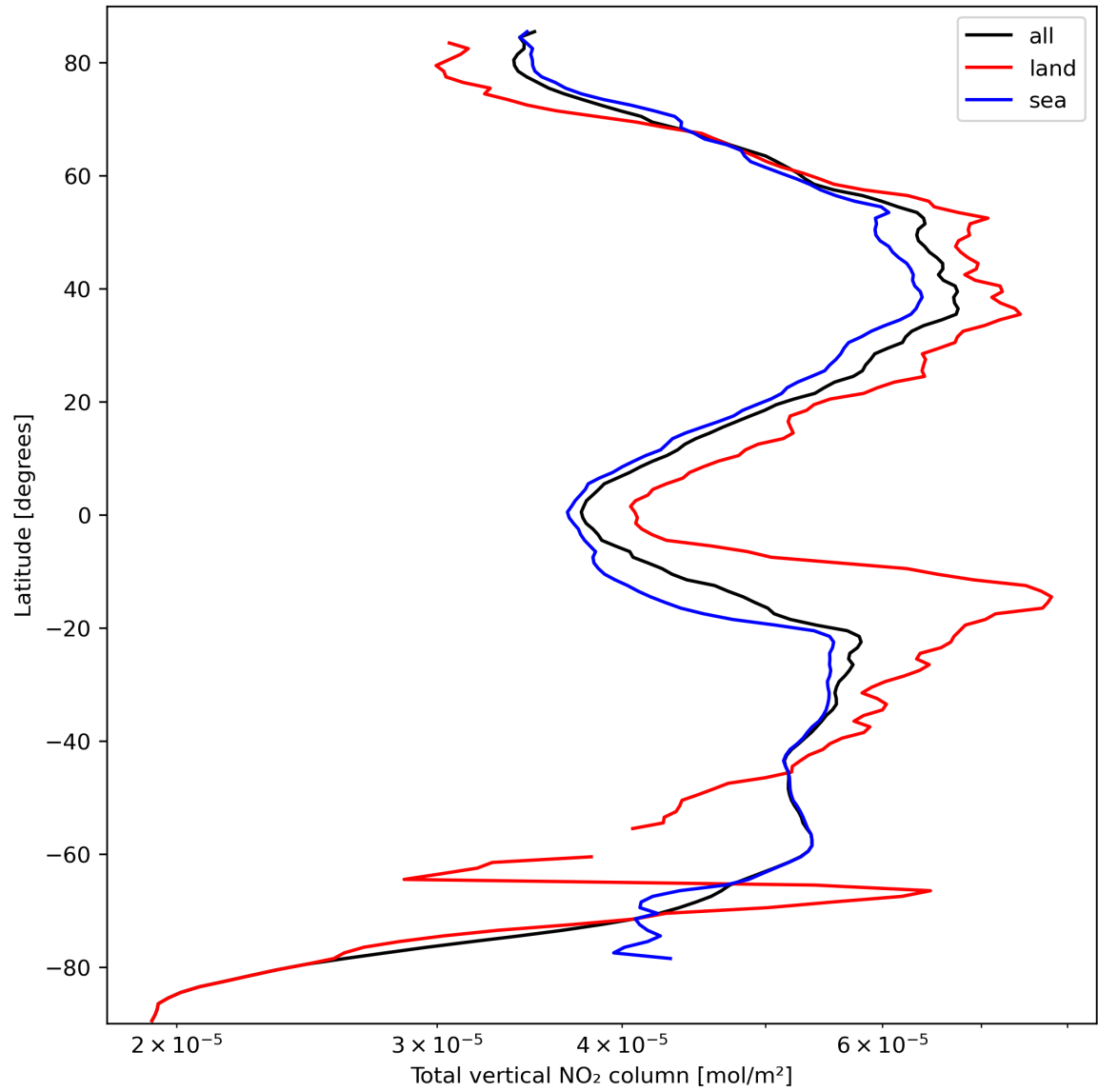
Figure 21: Zonal average of “Total vertical NO 2 column” for 2023-09-29 to 2023-10-01.
