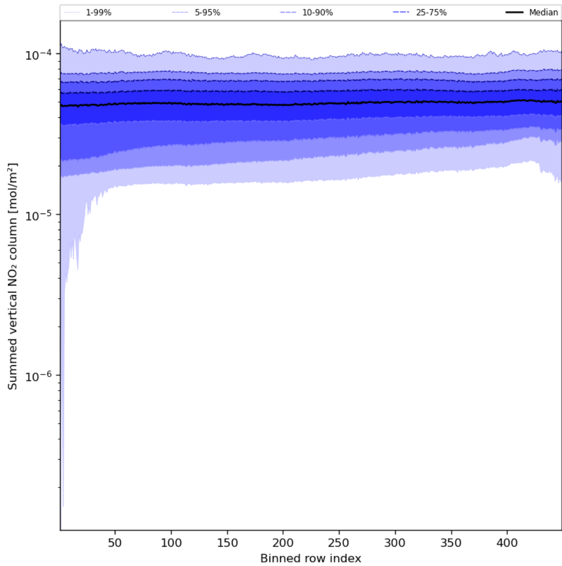
Figure 57: Along track statistics of “Summed vertical NO 2 column” for 2023-09-29 to 2023-10-01
