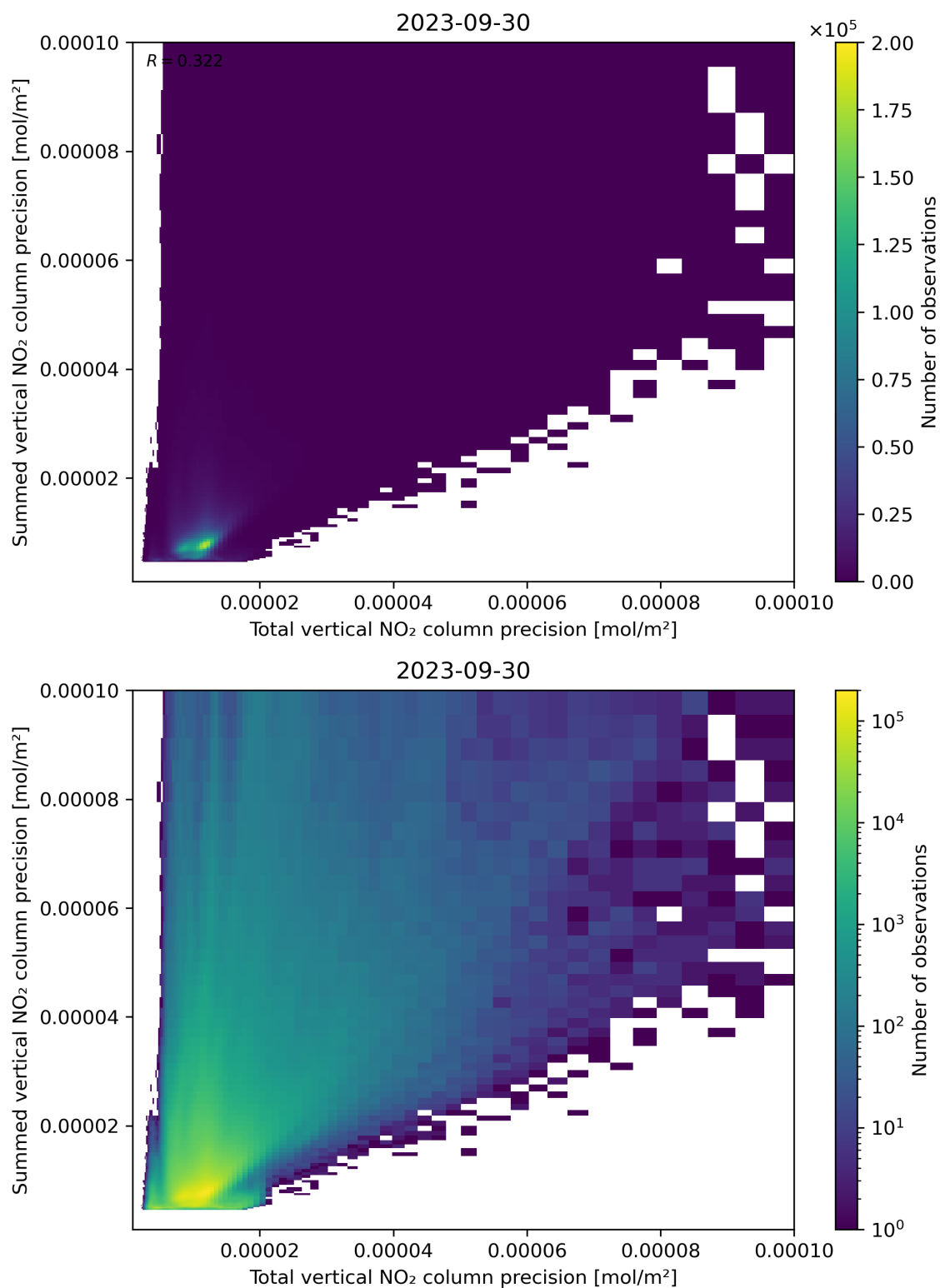
Figure 118: Scatter density plot of “Total vertical NO 2 column precision” against “Summed vertical NO 2 column precision” for 2023-09-29 to 2023-10-01.
