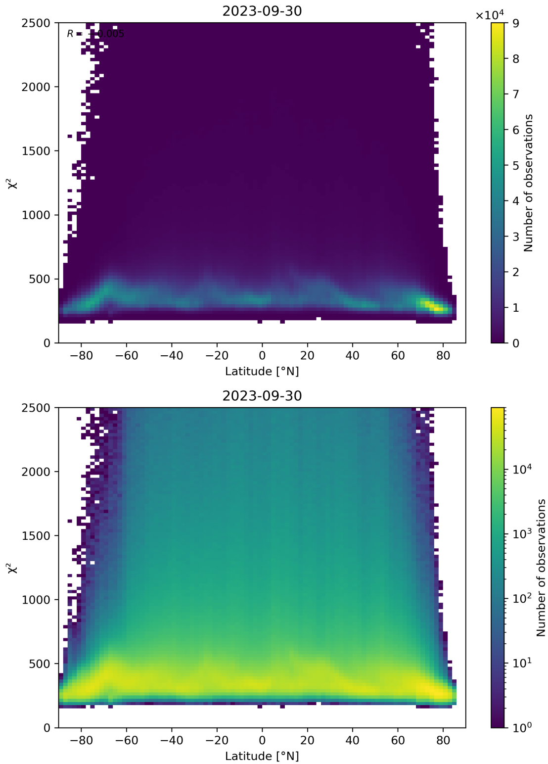
Figure 86: Scatter density plot of “Latitude” against “ \chi^2 ” for 2023-09-29 to 2023-10-01.
