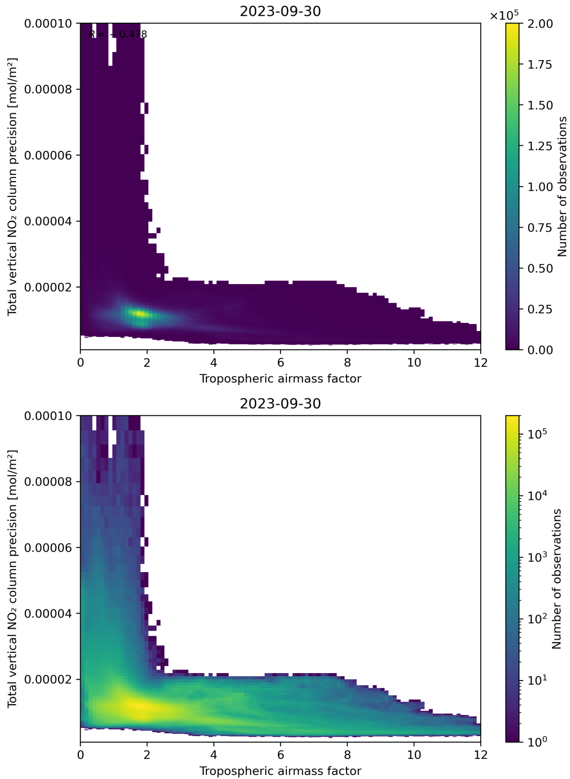
Figure 78: Scatter density plot of “Tropospheric air mass factor” against “Total vertical NO 2 column precision” for 2023-09-29 to 2023-10-01.
