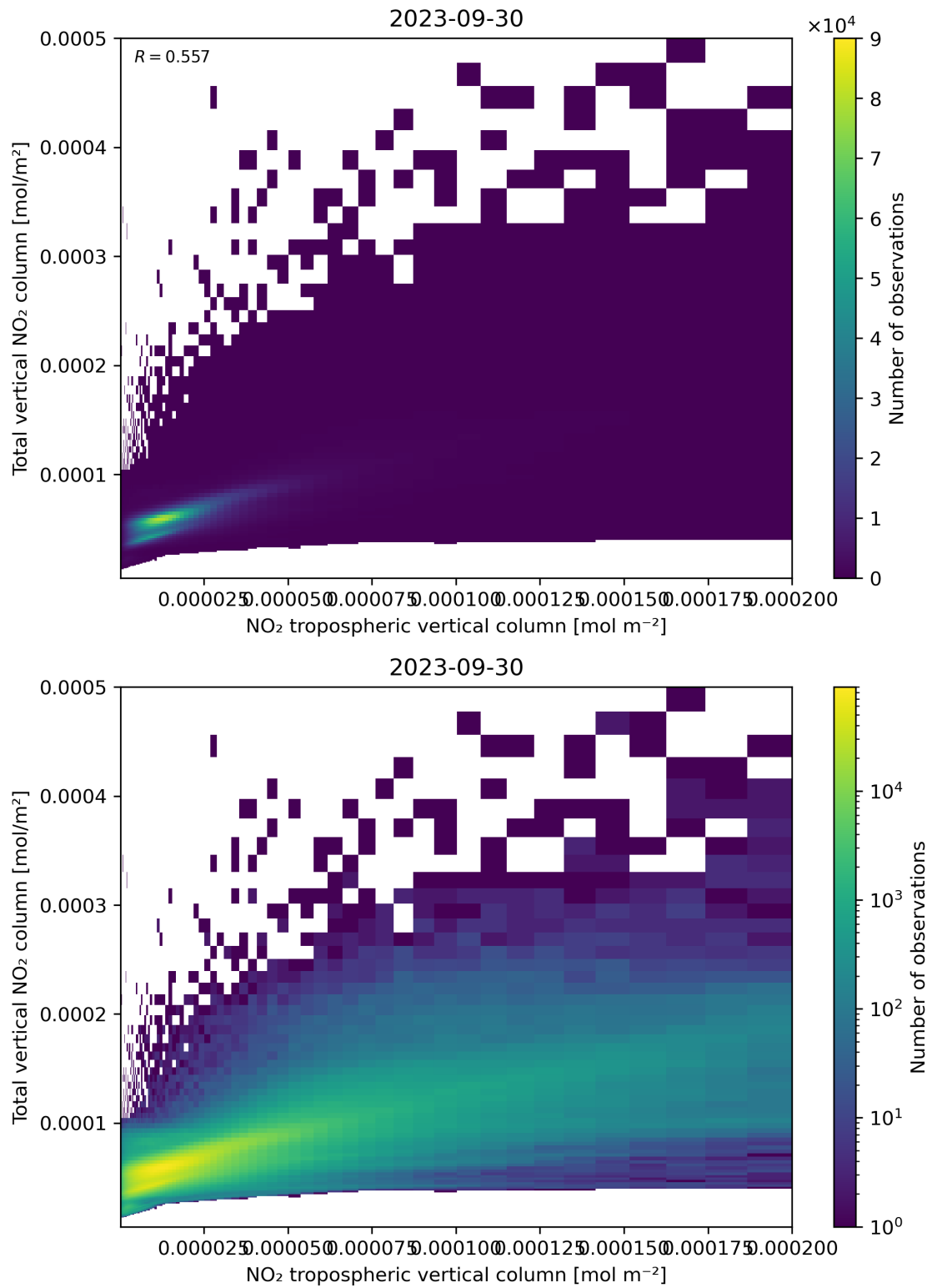
Figure 128: Scatter density plot of “NO 2 tropospheric vertical column” against “Total vertical NO 2 column” for 2023-09-29 to 2023-10-01.
