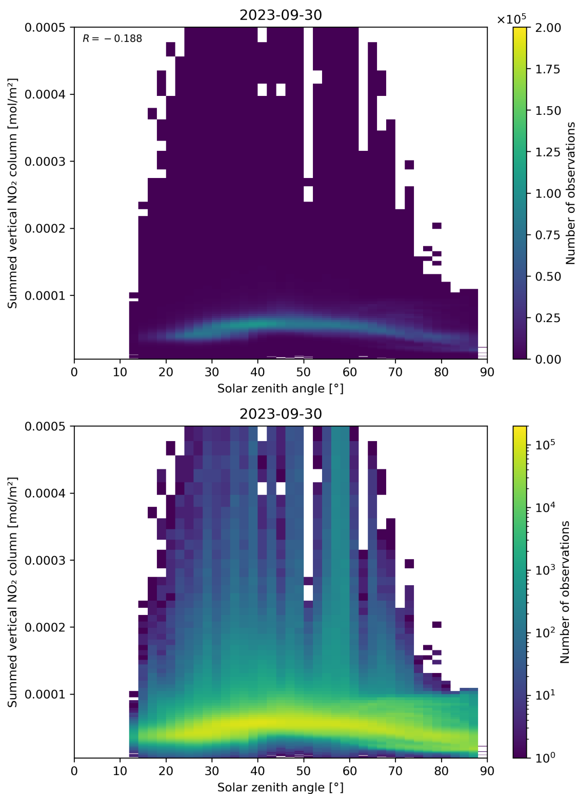
Figure 151: Scatter density plot of “Solar zenith angle” against “Summed vertical NO 2 column” for 2023-09-29 to 2023-10-01.
