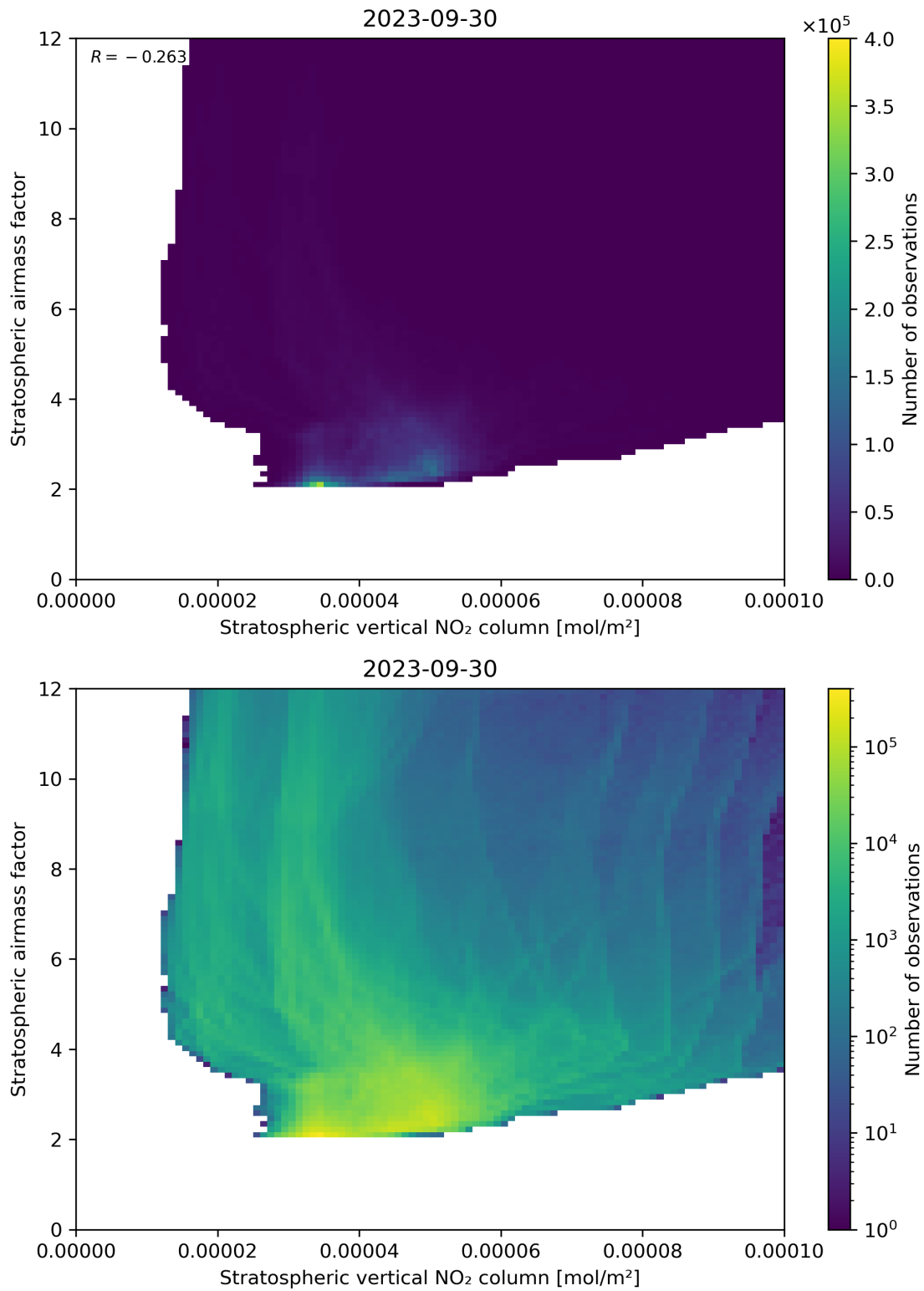
Figure 96: Scatter density plot of “Stratospheric vertical NO 2 column” against “Stratospheric airmass factor” for 2023-09-29 to 2023-10-01.
