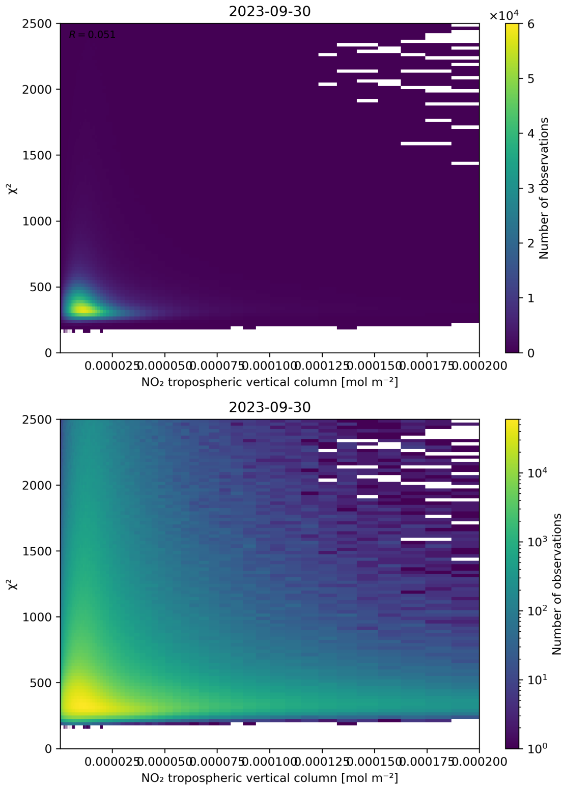
Figure 124: Scatter density plot of “NO 2 tropospheric vertical column” against “ \chi^2 ” for 2023-09-29 to 2023-10-01.
