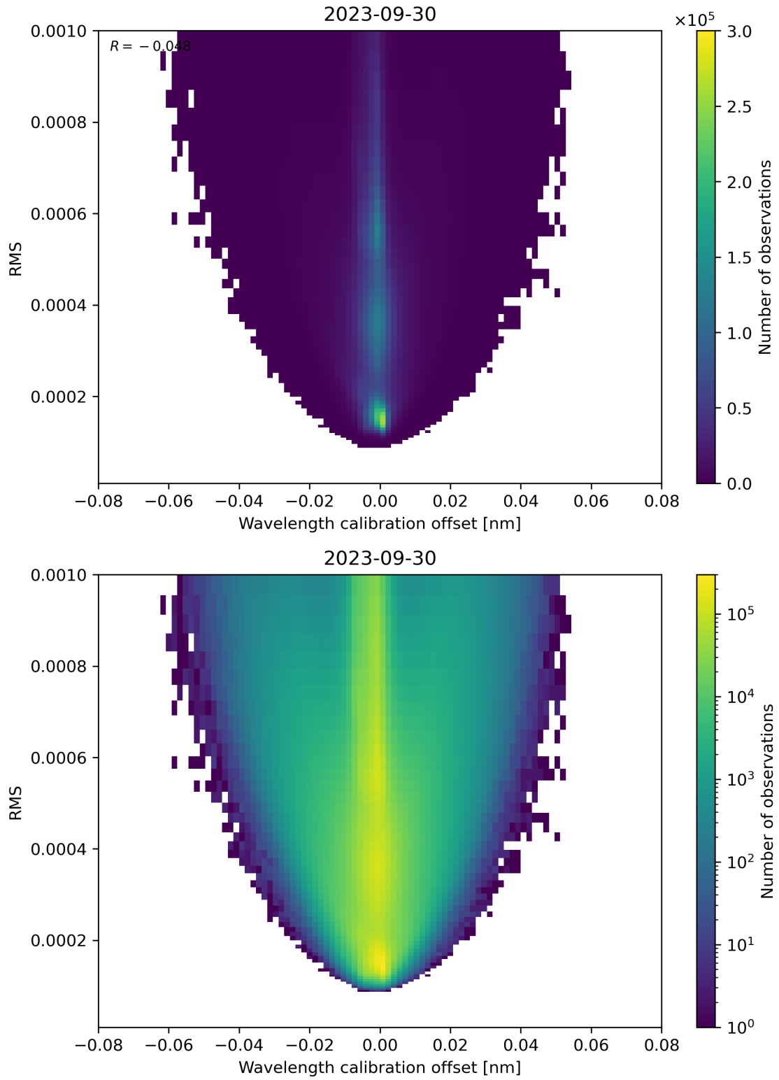
Figure 181: Scatter density plot of “Wavelength calibration offset” against “RMS” for 2023-09-29 to 2023-10-01.
