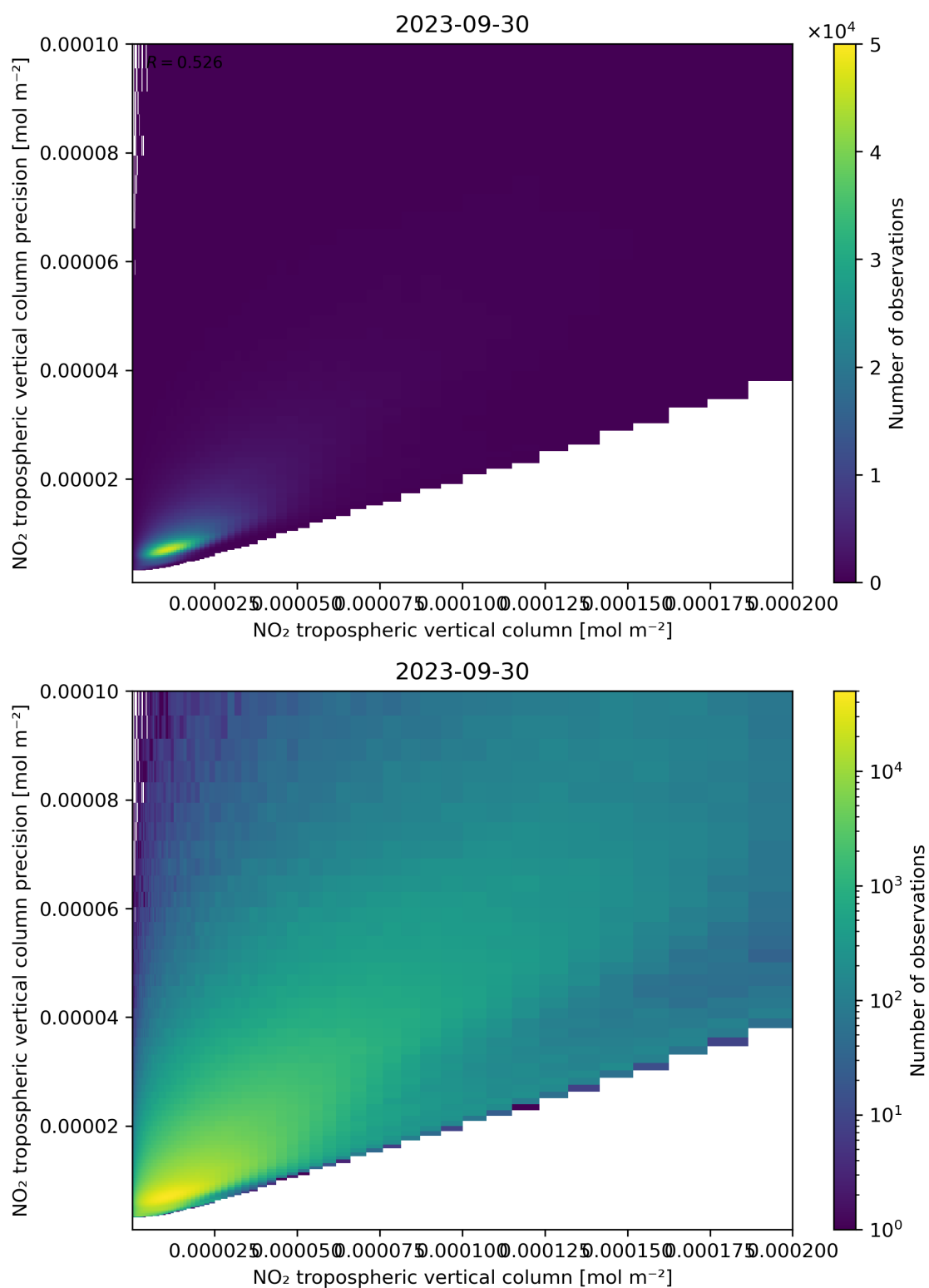
Figure 130: Scatter density plot of “NO 2 tropospheric vertical column” against “NO 2 tropospheric vertical column precision” for 2023-09-29 to 2023-10-01.
