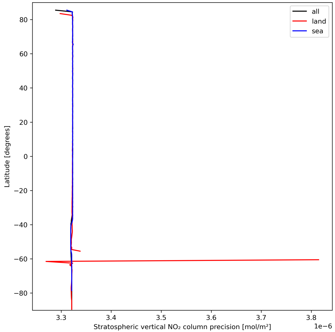
Figure 20: Zonal average of “Stratospheric vertical NO 2 column precision” for 2023-09-29 to 2023-10-01.
