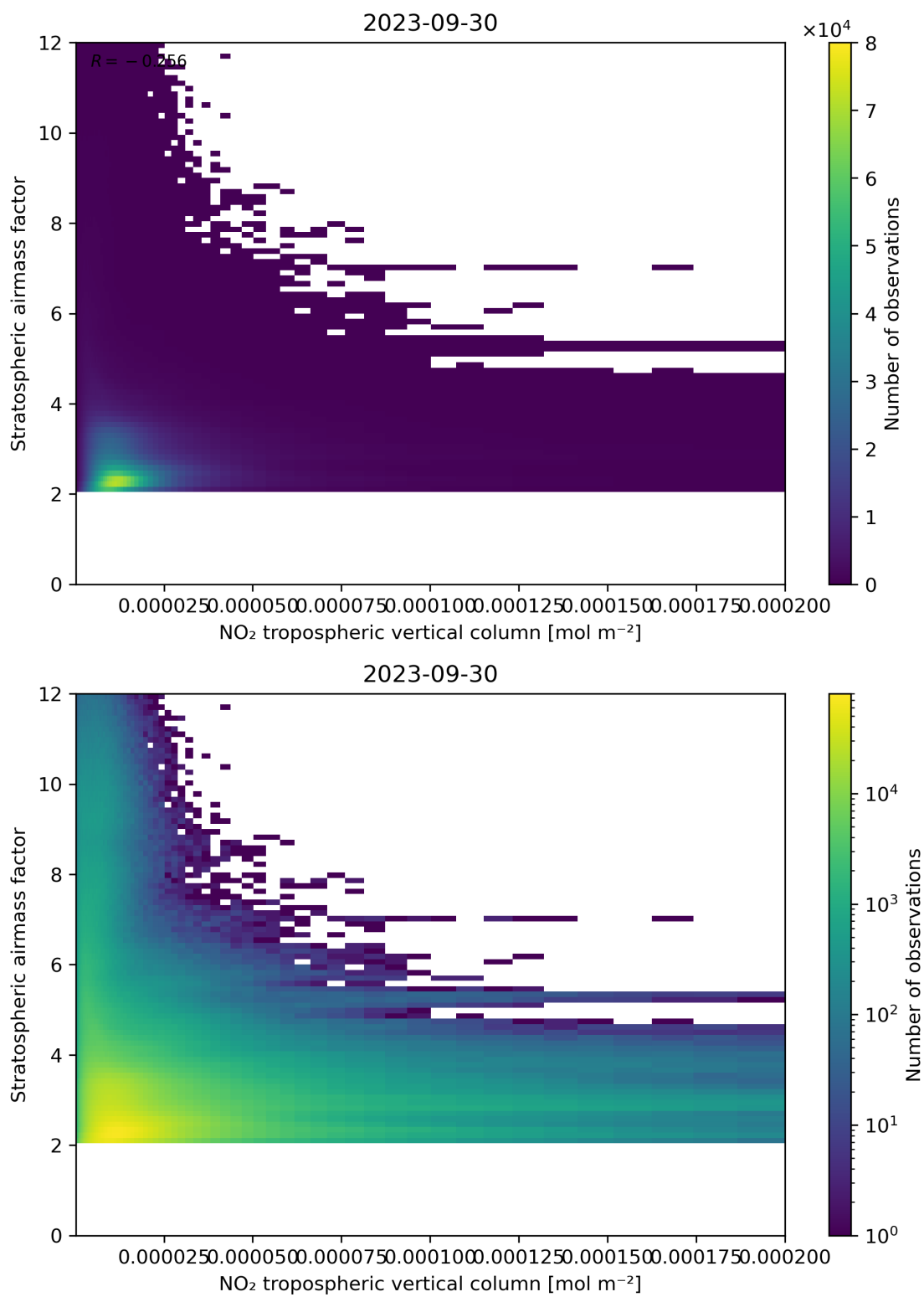
Figure 121: Scatter density plot of “NO 2 tropospheric vertical column” against “Stratospheric air mass factor” for 2023-09-29 to 2023-10-01.
