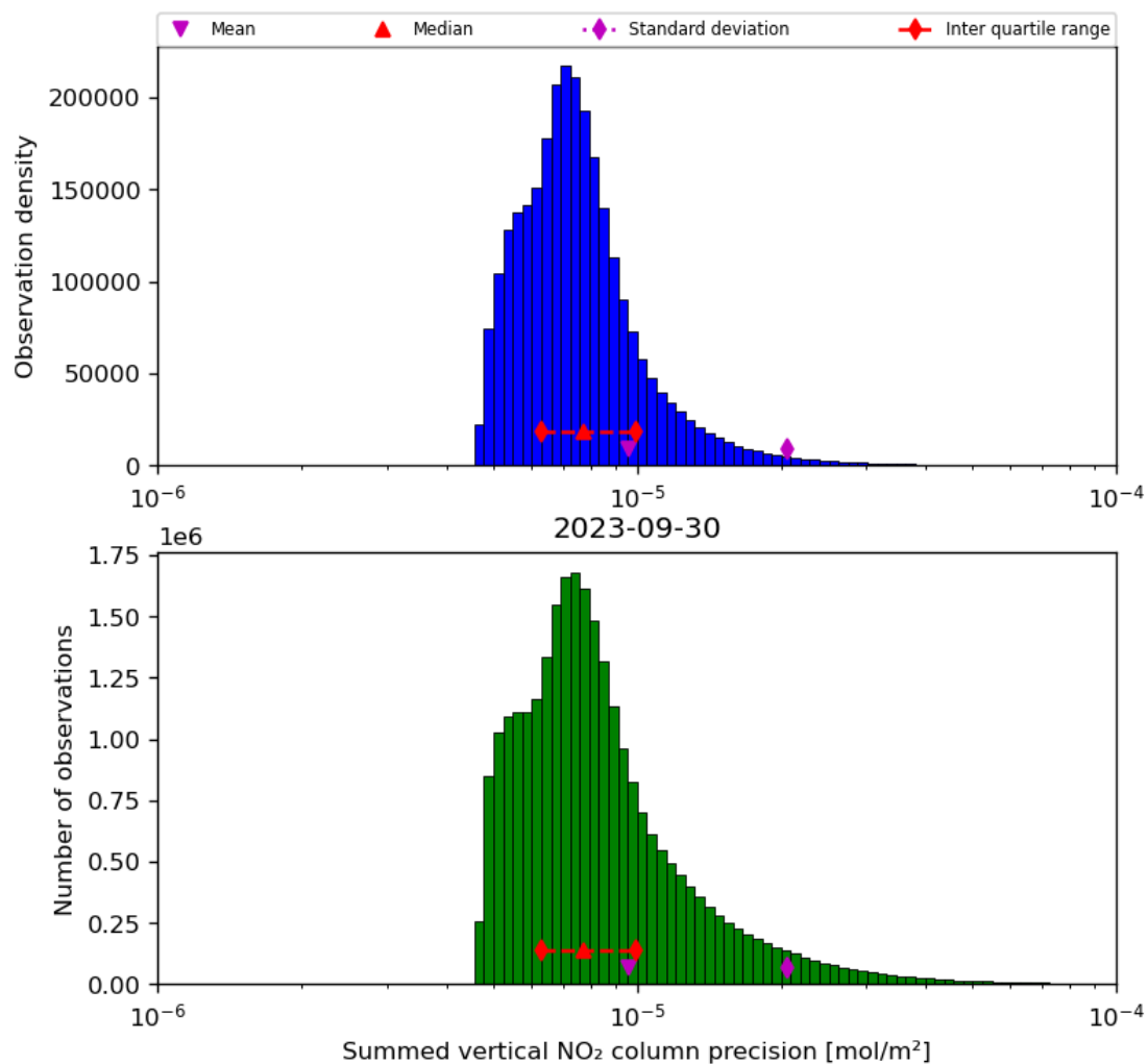
Figure 41: Histogram of “Summed vertical NO 2 column precision” for 2023-09-29 to 2023-10-01
