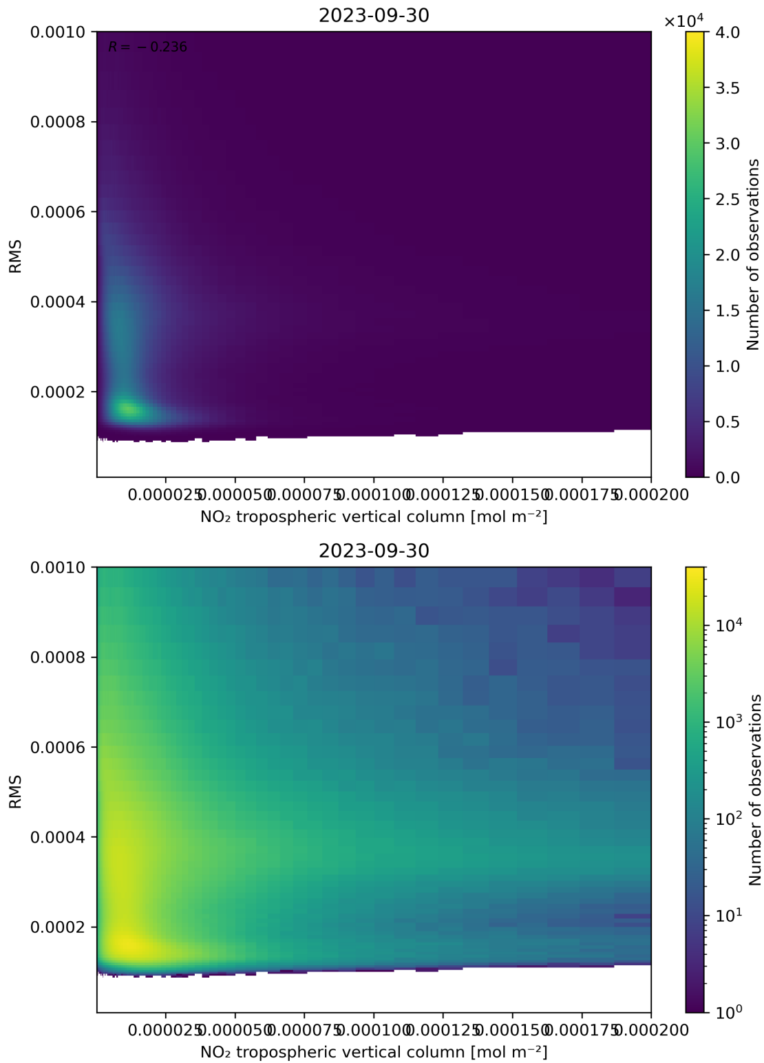
Figure 142: Scatter density plot of “NO 2 tropospheric vertical column” against “RMS” for 2023-09-29 to 2023-10-01.
