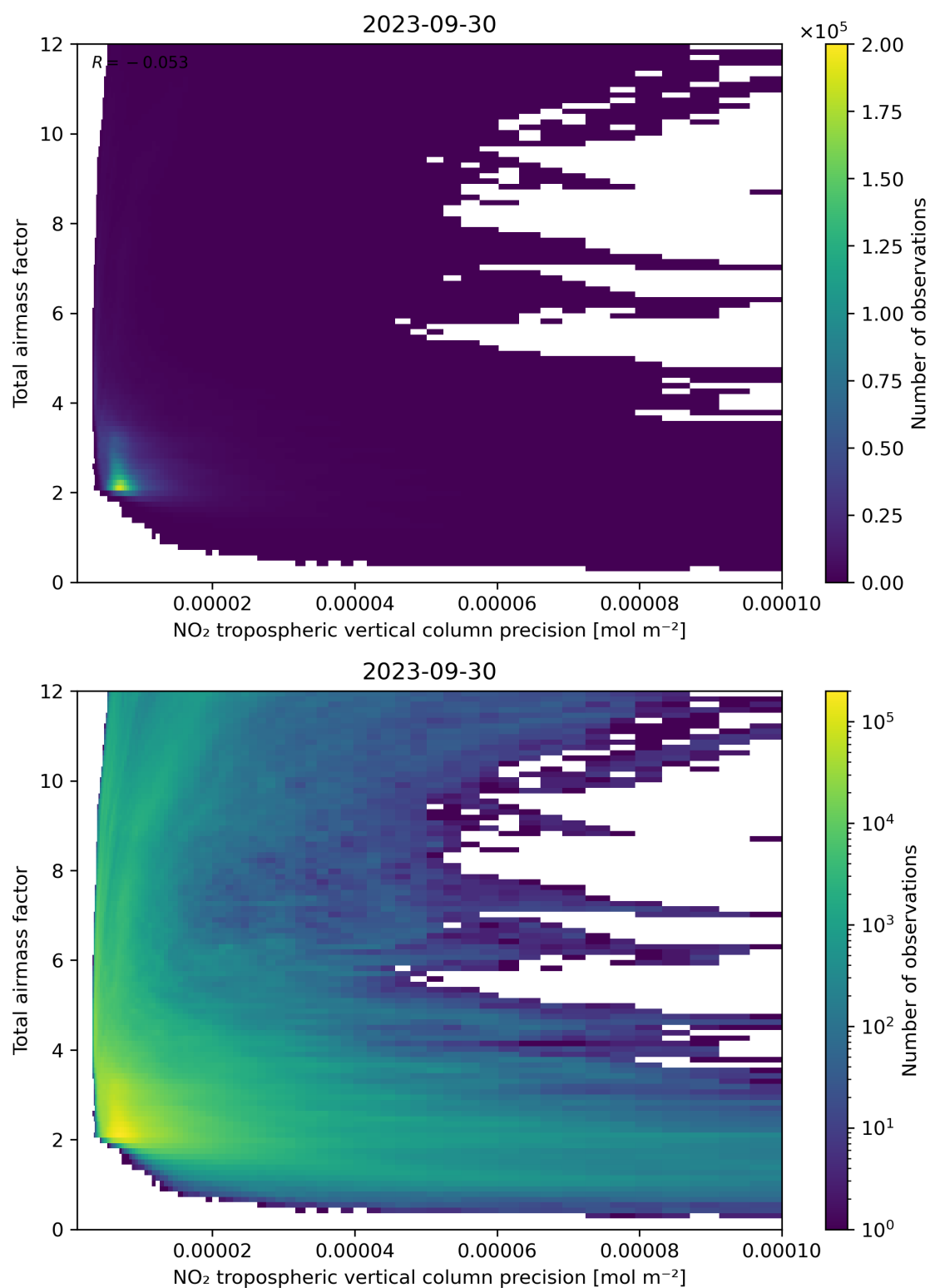
Figure 132: Scatter density plot of “NO 2 tropospheric vertical column precision” against “Total air mass factor” for 2023-09-29 to 2023-10-01.
