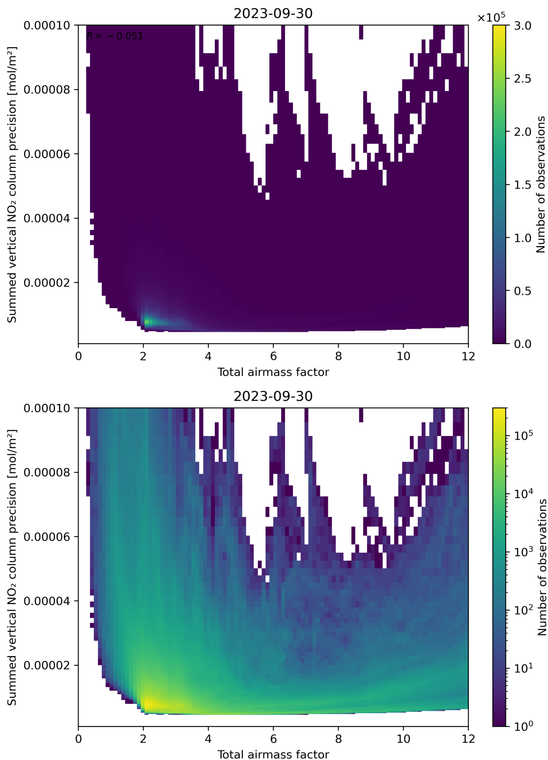
Figure 66: Scatter density plot of “Total airmass factor” against “Summed vertical NO 2 column precision” for 2023-09-29 to 2023-10-01.
