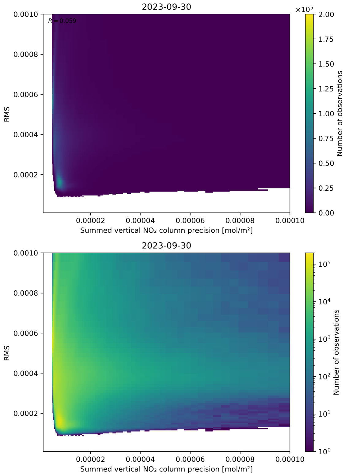
Figure 108: Scatter density plot of “Summed vertical NO 2 column precision” against “RMS” for 2023-09-29 to 2023-10-01.
