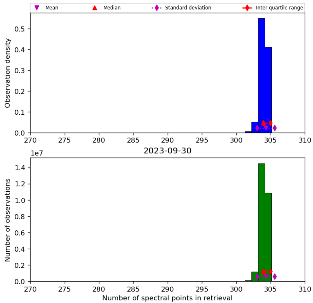
Figure 33: Histogram of “Number of spectral points in retrieval” for 2023-09-29 to 2023-10-01
