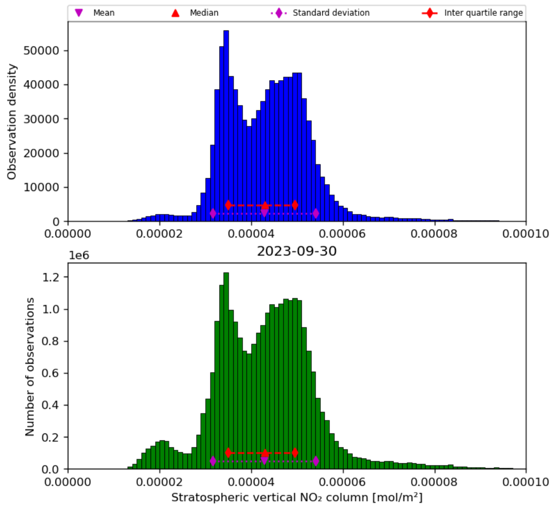
Figure 36: Histogram of “Stratospheric vertical NO 2 column” for 2023-09-29 to 2023-10-01
