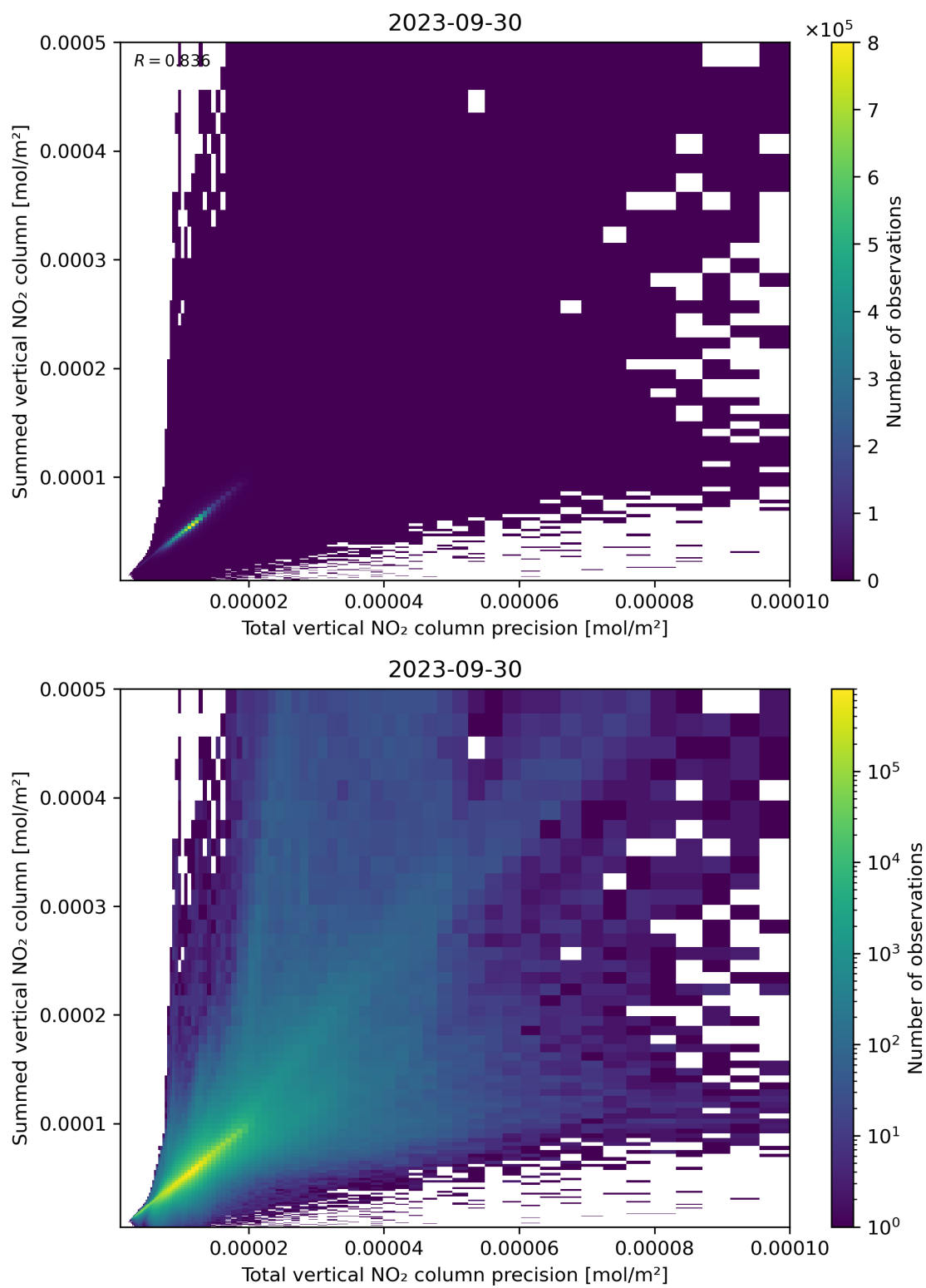
Figure 117: Scatter density plot of “Total vertical NO 2 column precision” against “Summed vertical NO 2 column” for 2023-09-29 to 2023-10-01.
