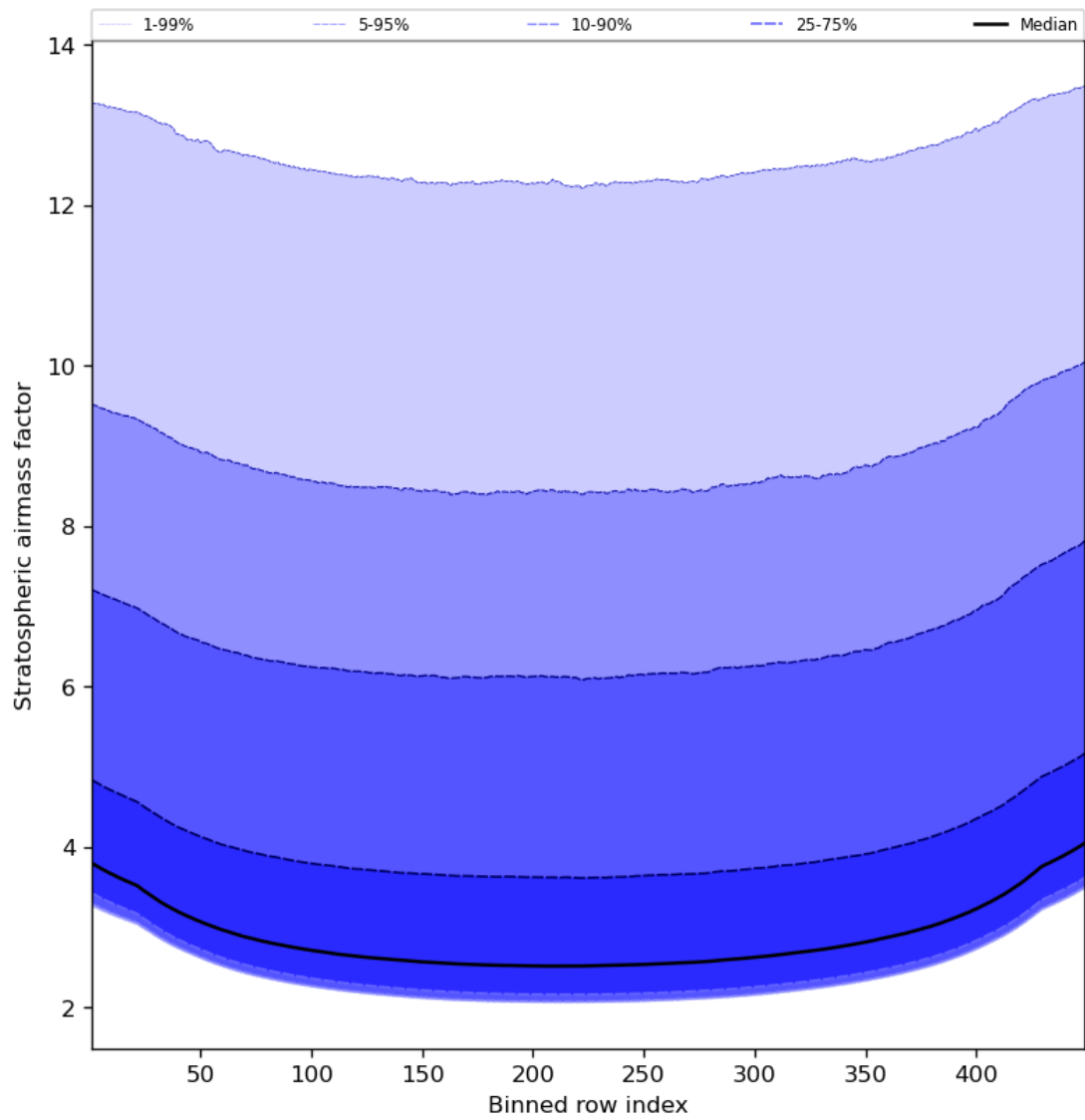
Figure 61: Along track statistics of “Stratospheric air mass factor” for 2023-09-29 to 2023-10-01
