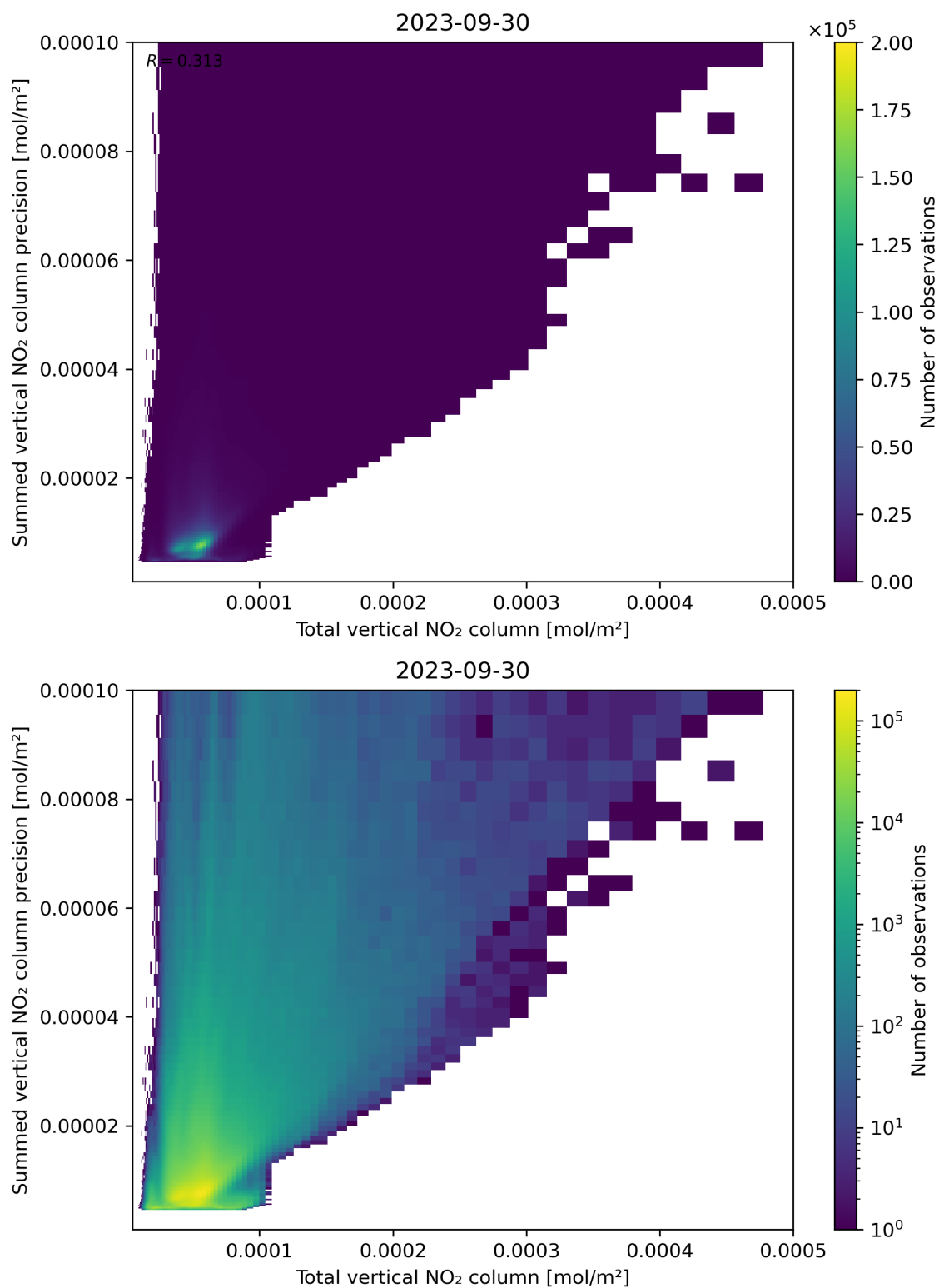
Figure 113: Scatter density plot of “Total vertical NO 2 column” against “Summed vertical NO 2 column precision” for 2023-09-29 to 2023-10-01.
