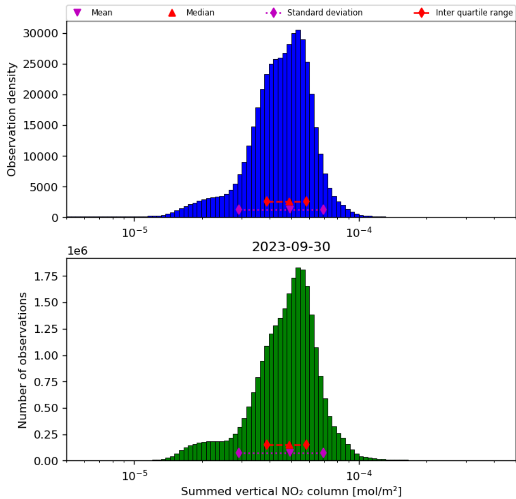
Figure 40: Histogram of “Summed vertical NO 2 column” for 2023-09-29 to 2023-10-01
