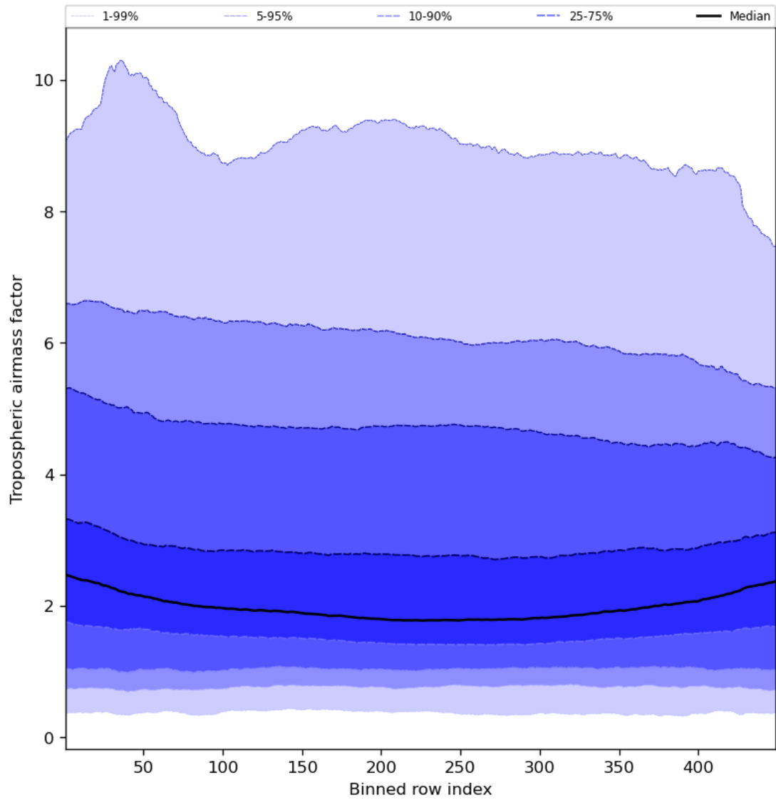
Figure 48: Along track statistics of “Tropospheric air mass factor” for 2023-09-29 to 2023-10-01
