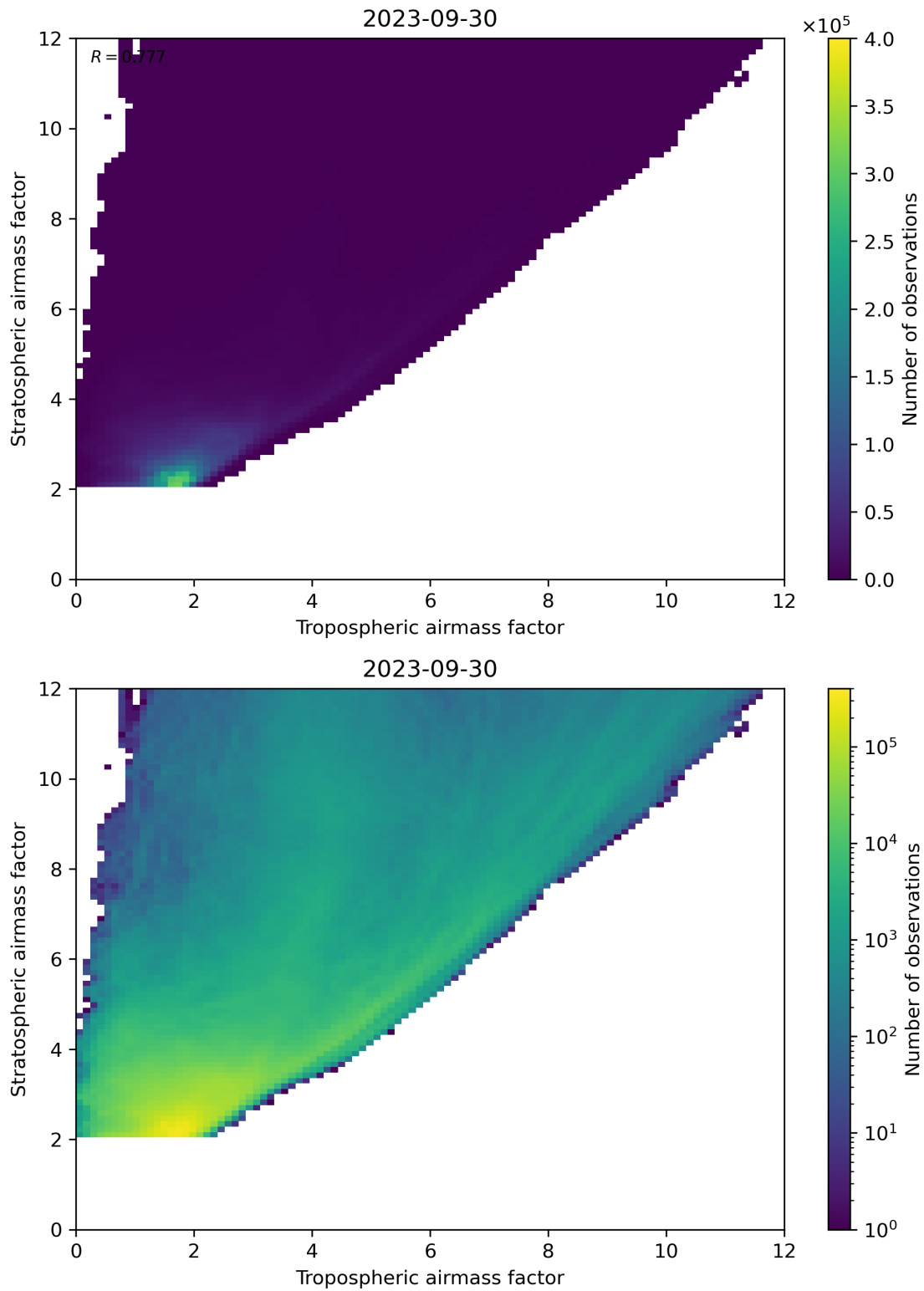
Figure 71: Scatter density plot of “Tropospheric airmass factor” against “Stratospheric airmass factor” for 2023-09-29 to 2023-10-01.
