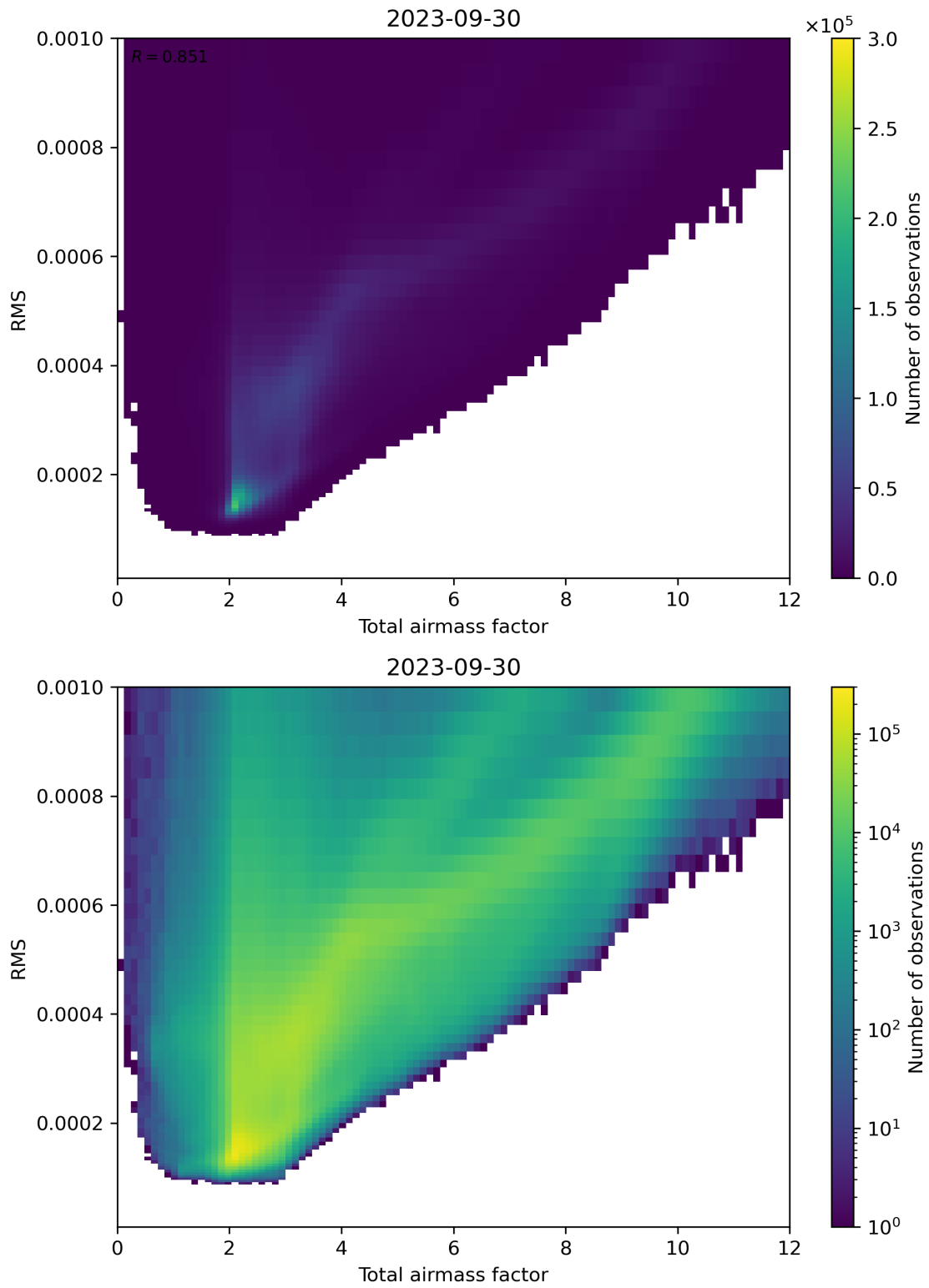
Figure 69: Scatter density plot of “Total airmass factor” against “RMS” for 2023-09-29 to 2023-10-01.
