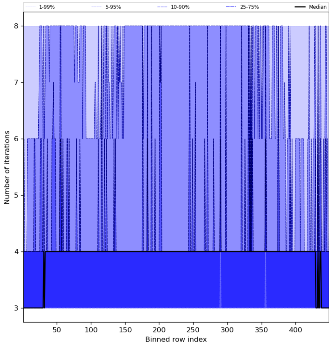
Figure 51: Along track statistics of “Number of iterations” for 2023-09-29 to 2023-10-01
