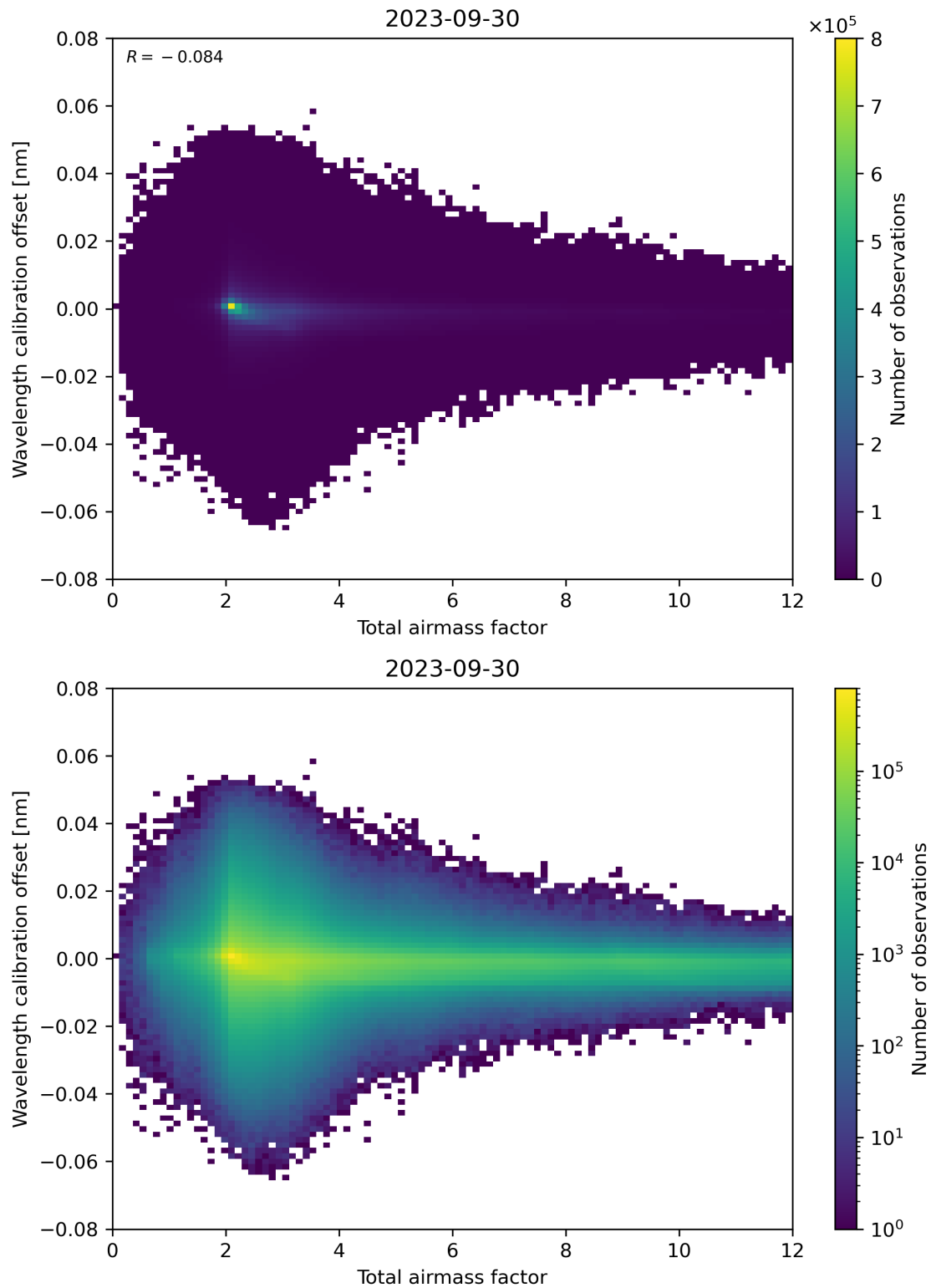
Figure 70: Scatter density plot of “Total airmass factor” against “Wavelength calibration offset” for 2023-09-29 to 2023-10-01.
