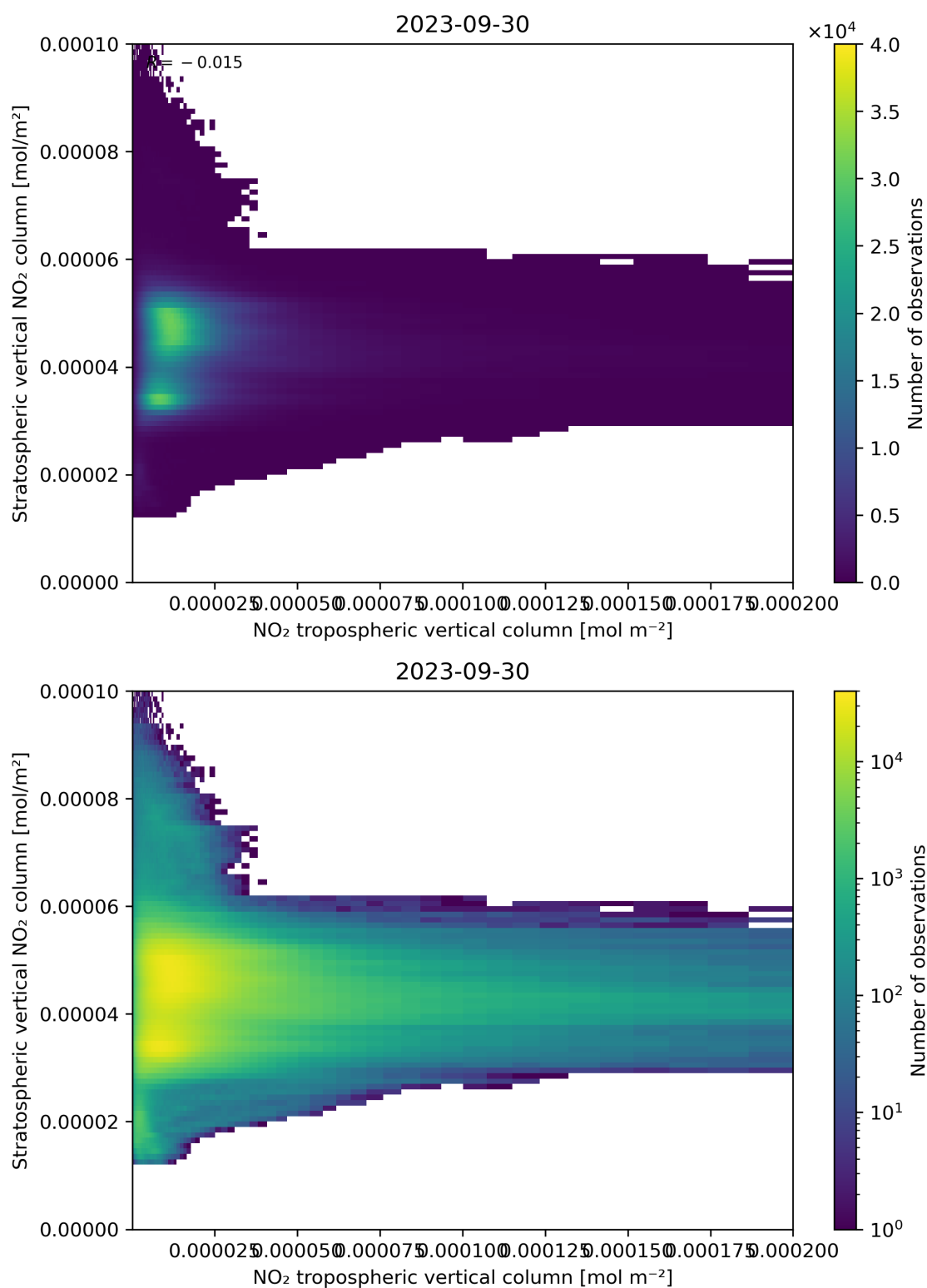
Figure 125: Scatter density plot of “NO 2 tropospheric vertical column” against “Stratospheric vertical NO 2 column” for 2023-09-29 to 2023-10-01.
