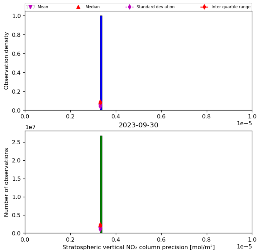
Figure 37: Histogram of “Stratospheric vertical NO 2 column precision” for 2023-09-29 to 2023-10-01
