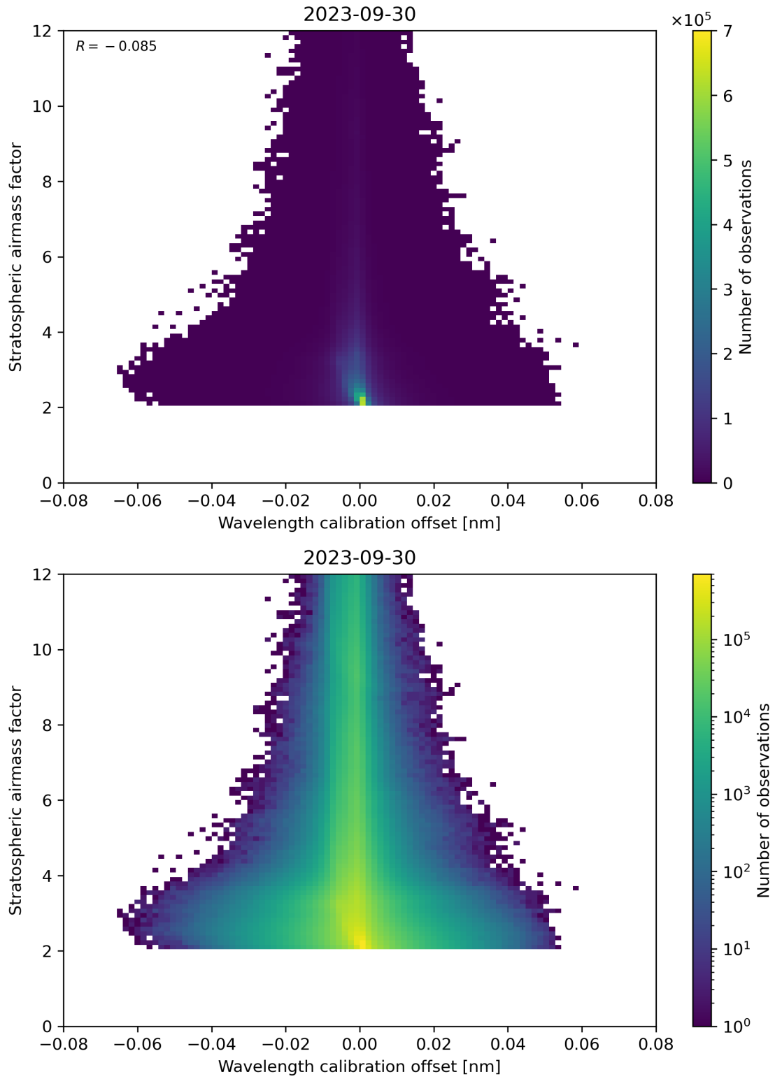
Figure 174: Scatter density plot of “Wavelength calibration offset” against “Stratospheric airmass factor” for 2023-09-29 to 2023-10-01.
