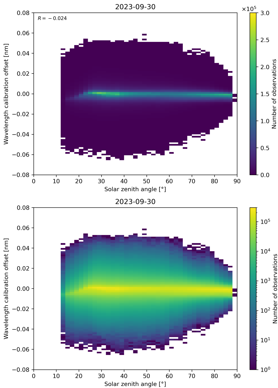
Figure 158: Scatter density plot of “Solar zenith angle” against “Wavelength calibration offset” for 2023-09-29 to 2023-10-01.
