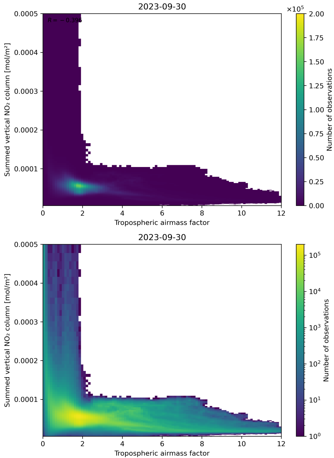
Figure 75: Scatter density plot of “Tropospheric air mass factor” against “Summed vertical NO 2 column” for 2023-09-29 to 2023-10-01.
