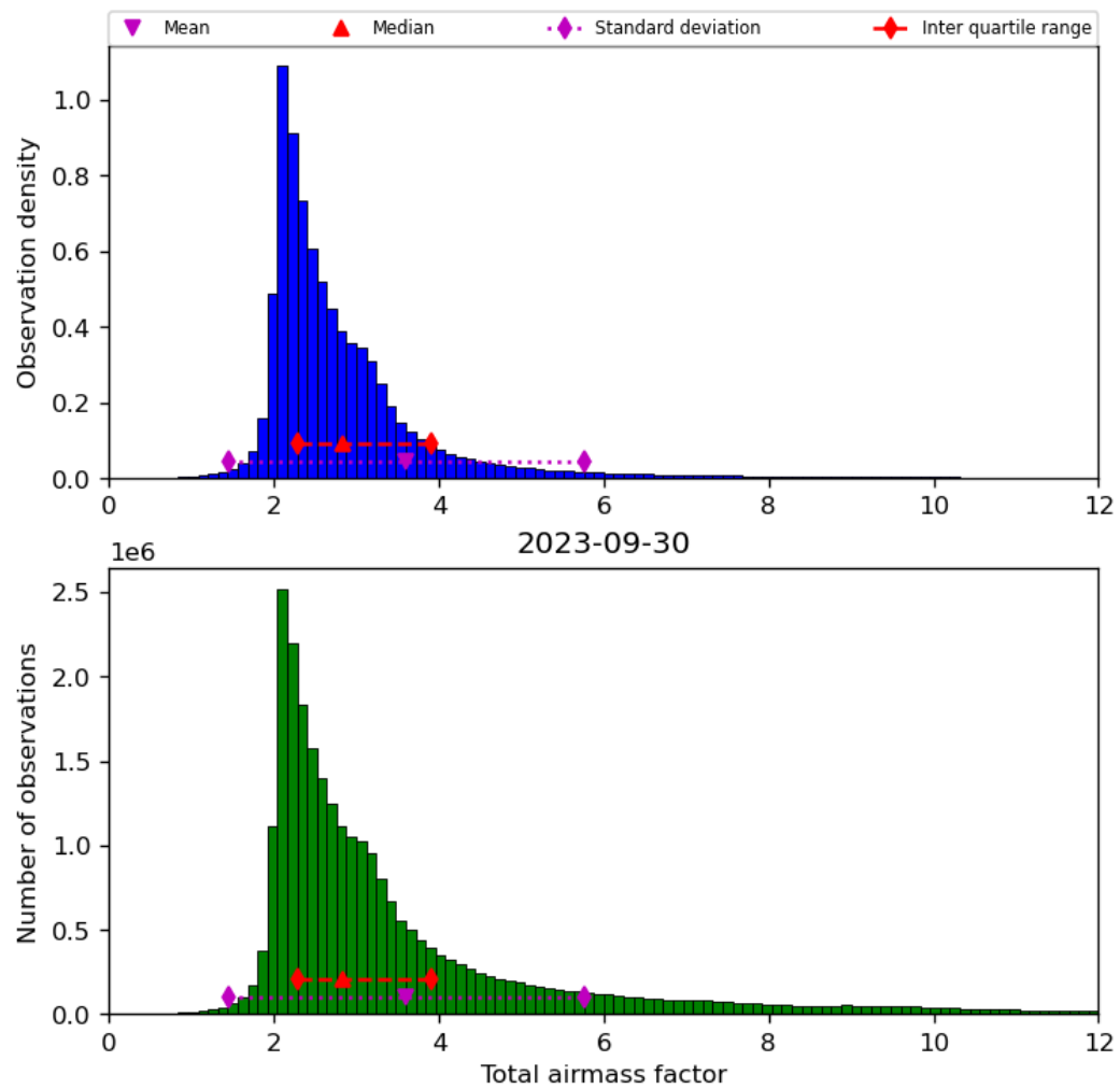
Figure 32: Histogram of “Total airmass factor” for 2023-09-29 to 2023-10-01
