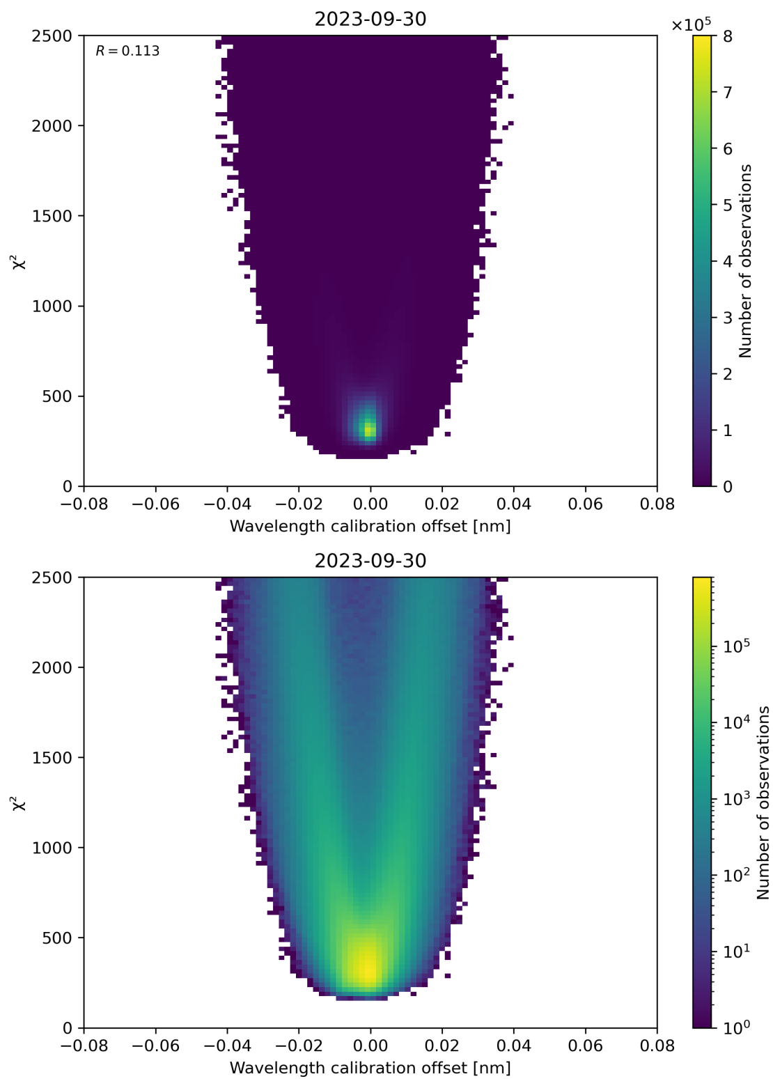
Figure 175: Scatter density plot of “Wavelength calibration offset” against “ \chi^2 ” for 2023-09-29 to 2023-10-01.
