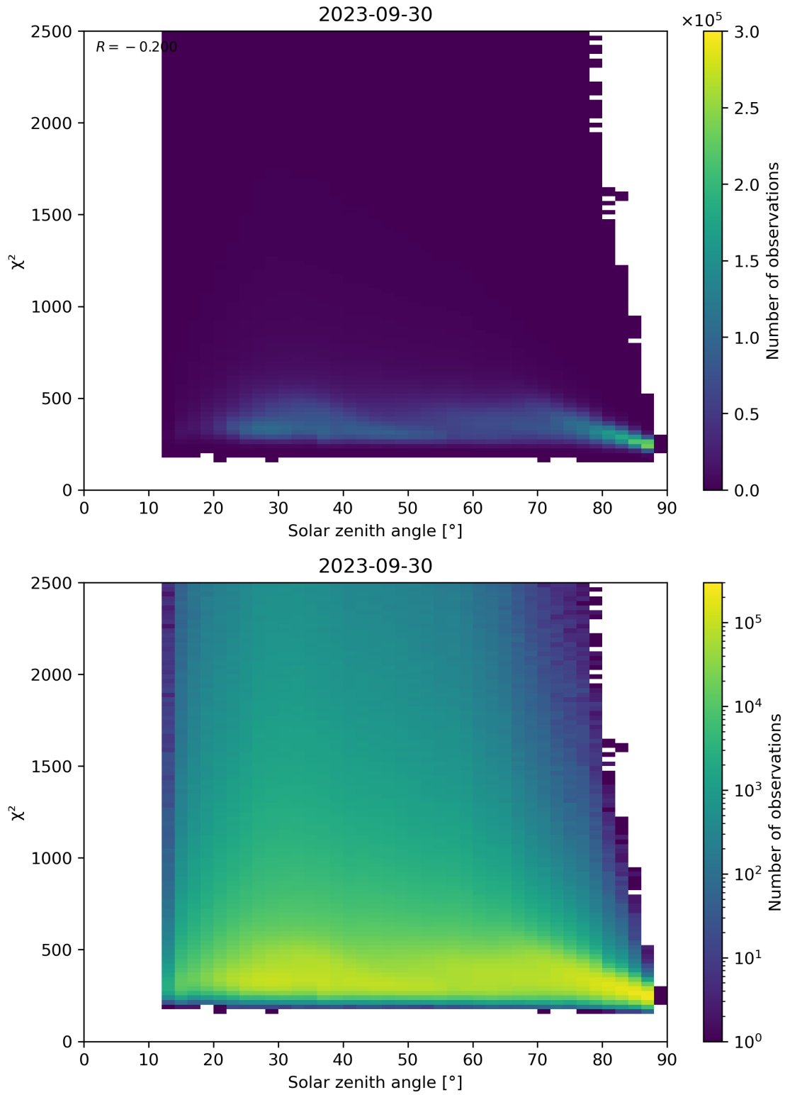
Figure 148: Scatter density plot of “Solar zenith angle” against “ \chi^2 ” for 2023-09-29 to 2023-10-01.
