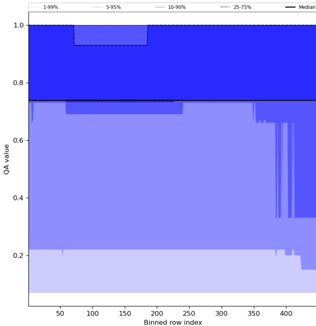
Figure 45: Along track statistics of “QA value” for 2023-09-29 to 2023-10-01
