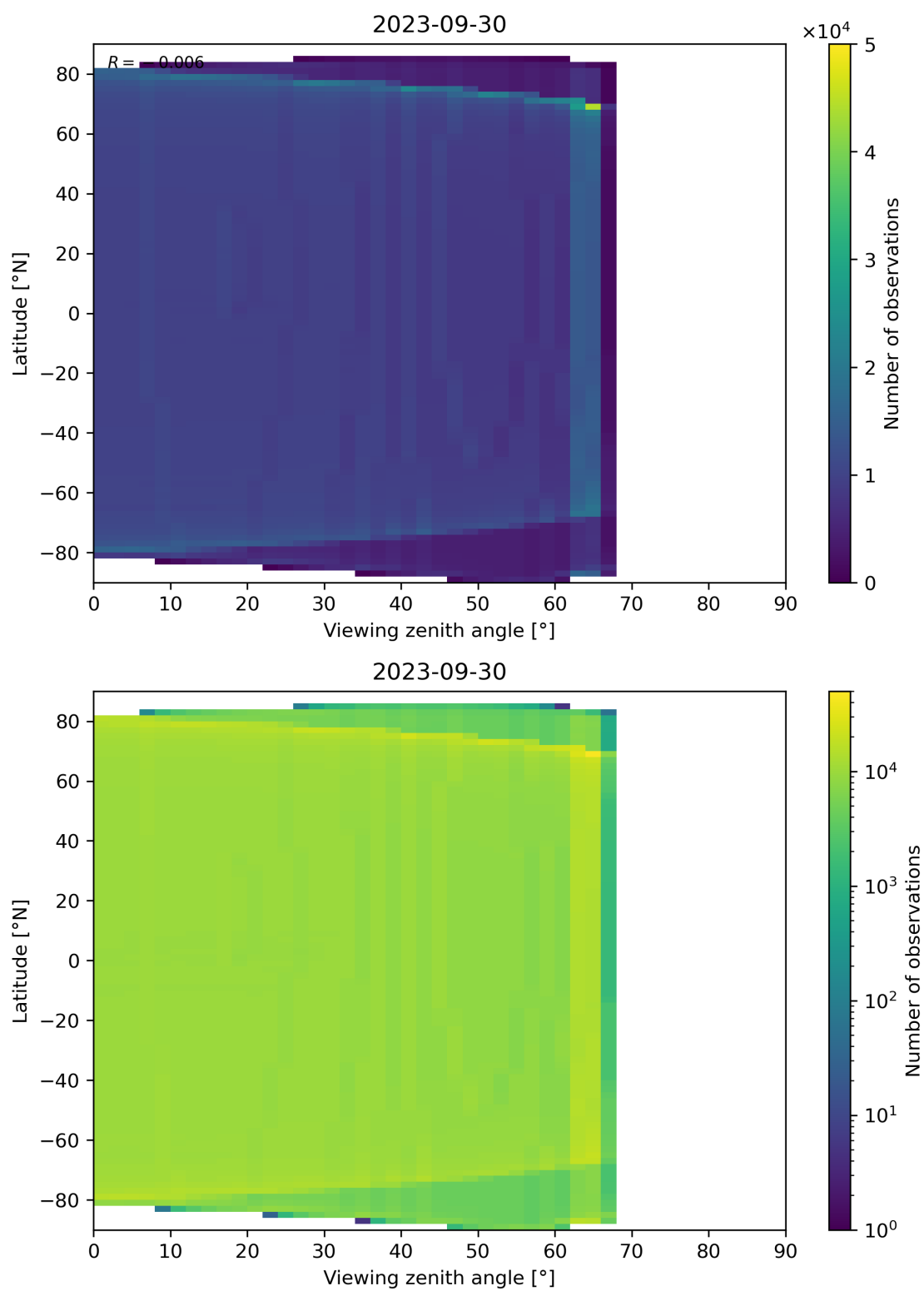
Figure 163: Scatter density plot of “Viewing zenith angle” against “Latitude” for 2023-09-29 to 2023-10-01.
