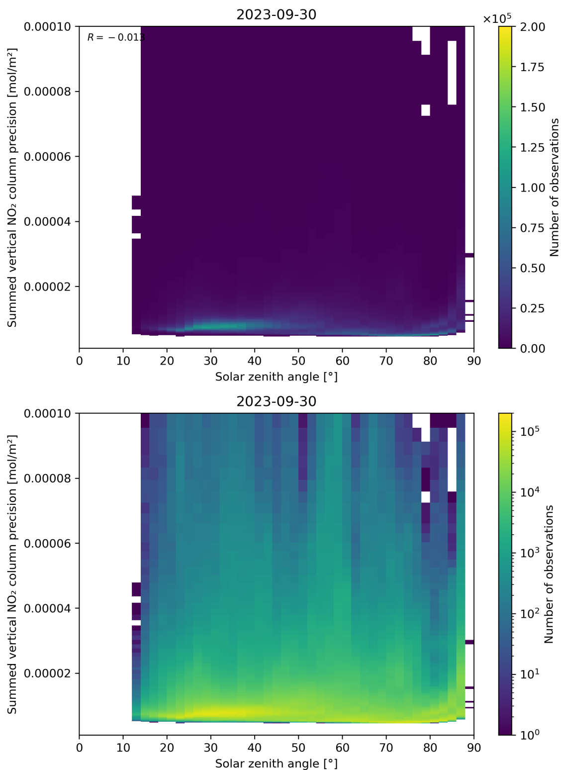
Figure 152: Scatter density plot of “Solar zenith angle” against “Summed vertical NO 2 column precision” for 2023-09-29 to 2023-10-01.
