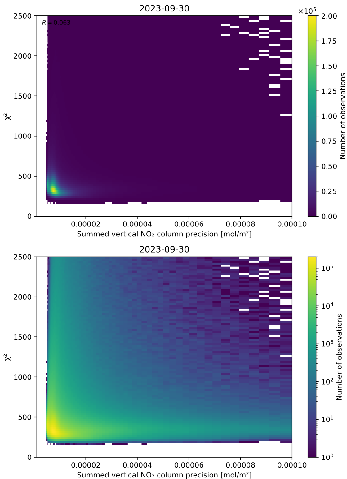
Figure 107: Scatter density plot of “Summed vertical NO 2 column precision” against “ \chi^2 ” for 2023-09-29 to 2023-10-01.
