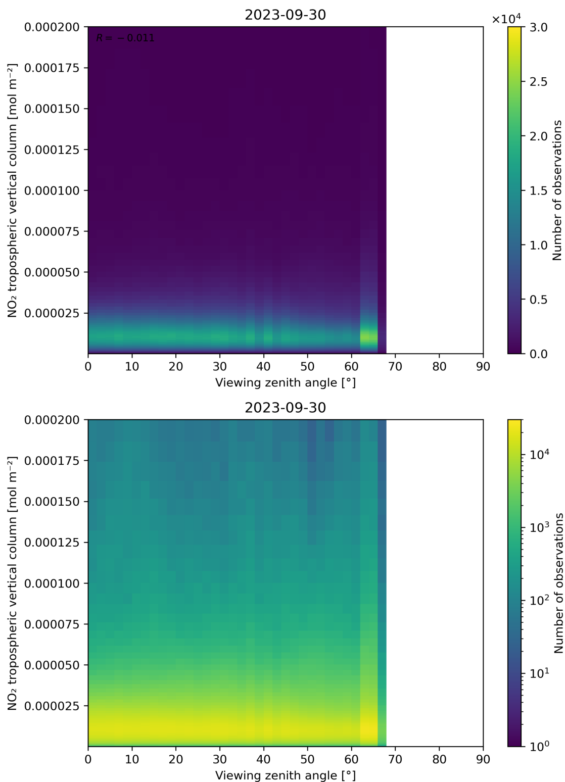
Figure 169: Scatter density plot of “Viewing zenith angle” against “NO 2 tropospheric vertical column” for 2023-09-29 to 2023-10-01.
