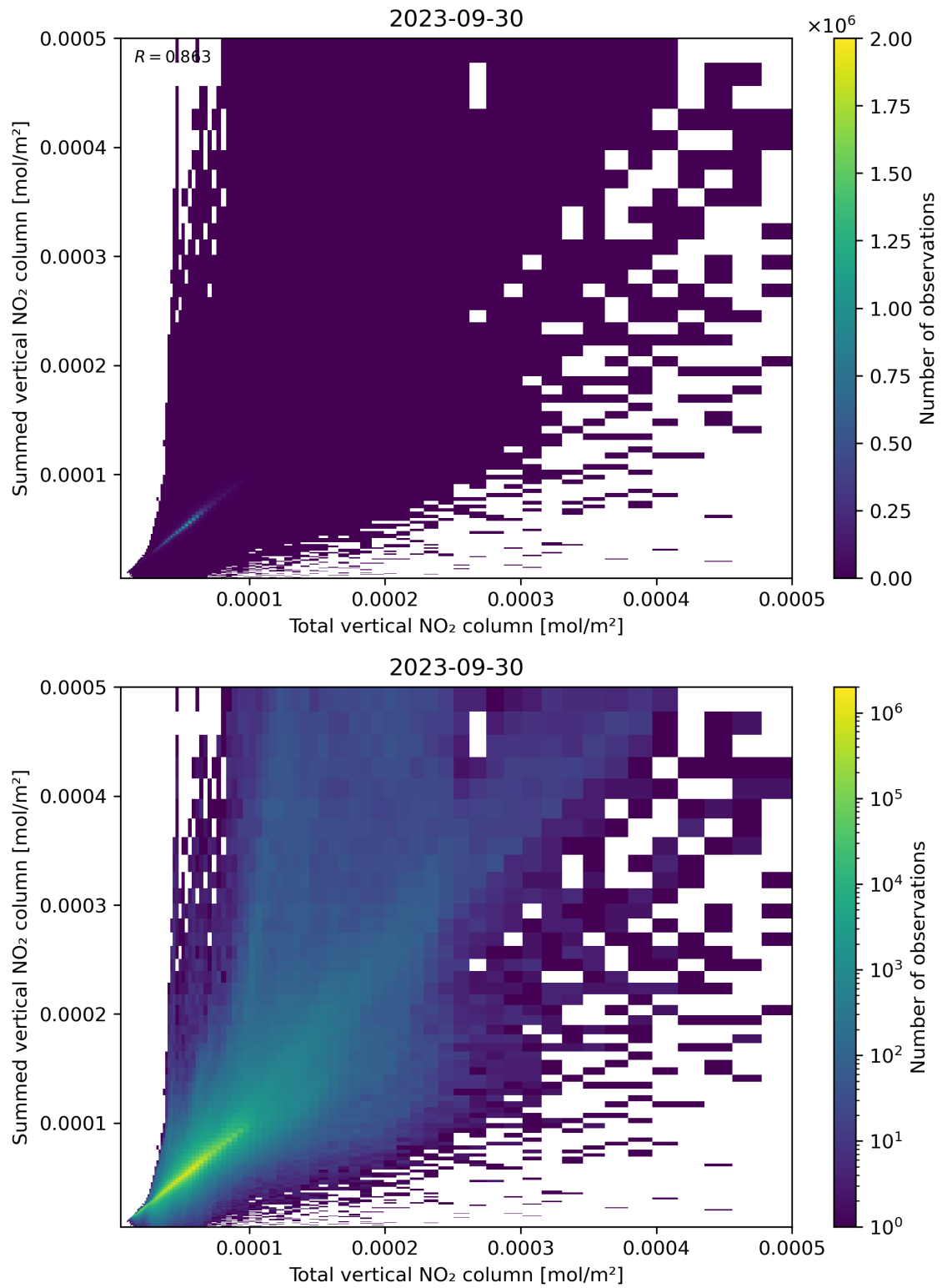
Figure 112: Scatter density plot of “Total vertical NO 2 column” against “Summed vertical NO 2 column” for 2023-09-29 to 2023-10-01.
