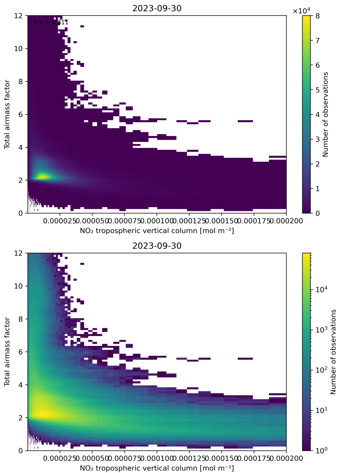
Figure 122: Scatter density plot of “NO 2 tropospheric vertical column” against “Total air mass factor” for 2023-09-29 to 2023-10-01.
