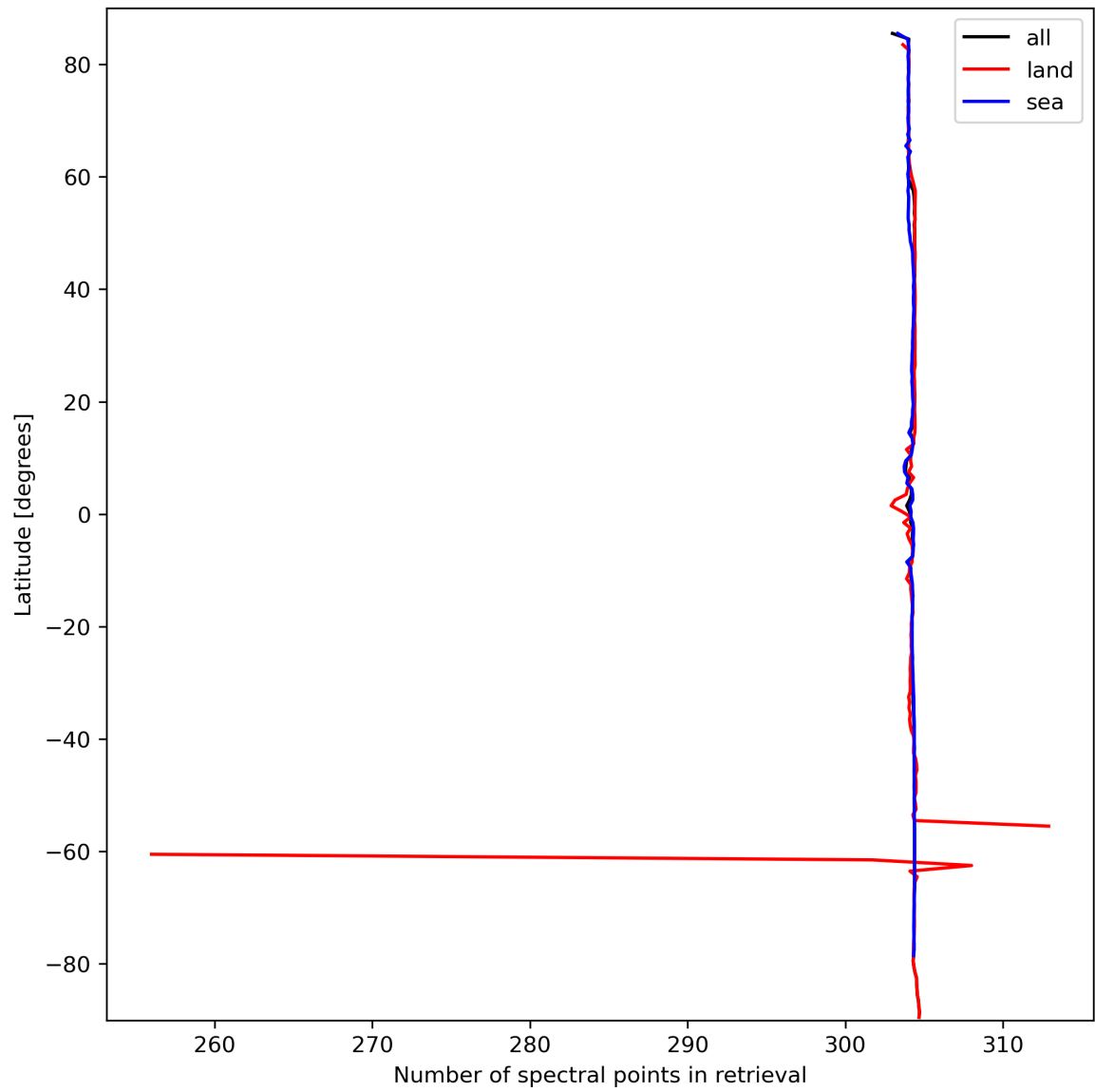
Figure 16: Zonal average of “Number of spectral points in retrieval” for 2023-09-29 to 2023-10-01.
