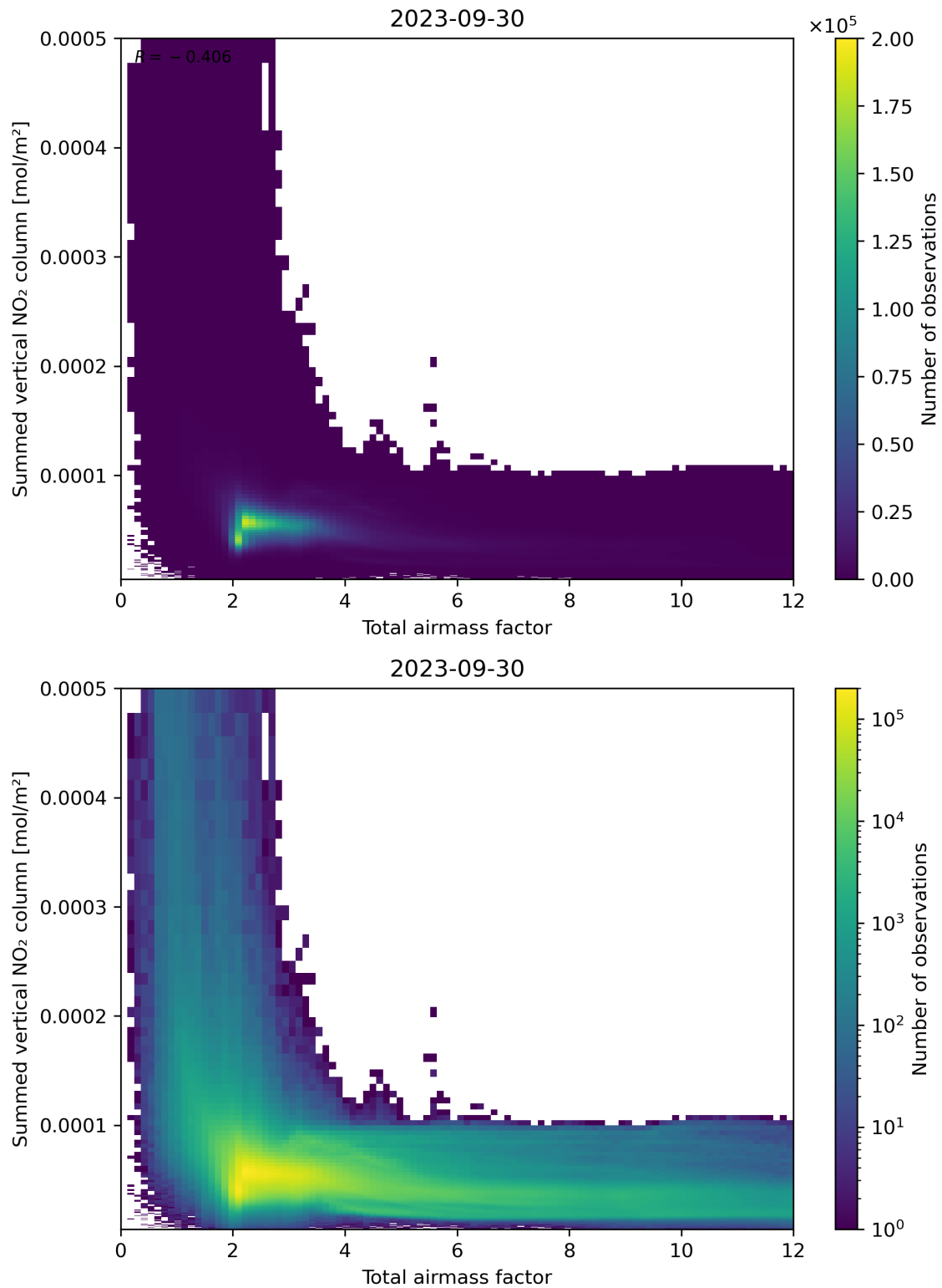
Figure 65: Scatter density plot of “Total airmass factor” against “Summed vertical NO 2 column” for 2023-09-29 to 2023-10-01.
