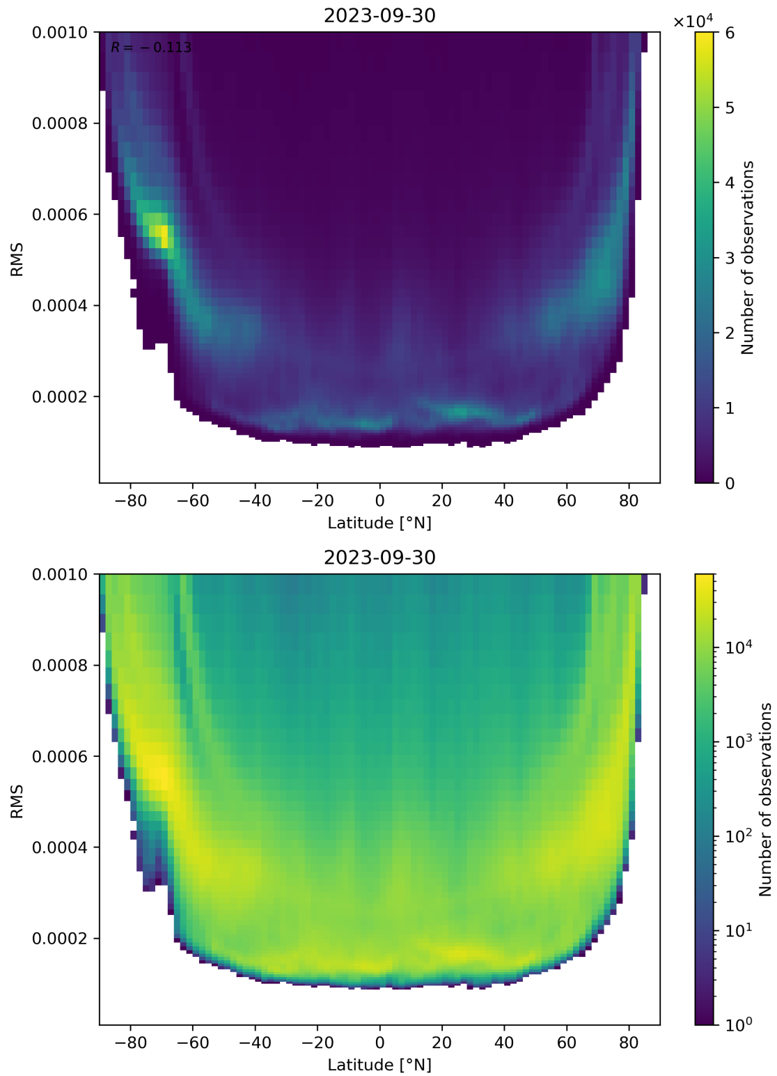
Figure 94: Scatter density plot of “Latitude” against “RMS” for 2023-09-29 to 2023-10-01.
