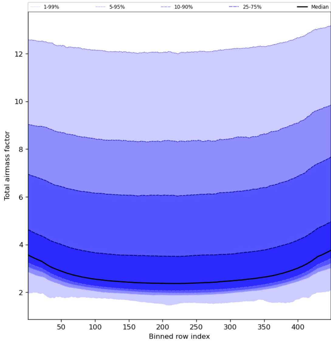
Figure 49: Along track statistics of “Total airmass factor” for 2023-09-29 to 2023-10-01
