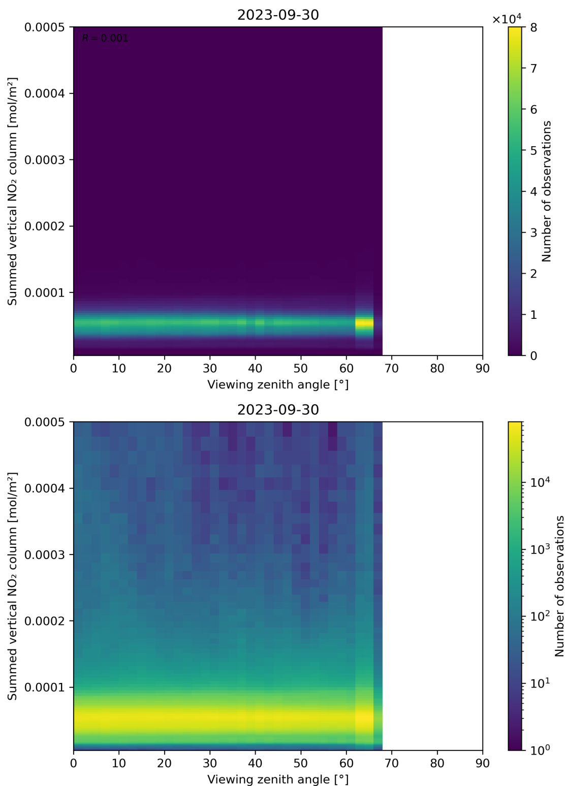
Figure 165: Scatter density plot of “Viewing zenith angle” against “Summed vertical NO 2 column” for 2023-09-29 to 2023-10-01.
