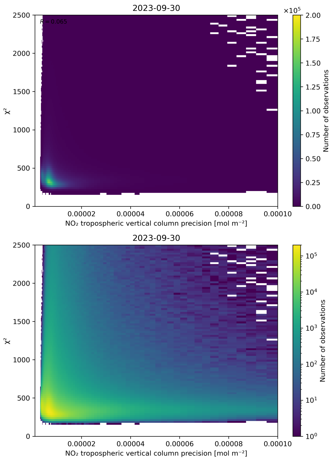
Figure 134: Scatter density plot of “NO 2 tropospheric vertical column precision” against “ \chi^2 ” for 2023-09-29 to 2023-10-01.
