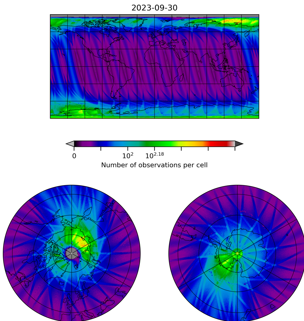
Figure 10: Map of the number of observations for 2023-09-29 to 2023-10-01
