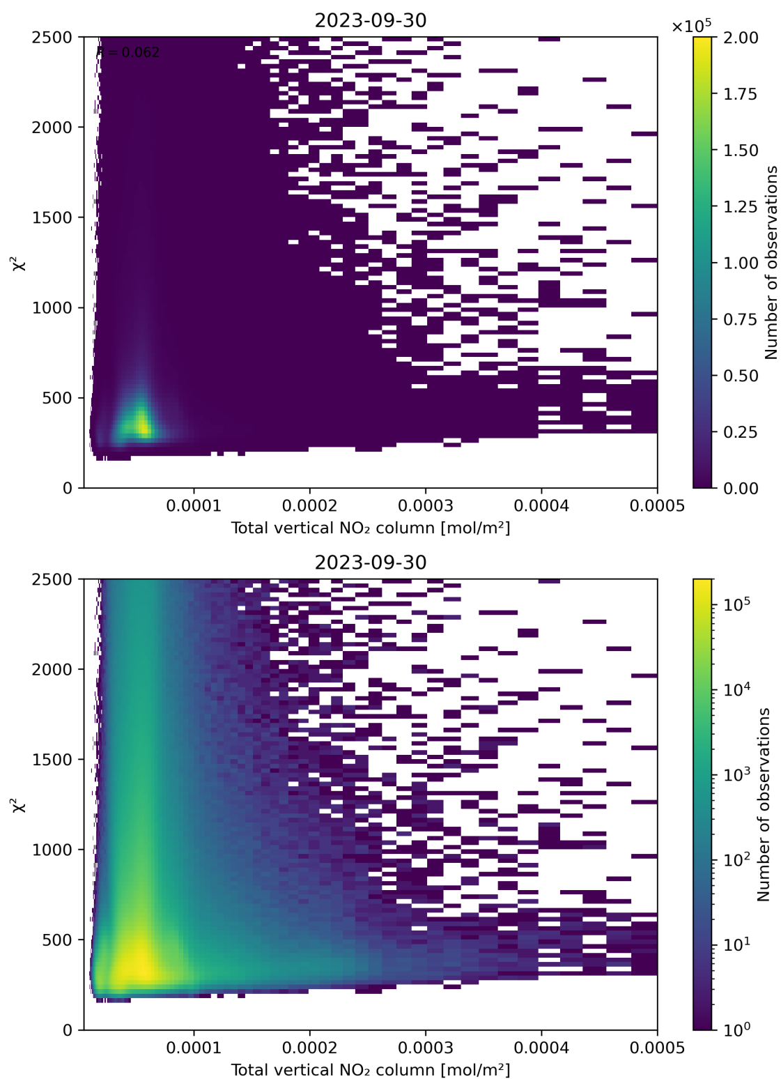
Figure 111: Scatter density plot of “Total vertical NO 2 column” against “ \chi^2 ” for 2023-09-29 to 2023-10-01.
