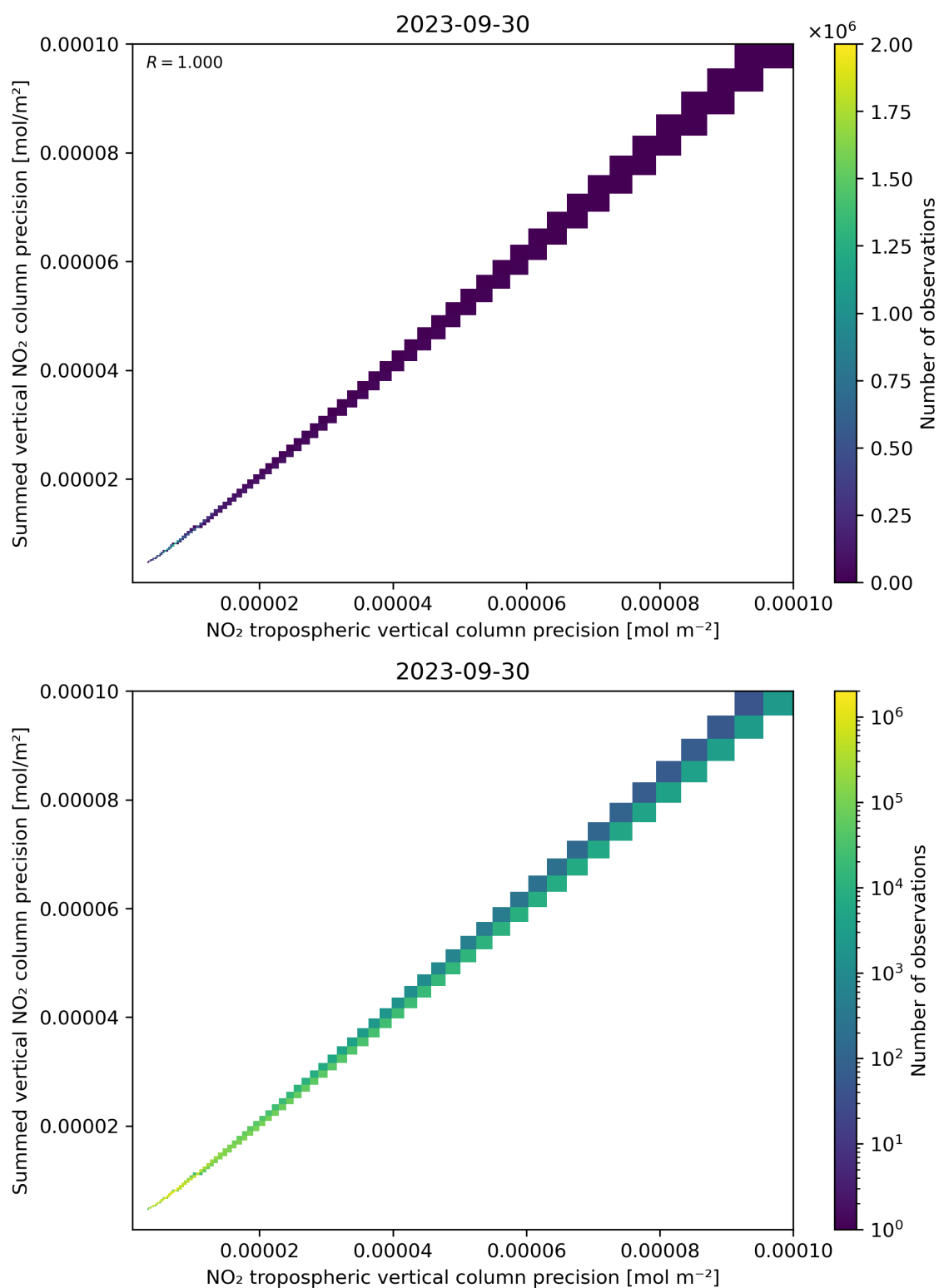
Figure 137: Scatter density plot of “NO 2 tropospheric vertical column precision” against “Summed vertical NO 2 column precision” for 2023-09-29 to 2023-10-01.
