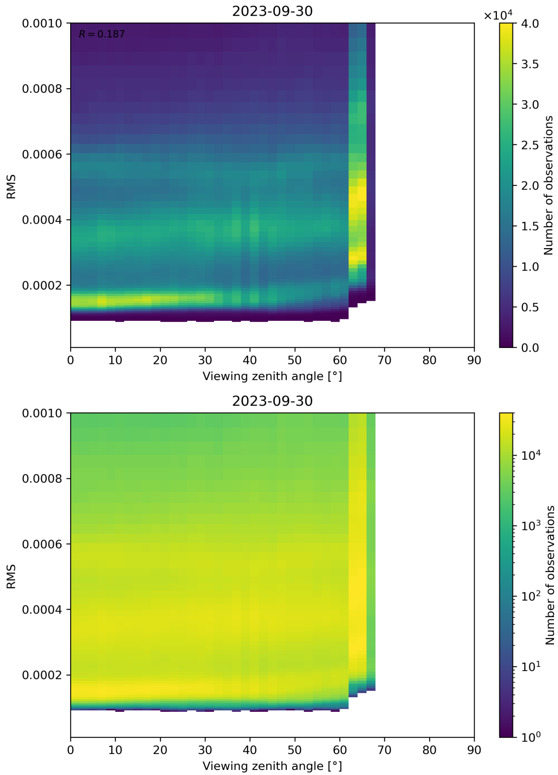
Figure 171: Scatter density plot of “Viewing zenith angle” against “RMS” for 2023-09-29 to 2023-10-01.
