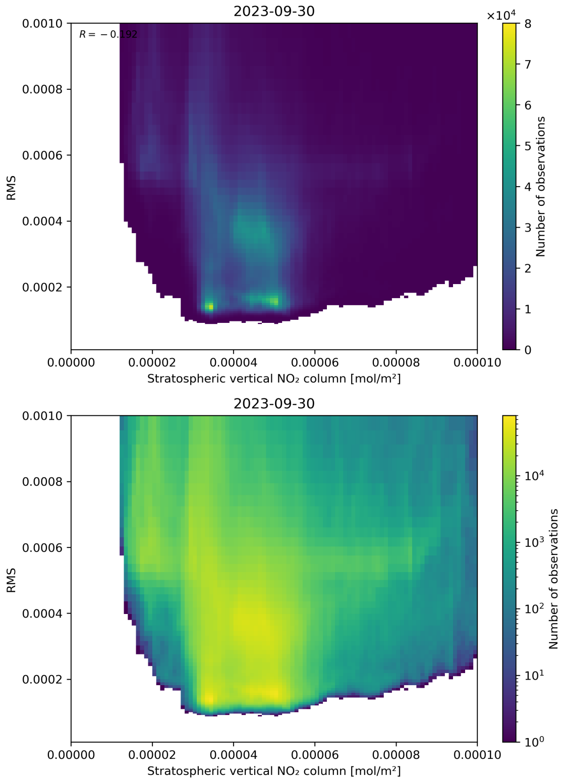
Figure 102: Scatter density plot of “Stratospheric vertical NO 2 column” against “RMS” for 2023-09-29 to 2023-10-01.
