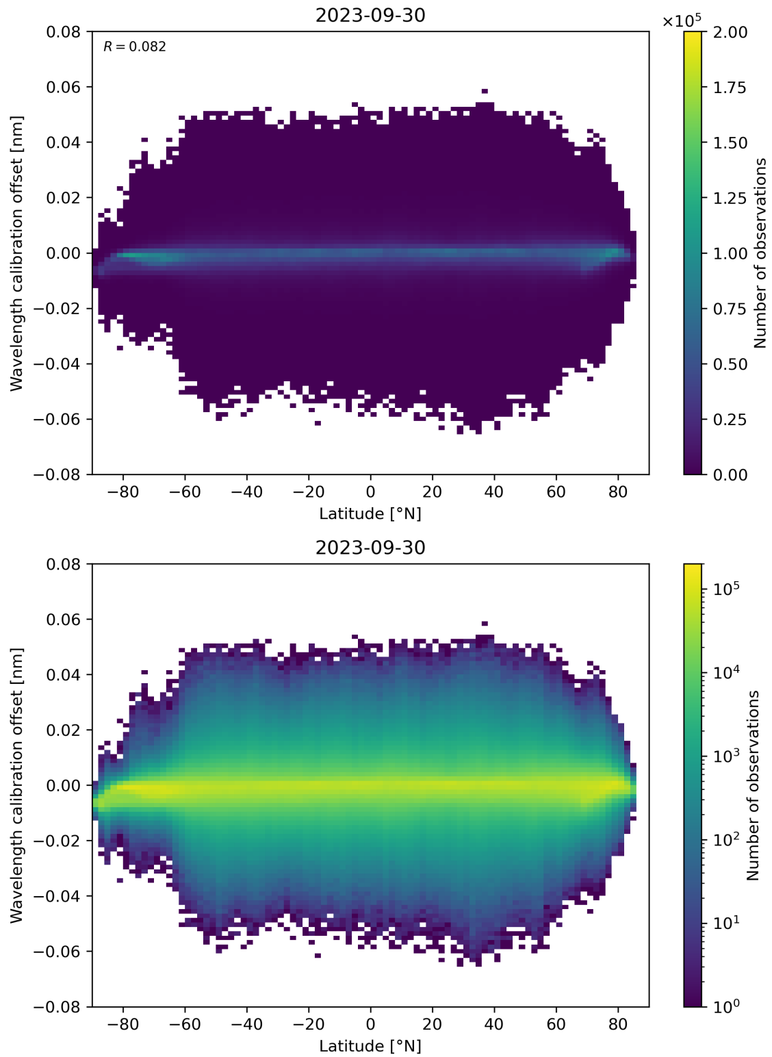
Figure 95: Scatter density plot of “Latitude” against “Wavelength calibration offset” for 2023-09-29 to 2023-10-01.
