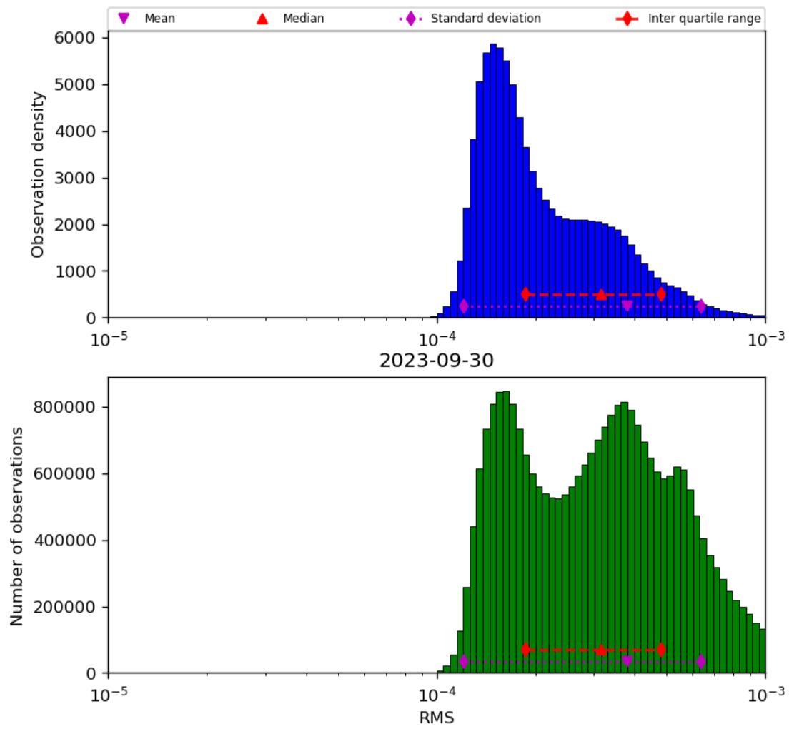
Figure 43: Histogram of “RMS” for 2023-09-29 to 2023-10-01
