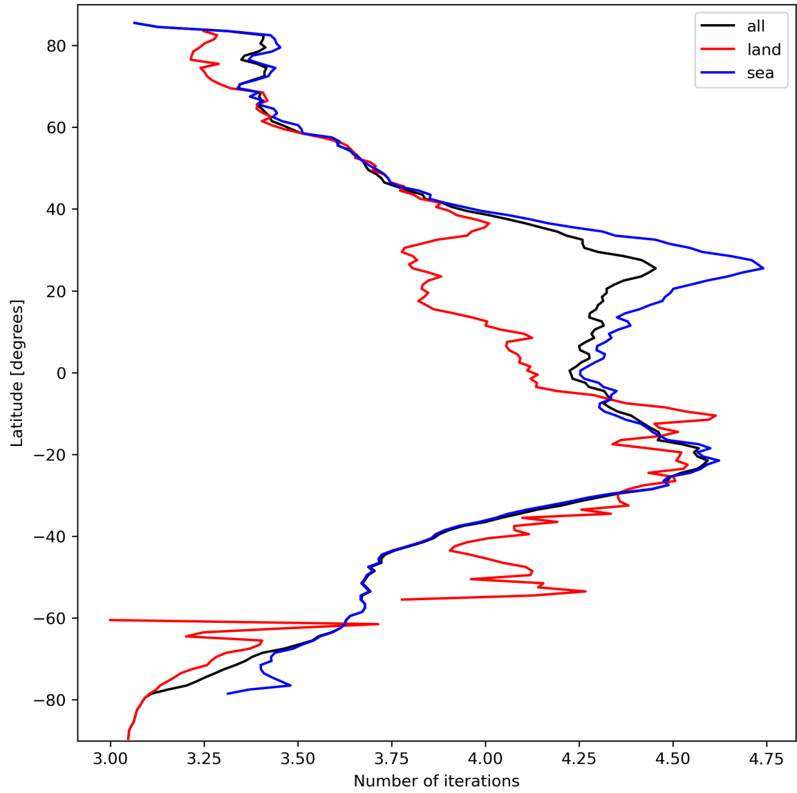
Figure 17: Zonal average of “Number of iterations” for 2023-09-29 to 2023-10-01.
