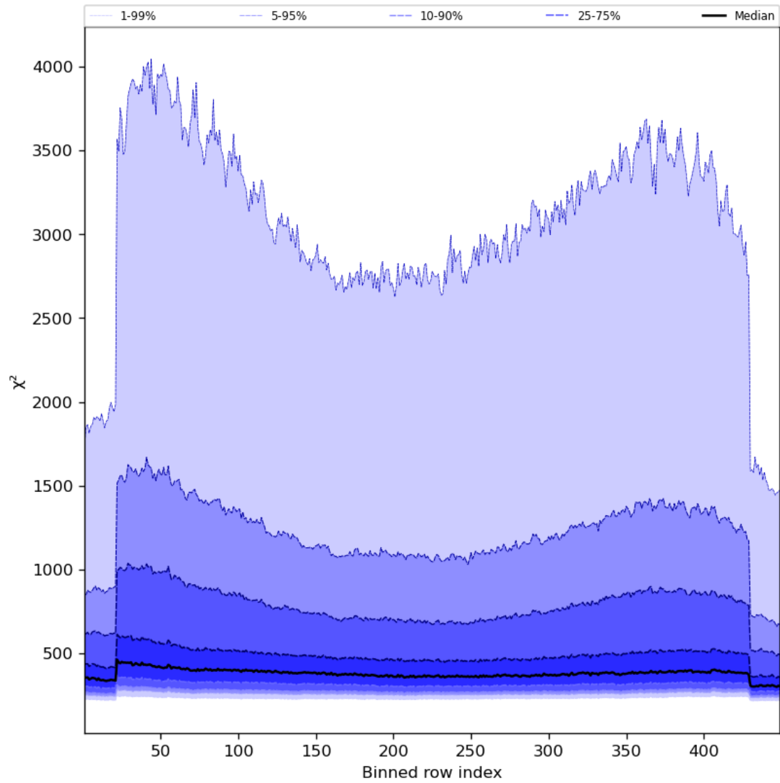
Figure 59: Along track statistics of “ \chi^2 ” for 2023-09-29 to 2023-10-01
