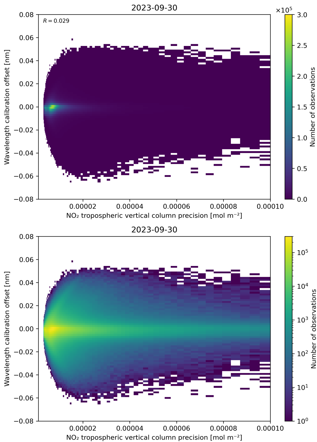
Figure 141: Scatter density plot of “NO 2 tropospheric vertical column precision” against “Wavelength calibration offset” for 2023-09-29 to 2023-10-01.
