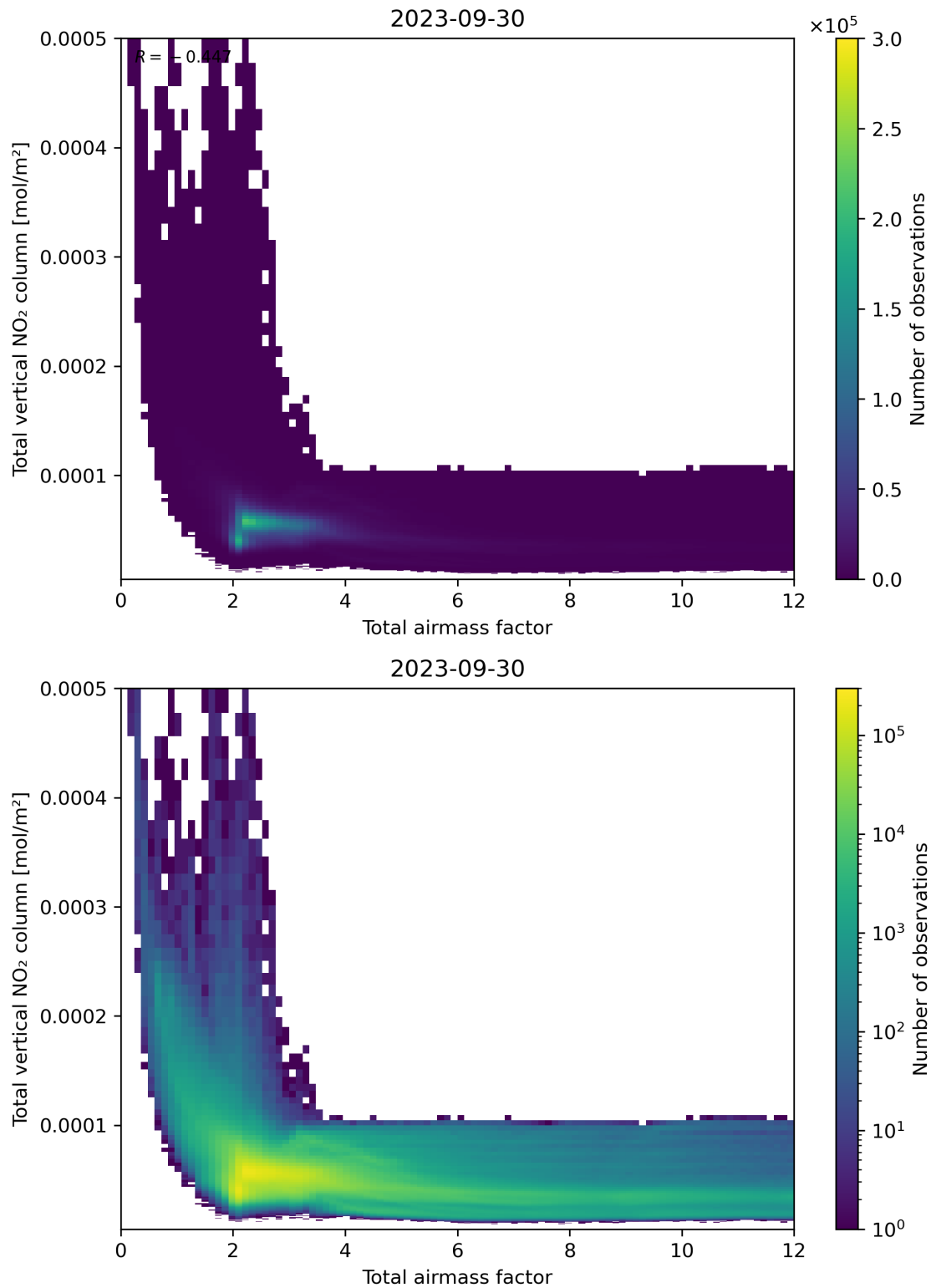
Figure 67: Scatter density plot of “Total airmass factor” against “Total vertical NO 2 column” for 2023-09-29 to 2023-10-01.
