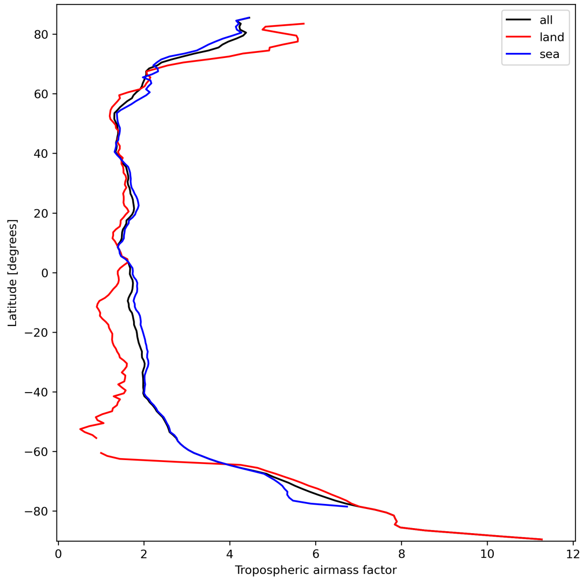
Figure 14: Zonal average of “Tropospheric airmass factor” for 2023-09-29 to 2023-10-01.
