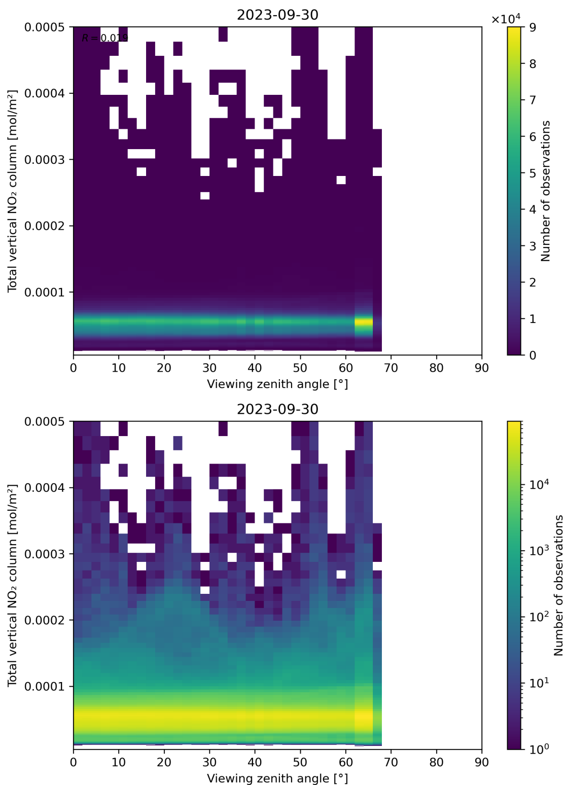
Figure 167: Scatter density plot of “Viewing zenith angle” against “Total vertical NO 2 column” for 2023-09-29 to 2023-10-01.
