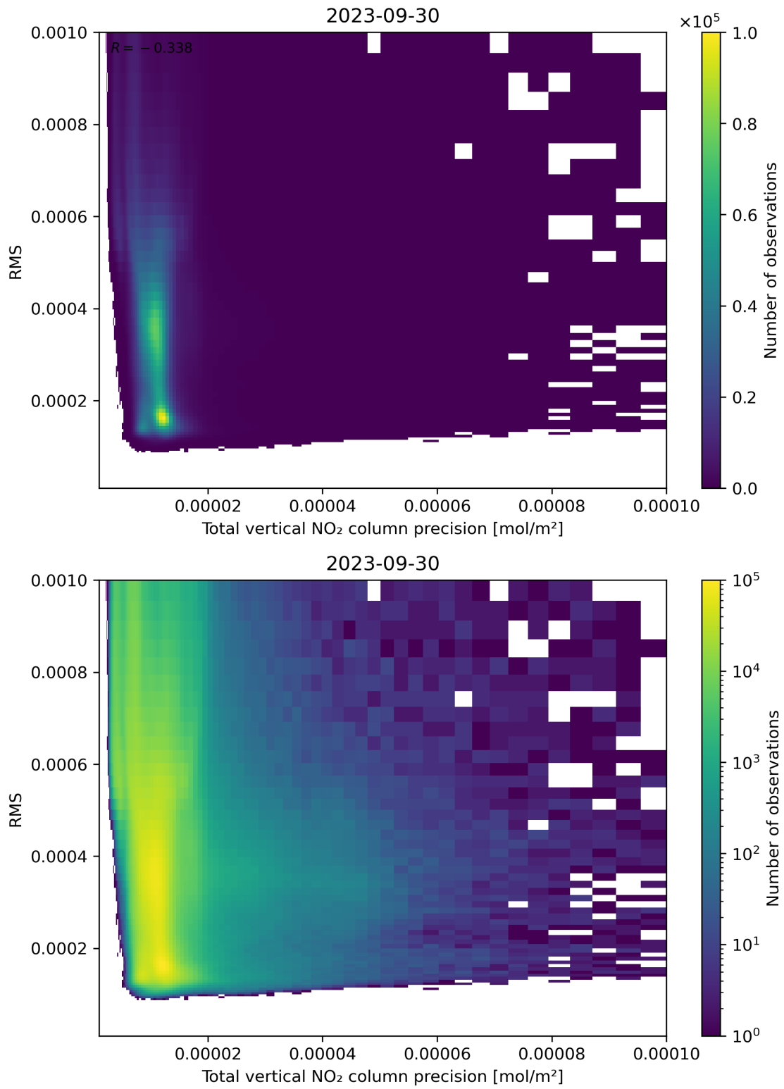
Figure 119: Scatter density plot of “Total vertical NO 2 column precision” against “RMS” for 2023-09-29 to 2023-10-01.
