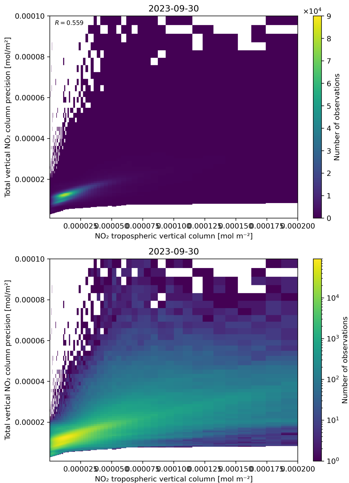
Figure 129: Scatter density plot of “NO 2 tropospheric vertical column” against “Total vertical NO 2 column precision” for 2023-09-29 to 2023-10-01.
