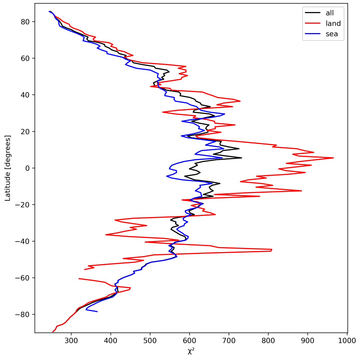
Figure 25: Zonal average of “ \chi^2 ” for 2023-09-29 to 2023-10-01.
