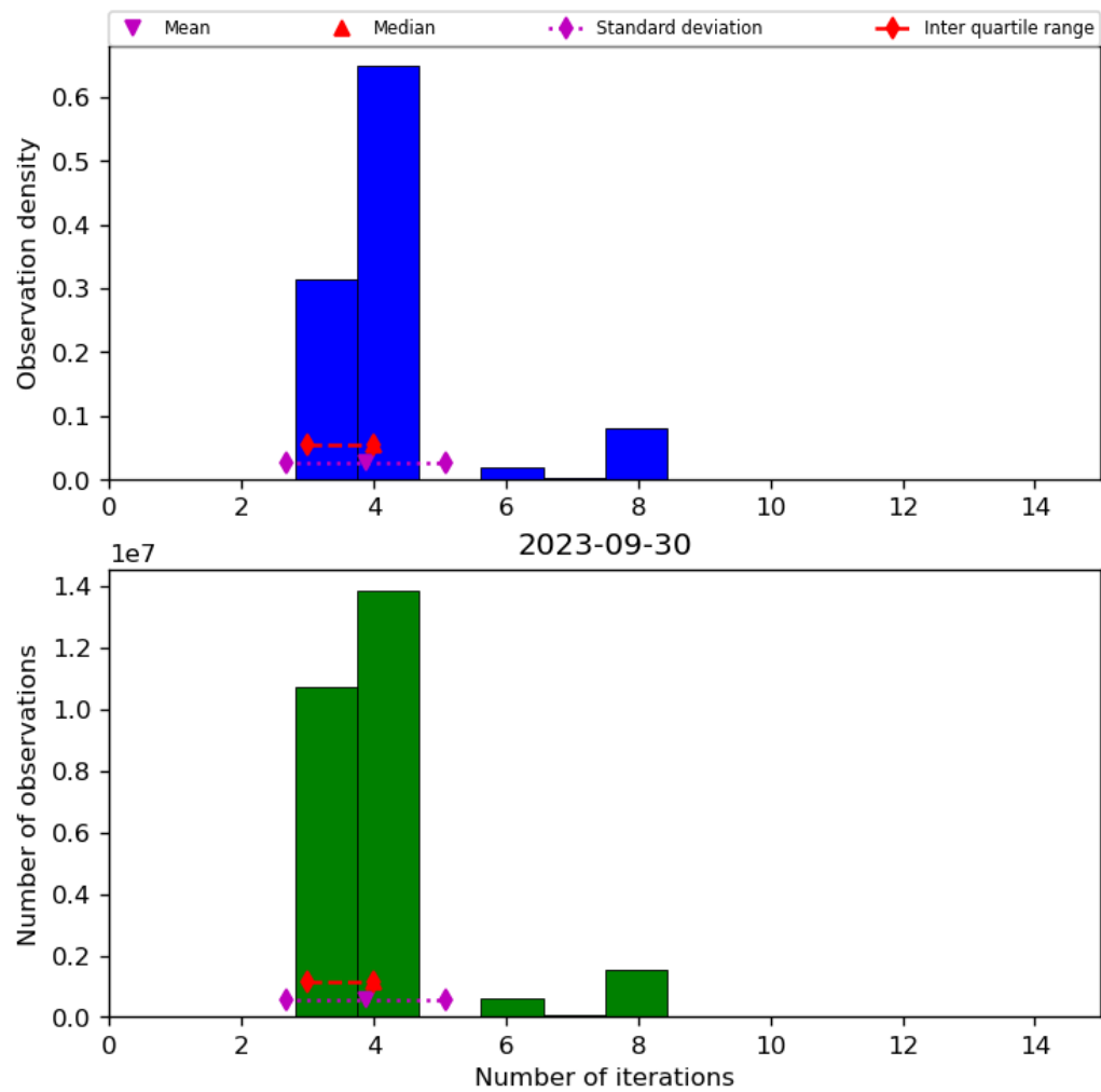
Figure 34: Histogram of “Number of iterations” for 2023-09-29 to 2023-10-01
