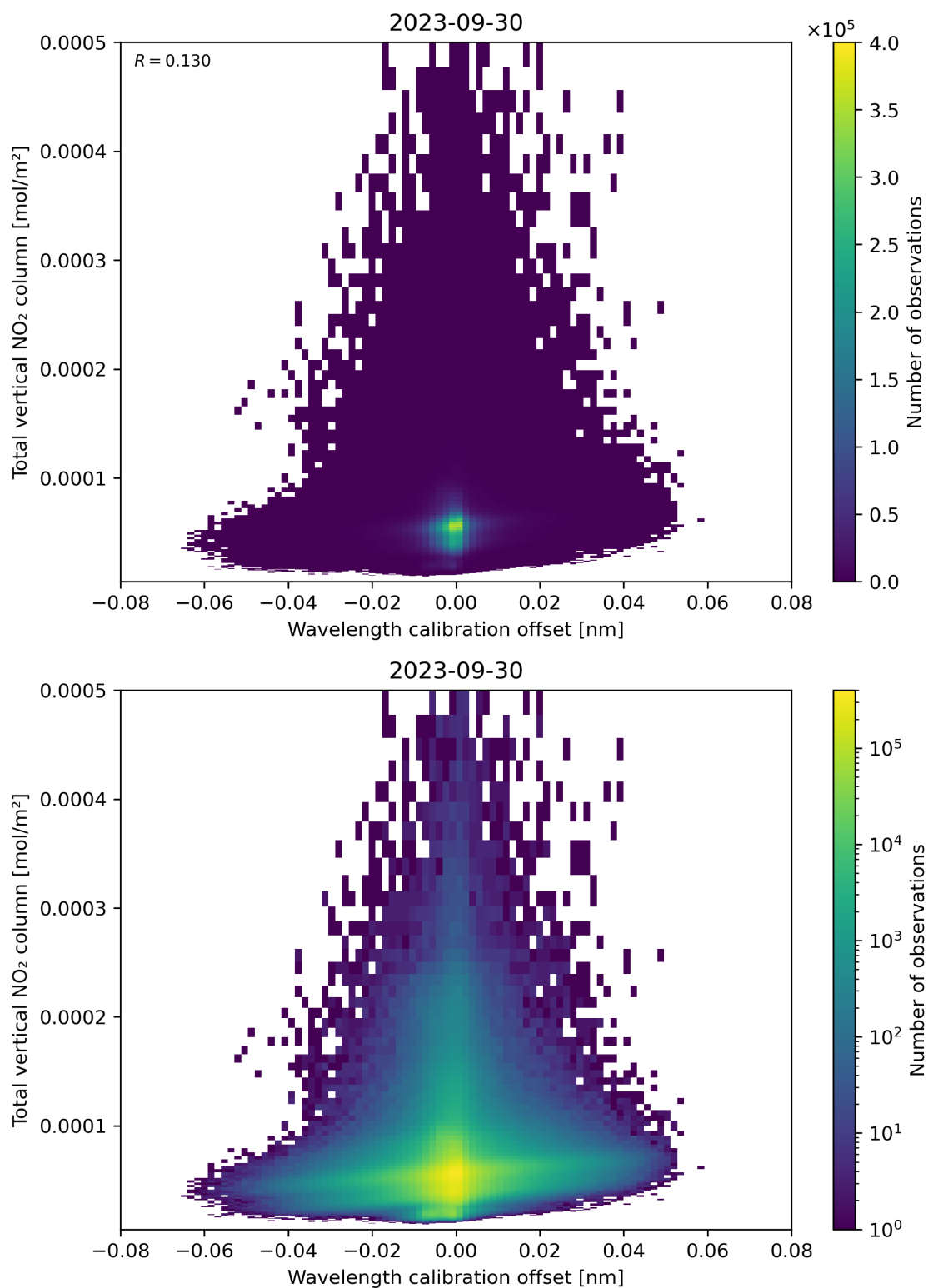
Figure 179: Scatter density plot of “Wavelength calibration offset” against “Total vertical NO 2 column” for 2023-09-29 to 2023-10-01.
