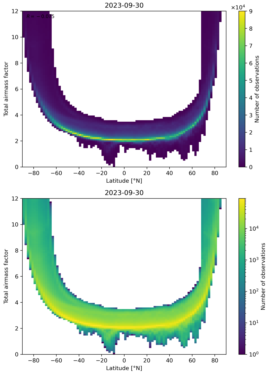
Figure 84: Scatter density plot of “Latitude” against “Total airmass factor” for 2023-09-29 to 2023-10-01.
