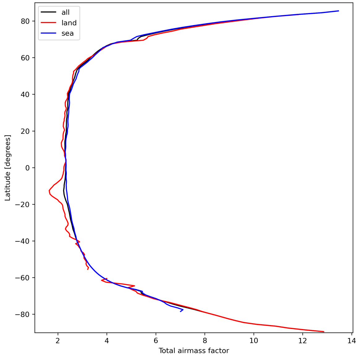
Figure 15: Zonal average of “Total airmass factor” for 2023-09-29 to 2023-10-01.
