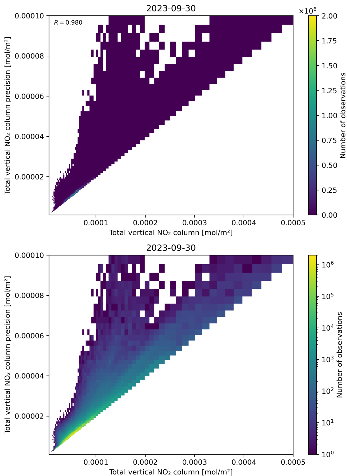
Figure 114: Scatter density plot of “Total vertical NO 2 column” against “Total vertical NO 2 column precision” for 2023-09-29 to 2023-10-01.
