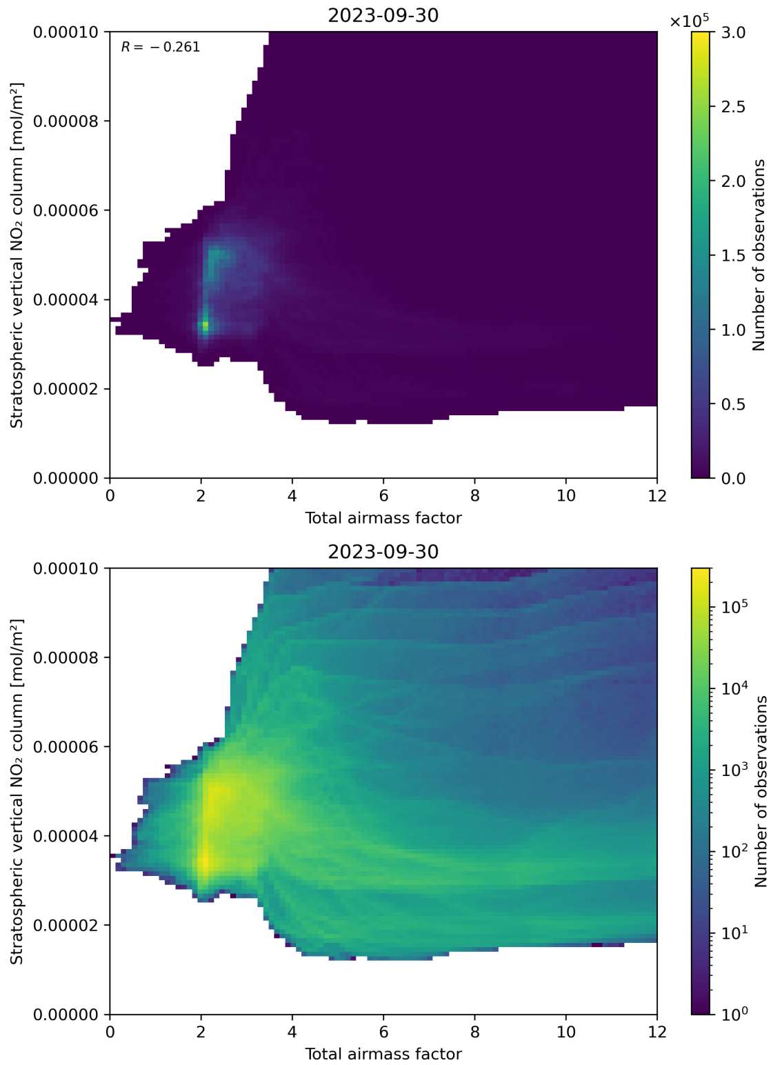
Figure 64: Scatter density plot of “Total airmass factor” against “Stratospheric vertical \text{NO}_2 column” for 2023-09-29 to 2023-10-01.
