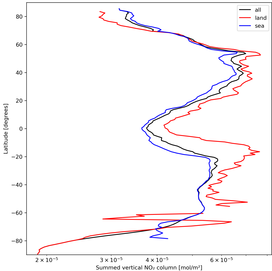
Figure 23: Zonal average of “Summed vertical NO 2 column” for 2023-09-29 to 2023-10-01.
