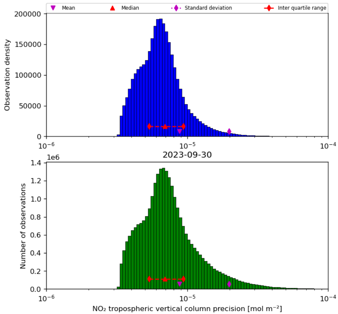
Figure 30: Histogram of “NO 2 tropospheric vertical column precision” for 2023-09-29 to 2023-10-01
