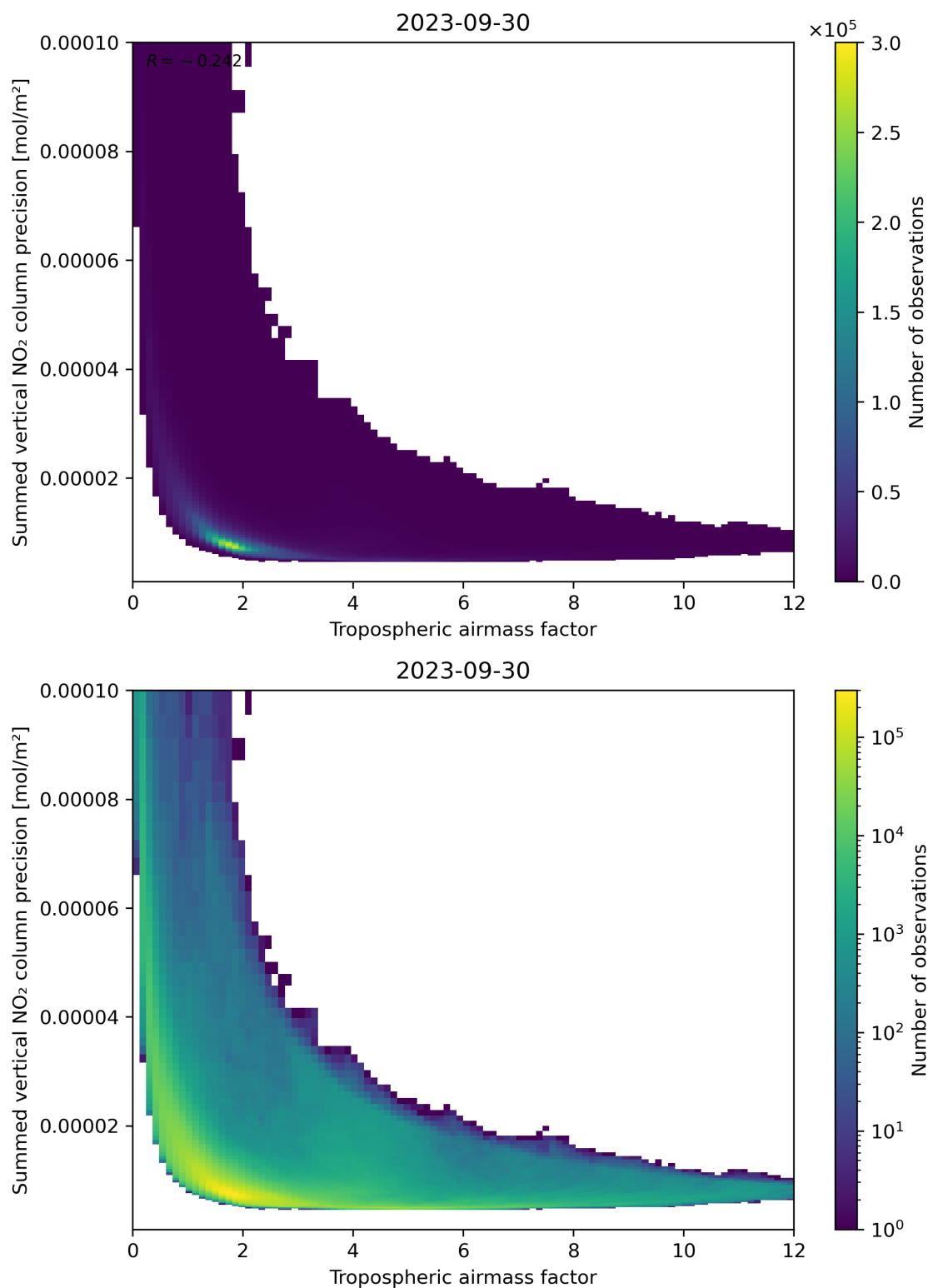
Figure 76: Scatter density plot of “Tropospheric air mass factor” against “Summed vertical NO 2 column precision” for 2023-09-29 to 2023-10-01.
