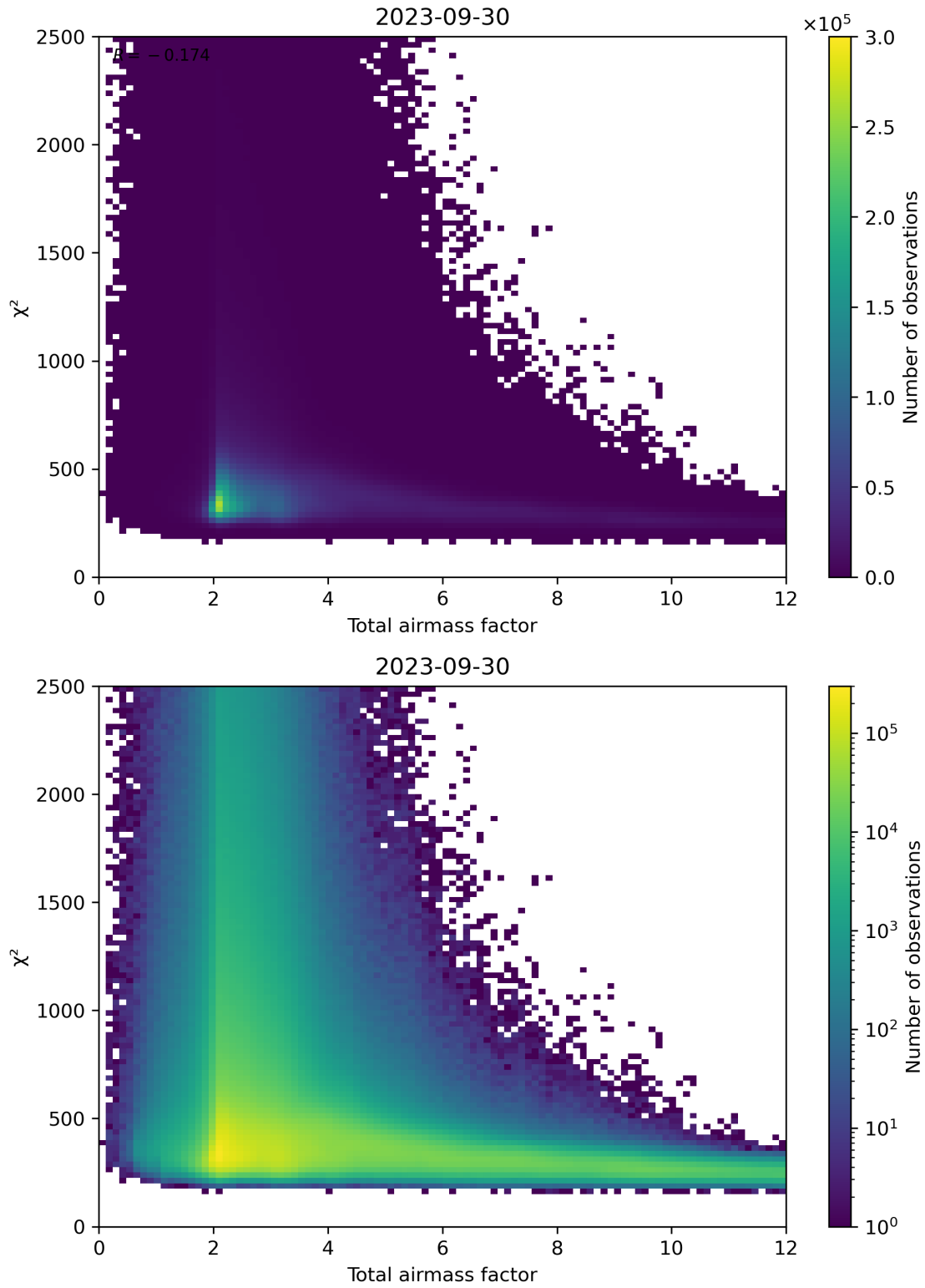
Figure 63: Scatter density plot of “Total airmass factor” against “ \chi^2 ” for 2023-09-29 to 2023-10-01.
