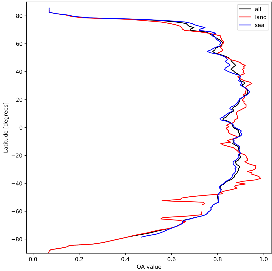
Figure 11: Zonal average of “QA value” for 2023-09-29 to 2023-10-01.
