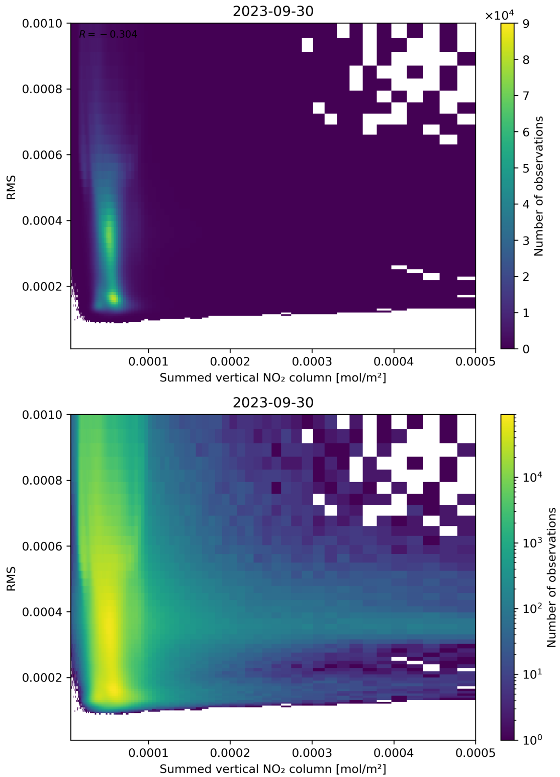
Figure 109: Scatter density plot of “Summed vertical NO 2 column” against “RMS” for 2023-09-29 to 2023-10-01.
