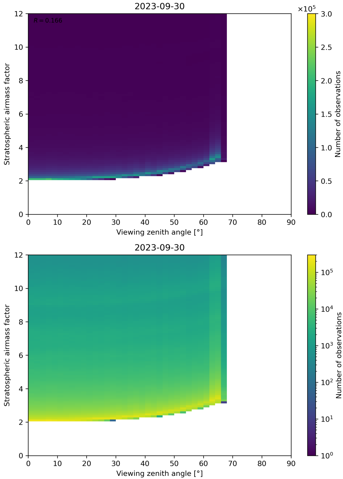
Figure 159: Scatter density plot of “Viewing zenith angle” against “Stratospheric airmass factor” for 2023-09-29 to 2023-10-01.
