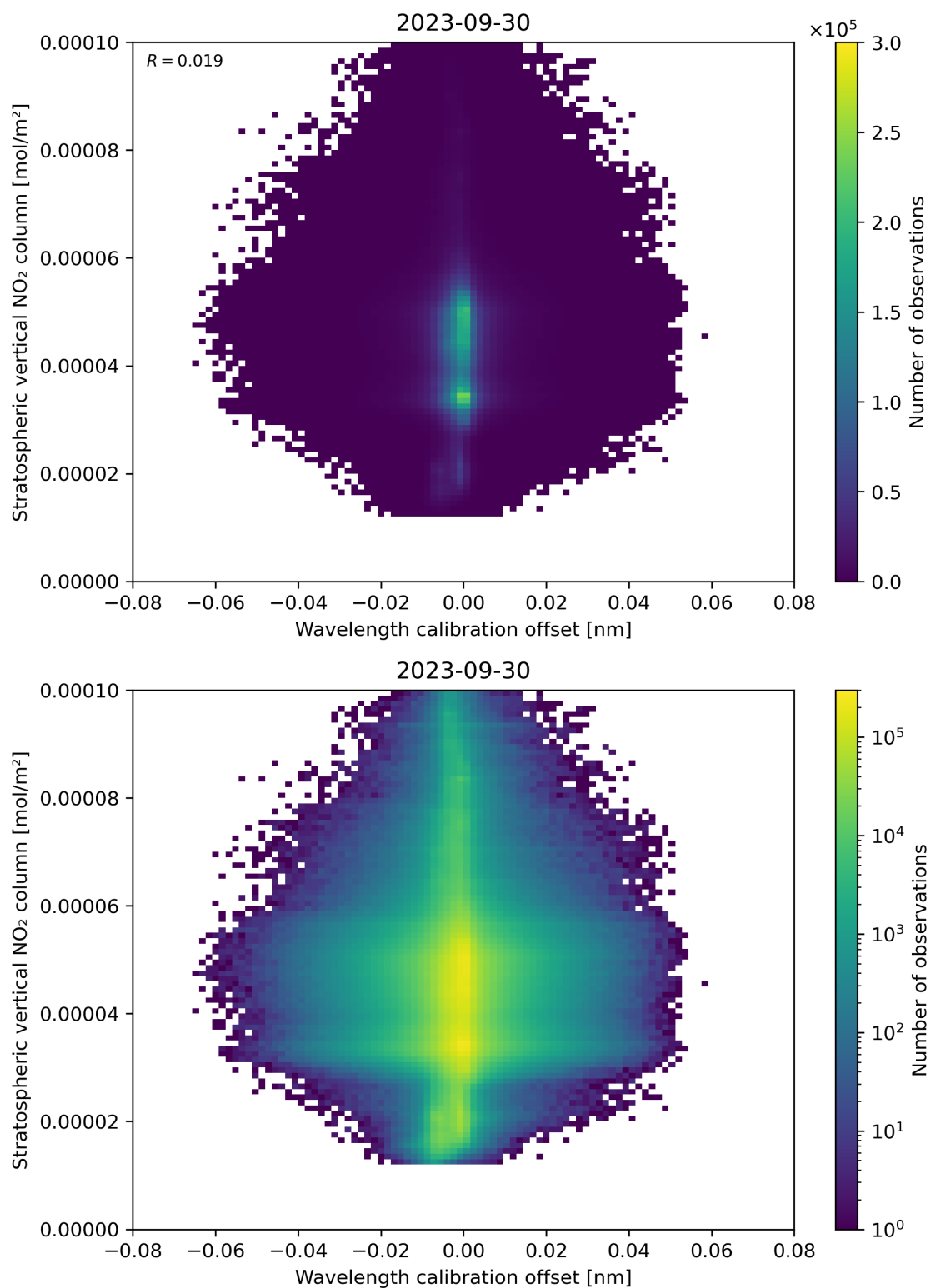
Figure 176: Scatter density plot of “Wavelength calibration offset” against “Stratospheric vertical NO 2 column” for 2023-09-29 to 2023-10-01.
