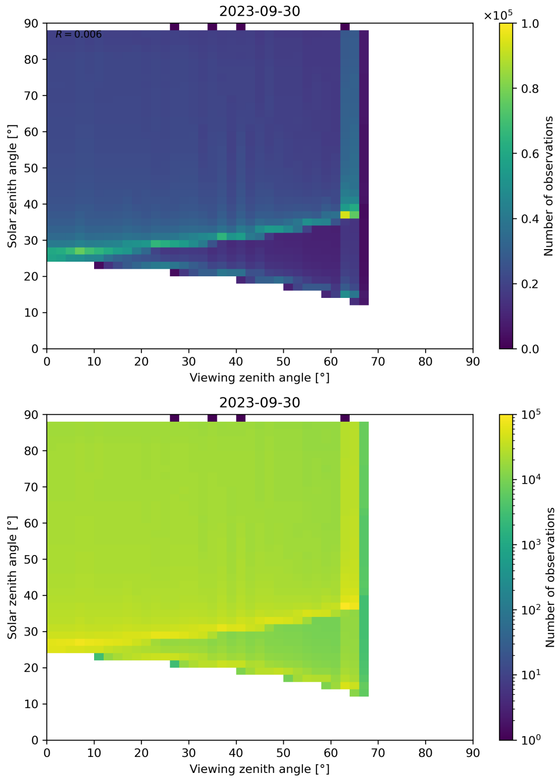
Figure 172: Scatter density plot of “Viewing zenith angle” against “Solar zenith angle” for 2023-09-29 to 2023-10-01.
