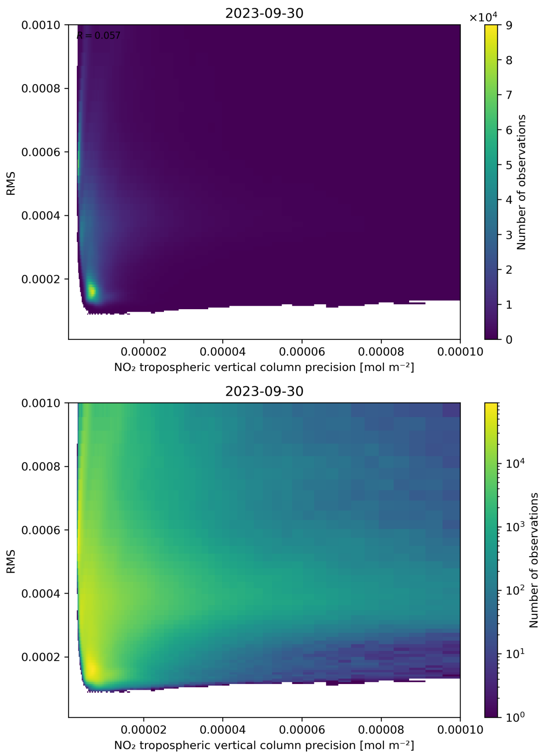
Figure 140: Scatter density plot of “NO 2 tropospheric vertical column precision” against “RMS” for 2023-09-29 to 2023-10-01.
