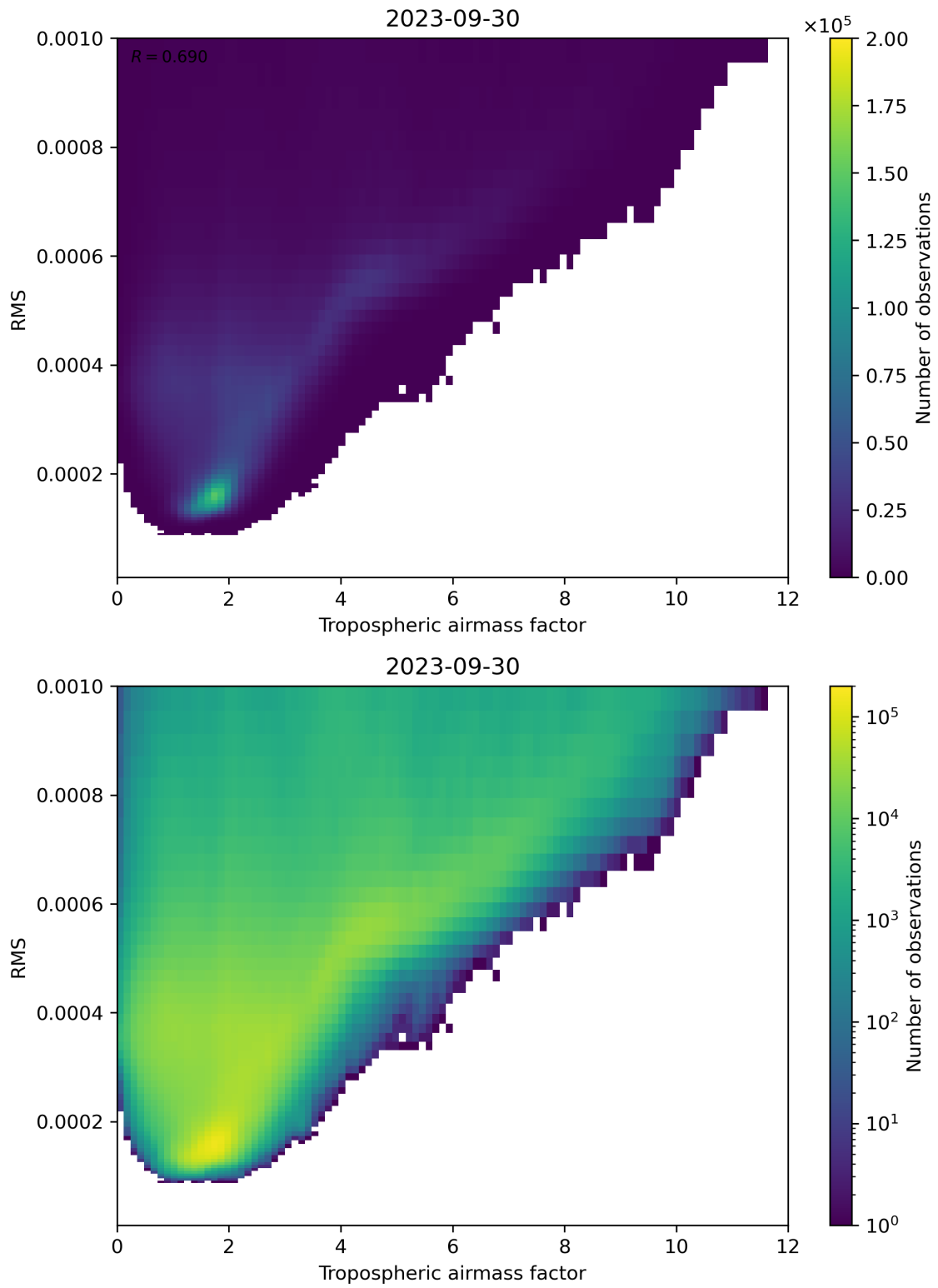
Figure 79: Scatter density plot of “Tropospheric airmass factor” against “RMS” for 2023-09-29 to 2023-10-01.
