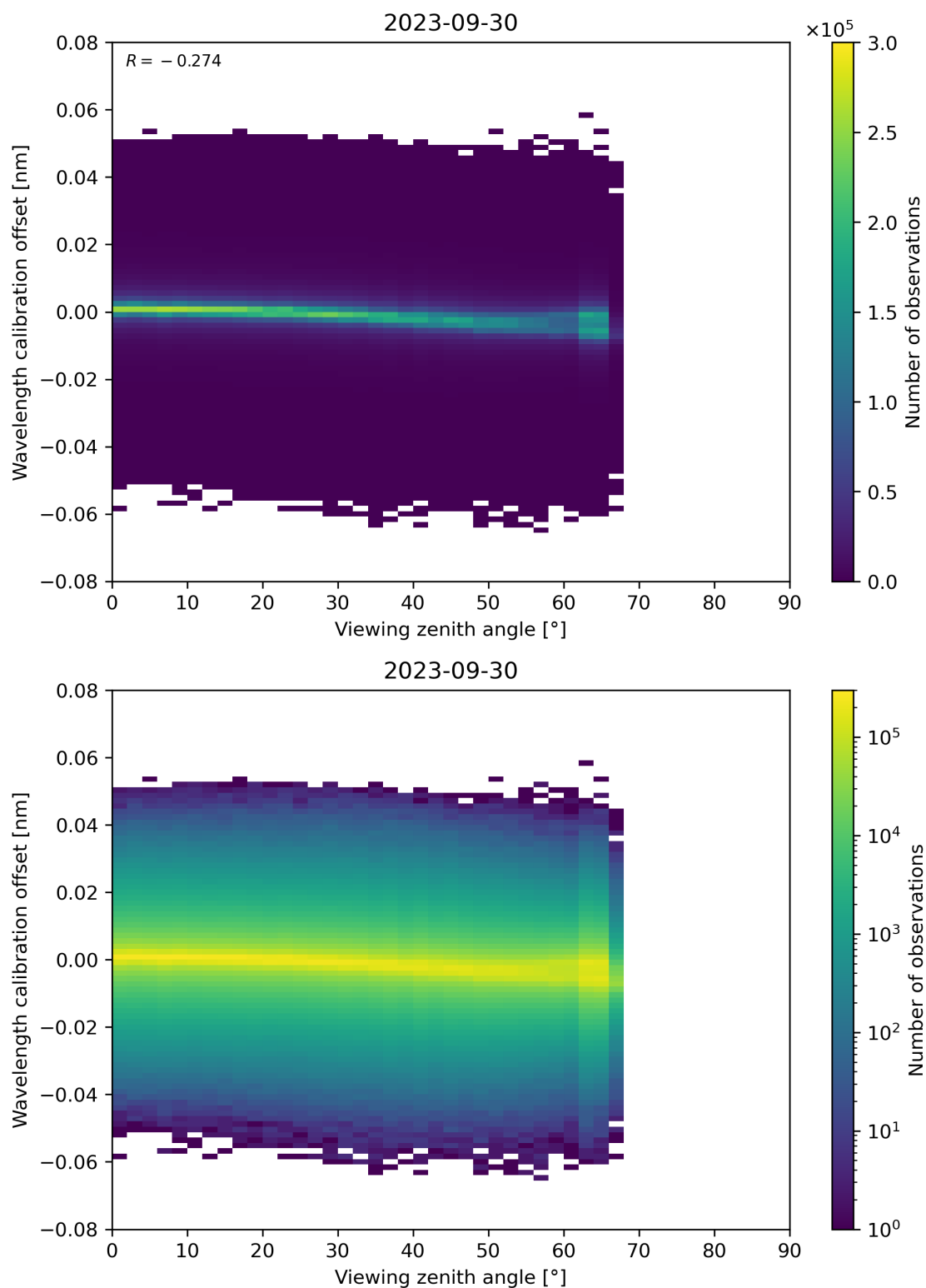
Figure 173: Scatter density plot of “Viewing zenith angle” against “Wavelength calibration offset” for 2023-09-29 to 2023-10-01.
