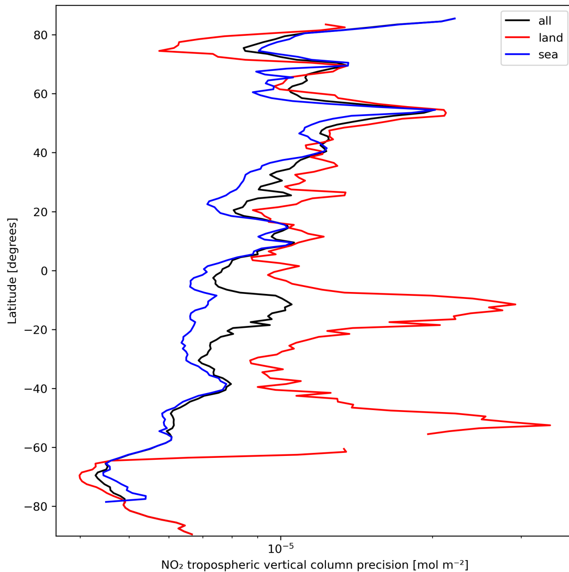
Figure 13: Zonal average of “NO 2 tropospheric vertical column precision” for 2023-09-29 to 2023-10-01.
