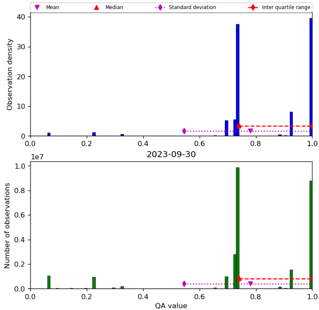
Figure 28: Histogram of “QA value” for 2023-09-29 to 2023-10-01
