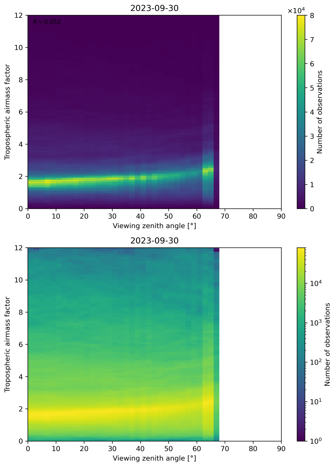
Figure 161: Scatter density plot of “Viewing zenith angle” against “Tropospheric airmass factor” for 2023-09-29 to 2023-10-01.
