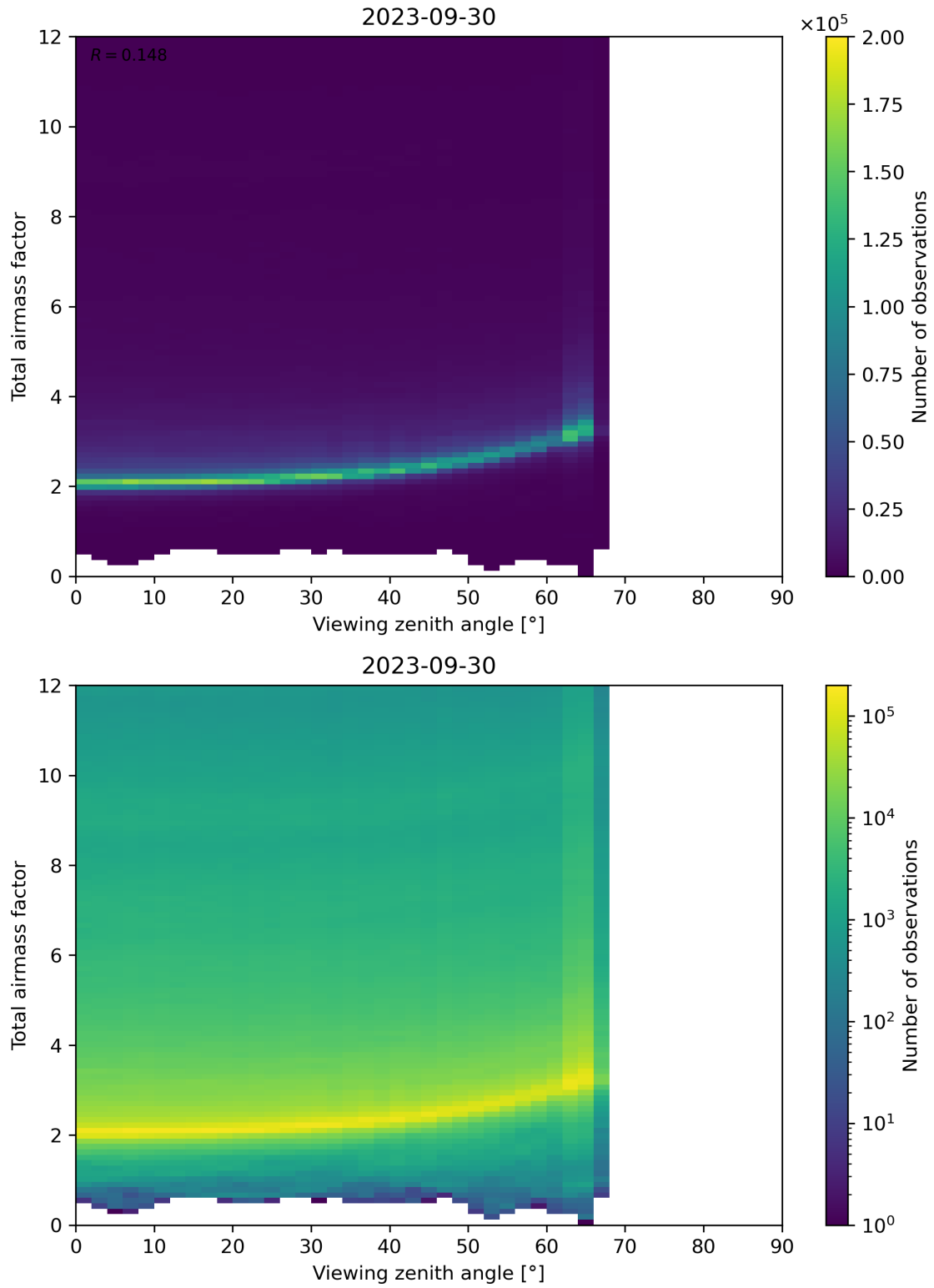
Figure 160: Scatter density plot of “Viewing zenith angle” against “Total airmass factor” for 2023-09-29 to 2023-10-01.
