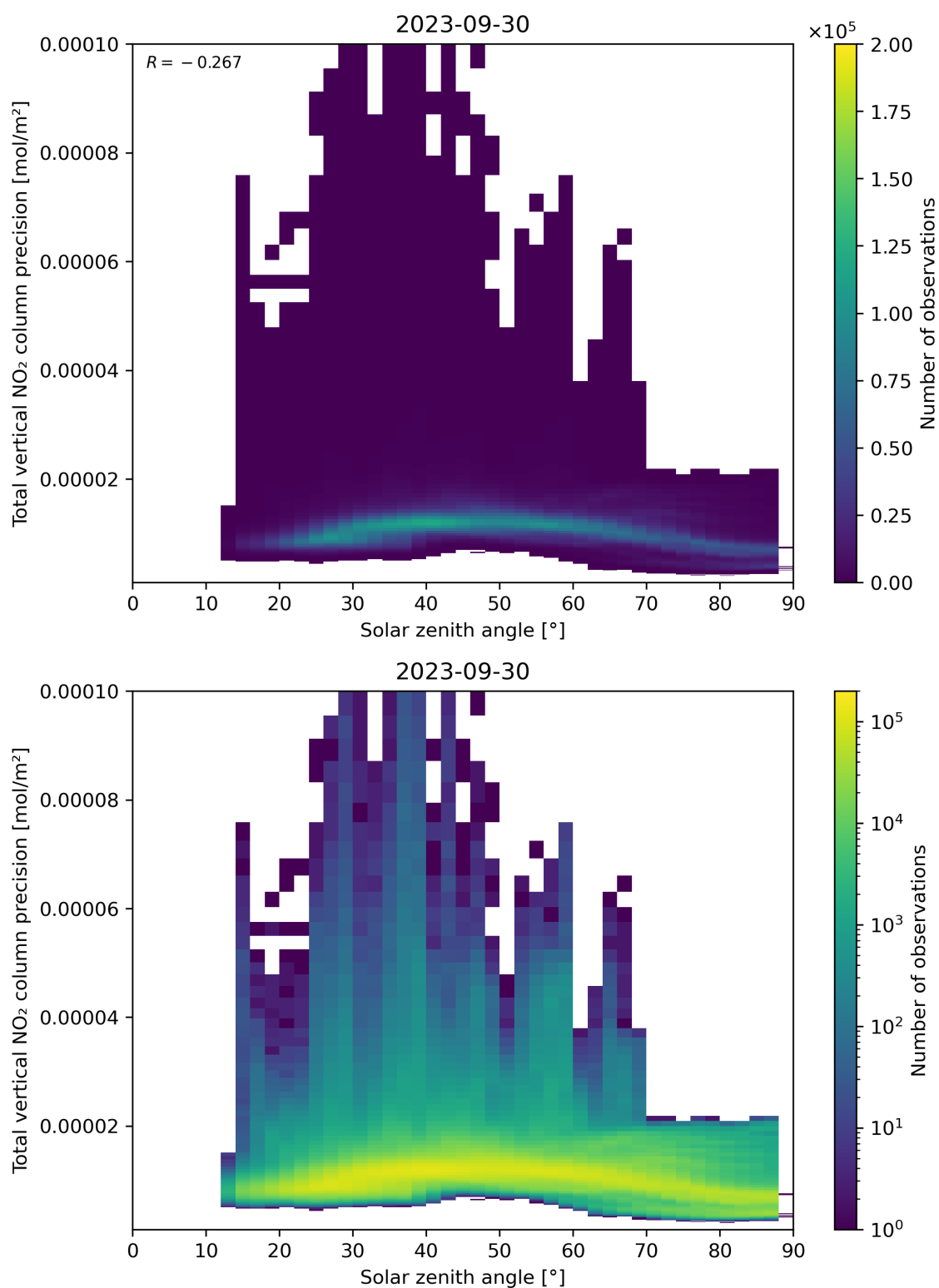
Figure 154: Scatter density plot of “Solar zenith angle” against “Total vertical NO 2 column precision” for 2023-09-29 to 2023-10-01.
