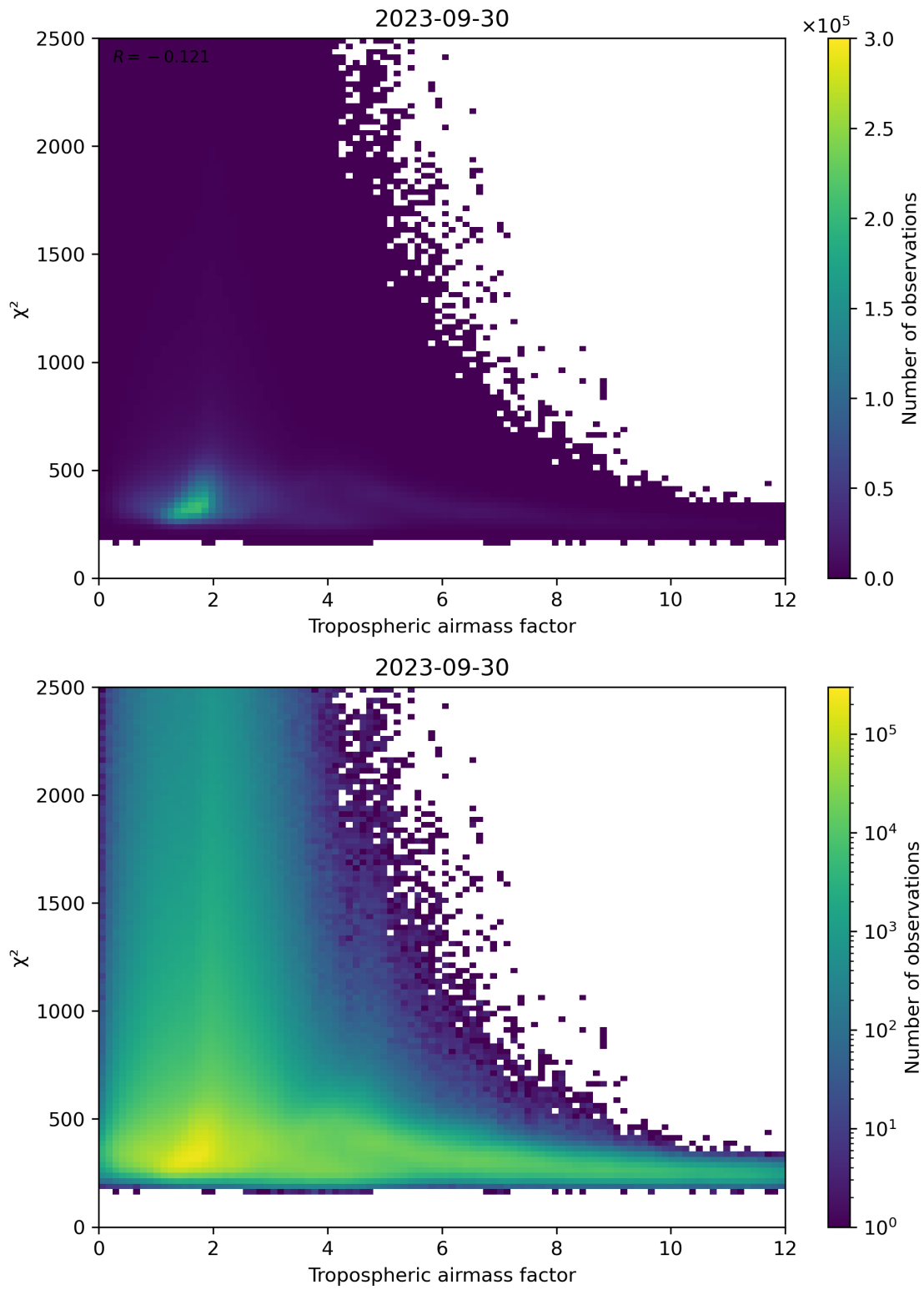
Figure 73: Scatter density plot of “Tropospheric airmass factor” against “ \chi^2 ” for 2023-09-29 to 2023-10-01.
