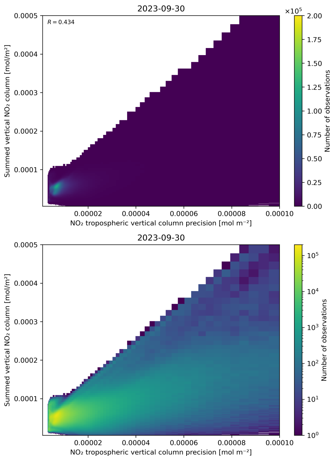
Figure 136: Scatter density plot of “NO 2 tropospheric vertical column precision” against “Summed vertical NO 2 column” for 2023-09-29 to 2023-10-01.
