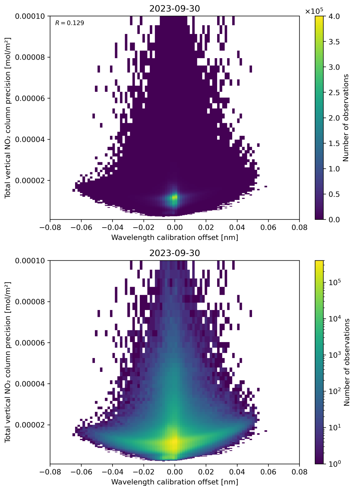
Figure 180: Scatter density plot of “Wavelength calibration offset” against “Total vertical NO 2 column precision” for 2023-09-29 to 2023-10-01.
