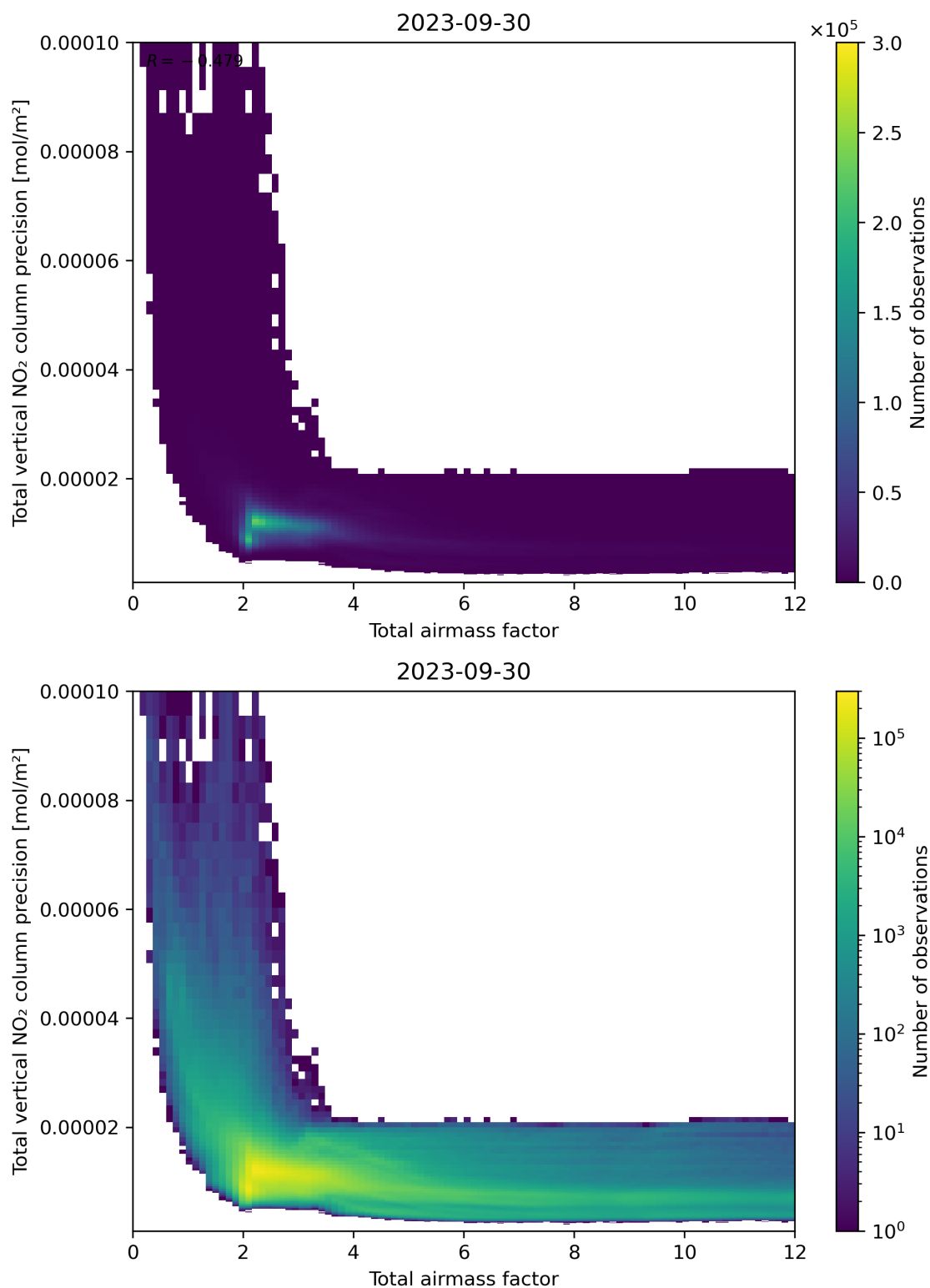
Figure 68: Scatter density plot of “Total airmass factor” against “Total vertical NO 2 column precision” for 2023-09-29 to 2023-10-01.
