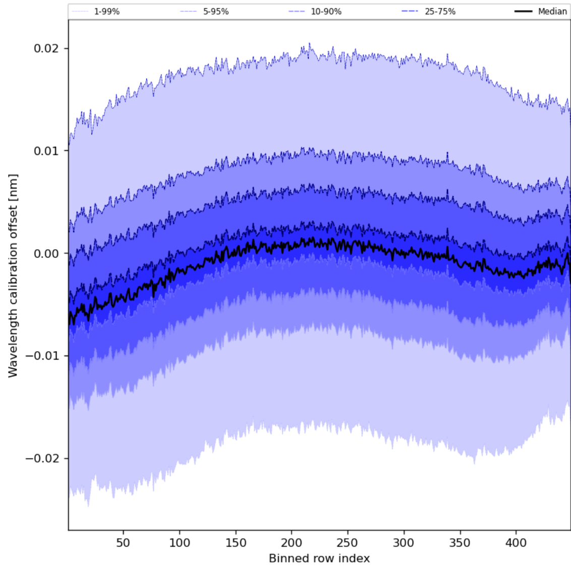
Figure 52: Along track statistics of “Wavelength calibration offset” for 2023-09-29 to 2023-10-01
