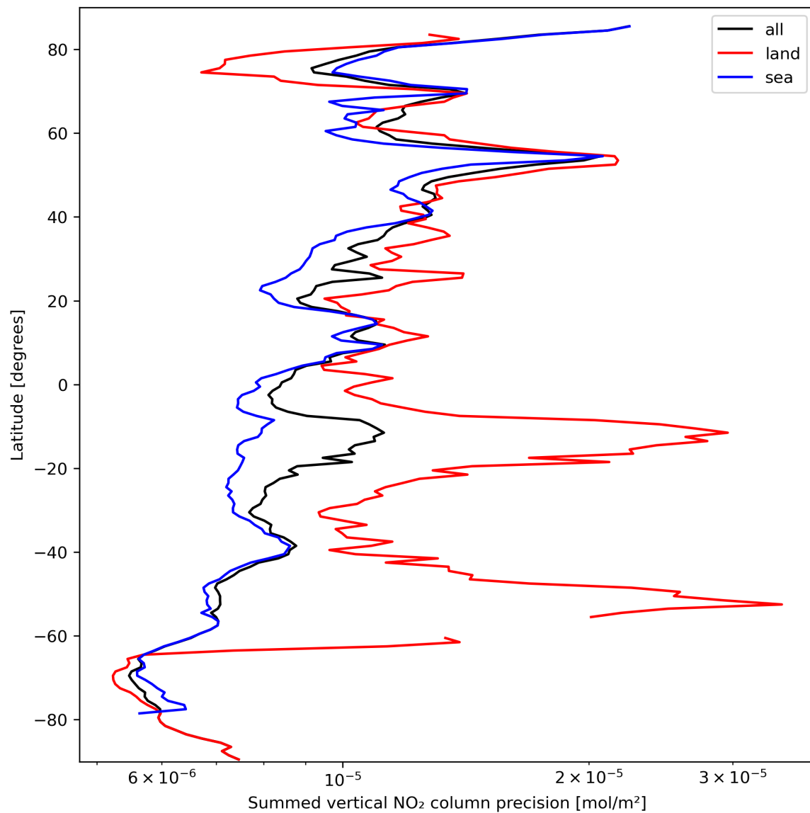
Figure 24: Zonal average of “Summed vertical NO 2 column precision” for 2023-09-29 to 2023-10-01.
