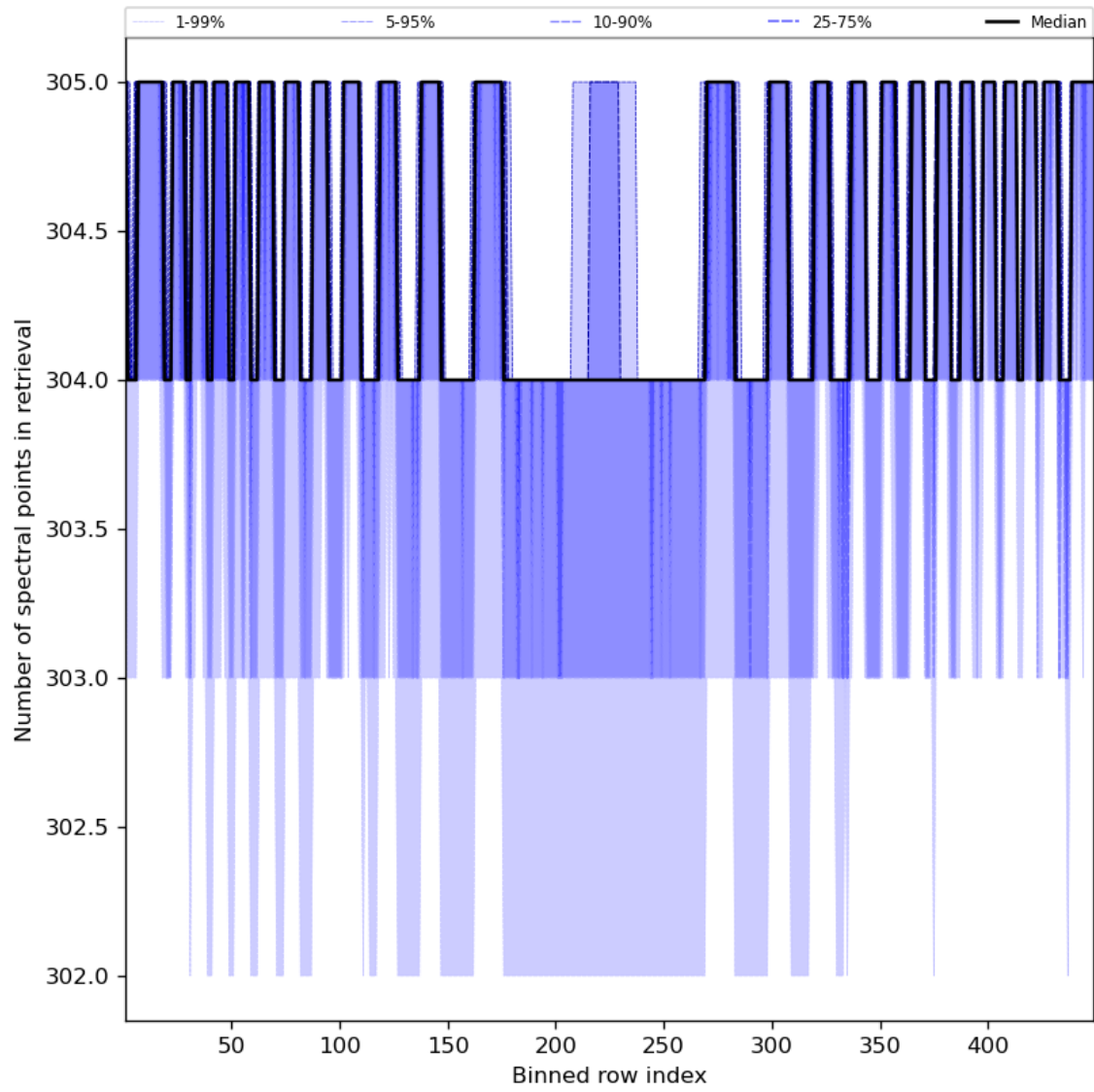
Figure 50: Along track statistics of “Number of spectral points in retrieval” for 2023-09-29 to 2023-10-01
