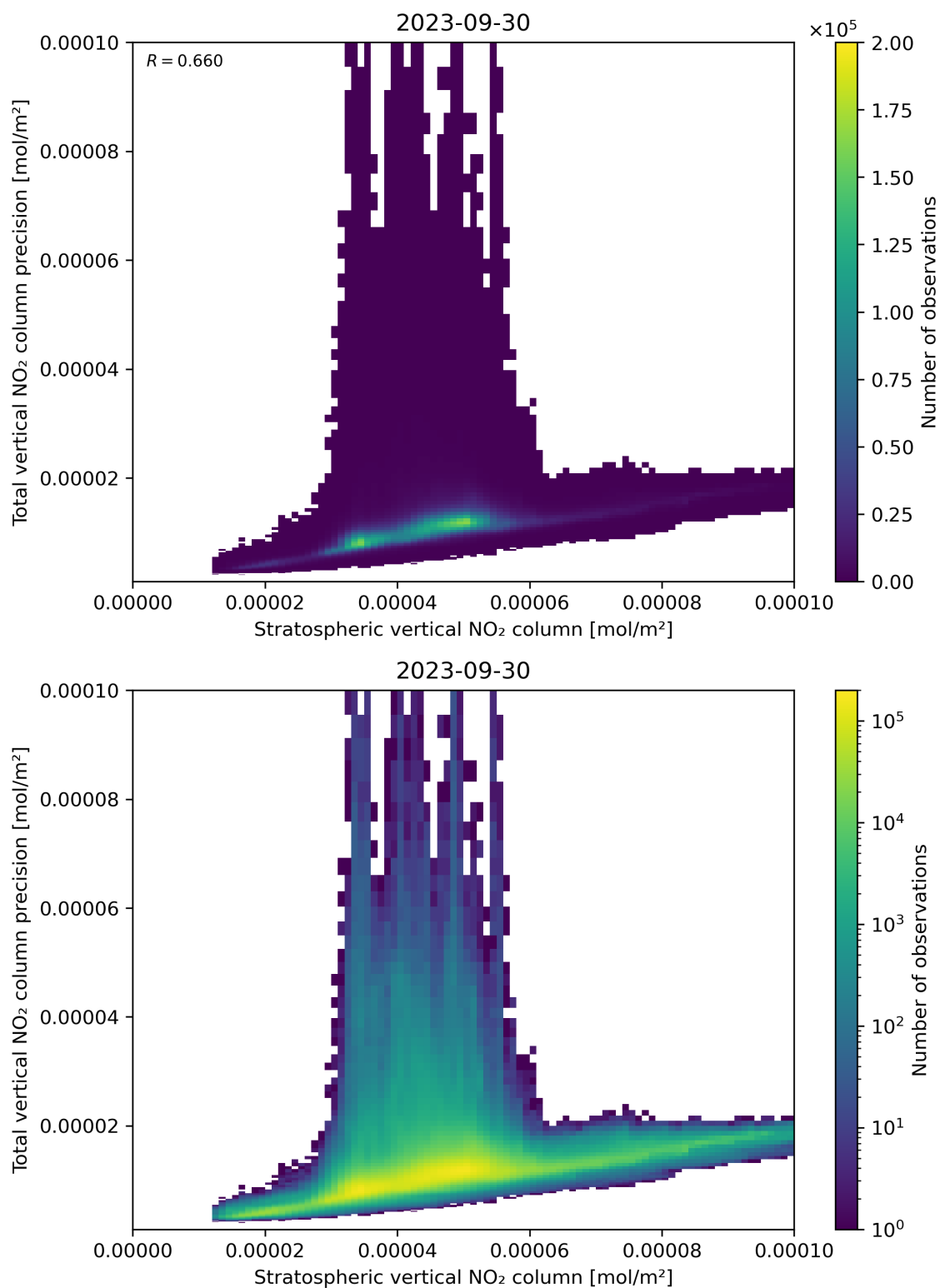
Figure 101: Scatter density plot of “Stratospheric vertical NO 2 column” against “Total vertical NO 2 column precision” for 2023-09-29 to 2023-10-01.
