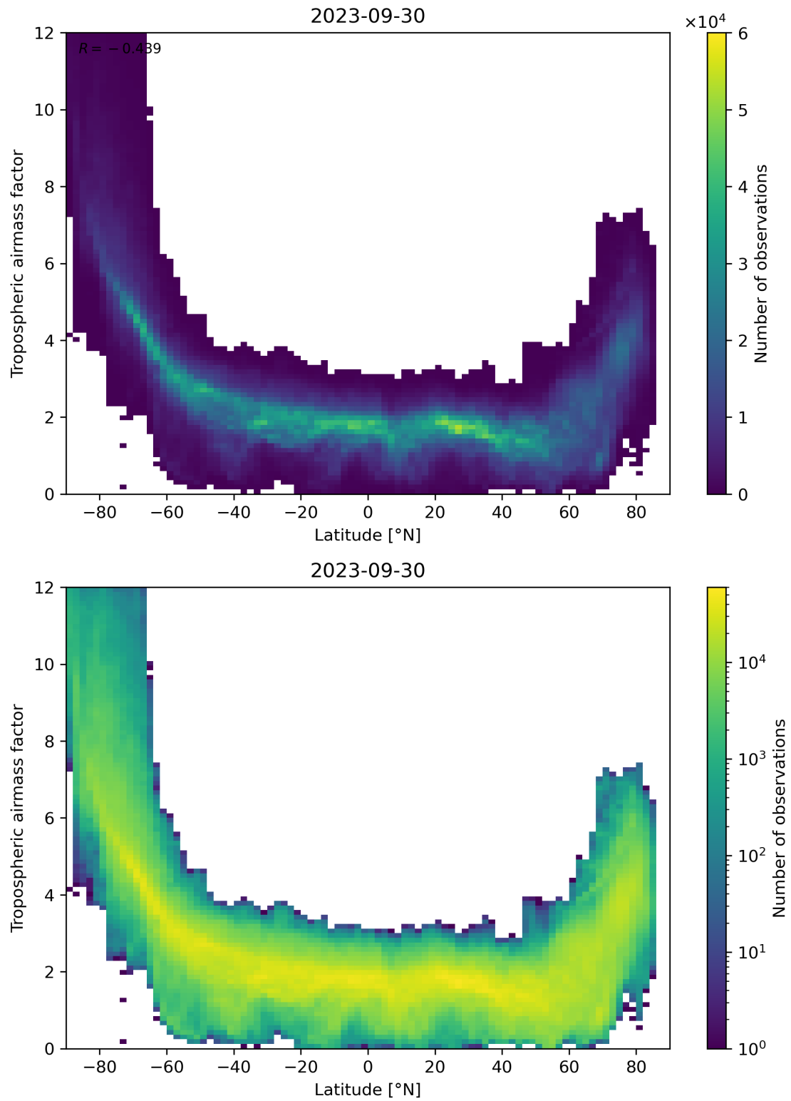
Figure 85: Scatter density plot of “Latitude” against “Tropospheric air mass factor” for 2023-09-29 to 2023-10-01.
