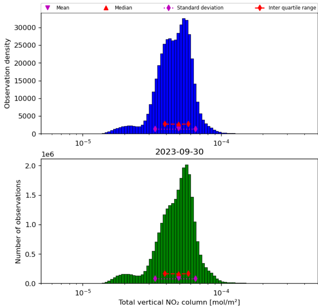
Figure 38: Histogram of “Total vertical NO 2 column” for 2023-09-29 to 2023-10-01
