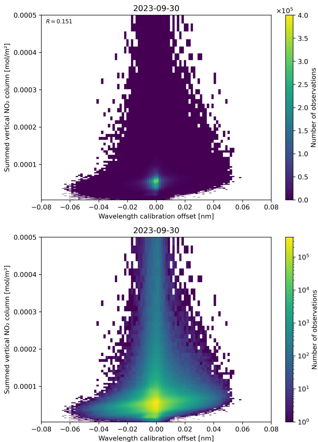
Figure 177: Scatter density plot of “Wavelength calibration offset” against “Summed vertical NO 2 column” for 2023-09-29 to 2023-10-01.
