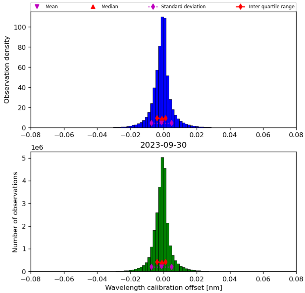
Figure 35: Histogram of “Wavelength calibration offset” for 2023-09-29 to 2023-10-01
