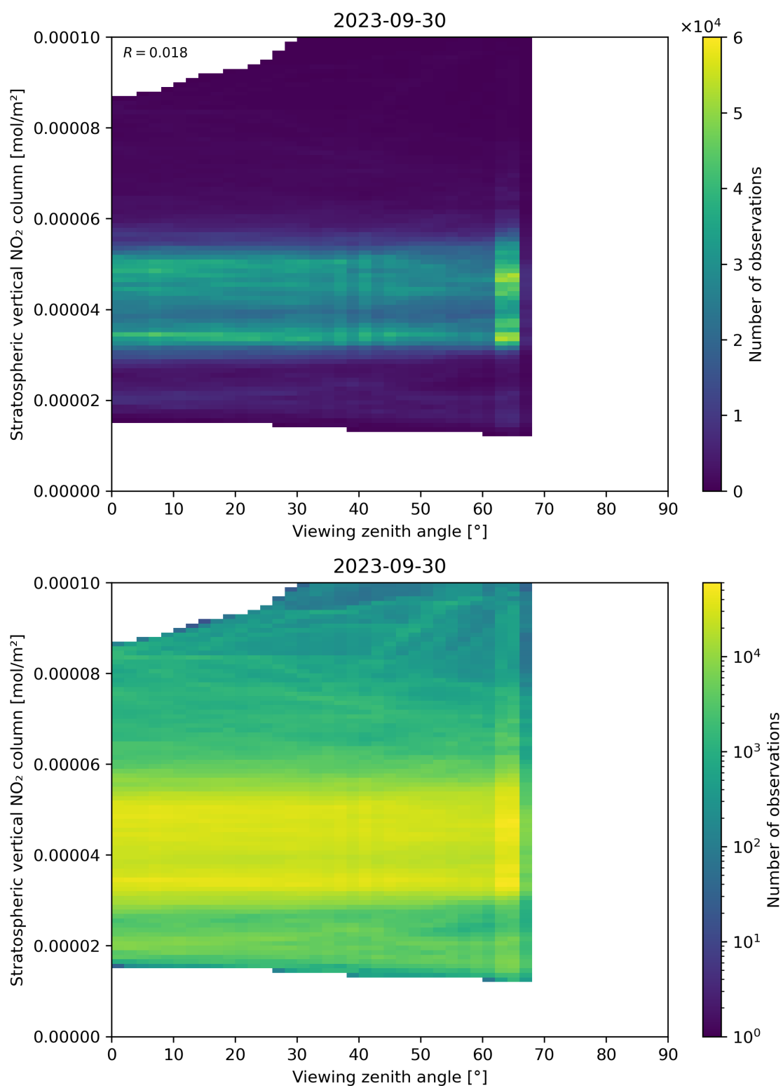
Figure 164: Scatter density plot of “Viewing zenith angle” against “Stratospheric vertical NO 2 column” for 2023-09-29 to 2023-10-01.
