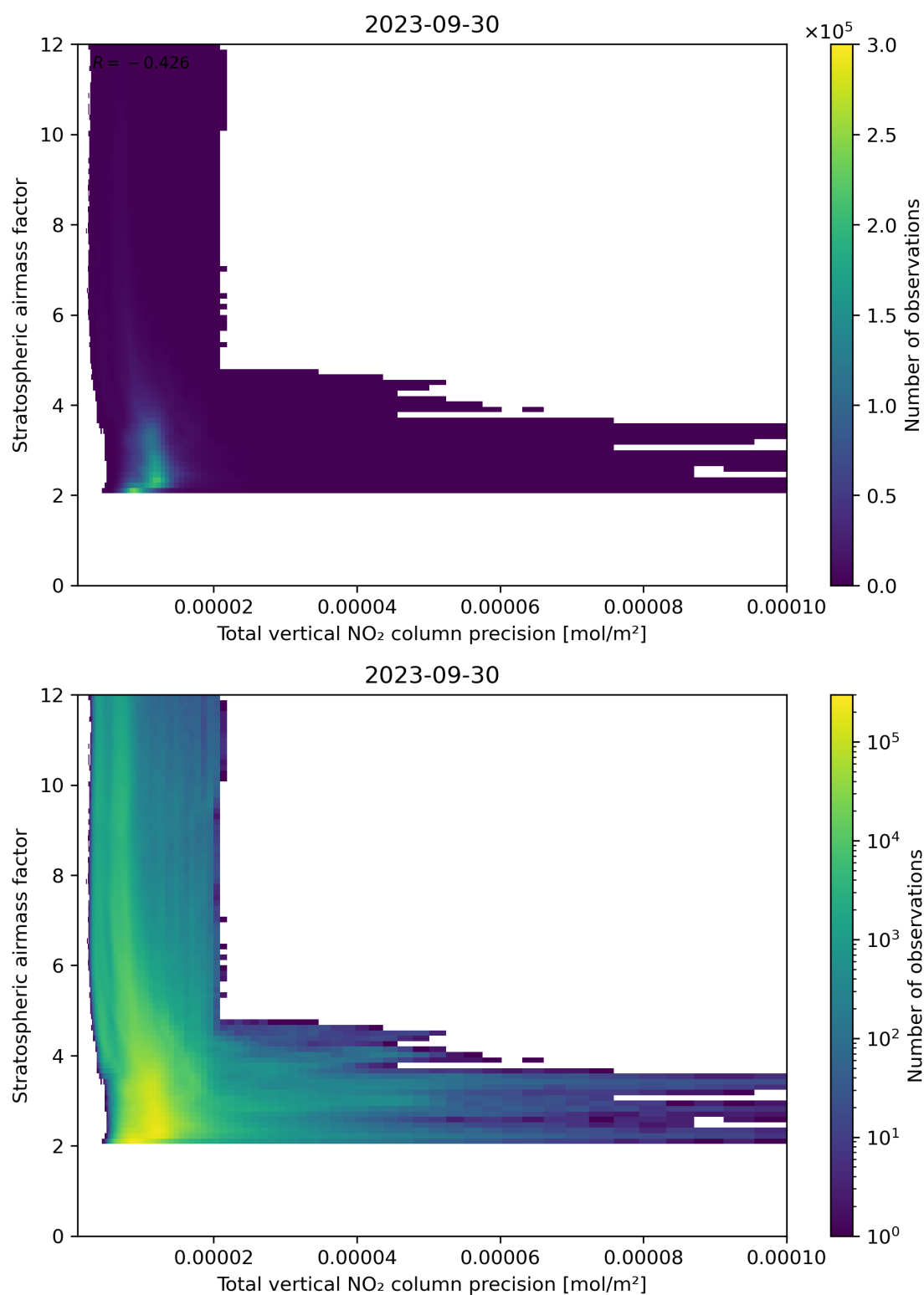
Figure 115: Scatter density plot of “Total vertical NO 2 column precision” against “Stratospheric air mass factor” for 2023-09-29 to 2023-10-01.
