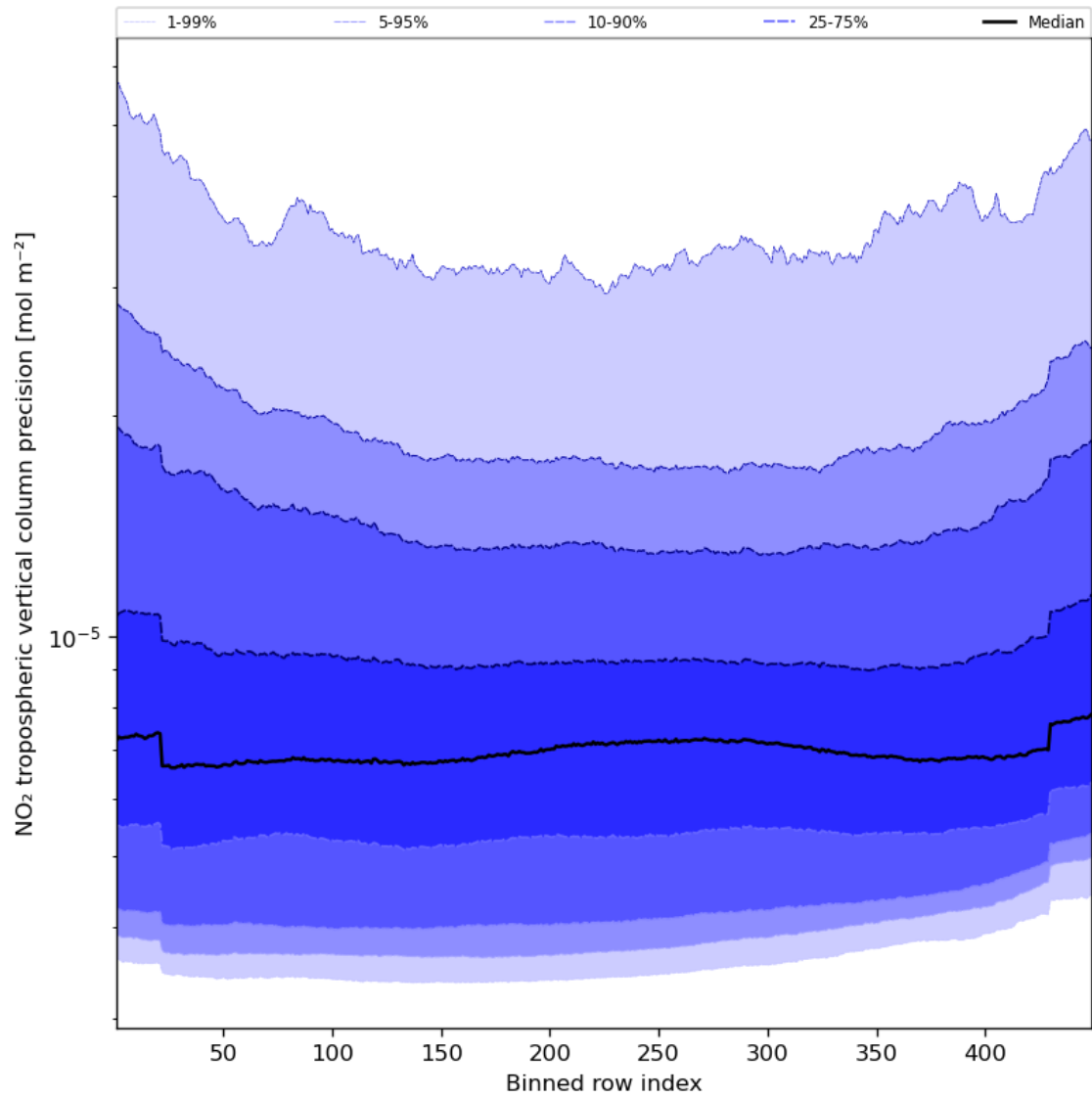
Figure 47: Along track statistics of “NO 2 tropospheric vertical column precision” for 2023-09-29 to 2023-10-01
