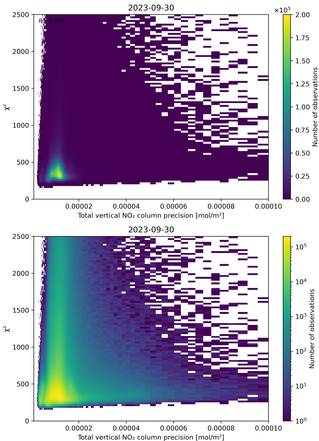
Figure 116: Scatter density plot of “Total vertical NO 2 column precision” against “ \chi^2 ” for 2023-09-29 to 2023-10-01.
