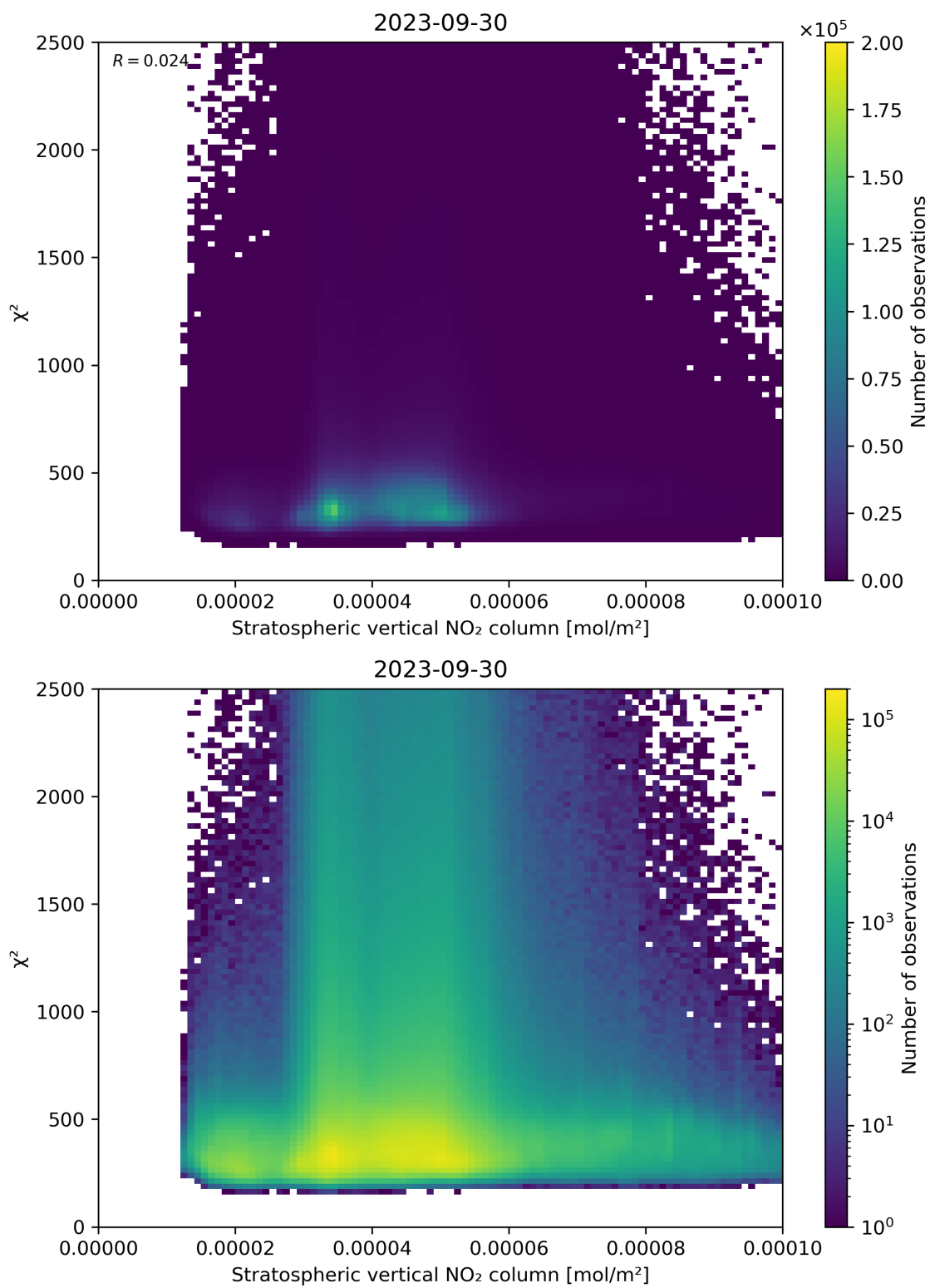
Figure 97: Scatter density plot of “Stratospheric vertical NO 2 column” against “ \chi^2 ” for 2023-09-29 to 2023-10-01.
