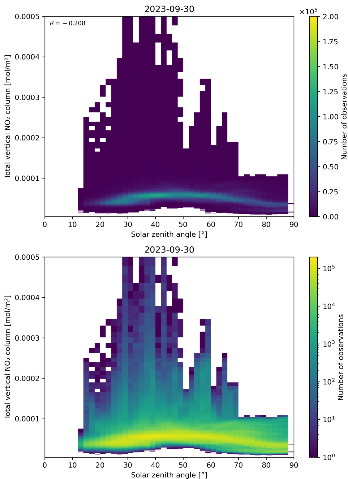
Figure 153: Scatter density plot of “Solar zenith angle” against “Total vertical NO 2 column” for 2023-09-29 to 2023-10-01.
