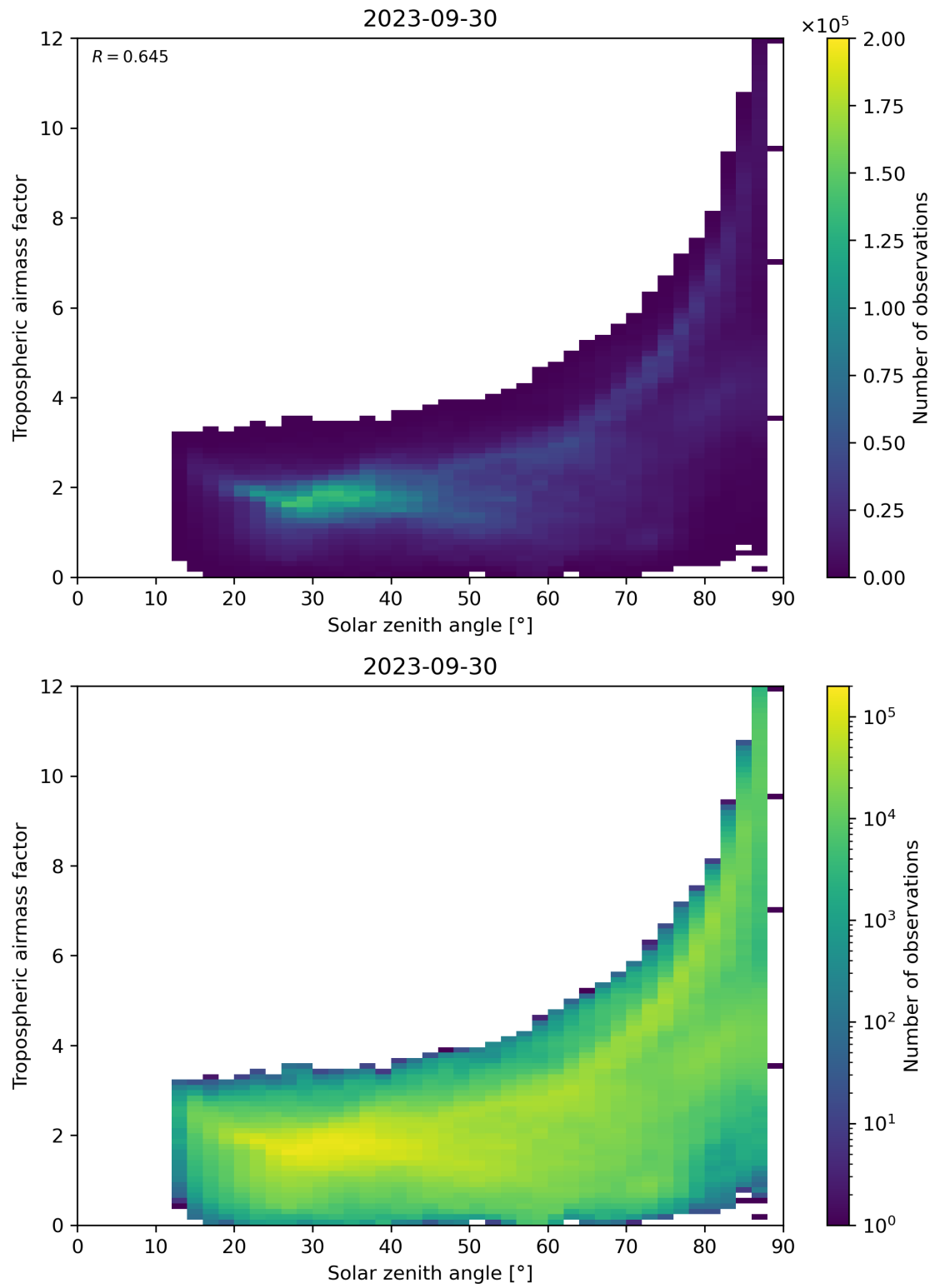
Figure 147: Scatter density plot of “Solar zenith angle” against “Tropospheric airmass factor” for 2023-09-29 to 2023-10-01.
