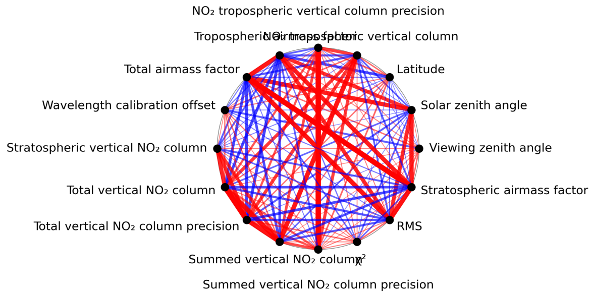
Figure 1: Map of correlation graph for 2023-09-29 to 2023-10-01.
