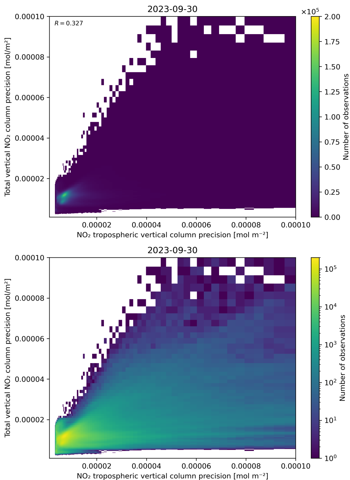
Figure 139: Scatter density plot of “NO 2 tropospheric vertical column precision” against “Total vertical NO 2 column precision” for 2023-09-29 to 2023-10-01.
