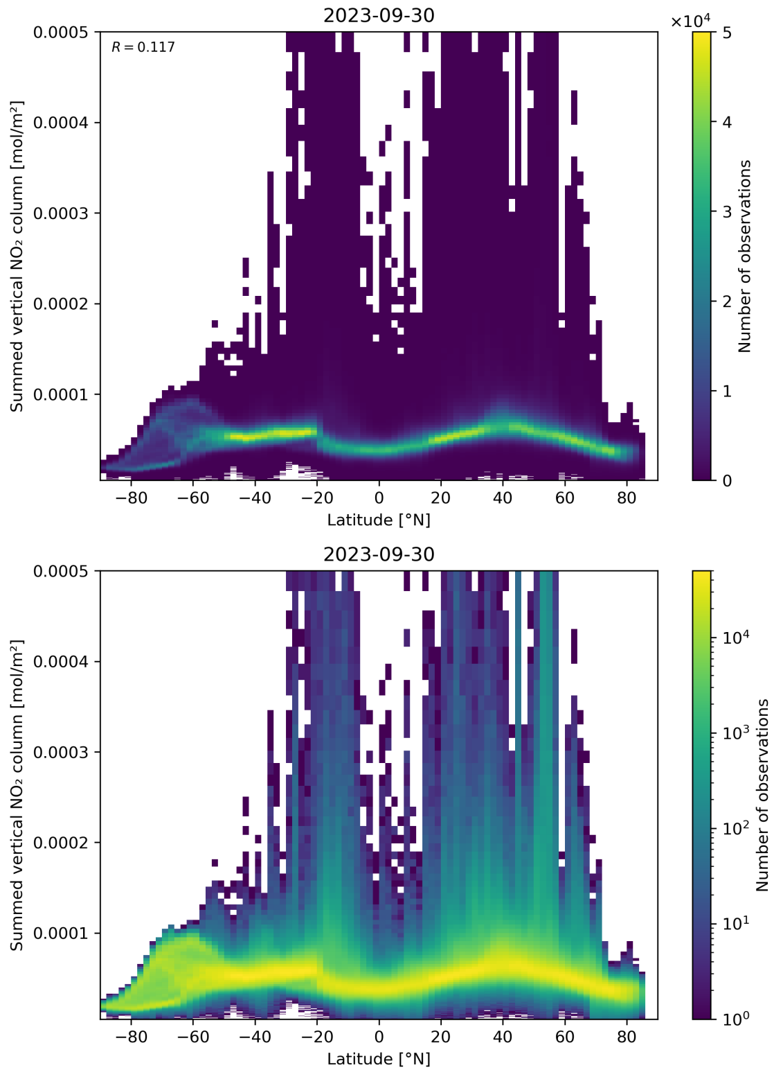
Figure 88: Scatter density plot of “Latitude” against “Summed vertical NO 2 column” for 2023-09-29 to 2023-10-01.
