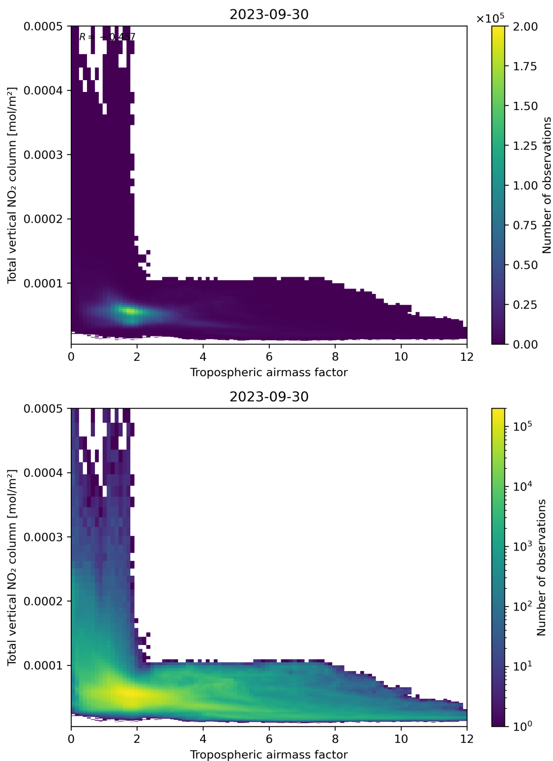
Figure 77: Scatter density plot of “Tropospheric airmass factor” against “Total vertical NO 2 column” for 2023-09-29 to 2023-10-01.
