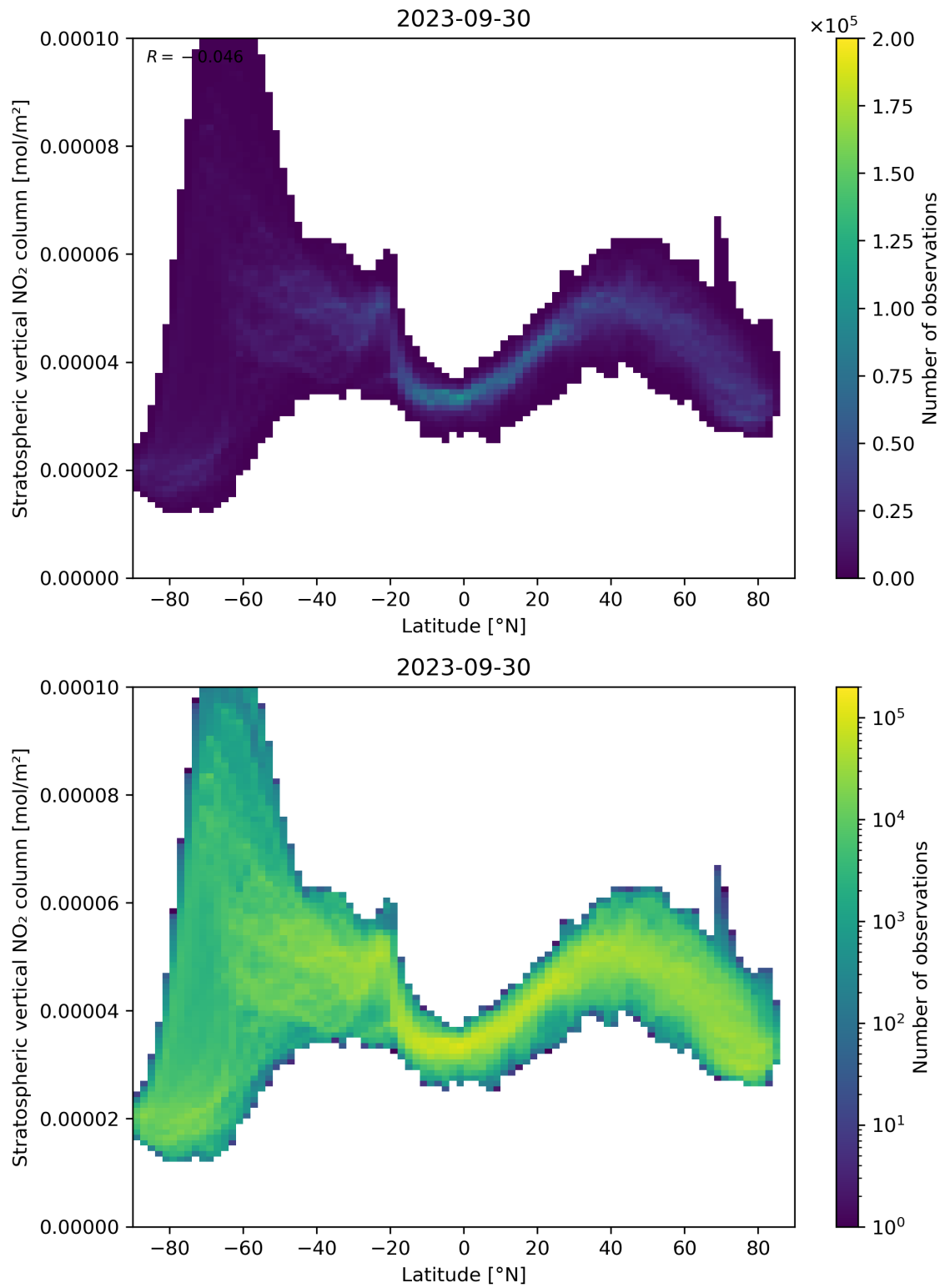
Figure 87: Scatter density plot of “Latitude” against “Stratospheric vertical NO 2 column” for 2023-09-29 to 2023-10-01.
