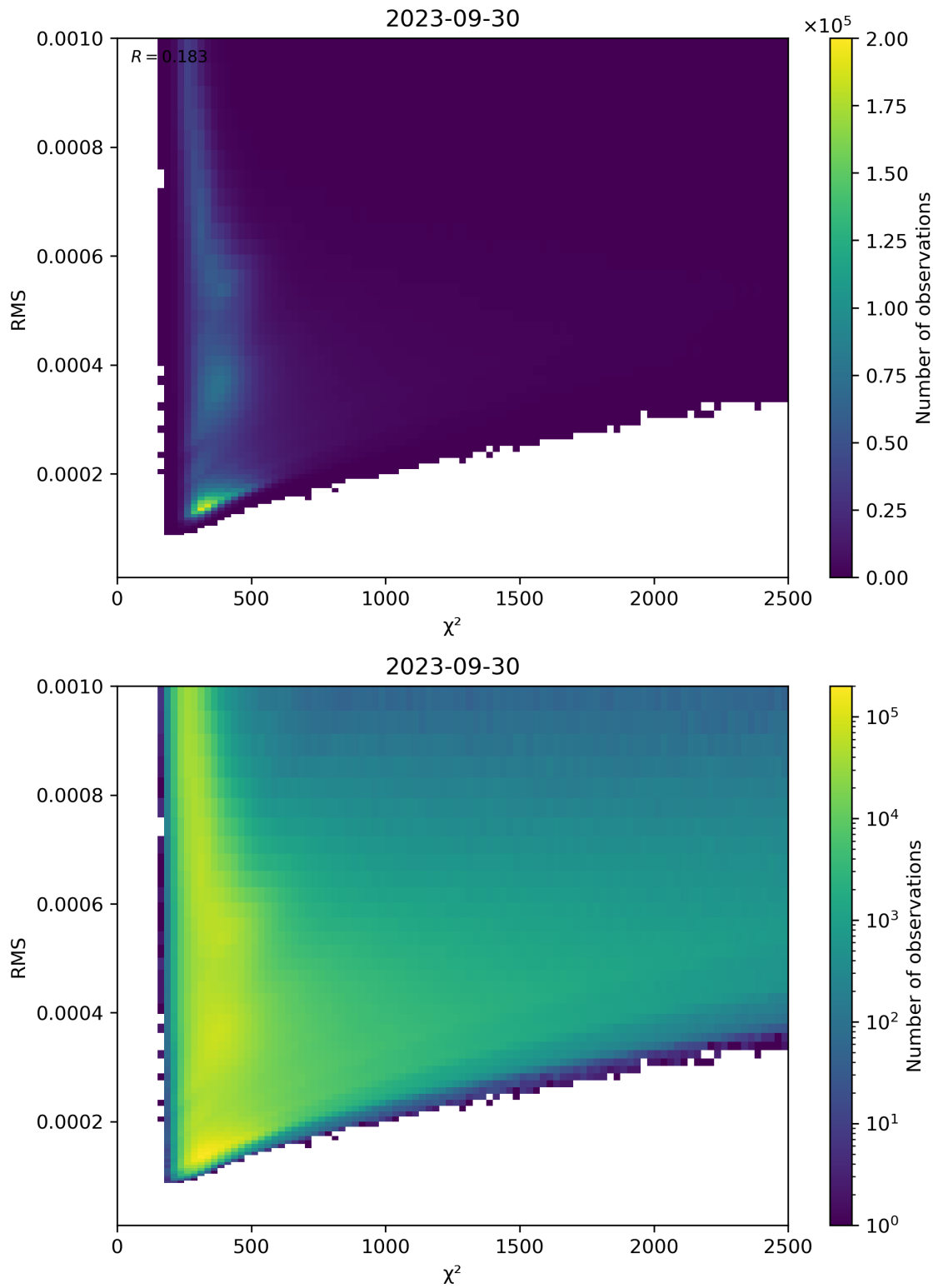
Figure 82: Scatter density plot of “ \chi^2 ” against “RMS” for 2023-09-29 to 2023-10-01.
