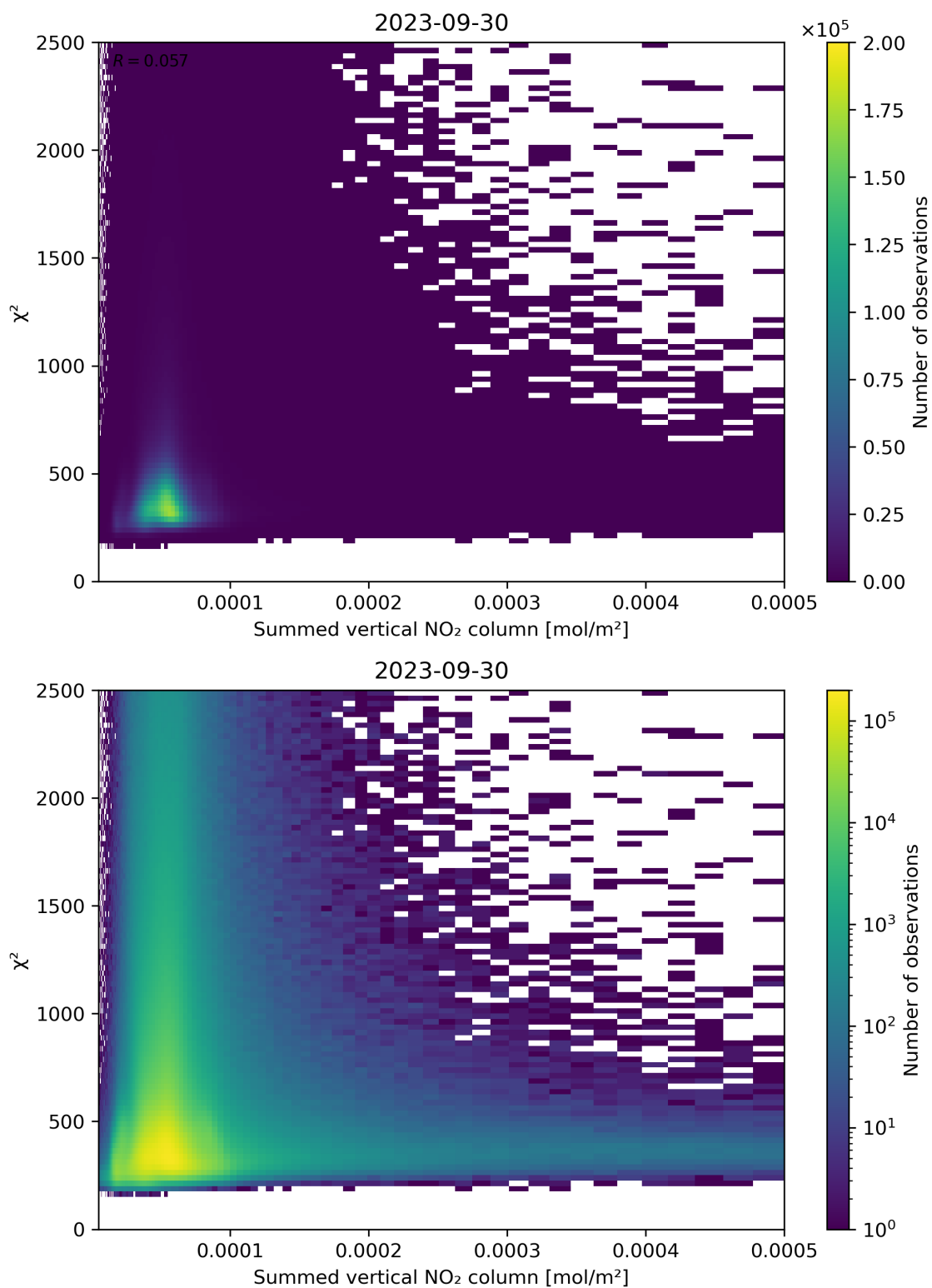
Figure 104: Scatter density plot of “Summed vertical NO 2 column” against “ \chi^2 ” for 2023-09-29 to 2023-10-01.
