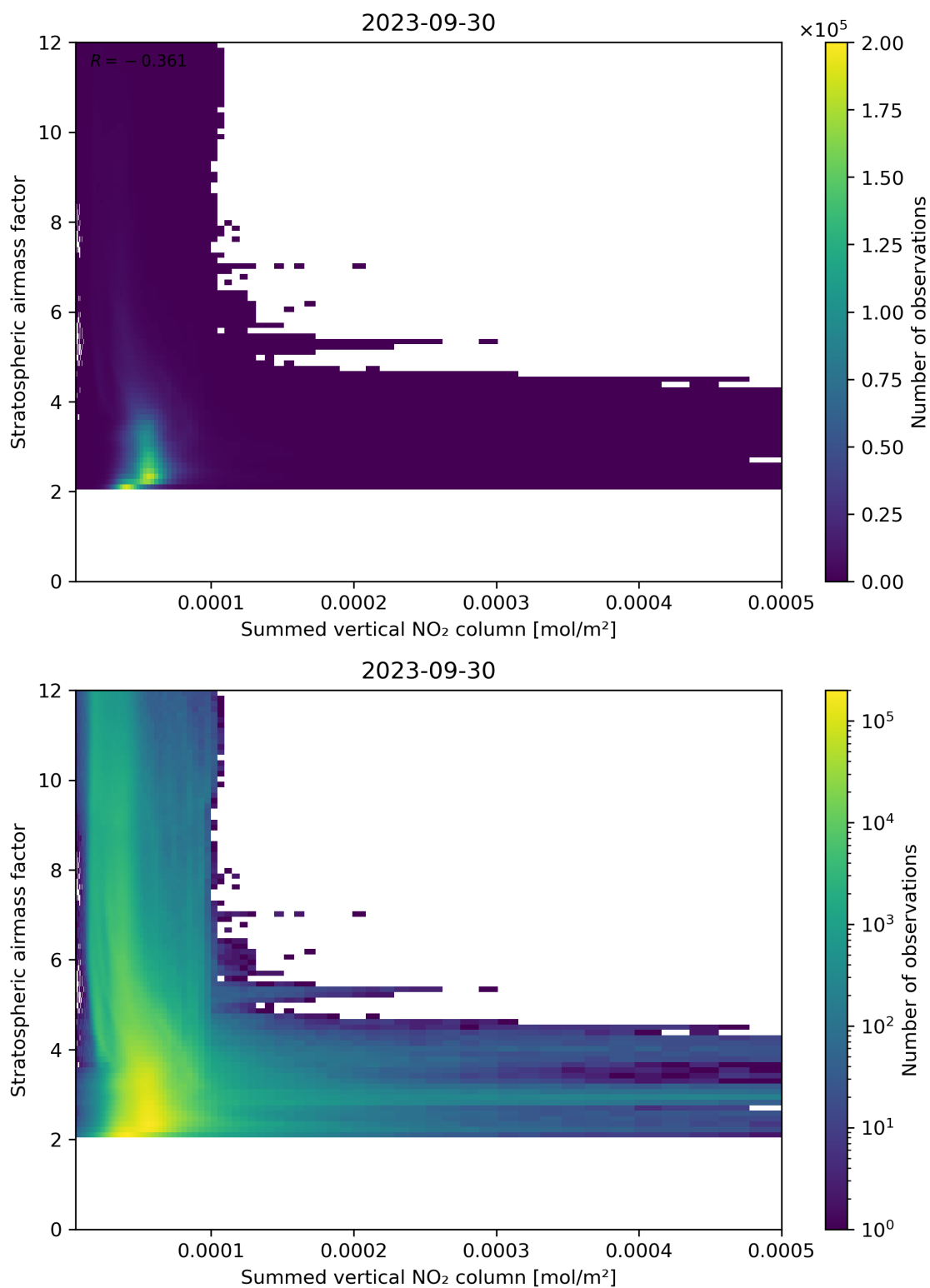
Figure 103: Scatter density plot of “Summed vertical NO 2 column” against “Stratospheric airmass factor” for 2023-09-29 to 2023-10-01.
