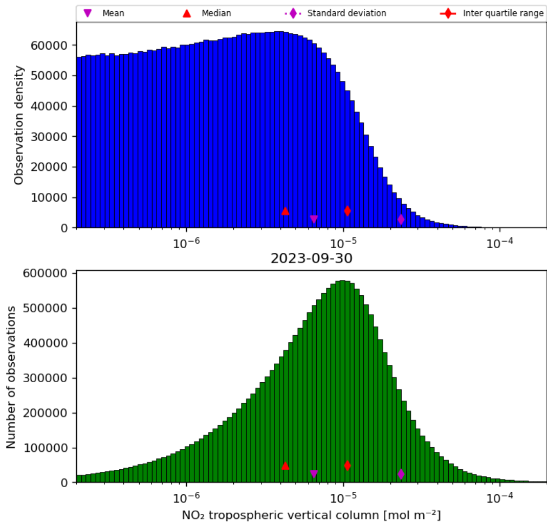
Figure 29: Histogram of “NO 2 tropospheric vertical column” for 2023-09-29 to 2023-10-01
