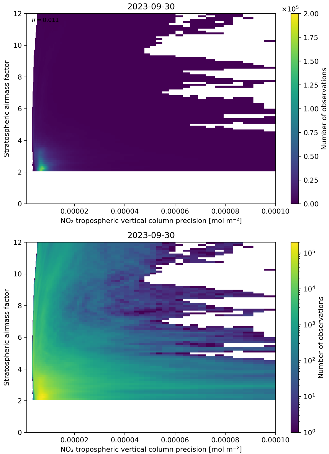
Figure 131: Scatter density plot of “NO 2 tropospheric vertical column precision” against “Stratospheric airmass factor” for 2023-09-29 to 2023-10-01.
