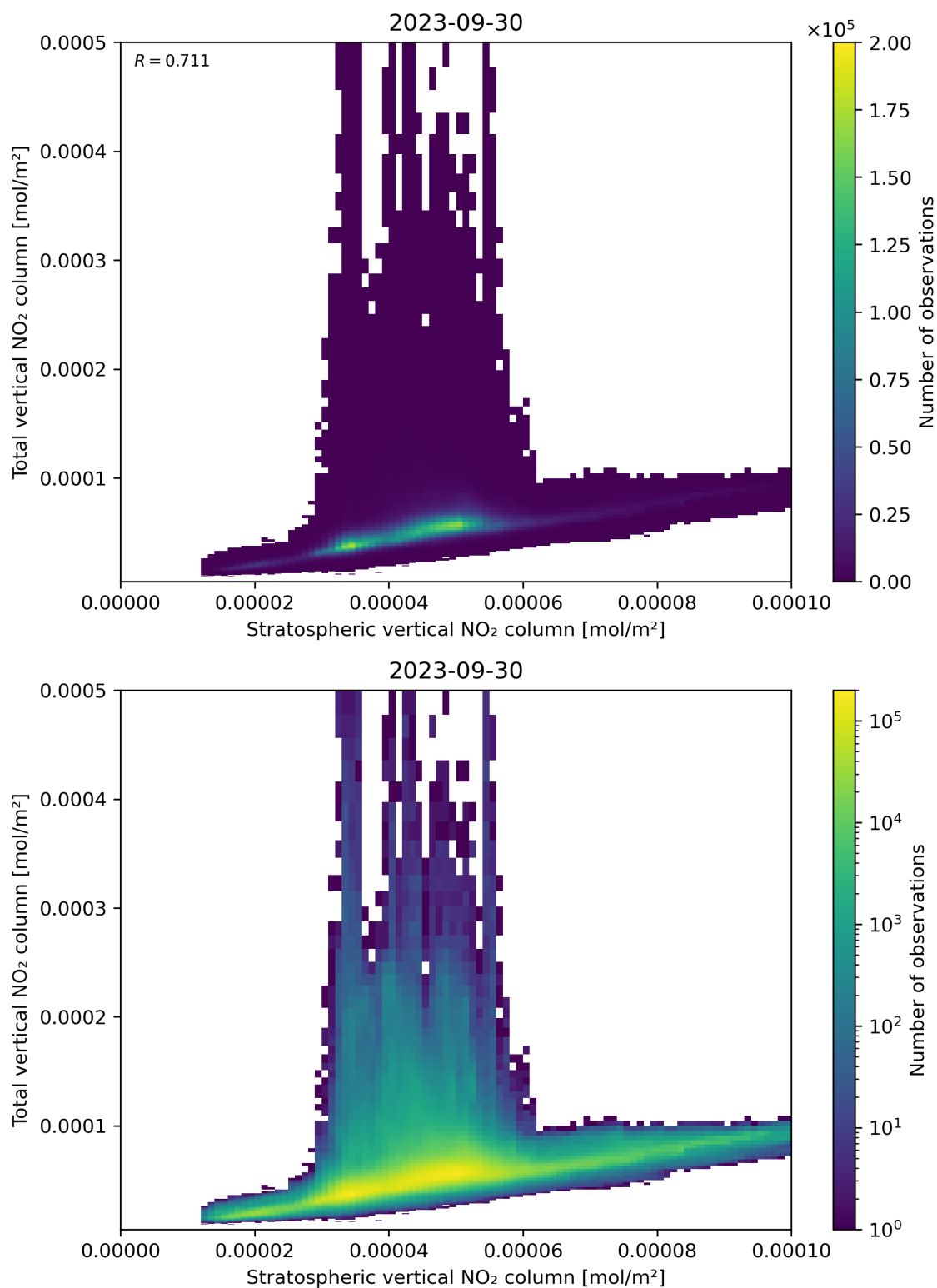
Figure 100: Scatter density plot of “Stratospheric vertical NO 2 column” against “Total vertical NO 2 column” for 2023-09-29 to 2023-10-01.
