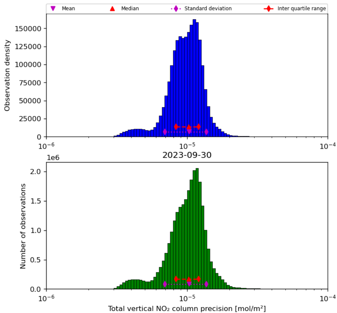
Figure 39: Histogram of “Total vertical NO 2 column precision” for 2023-09-29 to 2023-10-01
