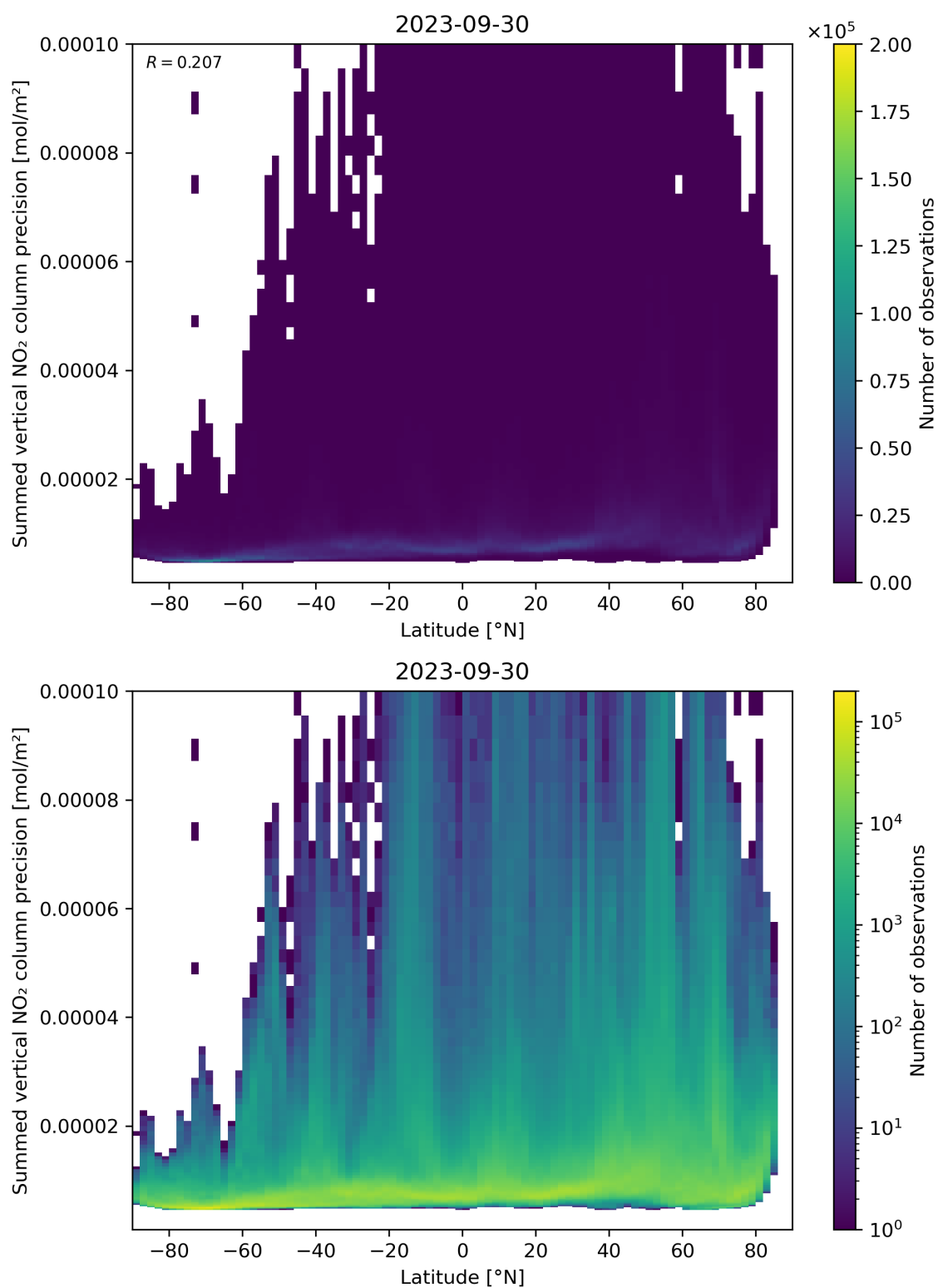
Figure 89: Scatter density plot of “Latitude” against “Summed vertical NO 2 column precision” for 2023-09-29 to 2023-10-01.
