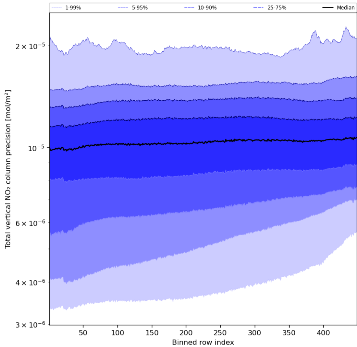
Figure 56: Along track statistics of “Total vertical NO 2 column precision” for 2023-09-29 to 2023-10-01
