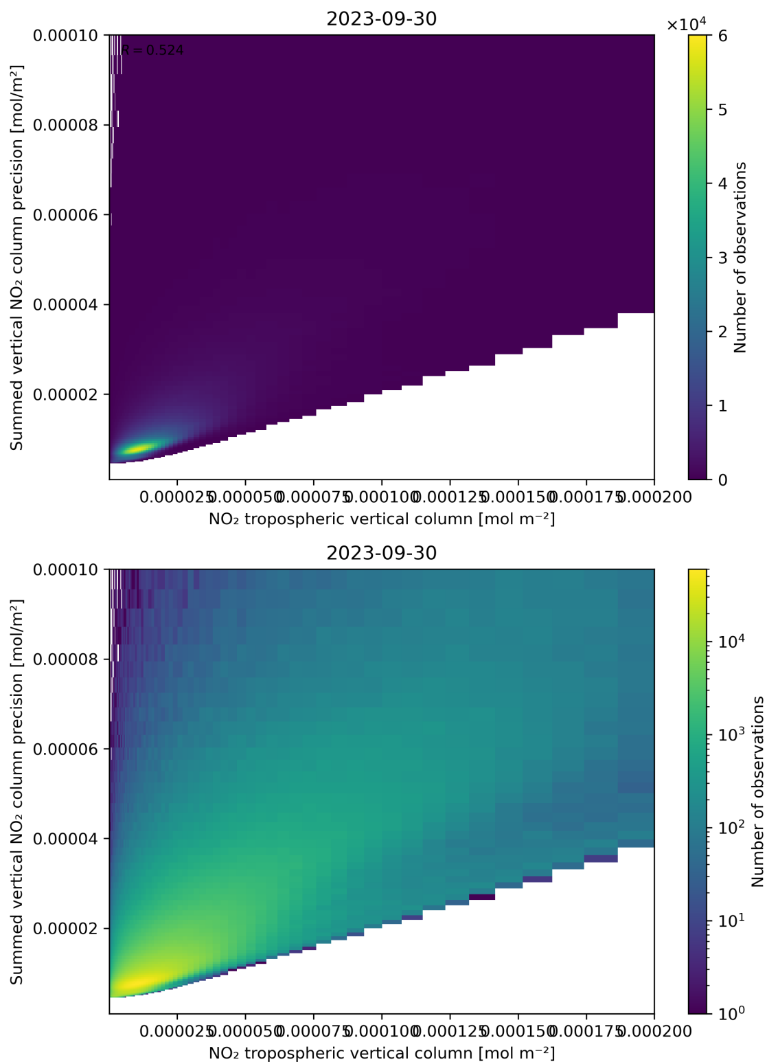
Figure 127: Scatter density plot of “NO 2 tropospheric vertical column” against “Summed vertical NO 2 column precision” for 2023-09-29 to 2023-10-01.
