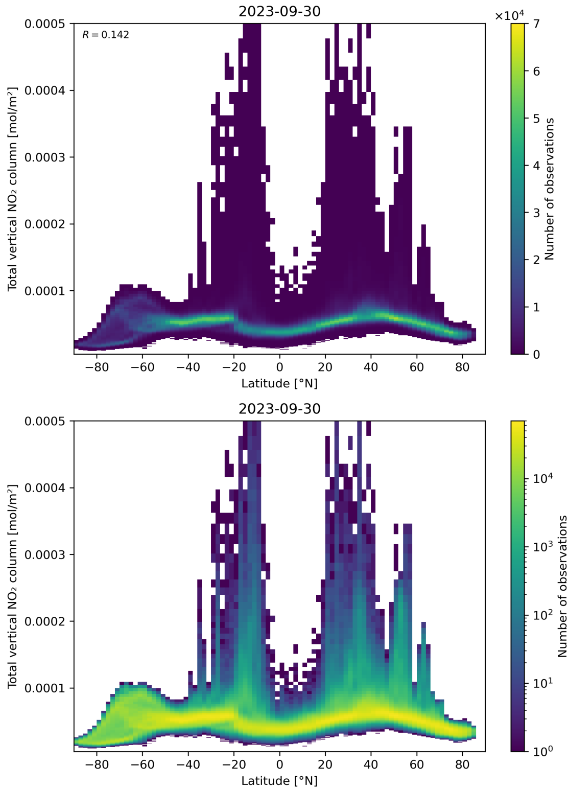
Figure 90: Scatter density plot of “Latitude” against “Total vertical NO 2 column” for 2023-09-29 to 2023-10-01.
