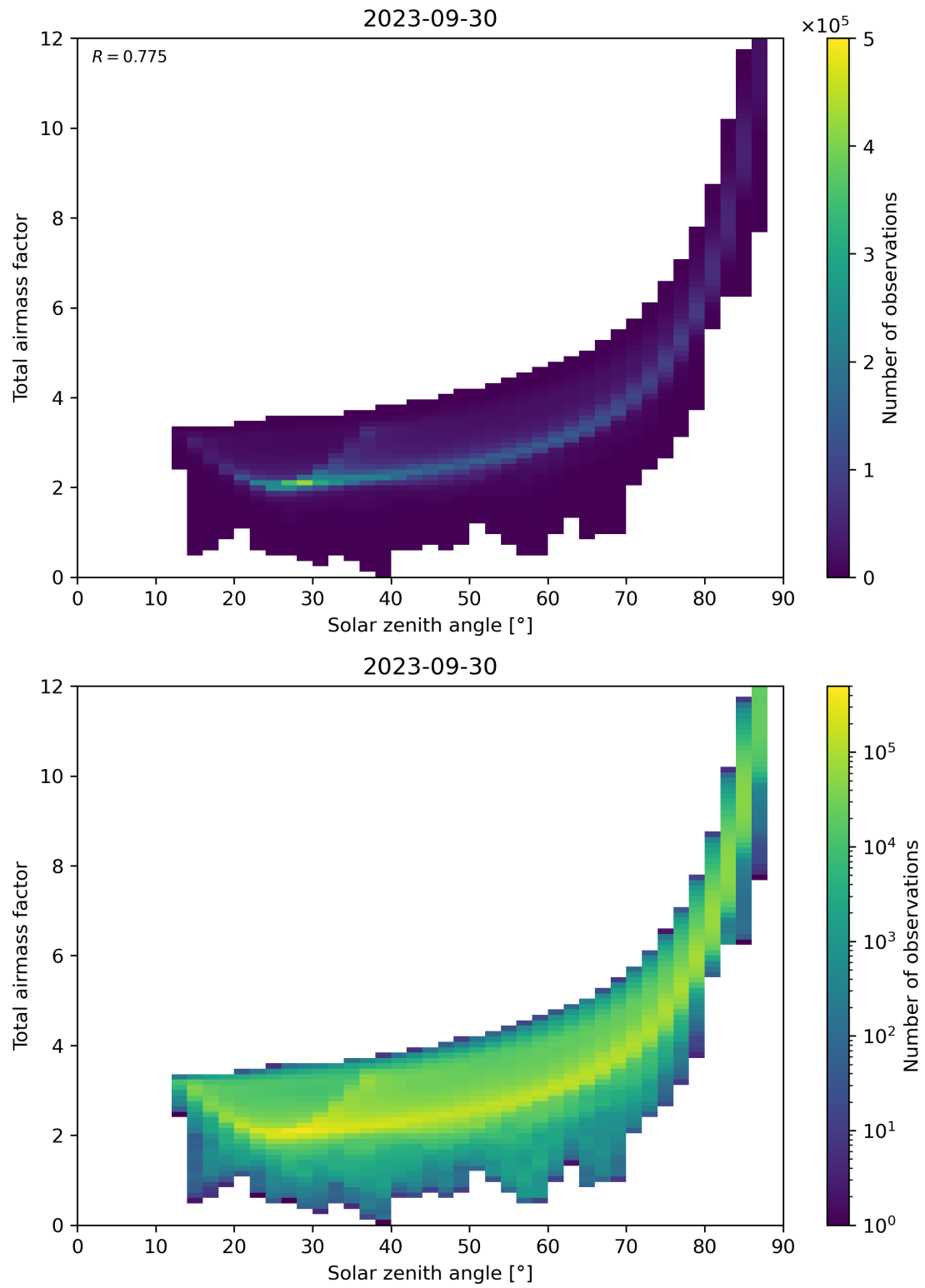
Figure 146: Scatter density plot of “Solar zenith angle” against “Total airmass factor” for 2023-09-29 to 2023-10-01.
