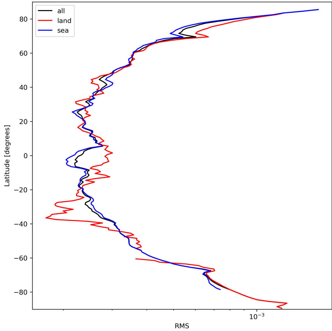
Figure 26: Zonal average of “RMS” for 2023-09-29 to 2023-10-01.
