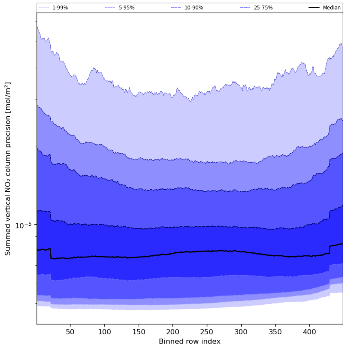
Figure 58: Along track statistics of “Summed vertical NO 2 column precision” for 2023-09-29 to 2023-10-01
