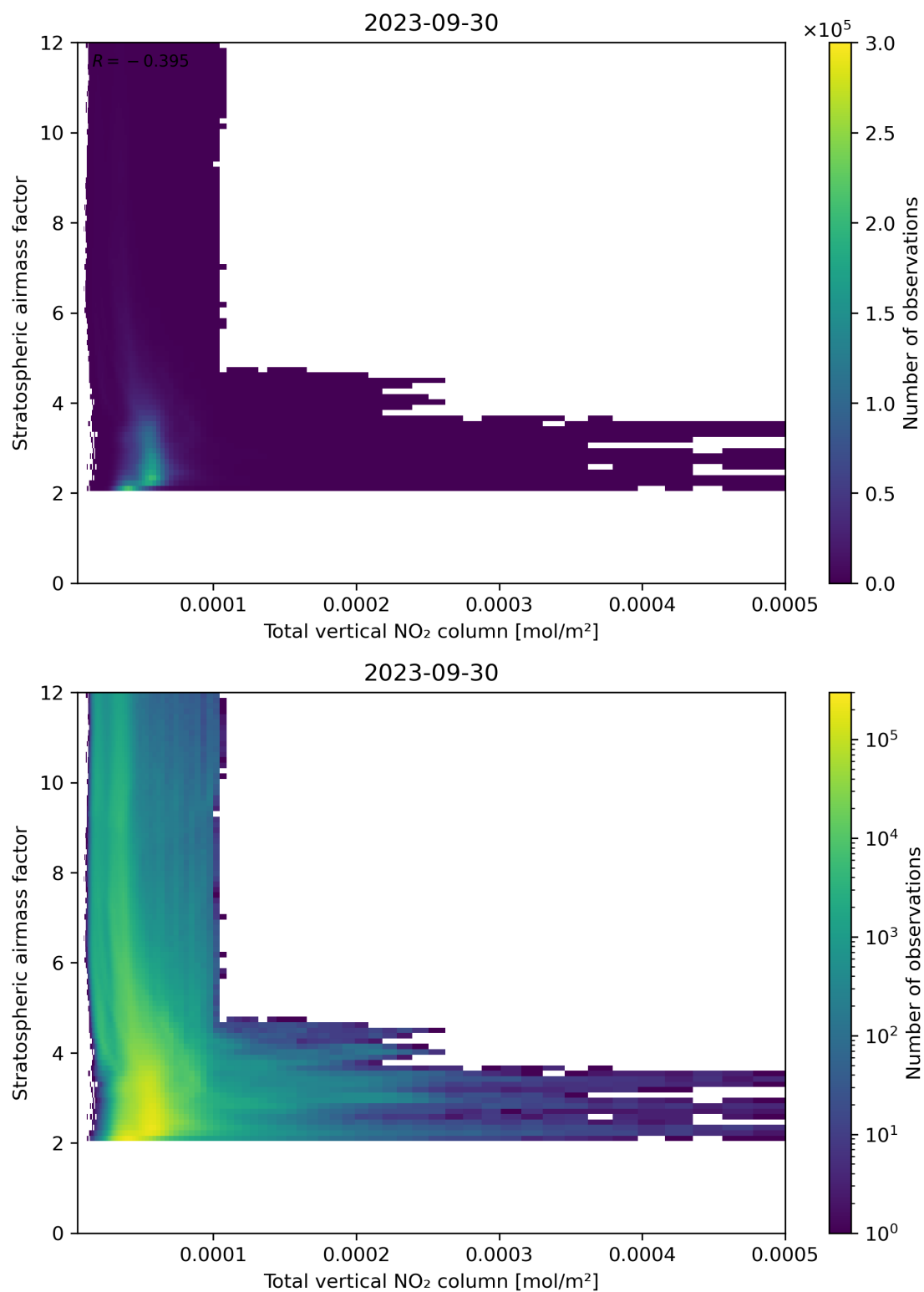
Figure 110: Scatter density plot of “Total vertical NO 2 column” against “Stratospheric airmass factor” for 2023-09-29 to 2023-10-01.
