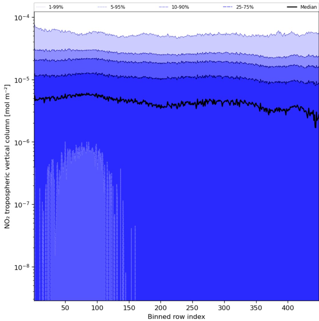
Figure 46: Along track statistics of “NO 2 tropospheric vertical column” for 2023-09-29 to 2023-10-01
