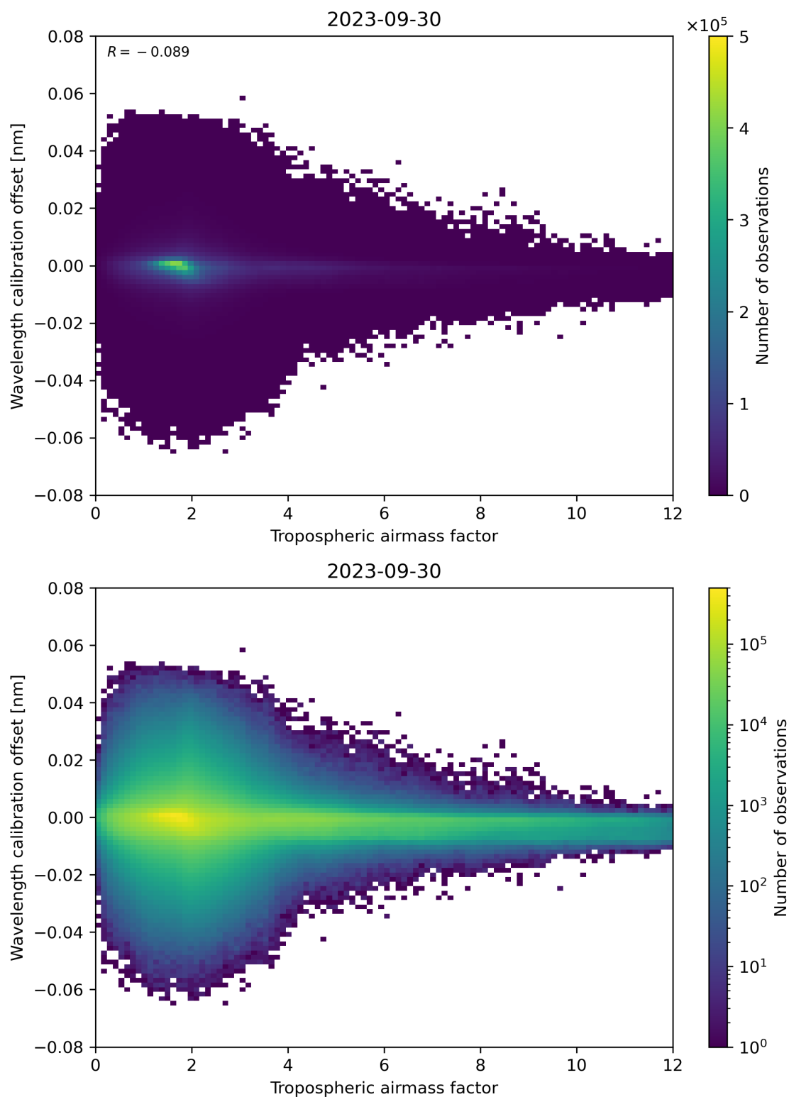
Figure 80: Scatter density plot of “Tropospheric airmass factor” against “Wavelength calibration offset” for 2023-09-29 to 2023-10-01.
