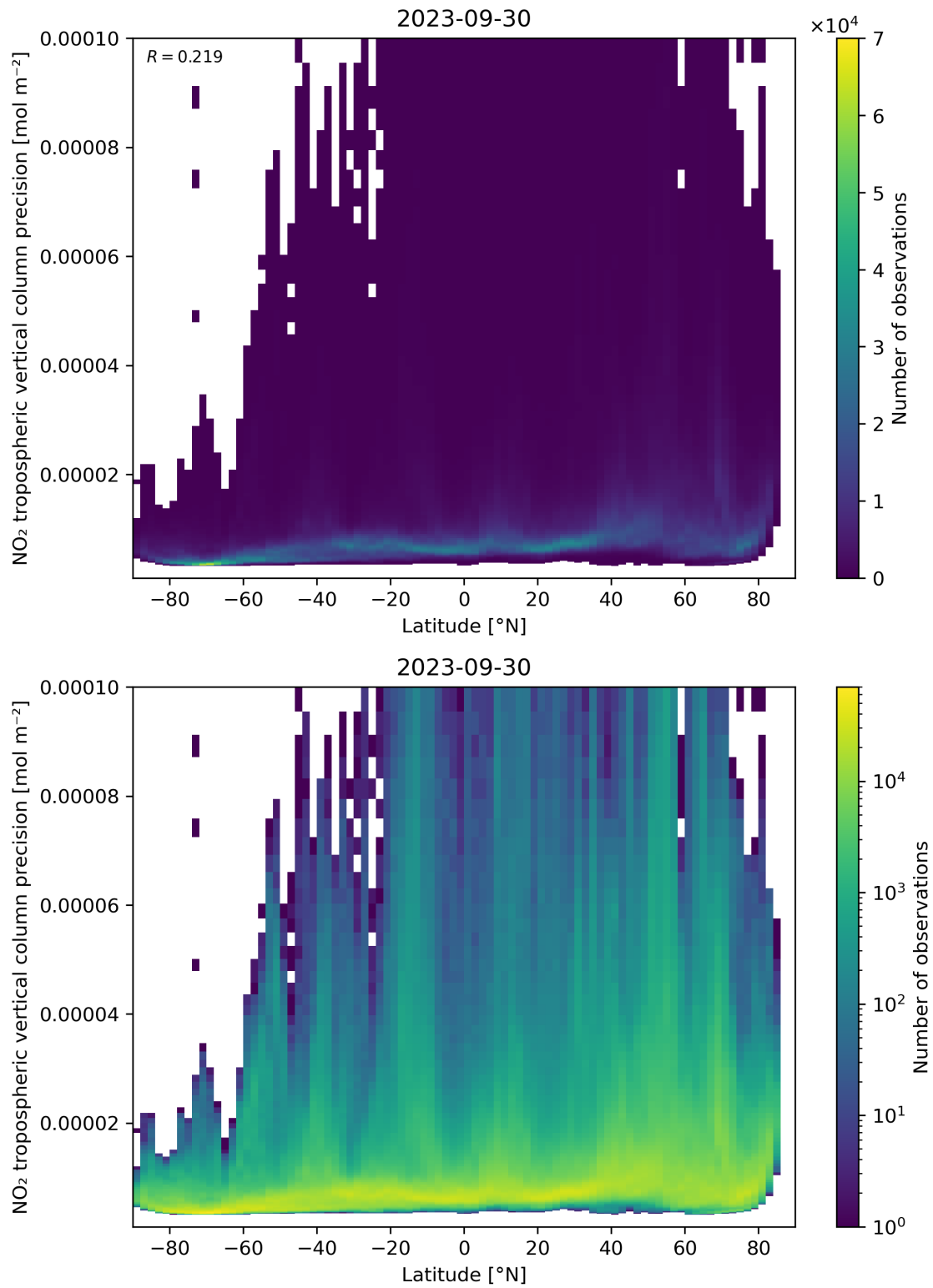
Figure 93: Scatter density plot of “Latitude” against “NO 2 tropospheric vertical column precision” for 2023-09-29 to 2023-10-01.
