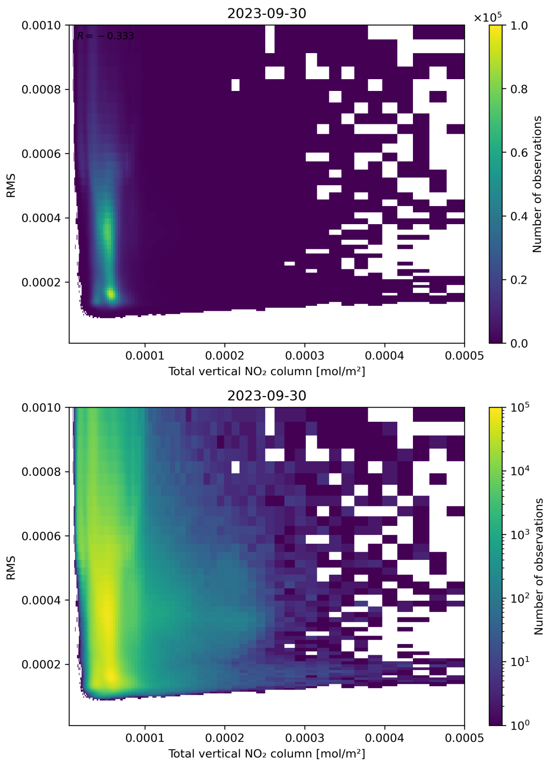
Figure 120: Scatter density plot of “Total vertical NO 2 column” against “RMS” for 2023-09-29 to 2023-10-01.
