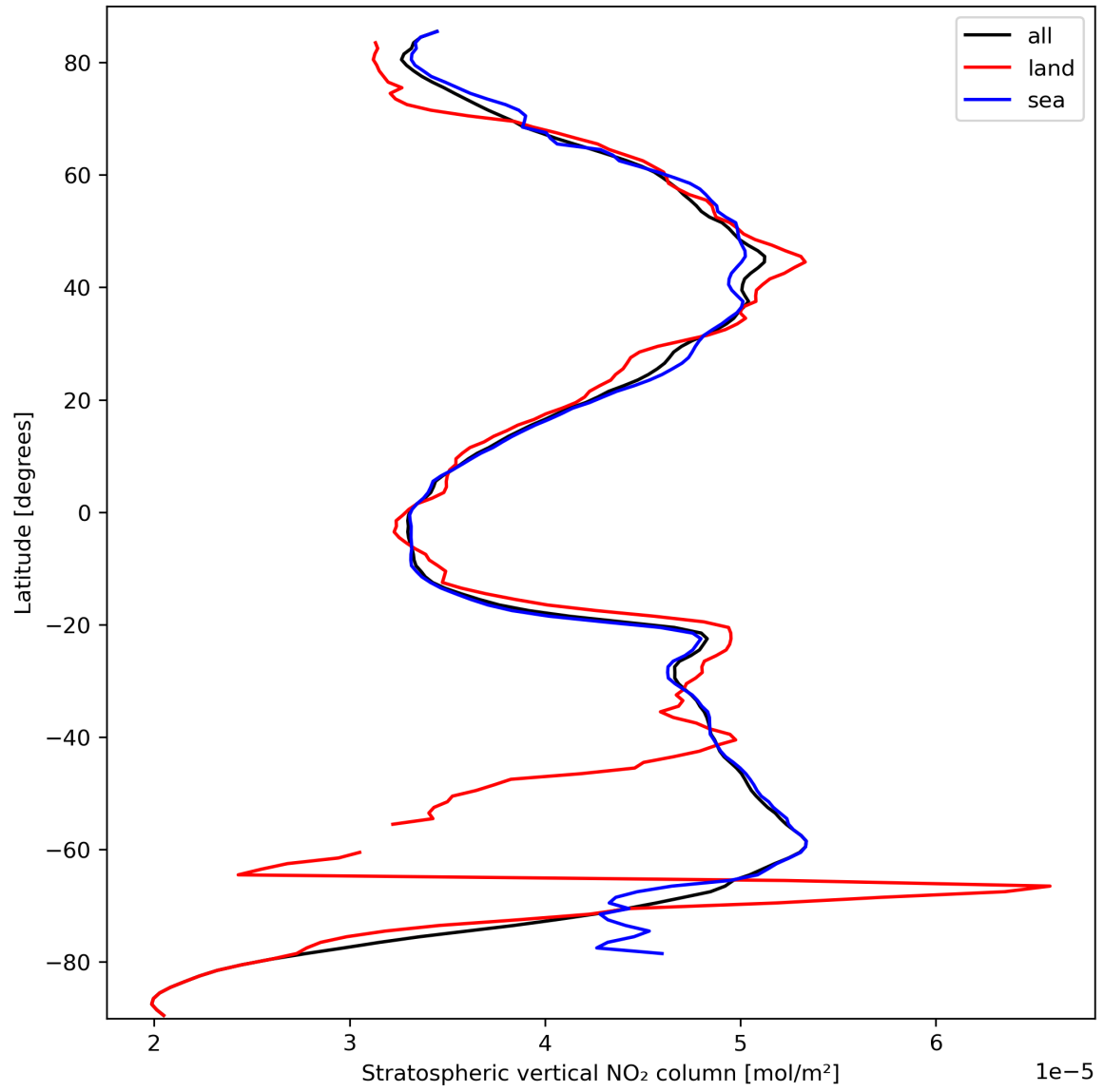
Figure 19: Zonal average of “Stratospheric vertical NO 2 column” for 2023-09-29 to 2023-10-01.
