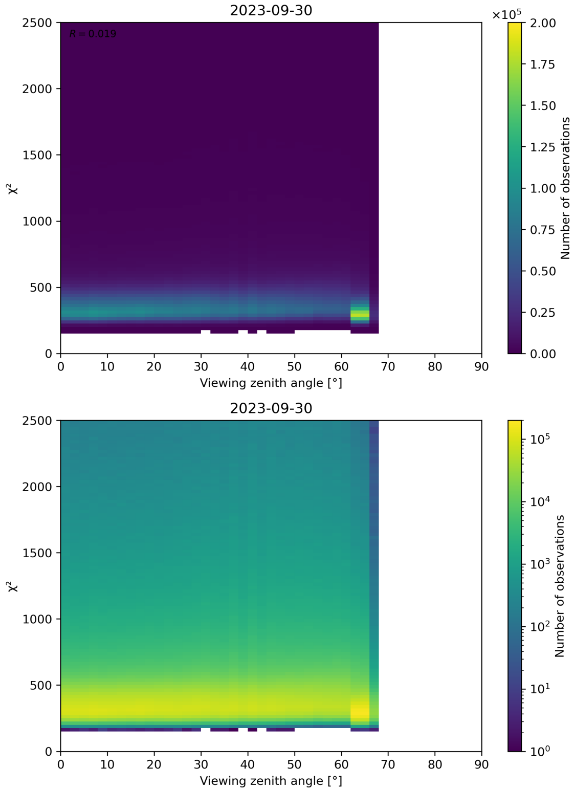
Figure 162: Scatter density plot of “Viewing zenith angle” against “ \chi^2 ” for 2023-09-29 to 2023-10-01.
