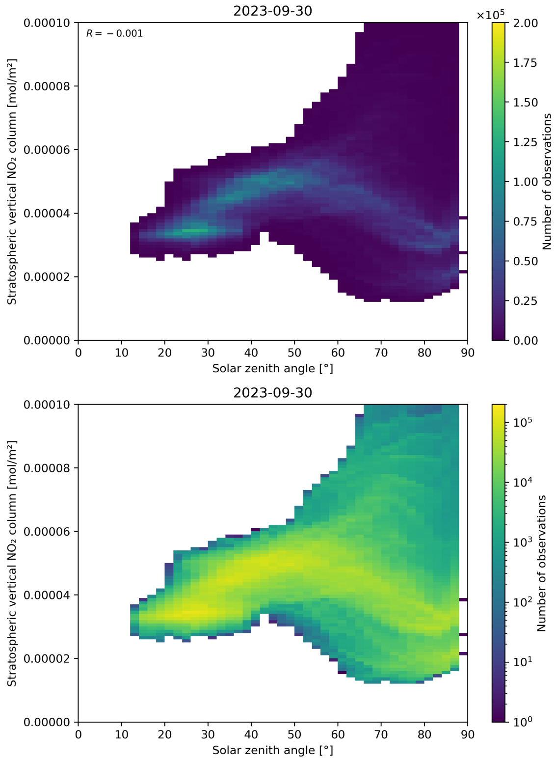
Figure 150: Scatter density plot of “Solar zenith angle” against “Stratospheric vertical NO 2 column” for 2023-09-29 to 2023-10-01.
