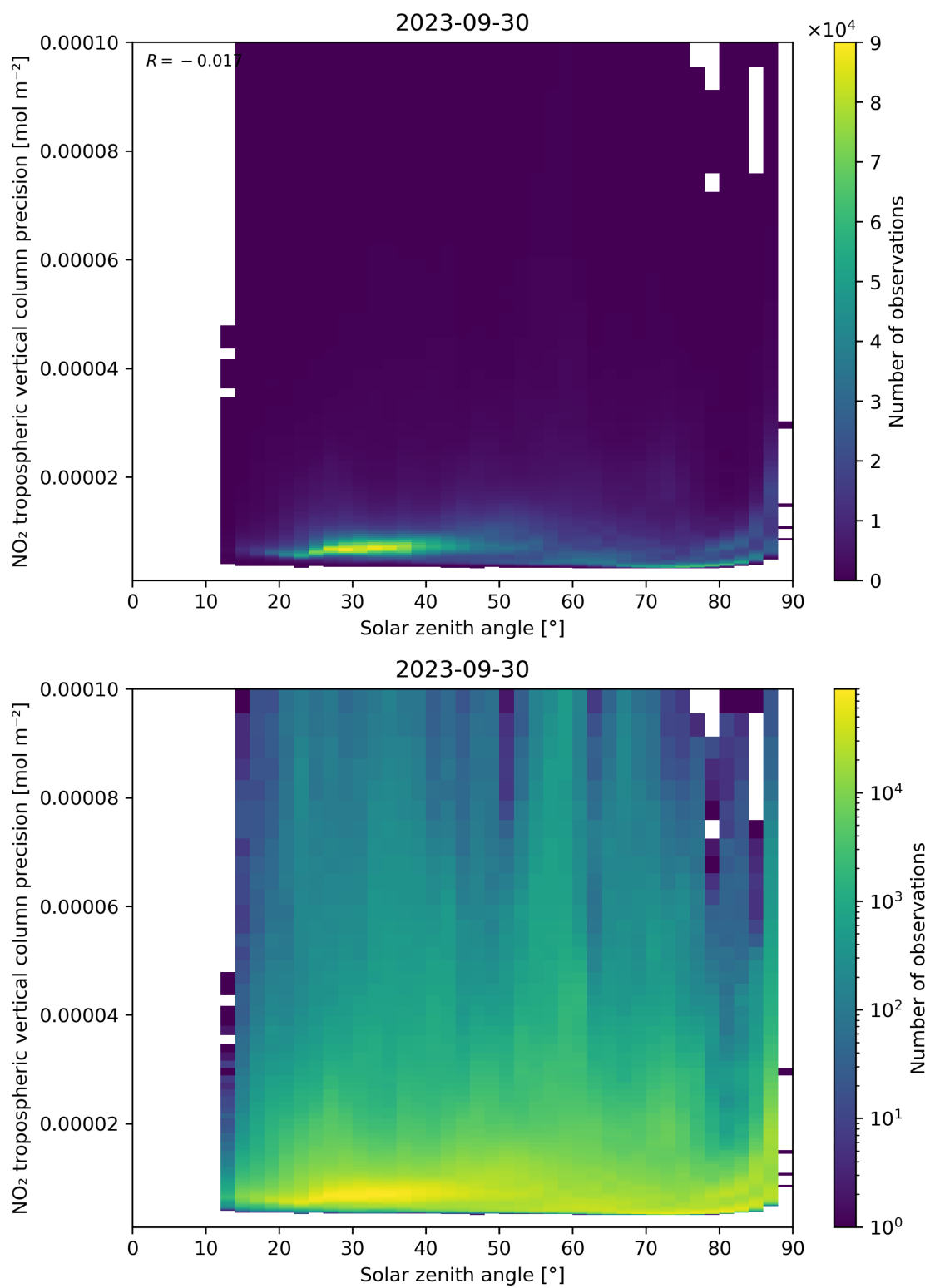
Figure 156: Scatter density plot of “Solar zenith angle” against “NO 2 tropospheric vertical column precision” for 2023-09-29 to 2023-10-01.
