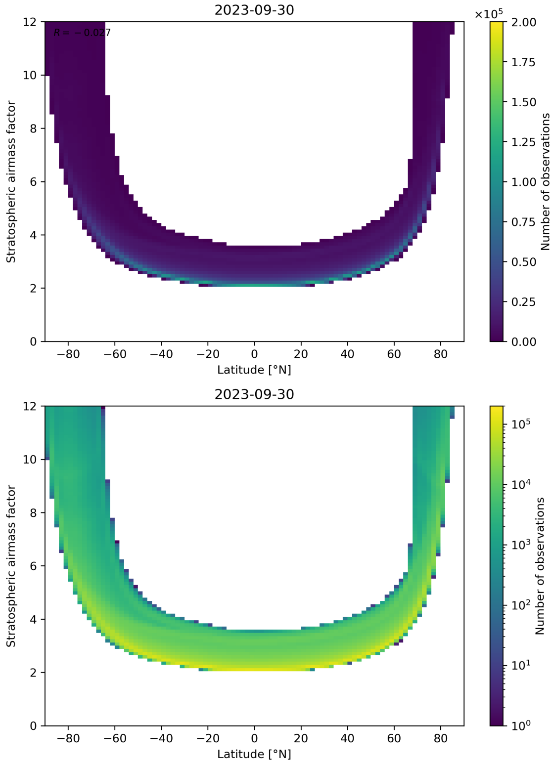
Figure 83: Scatter density plot of “Latitude” against “Stratospheric airmass factor” for 2023-09-29 to 2023-10-01.
