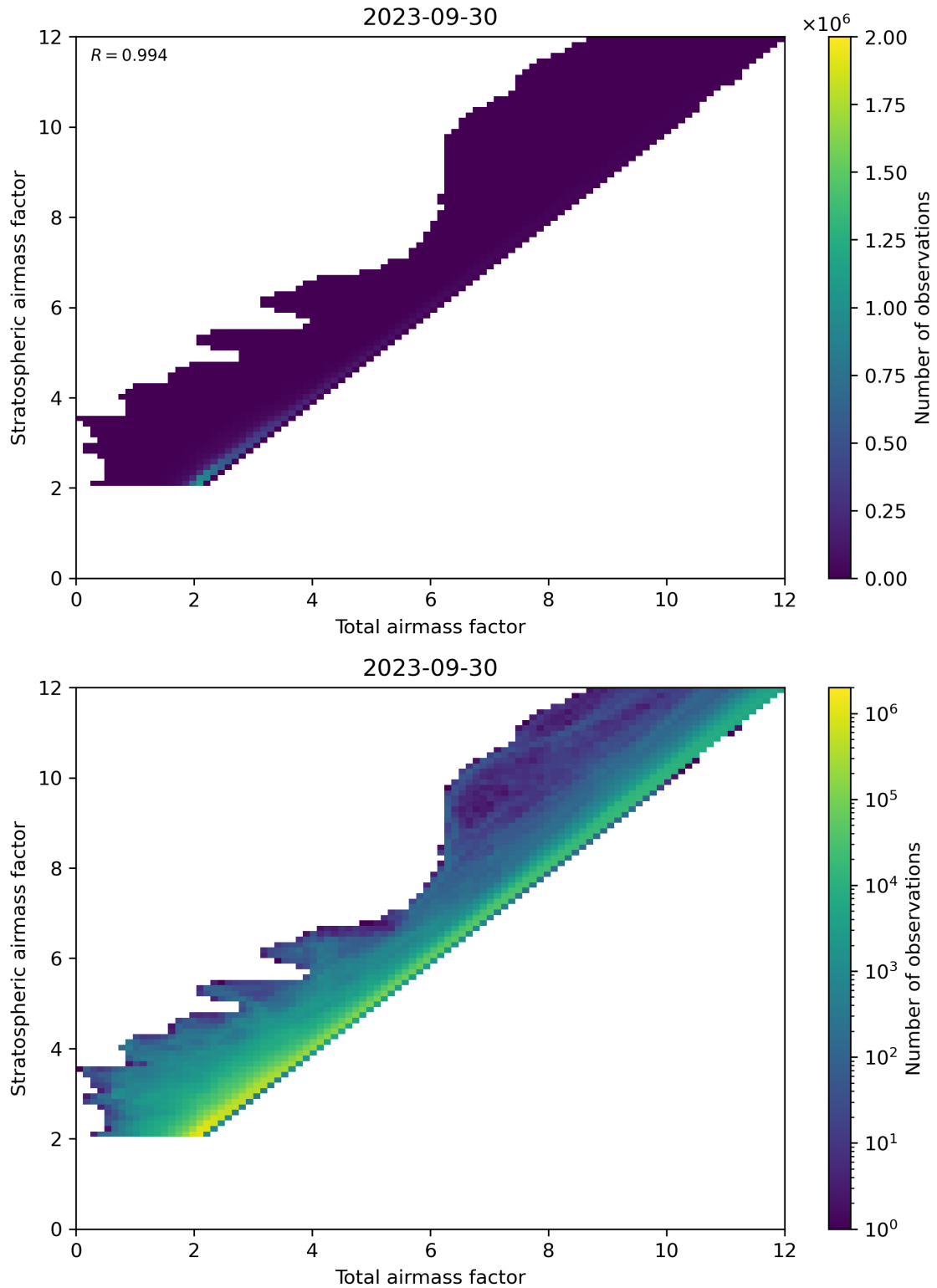
Figure 62: Scatter density plot of “Total airmass factor” against “Stratospheric airmass factor” for 2023-09-29 to 2023-10-01.
