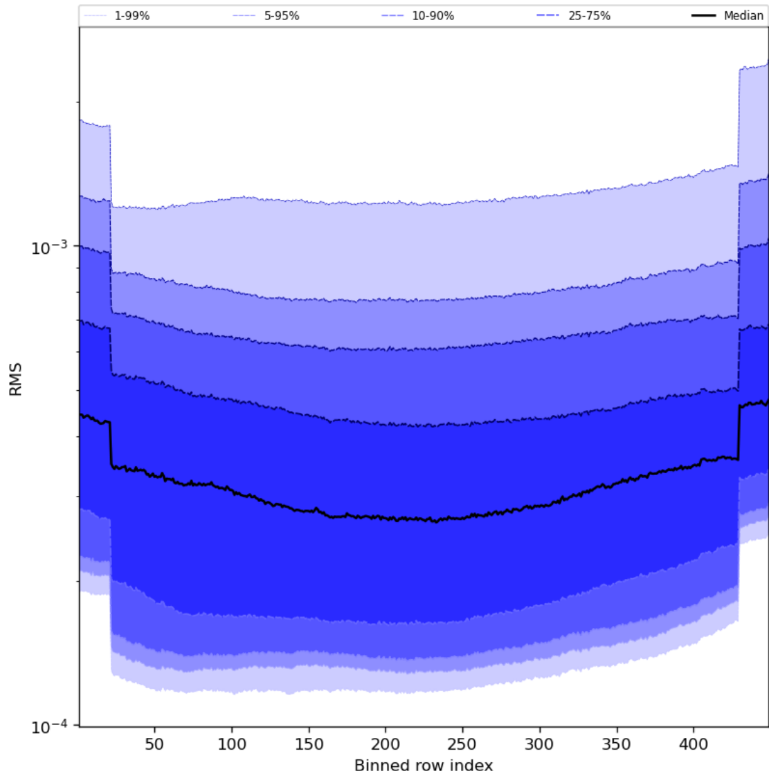
Figure 60: Along track statistics of “RMS” for 2023-09-29 to 2023-10-01
