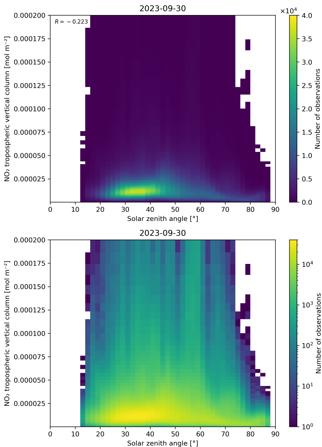
Figure 155: Scatter density plot of “Solar zenith angle” against “NO 2 tropospheric vertical column” for 2023-09-29 to 2023-10-01.
