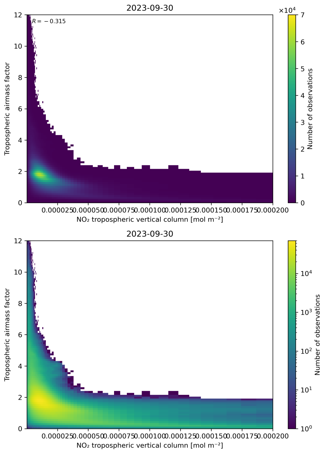
Figure 123: Scatter density plot of “NO 2 tropospheric vertical column” against “Tropospheric airmass factor” for 2023-09-29 to 2023-10-01.
