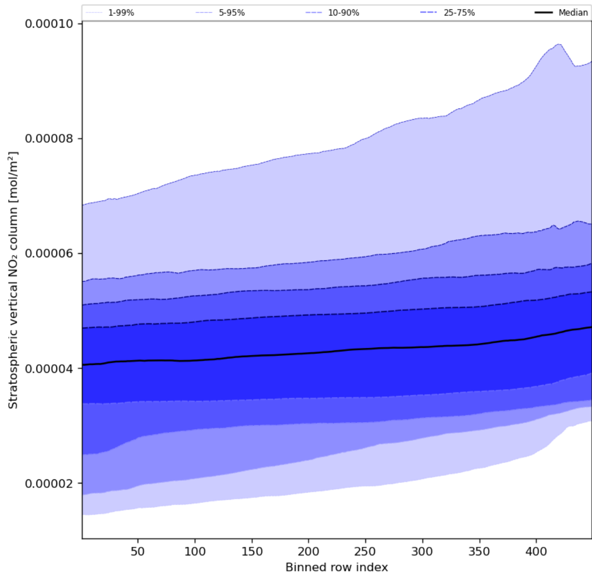
Figure 53: Along track statistics of “Stratospheric vertical NO 2 column” for 2023-09-29 to 2023-10-01
