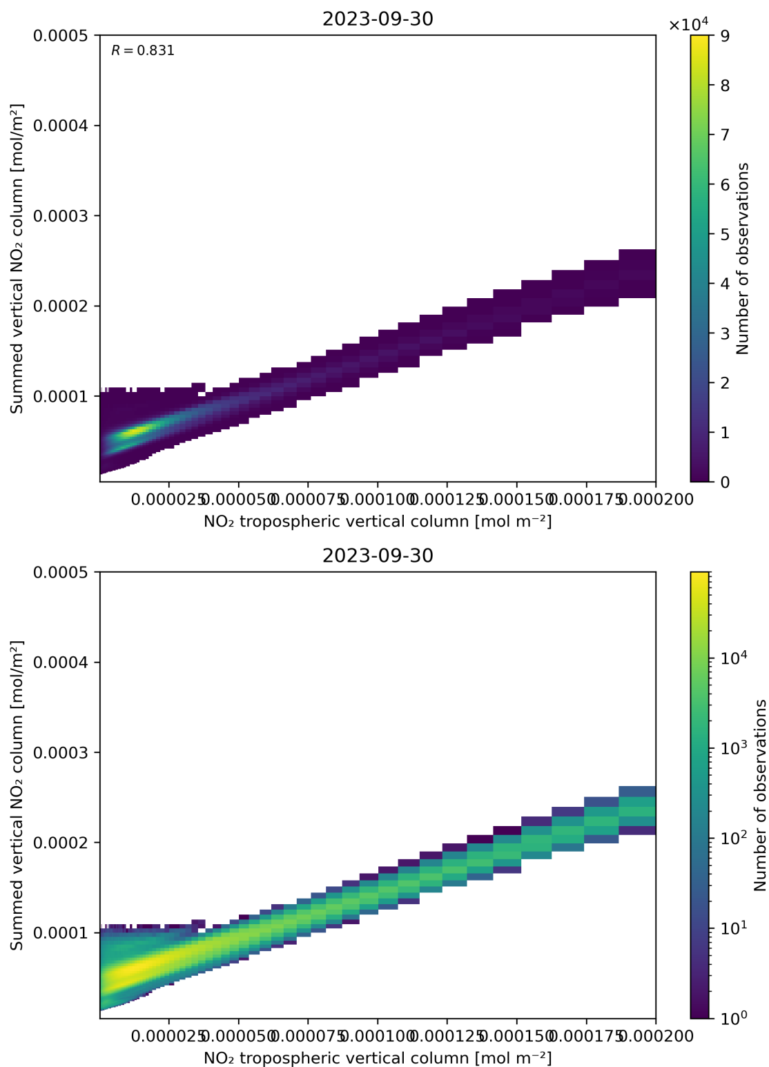
Figure 126: Scatter density plot of “NO 2 tropospheric vertical column” against “Summed vertical NO 2 column” for 2023-09-29 to 2023-10-01.
