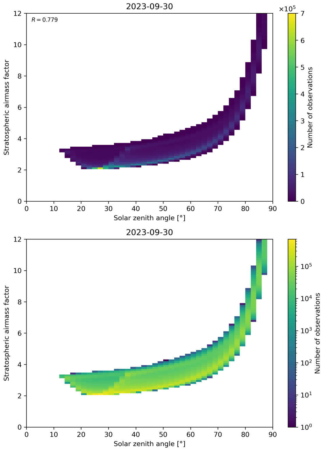
Figure 145: Scatter density plot of “Solar zenith angle” against “Stratospheric airmass factor” for 2023-09-29 to 2023-10-01.
