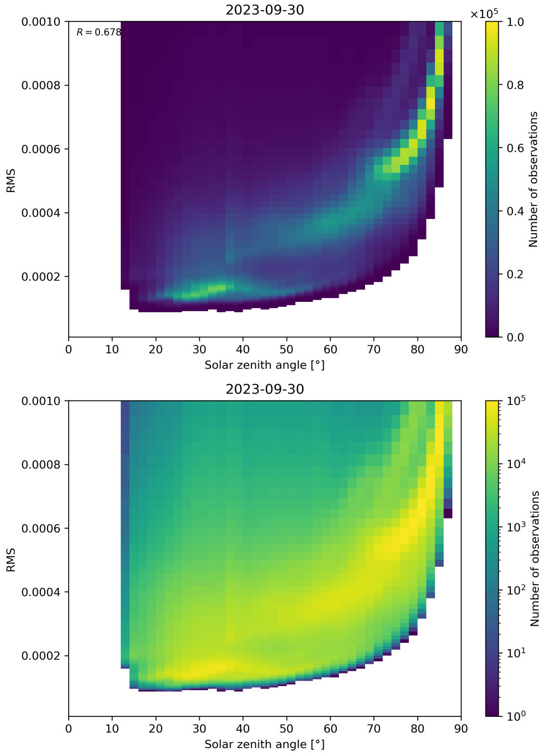
Figure 157: Scatter density plot of “Solar zenith angle” against “RMS” for 2023-09-29 to 2023-10-01.
