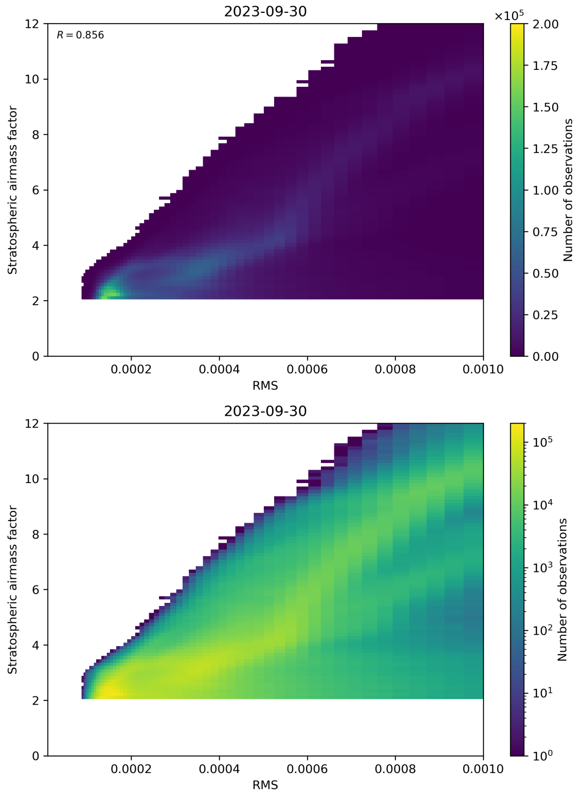
Figure 144: Scatter density plot of “RMS” against “Stratospheric airmass factor” for 2023-09-29 to 2023-10-01.
