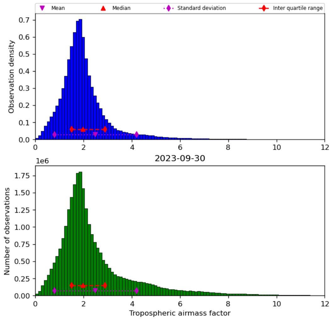
Figure 31: Histogram of “Tropospheric airmass factor” for 2023-09-29 to 2023-10-01
