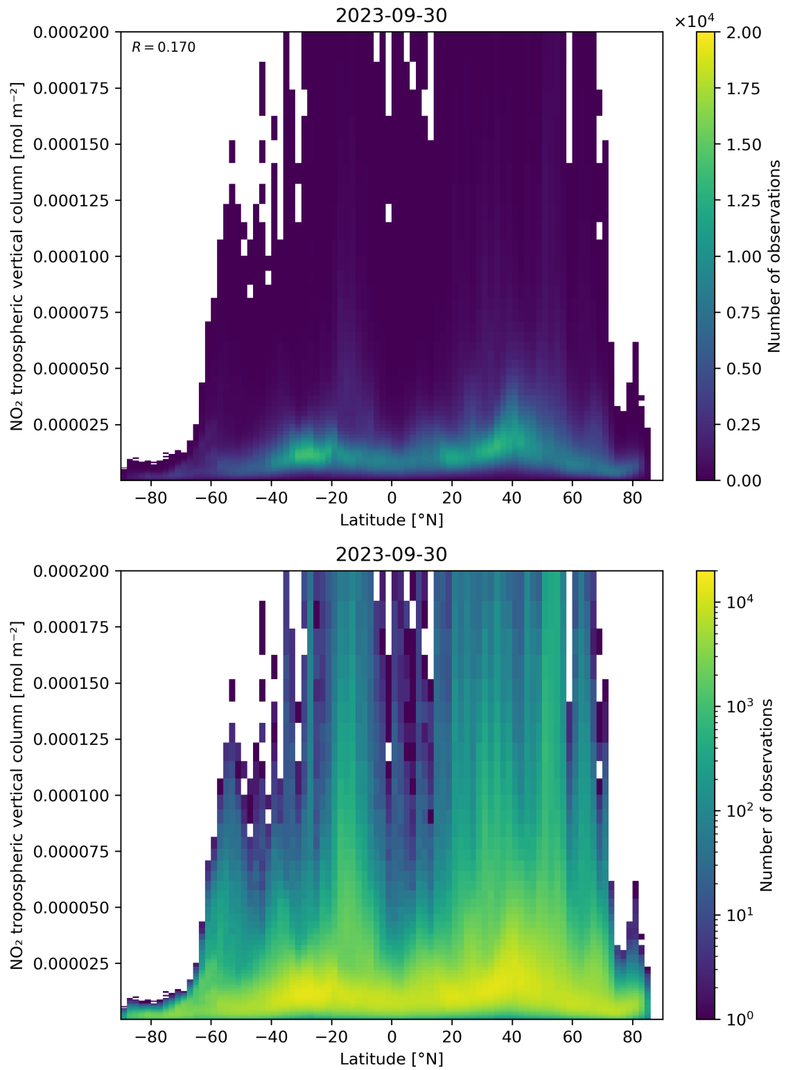
Figure 92: Scatter density plot of “Latitude” against “NO 2 tropospheric vertical column” for 2023-09-29 to 2023-10-01.
