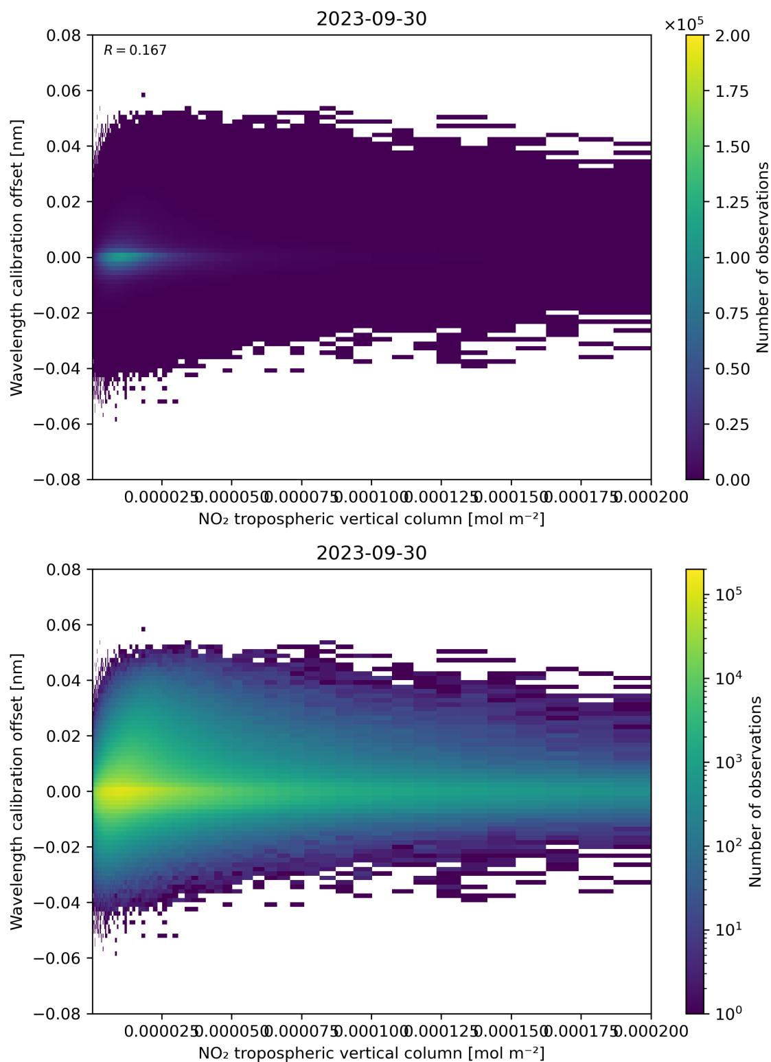
Figure 143: Scatter density plot of “NO 2 tropospheric vertical column” against “Wavelength calibration offset” for 2023-09-29 to 2023-10-01.
