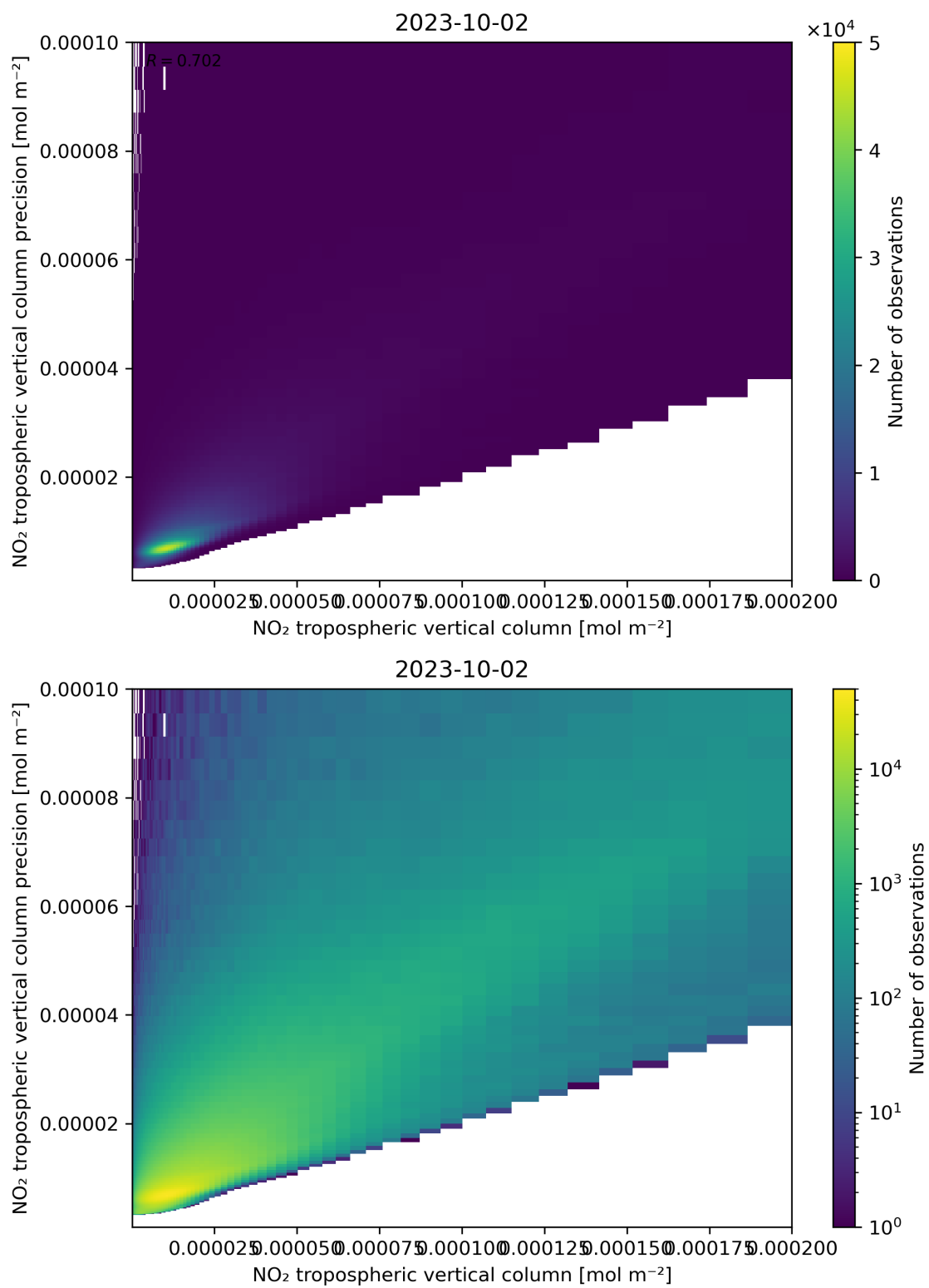
Figure 130: Scatter density plot of “NO 2 tropospheric vertical column” against “NO 2 tropospheric vertical column precision” for 2023-10-01 to 2023-10-03.
