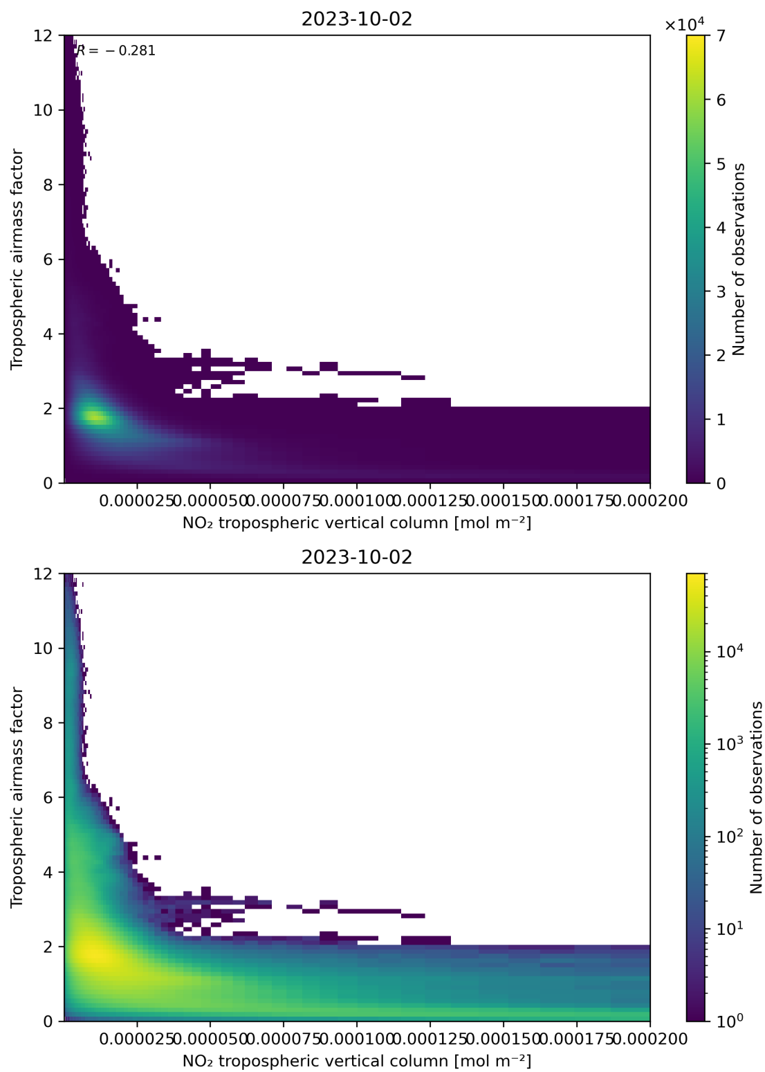
Figure 123: Scatter density plot of “NO 2 tropospheric vertical column” against “Tropospheric air mass factor” for 2023-10-01 to 2023-10-03.
