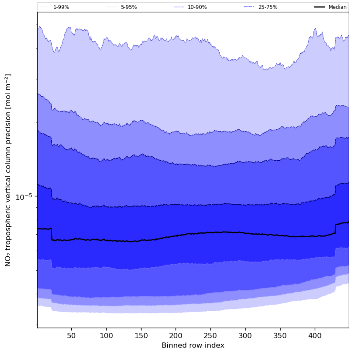
Figure 47: Along track statistics of “NO 2 tropospheric vertical column precision” for 2023-10-01 to 2023-10-03
