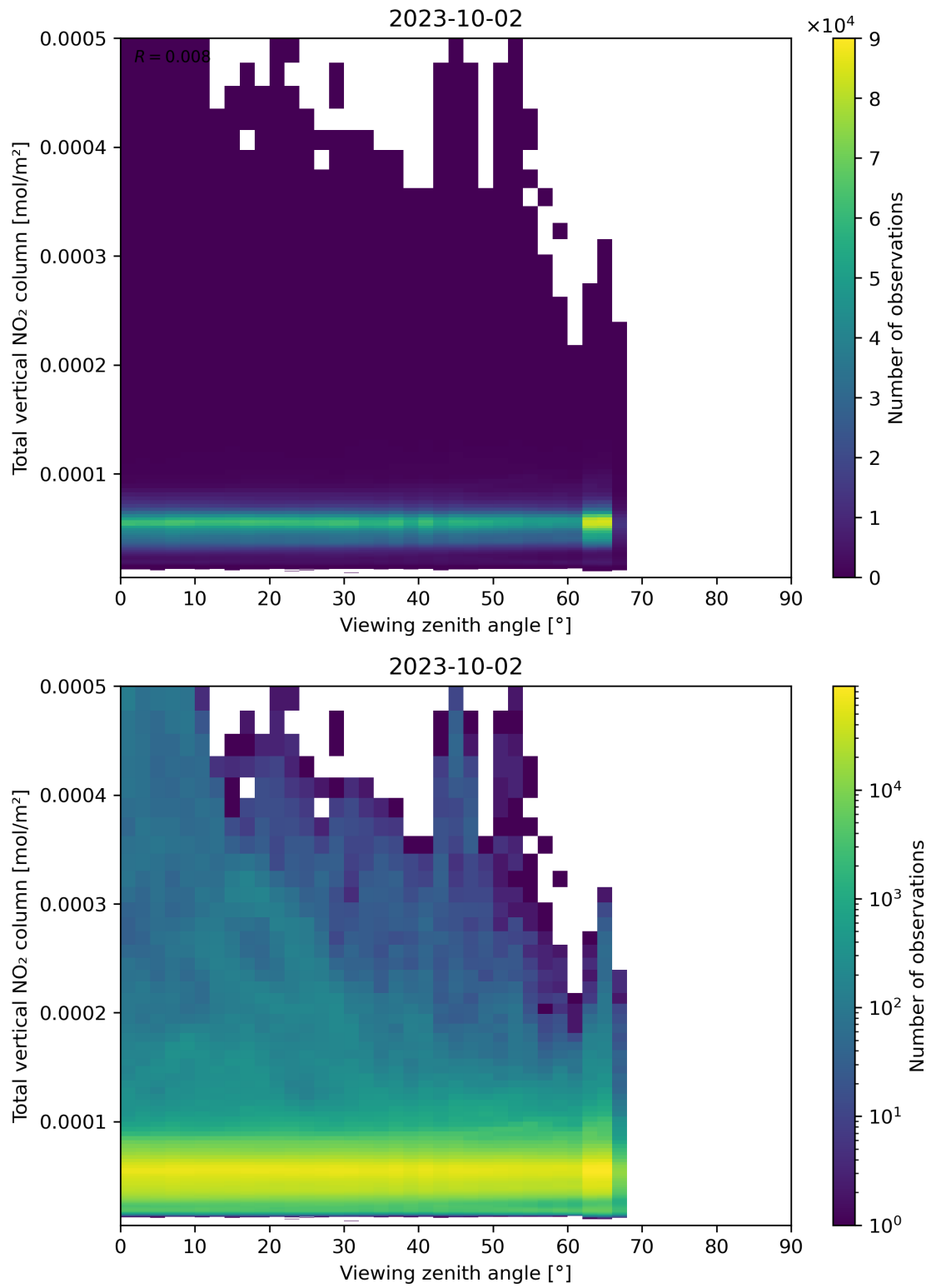
Figure 167: Scatter density plot of “Viewing zenith angle” against “Total vertical NO 2 column” for 2023-10-01 to 2023-10-03.
