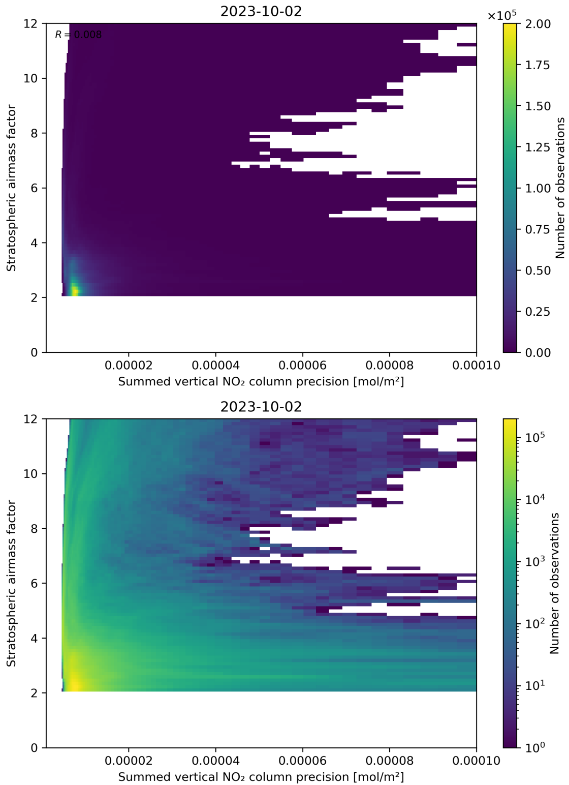
Figure 106: Scatter density plot of “Summed vertical NO 2 column precision” against “Stratospheric airmass factor” for 2023-10-01 to 2023-10-03.
