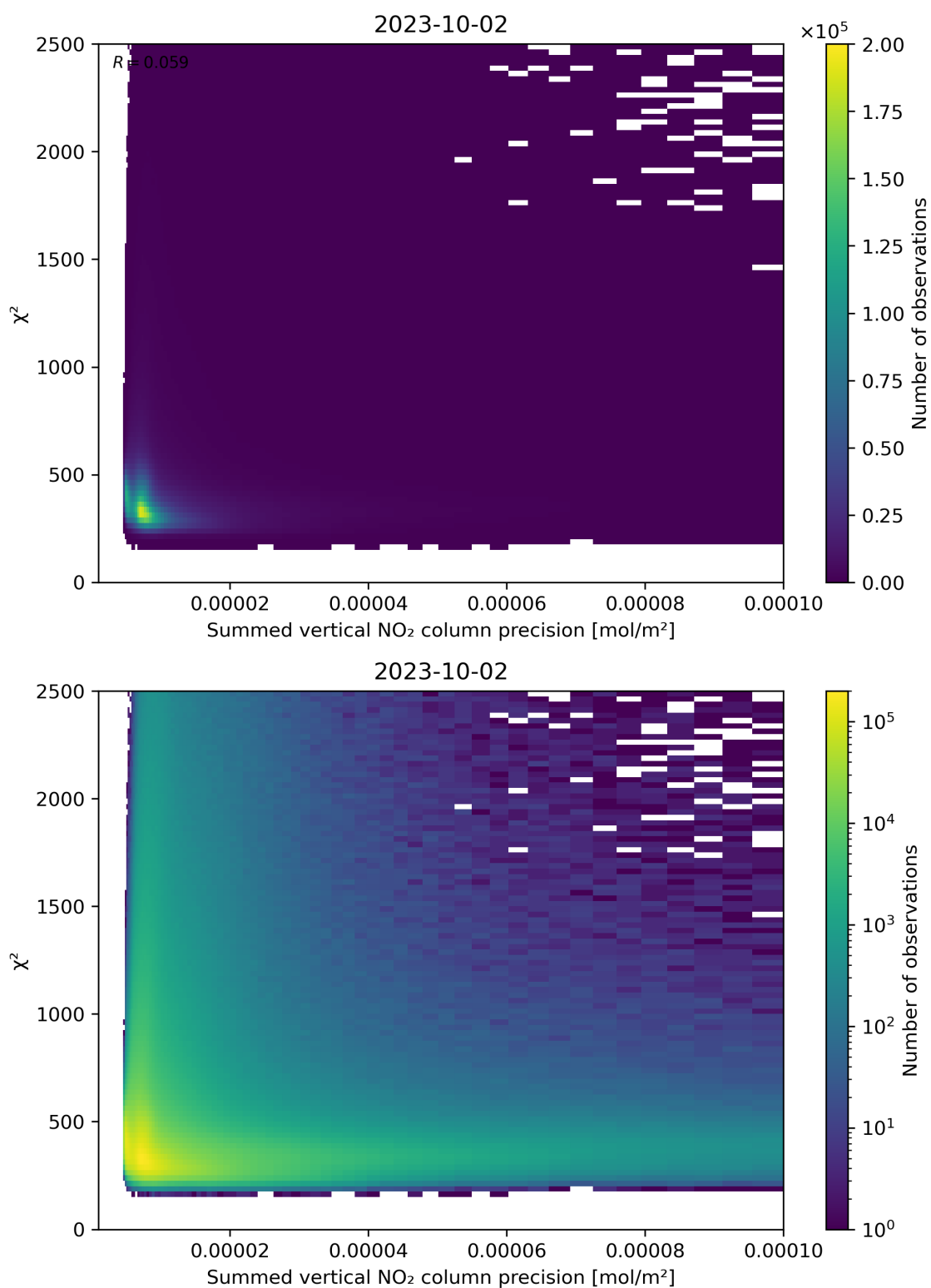
Figure 107: Scatter density plot of “Summed vertical NO 2 column precision” against “ \chi^2 ” for 2023-10-01 to 2023-10-03.
