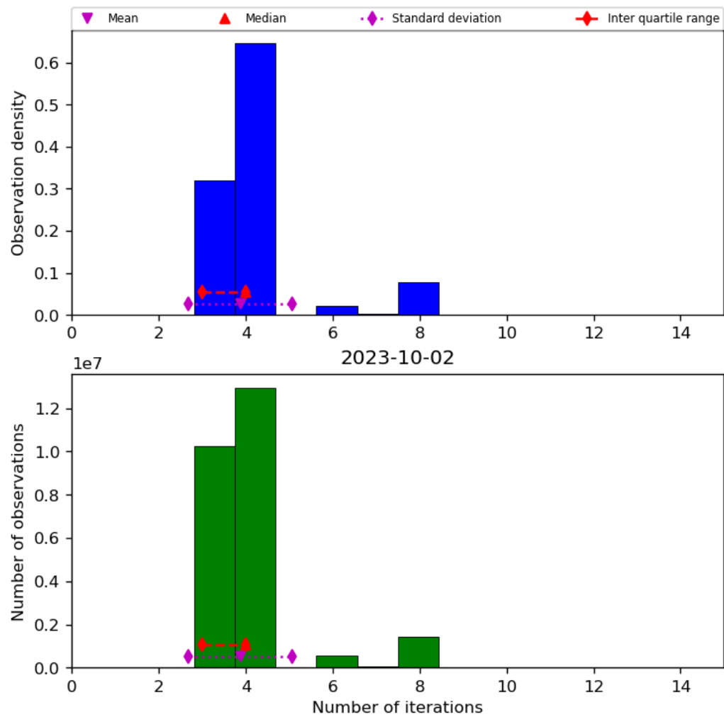
Figure 34: Histogram of “Number of iterations” for 2023-10-01 to 2023-10-03
