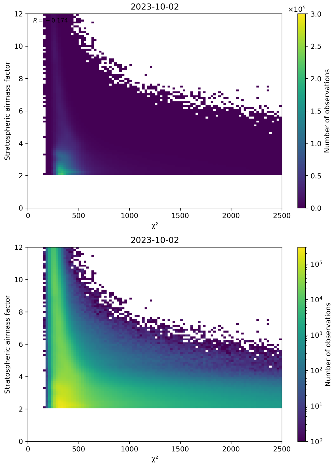
Figure 81: Scatter density plot of “ \chi^2 ” against “Stratospheric airmass factor” for 2023-10-01 to 2023-10-03.
