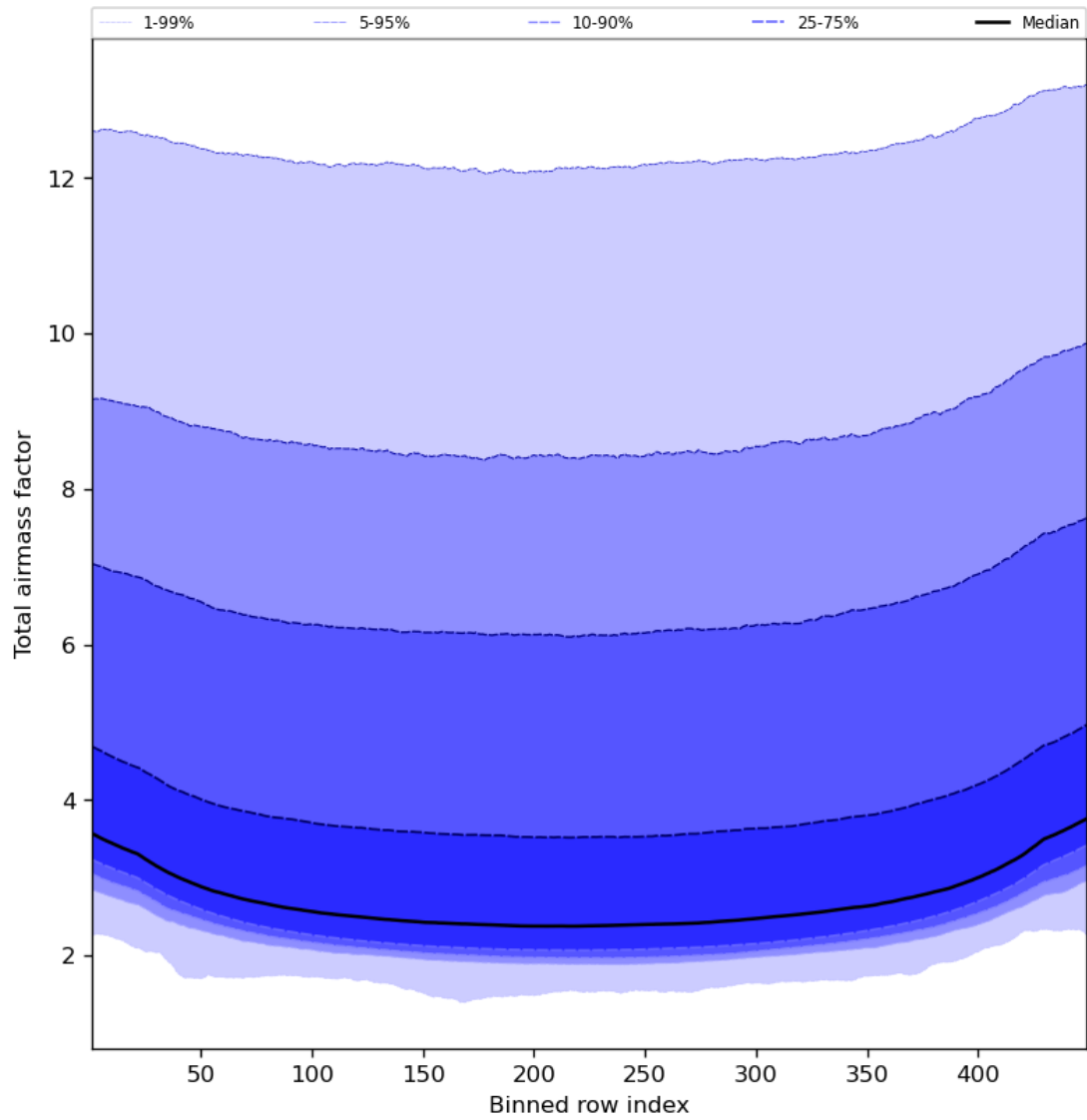
Figure 49: Along track statistics of “Total airmass factor” for 2023-10-01 to 2023-10-03
