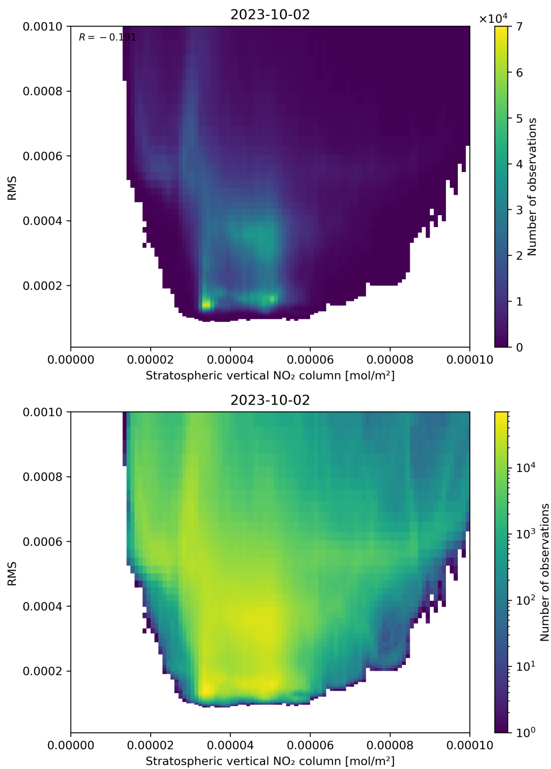
Figure 102: Scatter density plot of “Stratospheric vertical NO 2 column” against “RMS” for 2023-10-01 to 2023-10-03.
