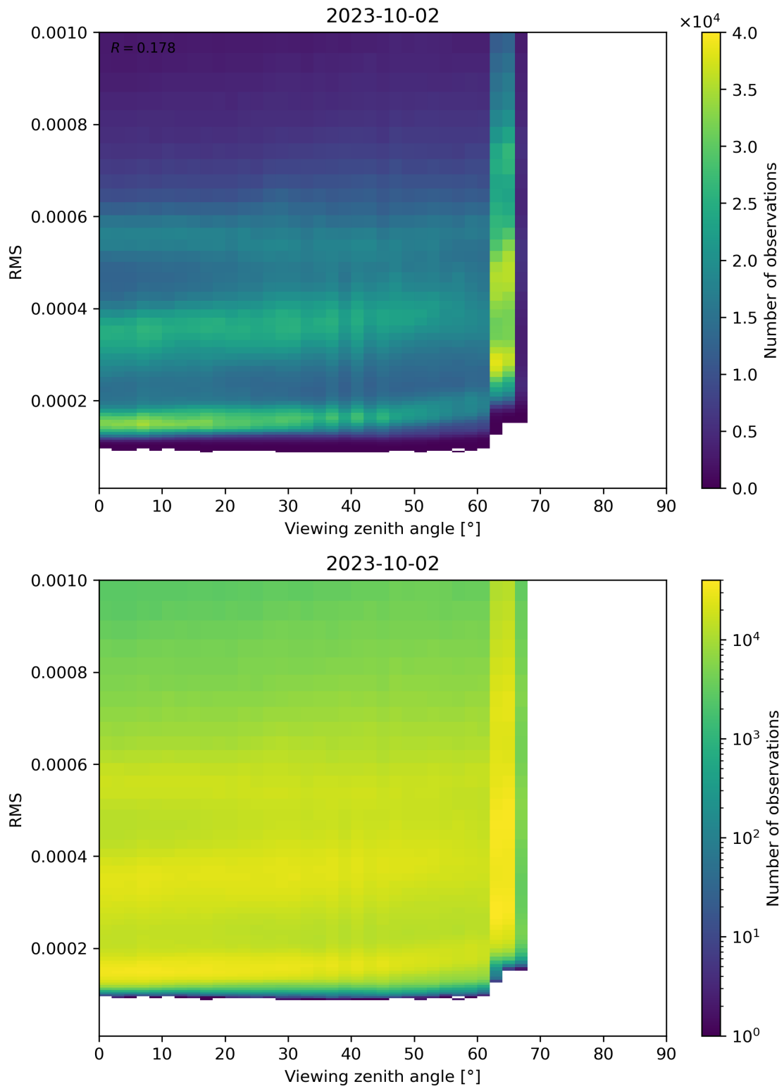
Figure 171: Scatter density plot of “Viewing zenith angle” against “RMS” for 2023-10-01 to 2023-10-03.
