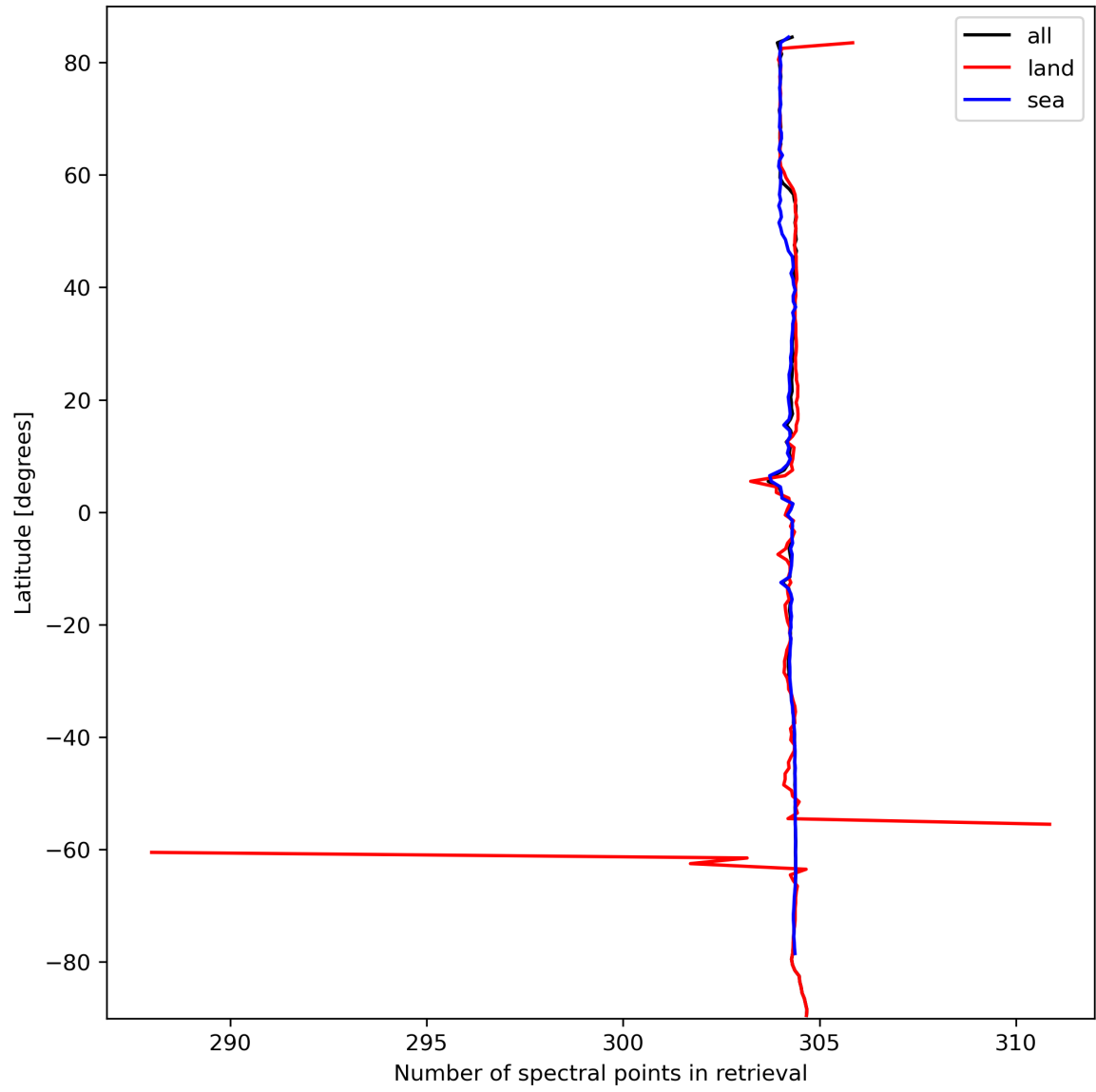
Figure 16: Zonal average of “Number of spectral points in retrieval” for 2023-10-01 to 2023-10-03.
