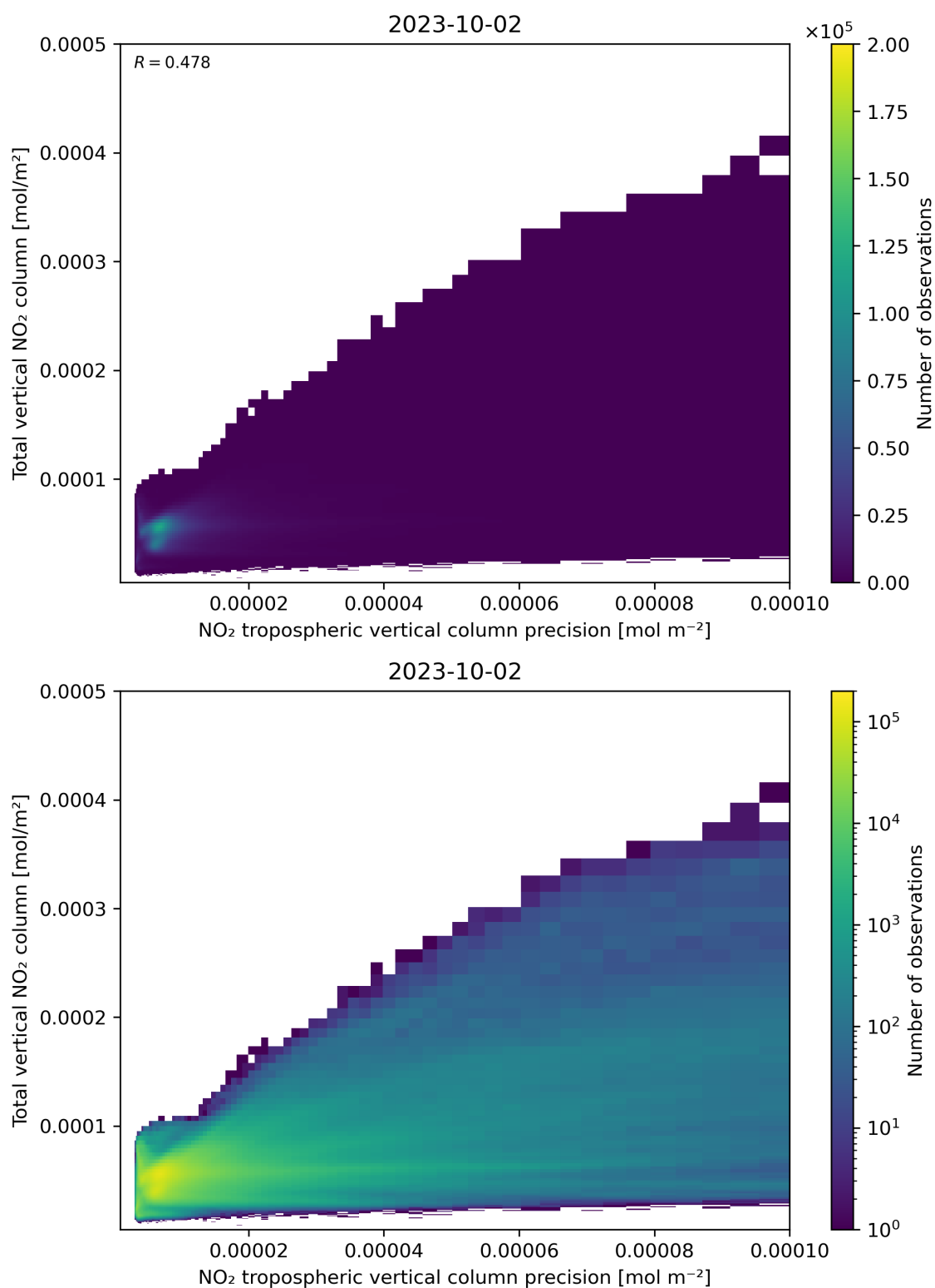
Figure 138: Scatter density plot of “NO 2 tropospheric vertical column precision” against “Total vertical NO 2 column” for 2023-10-01 to 2023-10-03.
