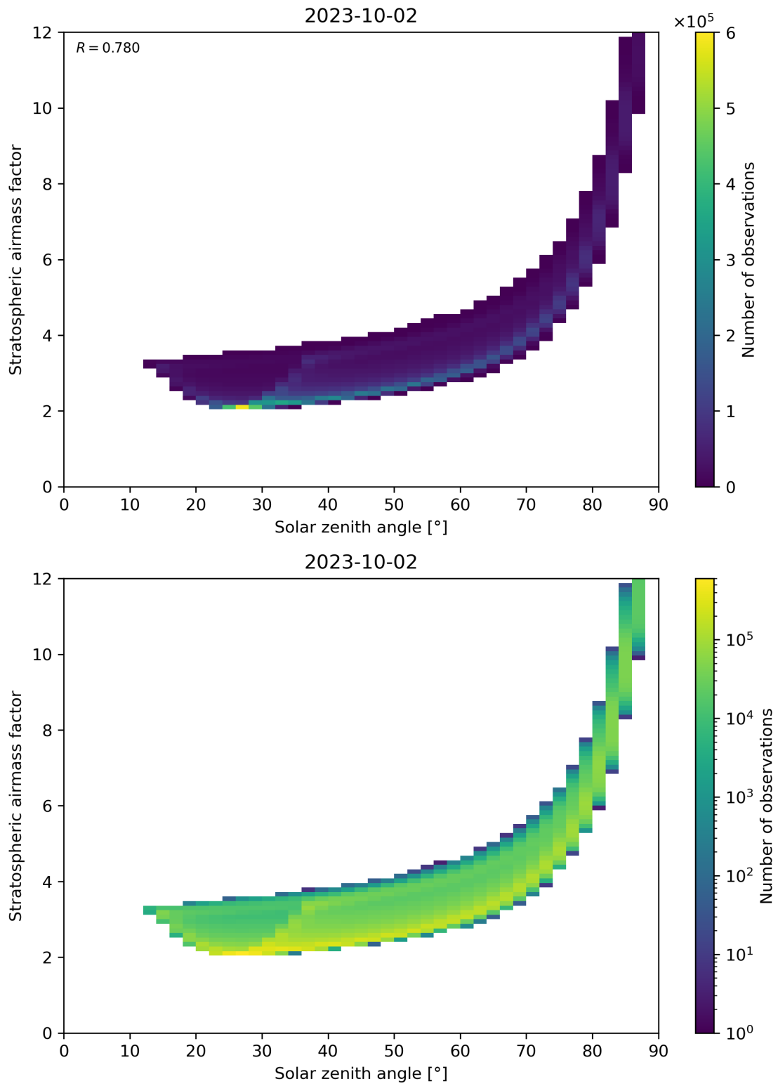
Figure 145: Scatter density plot of “Solar zenith angle” against “Stratospheric airmass factor” for 2023-10-01 to 2023-10-03.
