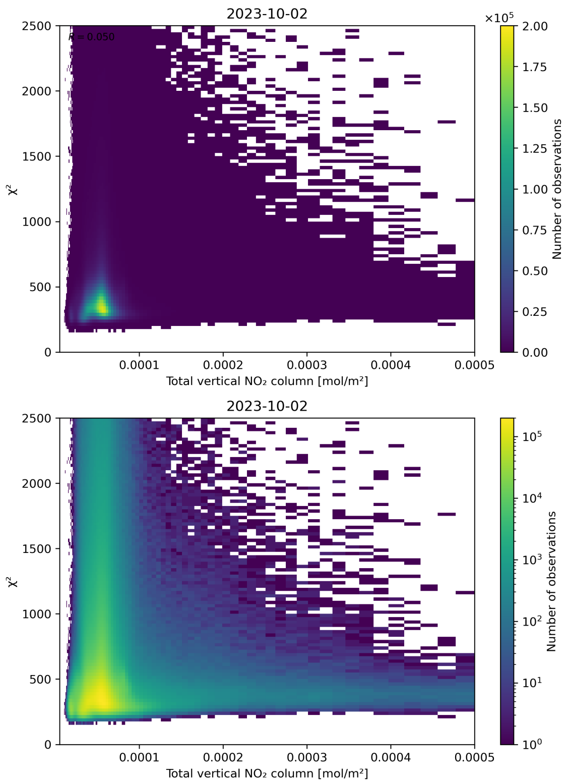
Figure 111: Scatter density plot of “Total vertical NO 2 column” against “ \chi^2 ” for 2023-10-01 to 2023-10-03.
