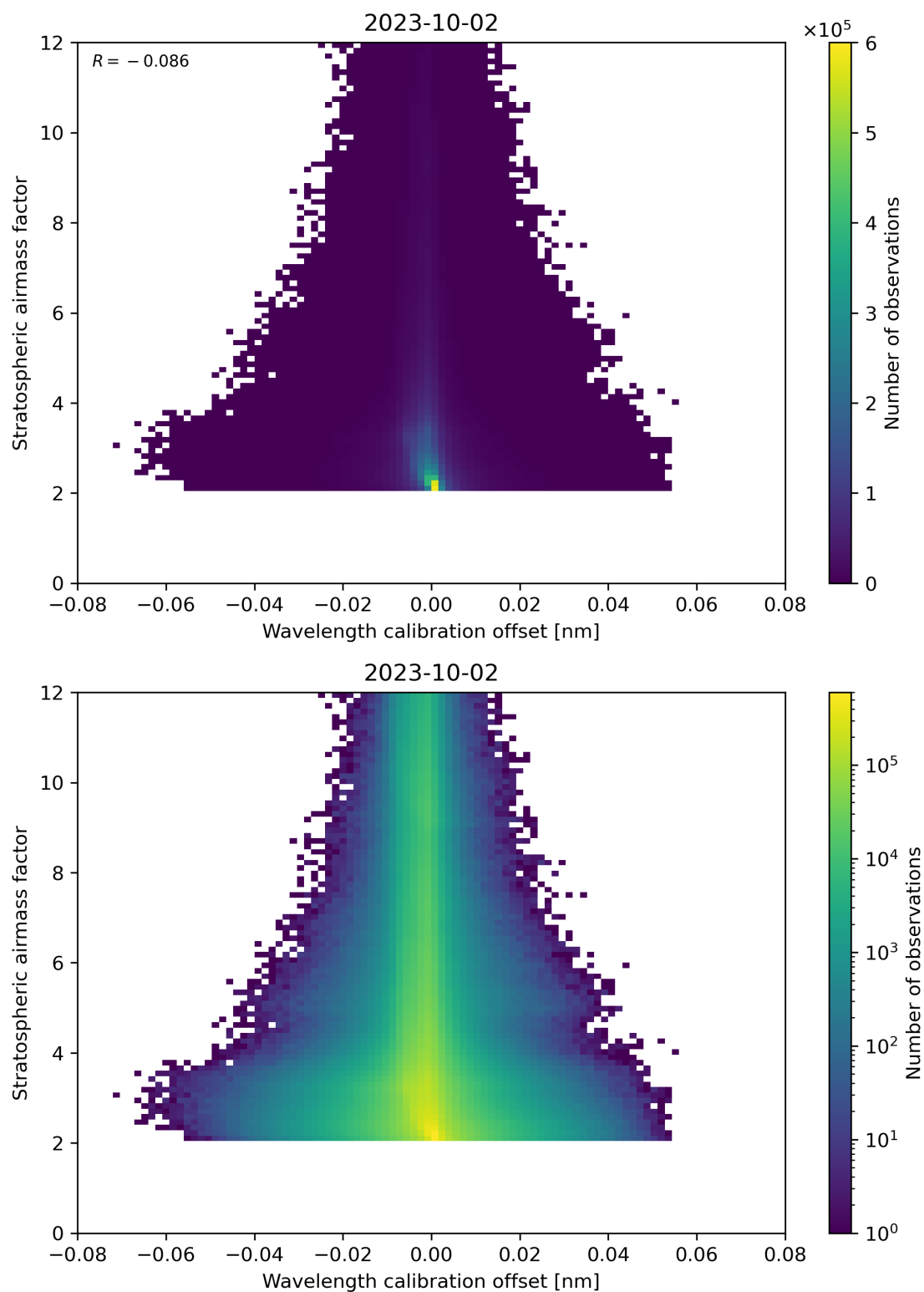
Figure 174: Scatter density plot of “Wavelength calibration offset” against “Stratospheric airmass factor” for 2023-10-01 to 2023-10-03.
