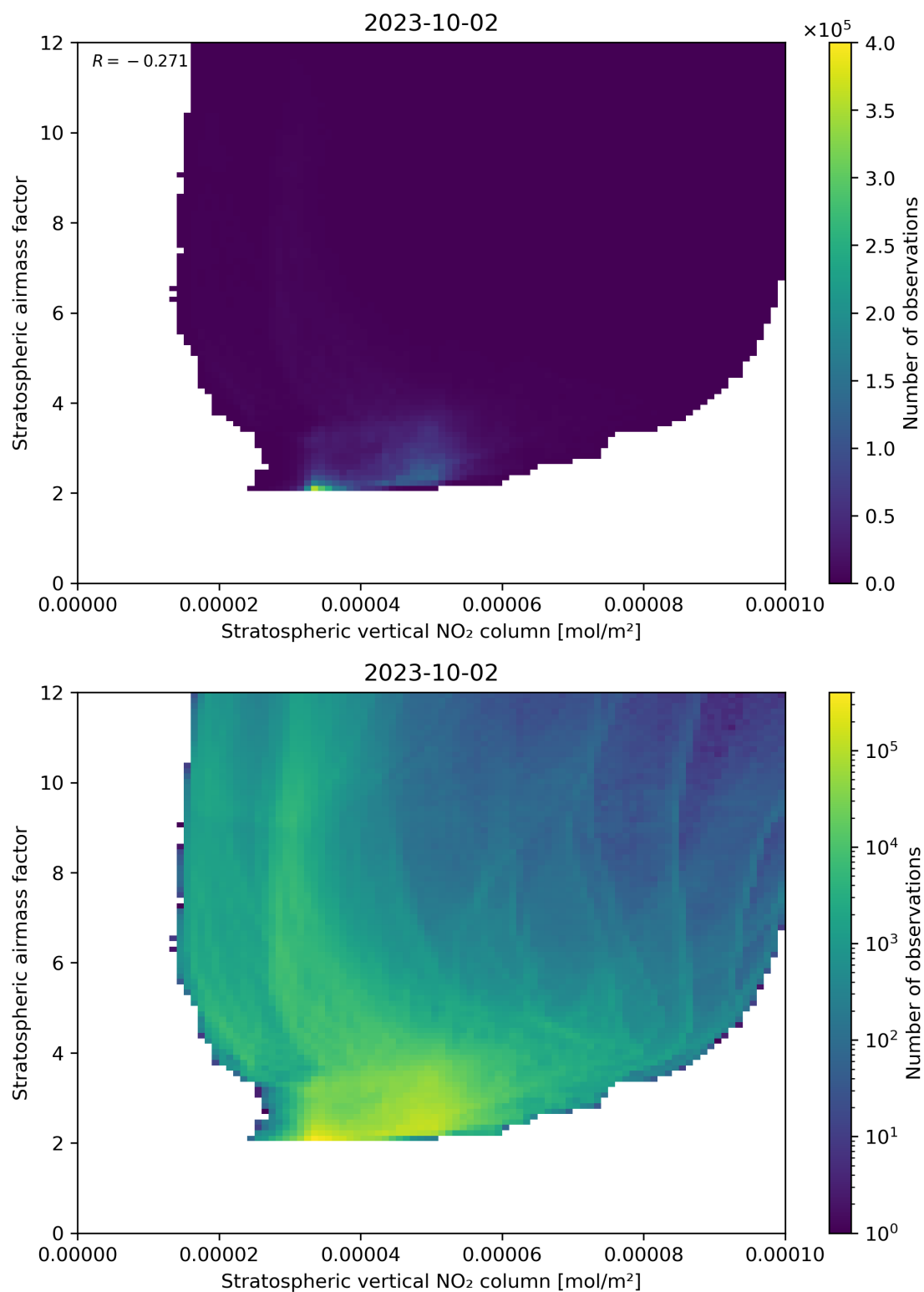
Figure 96: Scatter density plot of “Stratospheric vertical NO 2 column” against “Stratospheric airmass factor” for 2023-10-01 to 2023-10-03.
