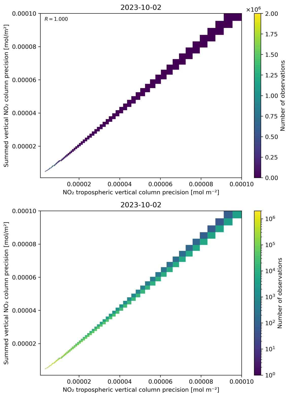
Figure 137: Scatter density plot of “NO 2 tropospheric vertical column precision” against “Summed vertical NO 2 column precision” for 2023-10-01 to 2023-10-03.
