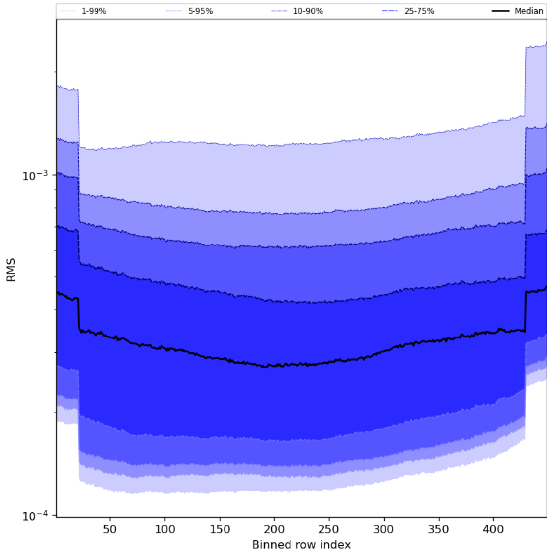
Figure 60: Along track statistics of “RMS” for 2023-10-01 to 2023-10-03
