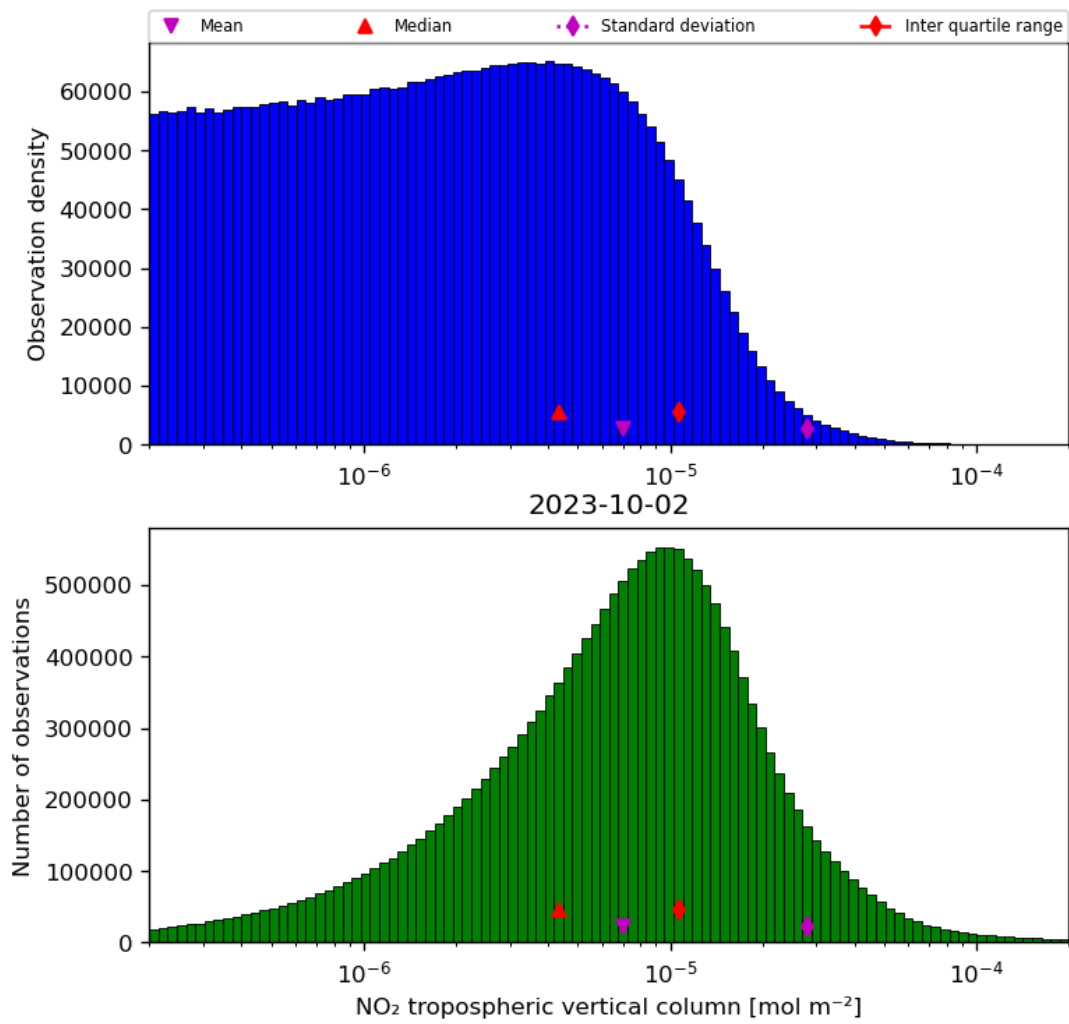
Figure 29: Histogram of “NO 2 tropospheric vertical column” for 2023-10-01 to 2023-10-03
