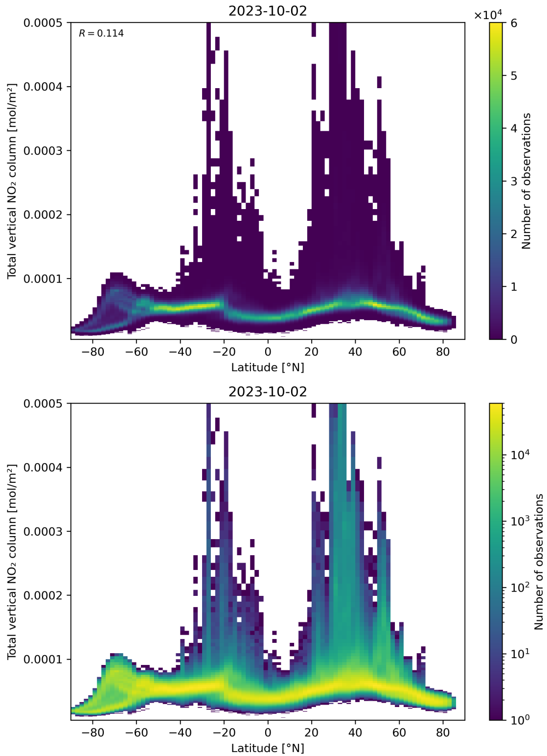
Figure 90: Scatter density plot of “Latitude” against “Total vertical NO 2 column” for 2023-10-01 to 2023-10-03.
