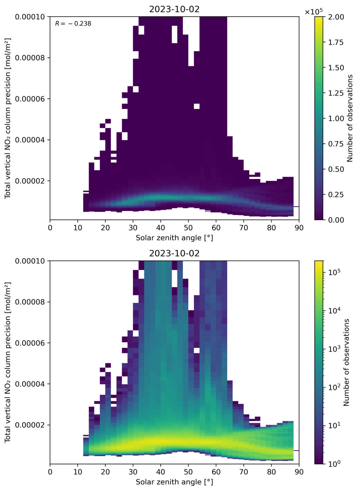
Figure 154: Scatter density plot of “Solar zenith angle” against “Total vertical NO 2 column precision” for 2023-10-01 to 2023-10-03.
