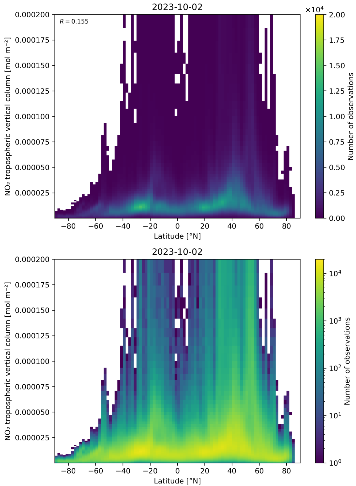
Figure 92: Scatter density plot of “Latitude” against “NO 2 tropospheric vertical column” for 2023-10-01 to 2023-10-03.
