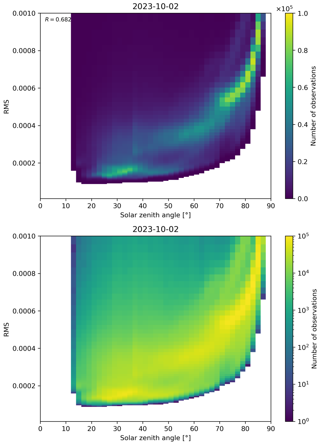
Figure 157: Scatter density plot of “Solar zenith angle” against “RMS” for 2023-10-01 to 2023-10-03.
