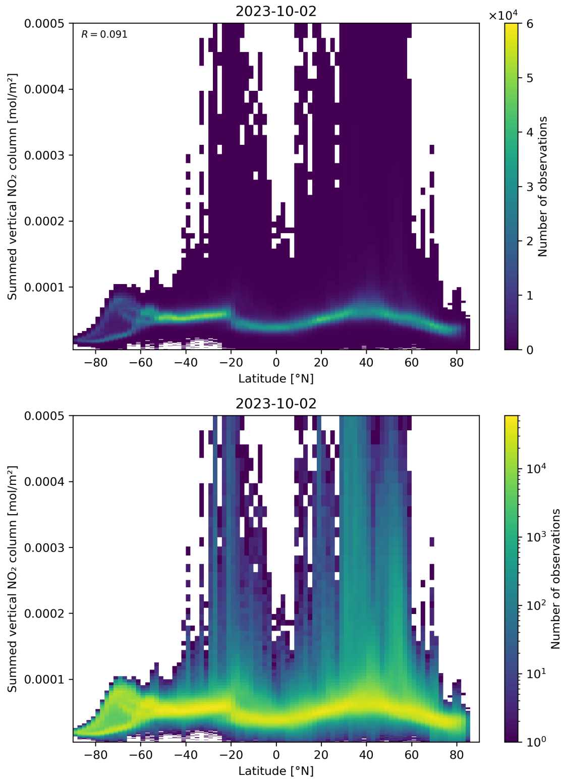
Figure 88: Scatter density plot of “Latitude” against “Summed vertical NO 2 column” for 2023-10-01 to 2023-10-03.
