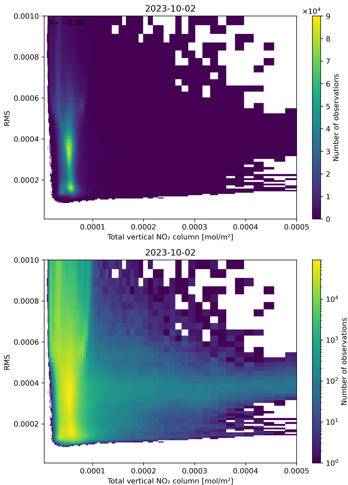
Figure 120: Scatter density plot of “Total vertical NO 2 column” against “RMS” for 2023-10-01 to 2023-10-03.
