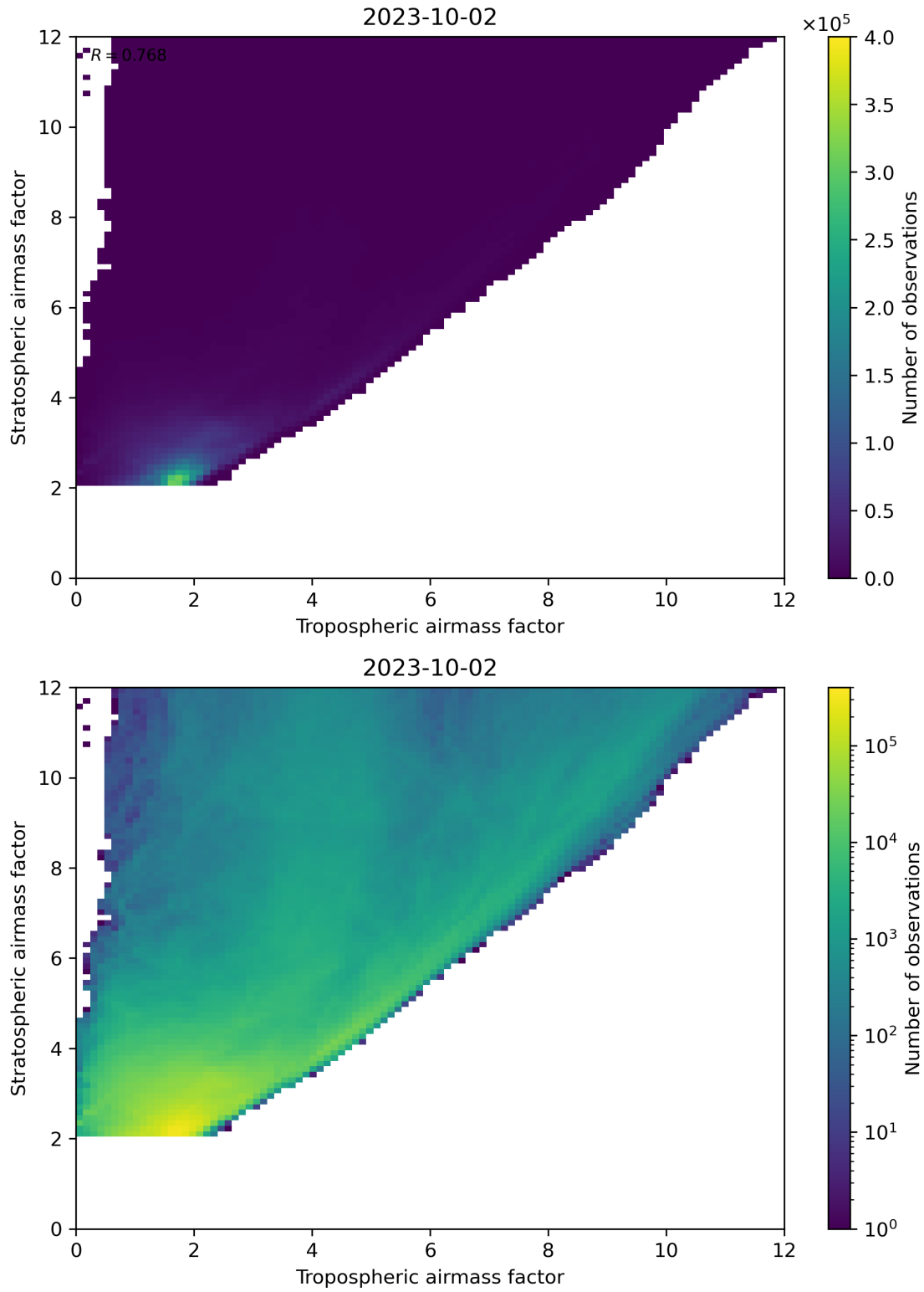
Figure 71: Scatter density plot of “Tropospheric airmass factor” against “Stratospheric airmass factor” for 2023-10-01 to 2023-10-03.
