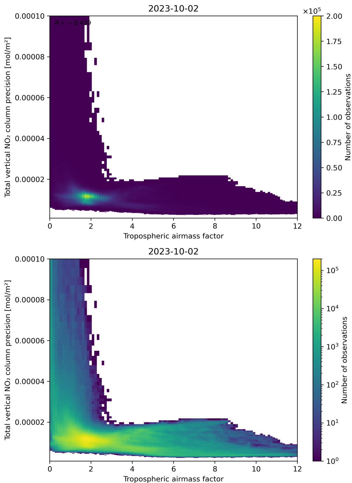
Figure 78: Scatter density plot of “Tropospheric air mass factor” against “Total vertical NO 2 column precision” for 2023-10-01 to 2023-10-03.
