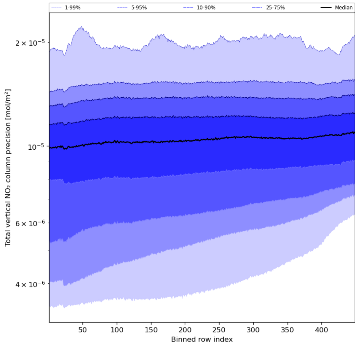
Figure 56: Along track statistics of “Total vertical NO 2 column precision” for 2023-10-01 to 2023-10-03
