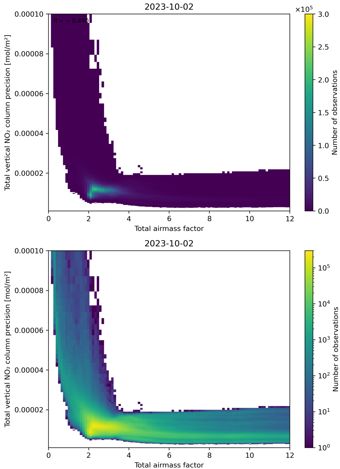
Figure 68: Scatter density plot of “Total airmass factor” against “Total vertical NO 2 column precision” for 2023-10-01 to 2023-10-03.
