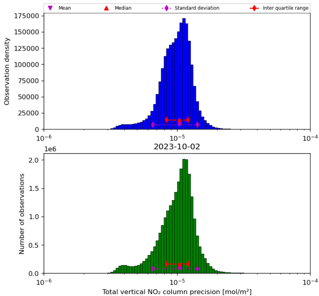
Figure 39: Histogram of “Total vertical NO 2 column precision” for 2023-10-01 to 2023-10-03
