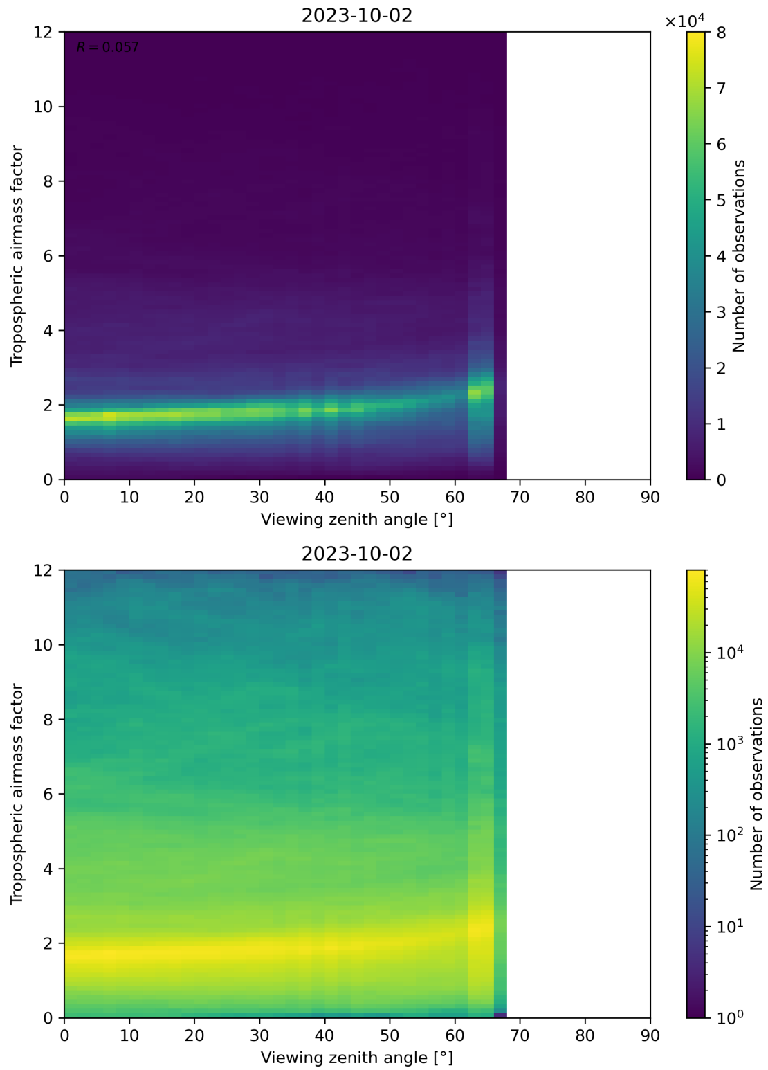
Figure 161: Scatter density plot of “Viewing zenith angle” against “Tropospheric airmass factor” for 2023-10-01 to 2023-10-03.
