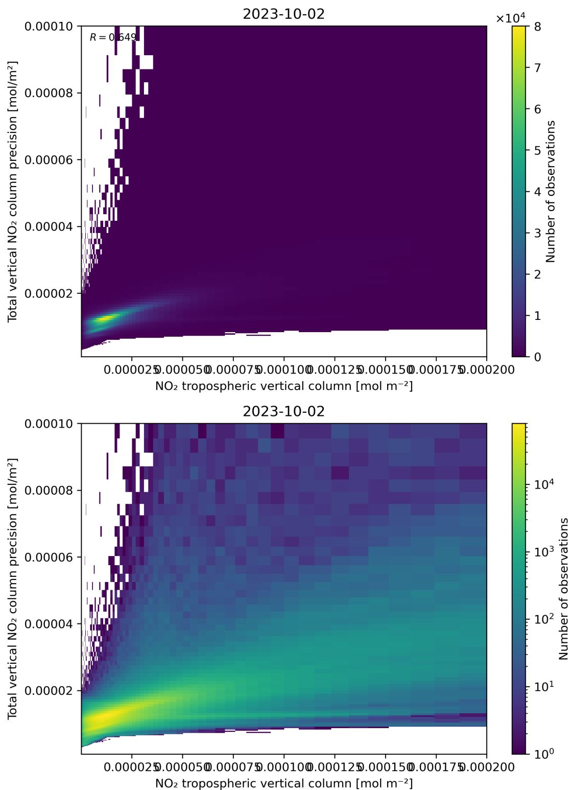
Figure 129: Scatter density plot of “NO 2 tropospheric vertical column” against “Total vertical NO 2 column precision” for 2023-10-01 to 2023-10-03.
