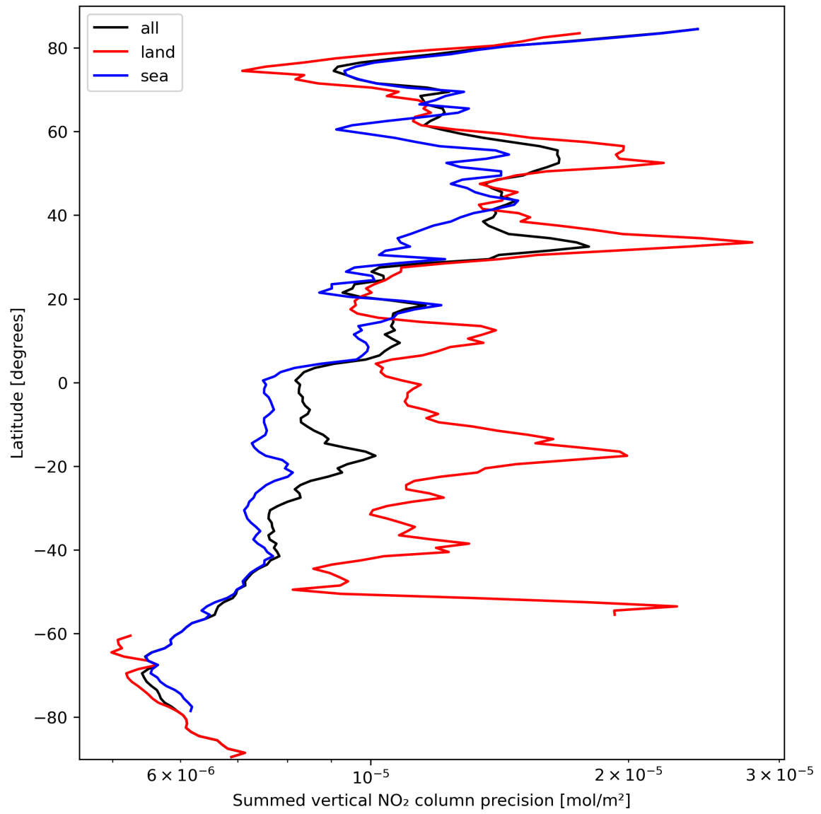
Figure 24: Zonal average of “Summed vertical NO 2 column precision” for 2023-10-01 to 2023-10-03.
