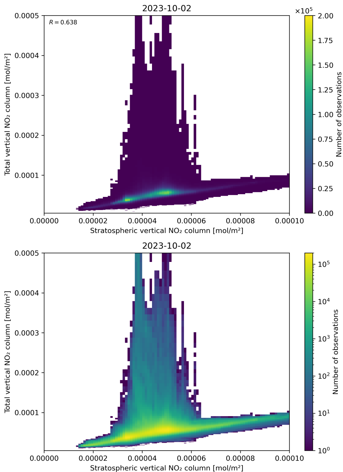
Figure 100: Scatter density plot of “Stratospheric vertical NO 2 column” against “Total vertical NO 2 column” for 2023-10-01 to 2023-10-03.
