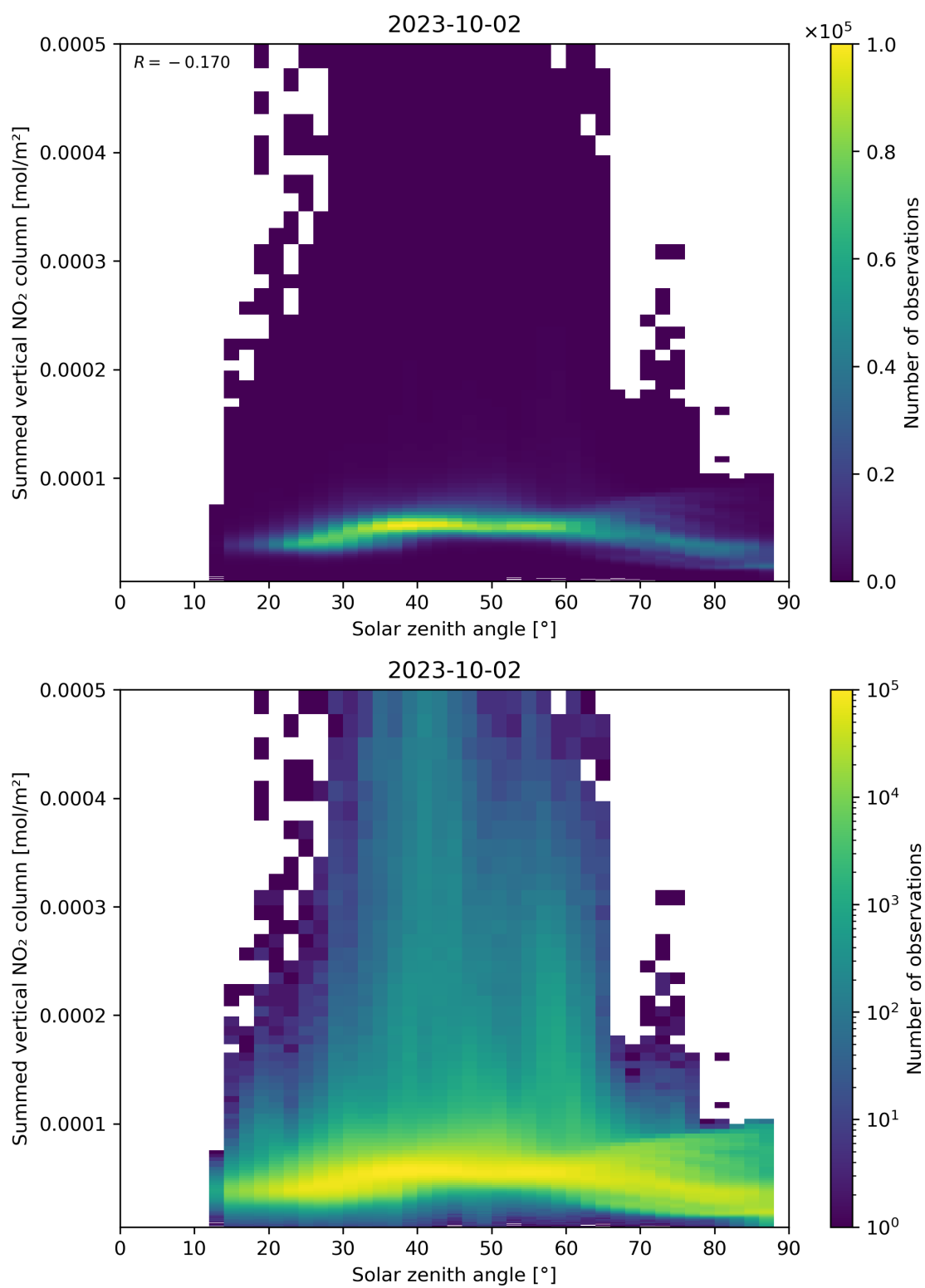
Figure 151: Scatter density plot of “Solar zenith angle” against “Summed vertical NO 2 column” for 2023-10-01 to 2023-10-03.
