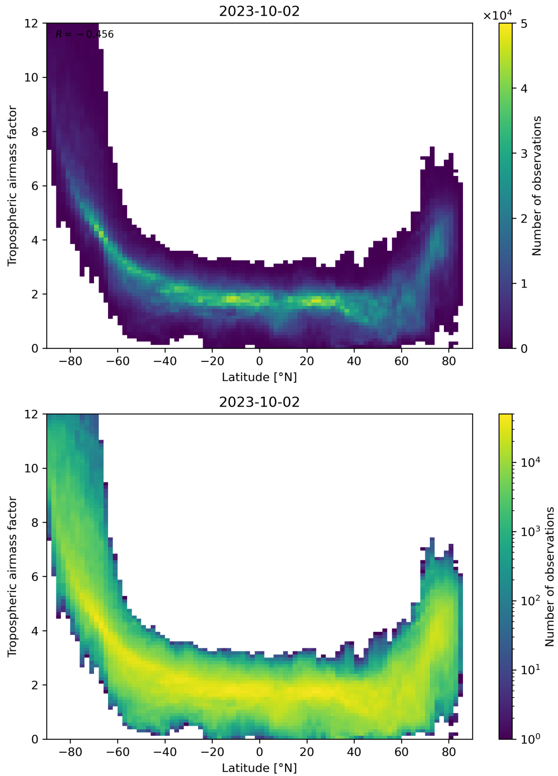
Figure 85: Scatter density plot of “Latitude” against “Tropospheric airmass factor” for 2023-10-01 to 2023-10-03.
