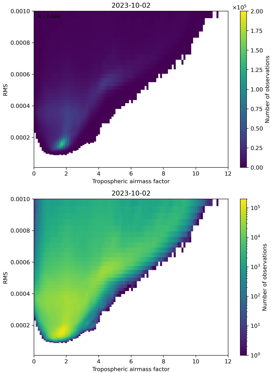
Figure 79: Scatter density plot of “Tropospheric airmass factor” against “RMS” for 2023-10-01 to 2023-10-03.
