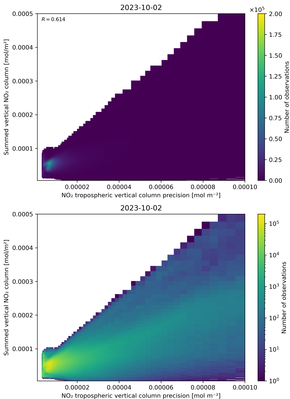
Figure 136: Scatter density plot of “NO 2 tropospheric vertical column precision” against “Summed vertical NO 2 column” for 2023-10-01 to 2023-10-03.
