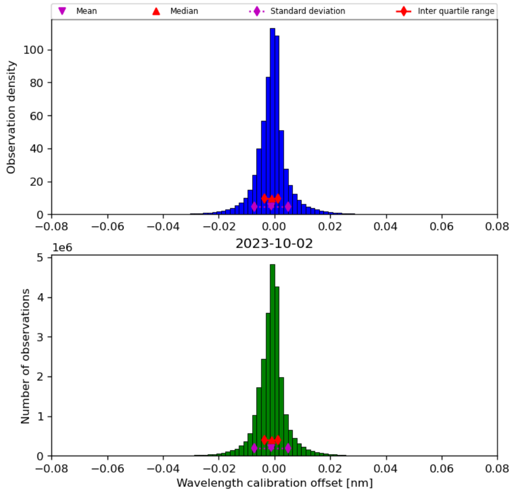
Figure 35: Histogram of “Wavelength calibration offset” for 2023-10-01 to 2023-10-03
