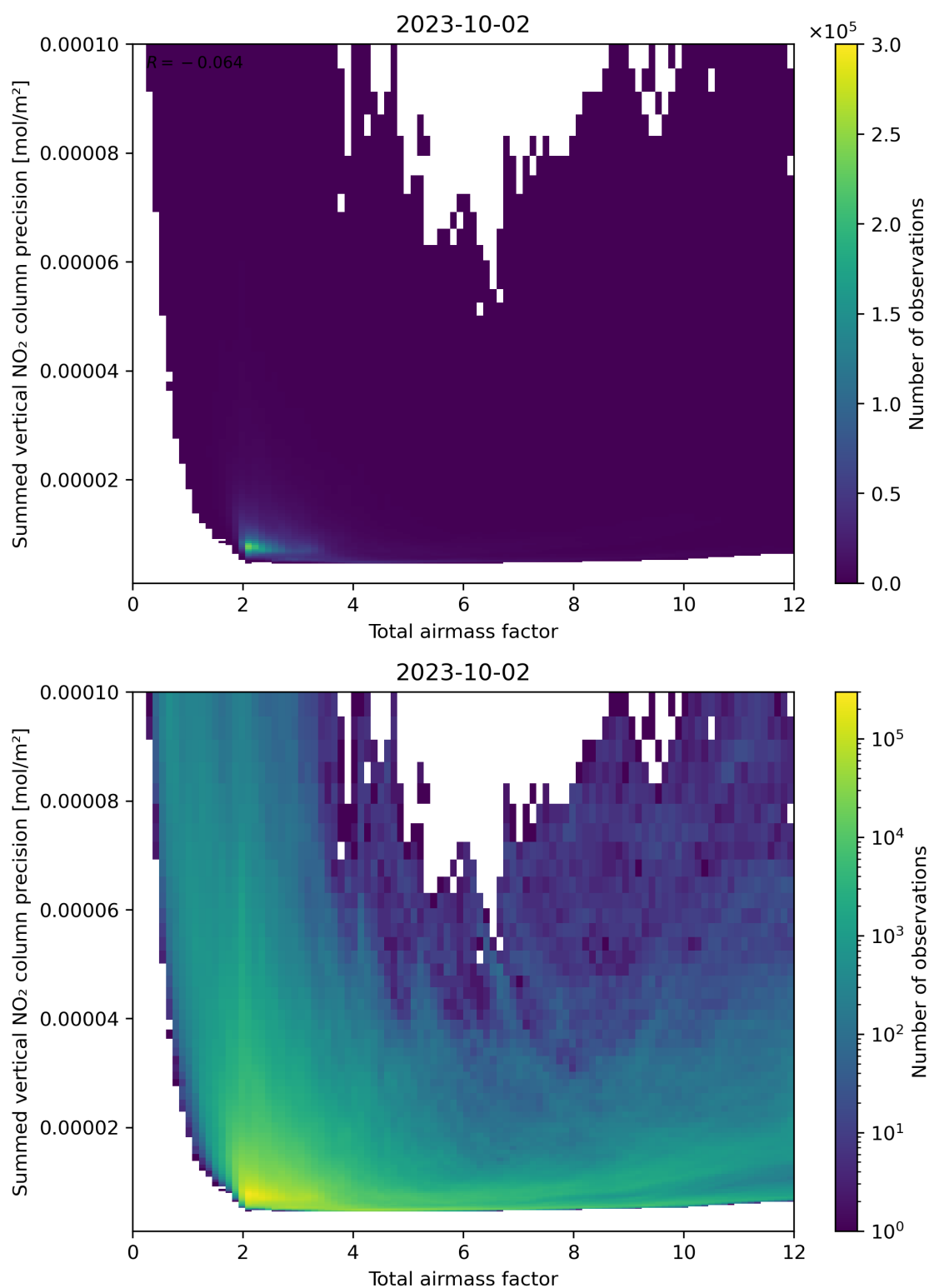
Figure 66: Scatter density plot of “Total airmass factor” against “Summed vertical NO 2 column precision” for 2023-10-01 to 2023-10-03.
