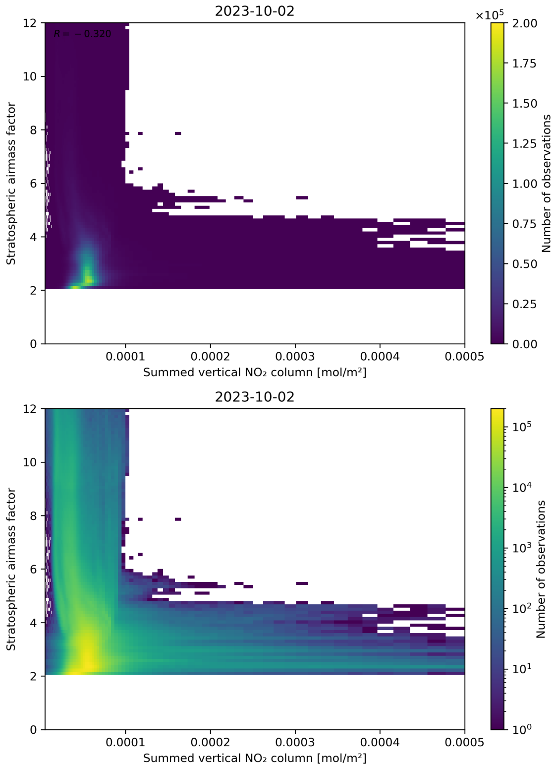
Figure 103: Scatter density plot of “Summed vertical NO 2 column” against “Stratospheric airmass factor” for 2023-10-01 to 2023-10-03.
