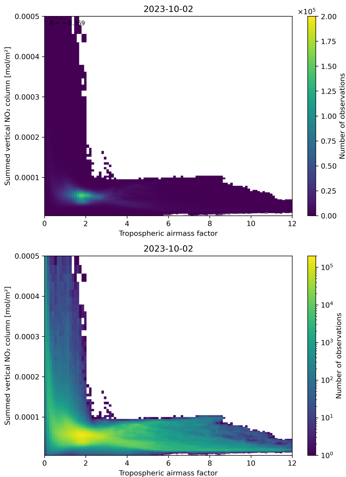
Figure 75: Scatter density plot of “Tropospheric airmass factor” against “Summed vertical NO 2 column” for 2023-10-01 to 2023-10-03.
