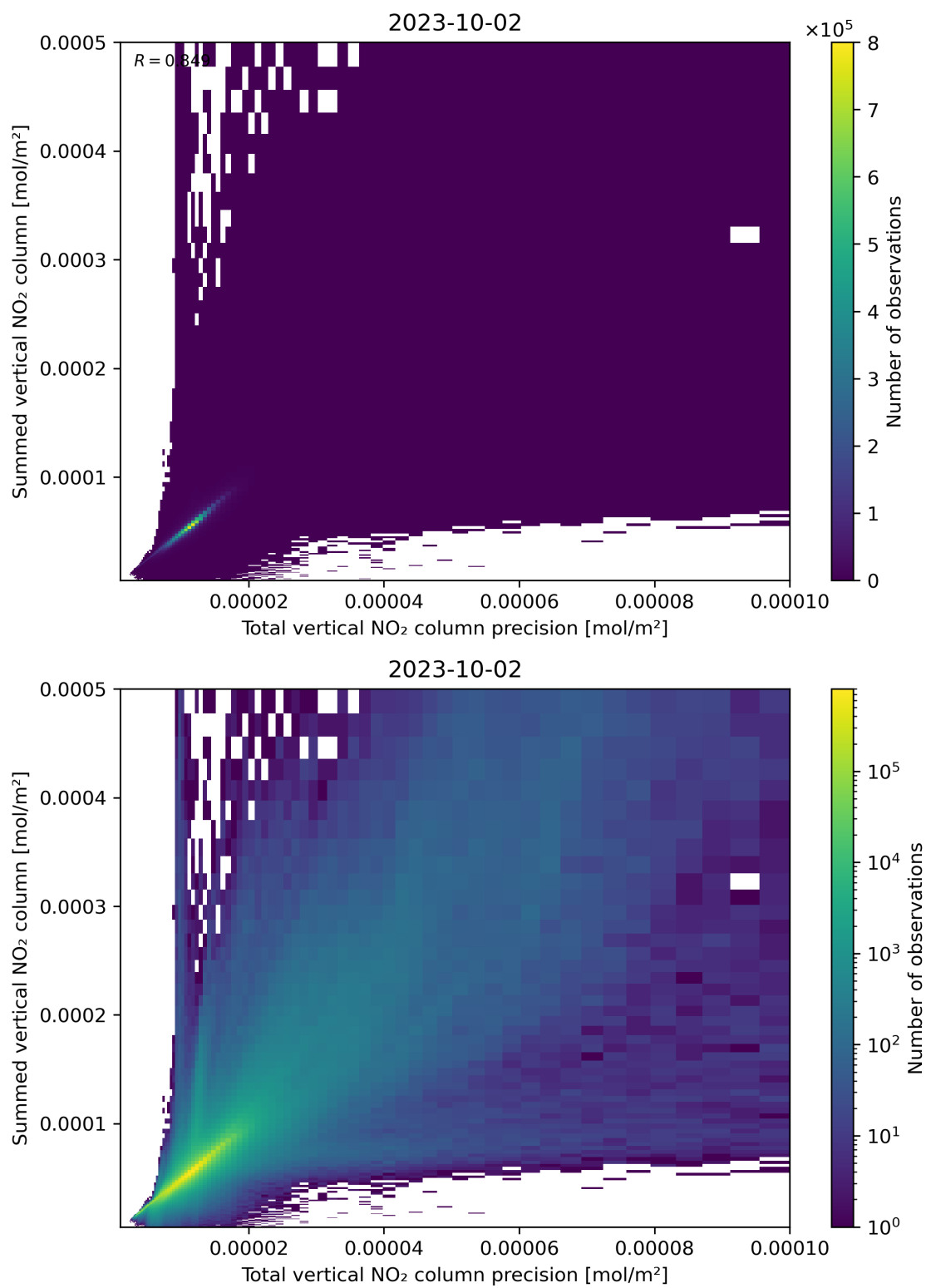
Figure 117: Scatter density plot of “Total vertical NO 2 column precision” against “Summed vertical NO 2 column” for 2023-10-01 to 2023-10-03.
