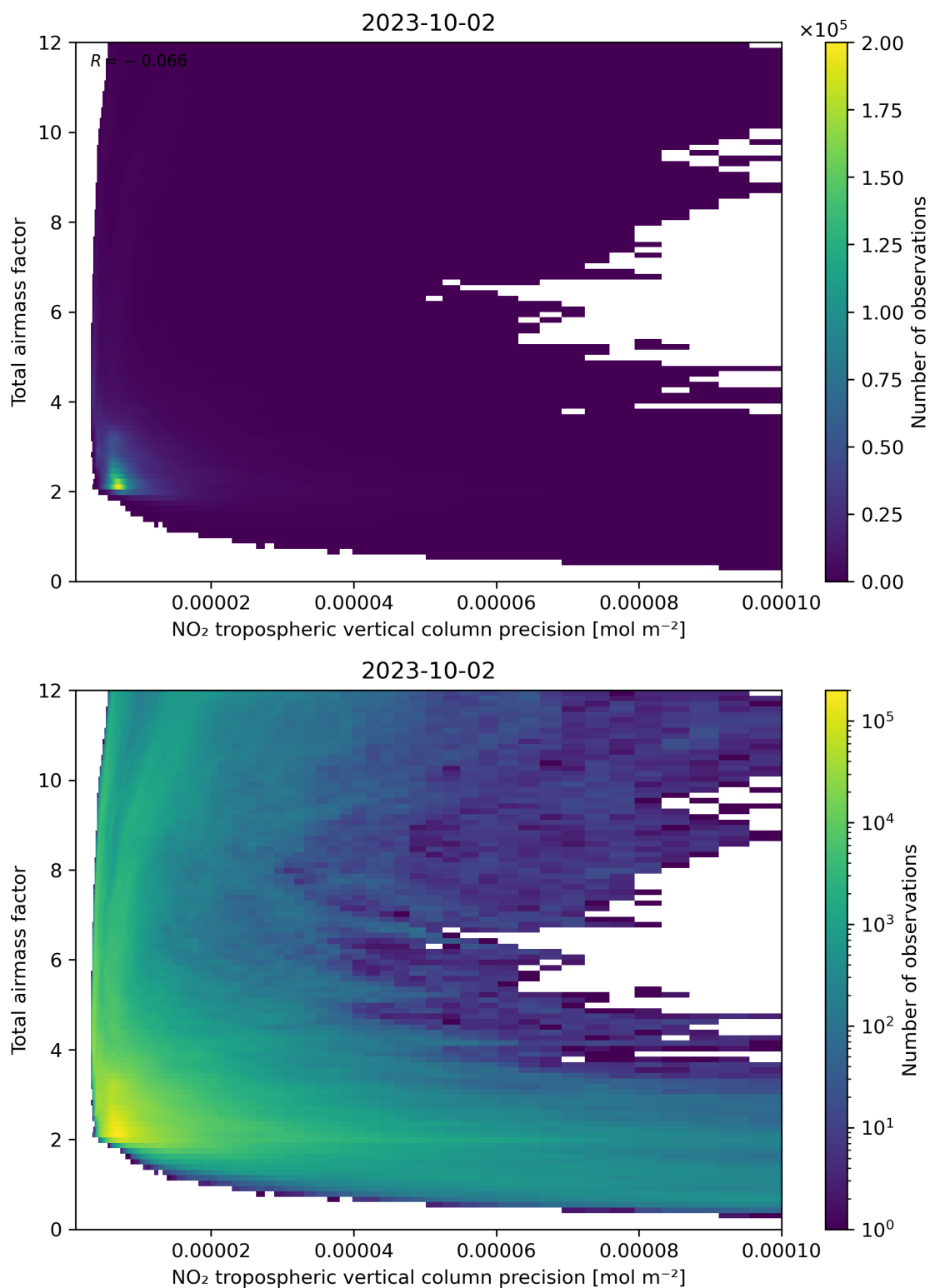
Figure 132: Scatter density plot of “NO 2 tropospheric vertical column precision” against “Total air mass factor” for 2023-10-01 to 2023-10-03.
