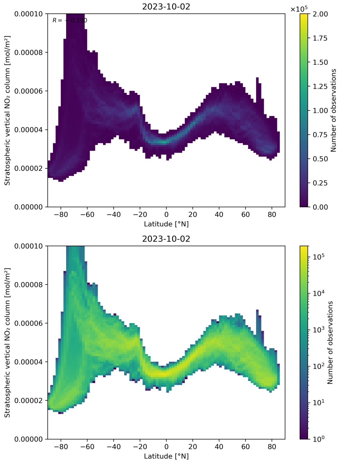
Figure 87: Scatter density plot of “Latitude” against “Stratospheric vertical NO 2 column” for 2023-10-01 to 2023-10-03.
