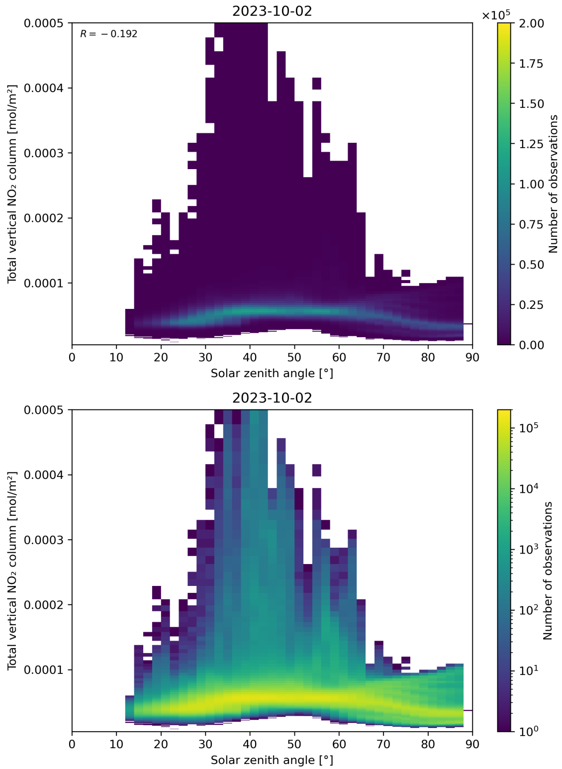
Figure 153: Scatter density plot of “Solar zenith angle” against “Total vertical NO 2 column” for 2023-10-01 to 2023-10-03.
