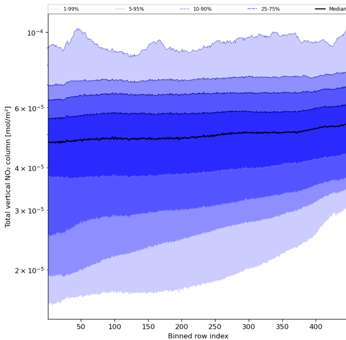
Figure 55: Along track statistics of “Total vertical NO 2 column” for 2023-10-01 to 2023-10-03
