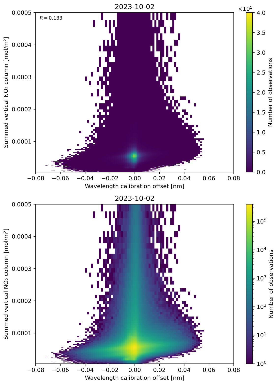
Figure 177: Scatter density plot of “Wavelength calibration offset” against “Summed vertical NO 2 column” for 2023-10-01 to 2023-10-03.
