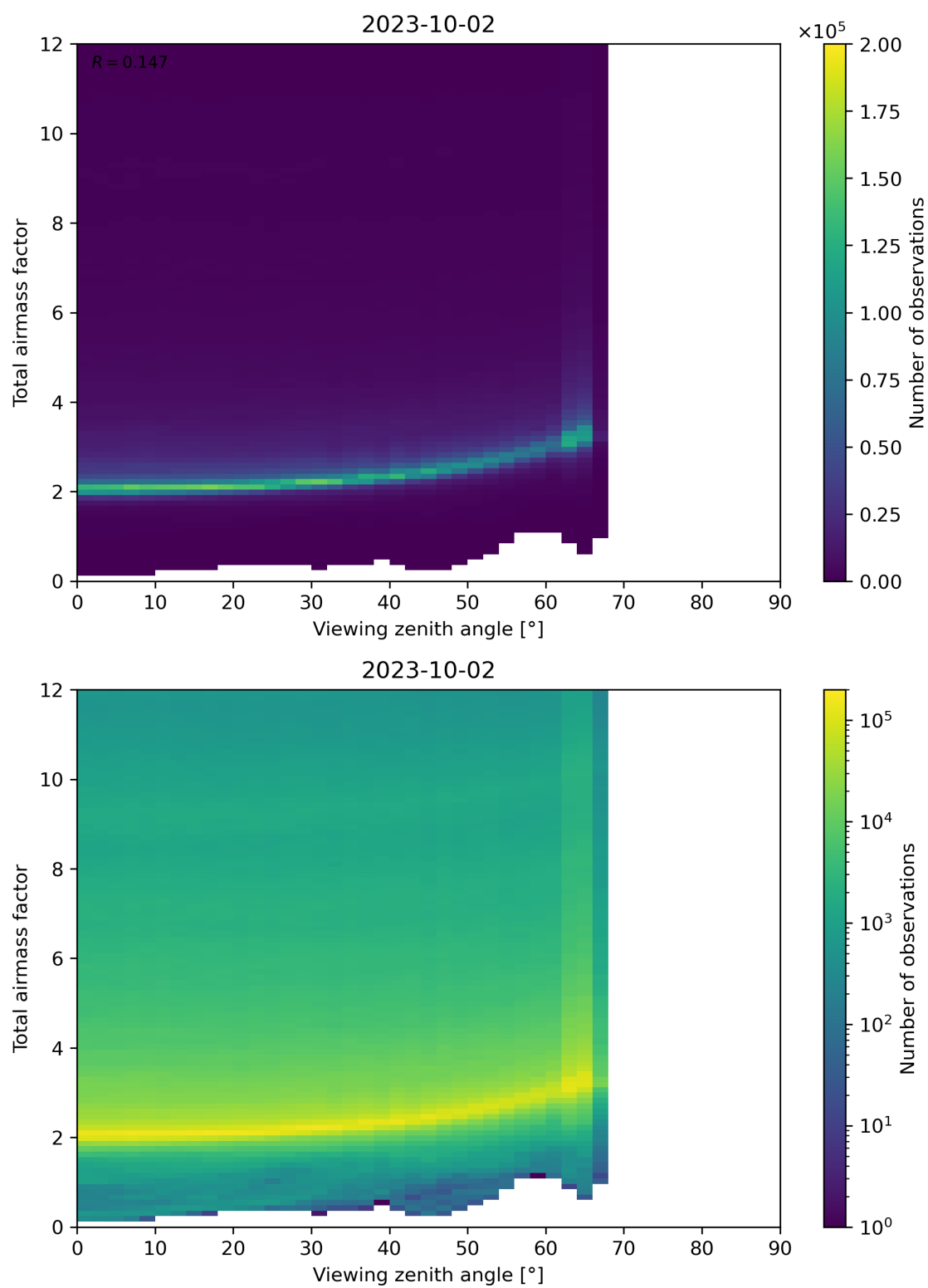
Figure 160: Scatter density plot of “Viewing zenith angle” against “Total airmass factor” for 2023-10-01 to 2023-10-03.
