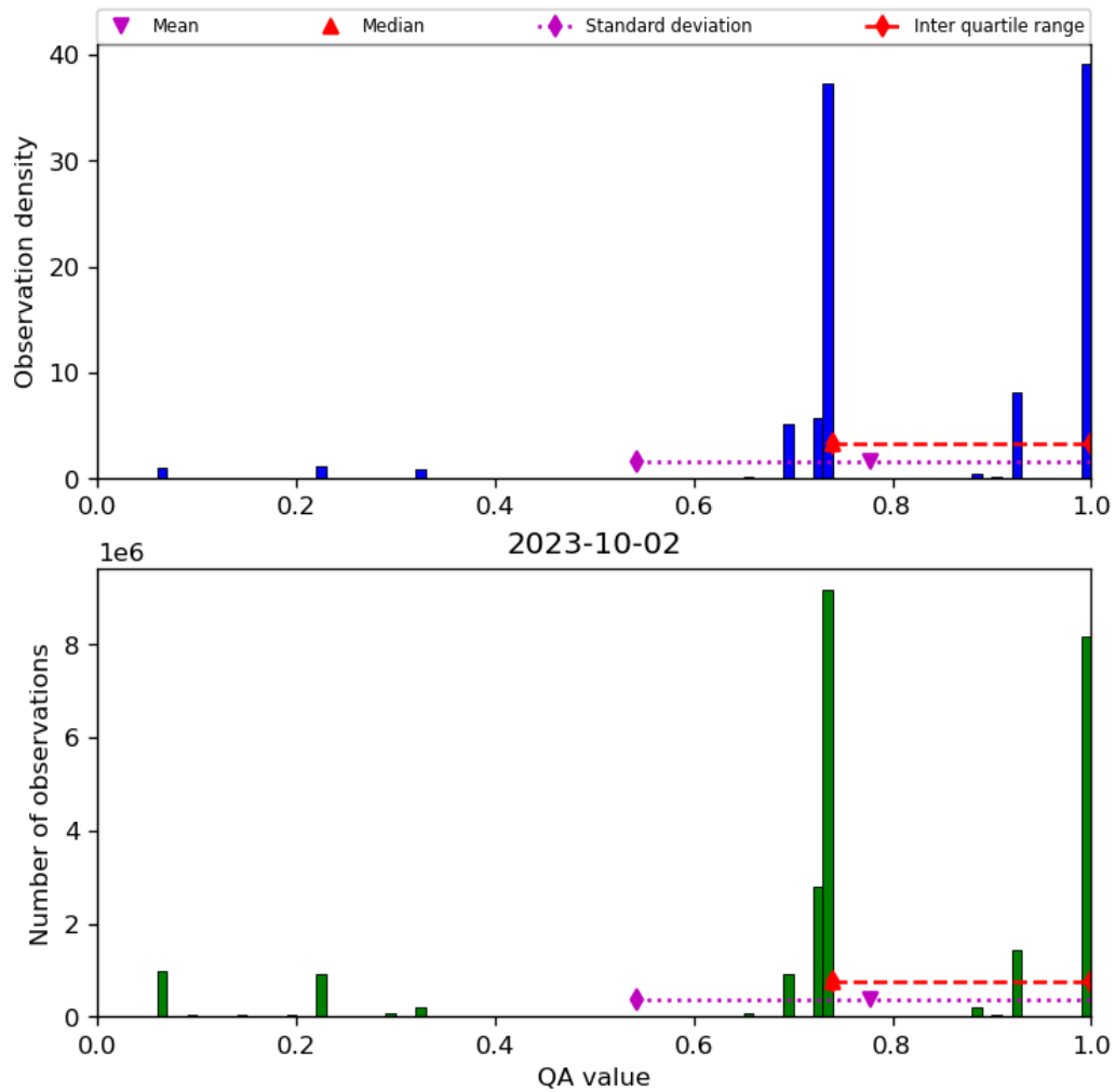
Figure 28: Histogram of “QA value” for 2023-10-01 to 2023-10-03
