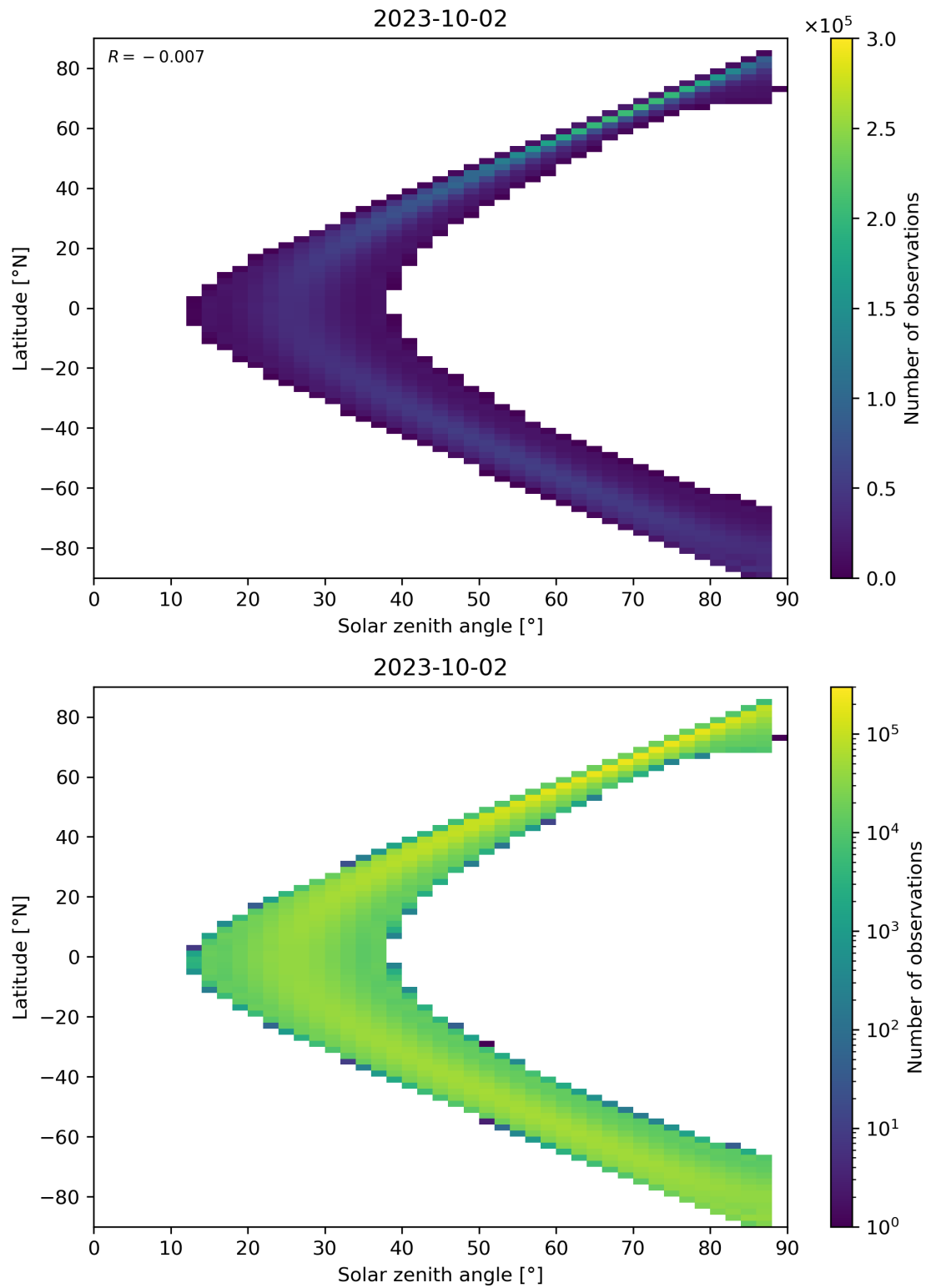
Figure 149: Scatter density plot of “Solar zenith angle” against “Latitude” for 2023-10-01 to 2023-10-03.
