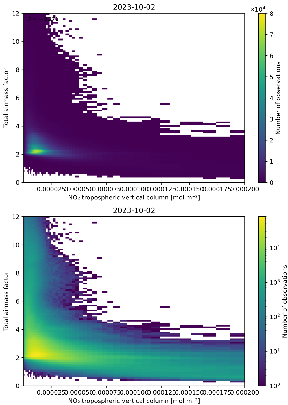
Figure 122: Scatter density plot of “NO 2 tropospheric vertical column” against “Total air mass factor” for 2023-10-01 to 2023-10-03.
