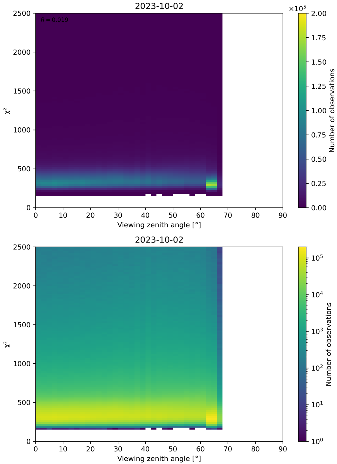
Figure 162: Scatter density plot of “Viewing zenith angle” against “ \chi^2 ” for 2023-10-01 to 2023-10-03.
