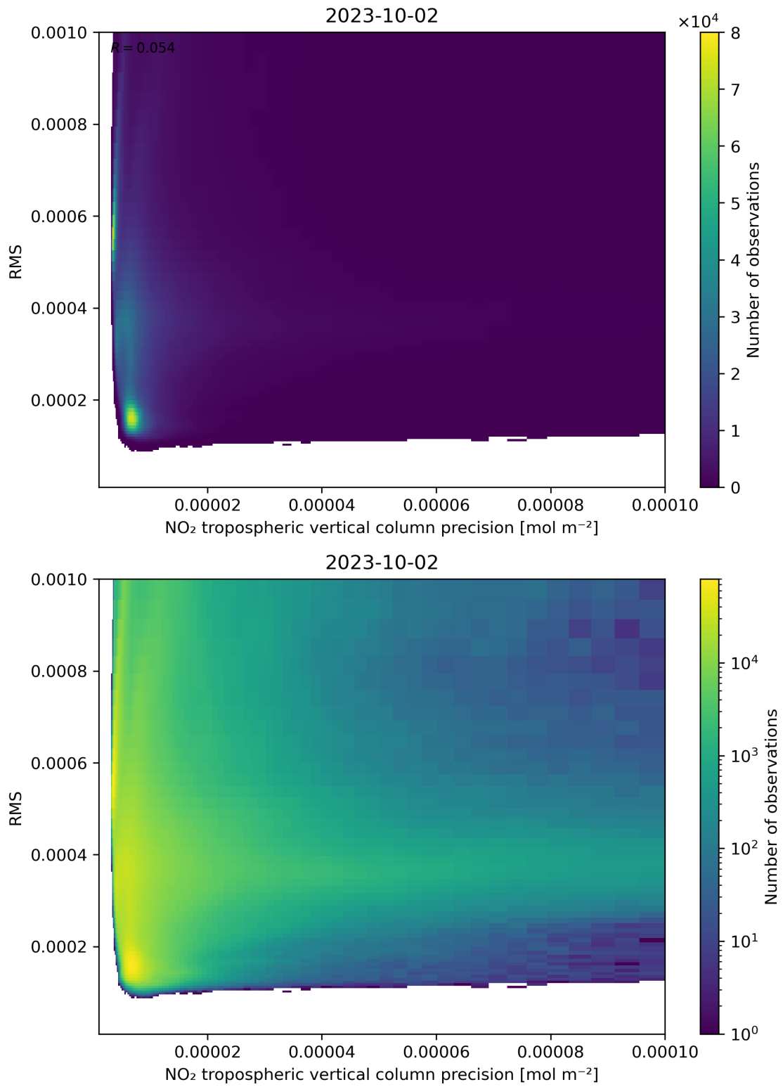
Figure 140: Scatter density plot of “NO 2 tropospheric vertical column precision” against “RMS” for 2023-10-01 to 2023-10-03.
