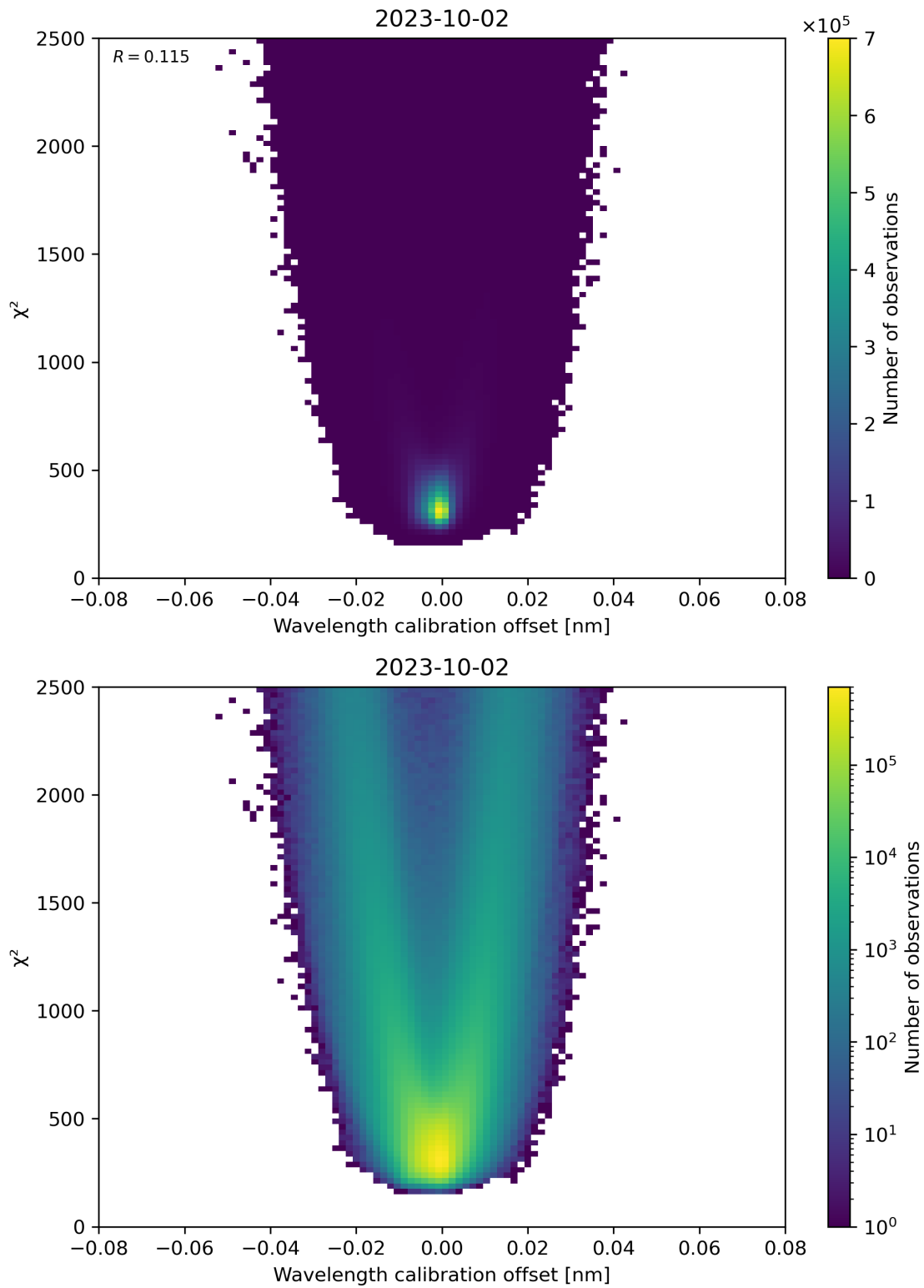
Figure 175: Scatter density plot of “Wavelength calibration offset” against “ \chi^2 ” for 2023-10-01 to 2023-10-03.
