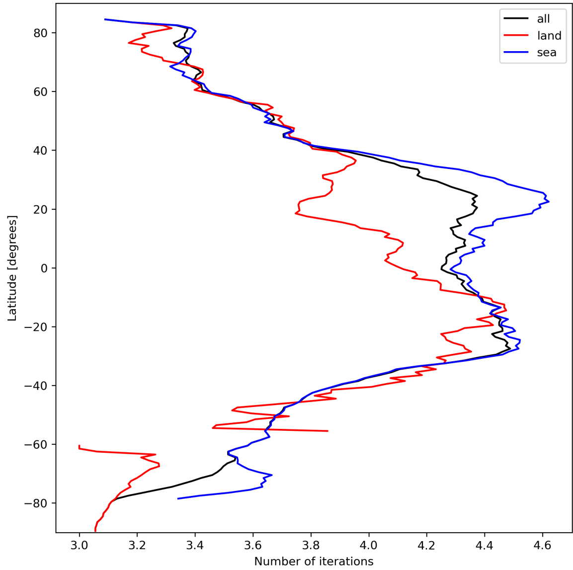
Figure 17: Zonal average of “Number of iterations” for 2023-10-01 to 2023-10-03.
