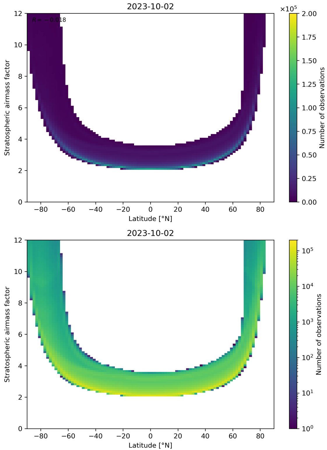
Figure 83: Scatter density plot of “Latitude” against “Stratospheric airmass factor” for 2023-10-01 to 2023-10-03.
