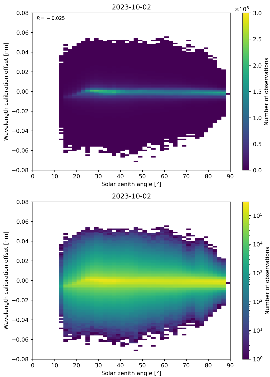
Figure 158: Scatter density plot of “Solar zenith angle” against “Wavelength calibration offset” for 2023-10-01 to 2023-10-03.
