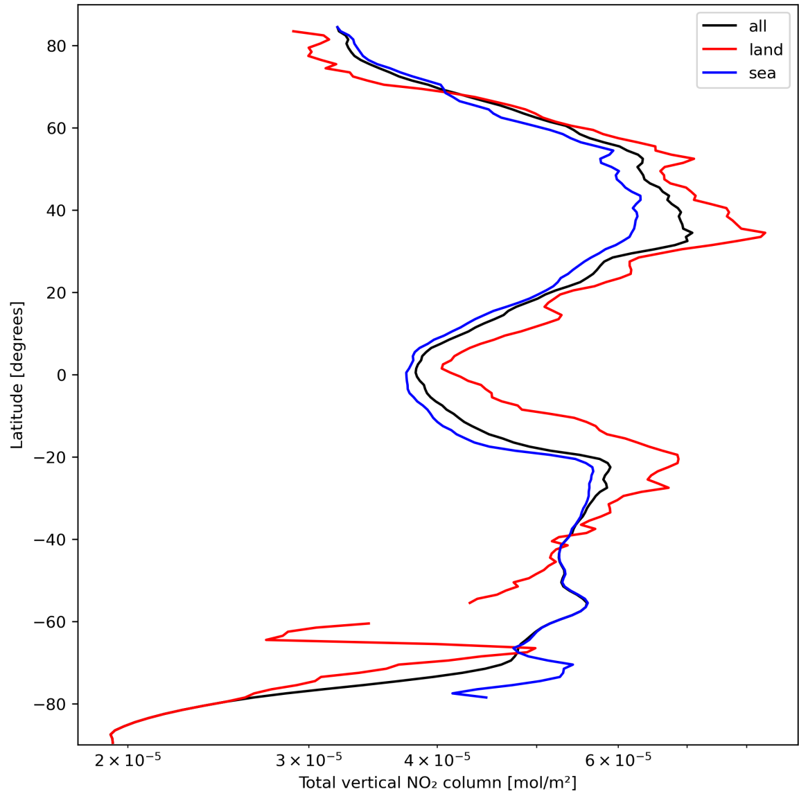
Figure 21: Zonal average of “Total vertical NO 2 column” for 2023-10-01 to 2023-10-03.
