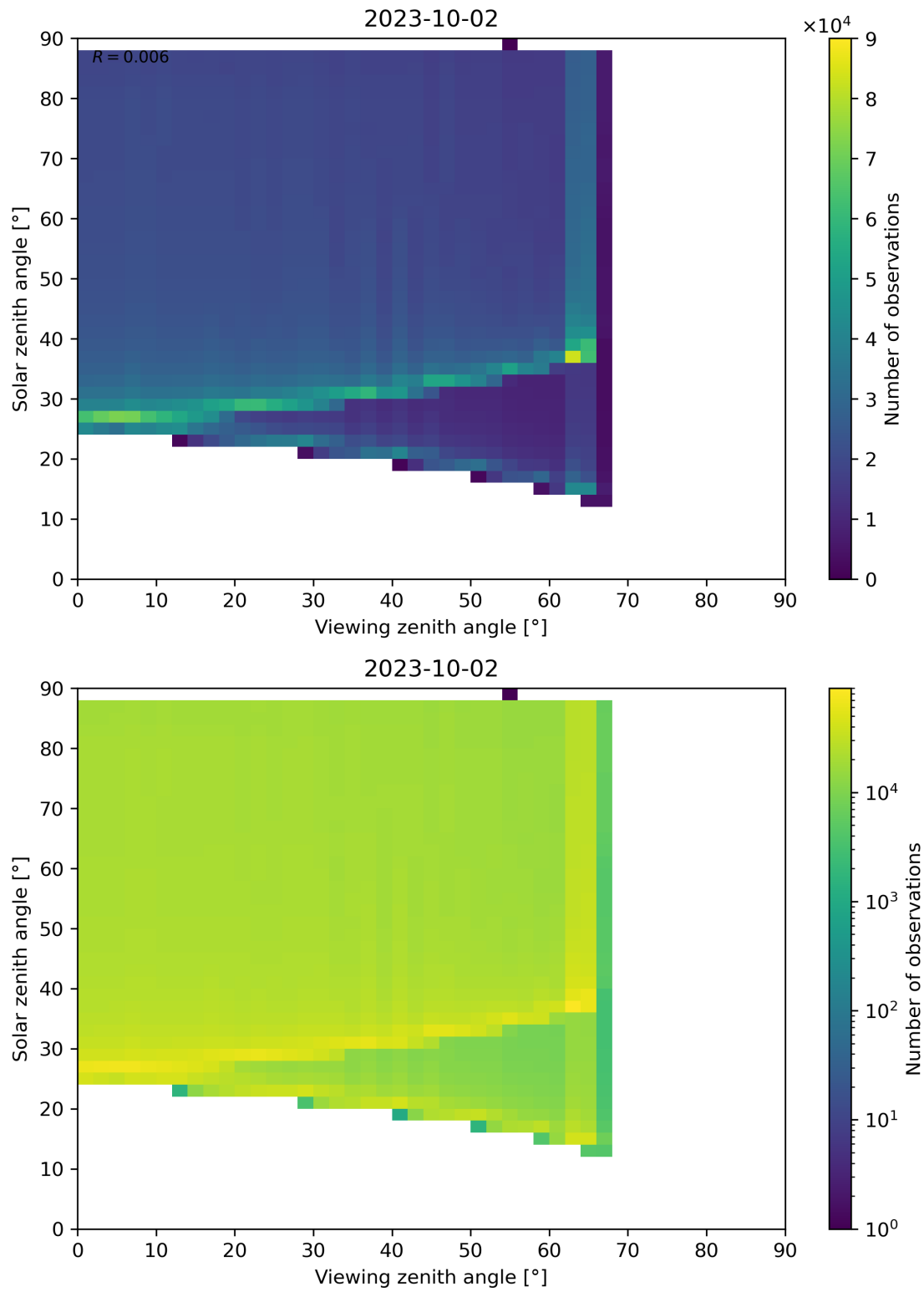
Figure 172: Scatter density plot of “Viewing zenith angle” against “Solar zenith angle” for 2023-10-01 to 2023-10-03.
