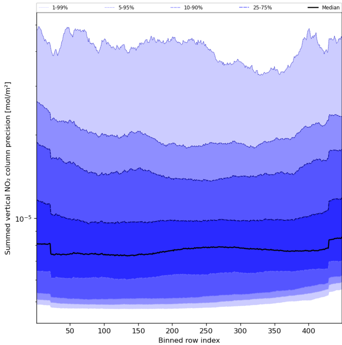
Figure 58: Along track statistics of “Summed vertical NO 2 column precision” for 2023-10-01 to 2023-10-03
