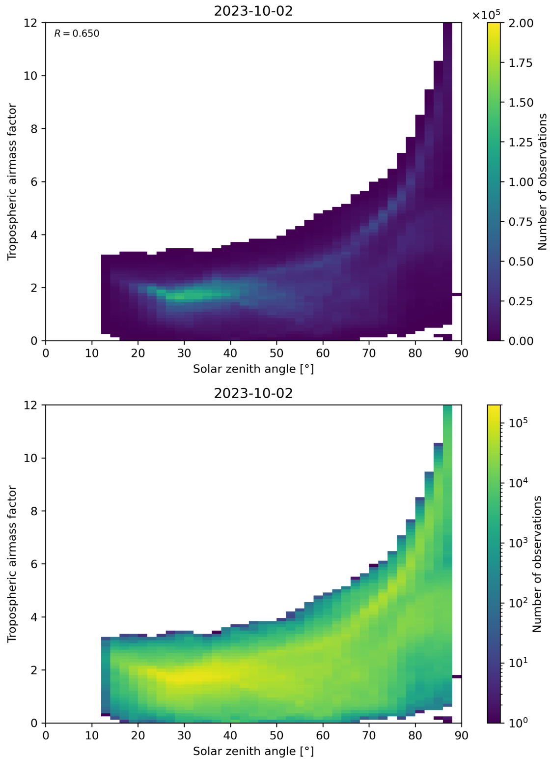
Figure 147: Scatter density plot of “Solar zenith angle” against “Tropospheric airmass factor” for 2023-10-01 to 2023-10-03.
