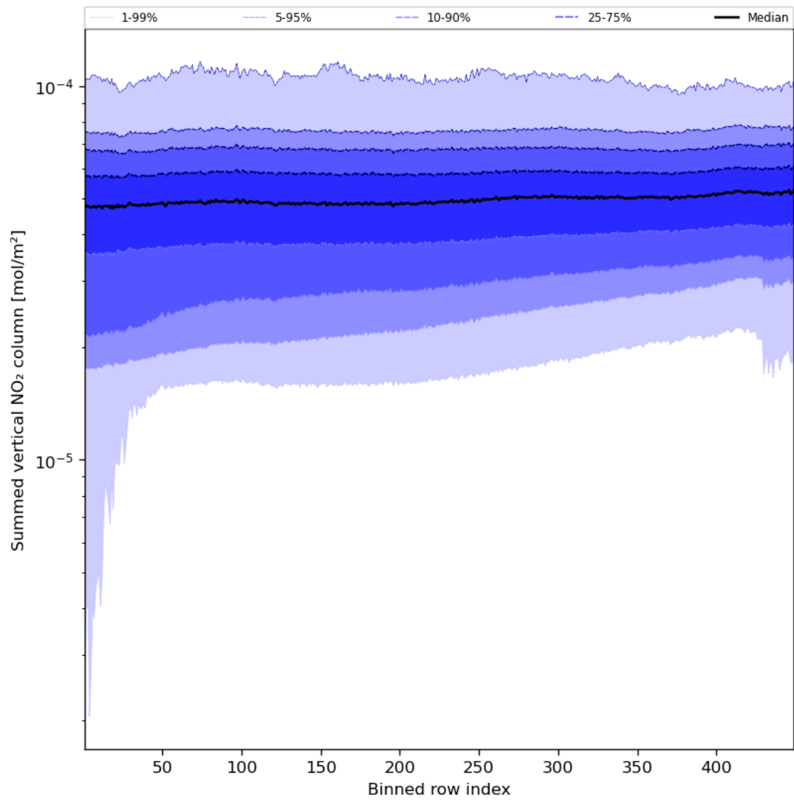
Figure 57: Along track statistics of “Summed vertical NO 2 column” for 2023-10-01 to 2023-10-03
