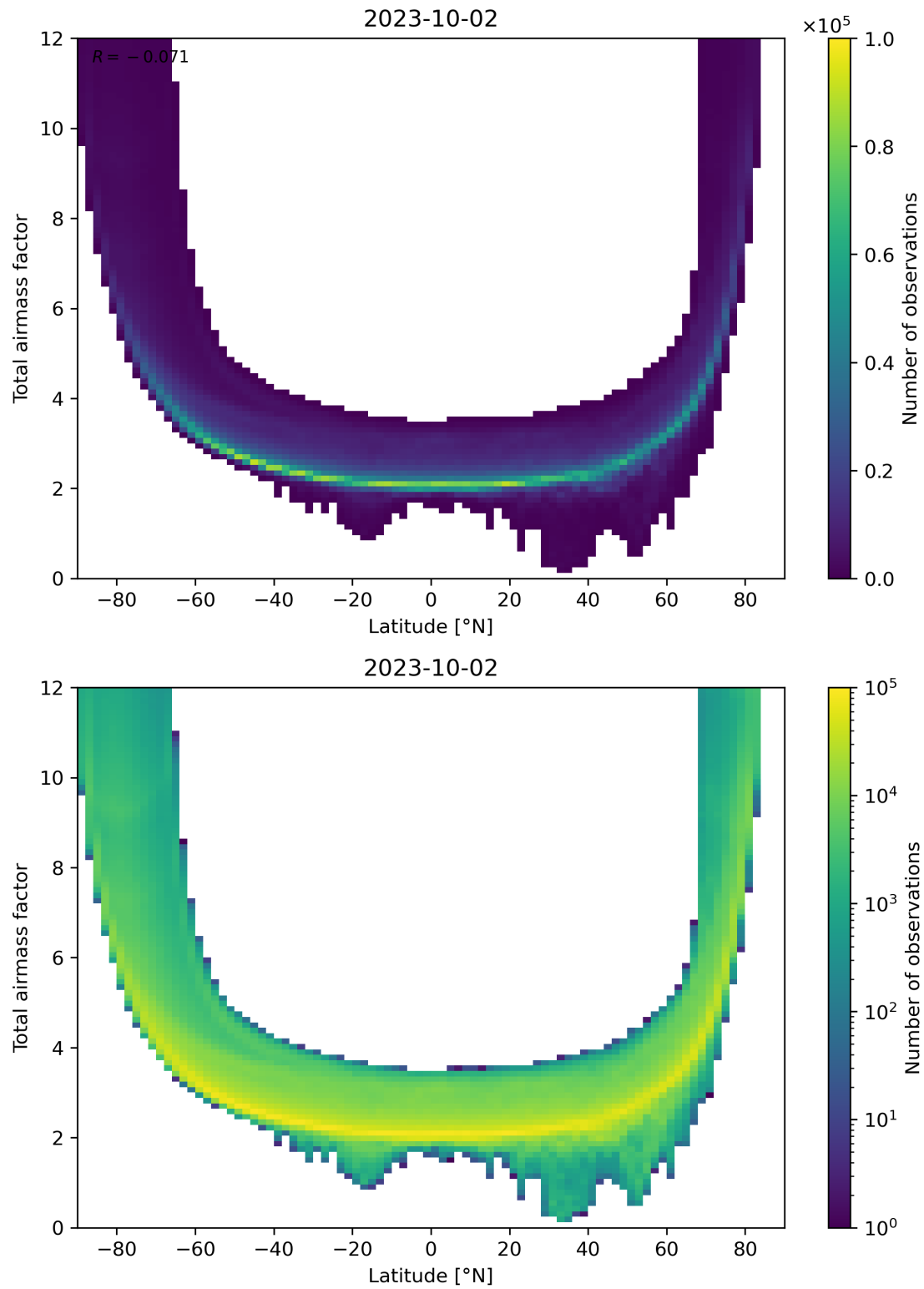
Figure 84: Scatter density plot of “Latitude” against “Total airmass factor” for 2023-10-01 to 2023-10-03.
