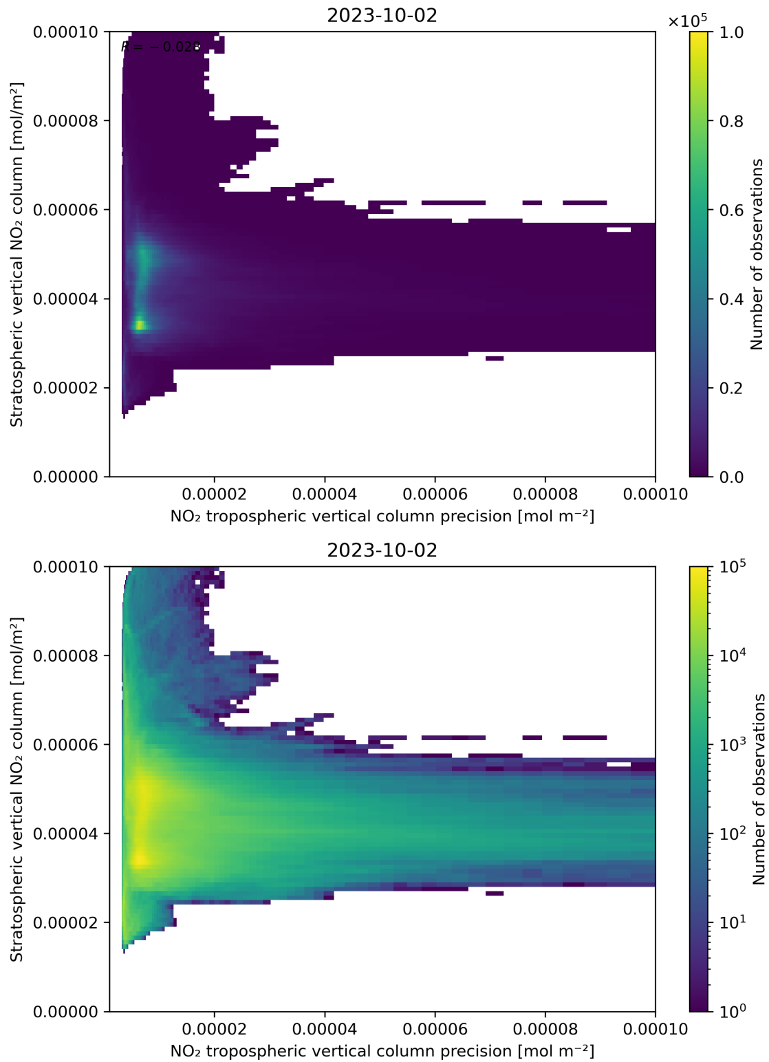
Figure 135: Scatter density plot of “NO 2 tropospheric vertical column precision” against “Stratospheric vertical NO 2 column” for 2023-10-01 to 2023-10-03.
