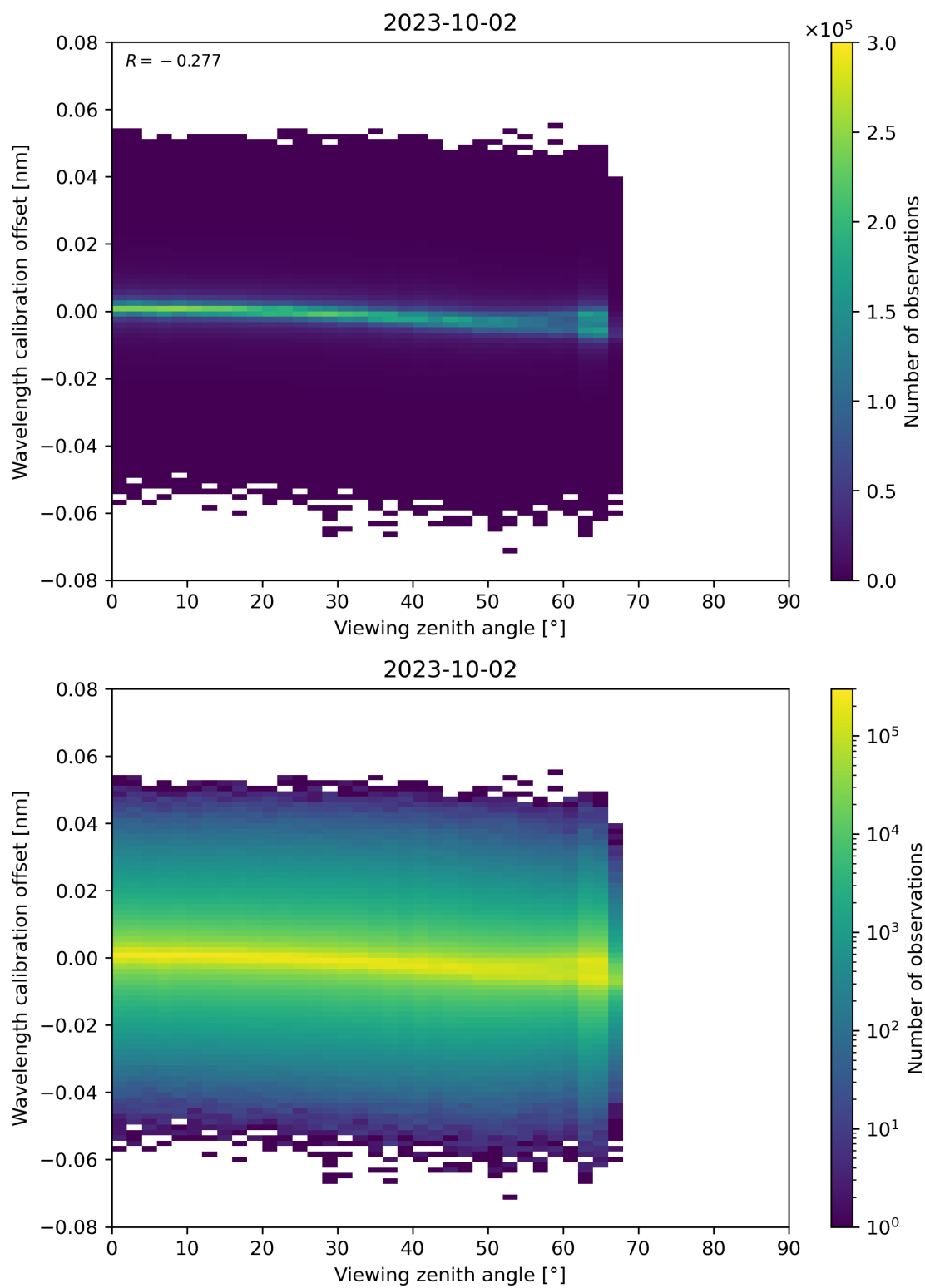
Figure 173: Scatter density plot of “Viewing zenith angle” against “Wavelength calibration offset” for 2023-10-01 to 2023-10-03.
