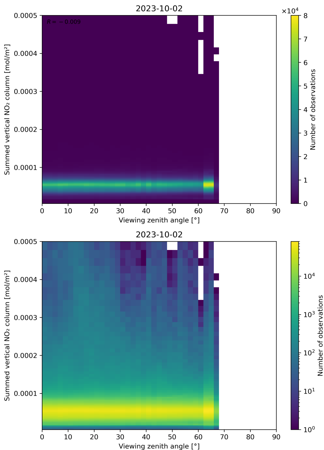
Figure 165: Scatter density plot of “Viewing zenith angle” against “Summed vertical NO 2 column” for 2023-10-01 to 2023-10-03.
