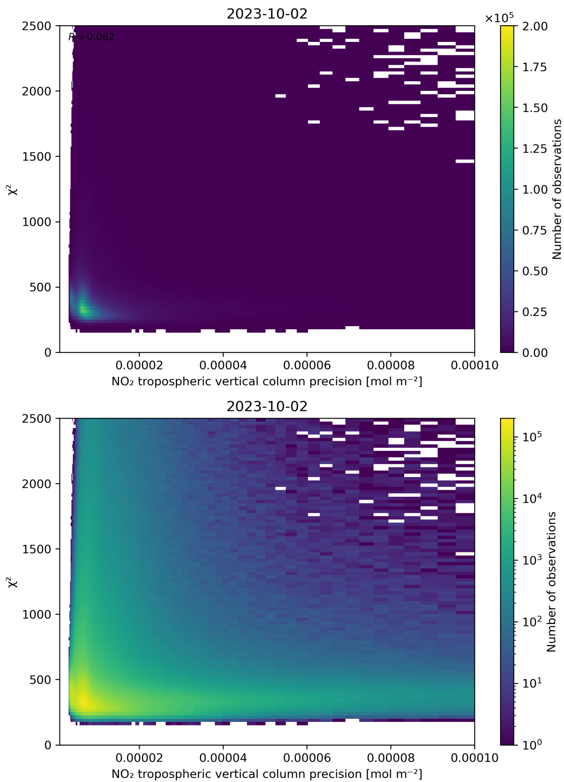
Figure 134: Scatter density plot of “NO 2 tropospheric vertical column precision” against “ \chi^2 ” for 2023-10-01 to 2023-10-03.
