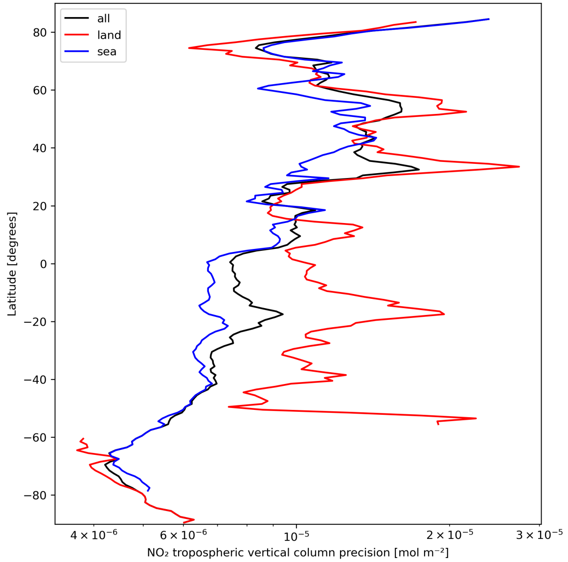
Figure 13: Zonal average of “NO 2 tropospheric vertical column precision” for 2023-10-01 to 2023-10-03.
