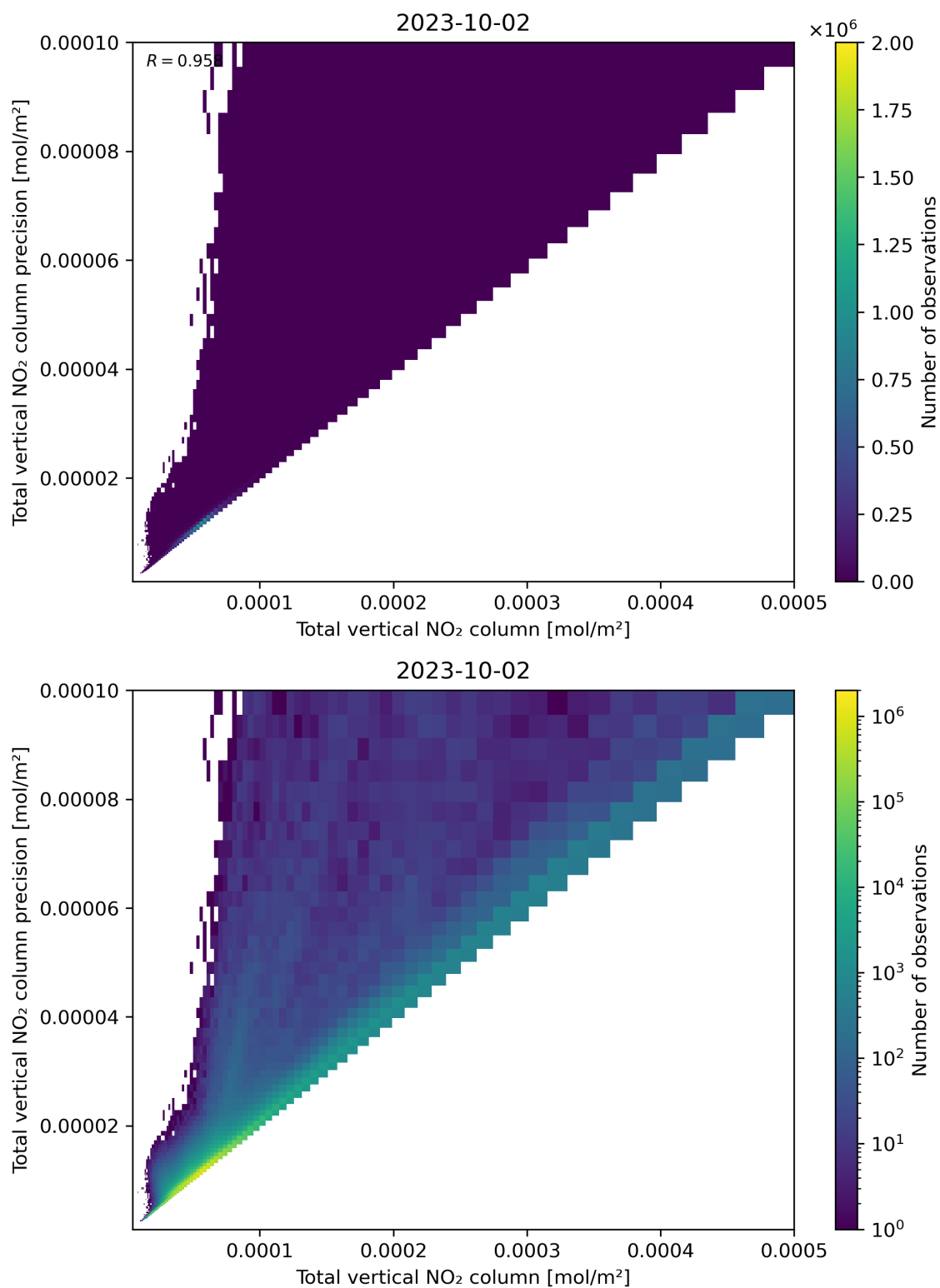
Figure 114: Scatter density plot of “Total vertical NO 2 column” against “Total vertical NO 2 column precision” for 2023-10-01 to 2023-10-03.
