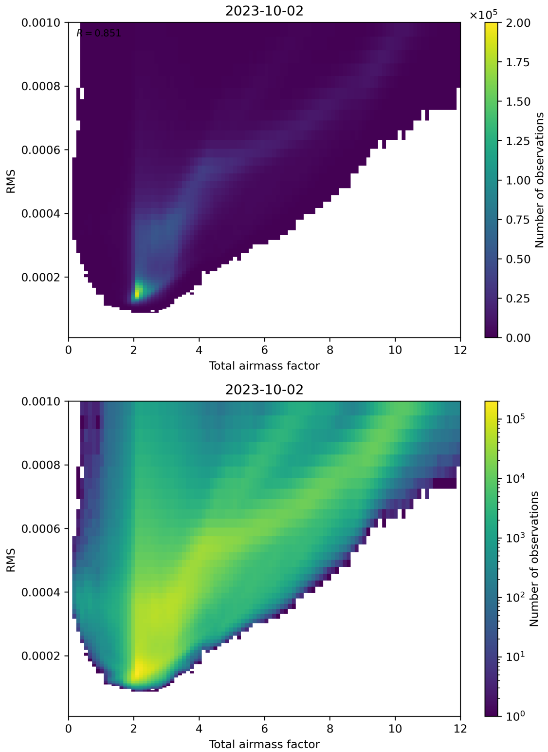
Figure 69: Scatter density plot of “Total airmass factor” against “RMS” for 2023-10-01 to 2023-10-03.
