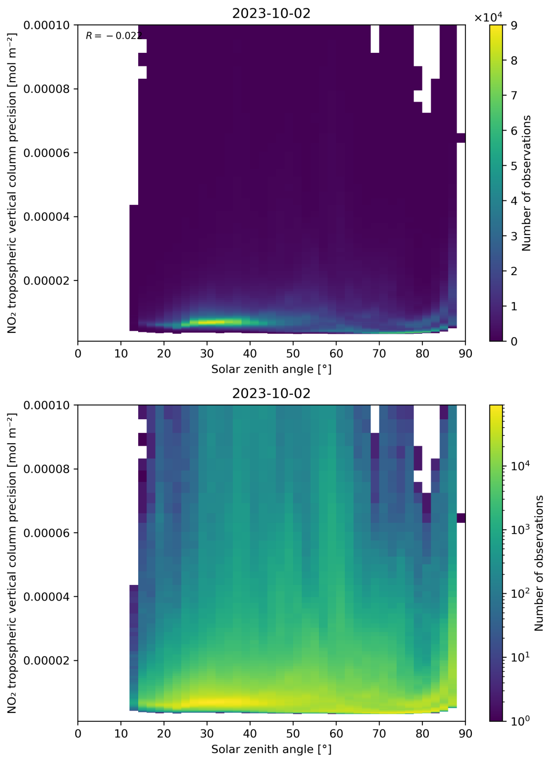
Figure 156: Scatter density plot of “Solar zenith angle” against “NO 2 tropospheric vertical column precision” for 2023-10-01 to 2023-10-03.
