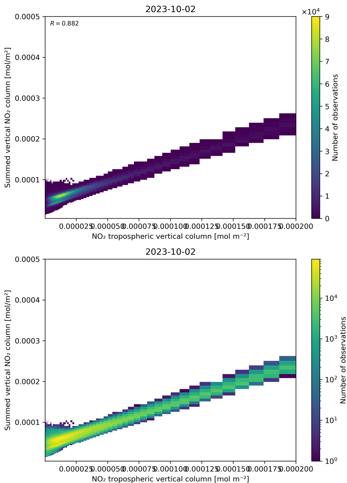
Figure 126: Scatter density plot of “NO 2 tropospheric vertical column” against “Summed vertical NO 2 column” for 2023-10-01 to 2023-10-03.
