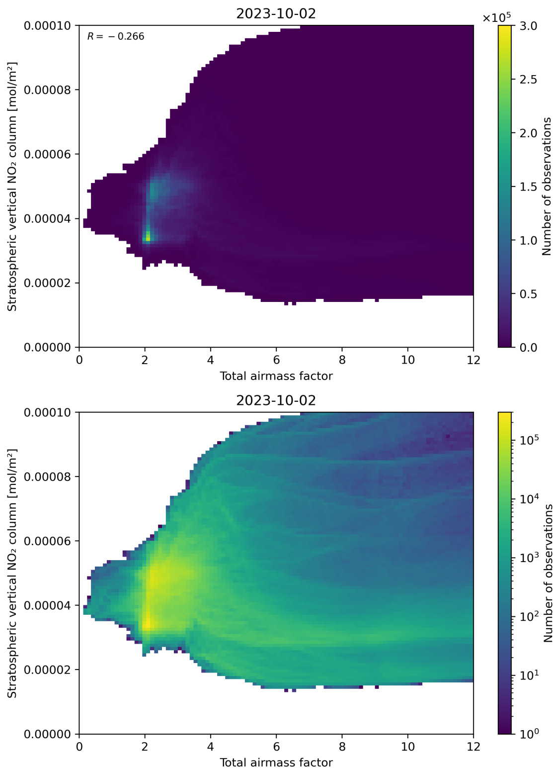
Figure 64: Scatter density plot of “Total airmass factor” against “Stratospheric vertical NO 2 column” for 2023-10-01 to 2023-10-03.
