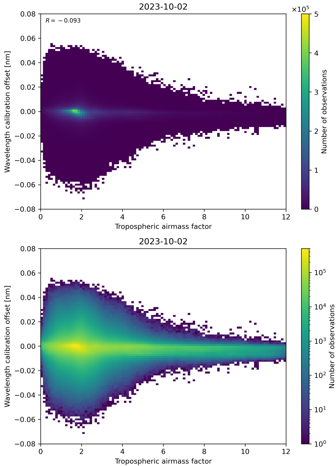
Figure 80: Scatter density plot of “Tropospheric airmass factor” against “Wavelength calibration offset” for 2023-10-01 to 2023-10-03.
