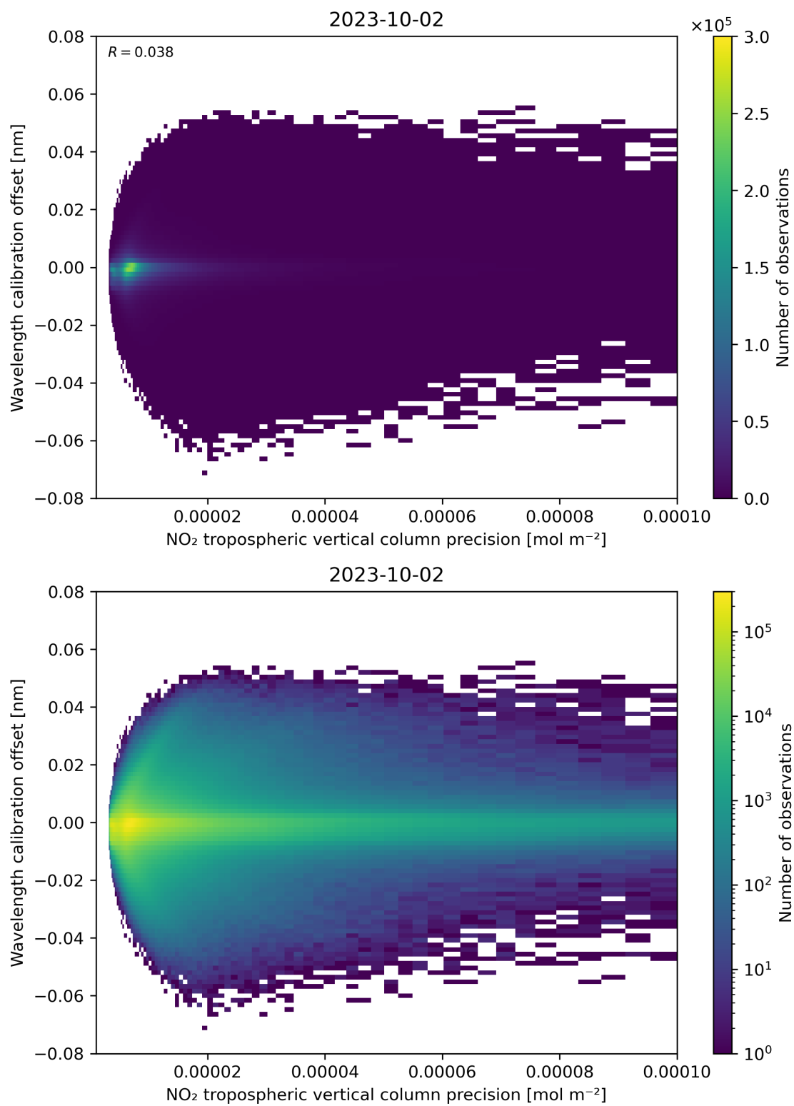
Figure 141: Scatter density plot of “NO 2 tropospheric vertical column precision” against “Wavelength calibration offset” for 2023-10-01 to 2023-10-03.
