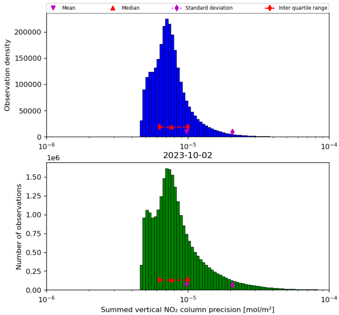
Figure 41: Histogram of "Summed vertical NO 2 column precision" for 2023-10-01 to 2023-10-03
