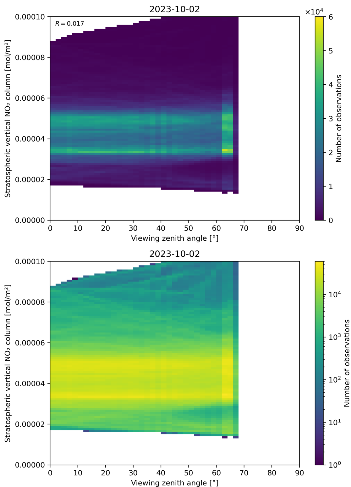
Figure 164: Scatter density plot of “Viewing zenith angle” against “Stratospheric vertical NO 2 column” for 2023-10-01 to 2023-10-03.
