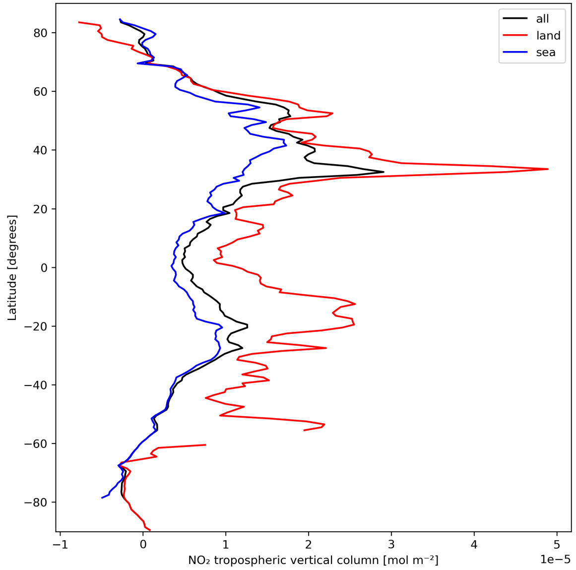
Figure 12: Zonal average of “NO 2 tropospheric vertical column” for 2023-10-01 to 2023-10-03.
