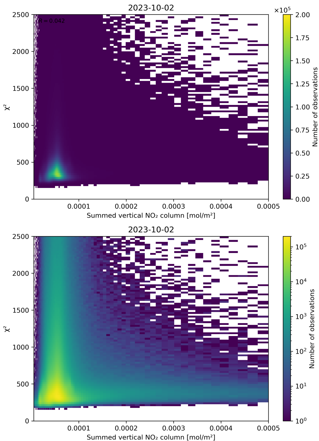
Figure 104: Scatter density plot of “Summed vertical NO 2 column” against “ \chi^2 ” for 2023-10-01 to 2023-10-03.
