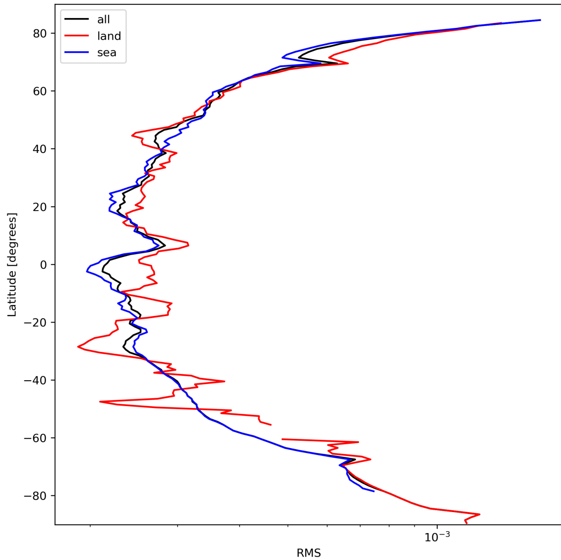
Figure 26: Zonal average of “RMS” for 2023-10-01 to 2023-10-03.
