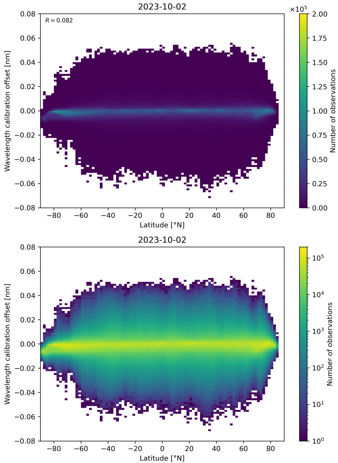
Figure 95: Scatter density plot of “Latitude” against “Wavelength calibration offset” for 2023-10-01 to 2023-10-03.
