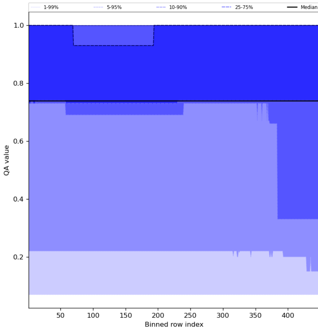
Figure 45: Along track statistics of “QA value” for 2023-10-01 to 2023-10-03
