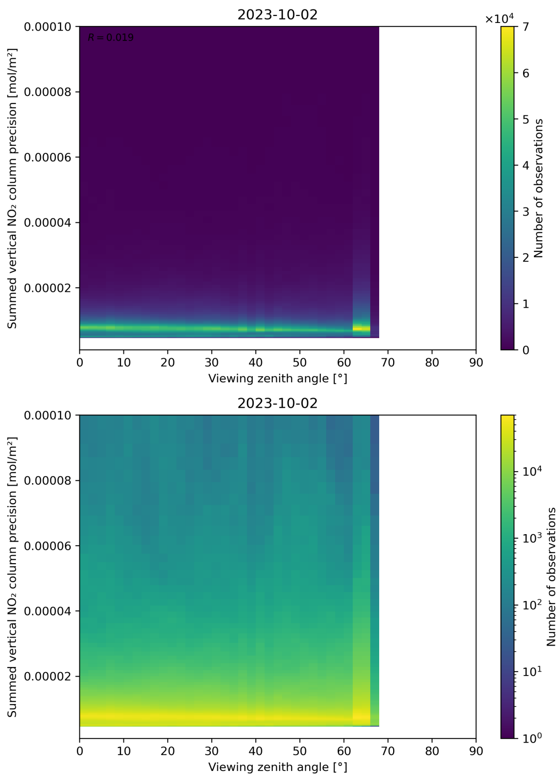
Figure 166: Scatter density plot of “Viewing zenith angle” against “Summed vertical NO 2 column precision” for 2023-10-01 to 2023-10-03.
