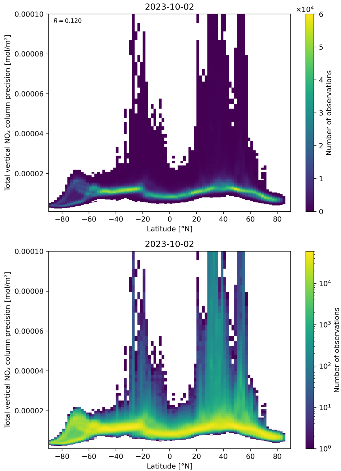
Figure 91: Scatter density plot of “Latitude” against “Total vertical NO 2 column precision” for 2023-10-01 to 2023-10-03.
