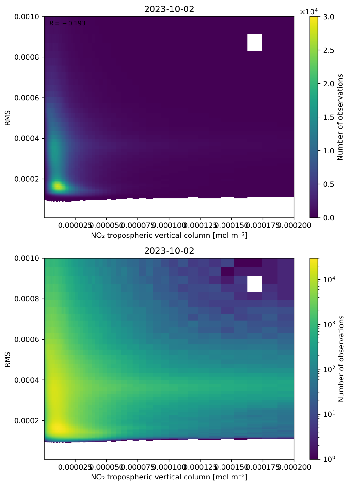
Figure 142: Scatter density plot of “NO 2 tropospheric vertical column” against “RMS” for 2023-10-01 to 2023-10-03.
