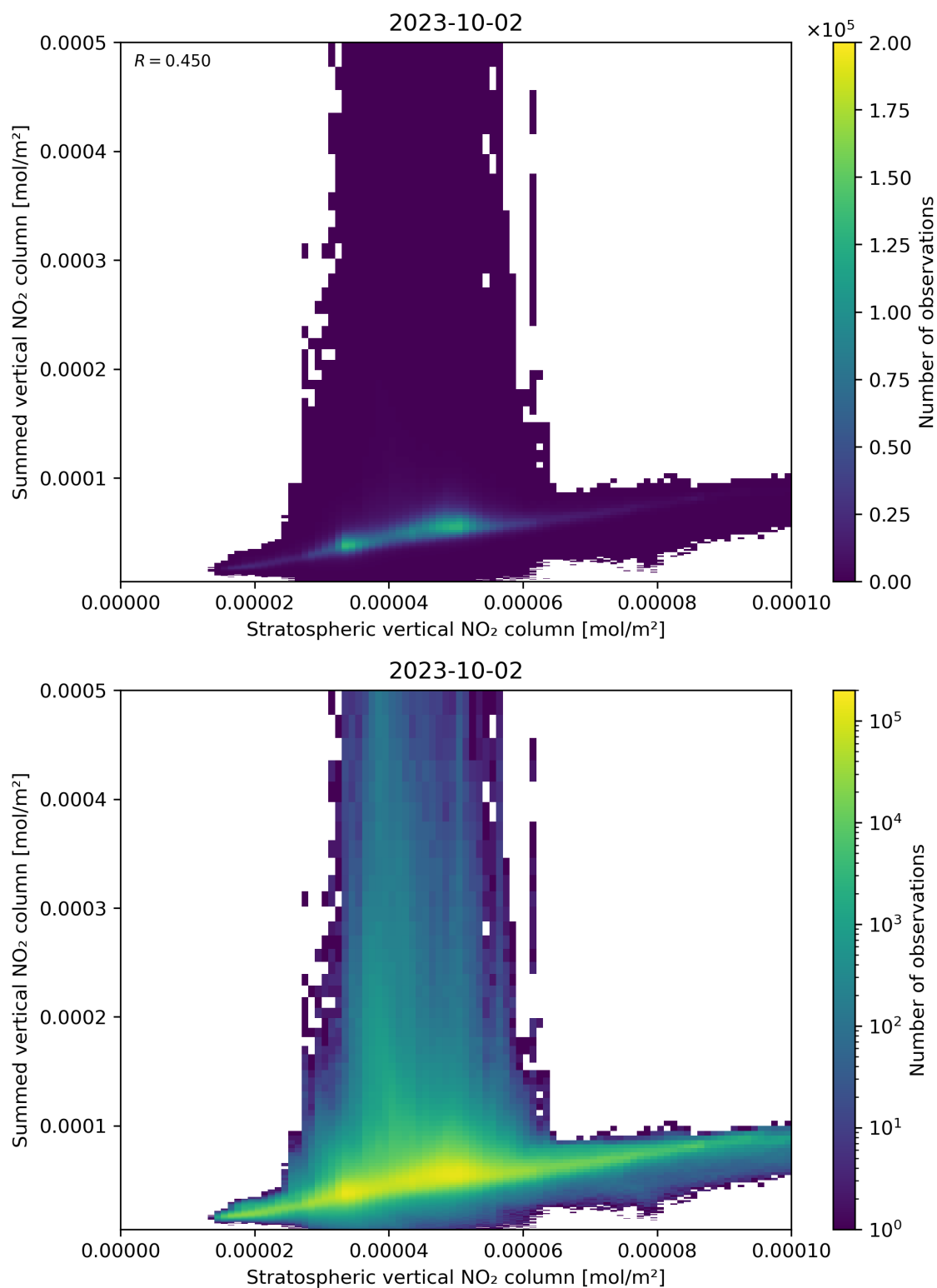
Figure 98: Scatter density plot of “Stratospheric vertical NO 2 column” against “Summed vertical NO 2 column” for 2023-10-01 to 2023-10-03.
