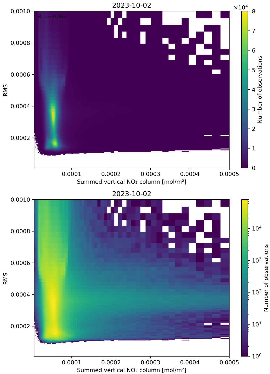
Figure 109: Scatter density plot of “Summed vertical NO 2 column” against “RMS” for 2023-10-01 to 2023-10-03.
