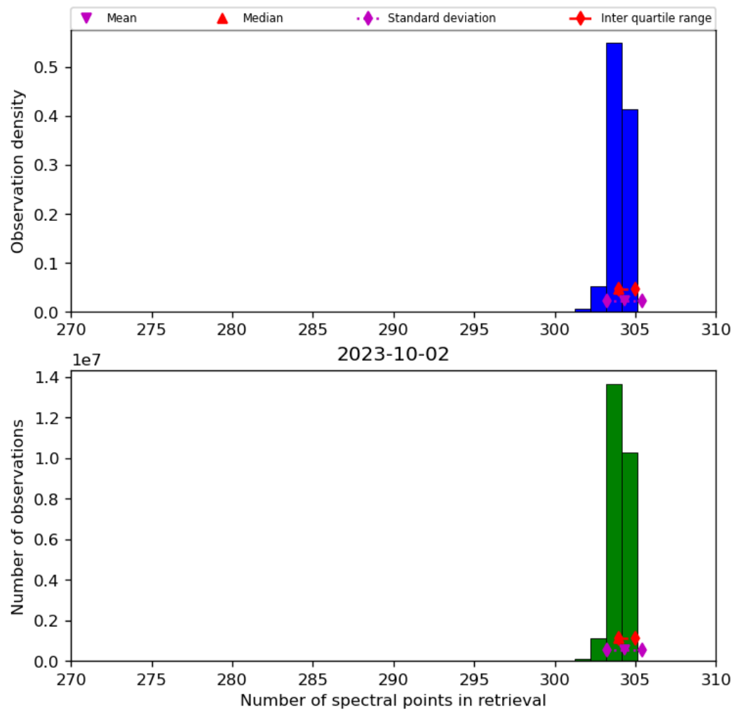
Figure 33: Histogram of “Number of spectral points in retrieval” for 2023-10-01 to 2023-10-03
