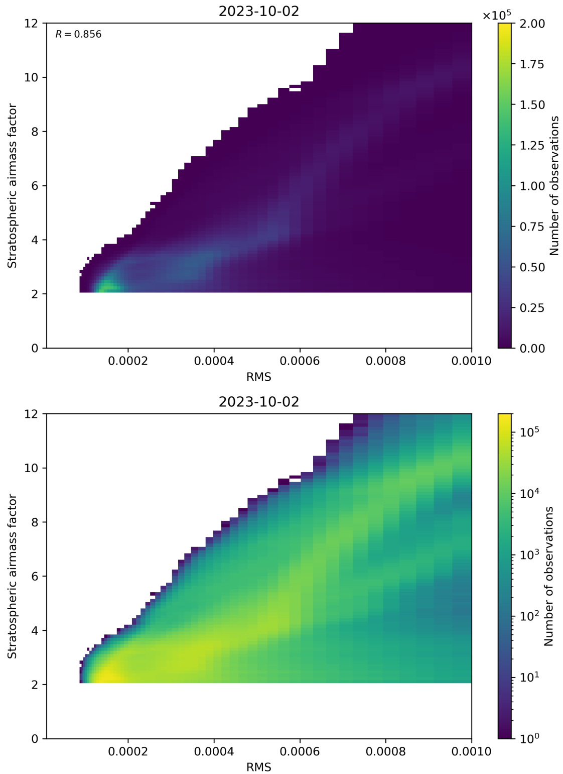
Figure 144: Scatter density plot of “RMS” against “Stratospheric airmass factor” for 2023-10-01 to 2023-10-03.
