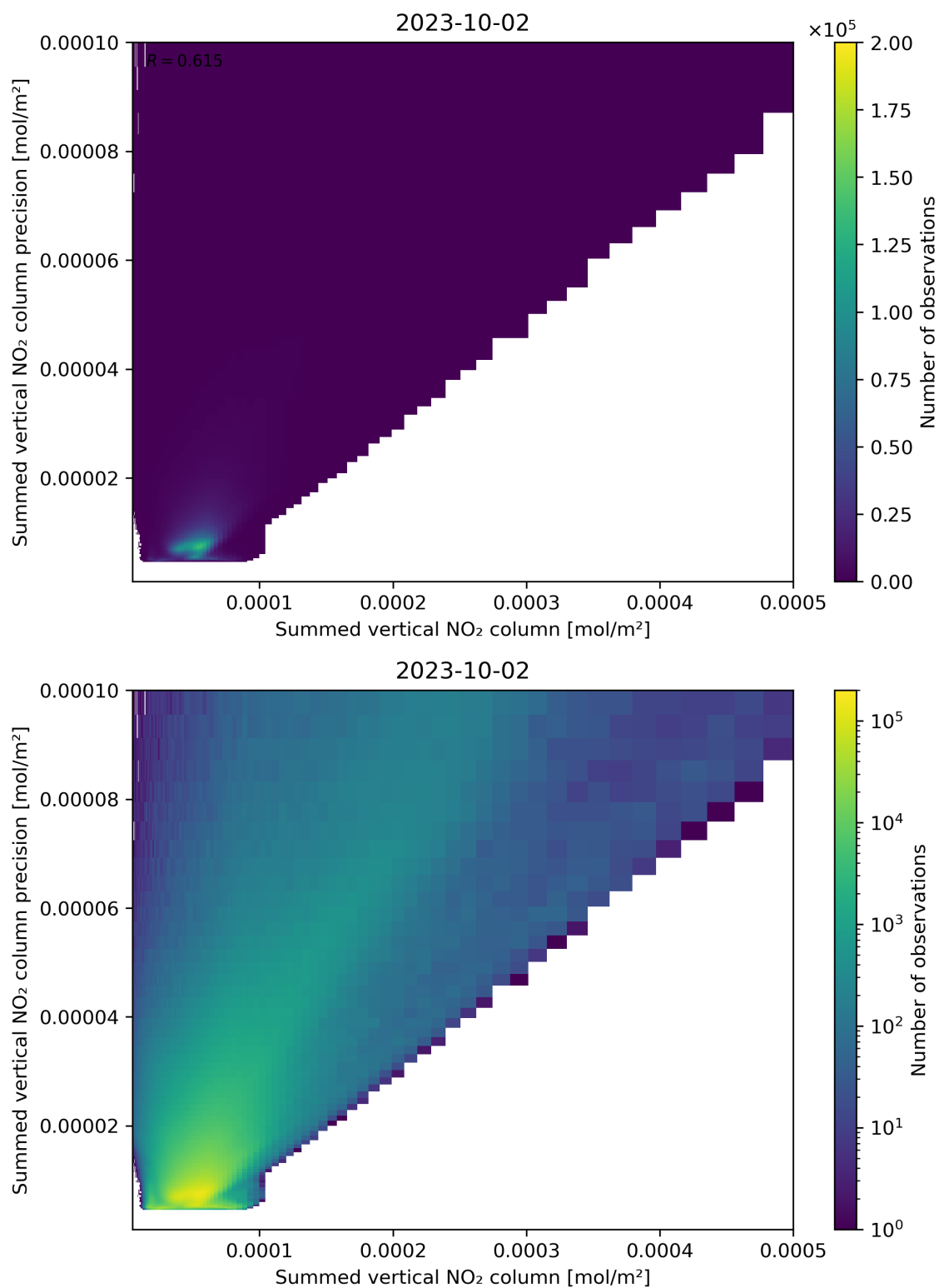
Figure 105: Scatter density plot of “Summed vertical NO 2 column” against “Summed vertical NO 2 column precision” for 2023-10-01 to 2023-10-03.
