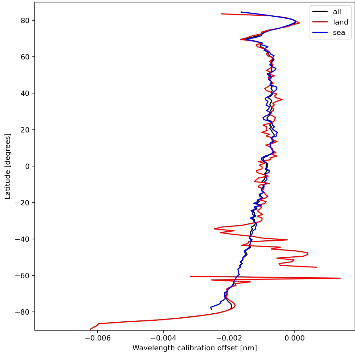
Figure 18: Zonal average of “Wavelength calibration offset” for 2023-10-01 to 2023-10-03.
