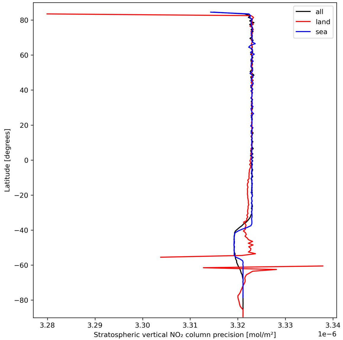
Figure 20: Zonal average of “Stratospheric vertical NO 2 column precision” for 2023-10-01 to 2023-10-03.
