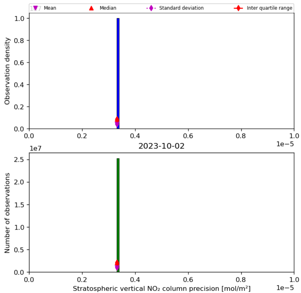
Figure 37: Histogram of “Stratospheric vertical NO 2 column precision” for 2023-10-01 to 2023-10-03
