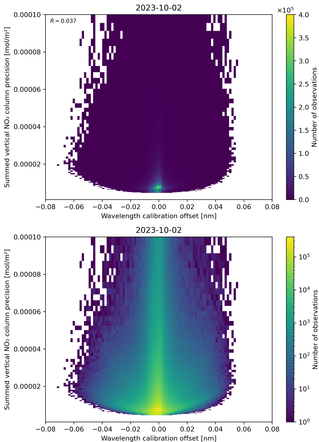
Figure 178: Scatter density plot of “Wavelength calibration offset” against “Summed vertical NO 2 column precision” for 2023-10-01 to 2023-10-03.
