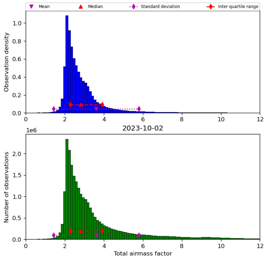
Figure 32: Histogram of “Total airmass factor” for 2023-10-01 to 2023-10-03
