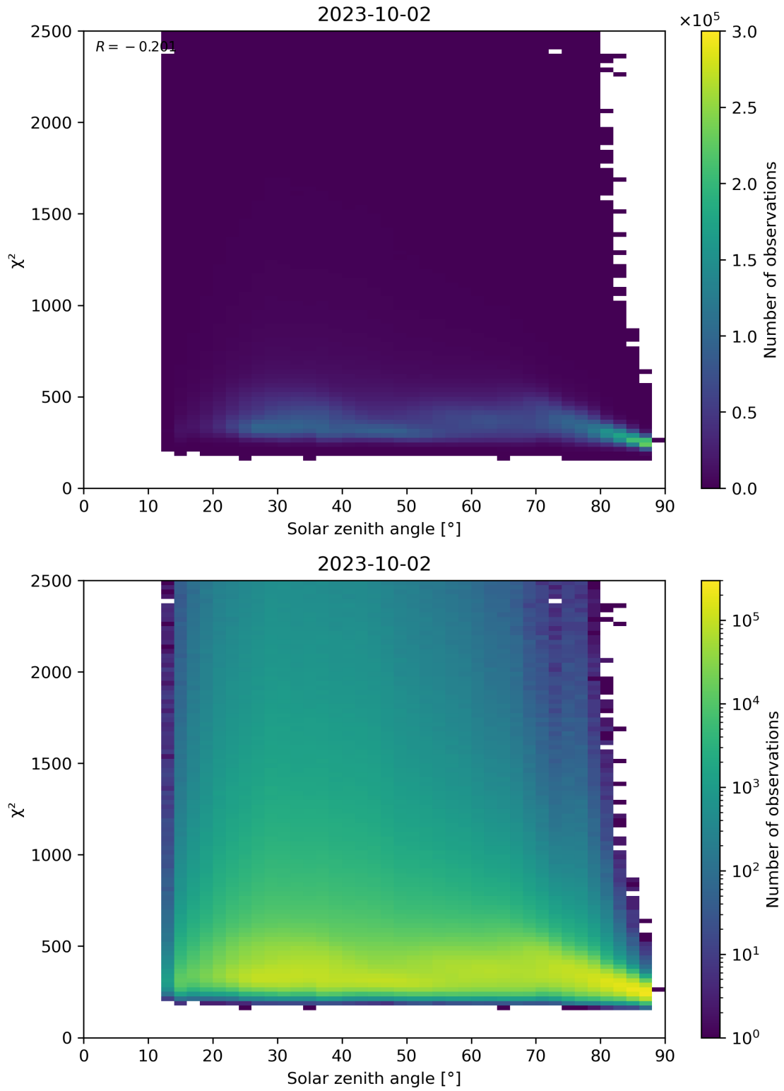
Figure 148: Scatter density plot of “Solar zenith angle” against “ \chi^2 ” for 2023-10-01 to 2023-10-03.
