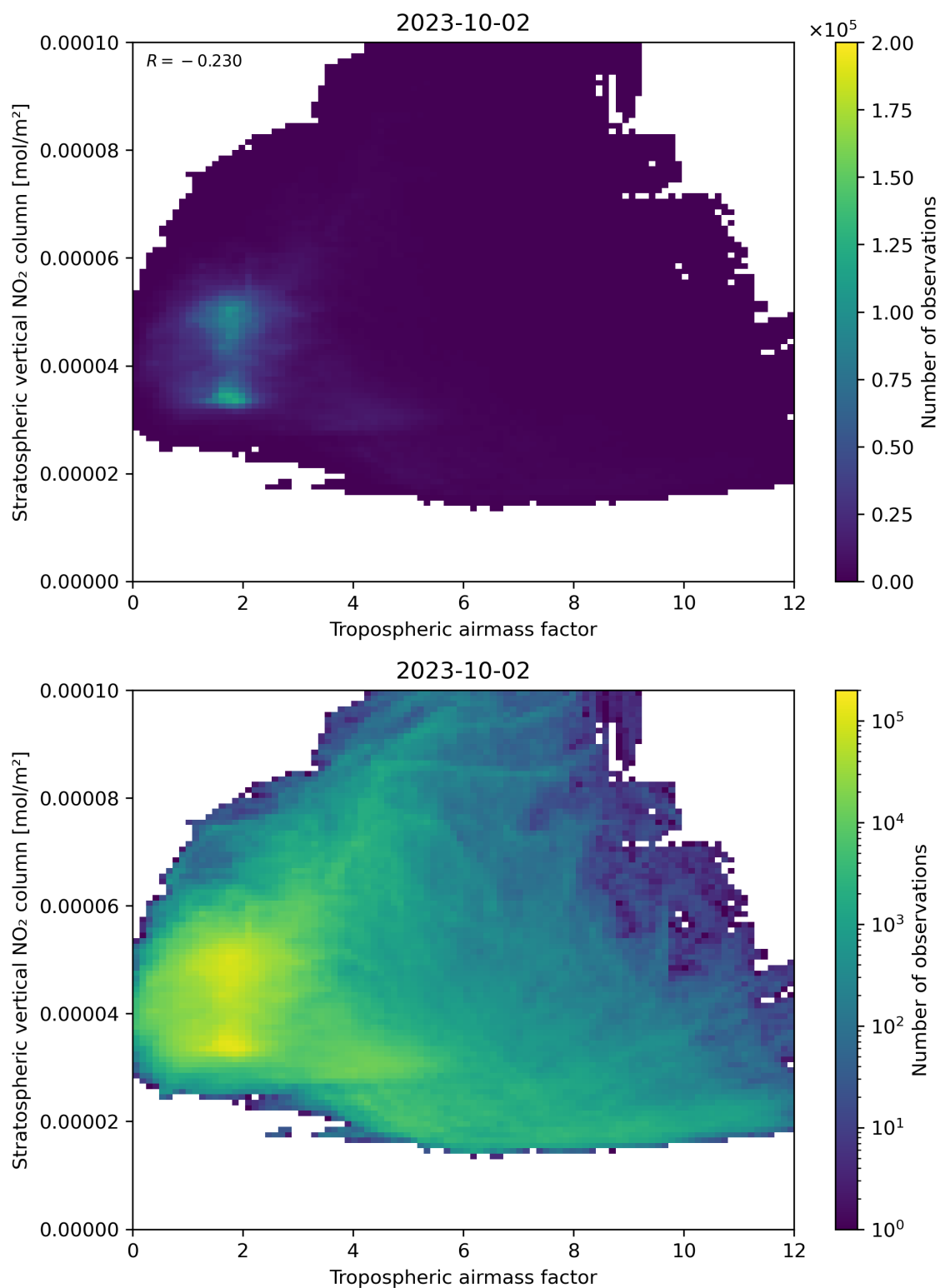
Figure 74: Scatter density plot of “Tropospheric air mass factor” against “Stratospheric vertical NO 2 column” for 2023-10-01 to 2023-10-03.
