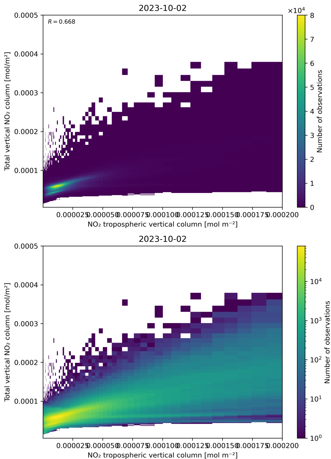
Figure 128: Scatter density plot of “NO 2 tropospheric vertical column” against “Total vertical NO 2 column” for 2023-10-01 to 2023-10-03.
