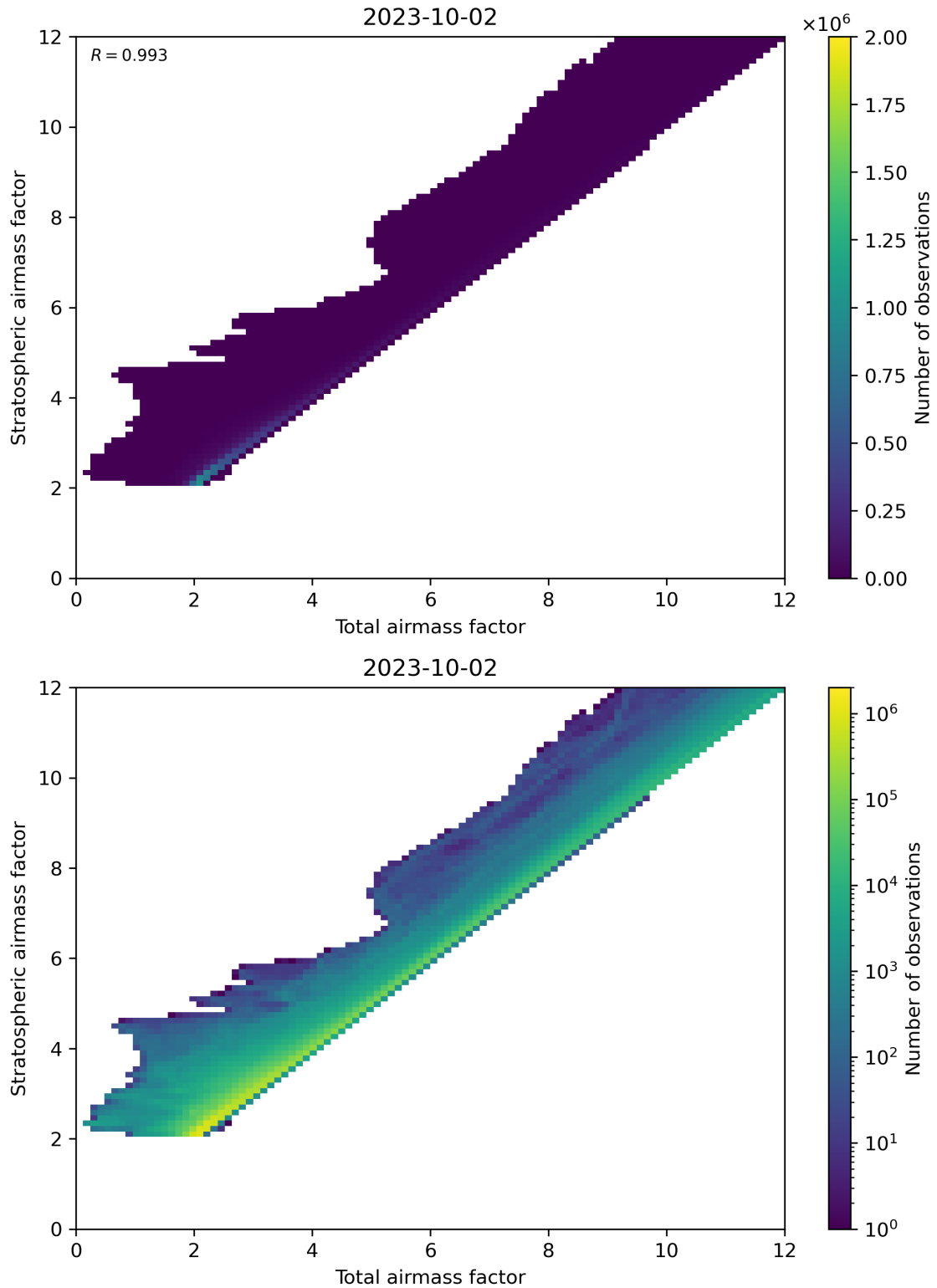
Figure 62: Scatter density plot of “Total airmass factor” against “Stratospheric airmass factor” for 2023-10-01 to 2023-10-03.
