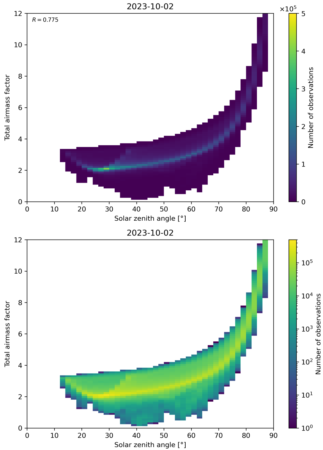
Figure 146: Scatter density plot of “Solar zenith angle” against “Total airmass factor” for 2023-10-01 to 2023-10-03.
