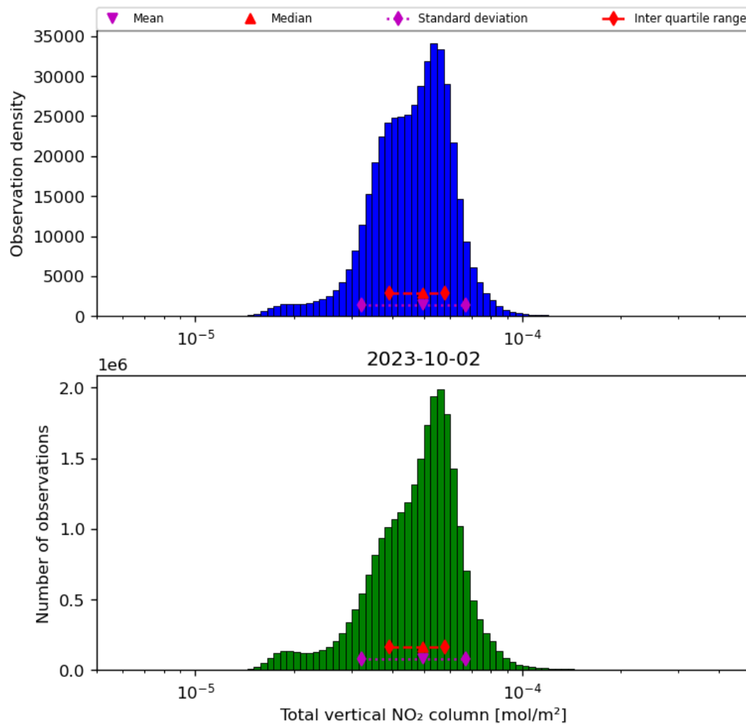
Figure 38: Histogram of “Total vertical NO 2 column” for 2023-10-01 to 2023-10-03
