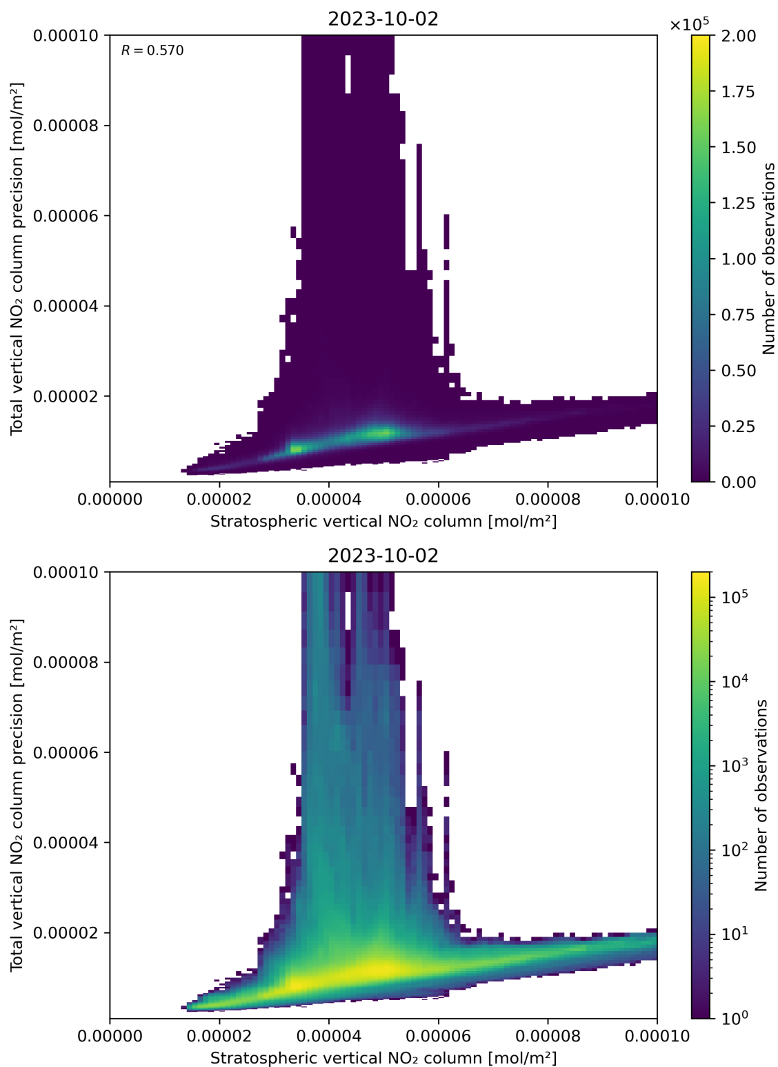
Figure 101: Scatter density plot of “Stratospheric vertical NO 2 column” against “Total vertical NO 2 column precision” for 2023-10-01 to 2023-10-03.
