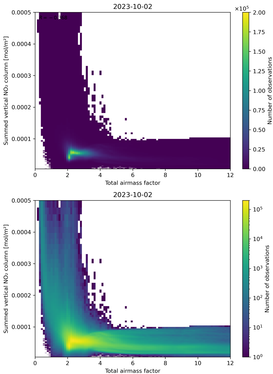
Figure 65: Scatter density plot of “Total airmass factor” against “Summed vertical NO 2 column” for 2023-10-01 to 2023-10-03.
