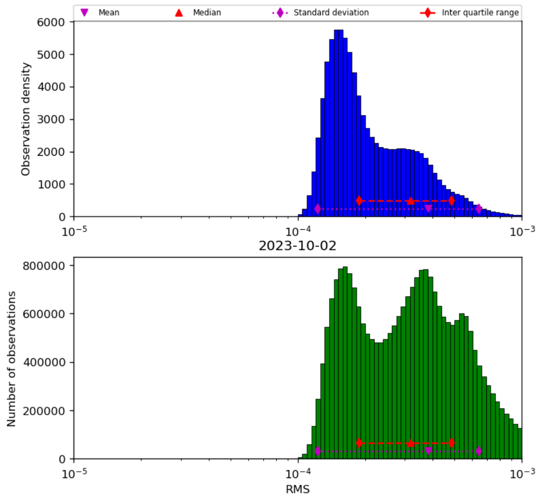
Figure 43: Histogram of “RMS” for 2023-10-01 to 2023-10-03
