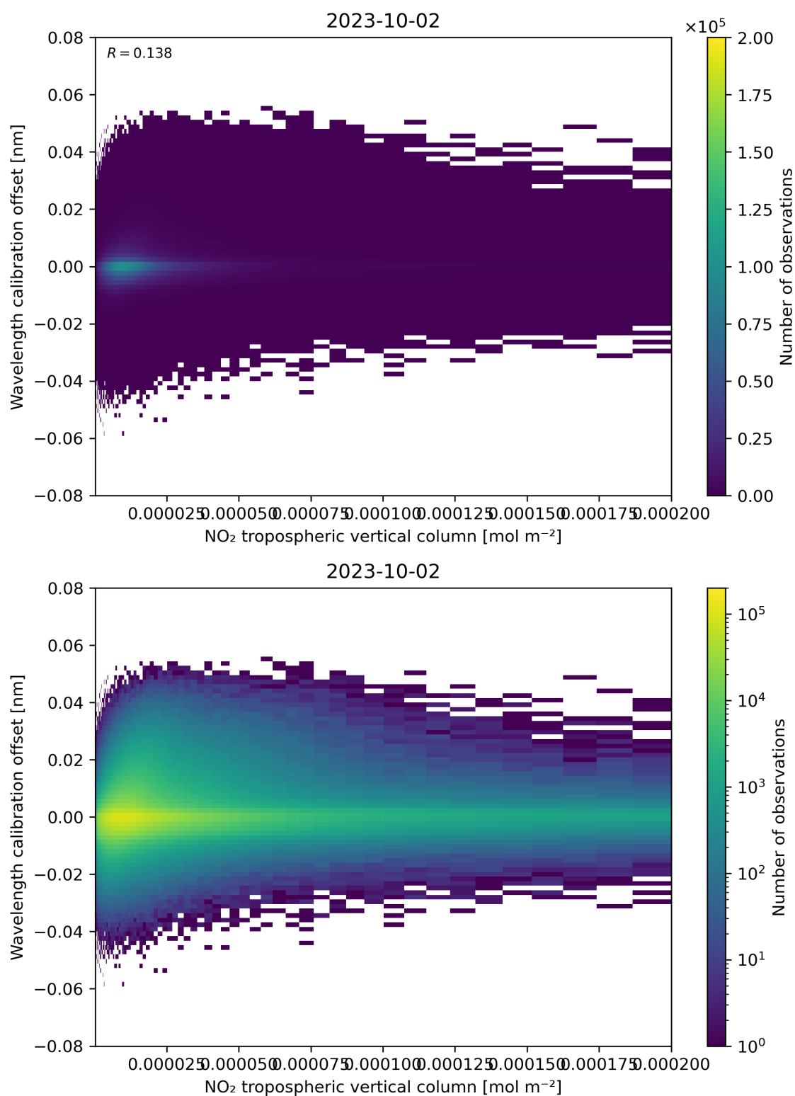
Figure 143: Scatter density plot of “NO 2 tropospheric vertical column” against “Wavelength calibration offset” for 2023-10-01 to 2023-10-03.
