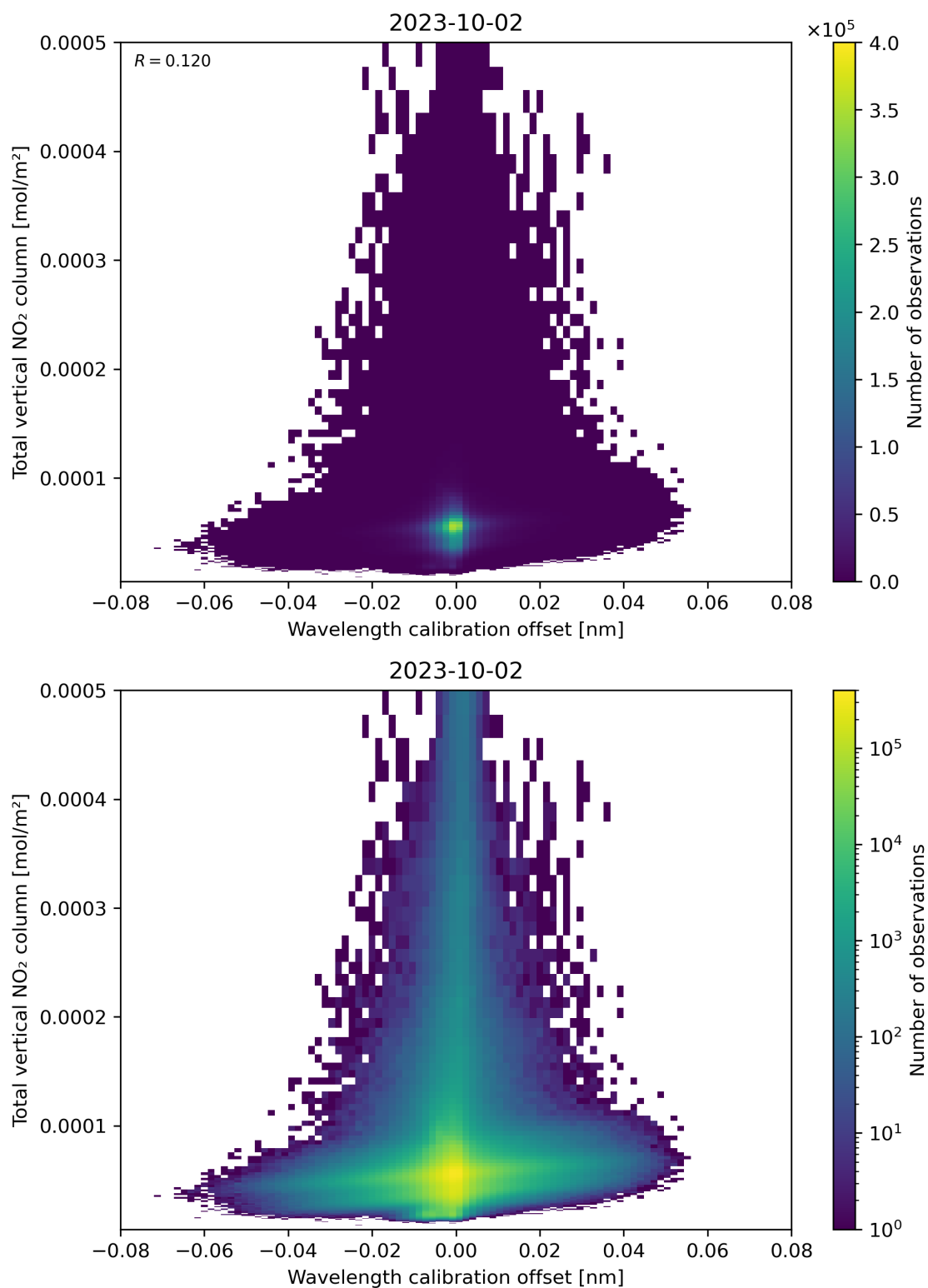
Figure 179: Scatter density plot of “Wavelength calibration offset” against “Total vertical NO 2 column” for 2023-10-01 to 2023-10-03.
