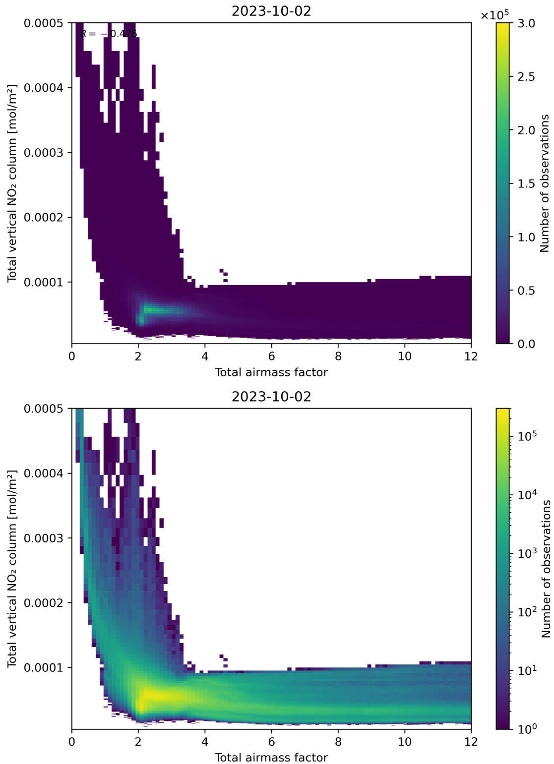
Figure 67: Scatter density plot of “Total airmass factor” against “Total vertical NO 2 column” for 2023-10-01 to 2023-10-03.
