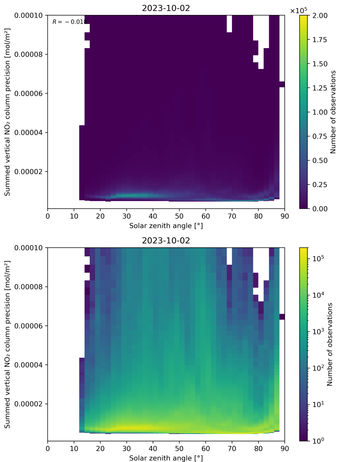
Figure 152: Scatter density plot of “Solar zenith angle” against “Summed vertical NO 2 column precision” for 2023-10-01 to 2023-10-03.
