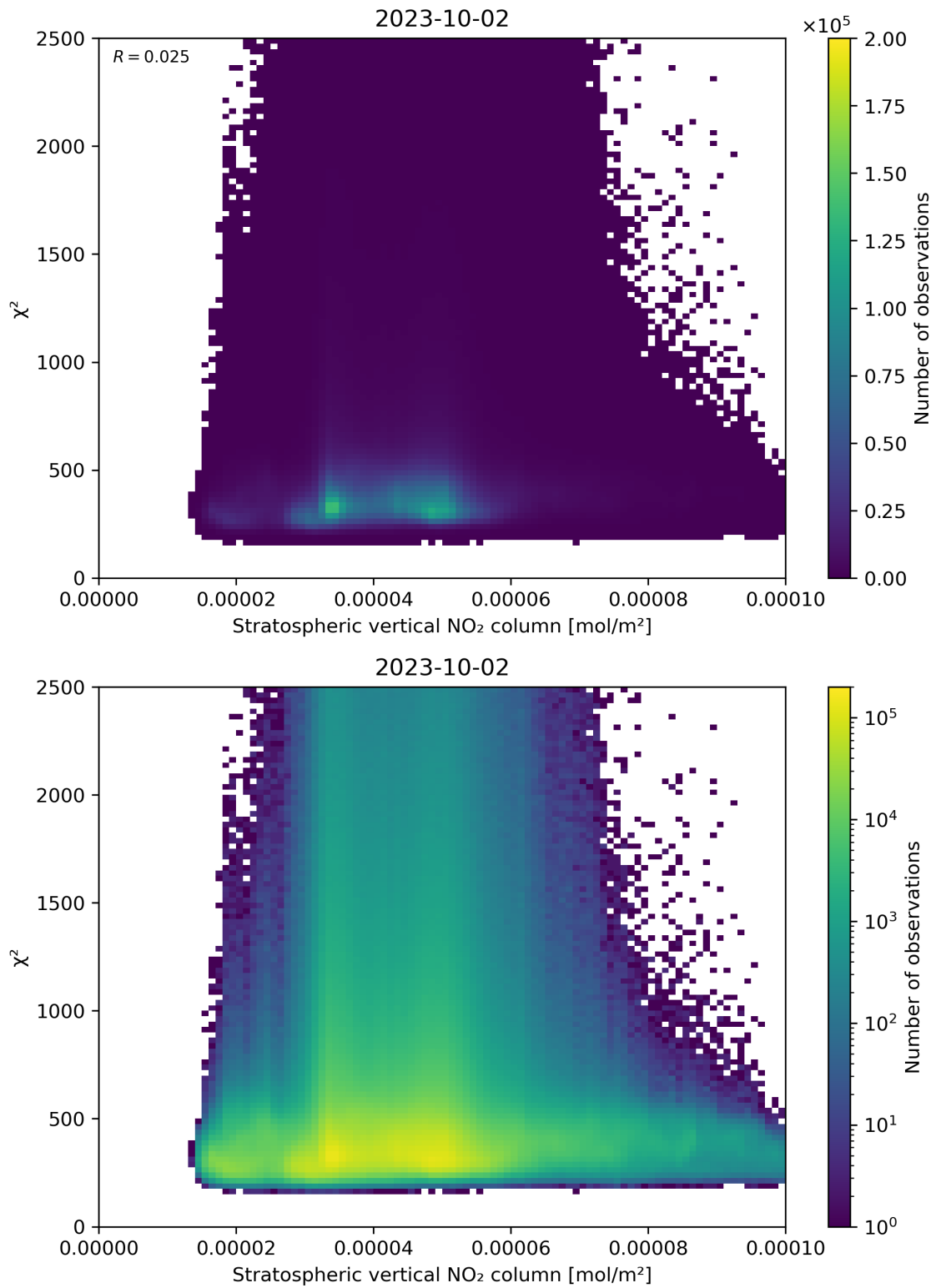
Figure 97: Scatter density plot of “Stratospheric vertical NO 2 column” against “ \chi^2 ” for 2023-10-01 to 2023-10-03.
