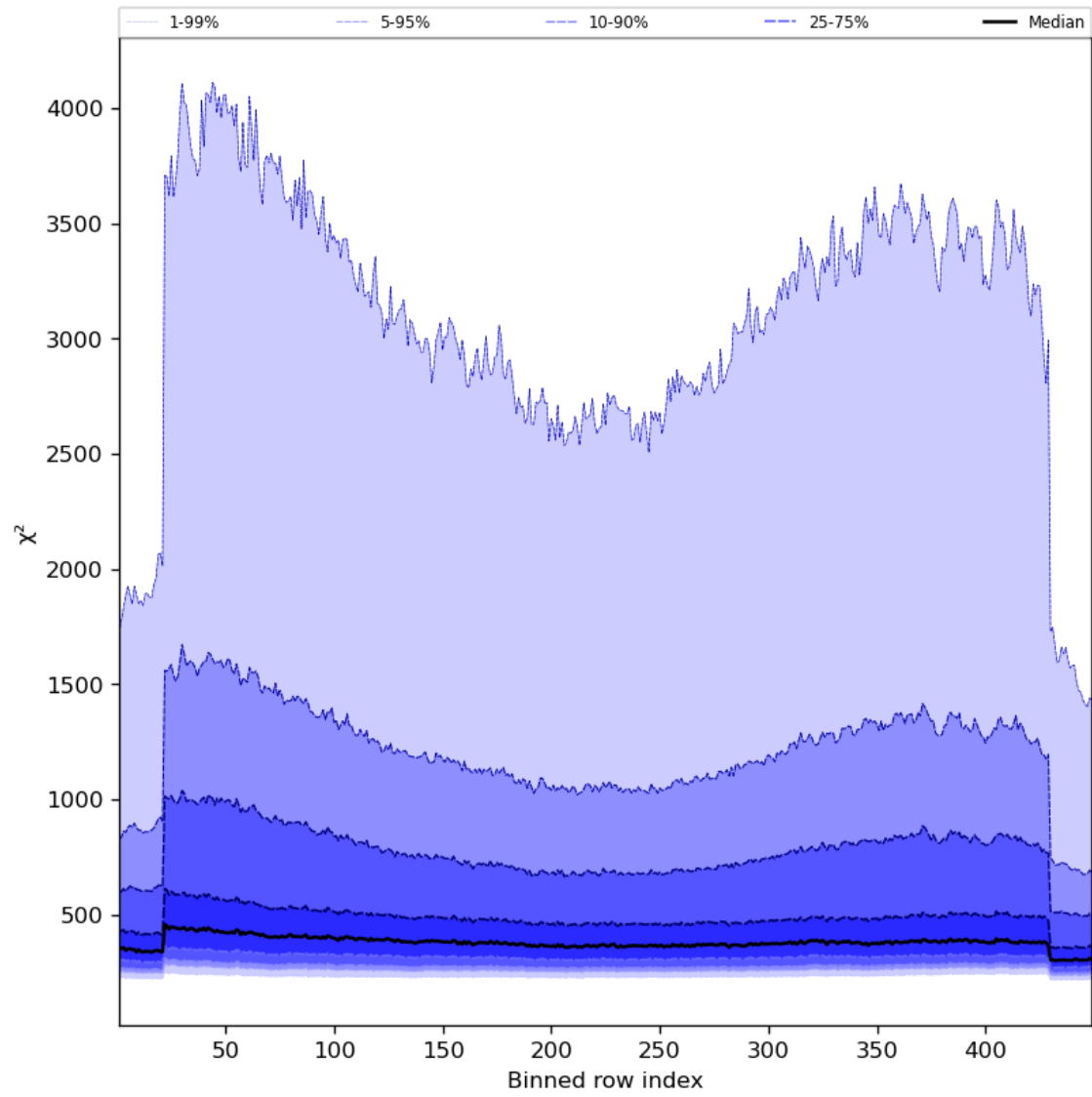
Figure 59: Along track statistics of “ \chi^2 ” for 2023-10-01 to 2023-10-03
