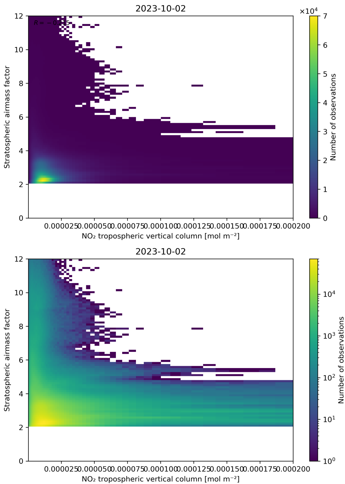
Figure 121: Scatter density plot of “NO 2 tropospheric vertical column” against “Stratospheric air mass factor” for 2023-10-01 to 2023-10-03.
