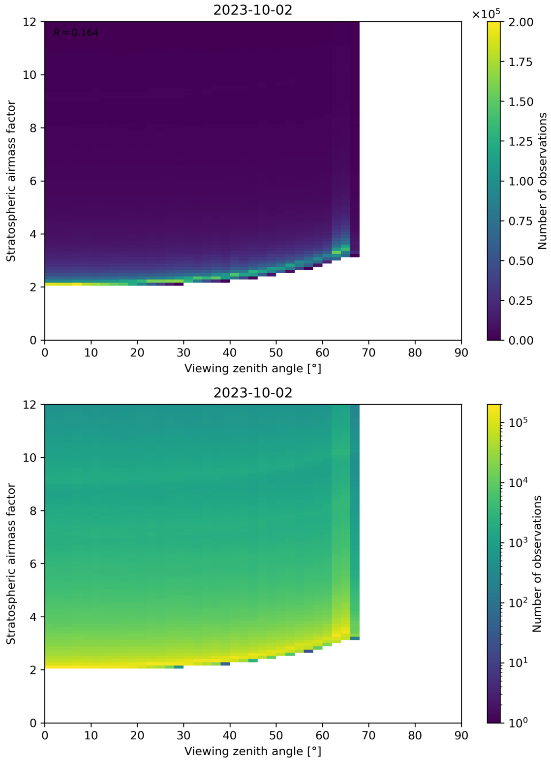
Figure 159: Scatter density plot of “Viewing zenith angle” against “Stratospheric airmass factor” for 2023-10-01 to 2023-10-03.
