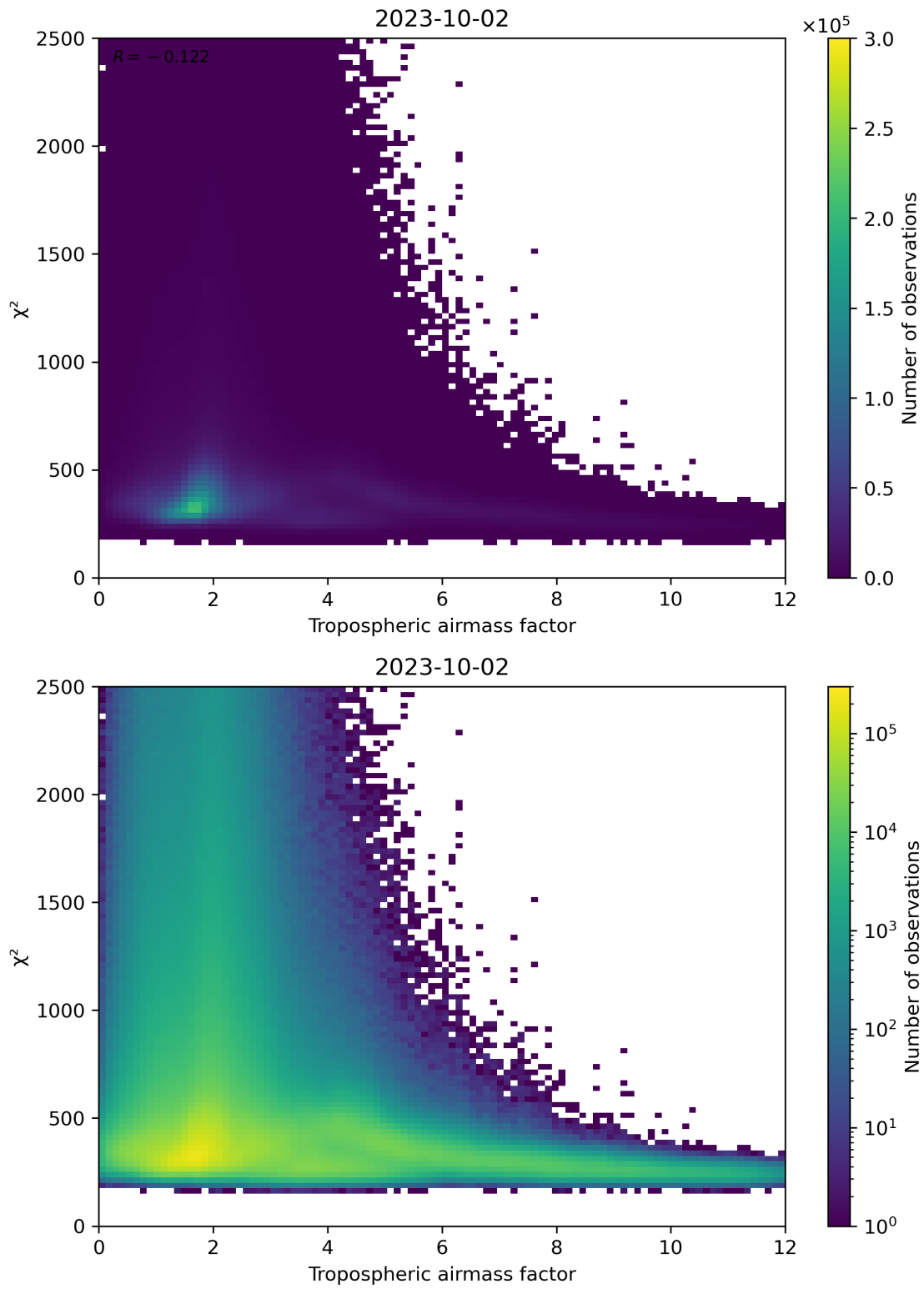
Figure 73: Scatter density plot of “Tropospheric airmass factor” against “ \chi^2 ” for 2023-10-01 to 2023-10-03.
