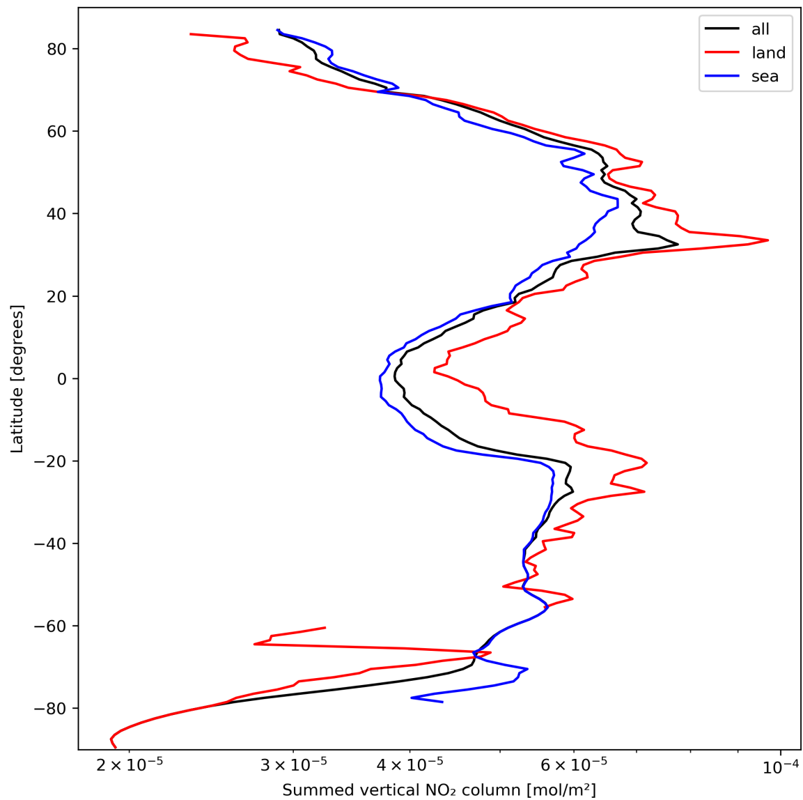
Figure 23: Zonal average of “Summed vertical NO 2 column” for 2023-10-01 to 2023-10-03.
