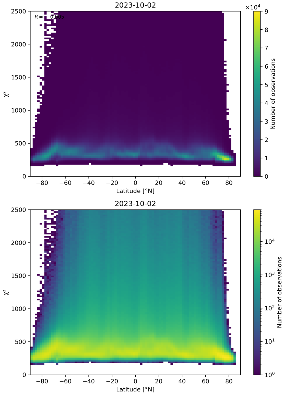
Figure 86: Scatter density plot of “Latitude” against “ \chi^2 ” for 2023-10-01 to 2023-10-03.
