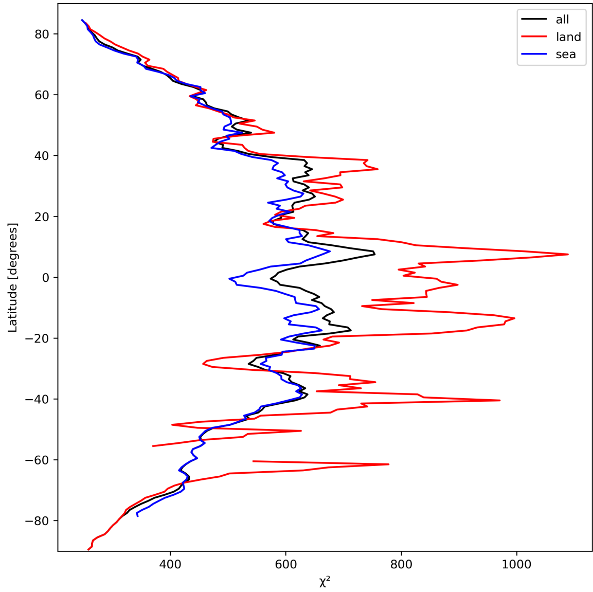
Figure 25: Zonal average of “ \chi^2 ” for 2023-10-01 to 2023-10-03.
