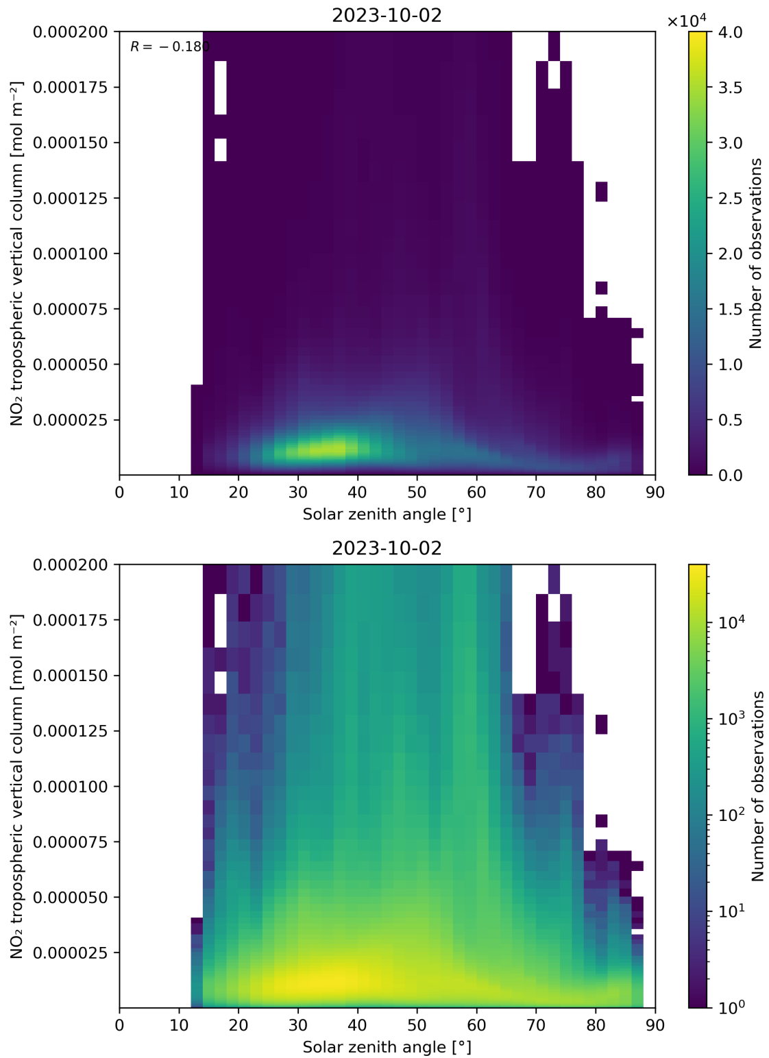
Figure 155: Scatter density plot of “Solar zenith angle” against “NO 2 tropospheric vertical column” for 2023-10-01 to 2023-10-03.
