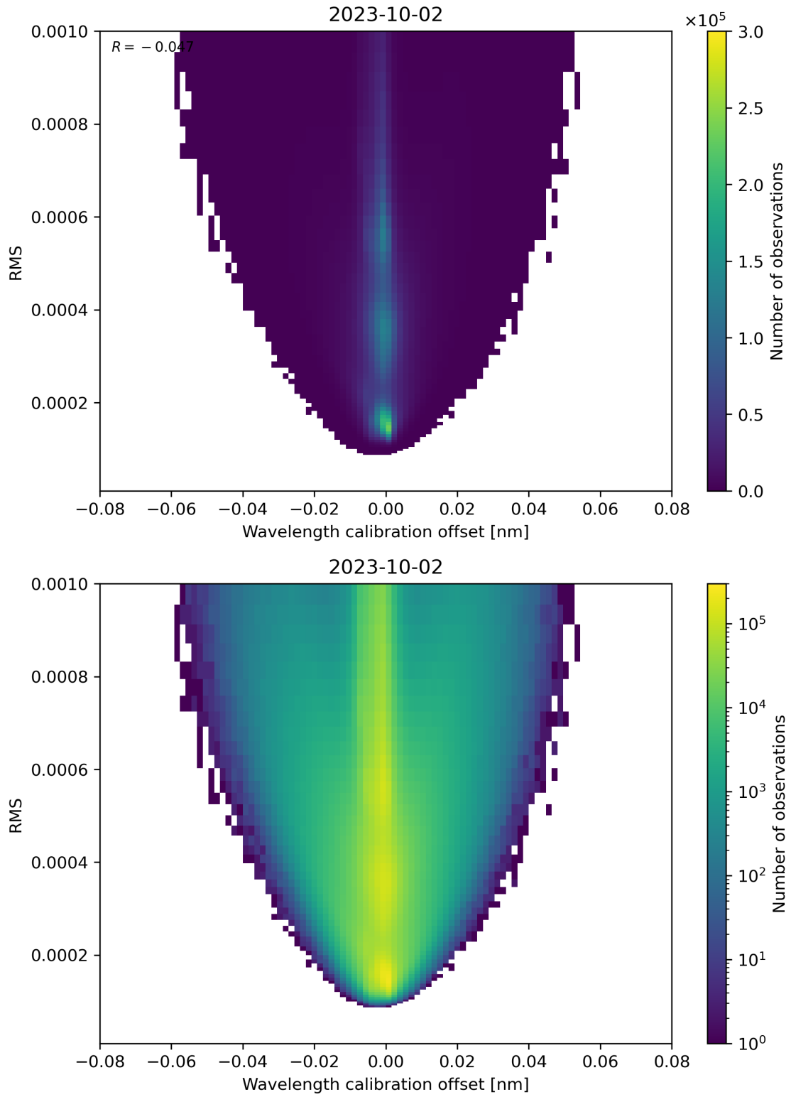
Figure 181: Scatter density plot of “Wavelength calibration offset” against “RMS” for 2023-10-01 to 2023-10-03.
