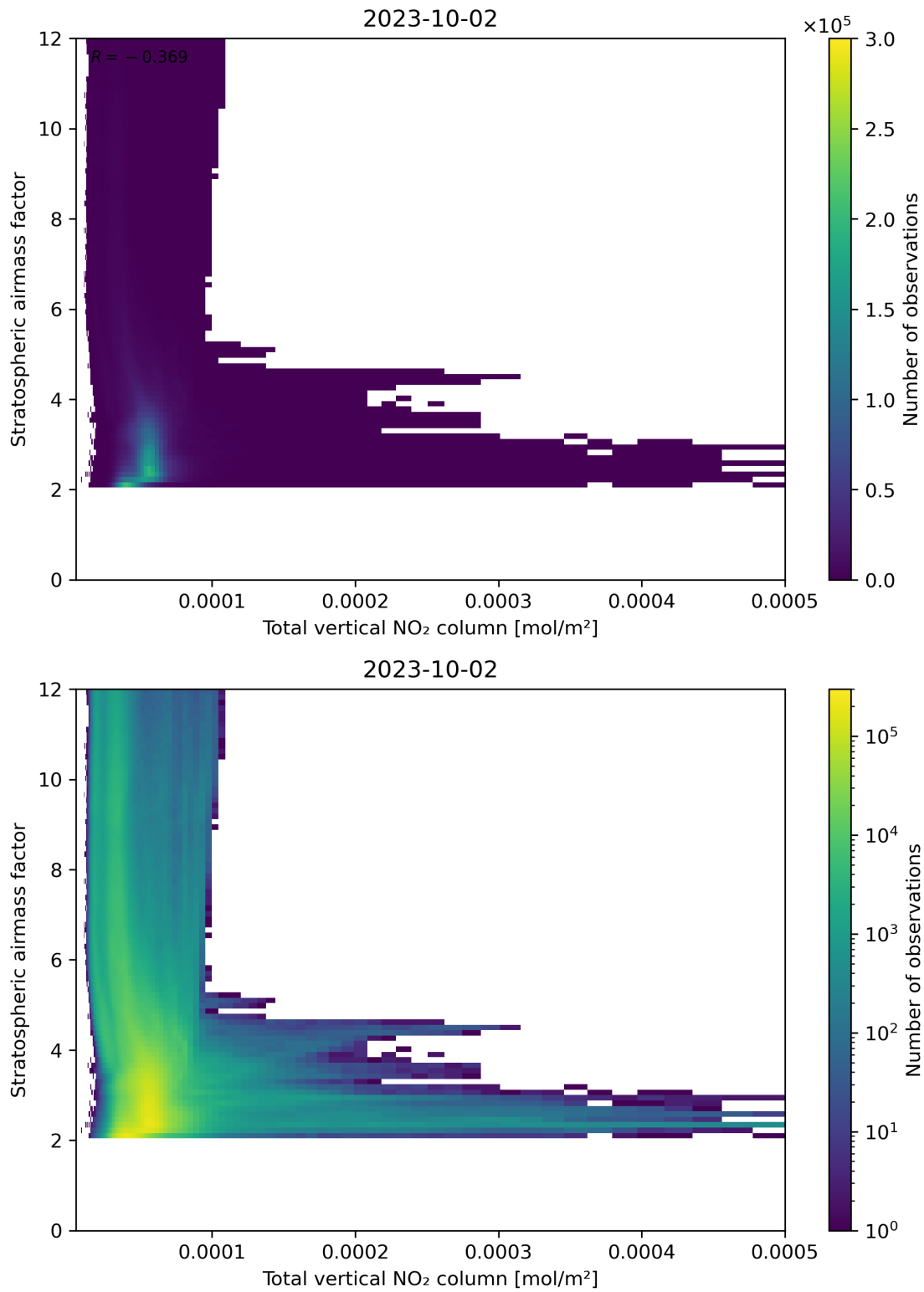
Figure 110: Scatter density plot of “Total vertical NO 2 column” against “Stratospheric airmass factor” for 2023-10-01 to 2023-10-03.
