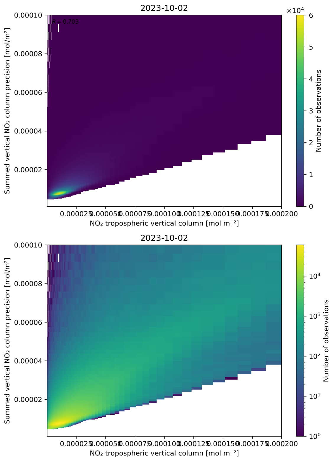
Figure 127: Scatter density plot of “NO 2 tropospheric vertical column” against “Summed vertical NO 2 column precision” for 2023-10-01 to 2023-10-03.
