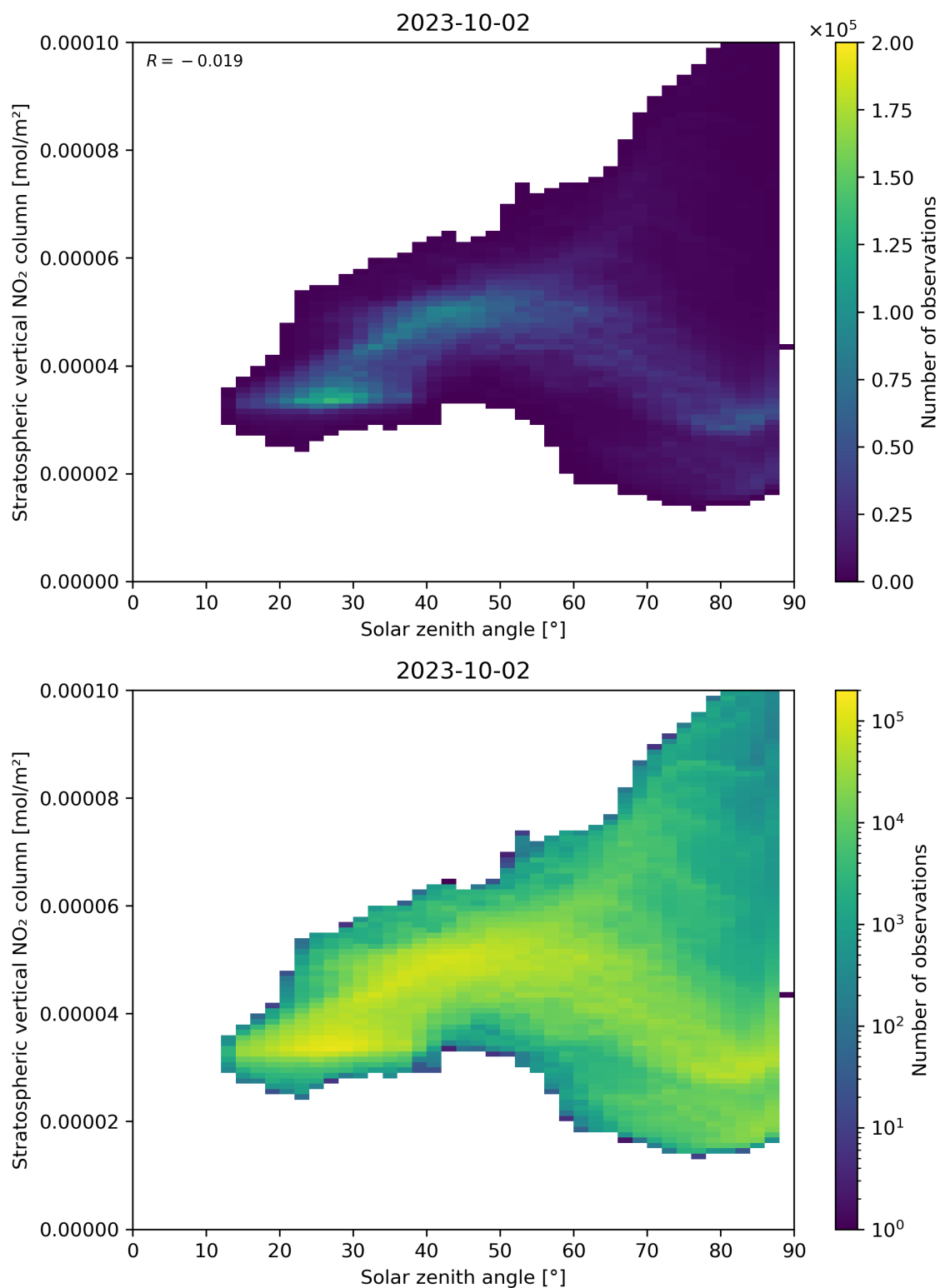
Figure 150: Scatter density plot of “Solar zenith angle” against “Stratospheric vertical NO 2 column” for 2023-10-01 to 2023-10-03.
