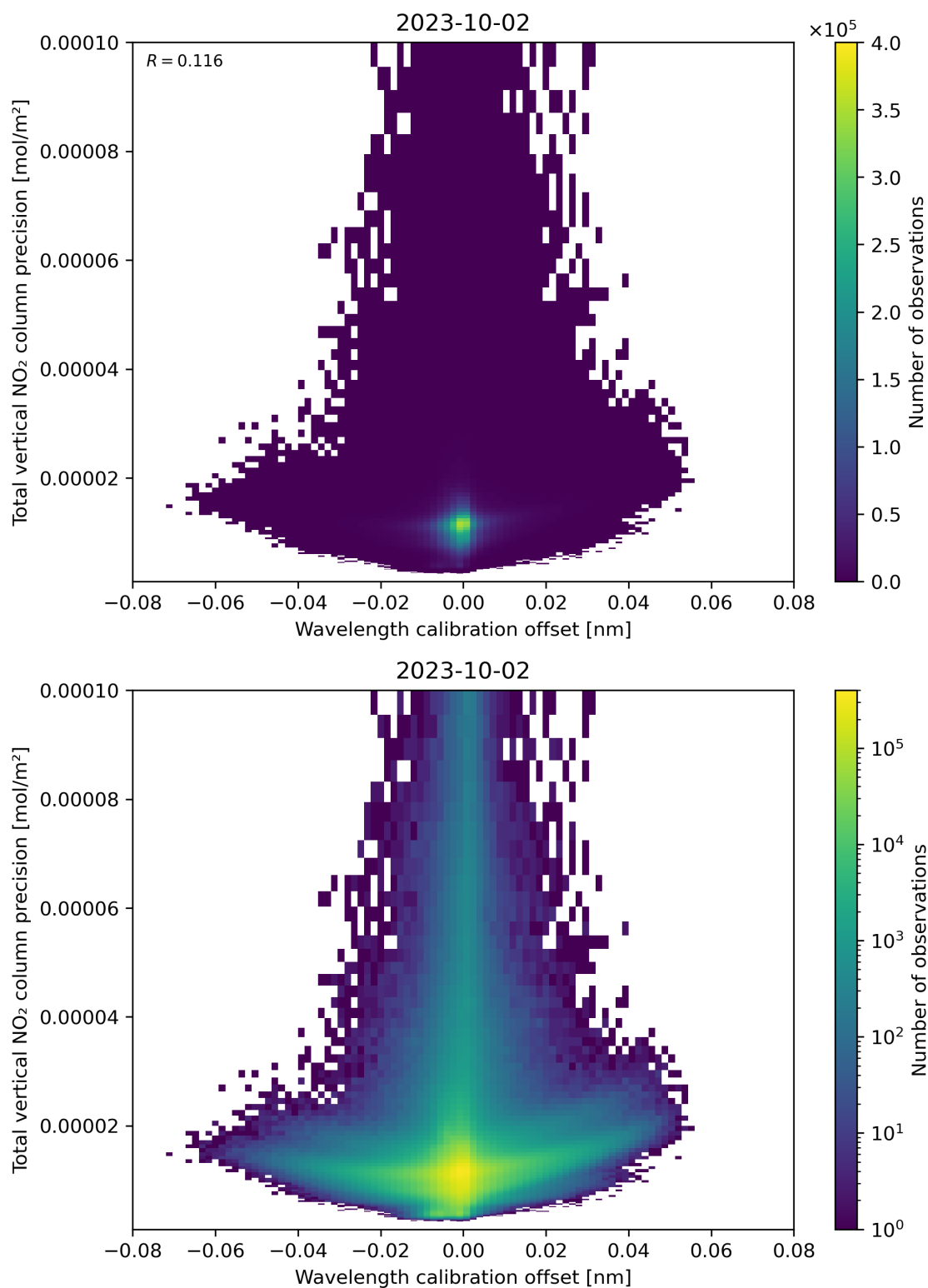
Figure 180: Scatter density plot of “Wavelength calibration offset” against “Total vertical NO 2 column precision” for 2023-10-01 to 2023-10-03.
