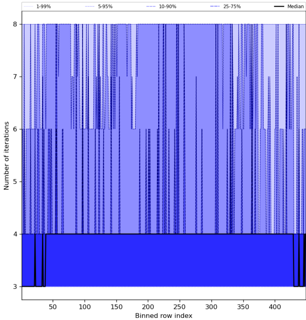
Figure 51: Along track statistics of “Number of iterations” for 2023-10-01 to 2023-10-03
