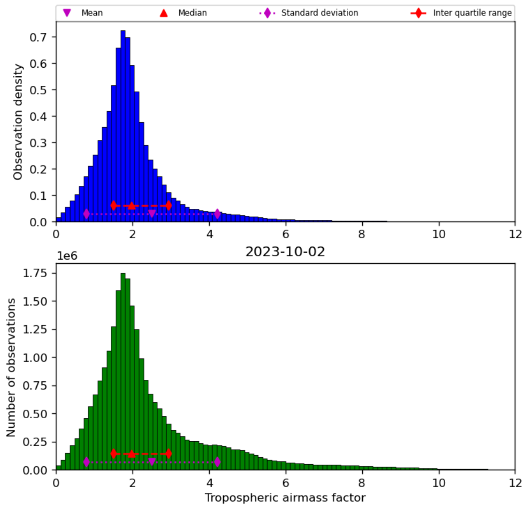
Figure 31: Histogram of “Tropospheric airmass factor” for 2023-10-01 to 2023-10-03
