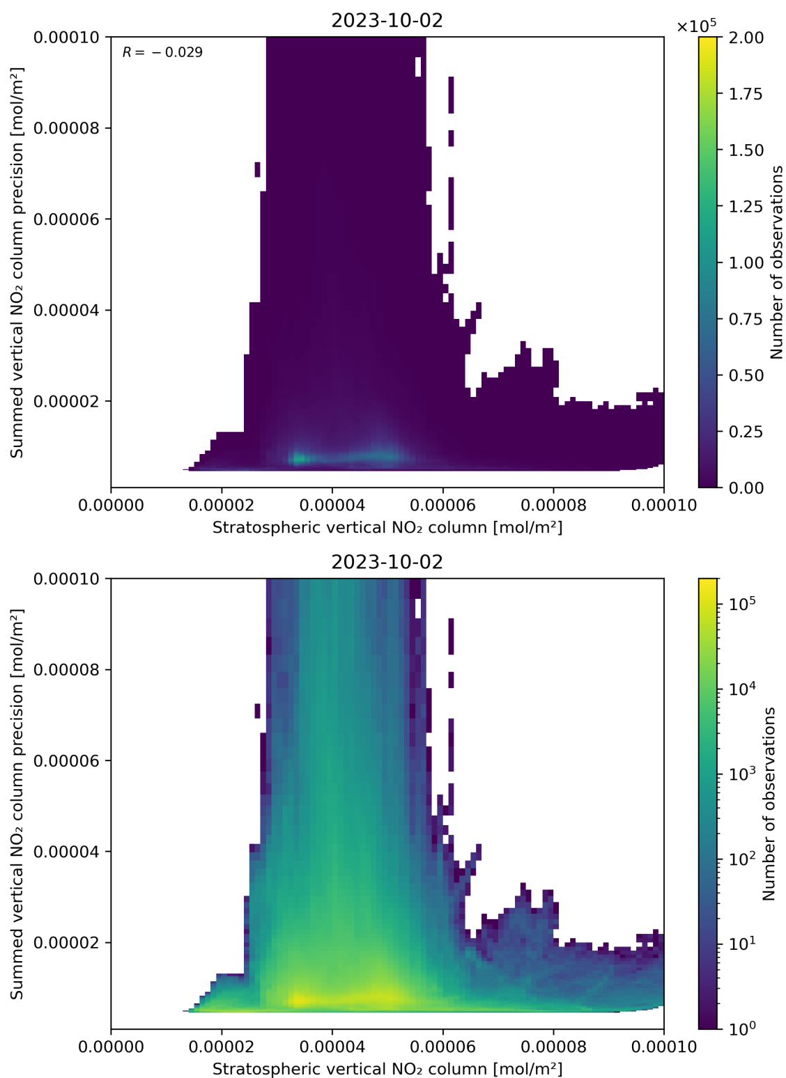
Figure 99: Scatter density plot of “Stratospheric vertical NO 2 column” against “Summed vertical NO 2 column precision” for 2023-10-01 to 2023-10-03.
