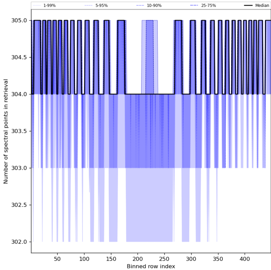
Figure 50: Along track statistics of “Number of spectral points in retrieval” for 2023-10-01 to 2023-10-03
