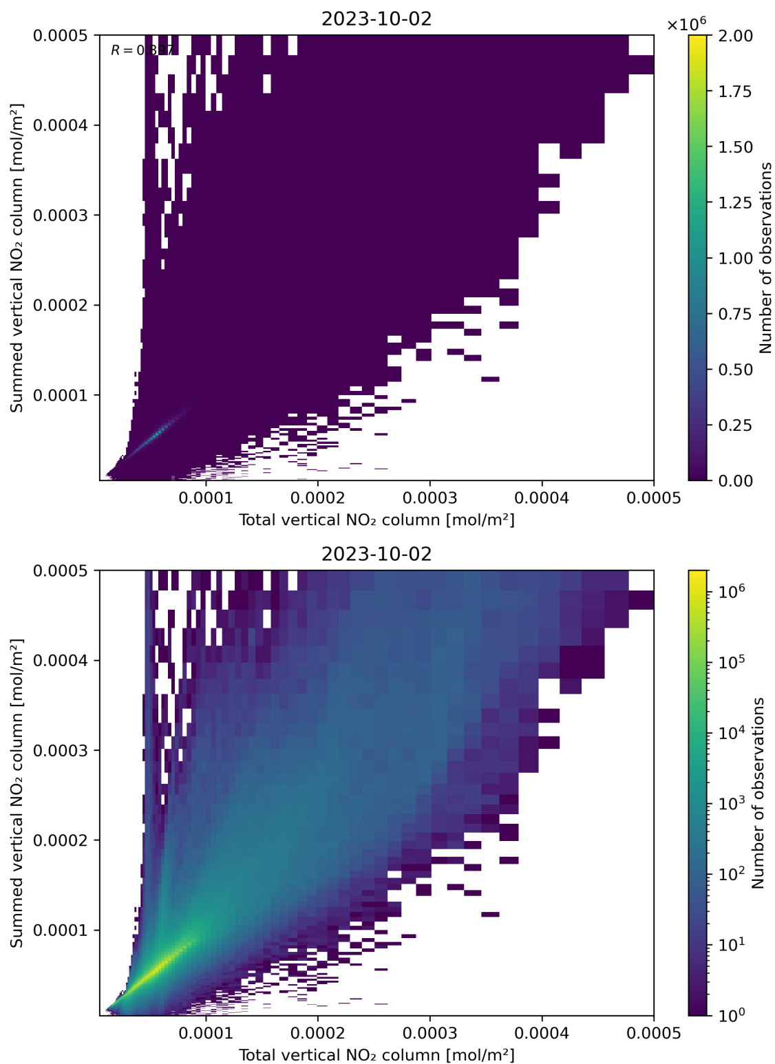
Figure 112: Scatter density plot of “Total vertical NO 2 column” against “Summed vertical NO 2 column” for 2023-10-01 to 2023-10-03.
