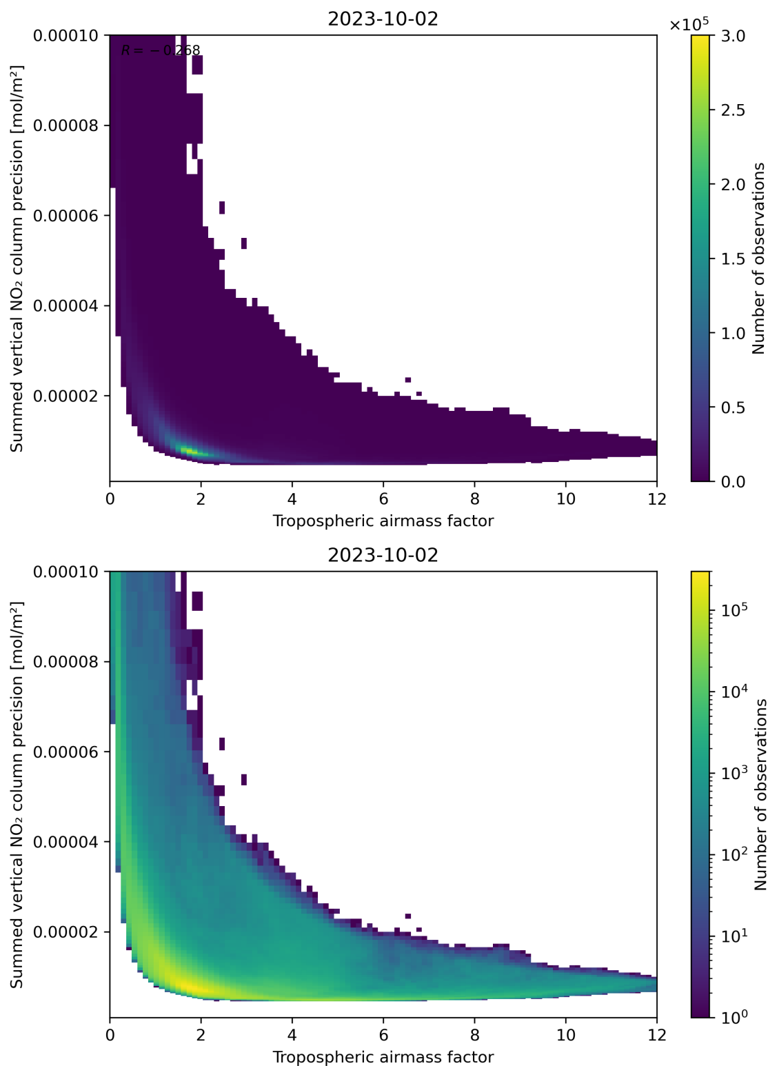
Figure 76: Scatter density plot of “Tropospheric air mass factor” against “Summed vertical NO 2 column precision” for 2023-10-01 to 2023-10-03.
