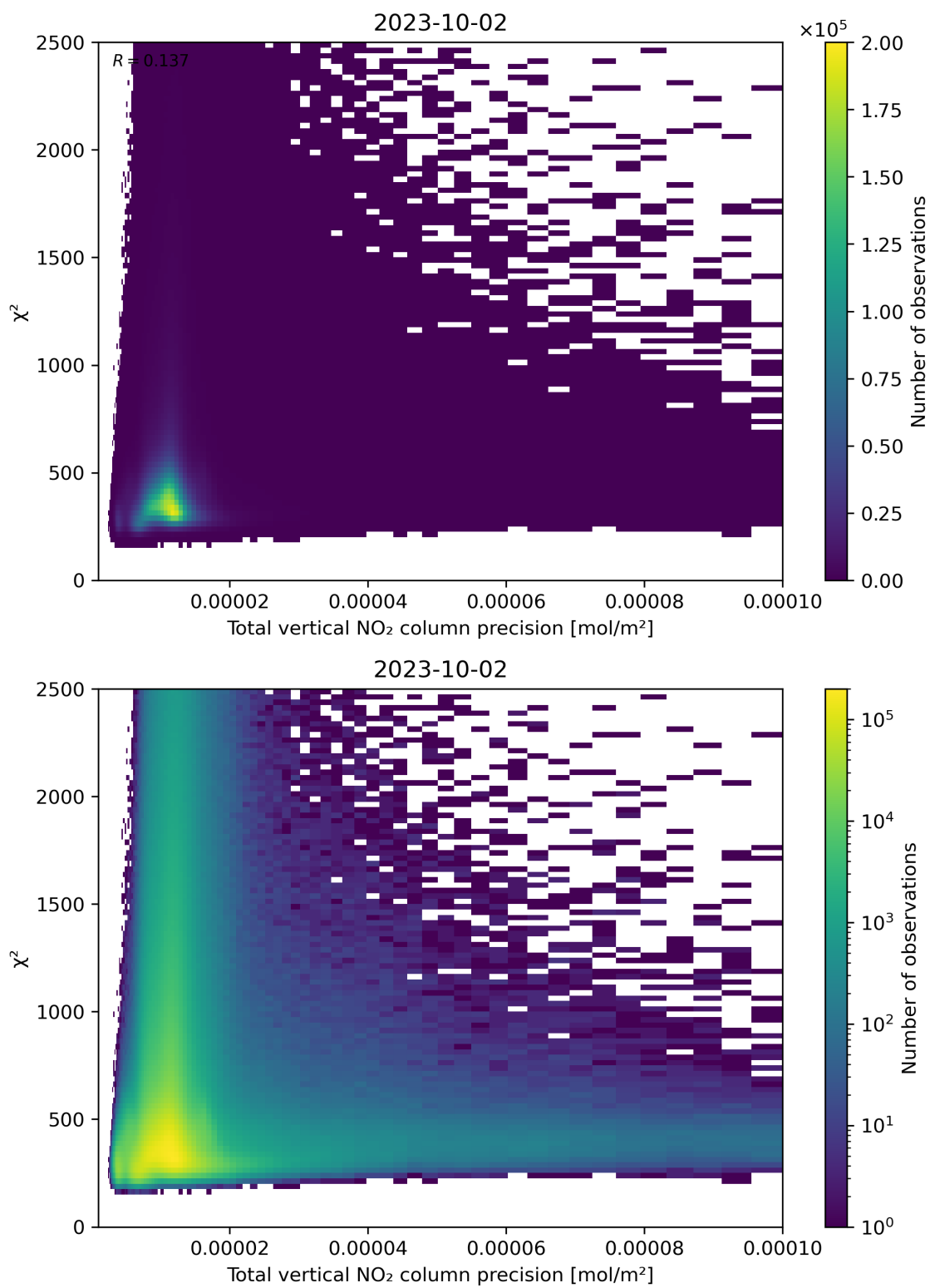
Figure 116: Scatter density plot of “Total vertical NO 2 column precision” against “ \chi^2 ” for 2023-10-01 to 2023-10-03.
