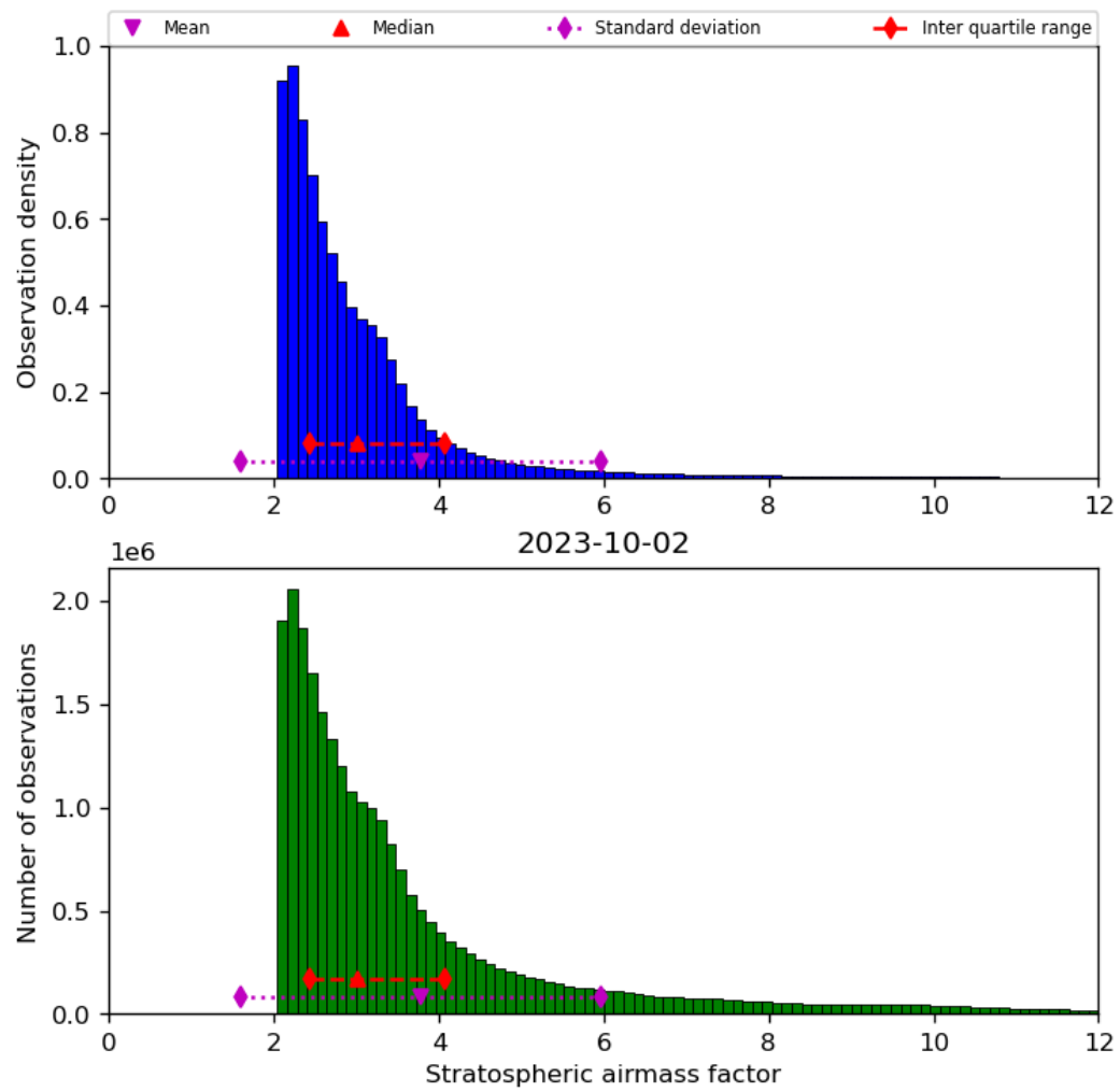
Figure 44: Histogram of “Stratospheric airmass factor” for 2023-10-01 to 2023-10-03
