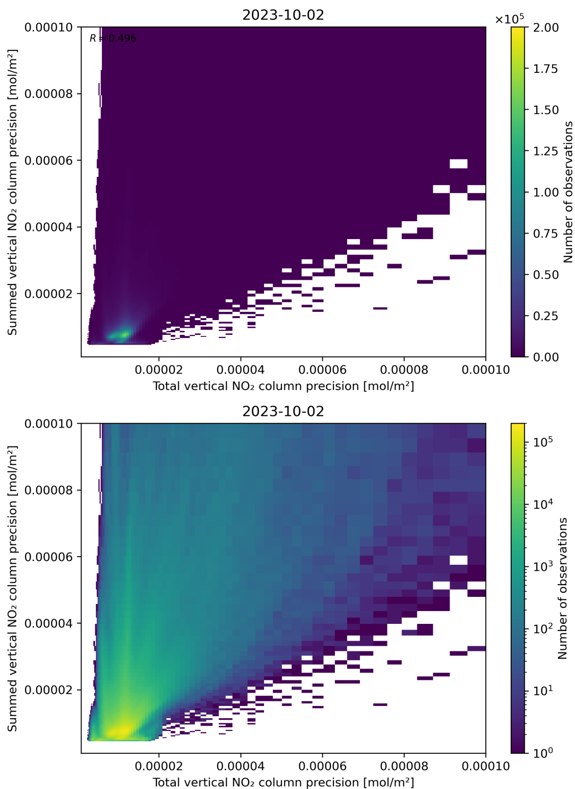
Figure 118: Scatter density plot of “Total vertical NO 2 column precision” against “Summed vertical NO 2 column precision” for 2023-10-01 to 2023-10-03.
