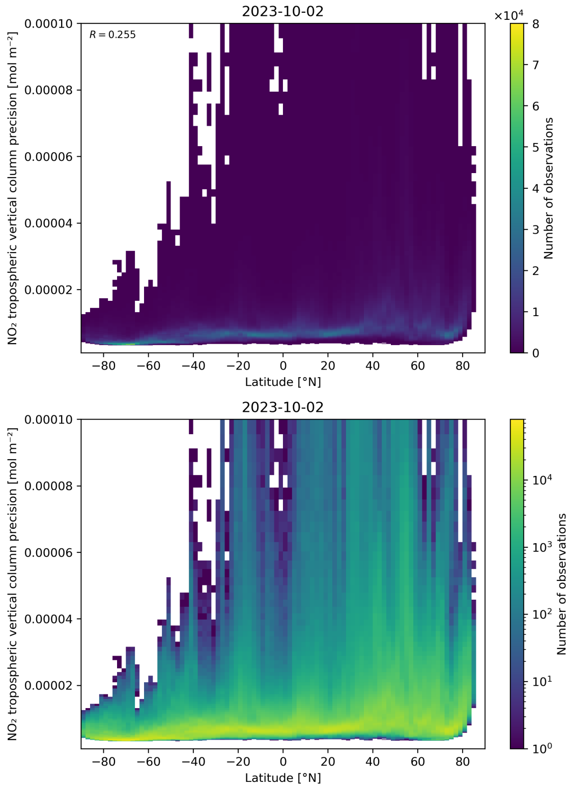
Figure 93: Scatter density plot of “Latitude” against “NO 2 tropospheric vertical column precision” for 2023-10-01 to 2023-10-03.
