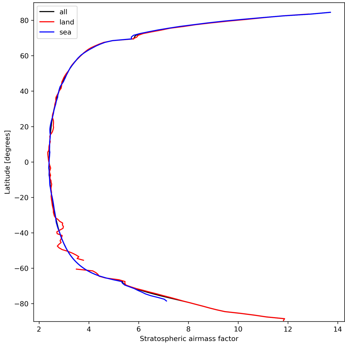
Figure 27: Zonal average of “Stratospheric air mass factor” for 2023-10-01 to 2023-10-03.
