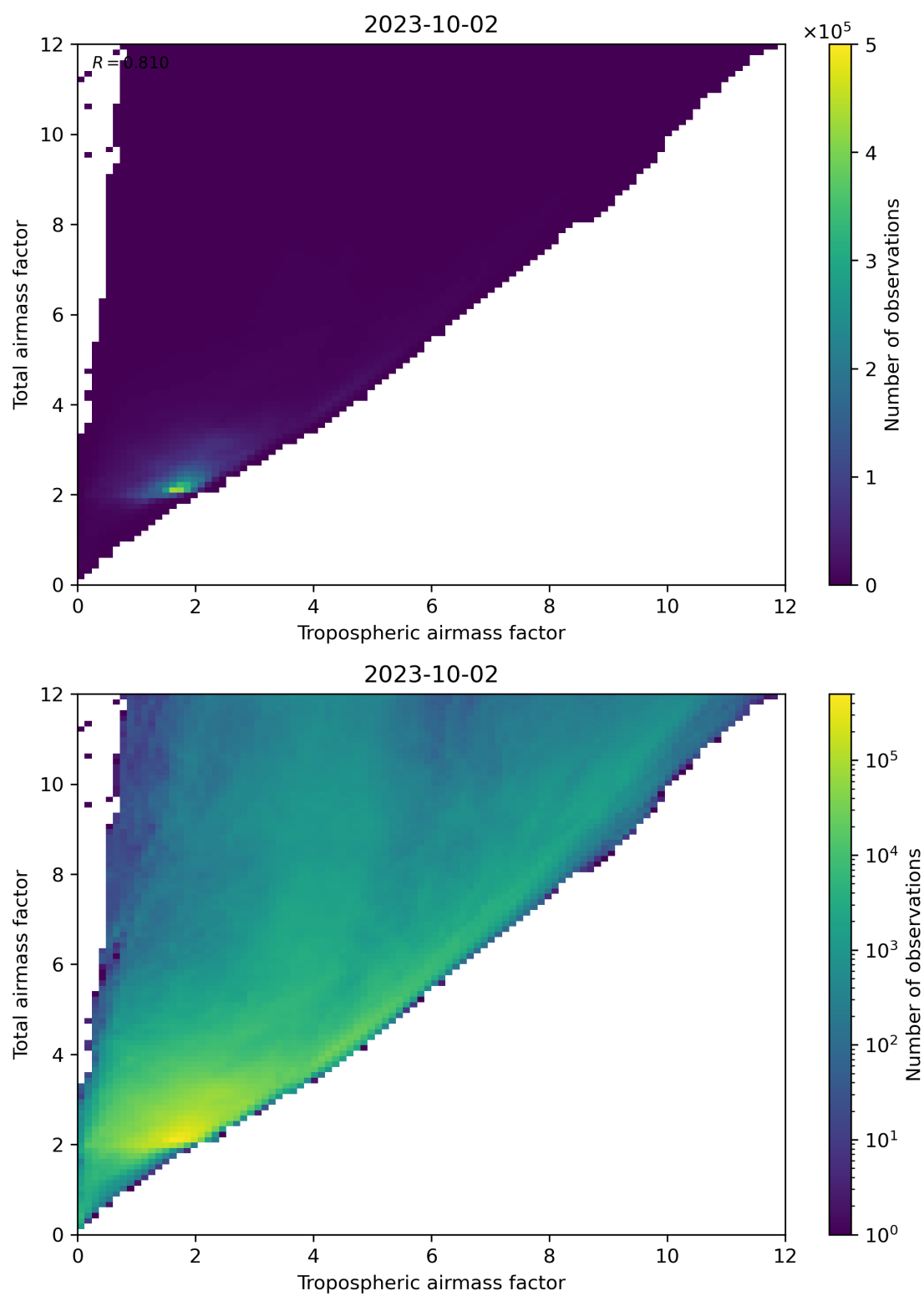
Figure 72: Scatter density plot of “Tropospheric airmass factor” against “Total airmass factor” for 2023-10-01 to 2023-10-03.
