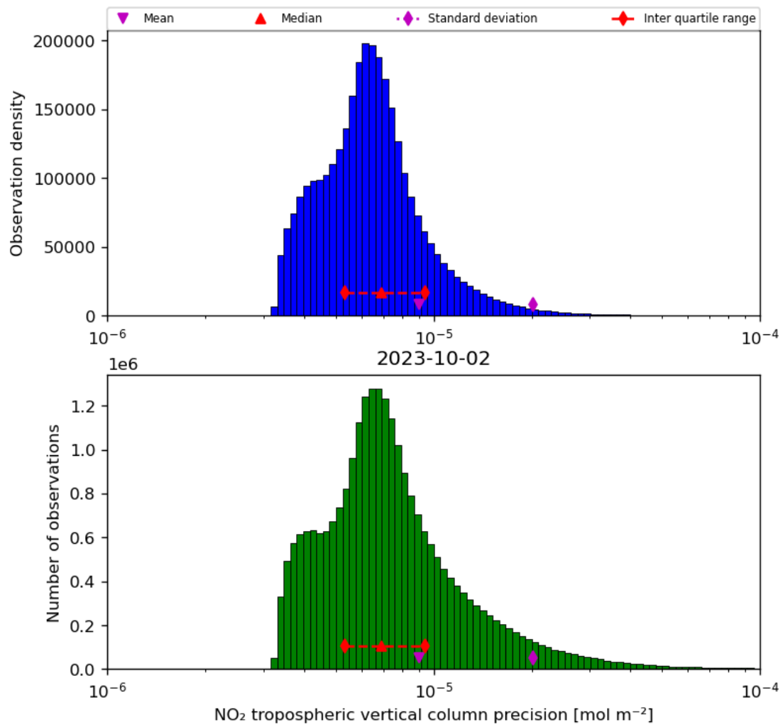
Figure 30: Histogram of “NO 2 tropospheric vertical column precision” for 2023-10-01 to 2023-10-03
