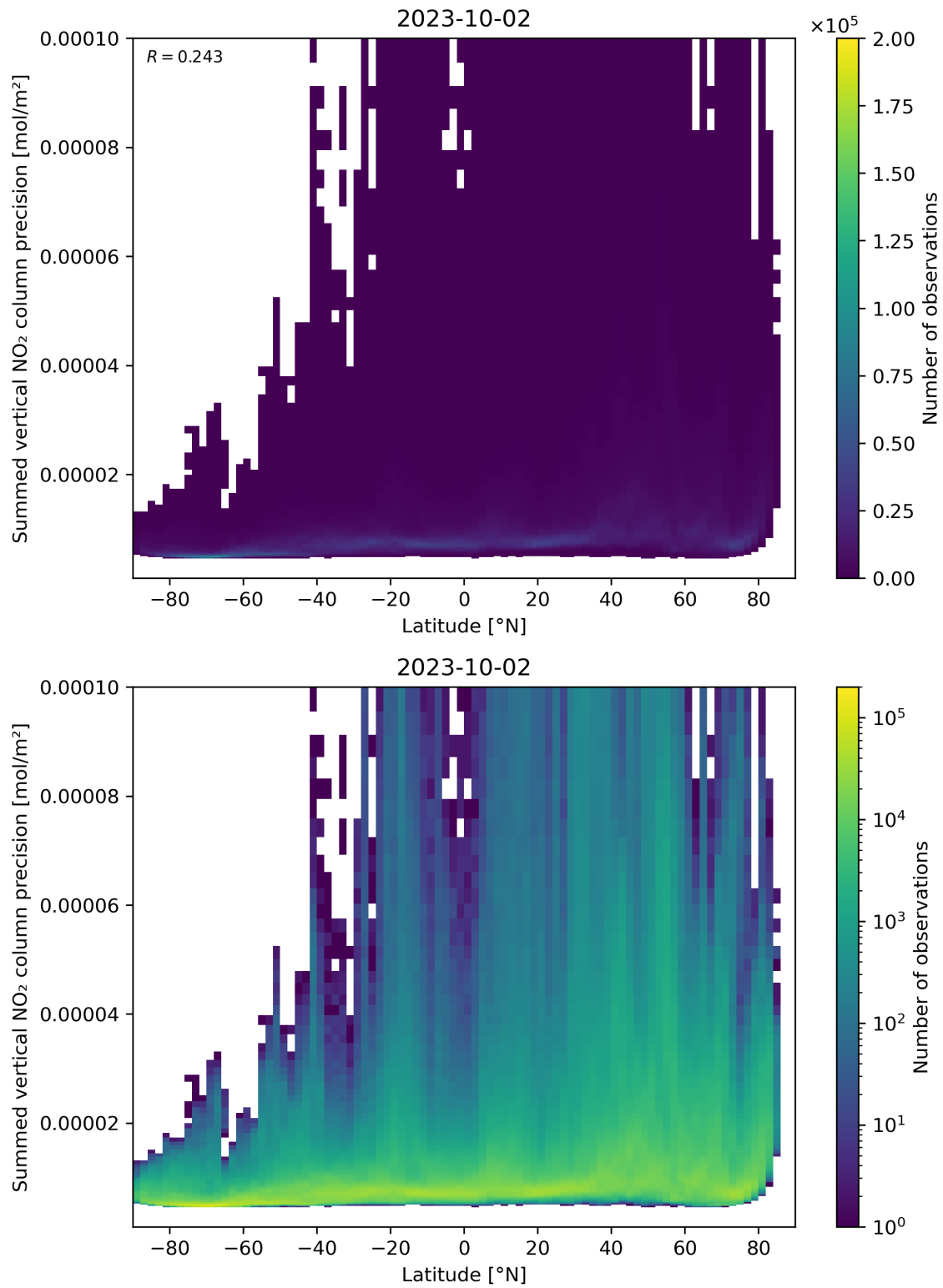
Figure 89: Scatter density plot of “Latitude” against “Summed vertical NO 2 column precision” for 2023-10-01 to 2023-10-03.
