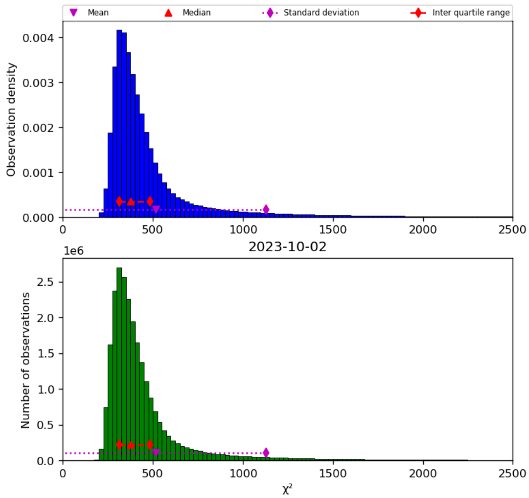
Figure 42: Histogram of “ \chi^2 ” for 2023-10-01 to 2023-10-03
