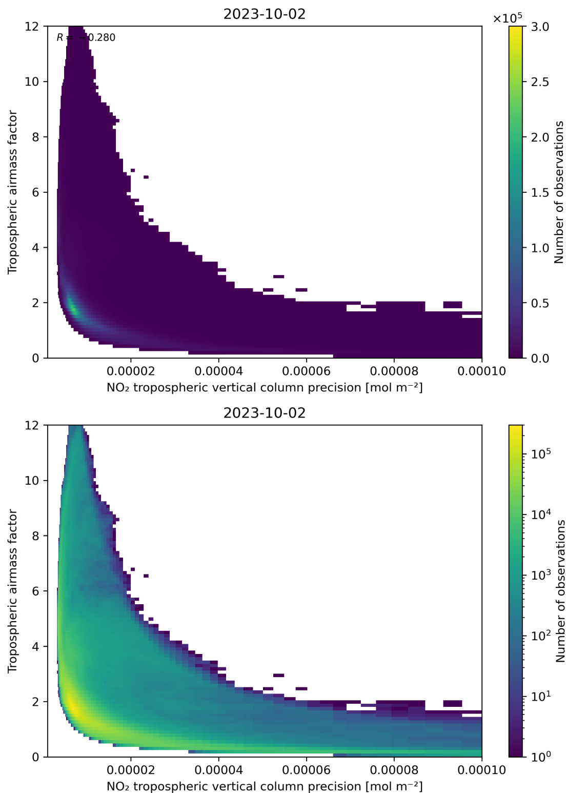
Figure 133: Scatter density plot of “NO 2 tropospheric vertical column precision” against “Tropospheric airmass factor” for 2023-10-01 to 2023-10-03.
