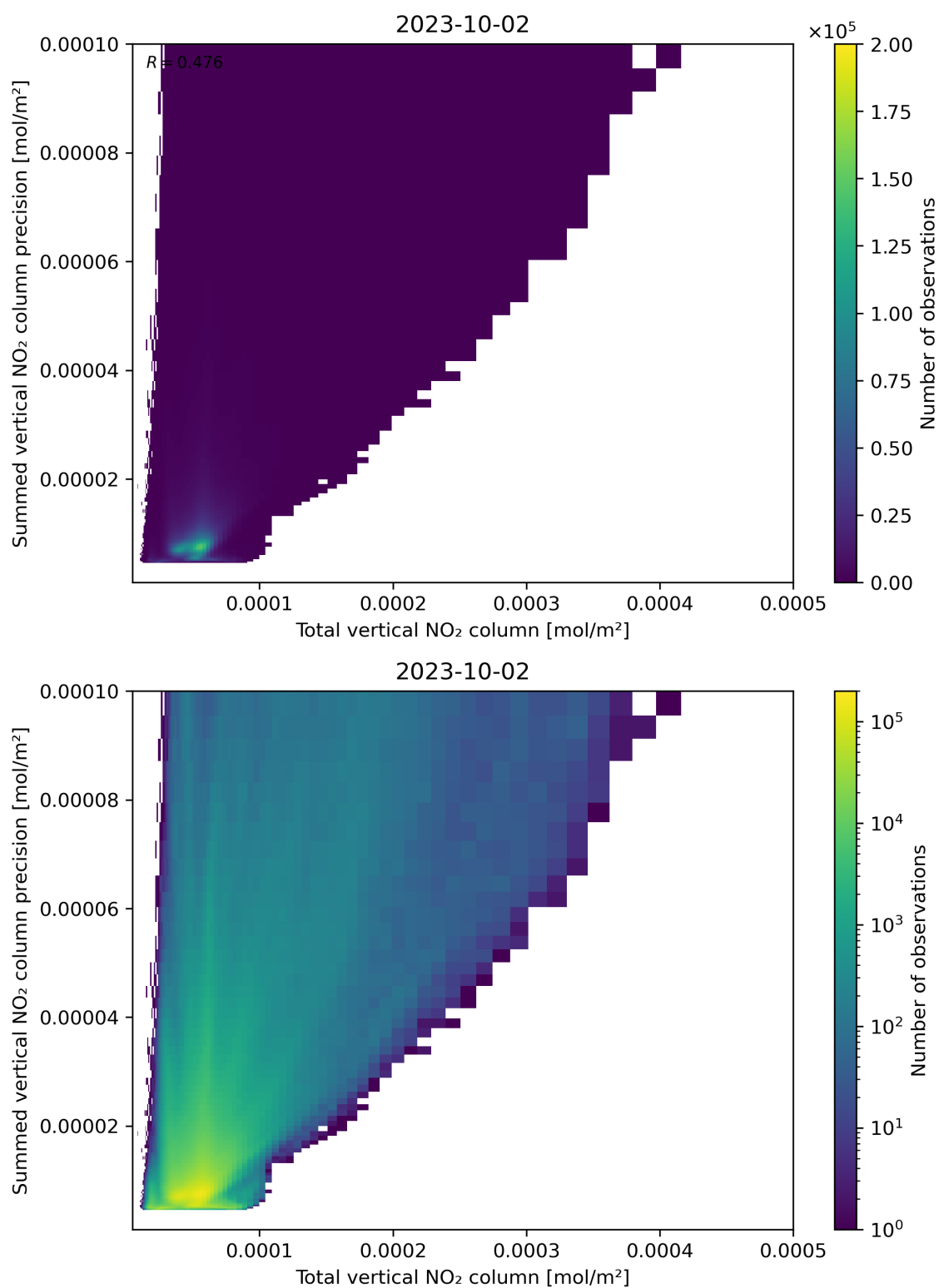
Figure 113: Scatter density plot of “Total vertical NO 2 column” against “Summed vertical NO 2 column precision” for 2023-10-01 to 2023-10-03.
