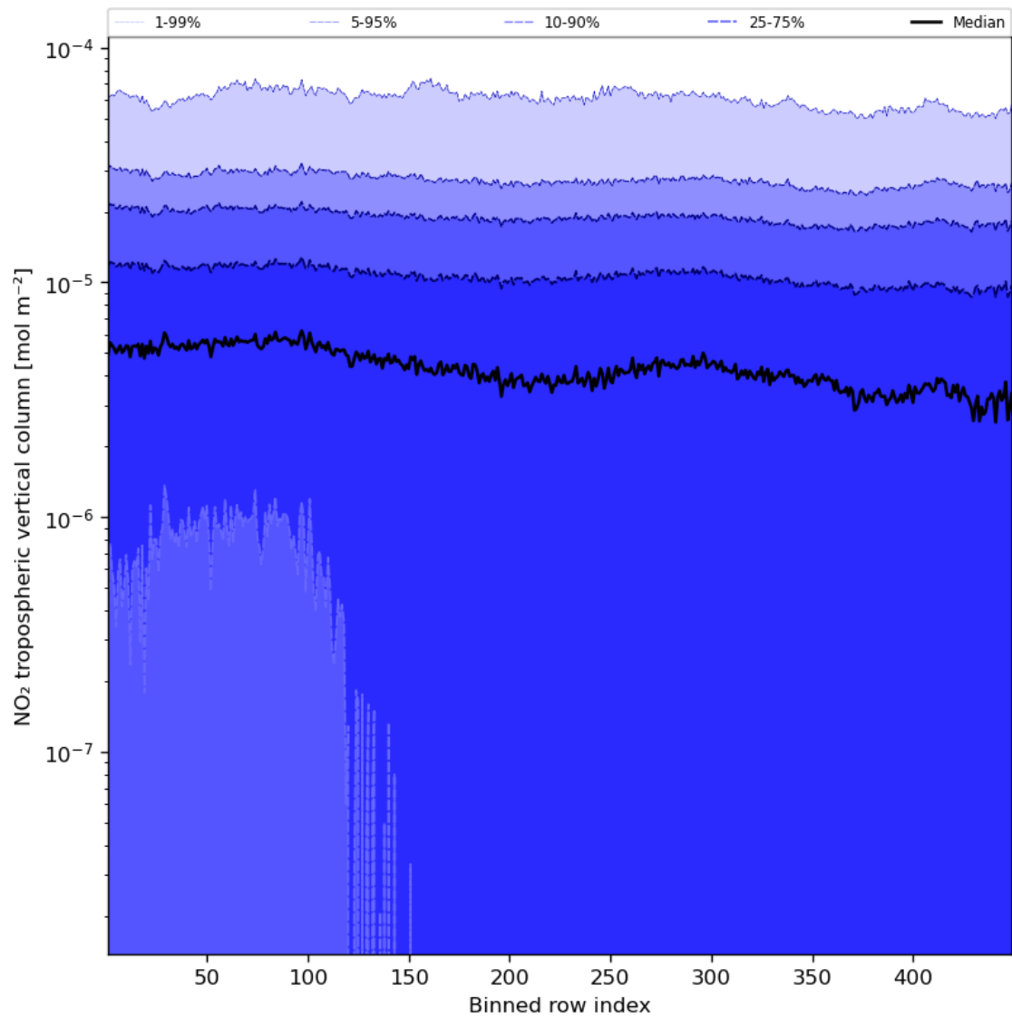
Figure 46: Along track statistics of “NO 2 tropospheric vertical column” for 2023-10-01 to 2023-10-03
