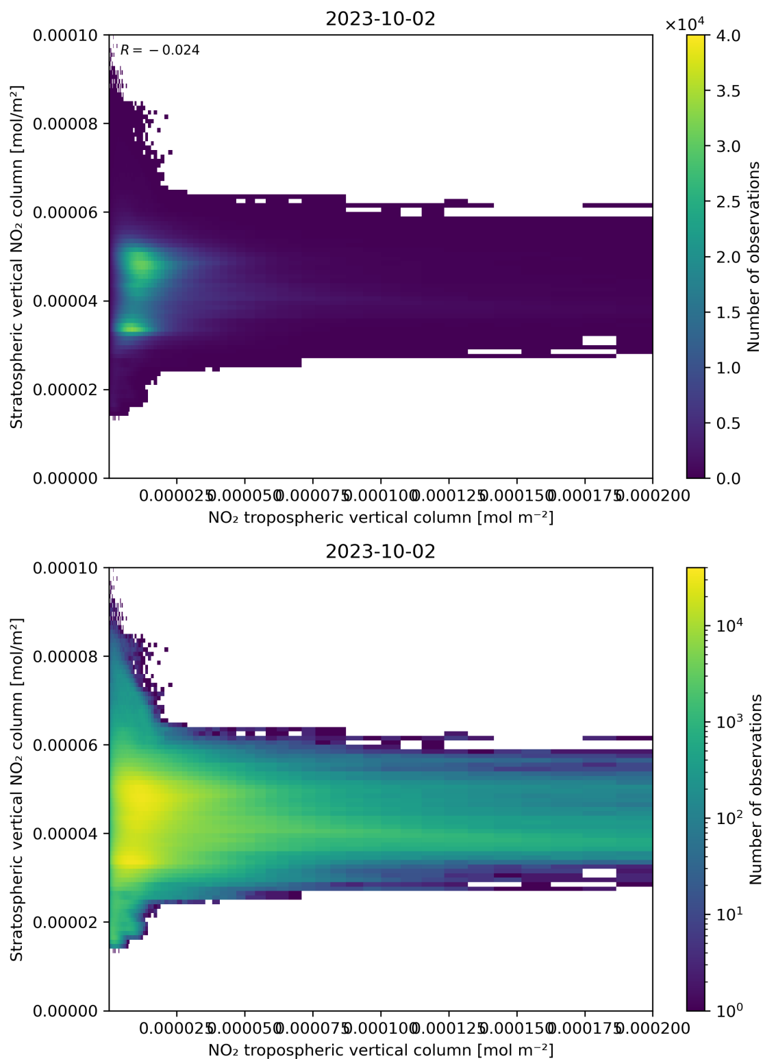
Figure 125: Scatter density plot of “NO 2 tropospheric vertical column” against “Stratospheric vertical NO 2 column” for 2023-10-01 to 2023-10-03.
