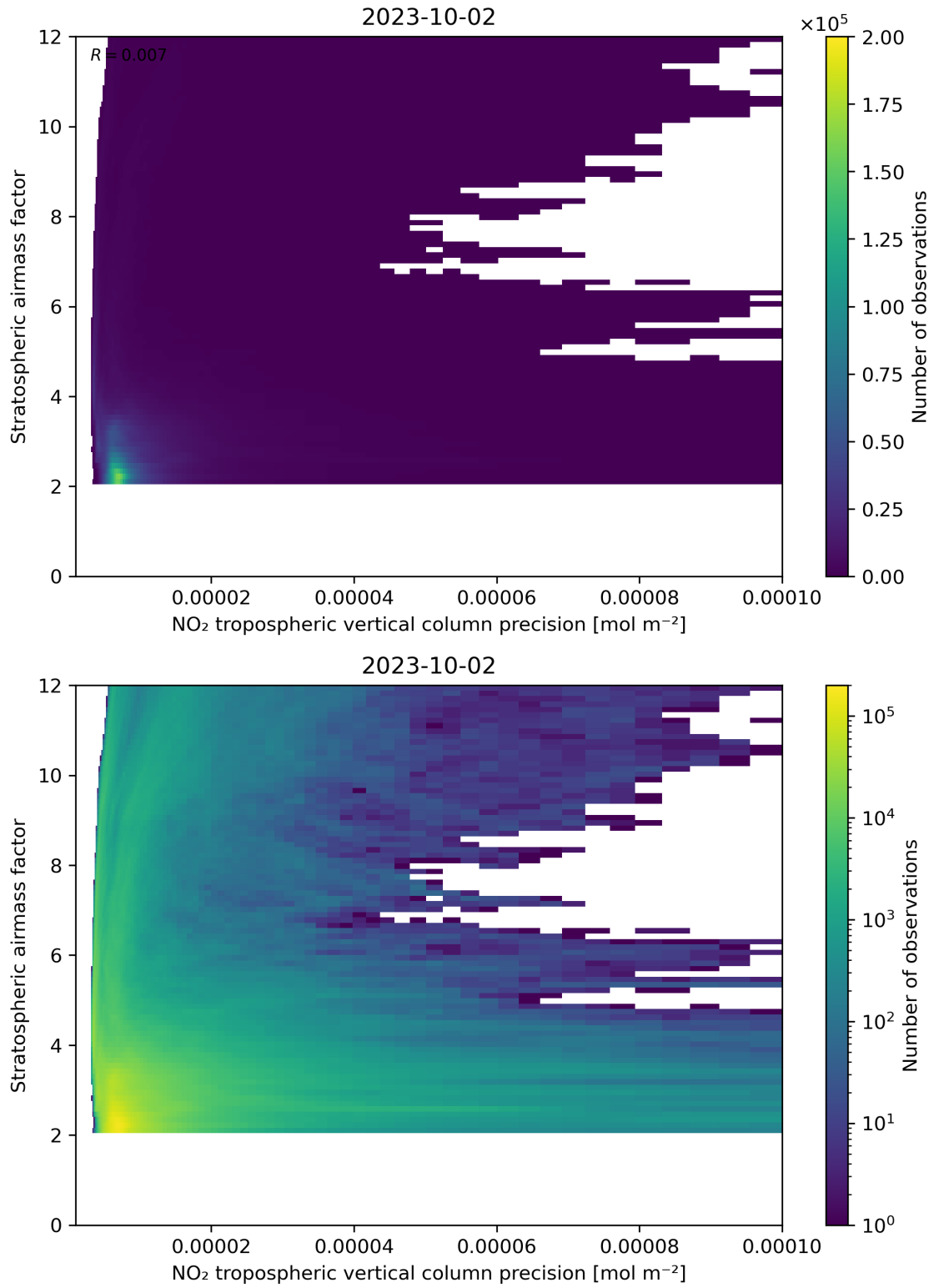
Figure 131: Scatter density plot of “NO 2 tropospheric vertical column precision” against “Stratospheric airmass factor” for 2023-10-01 to 2023-10-03.
