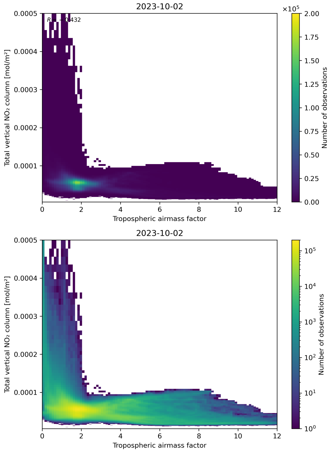
Figure 77: Scatter density plot of “Tropospheric airmass factor” against “Total vertical NO 2 column” for 2023-10-01 to 2023-10-03.
