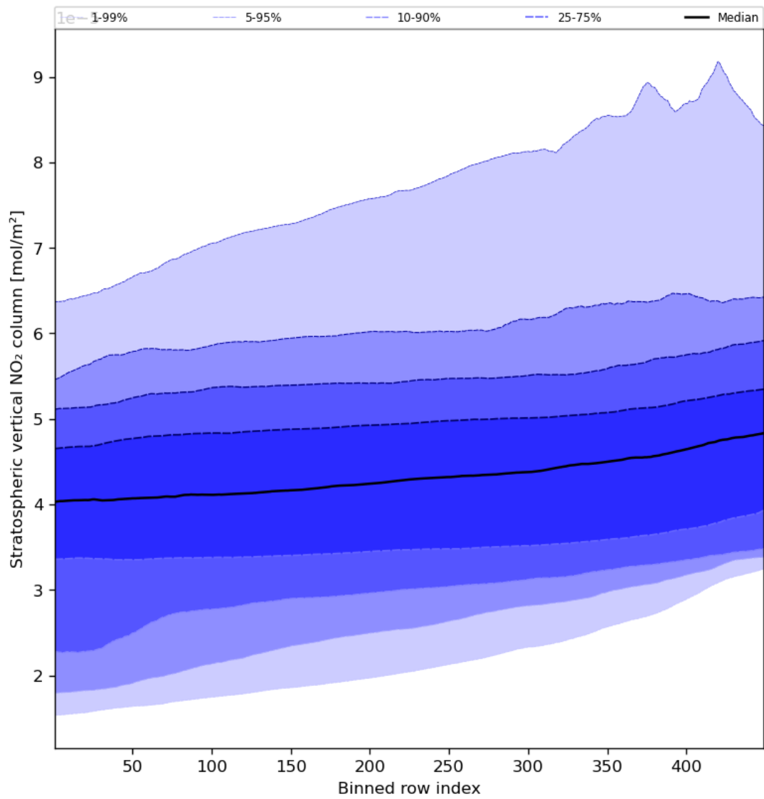
Figure 53: Along track statistics of “Stratospheric vertical NO 2 column” for 2023-10-01 to 2023-10-03
