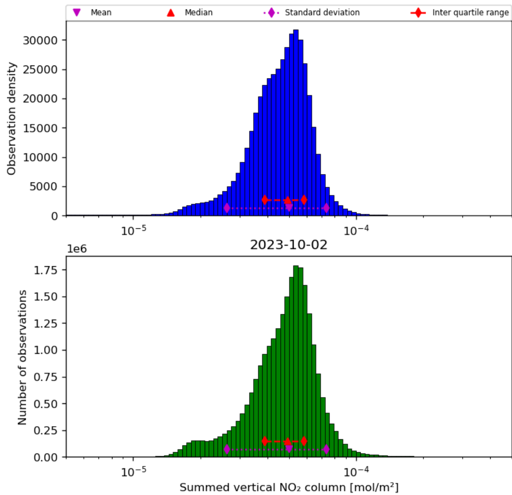
Figure 40: Histogram of “Summed vertical NO 2 column” for 2023-10-01 to 2023-10-03
