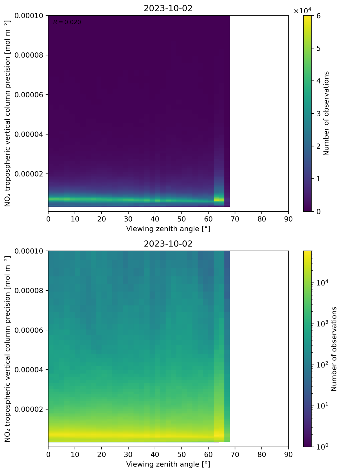
Figure 170: Scatter density plot of “Viewing zenith angle” against “NO 2 tropospheric vertical column precision” for 2023-10-01 to 2023-10-03.
