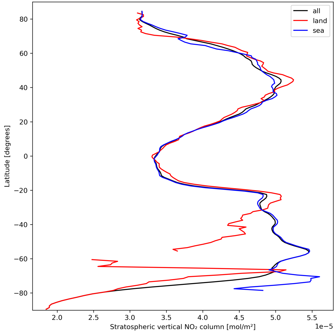
Figure 19: Zonal average of “Stratospheric vertical NO 2 column” for 2023-10-01 to 2023-10-03.
