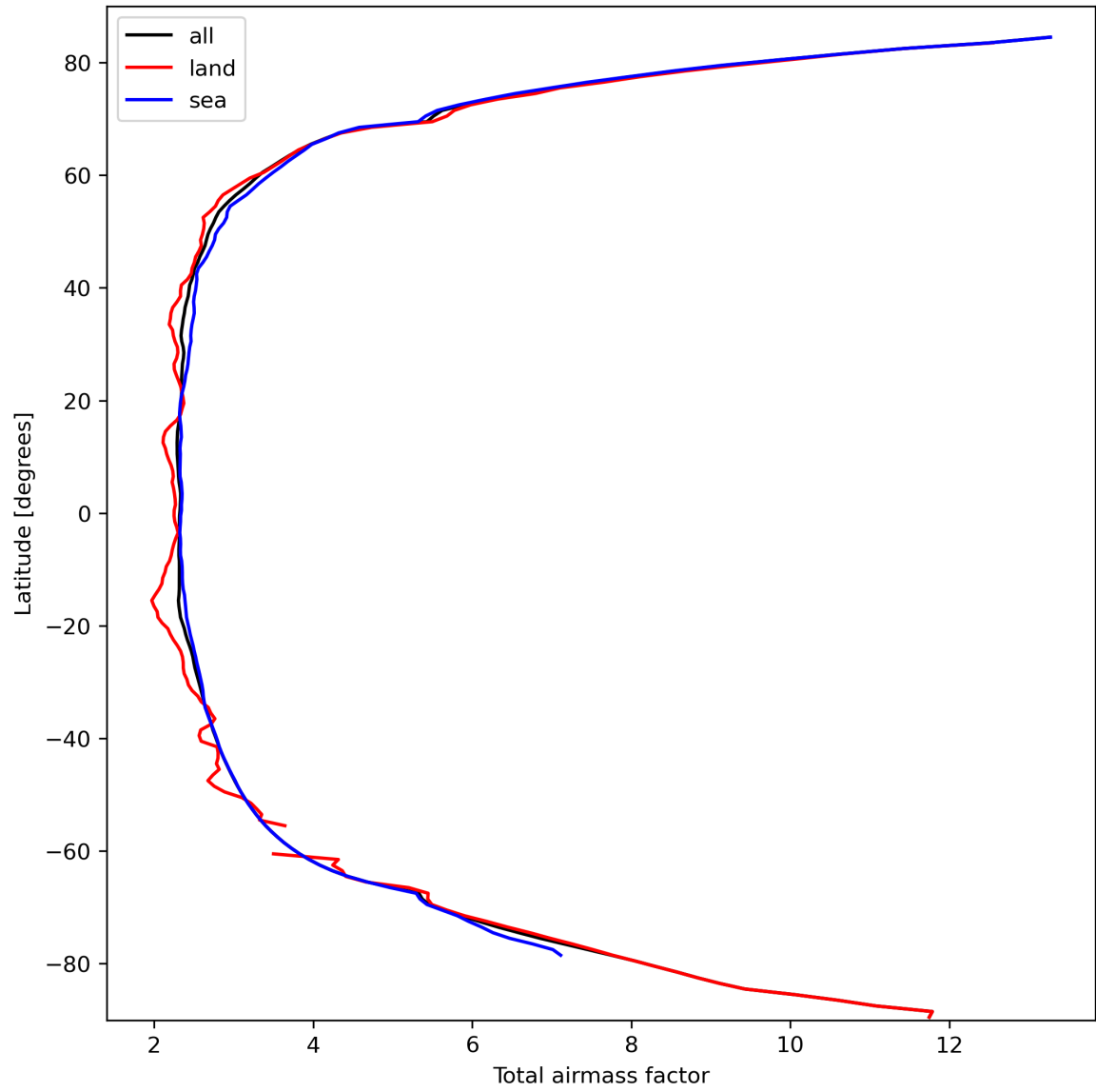
Figure 15: Zonal average of “Total airmass factor” for 2023-10-01 to 2023-10-03.
