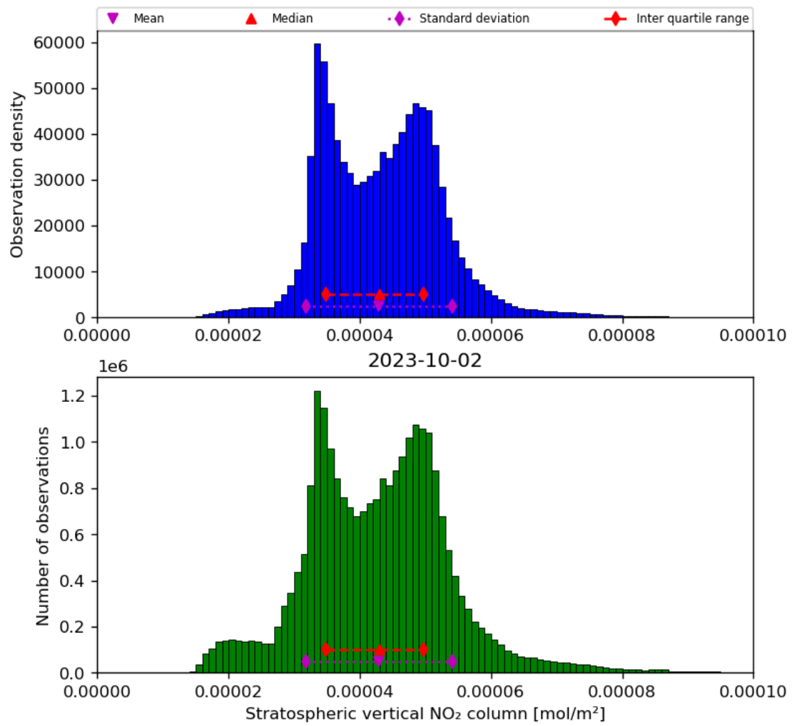
Figure 36: Histogram of “Stratospheric vertical NO 2 column” for 2023-10-01 to 2023-10-03
