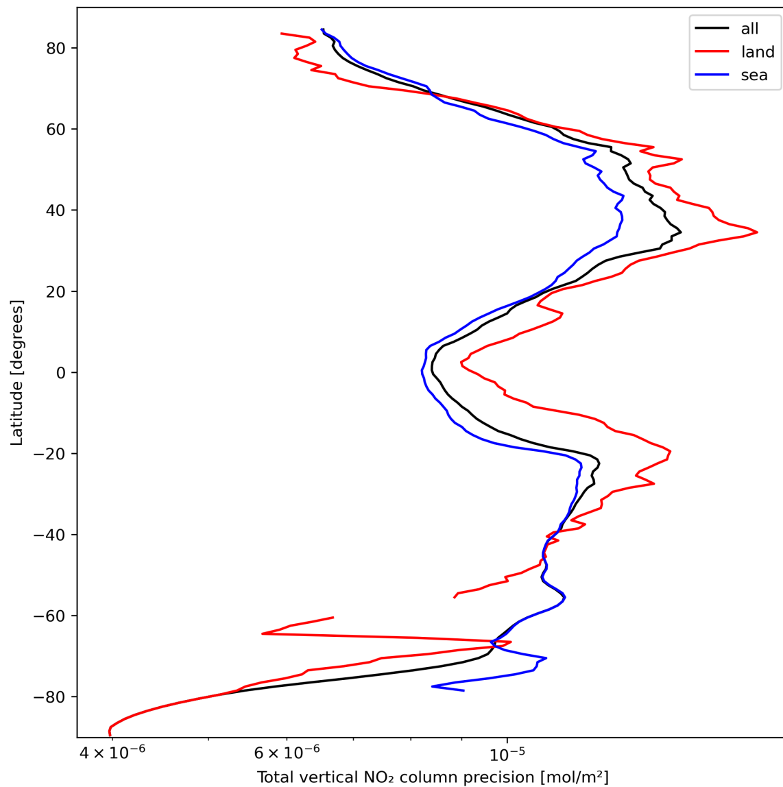
Figure 22: Zonal average of “Total vertical NO 2 column precision” for 2023-10-01 to 2023-10-03.
