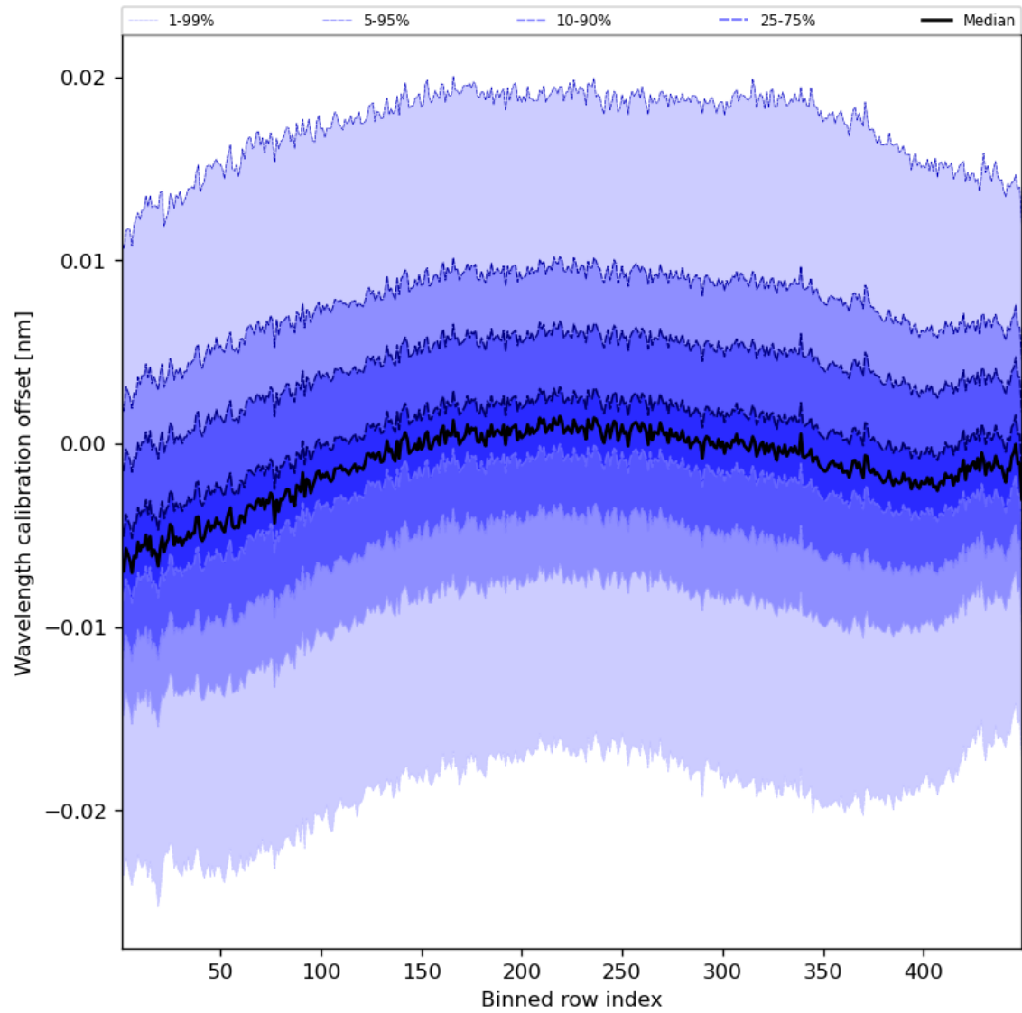
Figure 52: Along track statistics of “Wavelength calibration offset” for 2023-10-01 to 2023-10-03
