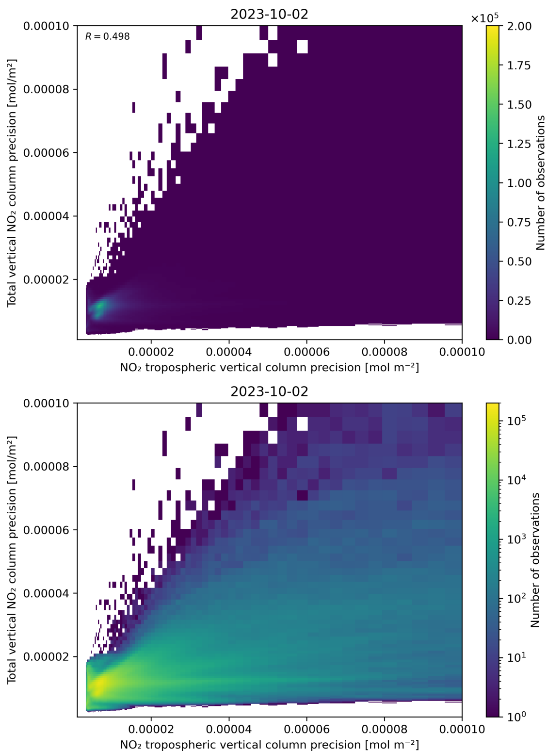
Figure 139: Scatter density plot of “NO 2 tropospheric vertical column precision” against “Total vertical NO 2 column precision” for 2023-10-01 to 2023-10-03.
