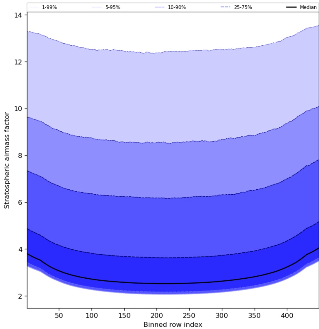
Figure 61: Along track statistics of “Stratospheric airmass factor” for 2023-10-01 to 2023-10-03
