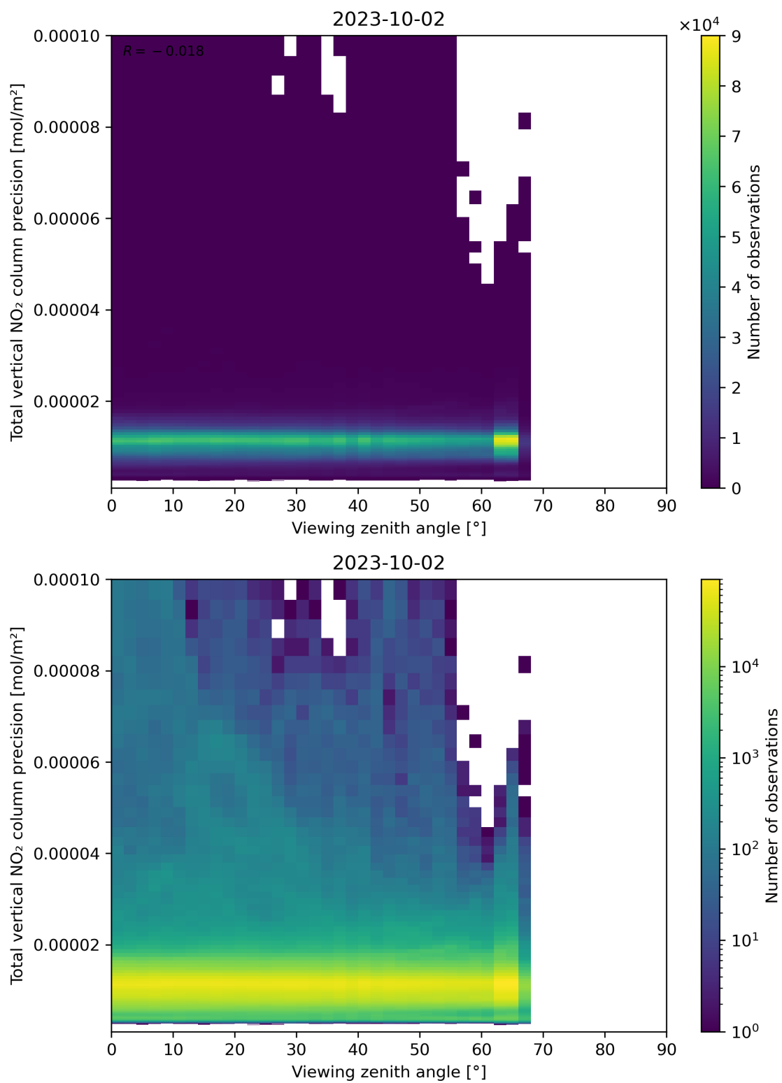
Figure 168: Scatter density plot of “Viewing zenith angle” against “Total vertical NO 2 column precision” for 2023-10-01 to 2023-10-03.
