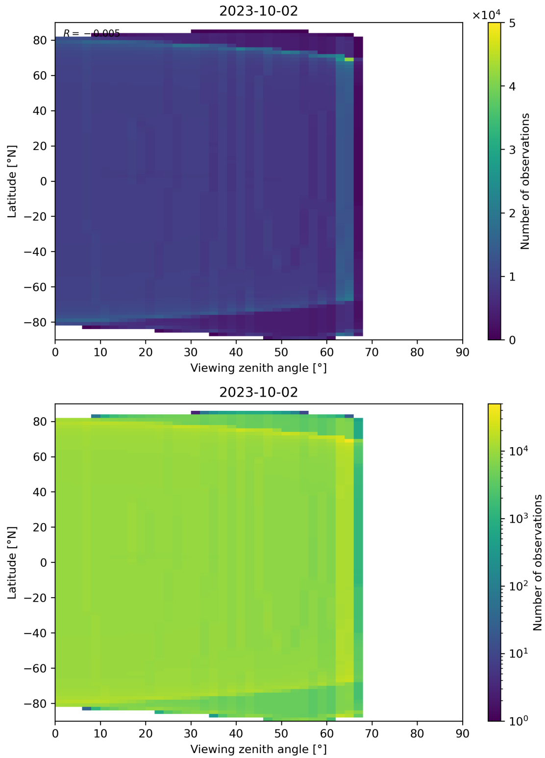
Figure 163: Scatter density plot of “Viewing zenith angle” against “Latitude” for 2023-10-01 to 2023-10-03.
