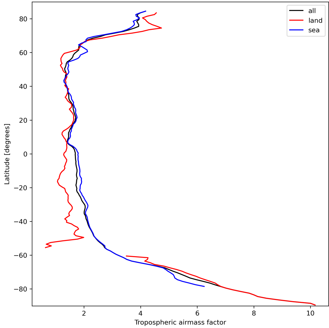
Figure 14: Zonal average of “Tropospheric airmass factor” for 2023-10-01 to 2023-10-03.
