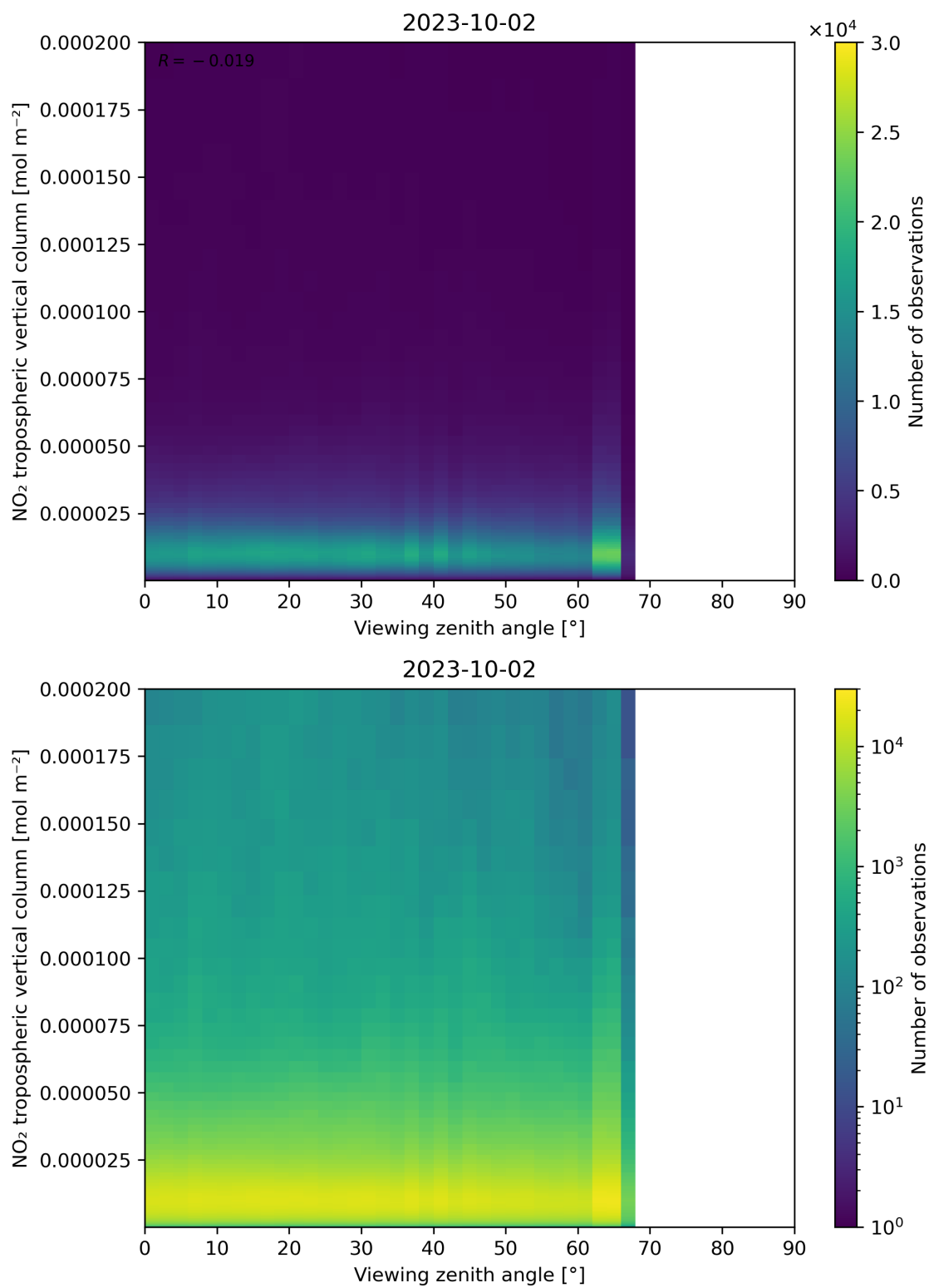
Figure 169: Scatter density plot of “Viewing zenith angle” against “NO 2 tropospheric vertical column” for 2023-10-01 to 2023-10-03.
