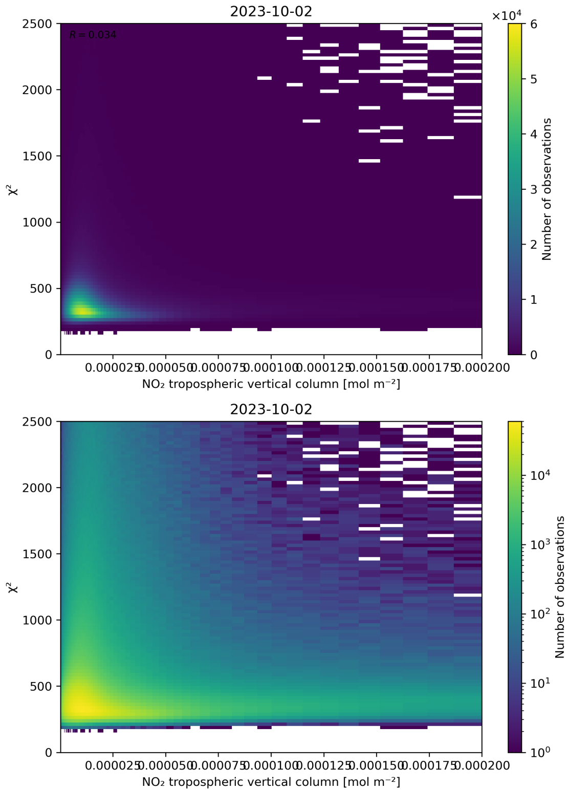
Figure 124: Scatter density plot of “NO 2 tropospheric vertical column” against “ \chi^2 ” for 2023-10-01 to 2023-10-03.
