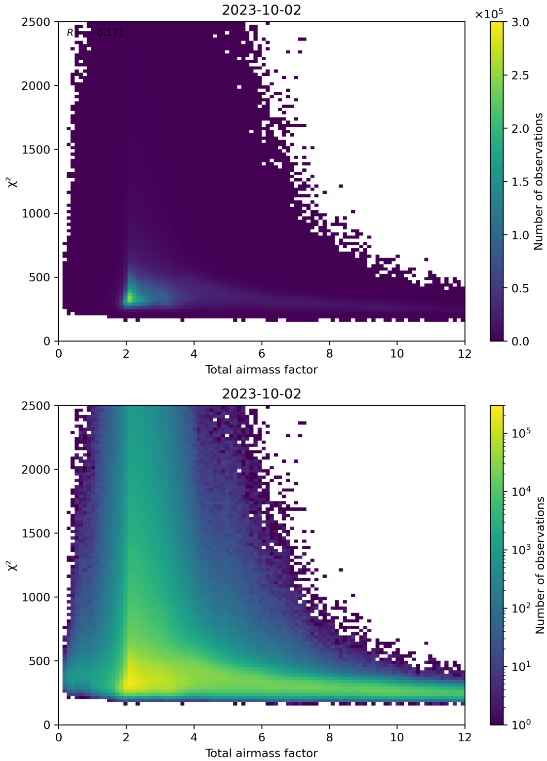
Figure 63: Scatter density plot of “Total airmass factor” against “ \chi^2 ” for 2023-10-01 to 2023-10-03.
