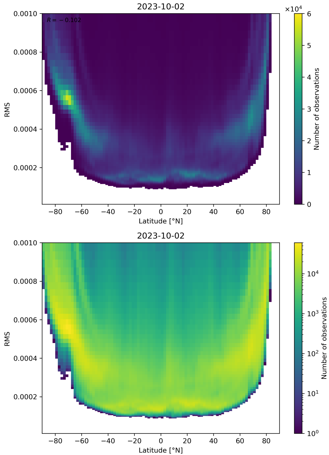
Figure 94: Scatter density plot of “Latitude” against “RMS” for 2023-10-01 to 2023-10-03.
