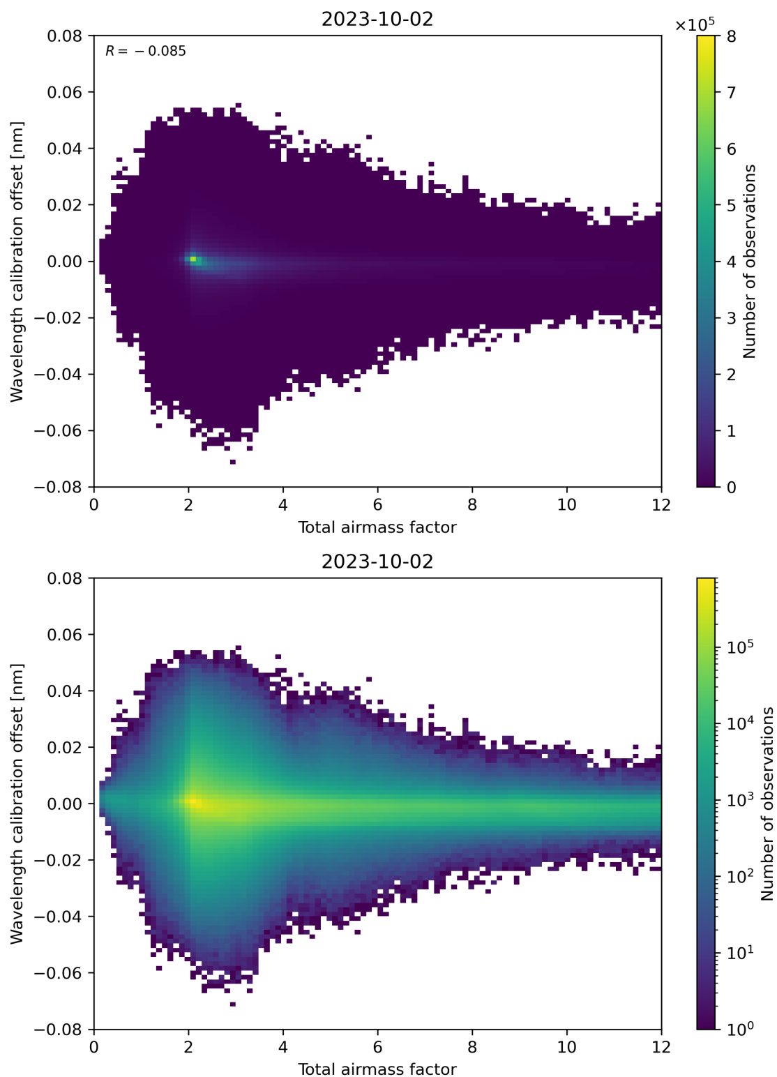
Figure 70: Scatter density plot of “Total airmass factor” against “Wavelength calibration offset” for 2023-10-01 to 2023-10-03.
