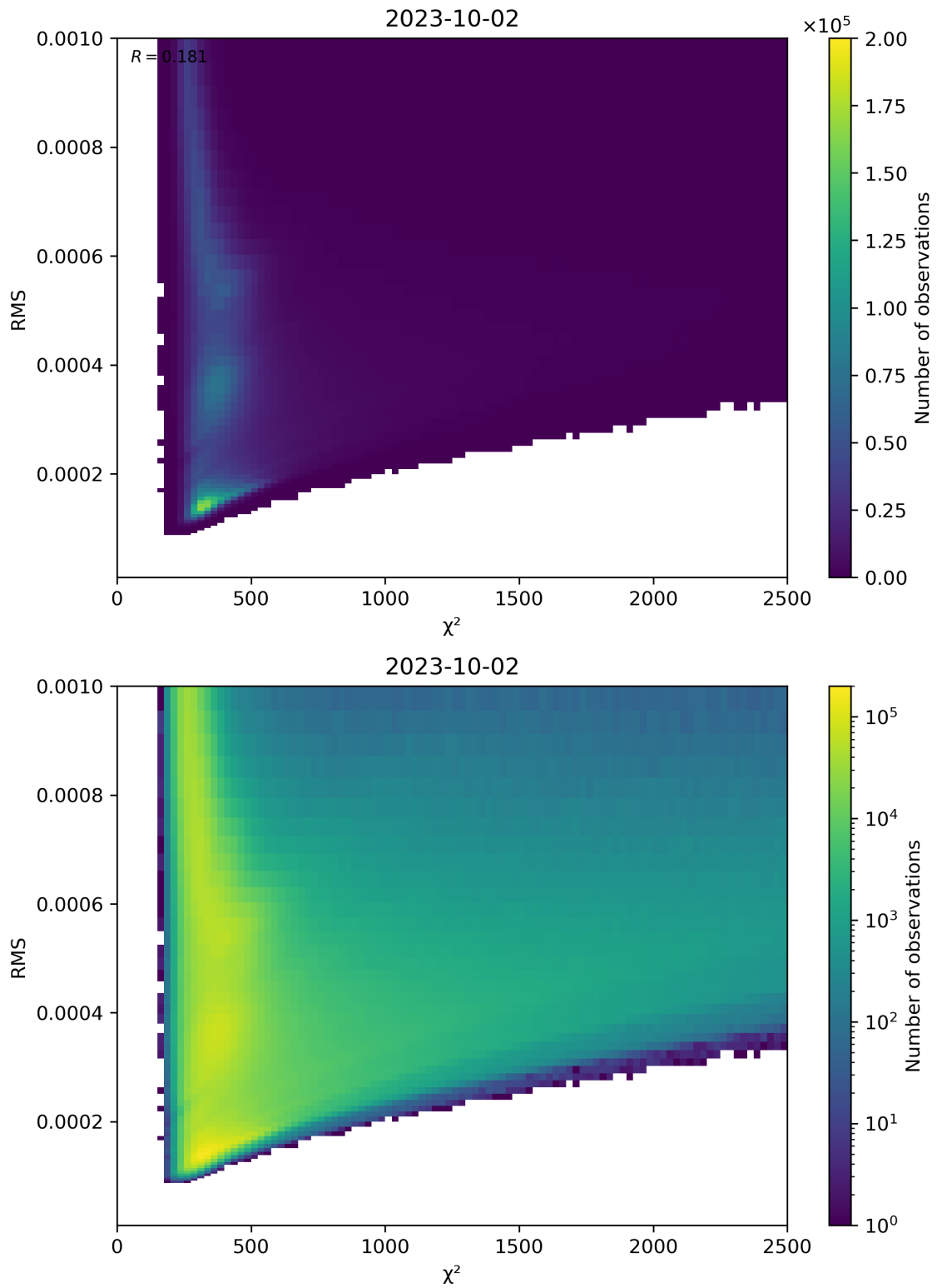
Figure 82: Scatter density plot of “ \chi^2 ” against “RMS” for 2023-10-01 to 2023-10-03.
