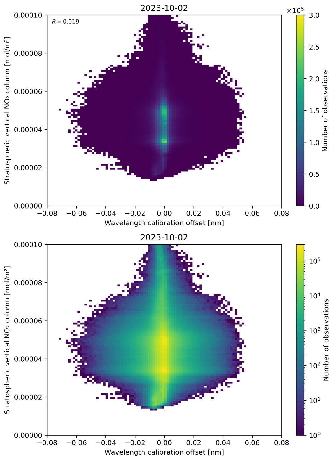
Figure 176: Scatter density plot of “Wavelength calibration offset” against “Stratospheric vertical NO 2 column” for 2023-10-01 to 2023-10-03.
