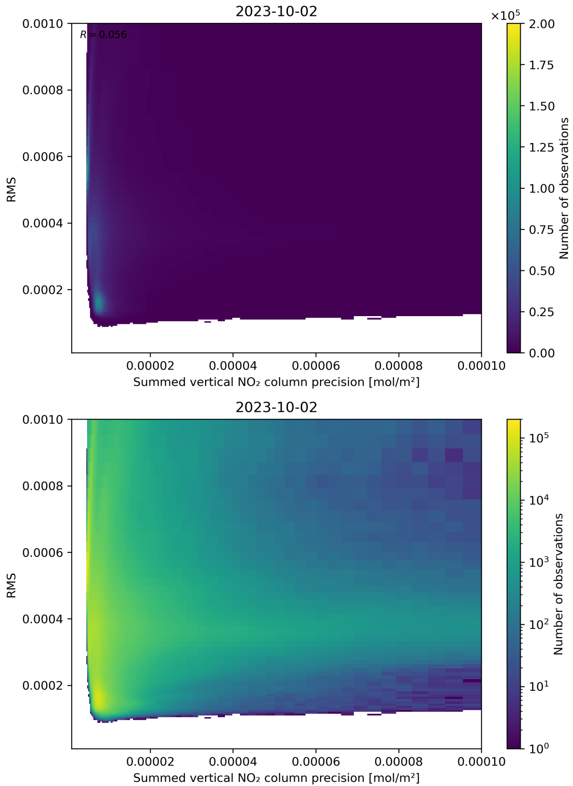
Figure 108: Scatter density plot of “Summed vertical NO 2 column precision” against “RMS” for 2023-10-01 to 2023-10-03.
