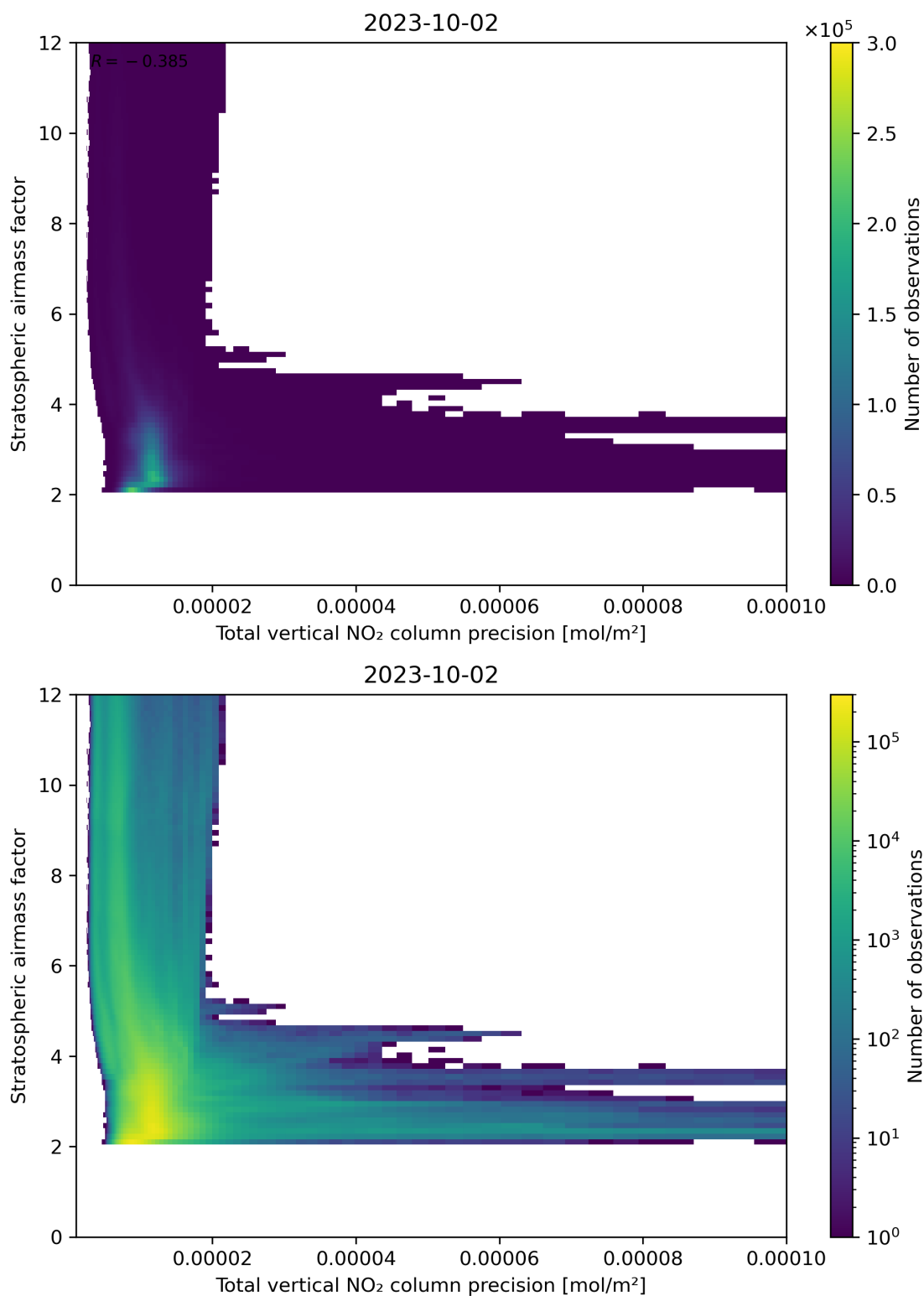
Figure 115: Scatter density plot of “Total vertical NO 2 column precision” against “Stratospheric airmass factor” for 2023-10-01 to 2023-10-03.
