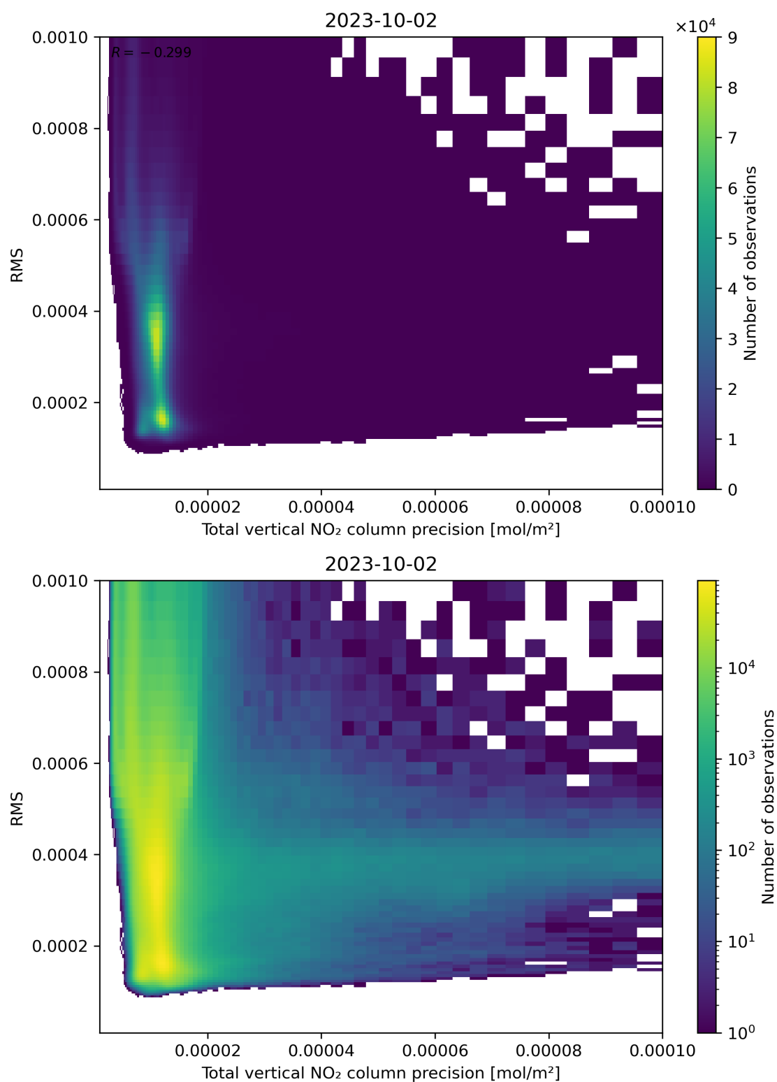
Figure 119: Scatter density plot of “Total vertical NO 2 column precision” against “RMS” for 2023-10-01 to 2023-10-03.
