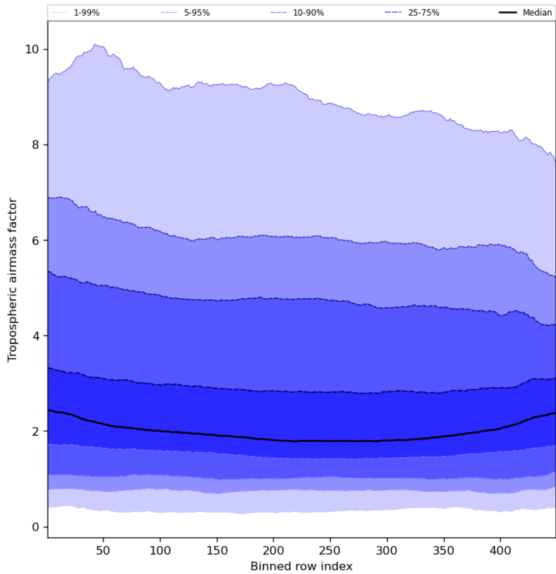
Figure 48: Along track statistics of “Tropospheric air mass factor” for 2023-10-01 to 2023-10-03
