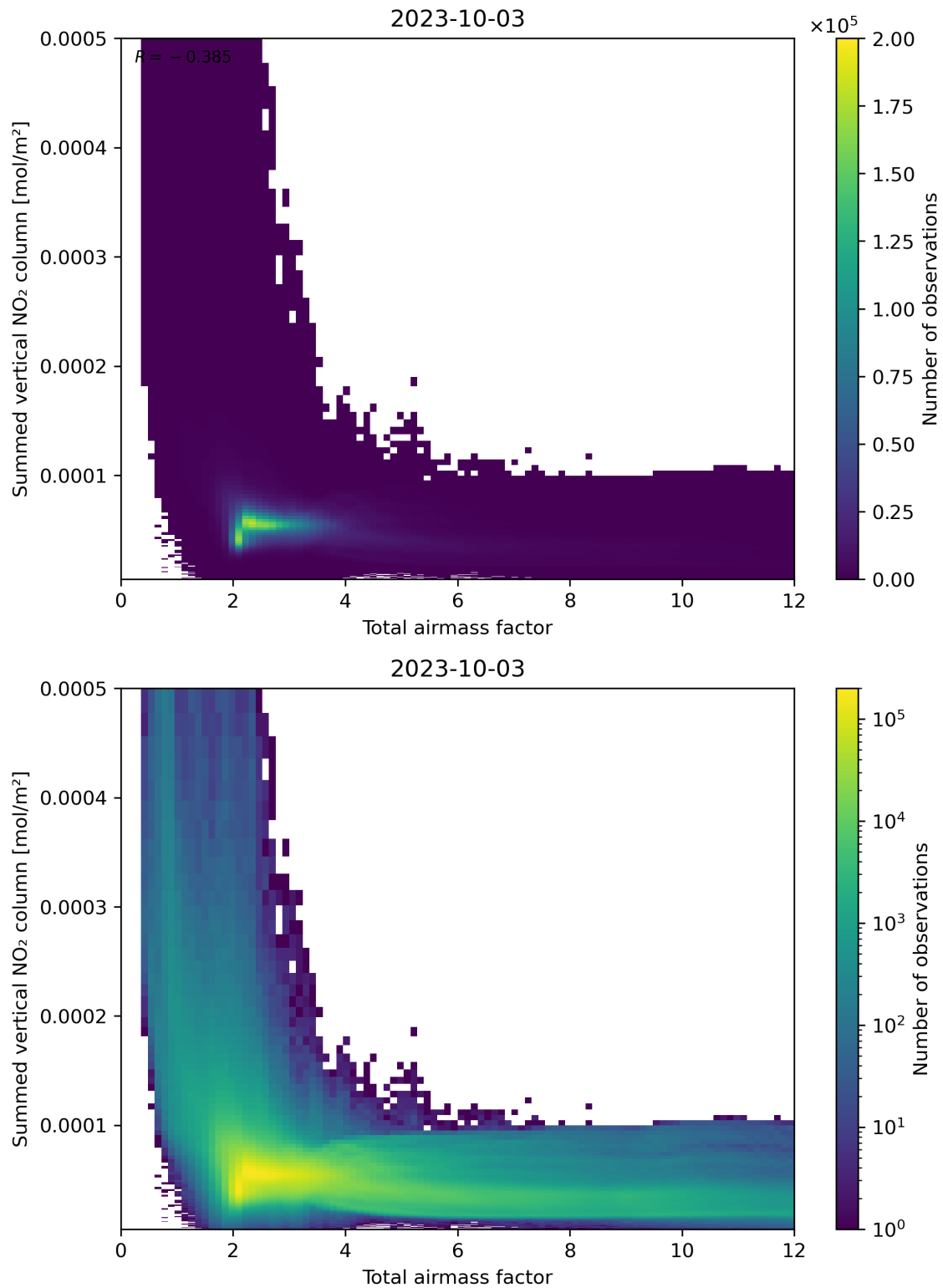
Figure 65: Scatter density plot of “Total airmass factor” against “Summed vertical NO 2 column” for 2023-10-02 to 2023-10-04.
