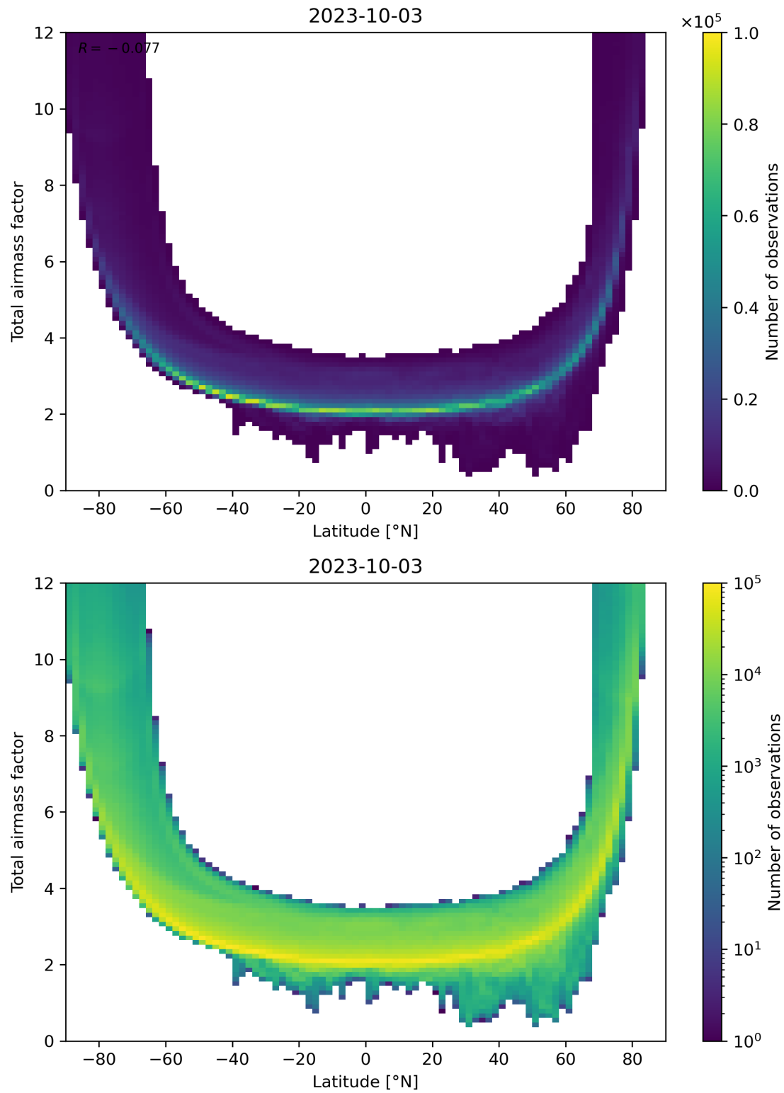
Figure 84: Scatter density plot of “Latitude” against “Total airmass factor” for 2023-10-02 to 2023-10-04.
