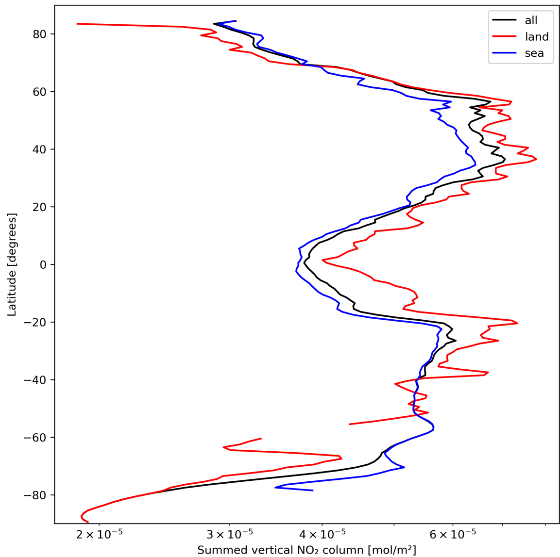
Figure 23: Zonal average of “Summed vertical NO 2 column” for 2023-10-02 to 2023-10-04.
