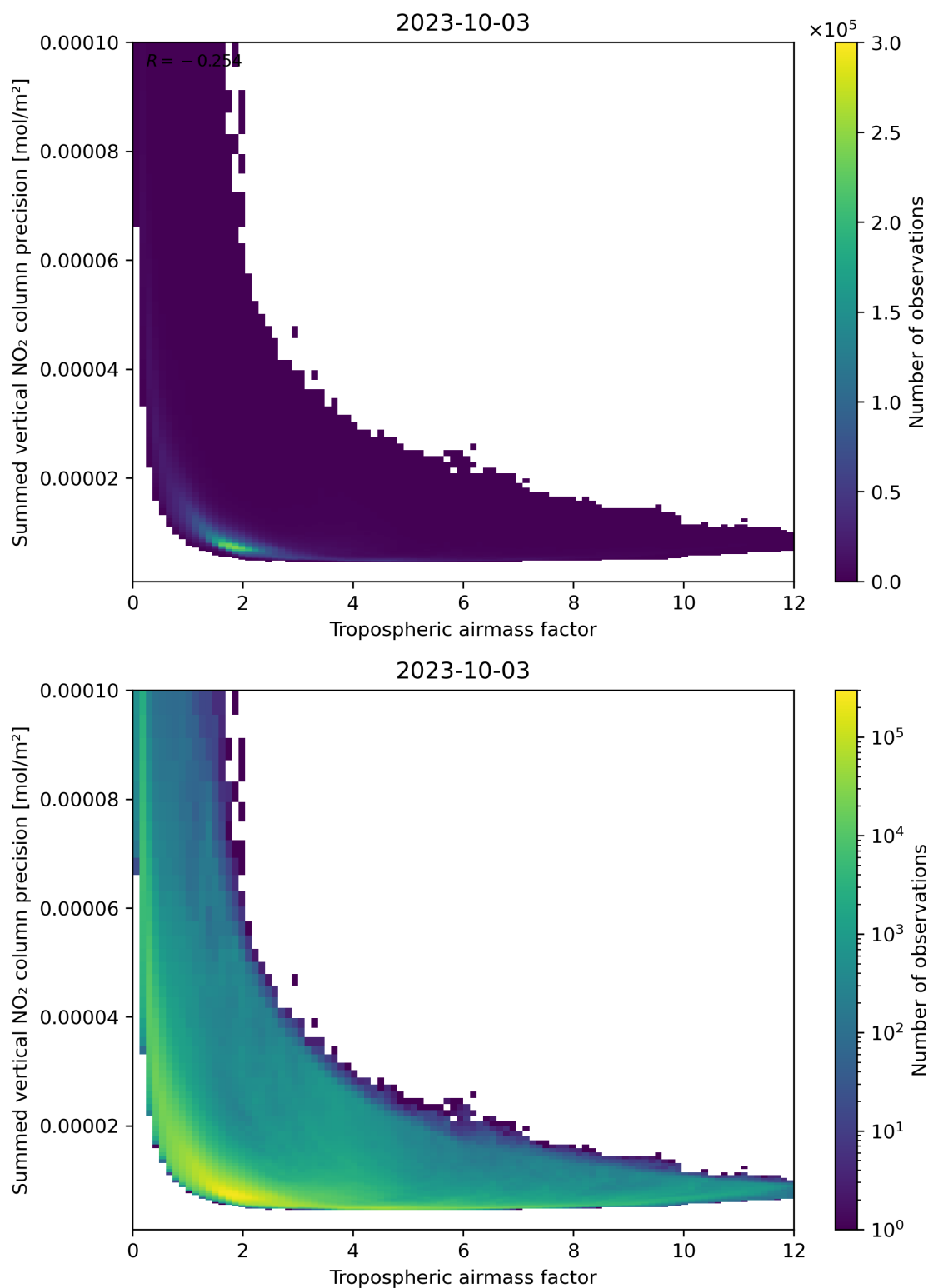
Figure 76: Scatter density plot of “Tropospheric air mass factor” against “Summed vertical NO 2 column precision” for 2023-10-02 to 2023-10-04.
