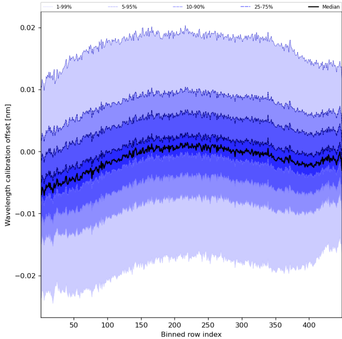
Figure 52: Along track statistics of “Wavelength calibration offset” for 2023-10-02 to 2023-10-04
