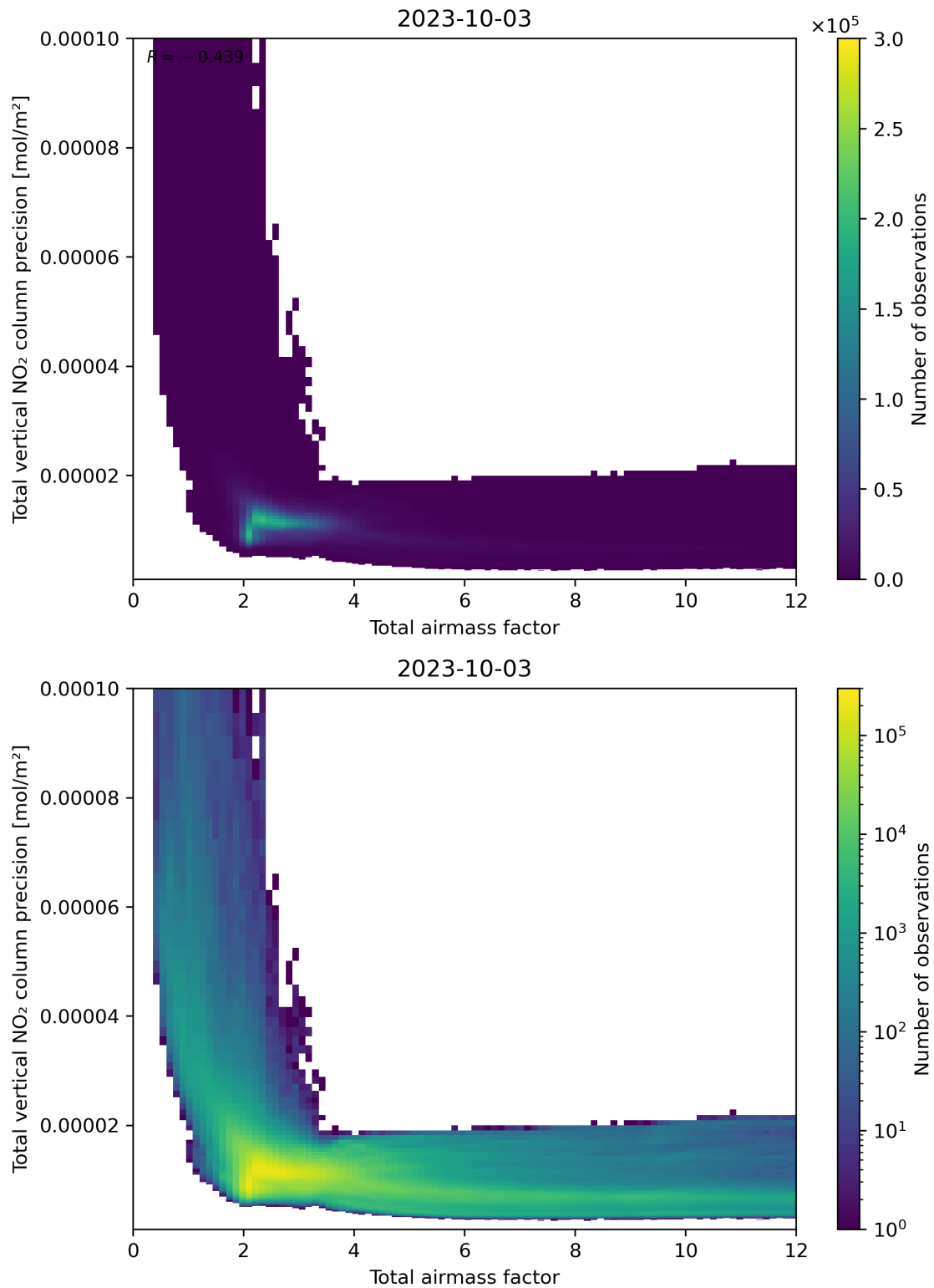
Figure 68: Scatter density plot of “Total airmass factor” against “Total vertical NO 2 column precision” for 2023-10-02 to 2023-10-04.
