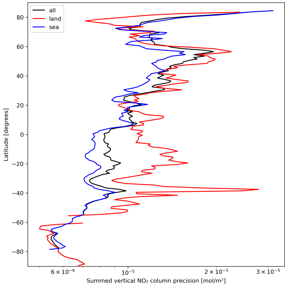
Figure 24: Zonal average of “Summed vertical NO 2 column precision” for 2023-10-02 to 2023-10-04.
