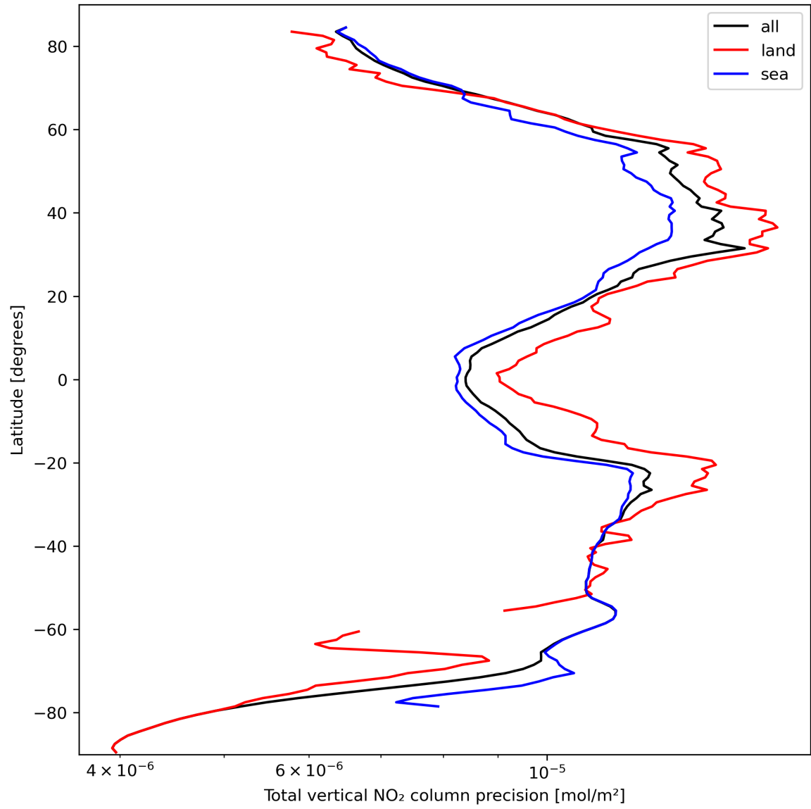
Figure 22: Zonal average of “Total vertical NO 2 column precision” for 2023-10-02 to 2023-10-04.
