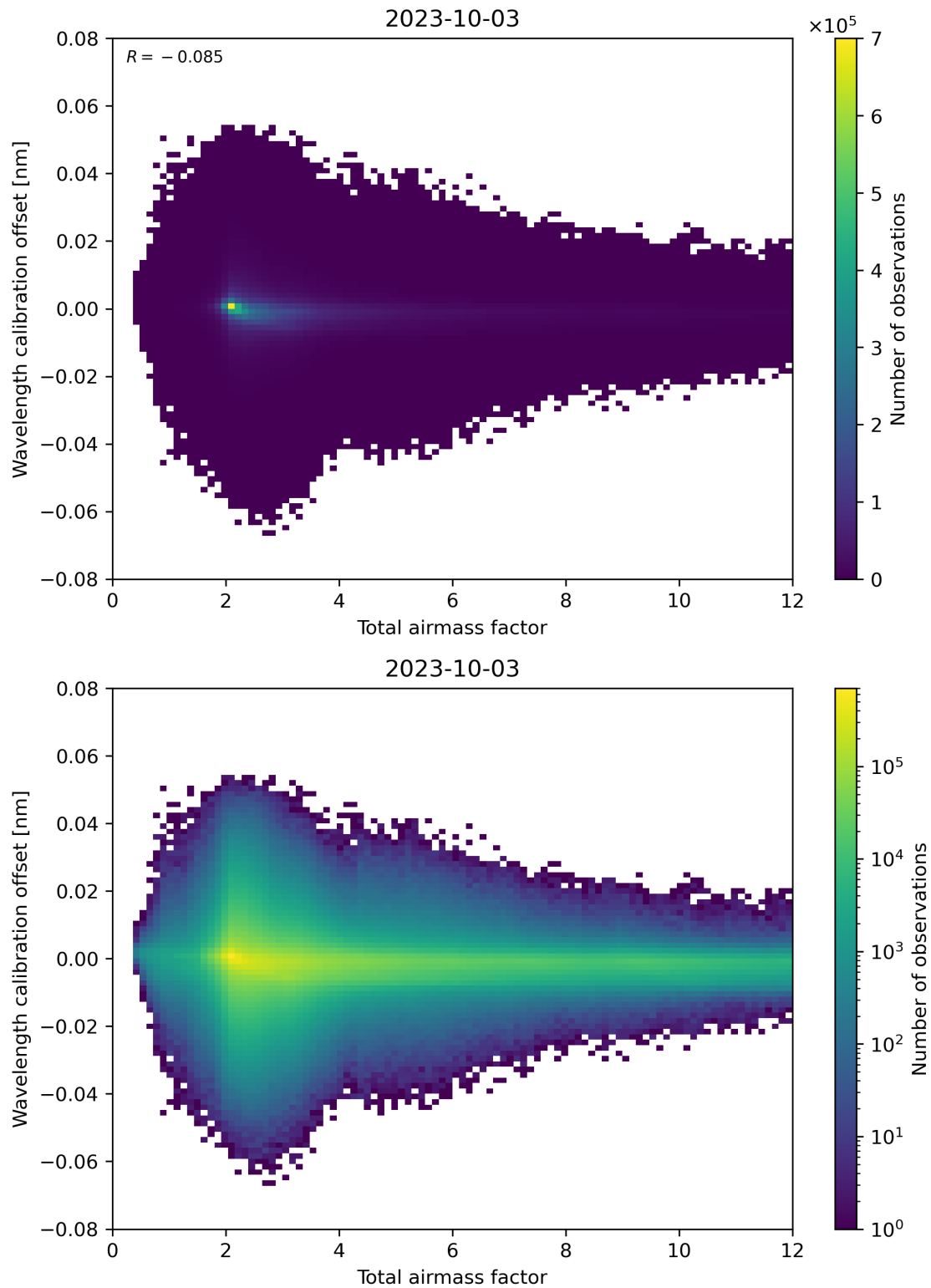
Figure 70: Scatter density plot of “Total airmass factor” against “Wavelength calibration offset” for 2023-10-02 to 2023-10-04.
