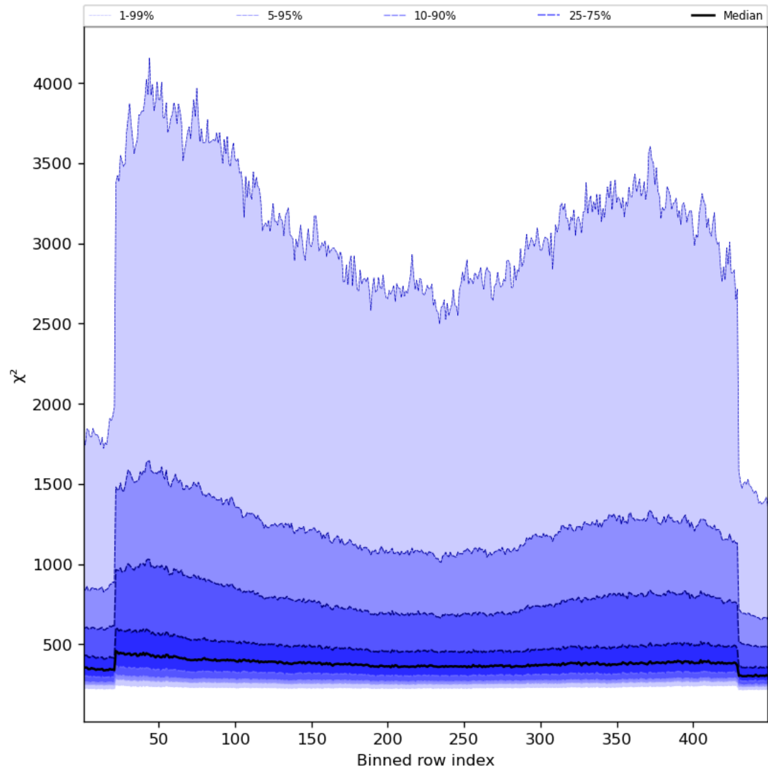
Figure 59: Along track statistics of “ \chi^2 ” for 2023-10-02 to 2023-10-04
