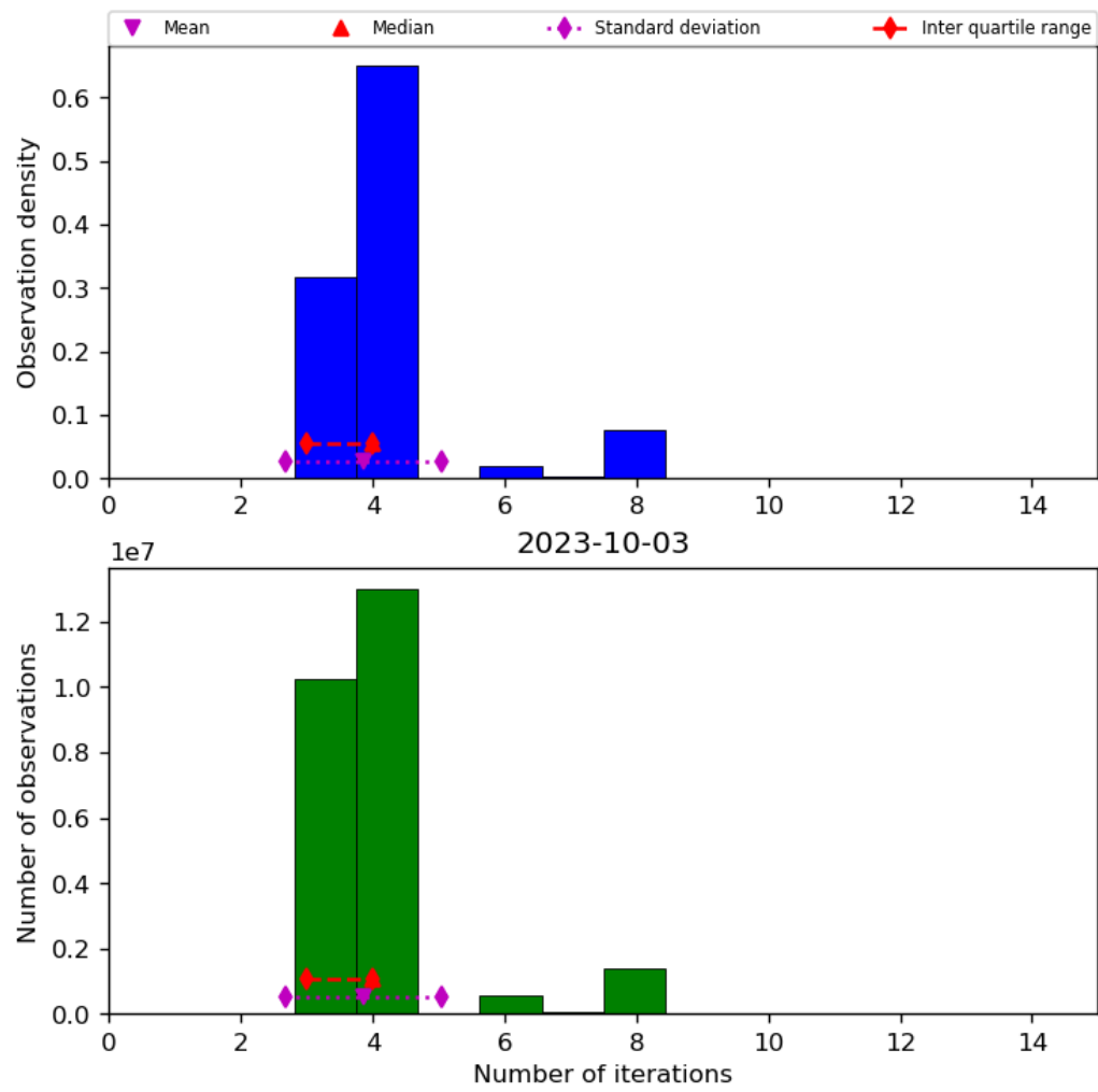
Figure 34: Histogram of “Number of iterations” for 2023-10-02 to 2023-10-04
