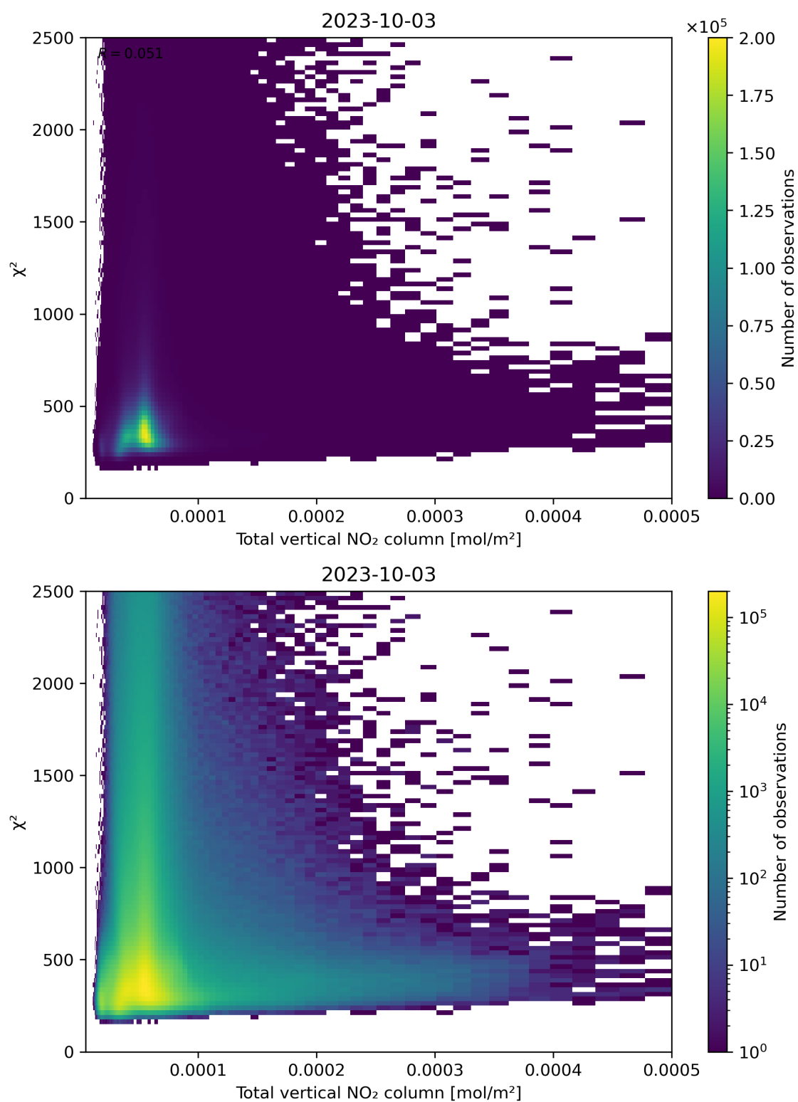
Figure 111: Scatter density plot of “Total vertical NO 2 column” against “ \chi^2 ” for 2023-10-02 to 2023-10-04.
