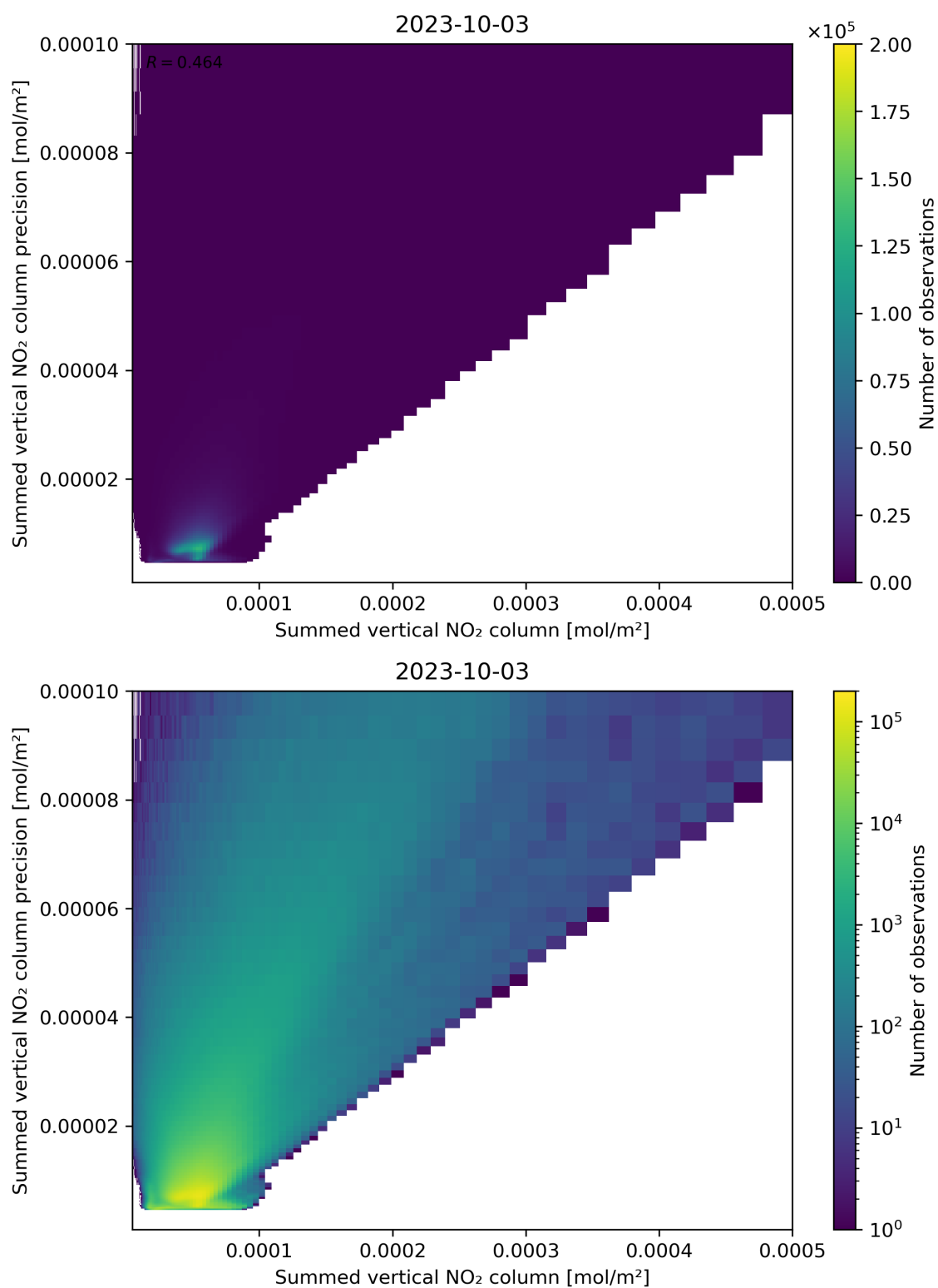
Figure 105: Scatter density plot of “Summed vertical NO 2 column” against “Summed vertical NO 2 column precision” for 2023-10-02 to 2023-10-04.
