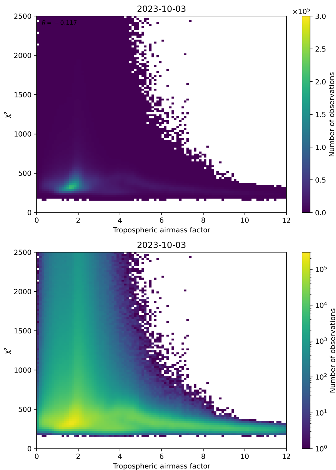
Figure 73: Scatter density plot of “Tropospheric airmass factor” against “ \chi^2 ” for 2023-10-02 to 2023-10-04.
