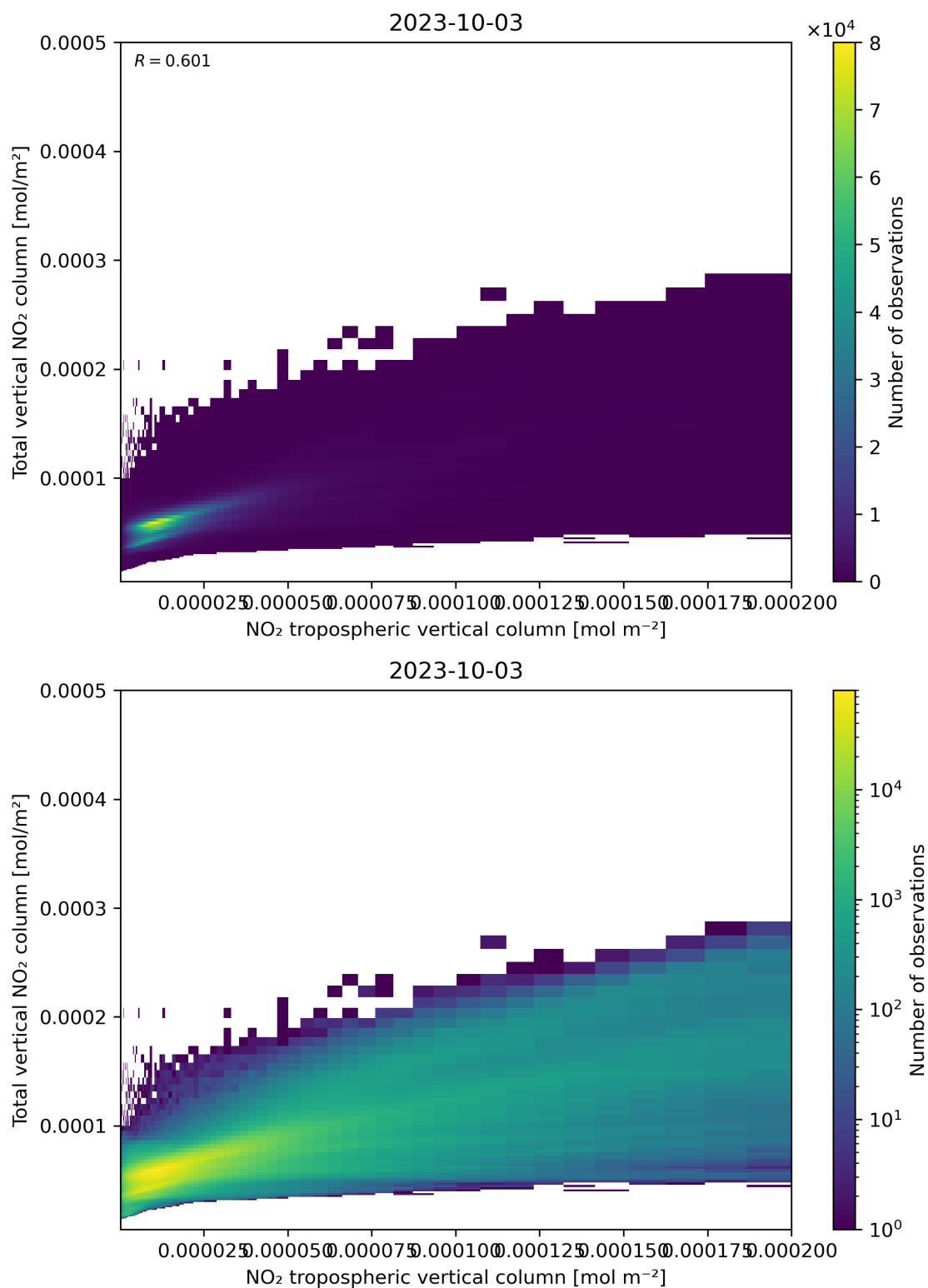
Figure 128: Scatter density plot of “NO 2 tropospheric vertical column” against “Total vertical NO 2 column” for 2023-10-02 to 2023-10-04.
