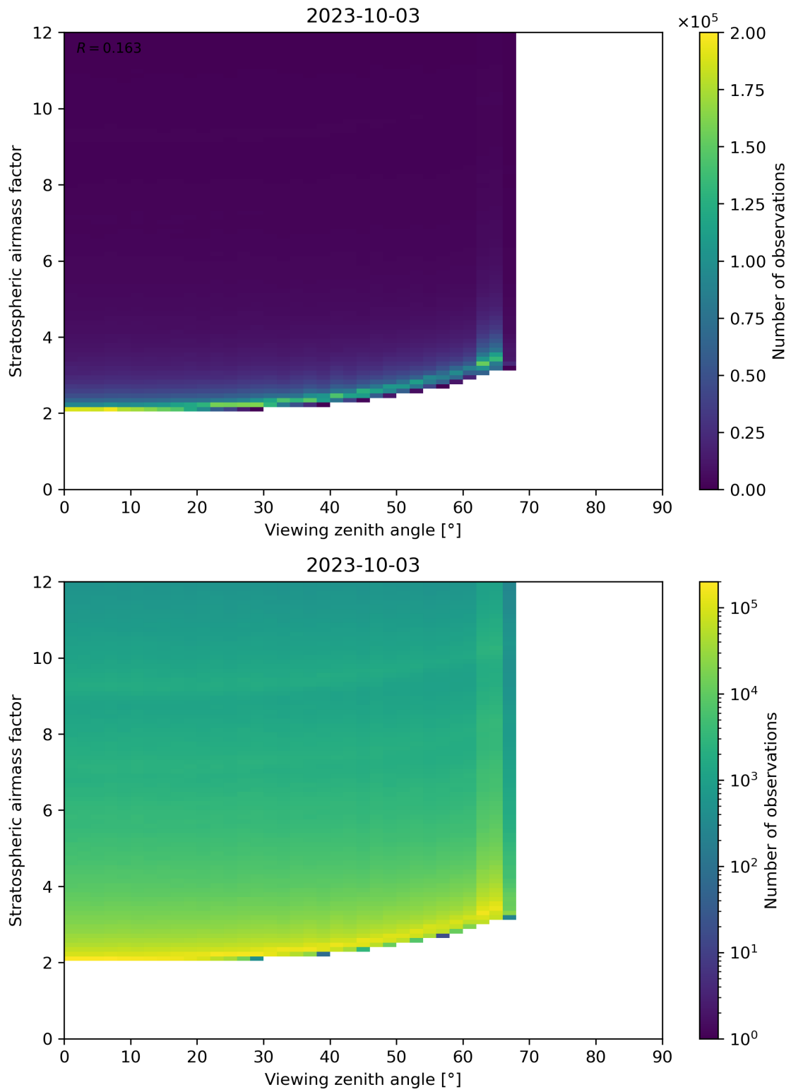
Figure 159: Scatter density plot of “Viewing zenith angle” against “Stratospheric airmass factor” for 2023-10-02 to 2023-10-04.
