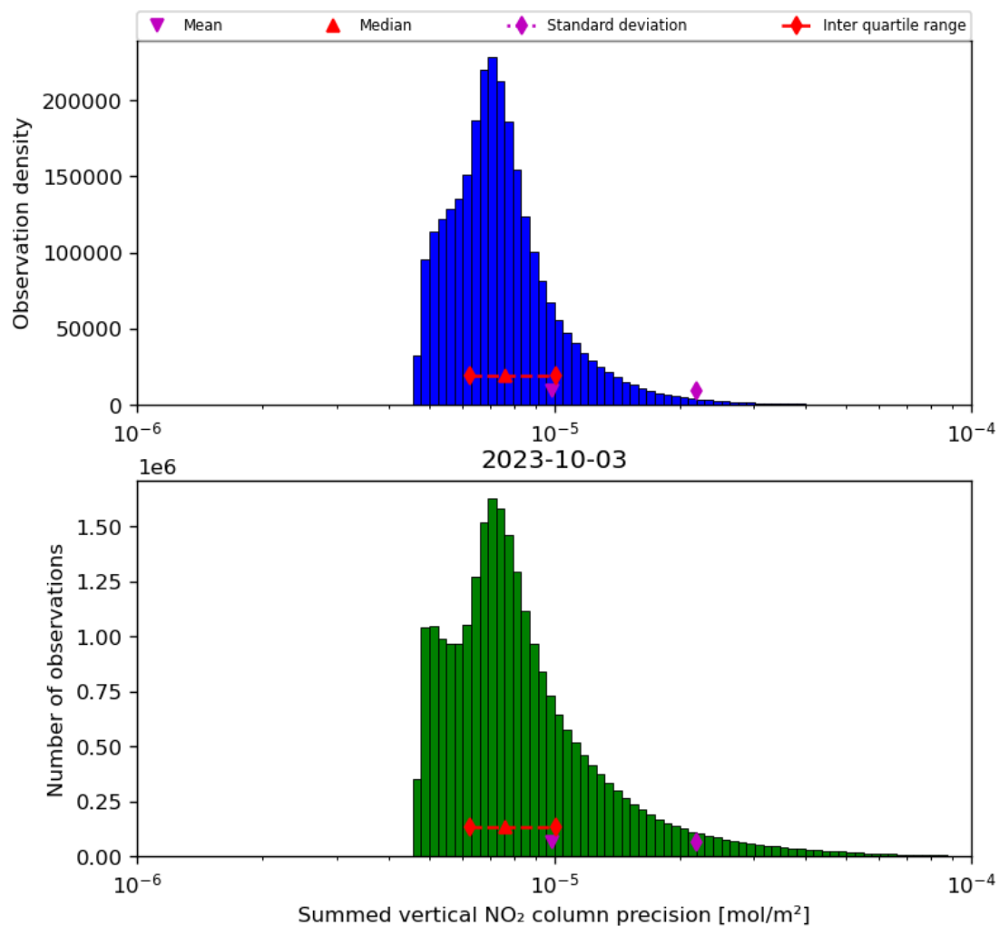
Figure 41: Histogram of “Summed vertical NO 2 column precision” for 2023-10-02 to 2023-10-04
