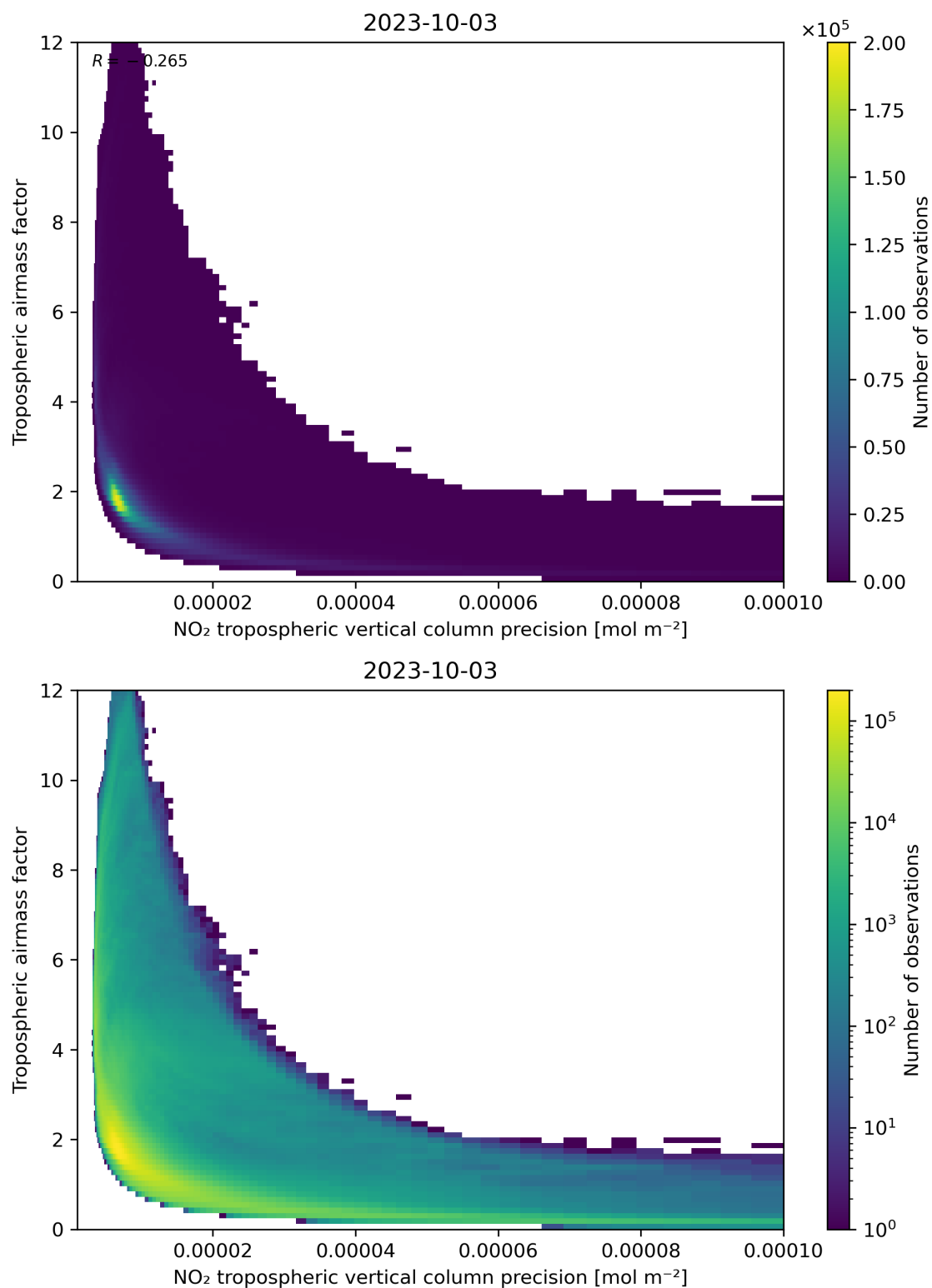
Figure 133: Scatter density plot of “NO 2 tropospheric vertical column precision” against “Tropospheric airmass factor” for 2023-10-02 to 2023-10-04.
