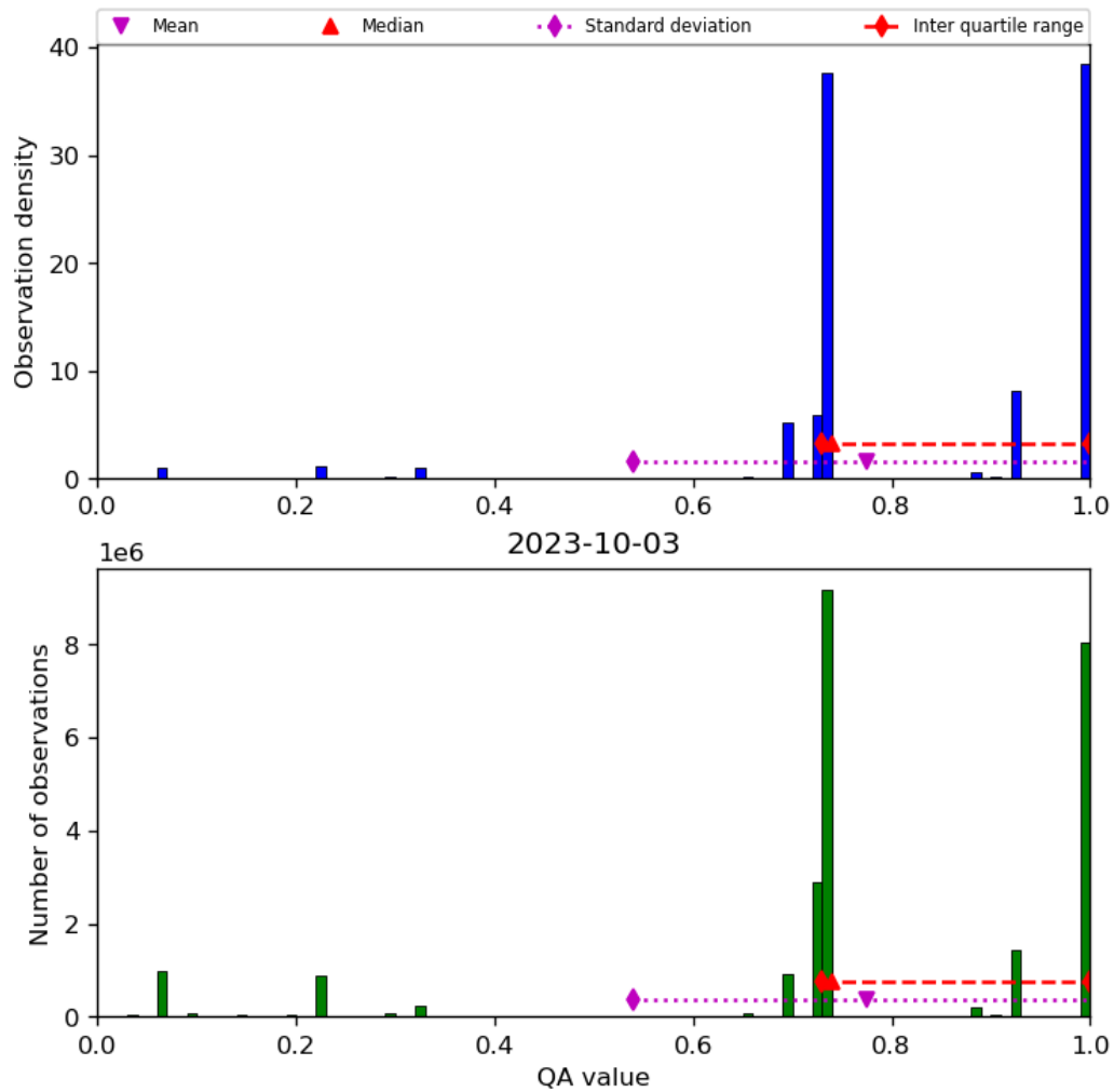
Figure 28: Histogram of “QA value” for 2023-10-02 to 2023-10-04
