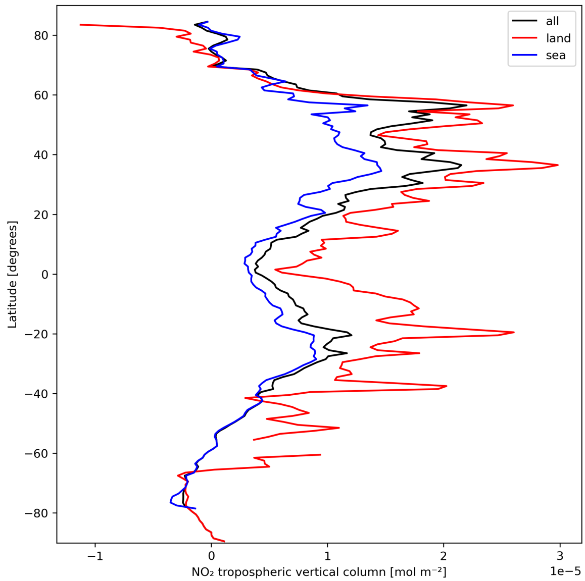
Figure 12: Zonal average of “NO 2 tropospheric vertical column” for 2023-10-02 to 2023-10-04.
