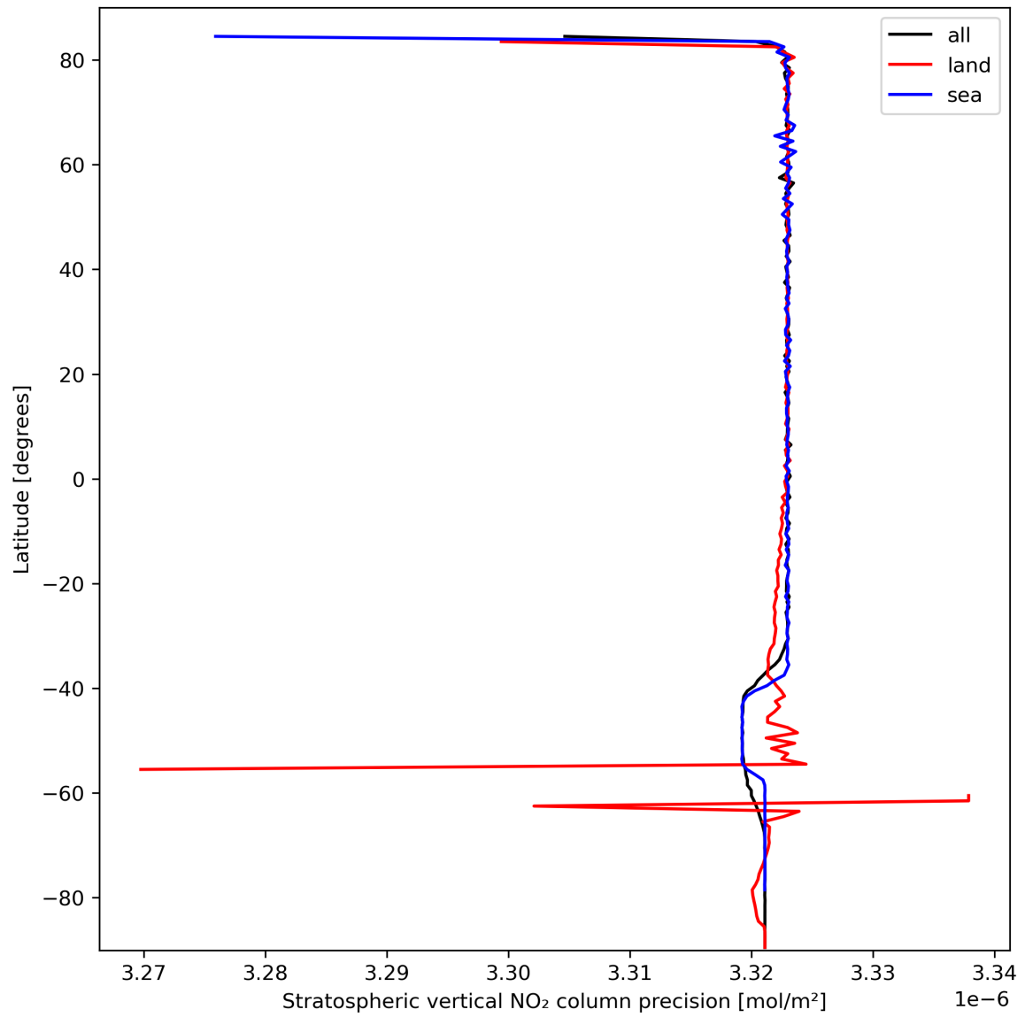
Figure 20: Zonal average of "Stratospheric vertical NO 2 column precision" for 2023-10-02 to 2023-10-04.
