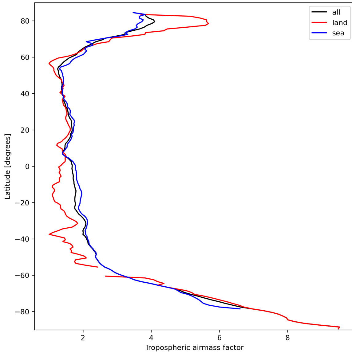
Figure 14: Zonal average of “Tropospheric airmass factor” for 2023-10-02 to 2023-10-04.
