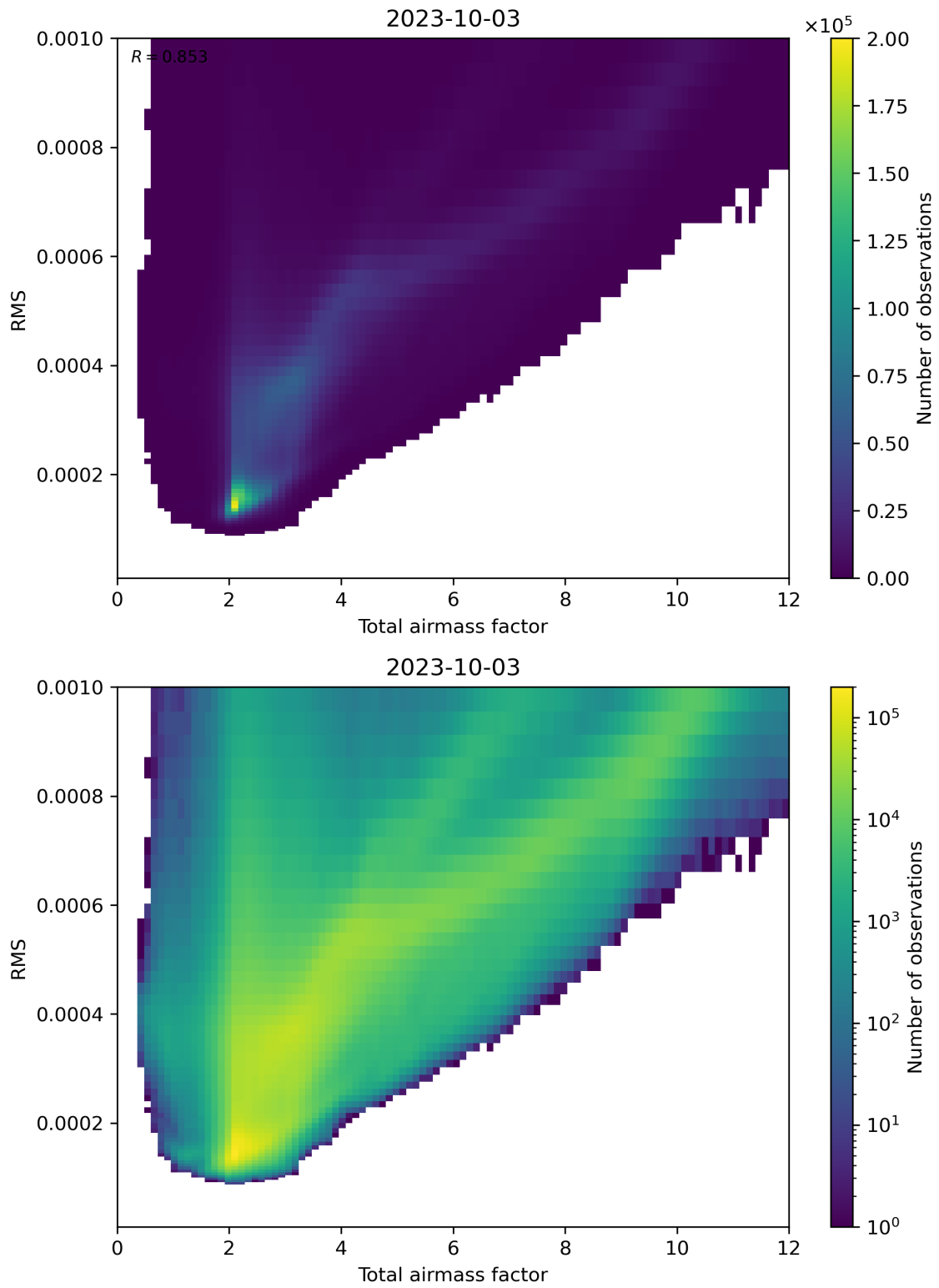
Figure 69: Scatter density plot of “Total airmass factor” against “RMS” for 2023-10-02 to 2023-10-04.
