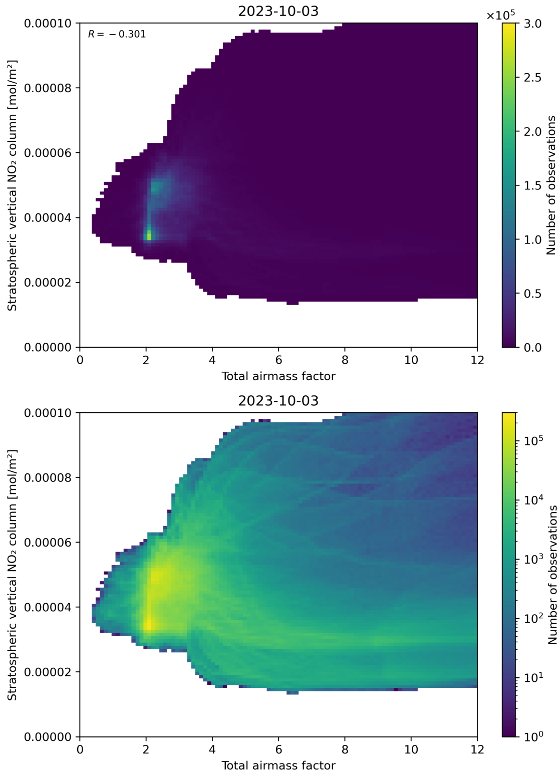
Figure 64: Scatter density plot of “Total airmass factor” against “Stratospheric vertical NO 2 column” for 2023-10-02 to 2023-10-04.
