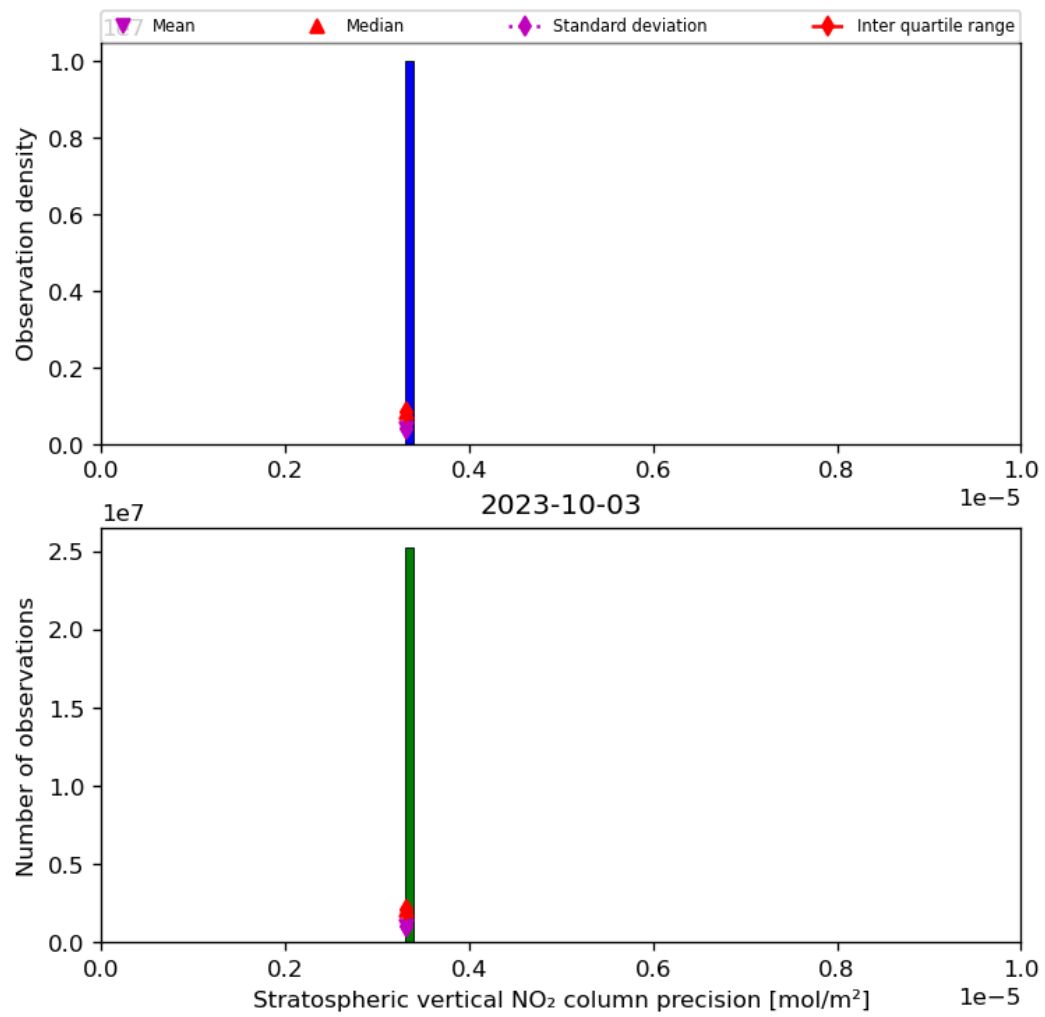
Figure 37: Histogram of “Stratospheric vertical NO 2 column precision” for 2023-10-02 to 2023-10-04
