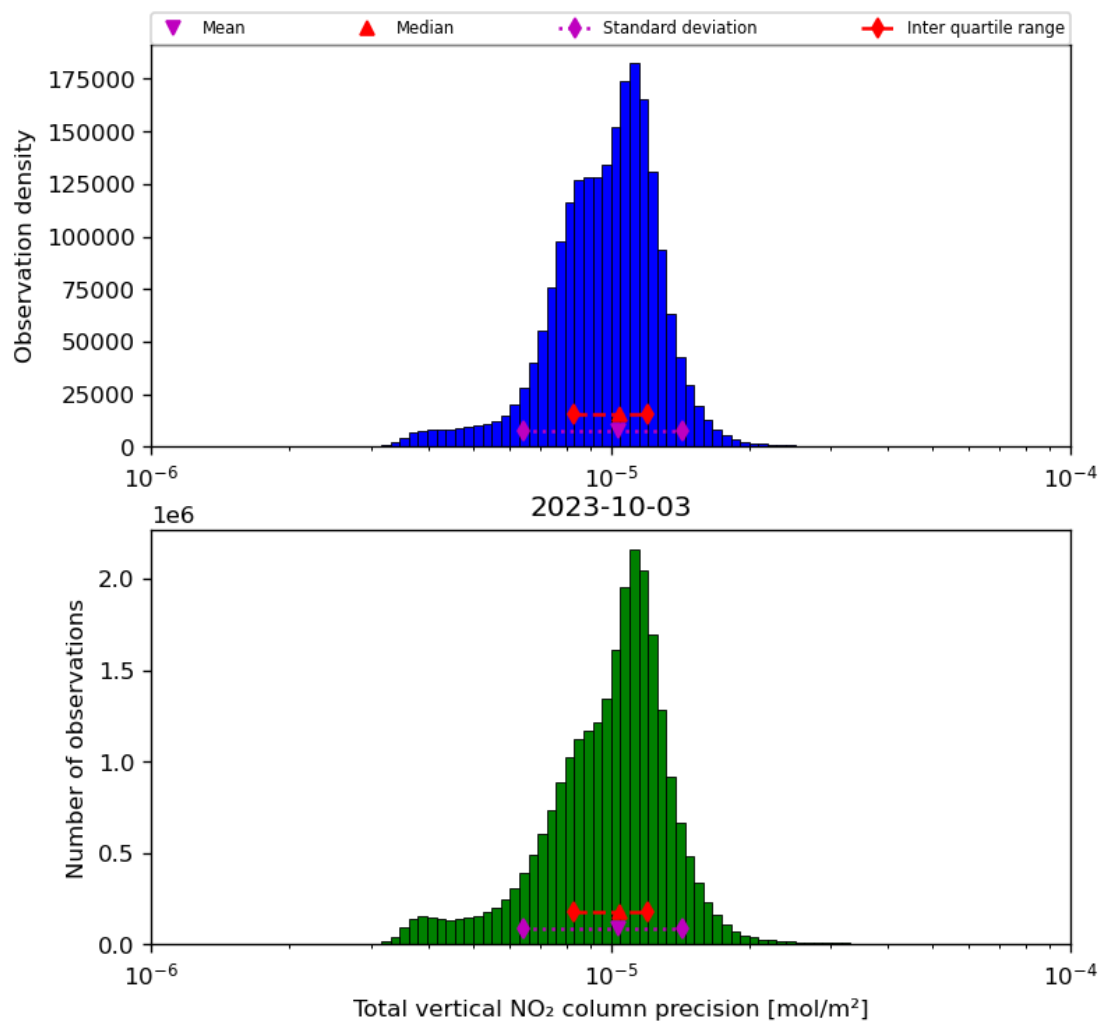
Figure 39: Histogram of "Total vertical NO 2 column precision" for 2023-10-02 to 2023-10-04
