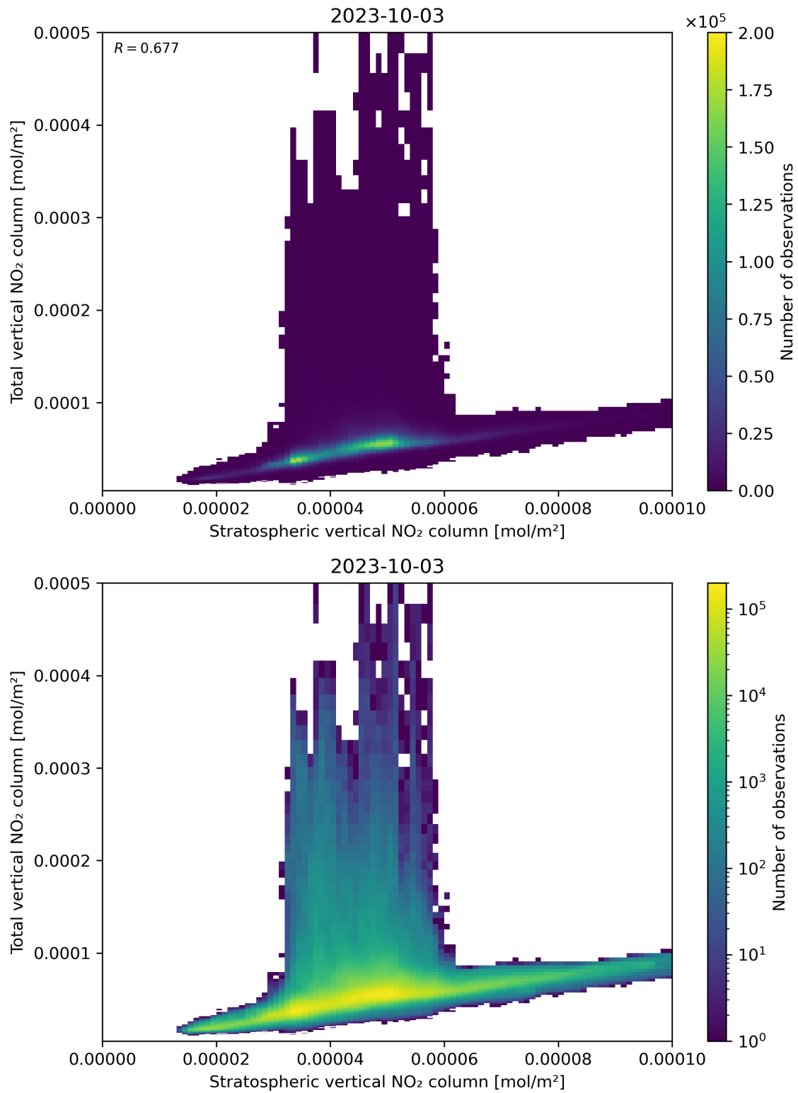
Figure 100: Scatter density plot of “Stratospheric vertical NO 2 column” against “Total vertical NO 2 column” for 2023-10-02 to 2023-10-04.
