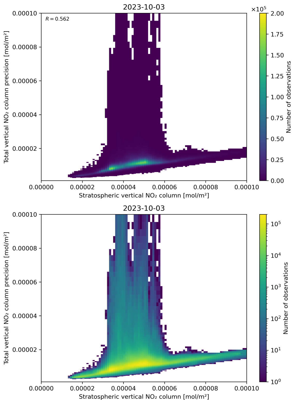
Figure 101: Scatter density plot of “Stratospheric vertical NO 2 column” against “Total vertical NO 2 column precision” for 2023-10-02 to 2023-10-04.
