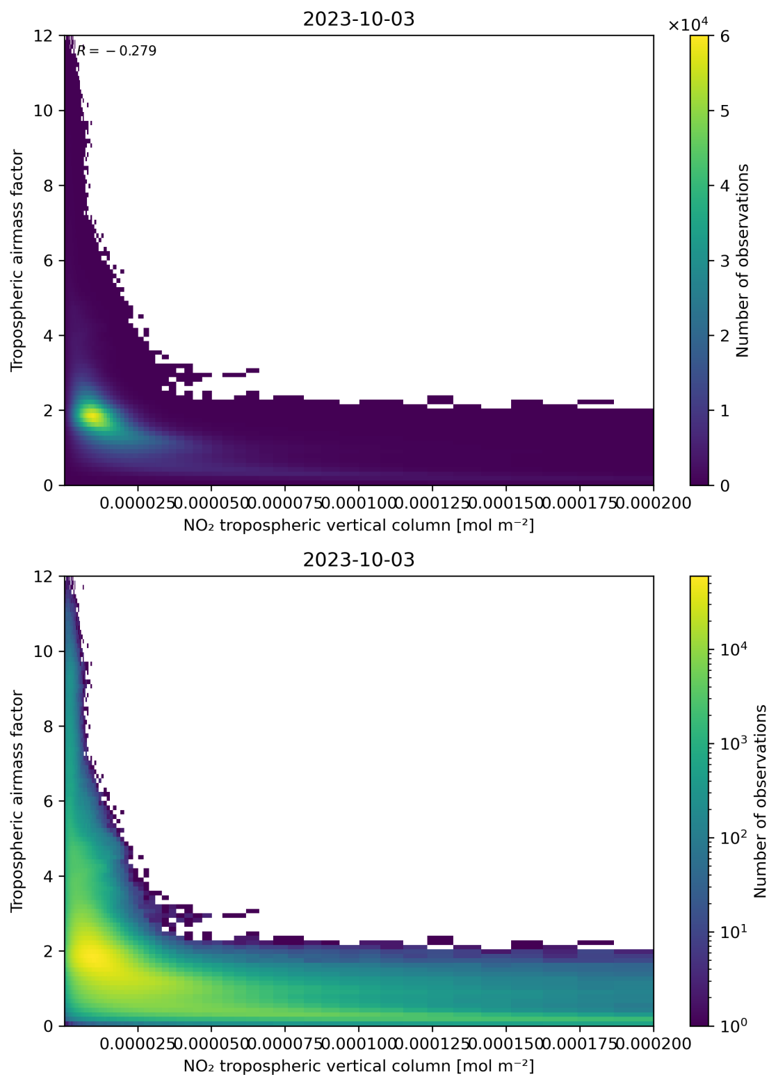
Figure 123: Scatter density plot of “NO 2 tropospheric vertical column” against “Tropospheric air mass factor” for 2023-10-02 to 2023-10-04.
