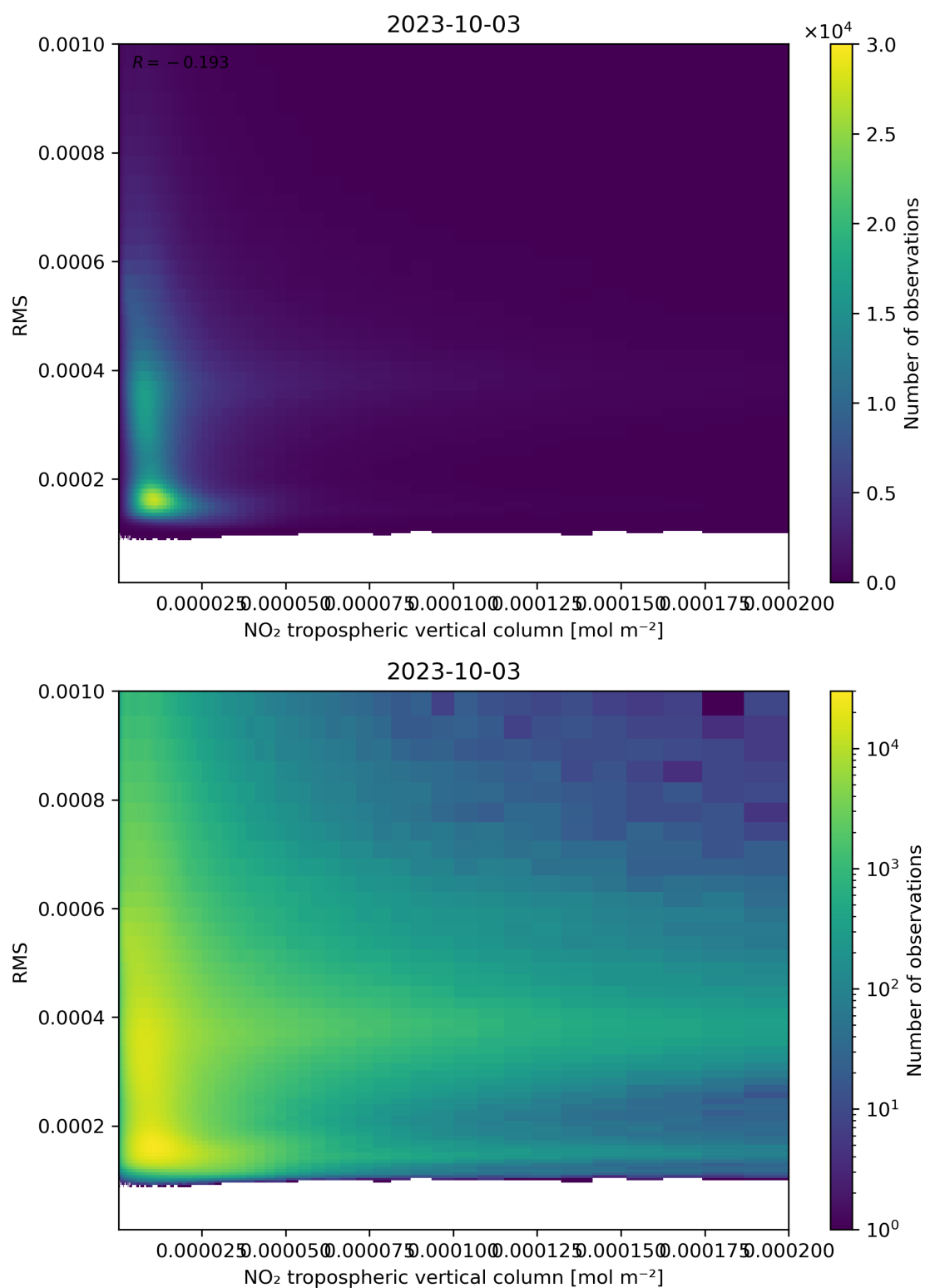
Figure 142: Scatter density plot of “NO 2 tropospheric vertical column” against “RMS” for 2023-10-02 to 2023-10-04.
