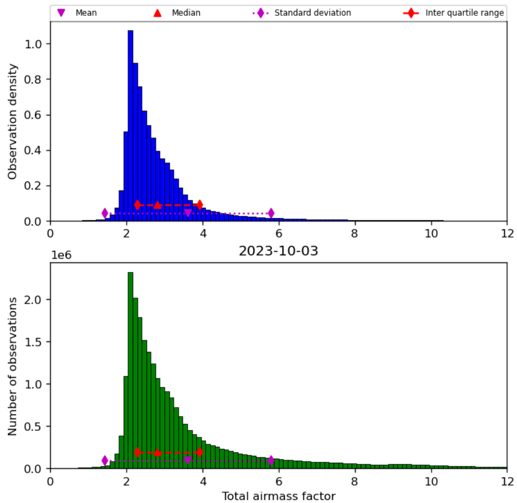
Figure 32: Histogram of “Total airmass factor” for 2023-10-02 to 2023-10-04
