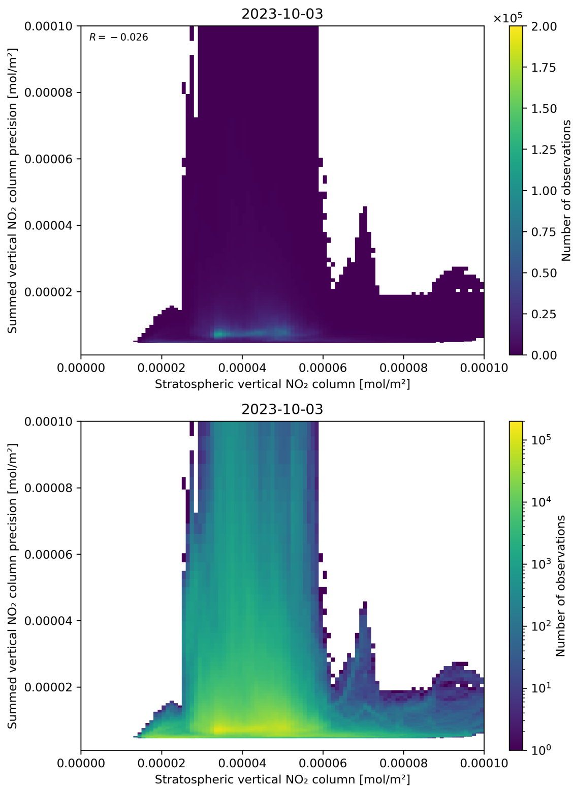
Figure 99: Scatter density plot of “Stratospheric vertical NO 2 column” against “Summed vertical NO 2 column precision” for 2023-10-02 to 2023-10-04.
