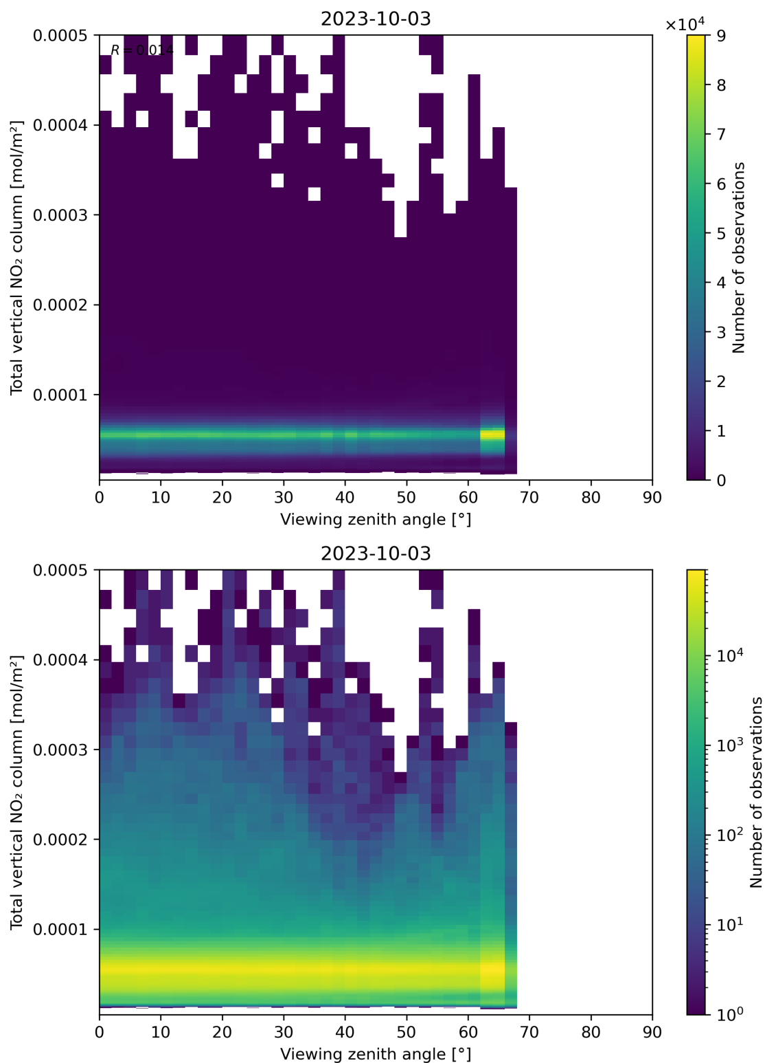
Figure 167: Scatter density plot of “Viewing zenith angle” against “Total vertical NO 2 column” for 2023-10-02 to 2023-10-04.
