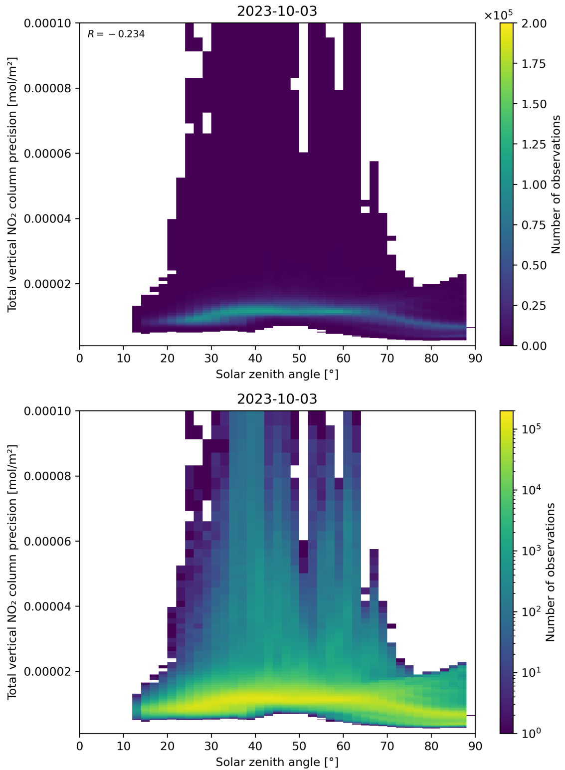
Figure 154: Scatter density plot of “Solar zenith angle” against “Total vertical NO 2 column precision” for 2023-10-02 to 2023-10-04.
