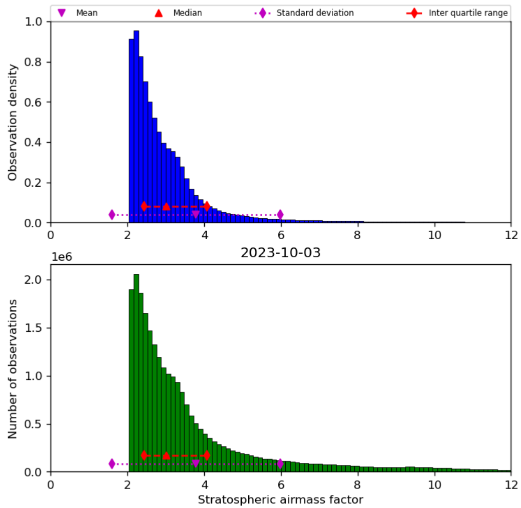
Figure 44: Histogram of “Stratospheric airmass factor” for 2023-10-02 to 2023-10-04
