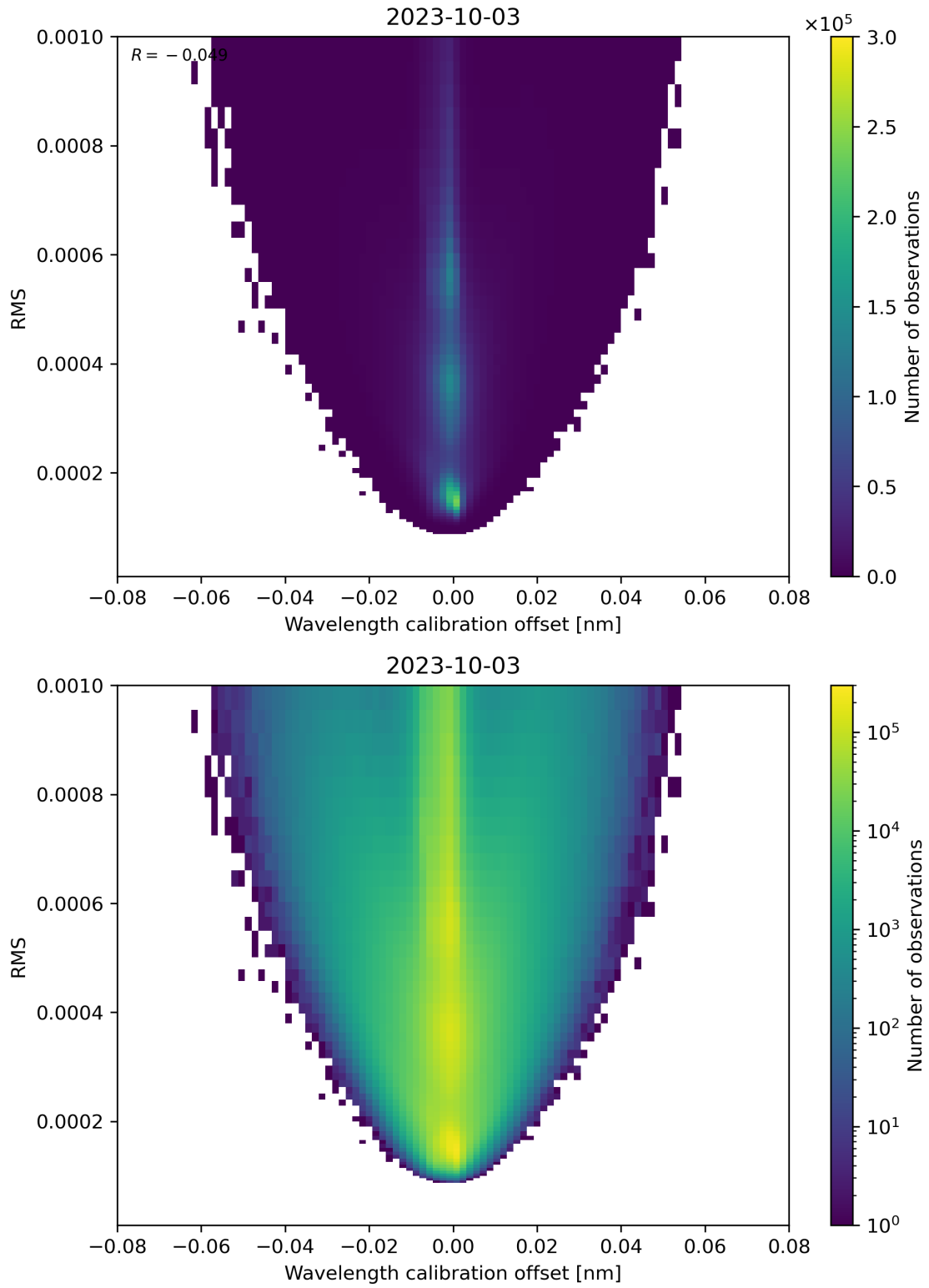
Figure 181: Scatter density plot of “Wavelength calibration offset” against “RMS” for 2023-10-02 to 2023-10-04.
