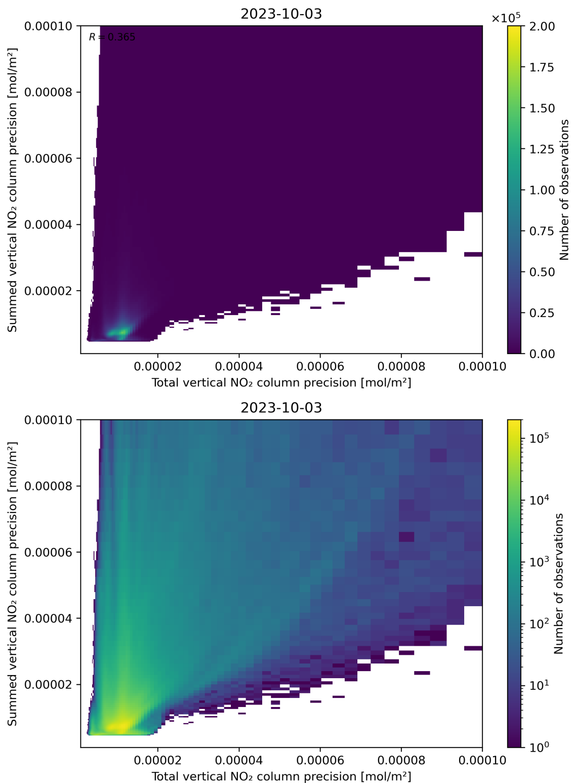
Figure 118: Scatter density plot of “Total vertical NO 2 column precision” against “Summed vertical NO 2 column precision” for 2023-10-02 to 2023-10-04.
