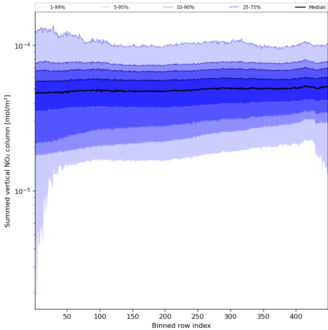
Figure 57: Along track statistics of “Summed vertical NO 2 column” for 2023-10-02 to 2023-10-04
