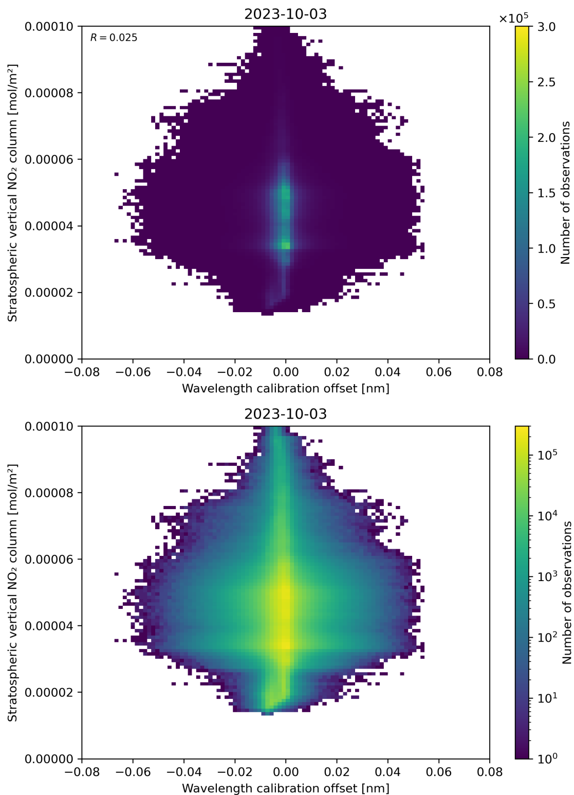
Figure 176: Scatter density plot of “Wavelength calibration offset” against “Stratospheric vertical NO 2 column” for 2023-10-02 to 2023-10-04.
