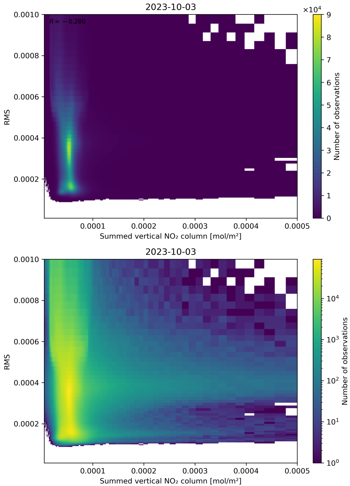
Figure 109: Scatter density plot of “Summed vertical NO 2 column” against “RMS” for 2023-10-02 to 2023-10-04.
