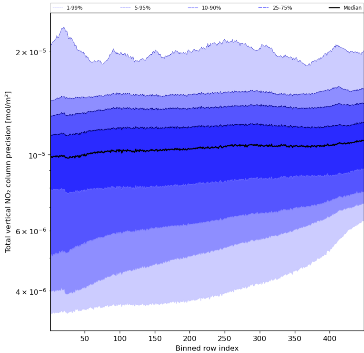
Figure 56: Along track statistics of “Total vertical NO 2 column precision” for 2023-10-02 to 2023-10-04
