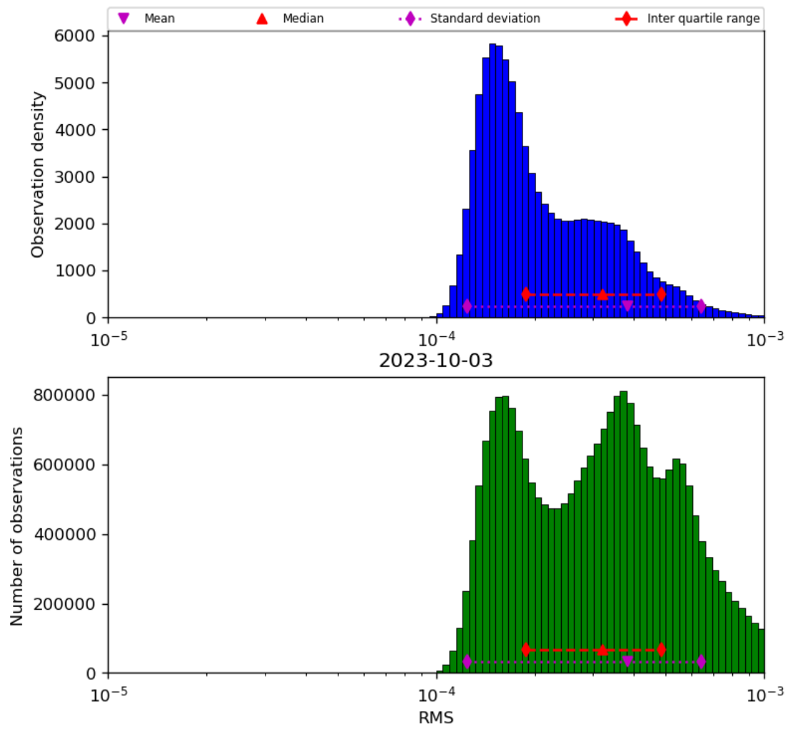
Figure 43: Histogram of “RMS” for 2023-10-02 to 2023-10-04
