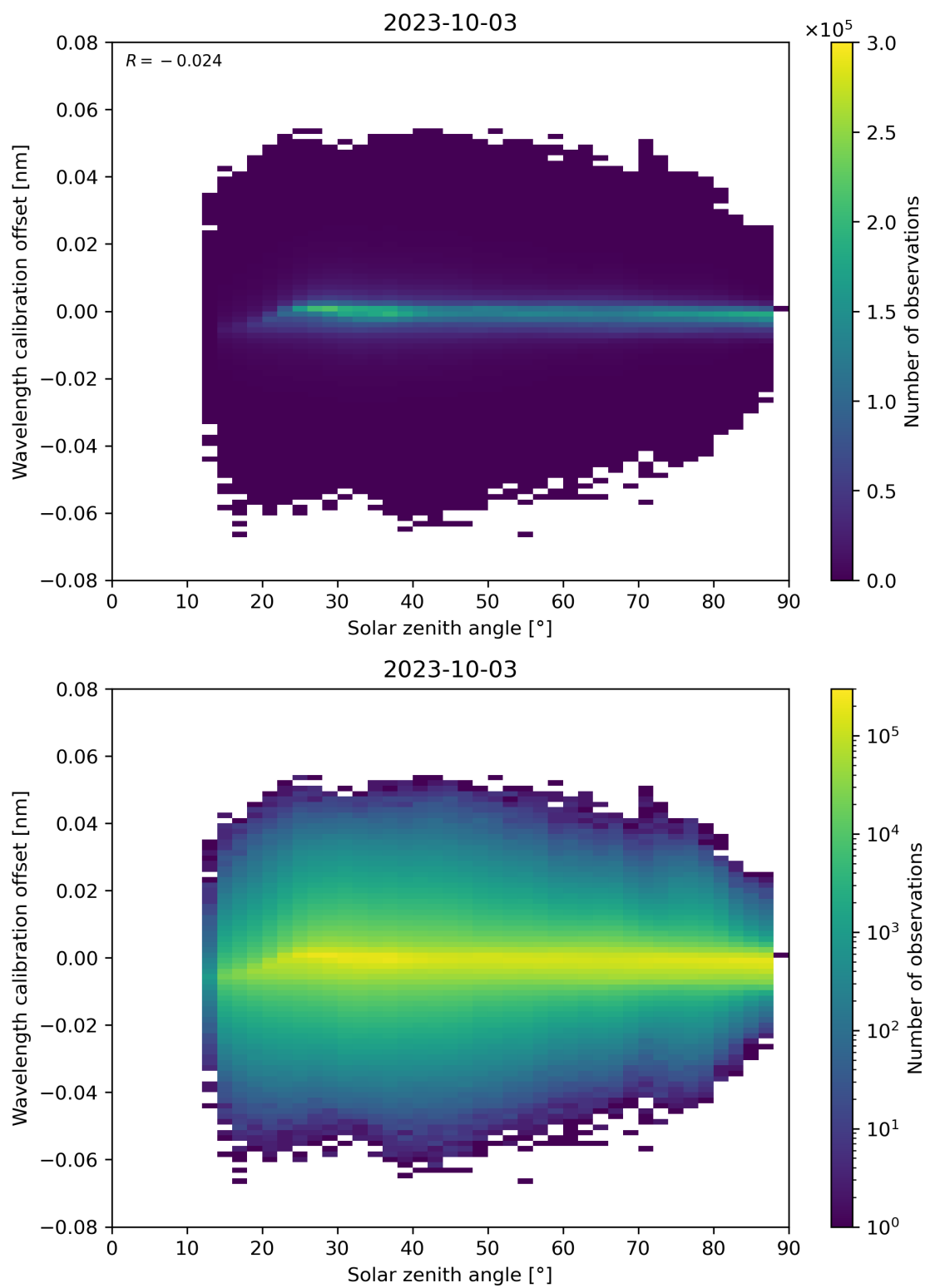
Figure 158: Scatter density plot of “Solar zenith angle” against “Wavelength calibration offset” for 2023-10-02 to 2023-10-04.
