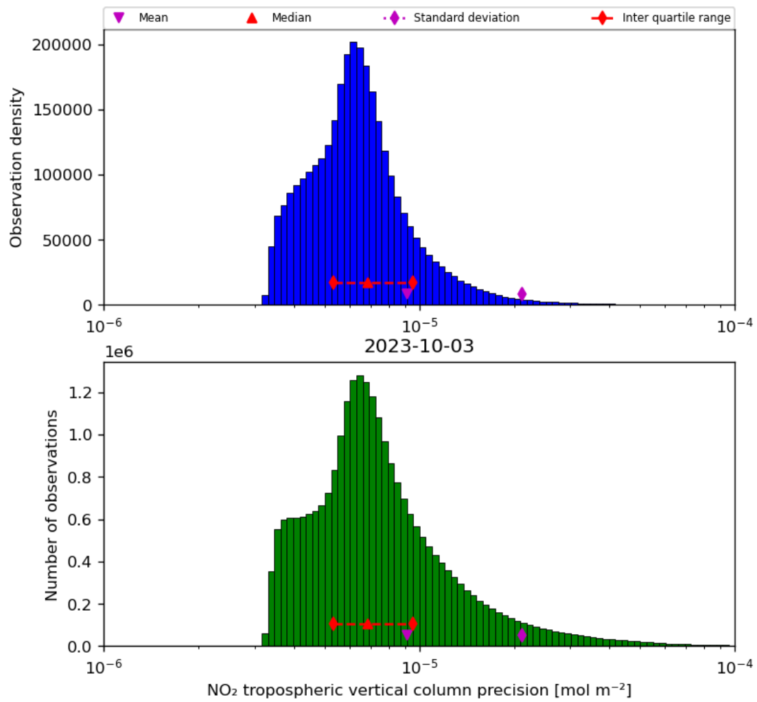
Figure 30: Histogram of “NO 2 tropospheric vertical column precision” for 2023-10-02 to 2023-10-04
