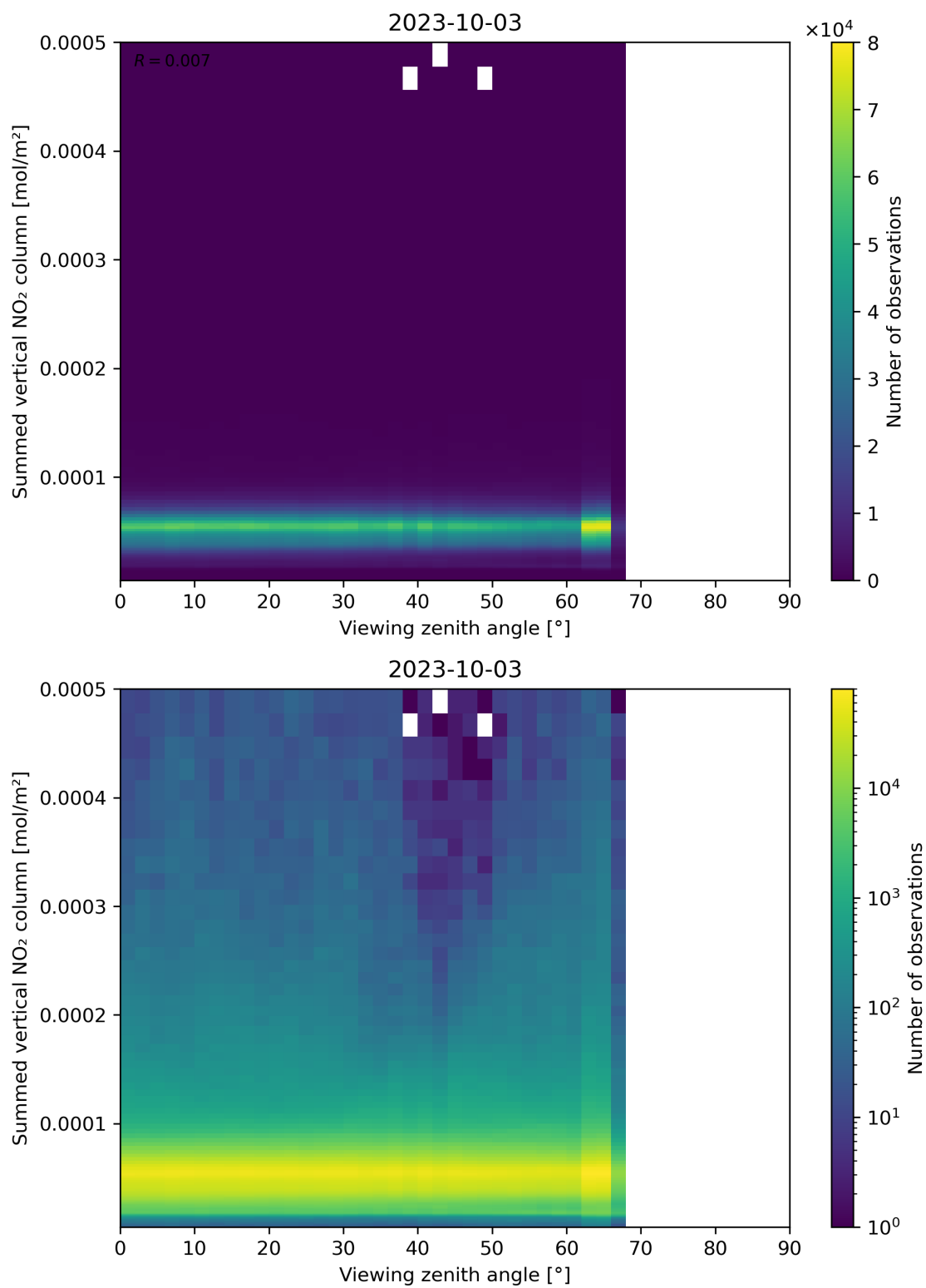
Figure 165: Scatter density plot of “Viewing zenith angle” against “Summed vertical NO 2 column” for 2023-10-02 to 2023-10-04.
