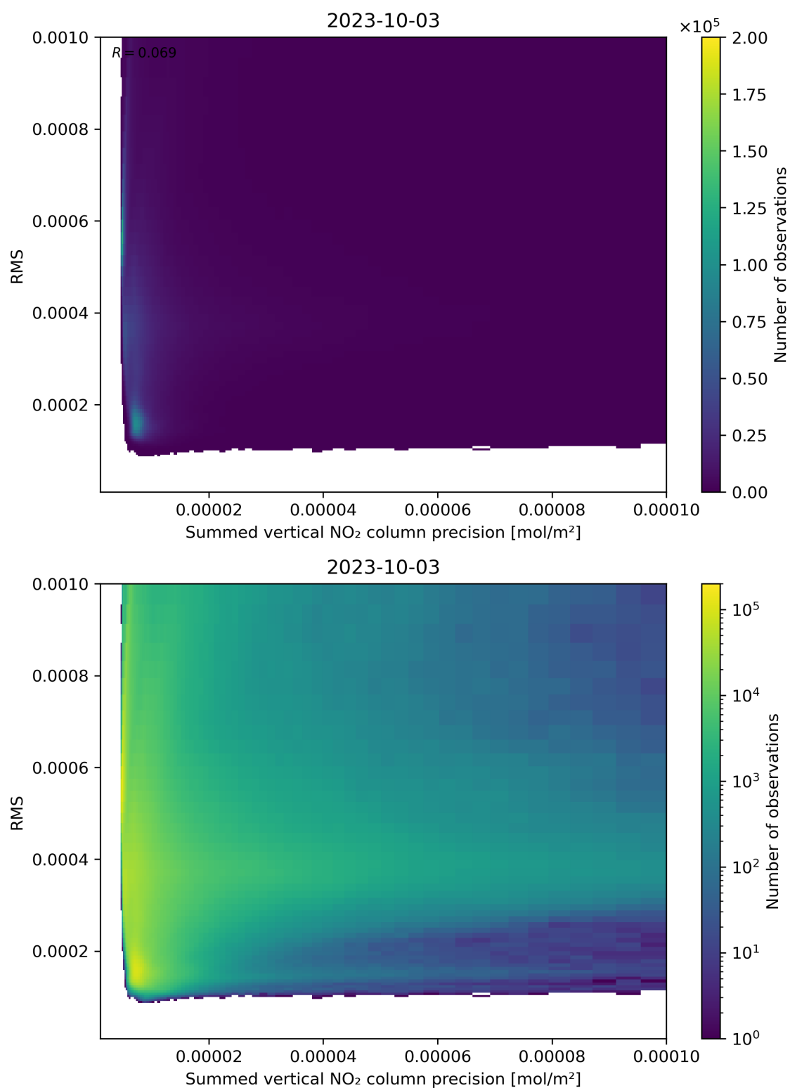
Figure 108: Scatter density plot of “Summed vertical NO 2 column precision” against “RMS” for 2023-10-02 to 2023-10-04.
