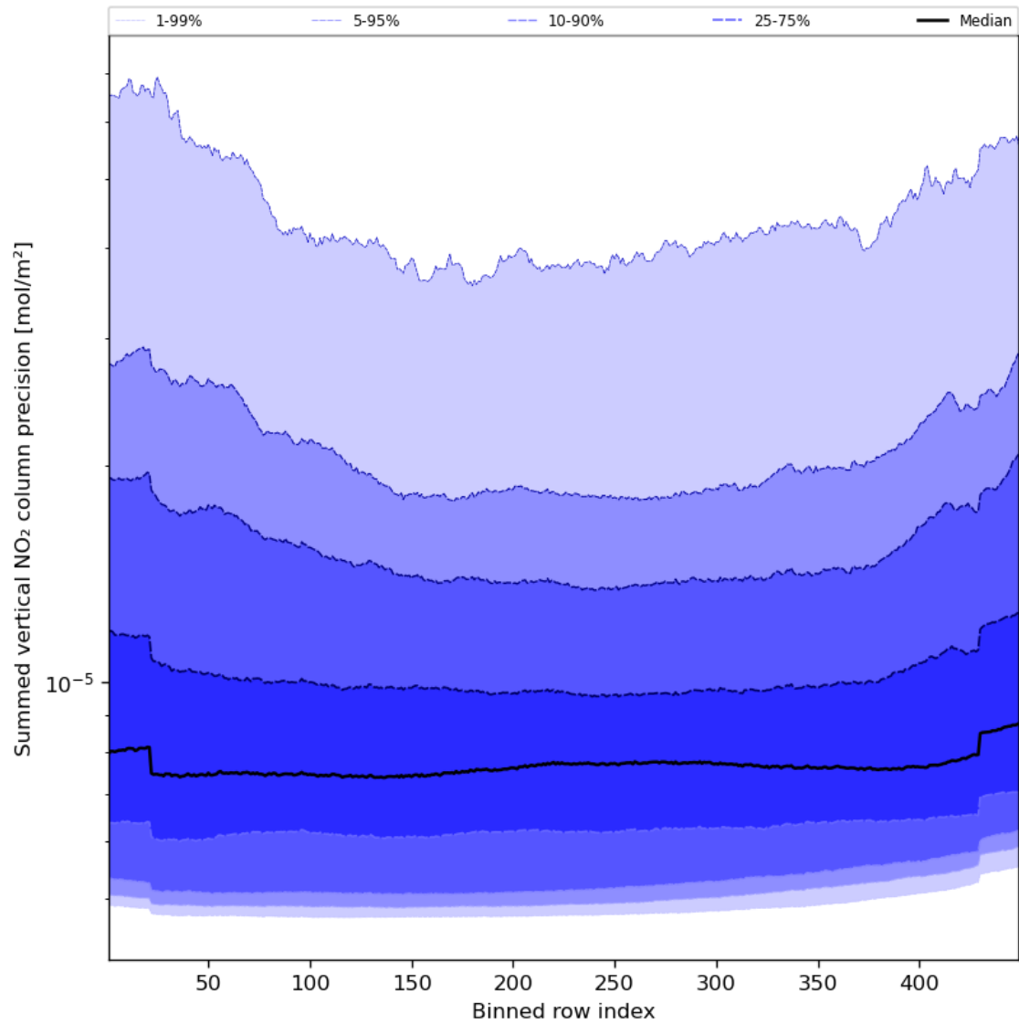
Figure 58: Along track statistics of “Summed vertical NO 2 column precision” for 2023-10-02 to 2023-10-04
