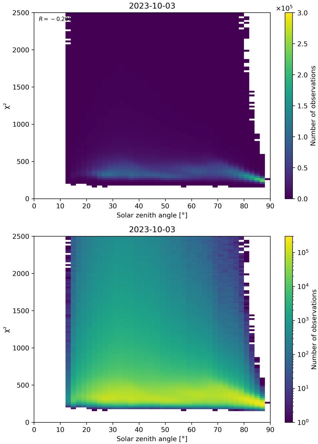
Figure 148: Scatter density plot of “Solar zenith angle” against “ \chi^2 ” for 2023-10-02 to 2023-10-04.
