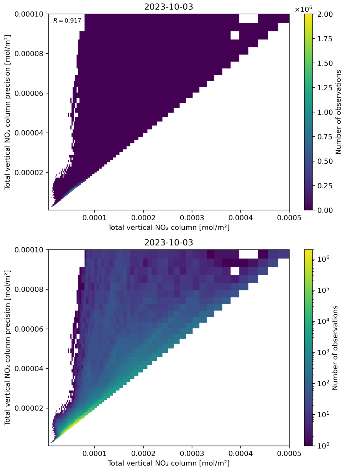
Figure 114: Scatter density plot of “Total vertical NO 2 column” against “Total vertical NO 2 column precision” for 2023-10-02 to 2023-10-04.
