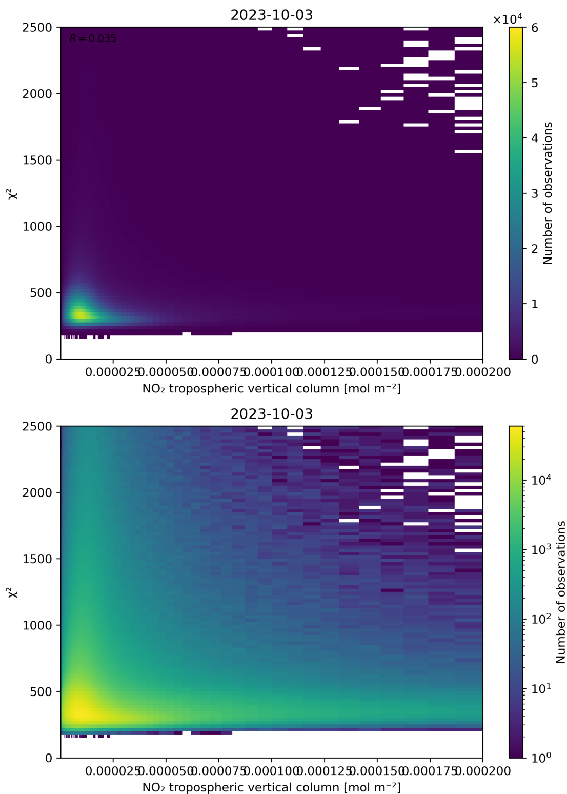
Figure 124: Scatter density plot of “NO 2 tropospheric vertical column” against “ \chi^2 ” for 2023-10-02 to 2023-10-04.
