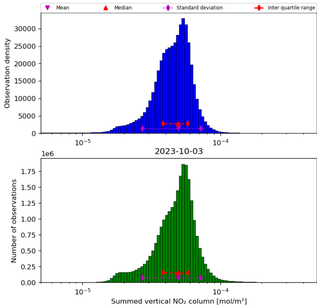
Figure 40: Histogram of “Summed vertical NO 2 column” for 2023-10-02 to 2023-10-04
