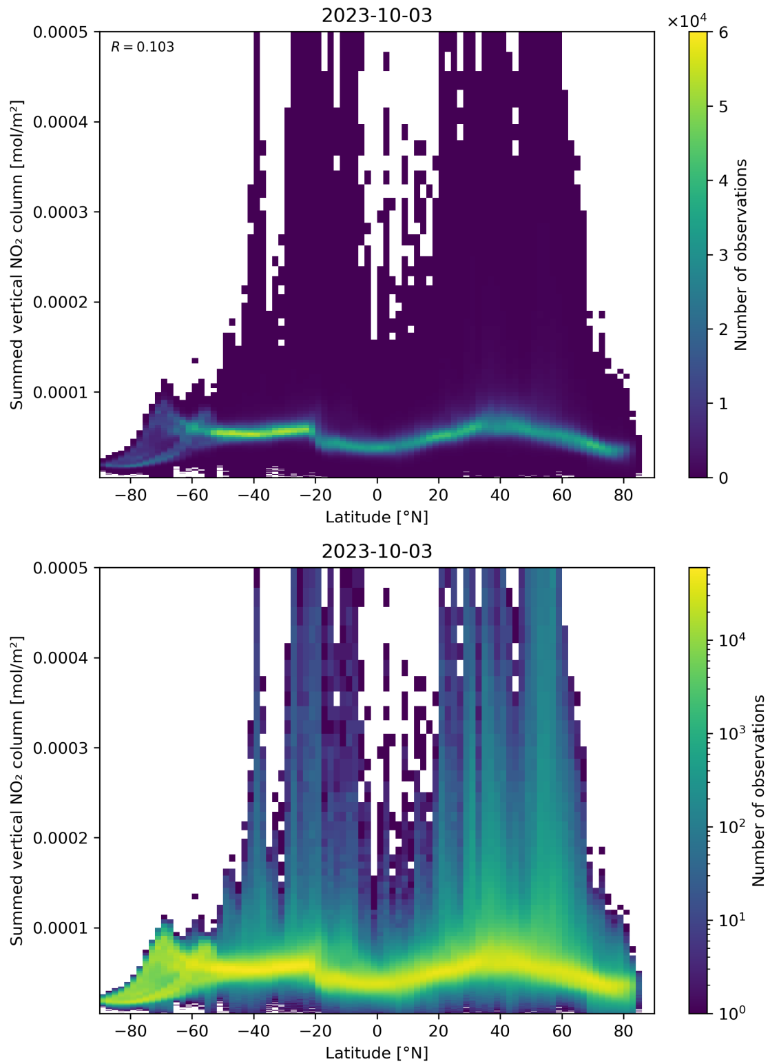
Figure 88: Scatter density plot of “Latitude” against “Summed vertical NO 2 column” for 2023-10-02 to 2023-10-04.
