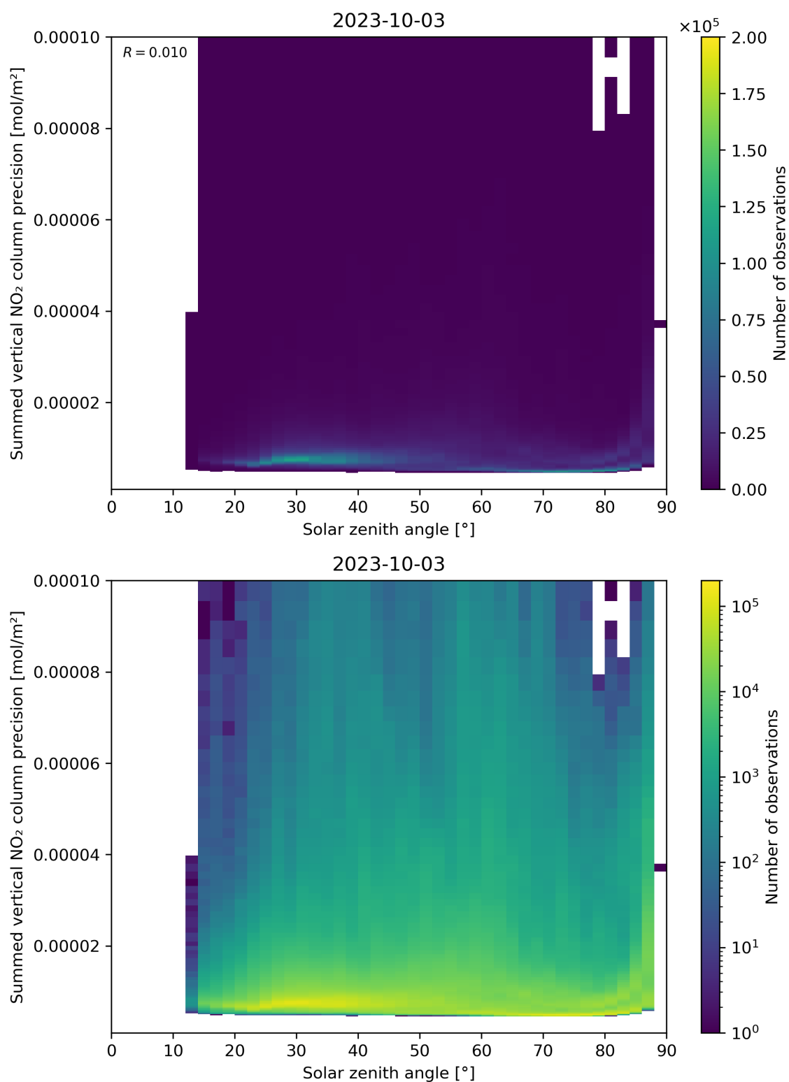
Figure 152: Scatter density plot of “Solar zenith angle” against “Summed vertical NO 2 column precision” for 2023-10-02 to 2023-10-04.
