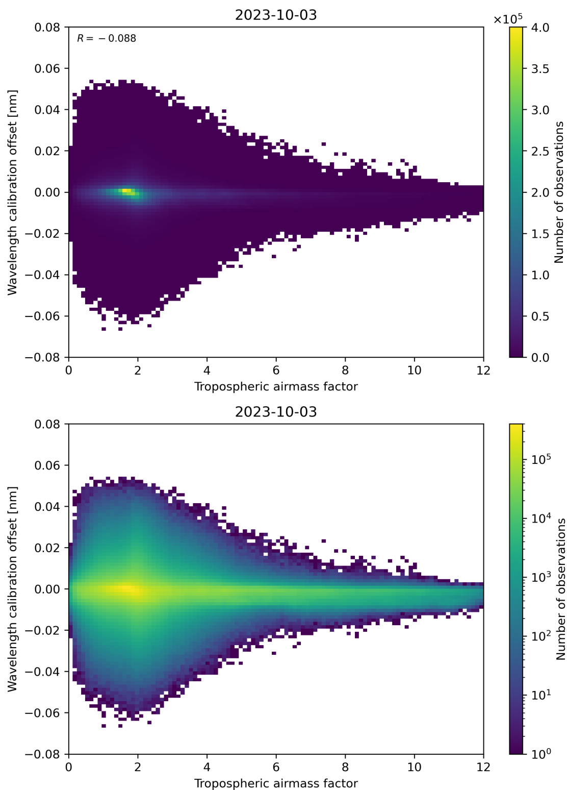
Figure 80: Scatter density plot of “Tropospheric airmass factor” against “Wavelength calibration offset” for 2023-10-02 to 2023-10-04.
