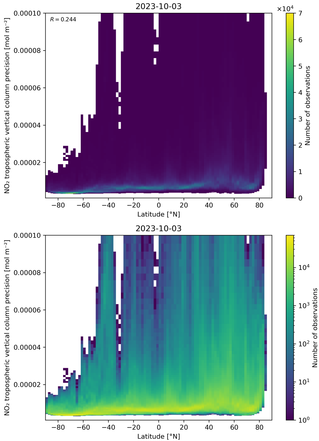
Figure 93: Scatter density plot of “Latitude” against “NO 2 tropospheric vertical column precision” for 2023-10-02 to 2023-10-04.
