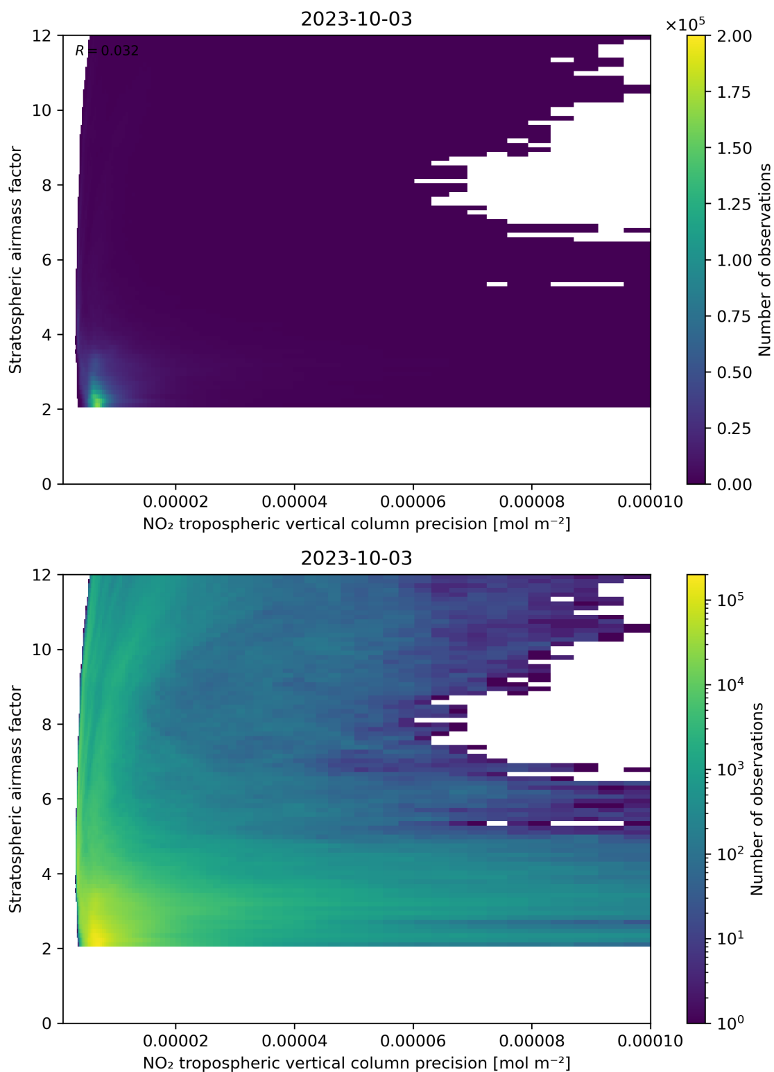
Figure 131: Scatter density plot of “NO 2 tropospheric vertical column precision” against “Stratospheric airmass factor” for 2023-10-02 to 2023-10-04.
