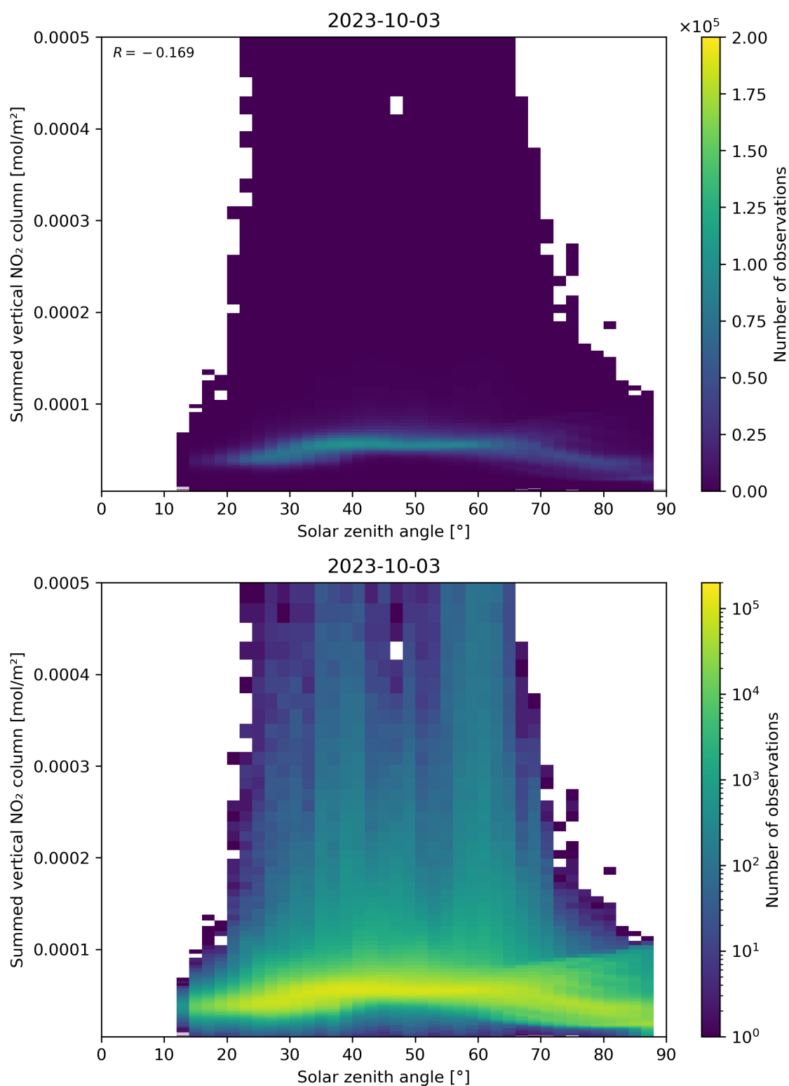
Figure 151: Scatter density plot of “Solar zenith angle” against “Summed vertical NO 2 column” for 2023-10-02 to 2023-10-04.
