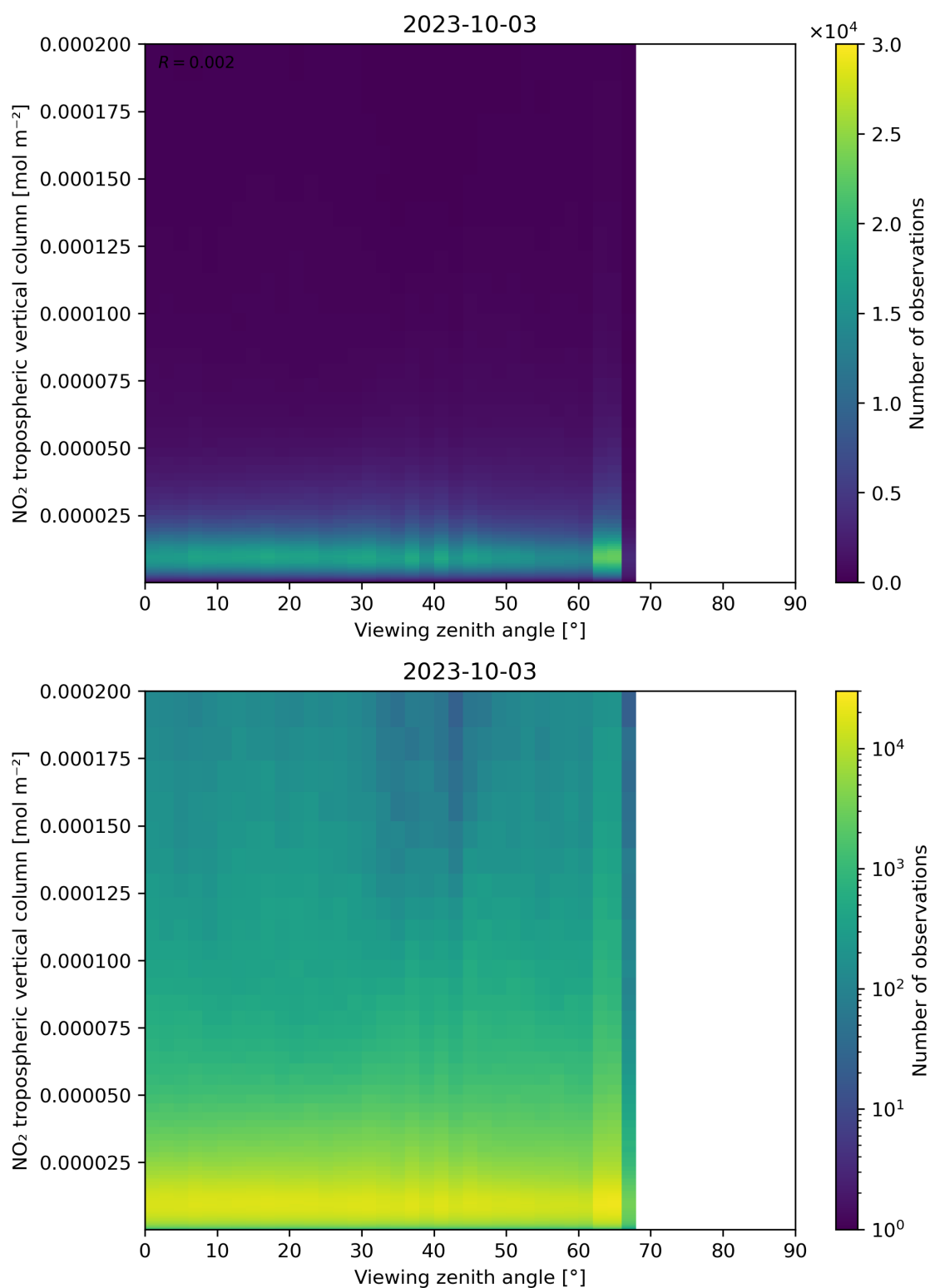
Figure 169: Scatter density plot of “Viewing zenith angle” against “NO 2 tropospheric vertical column” for 2023-10-02 to 2023-10-04.
