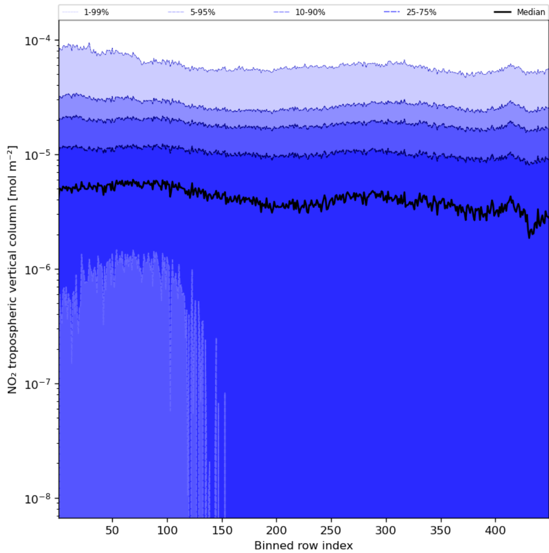
Figure 46: Along track statistics of “NO 2 tropospheric vertical column” for 2023-10-02 to 2023-10-04
