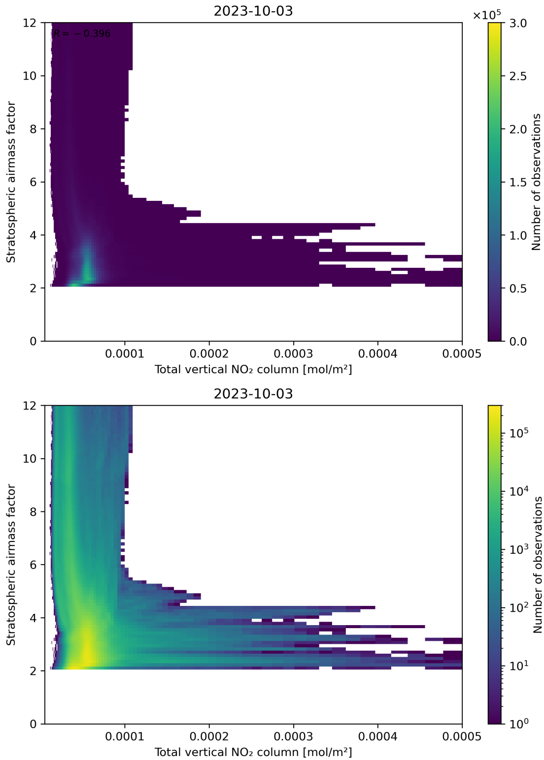
Figure 110: Scatter density plot of “Total vertical NO 2 column” against “Stratospheric airmass factor” for 2023-10-02 to 2023-10-04.
