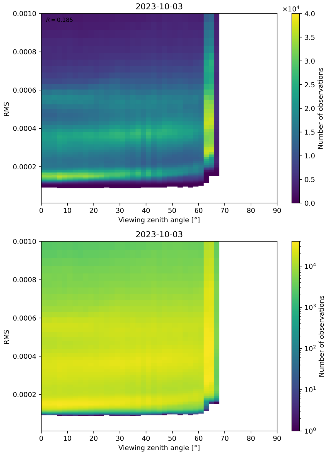
Figure 171: Scatter density plot of “Viewing zenith angle” against “RMS” for 2023-10-02 to 2023-10-04.
