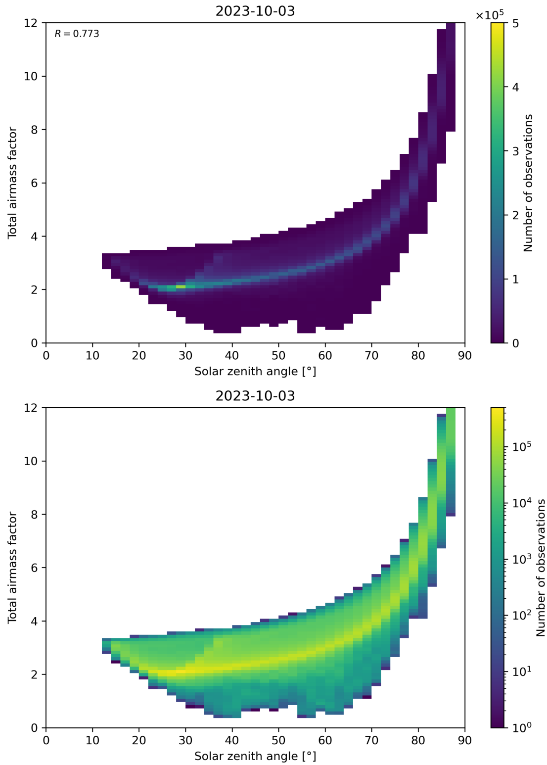
Figure 146: Scatter density plot of “Solar zenith angle” against “Total airmass factor” for 2023-10-02 to 2023-10-04.
