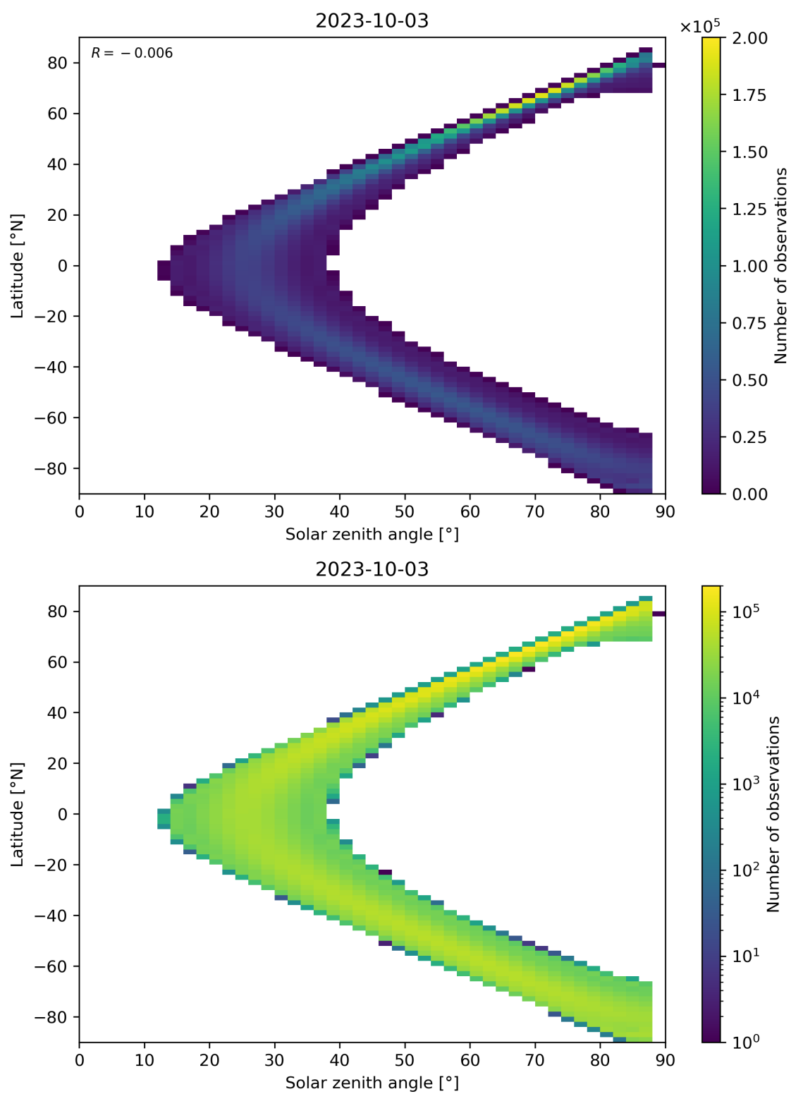
Figure 149: Scatter density plot of “Solar zenith angle” against “Latitude” for 2023-10-02 to 2023-10-04.
