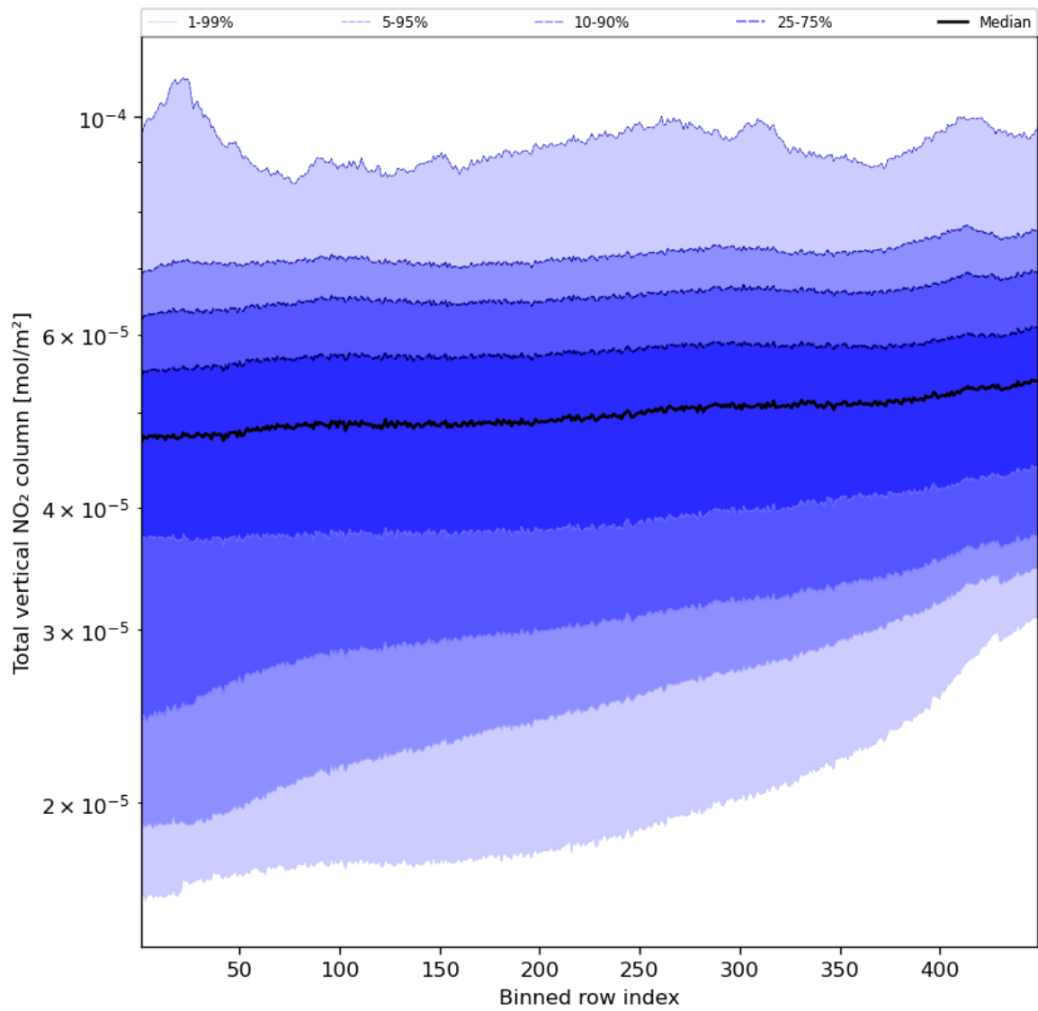
Figure 55: Along track statistics of “Total vertical NO 2 column” for 2023-10-02 to 2023-10-04
