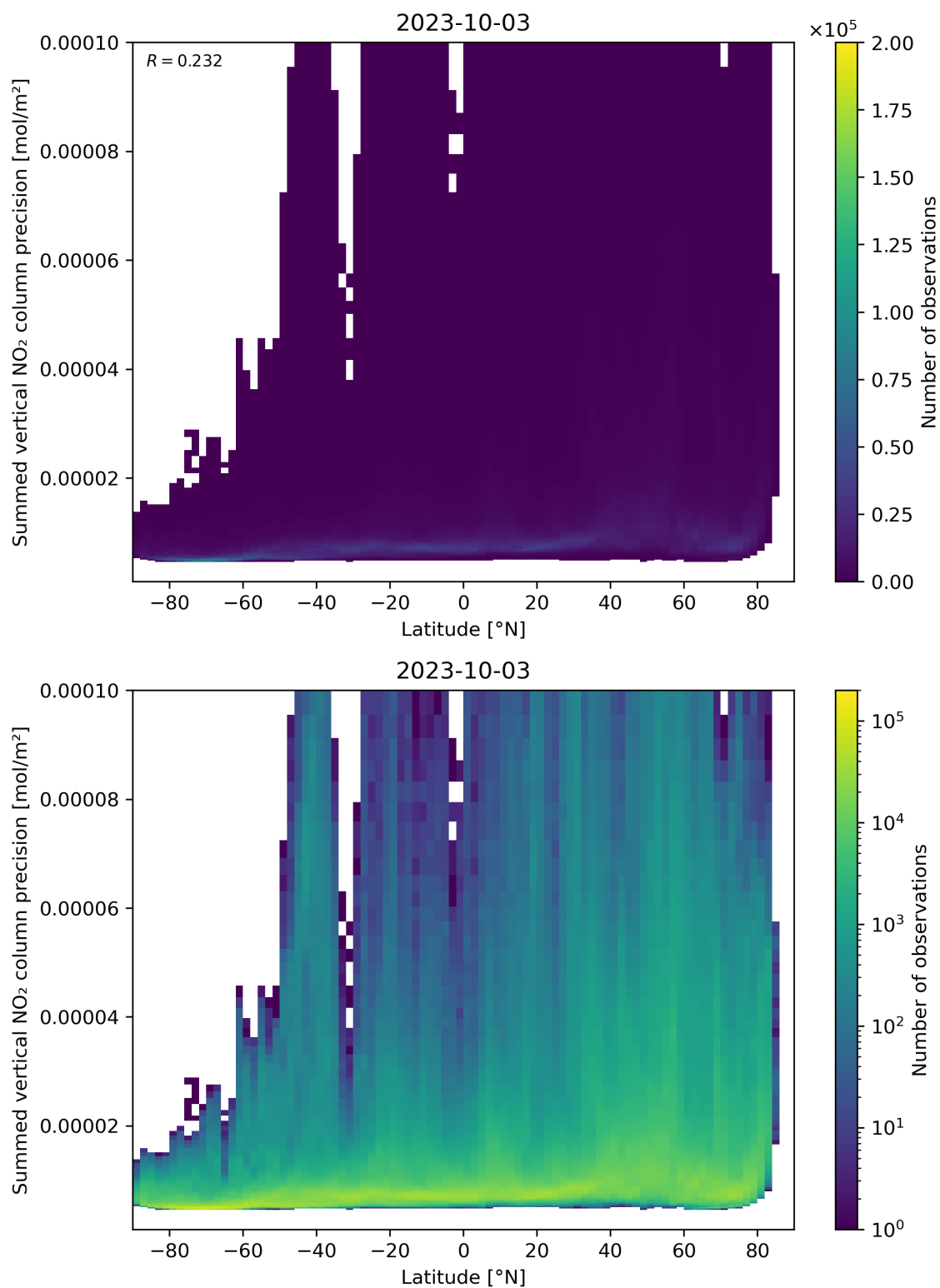
Figure 89: Scatter density plot of “Latitude” against “Summed vertical NO 2 column precision” for 2023-10-02 to 2023-10-04.
