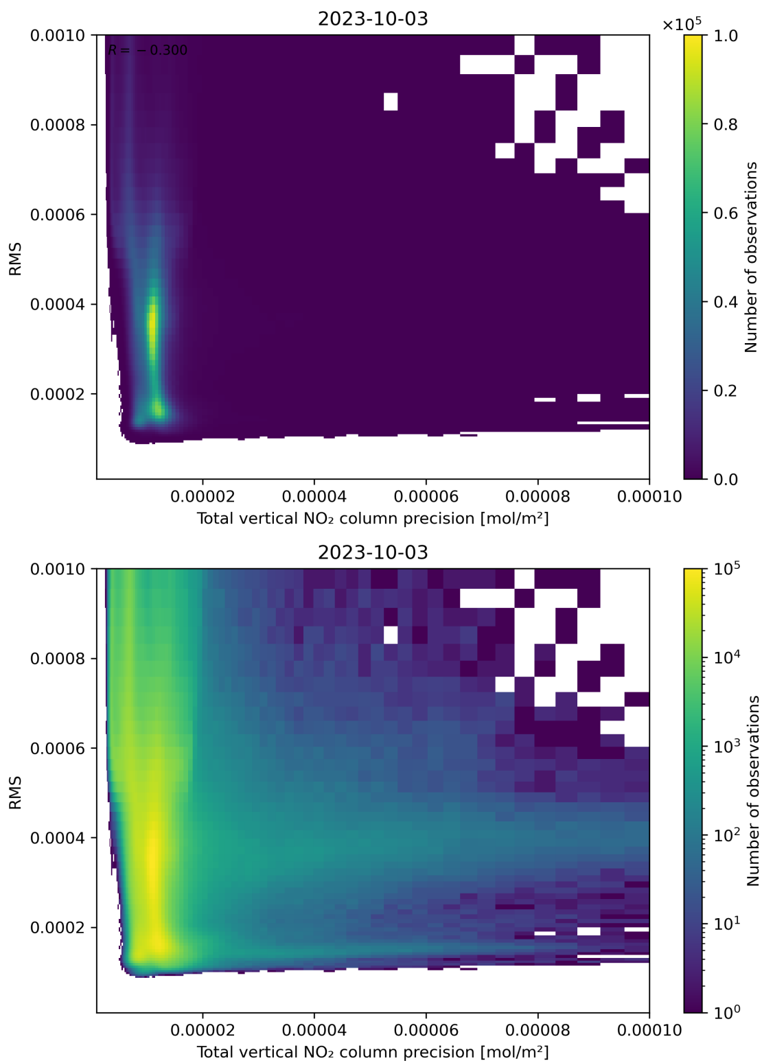
Figure 119: Scatter density plot of “Total vertical NO 2 column precision” against “RMS” for 2023-10-02 to 2023-10-04.
