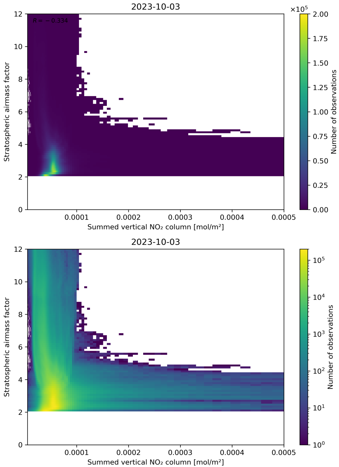
Figure 103: Scatter density plot of “Summed vertical NO 2 column” against “Stratospheric airmass factor” for 2023-10-02 to 2023-10-04.
