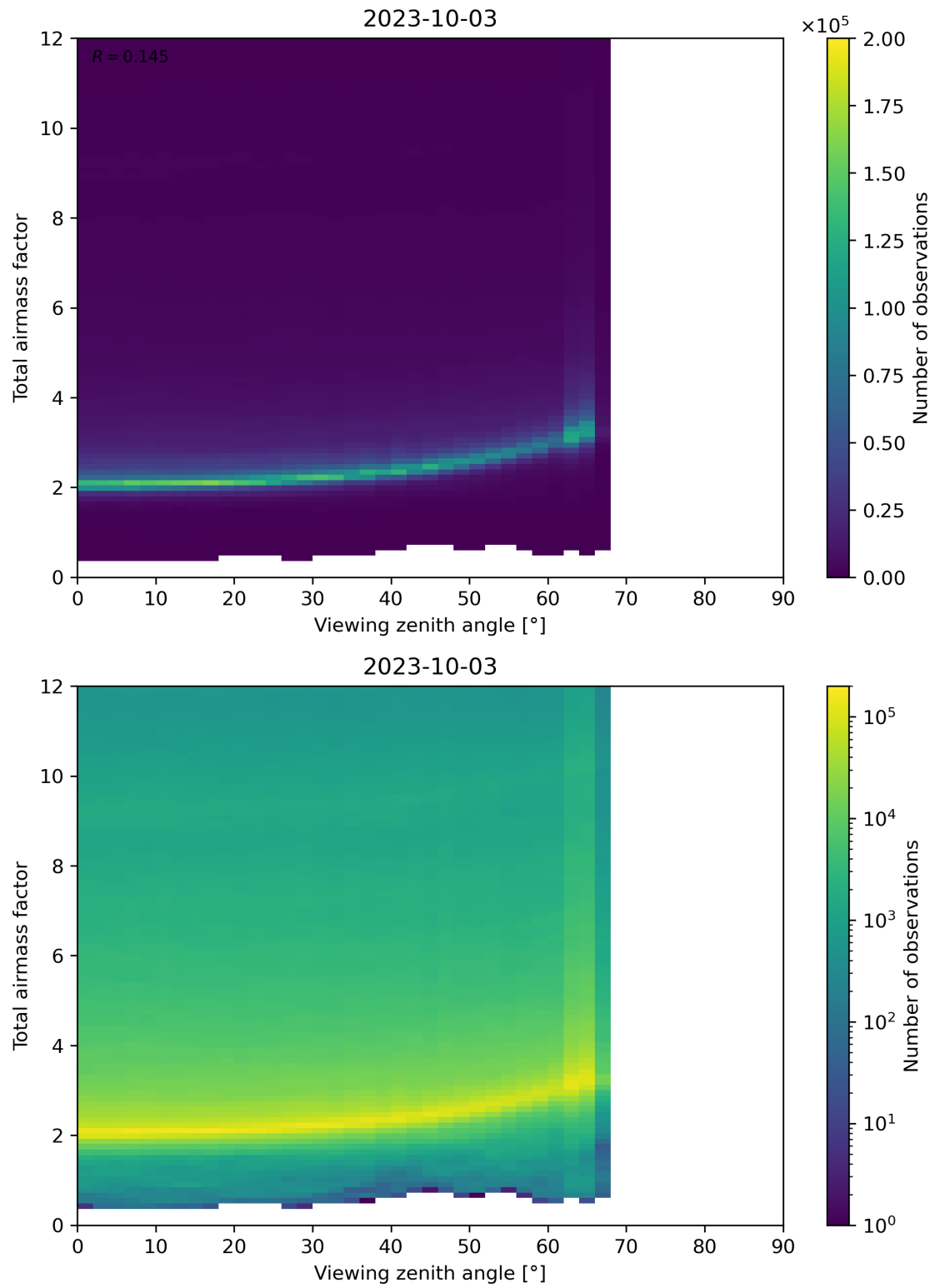
Figure 160: Scatter density plot of “Viewing zenith angle” against “Total airmass factor” for 2023-10-02 to 2023-10-04.
