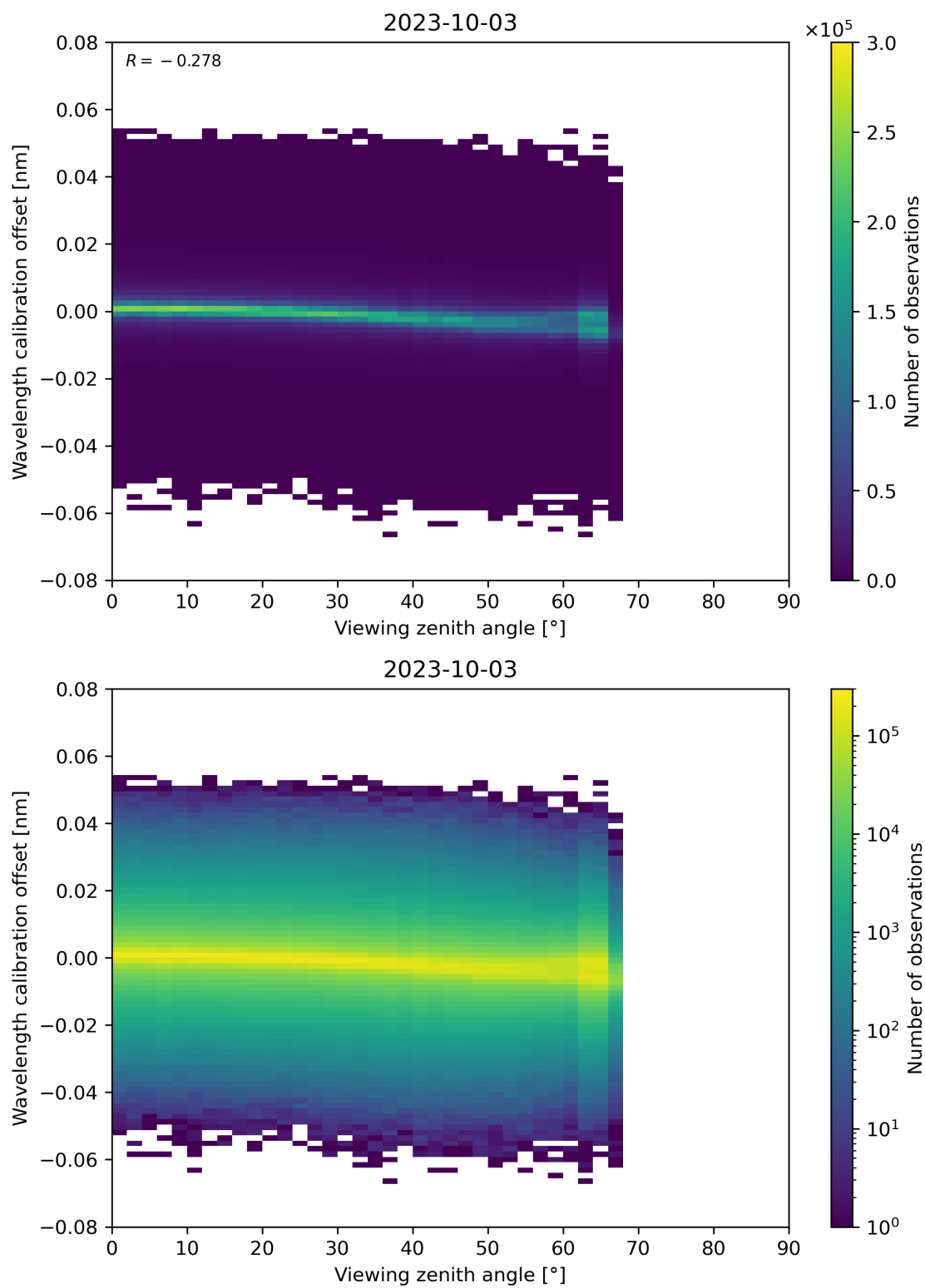
Figure 173: Scatter density plot of “Viewing zenith angle” against “Wavelength calibration offset” for 2023-10-02 to 2023-10-04.
