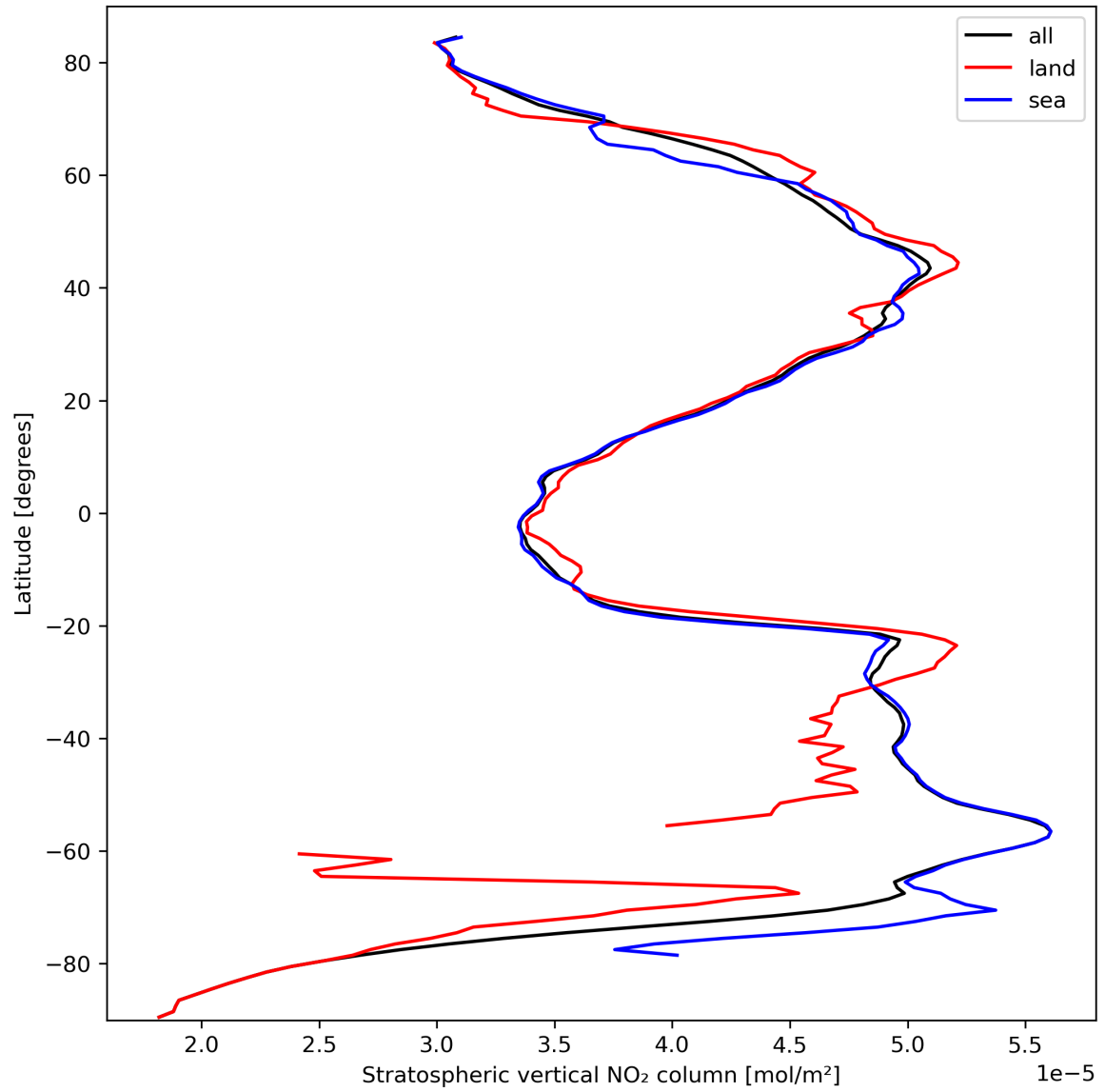
Figure 19: Zonal average of “Stratospheric vertical NO 2 column” for 2023-10-02 to 2023-10-04.
