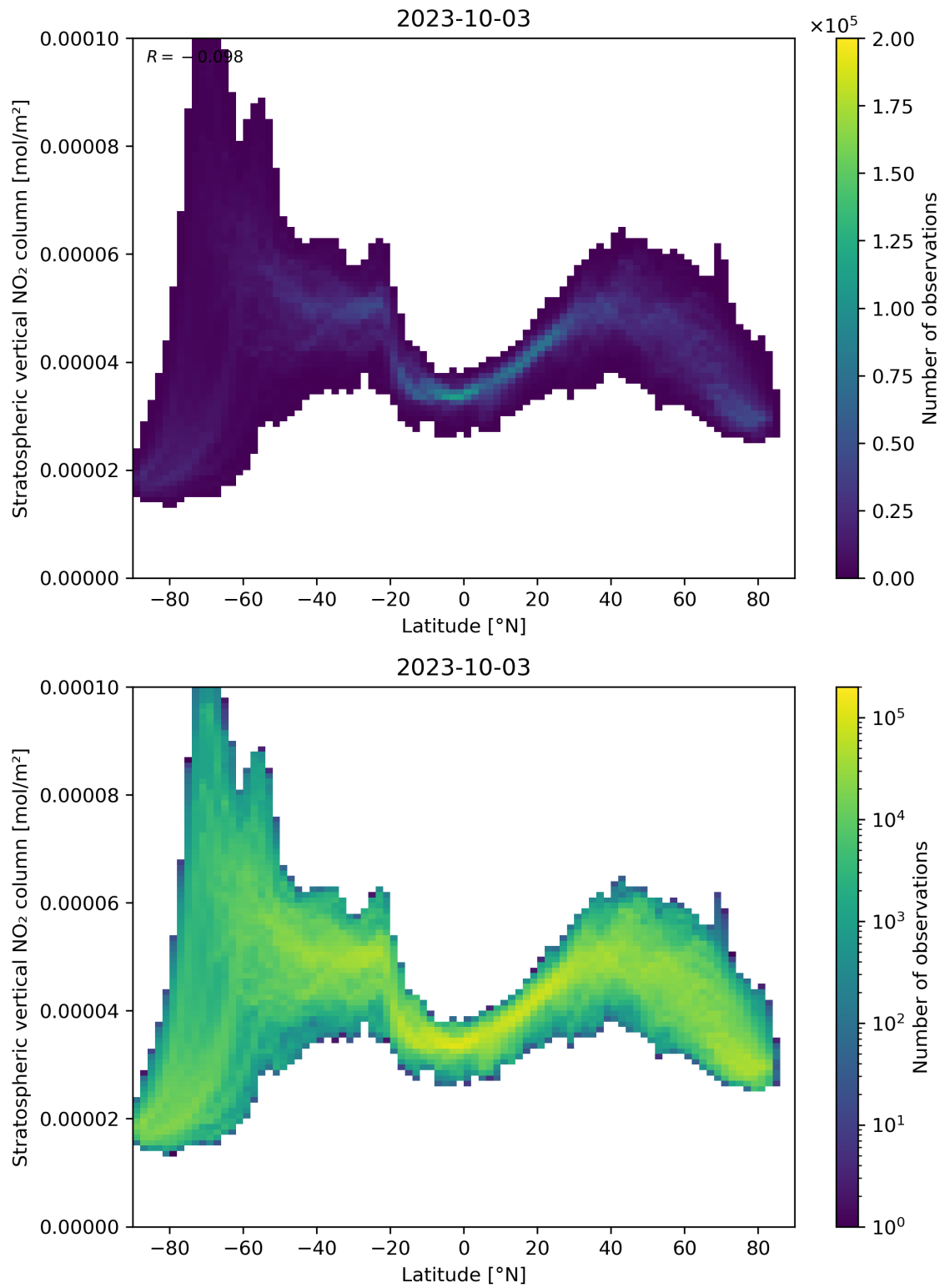
Figure 87: Scatter density plot of “Latitude” against “Stratospheric vertical NO 2 column” for 2023-10-02 to 2023-10-04.
