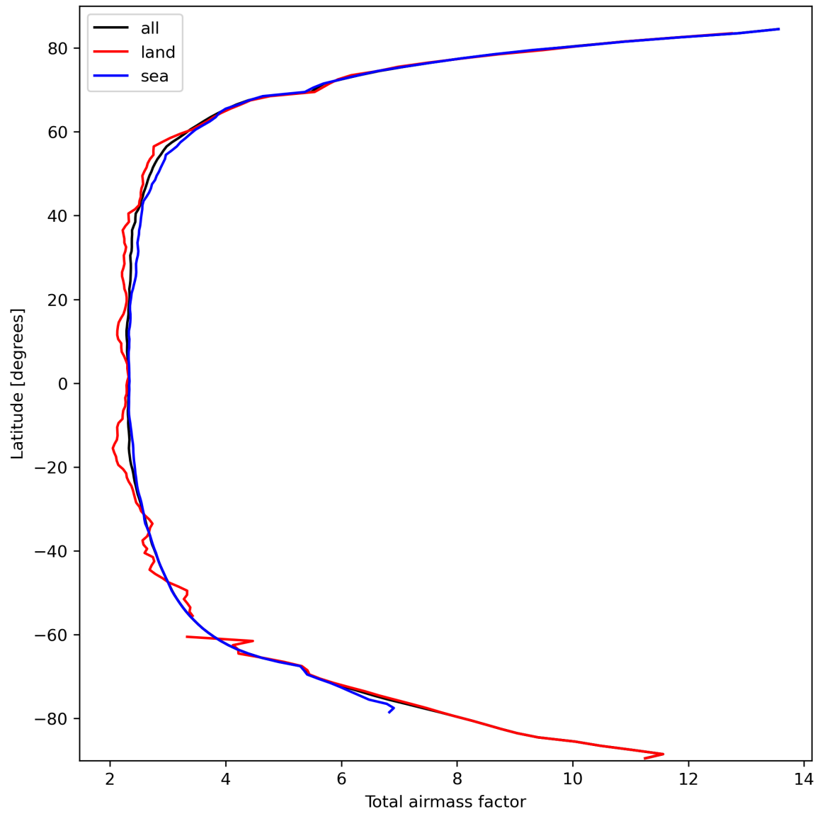
Figure 15: Zonal average of “Total airmass factor” for 2023-10-02 to 2023-10-04.
