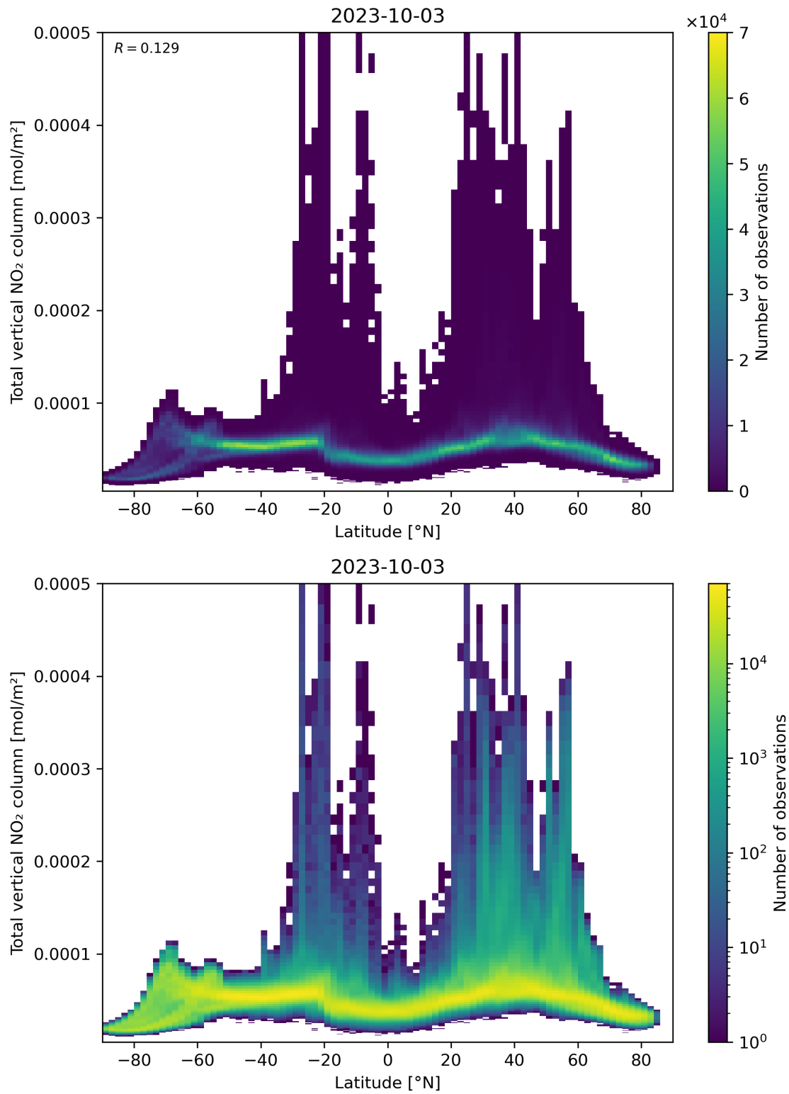
Figure 90: Scatter density plot of “Latitude” against “Total vertical NO 2 column” for 2023-10-02 to 2023-10-04.
