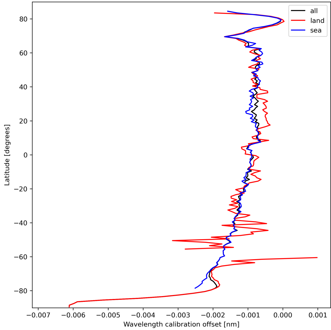
Figure 18: Zonal average of “Wavelength calibration offset” for 2023-10-02 to 2023-10-04.
