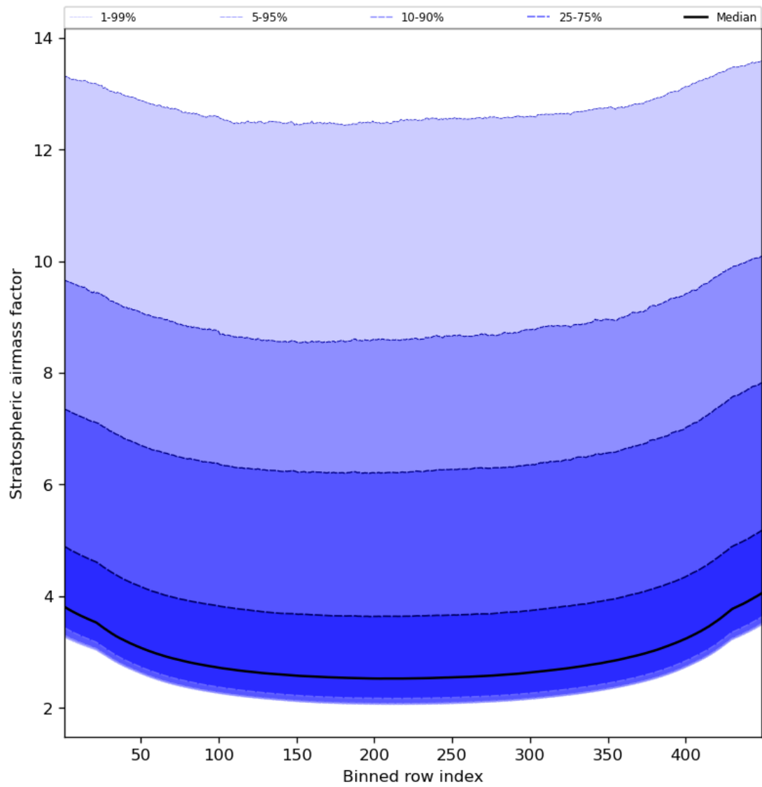
Figure 61: Along track statistics of “Stratospheric air mass factor” for 2023-10-02 to 2023-10-04
