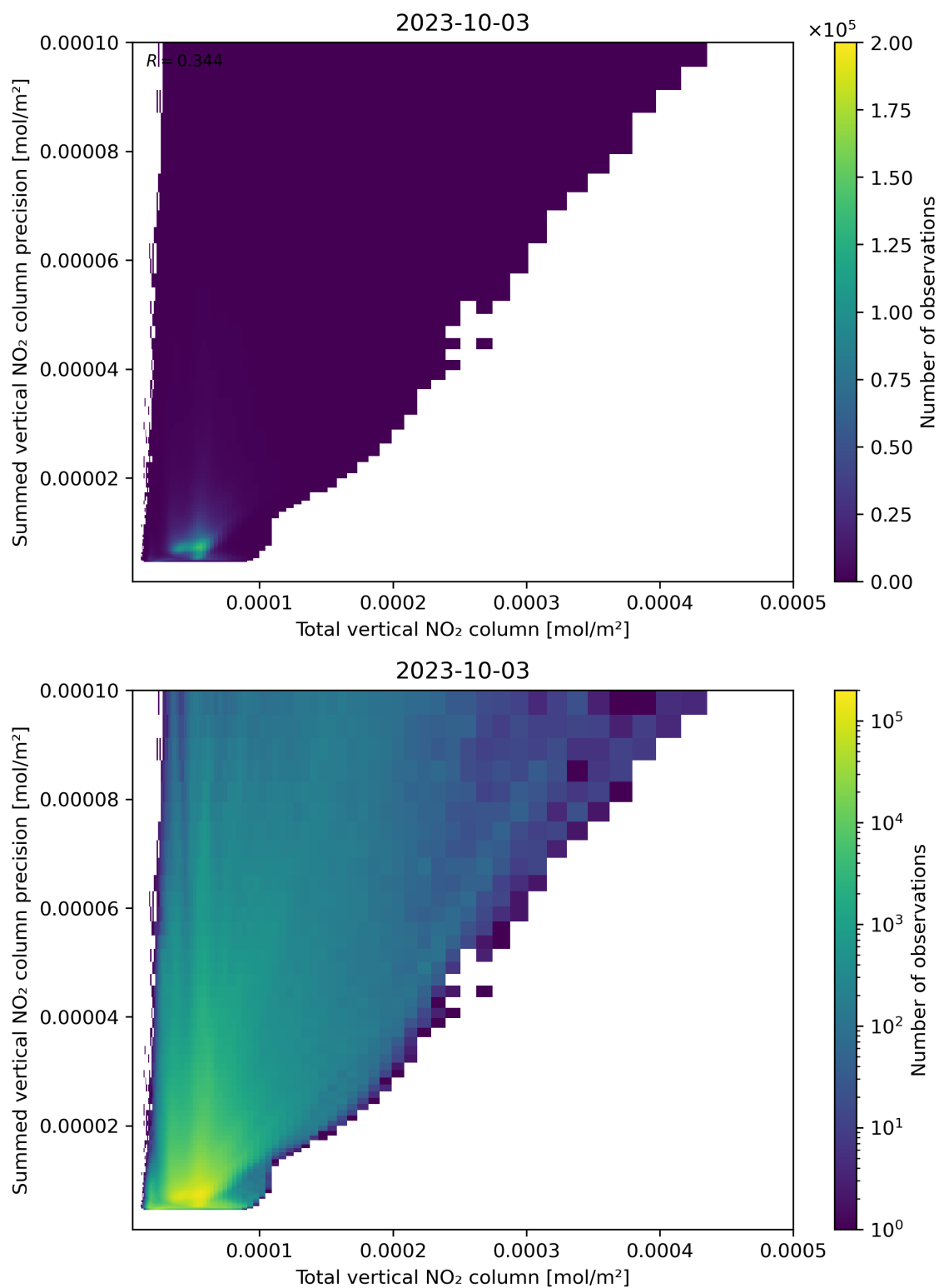
Figure 113: Scatter density plot of “Total vertical NO 2 column” against “Summed vertical NO 2 column precision” for 2023-10-02 to 2023-10-04.
