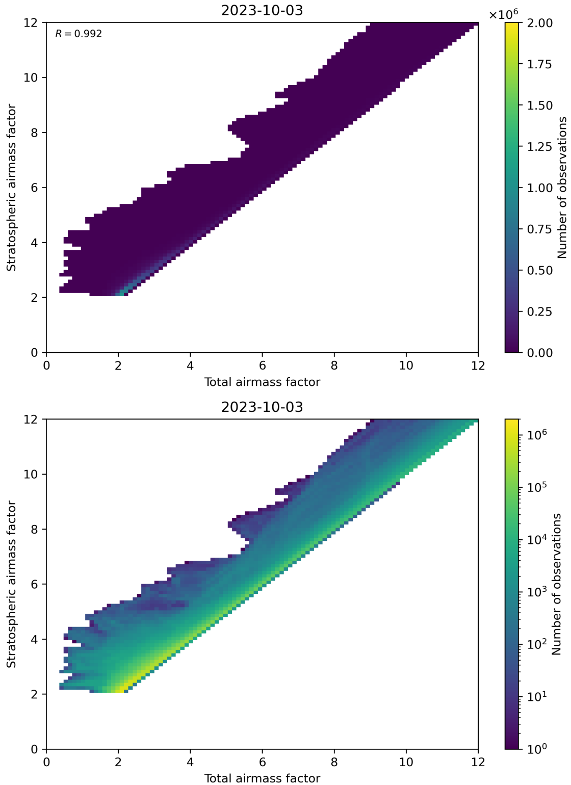
Figure 62: Scatter density plot of “Total air mass factor” against “Stratospheric air mass factor” for 2023-10-02 to 2023-10-04.
