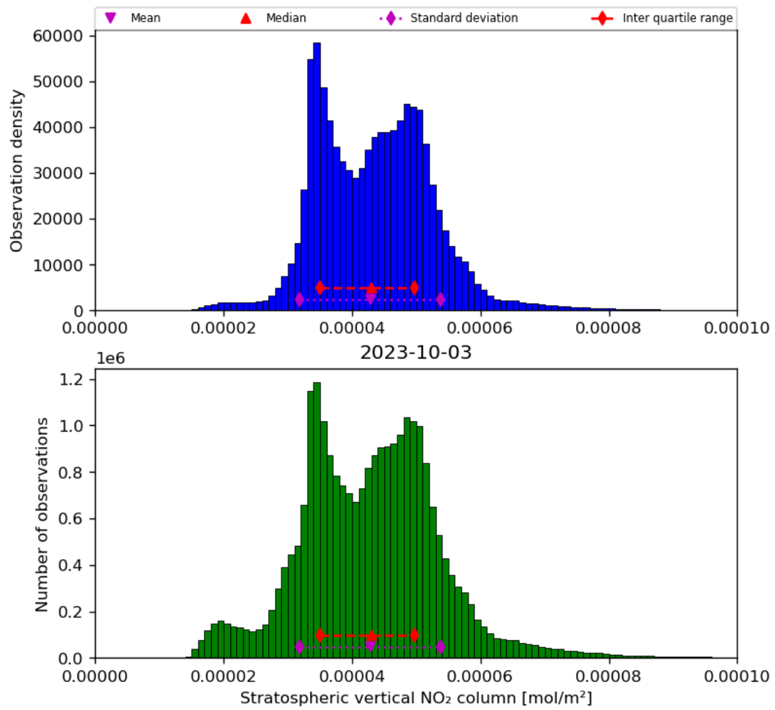
Figure 36: Histogram of “Stratospheric vertical NO 2 column” for 2023-10-02 to 2023-10-04
