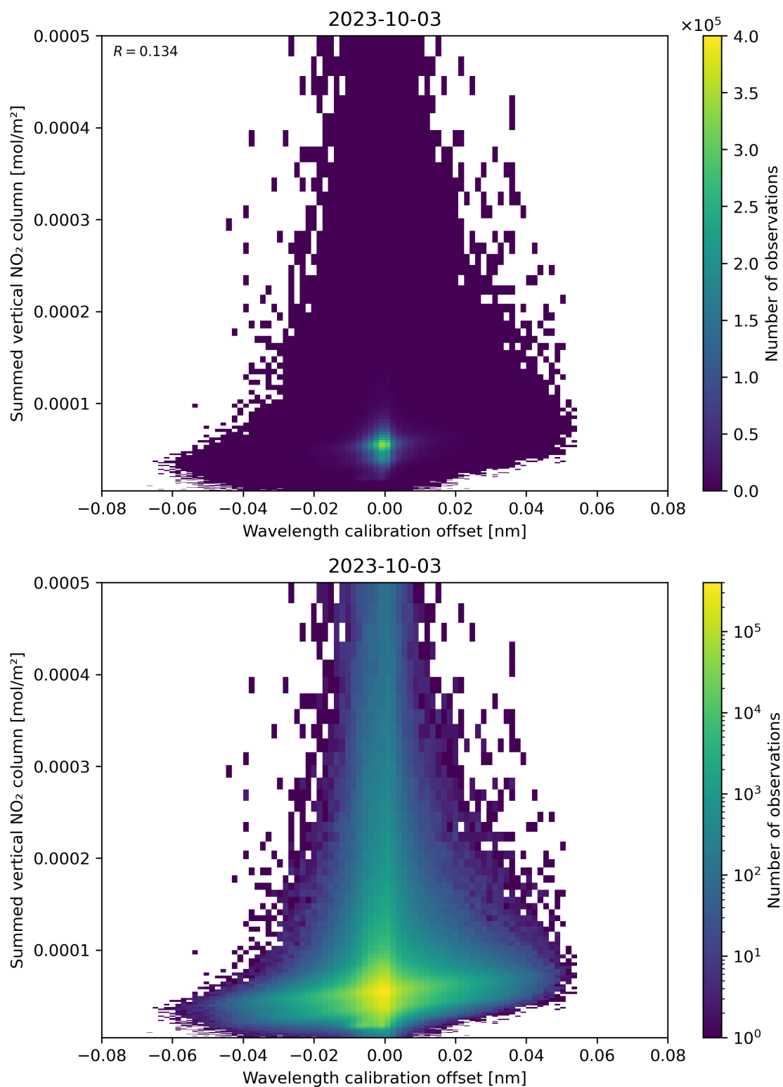
Figure 177: Scatter density plot of “Wavelength calibration offset” against “Summed vertical NO 2 column” for 2023-10-02 to 2023-10-04.
