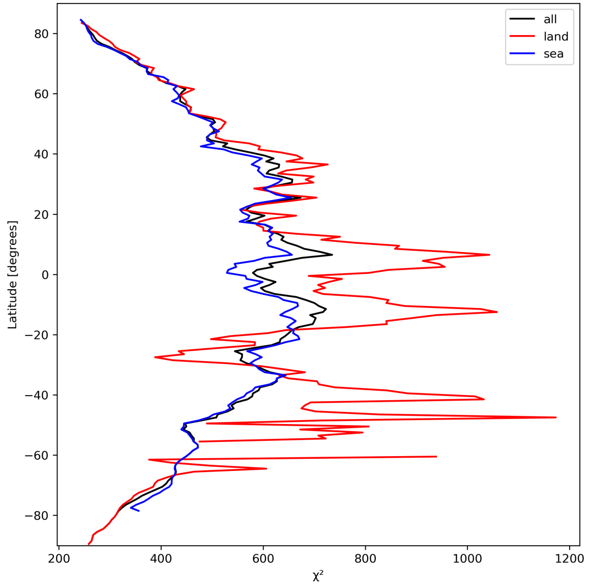
Figure 25: Zonal average of “ \chi^2 ” for 2023-10-02 to 2023-10-04.
