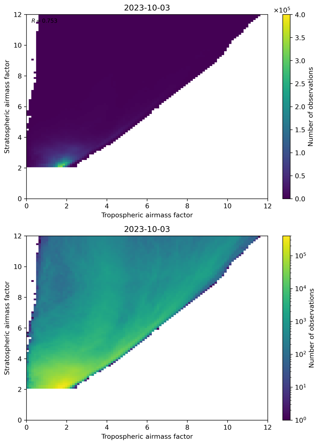
Figure 71: Scatter density plot of “Tropospheric airmass factor” against “Stratospheric airmass factor” for 2023-10-02 to 2023-10-04.
