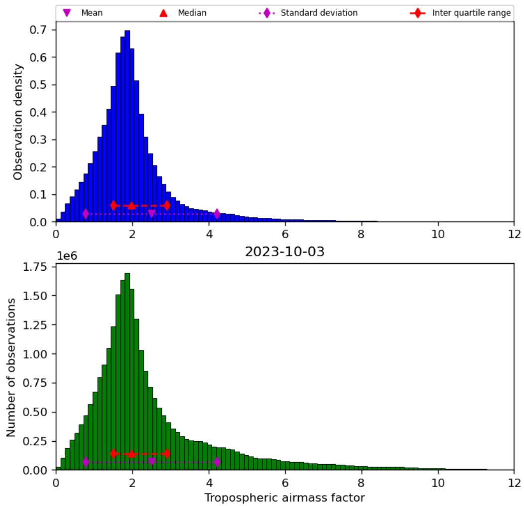
Figure 31: Histogram of “Tropospheric airmass factor” for 2023-10-02 to 2023-10-04
