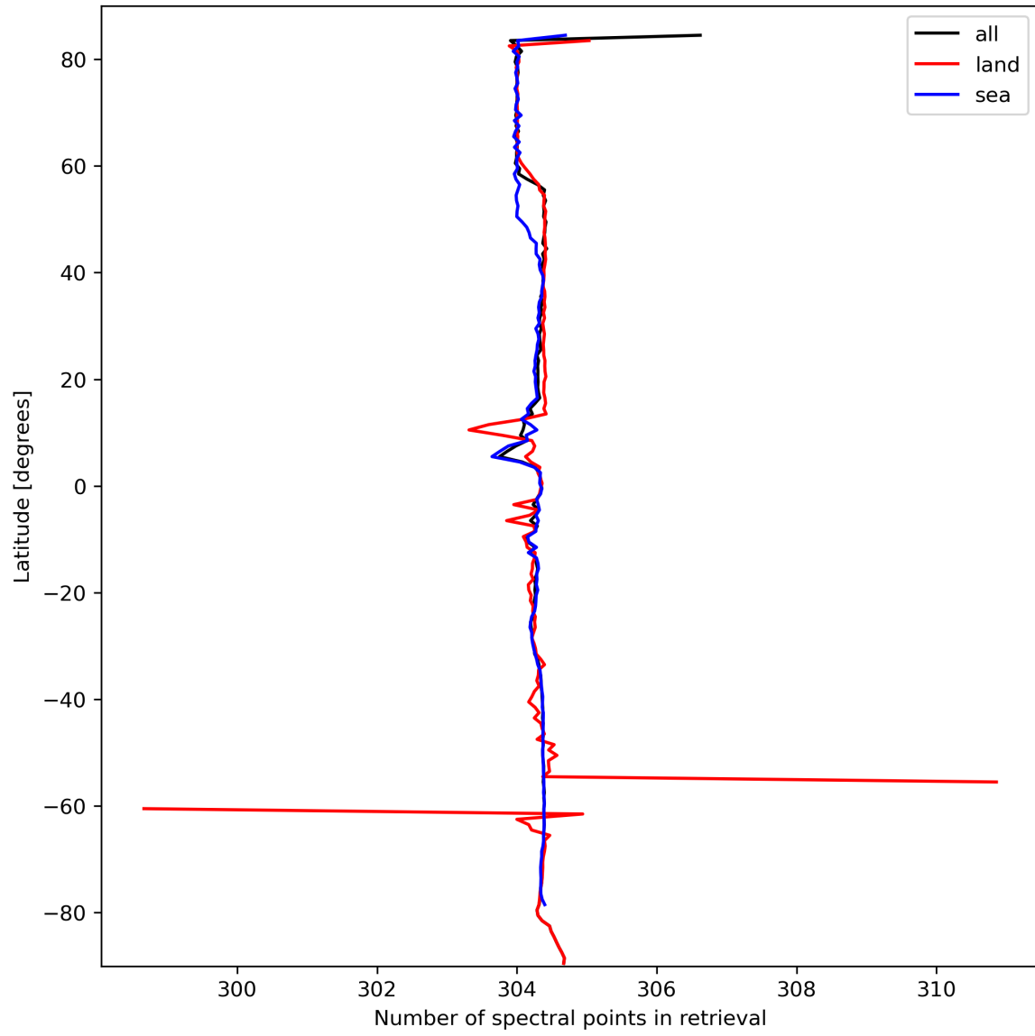
Figure 16: Zonal average of “Number of spectral points in retrieval” for 2023-10-02 to 2023-10-04.
