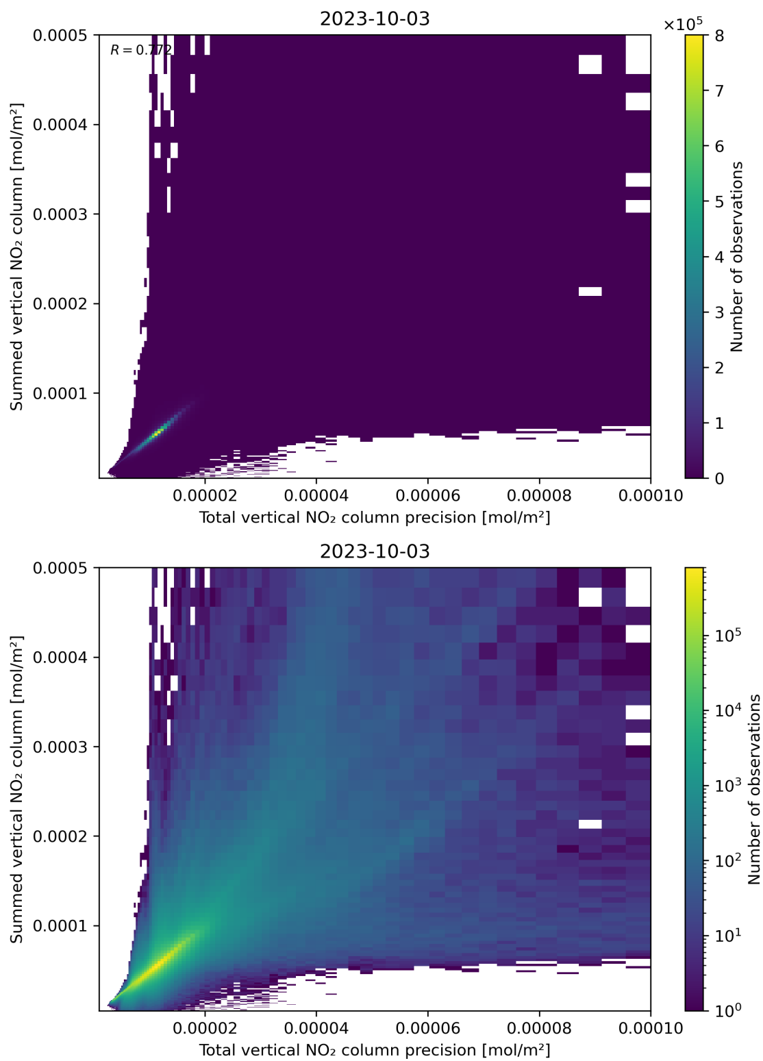
Figure 117: Scatter density plot of “Total vertical NO 2 column precision” against “Summed vertical NO 2 column” for 2023-10-02 to 2023-10-04.
