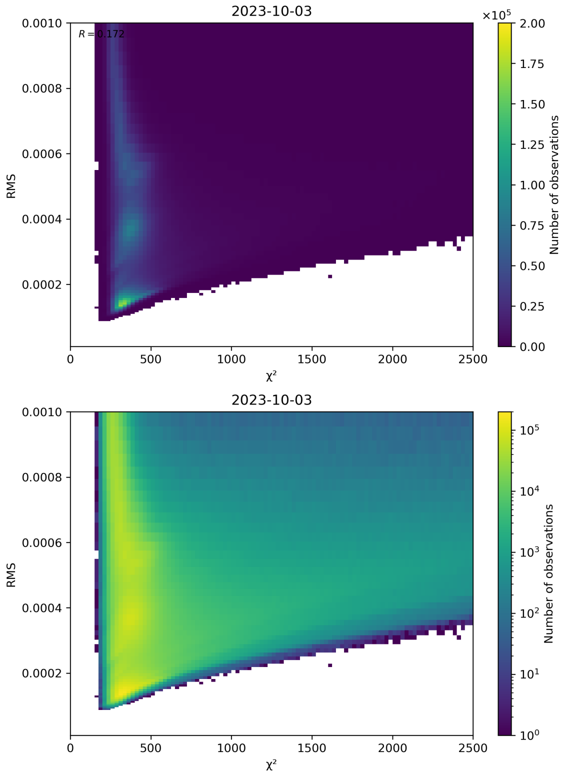
Figure 82: Scatter density plot of “ \chi^2 ” against “RMS” for 2023-10-02 to 2023-10-04.
