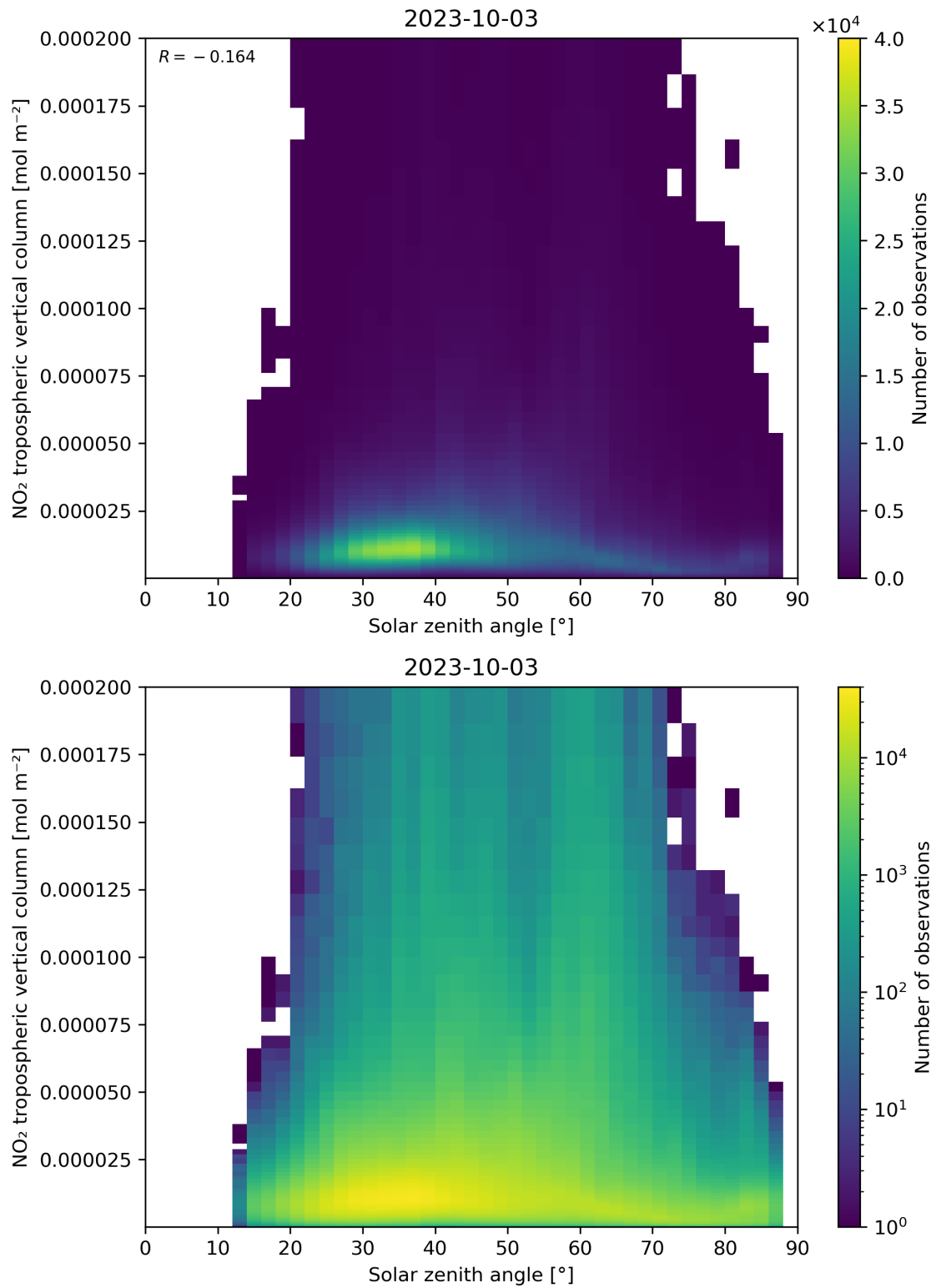
Figure 155: Scatter density plot of “Solar zenith angle” against “NO 2 tropospheric vertical column” for 2023-10-02 to 2023-10-04.
