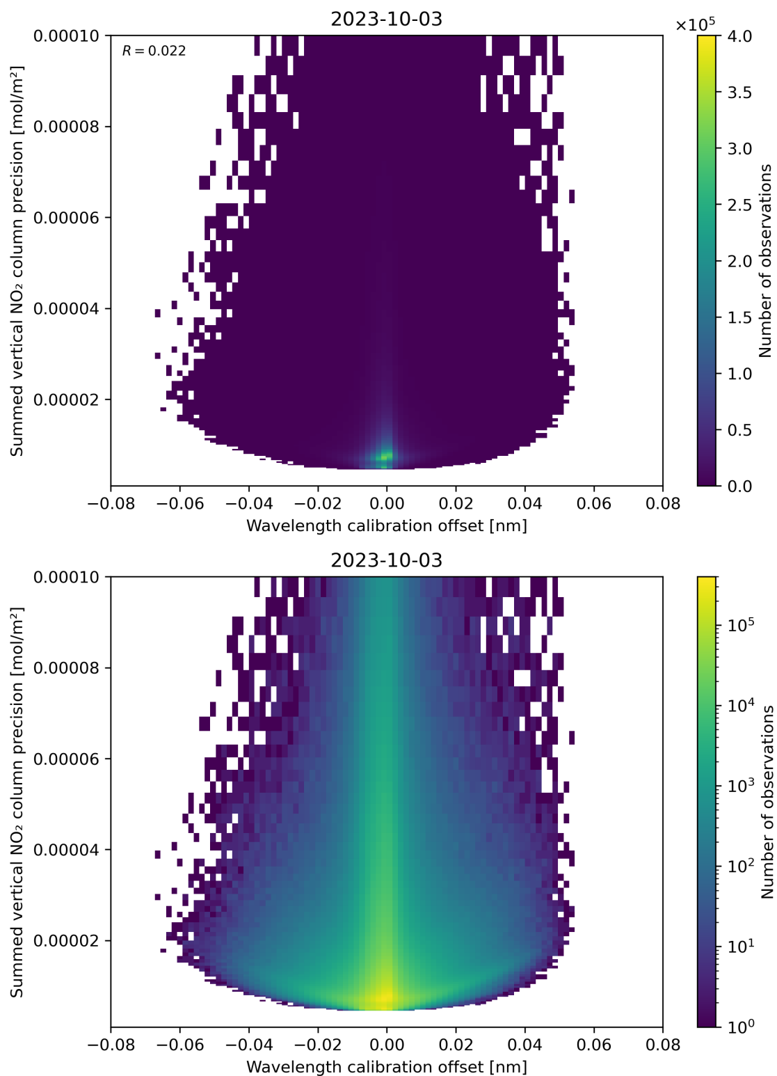
Figure 178: Scatter density plot of “Wavelength calibration offset” against “Summed vertical NO 2 column precision” for 2023-10-02 to 2023-10-04.
