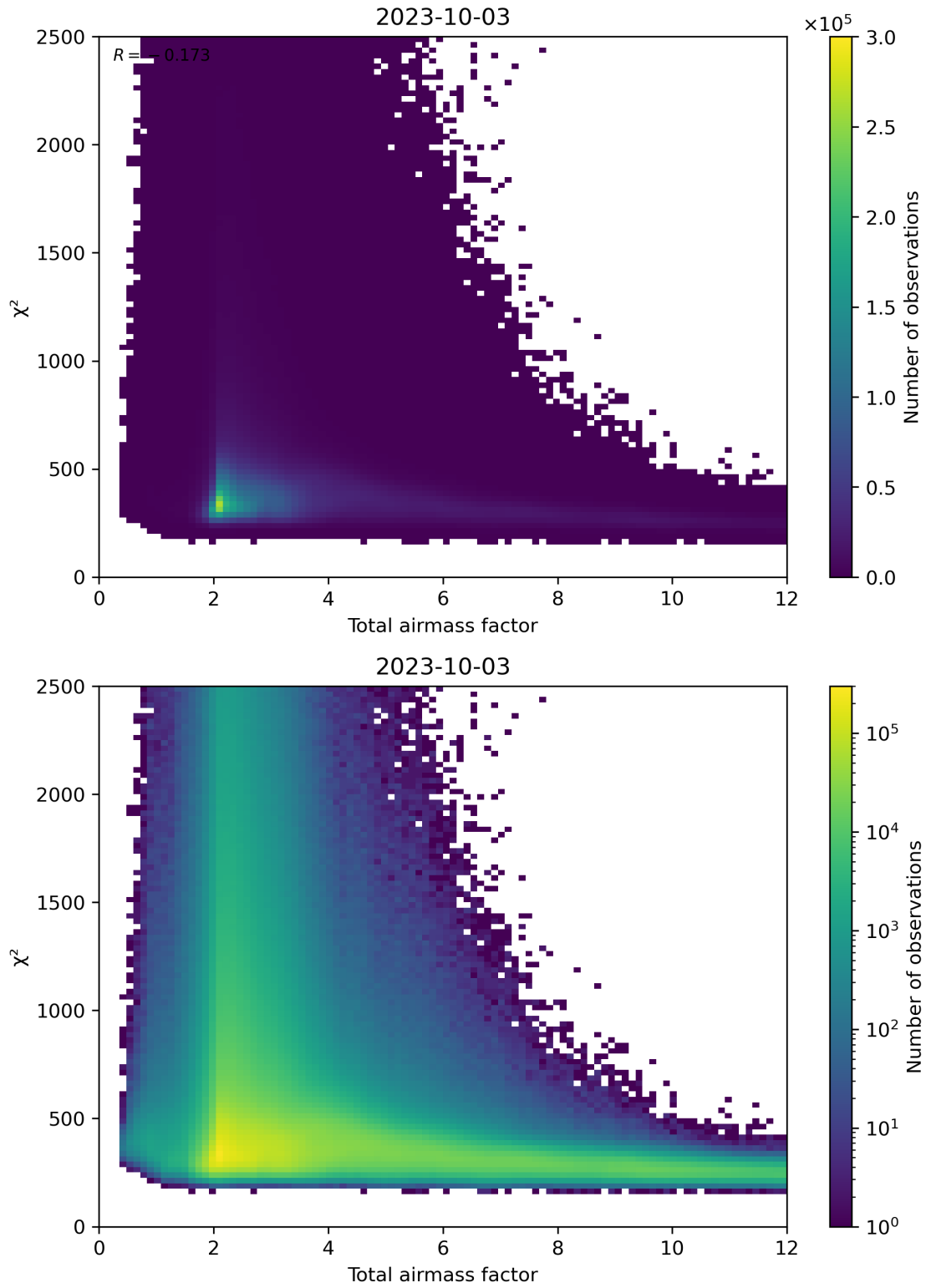
Figure 63: Scatter density plot of “Total airmass factor” against “ \chi^2 ” for 2023-10-02 to 2023-10-04.
