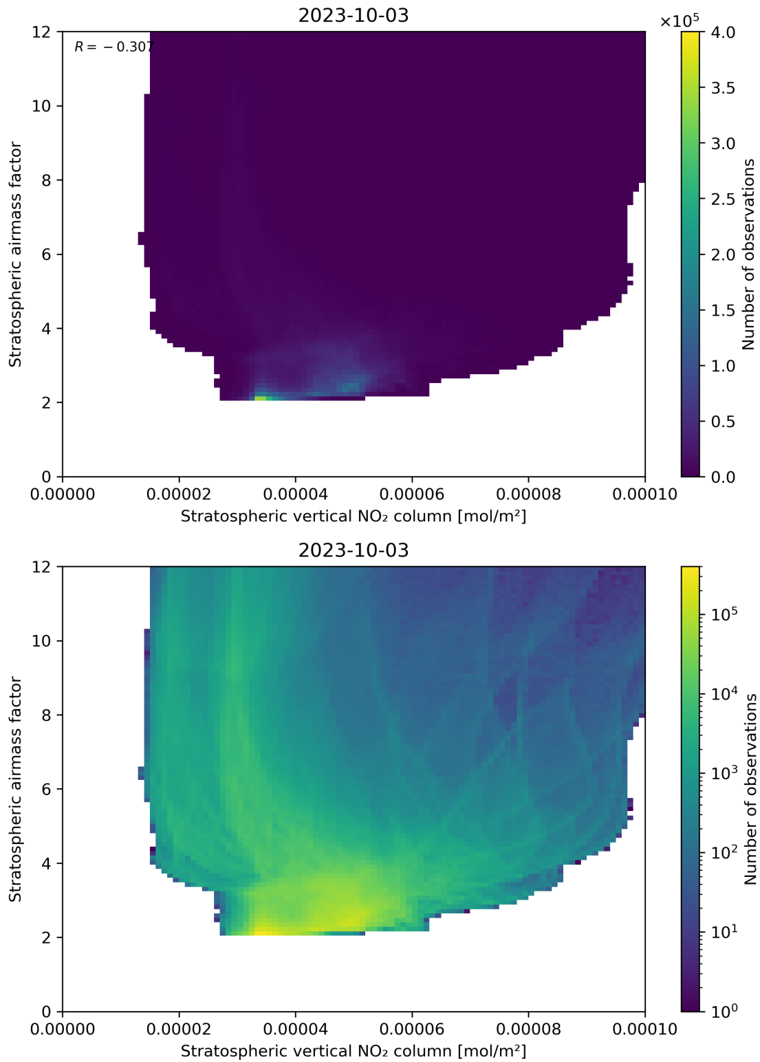
Figure 96: Scatter density plot of “Stratospheric vertical NO 2 column” against “Stratospheric airmass factor” for 2023-10-02 to 2023-10-04.
