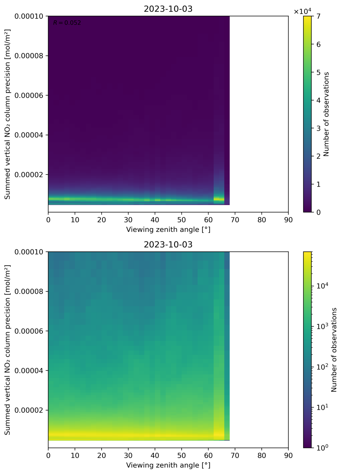
Figure 166: Scatter density plot of “Viewing zenith angle” against “Summed vertical NO 2 column precision” for 2023-10-02 to 2023-10-04.
