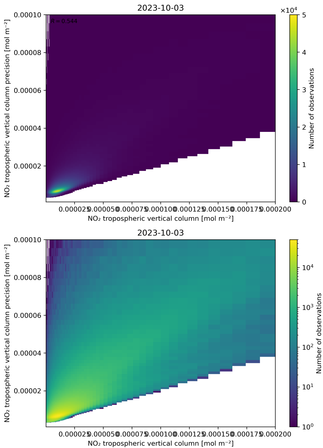
Figure 130: Scatter density plot of “NO 2 tropospheric vertical column” against “NO 2 tropospheric vertical column precision” for 2023-10-02 to 2023-10-04.
