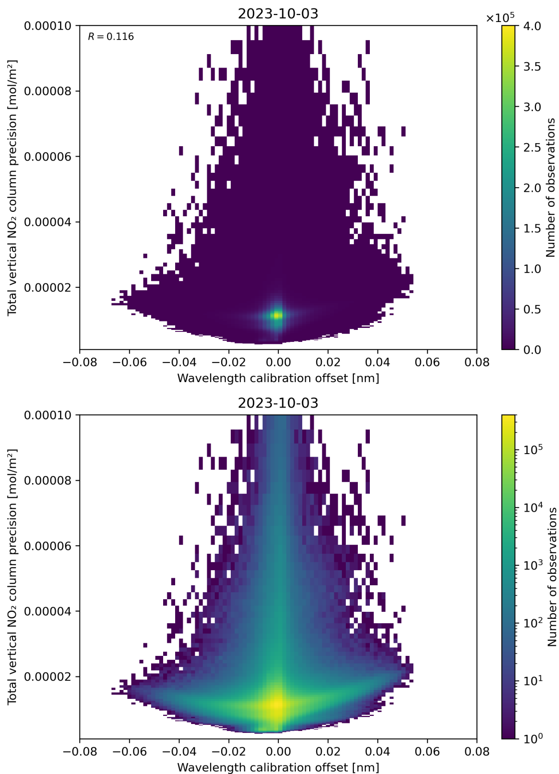
Figure 180: Scatter density plot of “Wavelength calibration offset” against “Total vertical NO 2 column precision” for 2023-10-02 to 2023-10-04.
