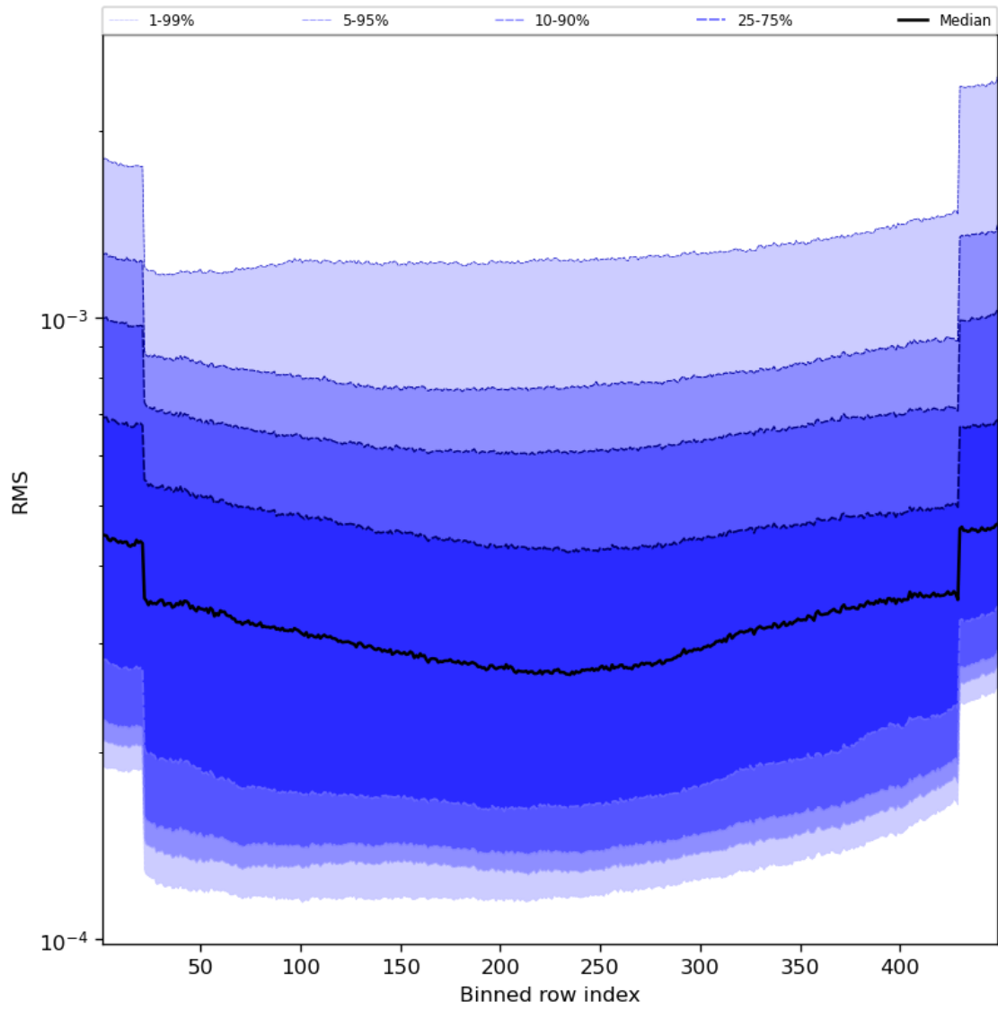
Figure 60: Along track statistics of “RMS” for 2023-10-02 to 2023-10-04
