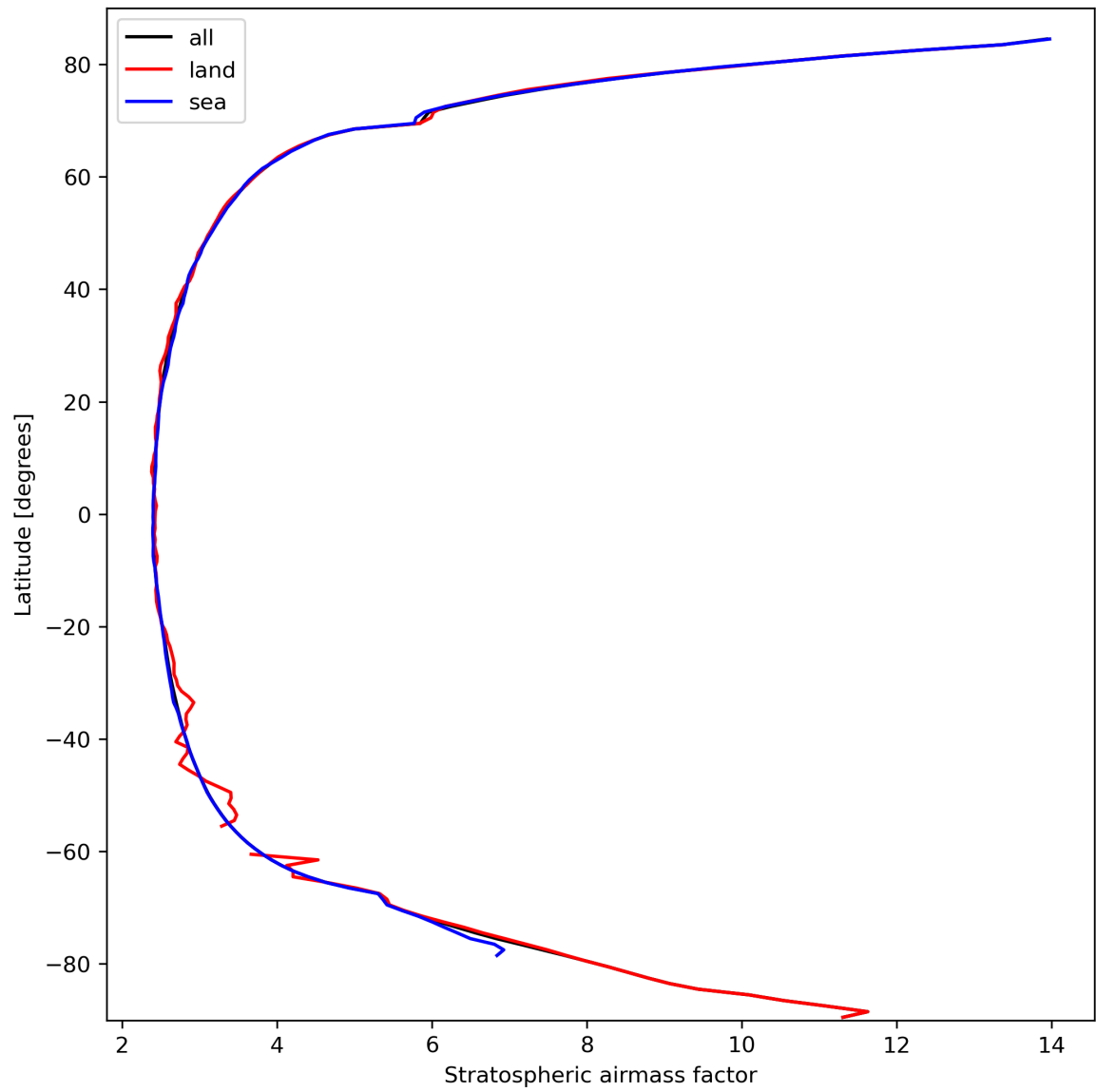
Figure 27: Zonal average of “Stratospheric air mass factor” for 2023-10-02 to 2023-10-04.
