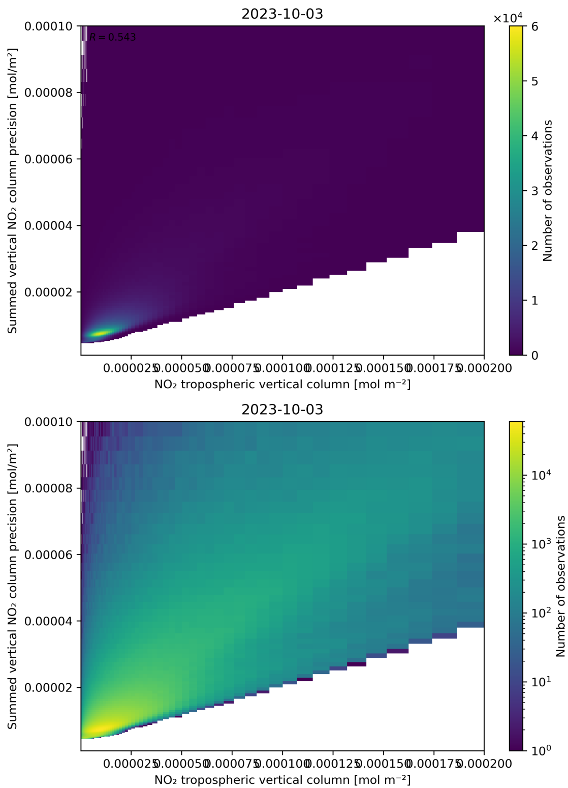
Figure 127: Scatter density plot of “NO 2 tropospheric vertical column” against “Summed vertical NO 2 column precision” for 2023-10-02 to 2023-10-04.
