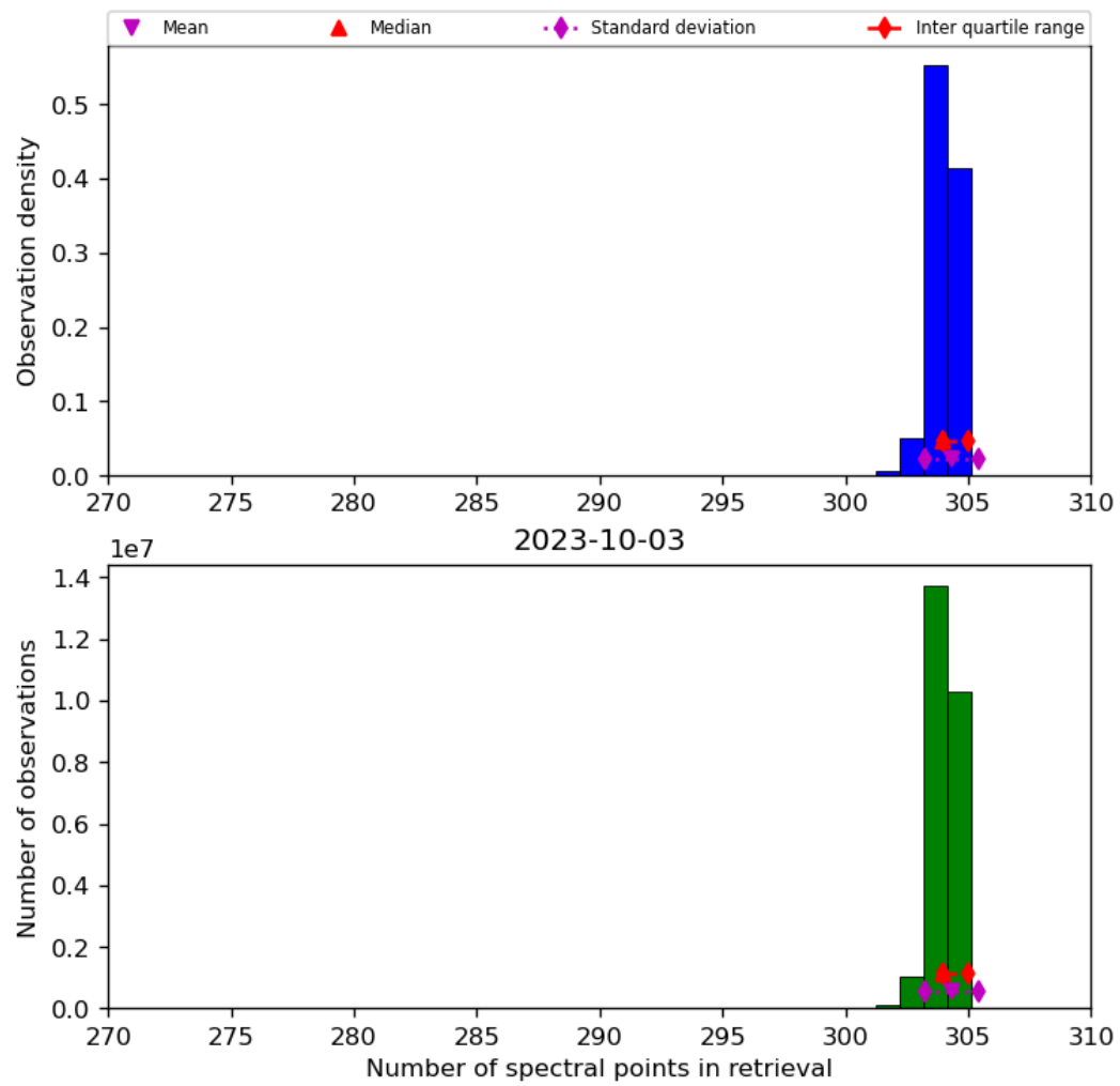
Figure 33: Histogram of “Number of spectral points in retrieval” for 2023-10-02 to 2023-10-04
