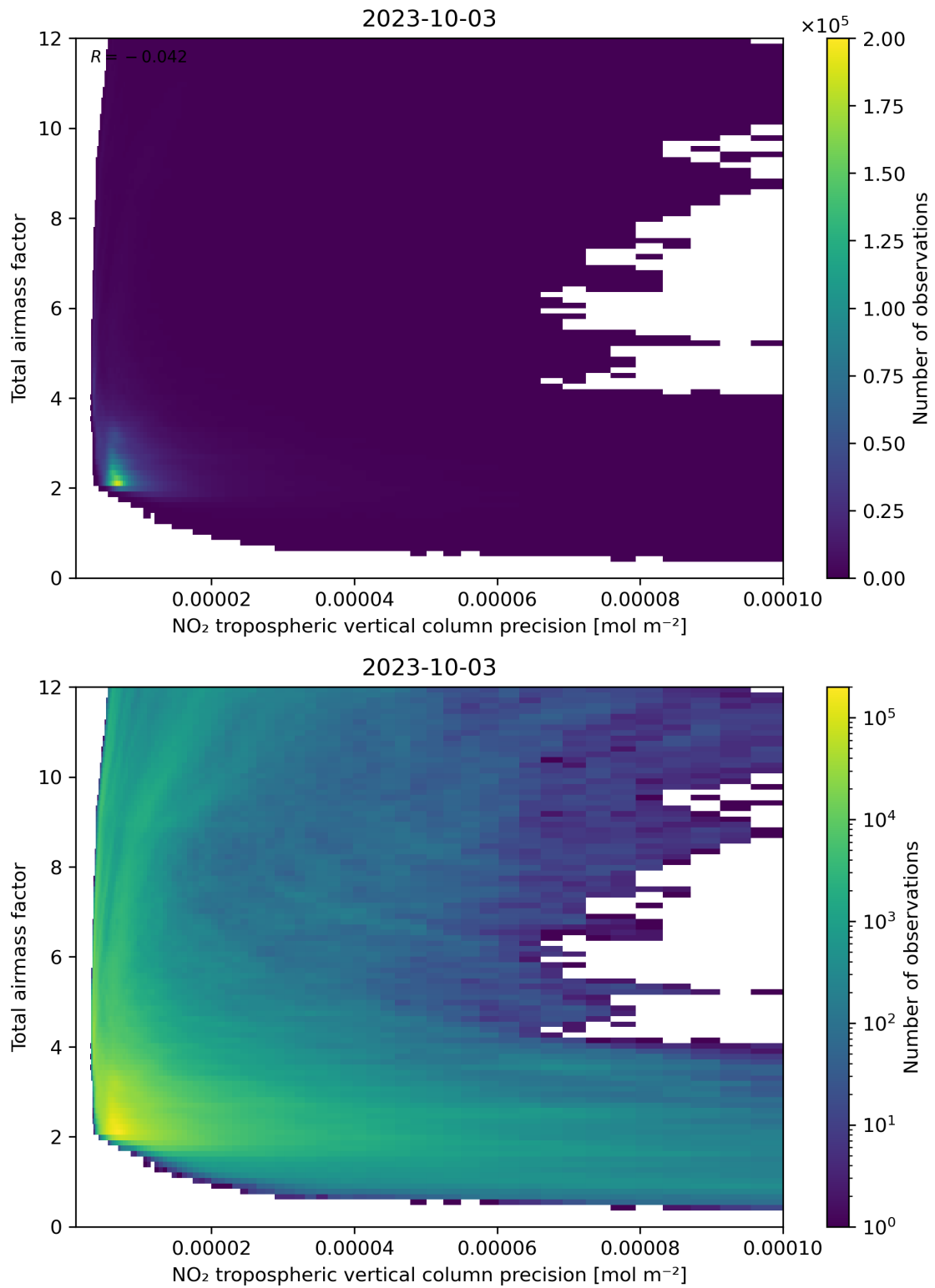
Figure 132: Scatter density plot of “NO 2 tropospheric vertical column precision” against “Total air mass factor” for 2023-10-02 to 2023-10-04.
