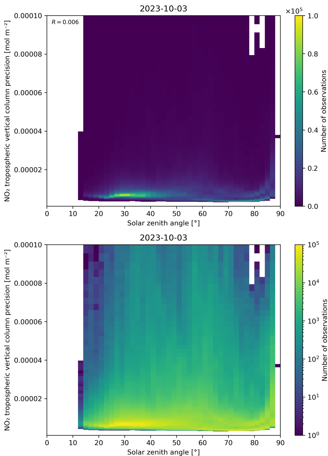
Figure 156: Scatter density plot of “Solar zenith angle” against “NO 2 tropospheric vertical column precision” for 2023-10-02 to 2023-10-04.
