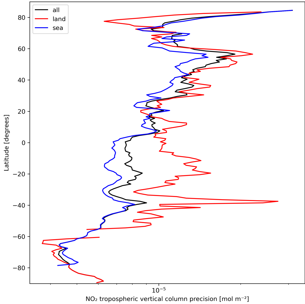
Figure 13: Zonal average of “NO 2 tropospheric vertical column precision” for 2023-10-02 to 2023-10-04.
