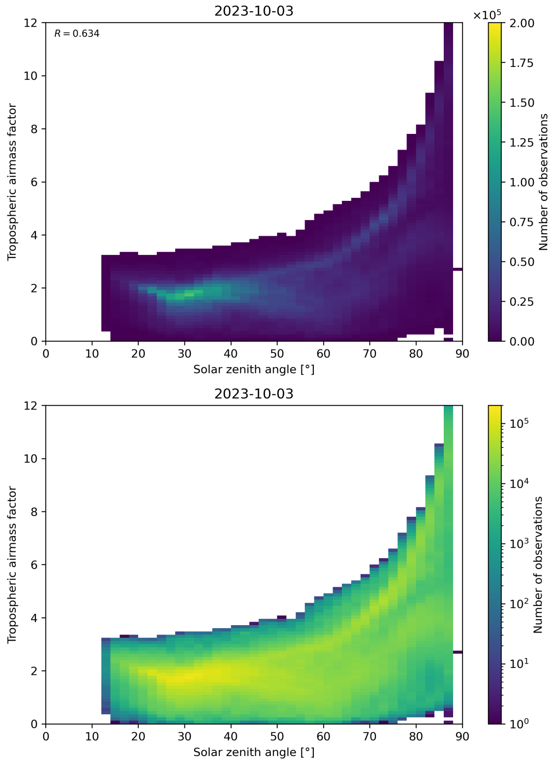
Figure 147: Scatter density plot of “Solar zenith angle” against “Tropospheric airmass factor” for 2023-10-02 to 2023-10-04.
