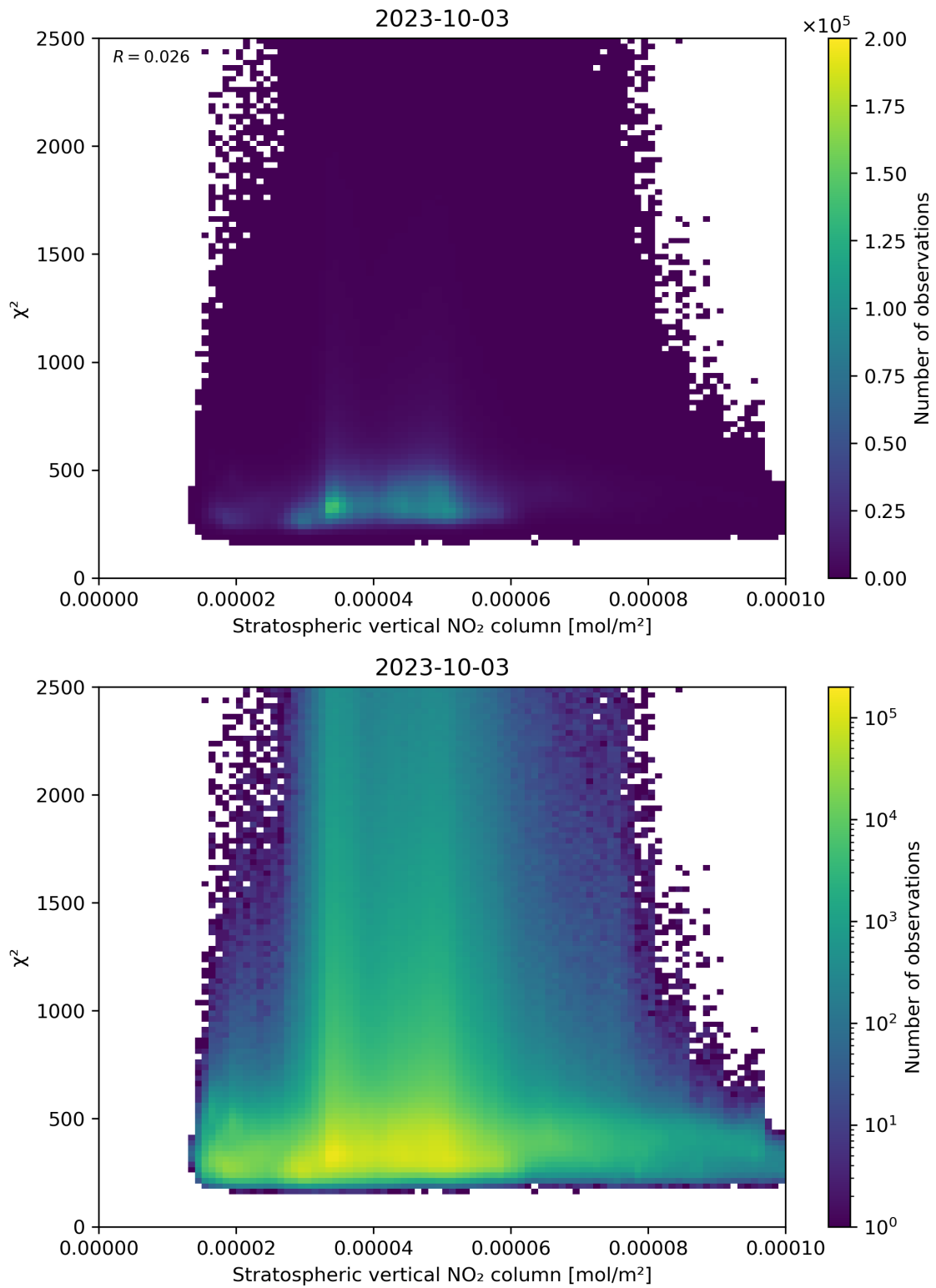
Figure 97: Scatter density plot of “Stratospheric vertical NO 2 column” against “ \chi^2 ” for 2023-10-02 to 2023-10-04.
