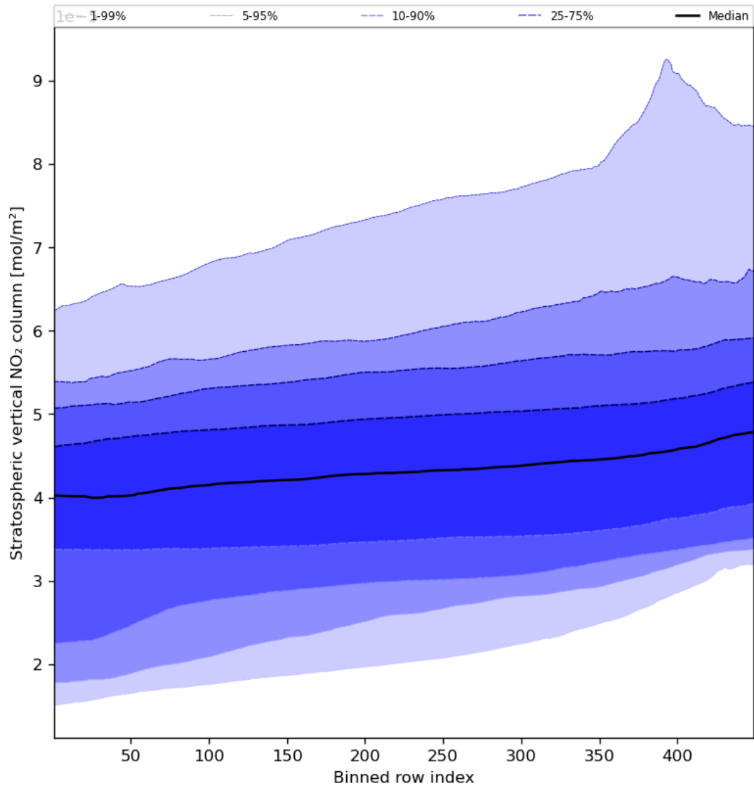
Figure 53: Along track statistics of “Stratospheric vertical NO 2 column” for 2023-10-02 to 2023-10-04
