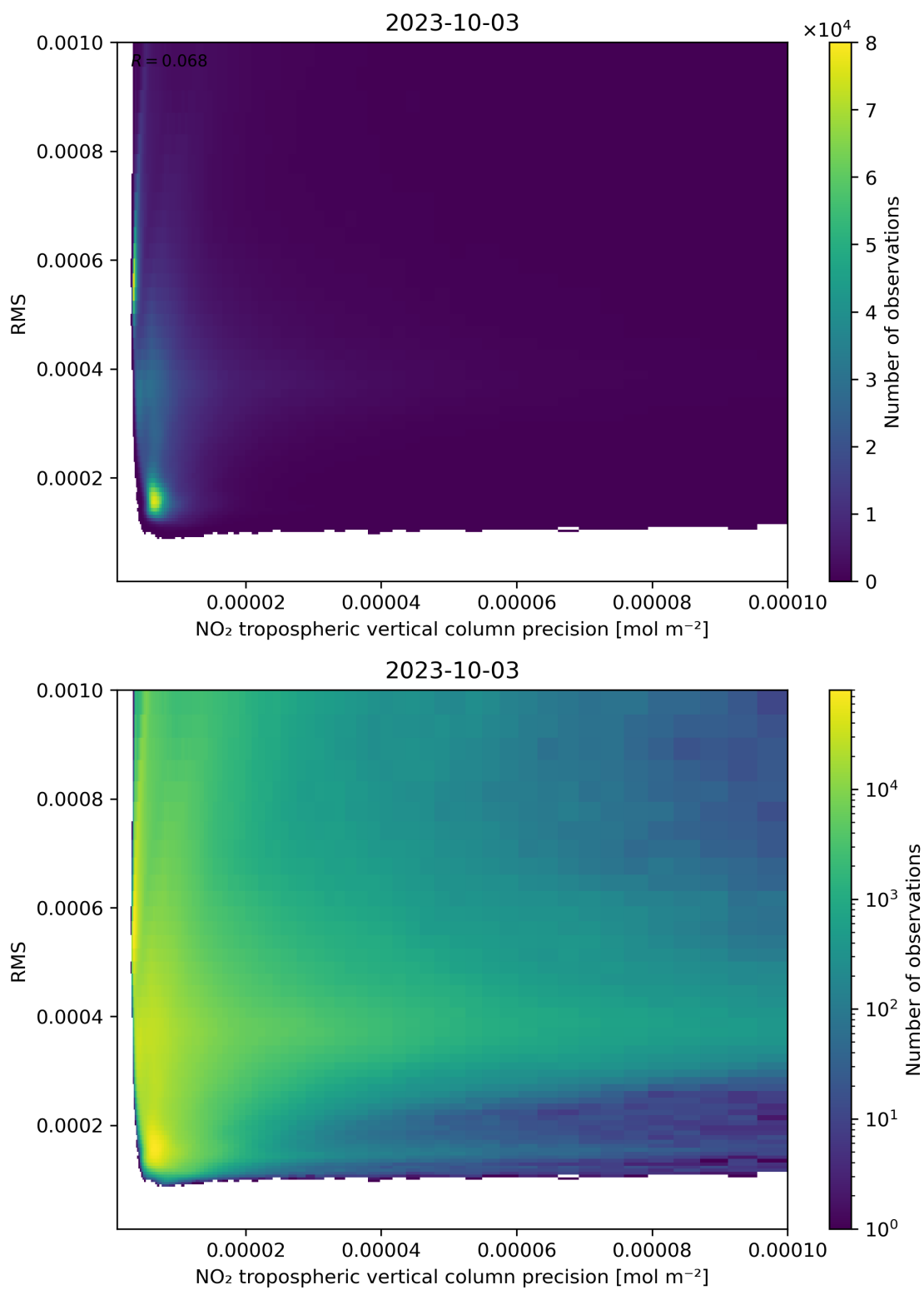
Figure 140: Scatter density plot of “NO 2 tropospheric vertical column precision” against “RMS” for 2023-10-02 to 2023-10-04.
