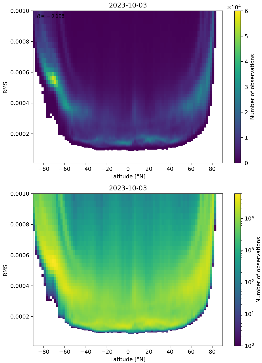
Figure 94: Scatter density plot of “Latitude” against “RMS” for 2023-10-02 to 2023-10-04.
