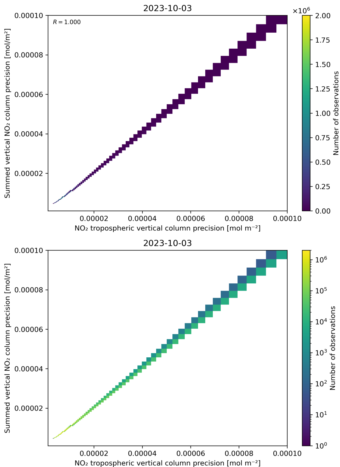
Figure 137: Scatter density plot of “NO 2 tropospheric vertical column precision” against “Summed vertical NO 2 column precision” for 2023-10-02 to 2023-10-04.
