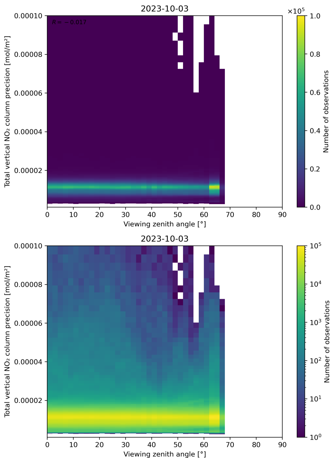
Figure 168: Scatter density plot of “Viewing zenith angle” against “Total vertical NO 2 column precision” for 2023-10-02 to 2023-10-04.
