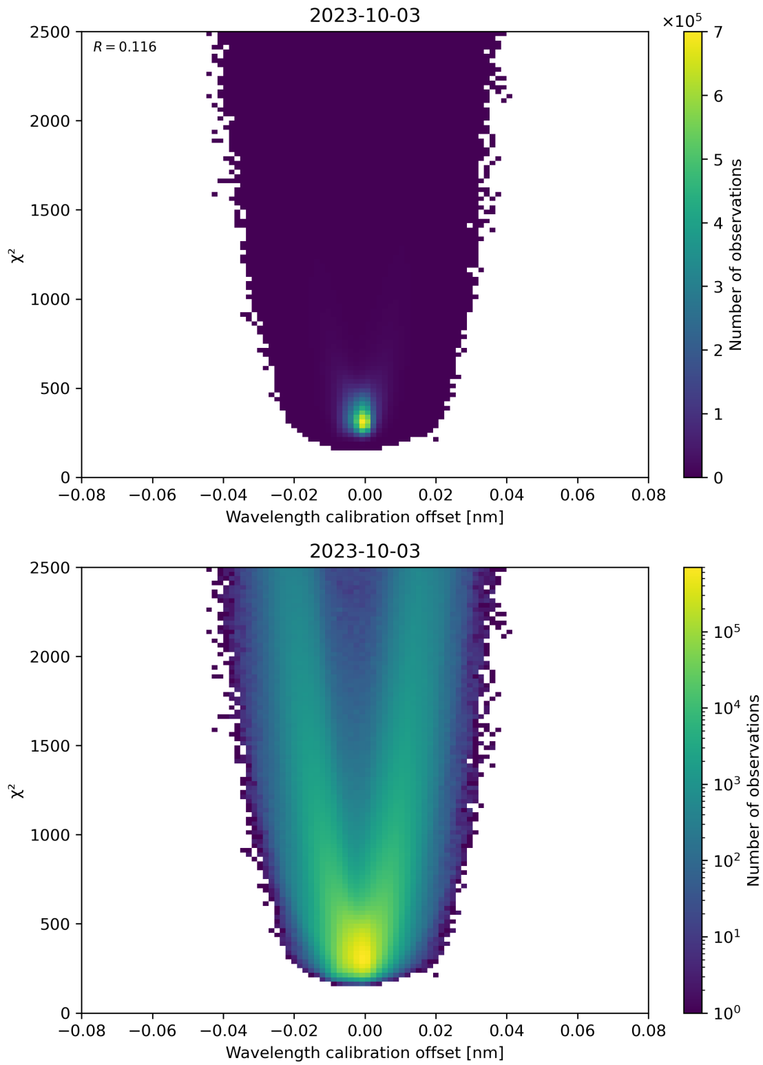
Figure 175: Scatter density plot of “Wavelength calibration offset” against “ \chi^2 ” for 2023-10-02 to 2023-10-04.
