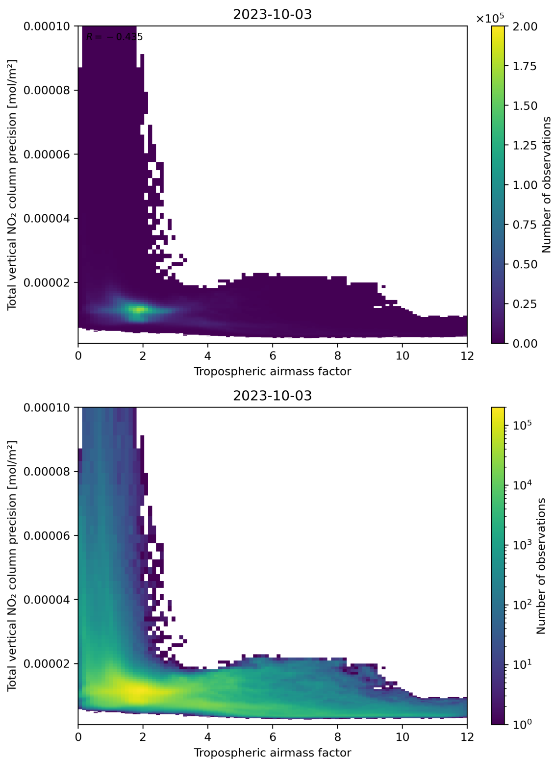
Figure 78: Scatter density plot of “Tropospheric air mass factor” against “Total vertical NO 2 column precision” for 2023-10-02 to 2023-10-04.
