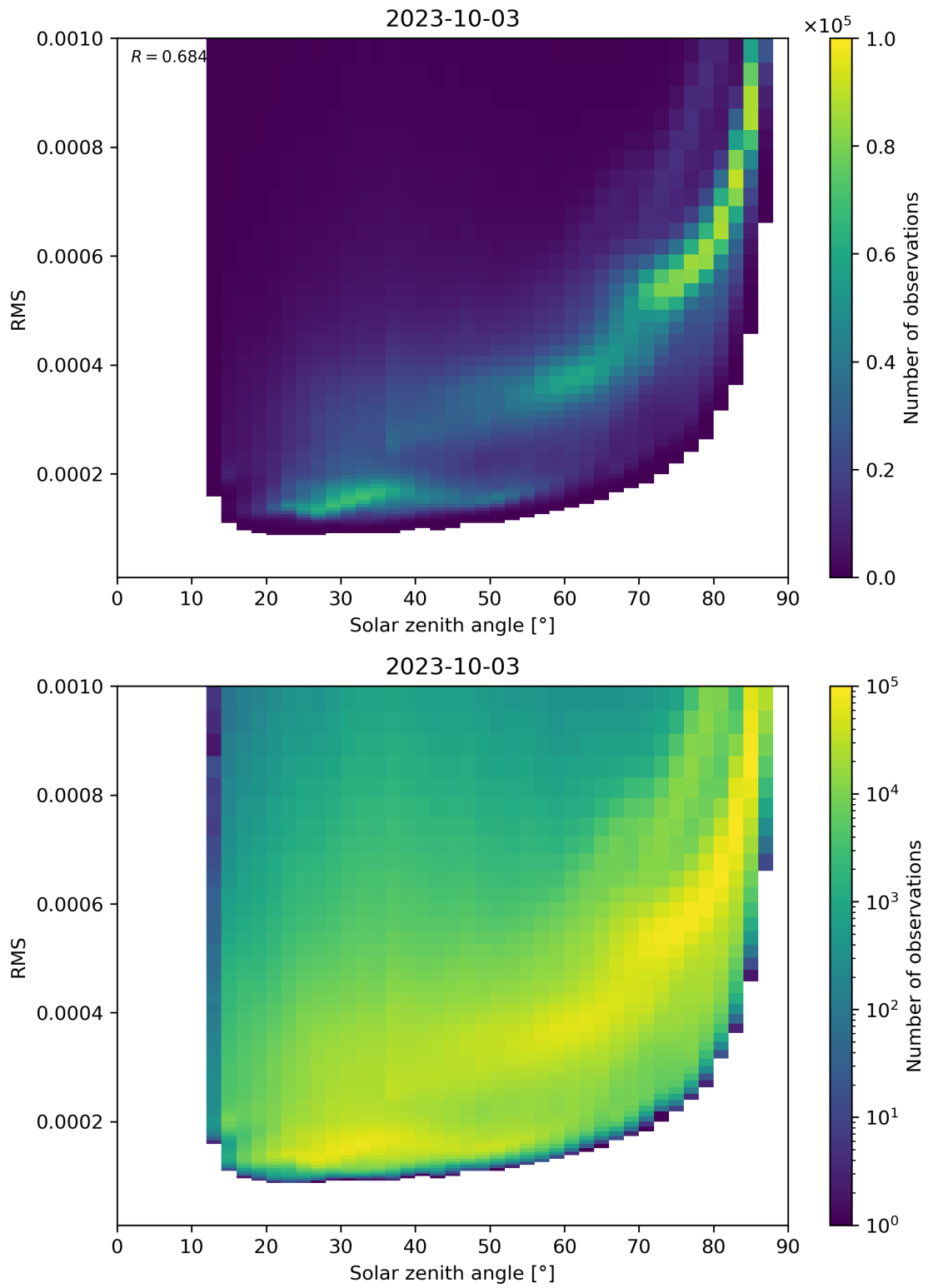
Figure 157: Scatter density plot of “Solar zenith angle” against “RMS” for 2023-10-02 to 2023-10-04.
