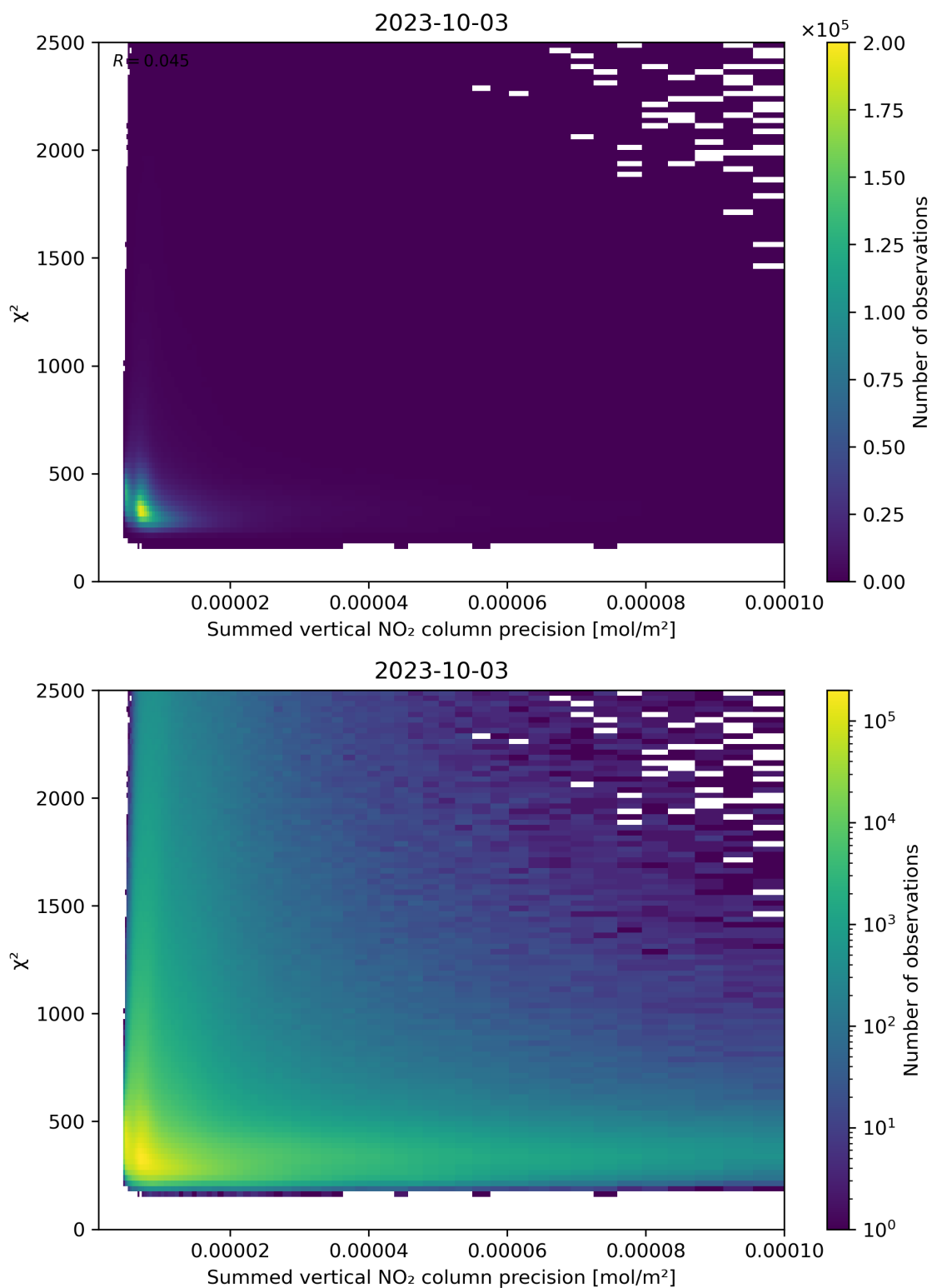
Figure 107: Scatter density plot of “Summed vertical NO 2 column precision” against “ \chi^2 ” for 2023-10-02 to 2023-10-04.
