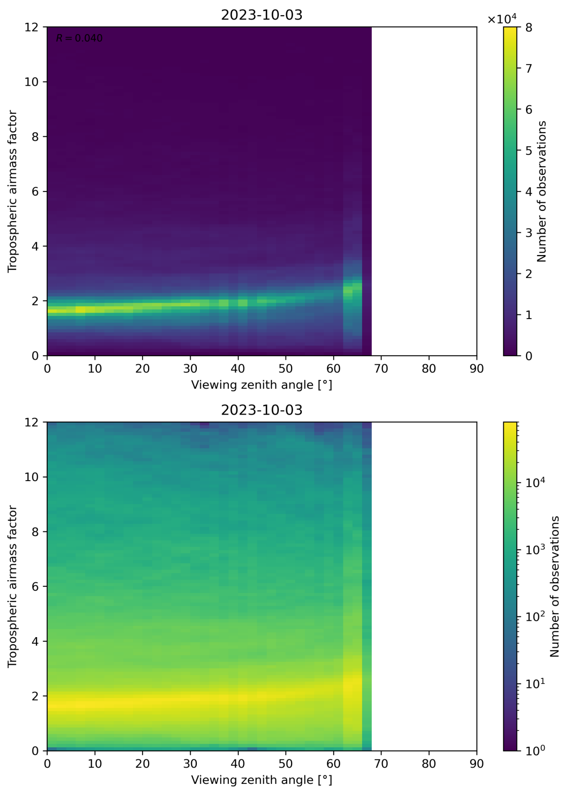
Figure 161: Scatter density plot of “Viewing zenith angle” against “Tropospheric airmass factor” for 2023-10-02 to 2023-10-04.
