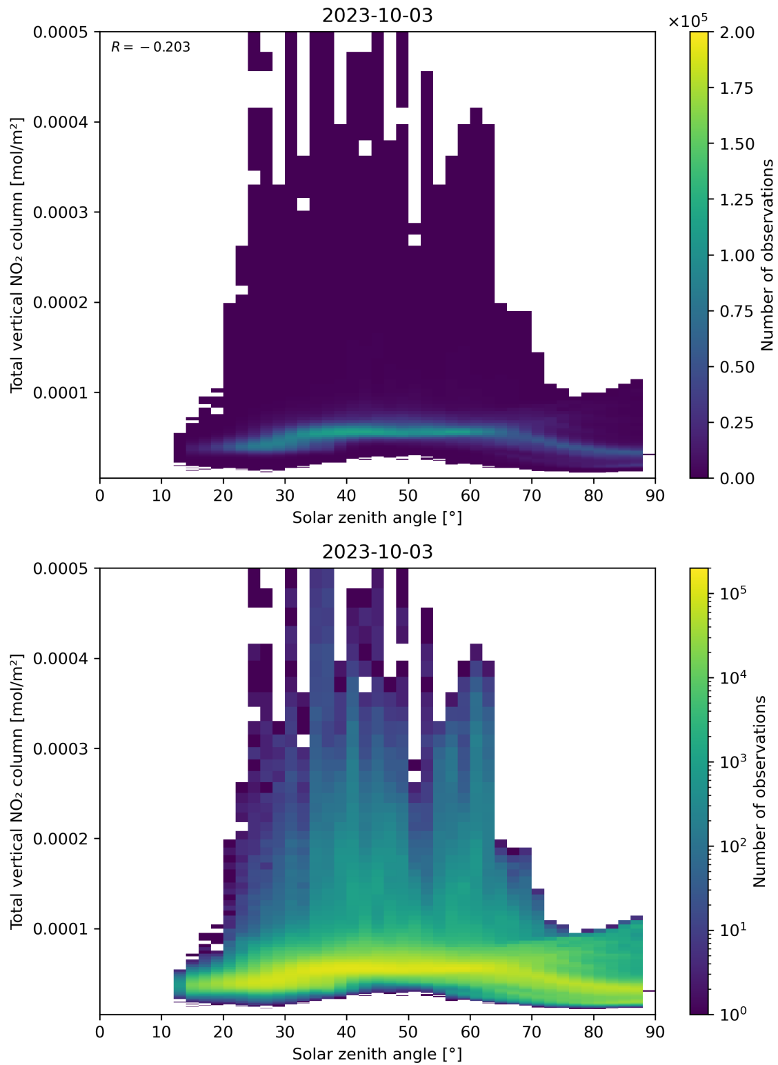
Figure 153: Scatter density plot of “Solar zenith angle” against “Total vertical NO 2 column” for 2023-10-02 to 2023-10-04.
