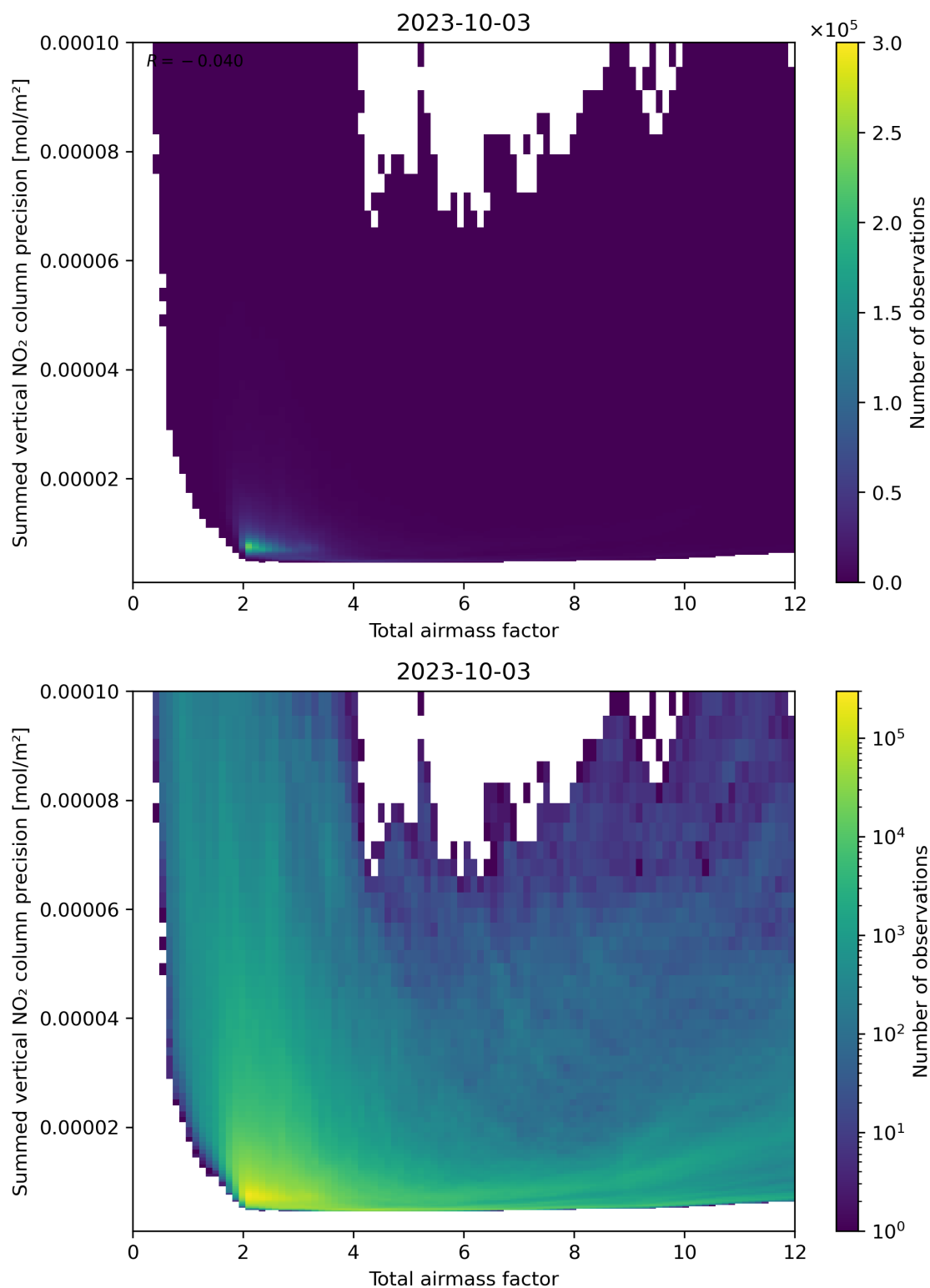
Figure 66: Scatter density plot of “Total airmass factor” against “Summed vertical NO 2 column precision” for 2023-10-02 to 2023-10-04.
