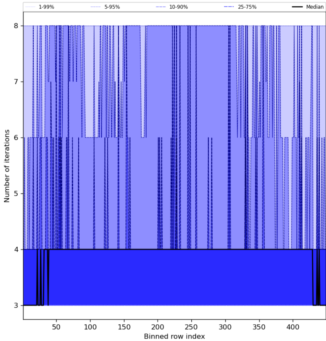
Figure 51: Along track statistics of “Number of iterations” for 2023-10-02 to 2023-10-04
