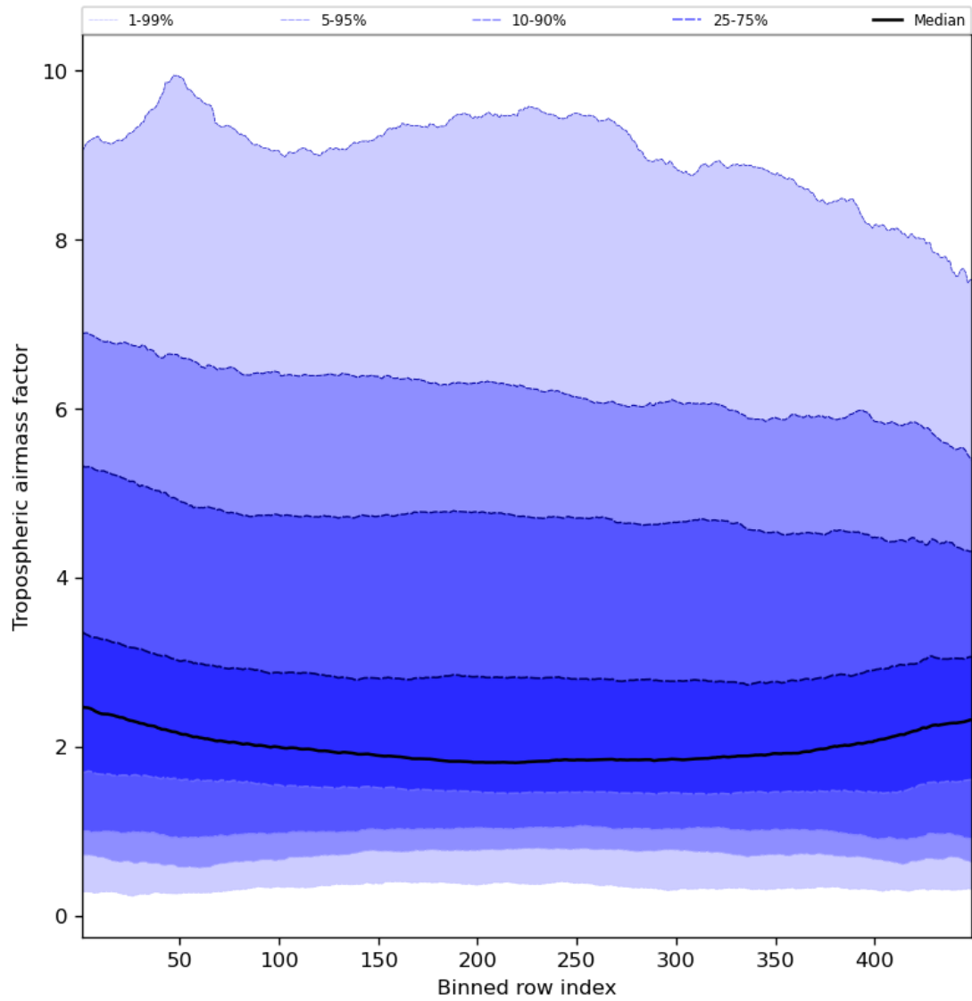
Figure 48: Along track statistics of “Tropospheric air mass factor” for 2023-10-02 to 2023-10-04
