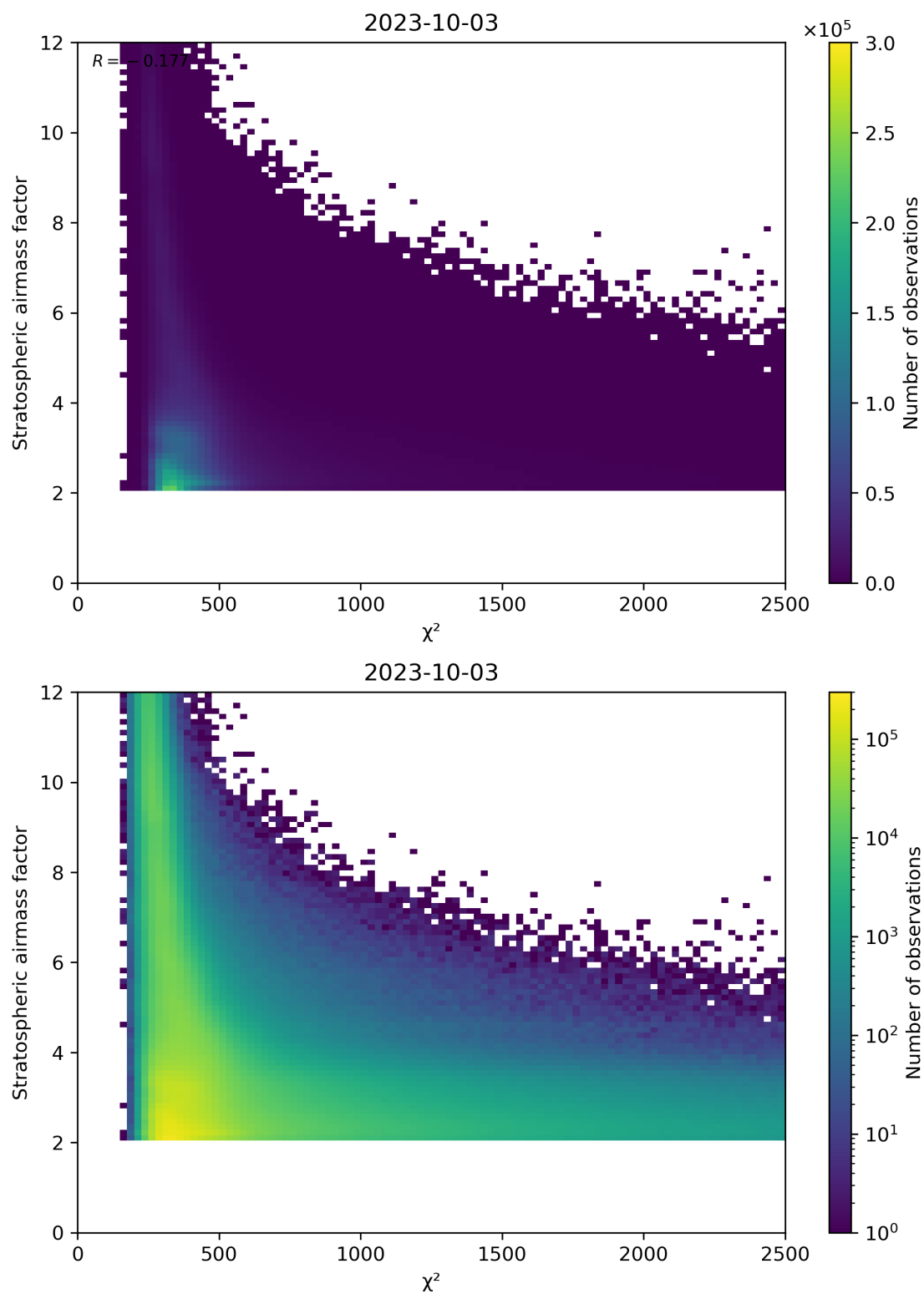
Figure 81: Scatter density plot of “ \chi^2 ” against “Stratospheric airmass factor” for 2023-10-02 to 2023-10-04.
