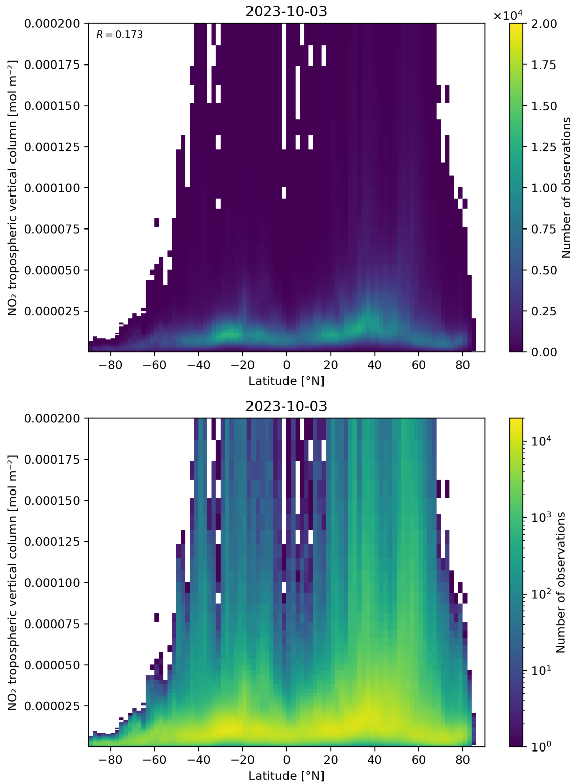
Figure 92: Scatter density plot of “Latitude” against “NO 2 tropospheric vertical column” for 2023-10-02 to 2023-10-04.
