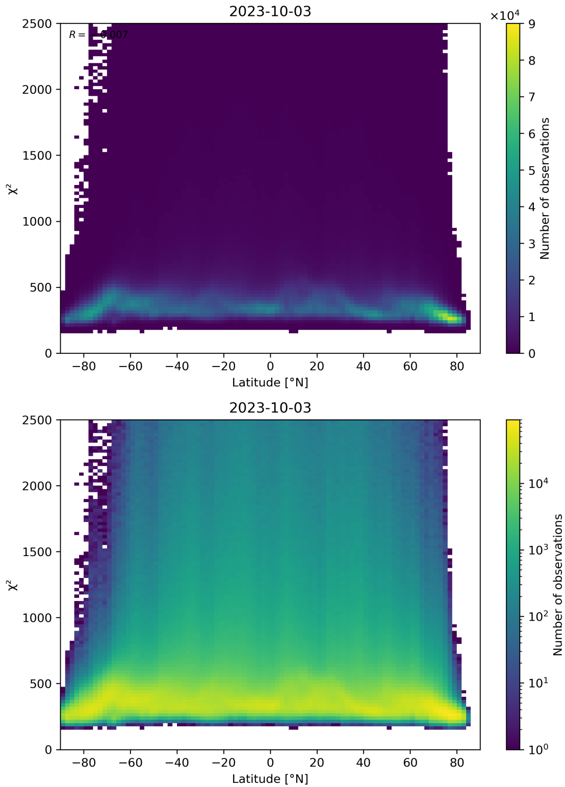
Figure 86: Scatter density plot of “Latitude” against “ \chi^2 ” for 2023-10-02 to 2023-10-04.
