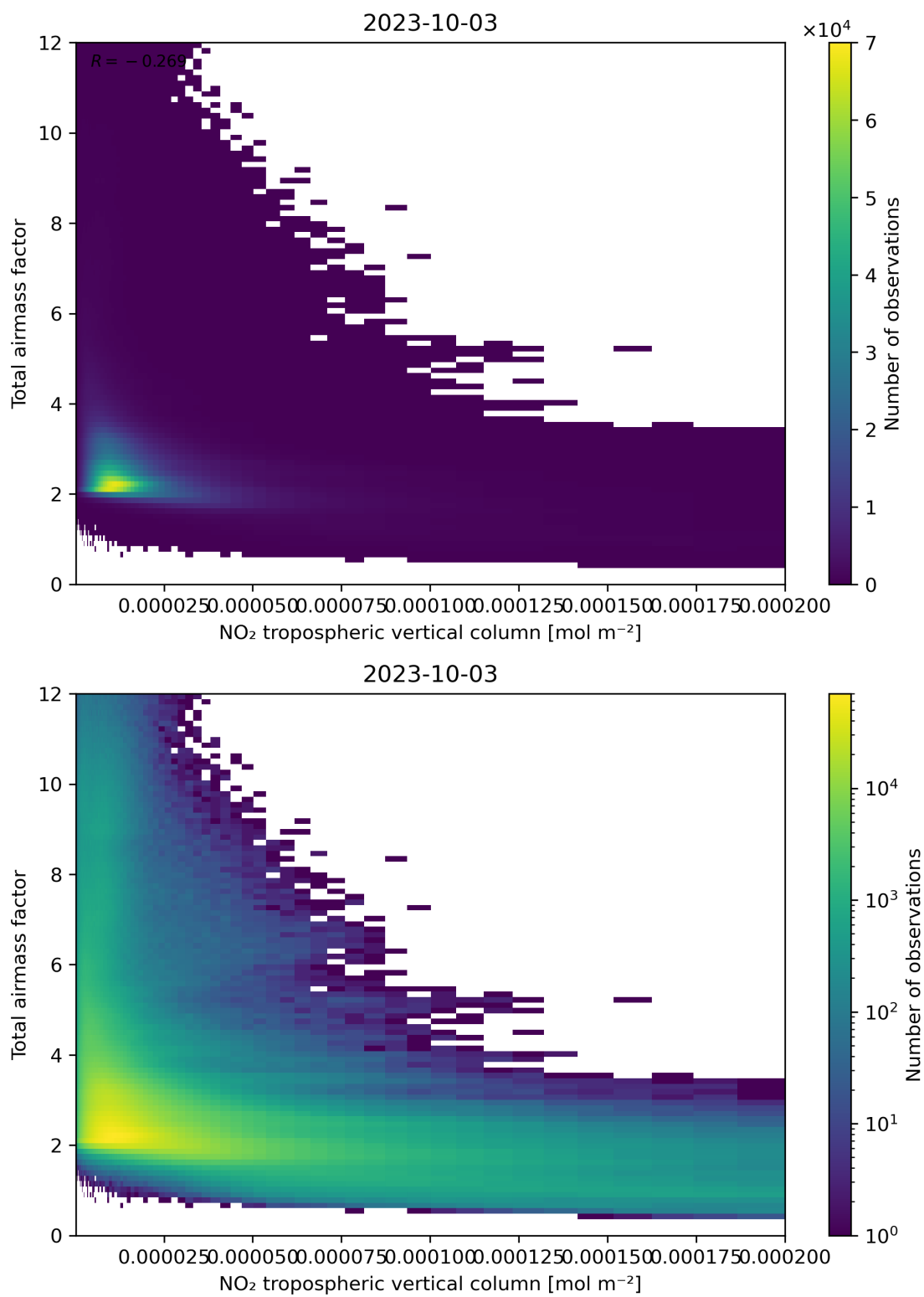
Figure 122: Scatter density plot of “NO 2 tropospheric vertical column” against “Total air mass factor” for 2023-10-02 to 2023-10-04.
