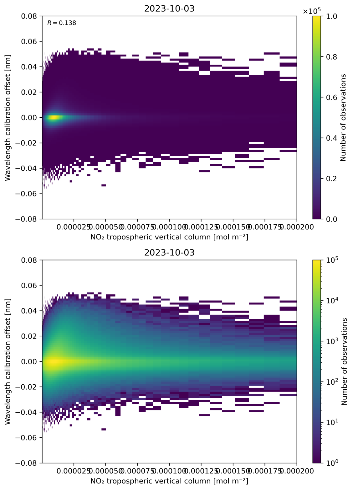
Figure 143: Scatter density plot of “NO 2 tropospheric vertical column” against “Wavelength calibration offset” for 2023-10-02 to 2023-10-04.
