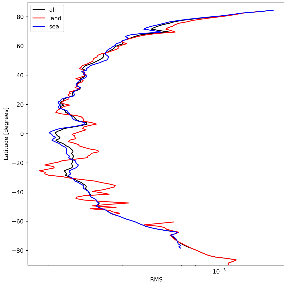
Figure 26: Zonal average of “RMS” for 2023-10-02 to 2023-10-04.
