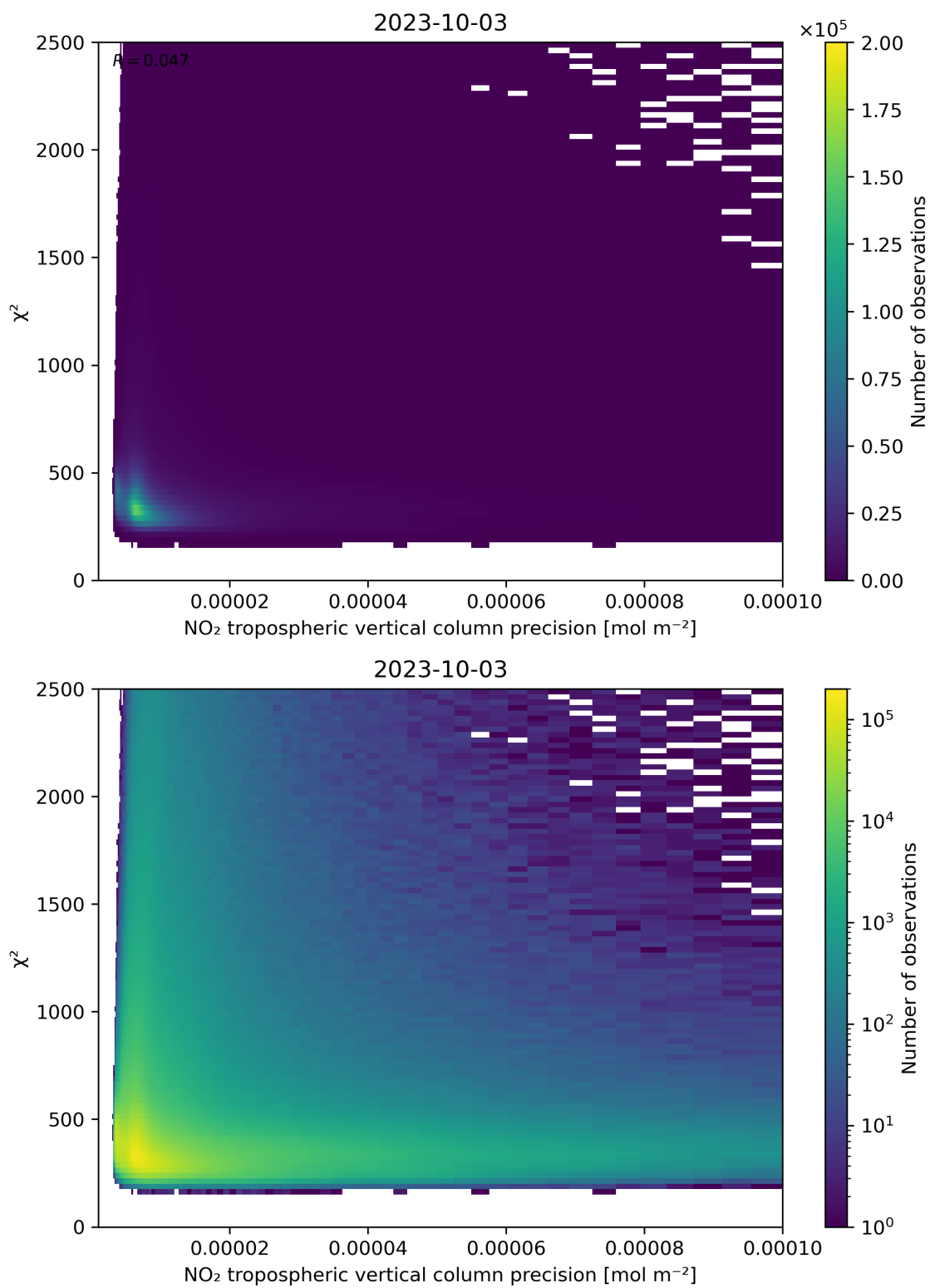
Figure 134: Scatter density plot of “NO 2 tropospheric vertical column precision” against “ \chi^2 ” for 2023-10-02 to 2023-10-04.
