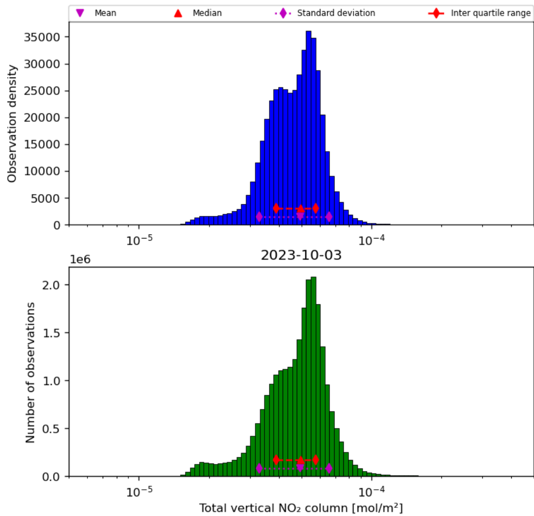
Figure 38: Histogram of “Total vertical NO 2 column” for 2023-10-02 to 2023-10-04
