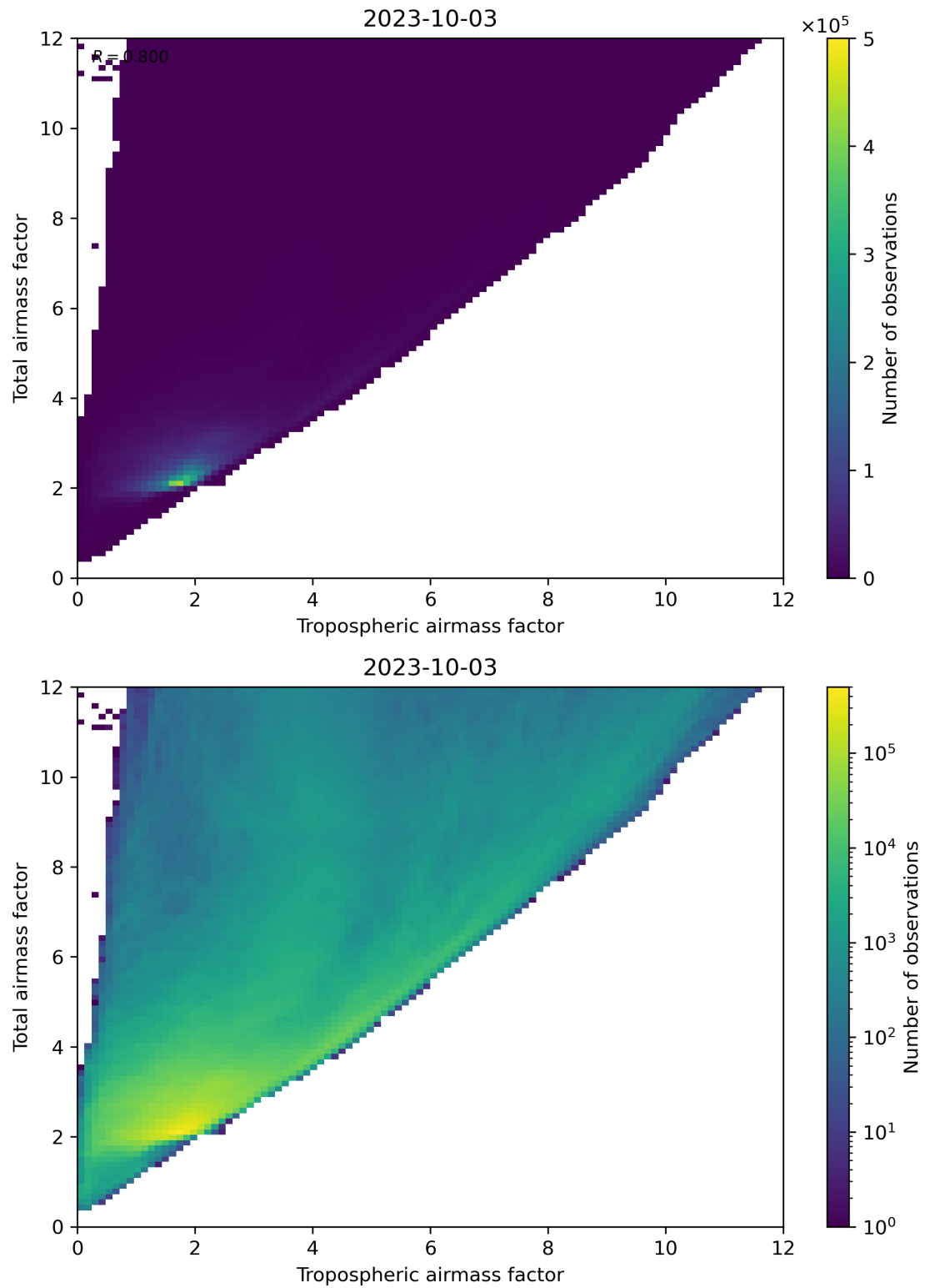
Figure 72: Scatter density plot of “Tropospheric airmass factor” against “Total airmass factor” for 2023-10-02 to 2023-10-04.
