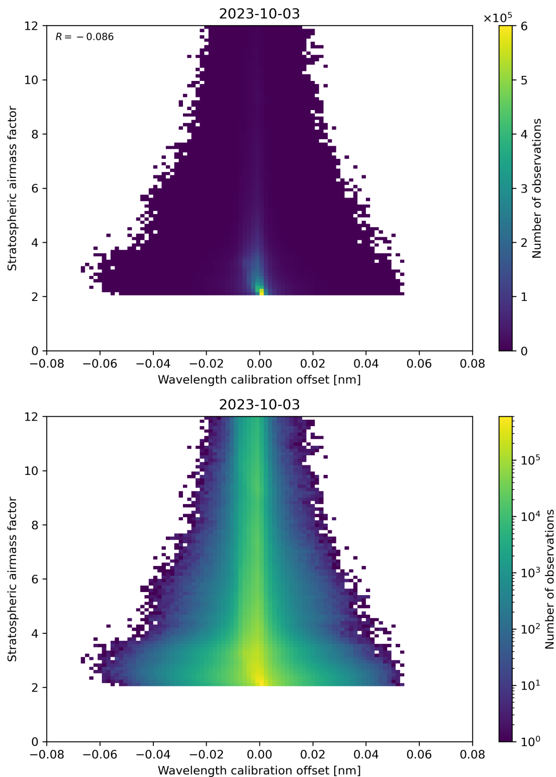
Figure 174: Scatter density plot of “Wavelength calibration offset” against “Stratospheric airmass factor” for 2023-10-02 to 2023-10-04.
