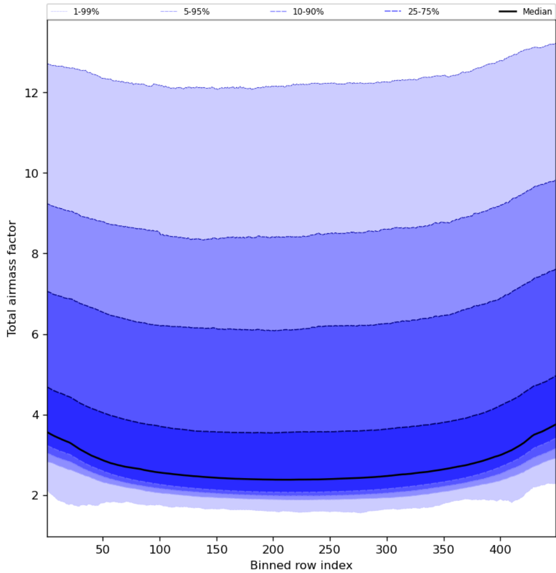
Figure 49: Along track statistics of “Total airmass factor” for 2023-10-02 to 2023-10-04
