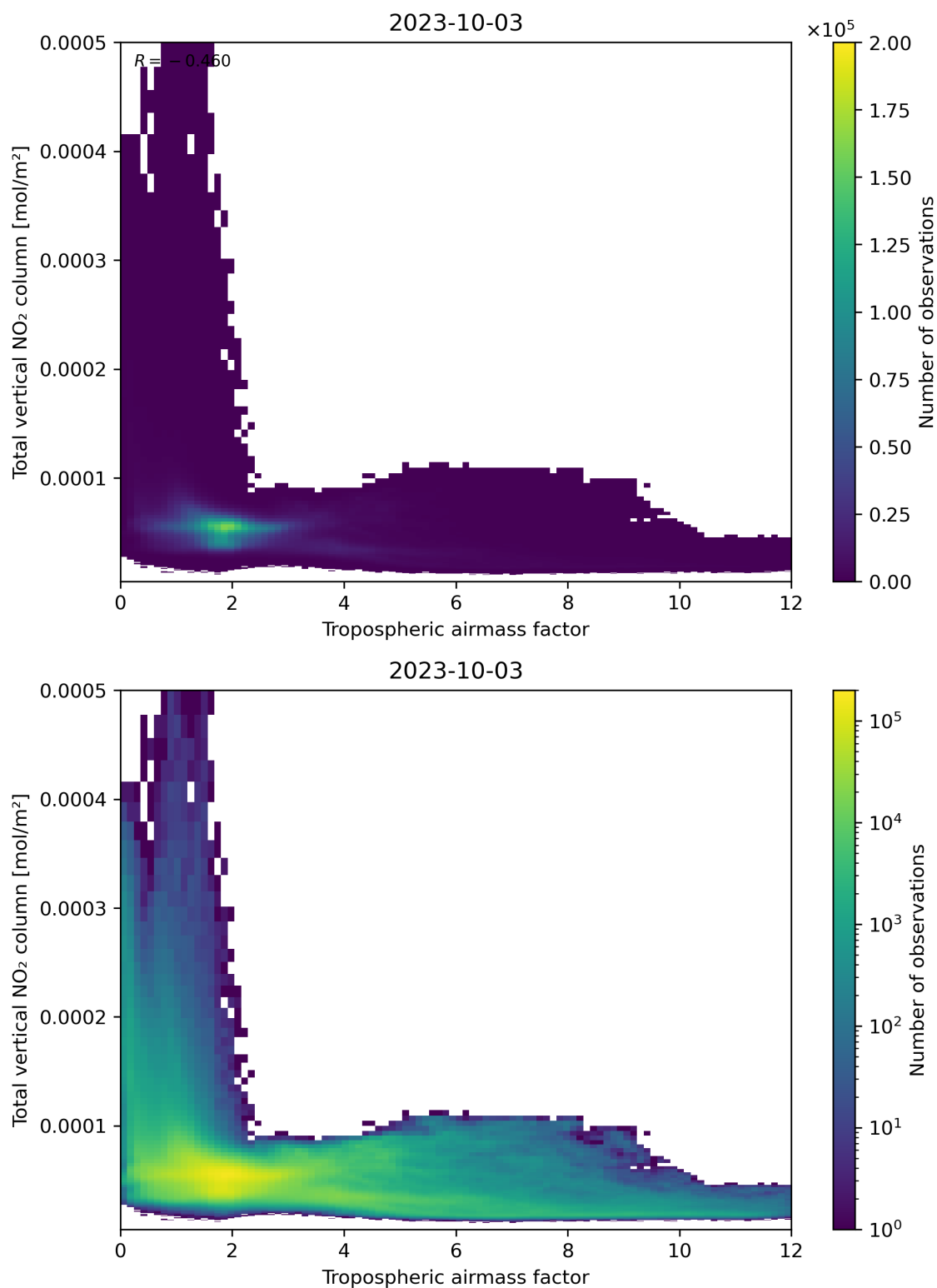
Figure 77: Scatter density plot of “Tropospheric airmass factor” against “Total vertical NO 2 column” for 2023-10-02 to 2023-10-04.
