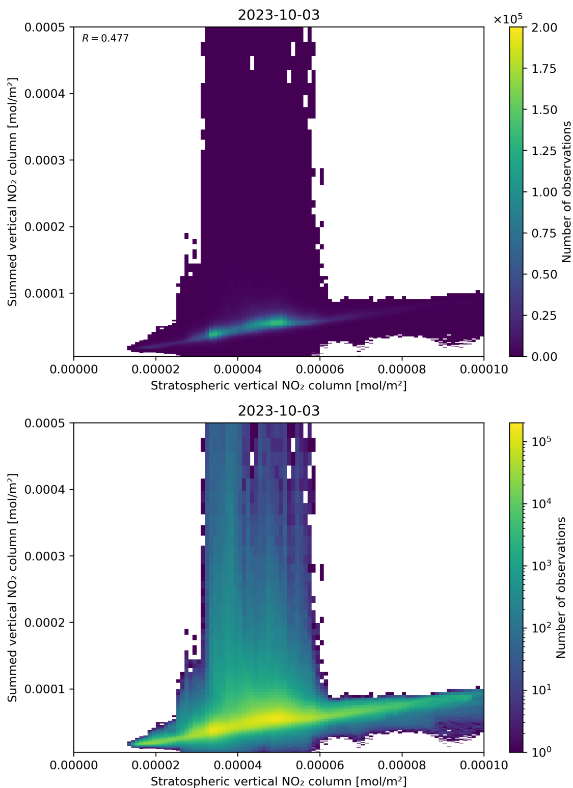
Figure 98: Scatter density plot of “Stratospheric vertical NO 2 column” against “Summed vertical NO 2 column” for 2023-10-02 to 2023-10-04.
