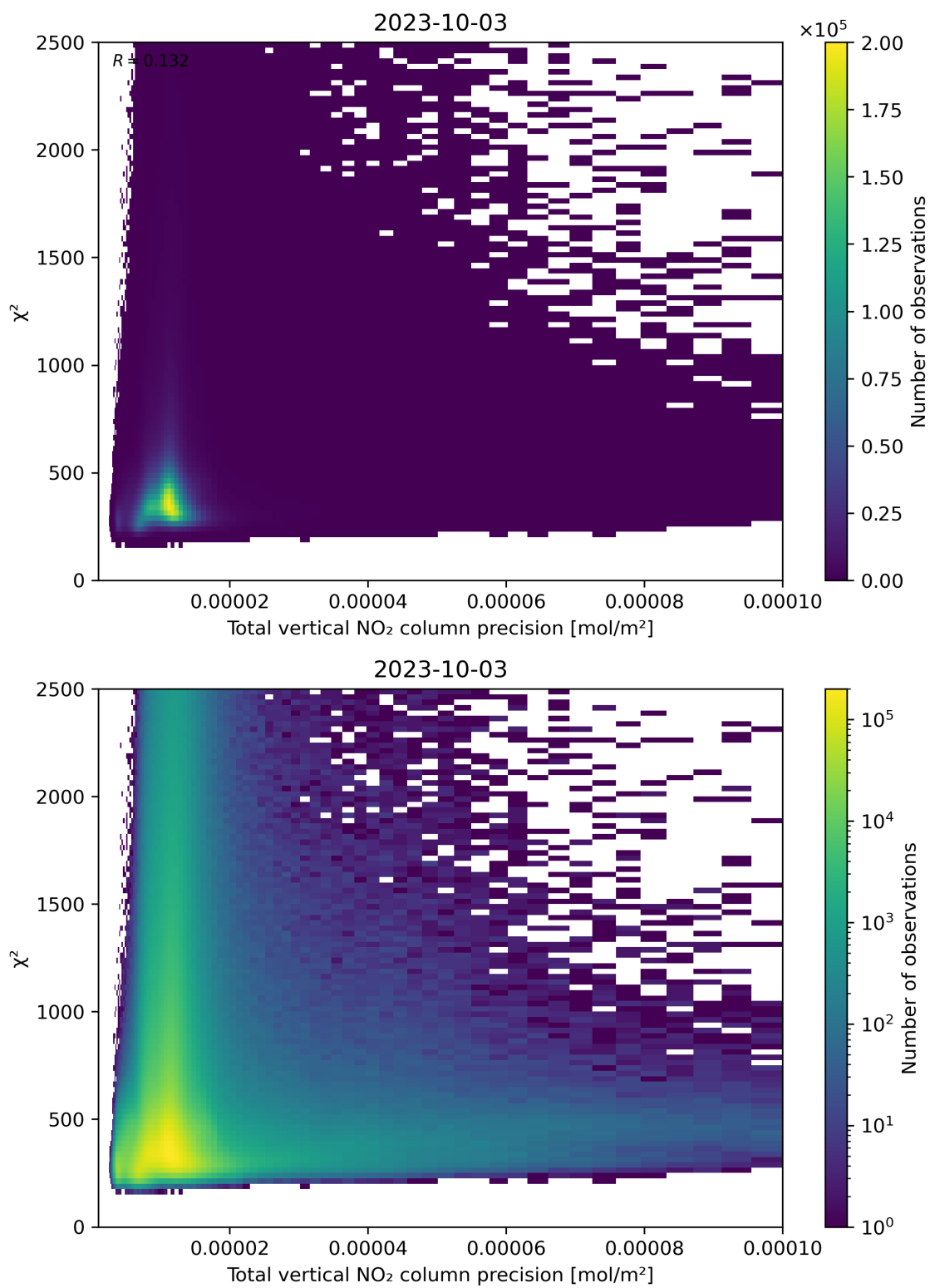
Figure 116: Scatter density plot of “Total vertical NO 2 column precision” against “ \chi^2 ” for 2023-10-02 to 2023-10-04.
