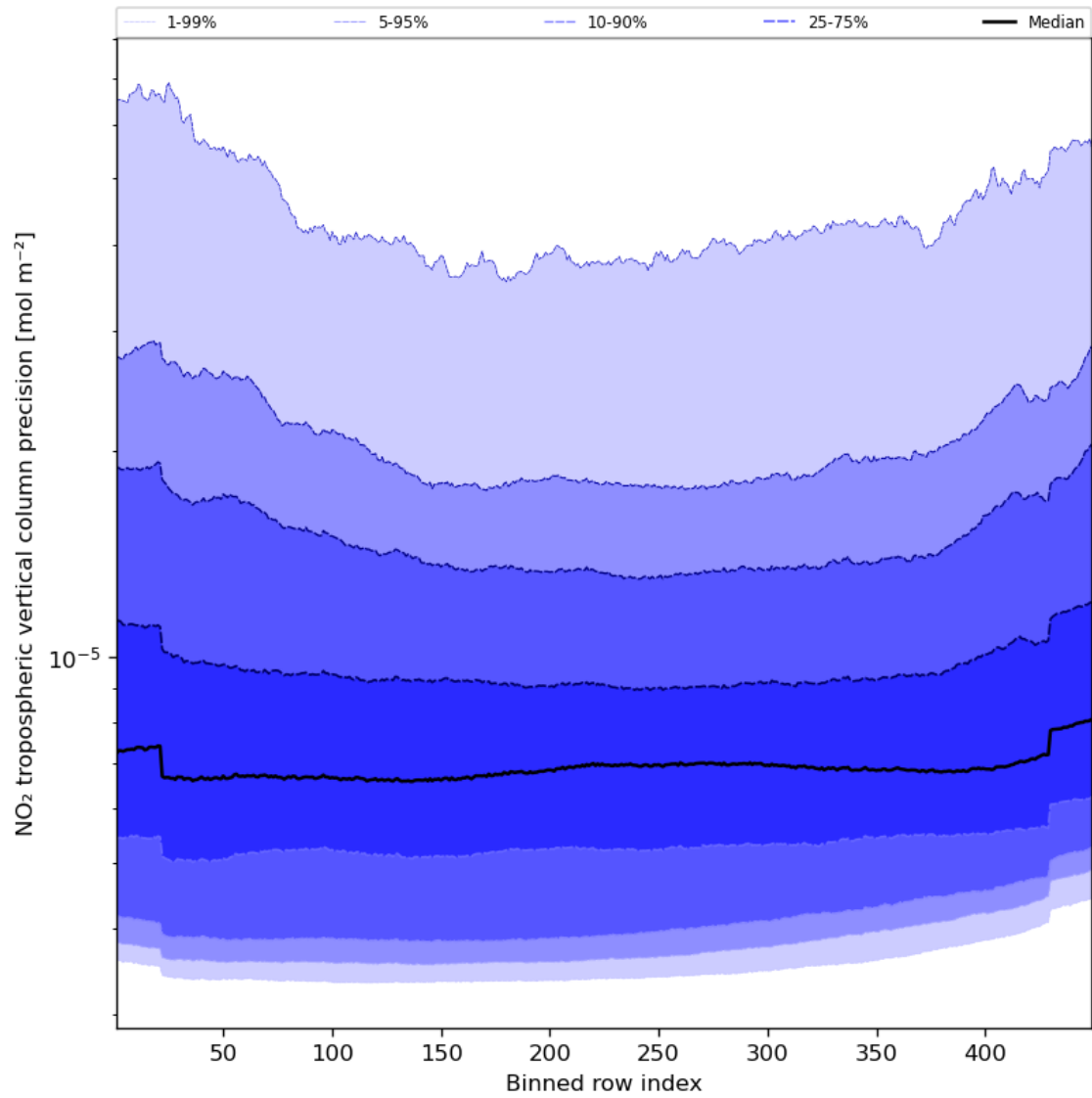
Figure 47: Along track statistics of “NO 2 tropospheric vertical column precision” for 2023-10-02 to 2023-10-04
