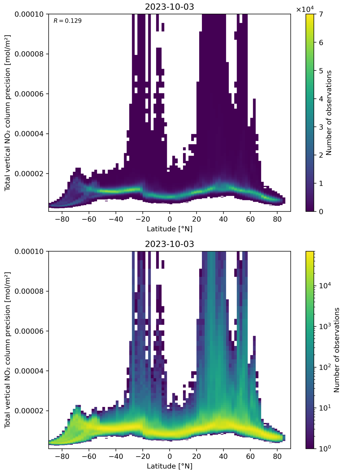
Figure 91: Scatter density plot of “Latitude” against “Total vertical NO 2 column precision” for 2023-10-02 to 2023-10-04.
