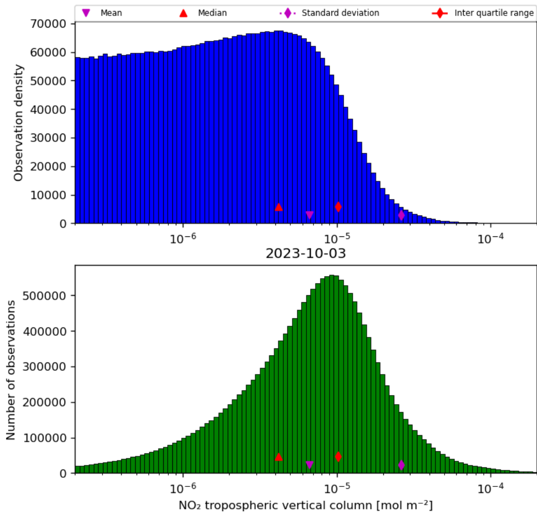
Figure 29: Histogram of “NO 2 tropospheric vertical column” for 2023-10-02 to 2023-10-04
