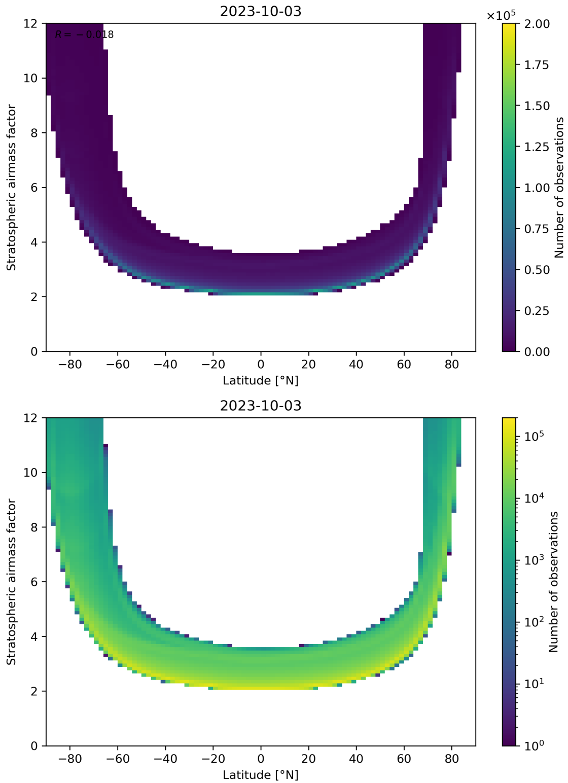
Figure 83: Scatter density plot of “Latitude” against “Stratospheric air mass factor” for 2023-10-02 to 2023-10-04.
