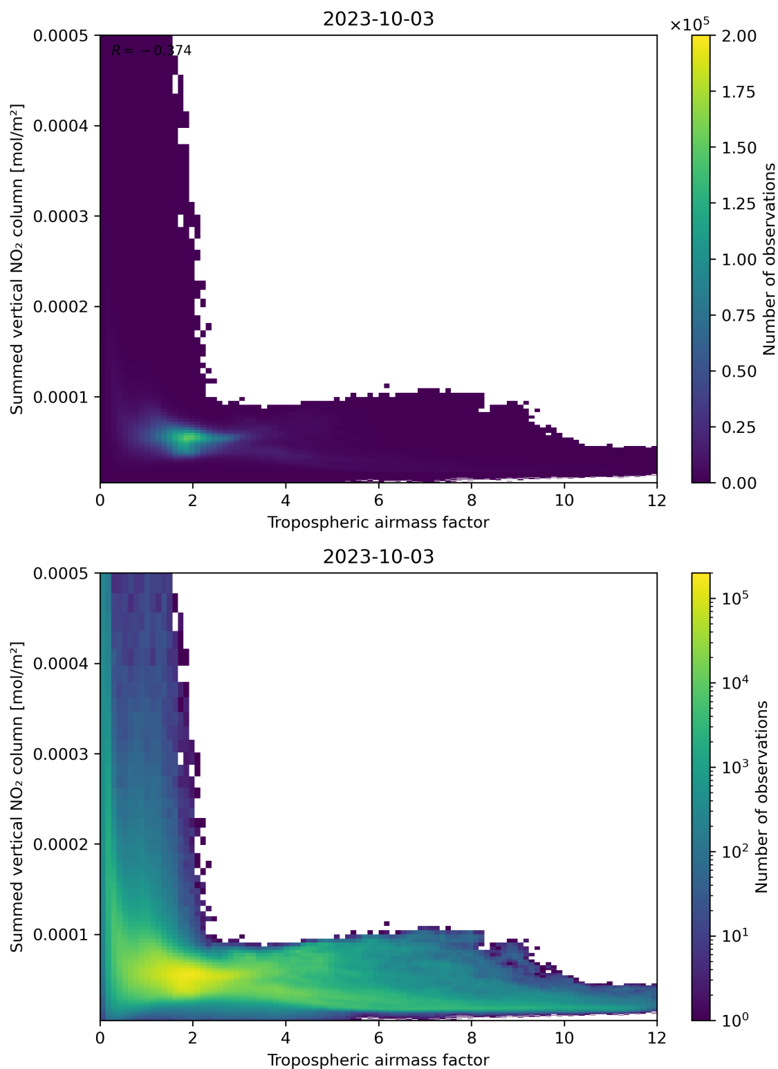
Figure 75: Scatter density plot of “Tropospheric airmass factor” against “Summed vertical NO 2 column” for 2023-10-02 to 2023-10-04.
