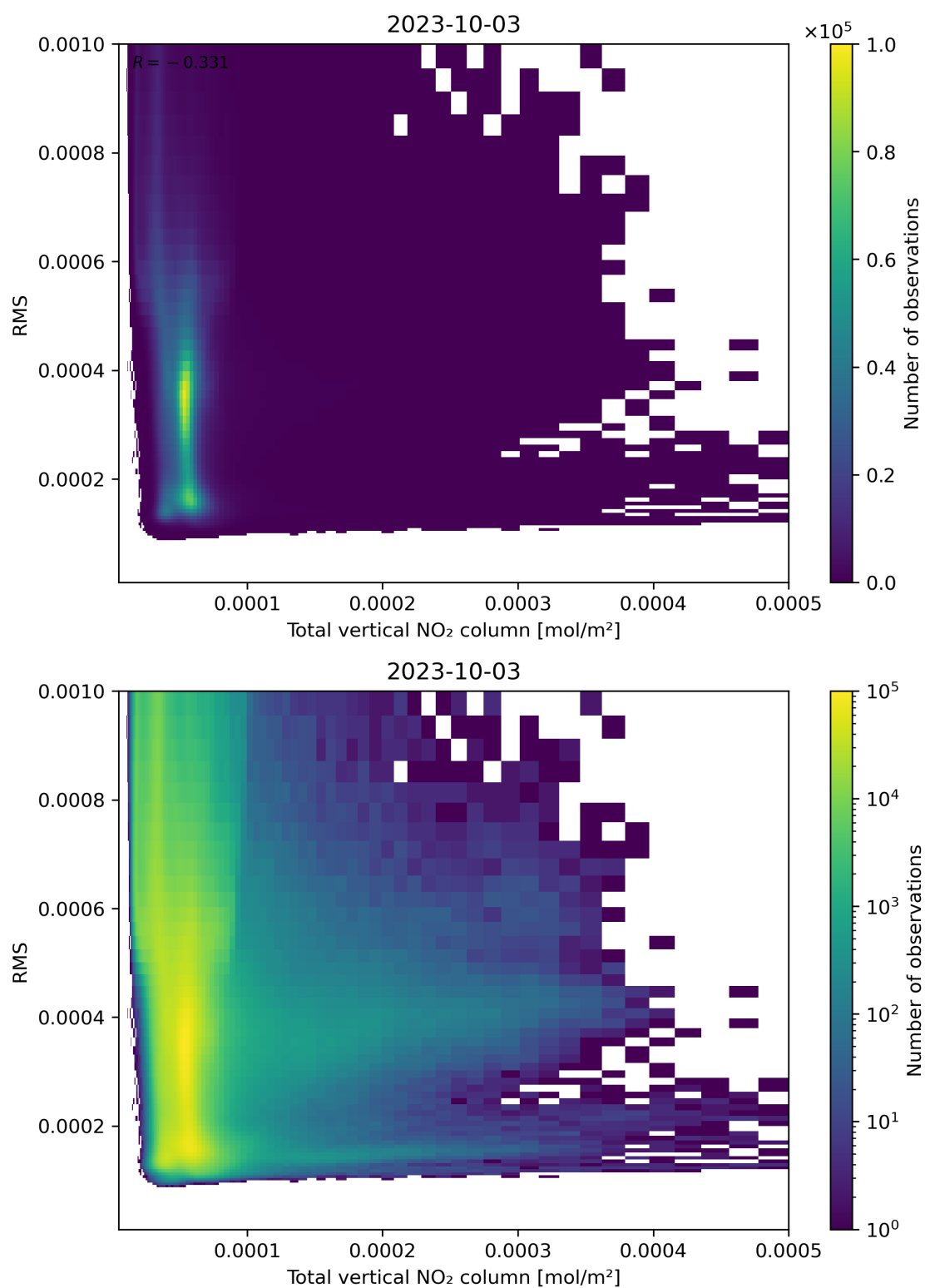
Figure 120: Scatter density plot of “Total vertical NO 2 column” against “RMS” for 2023-10-02 to 2023-10-04.
