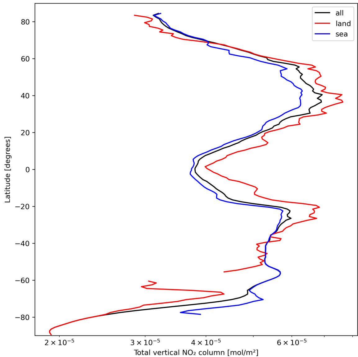
Figure 21: Zonal average of “Total vertical NO 2 column” for 2023-10-02 to 2023-10-04.
