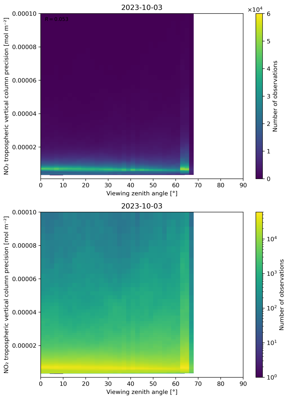
Figure 170: Scatter density plot of “Viewing zenith angle” against “NO 2 tropospheric vertical column precision” for 2023-10-02 to 2023-10-04.
