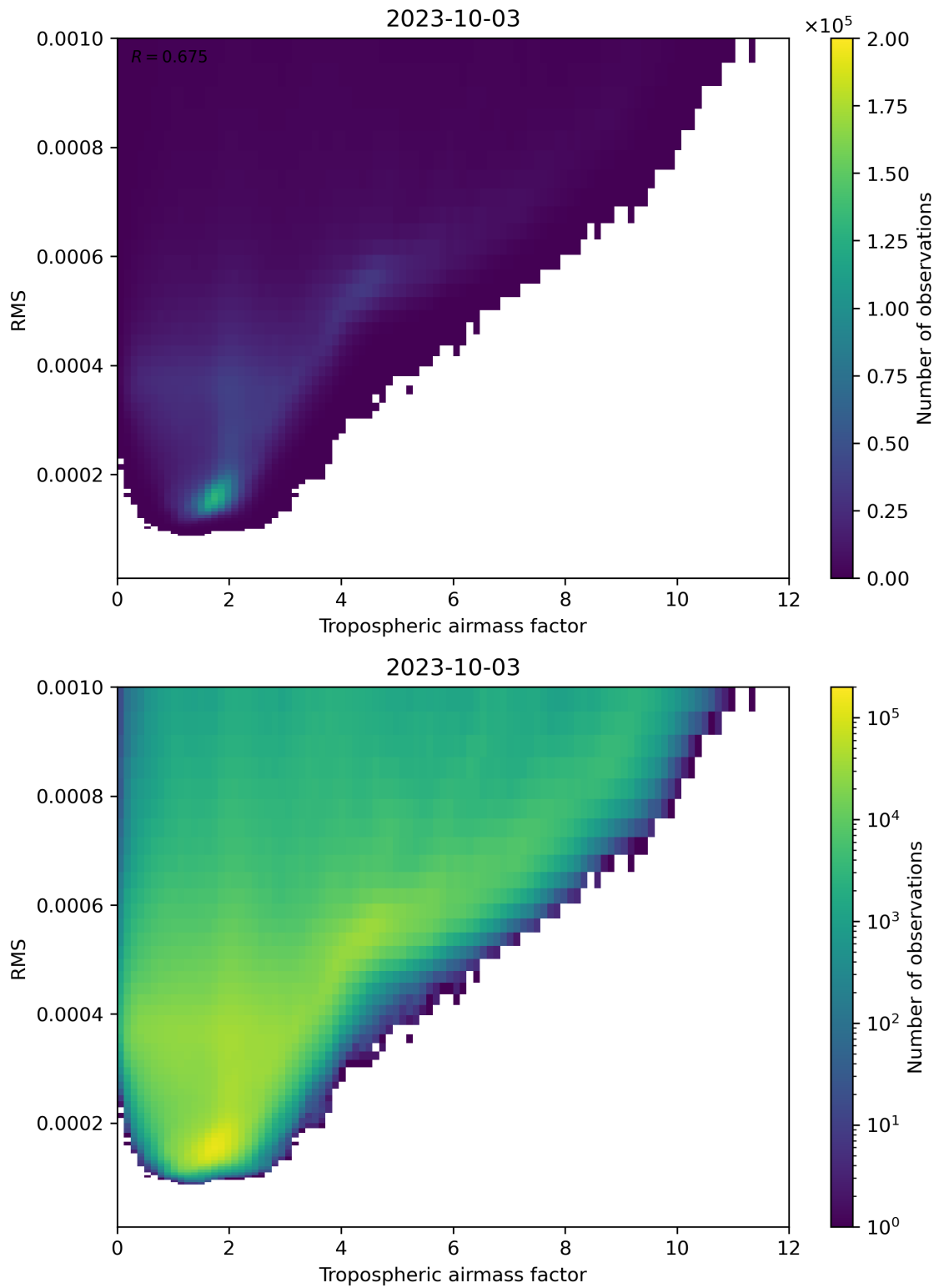
Figure 79: Scatter density plot of “Tropospheric airmass factor” against “RMS” for 2023-10-02 to 2023-10-04.
