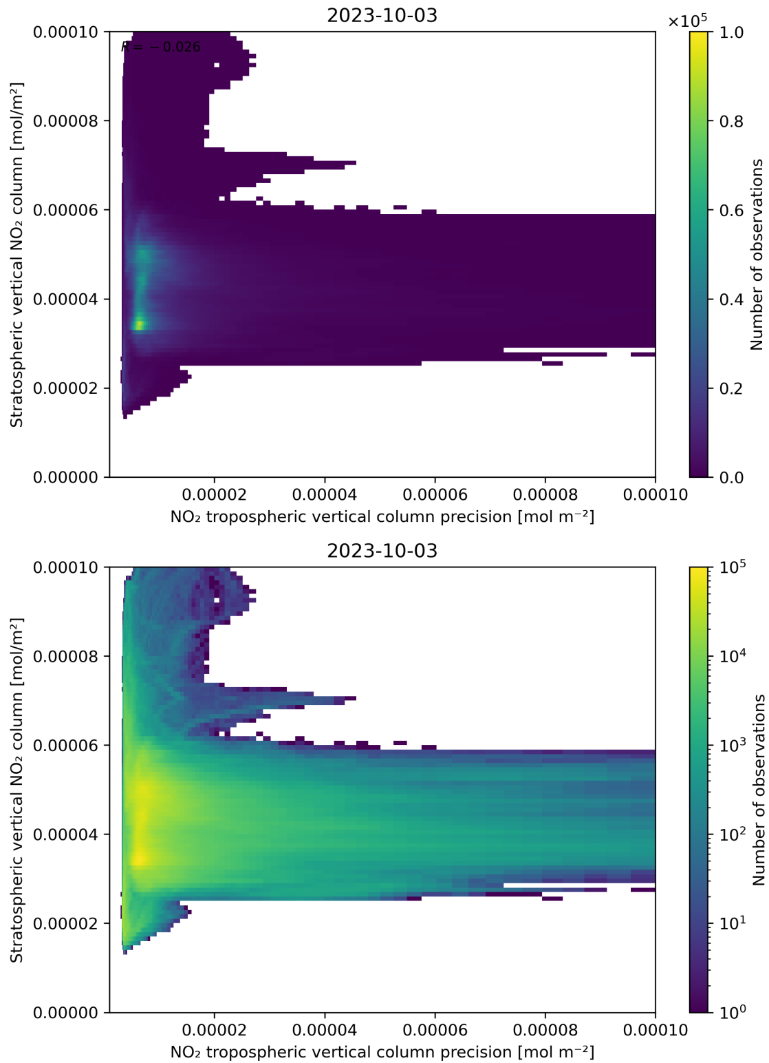
Figure 135: Scatter density plot of “NO 2 tropospheric vertical column precision” against “Stratospheric vertical NO 2 column” for 2023-10-02 to 2023-10-04.
