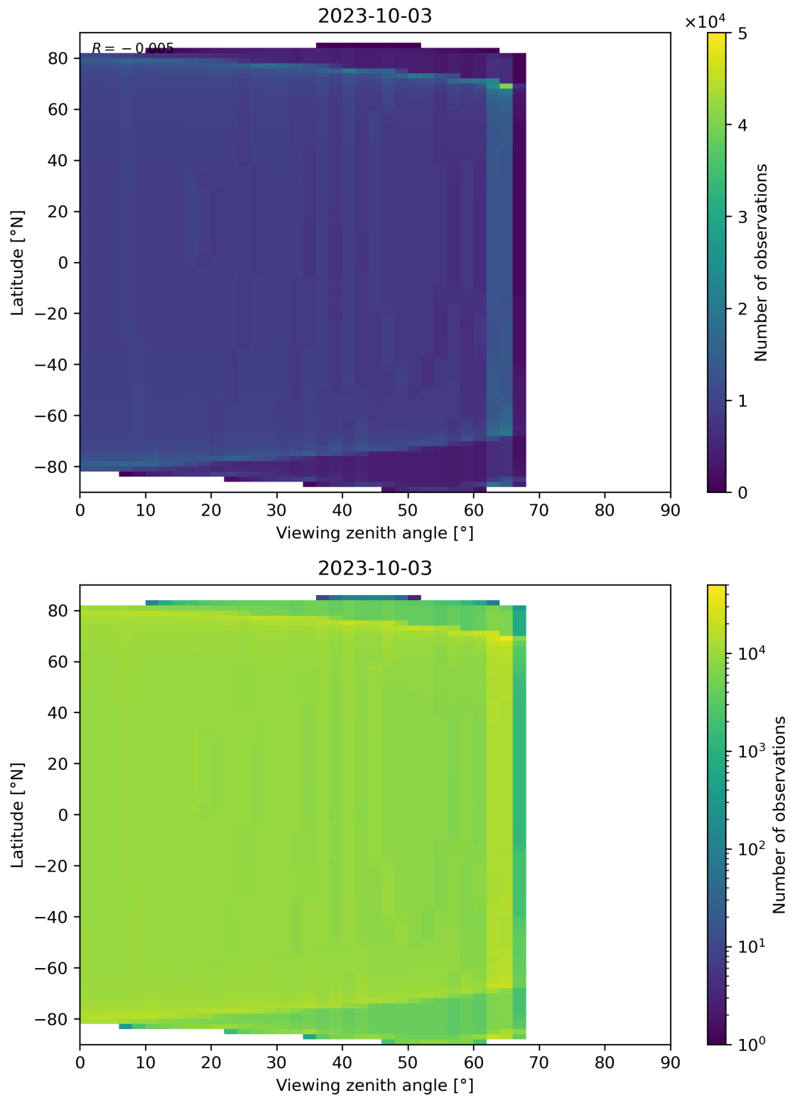
Figure 163: Scatter density plot of “Viewing zenith angle” against “Latitude” for 2023-10-02 to 2023-10-04.
