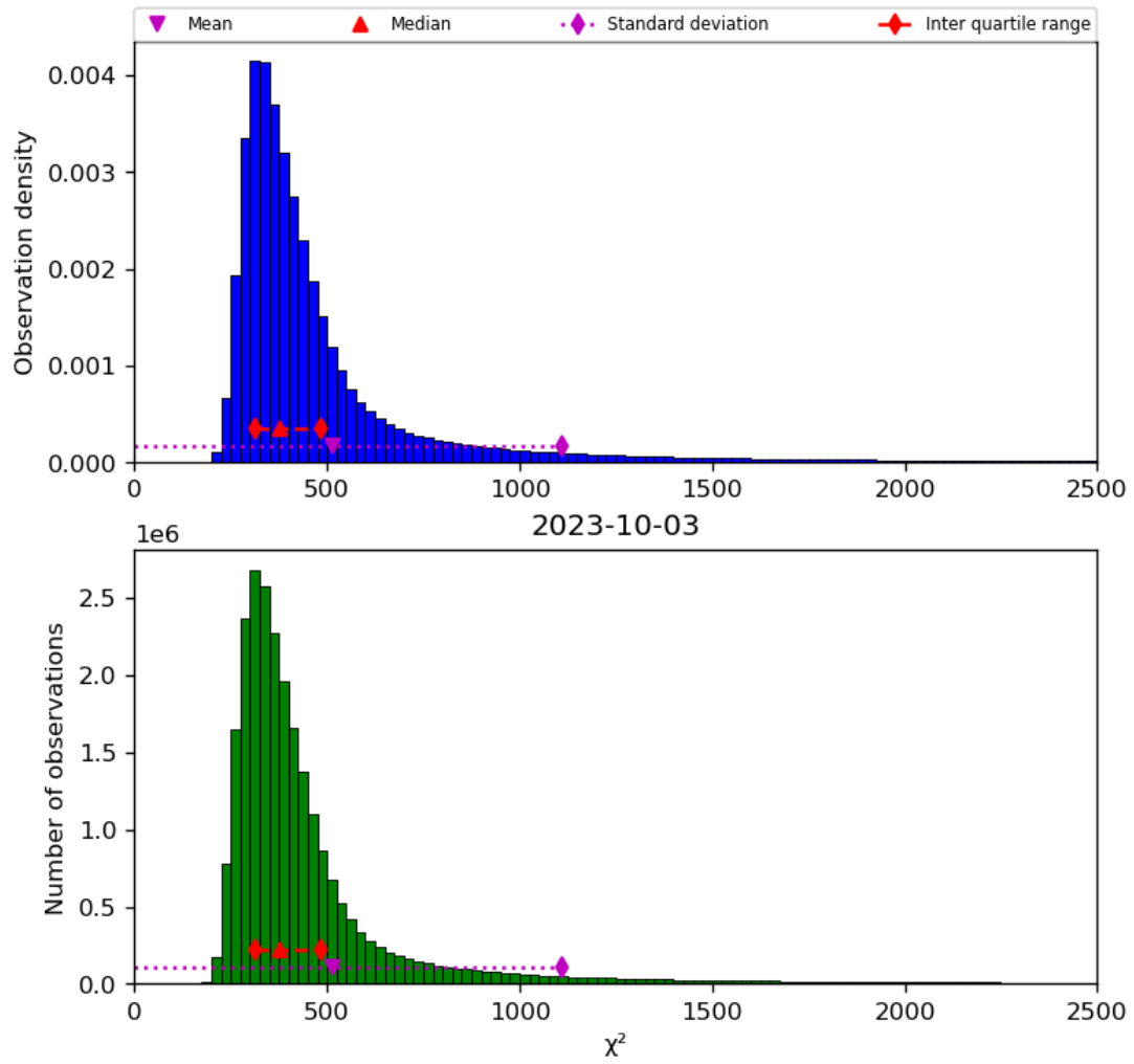
Figure 42: Histogram of “ \chi^2 ” for 2023-10-02 to 2023-10-04
