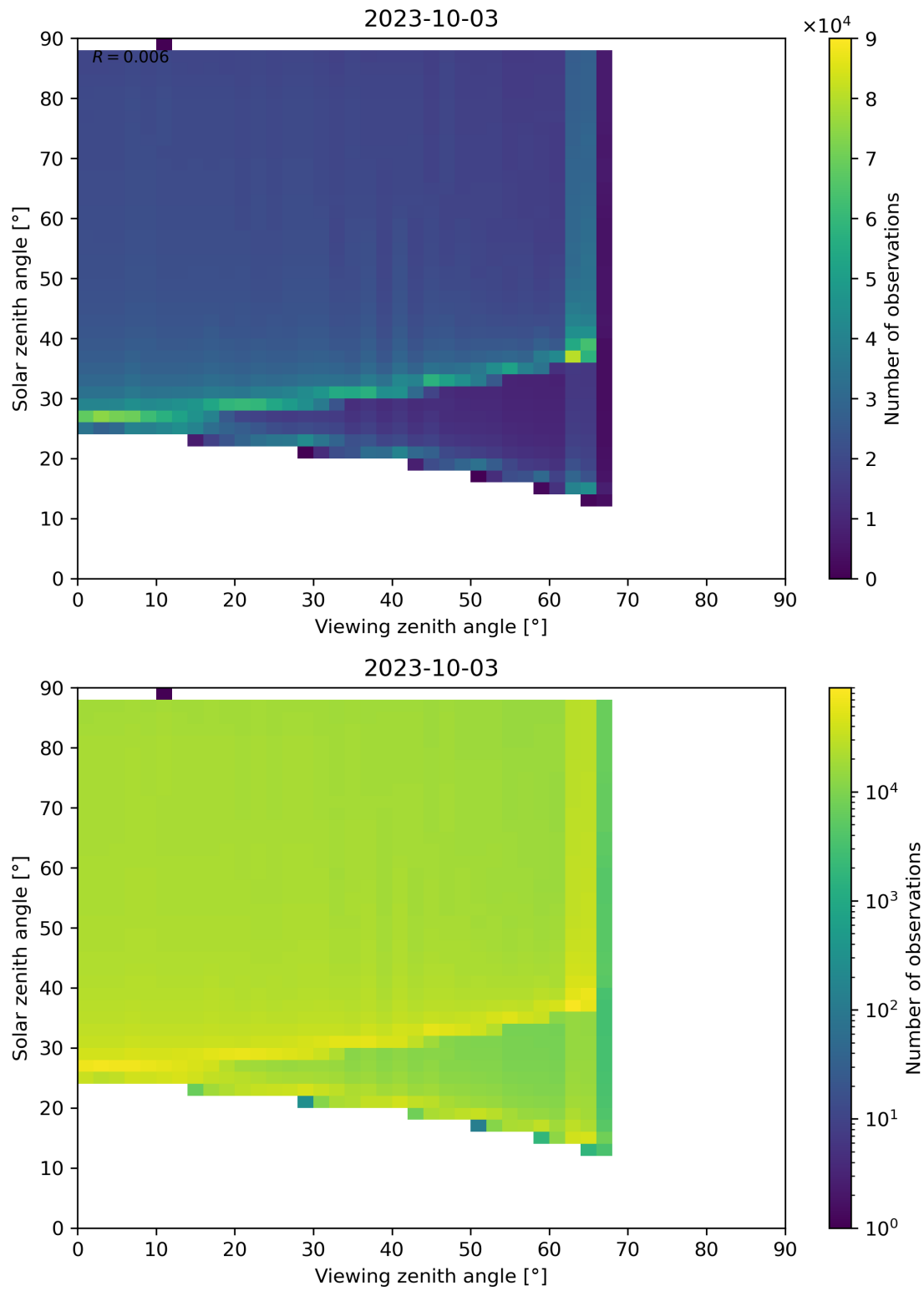
Figure 172: Scatter density plot of “Viewing zenith angle” against “Solar zenith angle” for 2023-10-02 to 2023-10-04.
