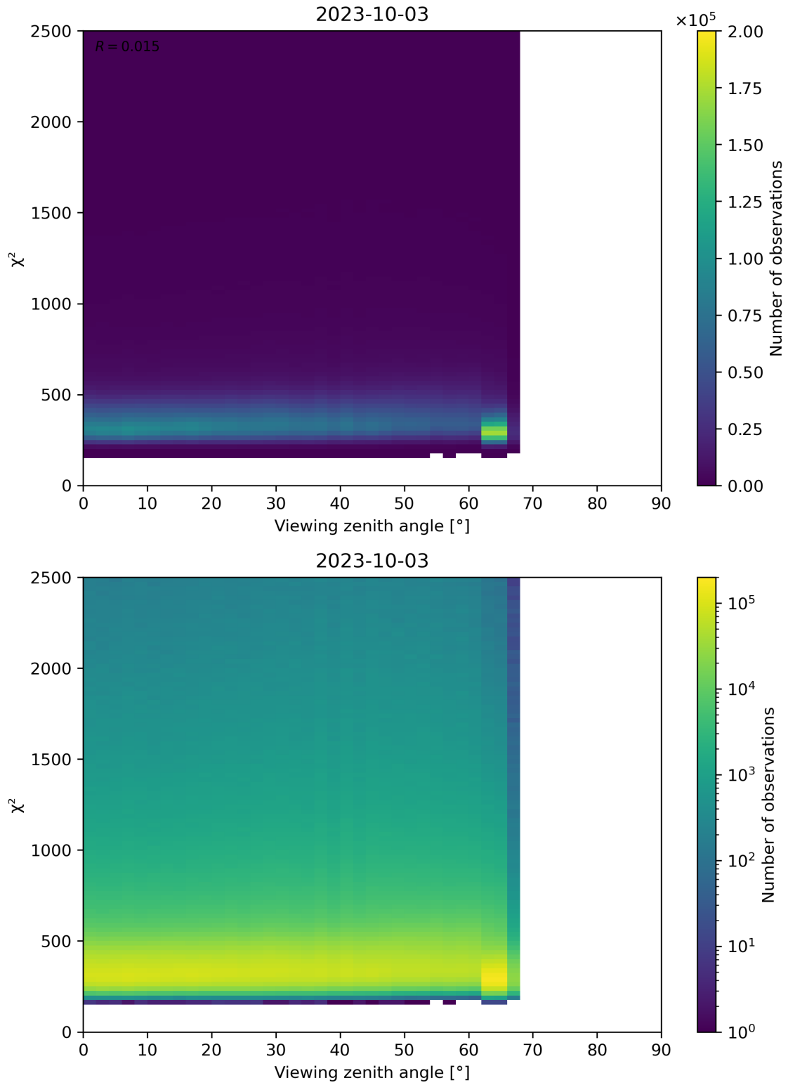
Figure 162: Scatter density plot of “Viewing zenith angle” against “ \chi^2 ” for 2023-10-02 to 2023-10-04.
