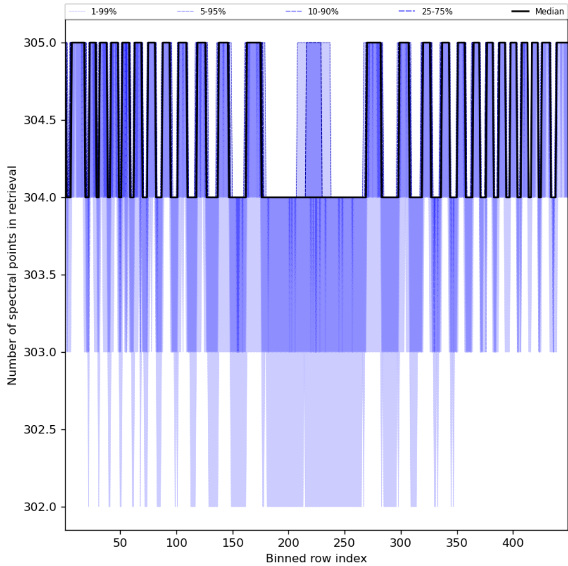
Figure 50: Along track statistics of “Number of spectral points in retrieval” for 2023-10-02 to 2023-10-04
