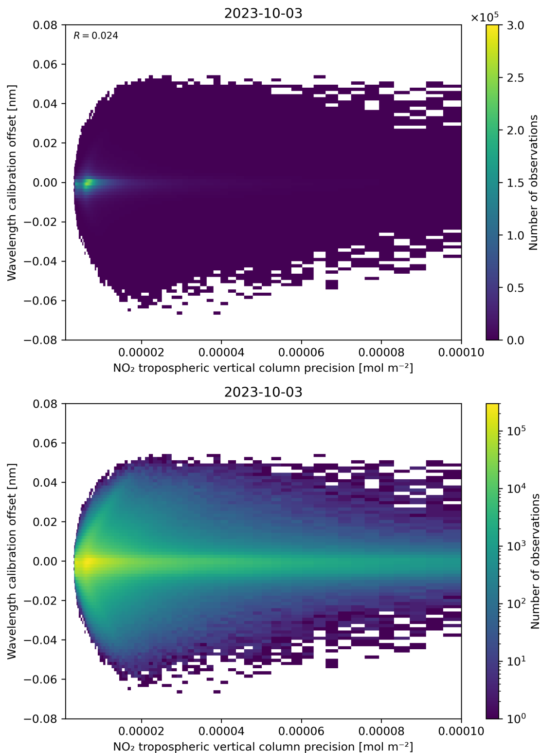
Figure 141: Scatter density plot of “NO 2 tropospheric vertical column precision” against “Wavelength calibration offset” for 2023-10-02 to 2023-10-04.
