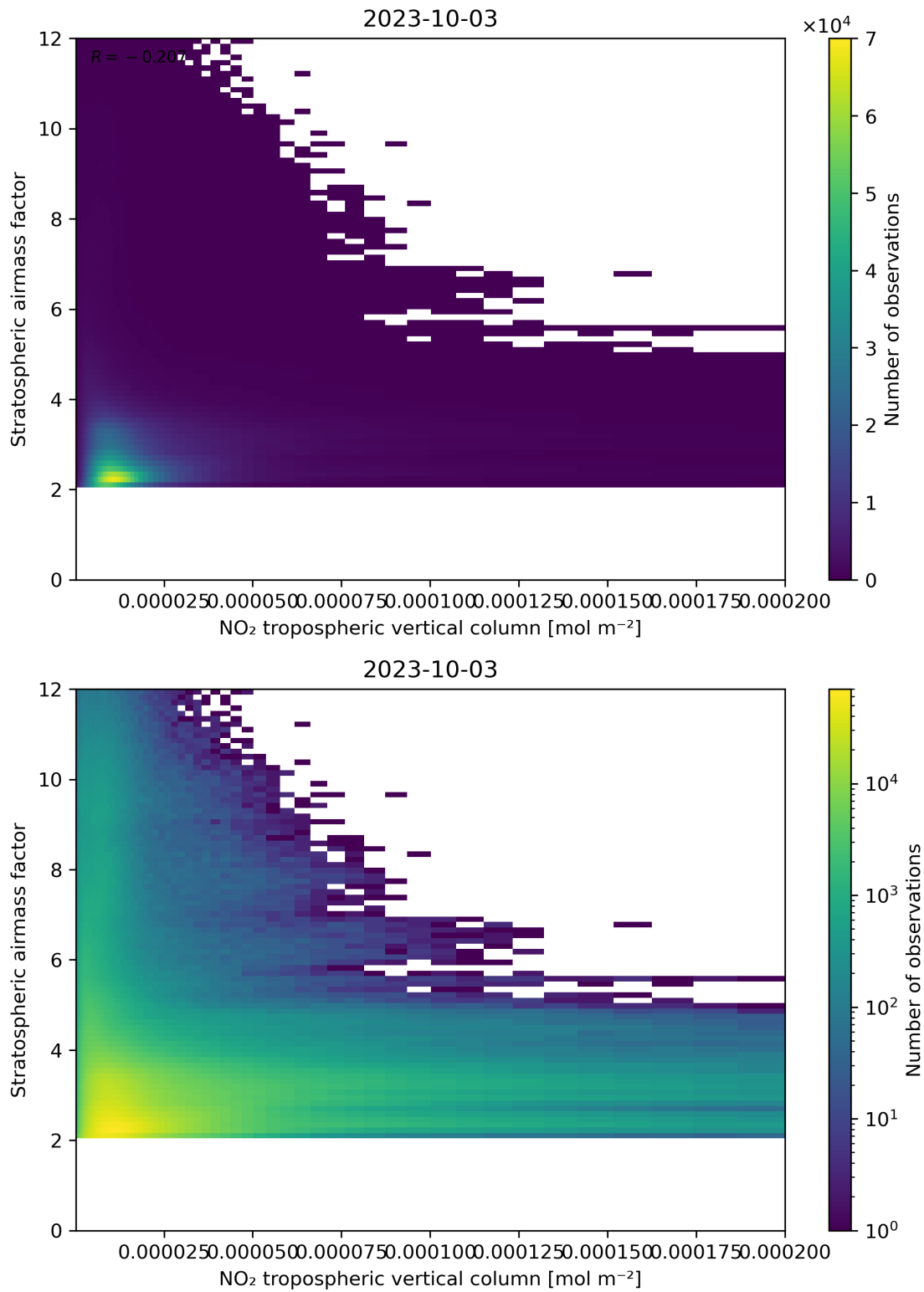
Figure 121: Scatter density plot of “NO 2 tropospheric vertical column” against “Stratospheric air mass factor” for 2023-10-02 to 2023-10-04.
