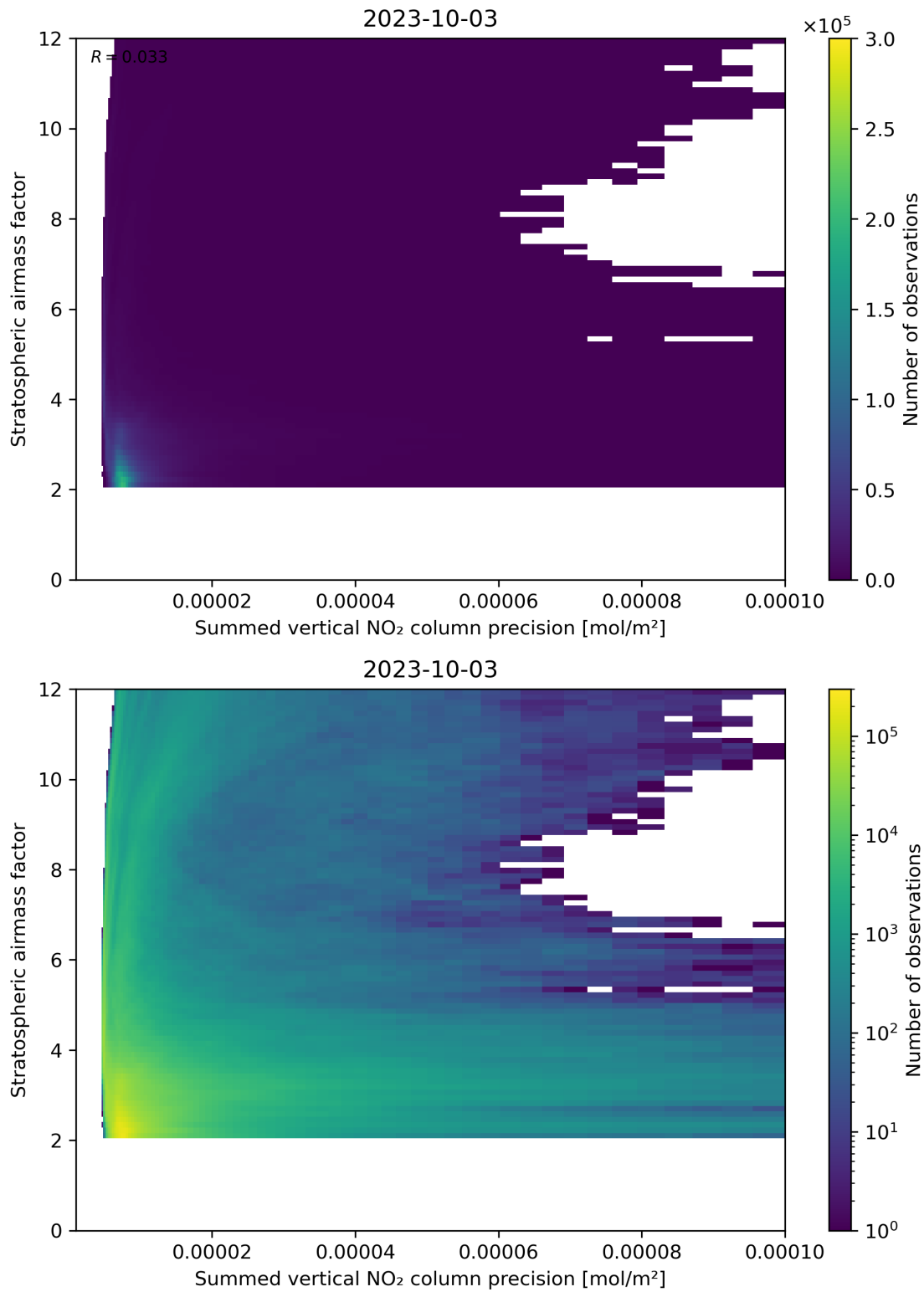
Figure 106: Scatter density plot of “Summed vertical NO 2 column precision” against “Stratospheric airmass factor” for 2023-10-02 to 2023-10-04.
