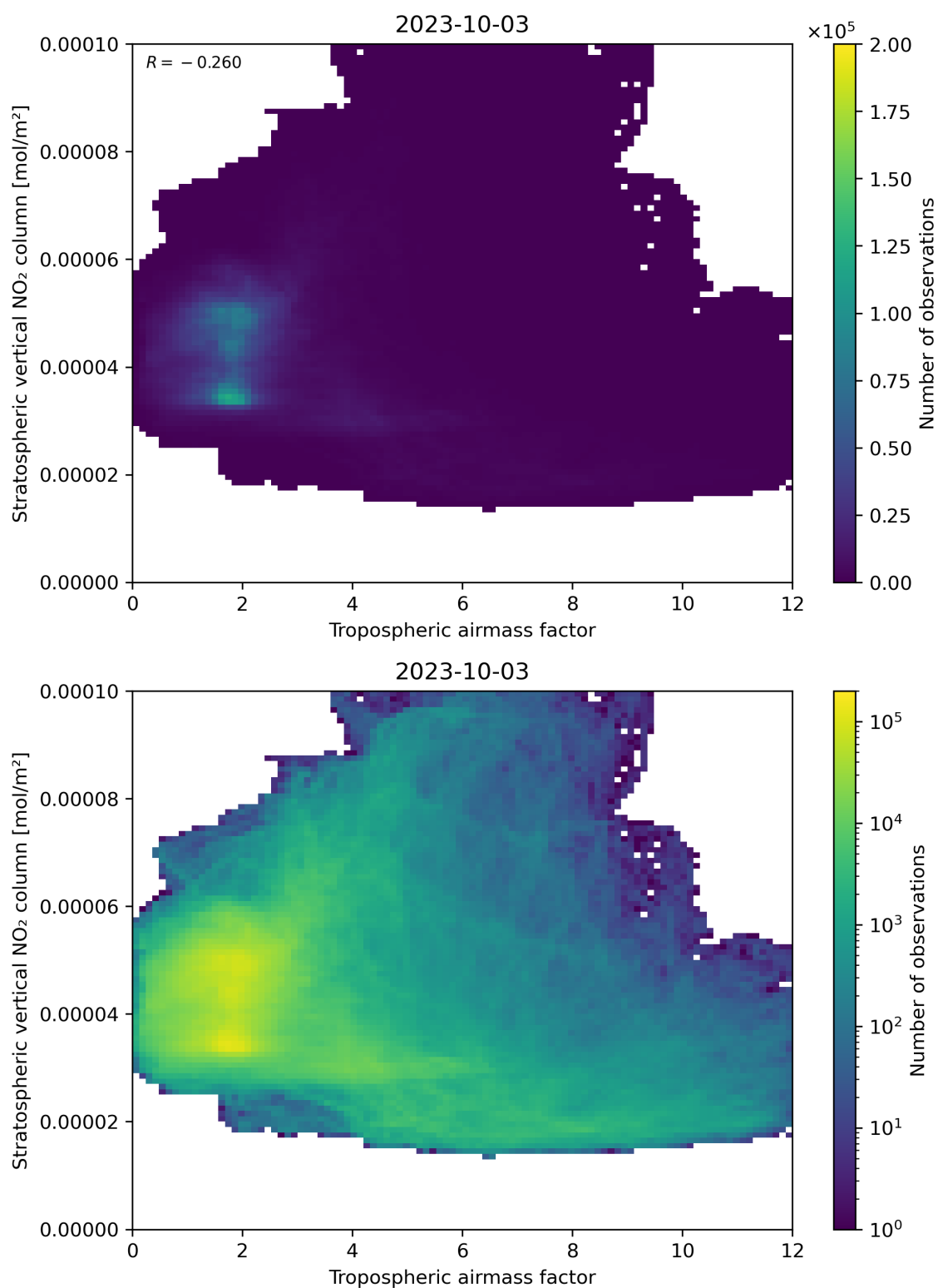
Figure 74: Scatter density plot of “Tropospheric air mass factor” against “Stratospheric vertical NO 2 column” for 2023-10-02 to 2023-10-04.
