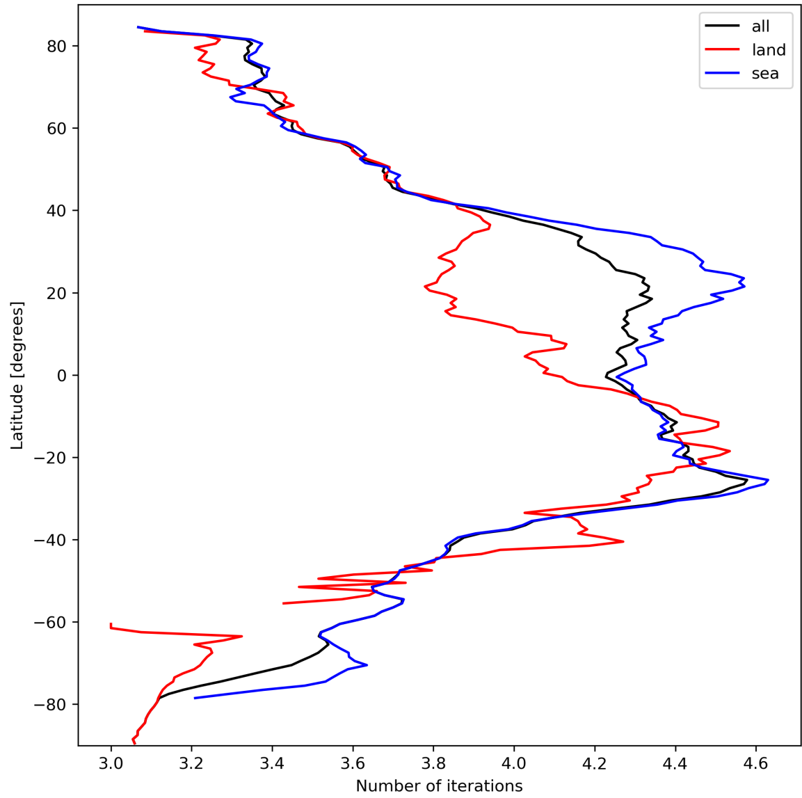
Figure 17: Zonal average of “Number of iterations” for 2023-10-02 to 2023-10-04.
