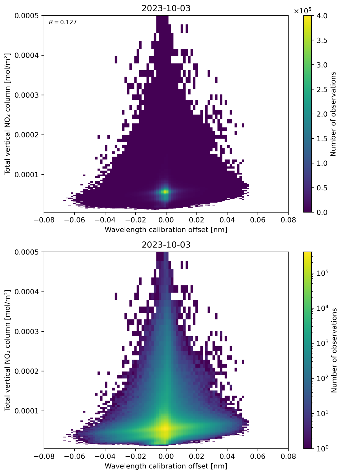
Figure 179: Scatter density plot of “Wavelength calibration offset” against “Total vertical NO 2 column” for 2023-10-02 to 2023-10-04.
