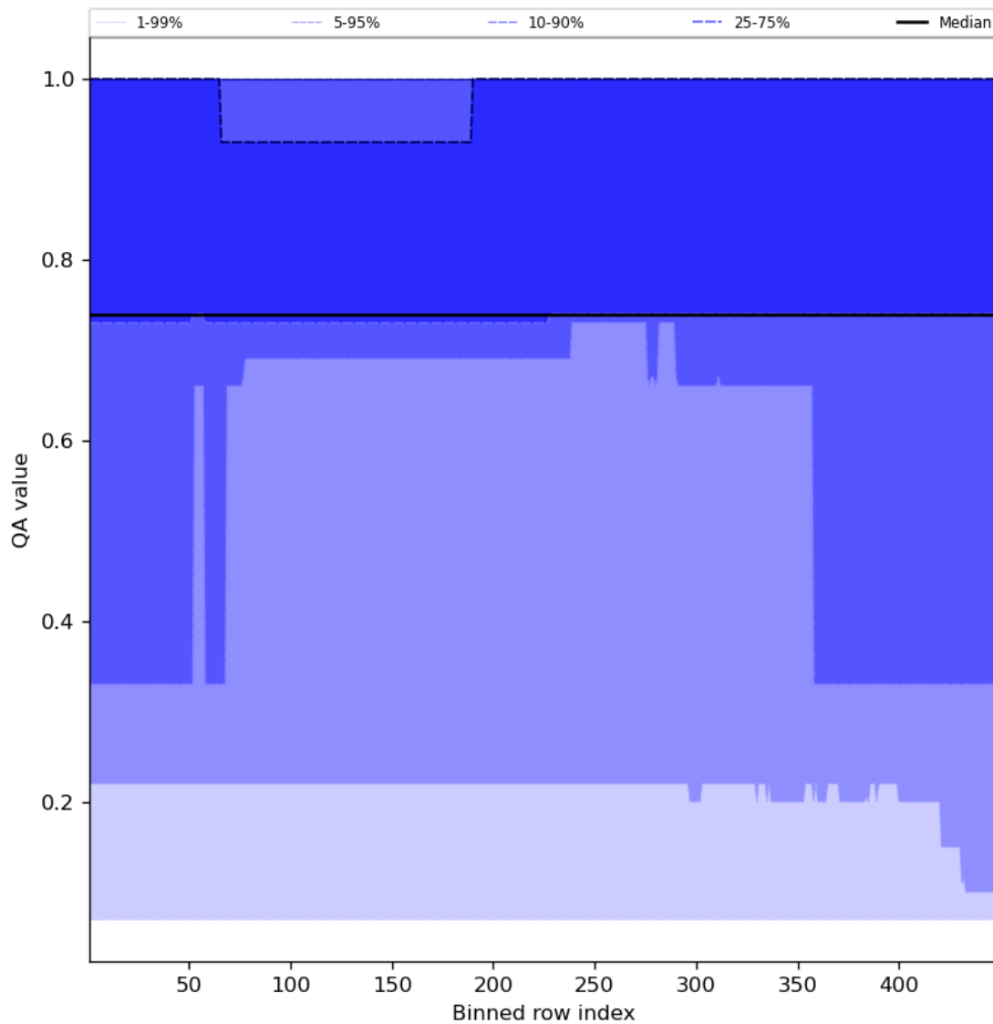
Figure 45: Along track statistics of “QA value” for 2023-10-02 to 2023-10-04
