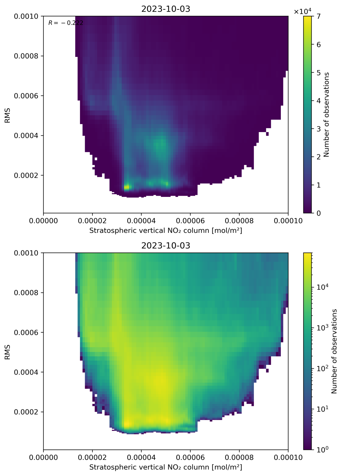
Figure 102: Scatter density plot of “Stratospheric vertical NO 2 column” against “RMS” for 2023-10-02 to 2023-10-04.
