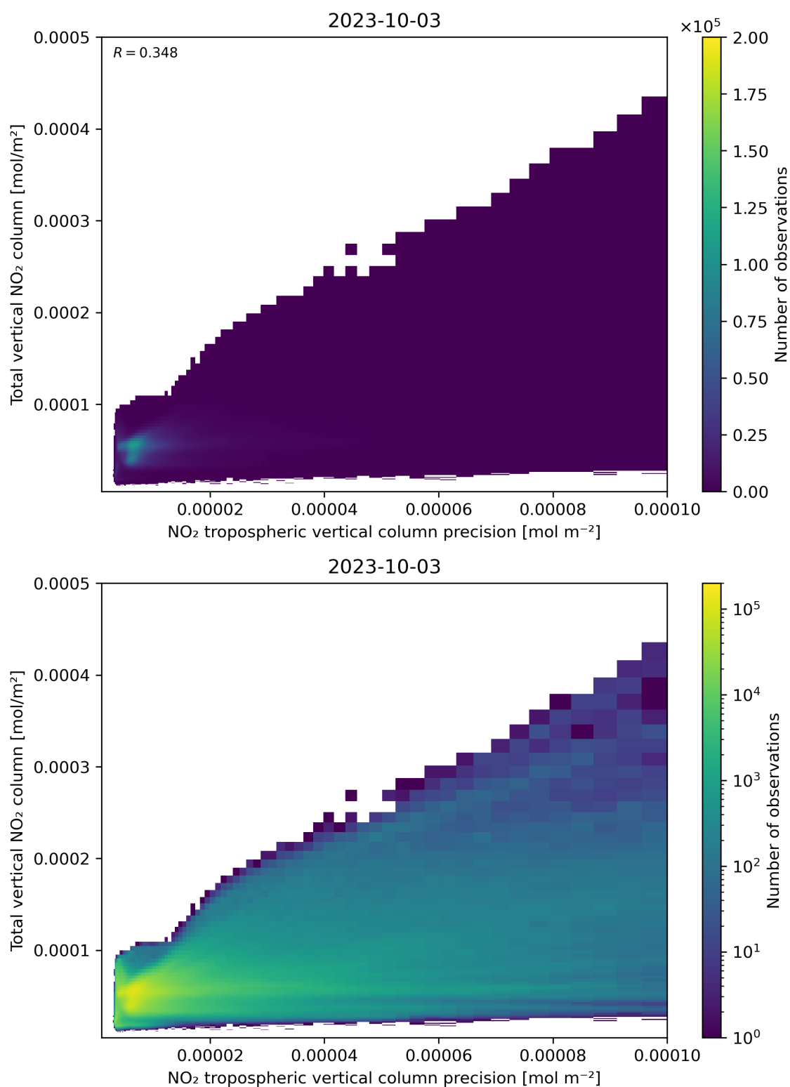
Figure 138: Scatter density plot of “NO 2 tropospheric vertical column precision” against “Total vertical NO 2 column” for 2023-10-02 to 2023-10-04.
