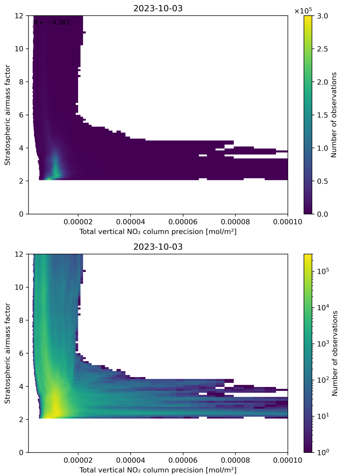
Figure 115: Scatter density plot of “Total vertical NO 2 column precision” against “Stratospheric air mass factor” for 2023-10-02 to 2023-10-04.
