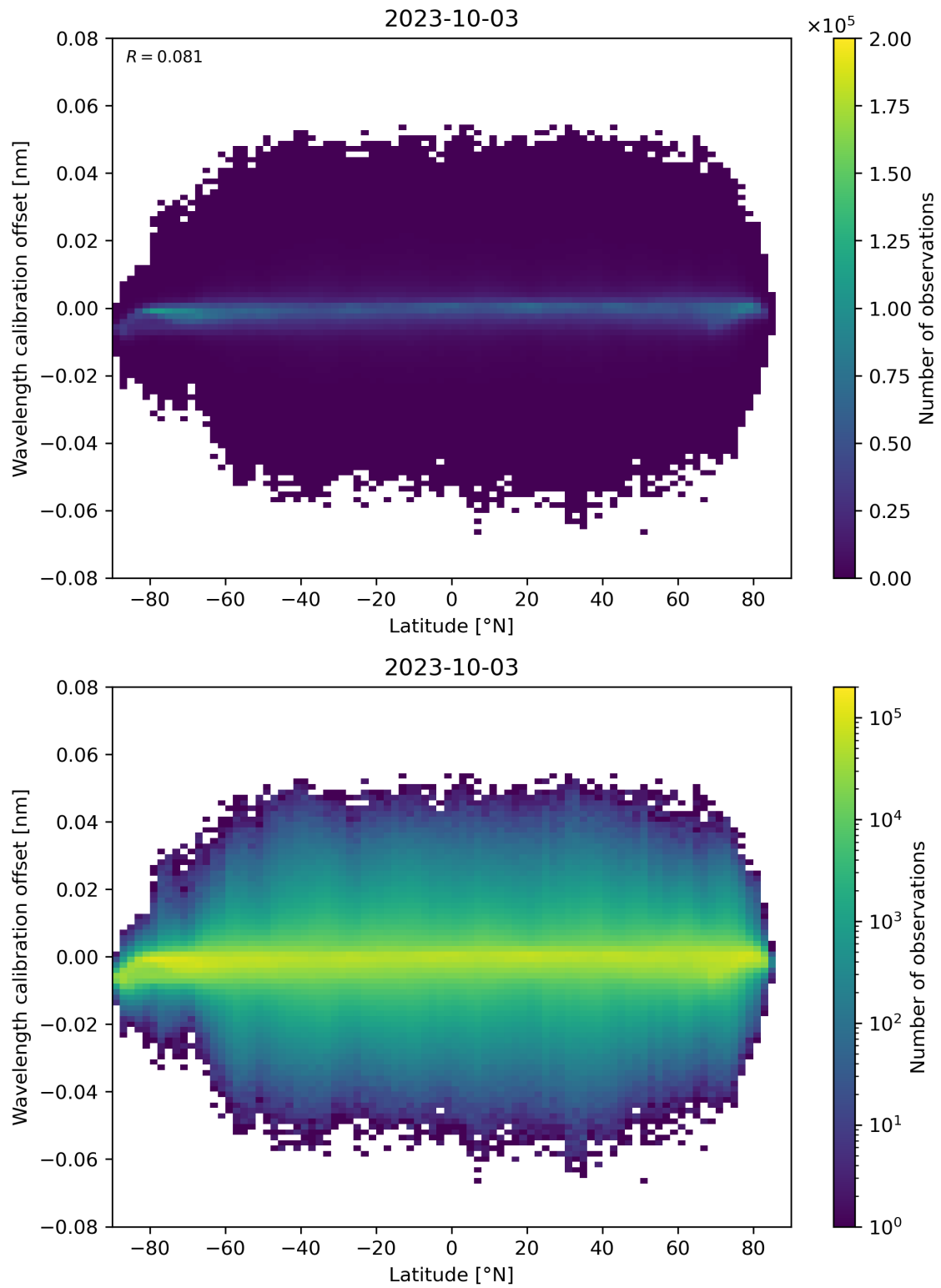
Figure 95: Scatter density plot of “Latitude” against “Wavelength calibration offset” for 2023-10-02 to 2023-10-04.
