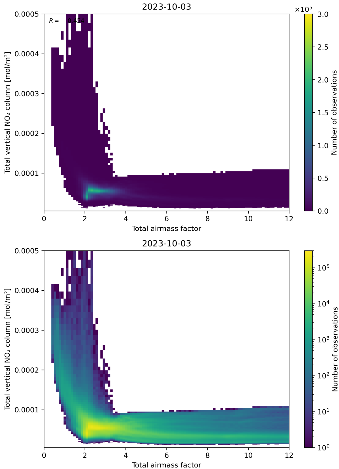
Figure 67: Scatter density plot of “Total airmass factor” against “Total vertical NO 2 column” for 2023-10-02 to 2023-10-04.
