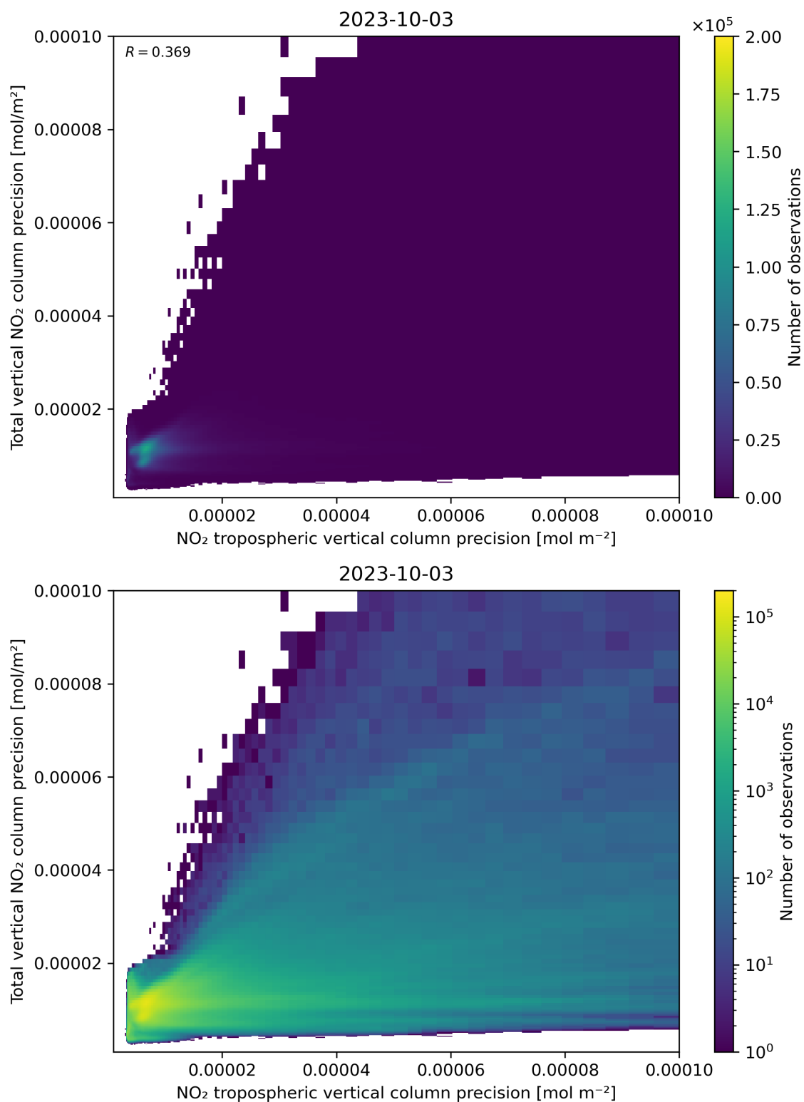
Figure 139: Scatter density plot of “NO 2 tropospheric vertical column precision” against “Total vertical NO 2 column precision” for 2023-10-02 to 2023-10-04.
