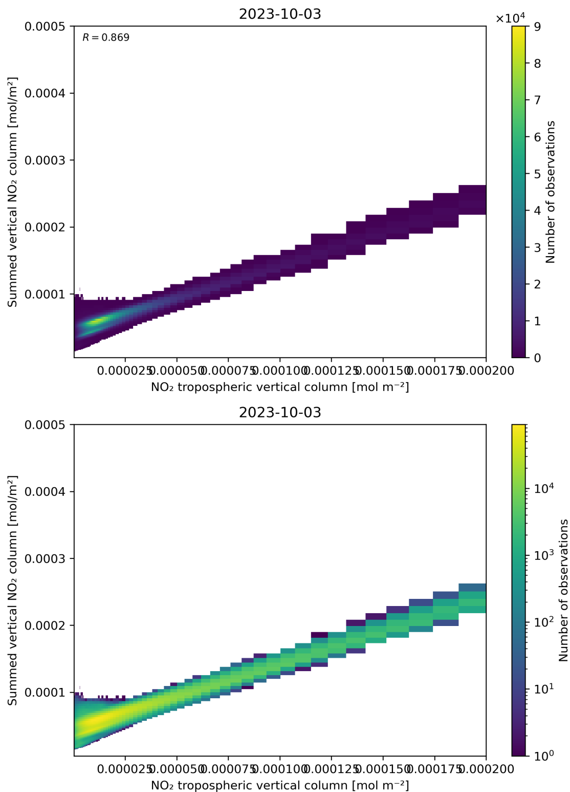
Figure 126: Scatter density plot of “NO 2 tropospheric vertical column” against “Summed vertical NO 2 column” for 2023-10-02 to 2023-10-04.
