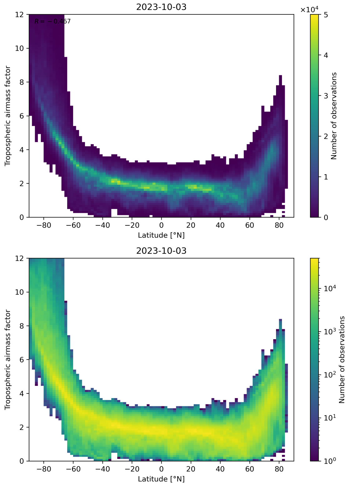
Figure 85: Scatter density plot of “Latitude” against “Tropospheric airmass factor” for 2023-10-02 to 2023-10-04.
