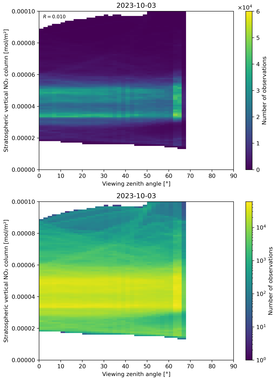
Figure 164: Scatter density plot of “Viewing zenith angle” against “Stratospheric vertical NO 2 column” for 2023-10-02 to 2023-10-04.
