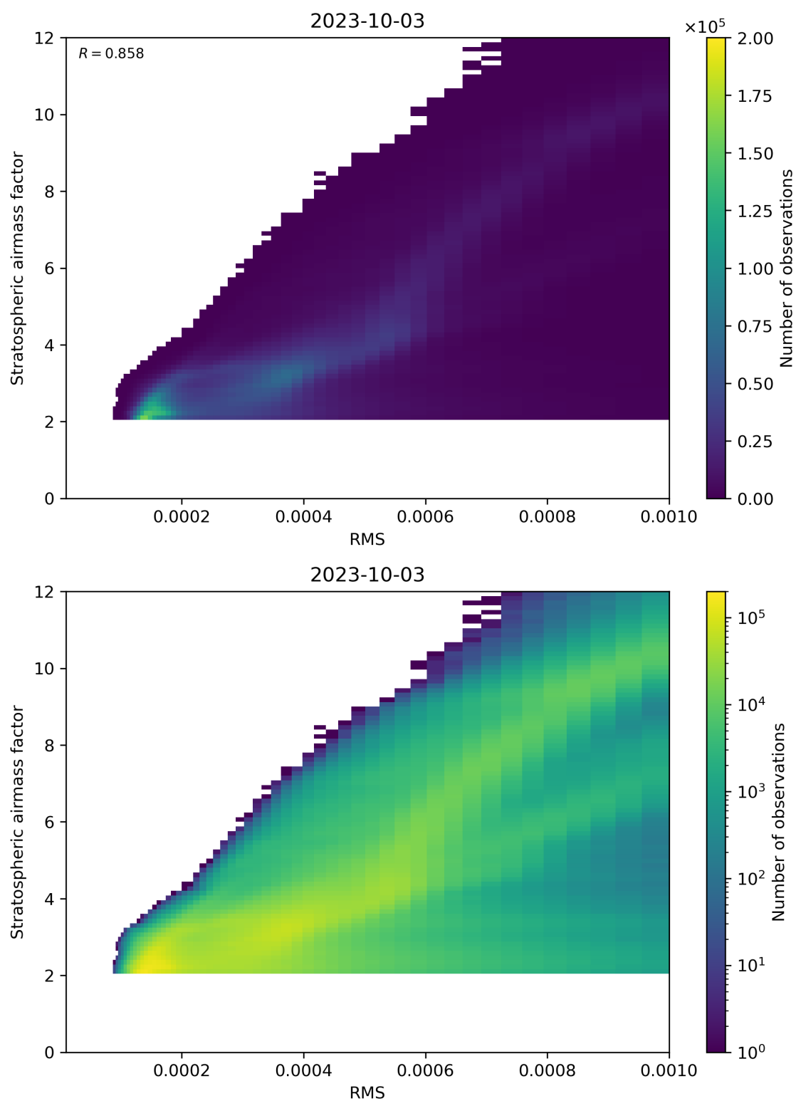
Figure 144: Scatter density plot of “RMS” against “Stratospheric airmass factor” for 2023-10-02 to 2023-10-04.
