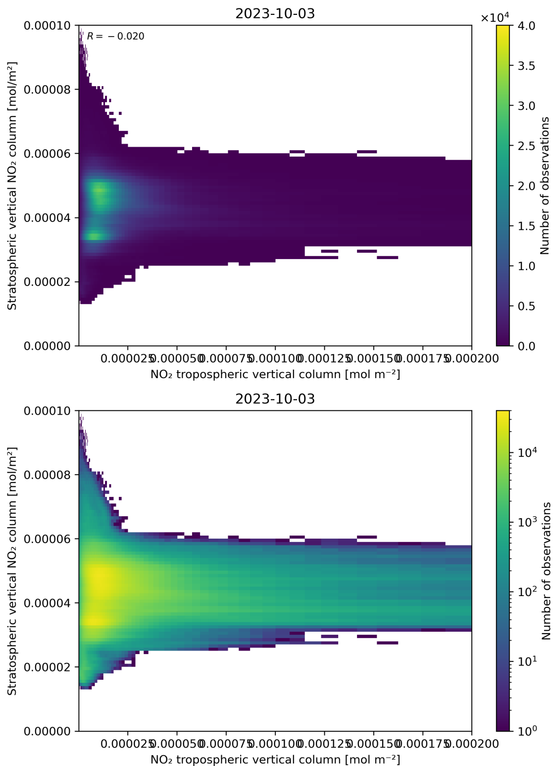
Figure 125: Scatter density plot of “NO 2 tropospheric vertical column” against “Stratospheric vertical NO 2 column” for 2023-10-02 to 2023-10-04.
