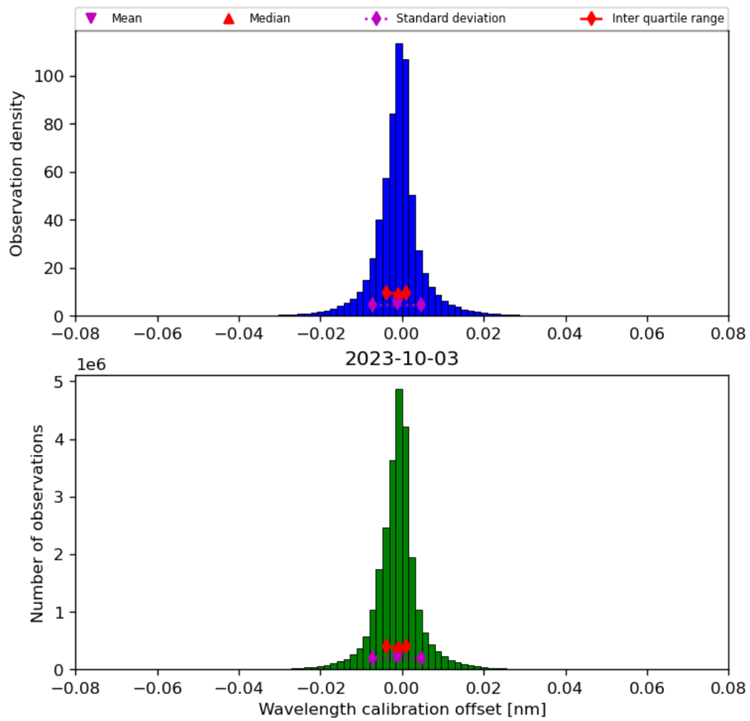
Figure 35: Histogram of “Wavelength calibration offset” for 2023-10-02 to 2023-10-04
