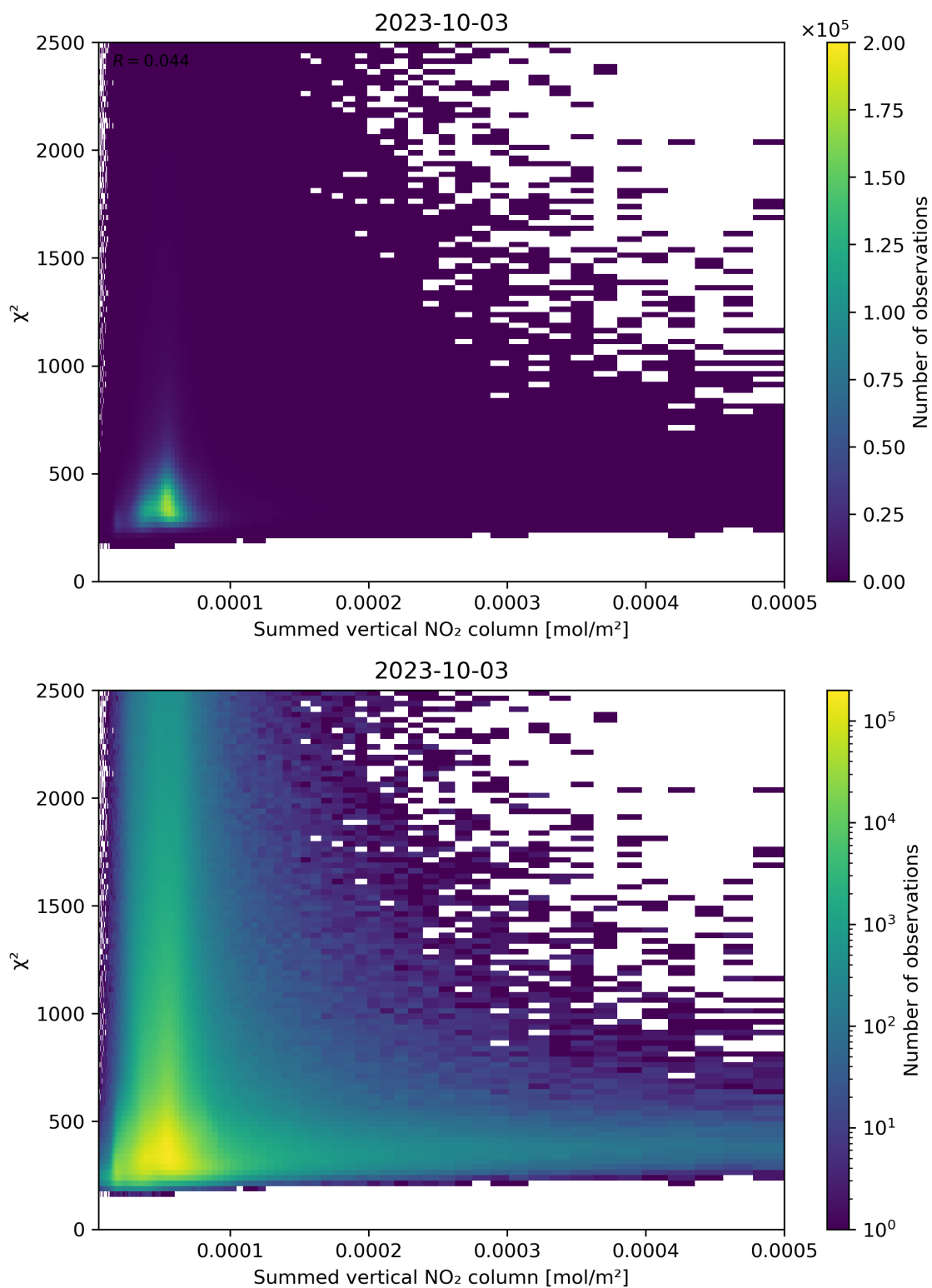
Figure 104: Scatter density plot of “Summed vertical NO 2 column” against “ \chi^2 ” for 2023-10-02 to 2023-10-04.
