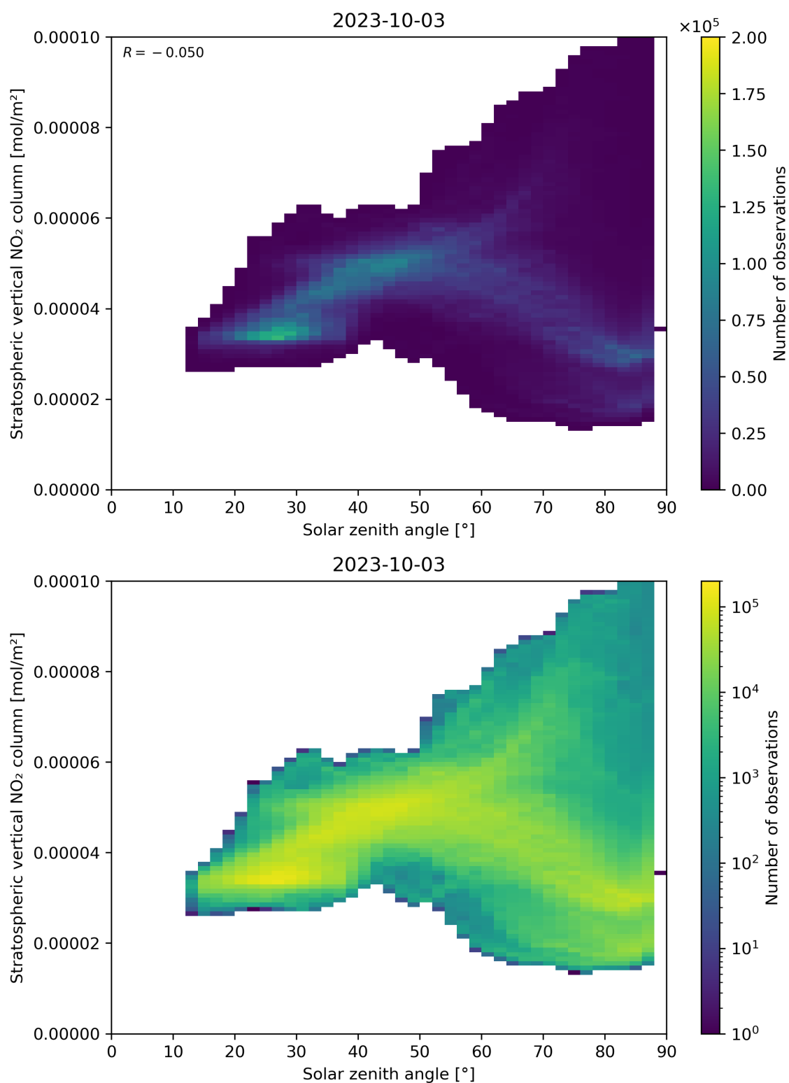
Figure 150: Scatter density plot of “Solar zenith angle” against “Stratospheric vertical NO 2 column” for 2023-10-02 to 2023-10-04.
