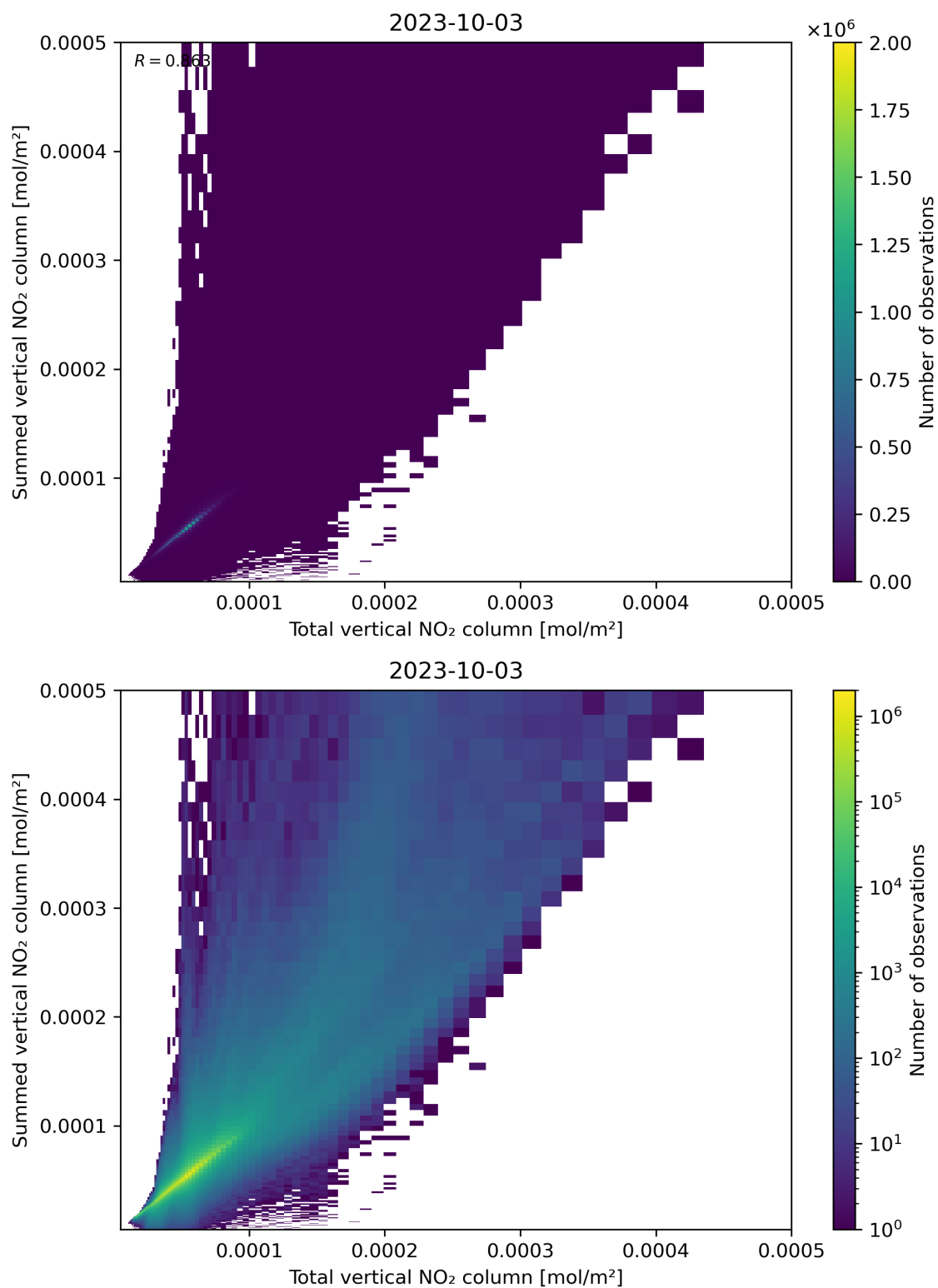
Figure 112: Scatter density plot of “Total vertical NO 2 column” against “Summed vertical NO 2 column” for 2023-10-02 to 2023-10-04.
