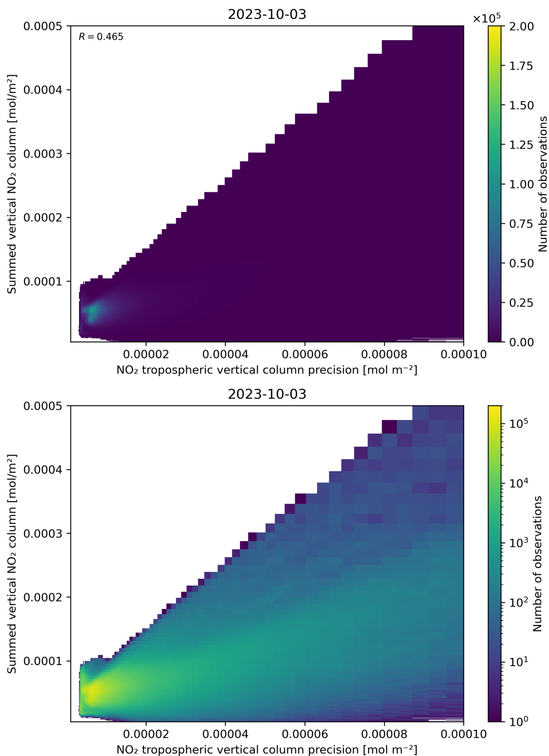
Figure 136: Scatter density plot of “NO 2 tropospheric vertical column precision” against “Summed vertical NO 2 column” for 2023-10-02 to 2023-10-04.
