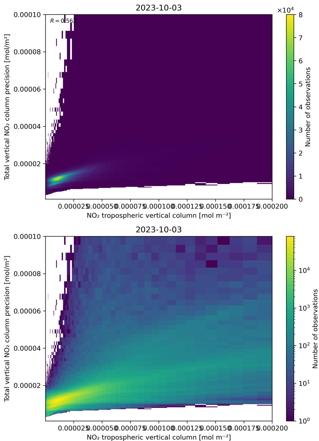
Figure 129: Scatter density plot of “NO 2 tropospheric vertical column” against “Total vertical NO 2 column precision” for 2023-10-02 to 2023-10-04.
