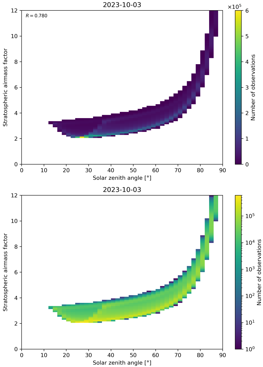
Figure 145: Scatter density plot of “Solar zenith angle” against “Stratospheric airmass factor” for 2023-10-02 to 2023-10-04.
