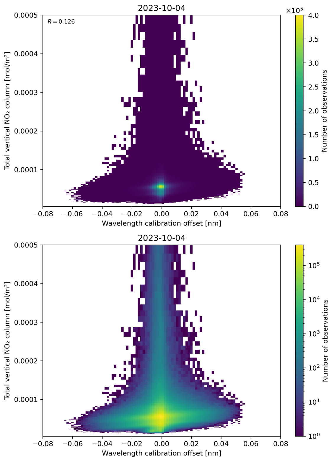
Figure 179: Scatter density plot of “Wavelength calibration offset” against “Total vertical NO 2 column” for 2023-10-03 to 2023-10-05.
