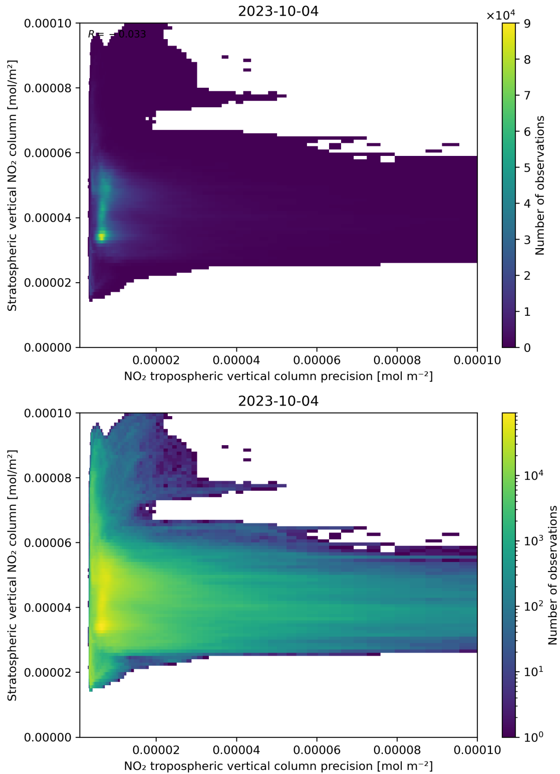
Figure 135: Scatter density plot of “NO 2 tropospheric vertical column precision” against “Stratospheric vertical NO 2 column” for 2023-10-03 to 2023-10-05.
