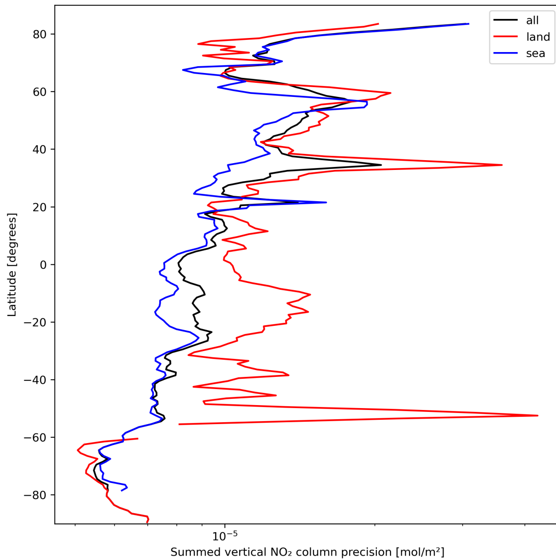
Figure 24: Zonal average of “Summed vertical NO 2 column precision” for 2023-10-03 to 2023-10-05.
