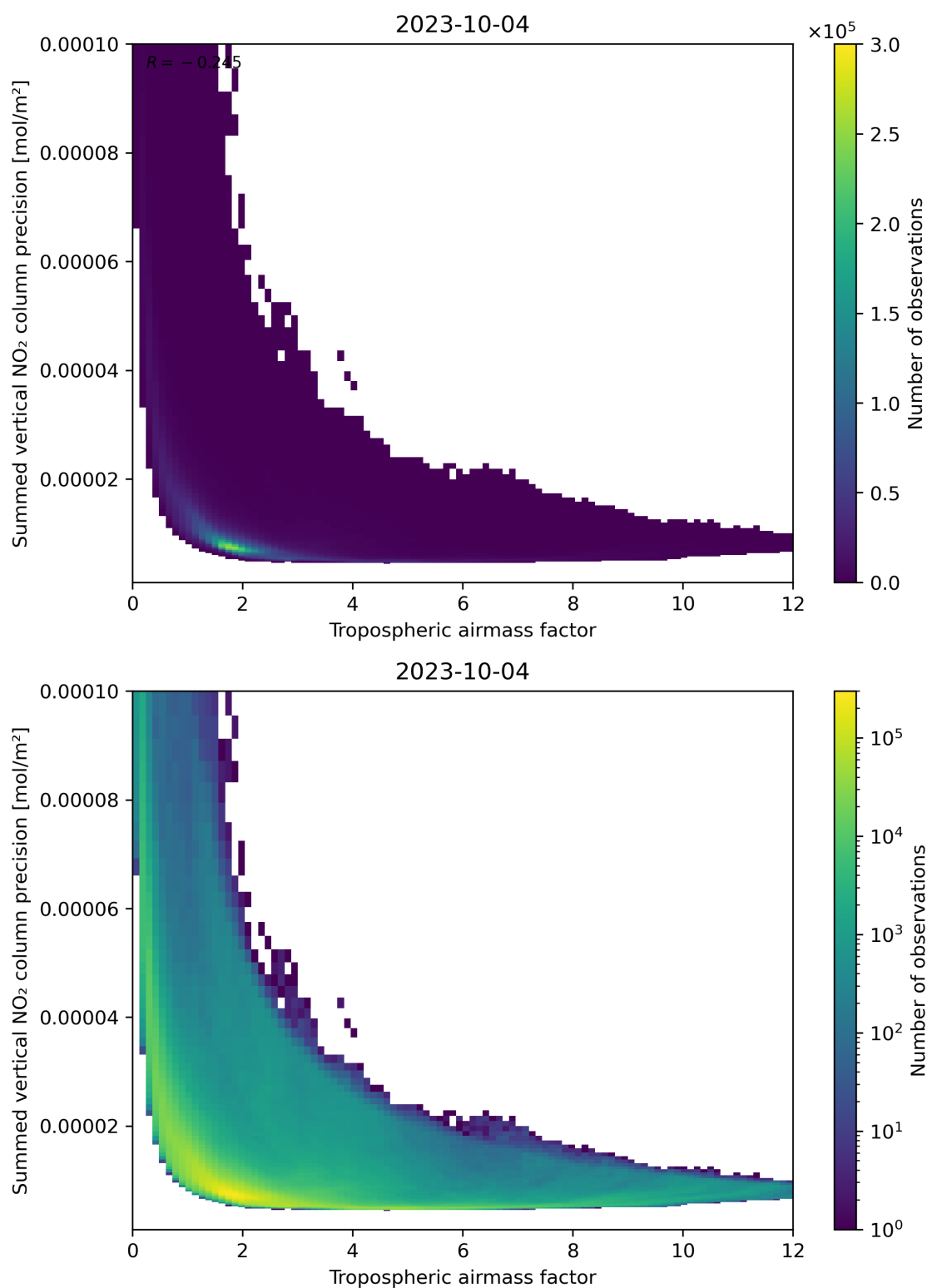
Figure 76: Scatter density plot of “Tropospheric air mass factor” against “Summed vertical NO 2 column precision” for 2023-10-03 to 2023-10-05.
