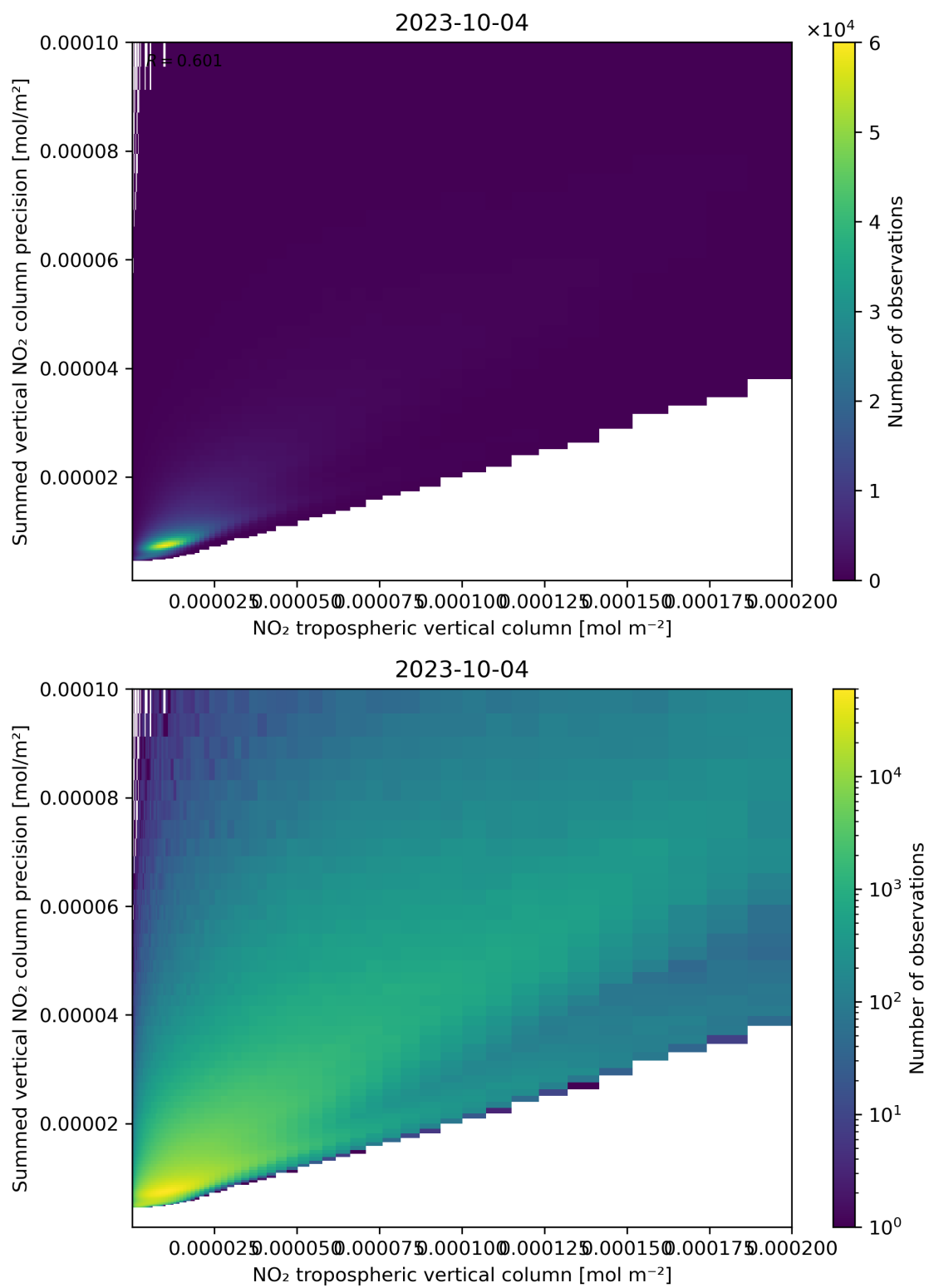
Figure 127: Scatter density plot of “NO 2 tropospheric vertical column” against “Summed vertical NO 2 column precision” for 2023-10-03 to 2023-10-05.
