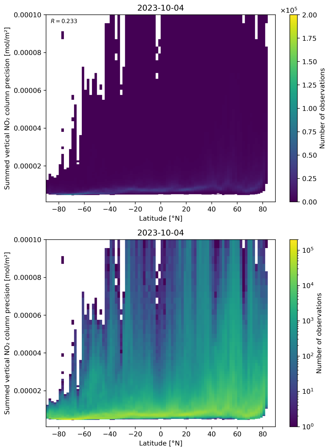
Figure 89: Scatter density plot of “Latitude” against “Summed vertical NO 2 column precision” for 2023-10-03 to 2023-10-05.
