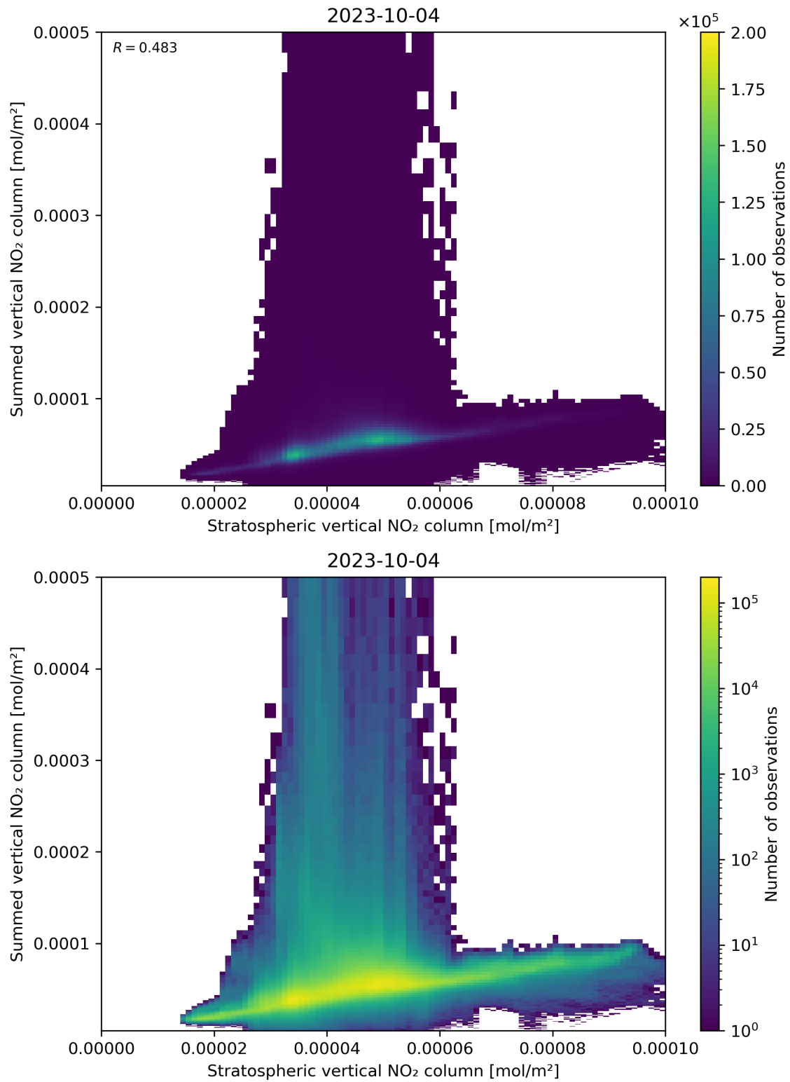
Figure 98: Scatter density plot of “Stratospheric vertical NO 2 column” against “Summed vertical NO 2 column” for 2023-10-03 to 2023-10-05.
