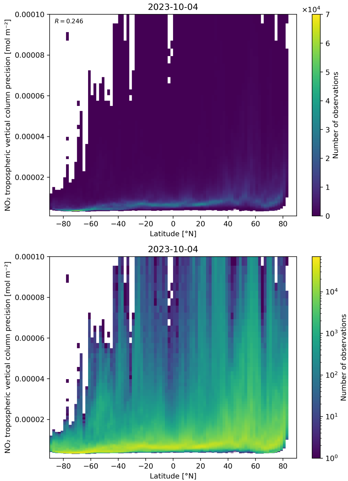
Figure 93: Scatter density plot of “Latitude” against “NO 2 tropospheric vertical column precision” for 2023-10-03 to 2023-10-05.
