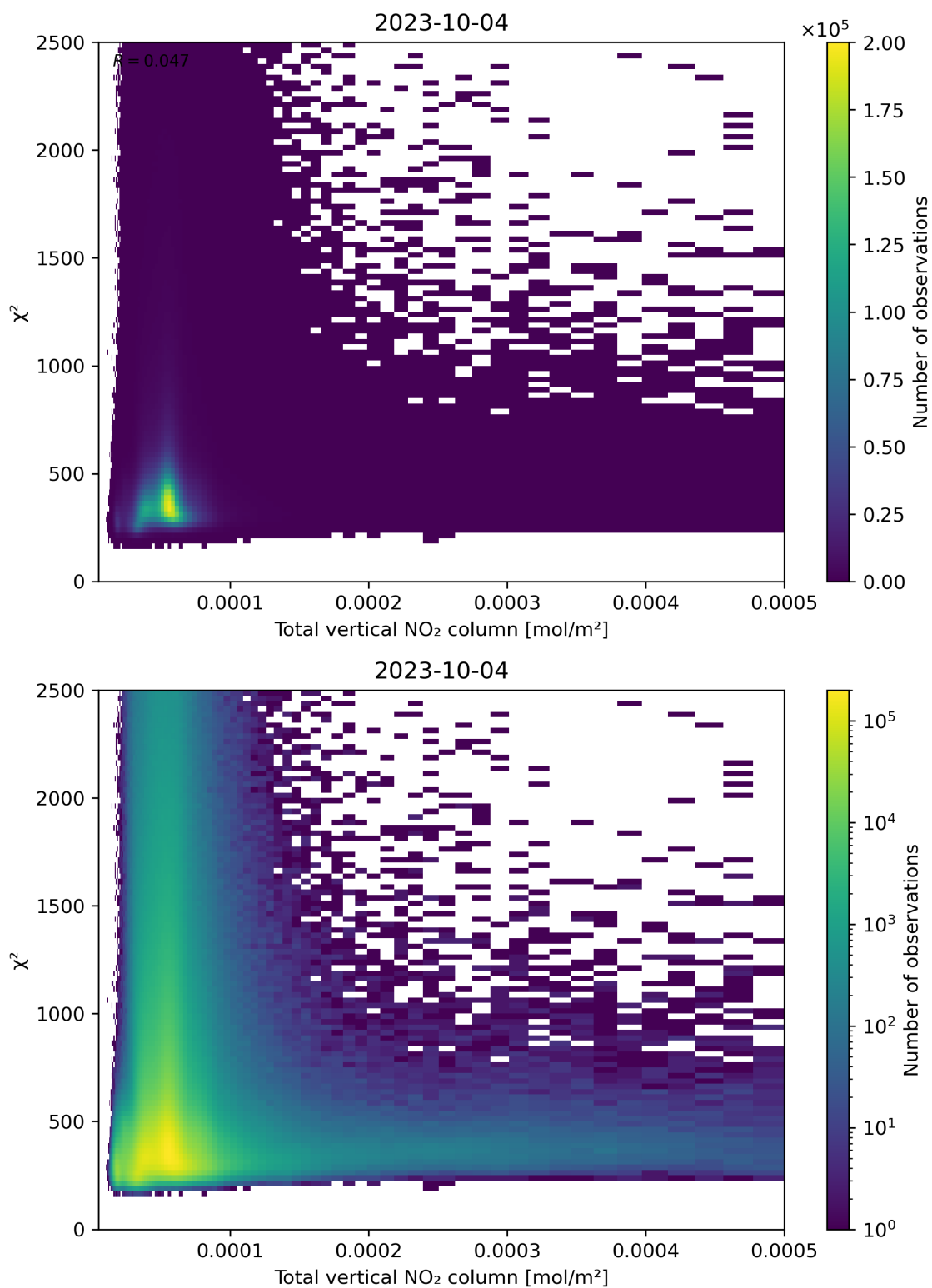
Figure 111: Scatter density plot of “Total vertical NO 2 column” against “ \chi^2 ” for 2023-10-03 to 2023-10-05.
