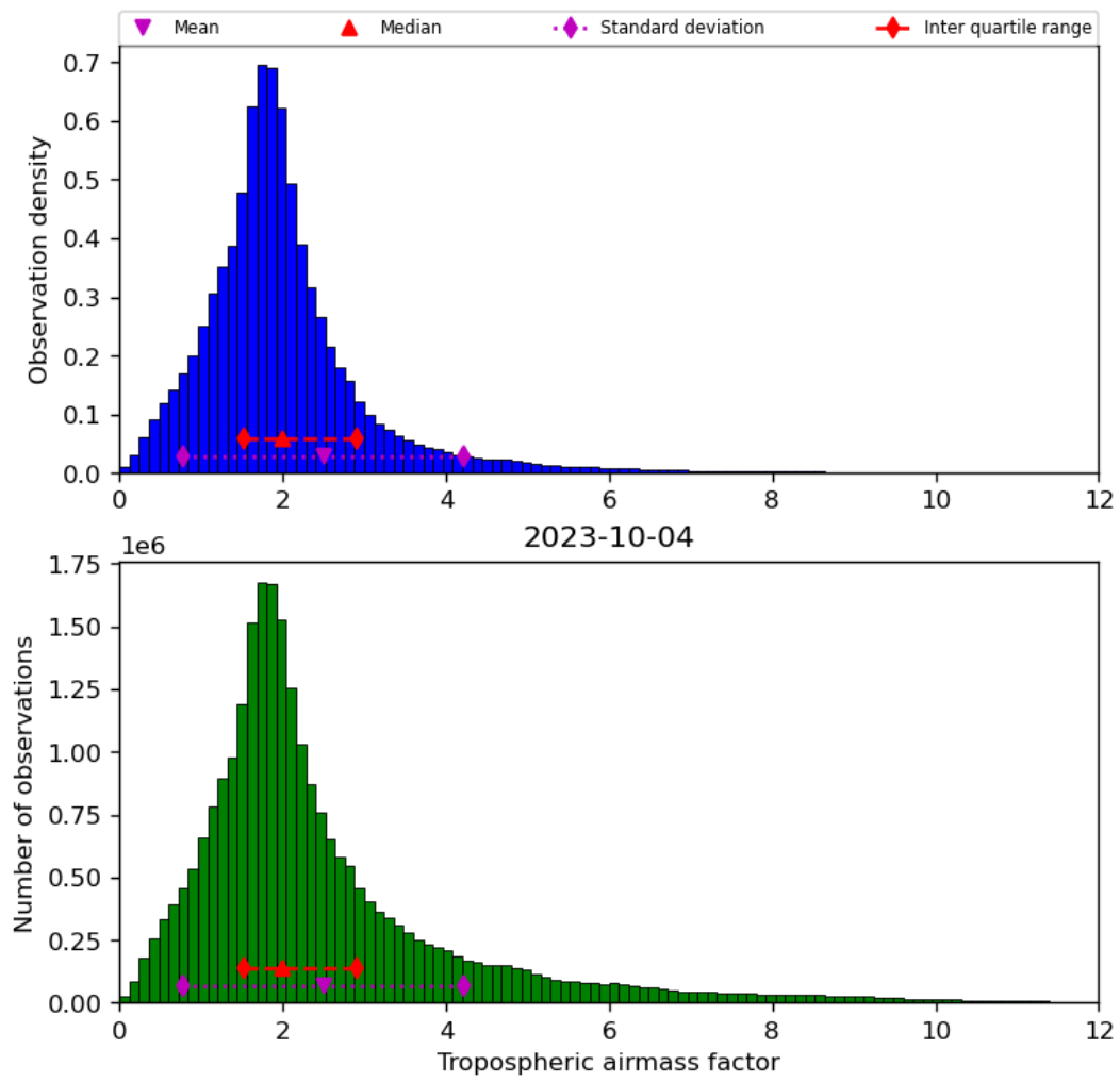
Figure 31: Histogram of “Tropospheric airmass factor” for 2023-10-03 to 2023-10-05
