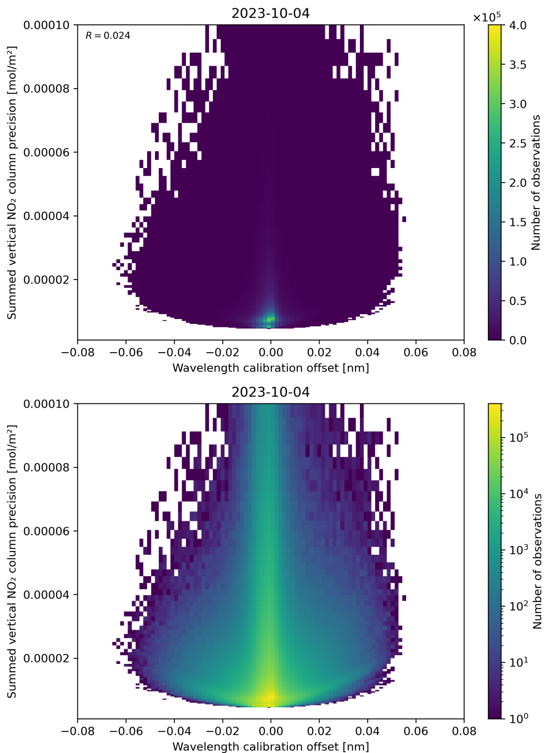
Figure 178: Scatter density plot of “Wavelength calibration offset” against “Summed vertical NO 2 column precision” for 2023-10-03 to 2023-10-05.
