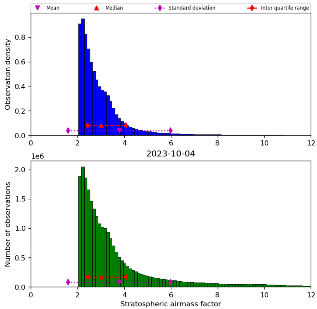
Figure 44: Histogram of “Stratospheric airmass factor” for 2023-10-03 to 2023-10-05
