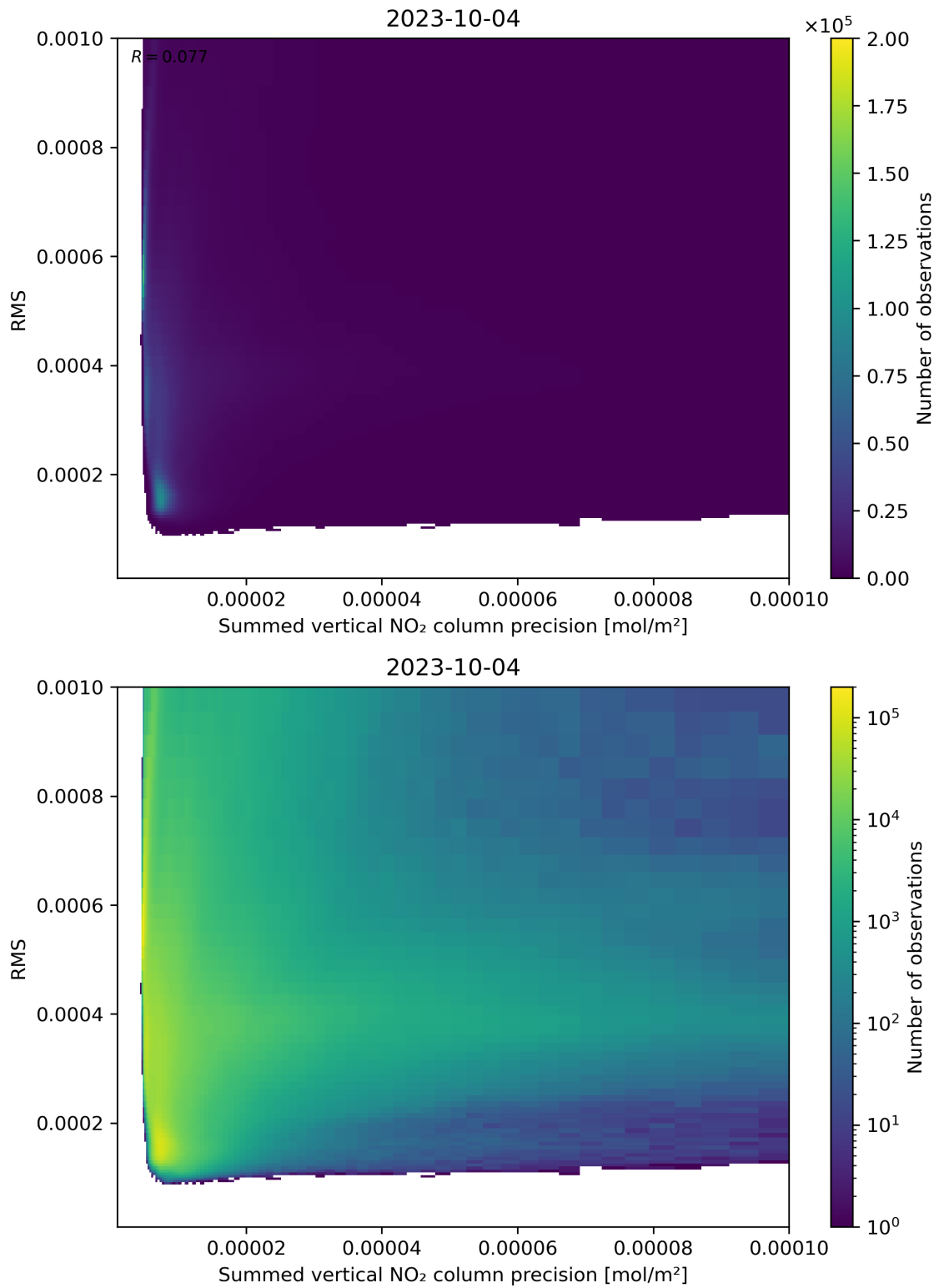
Figure 108: Scatter density plot of “Summed vertical NO 2 column precision” against “RMS” for 2023-10-03 to 2023-10-05.
