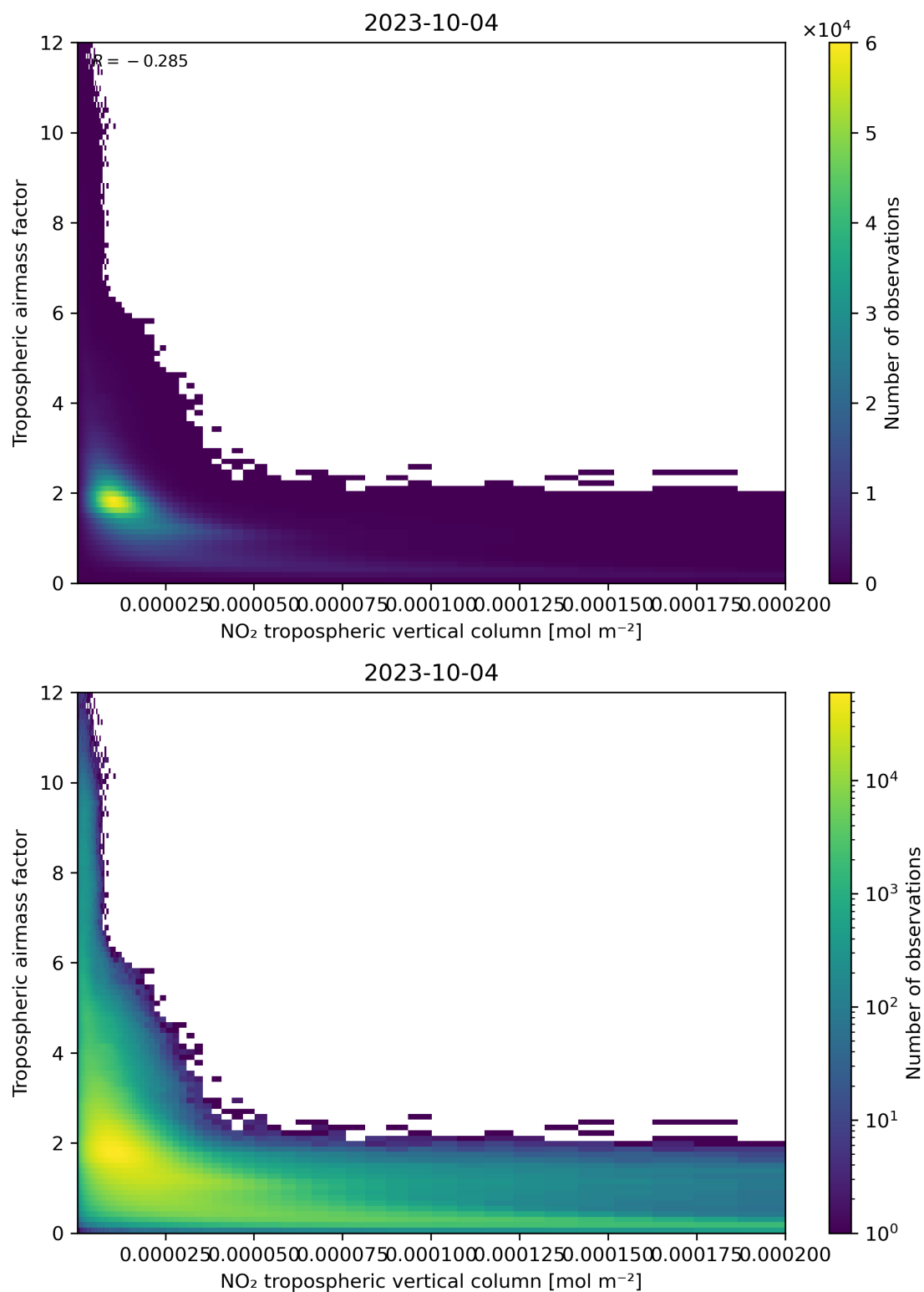
Figure 123: Scatter density plot of “NO 2 tropospheric vertical column” against “Tropospheric airmass factor” for 2023-10-03 to 2023-10-05.
