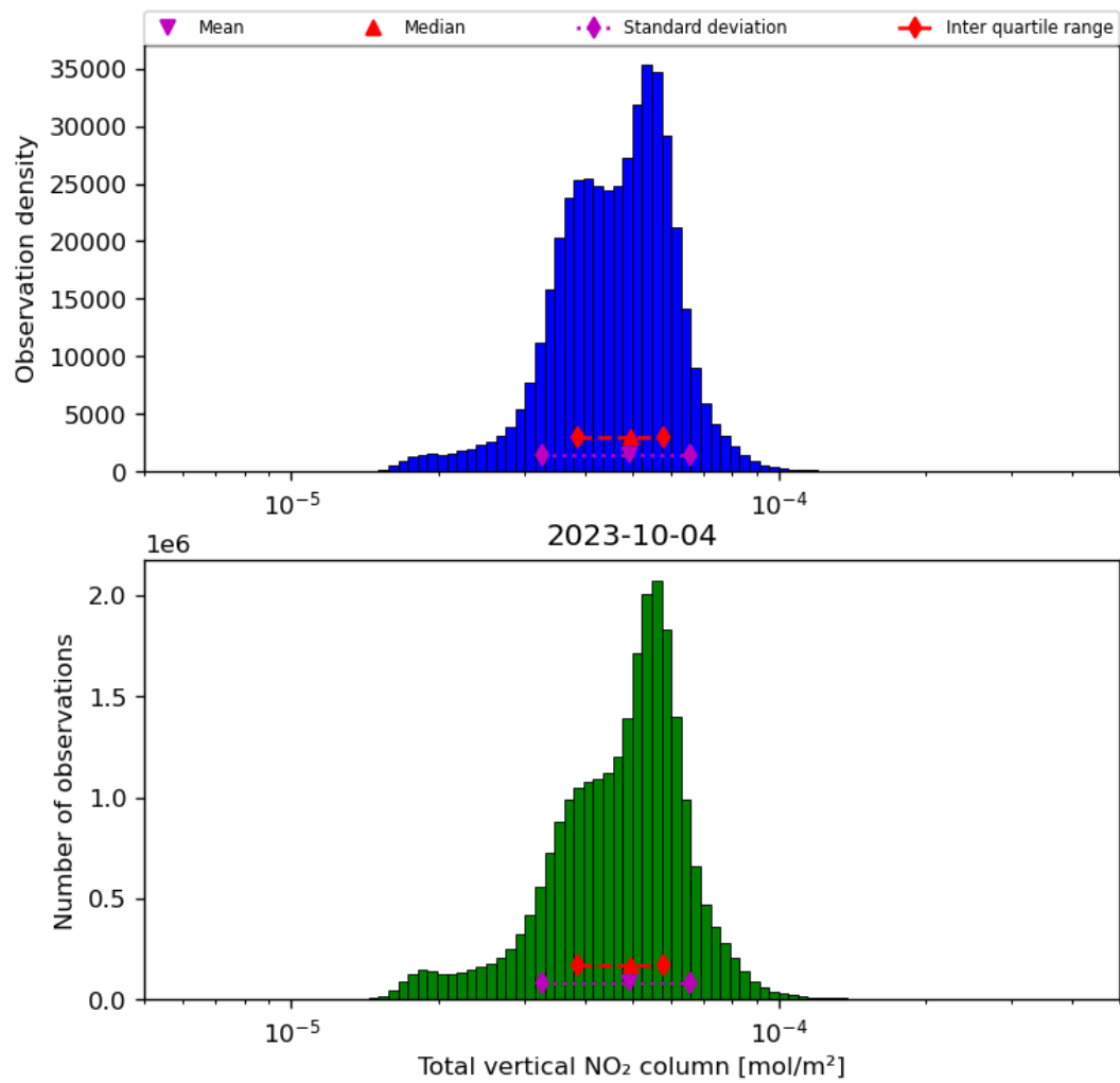
Figure 38: Histogram of “Total vertical NO 2 column” for 2023-10-03 to 2023-10-05
