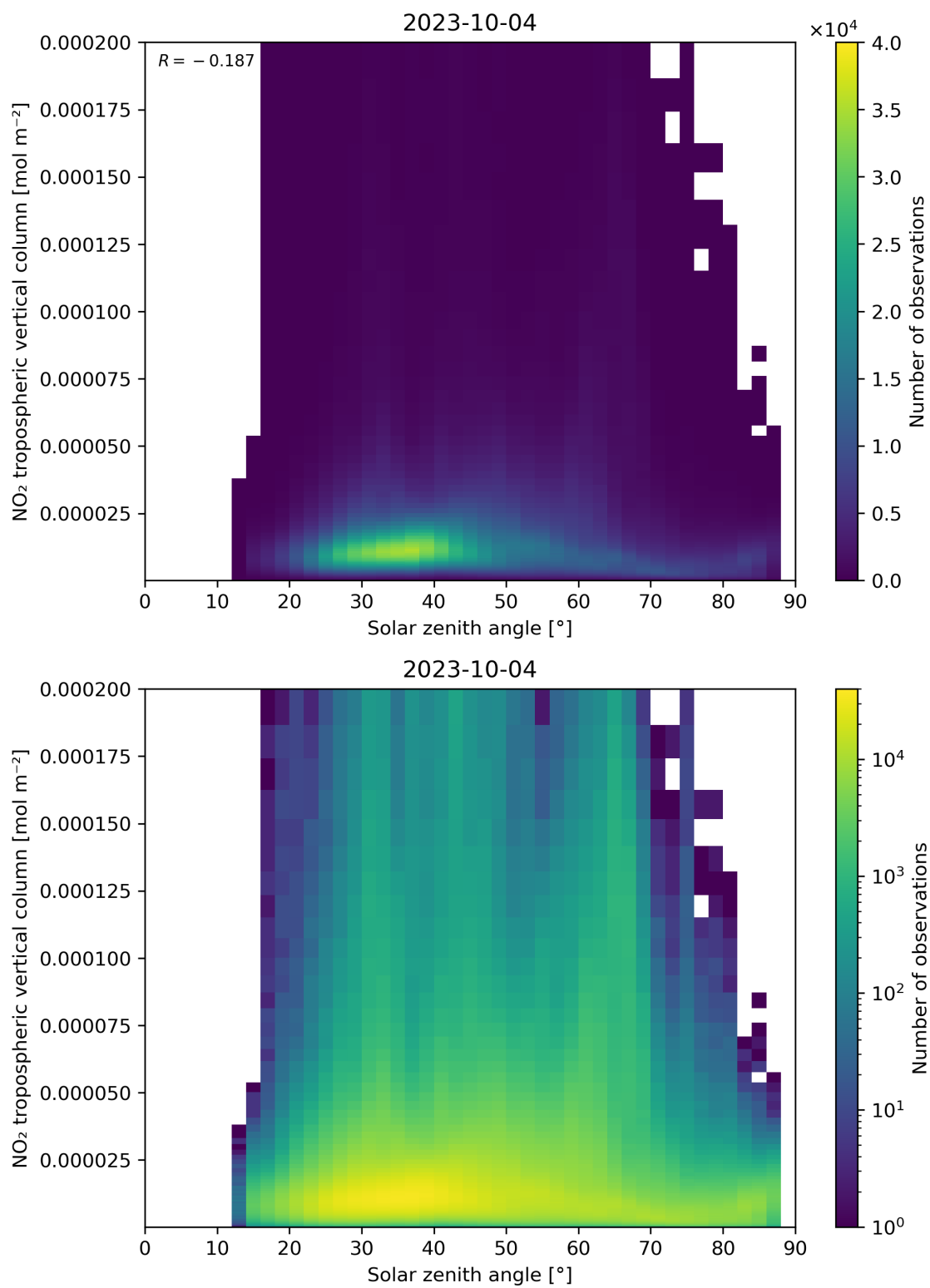
Figure 155: Scatter density plot of “Solar zenith angle” against “NO 2 tropospheric vertical column” for 2023-10-03 to 2023-10-05.
