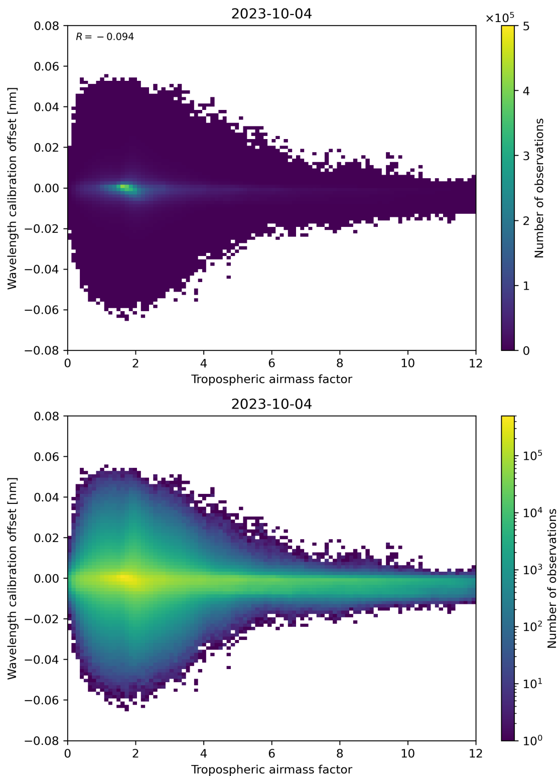
Figure 80: Scatter density plot of “Tropospheric air mass factor” against “Wavelength calibration offset” for 2023-10-03 to 2023-10-05.
