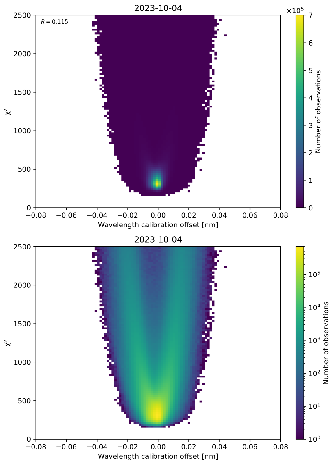
Figure 175: Scatter density plot of “Wavelength calibration offset” against “ \chi^2 ” for 2023-10-03 to 2023-10-05.
