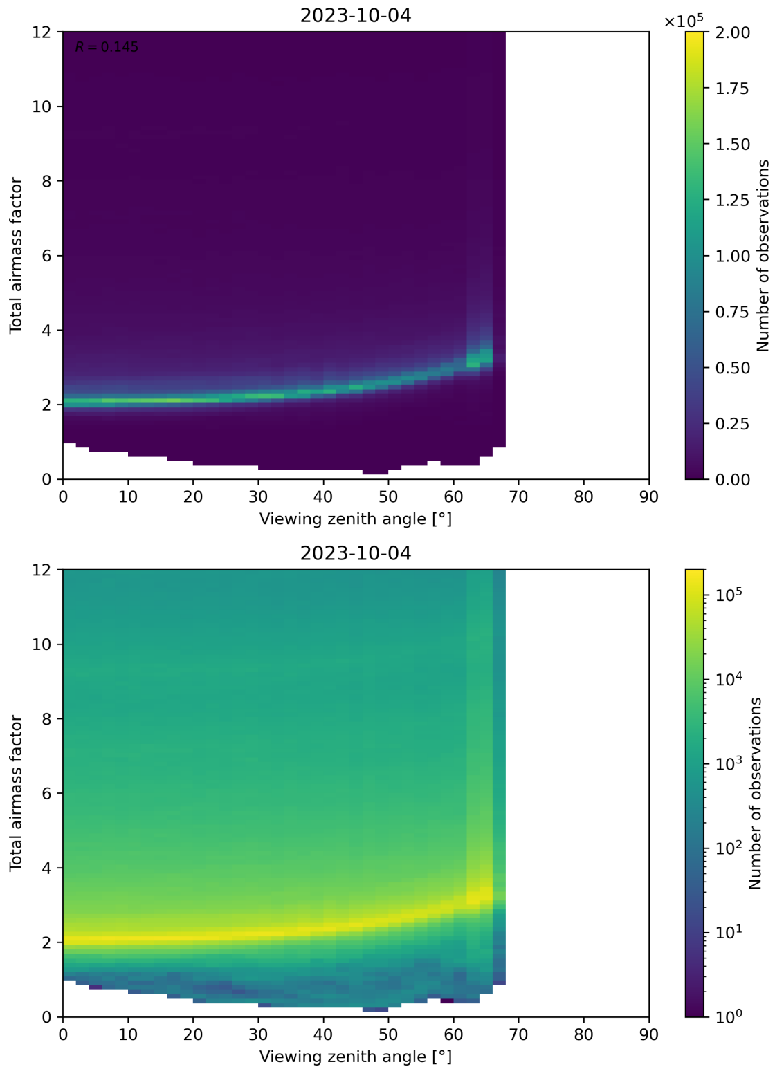
Figure 160: Scatter density plot of “Viewing zenith angle” against “Total airmass factor” for 2023-10-03 to 2023-10-05.
