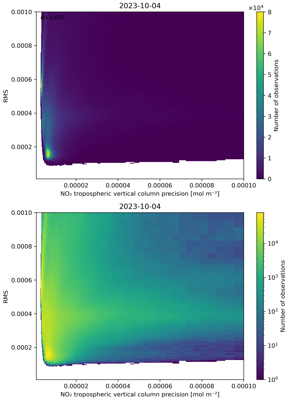
Figure 140: Scatter density plot of “NO 2 tropospheric vertical column precision” against “RMS” for 2023-10-03 to 2023-10-05.
