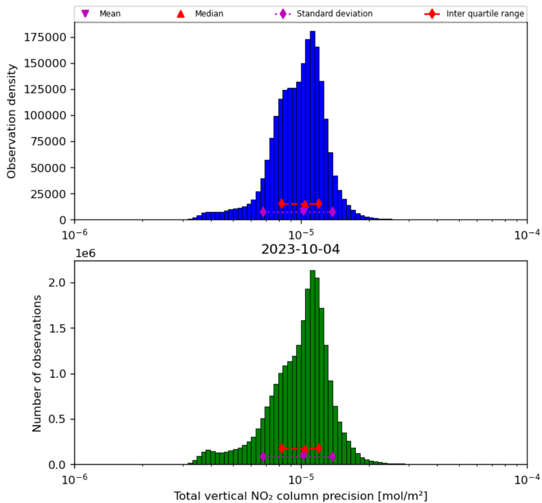
Figure 39: Histogram of "Total vertical NO 2 column precision" for 2023-10-03 to 2023-10-05
