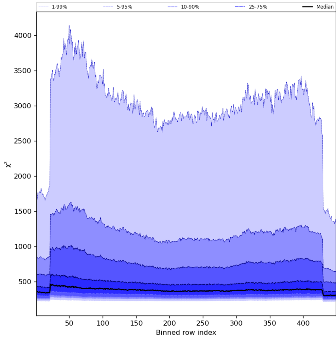
Figure 59: Along track statistics of “ \chi^2 ” for 2023-10-03 to 2023-10-05
