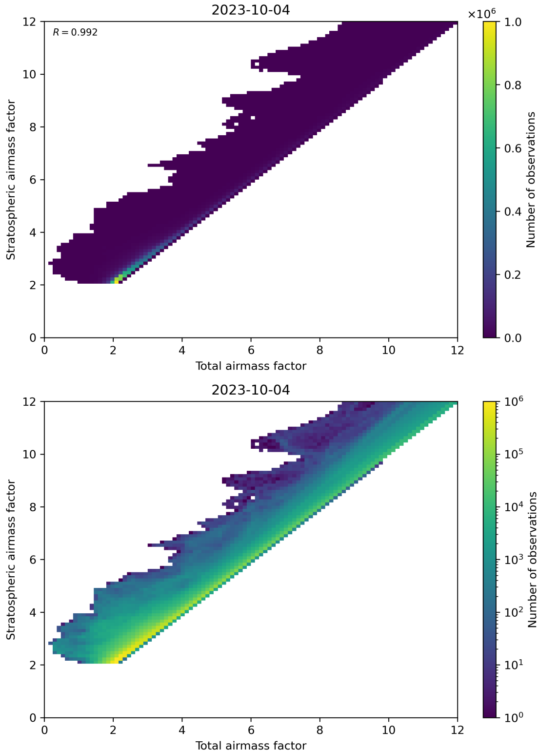
Figure 62: Scatter density plot of “Total airmass factor” against “Stratospheric airmass factor” for 2023-10-03 to 2023-10-05.
