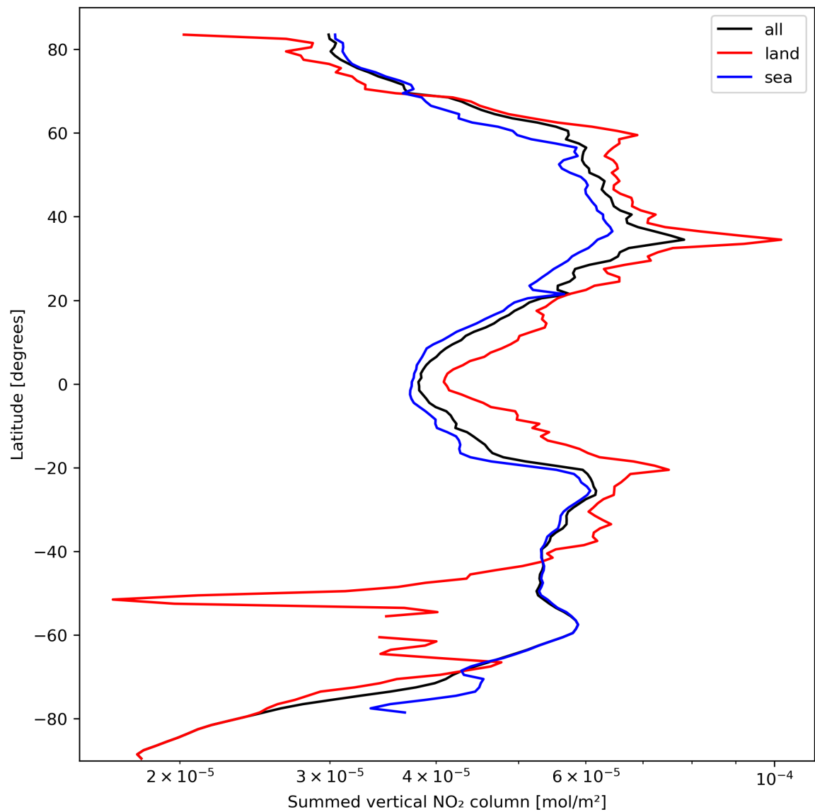
Figure 23: Zonal average of “Summed vertical NO 2 column” for 2023-10-03 to 2023-10-05.
