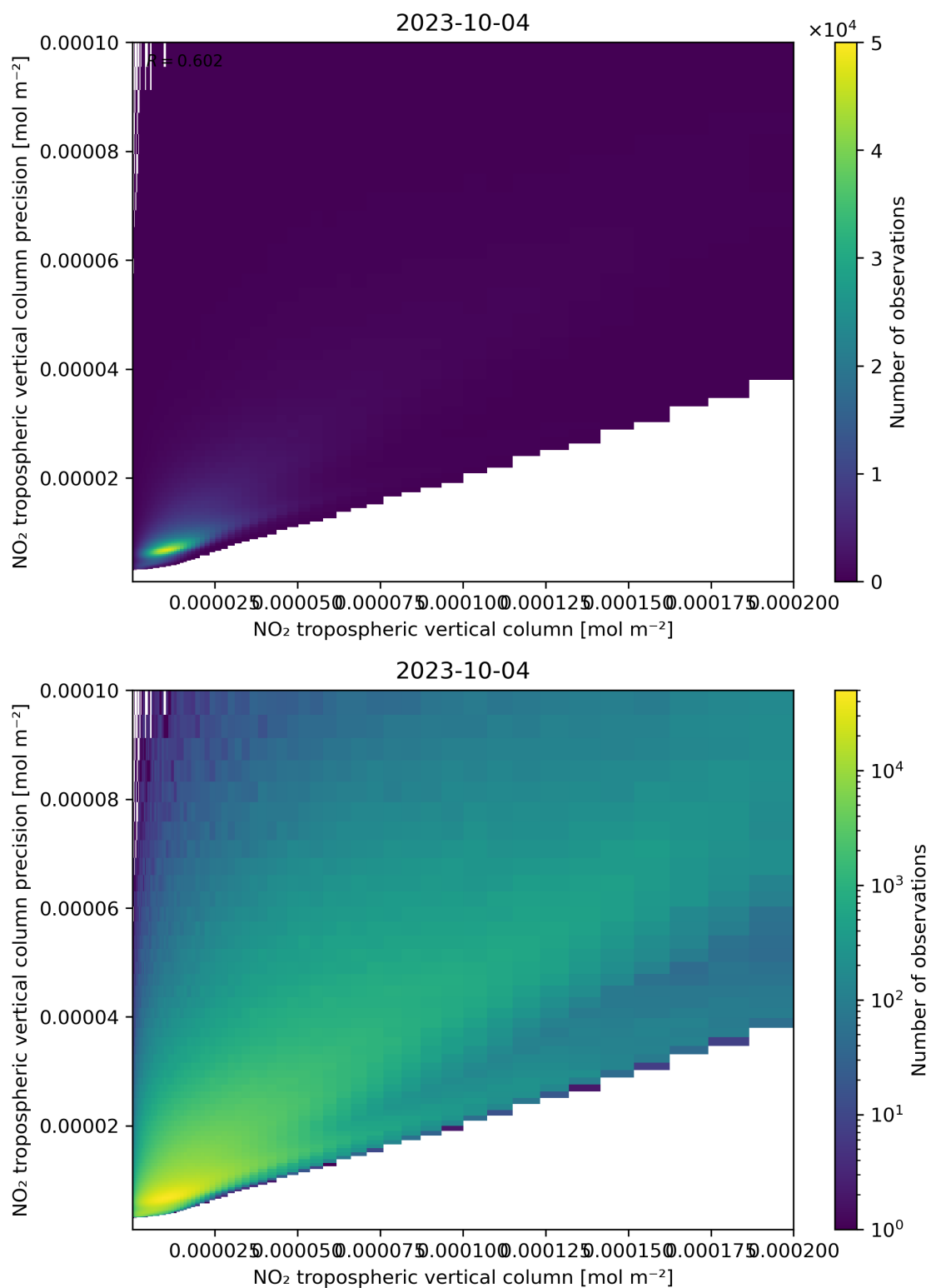
Figure 130: Scatter density plot of “NO 2 tropospheric vertical column” against “NO 2 tropospheric vertical column precision” for 2023-10-03 to 2023-10-05.
