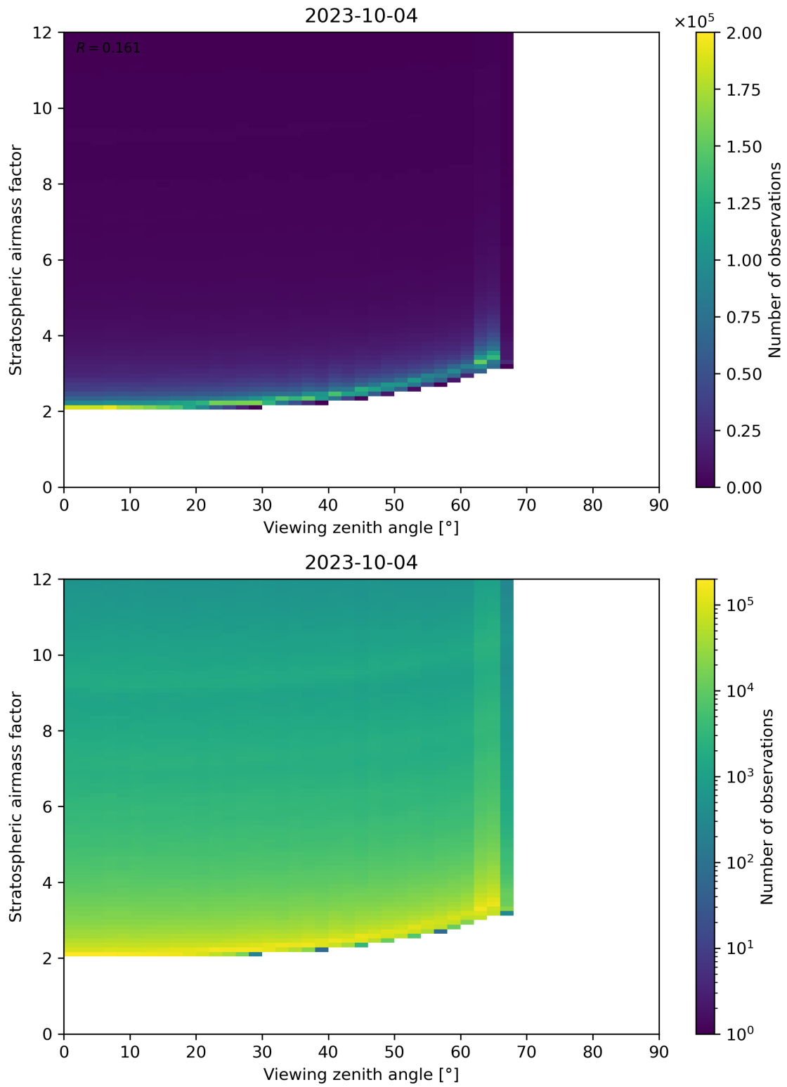
Figure 159: Scatter density plot of “Viewing zenith angle” against “Stratospheric airmass factor” for 2023-10-03 to 2023-10-05.
