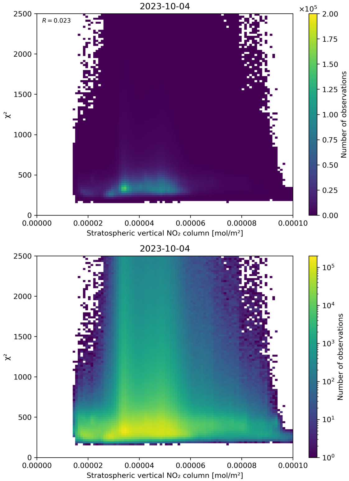
Figure 97: Scatter density plot of “Stratospheric vertical NO 2 column” against “ \chi^2 ” for 2023-10-03 to 2023-10-05.
