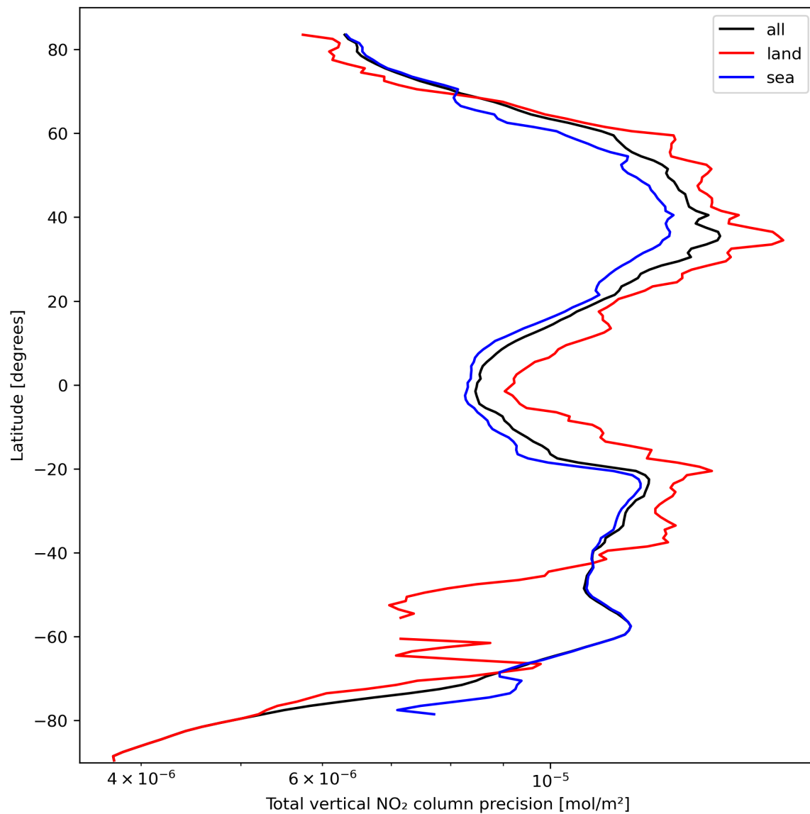
Figure 22: Zonal average of “Total vertical NO 2 column precision” for 2023-10-03 to 2023-10-05.
