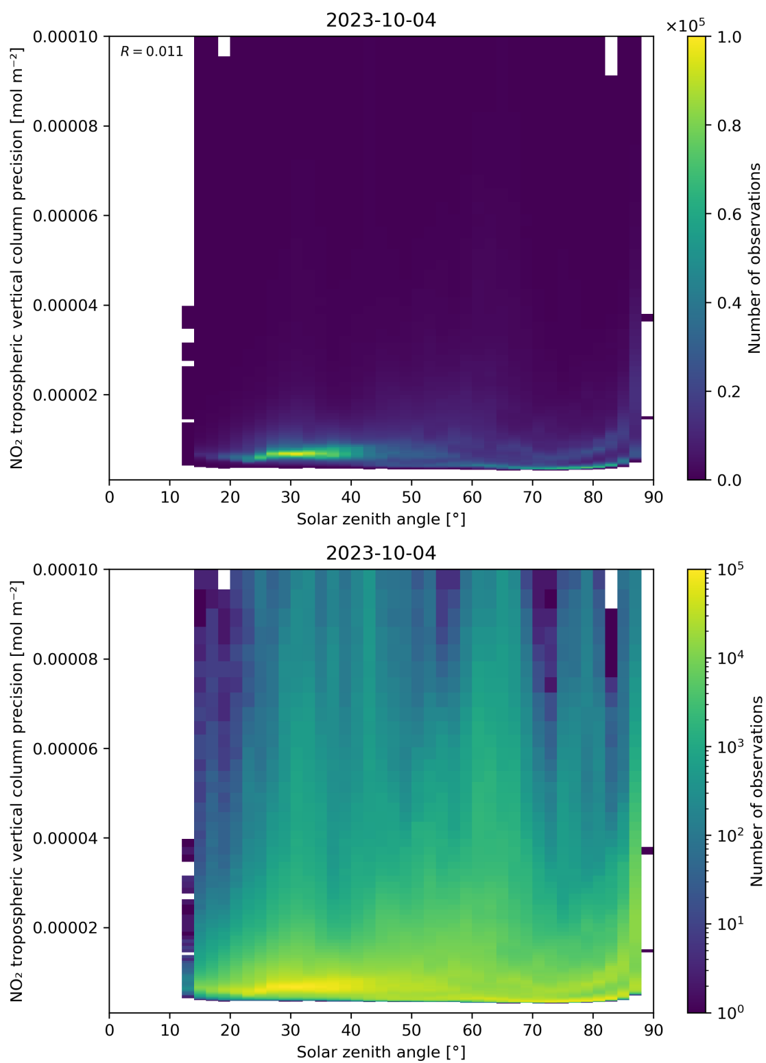
Figure 156: Scatter density plot of “Solar zenith angle” against “NO 2 tropospheric vertical column precision” for 2023-10-03 to 2023-10-05.
