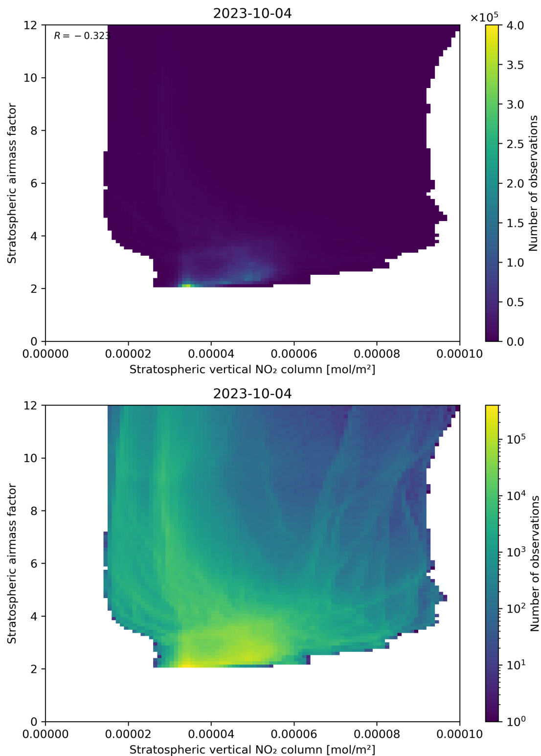
Figure 96: Scatter density plot of “Stratospheric vertical NO 2 column” against “Stratospheric airmass factor” for 2023-10-03 to 2023-10-05.
