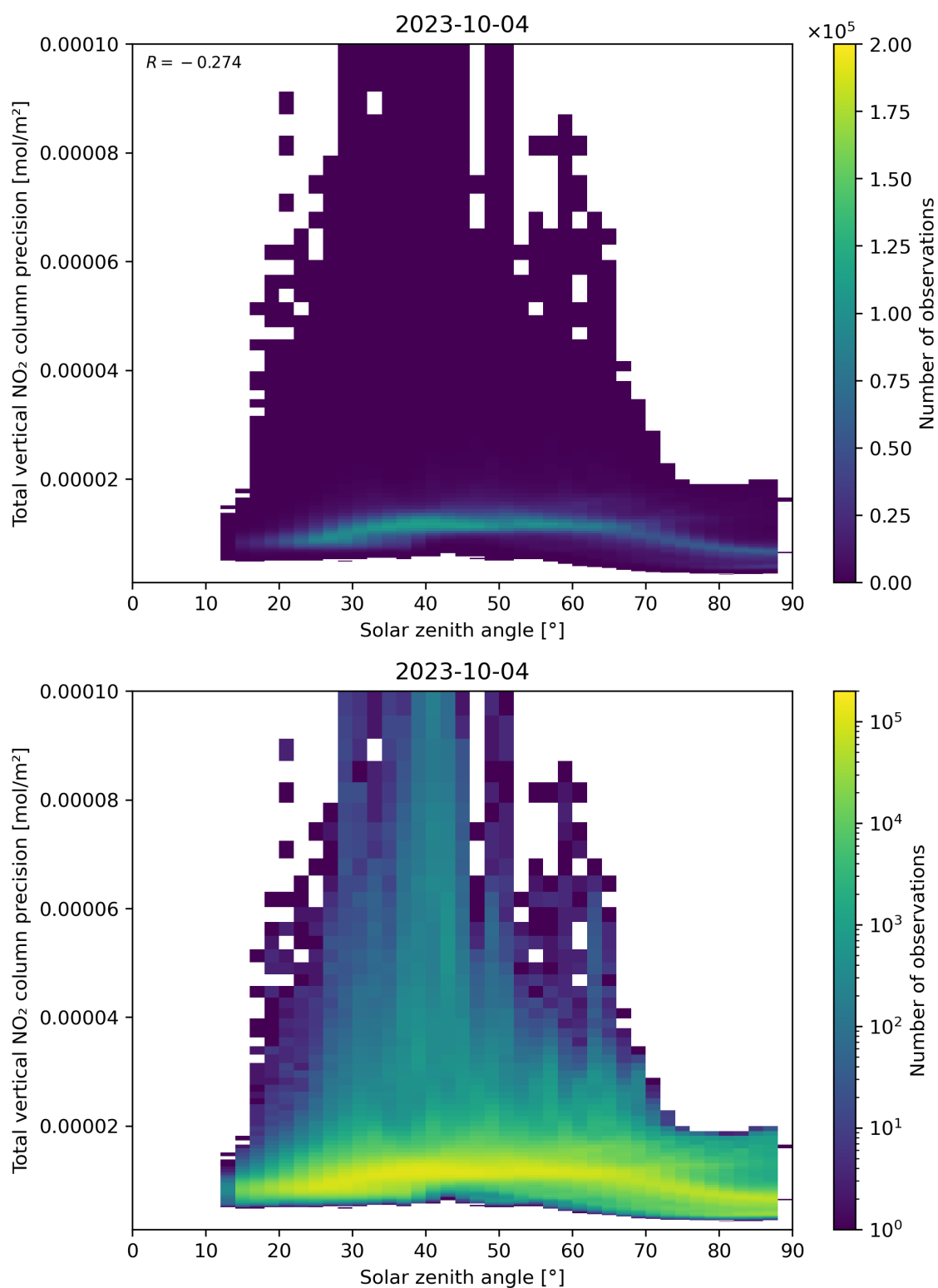
Figure 154: Scatter density plot of “Solar zenith angle” against “Total vertical NO 2 column precision” for 2023-10-03 to 2023-10-05.
