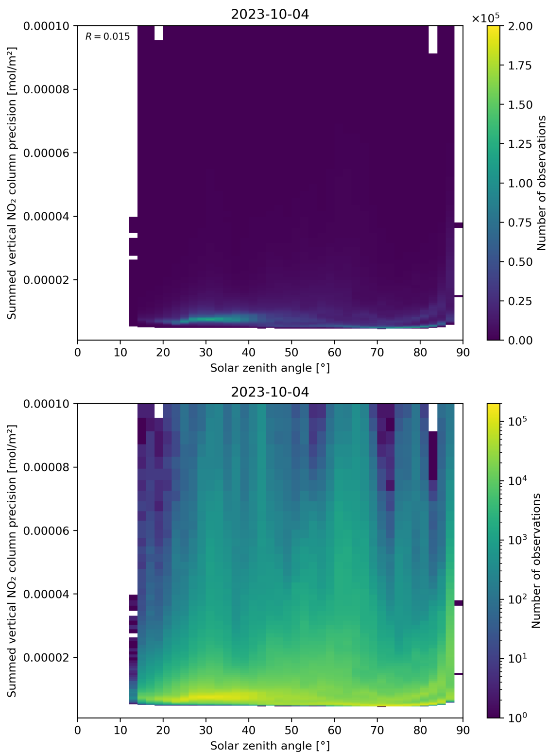
Figure 152: Scatter density plot of “Solar zenith angle” against “Summed vertical NO 2 column precision” for 2023-10-03 to 2023-10-05.
