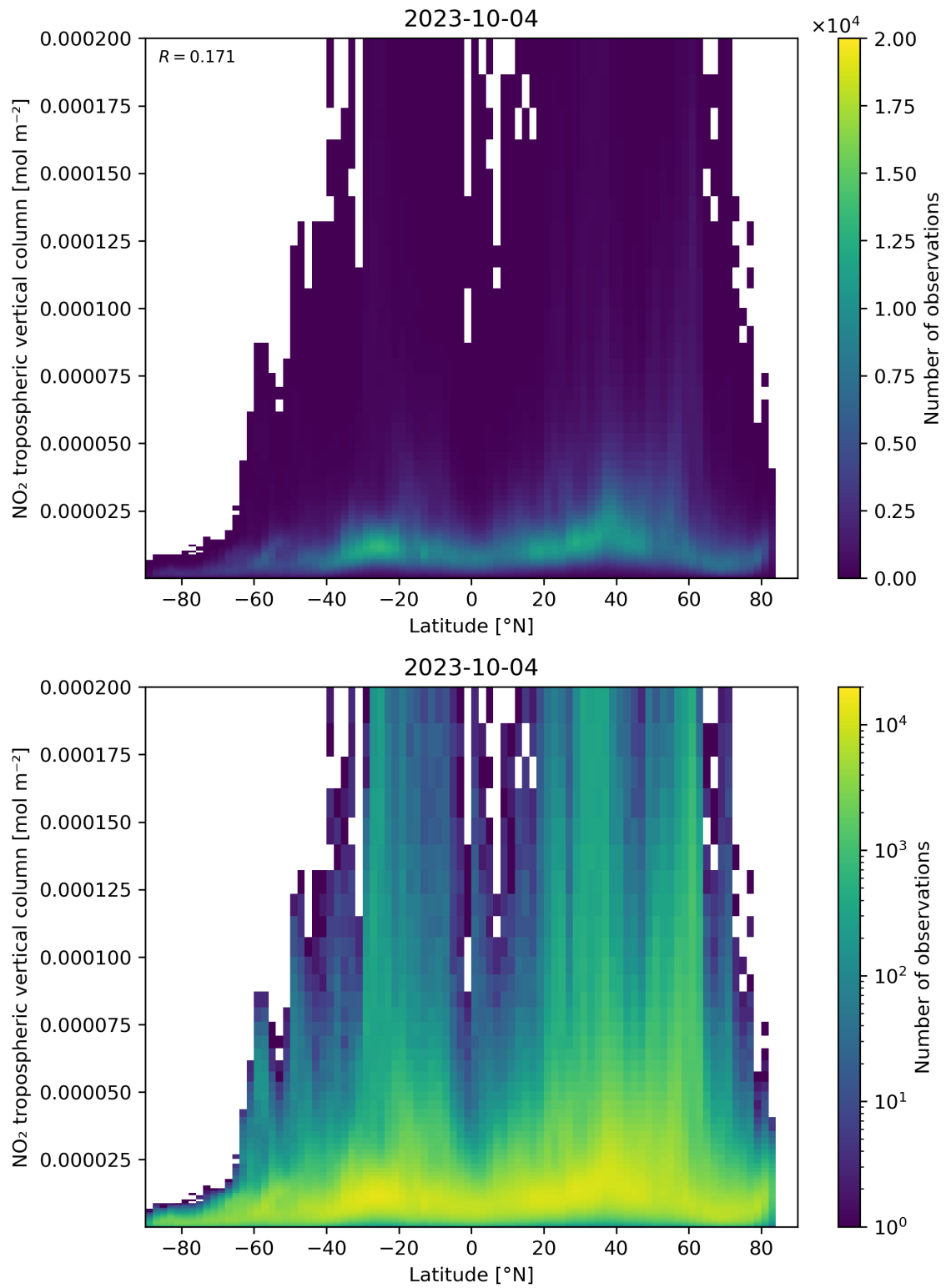
Figure 92: Scatter density plot of “Latitude” against “NO 2 tropospheric vertical column” for 2023-10-03 to 2023-10-05.
