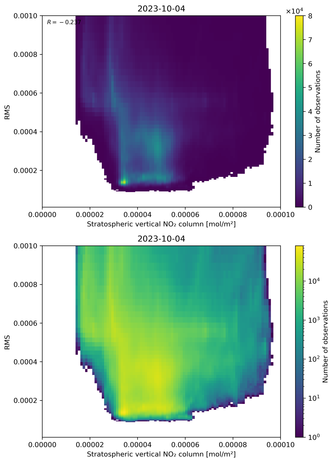
Figure 102: Scatter density plot of “Stratospheric vertical NO 2 column” against “RMS” for 2023-10-03 to 2023-10-05.
