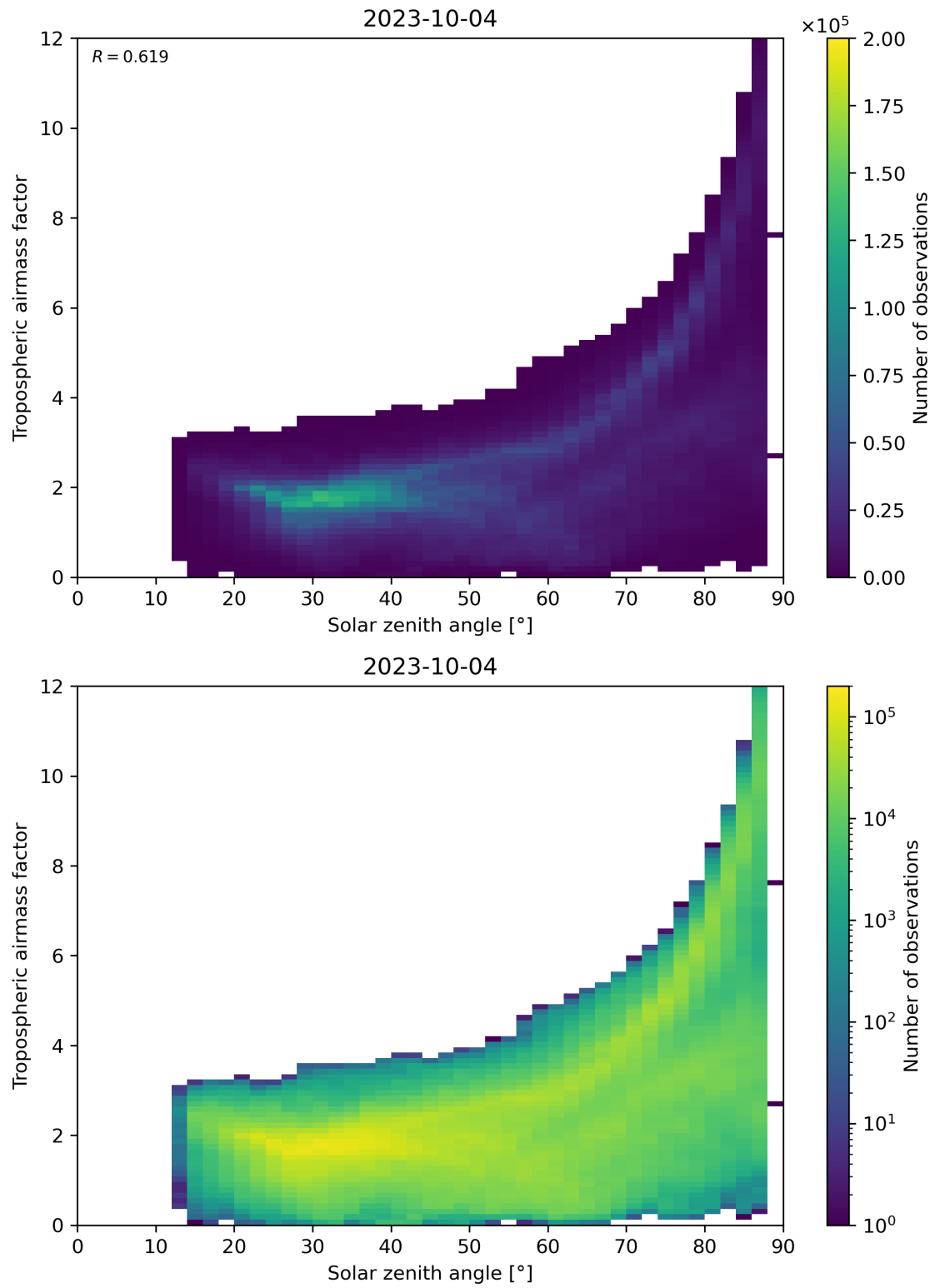
Figure 147: Scatter density plot of “Solar zenith angle” against “Tropospheric airmass factor” for 2023-10-03 to 2023-10-05.
