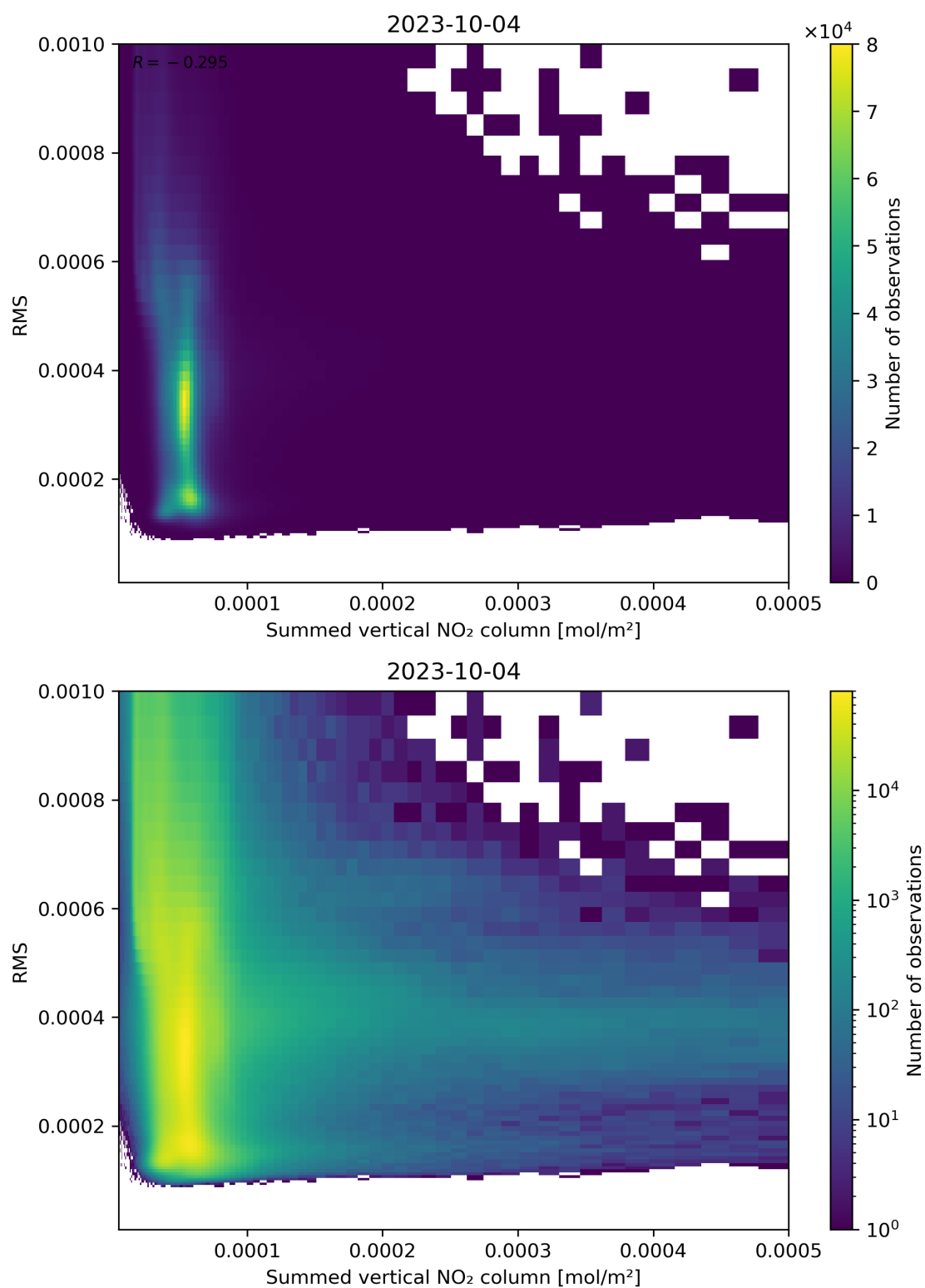
Figure 109: Scatter density plot of “Summed vertical NO 2 column” against “RMS” for 2023-10-03 to 2023-10-05.
