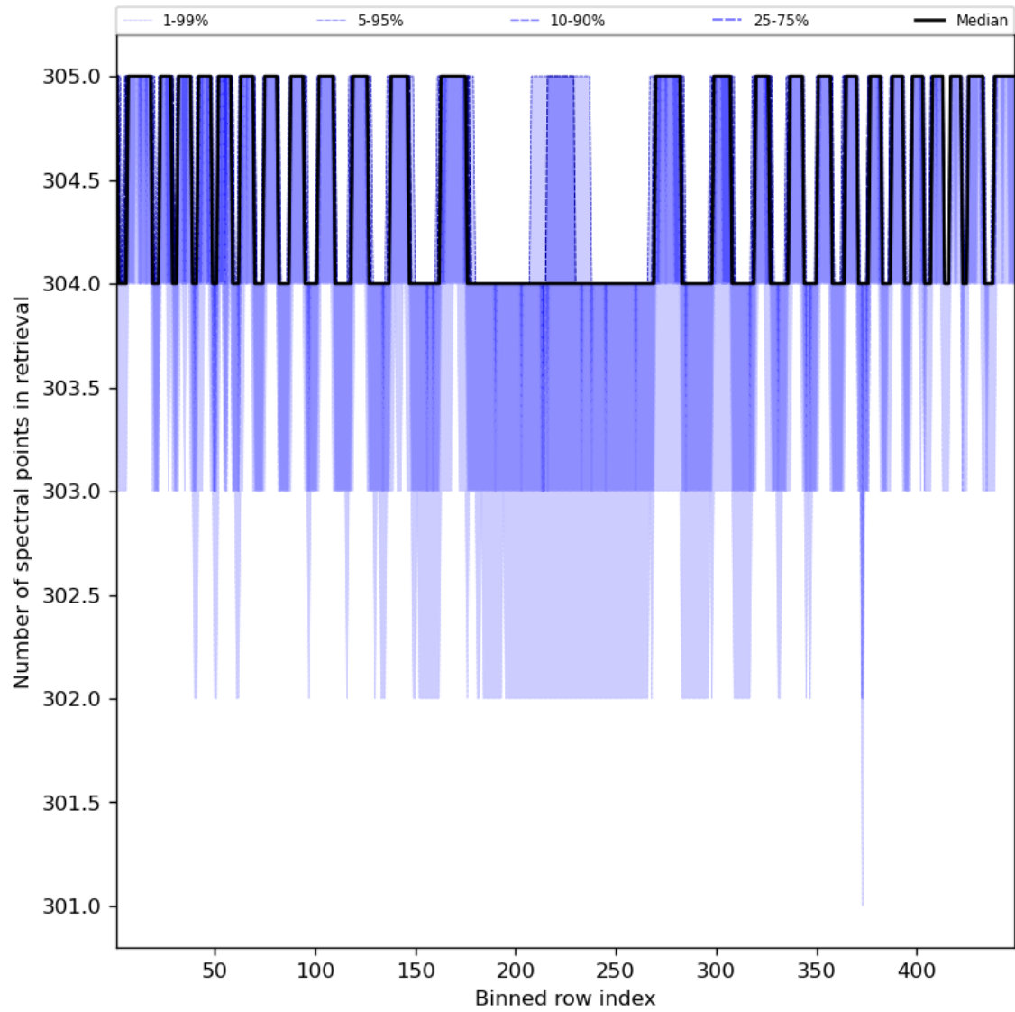
Figure 50: Along track statistics of “Number of spectral points in retrieval” for 2023-10-03 to 2023-10-05
