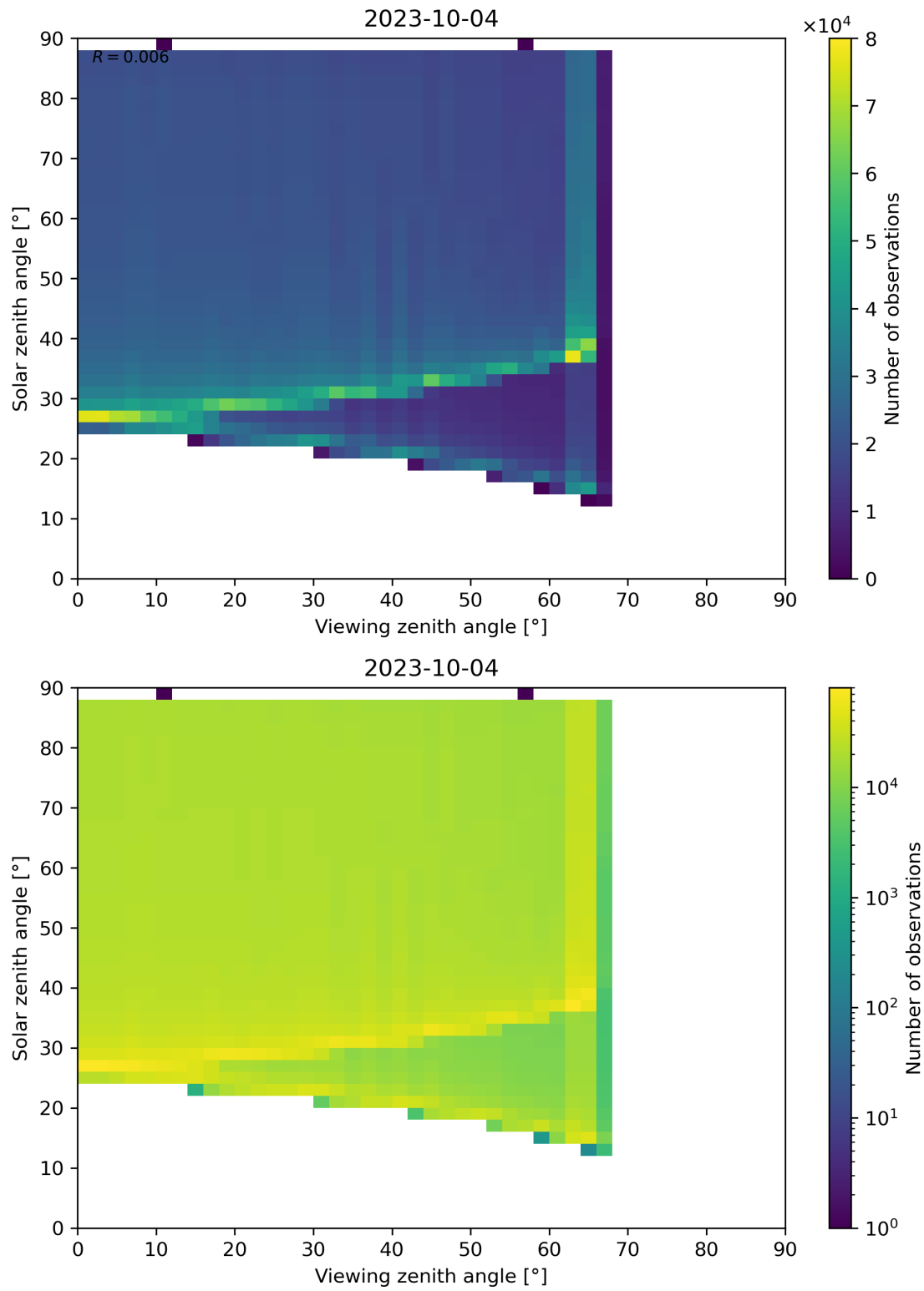
Figure 172: Scatter density plot of “Viewing zenith angle” against “Solar zenith angle” for 2023-10-03 to 2023-10-05.
