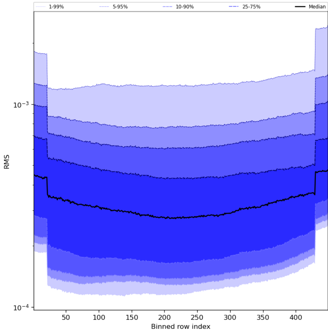
Figure 60: Along track statistics of “RMS” for 2023-10-03 to 2023-10-05
