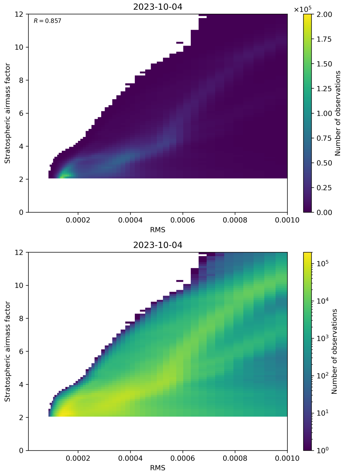
Figure 144: Scatter density plot of “RMS” against “Stratospheric airmass factor” for 2023-10-03 to 2023-10-05.
