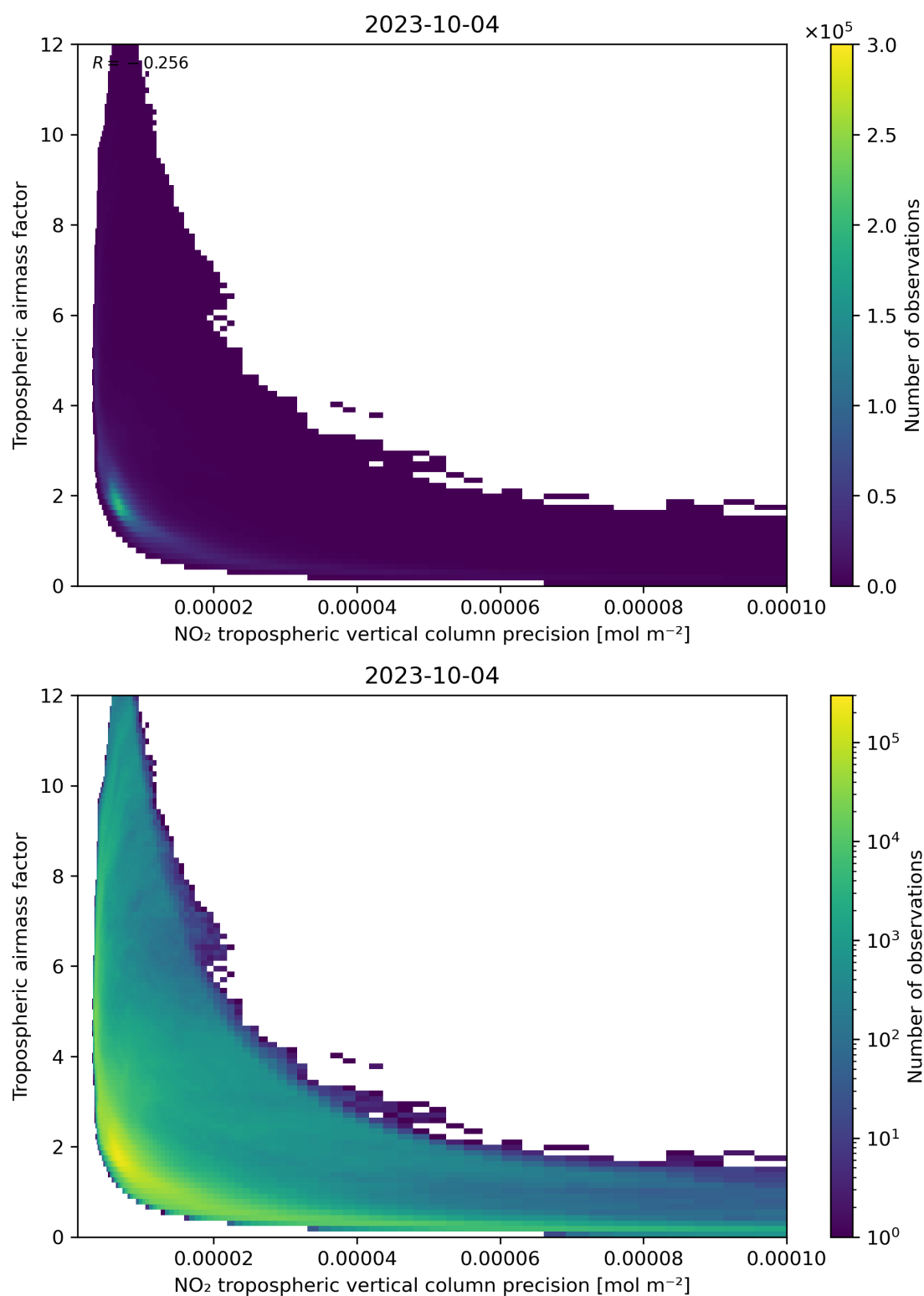
Figure 133: Scatter density plot of “NO 2 tropospheric vertical column precision” against “Tropospheric air mass factor” for 2023-10-03 to 2023-10-05.
