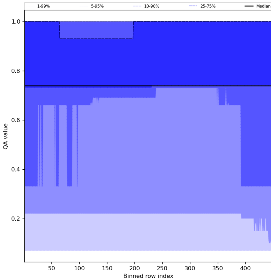
Figure 45: Along track statistics of “QA value” for 2023-10-03 to 2023-10-05
