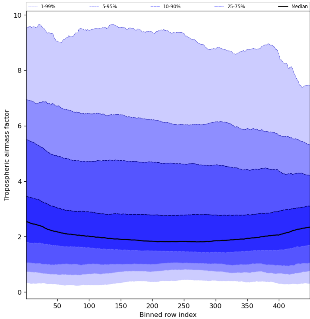
Figure 48: Along track statistics of “Tropospheric air mass factor” for 2023-10-03 to 2023-10-05
