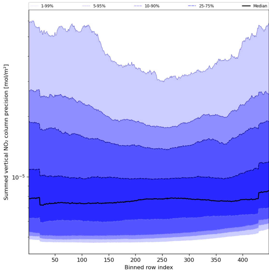
Figure 58: Along track statistics of “Summed vertical NO 2 column precision” for 2023-10-03 to 2023-10-05
