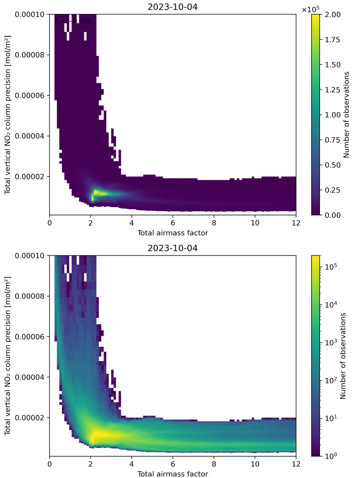
Figure 68: Scatter density plot of “Total airmass factor” against “Total vertical NO 2 column precision” for 2023-10-03 to 2023-10-05.
