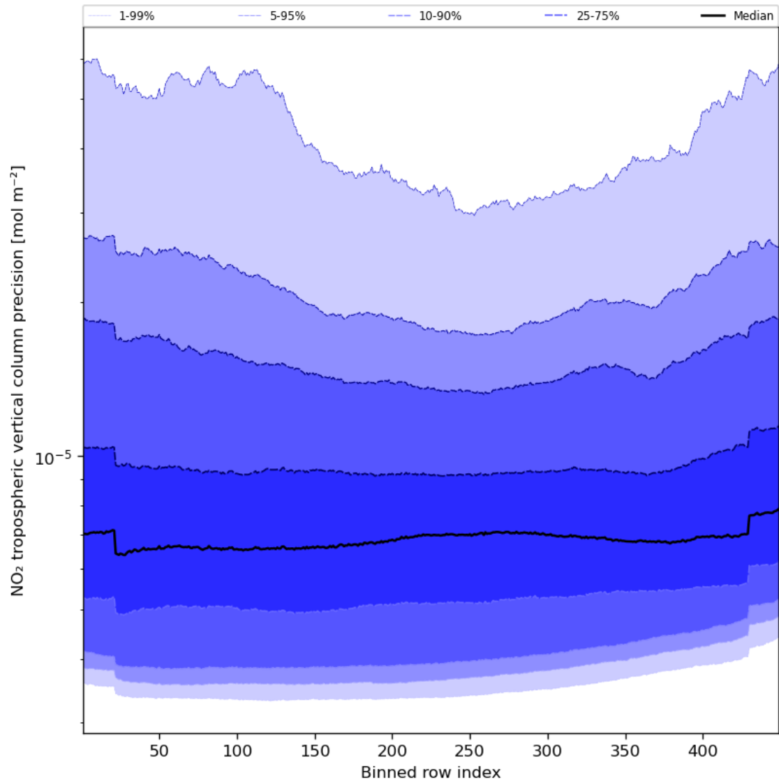
Figure 47: Along track statistics of “NO 2 tropospheric vertical column precision” for 2023-10-03 to 2023-10-05
