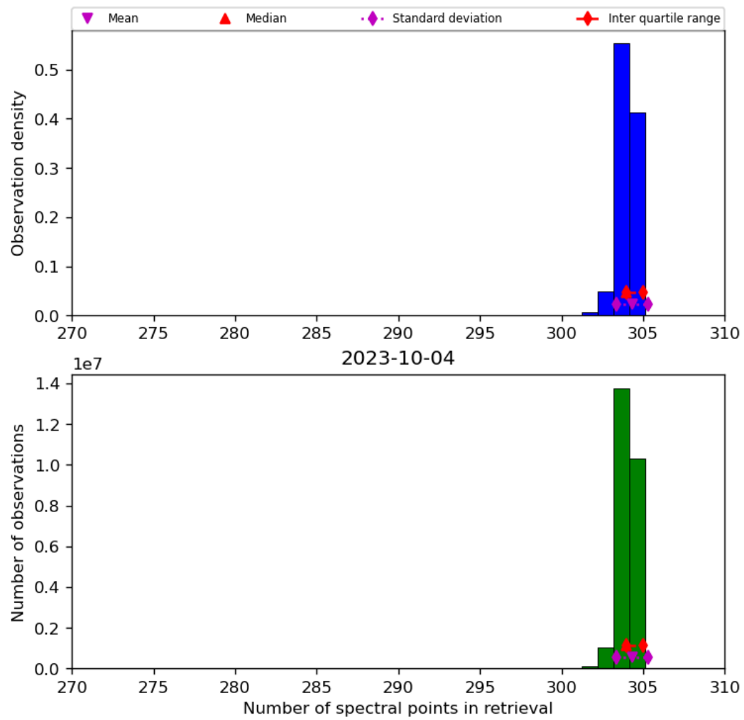
Figure 33: Histogram of “Number of spectral points in retrieval” for 2023-10-03 to 2023-10-05
