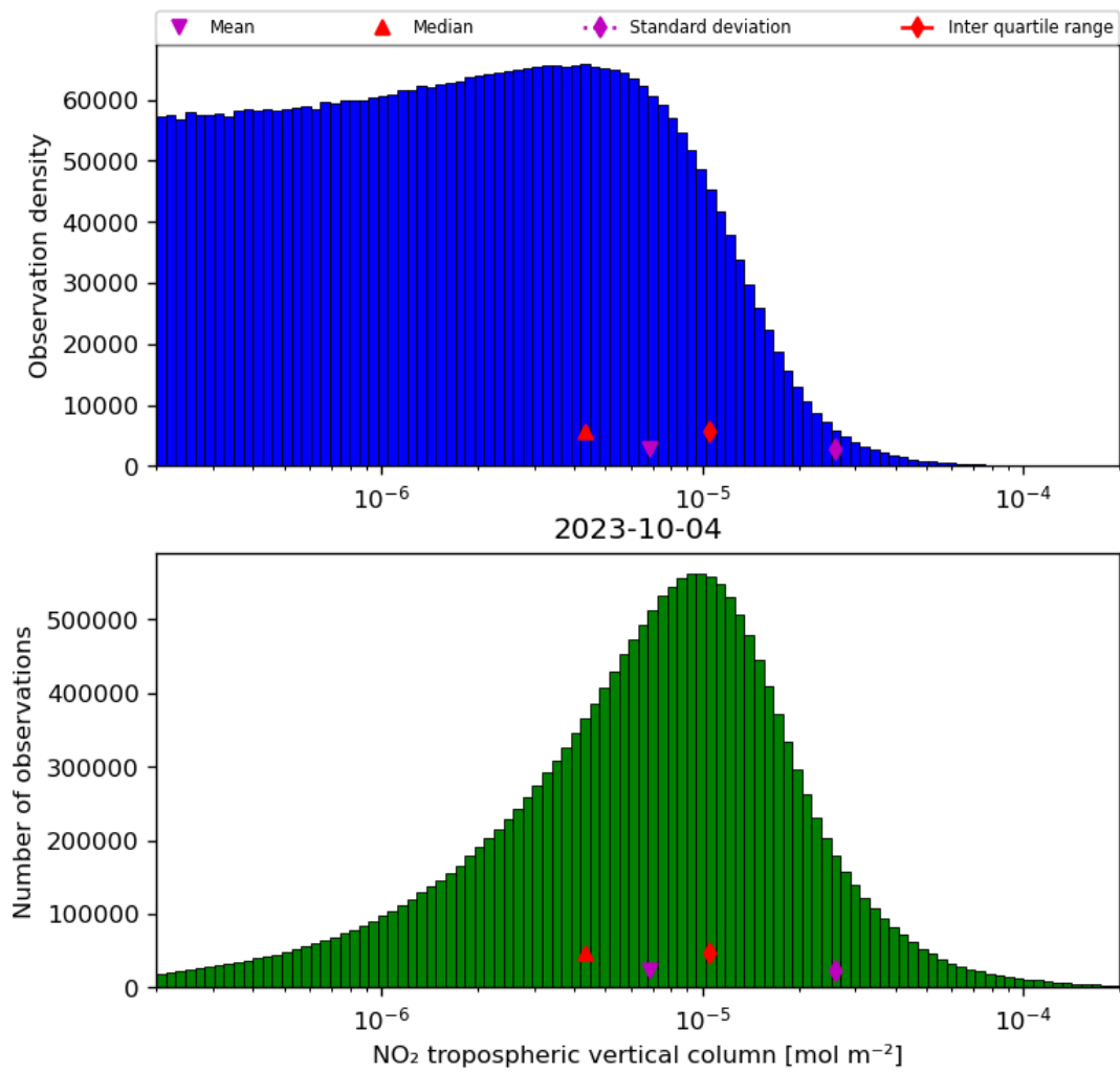
Figure 29: Histogram of “ \text{NO}_2 tropospheric vertical column” for 2023-10-03 to 2023-10-05
