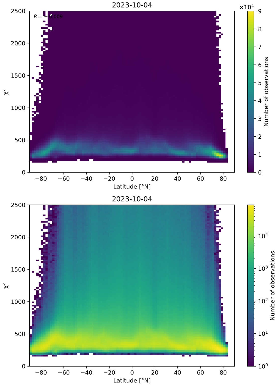
Figure 86: Scatter density plot of “Latitude” against “ \chi^2 ” for 2023-10-03 to 2023-10-05.
