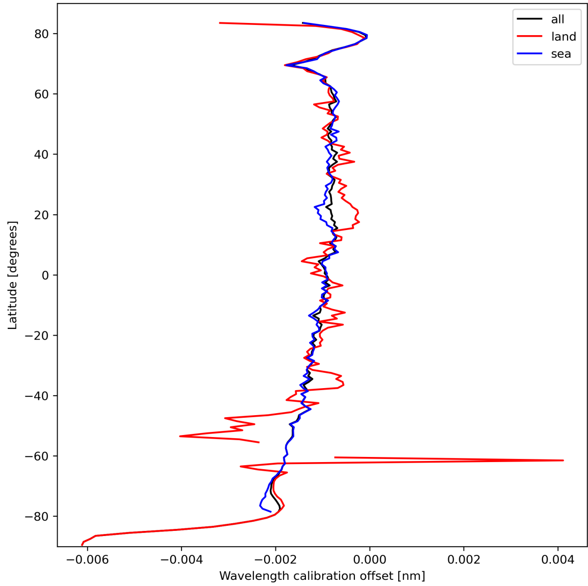
Figure 18: Zonal average of “Wavelength calibration offset” for 2023-10-03 to 2023-10-05.
