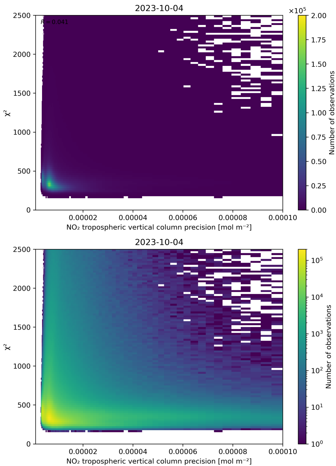
Figure 134: Scatter density plot of “NO 2 tropospheric vertical column precision” against “ \chi^2 ” for 2023-10-03 to 2023-10-05.
