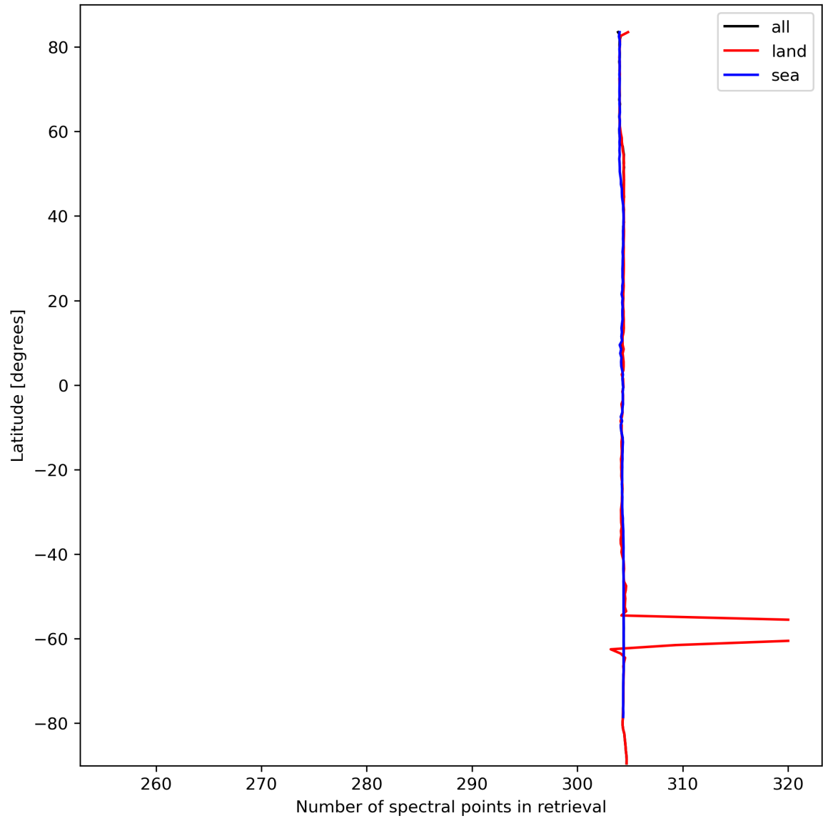
Figure 16: Zonal average of “Number of spectral points in retrieval” for 2023-10-03 to 2023-10-05.
