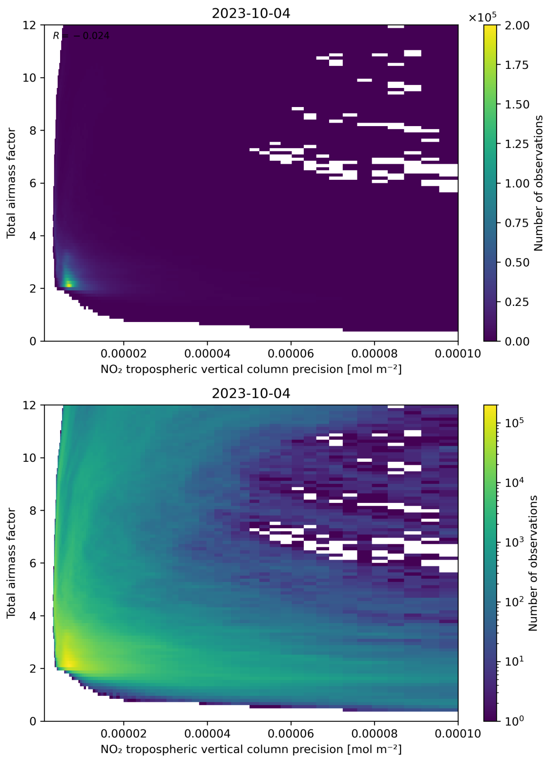
Figure 132: Scatter density plot of “NO 2 tropospheric vertical column precision” against “Total air mass factor” for 2023-10-03 to 2023-10-05.
