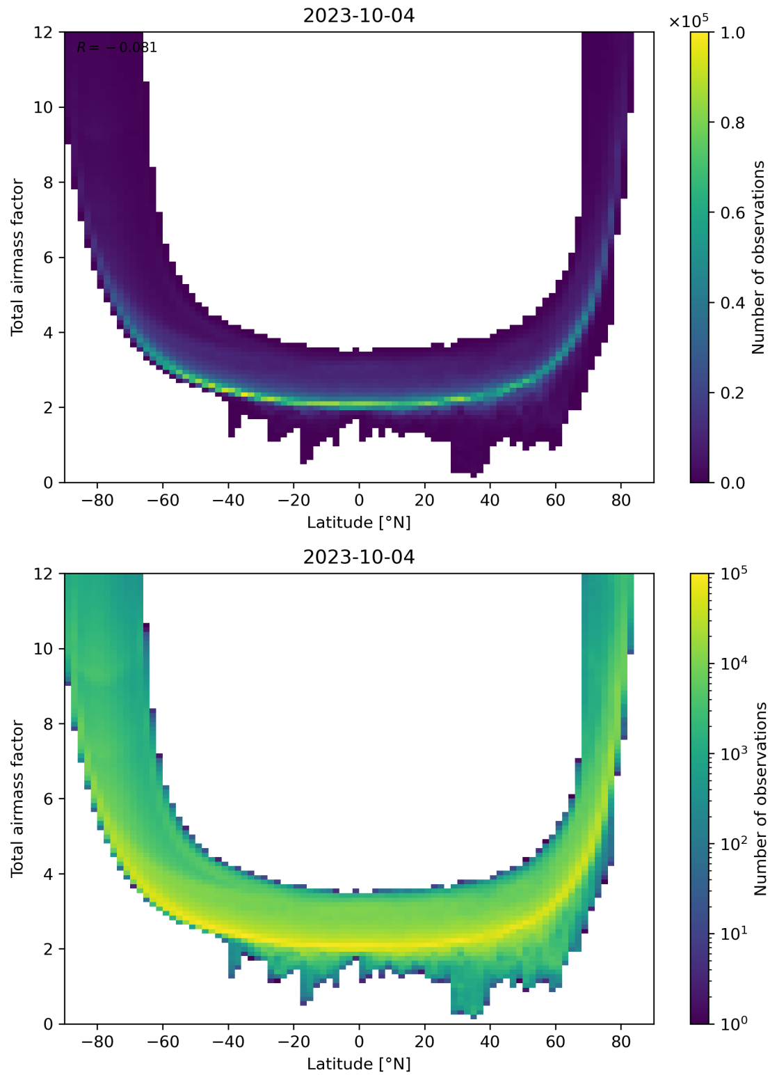
Figure 84: Scatter density plot of “Latitude” against “Total airmass factor” for 2023-10-03 to 2023-10-05.
