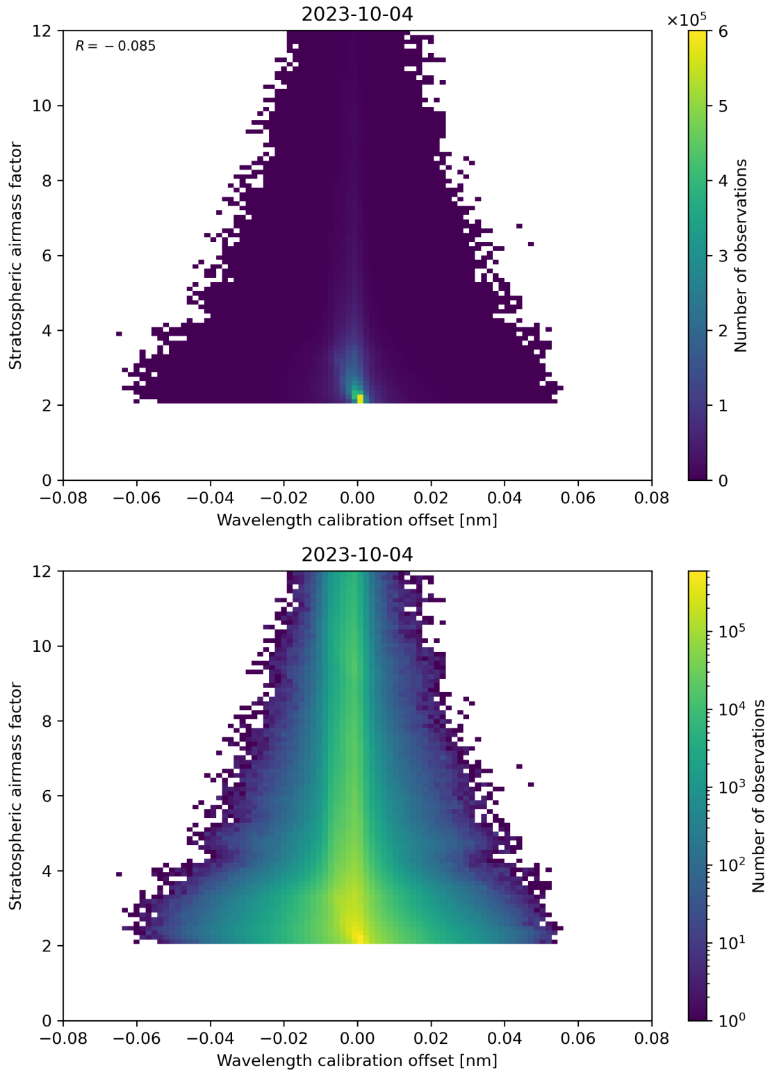
Figure 174: Scatter density plot of “Wavelength calibration offset” against “Stratospheric airmass factor” for 2023-10-03 to 2023-10-05.
