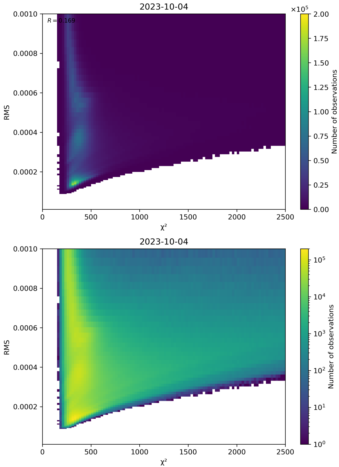
Figure 82: Scatter density plot of “ \chi^2 ” against “RMS” for 2023-10-03 to 2023-10-05.
