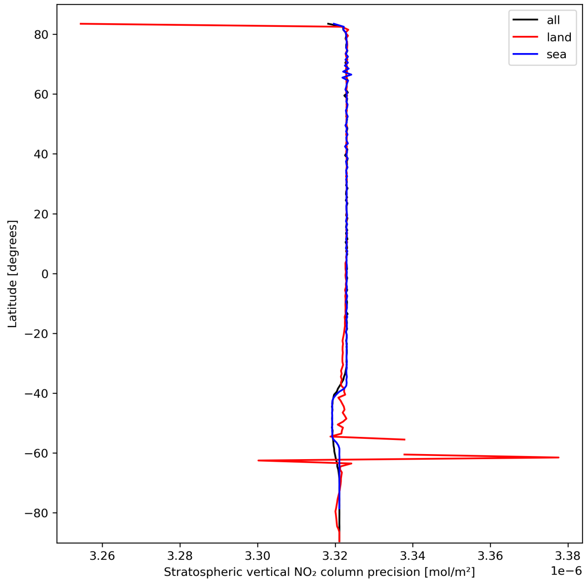
Figure 20: Zonal average of “Stratospheric vertical NO 2 column precision” for 2023-10-03 to 2023-10-05.
