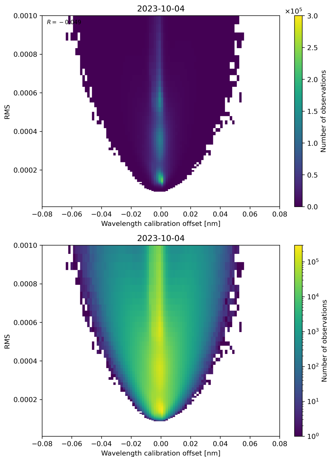
Figure 181: Scatter density plot of “Wavelength calibration offset” against “RMS” for 2023-10-03 to 2023-10-05.
