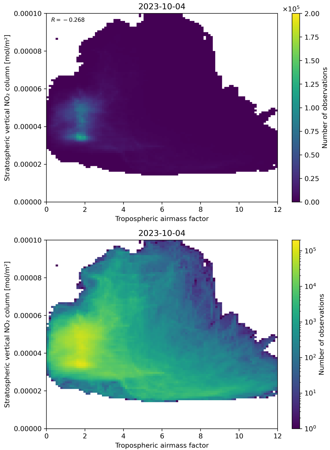
Figure 74: Scatter density plot of “Tropospheric air mass factor” against “Stratospheric vertical NO 2 column” for 2023-10-03 to 2023-10-05.
