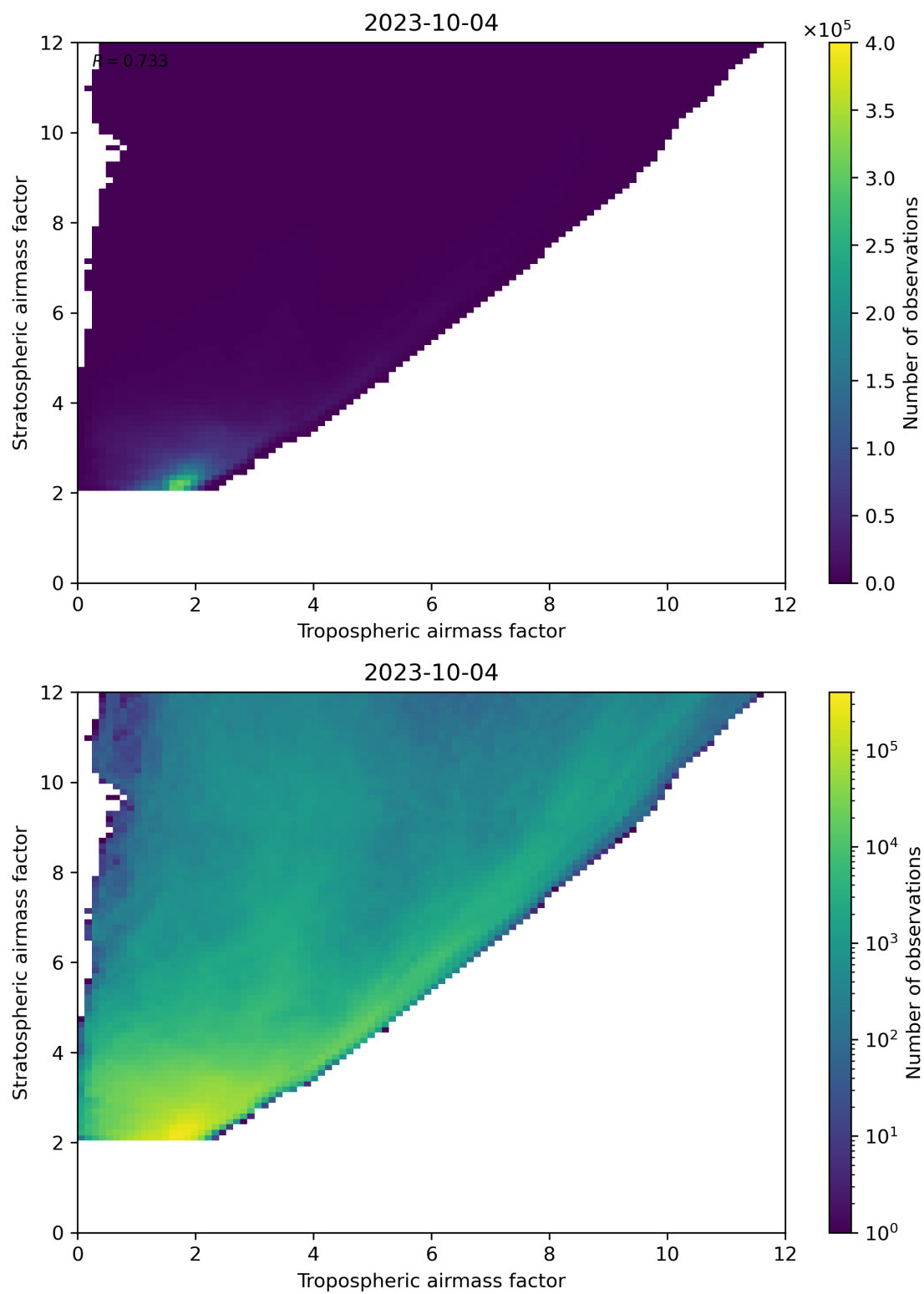
Figure 71: Scatter density plot of “Tropospheric airmass factor” against “Stratospheric airmass factor” for 2023-10-03 to 2023-10-05.
