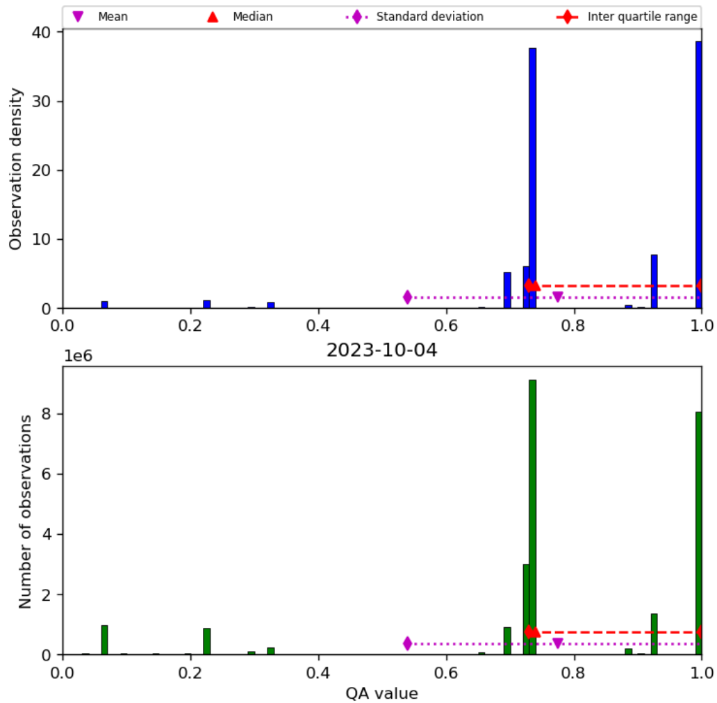
Figure 28: Histogram of “QA value” for 2023-10-03 to 2023-10-05
