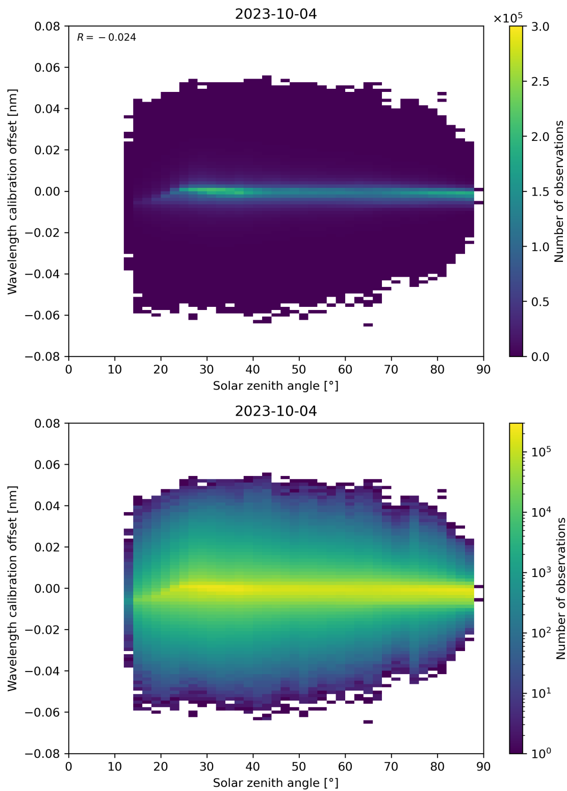
Figure 158: Scatter density plot of “Solar zenith angle” against “Wavelength calibration offset” for 2023-10-03 to 2023-10-05.
