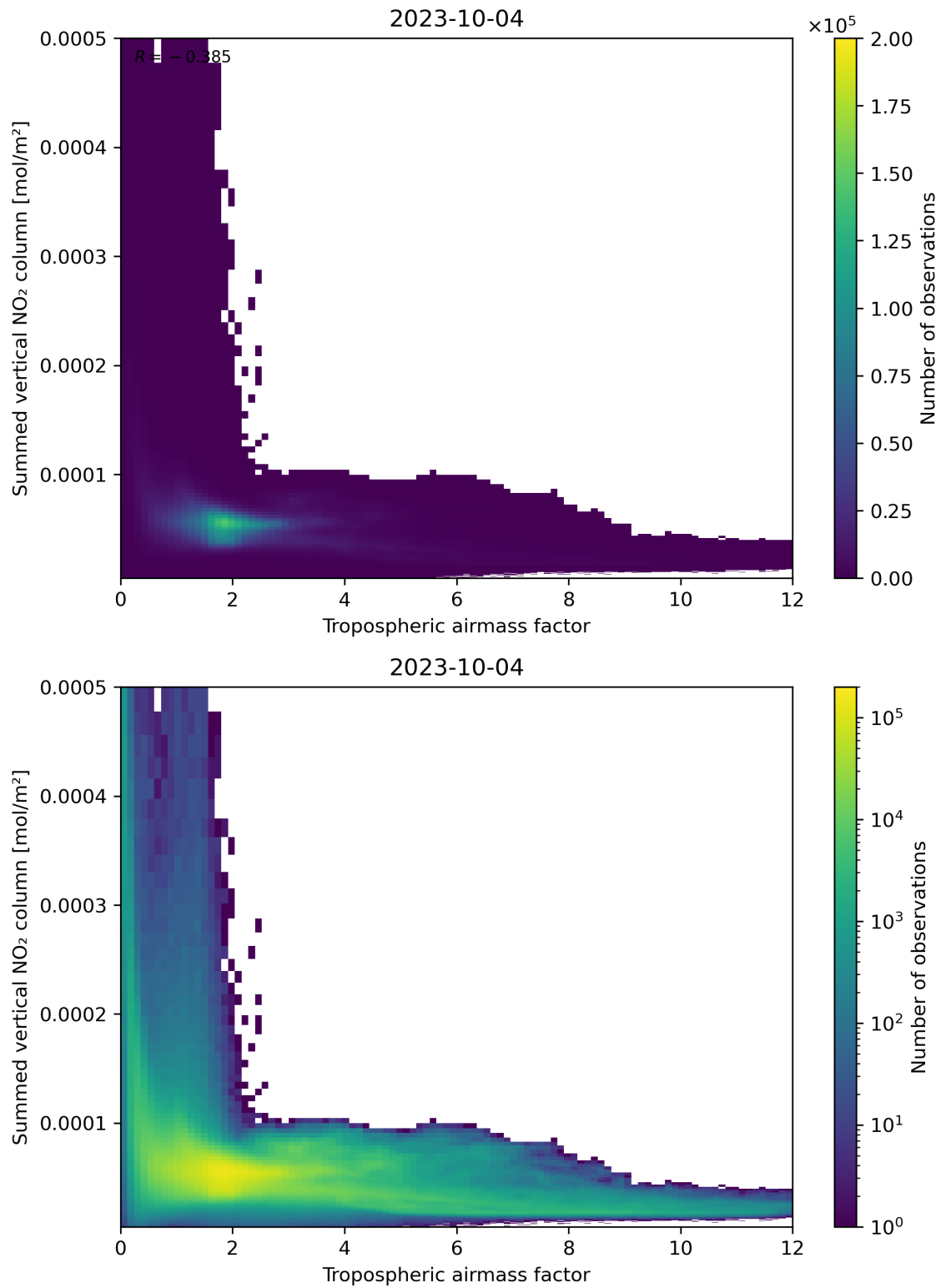
Figure 75: Scatter density plot of “Tropospheric air mass factor” against “Summed vertical NO 2 column” for 2023-10-03 to 2023-10-05.
