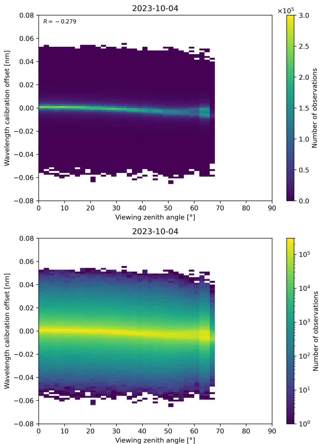
Figure 173: Scatter density plot of “Viewing zenith angle” against “Wavelength calibration offset” for 2023-10-03 to 2023-10-05.
