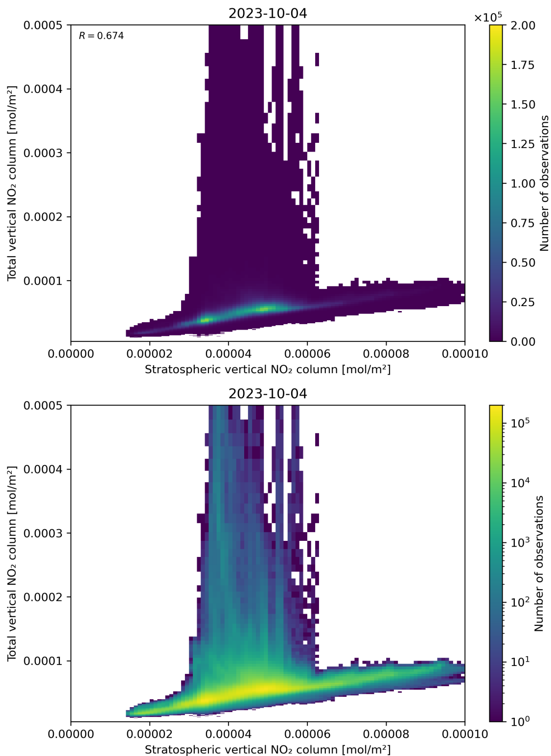
Figure 100: Scatter density plot of “Stratospheric vertical NO 2 column” against “Total vertical NO 2 column” for 2023-10-03 to 2023-10-05.
