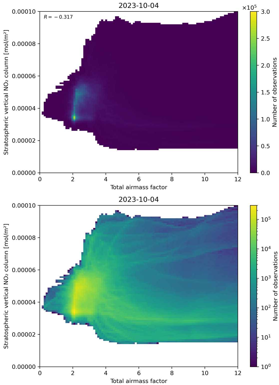
Figure 64: Scatter density plot of “Total airmass factor” against “Stratospheric vertical NO 2 column” for 2023-10-03 to 2023-10-05.
