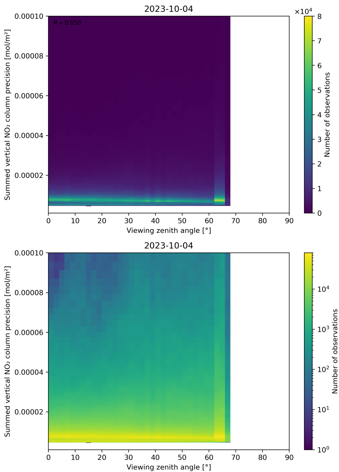
Figure 166: Scatter density plot of “Viewing zenith angle” against “Summed vertical NO 2 column precision” for 2023-10-03 to 2023-10-05.
