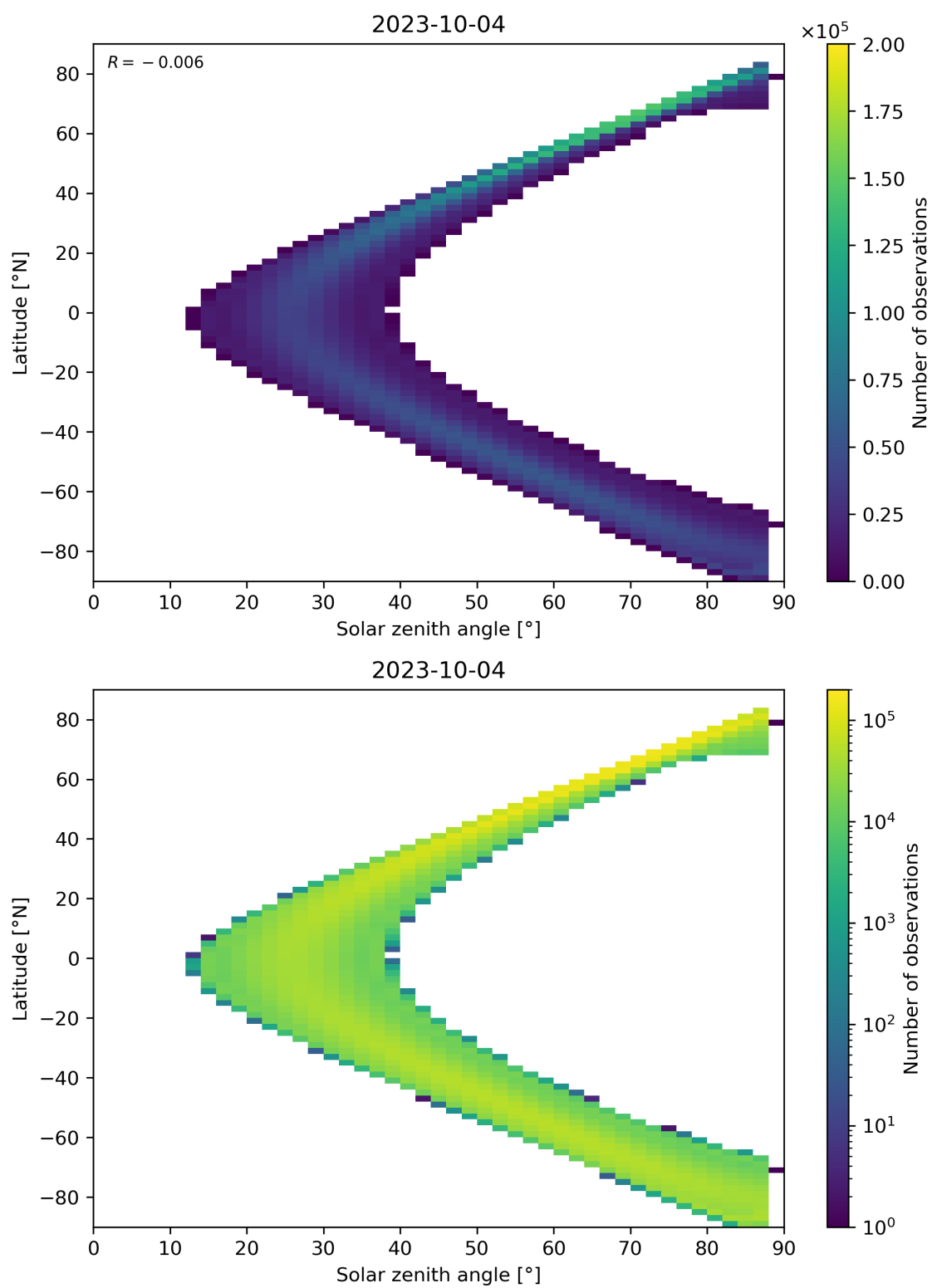
Figure 149: Scatter density plot of “Solar zenith angle” against “Latitude” for 2023-10-03 to 2023-10-05.
