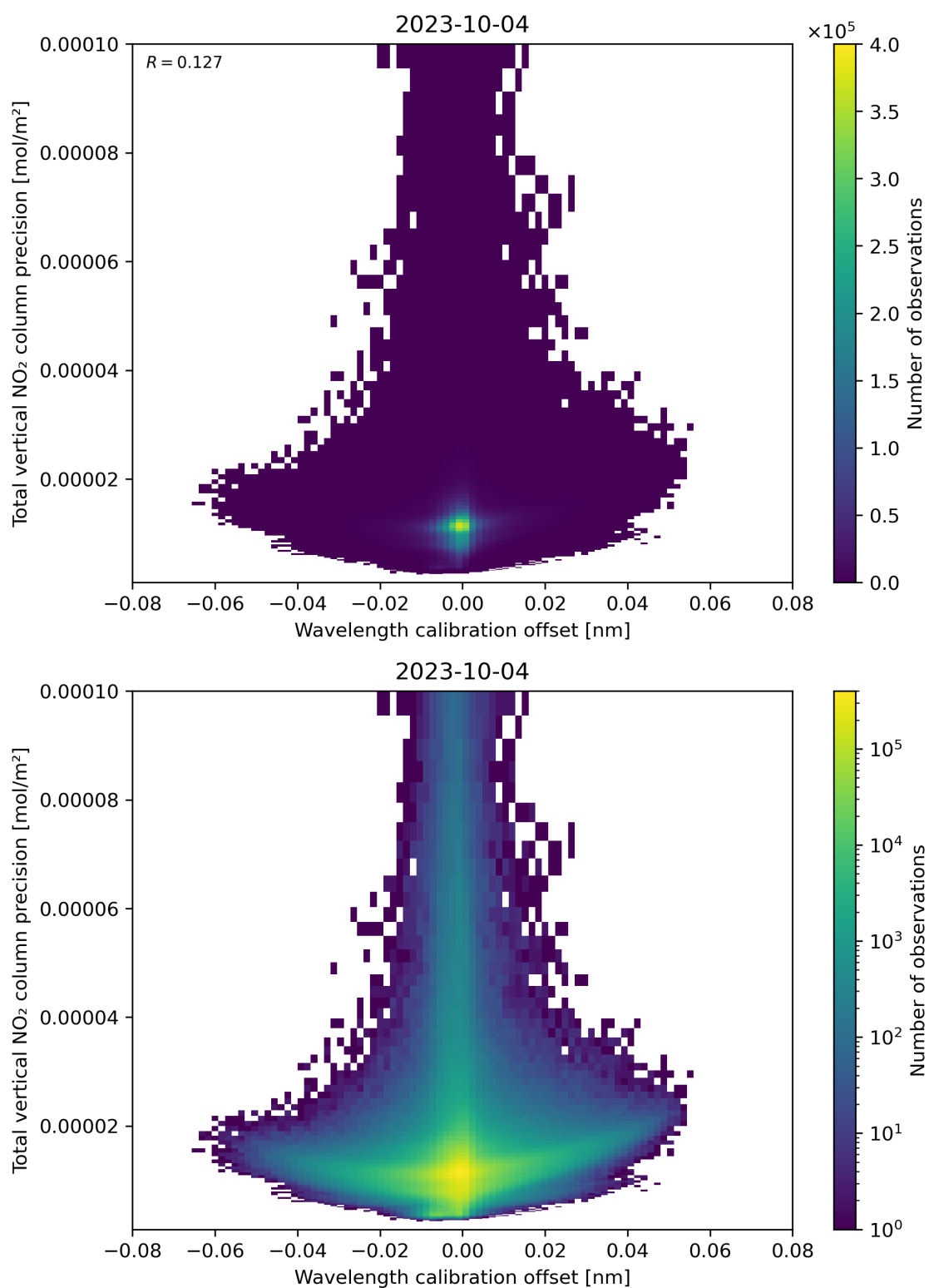
Figure 180: Scatter density plot of “Wavelength calibration offset” against “Total vertical NO 2 column precision” for 2023-10-03 to 2023-10-05.
