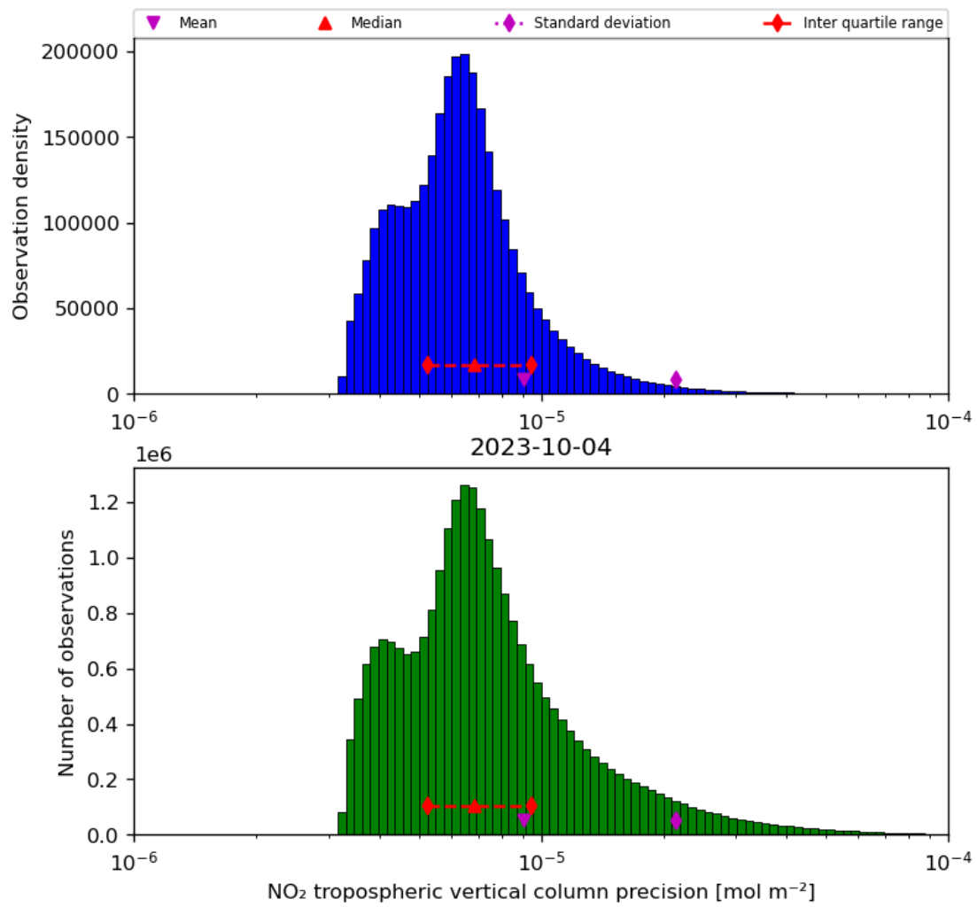
Figure 30: Histogram of “NO 2 tropospheric vertical column precision” for 2023-10-03 to 2023-10-05
