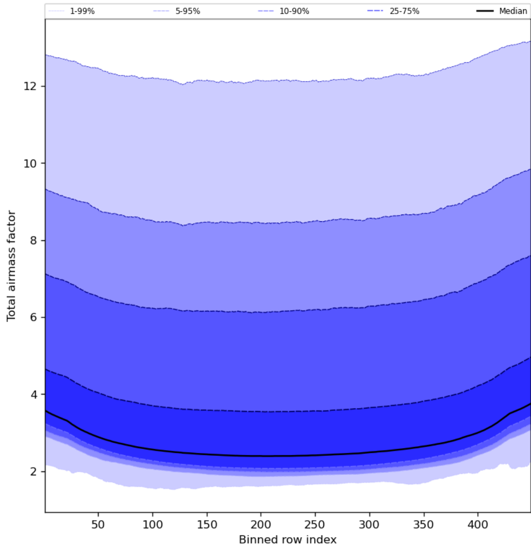
Figure 49: Along track statistics of “Total airmass factor” for 2023-10-03 to 2023-10-05
