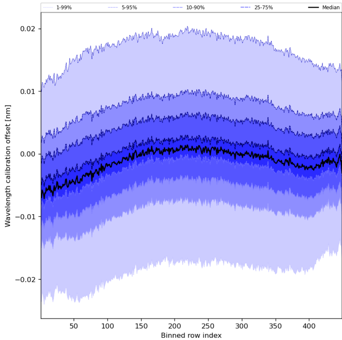
Figure 52: Along track statistics of “Wavelength calibration offset” for 2023-10-03 to 2023-10-05
