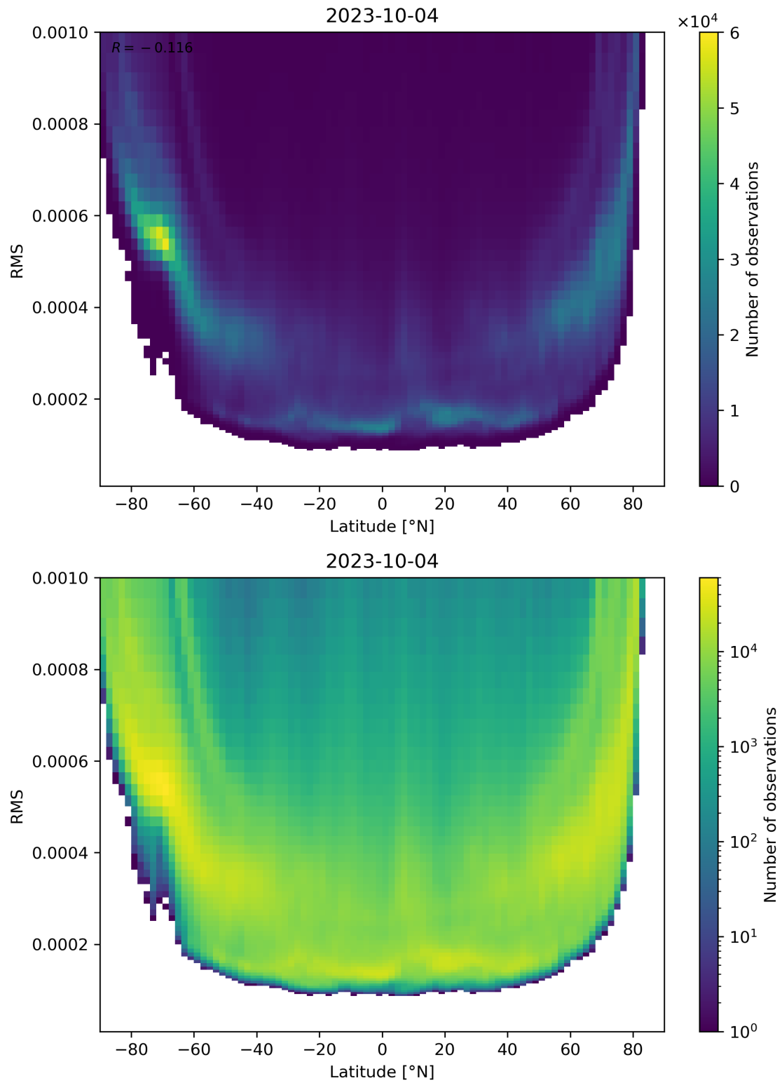
Figure 94: Scatter density plot of “Latitude” against “RMS” for 2023-10-03 to 2023-10-05.
