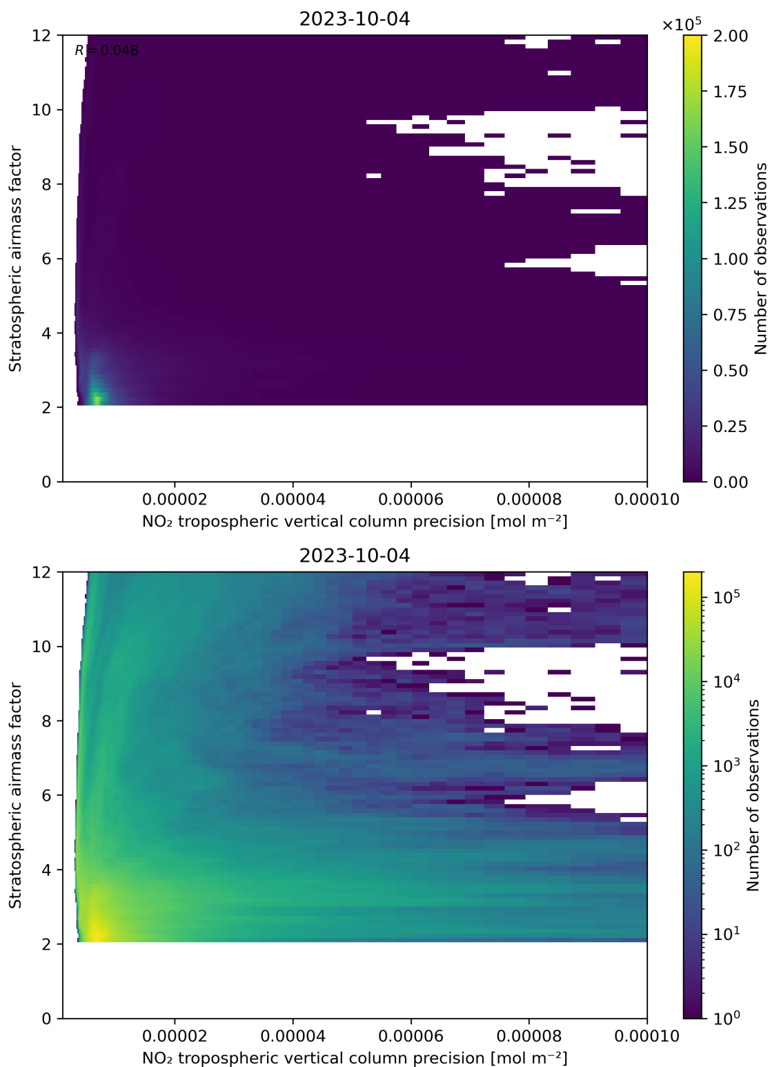
Figure 131: Scatter density plot of “NO 2 tropospheric vertical column precision” against “Stratospheric airmass factor” for 2023-10-03 to 2023-10-05.
