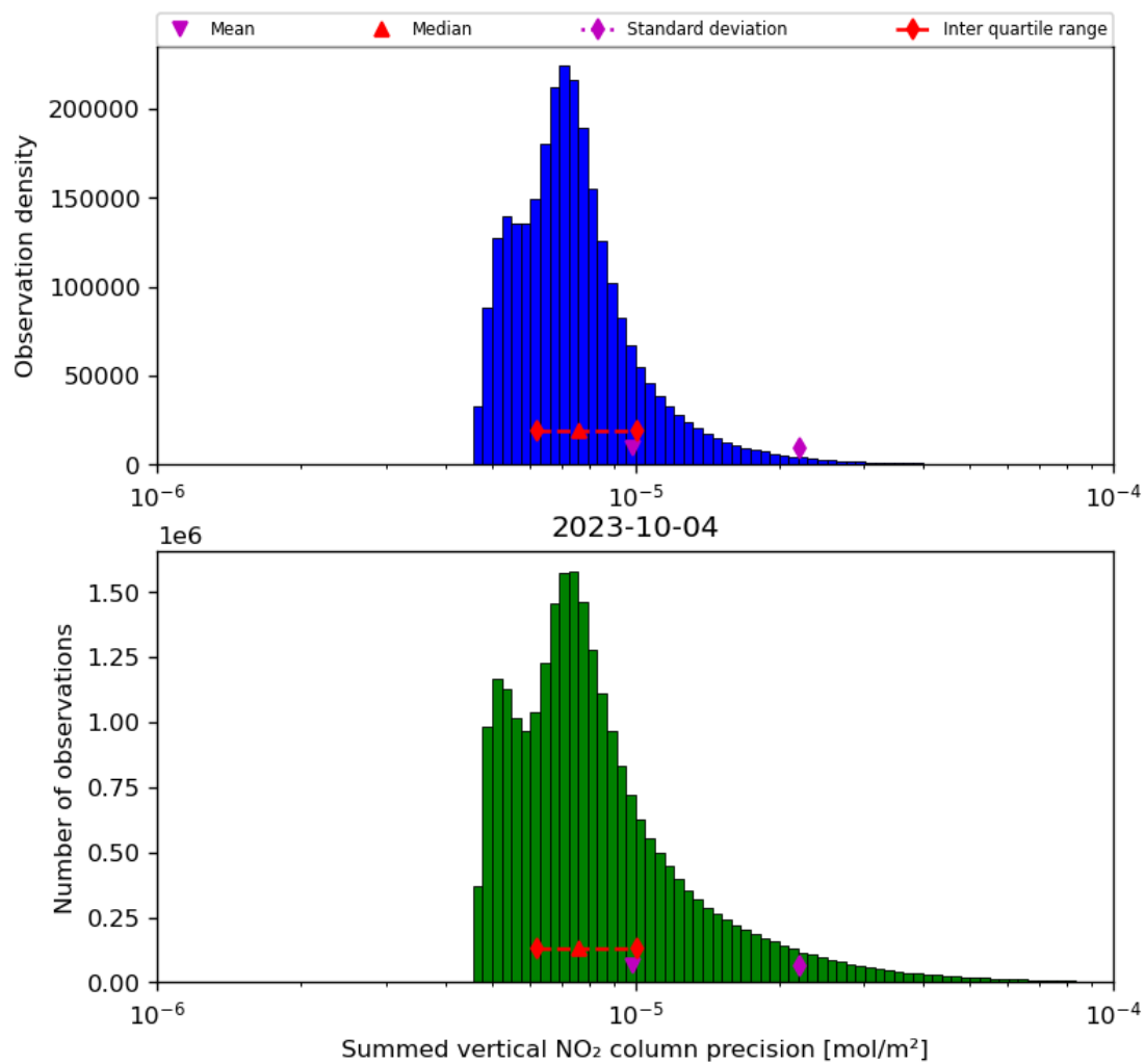
Figure 41: Histogram of "Summed vertical NO 2 column precision" for 2023-10-03 to 2023-10-05
