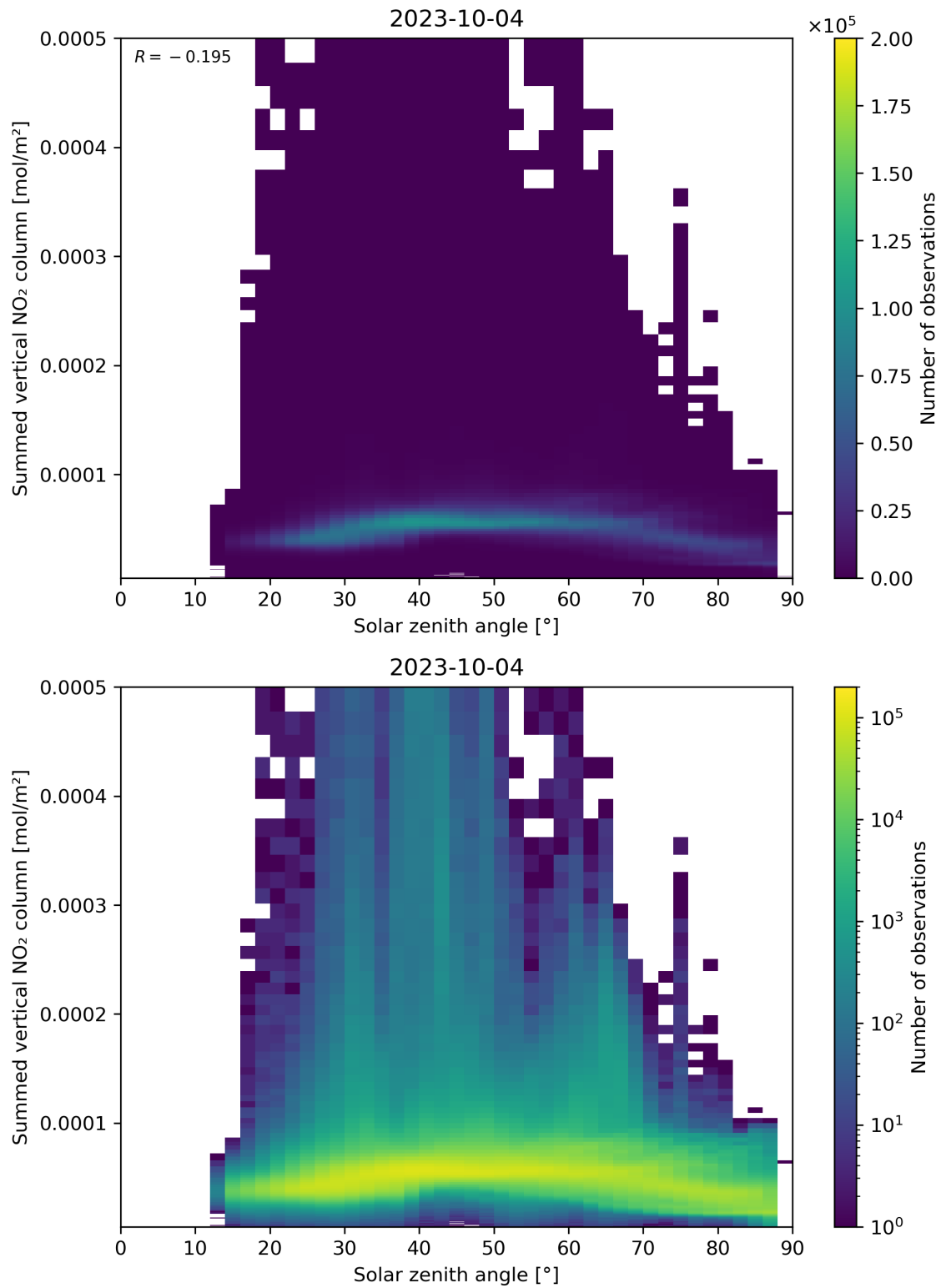
Figure 151: Scatter density plot of “Solar zenith angle” against “Summed vertical NO 2 column” for 2023-10-03 to 2023-10-05.
