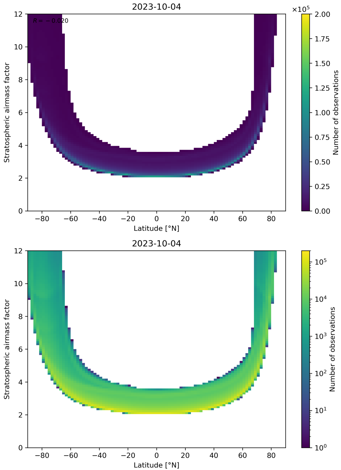
Figure 83: Scatter density plot of “Latitude” against “Stratospheric airmass factor” for 2023-10-03 to 2023-10-05.
