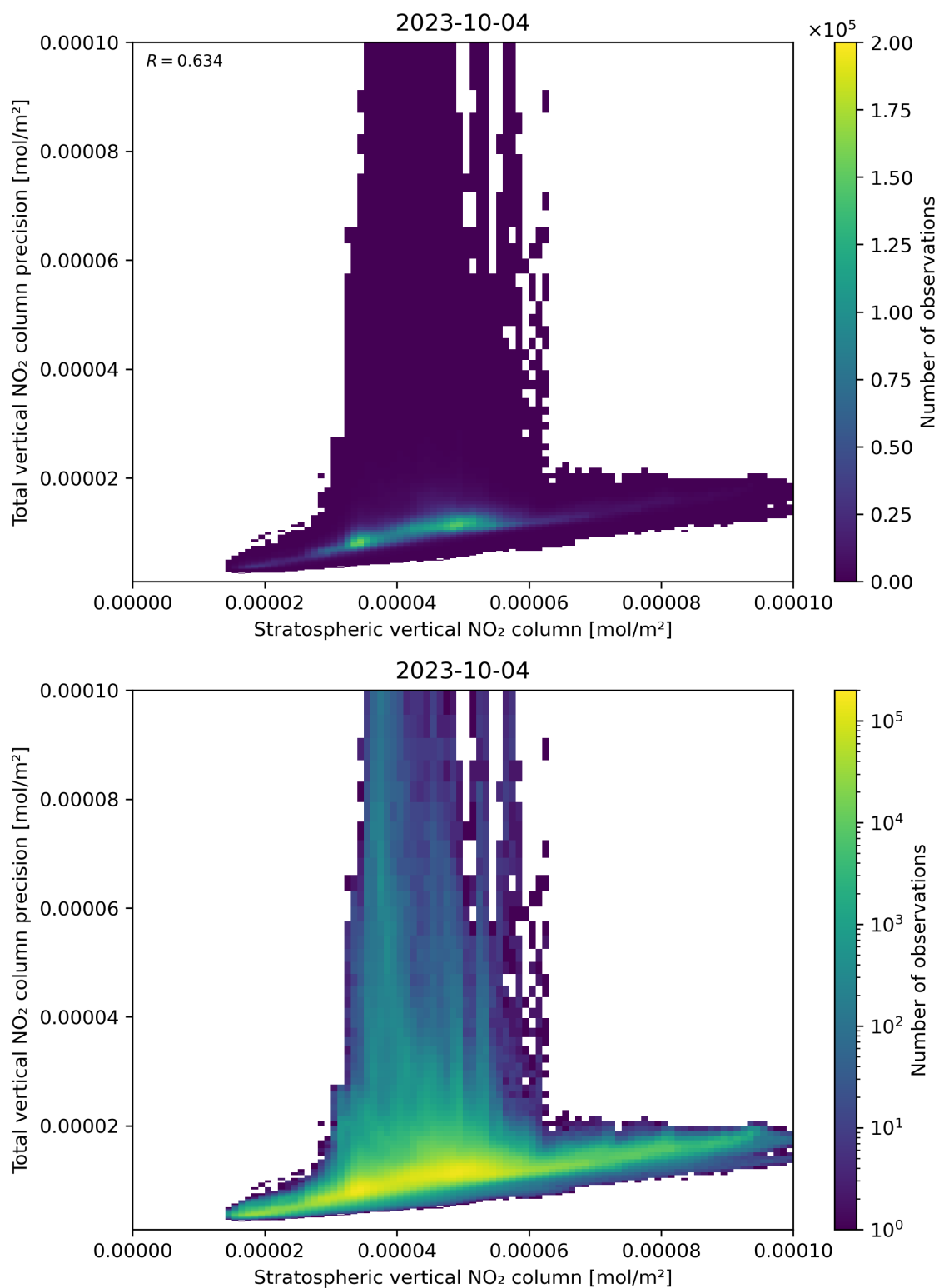
Figure 101: Scatter density plot of “Stratospheric vertical NO 2 column” against “Total vertical NO 2 column precision” for 2023-10-03 to 2023-10-05.
