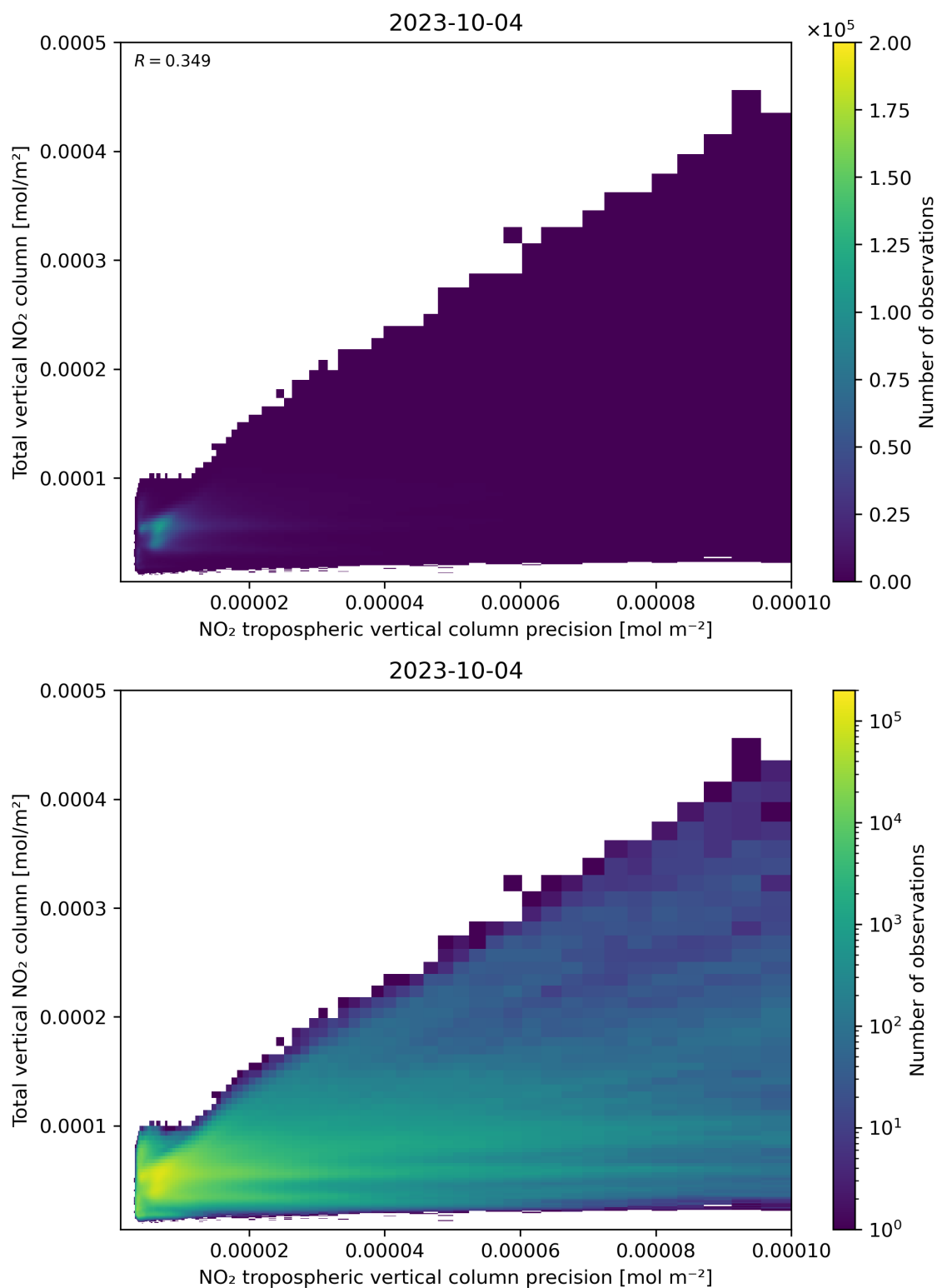
Figure 138: Scatter density plot of “NO 2 tropospheric vertical column precision” against “Total vertical NO 2 column” for 2023-10-03 to 2023-10-05.
