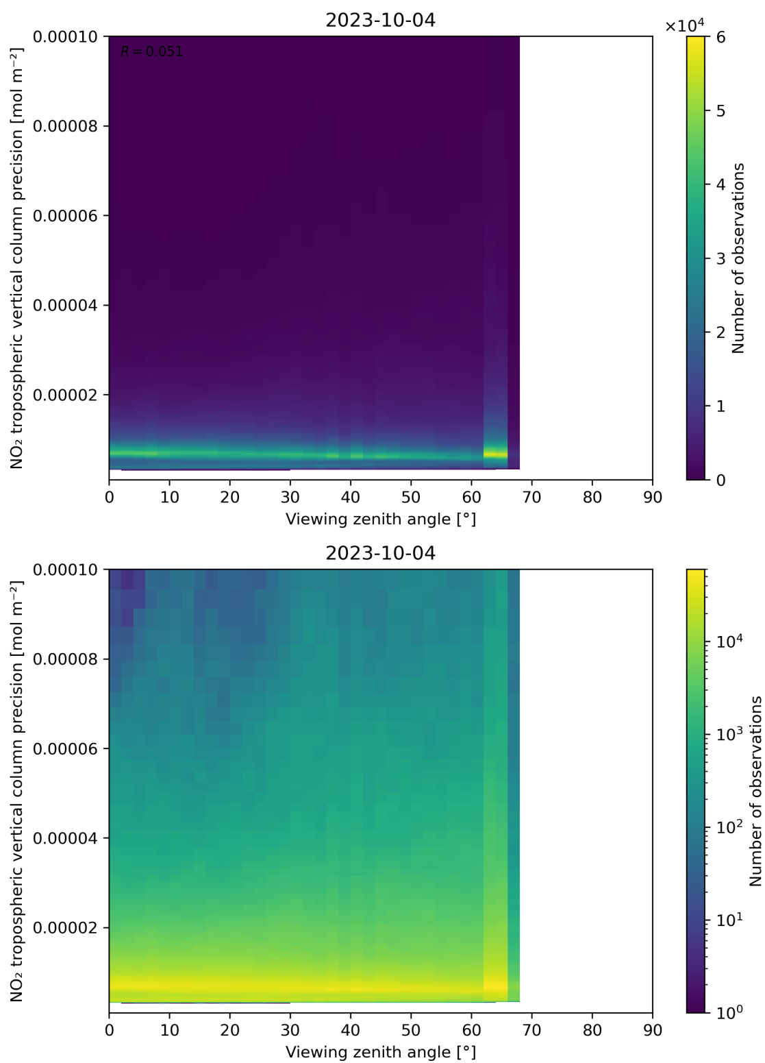
Figure 170: Scatter density plot of “Viewing zenith angle” against “NO 2 tropospheric vertical column precision” for 2023-10-03 to 2023-10-05.
