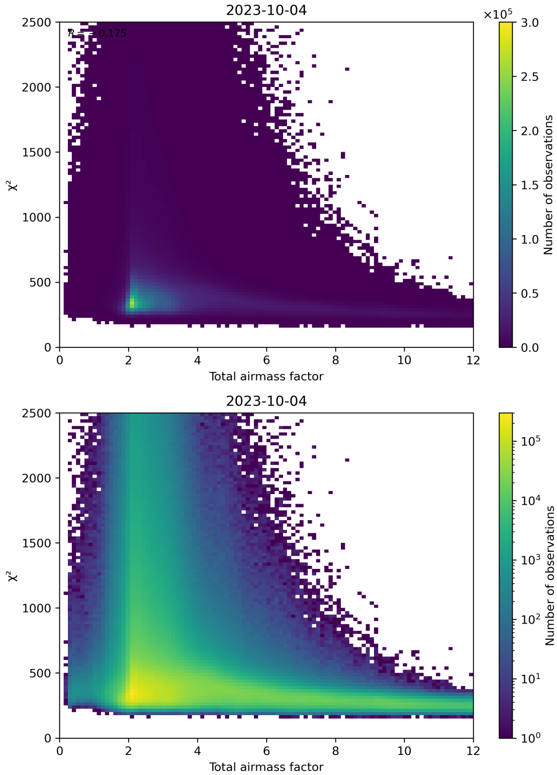
Figure 63: Scatter density plot of “Total airmass factor” against “ \chi^2 ” for 2023-10-03 to 2023-10-05.
