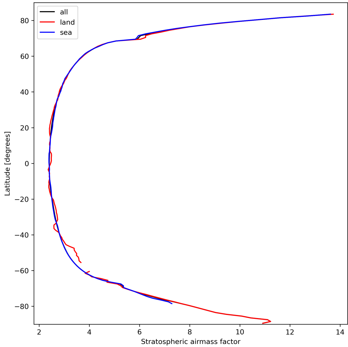
Figure 27: Zonal average of “Stratospheric airmass factor” for 2023-10-03 to 2023-10-05.
