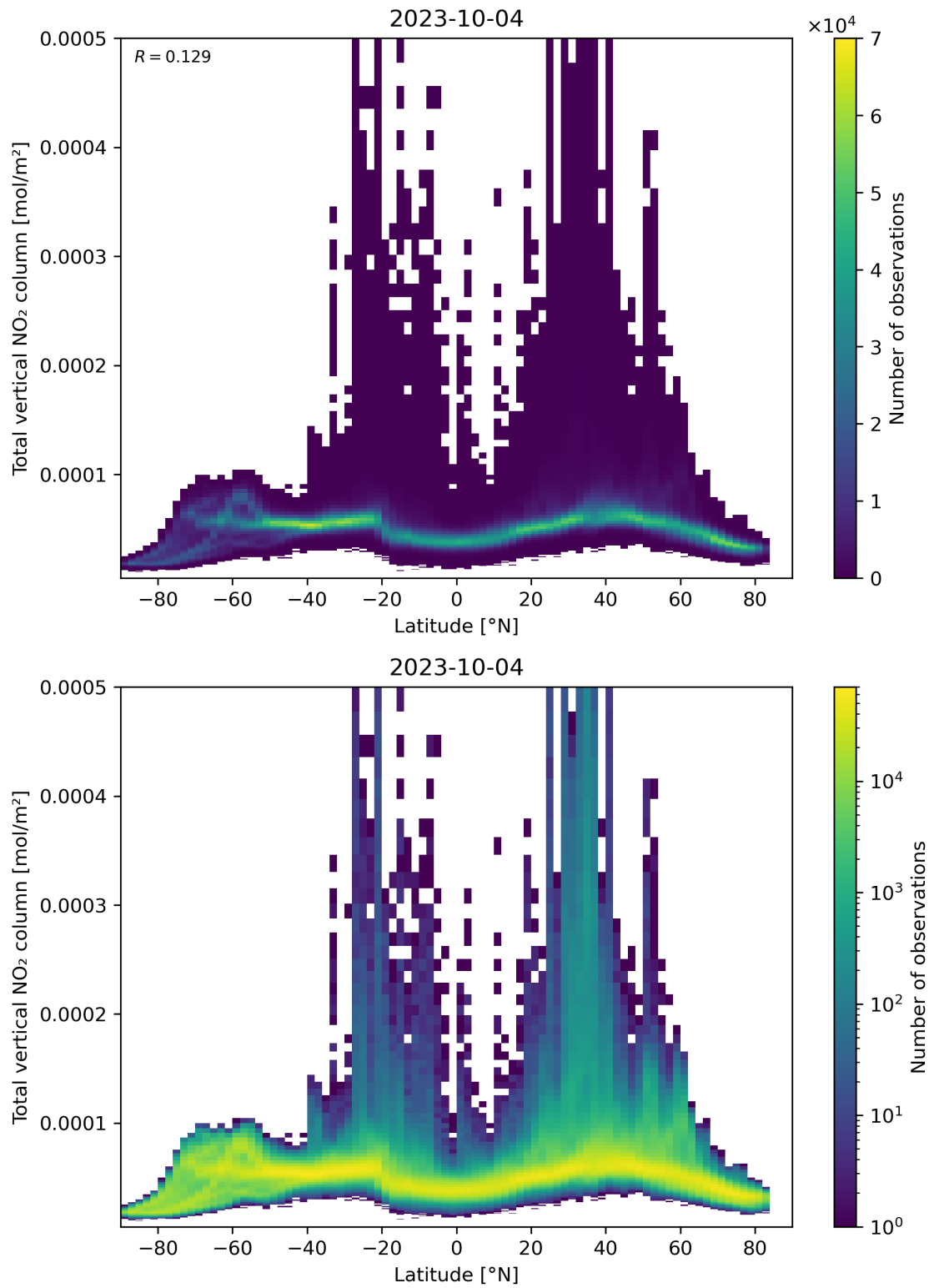
Figure 90: Scatter density plot of “Latitude” against “Total vertical NO 2 column” for 2023-10-03 to 2023-10-05.
