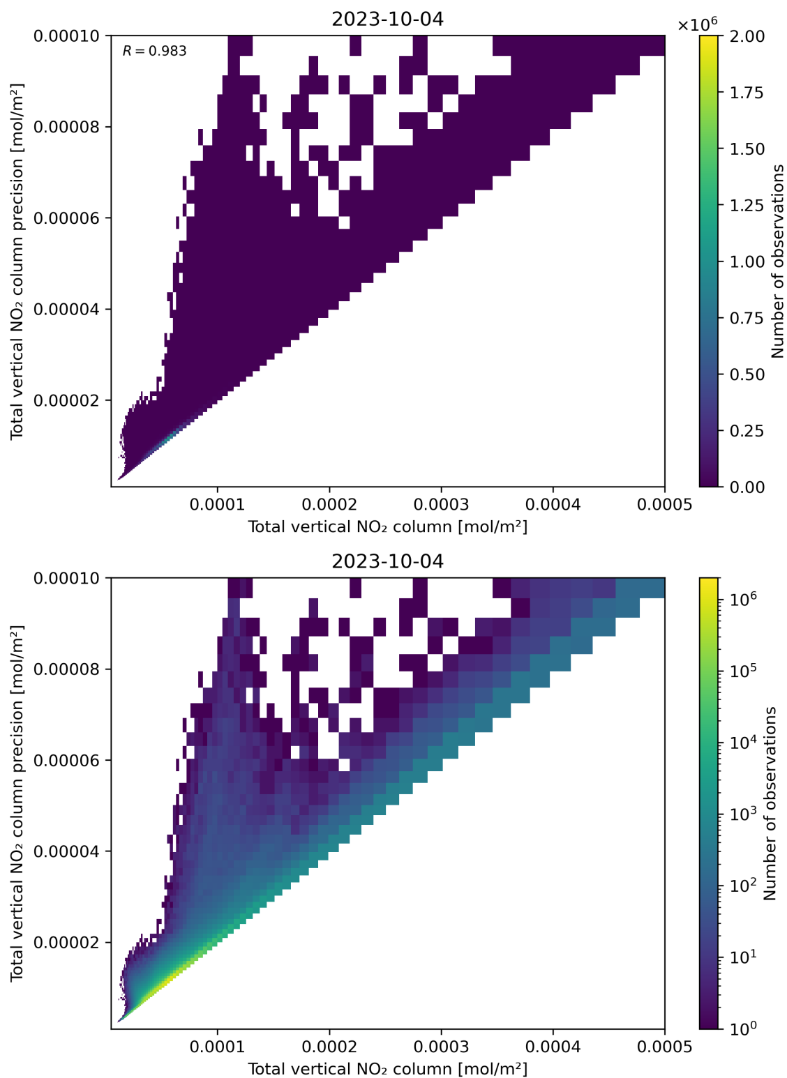
Figure 114: Scatter density plot of “Total vertical NO 2 column” against “Total vertical NO 2 column precision” for 2023-10-03 to 2023-10-05.
