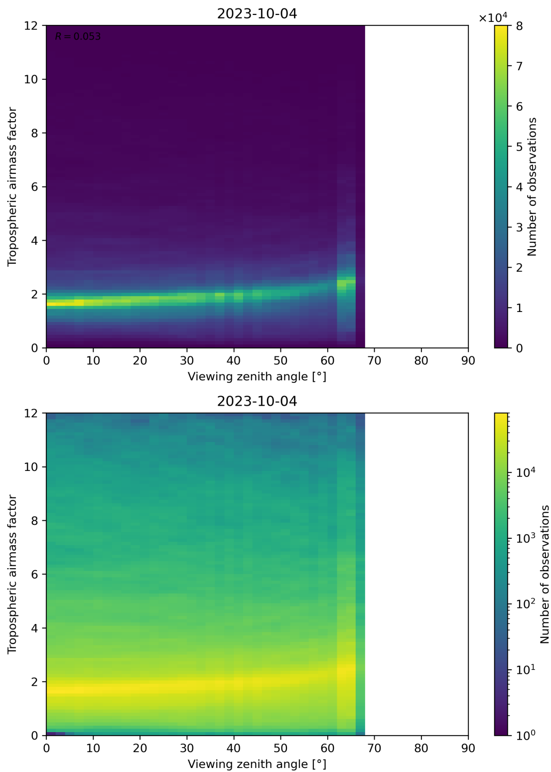
Figure 161: Scatter density plot of “Viewing zenith angle” against “Tropospheric airmass factor” for 2023-10-03 to 2023-10-05.
