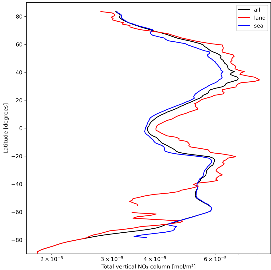
Figure 21: Zonal average of “Total vertical NO 2 column” for 2023-10-03 to 2023-10-05.
