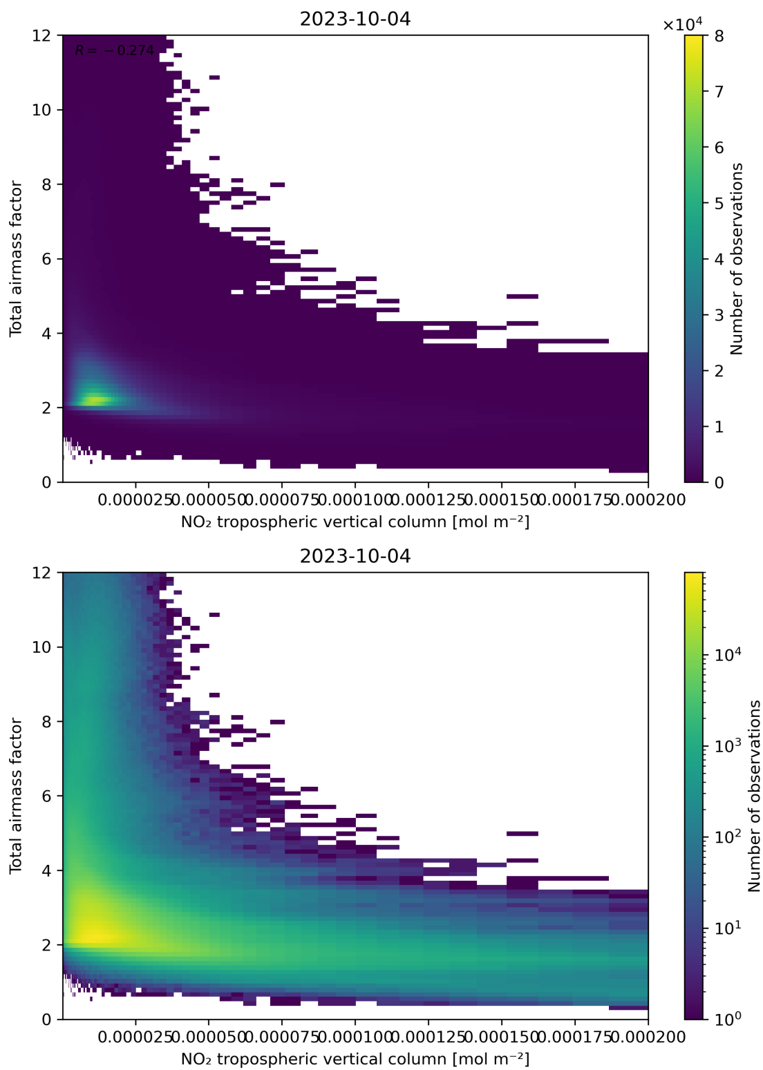
Figure 122: Scatter density plot of “NO 2 tropospheric vertical column” against “Total air mass factor” for 2023-10-03 to 2023-10-05.
