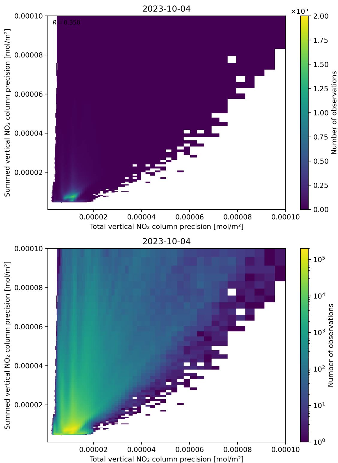
Figure 118: Scatter density plot of “Total vertical NO 2 column precision” against “Summed vertical NO 2 column precision” for 2023-10-03 to 2023-10-05.
