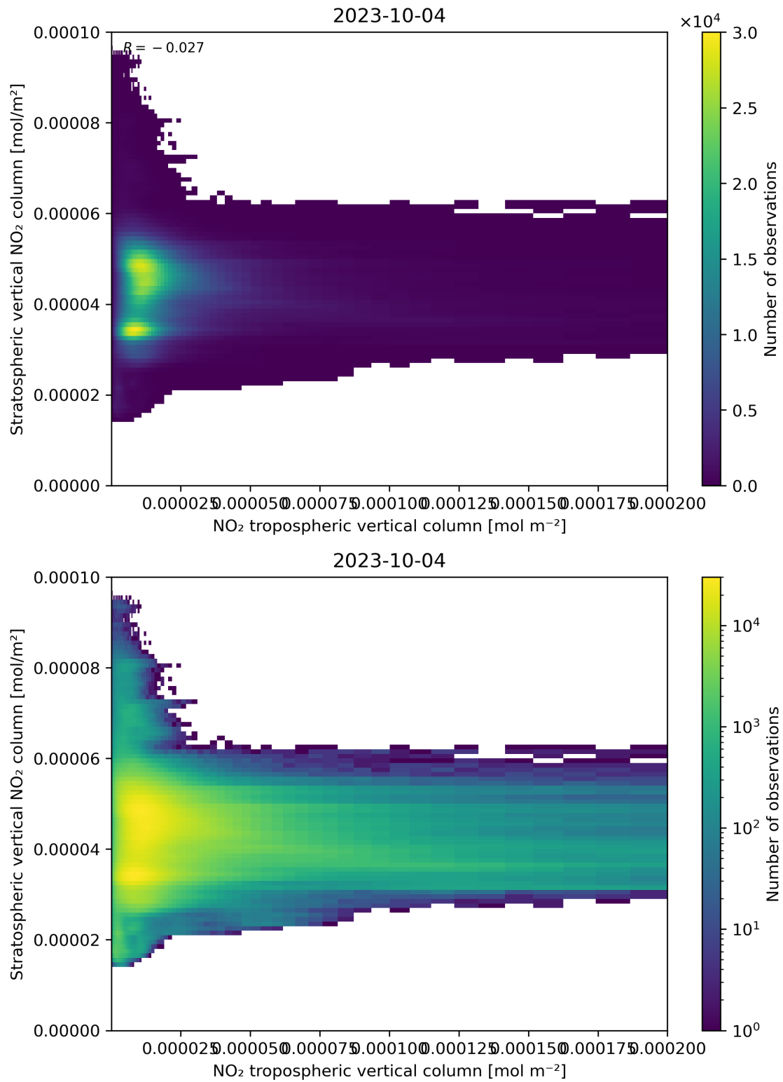
Figure 125: Scatter density plot of “NO 2 tropospheric vertical column” against “Stratospheric vertical NO 2 column” for 2023-10-03 to 2023-10-05.
