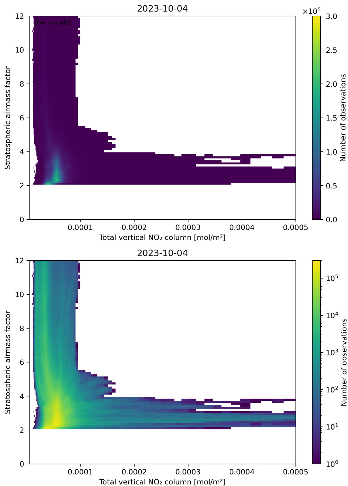
Figure 110: Scatter density plot of “Total vertical NO 2 column” against “Stratospheric airmass factor” for 2023-10-03 to 2023-10-05.
