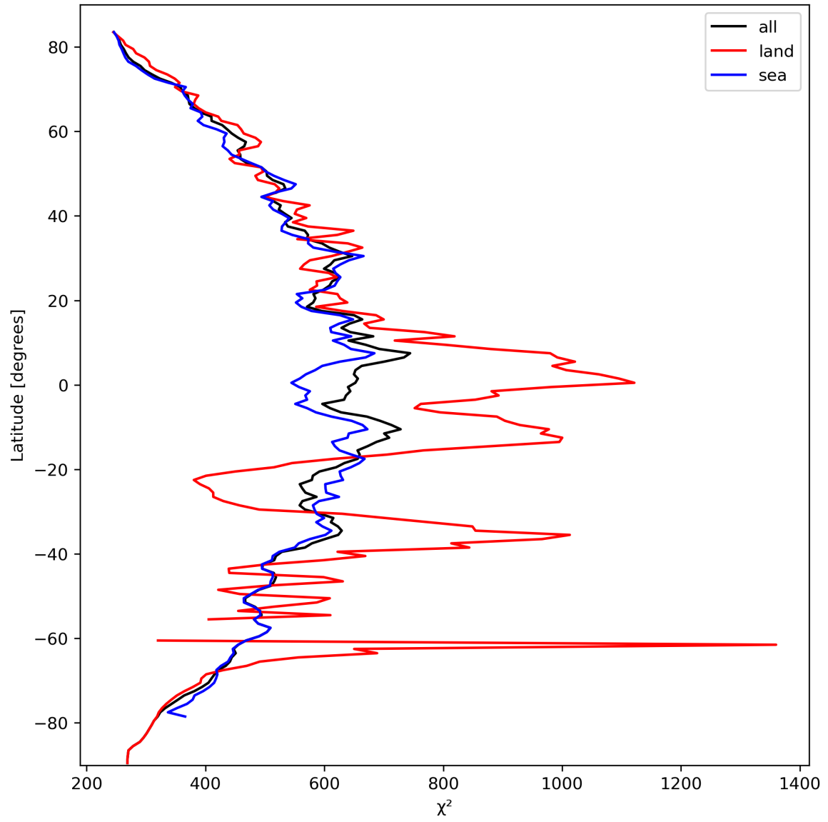
Figure 25: Zonal average of “ \chi^2 ” for 2023-10-03 to 2023-10-05.
