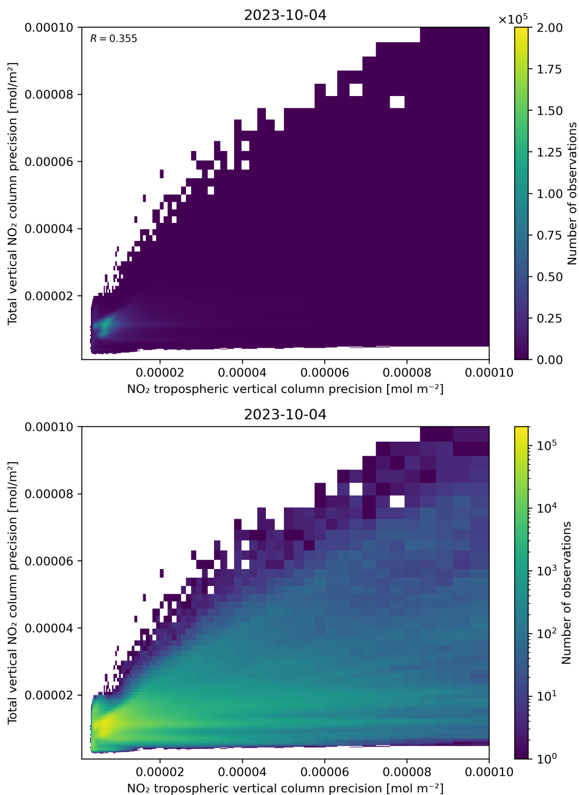
Figure 139: Scatter density plot of “NO 2 tropospheric vertical column precision” against “Total vertical NO 2 column precision” for 2023-10-03 to 2023-10-05.
