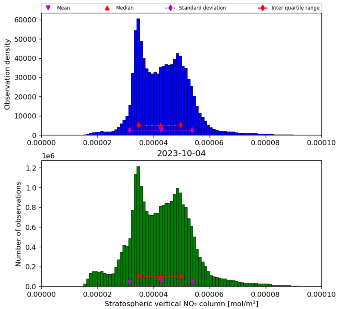
Figure 36: Histogram of “Stratospheric vertical NO 2 column” for 2023-10-03 to 2023-10-05
