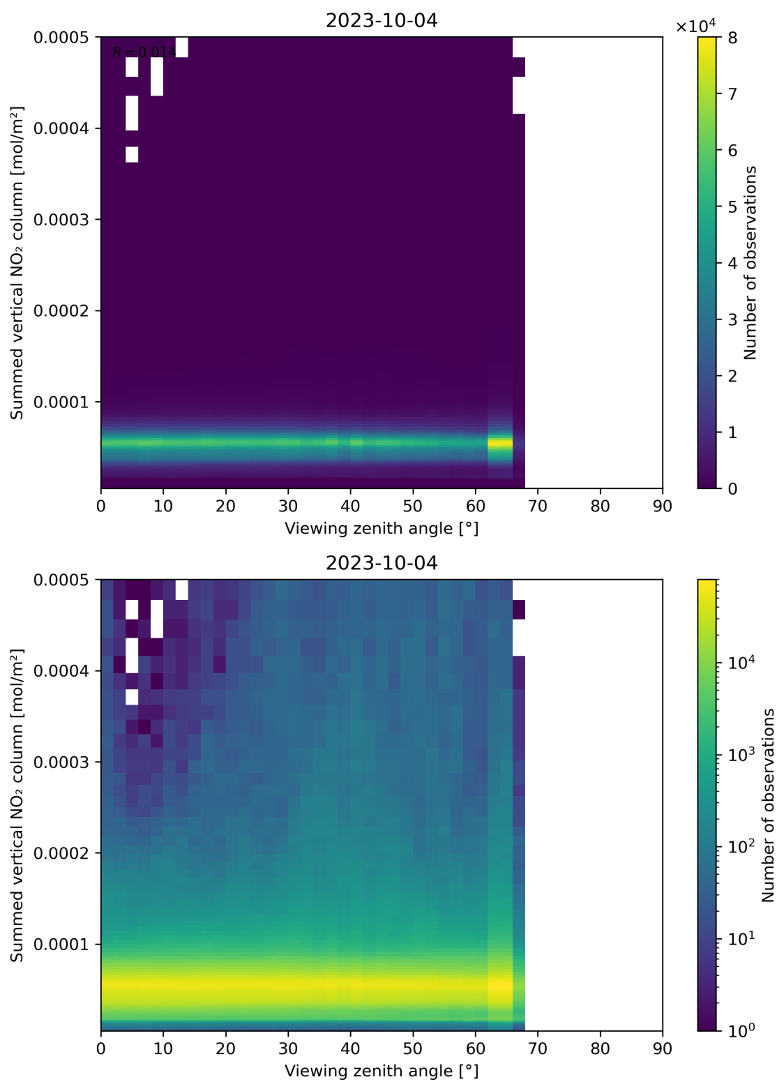
Figure 165: Scatter density plot of “Viewing zenith angle” against “Summed vertical NO 2 column” for 2023-10-03 to 2023-10-05.
