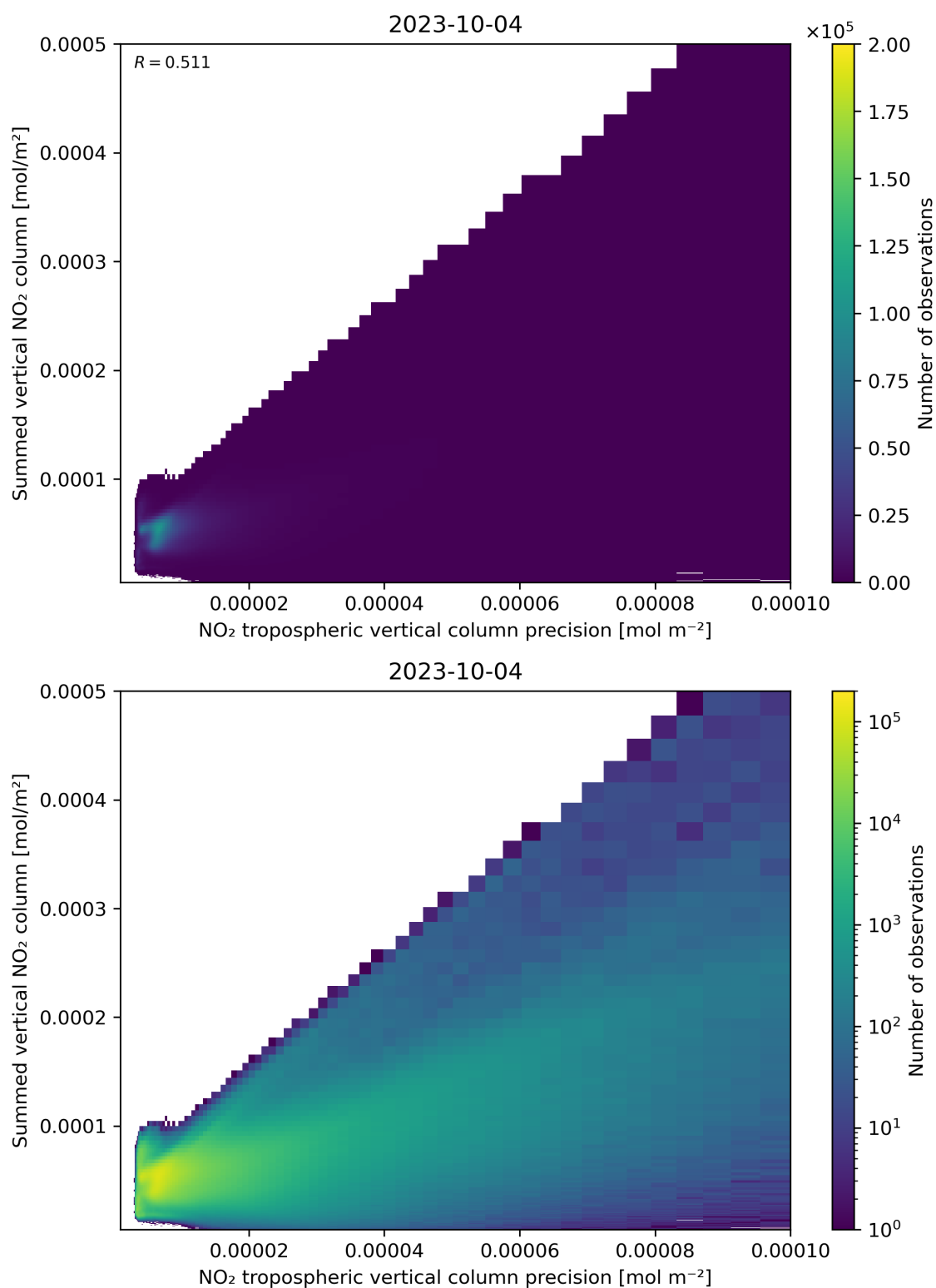
Figure 136: Scatter density plot of “NO 2 tropospheric vertical column precision” against “Summed vertical NO 2 column” for 2023-10-03 to 2023-10-05.
