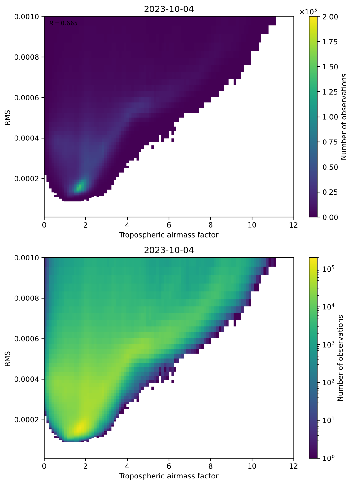
Figure 79: Scatter density plot of “Tropospheric airmass factor” against “RMS” for 2023-10-03 to 2023-10-05.
