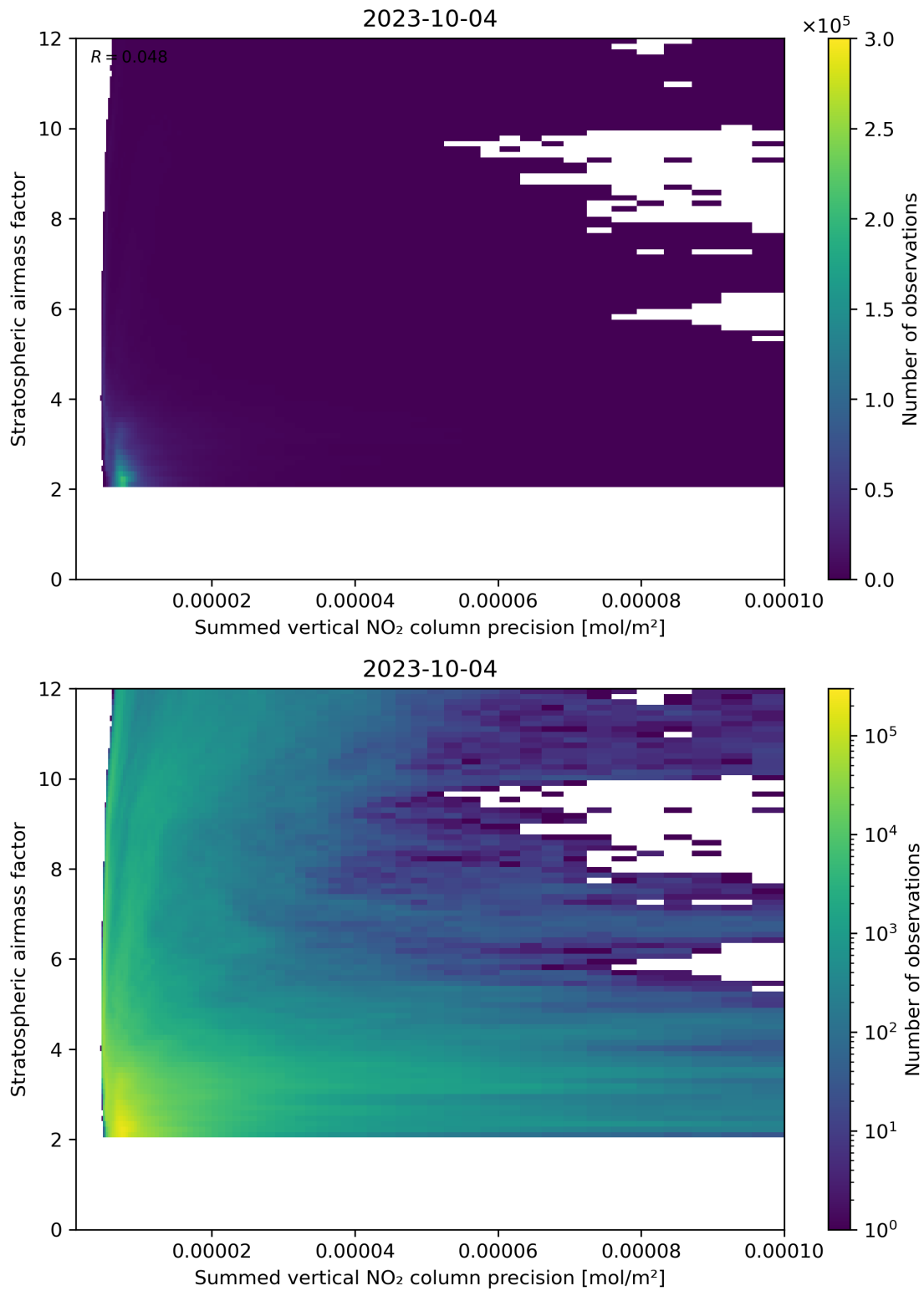
Figure 106: Scatter density plot of “Summed vertical NO 2 column precision” against “Stratospheric airmass factor” for 2023-10-03 to 2023-10-05.
