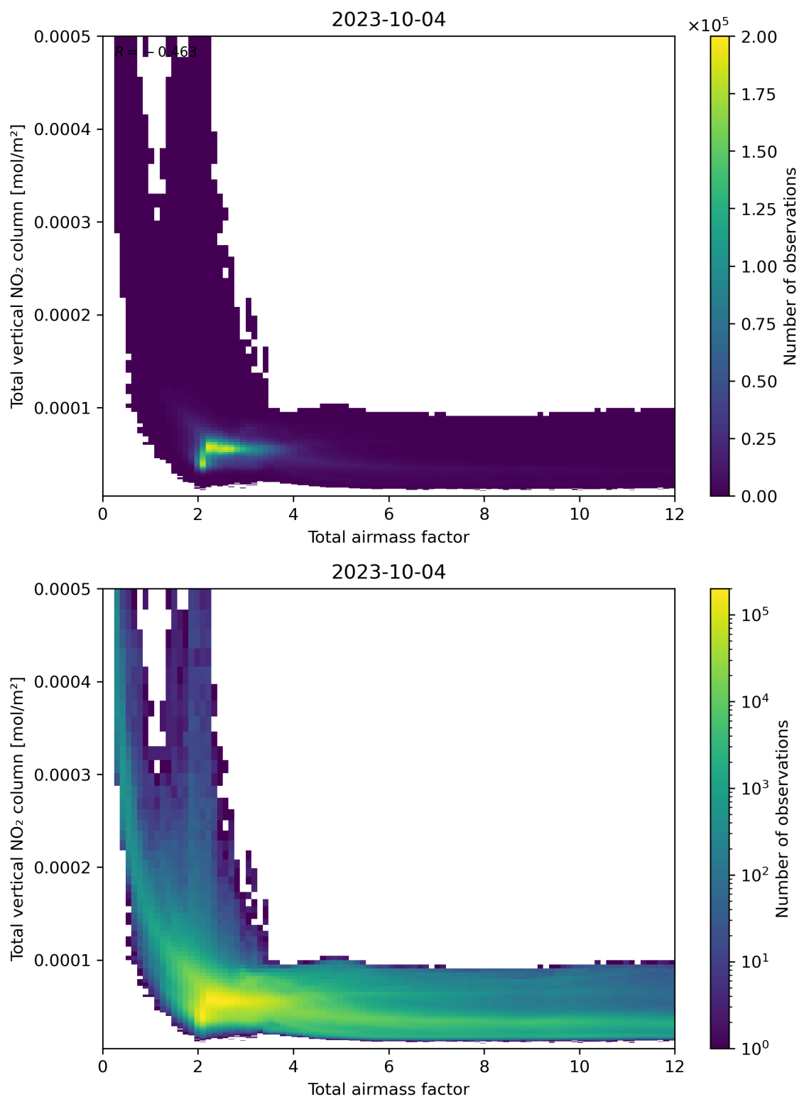
Figure 67: Scatter density plot of “Total airmass factor” against “Total vertical NO 2 column” for 2023-10-03 to 2023-10-05.
