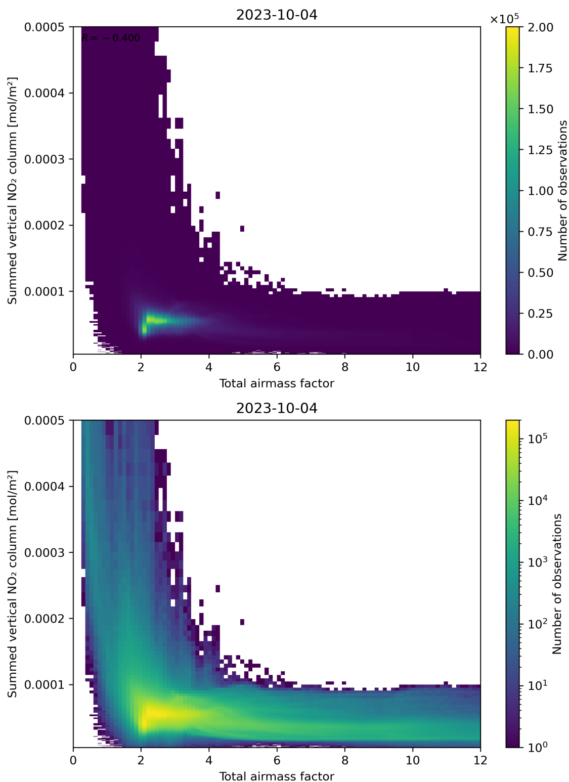
Figure 65: Scatter density plot of “Total airmass factor” against “Summed vertical NO 2 column” for 2023-10-03 to 2023-10-05.
