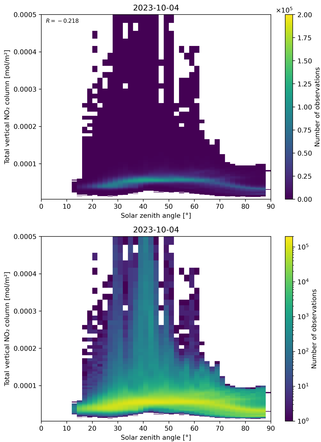
Figure 153: Scatter density plot of “Solar zenith angle” against “Total vertical NO 2 column” for 2023-10-03 to 2023-10-05.
