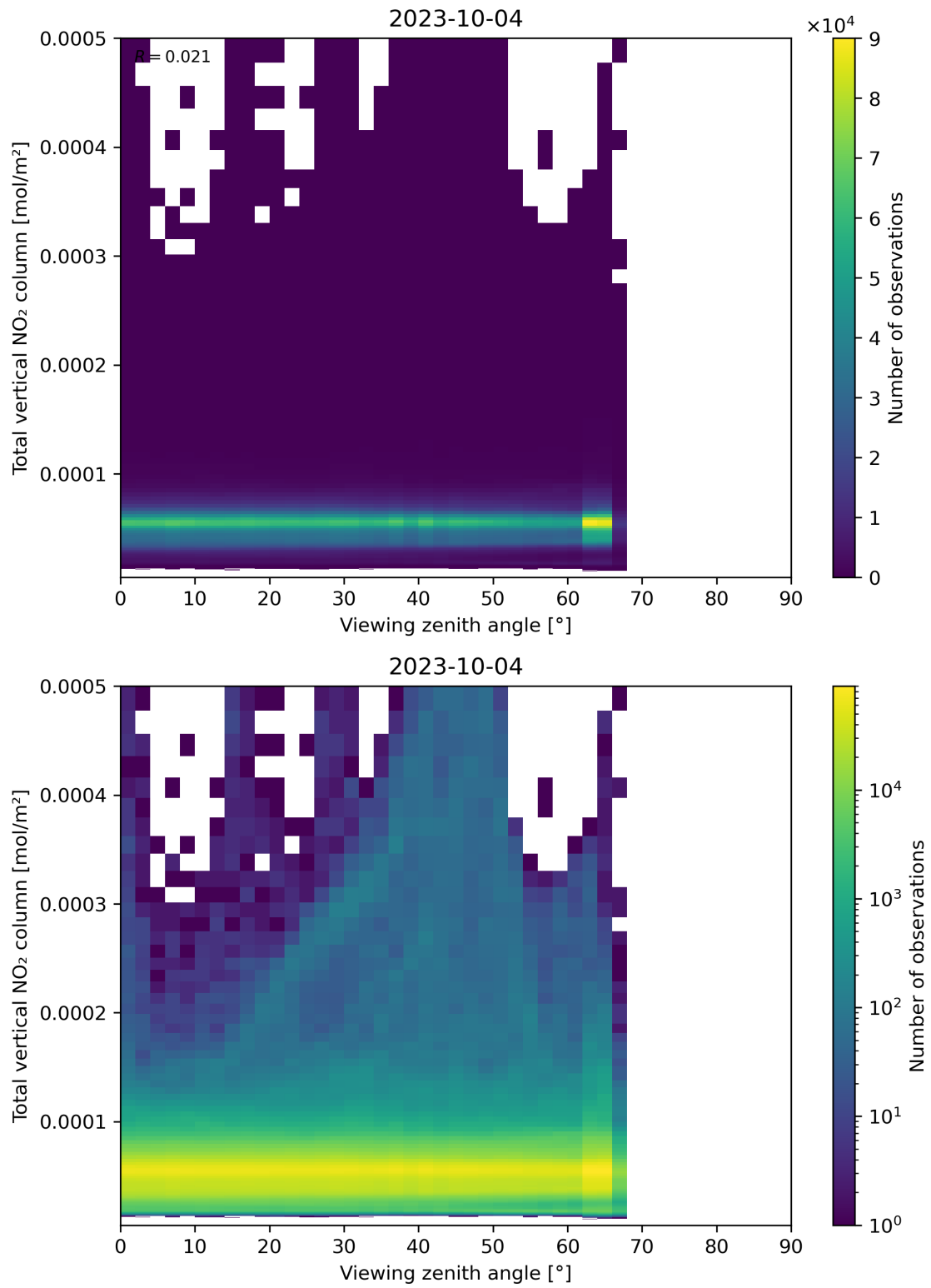
Figure 167: Scatter density plot of “Viewing zenith angle” against “Total vertical NO 2 column” for 2023-10-03 to 2023-10-05.
