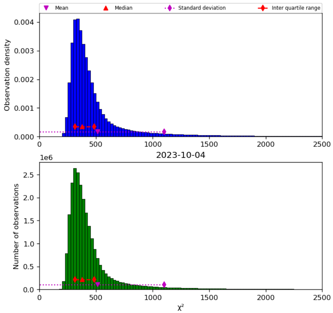
Figure 42: Histogram of “ \chi^2 ” for 2023-10-03 to 2023-10-05
