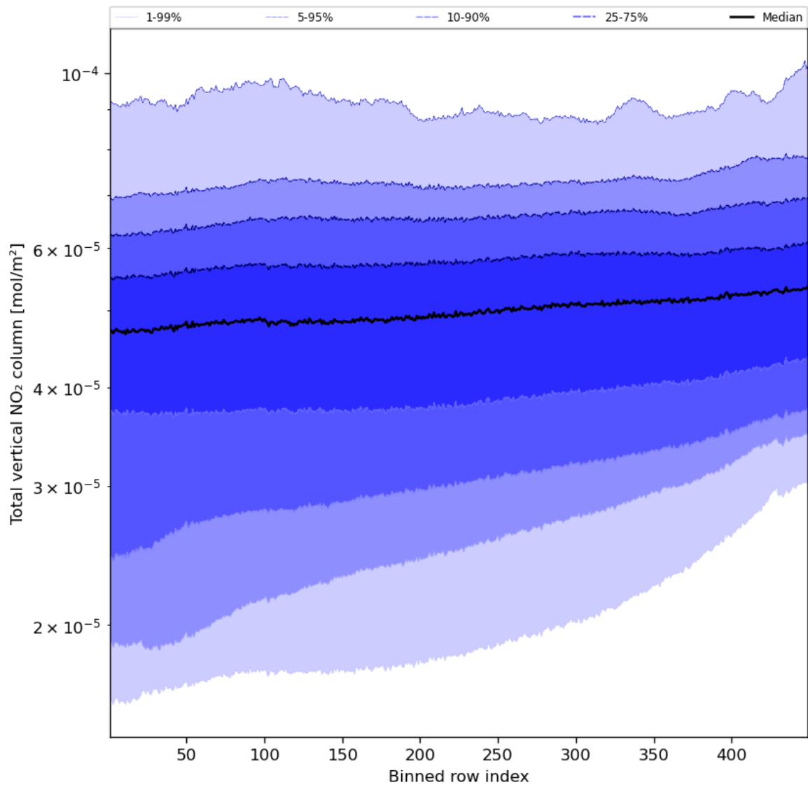
Figure 55: Along track statistics of “Total vertical NO 2 column” for 2023-10-03 to 2023-10-05
