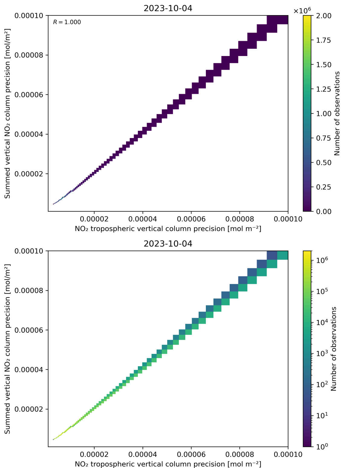
Figure 137: Scatter density plot of “NO 2 tropospheric vertical column precision” against “Summed vertical NO 2 column precision” for 2023-10-03 to 2023-10-05.
