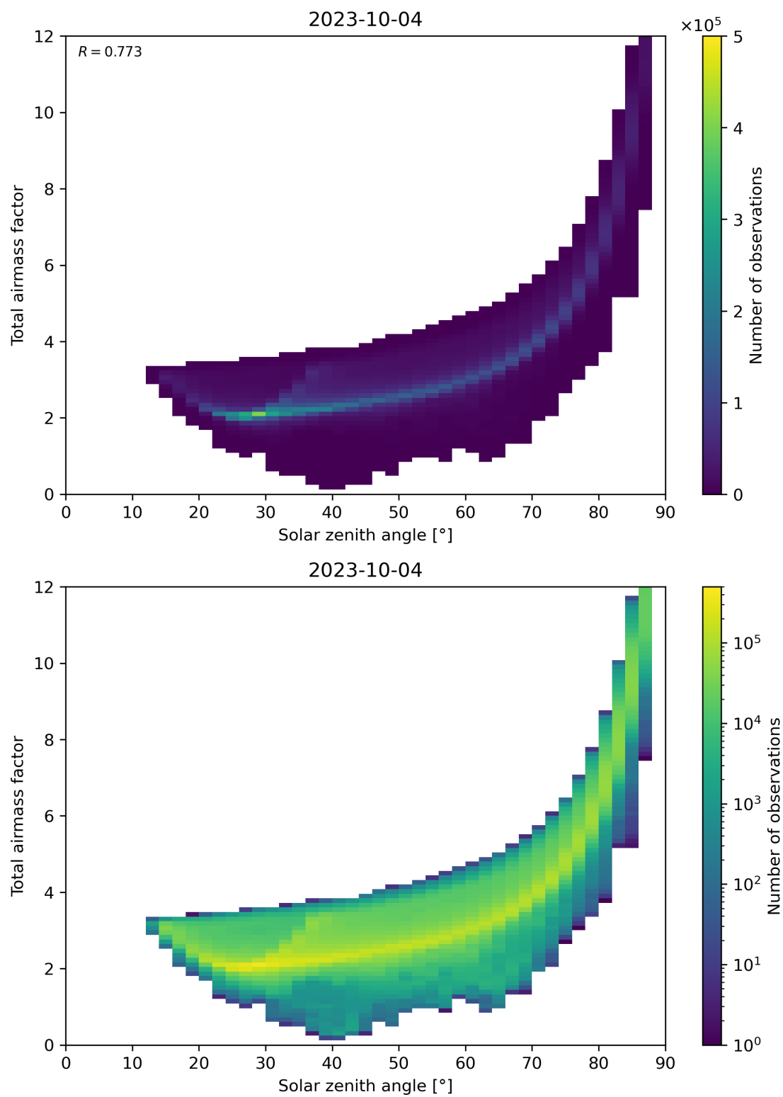
Figure 146: Scatter density plot of “Solar zenith angle” against “Total airmass factor” for 2023-10-03 to 2023-10-05.
