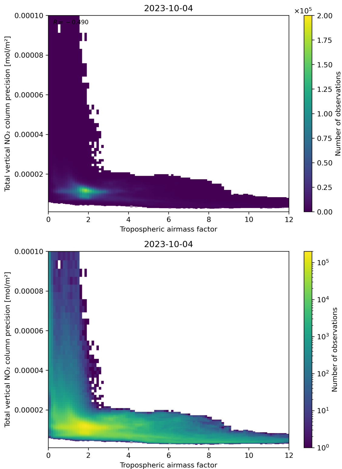
Figure 78: Scatter density plot of “Tropospheric air mass factor” against “Total vertical NO 2 column precision” for 2023-10-03 to 2023-10-05.
