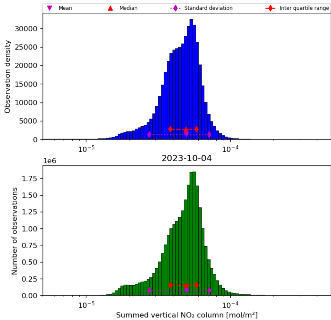
Figure 40: Histogram of “Summed vertical NO 2 column” for 2023-10-03 to 2023-10-05
