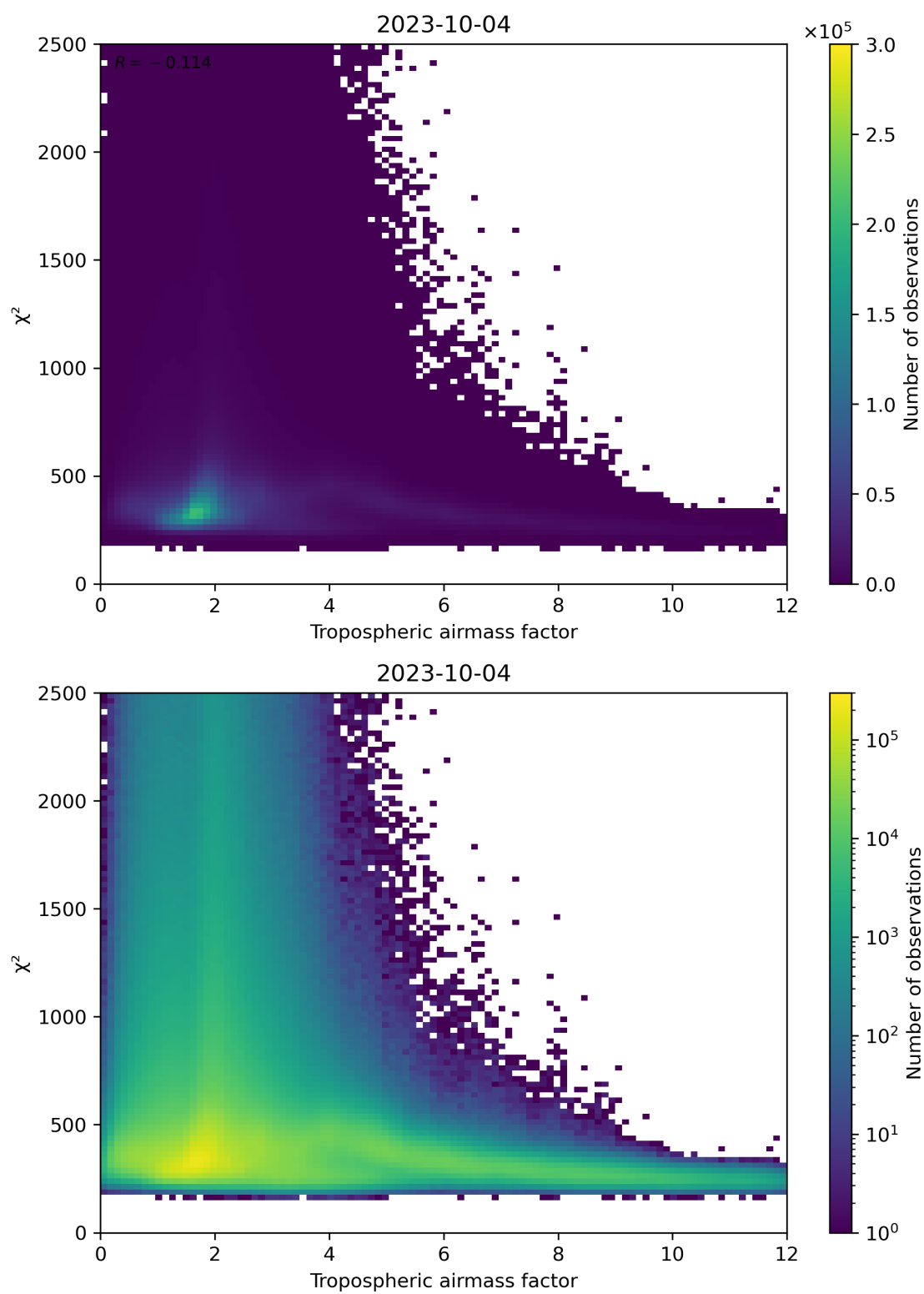
Figure 73: Scatter density plot of “Tropospheric airmass factor” against “ \chi^2 ” for 2023-10-03 to 2023-10-05.
