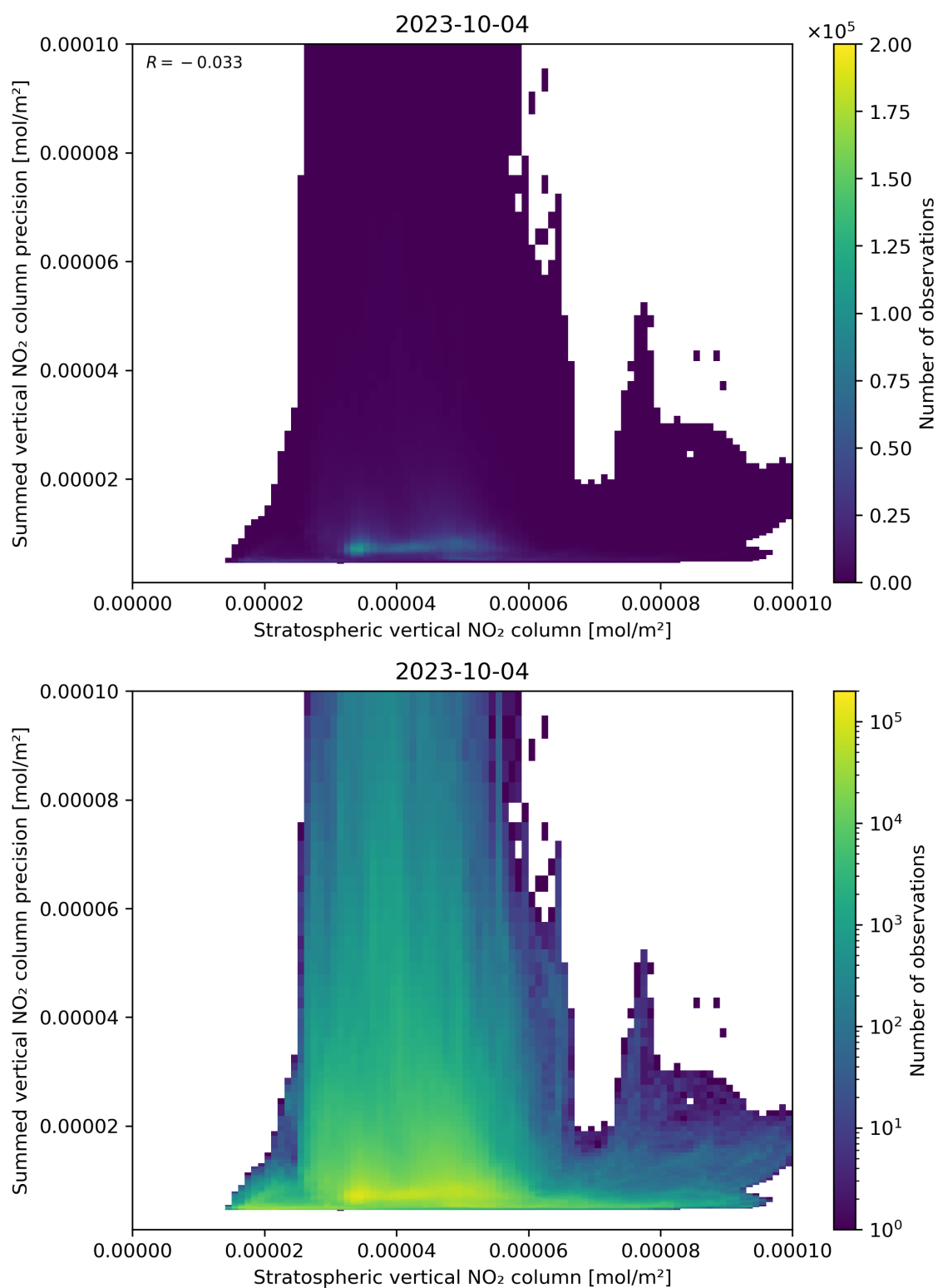
Figure 99: Scatter density plot of “Stratospheric vertical NO 2 column” against “Summed vertical NO 2 column precision” for 2023-10-03 to 2023-10-05.
