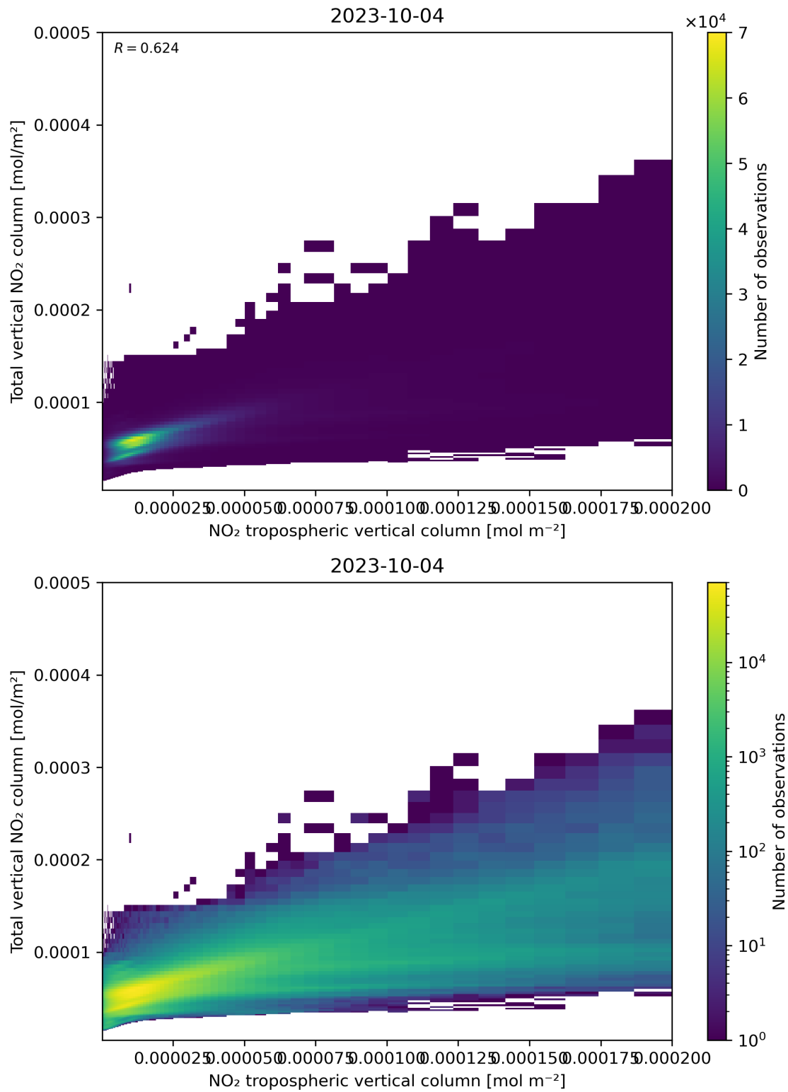
Figure 128: Scatter density plot of “NO 2 tropospheric vertical column” against “Total vertical NO 2 column” for 2023-10-03 to 2023-10-05.
