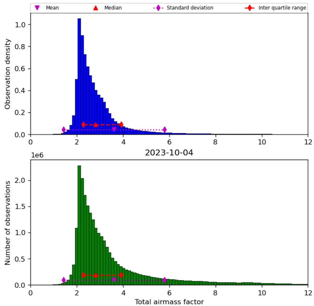
Figure 32: Histogram of “Total airmass factor” for 2023-10-03 to 2023-10-05
