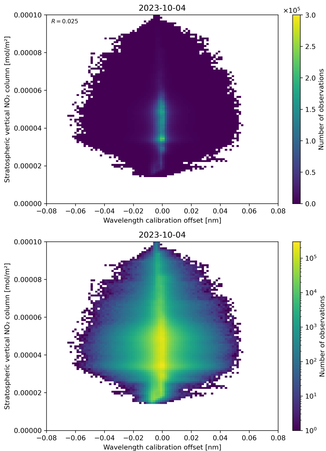
Figure 176: Scatter density plot of “Wavelength calibration offset” against “Stratospheric vertical NO 2 column” for 2023-10-03 to 2023-10-05.
