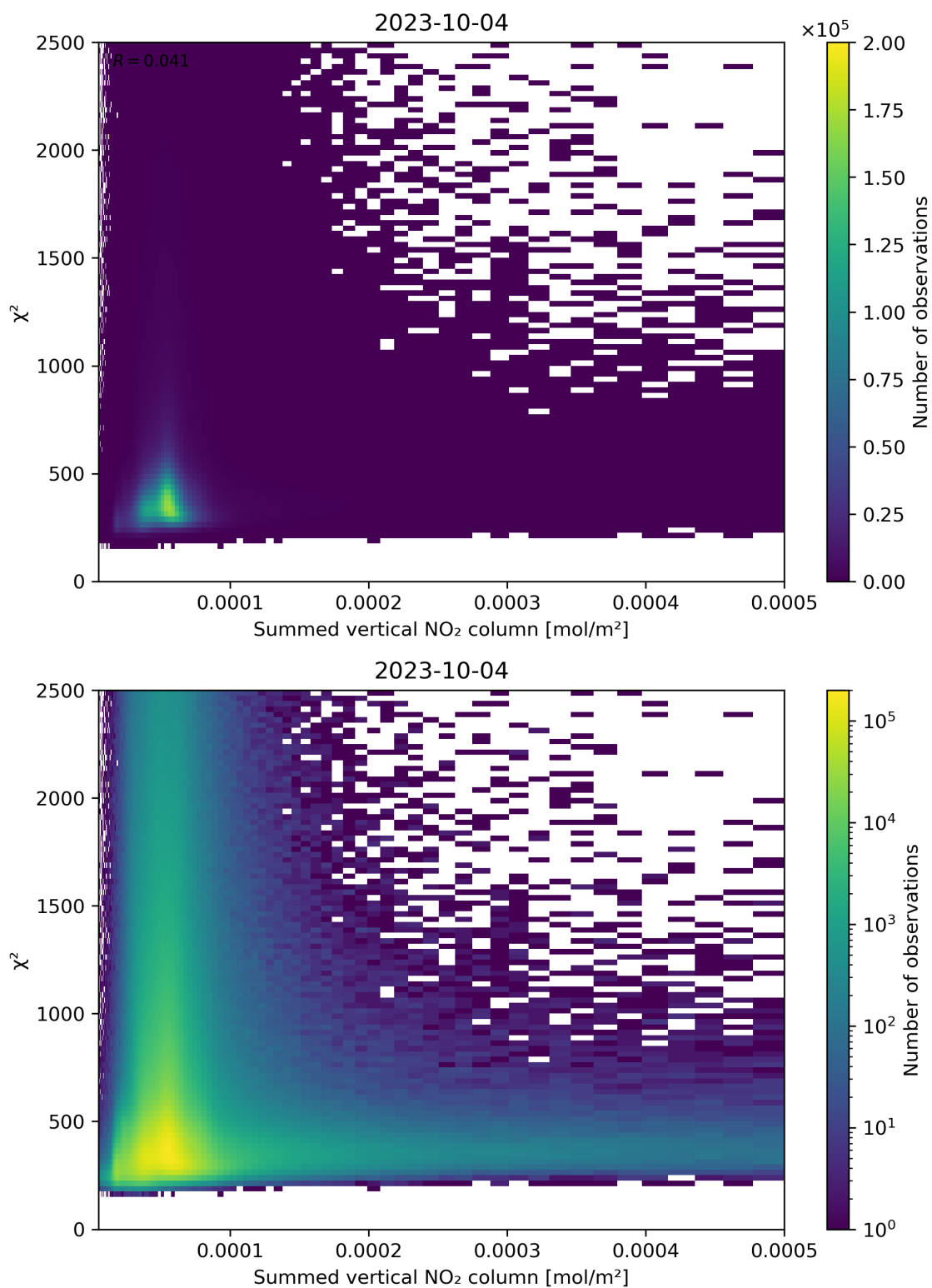
Figure 104: Scatter density plot of “Summed vertical NO 2 column” against “ \chi^2 ” for 2023-10-03 to 2023-10-05.
