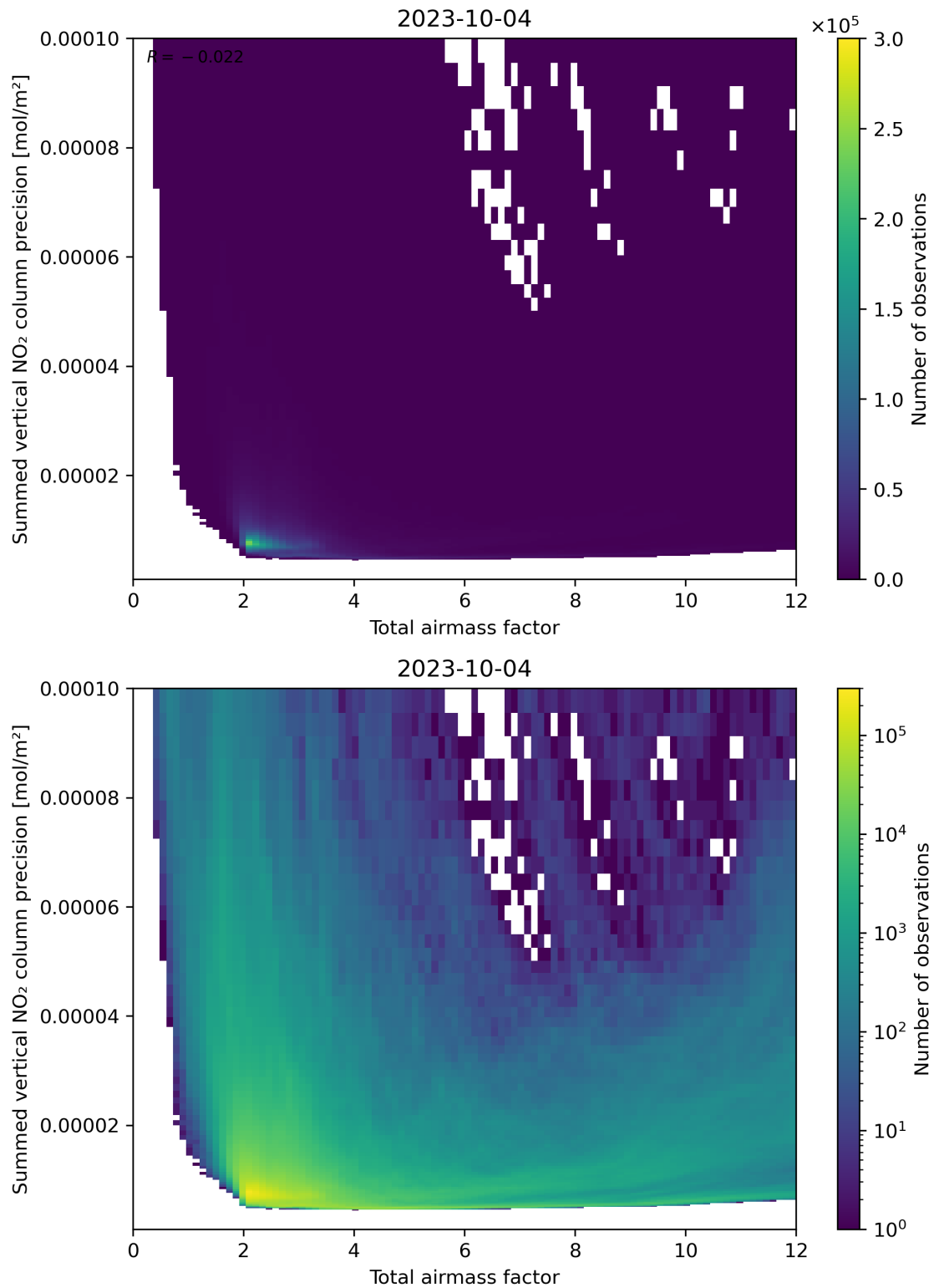
Figure 66: Scatter density plot of “Total airmass factor” against “Summed vertical NO 2 column precision” for 2023-10-03 to 2023-10-05.
