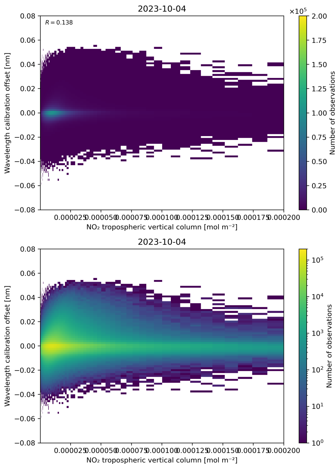
Figure 143: Scatter density plot of “NO 2 tropospheric vertical column” against “Wavelength calibration offset” for 2023-10-03 to 2023-10-05.
