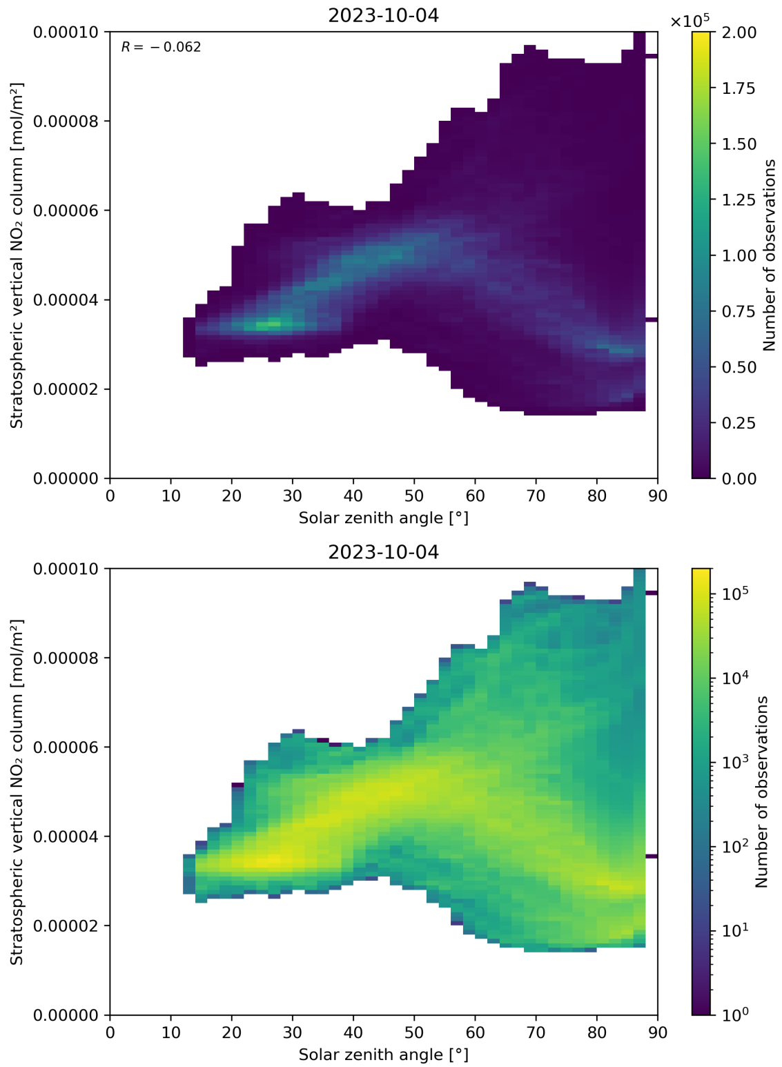
Figure 150: Scatter density plot of “Solar zenith angle” against “Stratospheric vertical NO 2 column” for 2023-10-03 to 2023-10-05.
