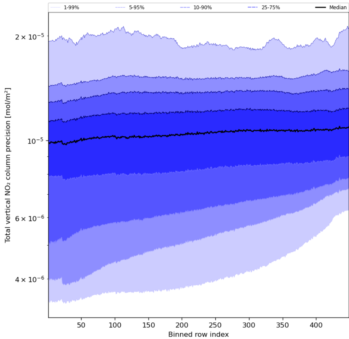
Figure 56: Along track statistics of “Total vertical NO 2 column precision” for 2023-10-03 to 2023-10-05
