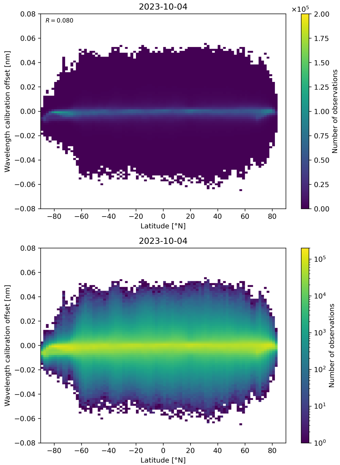
Figure 95: Scatter density plot of “Latitude” against “Wavelength calibration offset” for 2023-10-03 to 2023-10-05.
