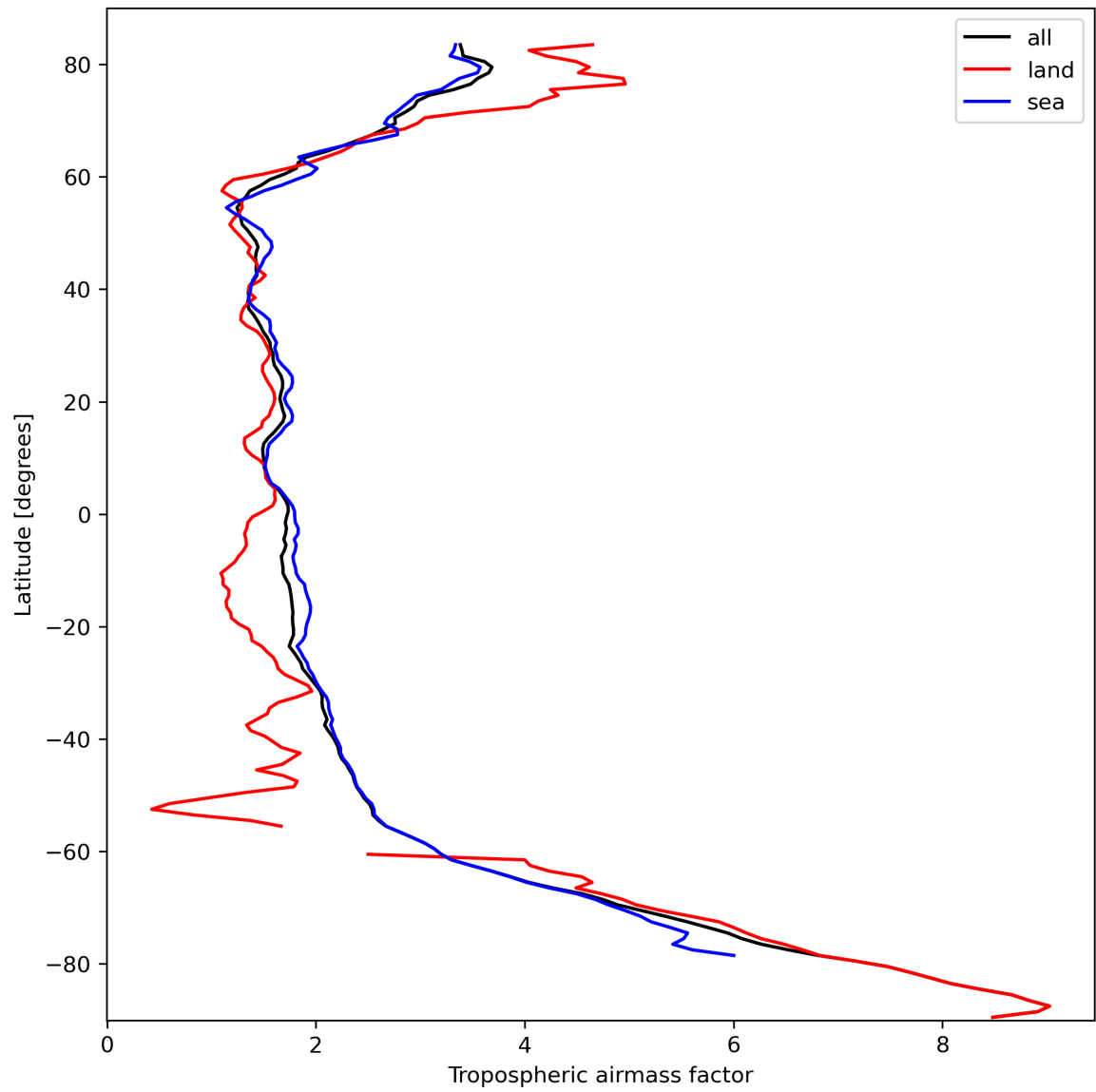
Figure 14: Zonal average of “Tropospheric airmass factor” for 2023-10-03 to 2023-10-05.
