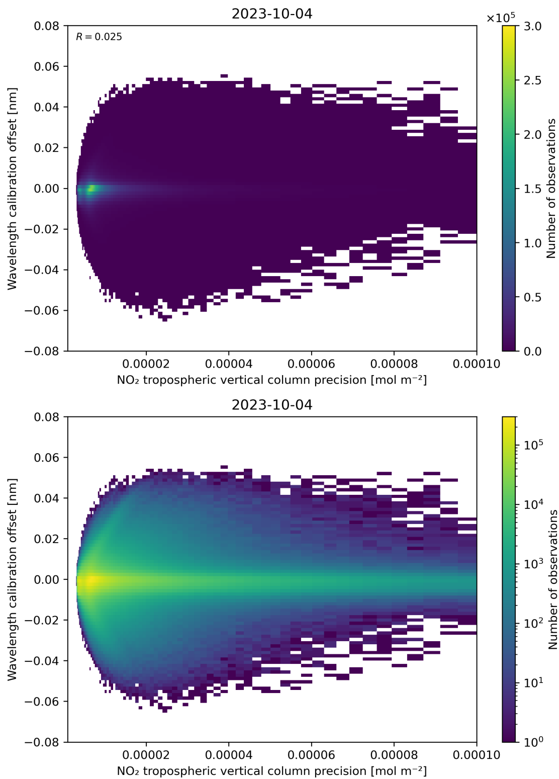
Figure 141: Scatter density plot of “NO 2 tropospheric vertical column precision” against “Wavelength calibration offset” for 2023-10-03 to 2023-10-05.
