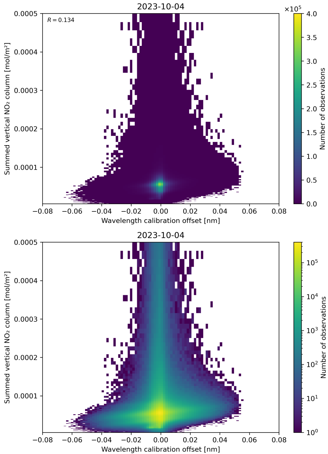
Figure 177: Scatter density plot of “Wavelength calibration offset” against “Summed vertical NO 2 column” for 2023-10-03 to 2023-10-05.
