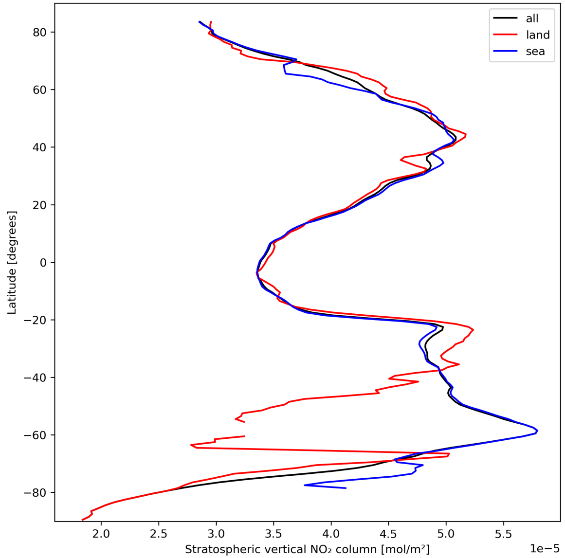
Figure 19: Zonal average of “Stratospheric vertical NO 2 column” for 2023-10-03 to 2023-10-05.
