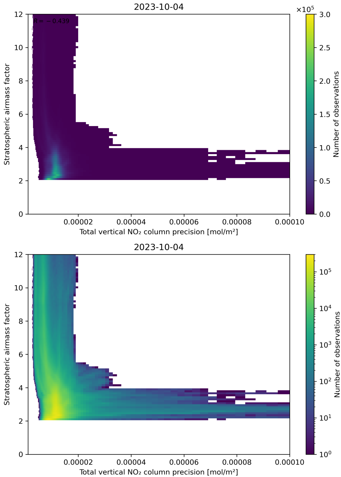
Figure 115: Scatter density plot of “Total vertical NO 2 column precision” against “Stratospheric air mass factor” for 2023-10-03 to 2023-10-05.
