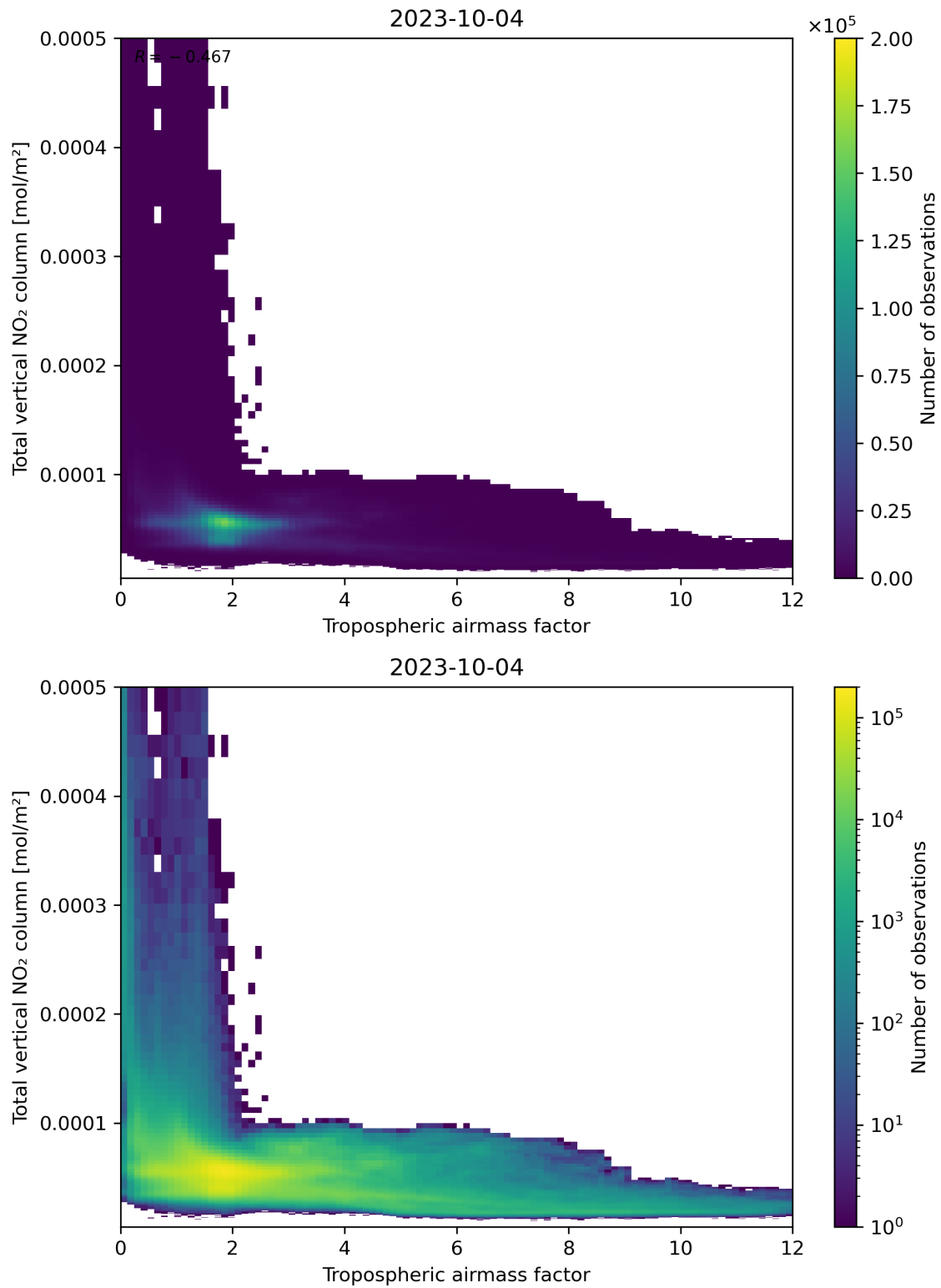
Figure 77: Scatter density plot of “Tropospheric airmass factor” against “Total vertical NO 2 column” for 2023-10-03 to 2023-10-05.
