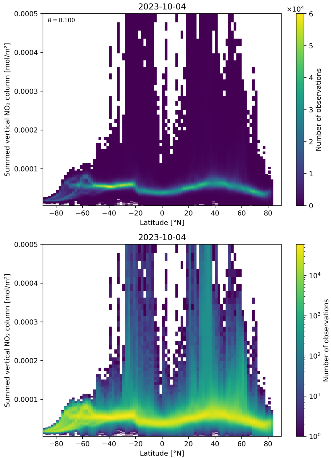
Figure 88: Scatter density plot of “Latitude” against “Summed vertical NO 2 column” for 2023-10-03 to 2023-10-05.
