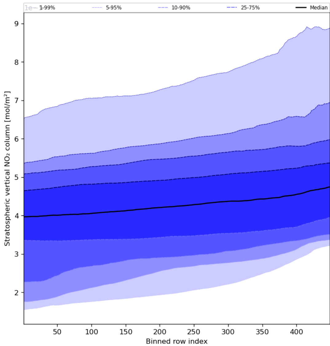
Figure 53: Along track statistics of “Stratospheric vertical NO 2 column” for 2023-10-03 to 2023-10-05
