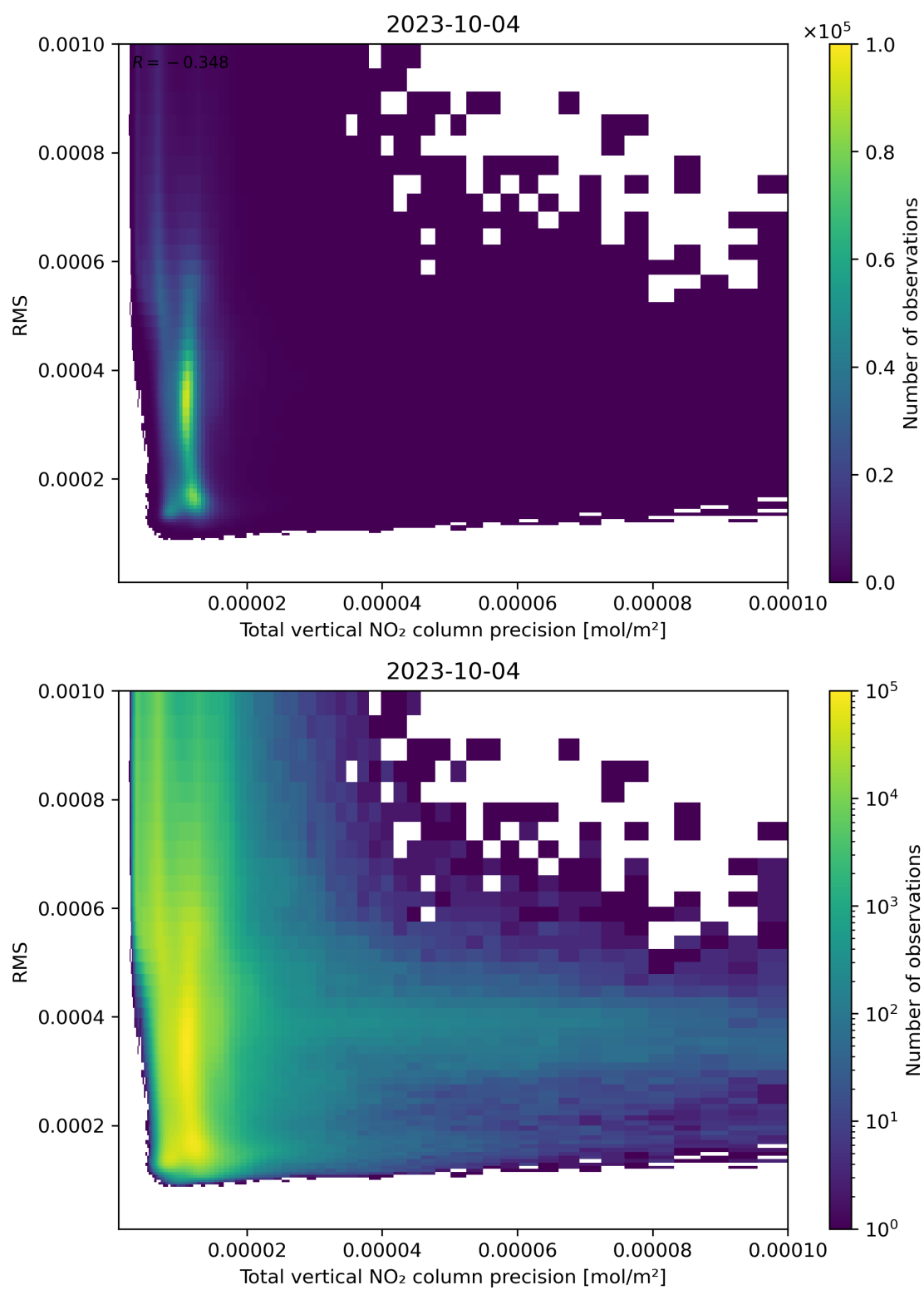
Figure 119: Scatter density plot of “Total vertical NO 2 column precision” against “RMS” for 2023-10-03 to 2023-10-05.
