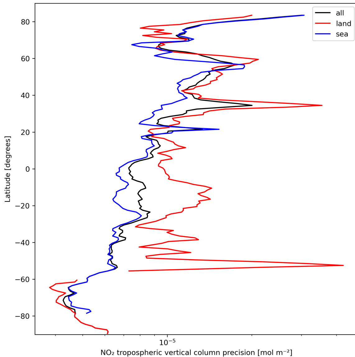
Figure 13: Zonal average of “NO 2 tropospheric vertical column precision” for 2023-10-03 to 2023-10-05.
