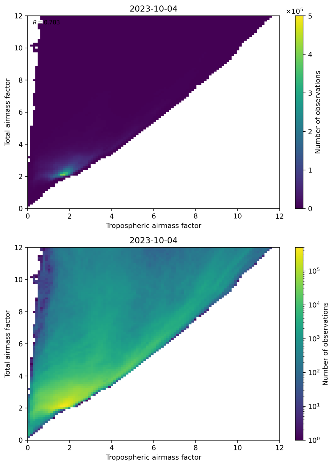
Figure 72: Scatter density plot of “Tropospheric airmass factor” against “Total airmass factor” for 2023-10-03 to 2023-10-05.
