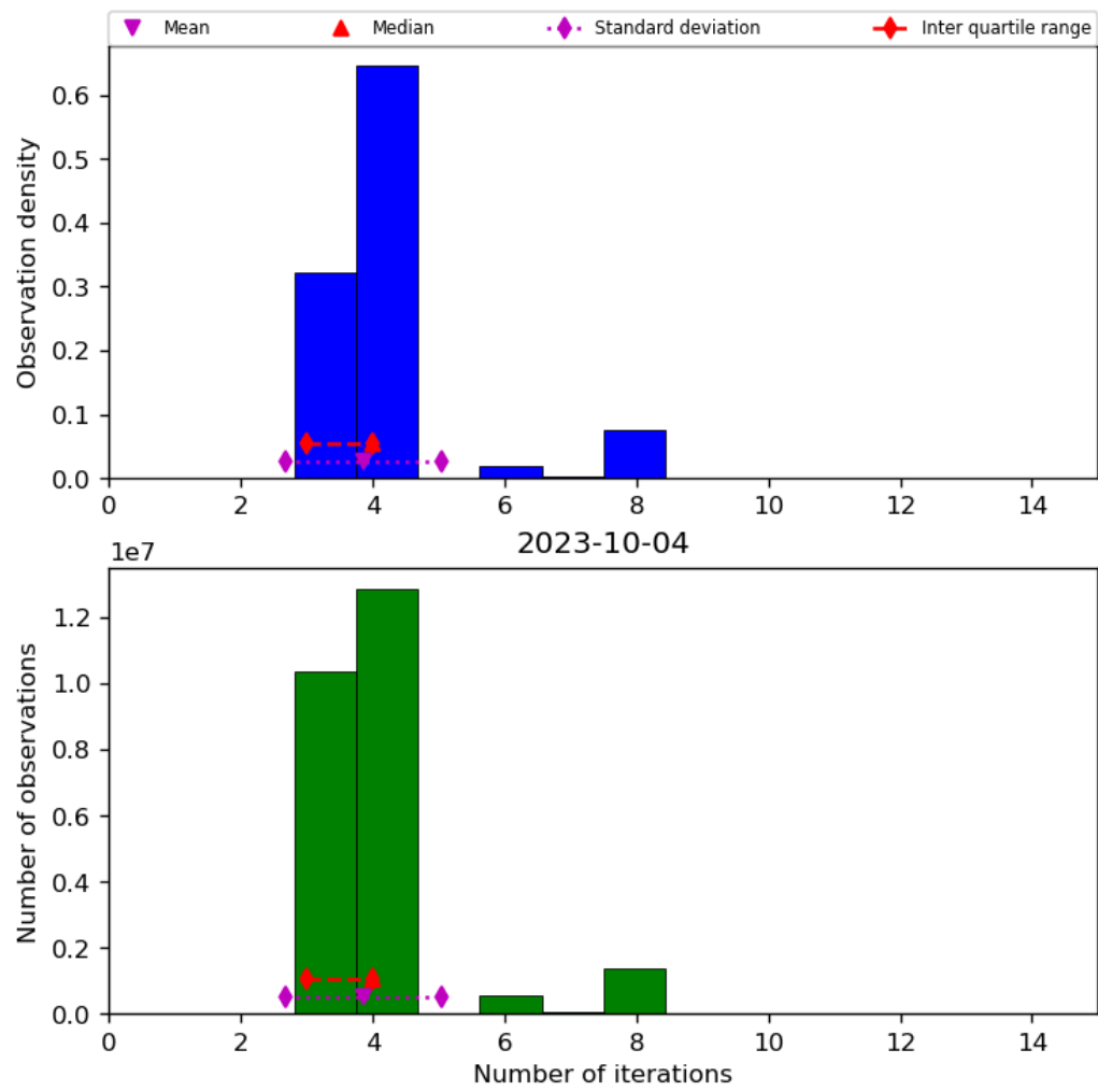
Figure 34: Histogram of “Number of iterations” for 2023-10-03 to 2023-10-05
