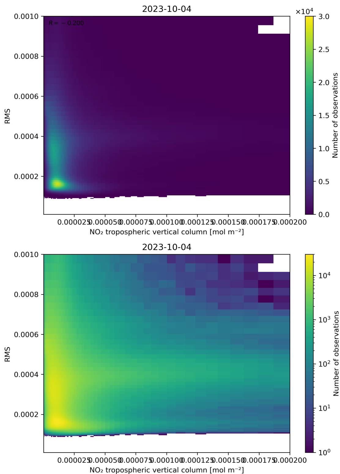
Figure 142: Scatter density plot of “NO 2 tropospheric vertical column” against “RMS” for 2023-10-03 to 2023-10-05.
