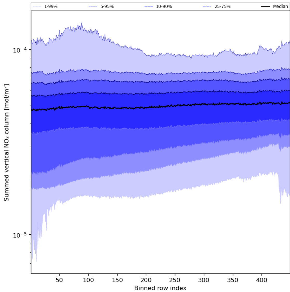
Figure 57: Along track statistics of “Summed vertical NO 2 column” for 2023-10-03 to 2023-10-05
