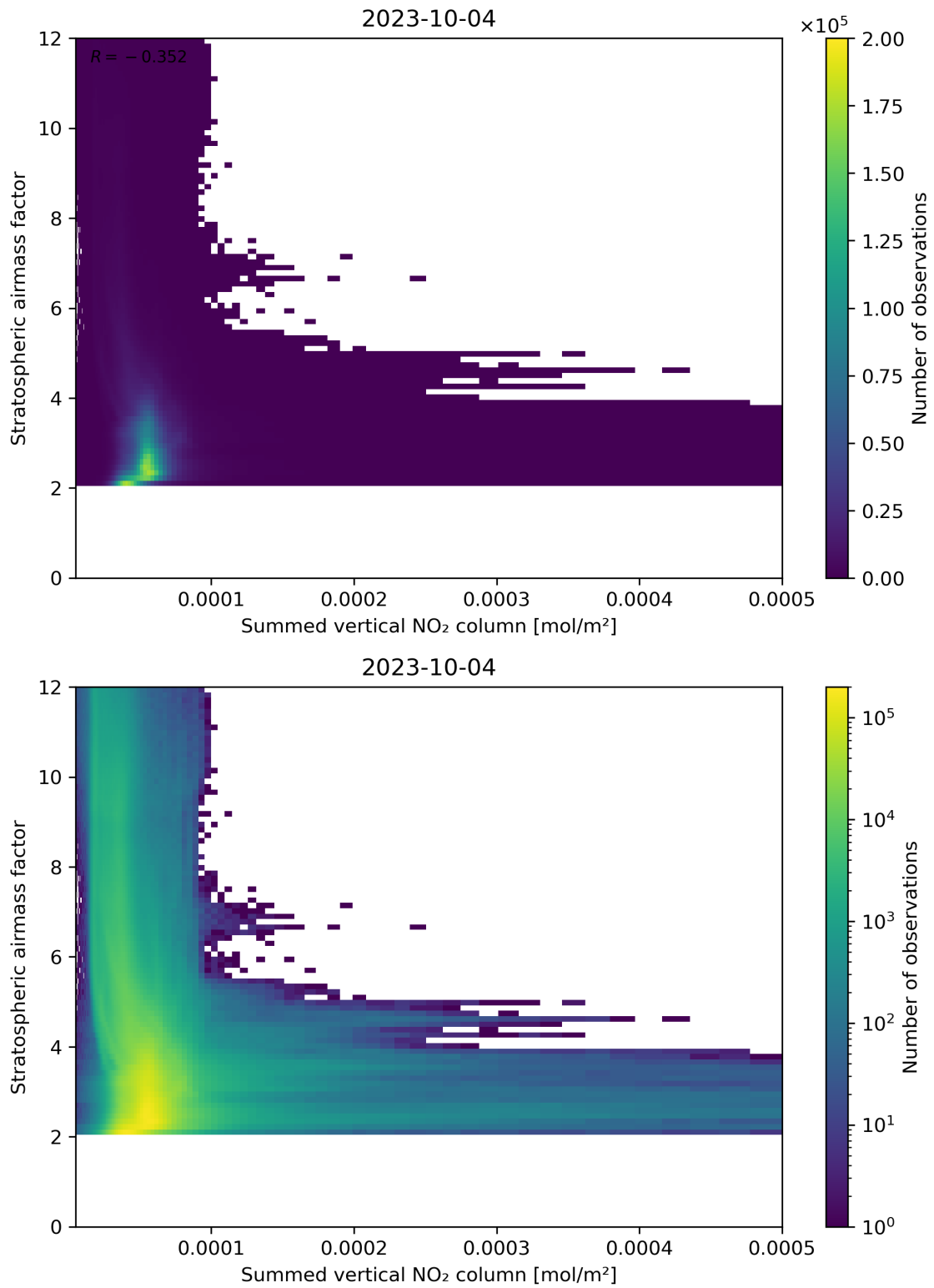
Figure 103: Scatter density plot of “Summed vertical NO 2 column” against “Stratospheric air mass factor” for 2023-10-03 to 2023-10-05.
