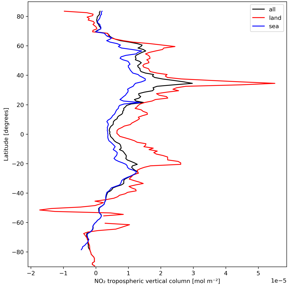
Figure 12: Zonal average of “NO 2 tropospheric vertical column” for 2023-10-03 to 2023-10-05.
