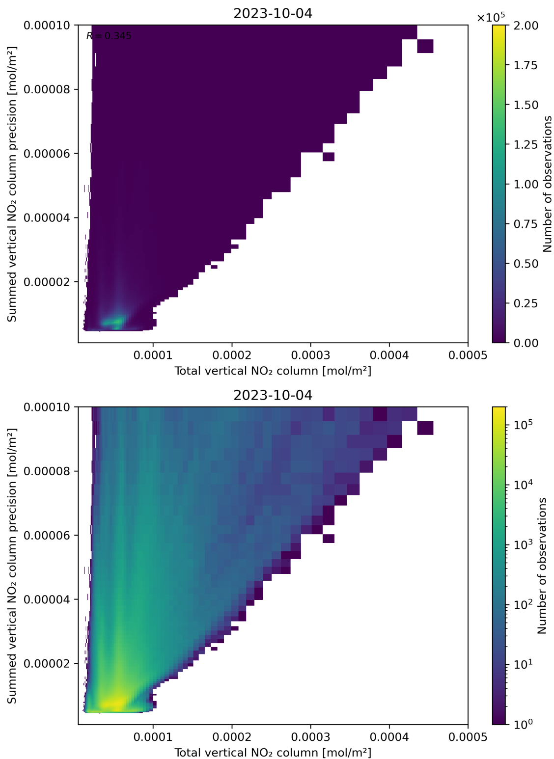
Figure 113: Scatter density plot of “Total vertical NO 2 column” against “Summed vertical NO 2 column precision” for 2023-10-03 to 2023-10-05.
