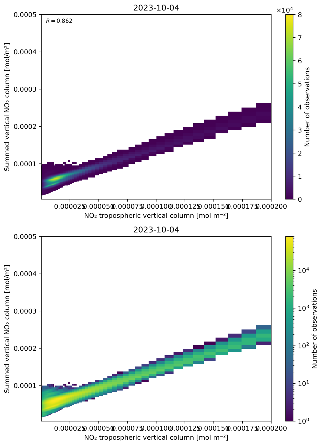
Figure 126: Scatter density plot of “NO 2 tropospheric vertical column” against “Summed vertical NO 2 column” for 2023-10-03 to 2023-10-05.
