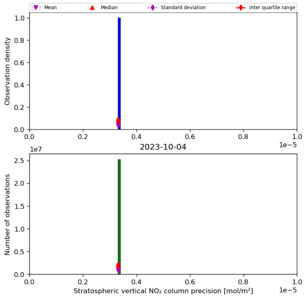
Figure 37: Histogram of “Stratospheric vertical NO 2 column precision” for 2023-10-03 to 2023-10-05
