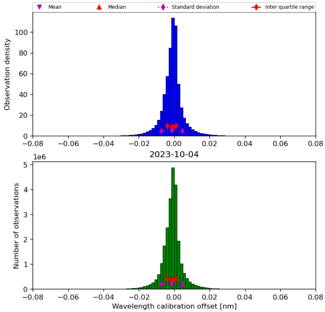
Figure 35: Histogram of “Wavelength calibration offset” for 2023-10-03 to 2023-10-05
