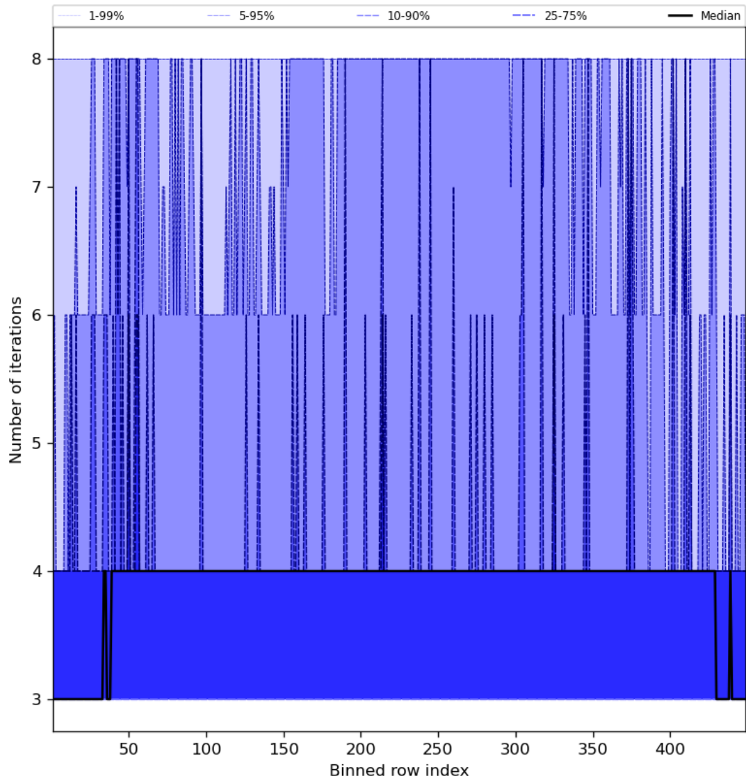
Figure 51: Along track statistics of “Number of iterations” for 2023-10-03 to 2023-10-05
