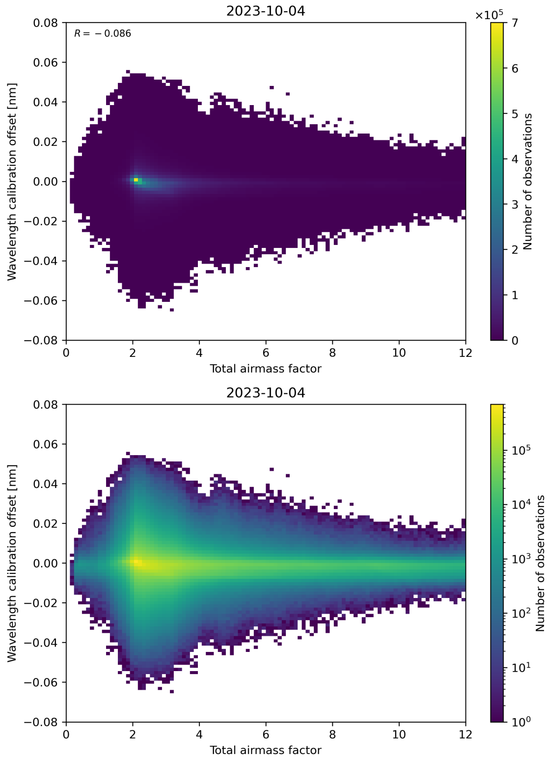
Figure 70: Scatter density plot of “Total airmass factor” against “Wavelength calibration offset” for 2023-10-03 to 2023-10-05.
