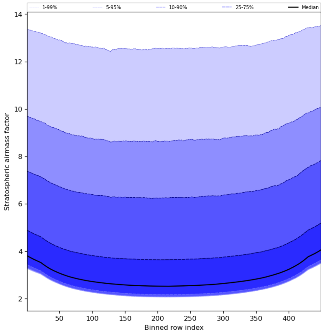
Figure 61: Along track statistics of “Stratospheric airmass factor” for 2023-10-03 to 2023-10-05
