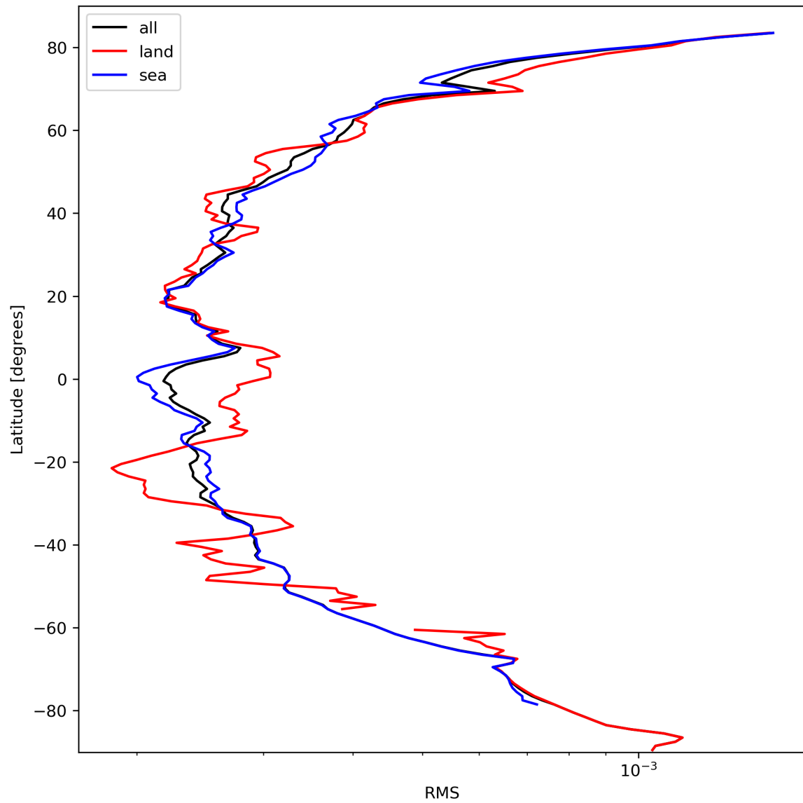
Figure 26: Zonal average of “RMS” for 2023-10-03 to 2023-10-05.
