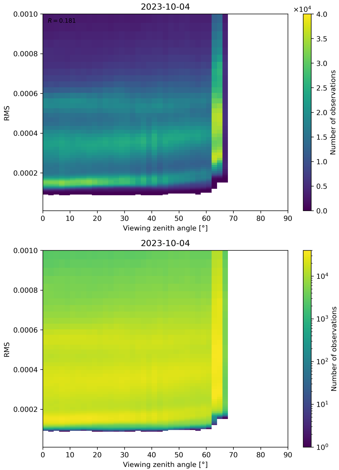
Figure 171: Scatter density plot of “Viewing zenith angle” against “RMS” for 2023-10-03 to 2023-10-05.
