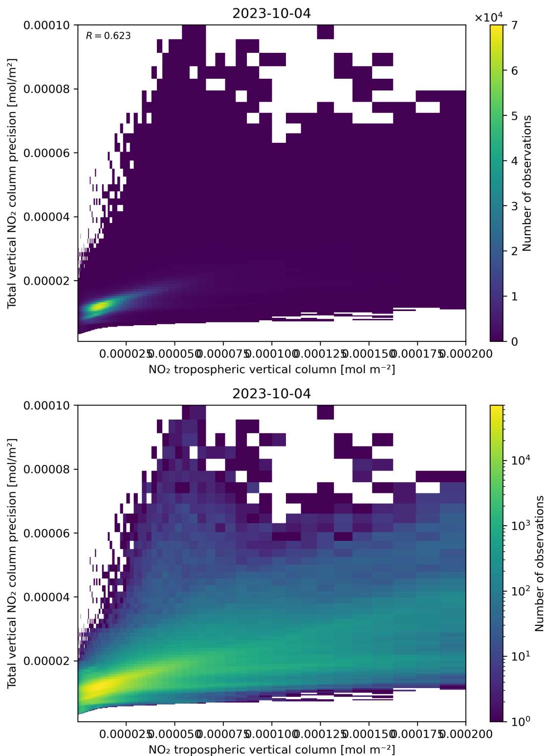
Figure 129: Scatter density plot of “NO 2 tropospheric vertical column” against “Total vertical NO 2 column precision” for 2023-10-03 to 2023-10-05.
