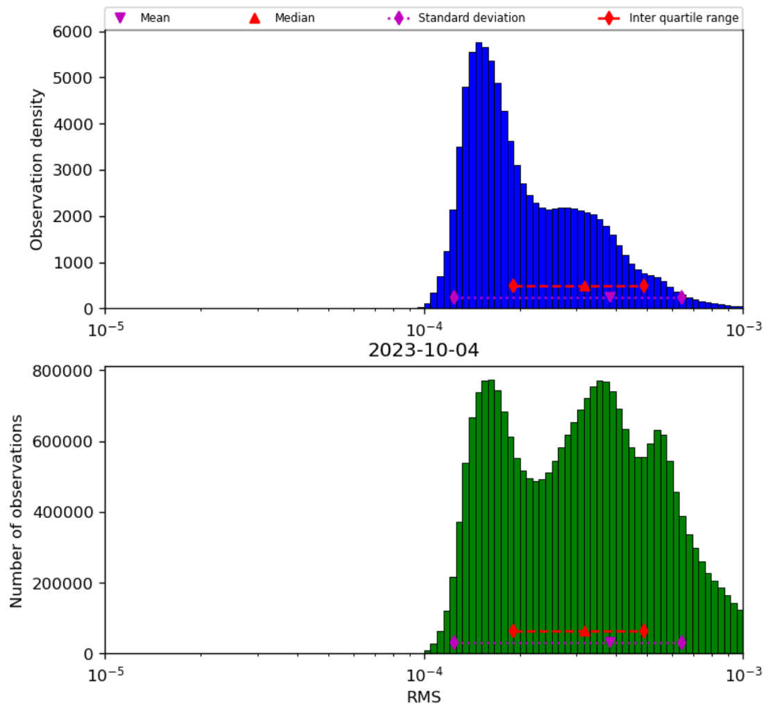
Figure 43: Histogram of “RMS” for 2023-10-03 to 2023-10-05
