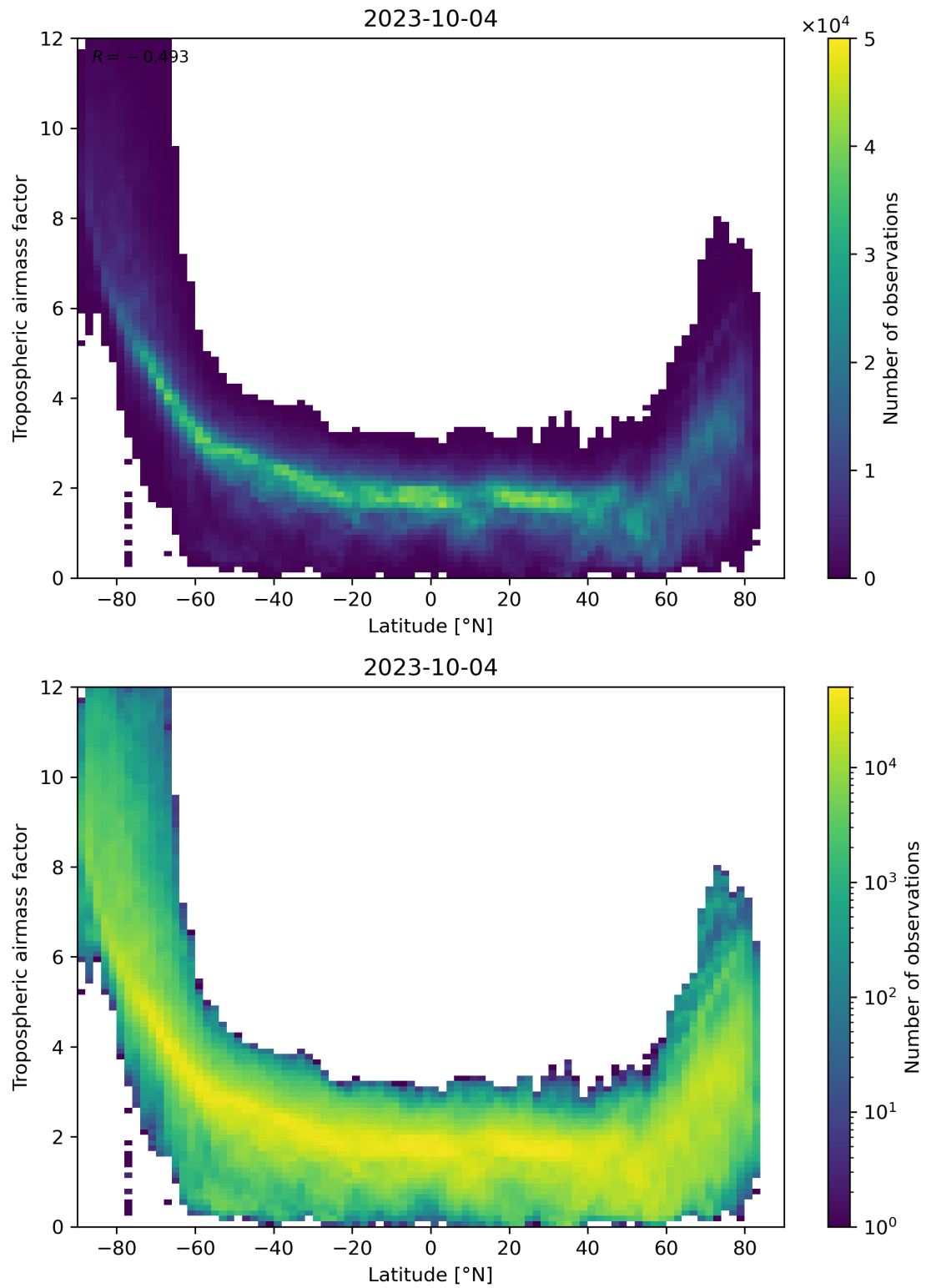
Figure 85: Scatter density plot of “Latitude” against “Tropospheric airmass factor” for 2023-10-03 to 2023-10-05.
