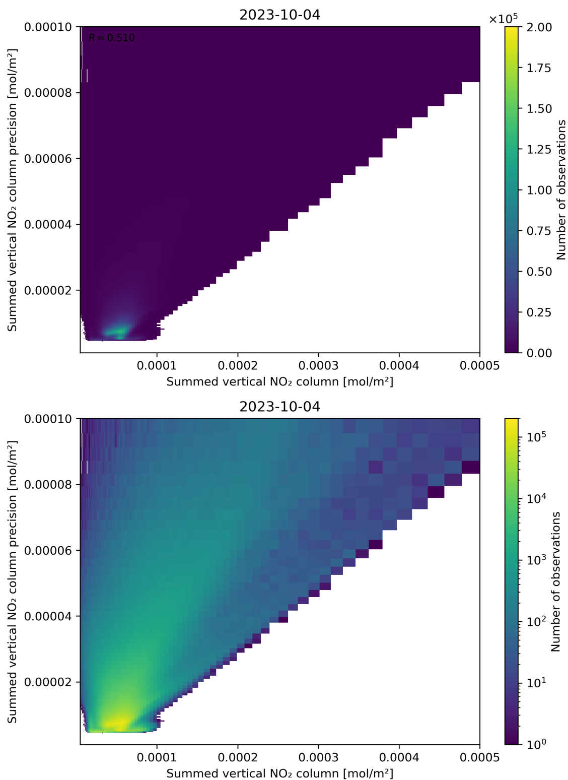
Figure 105: Scatter density plot of “Summed vertical NO 2 column” against “Summed vertical NO 2 column precision” for 2023-10-03 to 2023-10-05.
