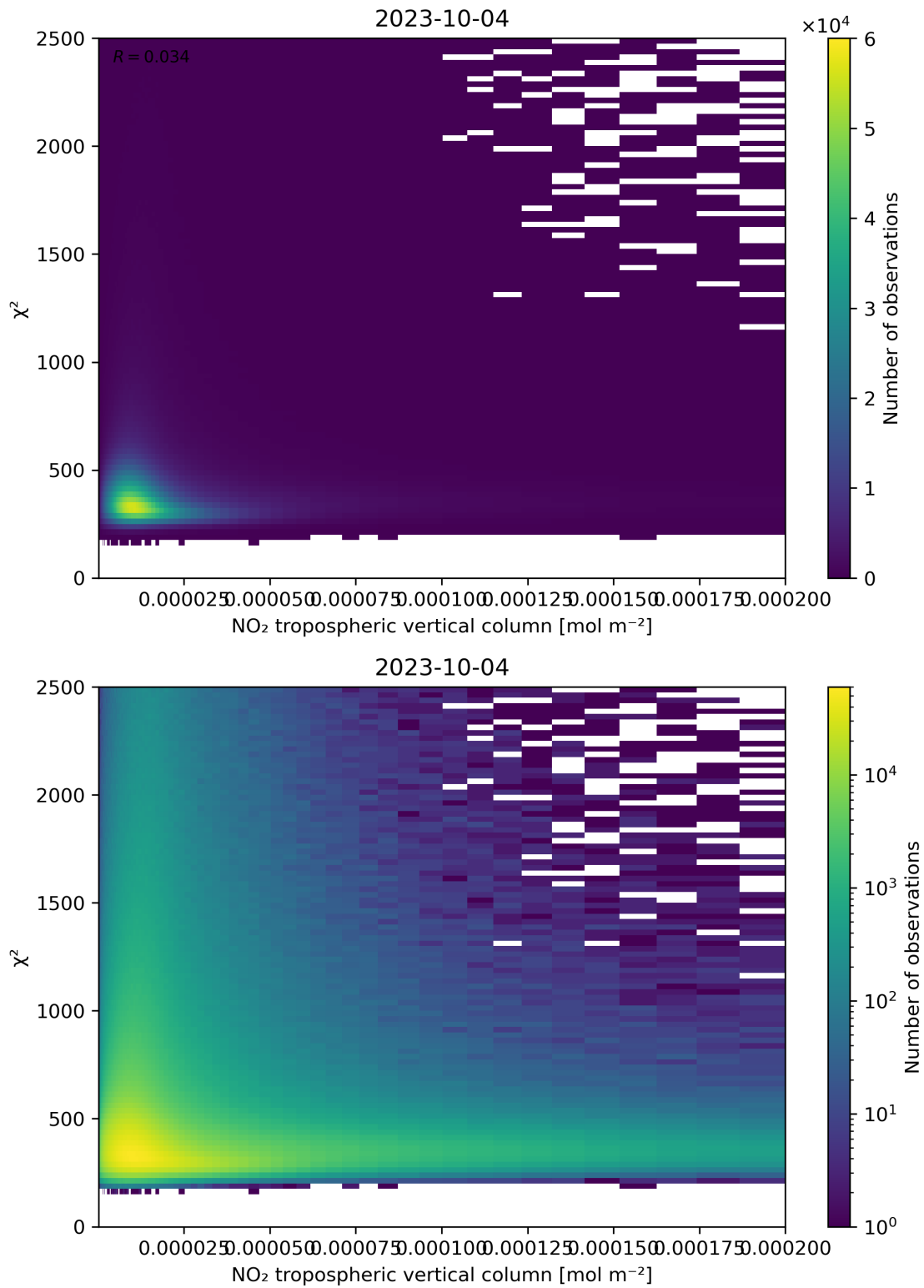
Figure 124: Scatter density plot of “NO 2 tropospheric vertical column” against “ \chi^2 ” for 2023-10-03 to 2023-10-05.
