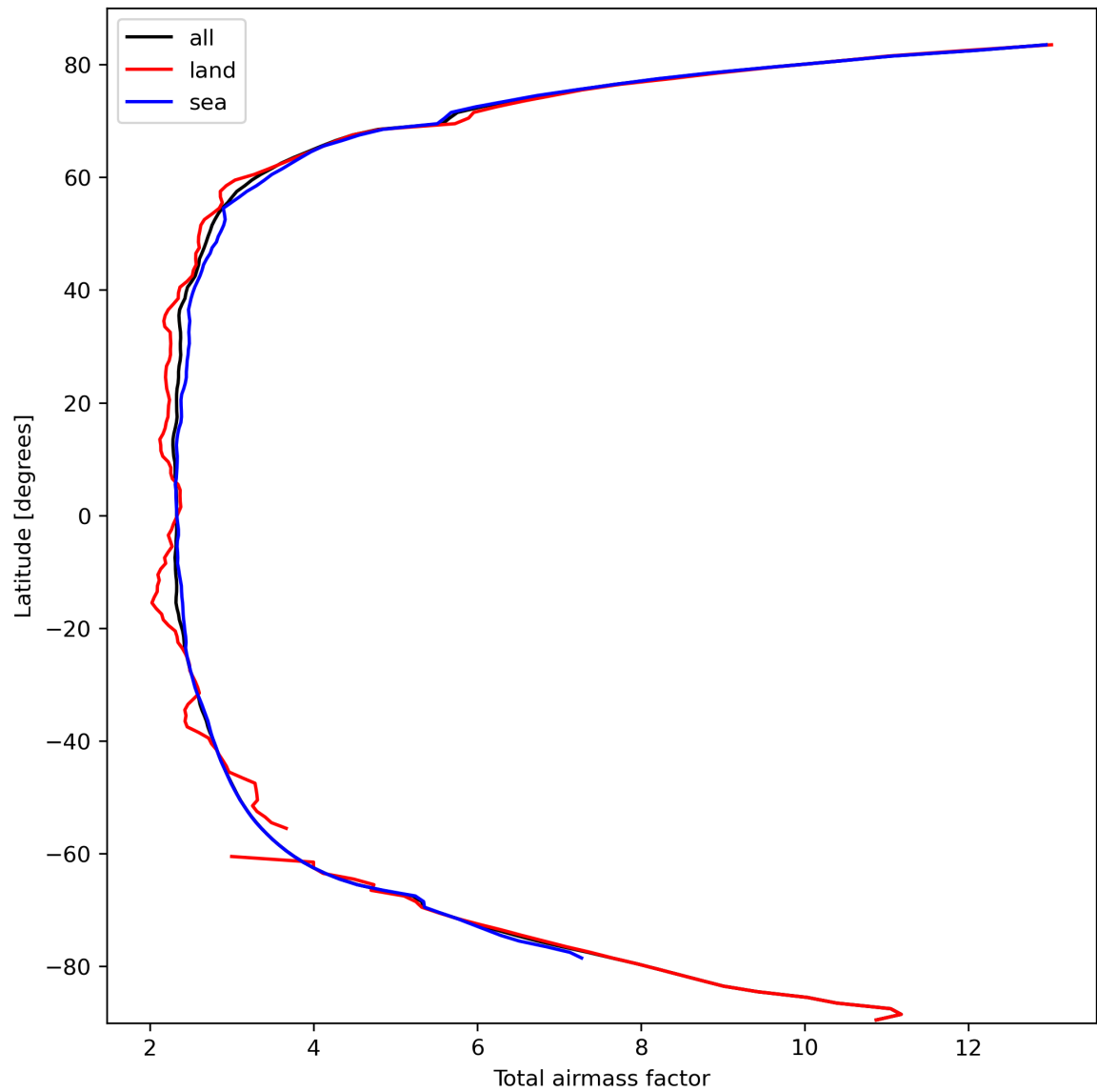
Figure 15: Zonal average of “Total airmass factor” for 2023-10-03 to 2023-10-05.
