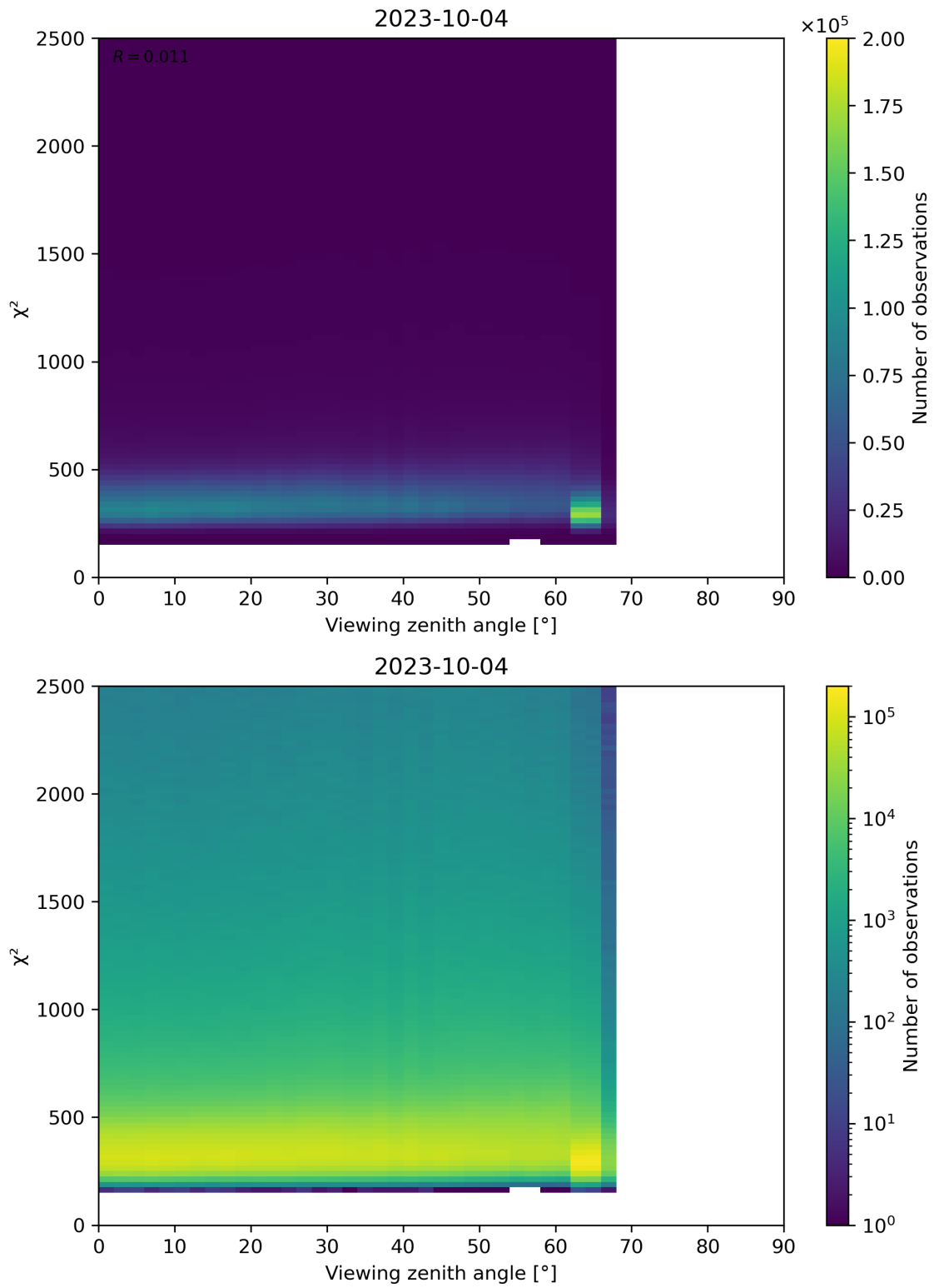
Figure 162: Scatter density plot of “Viewing zenith angle” against “ \chi^2 ” for 2023-10-03 to 2023-10-05.
