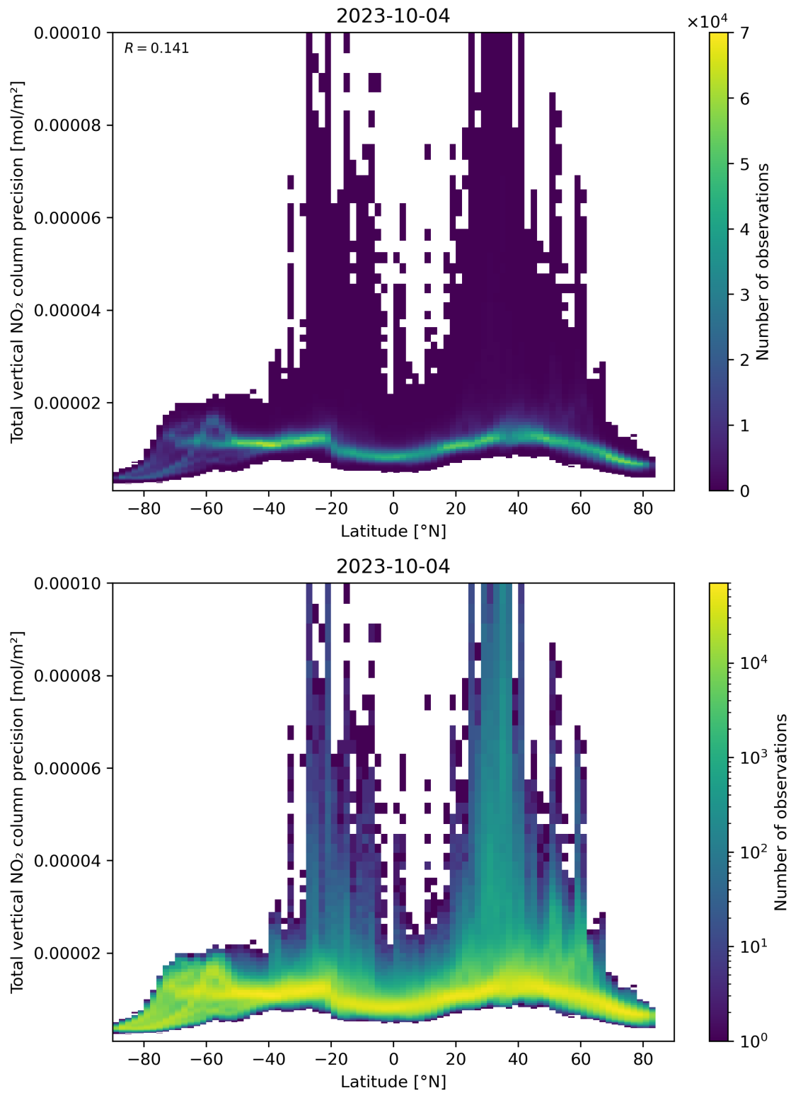
Figure 91: Scatter density plot of “Latitude” against “Total vertical NO 2 column precision” for 2023-10-03 to 2023-10-05.
