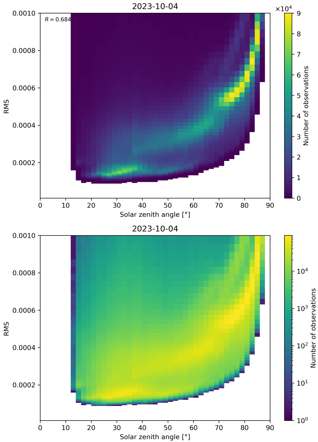
Figure 157: Scatter density plot of “Solar zenith angle” against “RMS” for 2023-10-03 to 2023-10-05.
