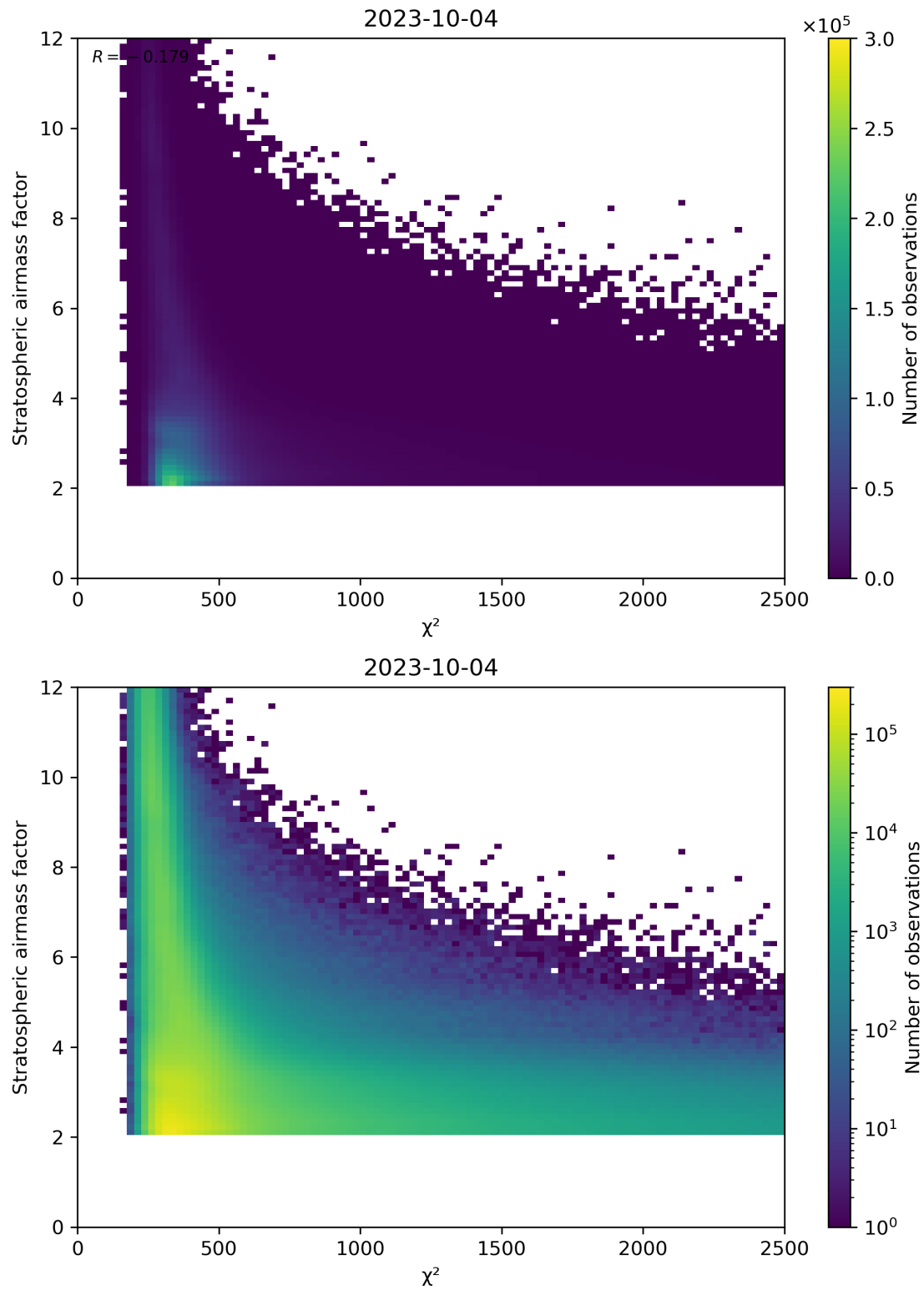
Figure 81: Scatter density plot of “ \chi^2 ” against “Stratospheric airmass factor” for 2023-10-03 to 2023-10-05.
