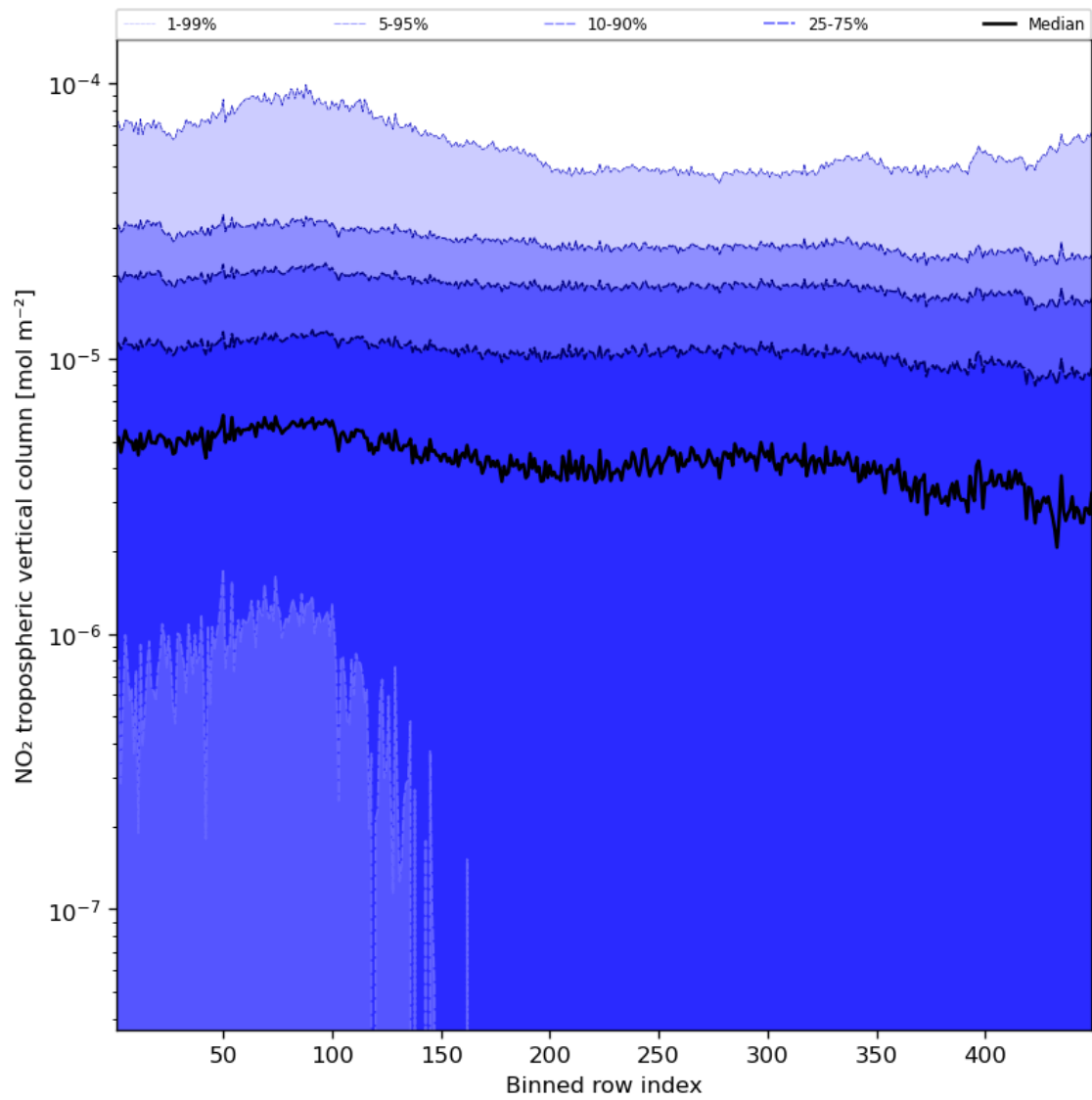
Figure 46: Along track statistics of “NO 2 tropospheric vertical column” for 2023-10-03 to 2023-10-05
