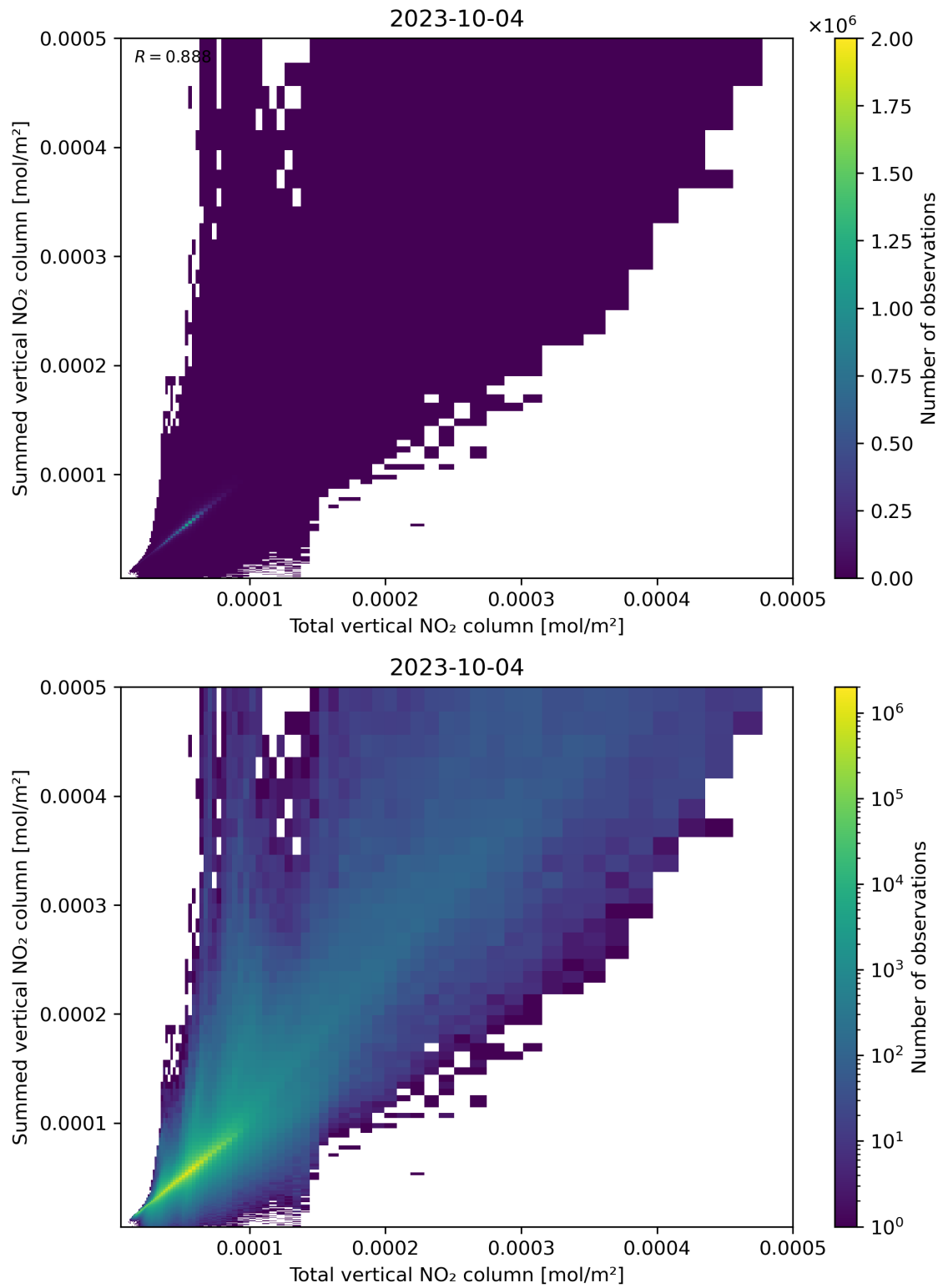
Figure 112: Scatter density plot of “Total vertical NO 2 column” against “Summed vertical NO 2 column” for 2023-10-03 to 2023-10-05.
