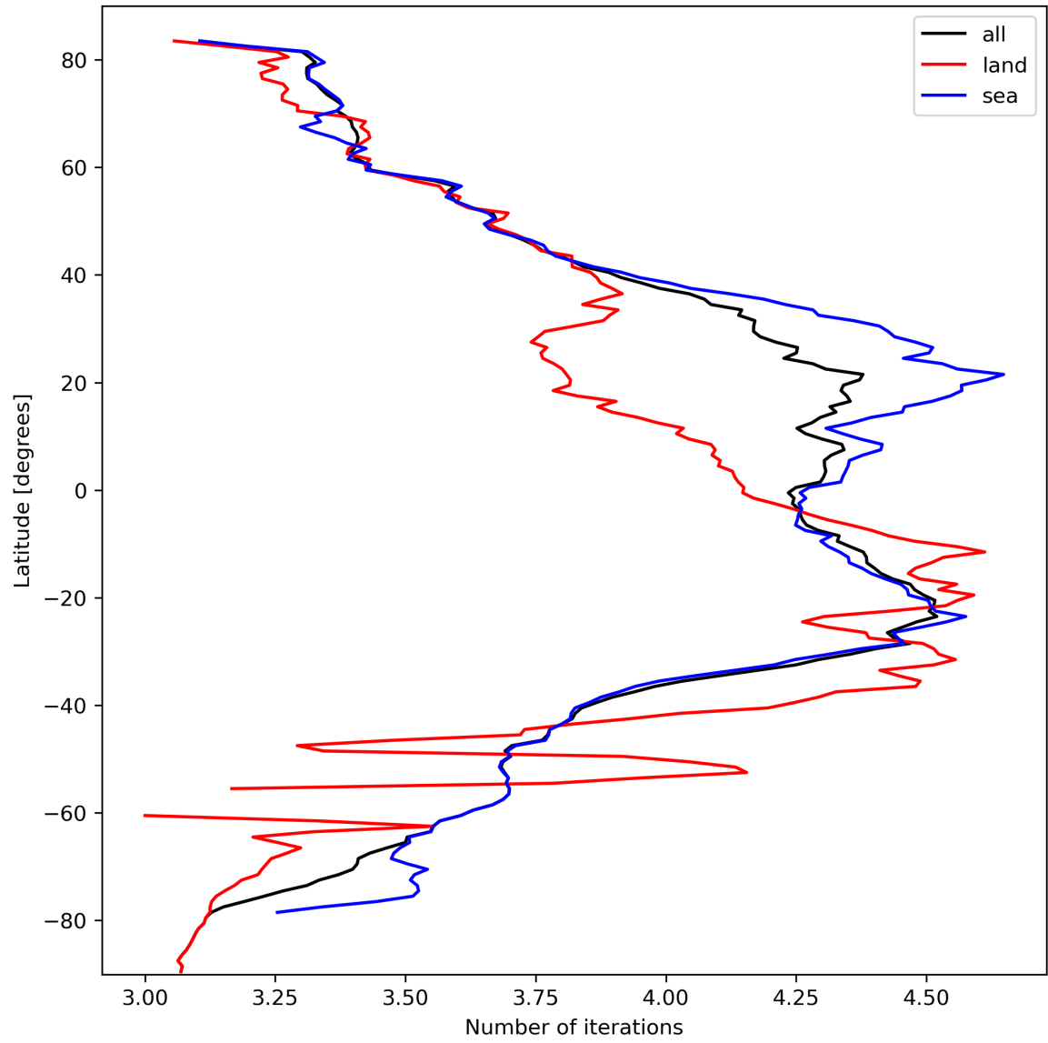
Figure 17: Zonal average of “Number of iterations” for 2023-10-03 to 2023-10-05.
