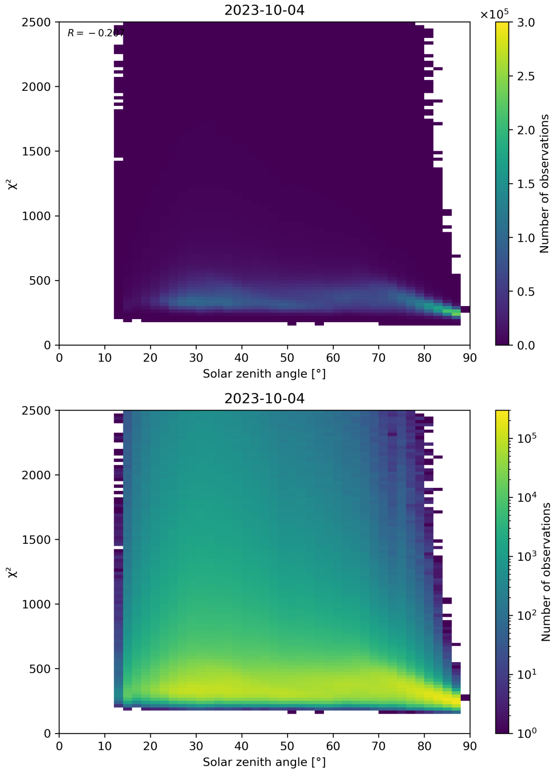
Figure 148: Scatter density plot of “Solar zenith angle” against “ \chi^2 ” for 2023-10-03 to 2023-10-05.
