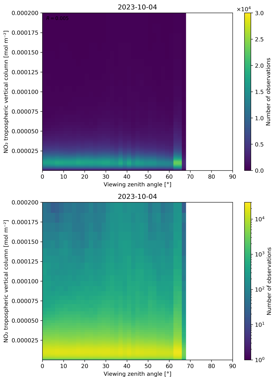
Figure 169: Scatter density plot of “Viewing zenith angle” against “NO 2 tropospheric vertical column” for 2023-10-03 to 2023-10-05.
