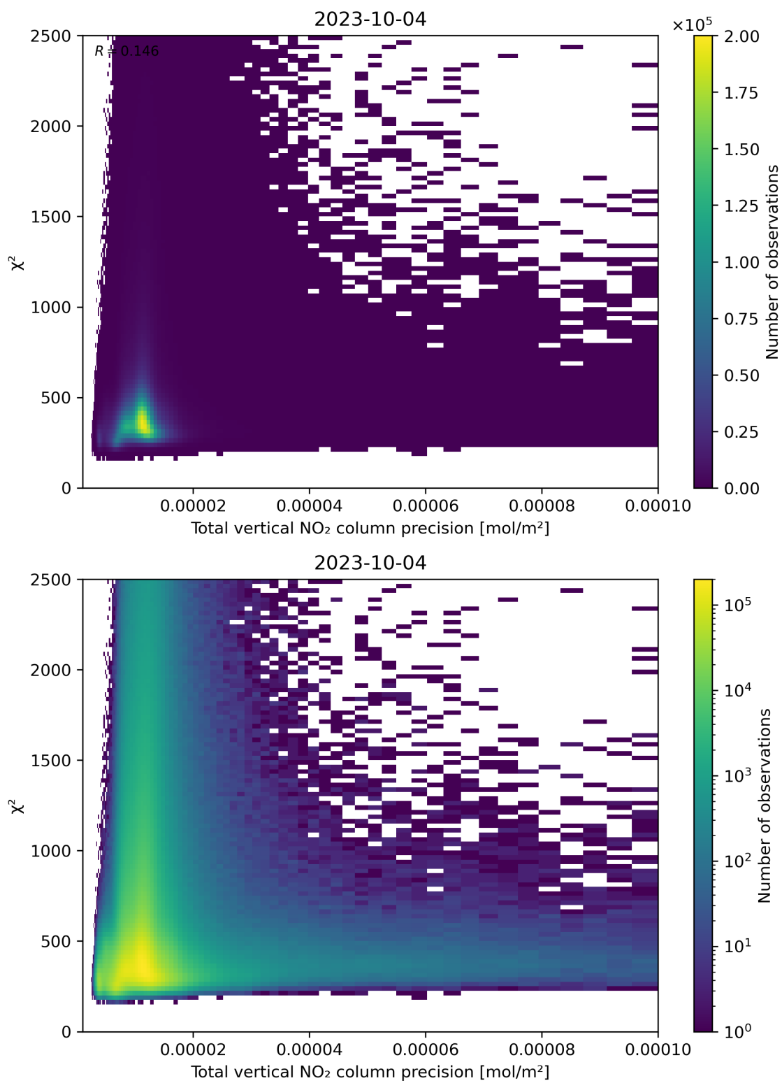
Figure 116: Scatter density plot of “Total vertical NO 2 column precision” against “ \chi^2 ” for 2023-10-03 to 2023-10-05.
