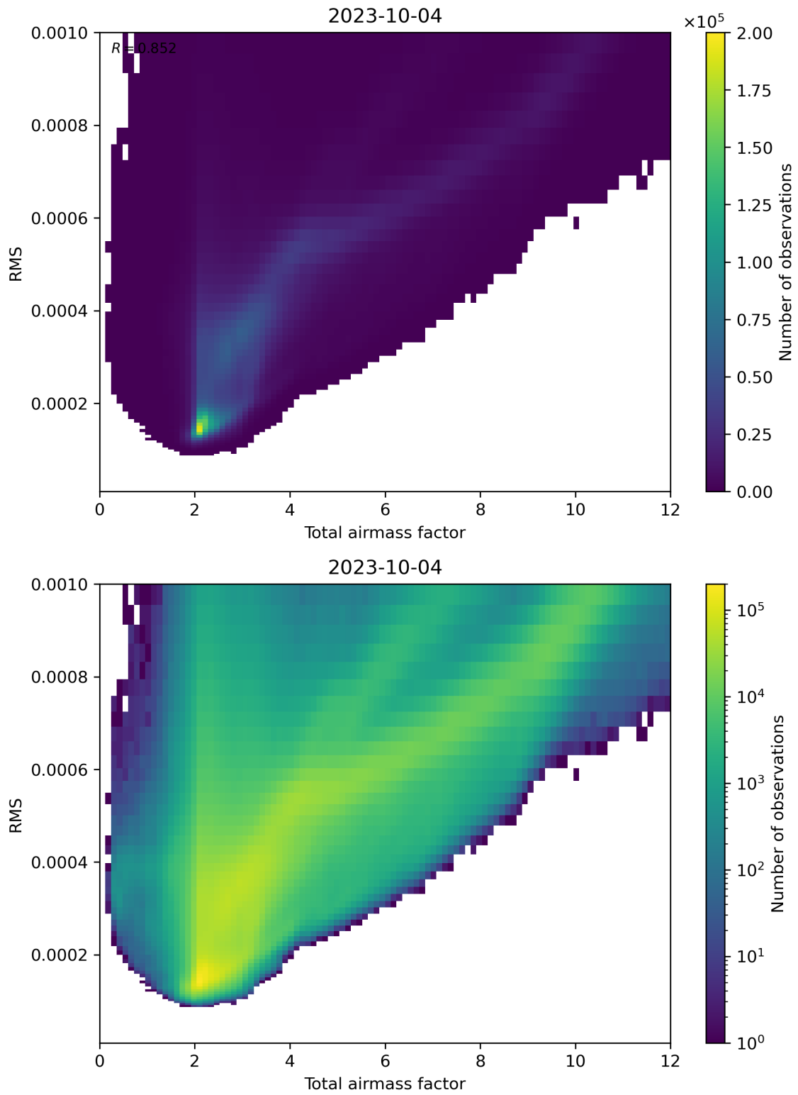
Figure 69: Scatter density plot of “Total airmass factor” against “RMS” for 2023-10-03 to 2023-10-05.
