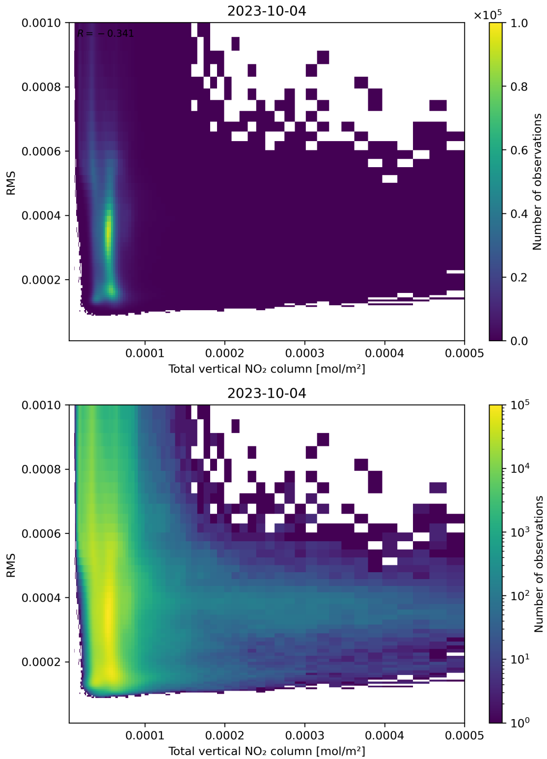
Figure 120: Scatter density plot of “Total vertical NO 2 column” against “RMS” for 2023-10-03 to 2023-10-05.
