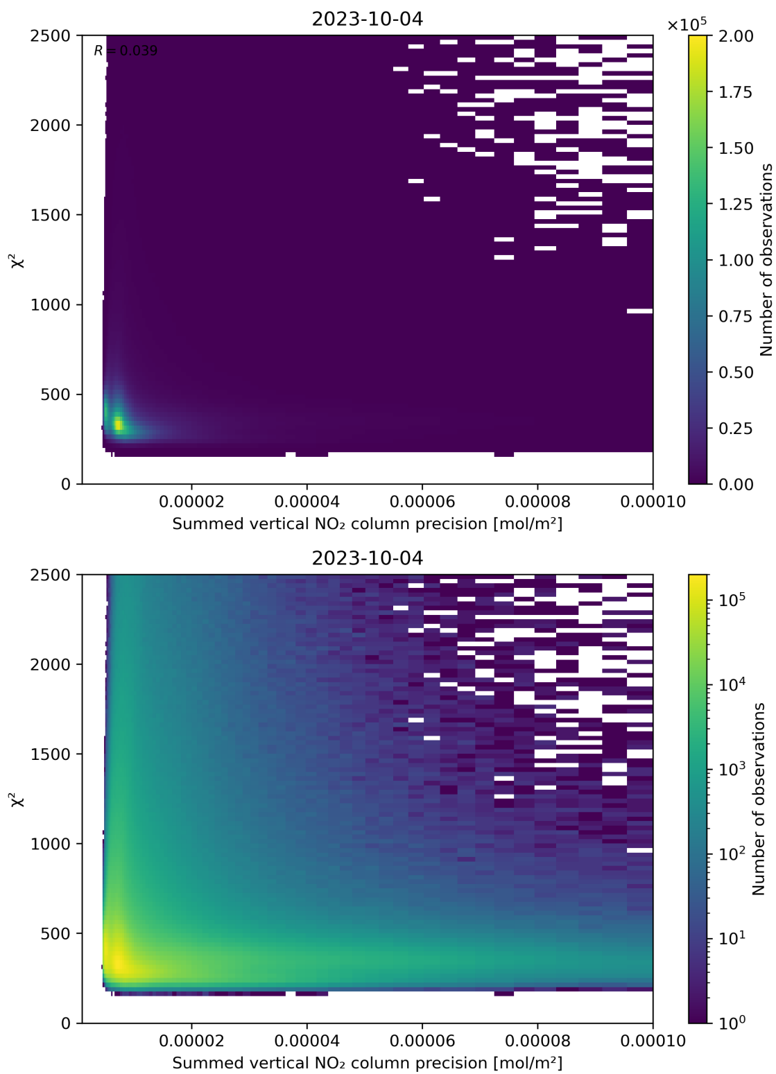
Figure 107: Scatter density plot of “Summed vertical NO 2 column precision” against “ \chi^2 ” for 2023-10-03 to 2023-10-05.
