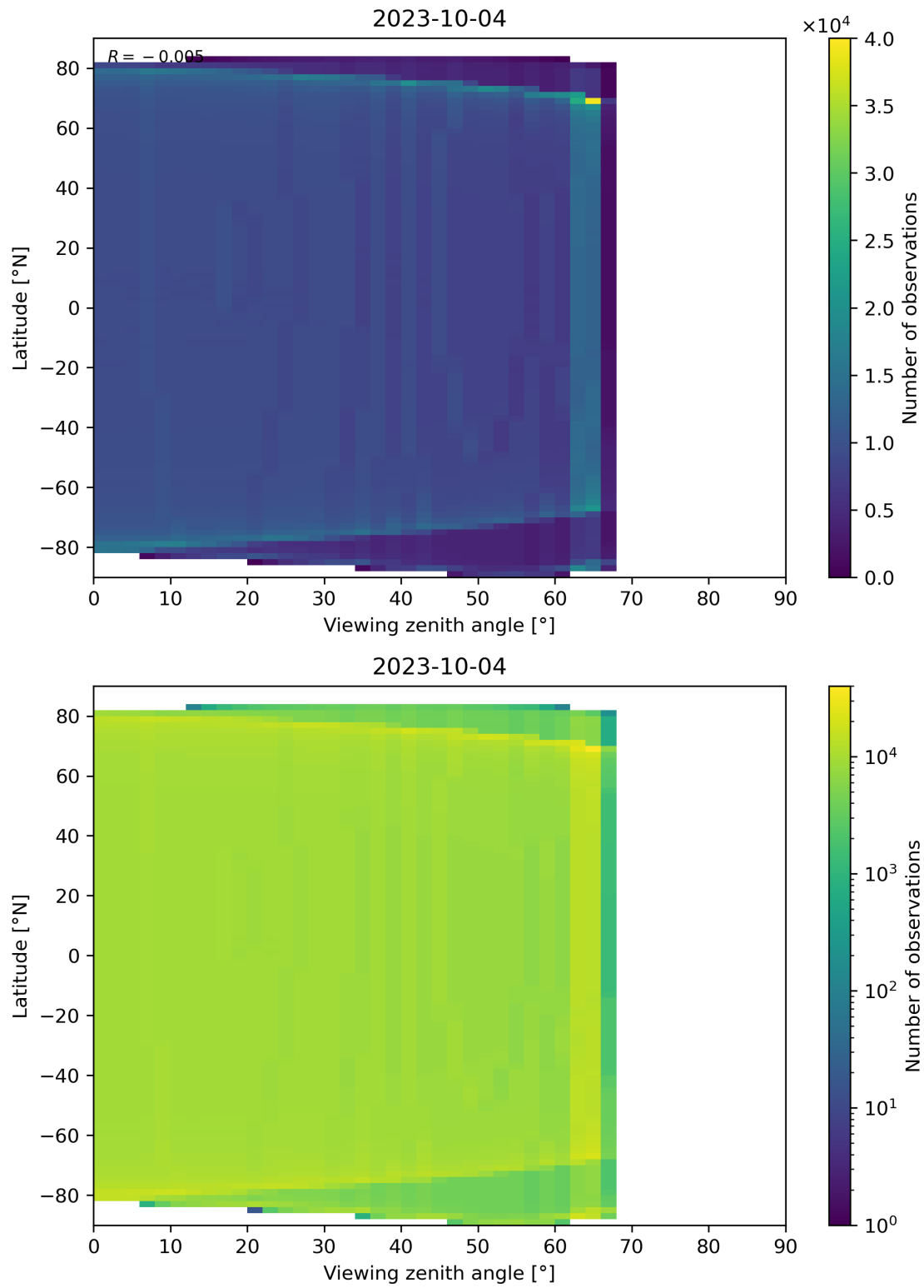
Figure 163: Scatter density plot of “Viewing zenith angle” against “Latitude” for 2023-10-03 to 2023-10-05.
