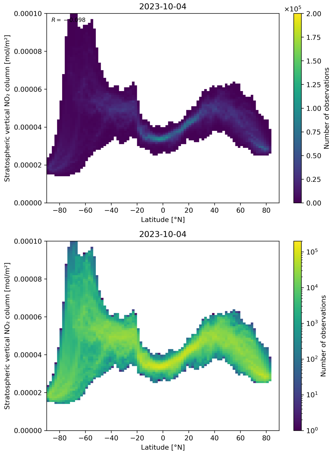
Figure 87: Scatter density plot of “Latitude” against “Stratospheric vertical NO 2 column” for 2023-10-03 to 2023-10-05.
