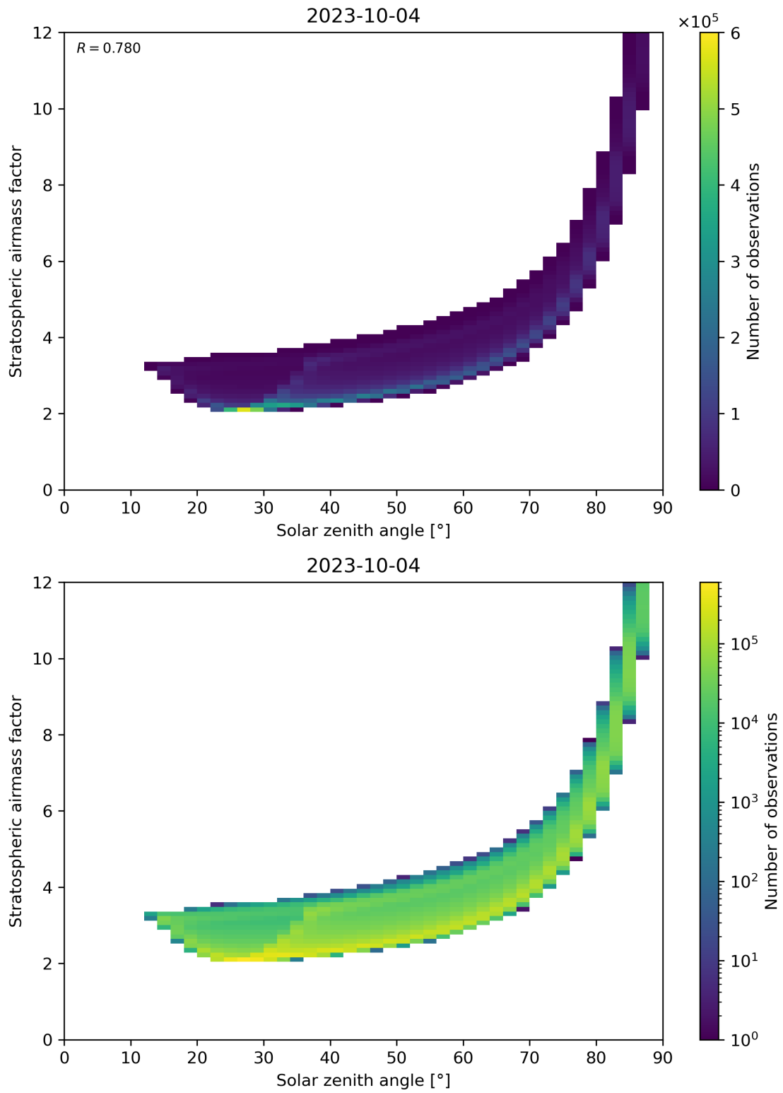
Figure 145: Scatter density plot of “Solar zenith angle” against “Stratospheric airmass factor” for 2023-10-03 to 2023-10-05.
