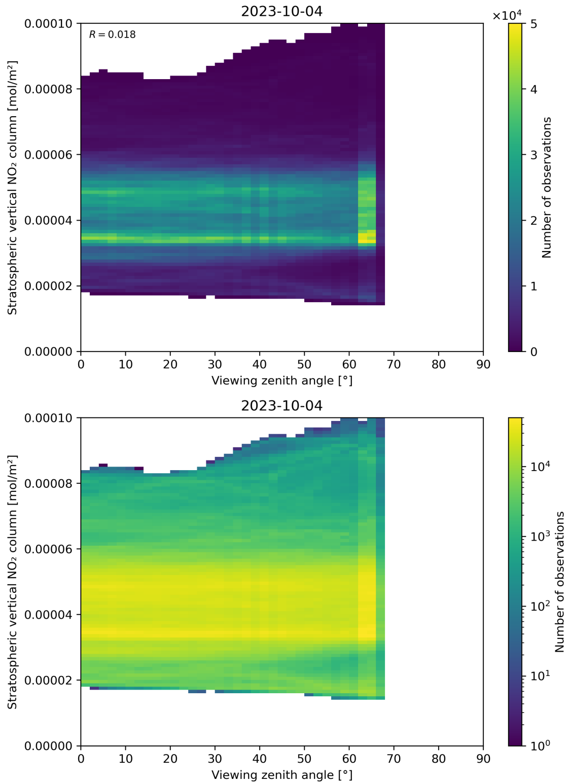
Figure 164: Scatter density plot of “Viewing zenith angle” against “Stratospheric vertical NO 2 column” for 2023-10-03 to 2023-10-05.
