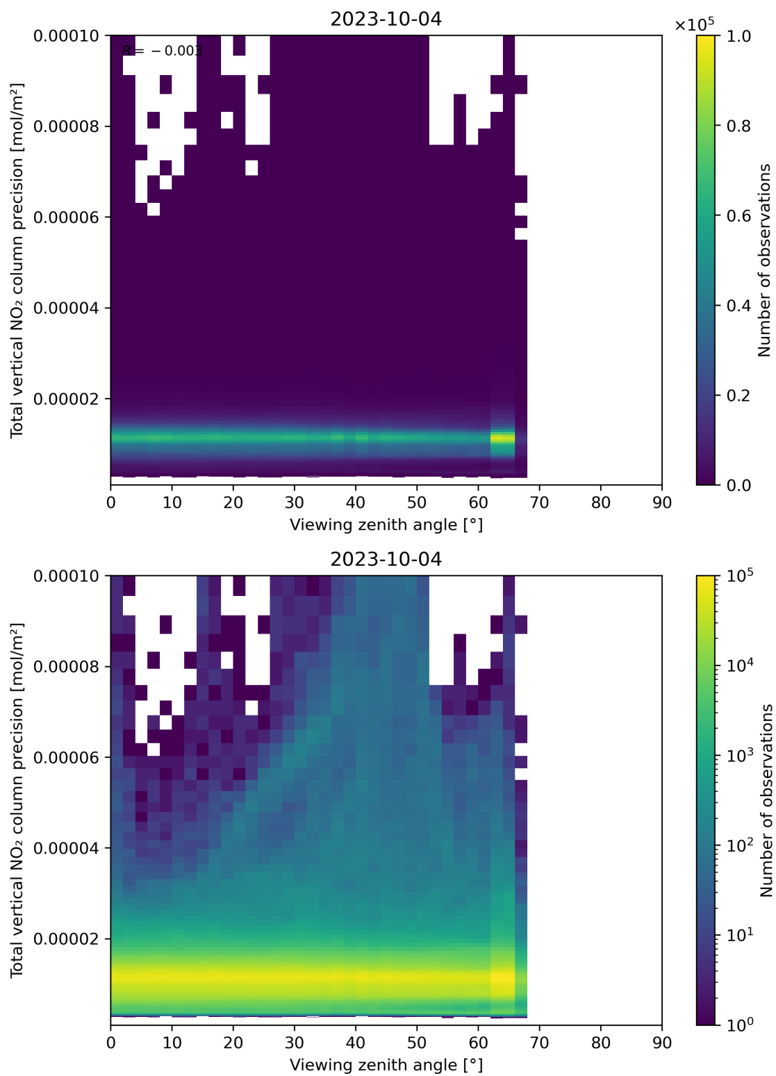
Figure 168: Scatter density plot of “Viewing zenith angle” against “Total vertical NO 2 column precision” for 2023-10-03 to 2023-10-05.
