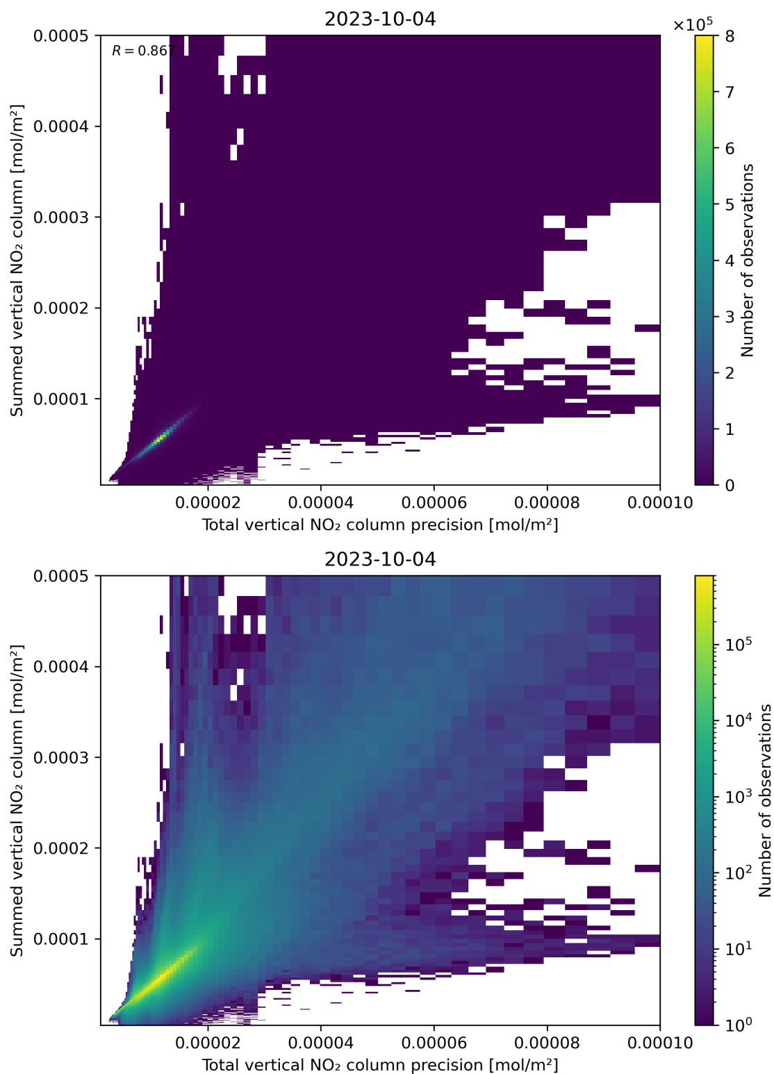
Figure 117: Scatter density plot of “Total vertical NO 2 column precision” against “Summed vertical NO 2 column” for 2023-10-03 to 2023-10-05.
