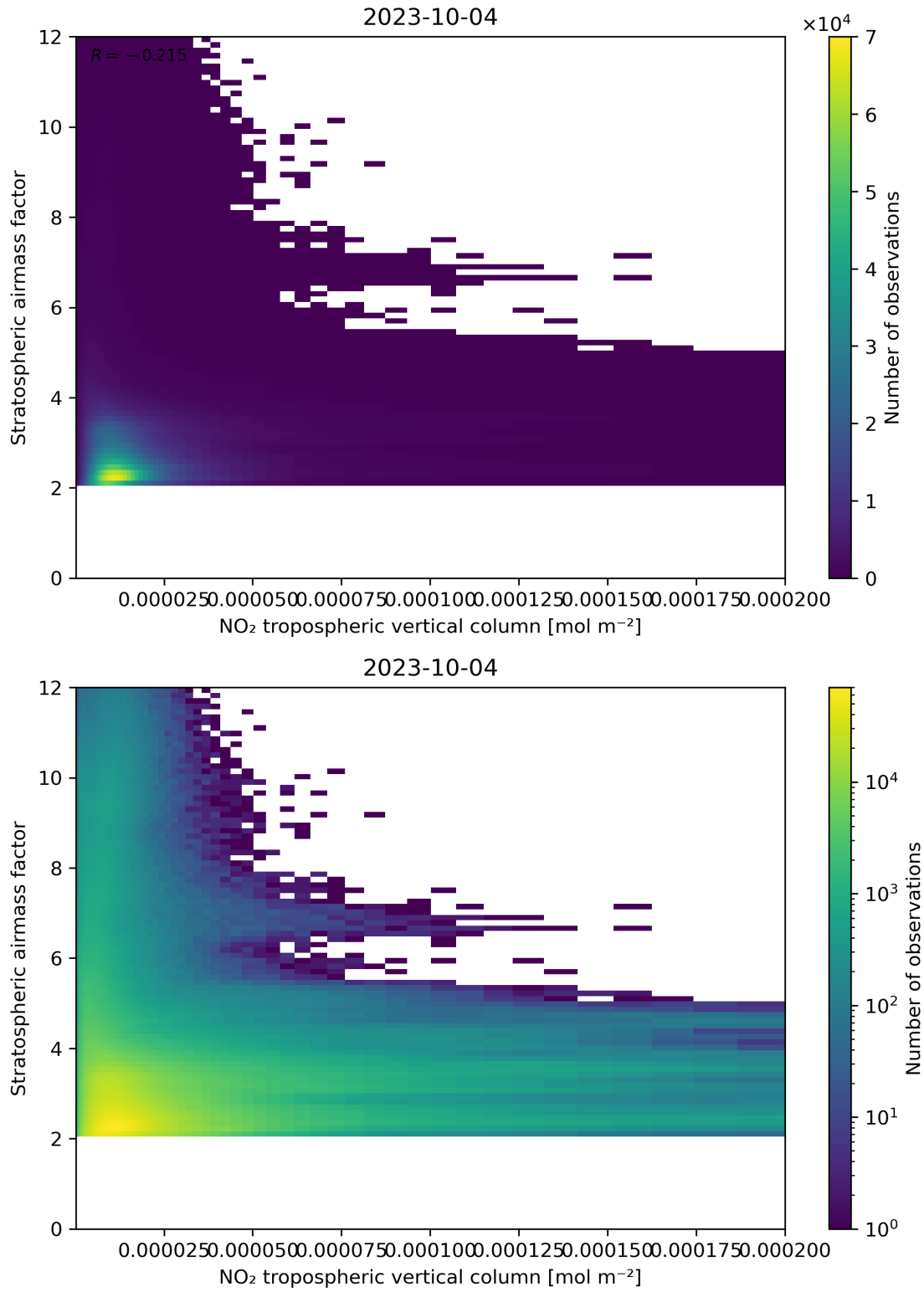
Figure 121: Scatter density plot of “NO 2 tropospheric vertical column” against “Stratospheric airmass factor” for 2023-10-03 to 2023-10-05.
