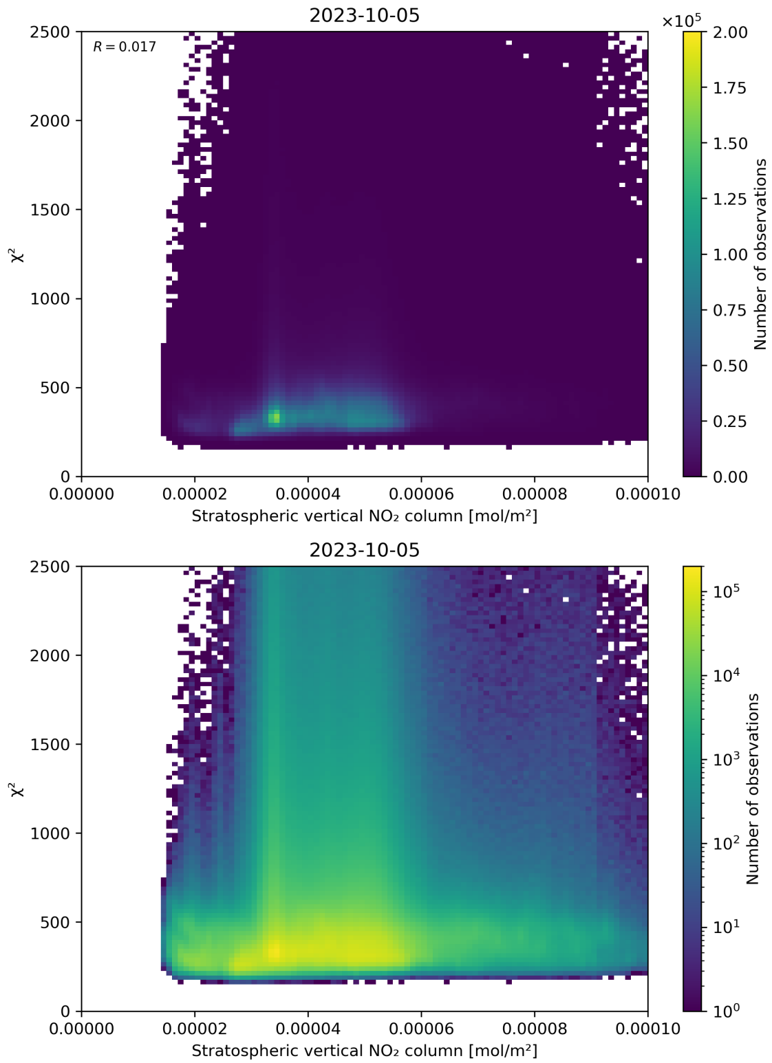
Figure 97: Scatter density plot of “Stratospheric vertical NO 2 column” against “ \chi^2 ” for 2023-10-04 to 2023-10-06.
