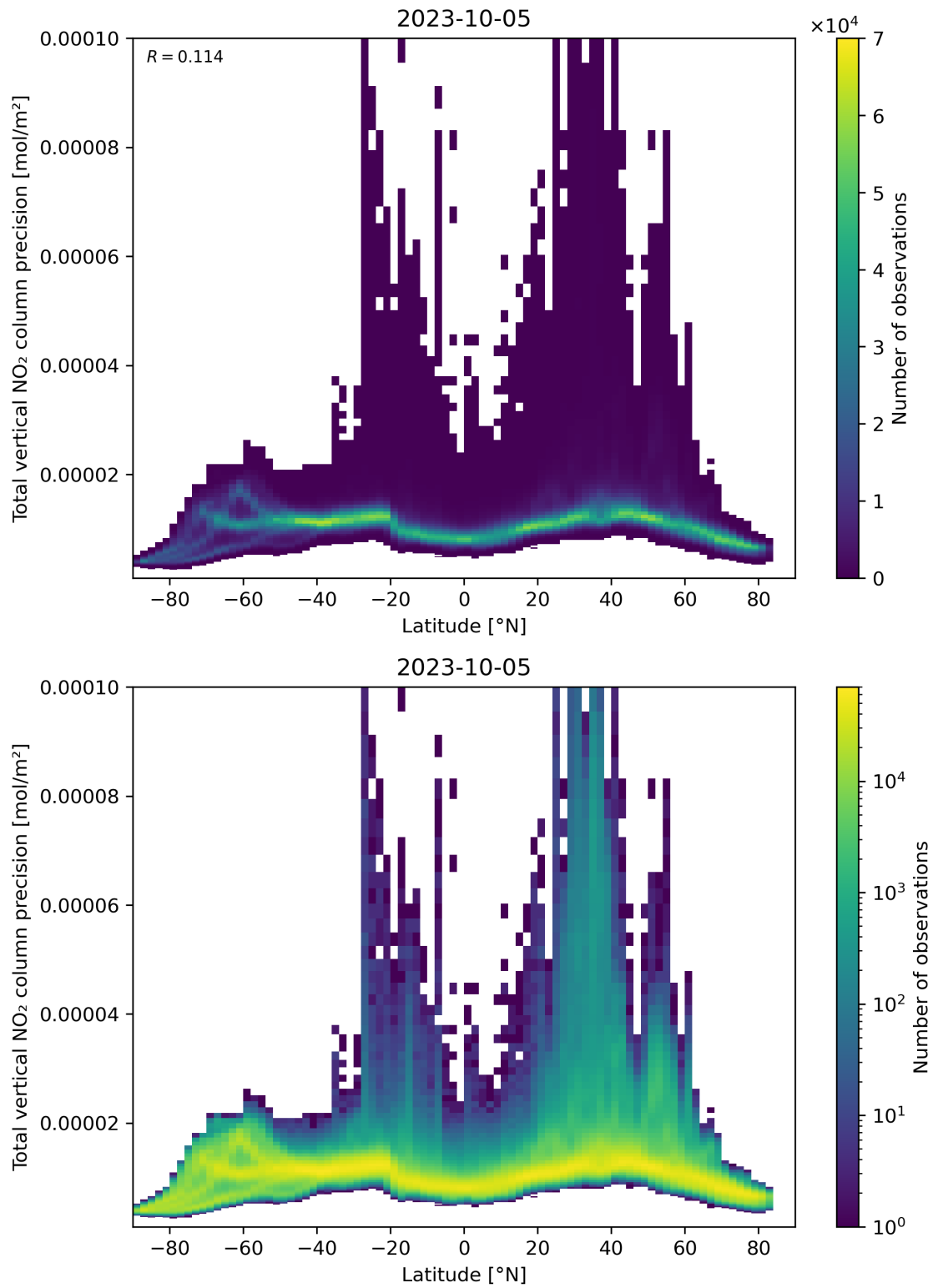
Figure 91: Scatter density plot of “Latitude” against “Total vertical NO 2 column precision” for 2023-10-04 to 2023-10-06.
