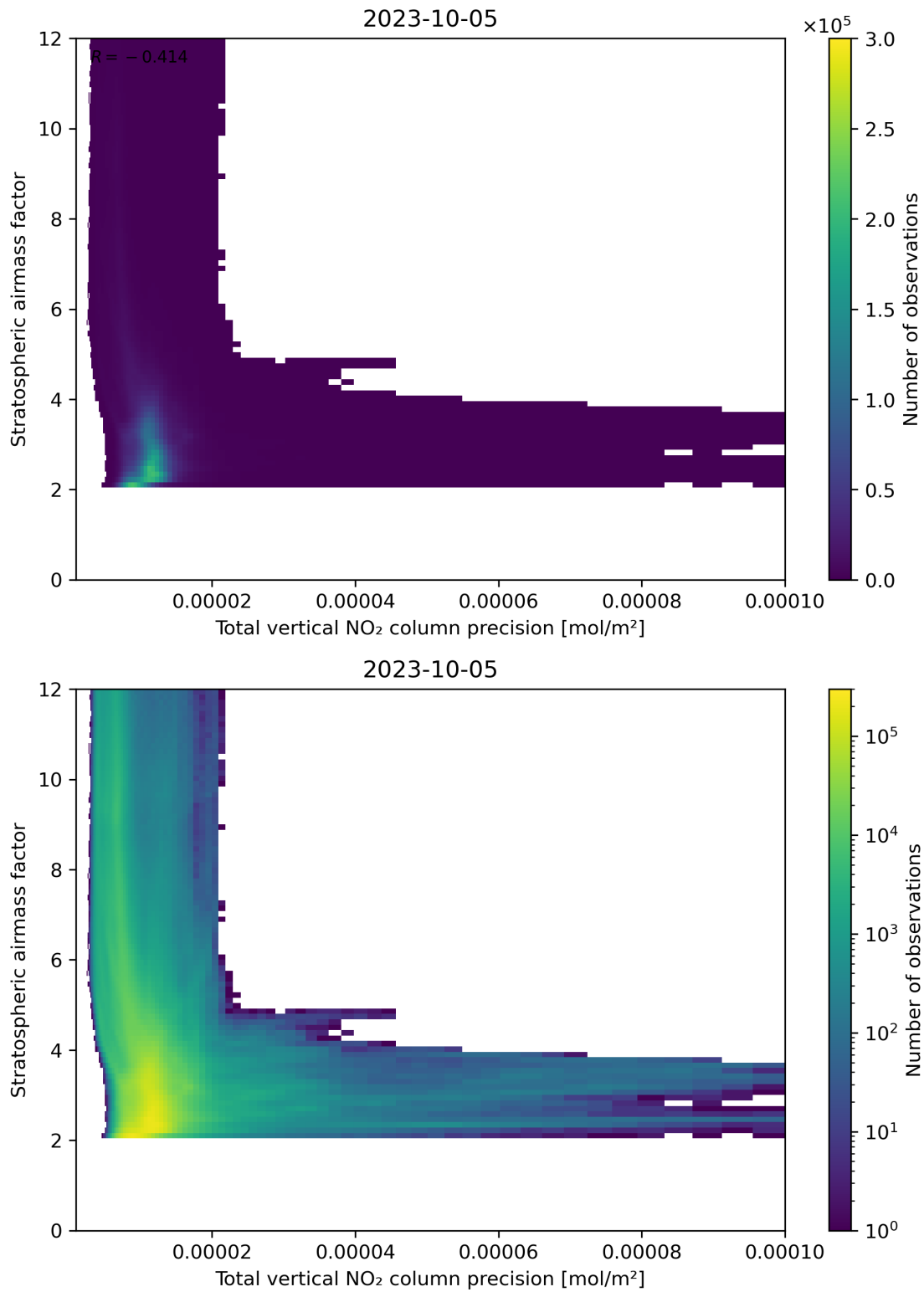
Figure 115: Scatter density plot of “Total vertical NO 2 column precision” against “Stratospheric airmass factor” for 2023-10-04 to 2023-10-06.
