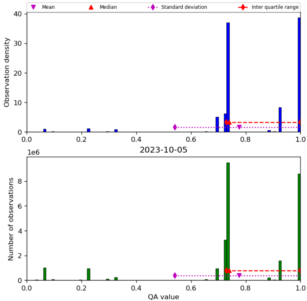
Figure 28: Histogram of “QA value” for 2023-10-04 to 2023-10-06
