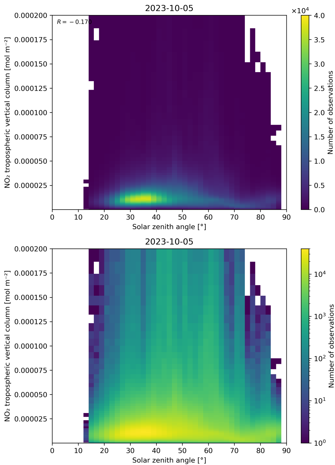
Figure 155: Scatter density plot of “Solar zenith angle” against “NO 2 tropospheric vertical column” for 2023-10-04 to 2023-10-06.
