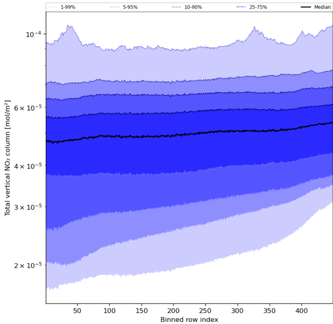
Figure 55: Along track statistics of “Total vertical NO 2 column” for 2023-10-04 to 2023-10-06
