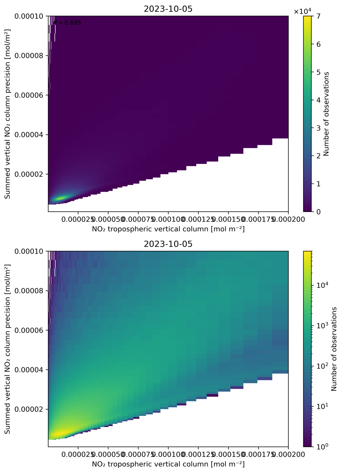
Figure 127: Scatter density plot of “NO 2 tropospheric vertical column” against “Summed vertical NO 2 column precision” for 2023-10-04 to 2023-10-06.
