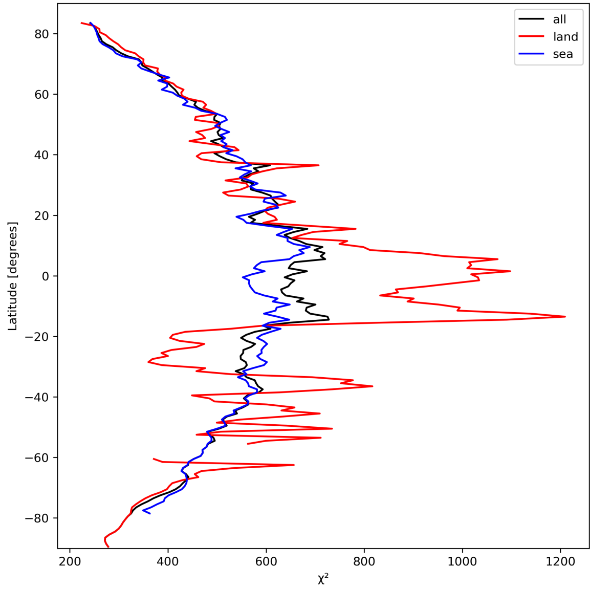
Figure 25: Zonal average of “ \chi^2 ” for 2023-10-04 to 2023-10-06.
