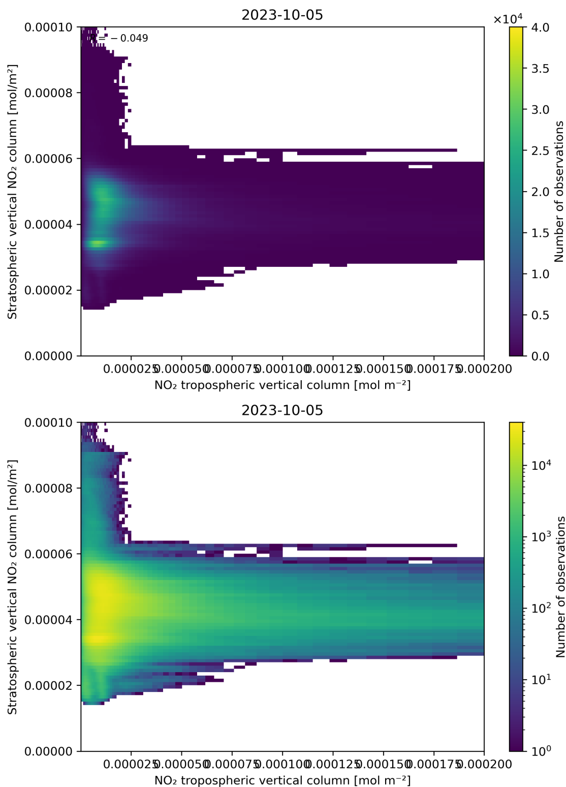
Figure 125: Scatter density plot of “NO 2 tropospheric vertical column” against “Stratospheric vertical NO 2 column” for 2023-10-04 to 2023-10-06.
