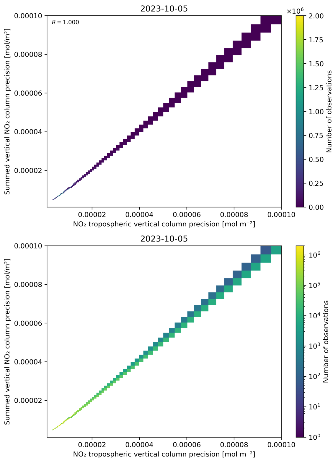
Figure 137: Scatter density plot of “NO 2 tropospheric vertical column precision” against “Summed vertical NO 2 column precision” for 2023-10-04 to 2023-10-06.
