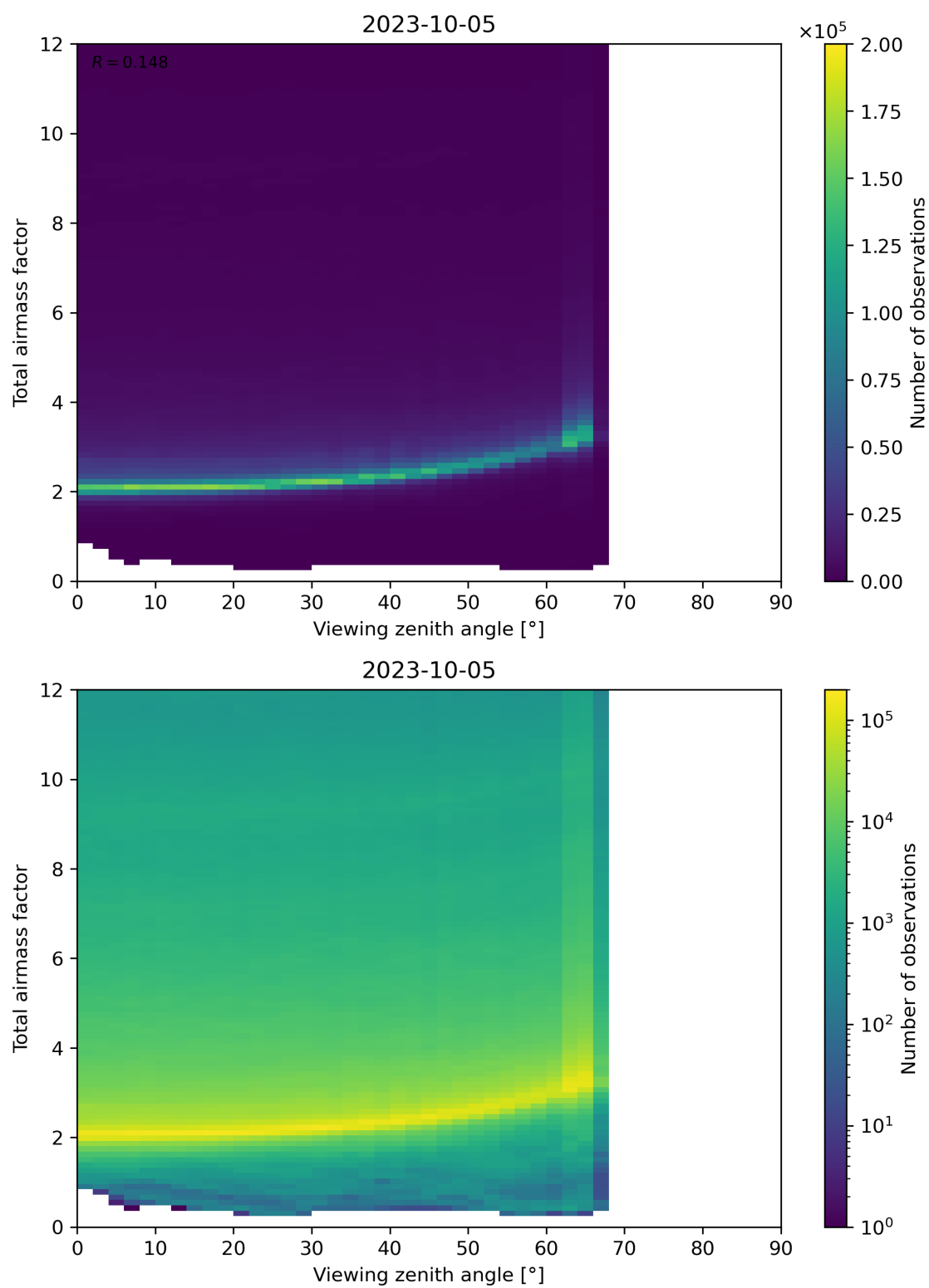
Figure 160: Scatter density plot of “Viewing zenith angle” against “Total airmass factor” for 2023-10-04 to 2023-10-06.
