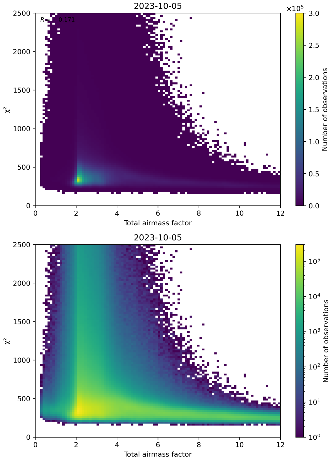
Figure 63: Scatter density plot of “Total airmass factor” against “ \chi^2 ” for 2023-10-04 to 2023-10-06.
