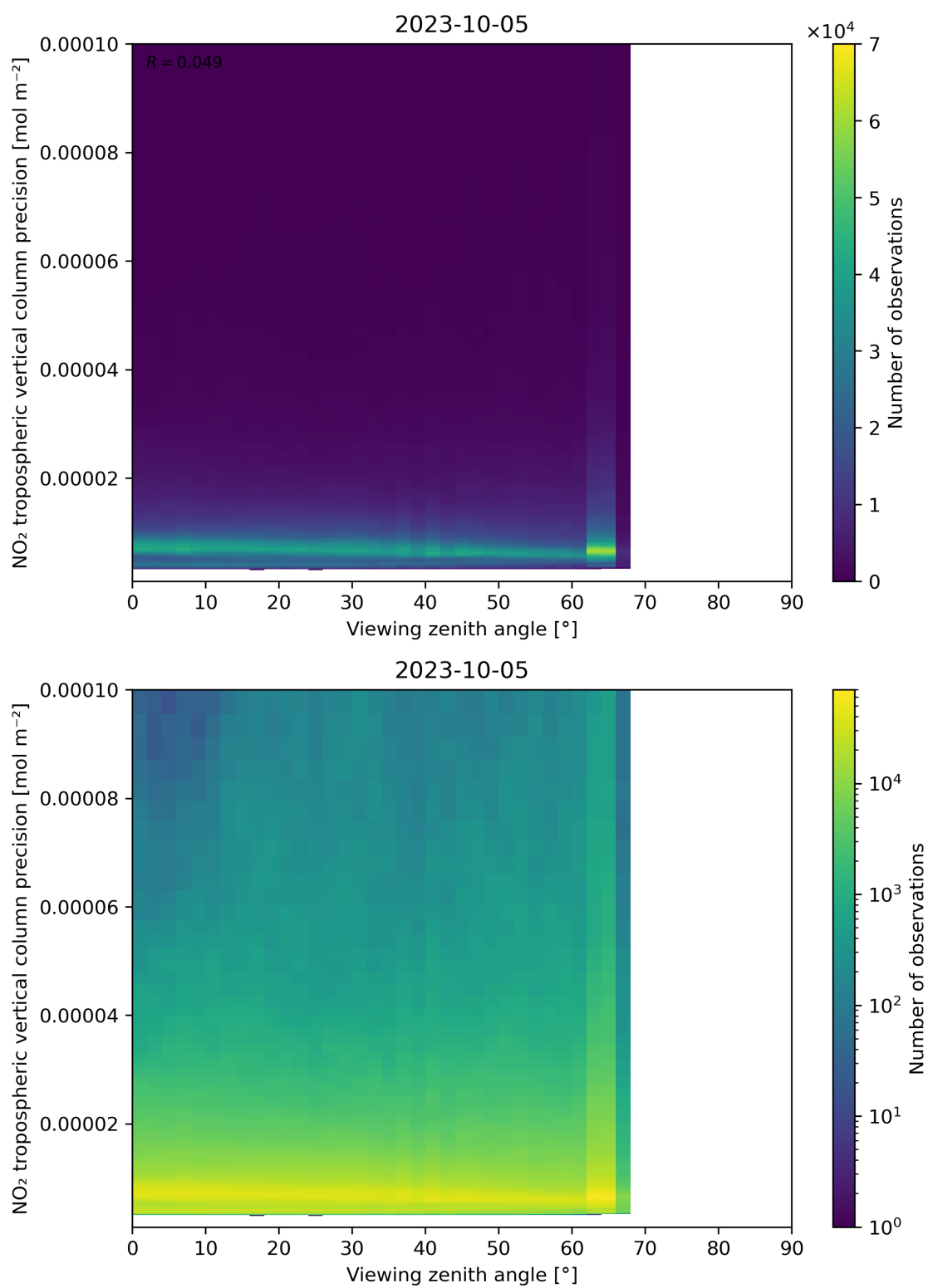
Figure 170: Scatter density plot of “Viewing zenith angle” against “NO 2 tropospheric vertical column precision” for 2023-10-04 to 2023-10-06.
