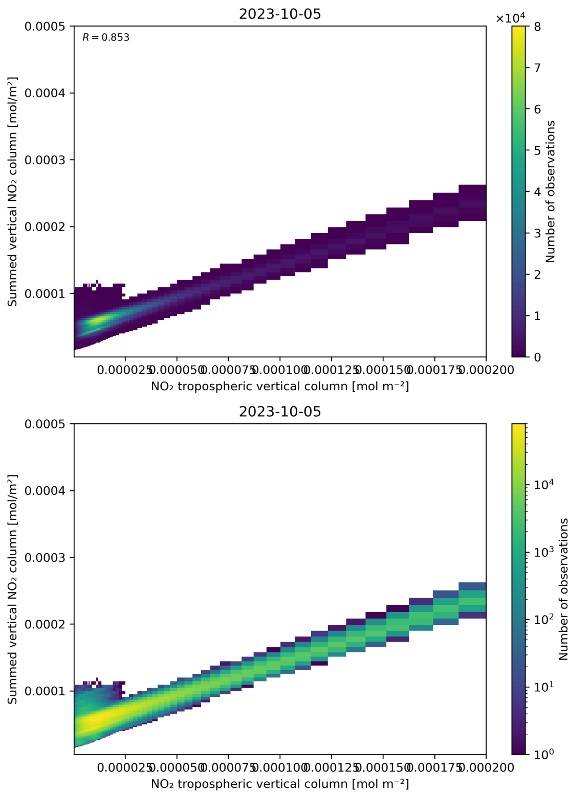
Figure 126: Scatter density plot of “NO 2 tropospheric vertical column” against “Summed vertical NO 2 column” for 2023-10-04 to 2023-10-06.
