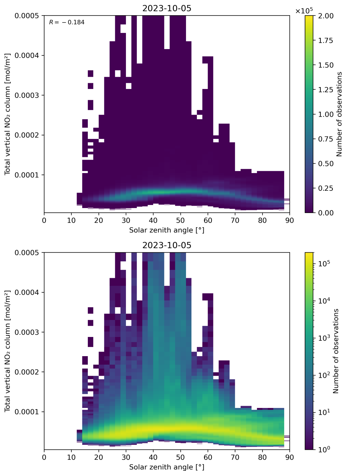
Figure 153: Scatter density plot of “Solar zenith angle” against “Total vertical NO 2 column” for 2023-10-04 to 2023-10-06.
