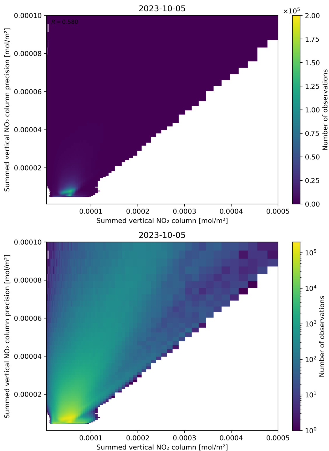
Figure 105: Scatter density plot of “Summed vertical NO 2 column” against “Summed vertical NO 2 column precision” for 2023-10-04 to 2023-10-06.
