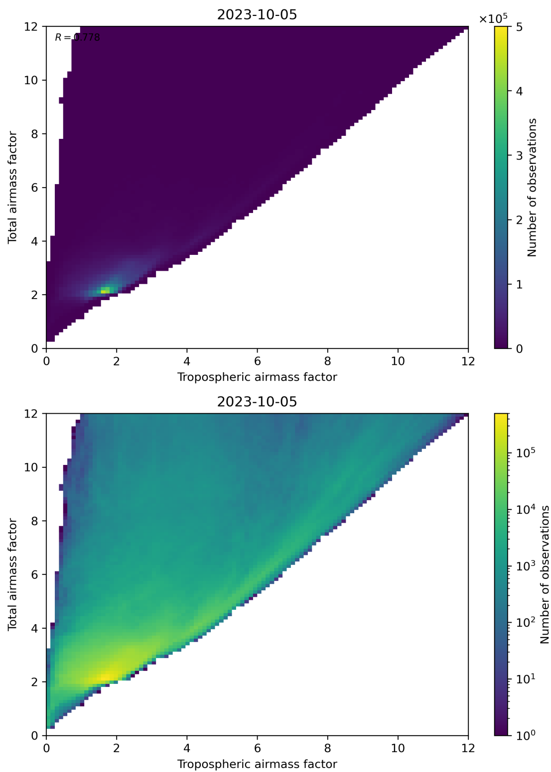
Figure 72: Scatter density plot of “Tropospheric airmass factor” against “Total airmass factor” for 2023-10-04 to 2023-10-06.
