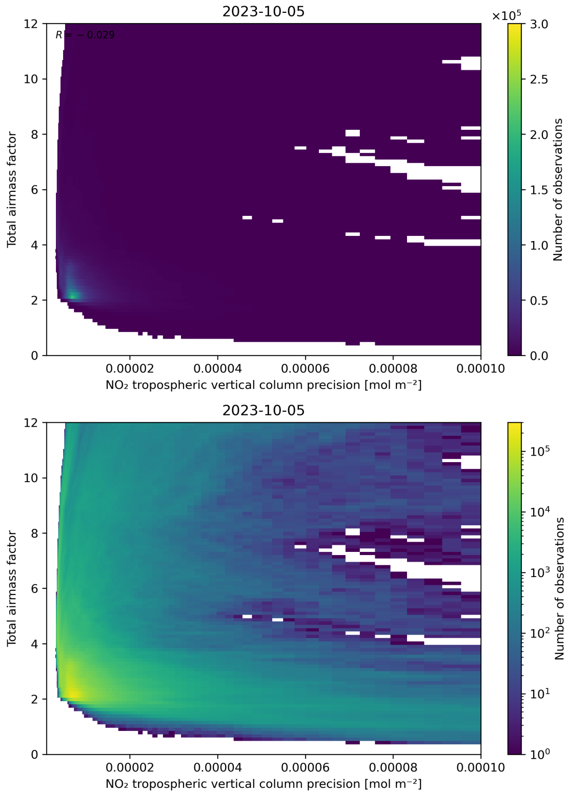
Figure 132: Scatter density plot of “NO 2 tropospheric vertical column precision” against “Total air mass factor” for 2023-10-04 to 2023-10-06.
