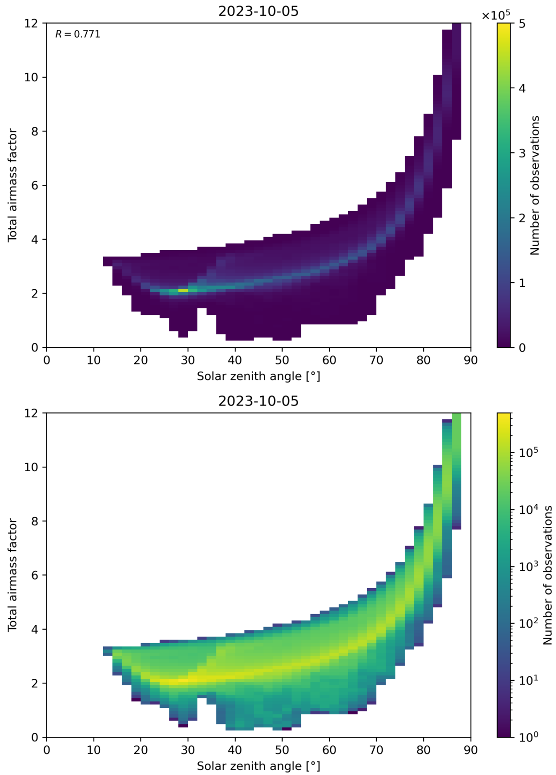
Figure 146: Scatter density plot of “Solar zenith angle” against “Total air mass factor” for 2023-10-04 to 2023-10-06.
