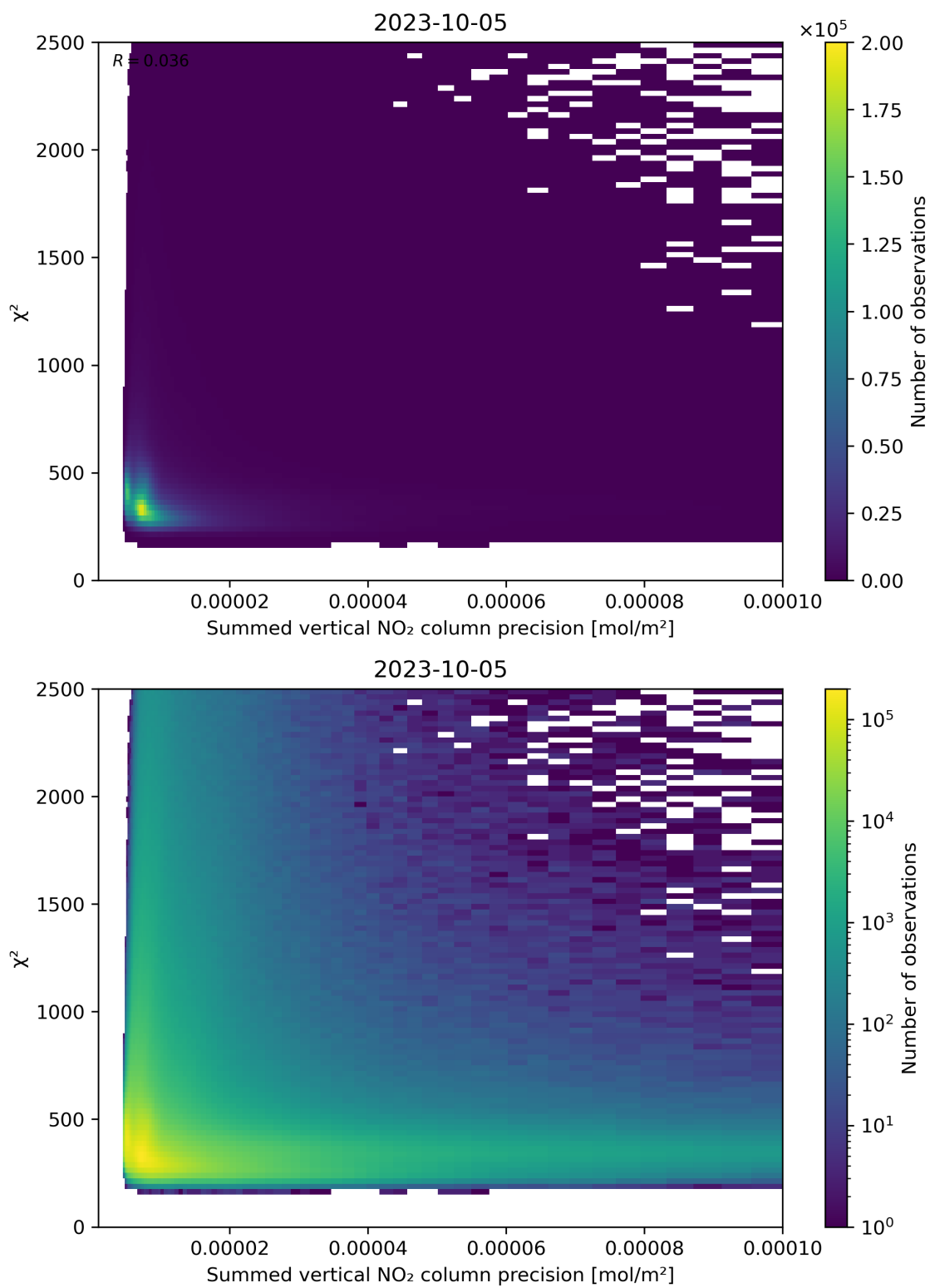
Figure 107: Scatter density plot of “Summed vertical NO 2 column precision” against “ \chi^2 ” for 2023-10-04 to 2023-10-06.
