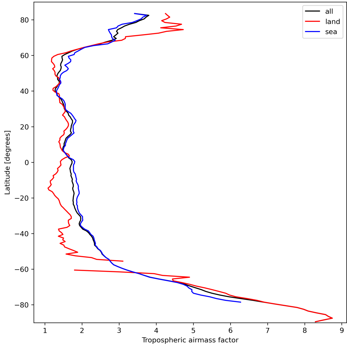
Figure 14: Zonal average of “Tropospheric air mass factor” for 2023-10-04 to 2023-10-06.
