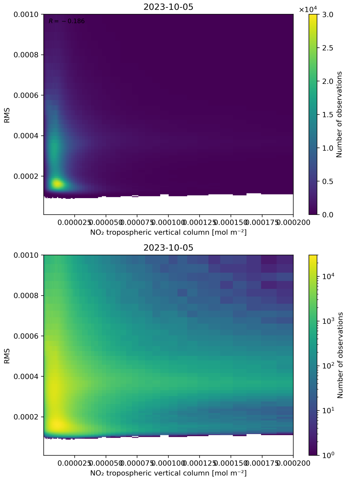
Figure 142: Scatter density plot of “NO 2 tropospheric vertical column” against “RMS” for 2023-10-04 to 2023-10-06.
