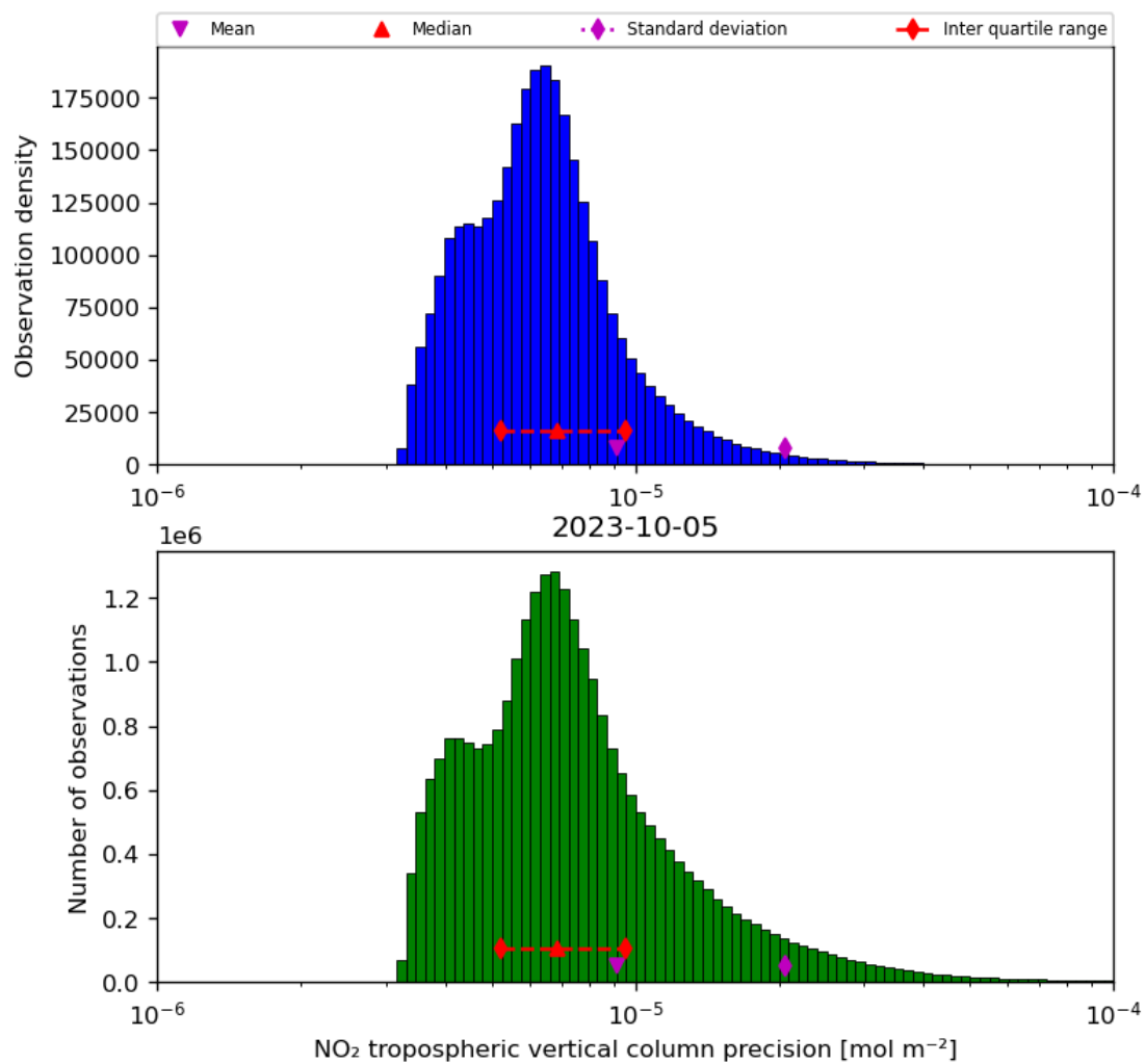
Figure 30: Histogram of “NO 2 tropospheric vertical column precision” for 2023-10-04 to 2023-10-06
