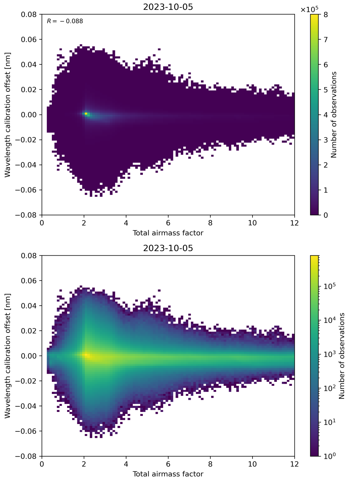
Figure 70: Scatter density plot of “Total airmass factor” against “Wavelength calibration offset” for 2023-10-04 to 2023-10-06.
