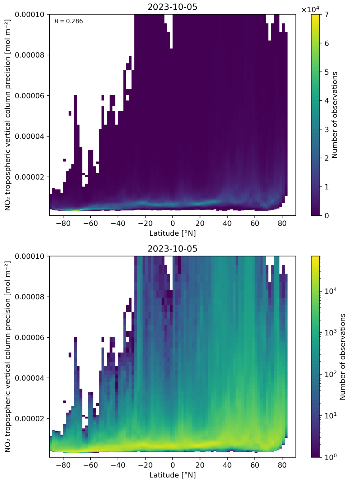
Figure 93: Scatter density plot of “Latitude” against “NO 2 tropospheric vertical column precision” for 2023-10-04 to 2023-10-06.
