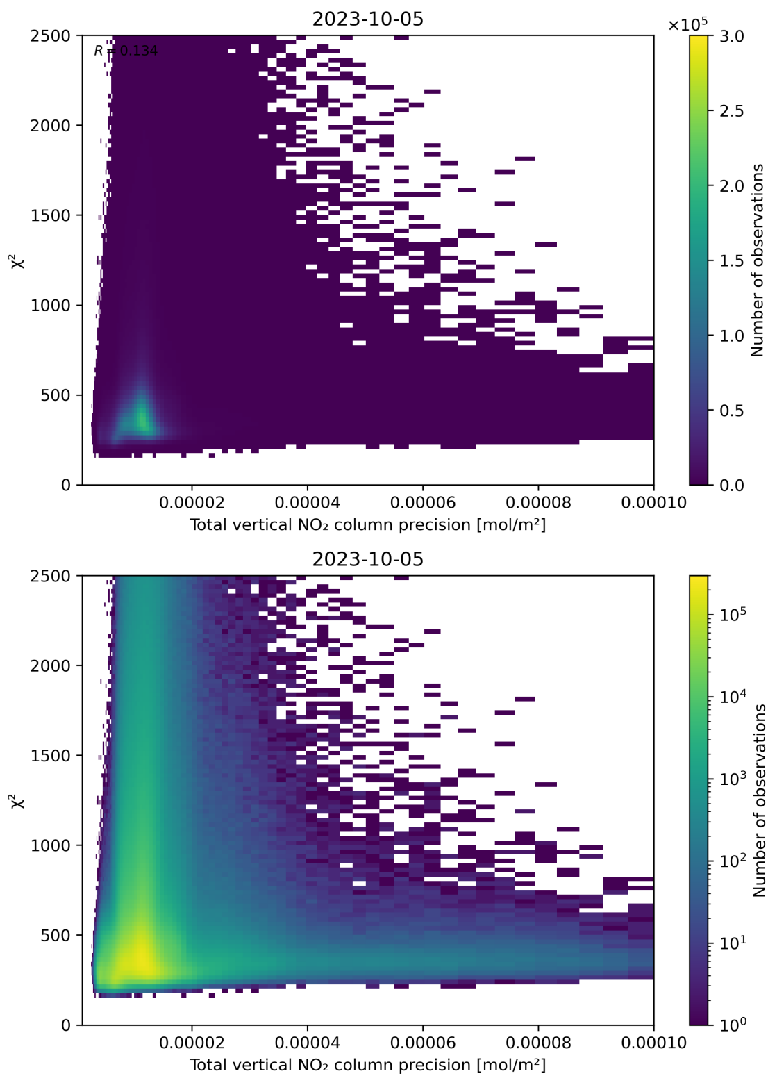
Figure 116: Scatter density plot of “Total vertical NO 2 column precision” against “ \chi^2 ” for 2023-10-04 to 2023-10-06.
