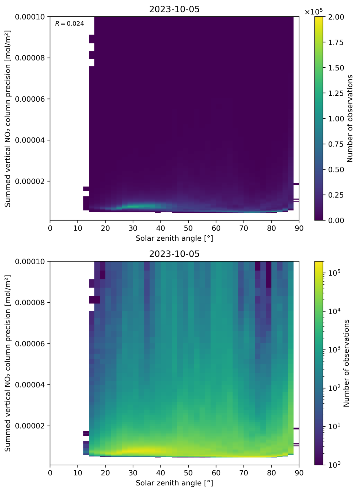
Figure 152: Scatter density plot of “Solar zenith angle” against “Summed vertical NO 2 column precision” for 2023-10-04 to 2023-10-06.
