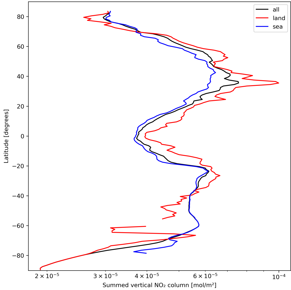
Figure 23: Zonal average of “Summed vertical NO 2 column” for 2023-10-04 to 2023-10-06.
