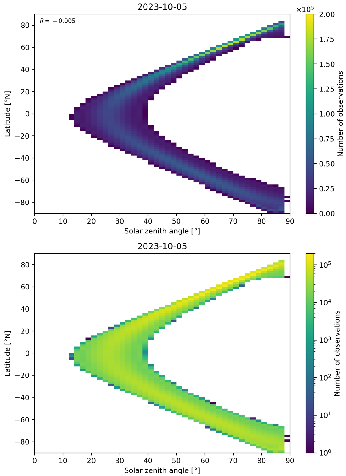
Figure 149: Scatter density plot of “Solar zenith angle” against “Latitude” for 2023-10-04 to 2023-10-06.
