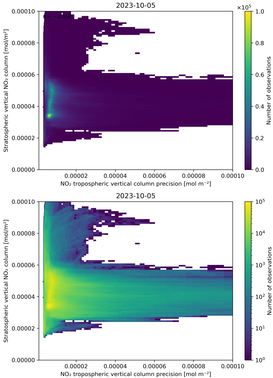
Figure 135: Scatter density plot of “NO 2 tropospheric vertical column precision” against “Stratospheric vertical NO 2 column” for 2023-10-04 to 2023-10-06.
