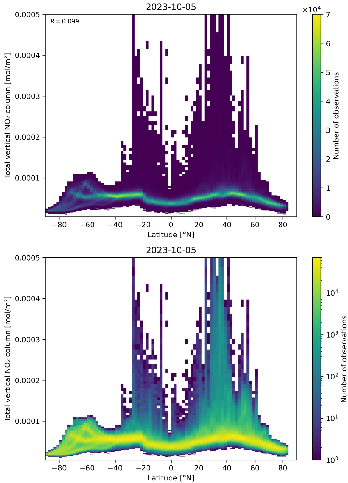
Figure 90: Scatter density plot of “Latitude” against “Total vertical NO 2 column” for 2023-10-04 to 2023-10-06.
