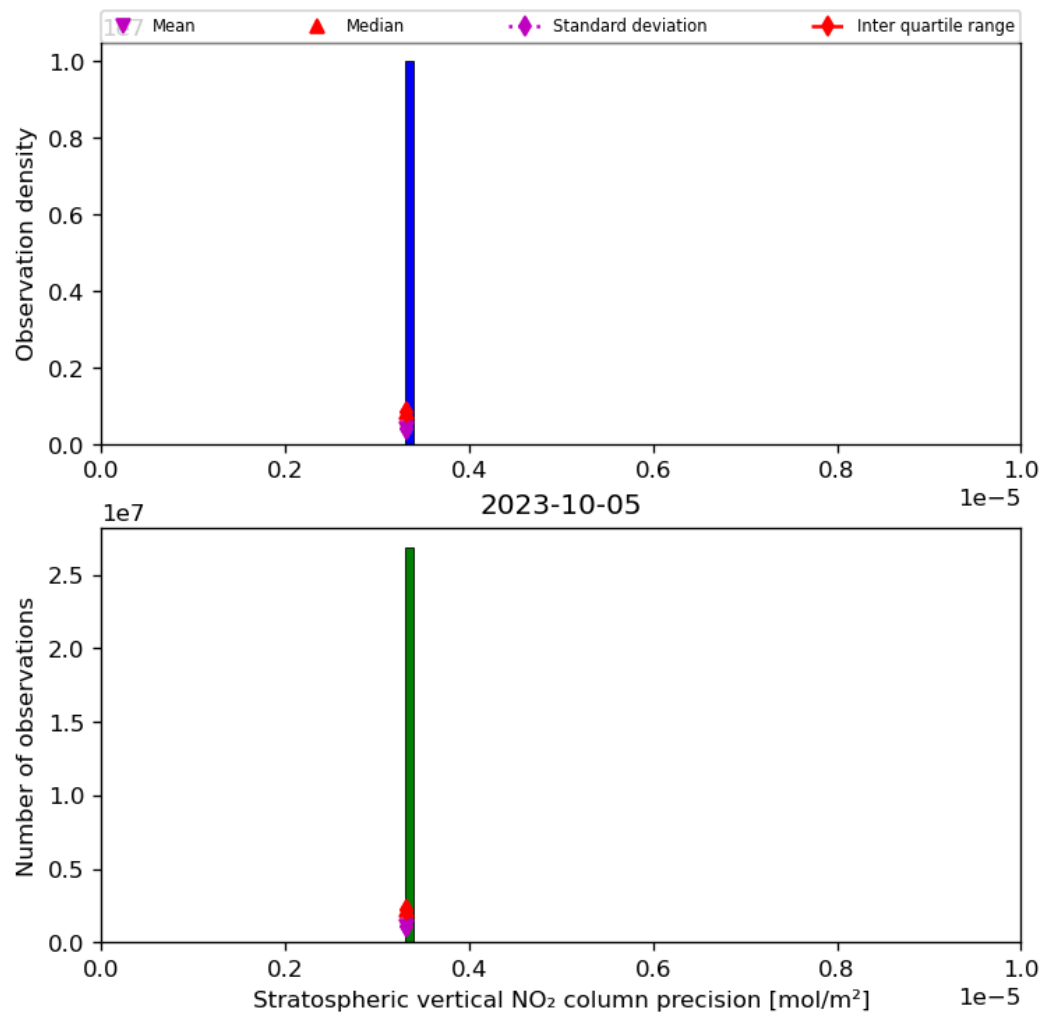
Figure 37: Histogram of “Stratospheric vertical NO 2 column precision” for 2023-10-04 to 2023-10-06
