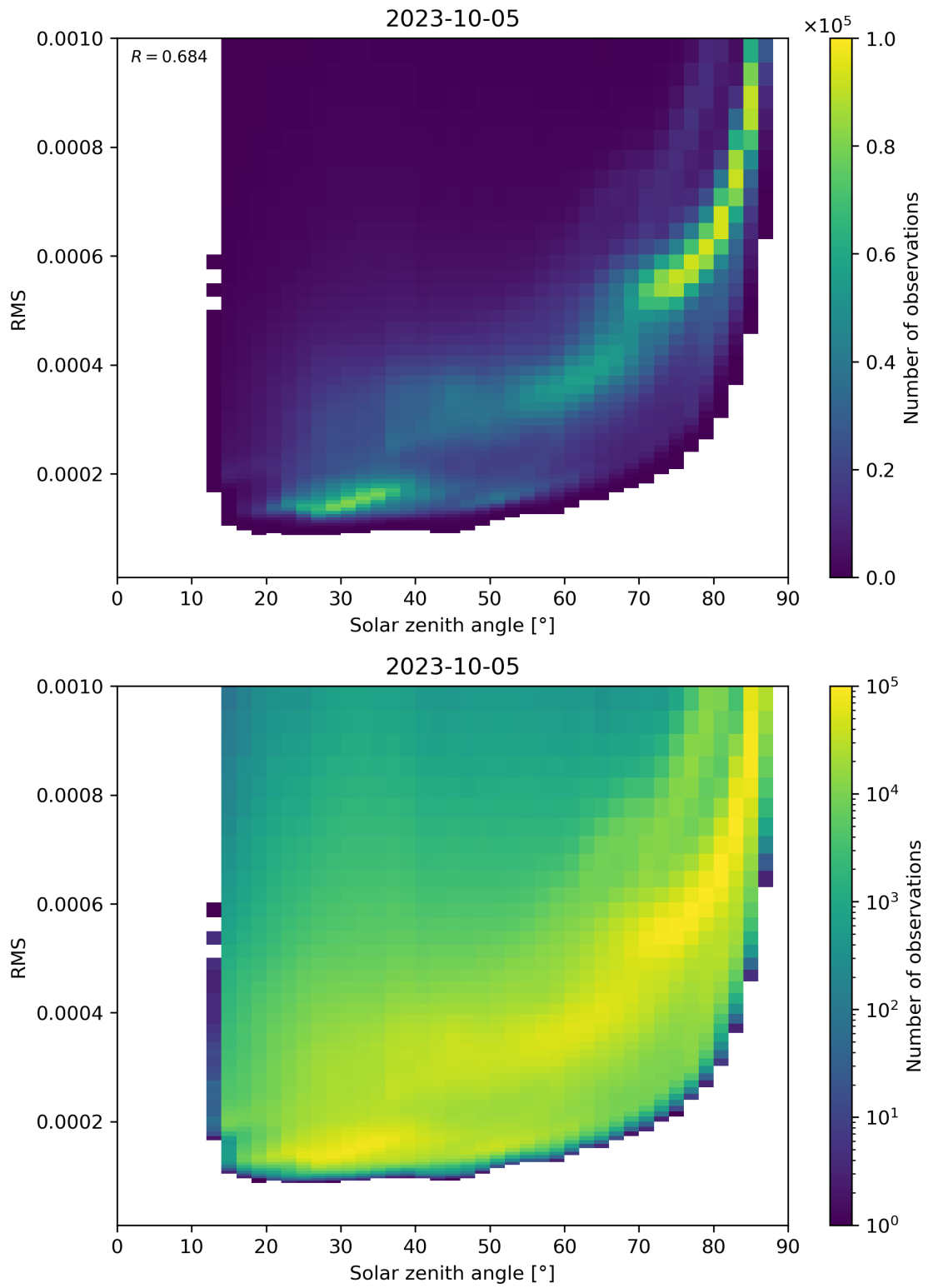
Figure 157: Scatter density plot of “Solar zenith angle” against “RMS” for 2023-10-04 to 2023-10-06.
