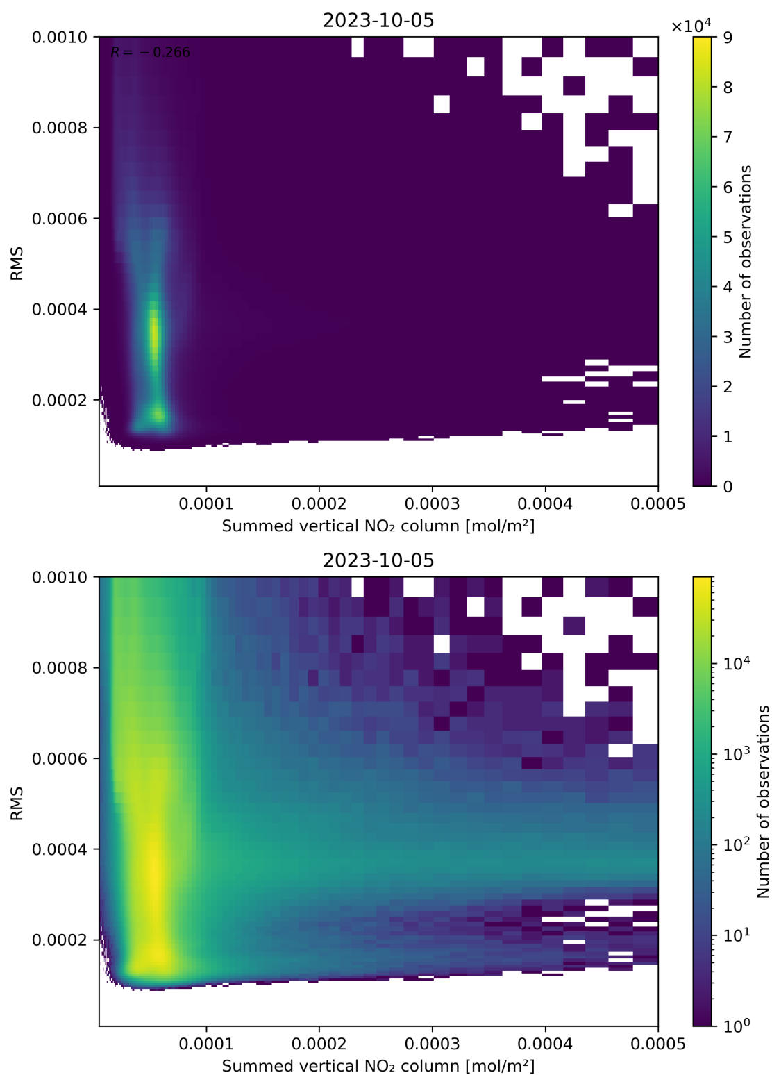
Figure 109: Scatter density plot of “Summed vertical NO 2 column” against “RMS” for 2023-10-04 to 2023-10-06.
