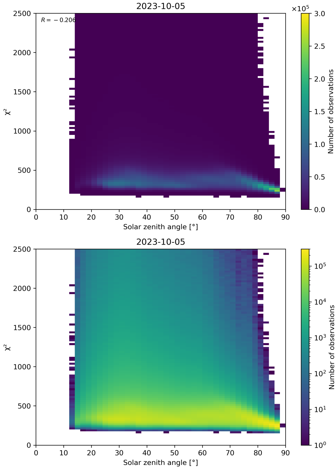
Figure 148: Scatter density plot of “Solar zenith angle” against “ \chi^2 ” for 2023-10-04 to 2023-10-06.
