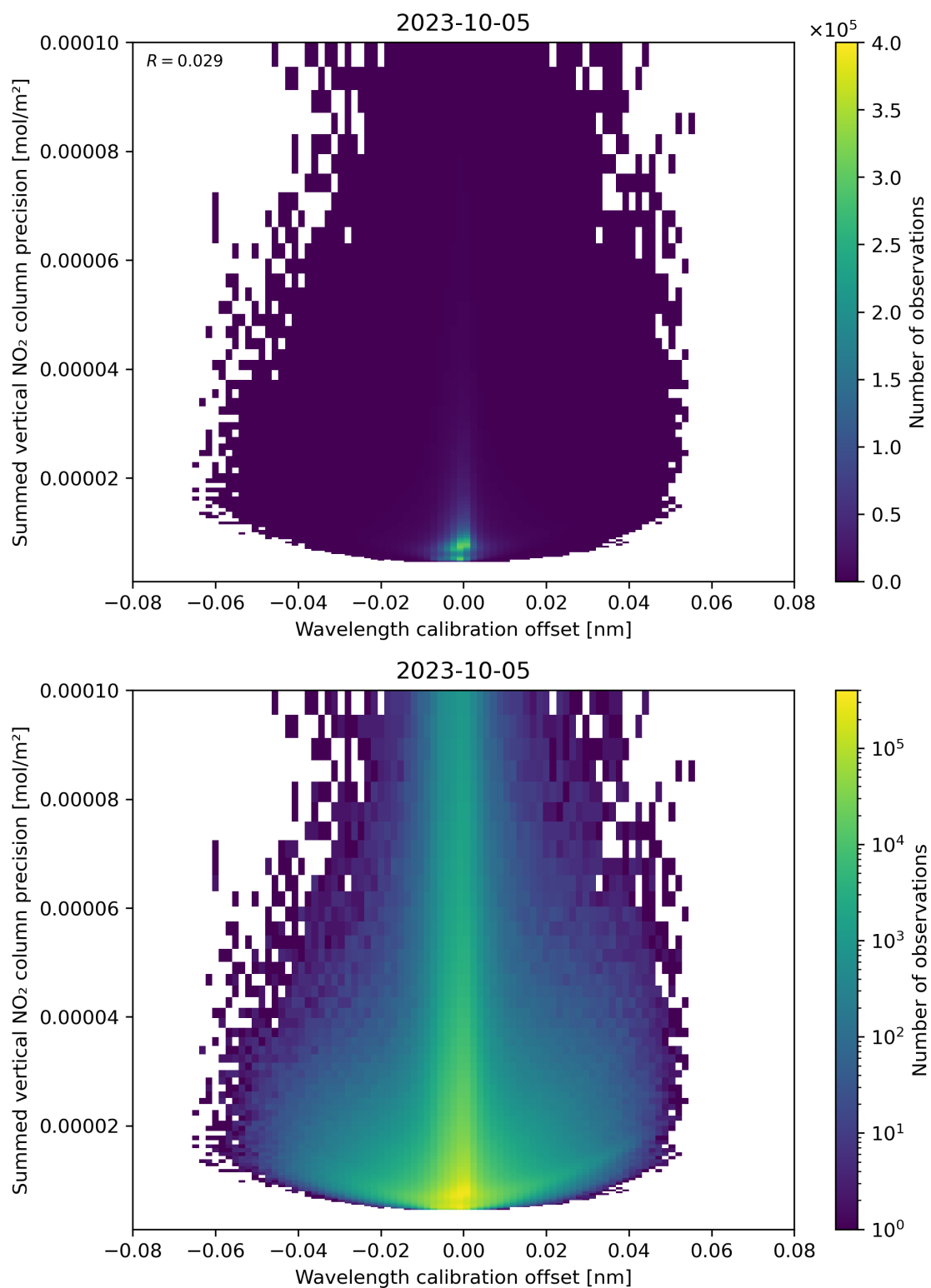
Figure 178: Scatter density plot of “Wavelength calibration offset” against “Summed vertical NO 2 column precision” for 2023-10-04 to 2023-10-06.
