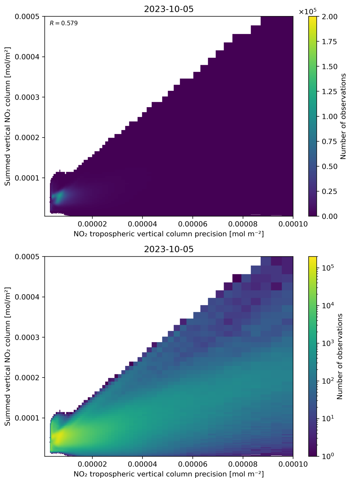
Figure 136: Scatter density plot of “NO 2 tropospheric vertical column precision” against “Summed vertical NO 2 column” for 2023-10-04 to 2023-10-06.
