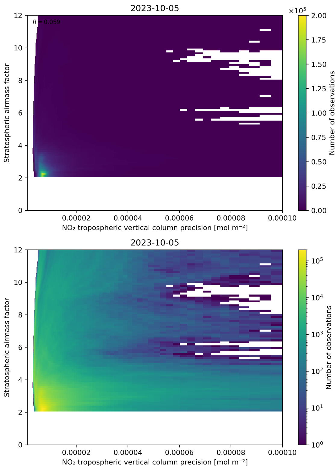
Figure 131: Scatter density plot of “NO 2 tropospheric vertical column precision” against “Stratospheric airmass factor” for 2023-10-04 to 2023-10-06.
