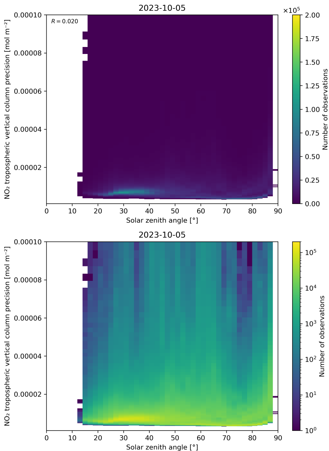
Figure 156: Scatter density plot of “Solar zenith angle” against “NO 2 tropospheric vertical column precision” for 2023-10-04 to 2023-10-06.
