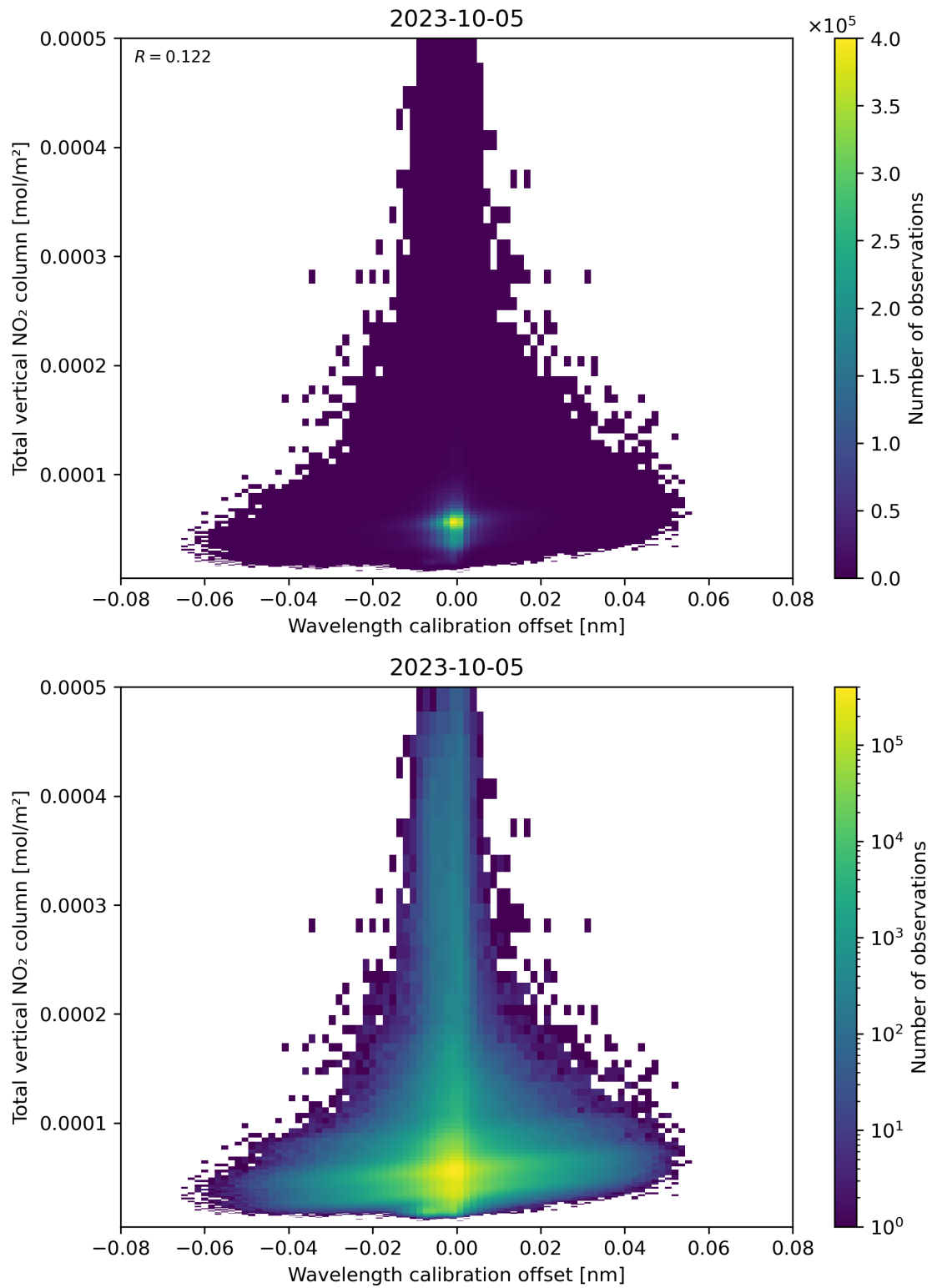
Figure 179: Scatter density plot of “Wavelength calibration offset” against “Total vertical NO 2 column” for 2023-10-04 to 2023-10-06.
