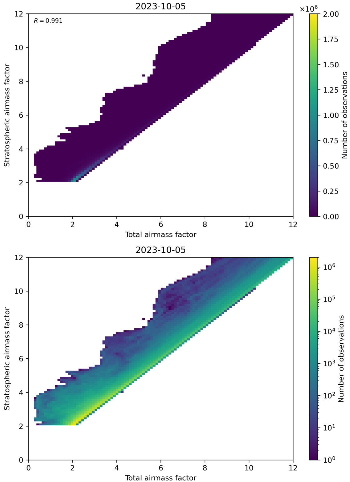
Figure 62: Scatter density plot of “Total airmass factor” against “Stratospheric airmass factor” for 2023-10-04 to 2023-10-06.
