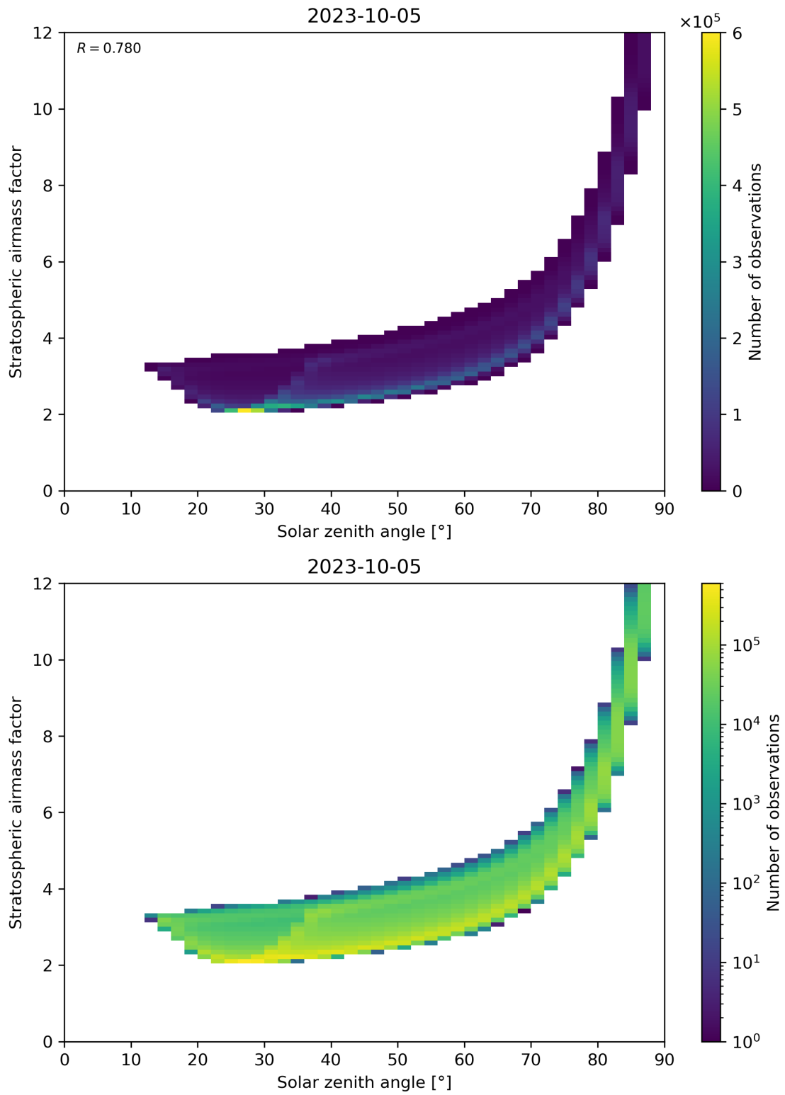
Figure 145: Scatter density plot of “Solar zenith angle” against “Stratospheric airmass factor” for 2023-10-04 to 2023-10-06.
