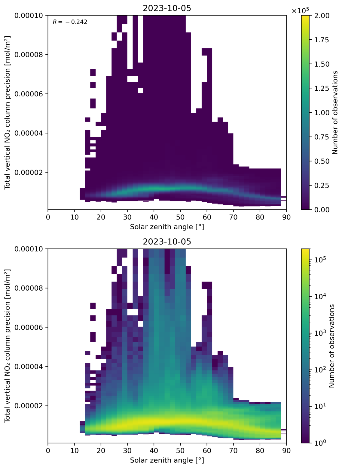
Figure 154: Scatter density plot of “Solar zenith angle” against “Total vertical NO 2 column precision” for 2023-10-04 to 2023-10-06.
