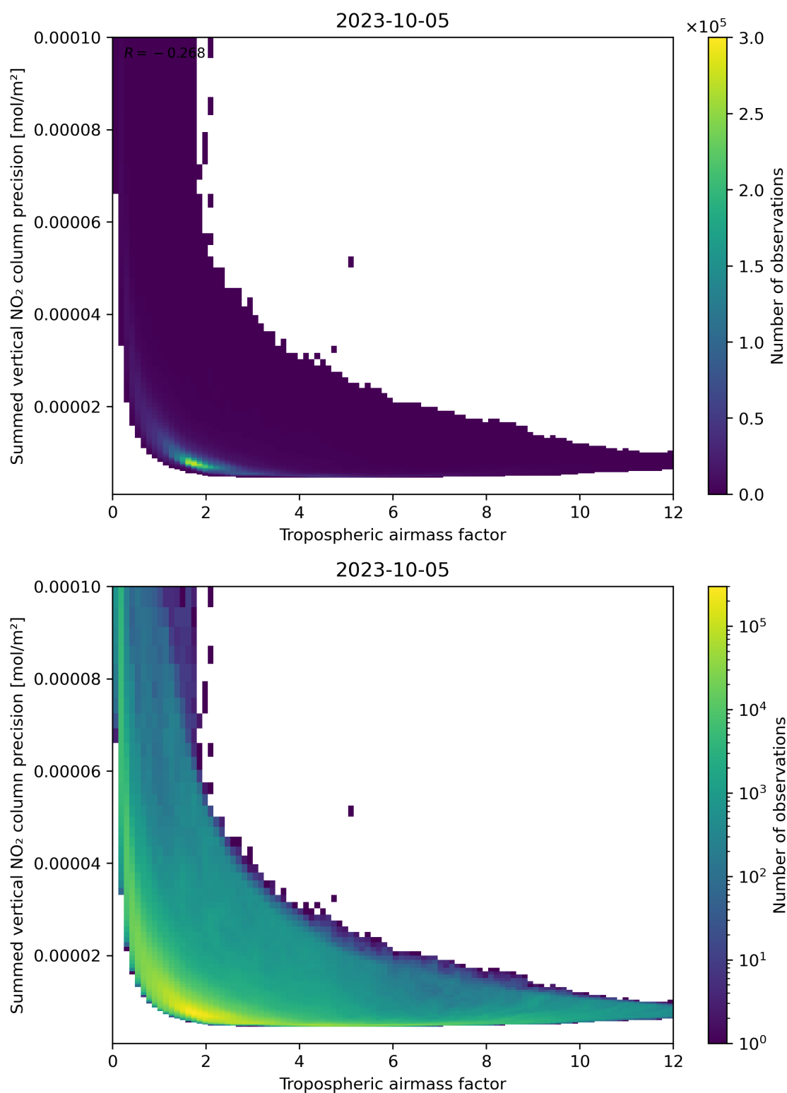
Figure 76: Scatter density plot of “Tropospheric air mass factor” against “Summed vertical NO 2 column precision” for 2023-10-04 to 2023-10-06.
