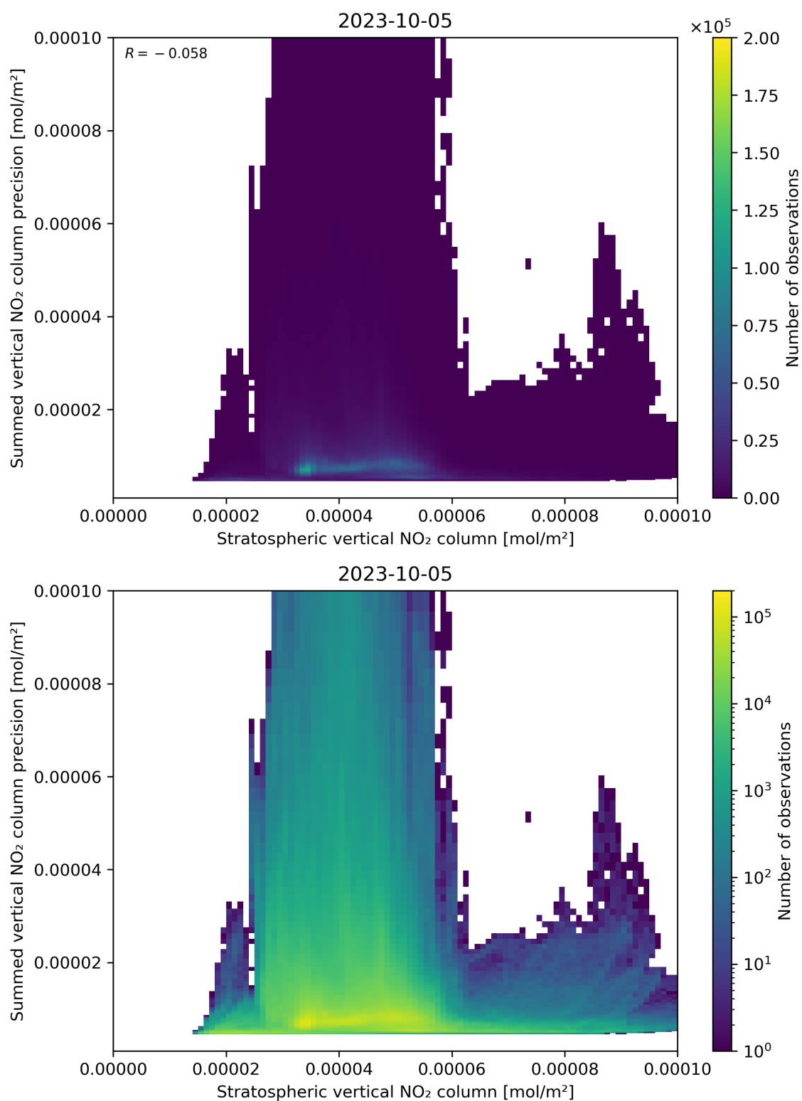
Figure 99: Scatter density plot of “Stratospheric vertical NO 2 column” against “Summed vertical NO 2 column precision” for 2023-10-04 to 2023-10-06.
