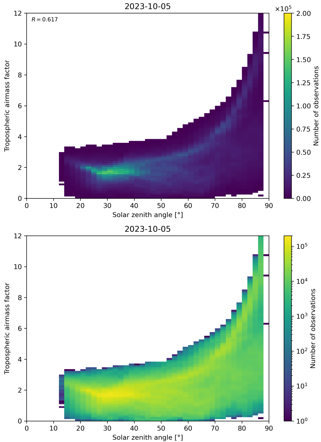
Figure 147: Scatter density plot of “Solar zenith angle” against “Tropospheric airmass factor” for 2023-10-04 to 2023-10-06.
