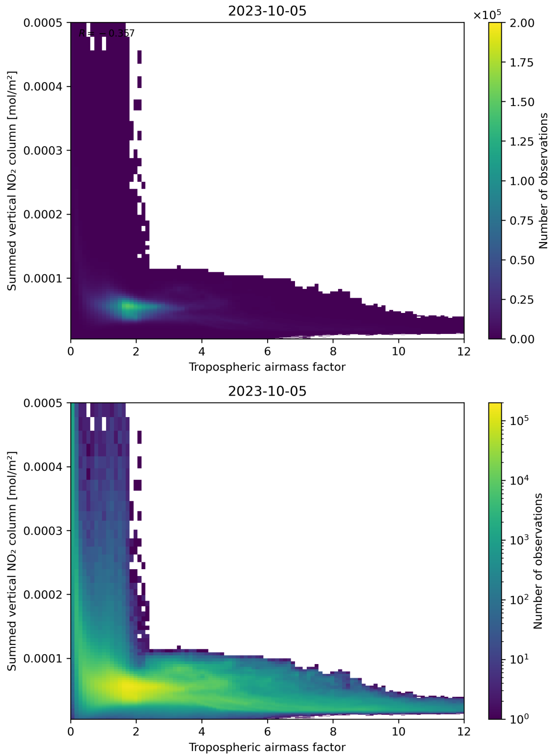
Figure 75: Scatter density plot of “Tropospheric airmass factor” against “Summed vertical NO 2 column” for 2023-10-04 to 2023-10-06.
