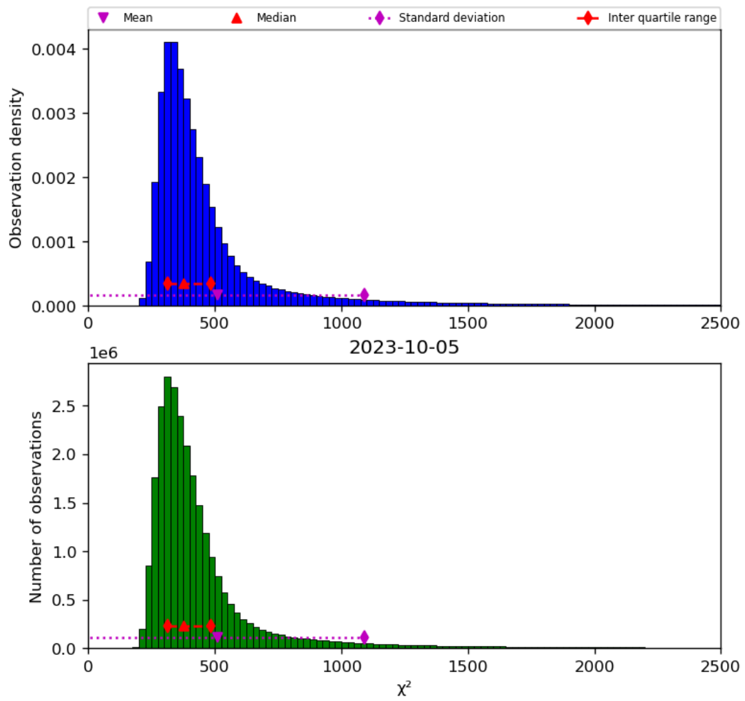
Figure 42: Histogram of “ \chi^2 ” for 2023-10-04 to 2023-10-06
