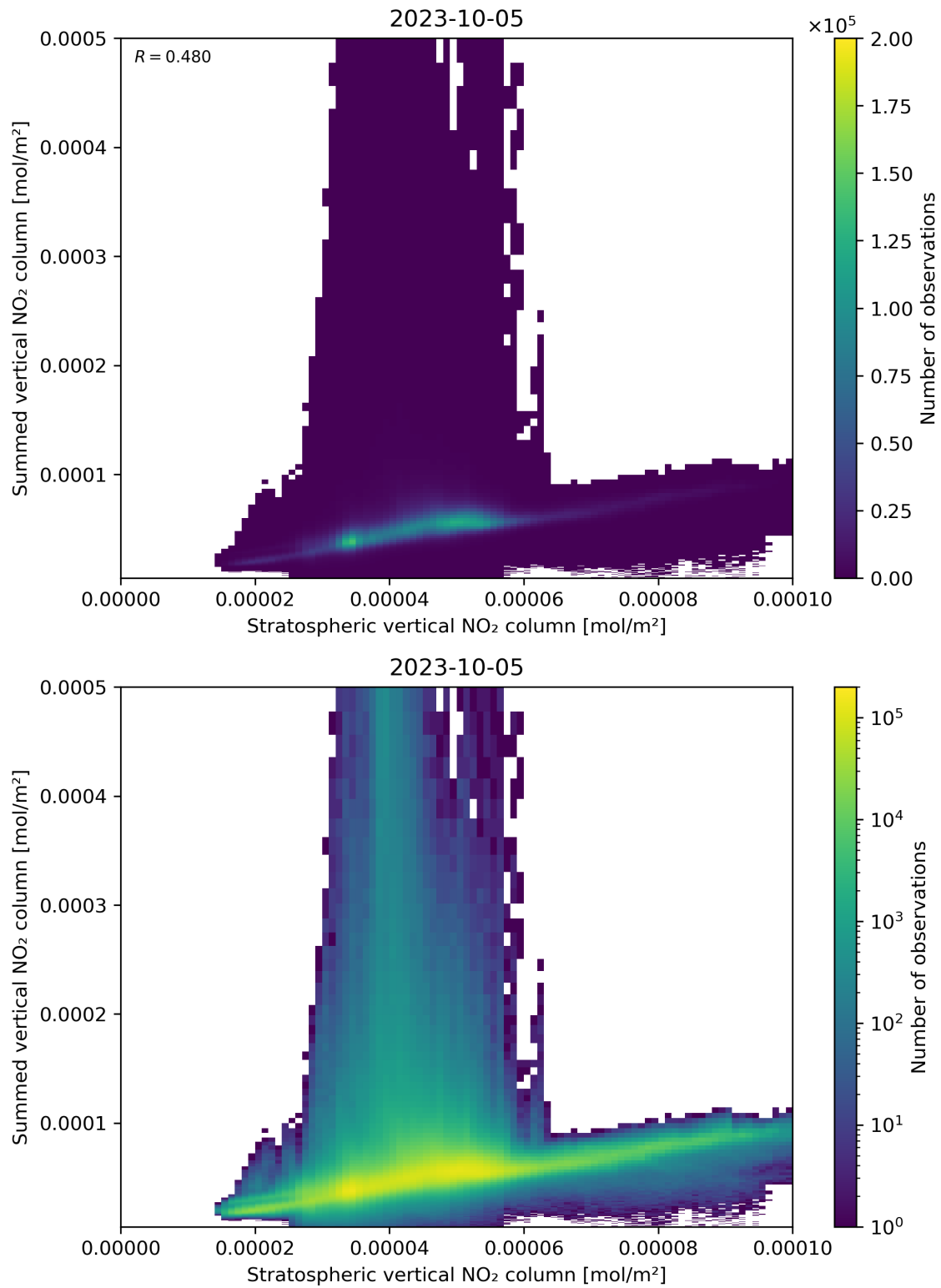
Figure 98: Scatter density plot of “Stratospheric vertical NO 2 column” against “Summed vertical NO 2 column” for 2023-10-04 to 2023-10-06.
