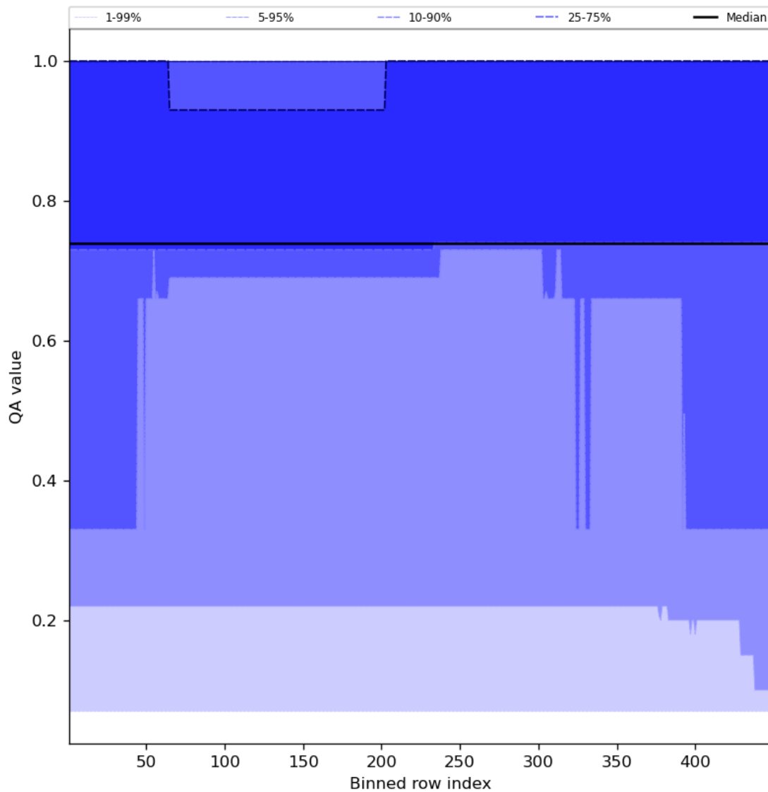
Figure 45: Along track statistics of “QA value” for 2023-10-04 to 2023-10-06
