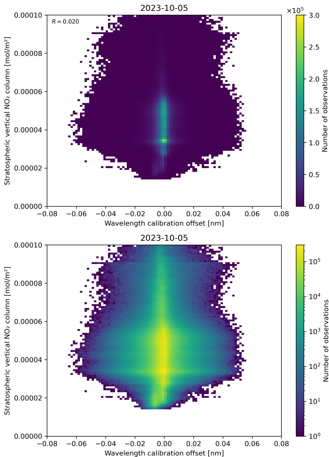
Figure 176: Scatter density plot of “Wavelength calibration offset” against “Stratospheric vertical NO 2 column” for 2023-10-04 to 2023-10-06.
