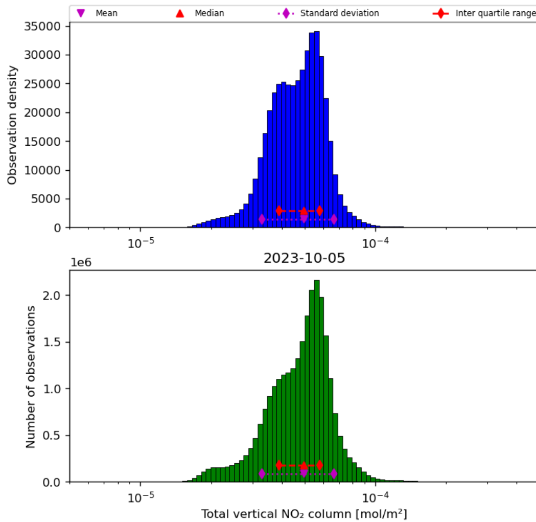
Figure 38: Histogram of “Total vertical NO 2 column” for 2023-10-04 to 2023-10-06
