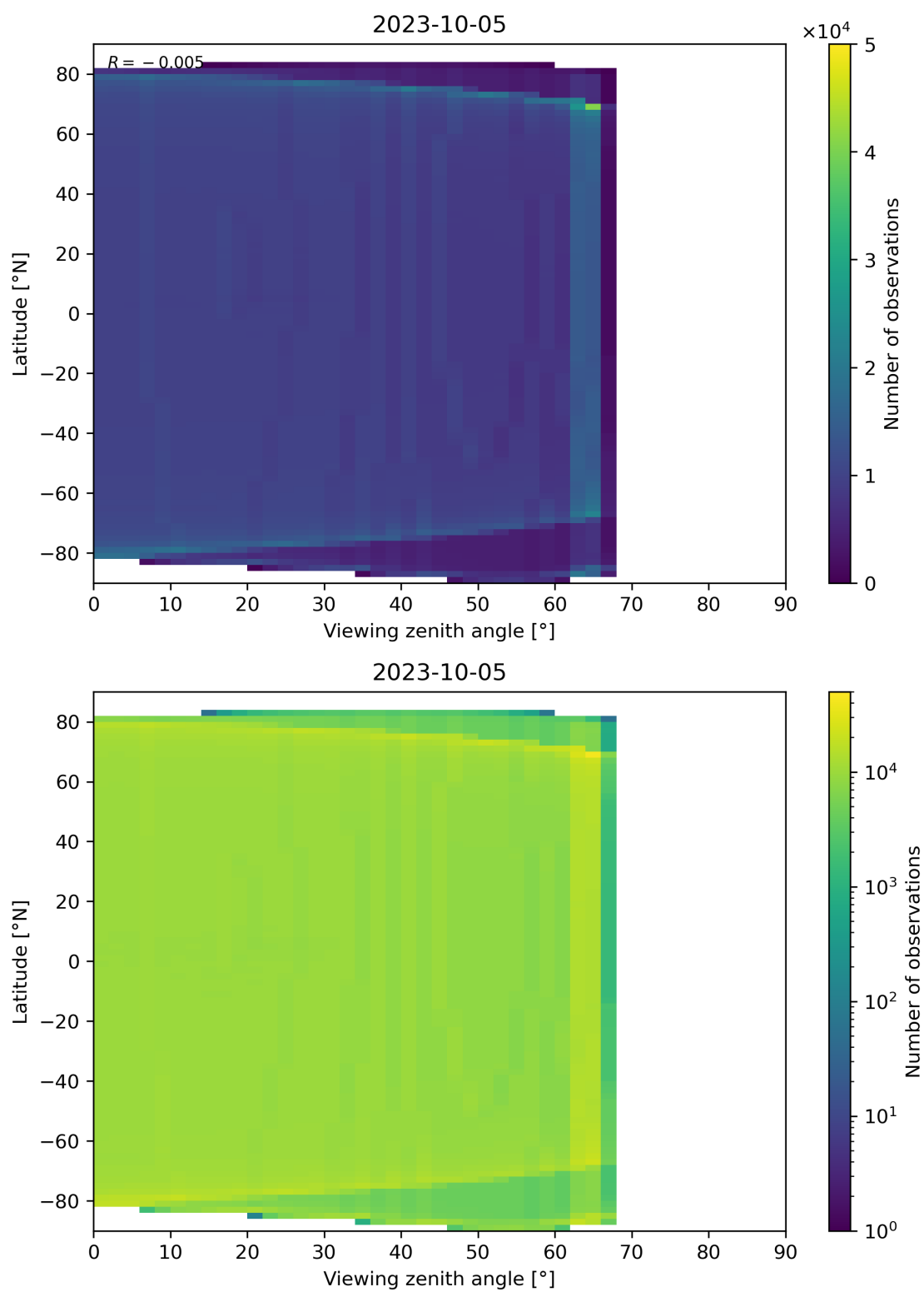
Figure 163: Scatter density plot of “Viewing zenith angle” against “Latitude” for 2023-10-04 to 2023-10-06.
