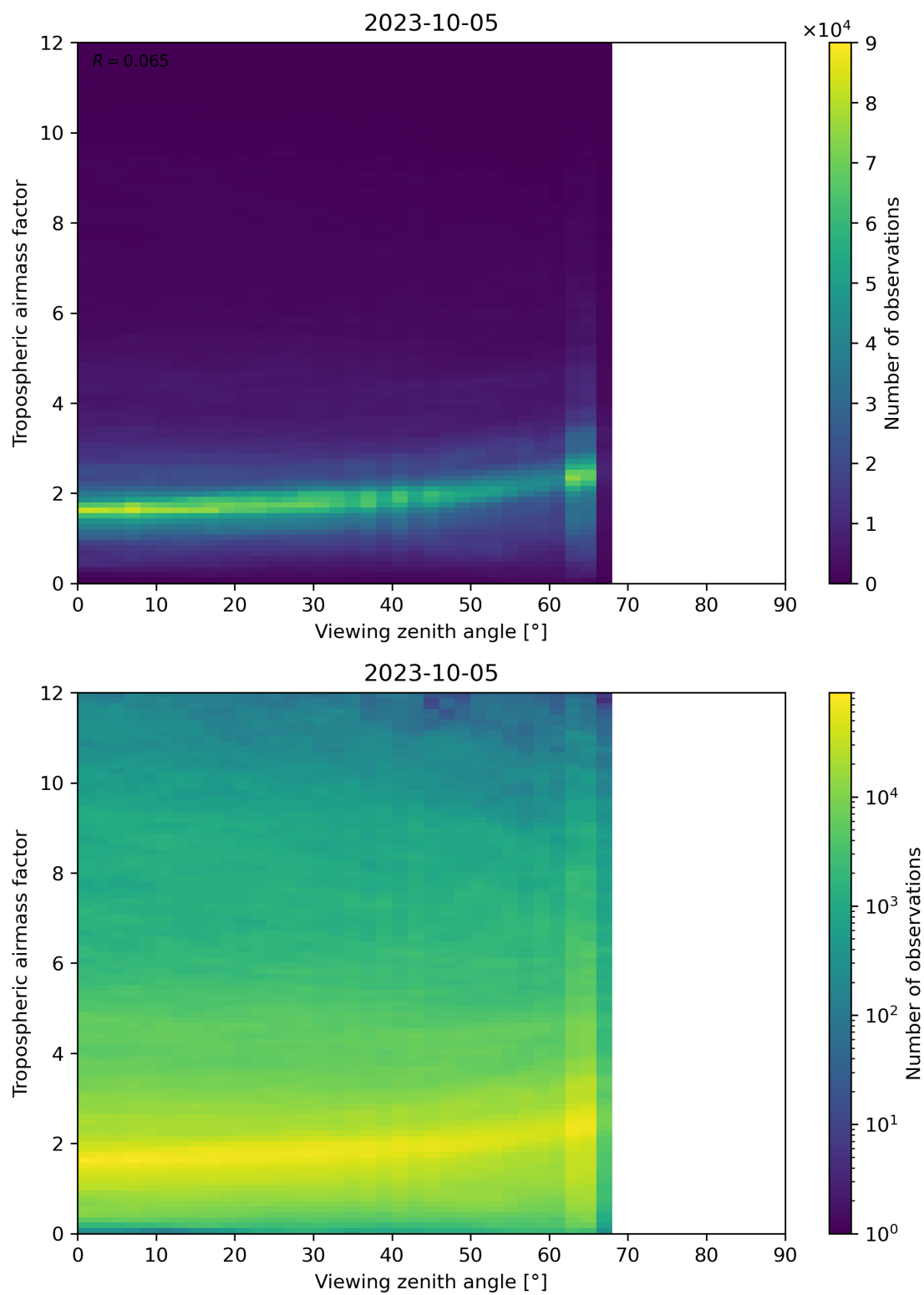
Figure 161: Scatter density plot of “Viewing zenith angle” against “Tropospheric airmass factor” for 2023-10-04 to 2023-10-06.
