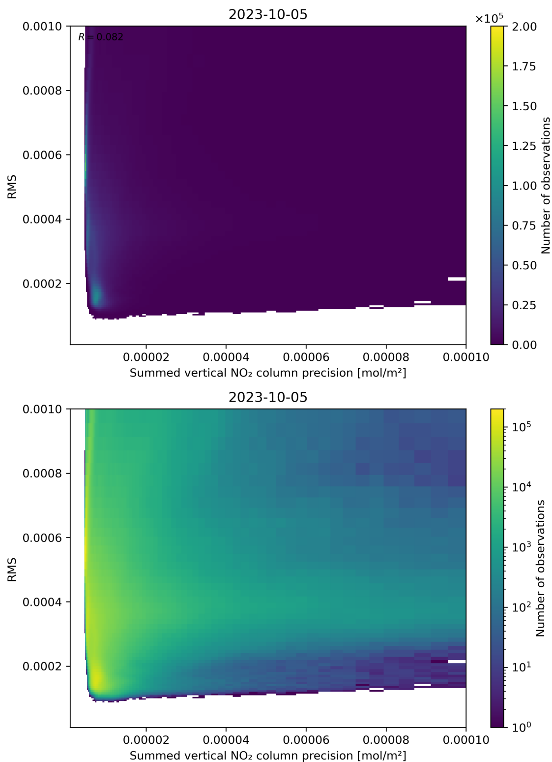
Figure 108: Scatter density plot of “Summed vertical NO 2 column precision” against “RMS” for 2023-10-04 to 2023-10-06.
