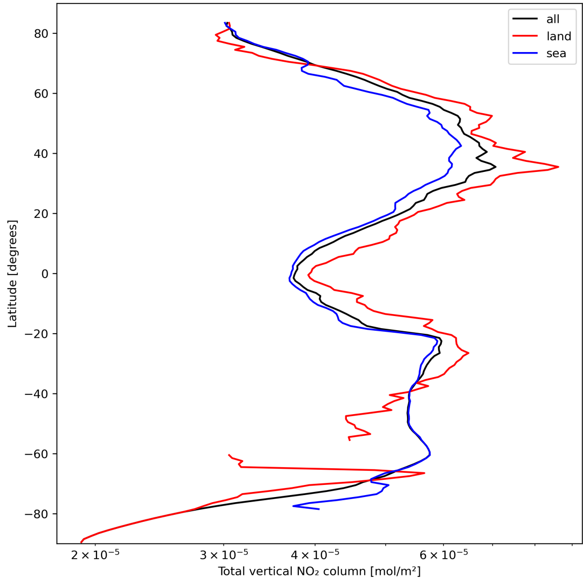
Figure 21: Zonal average of “Total vertical NO 2 column” for 2023-10-04 to 2023-10-06.
