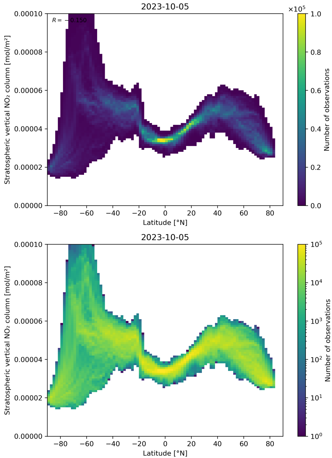
Figure 87: Scatter density plot of “Latitude” against “Stratospheric vertical NO 2 column” for 2023-10-04 to 2023-10-06.
