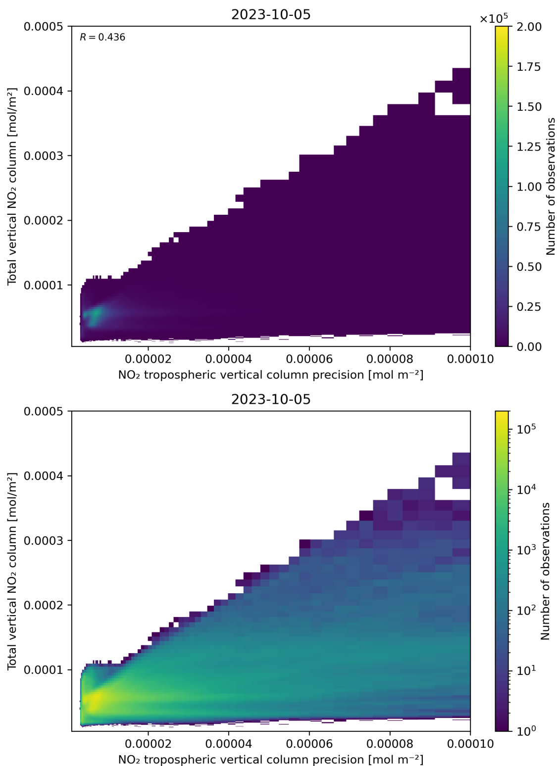
Figure 138: Scatter density plot of “NO 2 tropospheric vertical column precision” against “Total vertical NO 2 column” for 2023-10-04 to 2023-10-06.
