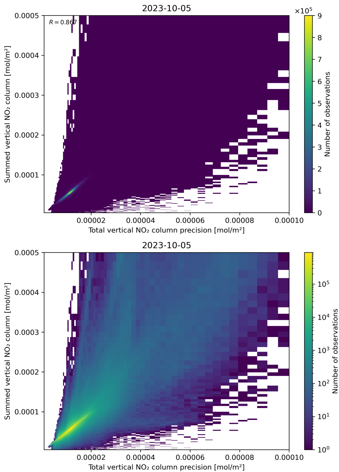
Figure 117: Scatter density plot of “Total vertical NO 2 column precision” against “Summed vertical NO 2 column” for 2023-10-04 to 2023-10-06.
