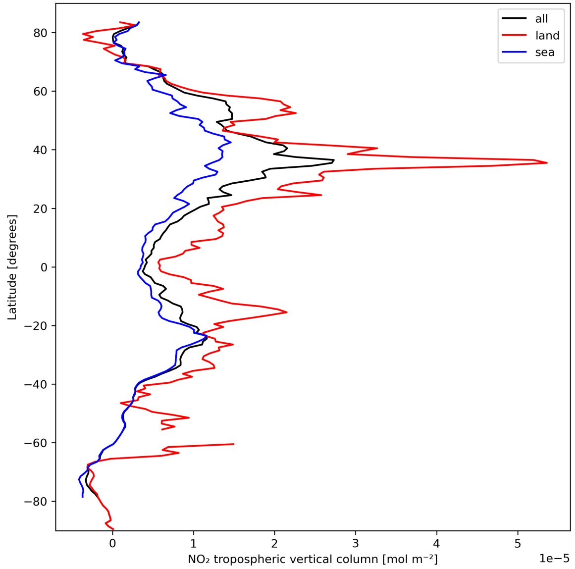
Figure 12: Zonal average of “NO 2 tropospheric vertical column” for 2023-10-04 to 2023-10-06.
