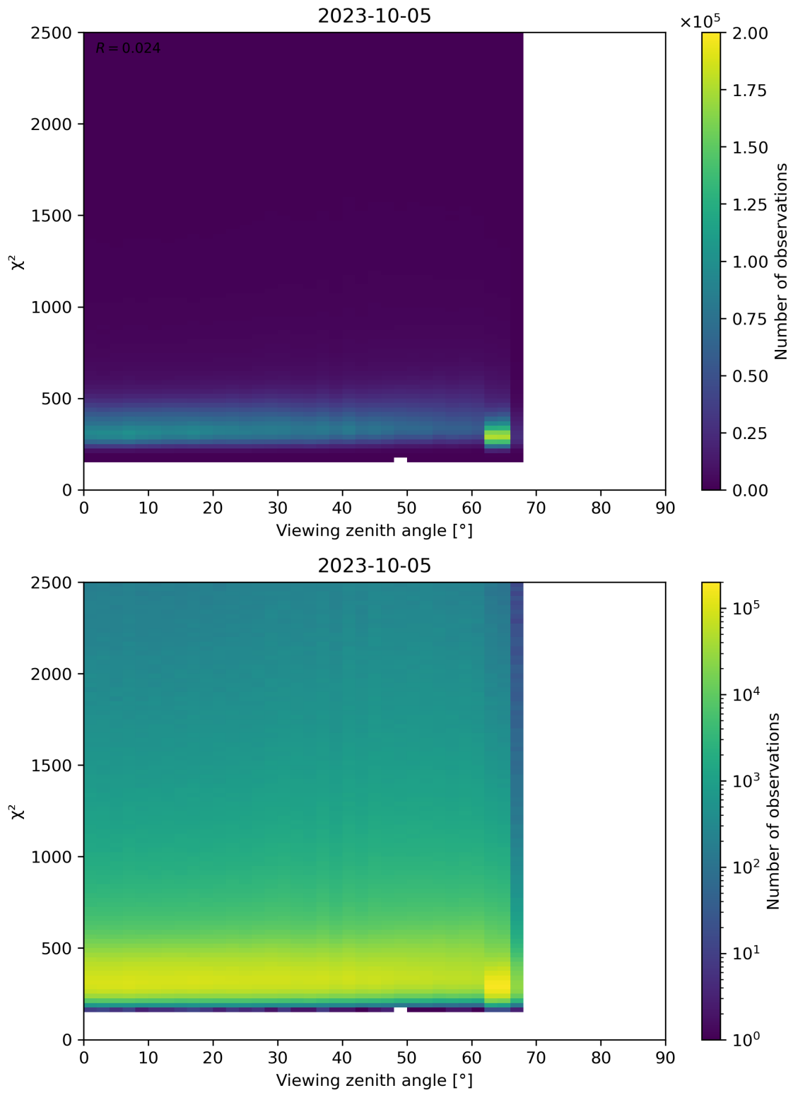
Figure 162: Scatter density plot of “Viewing zenith angle” against “ \chi^2 ” for 2023-10-04 to 2023-10-06.
