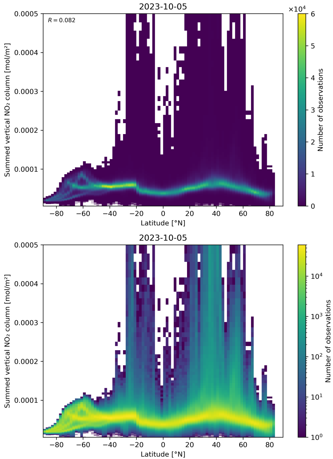
Figure 88: Scatter density plot of “Latitude” against “Summed vertical NO 2 column” for 2023-10-04 to 2023-10-06.
