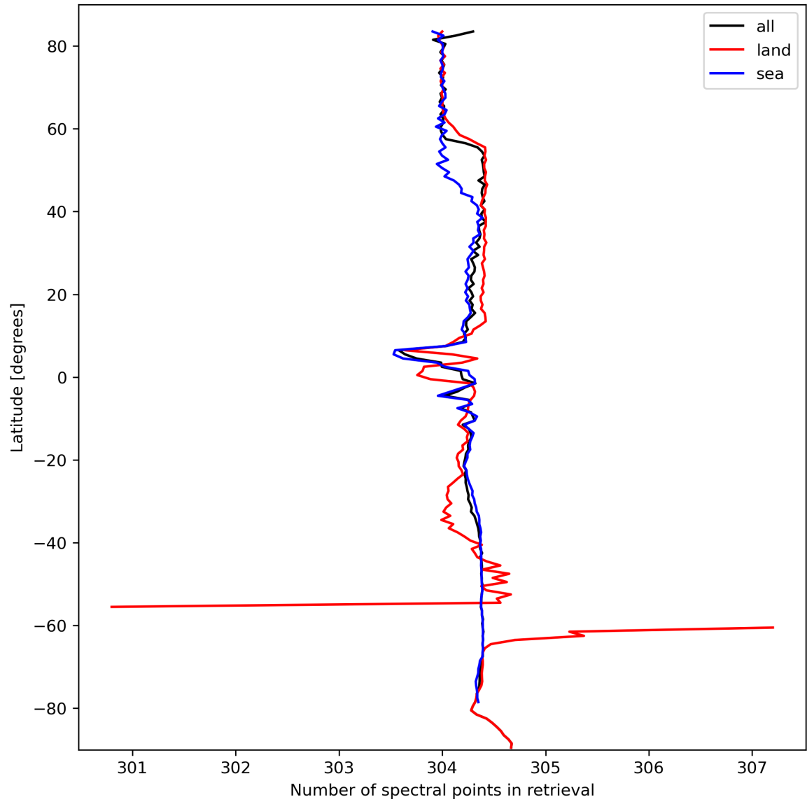
Figure 16: Zonal average of “Number of spectral points in retrieval” for 2023-10-04 to 2023-10-06.
