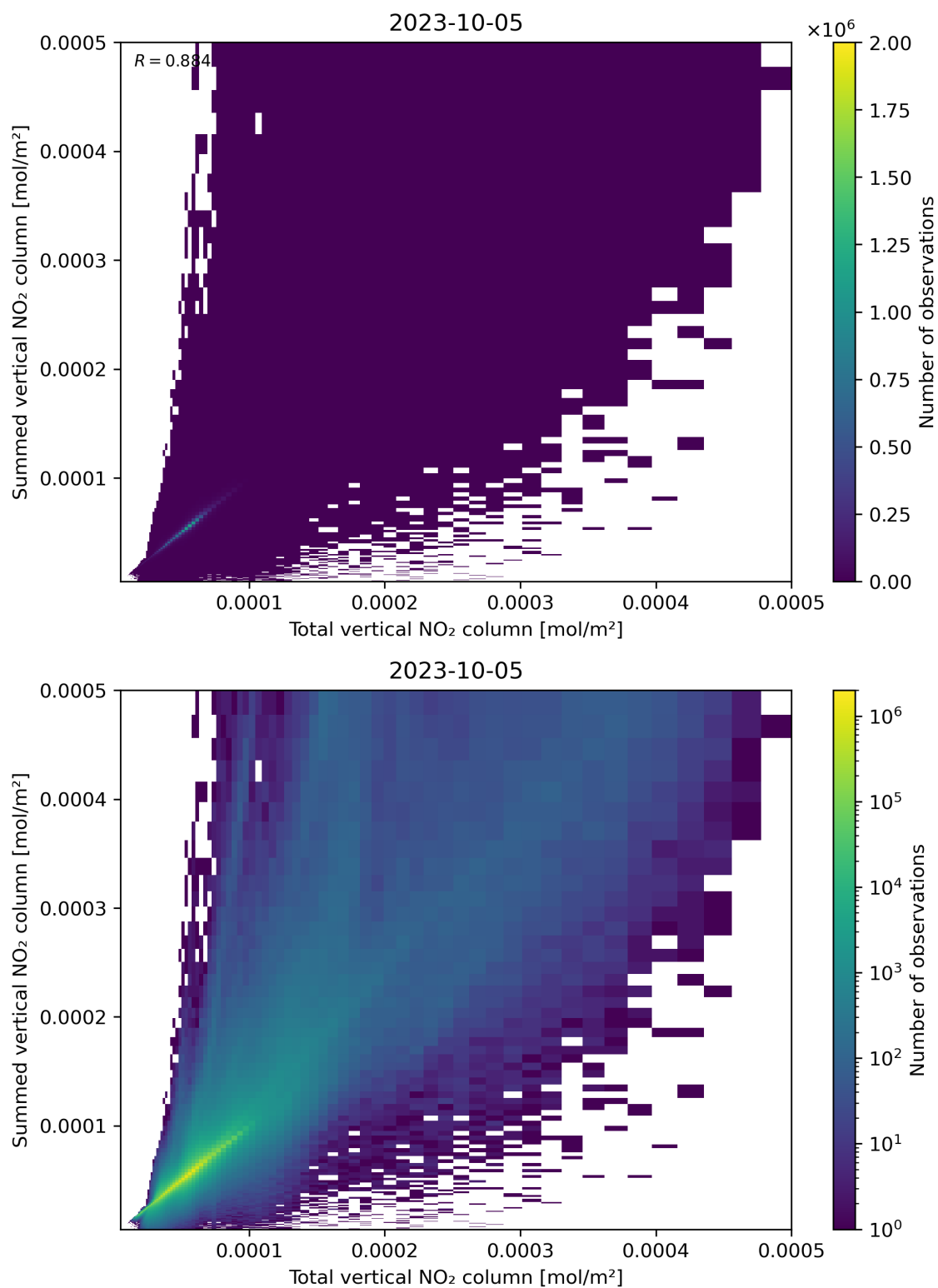
Figure 112: Scatter density plot of “Total vertical NO 2 column” against “Summed vertical NO 2 column” for 2023-10-04 to 2023-10-06.
