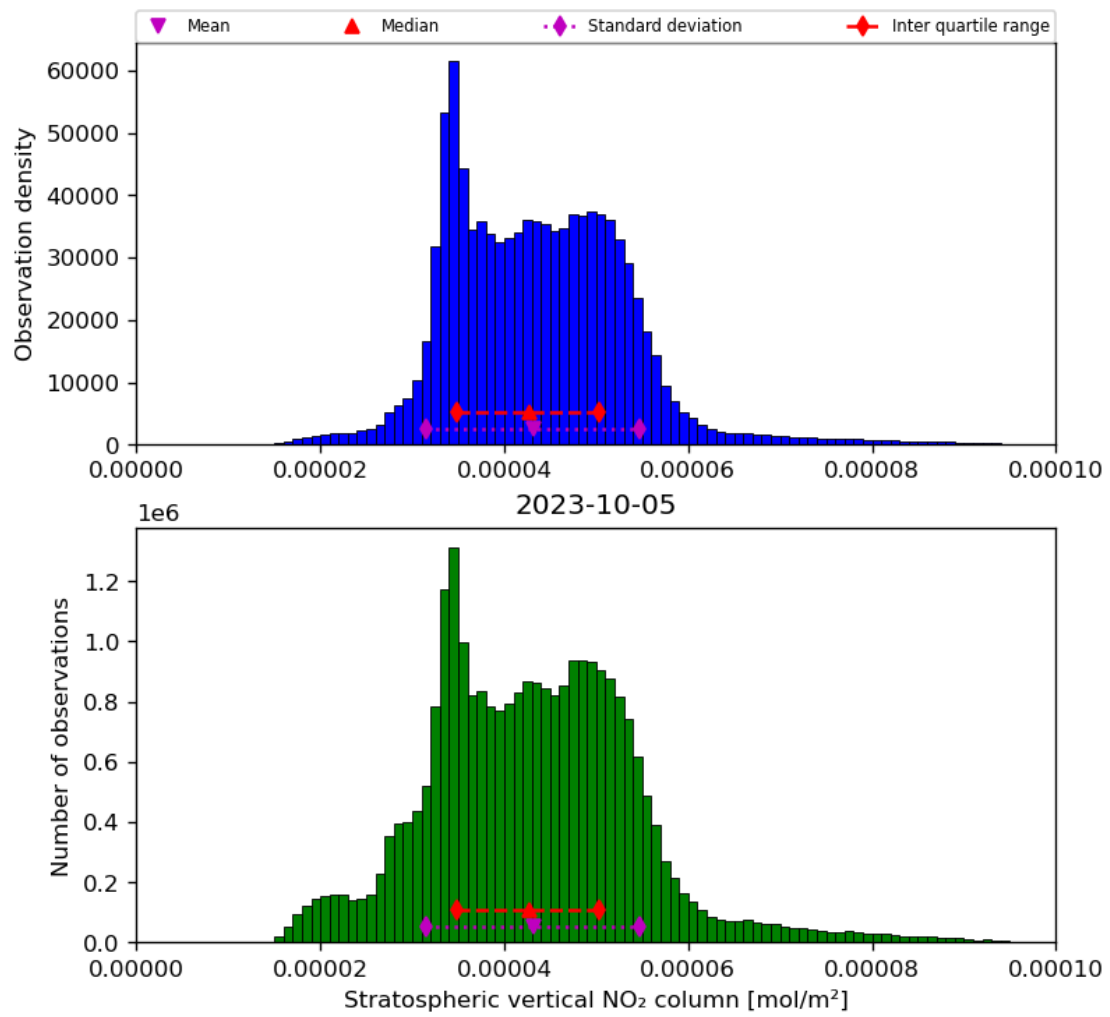
Figure 36: Histogram of “Stratospheric vertical NO 2 column” for 2023-10-04 to 2023-10-06
