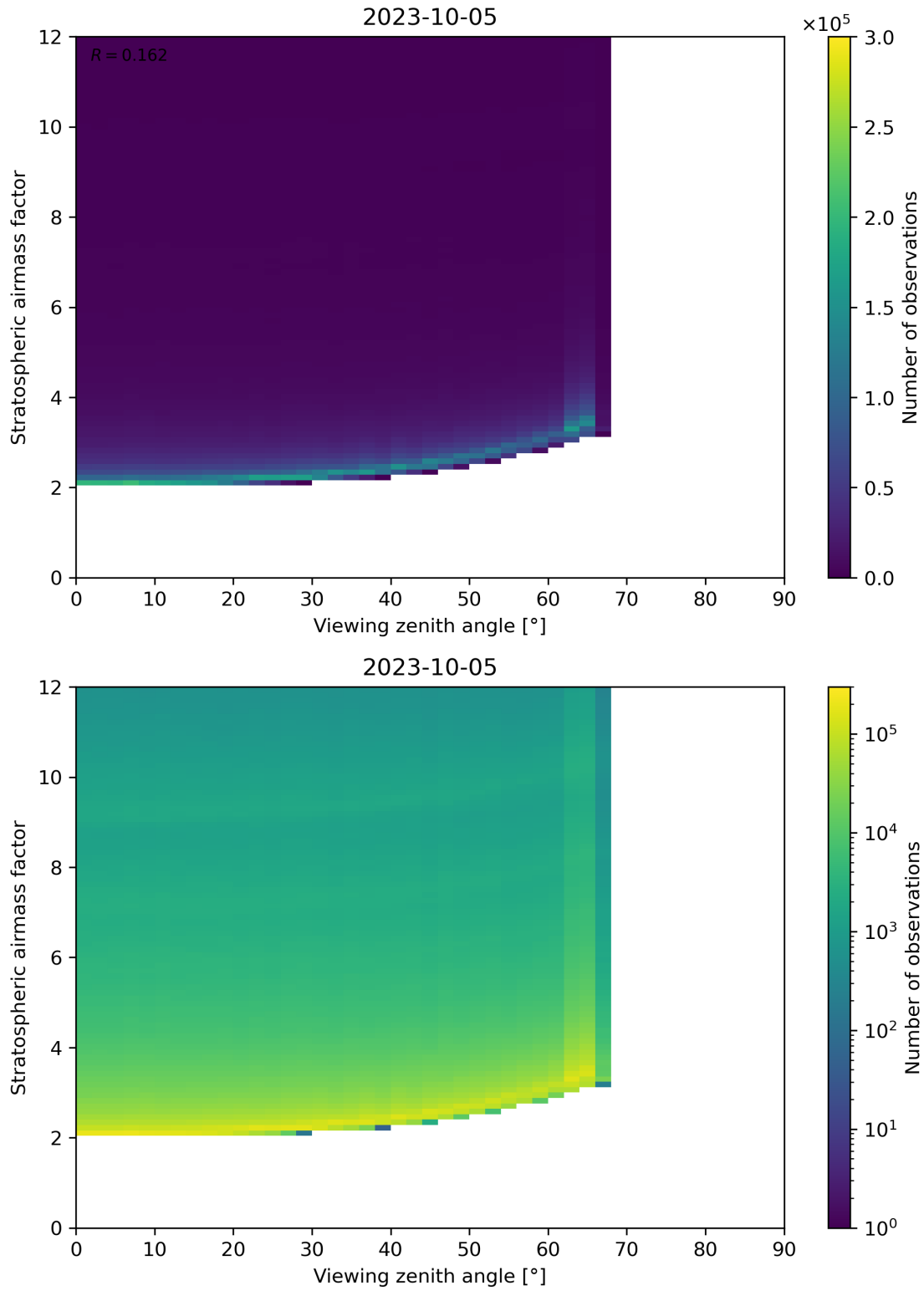
Figure 159: Scatter density plot of “Viewing zenith angle” against “Stratospheric airmass factor” for 2023-10-04 to 2023-10-06.
