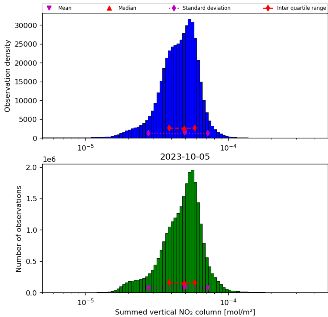
Figure 40: Histogram of “Summed vertical NO 2 column” for 2023-10-04 to 2023-10-06
