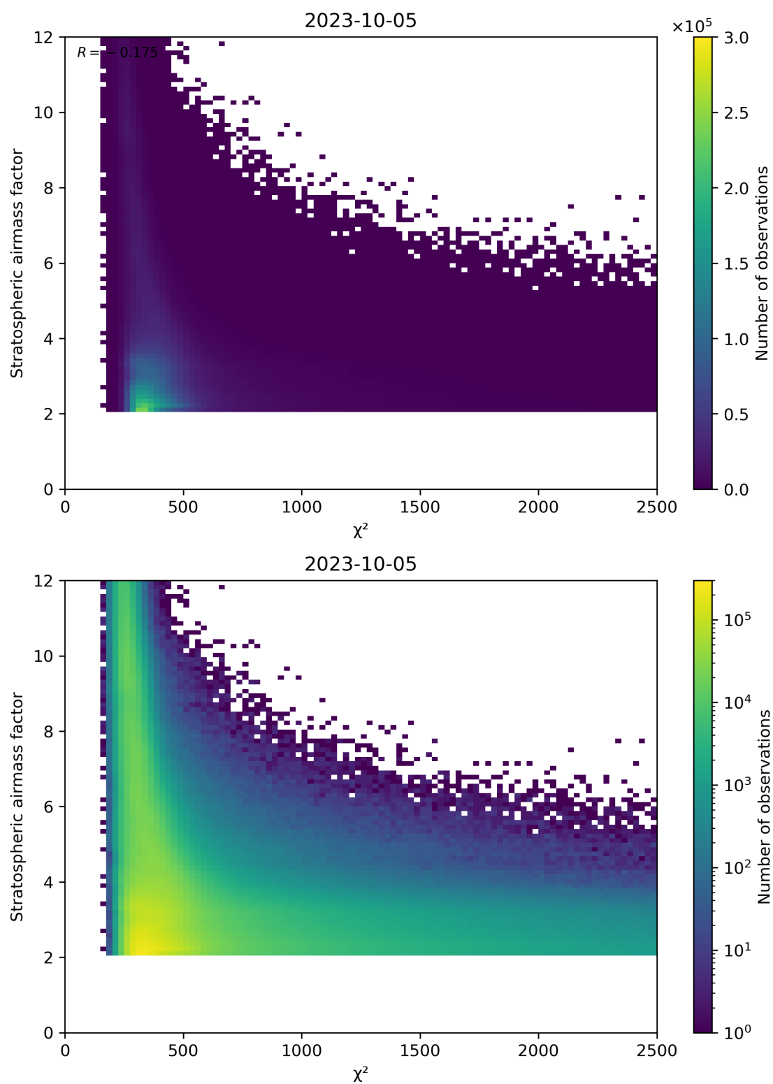
Figure 81: Scatter density plot of “ \chi^2 ” against “Stratospheric airmass factor” for 2023-10-04 to 2023-10-06.
