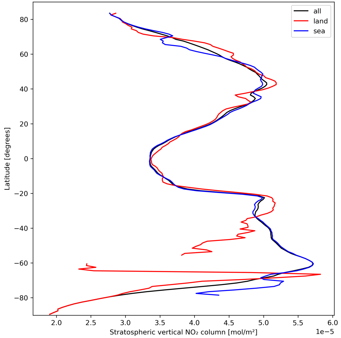
Figure 19: Zonal average of “Stratospheric vertical NO 2 column” for 2023-10-04 to 2023-10-06.
