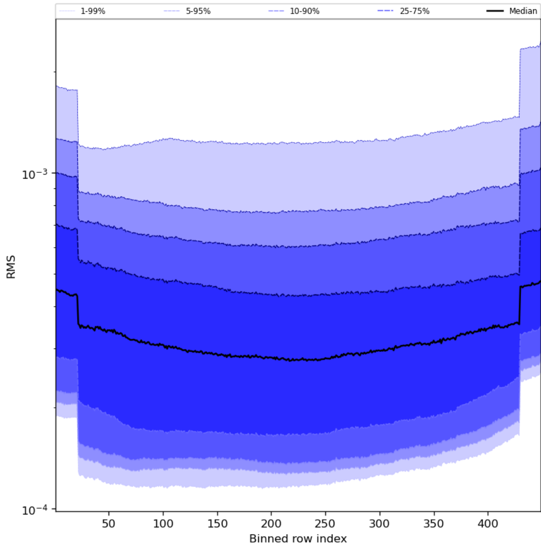
Figure 60: Along track statistics of “RMS” for 2023-10-04 to 2023-10-06
