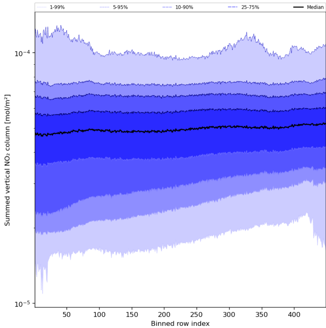
Figure 57: Along track statistics of “Summed vertical NO 2 column” for 2023-10-04 to 2023-10-06
