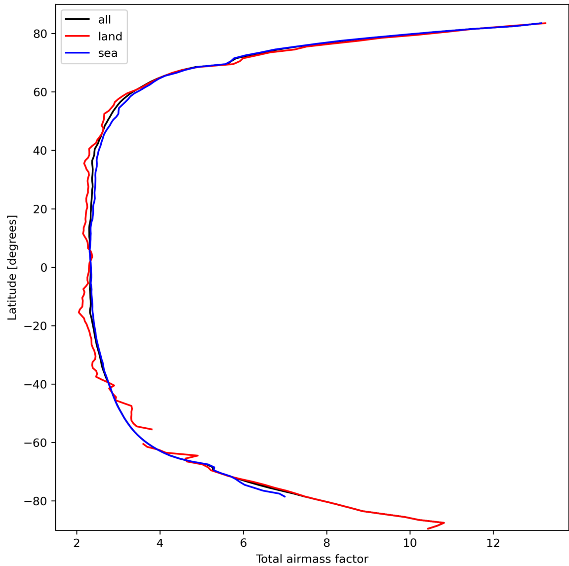
Figure 15: Zonal average of “Total airmass factor” for 2023-10-04 to 2023-10-06.
