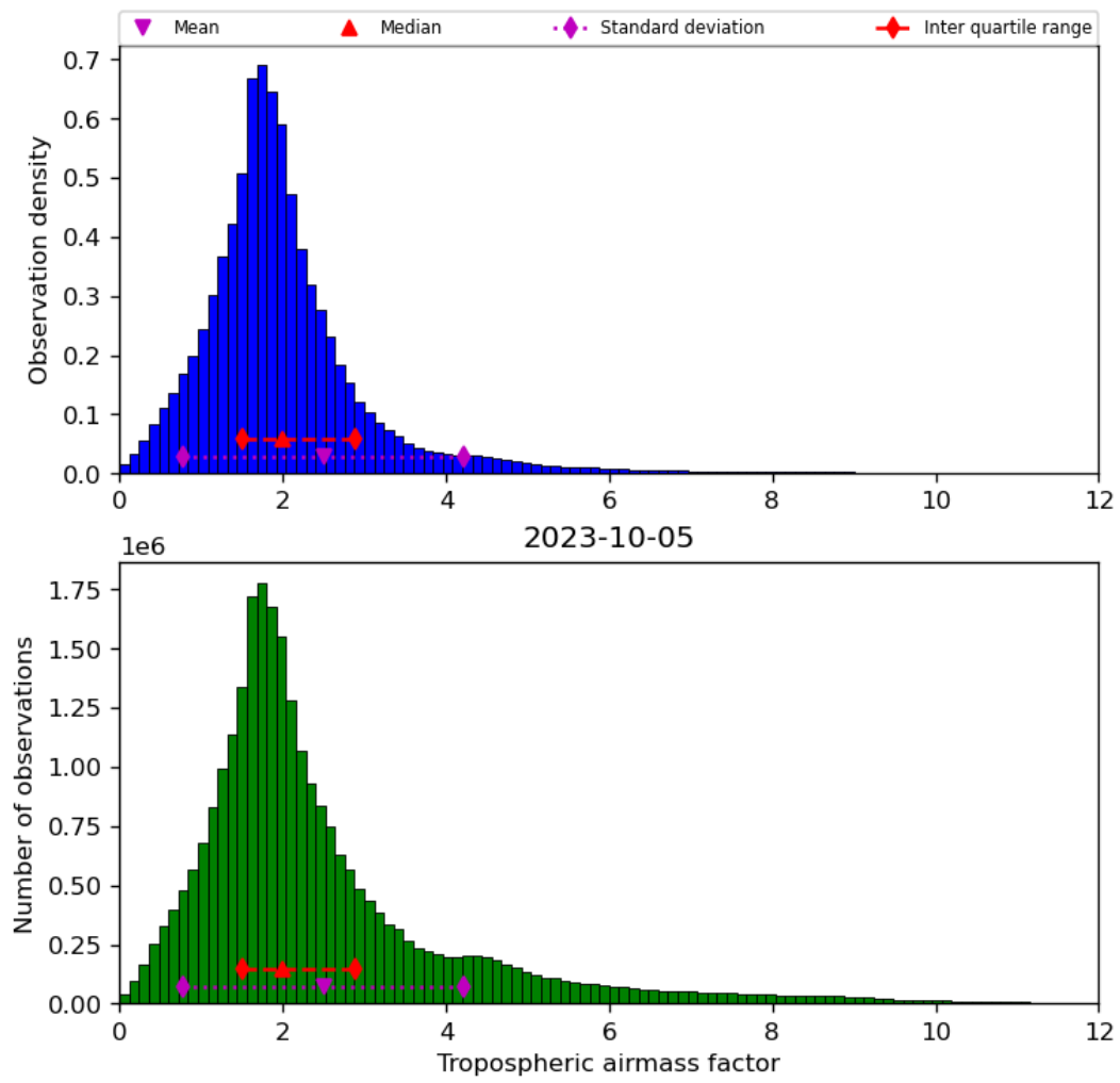
Figure 31: Histogram of “Tropospheric airmass factor” for 2023-10-04 to 2023-10-06
