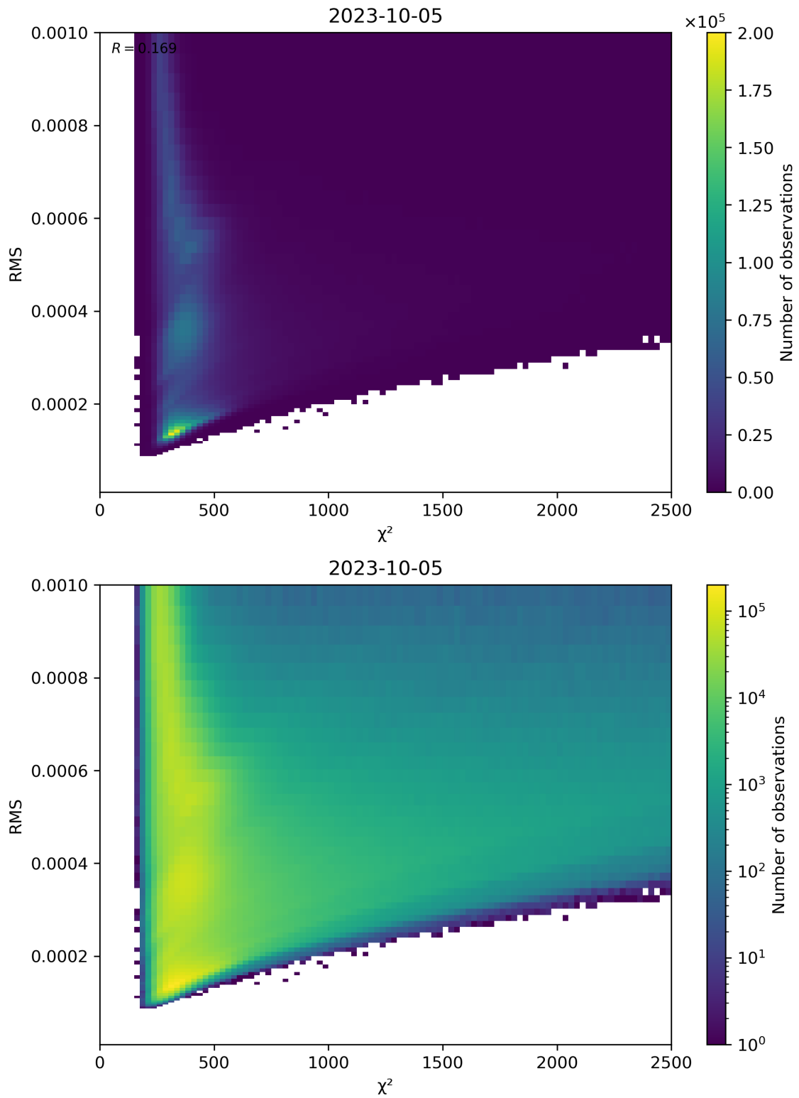
Figure 82: Scatter density plot of “ \chi^2 ” against “RMS” for 2023-10-04 to 2023-10-06.
