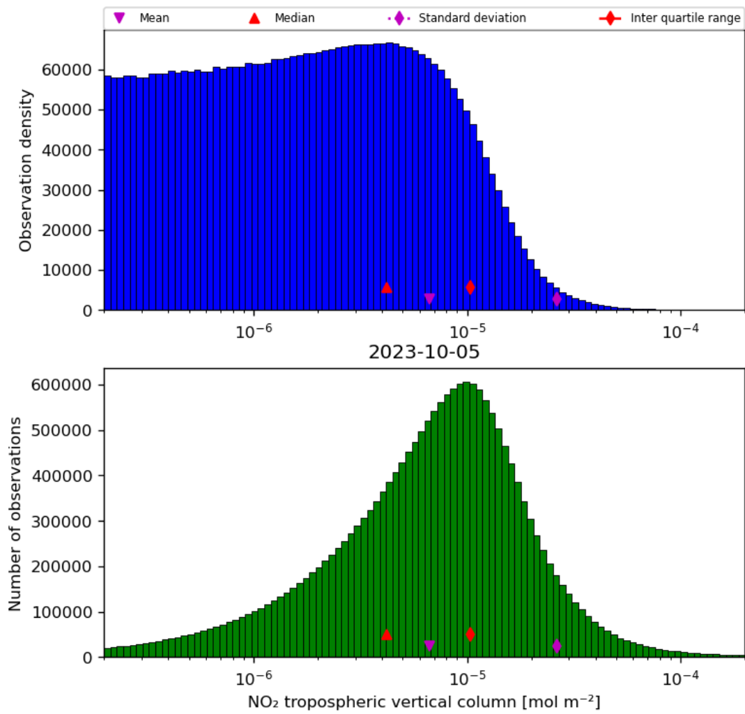
Figure 29: Histogram of “NO 2 tropospheric vertical column” for 2023-10-04 to 2023-10-06
