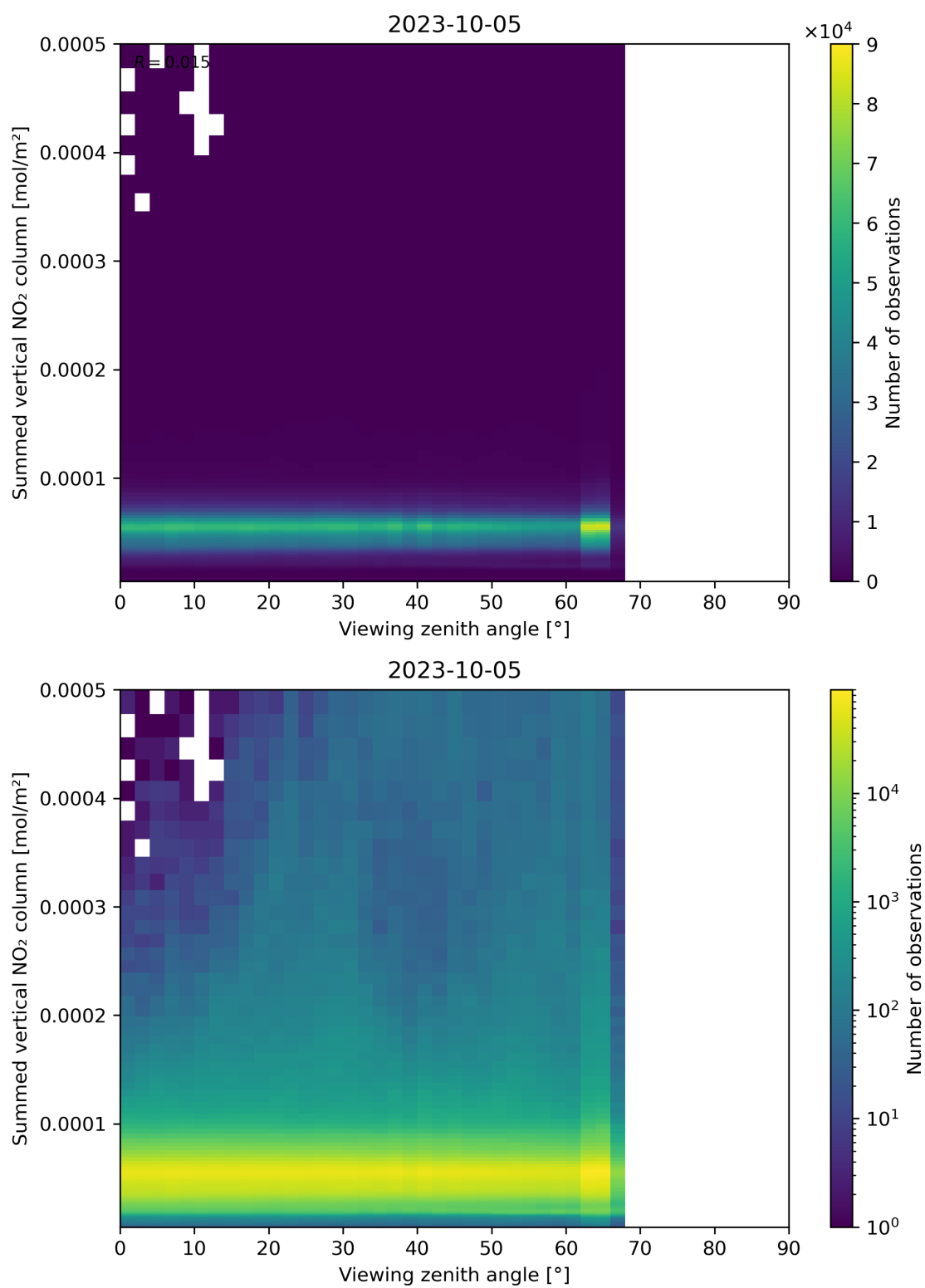
Figure 165: Scatter density plot of “Viewing zenith angle” against “Summed vertical NO 2 column” for 2023-10-04 to 2023-10-06.
