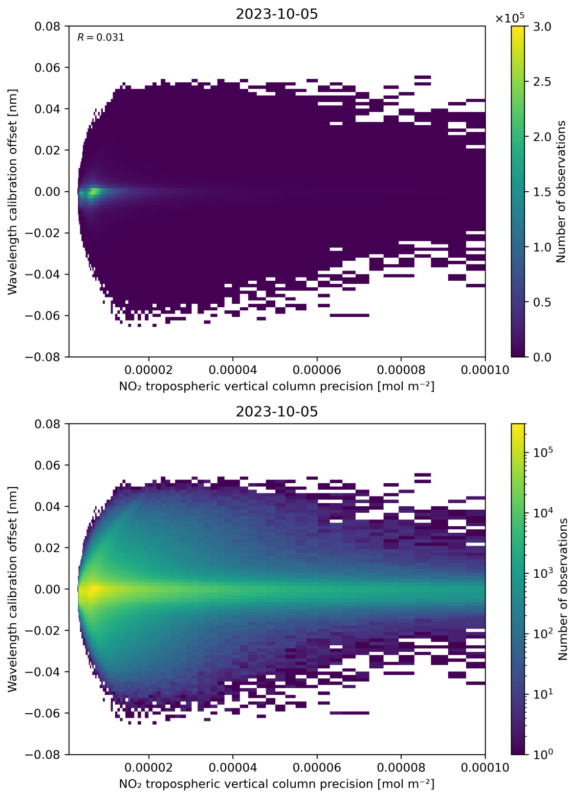
Figure 141: Scatter density plot of “NO 2 tropospheric vertical column precision” against “Wavelength calibration offset” for 2023-10-04 to 2023-10-06.
