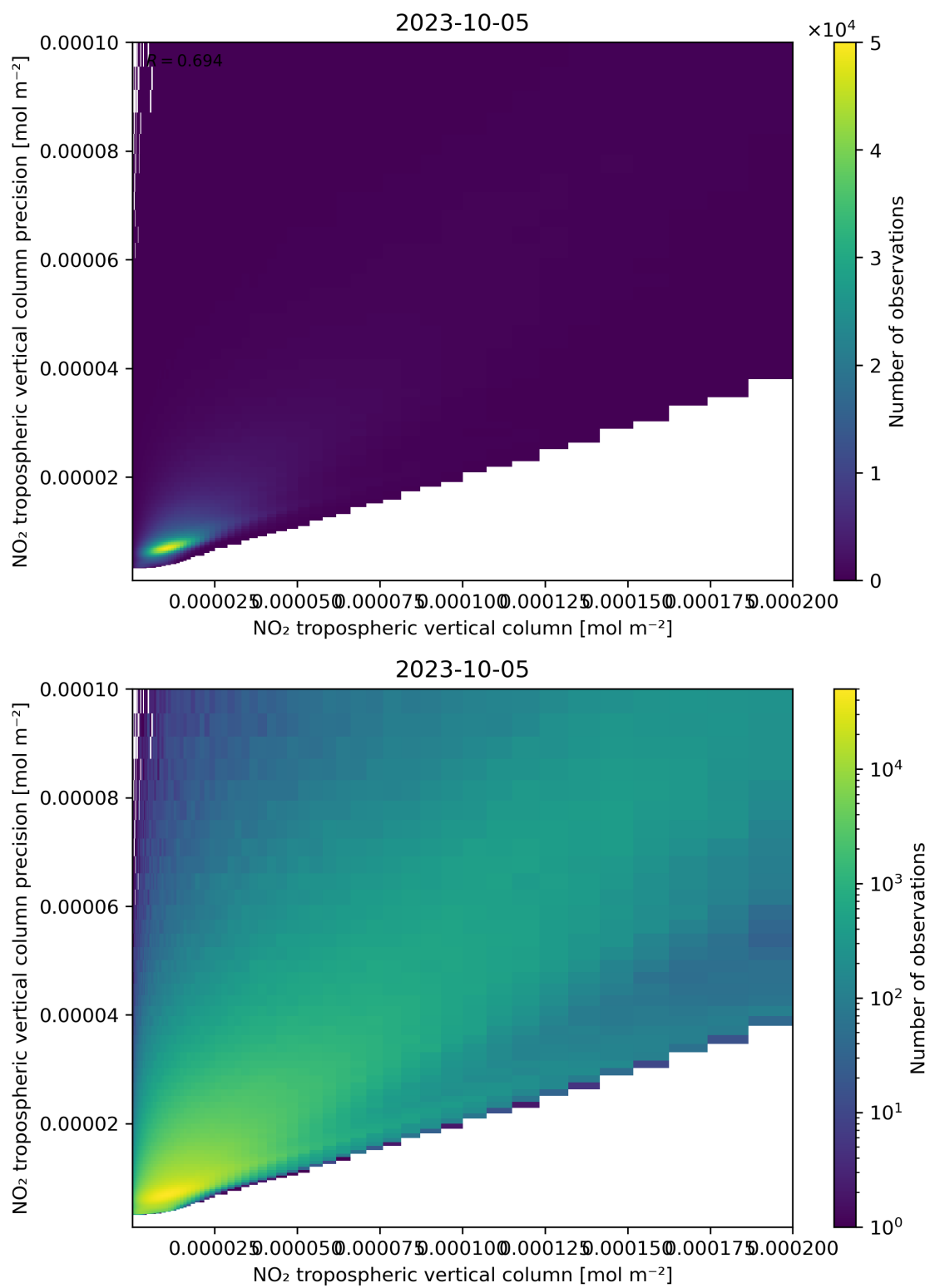
Figure 130: Scatter density plot of “NO 2 tropospheric vertical column” against “NO 2 tropospheric vertical column precision” for 2023-10-04 to 2023-10-06.
