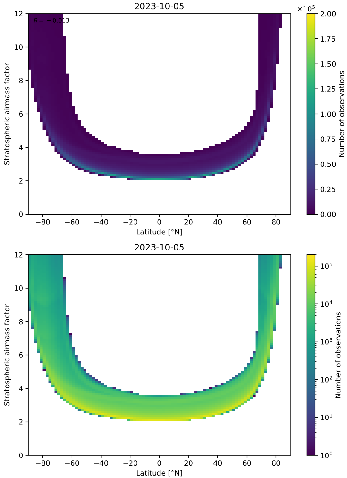
Figure 83: Scatter density plot of “Latitude” against “Stratospheric air mass factor” for 2023-10-04 to 2023-10-06.
