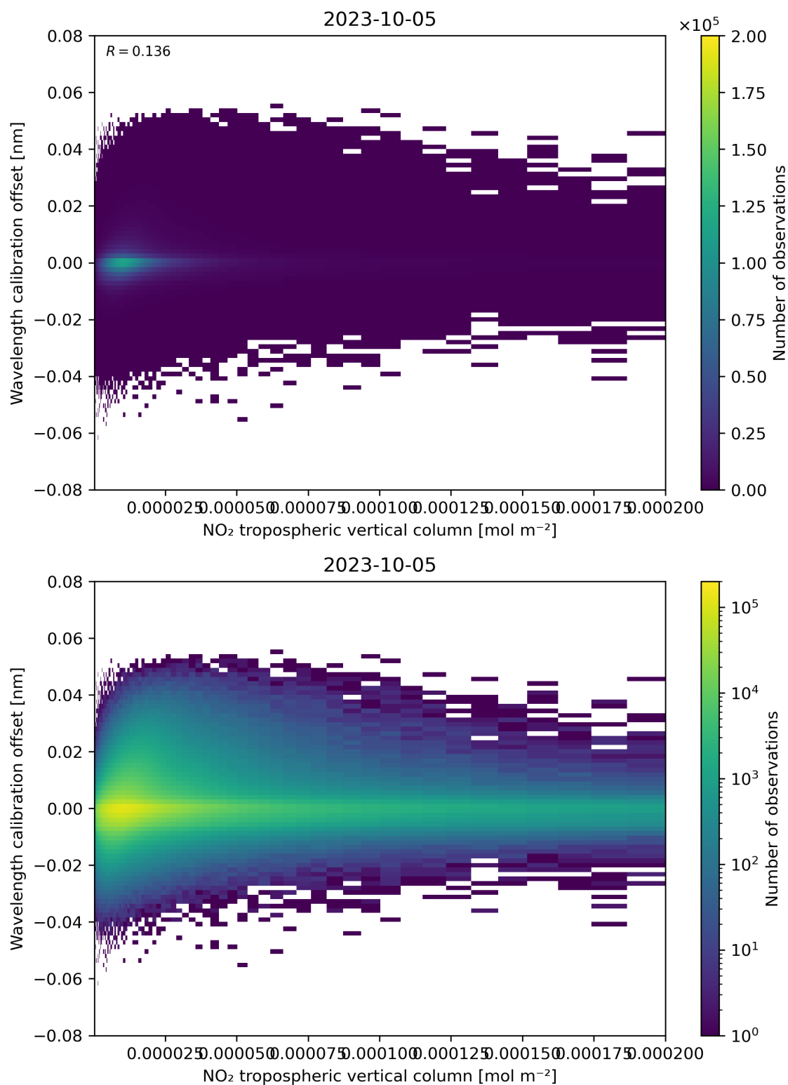
Figure 143: Scatter density plot of “NO 2 tropospheric vertical column” against “Wavelength calibration offset” for 2023-10-04 to 2023-10-06.
