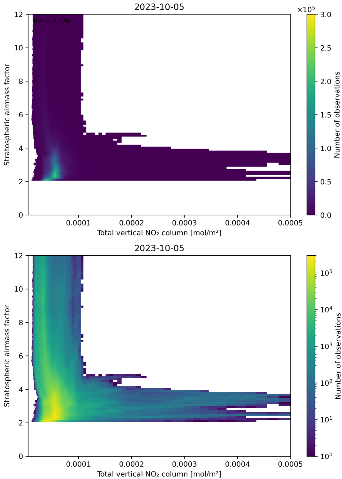
Figure 110: Scatter density plot of “Total vertical NO 2 column” against “Stratospheric airmass factor” for 2023-10-04 to 2023-10-06.
