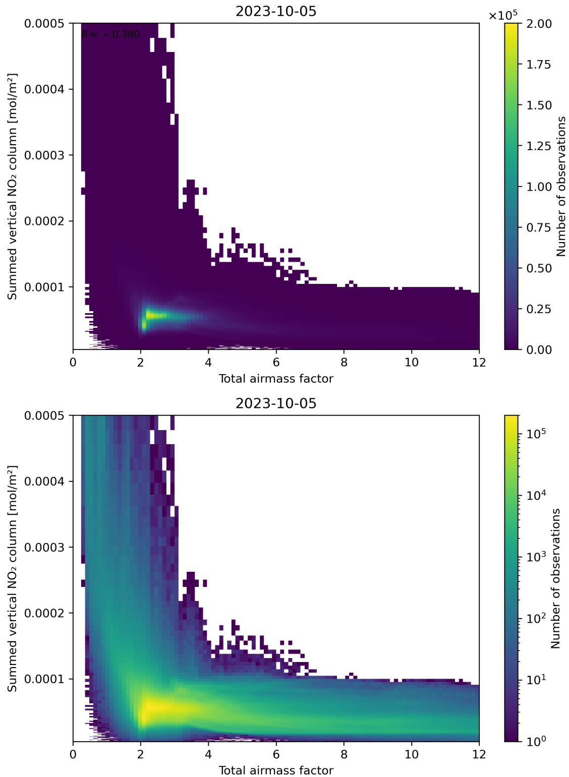
Figure 65: Scatter density plot of “Total airmass factor” against “Summed vertical NO 2 column” for 2023-10-04 to 2023-10-06.
