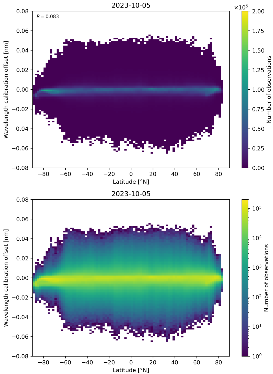
Figure 95: Scatter density plot of “Latitude” against “Wavelength calibration offset” for 2023-10-04 to 2023-10-06.
