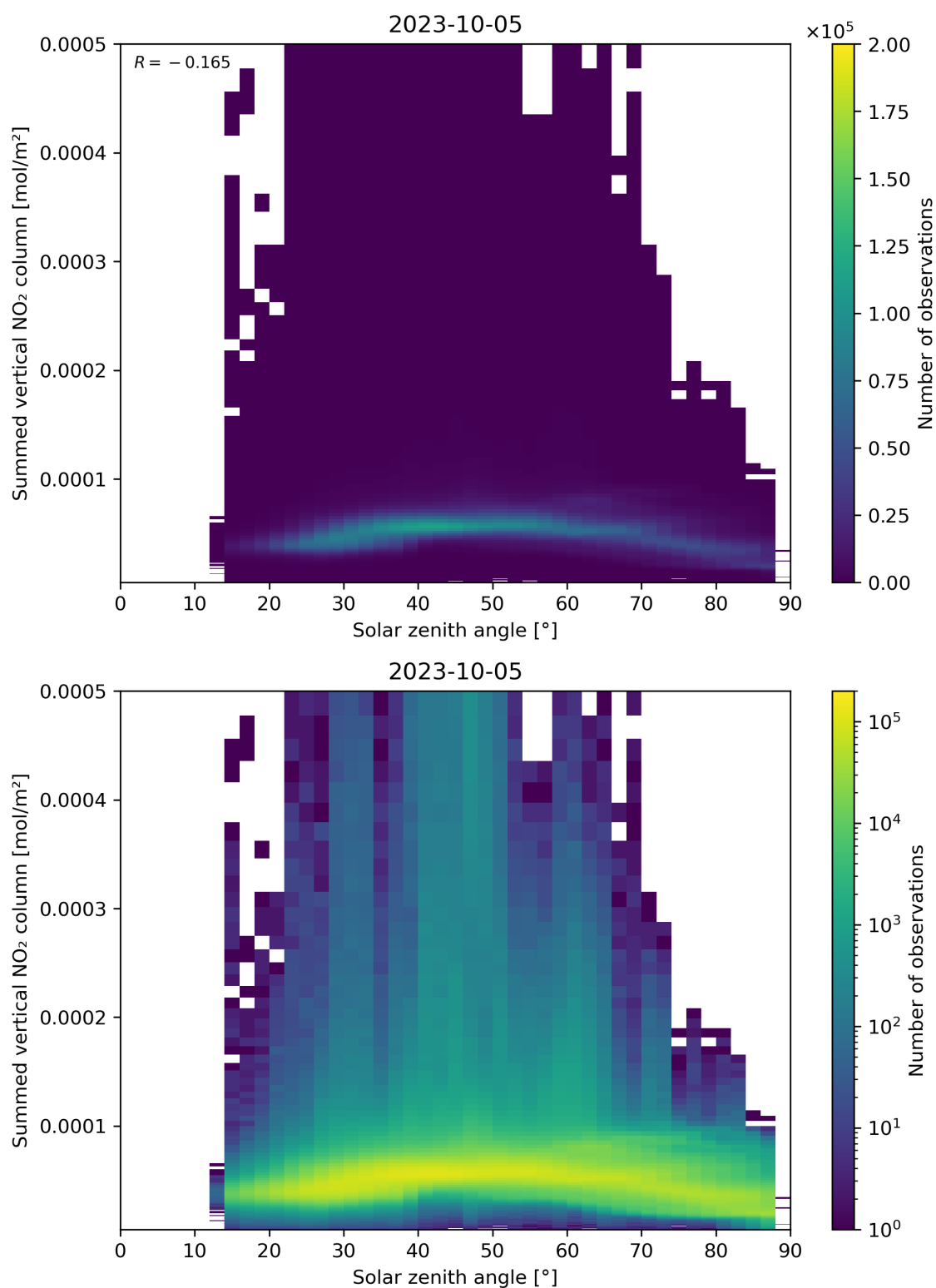
Figure 151: Scatter density plot of “Solar zenith angle” against “Summed vertical NO 2 column” for 2023-10-04 to 2023-10-06.
