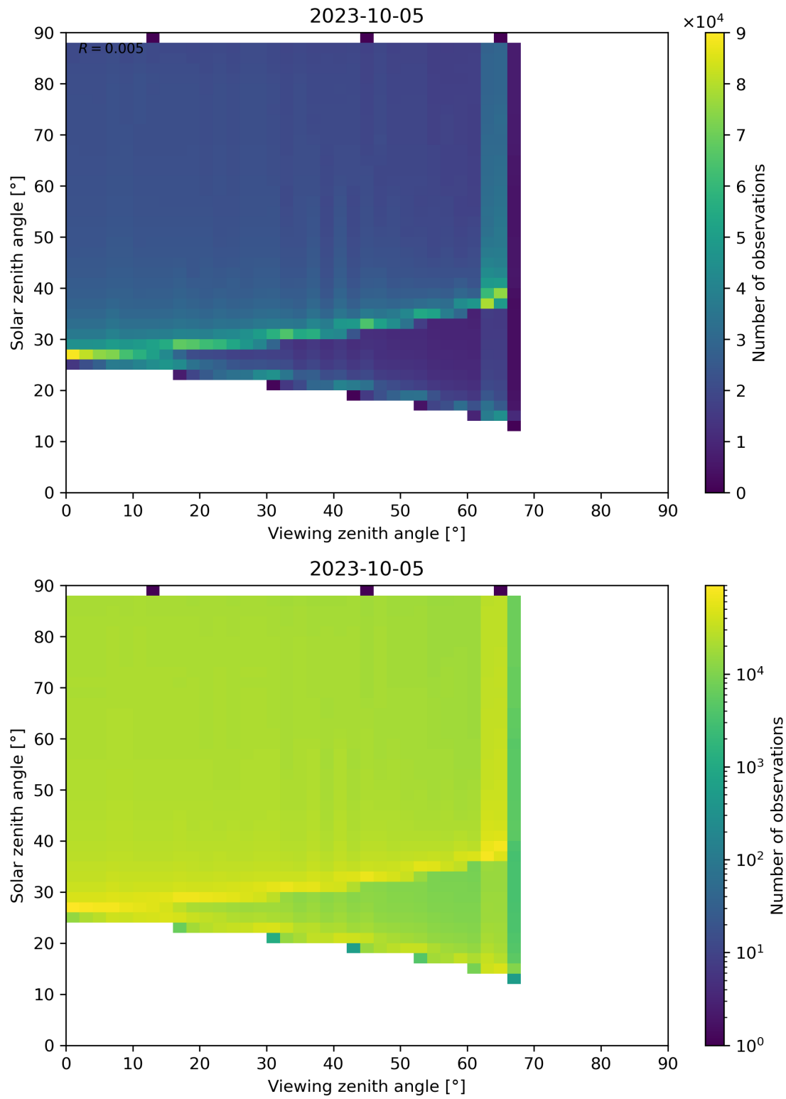
Figure 172: Scatter density plot of “Viewing zenith angle” against “Solar zenith angle” for 2023-10-04 to 2023-10-06.
