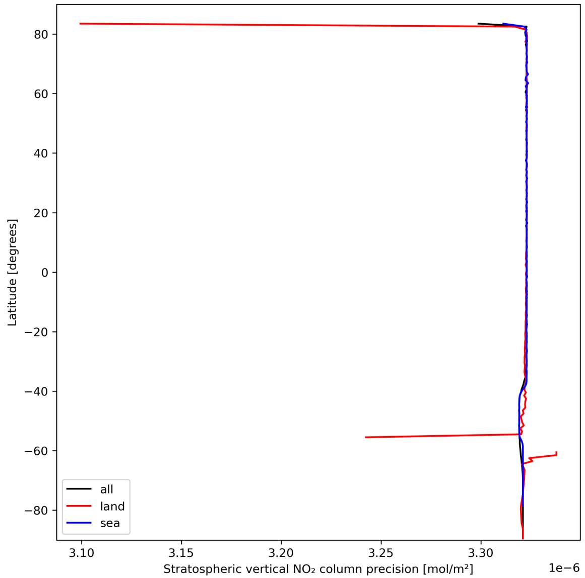
Figure 20: Zonal average of “Stratospheric vertical NO 2 column precision” for 2023-10-04 to 2023-10-06.
