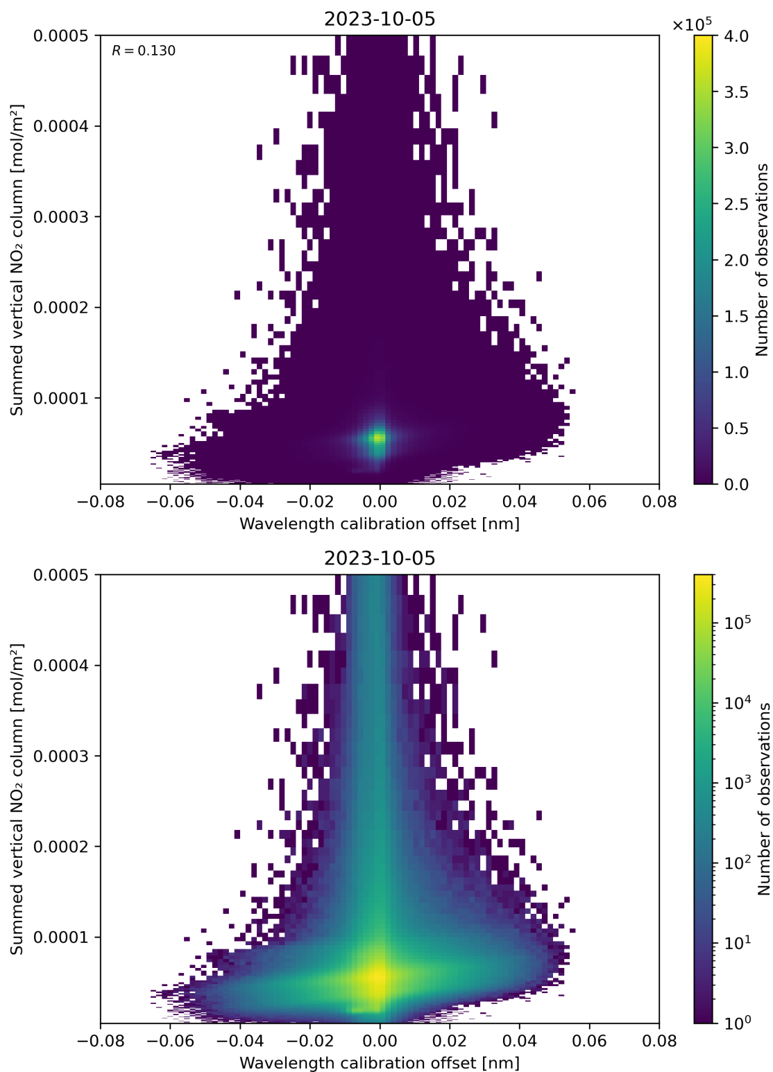
Figure 177: Scatter density plot of “Wavelength calibration offset” against “Summed vertical NO 2 column” for 2023-10-04 to 2023-10-06.
