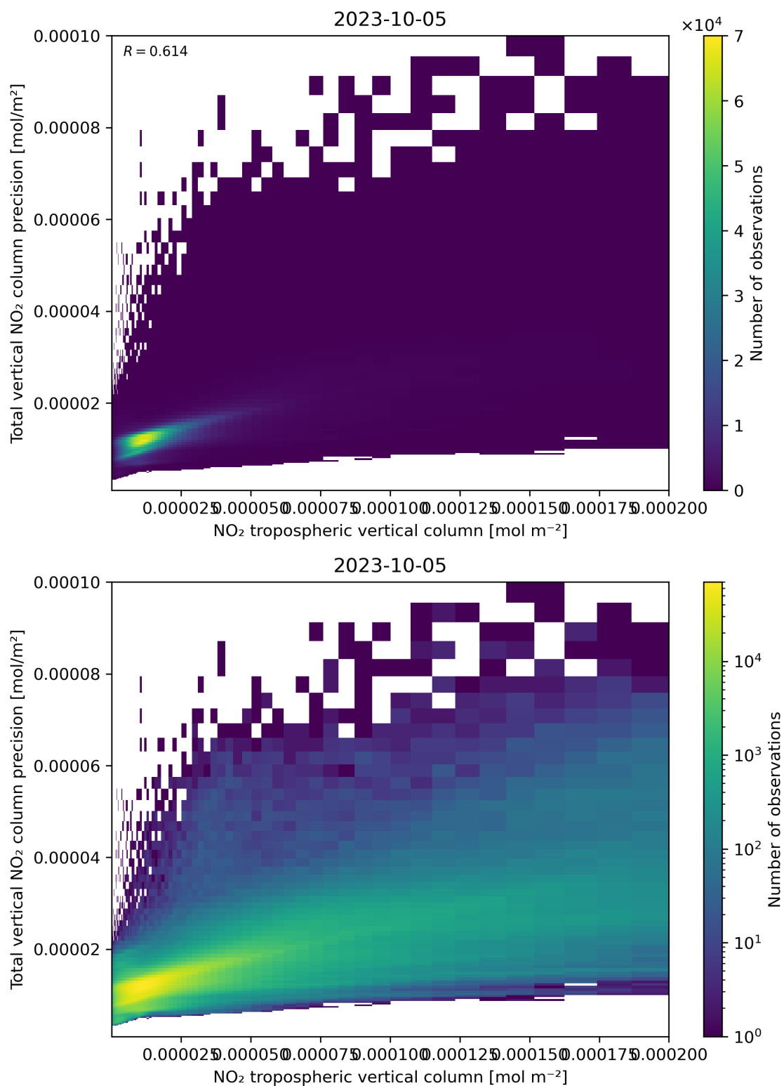
Figure 129: Scatter density plot of “NO 2 tropospheric vertical column” against “Total vertical NO 2 column precision” for 2023-10-04 to 2023-10-06.
