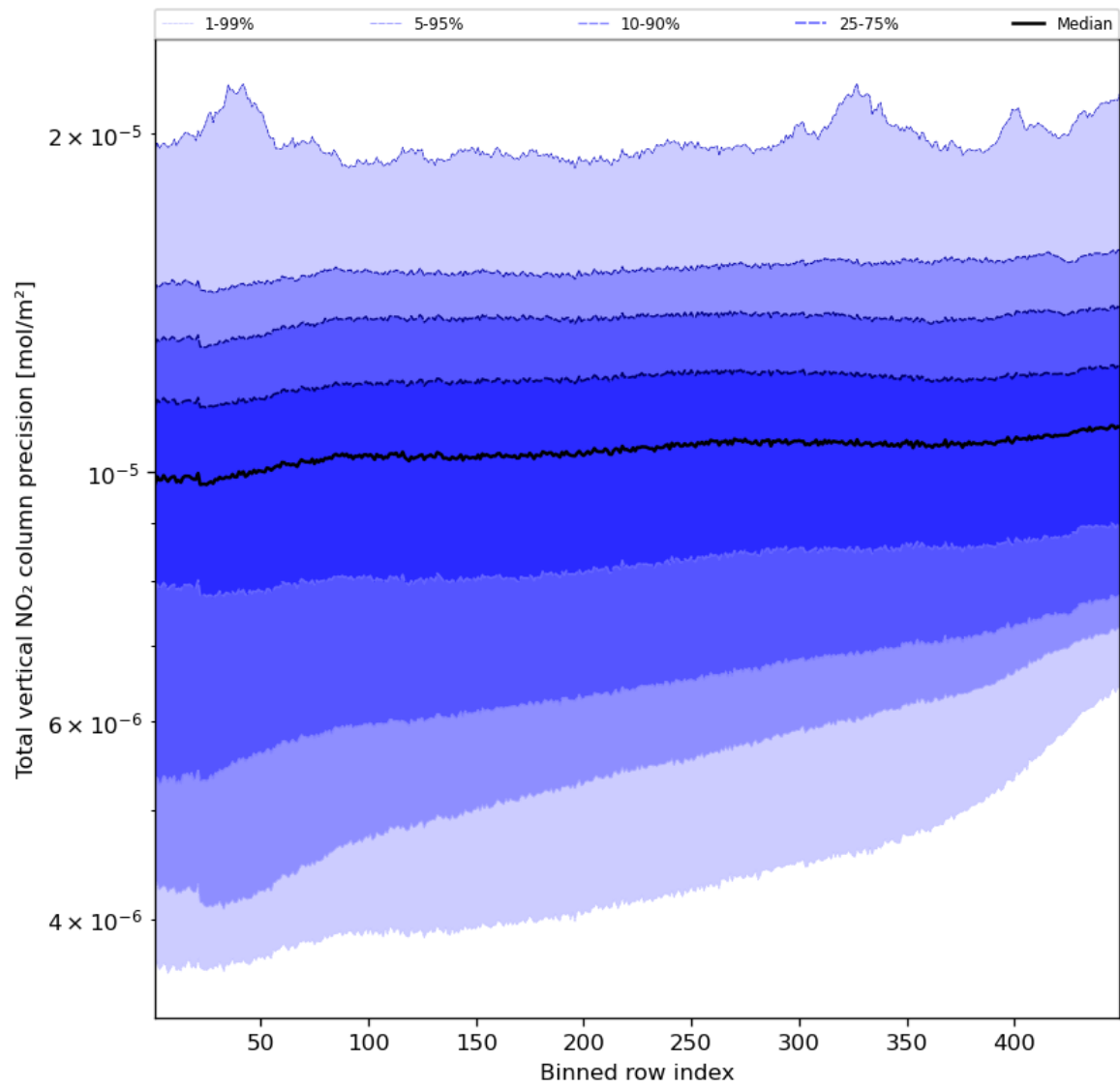
Figure 56: Along track statistics of “Total vertical NO 2 column precision” for 2023-10-04 to 2023-10-06
