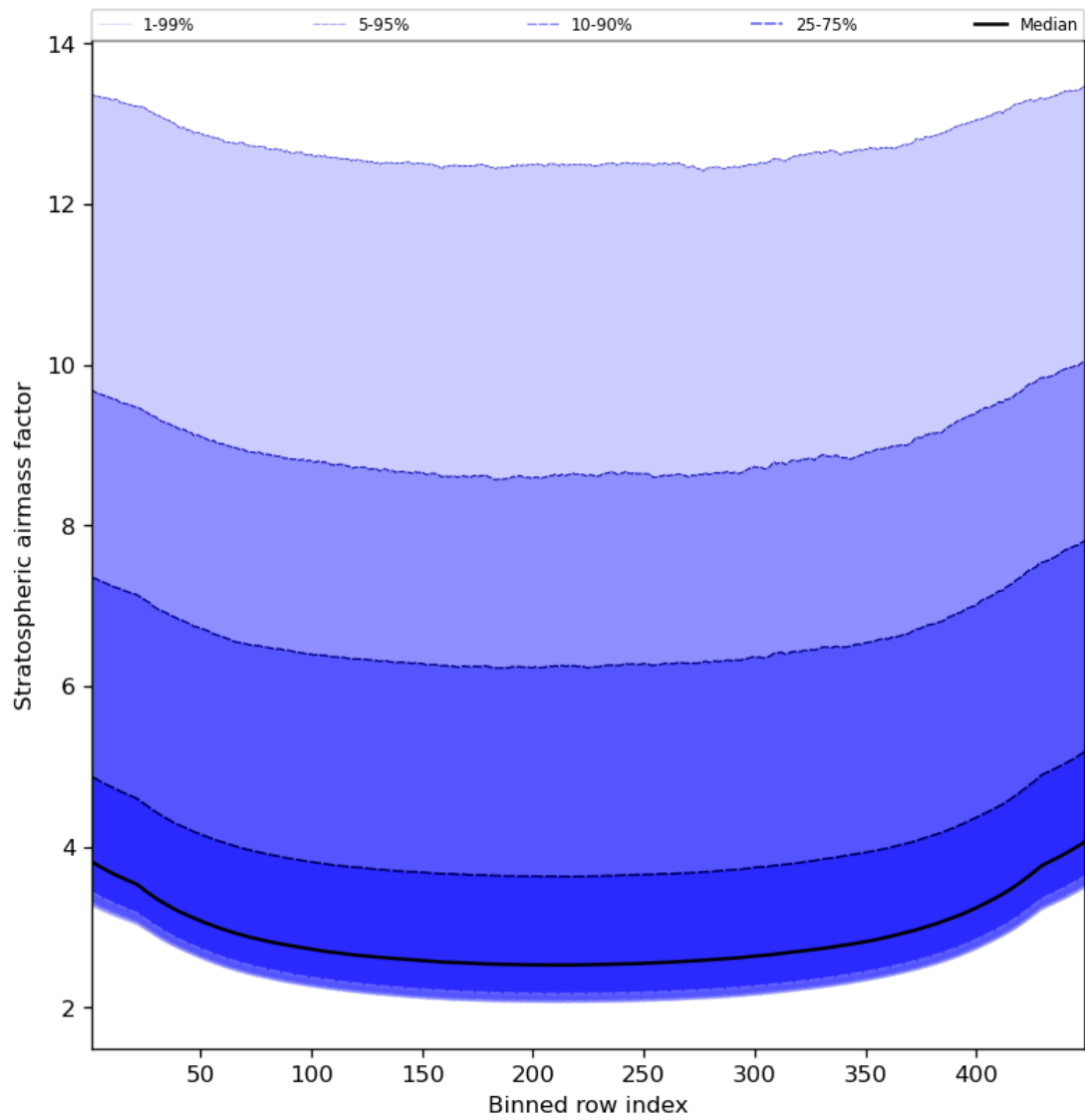
Figure 61: Along track statistics of “Stratospheric air mass factor” for 2023-10-04 to 2023-10-06
