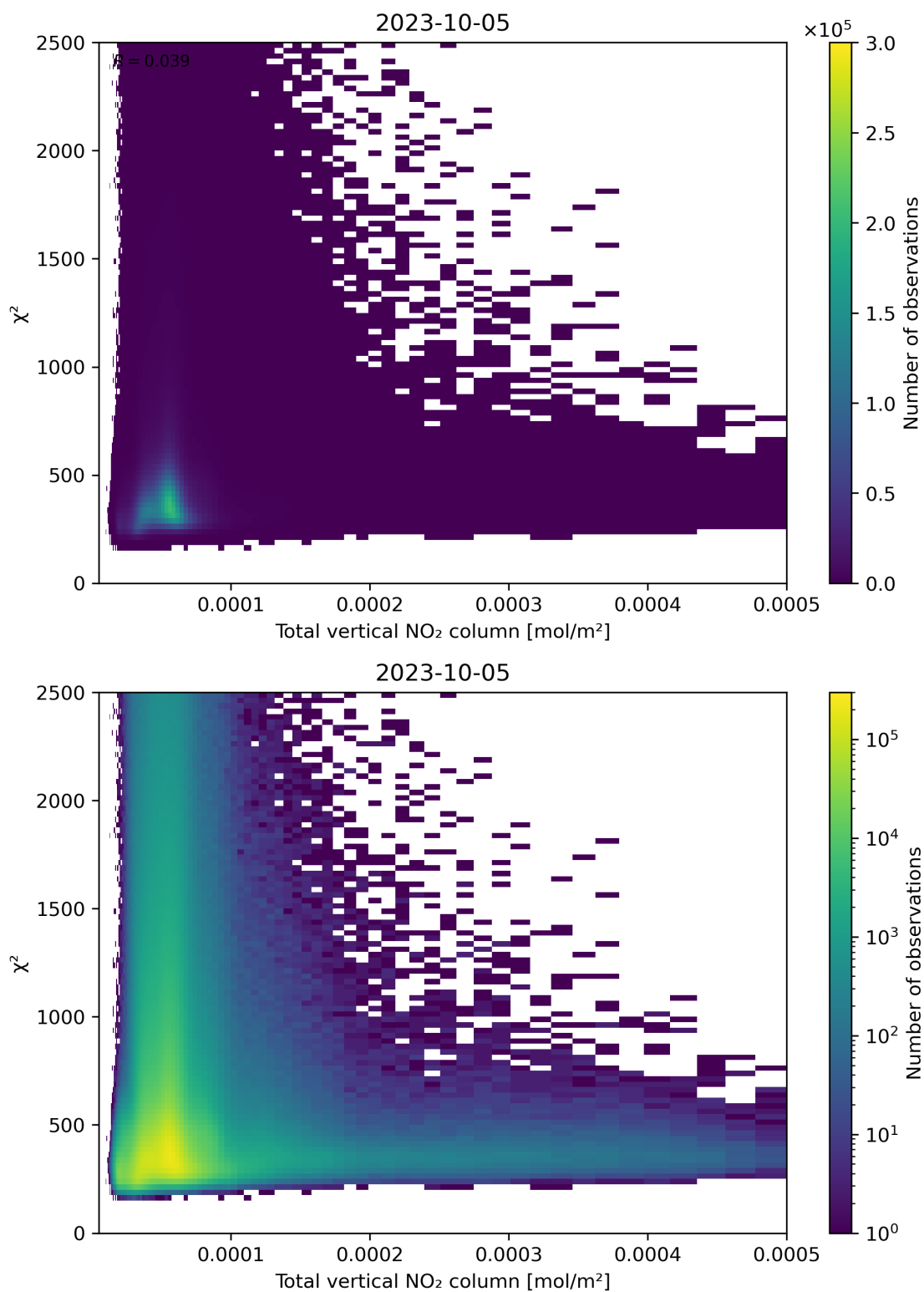
Figure 111: Scatter density plot of “Total vertical NO 2 column” against “ \chi^2 ” for 2023-10-04 to 2023-10-06.
