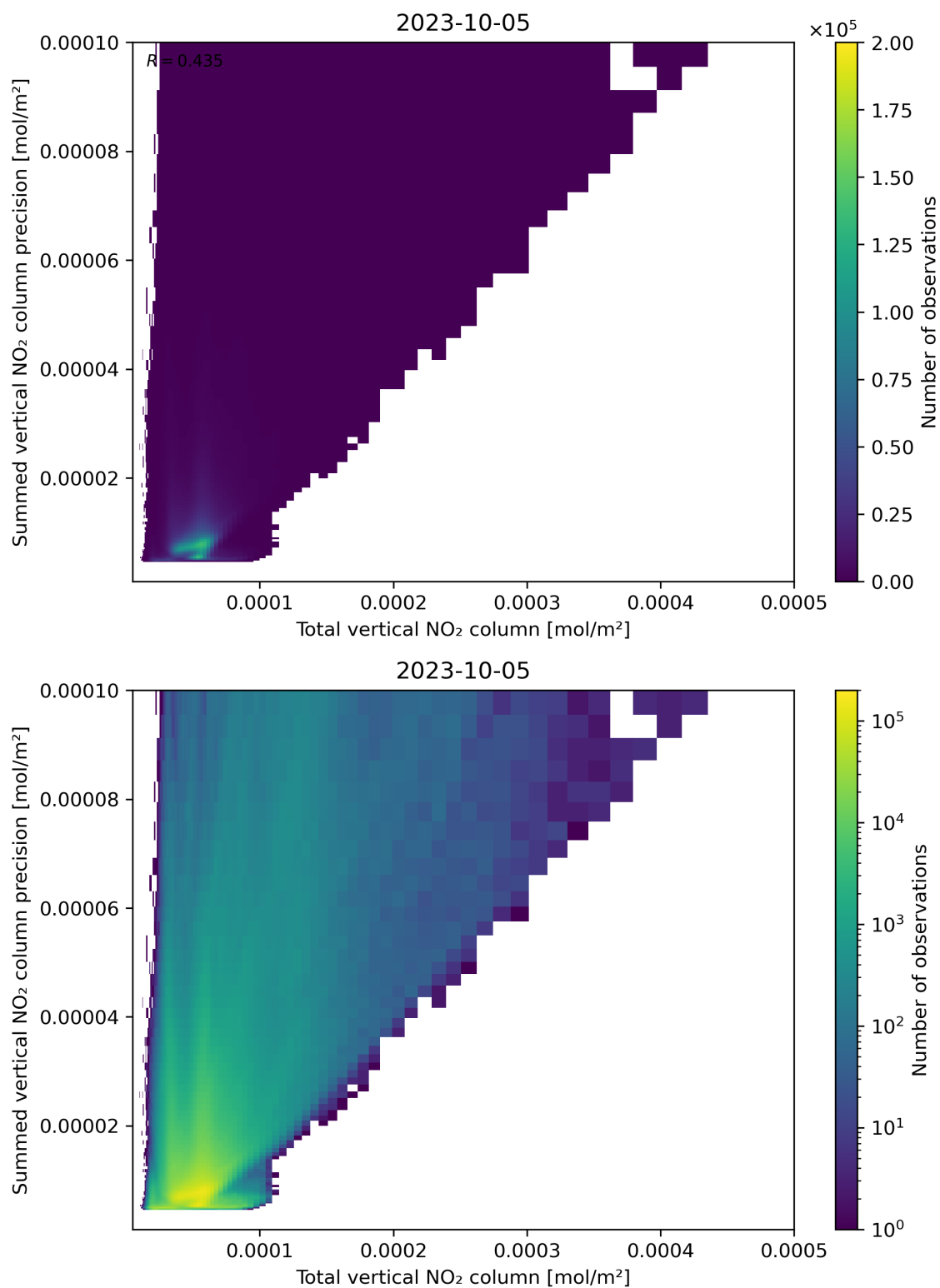
Figure 113: Scatter density plot of “Total vertical NO 2 column” against “Summed vertical NO 2 column precision” for 2023-10-04 to 2023-10-06.
