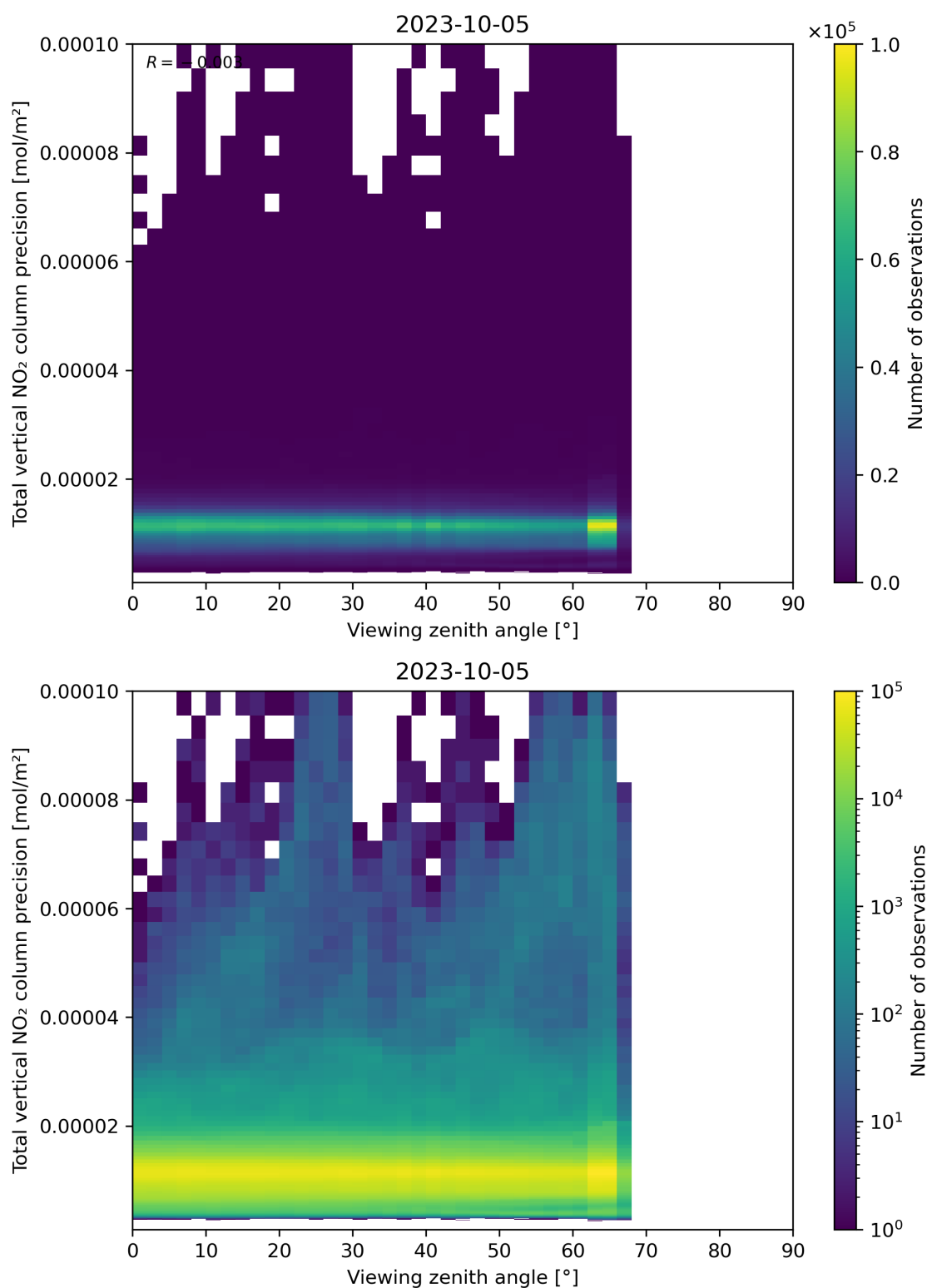
Figure 168: Scatter density plot of “Viewing zenith angle” against “Total vertical NO 2 column precision” for 2023-10-04 to 2023-10-06.
