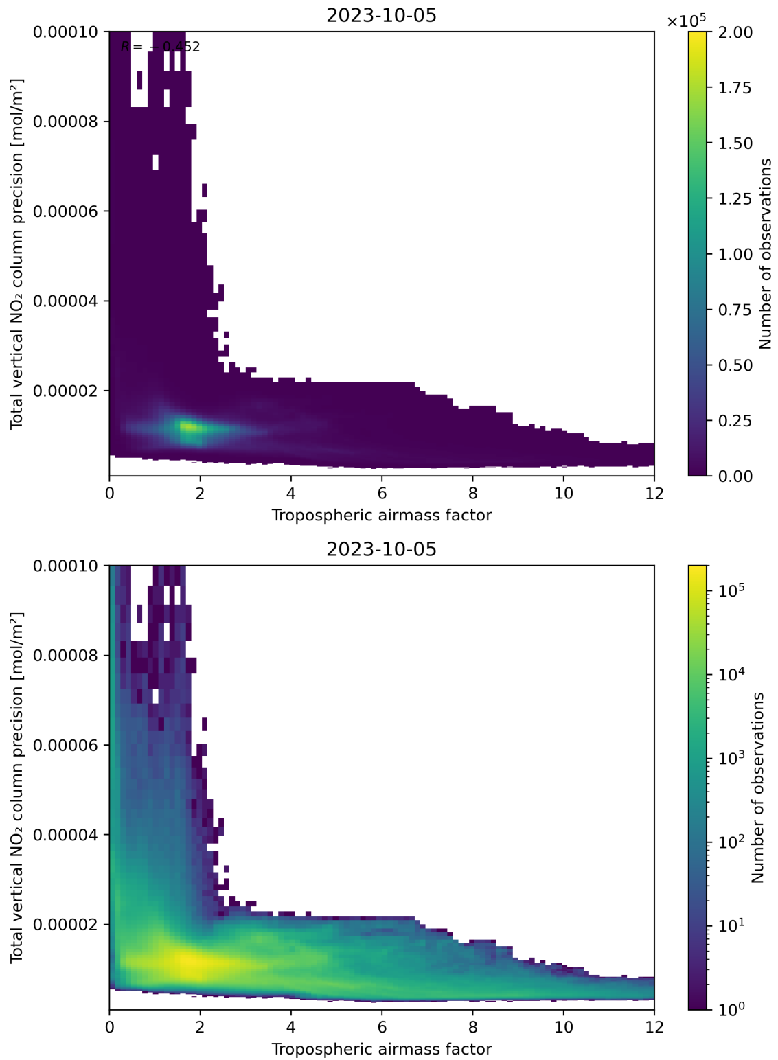
Figure 78: Scatter density plot of “Tropospheric air mass factor” against “Total vertical NO 2 column precision” for 2023-10-04 to 2023-10-06.
