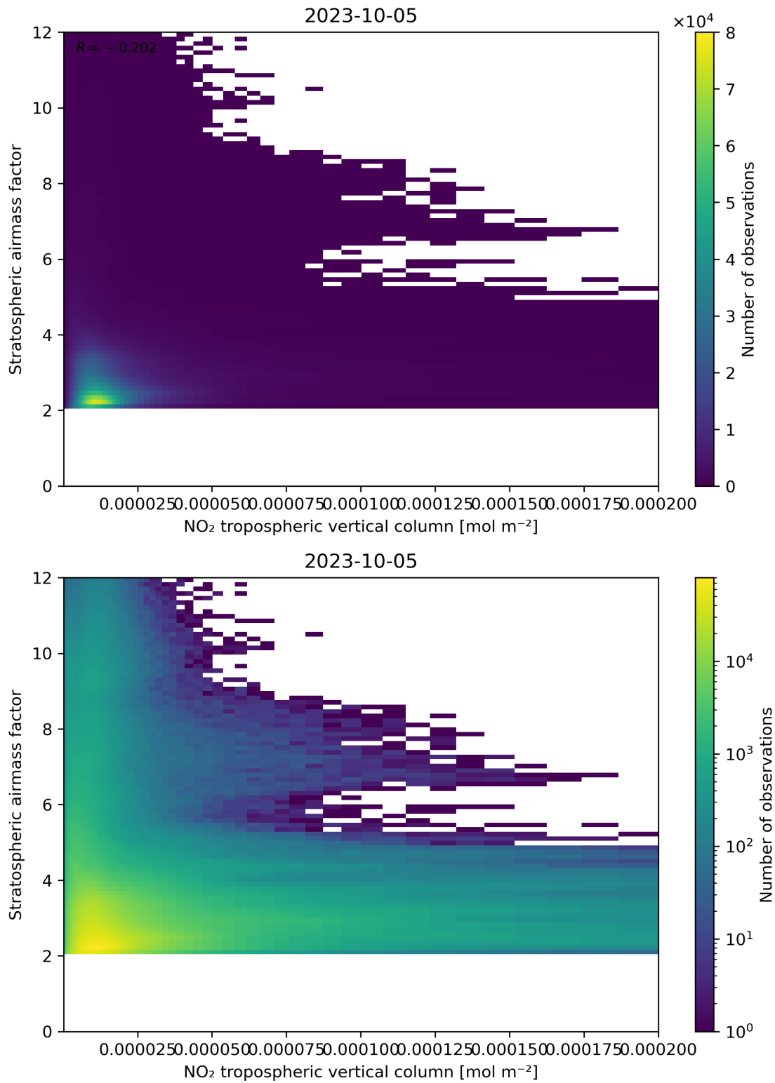
Figure 121: Scatter density plot of “NO 2 tropospheric vertical column” against “Stratospheric air mass factor” for 2023-10-04 to 2023-10-06.
