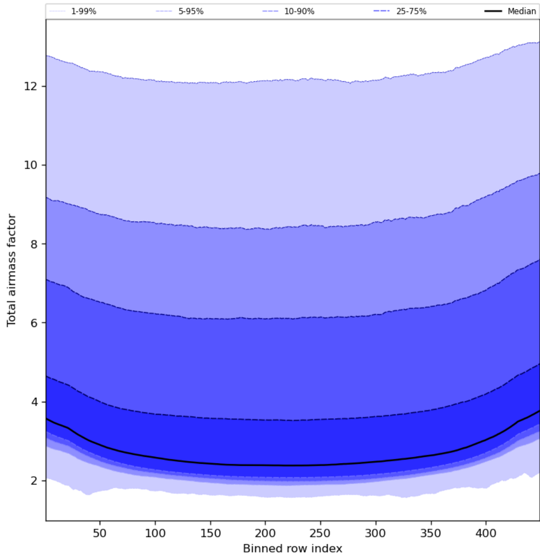
Figure 49: Along track statistics of “Total airmass factor” for 2023-10-04 to 2023-10-06
