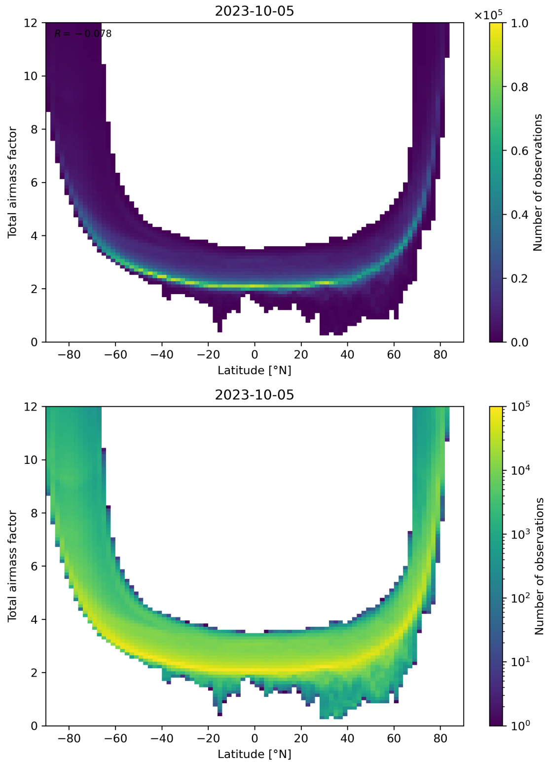
Figure 84: Scatter density plot of “Latitude” against “Total airmass factor” for 2023-10-04 to 2023-10-06.
