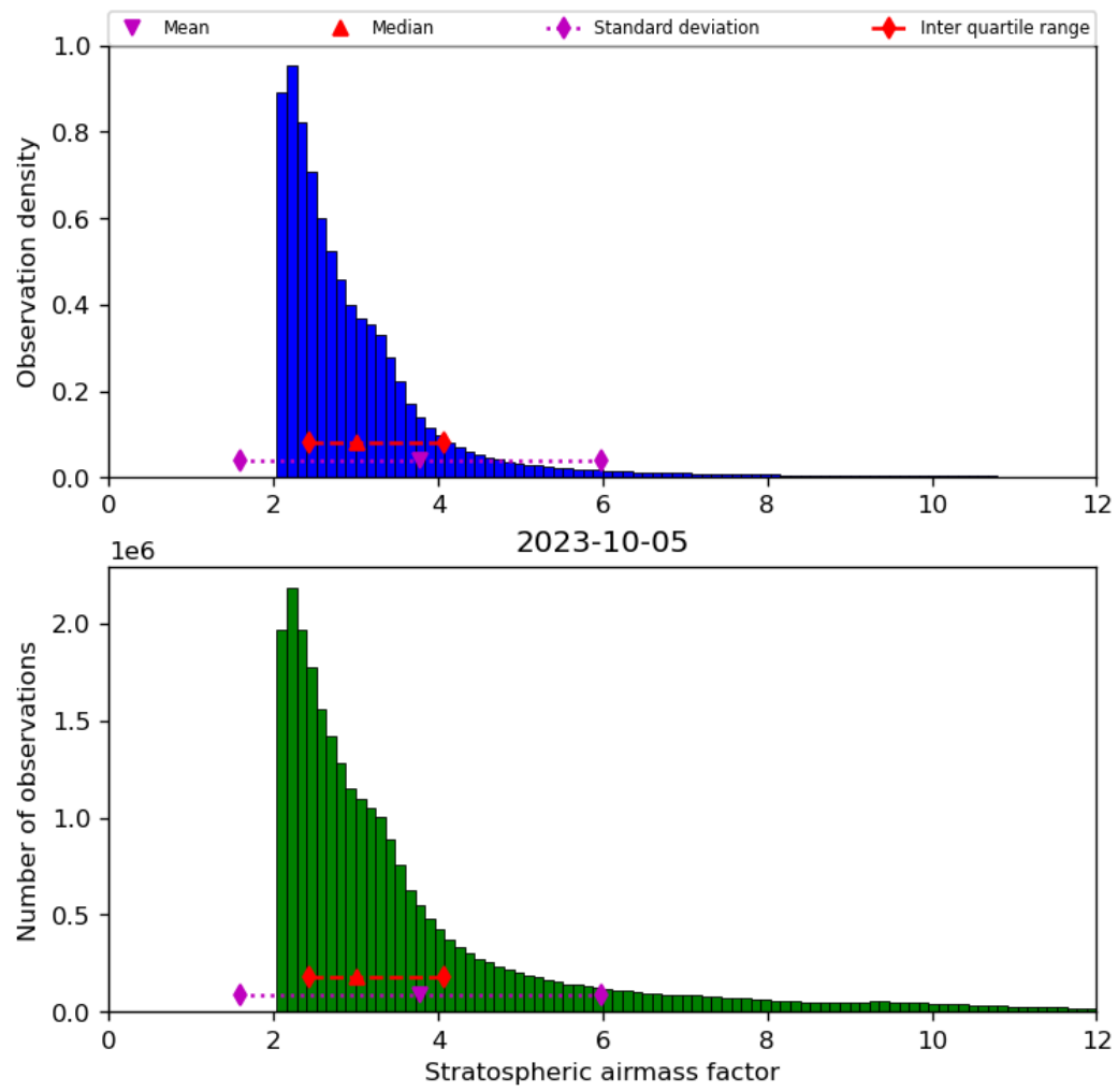
Figure 44: Histogram of “Stratospheric airmass factor” for 2023-10-04 to 2023-10-06
