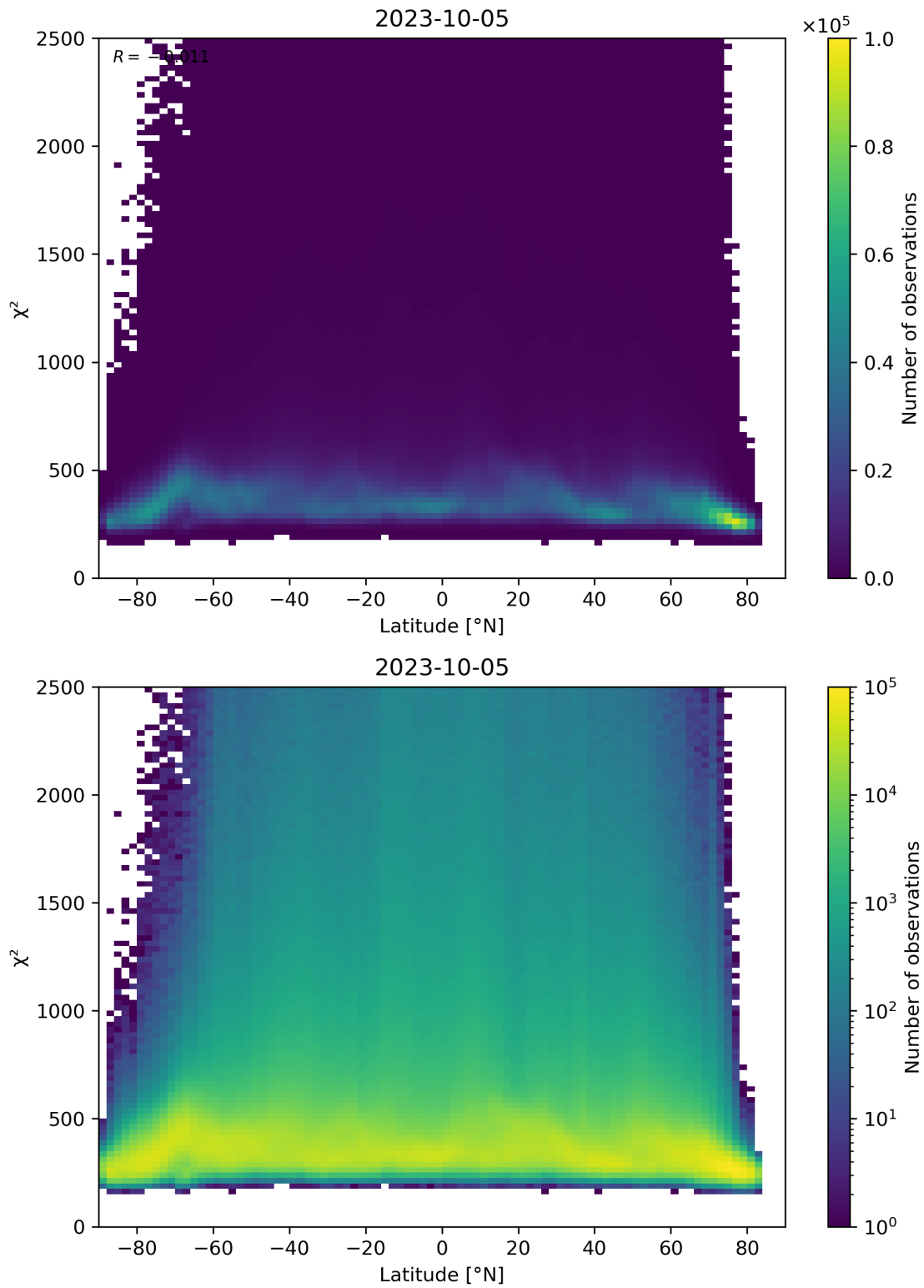
Figure 86: Scatter density plot of “Latitude” against “ \chi^2 ” for 2023-10-04 to 2023-10-06.
