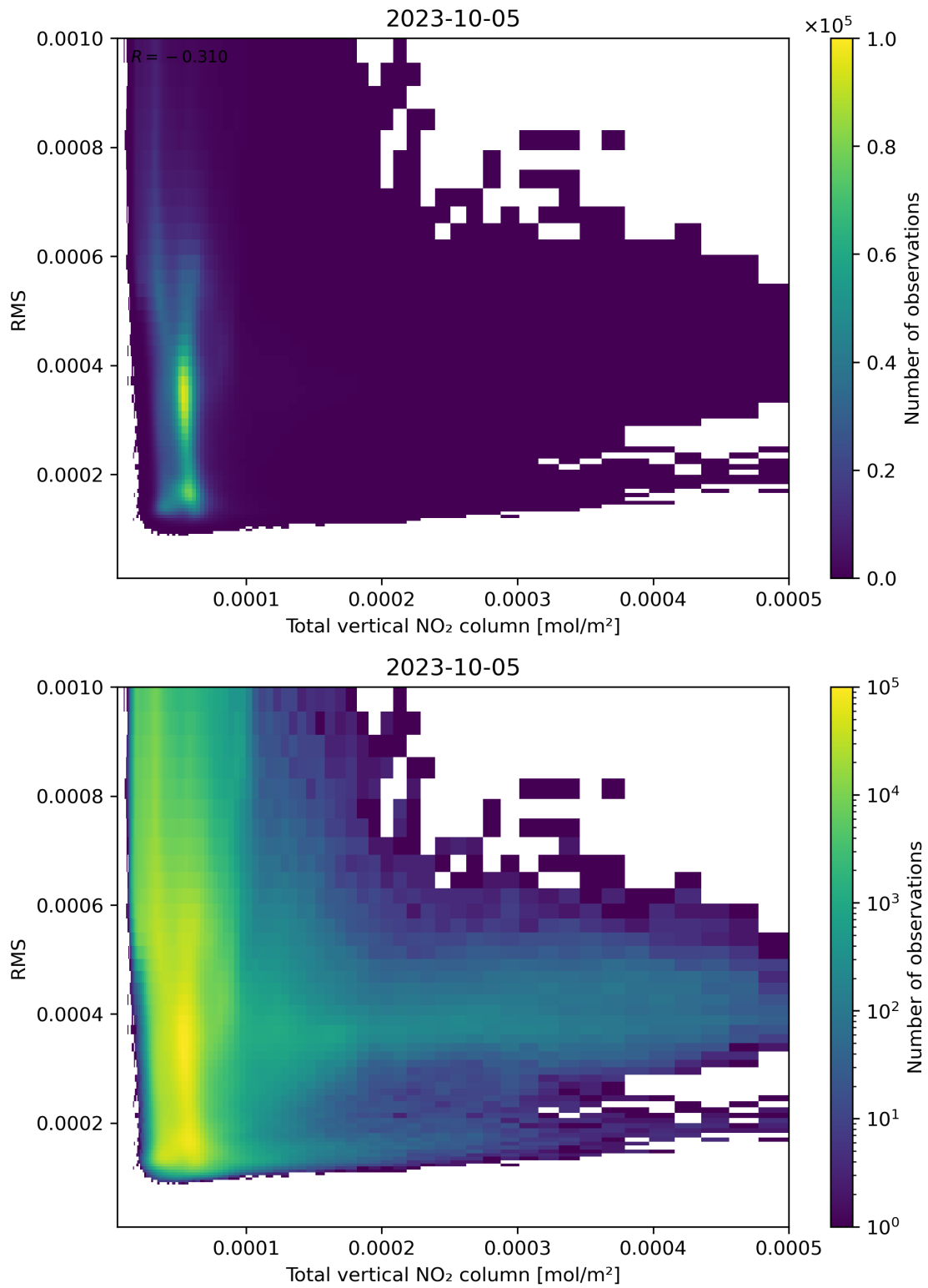
Figure 120: Scatter density plot of “Total vertical NO 2 column” against “RMS” for 2023-10-04 to 2023-10-06.
