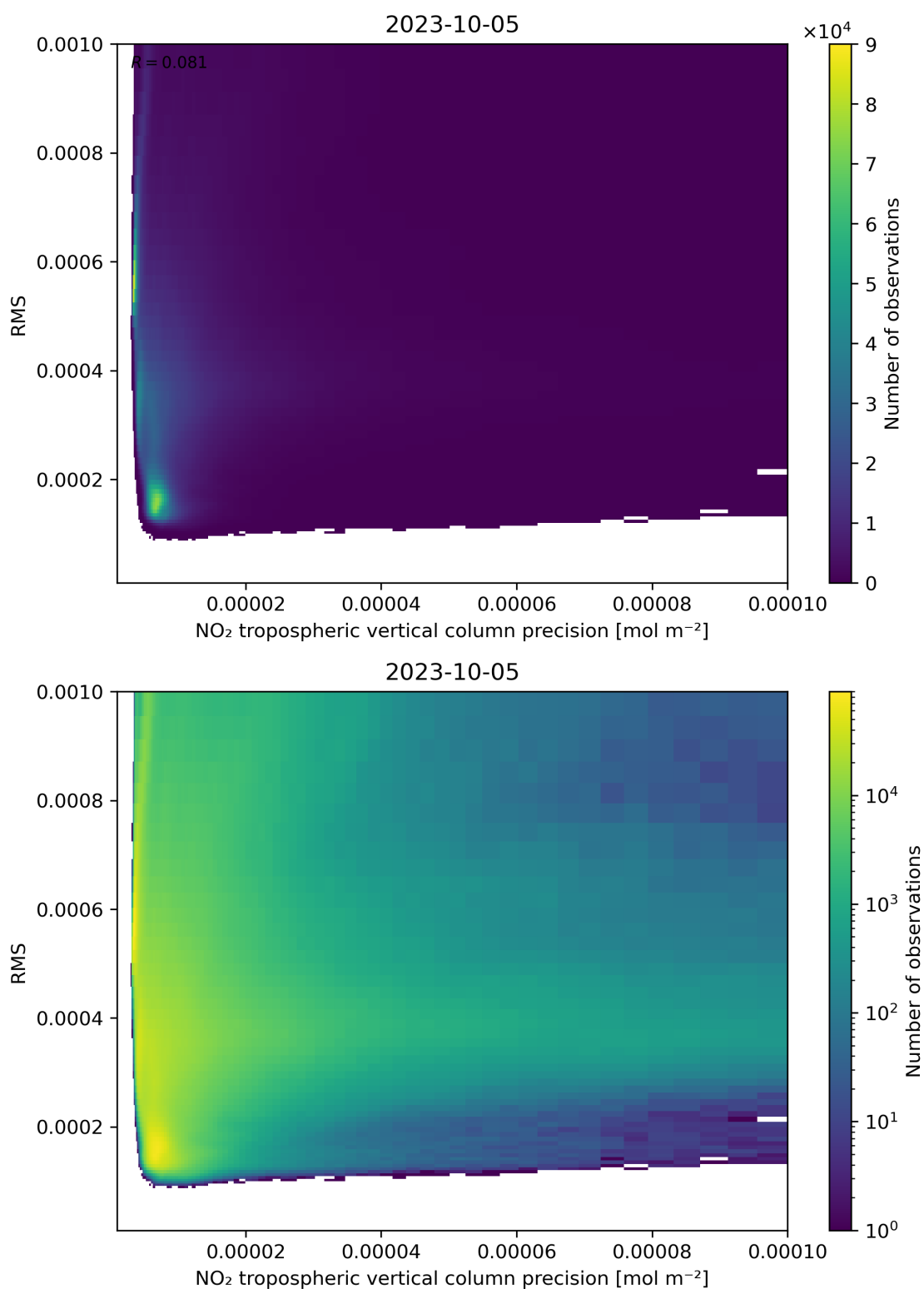
Figure 140: Scatter density plot of “NO 2 tropospheric vertical column precision” against “RMS” for 2023-10-04 to 2023-10-06.
