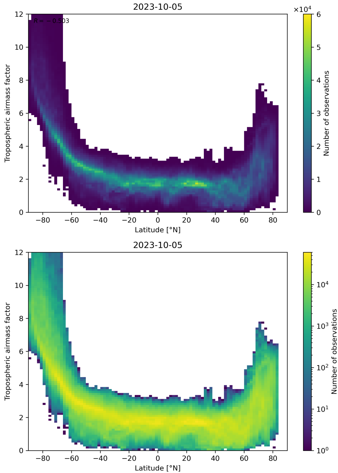
Figure 85: Scatter density plot of “Latitude” against “Tropospheric airmass factor” for 2023-10-04 to 2023-10-06.
