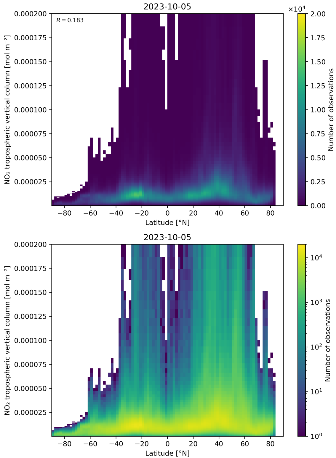
Figure 92: Scatter density plot of “Latitude” against “NO 2 tropospheric vertical column” for 2023-10-04 to 2023-10-06.
