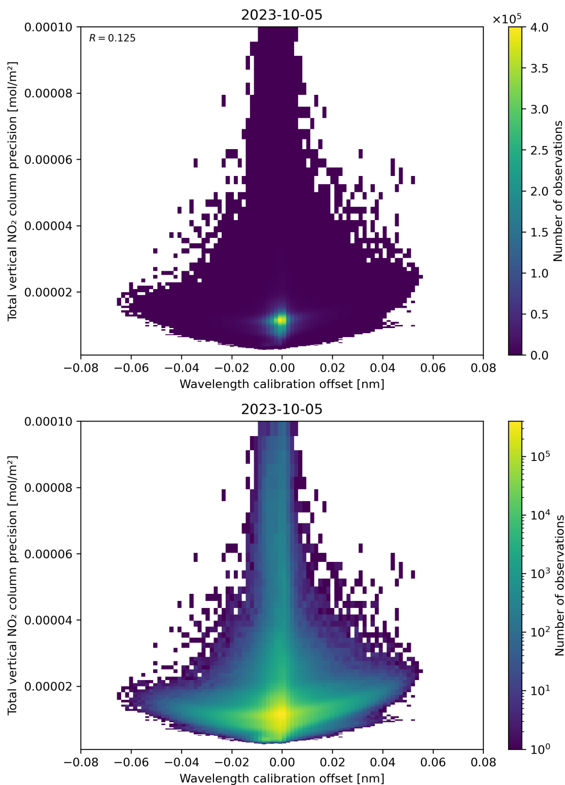
Figure 180: Scatter density plot of “Wavelength calibration offset” against “Total vertical NO 2 column precision” for 2023-10-04 to 2023-10-06.
