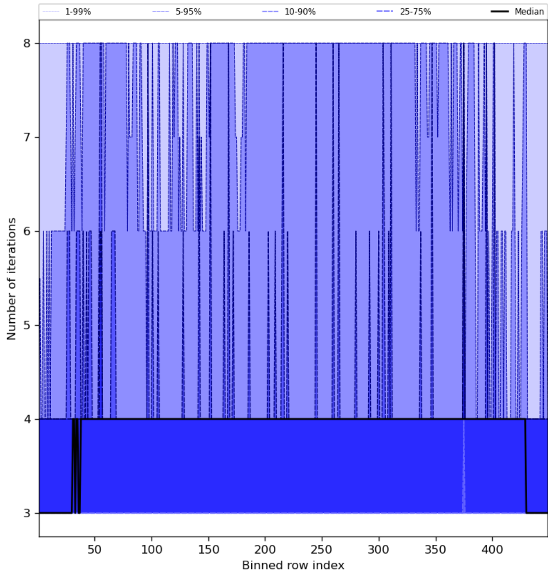
Figure 51: Along track statistics of “Number of iterations” for 2023-10-04 to 2023-10-06
