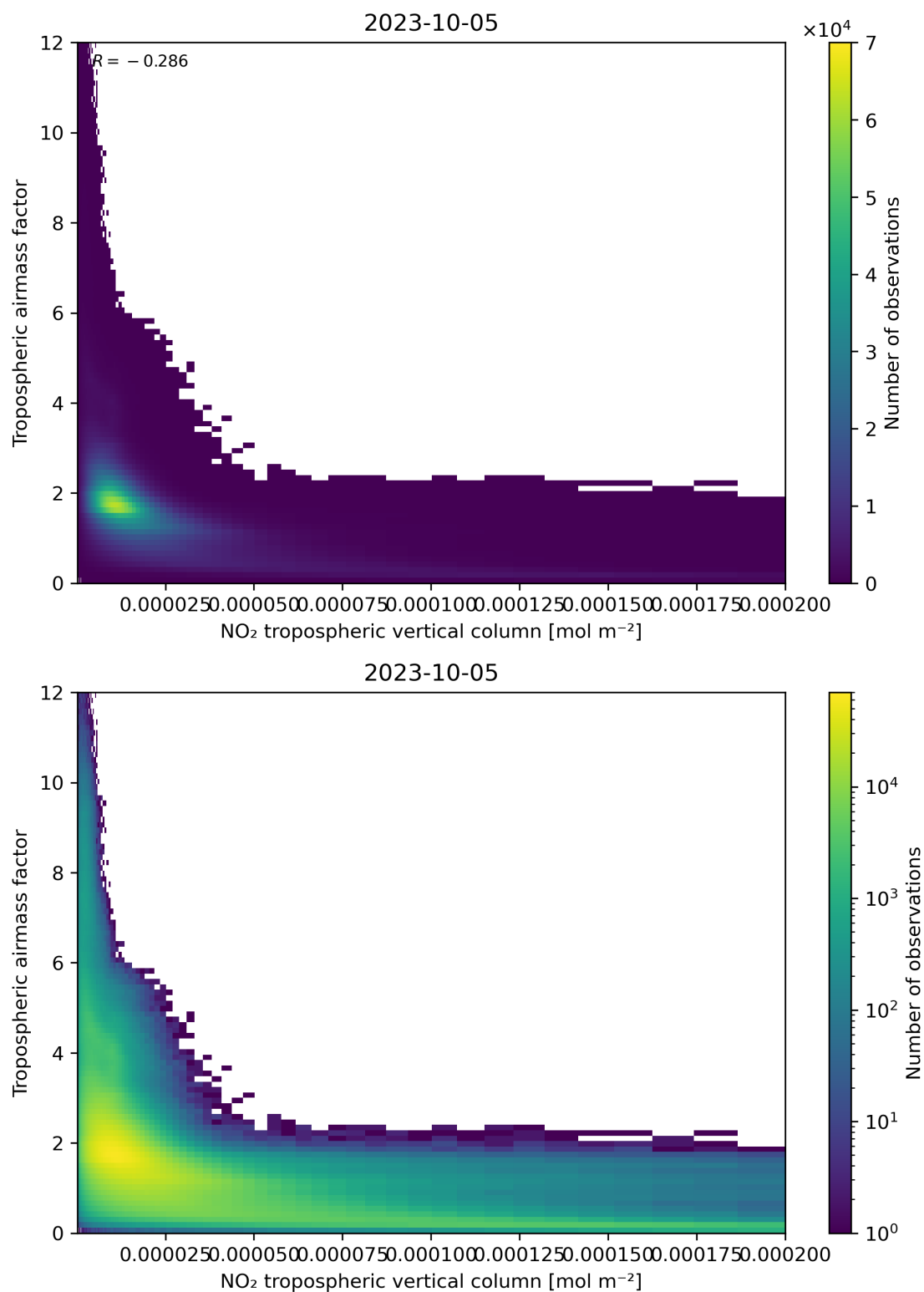
Figure 123: Scatter density plot of “NO 2 tropospheric vertical column” against “Tropospheric airmass factor” for 2023-10-04 to 2023-10-06.
