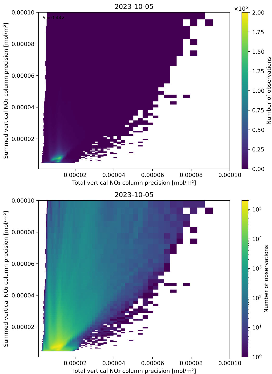
Figure 118: Scatter density plot of “Total vertical NO 2 column precision” against “Summed vertical NO 2 column precision” for 2023-10-04 to 2023-10-06.
