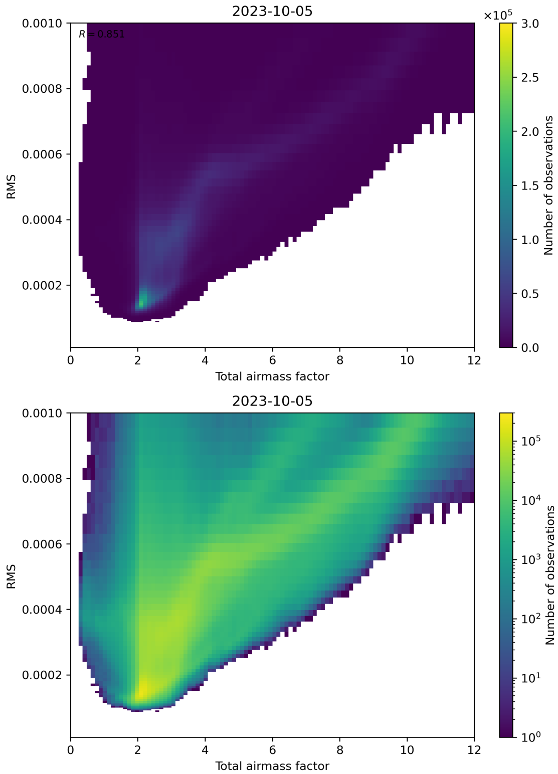
Figure 69: Scatter density plot of “Total airmass factor” against “RMS” for 2023-10-04 to 2023-10-06.
