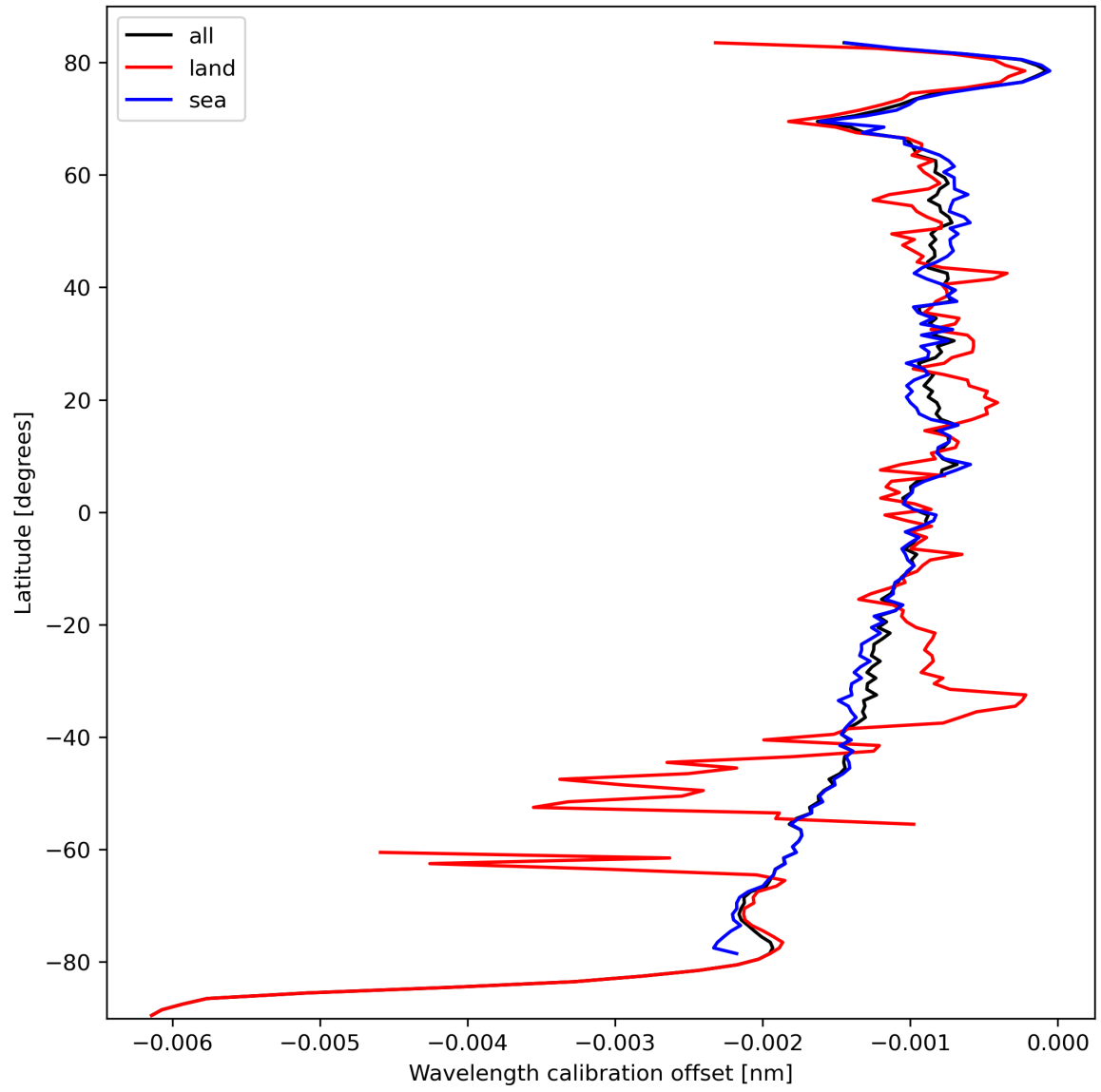
Figure 18: Zonal average of “Wavelength calibration offset” for 2023-10-04 to 2023-10-06.
