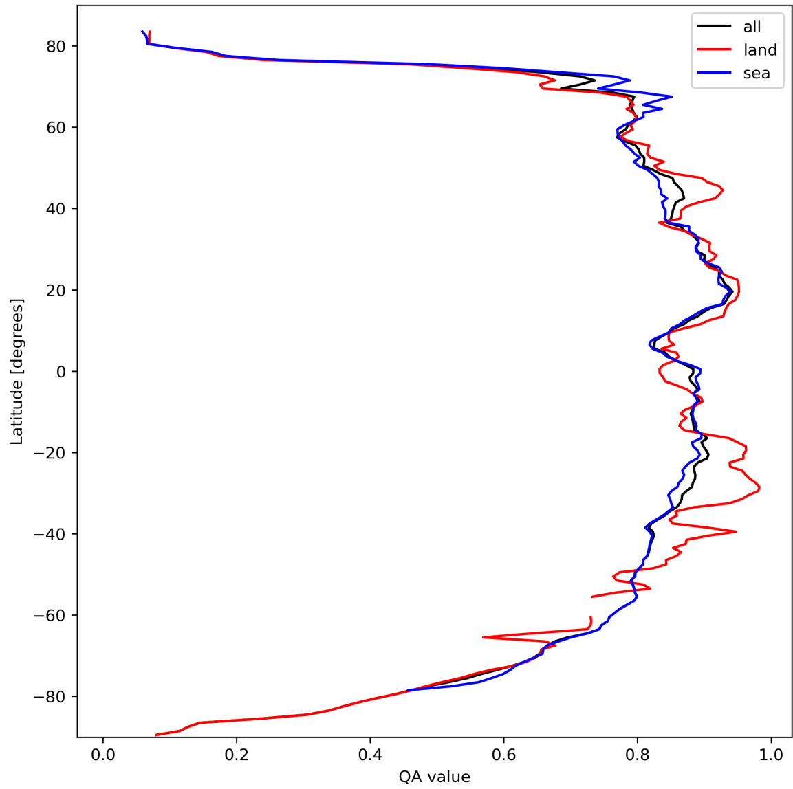
Figure 11: Zonal average of “QA value” for 2023-10-04 to 2023-10-06.
