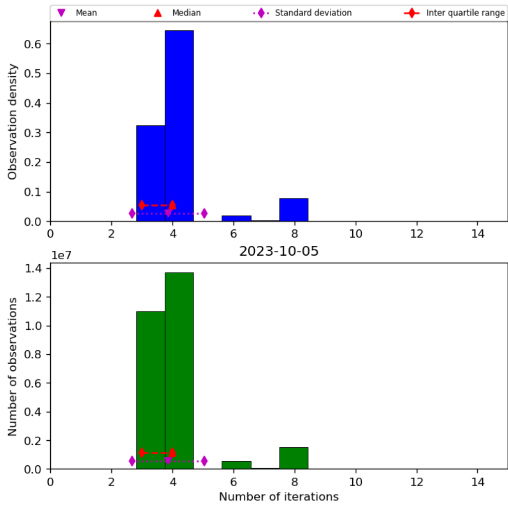
Figure 34: Histogram of “Number of iterations” for 2023-10-04 to 2023-10-06
