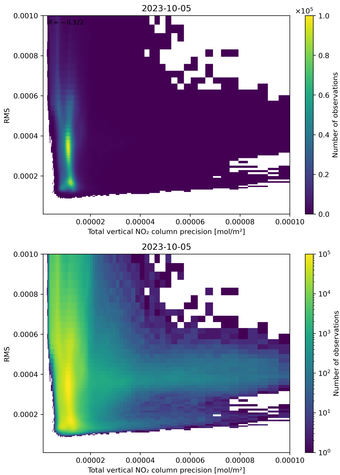
Figure 119: Scatter density plot of “Total vertical NO 2 column precision” against “RMS” for 2023-10-04 to 2023-10-06.
