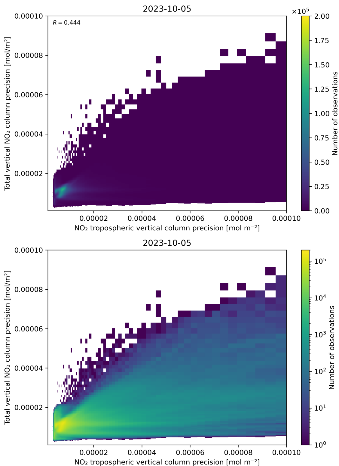
Figure 139: Scatter density plot of “NO 2 tropospheric vertical column precision” against “Total vertical NO 2 column precision” for 2023-10-04 to 2023-10-06.
