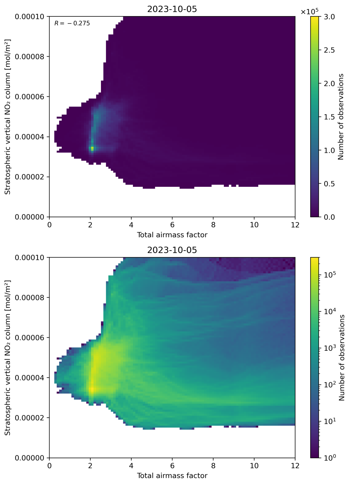
Figure 64: Scatter density plot of “Total airmass factor” against “Stratospheric vertical NO 2 column” for 2023-10-04 to 2023-10-06.
