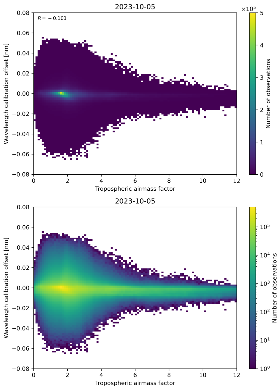
Figure 80: Scatter density plot of “Tropospheric airmass factor” against “Wavelength calibration offset” for 2023-10-04 to 2023-10-06.
