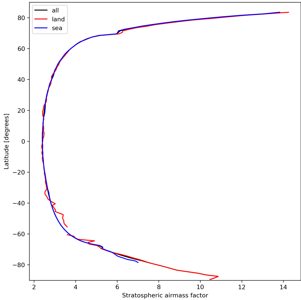
Figure 27: Zonal average of “Stratospheric air mass factor” for 2023-10-04 to 2023-10-06.
