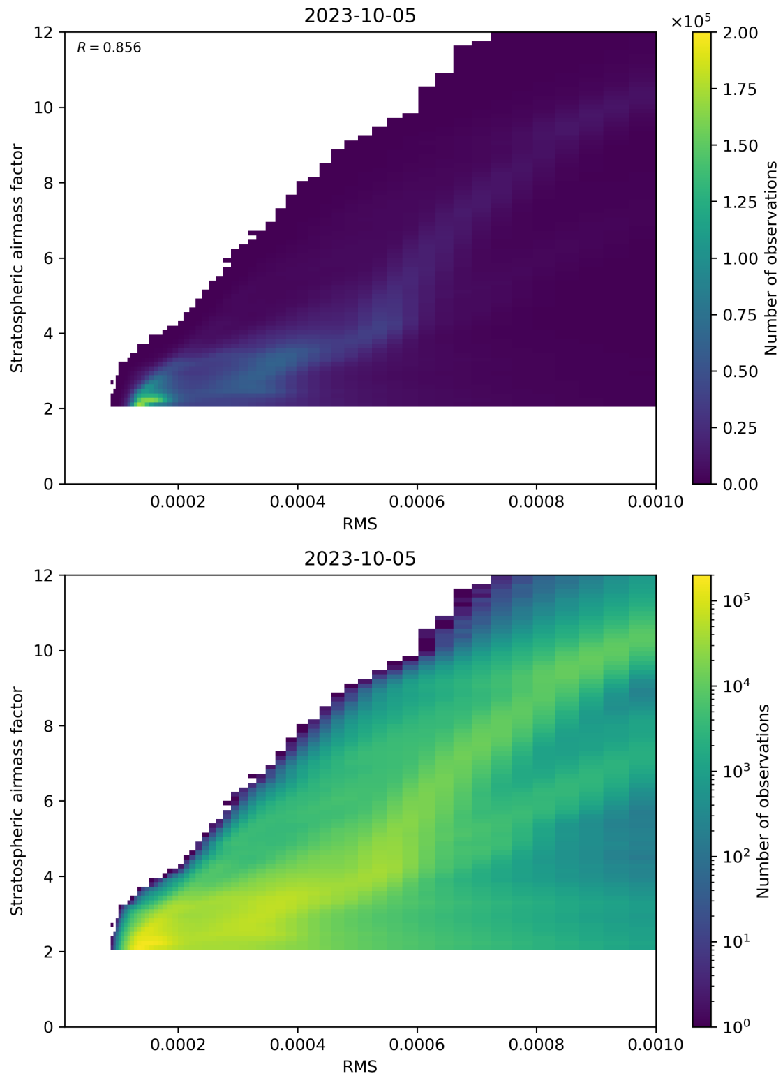
Figure 144: Scatter density plot of “RMS” against “Stratospheric airmass factor” for 2023-10-04 to 2023-10-06.
