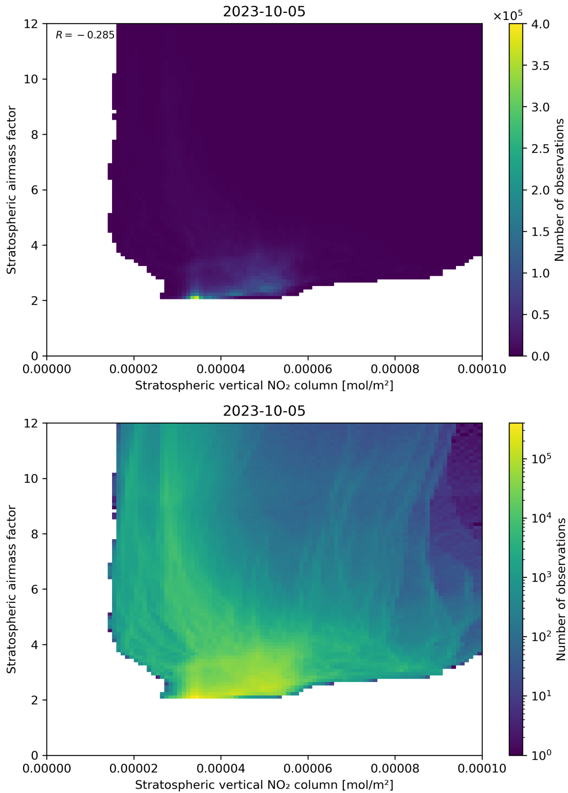
Figure 96: Scatter density plot of “Stratospheric vertical NO 2 column” against “Stratospheric airmass factor” for 2023-10-04 to 2023-10-06.
