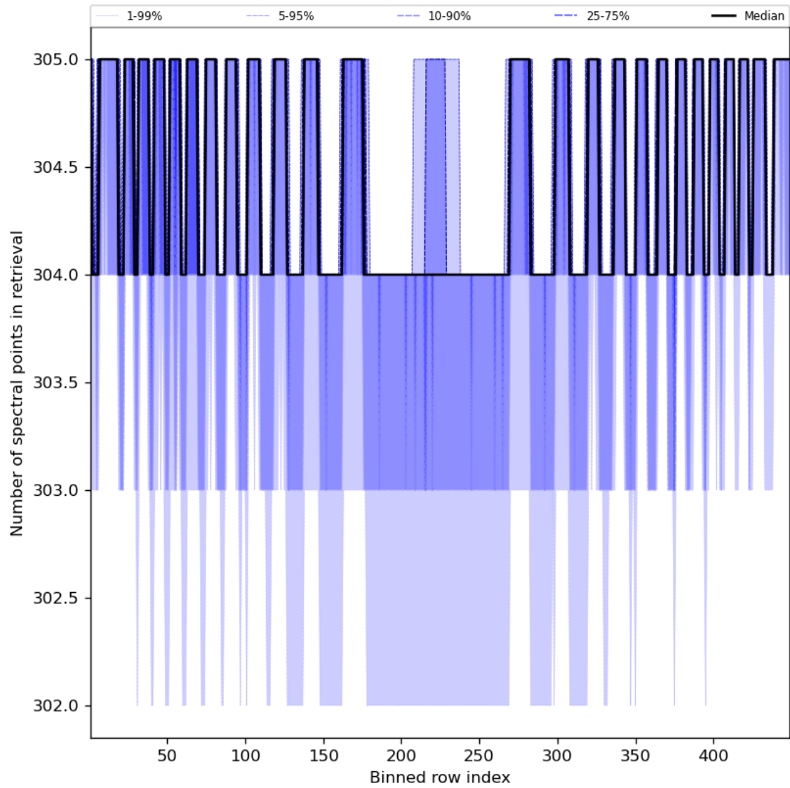
Figure 50: Along track statistics of “Number of spectral points in retrieval” for 2023-10-04 to 2023-10-06
