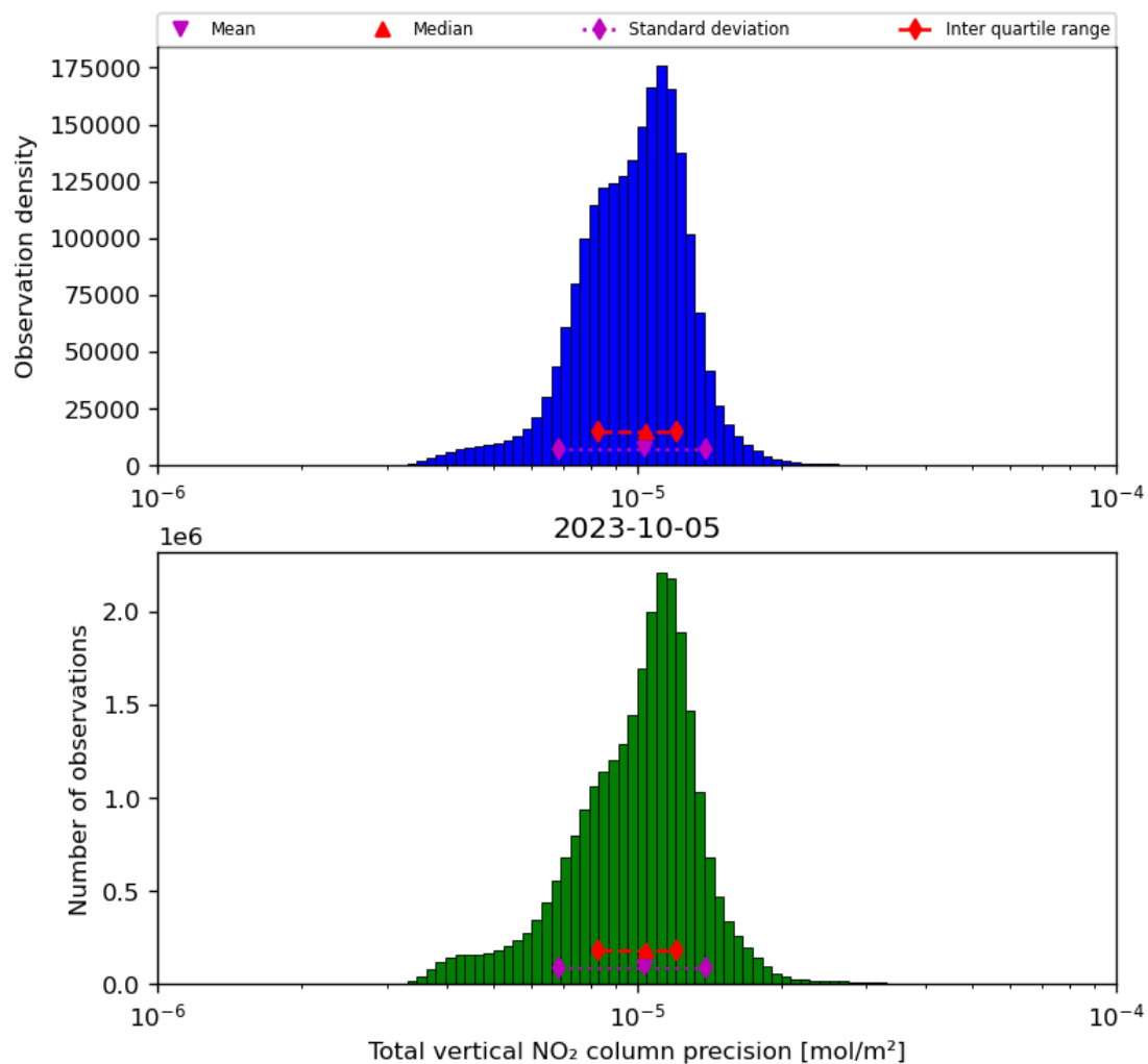
Figure 39: Histogram of “Total vertical NO 2 column precision” for 2023-10-04 to 2023-10-06
