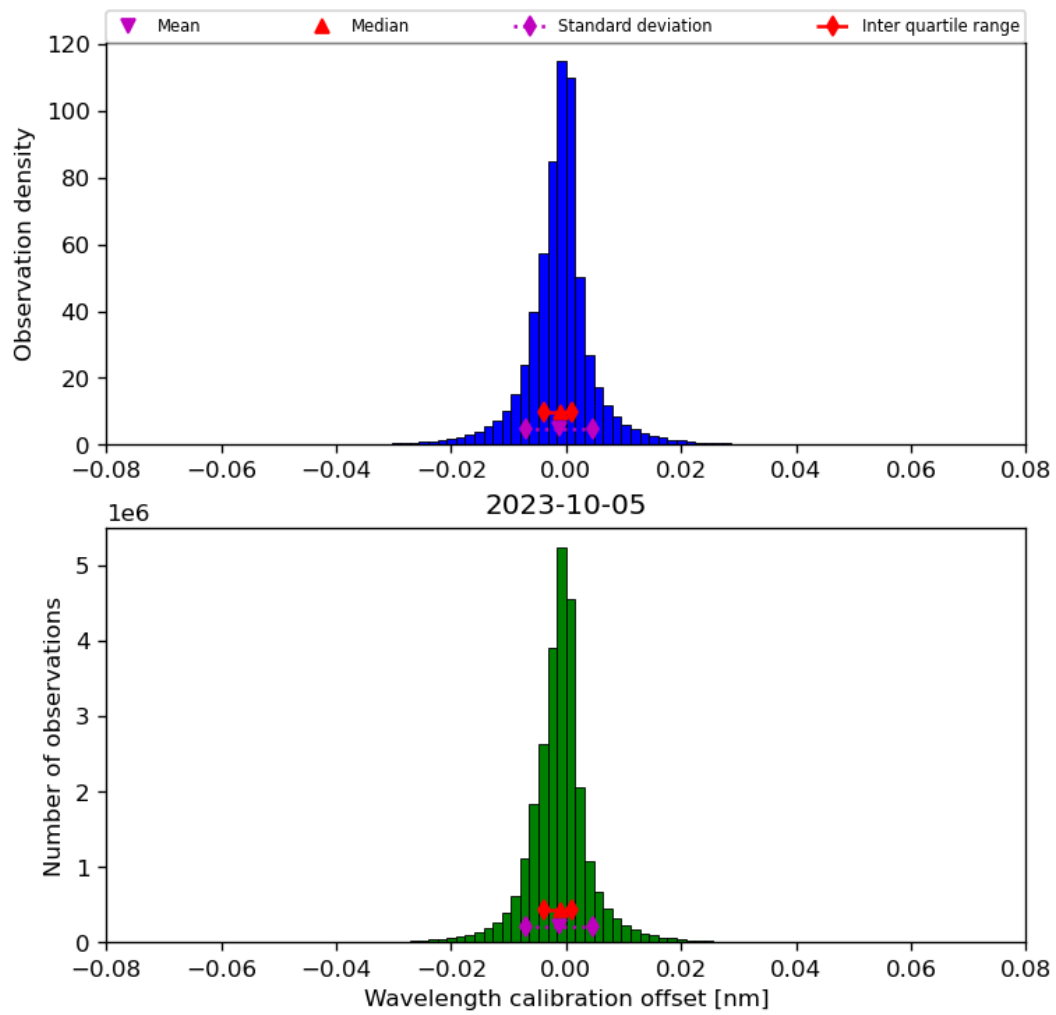
Figure 35: Histogram of “Wavelength calibration offset” for 2023-10-04 to 2023-10-06
