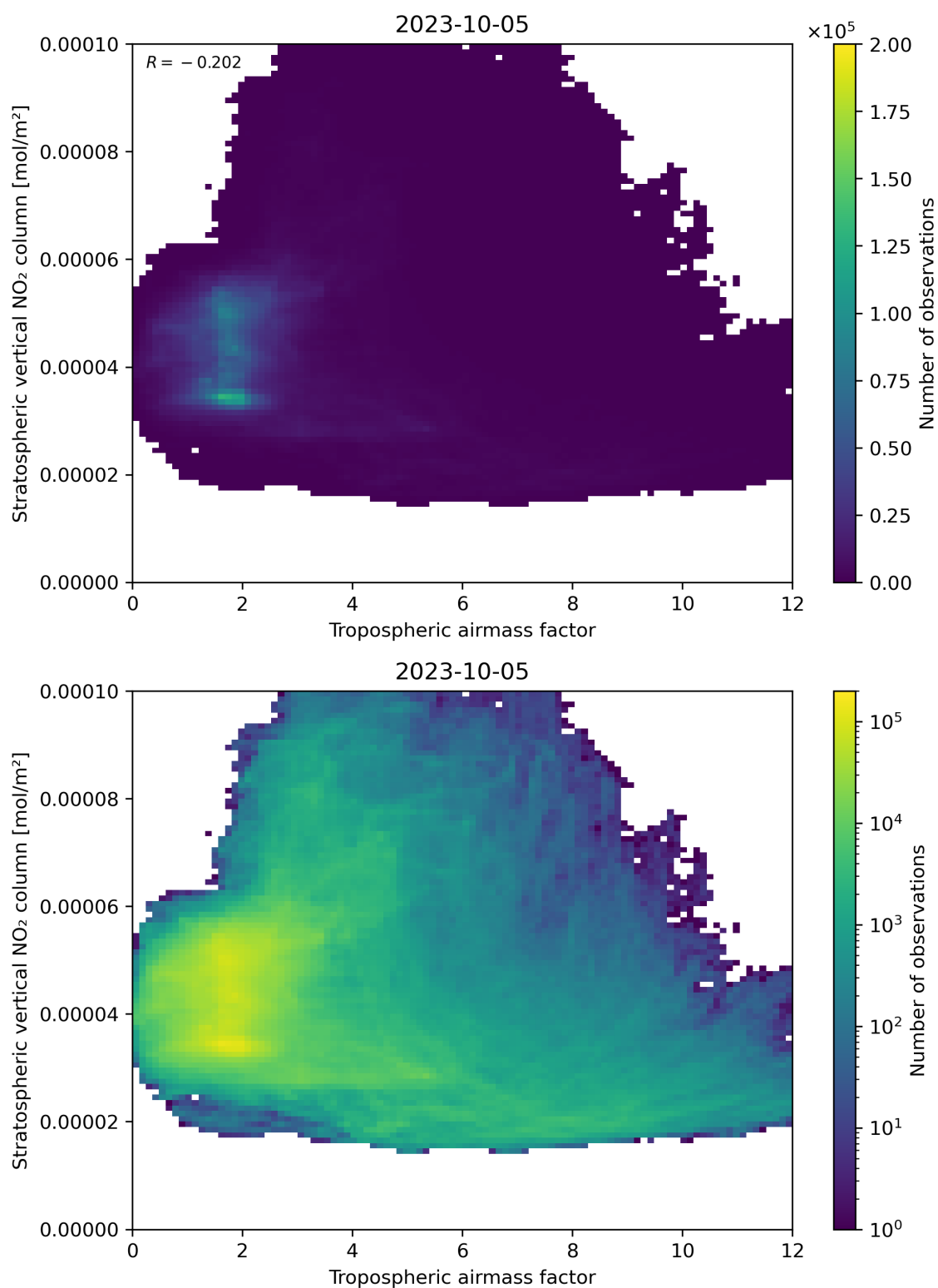
Figure 74: Scatter density plot of “Tropospheric air mass factor” against “Stratospheric vertical NO 2 column” for 2023-10-04 to 2023-10-06.
