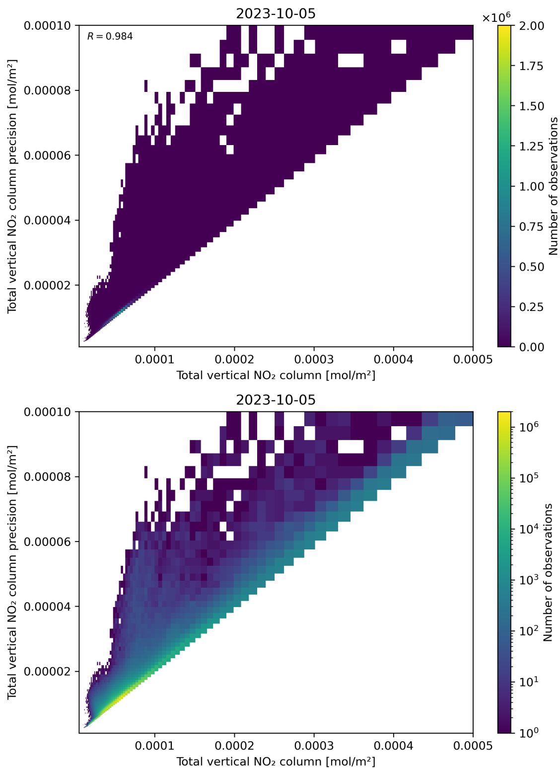
Figure 114: Scatter density plot of “Total vertical NO 2 column” against “Total vertical NO 2 column precision” for 2023-10-04 to 2023-10-06.
