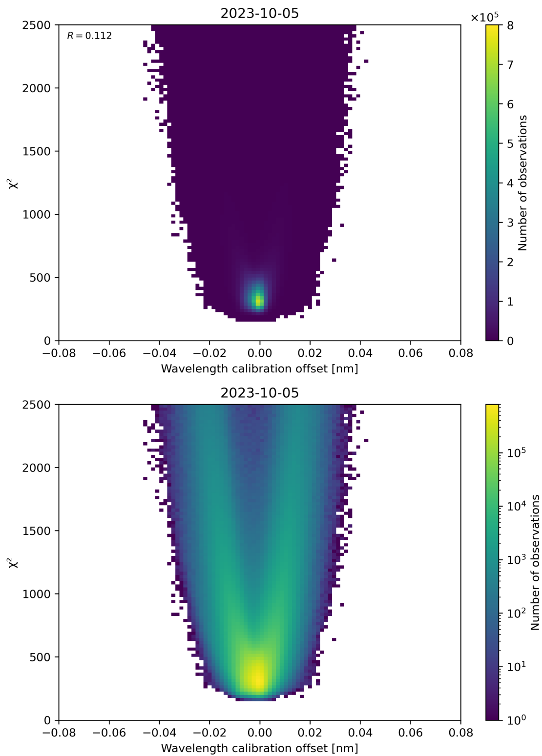
Figure 175: Scatter density plot of “Wavelength calibration offset” against “ \chi^2 ” for 2023-10-04 to 2023-10-06.
