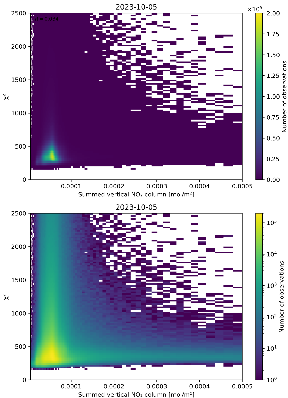
Figure 104: Scatter density plot of “Summed vertical NO 2 column” against “ \chi^2 ” for 2023-10-04 to 2023-10-06.
