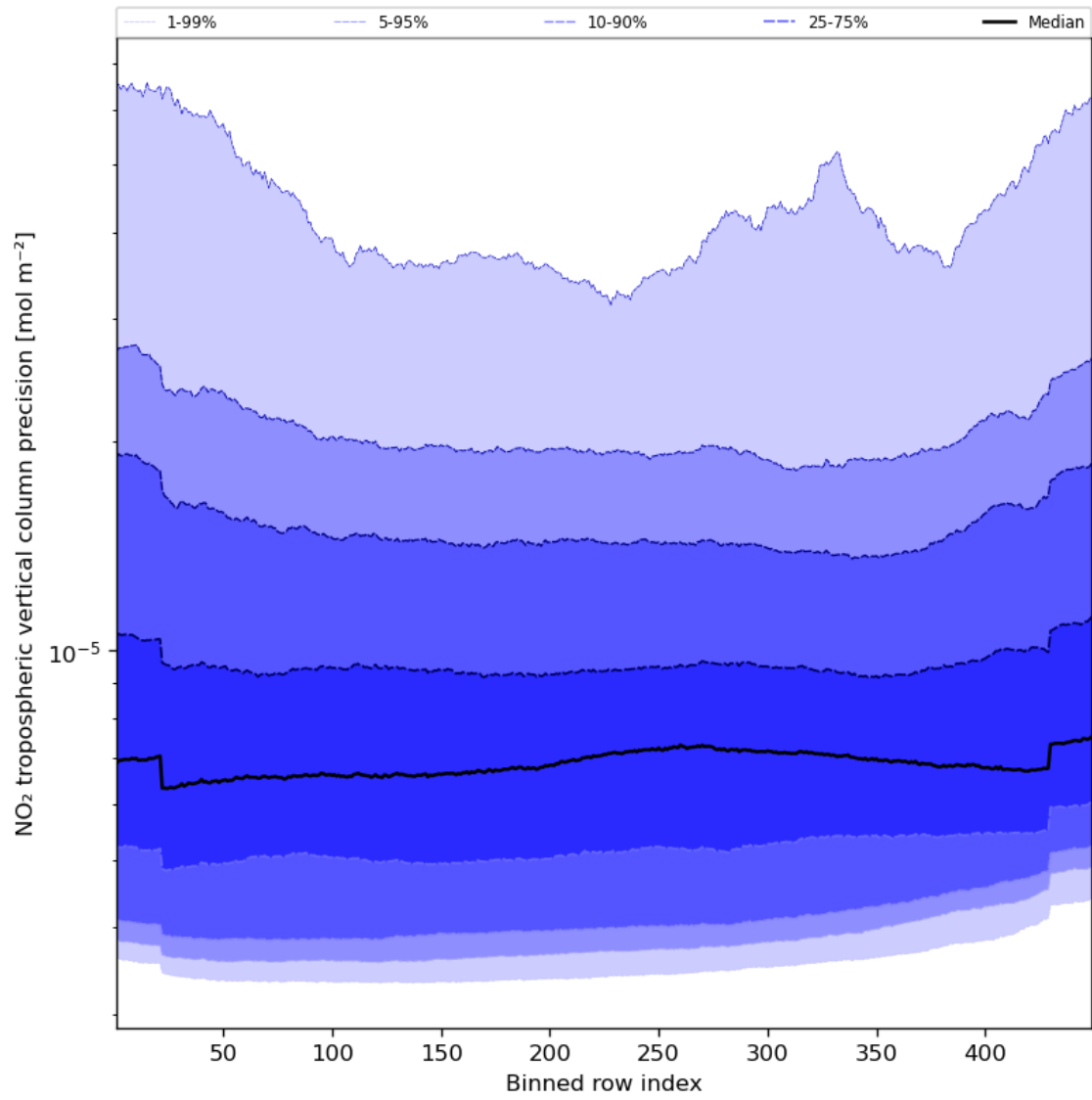
Figure 47: Along track statistics of “NO 2 tropospheric vertical column precision” for 2023-10-04 to 2023-10-06
