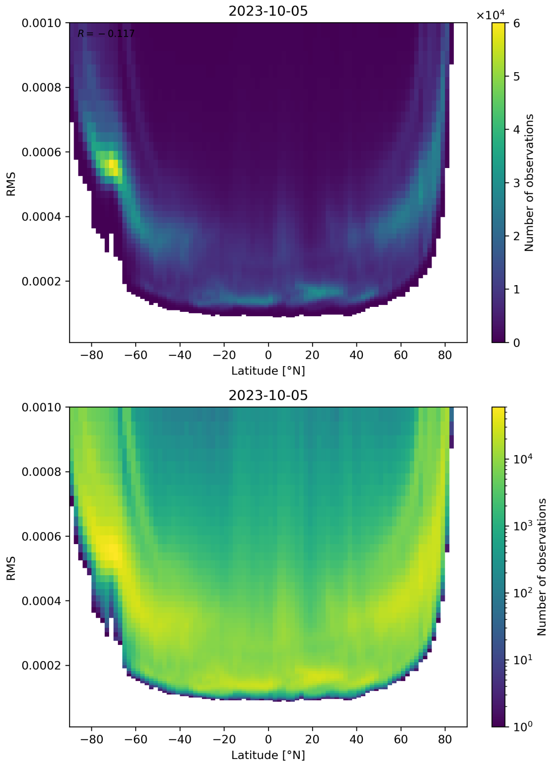
Figure 94: Scatter density plot of “Latitude” against “RMS” for 2023-10-04 to 2023-10-06.
