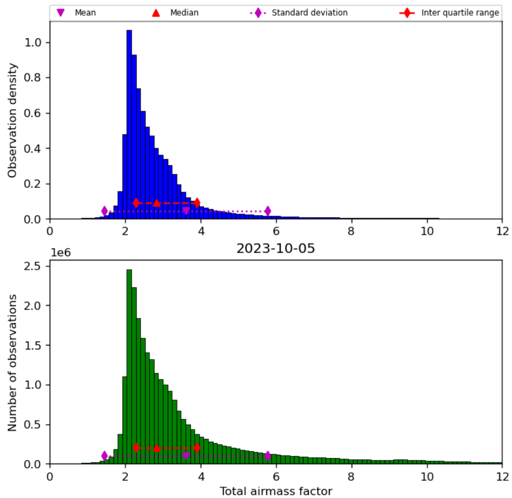
Figure 32: Histogram of “Total airmass factor” for 2023-10-04 to 2023-10-06
