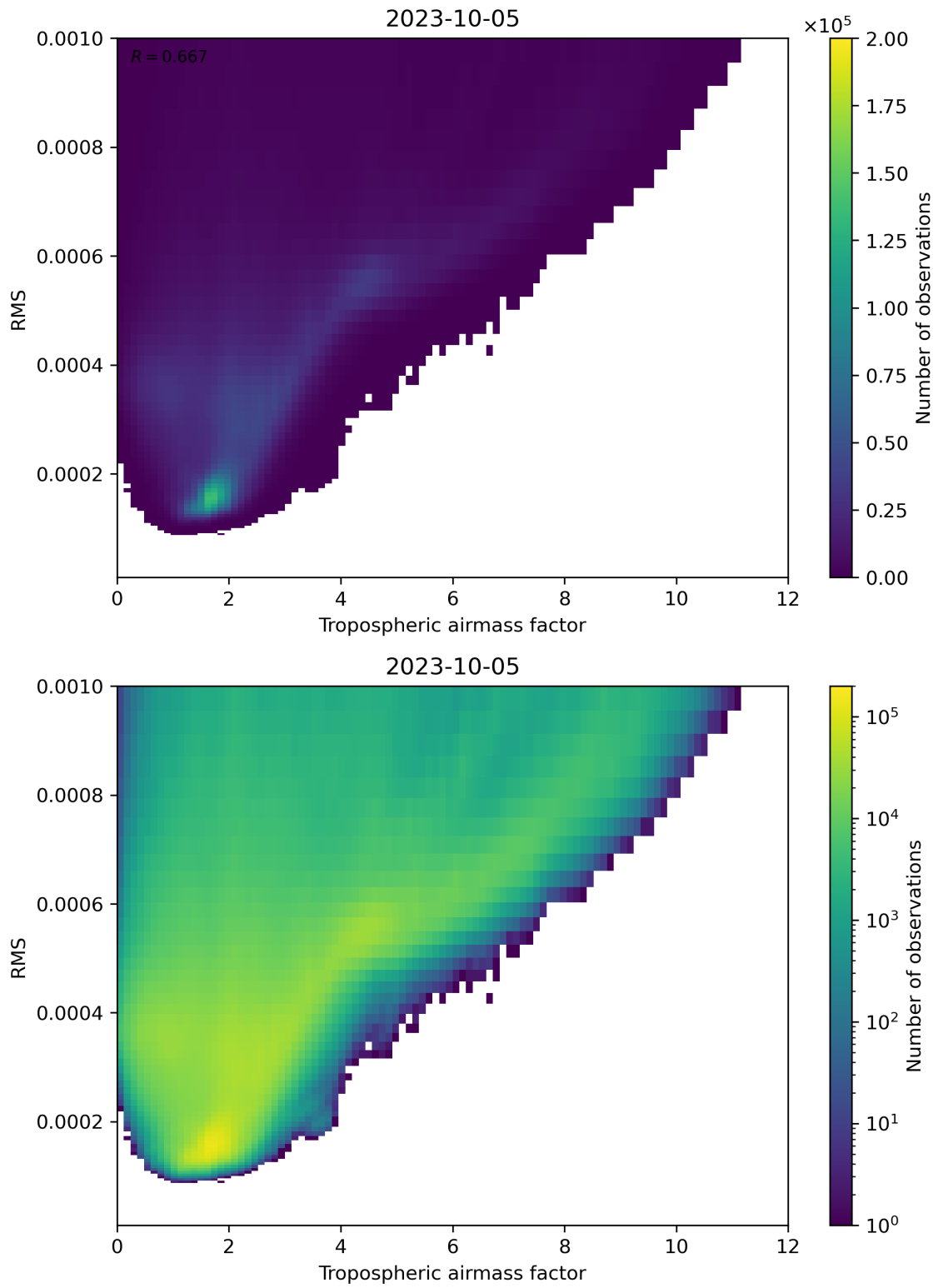
Figure 79: Scatter density plot of “Tropospheric airmass factor” against “RMS” for 2023-10-04 to 2023-10-06.
