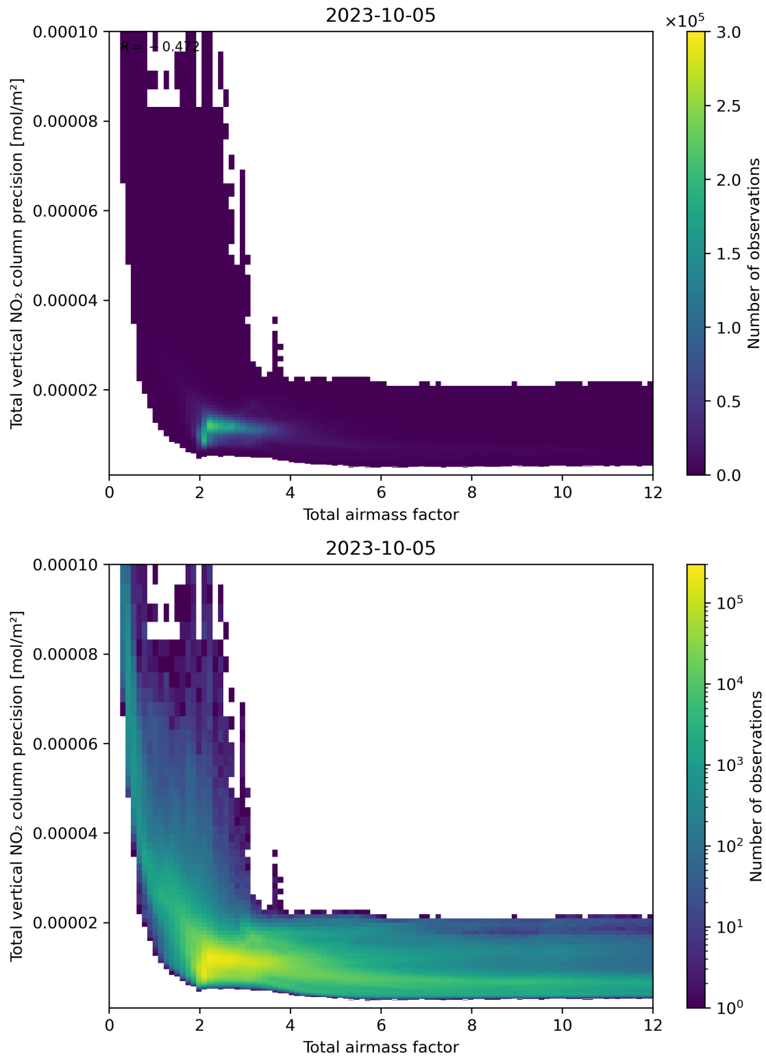
Figure 68: Scatter density plot of “Total airmass factor” against “Total vertical NO 2 column precision” for 2023-10-04 to 2023-10-06.
