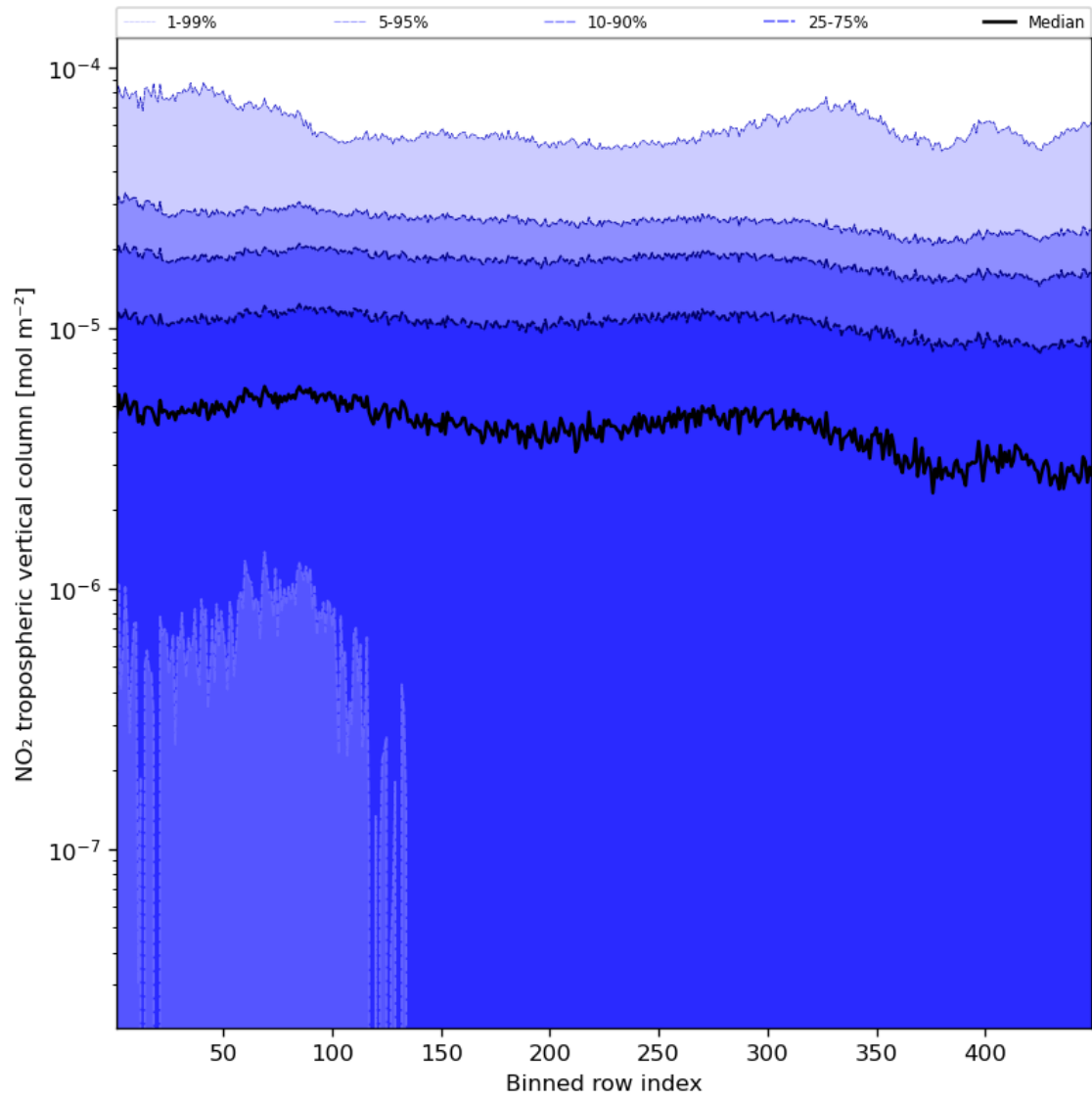
Figure 46: Along track statistics of “NO 2 tropospheric vertical column” for 2023-10-04 to 2023-10-06
