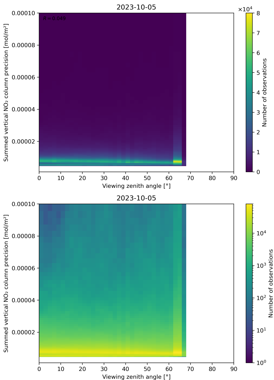
Figure 166: Scatter density plot of “Viewing zenith angle” against “Summed vertical NO 2 column precision” for 2023-10-04 to 2023-10-06.
