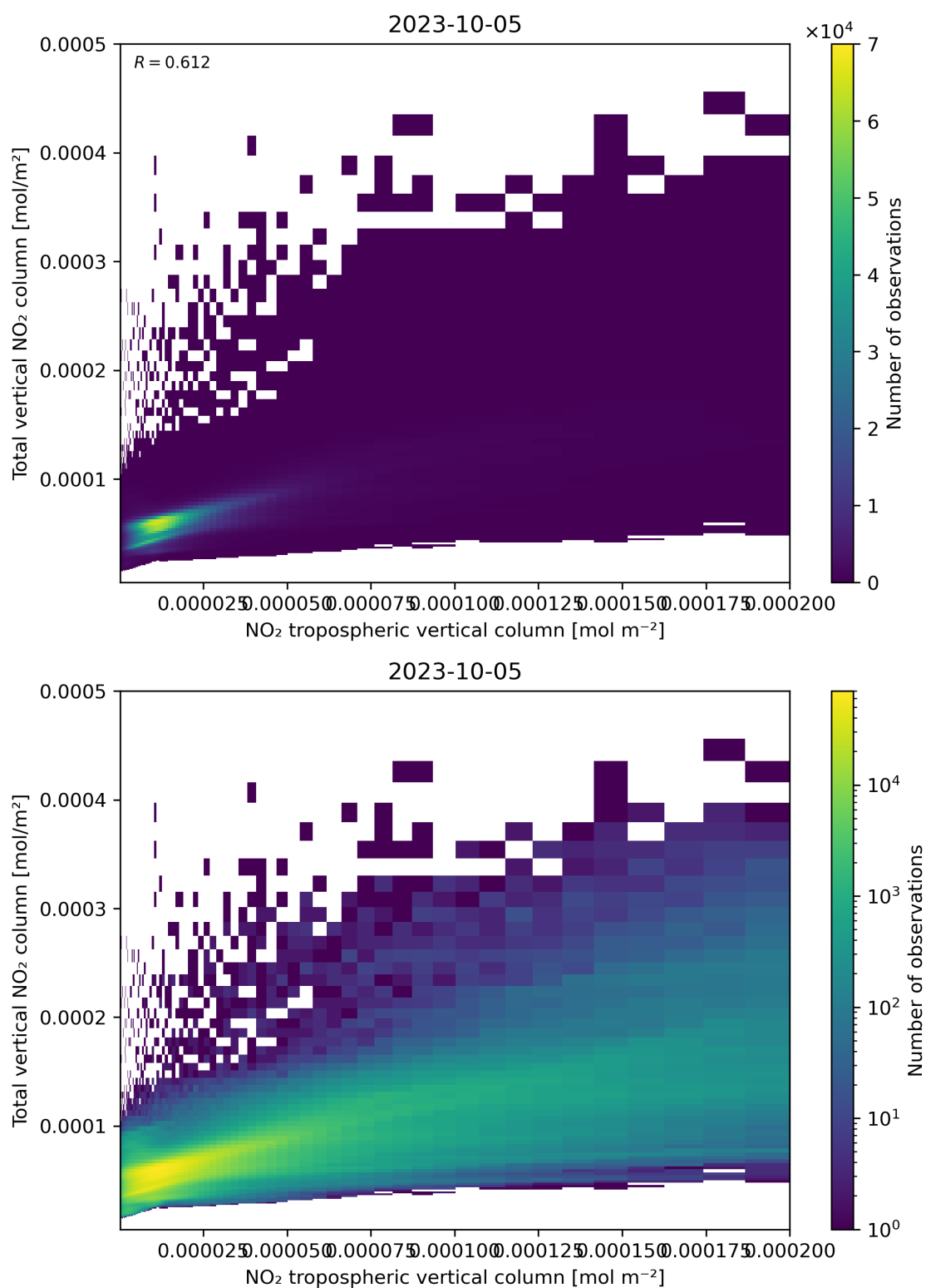
Figure 128: Scatter density plot of “NO 2 tropospheric vertical column” against “Total vertical NO 2 column” for 2023-10-04 to 2023-10-06.
