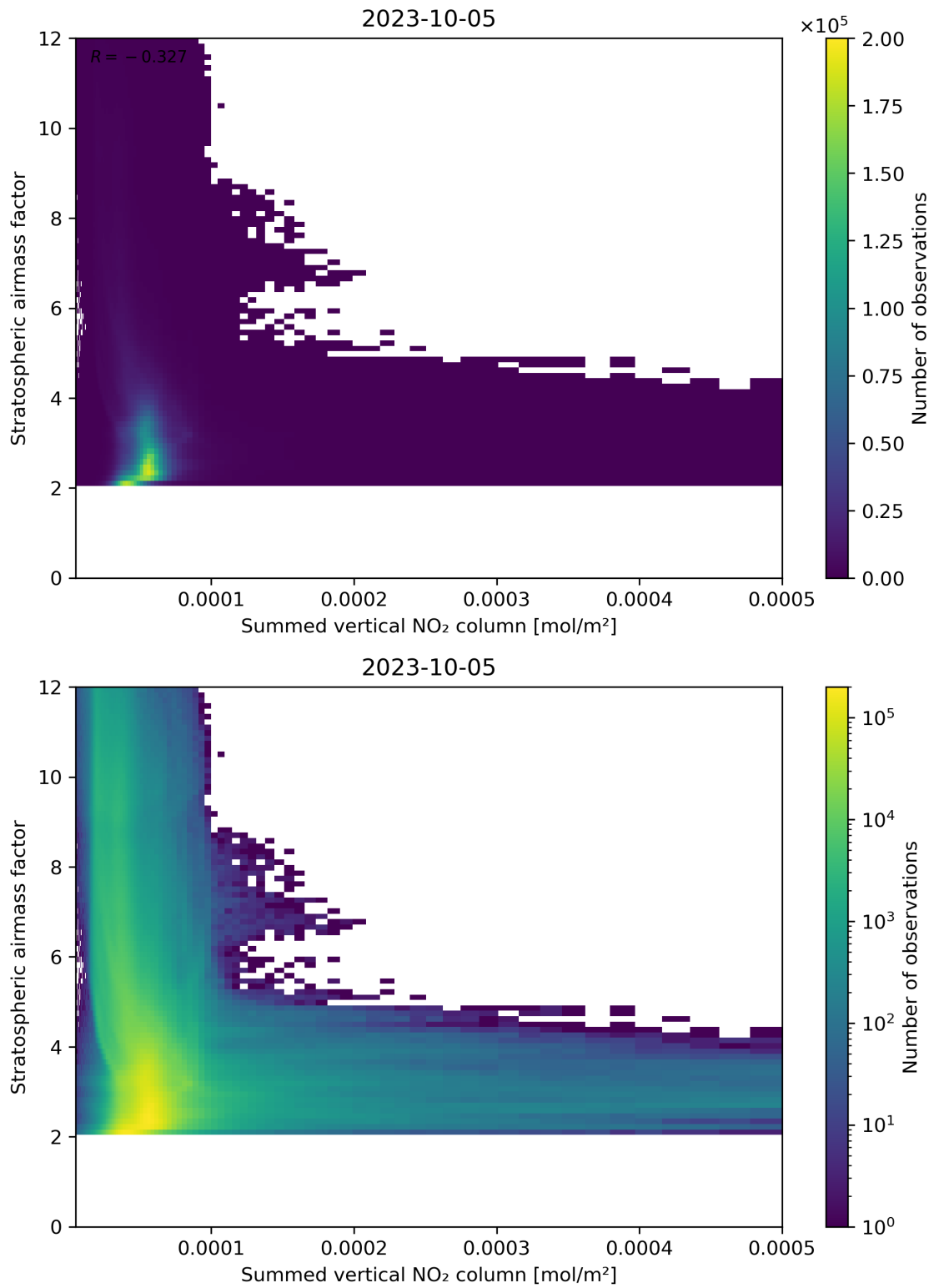
Figure 103: Scatter density plot of “Summed vertical NO 2 column” against “Stratospheric air mass factor” for 2023-10-04 to 2023-10-06.
