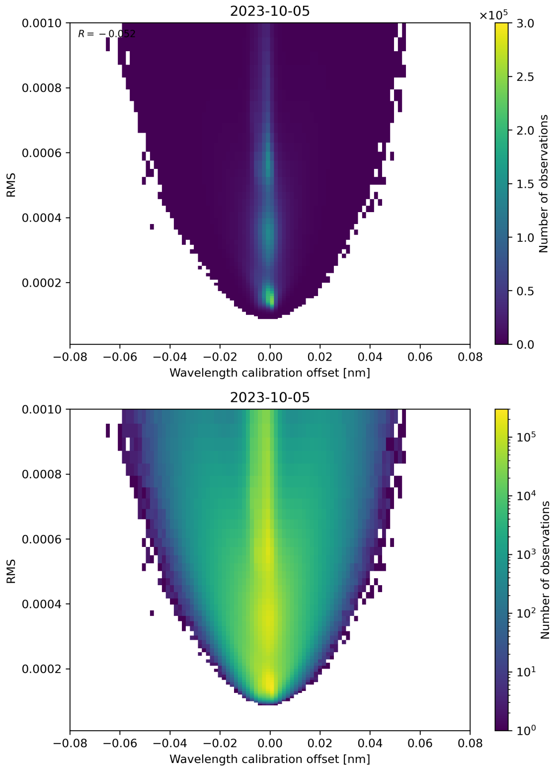
Figure 181: Scatter density plot of “Wavelength calibration offset” against “RMS” for 2023-10-04 to 2023-10-06.
