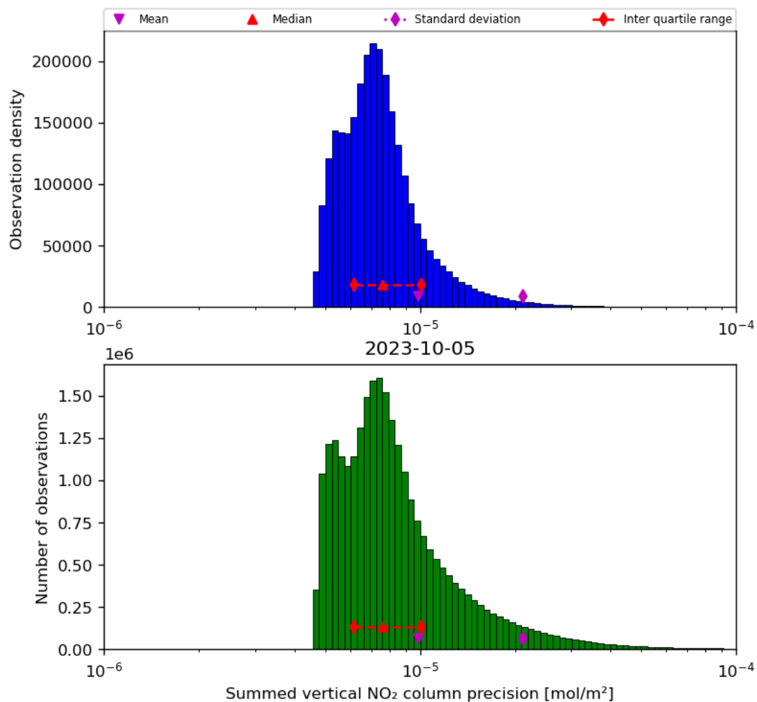
Figure 41: Histogram of “Summed vertical NO 2 column precision” for 2023-10-04 to 2023-10-06
