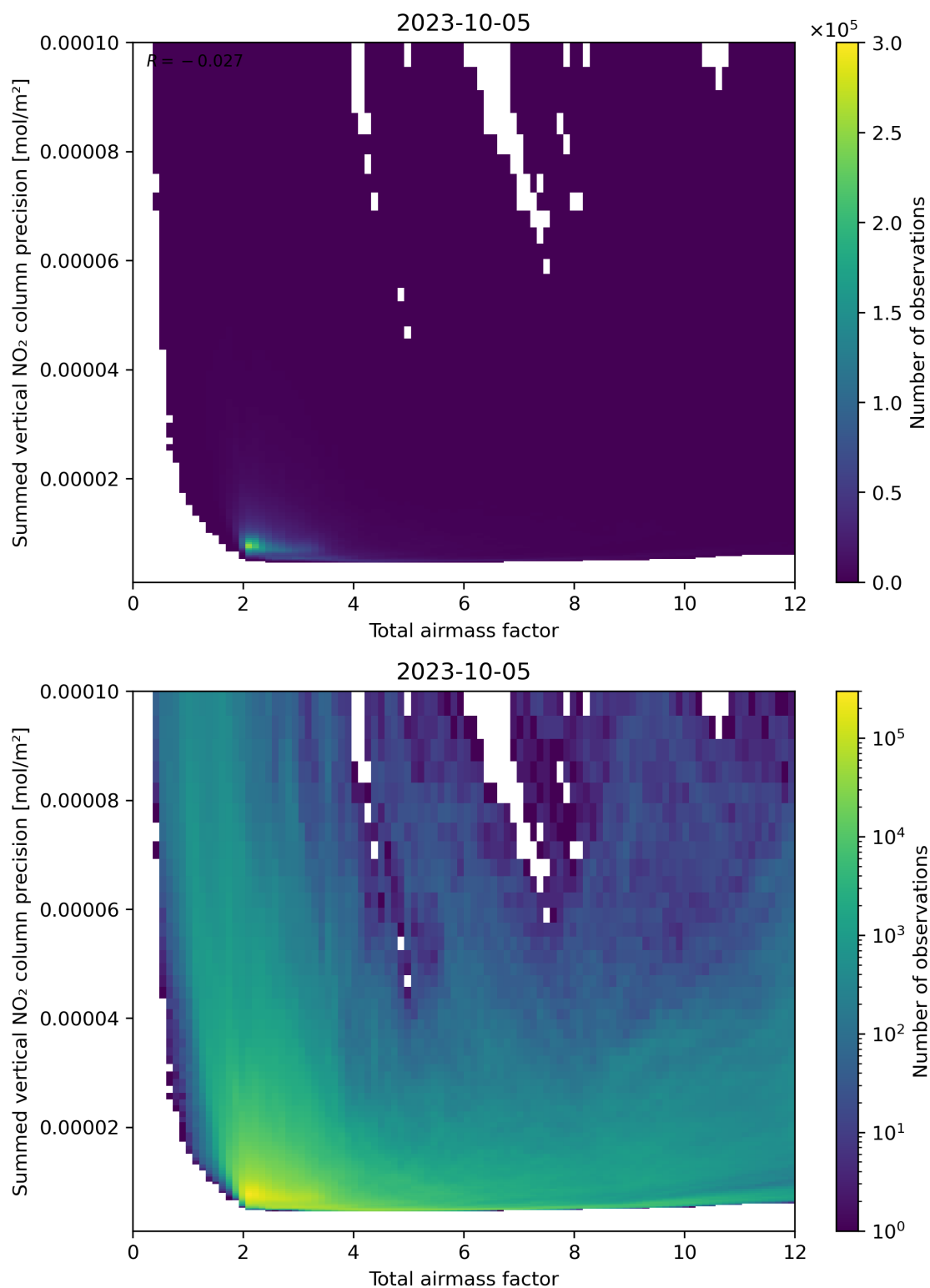
Figure 66: Scatter density plot of “Total airmass factor” against “Summed vertical NO 2 column precision” for 2023-10-04 to 2023-10-06.
