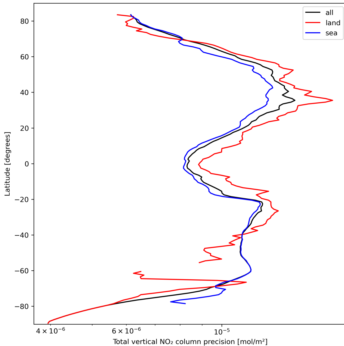
Figure 22: Zonal average of “Total vertical NO 2 column precision” for 2023-10-04 to 2023-10-06.
