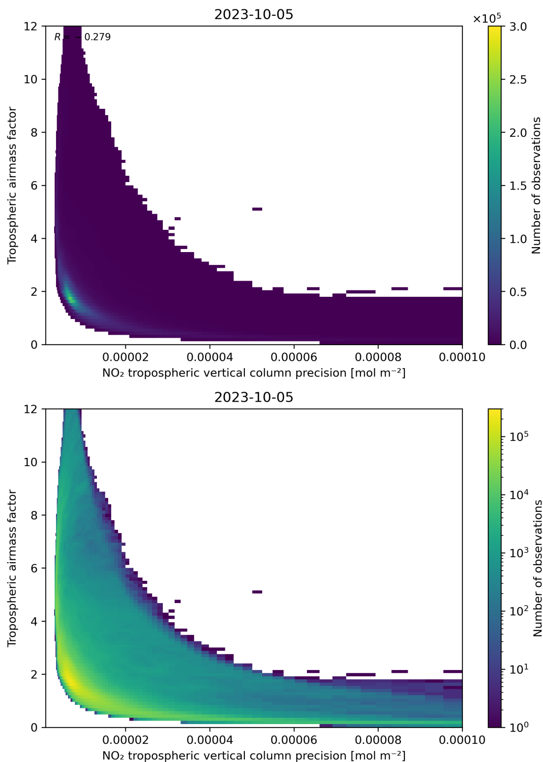
Figure 133: Scatter density plot of “NO 2 tropospheric vertical column precision” against “Tropospheric airmass factor” for 2023-10-04 to 2023-10-06.
