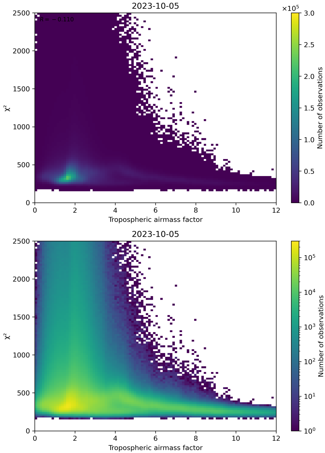
Figure 73: Scatter density plot of “Tropospheric airmass factor” against “ \chi^2 ” for 2023-10-04 to 2023-10-06.
