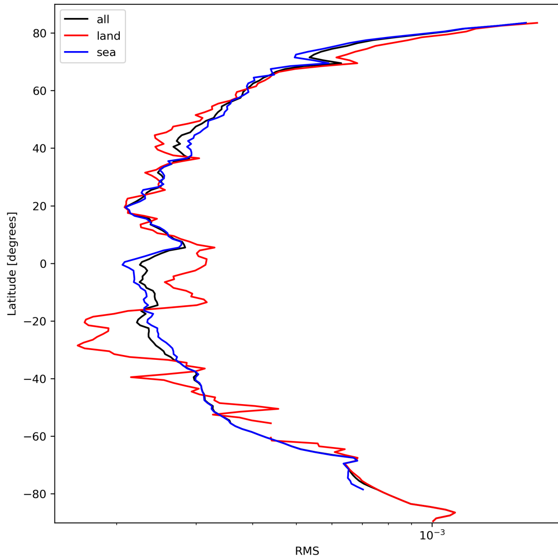
Figure 26: Zonal average of “RMS” for 2023-10-04 to 2023-10-06.
