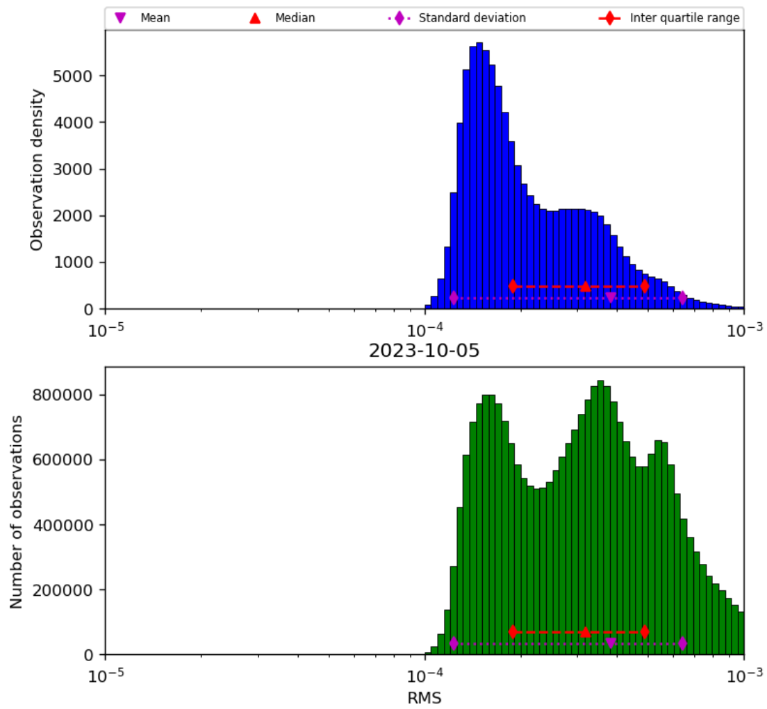
Figure 43: Histogram of “RMS” for 2023-10-04 to 2023-10-06
