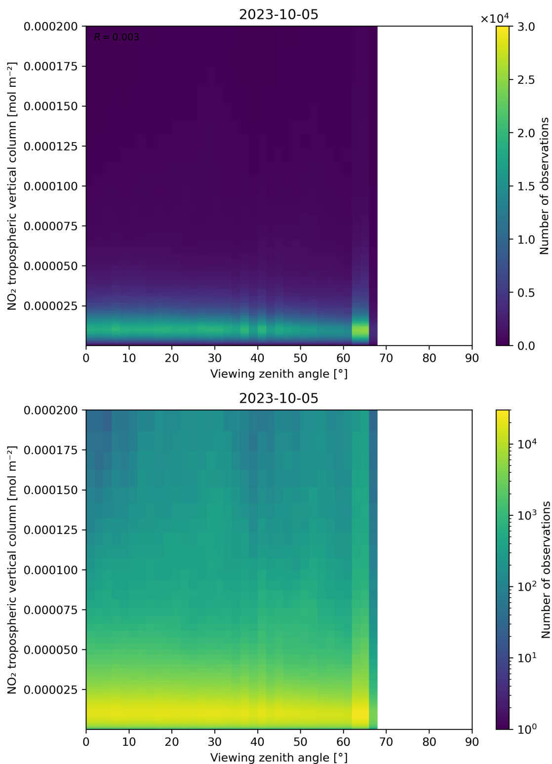
Figure 169: Scatter density plot of “Viewing zenith angle” against “NO 2 tropospheric vertical column” for 2023-10-04 to 2023-10-06.
