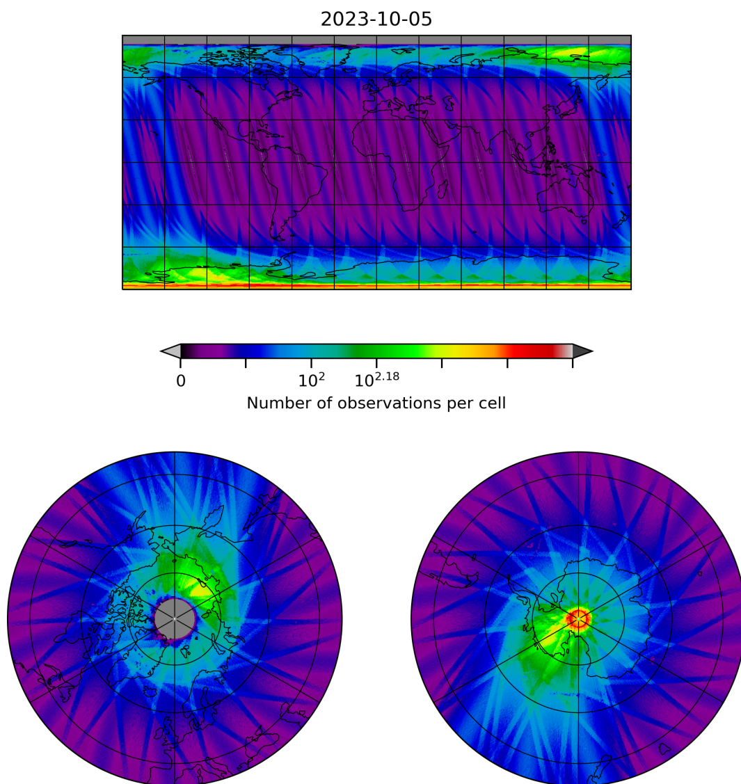
Figure 10: Map of the number of observations for 2023-10-04 to 2023-10-06
