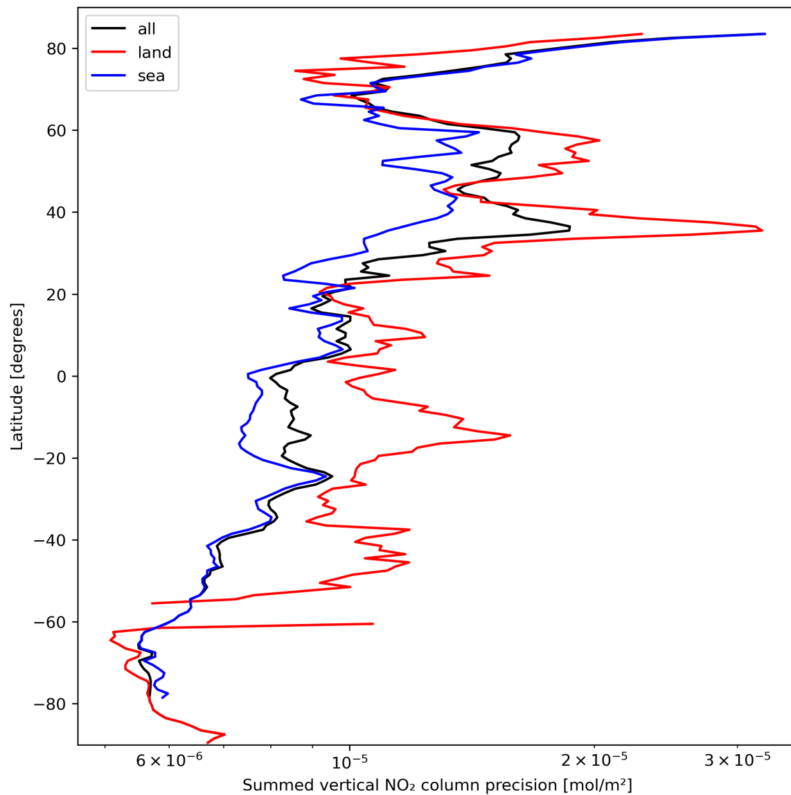
Figure 24: Zonal average of “Summed vertical NO 2 column precision” for 2023-10-04 to 2023-10-06.
