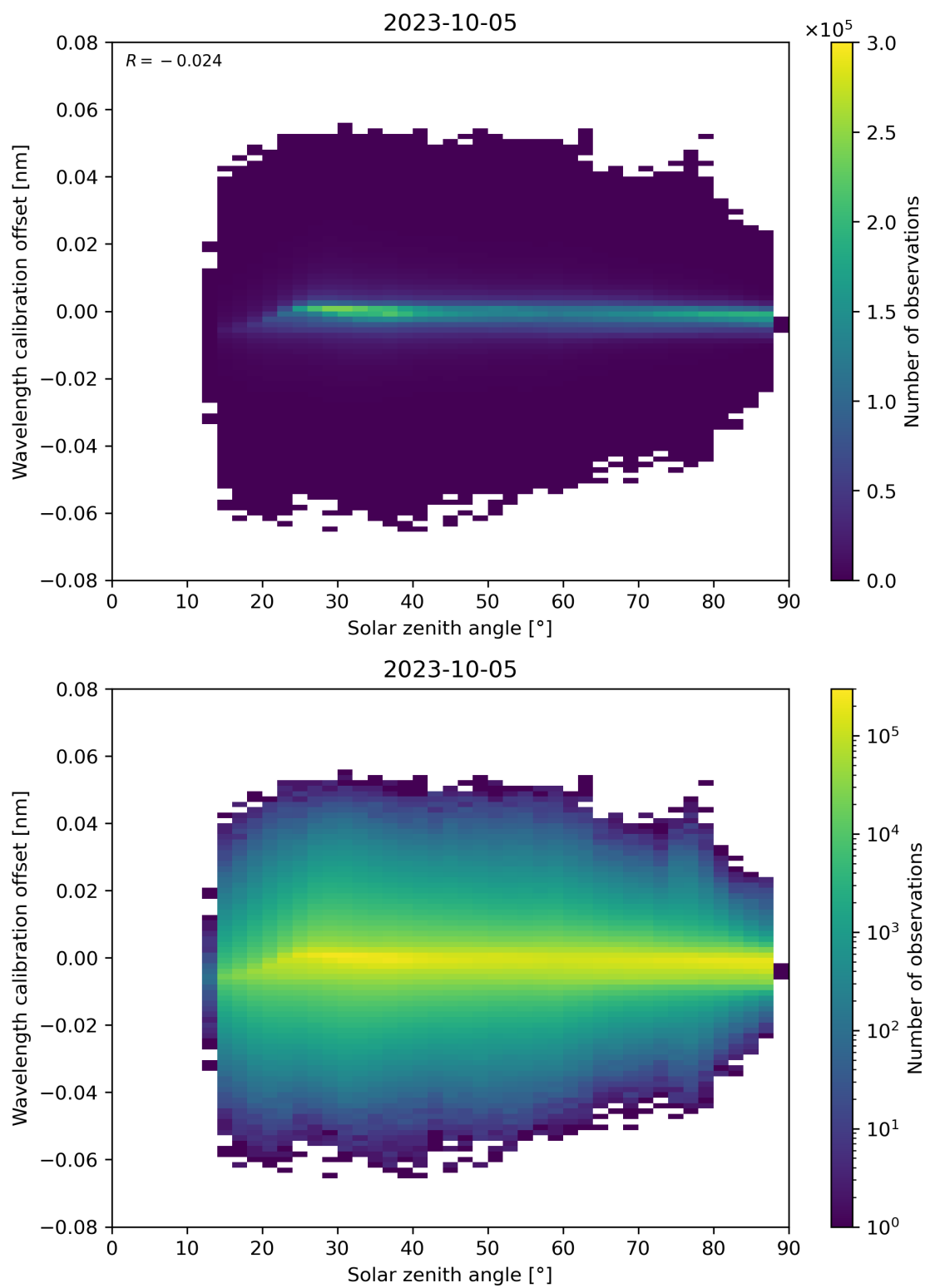
Figure 158: Scatter density plot of “Solar zenith angle” against “Wavelength calibration offset” for 2023-10-04 to 2023-10-06.
