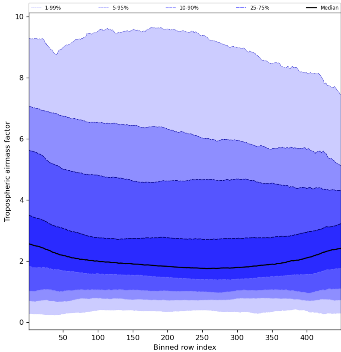
Figure 48: Along track statistics of “Tropospheric air mass factor” for 2023-10-04 to 2023-10-06
