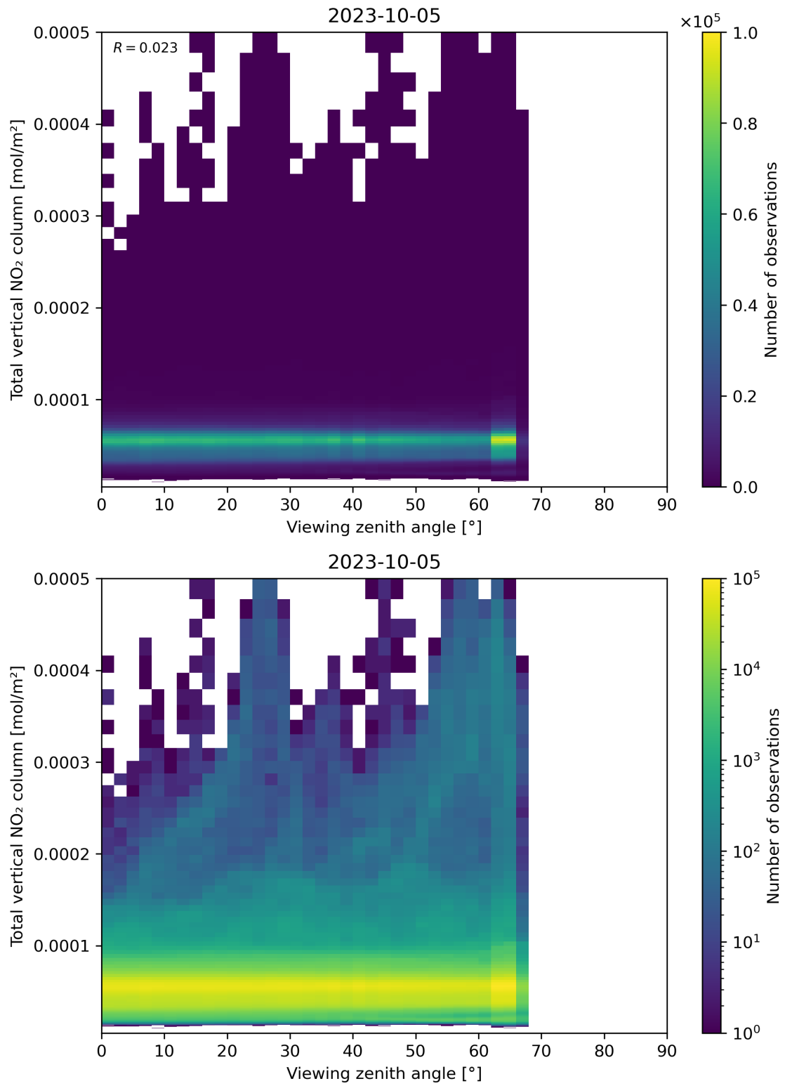
Figure 167: Scatter density plot of “Viewing zenith angle” against “Total vertical NO 2 column” for 2023-10-04 to 2023-10-06.
