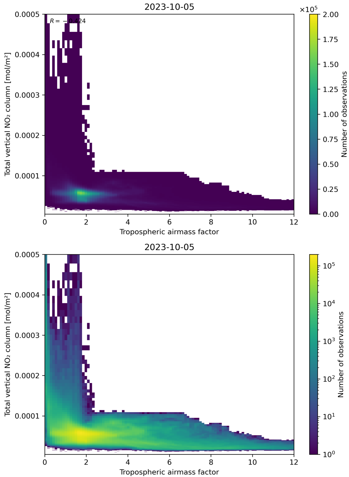
Figure 77: Scatter density plot of “Tropospheric airmass factor” against “Total vertical NO 2 column” for 2023-10-04 to 2023-10-06.
