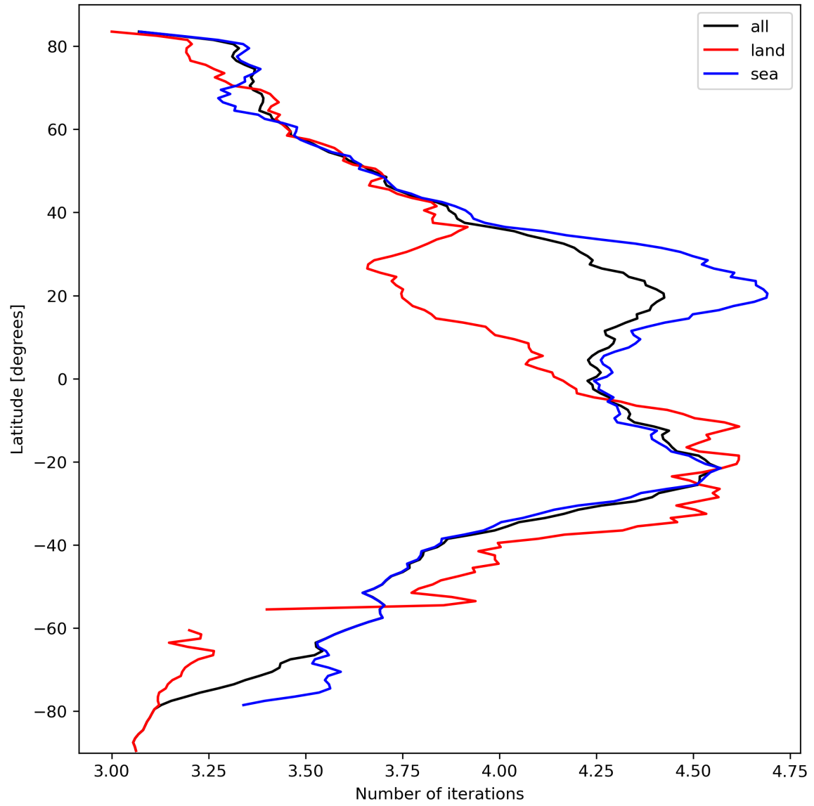
Figure 17: Zonal average of “Number of iterations” for 2023-10-04 to 2023-10-06.
