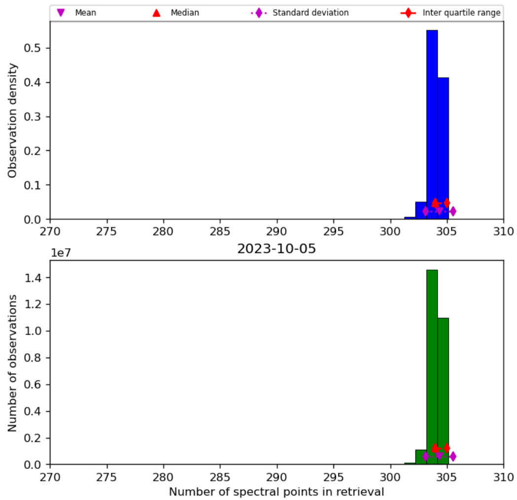
Figure 33: Histogram of “Number of spectral points in retrieval” for 2023-10-04 to 2023-10-06
