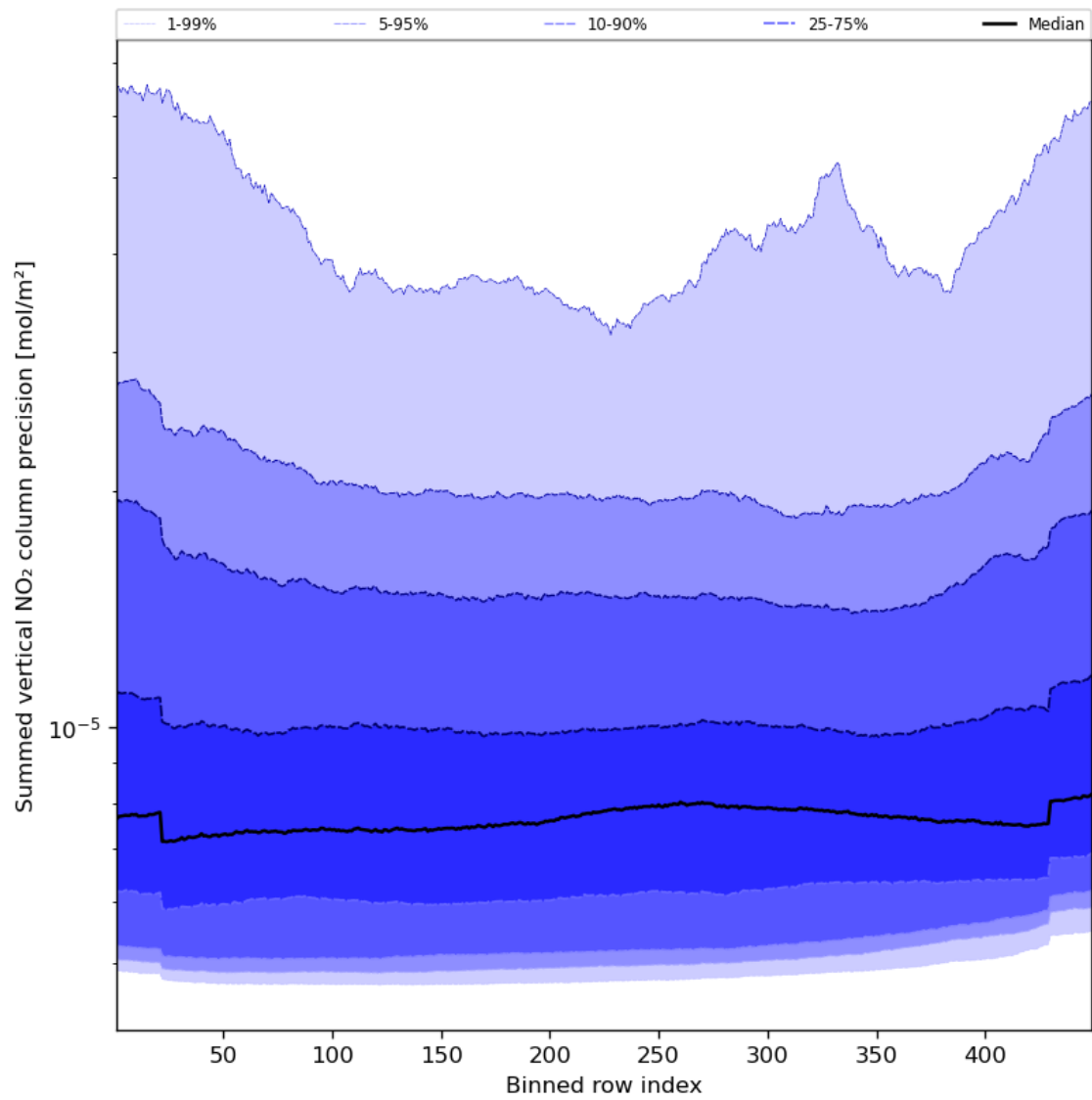
Figure 58: Along track statistics of “Summed vertical NO 2 column precision” for 2023-10-04 to 2023-10-06
