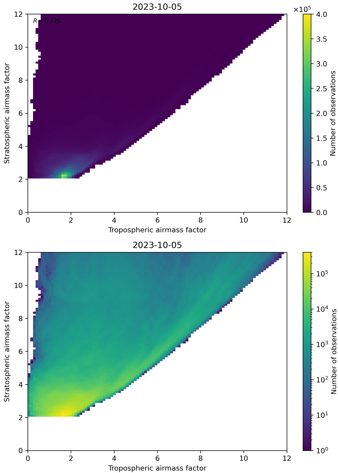
Figure 71: Scatter density plot of “Tropospheric airmass factor” against “Stratospheric airmass factor” for 2023-10-04 to 2023-10-06.
