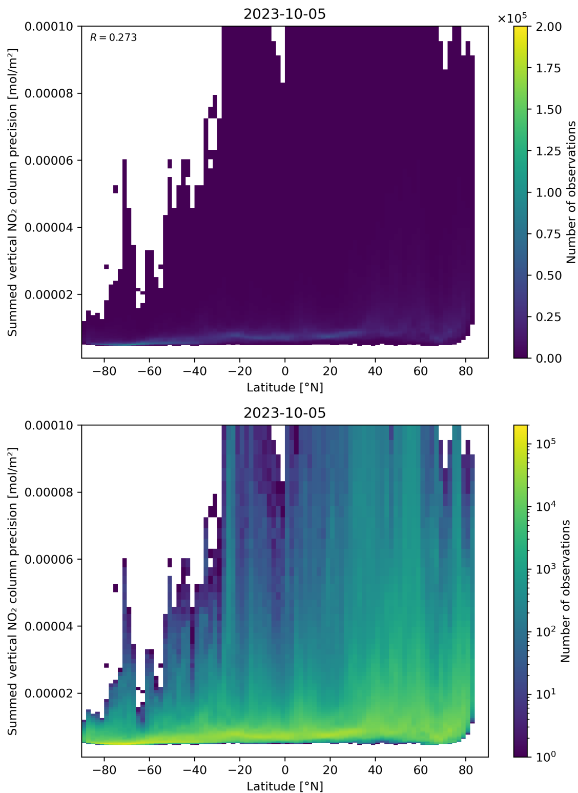
Figure 89: Scatter density plot of “Latitude” against “Summed vertical NO 2 column precision” for 2023-10-04 to 2023-10-06.
