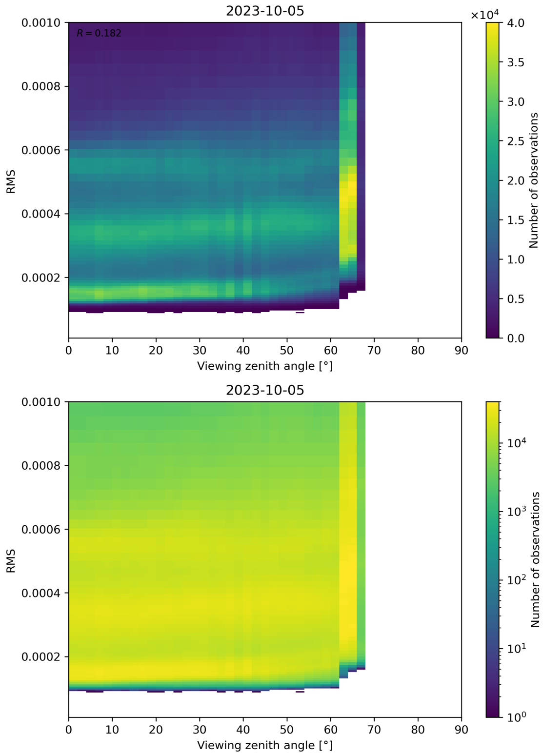
Figure 171: Scatter density plot of “Viewing zenith angle” against “RMS” for 2023-10-04 to 2023-10-06.
