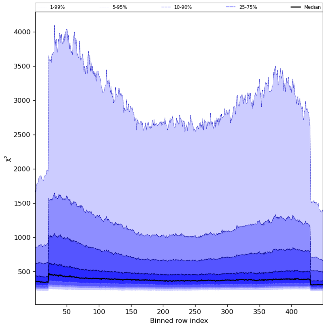
Figure 59: Along track statistics of “ \chi^2 ” for 2023-10-04 to 2023-10-06
