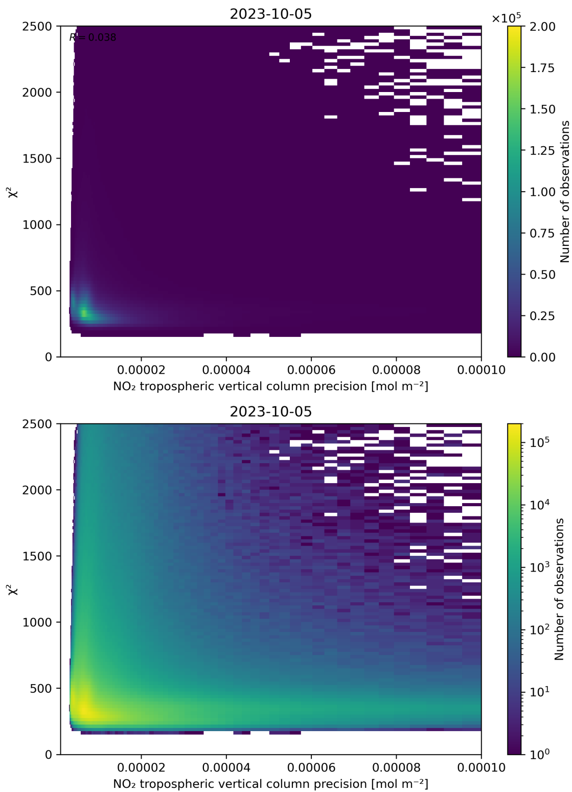
Figure 134: Scatter density plot of “NO 2 tropospheric vertical column precision” against “ \chi^2 ” for 2023-10-04 to 2023-10-06.
