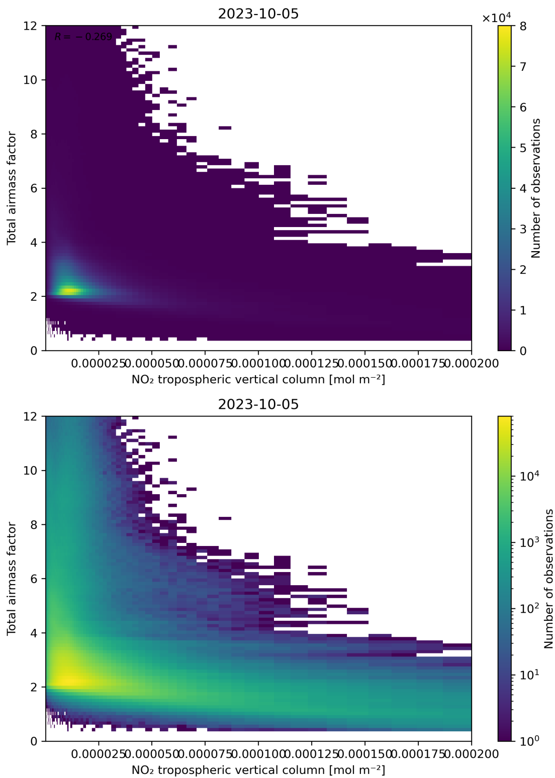
Figure 122: Scatter density plot of “NO 2 tropospheric vertical column” against “Total air mass factor” for 2023-10-04 to 2023-10-06.
