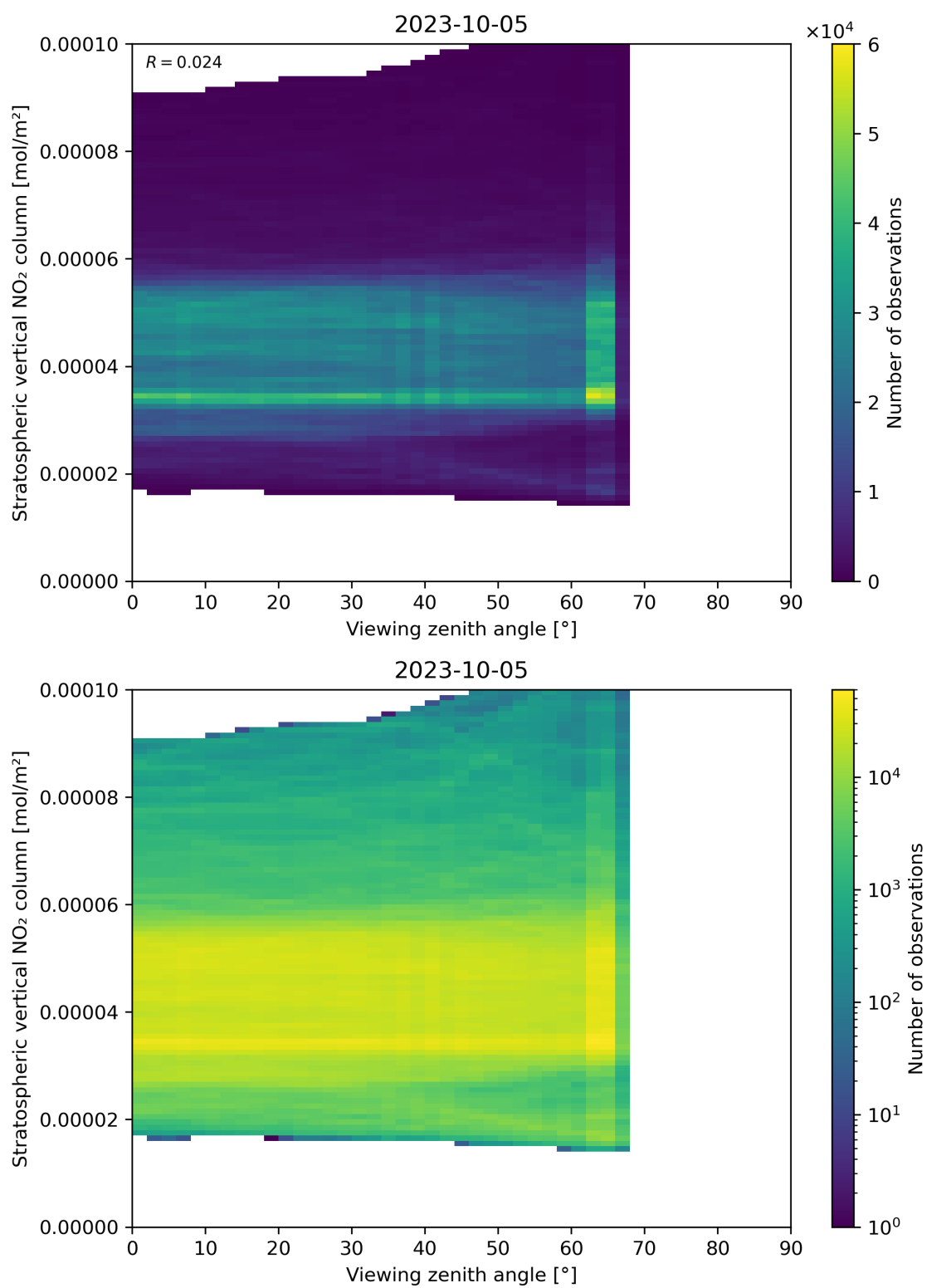
Figure 164: Scatter density plot of “Viewing zenith angle” against “Stratospheric vertical NO 2 column” for 2023-10-04 to 2023-10-06.
