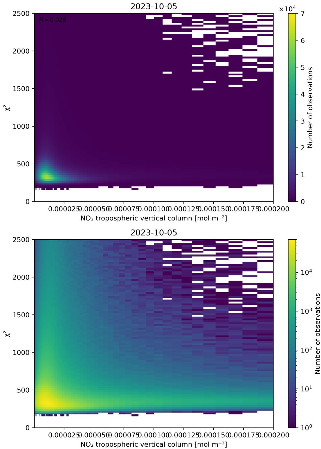
Figure 124: Scatter density plot of “NO 2 tropospheric vertical column” against “ \chi^2 ” for 2023-10-04 to 2023-10-06.
