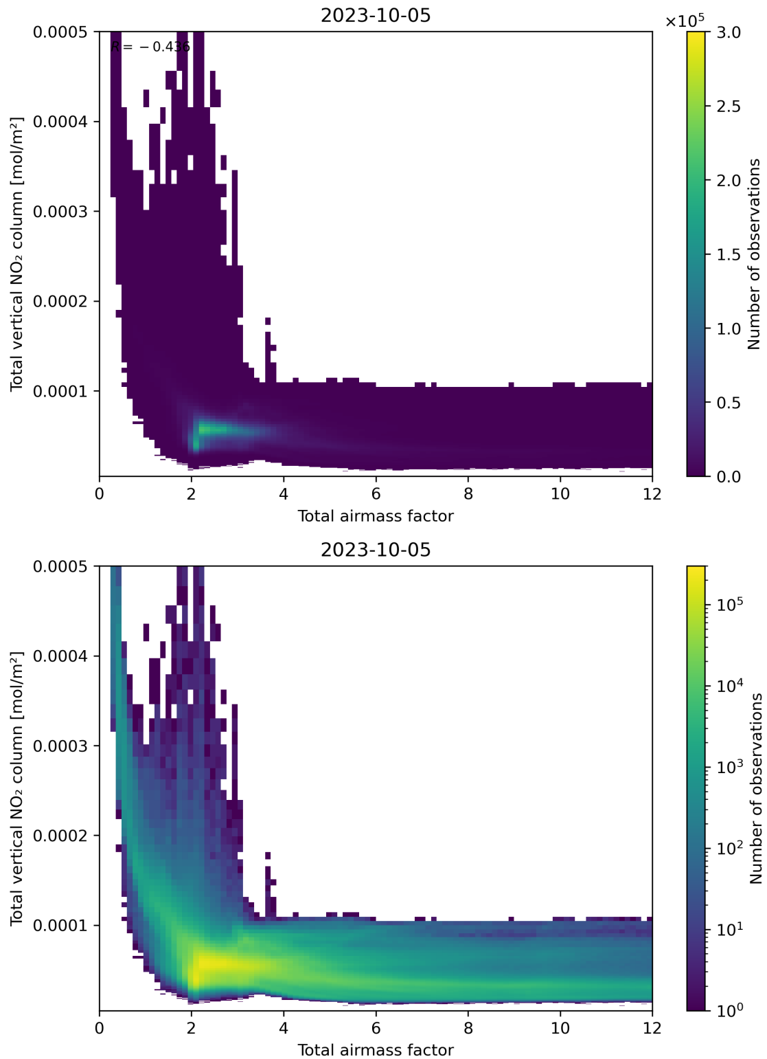
Figure 67: Scatter density plot of “Total airmass factor” against “Total vertical NO 2 column” for 2023-10-04 to 2023-10-06.
