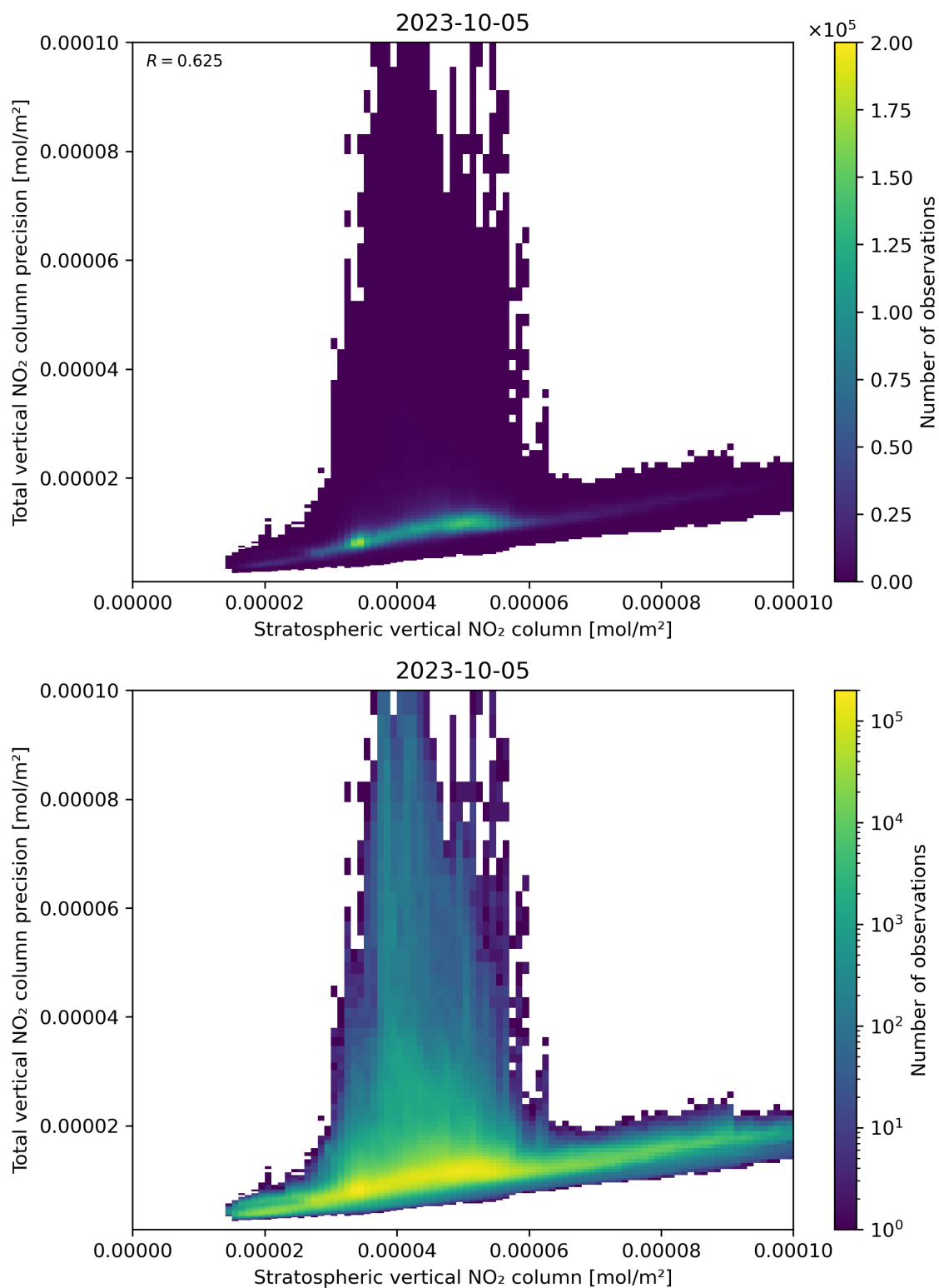
Figure 101: Scatter density plot of “Stratospheric vertical NO 2 column” against “Total vertical NO 2 column precision” for 2023-10-04 to 2023-10-06.
