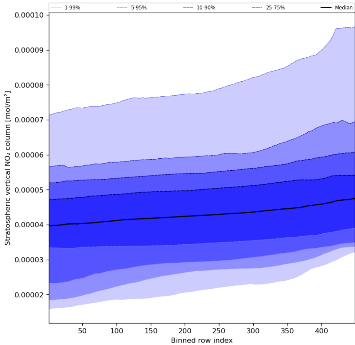
Figure 53: Along track statistics of “Stratospheric vertical NO 2 column” for 2023-10-04 to 2023-10-06
