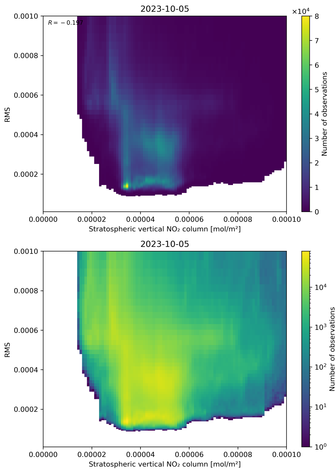
Figure 102: Scatter density plot of “Stratospheric vertical NO 2 column” against “RMS” for 2023-10-04 to 2023-10-06.
