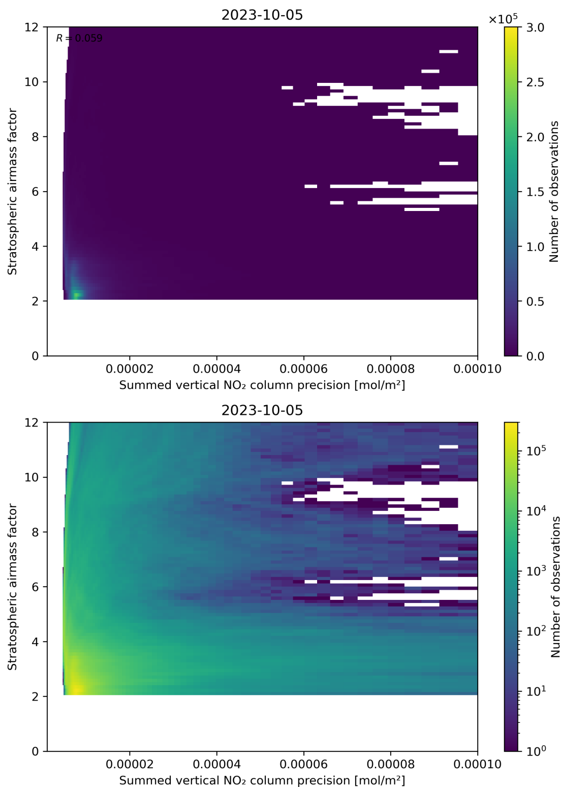
Figure 106: Scatter density plot of “Summed vertical NO 2 column precision” against “Stratospheric airmass factor” for 2023-10-04 to 2023-10-06.
