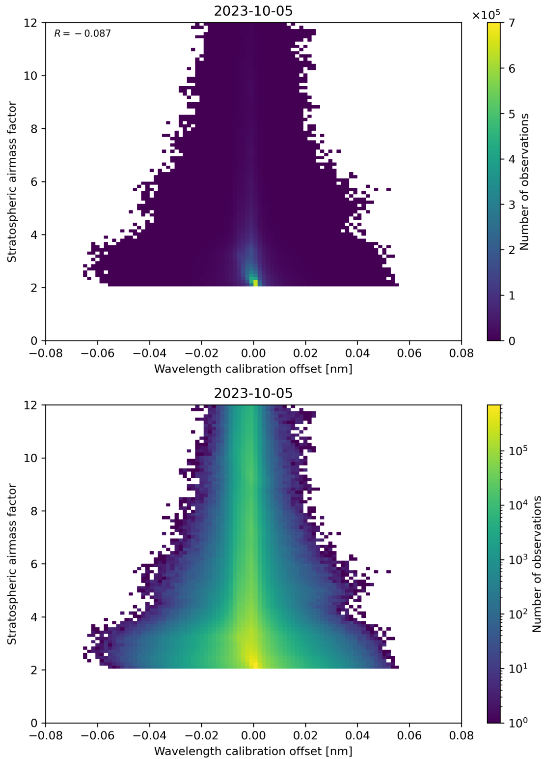
Figure 174: Scatter density plot of “Wavelength calibration offset” against “Stratospheric air mass factor” for 2023-10-04 to 2023-10-06.
