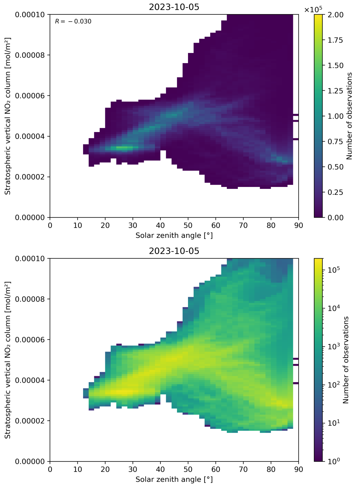
Figure 150: Scatter density plot of “Solar zenith angle” against “Stratospheric vertical NO 2 column” for 2023-10-04 to 2023-10-06.
