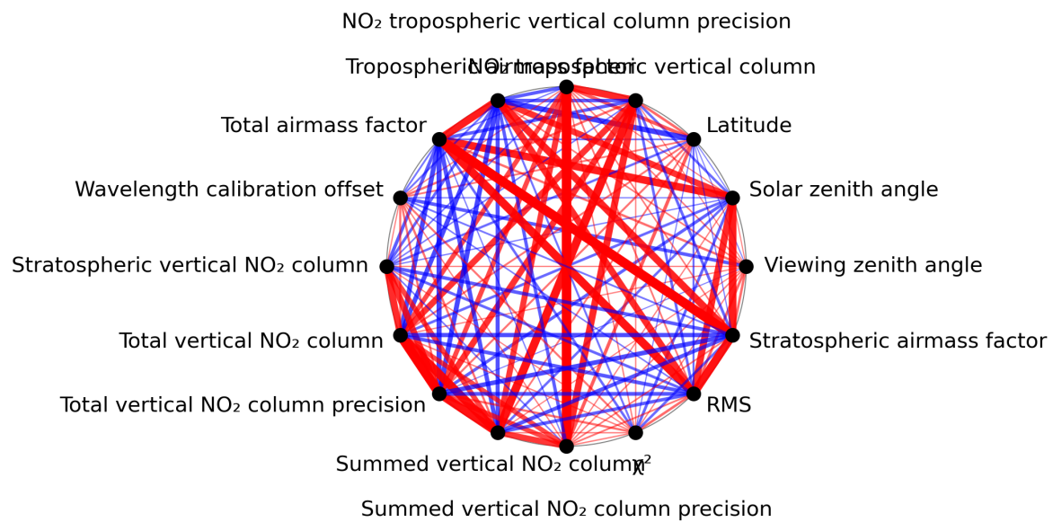
Figure 1: Map of correlation graph for 2023-10-04 to 2023-10-06.
