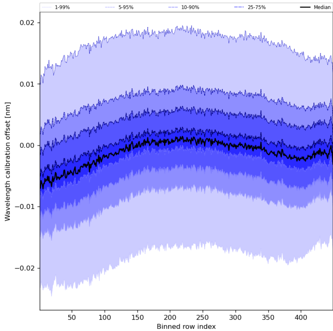
Figure 52: Along track statistics of “Wavelength calibration offset” for 2023-10-04 to 2023-10-06
