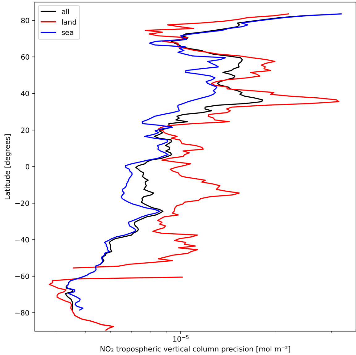
Figure 13: Zonal average of “NO 2 tropospheric vertical column precision” for 2023-10-04 to 2023-10-06.
