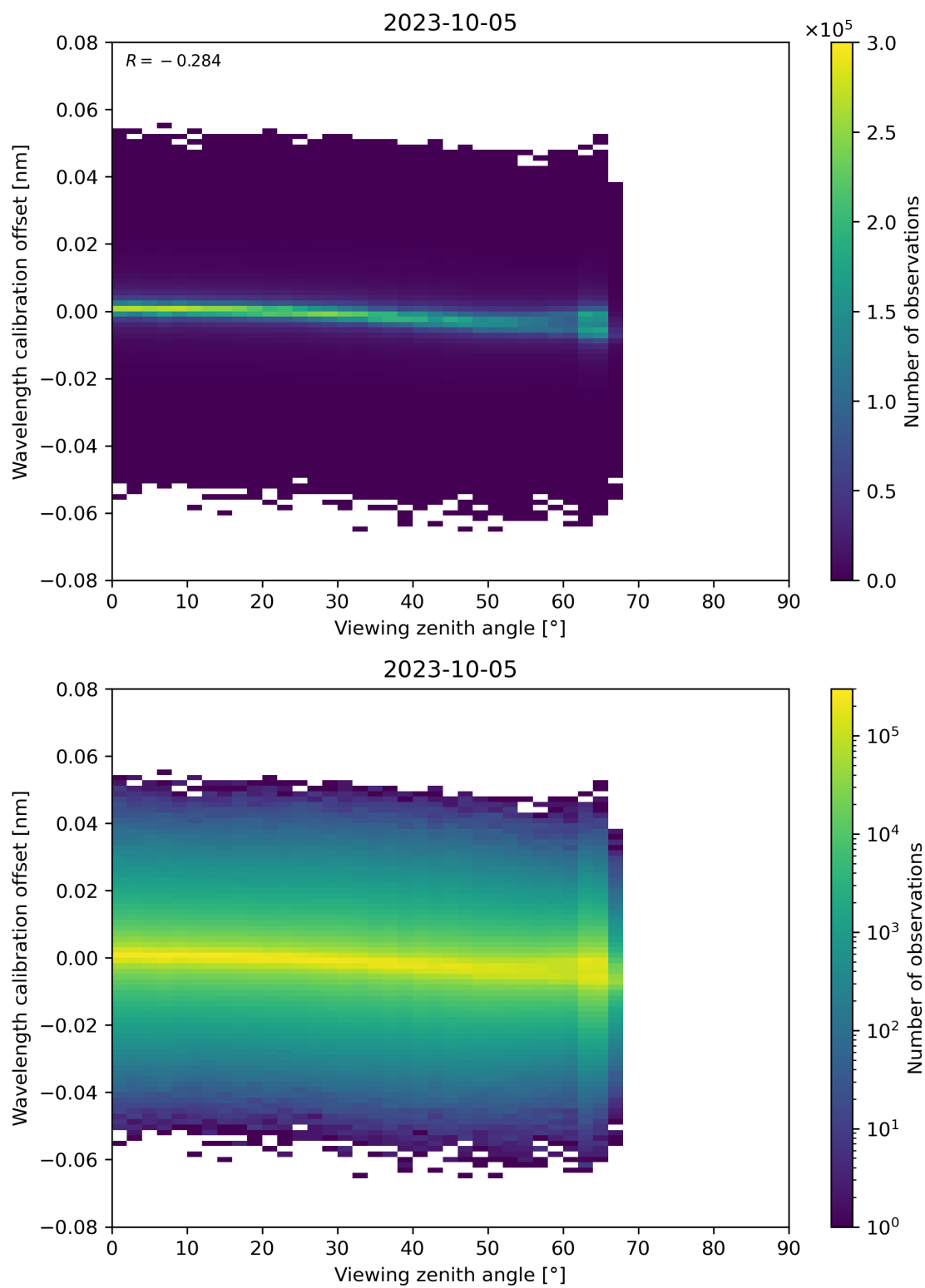
Figure 173: Scatter density plot of “Viewing zenith angle” against “Wavelength calibration offset” for 2023-10-04 to 2023-10-06.
