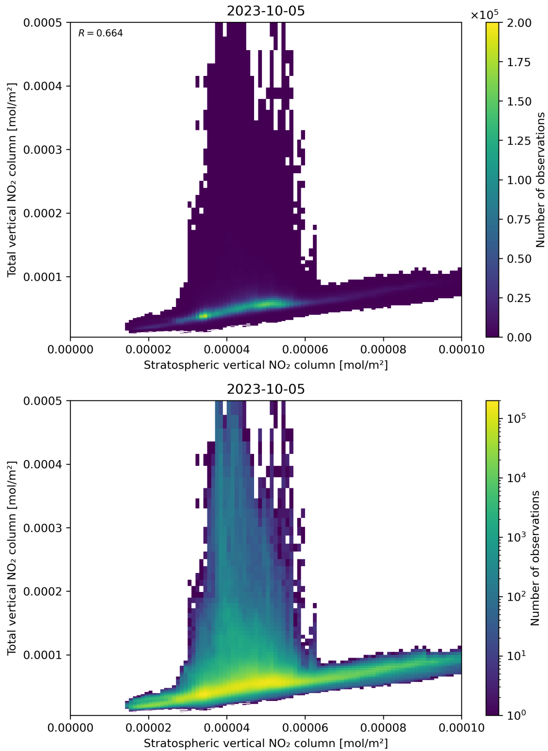
Figure 100: Scatter density plot of “Stratospheric vertical NO 2 column” against “Total vertical NO 2 column” for 2023-10-04 to 2023-10-06.
