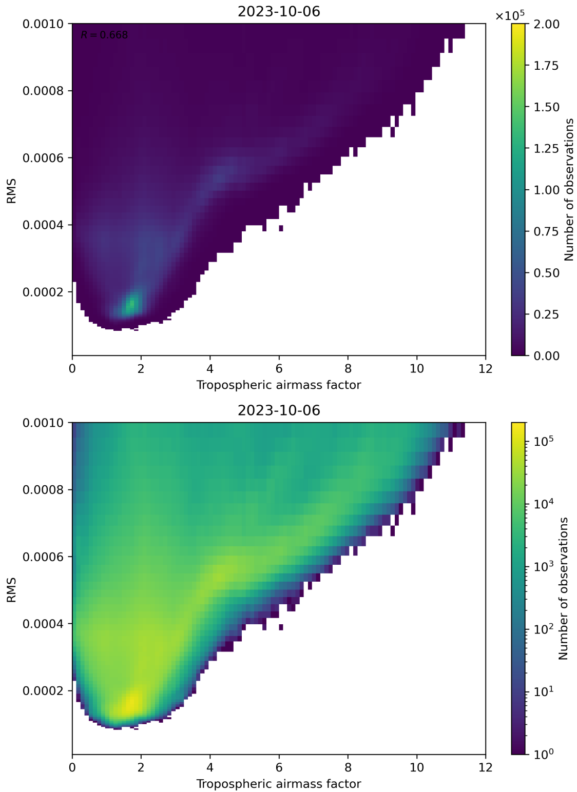
Figure 79: Scatter density plot of “Tropospheric airmass factor” against “RMS” for 2023-10-06 to 2023-10-07.
