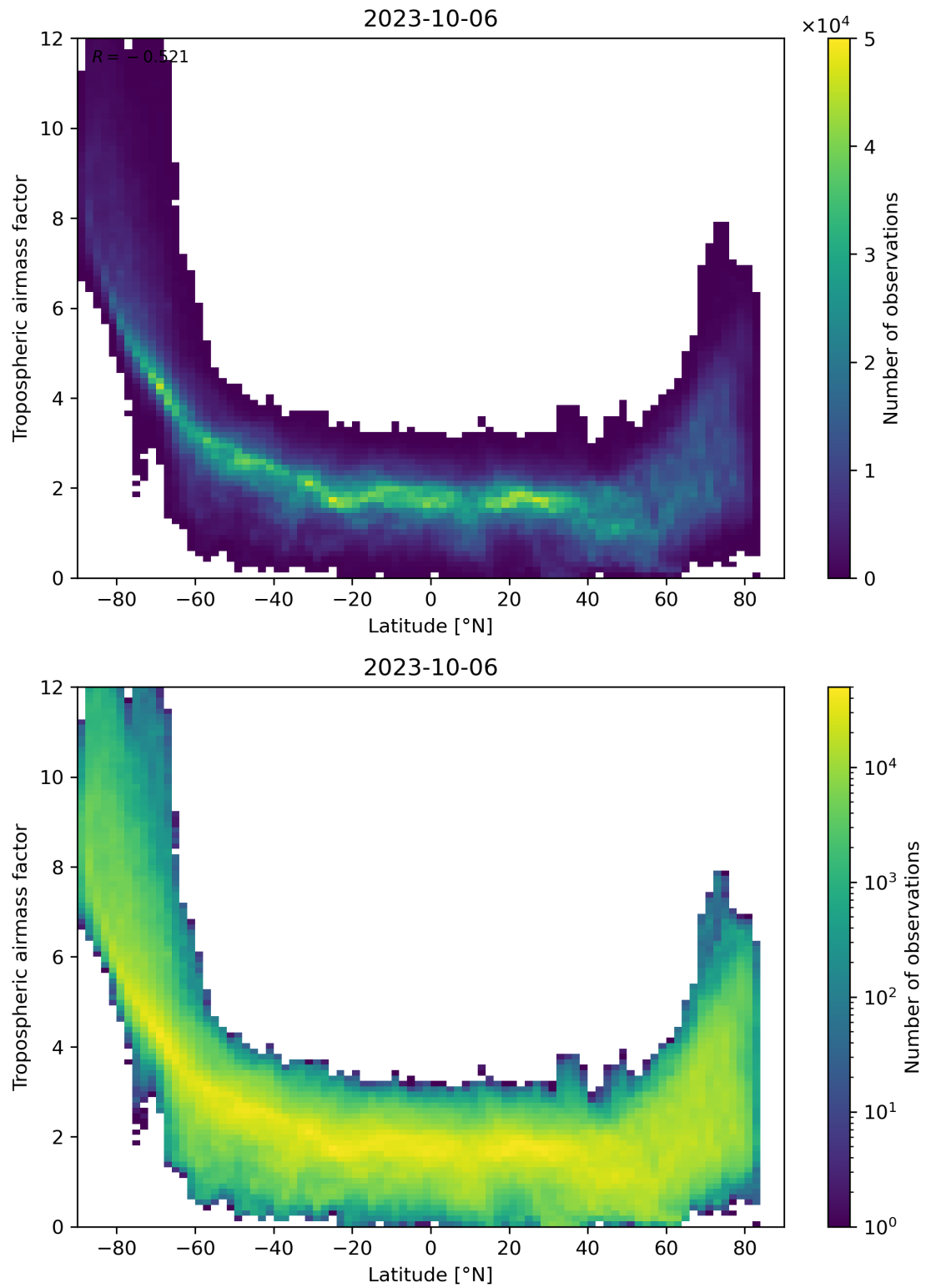
Figure 85: Scatter density plot of “Latitude” against “Tropospheric airmass factor” for 2023-10-06 to 2023-10-07.
