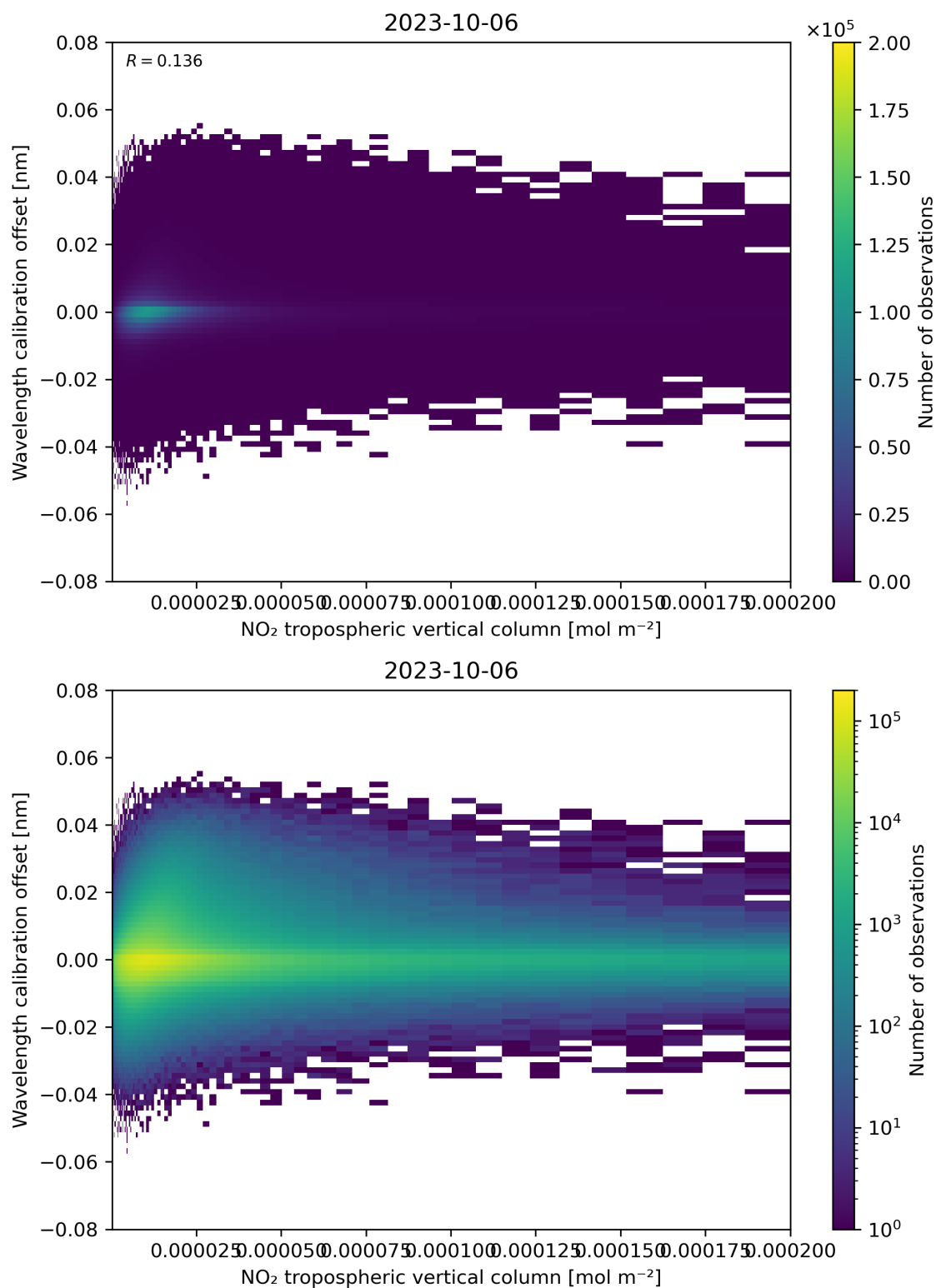
Figure 143: Scatter density plot of “NO 2 tropospheric vertical column” against “Wavelength calibration offset” for 2023-10-06 to 2023-10-07.
