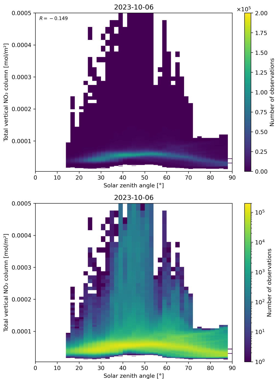
Figure 153: Scatter density plot of “Solar zenith angle” against “Total vertical NO 2 column” for 2023-10-06 to 2023-10-07.
