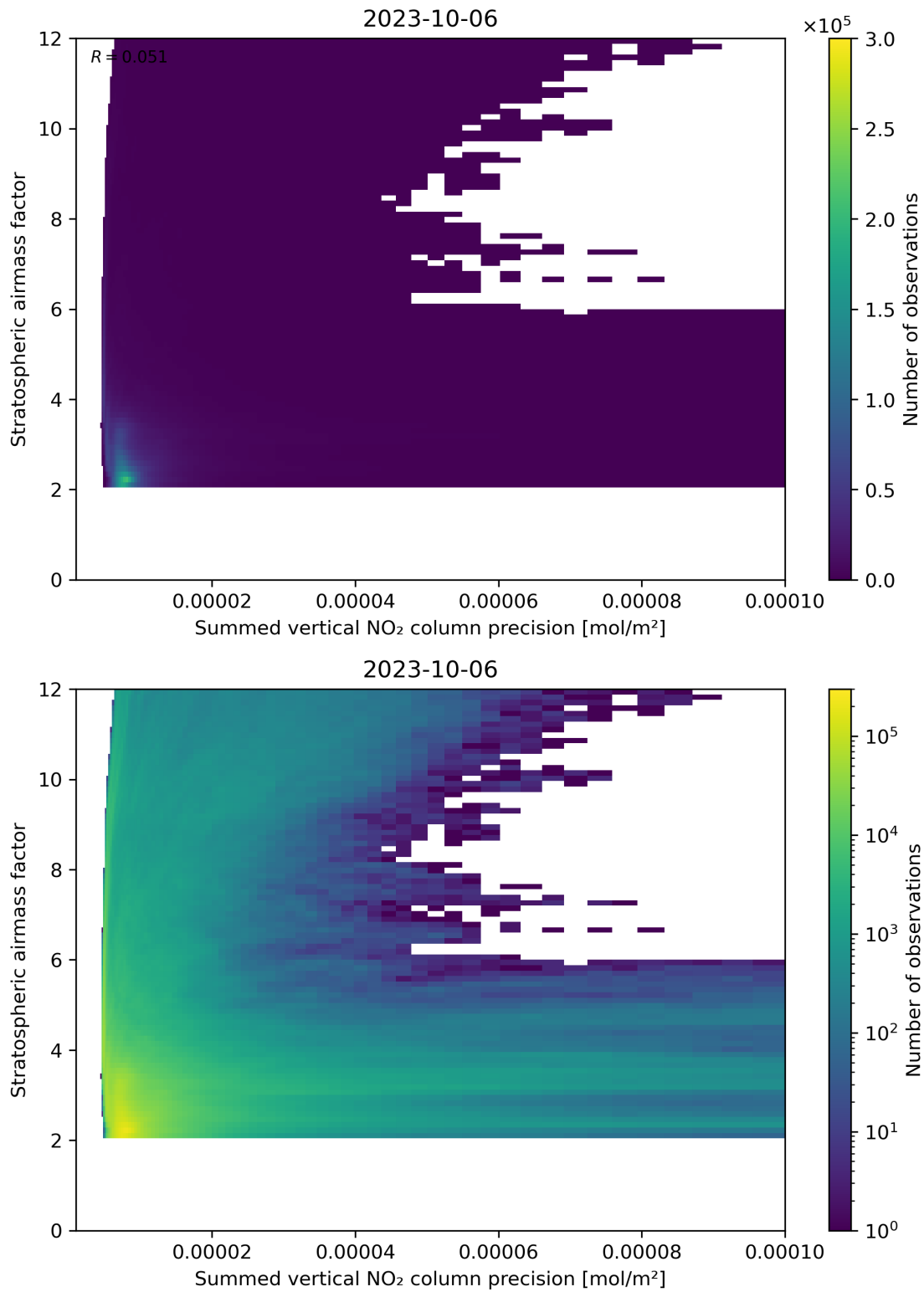
Figure 106: Scatter density plot of “Summed vertical NO 2 column precision” against “Stratospheric airmass factor” for 2023-10-06 to 2023-10-07.
