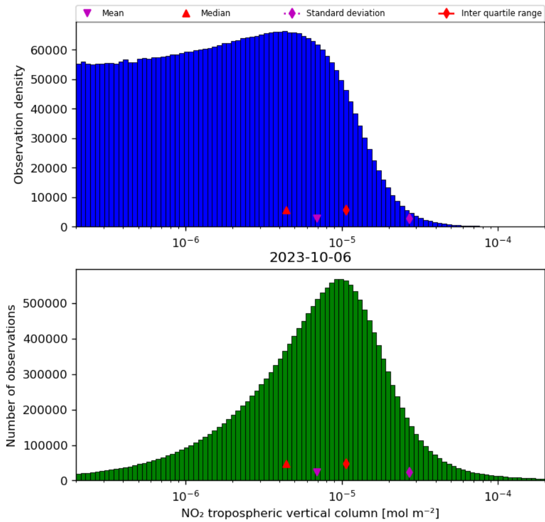
Figure 29: Histogram of “NO 2 tropospheric vertical column” for 2023-10-06 to 2023-10-07
