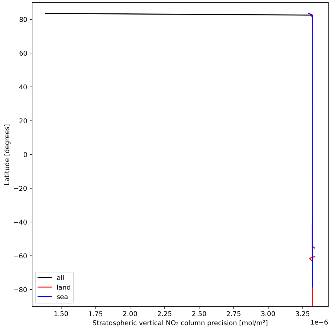
Figure 20: Zonal average of “Stratospheric vertical NO 2 column precision” for 2023-10-06 to 2023-10-07.
