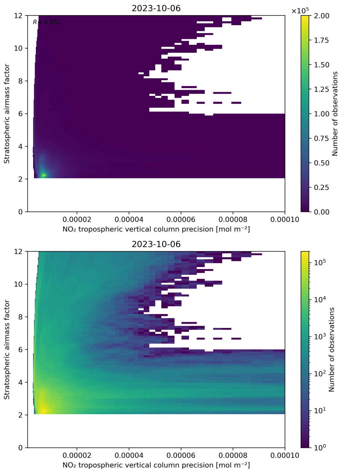
Figure 131: Scatter density plot of “NO 2 tropospheric vertical column precision” against “Stratospheric airmass factor” for 2023-10-06 to 2023-10-07.
