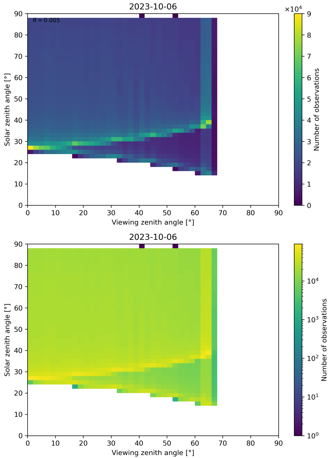
Figure 172: Scatter density plot of “Viewing zenith angle” against “Solar zenith angle” for 2023-10-06 to 2023-10-07.
