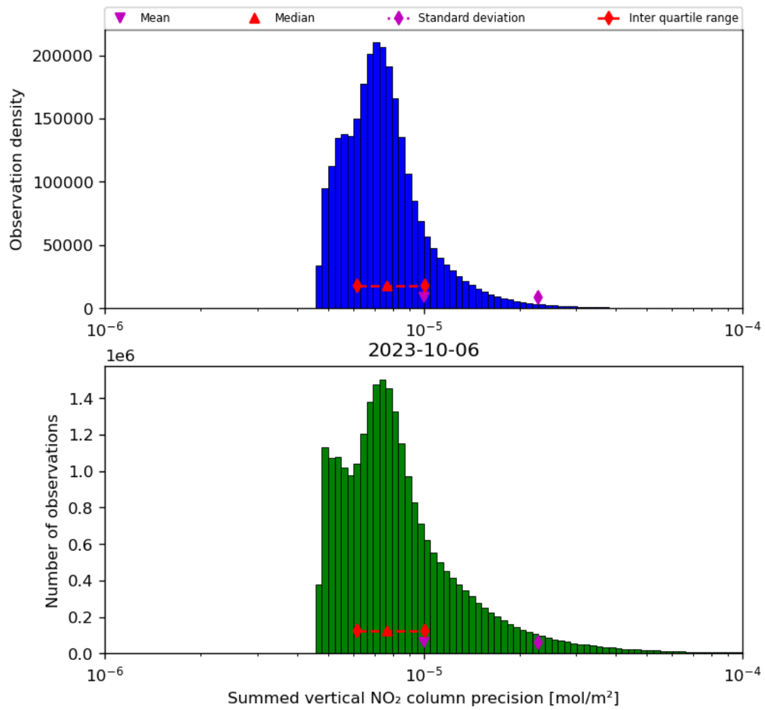
Figure 41: Histogram of “Summed vertical NO 2 column precision” for 2023-10-06 to 2023-10-07
