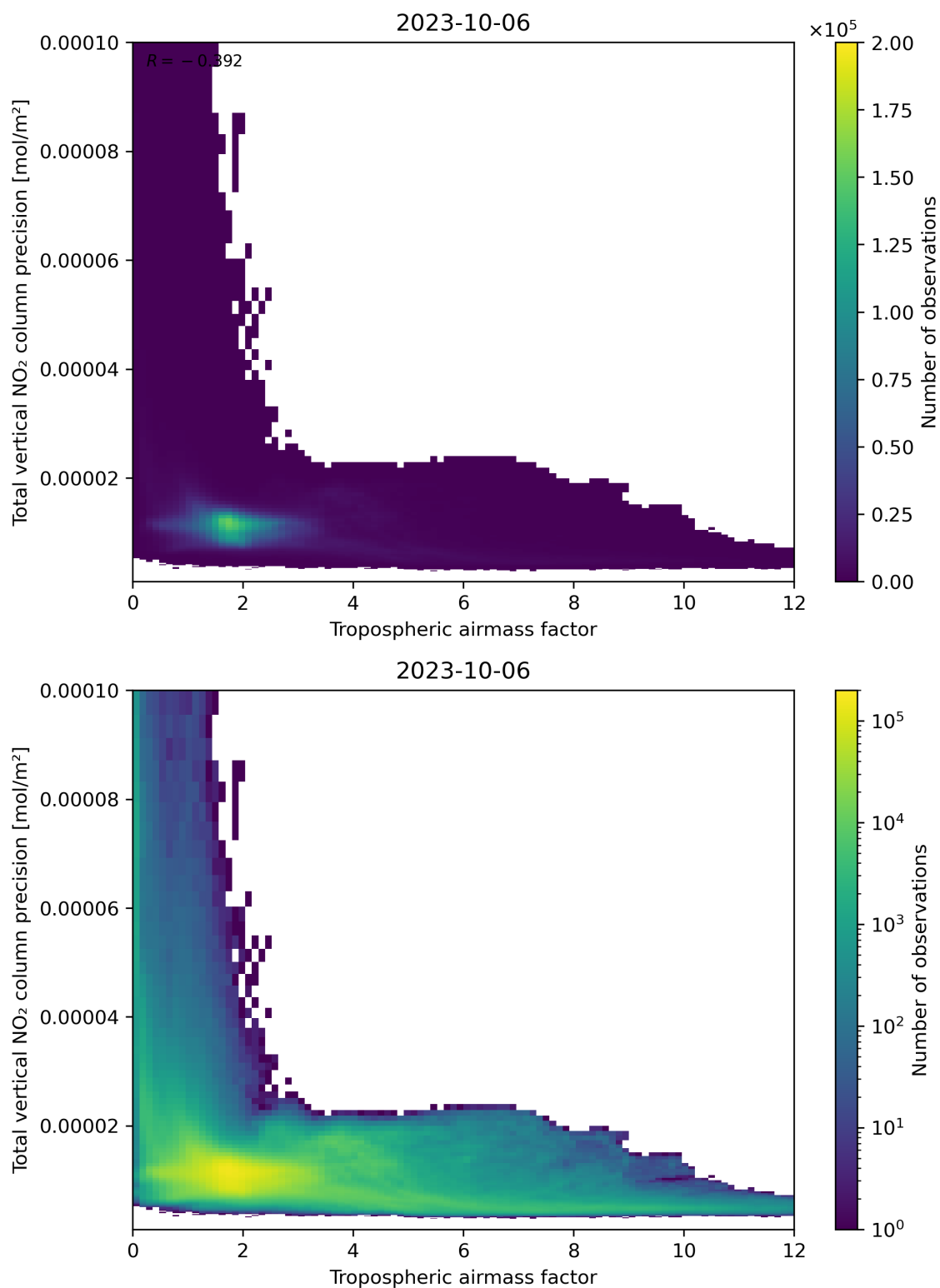
Figure 78: Scatter density plot of “Tropospheric air mass factor” against “Total vertical NO 2 column precision” for 2023-10-06 to 2023-10-07.
