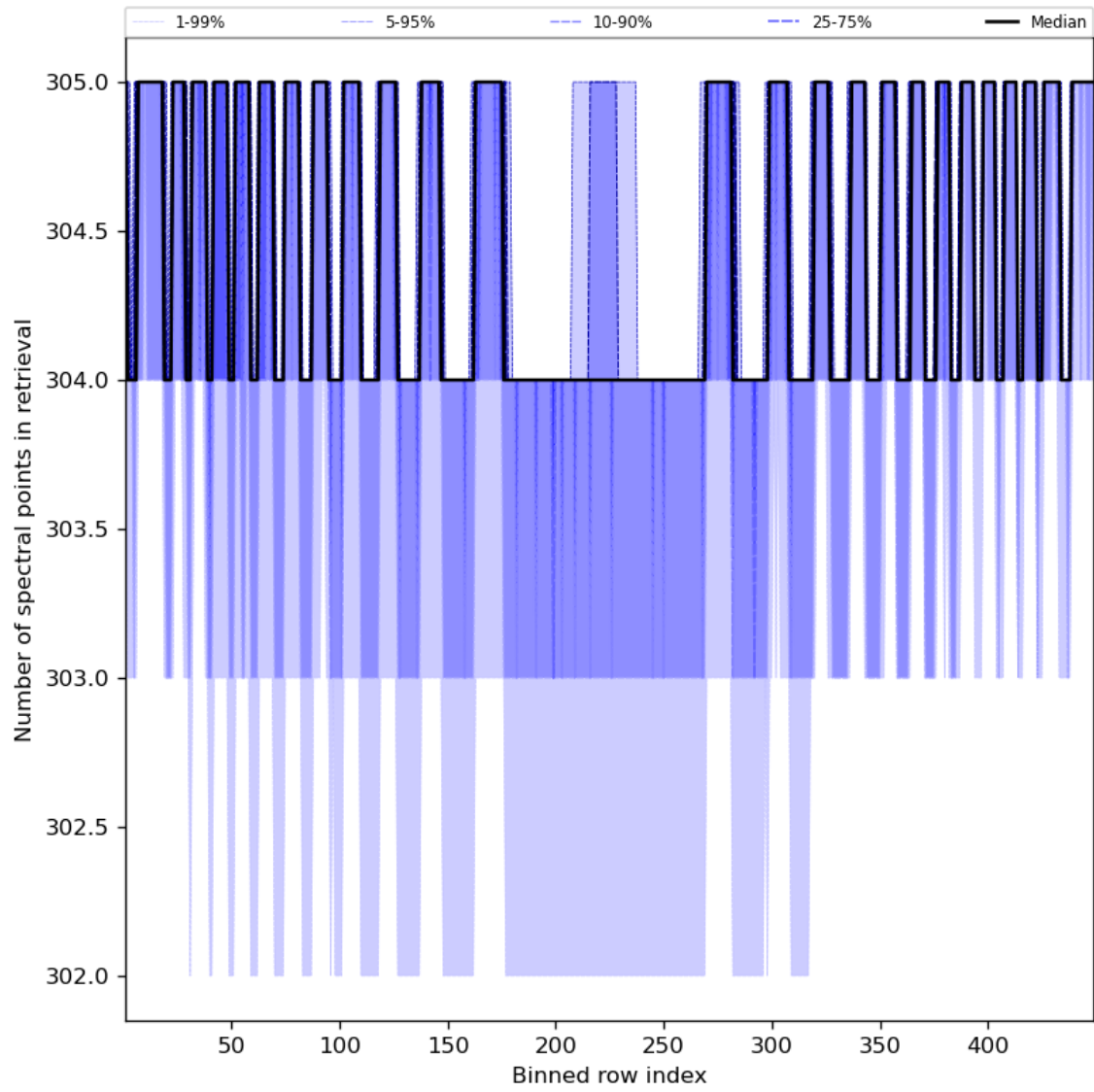
Figure 50: Along track statistics of “Number of spectral points in retrieval” for 2023-10-06 to 2023-10-07
