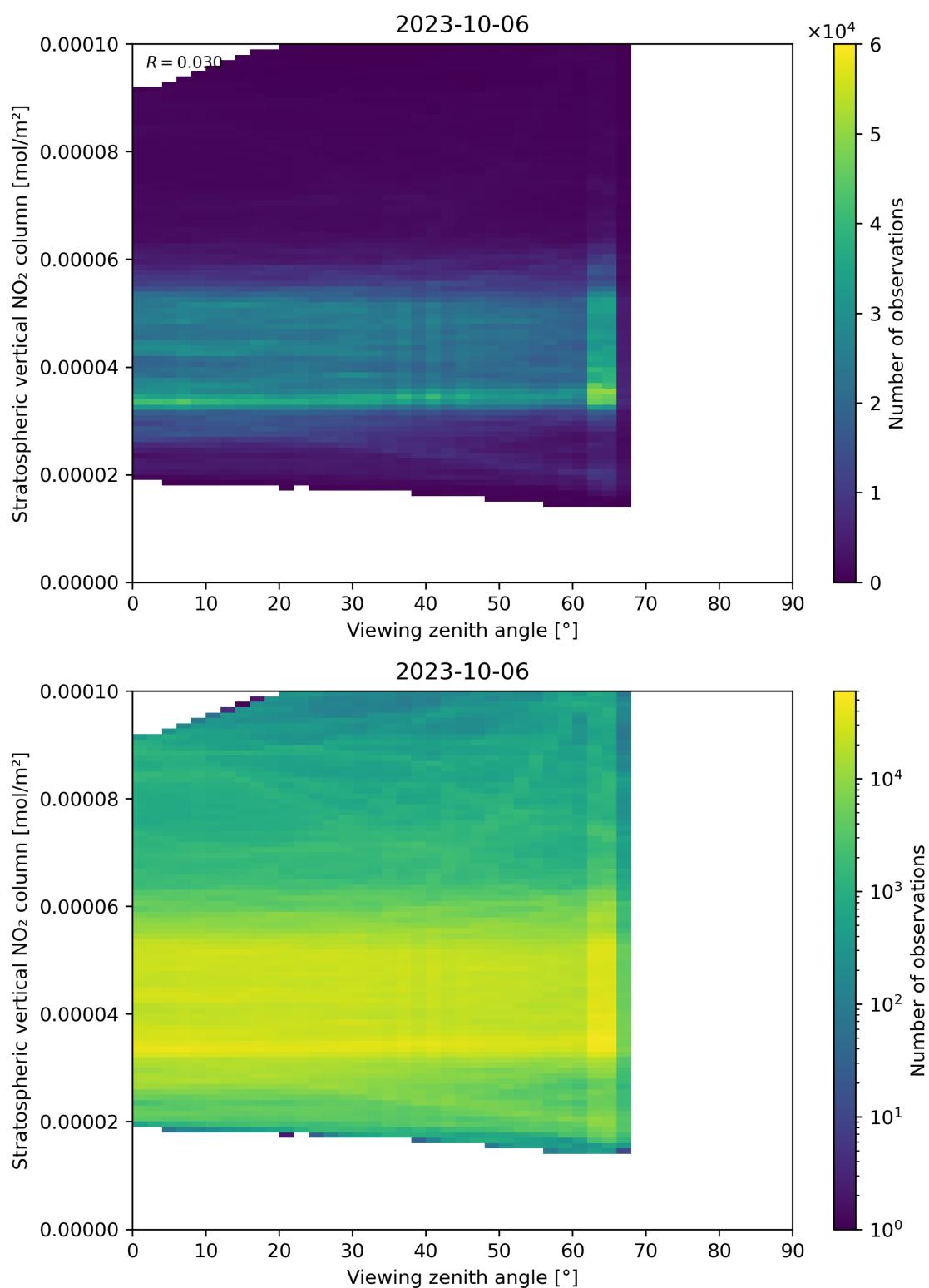
Figure 164: Scatter density plot of “Viewing zenith angle” against “Stratospheric vertical NO 2 column” for 2023-10-06 to 2023-10-07.
