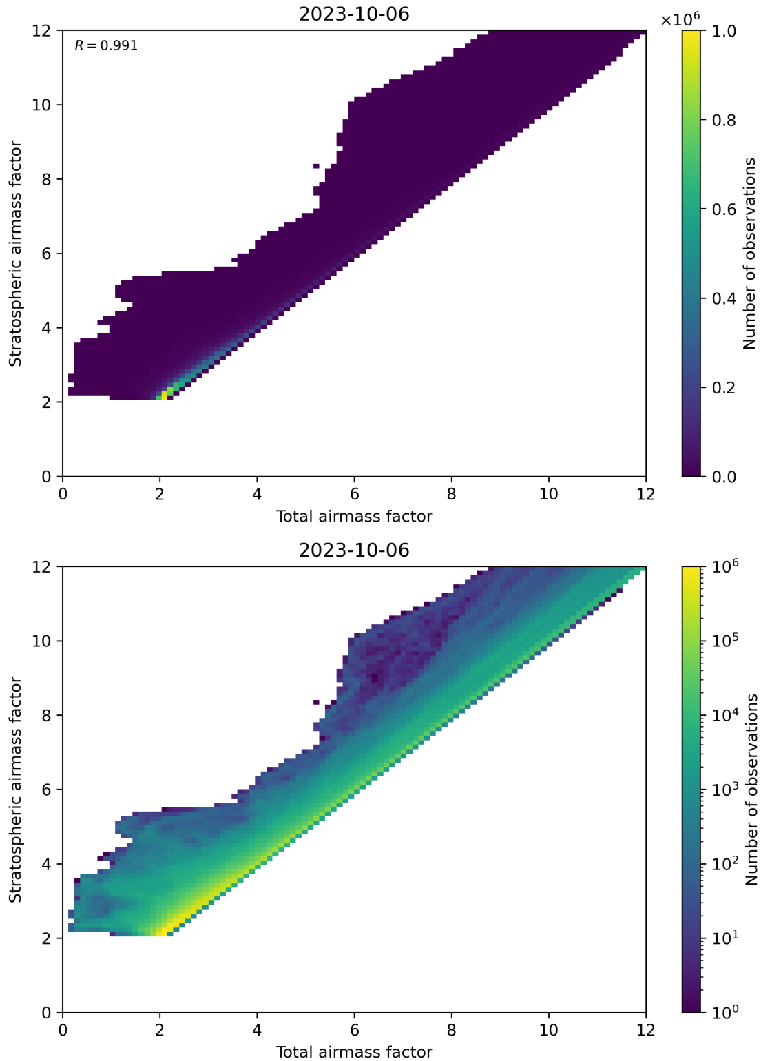
Figure 62: Scatter density plot of “Total airmass factor” against “Stratospheric airmass factor” for 2023-10-06 to 2023-10-07.
