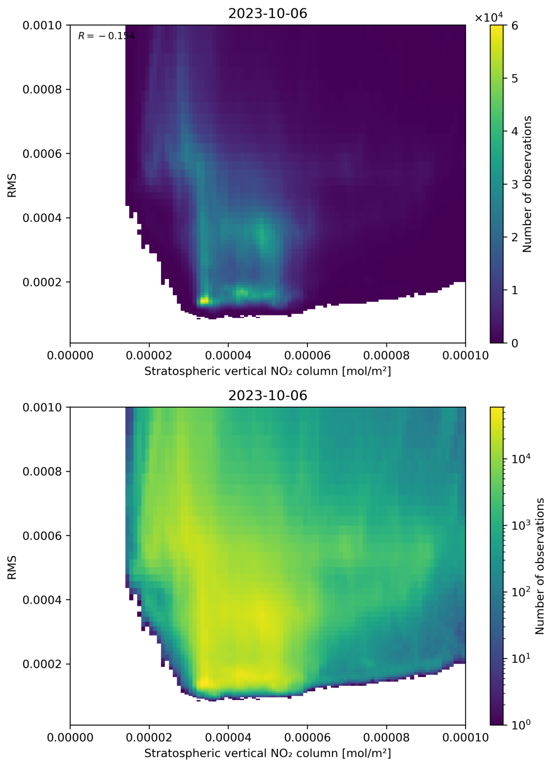
Figure 102: Scatter density plot of “Stratospheric vertical NO 2 column” against “RMS” for 2023-10-06 to 2023-10-07.
