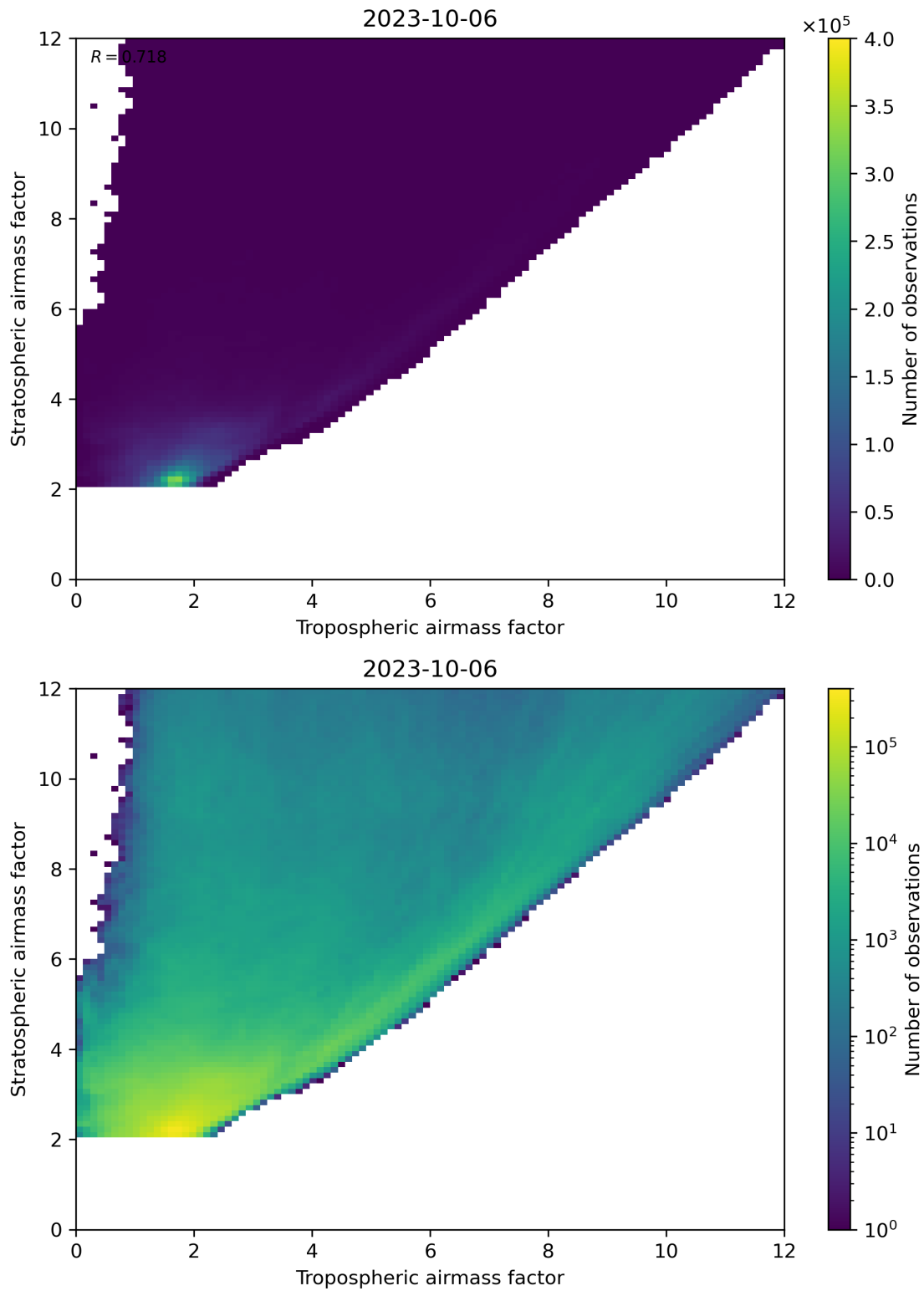
Figure 71: Scatter density plot of “Tropospheric airmass factor” against “Stratospheric airmass factor” for 2023-10-06 to 2023-10-07.
