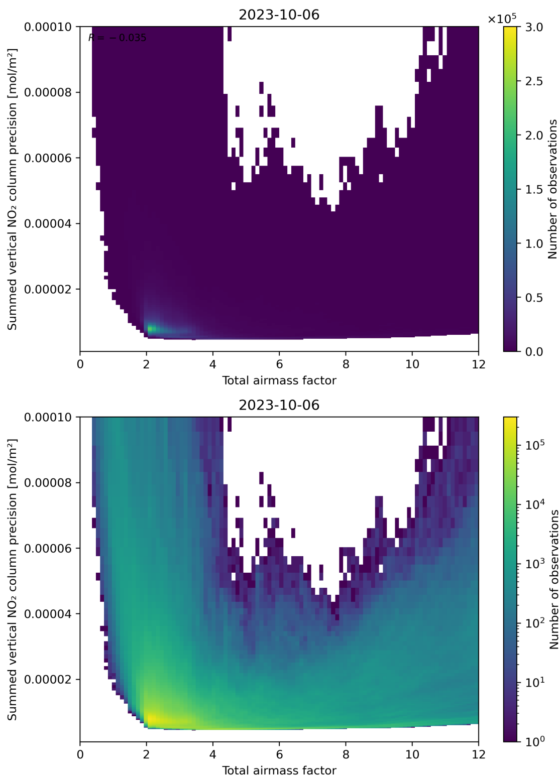
Figure 66: Scatter density plot of “Total airmass factor” against “Summed vertical NO 2 column precision” for 2023-10-06 to 2023-10-07.
