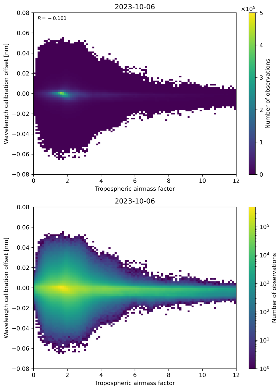
Figure 80: Scatter density plot of “Tropospheric airmass factor” against “Wavelength calibration offset” for 2023-10-06 to 2023-10-07.
