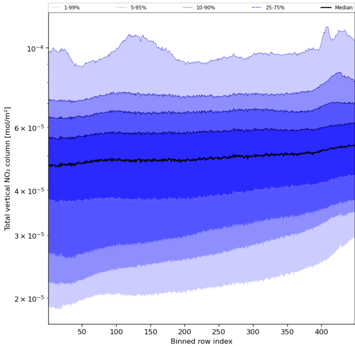
Figure 55: Along track statistics of “Total vertical NO 2 column” for 2023-10-06 to 2023-10-07
