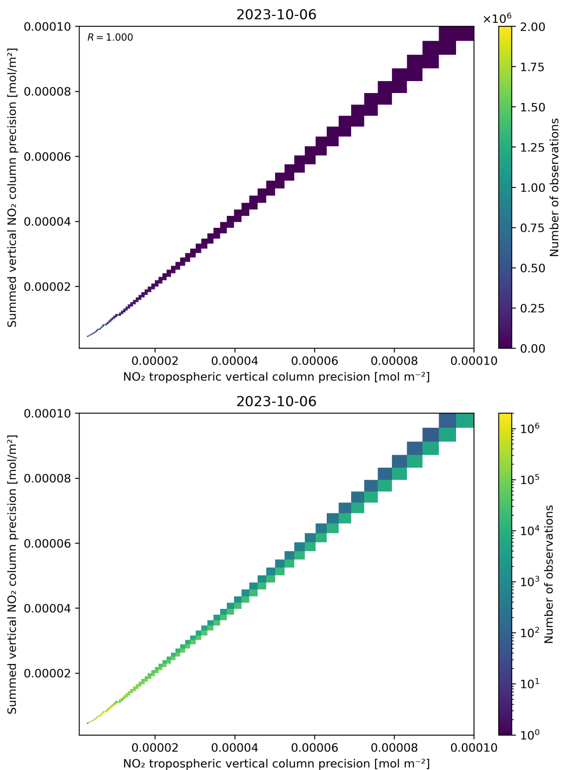
Figure 137: Scatter density plot of “NO 2 tropospheric vertical column precision” against “Summed vertical NO 2 column precision” for 2023-10-06 to 2023-10-07.
