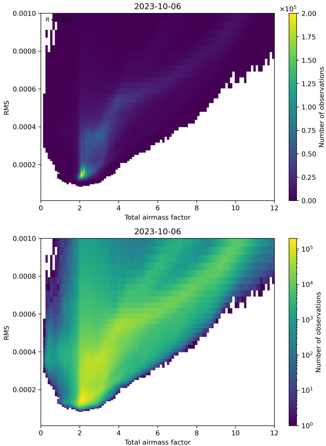
Figure 69: Scatter density plot of “Total airmass factor” against “RMS” for 2023-10-06 to 2023-10-07.
