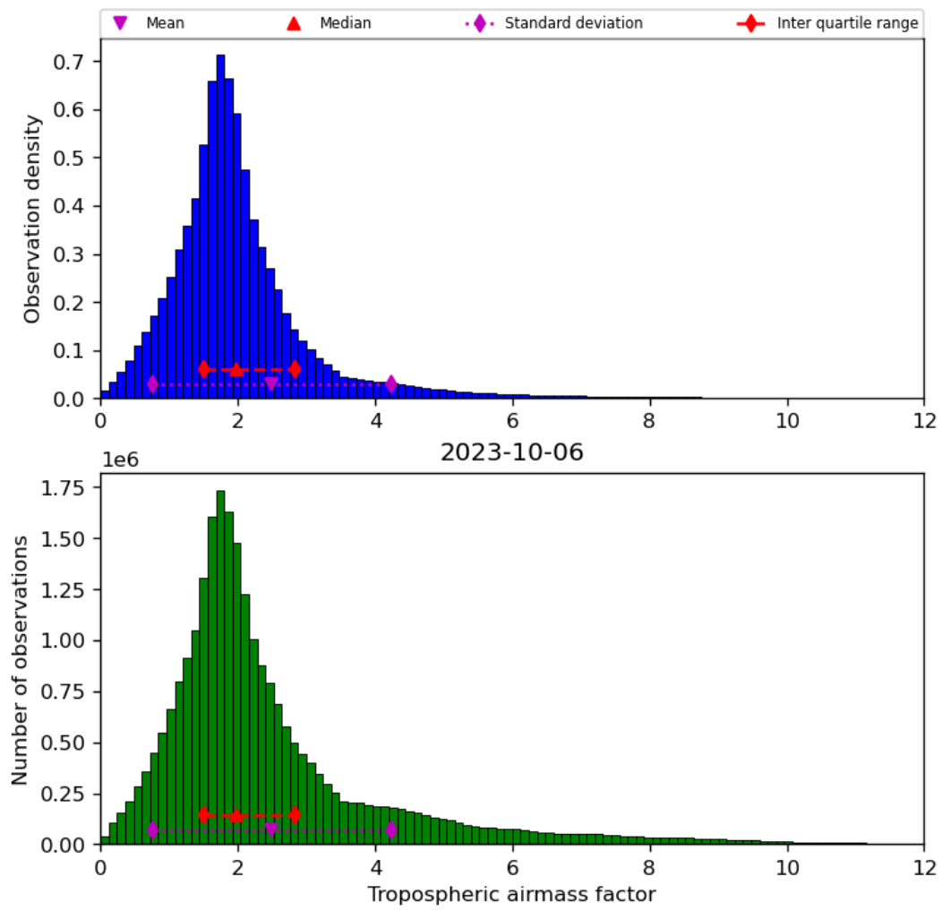
Figure 31: Histogram of “Tropospheric airmass factor” for 2023-10-06 to 2023-10-07
