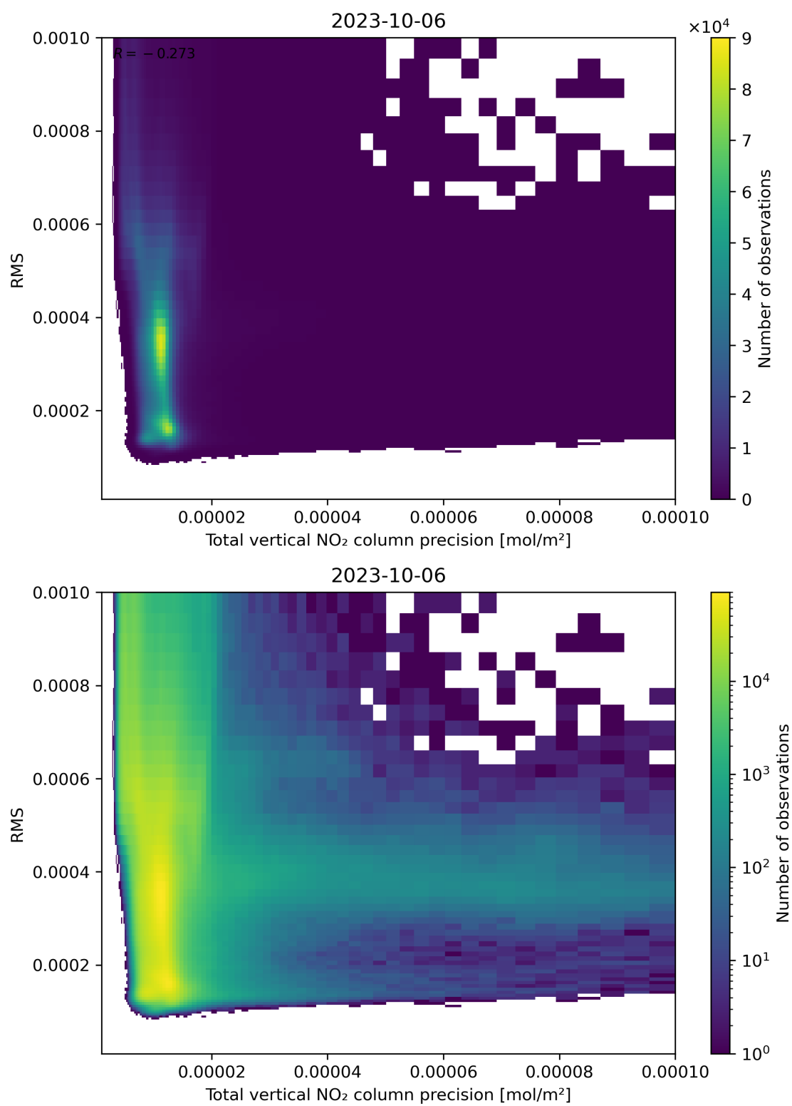
Figure 119: Scatter density plot of “Total vertical NO 2 column precision” against “RMS” for 2023-10-06 to 2023-10-07.
