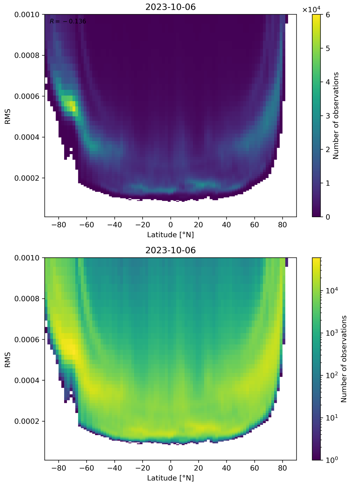
Figure 94: Scatter density plot of “Latitude” against “RMS” for 2023-10-06 to 2023-10-07.
