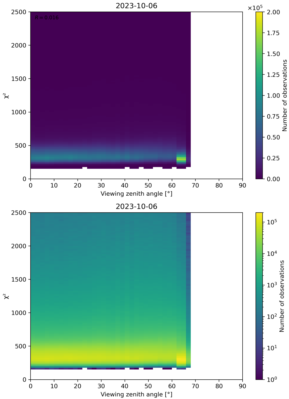
Figure 162: Scatter density plot of “Viewing zenith angle” against “ \chi^2 ” for 2023-10-06 to 2023-10-07.
