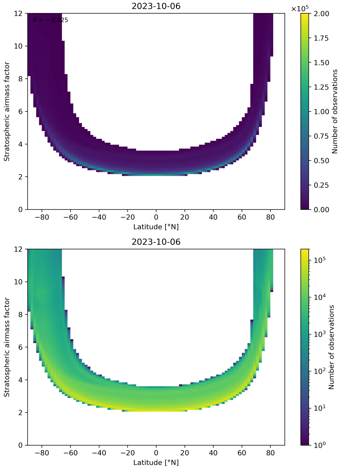
Figure 83: Scatter density plot of “Latitude” against “Stratospheric airmass factor” for 2023-10-06 to 2023-10-07.
