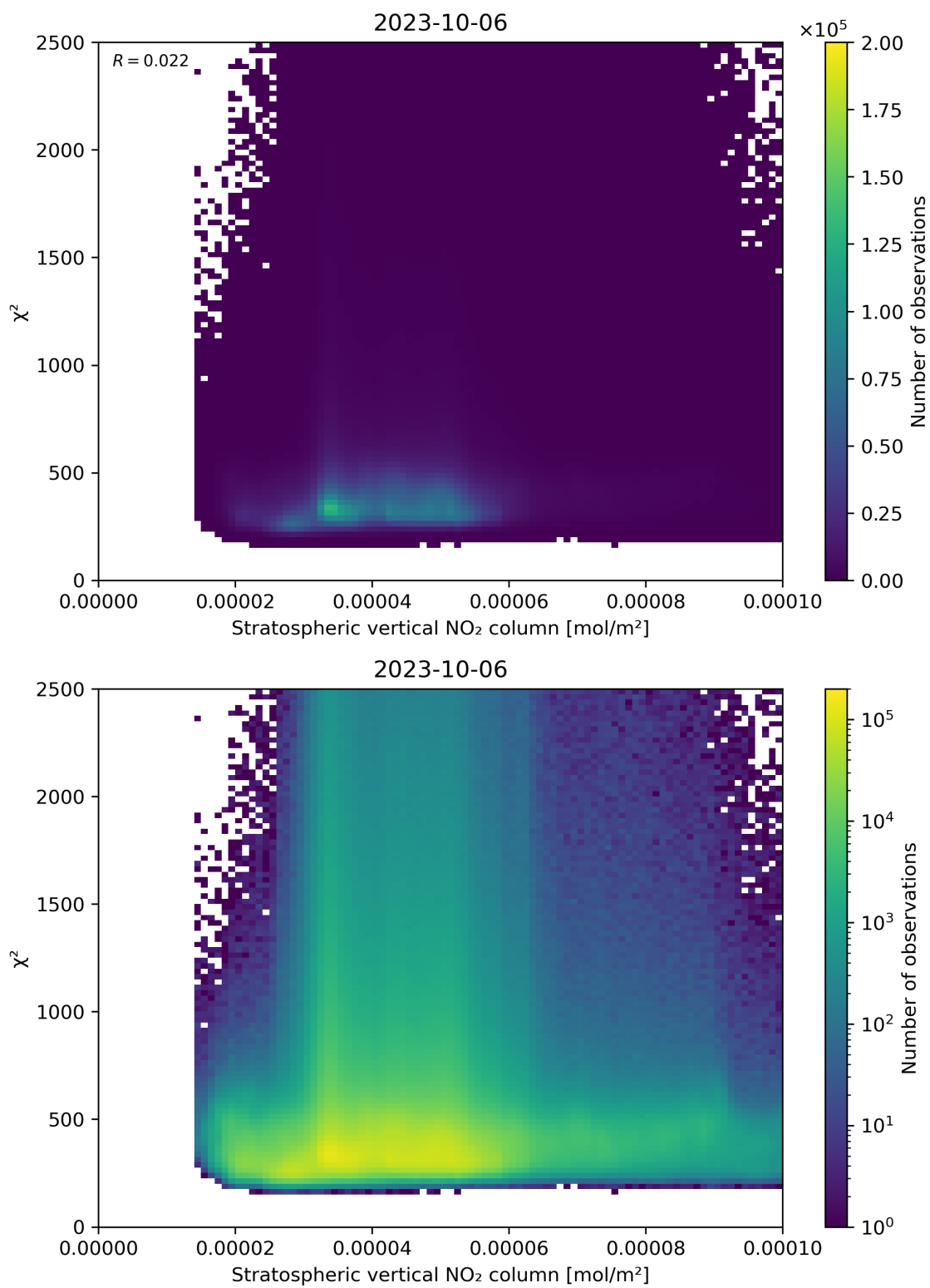
Figure 97: Scatter density plot of “Stratospheric vertical NO 2 column” against “ \chi^2 ” for 2023-10-06 to 2023-10-07.
