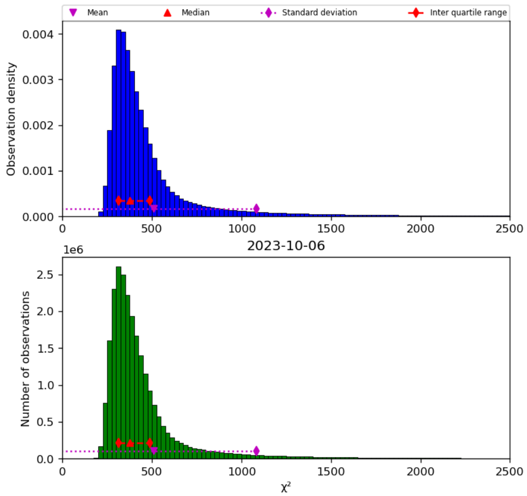
Figure 42: Histogram of “ \chi^2 ” for 2023-10-06 to 2023-10-07
