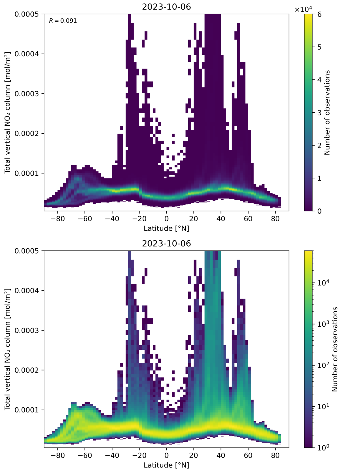
Figure 90: Scatter density plot of “Latitude” against “Total vertical NO 2 column” for 2023-10-06 to 2023-10-07.
