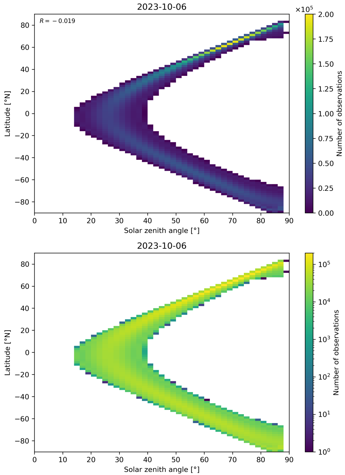
Figure 149: Scatter density plot of “Solar zenith angle” against “Latitude” for 2023-10-06 to 2023-10-07.
