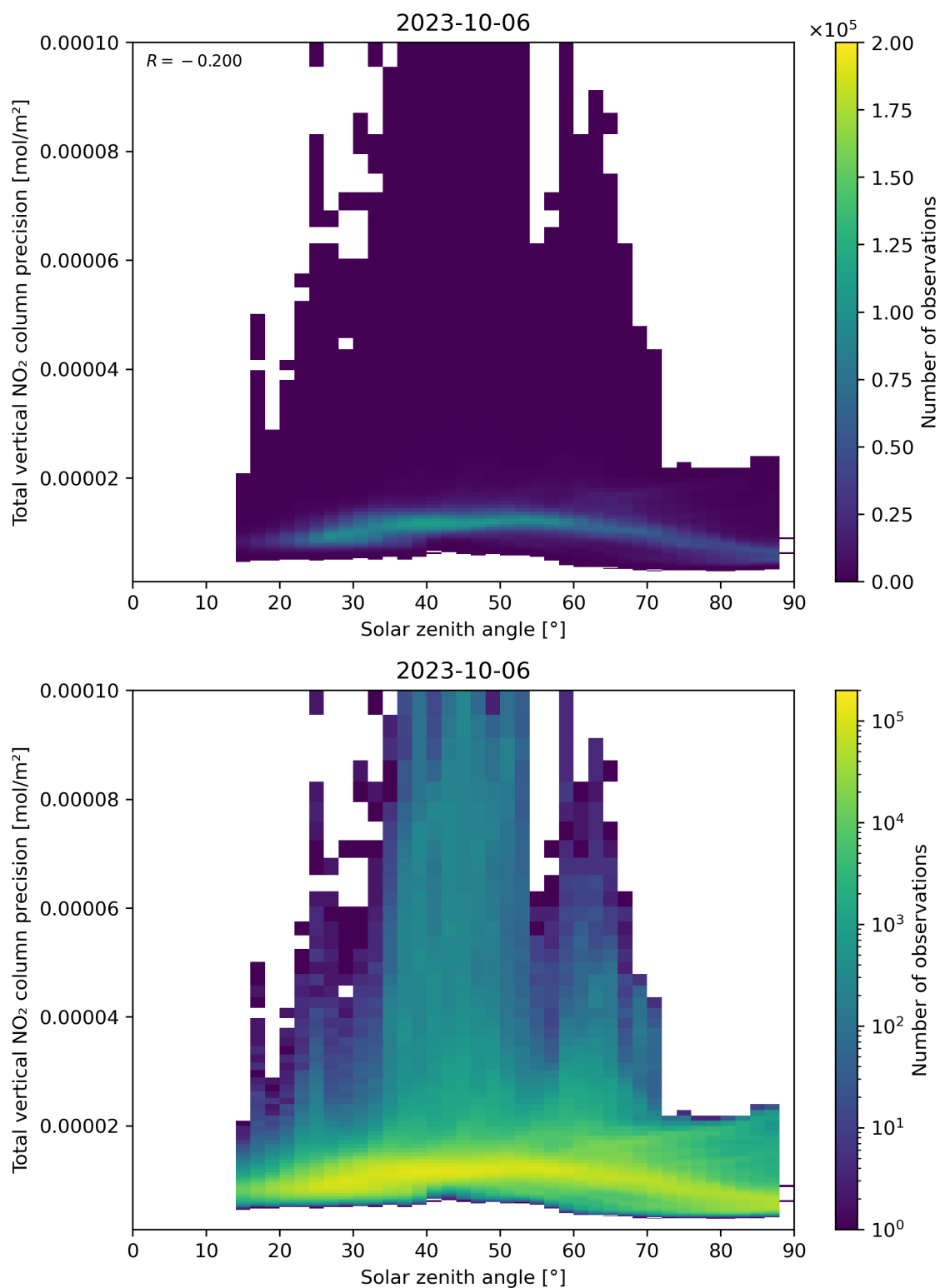
Figure 154: Scatter density plot of “Solar zenith angle” against “Total vertical NO 2 column precision” for 2023-10-06 to 2023-10-07.
