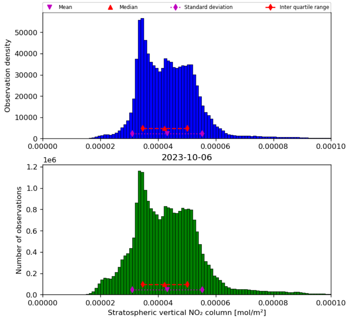
Figure 36: Histogram of “Stratospheric vertical NO 2 column” for 2023-10-06 to 2023-10-07
