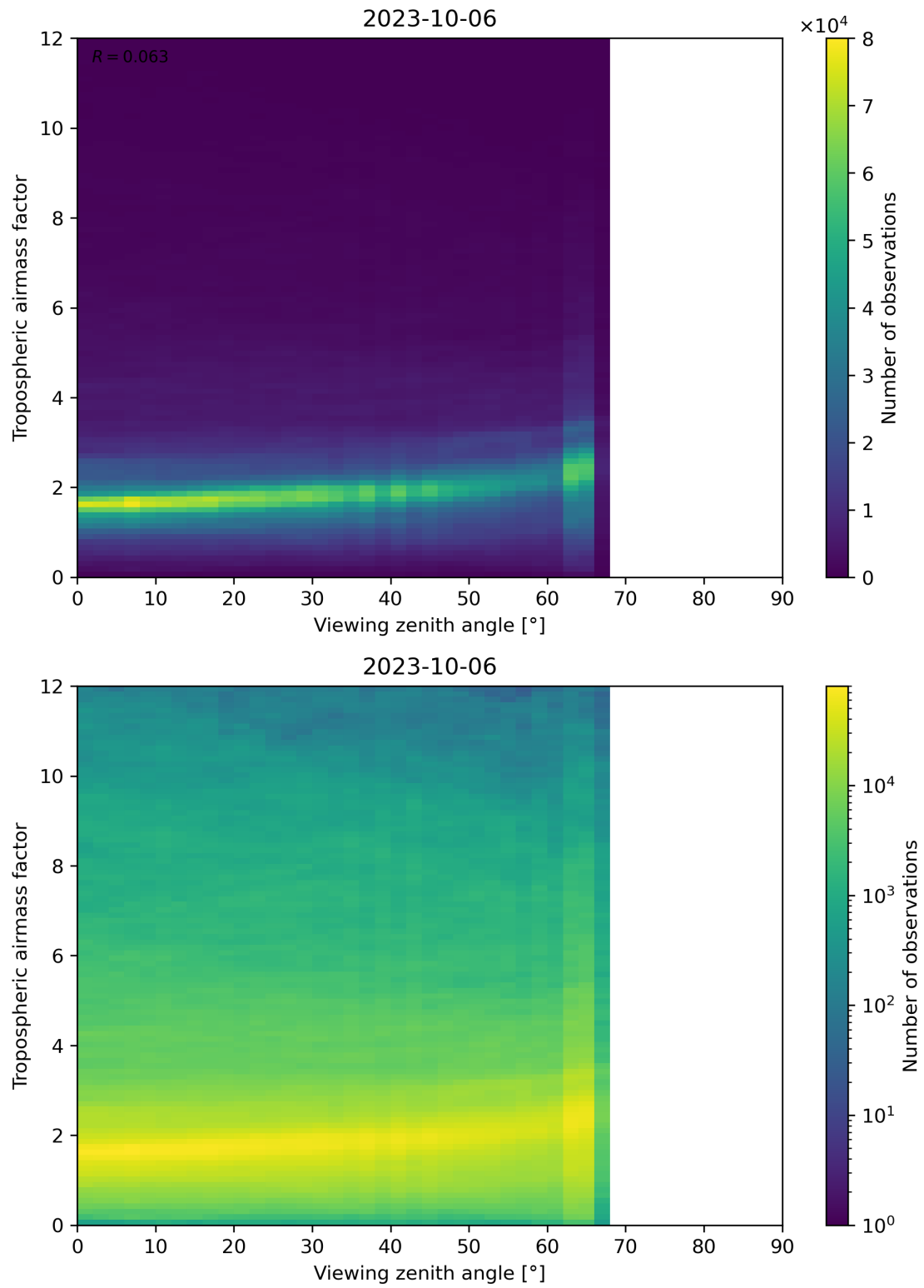
Figure 161: Scatter density plot of “Viewing zenith angle” against “Tropospheric airmass factor” for 2023-10-06 to 2023-10-07.
