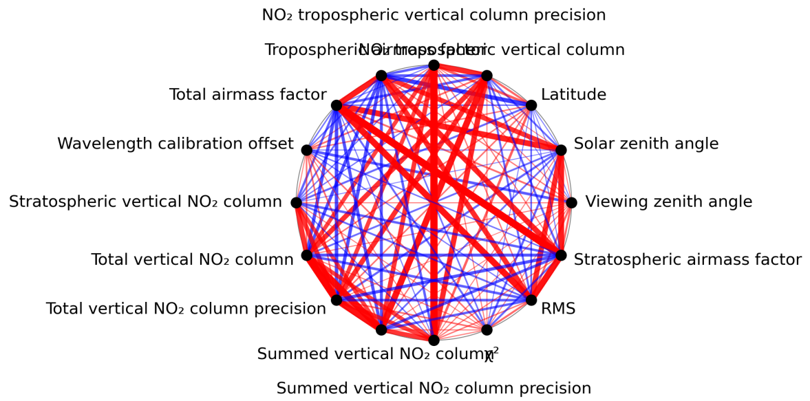
Figure 1: Map of correlation graph for 2023-10-06 to 2023-10-07.
