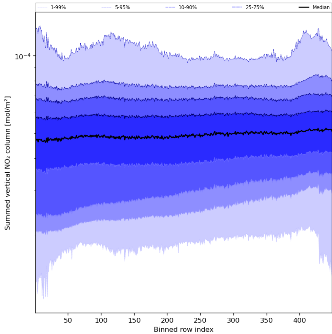
Figure 57: Along track statistics of “Summed vertical NO 2 column” for 2023-10-06 to 2023-10-07
