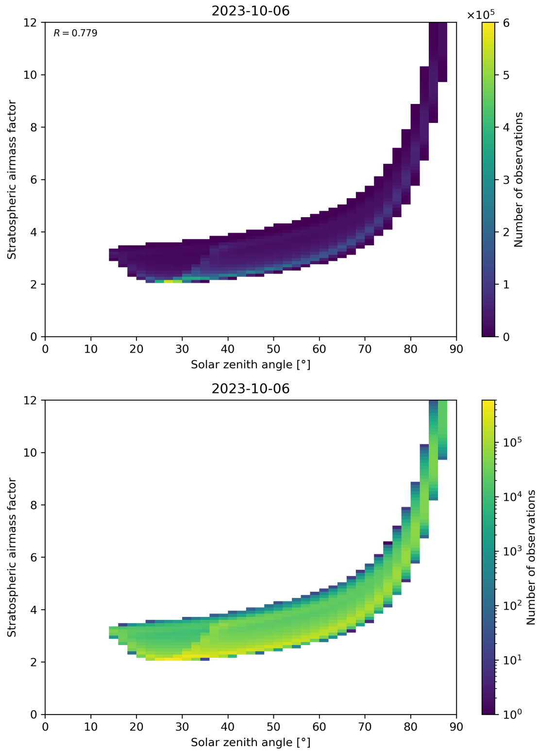
Figure 145: Scatter density plot of “Solar zenith angle” against “Stratospheric airmass factor” for 2023-10-06 to 2023-10-07.
