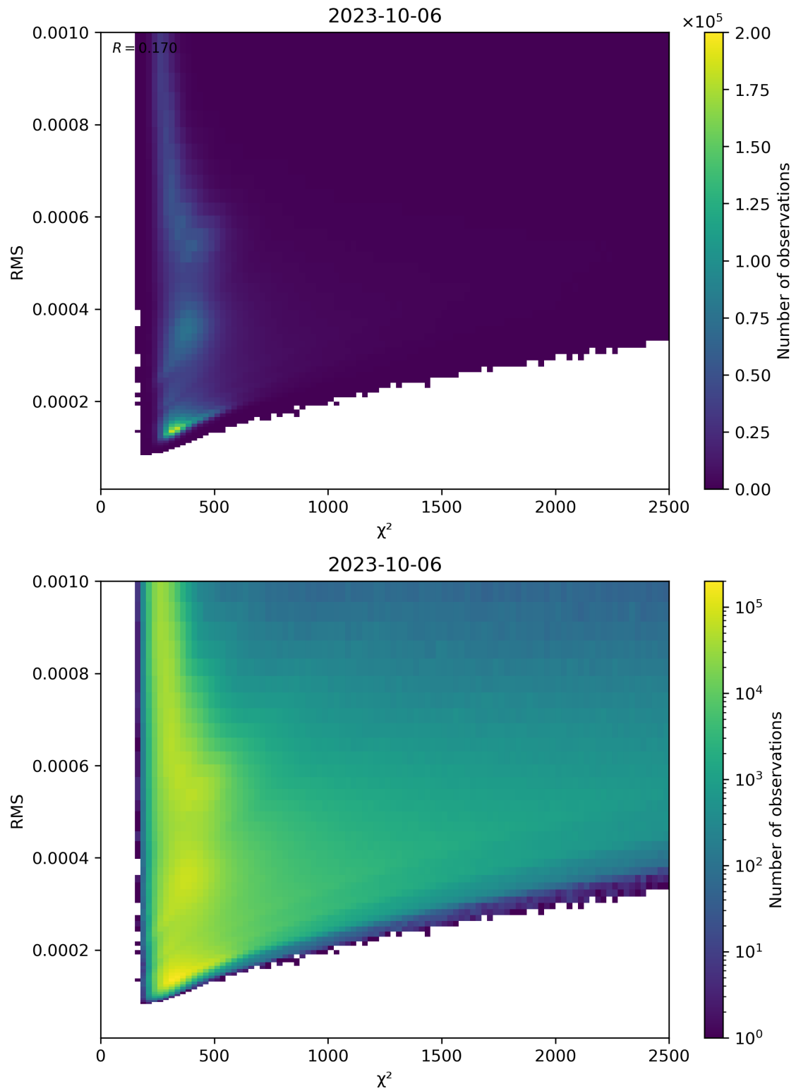
Figure 82: Scatter density plot of “ \chi^2 ” against “RMS” for 2023-10-06 to 2023-10-07.
