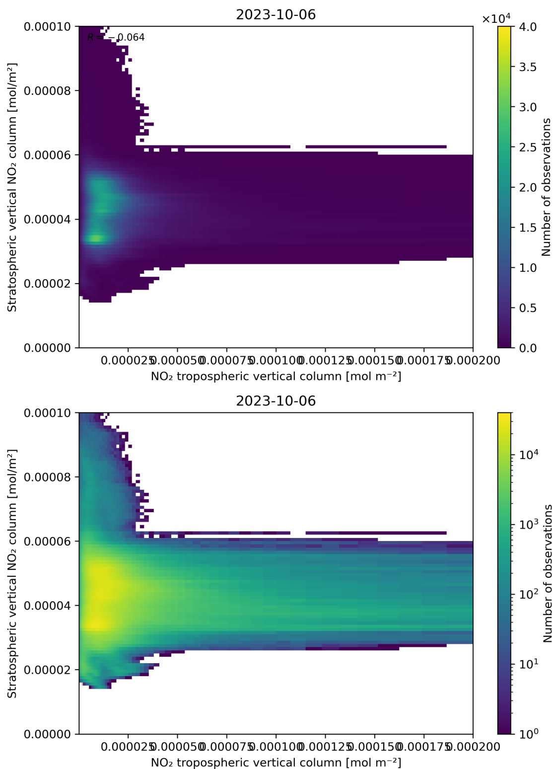
Figure 125: Scatter density plot of “NO 2 tropospheric vertical column” against “Stratospheric vertical NO 2 column” for 2023-10-06 to 2023-10-07.
