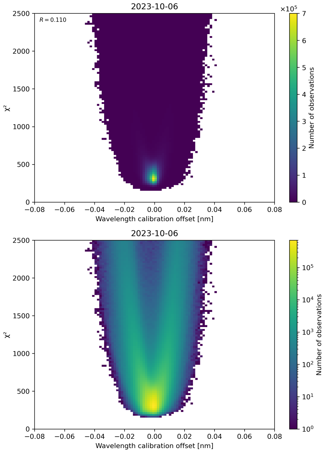
Figure 175: Scatter density plot of “Wavelength calibration offset” against “ \chi^2 ” for 2023-10-06 to 2023-10-07.
