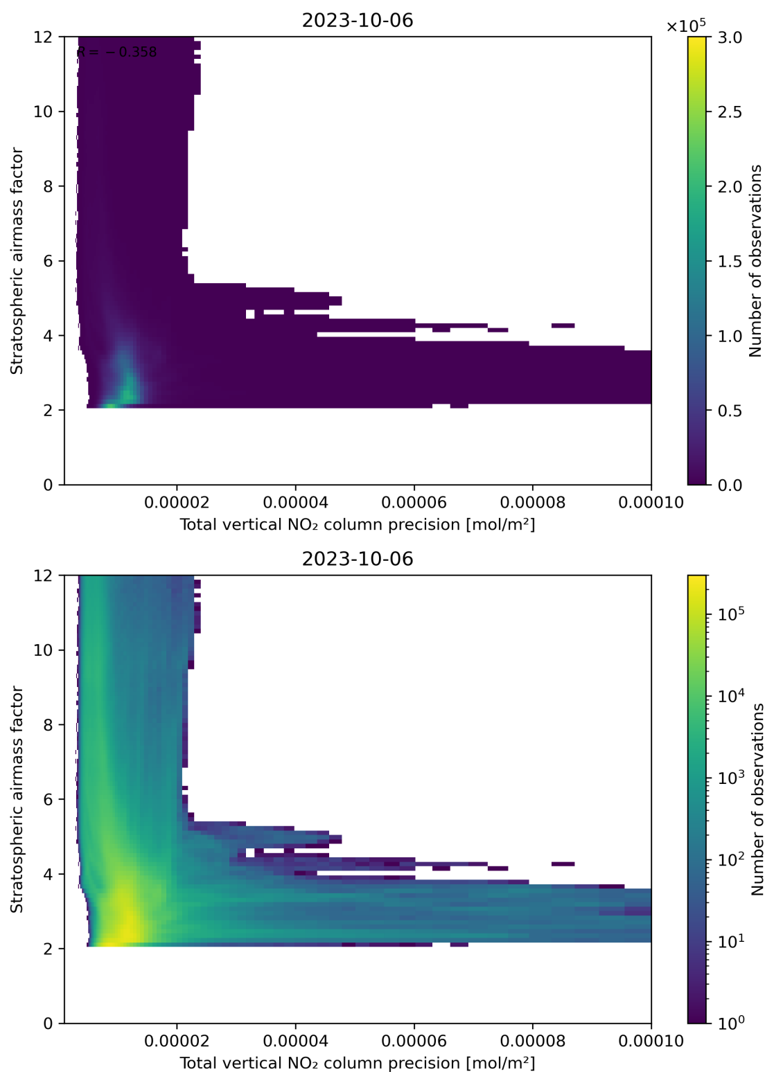
Figure 115: Scatter density plot of “Total vertical NO 2 column precision” against “Stratospheric airmass factor” for 2023-10-06 to 2023-10-07.
