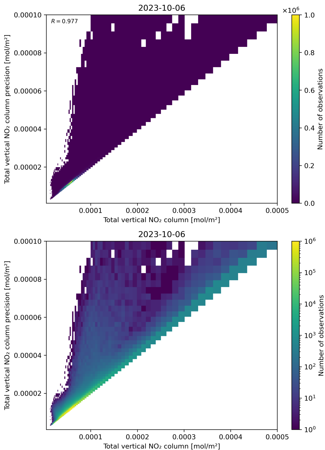
Figure 114: Scatter density plot of “Total vertical NO 2 column” against “Total vertical NO 2 column precision” for 2023-10-06 to 2023-10-07.
