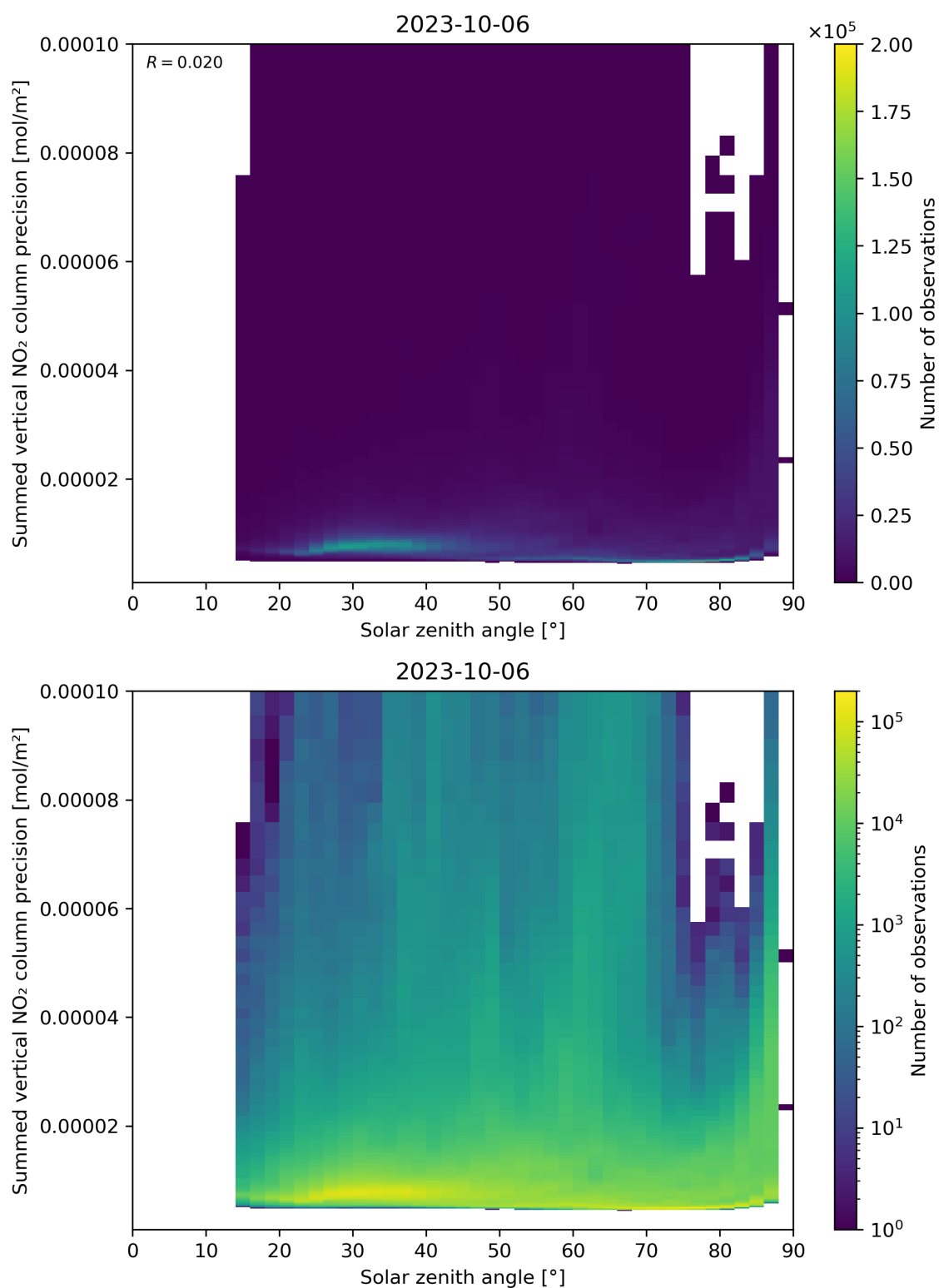
Figure 152: Scatter density plot of “Solar zenith angle” against “Summed vertical NO 2 column precision” for 2023-10-06 to 2023-10-07.
