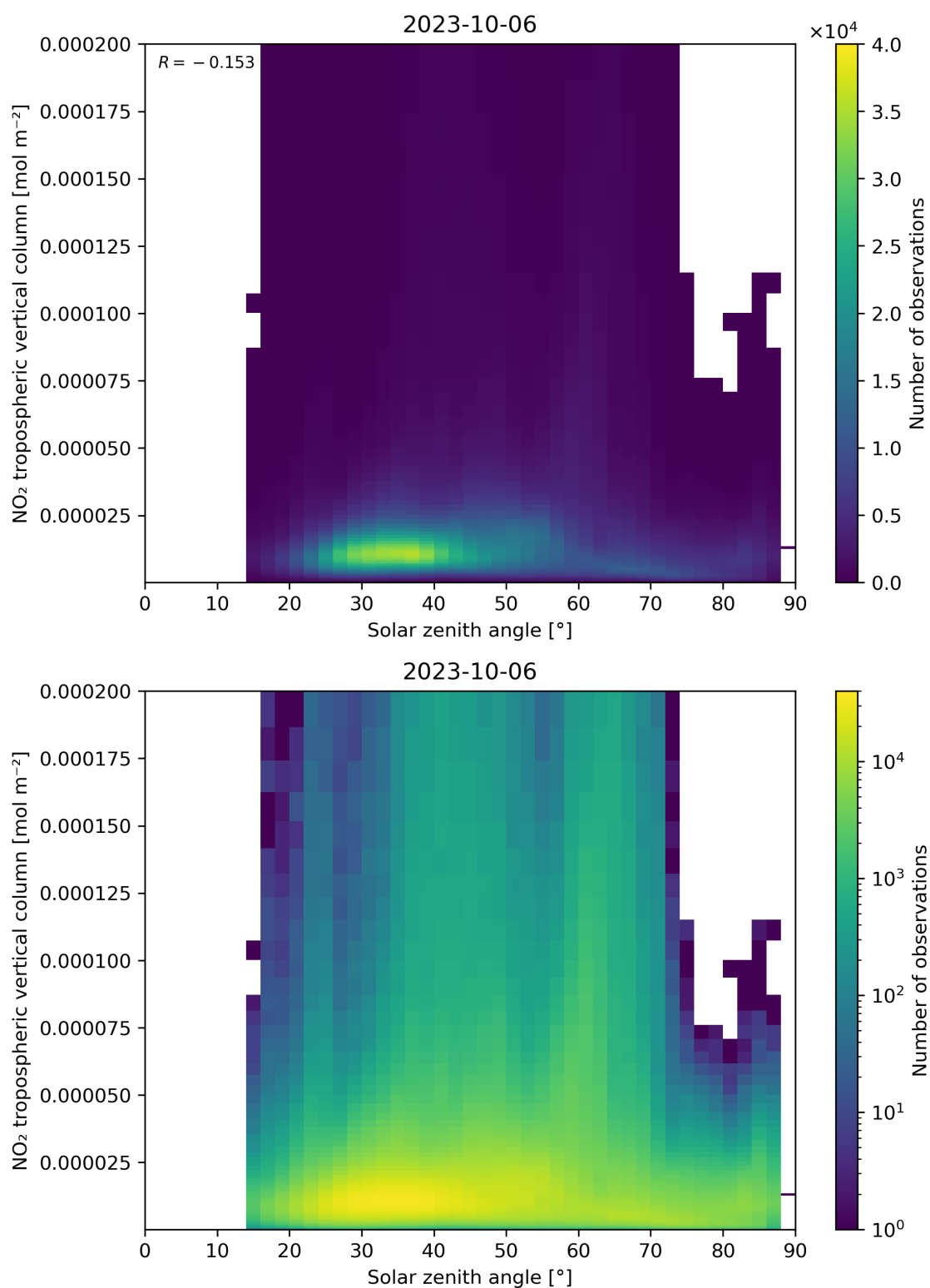
Figure 155: Scatter density plot of “Solar zenith angle” against “NO 2 tropospheric vertical column” for 2023-10-06 to 2023-10-07.
