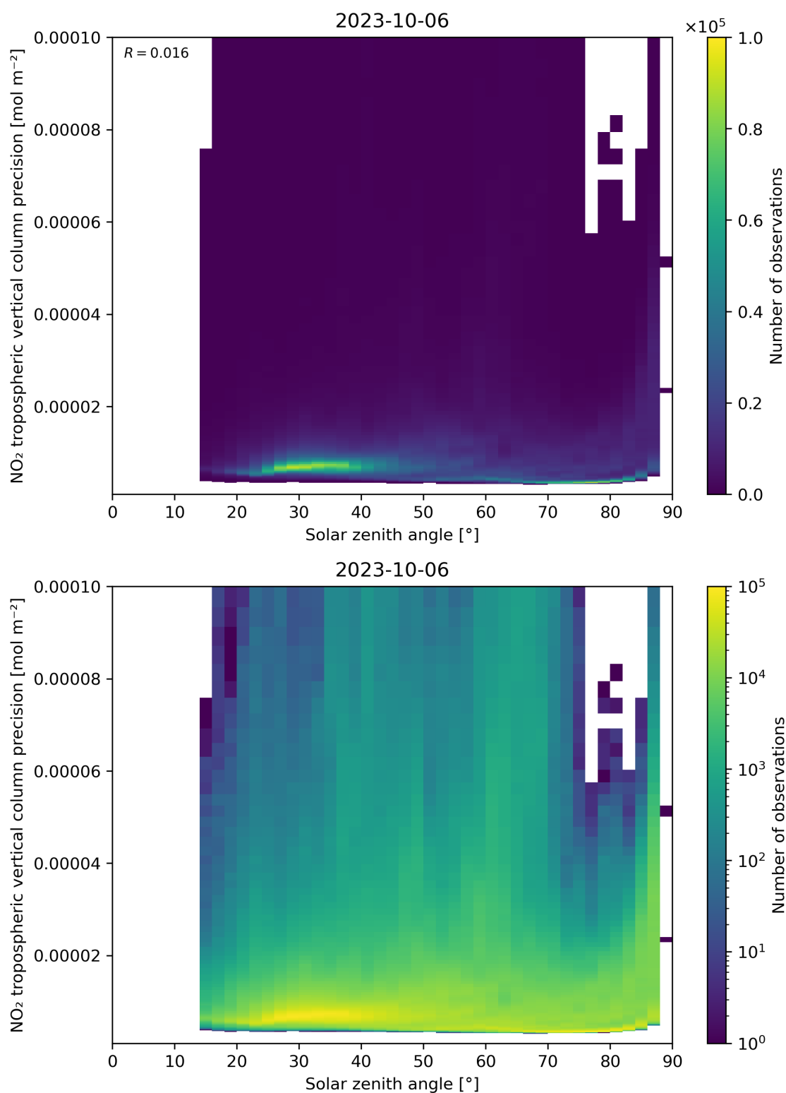
Figure 156: Scatter density plot of “Solar zenith angle” against “NO 2 tropospheric vertical column precision” for 2023-10-06 to 2023-10-07.
