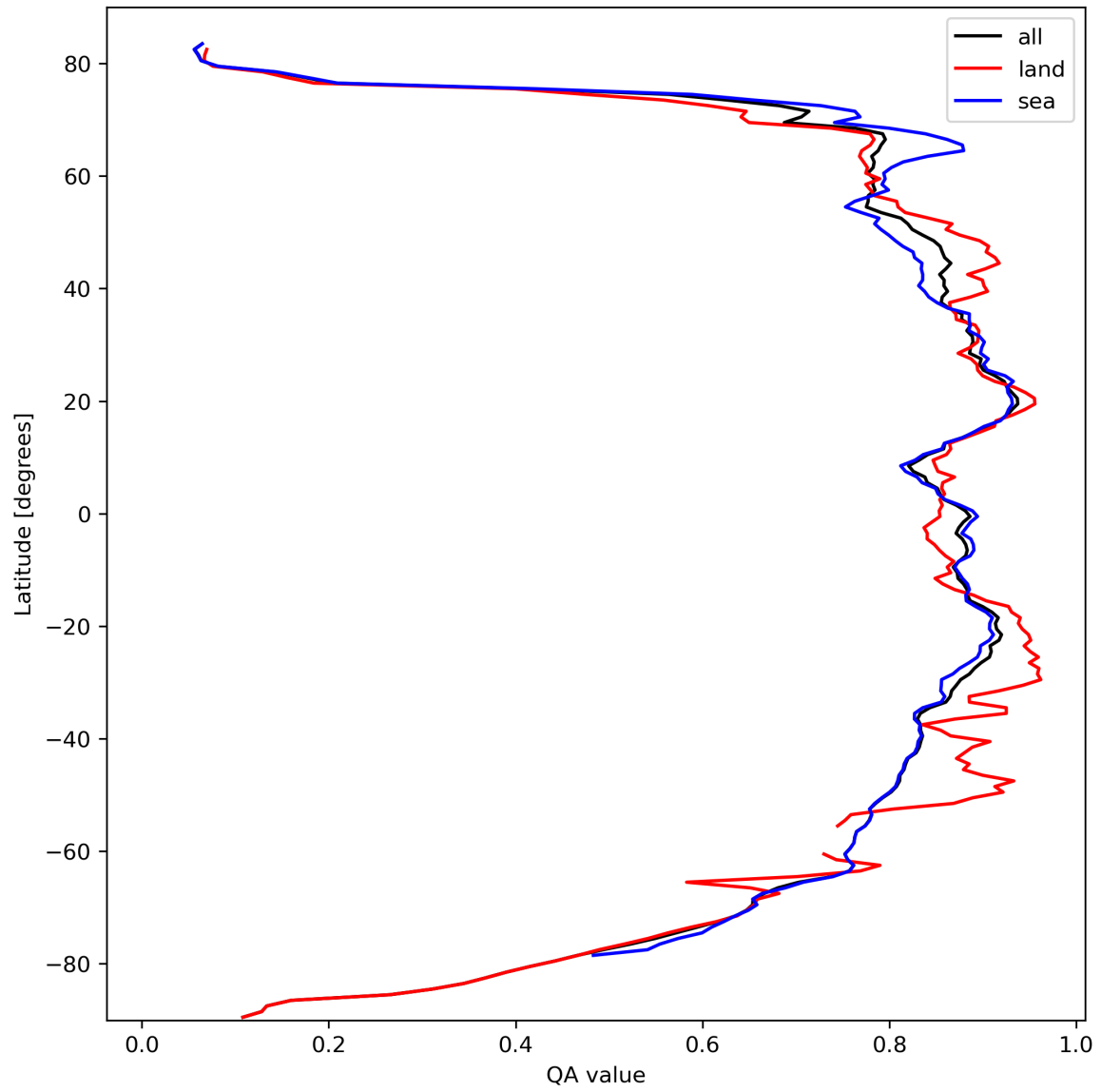
Figure 11: Zonal average of “QA value” for 2023-10-06 to 2023-10-07.
