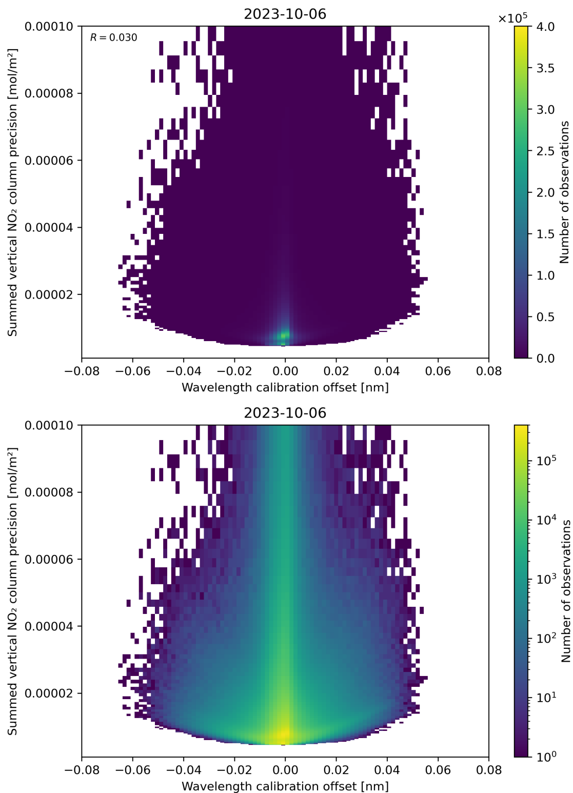
Figure 178: Scatter density plot of “Wavelength calibration offset” against “Summed vertical NO 2 column precision” for 2023-10-06 to 2023-10-07.
