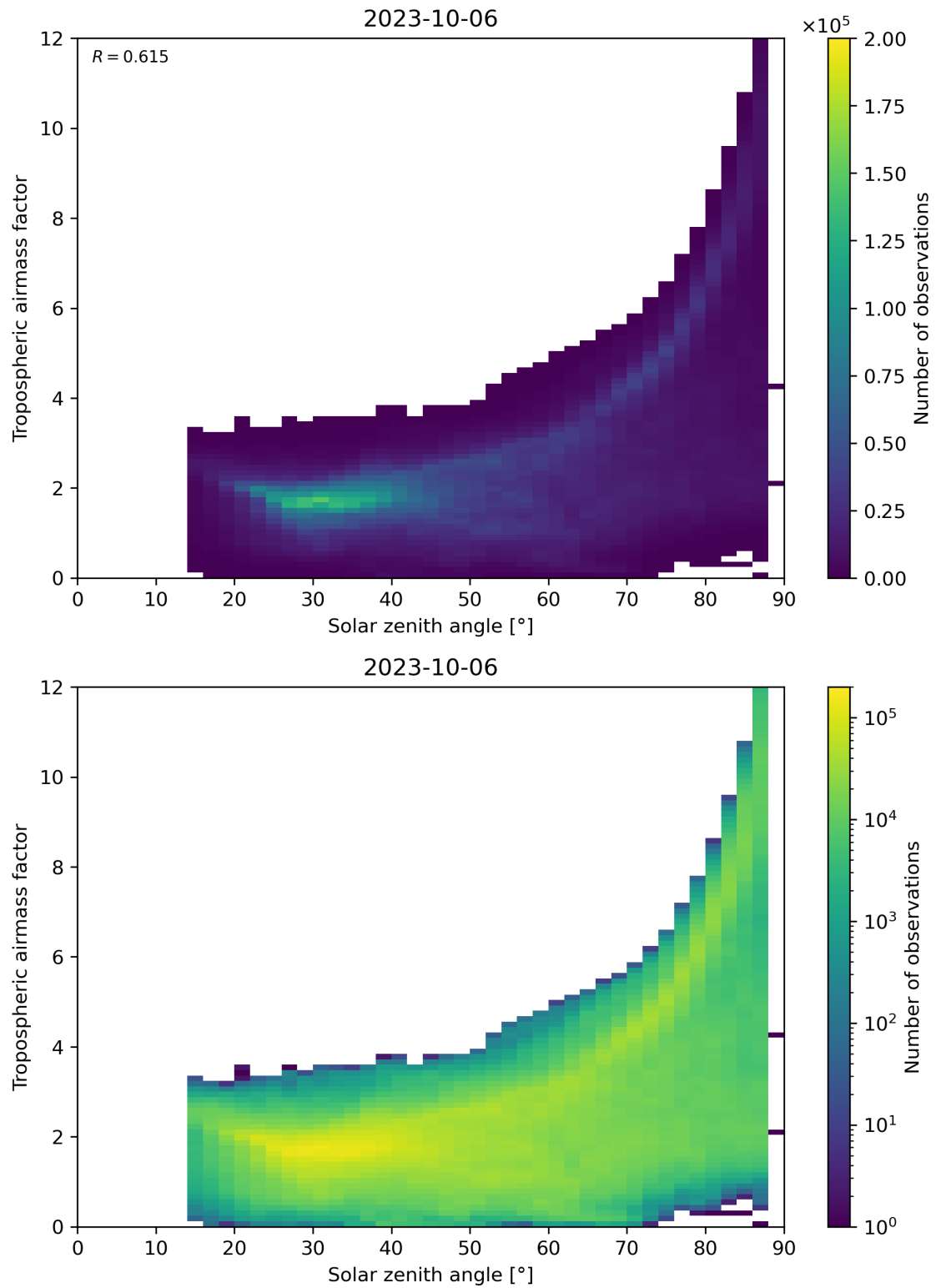
Figure 147: Scatter density plot of “Solar zenith angle” against “Tropospheric airmass factor” for 2023-10-06 to 2023-10-07.
