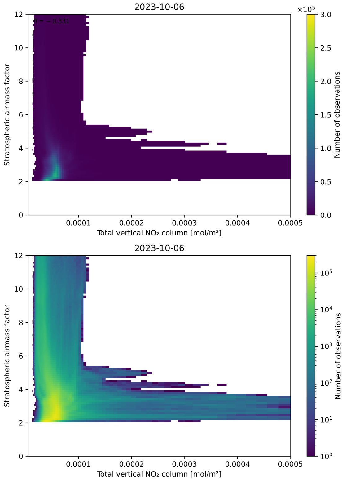
Figure 110: Scatter density plot of “Total vertical NO 2 column” against “Stratospheric airmass factor” for 2023-10-06 to 2023-10-07.
