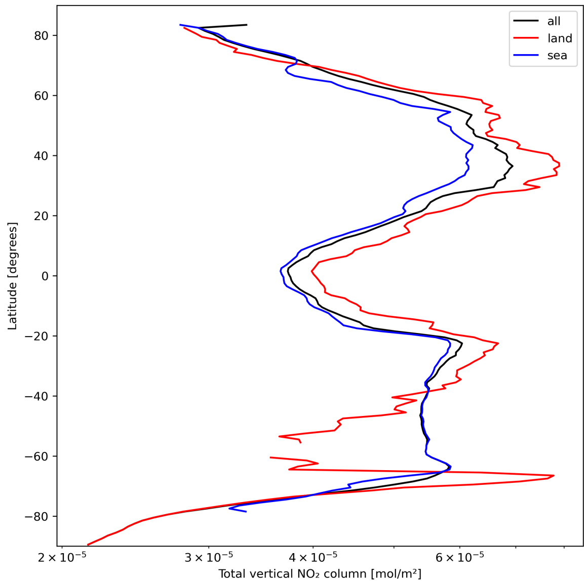
Figure 21: Zonal average of “Total vertical NO 2 column” for 2023-10-06 to 2023-10-07.
