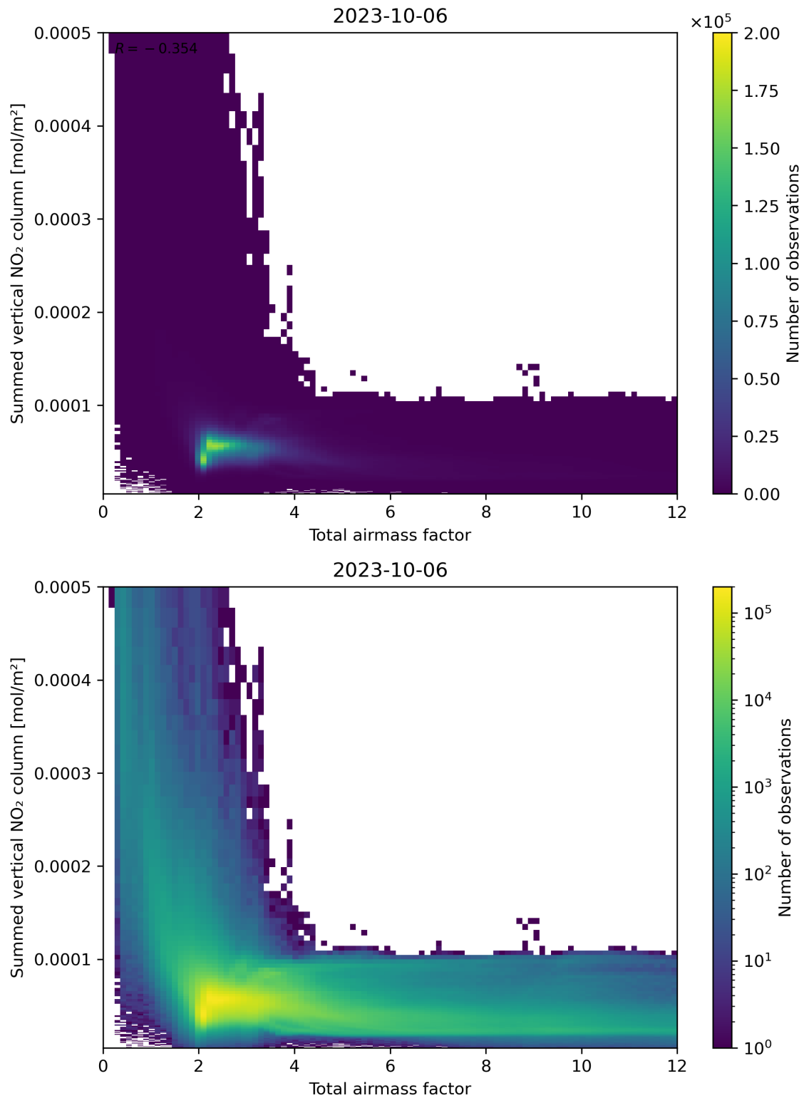
Figure 65: Scatter density plot of “Total airmass factor” against “Summed vertical NO 2 column” for 2023-10-06 to 2023-10-07.
