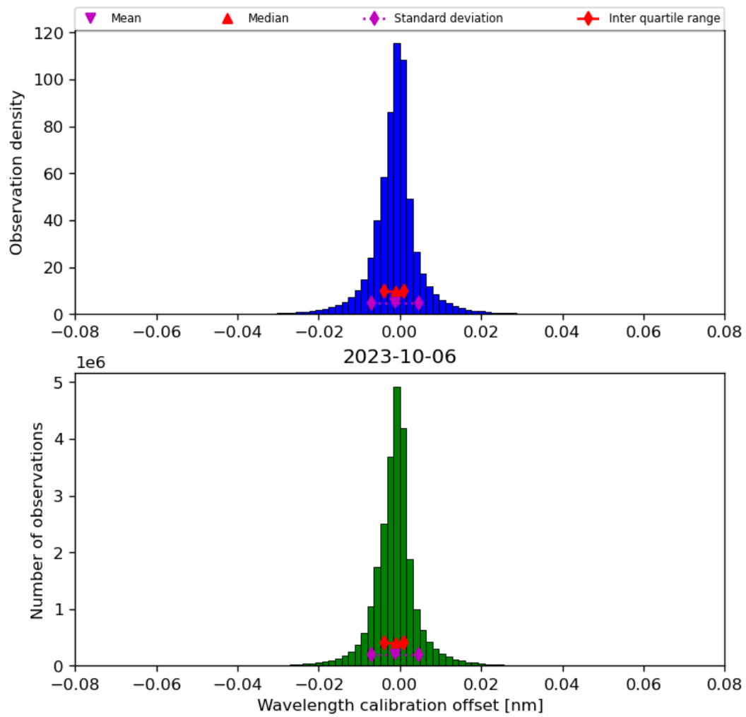
Figure 35: Histogram of “Wavelength calibration offset” for 2023-10-06 to 2023-10-07
