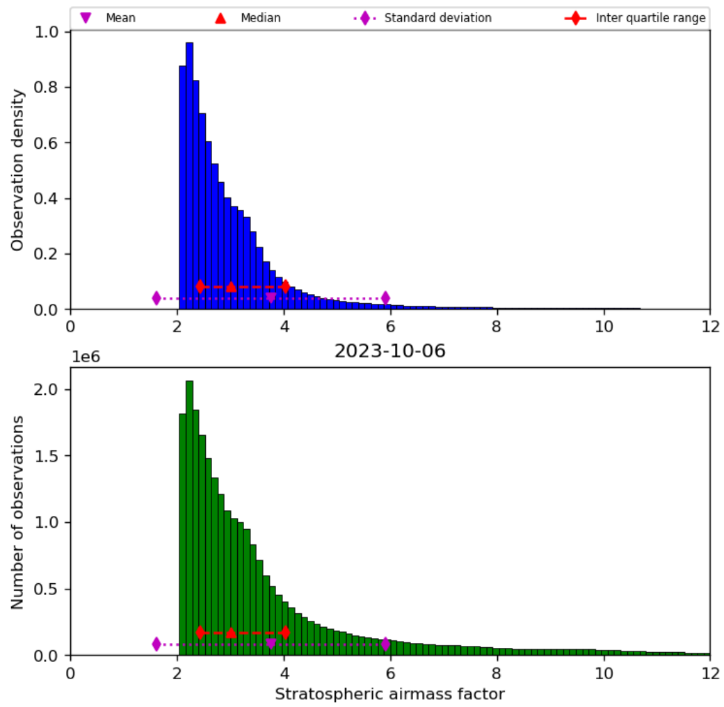
Figure 44: Histogram of “Stratospheric airmass factor” for 2023-10-06 to 2023-10-07
