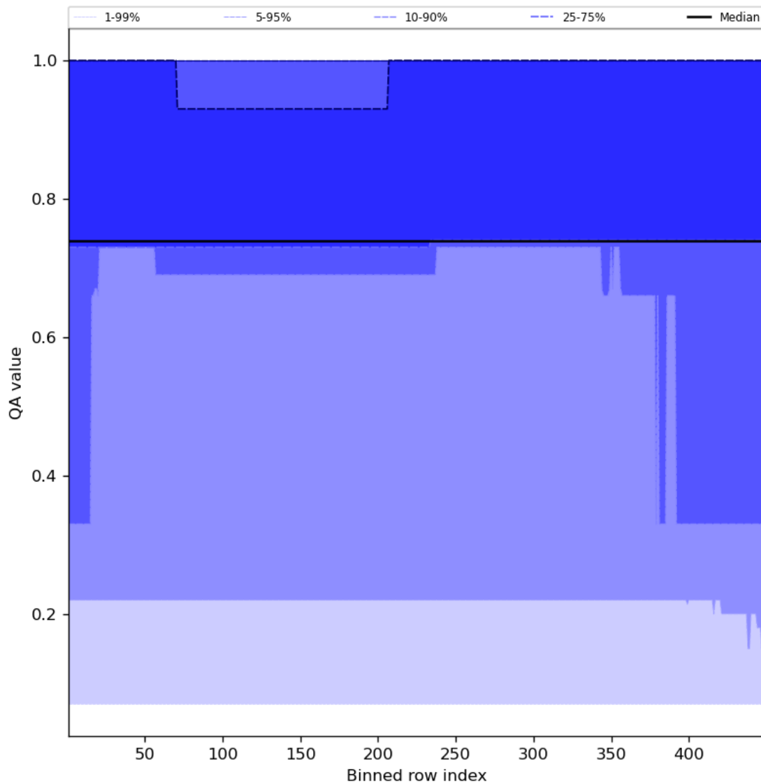
Figure 45: Along track statistics of “QA value” for 2023-10-06 to 2023-10-07
