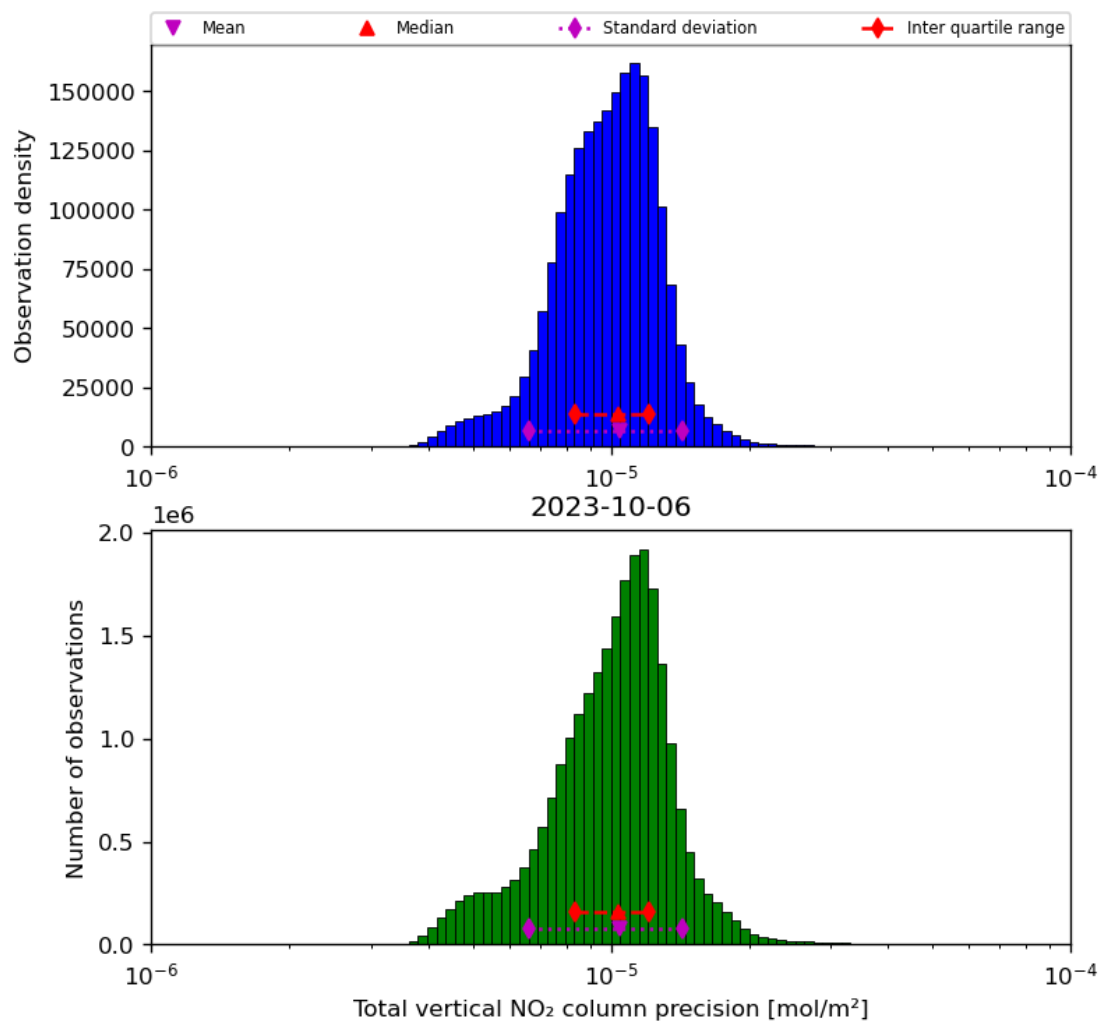
Figure 39: Histogram of “Total vertical NO 2 column precision” for 2023-10-06 to 2023-10-07
