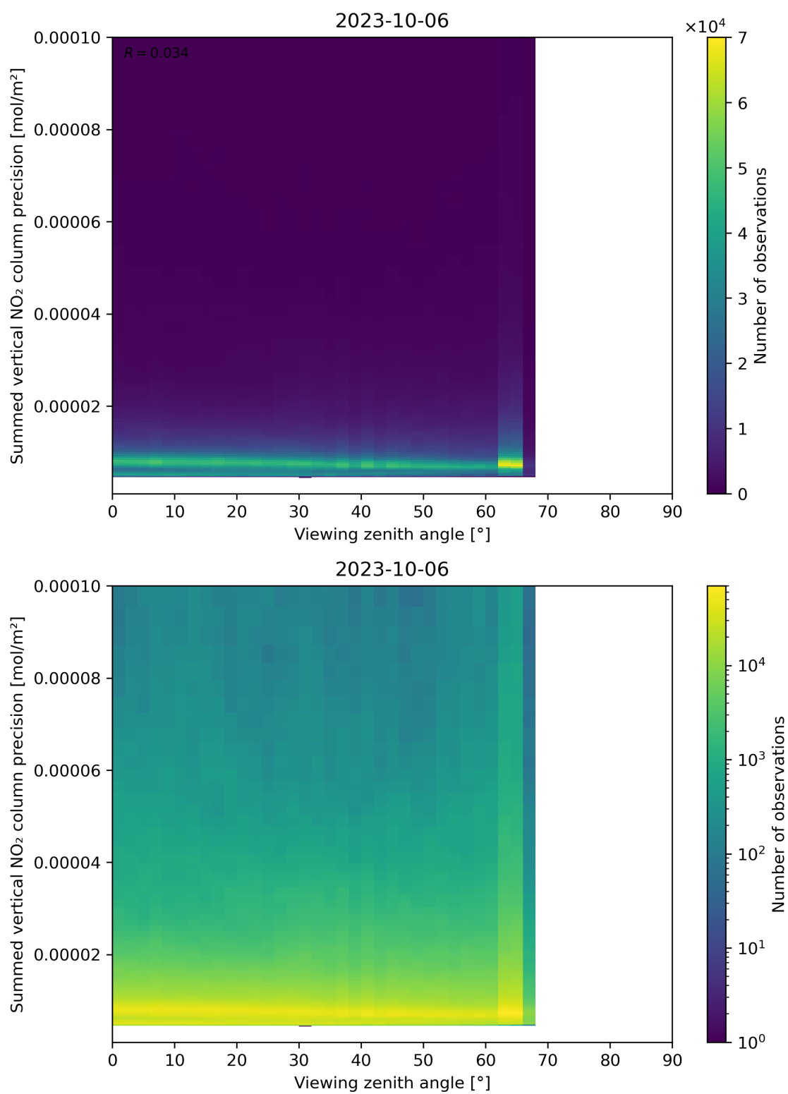
Figure 166: Scatter density plot of “Viewing zenith angle” against “Summed vertical NO 2 column precision” for 2023-10-06 to 2023-10-07.
