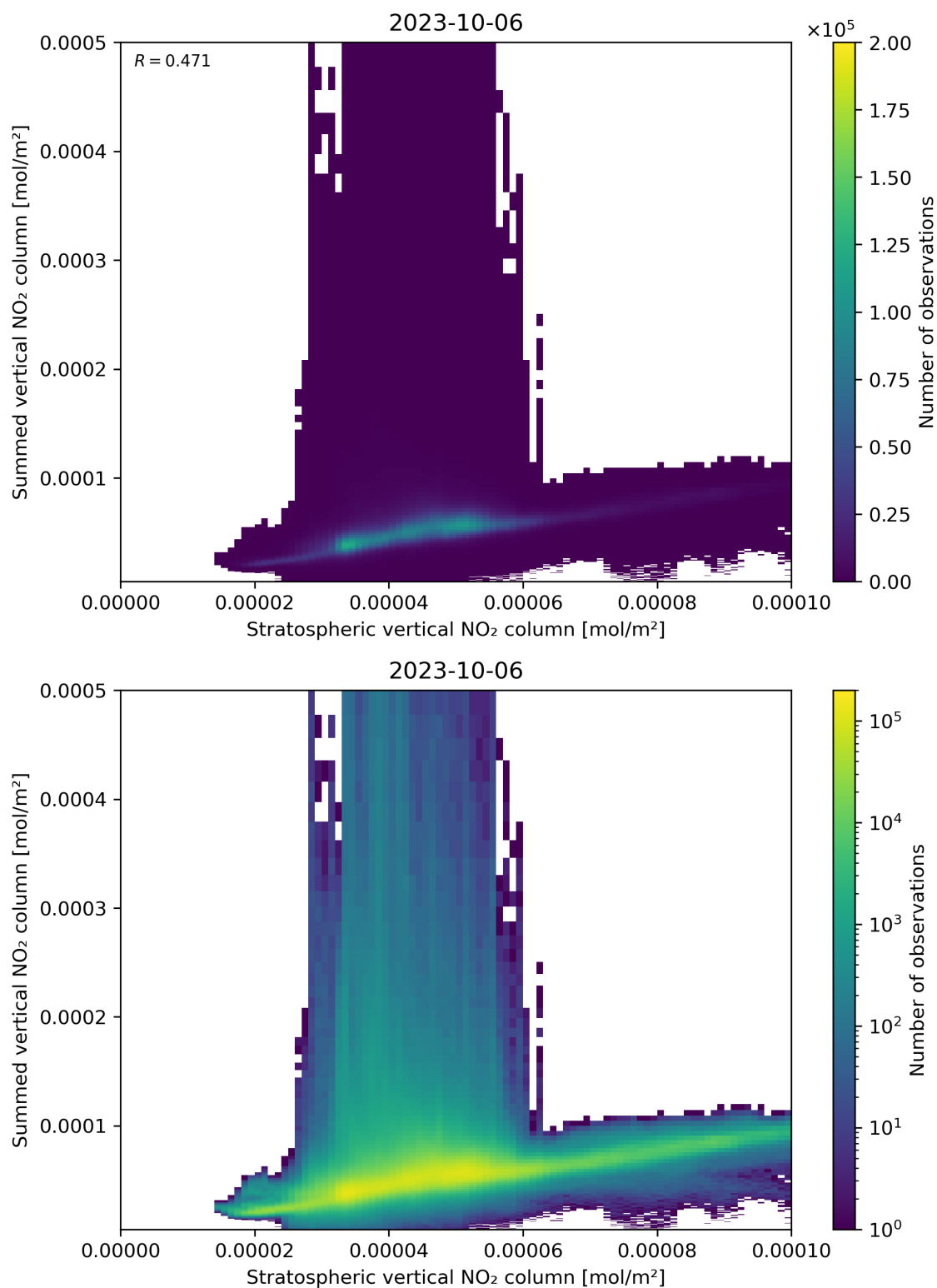
Figure 98: Scatter density plot of “Stratospheric vertical NO 2 column” against “Summed vertical NO 2 column” for 2023-10-06 to 2023-10-07.
