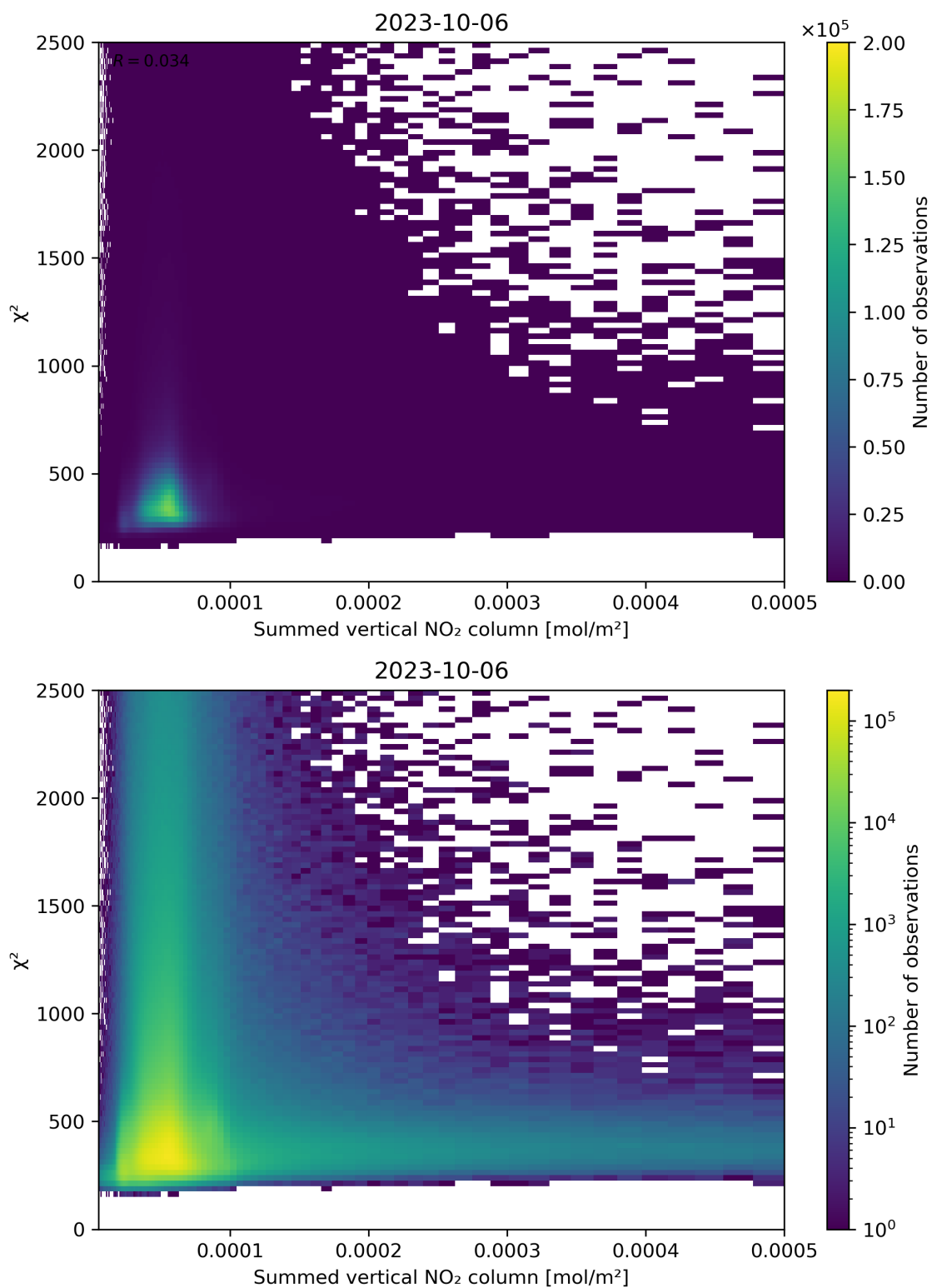
Figure 104: Scatter density plot of “Summed vertical NO 2 column” against “ \chi^2 ” for 2023-10-06 to 2023-10-07.
