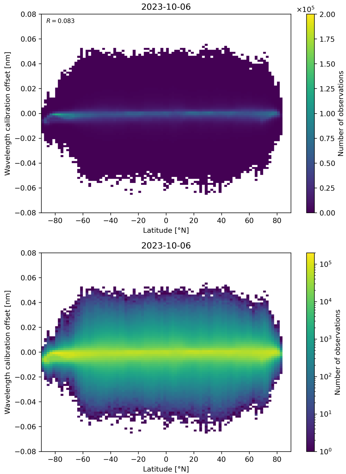
Figure 95: Scatter density plot of “Latitude” against “Wavelength calibration offset” for 2023-10-06 to 2023-10-07.
