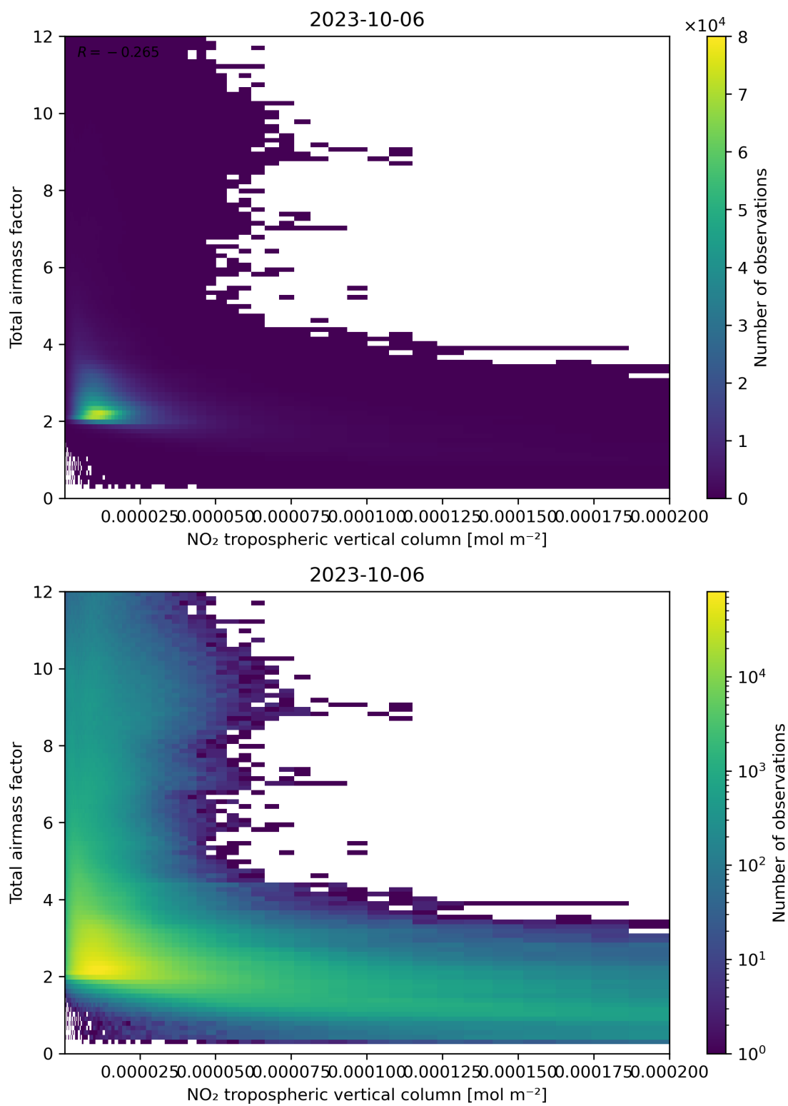
Figure 122: Scatter density plot of “NO 2 tropospheric vertical column” against “Total air mass factor” for 2023-10-06 to 2023-10-07.
