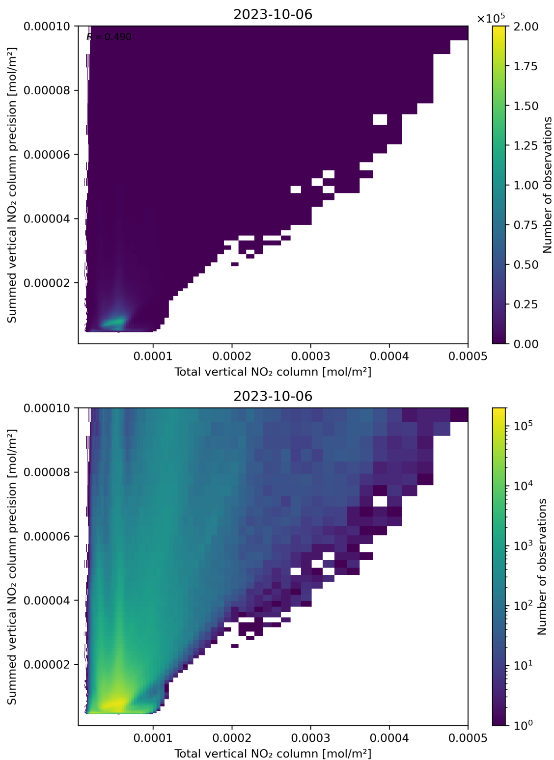
Figure 113: Scatter density plot of “Total vertical NO 2 column” against “Summed vertical NO 2 column precision” for 2023-10-06 to 2023-10-07.
