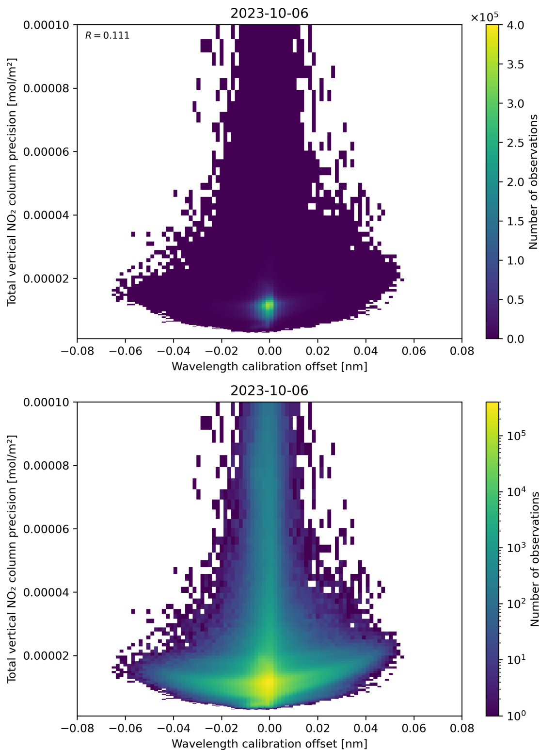
Figure 180: Scatter density plot of “Wavelength calibration offset” against “Total vertical NO 2 column precision” for 2023-10-06 to 2023-10-07.
