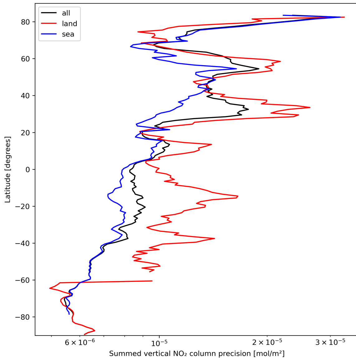
Figure 24: Zonal average of “Summed vertical NO 2 column precision” for 2023-10-06 to 2023-10-07.
