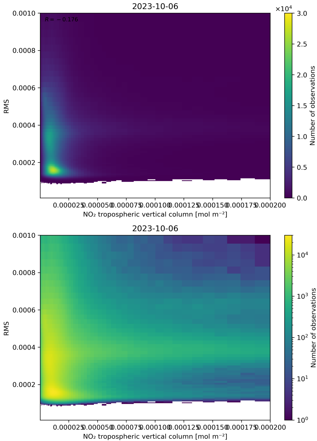
Figure 142: Scatter density plot of “NO 2 tropospheric vertical column” against “RMS” for 2023-10-06 to 2023-10-07.
