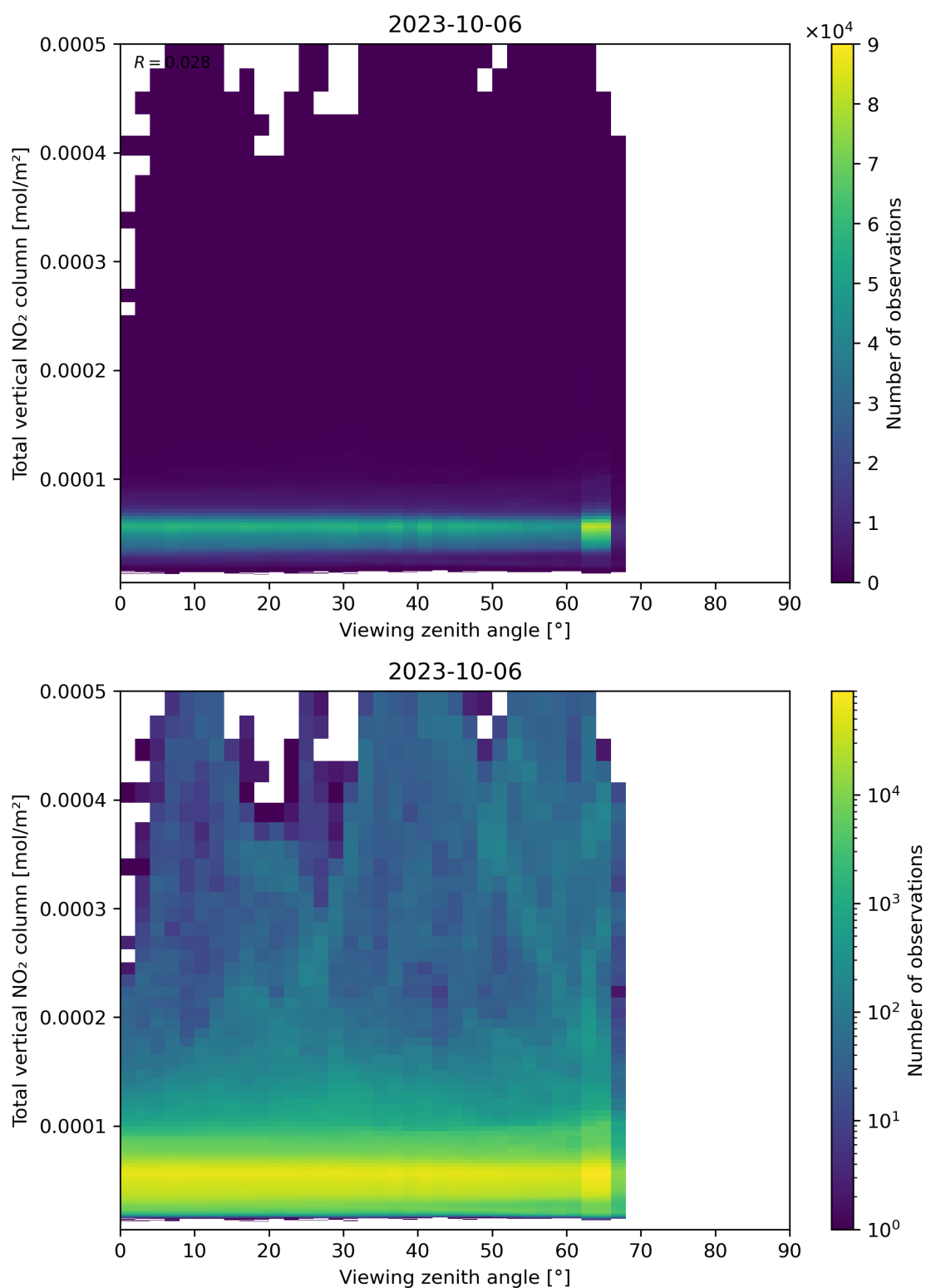
Figure 167: Scatter density plot of “Viewing zenith angle” against “Total vertical NO 2 column” for 2023-10-06 to 2023-10-07.
