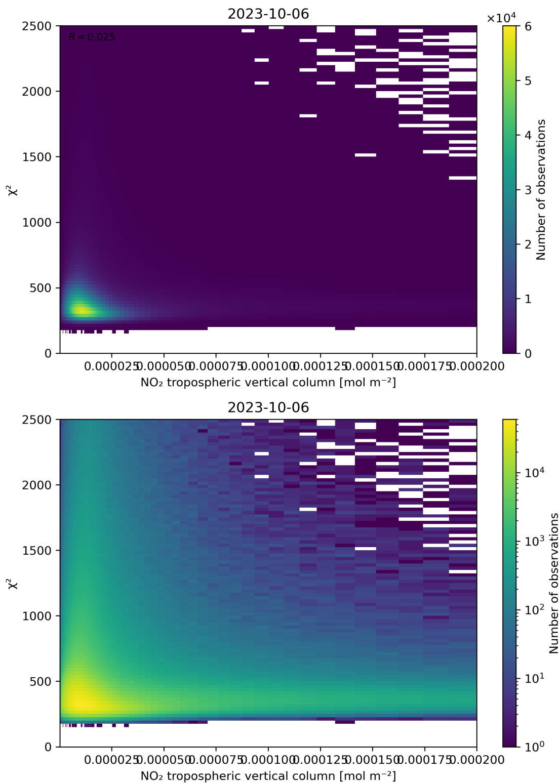
Figure 124: Scatter density plot of “NO 2 tropospheric vertical column” against “ \chi^2 ” for 2023-10-06 to 2023-10-07.
