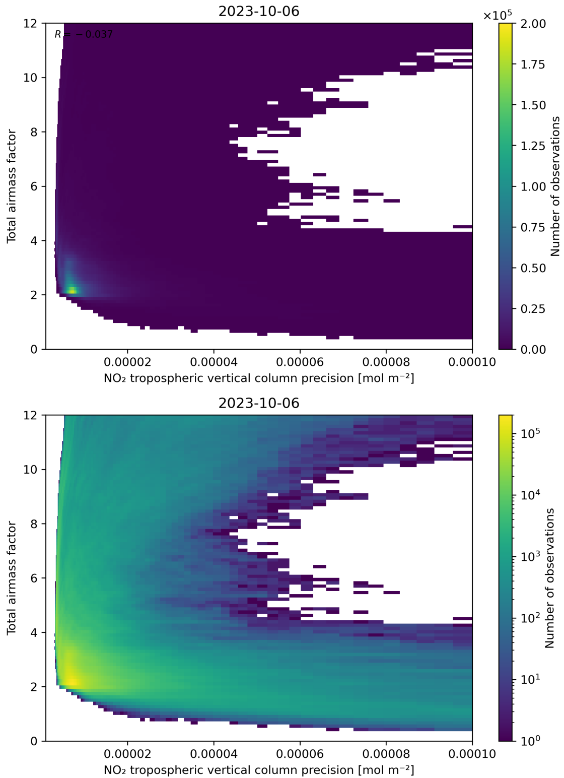
Figure 132: Scatter density plot of “NO 2 tropospheric vertical column precision” against “Total air mass factor” for 2023-10-06 to 2023-10-07.
