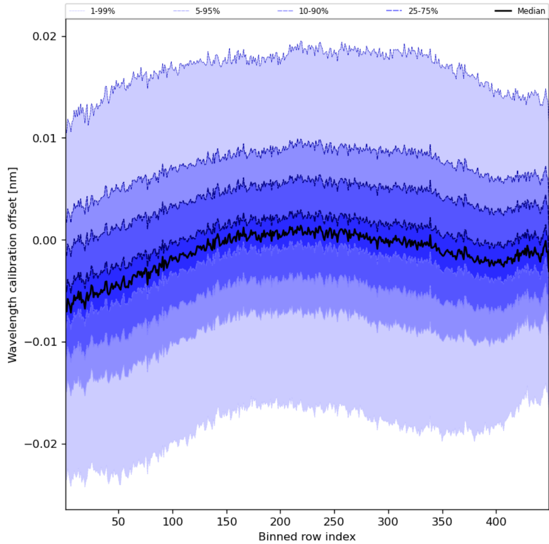
Figure 52: Along track statistics of “Wavelength calibration offset” for 2023-10-06 to 2023-10-07
