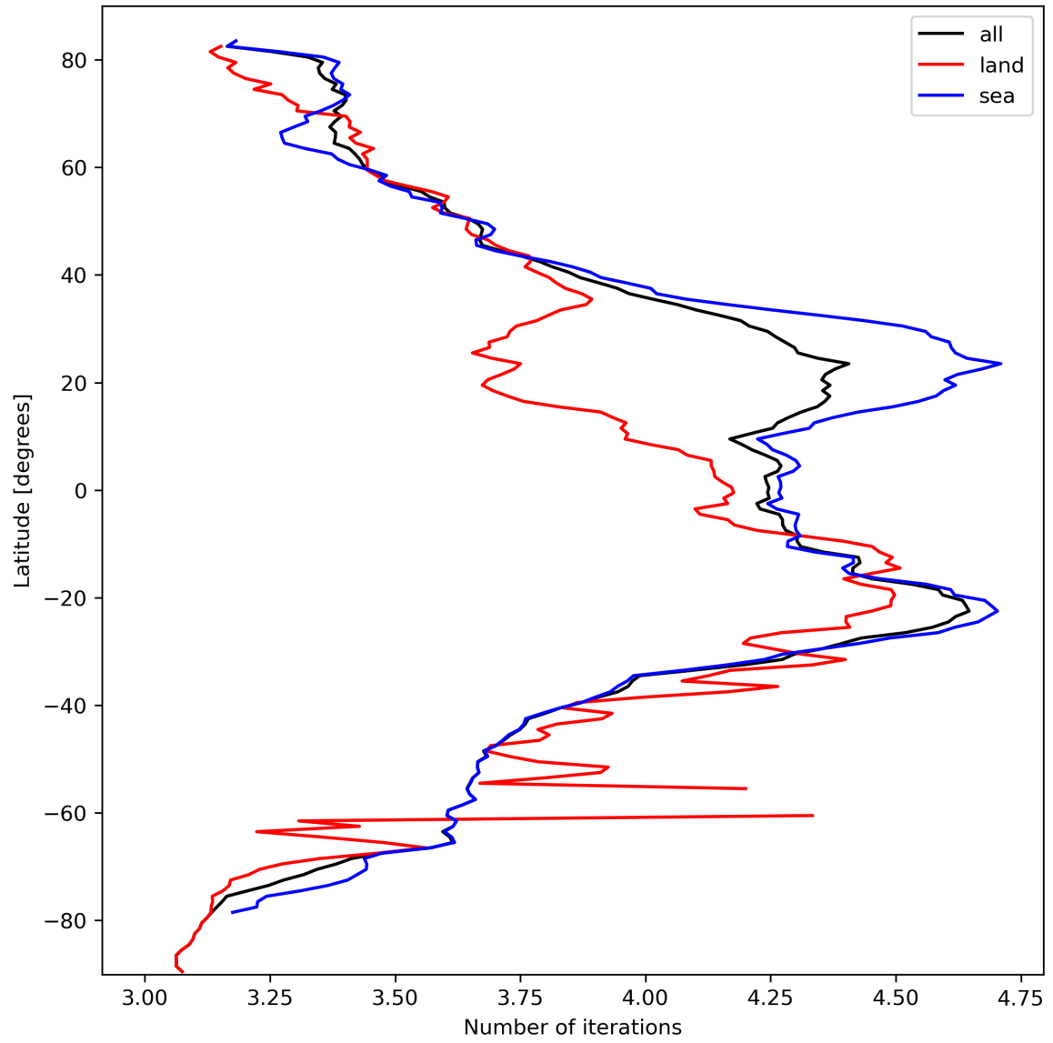
Figure 17: Zonal average of “Number of iterations” for 2023-10-06 to 2023-10-07.
