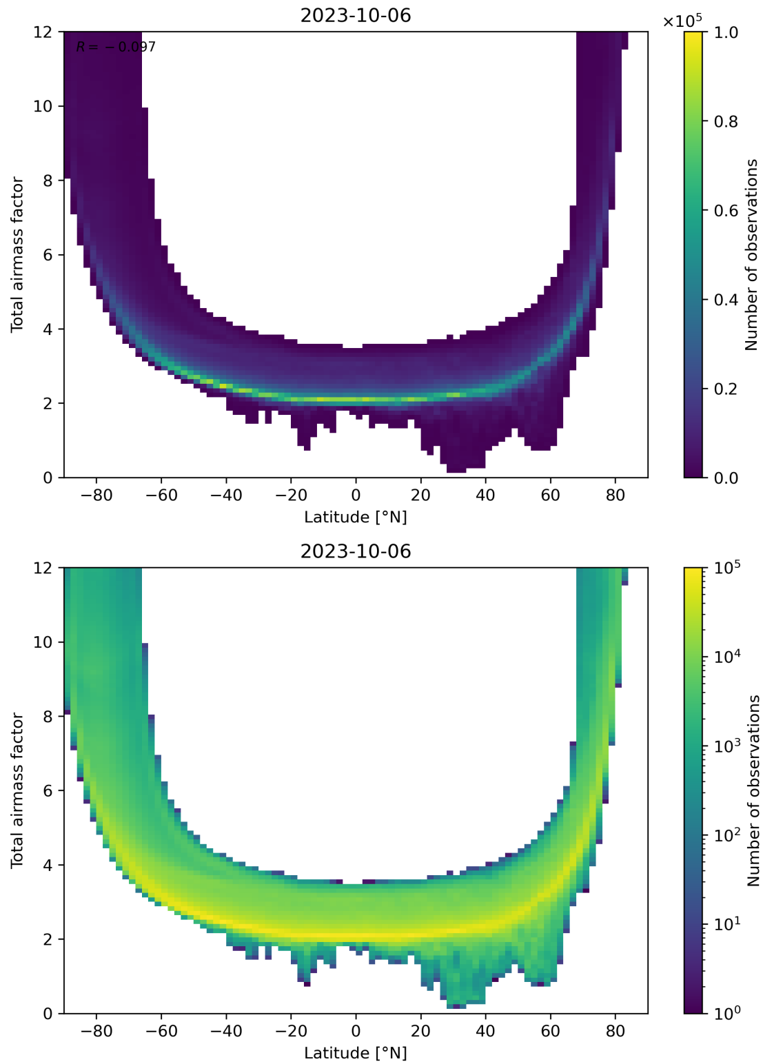
Figure 84: Scatter density plot of “Latitude” against “Total airmass factor” for 2023-10-06 to 2023-10-07.
