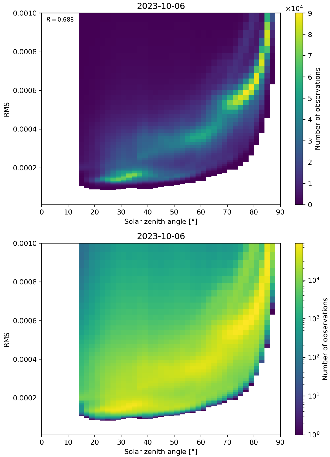
Figure 157: Scatter density plot of “Solar zenith angle” against “RMS” for 2023-10-06 to 2023-10-07.
