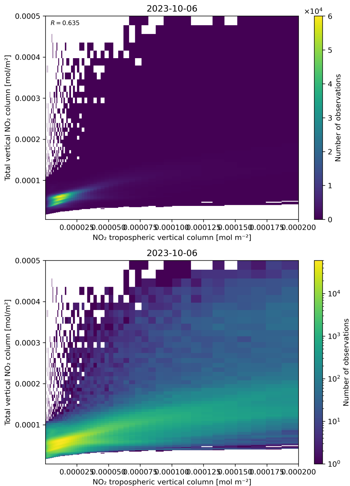
Figure 128: Scatter density plot of “NO 2 tropospheric vertical column” against “Total vertical NO 2 column” for 2023-10-06 to 2023-10-07.
