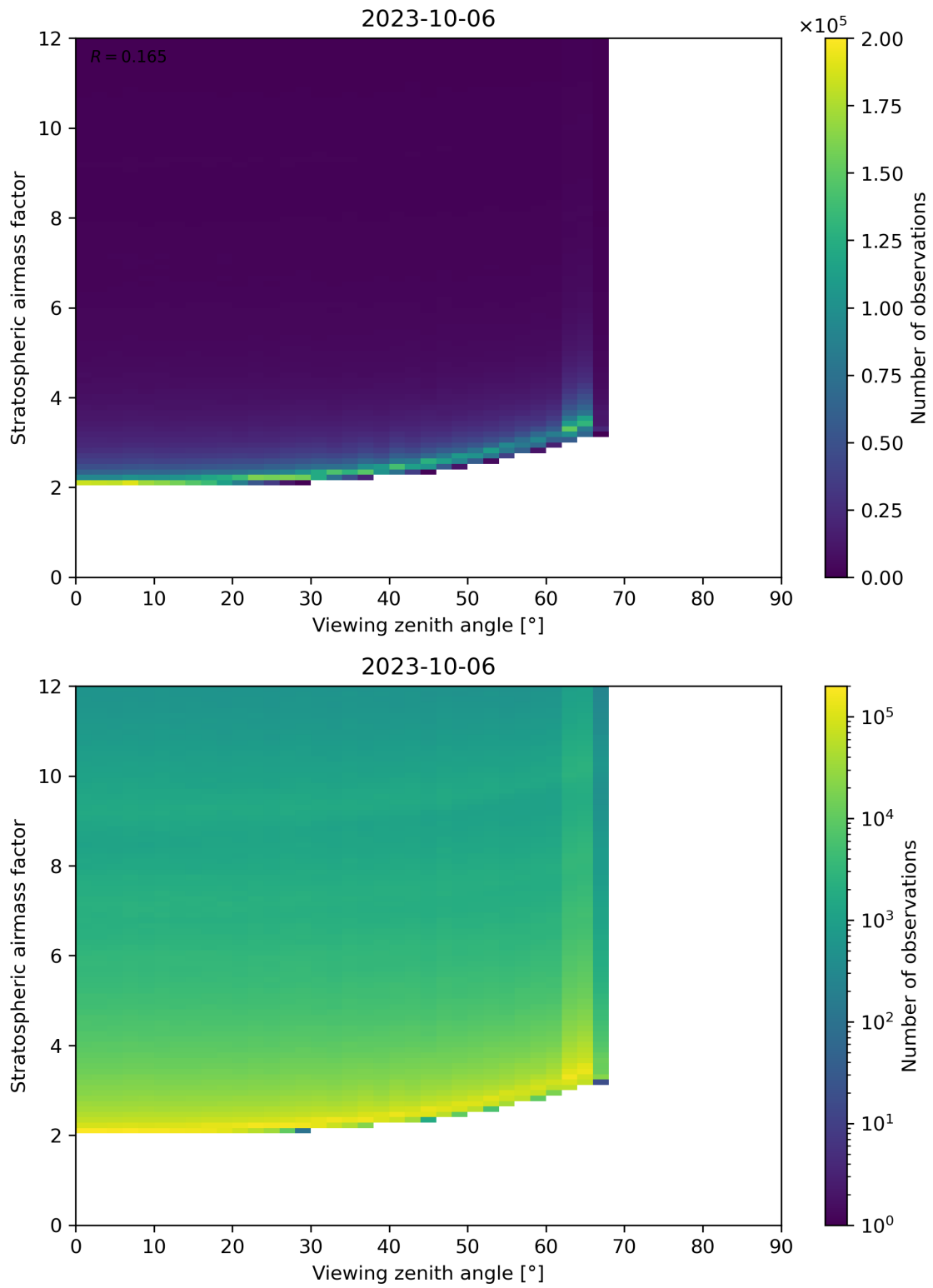
Figure 159: Scatter density plot of “Viewing zenith angle” against “Stratospheric airmass factor” for 2023-10-06 to 2023-10-07.
