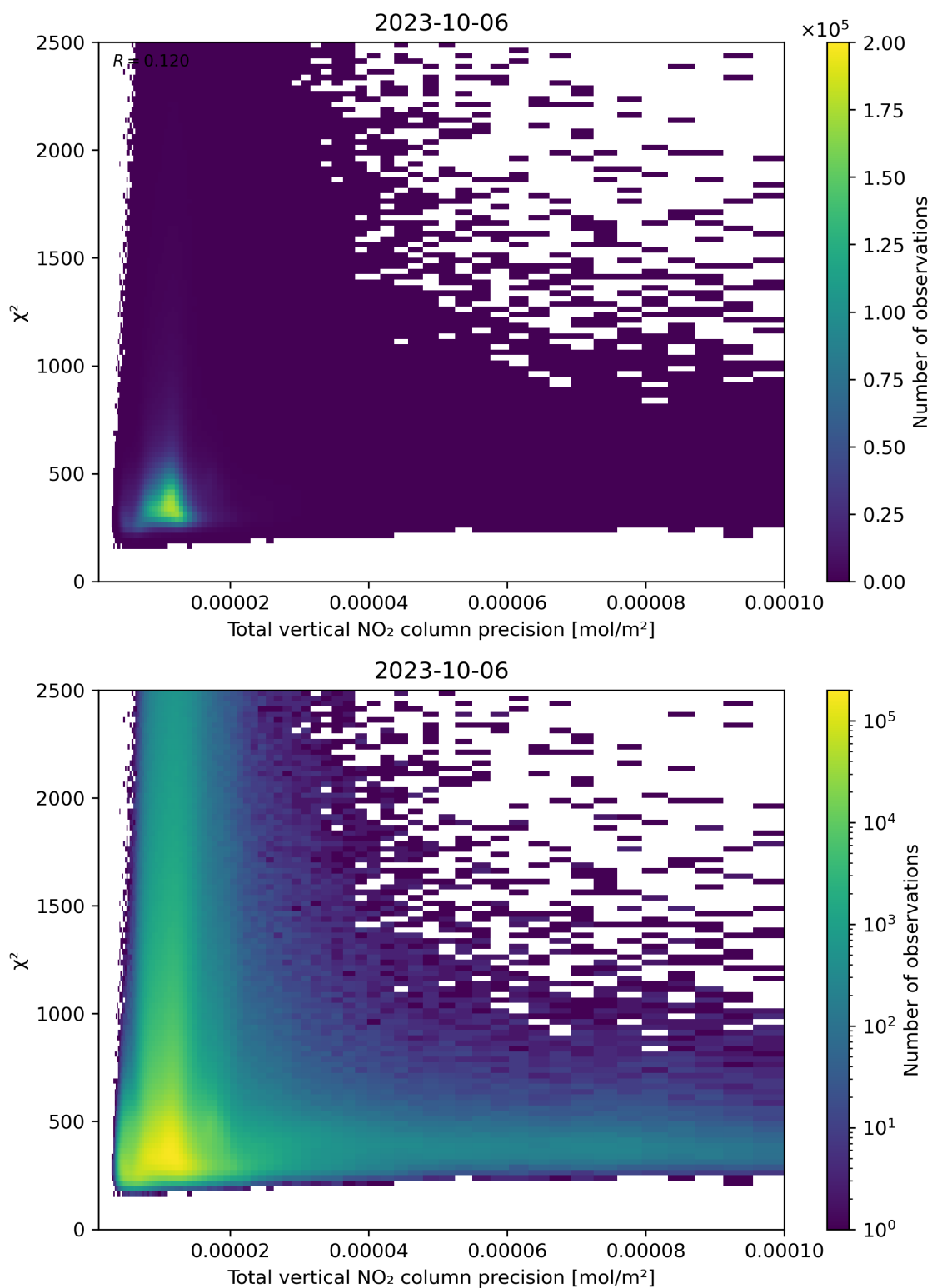
Figure 116: Scatter density plot of “Total vertical NO 2 column precision” against “ \chi^2 ” for 2023-10-06 to 2023-10-07.
