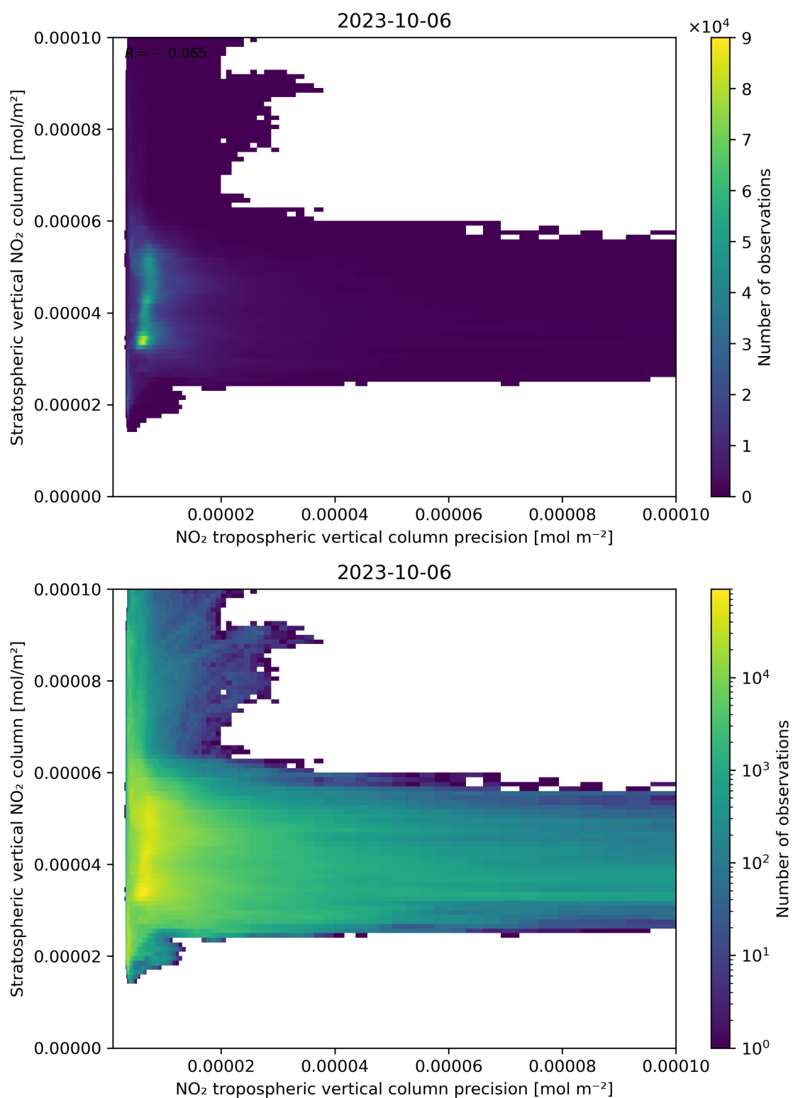
Figure 135: Scatter density plot of “NO 2 tropospheric vertical column precision” against “Stratospheric vertical NO 2 column” for 2023-10-06 to 2023-10-07.
