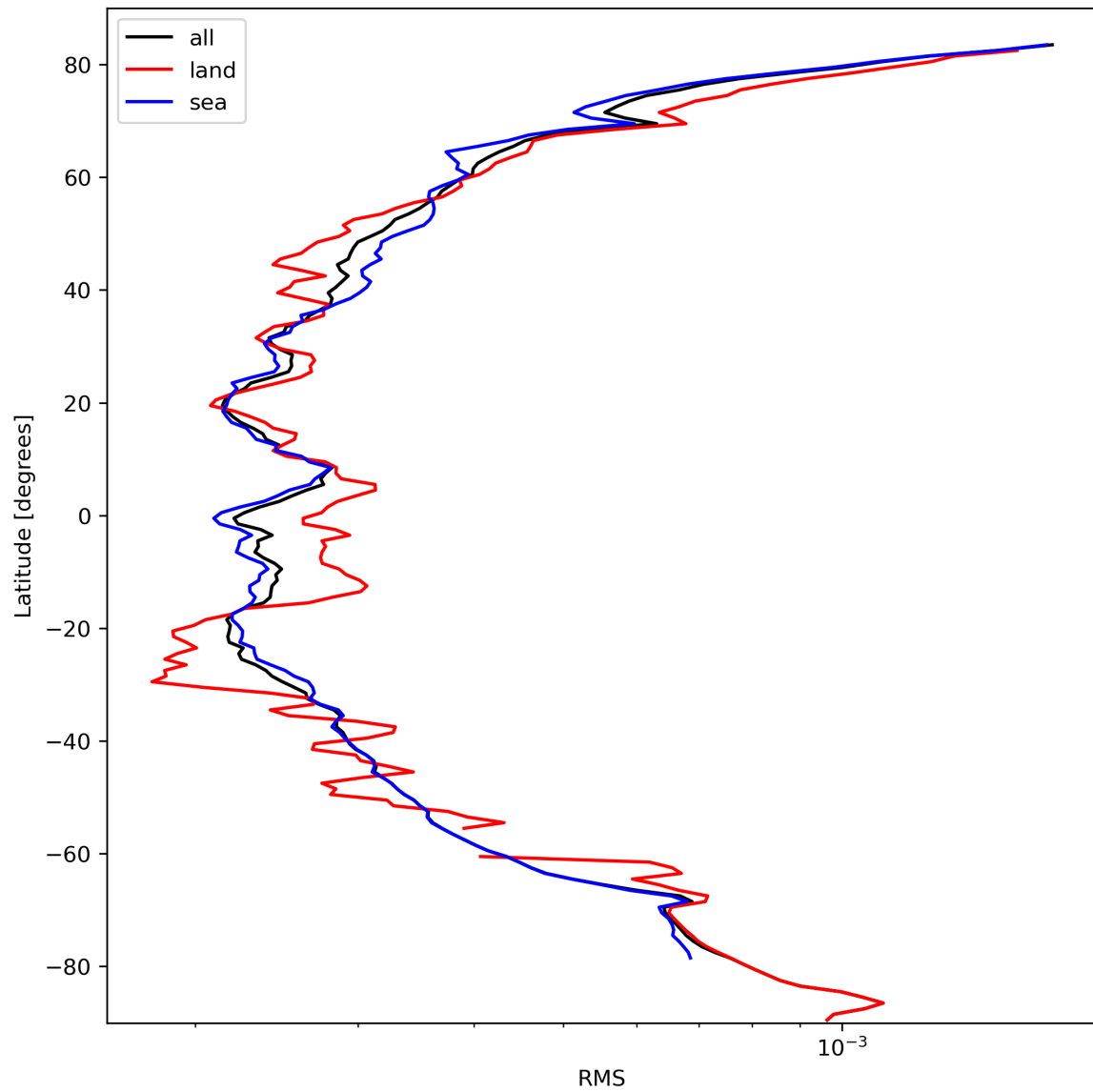
Figure 26: Zonal average of “RMS” for 2023-10-06 to 2023-10-07.
