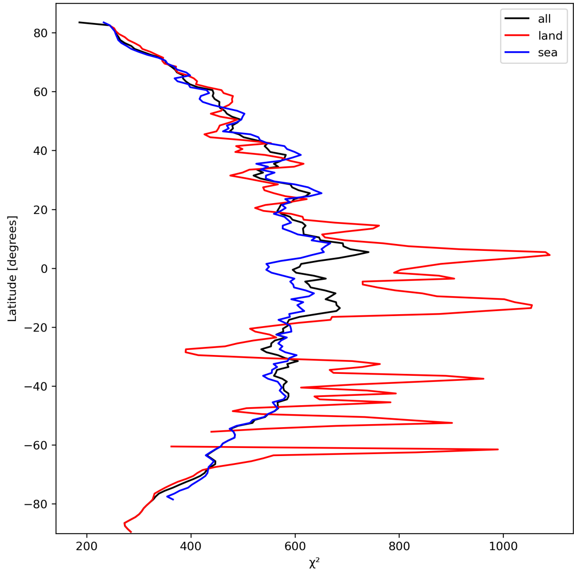
Figure 25: Zonal average of “ \chi^2 ” for 2023-10-06 to 2023-10-07.
