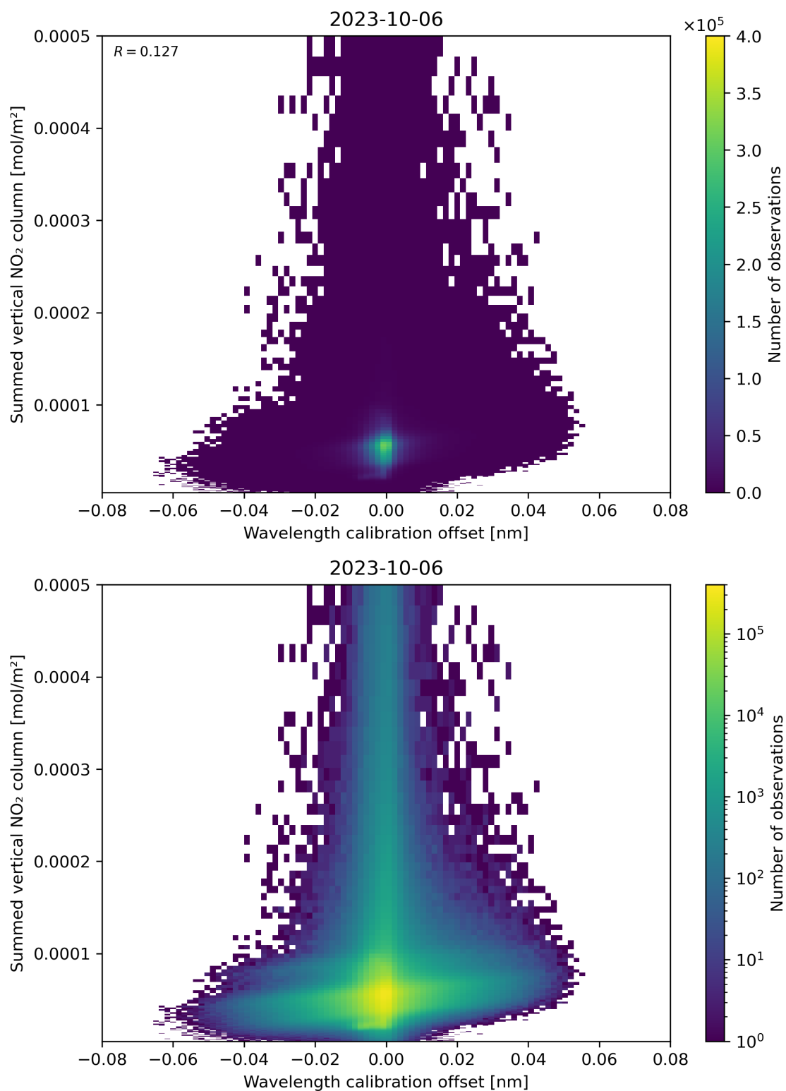
Figure 177: Scatter density plot of “Wavelength calibration offset” against “Summed vertical NO 2 column” for 2023-10-06 to 2023-10-07.
