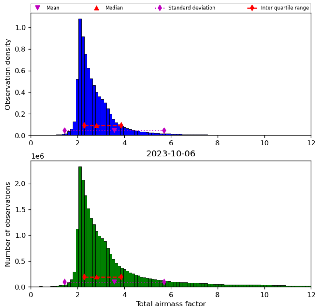
Figure 32: Histogram of “Total airmass factor” for 2023-10-06 to 2023-10-07
