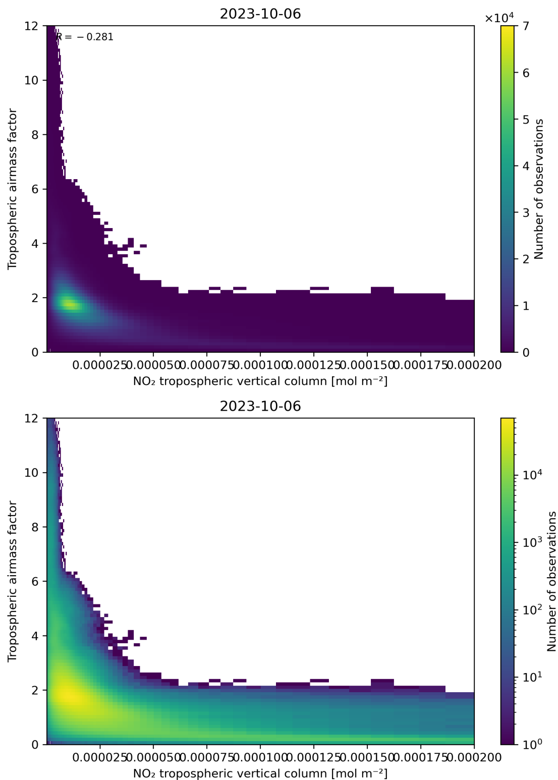
Figure 123: Scatter density plot of “NO 2 tropospheric vertical column” against “Tropospheric air mass factor” for 2023-10-06 to 2023-10-07.
