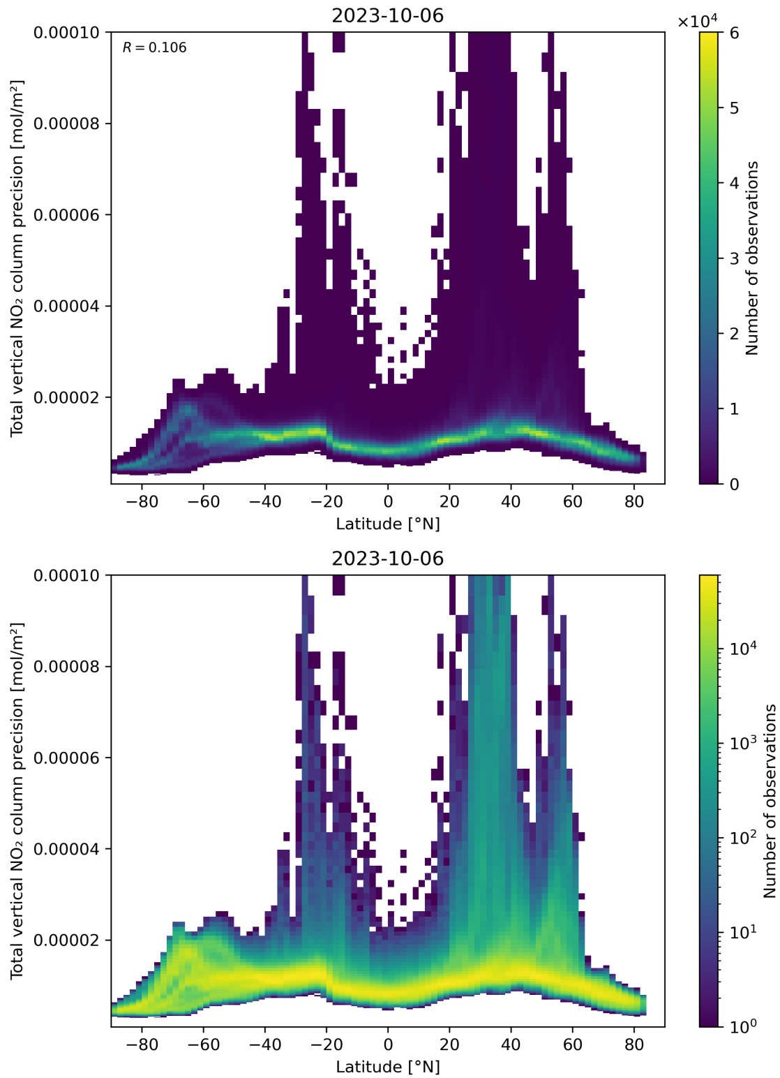
Figure 91: Scatter density plot of “Latitude” against “Total vertical NO 2 column precision” for 2023-10-06 to 2023-10-07.
