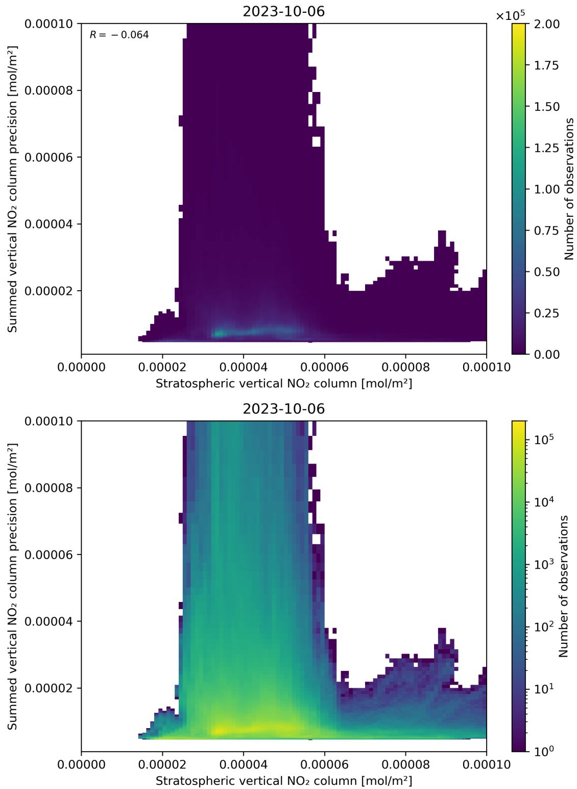
Figure 99: Scatter density plot of “Stratospheric vertical NO 2 column” against “Summed vertical NO 2 column precision” for 2023-10-06 to 2023-10-07.
