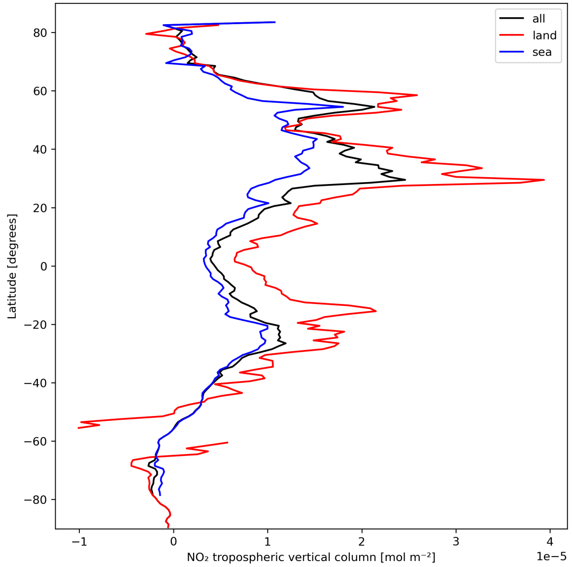
Figure 12: Zonal average of “NO 2 tropospheric vertical column” for 2023-10-06 to 2023-10-07.
