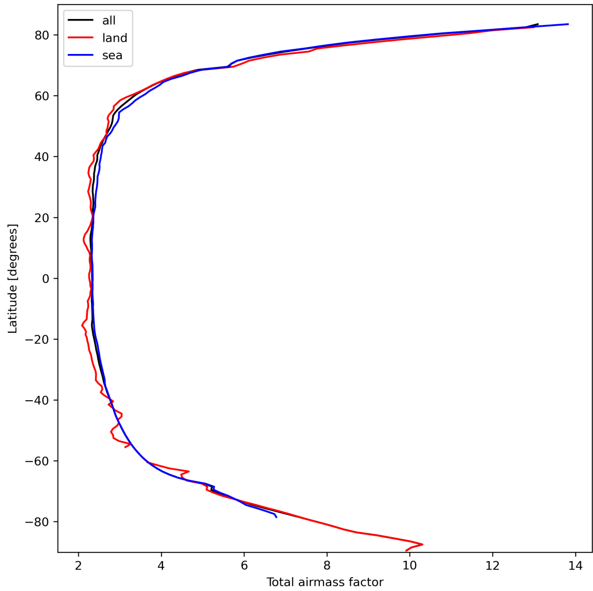
Figure 15: Zonal average of “Total airmass factor” for 2023-10-06 to 2023-10-07.
