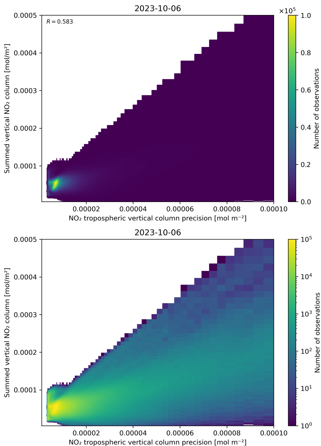
Figure 136: Scatter density plot of “NO 2 tropospheric vertical column precision” against “Summed vertical NO 2 column” for 2023-10-06 to 2023-10-07.
