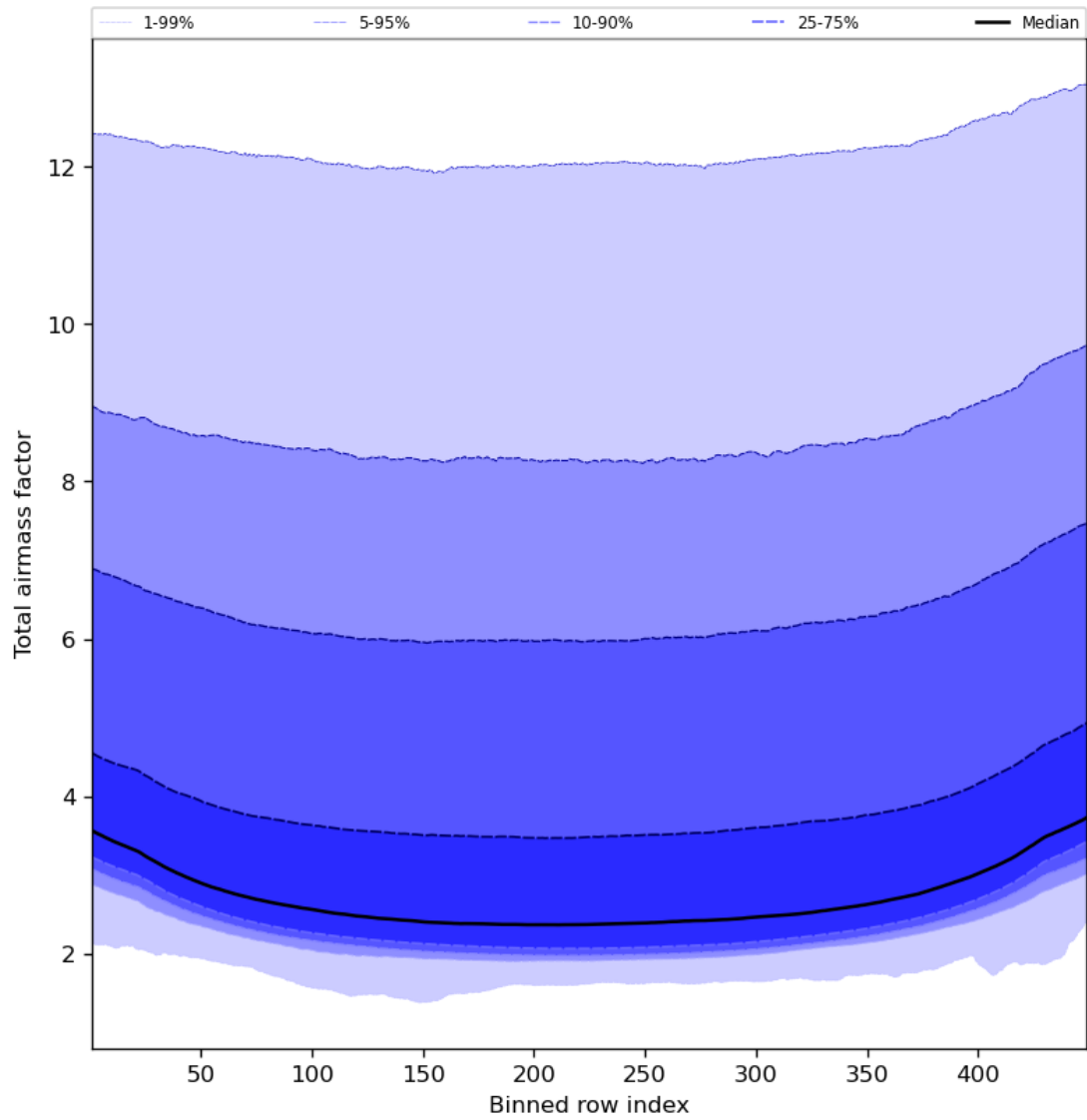
Figure 49: Along track statistics of “Total airmass factor” for 2023-10-06 to 2023-10-07
