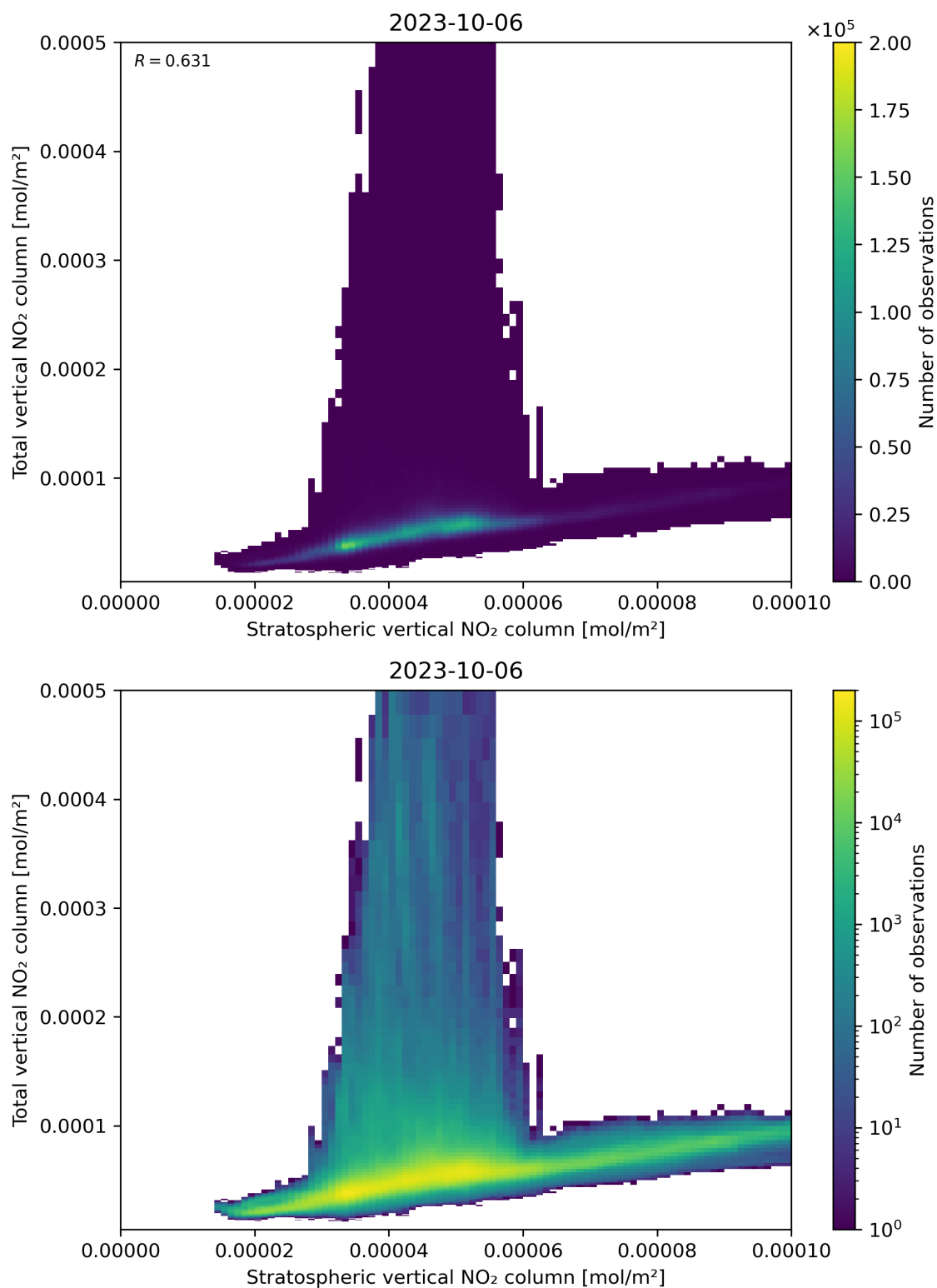
Figure 100: Scatter density plot of “Stratospheric vertical NO 2 column” against “Total vertical NO 2 column” for 2023-10-06 to 2023-10-07.
