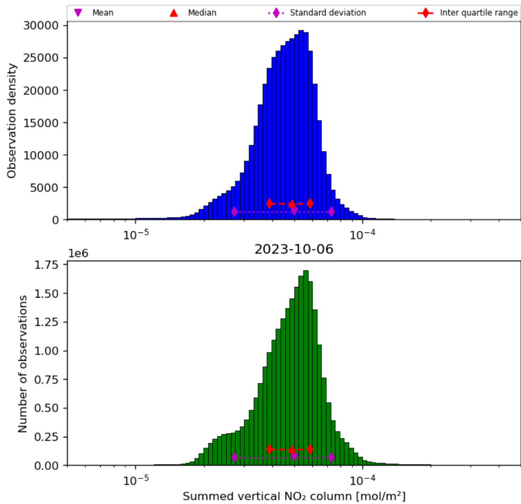
Figure 40: Histogram of “Summed vertical NO 2 column” for 2023-10-06 to 2023-10-07
