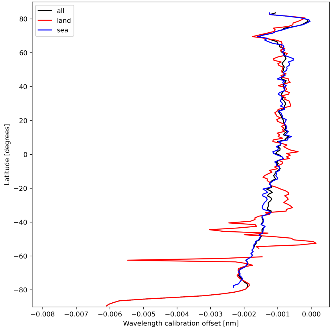
Figure 18: Zonal average of “Wavelength calibration offset” for 2023-10-06 to 2023-10-07.
