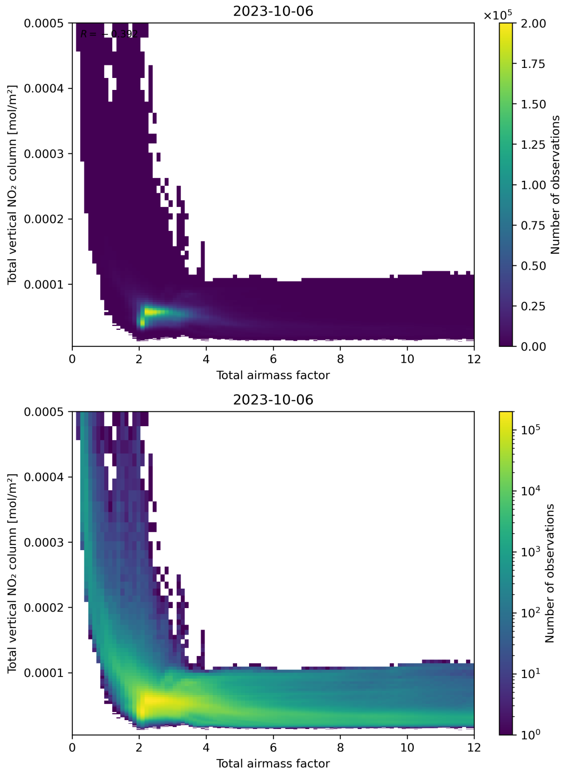
Figure 67: Scatter density plot of “Total airmass factor” against “Total vertical NO 2 column” for 2023-10-06 to 2023-10-07.
