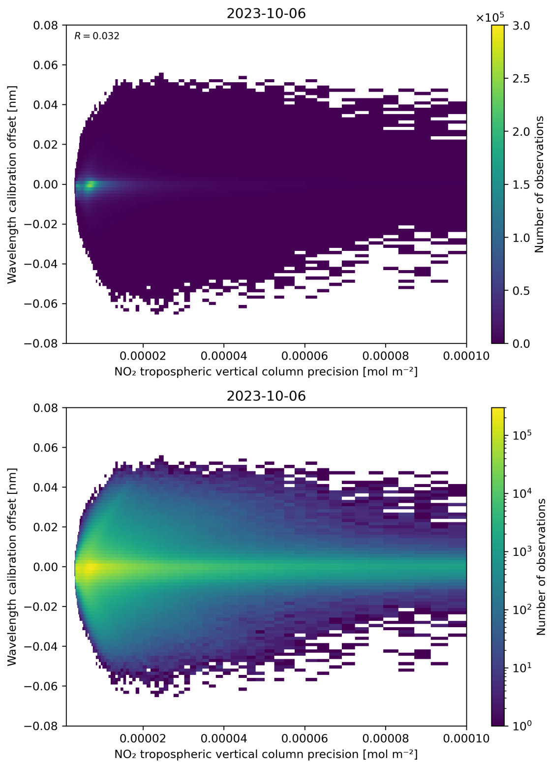
Figure 141: Scatter density plot of “NO 2 tropospheric vertical column precision” against “Wavelength calibration offset” for 2023-10-06 to 2023-10-07.
