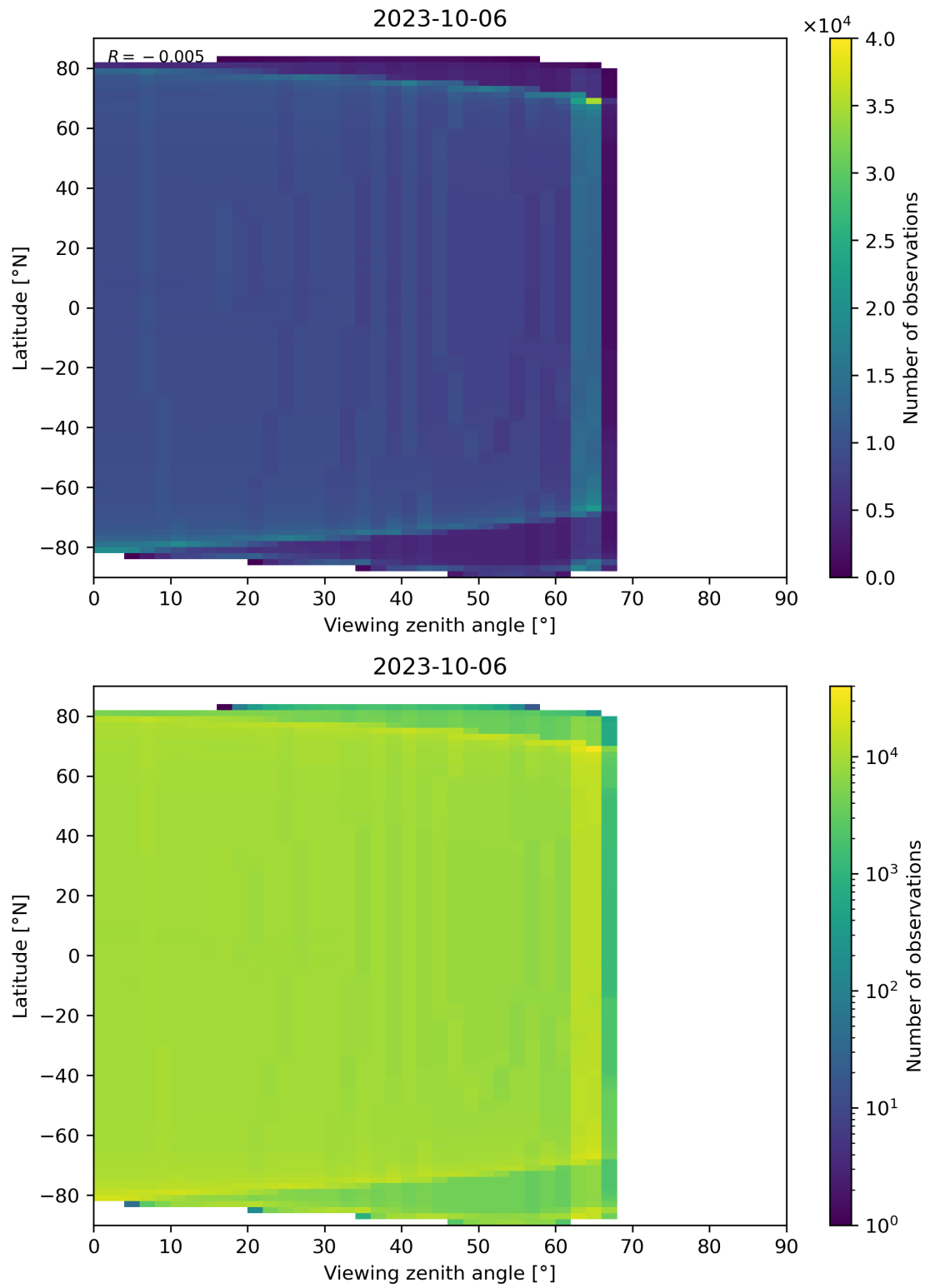
Figure 163: Scatter density plot of “Viewing zenith angle” against “Latitude” for 2023-10-06 to 2023-10-07.
