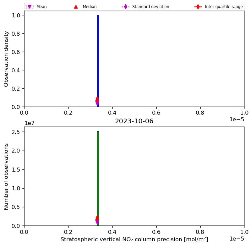
Figure 37: Histogram of “Stratospheric vertical NO 2 column precision” for 2023-10-06 to 2023-10-07
