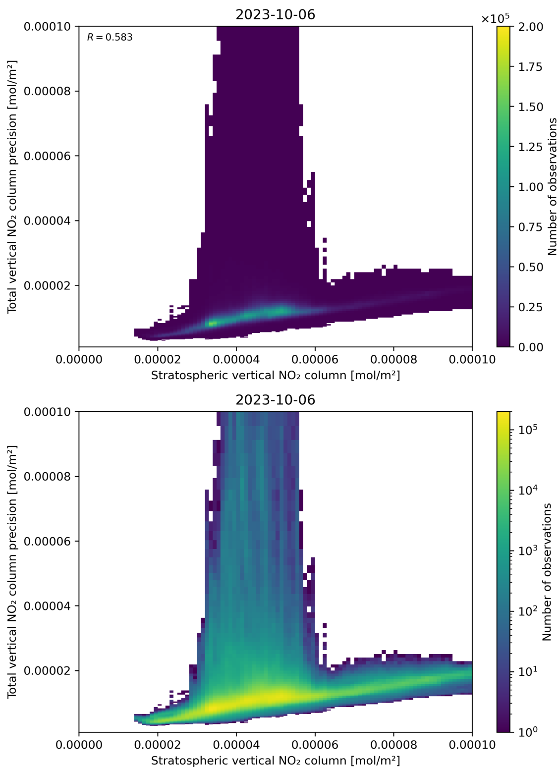
Figure 101: Scatter density plot of “Stratospheric vertical NO 2 column” against “Total vertical NO 2 column precision” for 2023-10-06 to 2023-10-07.
