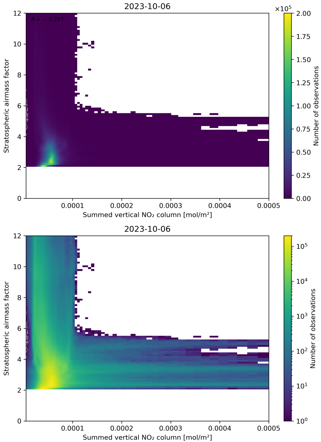
Figure 103: Scatter density plot of “Summed vertical NO 2 column” against “Stratospheric air mass factor” for 2023-10-06 to 2023-10-07.
