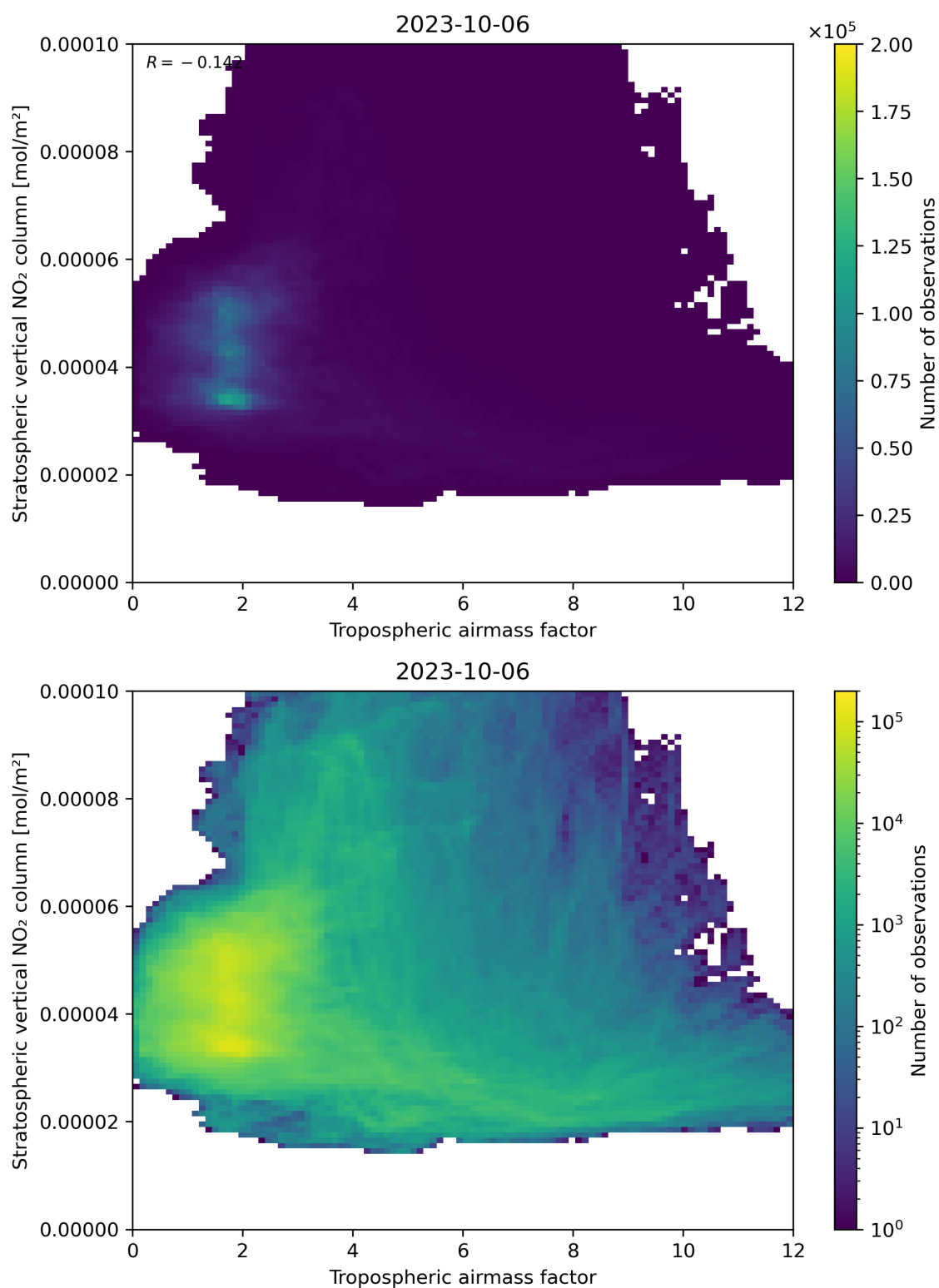
Figure 74: Scatter density plot of “Tropospheric air mass factor” against “Stratospheric vertical NO 2 column” for 2023-10-06 to 2023-10-07.
