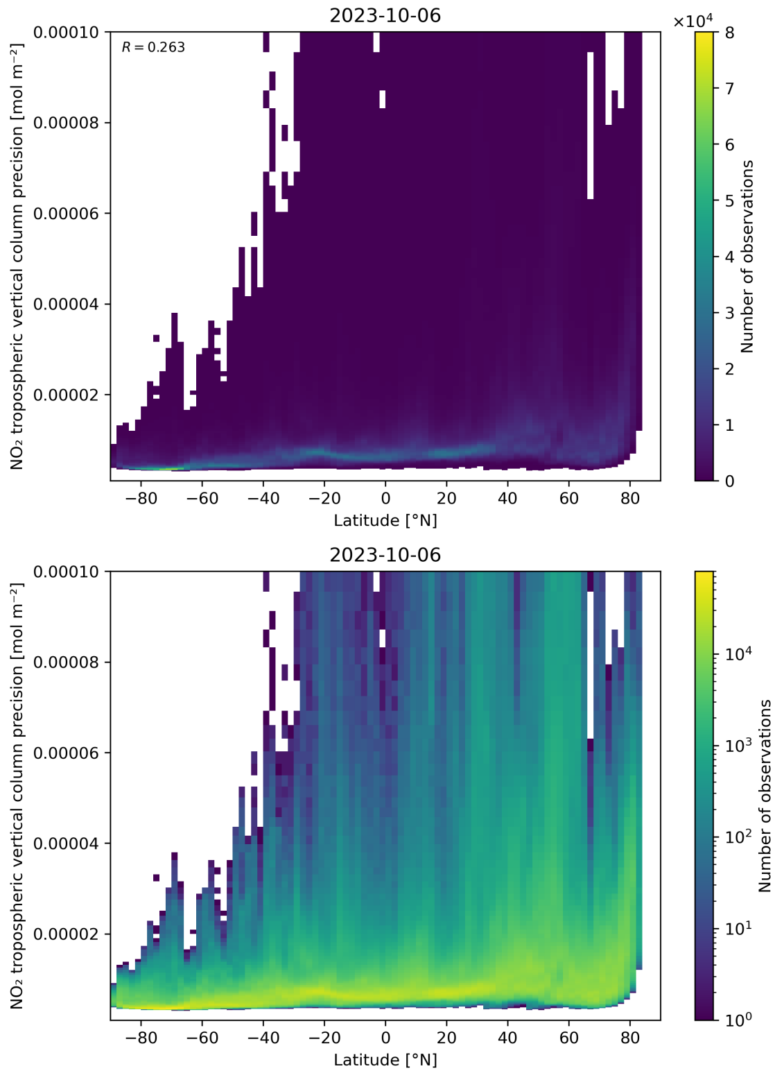
Figure 93: Scatter density plot of “Latitude” against “NO 2 tropospheric vertical column precision” for 2023-10-06 to 2023-10-07.
