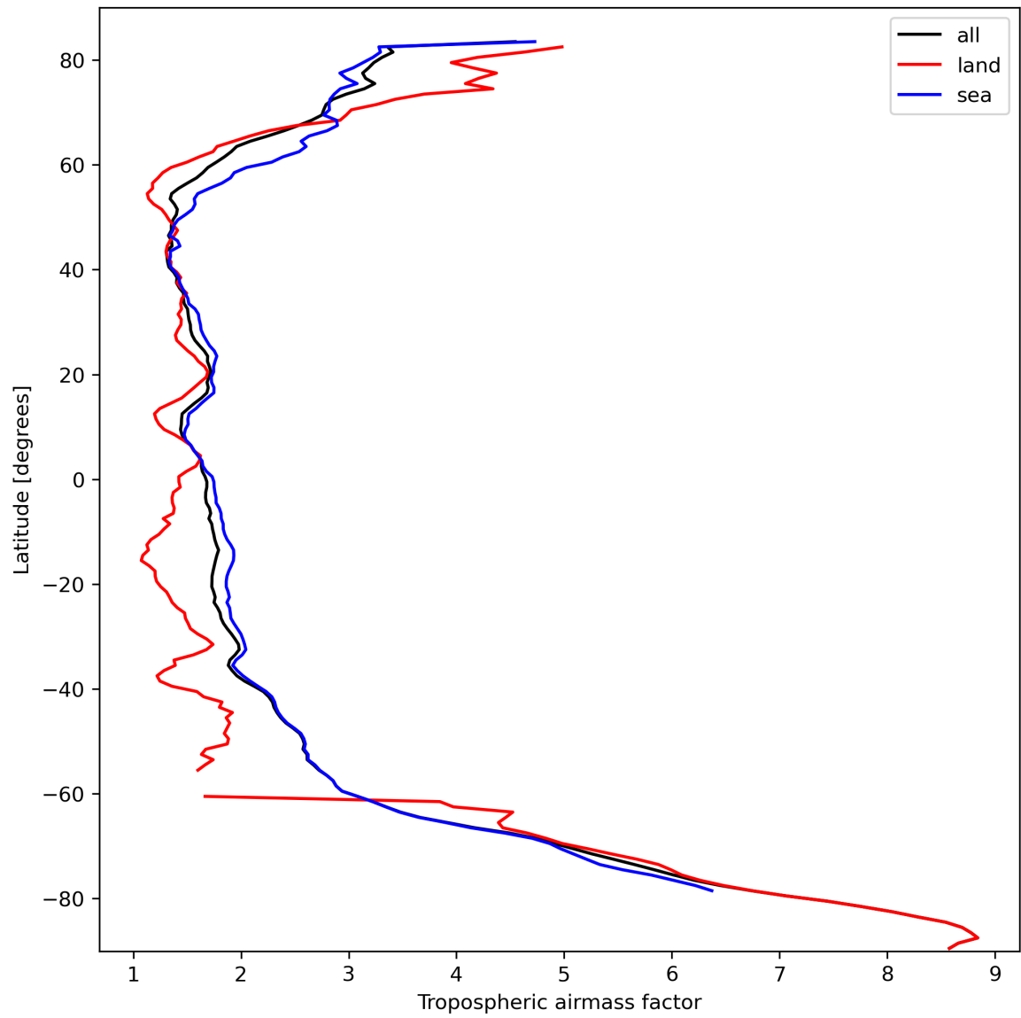
Figure 14: Zonal average of “Tropospheric air mass factor” for 2023-10-06 to 2023-10-07.
