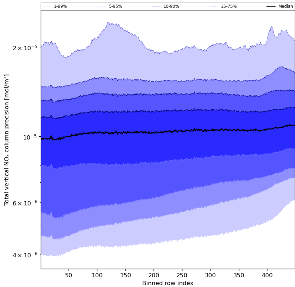
Figure 56: Along track statistics of "Total vertical NO 2 column precision" for 2023-10-06 to 2023-10-07
