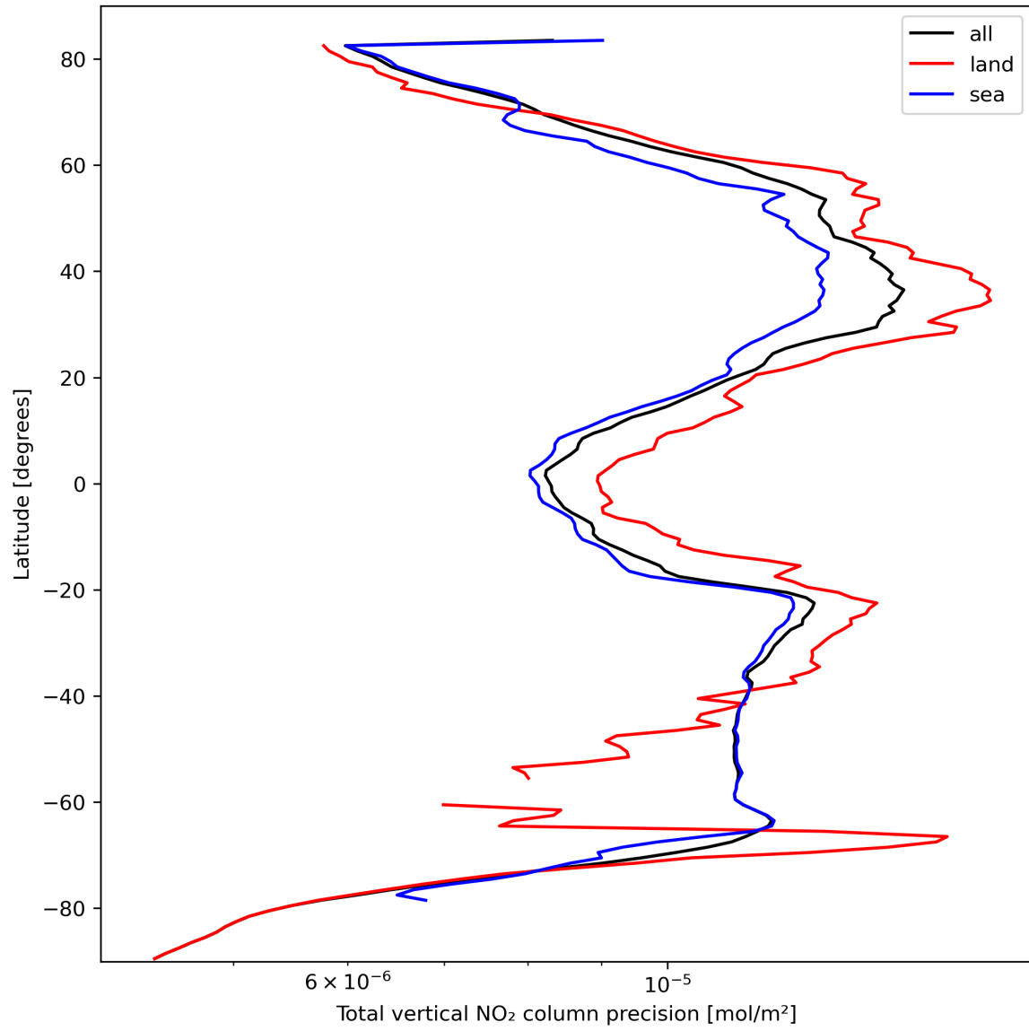
Figure 22: Zonal average of “Total vertical NO 2 column precision” for 2023-10-06 to 2023-10-07.
