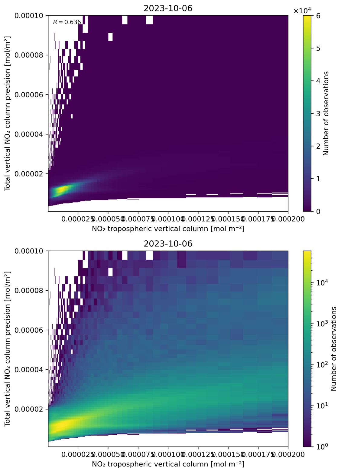
Figure 129: Scatter density plot of “NO 2 tropospheric vertical column” against “Total vertical NO 2 column precision” for 2023-10-06 to 2023-10-07.
