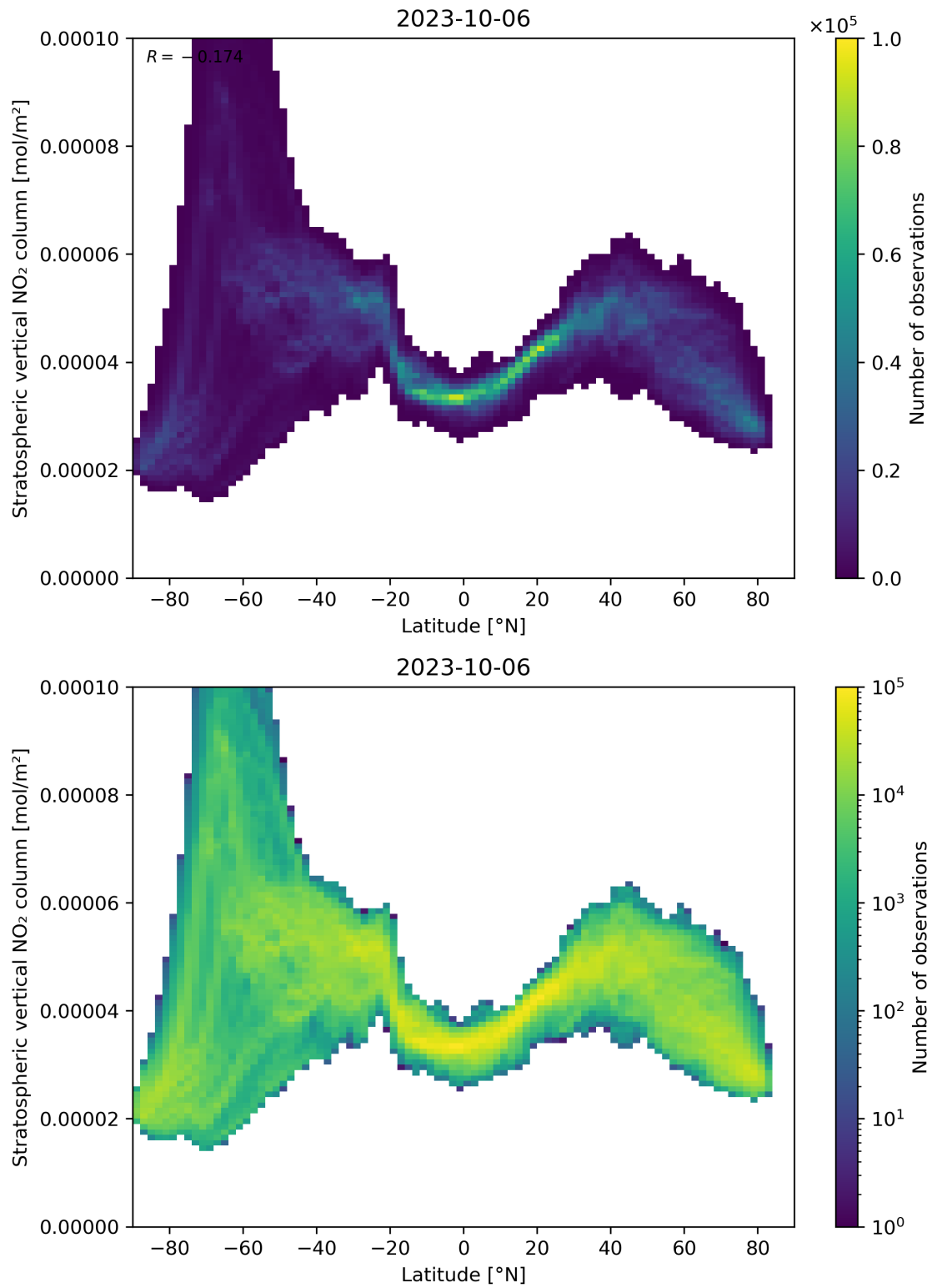
Figure 87: Scatter density plot of “Latitude” against “Stratospheric vertical NO 2 column” for 2023-10-06 to 2023-10-07.
