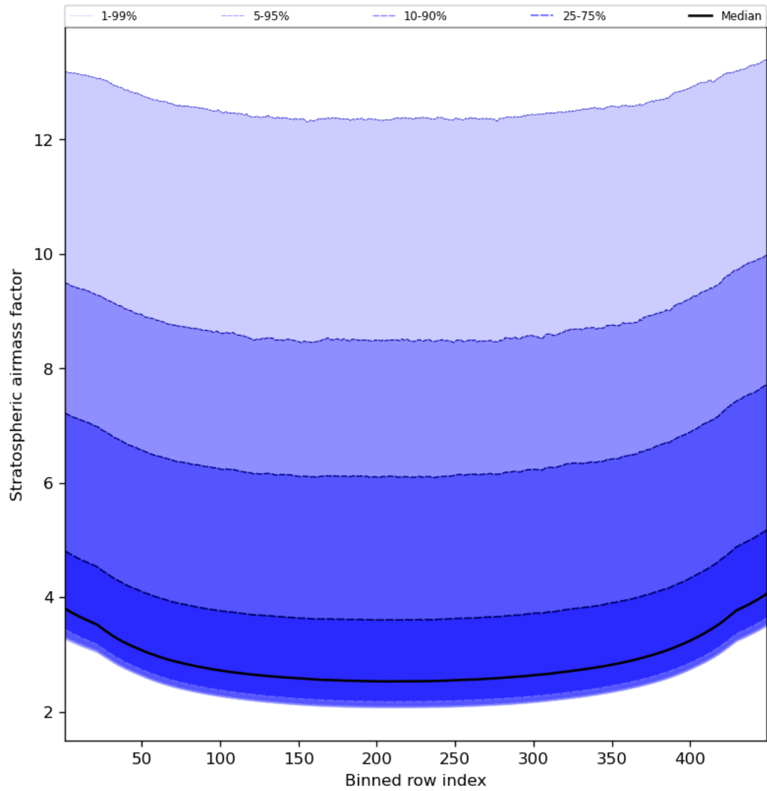
Figure 61: Along track statistics of “Stratospheric airmass factor” for 2023-10-06 to 2023-10-07
