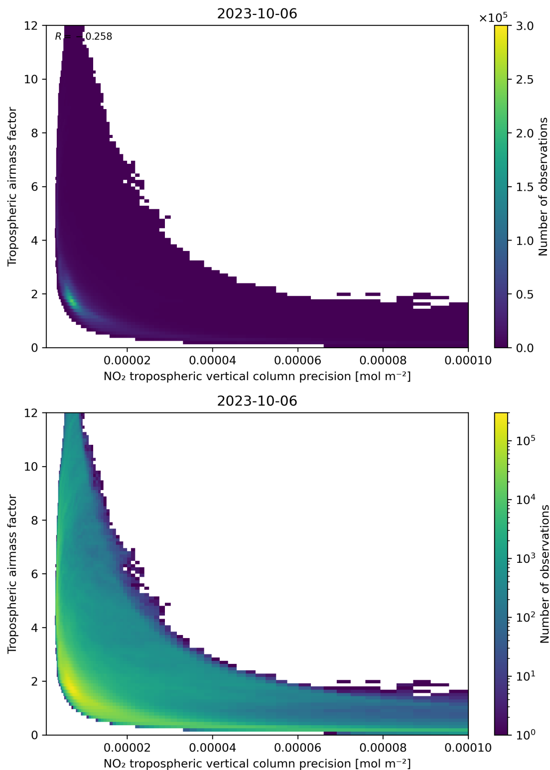
Figure 133: Scatter density plot of “NO 2 tropospheric vertical column precision” against “Tropospheric air mass factor” for 2023-10-06 to 2023-10-07.
