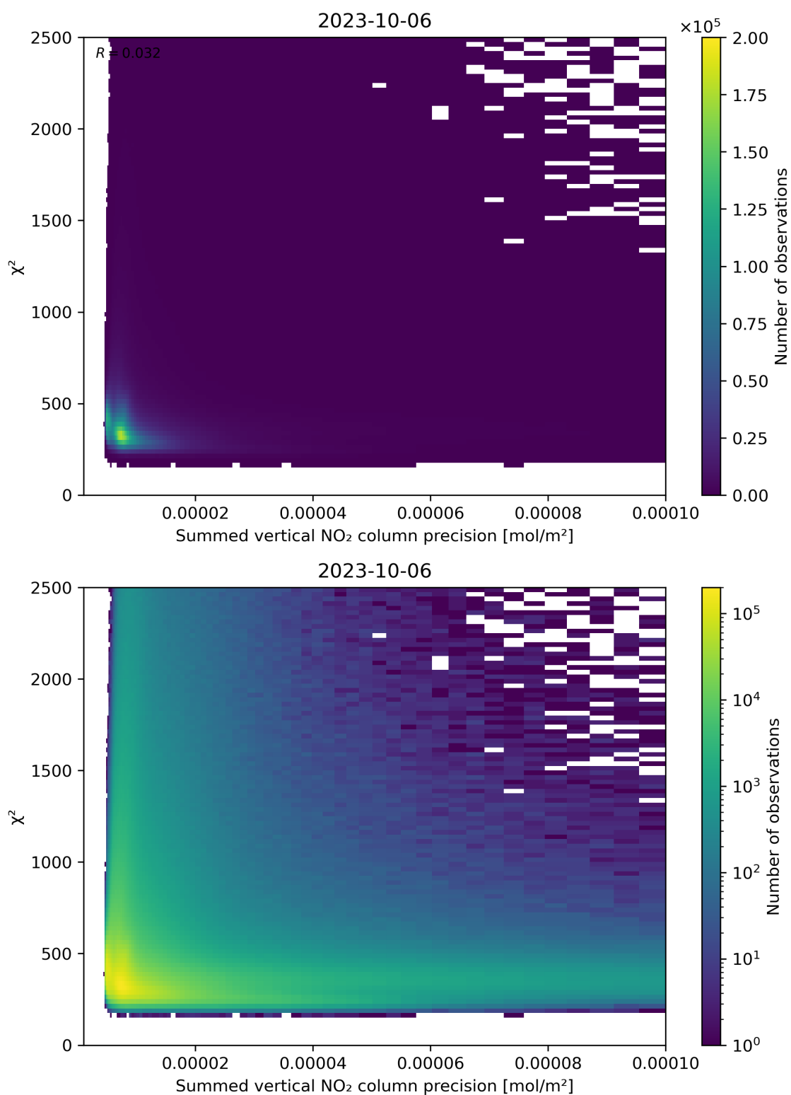
Figure 107: Scatter density plot of “Summed vertical NO 2 column precision” against “ \chi^2 ” for 2023-10-06 to 2023-10-07.
