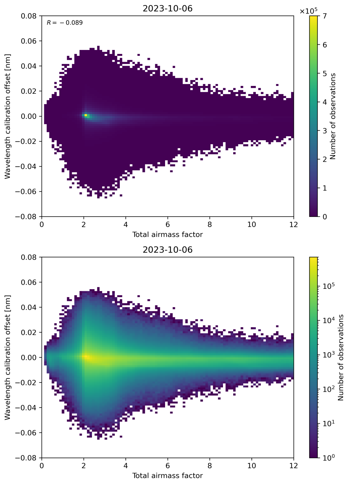
Figure 70: Scatter density plot of “Total airmass factor” against “Wavelength calibration offset” for 2023-10-06 to 2023-10-07.
