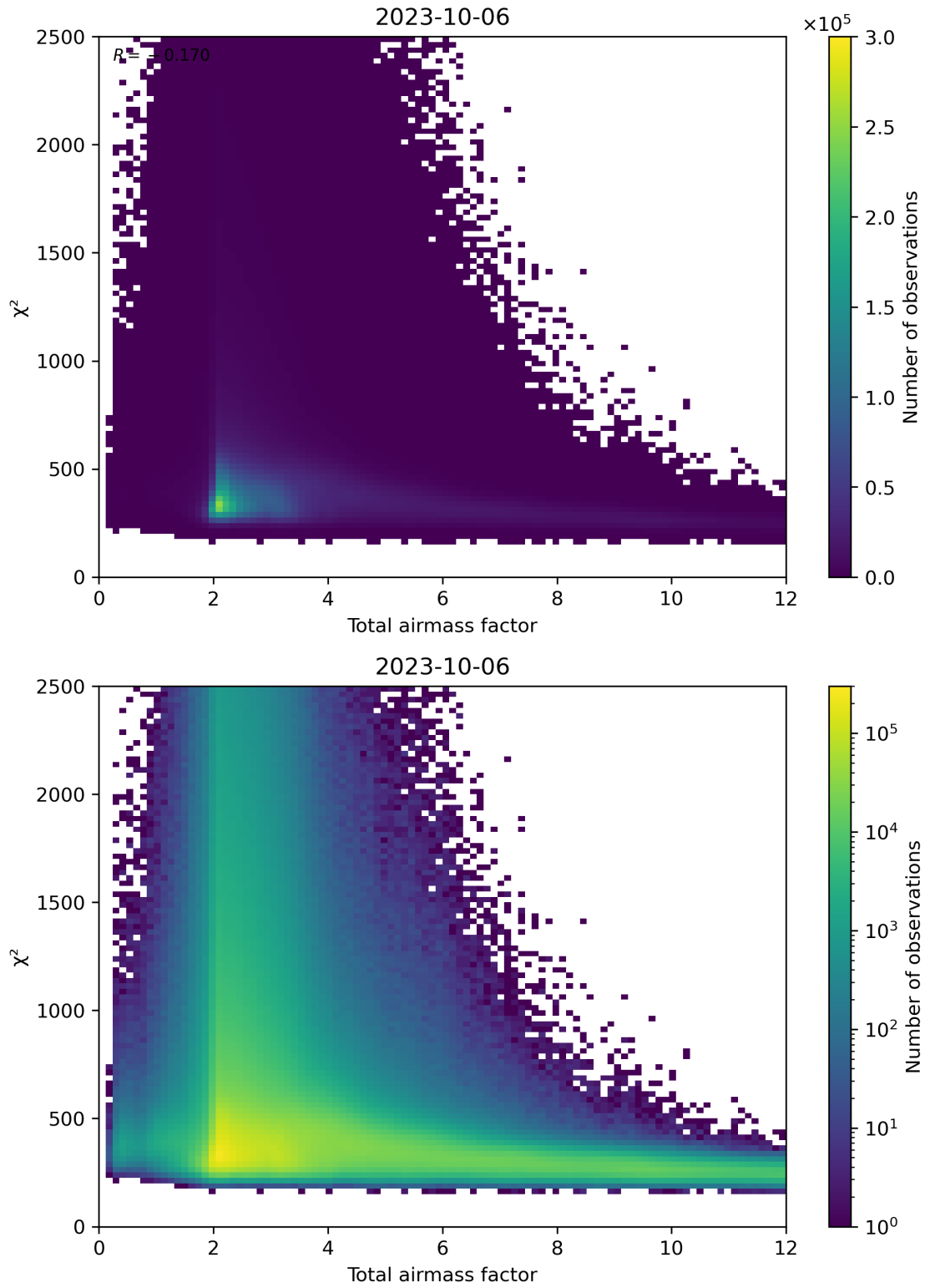
Figure 63: Scatter density plot of “Total airmass factor” against “ \chi^2 ” for 2023-10-06 to 2023-10-07.
