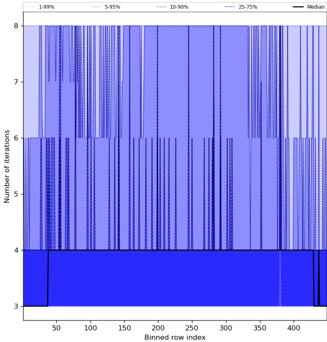
Figure 51: Along track statistics of “Number of iterations” for 2023-10-06 to 2023-10-07
