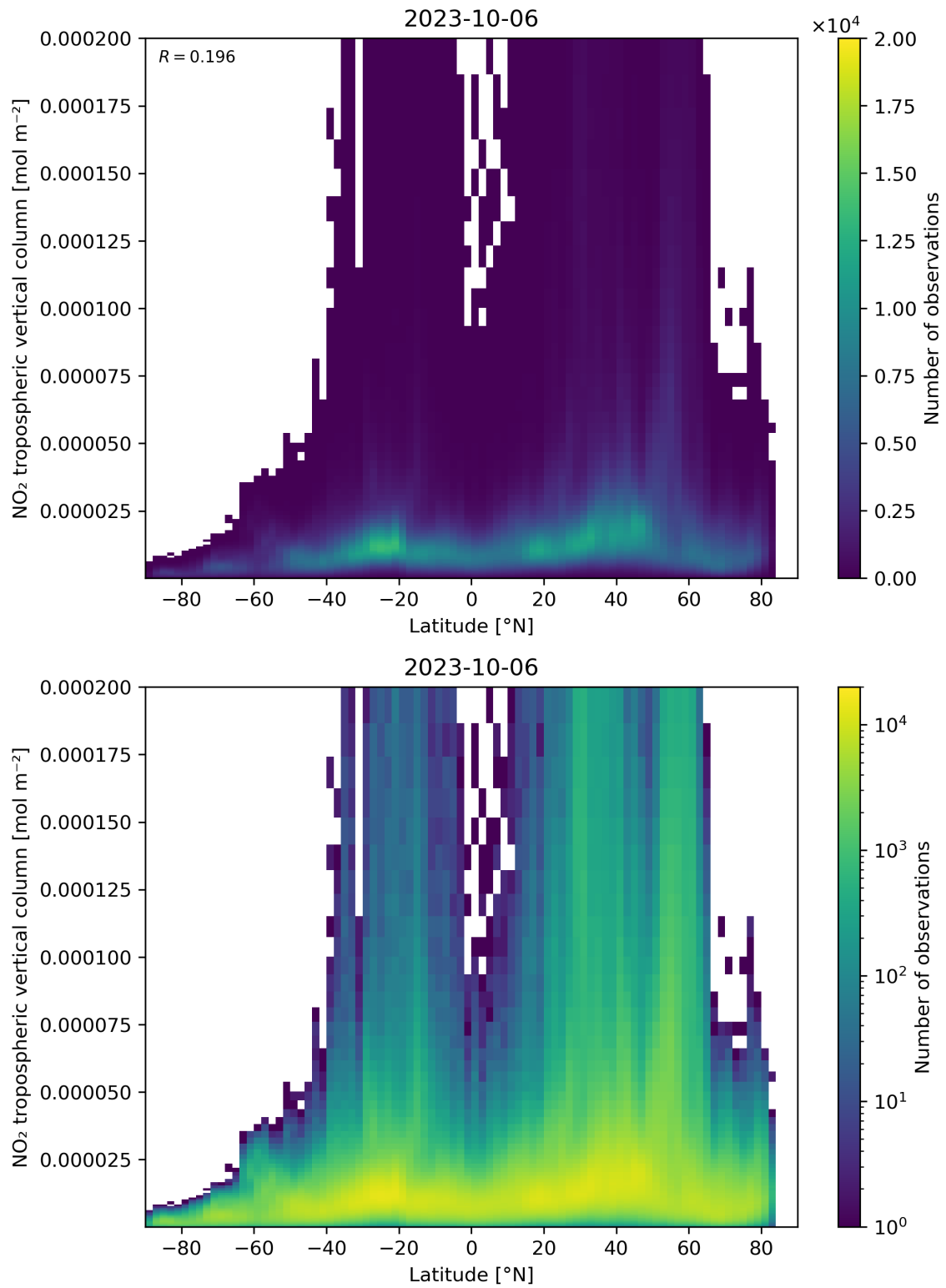
Figure 92: Scatter density plot of “Latitude” against “NO 2 tropospheric vertical column” for 2023-10-06 to 2023-10-07.
