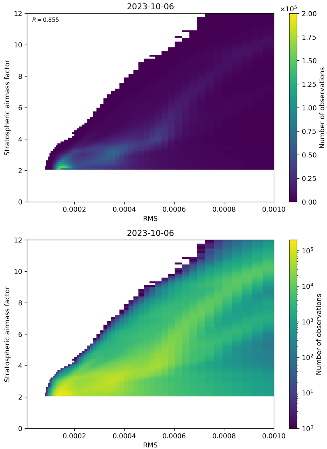
Figure 144: Scatter density plot of “RMS” against “Stratospheric airmass factor” for 2023-10-06 to 2023-10-07.
