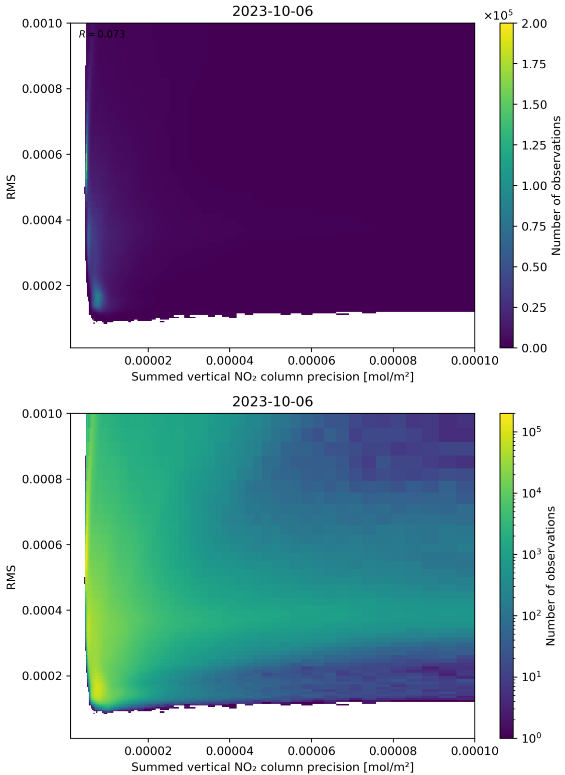
Figure 108: Scatter density plot of “Summed vertical NO 2 column precision” against “RMS” for 2023-10-06 to 2023-10-07.
