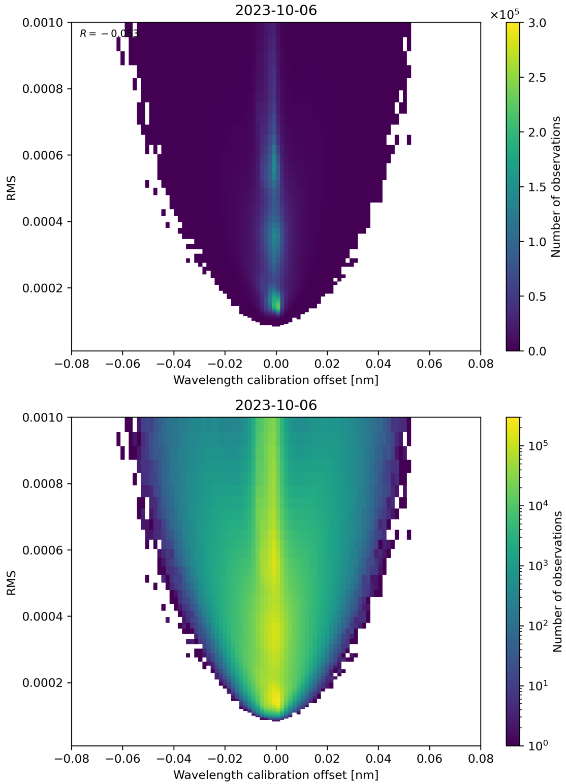
Figure 181: Scatter density plot of “Wavelength calibration offset” against “RMS” for 2023-10-06 to 2023-10-07.
