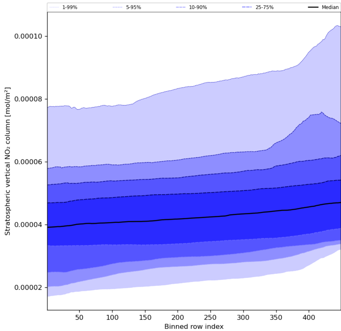
Figure 53: Along track statistics of “Stratospheric vertical NO 2 column” for 2023-10-06 to 2023-10-07
