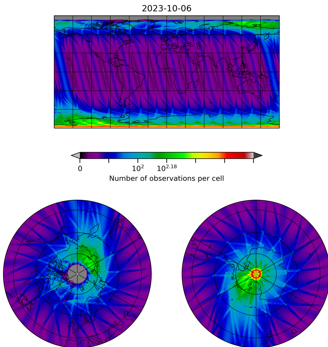
Figure 10: Map of the number of observations for 2023-10-06 to 2023-10-07
