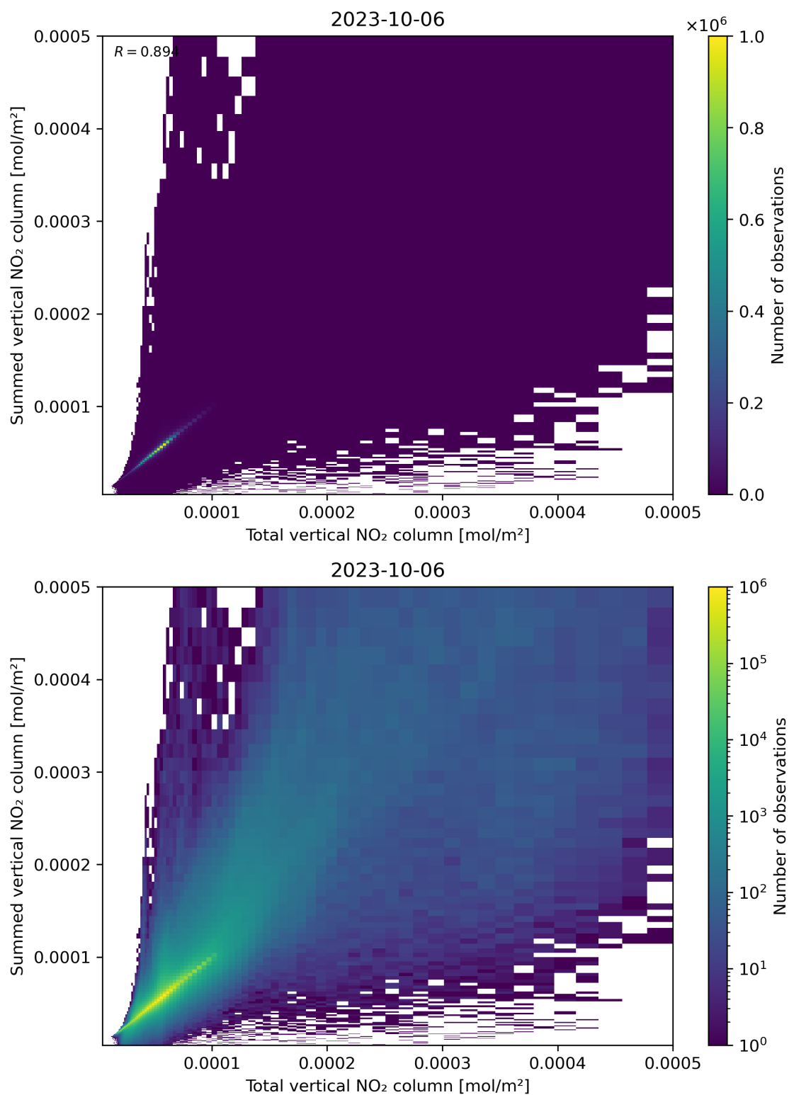
Figure 112: Scatter density plot of “Total vertical NO 2 column” against “Summed vertical NO 2 column” for 2023-10-06 to 2023-10-07.
