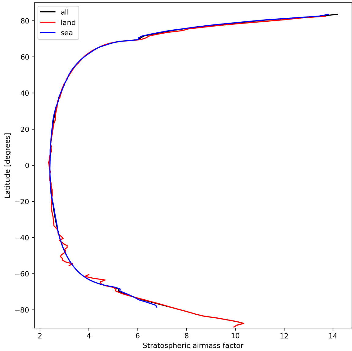
Figure 27: Zonal average of “Stratospheric air mass factor” for 2023-10-06 to 2023-10-07.
