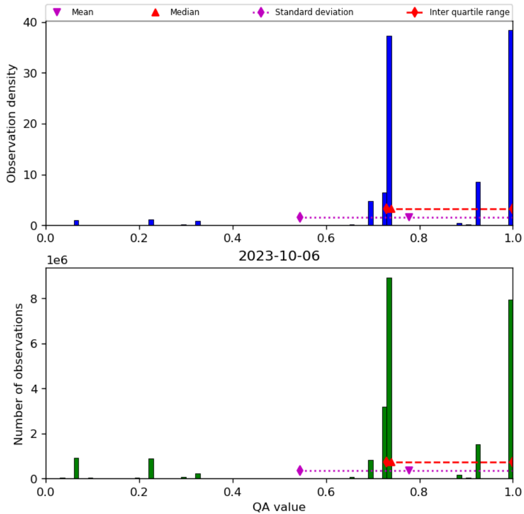
Figure 28: Histogram of “QA value” for 2023-10-06 to 2023-10-07
