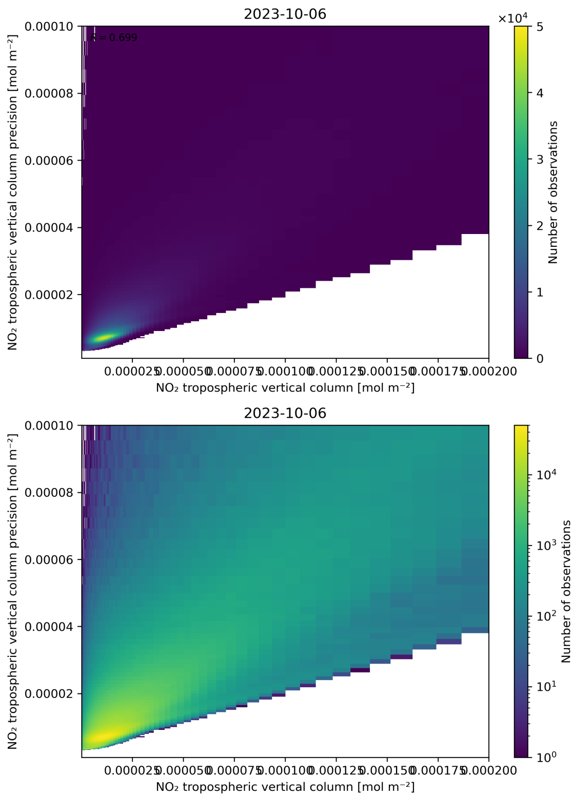
Figure 130: Scatter density plot of “NO 2 tropospheric vertical column” against “NO 2 tropospheric vertical column precision” for 2023-10-06 to 2023-10-07.
