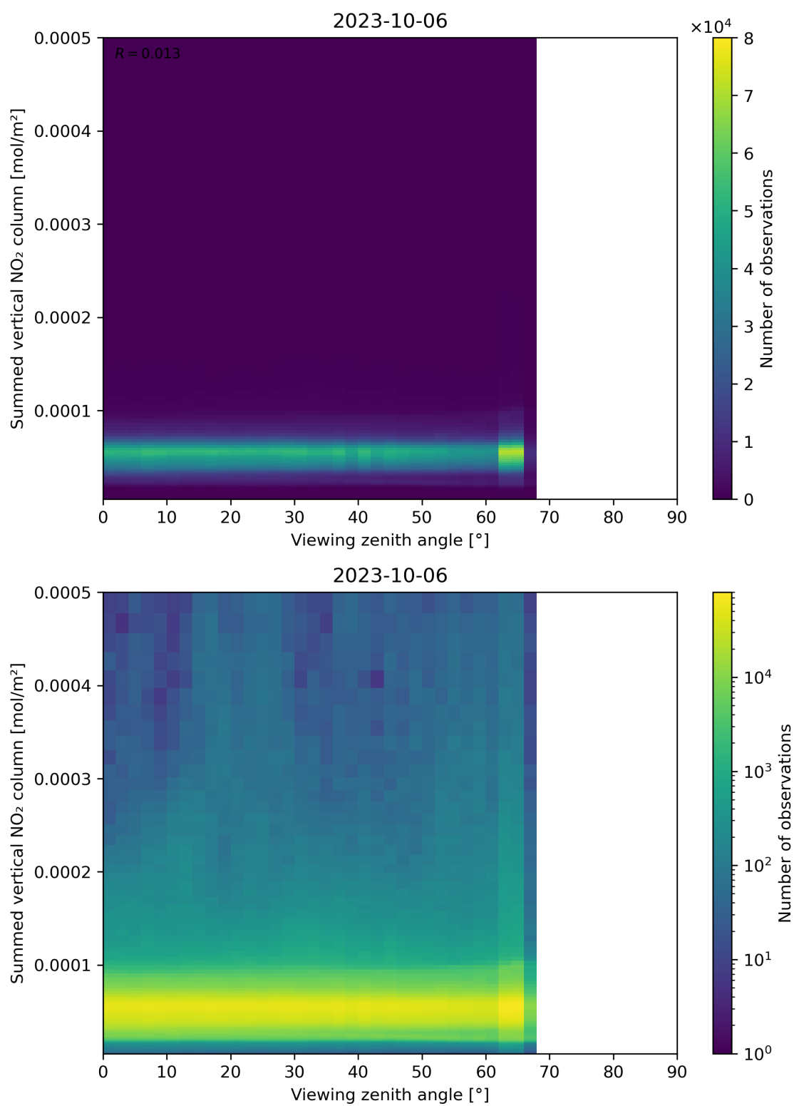
Figure 165: Scatter density plot of “Viewing zenith angle” against “Summed vertical NO 2 column” for 2023-10-06 to 2023-10-07.
