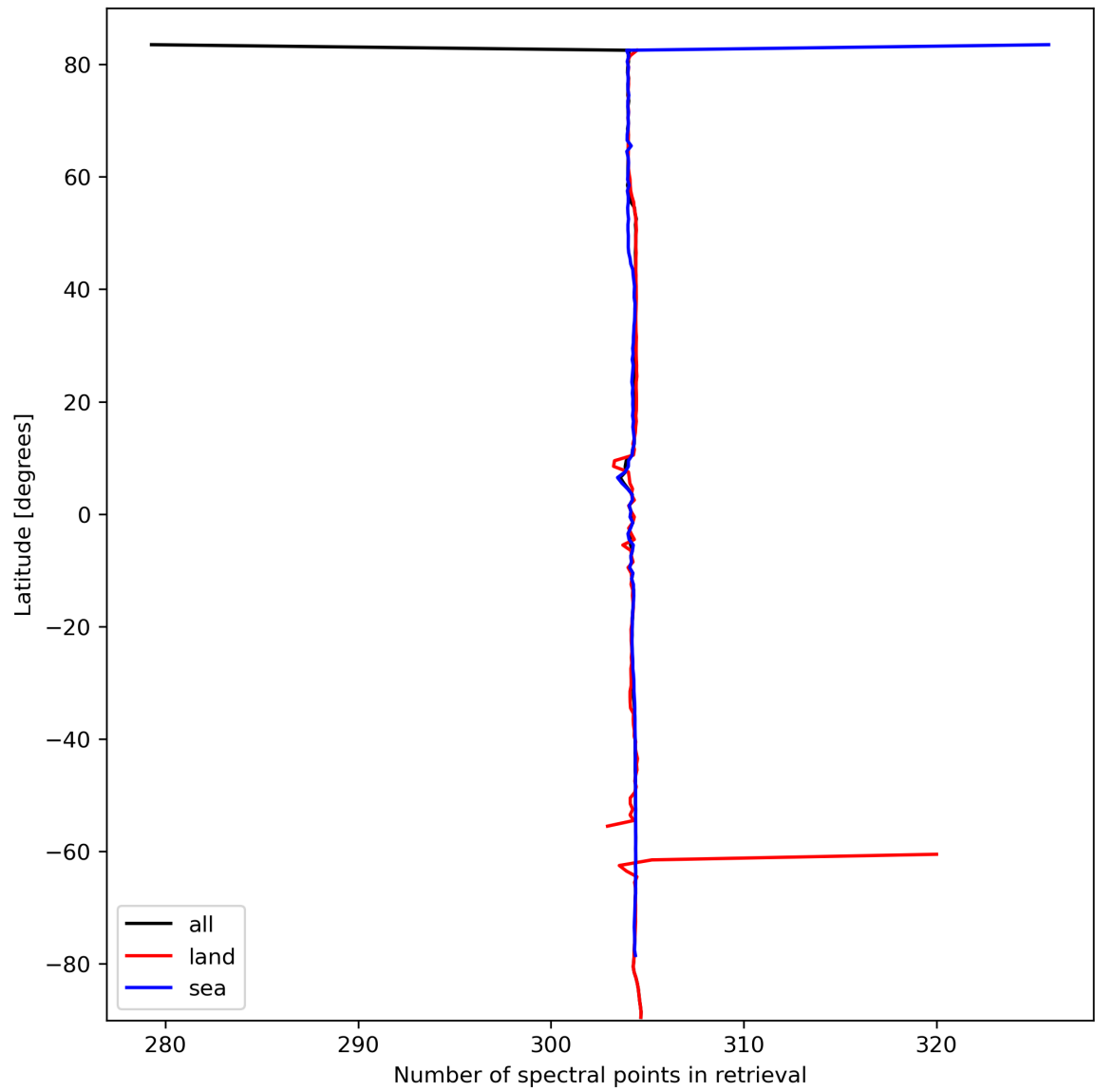
Figure 16: Zonal average of “Number of spectral points in retrieval” for 2023-10-06 to 2023-10-07.
