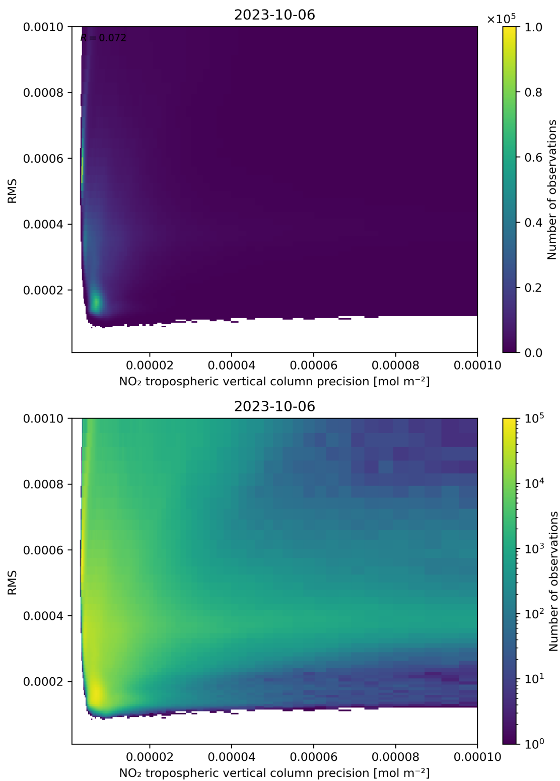
Figure 140: Scatter density plot of “NO 2 tropospheric vertical column precision” against “RMS” for 2023-10-06 to 2023-10-07.
