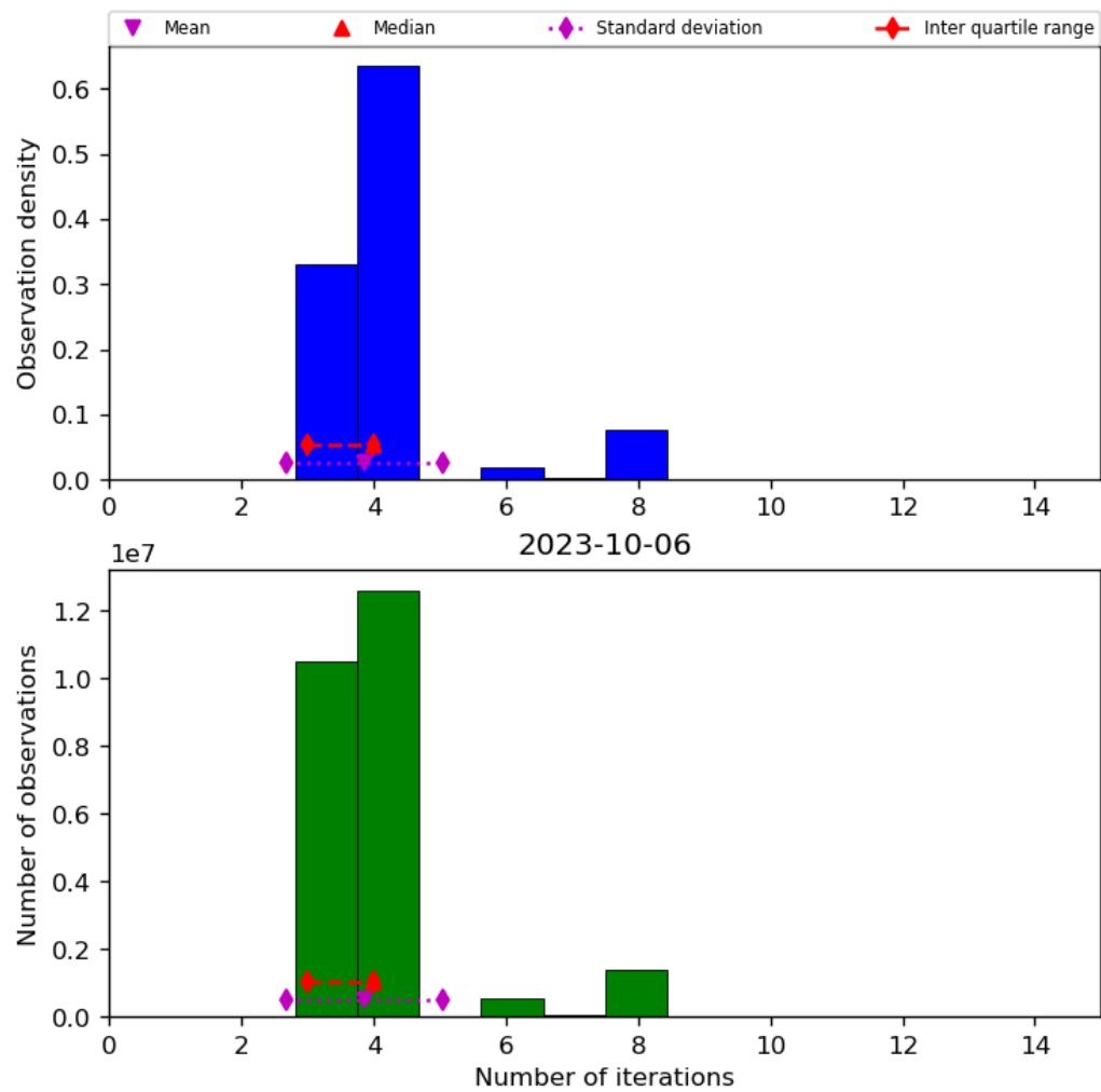
Figure 34: Histogram of “Number of iterations” for 2023-10-06 to 2023-10-07
