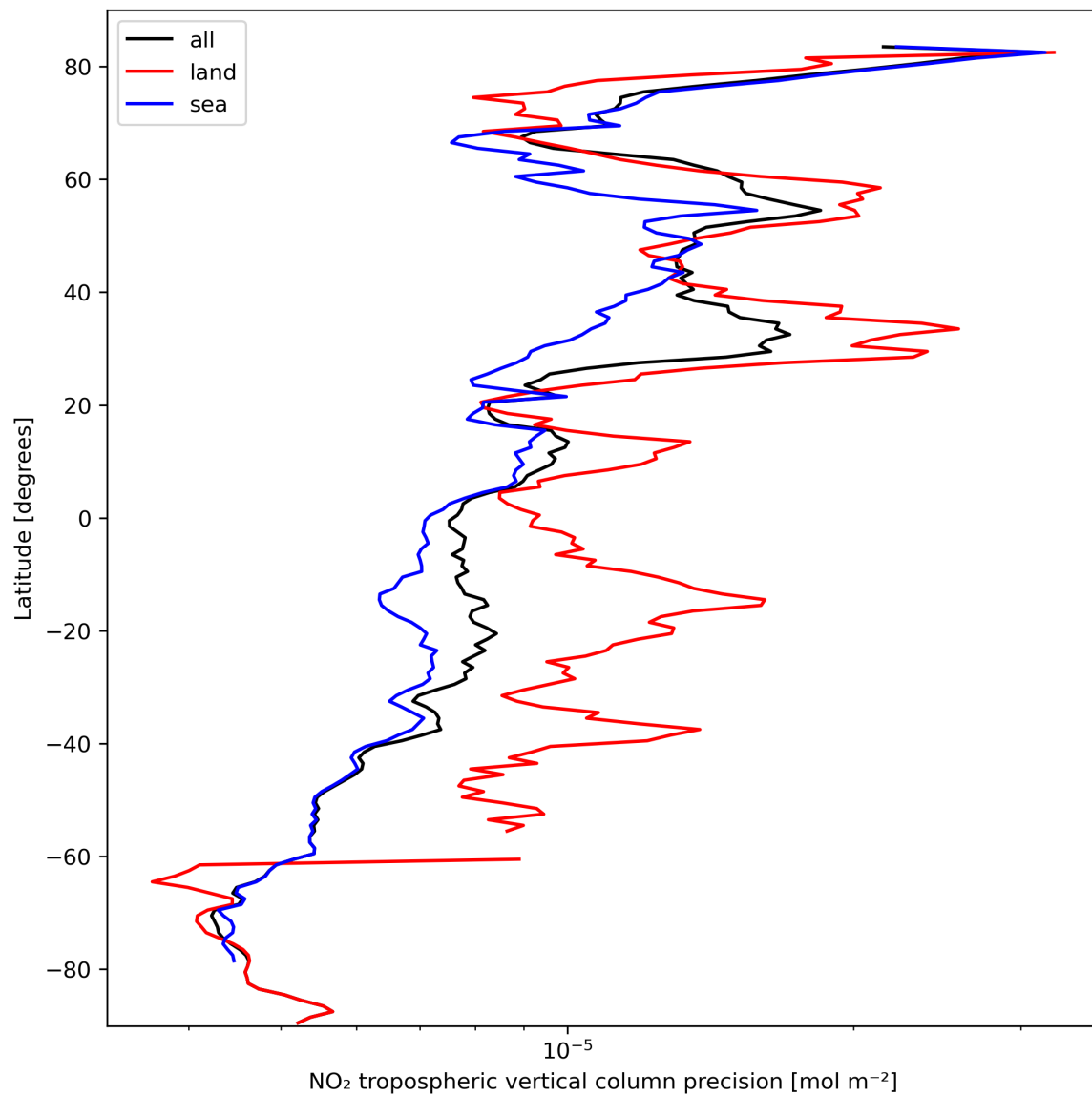
Figure 13: Zonal average of “NO 2 tropospheric vertical column precision” for 2023-10-06 to 2023-10-07.
