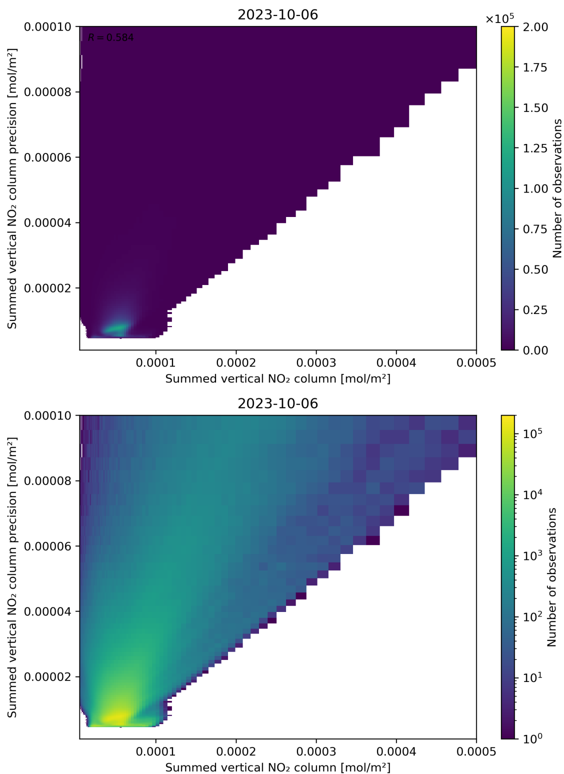
Figure 105: Scatter density plot of “Summed vertical NO 2 column” against “Summed vertical NO 2 column precision” for 2023-10-06 to 2023-10-07.
