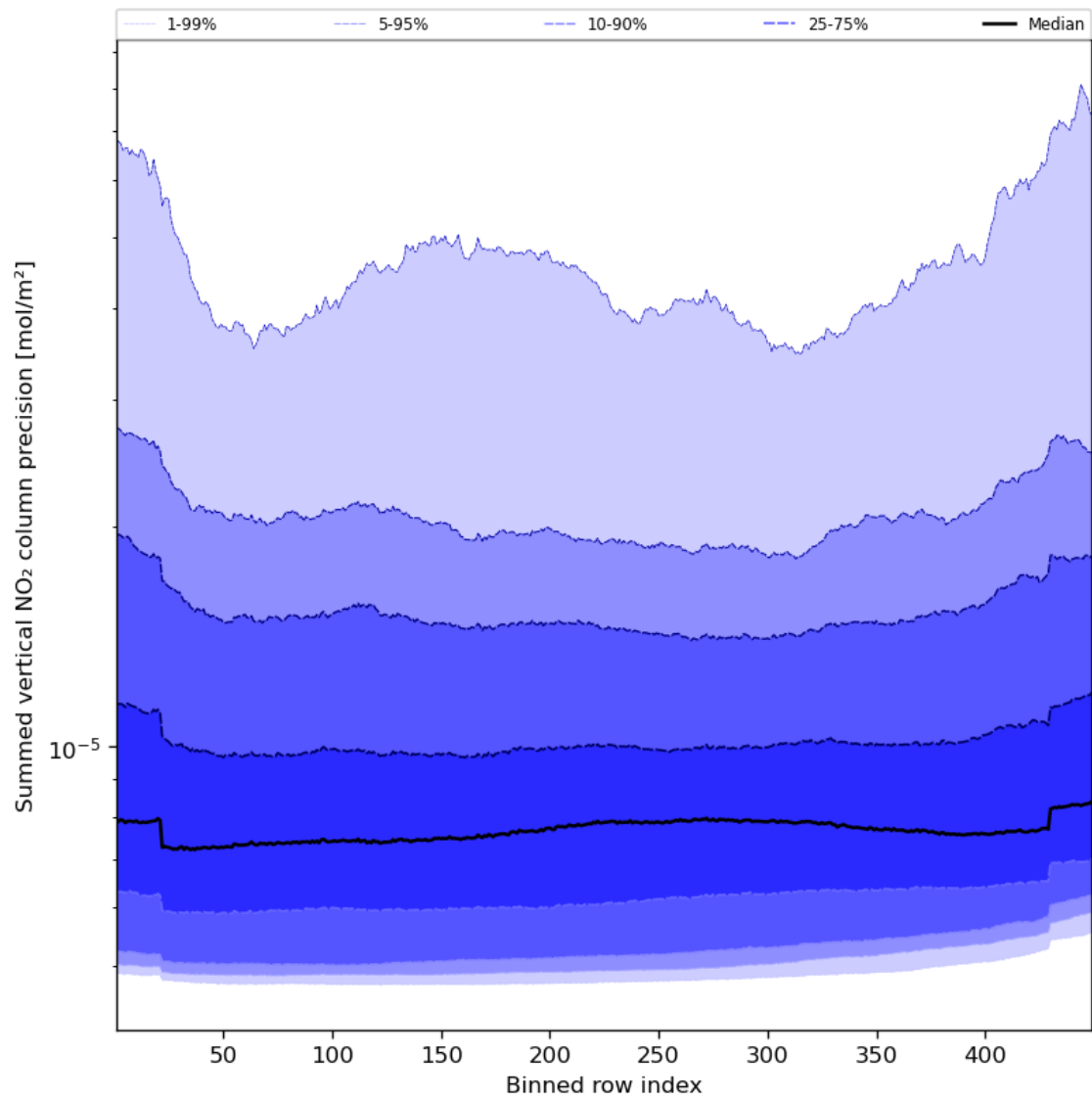
Figure 58: Along track statistics of “Summed vertical NO 2 column precision” for 2023-10-06 to 2023-10-07
