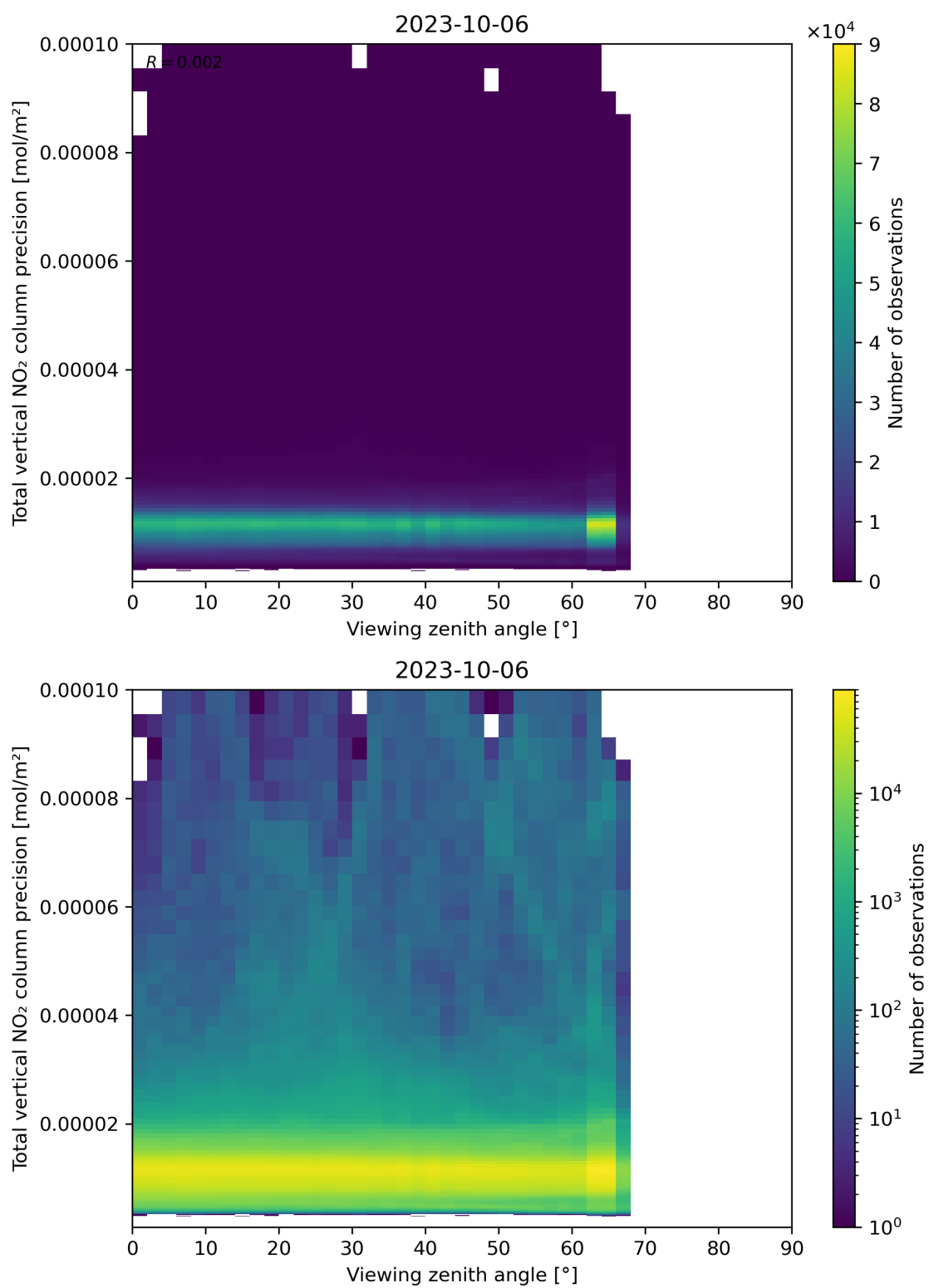
Figure 168: Scatter density plot of “Viewing zenith angle” against “Total vertical NO 2 column precision” for 2023-10-06 to 2023-10-07.
