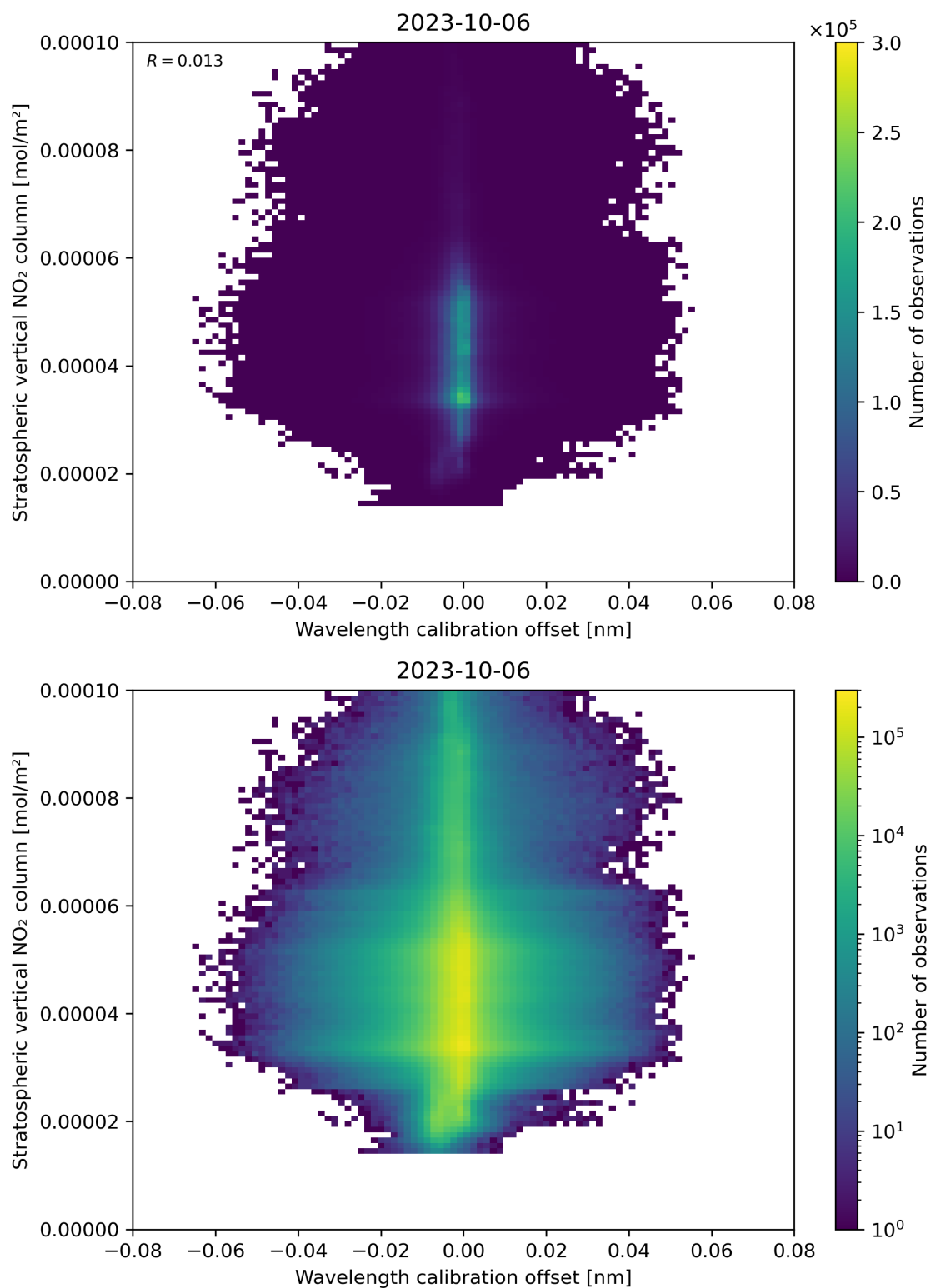
Figure 176: Scatter density plot of “Wavelength calibration offset” against “Stratospheric vertical NO 2 column” for 2023-10-06 to 2023-10-07.
