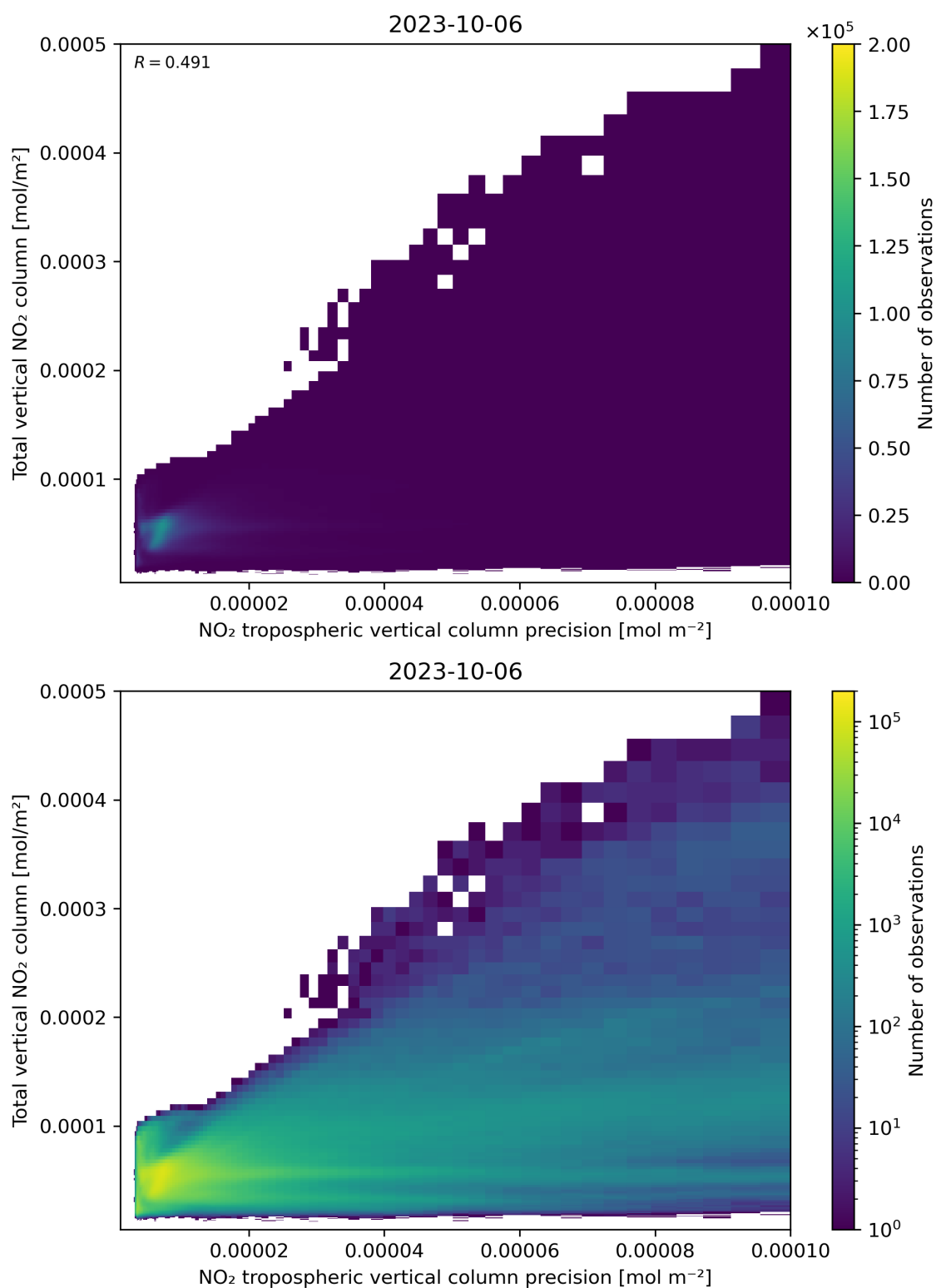
Figure 138: Scatter density plot of “NO 2 tropospheric vertical column precision” against “Total vertical NO 2 column” for 2023-10-06 to 2023-10-07.
