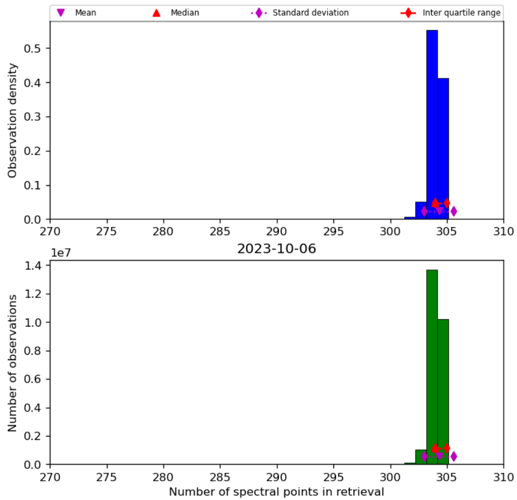
Figure 33: Histogram of “Number of spectral points in retrieval” for 2023-10-06 to 2023-10-07
