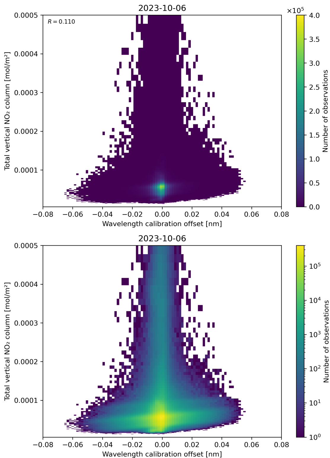
Figure 179: Scatter density plot of “Wavelength calibration offset” against “Total vertical NO 2 column” for 2023-10-06 to 2023-10-07.
