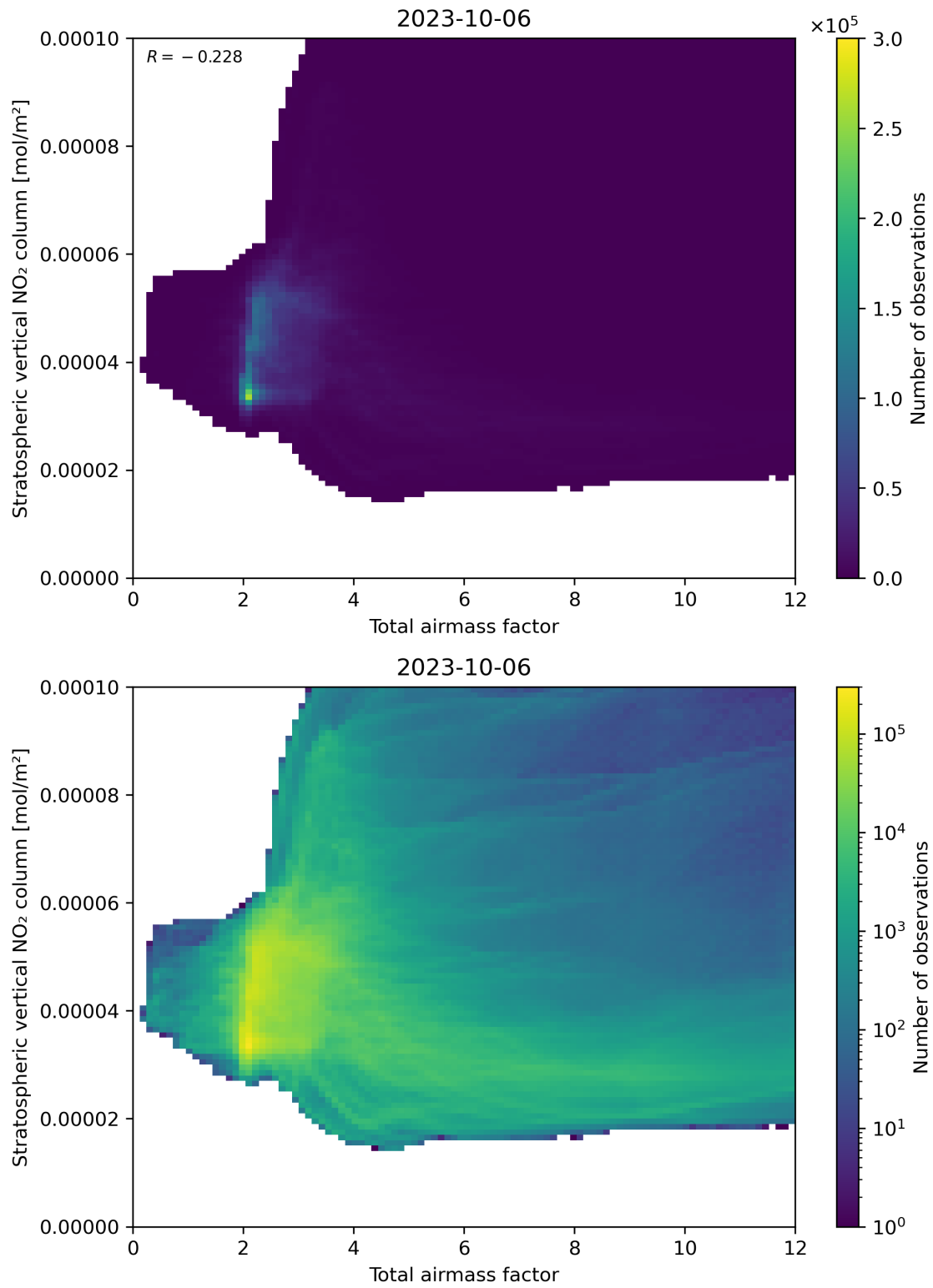
Figure 64: Scatter density plot of “Total airmass factor” against “Stratospheric vertical NO 2 column” for 2023-10-06 to 2023-10-07.
