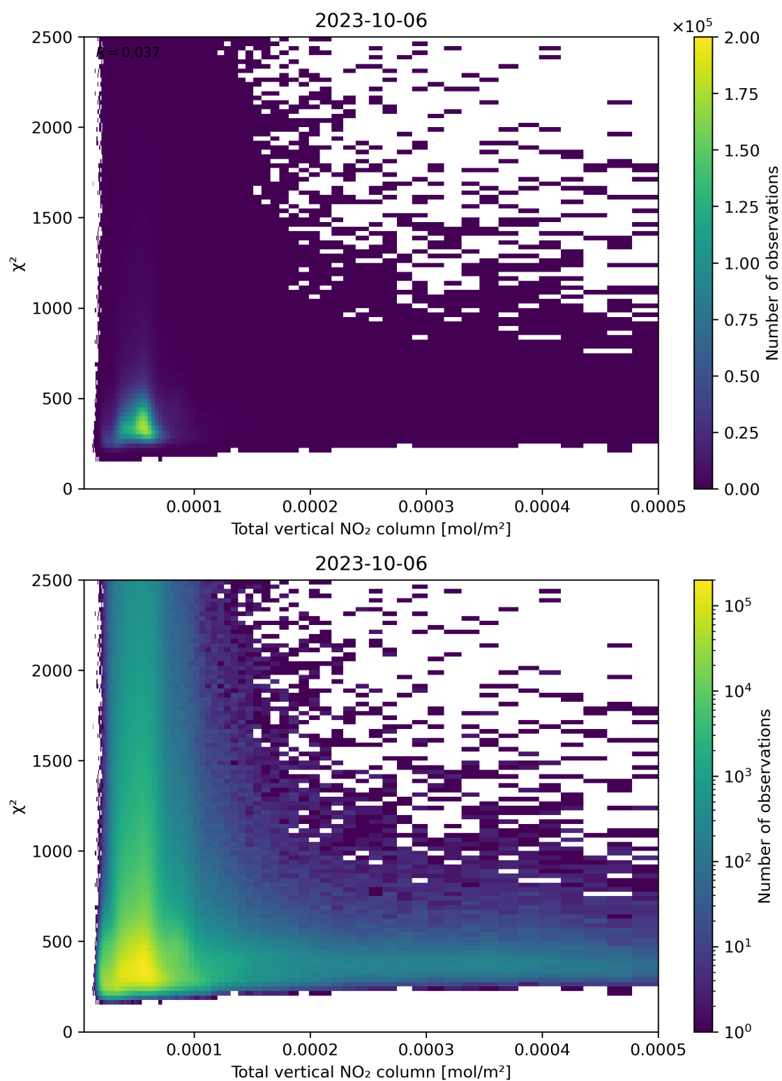
Figure 111: Scatter density plot of “Total vertical NO 2 column” against “ \chi^2 ” for 2023-10-06 to 2023-10-07.
