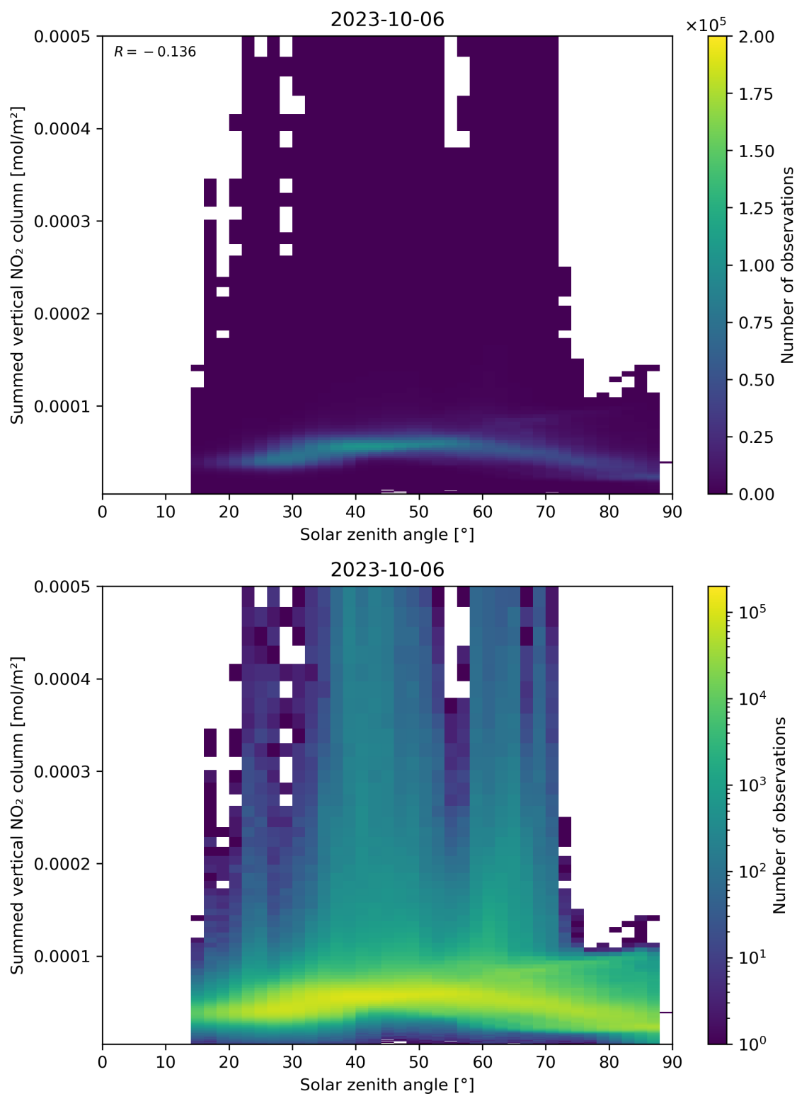
Figure 151: Scatter density plot of “Solar zenith angle” against “Summed vertical NO 2 column” for 2023-10-06 to 2023-10-07.
