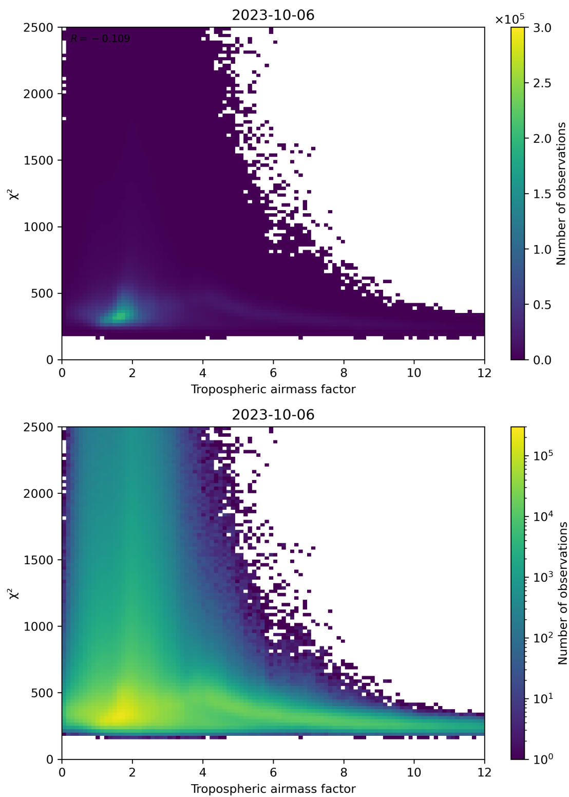
Figure 73: Scatter density plot of “Tropospheric airmass factor” against “ \chi^2 ” for 2023-10-06 to 2023-10-07.
