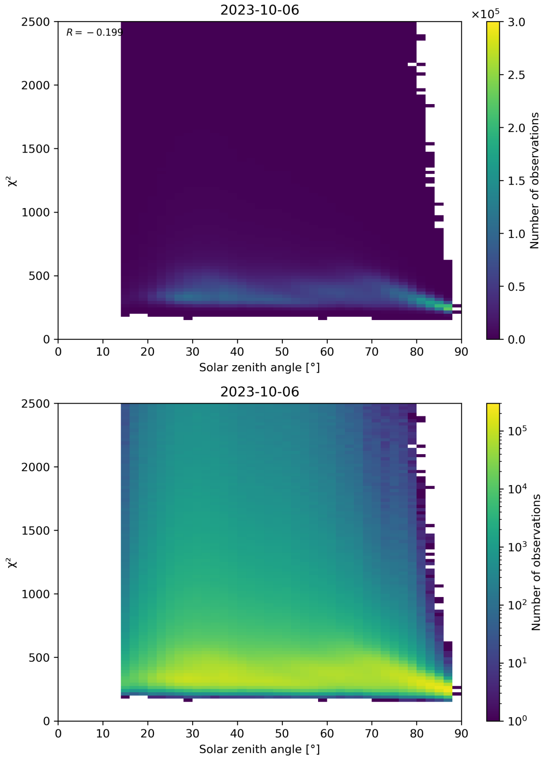
Figure 148: Scatter density plot of “Solar zenith angle” against “ \chi^2 ” for 2023-10-06 to 2023-10-07.
