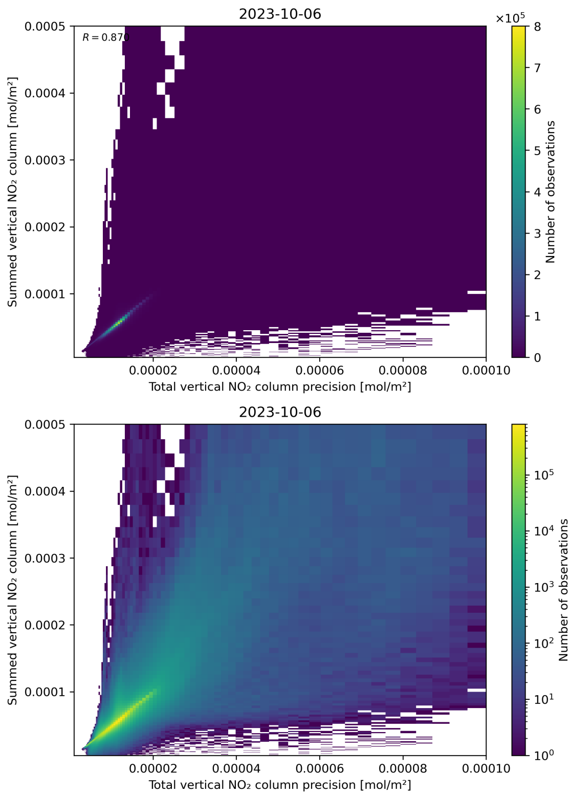
Figure 117: Scatter density plot of “Total vertical NO 2 column precision” against “Summed vertical NO 2 column” for 2023-10-06 to 2023-10-07.
