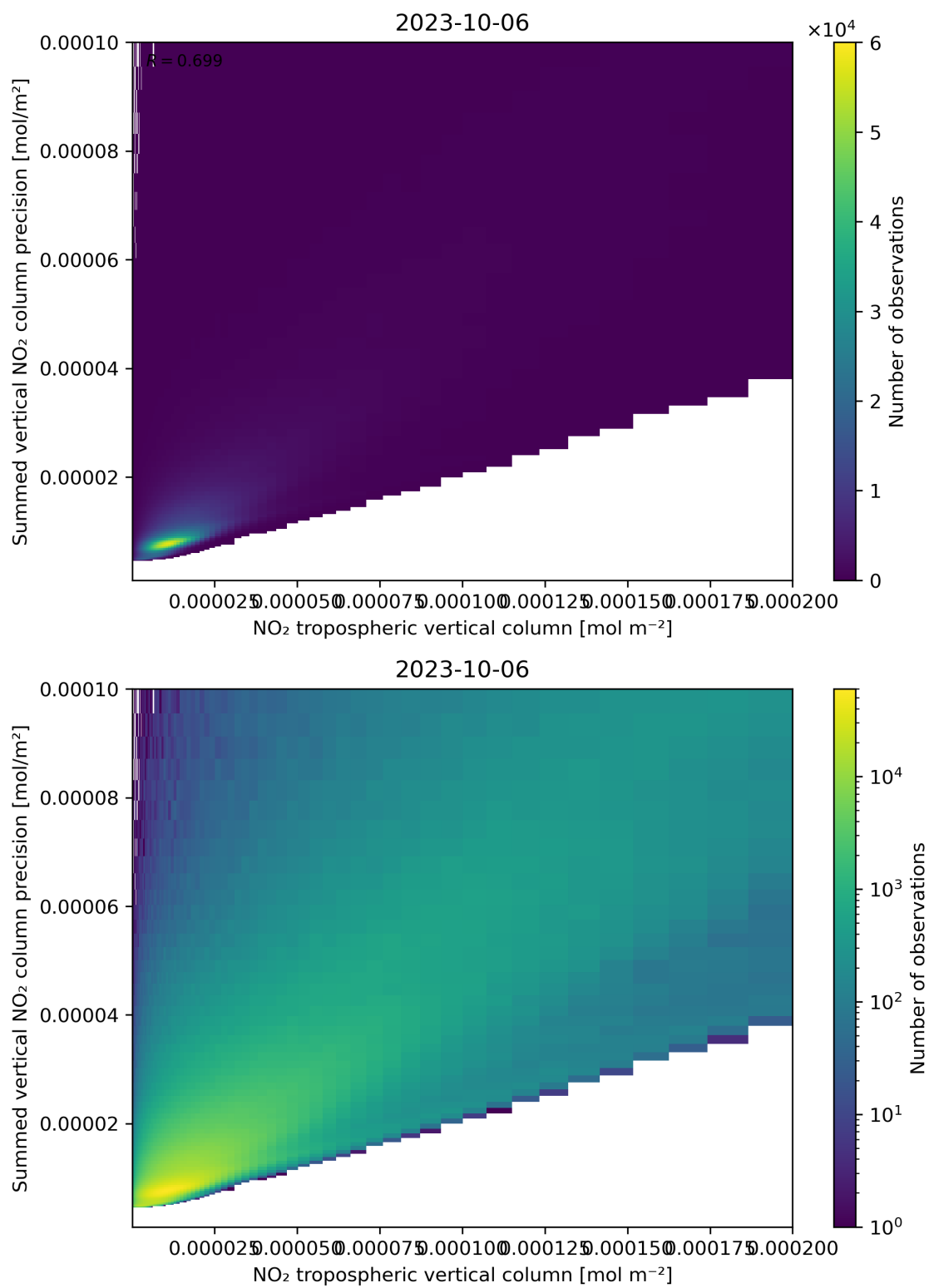
Figure 127: Scatter density plot of “NO 2 tropospheric vertical column” against “Summed vertical NO 2 column precision” for 2023-10-06 to 2023-10-07.
