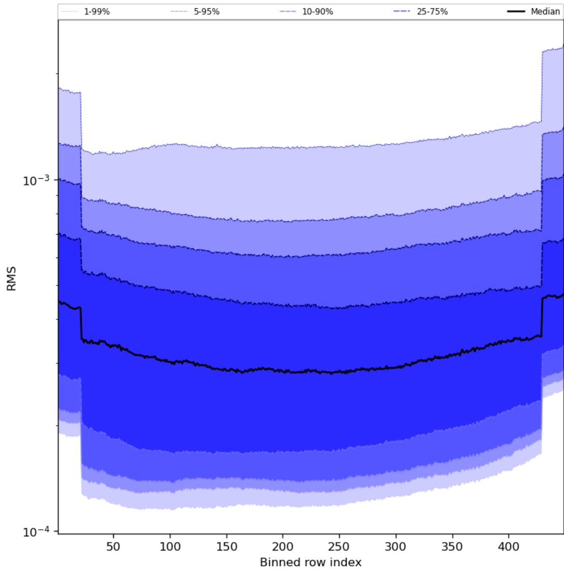
Figure 60: Along track statistics of “RMS” for 2023-10-06 to 2023-10-07
