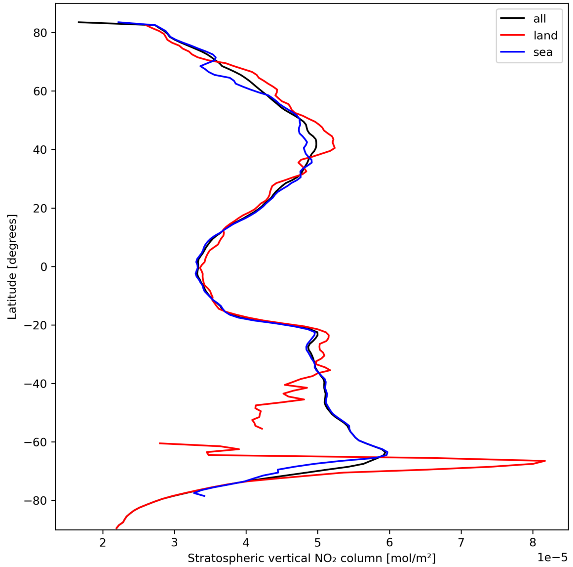
Figure 19: Zonal average of “Stratospheric vertical NO 2 column” for 2023-10-06 to 2023-10-07.
