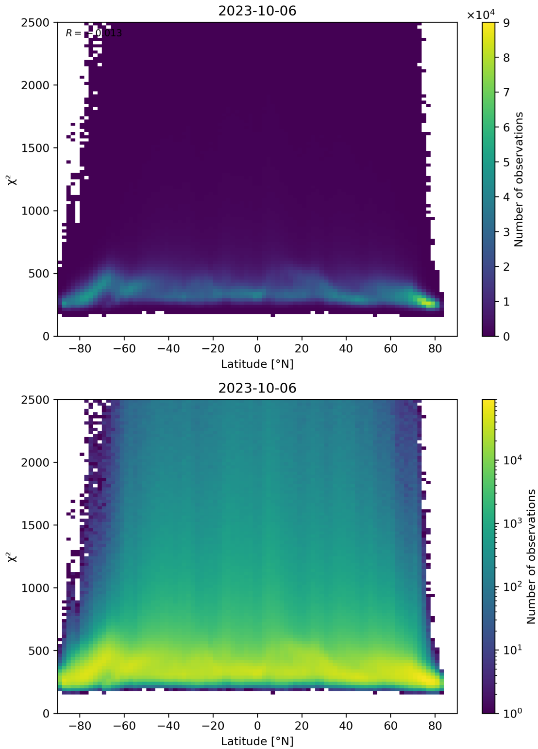
Figure 86: Scatter density plot of “Latitude” against “ \chi^2 ” for 2023-10-06 to 2023-10-07.
