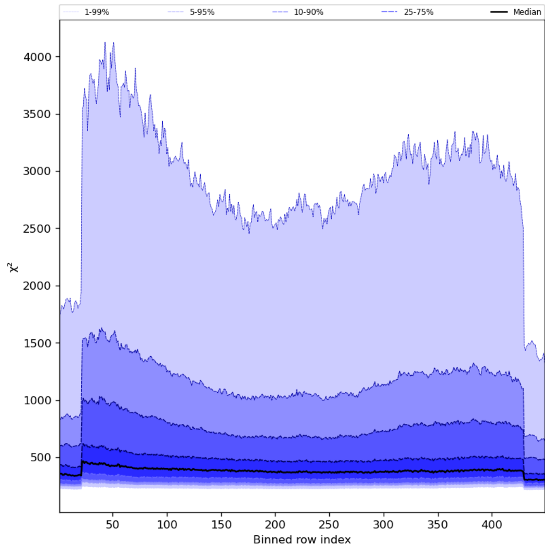
Figure 59: Along track statistics of “ \chi^2 ” for 2023-10-06 to 2023-10-07
