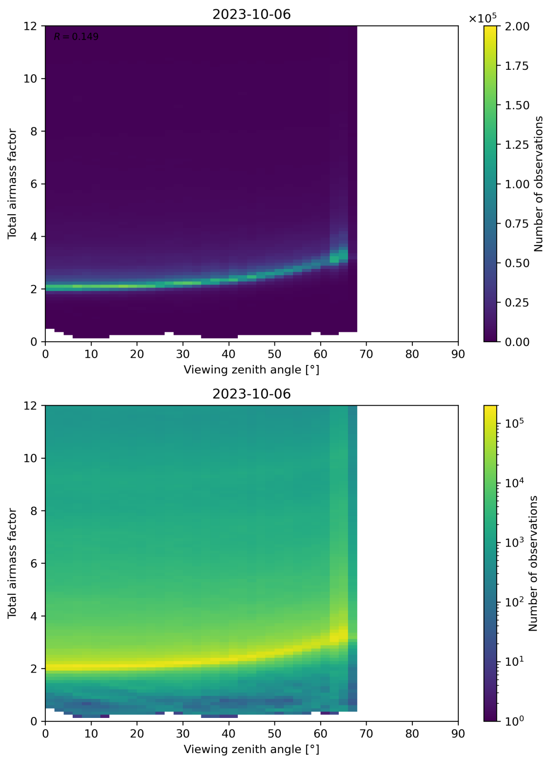
Figure 160: Scatter density plot of “Viewing zenith angle” against “Total airmass factor” for 2023-10-06 to 2023-10-07.
