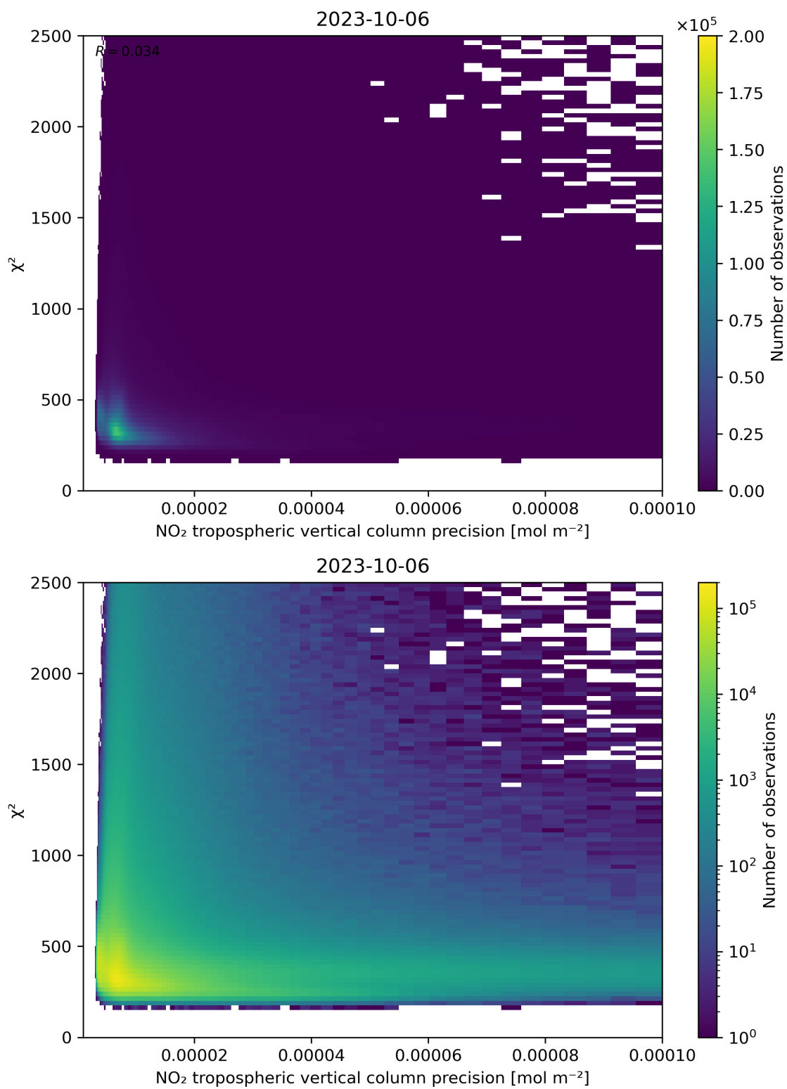
Figure 134: Scatter density plot of “NO 2 tropospheric vertical column precision” against “ \chi^2 ” for 2023-10-06 to 2023-10-07.
