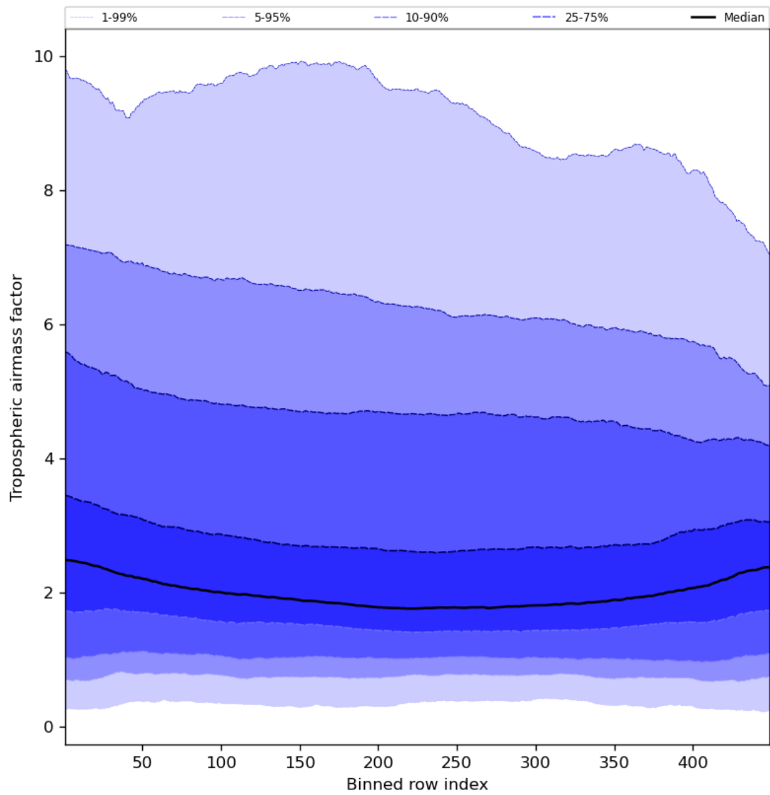
Figure 48: Along track statistics of “Tropospheric air mass factor” for 2023-10-06 to 2023-10-07
