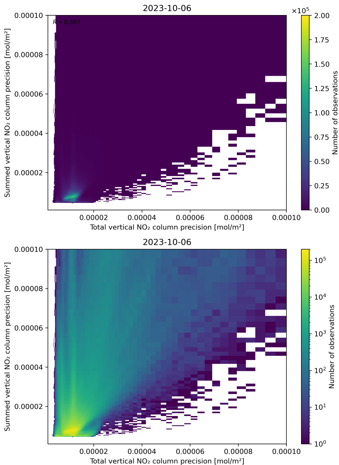
Figure 118: Scatter density plot of “Total vertical NO 2 column precision” against “Summed vertical NO 2 column precision” for 2023-10-06 to 2023-10-07.
