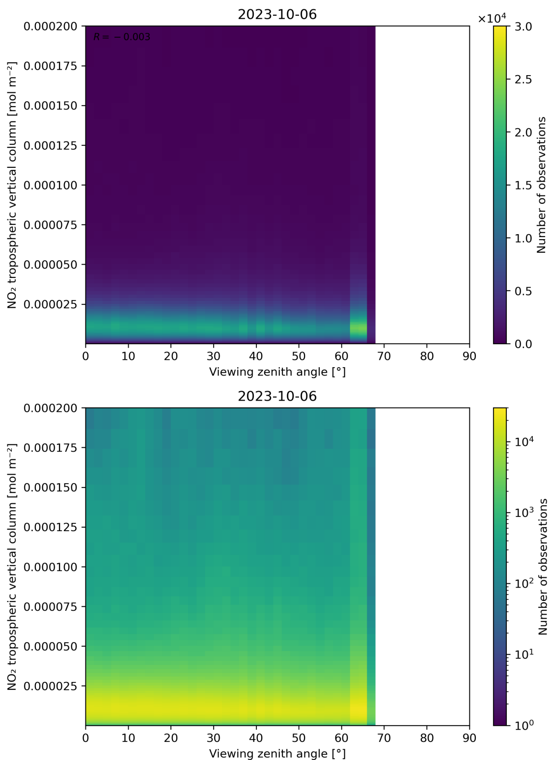
Figure 169: Scatter density plot of “Viewing zenith angle” against “NO 2 tropospheric vertical column” for 2023-10-06 to 2023-10-07.
