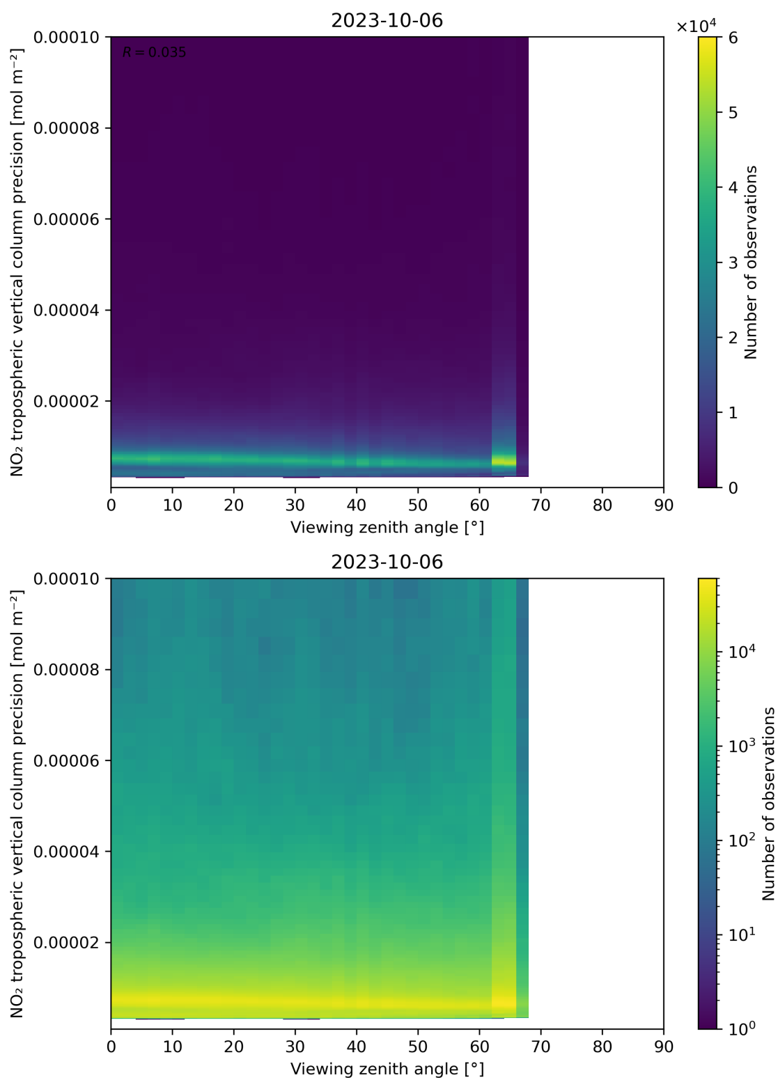
Figure 170: Scatter density plot of “Viewing zenith angle” against “NO 2 tropospheric vertical column precision” for 2023-10-06 to 2023-10-07.
