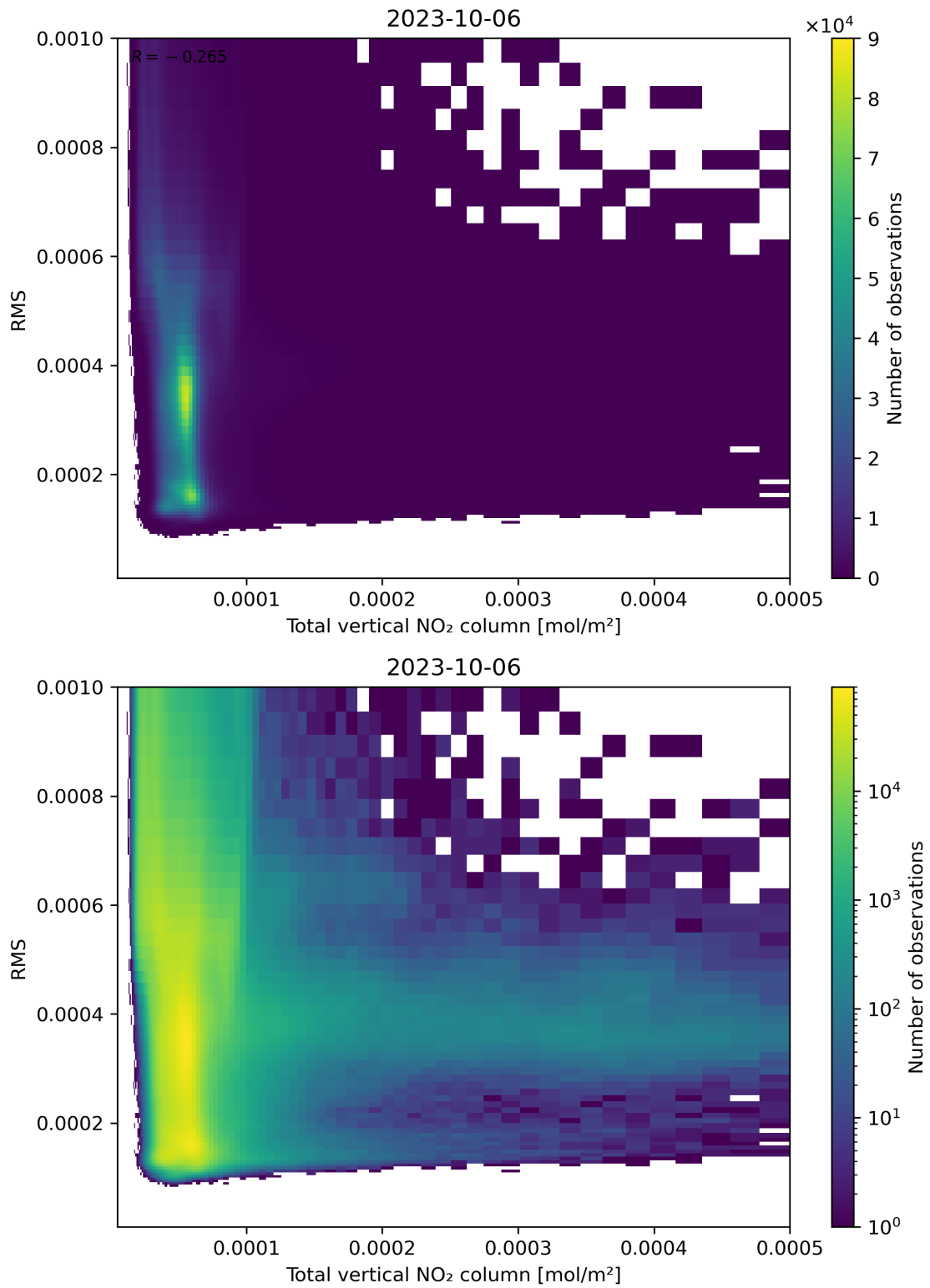
Figure 120: Scatter density plot of “Total vertical NO 2 column” against “RMS” for 2023-10-06 to 2023-10-07.
