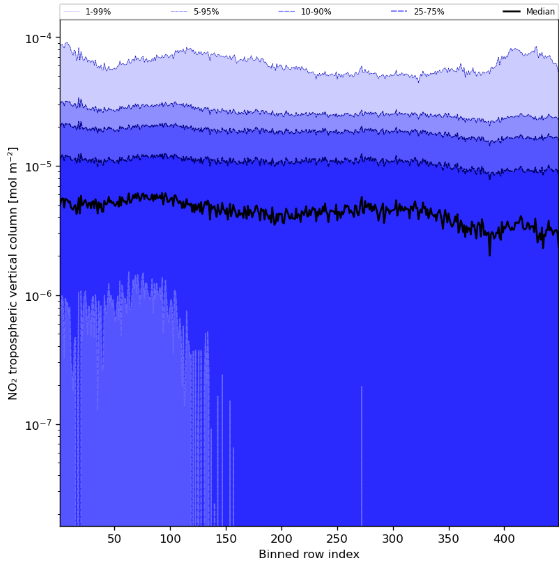
Figure 46: Along track statistics of “NO 2 tropospheric vertical column” for 2023-10-06 to 2023-10-07
