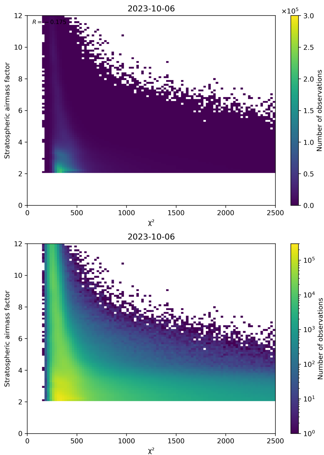
Figure 81: Scatter density plot of “ \chi^2 ” against “Stratospheric airmass factor” for 2023-10-06 to 2023-10-07.
