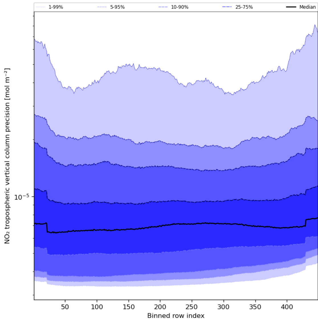
Figure 47: Along track statistics of “NO 2 tropospheric vertical column precision” for 2023-10-06 to 2023-10-07
