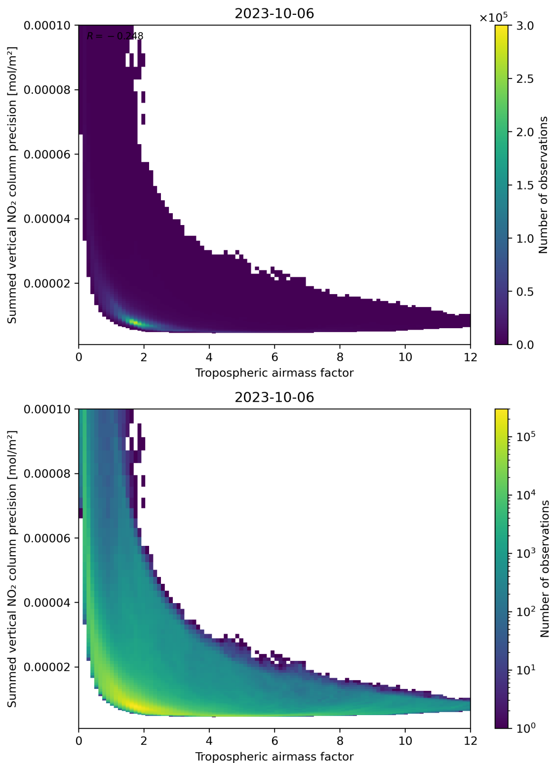
Figure 76: Scatter density plot of “Tropospheric air mass factor” against “Summed vertical NO 2 column precision” for 2023-10-06 to 2023-10-07.
