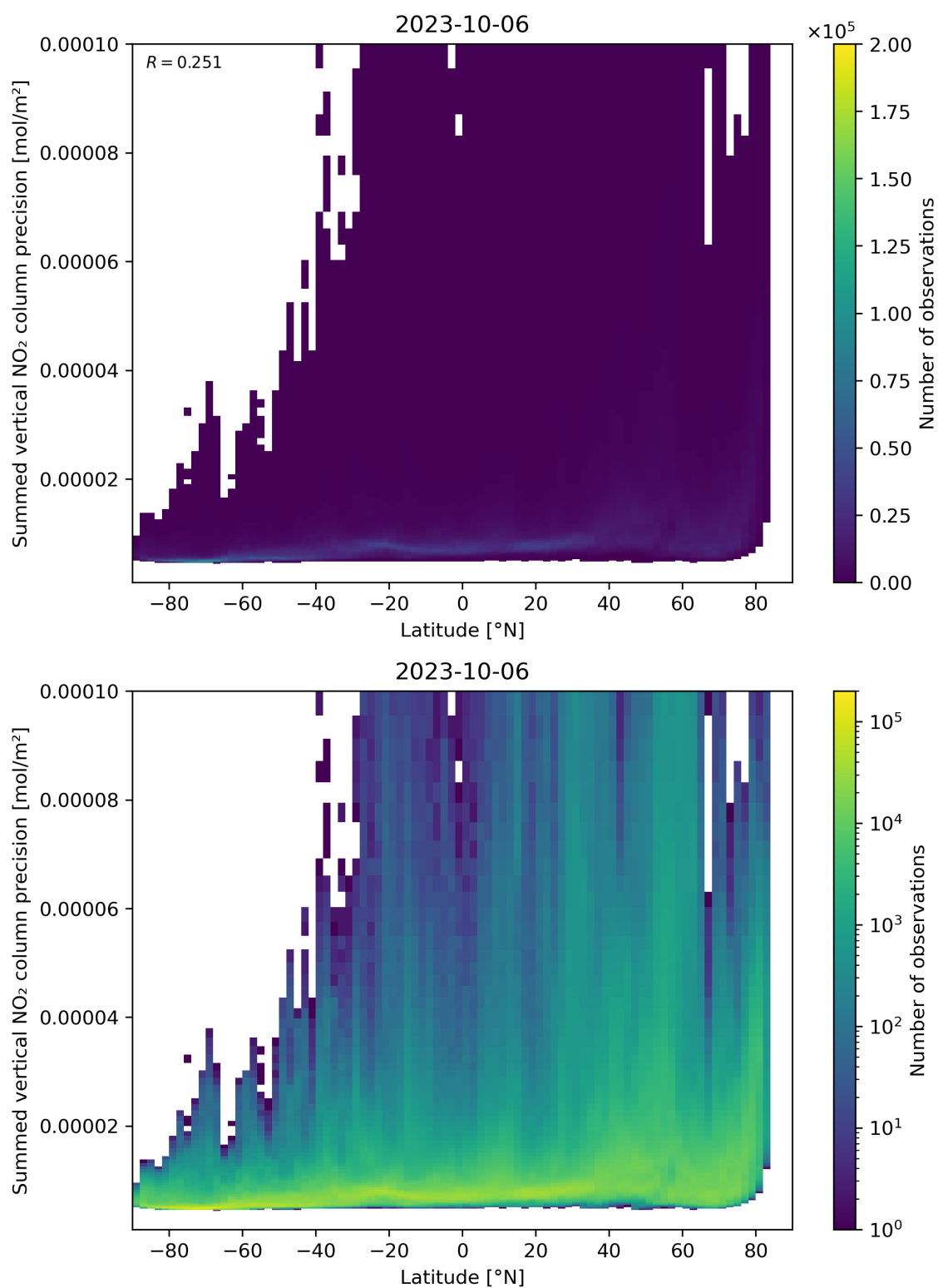
Figure 89: Scatter density plot of “Latitude” against “Summed vertical NO 2 column precision” for 2023-10-06 to 2023-10-07.
