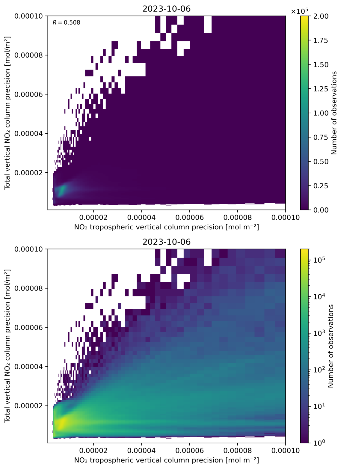
Figure 139: Scatter density plot of “NO 2 tropospheric vertical column precision” against “Total vertical NO 2 column precision” for 2023-10-06 to 2023-10-07.
