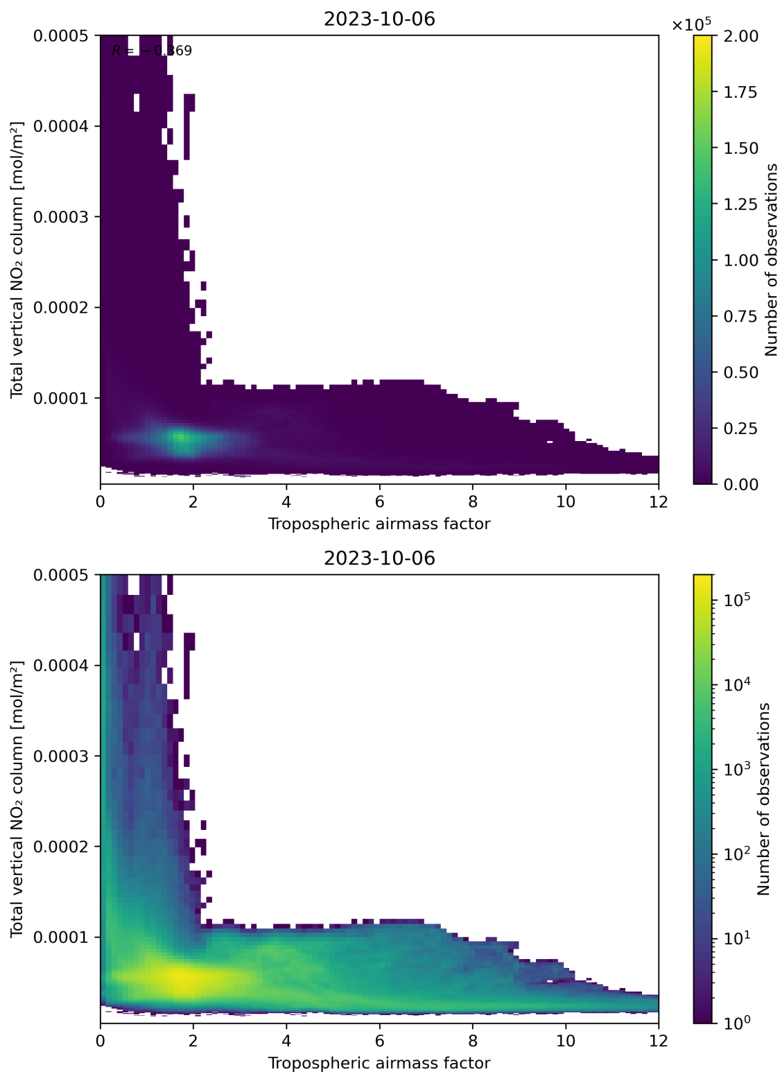
Figure 77: Scatter density plot of “Tropospheric airmass factor” against “Total vertical NO 2 column” for 2023-10-06 to 2023-10-07.
