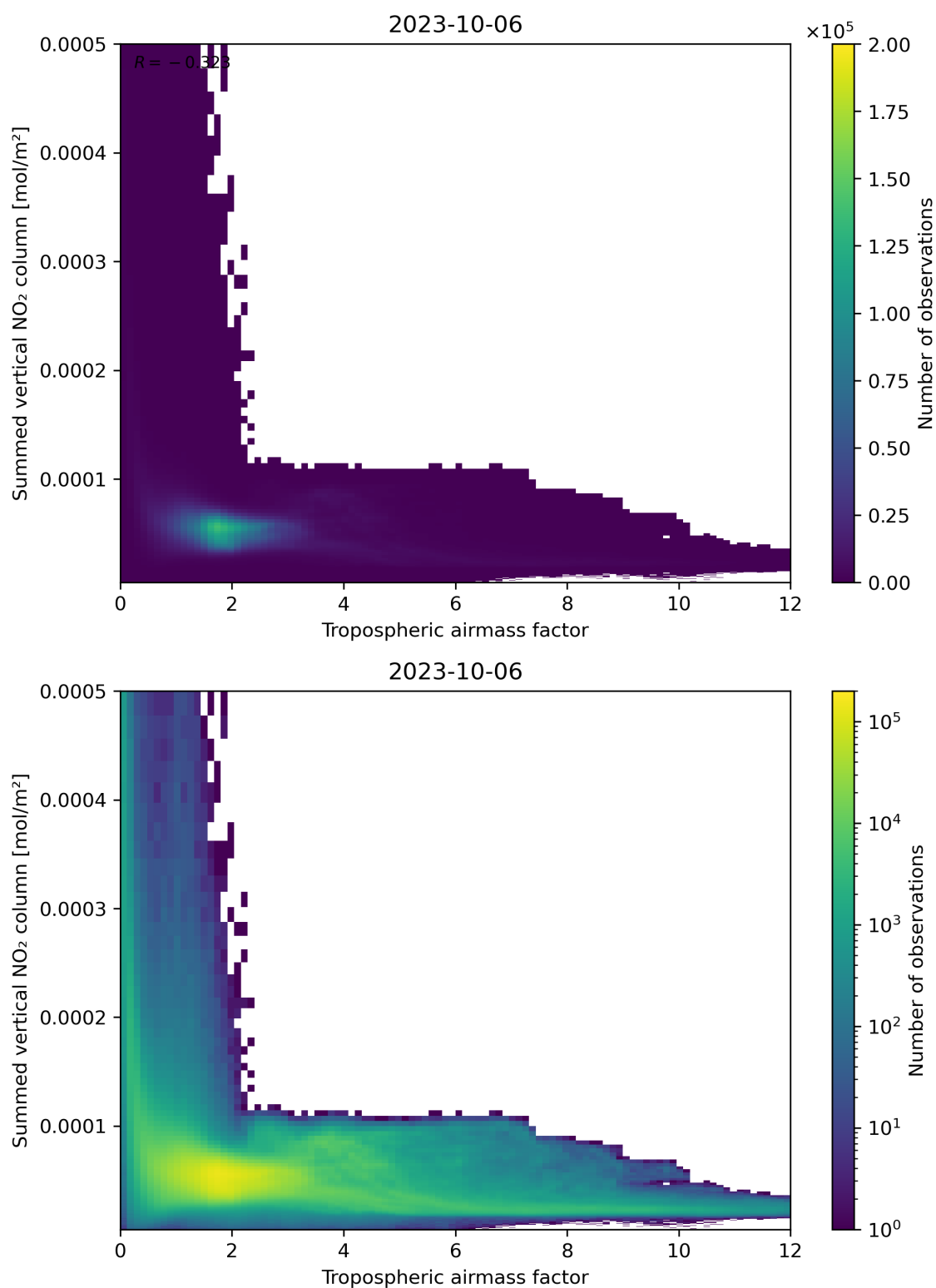
Figure 75: Scatter density plot of “Tropospheric airmass factor” against “Summed vertical NO 2 column” for 2023-10-06 to 2023-10-07.
