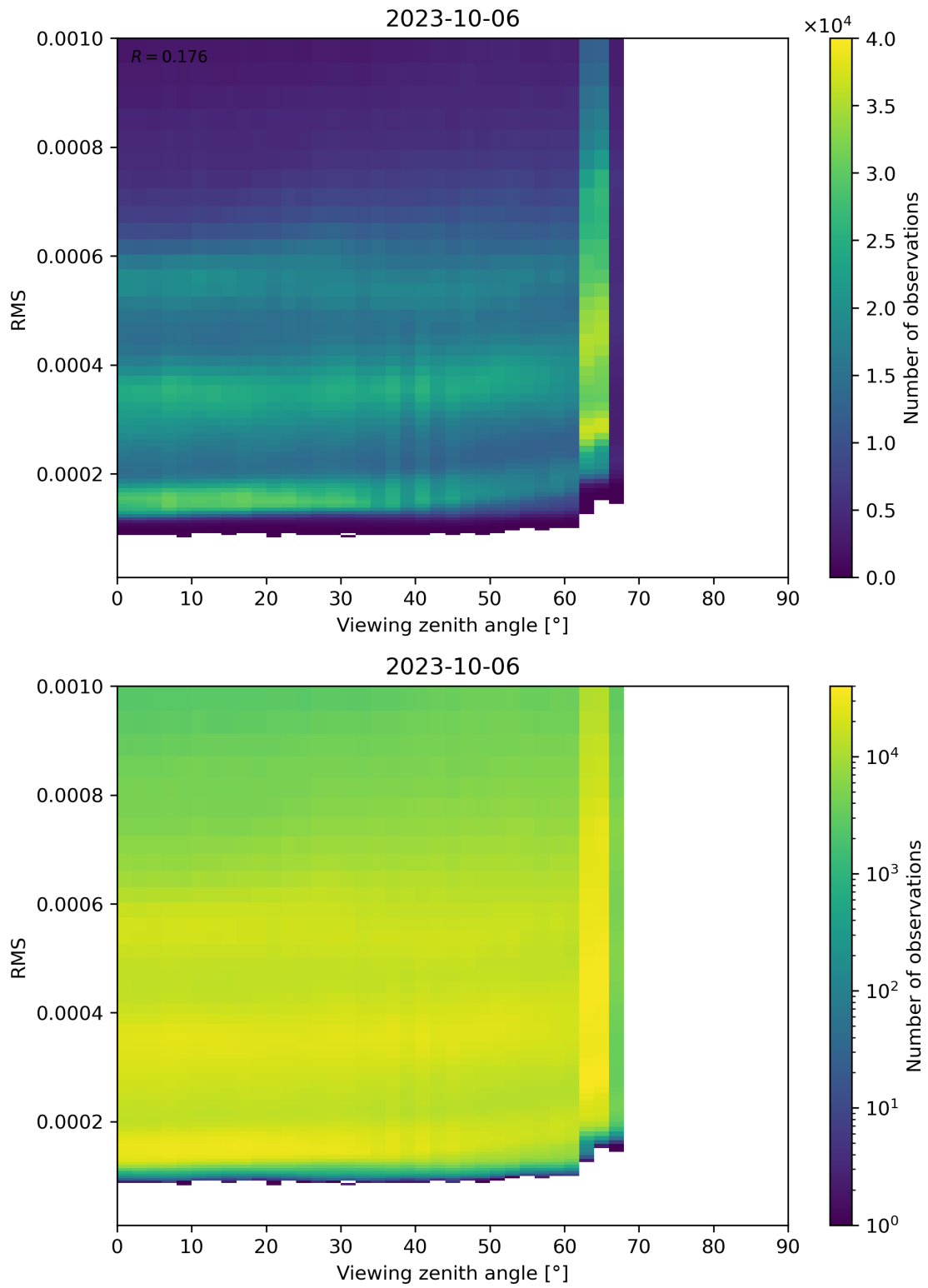
Figure 171: Scatter density plot of “Viewing zenith angle” against “RMS” for 2023-10-06 to 2023-10-07.
