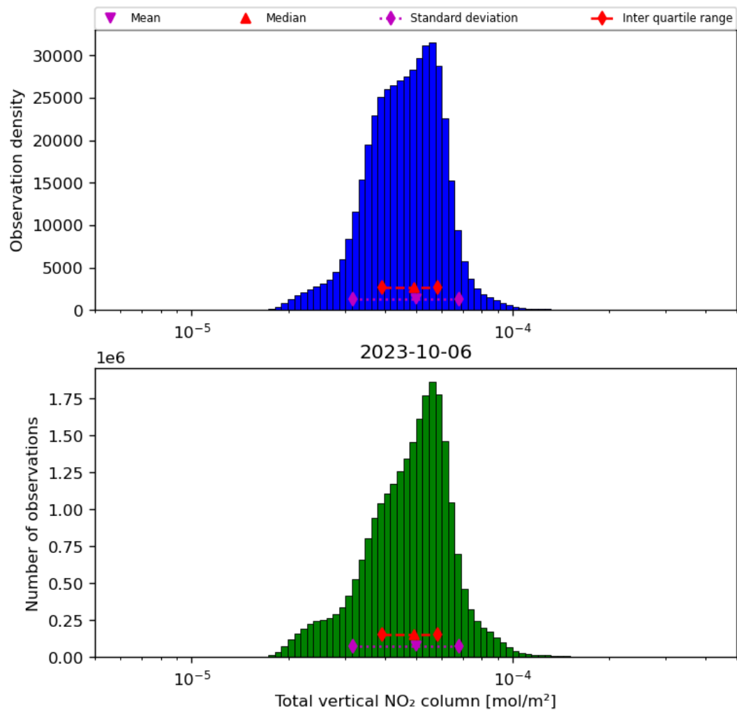
Figure 38: Histogram of “Total vertical NO 2 column” for 2023-10-06 to 2023-10-07
