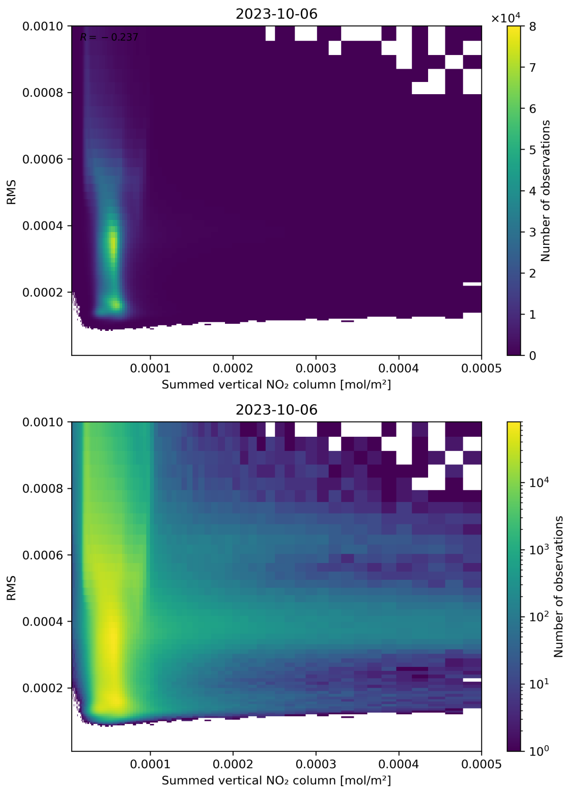
Figure 109: Scatter density plot of “Summed vertical NO 2 column” against “RMS” for 2023-10-06 to 2023-10-07.
