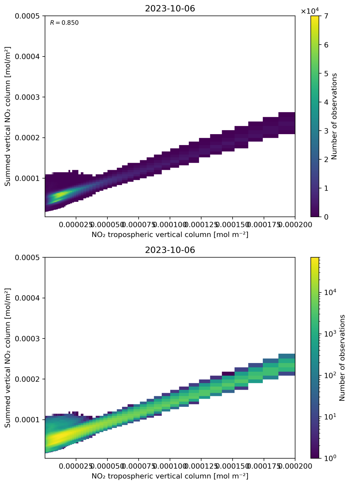
Figure 126: Scatter density plot of “NO 2 tropospheric vertical column” against “Summed vertical NO 2 column” for 2023-10-06 to 2023-10-07.
