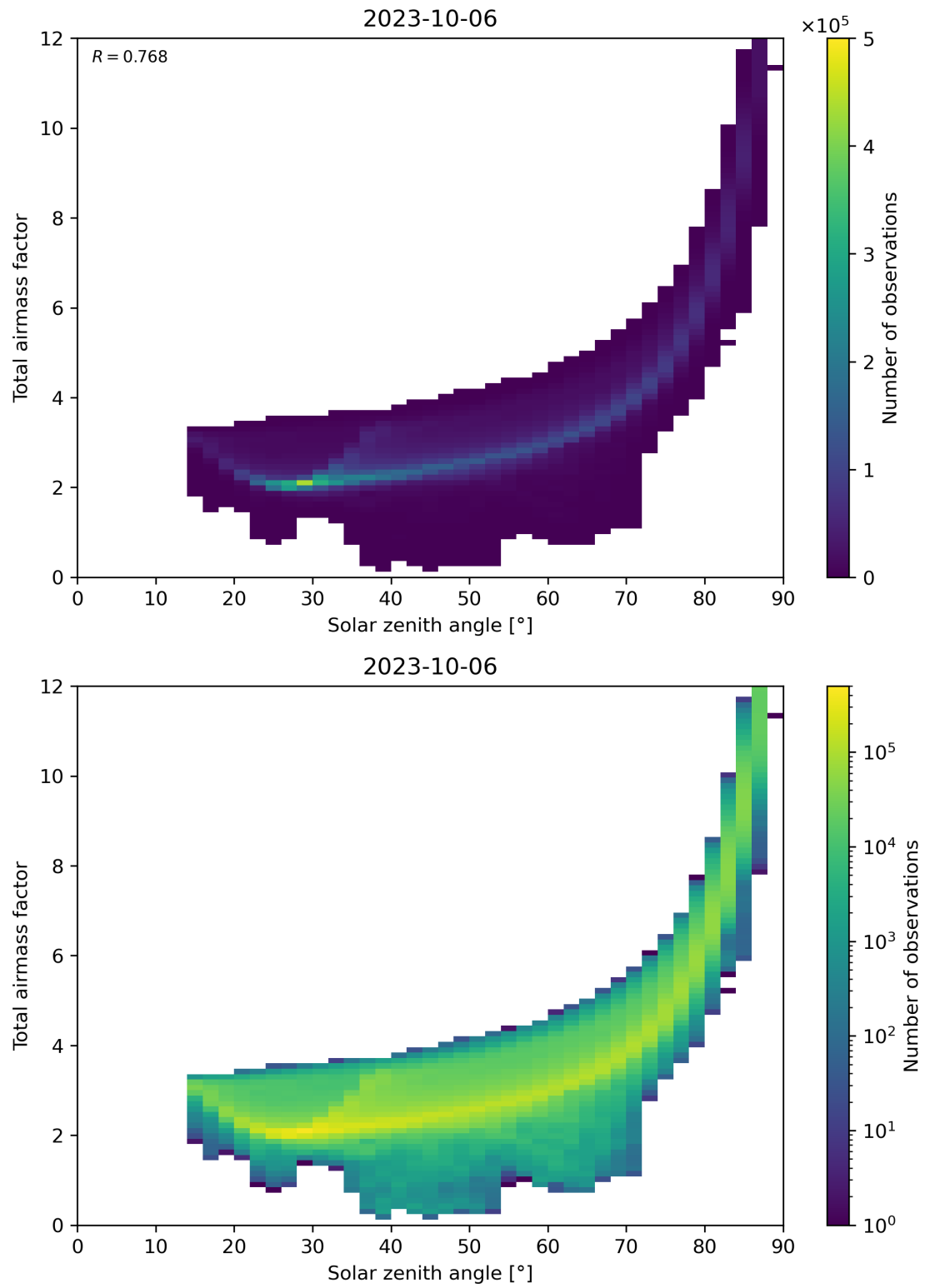
Figure 146: Scatter density plot of “Solar zenith angle” against “Total air mass factor” for 2023-10-06 to 2023-10-07.
