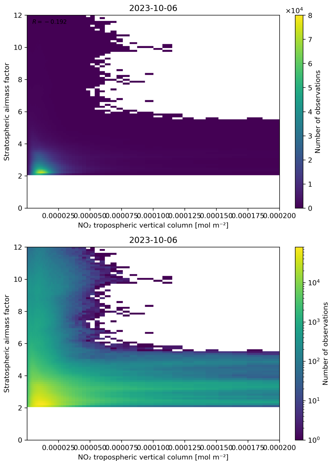
Figure 121: Scatter density plot of “NO 2 tropospheric vertical column” against “Stratospheric air mass factor” for 2023-10-06 to 2023-10-07.
