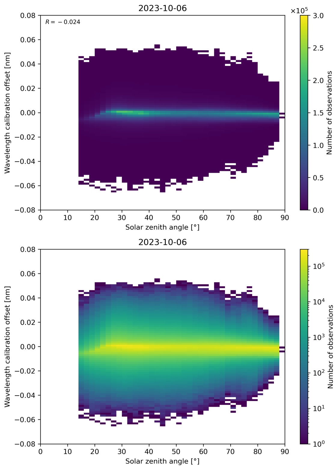
Figure 158: Scatter density plot of “Solar zenith angle” against “Wavelength calibration offset” for 2023-10-06 to 2023-10-07.
