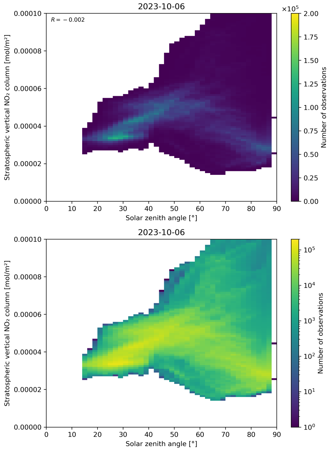
Figure 150: Scatter density plot of “Solar zenith angle” against “Stratospheric vertical NO 2 column” for 2023-10-06 to 2023-10-07.
