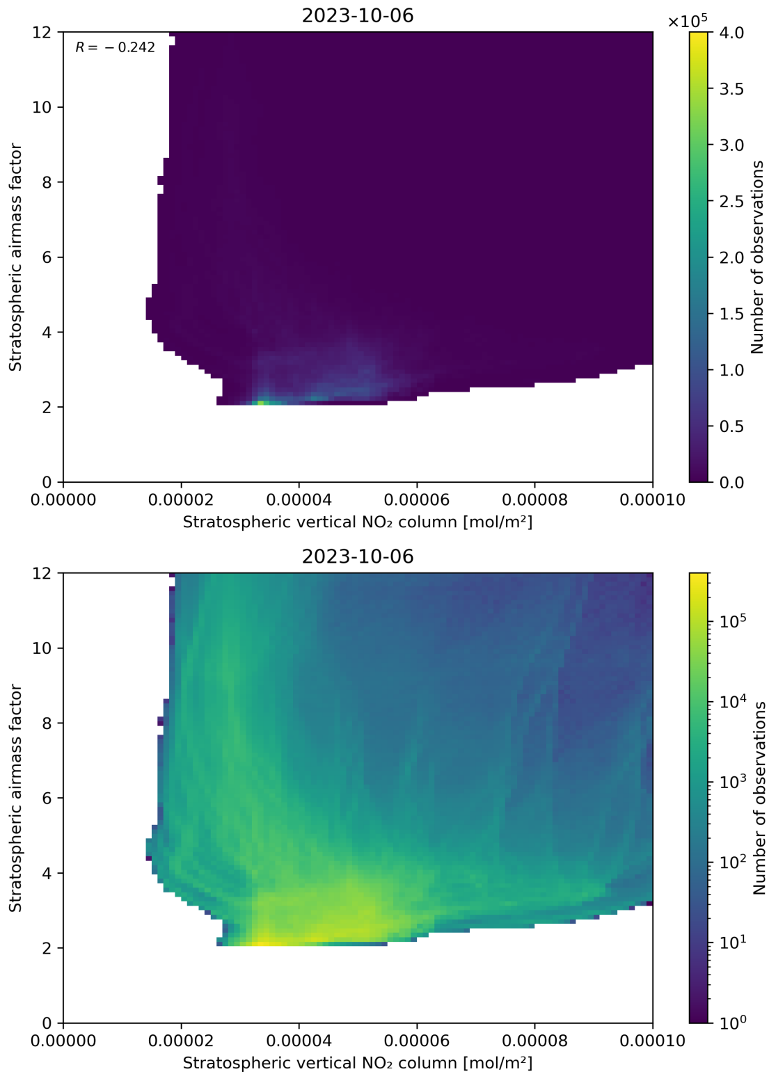
Figure 96: Scatter density plot of “Stratospheric vertical NO 2 column” against “Stratospheric airmass factor” for 2023-10-06 to 2023-10-07.
