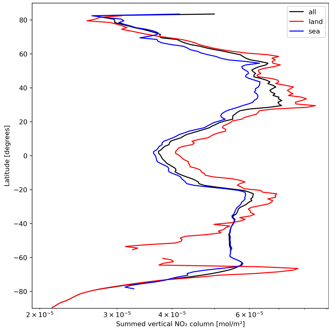
Figure 23: Zonal average of “Summed vertical NO 2 column” for 2023-10-06 to 2023-10-07.
