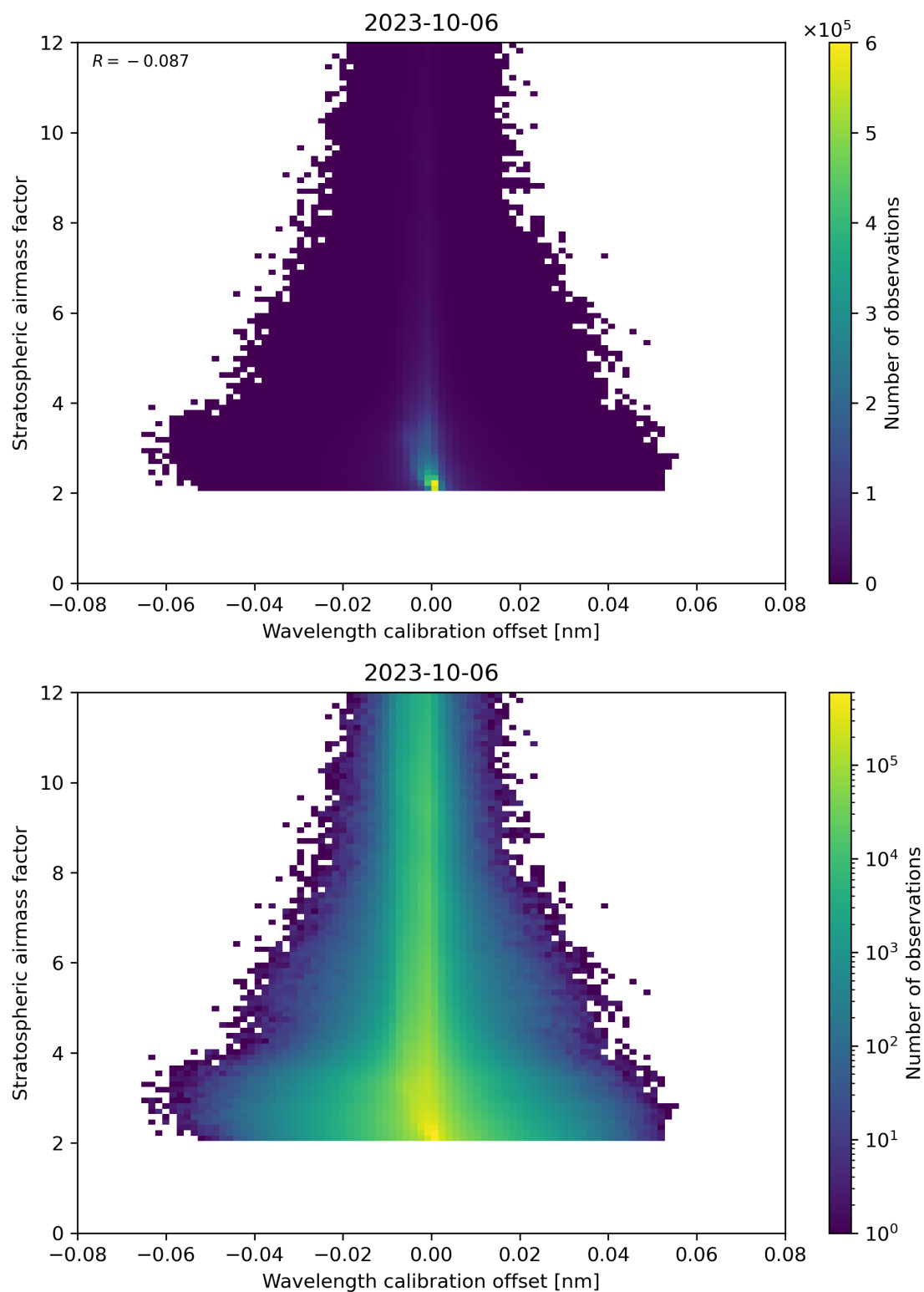
Figure 174: Scatter density plot of “Wavelength calibration offset” against “Stratospheric airmass factor” for 2023-10-06 to 2023-10-07.
