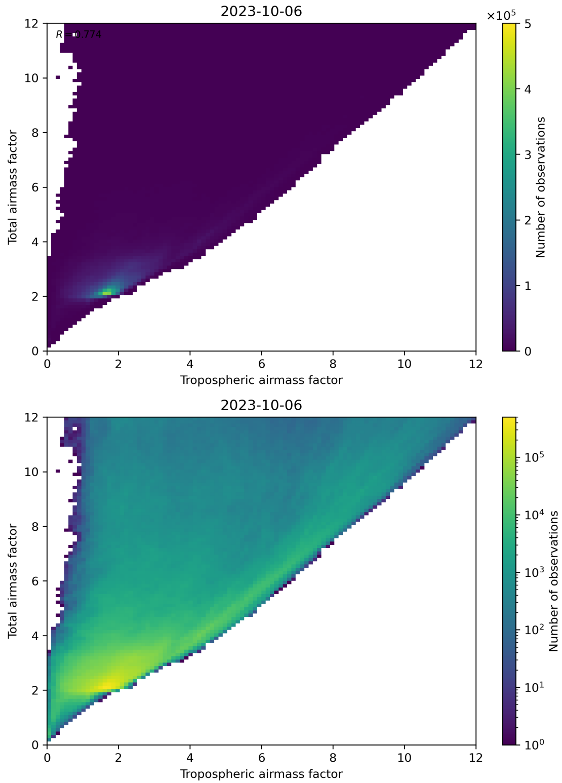
Figure 72: Scatter density plot of “Tropospheric airmass factor” against “Total airmass factor” for 2023-10-06 to 2023-10-07.
