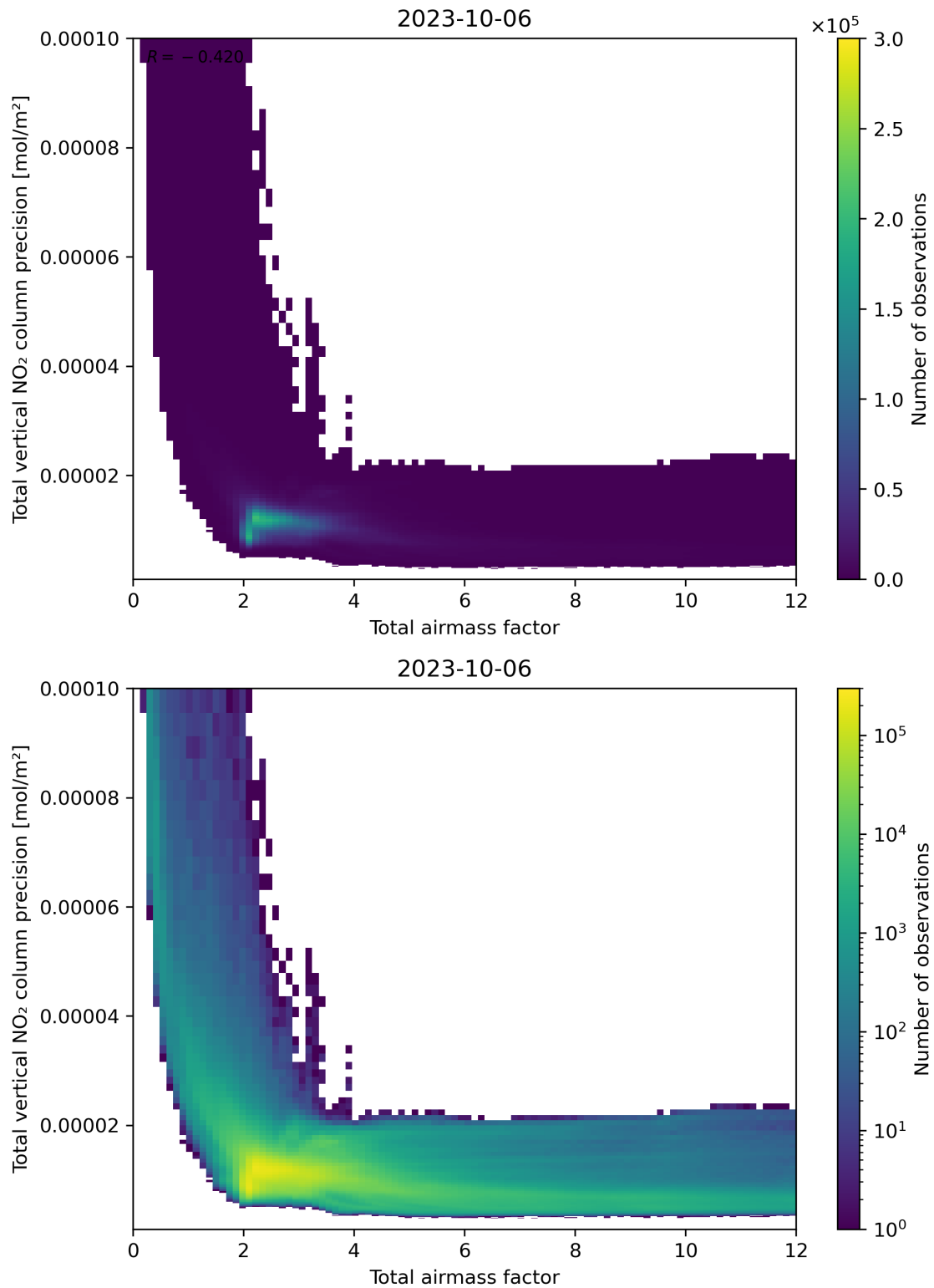
Figure 68: Scatter density plot of “Total airmass factor” against “Total vertical NO 2 column precision” for 2023-10-06 to 2023-10-07.
