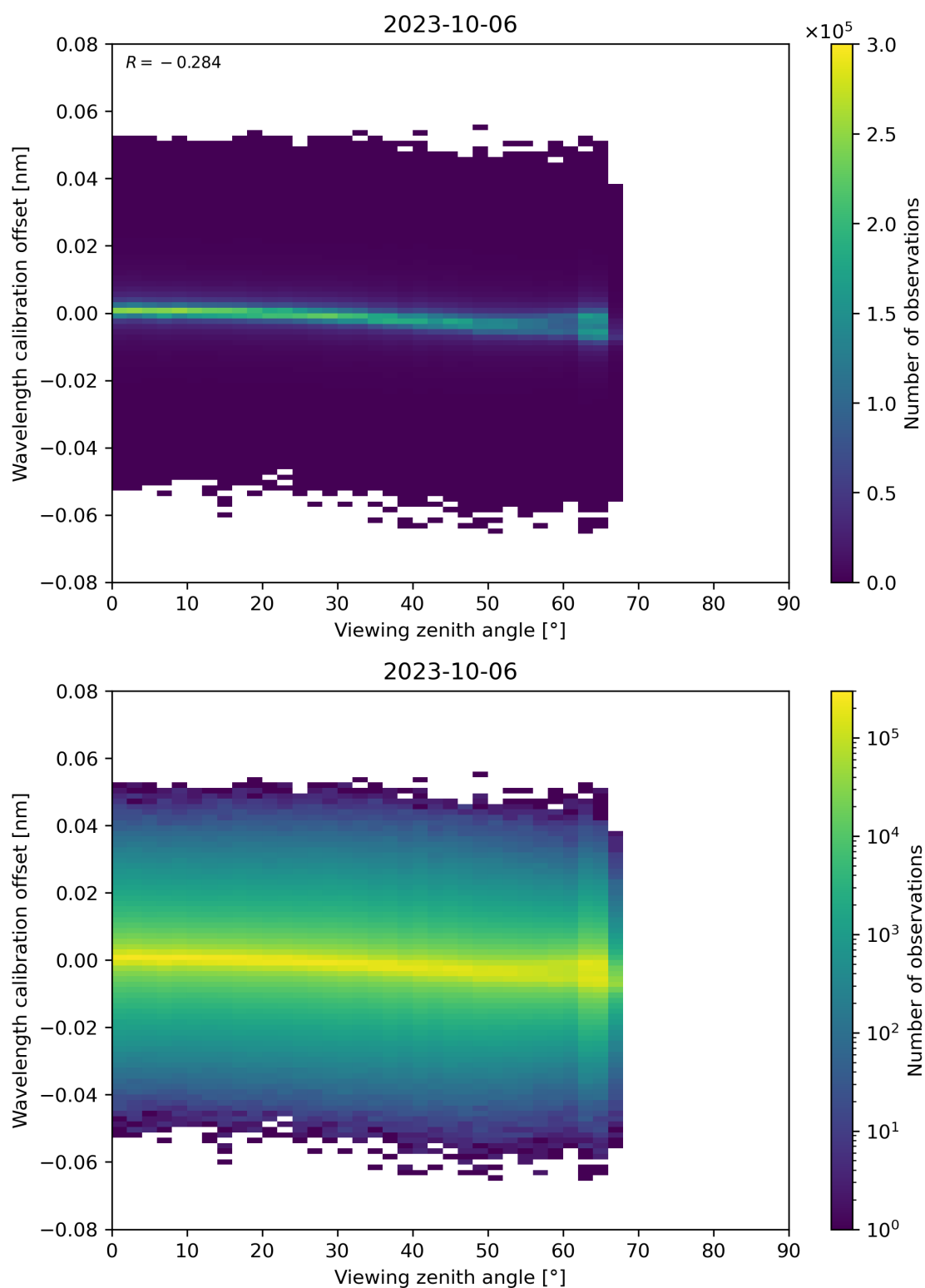
Figure 173: Scatter density plot of “Viewing zenith angle” against “Wavelength calibration offset” for 2023-10-06 to 2023-10-07.
