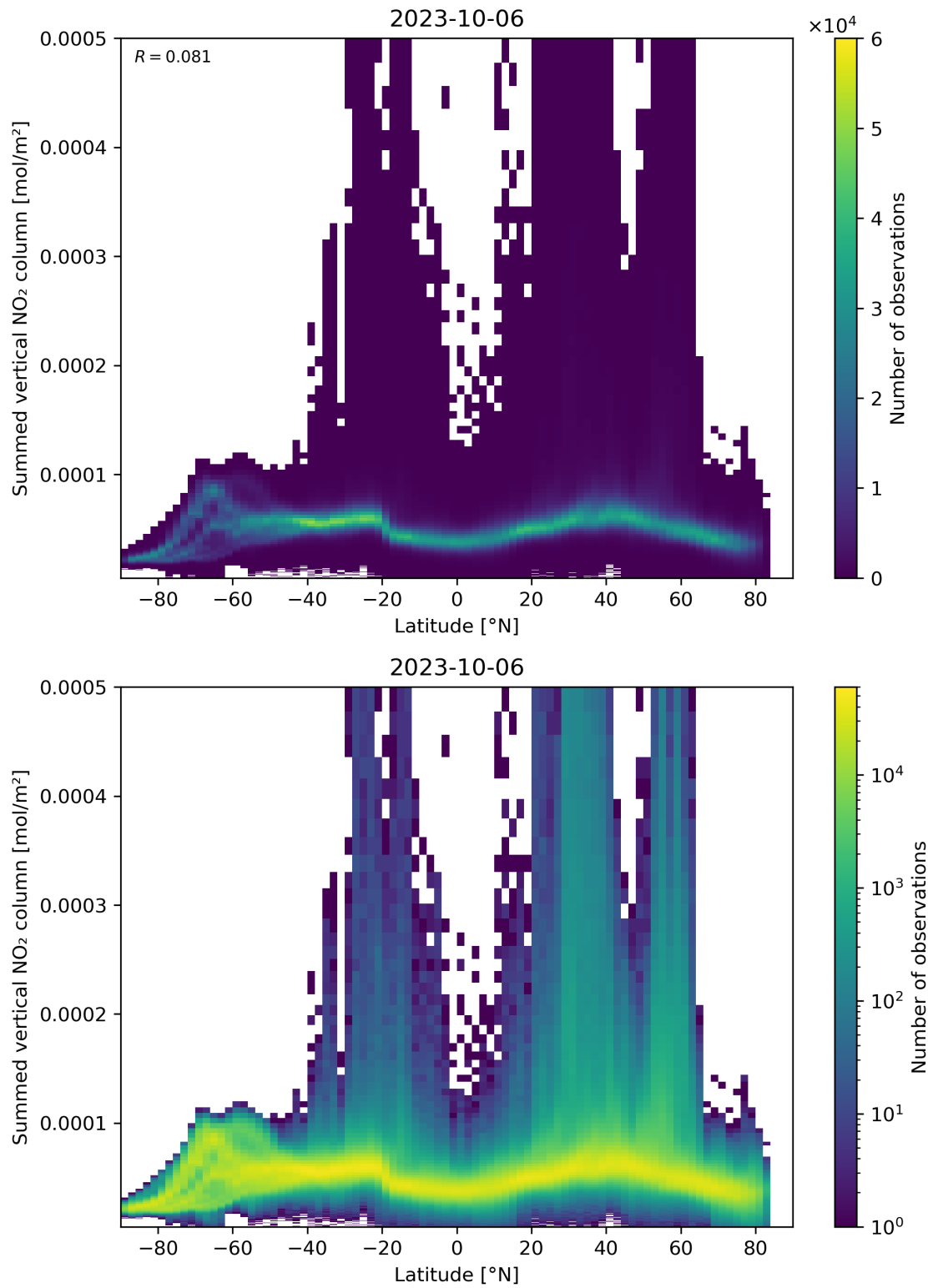
Figure 88: Scatter density plot of “Latitude” against “Summed vertical NO 2 column” for 2023-10-06 to 2023-10-07.
