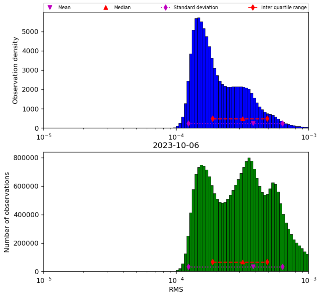
Figure 43: Histogram of “RMS” for 2023-10-06 to 2023-10-07
