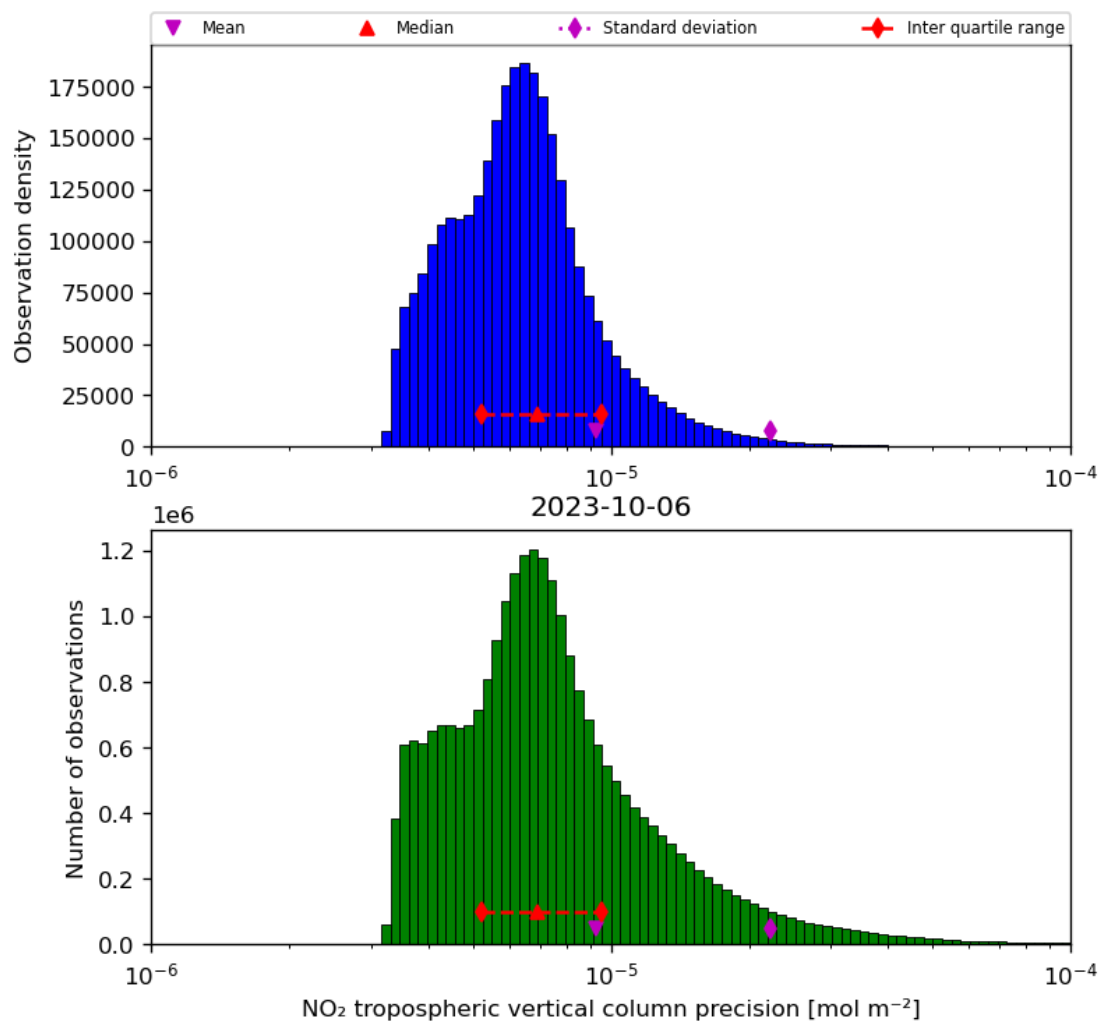
Figure 30: Histogram of “NO 2 tropospheric vertical column precision” for 2023-10-06 to 2023-10-07
