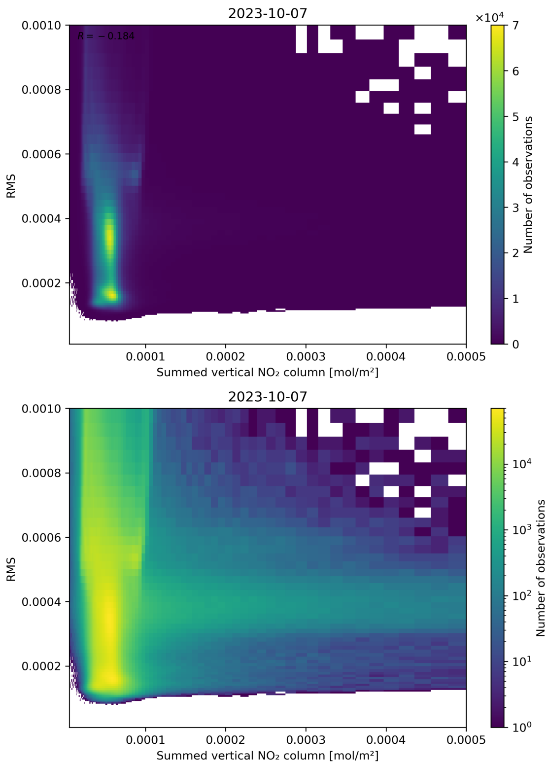
Figure 109: Scatter density plot of “Summed vertical NO 2 column” against “RMS” for 2023-10-06 to 2023-10-08.
