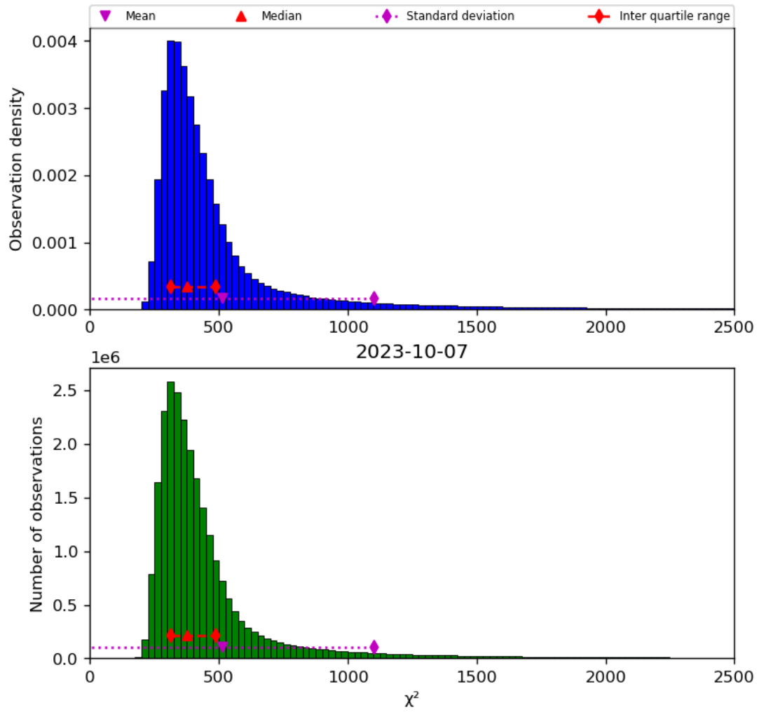
Figure 42: Histogram of “ \chi^2 ” for 2023-10-06 to 2023-10-08
