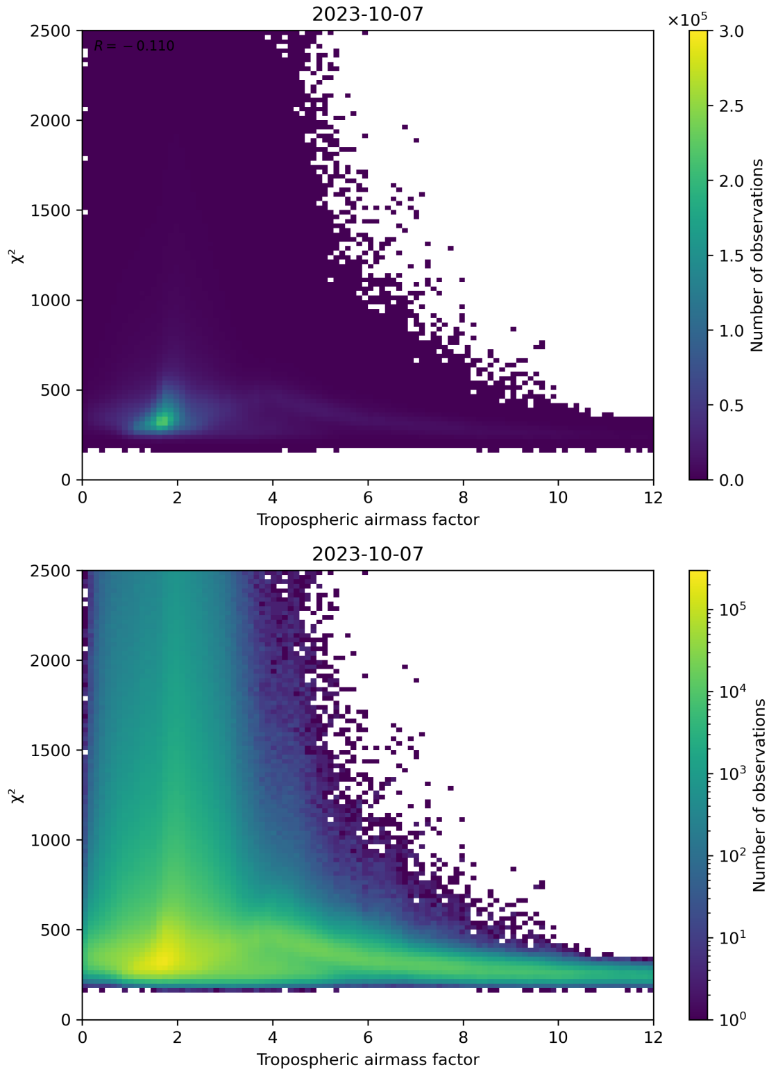
Figure 73: Scatter density plot of “Tropospheric airmass factor” against “ \chi^2 ” for 2023-10-06 to 2023-10-08.
