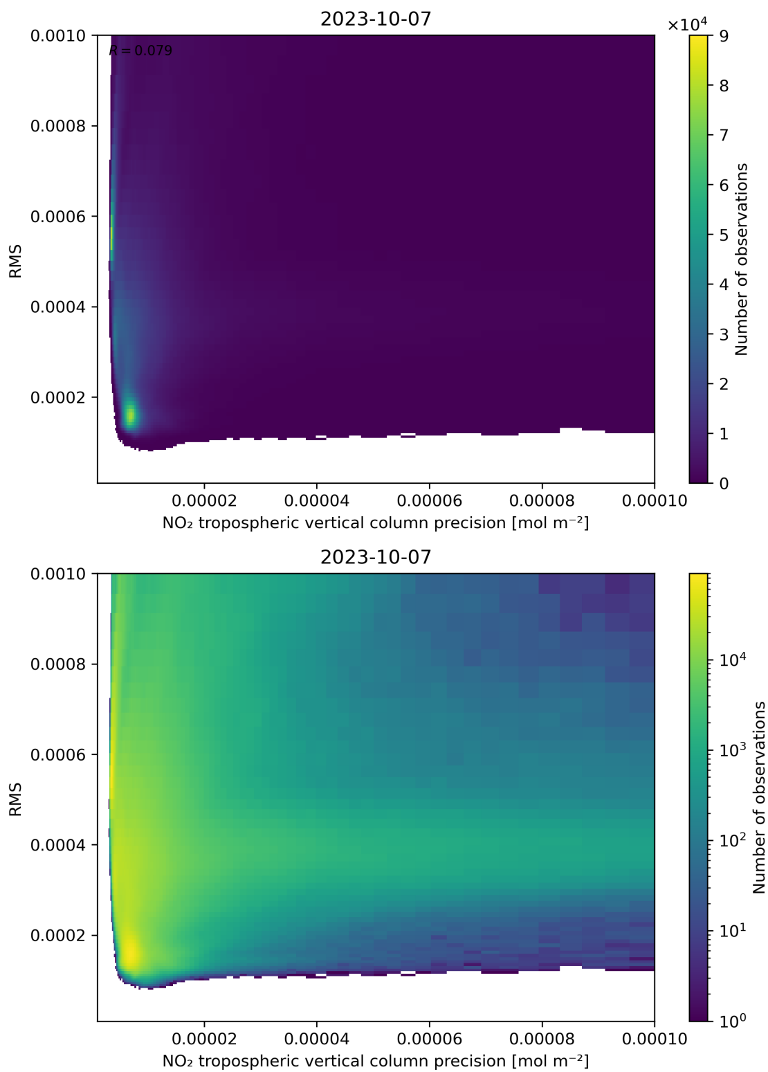
Figure 140: Scatter density plot of “NO 2 tropospheric vertical column precision” against “RMS” for 2023-10-06 to 2023-10-08.
