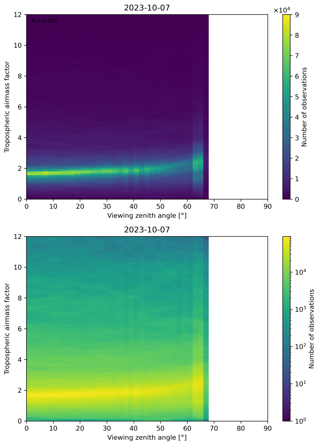
Figure 161: Scatter density plot of “Viewing zenith angle” against “Tropospheric airmass factor” for 2023-10-06 to 2023-10-08.
