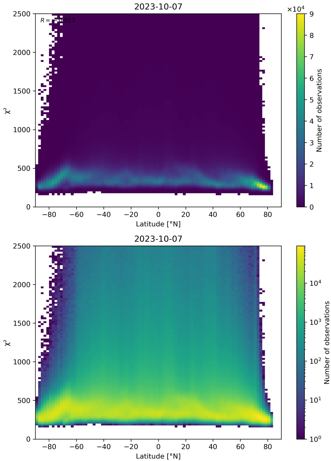
Figure 86: Scatter density plot of “Latitude” against “ \chi^2 ” for 2023-10-06 to 2023-10-08.
