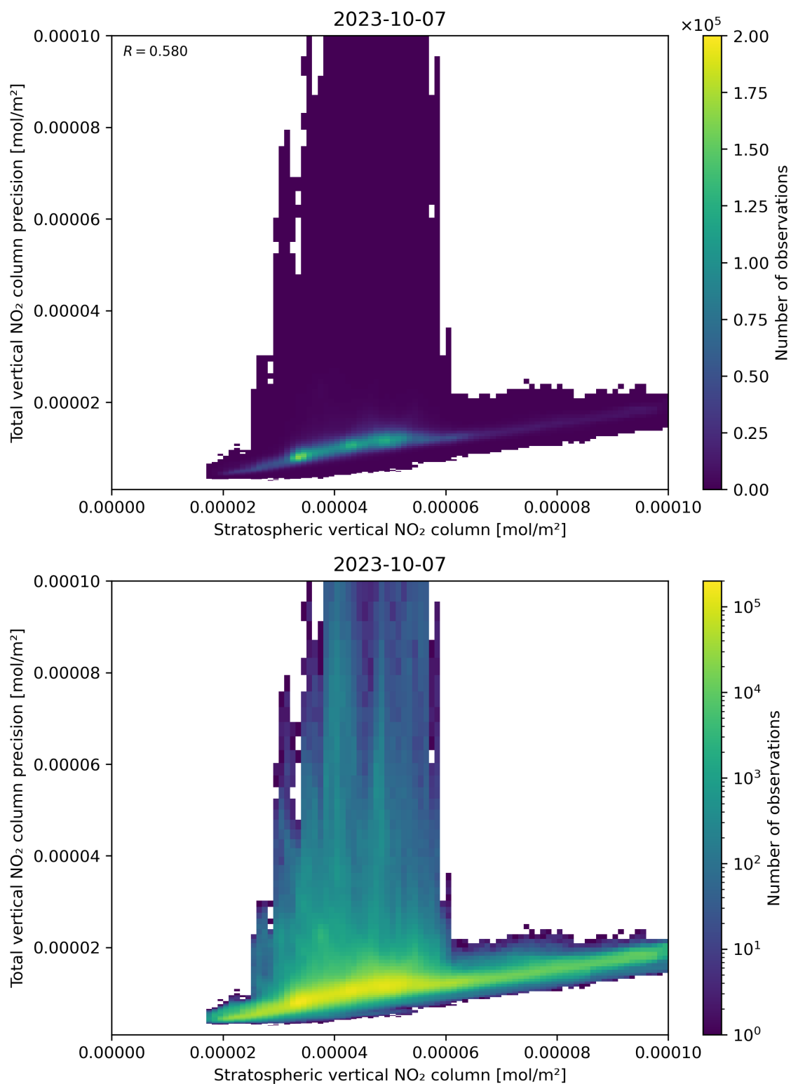
Figure 101: Scatter density plot of “Stratospheric vertical NO 2 column” against “Total vertical NO 2 column precision” for 2023-10-06 to 2023-10-08.
