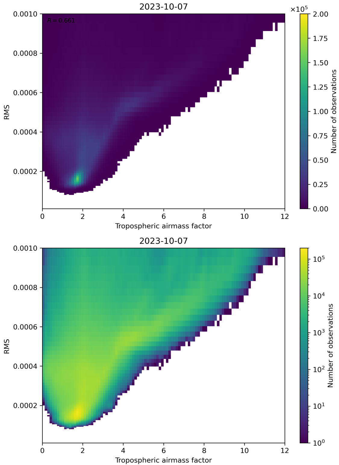
Figure 79: Scatter density plot of “Tropospheric airmass factor” against “RMS” for 2023-10-06 to 2023-10-08.
