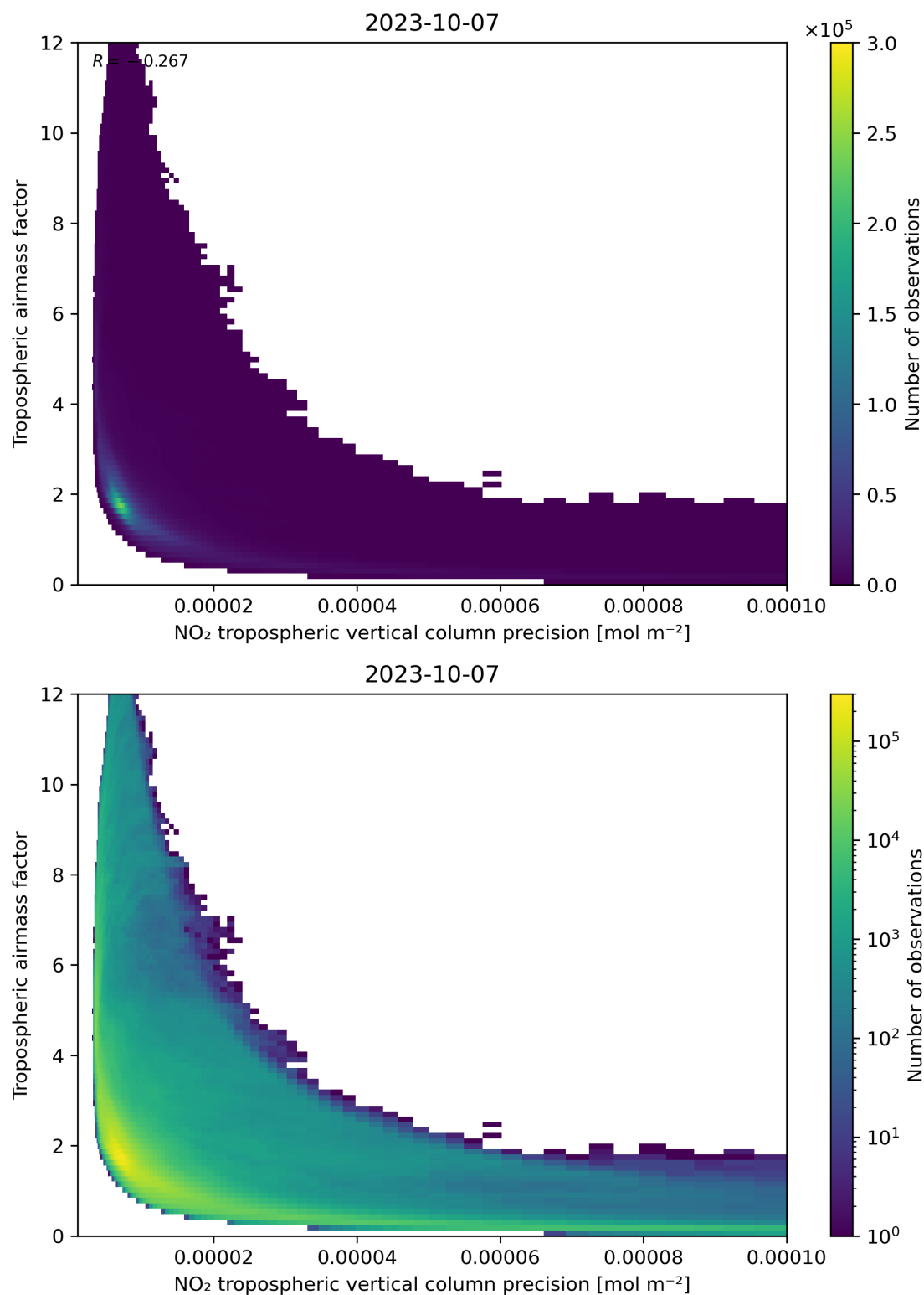
Figure 133: Scatter density plot of “NO 2 tropospheric vertical column precision” against “Tropospheric airmass factor” for 2023-10-06 to 2023-10-08.
