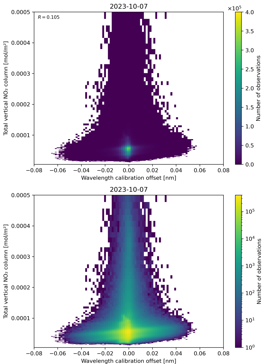
Figure 179: Scatter density plot of “Wavelength calibration offset” against “Total vertical NO 2 column” for 2023-10-06 to 2023-10-08.
