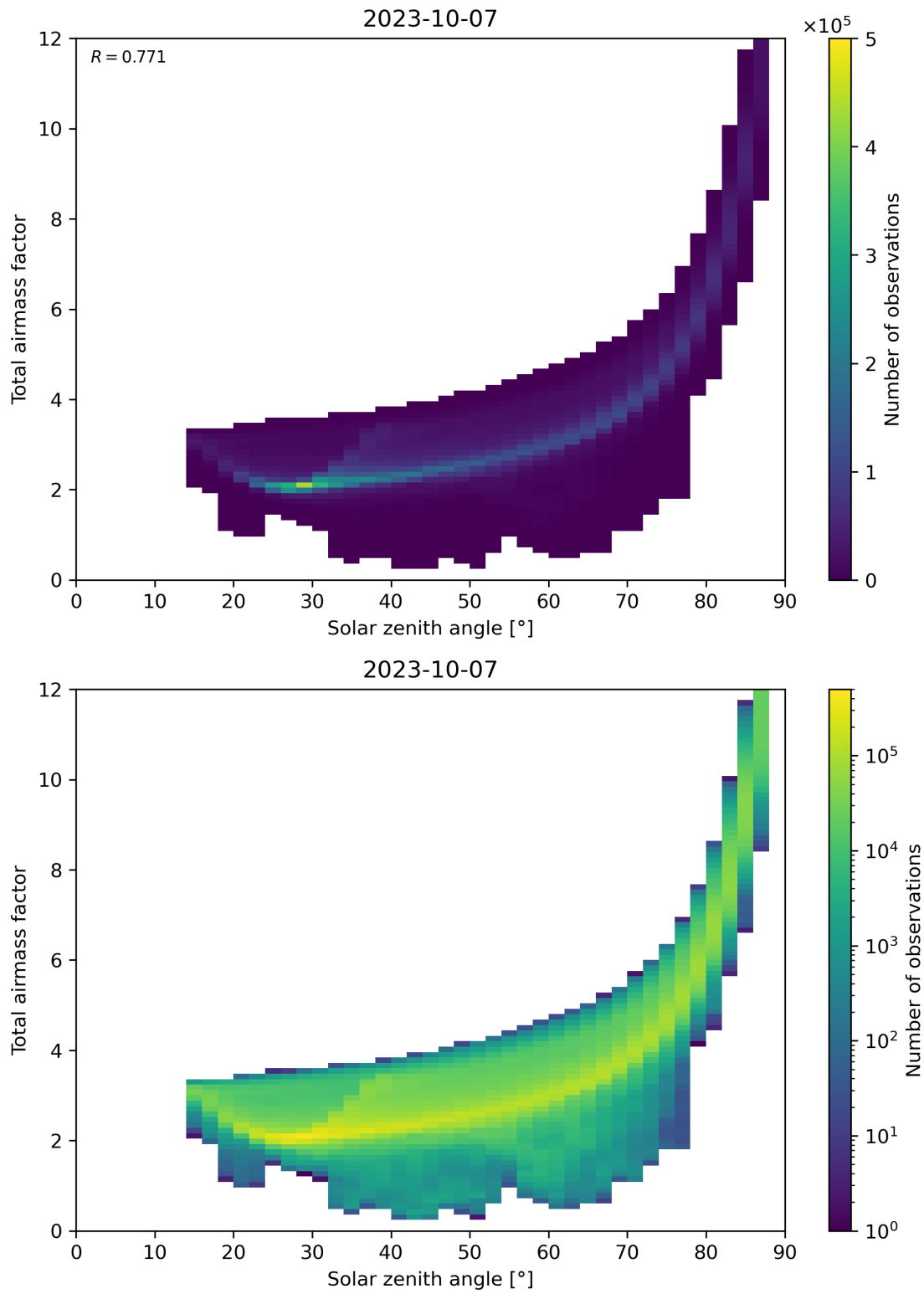
Figure 146: Scatter density plot of “Solar zenith angle” against “Total air mass factor” for 2023-10-06 to 2023-10-08.
