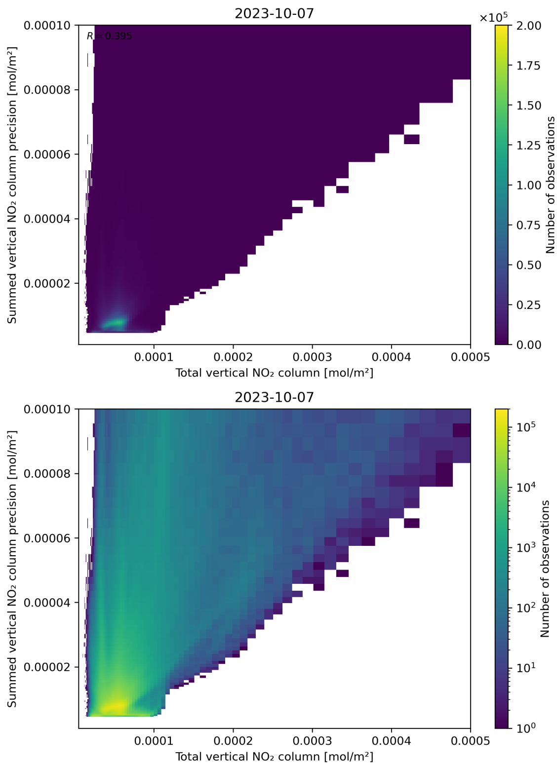
Figure 113: Scatter density plot of “Total vertical NO 2 column” against “Summed vertical NO 2 column precision” for 2023-10-06 to 2023-10-08.
