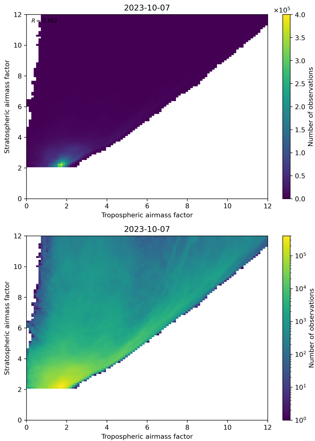
Figure 71: Scatter density plot of “Tropospheric airmass factor” against “Stratospheric airmass factor” for 2023-10-06 to 2023-10-08.
