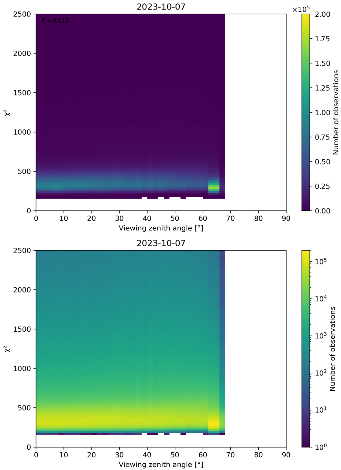
Figure 162: Scatter density plot of “Viewing zenith angle” against “ \chi^2 ” for 2023-10-06 to 2023-10-08.
