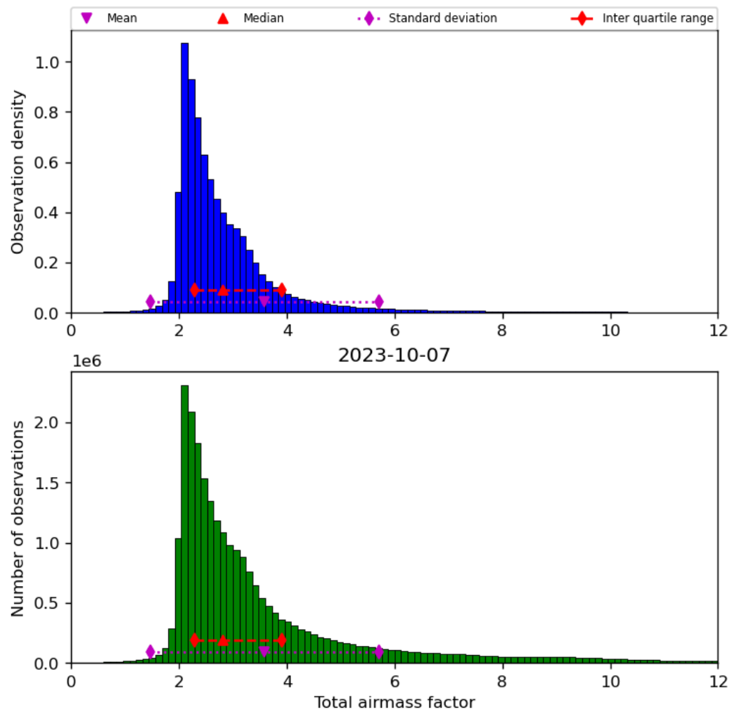
Figure 32: Histogram of “Total airmass factor” for 2023-10-06 to 2023-10-08
