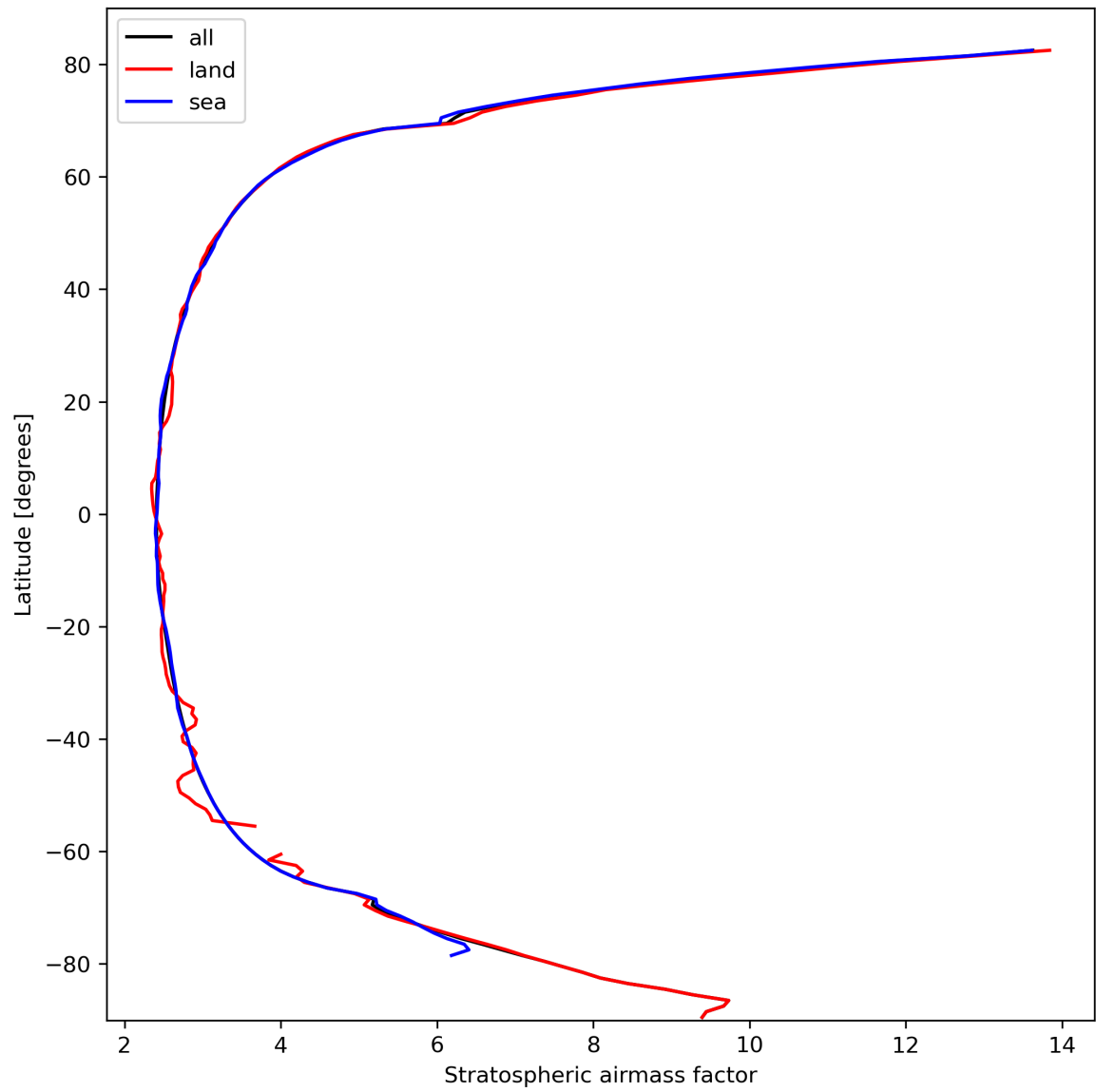
Figure 27: Zonal average of “Stratospheric air mass factor” for 2023-10-06 to 2023-10-08.
