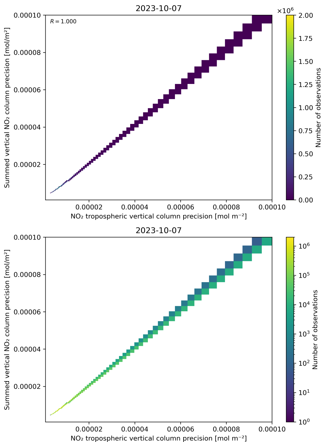
Figure 137: Scatter density plot of “NO 2 tropospheric vertical column precision” against “Summed vertical NO 2 column precision” for 2023-10-06 to 2023-10-08.
