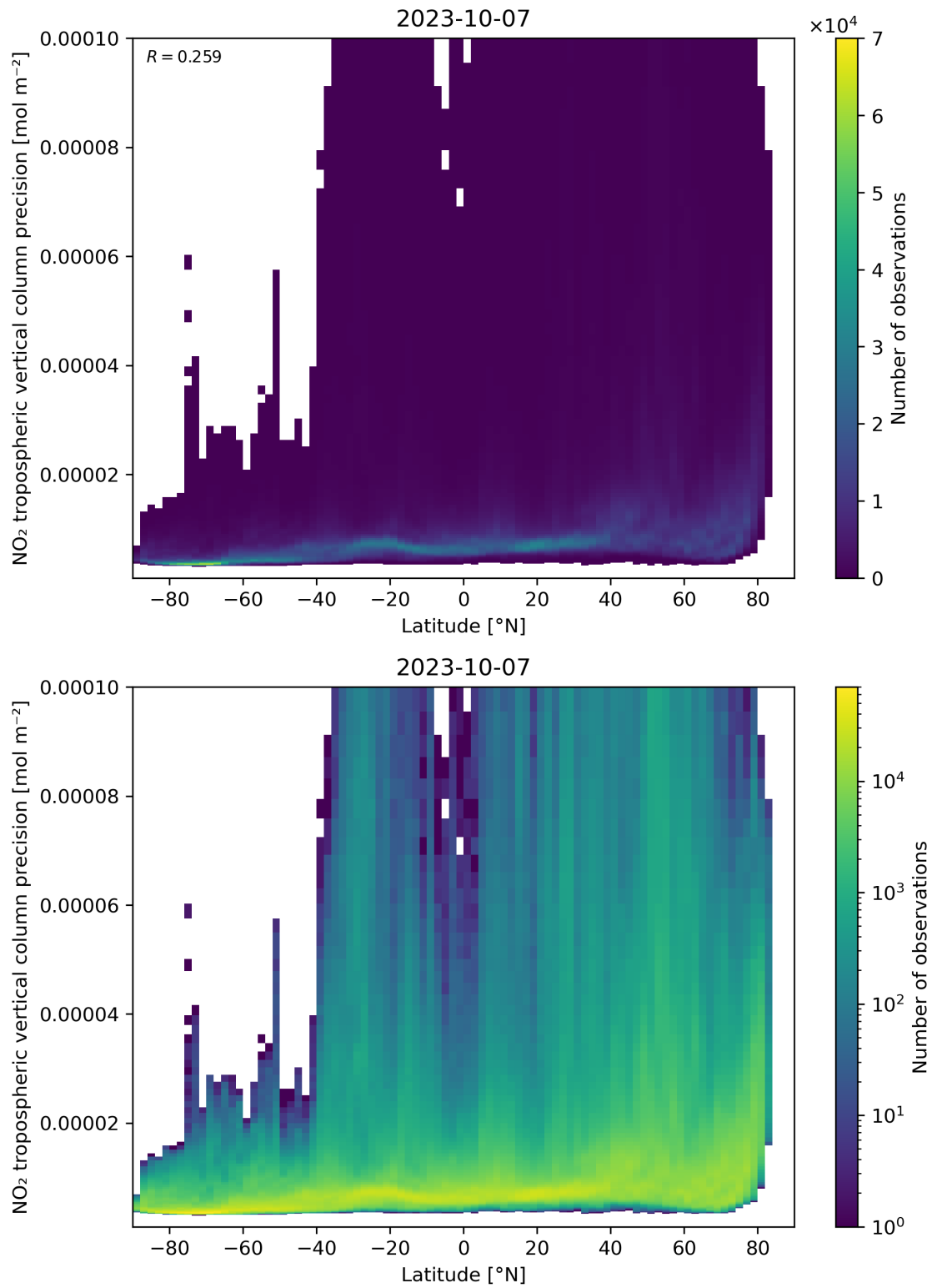
Figure 93: Scatter density plot of “Latitude” against “NO 2 tropospheric vertical column precision” for 2023-10-06 to 2023-10-08.
