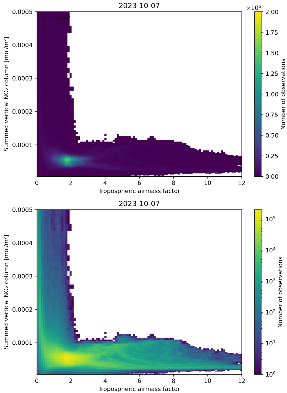
Figure 75: Scatter density plot of “Tropospheric airmass factor” against “Summed vertical NO 2 column” for 2023-10-06 to 2023-10-08.
