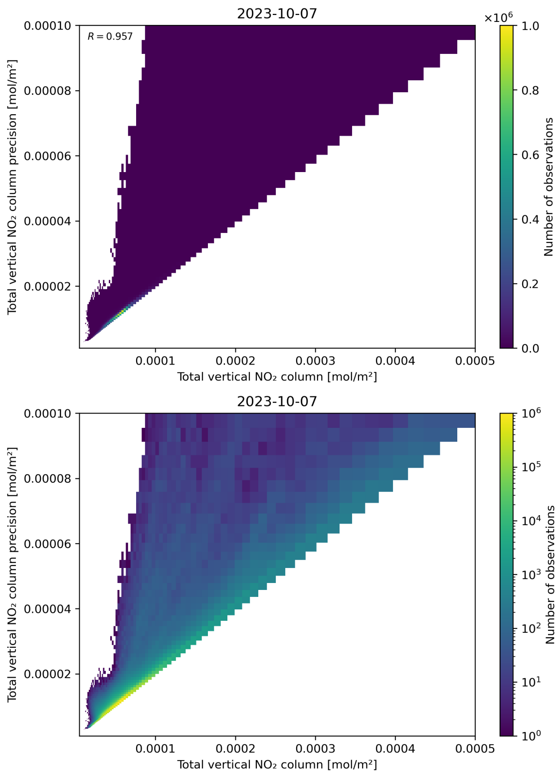
Figure 114: Scatter density plot of “Total vertical NO 2 column” against “Total vertical NO 2 column precision” for 2023-10-06 to 2023-10-08.
