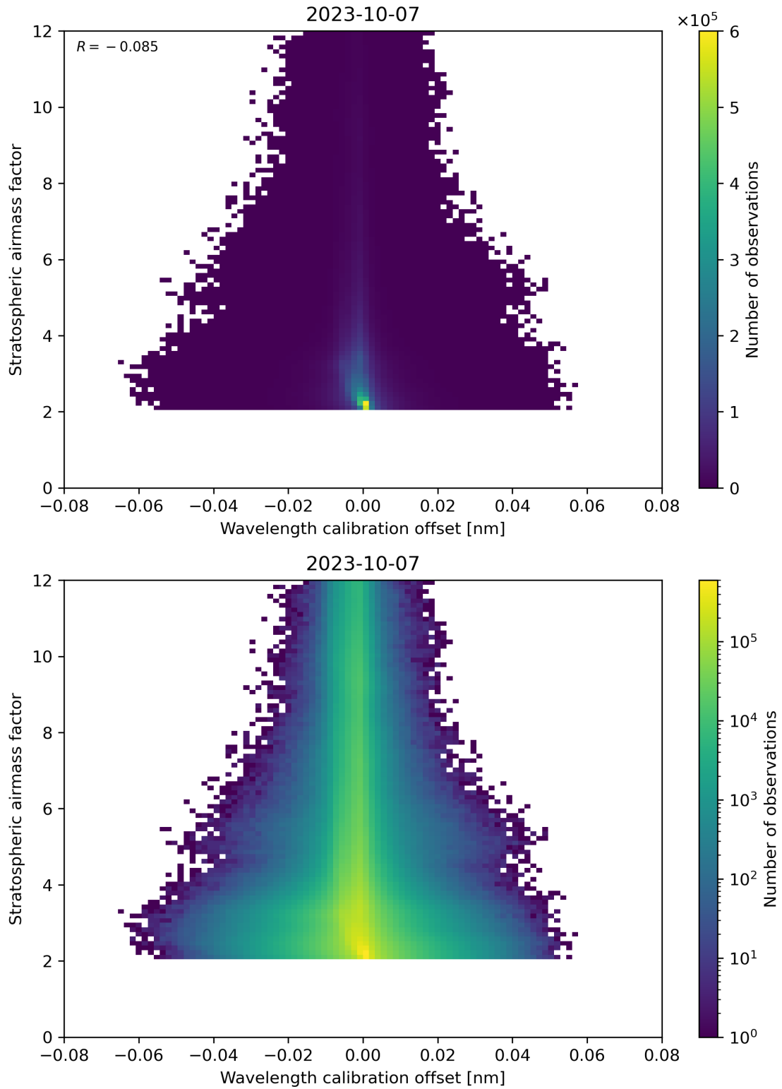
Figure 174: Scatter density plot of “Wavelength calibration offset” against “Stratospheric airmass factor” for 2023-10-06 to 2023-10-08.
