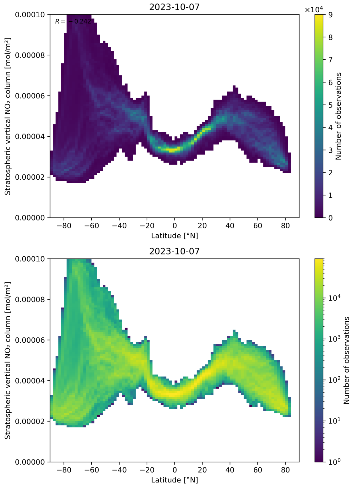
Figure 87: Scatter density plot of “Latitude” against “Stratospheric vertical NO 2 column” for 2023-10-06 to 2023-10-08.
