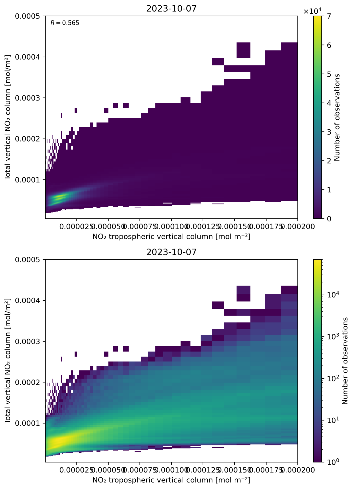
Figure 128: Scatter density plot of “NO 2 tropospheric vertical column” against “Total vertical NO 2 column” for 2023-10-06 to 2023-10-08.
