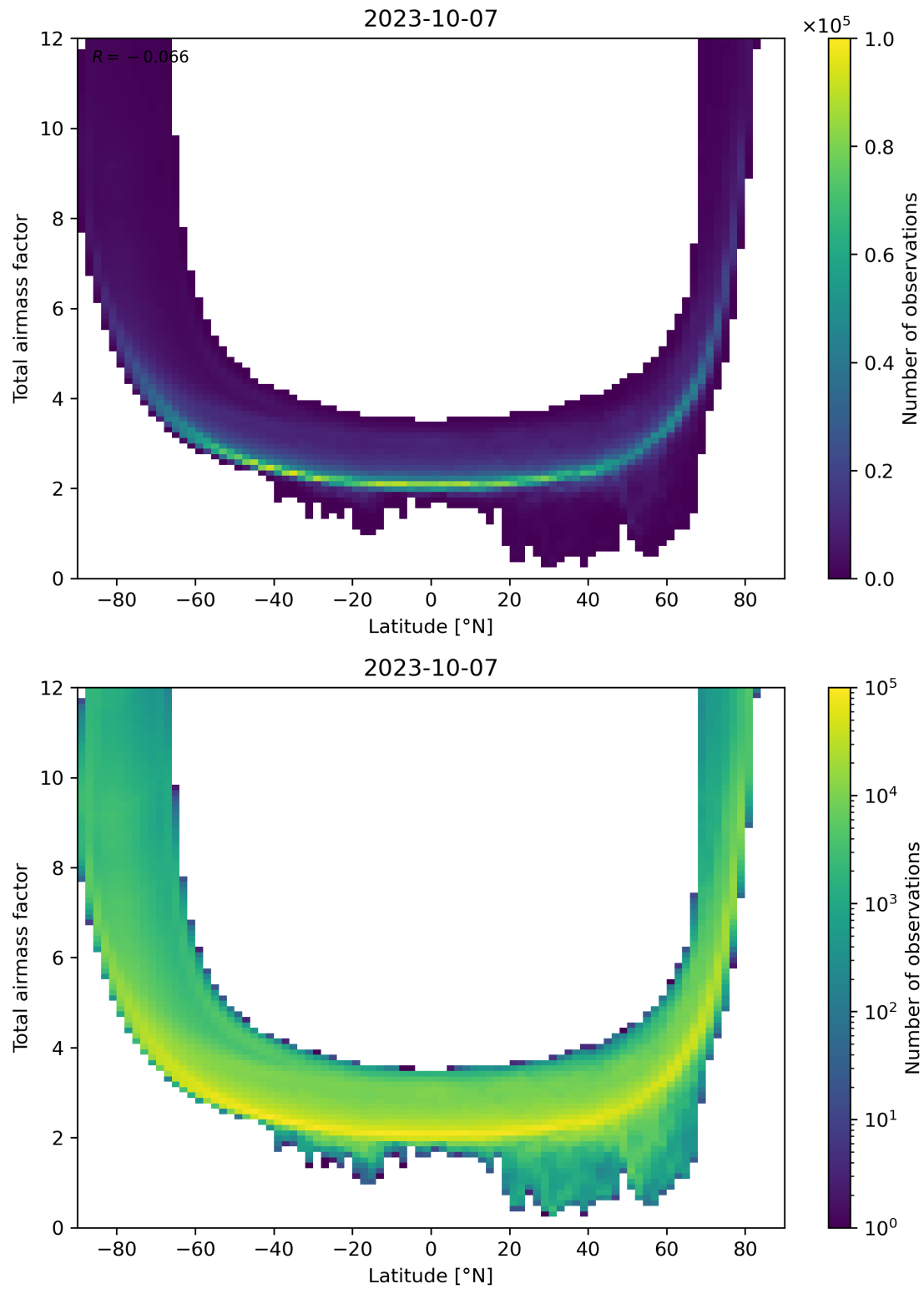
Figure 84: Scatter density plot of “Latitude” against “Total airmass factor” for 2023-10-06 to 2023-10-08.
