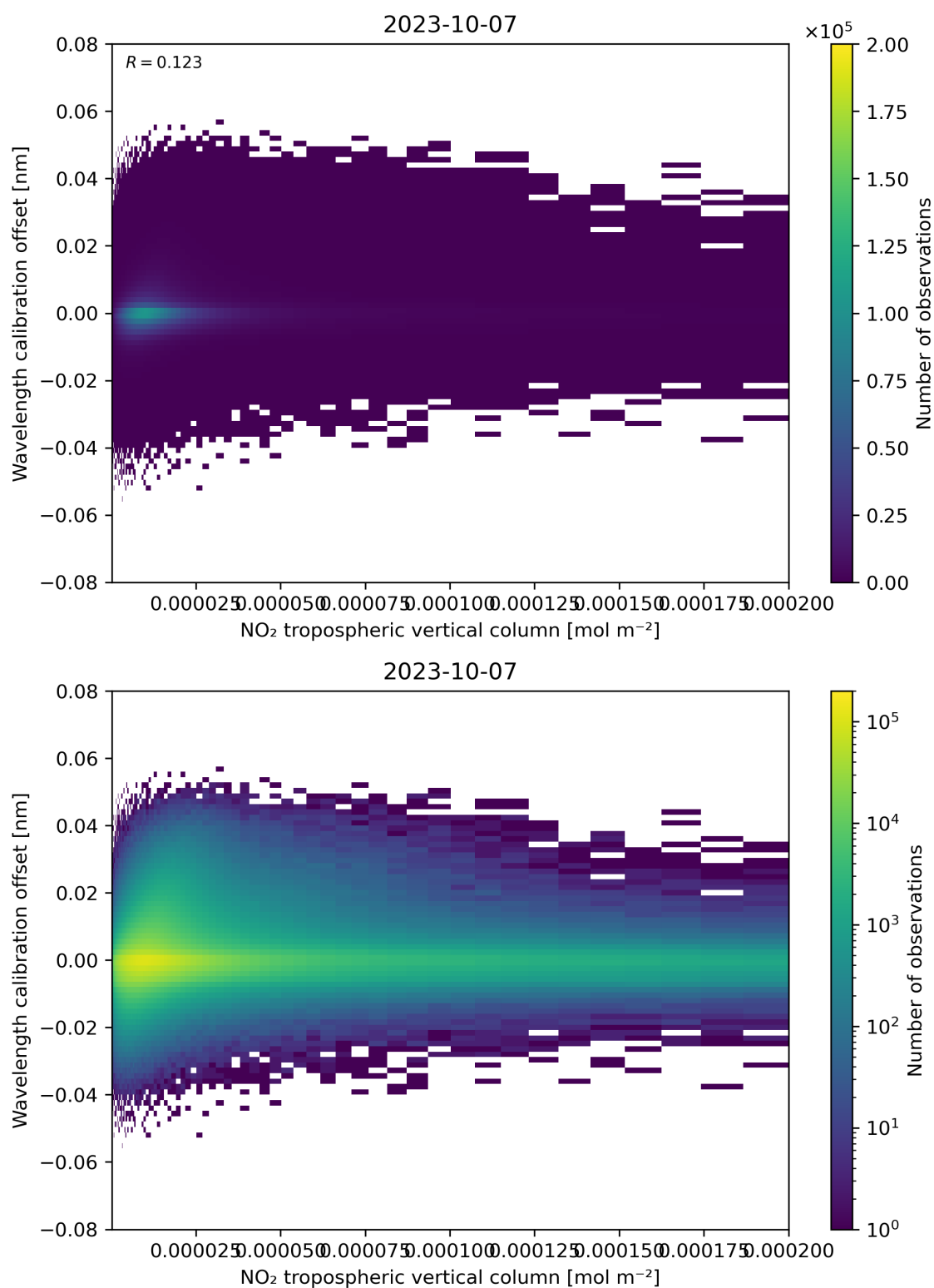
Figure 143: Scatter density plot of “NO 2 tropospheric vertical column” against “Wavelength calibration offset” for 2023-10-06 to 2023-10-08.
