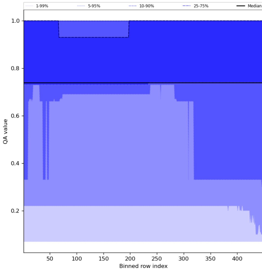
Figure 45: Along track statistics of “QA value” for 2023-10-06 to 2023-10-08
