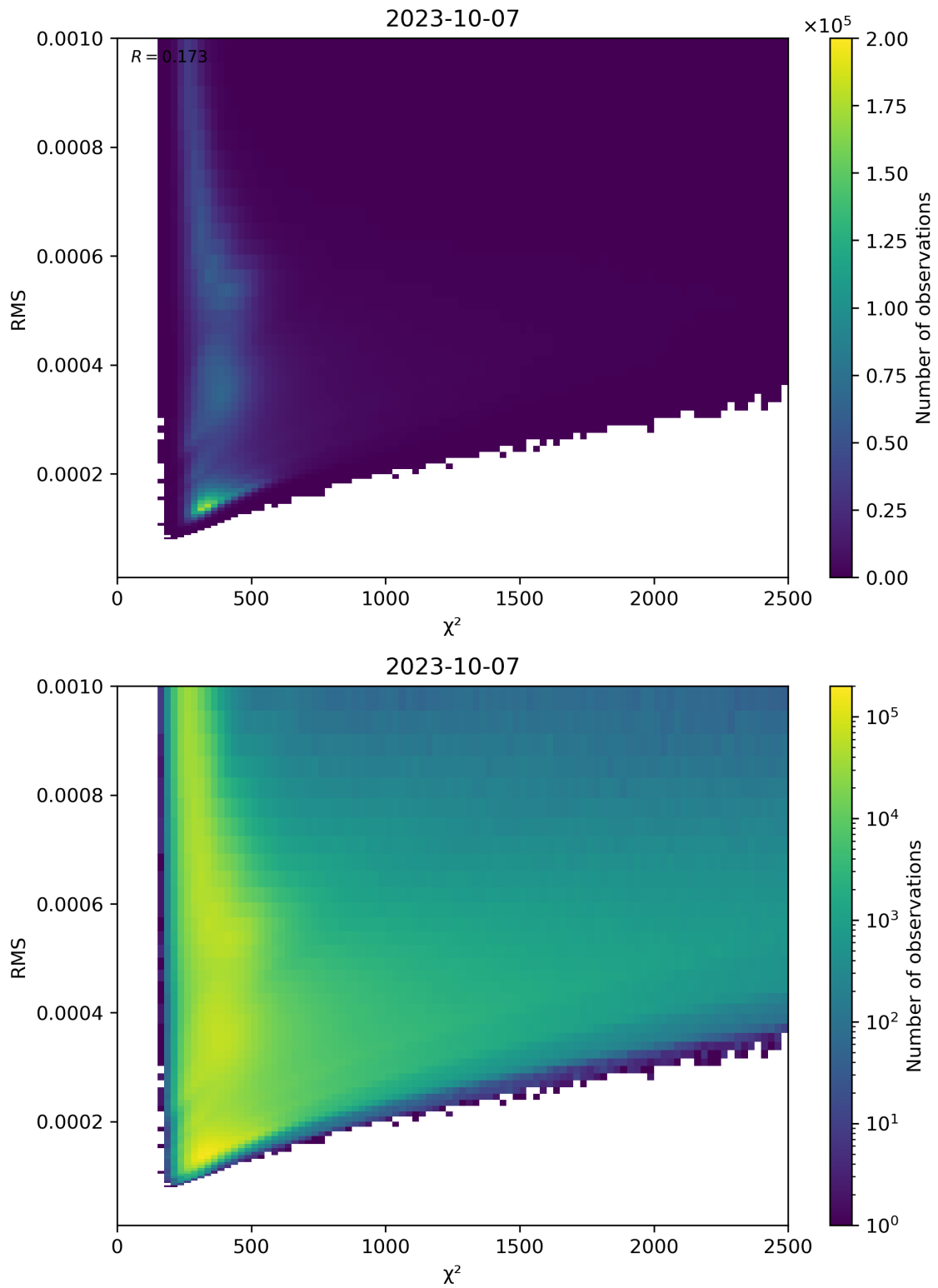
Figure 82: Scatter density plot of “ \chi^2 ” against “RMS” for 2023-10-06 to 2023-10-08.
