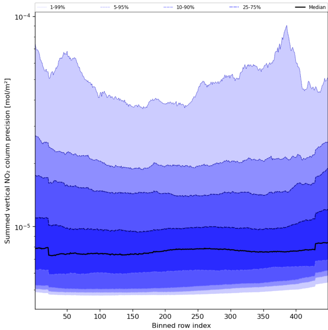
Figure 58: Along track statistics of “Summed vertical NO 2 column precision” for 2023-10-06 to 2023-10-08
