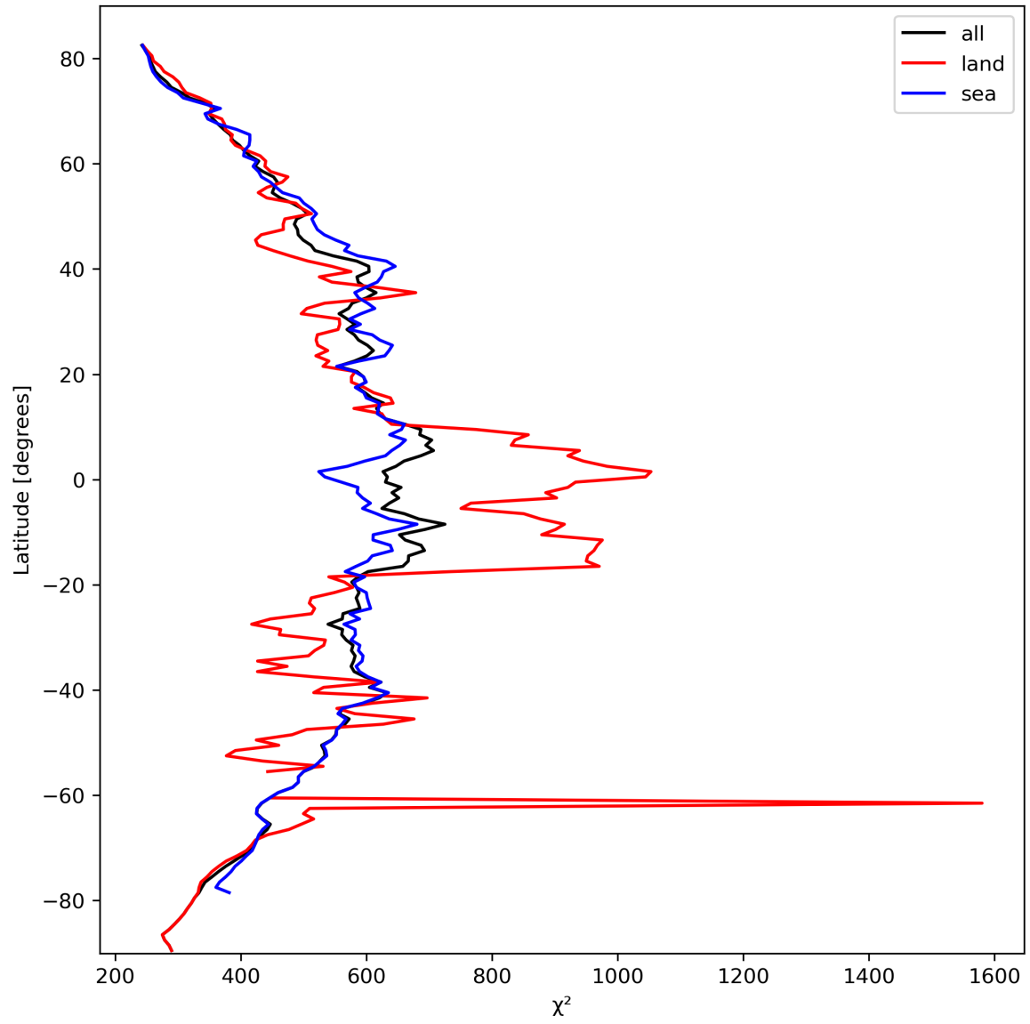
Figure 25: Zonal average of “ \chi^2 ” for 2023-10-06 to 2023-10-08.
