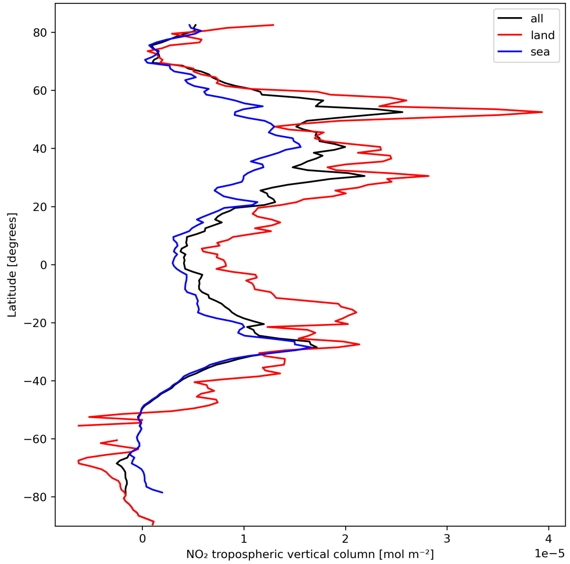
Figure 12: Zonal average of “NO 2 tropospheric vertical column” for 2023-10-06 to 2023-10-08.
