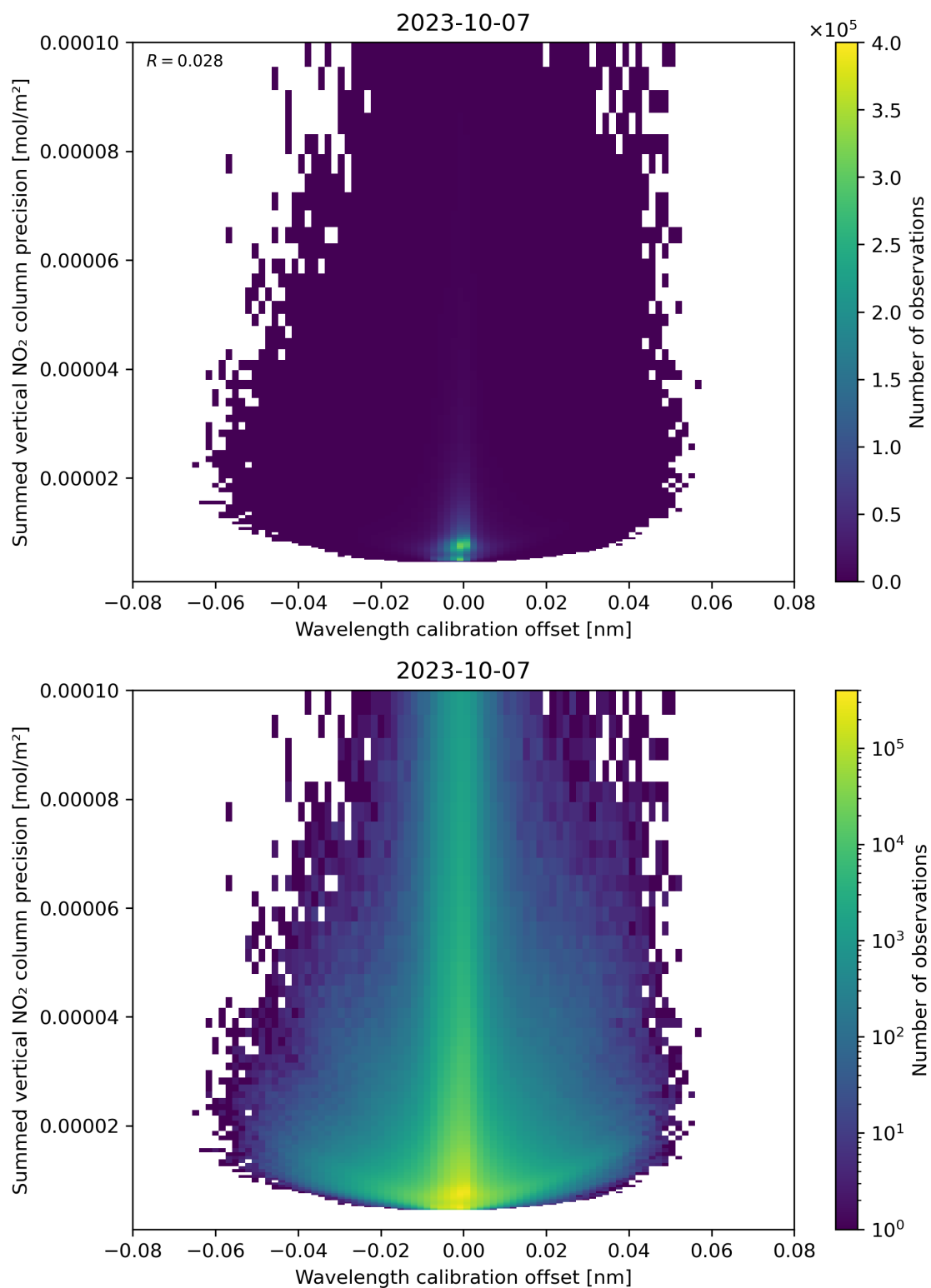
Figure 178: Scatter density plot of “Wavelength calibration offset” against “Summed vertical NO 2 column precision” for 2023-10-06 to 2023-10-08.
