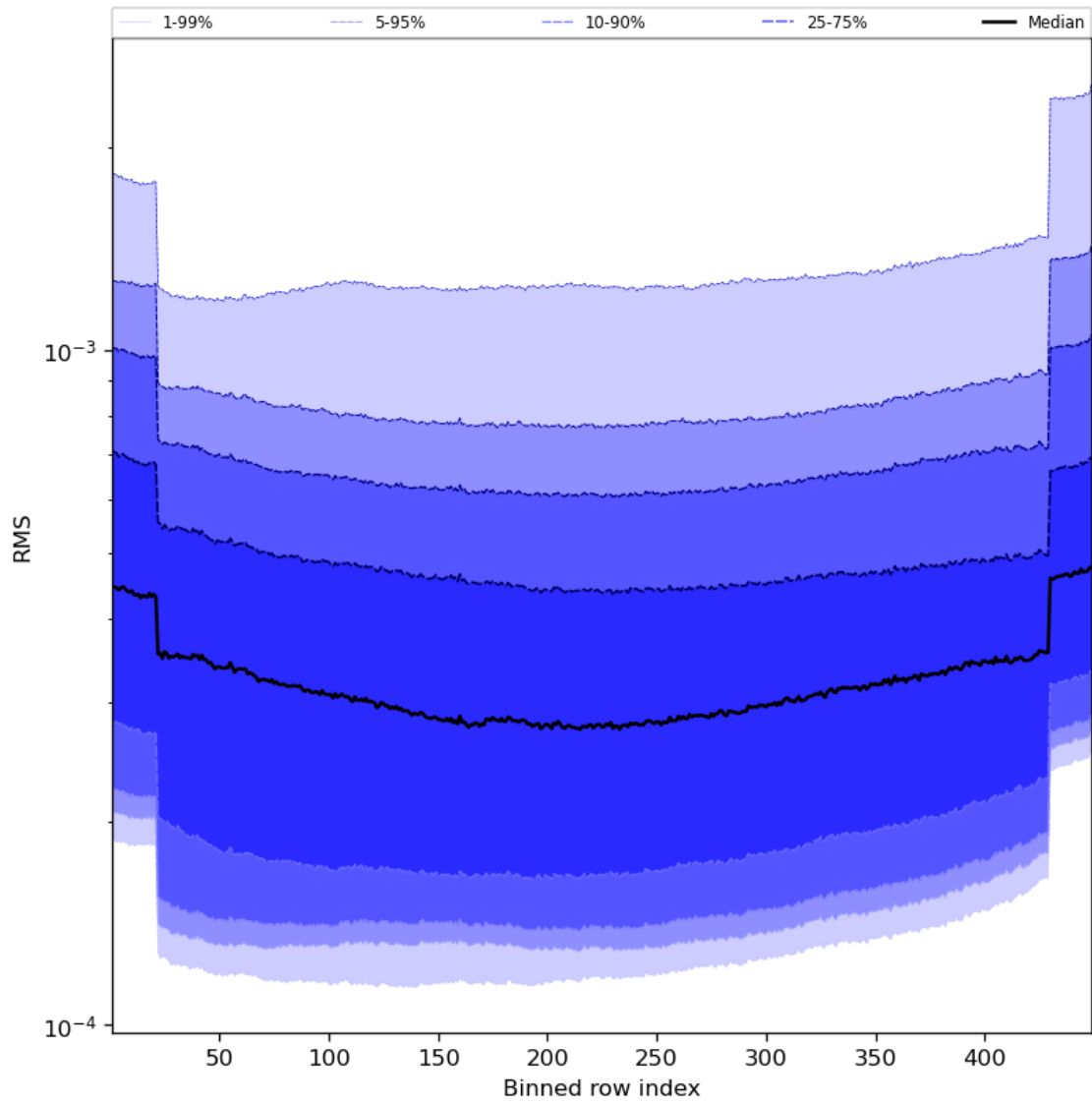
Figure 60: Along track statistics of “RMS” for 2023-10-06 to 2023-10-08
