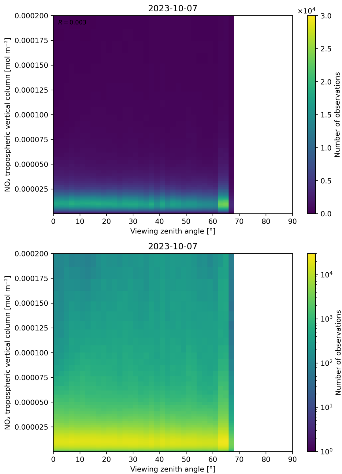
Figure 169: Scatter density plot of “Viewing zenith angle” against “NO 2 tropospheric vertical column” for 2023-10-06 to 2023-10-08.
