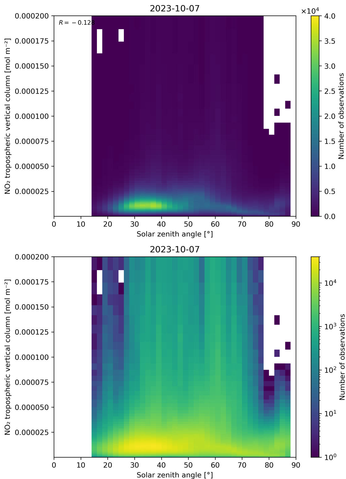
Figure 155: Scatter density plot of “Solar zenith angle” against “NO 2 tropospheric vertical column” for 2023-10-06 to 2023-10-08.
