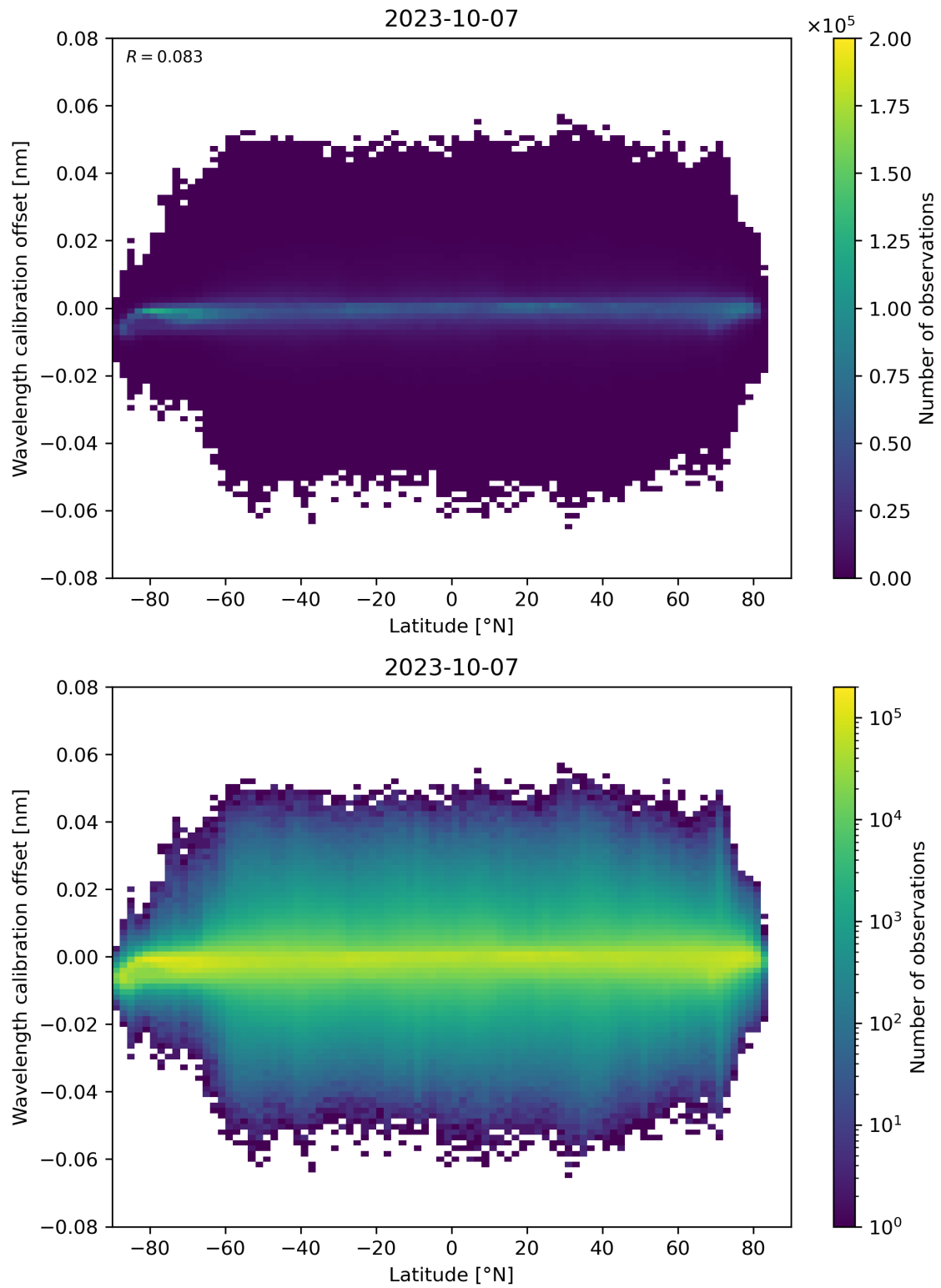
Figure 95: Scatter density plot of “Latitude” against “Wavelength calibration offset” for 2023-10-06 to 2023-10-08.
