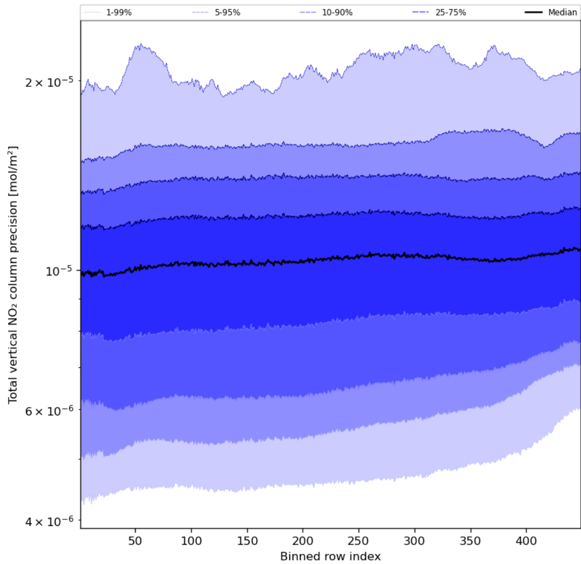
Figure 56: Along track statistics of “Total vertical NO 2 column precision” for 2023-10-06 to 2023-10-08
