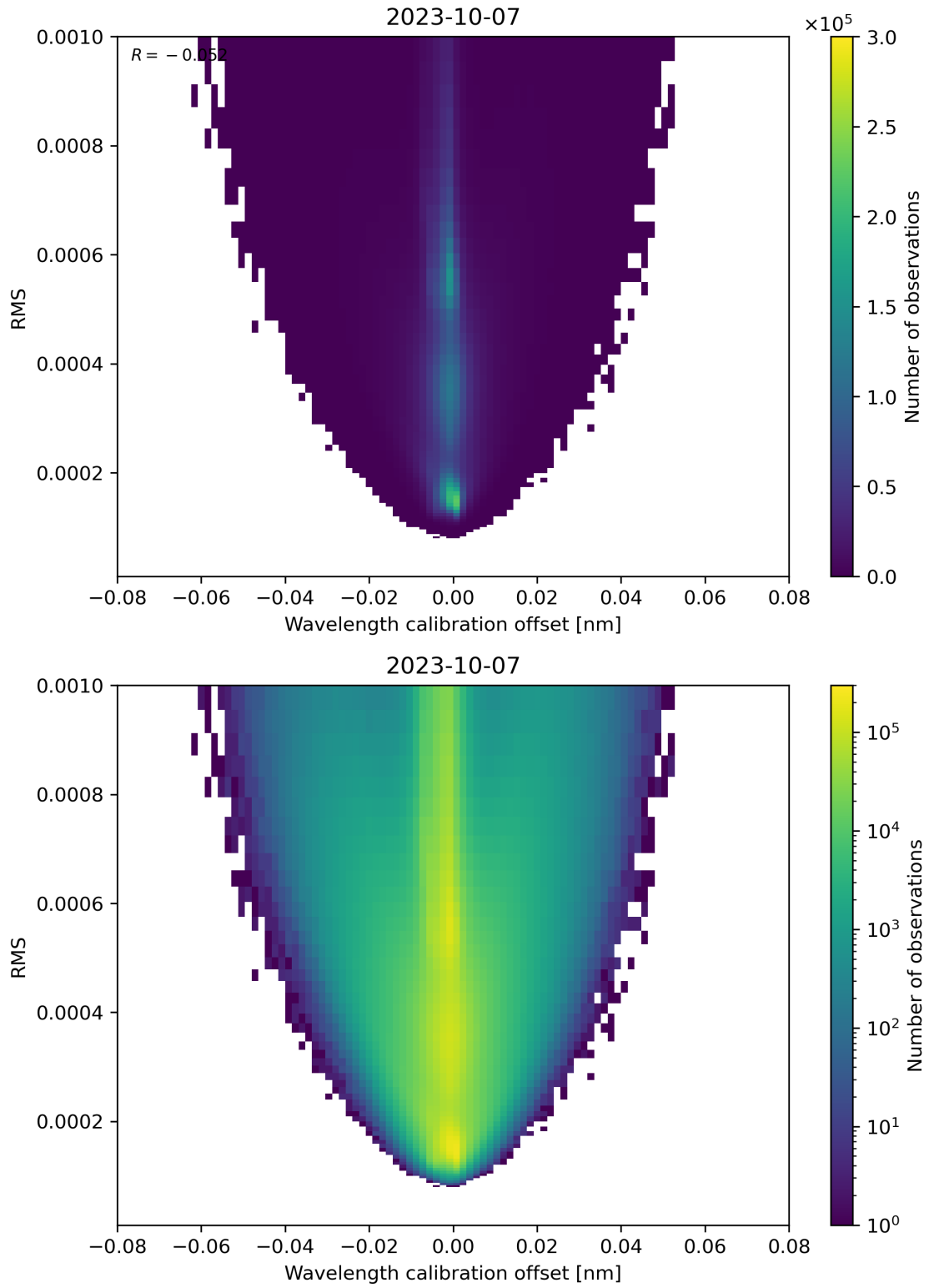
Figure 181: Scatter density plot of “Wavelength calibration offset” against “RMS” for 2023-10-06 to 2023-10-08.
