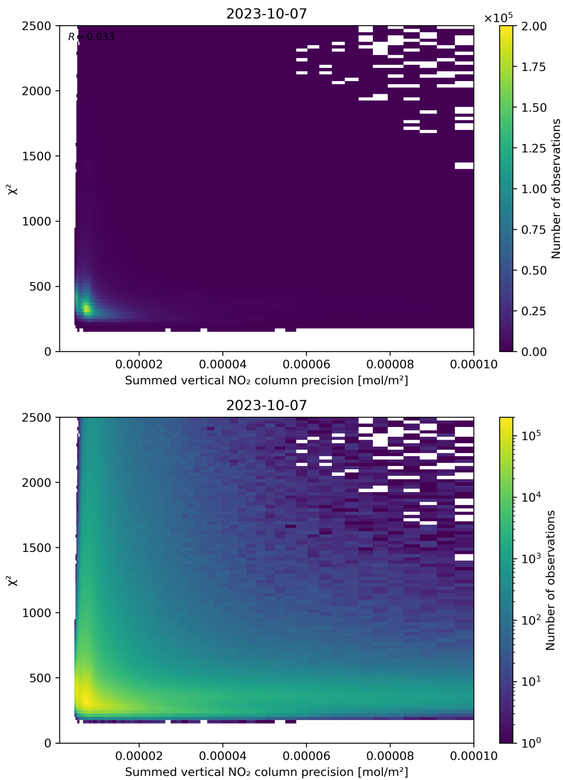
Figure 107: Scatter density plot of “Summed vertical NO 2 column precision” against “ \chi^2 ” for 2023-10-06 to 2023-10-08.
