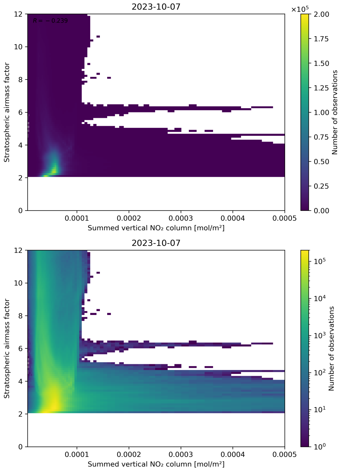
Figure 103: Scatter density plot of “Summed vertical NO 2 column” against “Stratospheric air mass factor” for 2023-10-06 to 2023-10-08.
