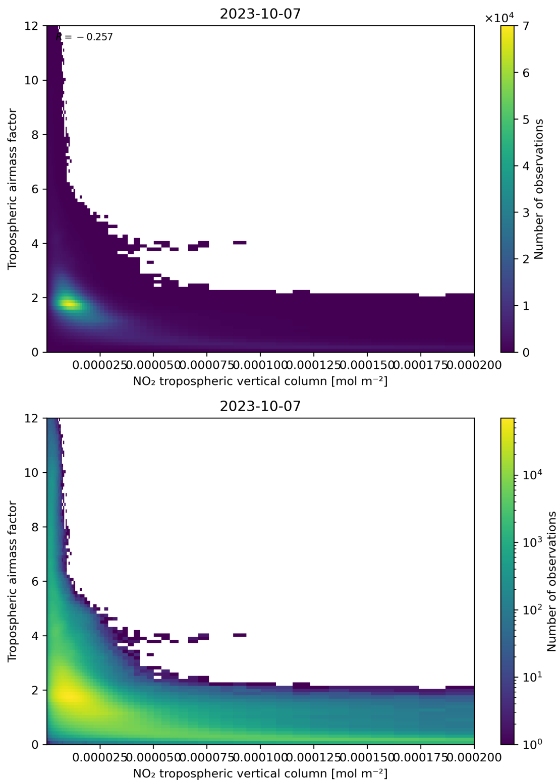
Figure 123: Scatter density plot of “NO 2 tropospheric vertical column” against “Tropospheric air mass factor” for 2023-10-06 to 2023-10-08.
