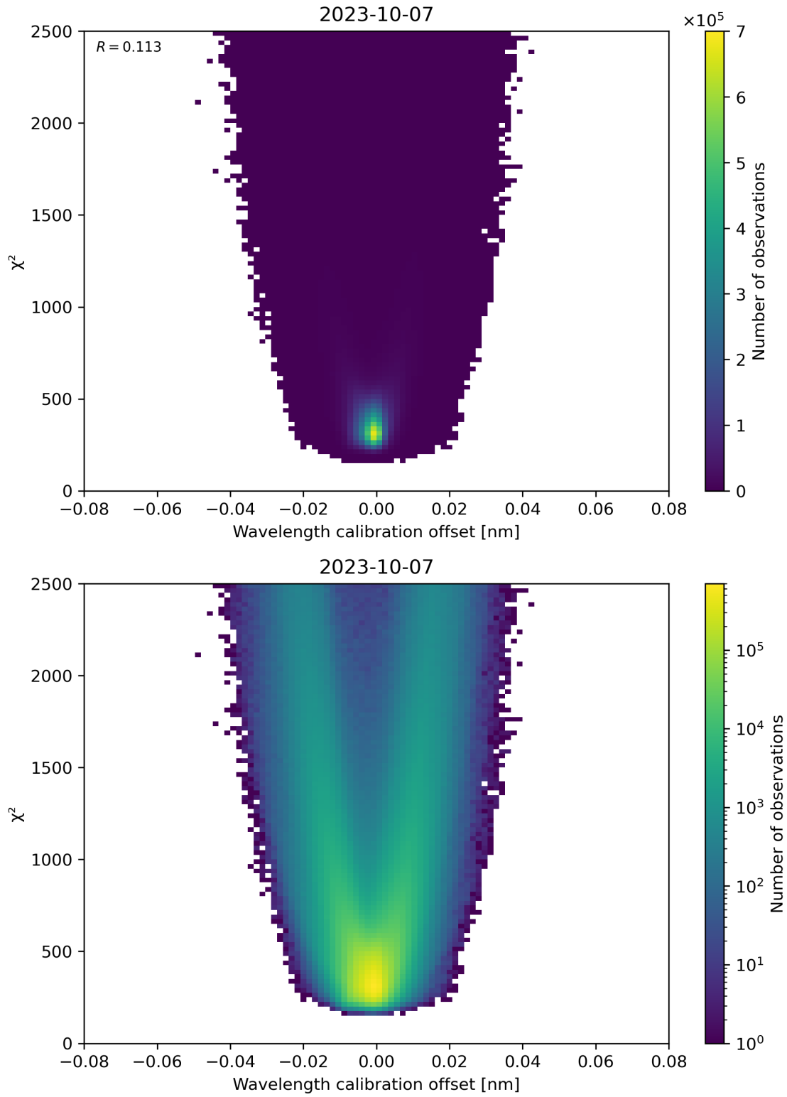
Figure 175: Scatter density plot of “Wavelength calibration offset” against “ \chi^2 ” for 2023-10-06 to 2023-10-08.
