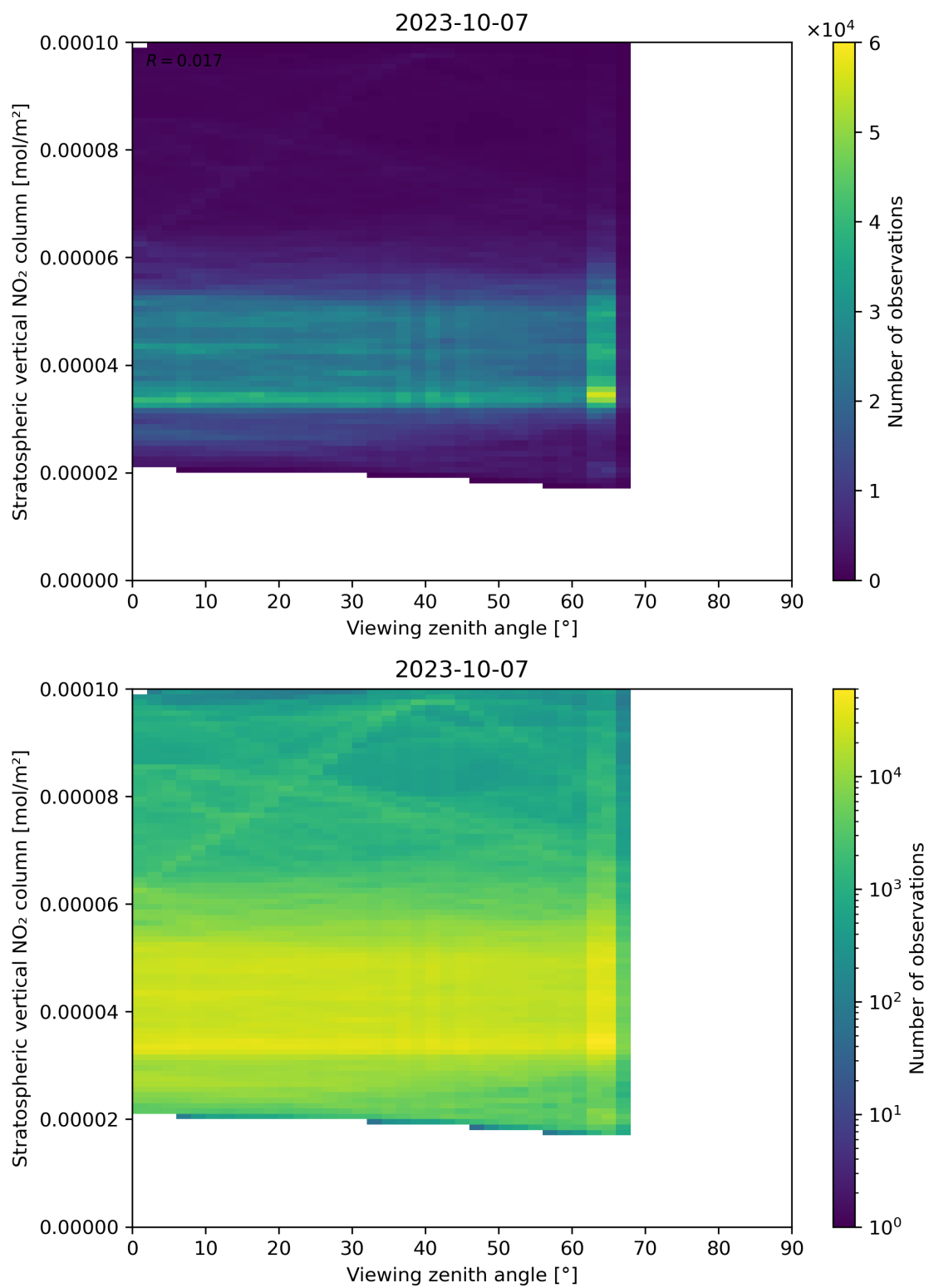
Figure 164: Scatter density plot of “Viewing zenith angle” against “Stratospheric vertical NO 2 column” for 2023-10-06 to 2023-10-08.
