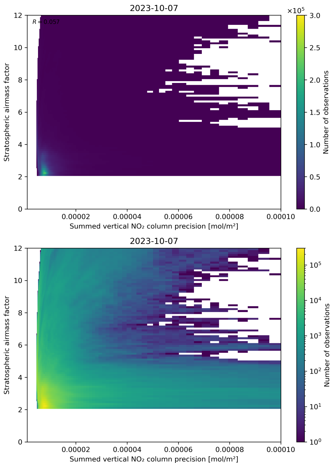
Figure 106: Scatter density plot of “Summed vertical NO 2 column precision” against “Stratospheric airmass factor” for 2023-10-06 to 2023-10-08.
