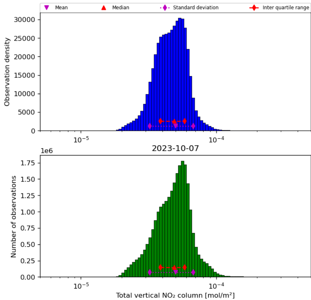
Figure 38: Histogram of “Total vertical NO 2 column” for 2023-10-06 to 2023-10-08
