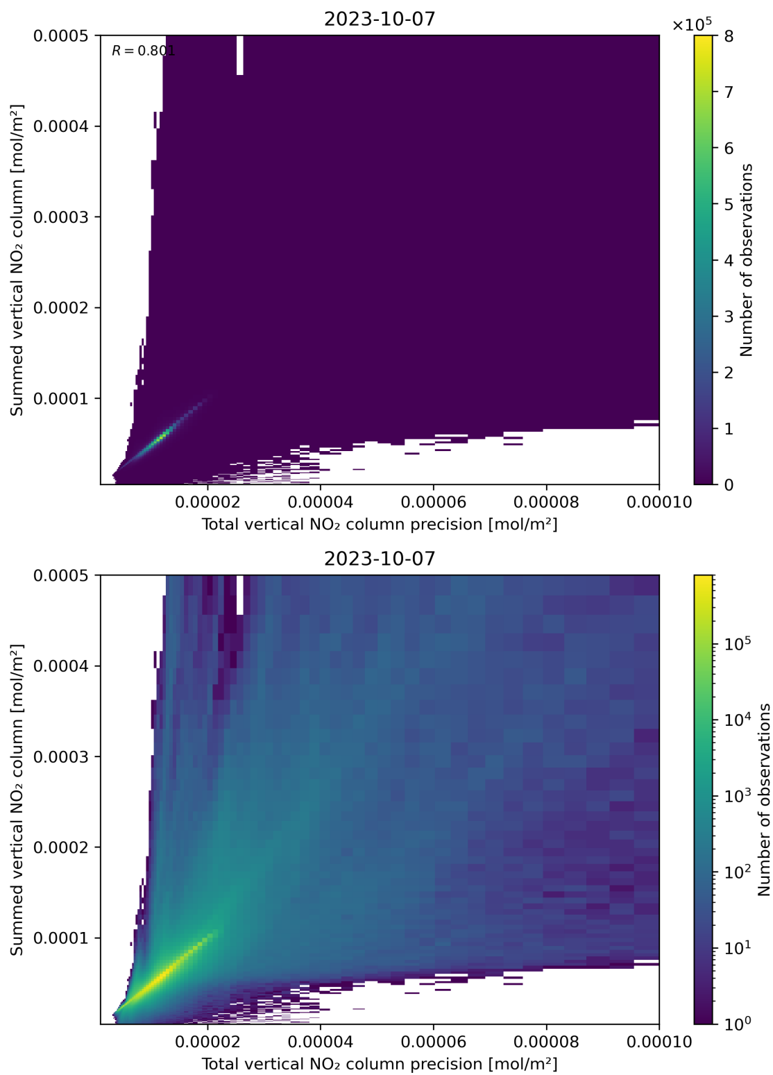
Figure 117: Scatter density plot of “Total vertical NO 2 column precision” against “Summed vertical NO 2 column” for 2023-10-06 to 2023-10-08.
