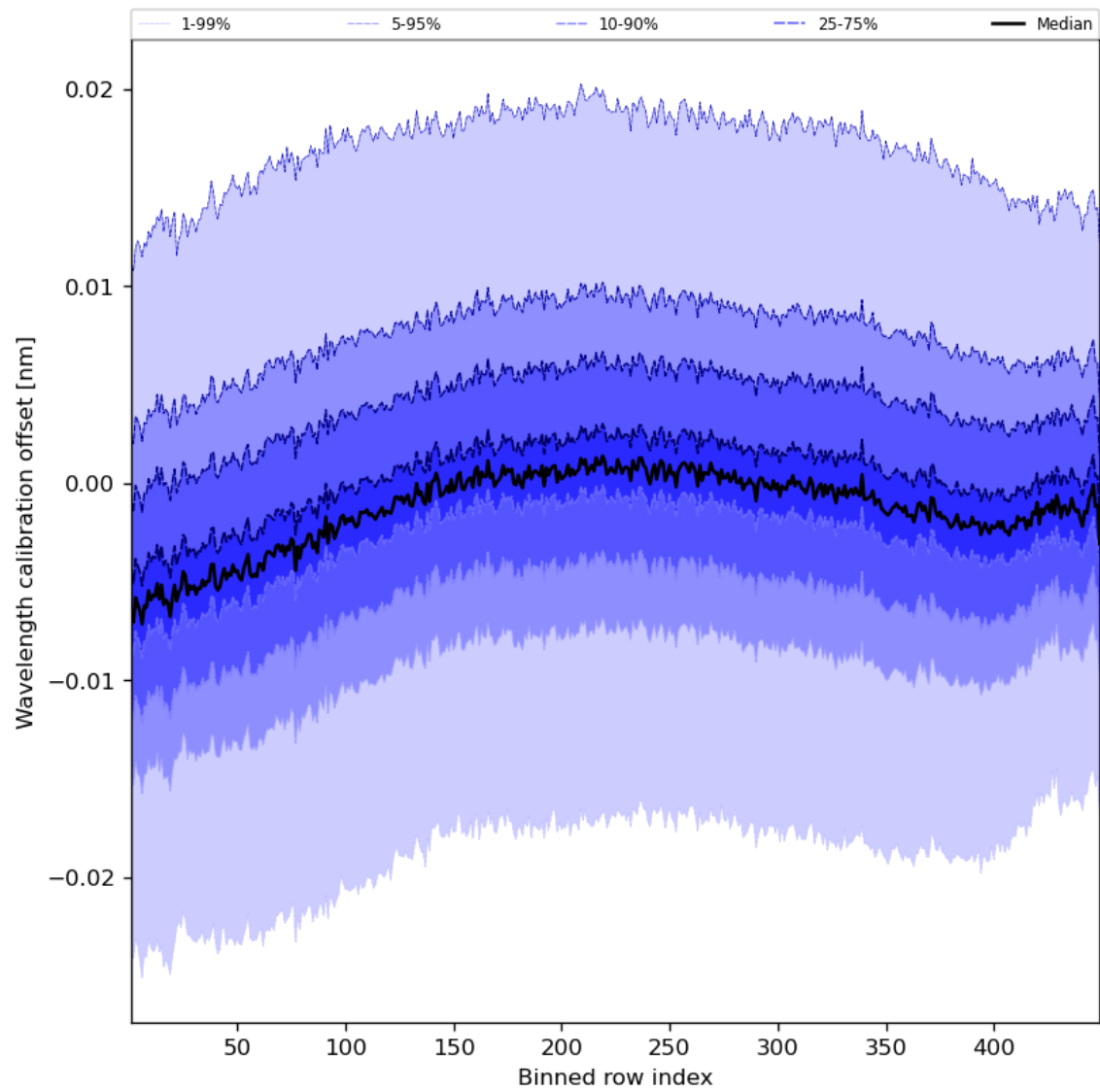
Figure 52: Along track statistics of “Wavelength calibration offset” for 2023-10-06 to 2023-10-08
