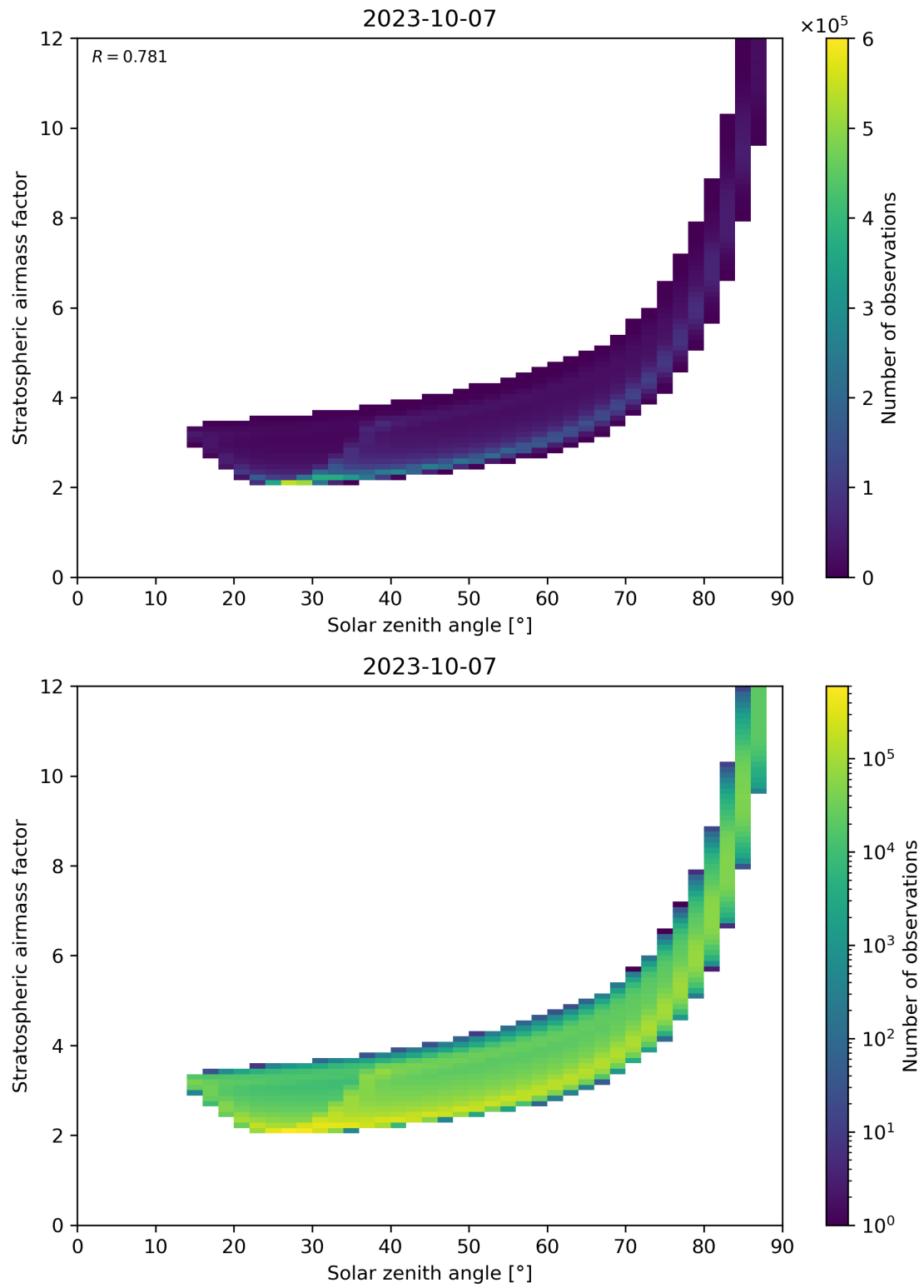
Figure 145: Scatter density plot of “Solar zenith angle” against “Stratospheric airmass factor” for 2023-10-06 to 2023-10-08.
