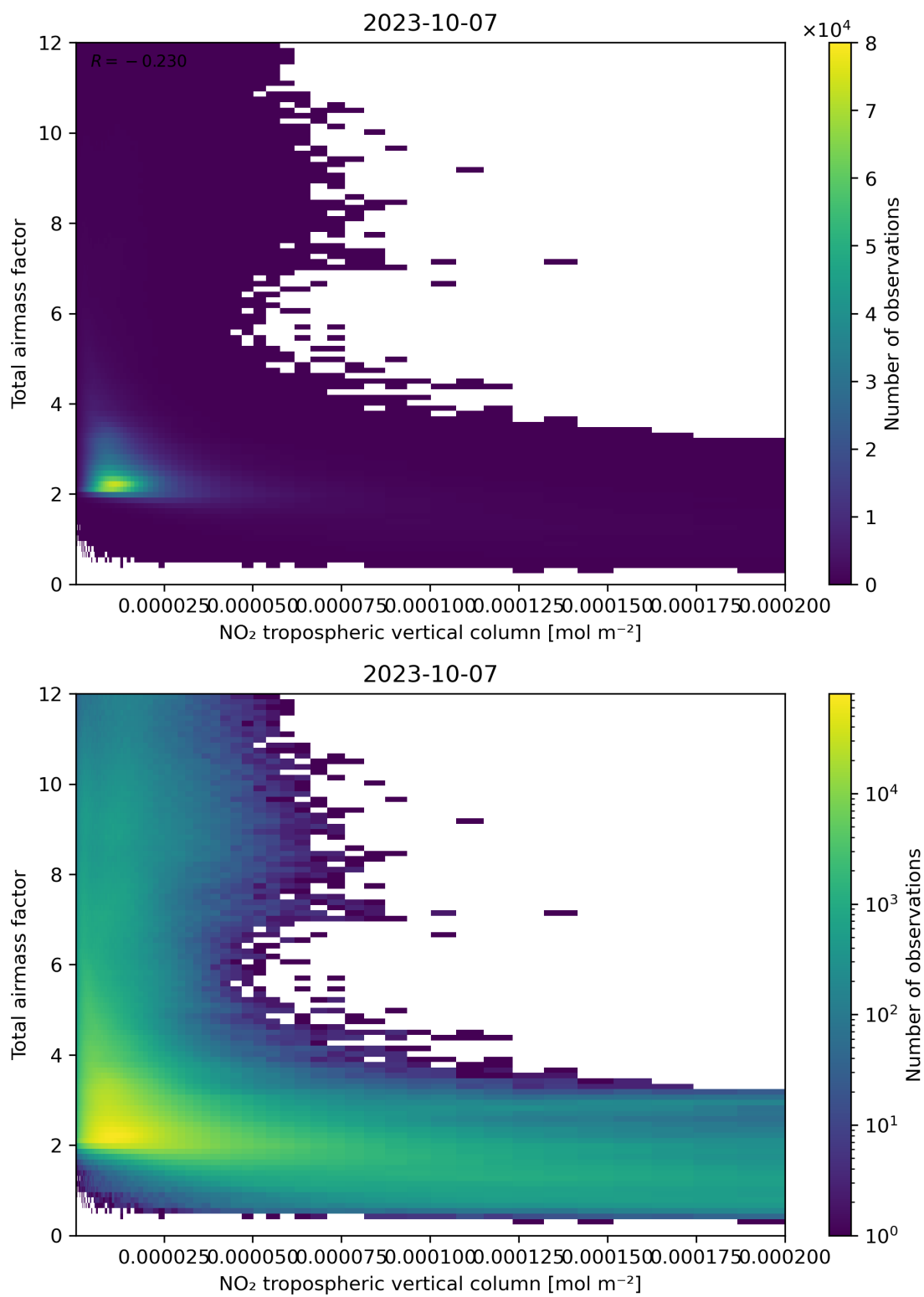
Figure 122: Scatter density plot of “NO 2 tropospheric vertical column” against “Total air mass factor” for 2023-10-06 to 2023-10-08.
