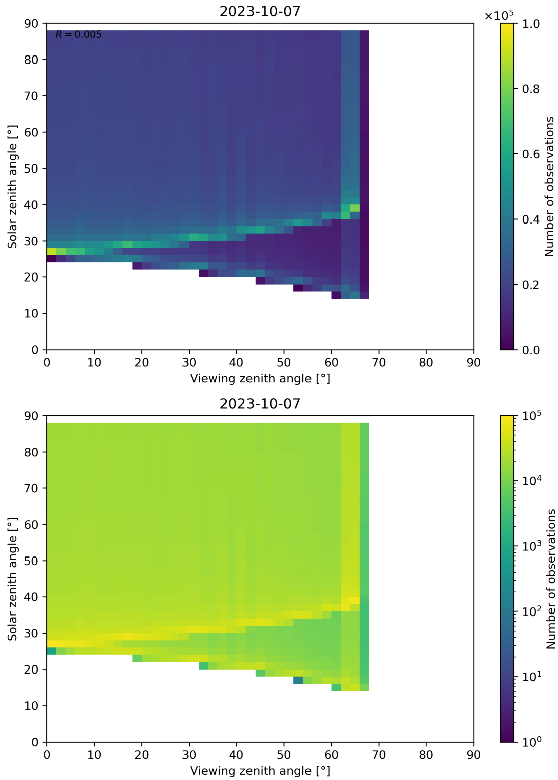
Figure 172: Scatter density plot of “Viewing zenith angle” against “Solar zenith angle” for 2023-10-06 to 2023-10-08.
