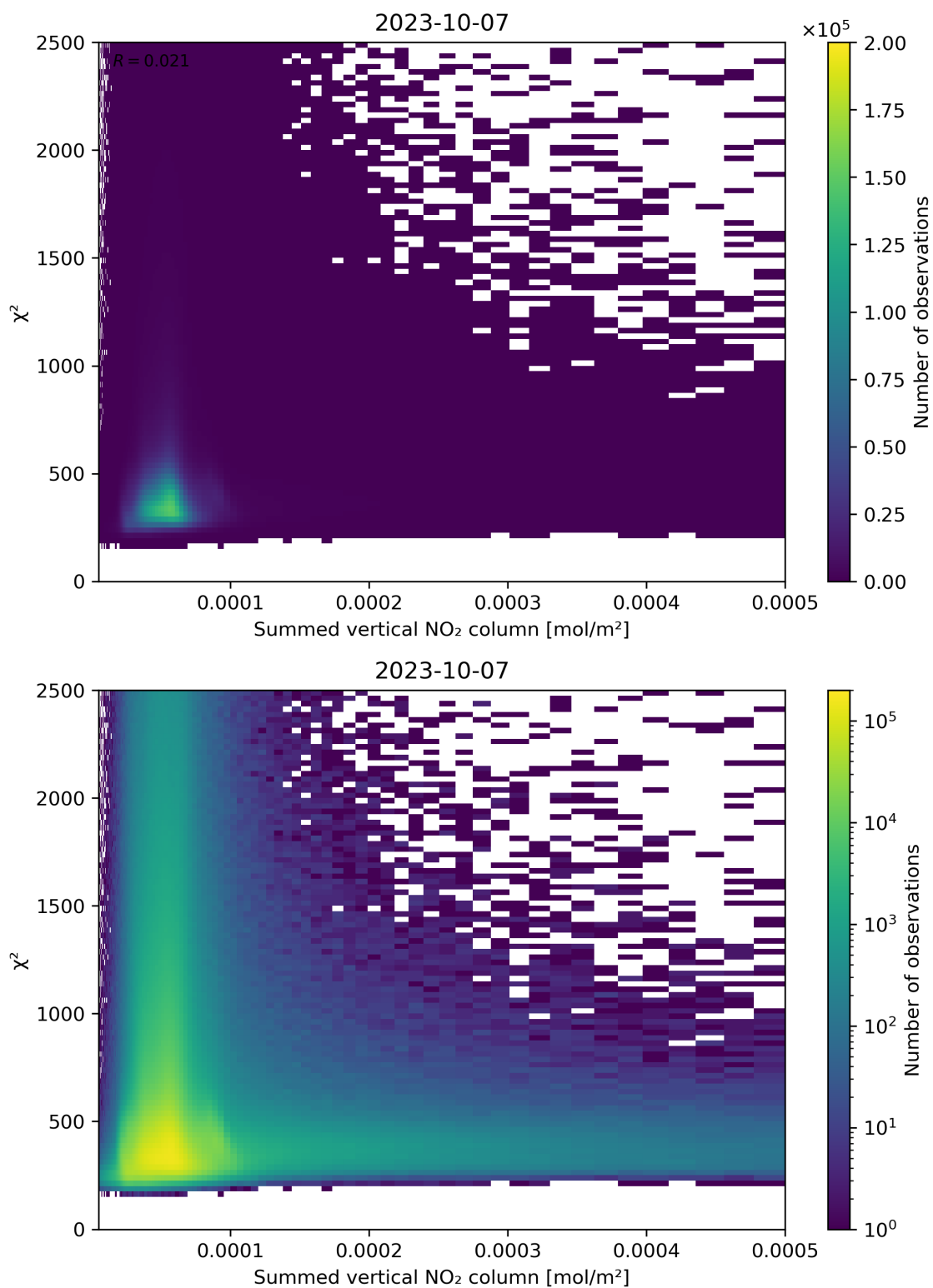
Figure 104: Scatter density plot of “Summed vertical NO 2 column” against “ \chi^2 ” for 2023-10-06 to 2023-10-08.
