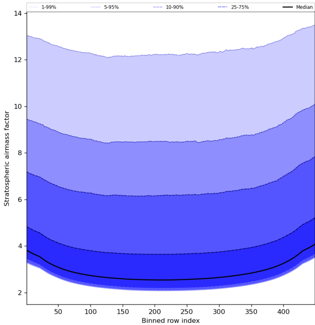
Figure 61: Along track statistics of “Stratospheric airmass factor” for 2023-10-06 to 2023-10-08
