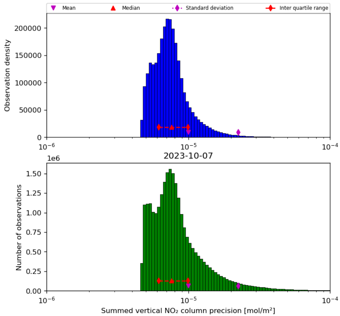
Figure 41: Histogram of "Summed vertical NO 2 column precision" for 2023-10-06 to 2023-10-08
