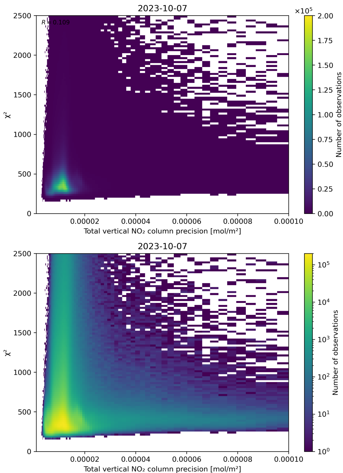
Figure 116: Scatter density plot of “Total vertical NO 2 column precision” against “ \chi^2 ” for 2023-10-06 to 2023-10-08.
