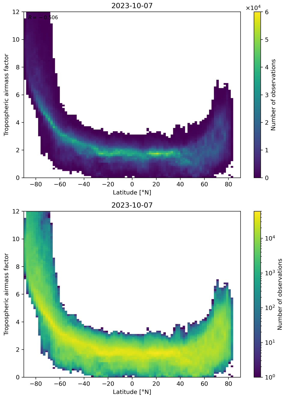
Figure 85: Scatter density plot of “Latitude” against “Tropospheric airmass factor” for 2023-10-06 to 2023-10-08.
