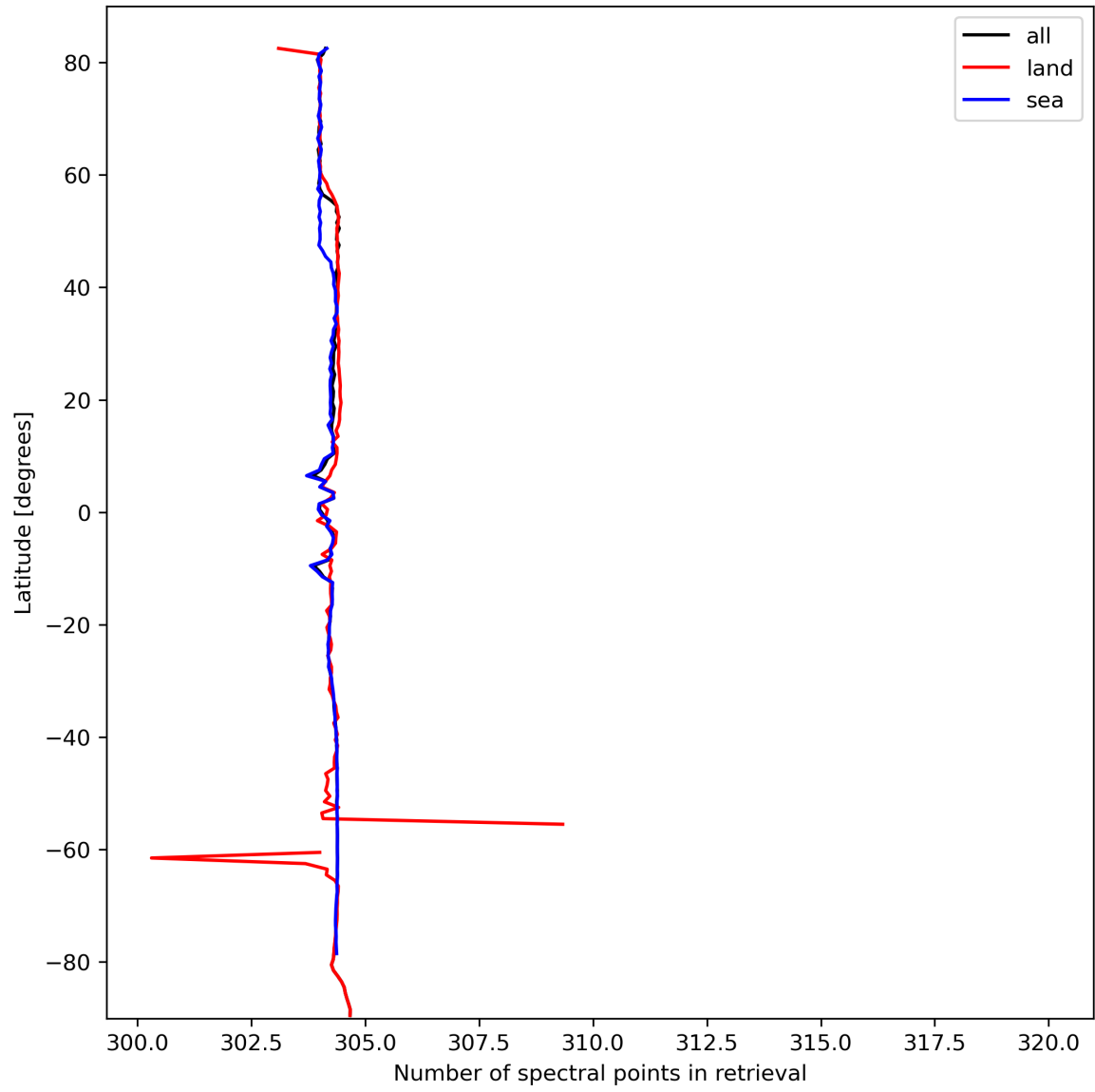
Figure 16: Zonal average of “Number of spectral points in retrieval” for 2023-10-06 to 2023-10-08.
