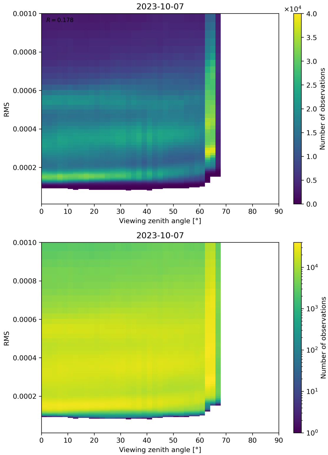
Figure 171: Scatter density plot of “Viewing zenith angle” against “RMS” for 2023-10-06 to 2023-10-08.
