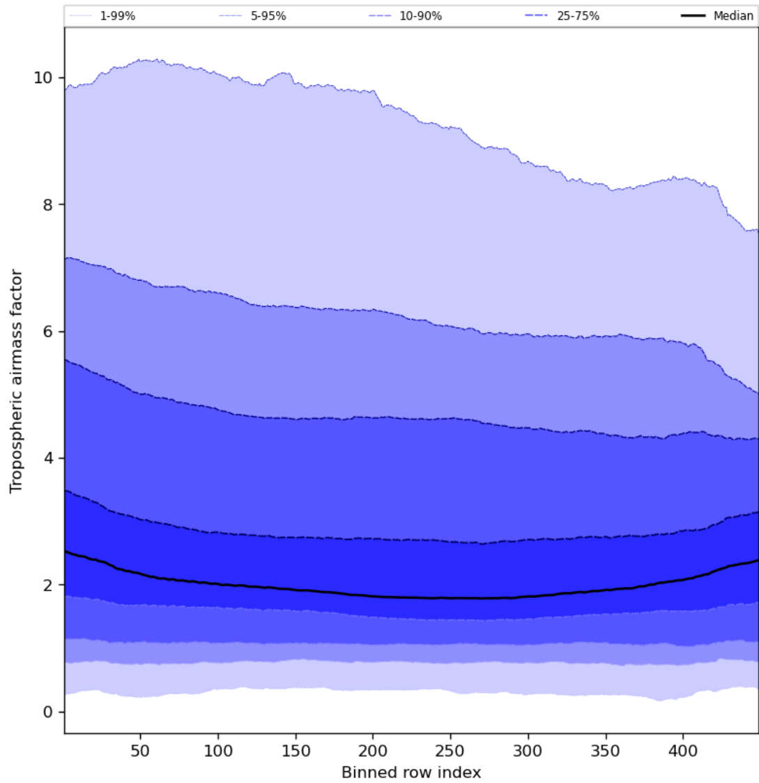
Figure 48: Along track statistics of “Tropospheric airmass factor” for 2023-10-06 to 2023-10-08
