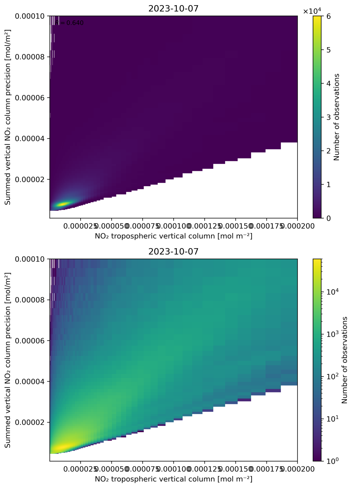
Figure 127: Scatter density plot of “NO 2 tropospheric vertical column” against “Summed vertical NO 2 column precision” for 2023-10-06 to 2023-10-08.
