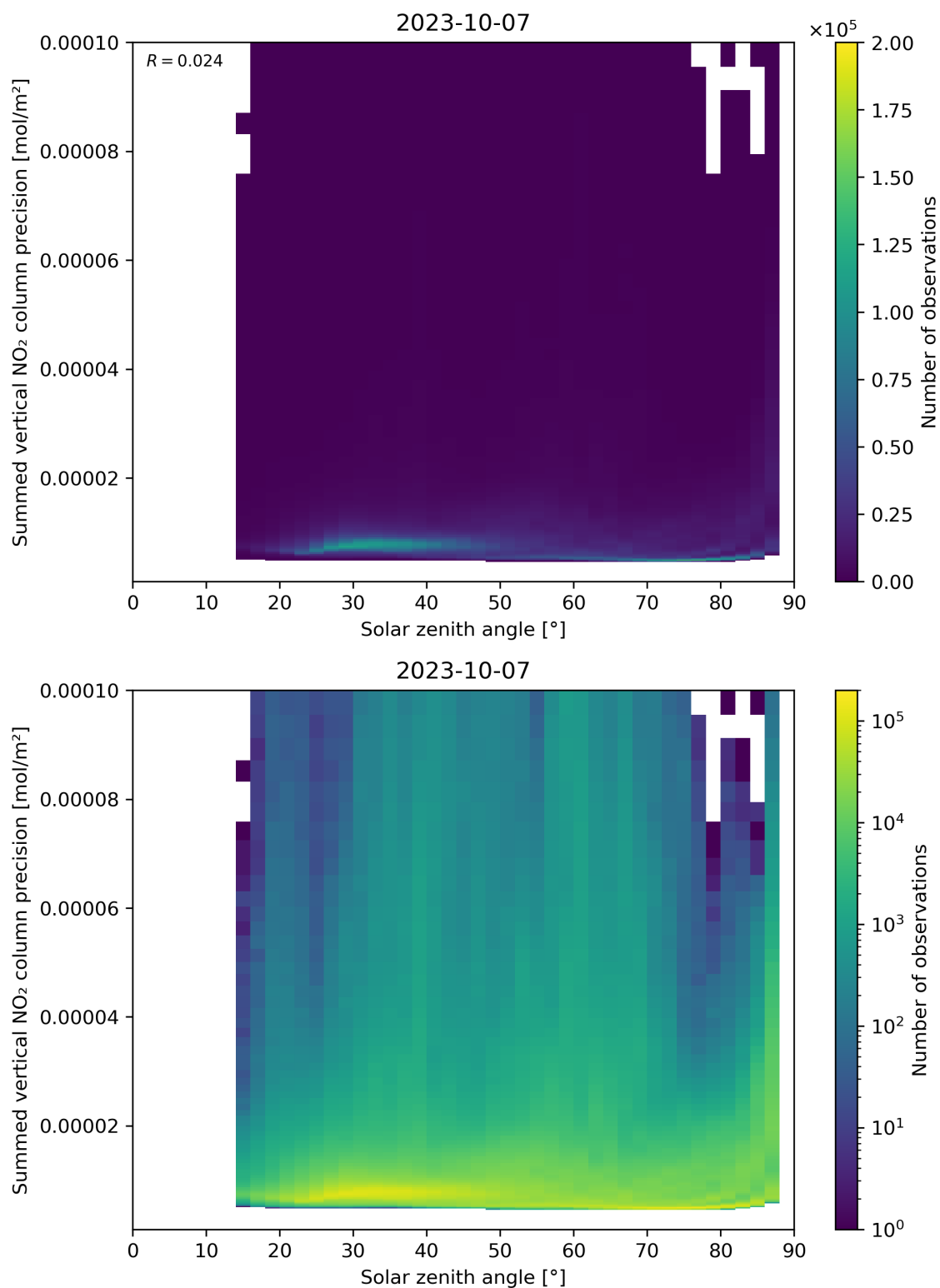
Figure 152: Scatter density plot of “Solar zenith angle” against “Summed vertical NO 2 column precision” for 2023-10-06 to 2023-10-08.
