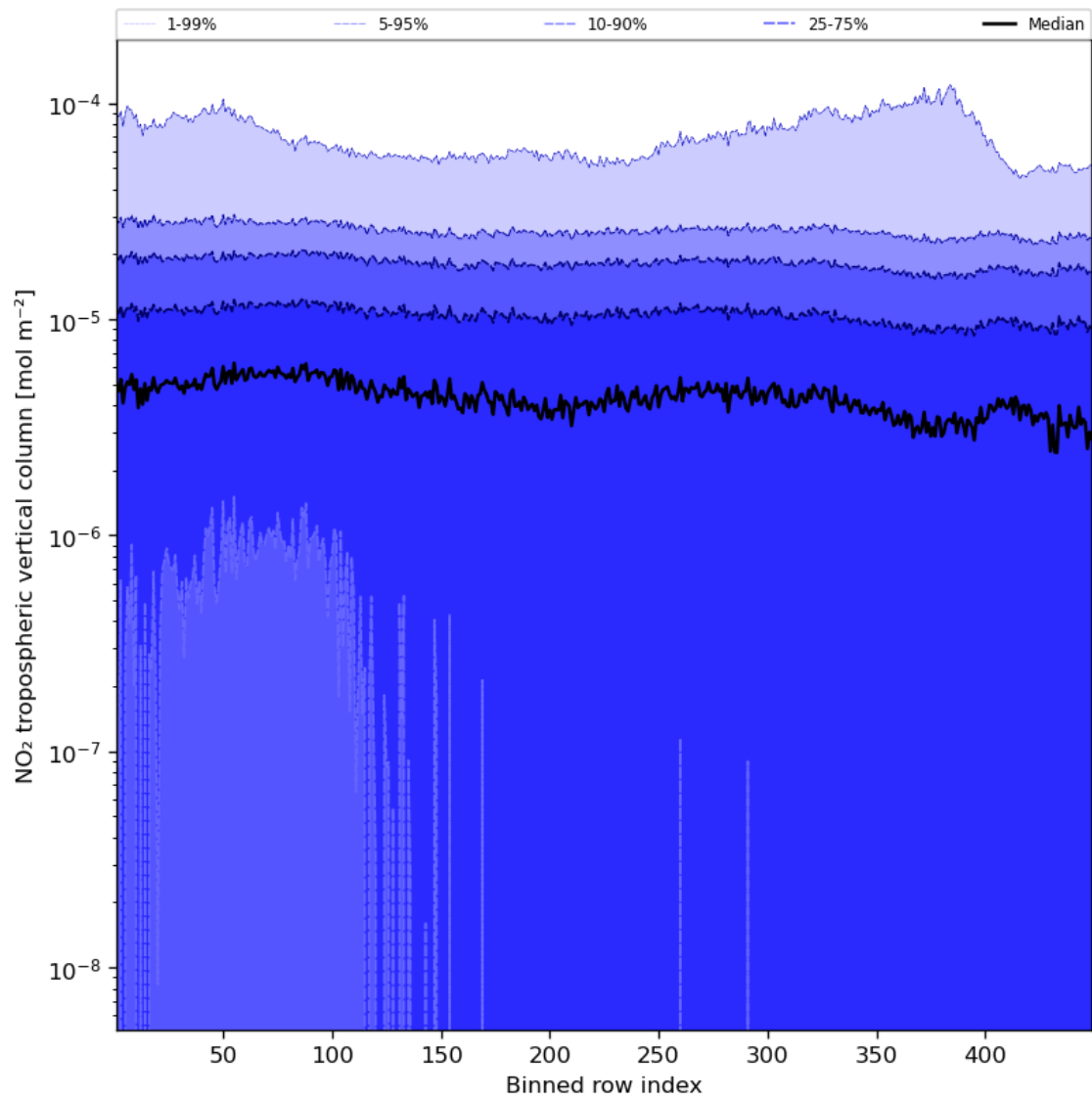
Figure 46: Along track statistics of “NO 2 tropospheric vertical column” for 2023-10-06 to 2023-10-08
