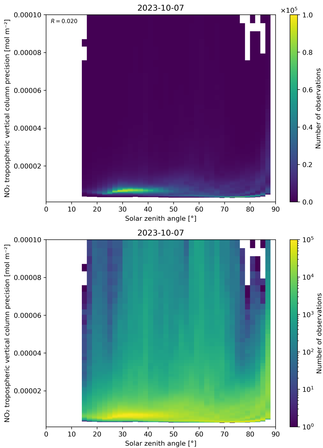
Figure 156: Scatter density plot of “Solar zenith angle” against “NO 2 tropospheric vertical column precision” for 2023-10-06 to 2023-10-08.
