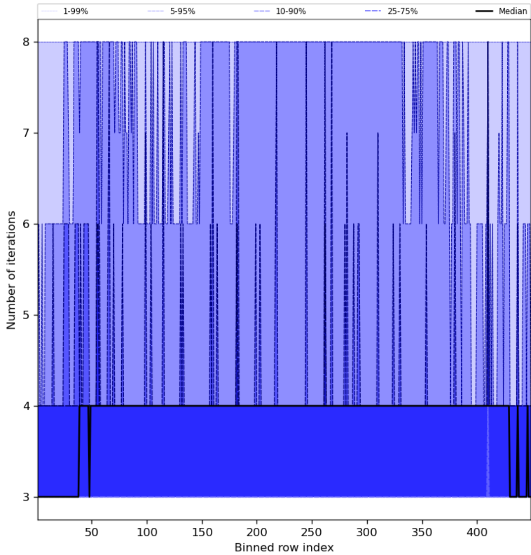
Figure 51: Along track statistics of “Number of iterations” for 2023-10-06 to 2023-10-08
