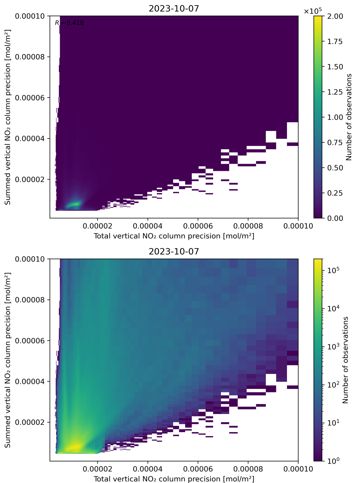
Figure 118: Scatter density plot of “Total vertical NO 2 column precision” against “Summed vertical NO 2 column precision” for 2023-10-06 to 2023-10-08.
