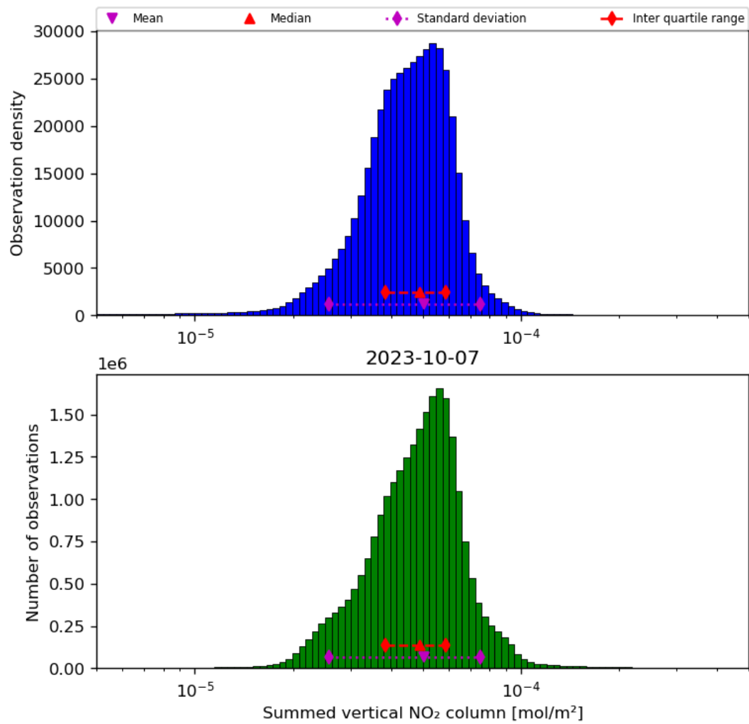
Figure 40: Histogram of “Summed vertical NO 2 column” for 2023-10-06 to 2023-10-08
