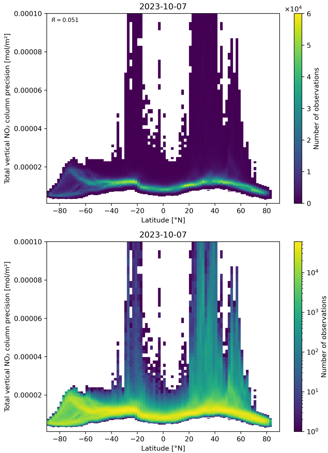
Figure 91: Scatter density plot of “Latitude” against “Total vertical NO 2 column precision” for 2023-10-06 to 2023-10-08.
