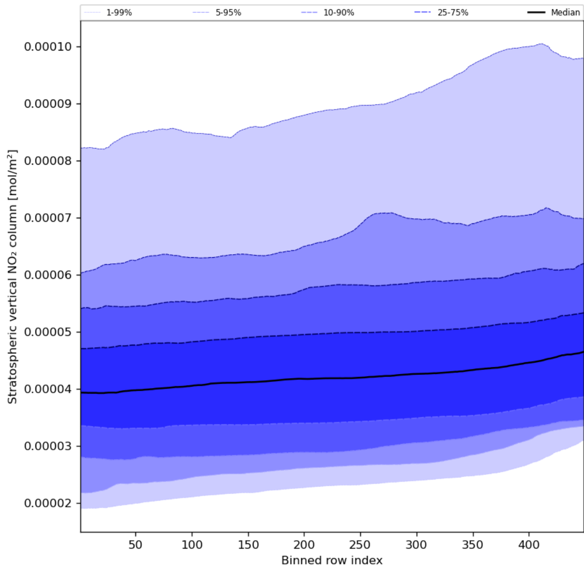
Figure 53: Along track statistics of “Stratospheric vertical NO 2 column” for 2023-10-06 to 2023-10-08
