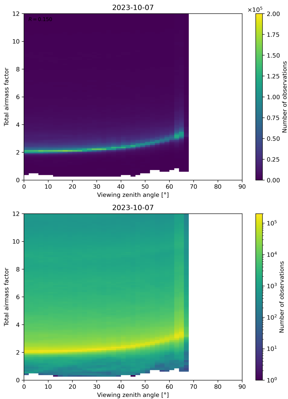
Figure 160: Scatter density plot of “Viewing zenith angle” against “Total airmass factor” for 2023-10-06 to 2023-10-08.
