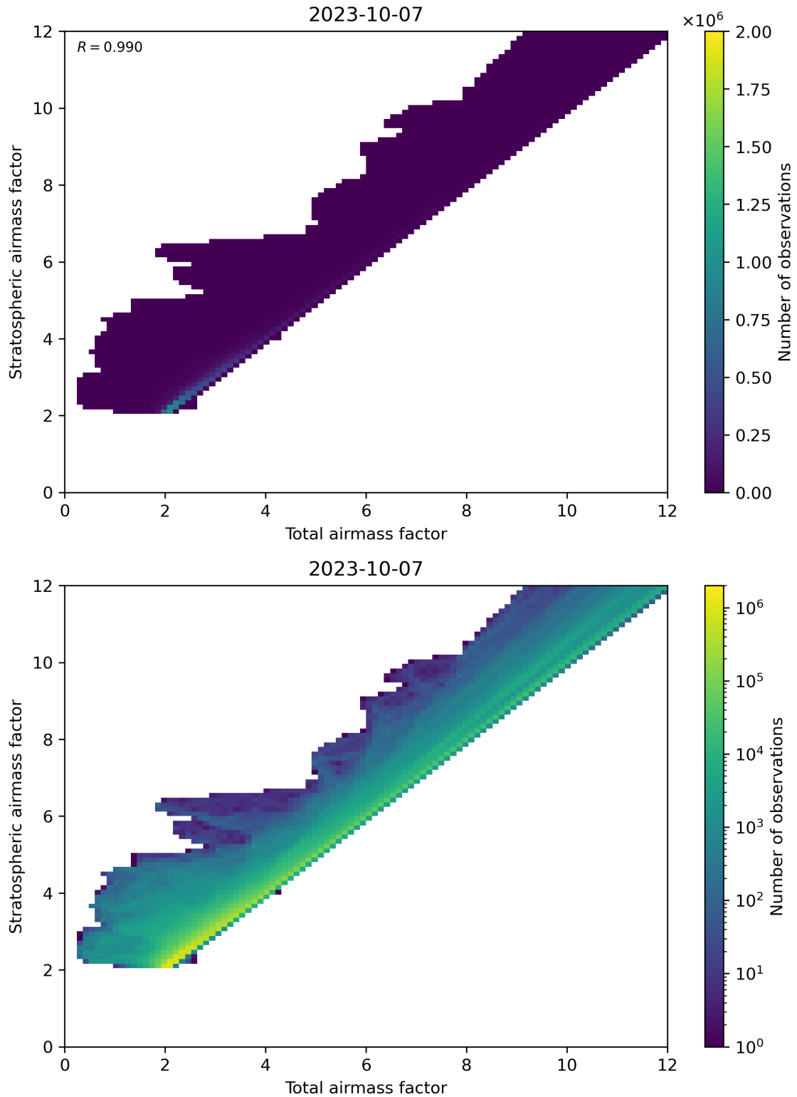
Figure 62: Scatter density plot of “Total airmass factor” against “Stratospheric airmass factor” for 2023-10-06 to 2023-10-08.
