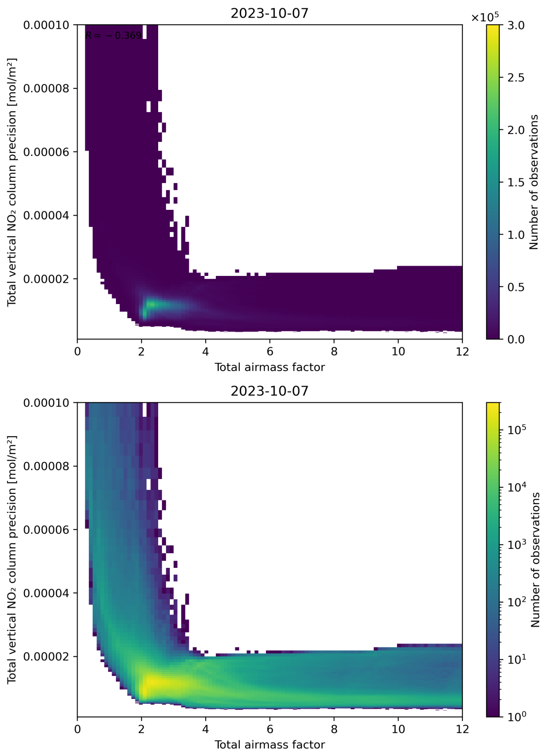
Figure 68: Scatter density plot of “Total airmass factor” against “Total vertical NO 2 column precision” for 2023-10-06 to 2023-10-08.
