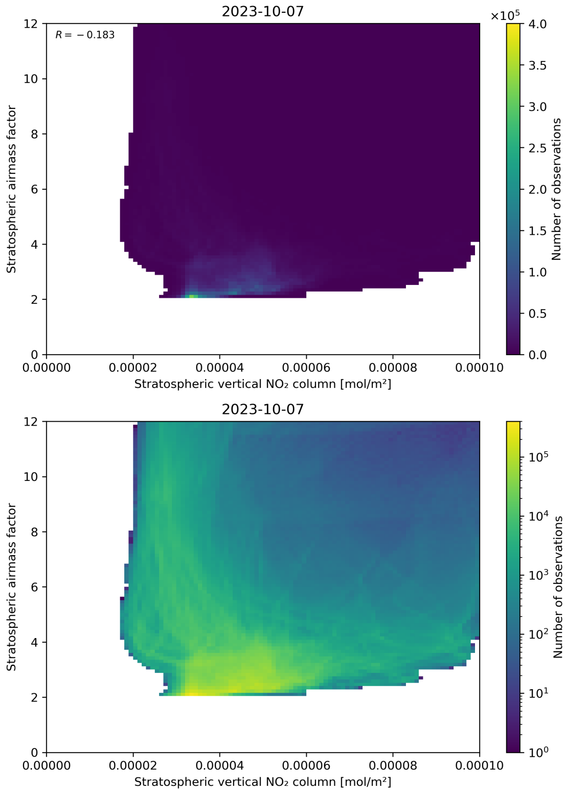
Figure 96: Scatter density plot of “Stratospheric vertical NO 2 column” against “Stratospheric airmass factor” for 2023-10-06 to 2023-10-08.
