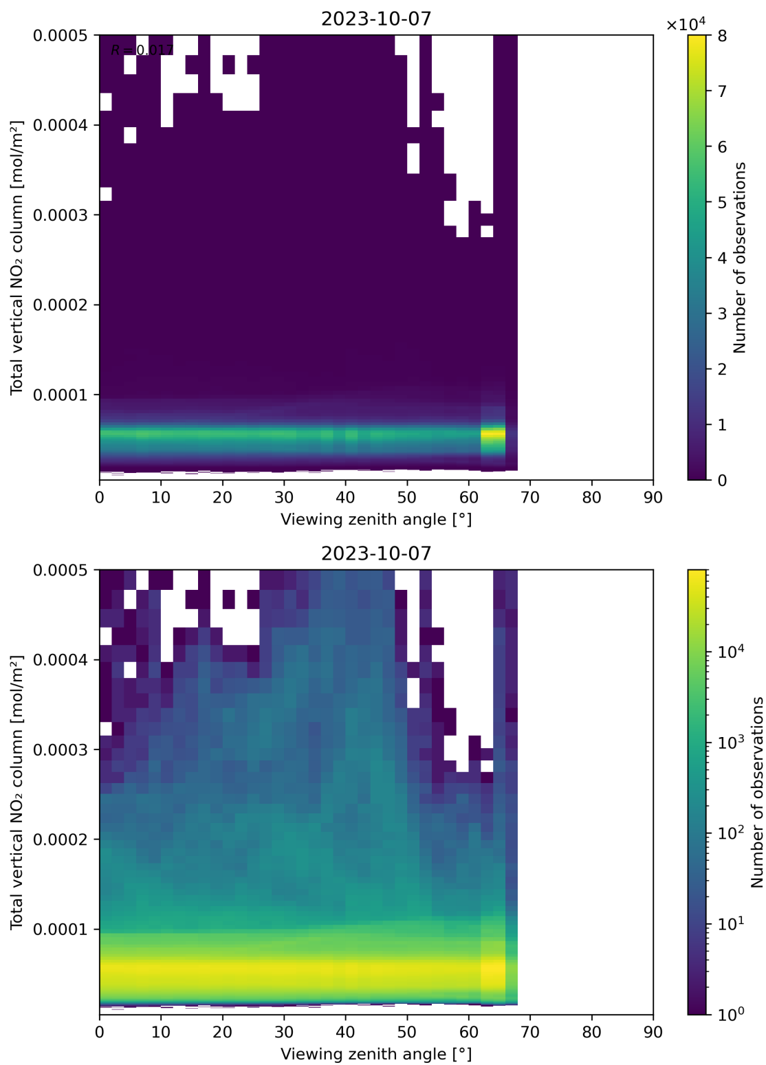
Figure 167: Scatter density plot of “Viewing zenith angle” against “Total vertical NO 2 column” for 2023-10-06 to 2023-10-08.
