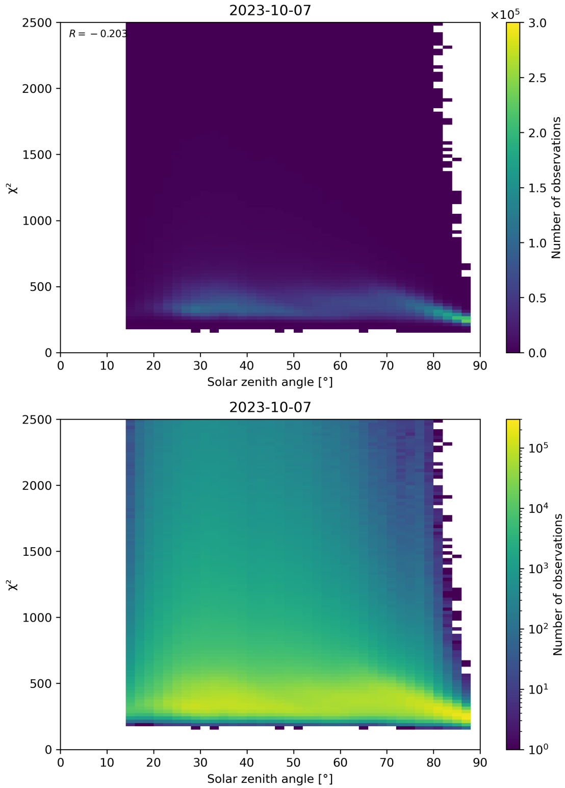
Figure 148: Scatter density plot of “Solar zenith angle” against “ \chi^2 ” for 2023-10-06 to 2023-10-08.
