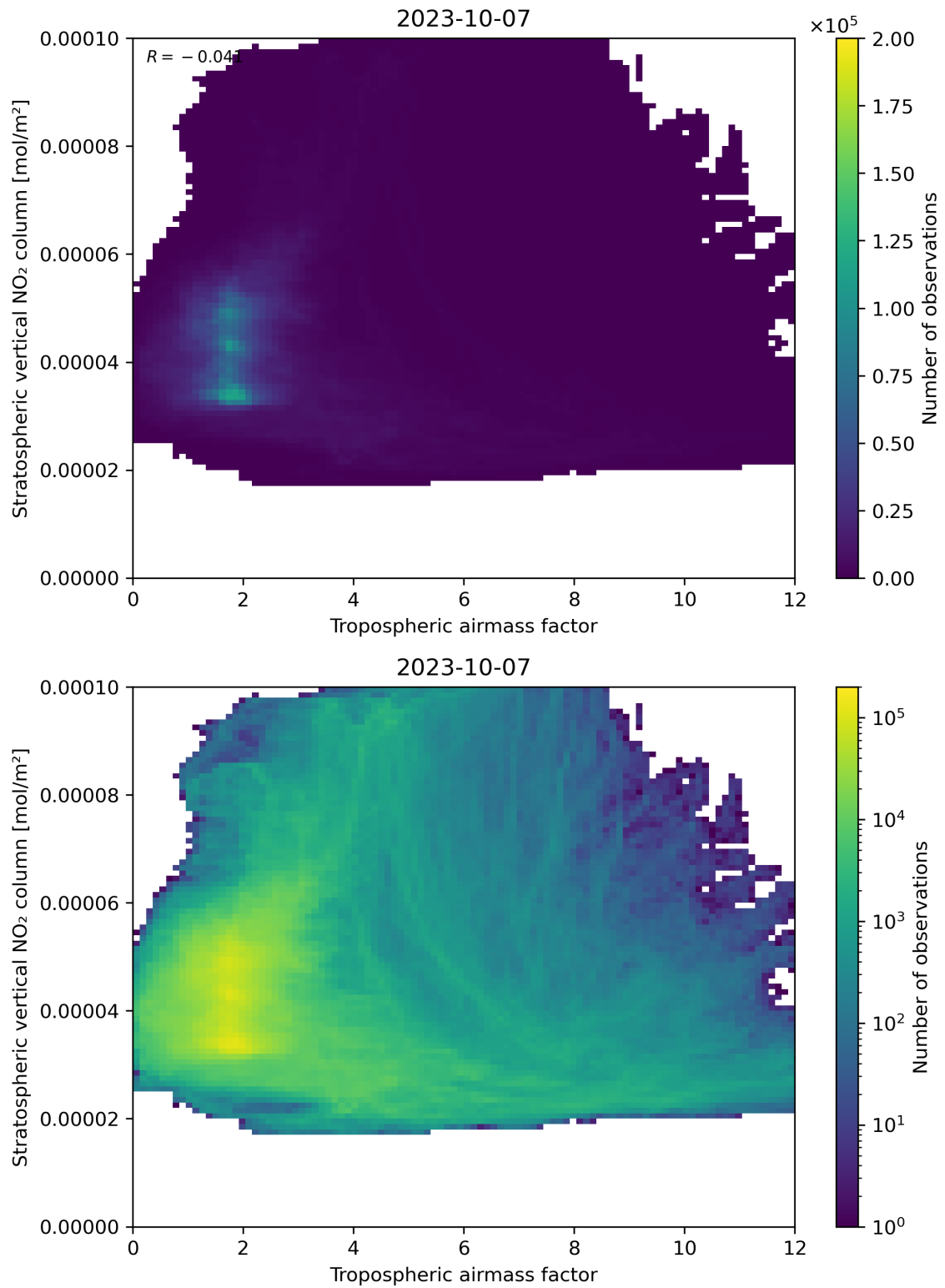
Figure 74: Scatter density plot of “Tropospheric air mass factor” against “Stratospheric vertical NO 2 column” for 2023-10-06 to 2023-10-08.
