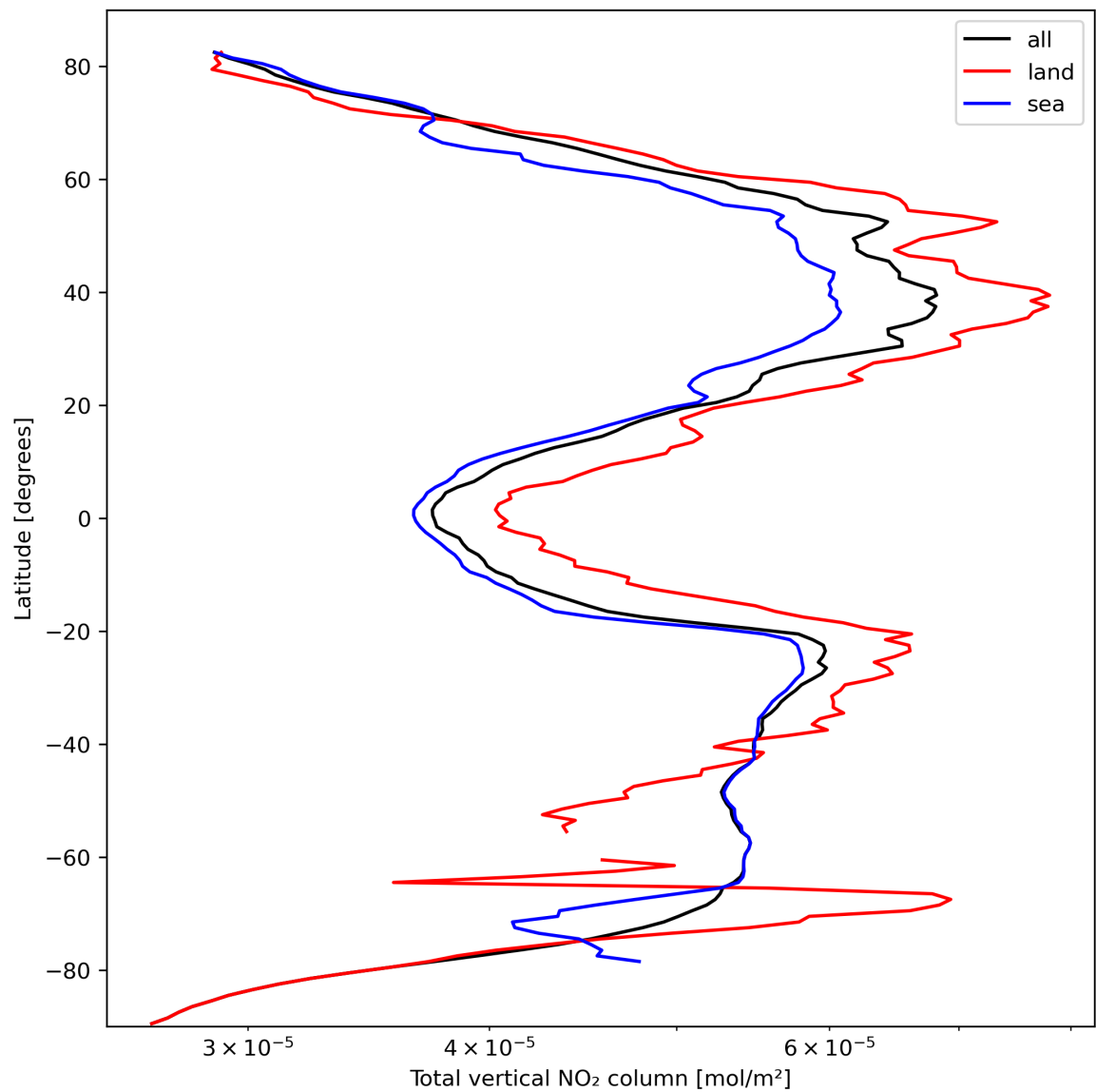
Figure 21: Zonal average of “Total vertical NO 2 column” for 2023-10-06 to 2023-10-08.
