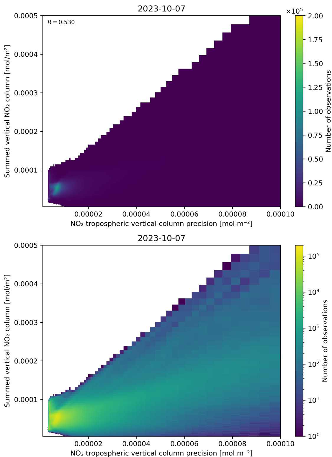
Figure 136: Scatter density plot of “NO 2 tropospheric vertical column precision” against “Summed vertical NO 2 column” for 2023-10-06 to 2023-10-08.
