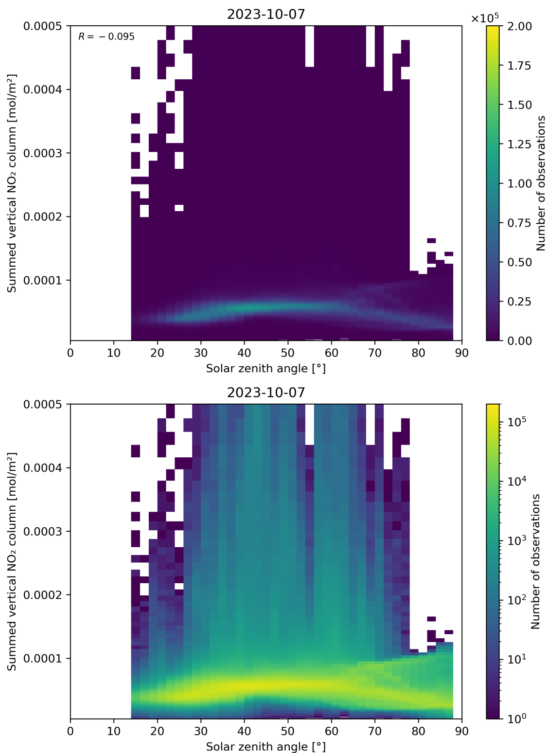
Figure 151: Scatter density plot of “Solar zenith angle” against “Summed vertical NO 2 column” for 2023-10-06 to 2023-10-08.
