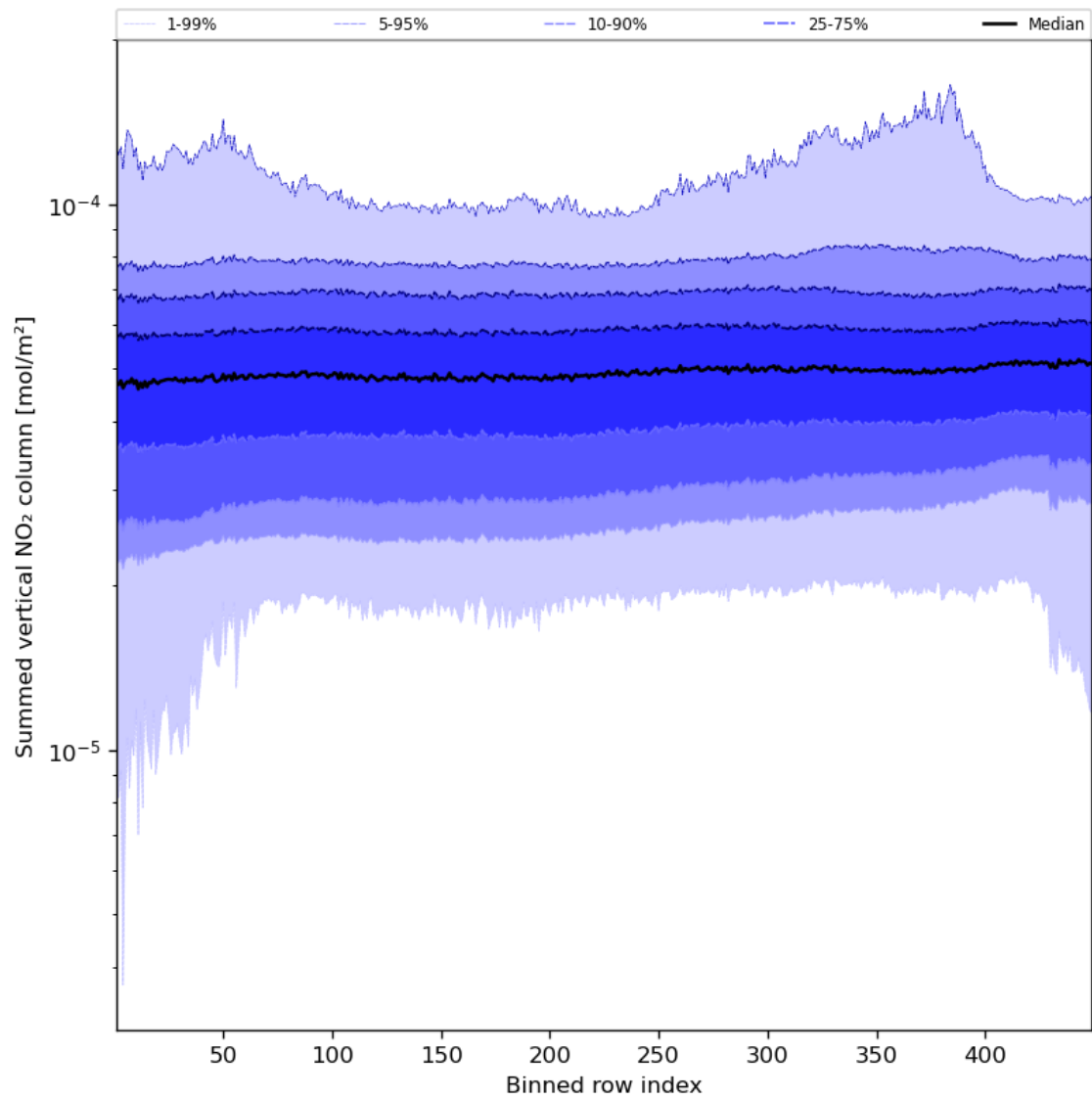
Figure 57: Along track statistics of “Summed vertical NO 2 column” for 2023-10-06 to 2023-10-08
