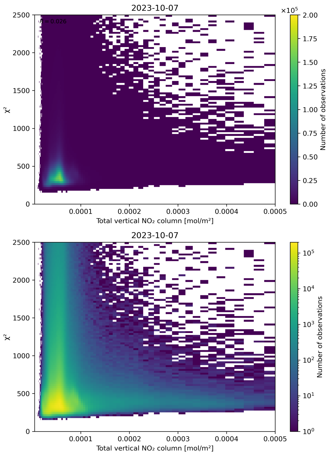
Figure 111: Scatter density plot of “Total vertical NO 2 column” against “ \chi^2 ” for 2023-10-06 to 2023-10-08.
