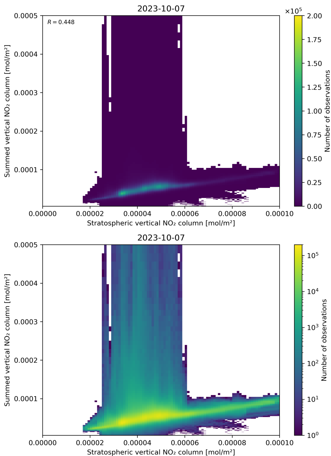
Figure 98: Scatter density plot of “Stratospheric vertical NO 2 column” against “Summed vertical NO 2 column” for 2023-10-06 to 2023-10-08.
