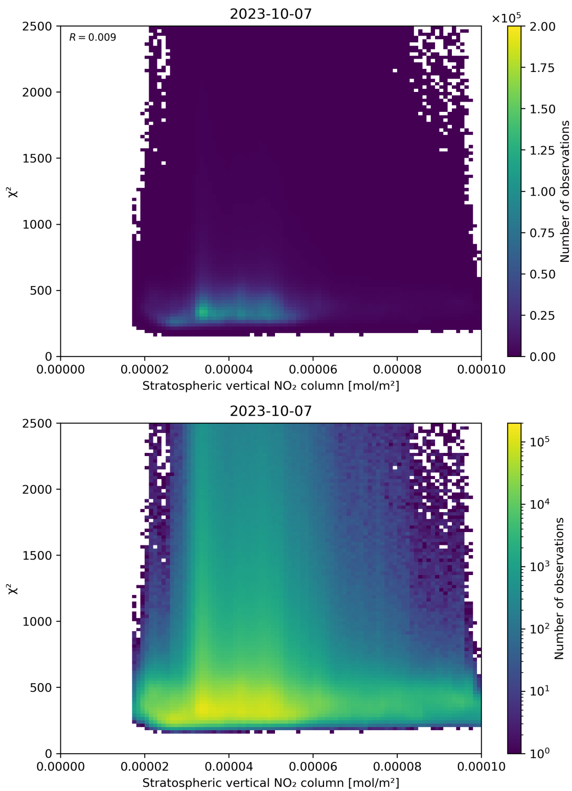
Figure 97: Scatter density plot of “Stratospheric vertical NO 2 column” against “ \chi^2 ” for 2023-10-06 to 2023-10-08.
