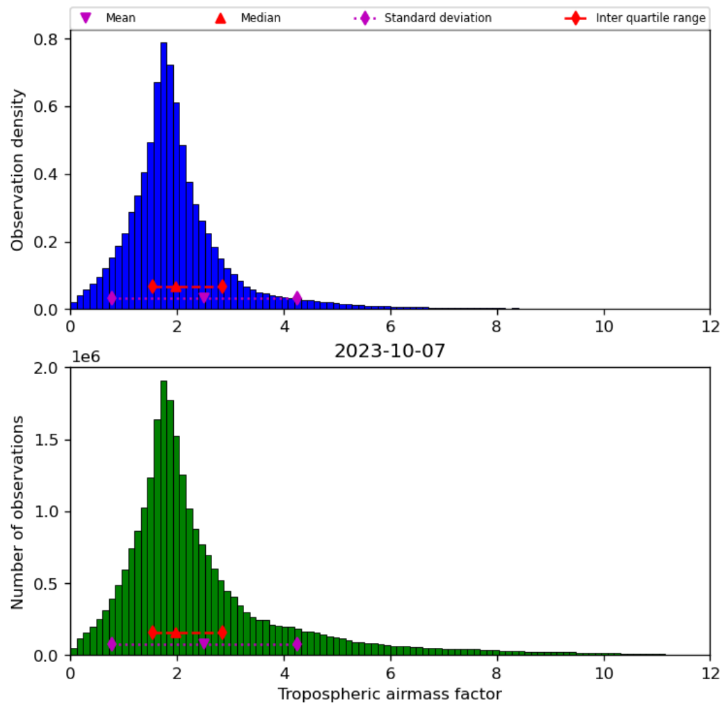
Figure 31: Histogram of “Tropospheric airmass factor” for 2023-10-06 to 2023-10-08
