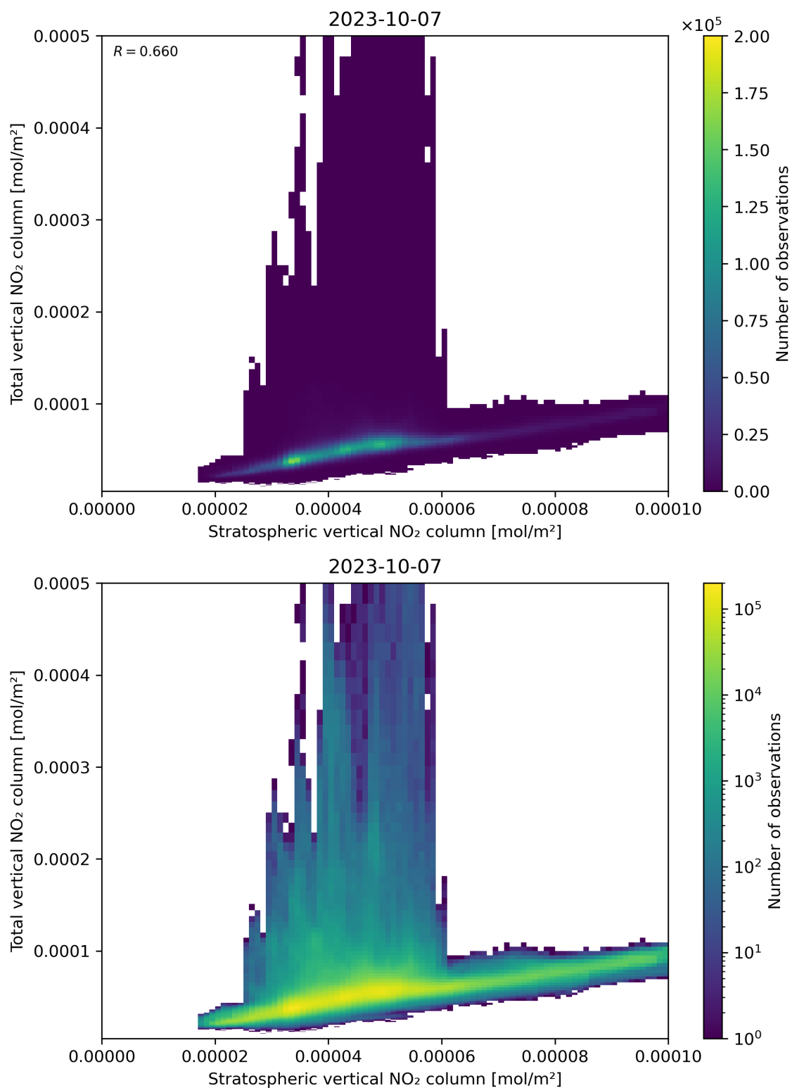
Figure 100: Scatter density plot of “Stratospheric vertical NO 2 column” against “Total vertical NO 2 column” for 2023-10-06 to 2023-10-08.
