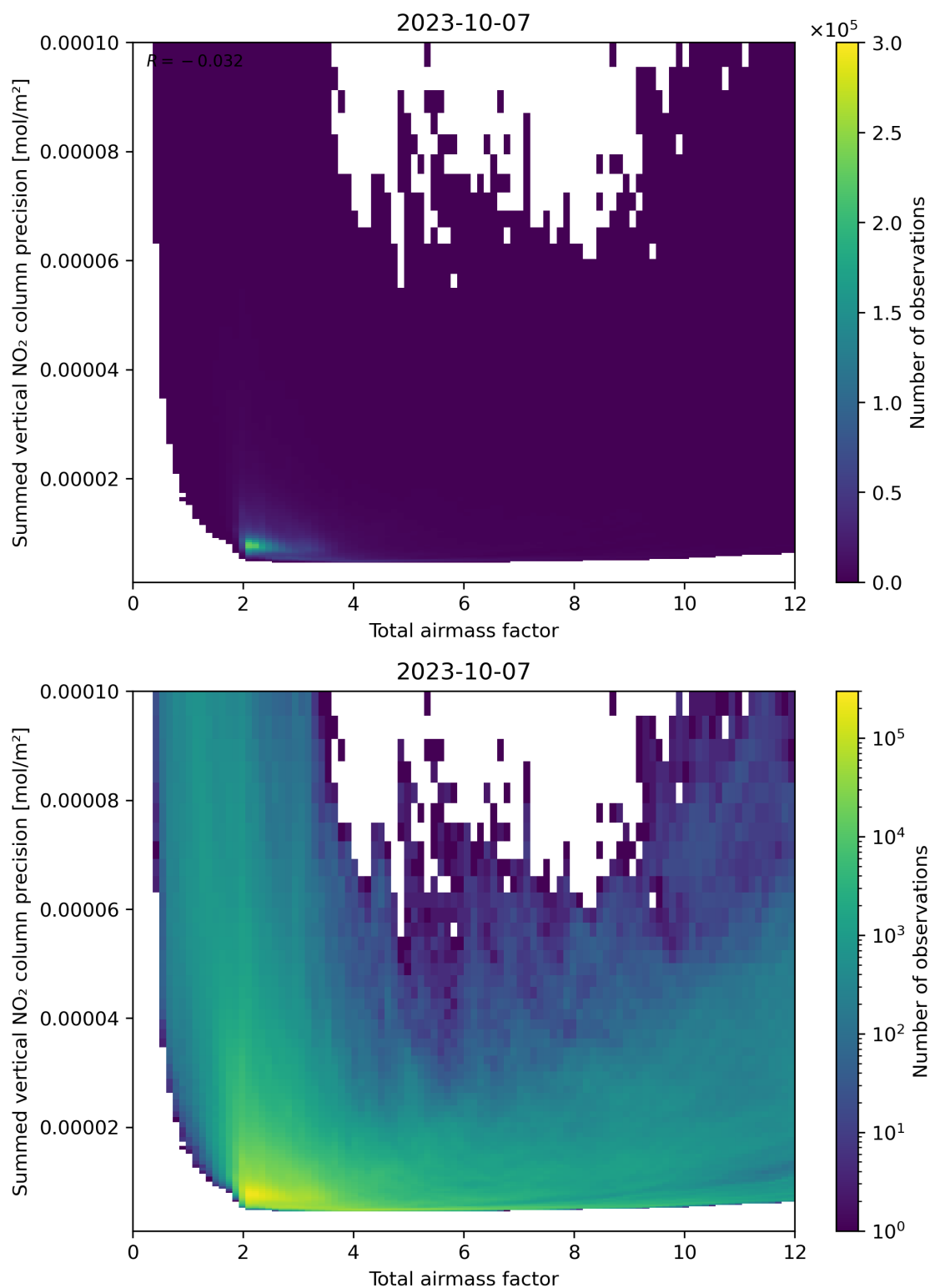
Figure 66: Scatter density plot of “Total airmass factor” against “Summed vertical NO 2 column precision” for 2023-10-06 to 2023-10-08.
