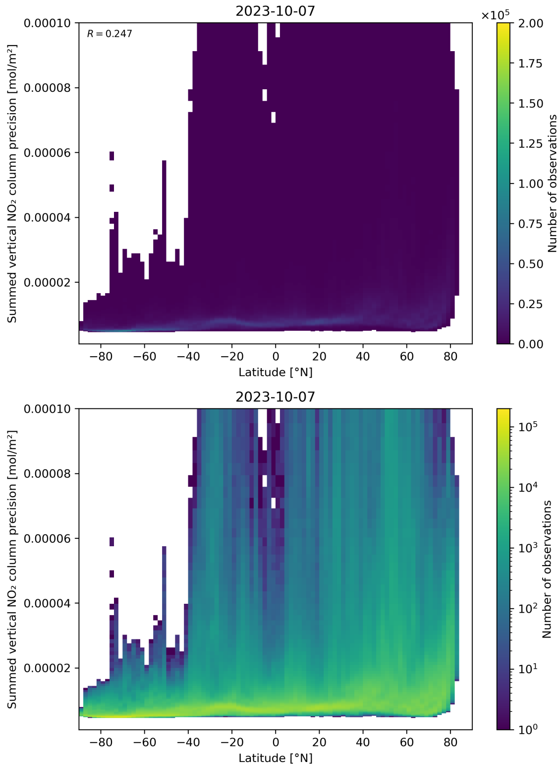
Figure 89: Scatter density plot of “Latitude” against “Summed vertical NO 2 column precision” for 2023-10-06 to 2023-10-08.
