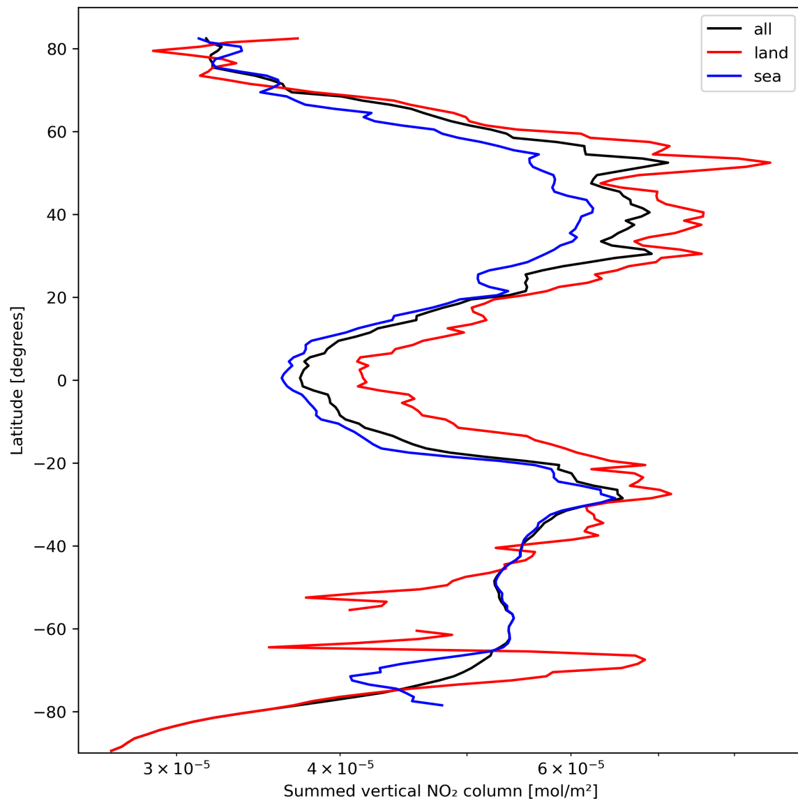
Figure 23: Zonal average of “Summed vertical NO 2 column” for 2023-10-06 to 2023-10-08.
