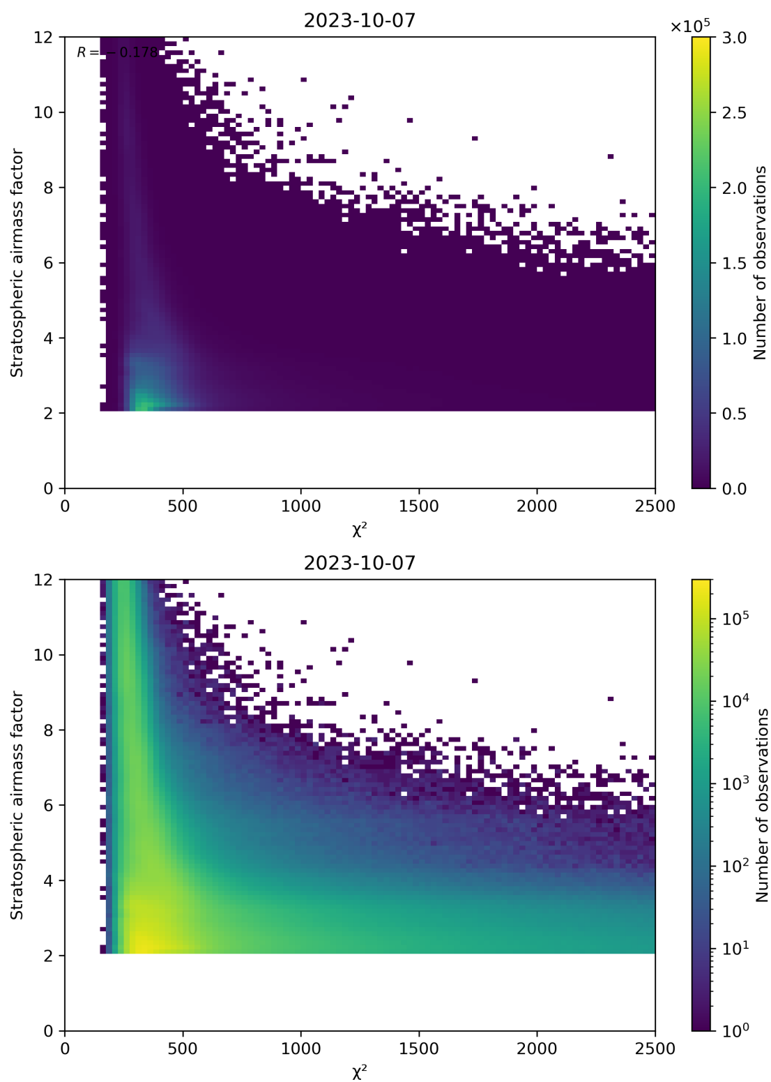
Figure 81: Scatter density plot of “ \chi^2 ” against “Stratospheric airmass factor” for 2023-10-06 to 2023-10-08.
