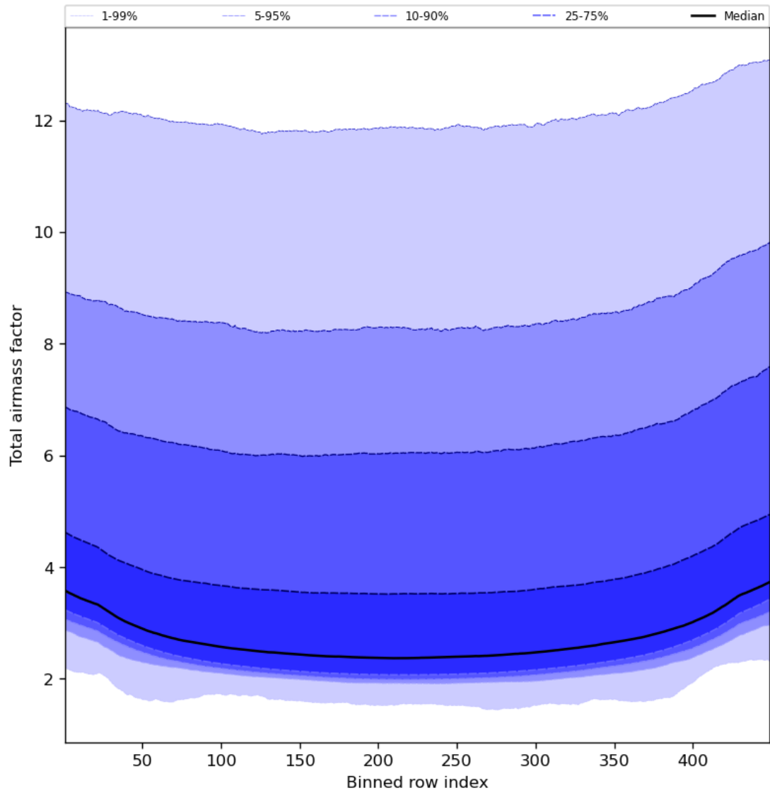
Figure 49: Along track statistics of “Total airmass factor” for 2023-10-06 to 2023-10-08
