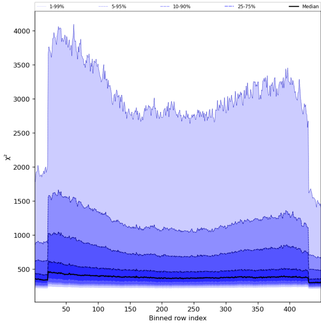
Figure 59: Along track statistics of “ \chi^2 ” for 2023-10-06 to 2023-10-08
