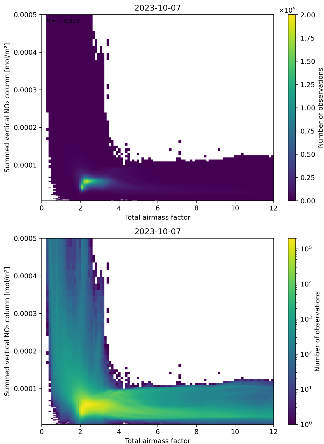
Figure 65: Scatter density plot of “Total airmass factor” against “Summed vertical NO 2 column” for 2023-10-06 to 2023-10-08.
