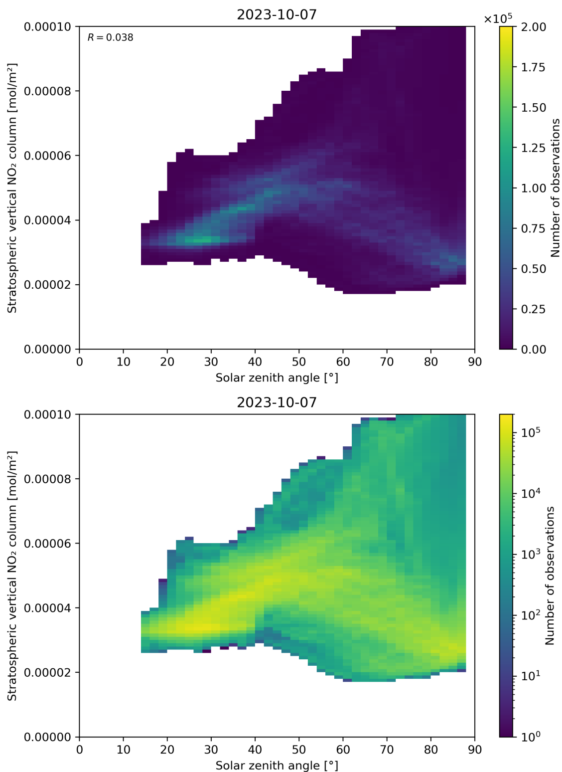
Figure 150: Scatter density plot of “Solar zenith angle” against “Stratospheric vertical NO 2 column” for 2023-10-06 to 2023-10-08.
