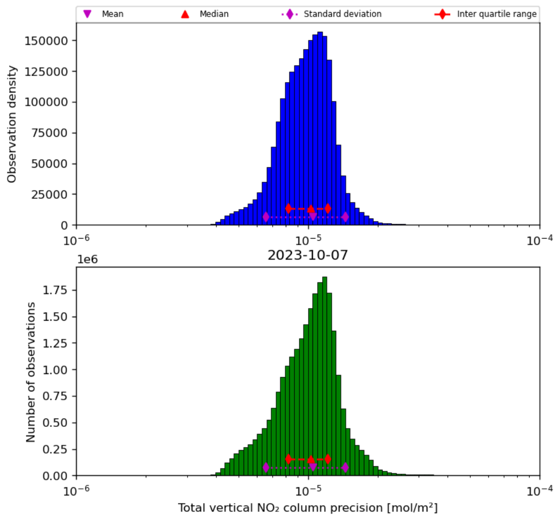
Figure 39: Histogram of “Total vertical NO 2 column precision” for 2023-10-06 to 2023-10-08
