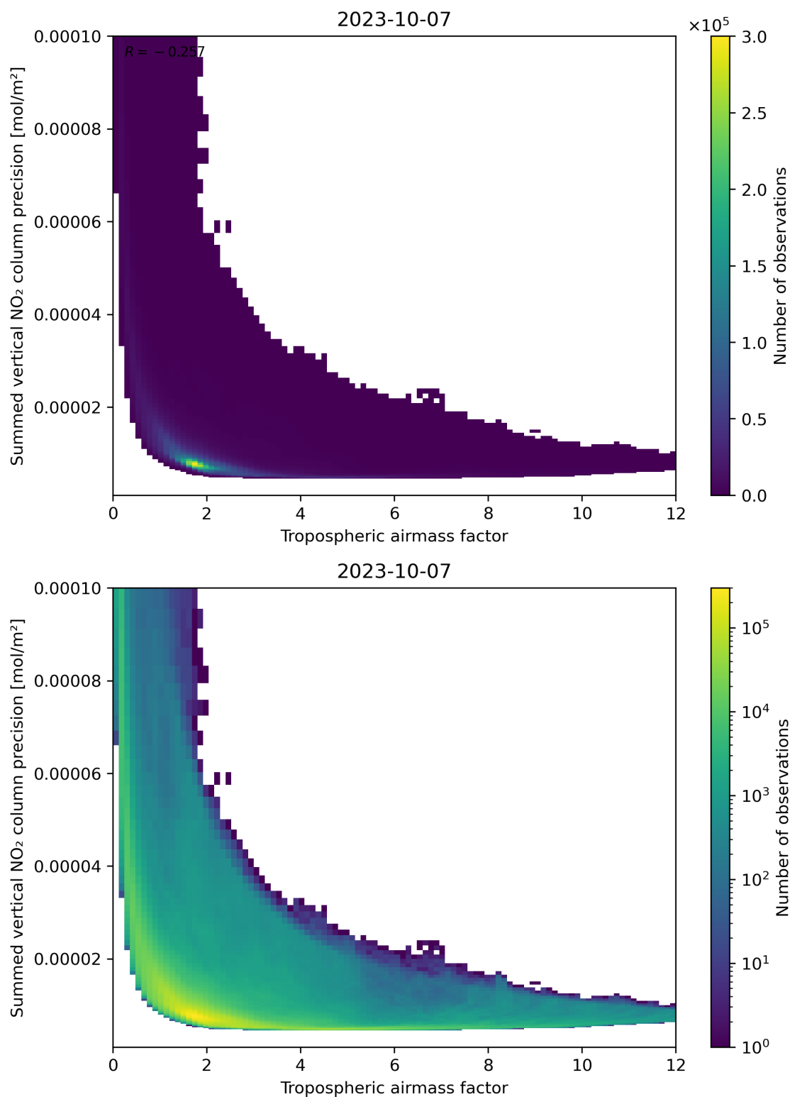
Figure 76: Scatter density plot of “Tropospheric air mass factor” against “Summed vertical NO 2 column precision” for 2023-10-06 to 2023-10-08.
