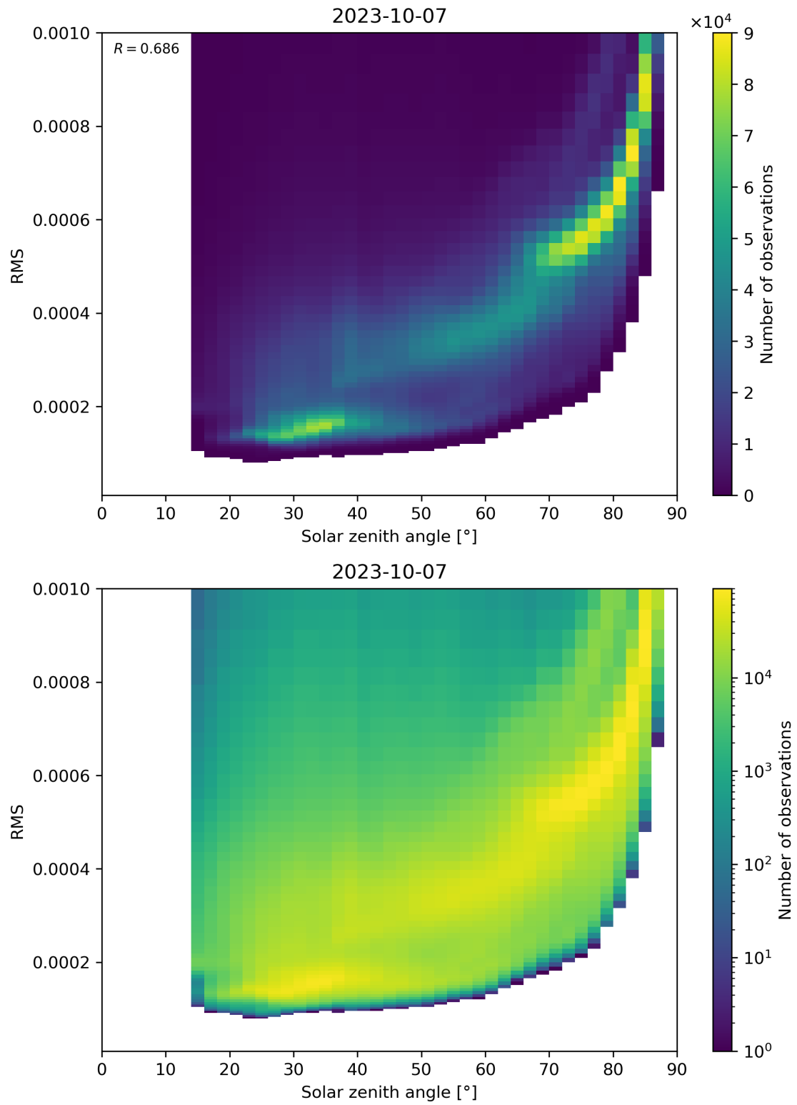
Figure 157: Scatter density plot of “Solar zenith angle” against “RMS” for 2023-10-06 to 2023-10-08.
