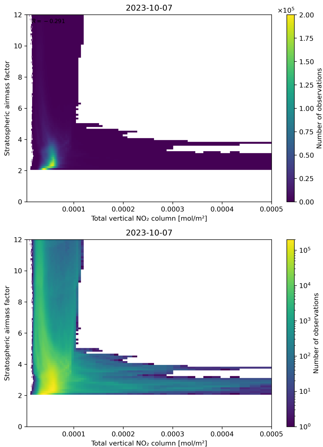
Figure 110: Scatter density plot of “Total vertical NO 2 column” against “Stratospheric airmass factor” for 2023-10-06 to 2023-10-08.
