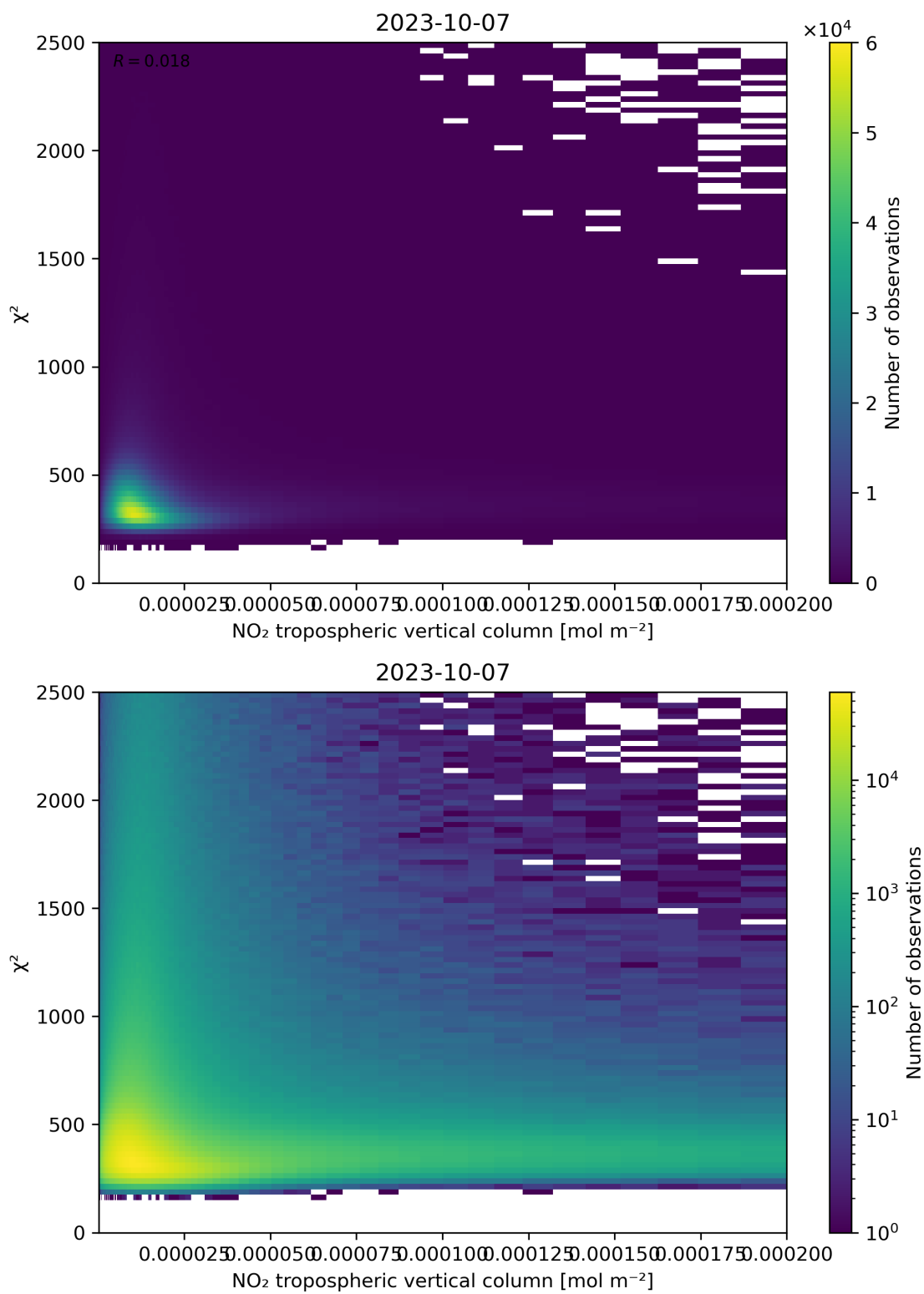
Figure 124: Scatter density plot of “NO 2 tropospheric vertical column” against “ \chi^2 ” for 2023-10-06 to 2023-10-08.
