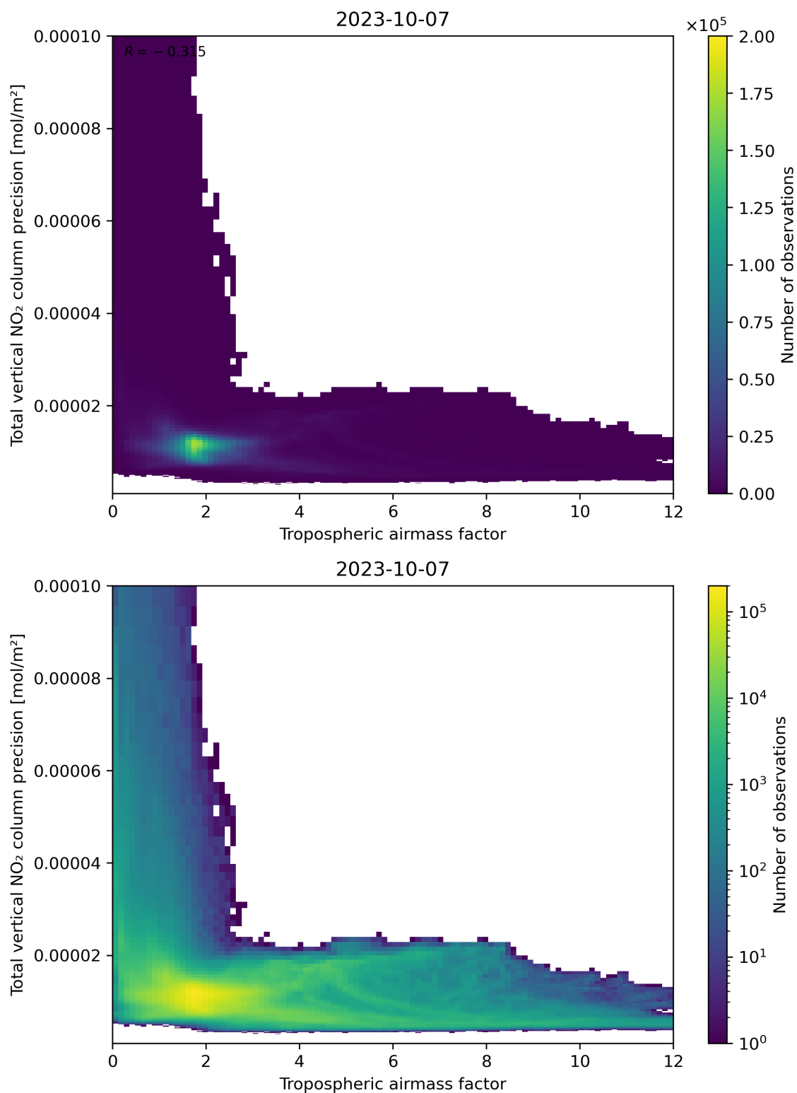
Figure 78: Scatter density plot of “Tropospheric air mass factor” against “Total vertical NO 2 column precision” for 2023-10-06 to 2023-10-08.
