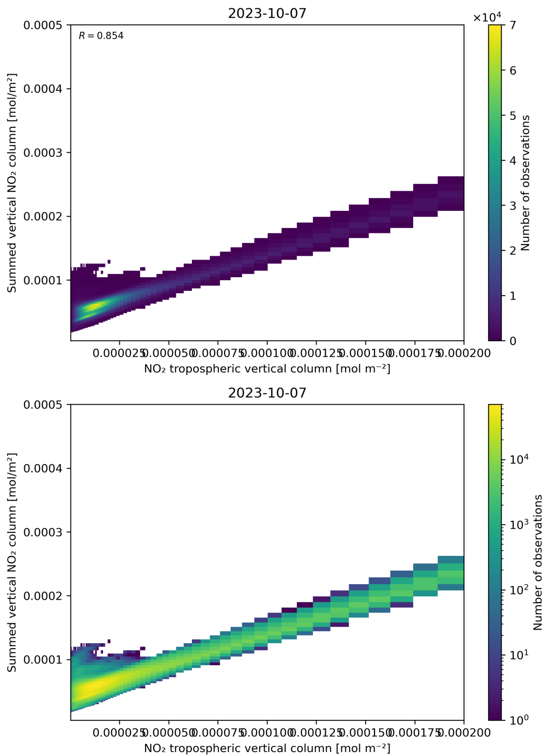
Figure 126: Scatter density plot of “NO 2 tropospheric vertical column” against “Summed vertical NO 2 column” for 2023-10-06 to 2023-10-08.
