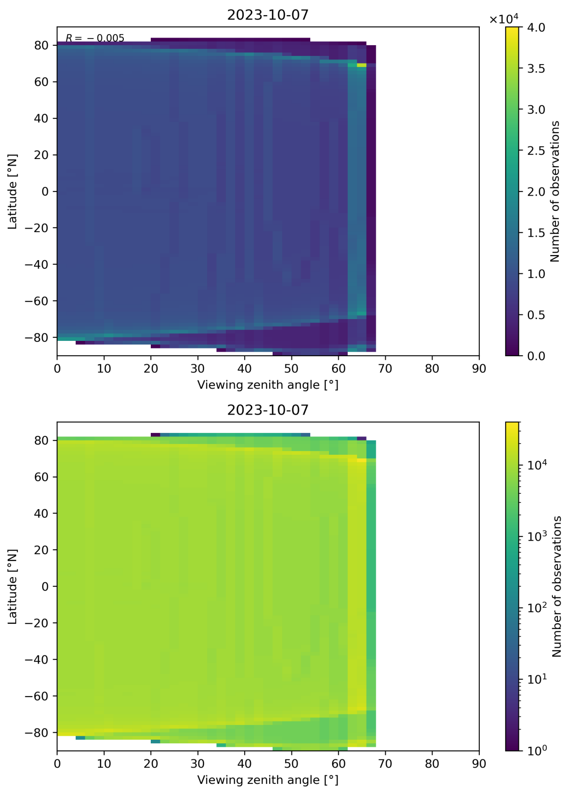
Figure 163: Scatter density plot of “Viewing zenith angle” against “Latitude” for 2023-10-06 to 2023-10-08.
