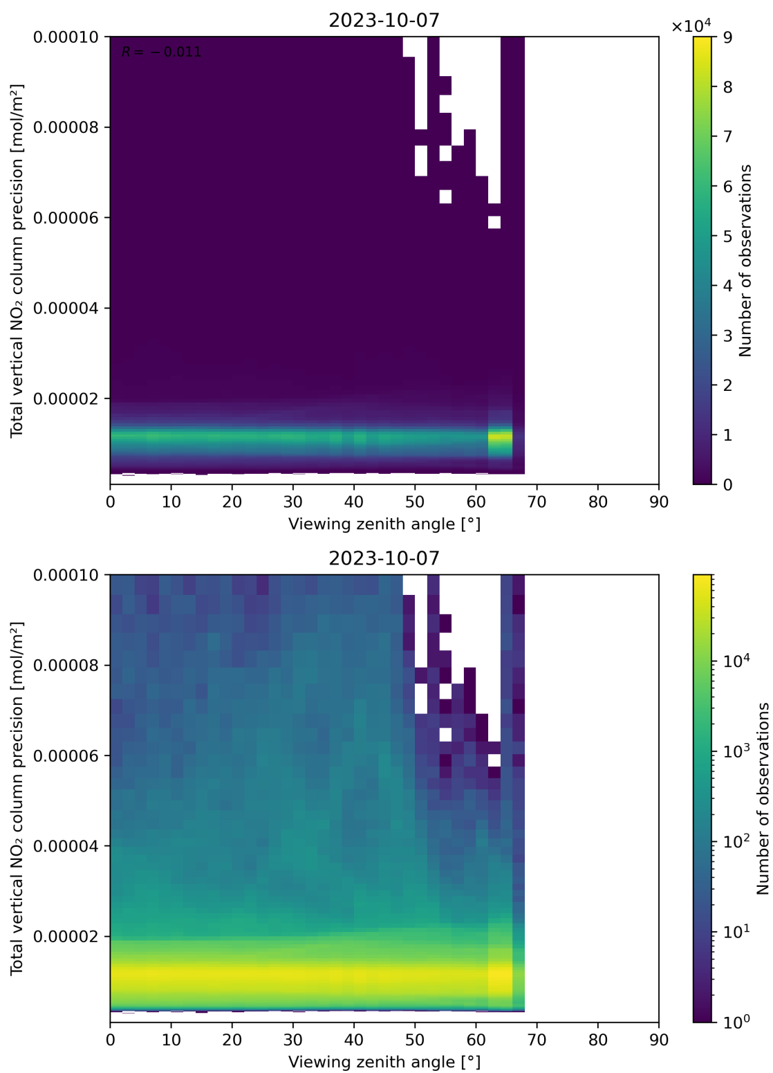
Figure 168: Scatter density plot of “Viewing zenith angle” against “Total vertical NO 2 column precision” for 2023-10-06 to 2023-10-08.
