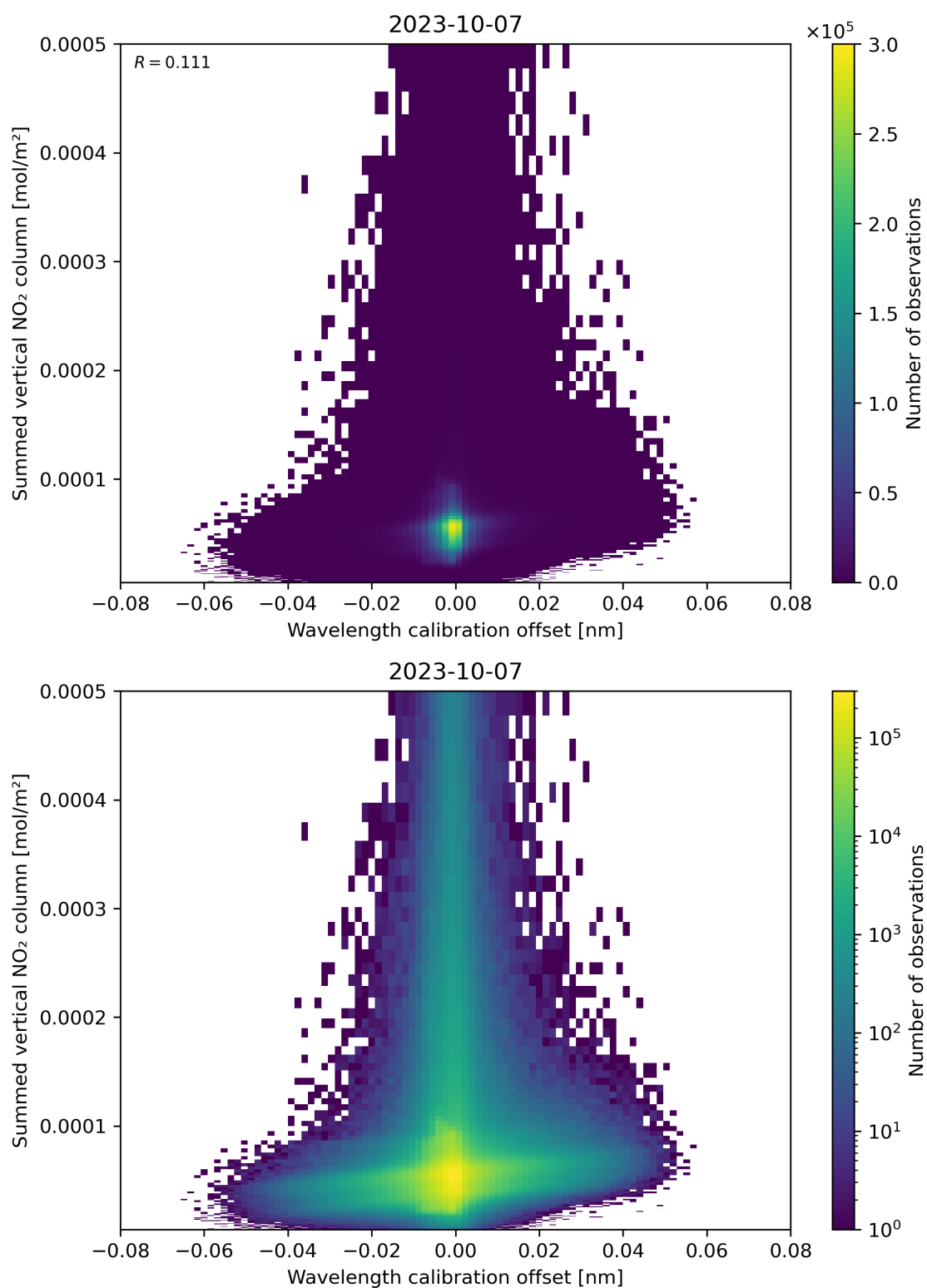
Figure 177: Scatter density plot of “Wavelength calibration offset” against “Summed vertical NO 2 column” for 2023-10-06 to 2023-10-08.
