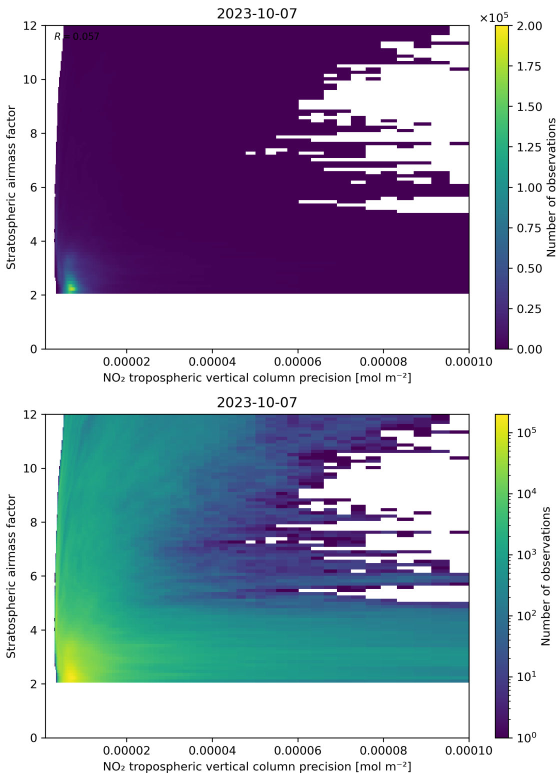
Figure 131: Scatter density plot of “NO 2 tropospheric vertical column precision” against “Stratospheric airmass factor” for 2023-10-06 to 2023-10-08.
