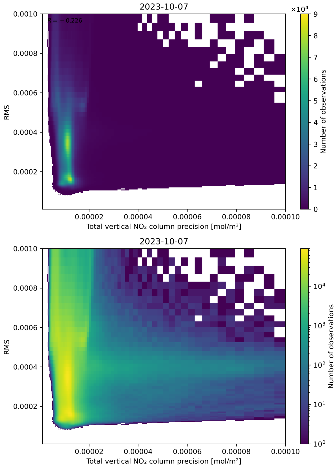
Figure 119: Scatter density plot of “Total vertical NO 2 column precision” against “RMS” for 2023-10-06 to 2023-10-08.
