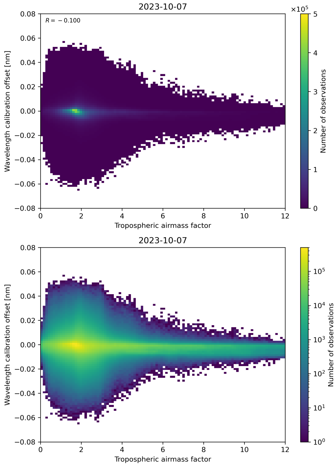
Figure 80: Scatter density plot of “Tropospheric airmass factor” against “Wavelength calibration offset” for 2023-10-06 to 2023-10-08.
