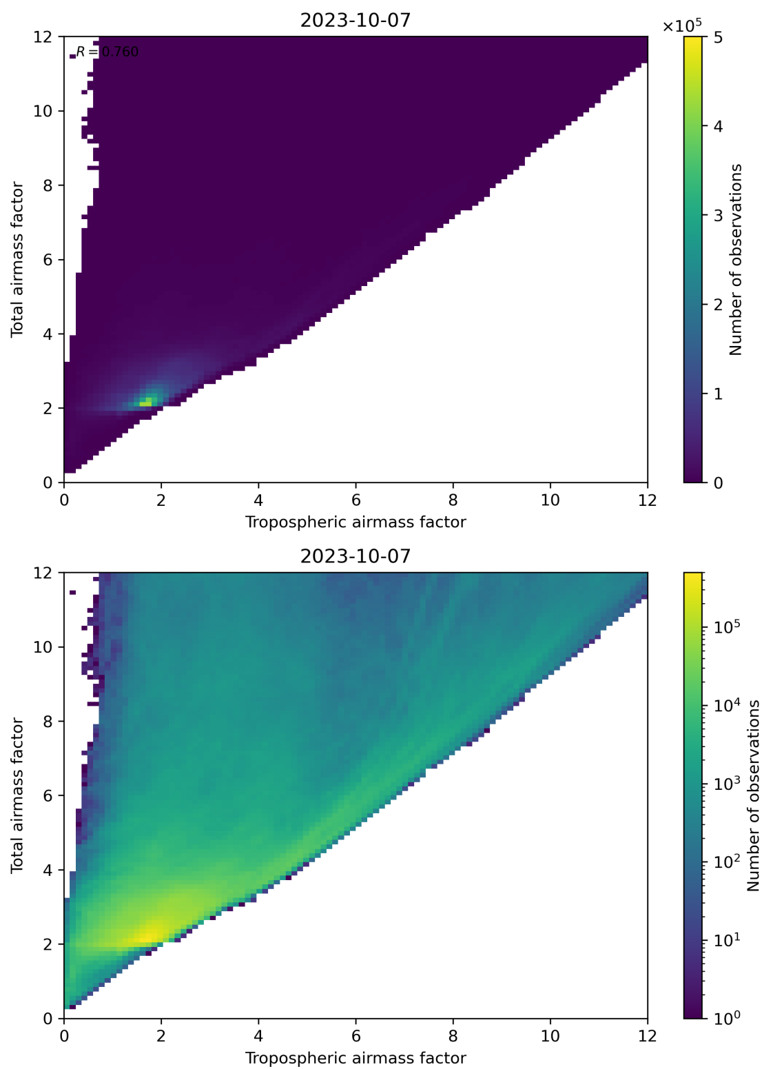
Figure 72: Scatter density plot of “Tropospheric airmass factor” against “Total airmass factor” for 2023-10-06 to 2023-10-08.
