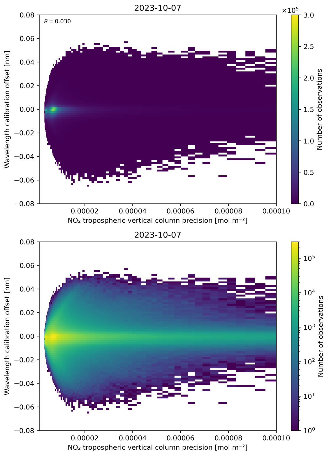
Figure 141: Scatter density plot of “NO 2 tropospheric vertical column precision” against “Wavelength calibration offset” for 2023-10-06 to 2023-10-08.
