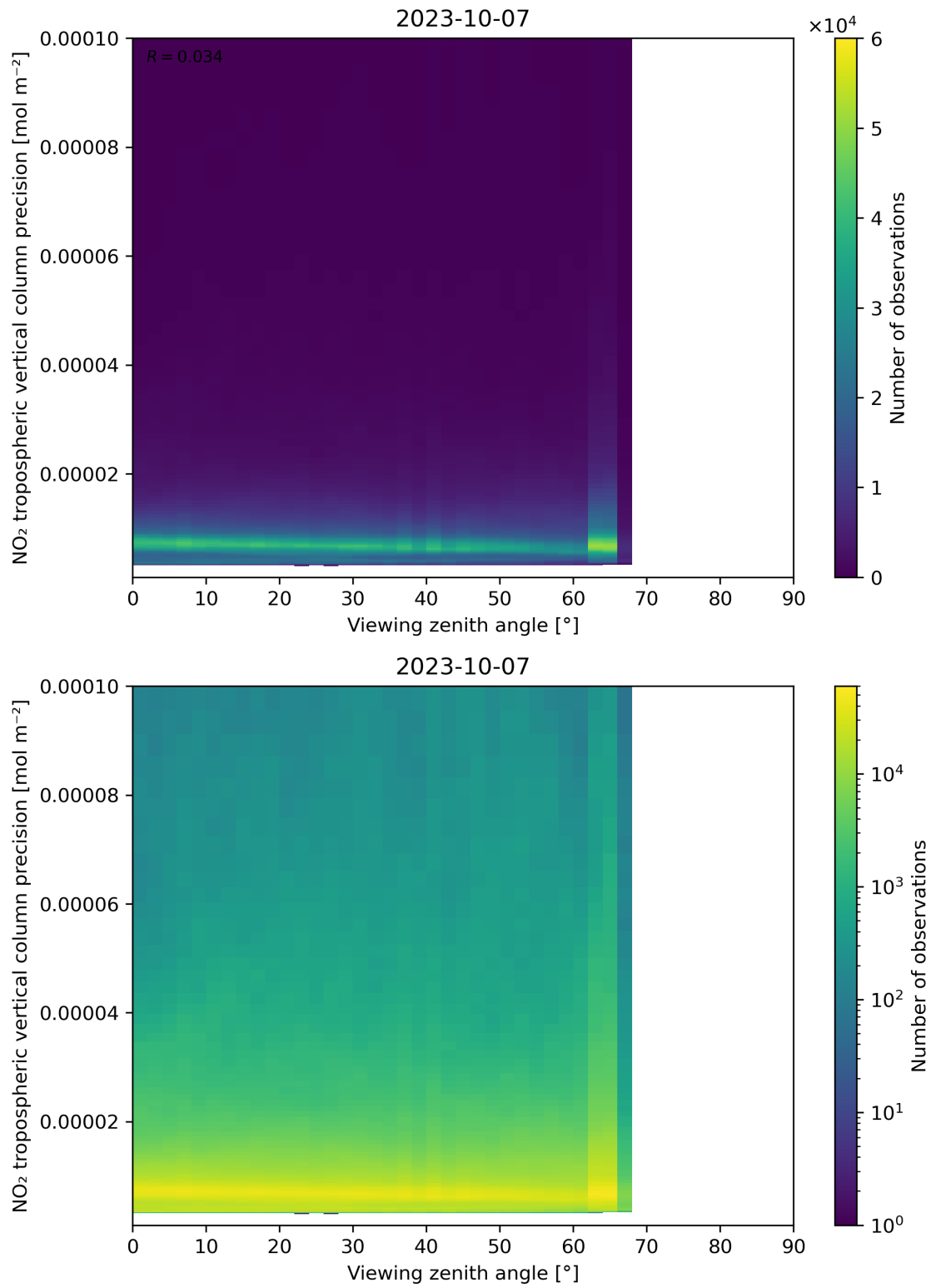
Figure 170: Scatter density plot of “Viewing zenith angle” against “NO 2 tropospheric vertical column precision” for 2023-10-06 to 2023-10-08.
