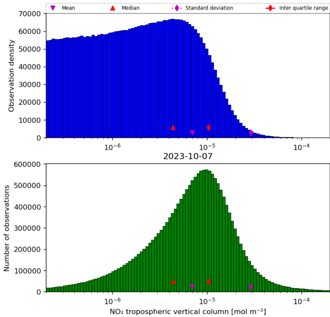
Figure 29: Histogram of “ \text{NO}_2 tropospheric vertical column” for 2023-10-06 to 2023-10-08
