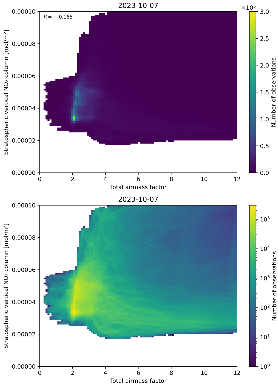
Figure 64: Scatter density plot of “Total airmass factor” against “Stratospheric vertical NO 2 column” for 2023-10-06 to 2023-10-08.
