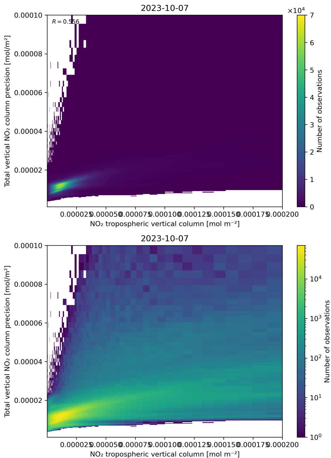
Figure 129: Scatter density plot of “NO 2 tropospheric vertical column” against “Total vertical NO 2 column precision” for 2023-10-06 to 2023-10-08.
