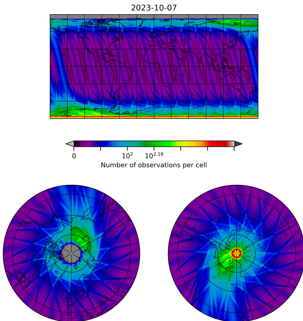
Figure 10: Map of the number of observations for 2023-10-06 to 2023-10-08
