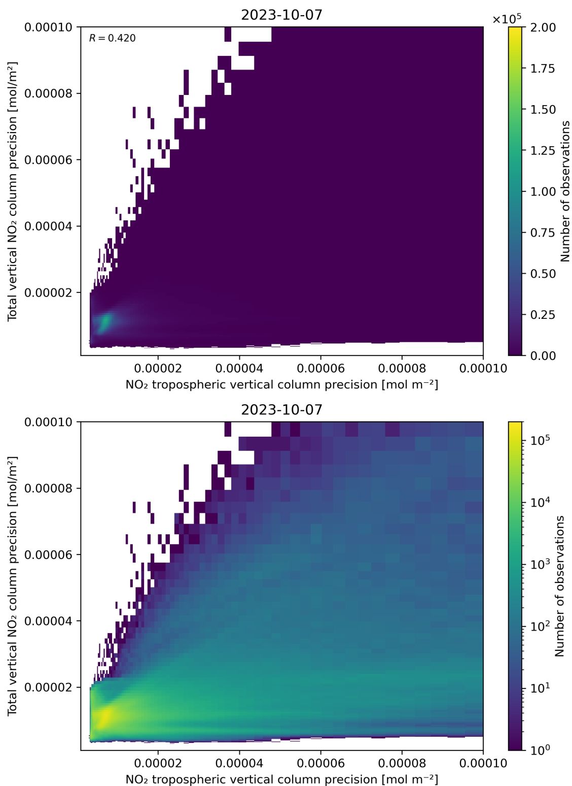
Figure 139: Scatter density plot of “NO 2 tropospheric vertical column precision” against “Total vertical NO 2 column precision” for 2023-10-06 to 2023-10-08.
