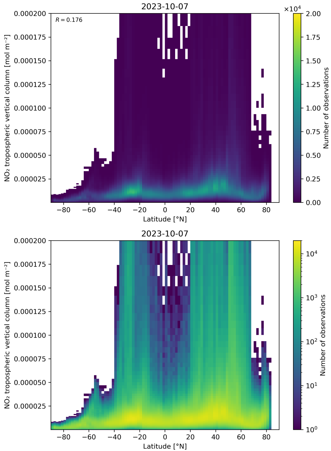
Figure 92: Scatter density plot of “Latitude” against “NO 2 tropospheric vertical column” for 2023-10-06 to 2023-10-08.
