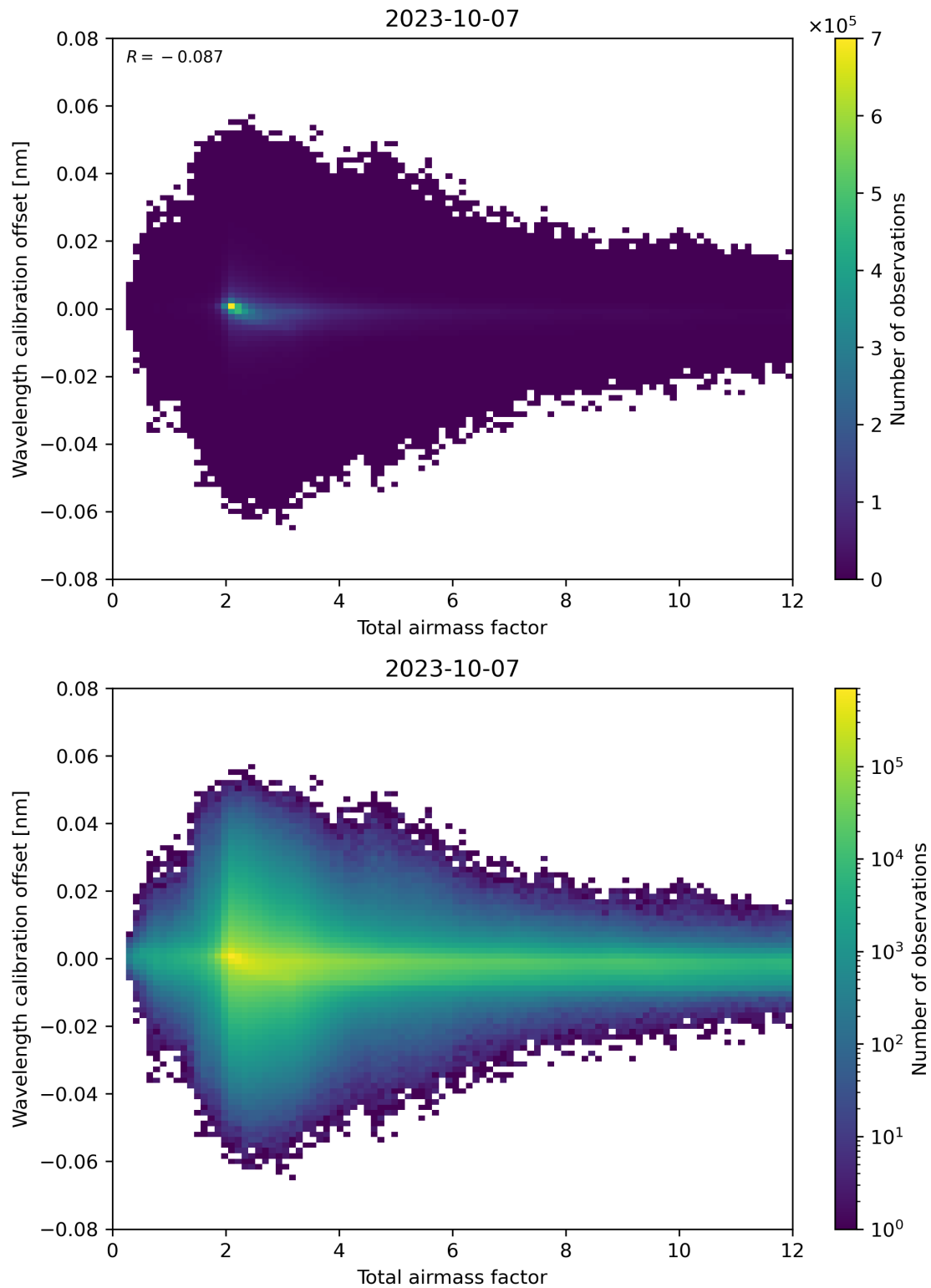
Figure 70: Scatter density plot of “Total airmass factor” against “Wavelength calibration offset” for 2023-10-06 to 2023-10-08.
