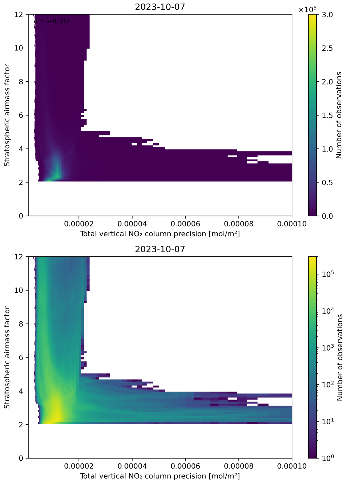
Figure 115: Scatter density plot of “Total vertical NO 2 column precision” against “Stratospheric airmass factor” for 2023-10-06 to 2023-10-08.
