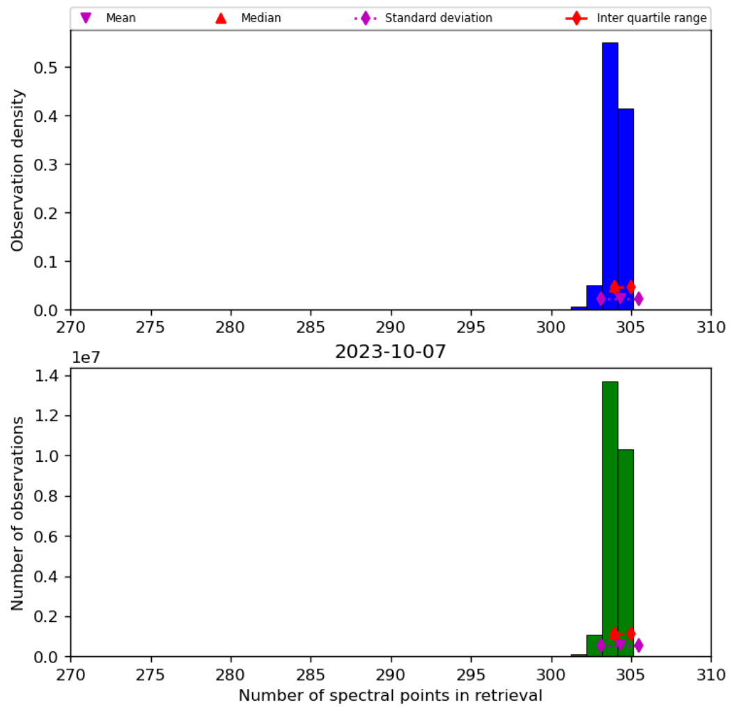
Figure 33: Histogram of “Number of spectral points in retrieval” for 2023-10-06 to 2023-10-08
