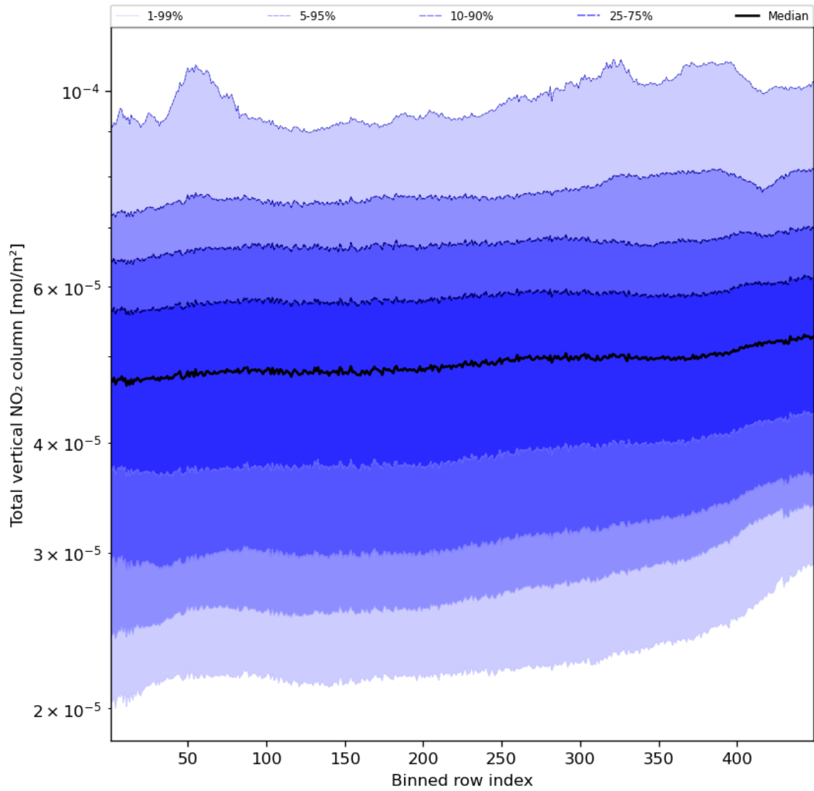
Figure 55: Along track statistics of “Total vertical NO 2 column” for 2023-10-06 to 2023-10-08
