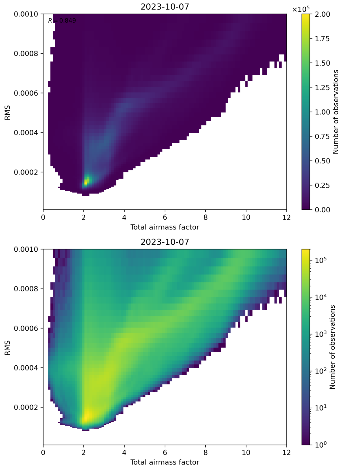
Figure 69: Scatter density plot of “Total airmass factor” against “RMS” for 2023-10-06 to 2023-10-08.
