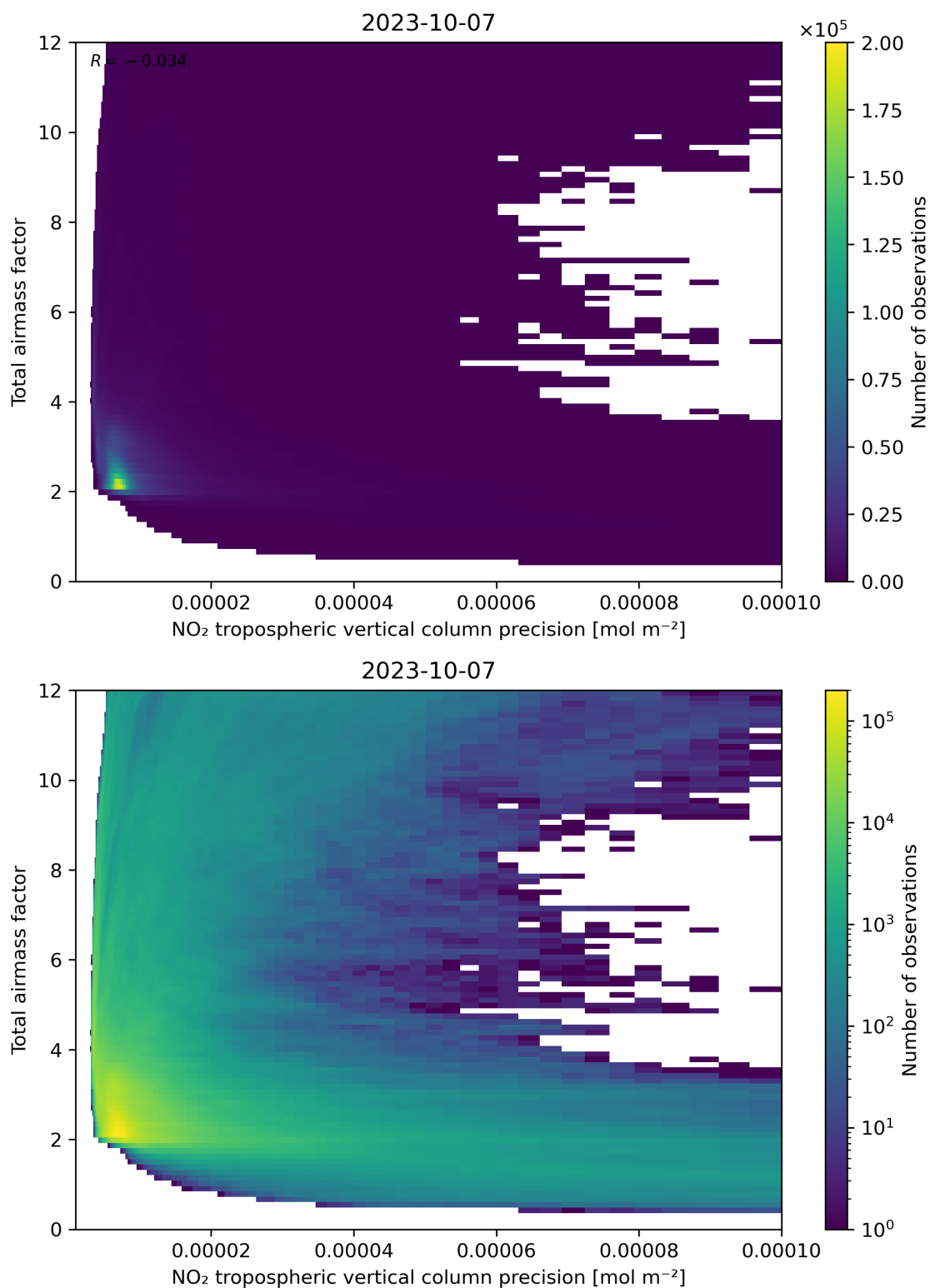
Figure 132: Scatter density plot of “NO 2 tropospheric vertical column precision” against “Total air mass factor” for 2023-10-06 to 2023-10-08.
