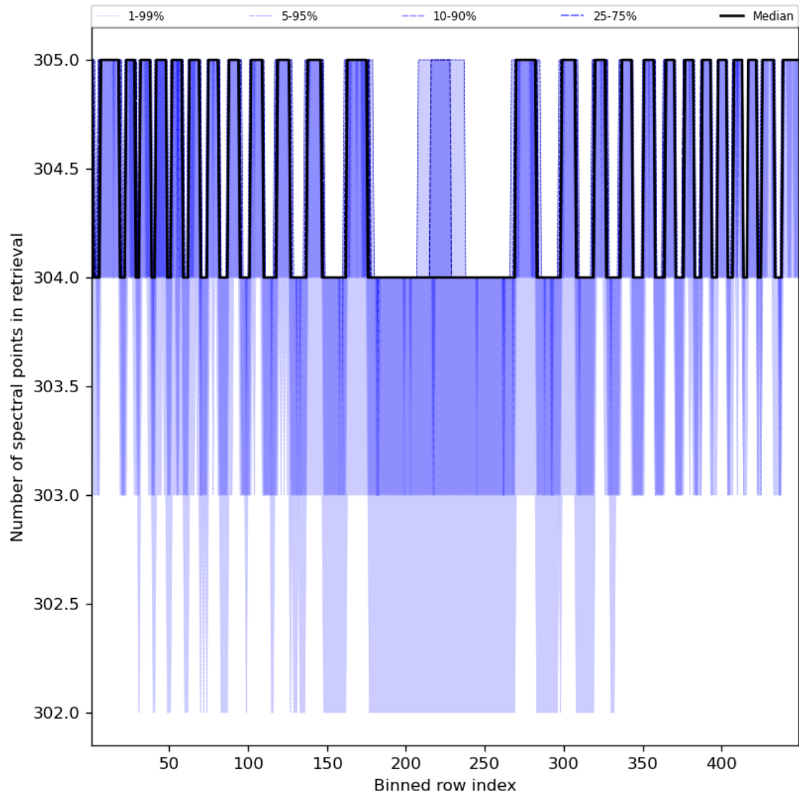
Figure 50: Along track statistics of “Number of spectral points in retrieval” for 2023-10-06 to 2023-10-08
