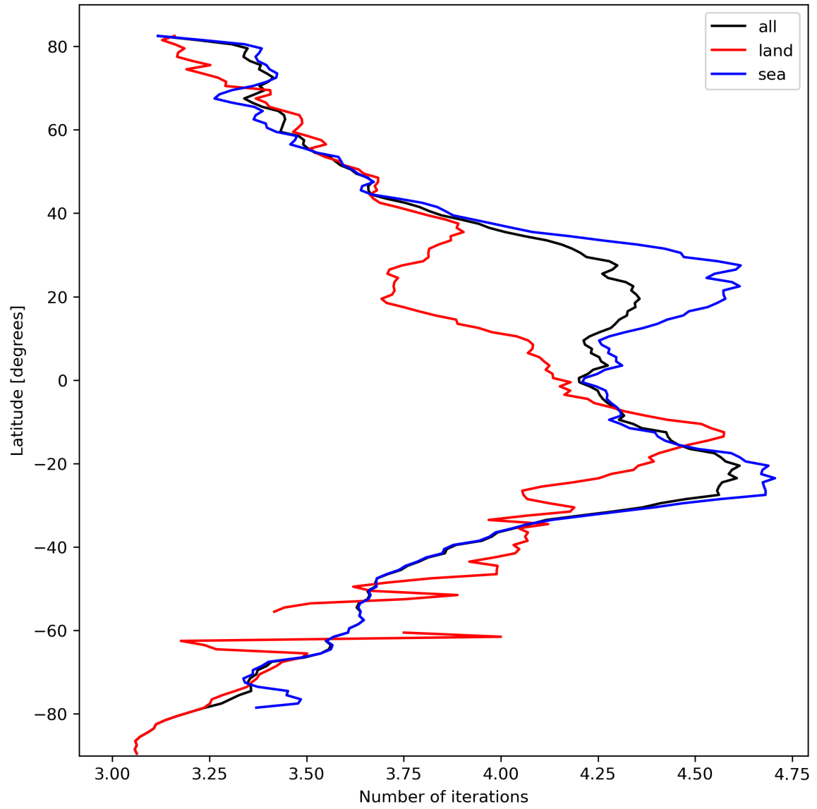
Figure 17: Zonal average of “Number of iterations” for 2023-10-06 to 2023-10-08.
