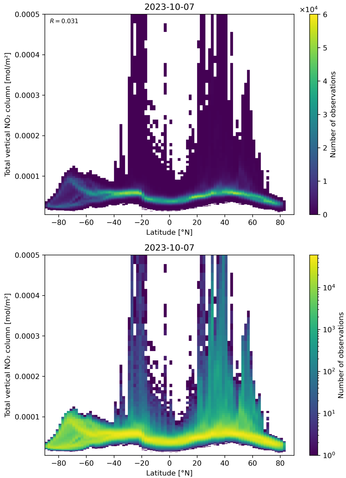
Figure 90: Scatter density plot of “Latitude” against “Total vertical NO 2 column” for 2023-10-06 to 2023-10-08.
