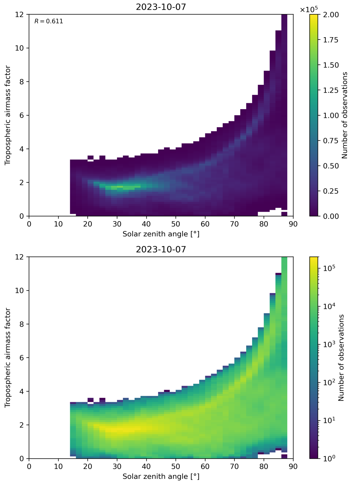
Figure 147: Scatter density plot of “Solar zenith angle” against “Tropospheric airmass factor” for 2023-10-06 to 2023-10-08.
