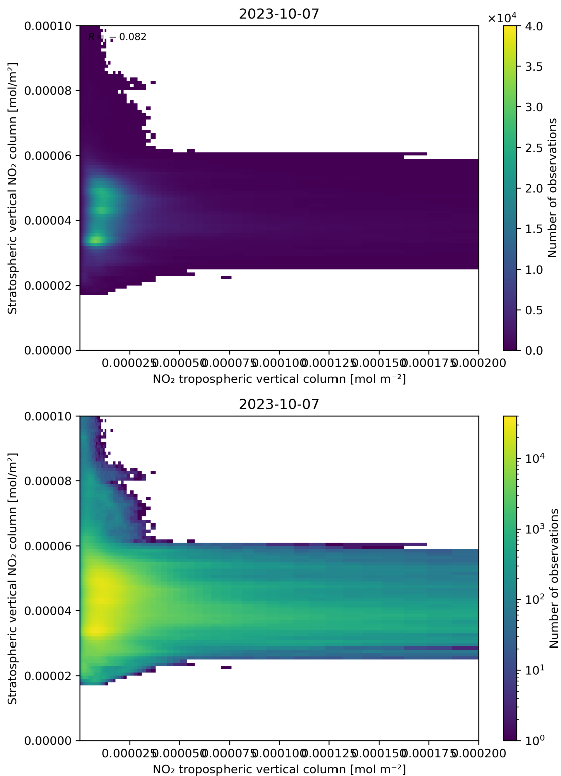
Figure 125: Scatter density plot of “NO 2 tropospheric vertical column” against “Stratospheric vertical NO 2 column” for 2023-10-06 to 2023-10-08.
