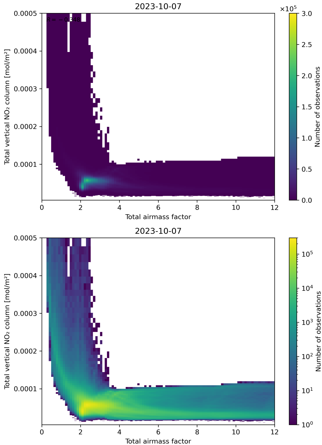
Figure 67: Scatter density plot of “Total airmass factor” against “Total vertical NO 2 column” for 2023-10-06 to 2023-10-08.
