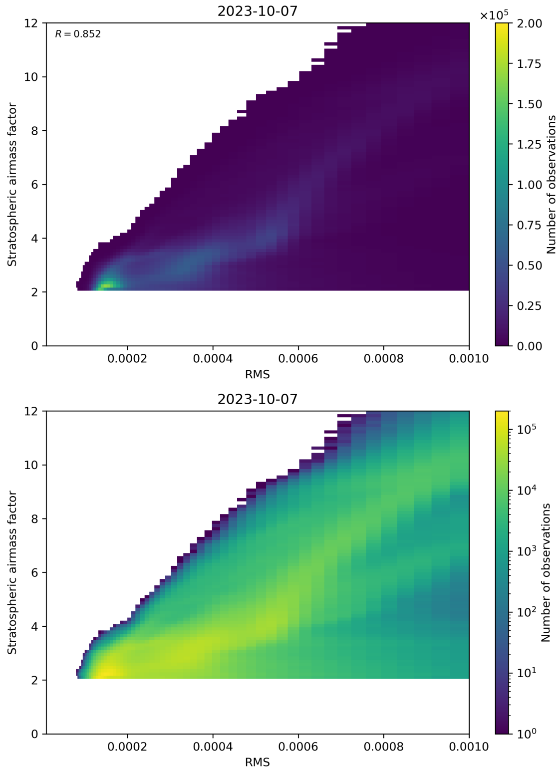
Figure 144: Scatter density plot of “RMS” against “Stratospheric airmass factor” for 2023-10-06 to 2023-10-08.
