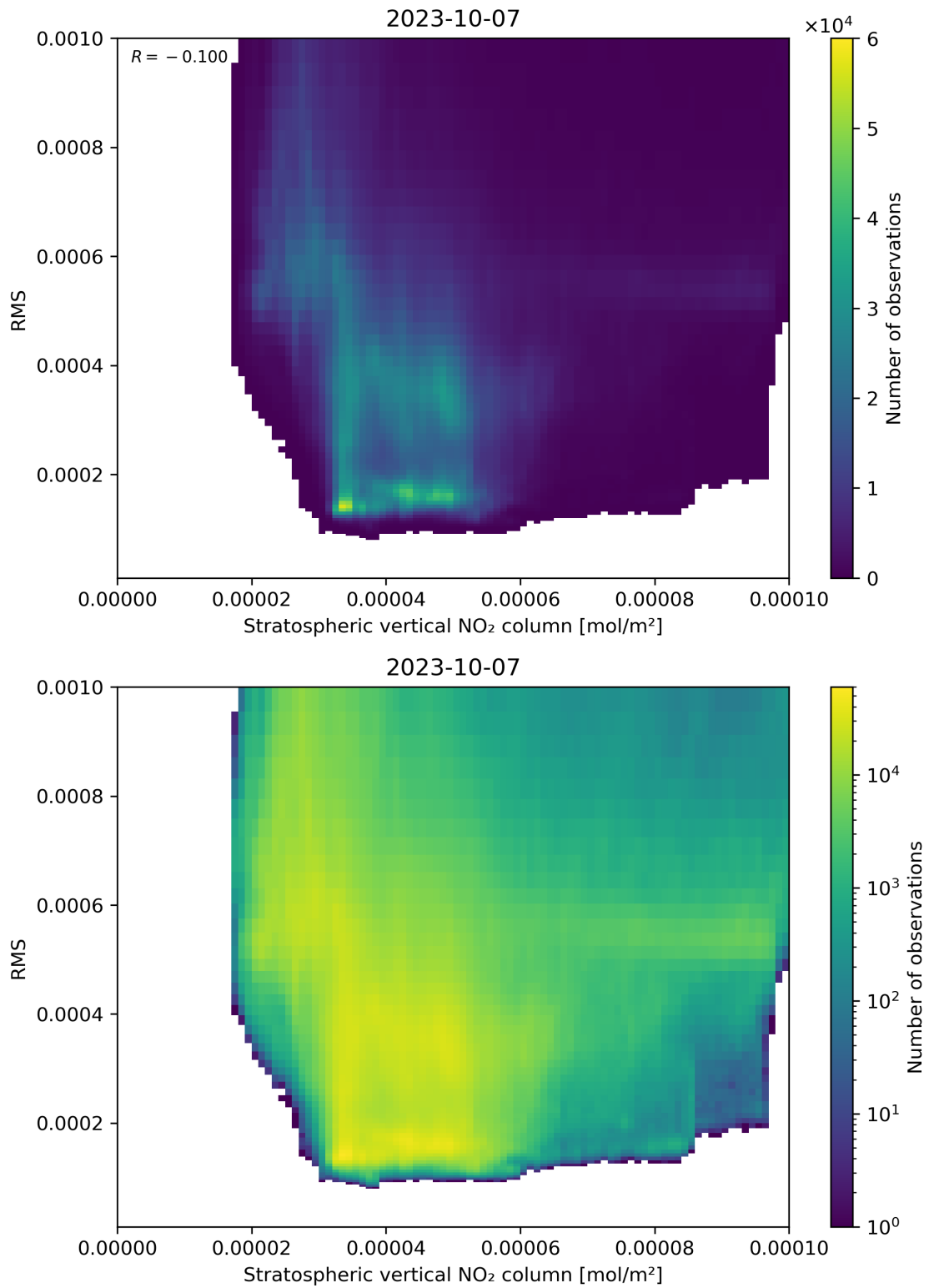
Figure 102: Scatter density plot of “Stratospheric vertical NO 2 column” against “RMS” for 2023-10-06 to 2023-10-08.
