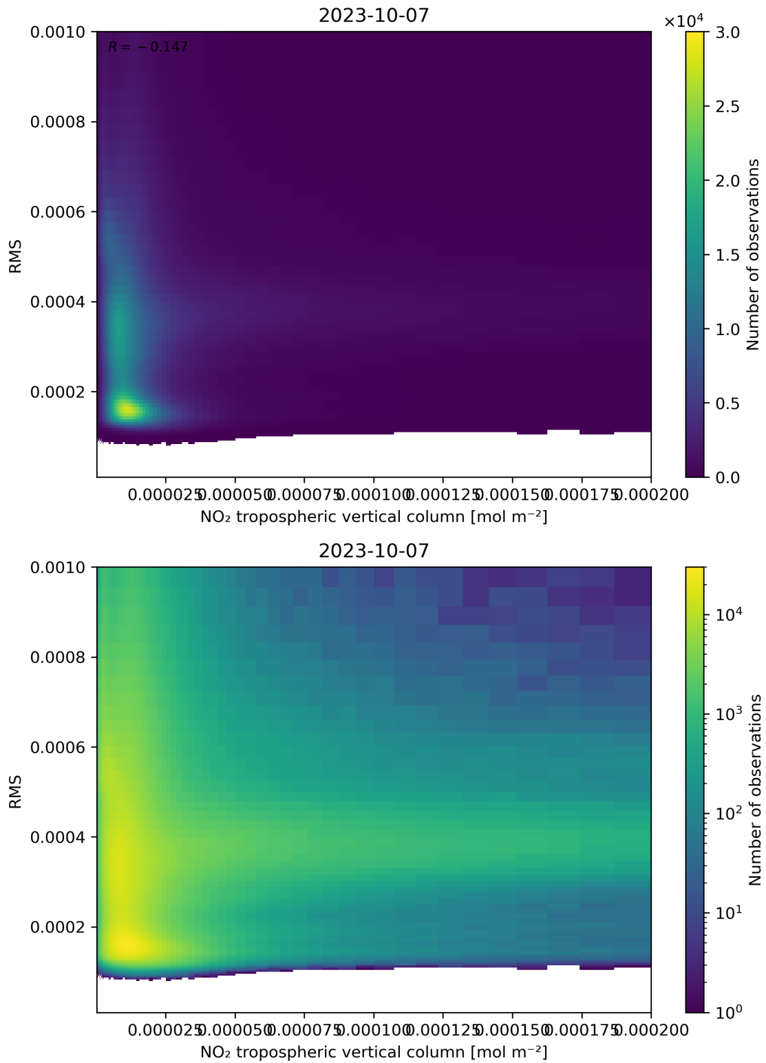
Figure 142: Scatter density plot of “NO 2 tropospheric vertical column” against “RMS” for 2023-10-06 to 2023-10-08.
