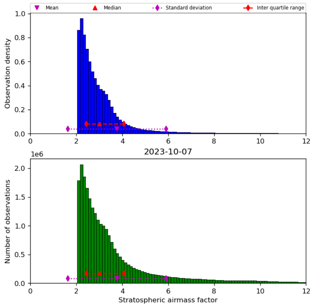
Figure 44: Histogram of “Stratospheric airmass factor” for 2023-10-06 to 2023-10-08
