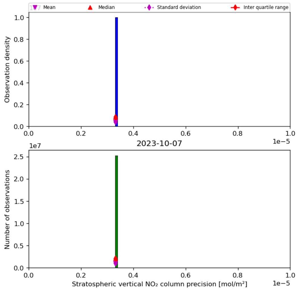
Figure 37: Histogram of “Stratospheric vertical NO 2 column precision” for 2023-10-06 to 2023-10-08
