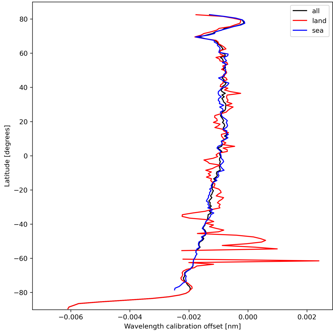
Figure 18: Zonal average of “Wavelength calibration offset” for 2023-10-06 to 2023-10-08.
