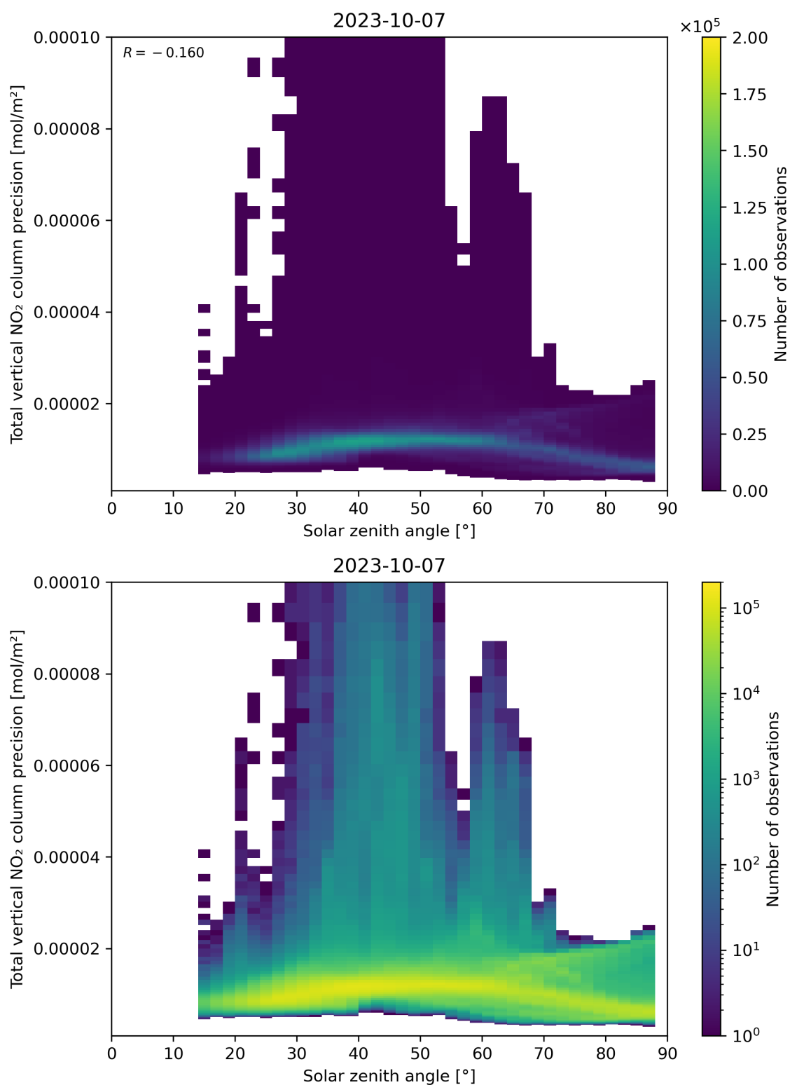
Figure 154: Scatter density plot of “Solar zenith angle” against “Total vertical NO 2 column precision” for 2023-10-06 to 2023-10-08.
