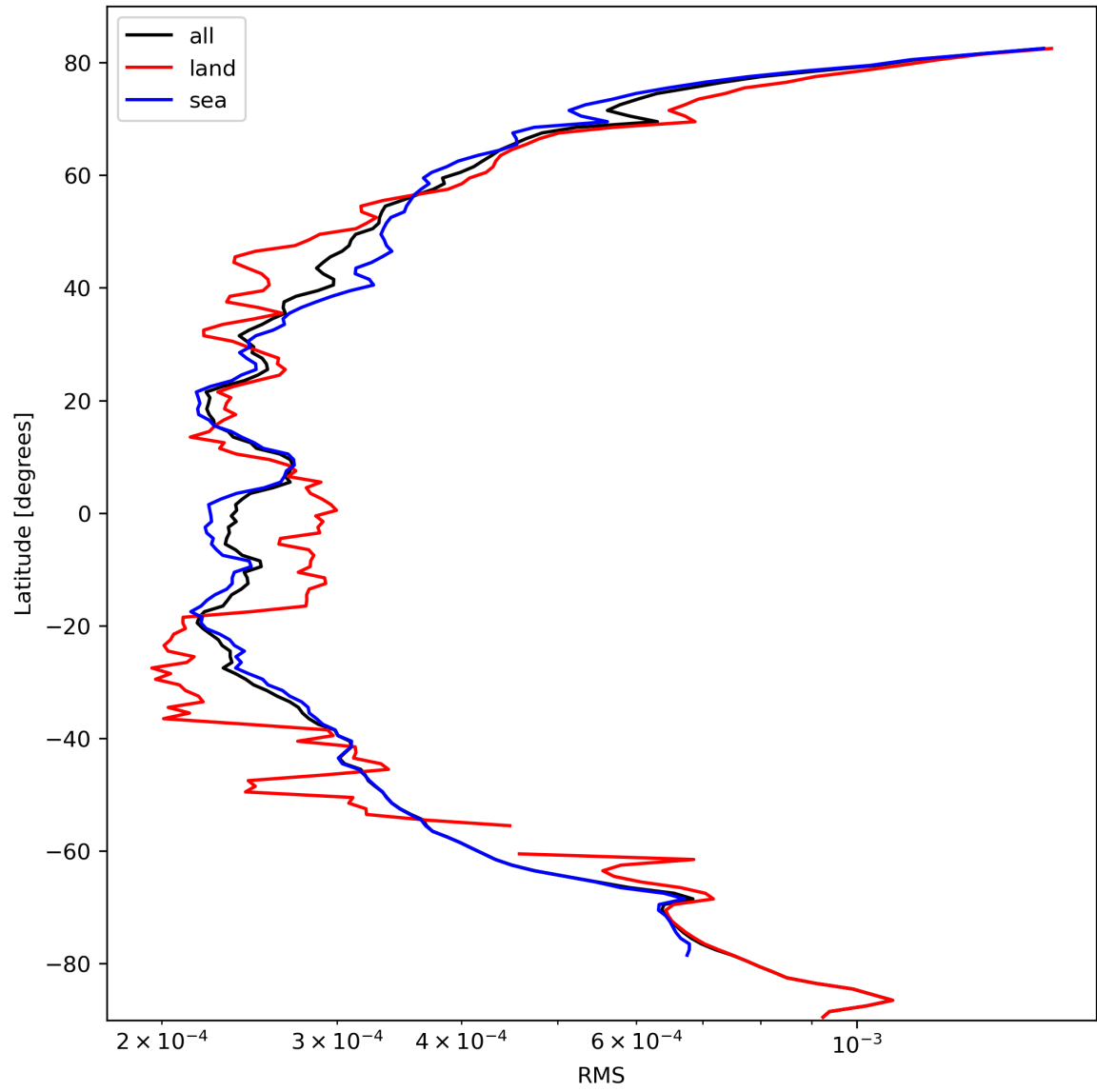
Figure 26: Zonal average of “RMS” for 2023-10-06 to 2023-10-08.
