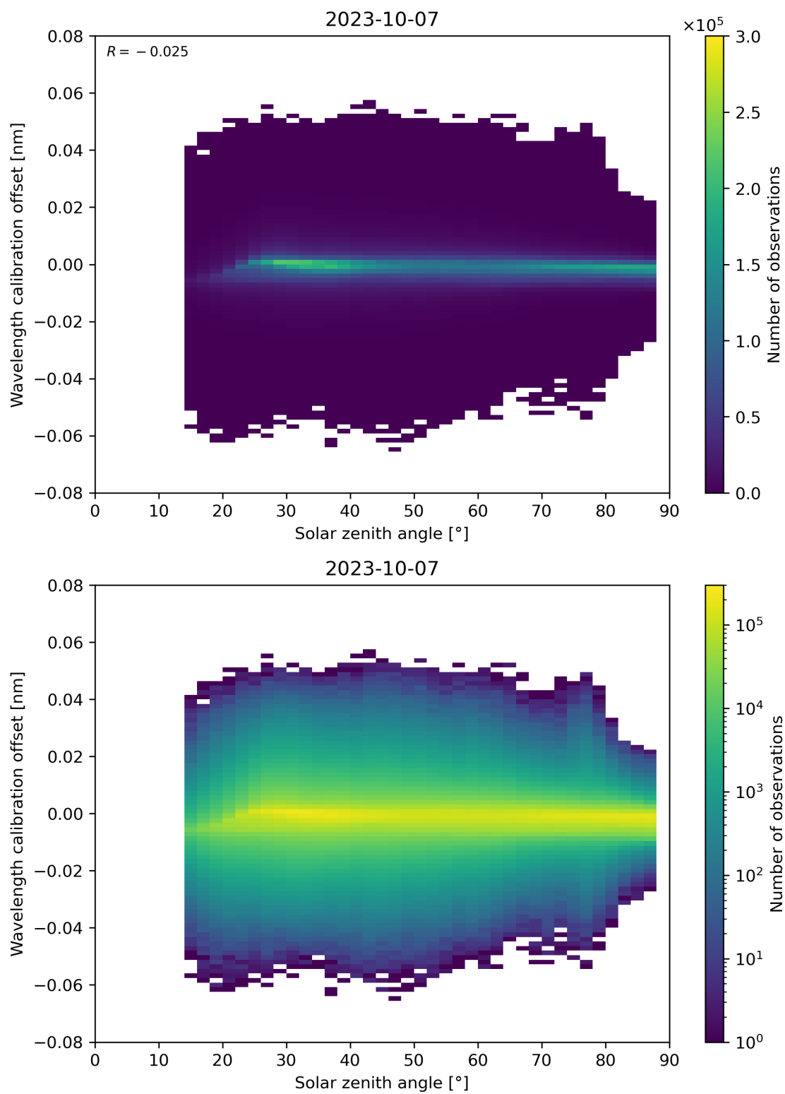
Figure 158: Scatter density plot of “Solar zenith angle” against “Wavelength calibration offset” for 2023-10-06 to 2023-10-08.
