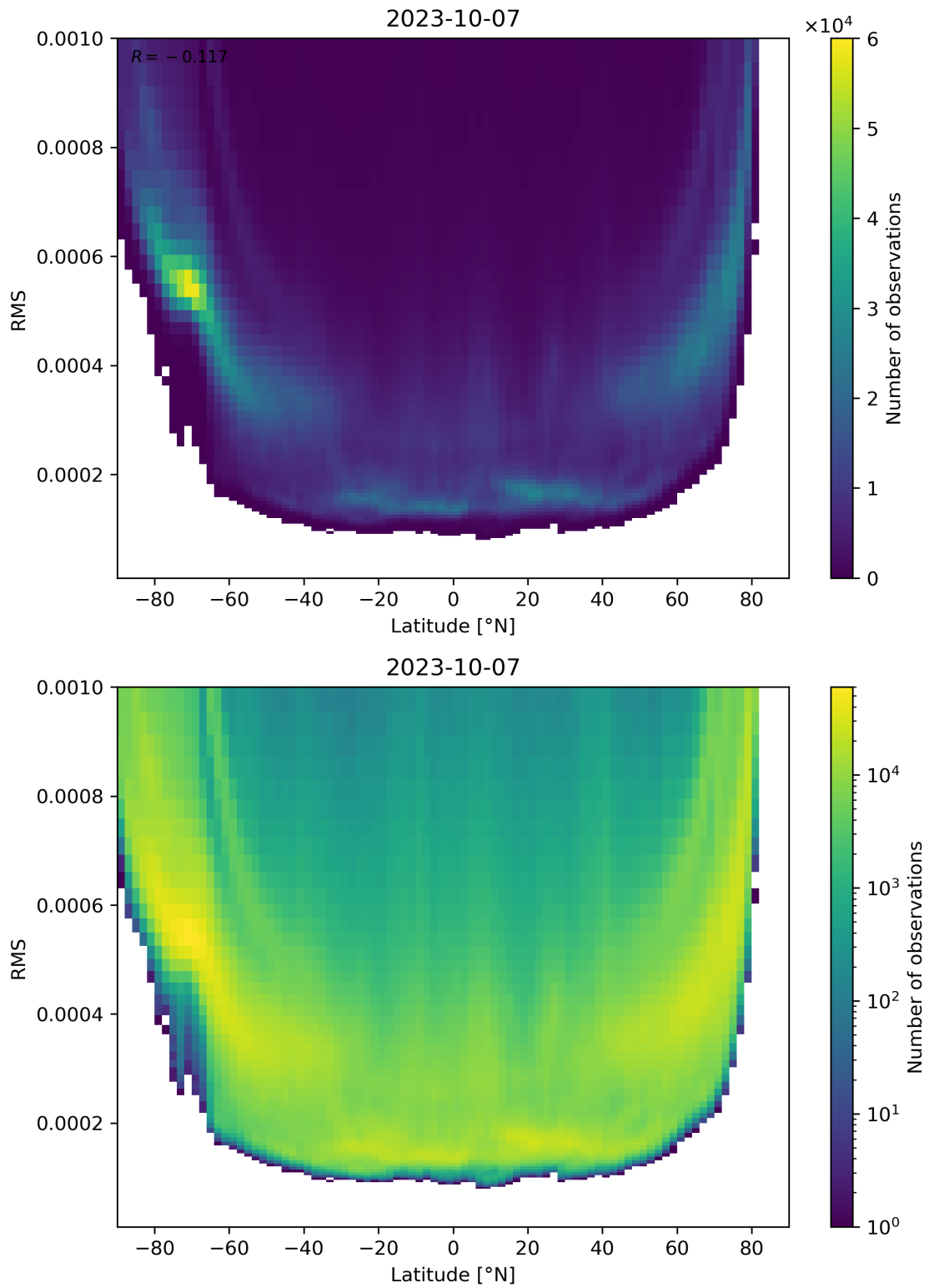
Figure 94: Scatter density plot of “Latitude” against “RMS” for 2023-10-06 to 2023-10-08.
