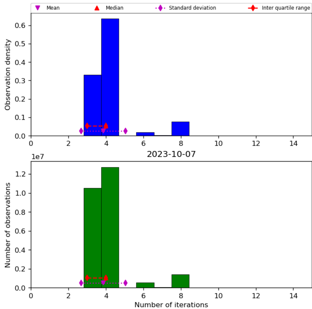
Figure 34: Histogram of “Number of iterations” for 2023-10-06 to 2023-10-08
