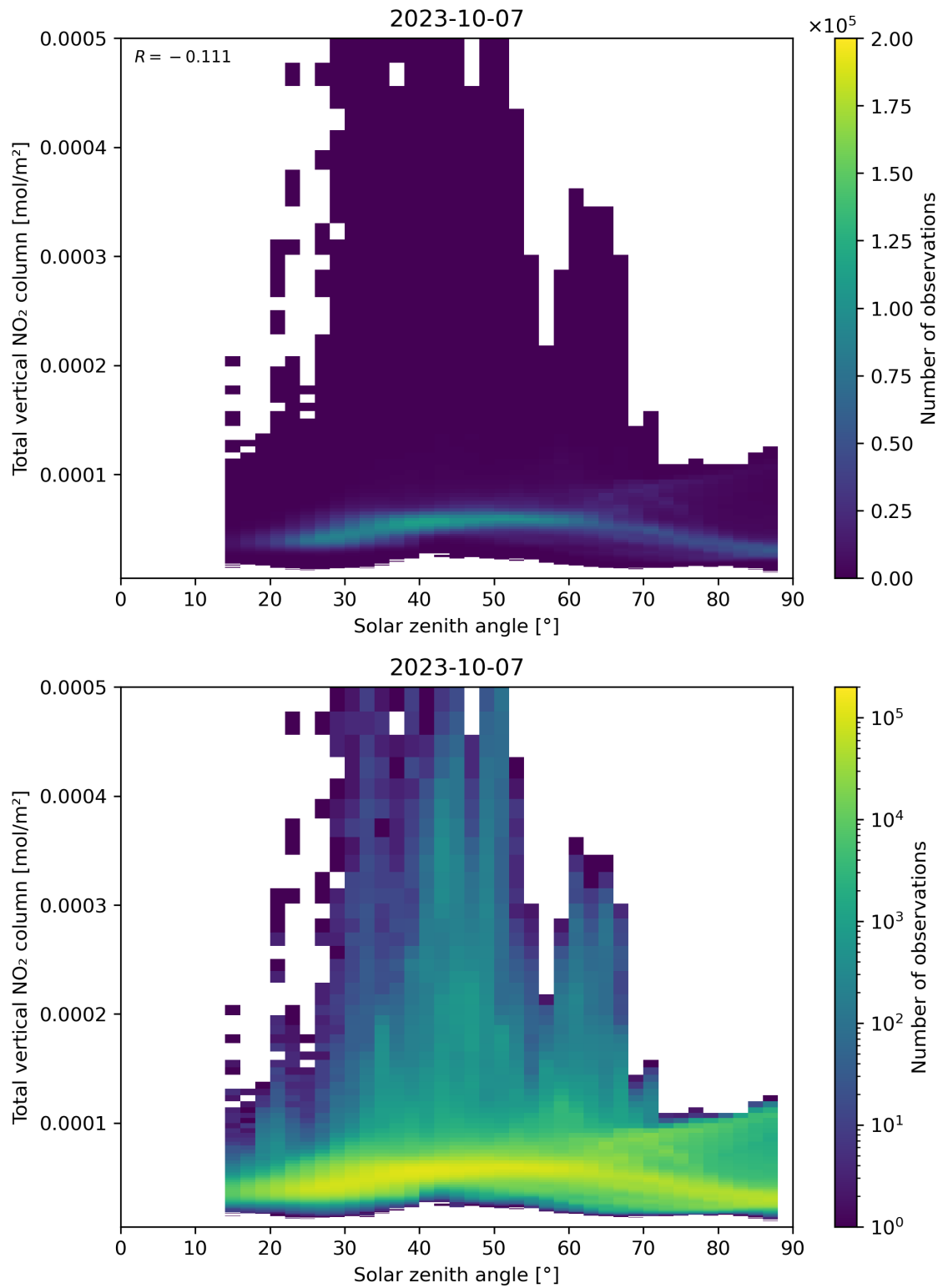
Figure 153: Scatter density plot of “Solar zenith angle” against “Total vertical NO 2 column” for 2023-10-06 to 2023-10-08.
