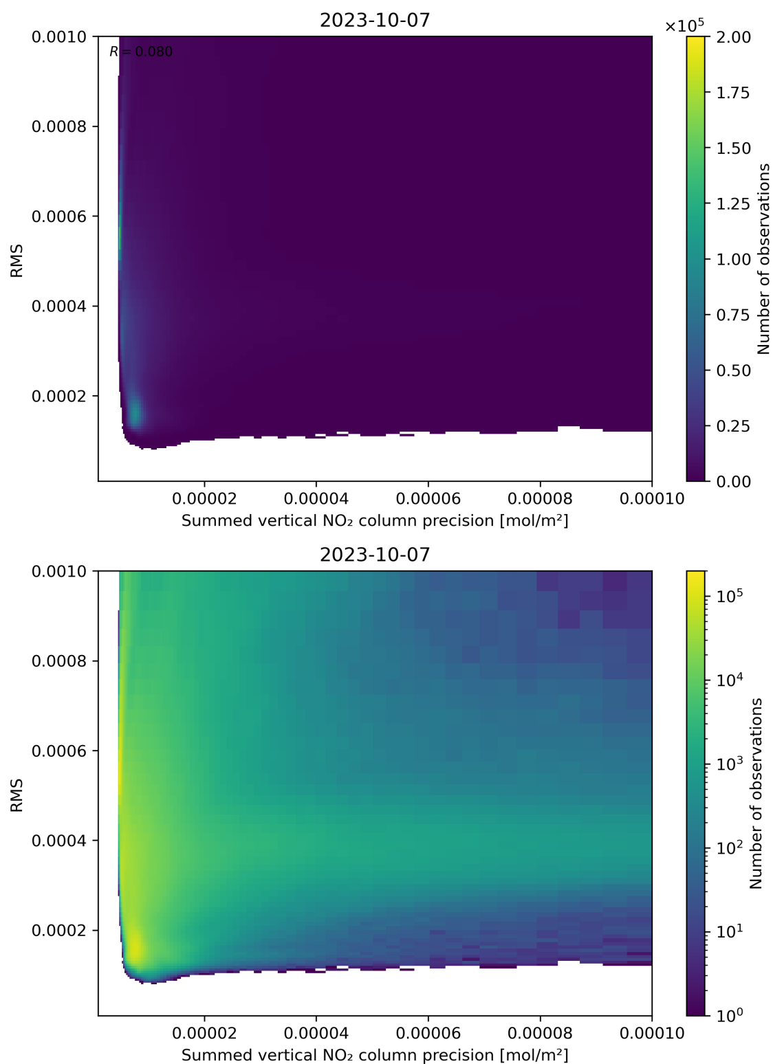
Figure 108: Scatter density plot of “Summed vertical NO 2 column precision” against “RMS” for 2023-10-06 to 2023-10-08.
