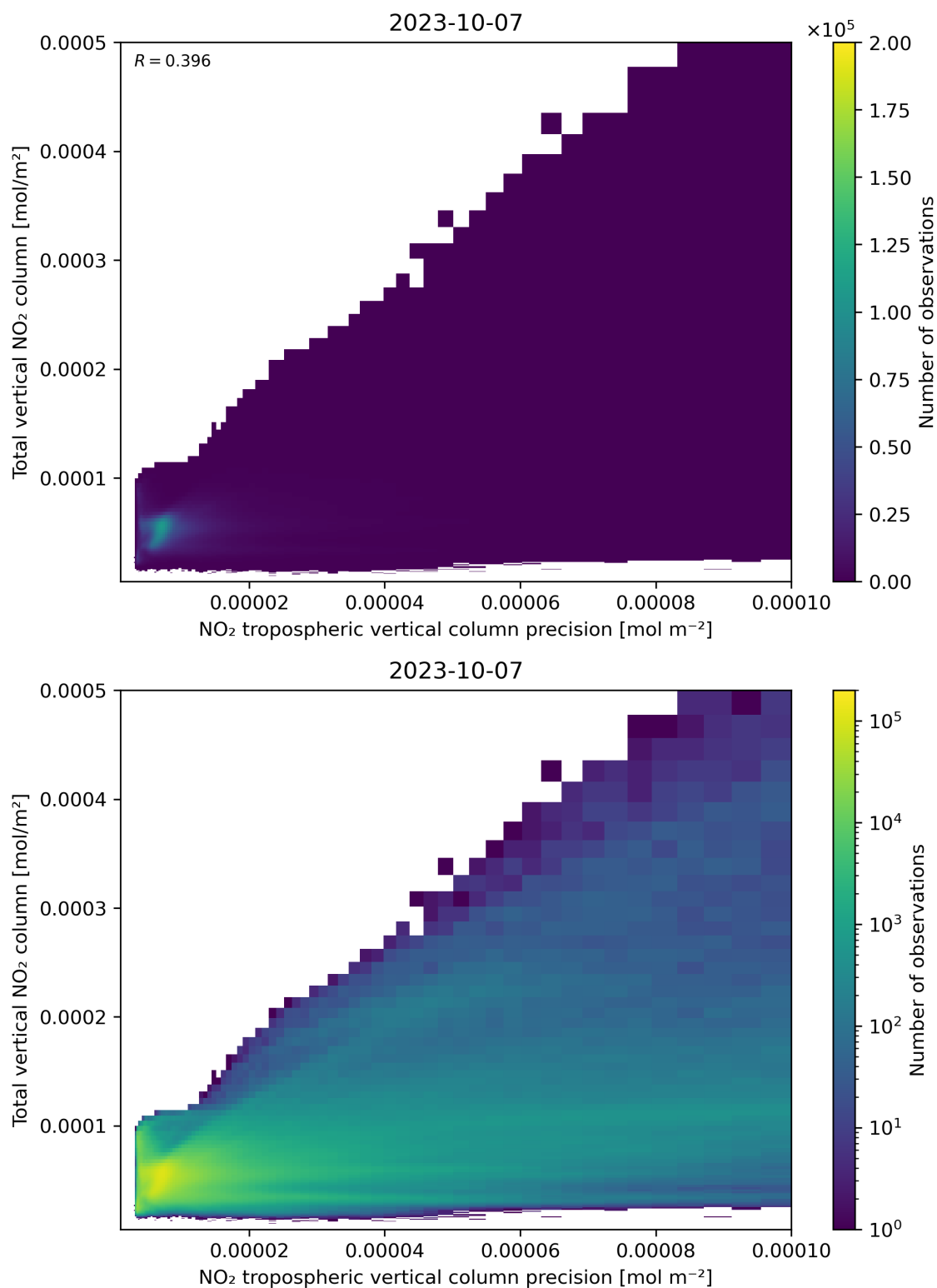
Figure 138: Scatter density plot of “NO 2 tropospheric vertical column precision” against “Total vertical NO 2 column” for 2023-10-06 to 2023-10-08.
