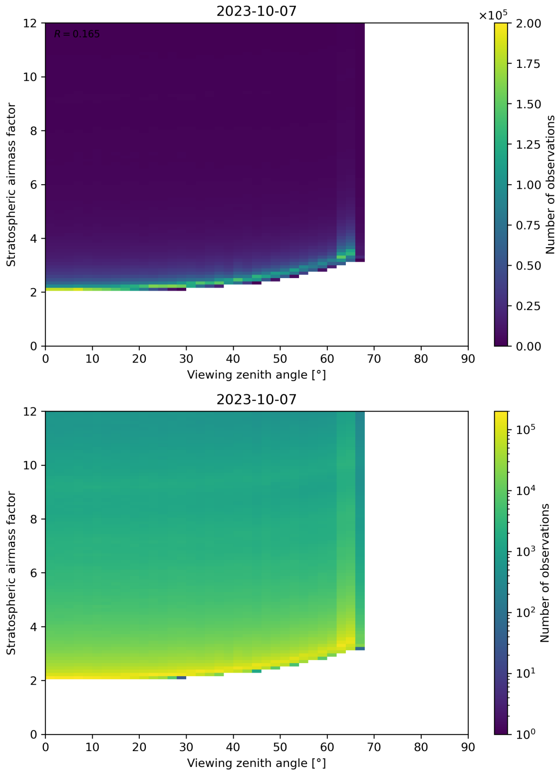
Figure 159: Scatter density plot of “Viewing zenith angle” against “Stratospheric airmass factor” for 2023-10-06 to 2023-10-08.
