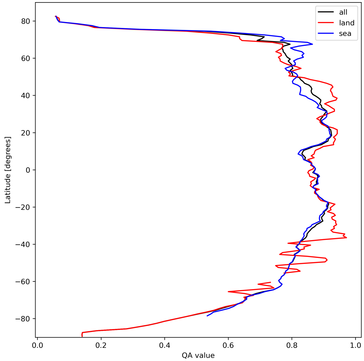
Figure 11: Zonal average of “QA value” for 2023-10-06 to 2023-10-08.
