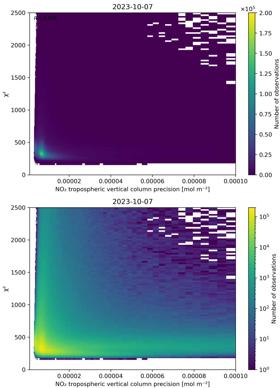
Figure 134: Scatter density plot of “NO 2 tropospheric vertical column precision” against “ \chi^2 ” for 2023-10-06 to 2023-10-08.
