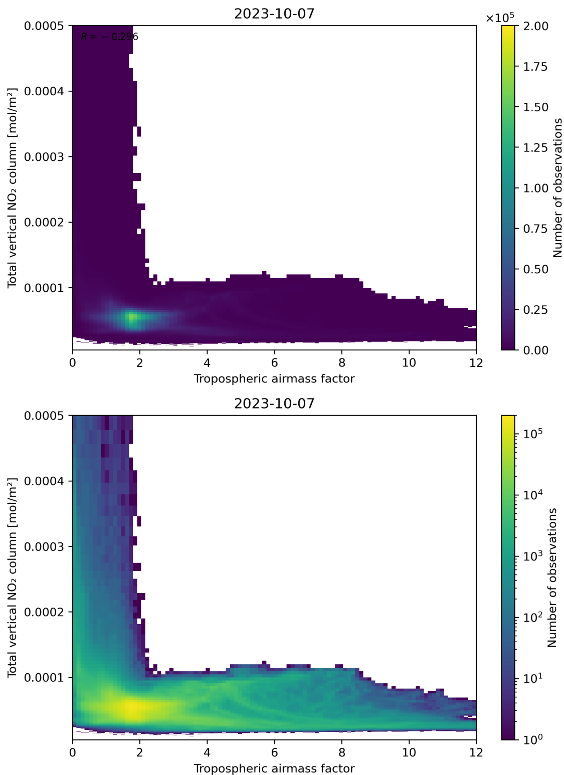
Figure 77: Scatter density plot of “Tropospheric airmass factor” against “Total vertical NO 2 column” for 2023-10-06 to 2023-10-08.
