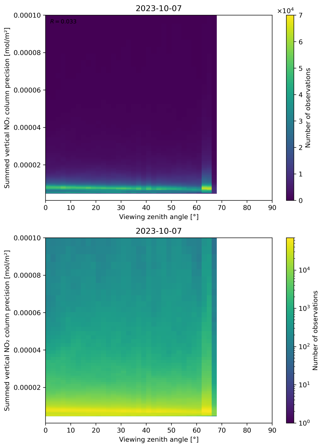
Figure 166: Scatter density plot of “Viewing zenith angle” against “Summed vertical NO 2 column precision” for 2023-10-06 to 2023-10-08.
