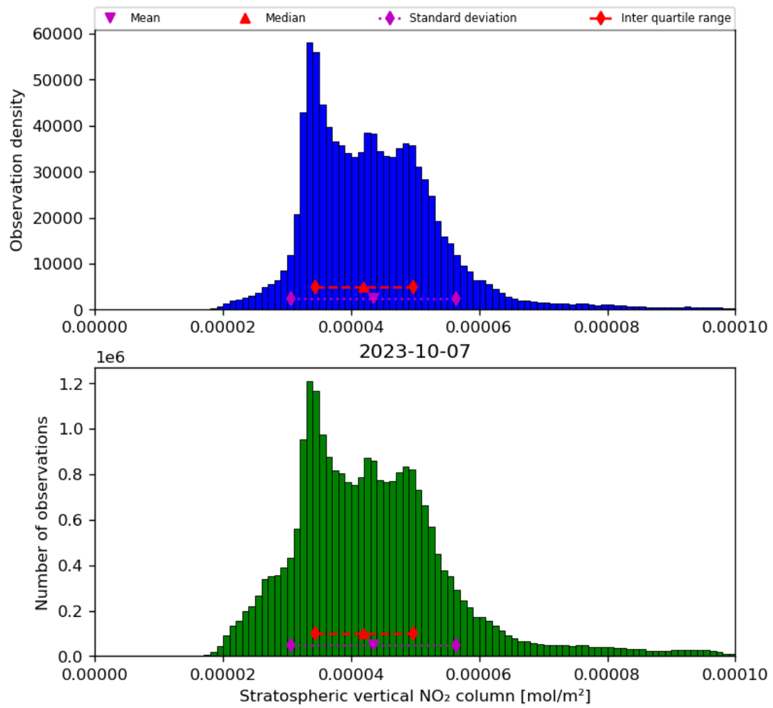
Figure 36: Histogram of “Stratospheric vertical NO 2 column” for 2023-10-06 to 2023-10-08
