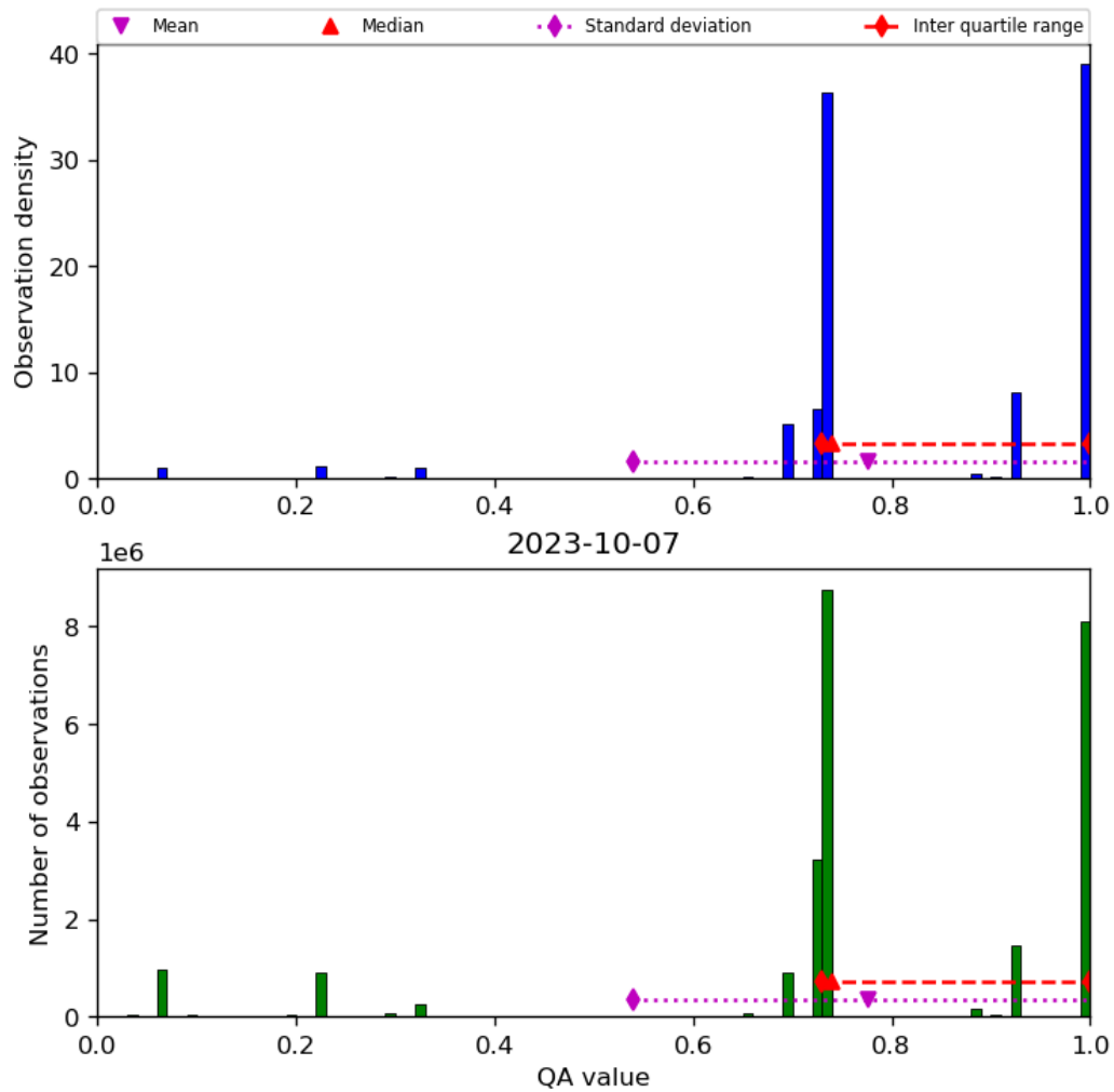
Figure 28: Histogram of “QA value” for 2023-10-06 to 2023-10-08
