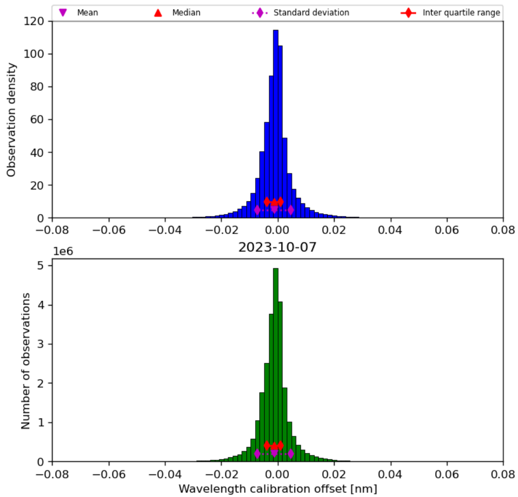
Figure 35: Histogram of “Wavelength calibration offset” for 2023-10-06 to 2023-10-08
