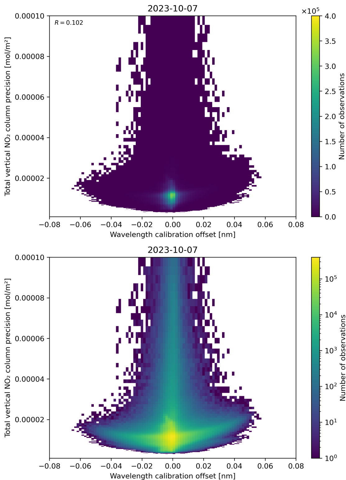
Figure 180: Scatter density plot of “Wavelength calibration offset” against “Total vertical NO 2 column precision” for 2023-10-06 to 2023-10-08.
