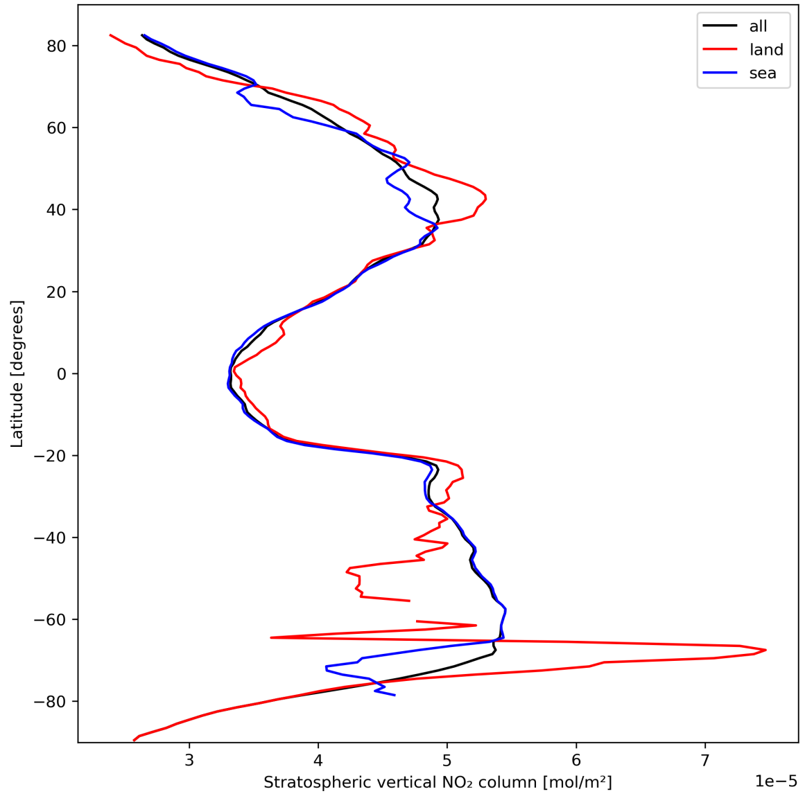
Figure 19: Zonal average of “Stratospheric vertical NO 2 column” for 2023-10-06 to 2023-10-08.
