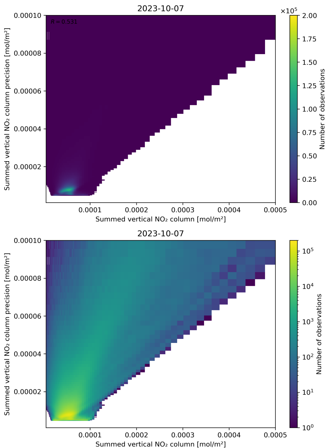
Figure 105: Scatter density plot of “Summed vertical NO 2 column” against “Summed vertical NO 2 column precision” for 2023-10-06 to 2023-10-08.
