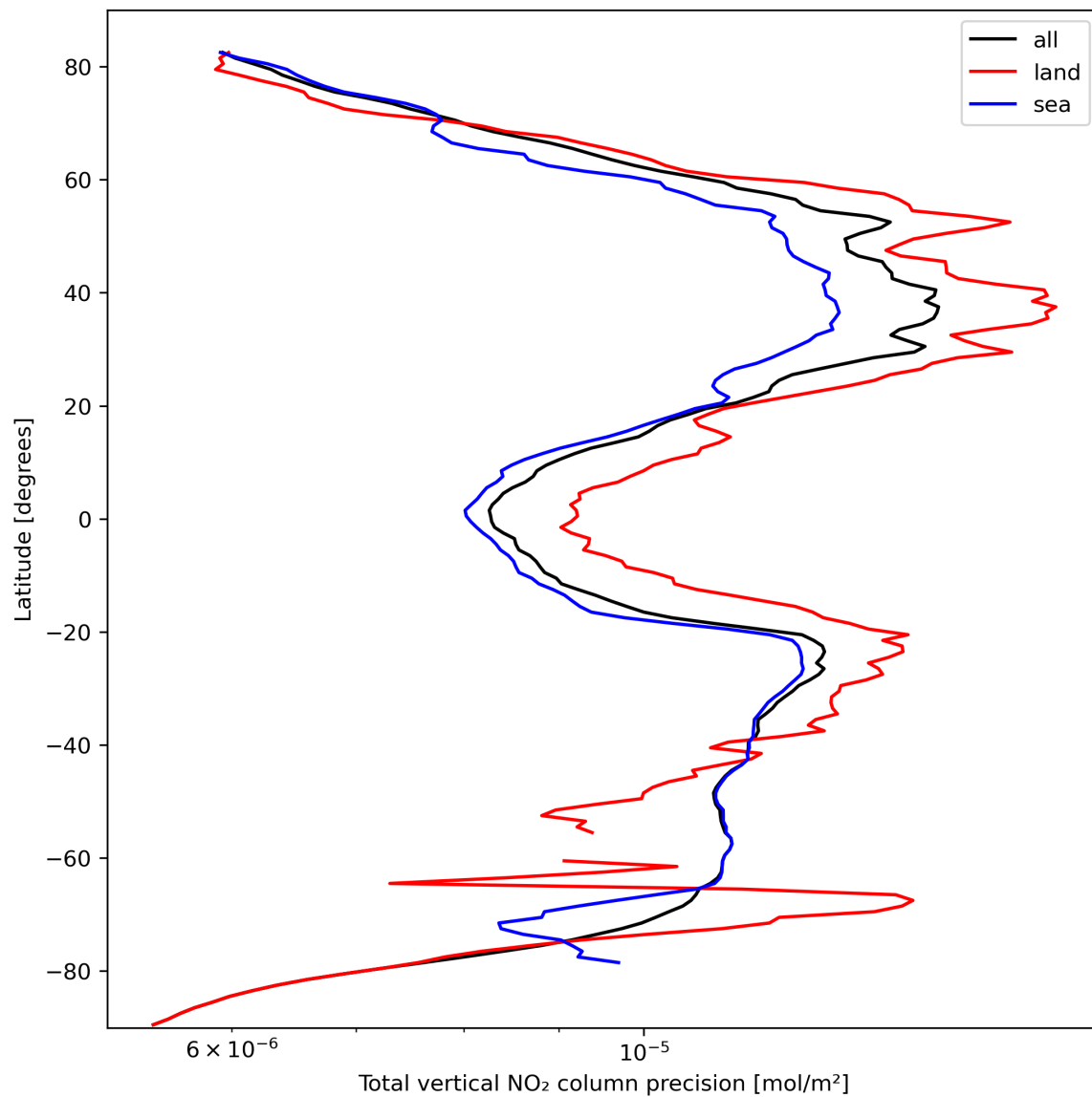
Figure 22: Zonal average of “Total vertical NO 2 column precision” for 2023-10-06 to 2023-10-08.
