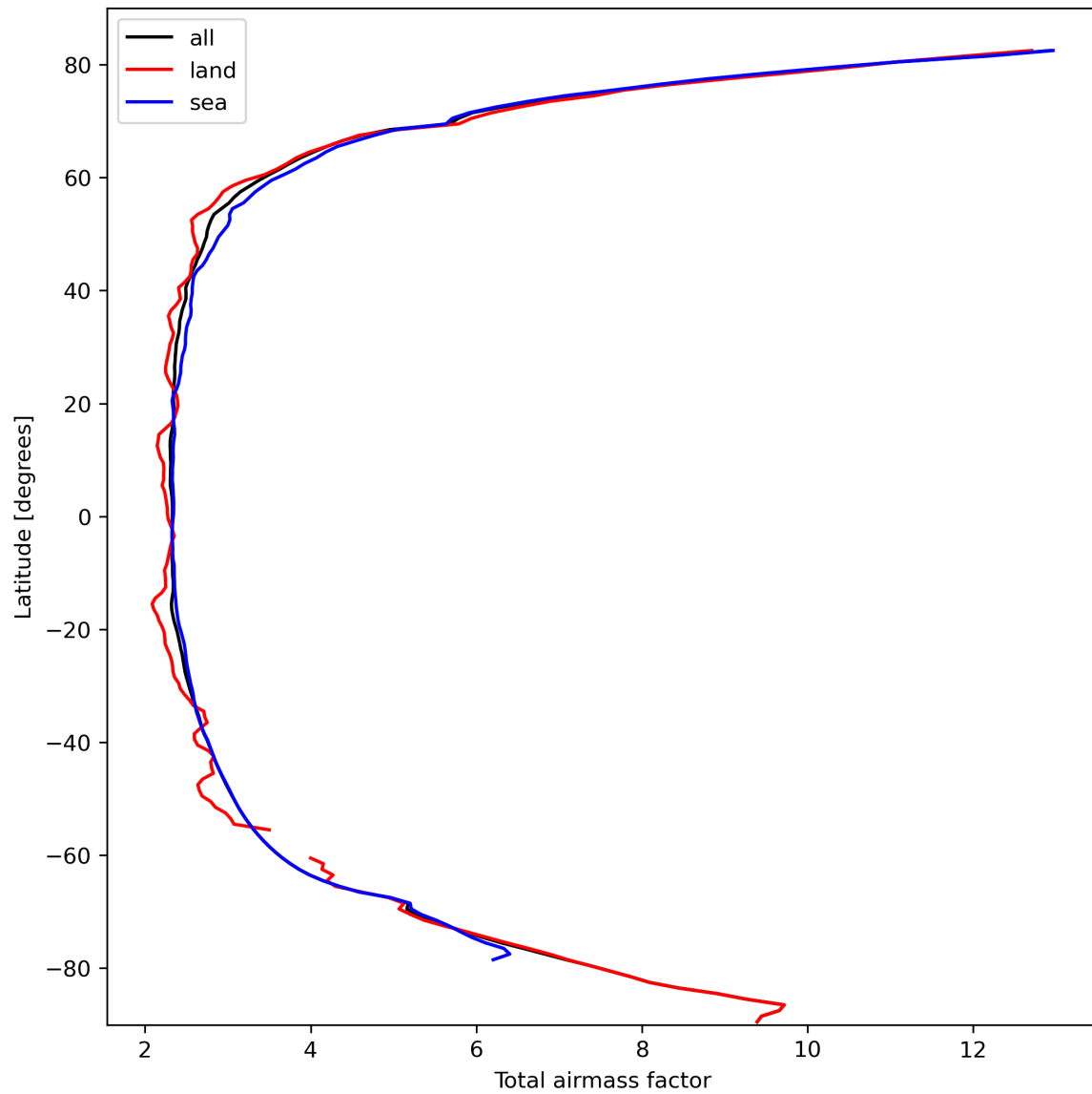
Figure 15: Zonal average of “Total airmass factor” for 2023-10-06 to 2023-10-08.
