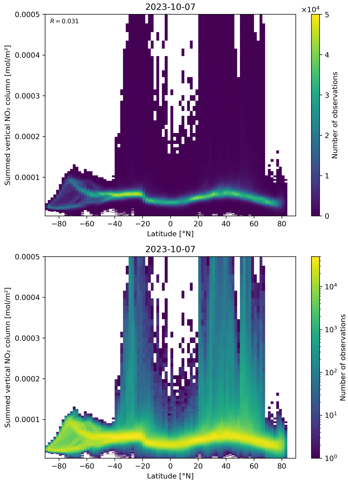
Figure 88: Scatter density plot of “Latitude” against “Summed vertical NO 2 column” for 2023-10-06 to 2023-10-08.
