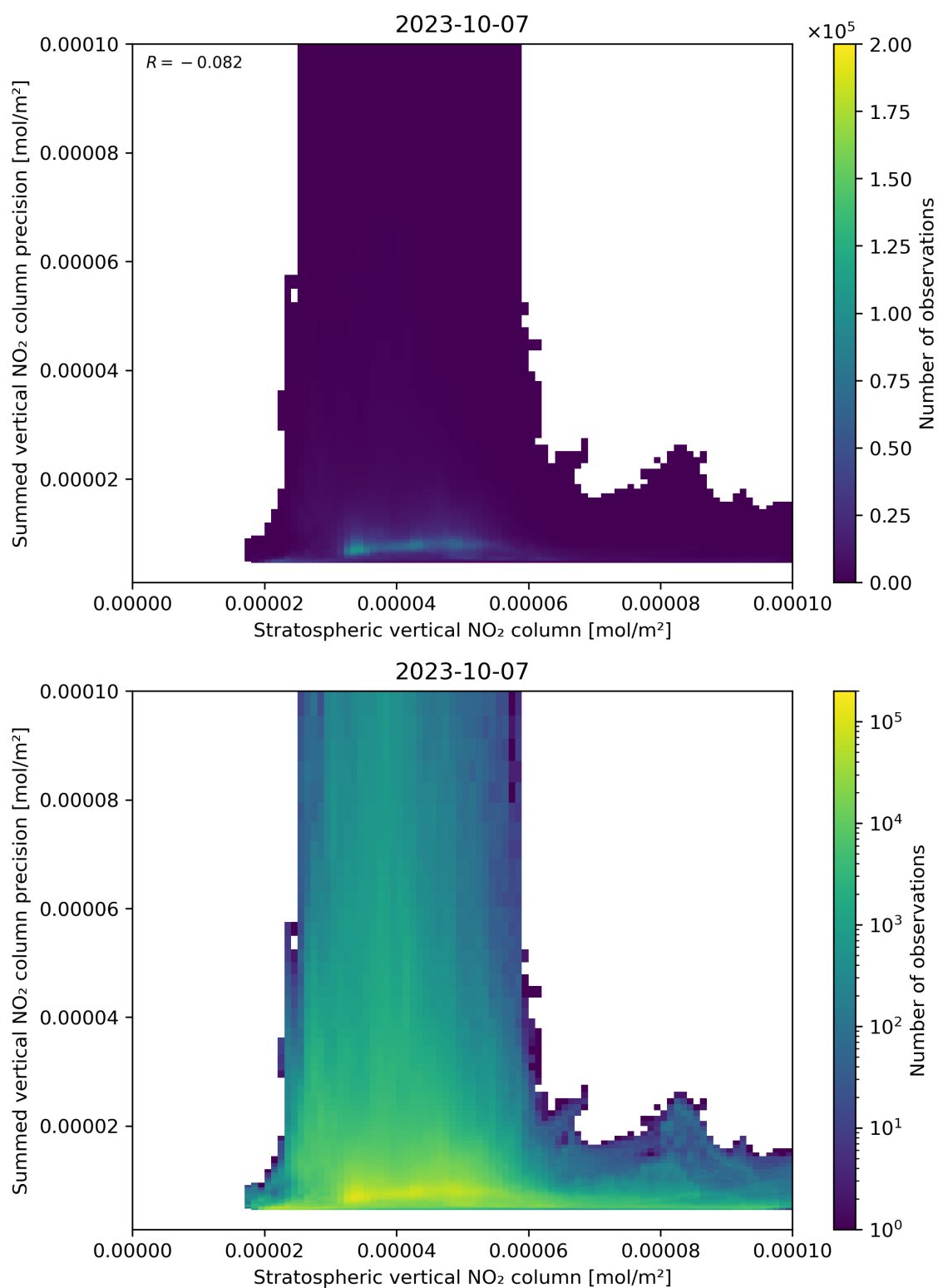
Figure 99: Scatter density plot of “Stratospheric vertical NO 2 column” against “Summed vertical NO 2 column precision” for 2023-10-06 to 2023-10-08.
