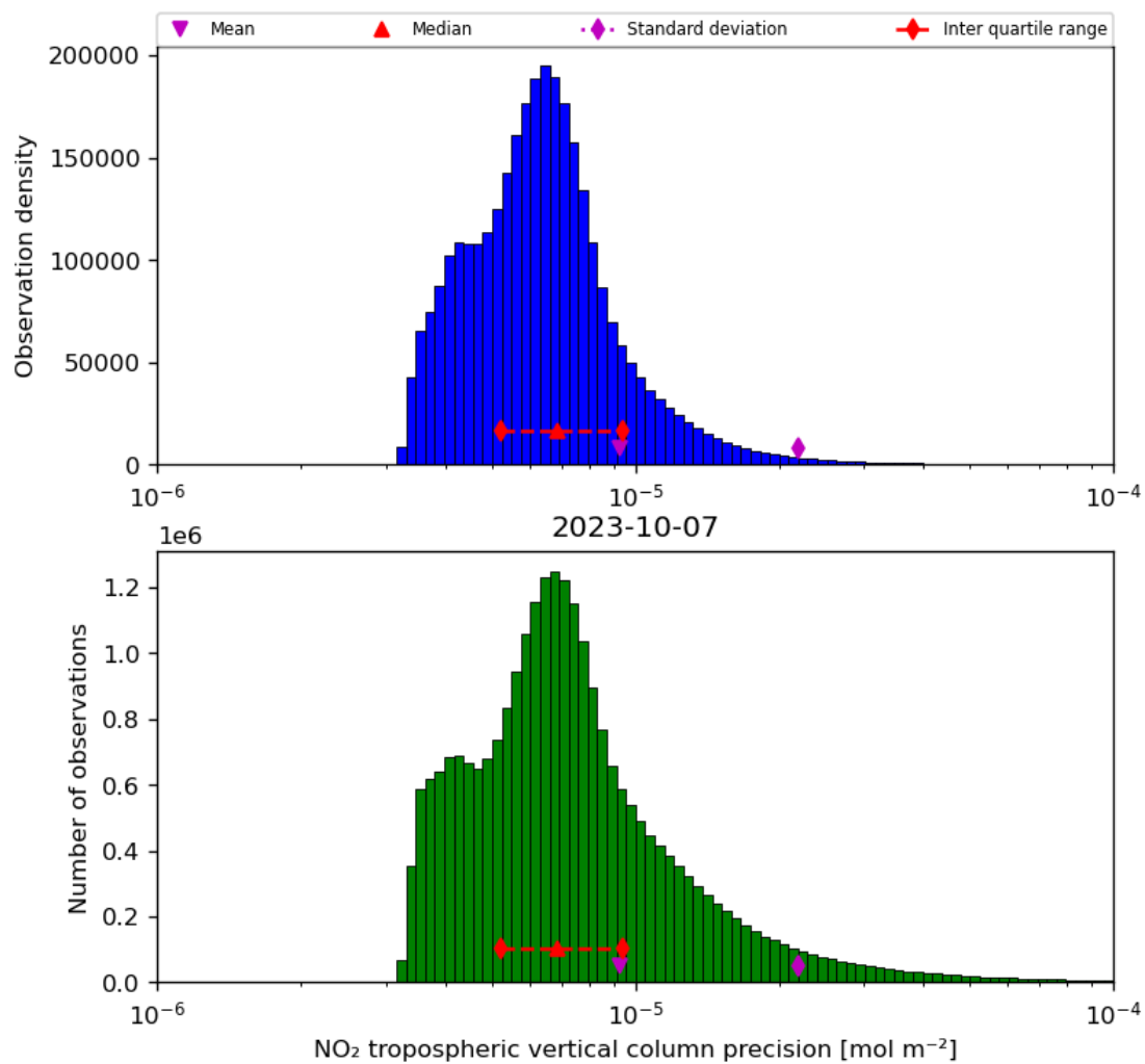
Figure 30: Histogram of “NO 2 tropospheric vertical column precision” for 2023-10-06 to 2023-10-08
