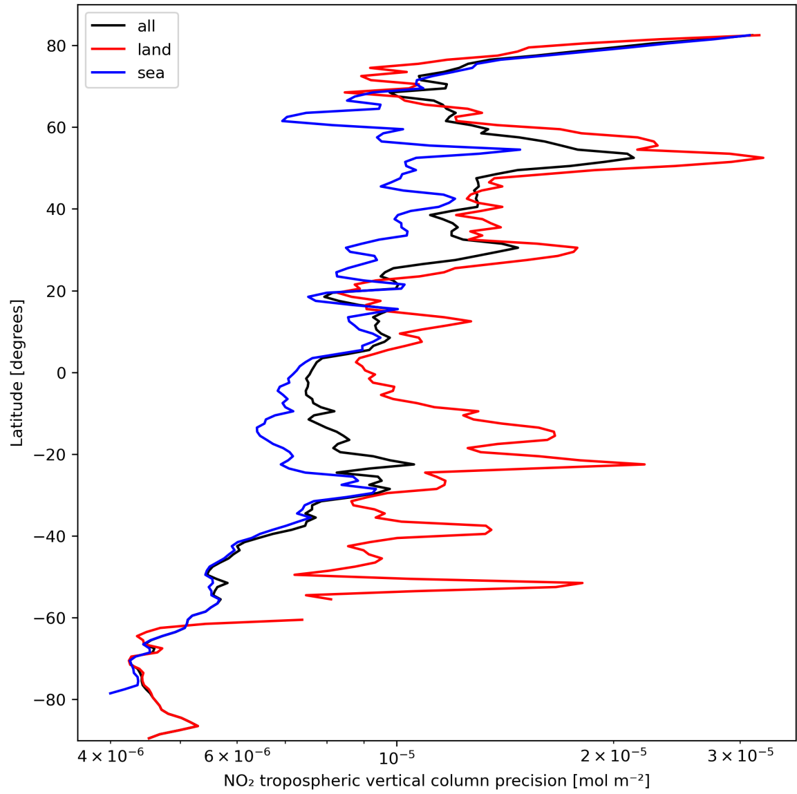
Figure 13: Zonal average of “NO 2 tropospheric vertical column precision” for 2023-10-06 to 2023-10-08.
