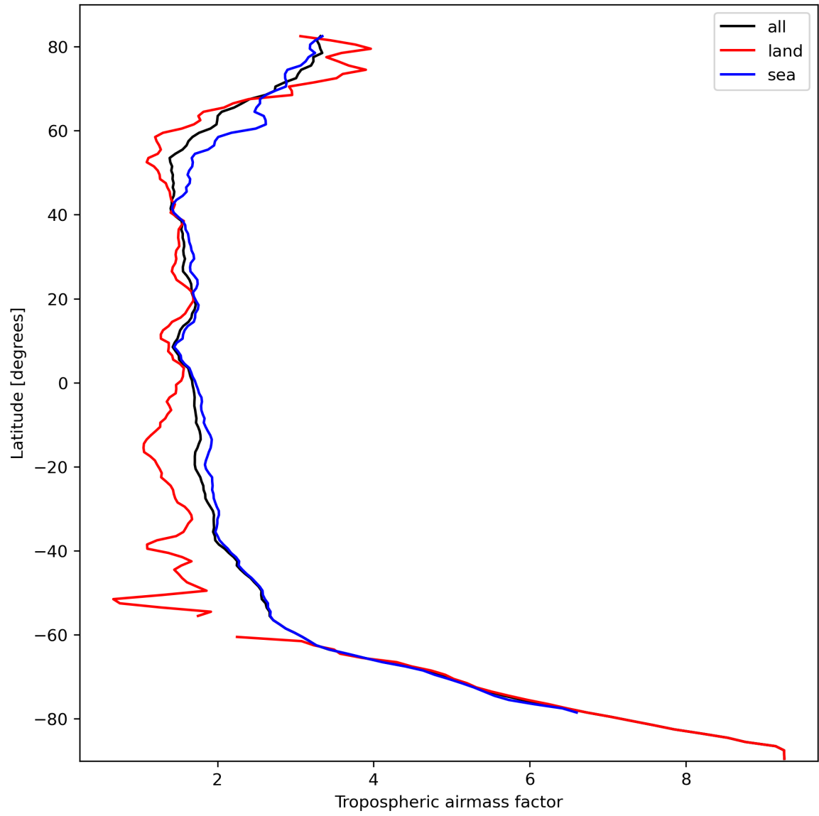
Figure 14: Zonal average of “Tropospheric airmass factor” for 2023-10-06 to 2023-10-08.
