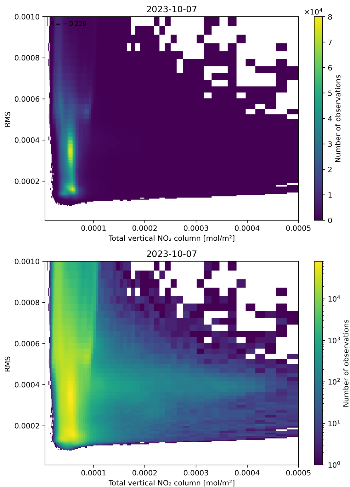
Figure 120: Scatter density plot of “Total vertical NO 2 column” against “RMS” for 2023-10-06 to 2023-10-08.
