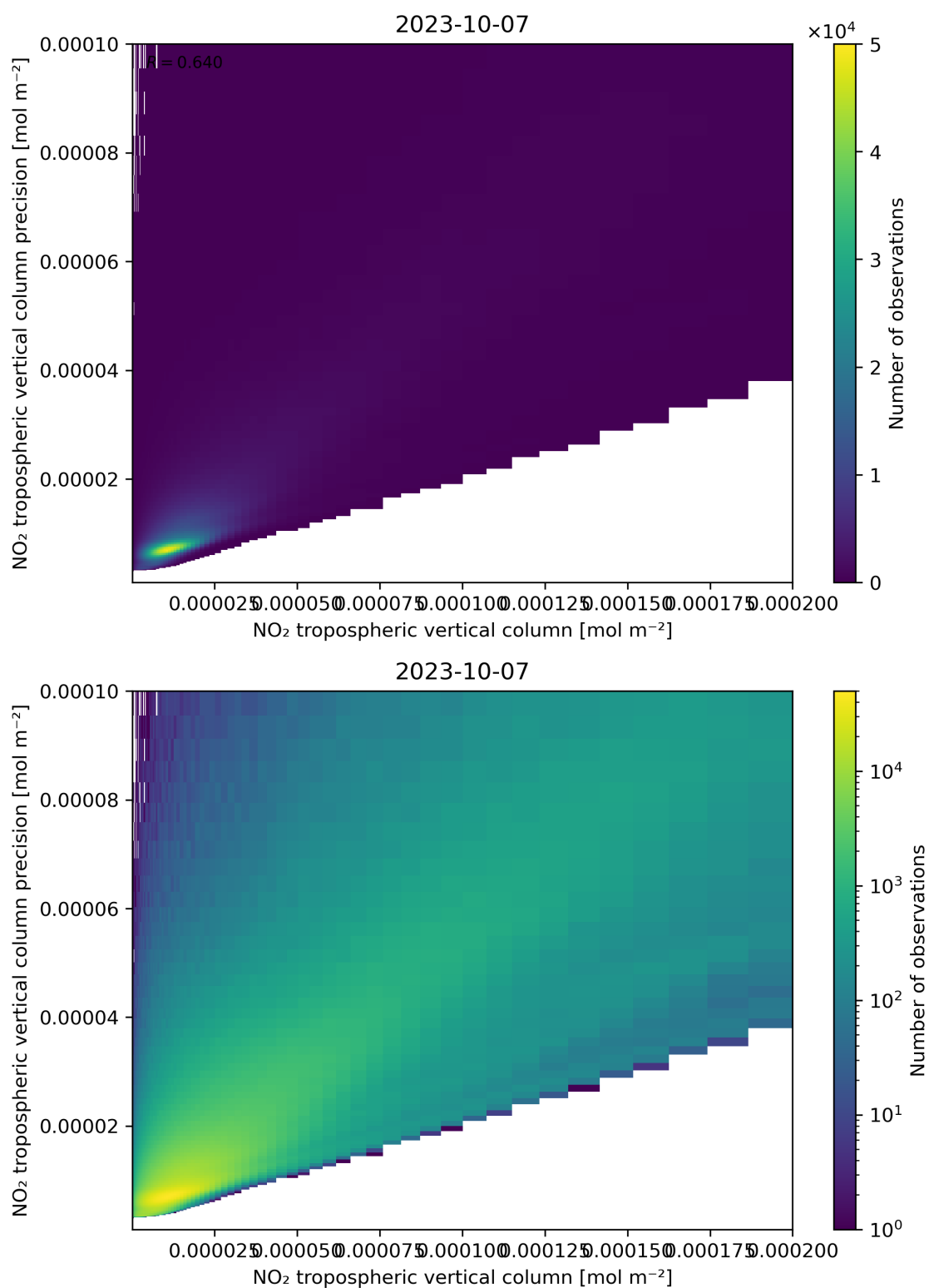
Figure 130: Scatter density plot of “NO 2 tropospheric vertical column” against “NO 2 tropospheric vertical column precision” for 2023-10-06 to 2023-10-08.
