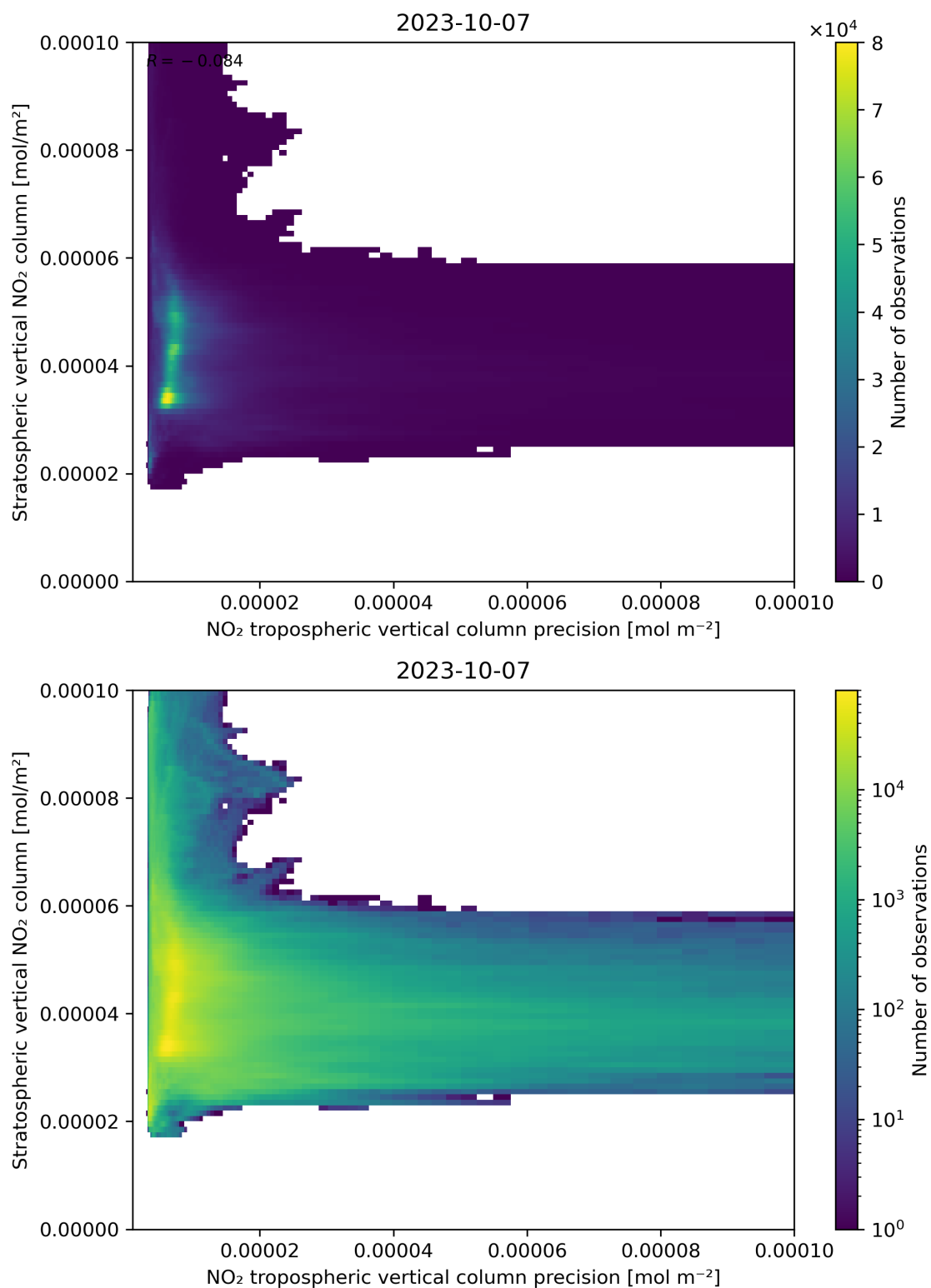
Figure 135: Scatter density plot of “NO 2 tropospheric vertical column precision” against “Stratospheric vertical NO 2 column” for 2023-10-06 to 2023-10-08.
