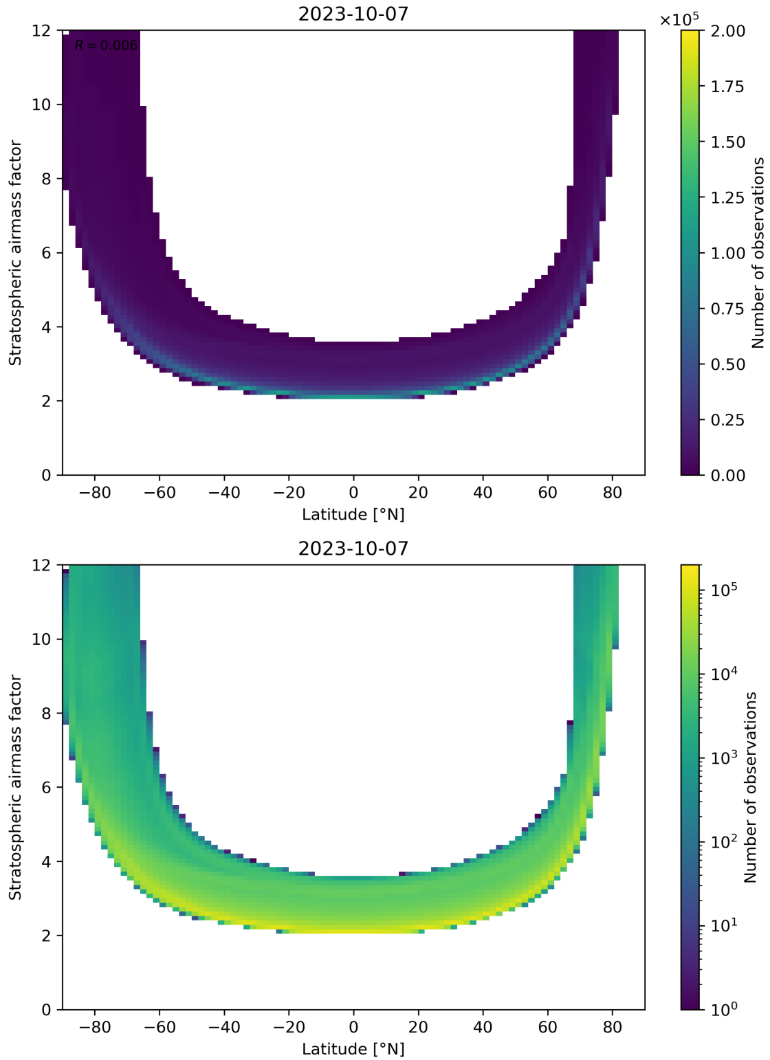
Figure 83: Scatter density plot of “Latitude” against “Stratospheric airmass factor” for 2023-10-06 to 2023-10-08.
