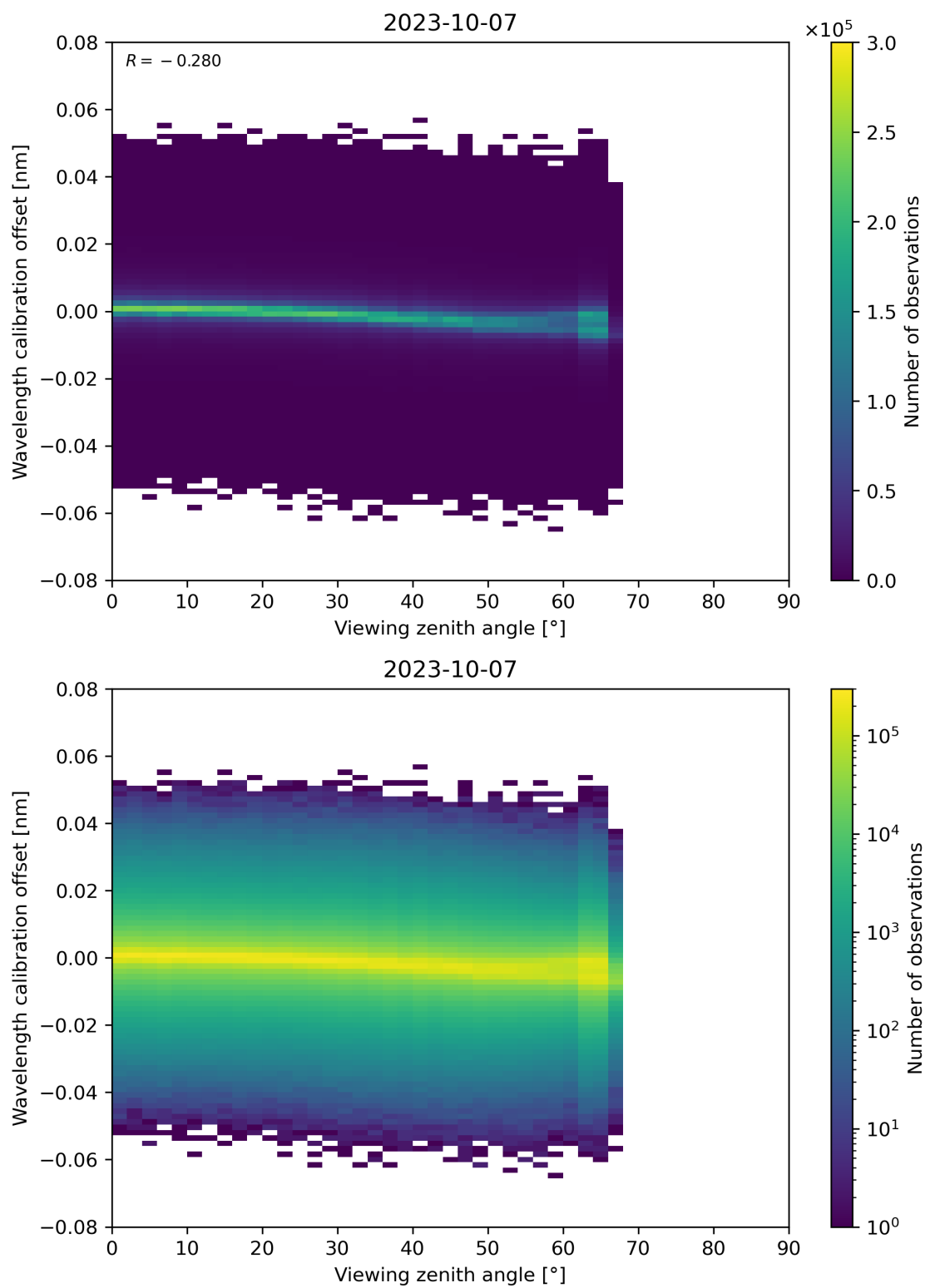
Figure 173: Scatter density plot of “Viewing zenith angle” against “Wavelength calibration offset” for 2023-10-06 to 2023-10-08.
