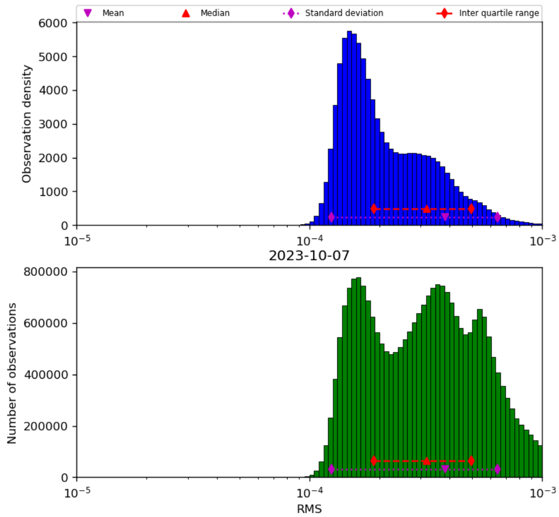
Figure 43: Histogram of “RMS” for 2023-10-06 to 2023-10-08
