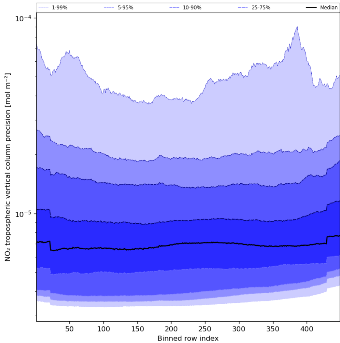
Figure 47: Along track statistics of “NO 2 tropospheric vertical column precision” for 2023-10-06 to 2023-10-08
