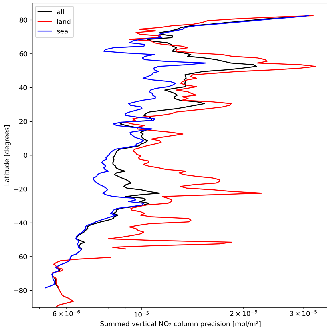
Figure 24: Zonal average of “Summed vertical NO 2 column precision” for 2023-10-06 to 2023-10-08.
