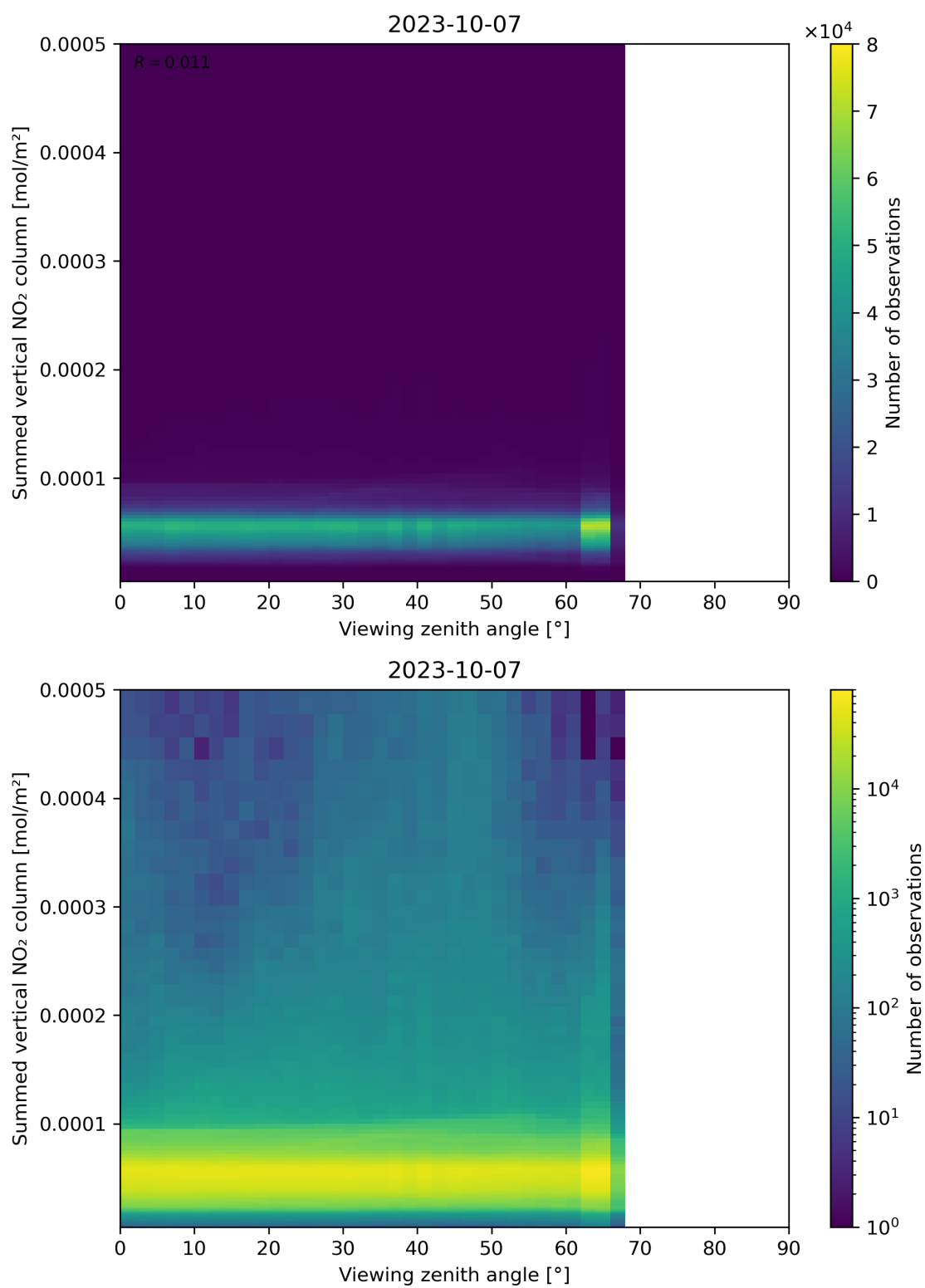
Figure 165: Scatter density plot of “Viewing zenith angle” against “Summed vertical NO 2 column” for 2023-10-06 to 2023-10-08.
