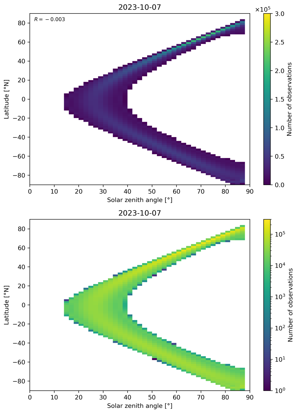
Figure 149: Scatter density plot of “Solar zenith angle” against “Latitude” for 2023-10-06 to 2023-10-08.
