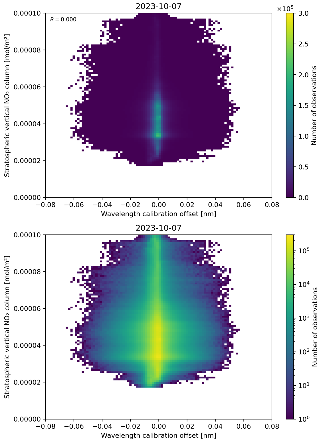
Figure 176: Scatter density plot of “Wavelength calibration offset” against “Stratospheric vertical NO 2 column” for 2023-10-06 to 2023-10-08.
