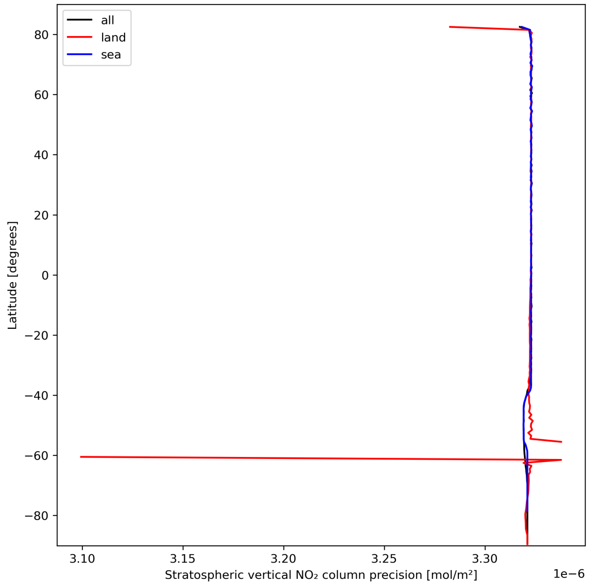
Figure 20: Zonal average of “Stratospheric vertical NO 2 column precision” for 2023-10-06 to 2023-10-08.
