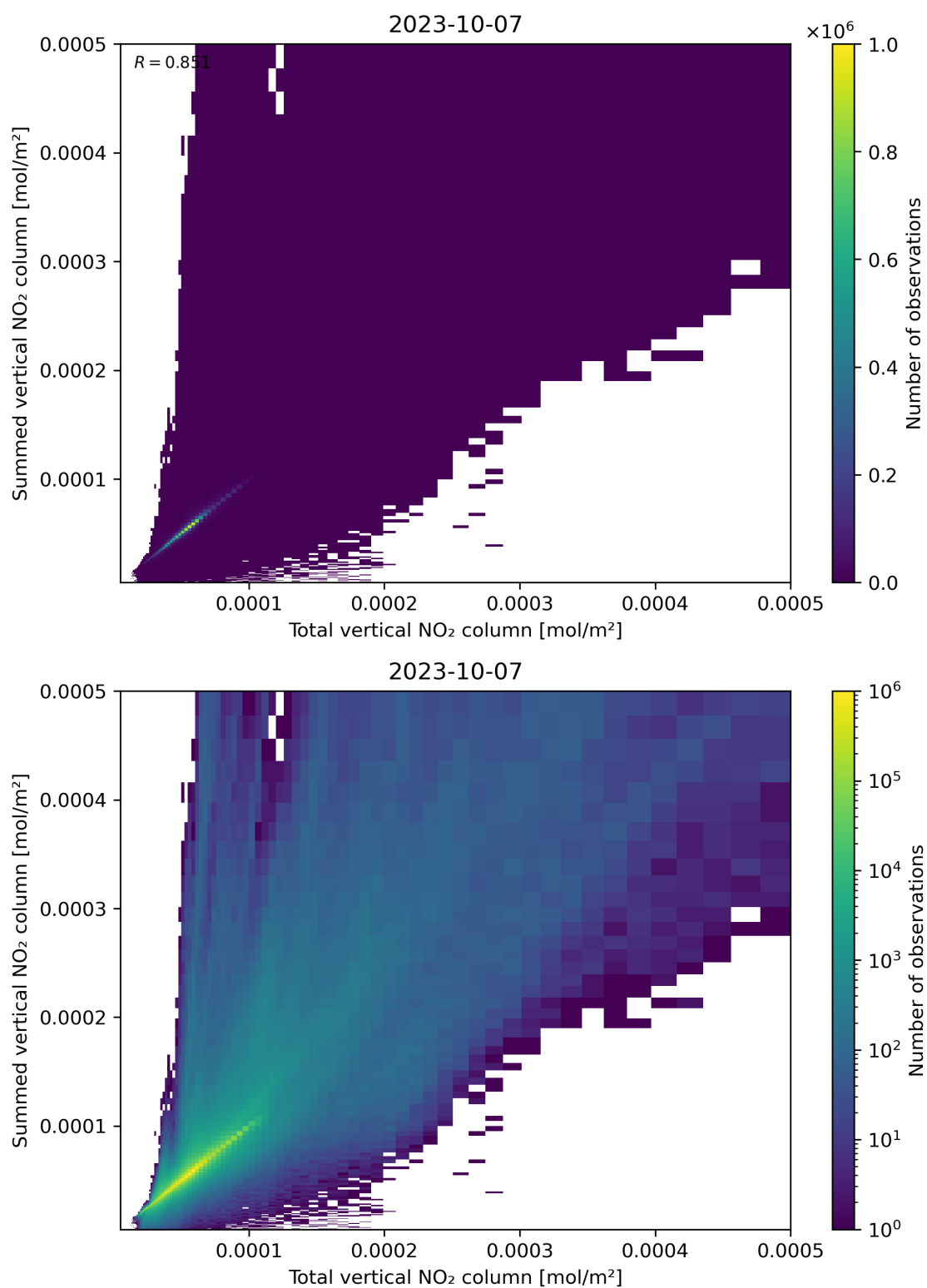
Figure 112: Scatter density plot of “Total vertical NO 2 column” against “Summed vertical NO 2 column” for 2023-10-06 to 2023-10-08.
