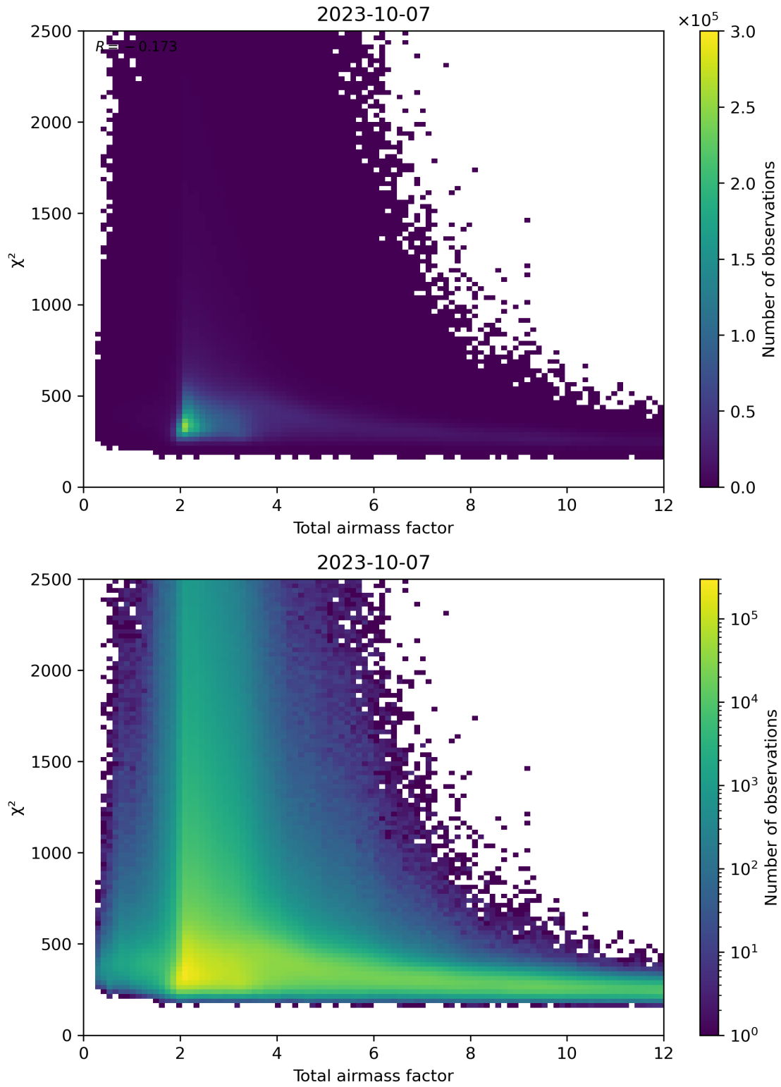
Figure 63: Scatter density plot of “Total airmass factor” against “ \chi^2 ” for 2023-10-06 to 2023-10-08.
