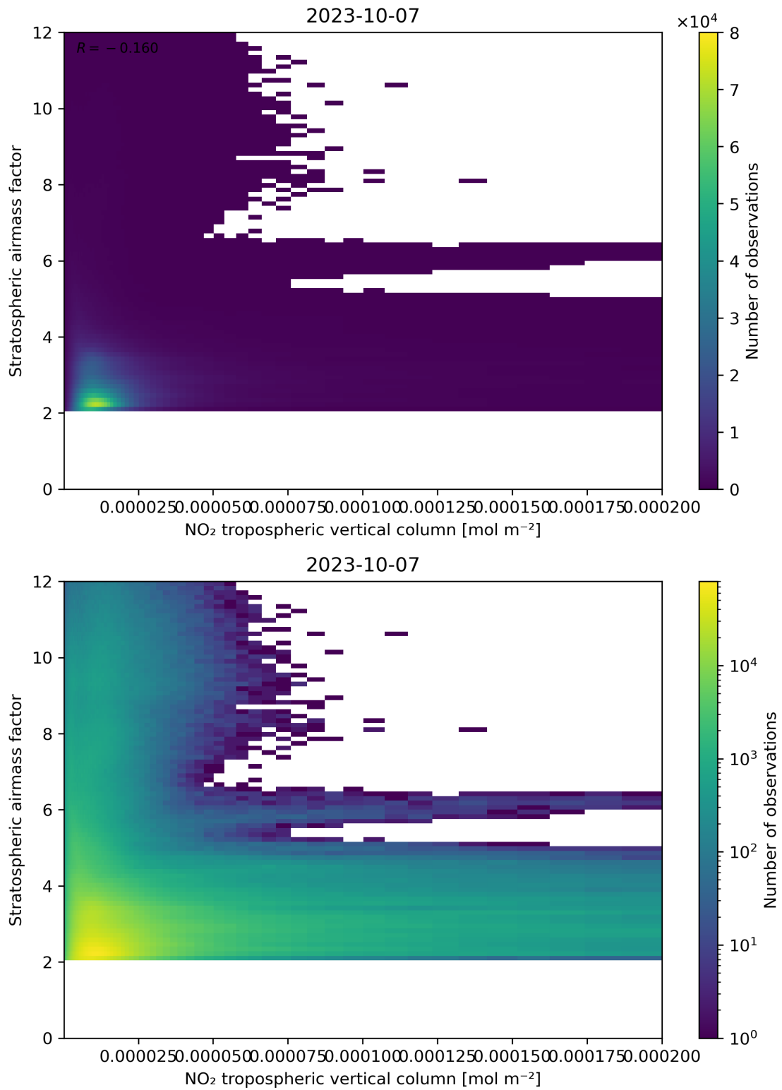
Figure 121: Scatter density plot of “NO 2 tropospheric vertical column” against “Stratospheric air mass factor” for 2023-10-06 to 2023-10-08.
