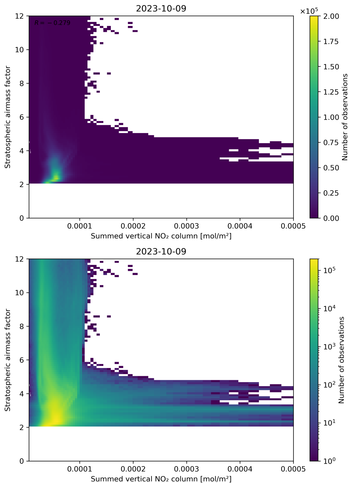
Figure 103: Scatter density plot of “Summed vertical NO 2 column” against “Stratospheric airmass factor” for 2023-10-08 to 2023-10-10.
