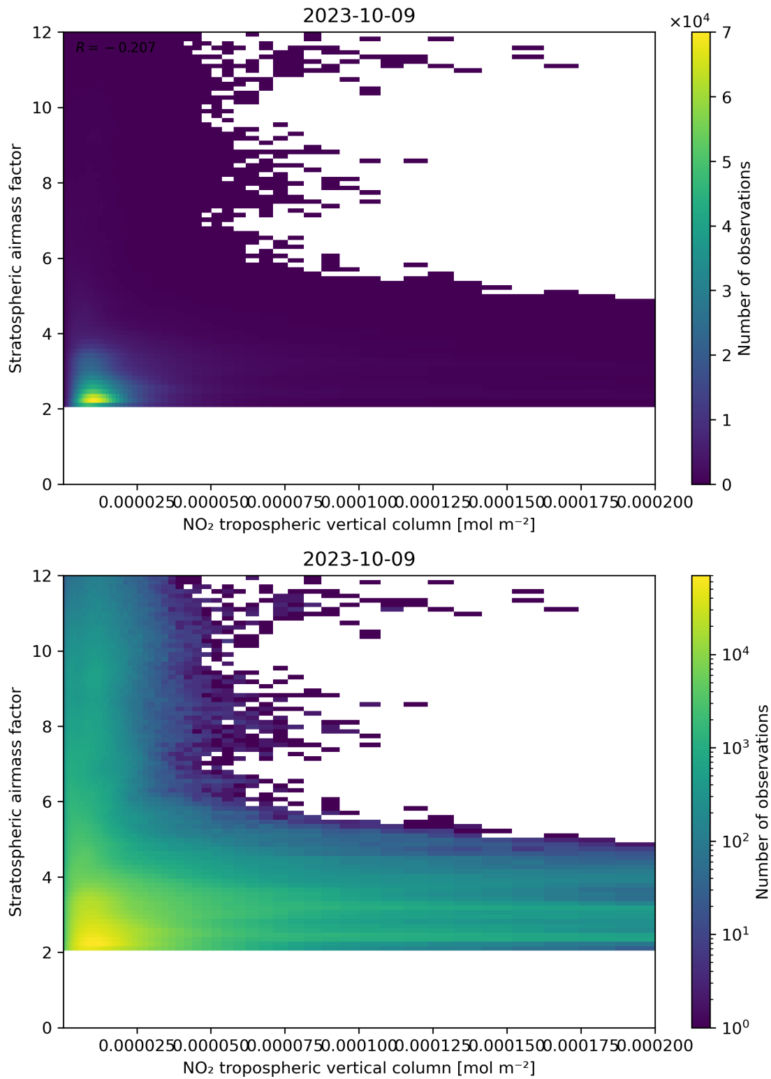
Figure 121: Scatter density plot of “NO 2 tropospheric vertical column” against “Stratospheric air mass factor” for 2023-10-08 to 2023-10-10.
