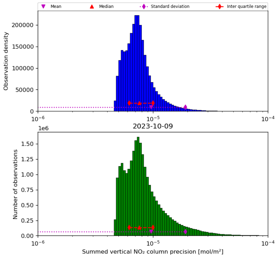
Figure 41: Histogram of “Summed vertical NO 2 column precision” for 2023-10-08 to 2023-10-10
