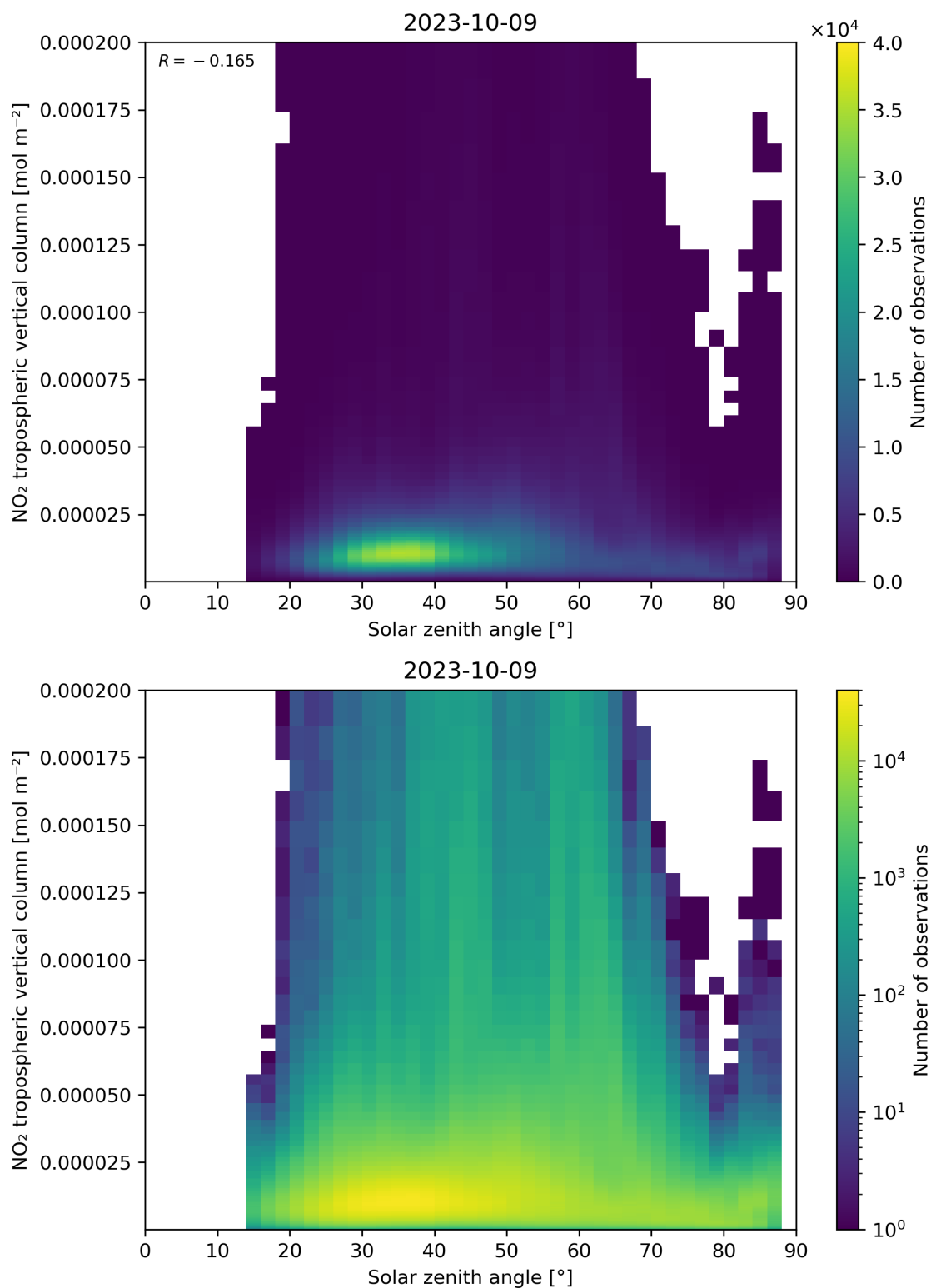
Figure 155: Scatter density plot of “Solar zenith angle” against “NO 2 tropospheric vertical column” for 2023-10-08 to 2023-10-10.
