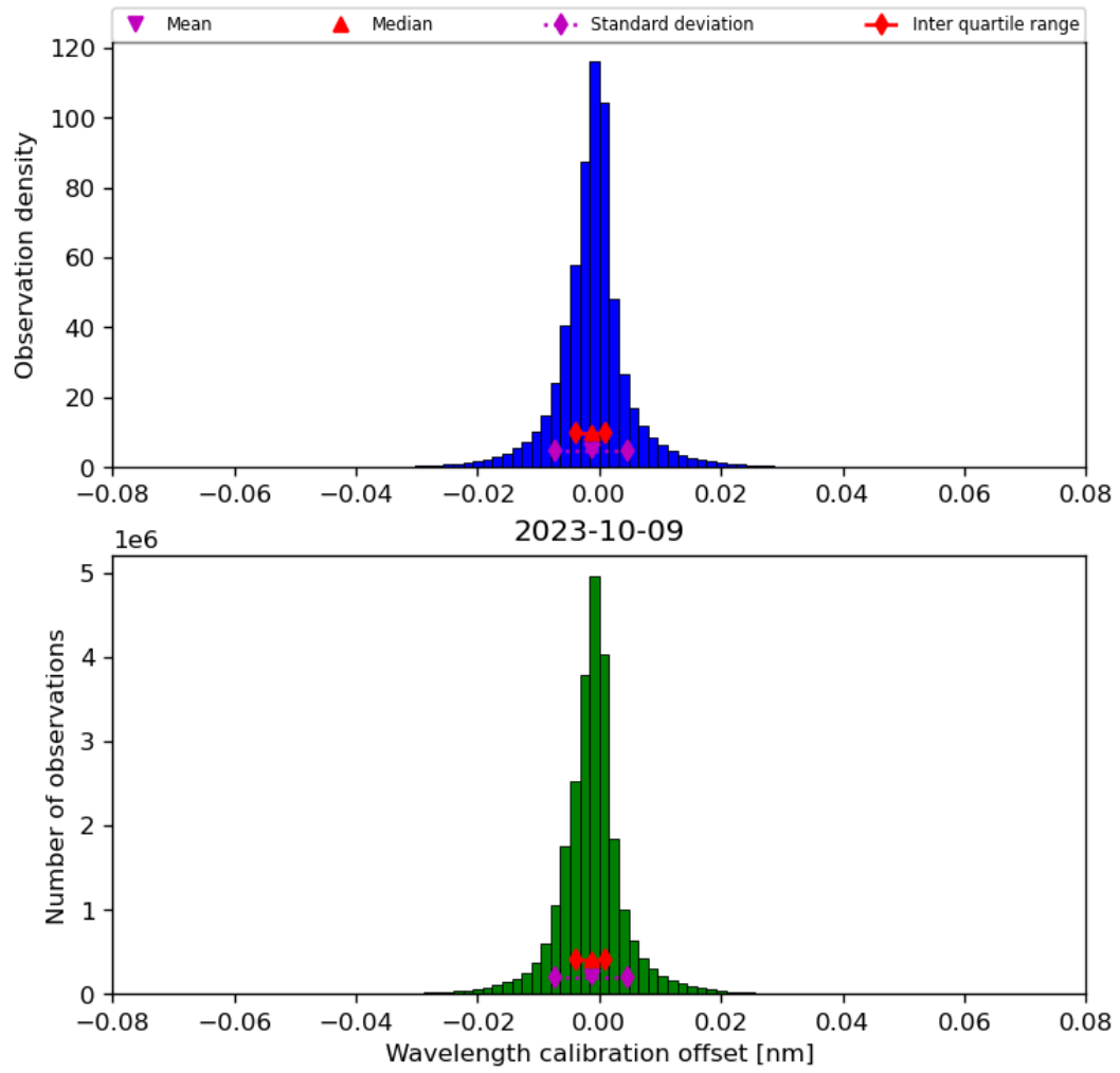
Figure 35: Histogram of “Wavelength calibration offset” for 2023-10-08 to 2023-10-10
