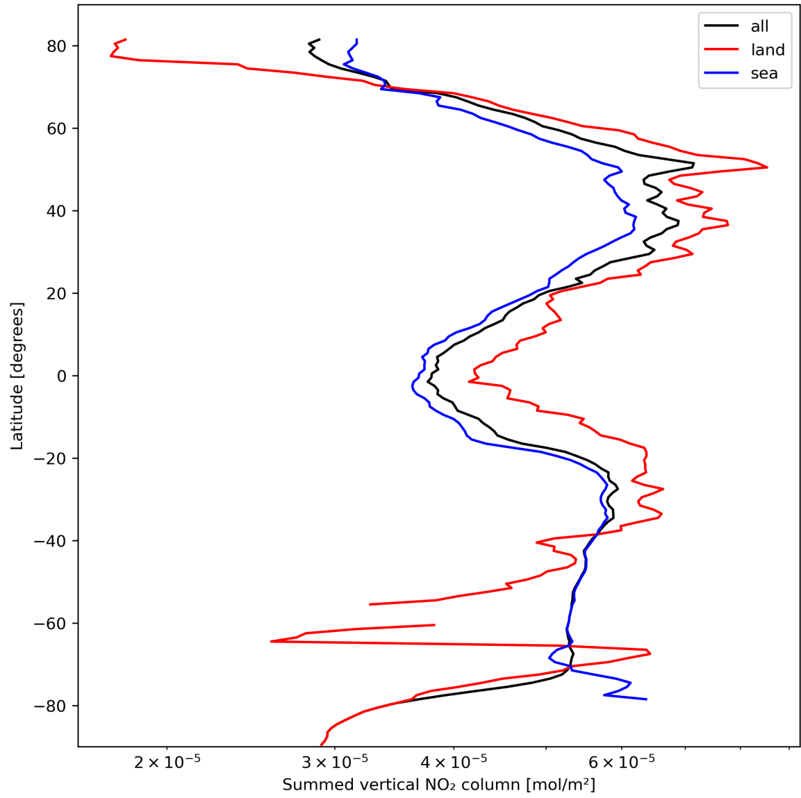
Figure 23: Zonal average of “Summed vertical NO 2 column” for 2023-10-08 to 2023-10-10.
