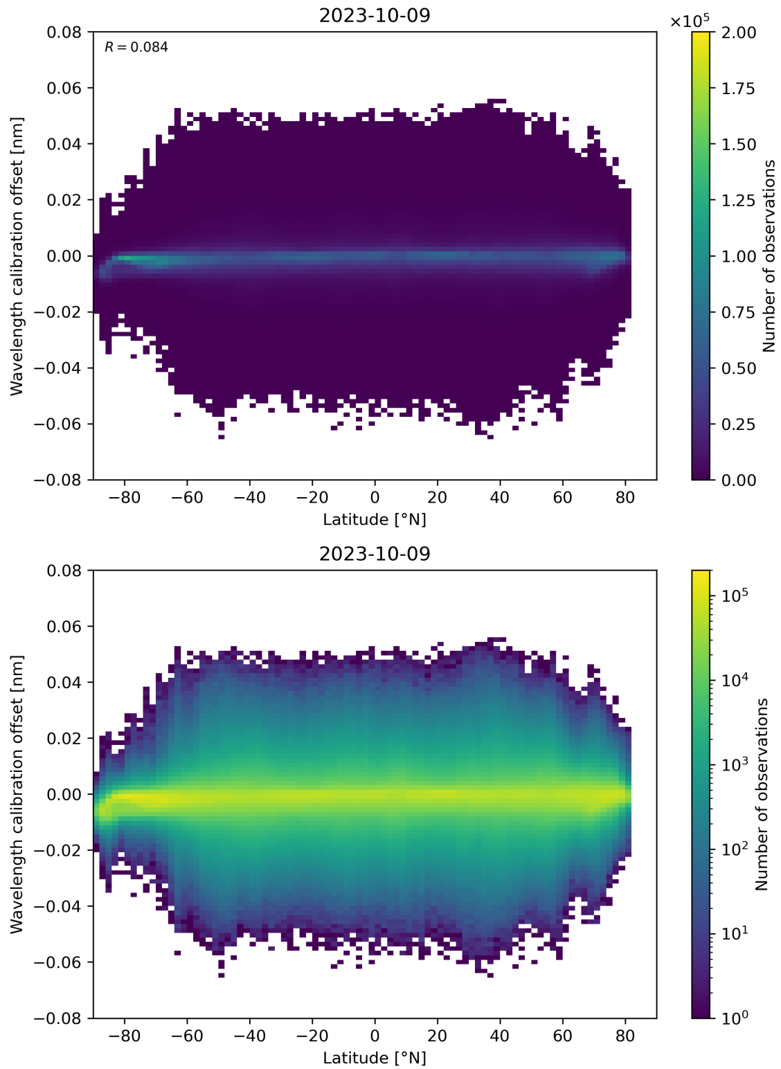
Figure 95: Scatter density plot of “Latitude” against “Wavelength calibration offset” for 2023-10-08 to 2023-10-10.
