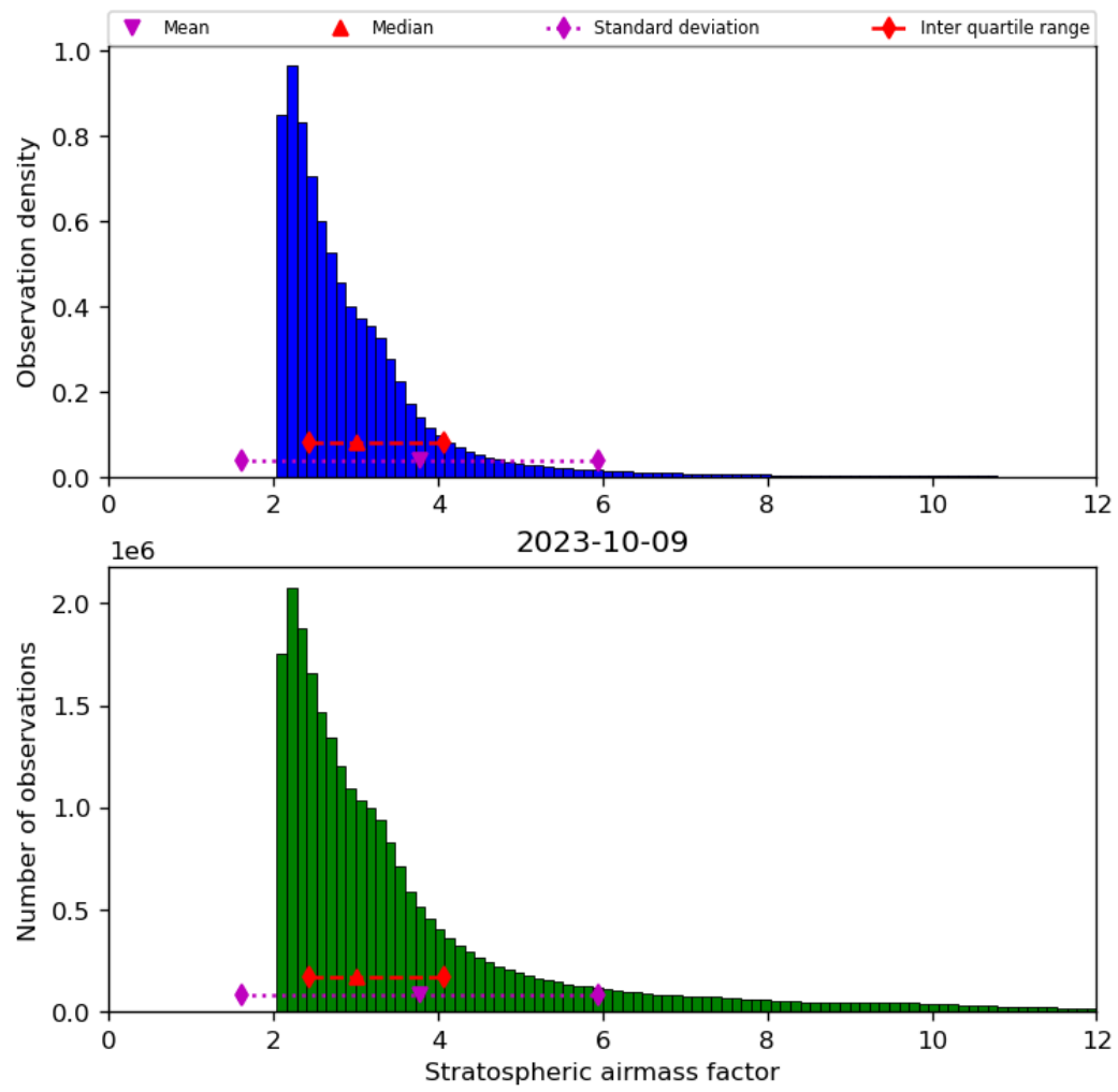
Figure 44: Histogram of “Stratospheric airmass factor” for 2023-10-08 to 2023-10-10
