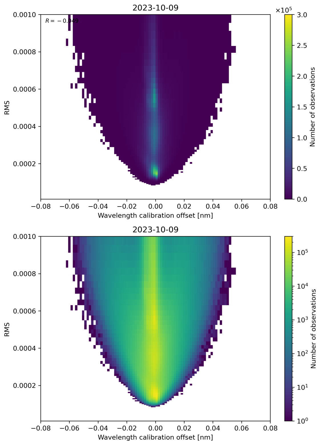
Figure 181: Scatter density plot of “Wavelength calibration offset” against “RMS” for 2023-10-08 to 2023-10-10.
