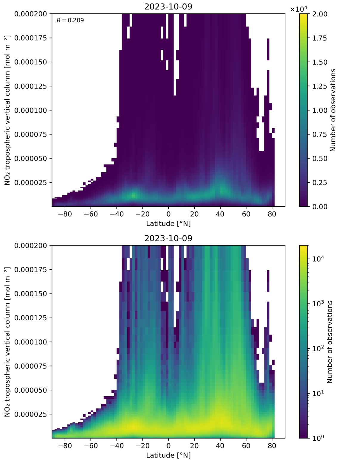
Figure 92: Scatter density plot of “Latitude” against “NO 2 tropospheric vertical column” for 2023-10-08 to 2023-10-10.
