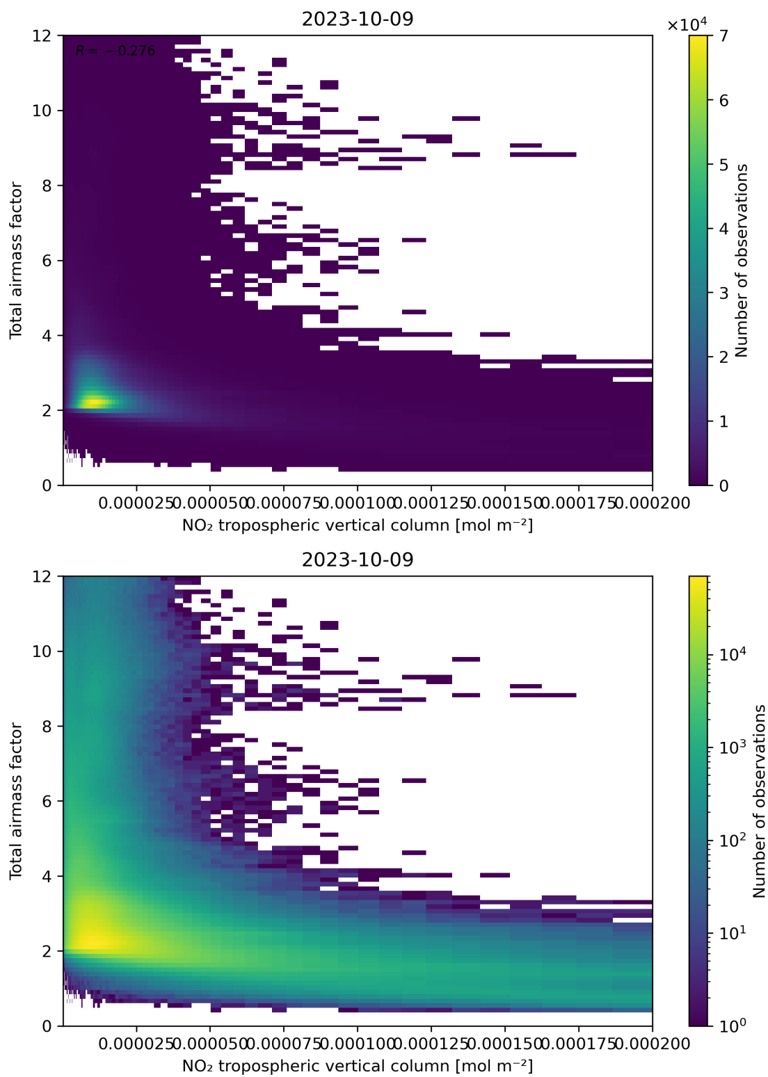
Figure 122: Scatter density plot of “NO 2 tropospheric vertical column” against “Total air mass factor” for 2023-10-08 to 2023-10-10.
