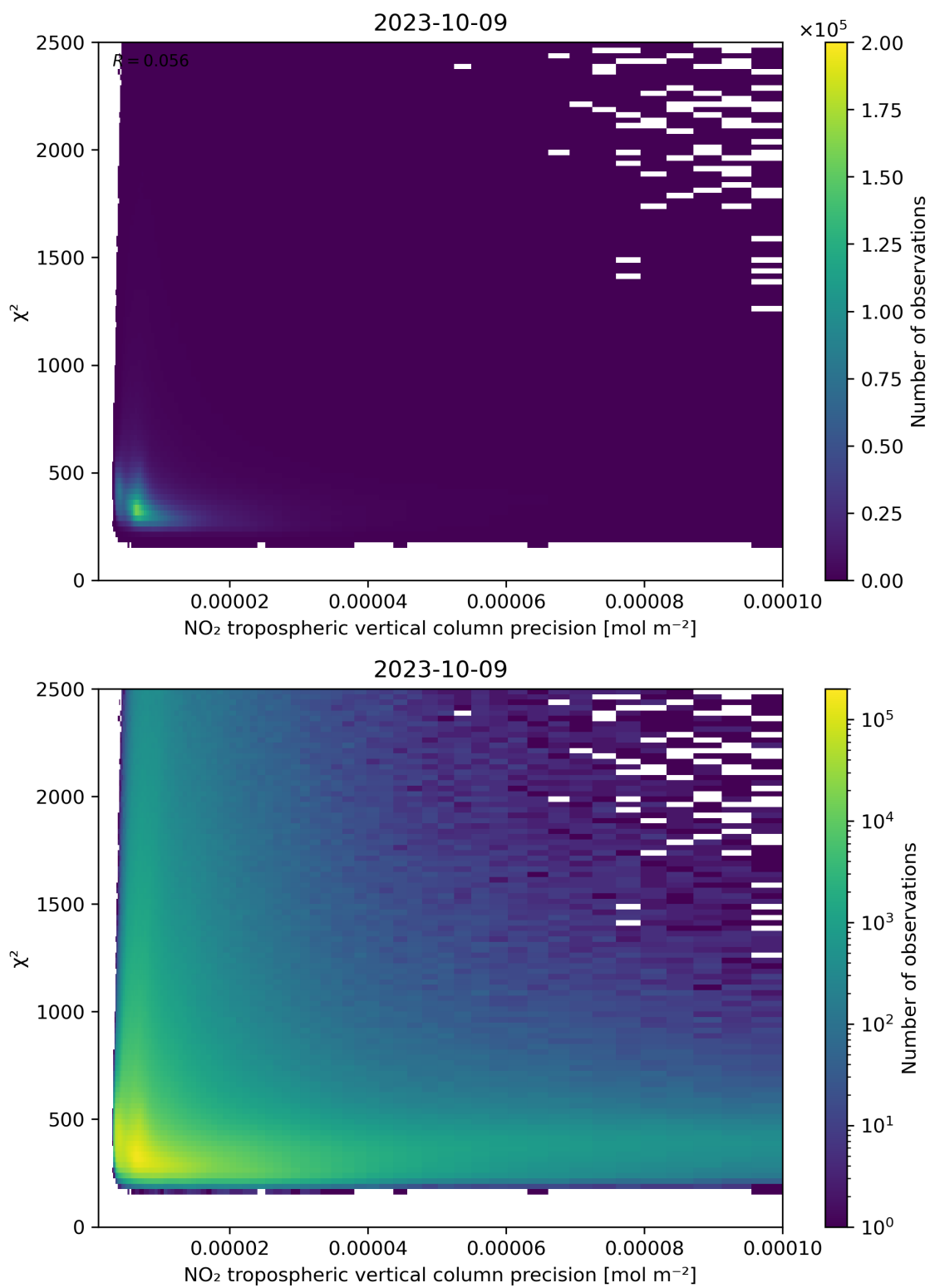
Figure 134: Scatter density plot of “NO 2 tropospheric vertical column precision” against “ \chi^2 ” for 2023-10-08 to 2023-10-10.
