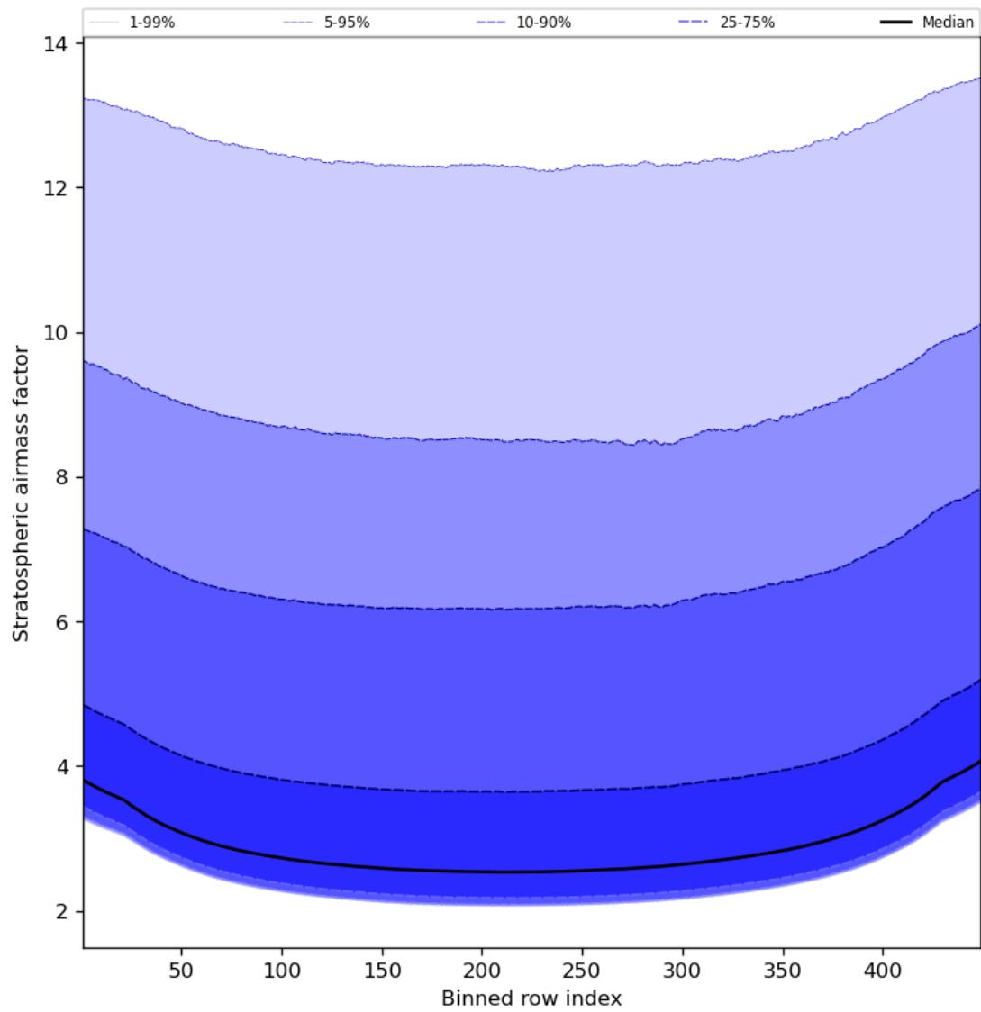
Figure 61: Along track statistics of “Stratospheric airmass factor” for 2023-10-08 to 2023-10-10
