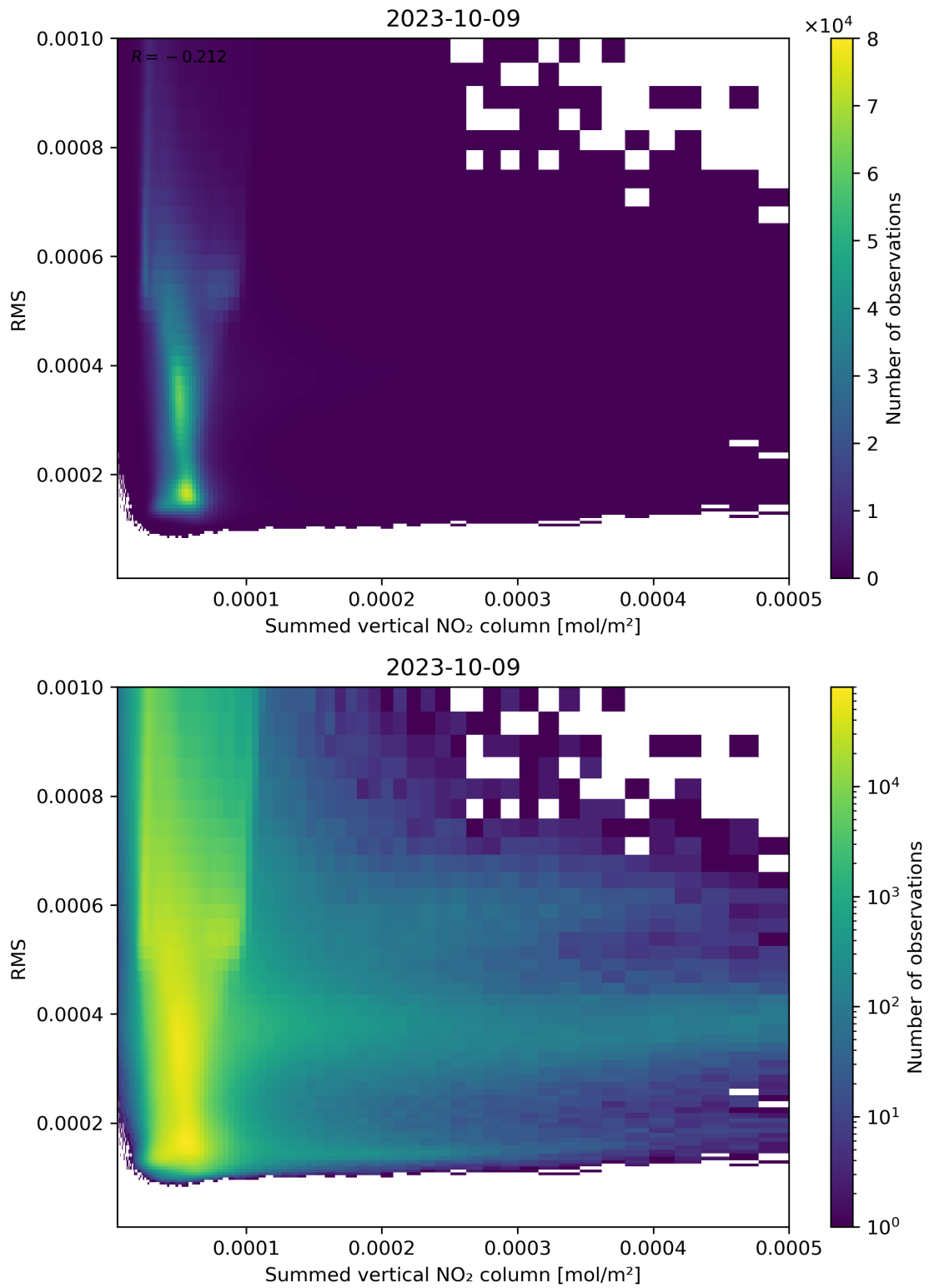
Figure 109: Scatter density plot of “Summed vertical NO 2 column” against “RMS” for 2023-10-08 to 2023-10-10.
