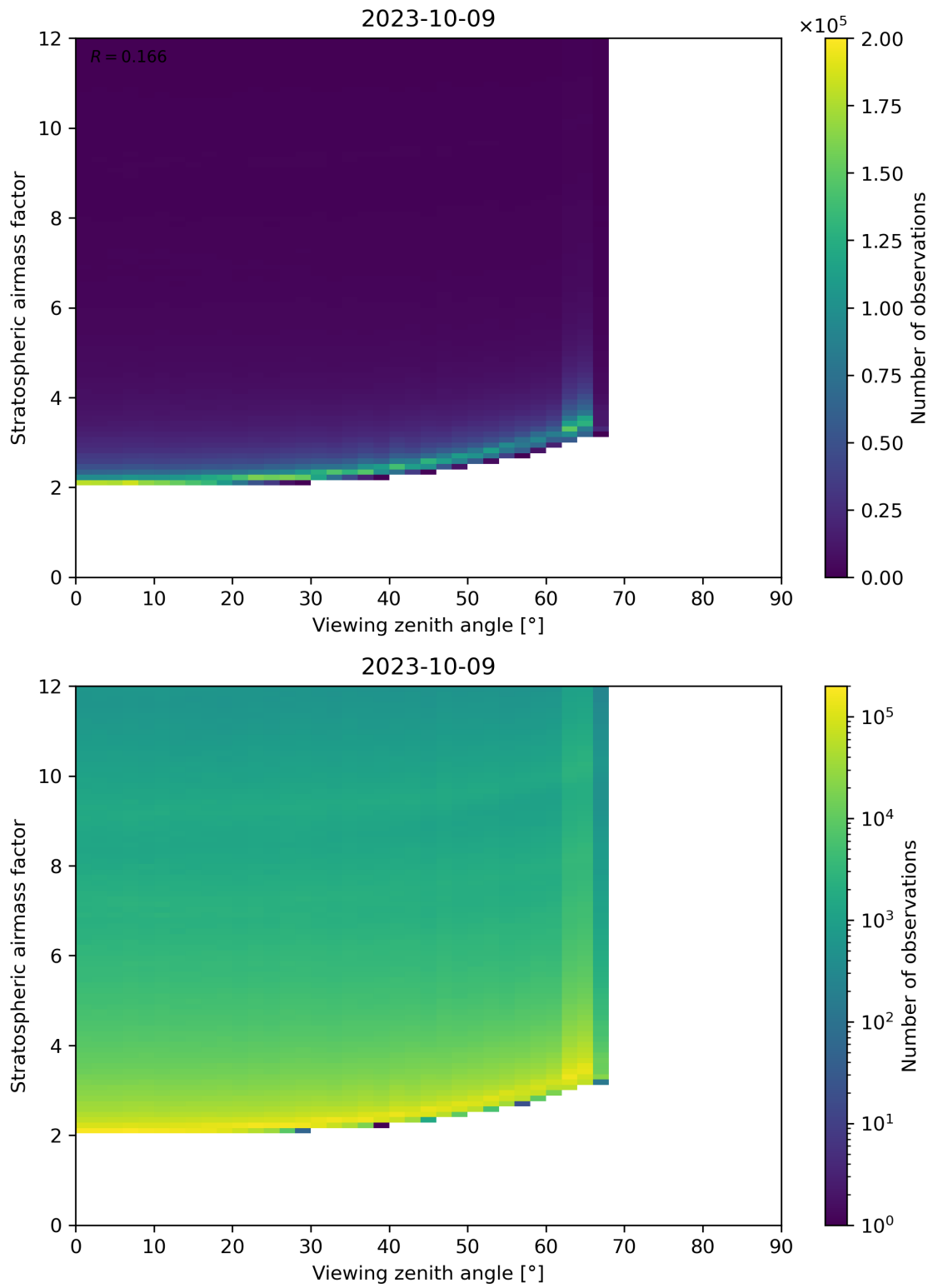
Figure 159: Scatter density plot of “Viewing zenith angle” against “Stratospheric airmass factor” for 2023-10-08 to 2023-10-10.
