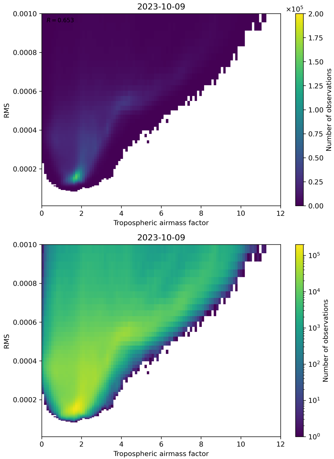
Figure 79: Scatter density plot of “Tropospheric airmass factor” against “RMS” for 2023-10-08 to 2023-10-10.
