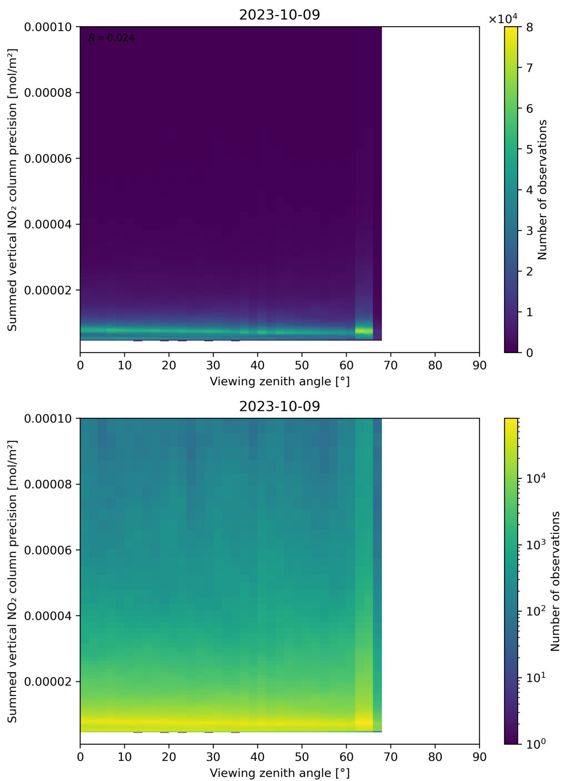
Figure 166: Scatter density plot of “Viewing zenith angle” against “Summed vertical NO 2 column precision” for 2023-10-08 to 2023-10-10.
