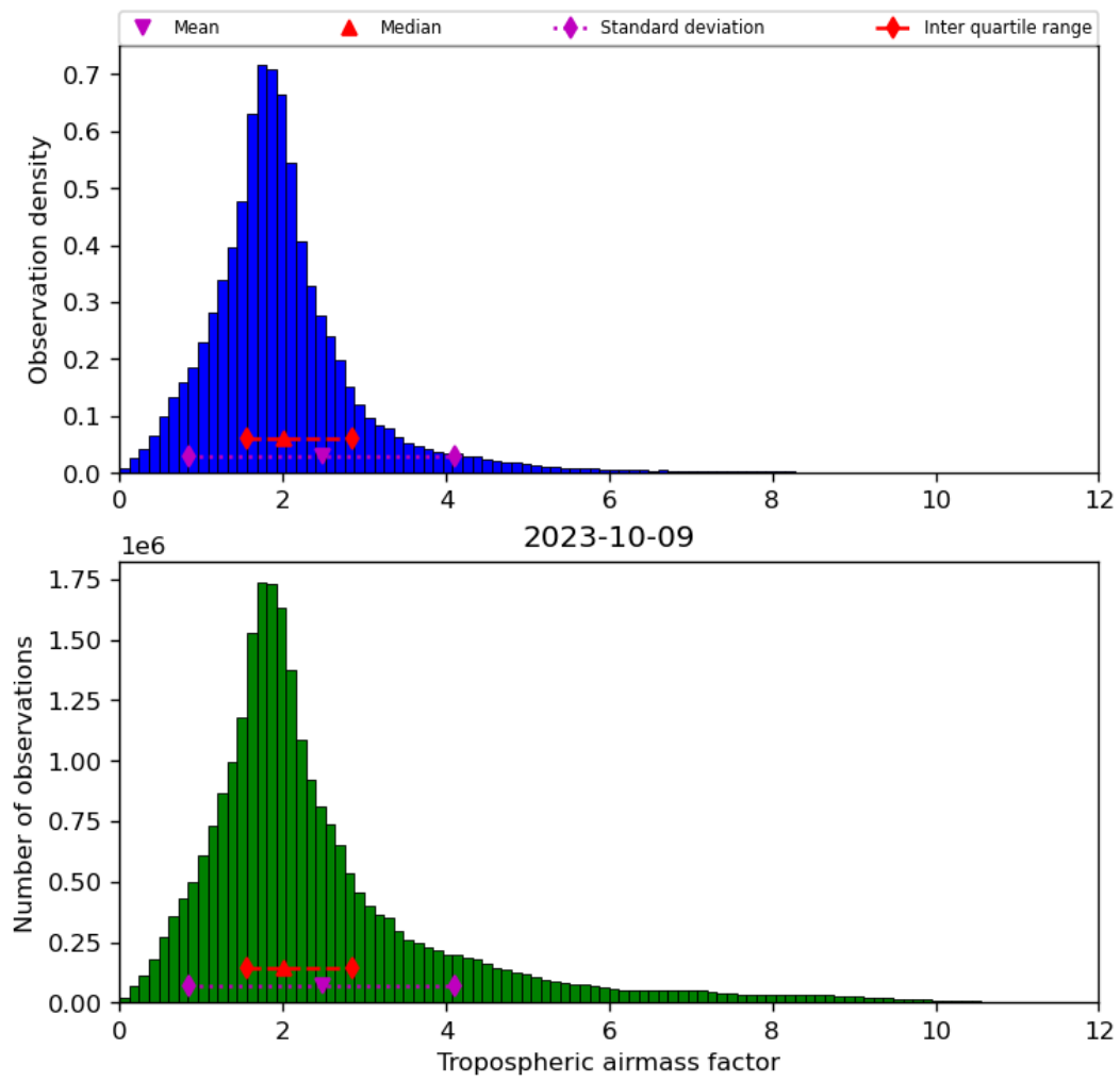
Figure 31: Histogram of “Tropospheric airmass factor” for 2023-10-08 to 2023-10-10
