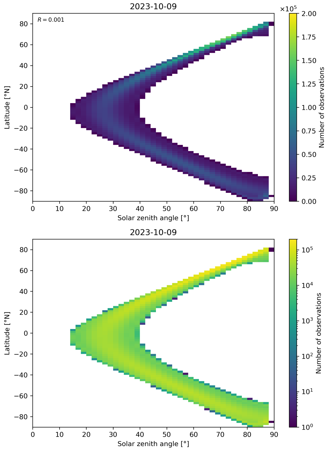
Figure 149: Scatter density plot of “Solar zenith angle” against “Latitude” for 2023-10-08 to 2023-10-10.
