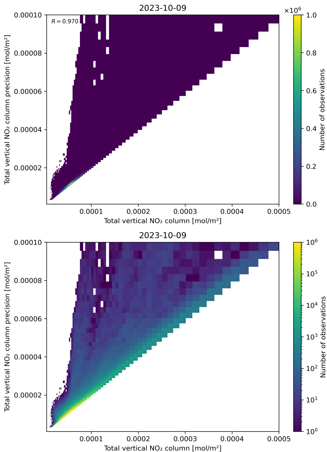
Figure 114: Scatter density plot of “Total vertical NO 2 column” against “Total vertical NO 2 column precision” for 2023-10-08 to 2023-10-10.
