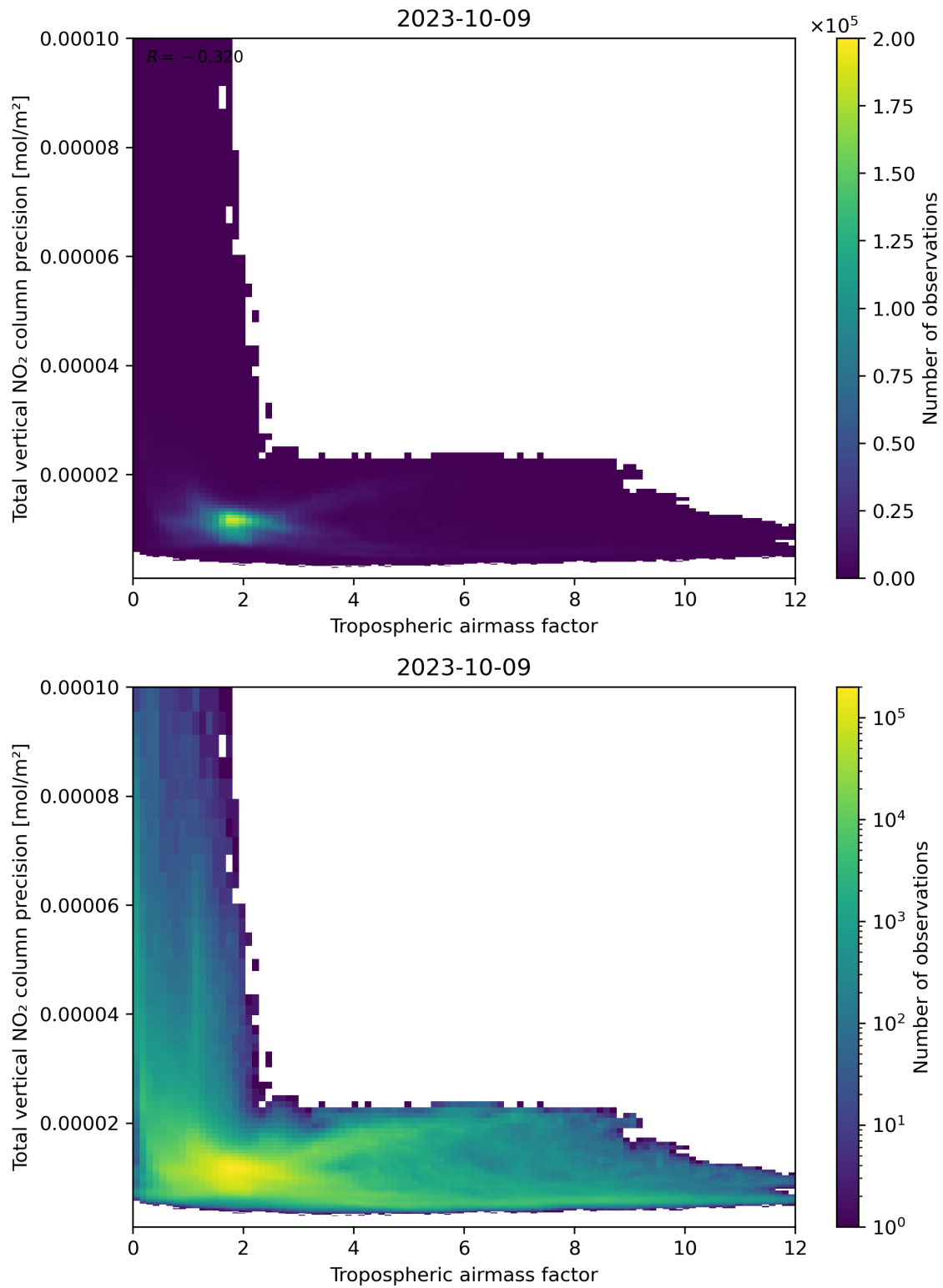
Figure 78: Scatter density plot of “Tropospheric air mass factor” against “Total vertical NO 2 column precision” for 2023-10-08 to 2023-10-10.
