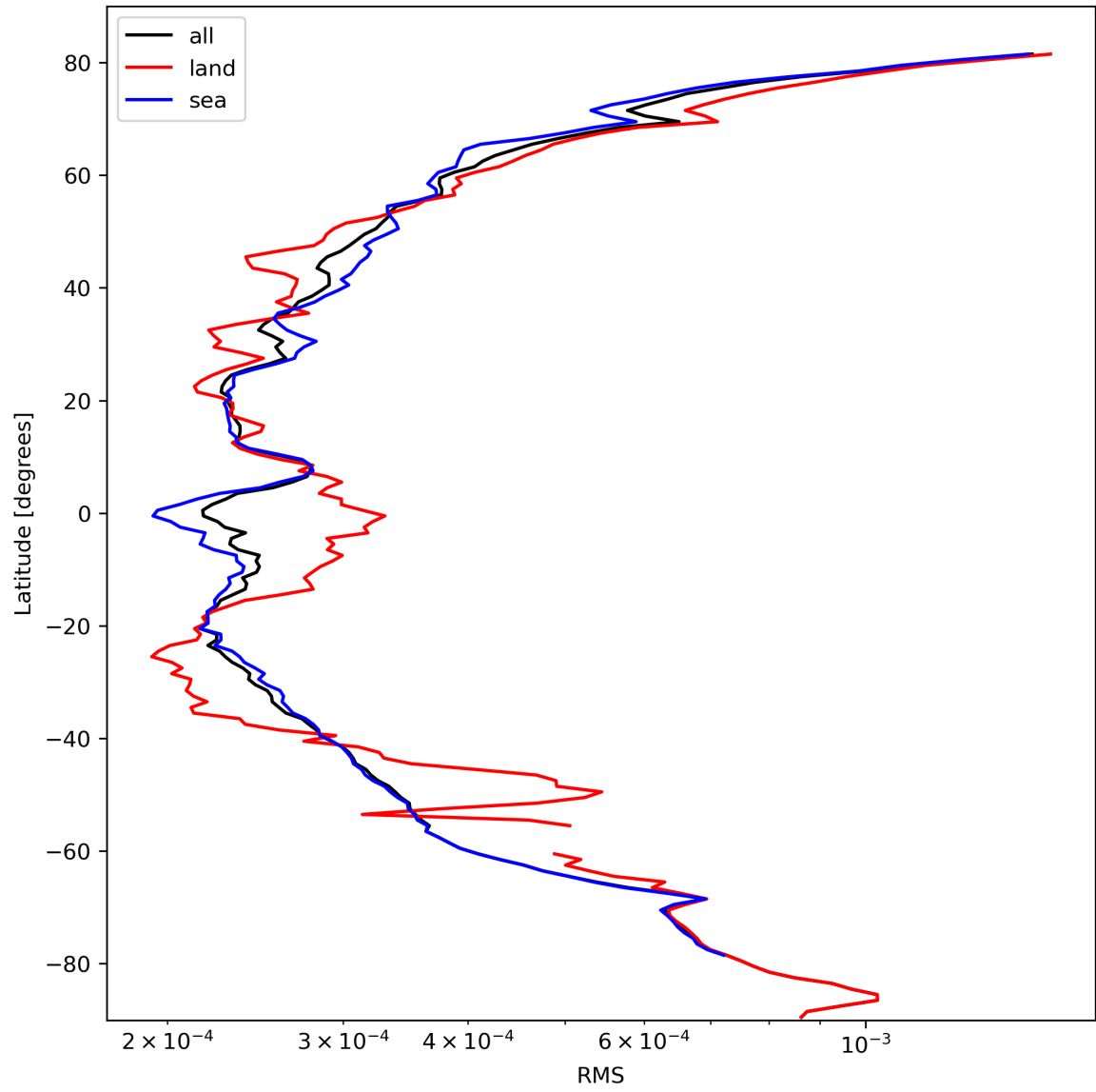
Figure 26: Zonal average of “RMS” for 2023-10-08 to 2023-10-10.
