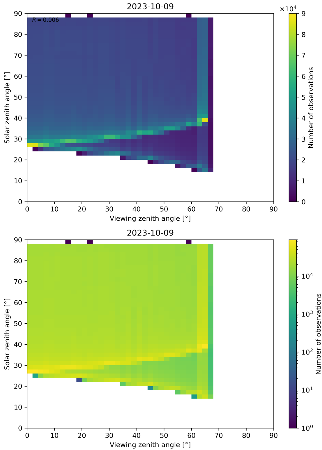
Figure 172: Scatter density plot of “Viewing zenith angle” against “Solar zenith angle” for 2023-10-08 to 2023-10-10.
