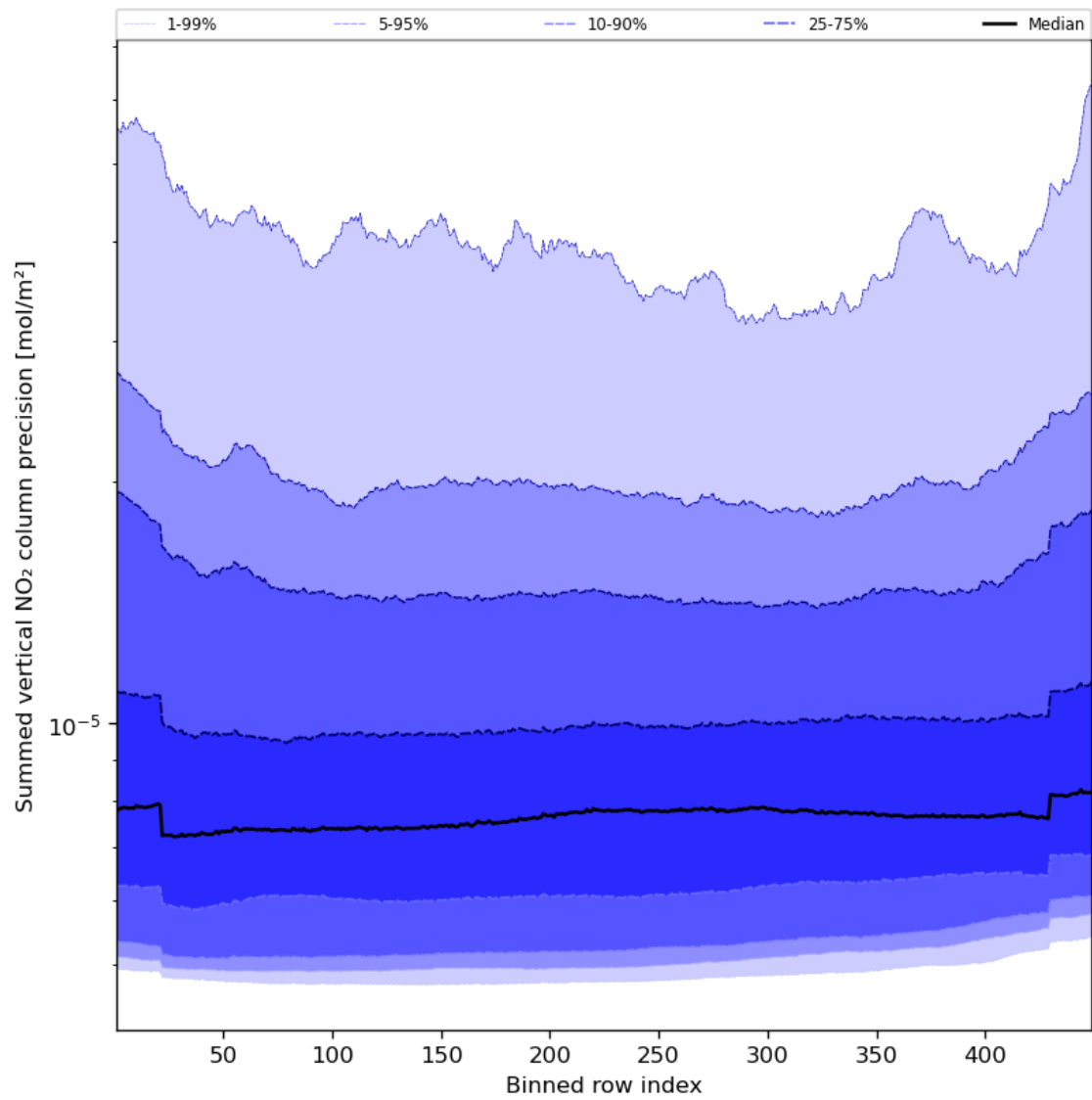
Figure 58: Along track statistics of “Summed vertical NO 2 column precision” for 2023-10-08 to 2023-10-10
