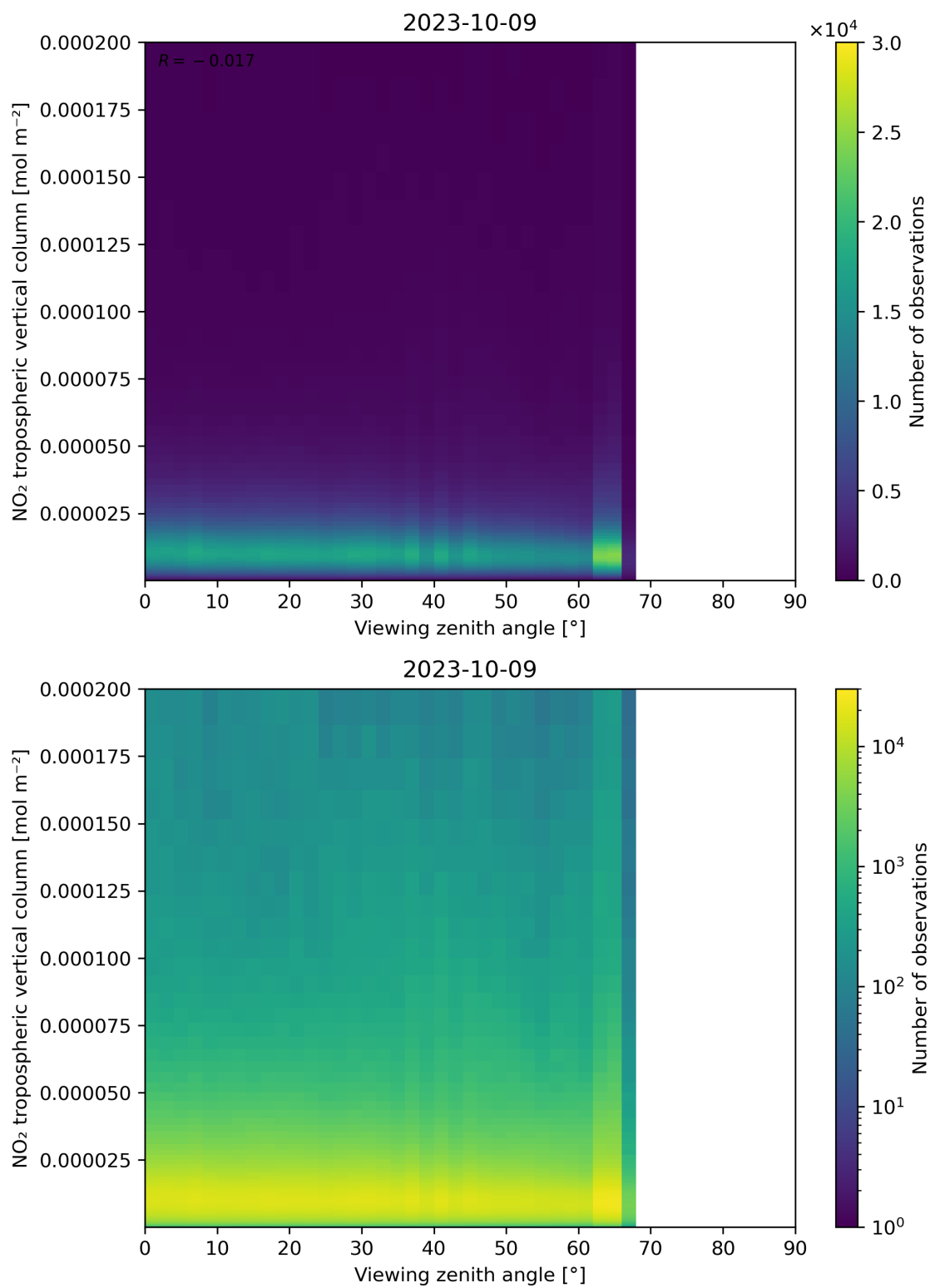
Figure 169: Scatter density plot of “Viewing zenith angle” against “NO 2 tropospheric vertical column” for 2023-10-08 to 2023-10-10.
