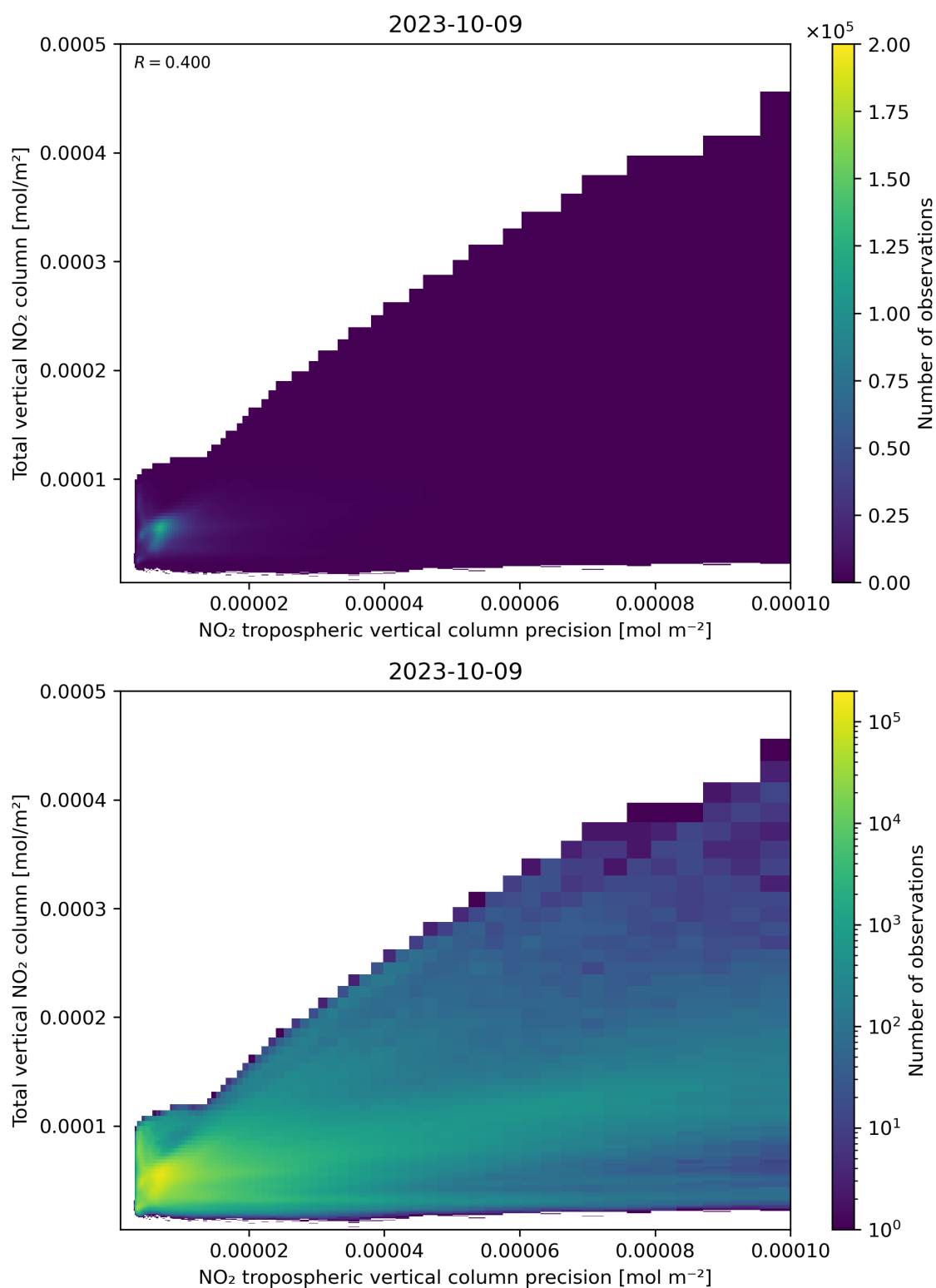
Figure 138: Scatter density plot of “NO 2 tropospheric vertical column precision” against “Total vertical NO 2 column” for 2023-10-08 to 2023-10-10.
