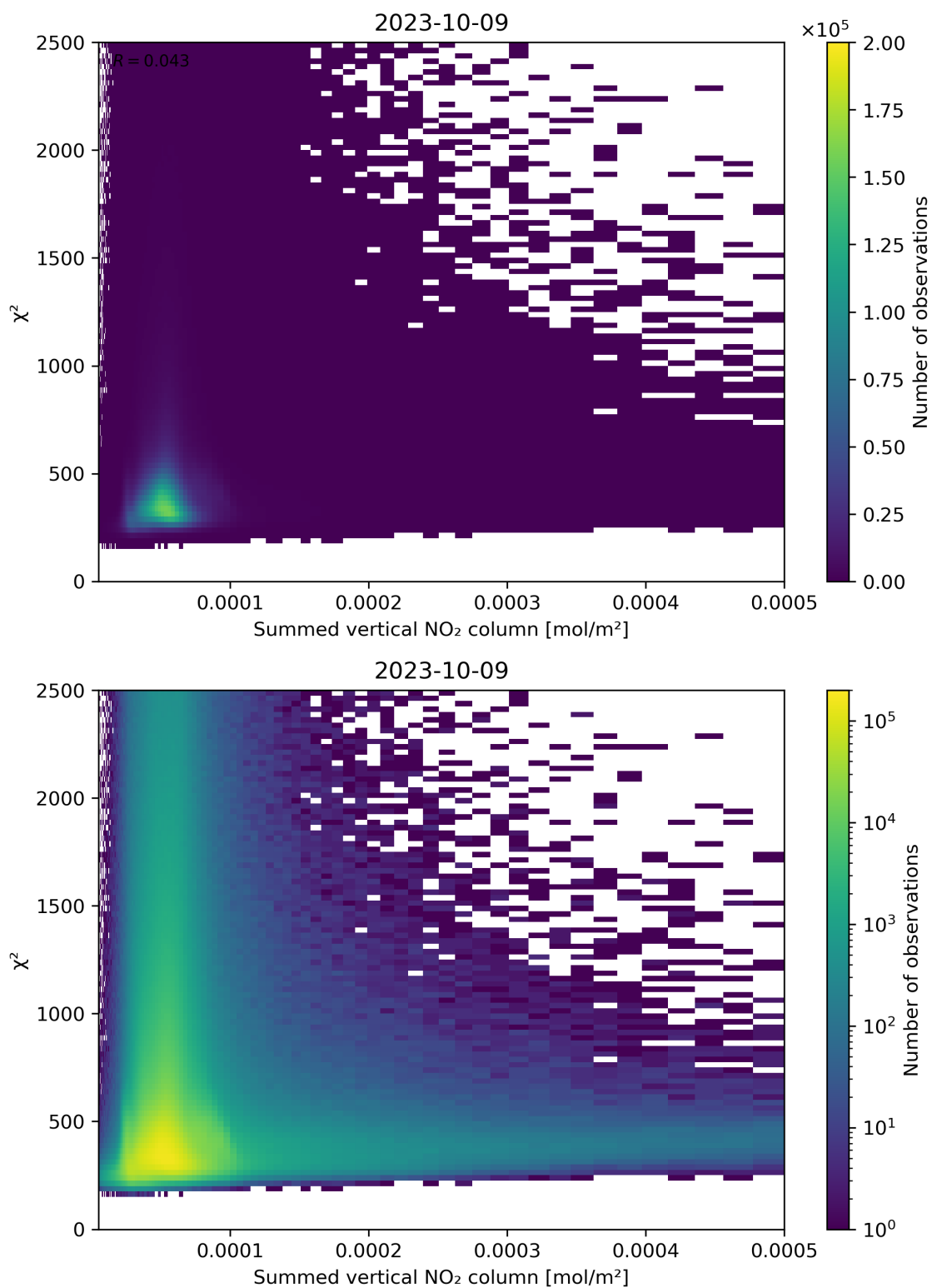
Figure 104: Scatter density plot of “Summed vertical NO 2 column” against “ \chi^2 ” for 2023-10-08 to 2023-10-10.
