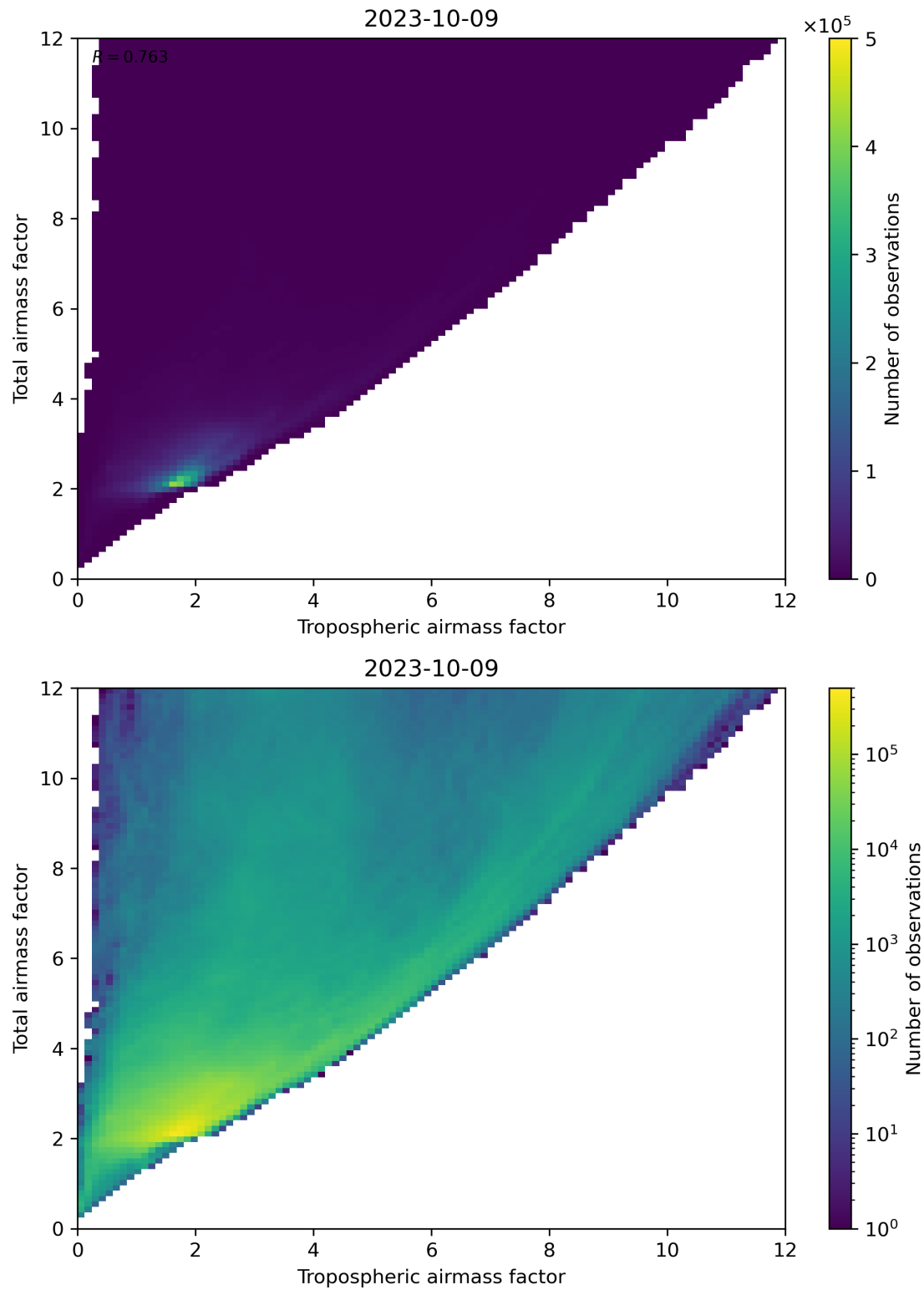
Figure 72: Scatter density plot of “Tropospheric airmass factor” against “Total airmass factor” for 2023-10-08 to 2023-10-10.
