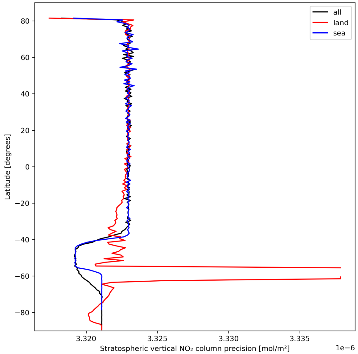
Figure 20: Zonal average of “Stratospheric vertical NO 2 column precision” for 2023-10-08 to 2023-10-10.
