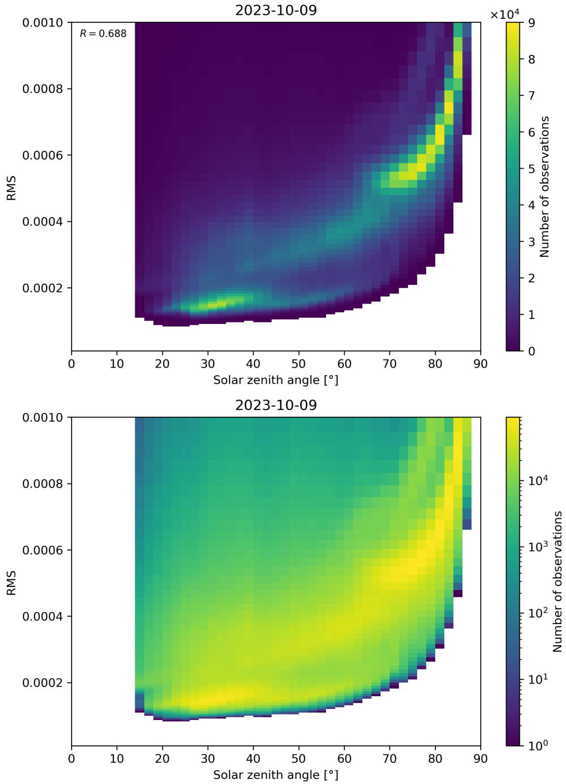
Figure 157: Scatter density plot of “Solar zenith angle” against “RMS” for 2023-10-08 to 2023-10-10.
