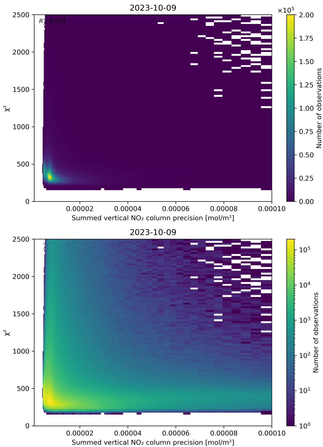
Figure 107: Scatter density plot of “Summed vertical NO 2 column precision” against “ \chi^2 ” for 2023-10-08 to 2023-10-10.
