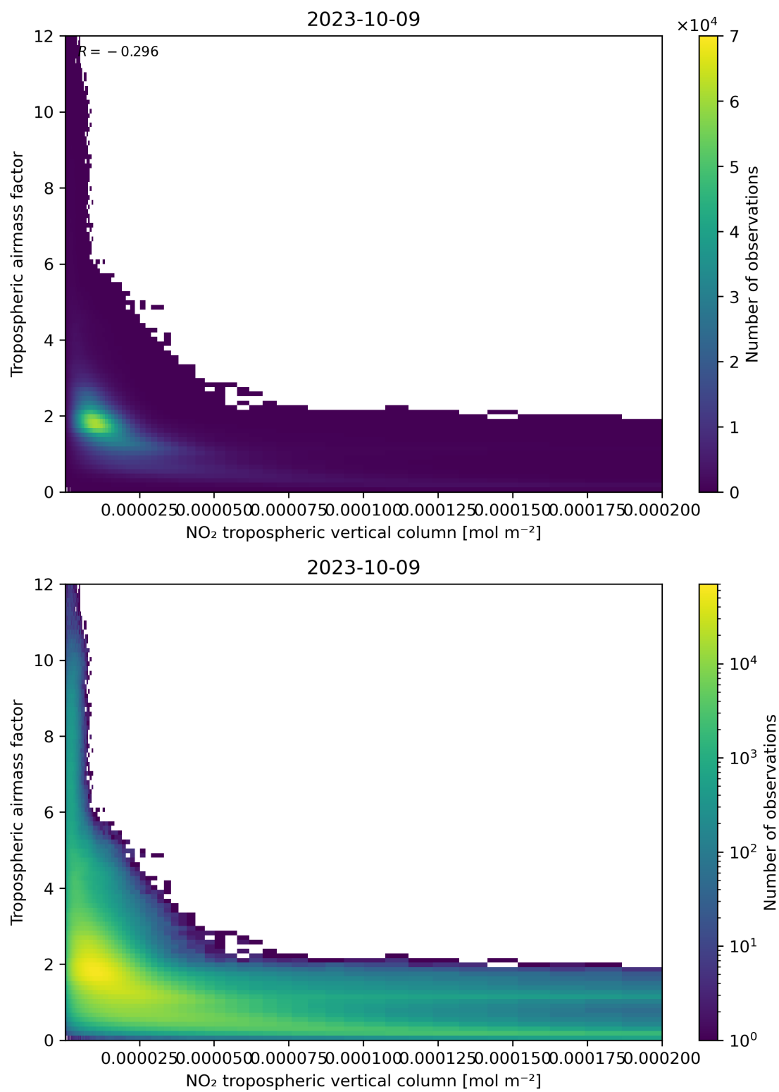
Figure 123: Scatter density plot of “NO 2 tropospheric vertical column” against “Tropospheric air mass factor” for 2023-10-08 to 2023-10-10.
