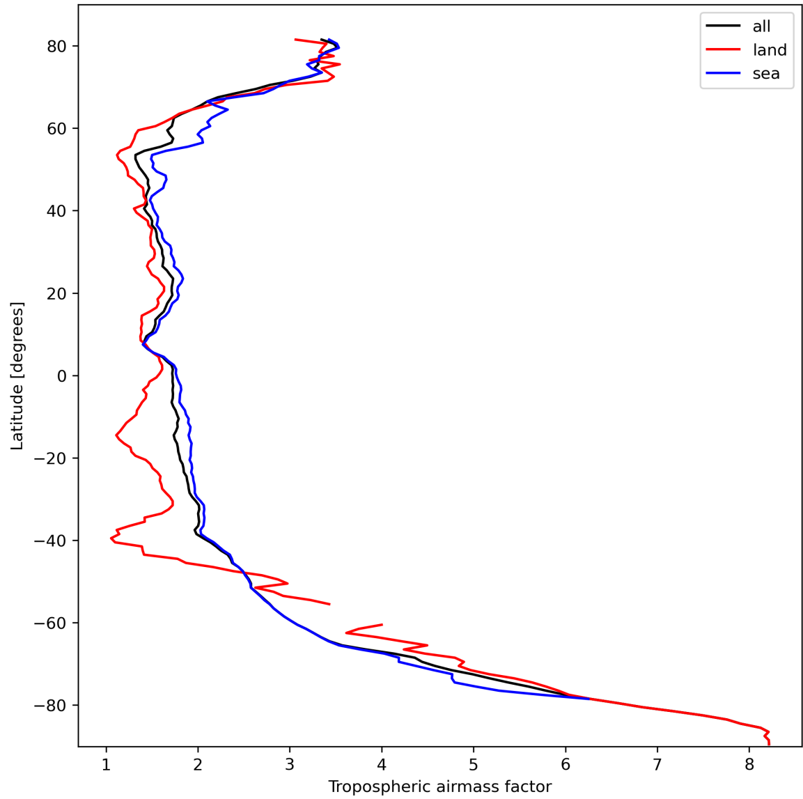
Figure 14: Zonal average of “Tropospheric airmass factor” for 2023-10-08 to 2023-10-10.
