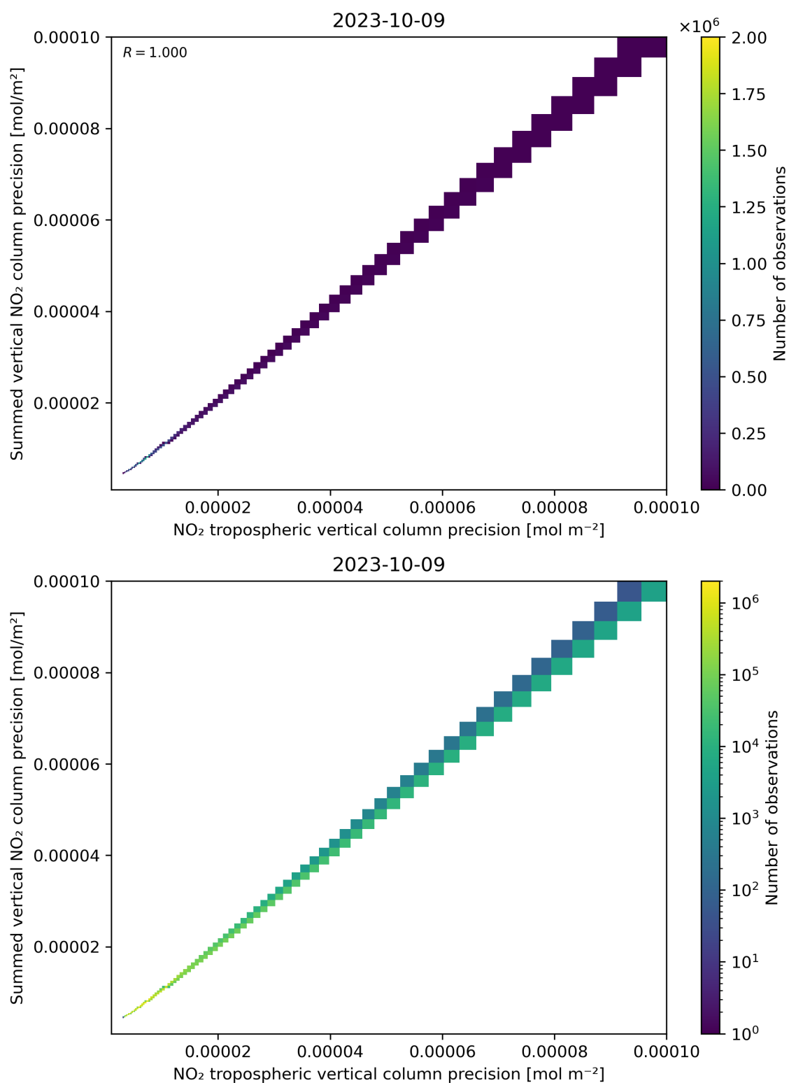
Figure 137: Scatter density plot of “NO 2 tropospheric vertical column precision” against “Summed vertical NO 2 column precision” for 2023-10-08 to 2023-10-10.
