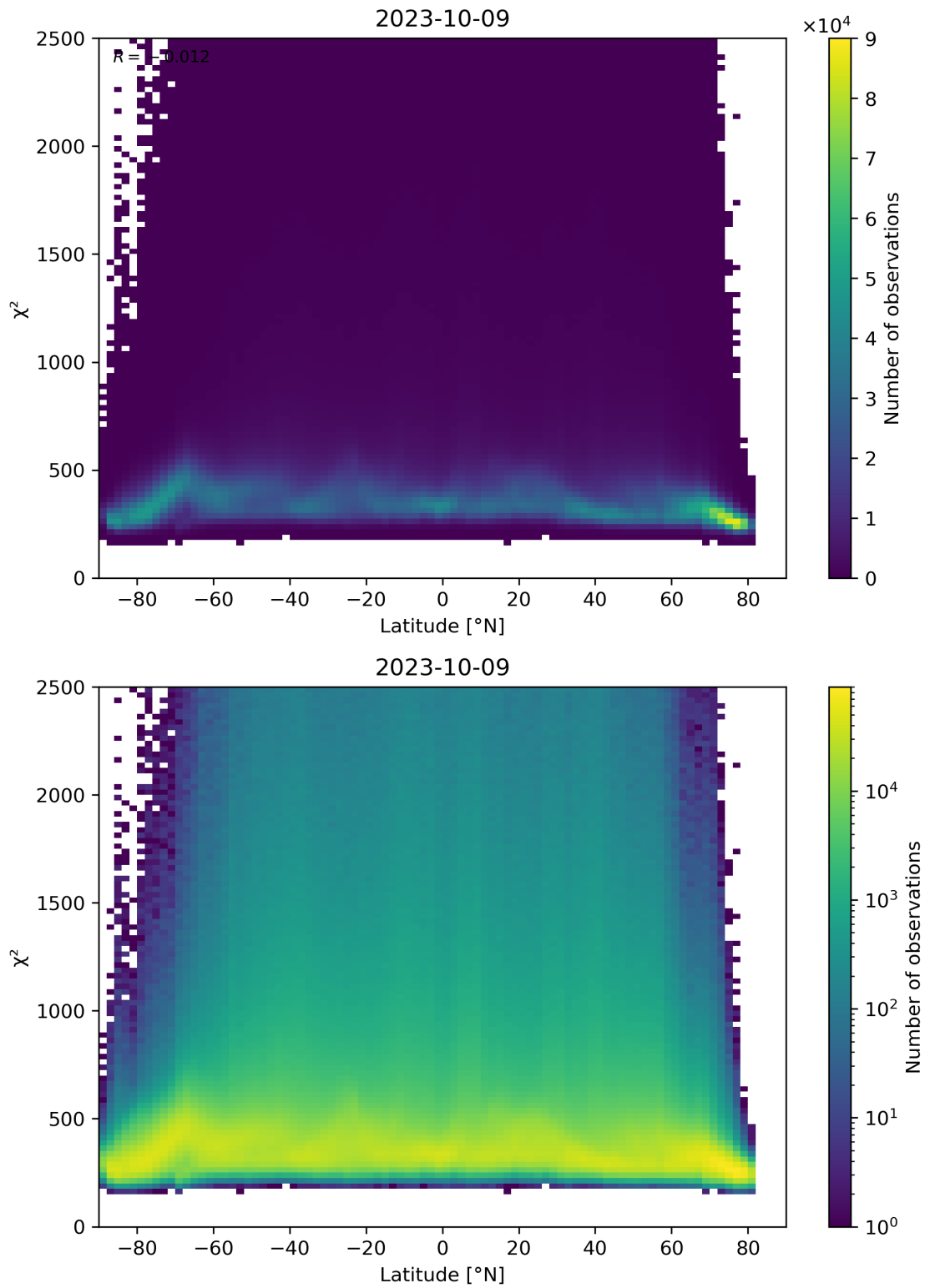
Figure 86: Scatter density plot of “Latitude” against “ \chi^2 ” for 2023-10-08 to 2023-10-10.
