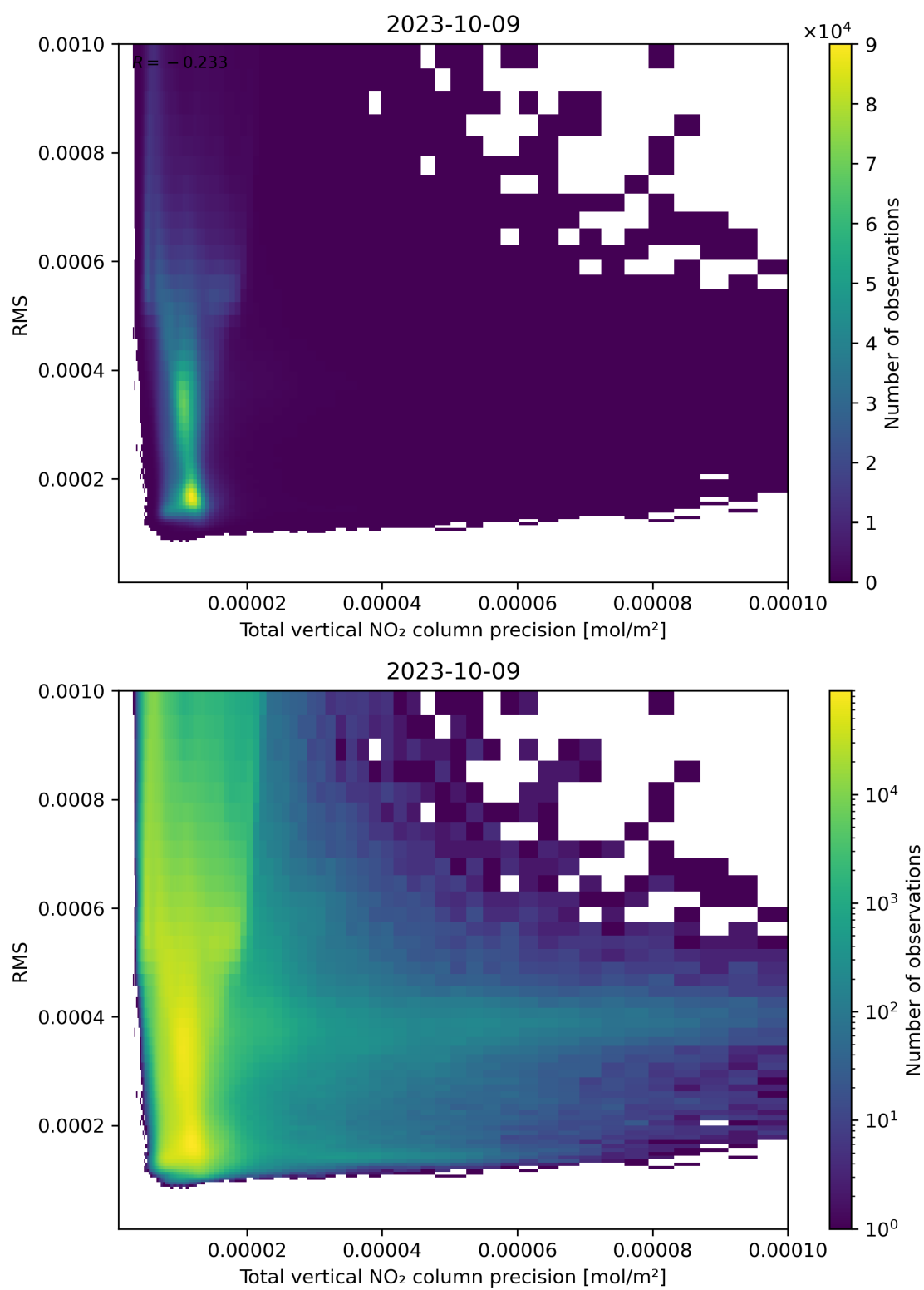
Figure 119: Scatter density plot of “Total vertical NO 2 column precision” against “RMS” for 2023-10-08 to 2023-10-10.
