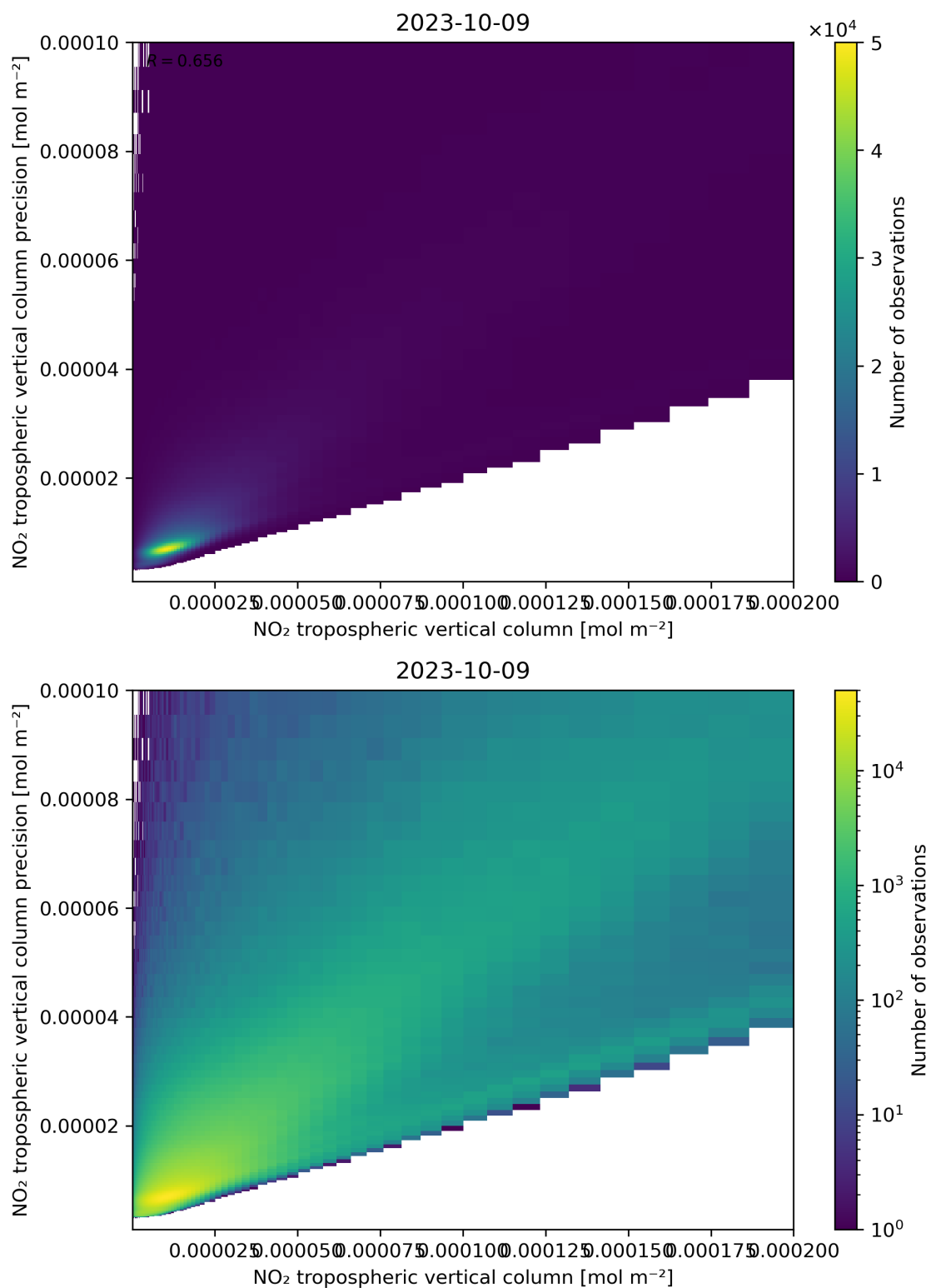
Figure 130: Scatter density plot of “NO 2 tropospheric vertical column” against “NO 2 tropospheric vertical column precision” for 2023-10-08 to 2023-10-10.
