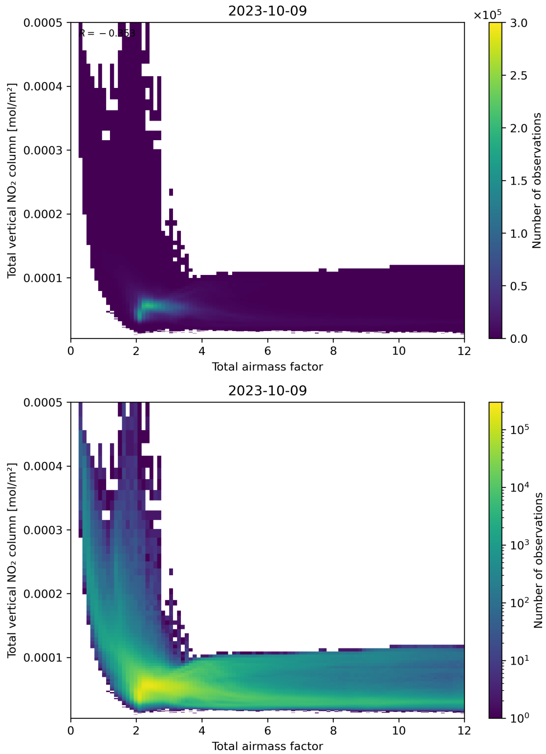
Figure 67: Scatter density plot of “Total airmass factor” against “Total vertical NO 2 column” for 2023-10-08 to 2023-10-10.
