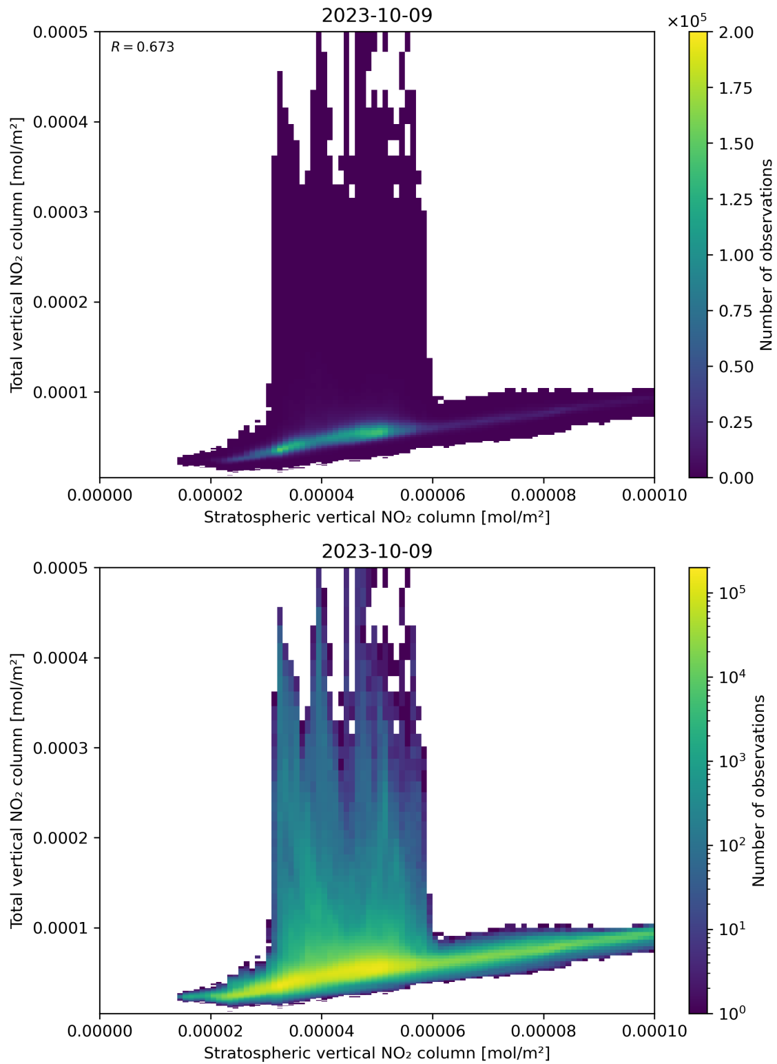
Figure 100: Scatter density plot of “Stratospheric vertical NO 2 column” against “Total vertical NO 2 column” for 2023-10-08 to 2023-10-10.
