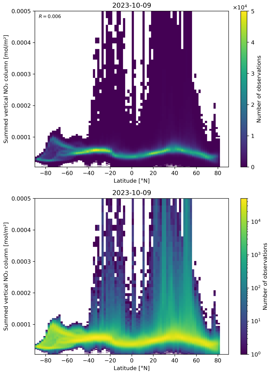
Figure 88: Scatter density plot of “Latitude” against “Summed vertical NO 2 column” for 2023-10-08 to 2023-10-10.
