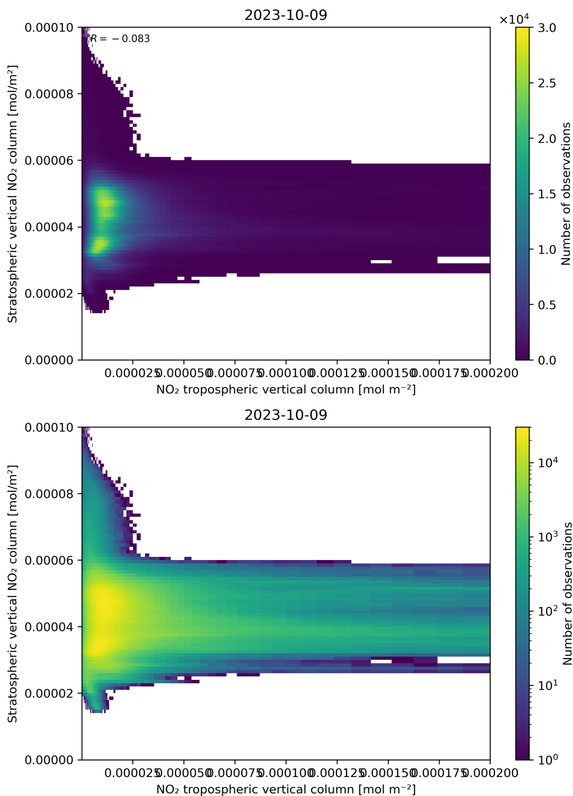
Figure 125: Scatter density plot of “NO 2 tropospheric vertical column” against “Stratospheric vertical NO 2 column” for 2023-10-08 to 2023-10-10.
