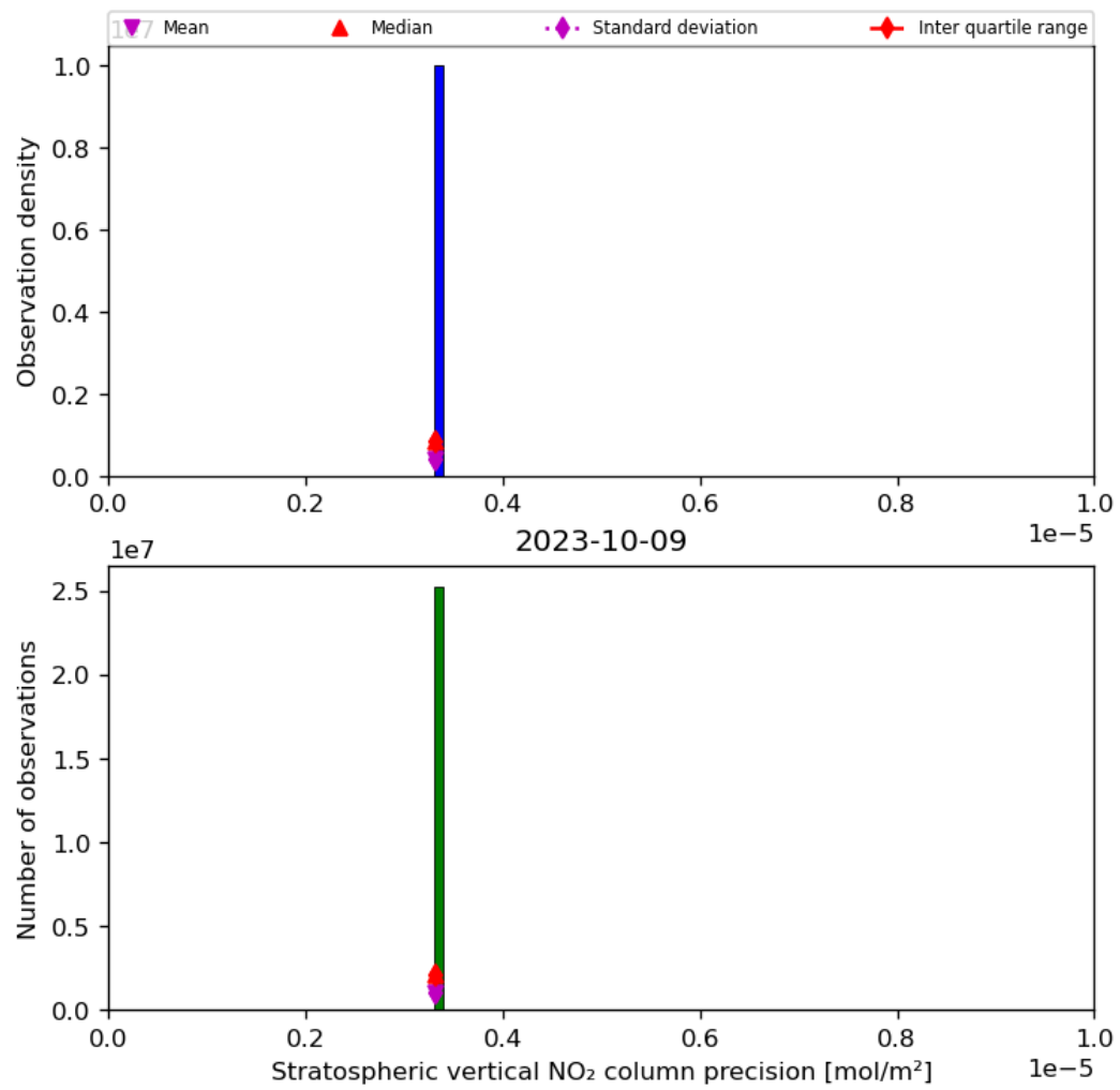
Figure 37: Histogram of “Stratospheric vertical NO 2 column precision” for 2023-10-08 to 2023-10-10
