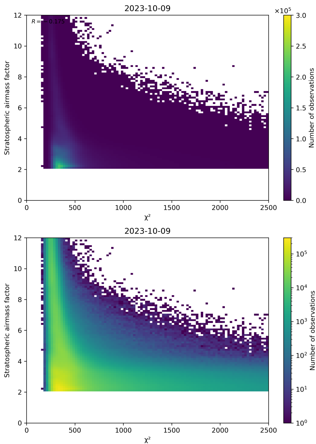
Figure 81: Scatter density plot of “ \chi^2 ” against “Stratospheric airmass factor” for 2023-10-08 to 2023-10-10.
