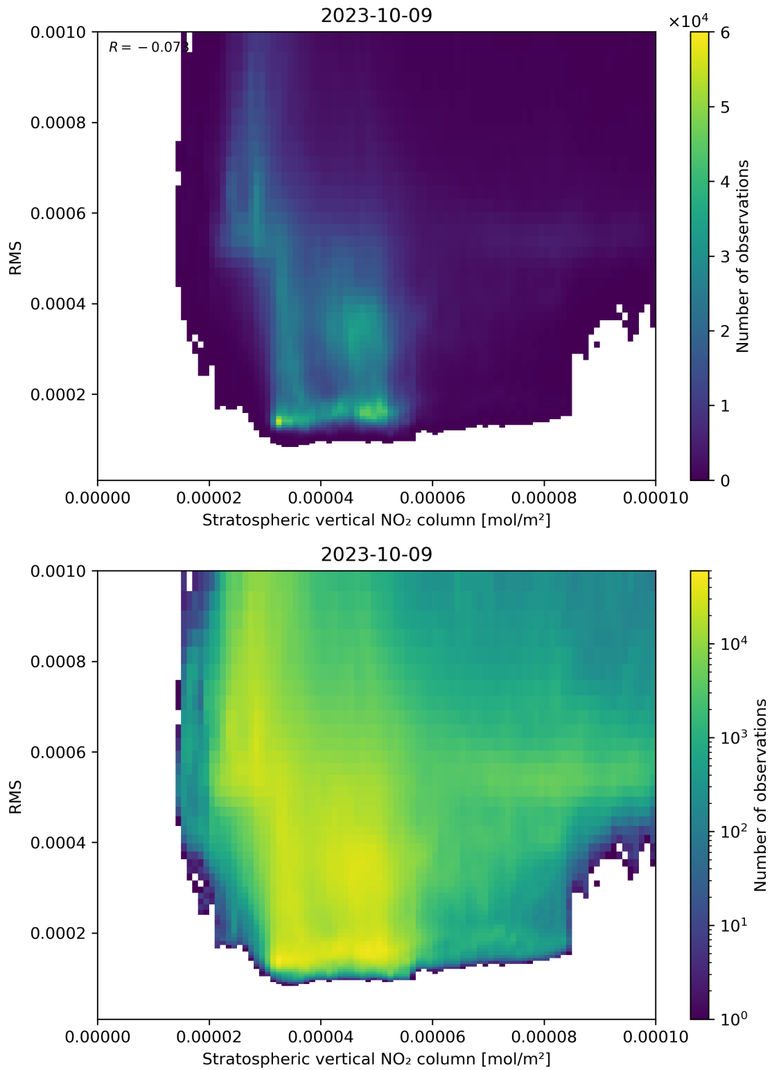
Figure 102: Scatter density plot of “Stratospheric vertical NO 2 column” against “RMS” for 2023-10-08 to 2023-10-10.
