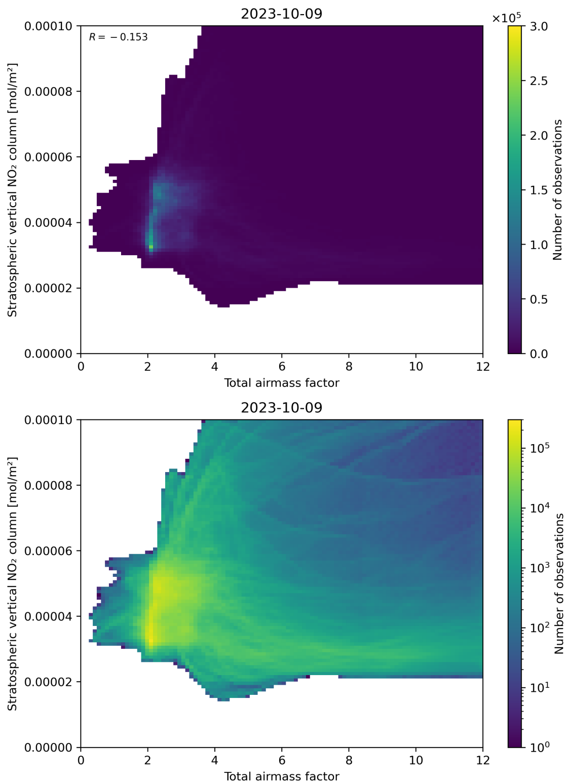
Figure 64: Scatter density plot of “Total airmass factor” against “Stratospheric vertical NO 2 column” for 2023-10-08 to 2023-10-10.
