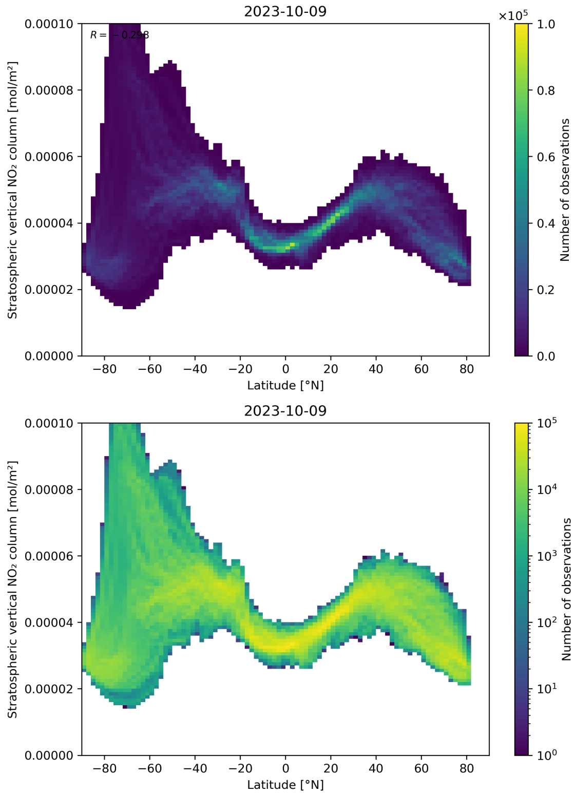
Figure 87: Scatter density plot of “Latitude” against “Stratospheric vertical NO 2 column” for 2023-10-08 to 2023-10-10.
