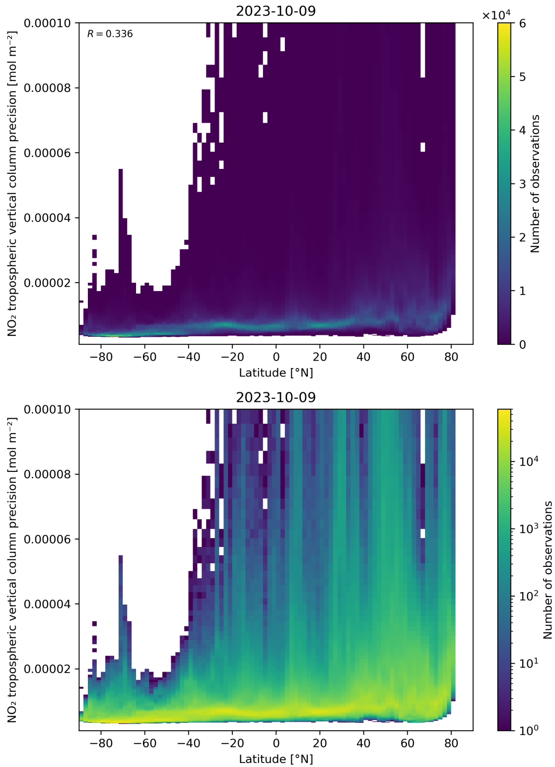
Figure 93: Scatter density plot of “Latitude” against “NO 2 tropospheric vertical column precision” for 2023-10-08 to 2023-10-10.
