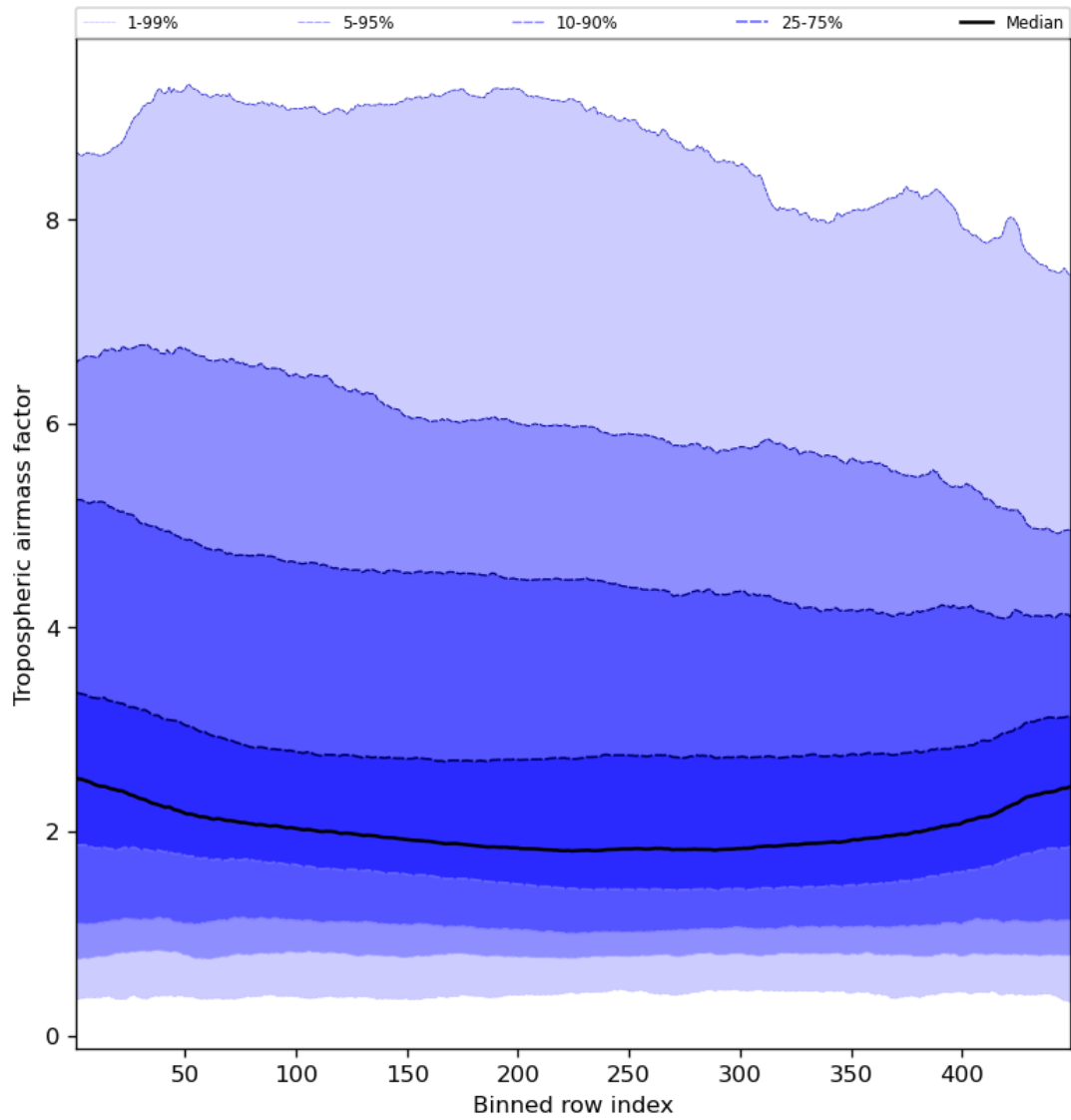
Figure 48: Along track statistics of “Tropospheric air mass factor” for 2023-10-08 to 2023-10-10
