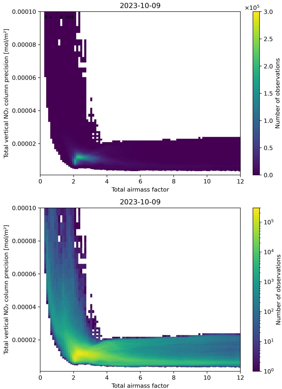
Figure 68: Scatter density plot of “Total airmass factor” against “Total vertical NO 2 column precision” for 2023-10-08 to 2023-10-10.
