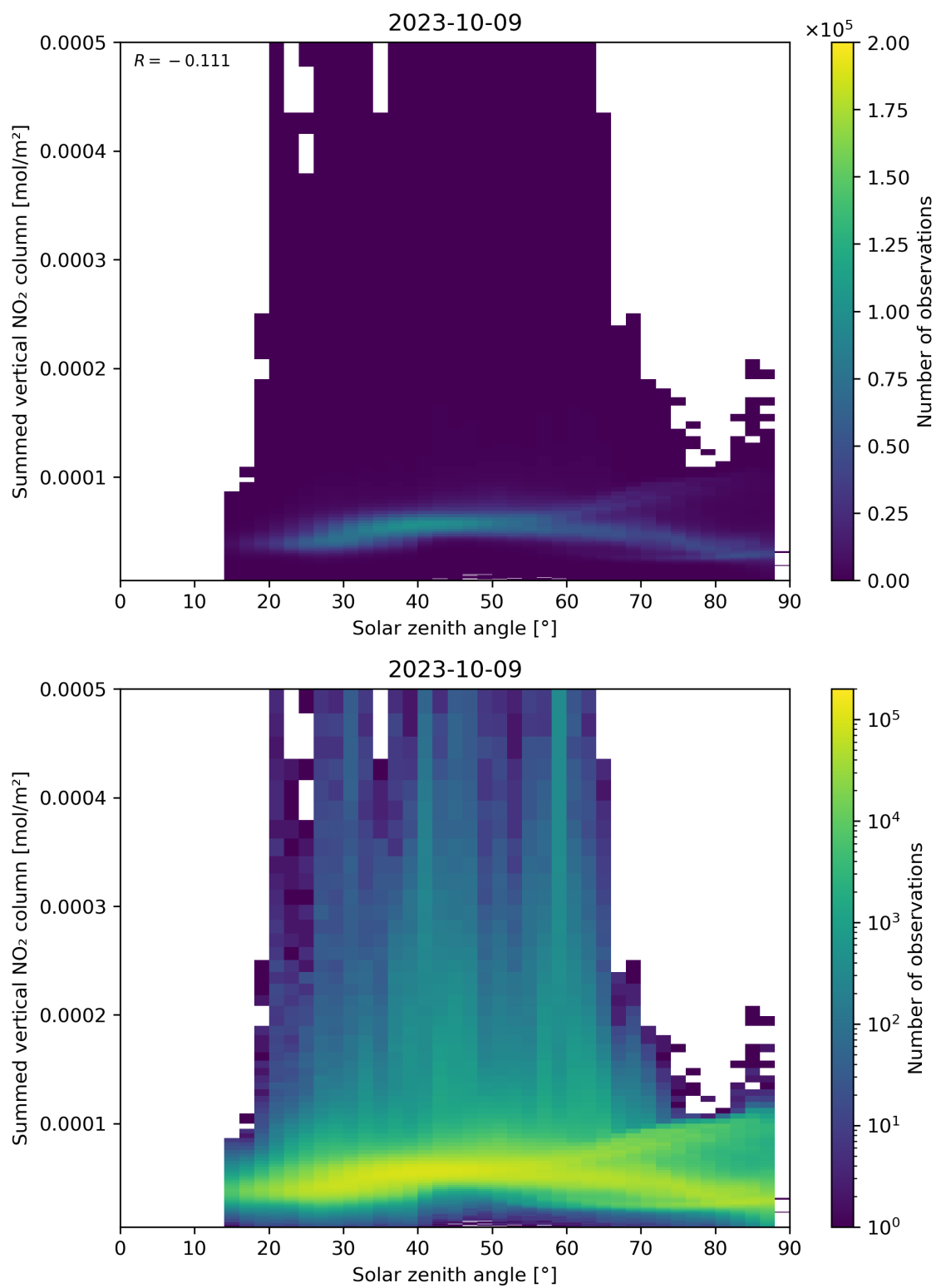
Figure 151: Scatter density plot of “Solar zenith angle” against “Summed vertical NO 2 column” for 2023-10-08 to 2023-10-10.
