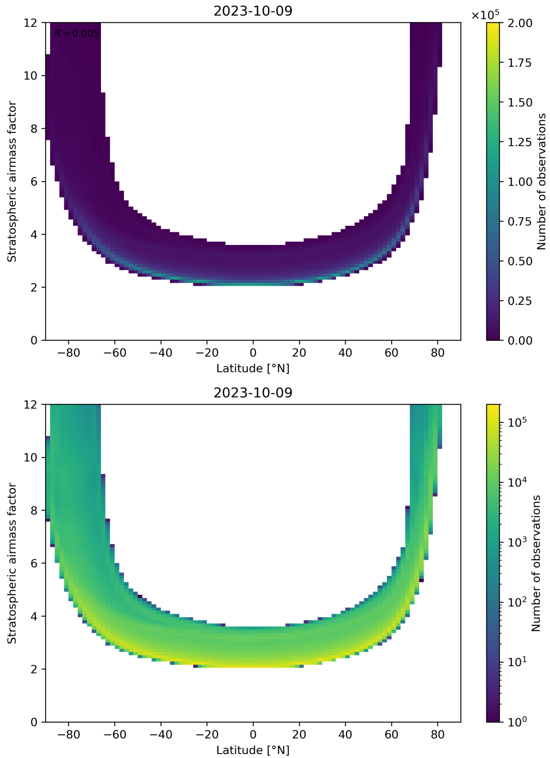
Figure 83: Scatter density plot of “Latitude” against “Stratospheric airmass factor” for 2023-10-08 to 2023-10-10.
