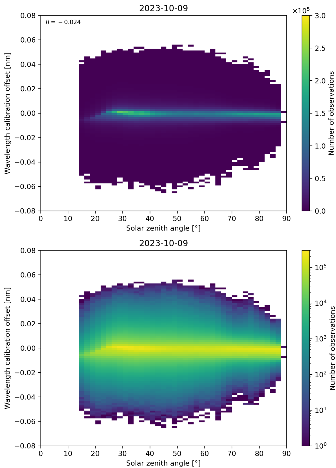
Figure 158: Scatter density plot of “Solar zenith angle” against “Wavelength calibration offset” for 2023-10-08 to 2023-10-10.
