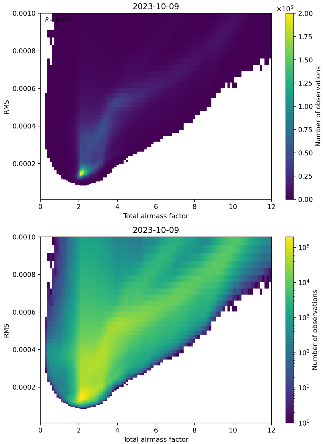
Figure 69: Scatter density plot of “Total airmass factor” against “RMS” for 2023-10-08 to 2023-10-10.
