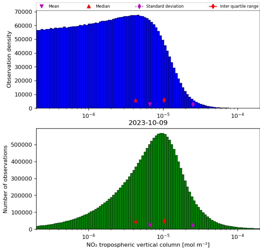
Figure 29: Histogram of “ \text{NO}_2 tropospheric vertical column” for 2023-10-08 to 2023-10-10
