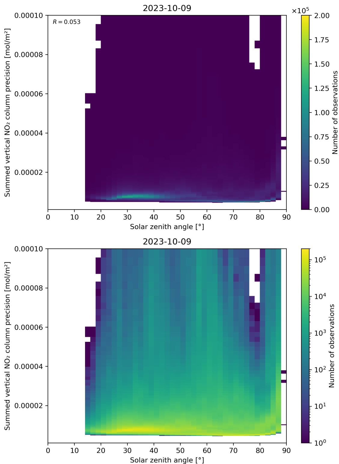
Figure 152: Scatter density plot of “Solar zenith angle” against “Summed vertical NO 2 column precision” for 2023-10-08 to 2023-10-10.
