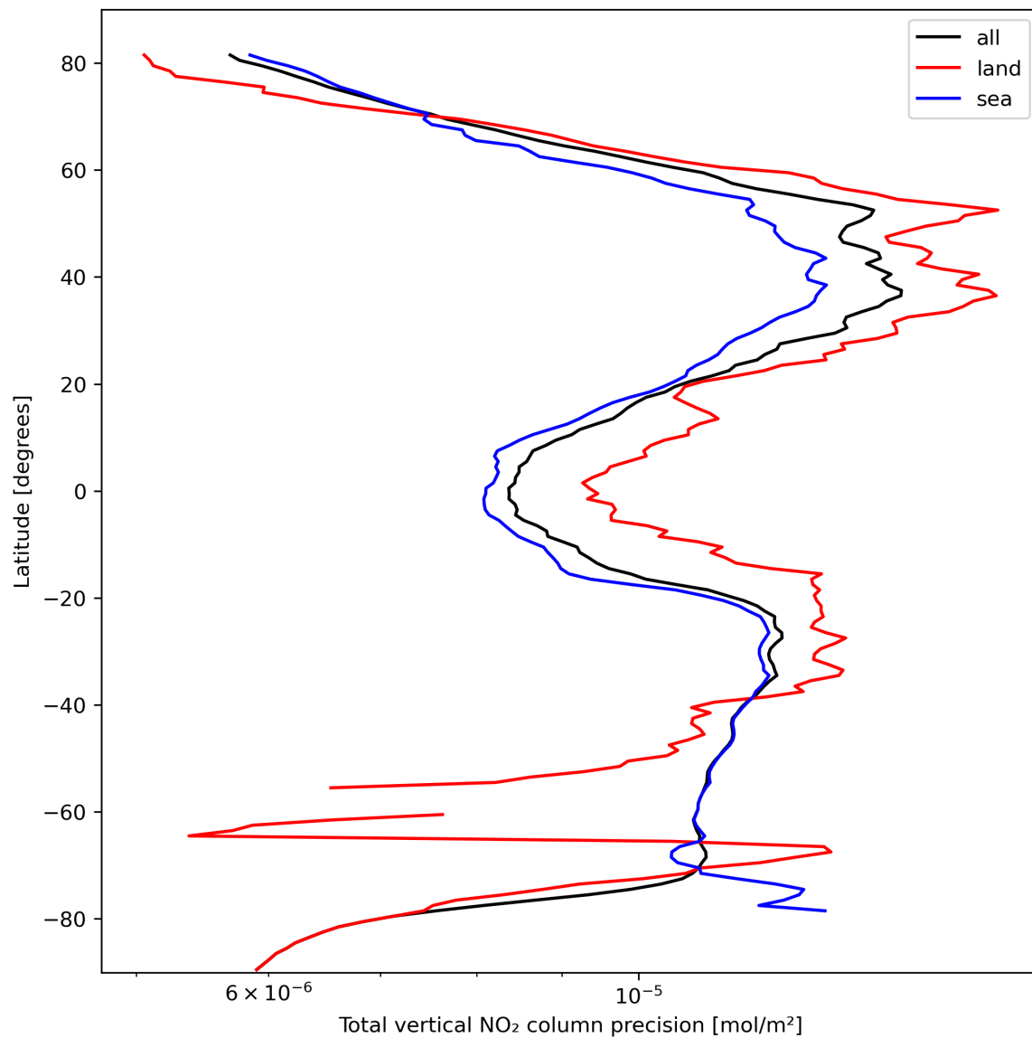
Figure 22: Zonal average of “Total vertical NO 2 column precision” for 2023-10-08 to 2023-10-10.
