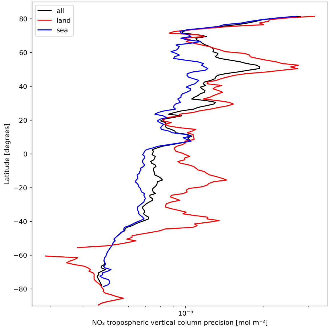
Figure 13: Zonal average of “NO 2 tropospheric vertical column precision” for 2023-10-08 to 2023-10-10.
