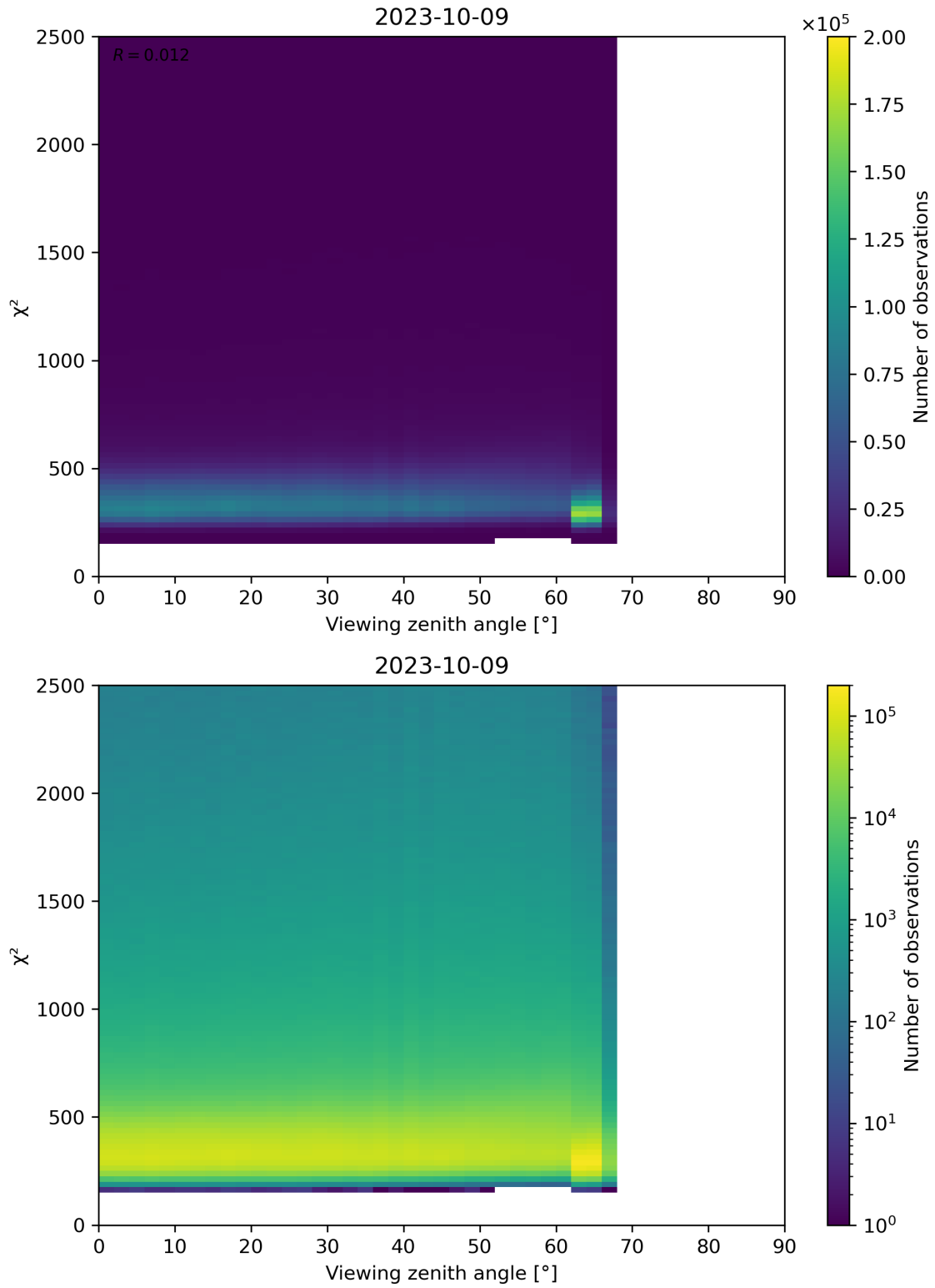
Figure 162: Scatter density plot of “Viewing zenith angle” against “ \chi^2 ” for 2023-10-08 to 2023-10-10.
