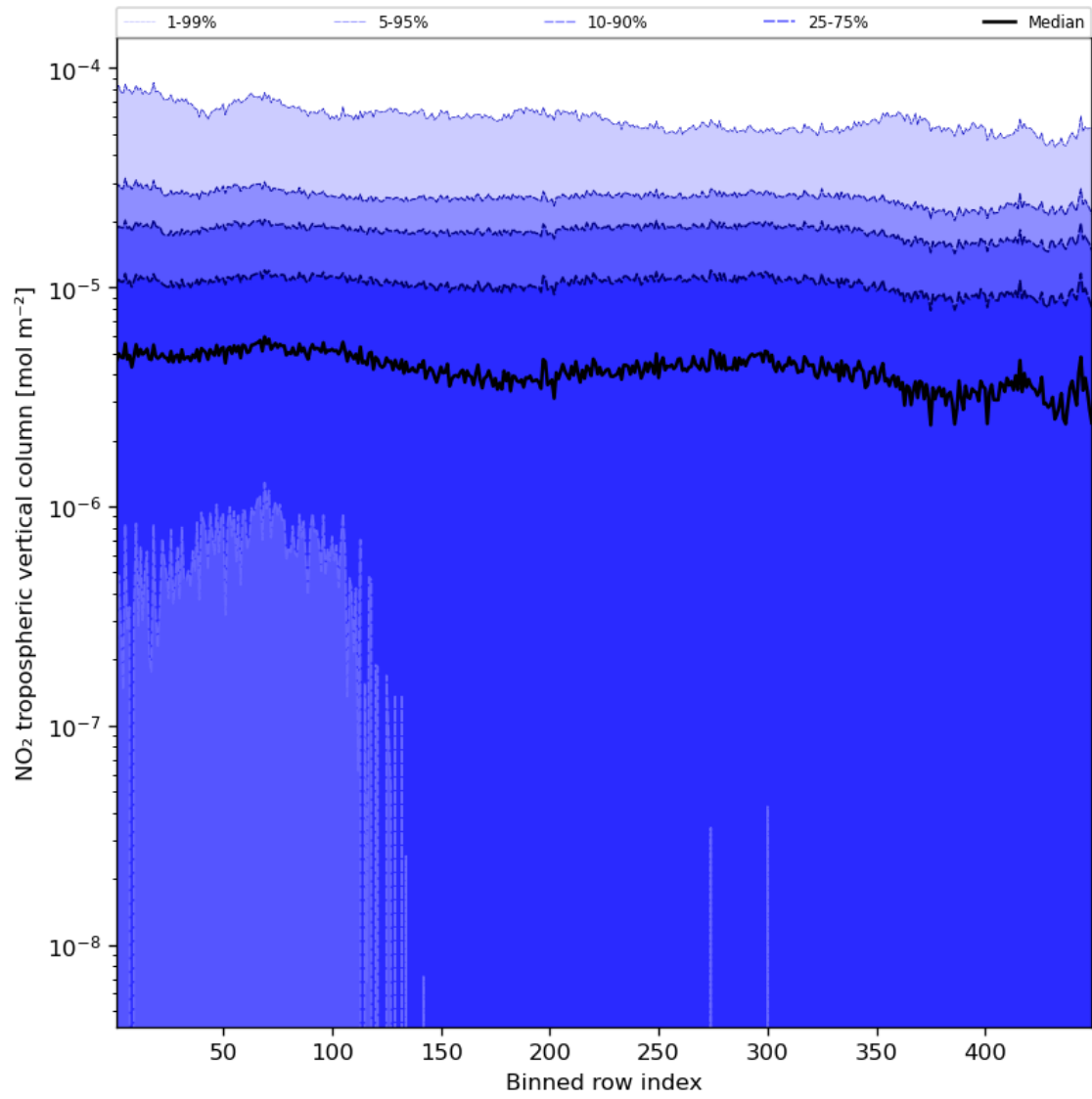
Figure 46: Along track statistics of “NO 2 tropospheric vertical column” for 2023-10-08 to 2023-10-10
