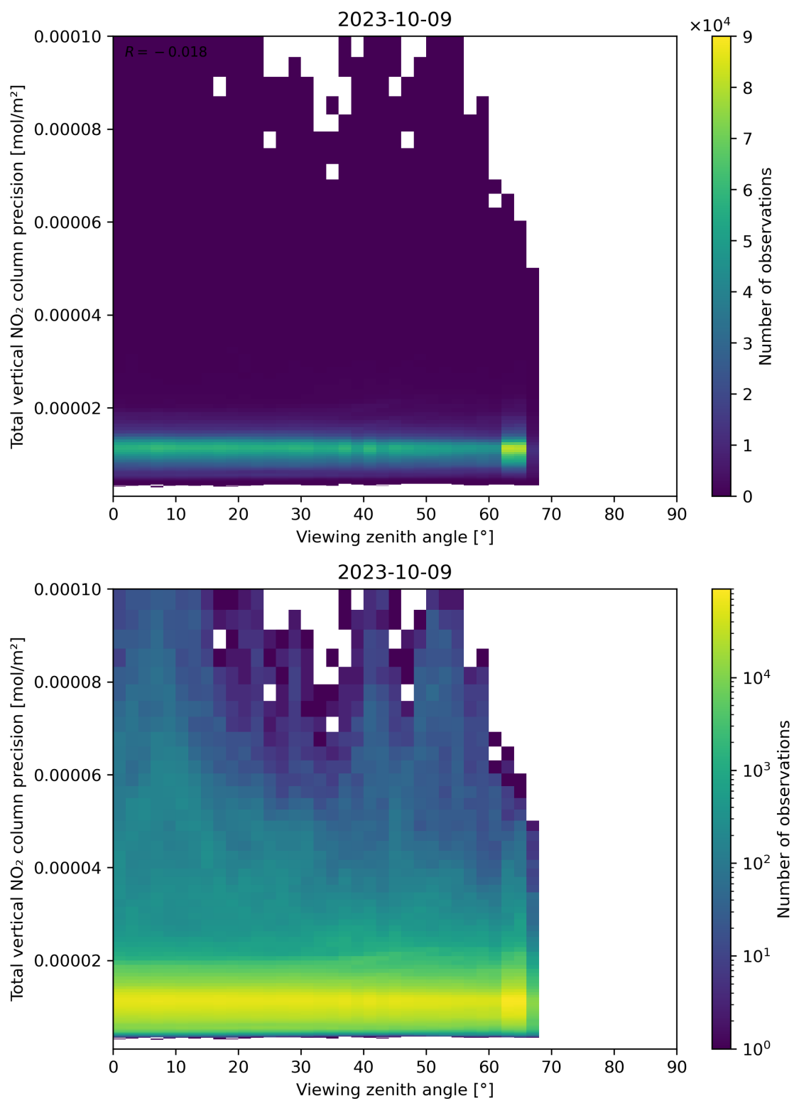
Figure 168: Scatter density plot of “Viewing zenith angle” against “Total vertical NO 2 column precision” for 2023-10-08 to 2023-10-10.
