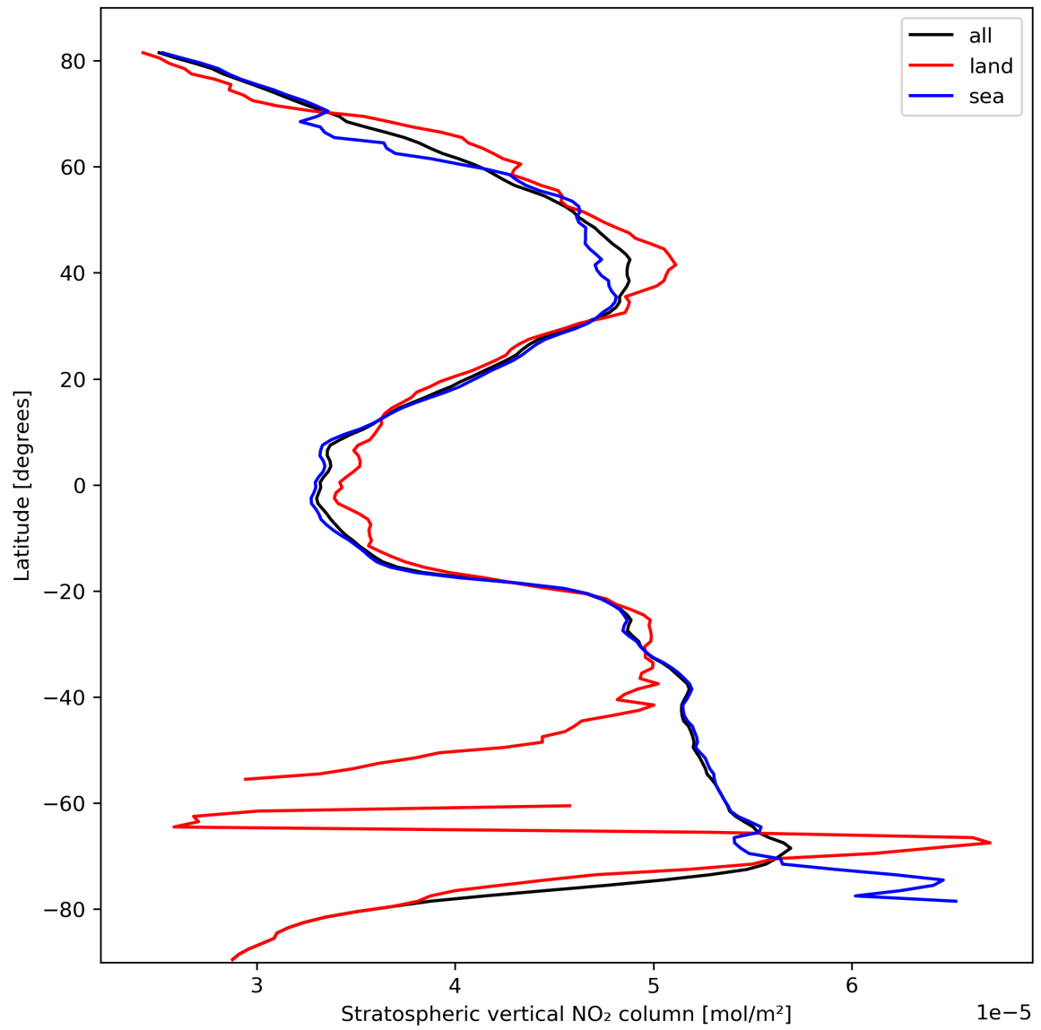
Figure 19: Zonal average of “Stratospheric vertical NO 2 column” for 2023-10-08 to 2023-10-10.
