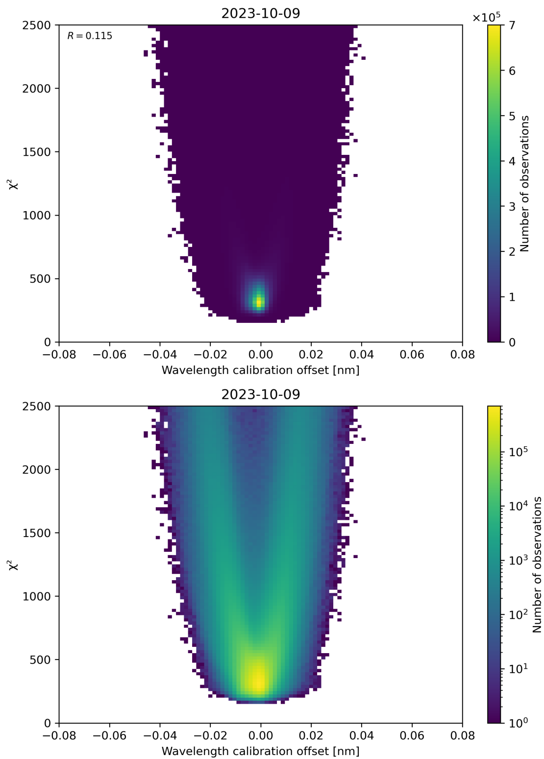
Figure 175: Scatter density plot of “Wavelength calibration offset” against “ \chi^2 ” for 2023-10-08 to 2023-10-10.
