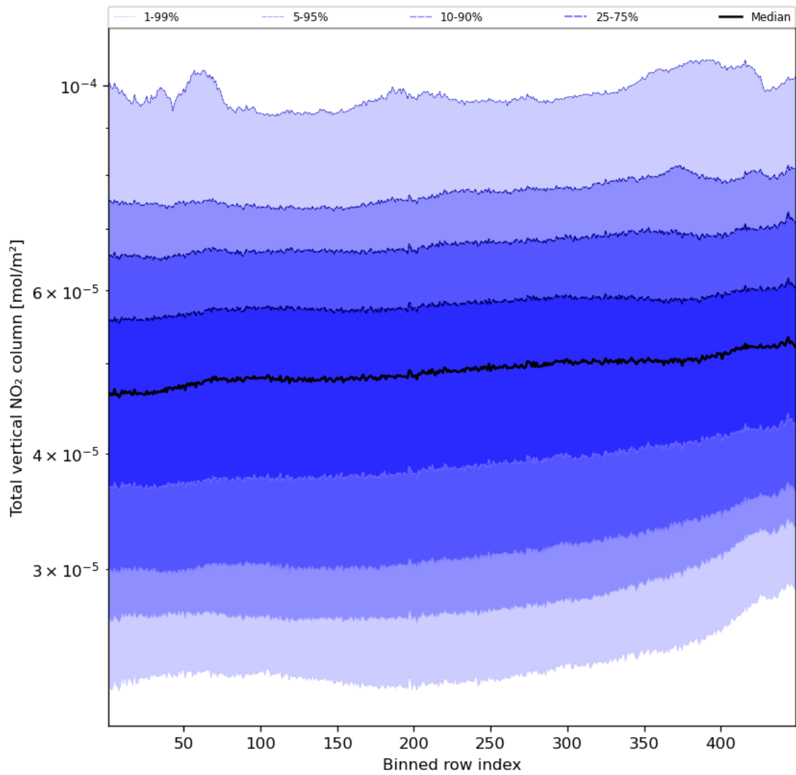
Figure 55: Along track statistics of “Total vertical NO 2 column” for 2023-10-08 to 2023-10-10
