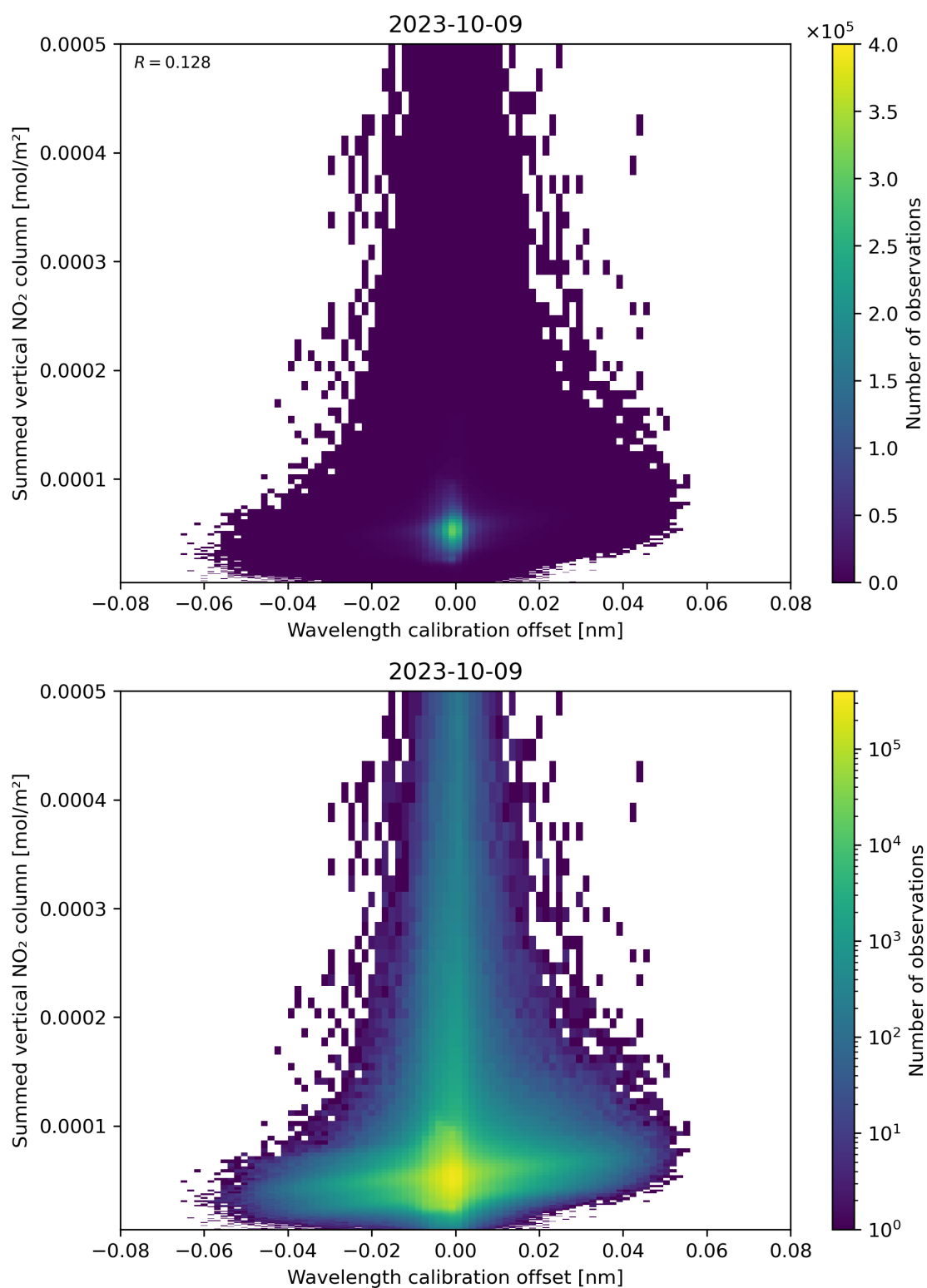
Figure 177: Scatter density plot of “Wavelength calibration offset” against “Summed vertical NO 2 column” for 2023-10-08 to 2023-10-10.
