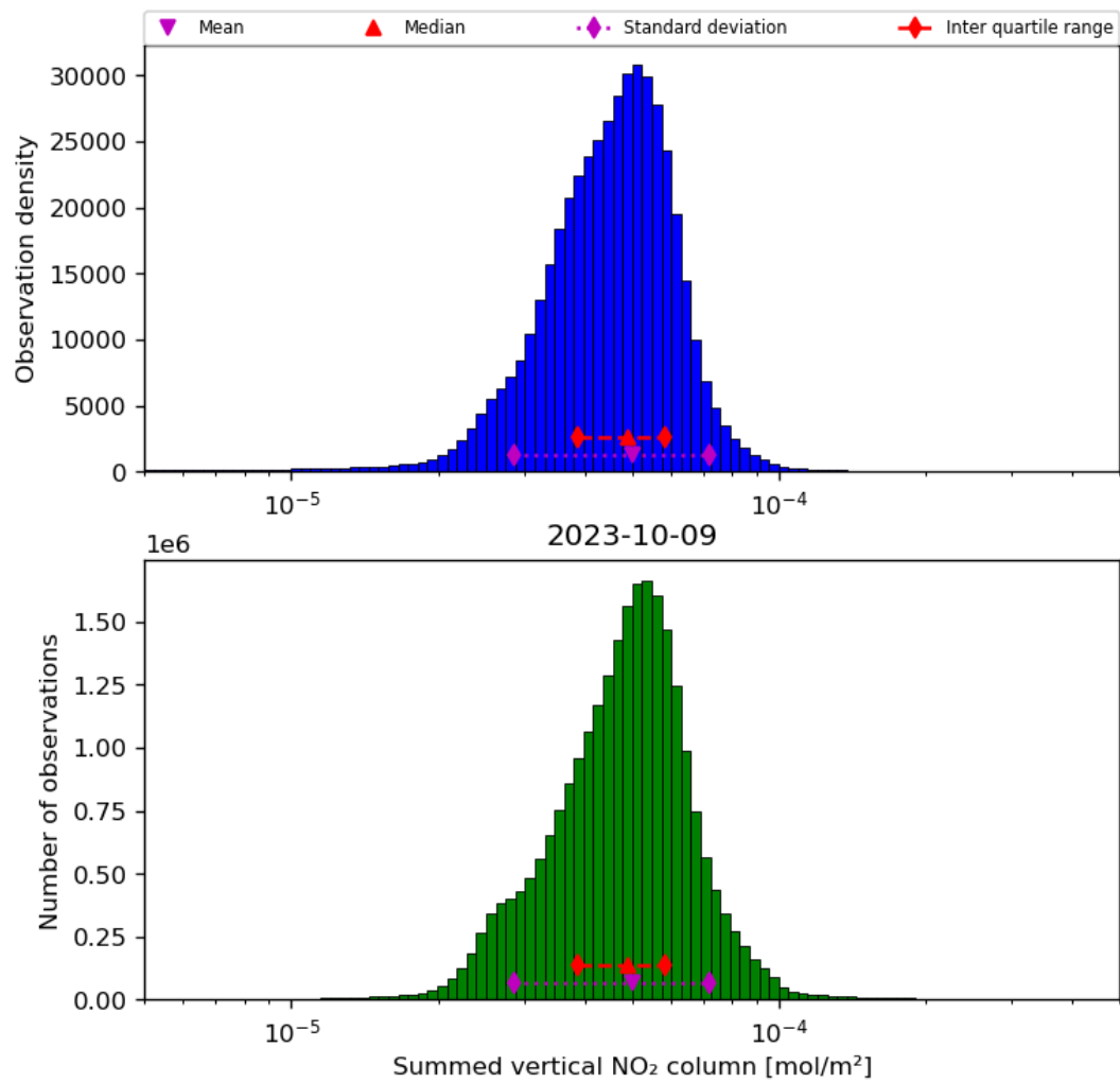
Figure 40: Histogram of “Summed vertical NO 2 column” for 2023-10-08 to 2023-10-10
