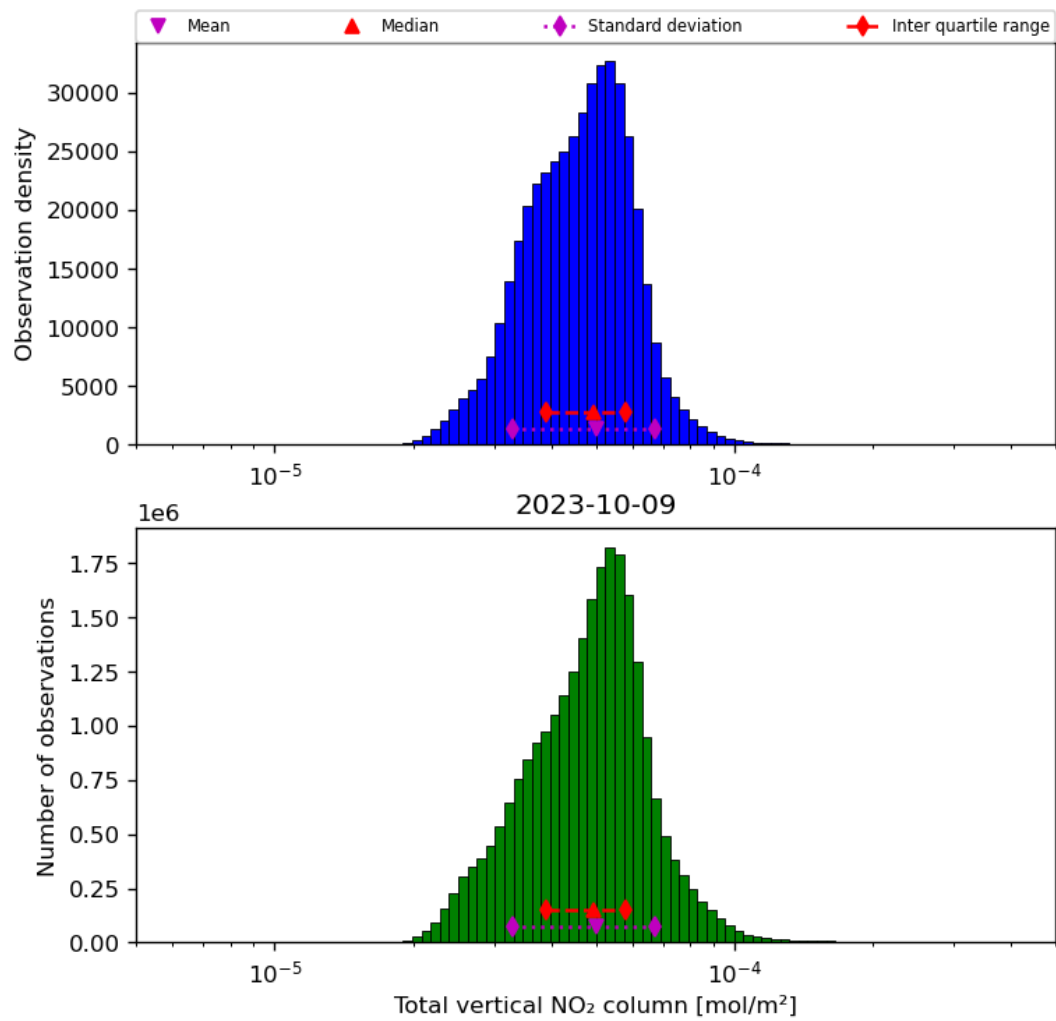
Figure 38: Histogram of “Total vertical NO 2 column” for 2023-10-08 to 2023-10-10
