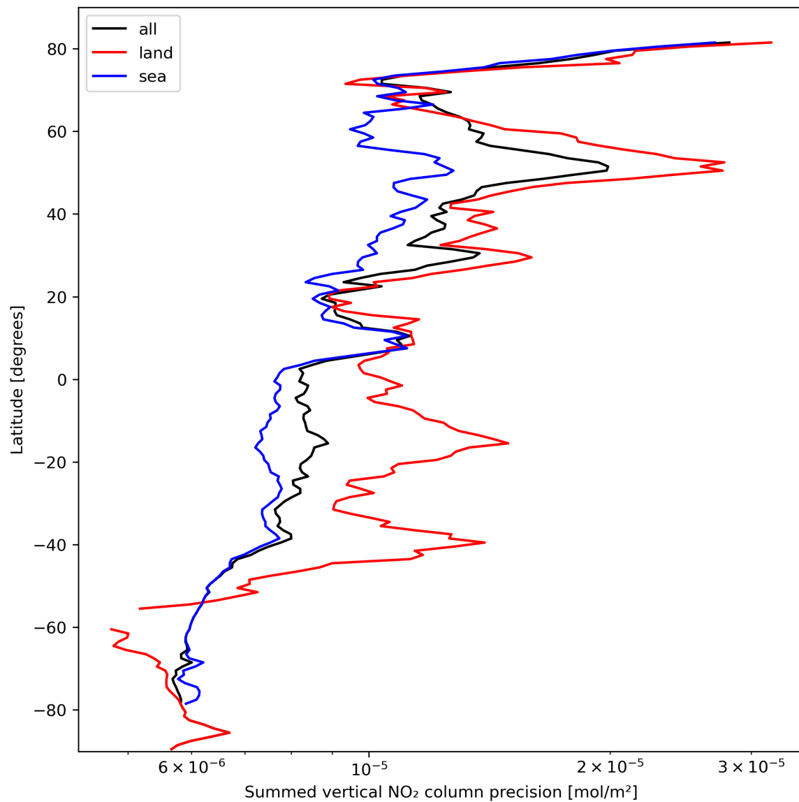
Figure 24: Zonal average of “Summed vertical NO 2 column precision” for 2023-10-08 to 2023-10-10.
