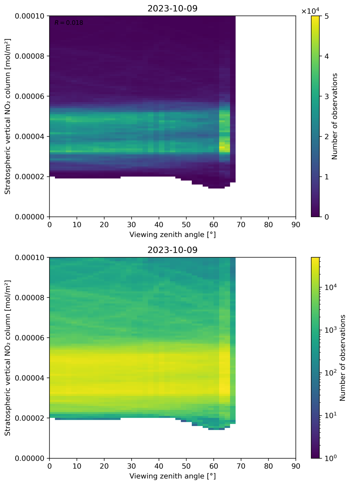
Figure 164: Scatter density plot of “Viewing zenith angle” against “Stratospheric vertical NO 2 column” for 2023-10-08 to 2023-10-10.
