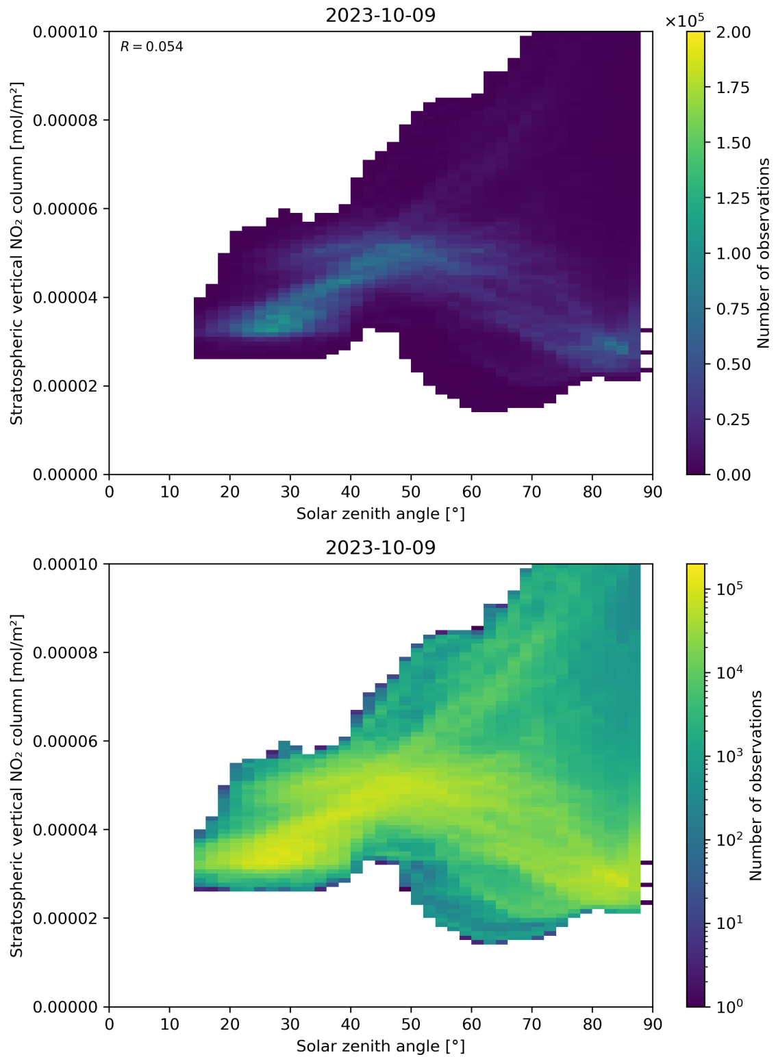
Figure 150: Scatter density plot of “Solar zenith angle” against “Stratospheric vertical NO 2 column” for 2023-10-08 to 2023-10-10.
