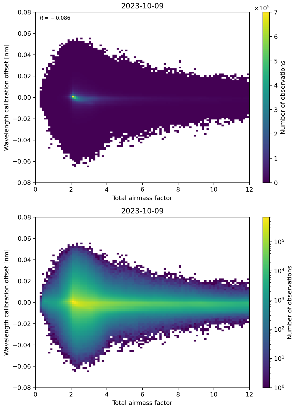
Figure 70: Scatter density plot of “Total airmass factor” against “Wavelength calibration offset” for 2023-10-08 to 2023-10-10.
