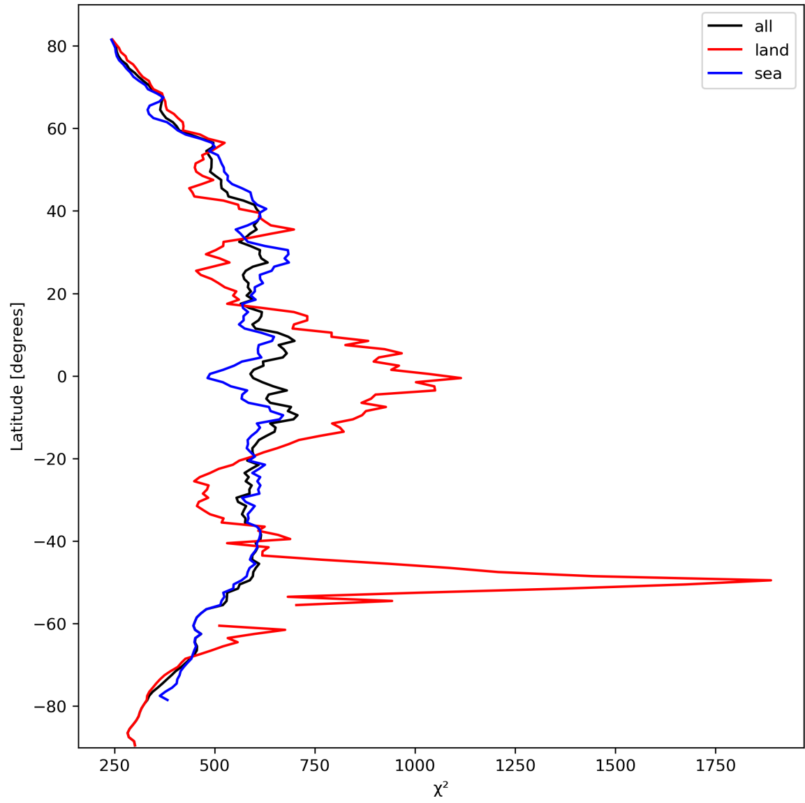
Figure 25: Zonal average of “ \chi^2 ” for 2023-10-08 to 2023-10-10.
