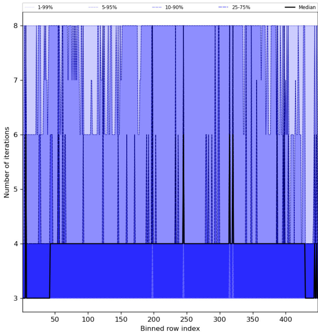
Figure 51: Along track statistics of “Number of iterations” for 2023-10-08 to 2023-10-10
