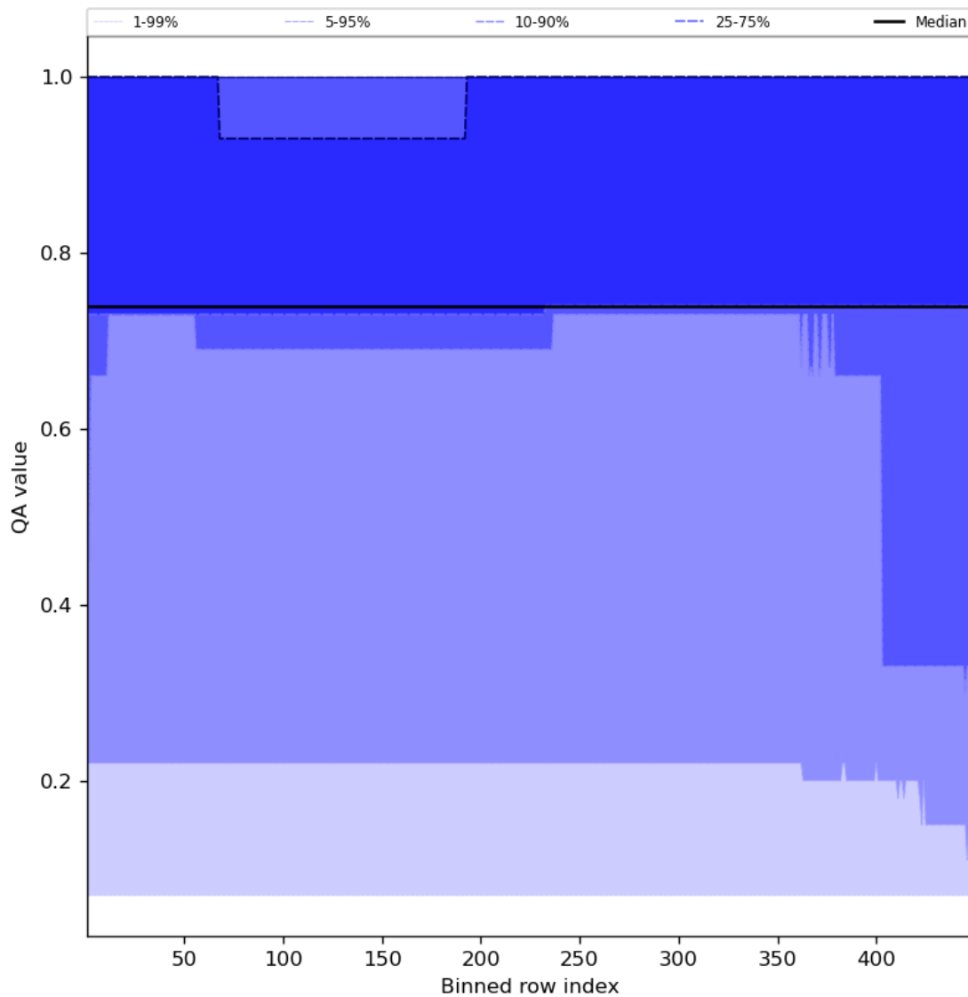
Figure 45: Along track statistics of "QA value" for 2023-10-08 to 2023-10-10
