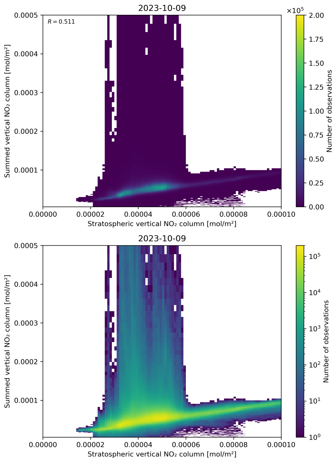
Figure 98: Scatter density plot of “Stratospheric vertical NO 2 column” against “Summed vertical NO 2 column” for 2023-10-08 to 2023-10-10.
