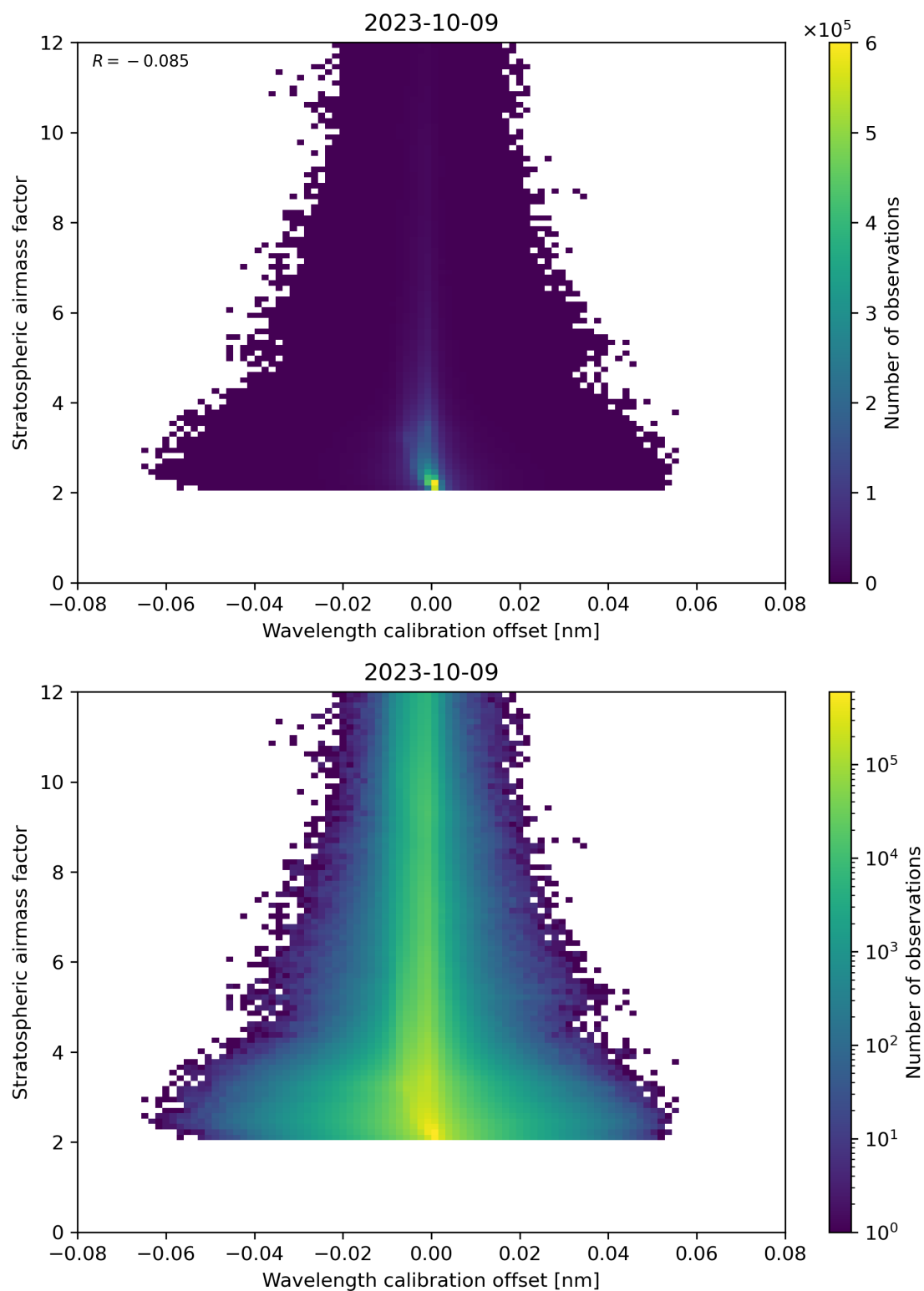
Figure 174: Scatter density plot of “Wavelength calibration offset” against “Stratospheric airmass factor” for 2023-10-08 to 2023-10-10.
