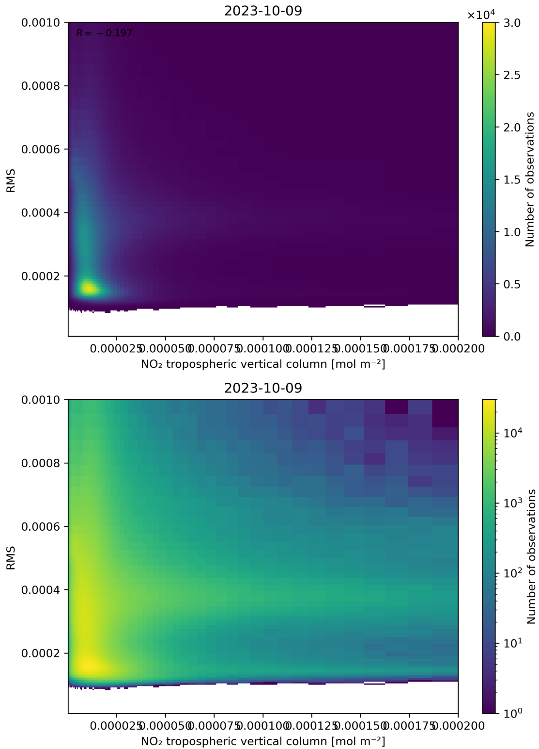
Figure 142: Scatter density plot of “NO 2 tropospheric vertical column” against “RMS” for 2023-10-08 to 2023-10-10.
