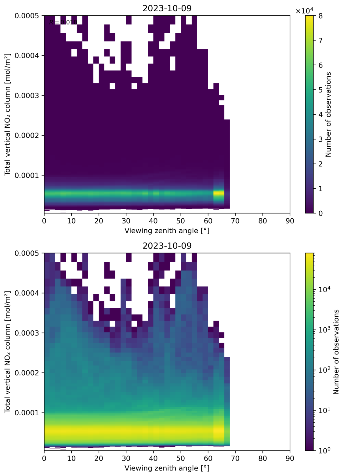
Figure 167: Scatter density plot of “Viewing zenith angle” against “Total vertical NO 2 column” for 2023-10-08 to 2023-10-10.
