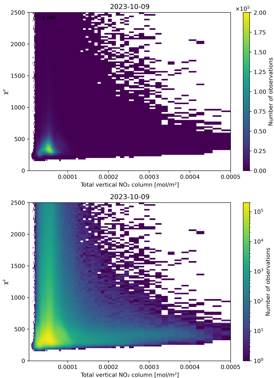
Figure 111: Scatter density plot of “Total vertical NO 2 column” against “ \chi^2 ” for 2023-10-08 to 2023-10-10.
