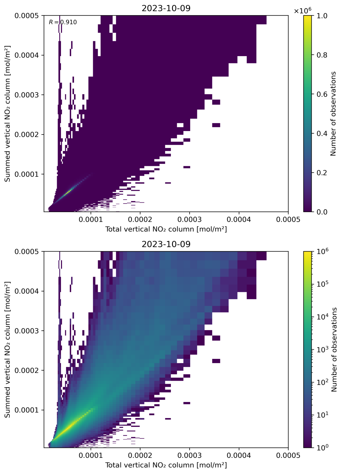
Figure 112: Scatter density plot of “Total vertical NO 2 column” against “Summed vertical NO 2 column” for 2023-10-08 to 2023-10-10.
