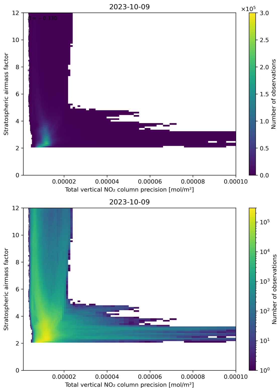
Figure 115: Scatter density plot of “Total vertical NO 2 column precision” against “Stratospheric airmass factor” for 2023-10-08 to 2023-10-10.
