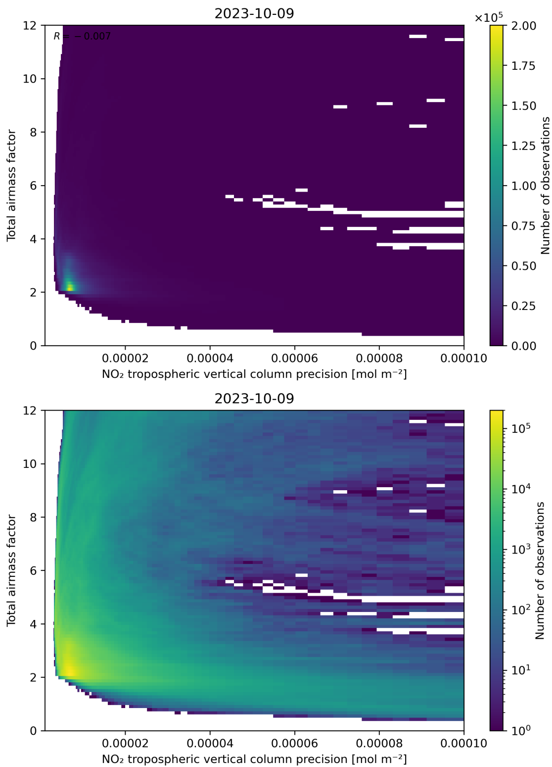
Figure 132: Scatter density plot of “NO 2 tropospheric vertical column precision” against “Total air mass factor” for 2023-10-08 to 2023-10-10.
