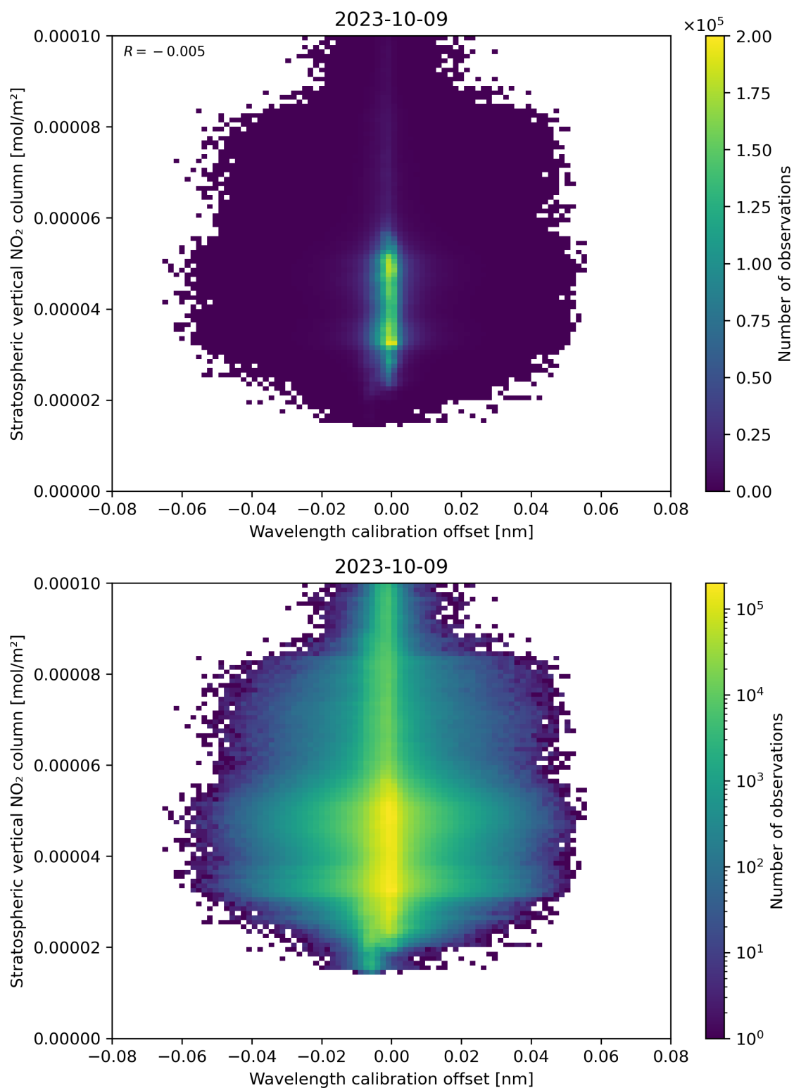
Figure 176: Scatter density plot of “Wavelength calibration offset” against “Stratospheric vertical NO 2 column” for 2023-10-08 to 2023-10-10.
