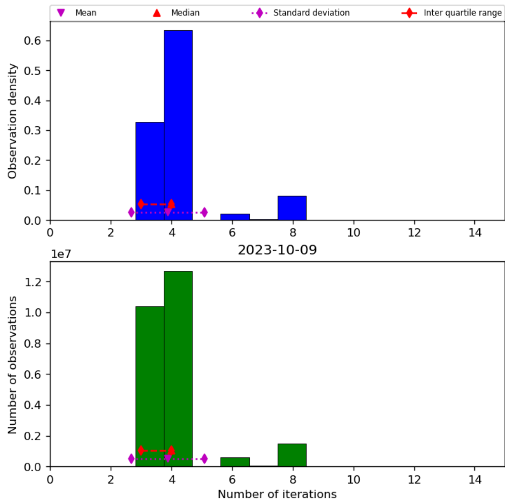
Figure 34: Histogram of "Number of iterations" for 2023-10-08 to 2023-10-10
