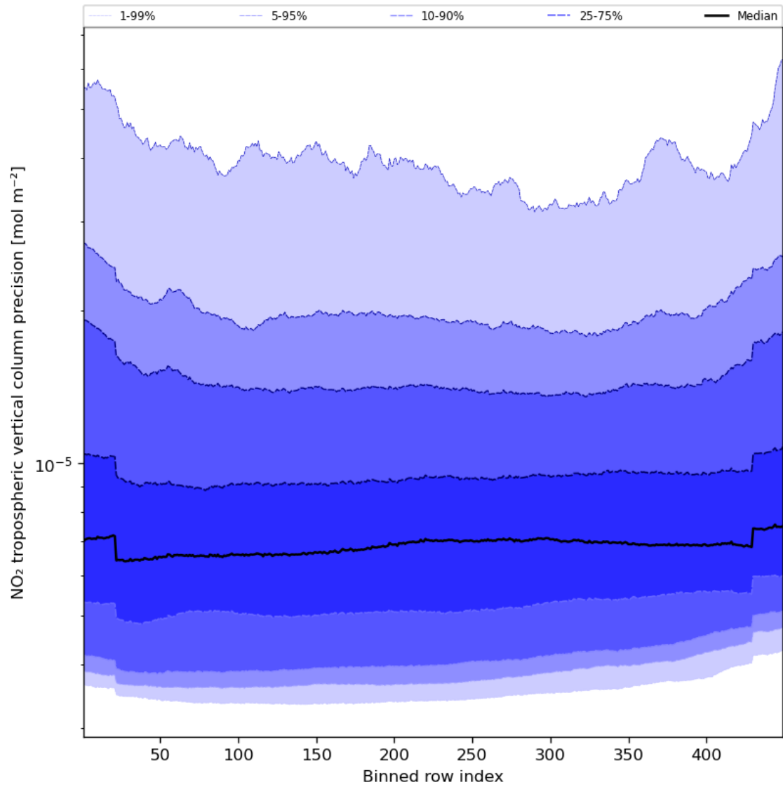
Figure 47: Along track statistics of “NO 2 tropospheric vertical column precision” for 2023-10-08 to 2023-10-10
