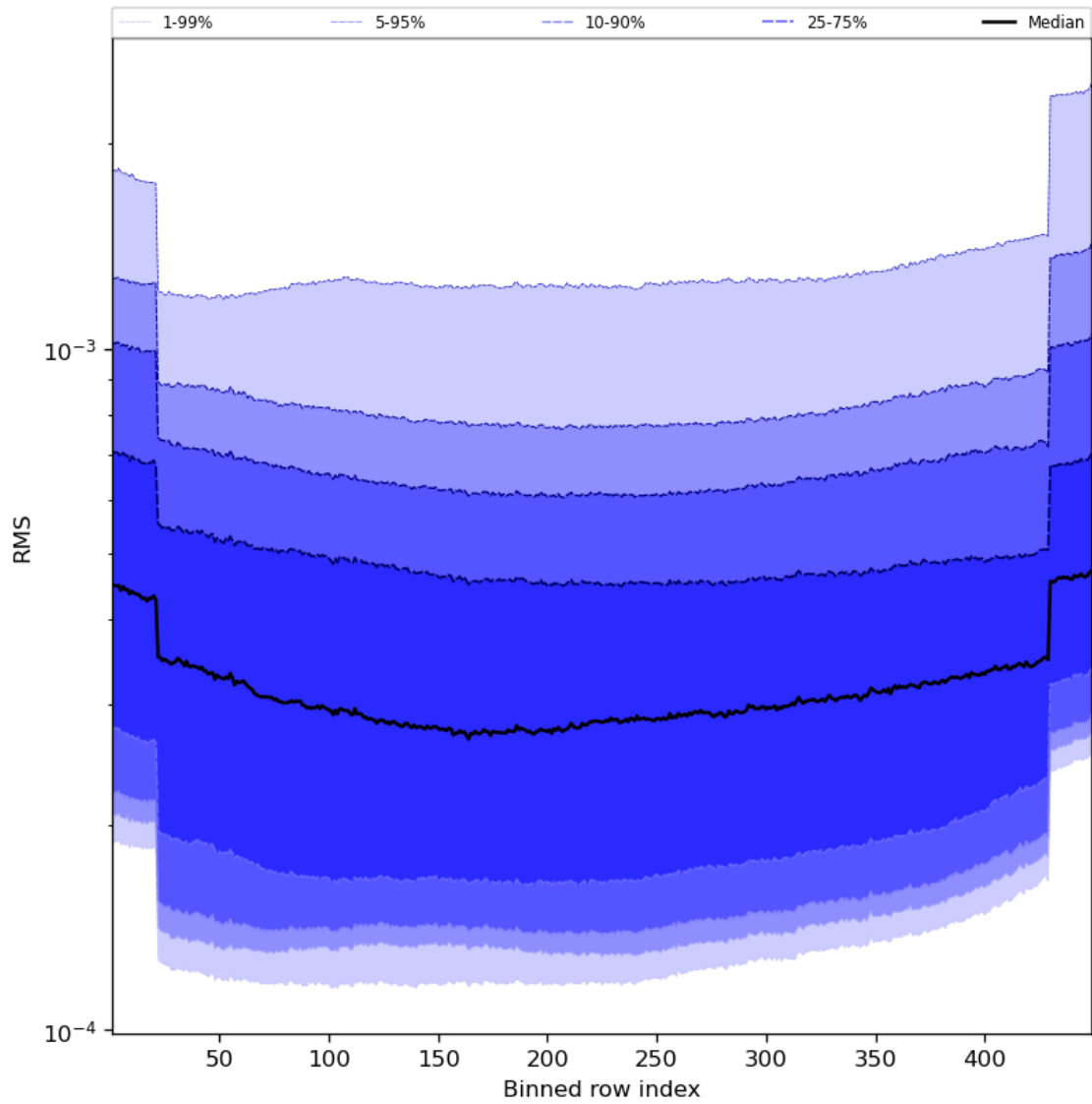
Figure 60: Along track statistics of “RMS” for 2023-10-08 to 2023-10-10
