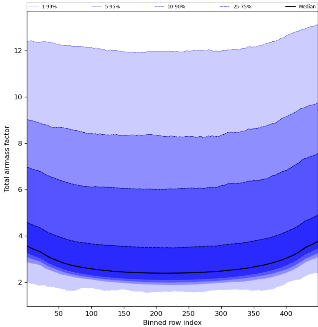
Figure 49: Along track statistics of “Total airmass factor” for 2023-10-08 to 2023-10-10
