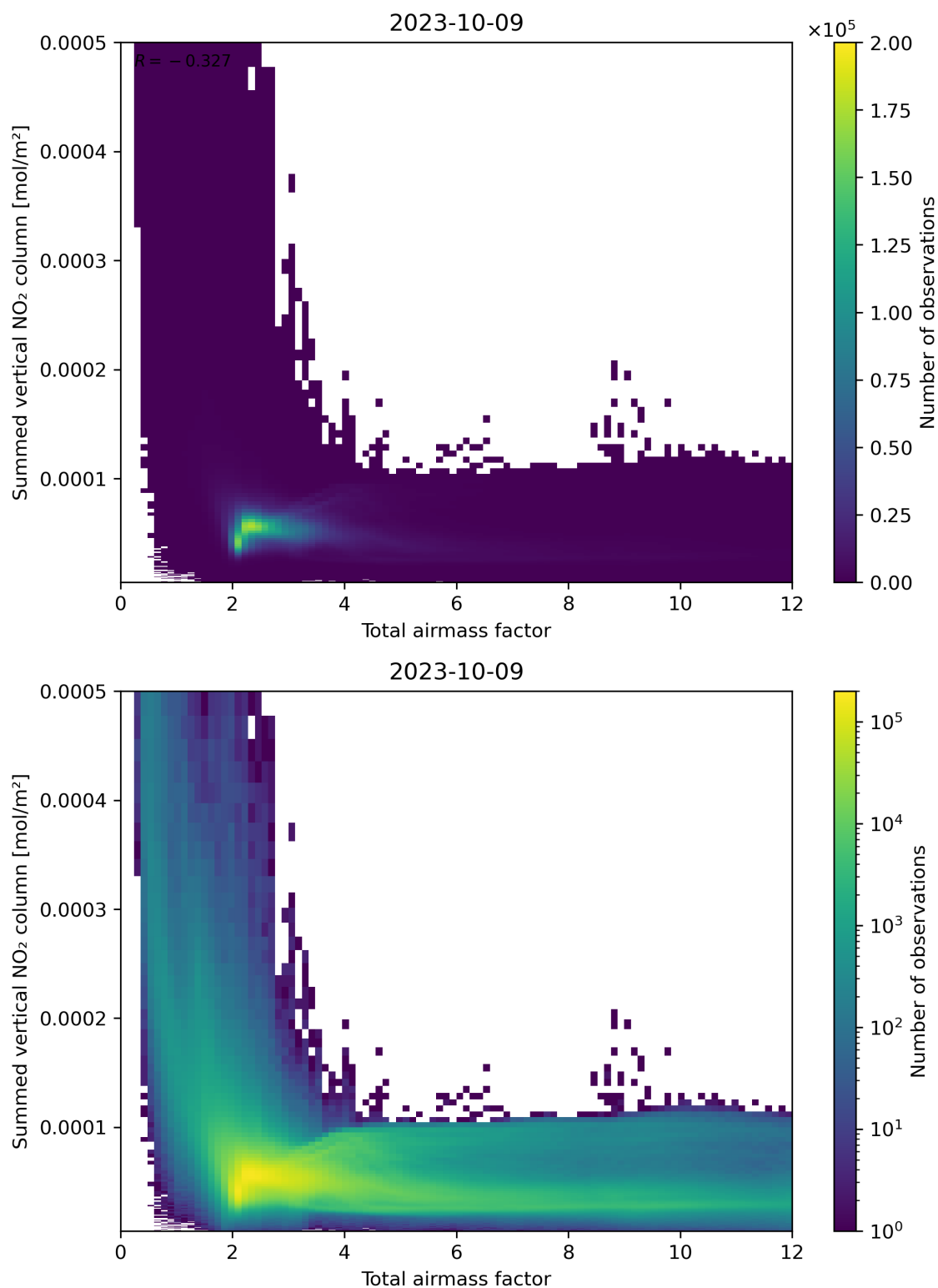
Figure 65: Scatter density plot of “Total airmass factor” against “Summed vertical NO 2 column” for 2023-10-08 to 2023-10-10.
