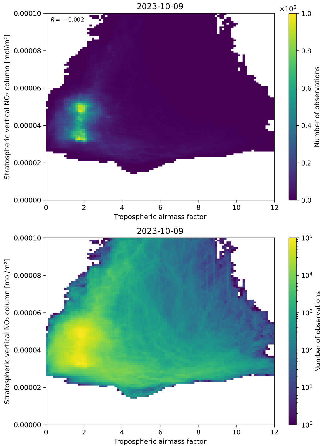
Figure 74: Scatter density plot of “Tropospheric air mass factor” against “Stratospheric vertical NO 2 column” for 2023-10-08 to 2023-10-10.
