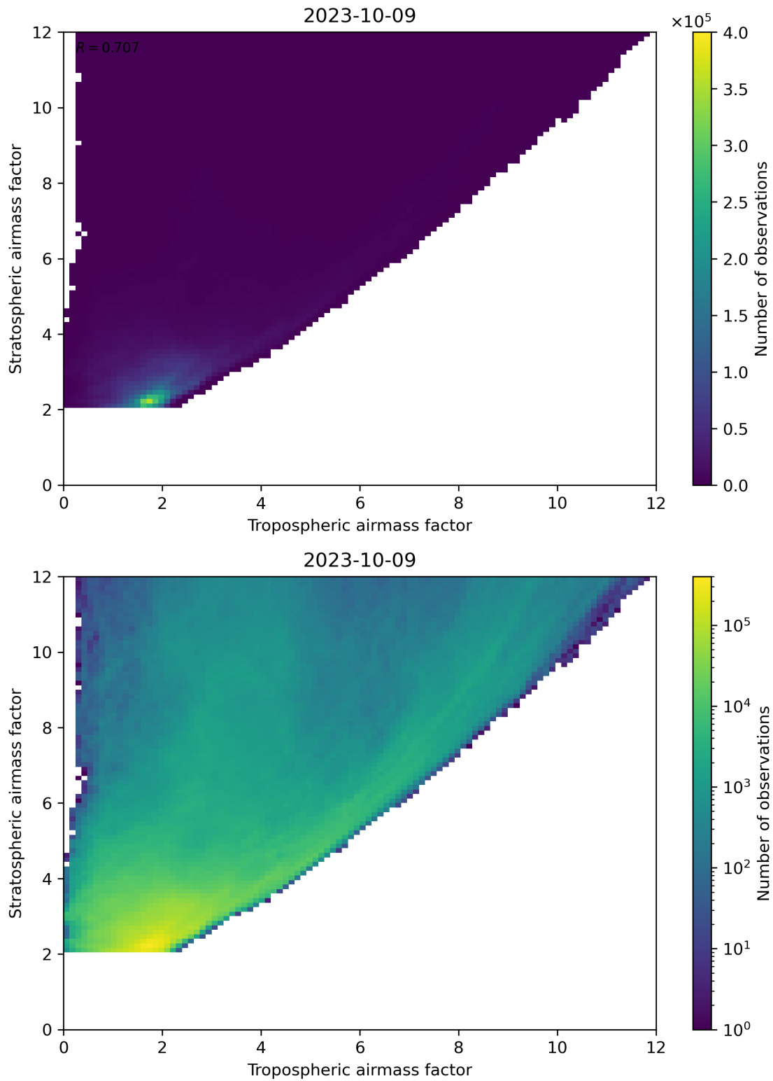
Figure 71: Scatter density plot of “Tropospheric airmass factor” against “Stratospheric airmass factor” for 2023-10-08 to 2023-10-10.
