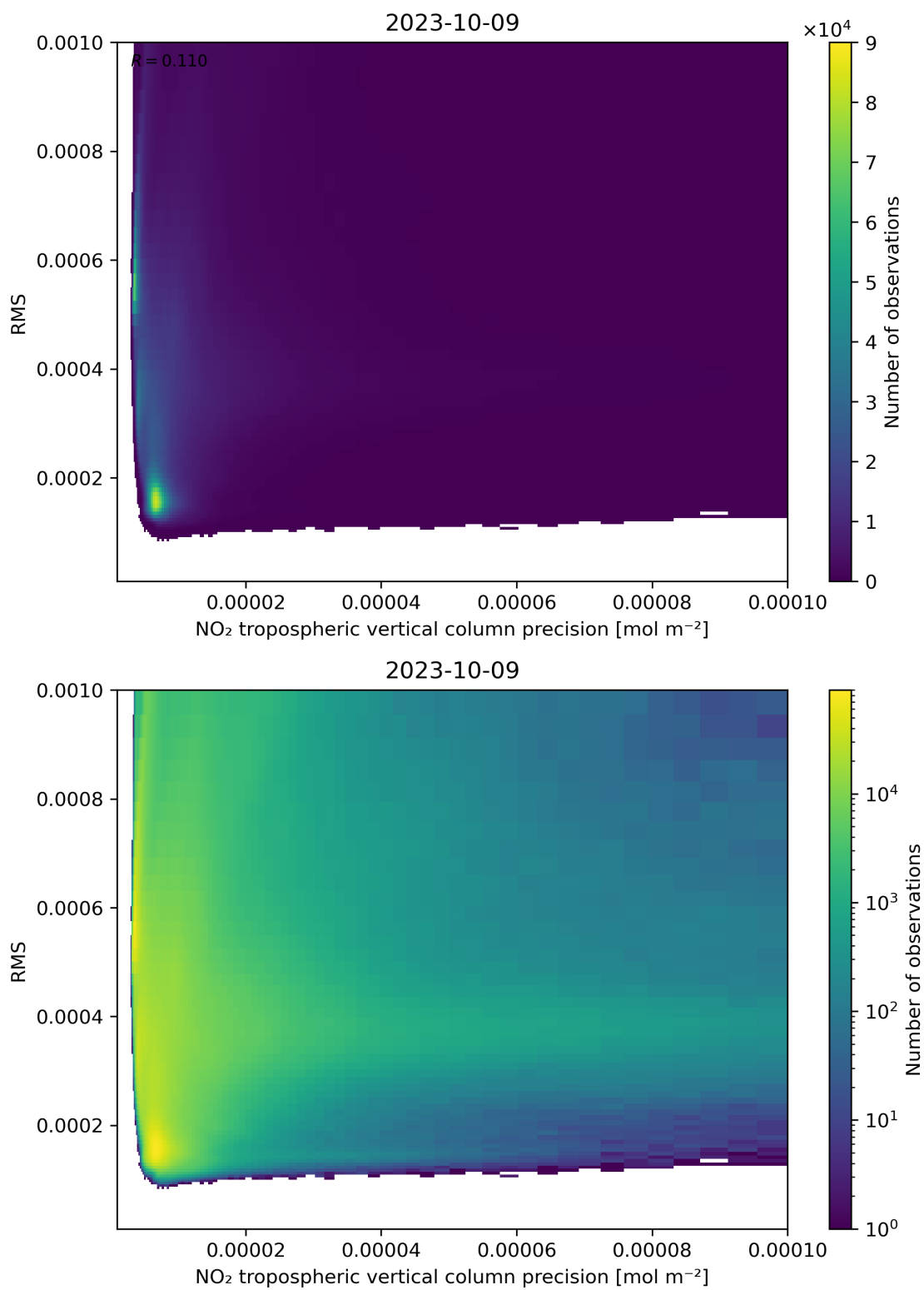
Figure 140: Scatter density plot of “NO 2 tropospheric vertical column precision” against “RMS” for 2023-10-08 to 2023-10-10.
