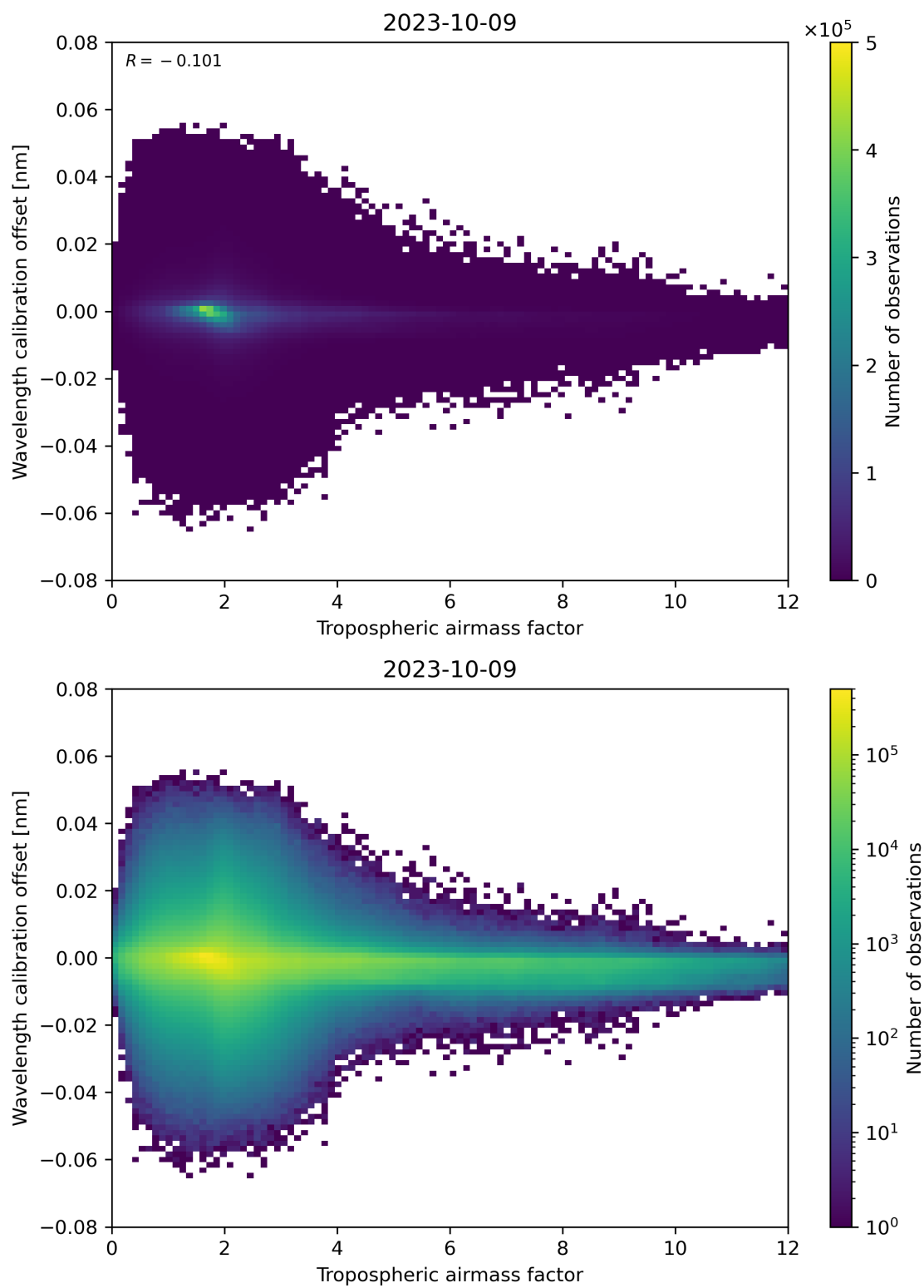
Figure 80: Scatter density plot of “Tropospheric airmass factor” against “Wavelength calibration offset” for 2023-10-08 to 2023-10-10.
