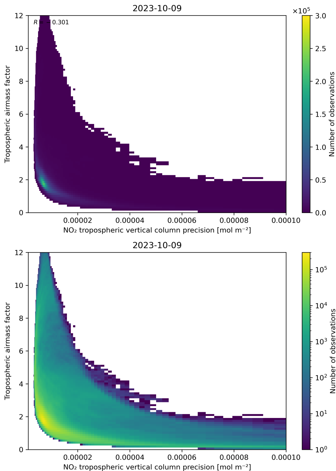
Figure 133: Scatter density plot of “NO 2 tropospheric vertical column precision” against “Tropospheric air mass factor” for 2023-10-08 to 2023-10-10.
