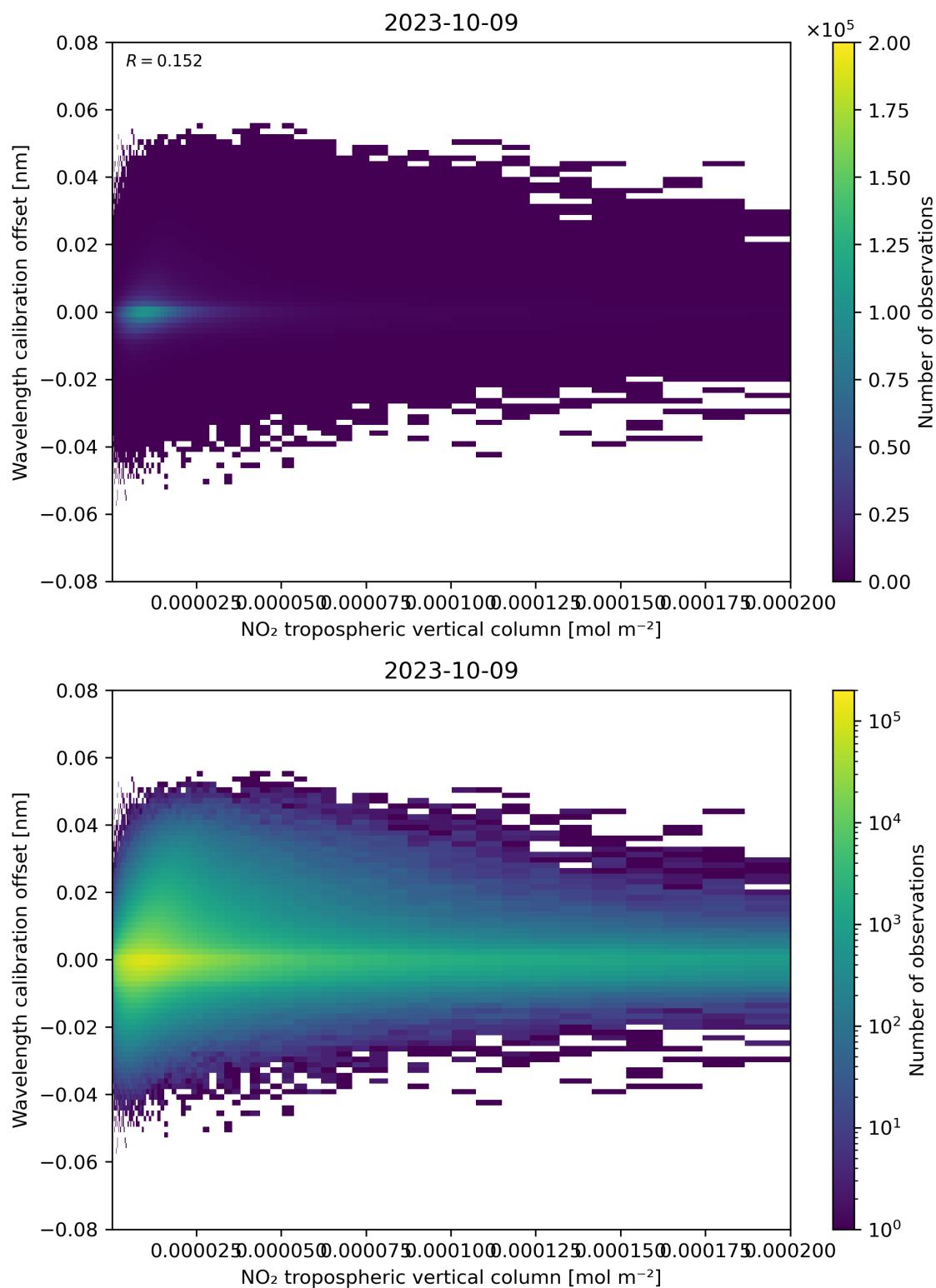
Figure 143: Scatter density plot of “NO 2 tropospheric vertical column” against “Wavelength calibration offset” for 2023-10-08 to 2023-10-10.
