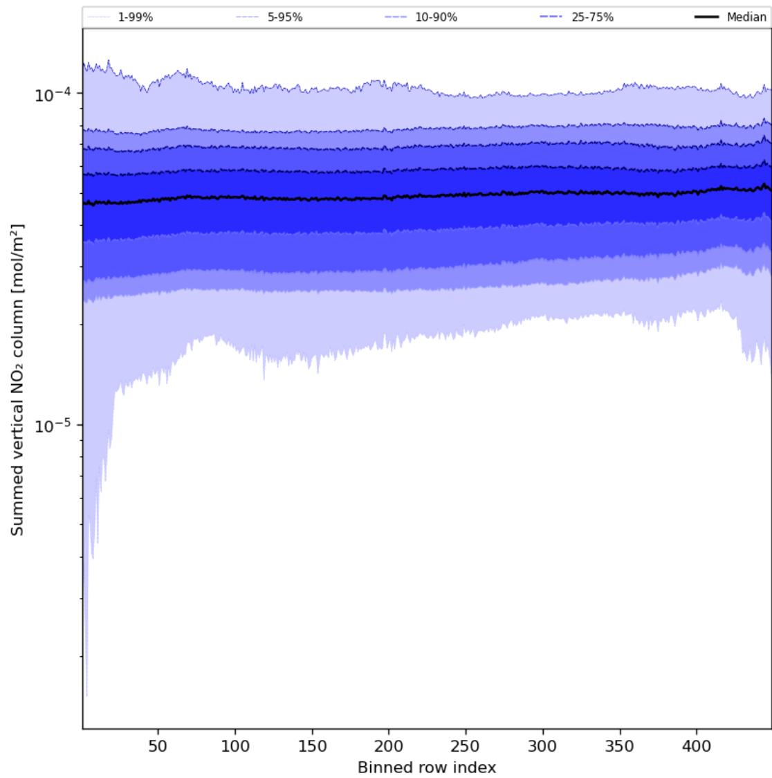
Figure 57: Along track statistics of “Summed vertical NO 2 column” for 2023-10-08 to 2023-10-10
