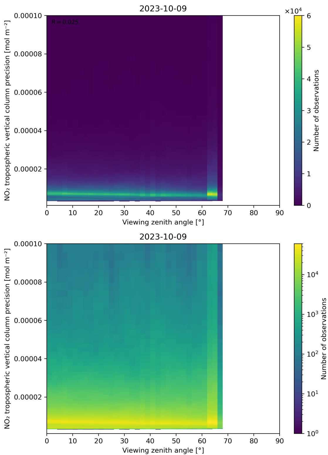
Figure 170: Scatter density plot of “Viewing zenith angle” against “NO 2 tropospheric vertical column precision” for 2023-10-08 to 2023-10-10.
