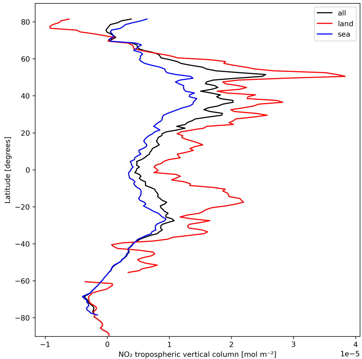
Figure 12: Zonal average of “NO 2 tropospheric vertical column” for 2023-10-08 to 2023-10-10.
