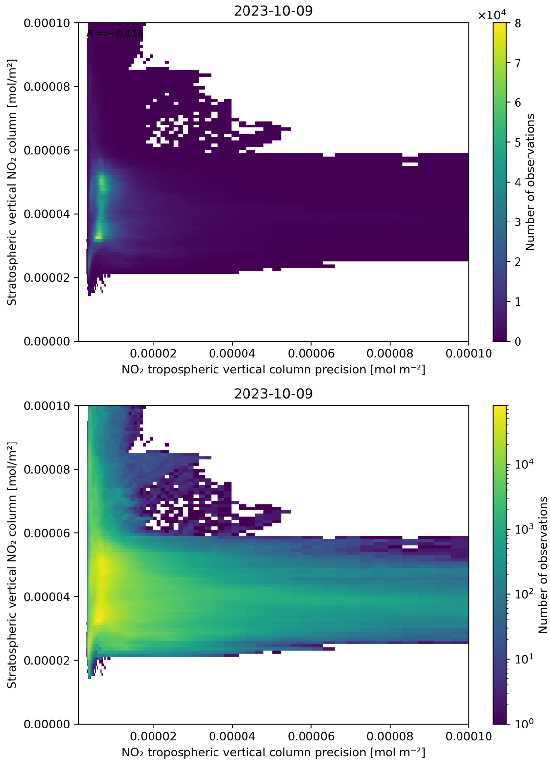
Figure 135: Scatter density plot of “NO 2 tropospheric vertical column precision” against “Stratospheric vertical NO 2 column” for 2023-10-08 to 2023-10-10.
