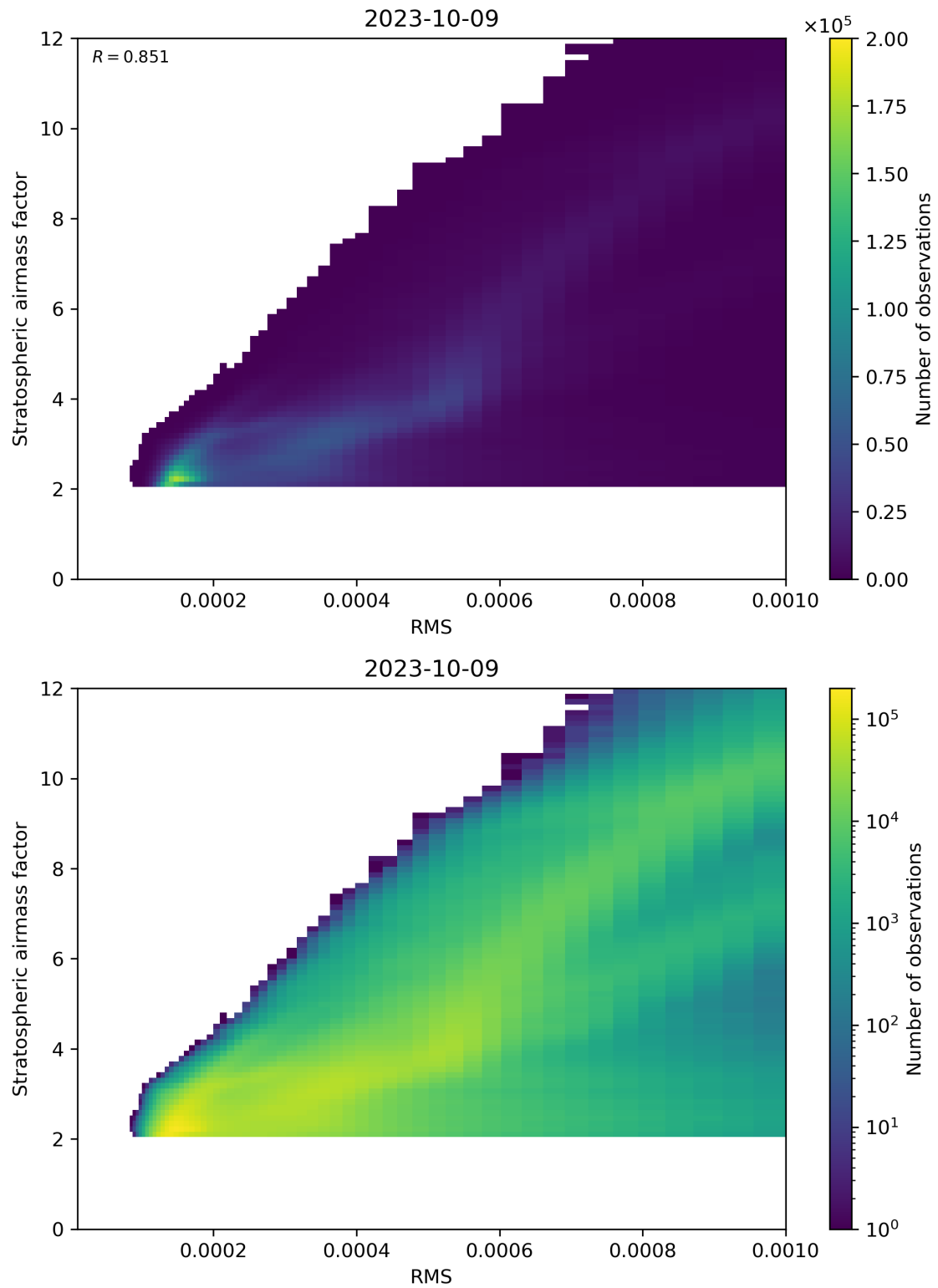
Figure 144: Scatter density plot of “RMS” against “Stratospheric airmass factor” for 2023-10-08 to 2023-10-10.
