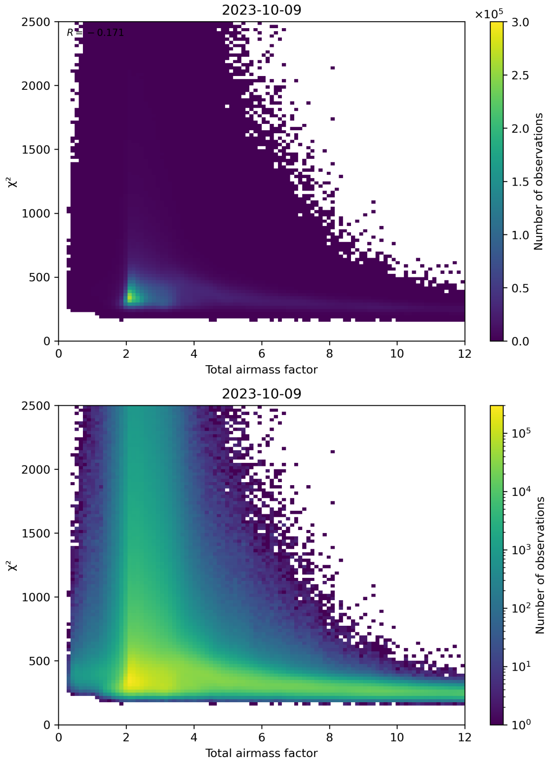
Figure 63: Scatter density plot of “Total airmass factor” against “ \chi^2 ” for 2023-10-08 to 2023-10-10.
