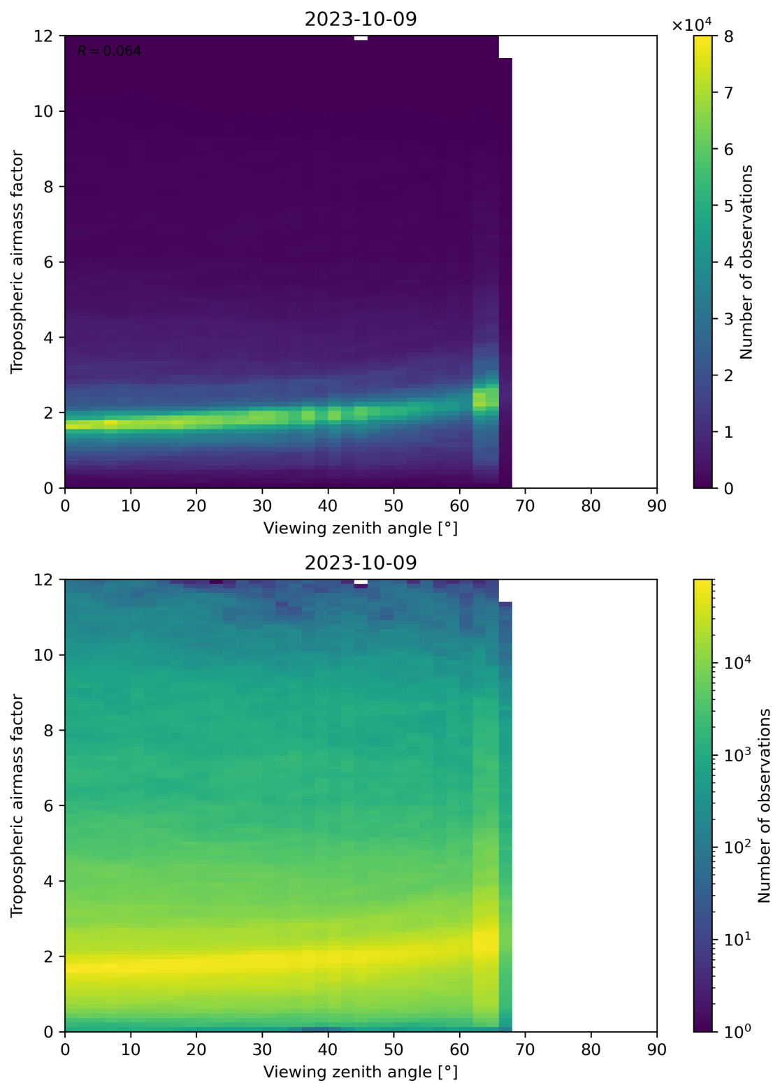
Figure 161: Scatter density plot of “Viewing zenith angle” against “Tropospheric airmass factor” for 2023-10-08 to 2023-10-10.
