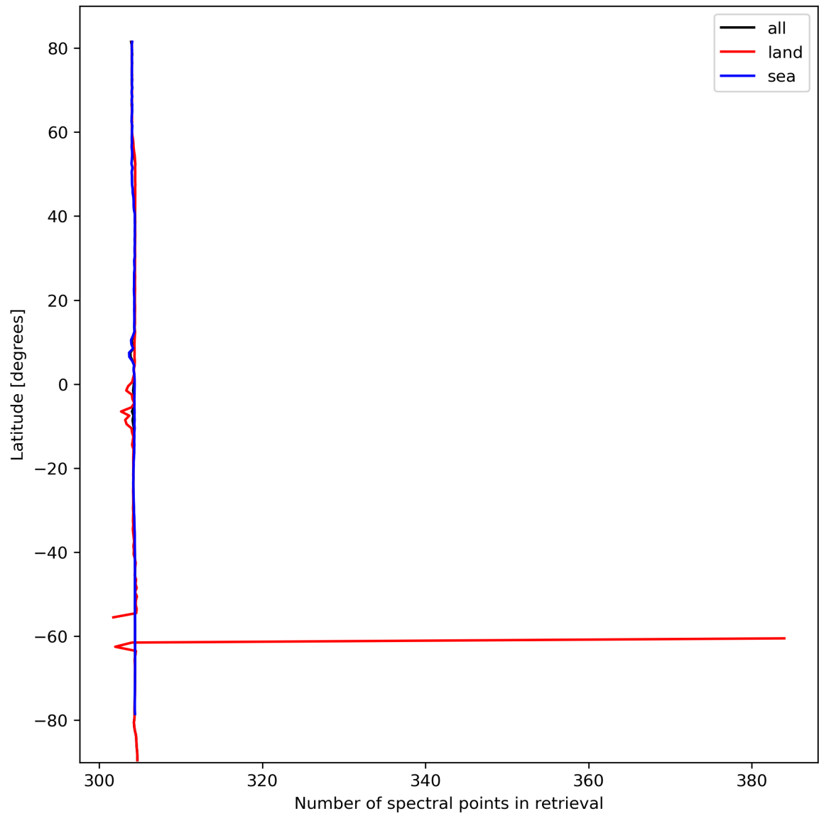
Figure 16: Zonal average of “Number of spectral points in retrieval” for 2023-10-08 to 2023-10-10.
