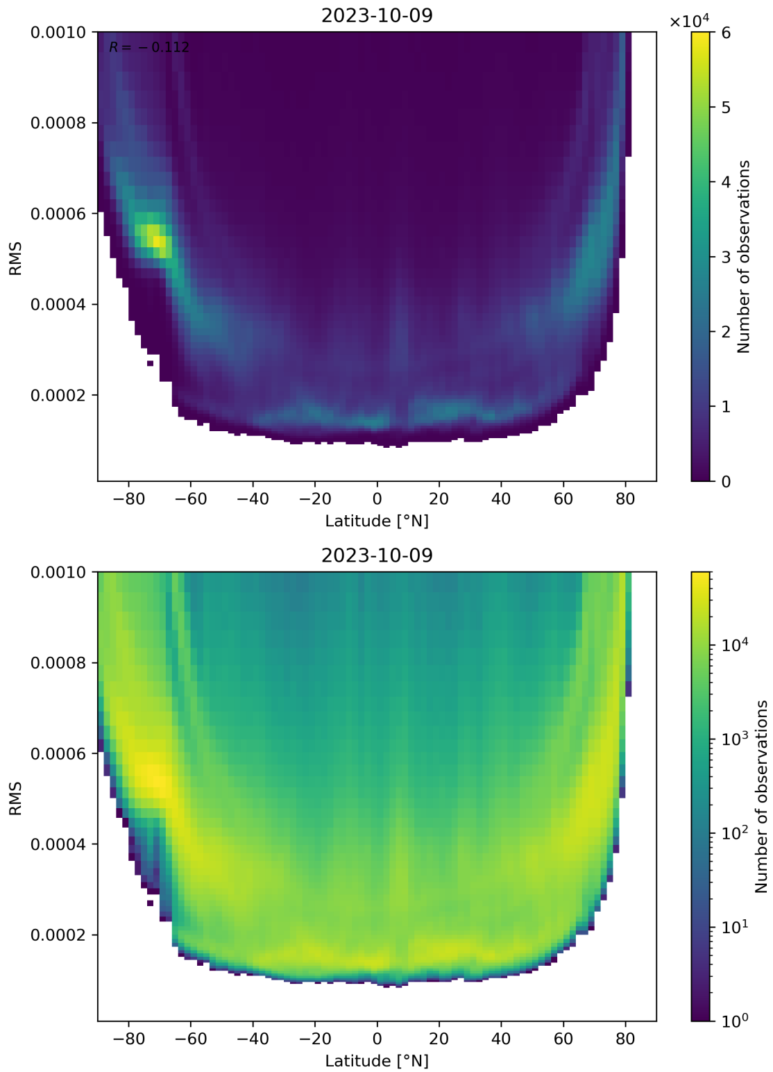
Figure 94: Scatter density plot of “Latitude” against “RMS” for 2023-10-08 to 2023-10-10.
