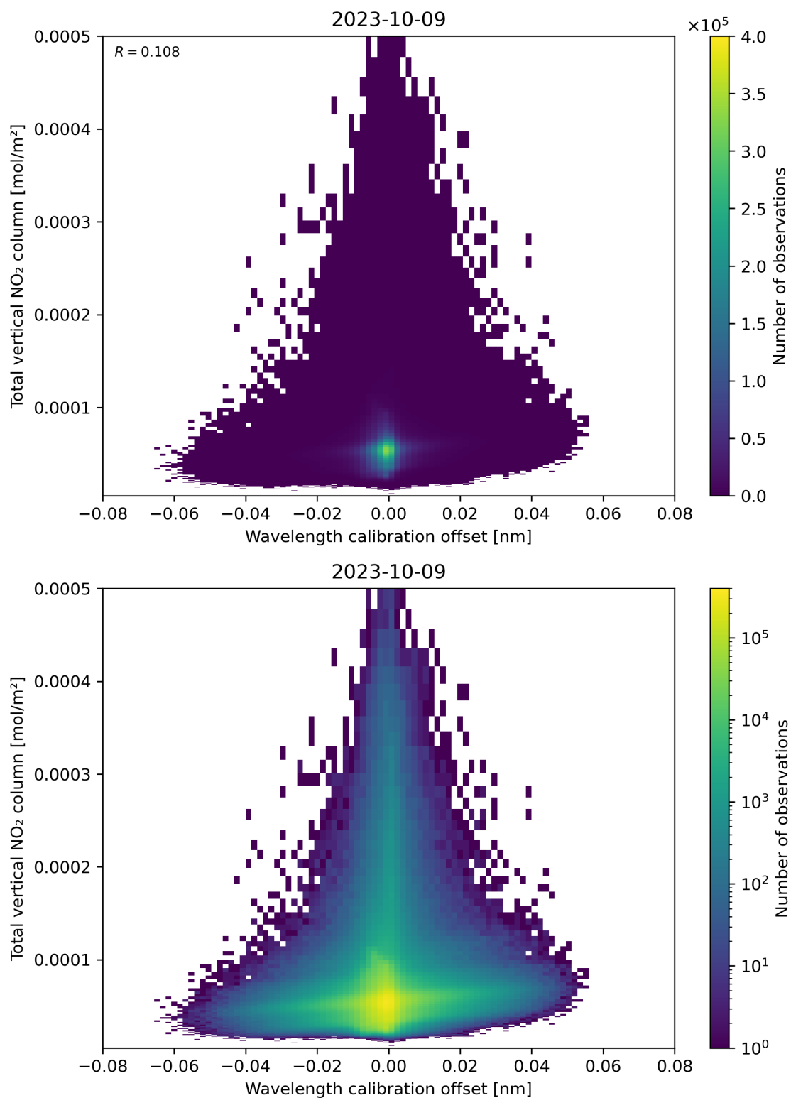
Figure 179: Scatter density plot of “Wavelength calibration offset” against “Total vertical NO 2 column” for 2023-10-08 to 2023-10-10.
