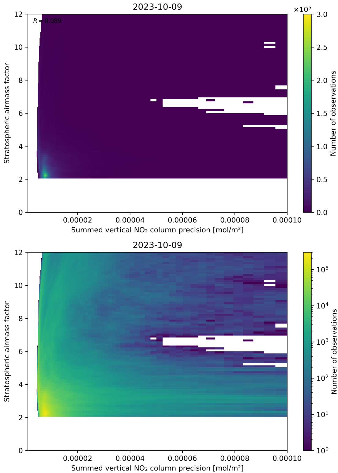
Figure 106: Scatter density plot of “Summed vertical NO 2 column precision” against “Stratospheric airmass factor” for 2023-10-08 to 2023-10-10.
