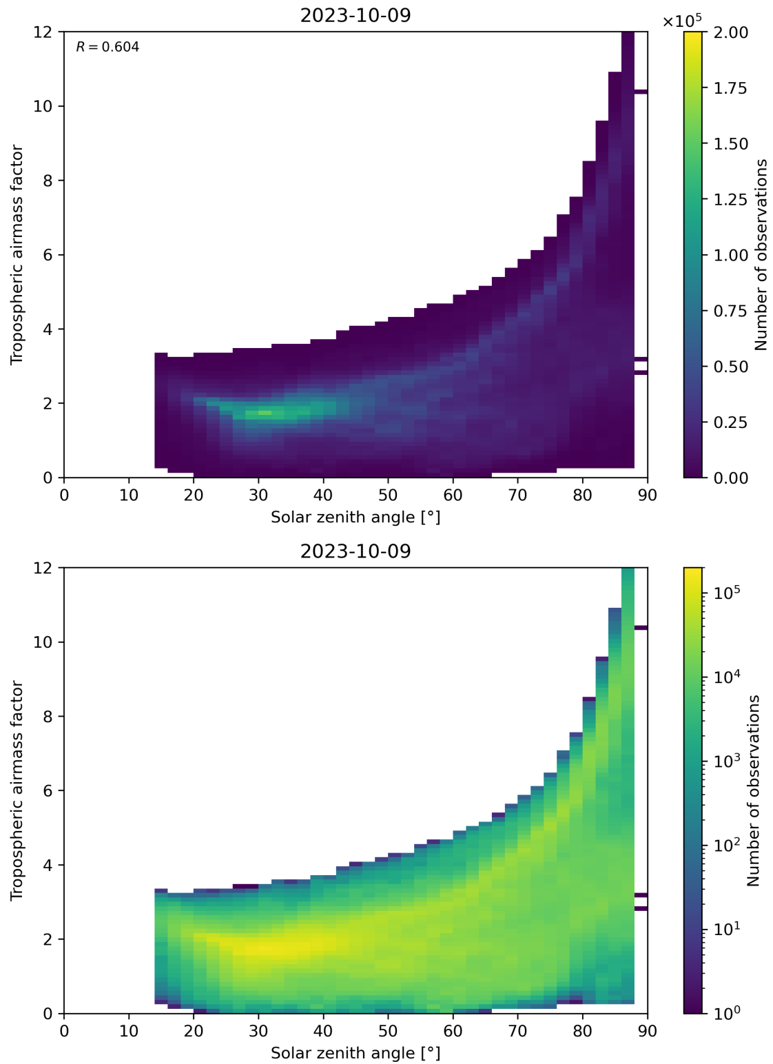
Figure 147: Scatter density plot of “Solar zenith angle” against “Tropospheric airmass factor” for 2023-10-08 to 2023-10-10.
