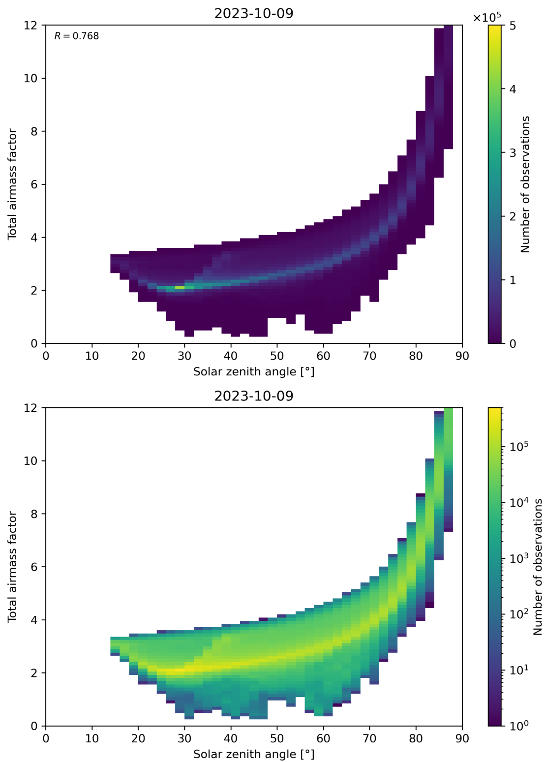
Figure 146: Scatter density plot of “Solar zenith angle” against “Total air mass factor” for 2023-10-08 to 2023-10-10.
