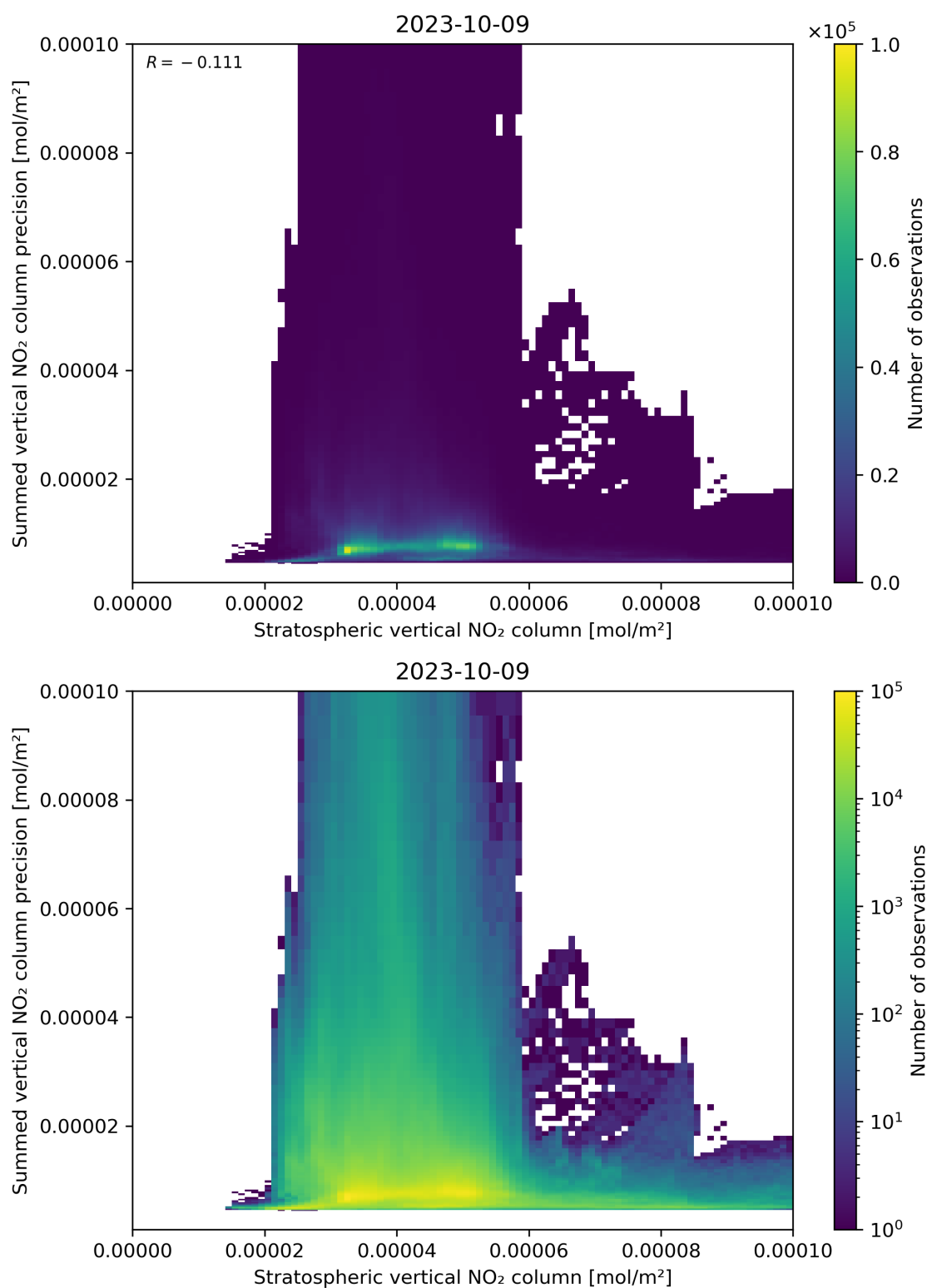
Figure 99: Scatter density plot of “Stratospheric vertical NO 2 column” against “Summed vertical NO 2 column precision” for 2023-10-08 to 2023-10-10.
