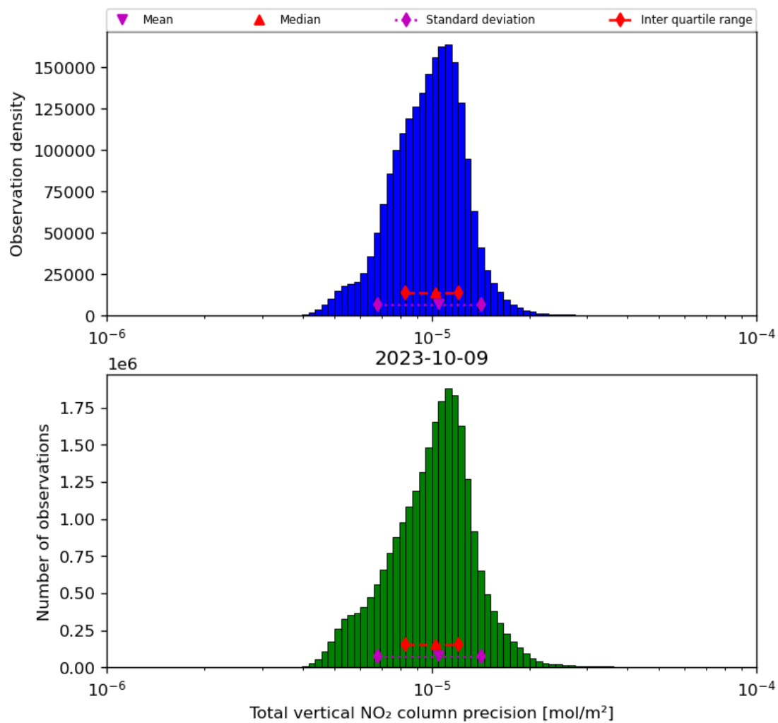
Figure 39: Histogram of "Total vertical NO 2 column precision" for 2023-10-08 to 2023-10-10
