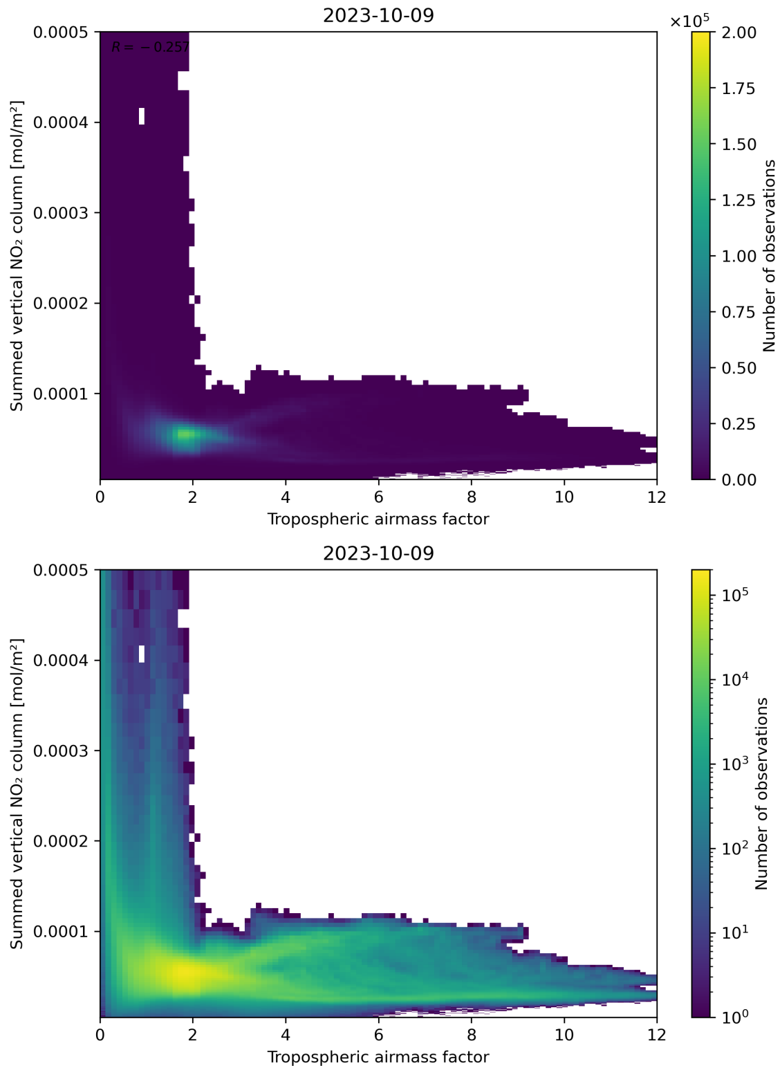
Figure 75: Scatter density plot of “Tropospheric airmass factor” against “Summed vertical NO 2 column” for 2023-10-08 to 2023-10-10.
