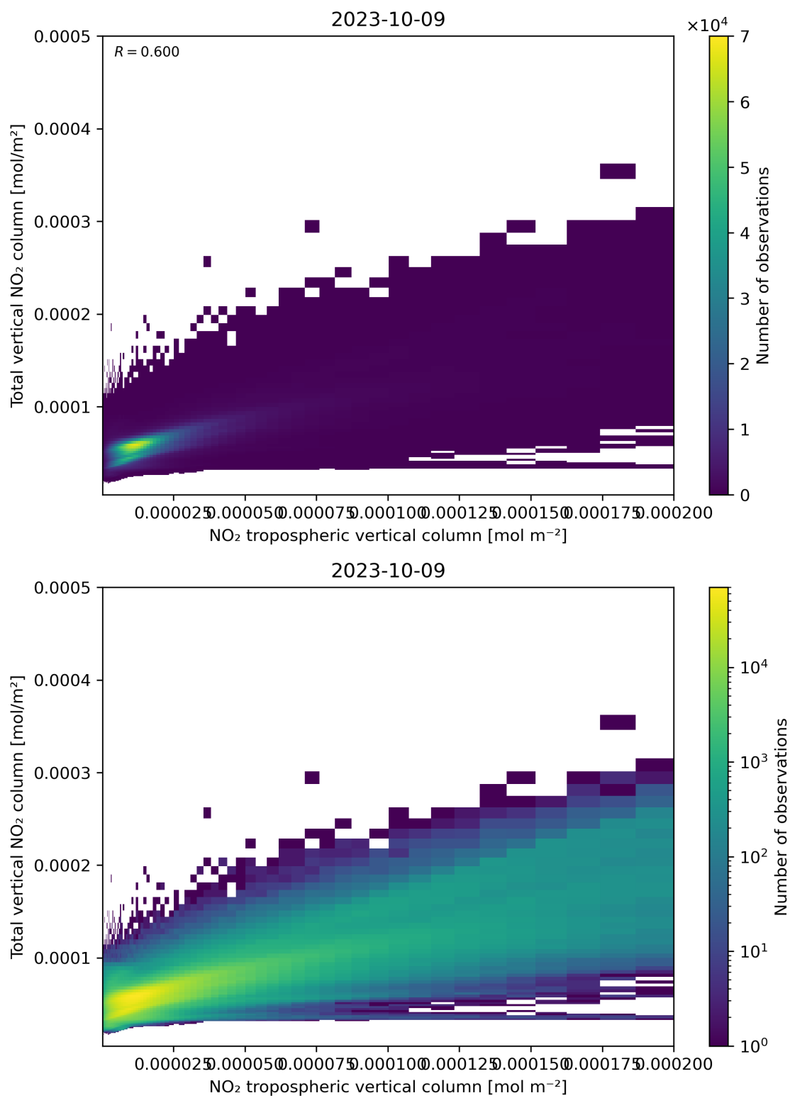
Figure 128: Scatter density plot of “NO 2 tropospheric vertical column” against “Total vertical NO 2 column” for 2023-10-08 to 2023-10-10.
