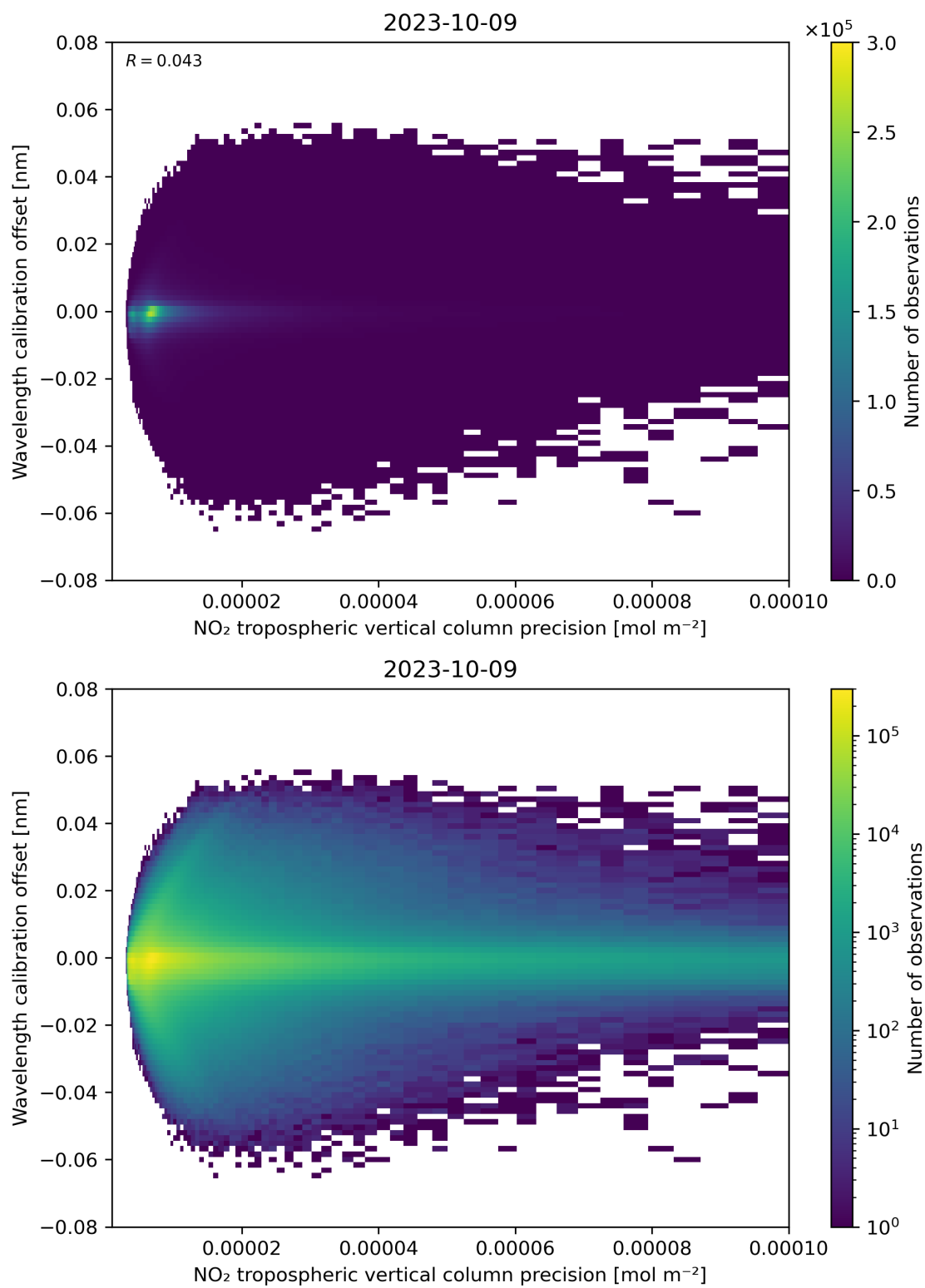
Figure 141: Scatter density plot of “NO 2 tropospheric vertical column precision” against “Wavelength calibration offset” for 2023-10-08 to 2023-10-10.
