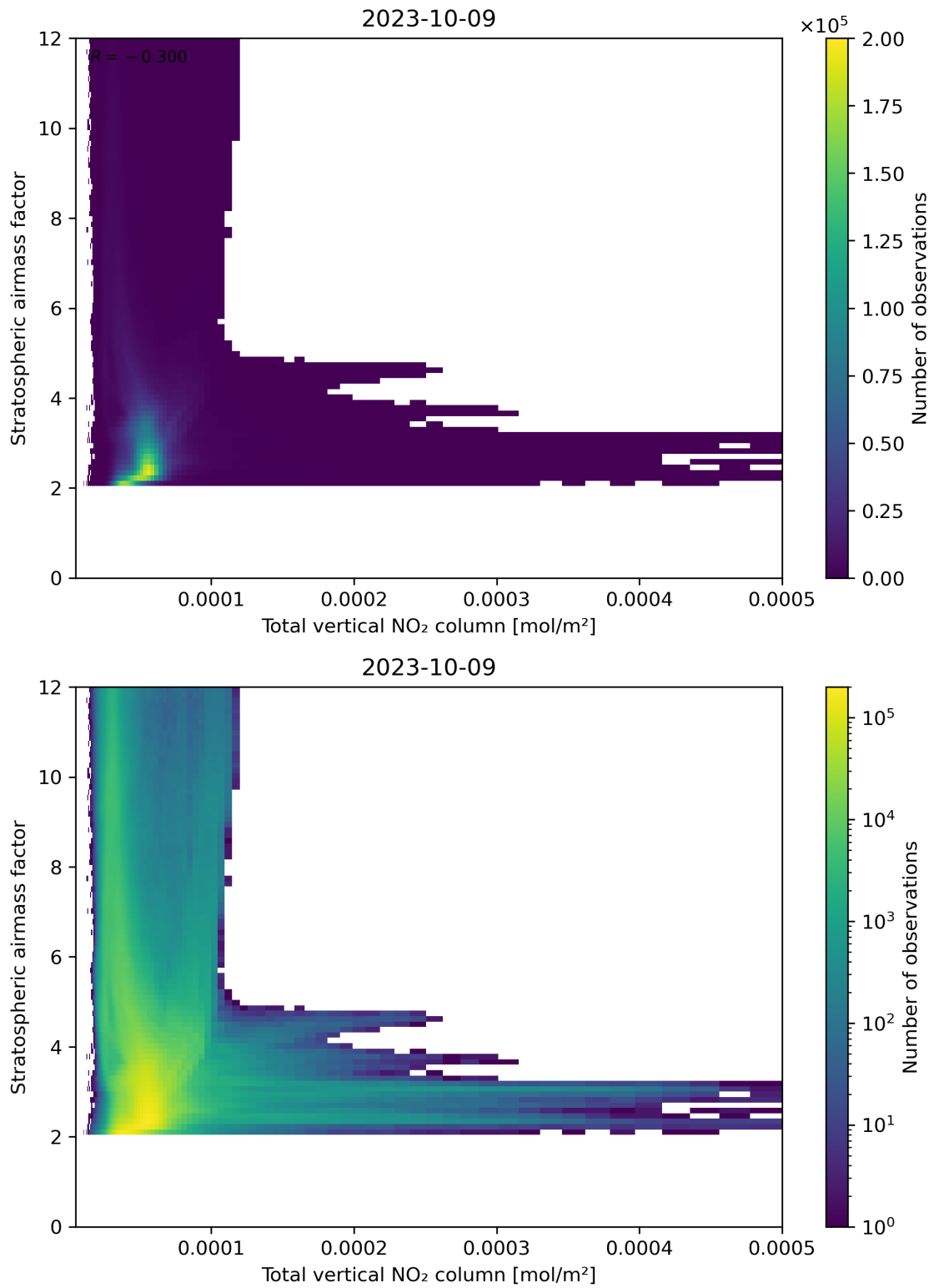
Figure 110: Scatter density plot of “Total vertical NO 2 column” against “Stratospheric airmass factor” for 2023-10-08 to 2023-10-10.
