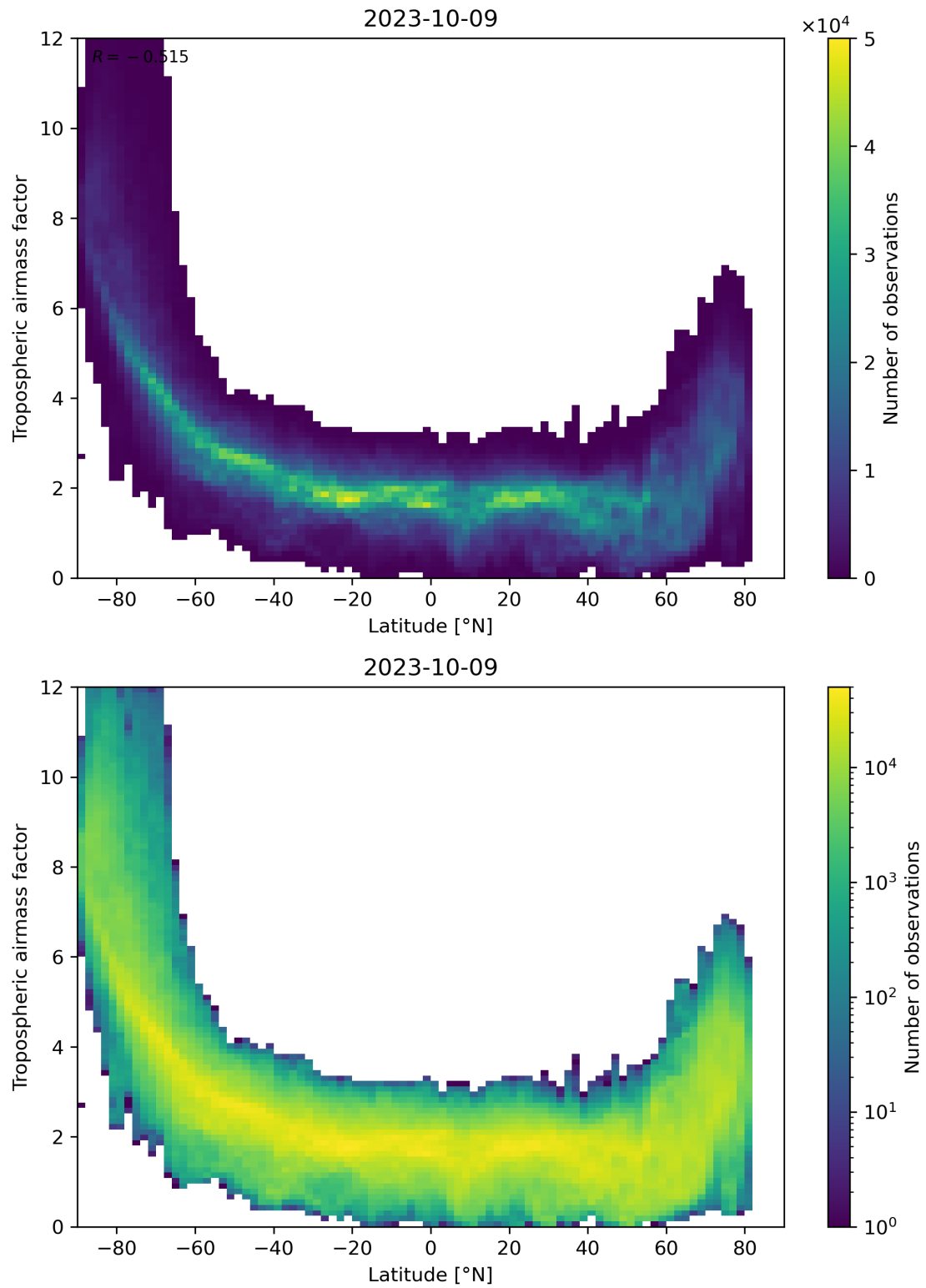
Figure 85: Scatter density plot of “Latitude” against “Tropospheric air mass factor” for 2023-10-08 to 2023-10-10.
