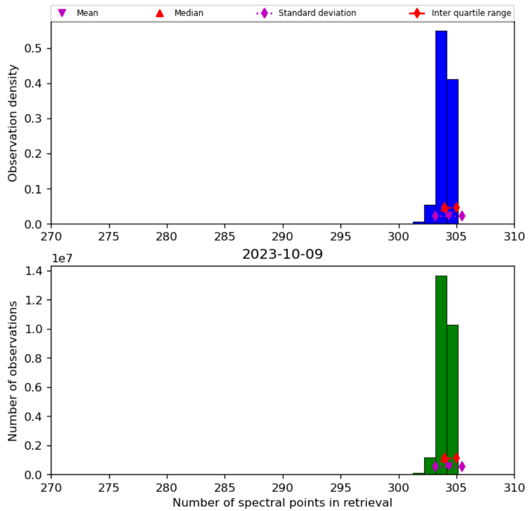
Figure 33: Histogram of “Number of spectral points in retrieval” for 2023-10-08 to 2023-10-10
