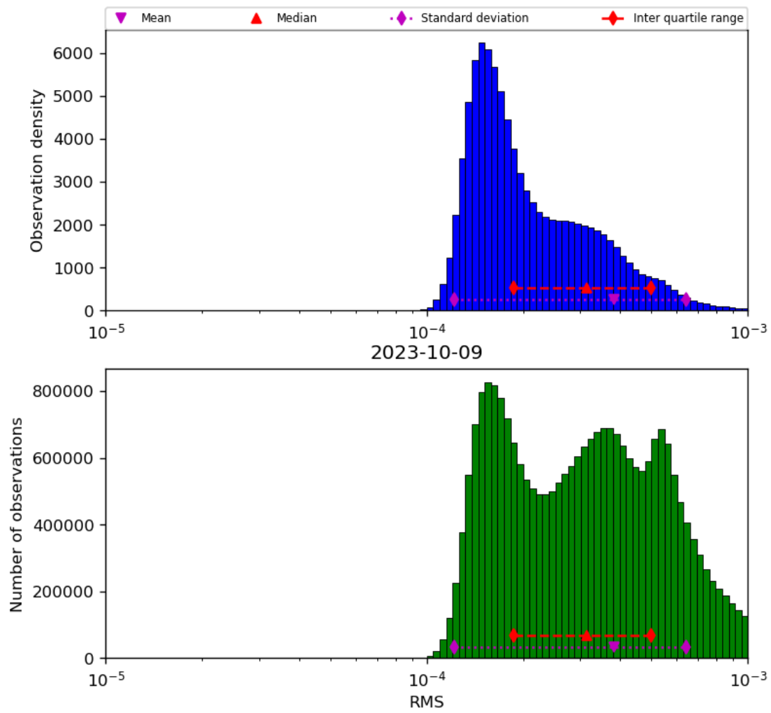
Figure 43: Histogram of “RMS” for 2023-10-08 to 2023-10-10
