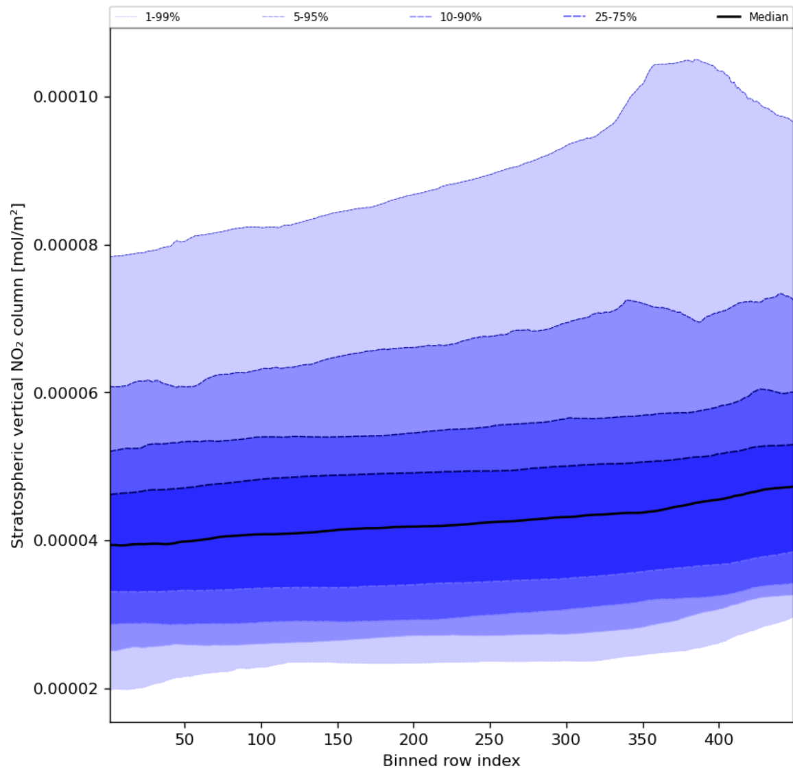
Figure 53: Along track statistics of “Stratospheric vertical NO 2 column” for 2023-10-08 to 2023-10-10
