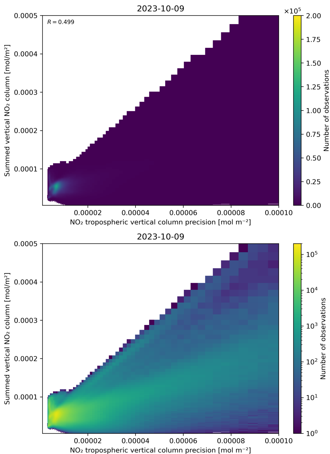
Figure 136: Scatter density plot of “NO 2 tropospheric vertical column precision” against “Summed vertical NO 2 column” for 2023-10-08 to 2023-10-10.
