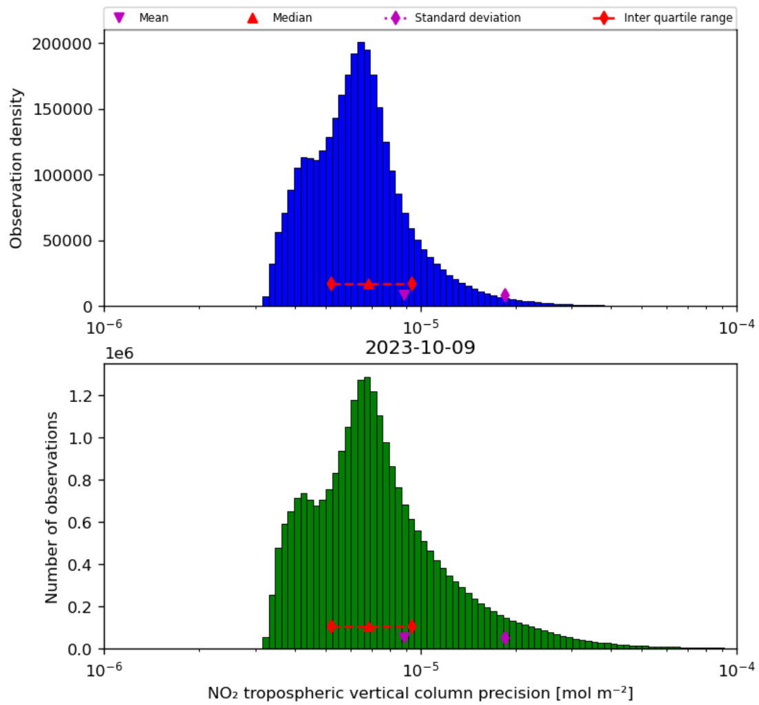
Figure 30: Histogram of “NO 2 tropospheric vertical column precision” for 2023-10-08 to 2023-10-10
