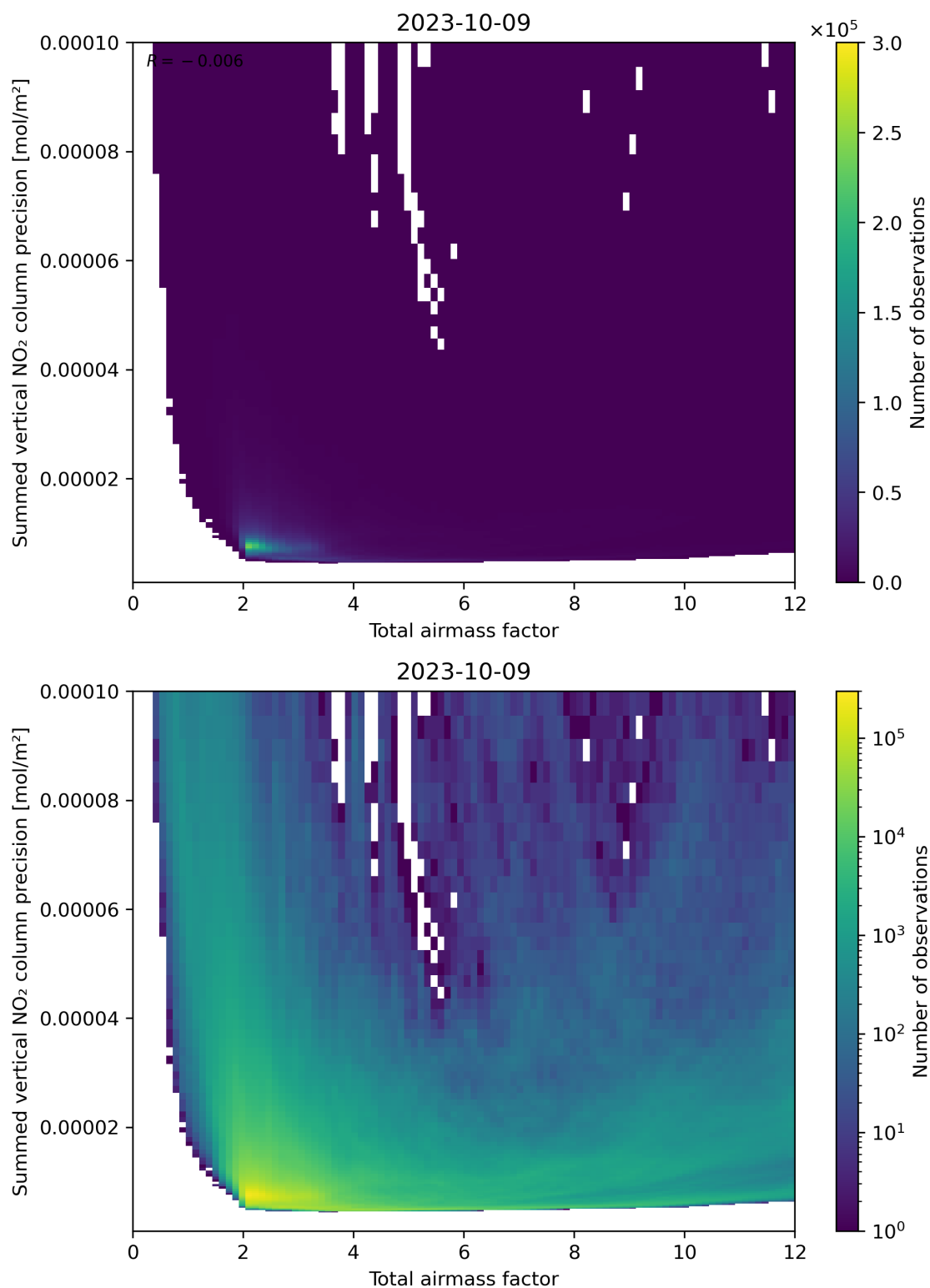
Figure 66: Scatter density plot of “Total airmass factor” against “Summed vertical NO 2 column precision” for 2023-10-08 to 2023-10-10.
