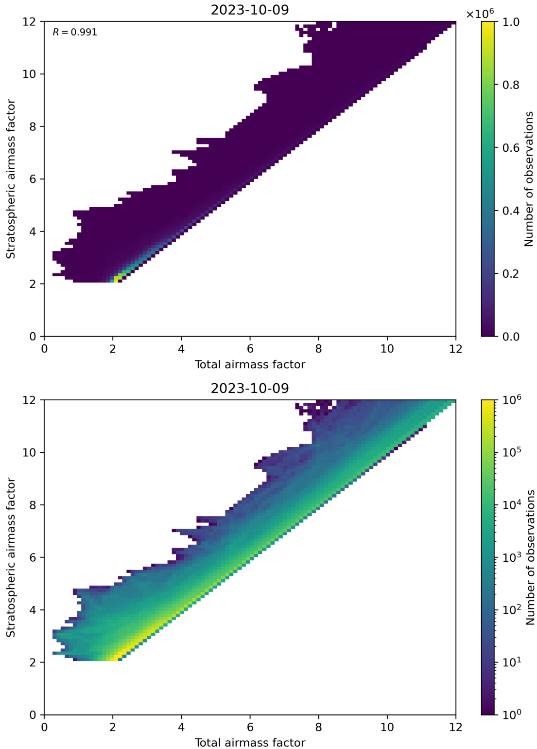
Figure 62: Scatter density plot of “Total airmass factor” against “Stratospheric airmass factor” for 2023-10-08 to 2023-10-10.
