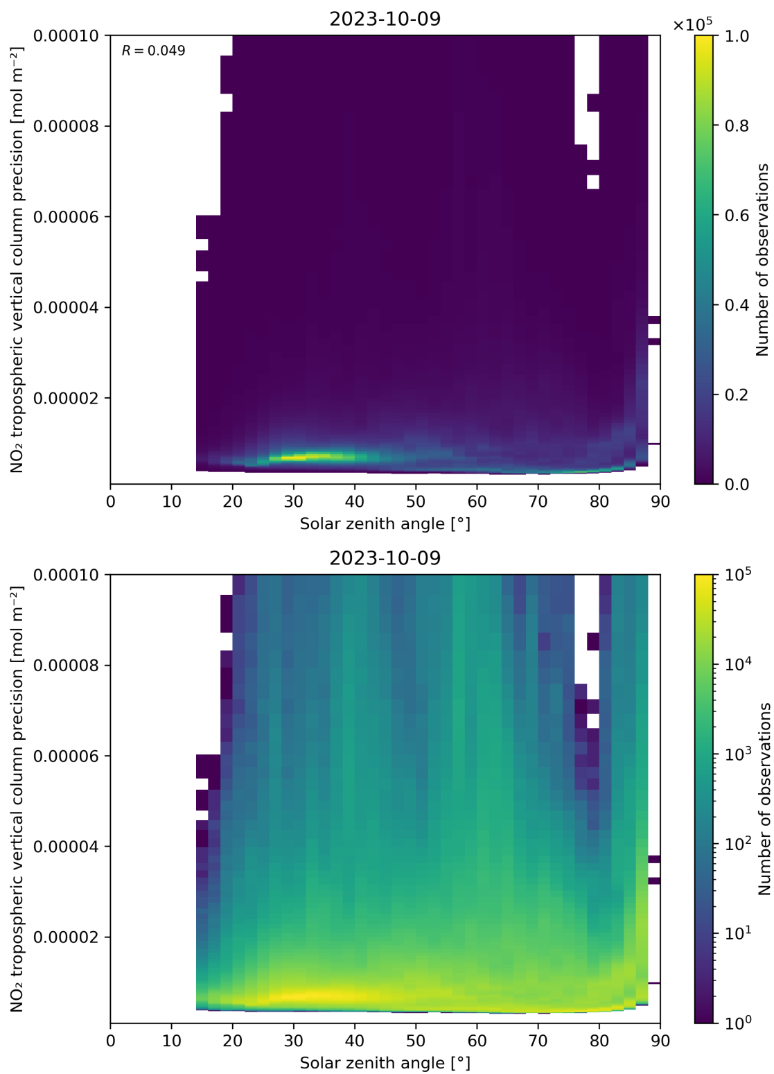
Figure 156: Scatter density plot of “Solar zenith angle” against “NO 2 tropospheric vertical column precision” for 2023-10-08 to 2023-10-10.
