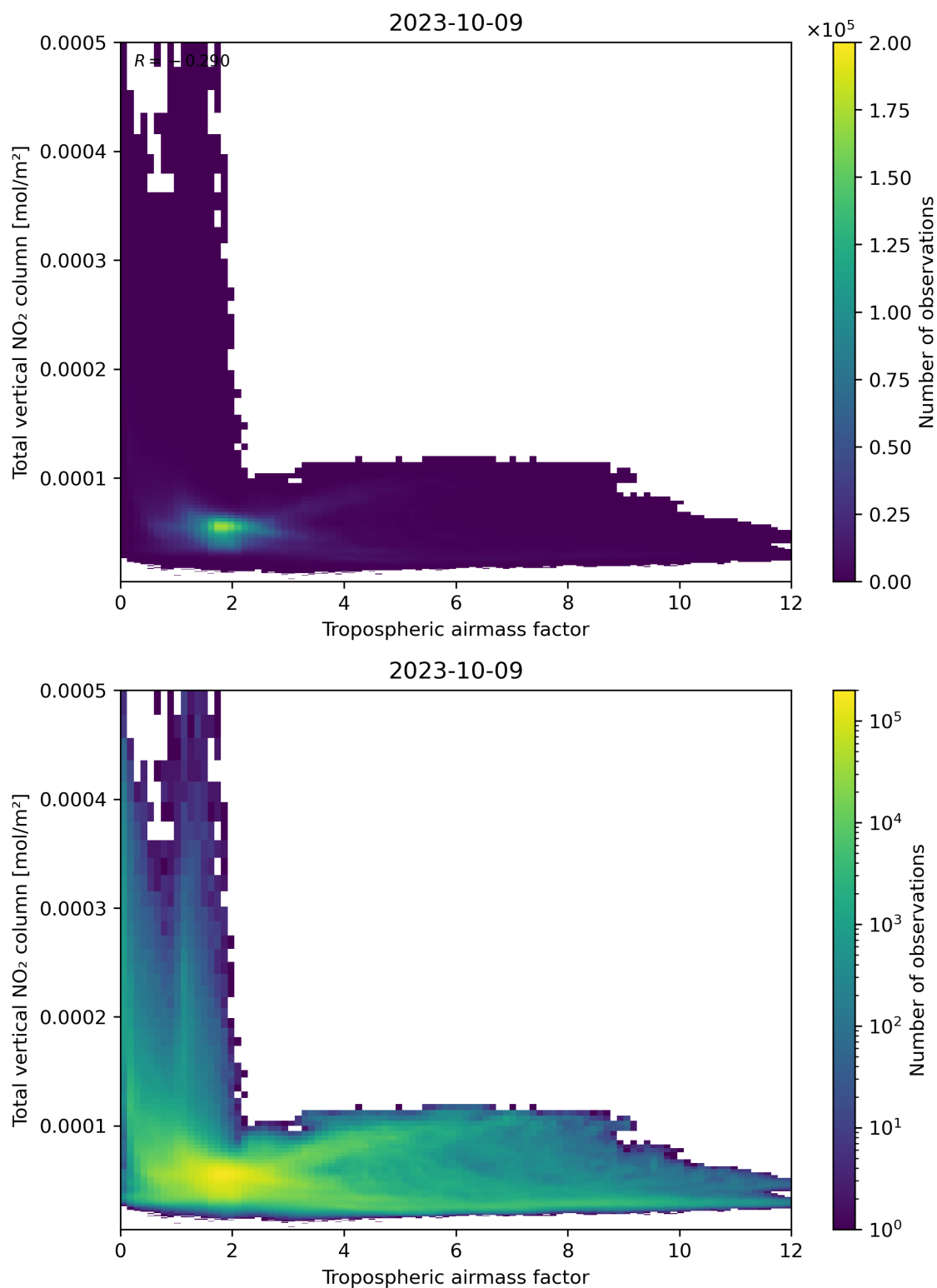
Figure 77: Scatter density plot of “Tropospheric airmass factor” against “Total vertical NO 2 column” for 2023-10-08 to 2023-10-10.
