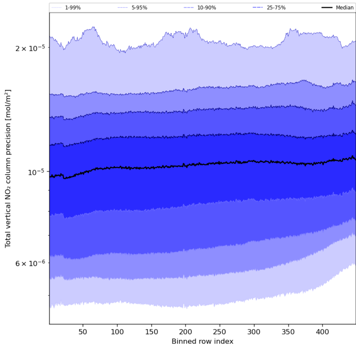
Figure 56: Along track statistics of “Total vertical NO 2 column precision” for 2023-10-08 to 2023-10-10
