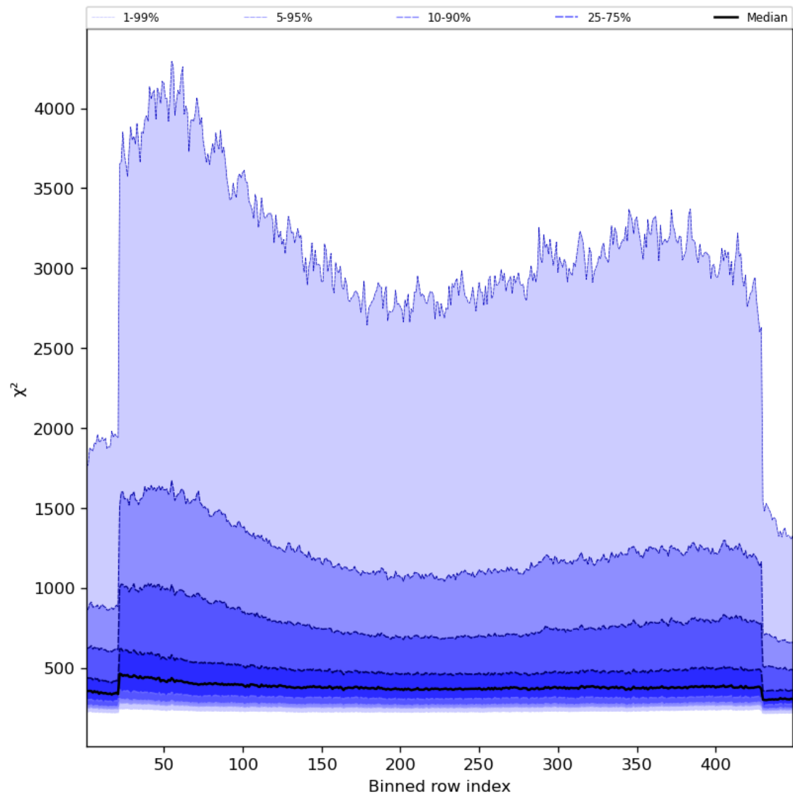
Figure 59: Along track statistics of “ \chi^2 ” for 2023-10-08 to 2023-10-10
