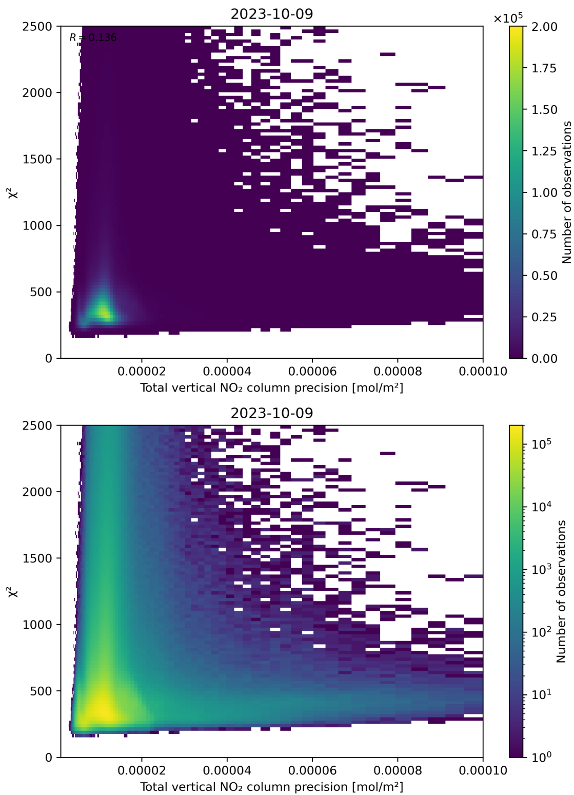
Figure 116: Scatter density plot of “Total vertical NO 2 column precision” against “ \chi^2 ” for 2023-10-08 to 2023-10-10.
