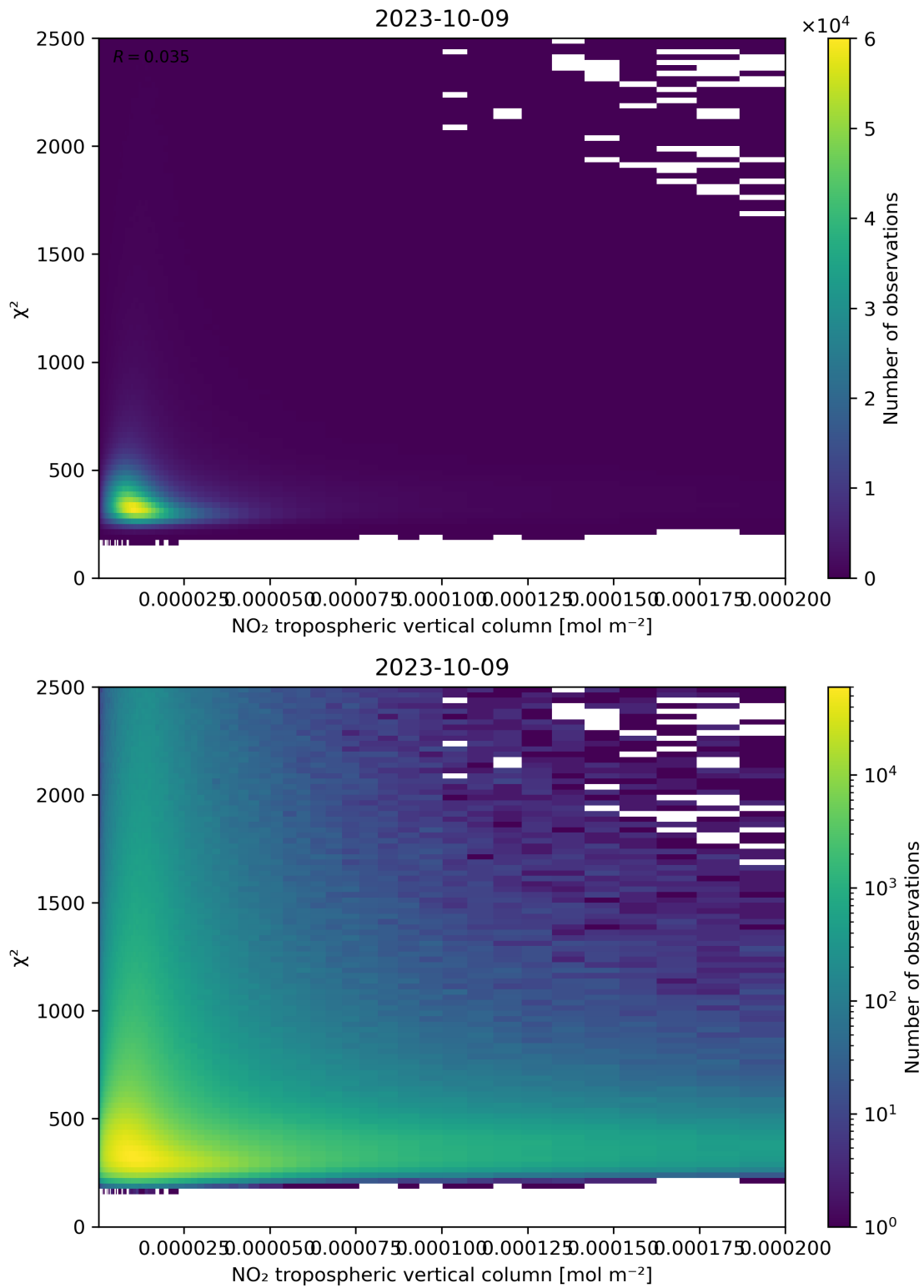
Figure 124: Scatter density plot of “NO 2 tropospheric vertical column” against “ \chi^2 ” for 2023-10-08 to 2023-10-10.
