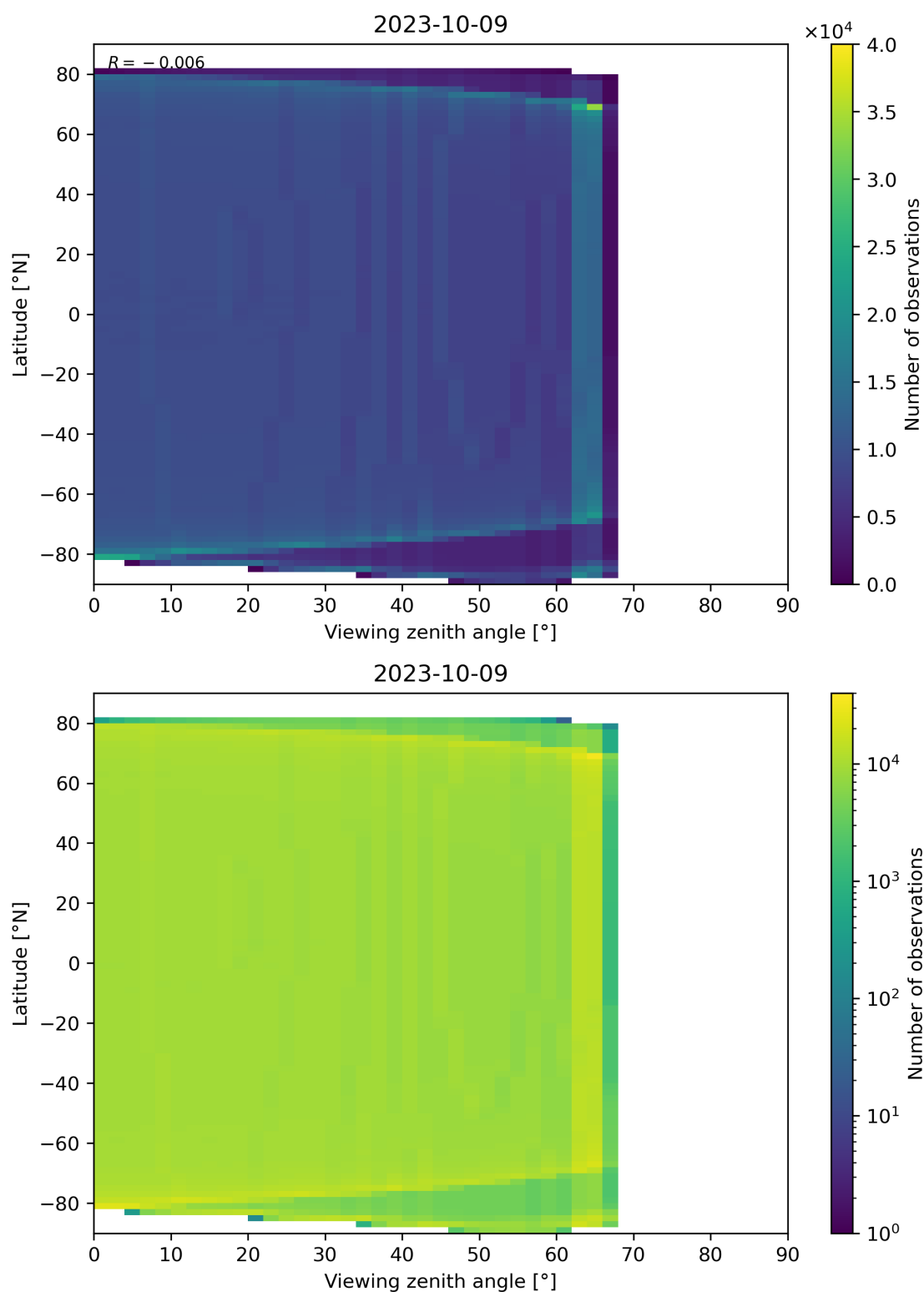
Figure 163: Scatter density plot of “Viewing zenith angle” against “Latitude” for 2023-10-08 to 2023-10-10.
