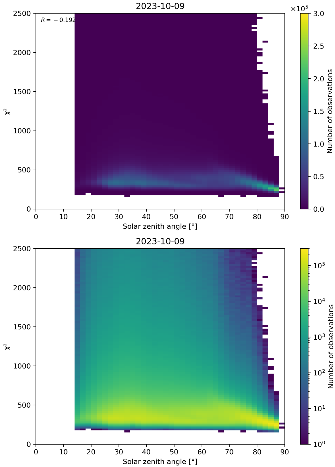
Figure 148: Scatter density plot of “Solar zenith angle” against “ \chi^2 ” for 2023-10-08 to 2023-10-10.
