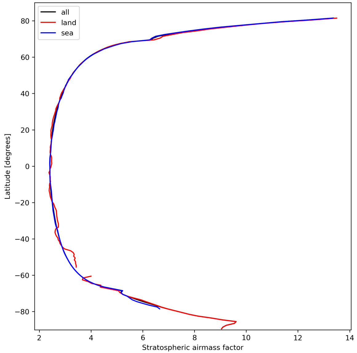
Figure 27: Zonal average of “Stratospheric airmass factor” for 2023-10-08 to 2023-10-10.
