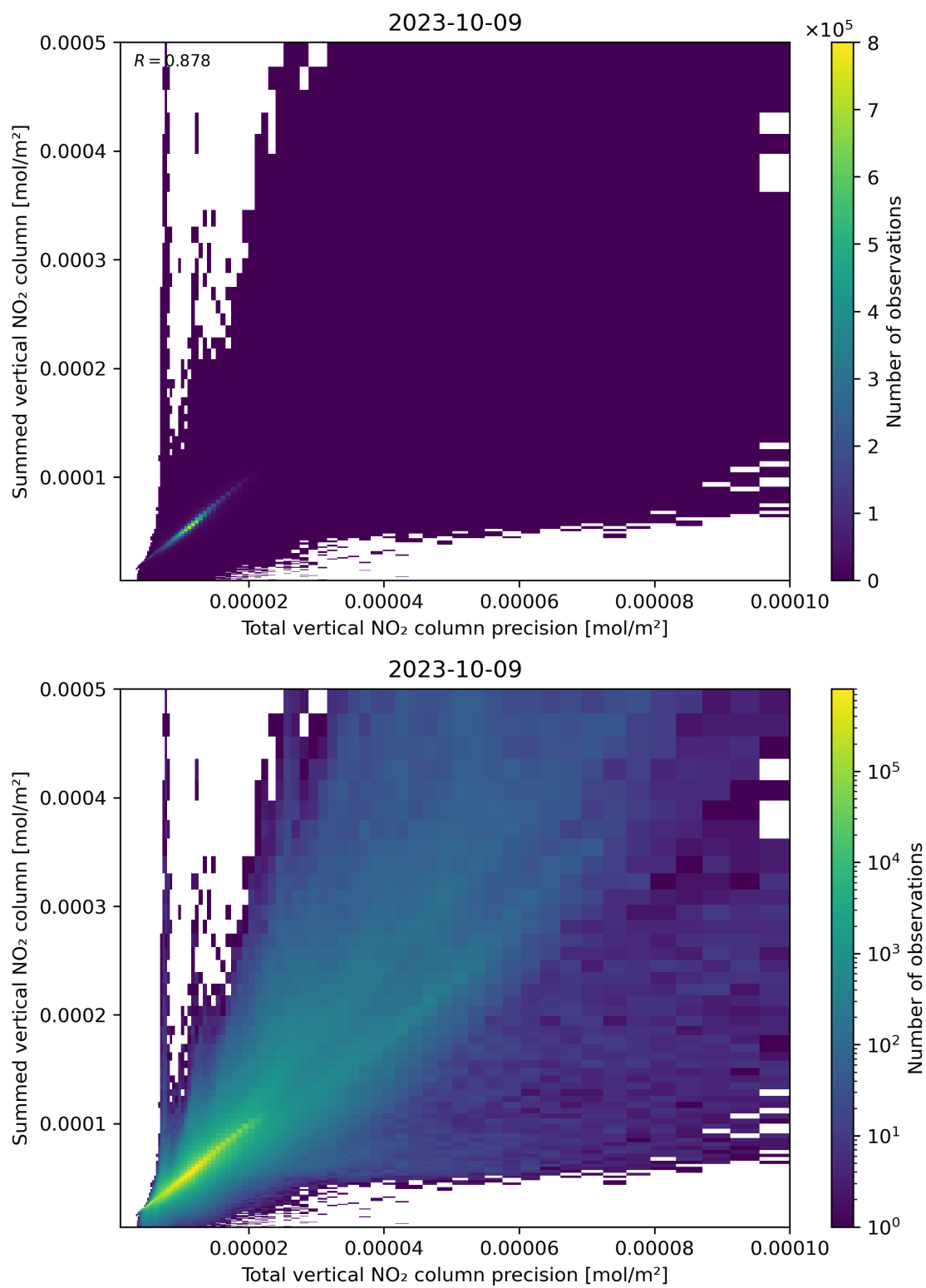
Figure 117: Scatter density plot of “Total vertical NO 2 column precision” against “Summed vertical NO 2 column” for 2023-10-08 to 2023-10-10.
