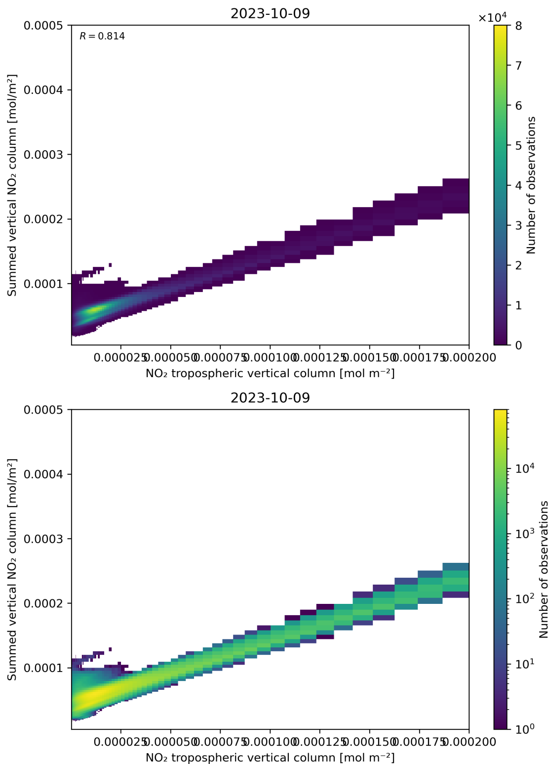
Figure 126: Scatter density plot of “NO 2 tropospheric vertical column” against “Summed vertical NO 2 column” for 2023-10-08 to 2023-10-10.
