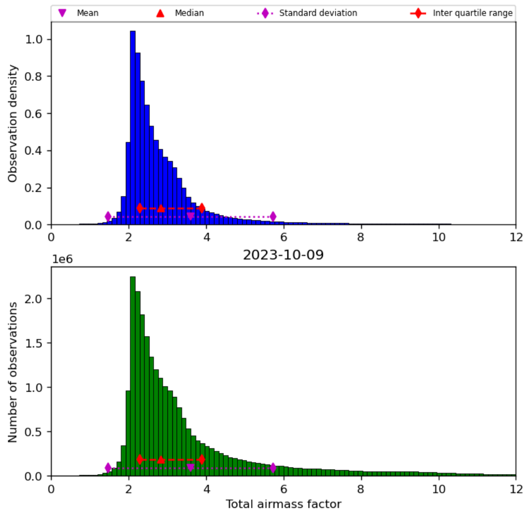
Figure 32: Histogram of “Total airmass factor” for 2023-10-08 to 2023-10-10
