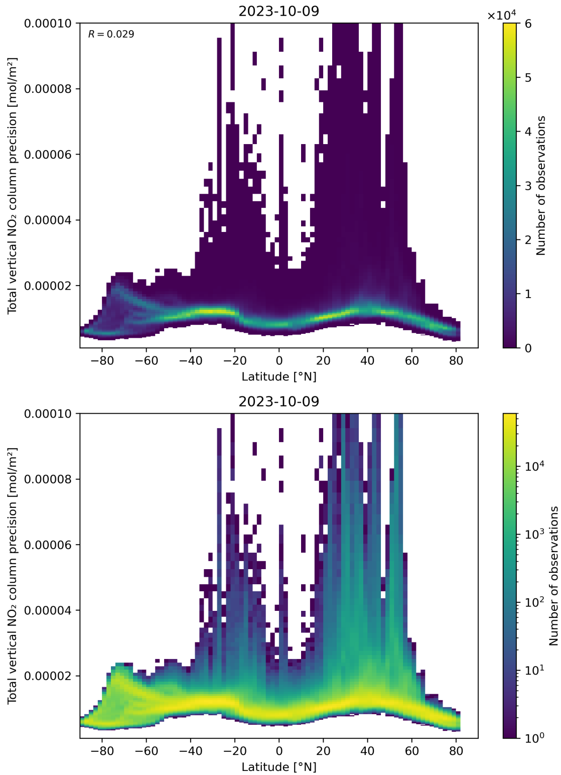
Figure 91: Scatter density plot of “Latitude” against “Total vertical NO 2 column precision” for 2023-10-08 to 2023-10-10.
