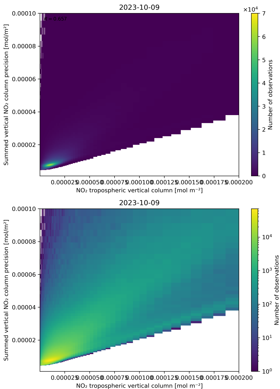
Figure 127: Scatter density plot of “NO 2 tropospheric vertical column” against “Summed vertical NO 2 column precision” for 2023-10-08 to 2023-10-10.
