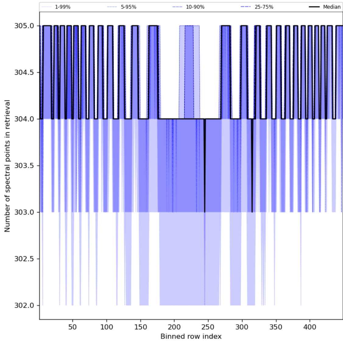
Figure 50: Along track statistics of “Number of spectral points in retrieval” for 2023-10-08 to 2023-10-10
