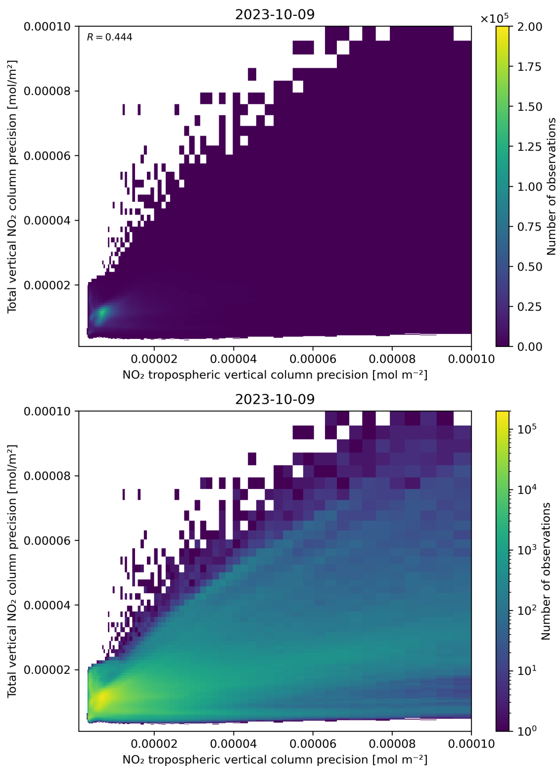
Figure 139: Scatter density plot of “NO 2 tropospheric vertical column precision” against “Total vertical NO 2 column precision” for 2023-10-08 to 2023-10-10.
