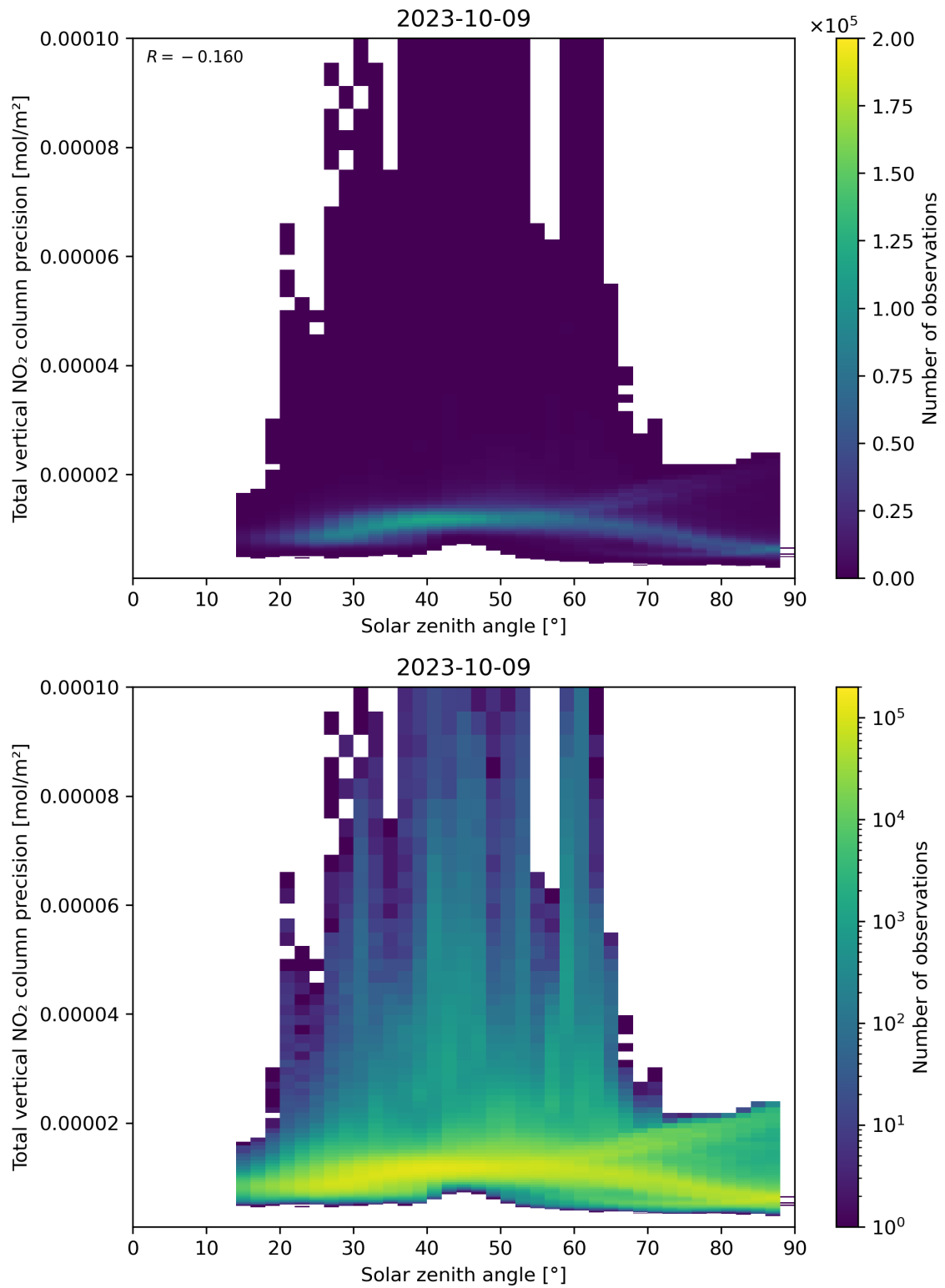
Figure 154: Scatter density plot of “Solar zenith angle” against “Total vertical NO 2 column precision” for 2023-10-08 to 2023-10-10.
