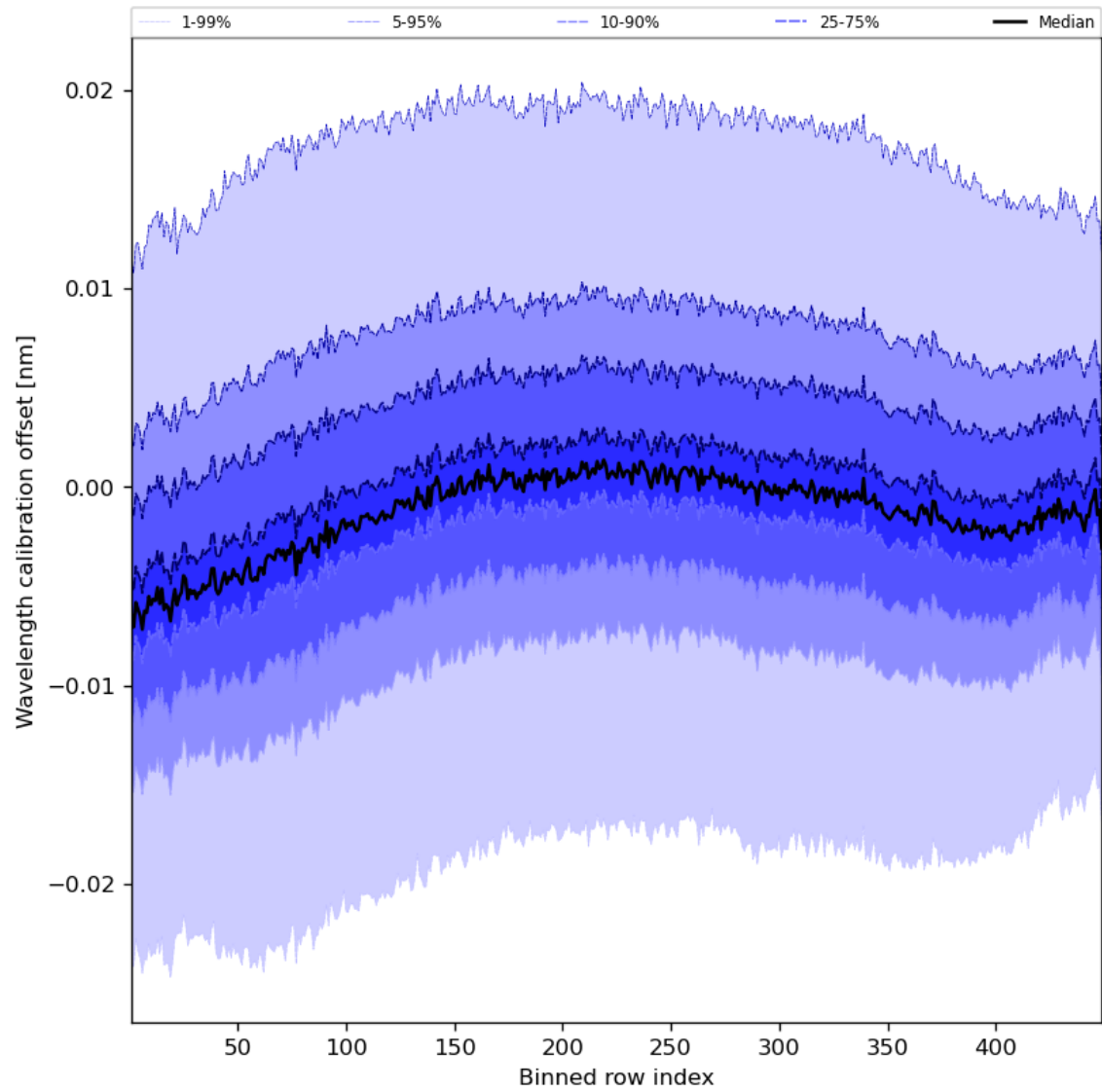
Figure 52: Along track statistics of “Wavelength calibration offset” for 2023-10-08 to 2023-10-10
