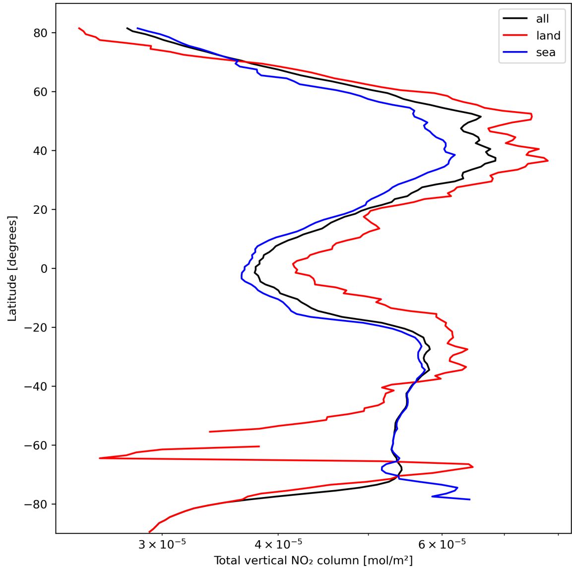
Figure 21: Zonal average of “Total vertical NO 2 column” for 2023-10-08 to 2023-10-10.
