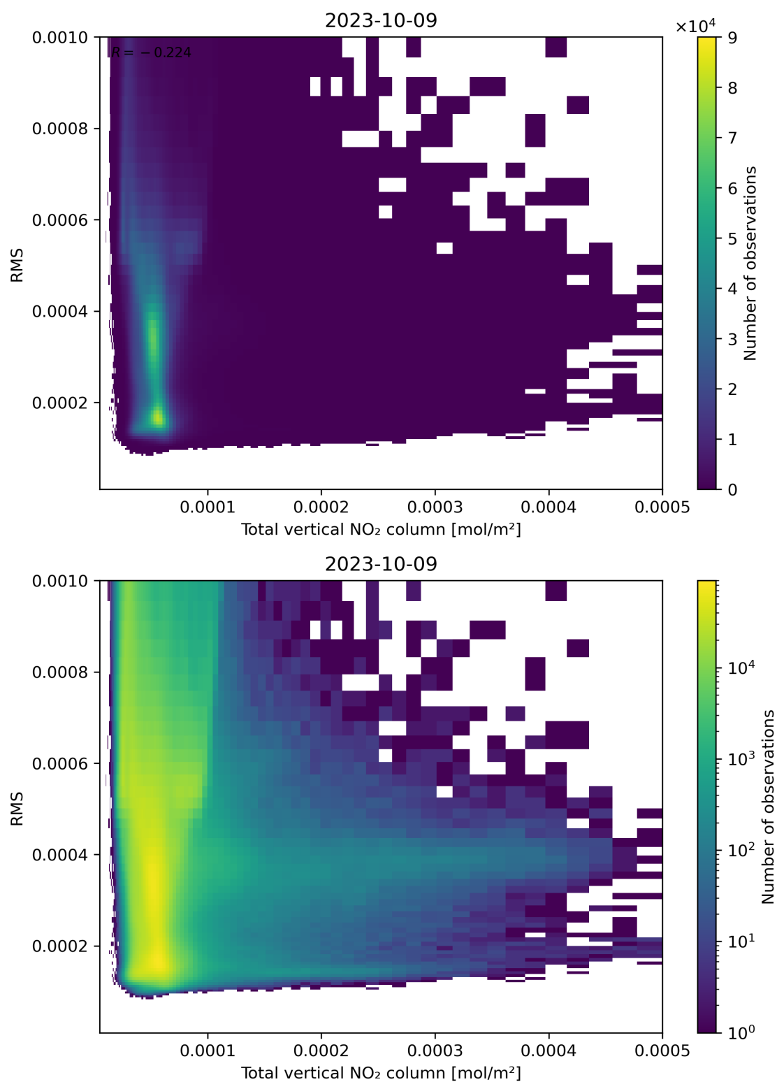
Figure 120: Scatter density plot of “Total vertical NO 2 column” against “RMS” for 2023-10-08 to 2023-10-10.
