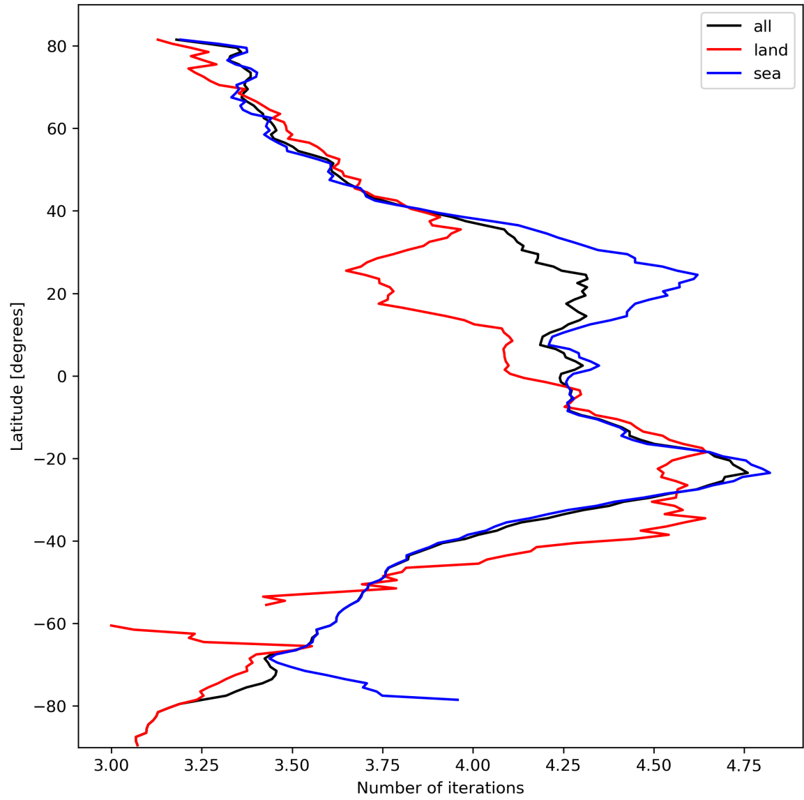
Figure 17: Zonal average of “Number of iterations” for 2023-10-08 to 2023-10-10.
