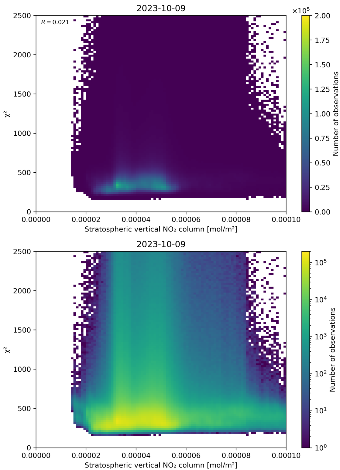
Figure 97: Scatter density plot of “Stratospheric vertical NO 2 column” against “ \chi^2 ” for 2023-10-08 to 2023-10-10.
