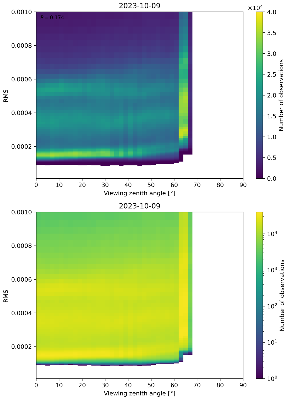
Figure 171: Scatter density plot of “Viewing zenith angle” against “RMS” for 2023-10-08 to 2023-10-10.
