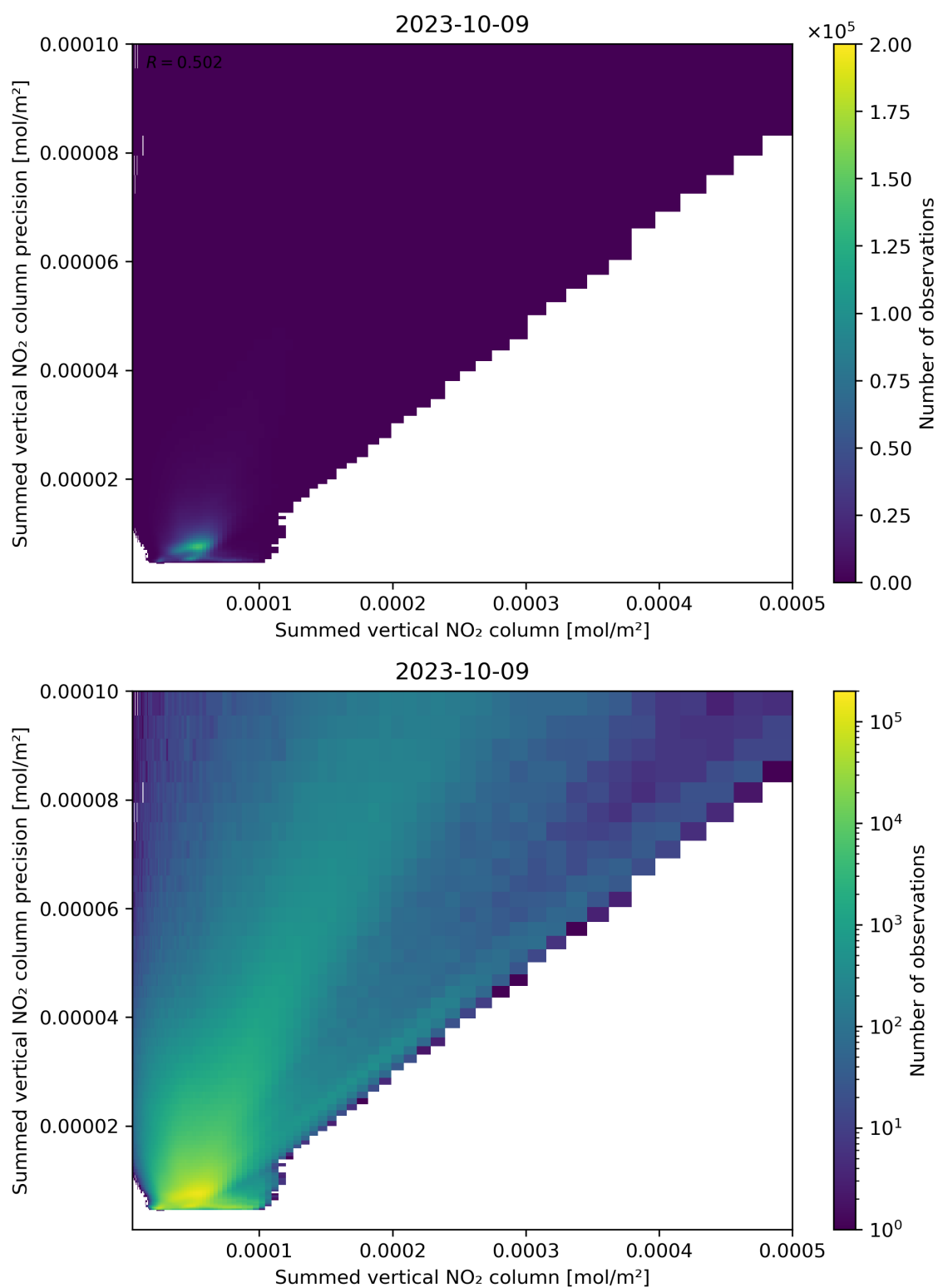
Figure 105: Scatter density plot of “Summed vertical NO 2 column” against “Summed vertical NO 2 column precision” for 2023-10-08 to 2023-10-10.
