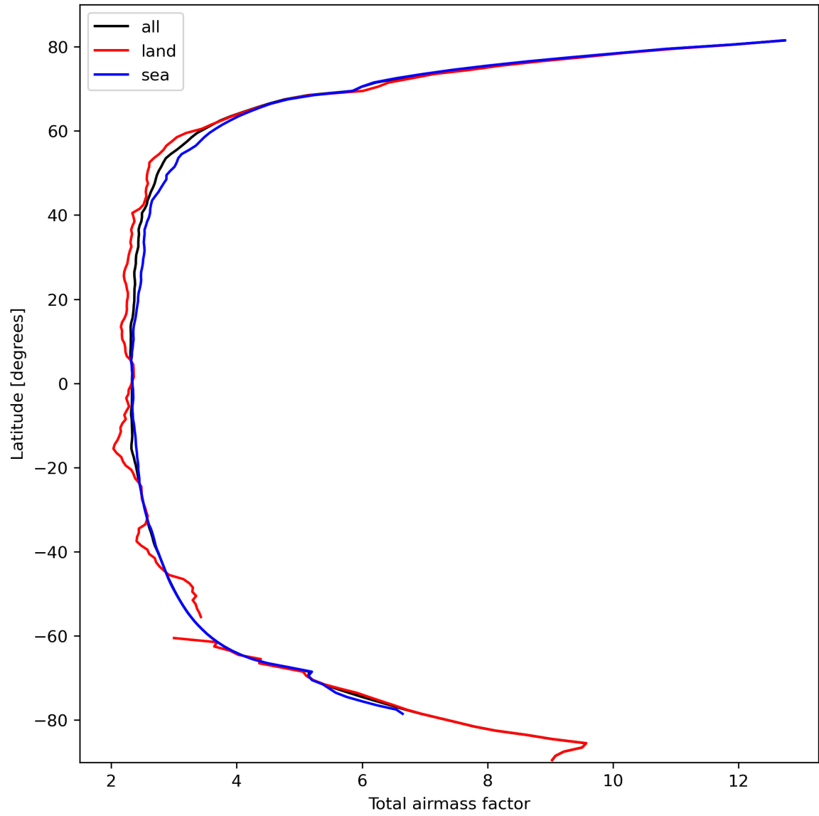
Figure 15: Zonal average of “Total airmass factor” for 2023-10-08 to 2023-10-10.
