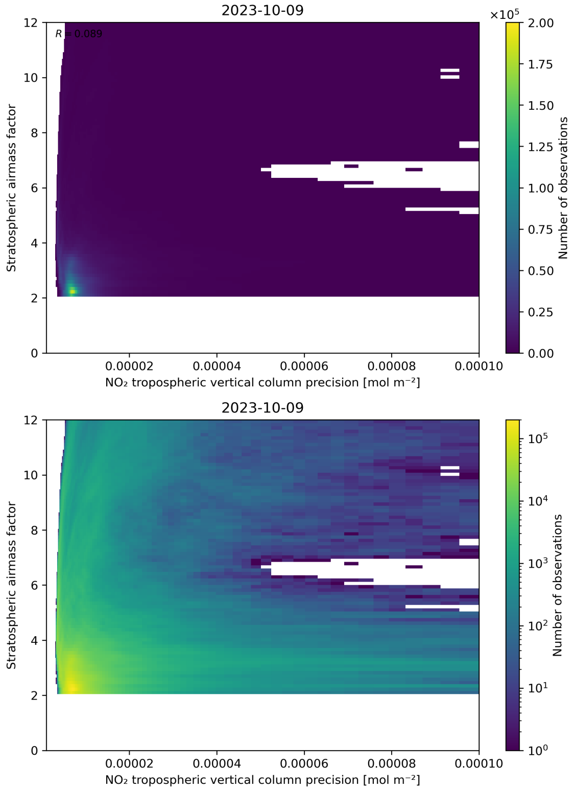
Figure 131: Scatter density plot of “NO 2 tropospheric vertical column precision” against “Stratospheric airmass factor” for 2023-10-08 to 2023-10-10.
