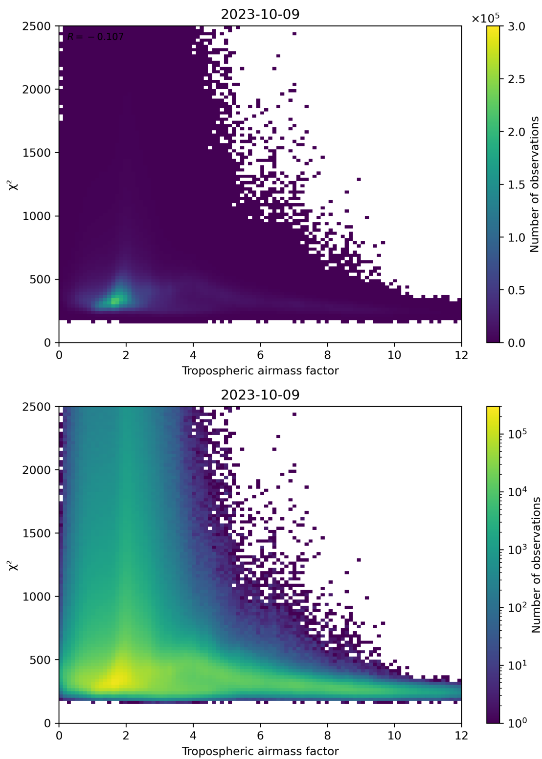
Figure 73: Scatter density plot of “Tropospheric airmass factor” against “ \chi^2 ” for 2023-10-08 to 2023-10-10.
