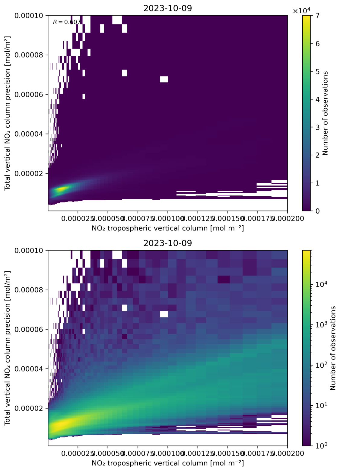
Figure 129: Scatter density plot of “NO 2 tropospheric vertical column” against “Total vertical NO 2 column precision” for 2023-10-08 to 2023-10-10.
