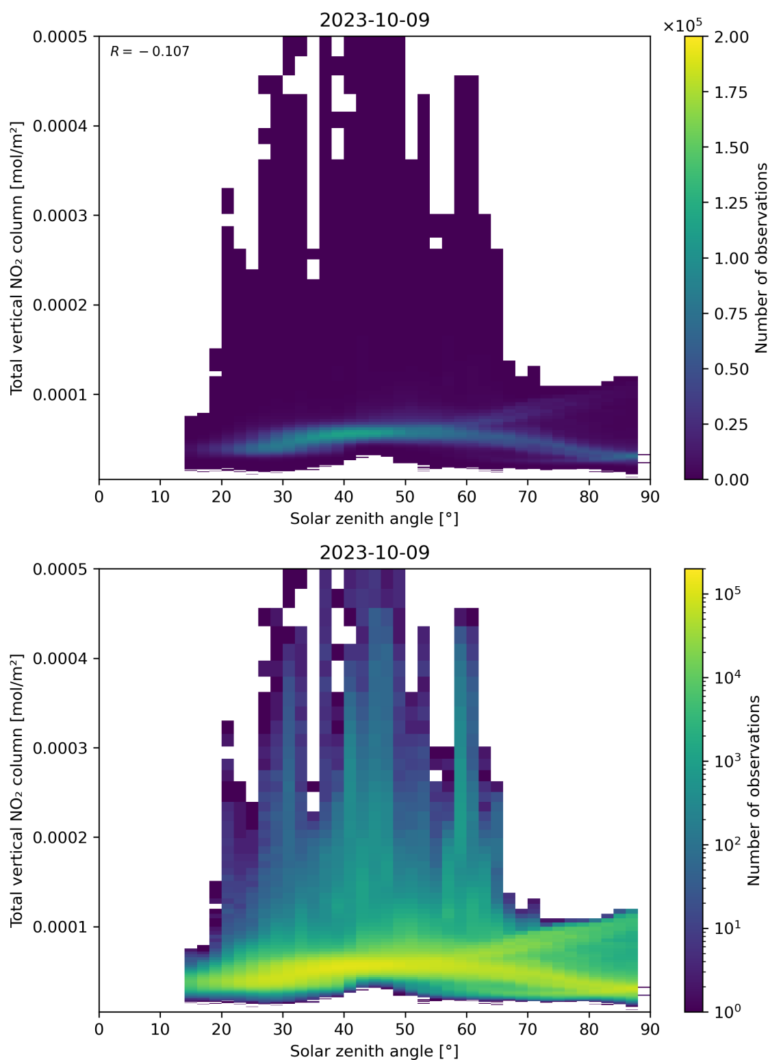
Figure 153: Scatter density plot of “Solar zenith angle” against “Total vertical NO 2 column” for 2023-10-08 to 2023-10-10.
