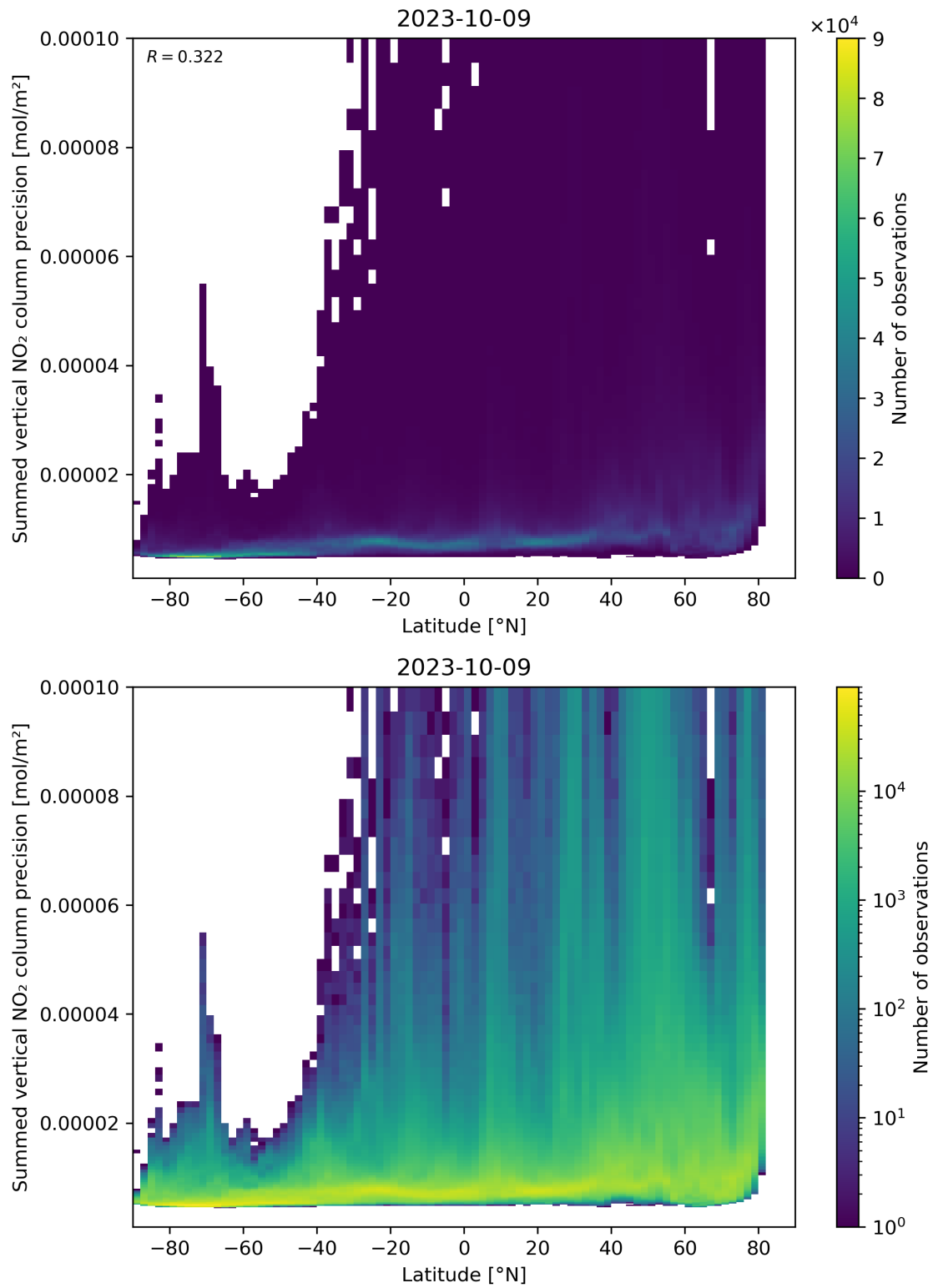
Figure 89: Scatter density plot of “Latitude” against “Summed vertical NO 2 column precision” for 2023-10-08 to 2023-10-10.
