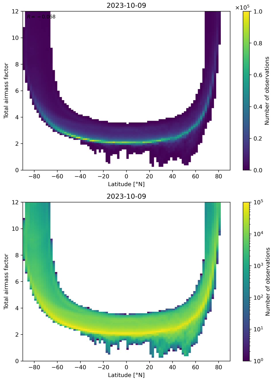
Figure 84: Scatter density plot of “Latitude” against “Total airmass factor” for 2023-10-08 to 2023-10-10.
