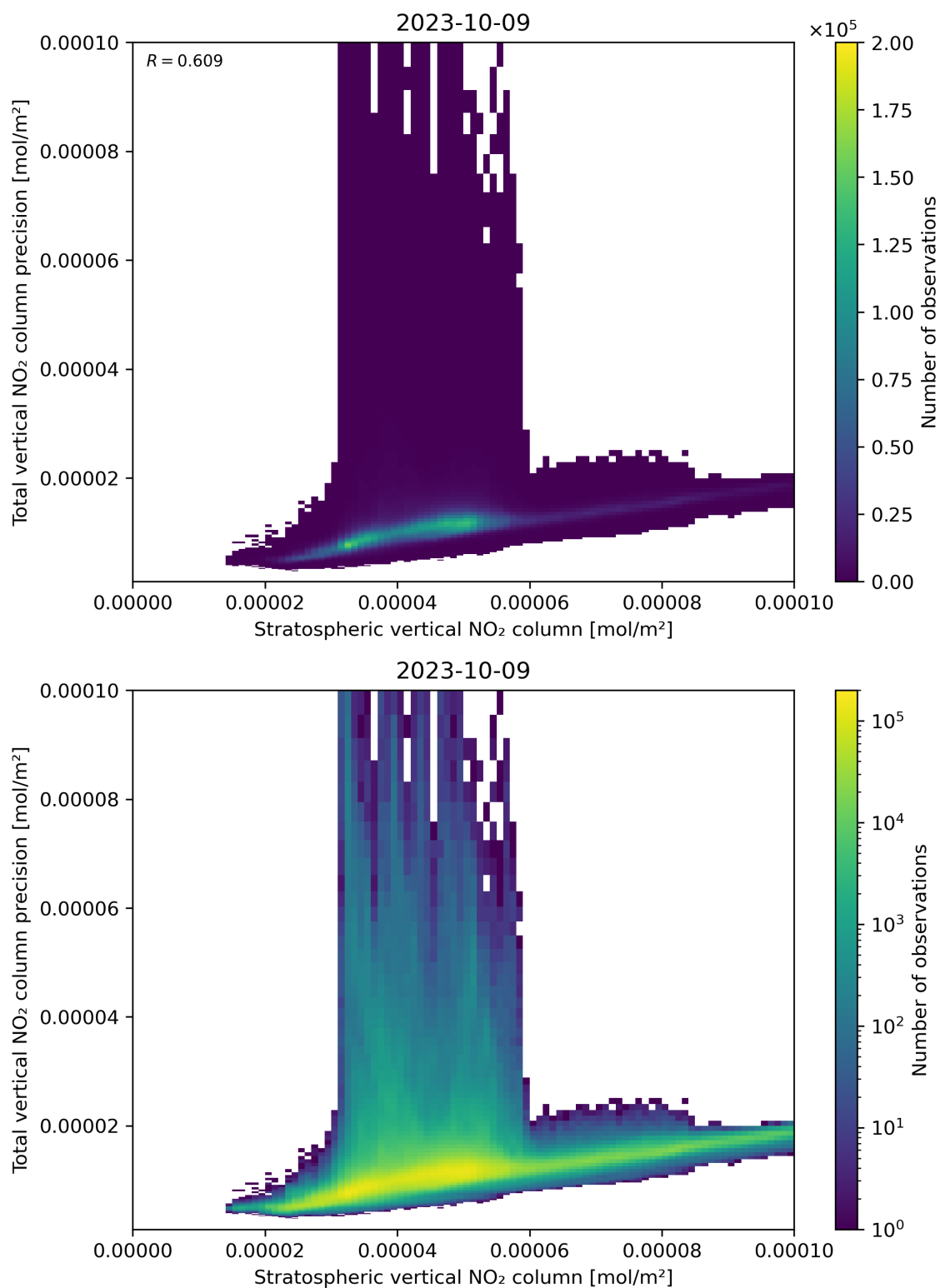
Figure 101: Scatter density plot of “Stratospheric vertical NO 2 column” against “Total vertical NO 2 column precision” for 2023-10-08 to 2023-10-10.
