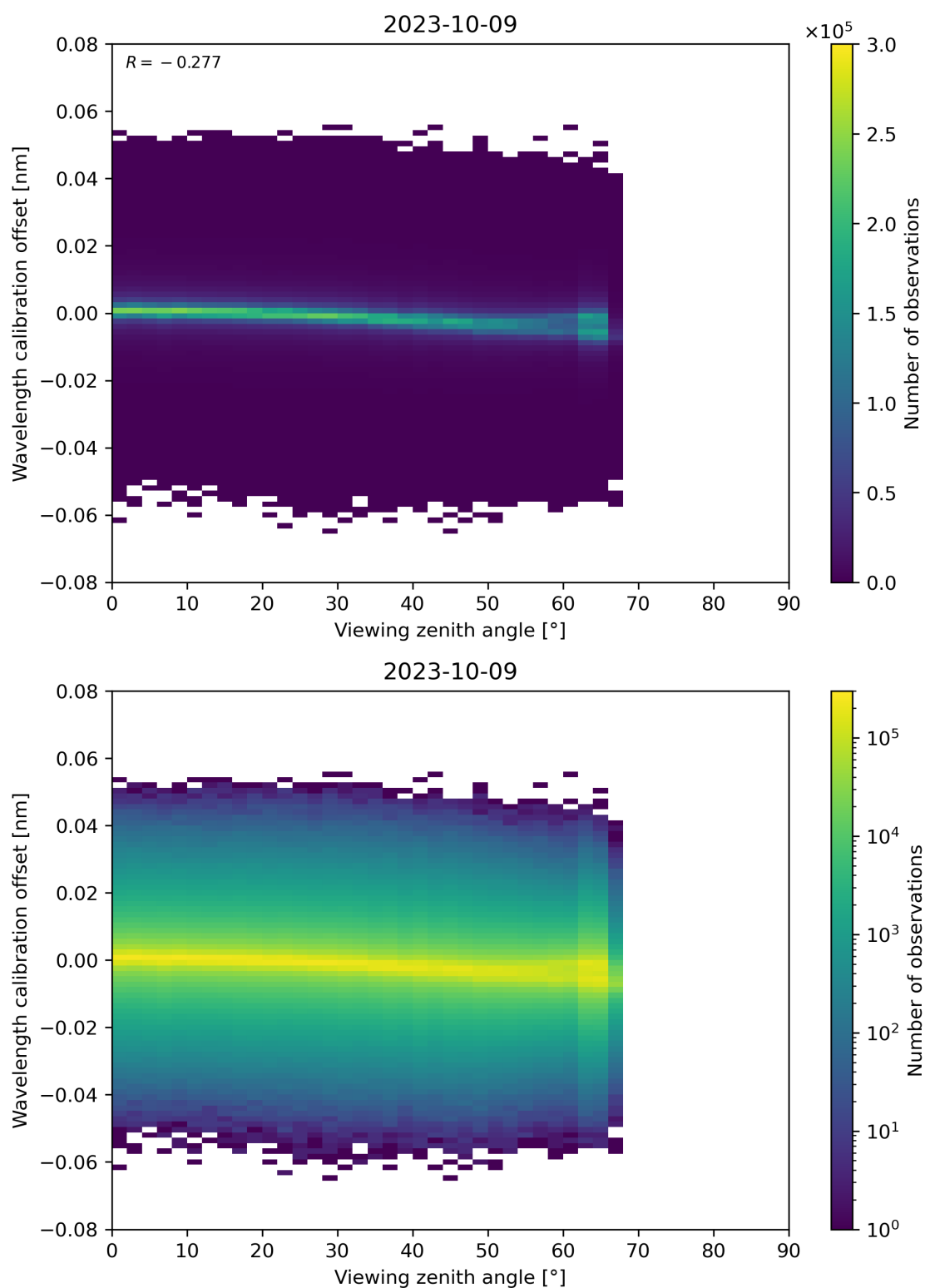
Figure 173: Scatter density plot of “Viewing zenith angle” against “Wavelength calibration offset” for 2023-10-08 to 2023-10-10.
