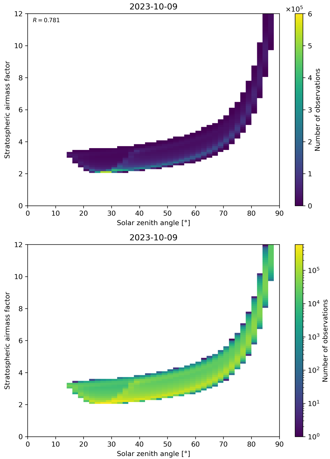
Figure 145: Scatter density plot of “Solar zenith angle” against “Stratospheric airmass factor” for 2023-10-08 to 2023-10-10.
