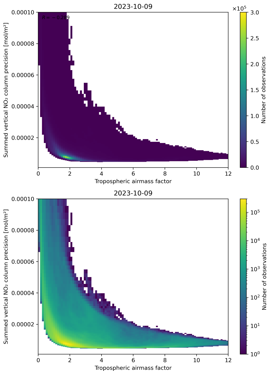
Figure 76: Scatter density plot of “Tropospheric air mass factor” against “Summed vertical NO 2 column precision” for 2023-10-08 to 2023-10-10.
