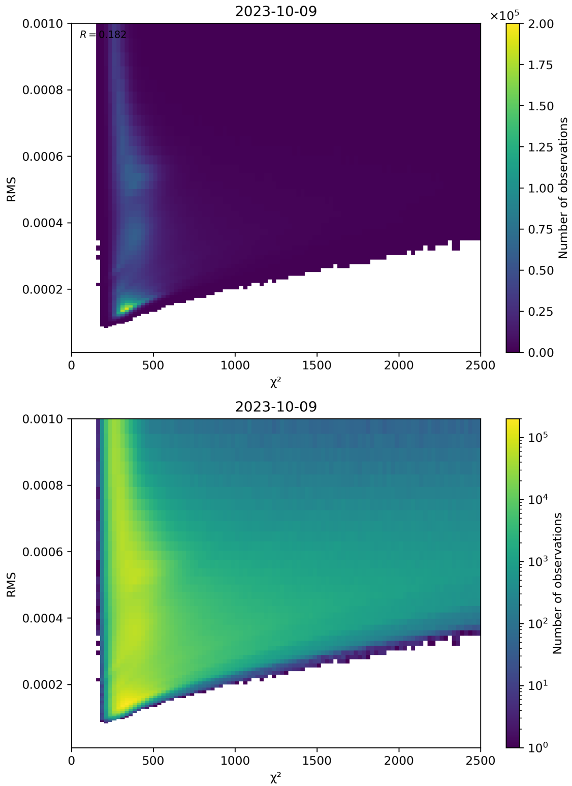
Figure 82: Scatter density plot of “ \chi^2 ” against “RMS” for 2023-10-08 to 2023-10-10.
