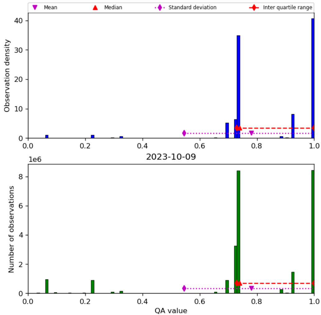
Figure 28: Histogram of “QA value” for 2023-10-08 to 2023-10-10
