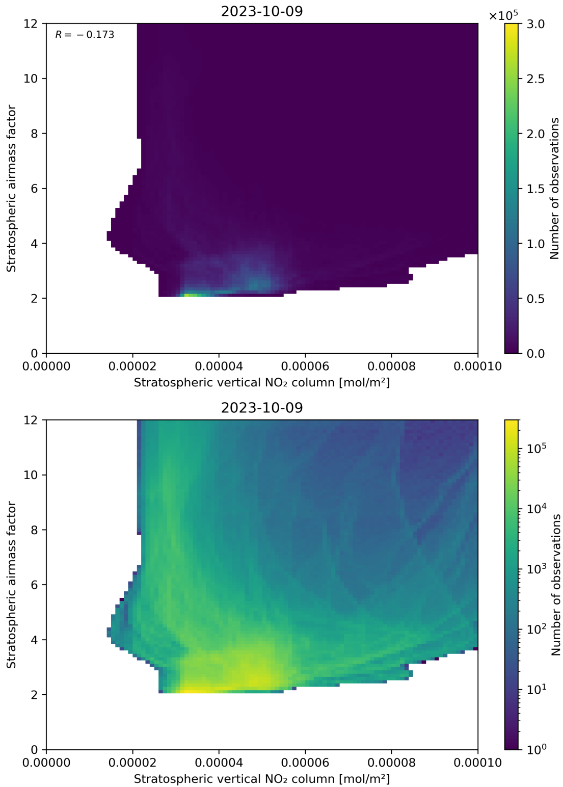
Figure 96: Scatter density plot of “Stratospheric vertical NO 2 column” against “Stratospheric airmass factor” for 2023-10-08 to 2023-10-10.
