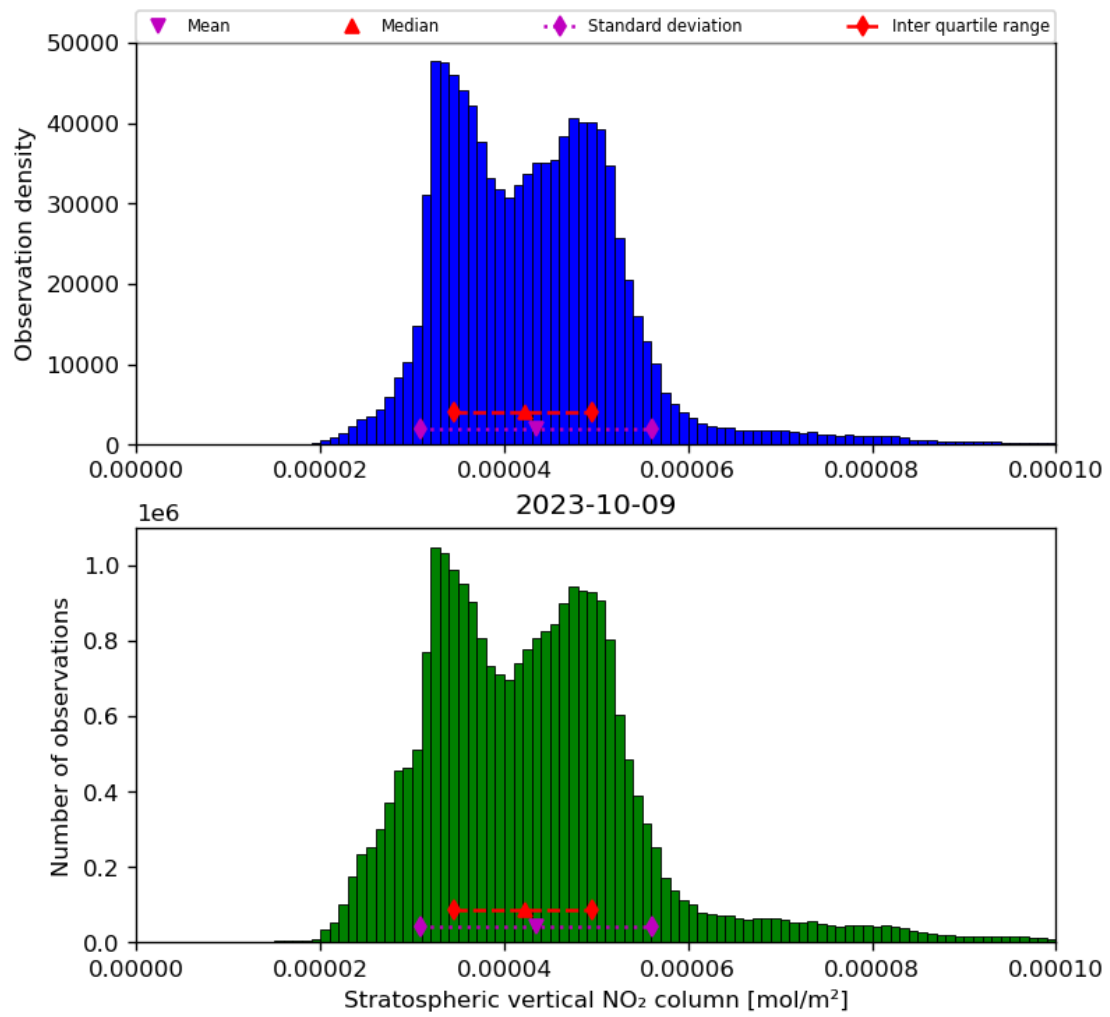
Figure 36: Histogram of “Stratospheric vertical NO 2 column” for 2023-10-08 to 2023-10-10
