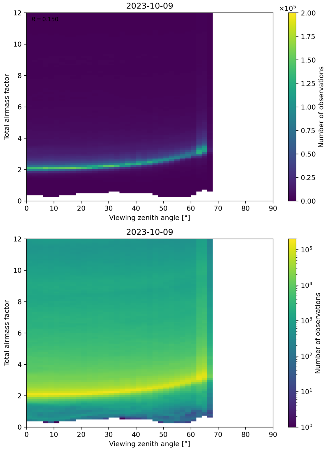
Figure 160: Scatter density plot of “Viewing zenith angle” against “Total airmass factor” for 2023-10-08 to 2023-10-10.
