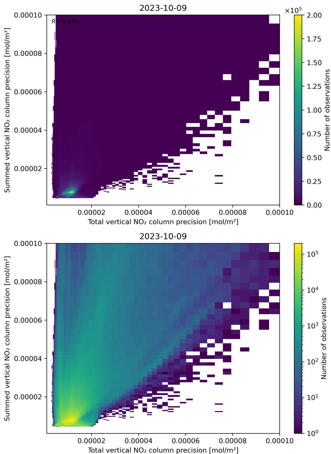
Figure 118: Scatter density plot of “Total vertical NO 2 column precision” against “Summed vertical NO 2 column precision” for 2023-10-08 to 2023-10-10.
