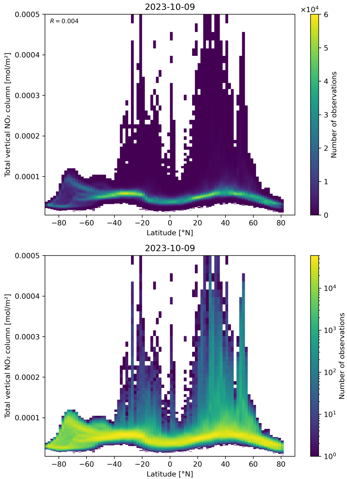
Figure 90: Scatter density plot of “Latitude” against “Total vertical NO 2 column” for 2023-10-08 to 2023-10-10.
