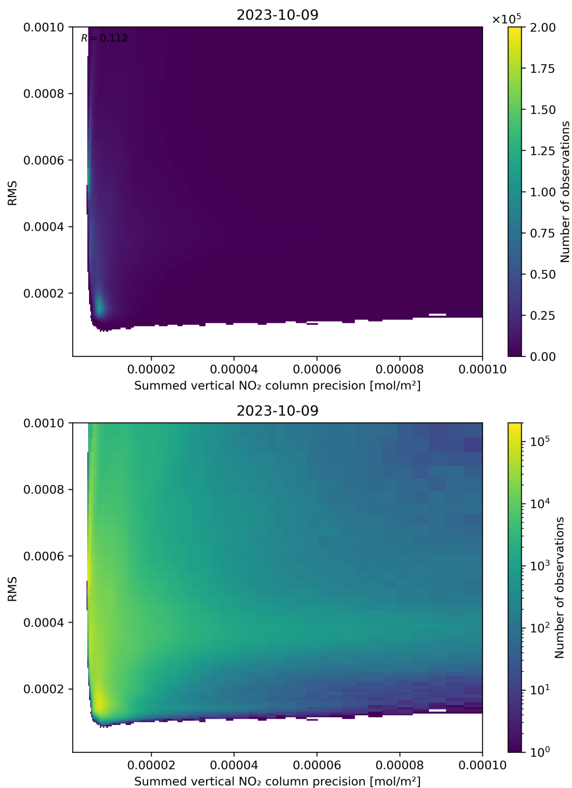
Figure 108: Scatter density plot of “Summed vertical NO 2 column precision” against “RMS” for 2023-10-08 to 2023-10-10.
