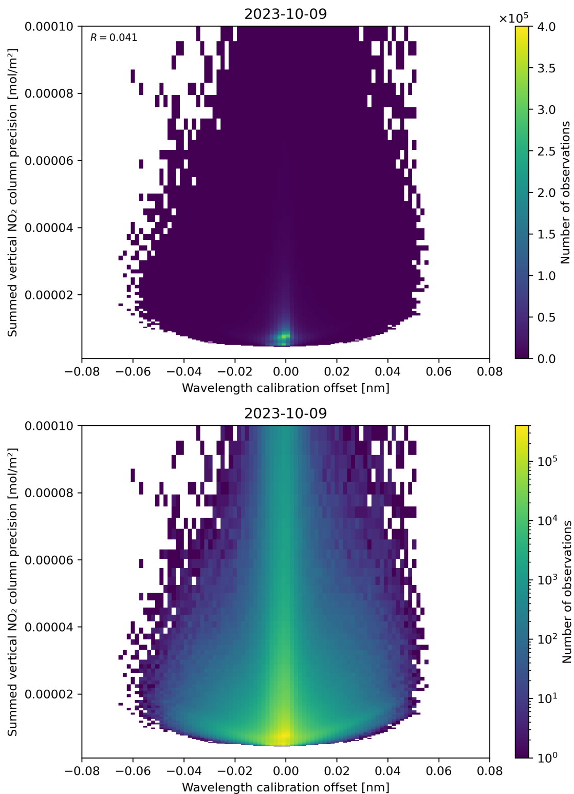
Figure 178: Scatter density plot of “Wavelength calibration offset” against “Summed vertical NO 2 column precision” for 2023-10-08 to 2023-10-10.
