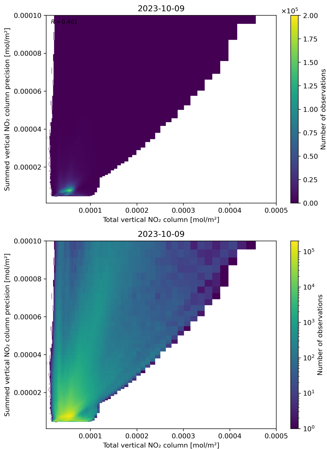
Figure 113: Scatter density plot of “Total vertical NO 2 column” against “Summed vertical NO 2 column precision” for 2023-10-08 to 2023-10-10.
