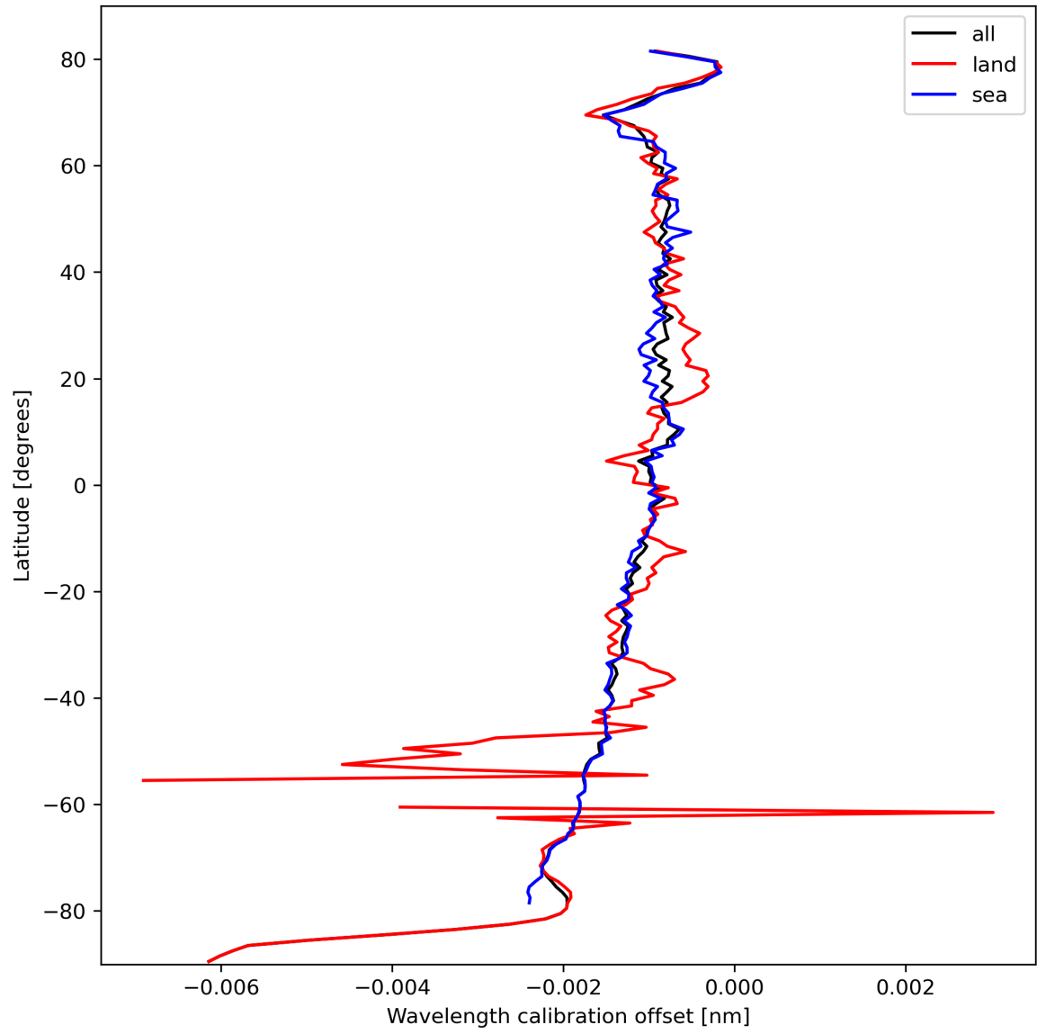
Figure 18: Zonal average of “Wavelength calibration offset” for 2023-10-08 to 2023-10-10.
