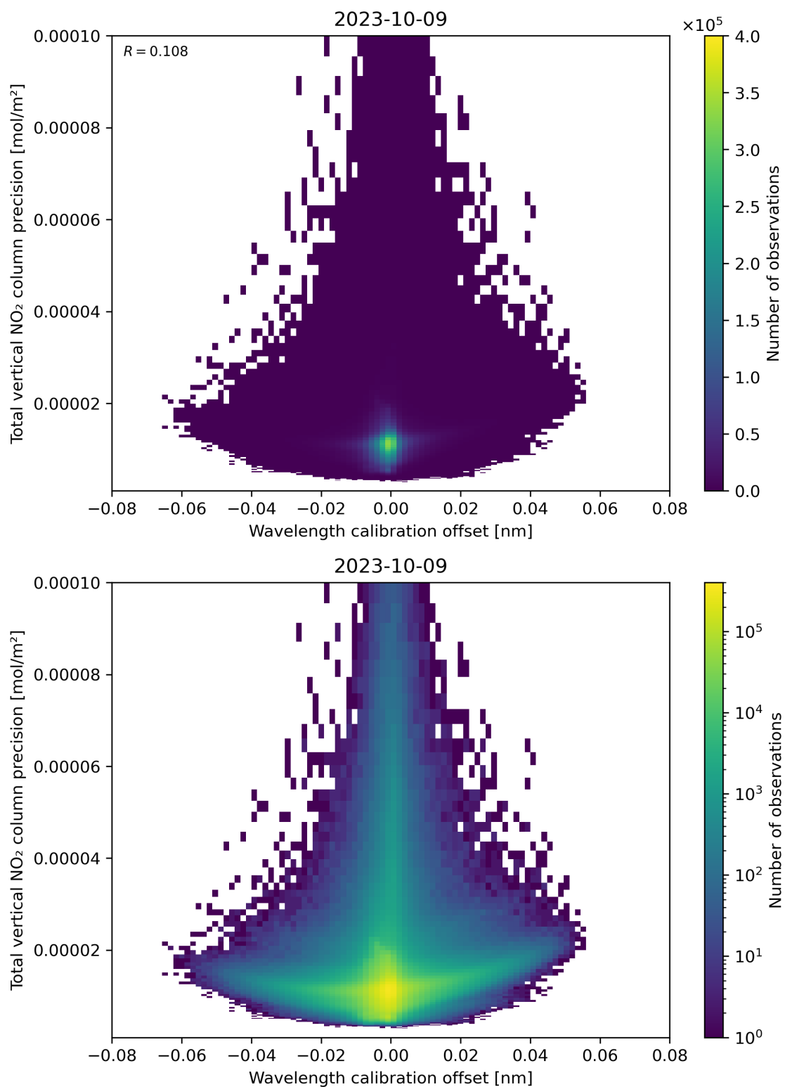
Figure 180: Scatter density plot of “Wavelength calibration offset” against “Total vertical NO 2 column precision” for 2023-10-08 to 2023-10-10.
