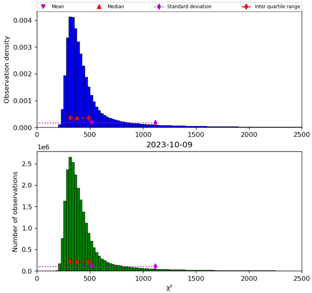
Figure 42: Histogram of “ \chi^2 ” for 2023-10-08 to 2023-10-10
