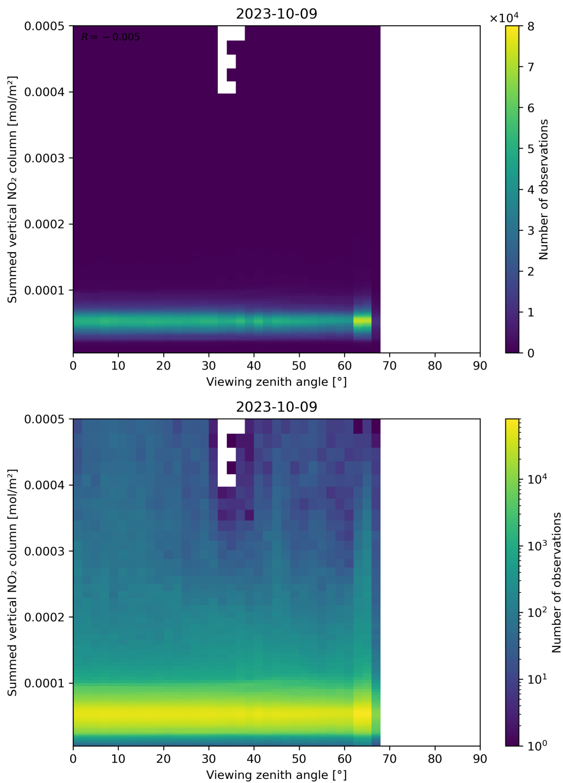
Figure 165: Scatter density plot of “Viewing zenith angle” against “Summed vertical NO 2 column” for 2023-10-08 to 2023-10-10.
