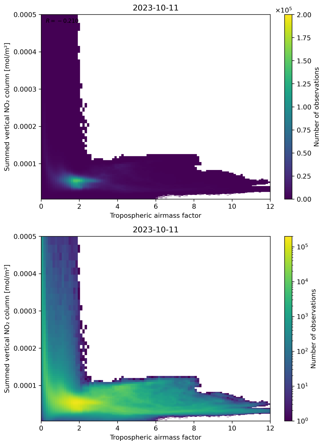
Figure 75: Scatter density plot of “Tropospheric air mass factor” against “Summed vertical NO 2 column” for 2023-10-10 to 2023-10-12.
