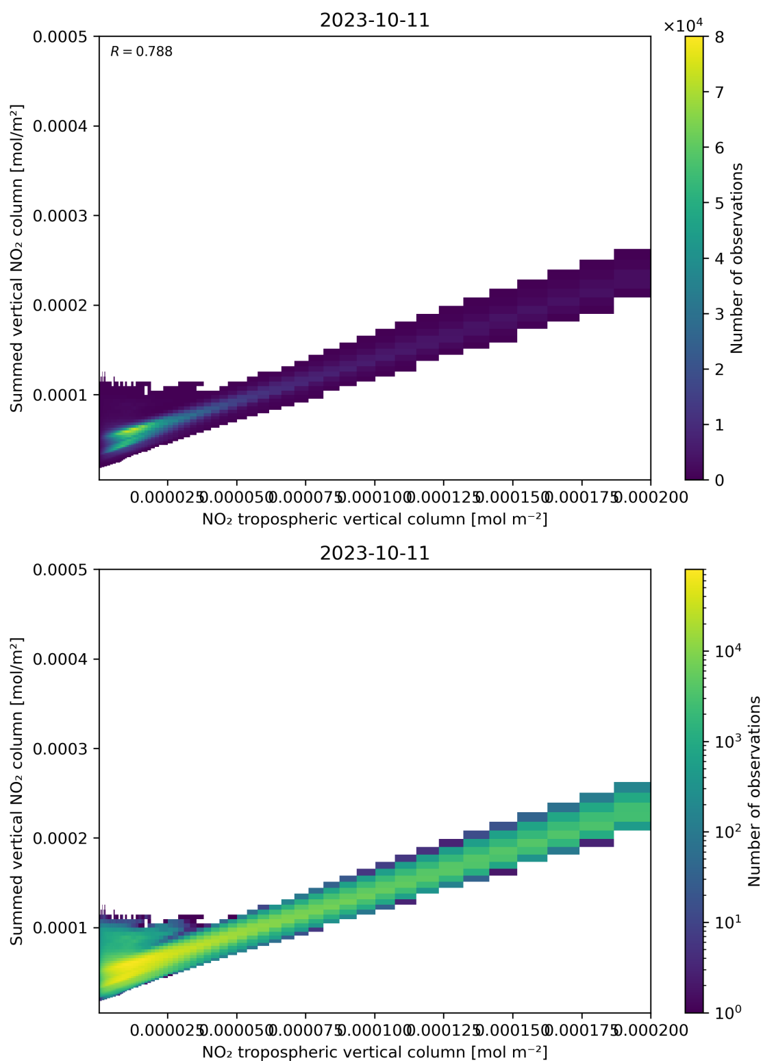
Figure 126: Scatter density plot of “NO 2 tropospheric vertical column” against “Summed vertical NO 2 column” for 2023-10-10 to 2023-10-12.
