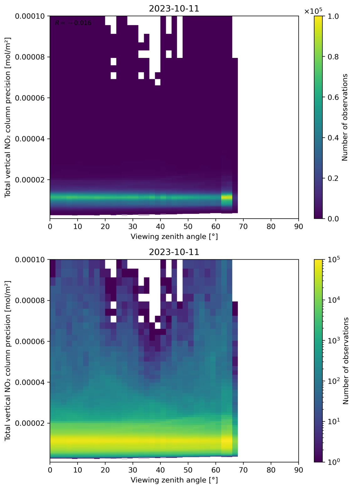
Figure 168: Scatter density plot of “Viewing zenith angle” against “Total vertical NO 2 column precision” for 2023-10-10 to 2023-10-12.
