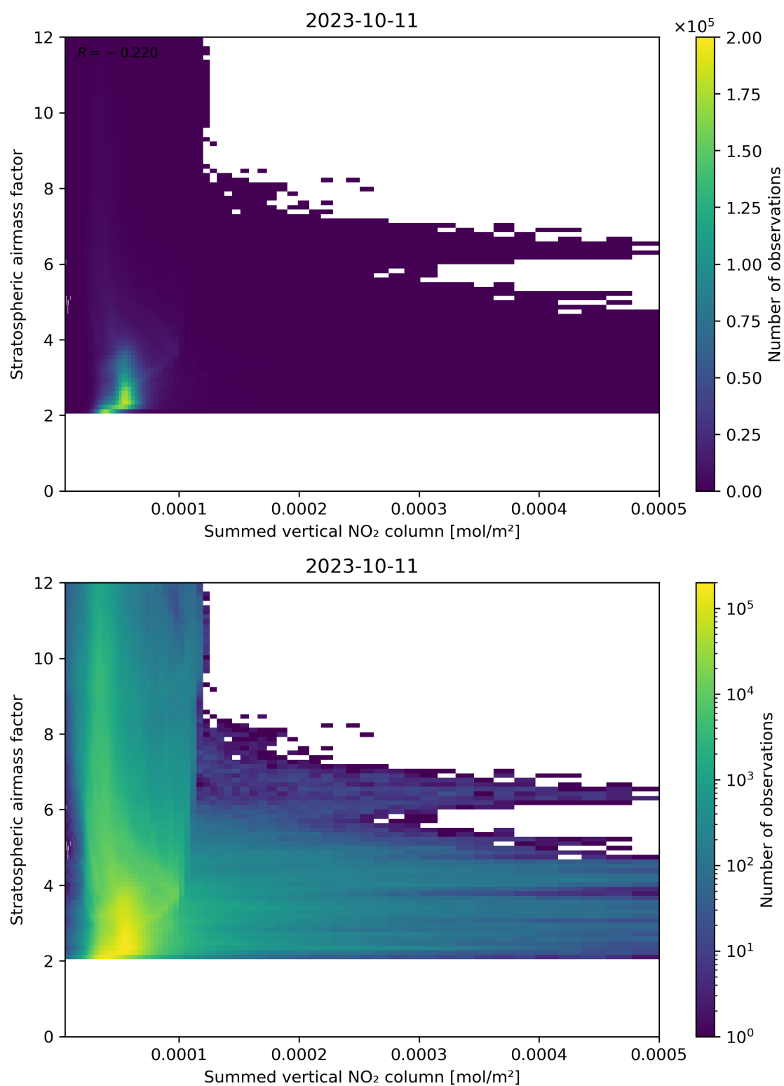
Figure 103: Scatter density plot of “Summed vertical NO 2 column” against “Stratospheric air mass factor” for 2023-10-10 to 2023-10-12.
