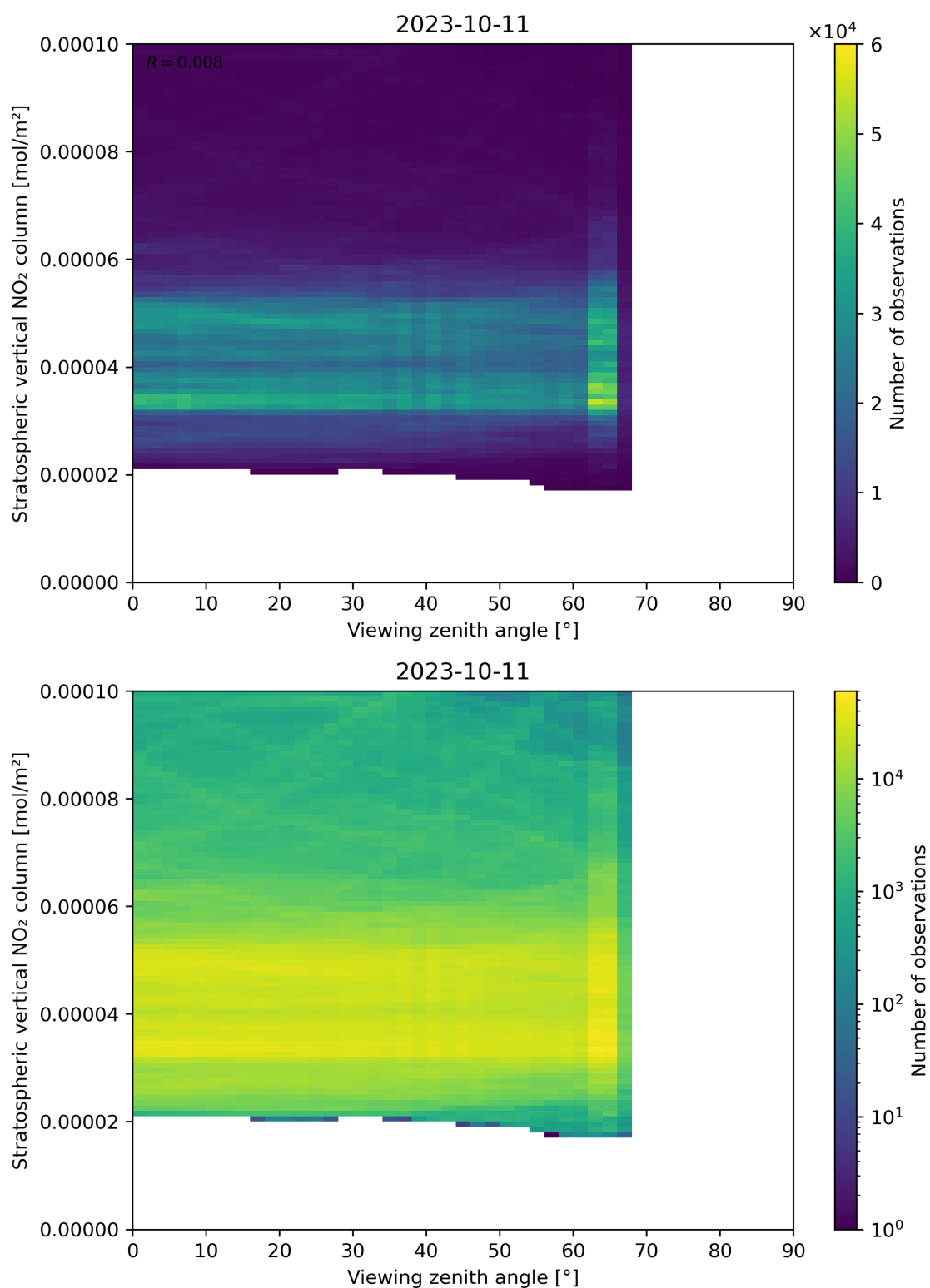
Figure 164: Scatter density plot of “Viewing zenith angle” against “Stratospheric vertical NO 2 column” for 2023-10-10 to 2023-10-12.
