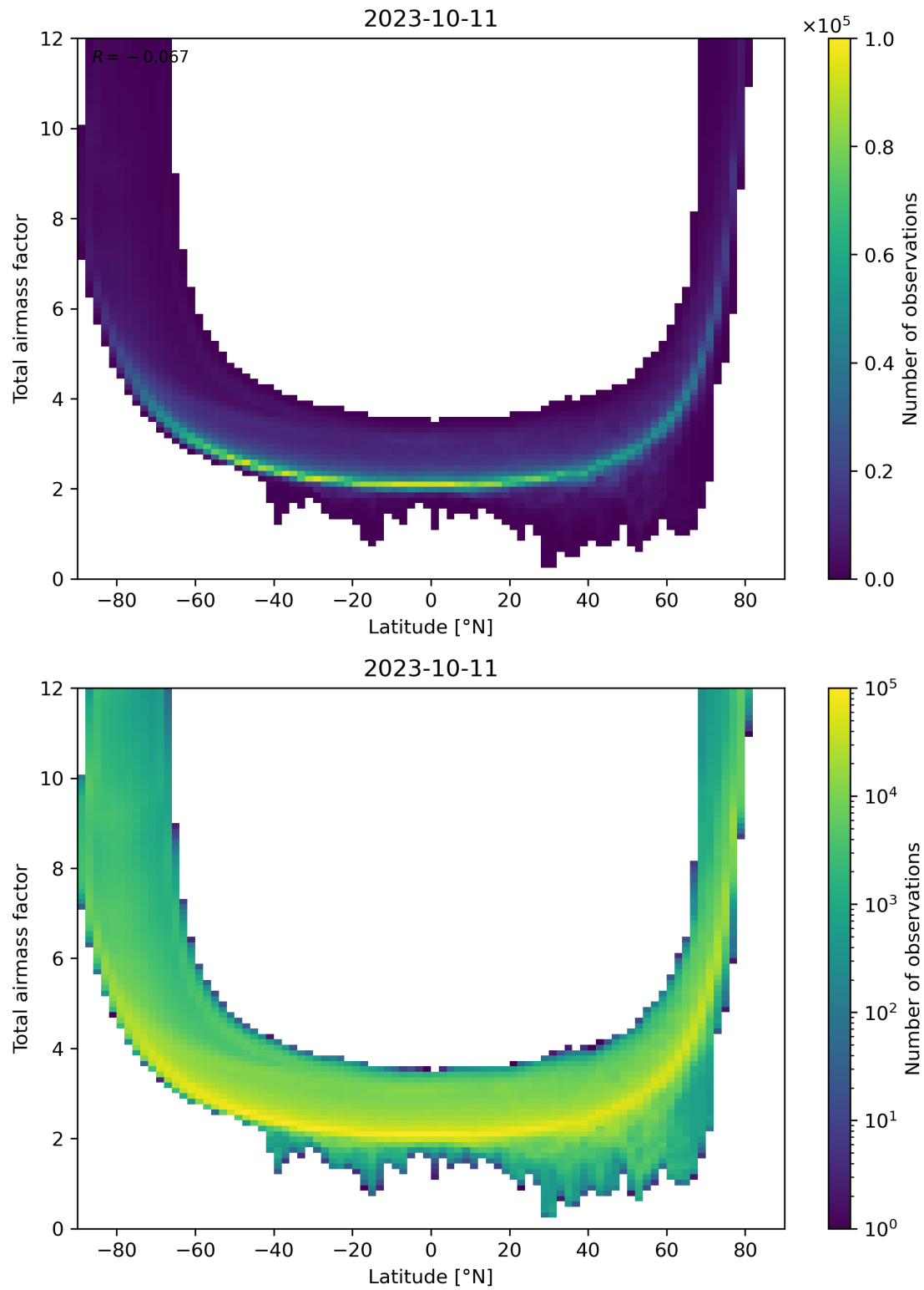
Figure 84: Scatter density plot of “Latitude” against “Total airmass factor” for 2023-10-10 to 2023-10-12.
