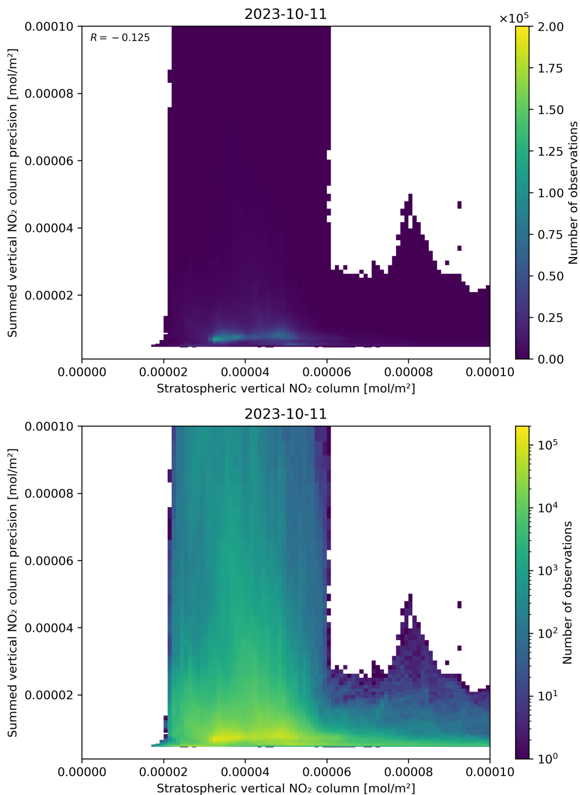
Figure 99: Scatter density plot of “Stratospheric vertical NO 2 column” against “Summed vertical NO 2 column precision” for 2023-10-10 to 2023-10-12.
