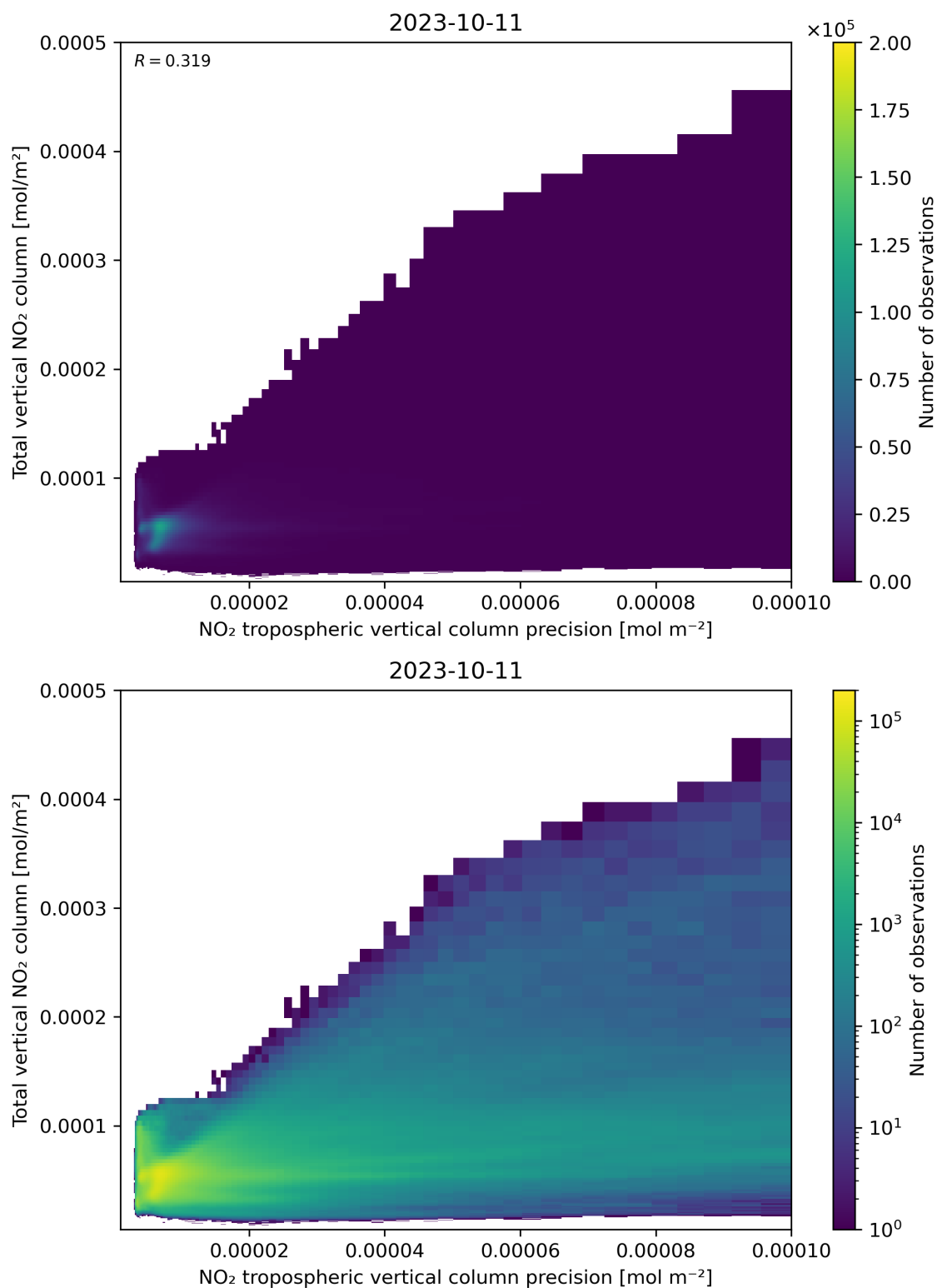
Figure 138: Scatter density plot of “NO 2 tropospheric vertical column precision” against “Total vertical NO 2 column” for 2023-10-10 to 2023-10-12.
