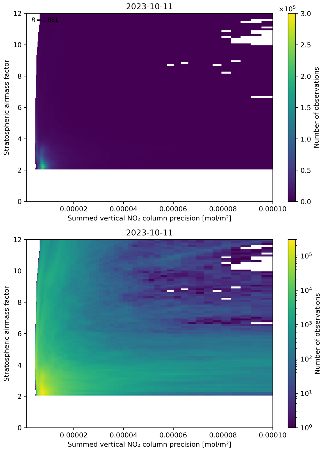
Figure 106: Scatter density plot of “Summed vertical NO 2 column precision” against “Stratospheric airmass factor” for 2023-10-10 to 2023-10-12.
