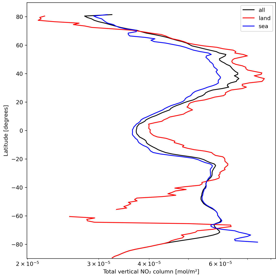
Figure 21: Zonal average of “Total vertical NO 2 column” for 2023-10-10 to 2023-10-12.
