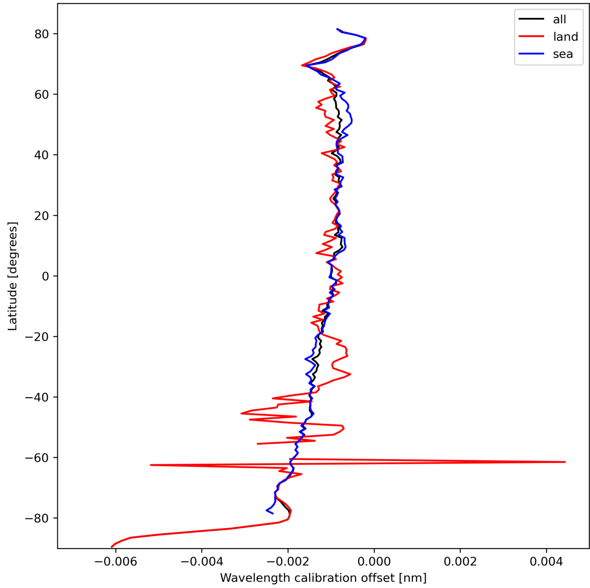
Figure 18: Zonal average of “Wavelength calibration offset” for 2023-10-10 to 2023-10-12.
