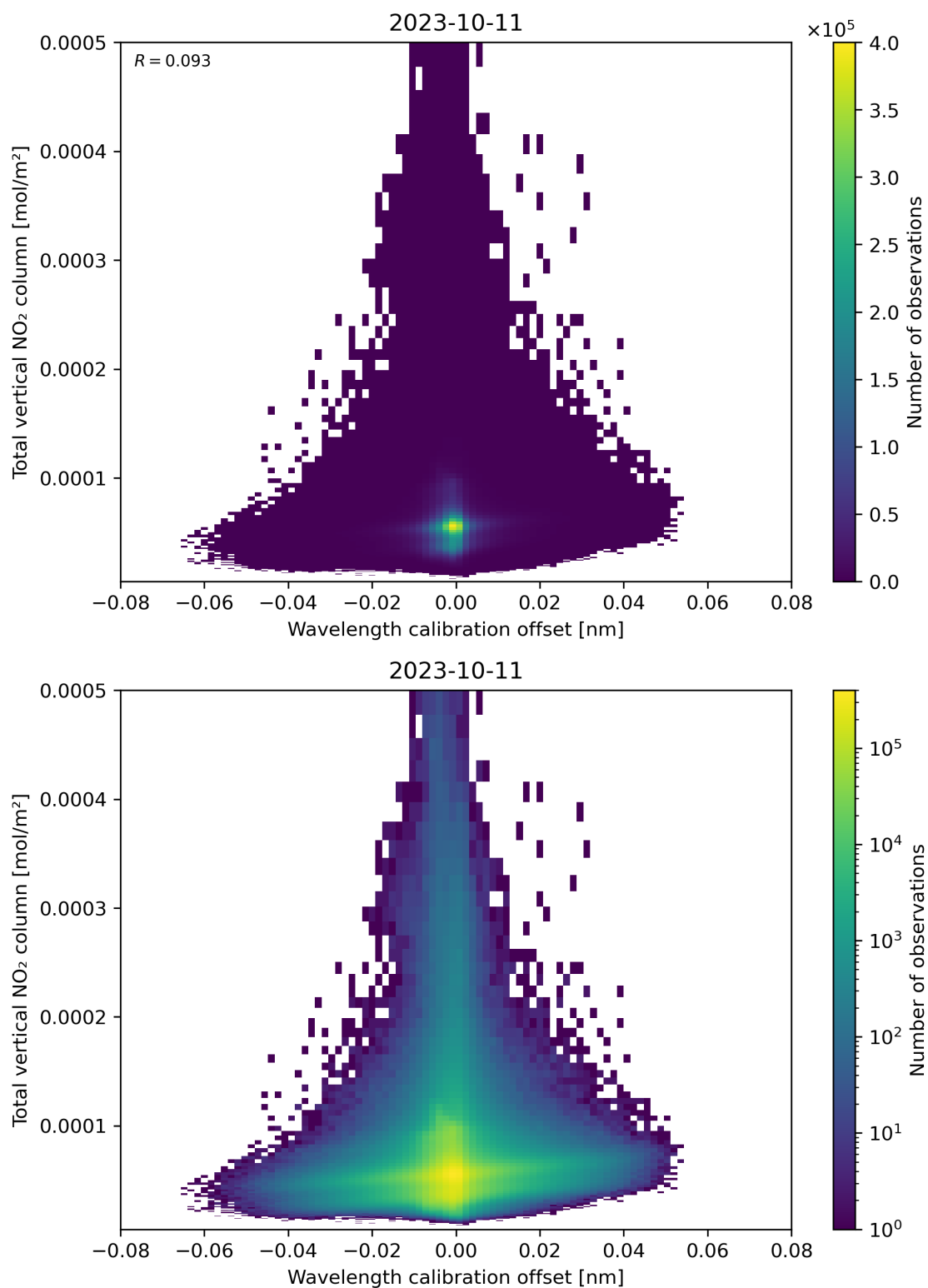
Figure 179: Scatter density plot of “Wavelength calibration offset” against “Total vertical NO 2 column” for 2023-10-10 to 2023-10-12.
