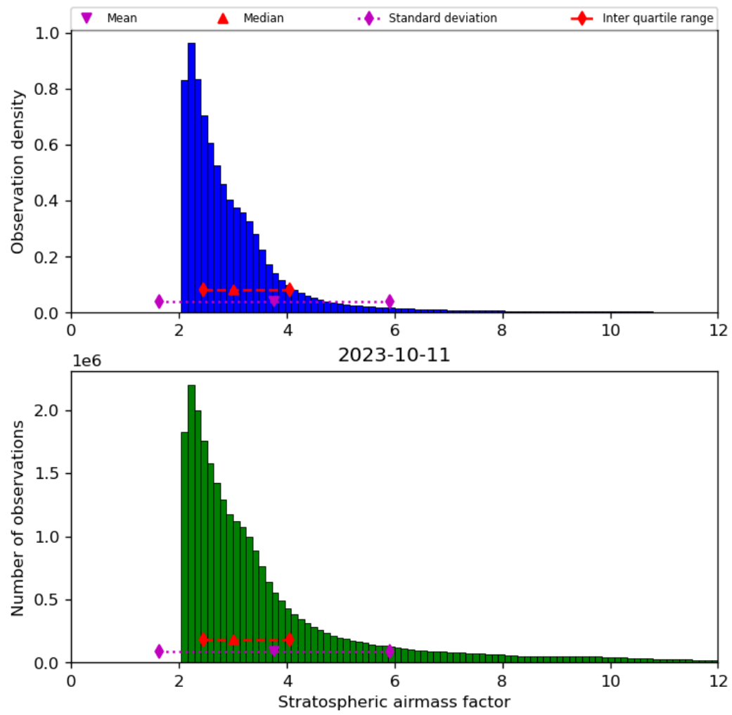
Figure 44: Histogram of “Stratospheric airmass factor” for 2023-10-10 to 2023-10-12
