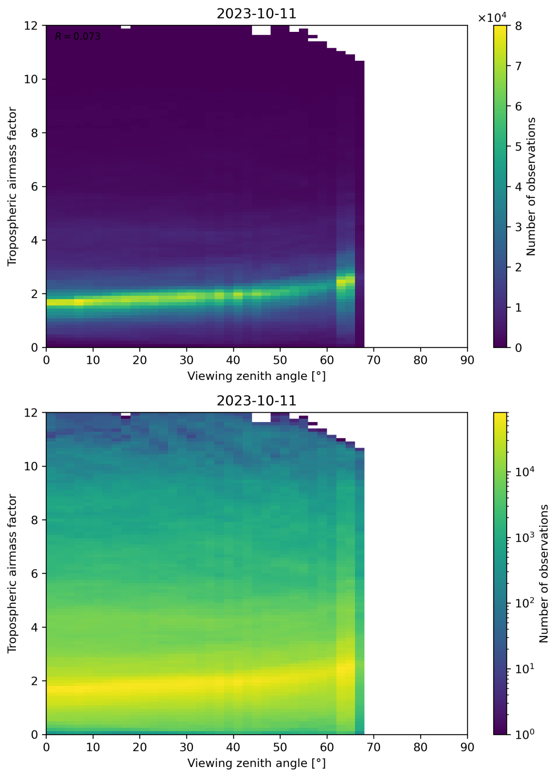
Figure 161: Scatter density plot of “Viewing zenith angle” against “Tropospheric airmass factor” for 2023-10-10 to 2023-10-12.
