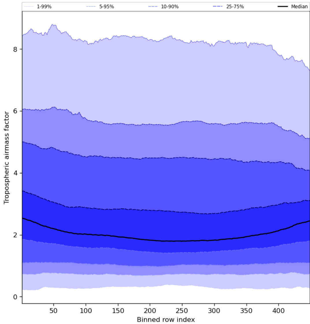
Figure 48: Along track statistics of “Tropospheric airmass factor” for 2023-10-10 to 2023-10-12
