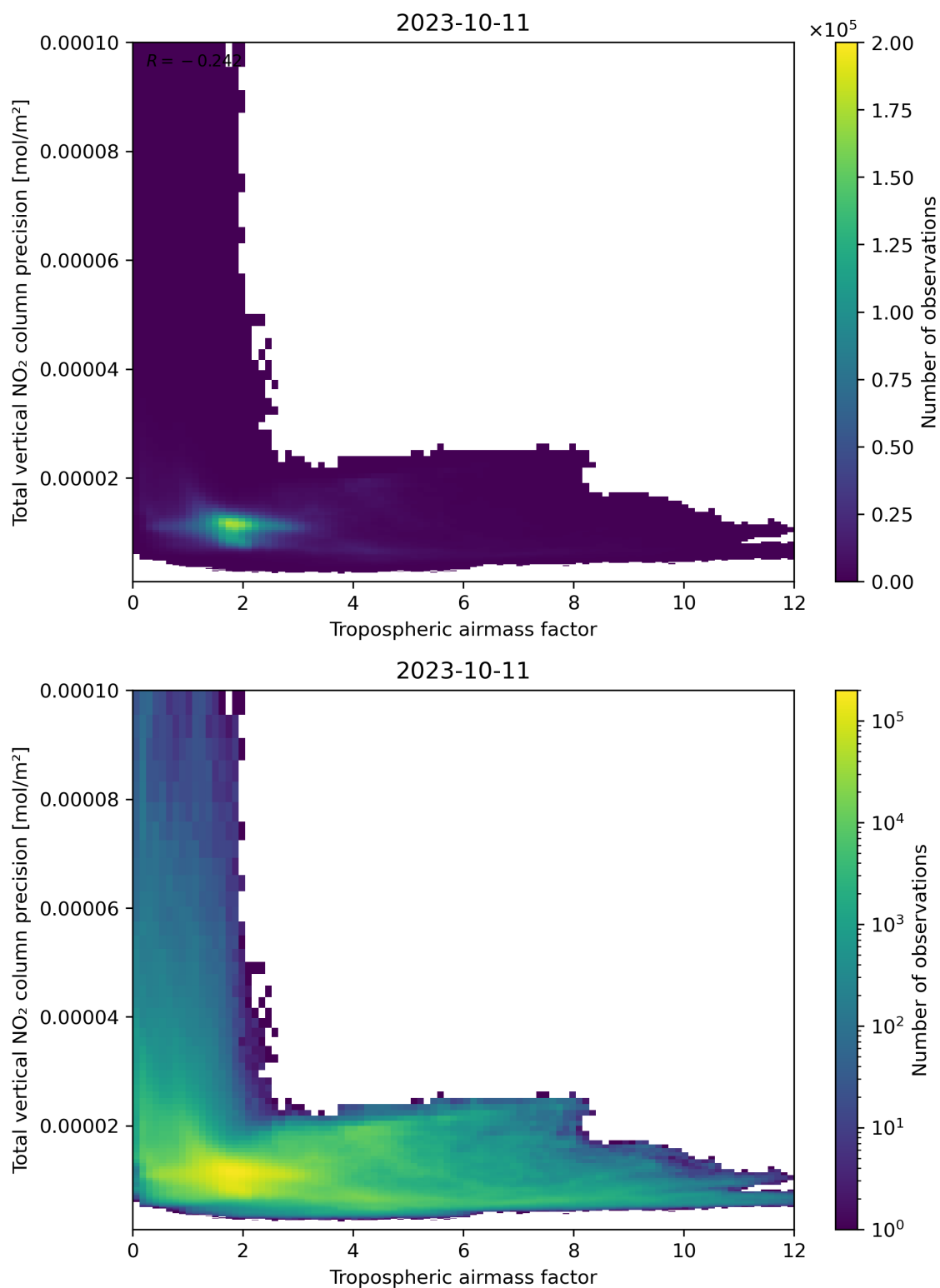
Figure 78: Scatter density plot of “Tropospheric air mass factor” against “Total vertical NO 2 column precision” for 2023-10-10 to 2023-10-12.
