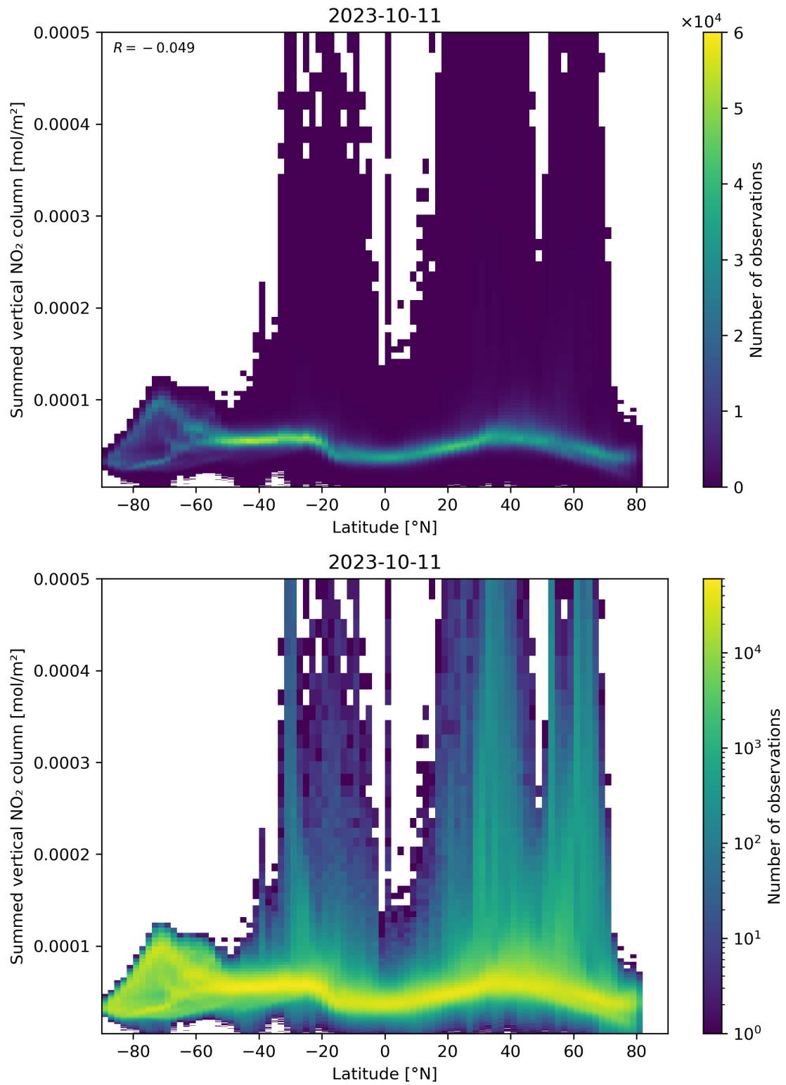
Figure 88: Scatter density plot of “Latitude” against “Summed vertical NO 2 column” for 2023-10-10 to 2023-10-12.
