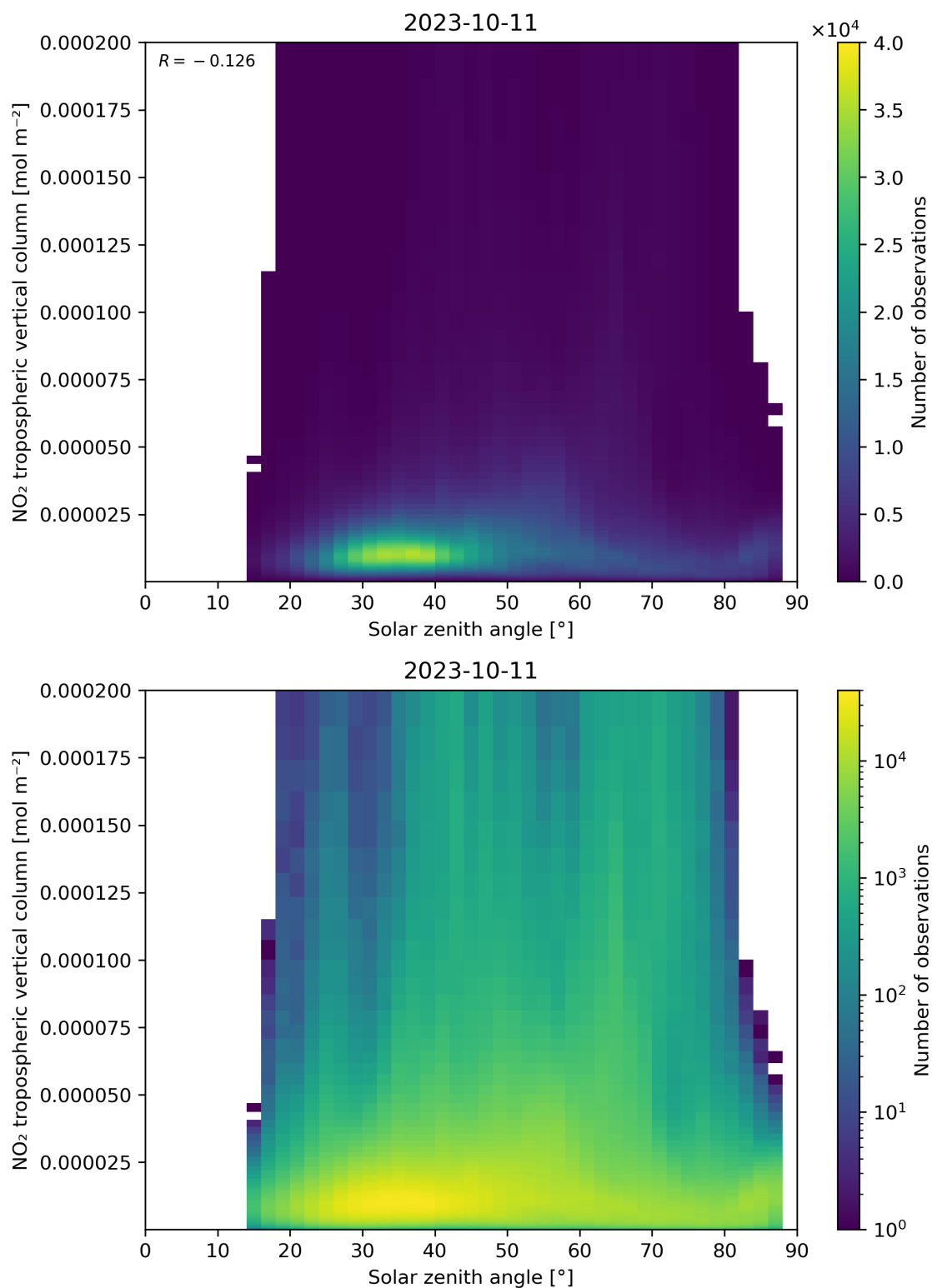
Figure 155: Scatter density plot of “Solar zenith angle” against “NO 2 tropospheric vertical column” for 2023-10-10 to 2023-10-12.
