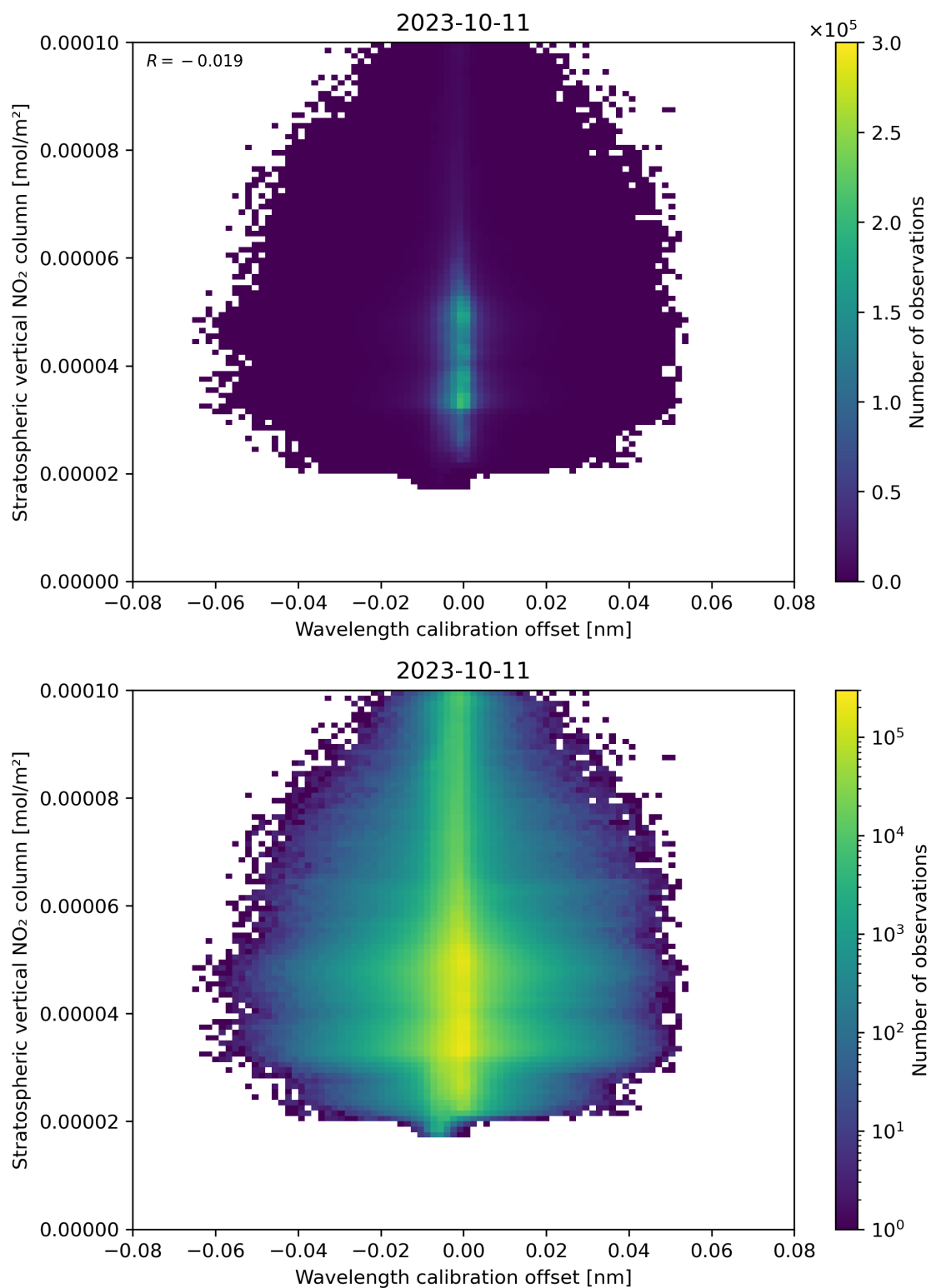
Figure 176: Scatter density plot of “Wavelength calibration offset” against “Stratospheric vertical NO 2 column” for 2023-10-10 to 2023-10-12.
