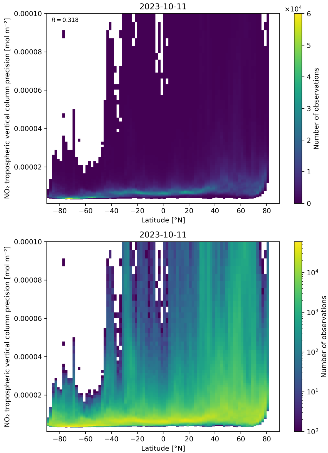
Figure 93: Scatter density plot of “Latitude” against “NO 2 tropospheric vertical column precision” for 2023-10-10 to 2023-10-12.
