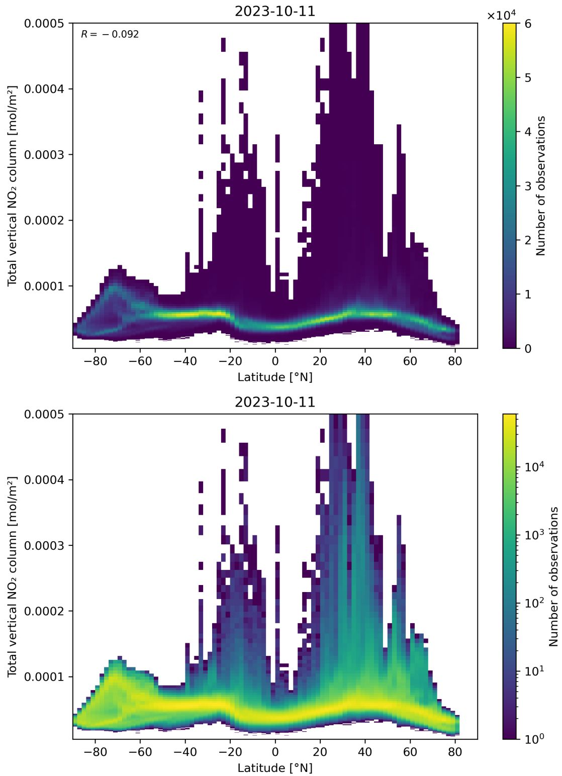
Figure 90: Scatter density plot of “Latitude” against “Total vertical NO 2 column” for 2023-10-10 to 2023-10-12.
