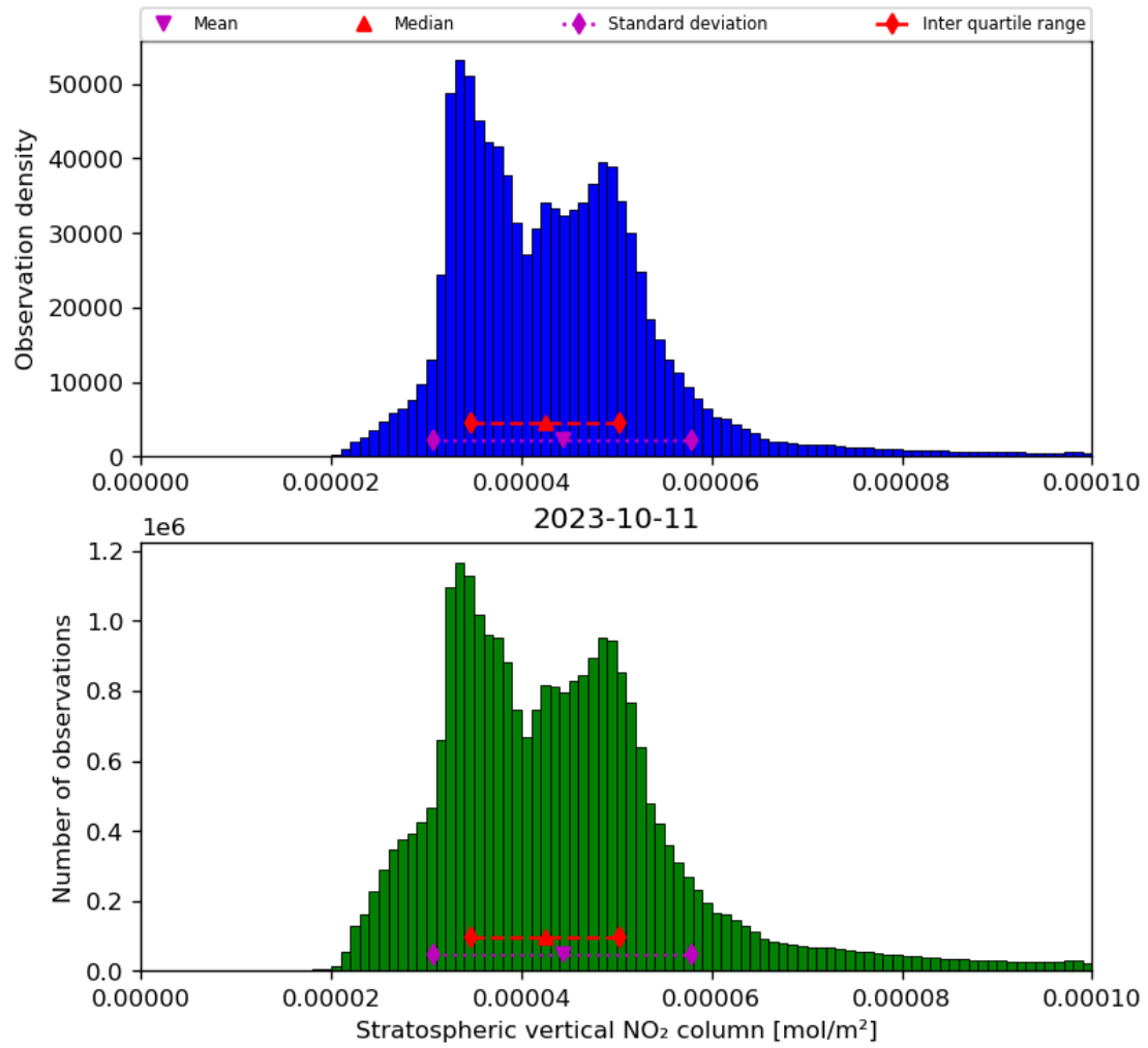
Figure 36: Histogram of “Stratospheric vertical NO 2 column” for 2023-10-10 to 2023-10-12
