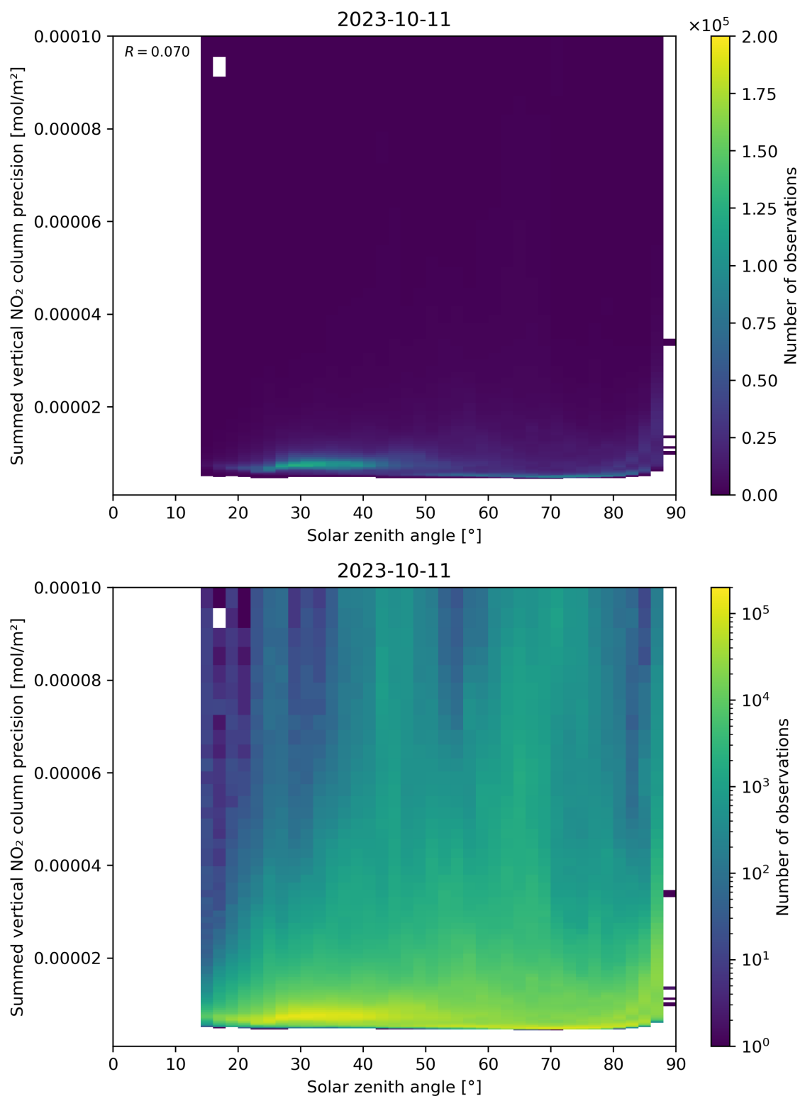
Figure 152: Scatter density plot of “Solar zenith angle” against “Summed vertical NO 2 column precision” for 2023-10-10 to 2023-10-12.
