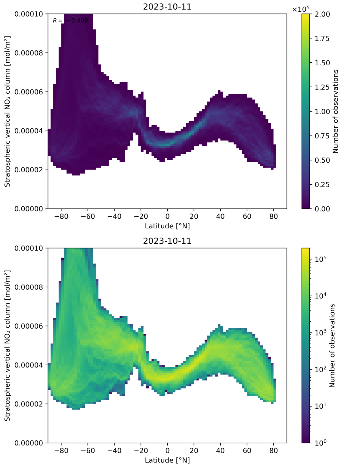
Figure 87: Scatter density plot of “Latitude” against “Stratospheric vertical NO 2 column” for 2023-10-10 to 2023-10-12.
