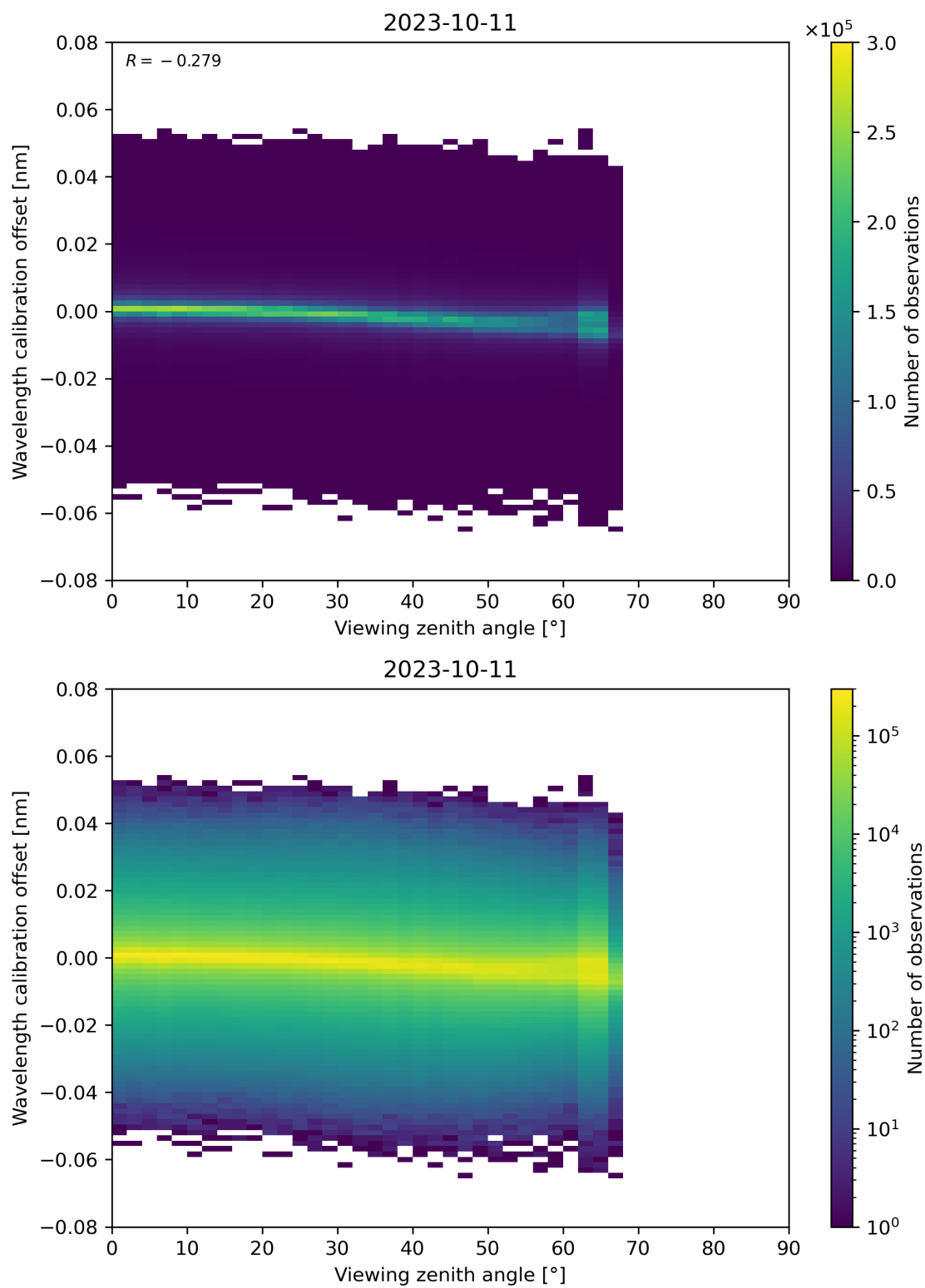
Figure 173: Scatter density plot of “Viewing zenith angle” against “Wavelength calibration offset” for 2023-10-10 to 2023-10-12.
