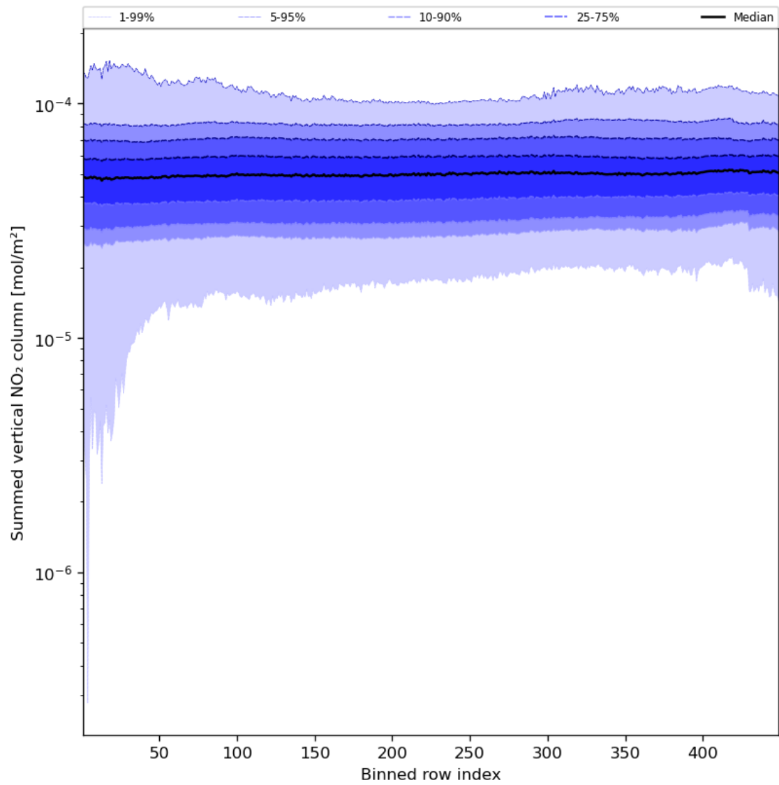
Figure 57: Along track statistics of “Summed vertical NO 2 column” for 2023-10-10 to 2023-10-12
