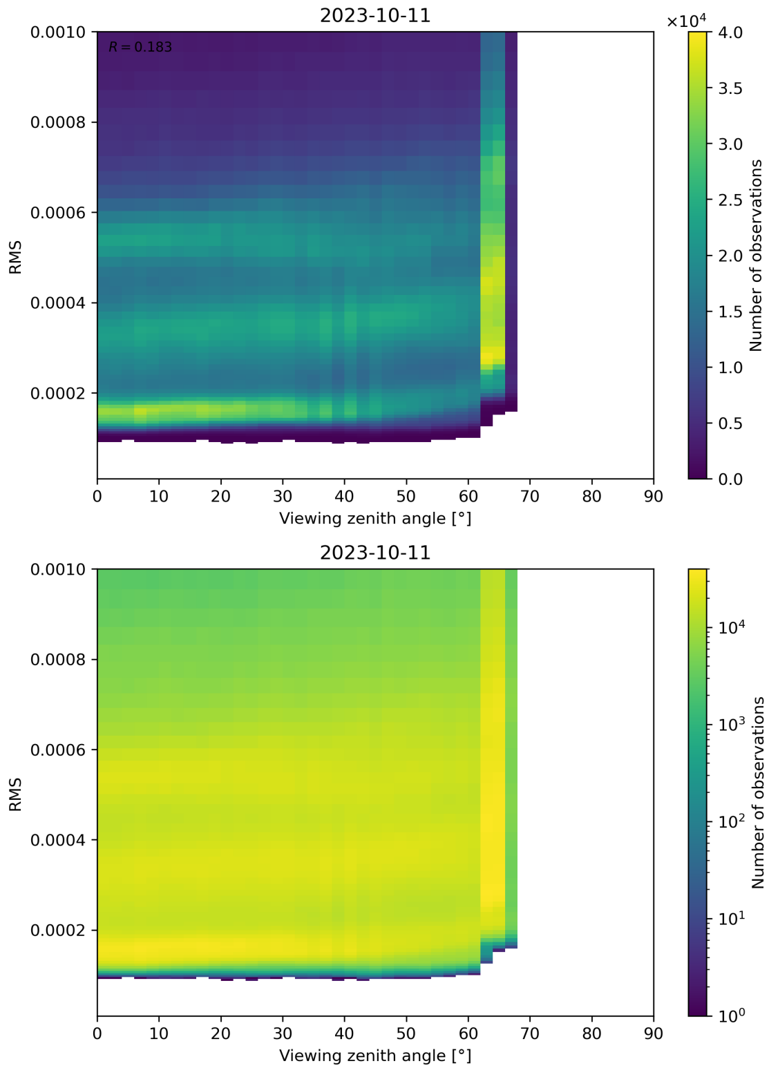
Figure 171: Scatter density plot of “Viewing zenith angle” against “RMS” for 2023-10-10 to 2023-10-12.
