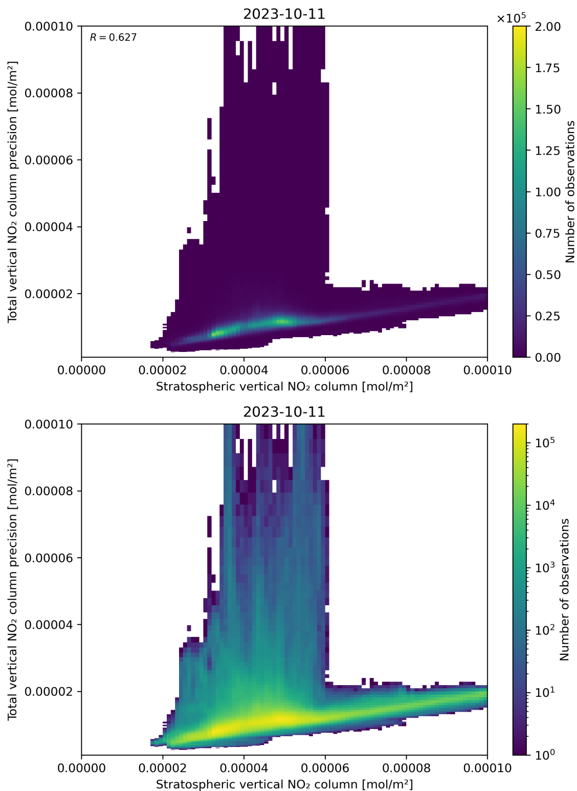
Figure 101: Scatter density plot of “Stratospheric vertical NO 2 column” against “Total vertical NO 2 column precision” for 2023-10-10 to 2023-10-12.
