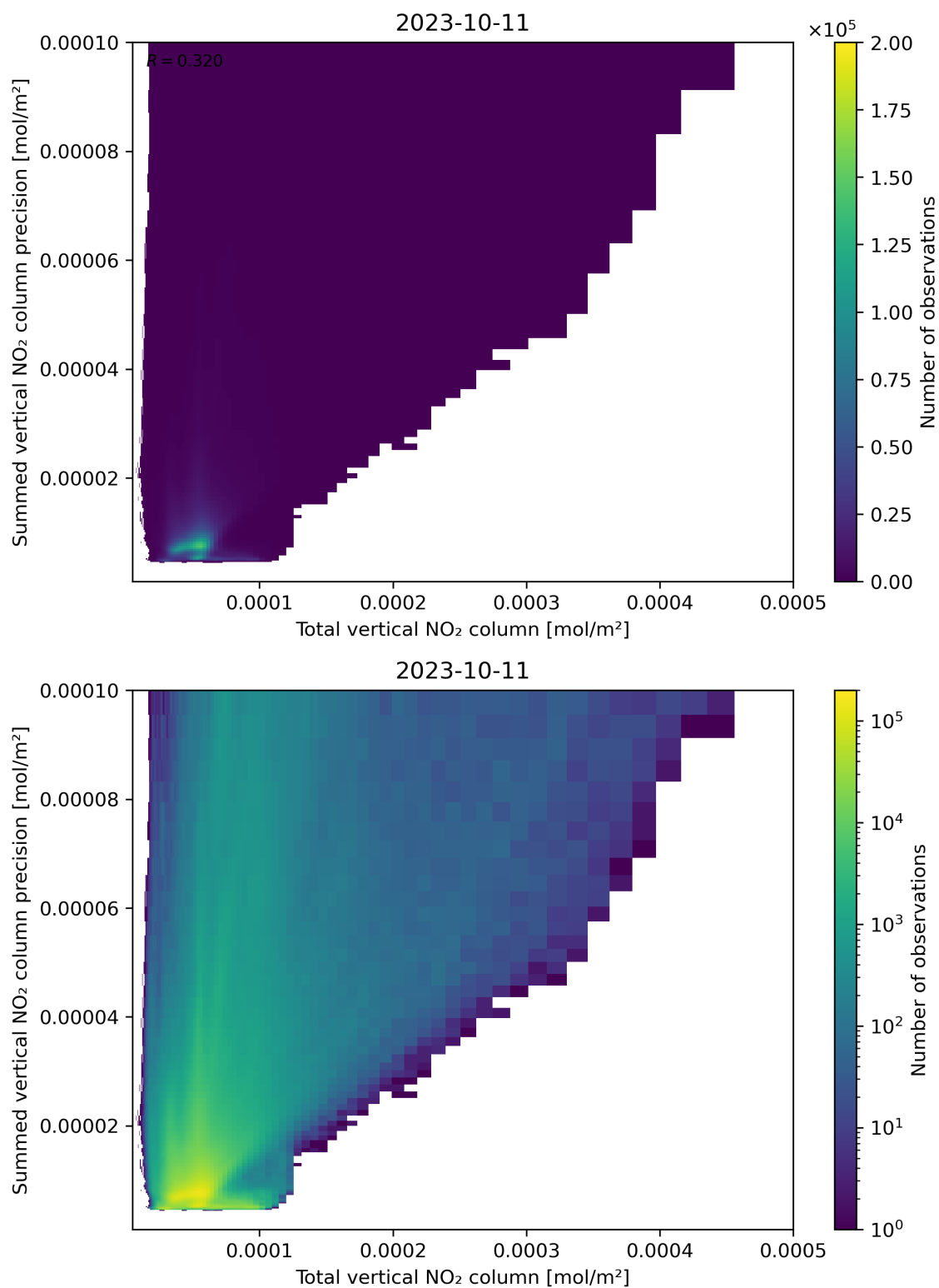
Figure 113: Scatter density plot of “Total vertical NO 2 column” against “Summed vertical NO 2 column precision” for 2023-10-10 to 2023-10-12.
