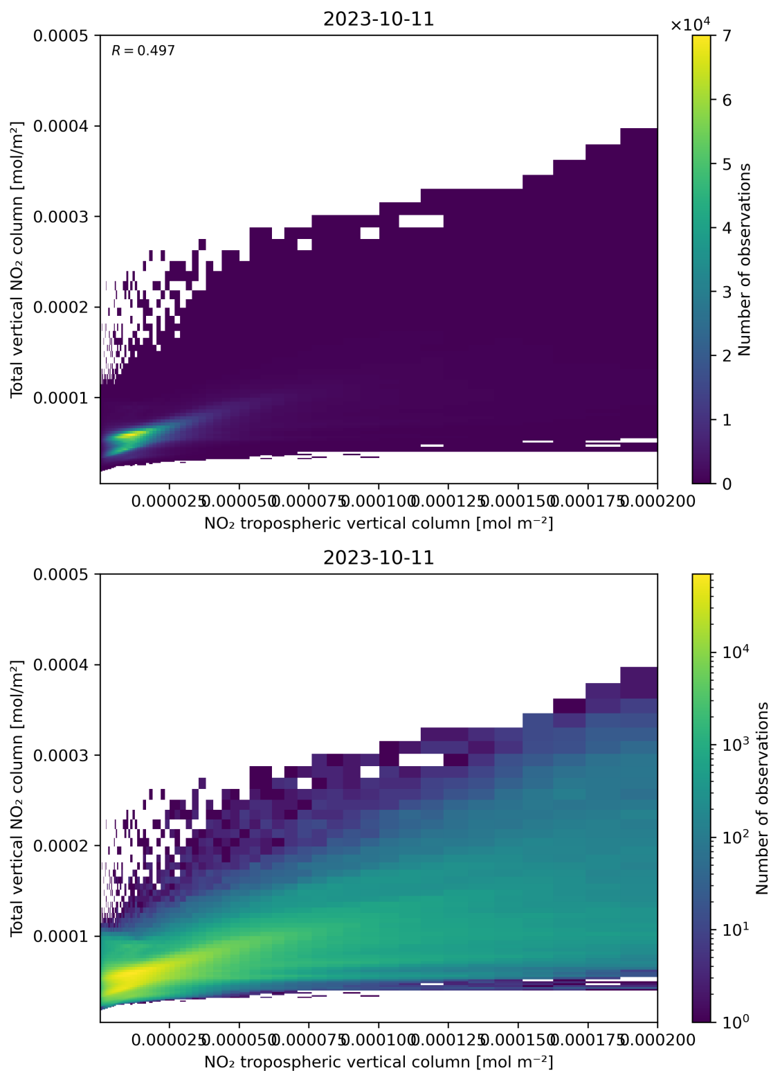
Figure 128: Scatter density plot of “NO 2 tropospheric vertical column” against “Total vertical NO 2 column” for 2023-10-10 to 2023-10-12.
