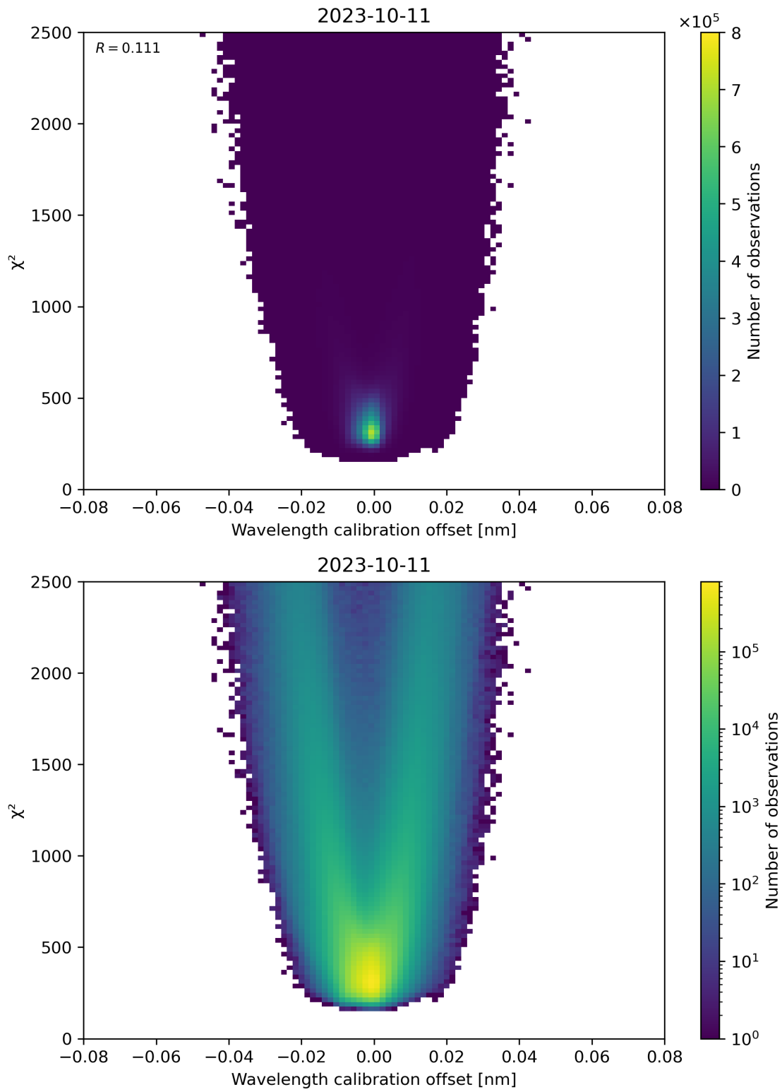
Figure 175: Scatter density plot of “Wavelength calibration offset” against “ \chi^2 ” for 2023-10-10 to 2023-10-12.
