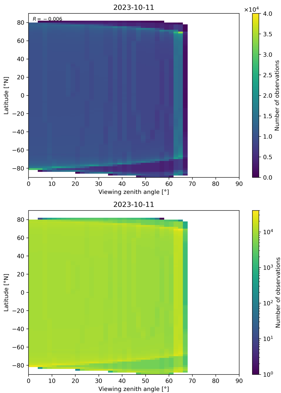
Figure 163: Scatter density plot of “Viewing zenith angle” against “Latitude” for 2023-10-10 to 2023-10-12.
