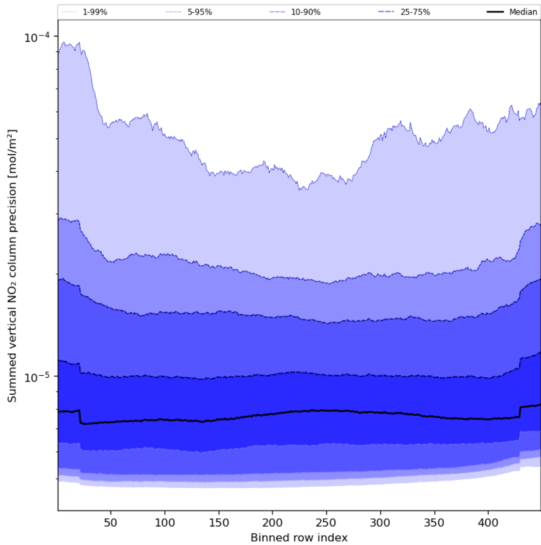
Figure 58: Along track statistics of “Summed vertical NO 2 column precision” for 2023-10-10 to 2023-10-12
