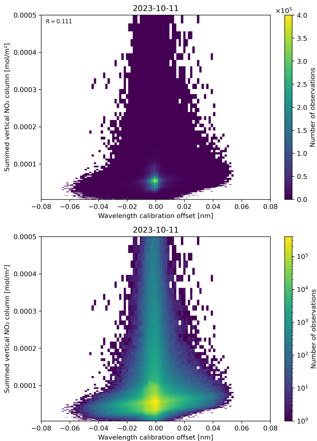
Figure 177: Scatter density plot of “Wavelength calibration offset” against “Summed vertical NO 2 column” for 2023-10-10 to 2023-10-12.
