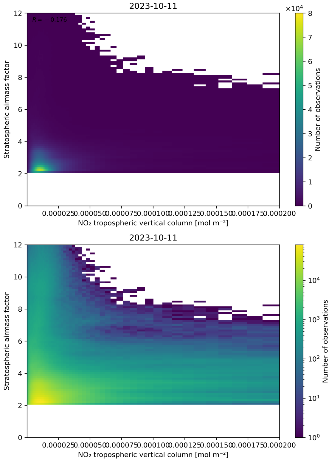
Figure 121: Scatter density plot of “NO 2 tropospheric vertical column” against “Stratospheric air mass factor” for 2023-10-10 to 2023-10-12.
