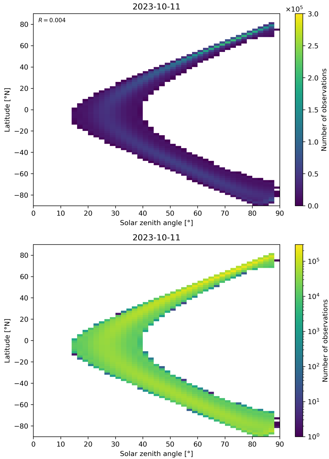
Figure 149: Scatter density plot of “Solar zenith angle” against “Latitude” for 2023-10-10 to 2023-10-12.
