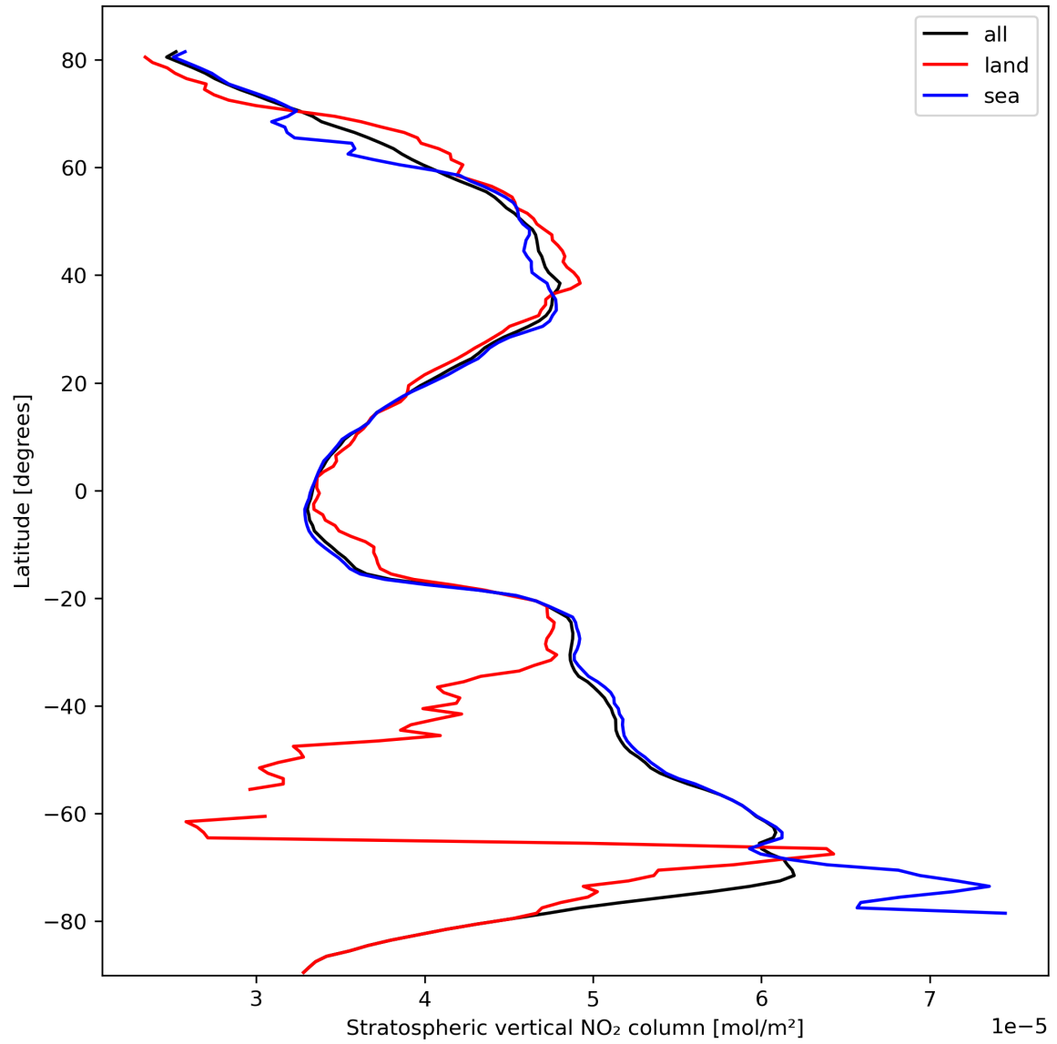
Figure 19: Zonal average of “Stratospheric vertical NO 2 column” for 2023-10-10 to 2023-10-12.
