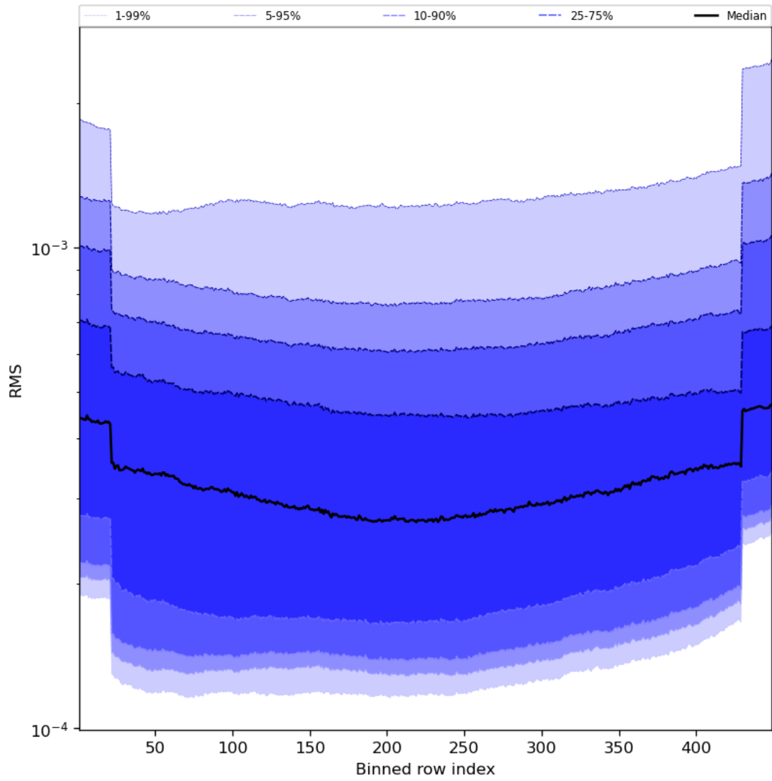
Figure 60: Along track statistics of “RMS” for 2023-10-10 to 2023-10-12
