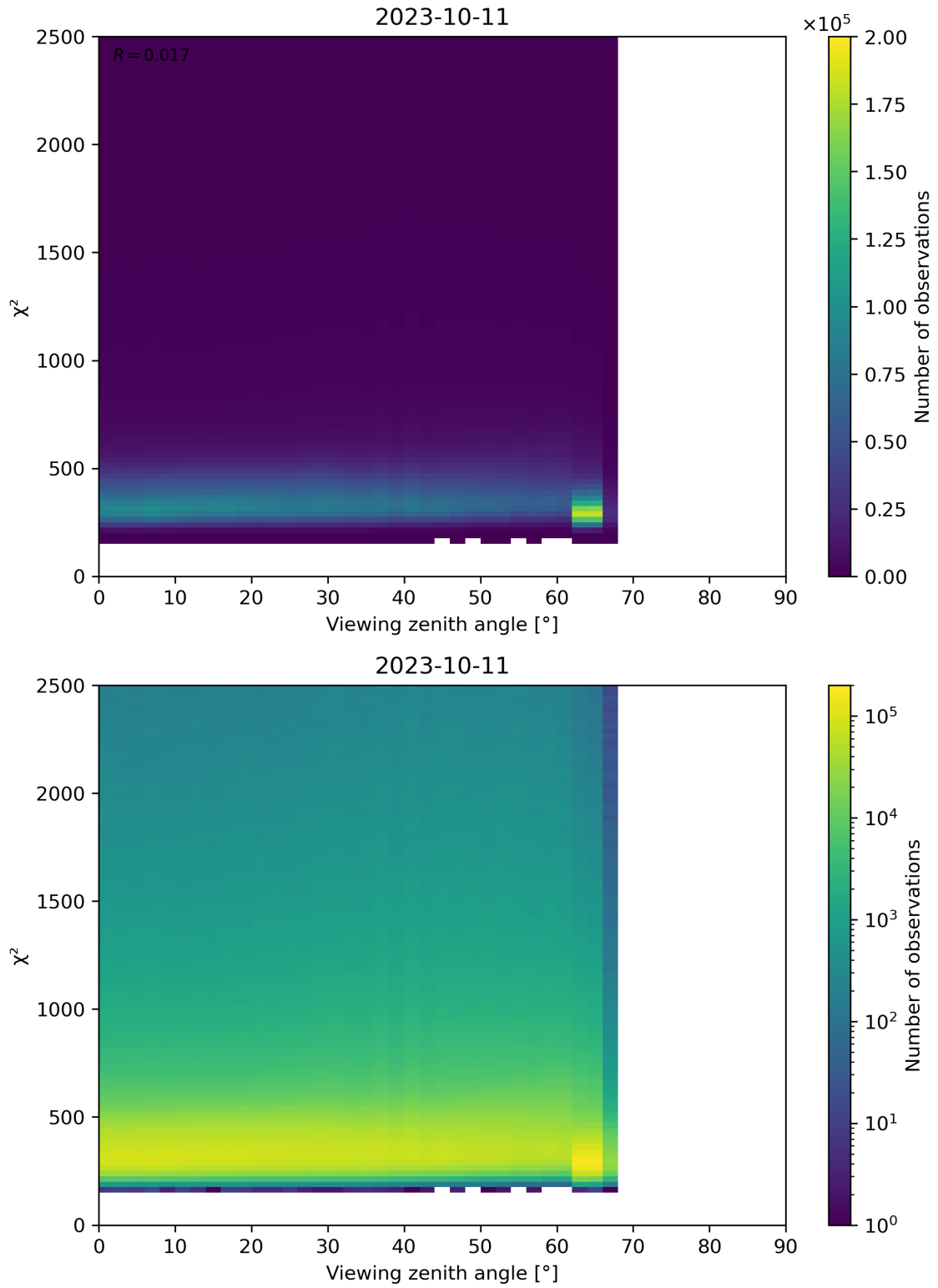
Figure 162: Scatter density plot of “Viewing zenith angle” against “ \chi^2 ” for 2023-10-10 to 2023-10-12.
