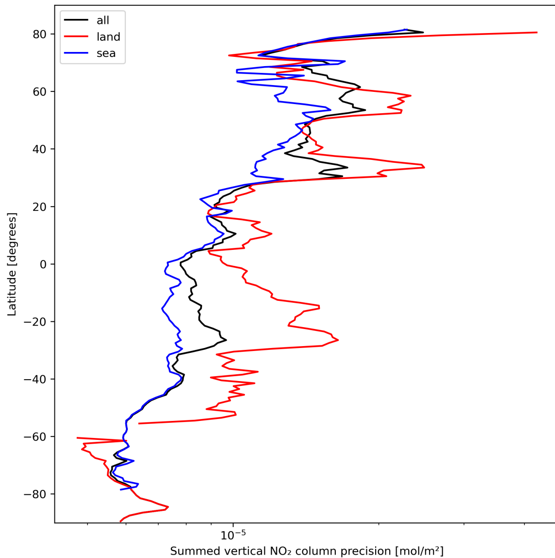
Figure 24: Zonal average of “Summed vertical NO 2 column precision” for 2023-10-10 to 2023-10-12.
