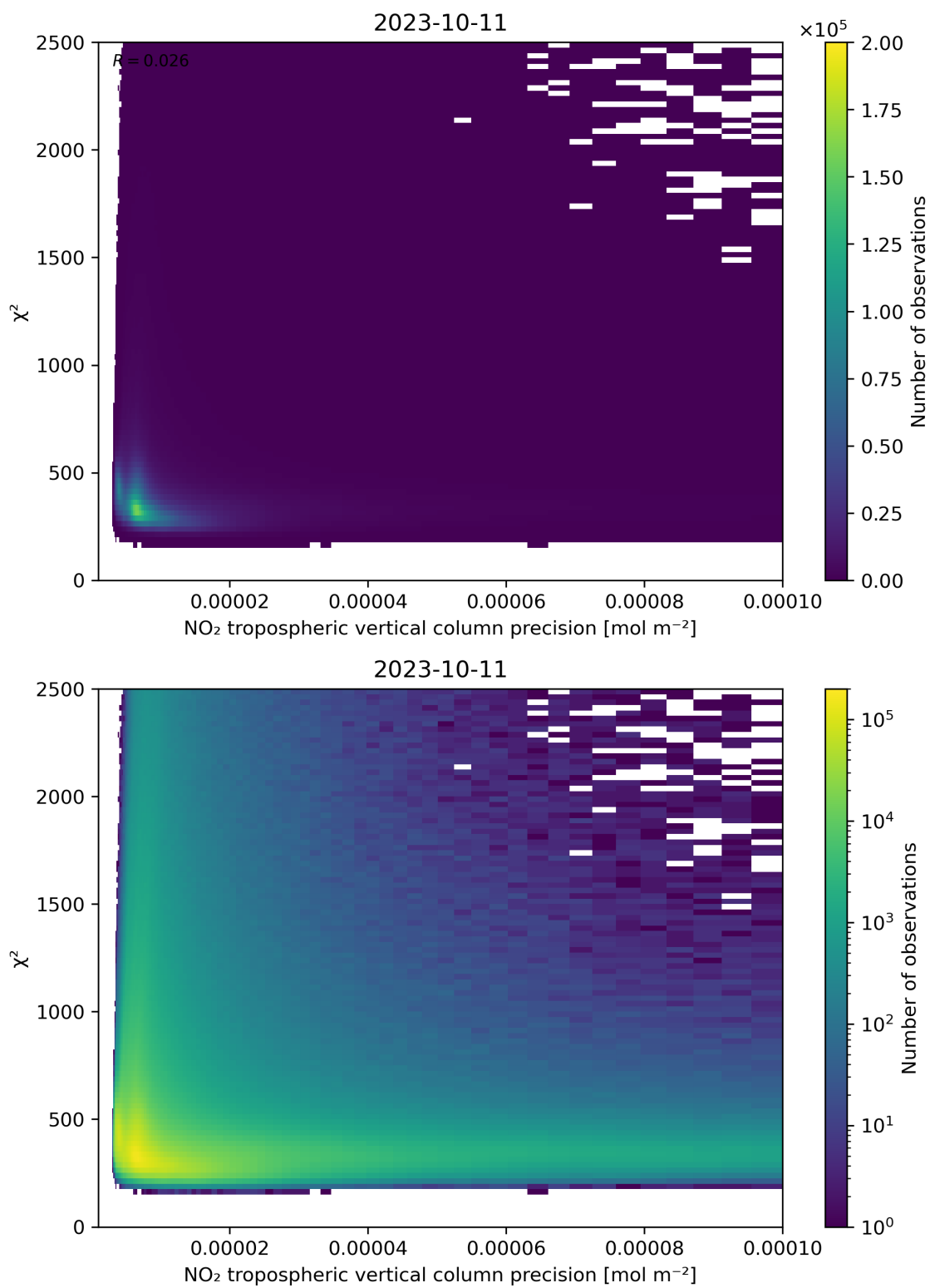
Figure 134: Scatter density plot of “NO 2 tropospheric vertical column precision” against “ \chi^2 ” for 2023-10-10 to 2023-10-12.
