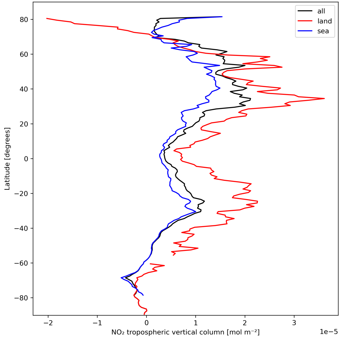
Figure 12: Zonal average of “NO 2 tropospheric vertical column” for 2023-10-10 to 2023-10-12.
