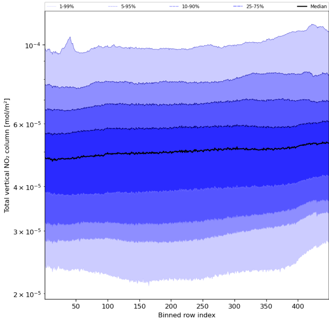
Figure 55: Along track statistics of “Total vertical NO 2 column” for 2023-10-10 to 2023-10-12
