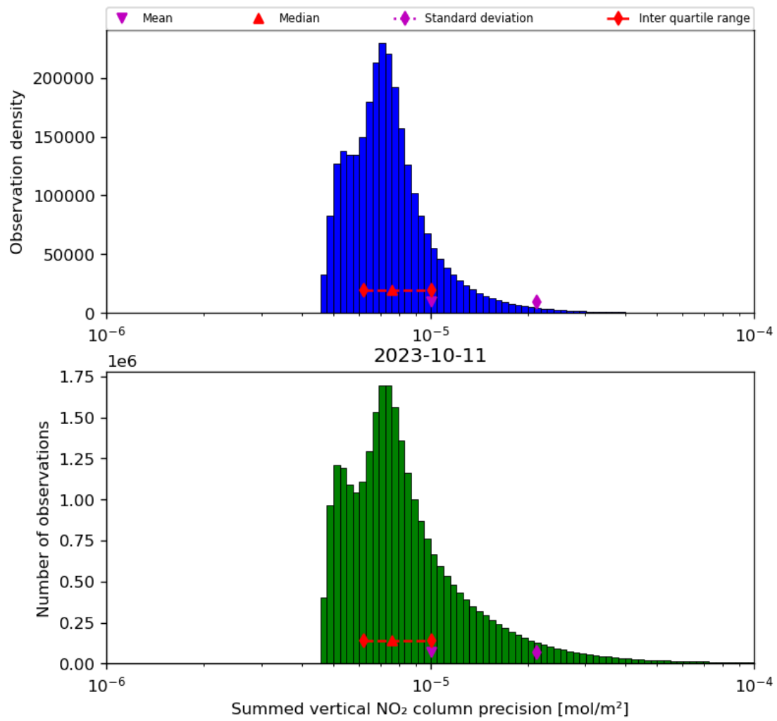
Figure 41: Histogram of “Summed vertical NO 2 column precision” for 2023-10-10 to 2023-10-12
