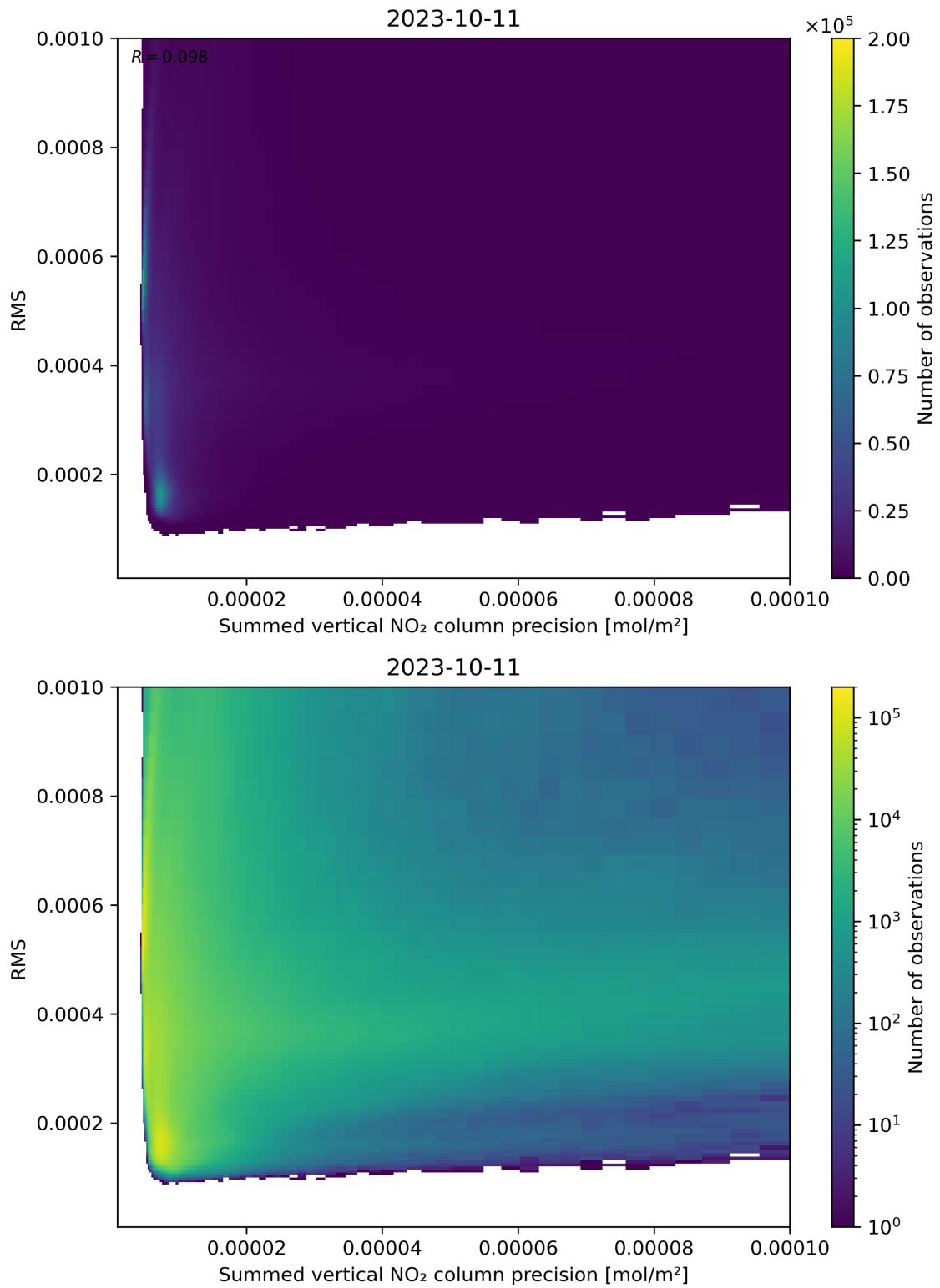
Figure 108: Scatter density plot of “Summed vertical NO 2 column precision” against “RMS” for 2023-10-10 to 2023-10-12.
