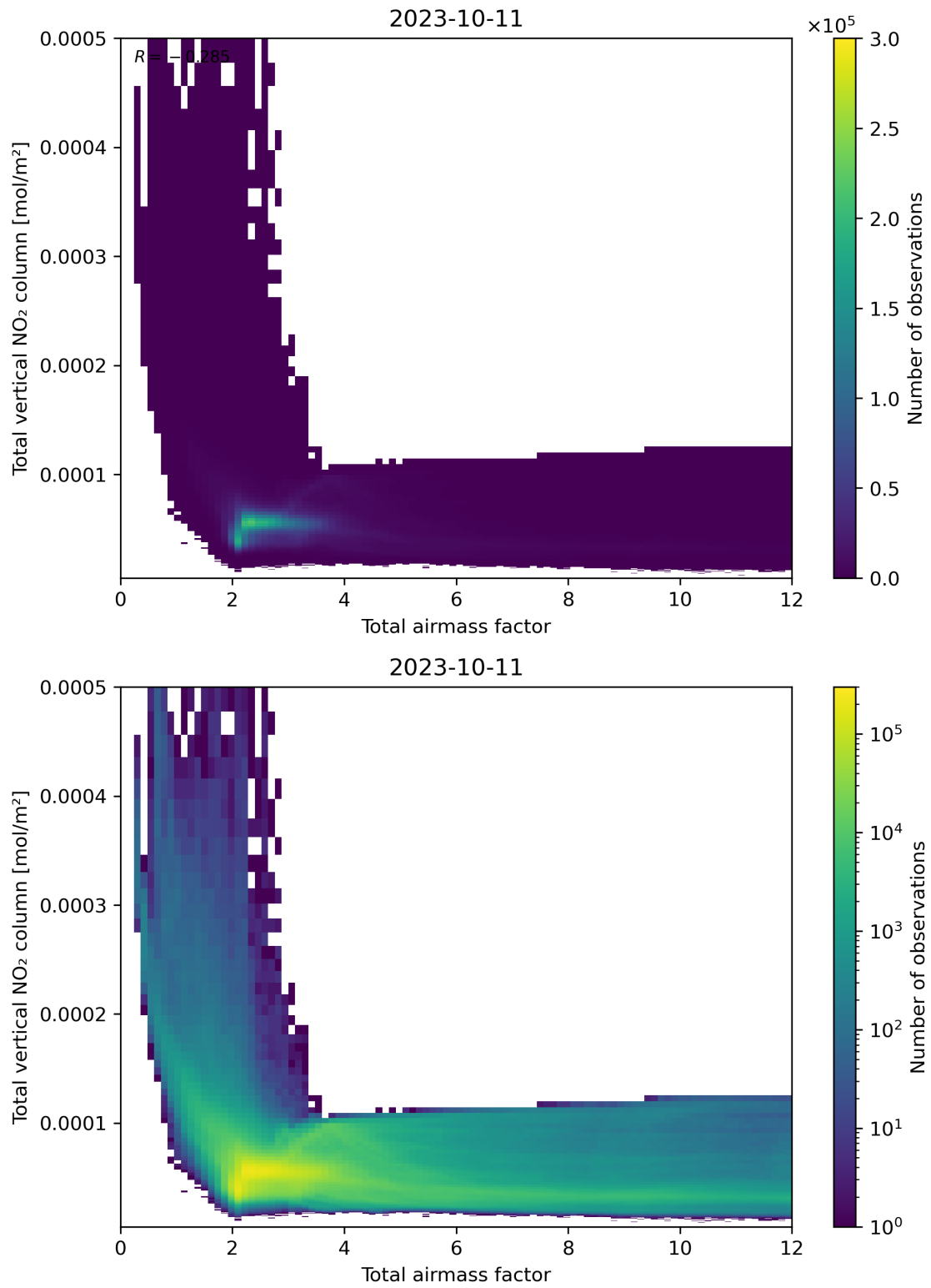
Figure 67: Scatter density plot of “Total air mass factor” against “Total vertical NO 2 column” for 2023-10-10 to 2023-10-12.
