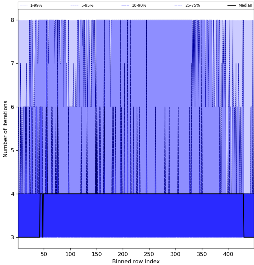
Figure 51: Along track statistics of “Number of iterations” for 2023-10-10 to 2023-10-12
