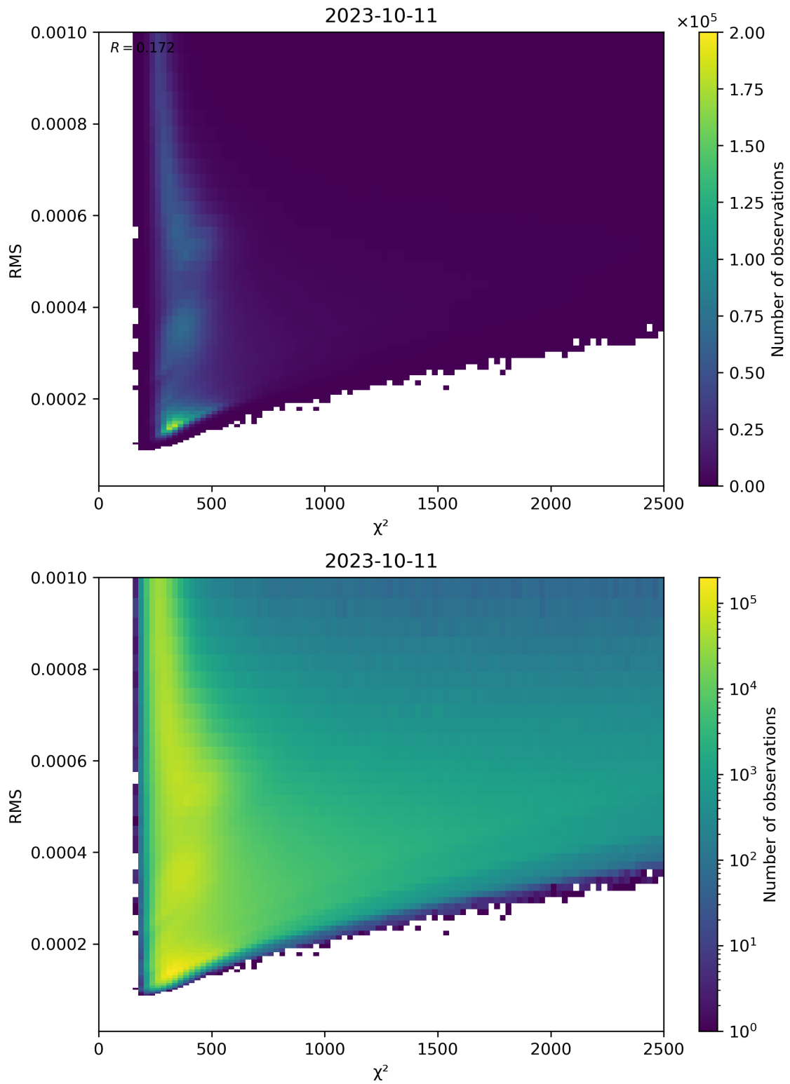
Figure 82: Scatter density plot of “ \chi^2 ” against “RMS” for 2023-10-10 to 2023-10-12.
