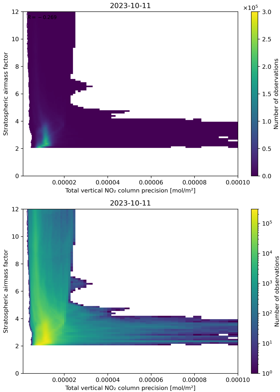
Figure 115: Scatter density plot of “Total vertical NO 2 column precision” against “Stratospheric airmass factor” for 2023-10-10 to 2023-10-12.
