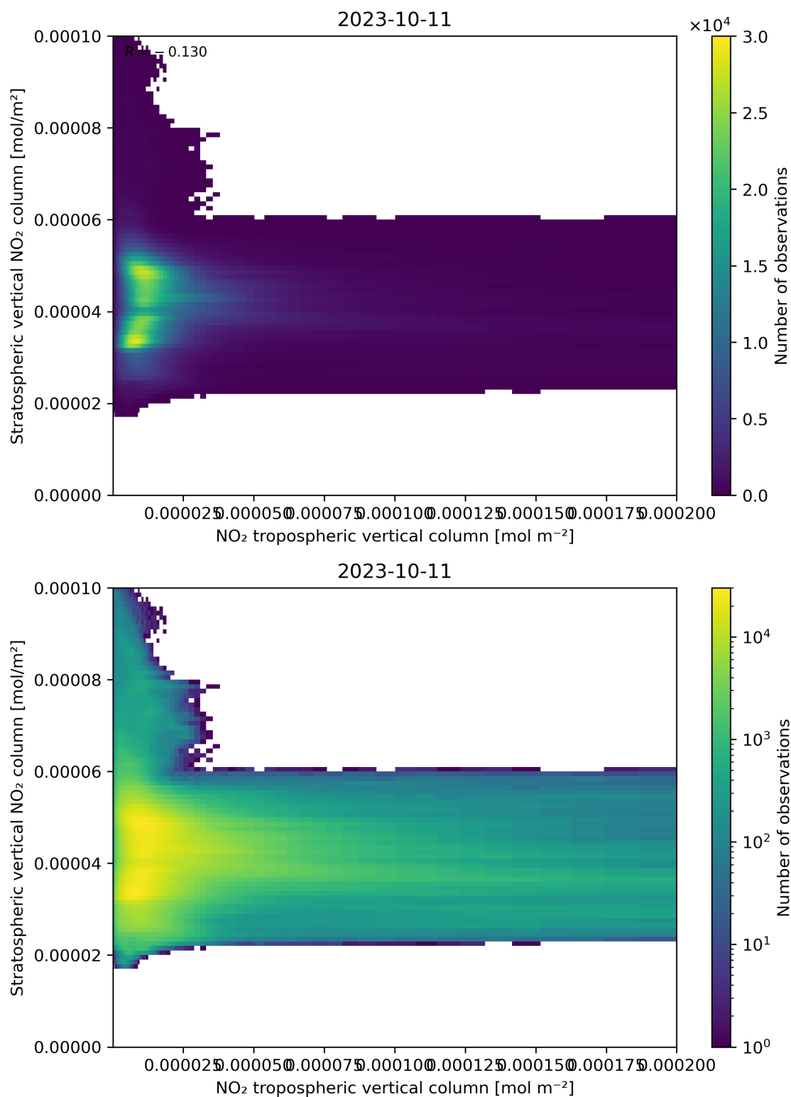
Figure 125: Scatter density plot of “NO 2 tropospheric vertical column” against “Stratospheric vertical NO 2 column” for 2023-10-10 to 2023-10-12.
