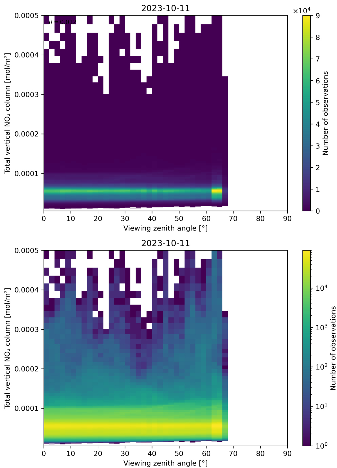
Figure 167: Scatter density plot of “Viewing zenith angle” against “Total vertical NO 2 column” for 2023-10-10 to 2023-10-12.
