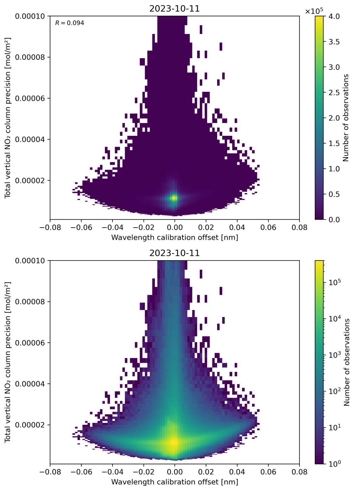
Figure 180: Scatter density plot of “Wavelength calibration offset” against “Total vertical NO 2 column precision” for 2023-10-10 to 2023-10-12.
