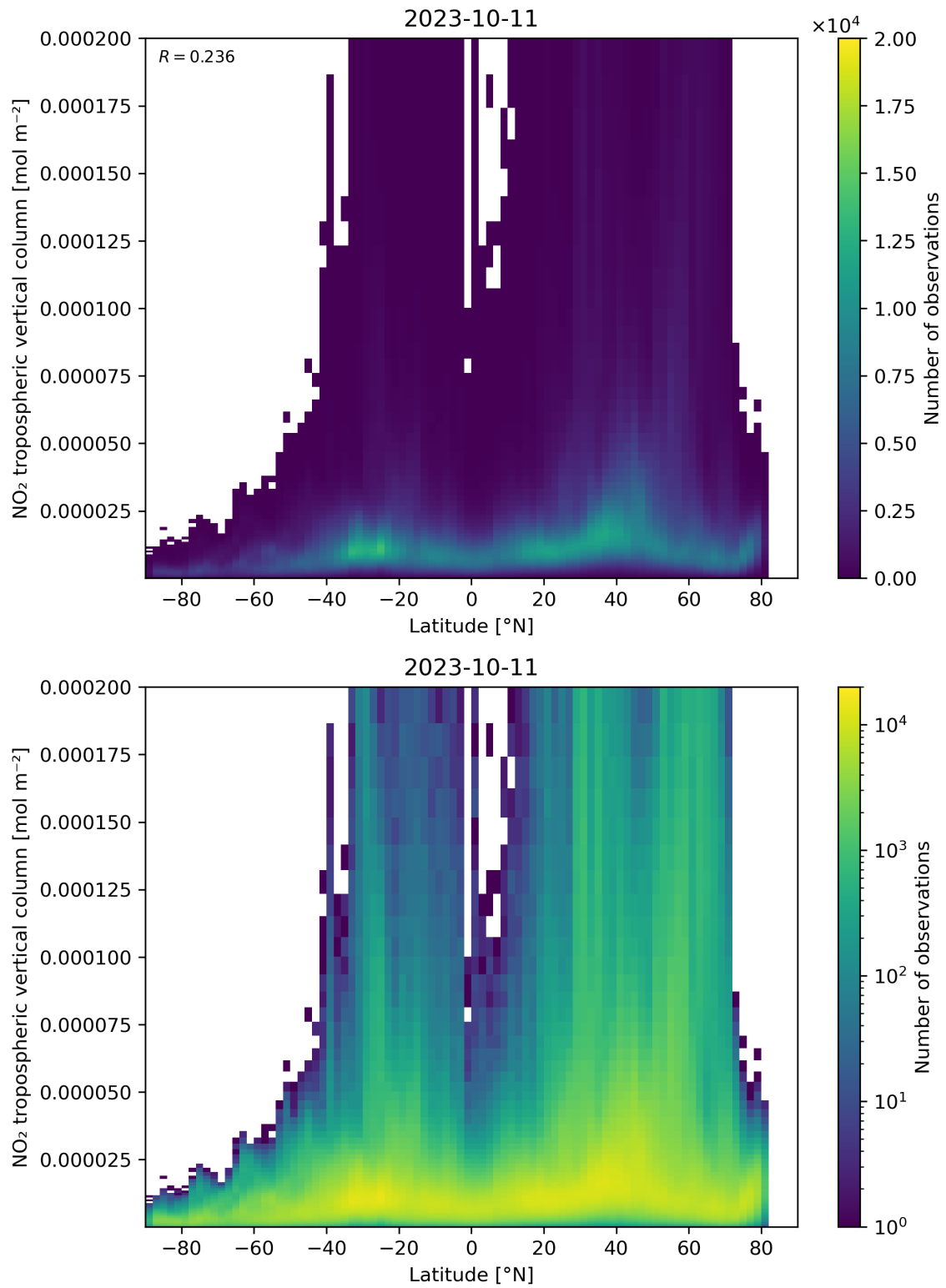
Figure 92: Scatter density plot of “Latitude” against “NO 2 tropospheric vertical column” for 2023-10-10 to 2023-10-12.
