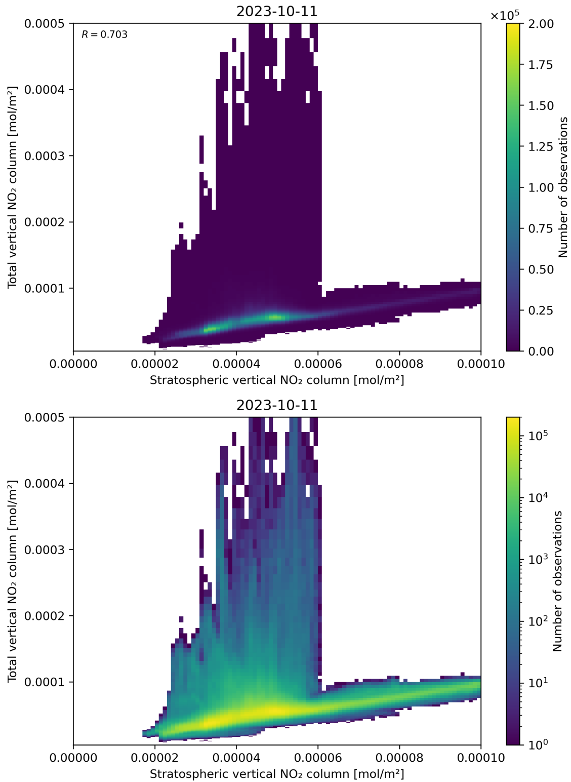
Figure 100: Scatter density plot of “Stratospheric vertical NO 2 column” against “Total vertical NO 2 column” for 2023-10-10 to 2023-10-12.
