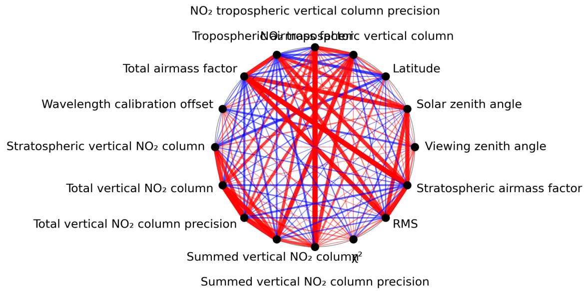
Figure 1: Map of correlation graph for 2023-10-10 to 2023-10-12.
