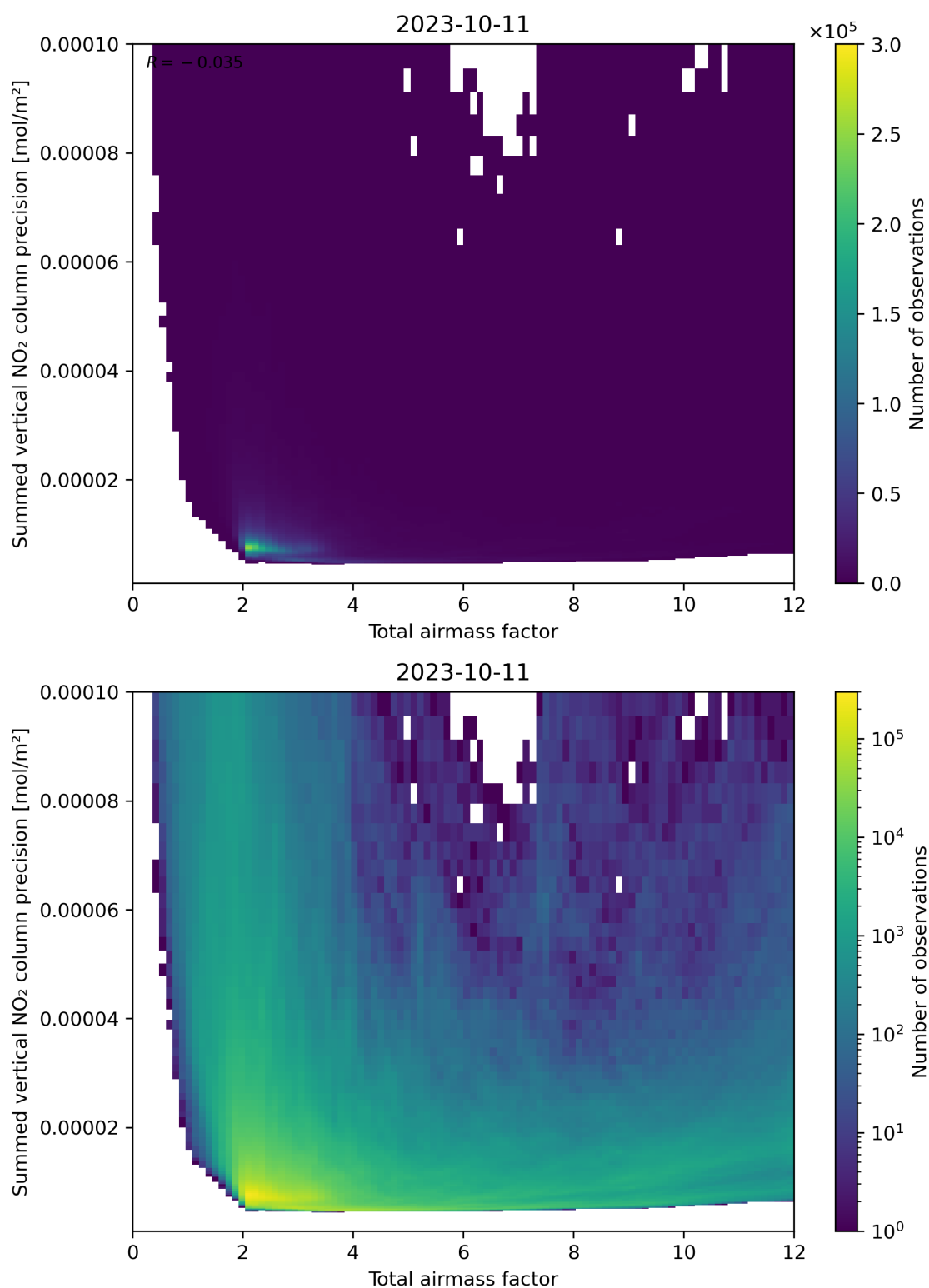
Figure 66: Scatter density plot of “Total airmass factor” against “Summed vertical NO 2 column precision” for 2023-10-10 to 2023-10-12.
