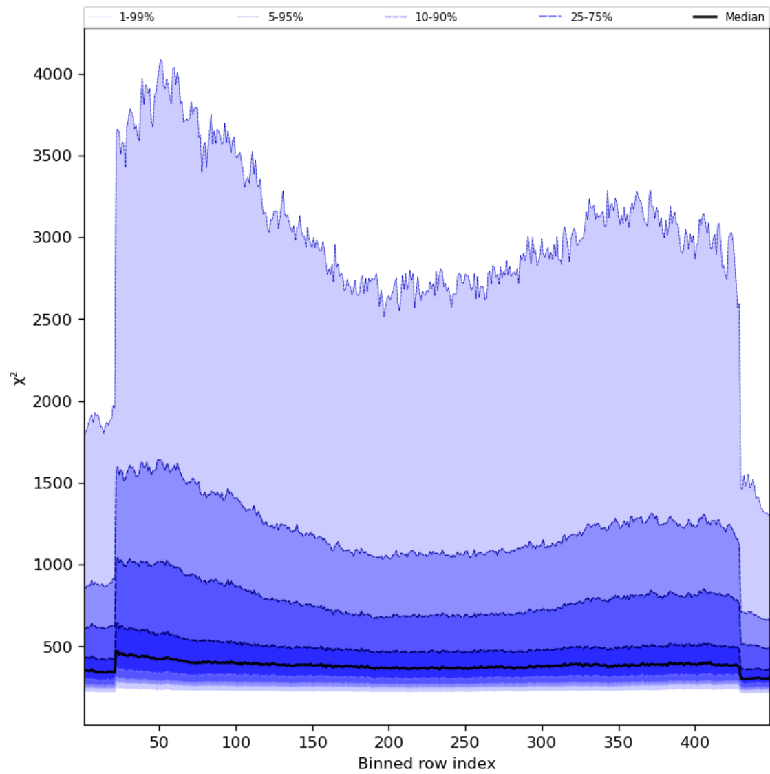
Figure 59: Along track statistics of “ \chi^2 ” for 2023-10-10 to 2023-10-12
