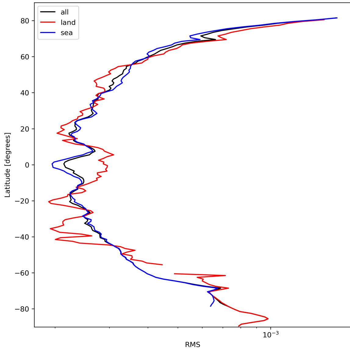
Figure 26: Zonal average of “RMS” for 2023-10-10 to 2023-10-12.
