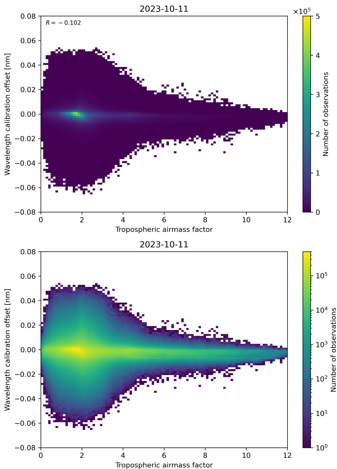
Figure 80: Scatter density plot of “Tropospheric airmass factor” against “Wavelength calibration offset” for 2023-10-10 to 2023-10-12.
