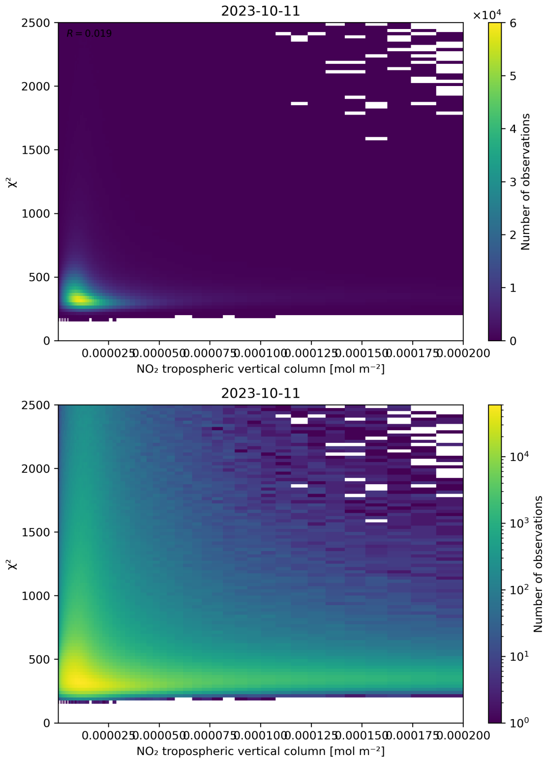
Figure 124: Scatter density plot of “NO 2 tropospheric vertical column” against “ \chi^2 ” for 2023-10-10 to 2023-10-12.
