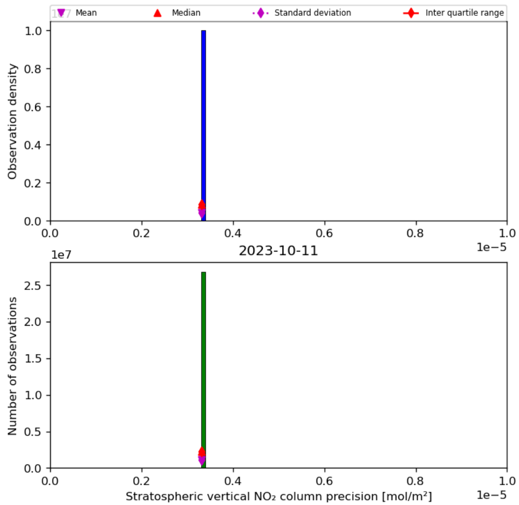
Figure 37: Histogram of “Stratospheric vertical NO 2 column precision” for 2023-10-10 to 2023-10-12
