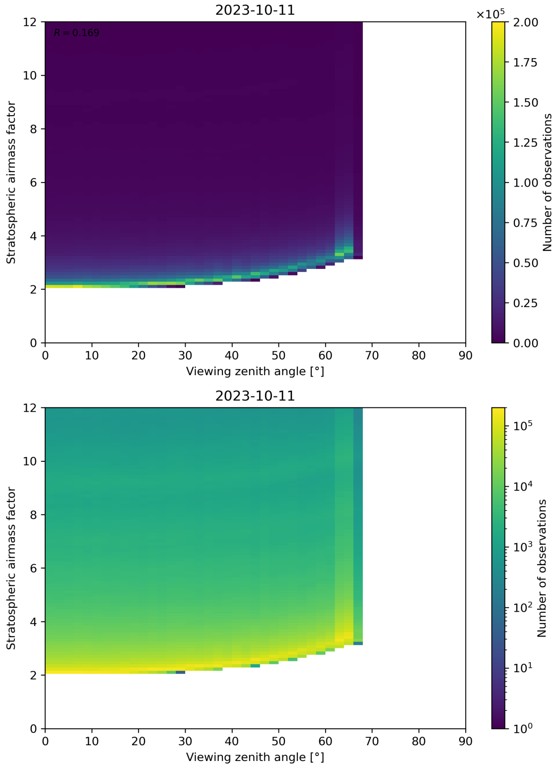
Figure 159: Scatter density plot of “Viewing zenith angle” against “Stratospheric airmass factor” for 2023-10-10 to 2023-10-12.
