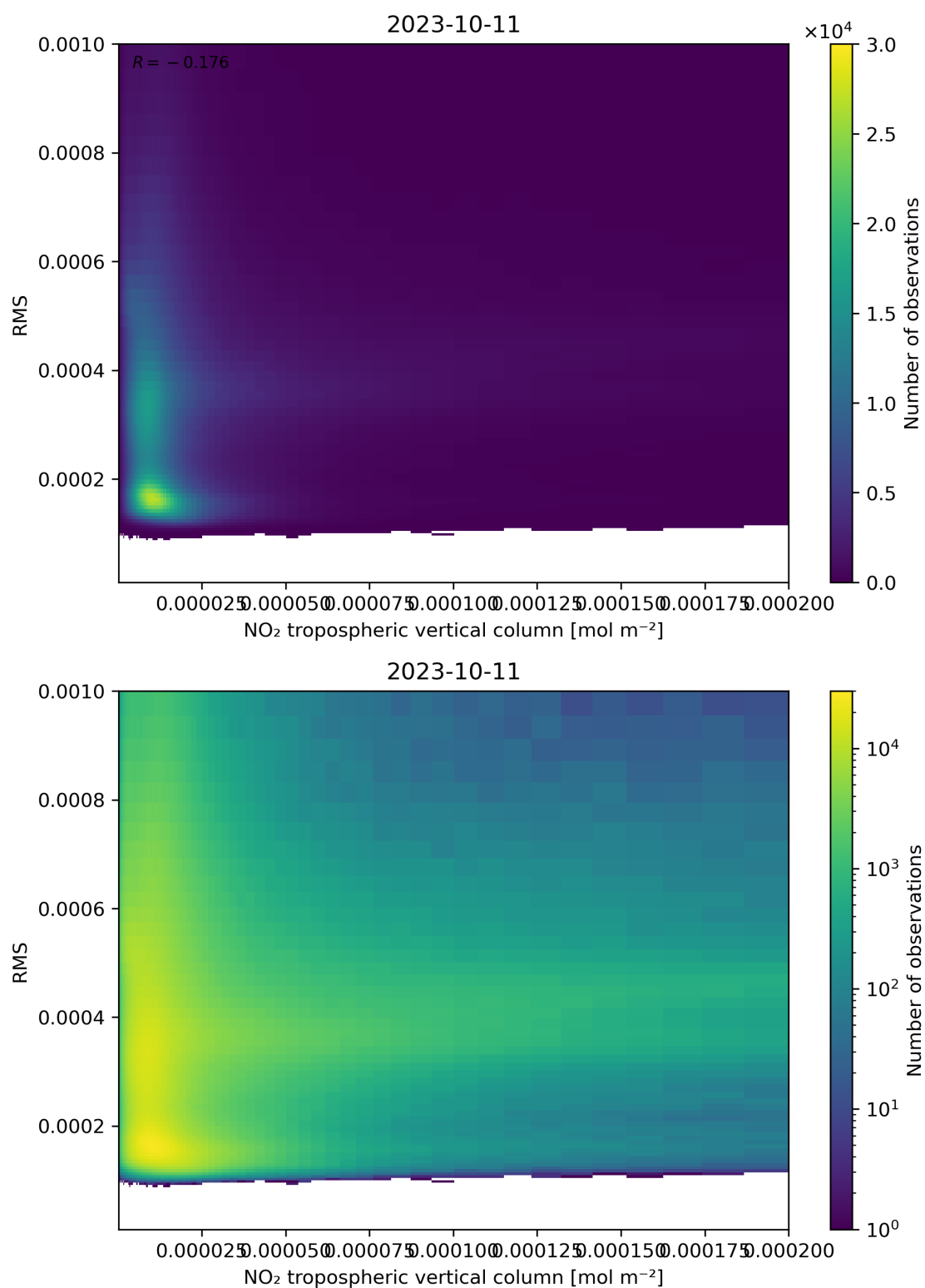
Figure 142: Scatter density plot of “NO 2 tropospheric vertical column” against “RMS” for 2023-10-10 to 2023-10-12.
