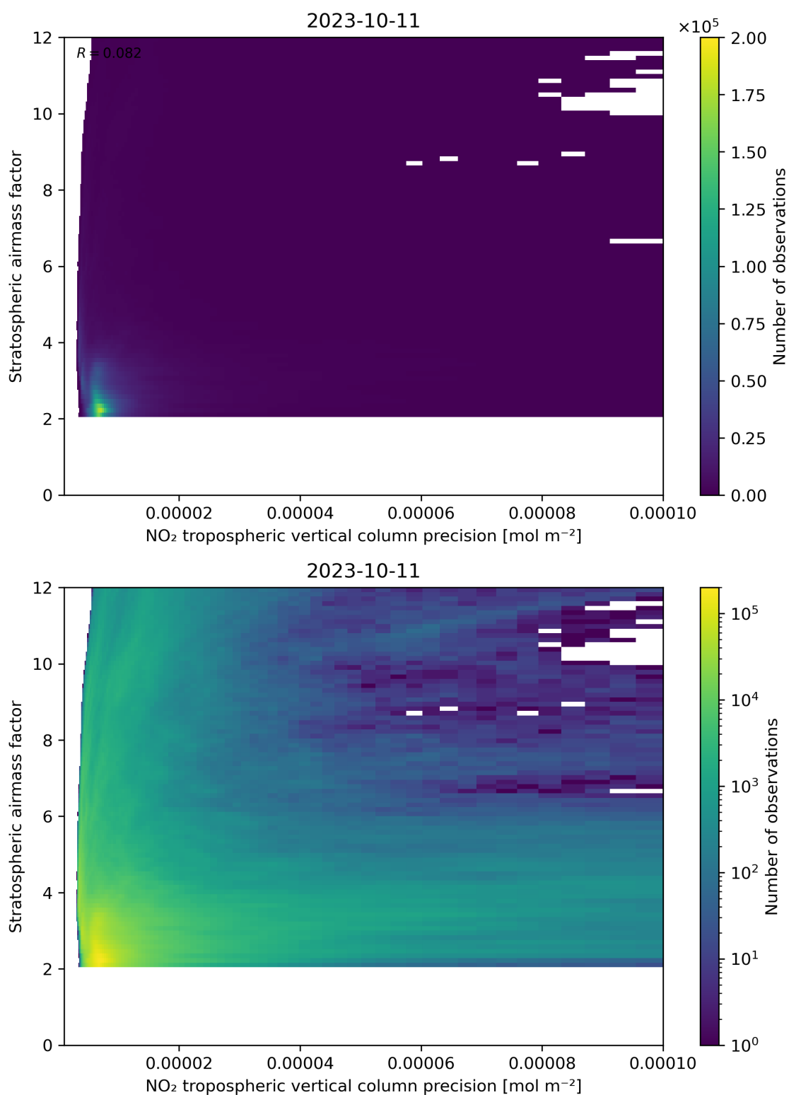
Figure 131: Scatter density plot of “NO 2 tropospheric vertical column precision” against “Stratospheric airmass factor” for 2023-10-10 to 2023-10-12.
