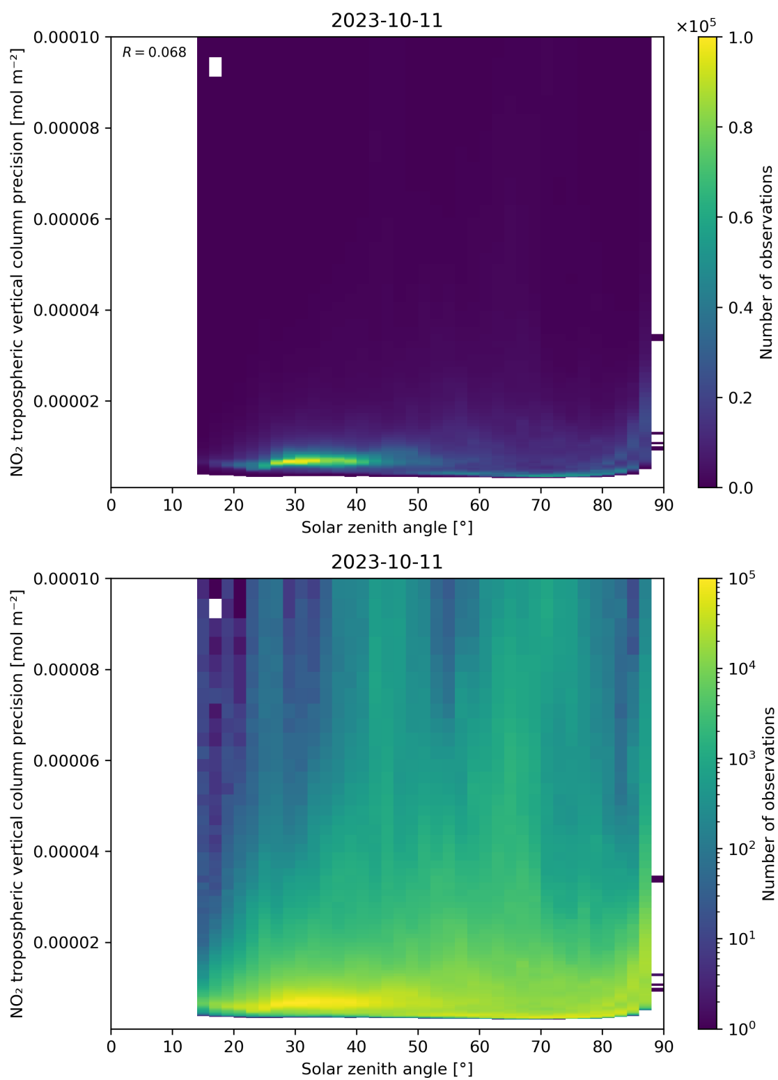
Figure 156: Scatter density plot of “Solar zenith angle” against “NO 2 tropospheric vertical column precision” for 2023-10-10 to 2023-10-12.
