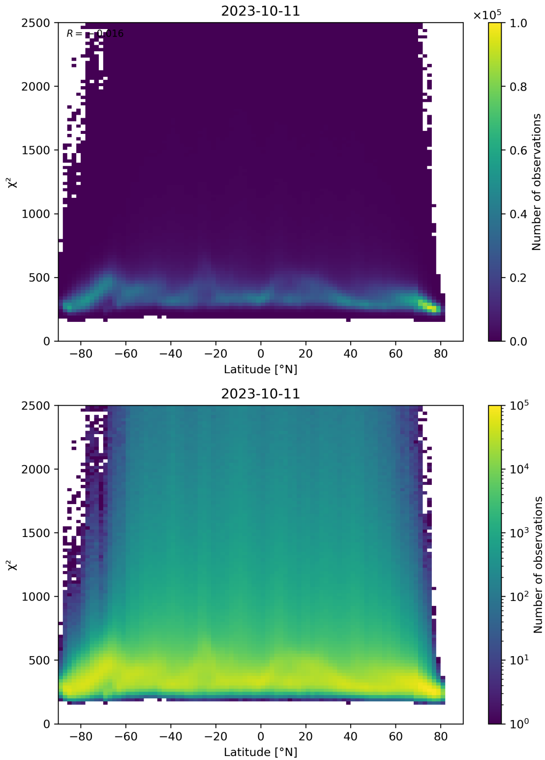
Figure 86: Scatter density plot of “Latitude” against “ \chi^2 ” for 2023-10-10 to 2023-10-12.
