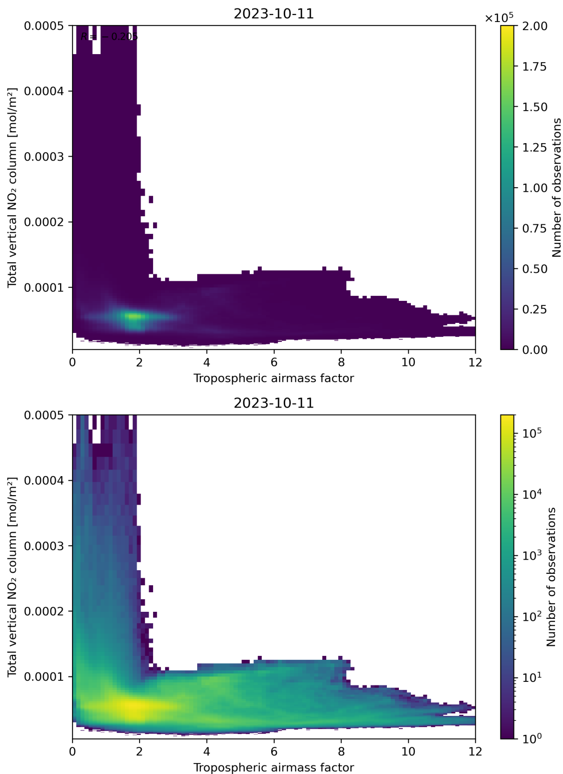
Figure 77: Scatter density plot of “Tropospheric airmass factor” against “Total vertical NO 2 column” for 2023-10-10 to 2023-10-12.
