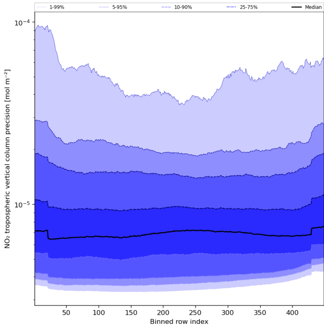
Figure 47: Along track statistics of “NO 2 tropospheric vertical column precision” for 2023-10-10 to 2023-10-12
