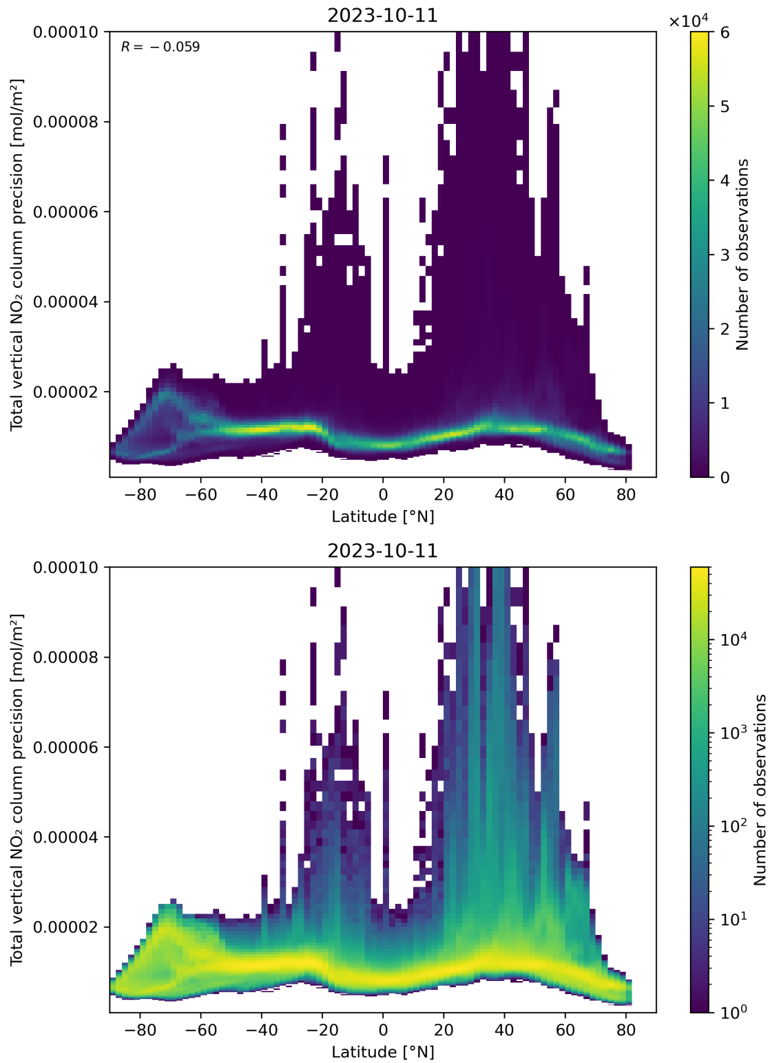
Figure 91: Scatter density plot of “Latitude” against “Total vertical NO 2 column precision” for 2023-10-10 to 2023-10-12.
