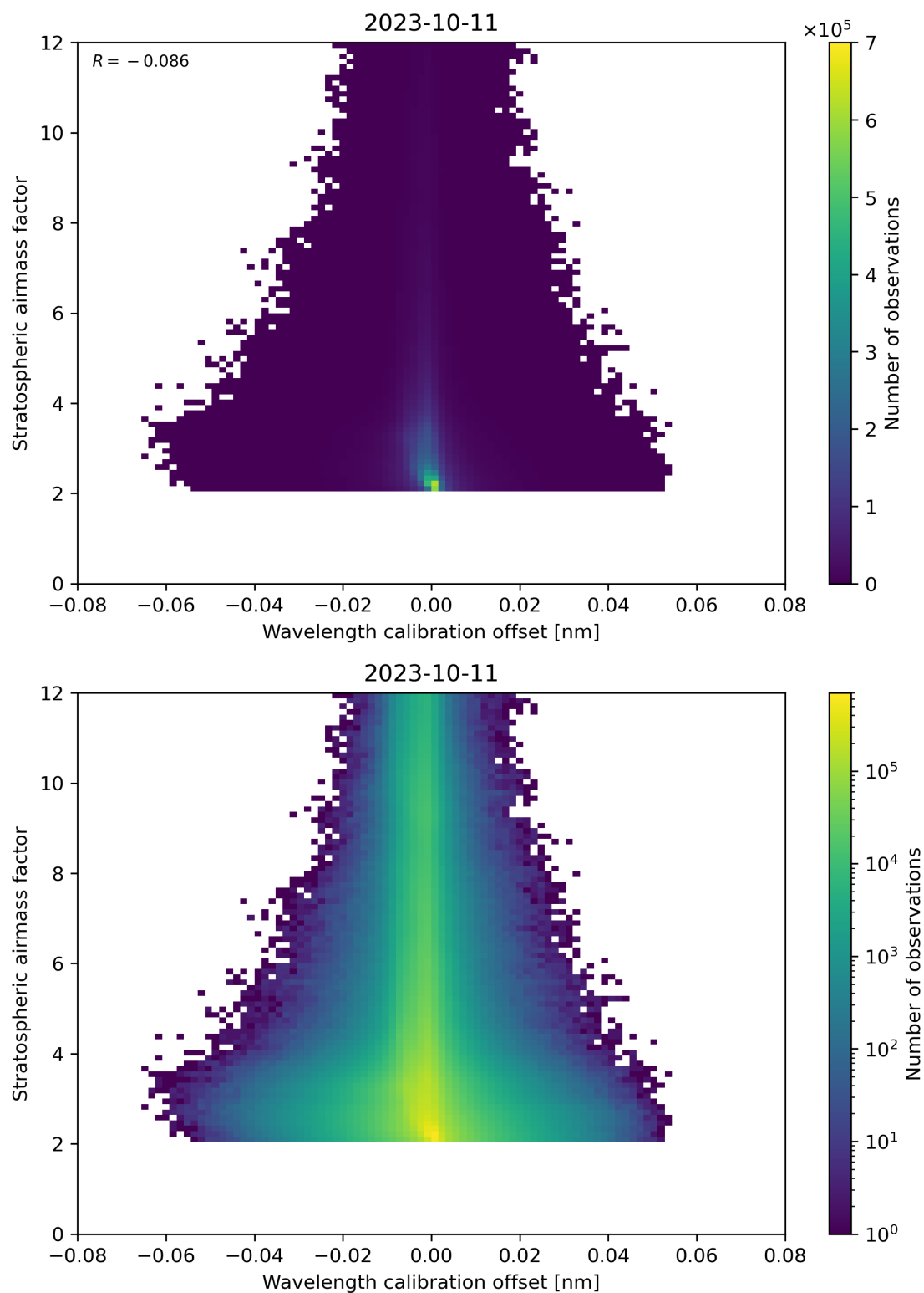
Figure 174: Scatter density plot of “Wavelength calibration offset” against “Stratospheric air mass factor” for 2023-10-10 to 2023-10-12.
