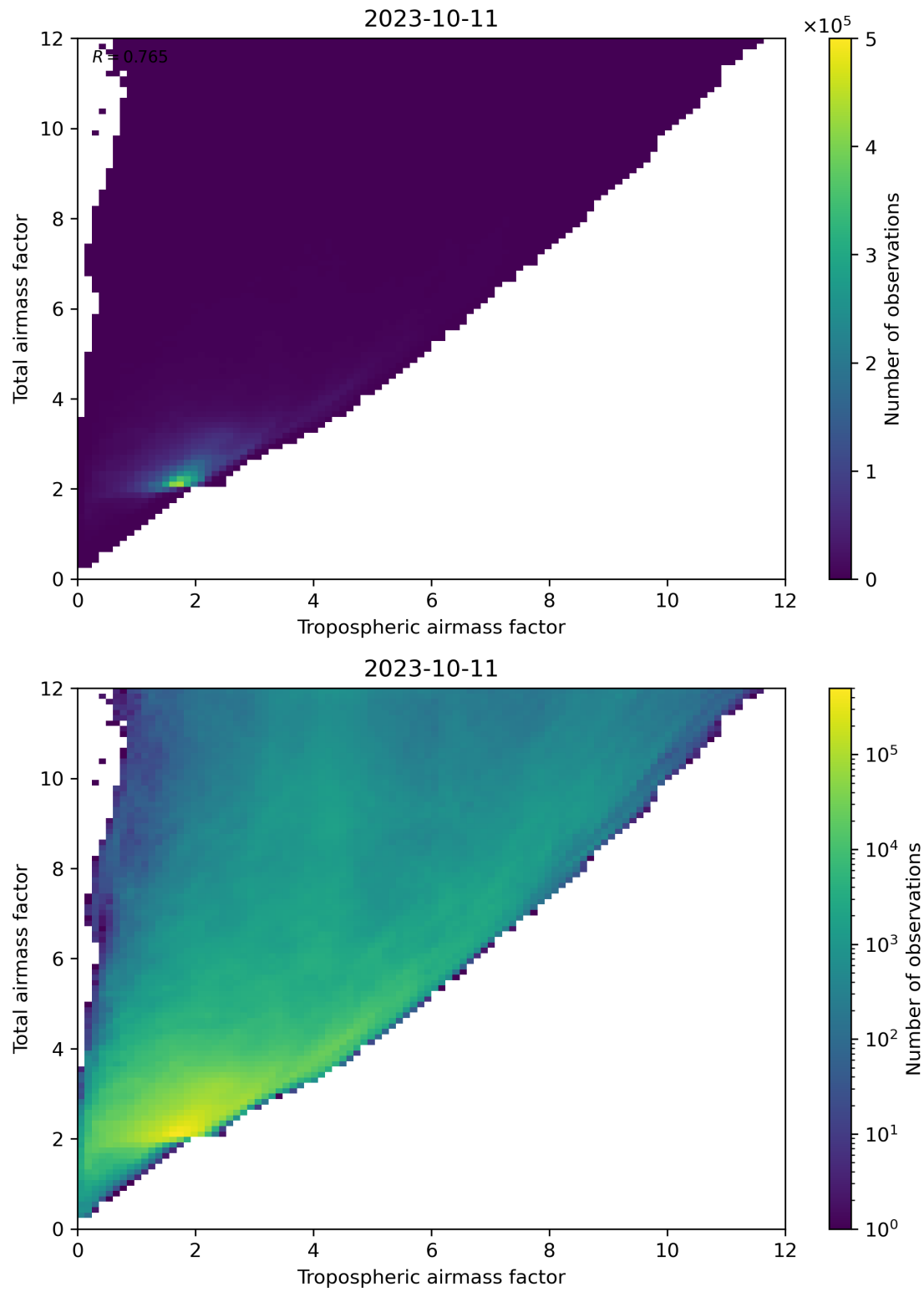
Figure 72: Scatter density plot of “Tropospheric airmass factor” against “Total airmass factor” for 2023-10-10 to 2023-10-12.
