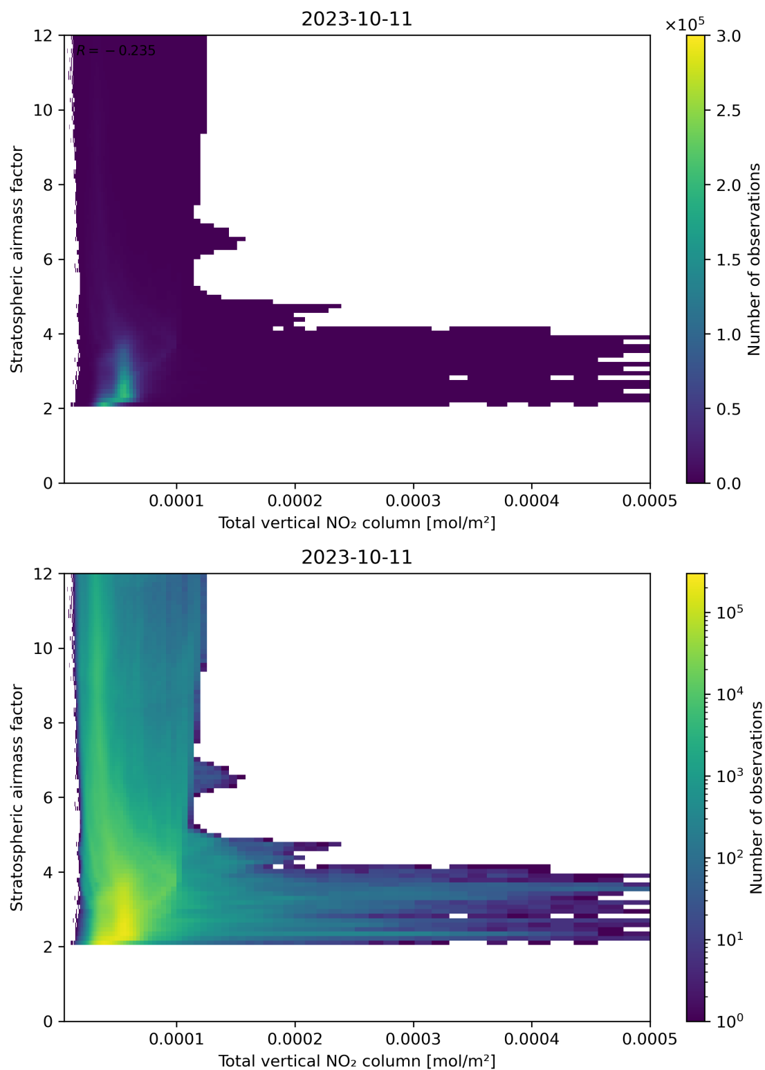
Figure 110: Scatter density plot of “Total vertical NO 2 column” against “Stratospheric airmass factor” for 2023-10-10 to 2023-10-12.
