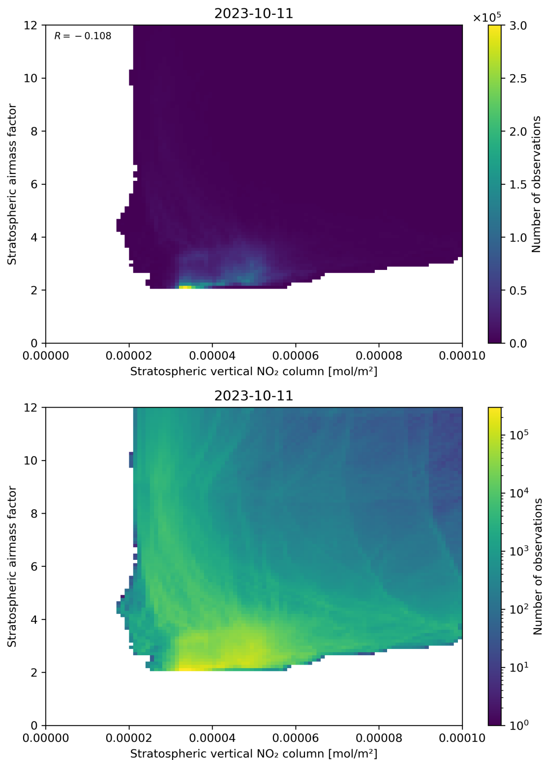
Figure 96: Scatter density plot of “Stratospheric vertical NO 2 column” against “Stratospheric airmass factor” for 2023-10-10 to 2023-10-12.
