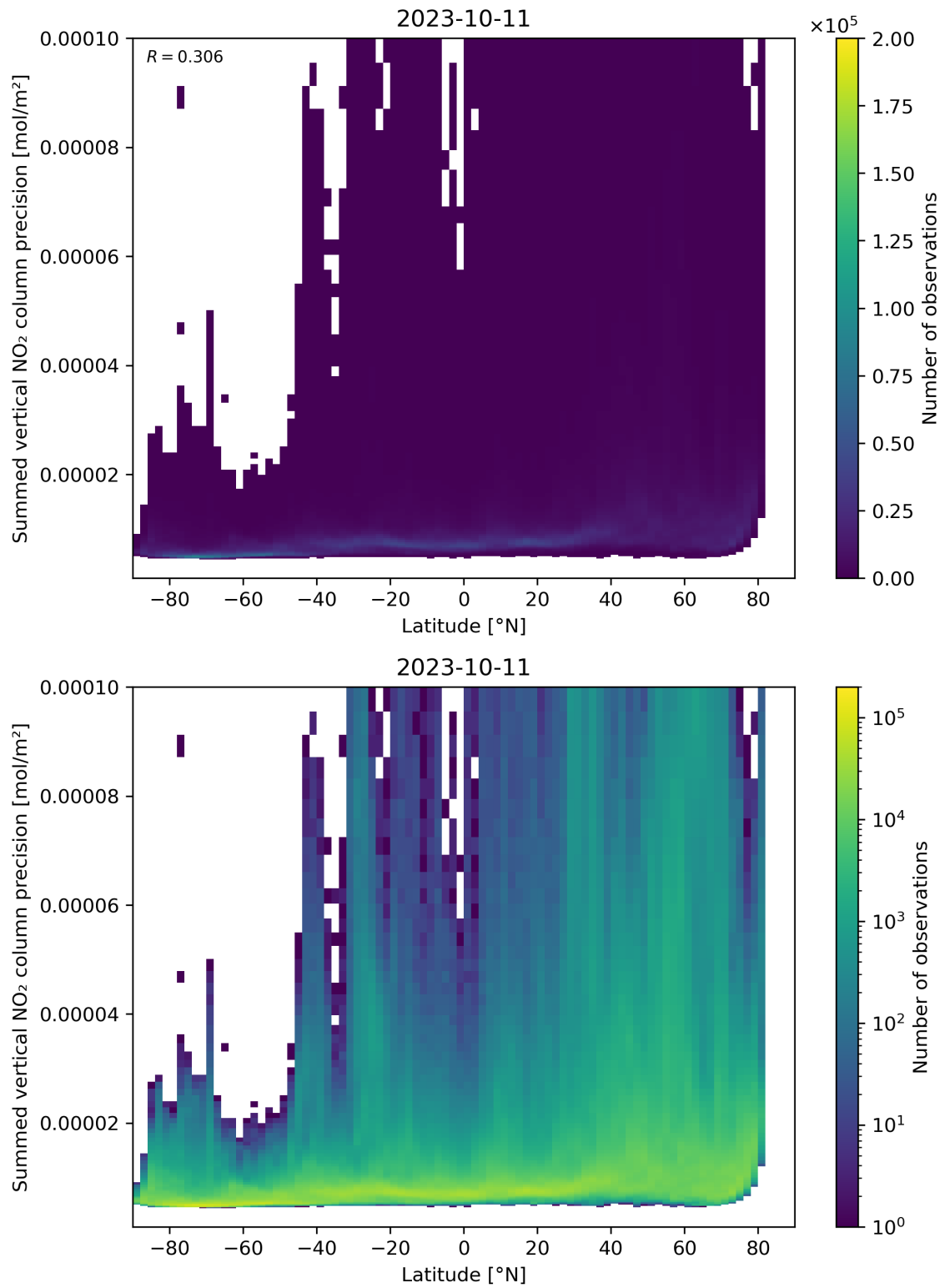
Figure 89: Scatter density plot of “Latitude” against “Summed vertical NO 2 column precision” for 2023-10-10 to 2023-10-12.
