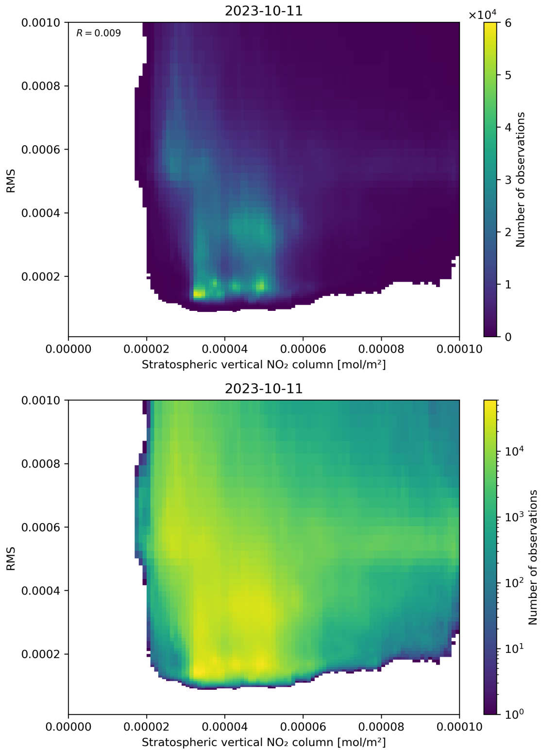
Figure 102: Scatter density plot of “Stratospheric vertical NO 2 column” against “RMS” for 2023-10-10 to 2023-10-12.
