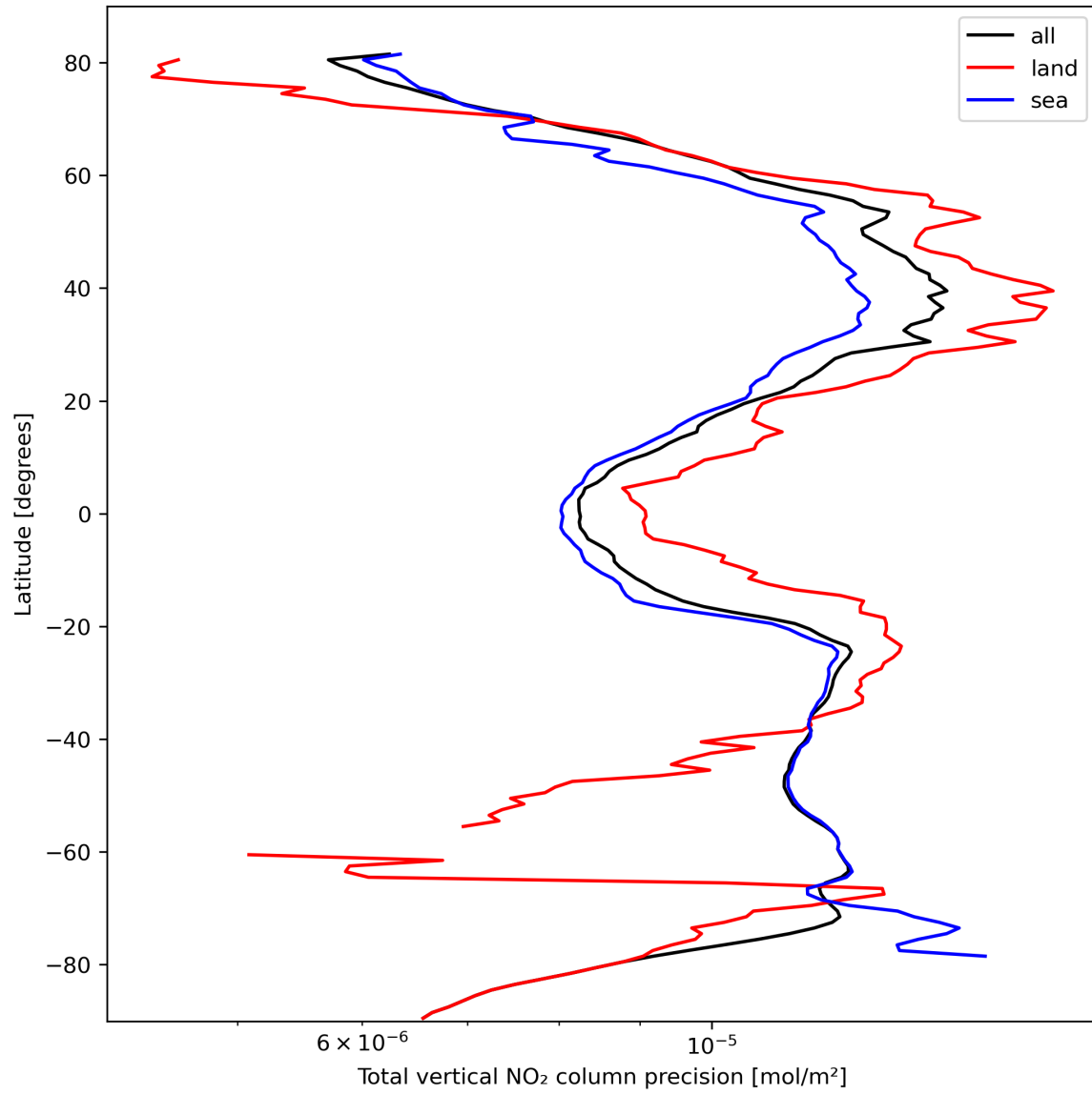
Figure 22: Zonal average of “Total vertical NO 2 column precision” for 2023-10-10 to 2023-10-12.
