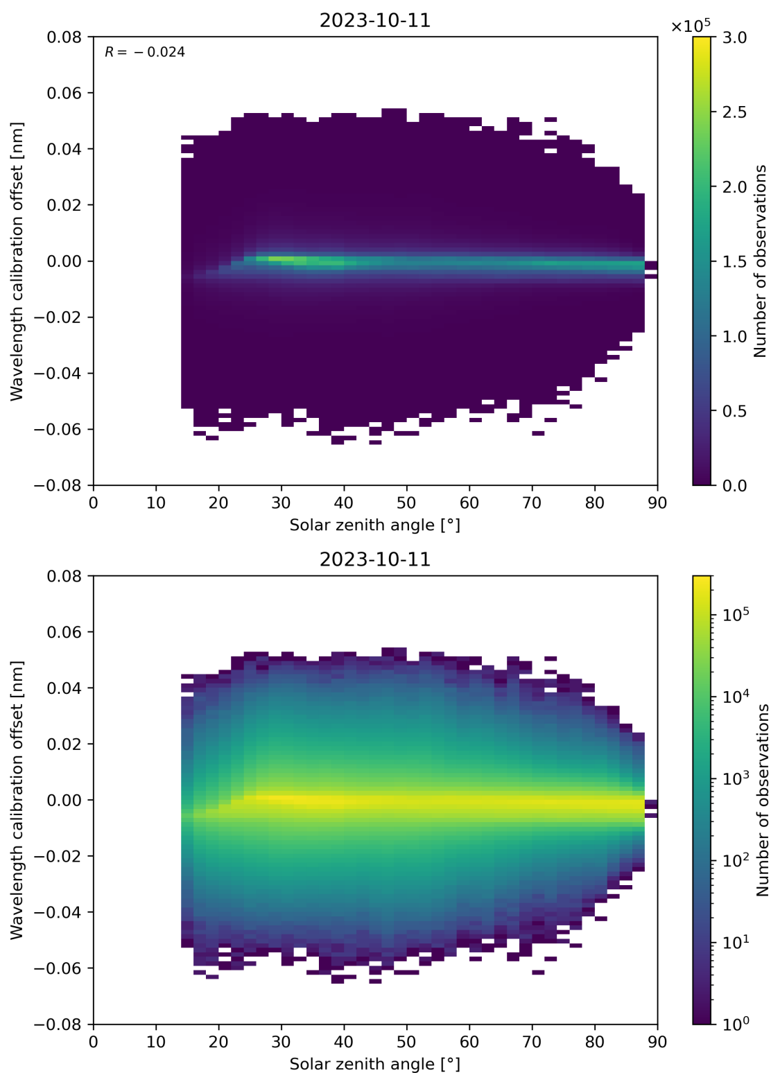
Figure 158: Scatter density plot of “Solar zenith angle” against “Wavelength calibration offset” for 2023-10-10 to 2023-10-12.
