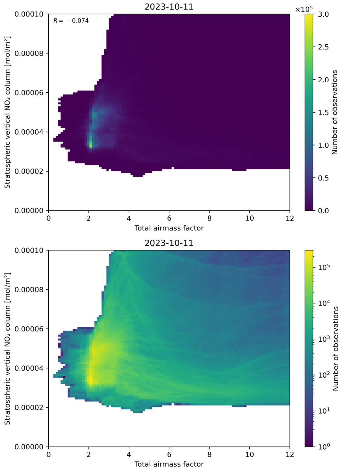
Figure 64: Scatter density plot of “Total airmass factor” against “Stratospheric vertical NO 2 column” for 2023-10-10 to 2023-10-12.
