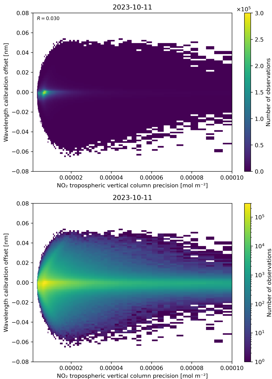
Figure 141: Scatter density plot of “NO 2 tropospheric vertical column precision” against “Wavelength calibration offset” for 2023-10-10 to 2023-10-12.
