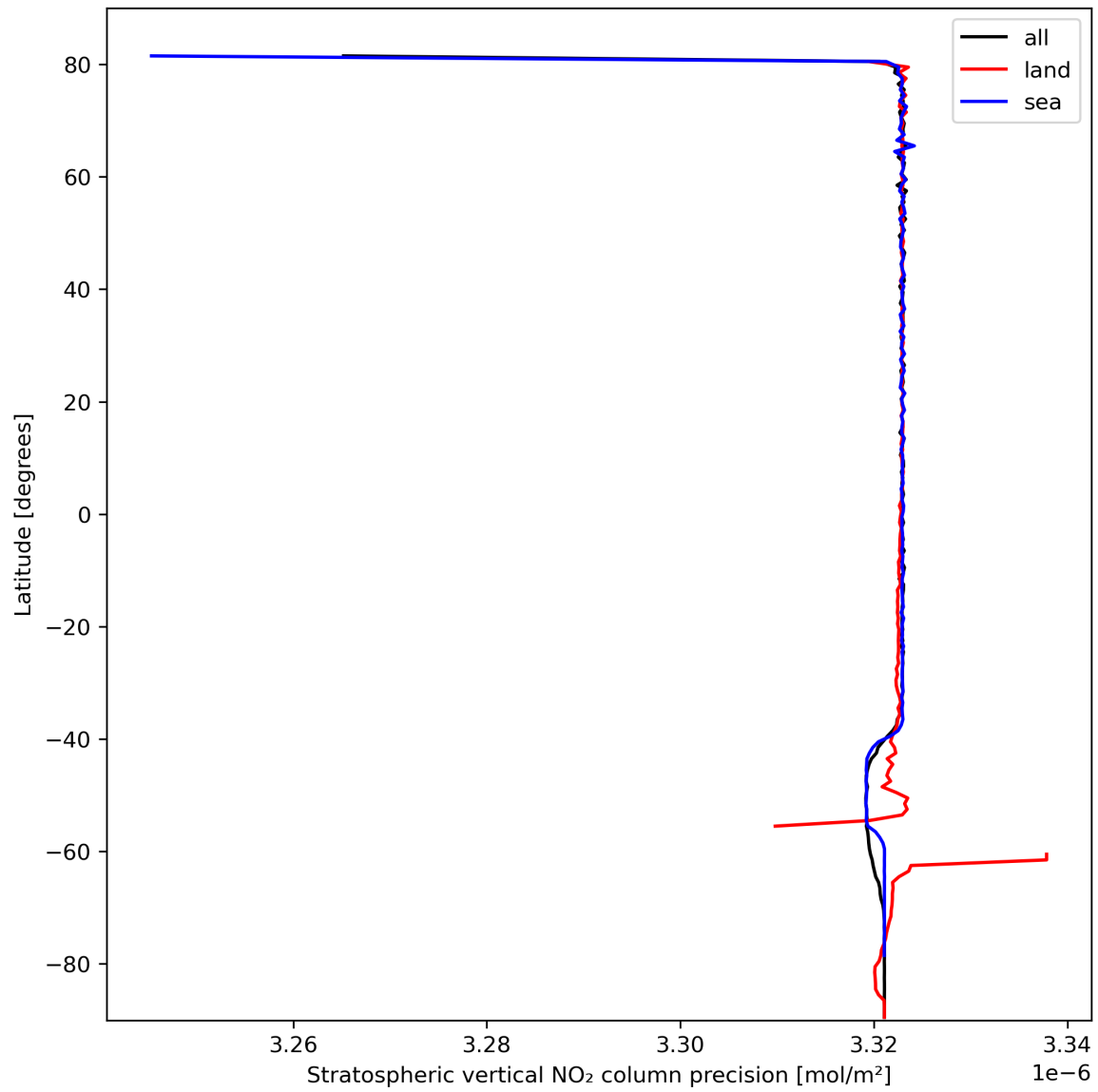
Figure 20: Zonal average of “Stratospheric vertical NO 2 column precision” for 2023-10-10 to 2023-10-12.
