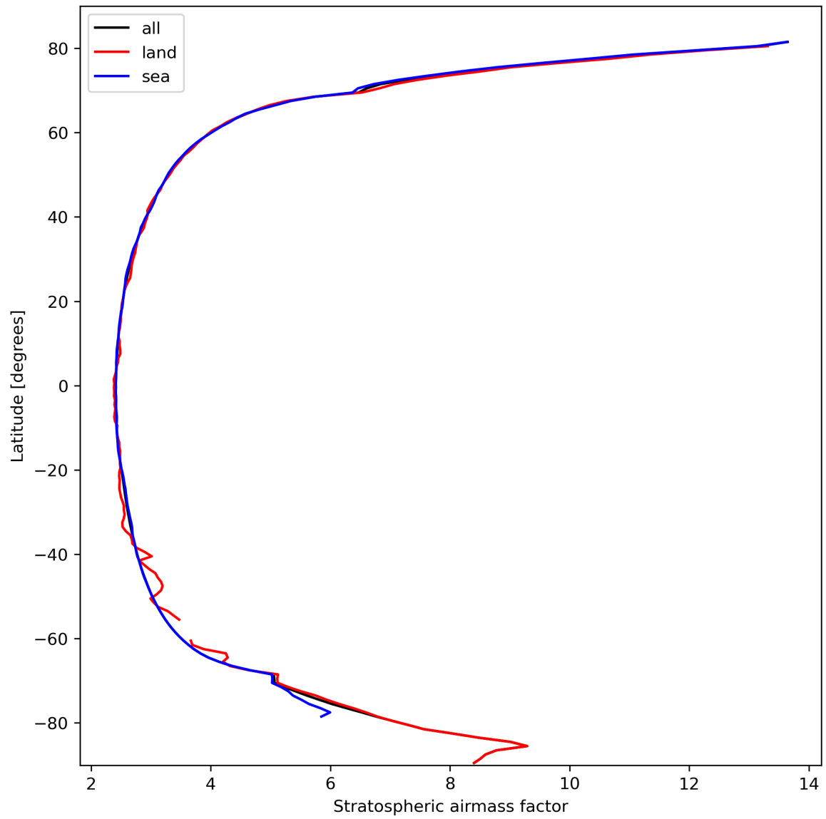
Figure 27: Zonal average of “Stratospheric air mass factor” for 2023-10-10 to 2023-10-12.
