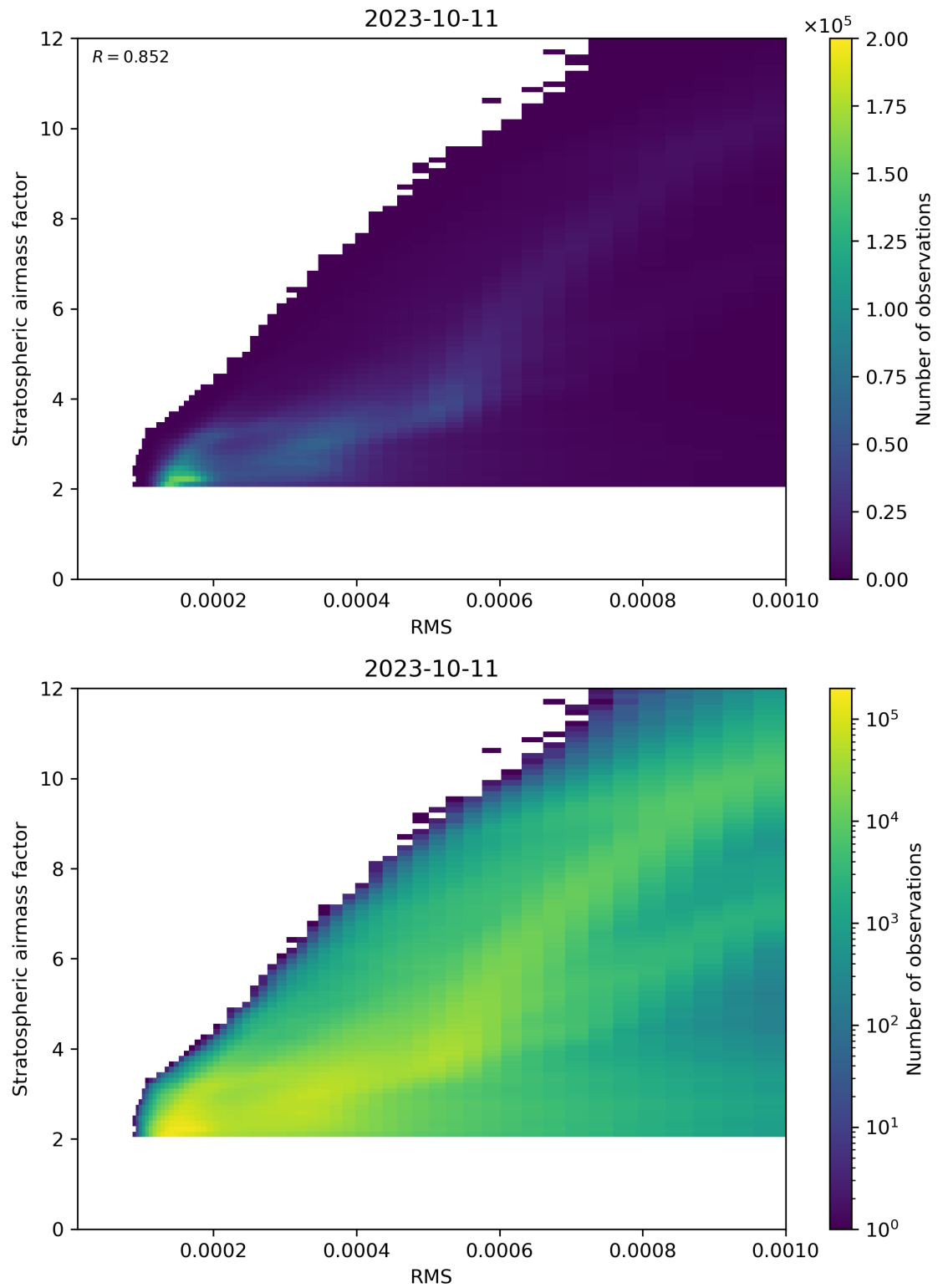
Figure 144: Scatter density plot of “RMS” against “Stratospheric airmass factor” for 2023-10-10 to 2023-10-12.
