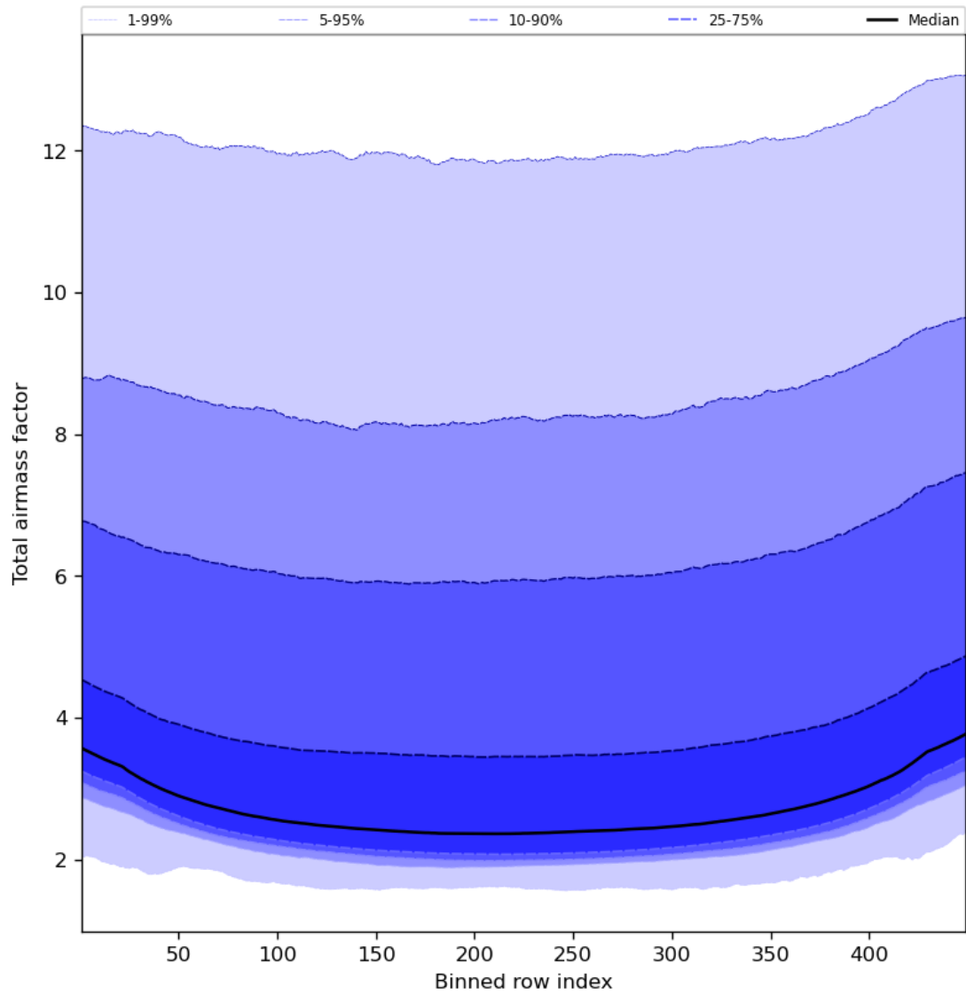
Figure 49: Along track statistics of “Total airmass factor” for 2023-10-10 to 2023-10-12
