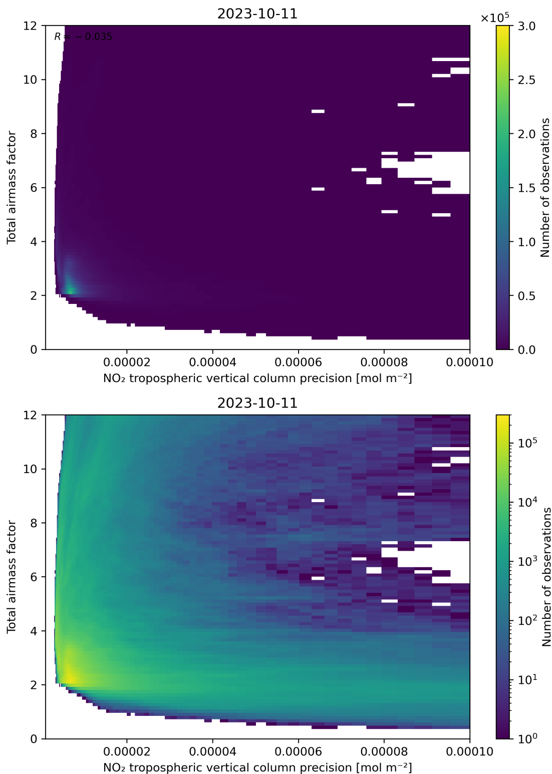
Figure 132: Scatter density plot of “NO 2 tropospheric vertical column precision” against “Total air mass factor” for 2023-10-10 to 2023-10-12.
