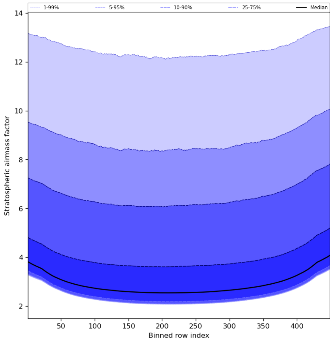
Figure 61: Along track statistics of “Stratospheric airmass factor” for 2023-10-10 to 2023-10-12
