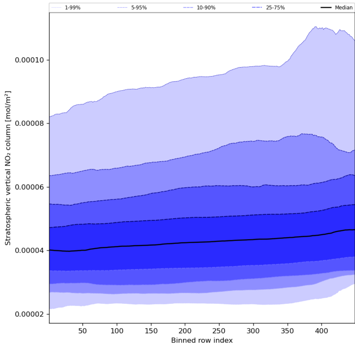
Figure 53: Along track statistics of “Stratospheric vertical NO 2 column” for 2023-10-10 to 2023-10-12
