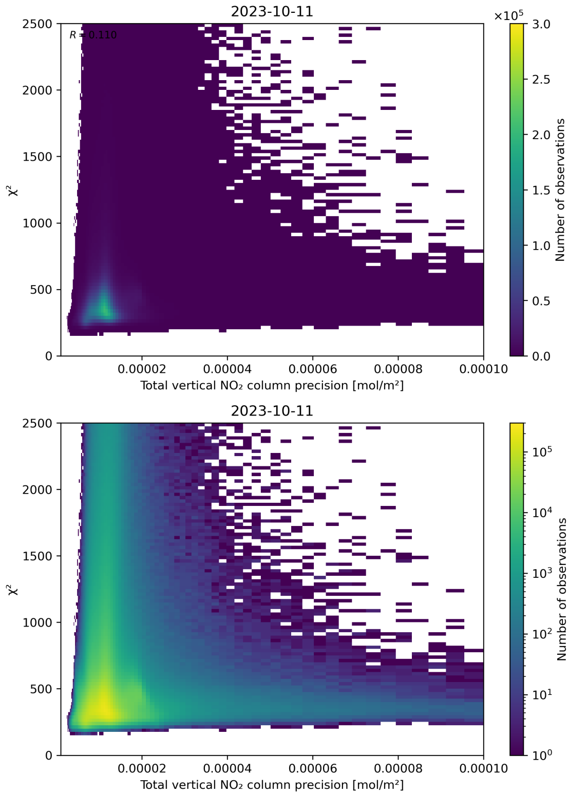
Figure 116: Scatter density plot of “Total vertical NO 2 column precision” against “ \chi^2 ” for 2023-10-10 to 2023-10-12.
