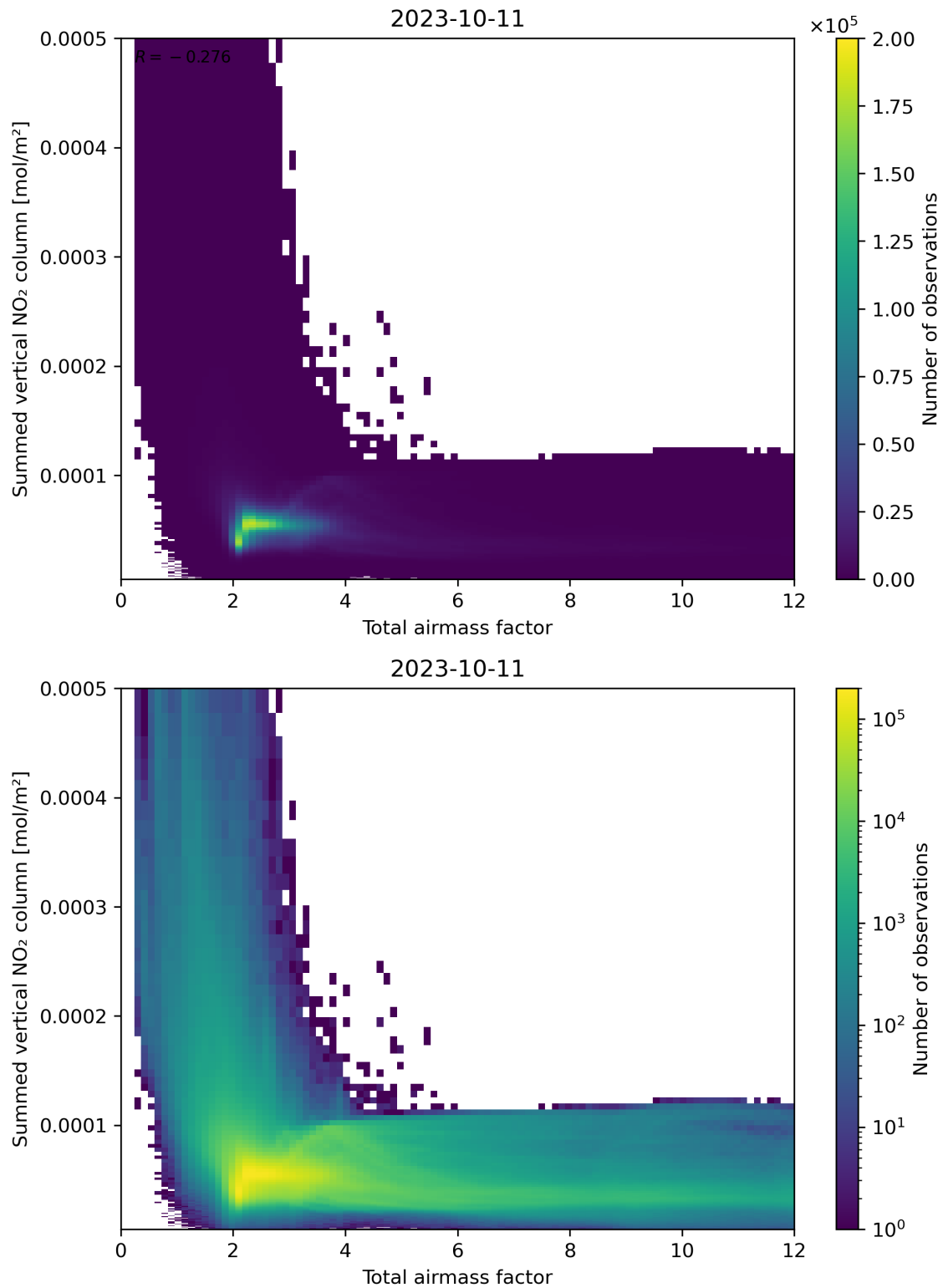
Figure 65: Scatter density plot of “Total airmass factor” against “Summed vertical NO 2 column” for 2023-10-10 to 2023-10-12.
