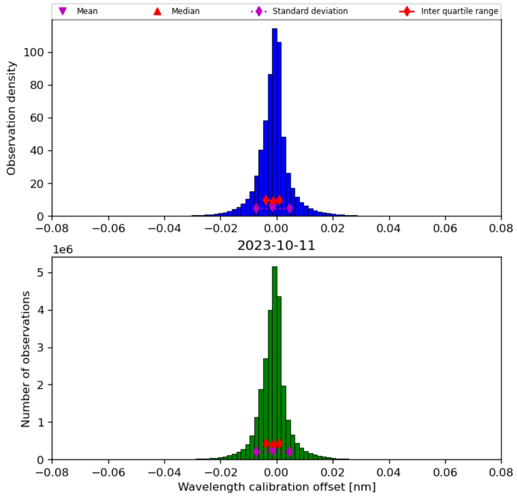
Figure 35: Histogram of “Wavelength calibration offset” for 2023-10-10 to 2023-10-12
