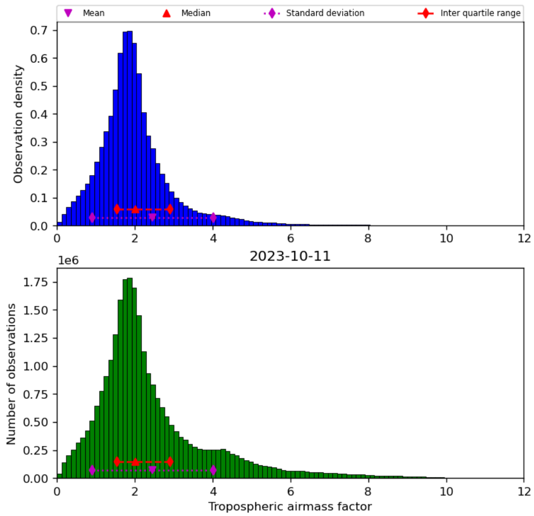
Figure 31: Histogram of “Tropospheric airmass factor” for 2023-10-10 to 2023-10-12
