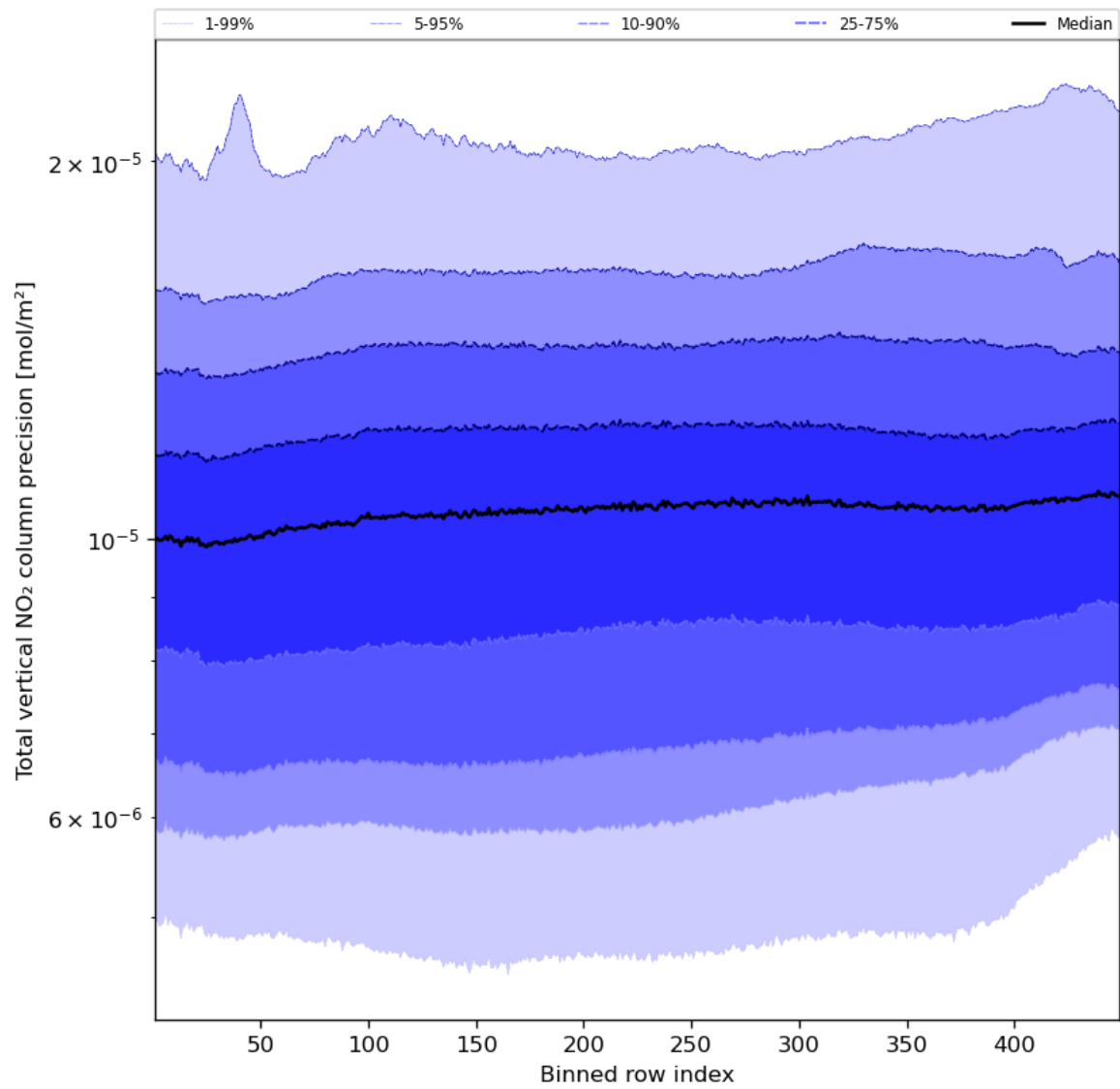
Figure 56: Along track statistics of “Total vertical NO 2 column precision” for 2023-10-10 to 2023-10-12
