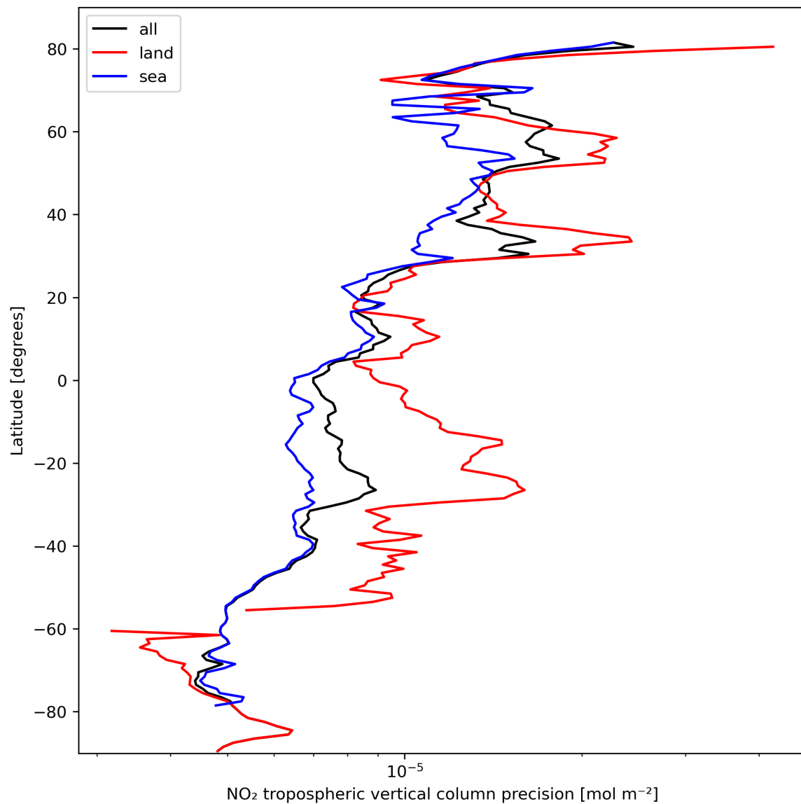
Figure 13: Zonal average of “NO 2 tropospheric vertical column precision” for 2023-10-10 to 2023-10-12.
