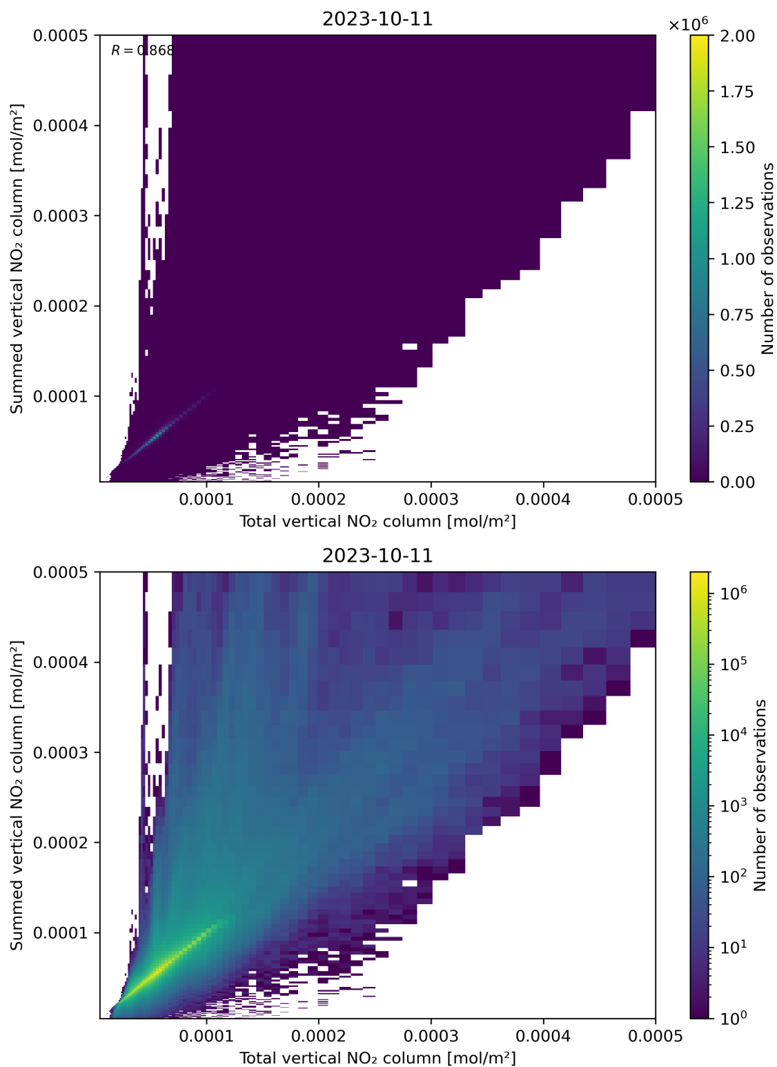
Figure 112: Scatter density plot of “Total vertical NO 2 column” against “Summed vertical NO 2 column” for 2023-10-10 to 2023-10-12.
