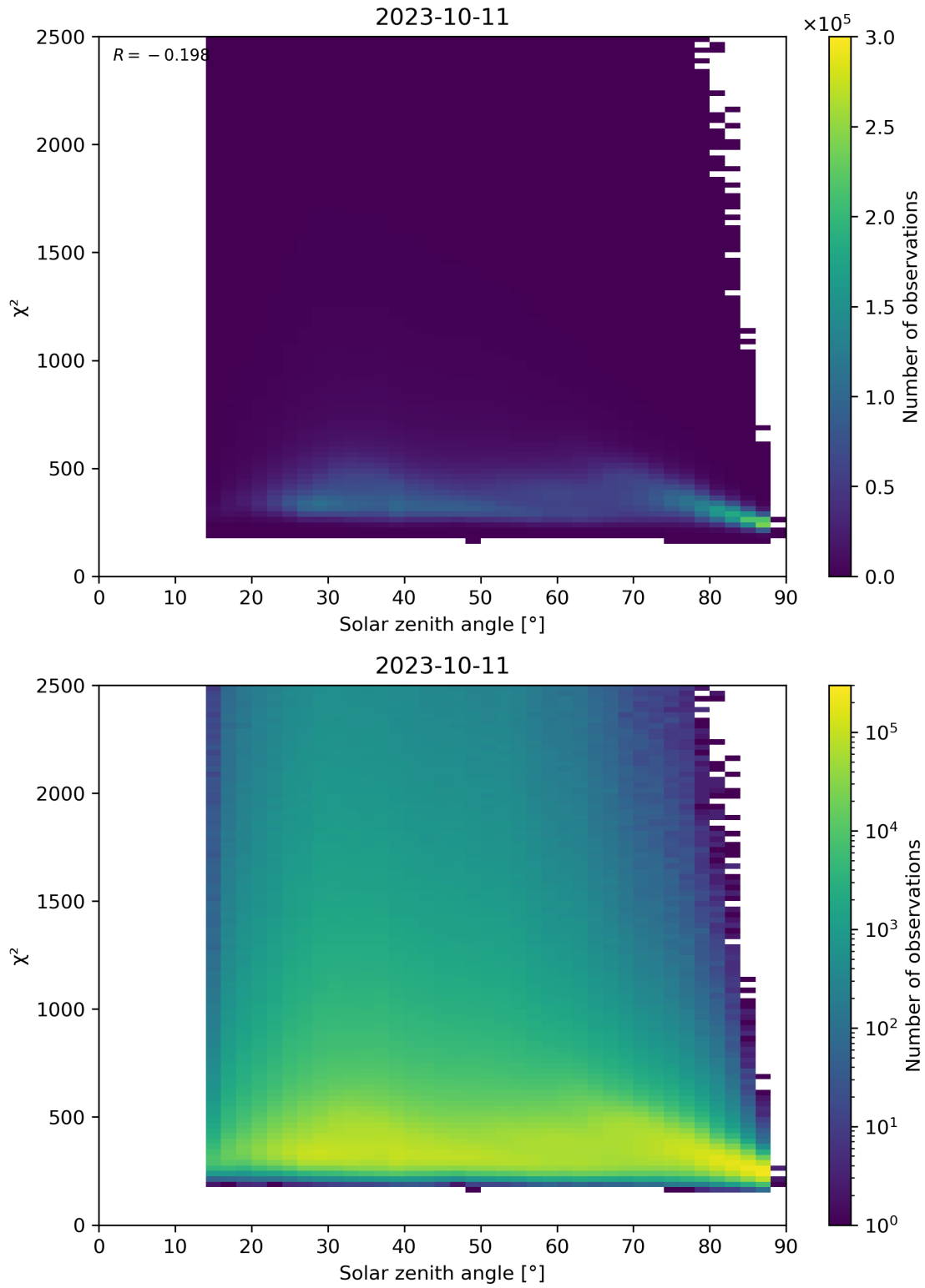
Figure 148: Scatter density plot of “Solar zenith angle” against “ \chi^2 ” for 2023-10-10 to 2023-10-12.
