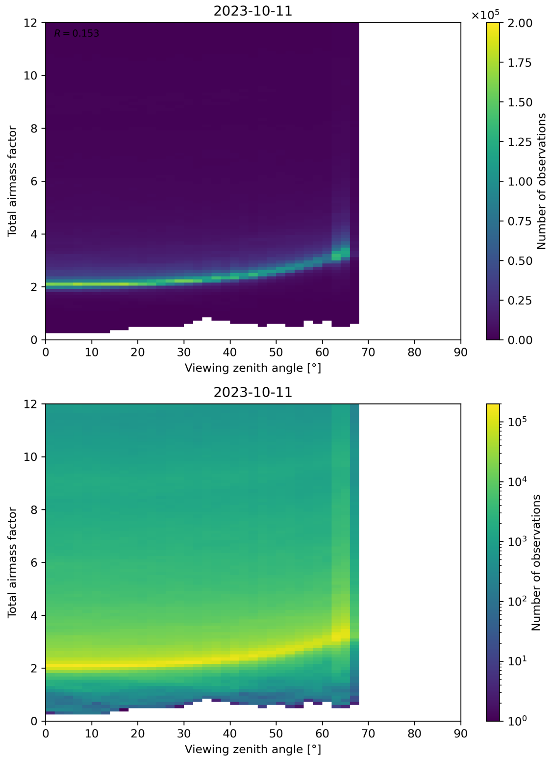
Figure 160: Scatter density plot of “Viewing zenith angle” against “Total airmass factor” for 2023-10-10 to 2023-10-12.
