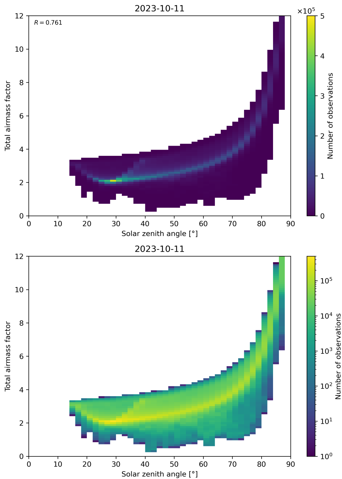
Figure 146: Scatter density plot of “Solar zenith angle” against “Total air mass factor” for 2023-10-10 to 2023-10-12.
