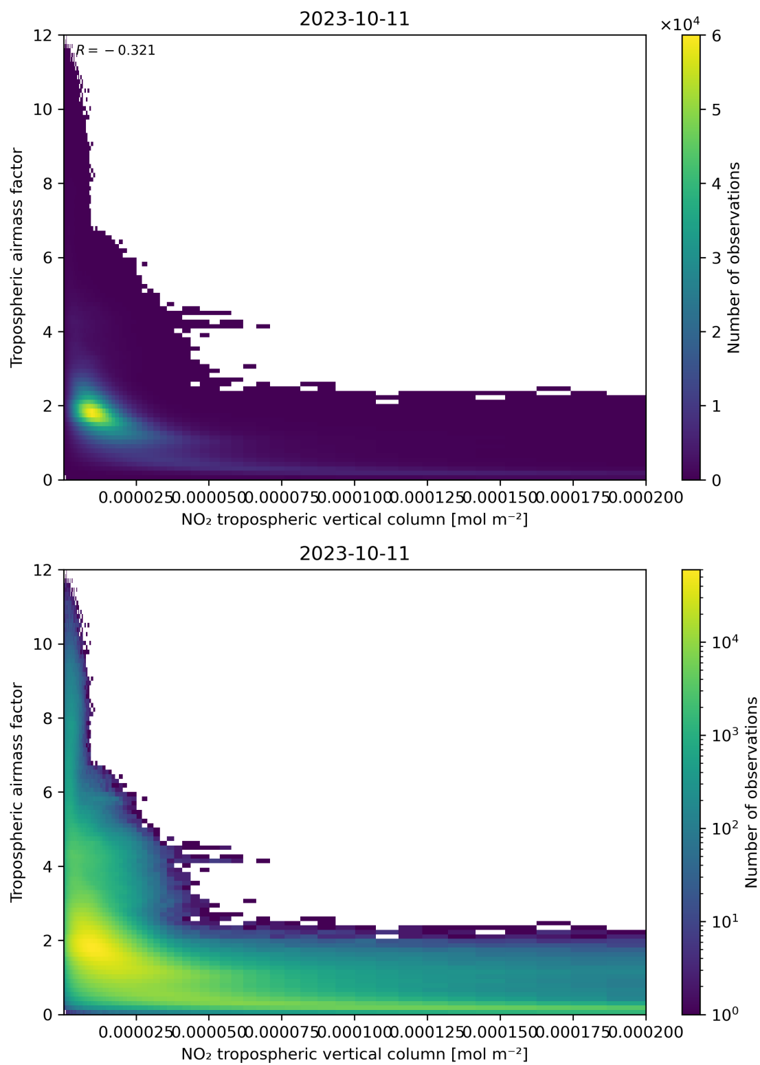
Figure 123: Scatter density plot of “NO 2 tropospheric vertical column” against “Tropospheric air mass factor” for 2023-10-10 to 2023-10-12.
