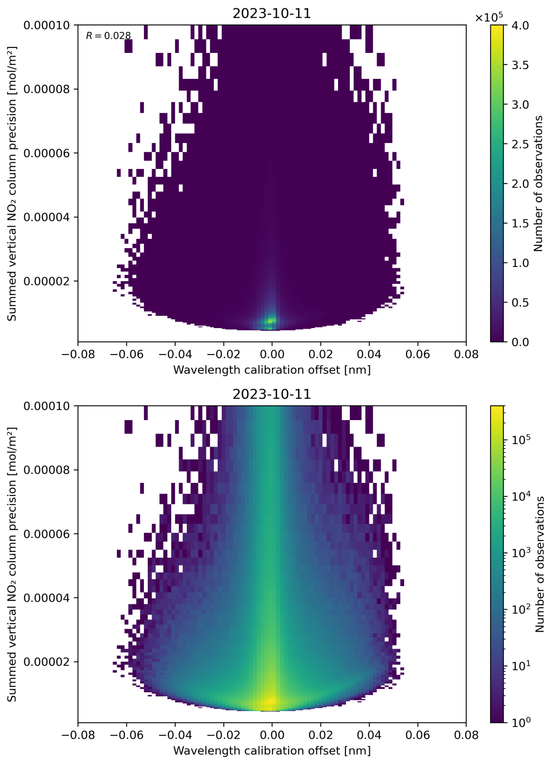
Figure 178: Scatter density plot of “Wavelength calibration offset” against “Summed vertical NO 2 column precision” for 2023-10-10 to 2023-10-12.
