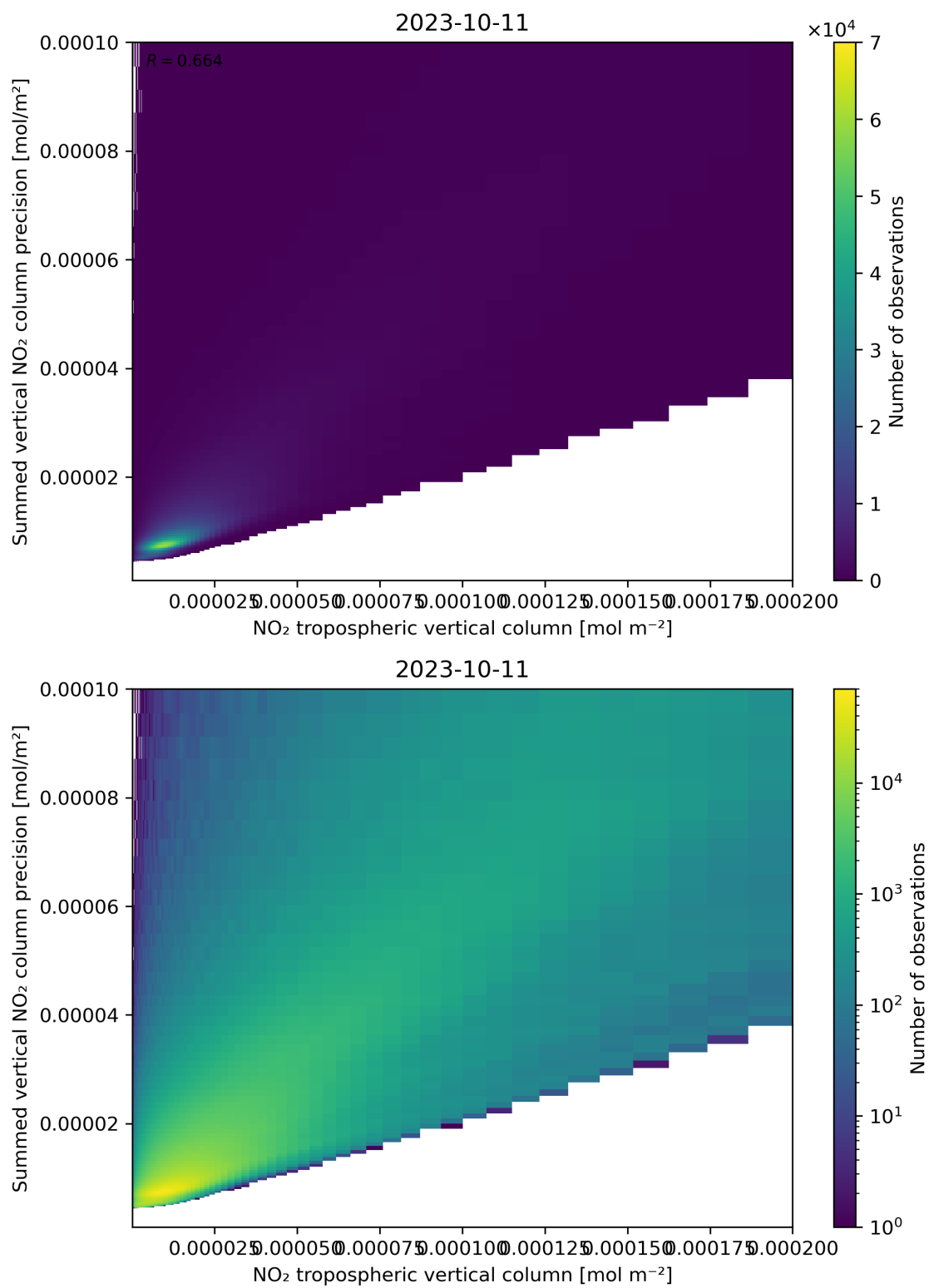
Figure 127: Scatter density plot of “NO 2 tropospheric vertical column” against “Summed vertical NO 2 column precision” for 2023-10-10 to 2023-10-12.
