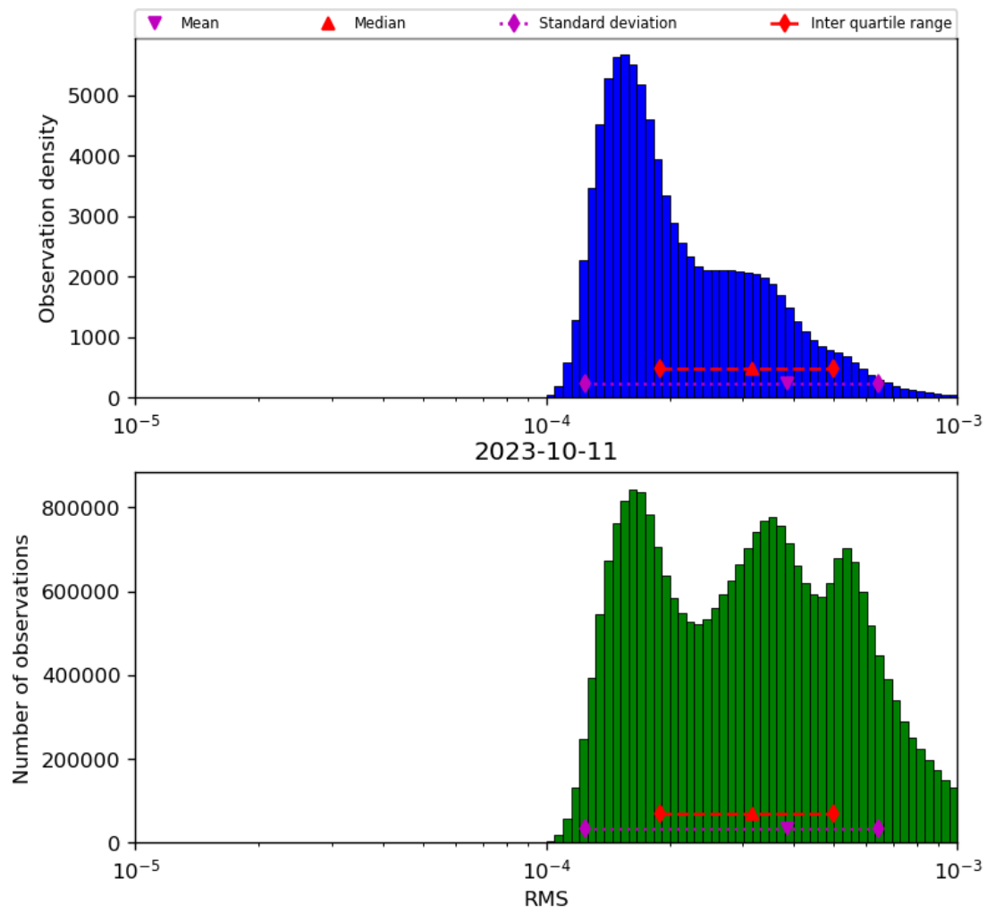
Figure 43: Histogram of “RMS” for 2023-10-10 to 2023-10-12
