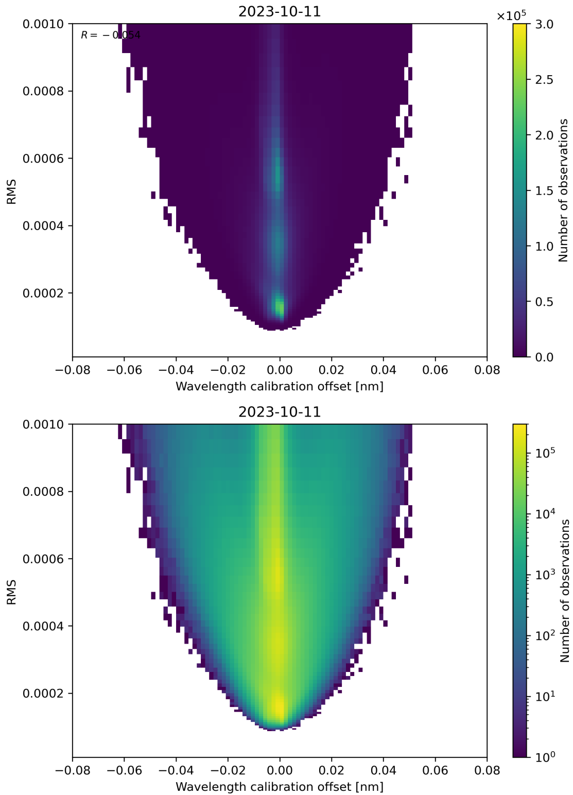
Figure 181: Scatter density plot of “Wavelength calibration offset” against “RMS” for 2023-10-10 to 2023-10-12.
