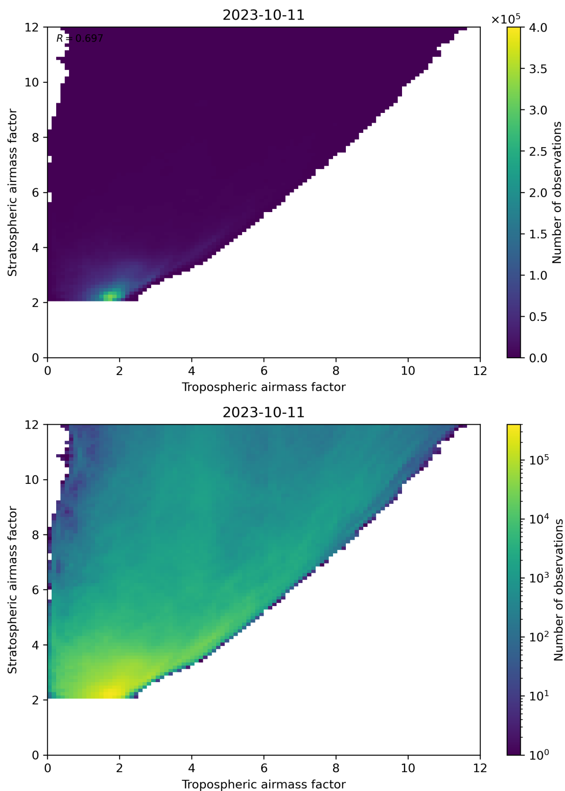
Figure 71: Scatter density plot of “Tropospheric airmass factor” against “Stratospheric airmass factor” for 2023-10-10 to 2023-10-12.
