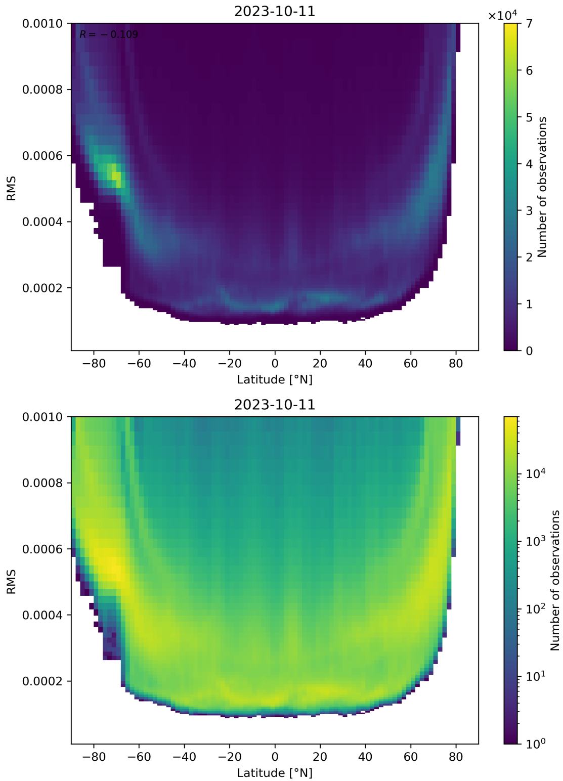
Figure 94: Scatter density plot of “Latitude” against “RMS” for 2023-10-10 to 2023-10-12.
