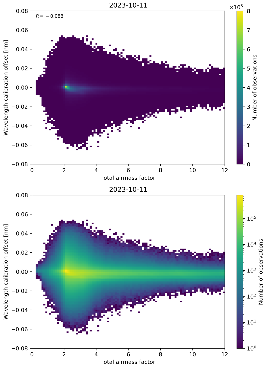
Figure 70: Scatter density plot of “Total airmass factor” against “Wavelength calibration offset” for 2023-10-10 to 2023-10-12.
