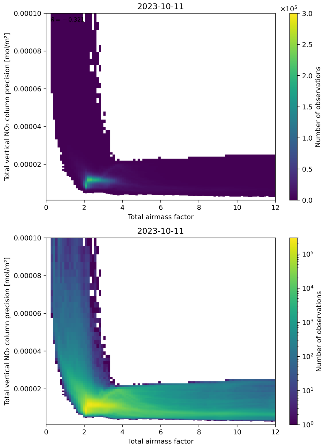
Figure 68: Scatter density plot of “Total airmass factor” against “Total vertical NO 2 column precision” for 2023-10-10 to 2023-10-12.
