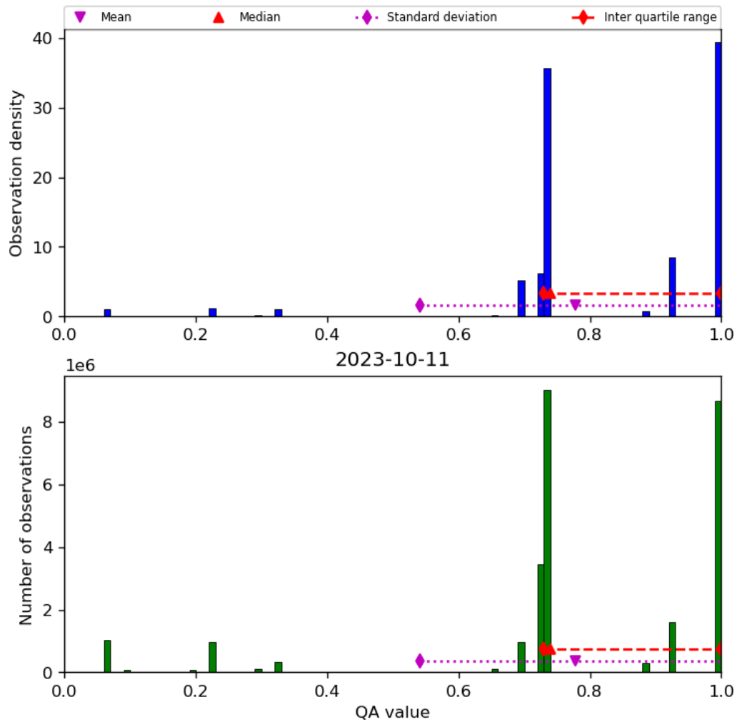
Figure 28: Histogram of “QA value” for 2023-10-10 to 2023-10-12
