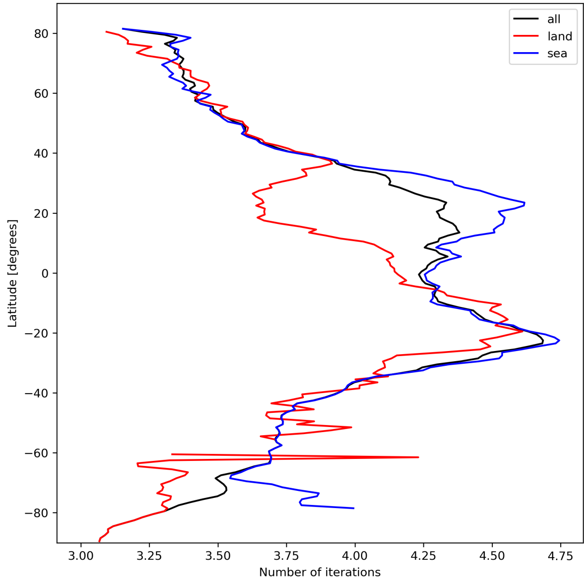
Figure 17: Zonal average of “Number of iterations” for 2023-10-10 to 2023-10-12.
