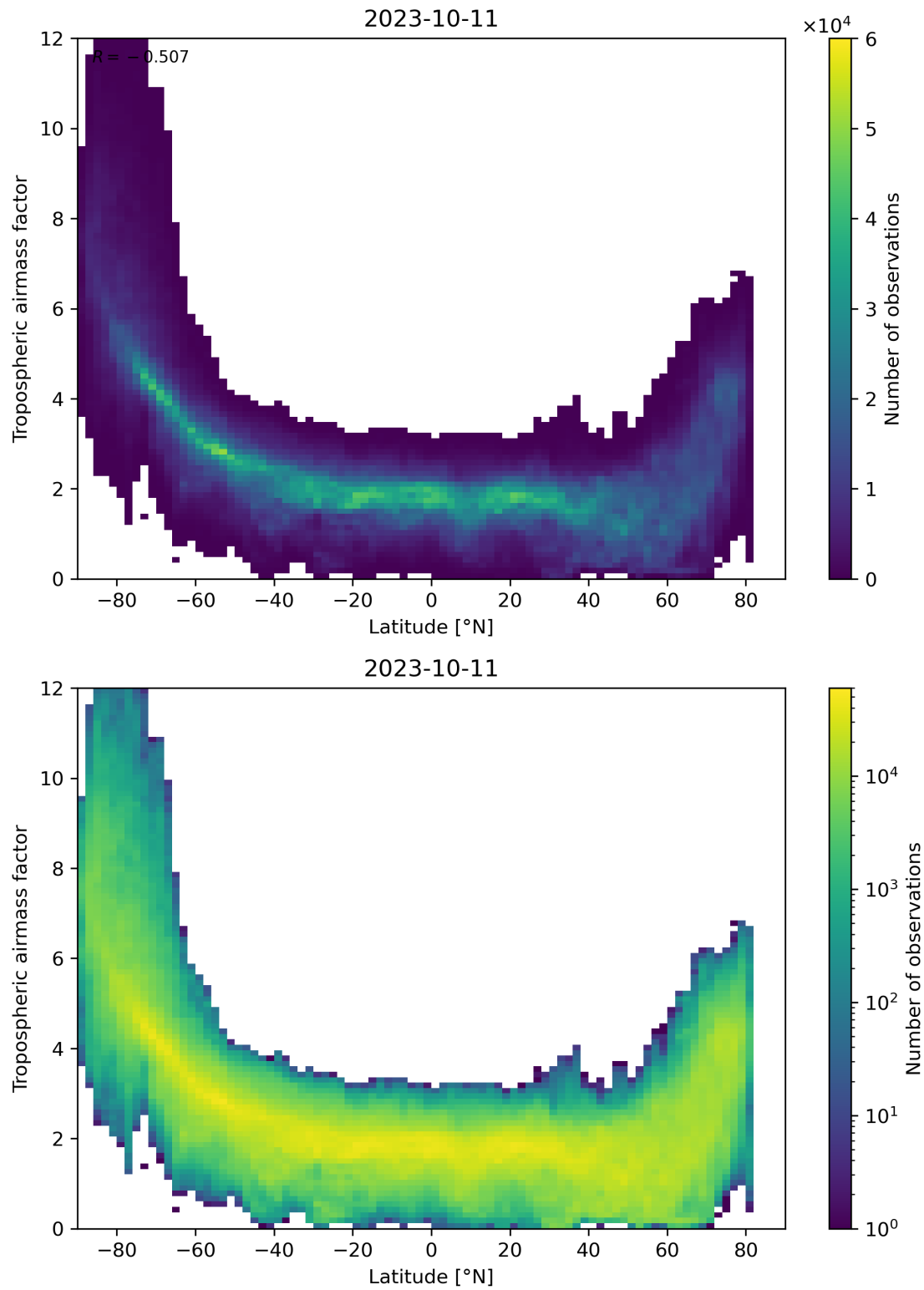
Figure 85: Scatter density plot of “Latitude” against “Tropospheric airmass factor” for 2023-10-10 to 2023-10-12.
