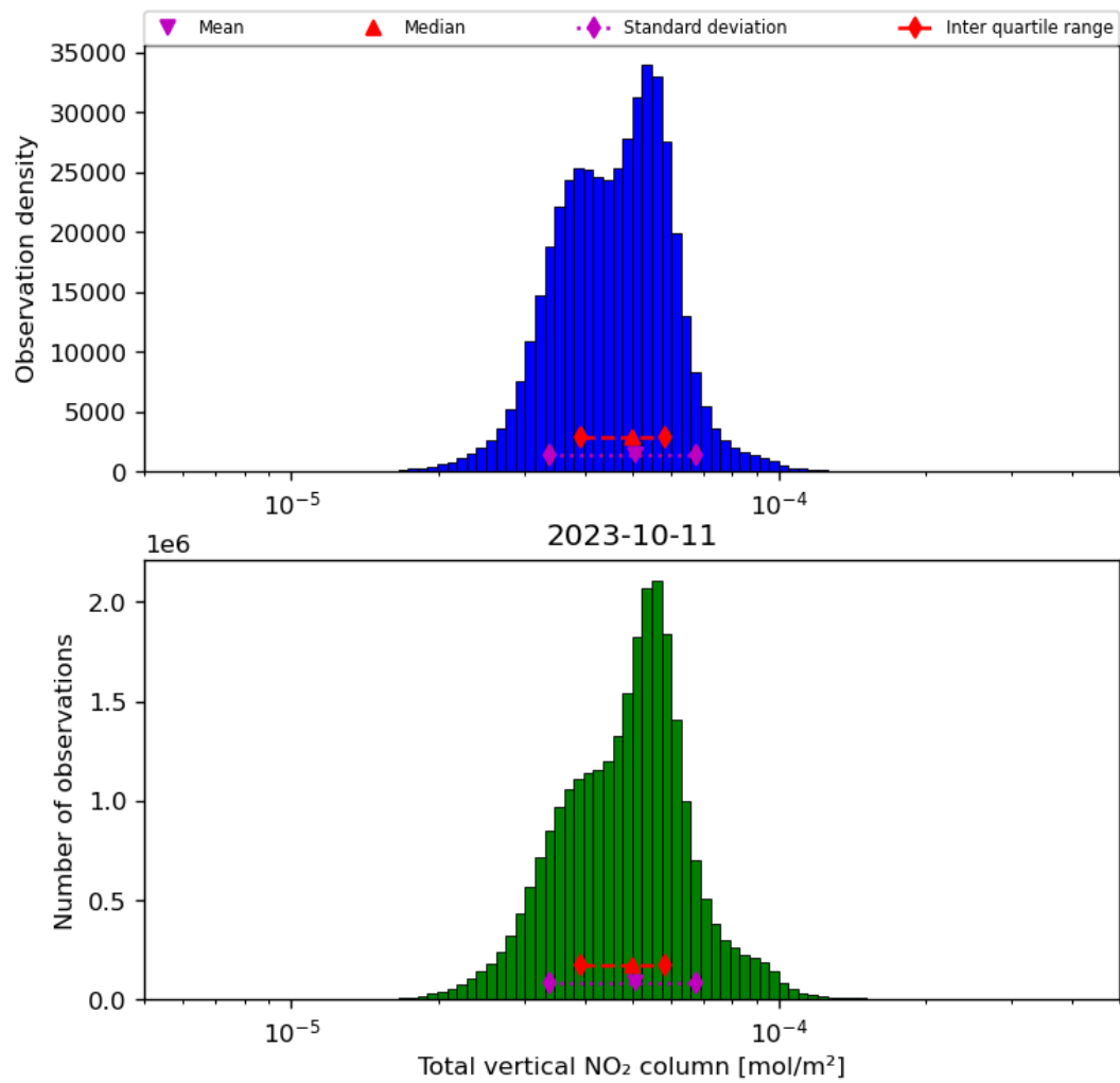
Figure 38: Histogram of “Total vertical NO 2 column” for 2023-10-10 to 2023-10-12
