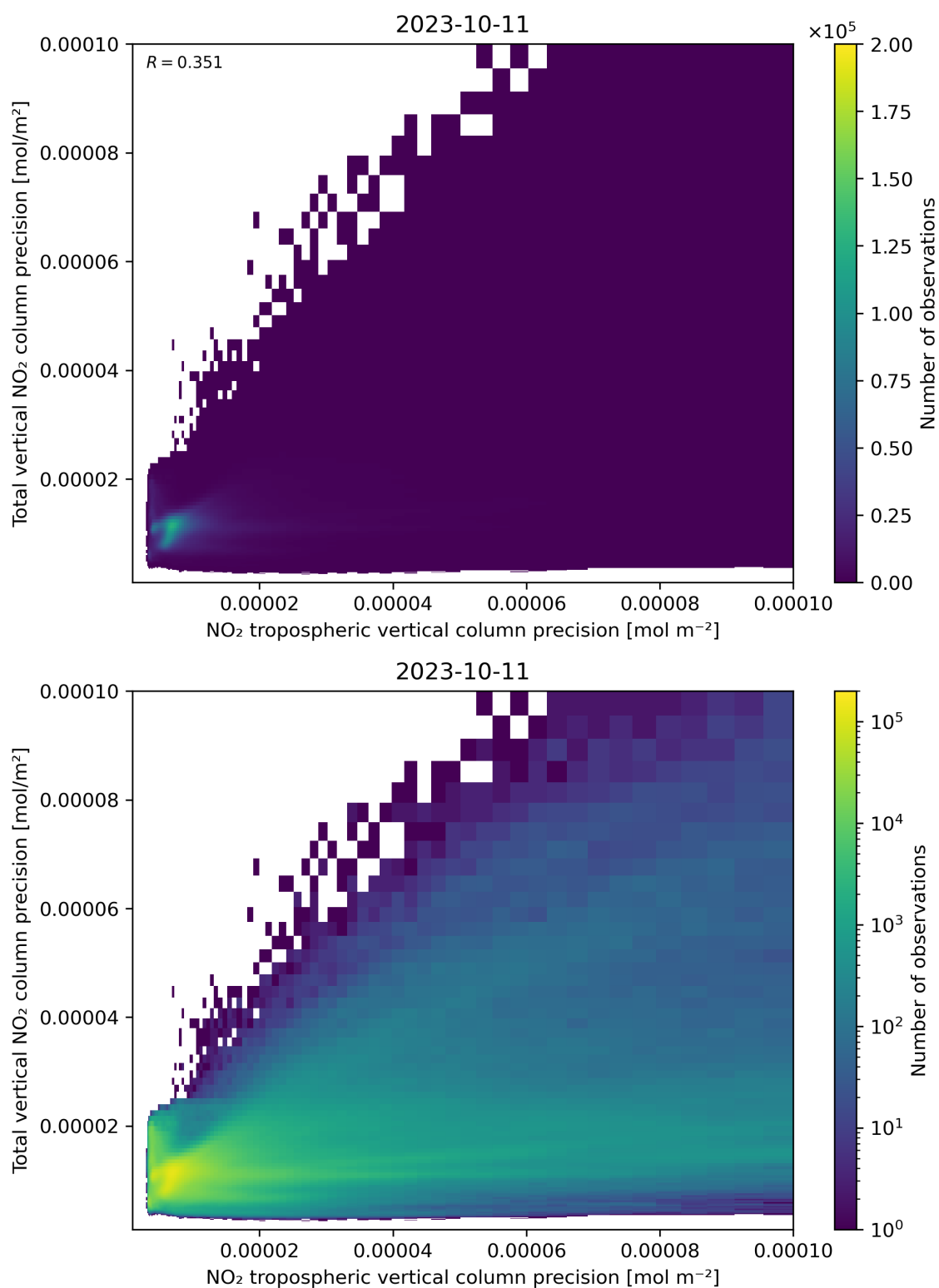
Figure 139: Scatter density plot of “NO 2 tropospheric vertical column precision” against “Total vertical NO 2 column precision” for 2023-10-10 to 2023-10-12.
