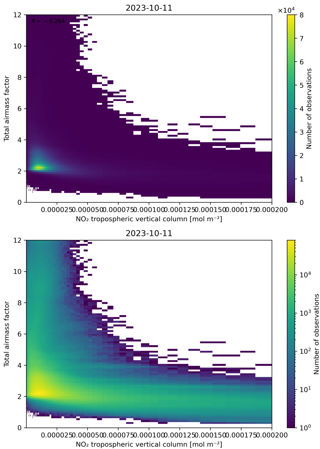
Figure 122: Scatter density plot of “NO 2 tropospheric vertical column” against “Total air mass factor” for 2023-10-10 to 2023-10-12.
