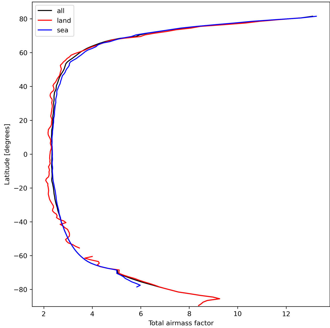
Figure 15: Zonal average of “Total airmass factor” for 2023-10-10 to 2023-10-12.
