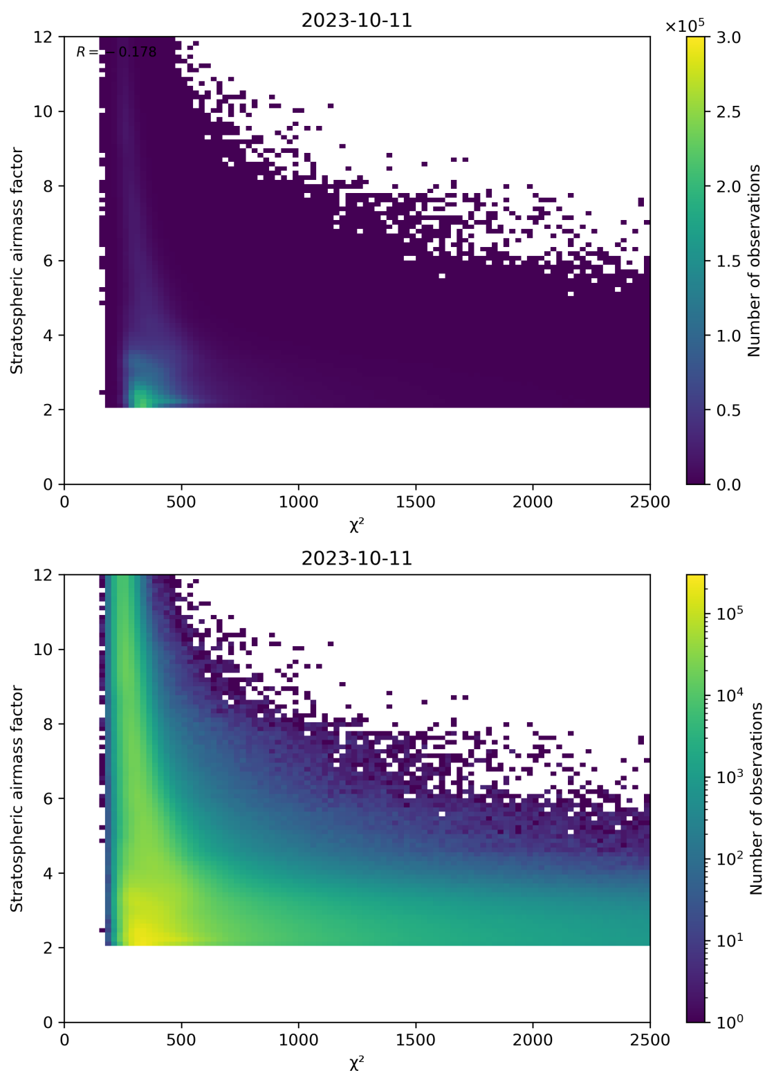
Figure 81: Scatter density plot of “ \chi^2 ” against “Stratospheric airmass factor” for 2023-10-10 to 2023-10-12.
