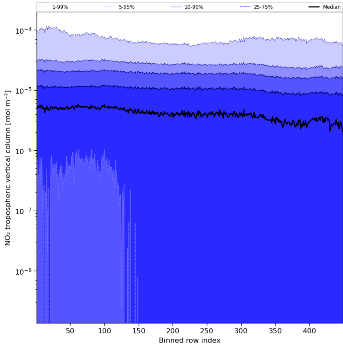
Figure 46: Along track statistics of “NO 2 tropospheric vertical column” for 2023-10-10 to 2023-10-12
