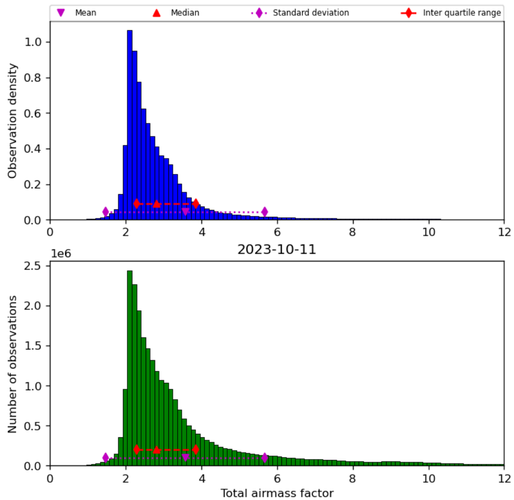
Figure 32: Histogram of “Total airmass factor” for 2023-10-10 to 2023-10-12
