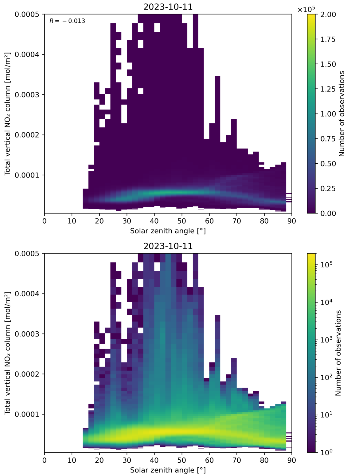
Figure 153: Scatter density plot of “Solar zenith angle” against “Total vertical NO 2 column” for 2023-10-10 to 2023-10-12.
