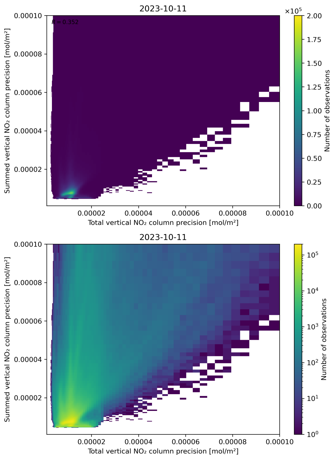
Figure 118: Scatter density plot of “Total vertical NO 2 column precision” against “Summed vertical NO 2 column precision” for 2023-10-10 to 2023-10-12.
