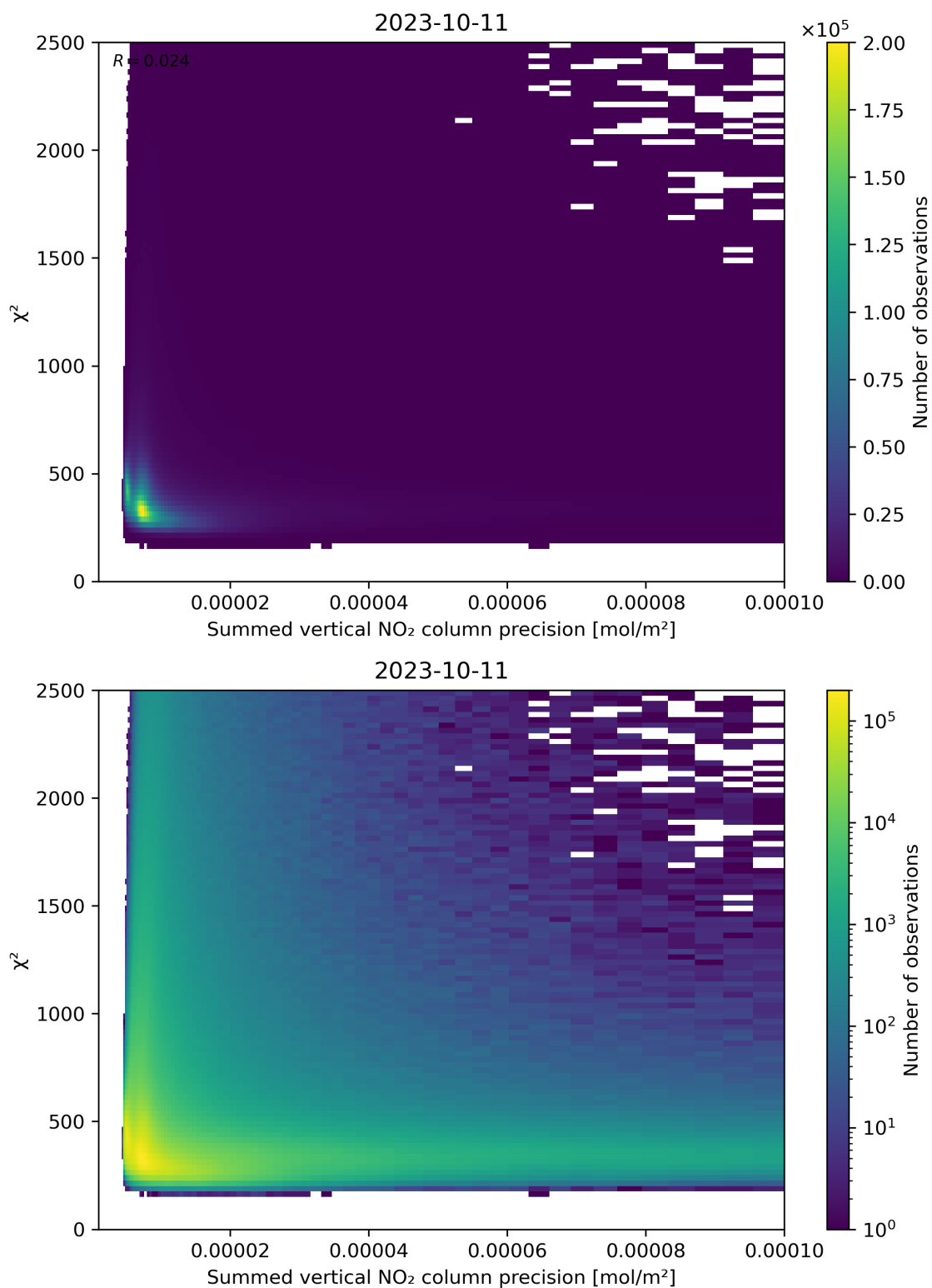
Figure 107: Scatter density plot of “Summed vertical NO 2 column precision” against “ \chi^2 ” for 2023-10-10 to 2023-10-12.
