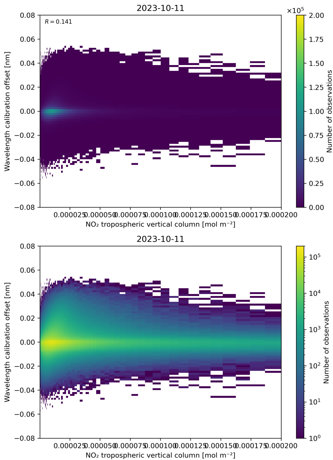
Figure 143: Scatter density plot of “NO 2 tropospheric vertical column” against “Wavelength calibration offset” for 2023-10-10 to 2023-10-12.
