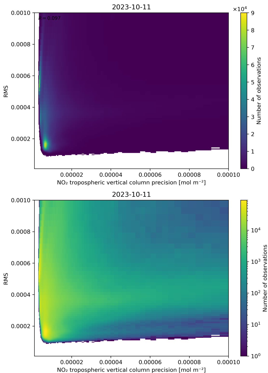
Figure 140: Scatter density plot of “NO 2 tropospheric vertical column precision” against “RMS” for 2023-10-10 to 2023-10-12.
