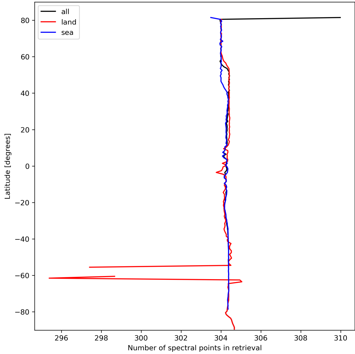
Figure 16: Zonal average of “Number of spectral points in retrieval” for 2023-10-10 to 2023-10-12.
