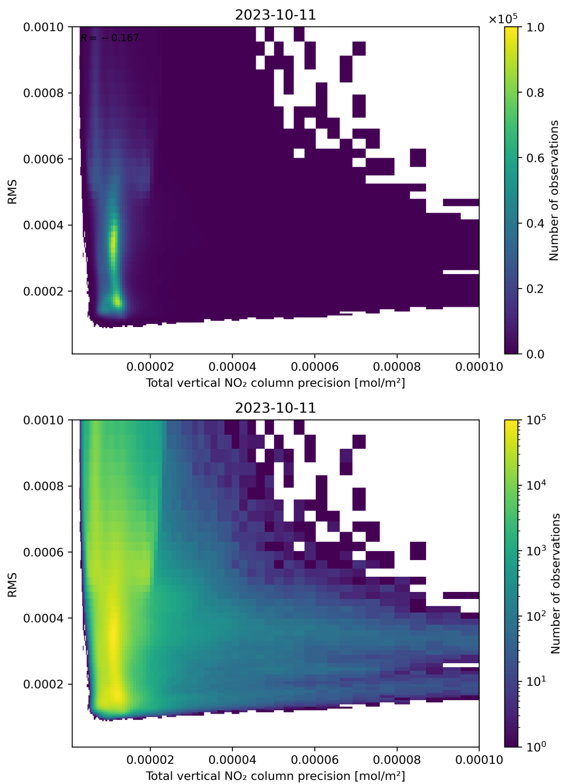
Figure 119: Scatter density plot of “Total vertical NO 2 column precision” against “RMS” for 2023-10-10 to 2023-10-12.
