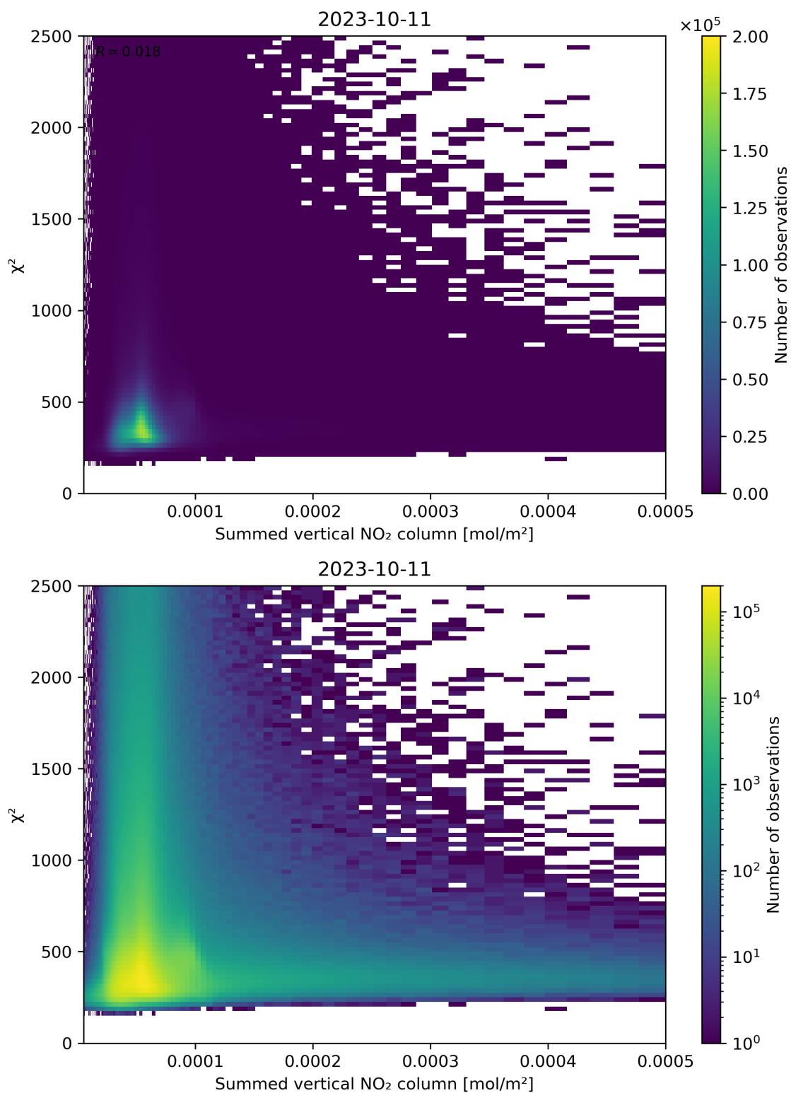
Figure 104: Scatter density plot of “Summed vertical NO 2 column” against “ \chi^2 ” for 2023-10-10 to 2023-10-12.
