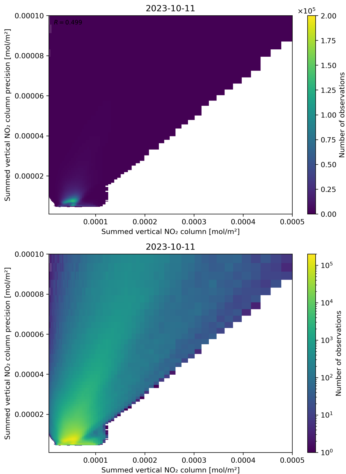
Figure 105: Scatter density plot of “Summed vertical NO 2 column” against “Summed vertical NO 2 column precision” for 2023-10-10 to 2023-10-12.
