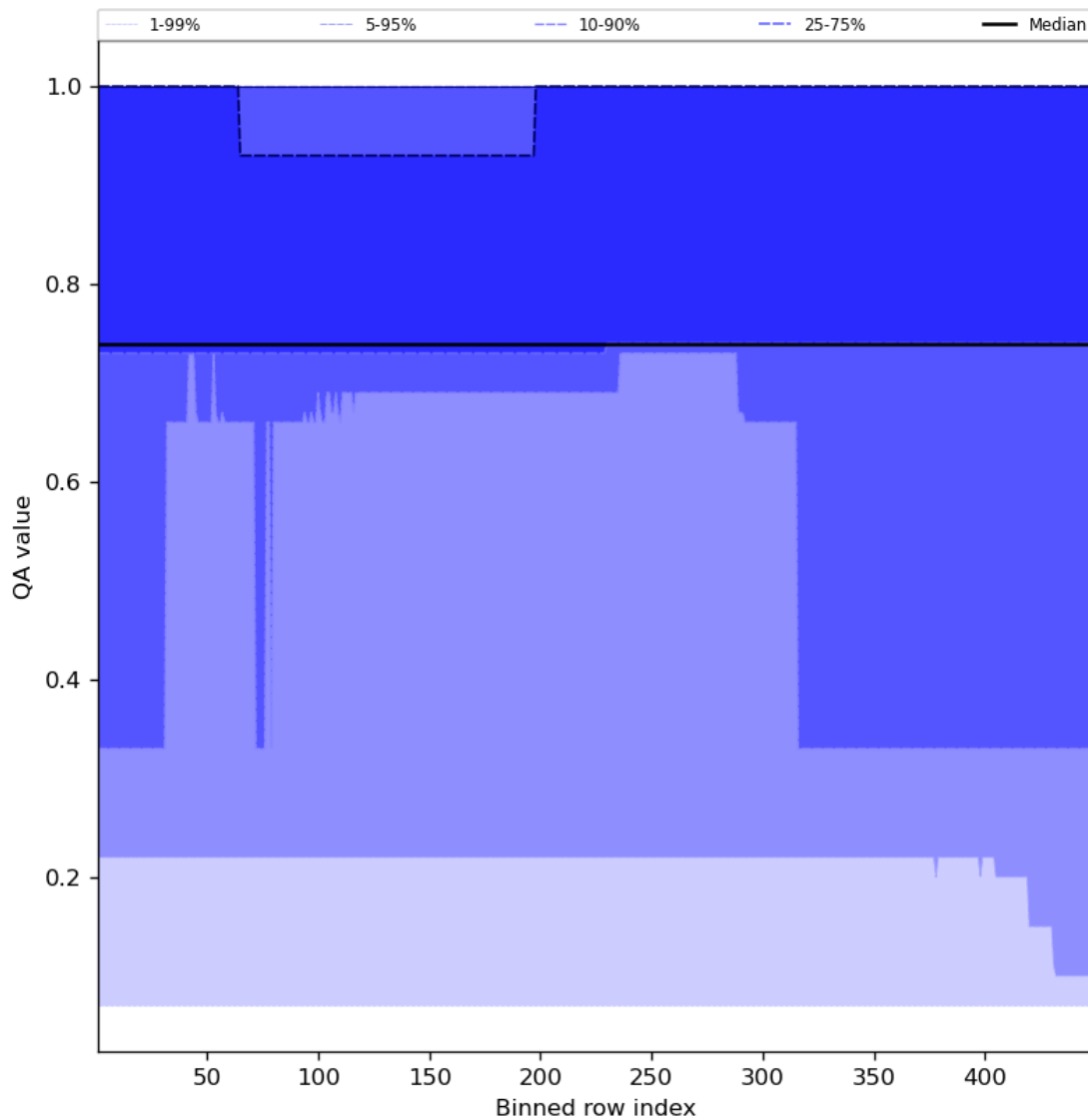
Figure 45: Along track statistics of “QA value” for 2023-10-10 to 2023-10-12
