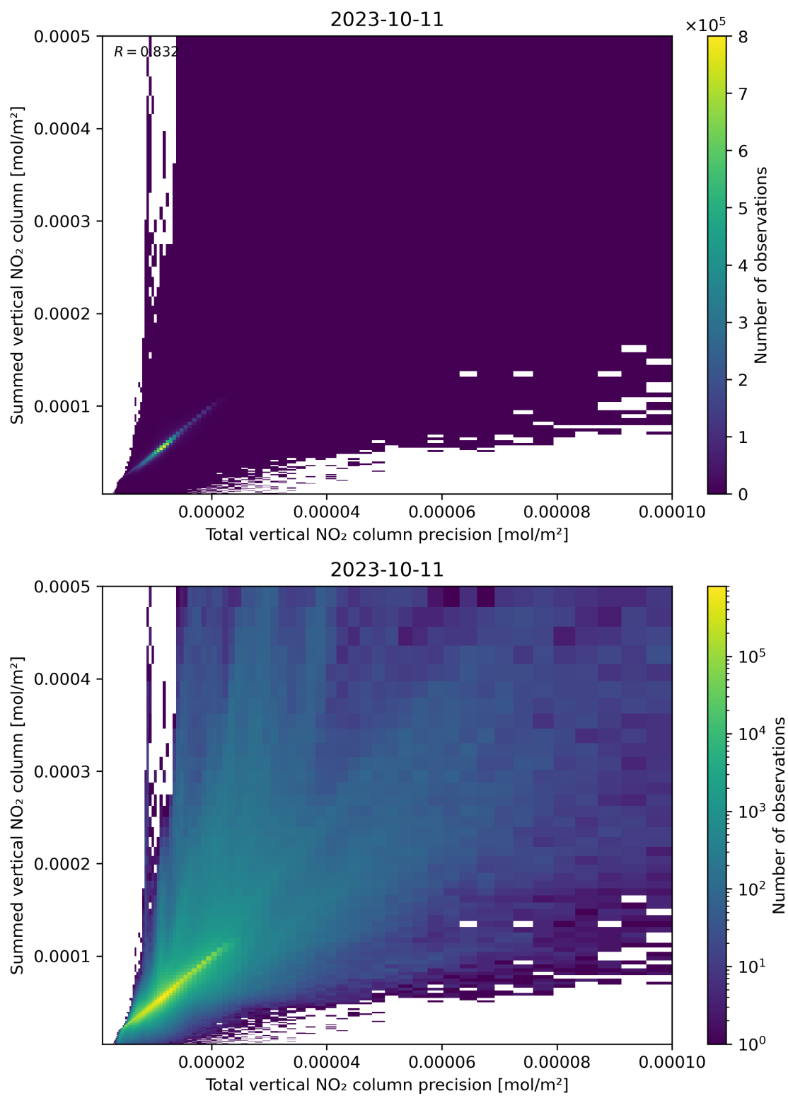
Figure 117: Scatter density plot of “Total vertical NO 2 column precision” against “Summed vertical NO 2 column” for 2023-10-10 to 2023-10-12.
