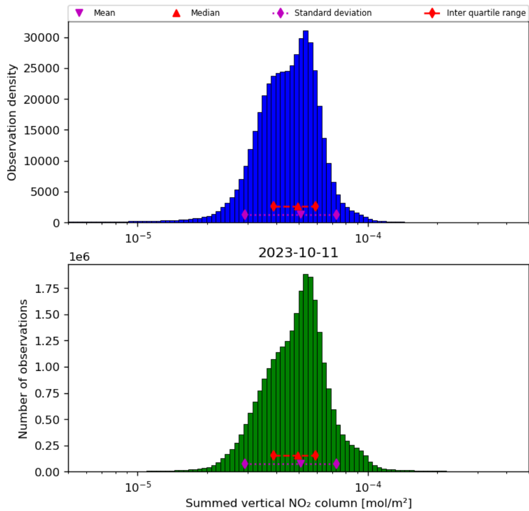
Figure 40: Histogram of “Summed vertical NO 2 column” for 2023-10-10 to 2023-10-12
