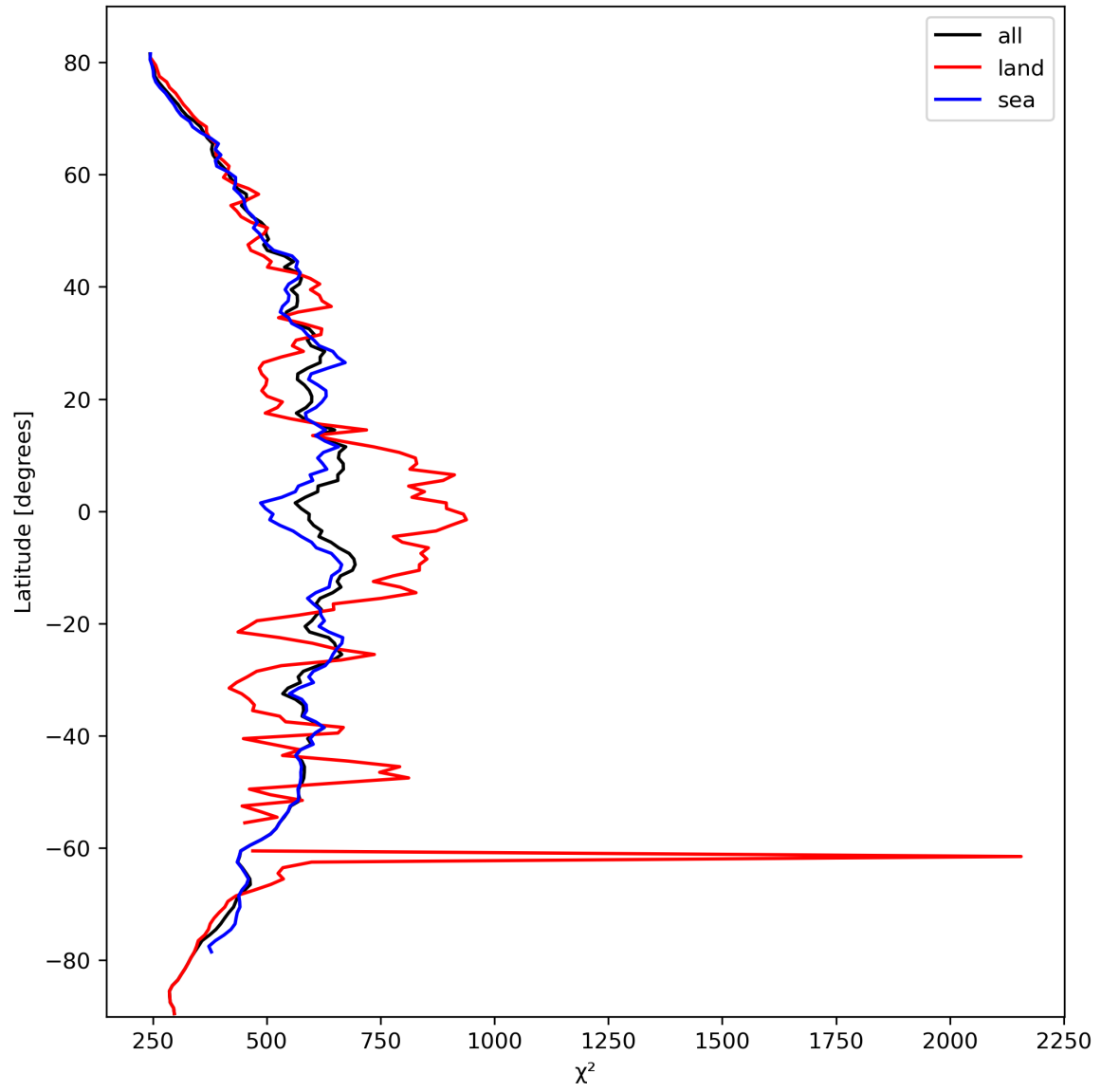
Figure 25: Zonal average of “ \chi^2 ” for 2023-10-10 to 2023-10-12.
