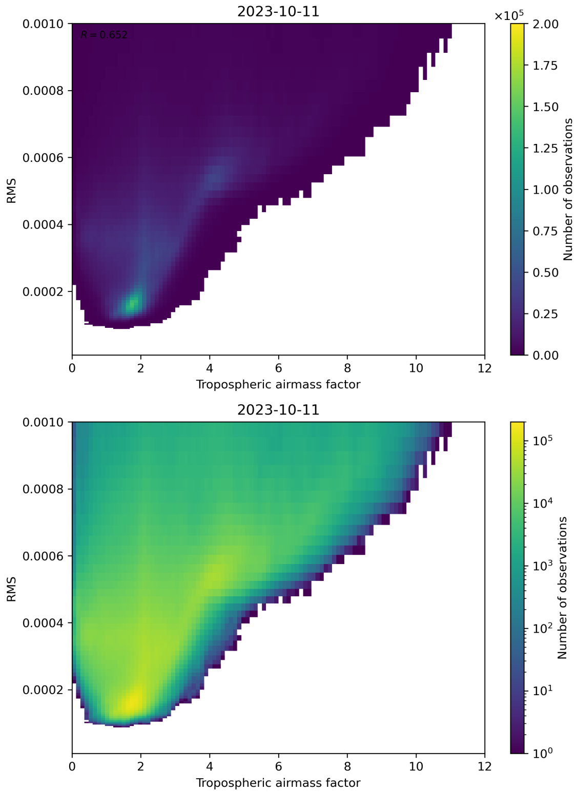
Figure 79: Scatter density plot of “Tropospheric airmass factor” against “RMS” for 2023-10-10 to 2023-10-12.
