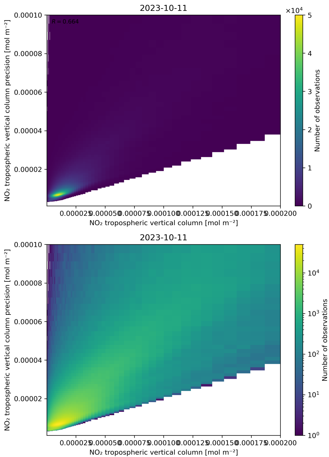
Figure 130: Scatter density plot of “NO 2 tropospheric vertical column” against “NO 2 tropospheric vertical column precision” for 2023-10-10 to 2023-10-12.
