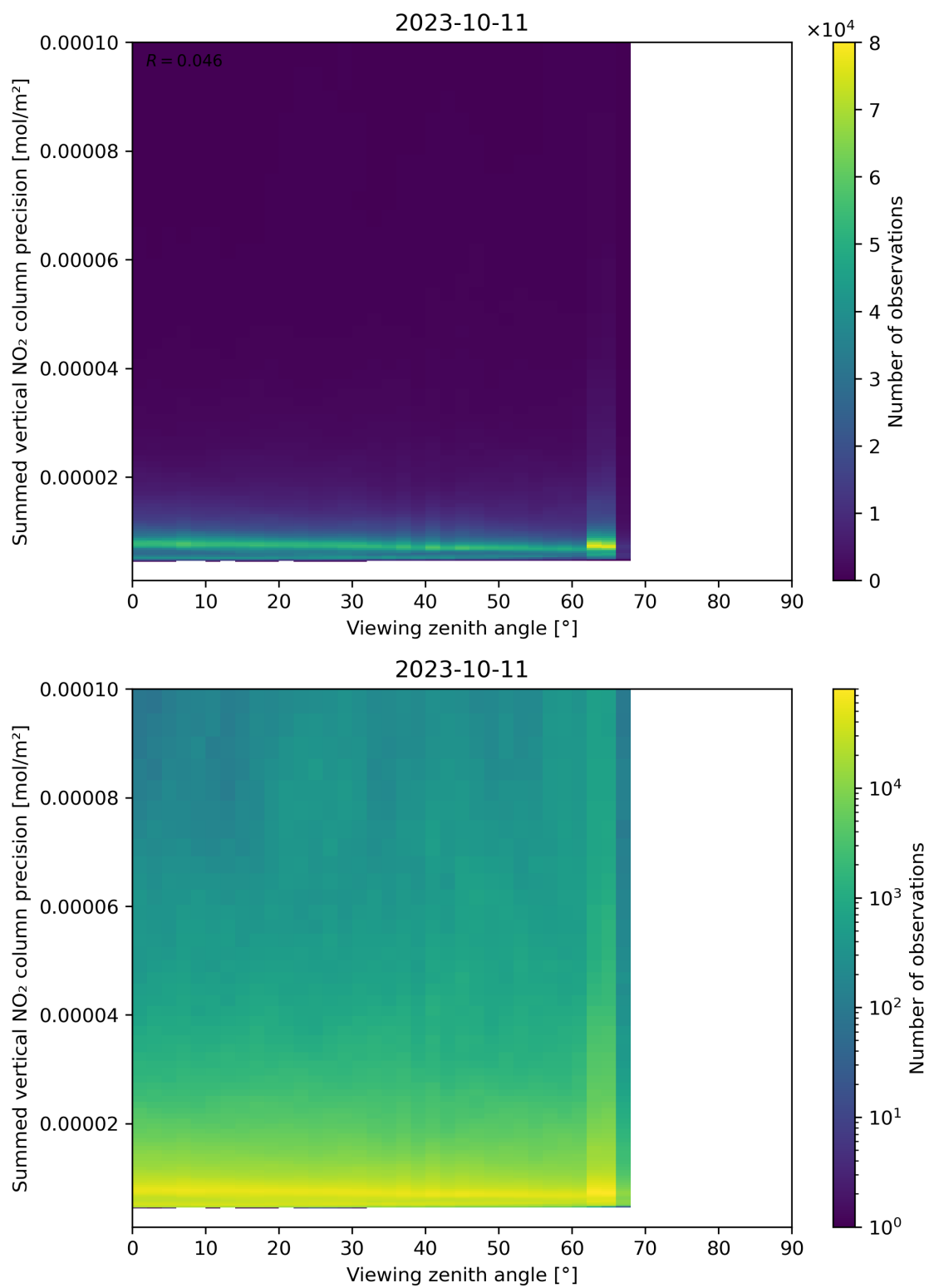
Figure 166: Scatter density plot of “Viewing zenith angle” against “Summed vertical NO 2 column precision” for 2023-10-10 to 2023-10-12.
