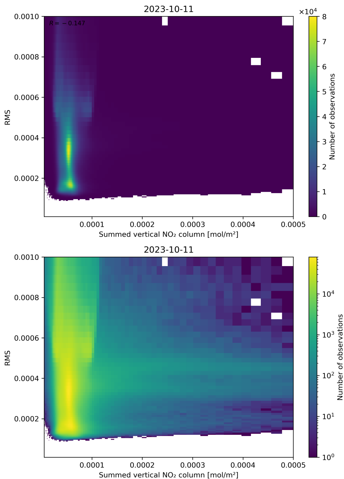
Figure 109: Scatter density plot of “Summed vertical NO 2 column” against “RMS” for 2023-10-10 to 2023-10-12.
