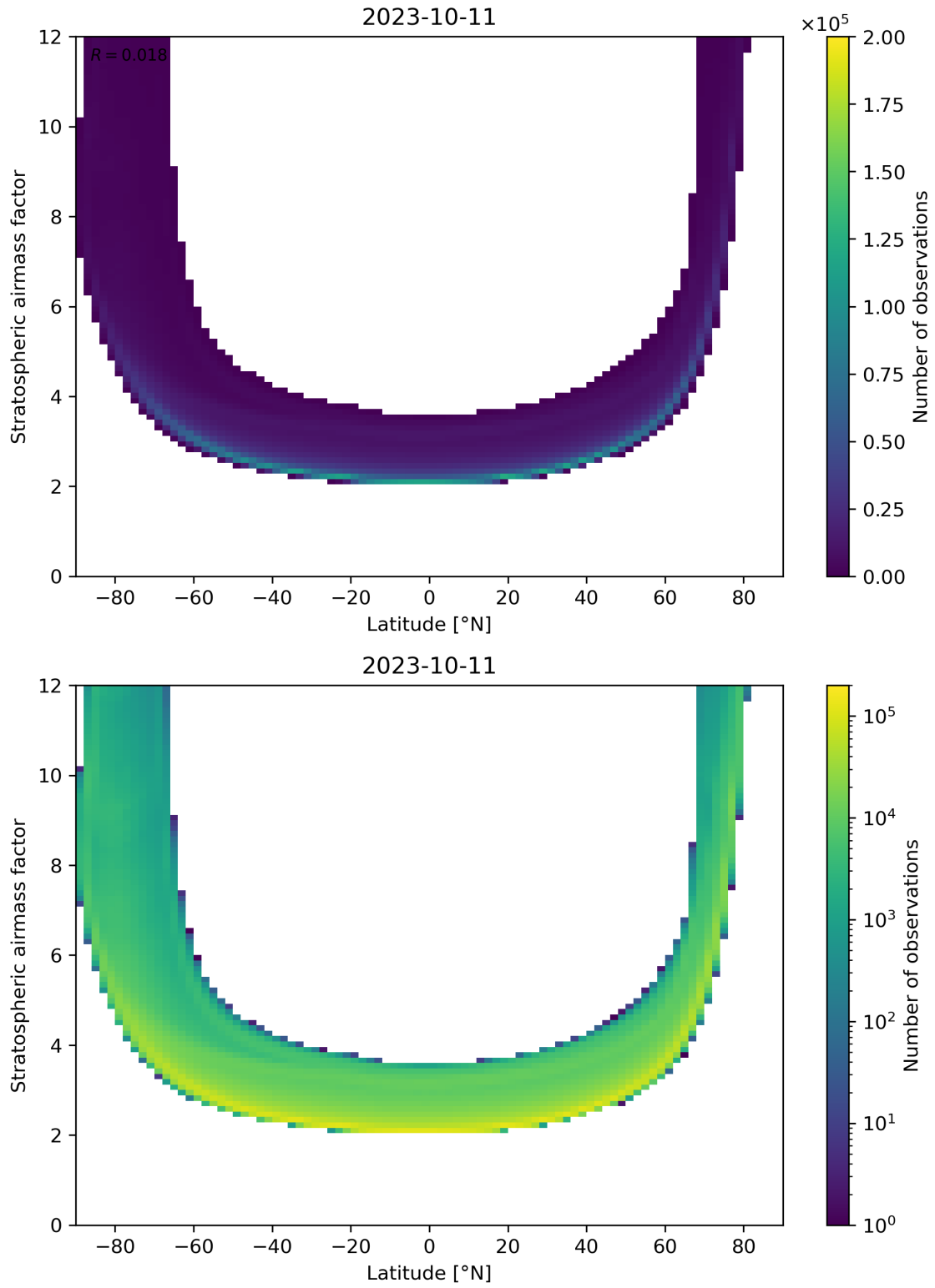
Figure 83: Scatter density plot of “Latitude” against “Stratospheric airmass factor” for 2023-10-10 to 2023-10-12.
