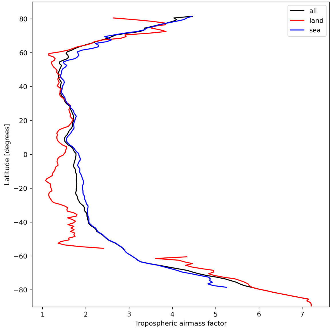
Figure 14: Zonal average of “Tropospheric airmass factor” for 2023-10-10 to 2023-10-12.
