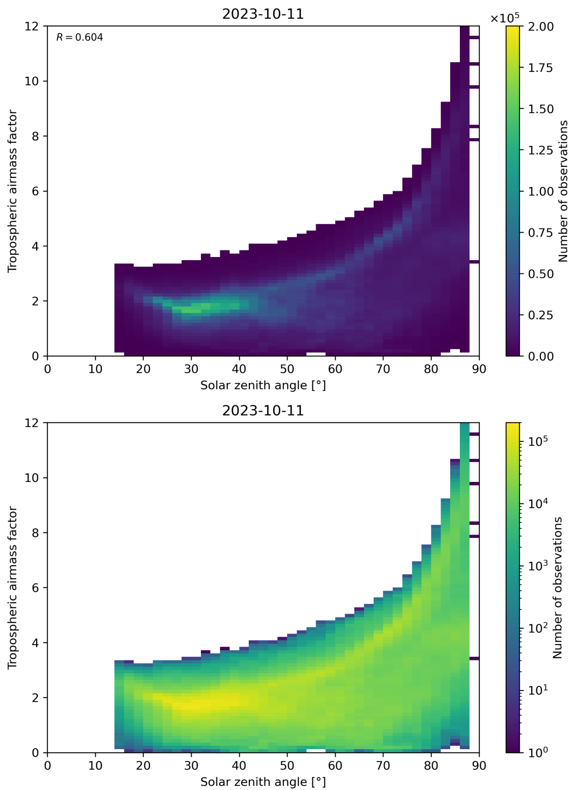
Figure 147: Scatter density plot of “Solar zenith angle” against “Tropospheric airmass factor” for 2023-10-10 to 2023-10-12.
