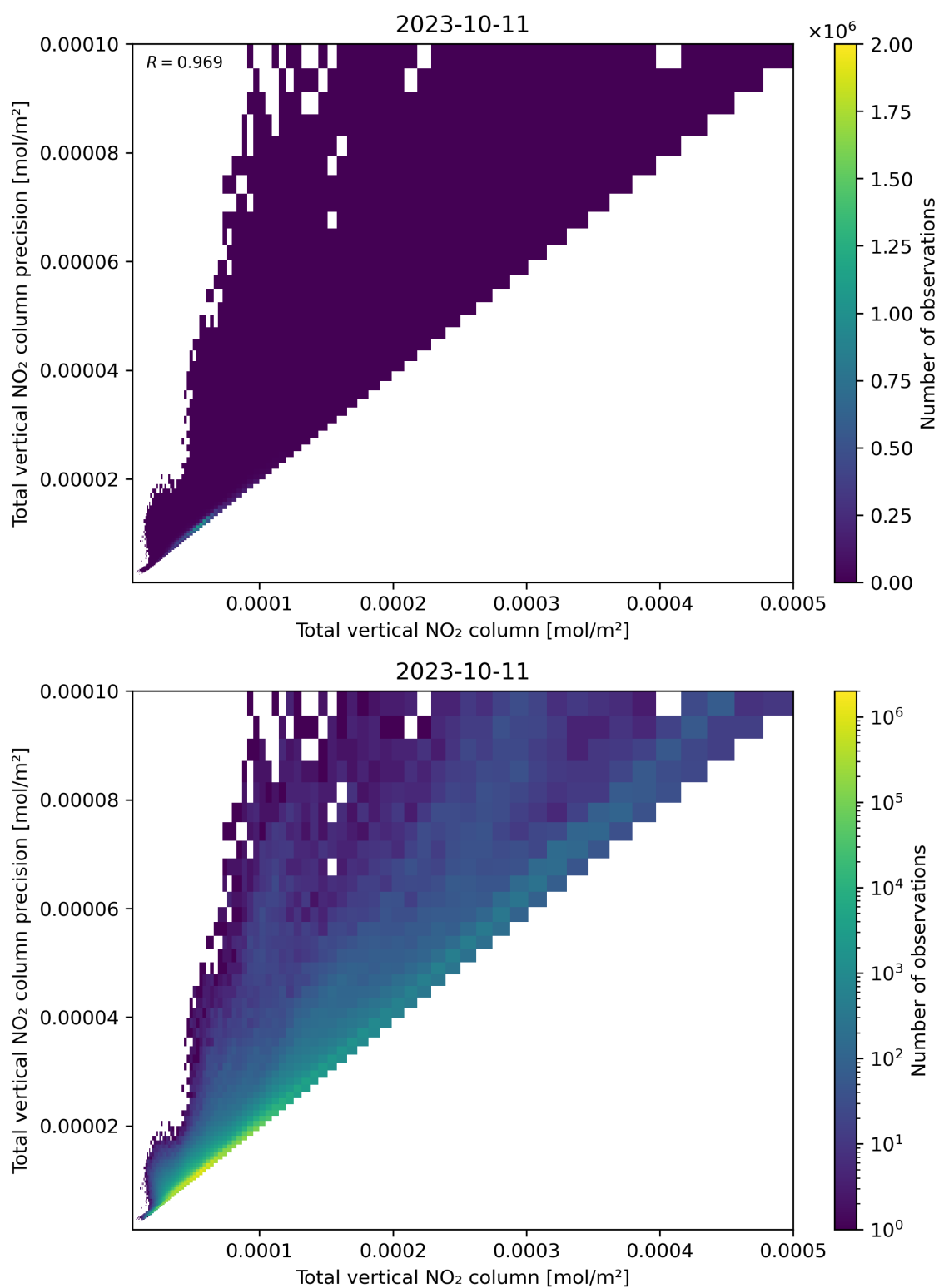
Figure 114: Scatter density plot of “Total vertical NO 2 column” against “Total vertical NO 2 column precision” for 2023-10-10 to 2023-10-12.
