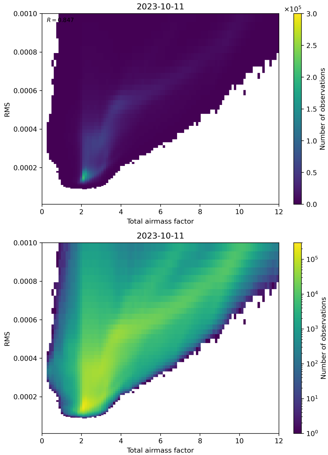
Figure 69: Scatter density plot of “Total airmass factor” against “RMS” for 2023-10-10 to 2023-10-12.
