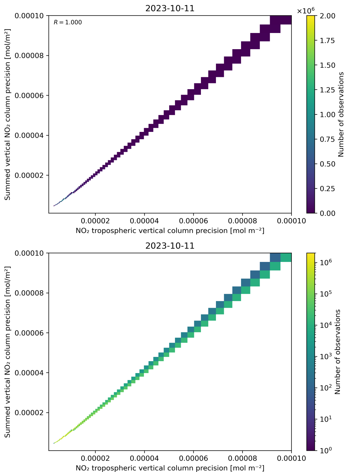
Figure 137: Scatter density plot of “NO 2 tropospheric vertical column precision” against “Summed vertical NO 2 column precision” for 2023-10-10 to 2023-10-12.
