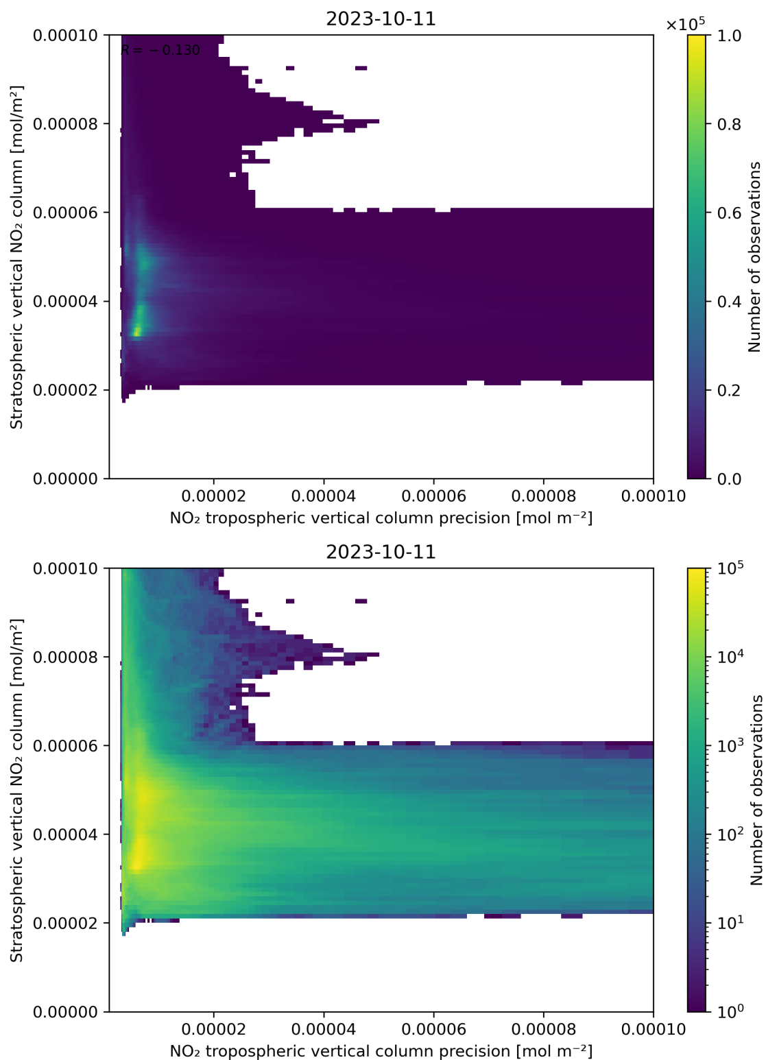
Figure 135: Scatter density plot of “NO 2 tropospheric vertical column precision” against “Stratospheric vertical NO 2 column” for 2023-10-10 to 2023-10-12.
