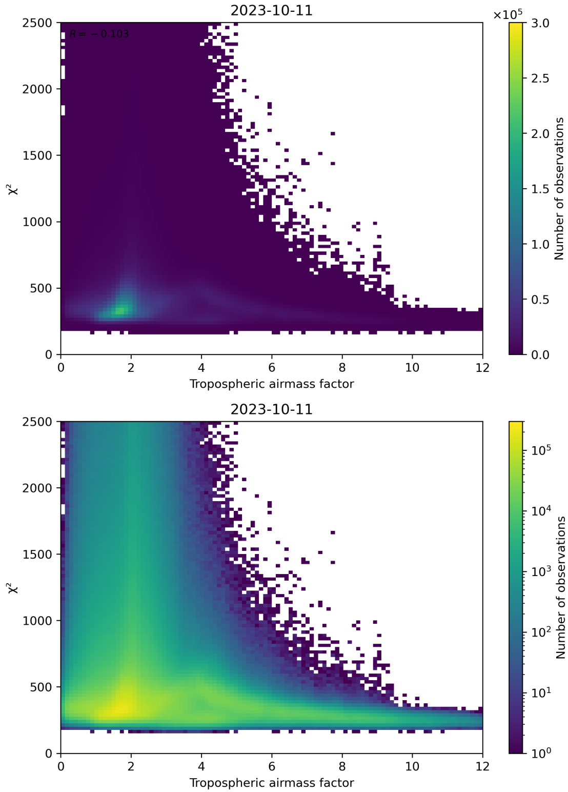
Figure 73: Scatter density plot of “Tropospheric airmass factor” against “ \chi^2 ” for 2023-10-10 to 2023-10-12.
