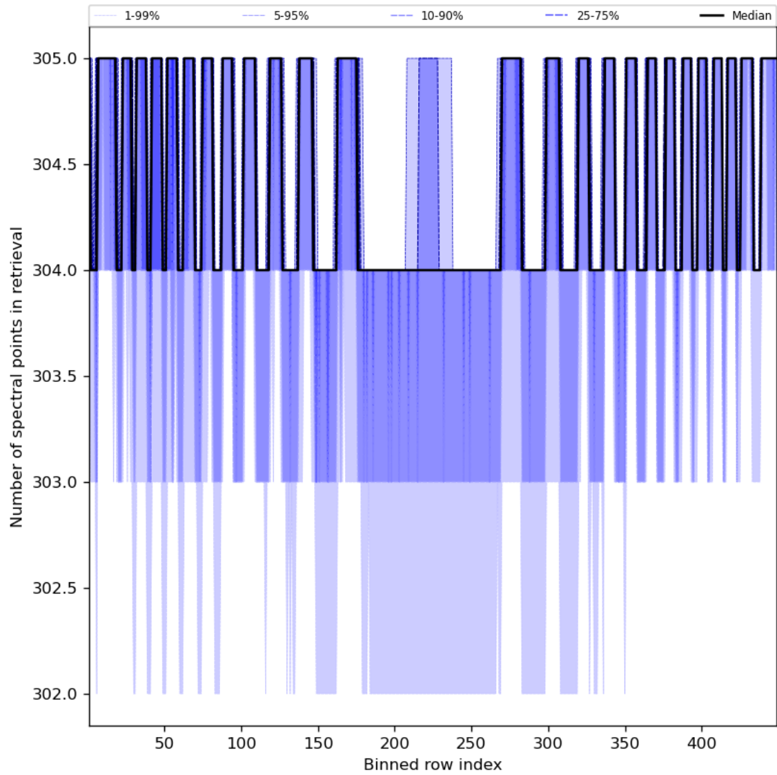
Figure 50: Along track statistics of “Number of spectral points in retrieval” for 2023-10-10 to 2023-10-12
