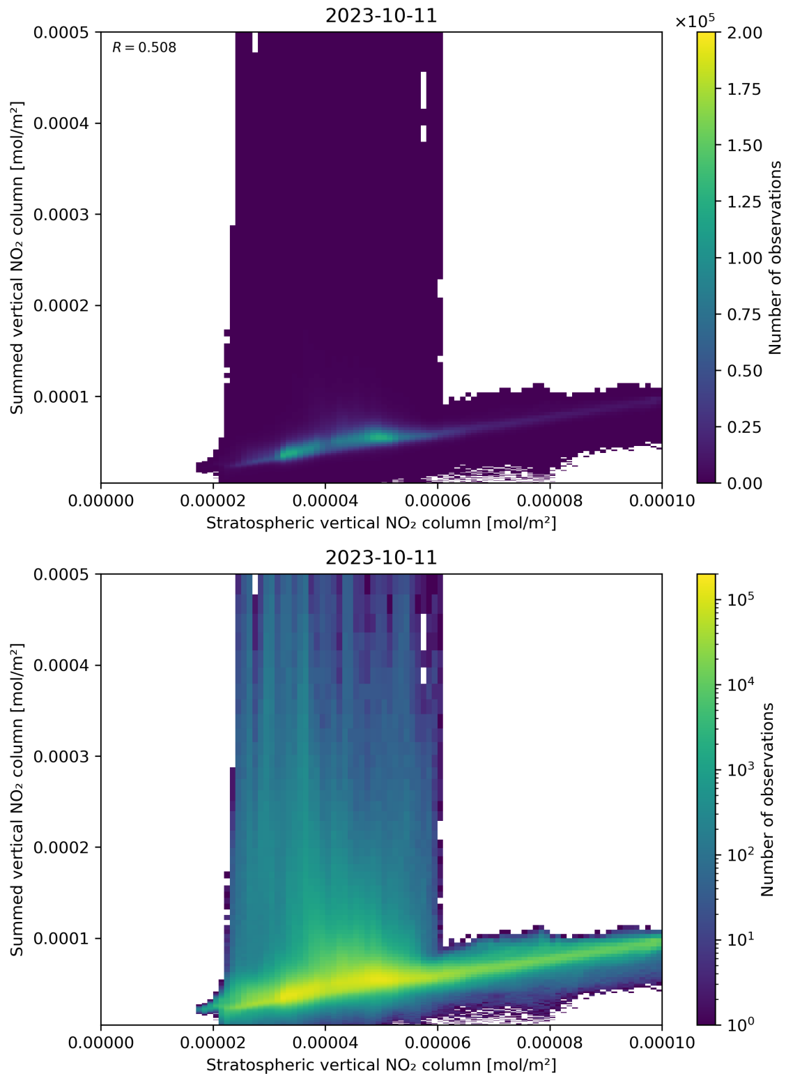
Figure 98: Scatter density plot of “Stratospheric vertical NO 2 column” against “Summed vertical NO 2 column” for 2023-10-10 to 2023-10-12.
