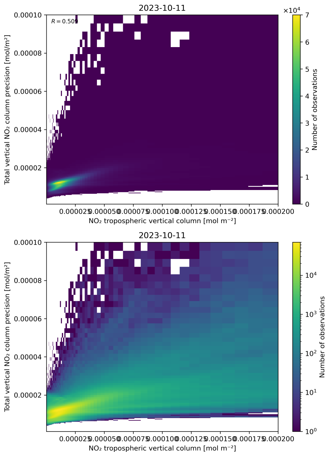
Figure 129: Scatter density plot of “NO 2 tropospheric vertical column” against “Total vertical NO 2 column precision” for 2023-10-10 to 2023-10-12.
