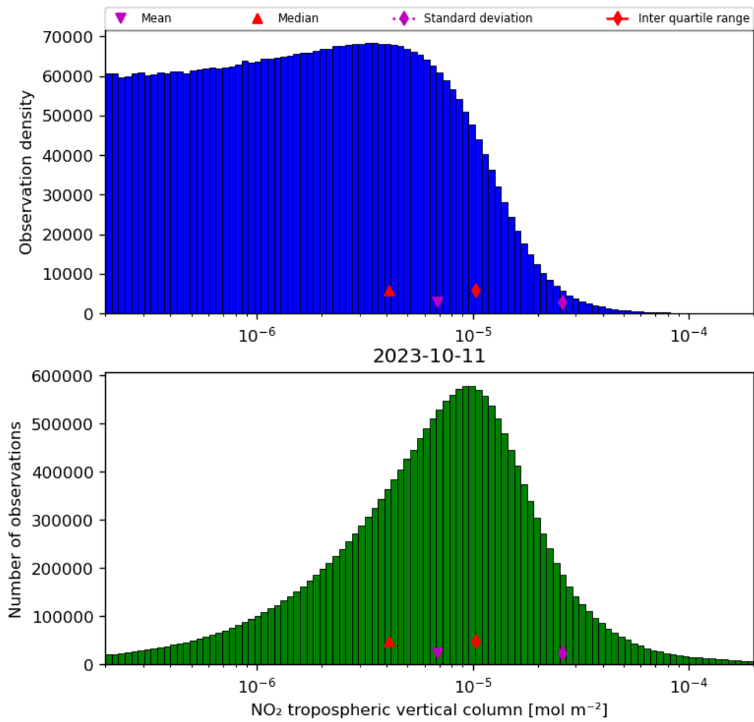
Figure 29: Histogram of “NO 2 tropospheric vertical column” for 2023-10-10 to 2023-10-12
