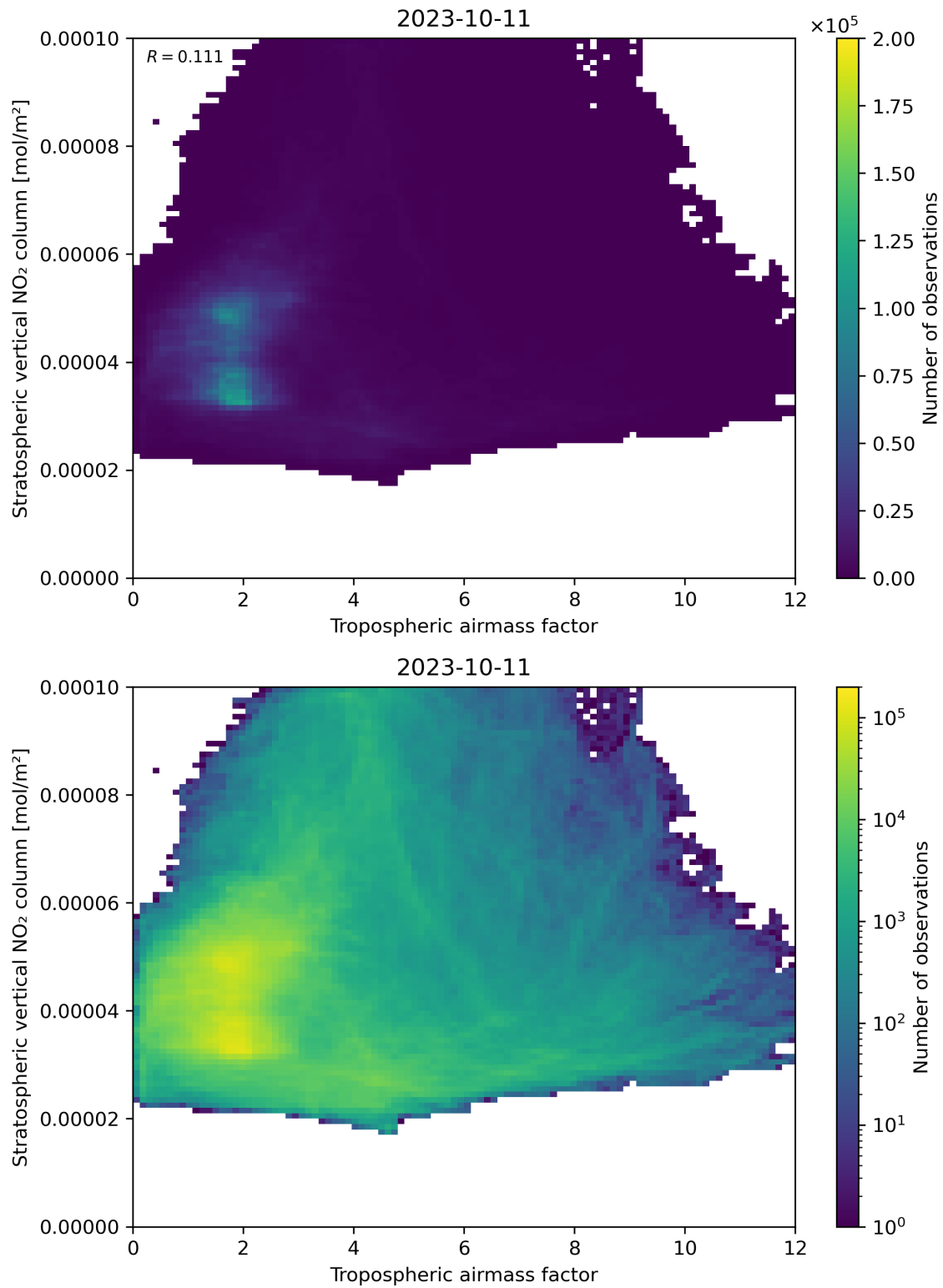
Figure 74: Scatter density plot of “Tropospheric air mass factor” against “Stratospheric vertical NO 2 column” for 2023-10-10 to 2023-10-12.
