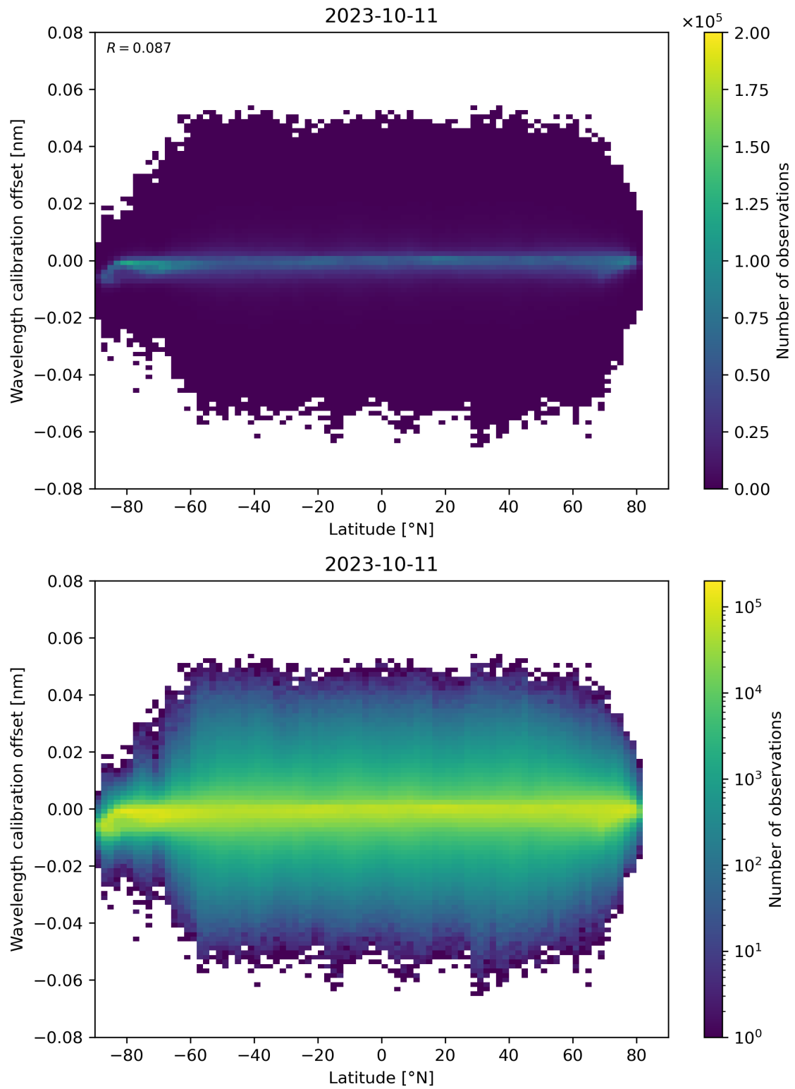
Figure 95: Scatter density plot of “Latitude” against “Wavelength calibration offset” for 2023-10-10 to 2023-10-12.
