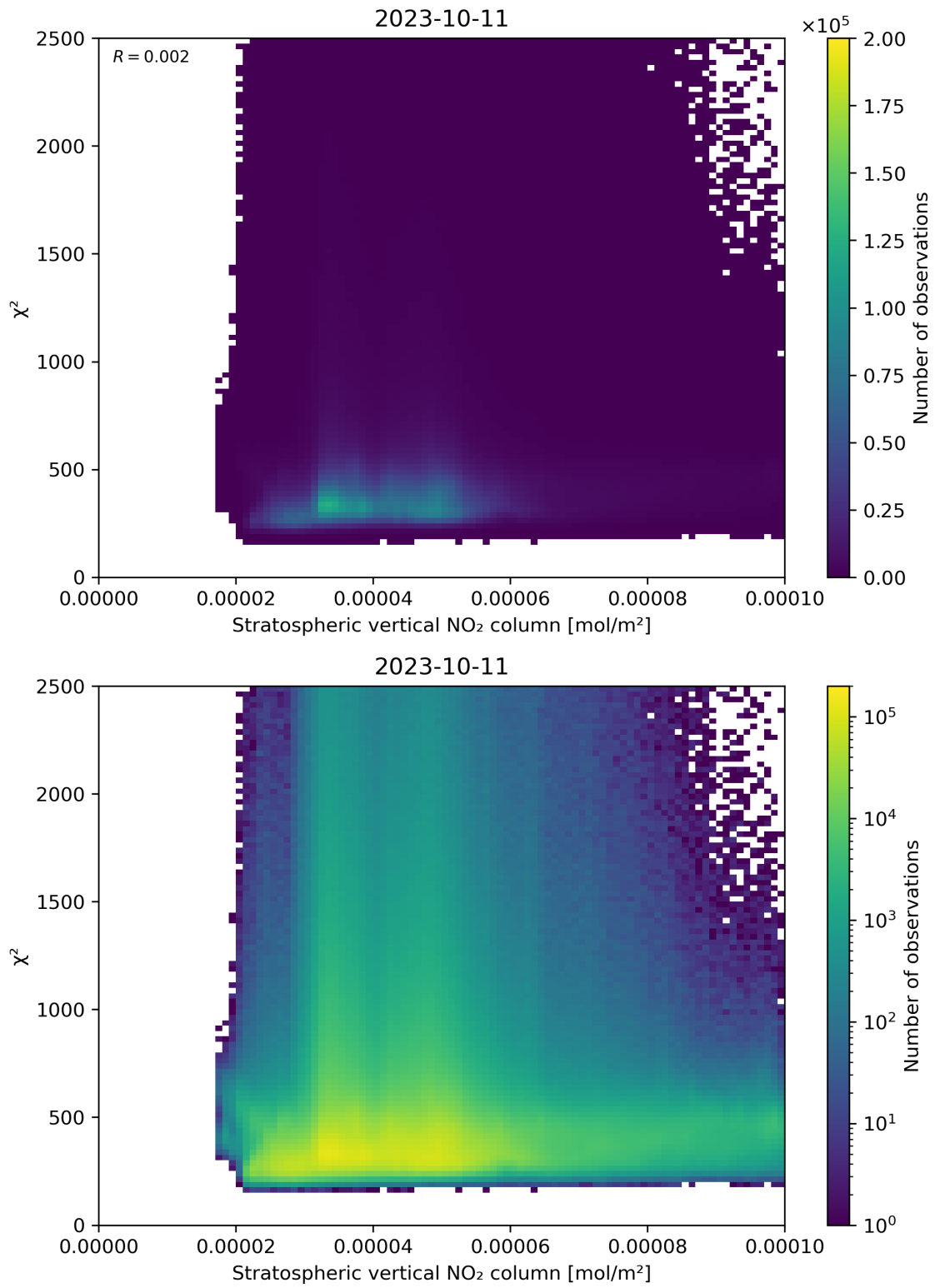
Figure 97: Scatter density plot of “Stratospheric vertical NO 2 column” against “ \chi^2 ” for 2023-10-10 to 2023-10-12.
