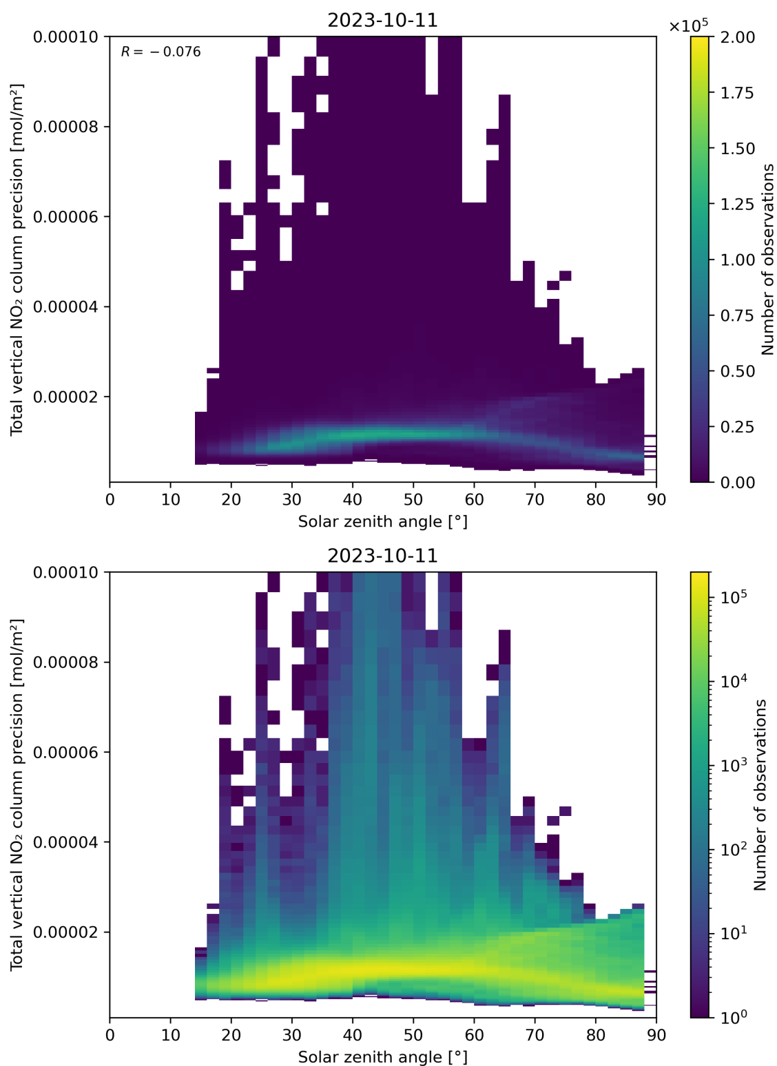
Figure 154: Scatter density plot of “Solar zenith angle” against “Total vertical NO 2 column precision” for 2023-10-10 to 2023-10-12.
