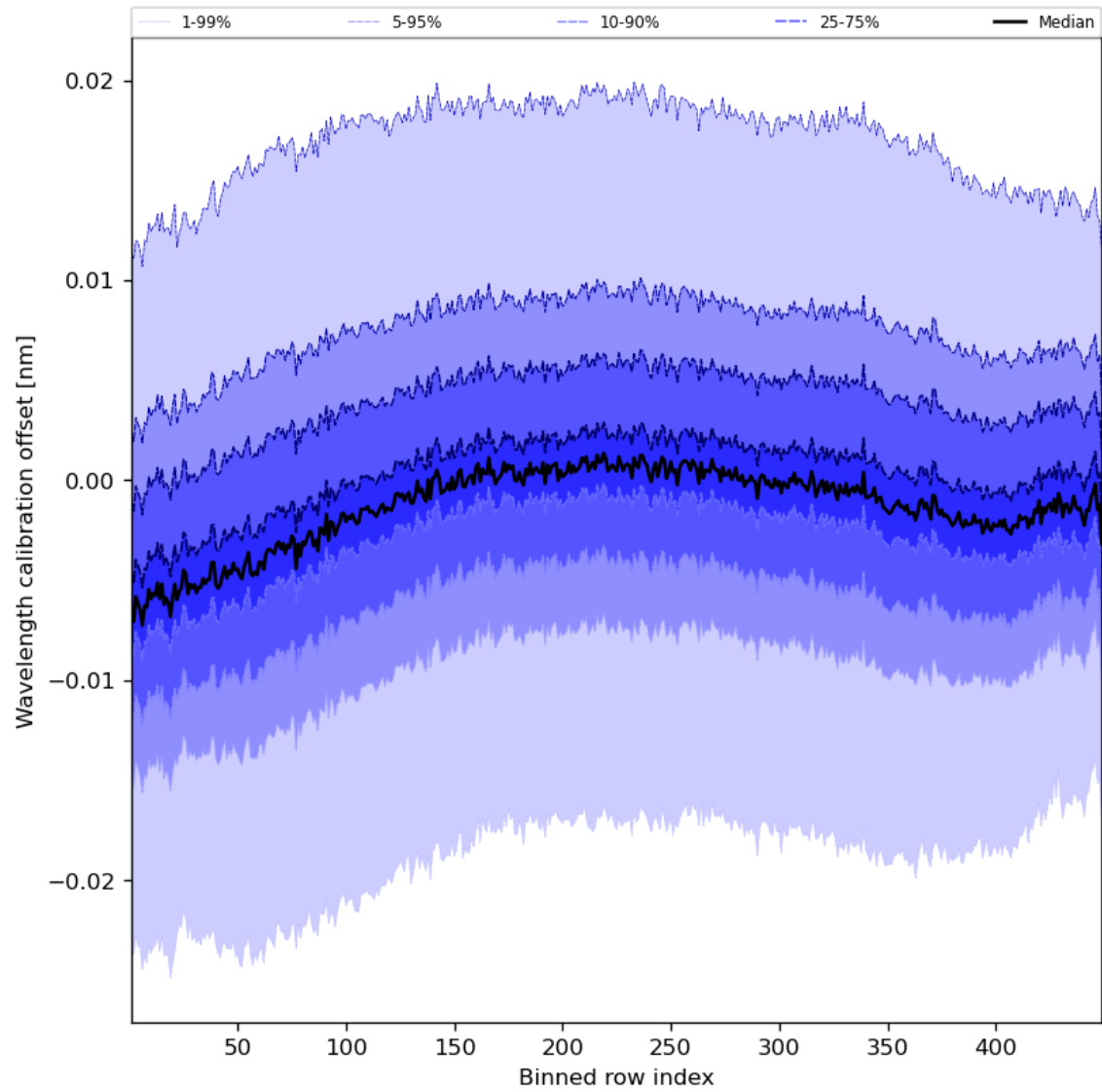
Figure 52: Along track statistics of “Wavelength calibration offset” for 2023-10-10 to 2023-10-12
