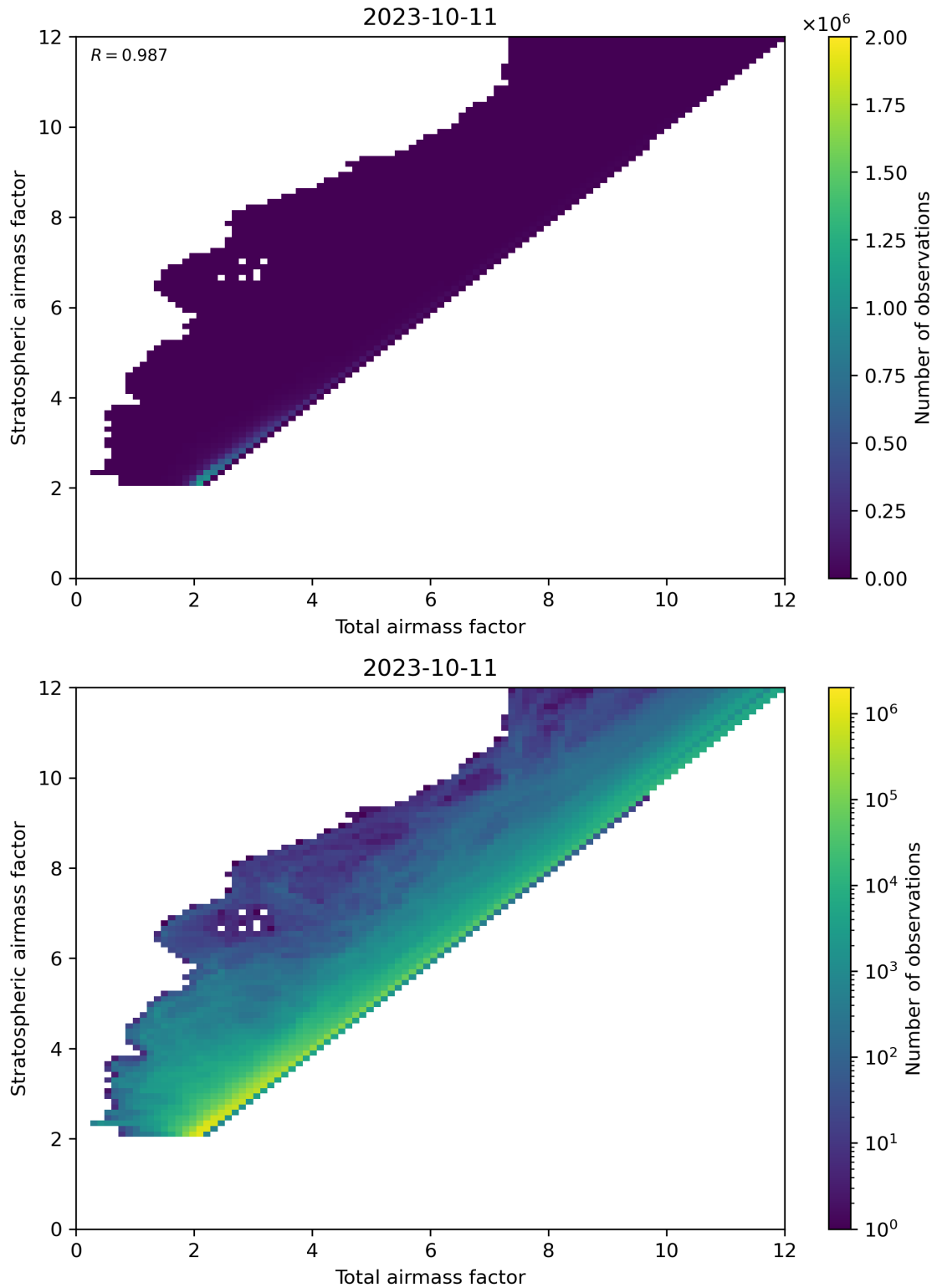
Figure 62: Scatter density plot of “Total airmass factor” against “Stratospheric airmass factor” for 2023-10-10 to 2023-10-12.
