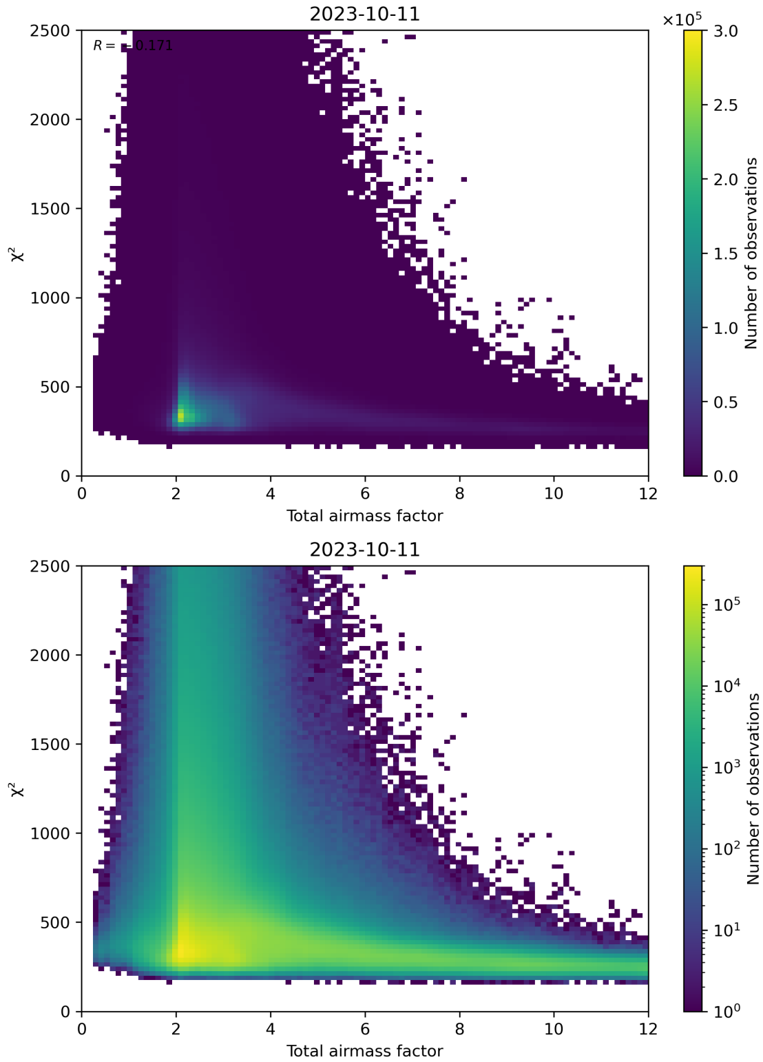
Figure 63: Scatter density plot of “Total airmass factor” against “ \chi^2 ” for 2023-10-10 to 2023-10-12.
