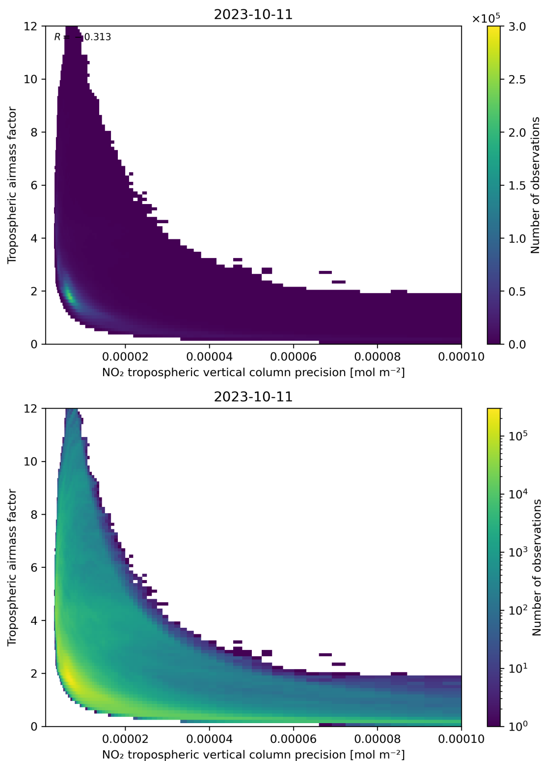
Figure 133: Scatter density plot of “NO 2 tropospheric vertical column precision” against “Tropospheric airmass factor” for 2023-10-10 to 2023-10-12.
