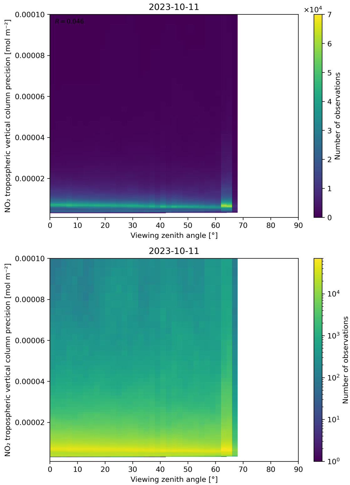
Figure 170: Scatter density plot of “Viewing zenith angle” against “NO 2 tropospheric vertical column precision” for 2023-10-10 to 2023-10-12.
