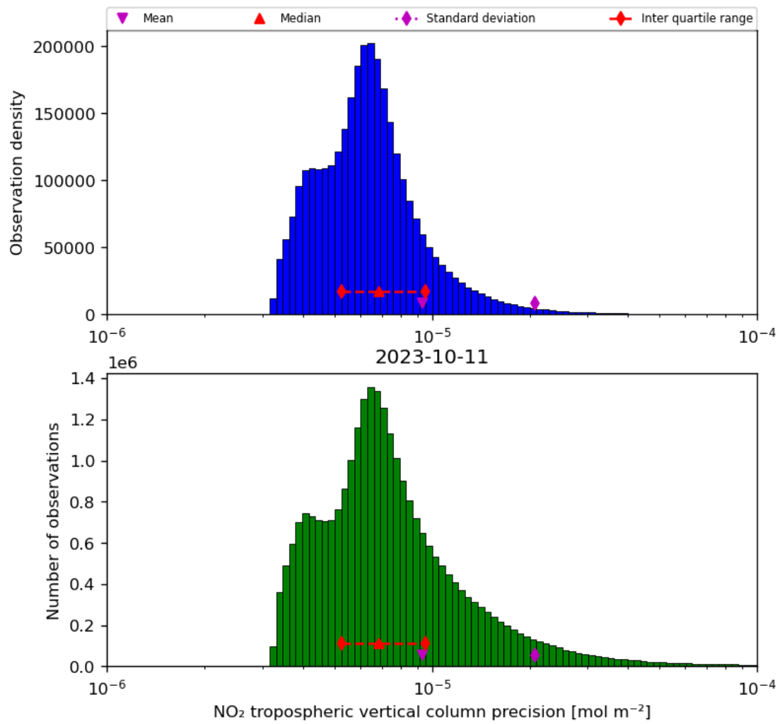
Figure 30: Histogram of “NO 2 tropospheric vertical column precision” for 2023-10-10 to 2023-10-12
