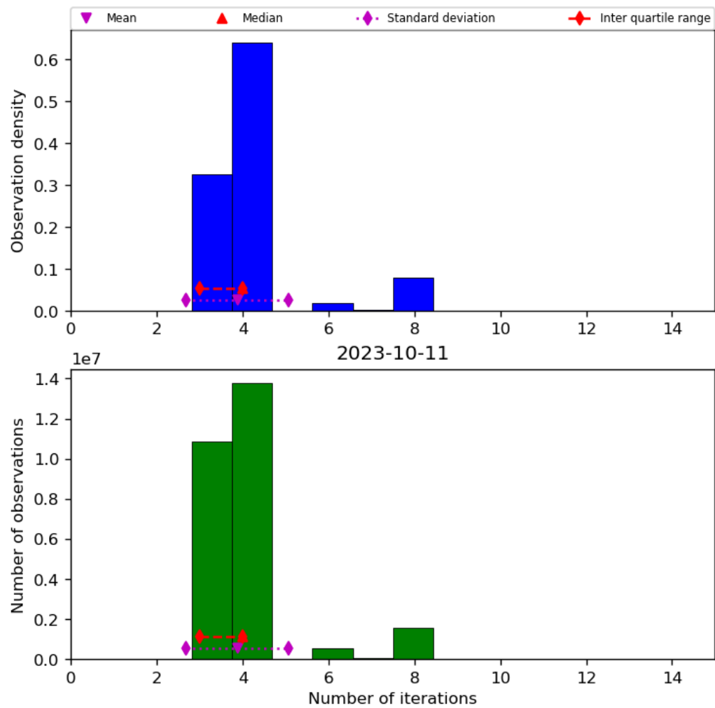
Figure 34: Histogram of “Number of iterations” for 2023-10-10 to 2023-10-12
