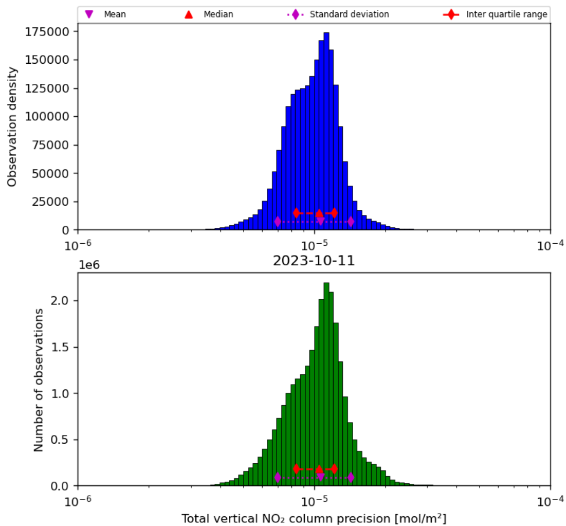
Figure 39: Histogram of “Total vertical NO 2 column precision” for 2023-10-10 to 2023-10-12
