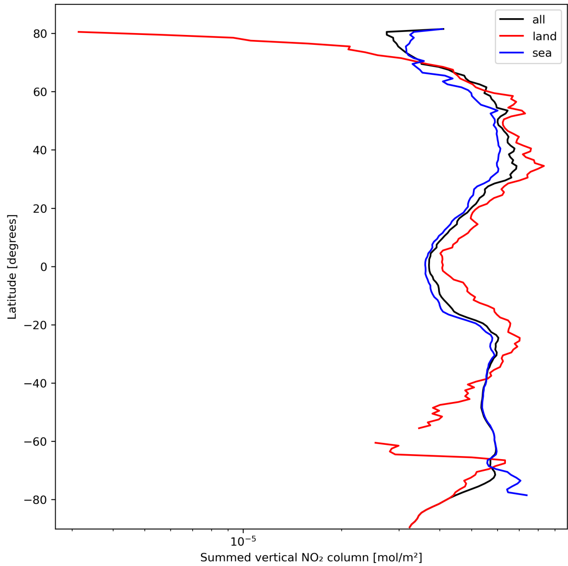
Figure 23: Zonal average of “Summed vertical NO 2 column” for 2023-10-10 to 2023-10-12.
