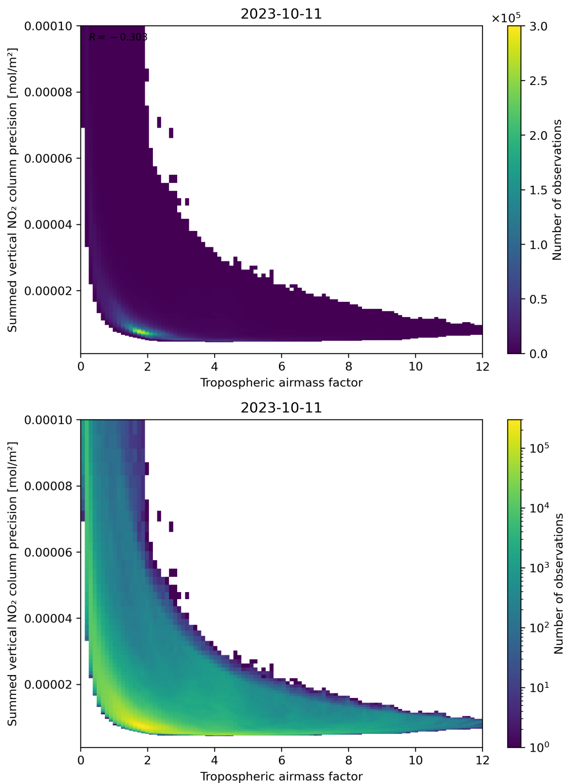
Figure 76: Scatter density plot of “Tropospheric air mass factor” against “Summed vertical NO 2 column precision” for 2023-10-10 to 2023-10-12.
