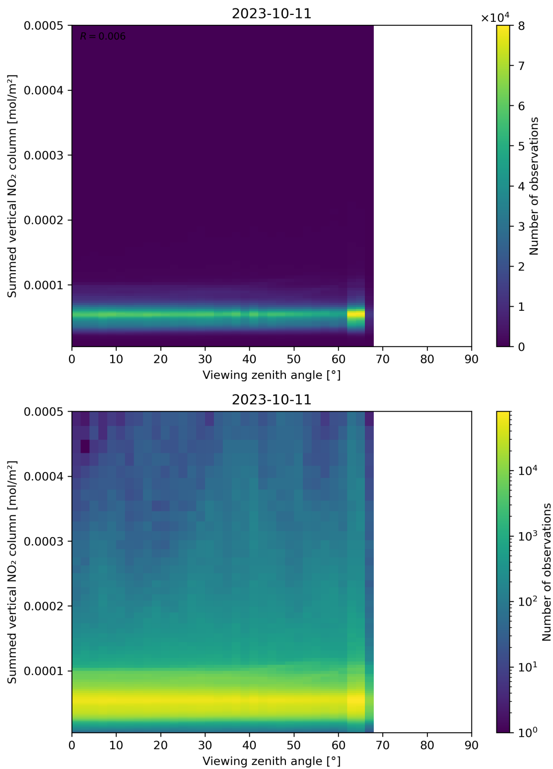
Figure 165: Scatter density plot of “Viewing zenith angle” against “Summed vertical NO 2 column” for 2023-10-10 to 2023-10-12.
