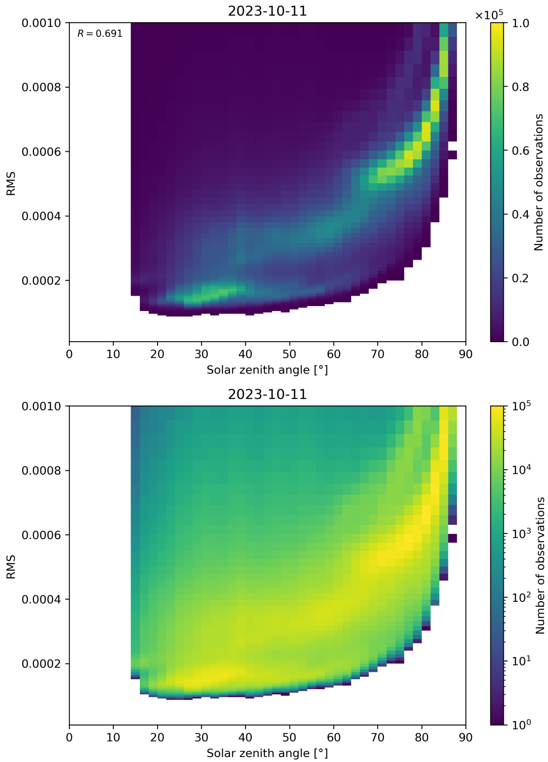
Figure 157: Scatter density plot of “Solar zenith angle” against “RMS” for 2023-10-10 to 2023-10-12.
