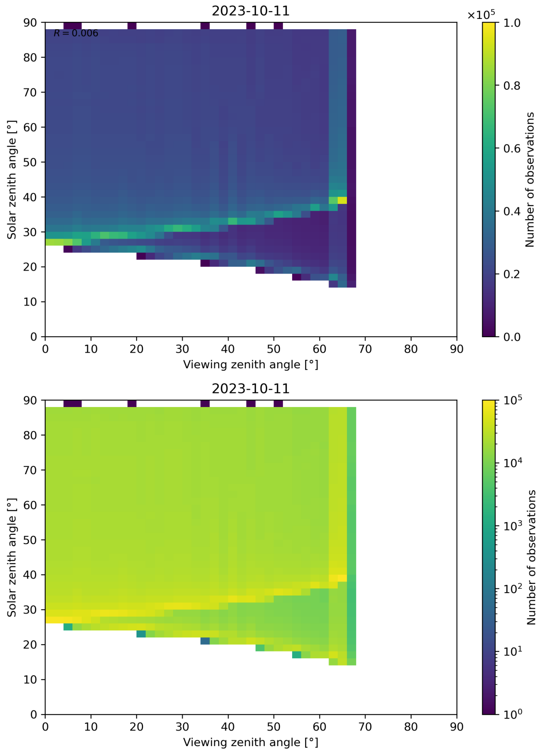
Figure 172: Scatter density plot of “Viewing zenith angle” against “Solar zenith angle” for 2023-10-10 to 2023-10-12.
