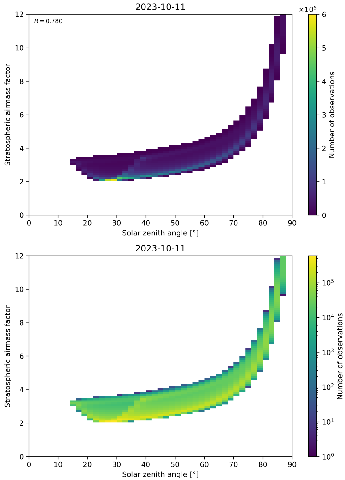
Figure 145: Scatter density plot of “Solar zenith angle” against “Stratospheric airmass factor” for 2023-10-10 to 2023-10-12.
