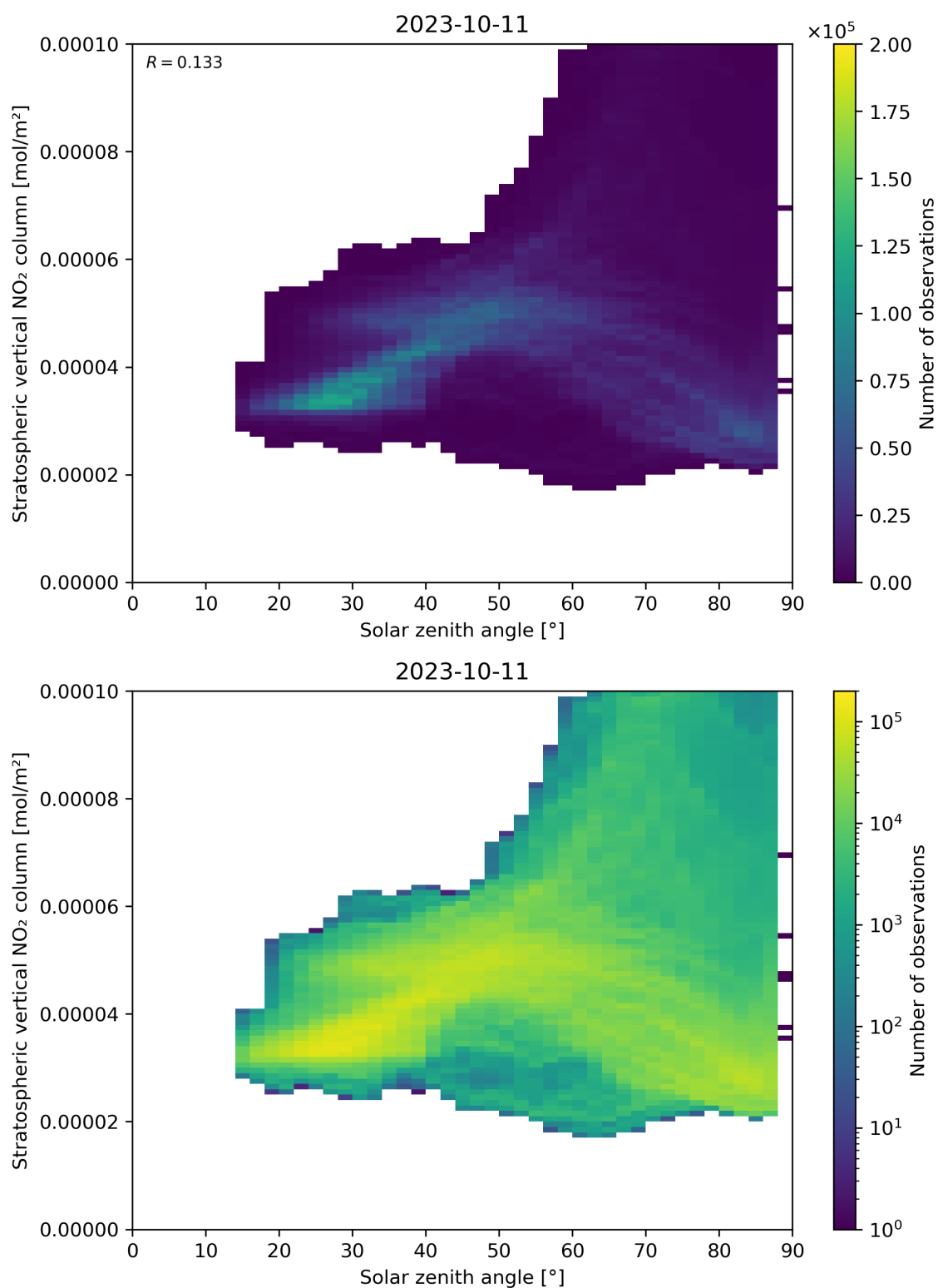
Figure 150: Scatter density plot of “Solar zenith angle” against “Stratospheric vertical NO 2 column” for 2023-10-10 to 2023-10-12.
