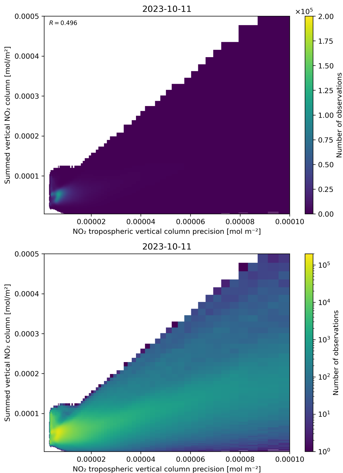
Figure 136: Scatter density plot of “NO 2 tropospheric vertical column precision” against “Summed vertical NO 2 column” for 2023-10-10 to 2023-10-12.
