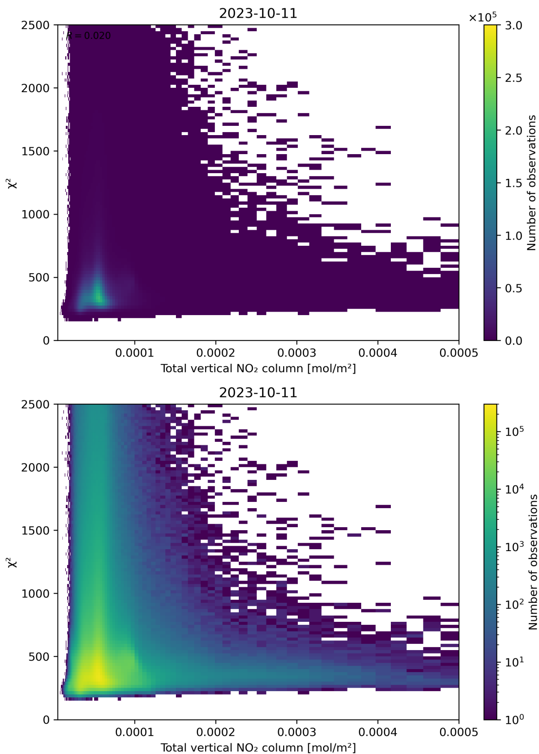
Figure 111: Scatter density plot of “Total vertical NO 2 column” against “ \chi^2 ” for 2023-10-10 to 2023-10-12.
