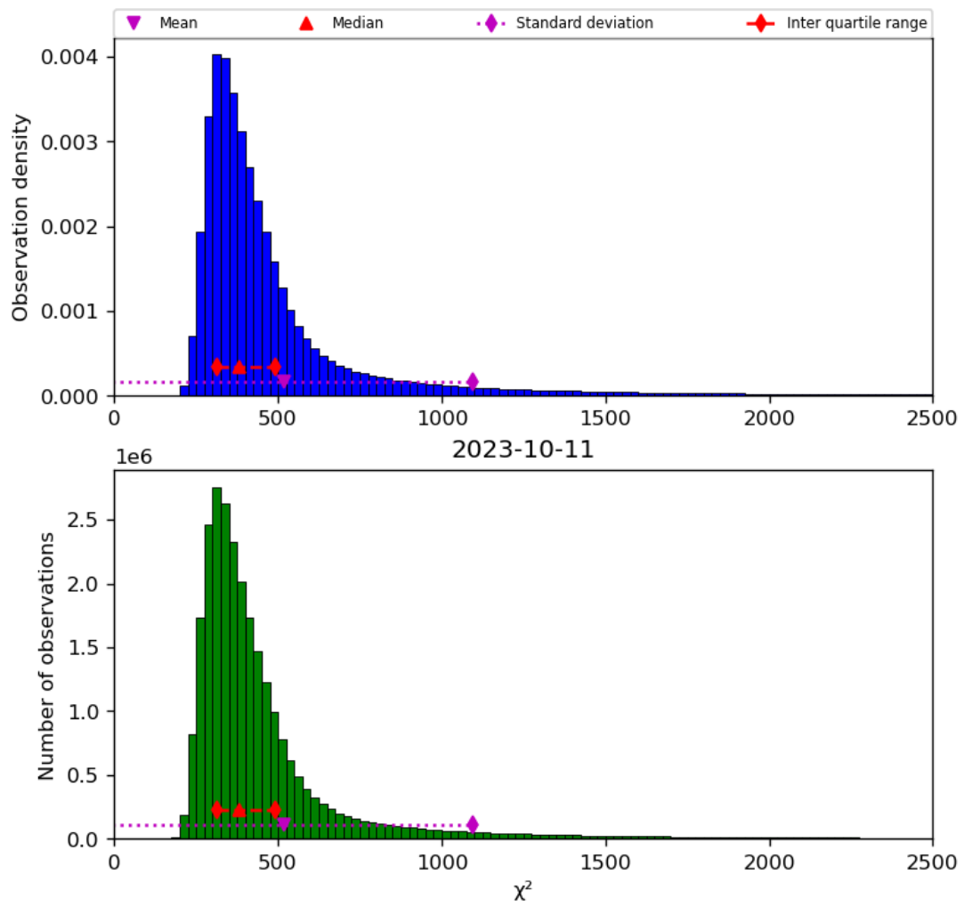
Figure 42: Histogram of “ \chi^2 ” for 2023-10-10 to 2023-10-12
