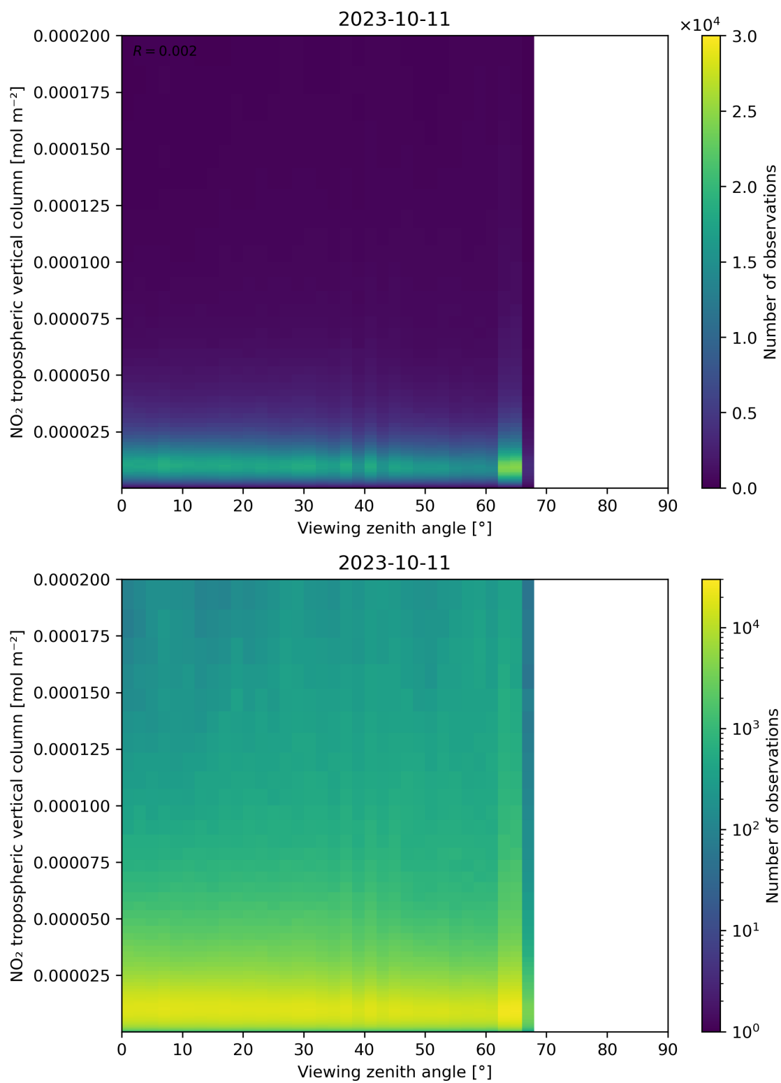
Figure 169: Scatter density plot of “Viewing zenith angle” against “NO 2 tropospheric vertical column” for 2023-10-10 to 2023-10-12.
