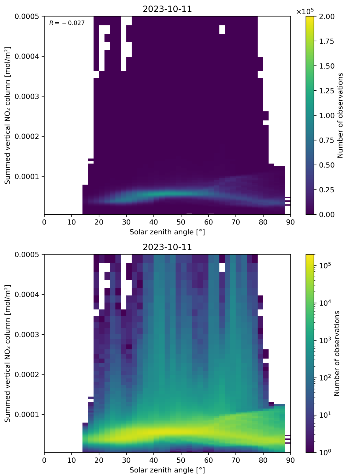
Figure 151: Scatter density plot of “Solar zenith angle” against “Summed vertical NO 2 column” for 2023-10-10 to 2023-10-12.
