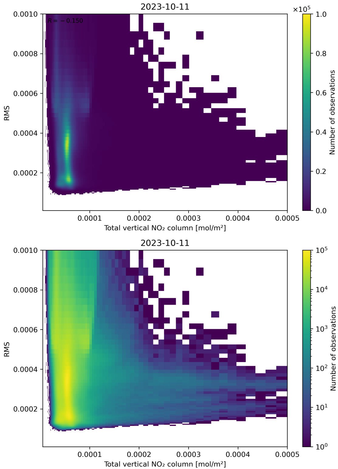
Figure 120: Scatter density plot of “Total vertical NO 2 column” against “RMS” for 2023-10-10 to 2023-10-12.
