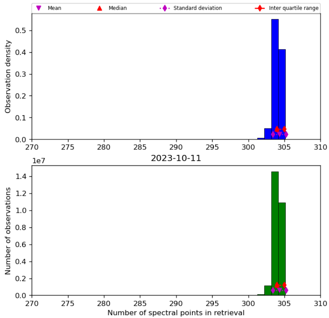
Figure 33: Histogram of “Number of spectral points in retrieval” for 2023-10-10 to 2023-10-12
