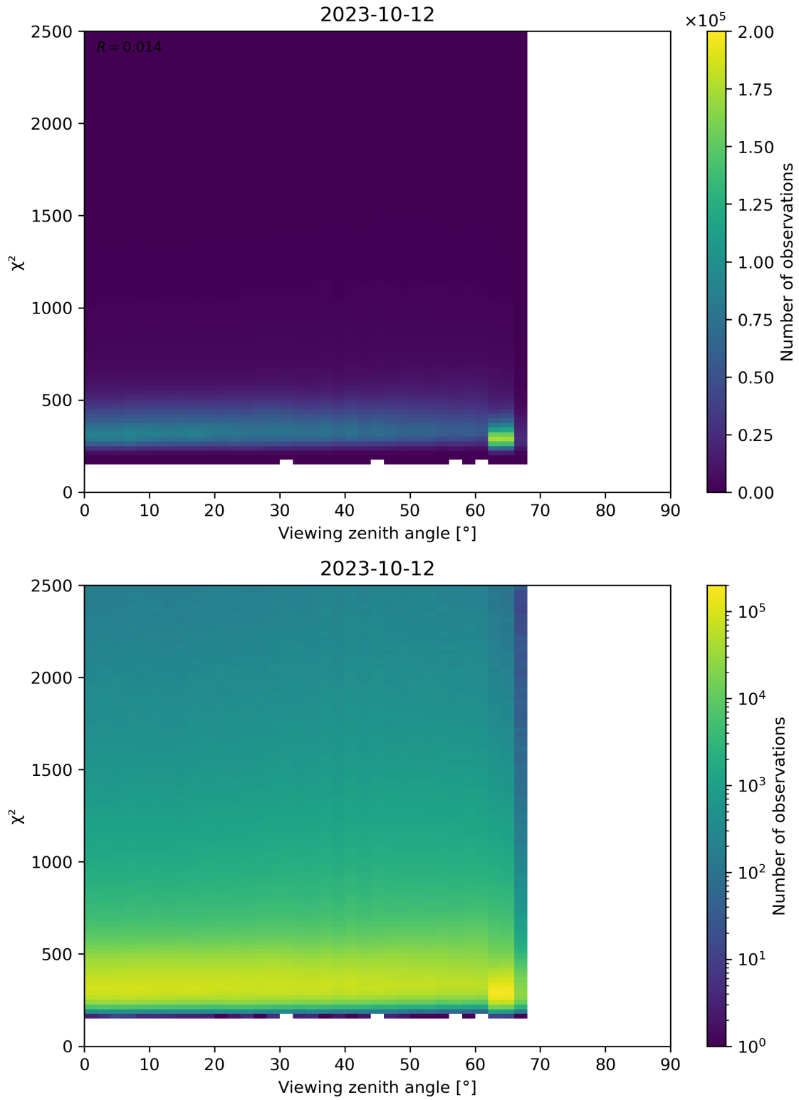
Figure 162: Scatter density plot of “Viewing zenith angle” against “ \chi^2 ” for 2023-10-12 to 2023-10-13.
