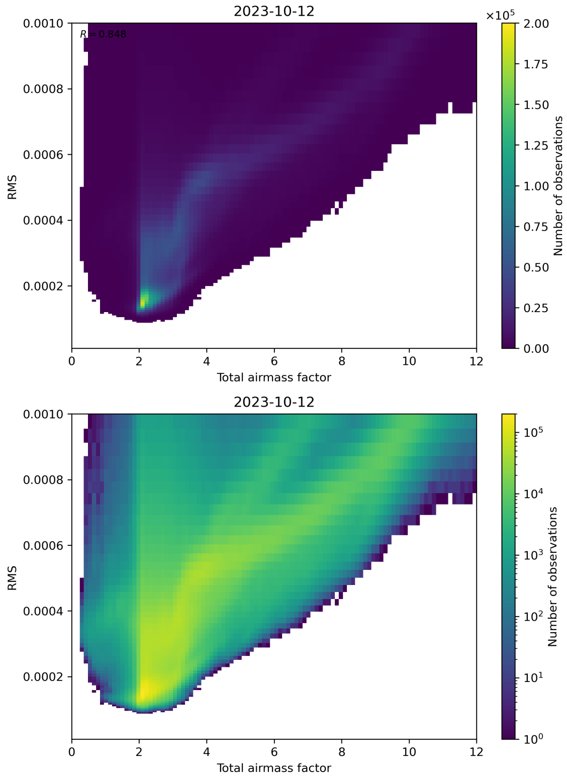
Figure 69: Scatter density plot of “Total airmass factor” against “RMS” for 2023-10-12 to 2023-10-13.
