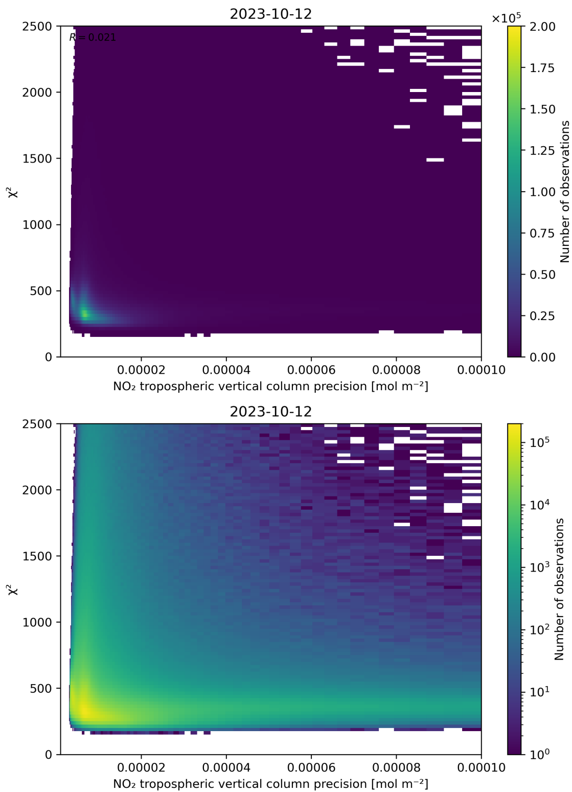
Figure 134: Scatter density plot of “NO 2 tropospheric vertical column precision” against “ \chi^2 ” for 2023-10-12 to 2023-10-13.
