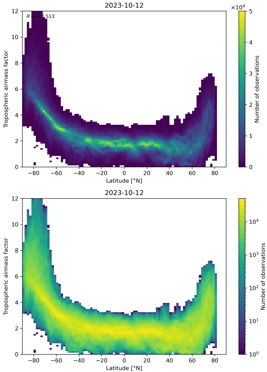
Figure 85: Scatter density plot of “Latitude” against “Tropospheric airmass factor” for 2023-10-12 to 2023-10-13.
