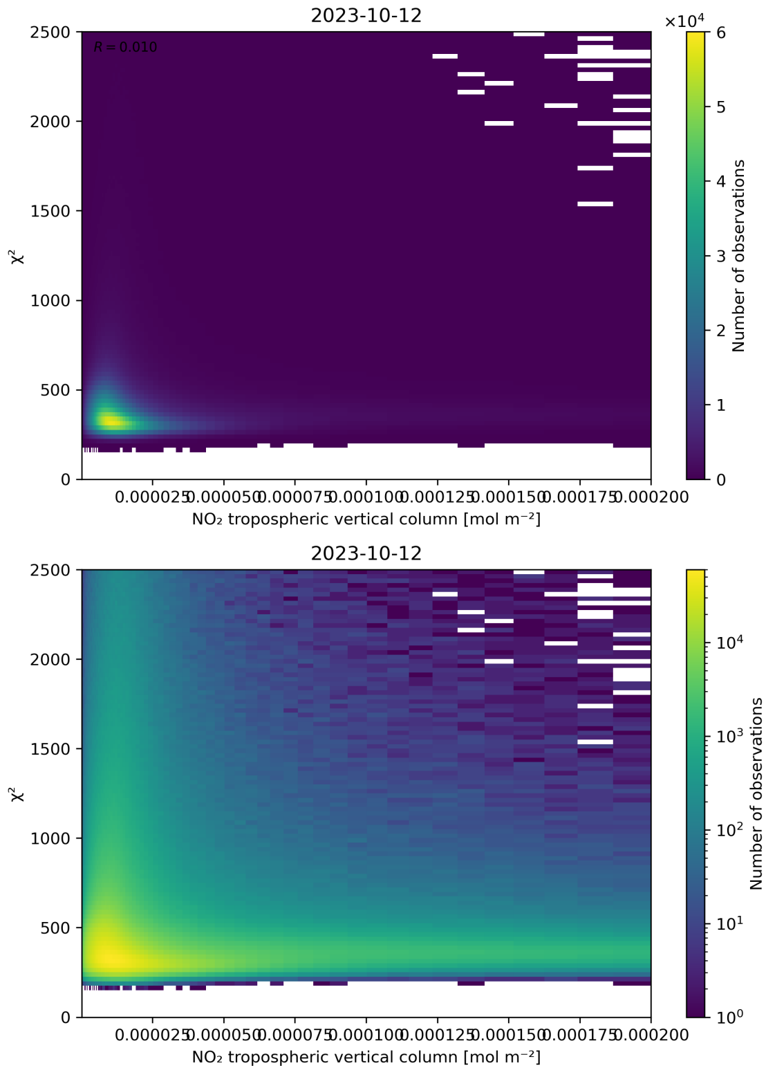
Figure 124: Scatter density plot of “NO 2 tropospheric vertical column” against “ \chi^2 ” for 2023-10-12 to 2023-10-13.
