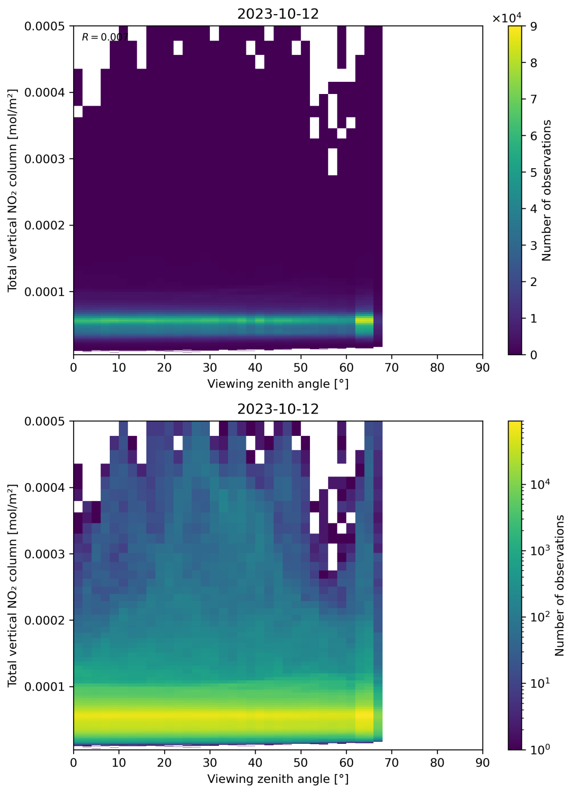
Figure 167: Scatter density plot of “Viewing zenith angle” against “Total vertical NO 2 column” for 2023-10-12 to 2023-10-13.
