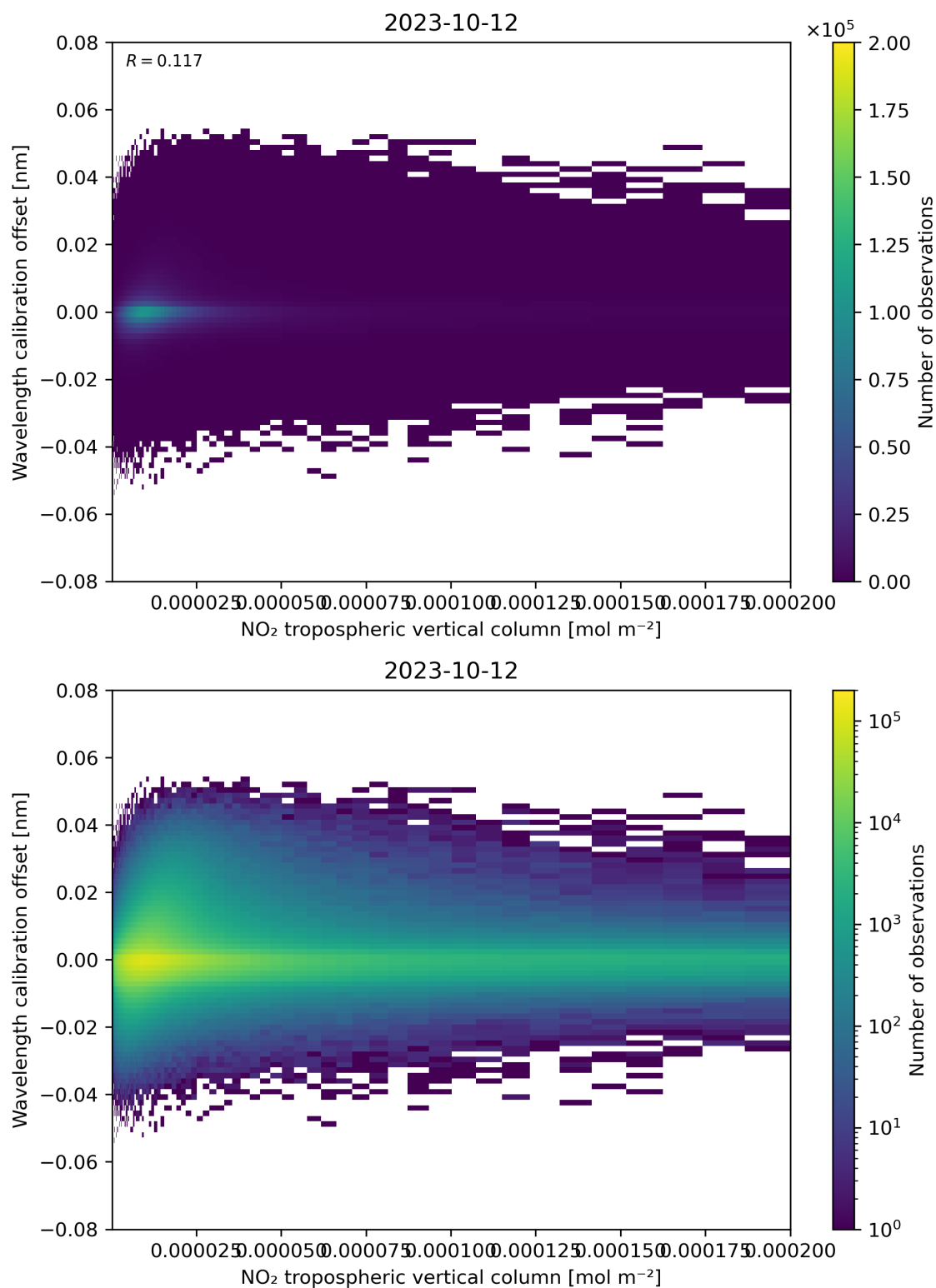
Figure 143: Scatter density plot of “NO 2 tropospheric vertical column” against “Wavelength calibration offset” for 2023-10-12 to 2023-10-13.
