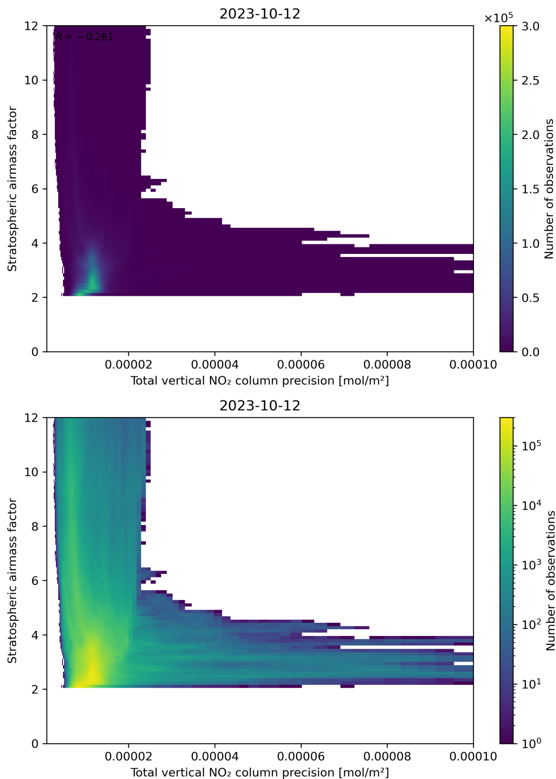
Figure 115: Scatter density plot of “Total vertical NO 2 column precision” against “Stratospheric air mass factor” for 2023-10-12 to 2023-10-13.
