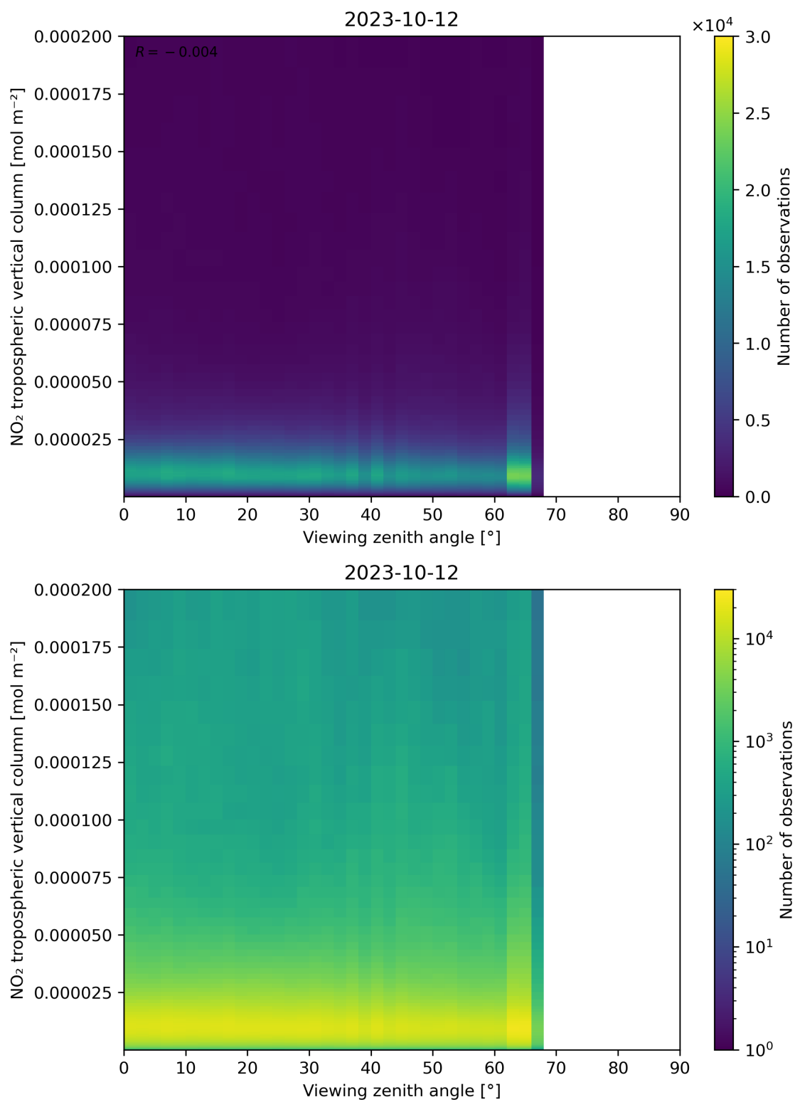
Figure 169: Scatter density plot of “Viewing zenith angle” against “NO 2 tropospheric vertical column” for 2023-10-12 to 2023-10-13.
