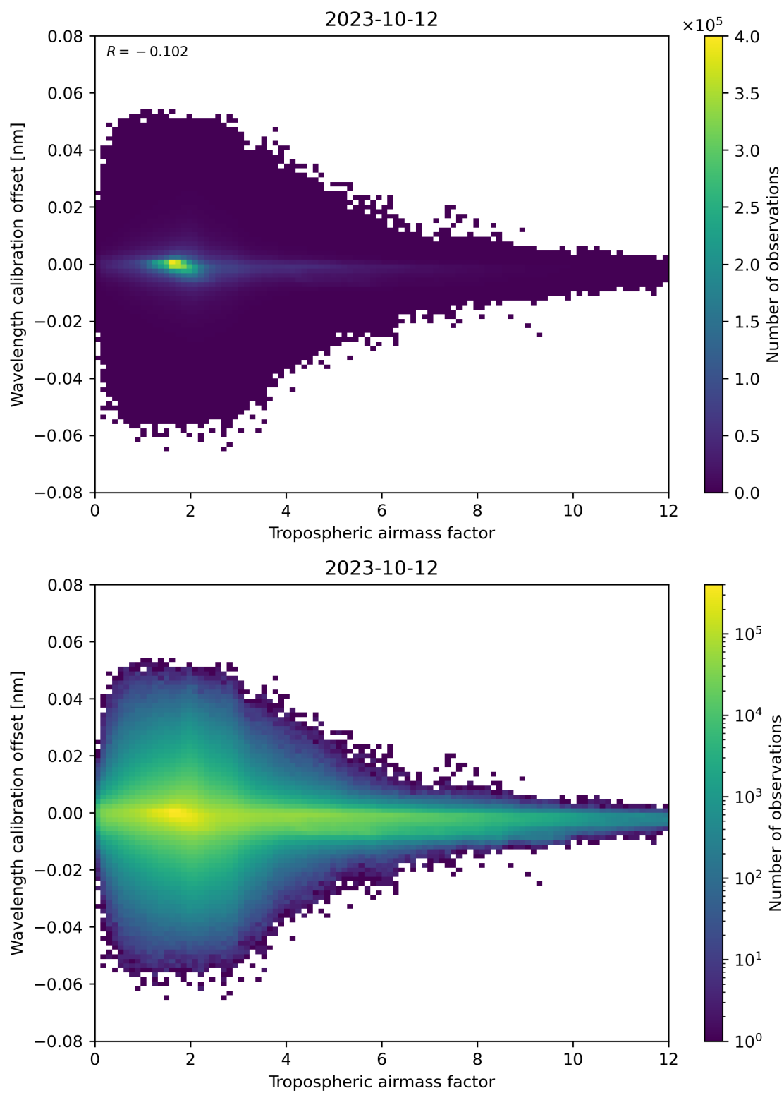
Figure 80: Scatter density plot of “Tropospheric airmass factor” against “Wavelength calibration offset” for 2023-10-12 to 2023-10-13.
