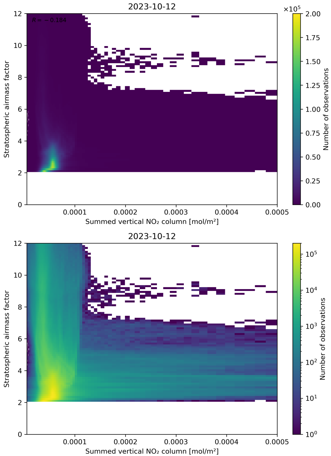
Figure 103: Scatter density plot of “Summed vertical NO 2 column” against “Stratospheric air mass factor” for 2023-10-12 to 2023-10-13.
