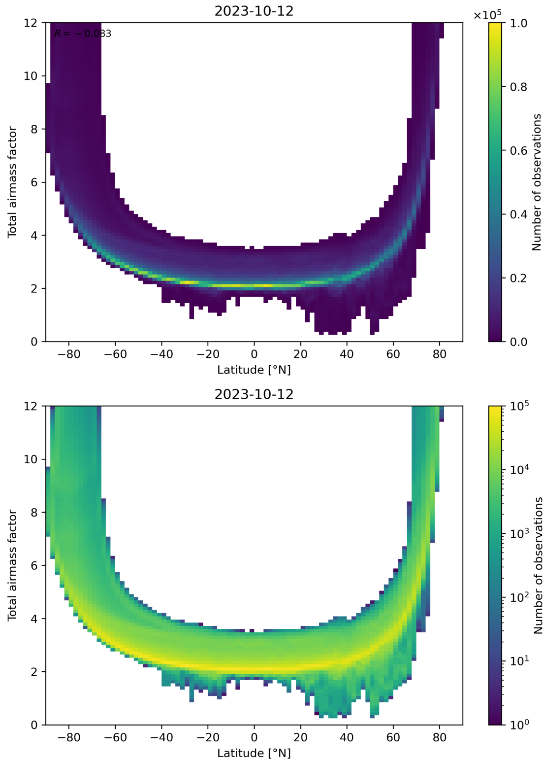
Figure 84: Scatter density plot of “Latitude” against “Total airmass factor” for 2023-10-12 to 2023-10-13.
