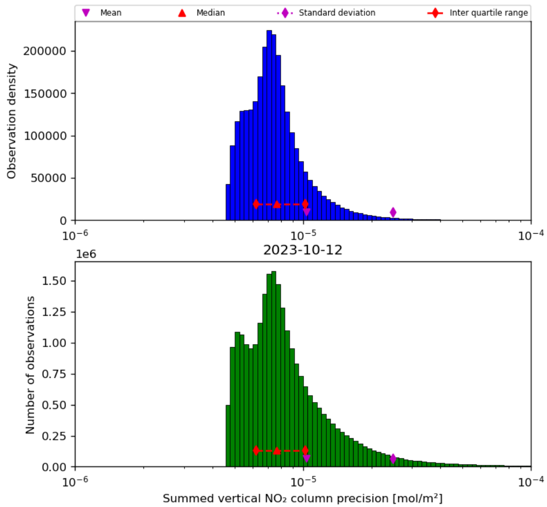
Figure 41: Histogram of “Summed vertical NO 2 column precision” for 2023-10-12 to 2023-10-13
