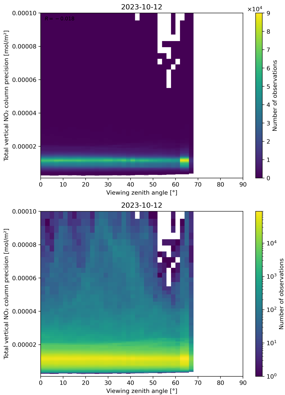
Figure 168: Scatter density plot of “Viewing zenith angle” against “Total vertical NO 2 column precision” for 2023-10-12 to 2023-10-13.
