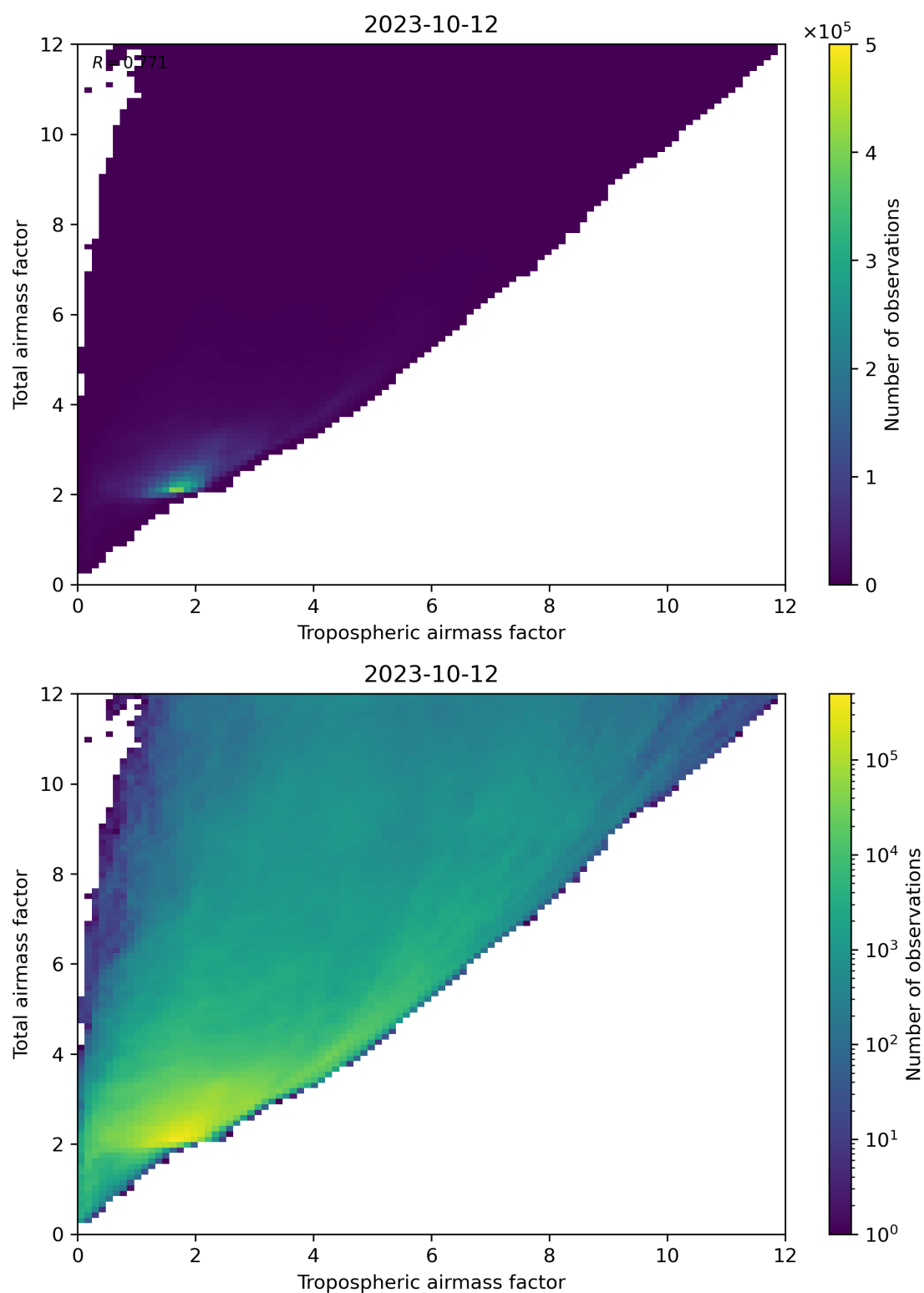
Figure 72: Scatter density plot of “Tropospheric airmass factor” against “Total airmass factor” for 2023-10-12 to 2023-10-13.
