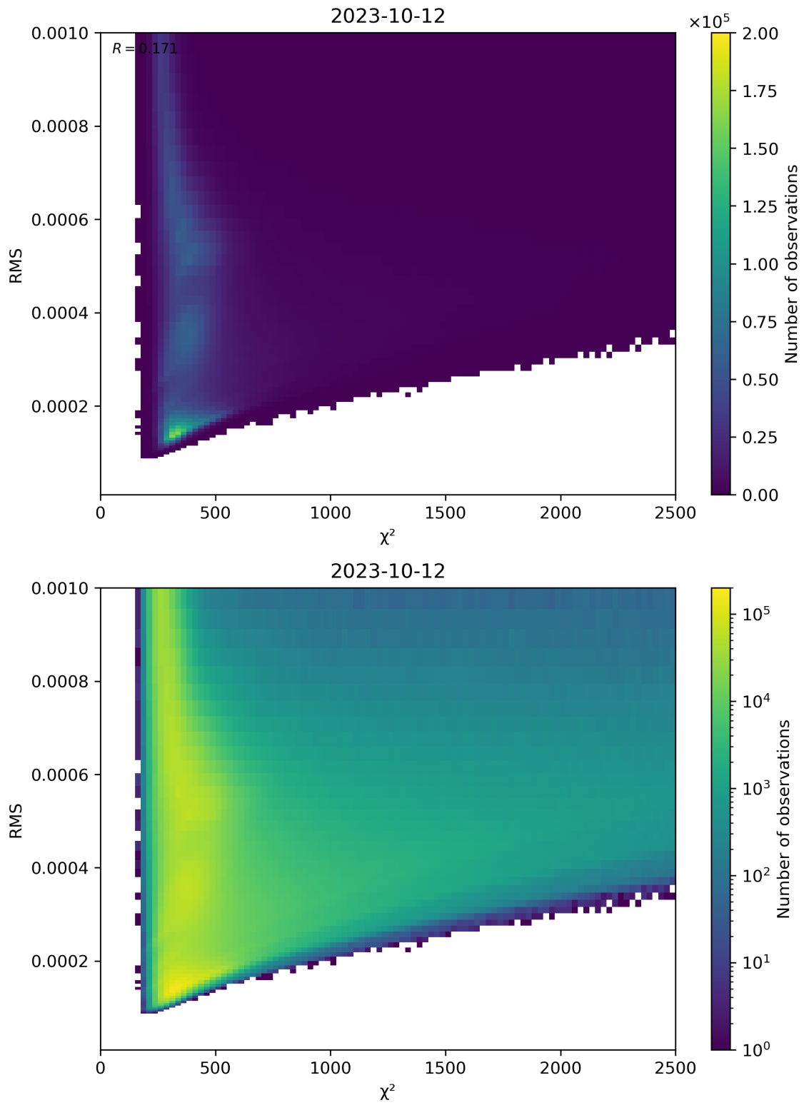
Figure 82: Scatter density plot of “ \chi^2 ” against “RMS” for 2023-10-12 to 2023-10-13.
