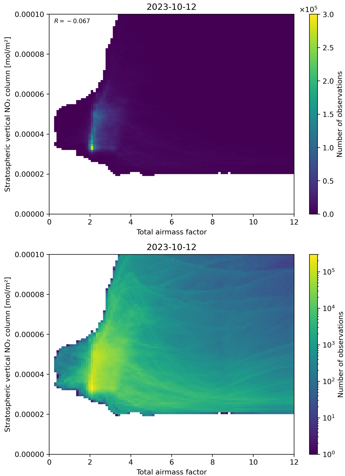
Figure 64: Scatter density plot of “Total airmass factor” against “Stratospheric vertical NO 2 column” for 2023-10-12 to 2023-10-13.
