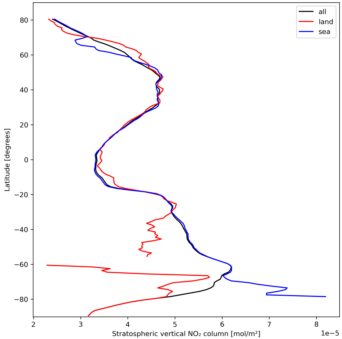
Figure 19: Zonal average of “Stratospheric vertical NO 2 column” for 2023-10-12 to 2023-10-13.
