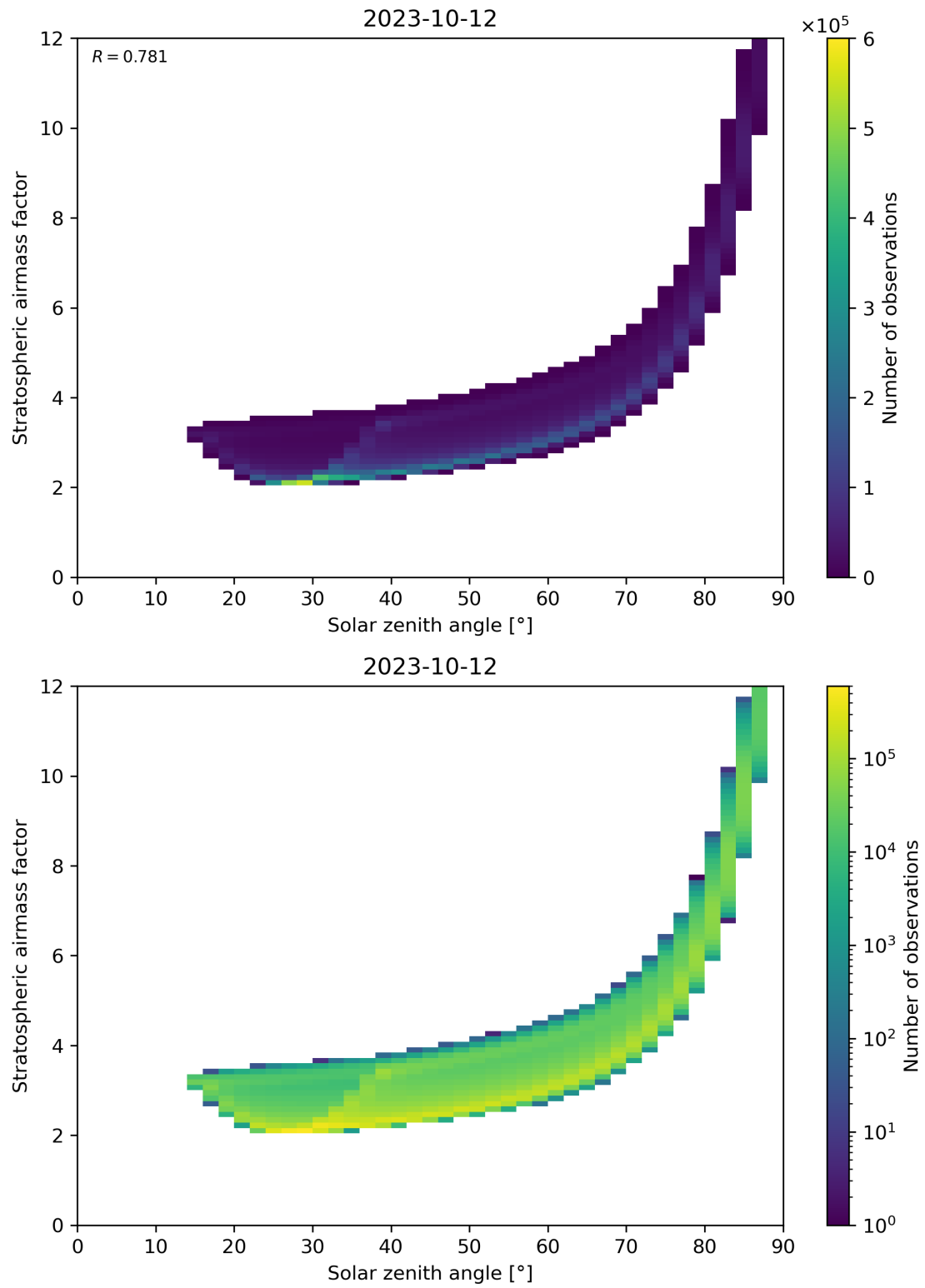
Figure 145: Scatter density plot of “Solar zenith angle” against “Stratospheric airmass factor” for 2023-10-12 to 2023-10-13.
