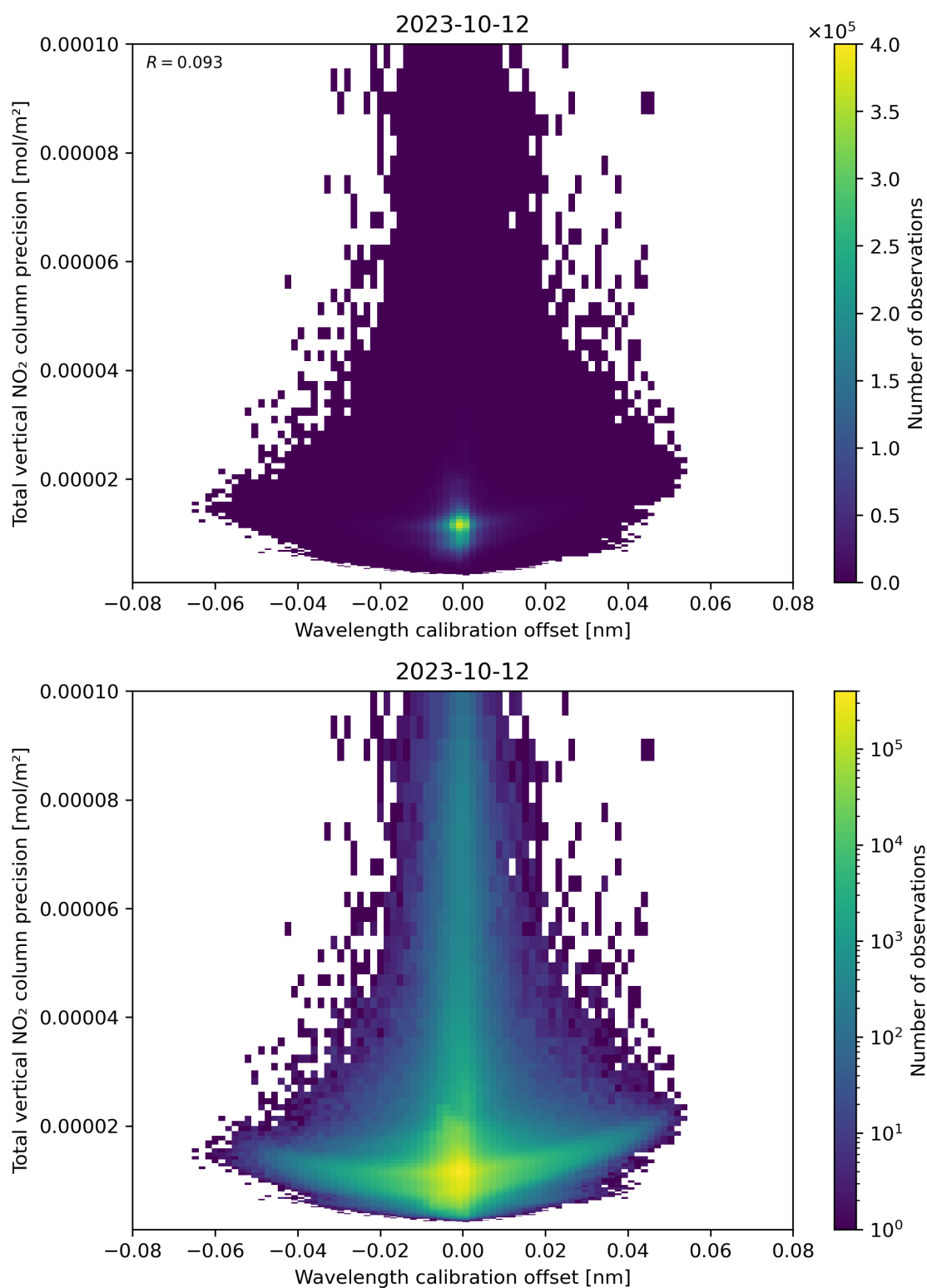
Figure 180: Scatter density plot of “Wavelength calibration offset” against “Total vertical NO 2 column precision” for 2023-10-12 to 2023-10-13.
