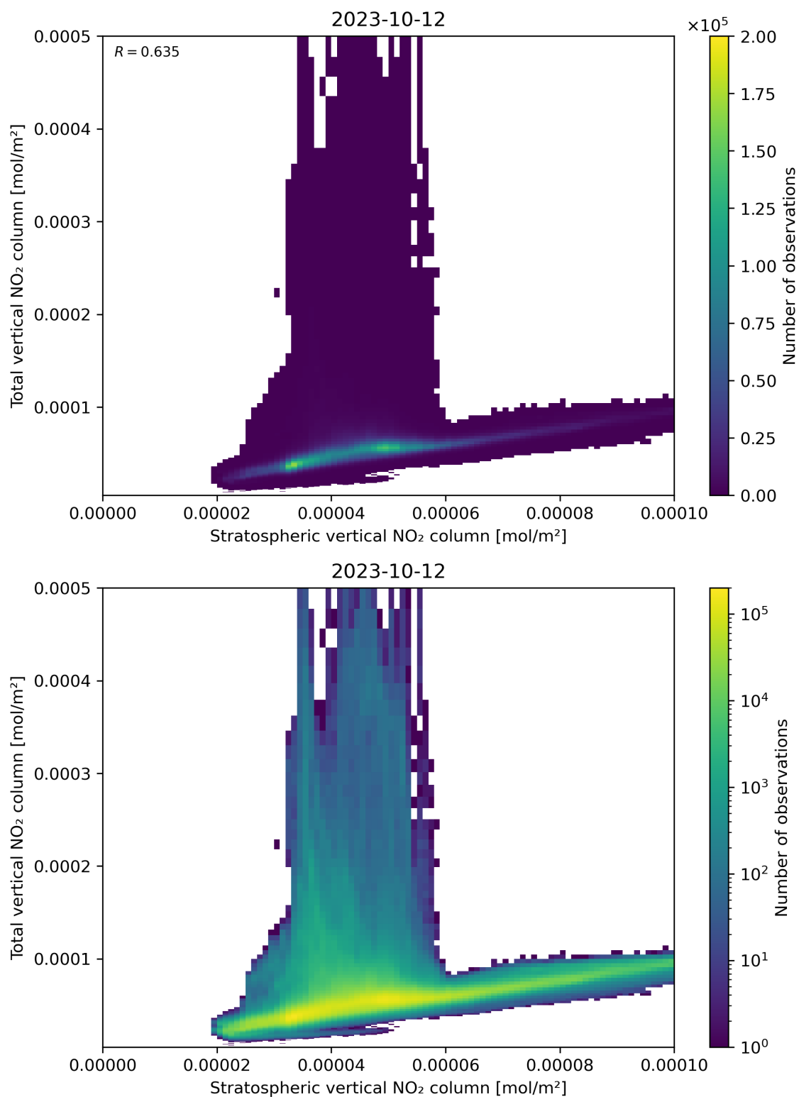
Figure 100: Scatter density plot of “Stratospheric vertical NO 2 column” against “Total vertical NO 2 column” for 2023-10-12 to 2023-10-13.
