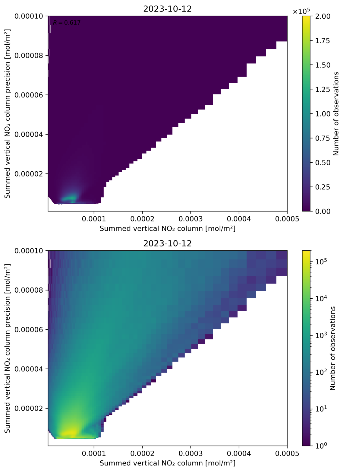
Figure 105: Scatter density plot of “Summed vertical NO 2 column” against “Summed vertical NO 2 column precision” for 2023-10-12 to 2023-10-13.
