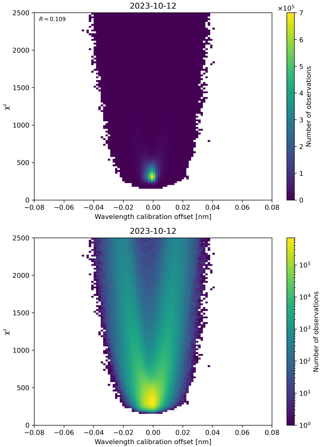
Figure 175: Scatter density plot of “Wavelength calibration offset” against “ \chi^2 ” for 2023-10-12 to 2023-10-13.
