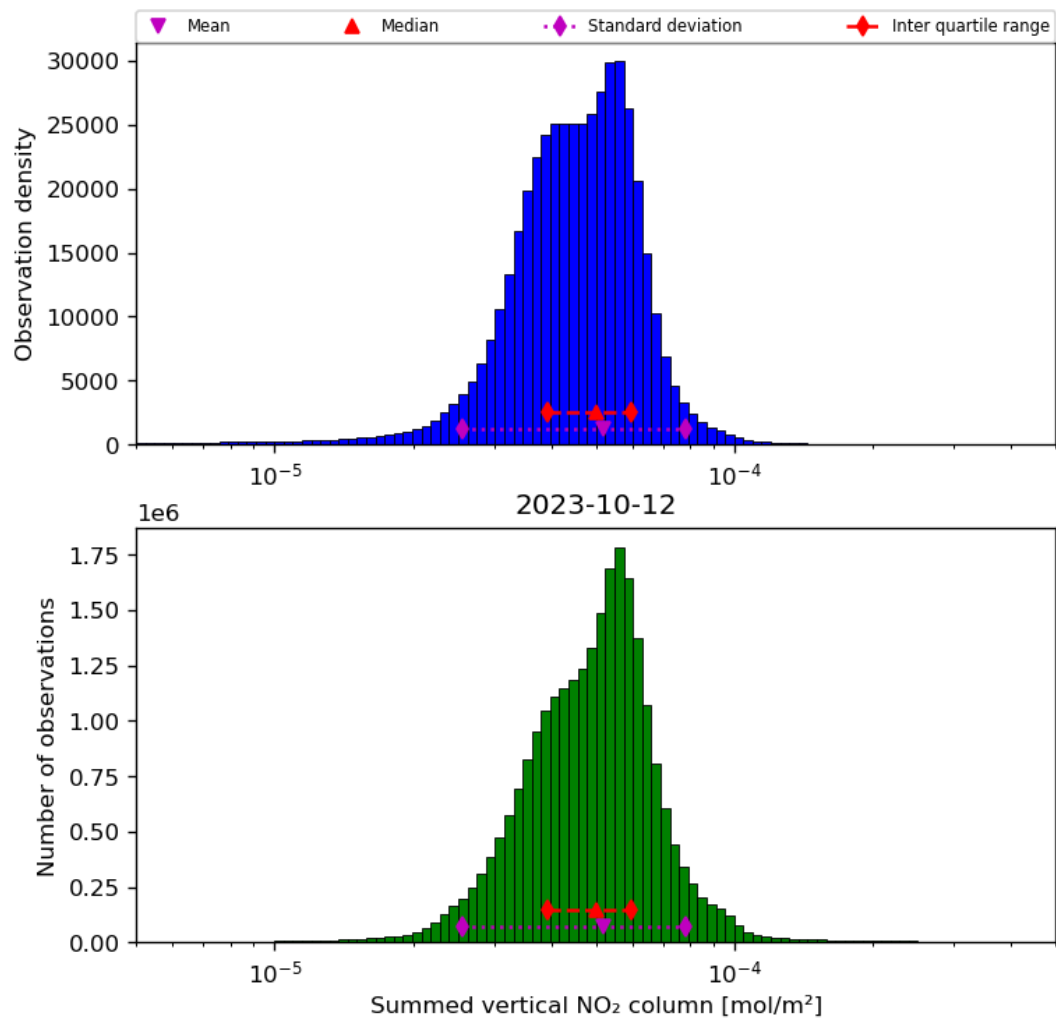
Figure 40: Histogram of “Summed vertical NO 2 column” for 2023-10-12 to 2023-10-13
