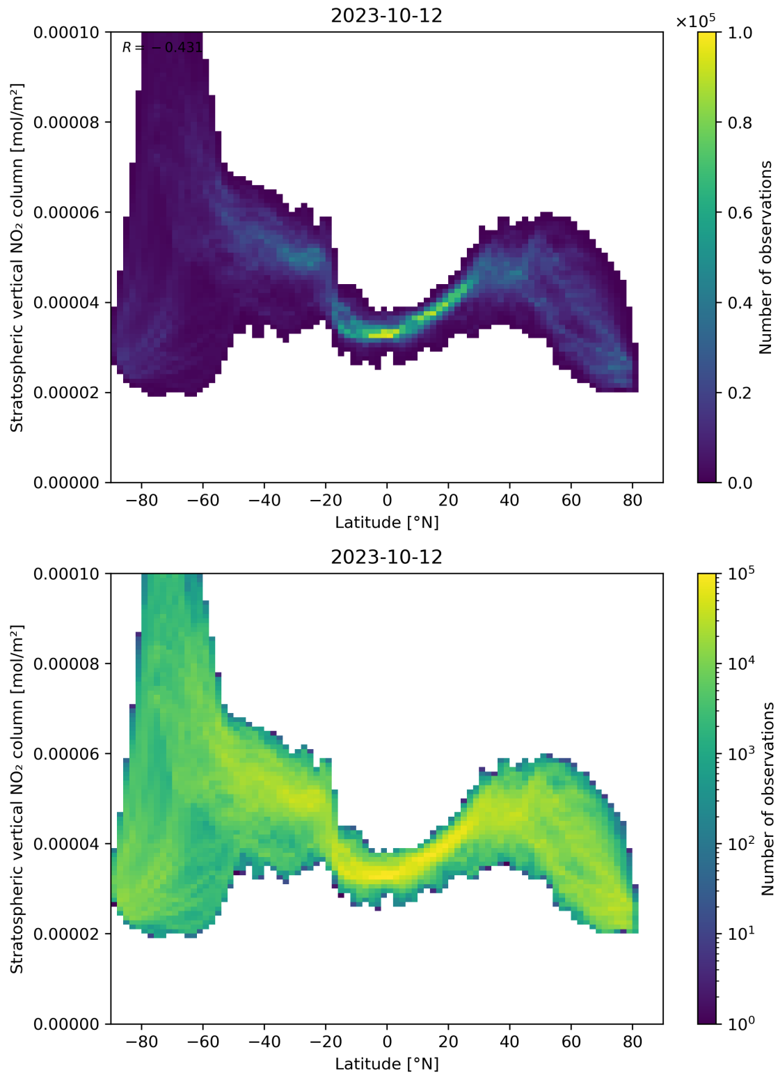
Figure 87: Scatter density plot of “Latitude” against “Stratospheric vertical NO 2 column” for 2023-10-12 to 2023-10-13.
