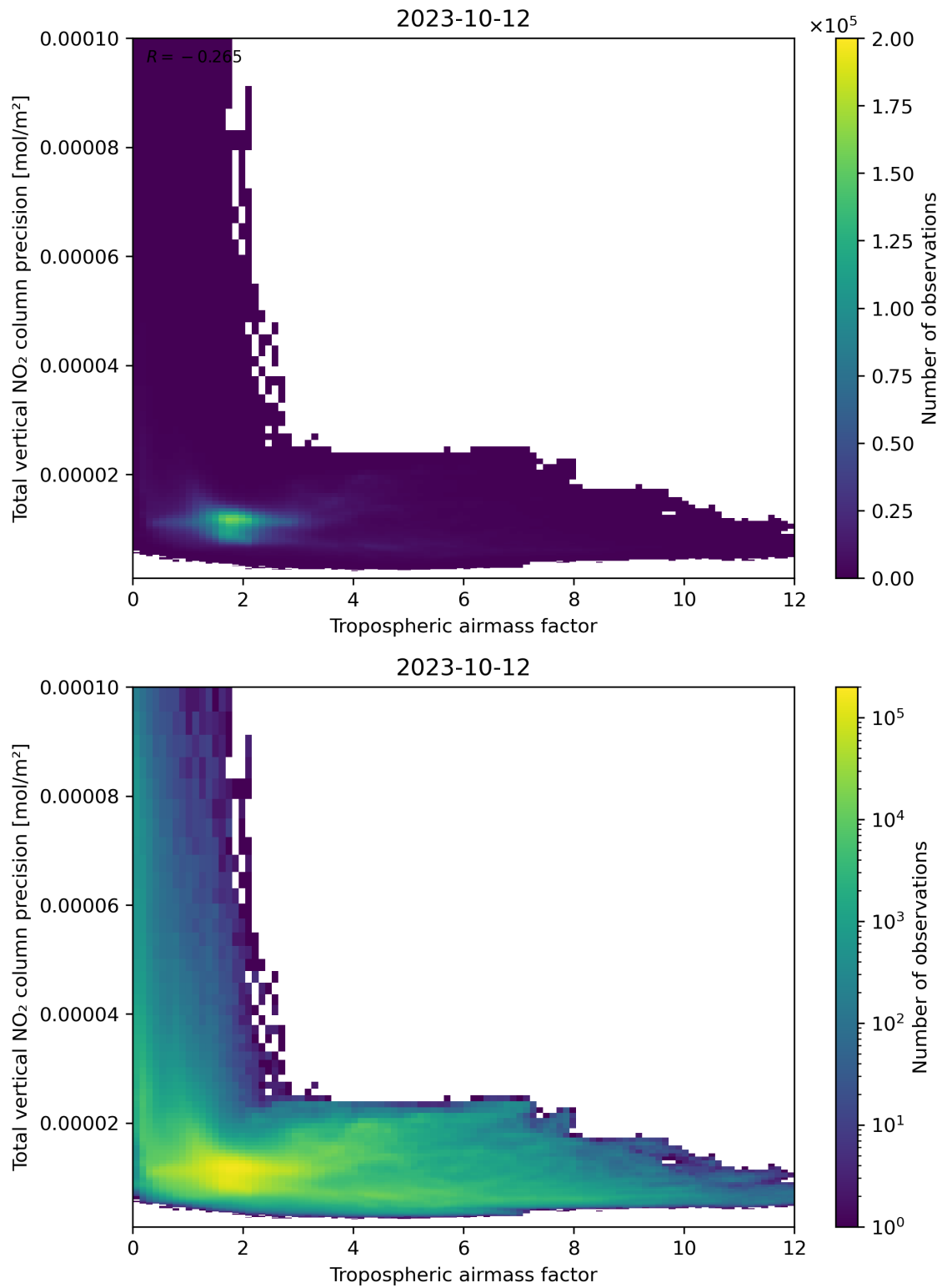
Figure 78: Scatter density plot of “Tropospheric air mass factor” against “Total vertical NO 2 column precision” for 2023-10-12 to 2023-10-13.
