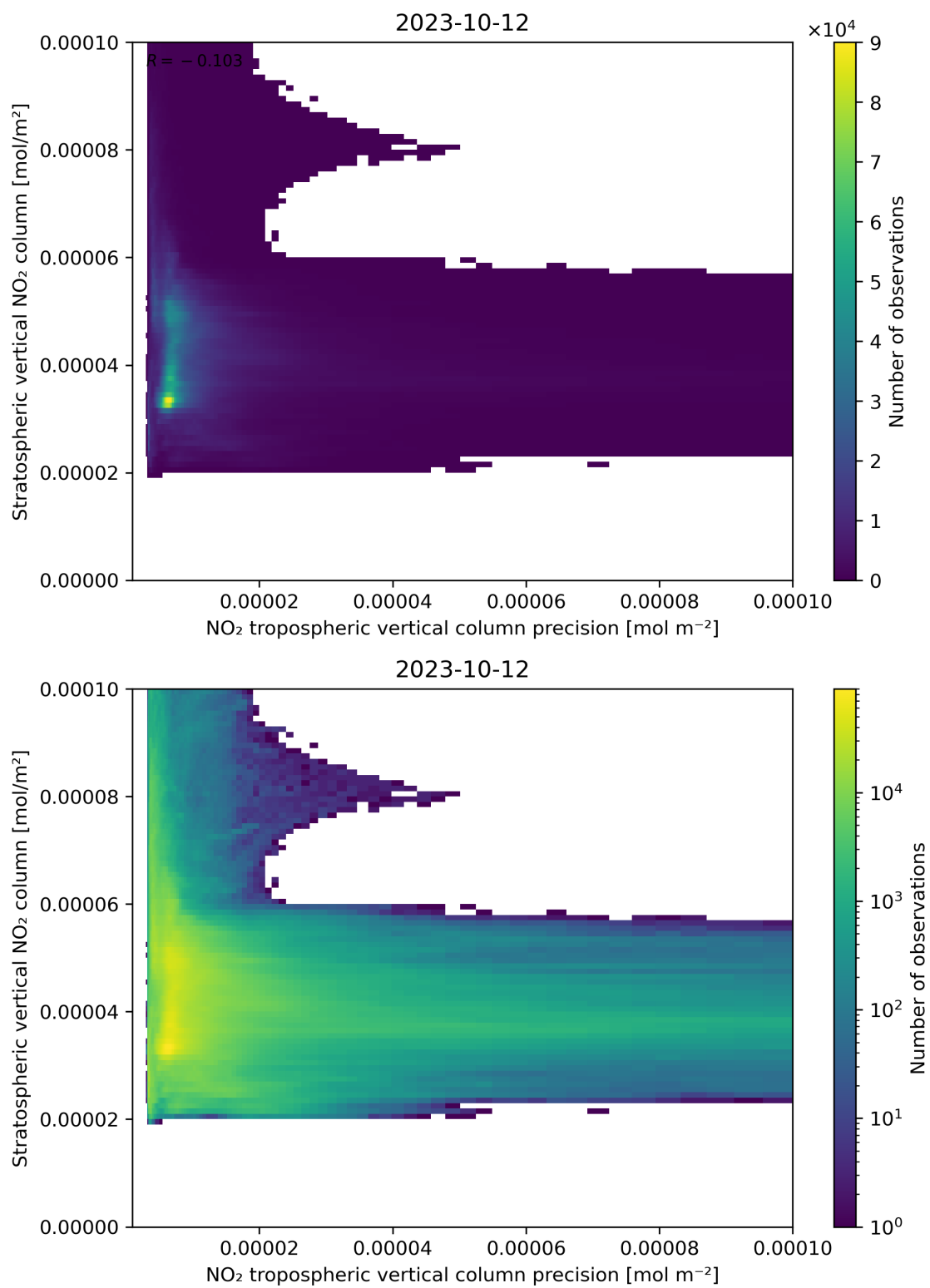
Figure 135: Scatter density plot of “NO 2 tropospheric vertical column precision” against “Stratospheric vertical NO 2 column” for 2023-10-12 to 2023-10-13.
