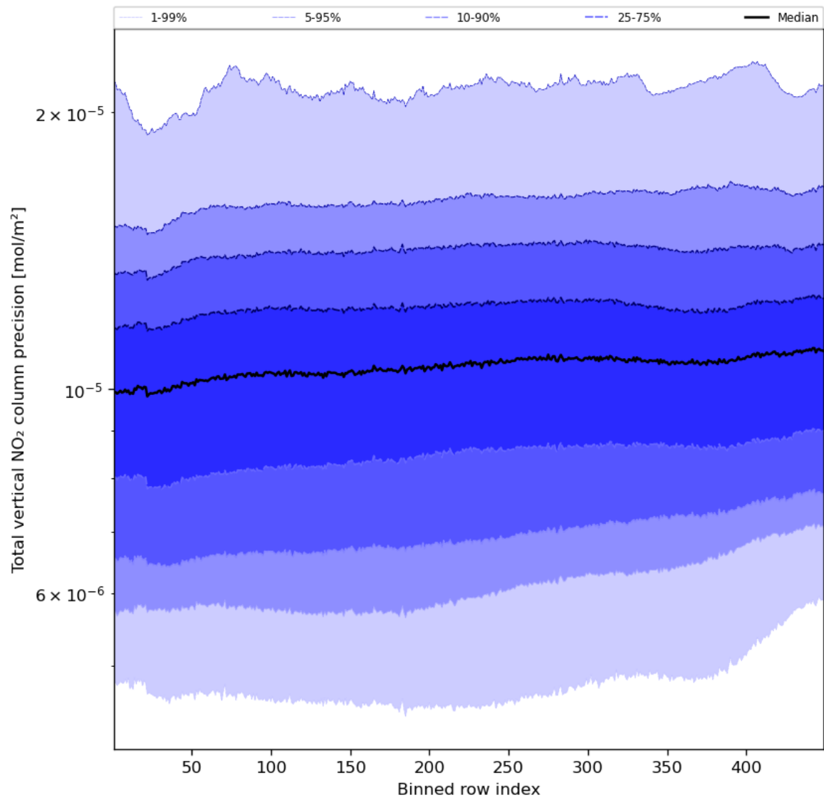
Figure 56: Along track statistics of “Total vertical NO 2 column precision” for 2023-10-12 to 2023-10-13
