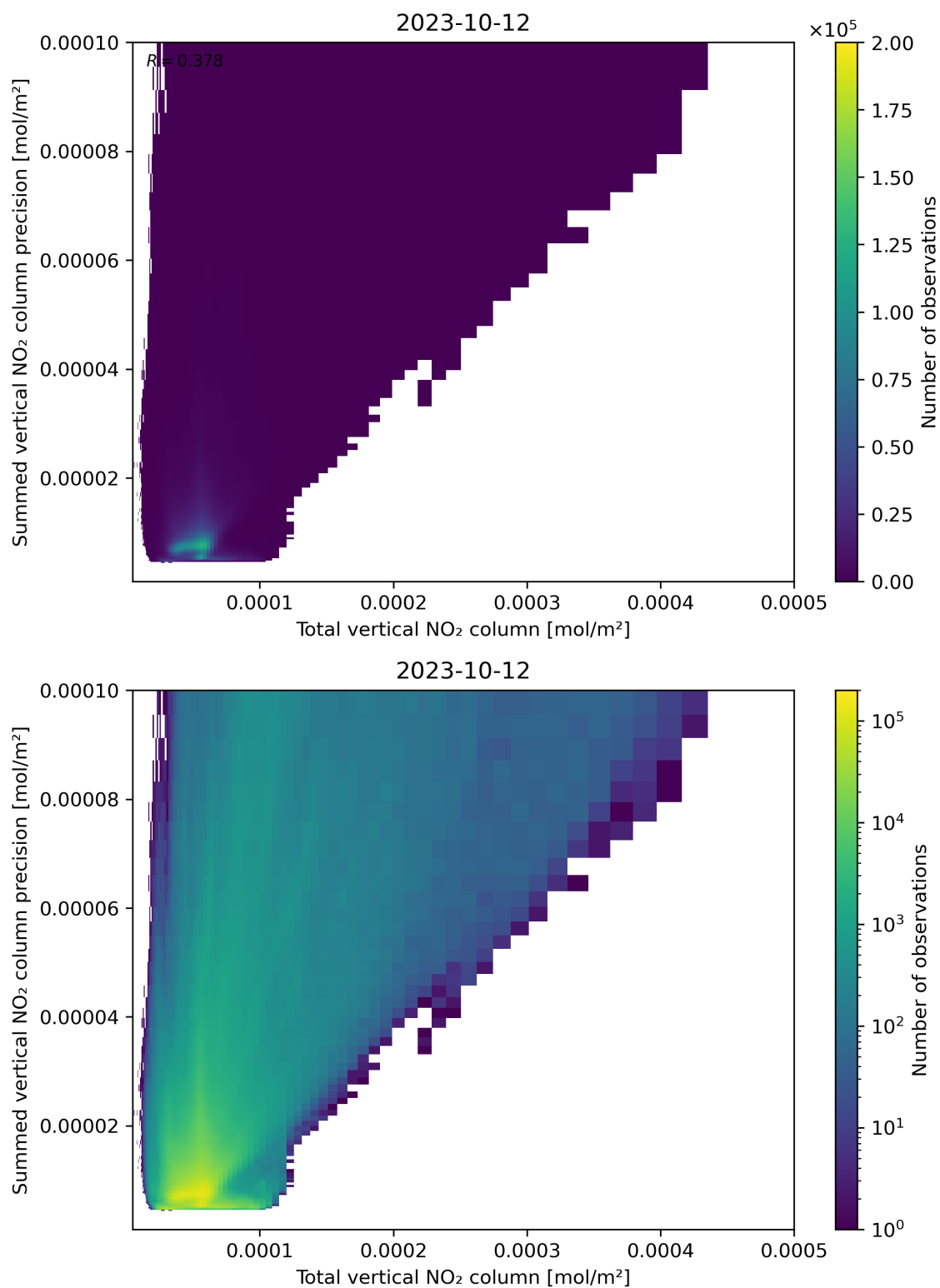
Figure 113: Scatter density plot of “Total vertical NO 2 column” against “Summed vertical NO 2 column precision” for 2023-10-12 to 2023-10-13.
