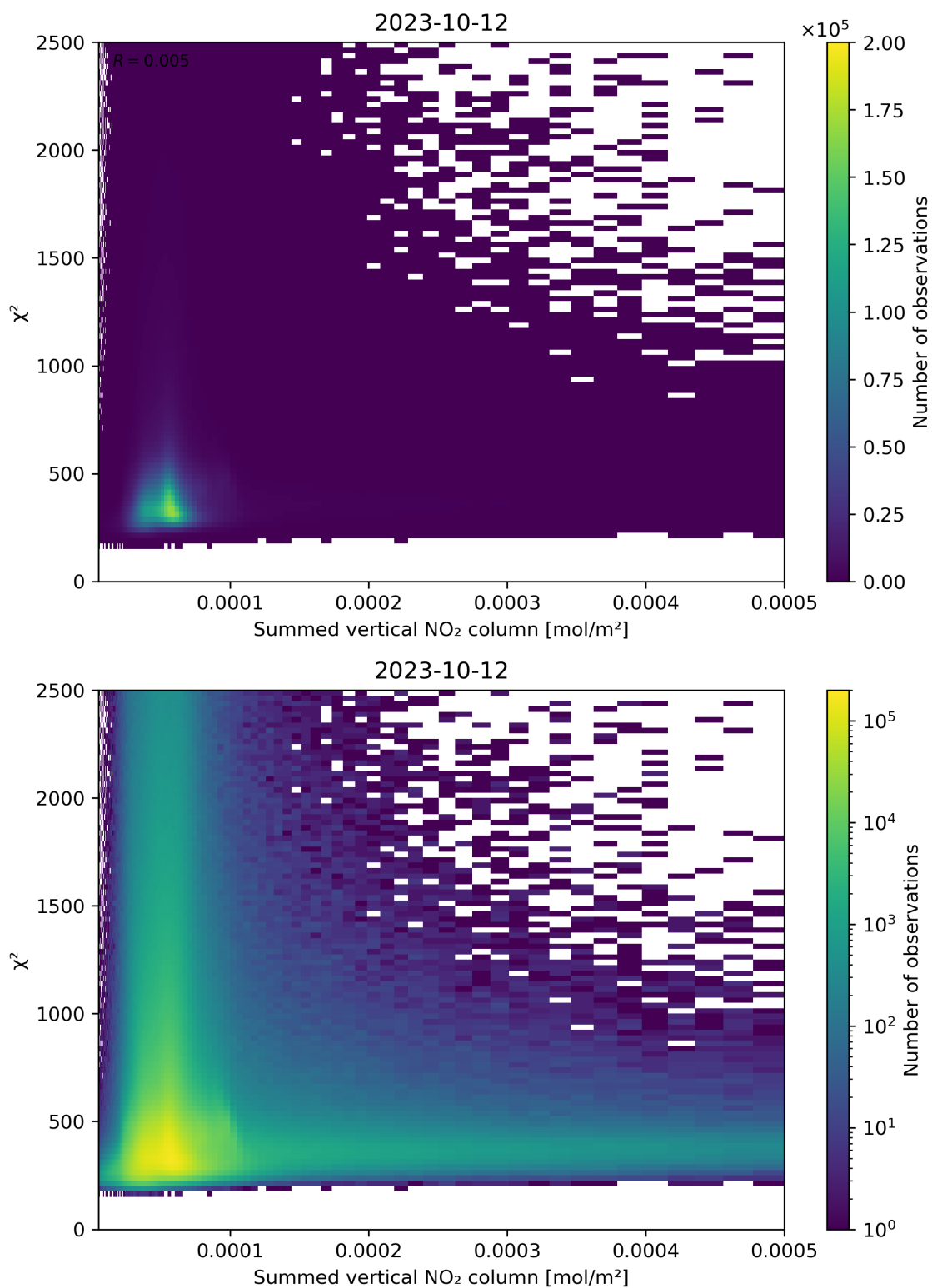
Figure 104: Scatter density plot of “Summed vertical NO 2 column” against “ \chi^2 ” for 2023-10-12 to 2023-10-13.
