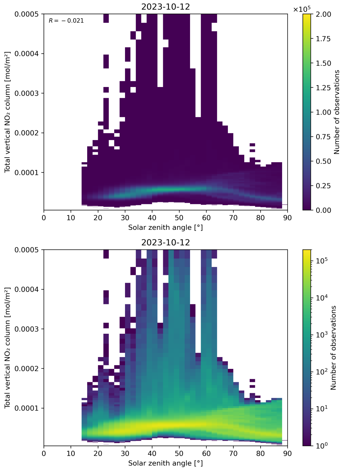
Figure 153: Scatter density plot of “Solar zenith angle” against “Total vertical NO 2 column” for 2023-10-12 to 2023-10-13.
