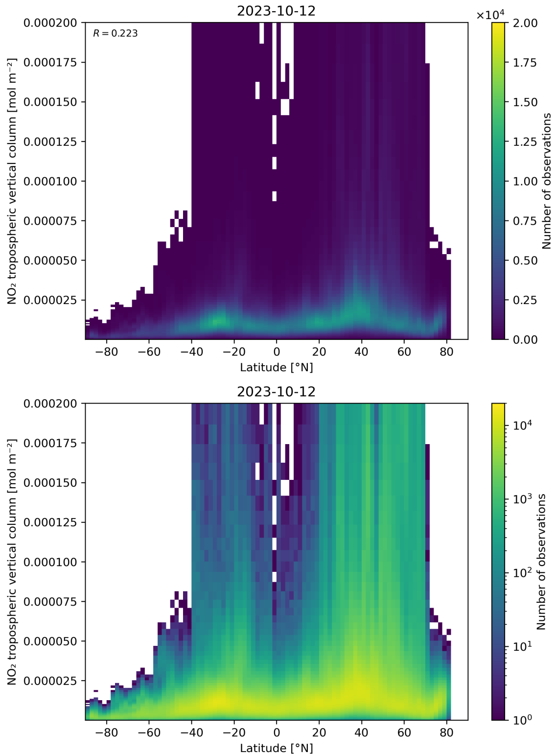
Figure 92: Scatter density plot of “Latitude” against “NO 2 tropospheric vertical column” for 2023-10-12 to 2023-10-13.
