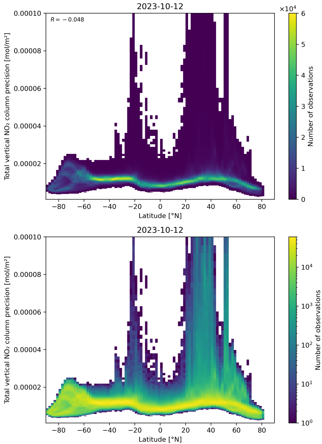
Figure 91: Scatter density plot of “Latitude” against “Total vertical NO 2 column precision” for 2023-10-12 to 2023-10-13.
