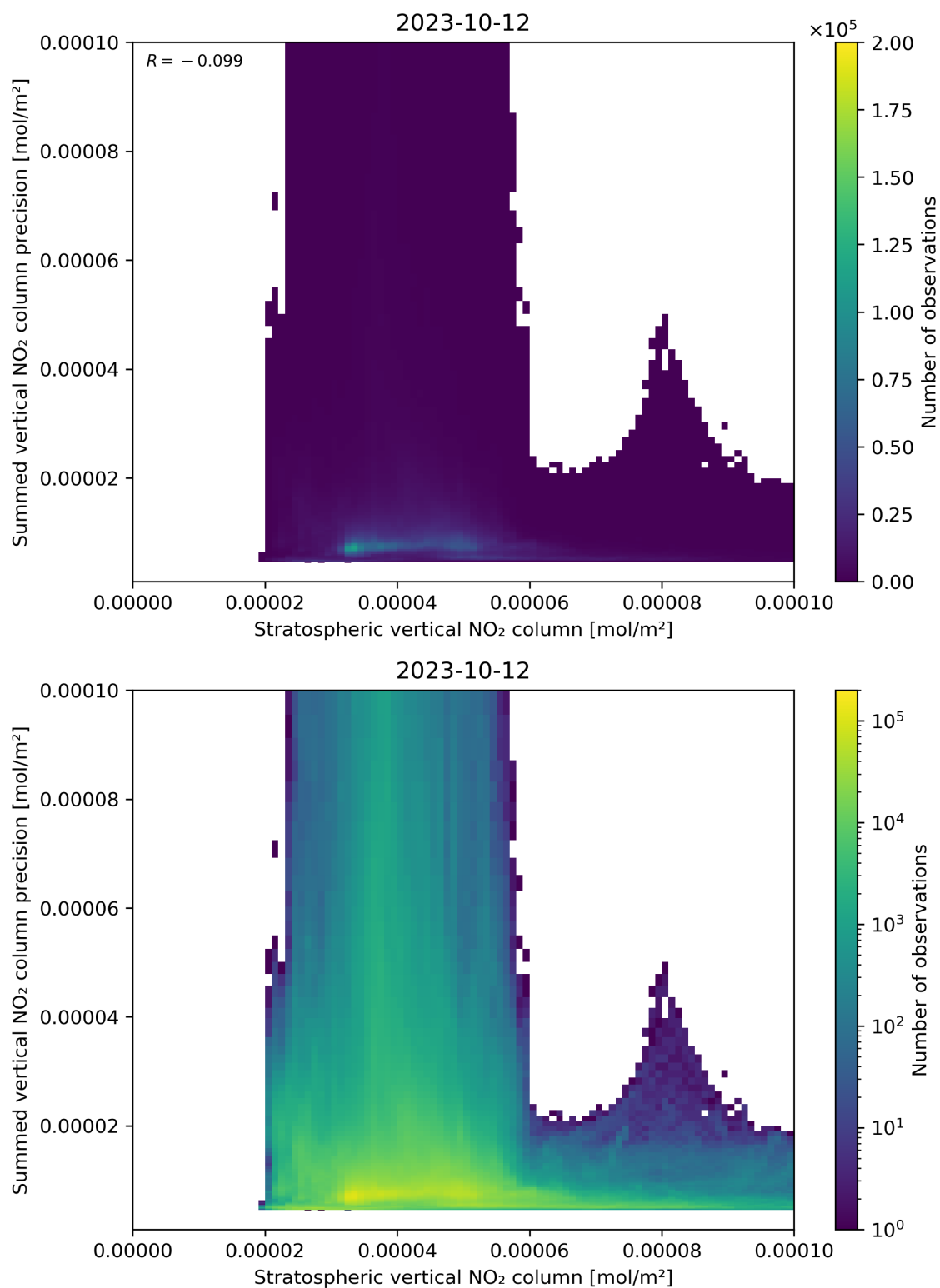
Figure 99: Scatter density plot of “Stratospheric vertical NO 2 column” against “Summed vertical NO 2 column precision” for 2023-10-12 to 2023-10-13.
