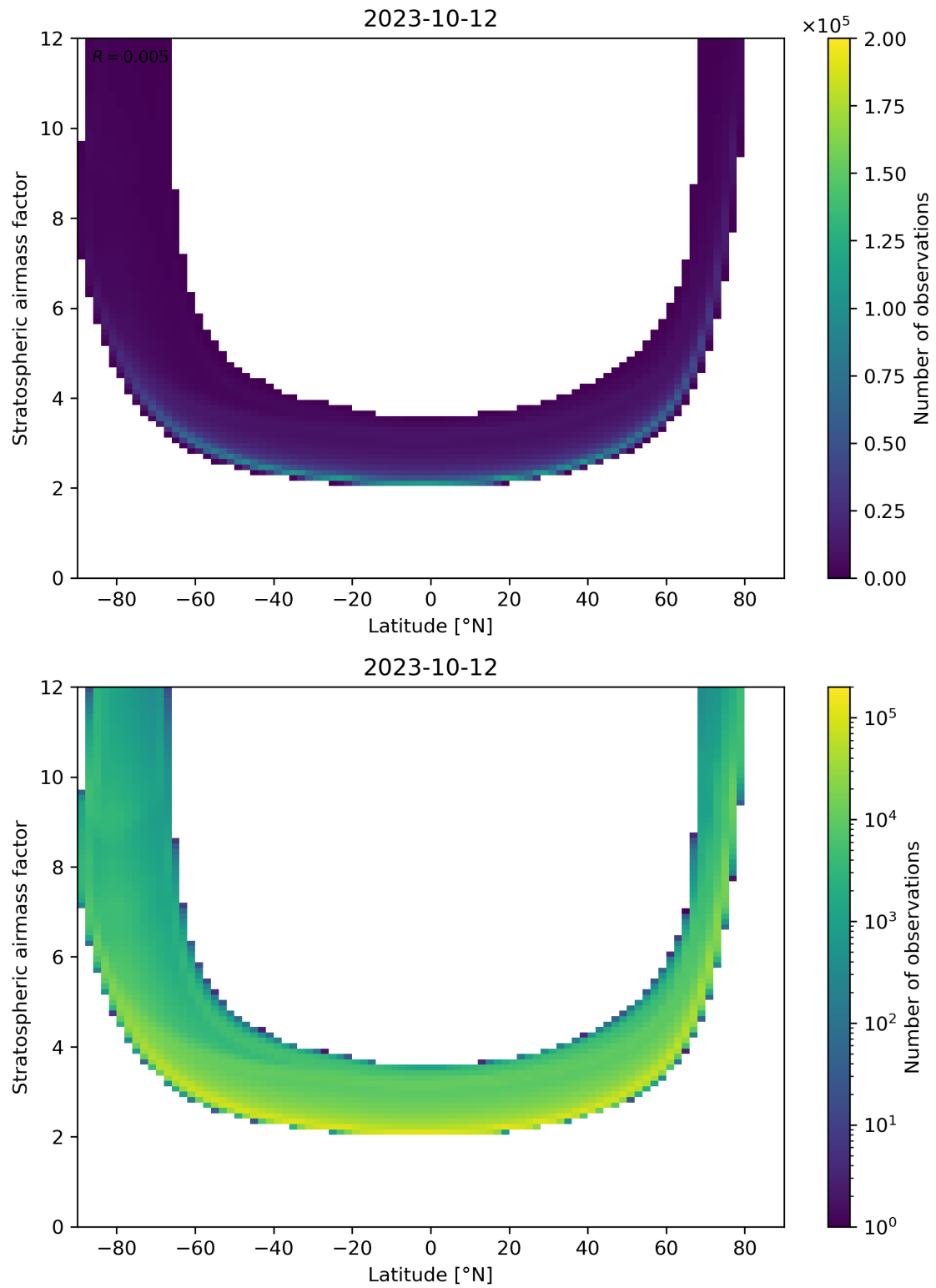
Figure 83: Scatter density plot of “Latitude” against “Stratospheric airmass factor” for 2023-10-12 to 2023-10-13.
