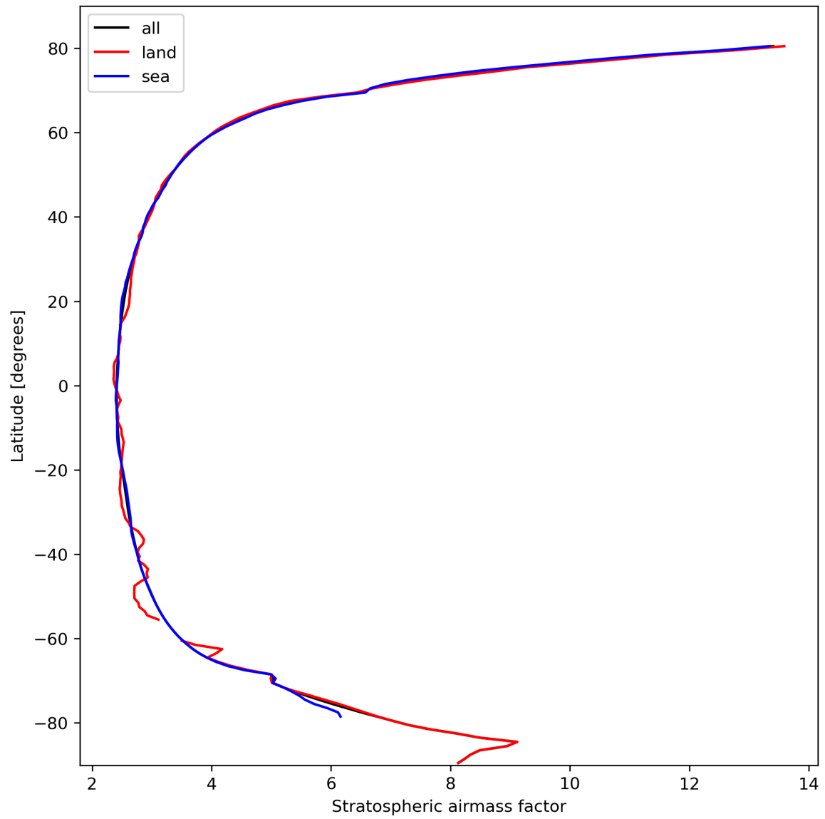
Figure 27: Zonal average of “Stratospheric airmass factor” for 2023-10-12 to 2023-10-13.
