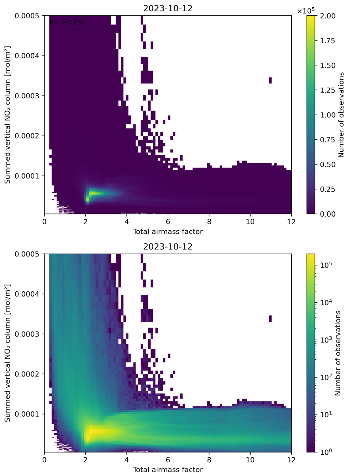
Figure 65: Scatter density plot of “Total airmass factor” against “Summed vertical NO 2 column” for 2023-10-12 to 2023-10-13.
