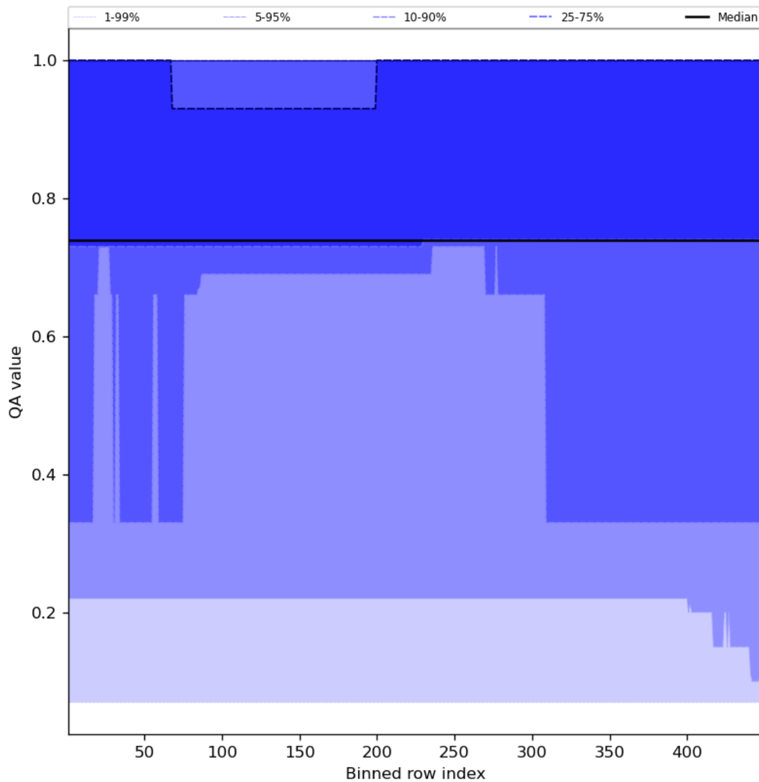
Figure 45: Along track statistics of “QA value” for 2023-10-12 to 2023-10-13
