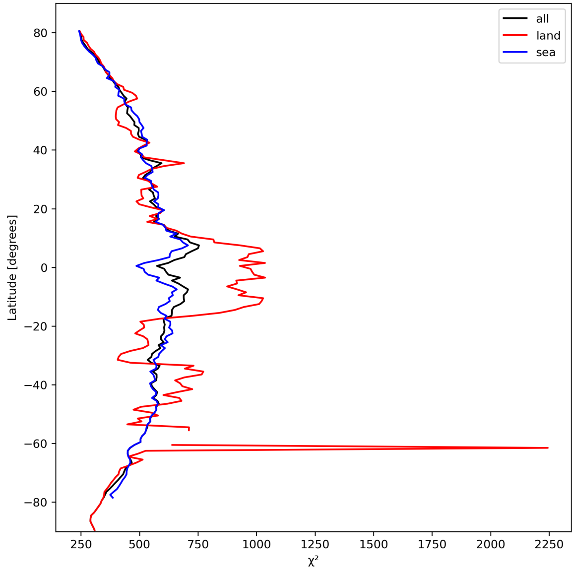
Figure 25: Zonal average of “ \chi^2 ” for 2023-10-12 to 2023-10-13.
