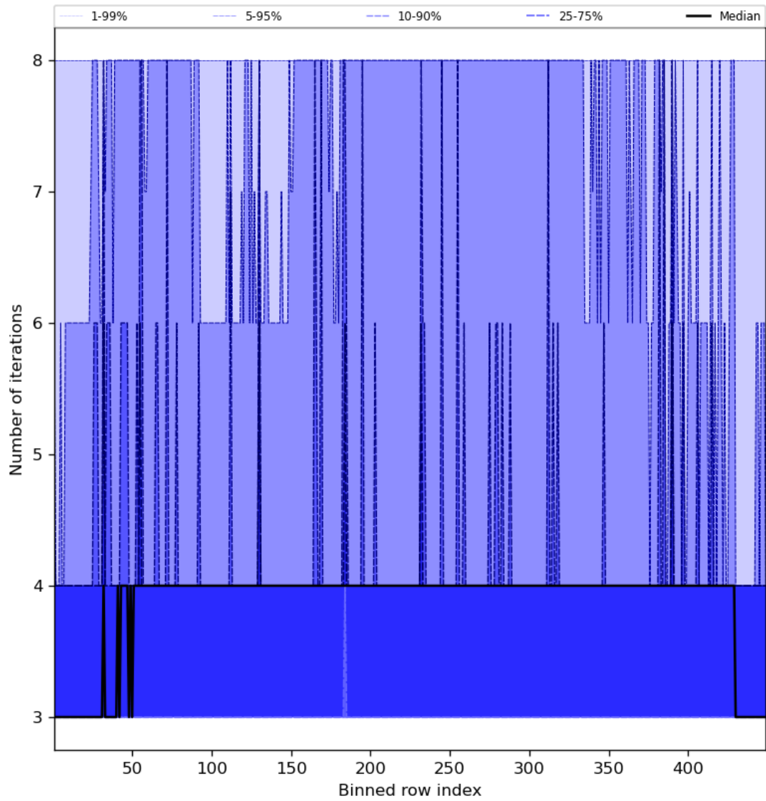
Figure 51: Along track statistics of “Number of iterations” for 2023-10-12 to 2023-10-13
