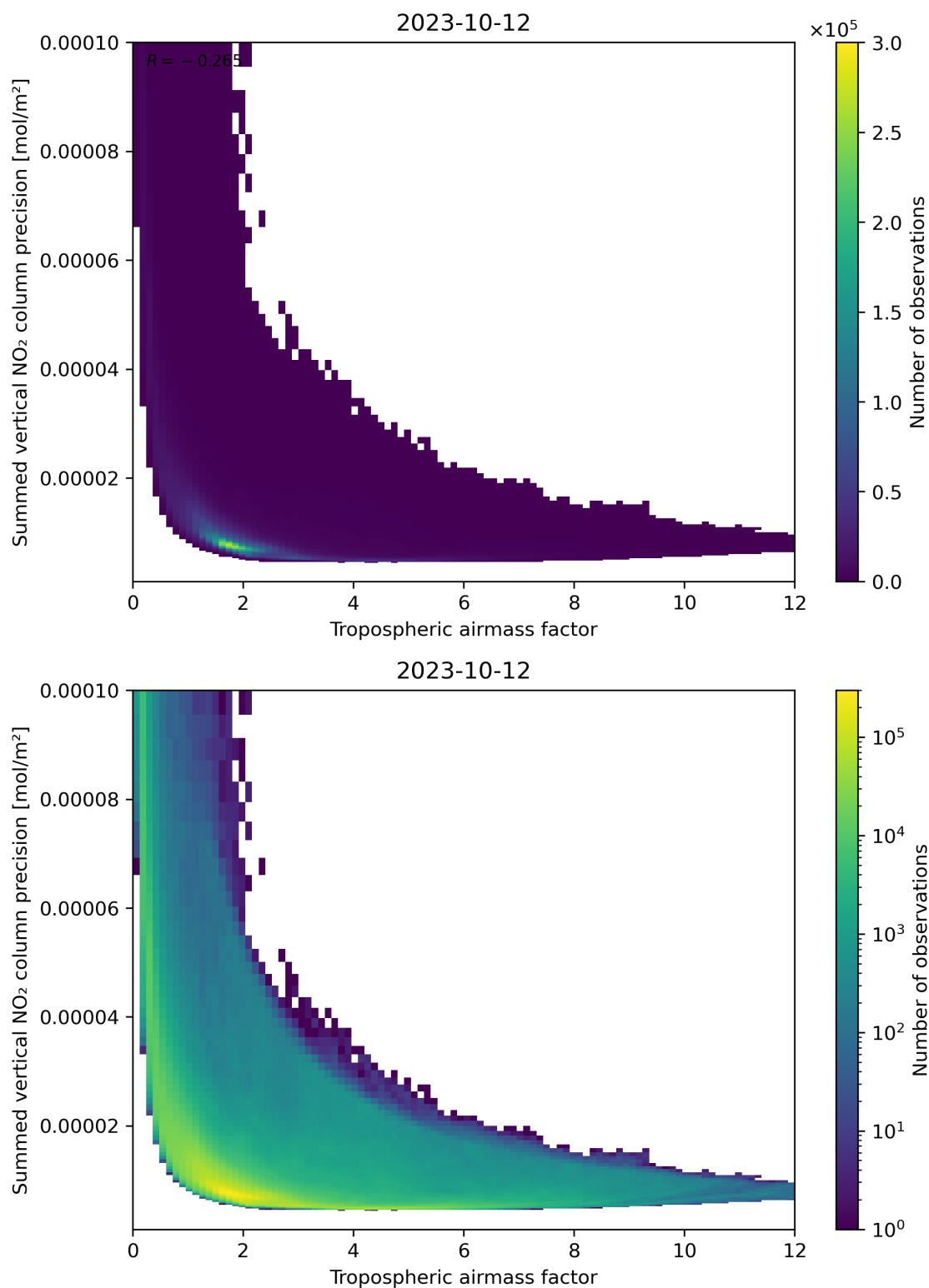
Figure 76: Scatter density plot of “Tropospheric air mass factor” against “Summed vertical NO 2 column precision” for 2023-10-12 to 2023-10-13.
