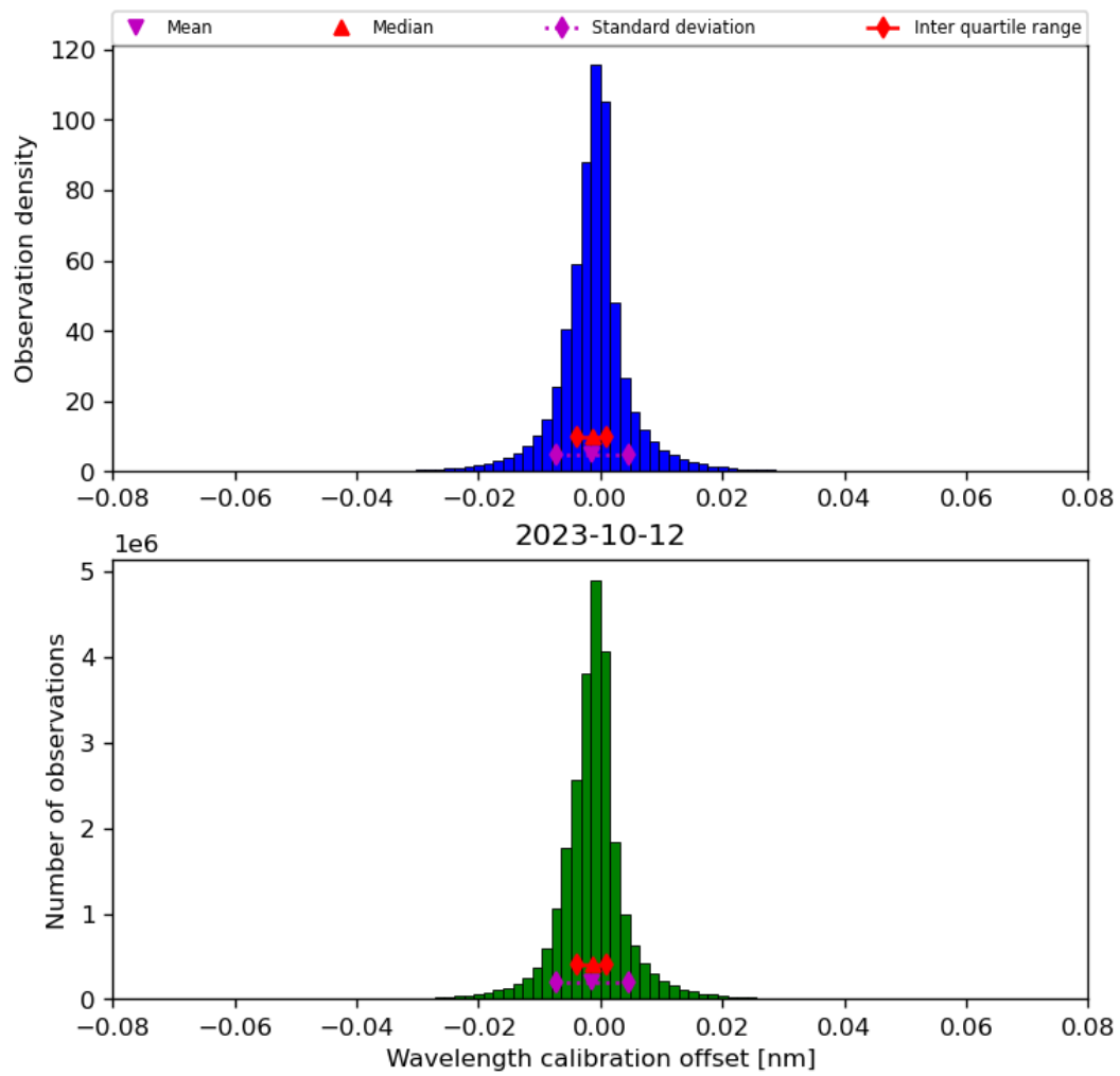
Figure 35: Histogram of “Wavelength calibration offset” for 2023-10-12 to 2023-10-13
