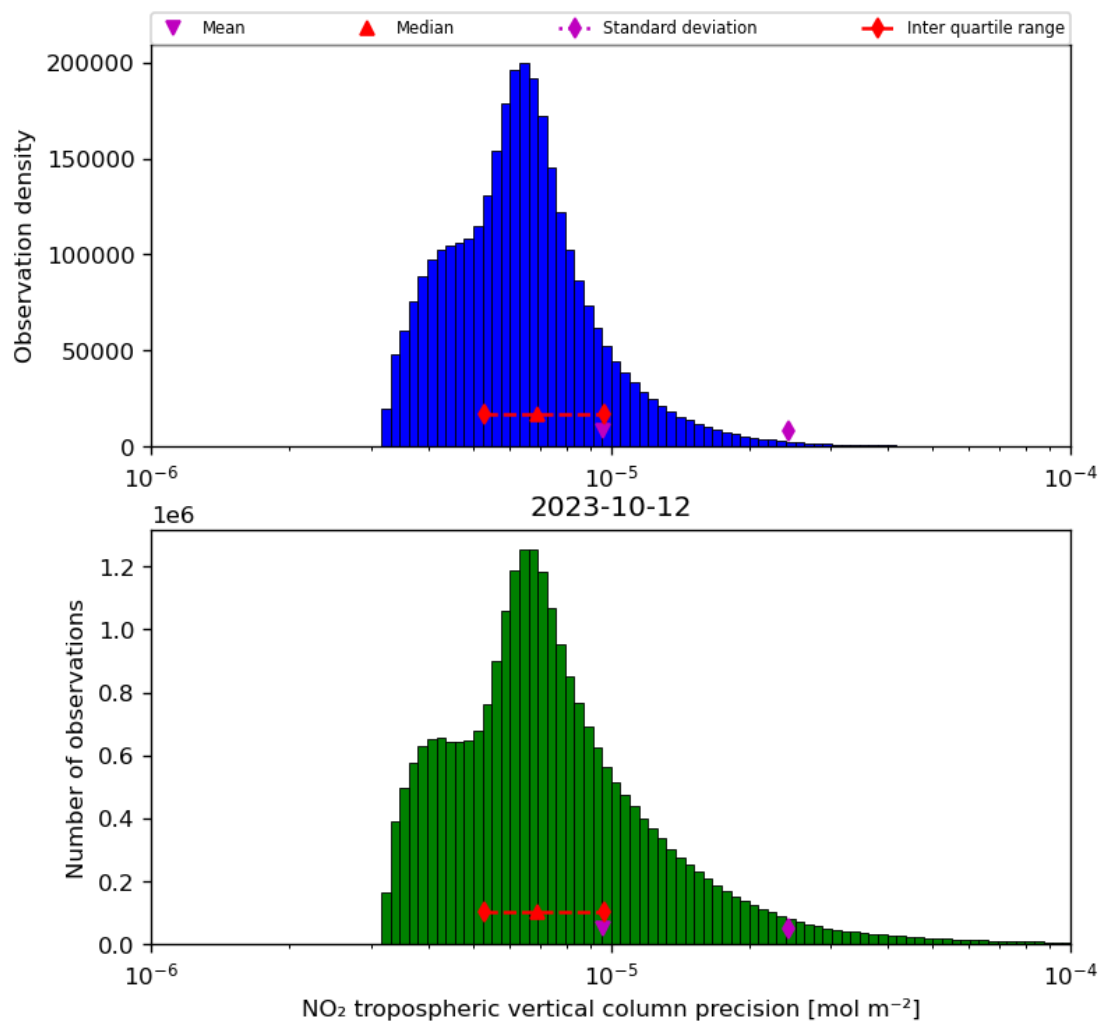
Figure 30: Histogram of “NO 2 tropospheric vertical column precision” for 2023-10-12 to 2023-10-13
