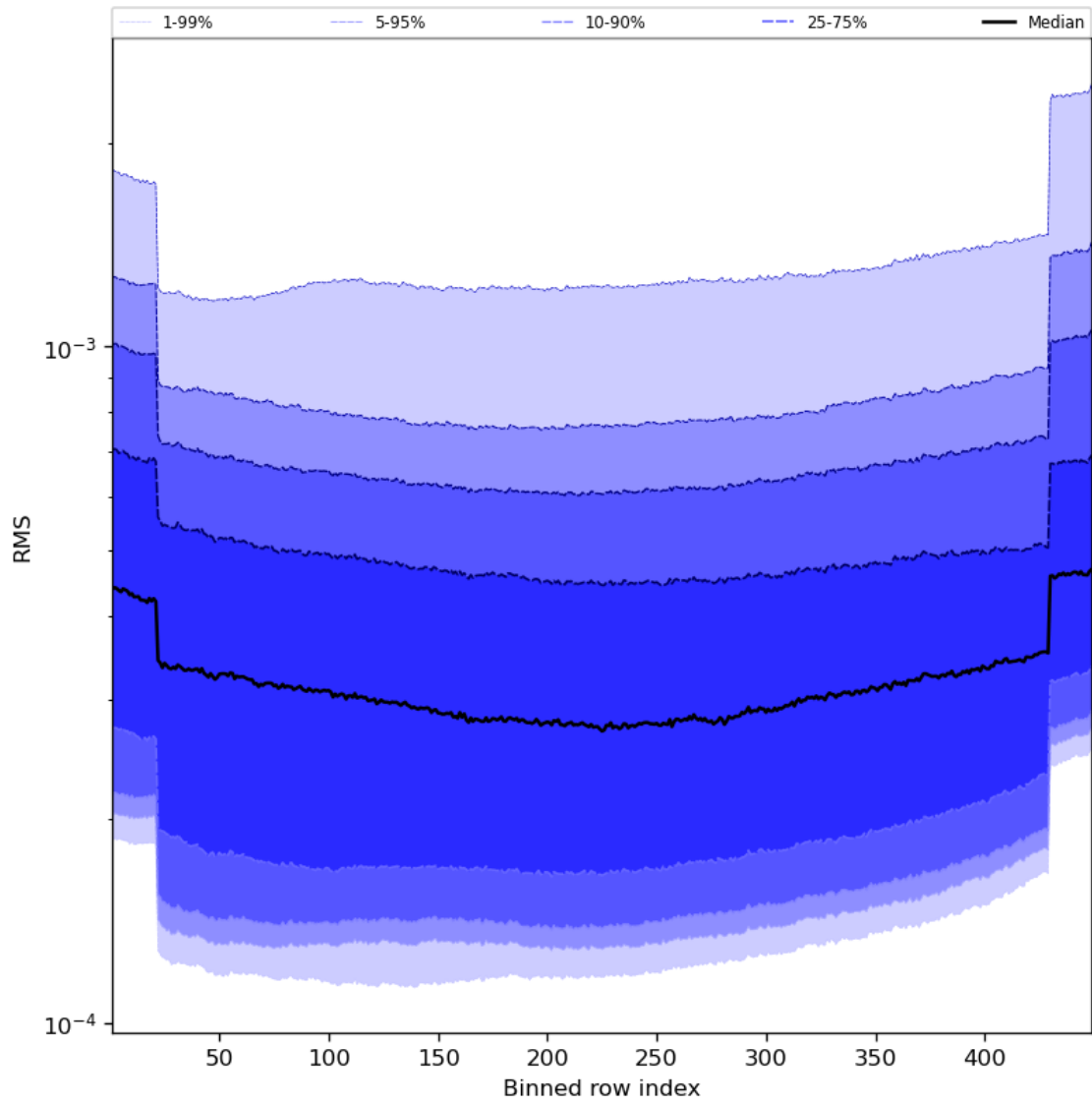
Figure 60: Along track statistics of “RMS” for 2023-10-12 to 2023-10-13
