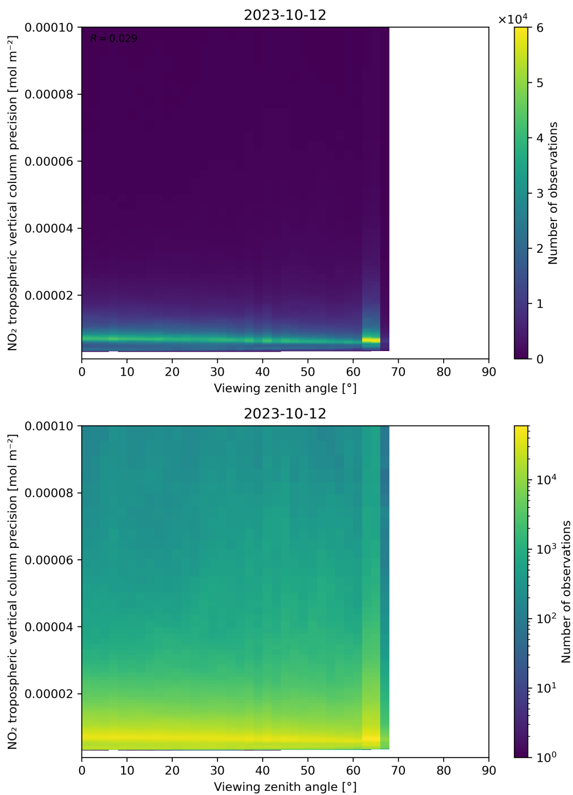
Figure 170: Scatter density plot of “Viewing zenith angle” against “NO 2 tropospheric vertical column precision” for 2023-10-12 to 2023-10-13.
