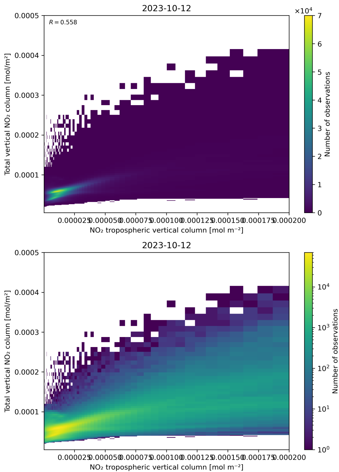
Figure 128: Scatter density plot of “NO 2 tropospheric vertical column” against “Total vertical NO 2 column” for 2023-10-12 to 2023-10-13.
