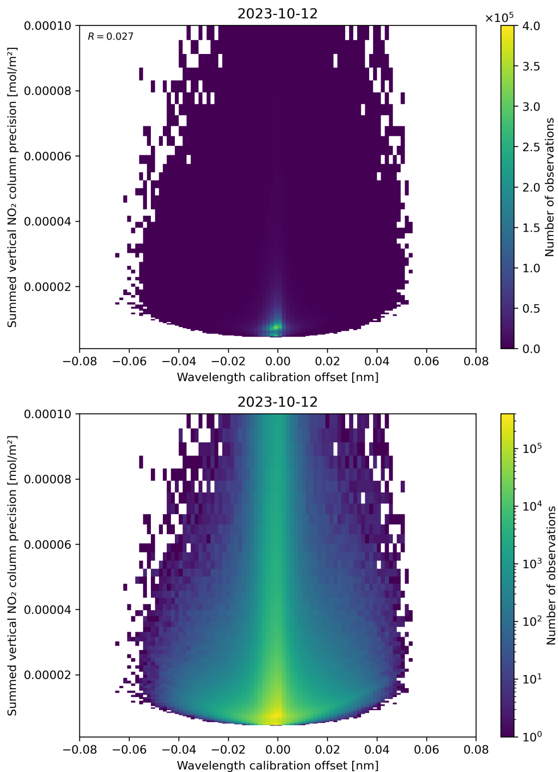
Figure 178: Scatter density plot of “Wavelength calibration offset” against “Summed vertical NO 2 column precision” for 2023-10-12 to 2023-10-13.
