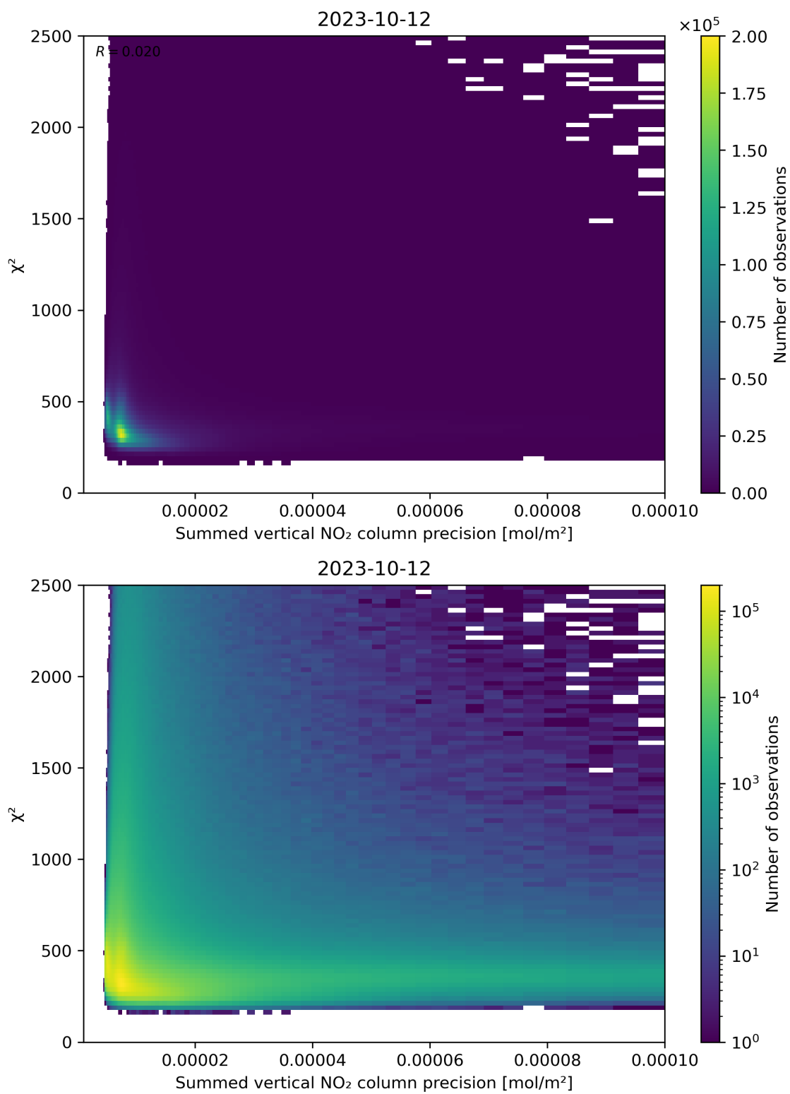
Figure 107: Scatter density plot of “Summed vertical NO 2 column precision” against “ \chi^2 ” for 2023-10-12 to 2023-10-13.
