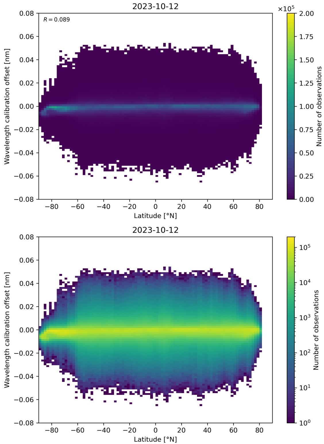
Figure 95: Scatter density plot of “Latitude” against “Wavelength calibration offset” for 2023-10-12 to 2023-10-13.
