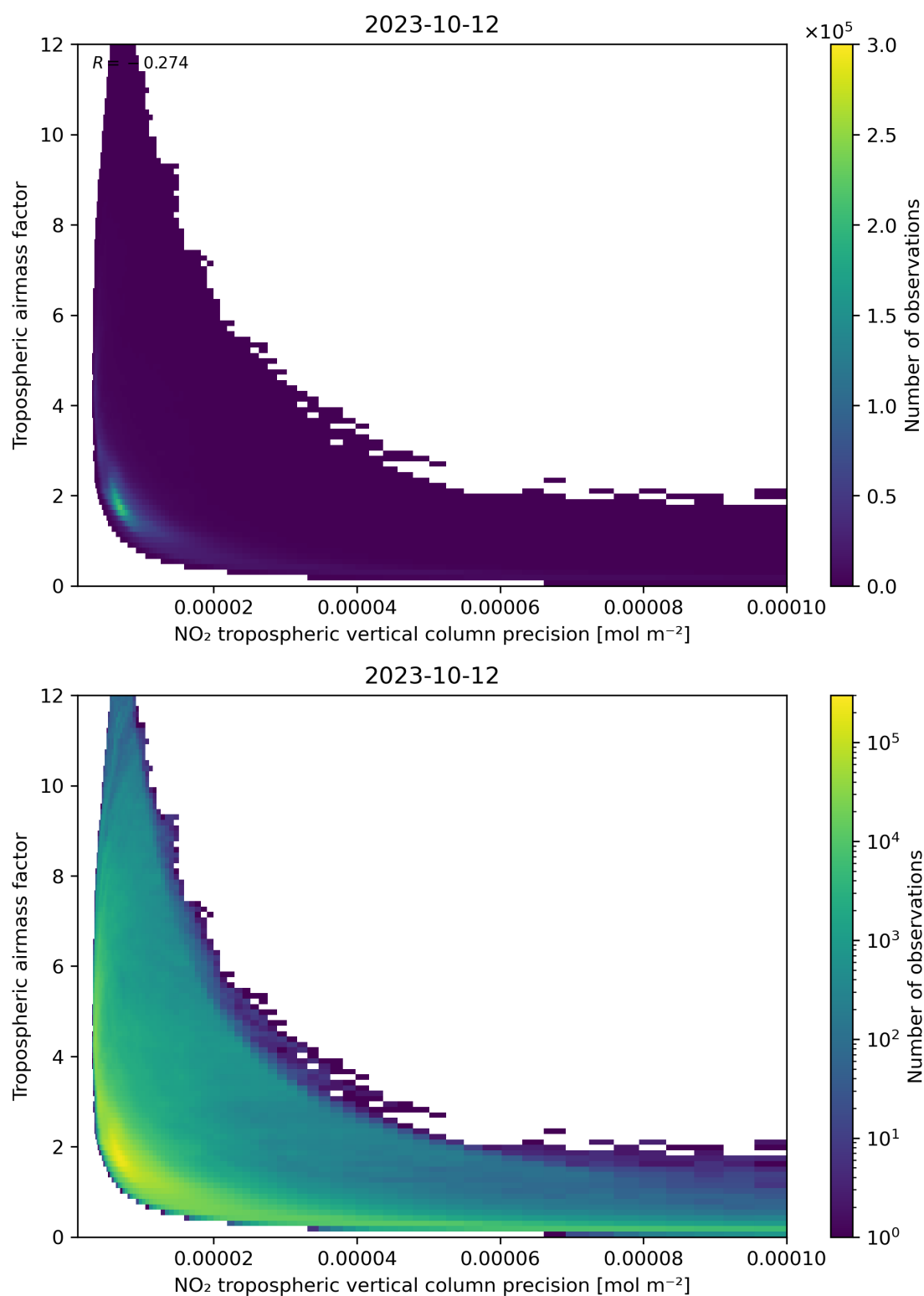
Figure 133: Scatter density plot of “NO 2 tropospheric vertical column precision” against “Tropospheric air mass factor” for 2023-10-12 to 2023-10-13.
