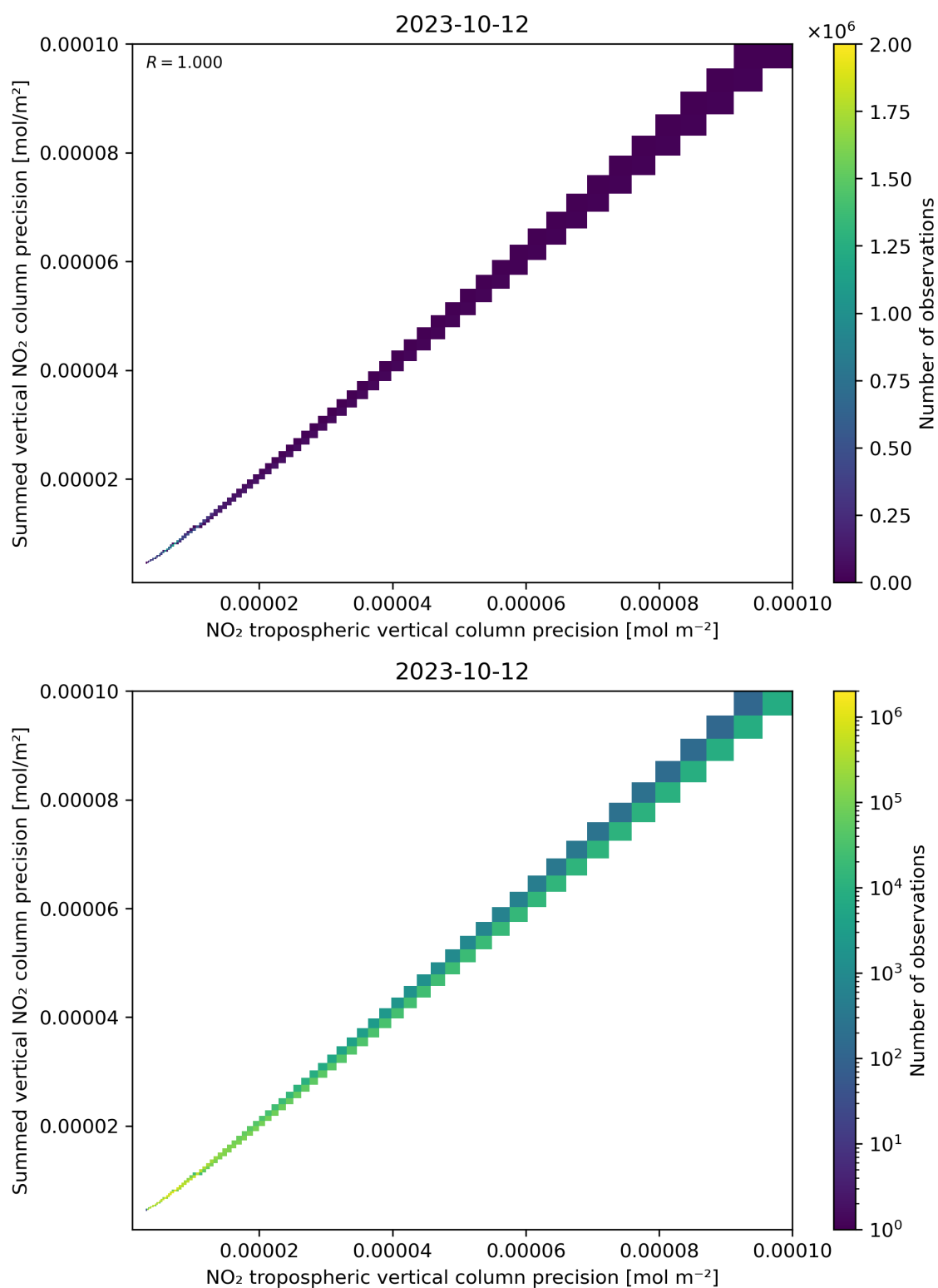
Figure 137: Scatter density plot of “NO 2 tropospheric vertical column precision” against “Summed vertical NO 2 column precision” for 2023-10-12 to 2023-10-13.
