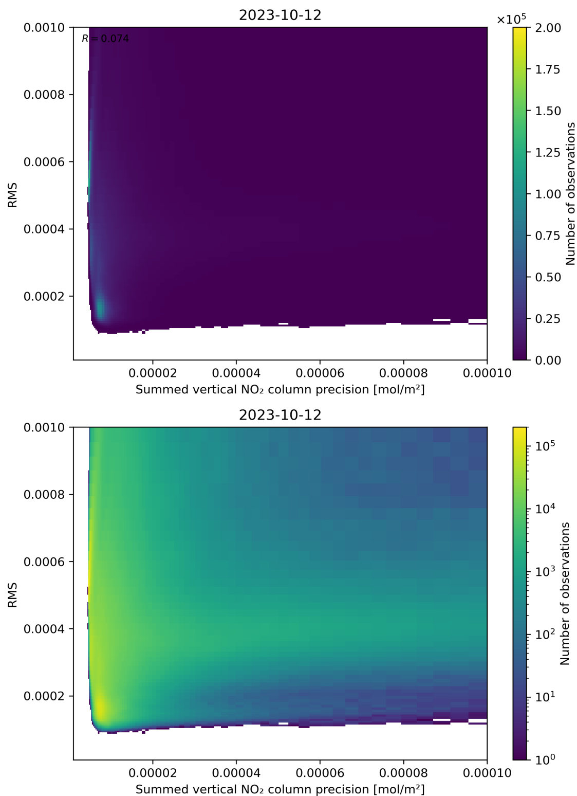
Figure 108: Scatter density plot of “Summed vertical NO 2 column precision” against “RMS” for 2023-10-12 to 2023-10-13.
