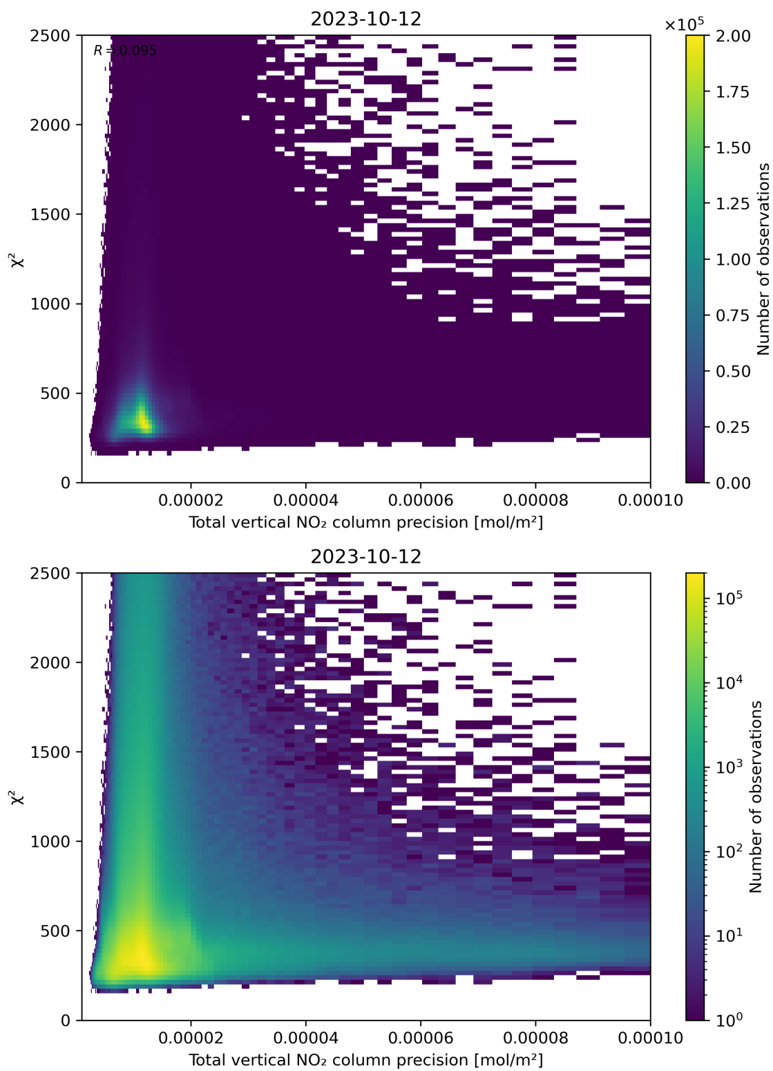
Figure 116: Scatter density plot of “Total vertical NO 2 column precision” against “ \chi^2 ” for 2023-10-12 to 2023-10-13.
