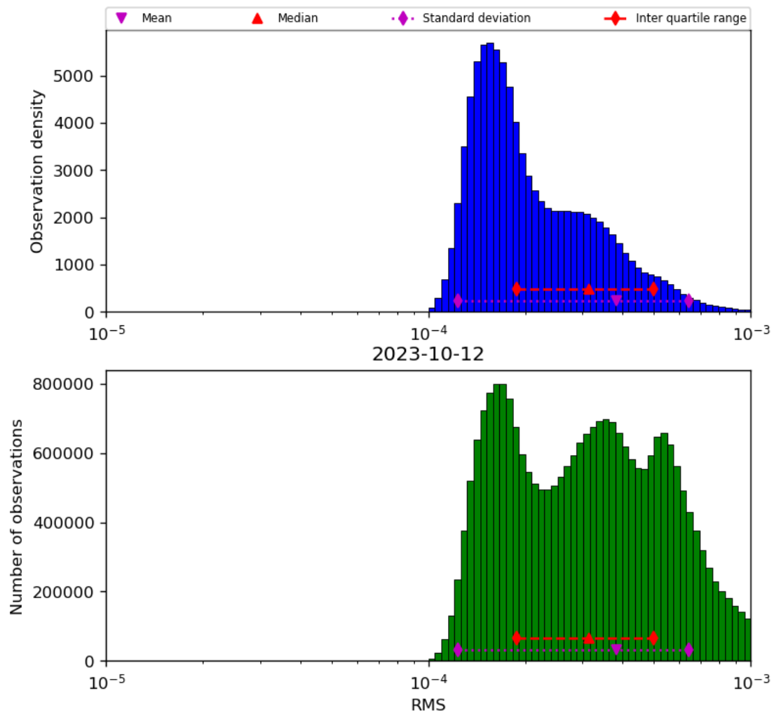
Figure 43: Histogram of “RMS” for 2023-10-12 to 2023-10-13
