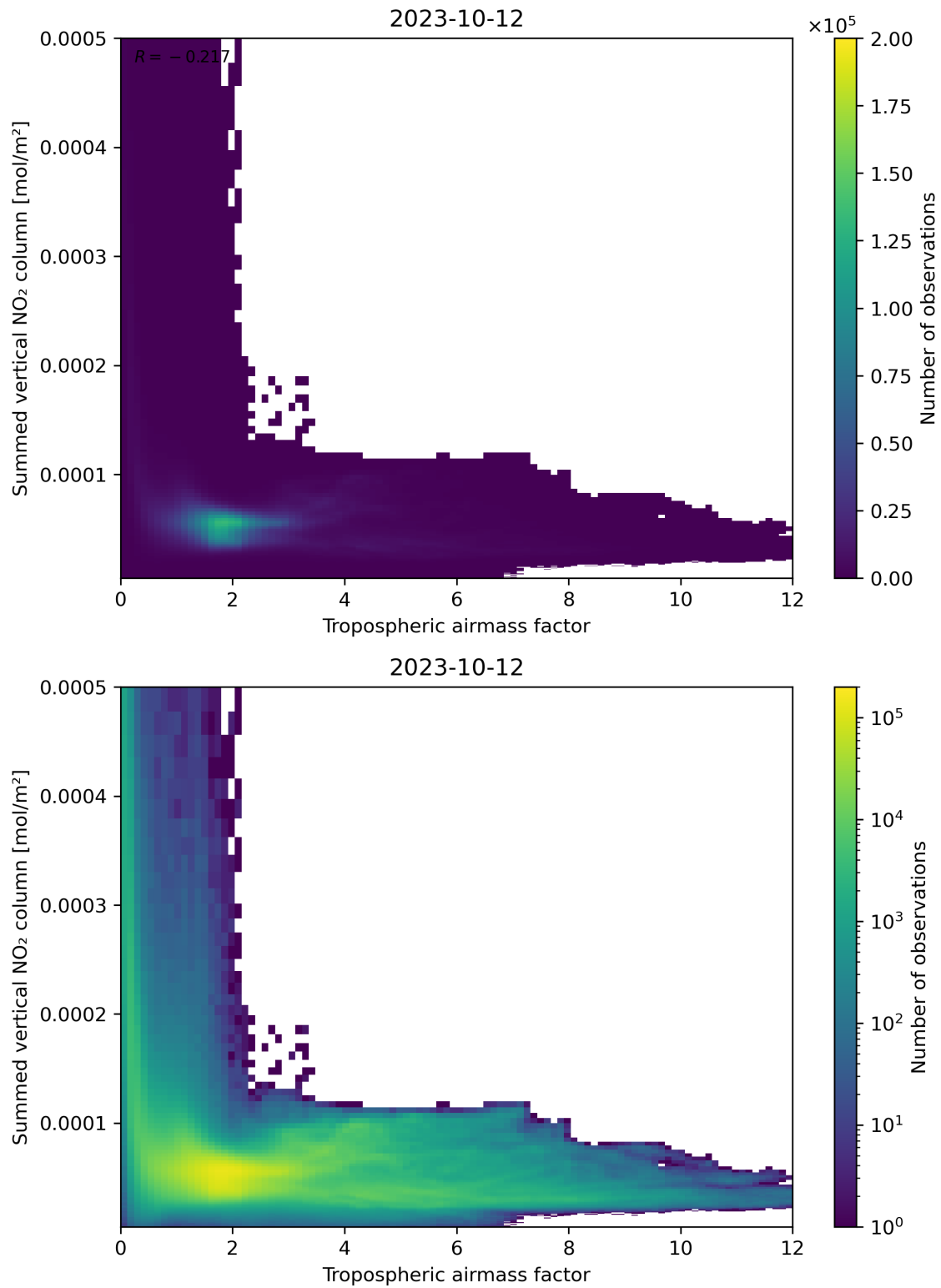
Figure 75: Scatter density plot of “Tropospheric airmass factor” against “Summed vertical NO 2 column” for 2023-10-12 to 2023-10-13.
