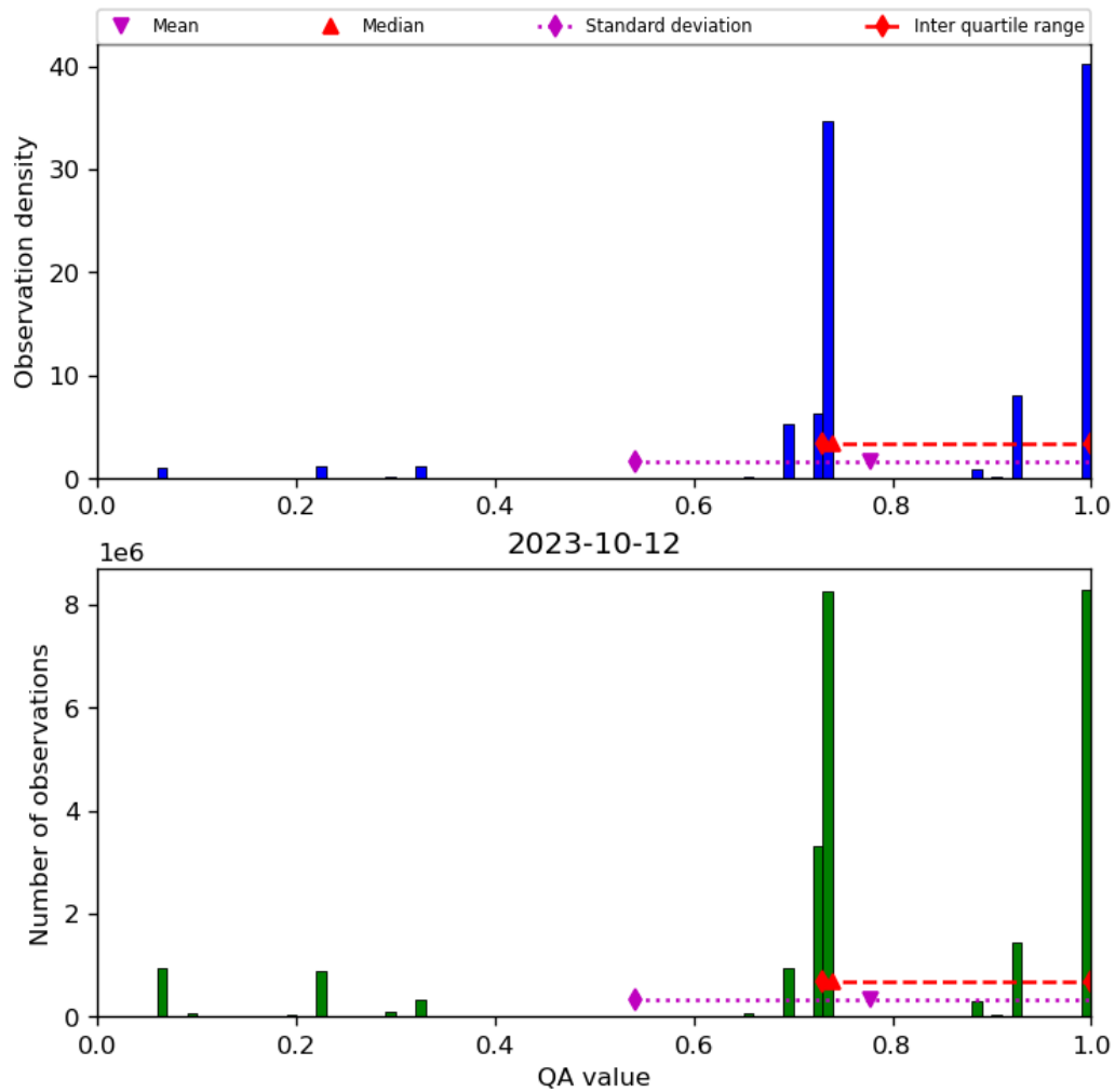
Figure 28: Histogram of “QA value” for 2023-10-12 to 2023-10-13
