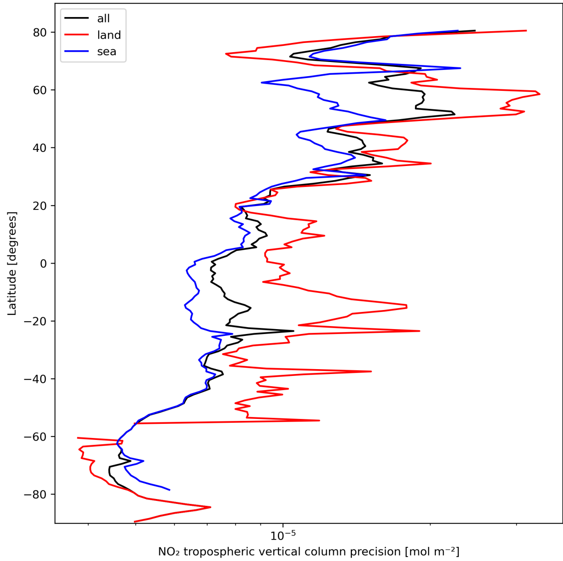
Figure 13: Zonal average of “NO 2 tropospheric vertical column precision” for 2023-10-12 to 2023-10-13.
