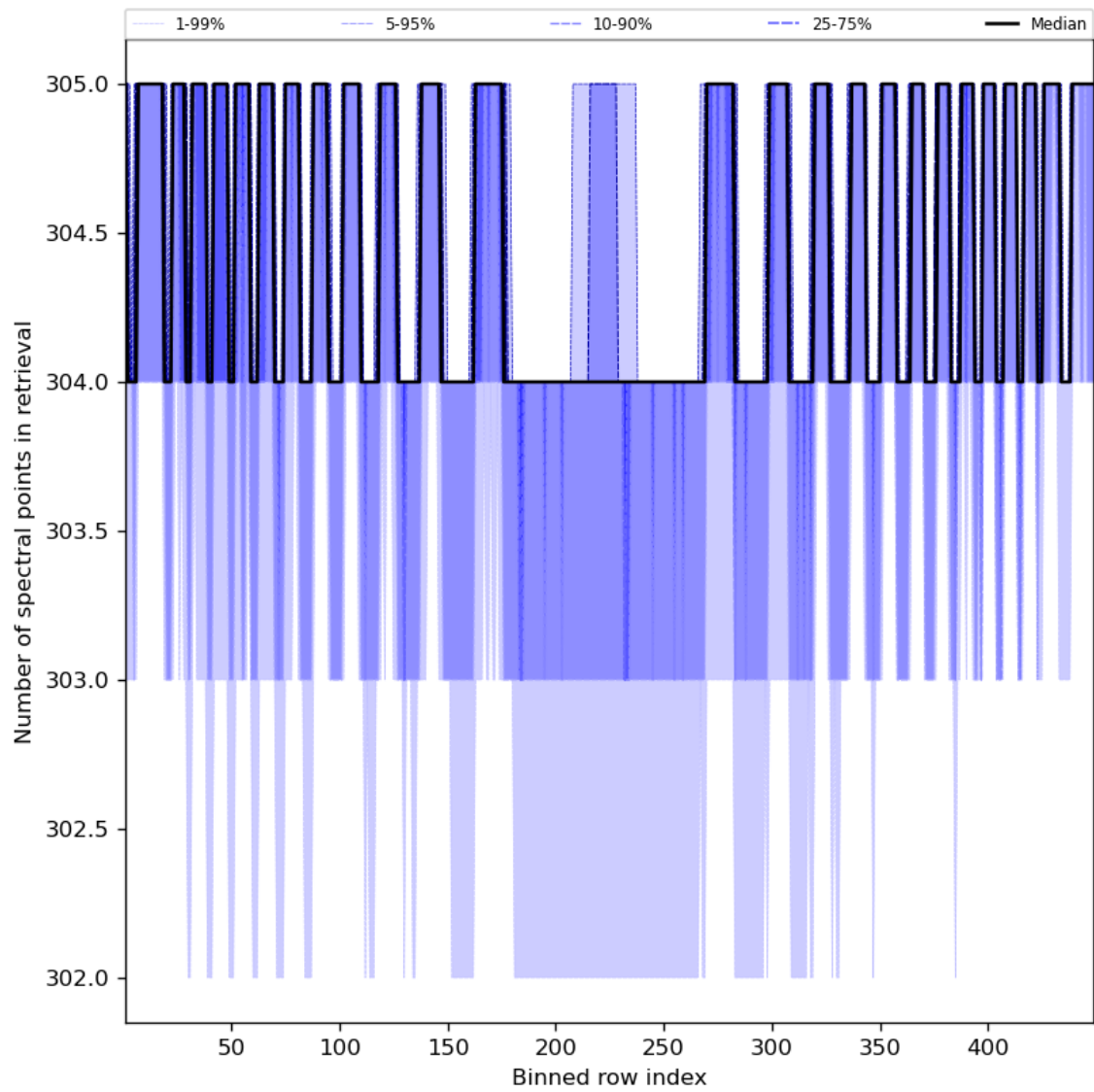
Figure 50: Along track statistics of “Number of spectral points in retrieval” for 2023-10-12 to 2023-10-13
