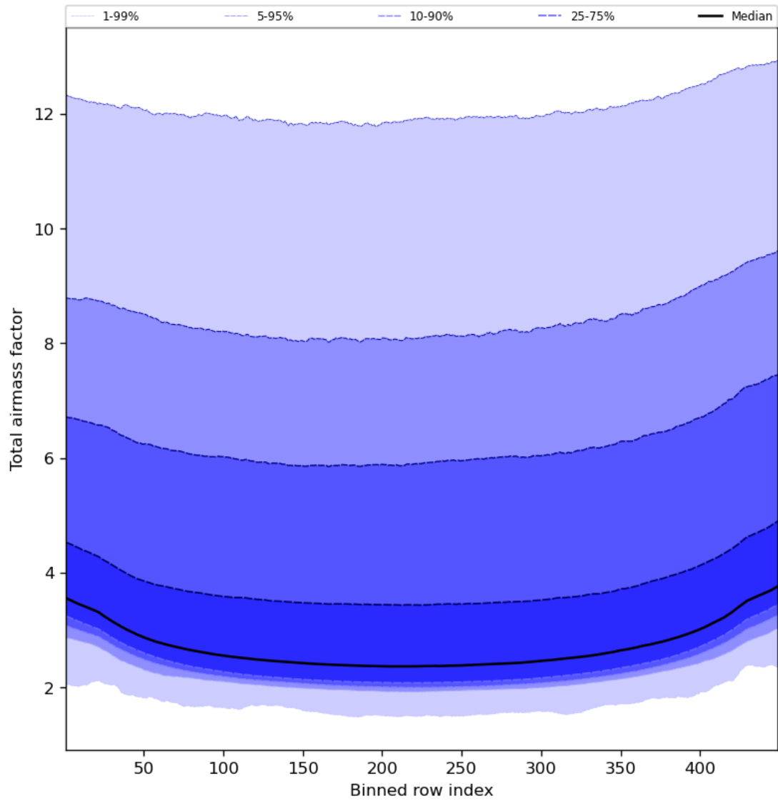
Figure 49: Along track statistics of “Total airmass factor” for 2023-10-12 to 2023-10-13
