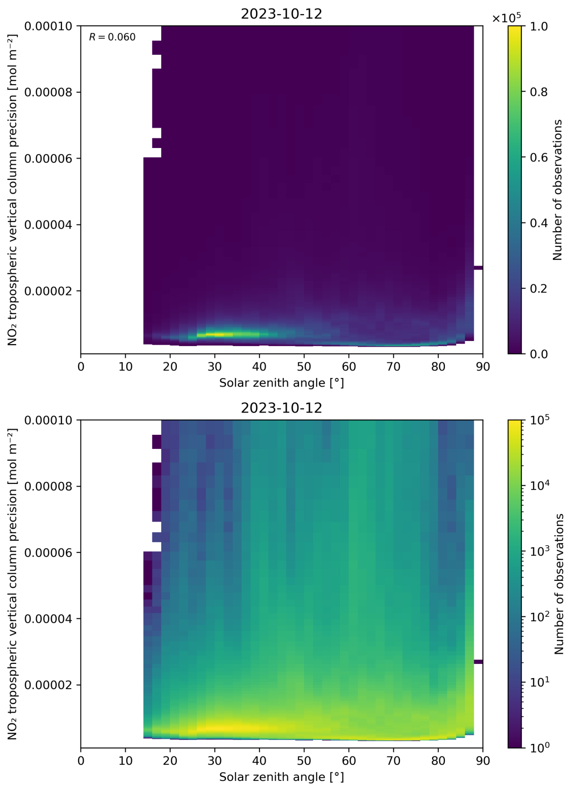
Figure 156: Scatter density plot of “Solar zenith angle” against “NO 2 tropospheric vertical column precision” for 2023-10-12 to 2023-10-13.
