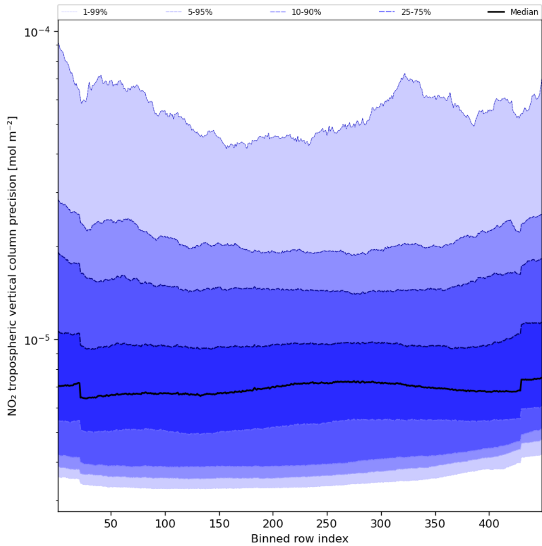
Figure 47: Along track statistics of “NO 2 tropospheric vertical column precision” for 2023-10-12 to 2023-10-13
