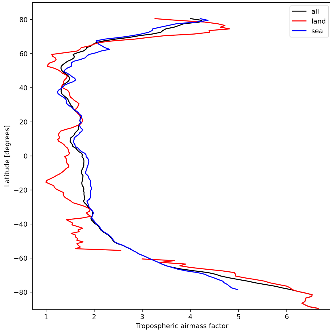
Figure 14: Zonal average of “Tropospheric airmass factor” for 2023-10-12 to 2023-10-13.
