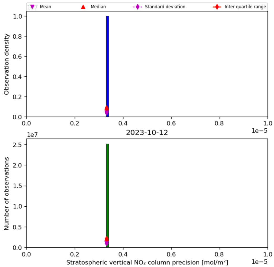
Figure 37: Histogram of “Stratospheric vertical NO 2 column precision” for 2023-10-12 to 2023-10-13
