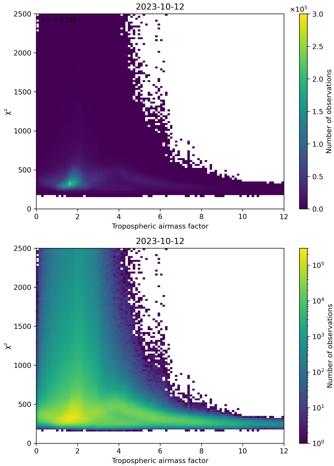
Figure 73: Scatter density plot of “Tropospheric airmass factor” against “ \chi^2 ” for 2023-10-12 to 2023-10-13.
