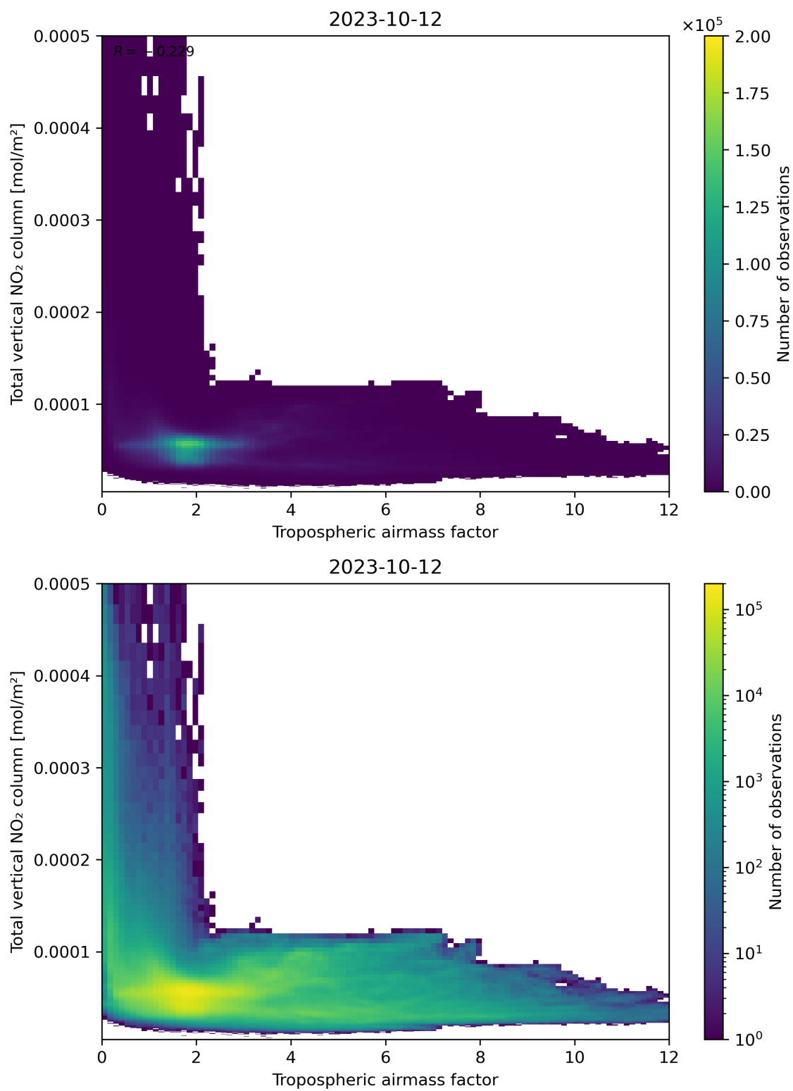
Figure 77: Scatter density plot of “Tropospheric airmass factor” against “Total vertical \text{NO}_2 column” for 2023-10-12 to 2023-10-13.
