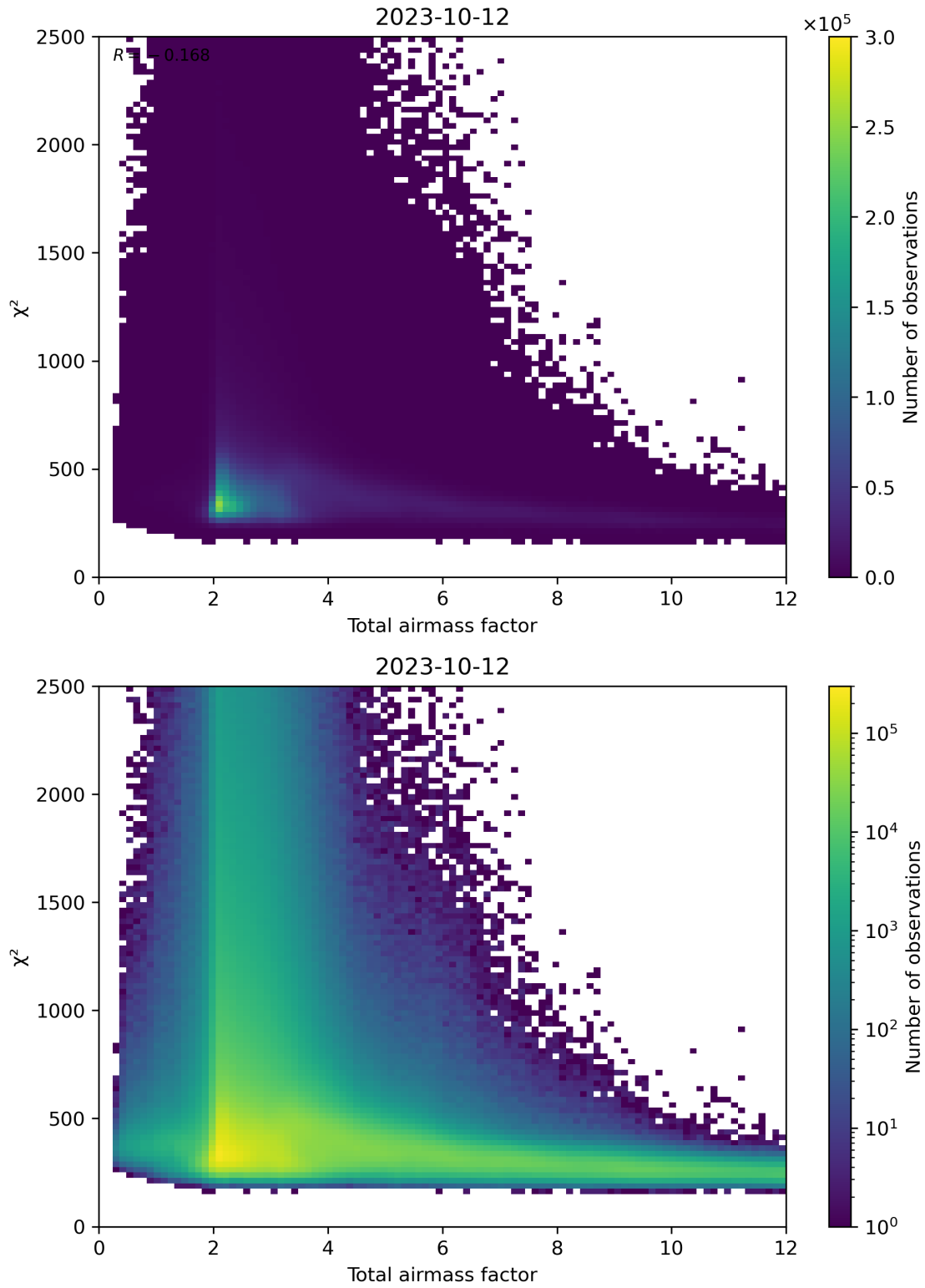
Figure 63: Scatter density plot of “Total airmass factor” against “ \chi^2 ” for 2023-10-12 to 2023-10-13.
