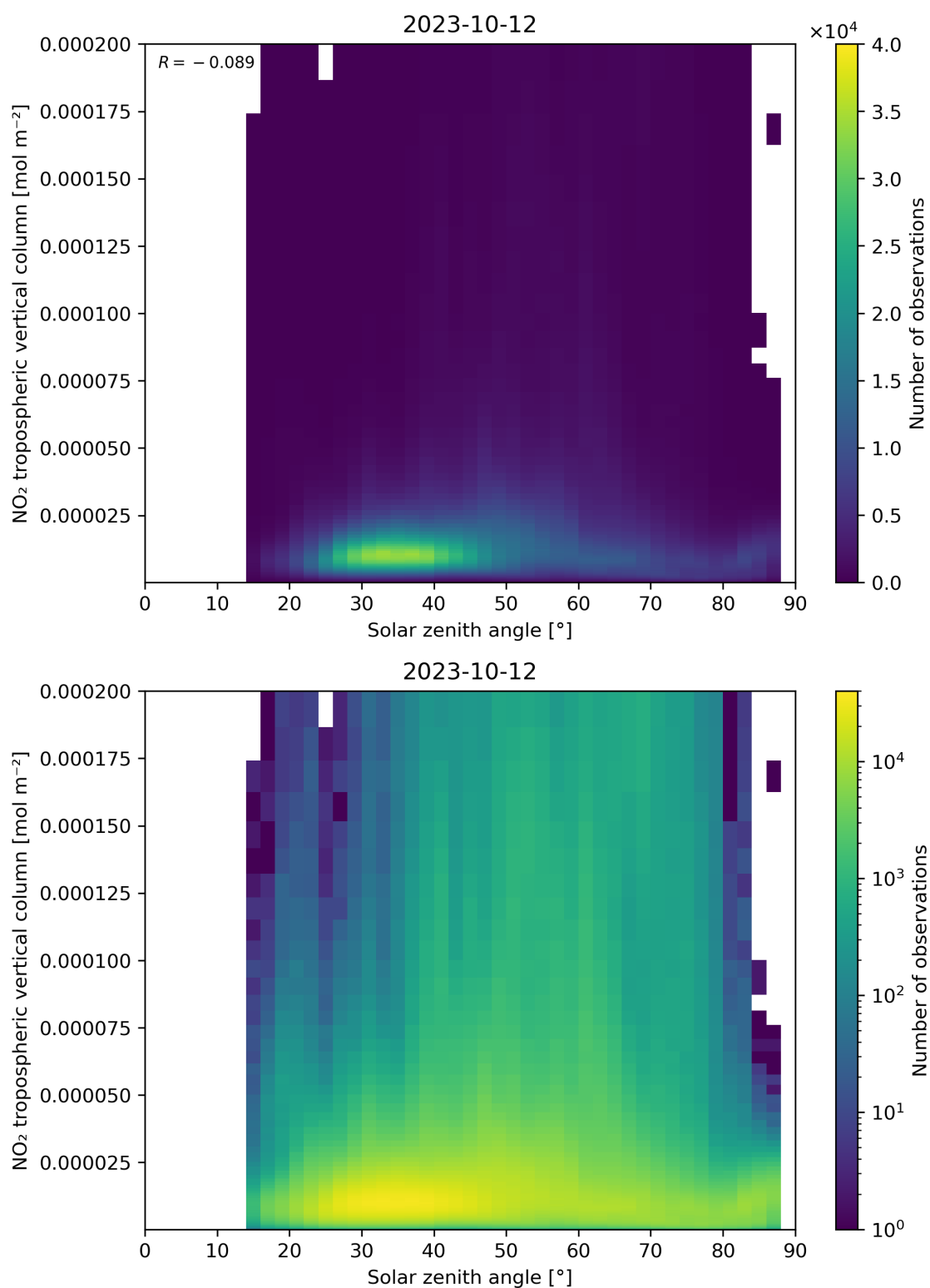
Figure 155: Scatter density plot of “Solar zenith angle” against “NO 2 tropospheric vertical column” for 2023-10-12 to 2023-10-13.
