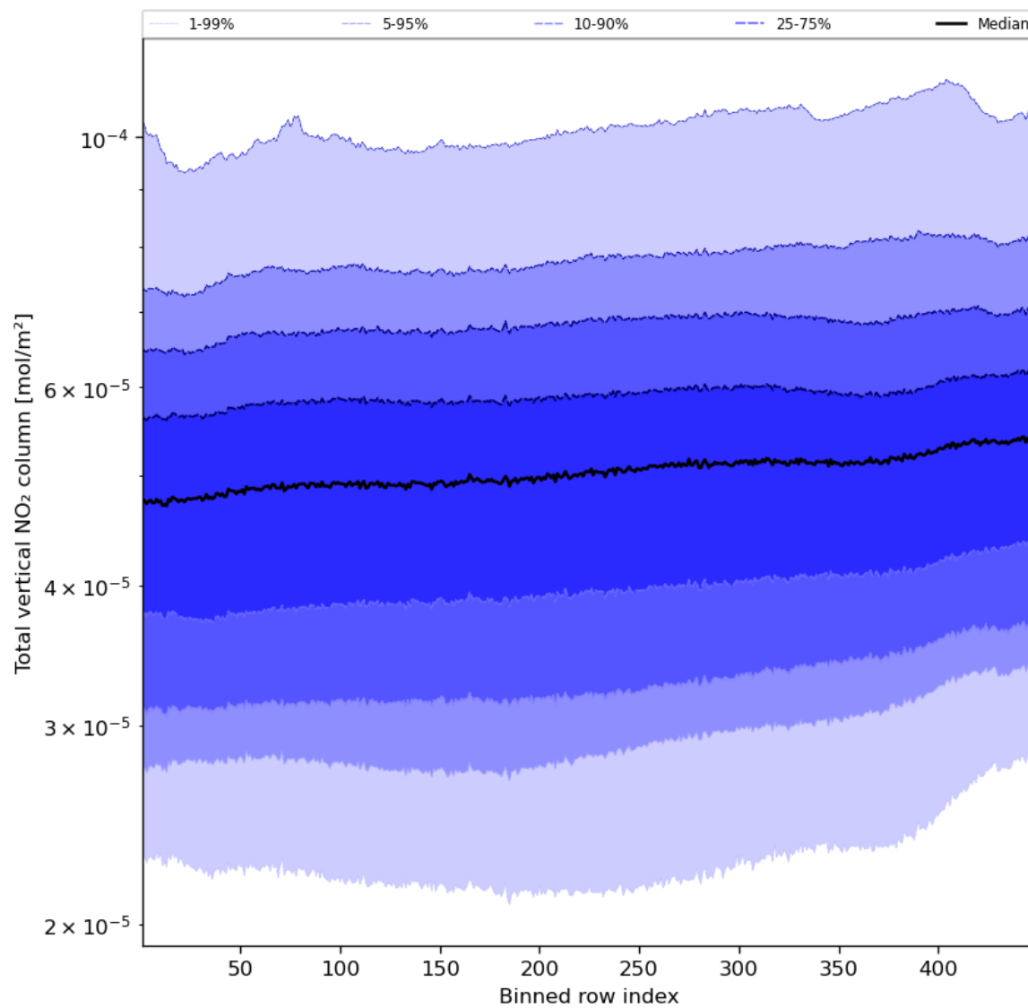
Figure 55: Along track statistics of “Total vertical NO 2 column” for 2023-10-12 to 2023-10-13
