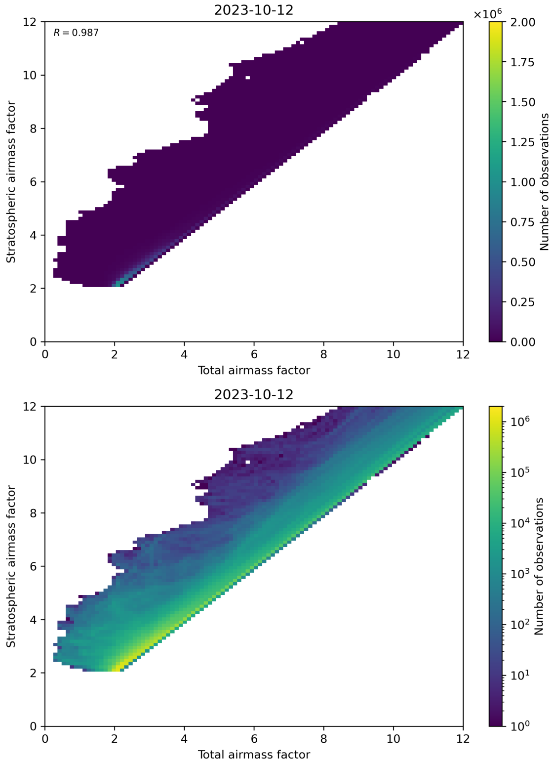
Figure 62: Scatter density plot of “Total airmass factor” against “Stratospheric airmass factor” for 2023-10-12 to 2023-10-13.
