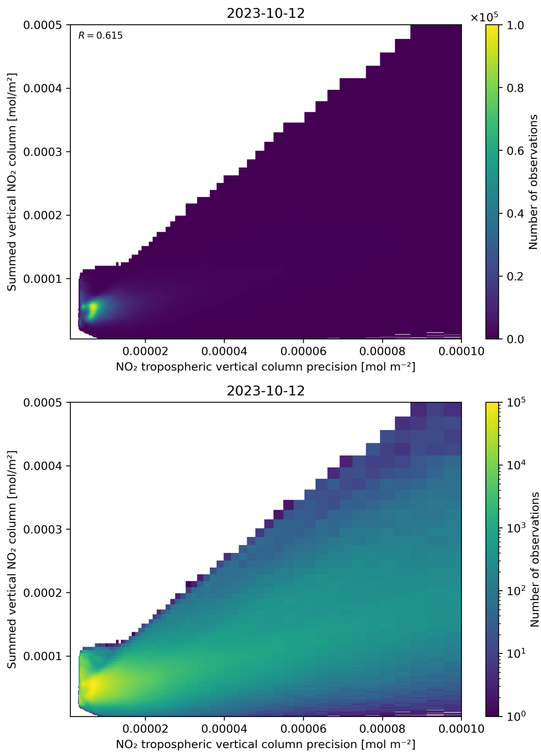
Figure 136: Scatter density plot of “NO 2 tropospheric vertical column precision” against “Summed vertical NO 2 column” for 2023-10-12 to 2023-10-13.
