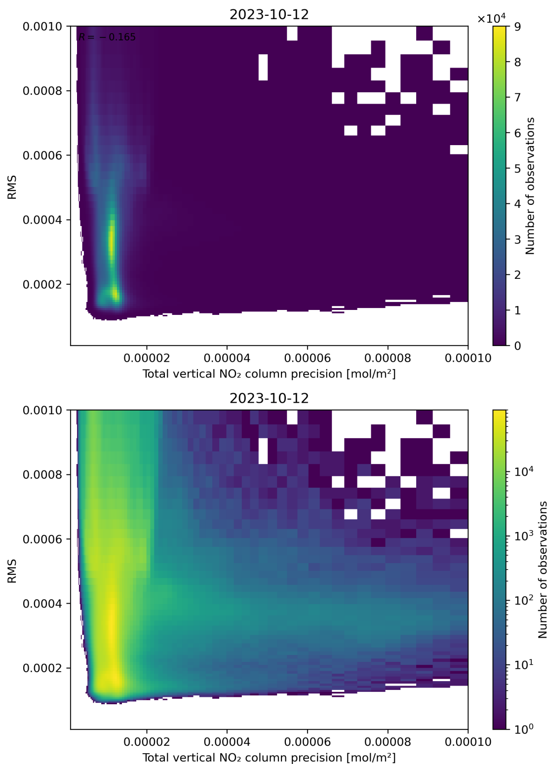
Figure 119: Scatter density plot of “Total vertical NO 2 column precision” against “RMS” for 2023-10-12 to 2023-10-13.
