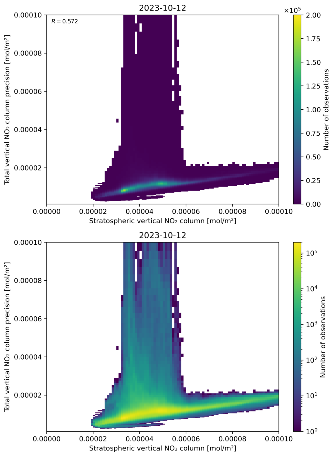
Figure 101: Scatter density plot of “Stratospheric vertical NO 2 column” against “Total vertical NO 2 column precision” for 2023-10-12 to 2023-10-13.
