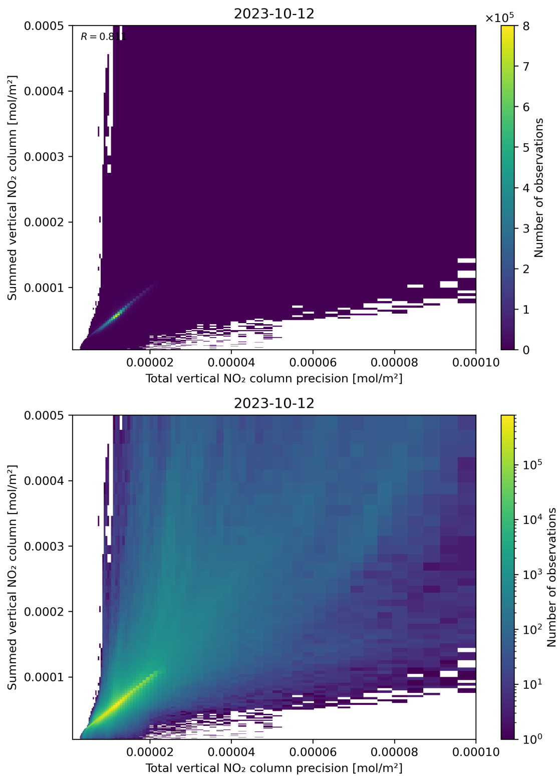
Figure 117: Scatter density plot of “Total vertical NO 2 column precision” against “Summed vertical NO 2 column” for 2023-10-12 to 2023-10-13.
