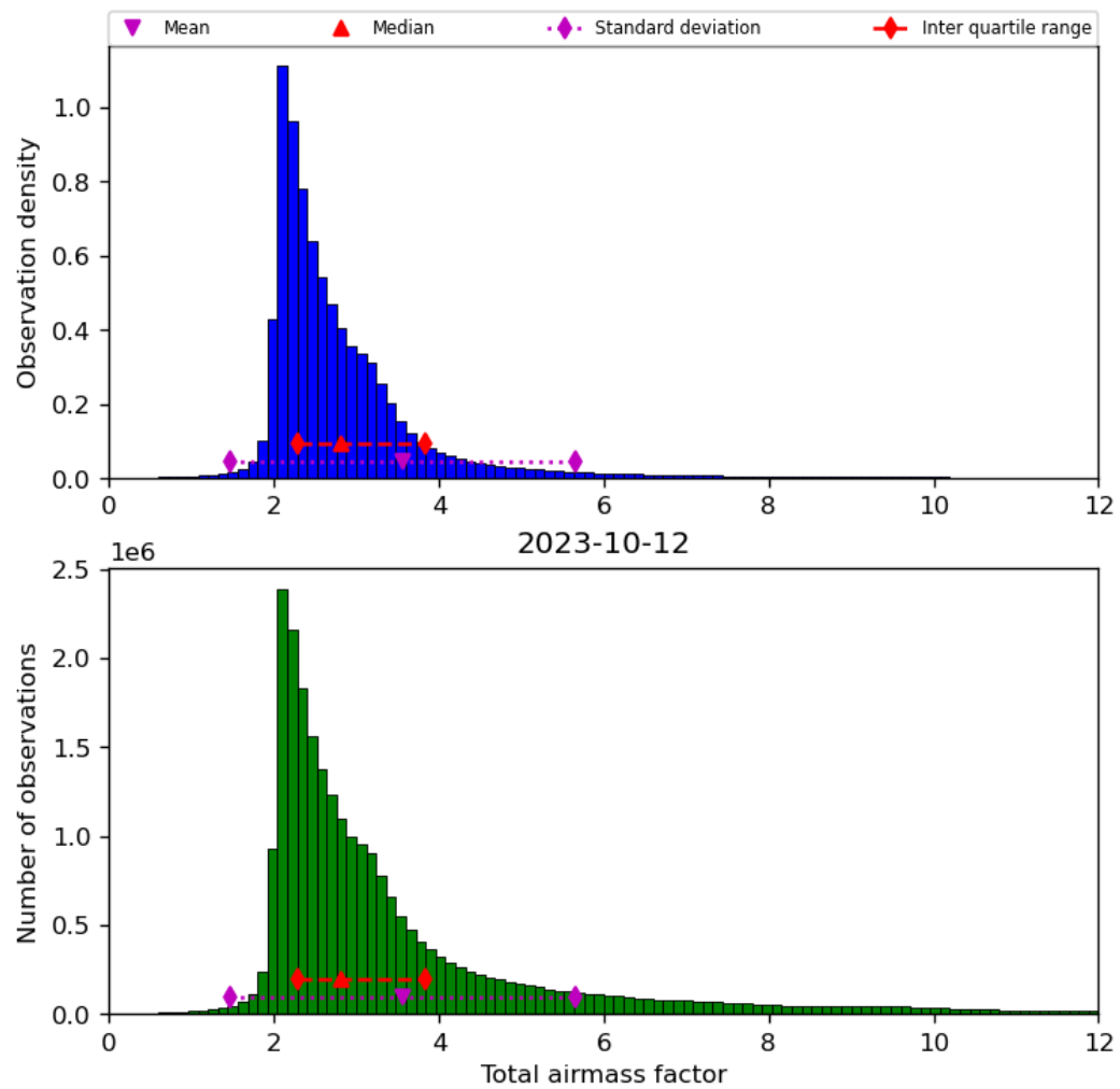
Figure 32: Histogram of “Total airmass factor” for 2023-10-12 to 2023-10-13
