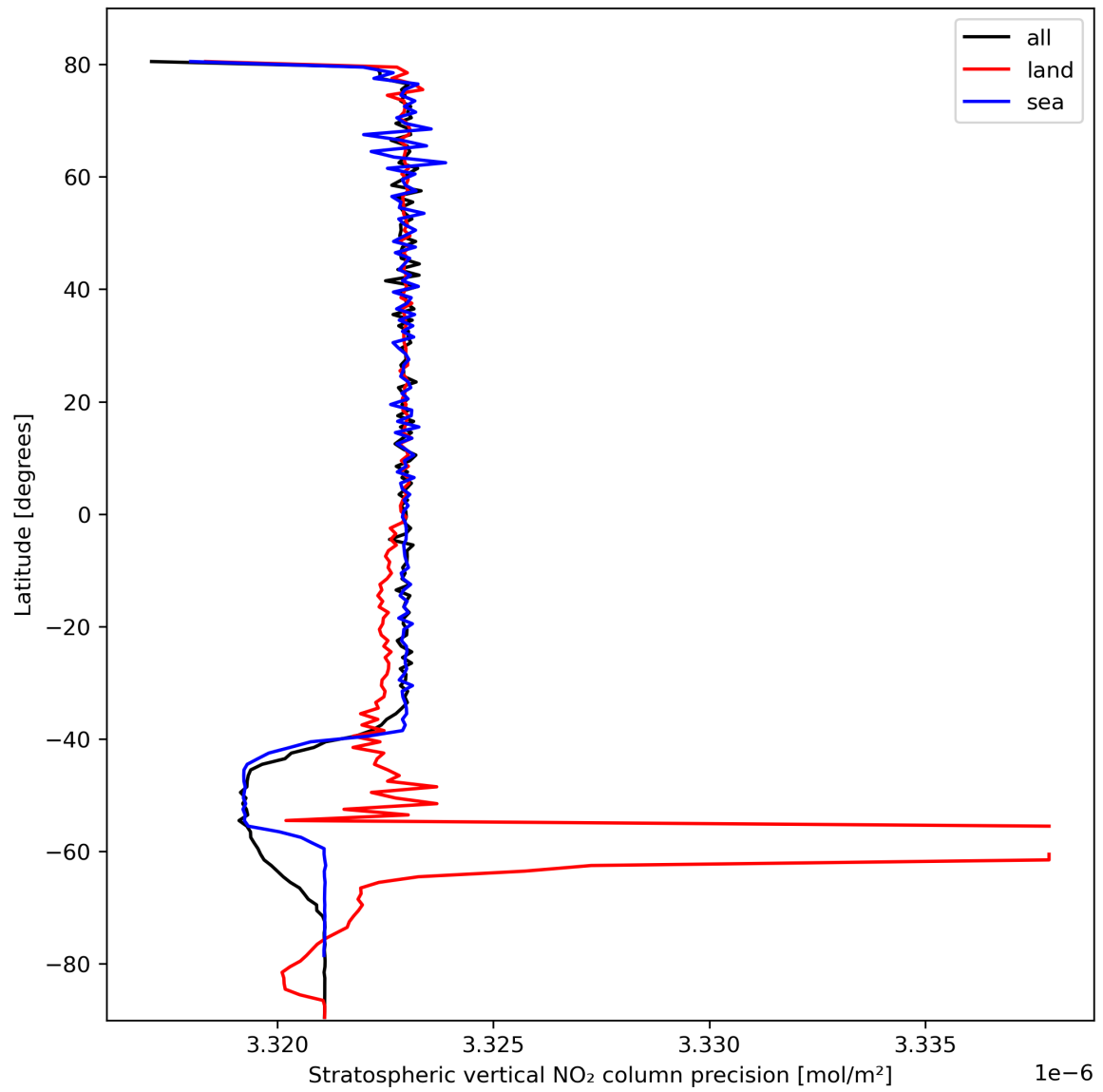
Figure 20: Zonal average of “Stratospheric vertical NO 2 column precision” for 2023-10-12 to 2023-10-13.
