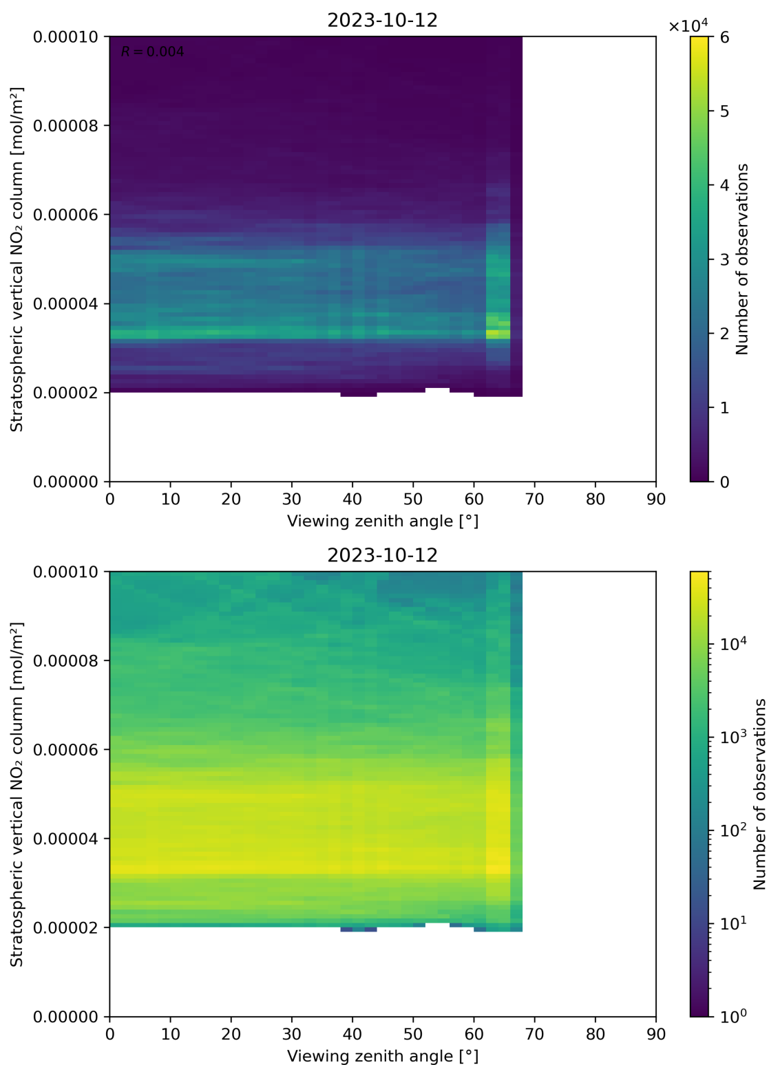
Figure 164: Scatter density plot of “Viewing zenith angle” against “Stratospheric vertical NO 2 column” for 2023-10-12 to 2023-10-13.
