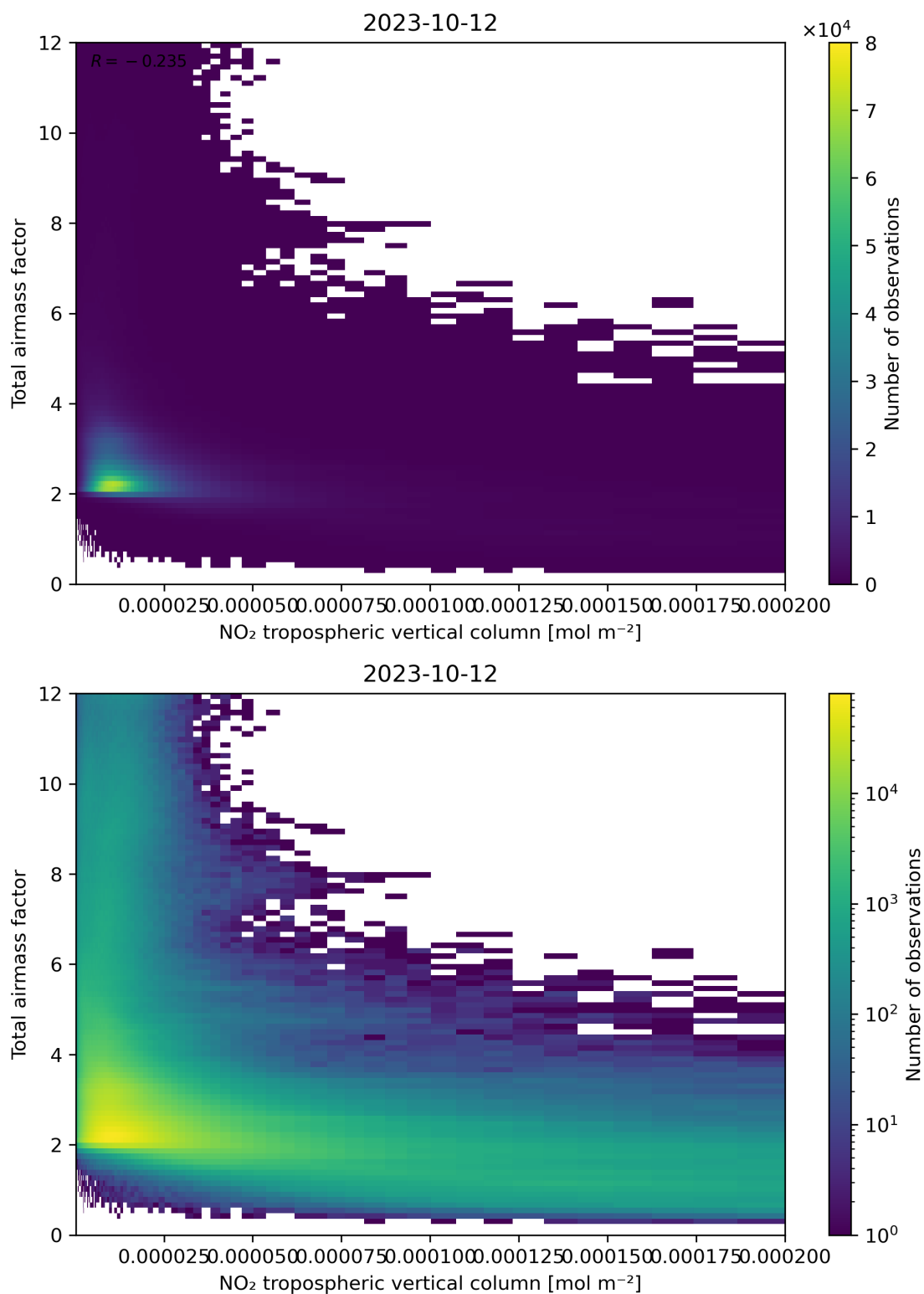
Figure 122: Scatter density plot of “NO 2 tropospheric vertical column” against “Total air mass factor” for 2023-10-12 to 2023-10-13.
