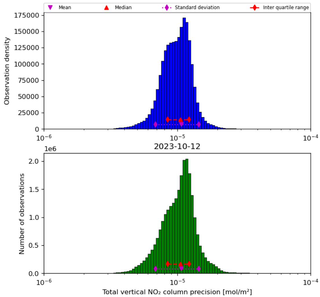
Figure 39: Histogram of “Total vertical NO 2 column precision” for 2023-10-12 to 2023-10-13
