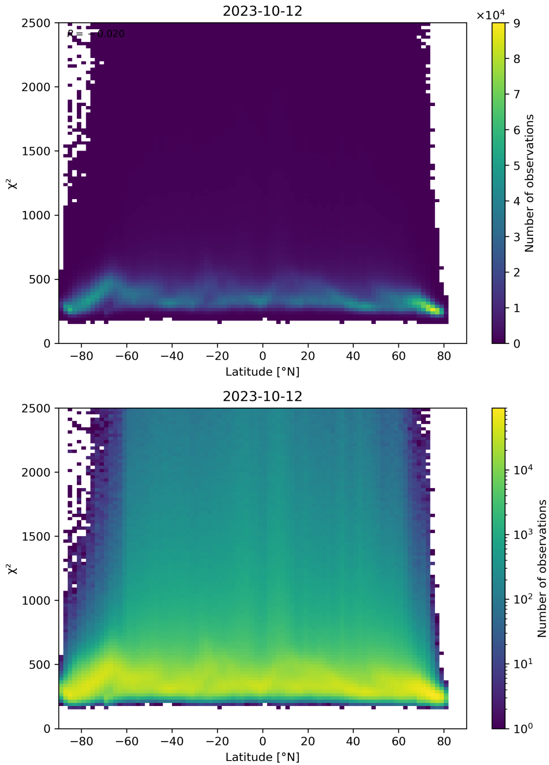
Figure 86: Scatter density plot of “Latitude” against “ \chi^2 ” for 2023-10-12 to 2023-10-13.
