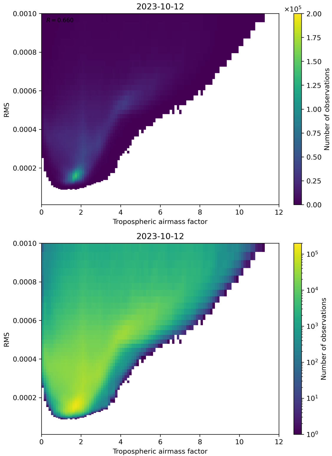
Figure 79: Scatter density plot of “Tropospheric airmass factor” against “RMS” for 2023-10-12 to 2023-10-13.
