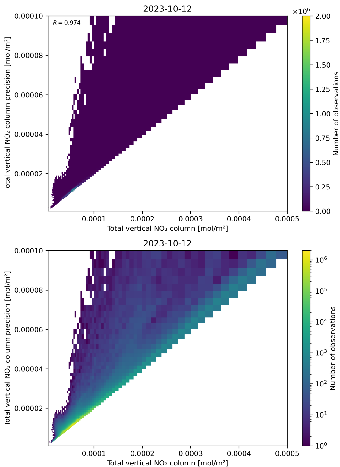
Figure 114: Scatter density plot of “Total vertical NO 2 column” against “Total vertical NO 2 column precision” for 2023-10-12 to 2023-10-13.
