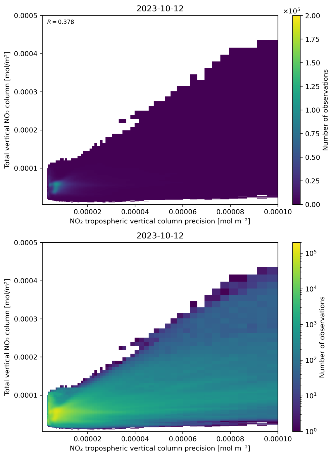
Figure 138: Scatter density plot of “NO 2 tropospheric vertical column precision” against “Total vertical NO 2 column” for 2023-10-12 to 2023-10-13.
