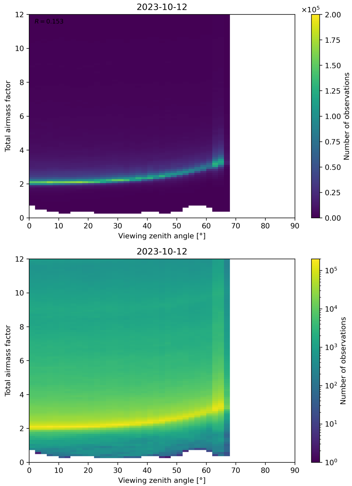
Figure 160: Scatter density plot of “Viewing zenith angle” against “Total airmass factor” for 2023-10-12 to 2023-10-13.
