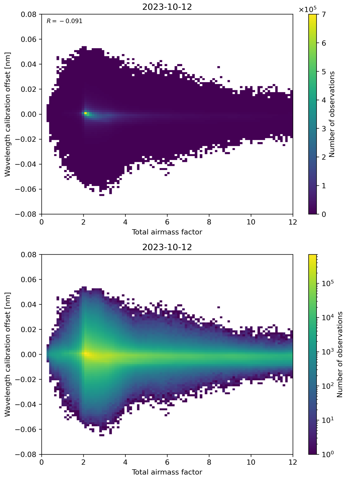
Figure 70: Scatter density plot of “Total airmass factor” against “Wavelength calibration offset” for 2023-10-12 to 2023-10-13.
