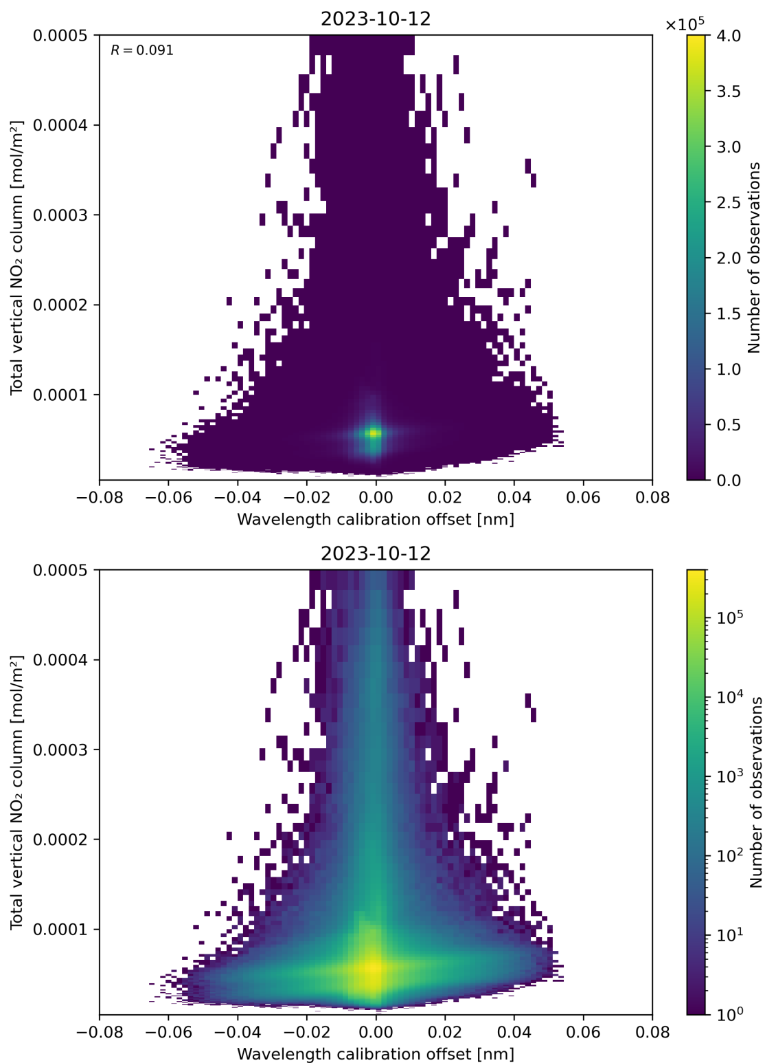
Figure 179: Scatter density plot of “Wavelength calibration offset” against “Total vertical NO 2 column” for 2023-10-12 to 2023-10-13.
