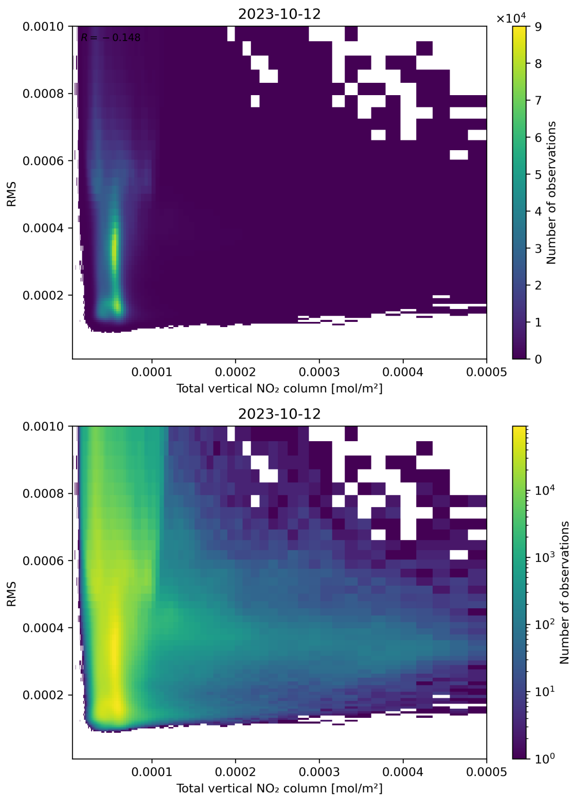
Figure 120: Scatter density plot of “Total vertical NO 2 column” against “RMS” for 2023-10-12 to 2023-10-13.
