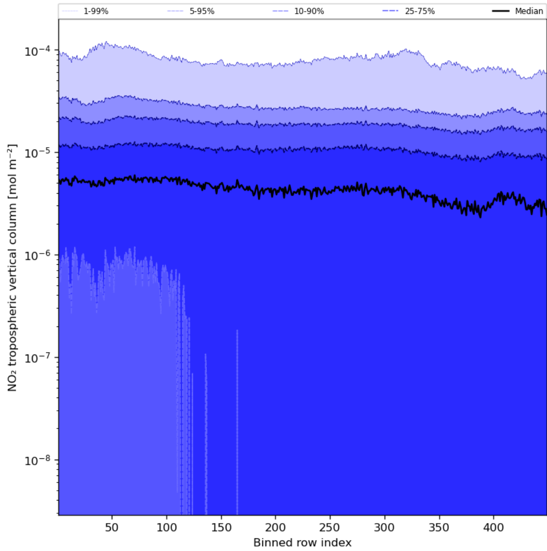
Figure 46: Along track statistics of “NO 2 tropospheric vertical column” for 2023-10-12 to 2023-10-13
