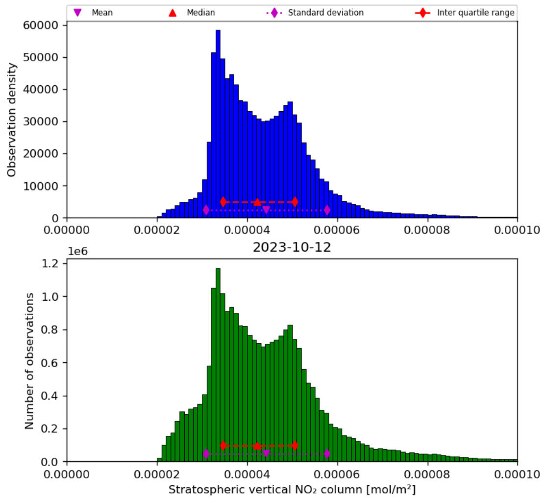
Figure 36: Histogram of “Stratospheric vertical NO 2 column” for 2023-10-12 to 2023-10-13
