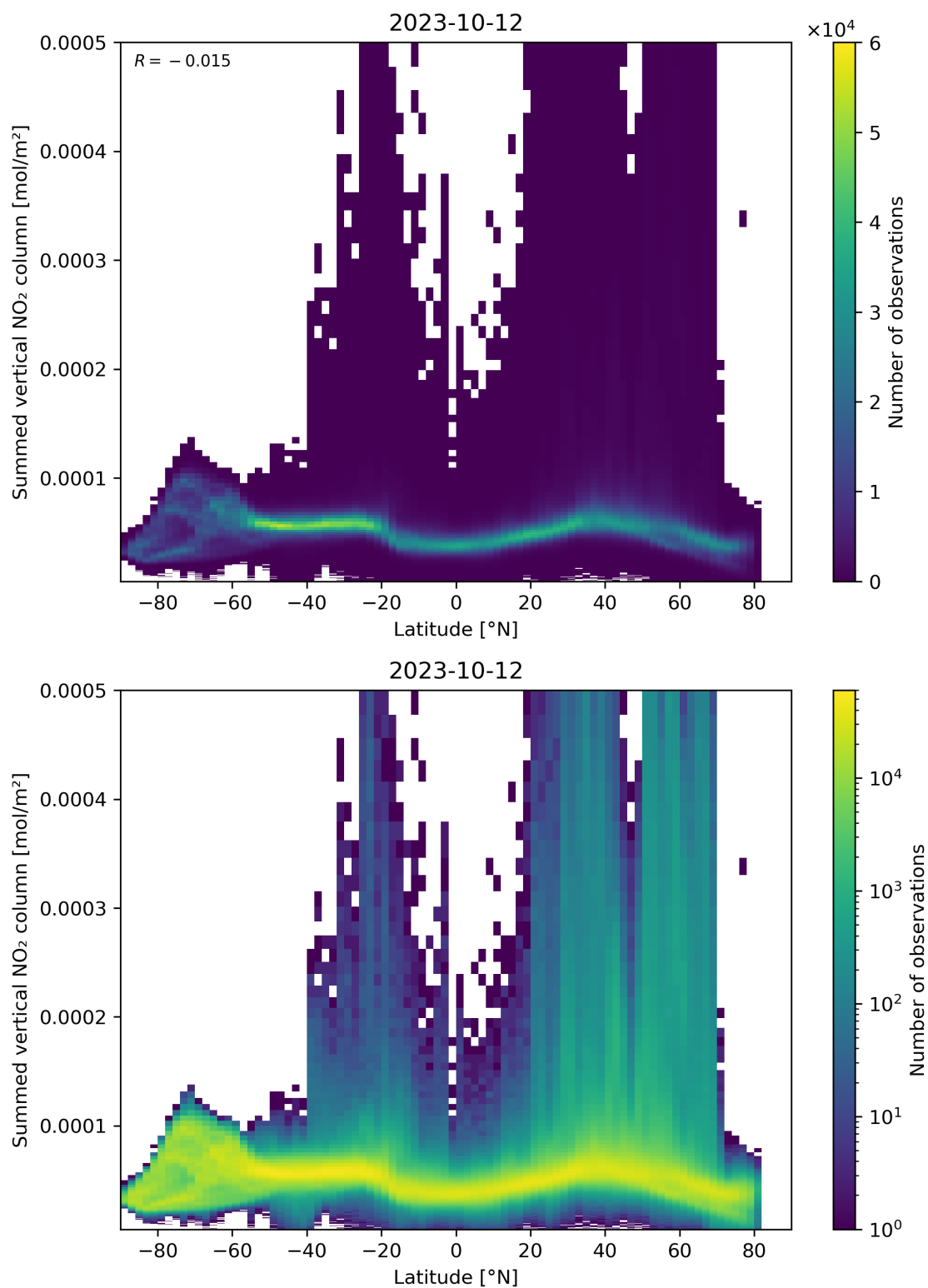
Figure 88: Scatter density plot of “Latitude” against “Summed vertical NO 2 column” for 2023-10-12 to 2023-10-13.
