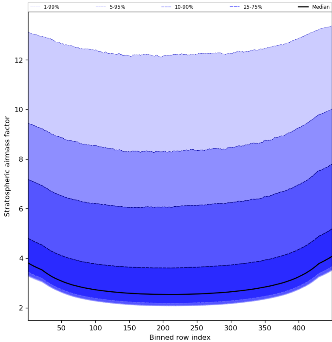
Figure 61: Along track statistics of “Stratospheric airmass factor” for 2023-10-12 to 2023-10-13
