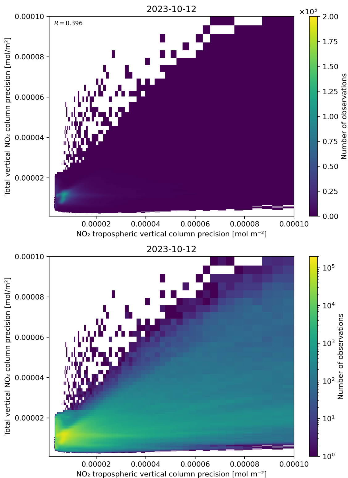
Figure 139: Scatter density plot of “NO 2 tropospheric vertical column precision” against “Total vertical NO 2 column precision” for 2023-10-12 to 2023-10-13.
