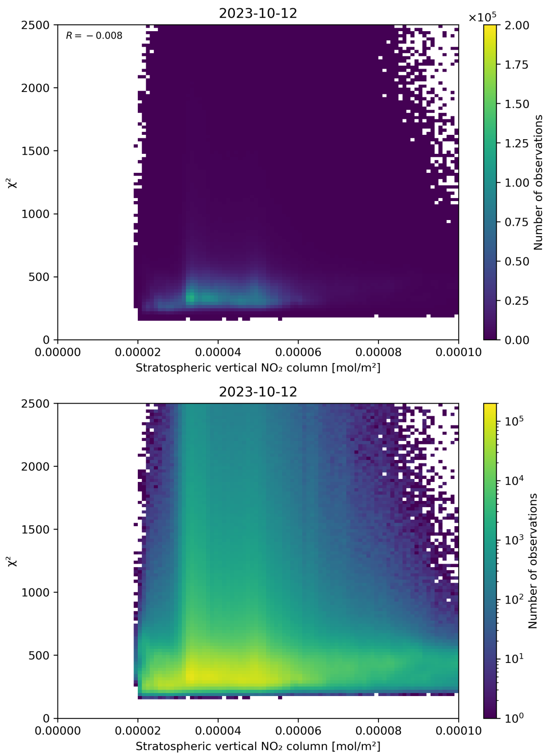
Figure 97: Scatter density plot of “Stratospheric vertical NO 2 column” against “ \chi^2 ” for 2023-10-12 to 2023-10-13.
