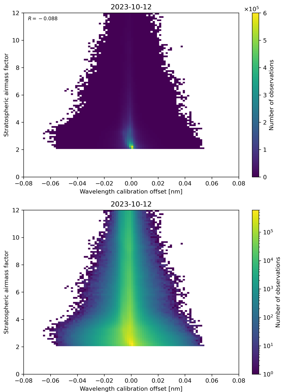
Figure 174: Scatter density plot of “Wavelength calibration offset” against “Stratospheric airmass factor” for 2023-10-12 to 2023-10-13.
