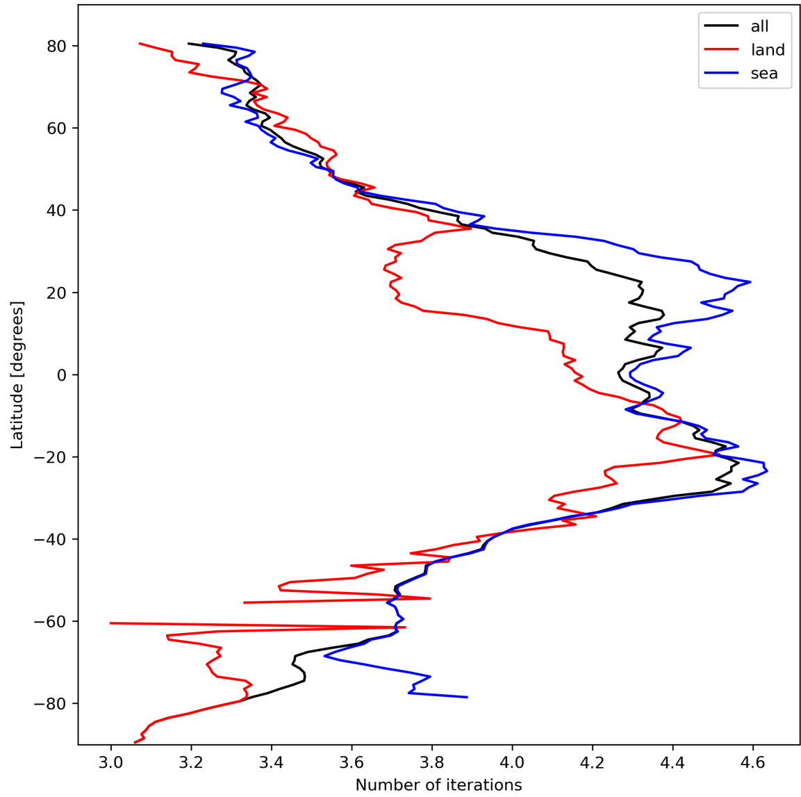
Figure 17: Zonal average of “Number of iterations” for 2023-10-12 to 2023-10-13.
