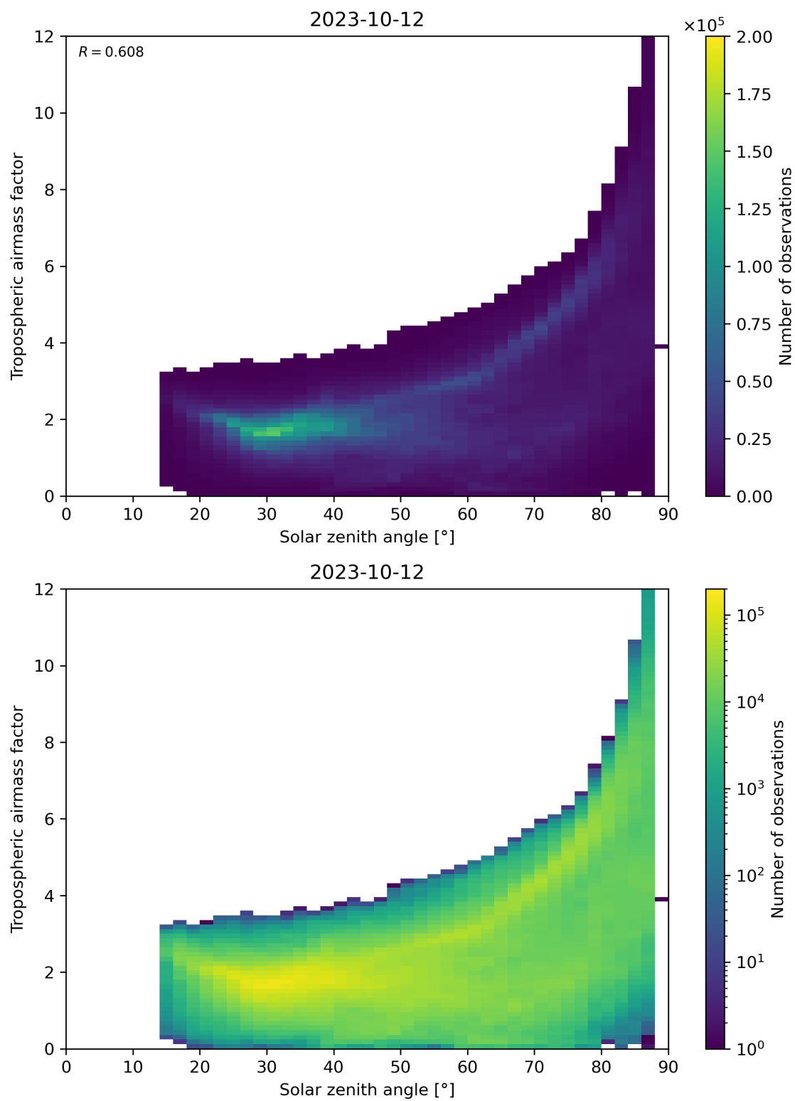
Figure 147: Scatter density plot of “Solar zenith angle” against “Tropospheric airmass factor” for 2023-10-12 to 2023-10-13.
