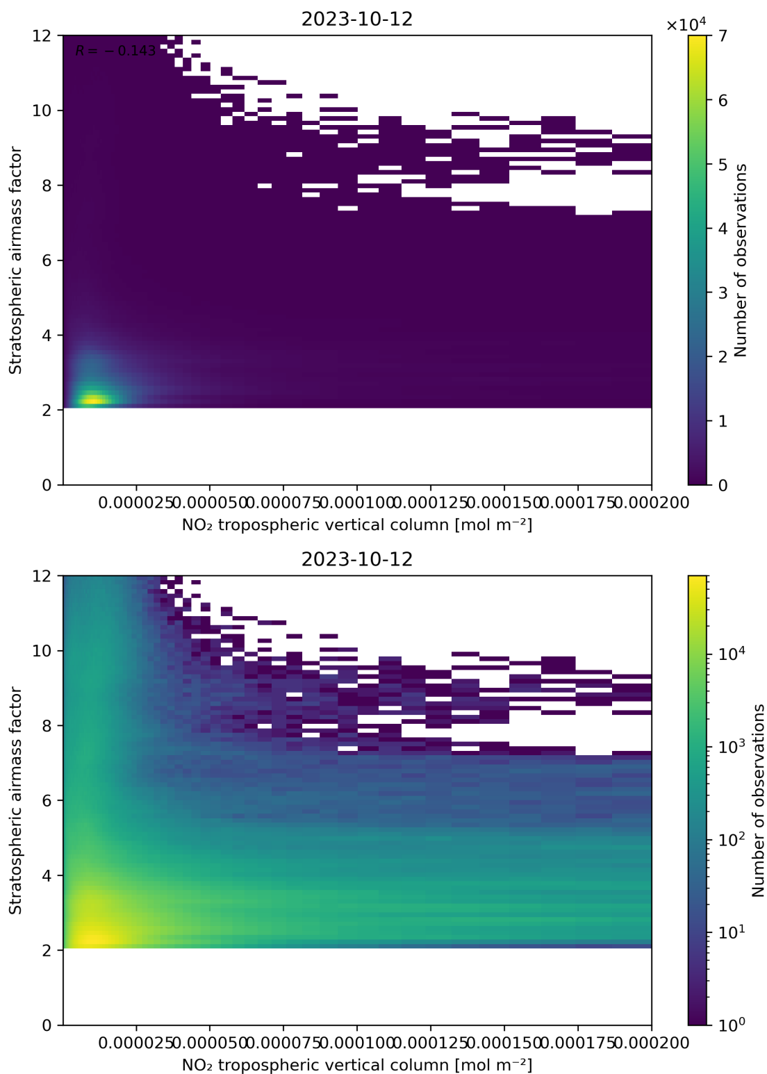
Figure 121: Scatter density plot of “NO 2 tropospheric vertical column” against “Stratospheric airmass factor” for 2023-10-12 to 2023-10-13.
