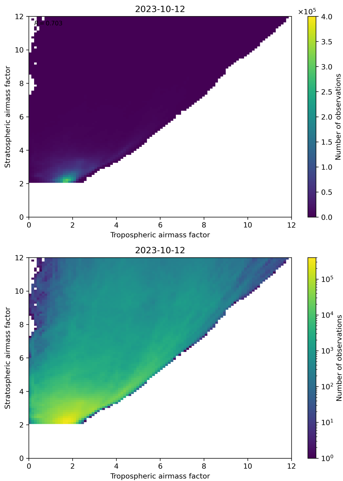
Figure 71: Scatter density plot of “Tropospheric airmass factor” against “Stratospheric airmass factor” for 2023-10-12 to 2023-10-13.
