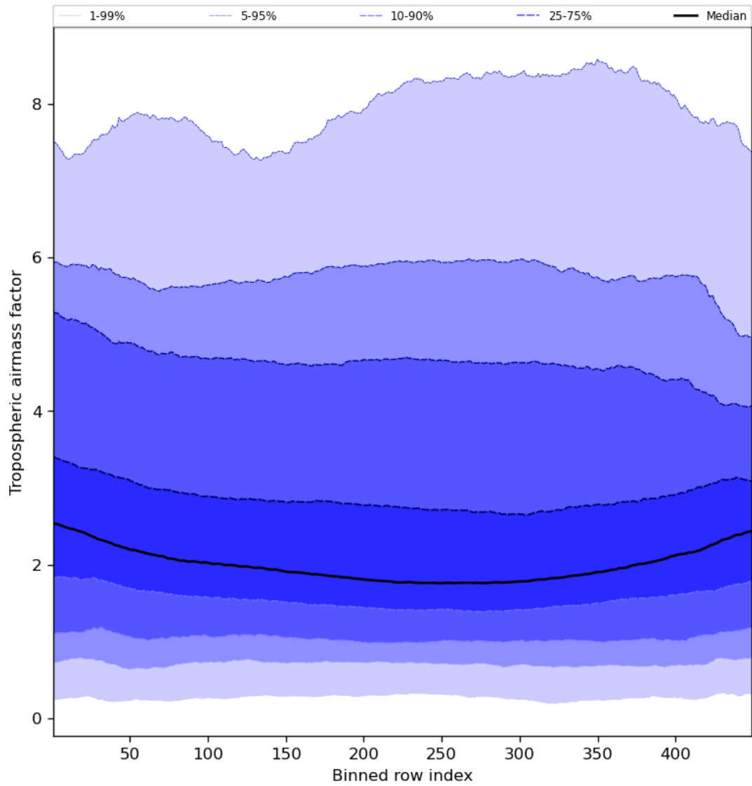
Figure 48: Along track statistics of “Tropospheric airmass factor” for 2023-10-12 to 2023-10-13
