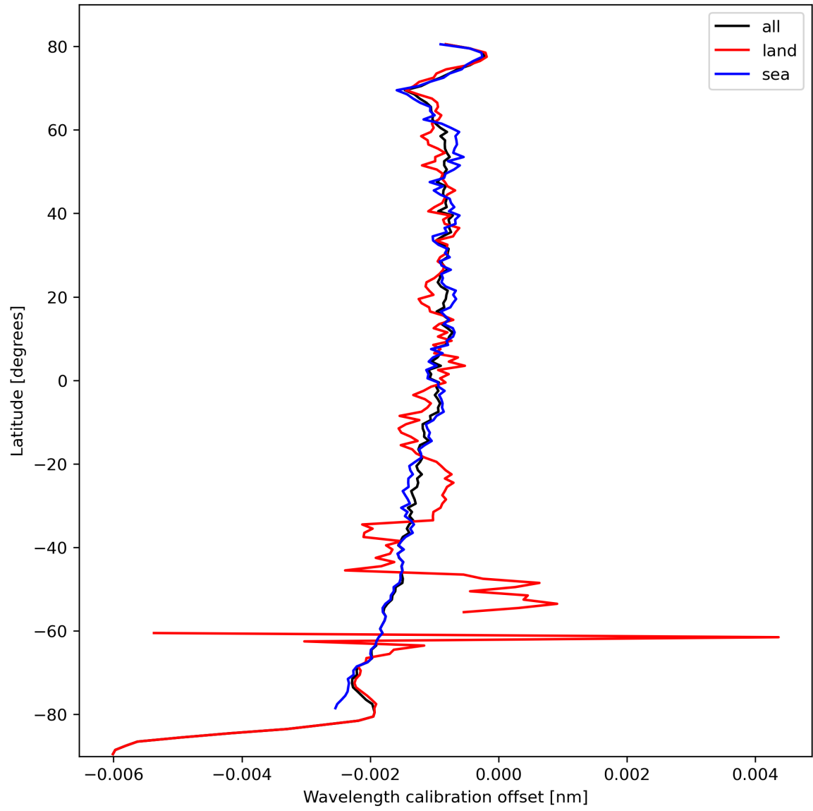
Figure 18: Zonal average of “Wavelength calibration offset” for 2023-10-12 to 2023-10-13.
