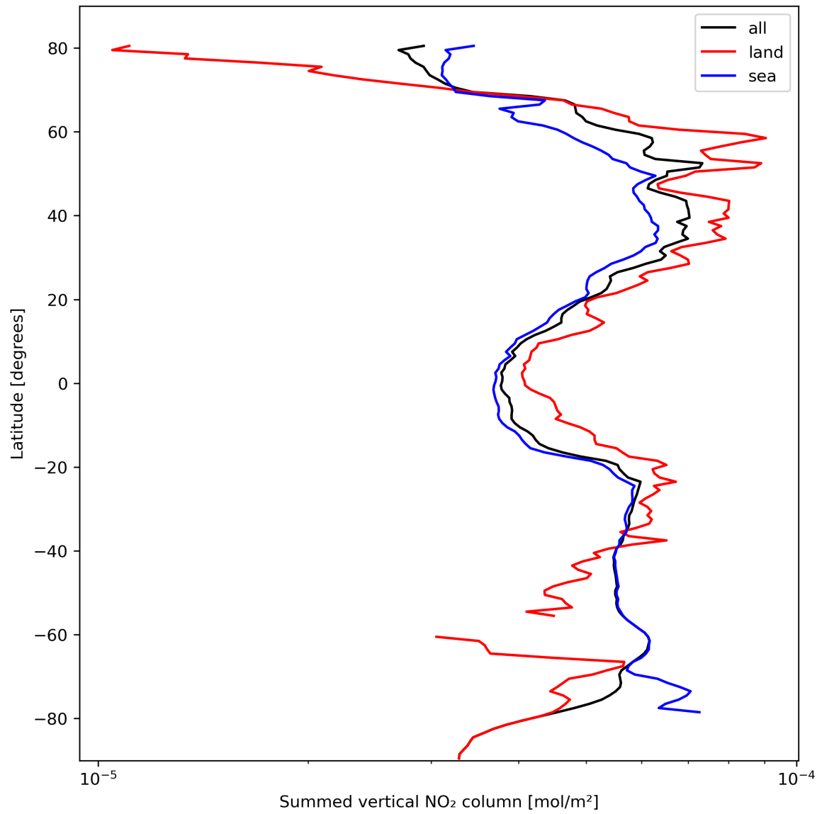
Figure 23: Zonal average of “Summed vertical NO 2 column” for 2023-10-12 to 2023-10-13.
