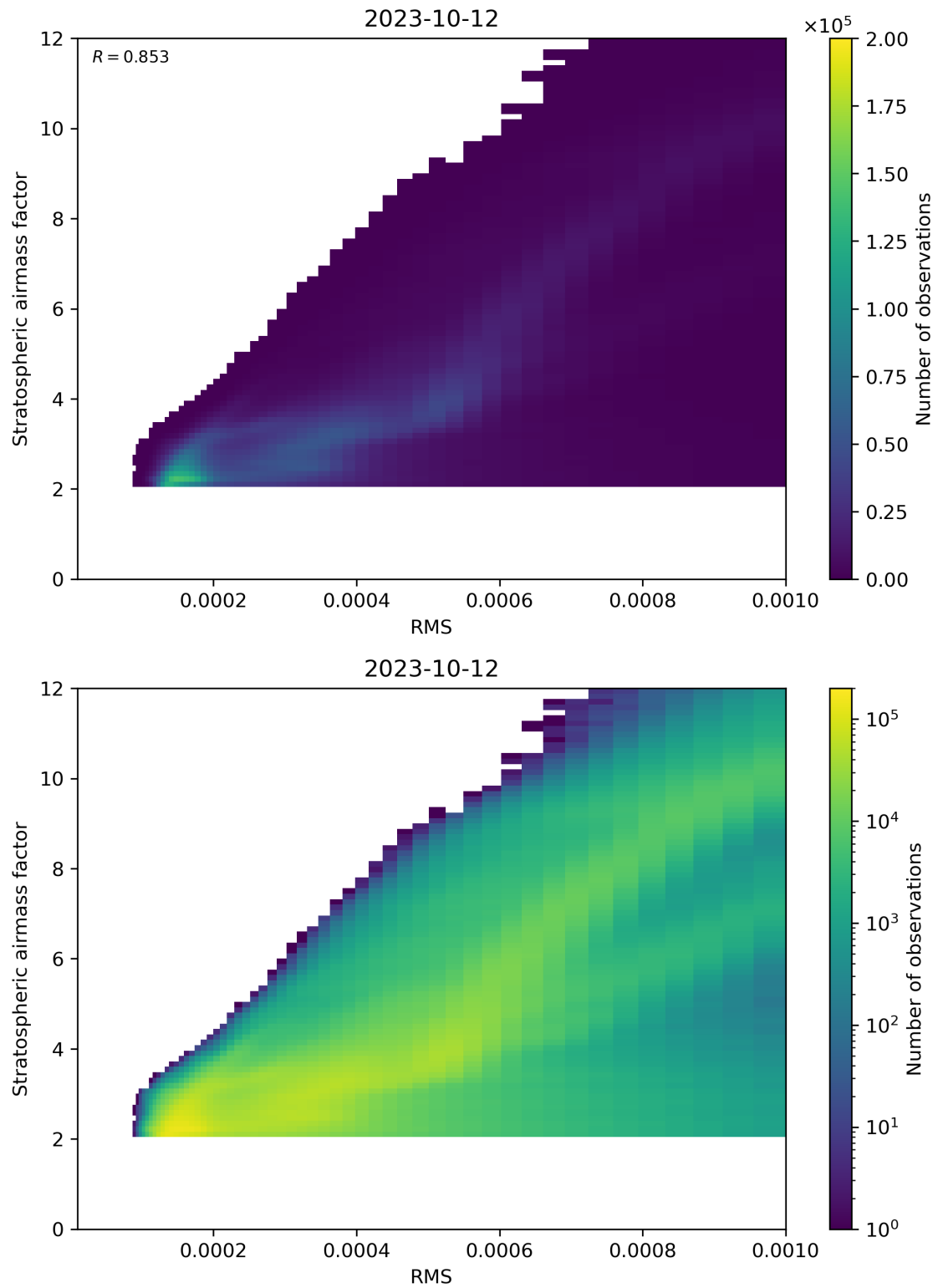
Figure 144: Scatter density plot of “RMS” against “Stratospheric airmass factor” for 2023-10-12 to 2023-10-13.
