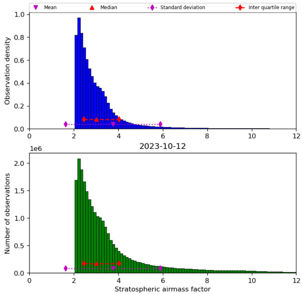
Figure 44: Histogram of “Stratospheric airmass factor” for 2023-10-12 to 2023-10-13
