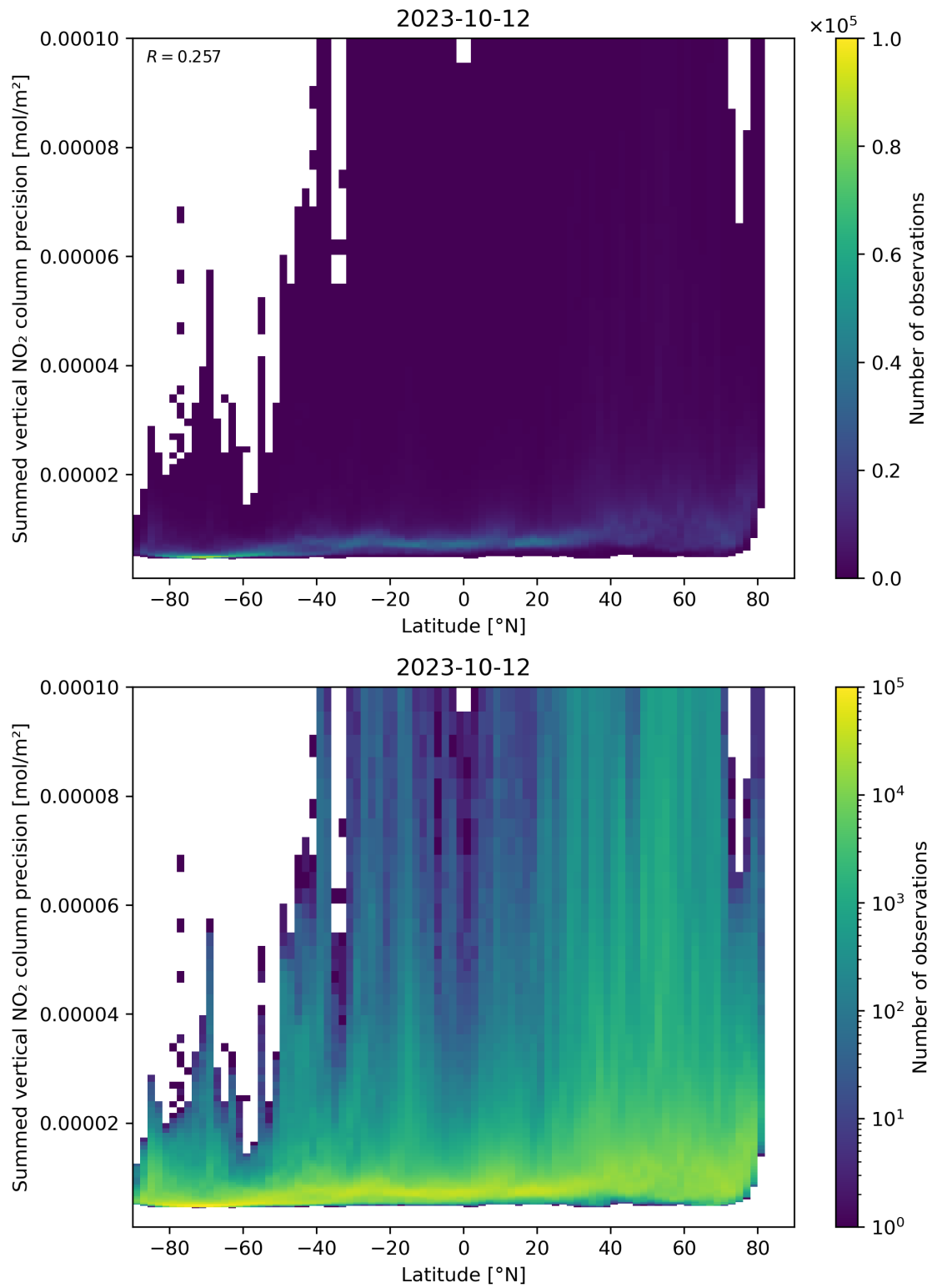
Figure 89: Scatter density plot of “Latitude” against “Summed vertical NO 2 column precision” for 2023-10-12 to 2023-10-13.
