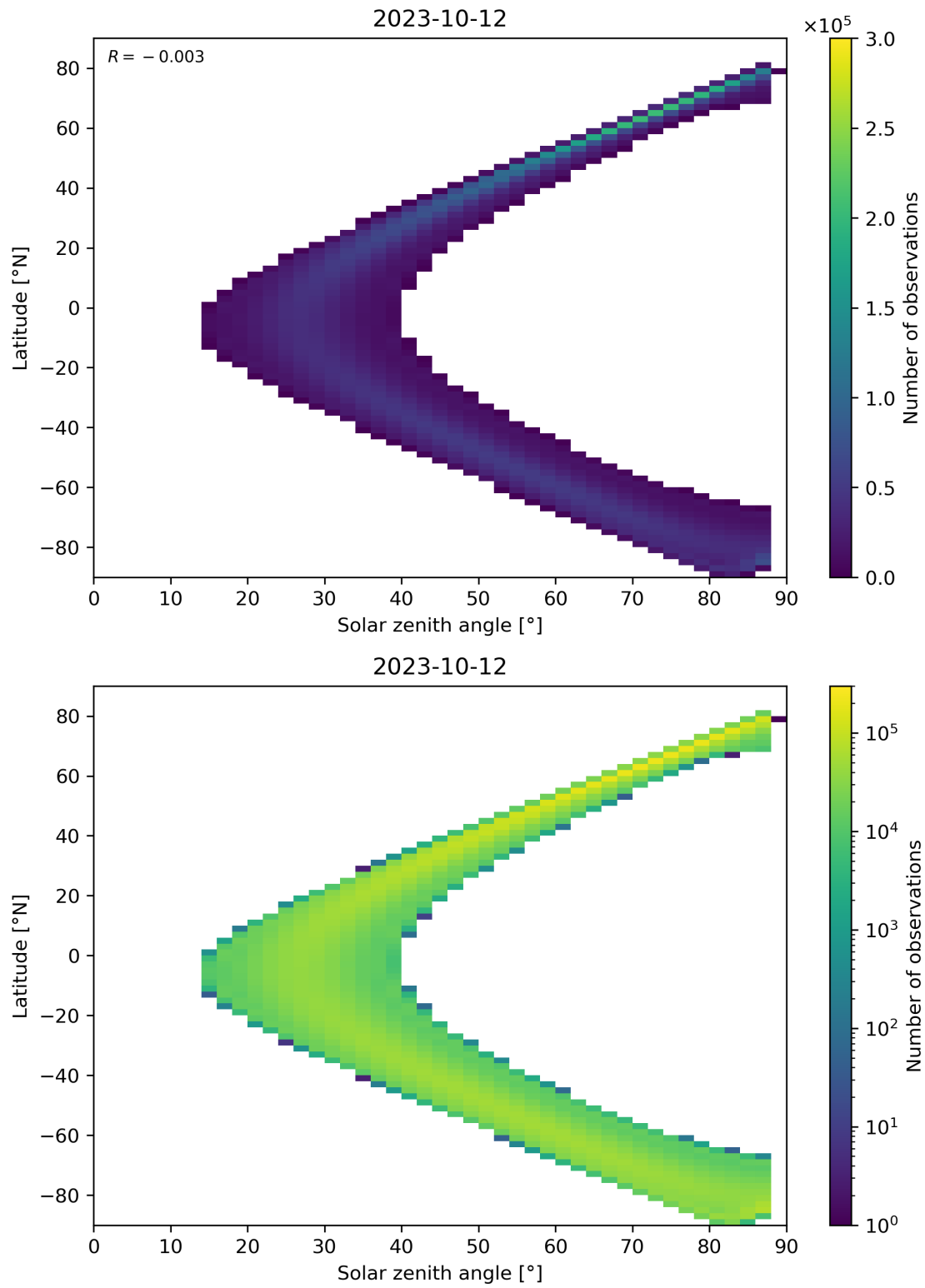
Figure 149: Scatter density plot of “Solar zenith angle” against “Latitude” for 2023-10-12 to 2023-10-13.
