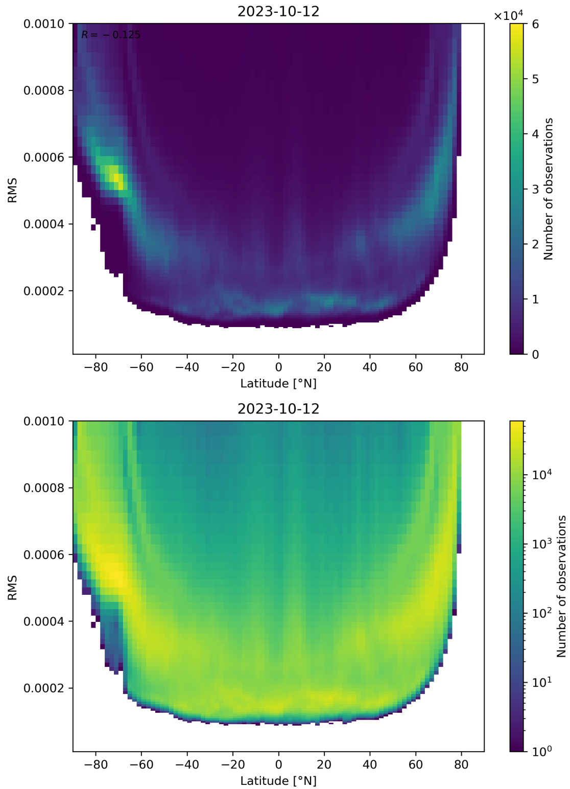
Figure 94: Scatter density plot of “Latitude” against “RMS” for 2023-10-12 to 2023-10-13.
