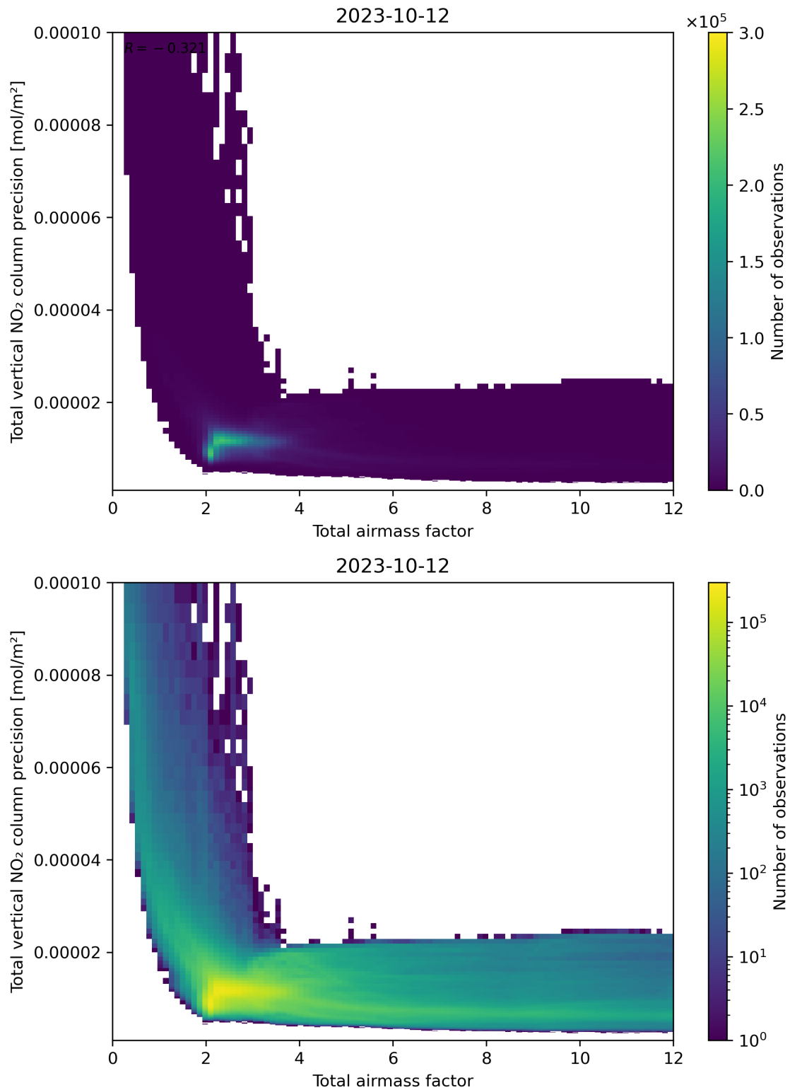
Figure 68: Scatter density plot of “Total airmass factor” against “Total vertical NO 2 column precision” for 2023-10-12 to 2023-10-13.
