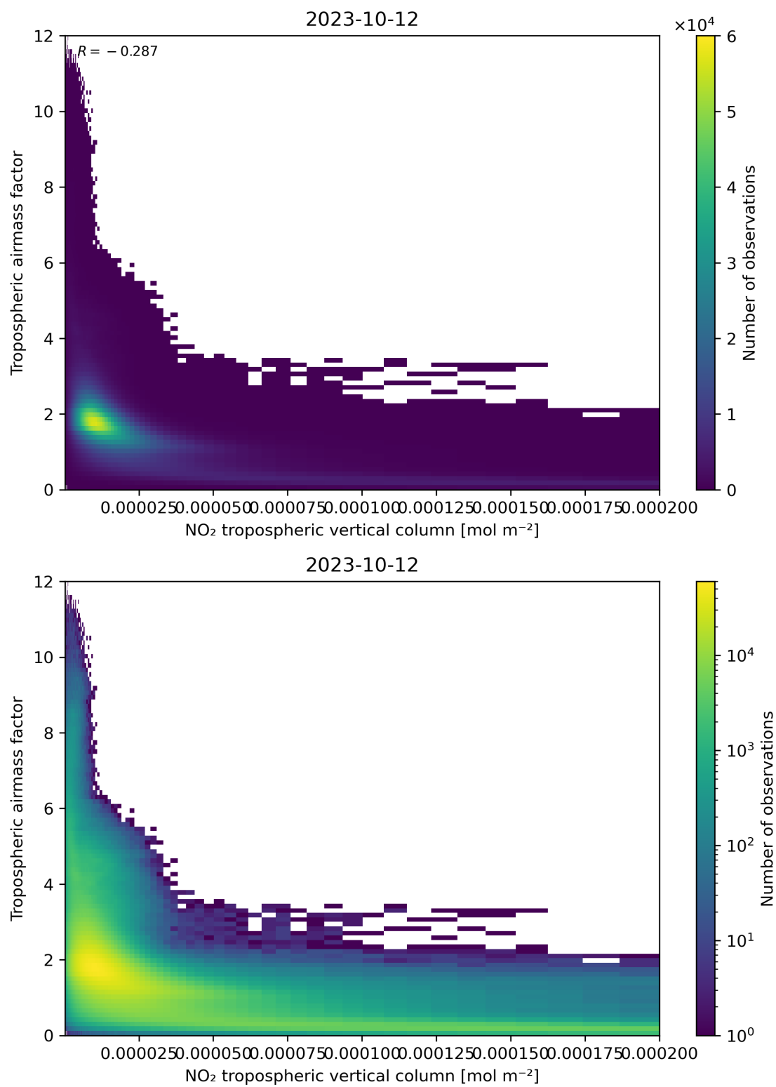
Figure 123: Scatter density plot of “NO 2 tropospheric vertical column” against “Tropospheric air mass factor” for 2023-10-12 to 2023-10-13.
