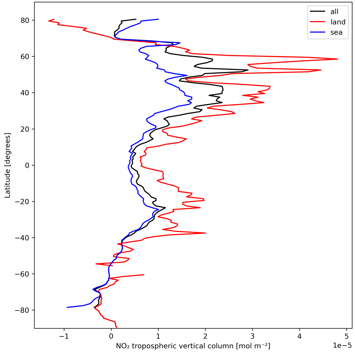
Figure 12: Zonal average of “NO 2 tropospheric vertical column” for 2023-10-12 to 2023-10-13.
