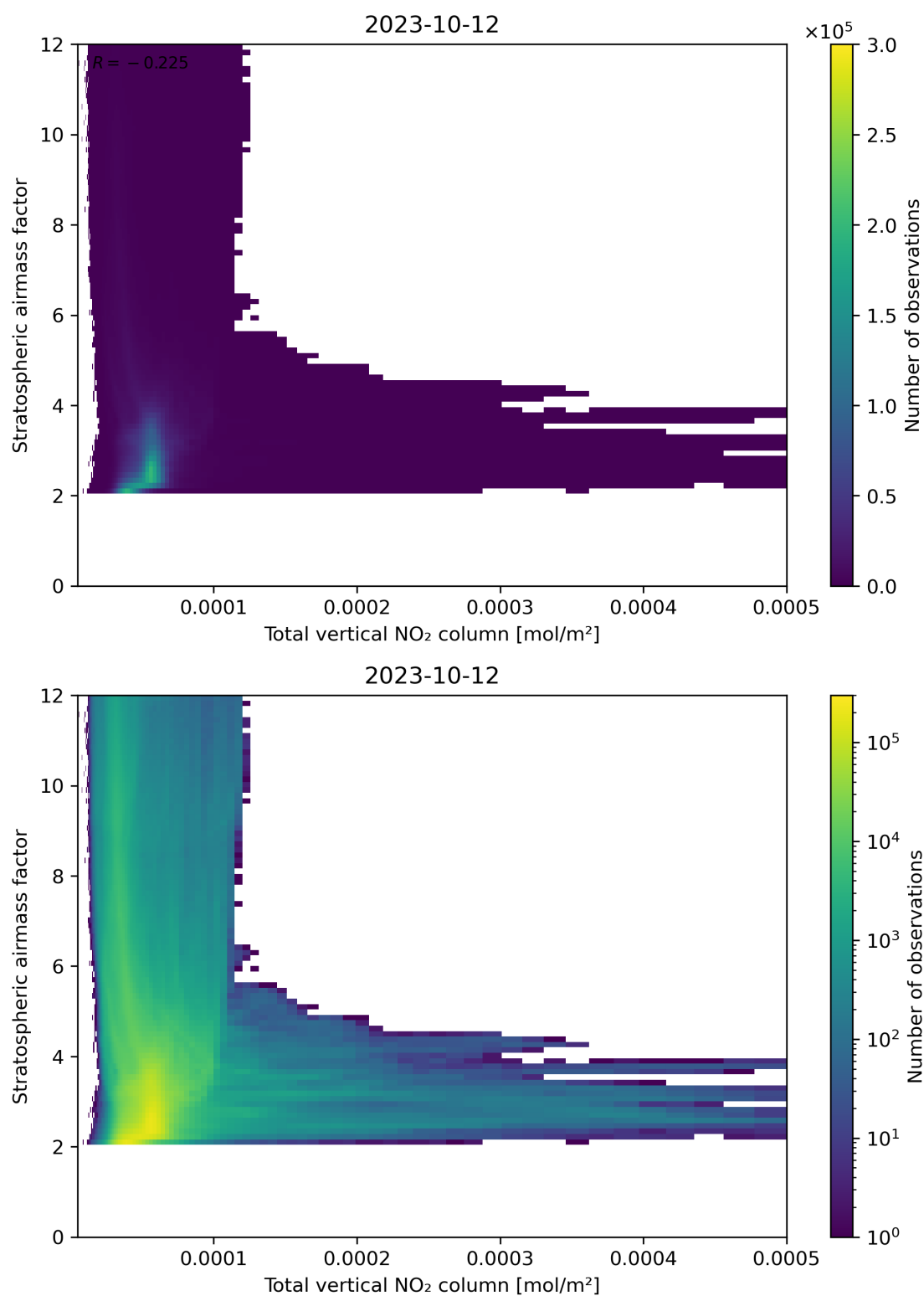
Figure 110: Scatter density plot of “Total vertical NO 2 column” against “Stratospheric airmass factor” for 2023-10-12 to 2023-10-13.
