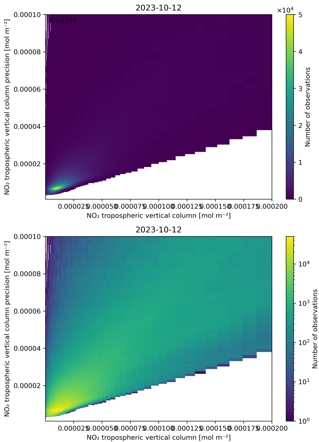
Figure 130: Scatter density plot of “NO 2 tropospheric vertical column” against “NO 2 tropospheric vertical column precision” for 2023-10-12 to 2023-10-13.
