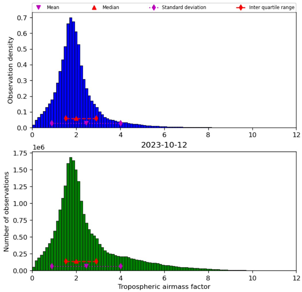
Figure 31: Histogram of “Tropospheric airmass factor” for 2023-10-12 to 2023-10-13
