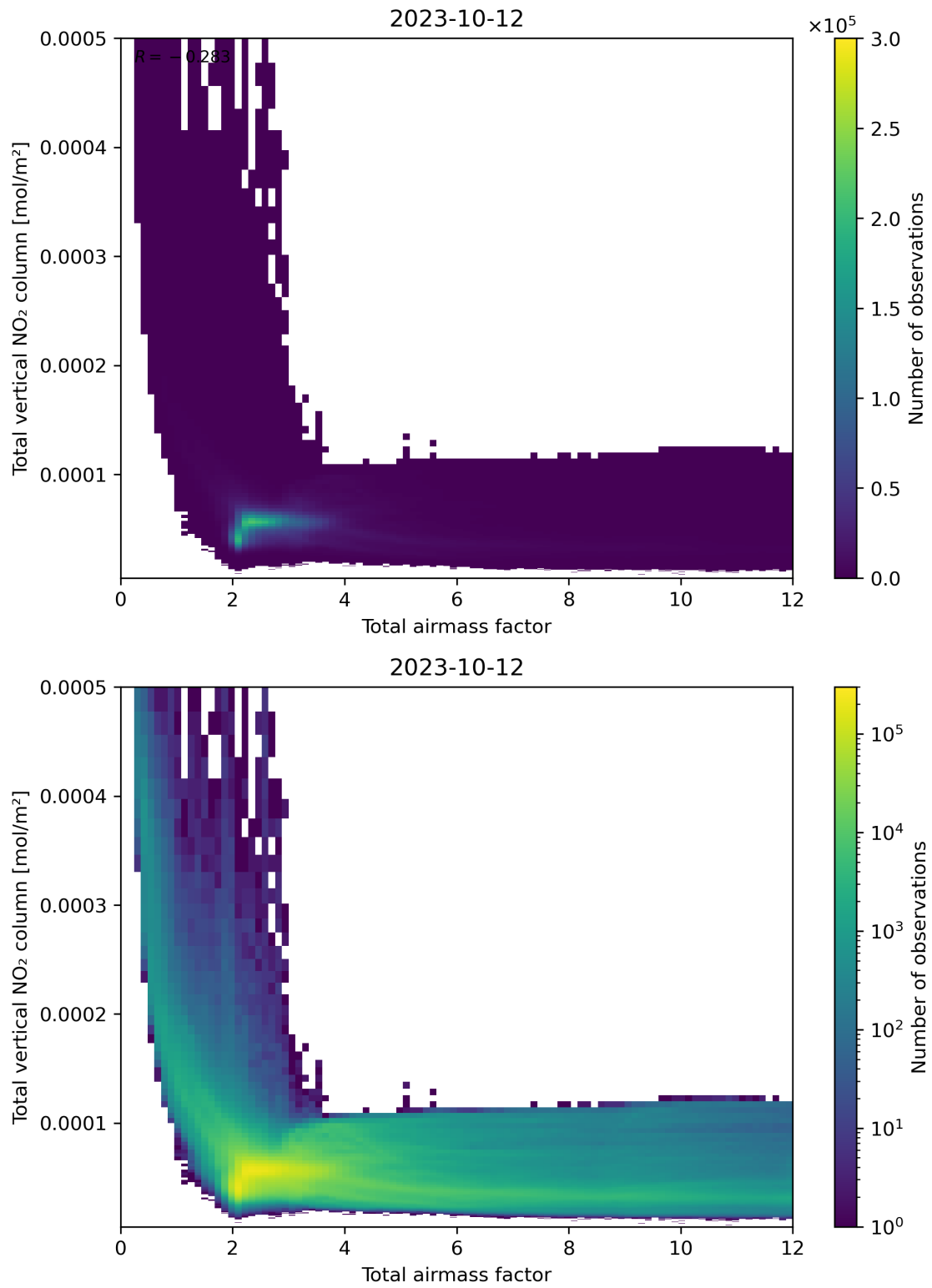
Figure 67: Scatter density plot of “Total airmass factor” against “Total vertical NO 2 column” for 2023-10-12 to 2023-10-13.
