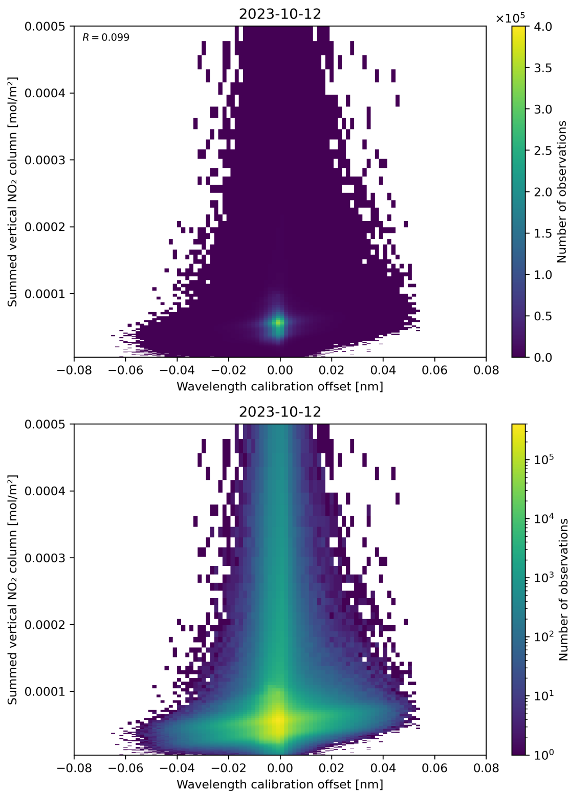
Figure 177: Scatter density plot of “Wavelength calibration offset” against “Summed vertical NO 2 column” for 2023-10-12 to 2023-10-13.
