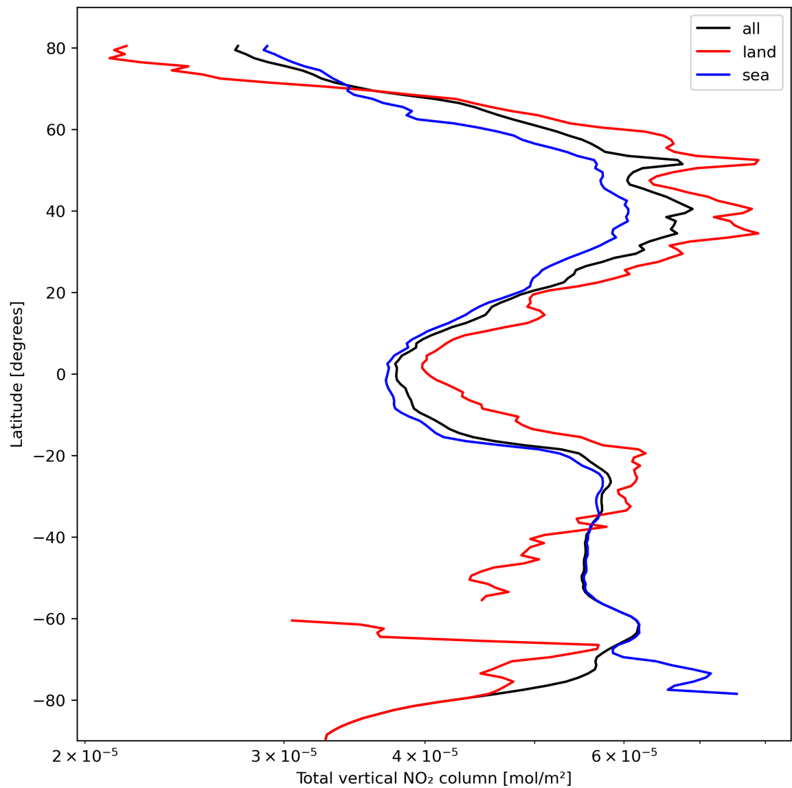
Figure 21: Zonal average of “Total vertical NO 2 column” for 2023-10-12 to 2023-10-13.
