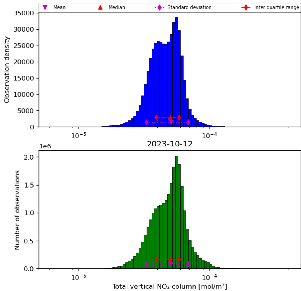
Figure 38: Histogram of “Total vertical NO 2 column” for 2023-10-12 to 2023-10-13
