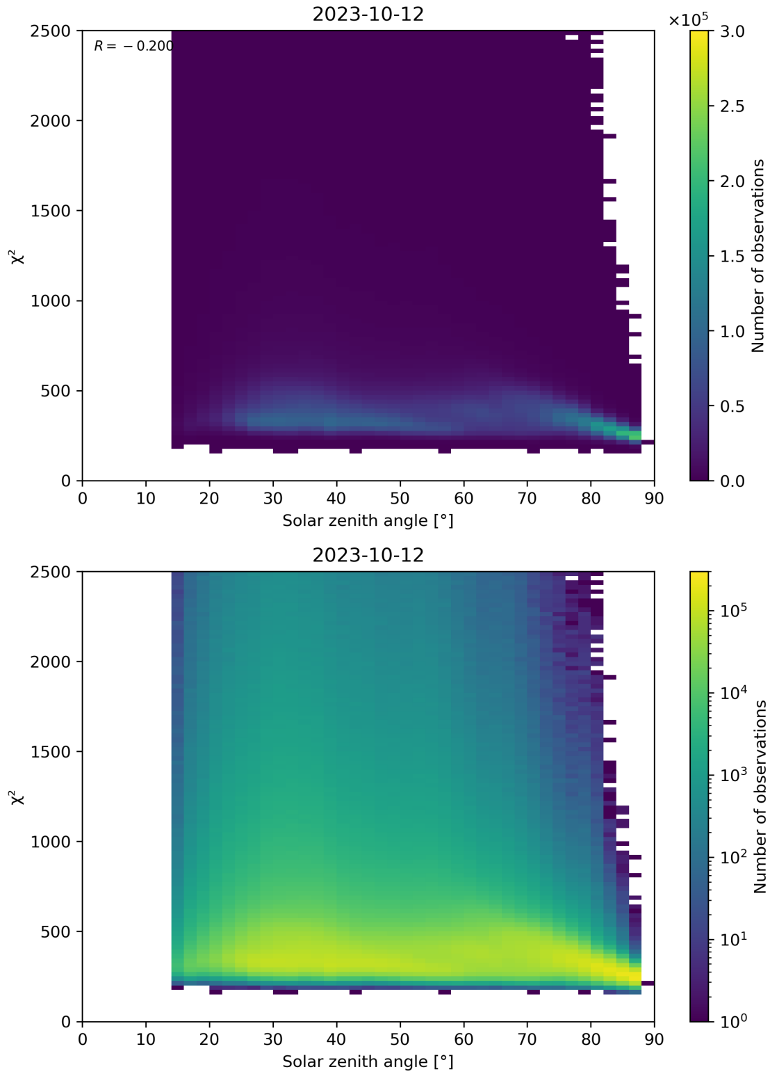
Figure 148: Scatter density plot of “Solar zenith angle” against “ \chi^2 ” for 2023-10-12 to 2023-10-13.
