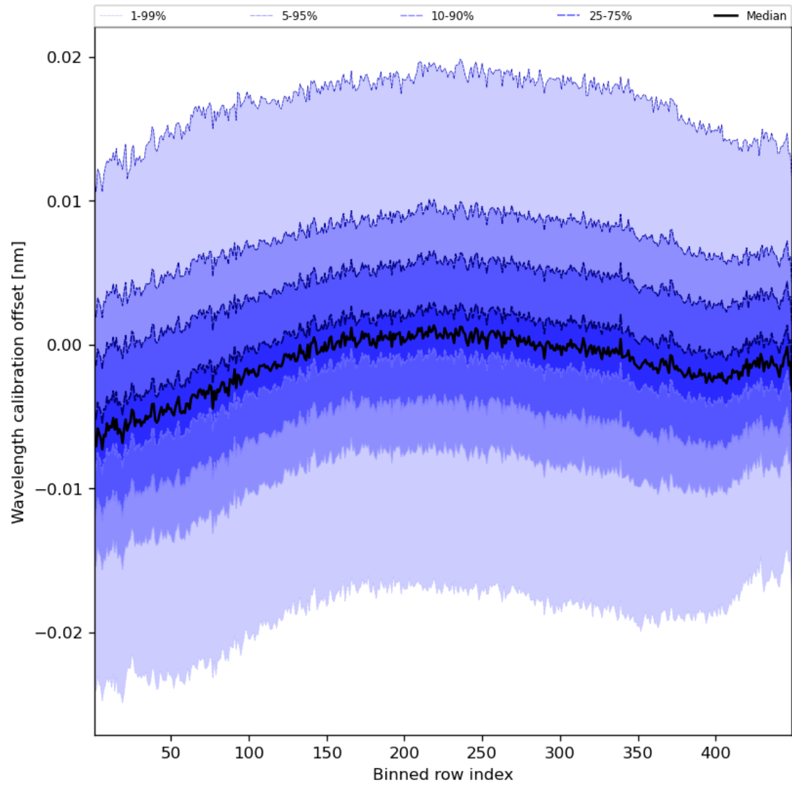
Figure 52: Along track statistics of “Wavelength calibration offset” for 2023-10-12 to 2023-10-13
