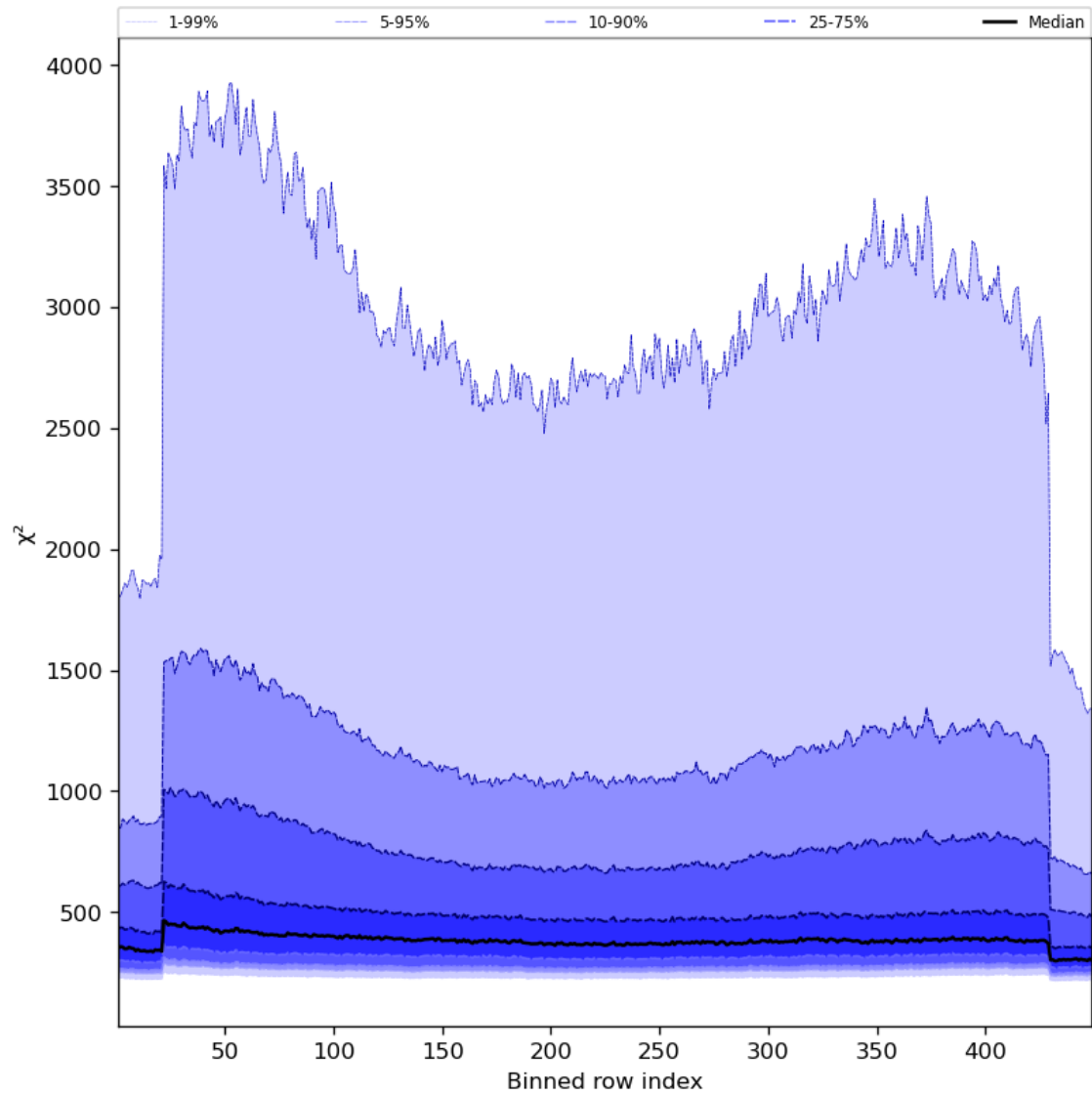
Figure 59: Along track statistics of “ \chi^2 ” for 2023-10-12 to 2023-10-13
