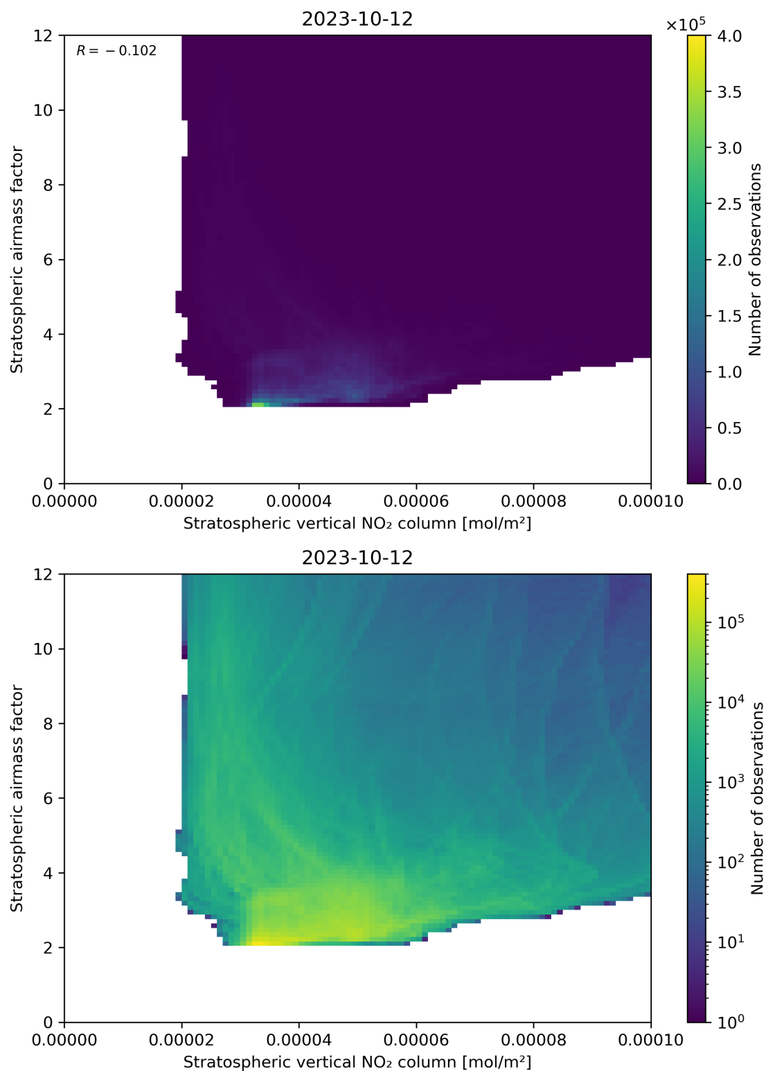
Figure 96: Scatter density plot of “Stratospheric vertical NO 2 column” against “Stratospheric airmass factor” for 2023-10-12 to 2023-10-13.
