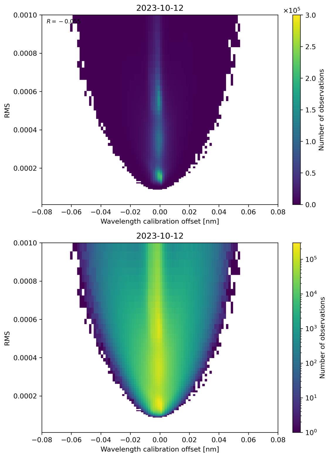
Figure 181: Scatter density plot of “Wavelength calibration offset” against “RMS” for 2023-10-12 to 2023-10-13.
