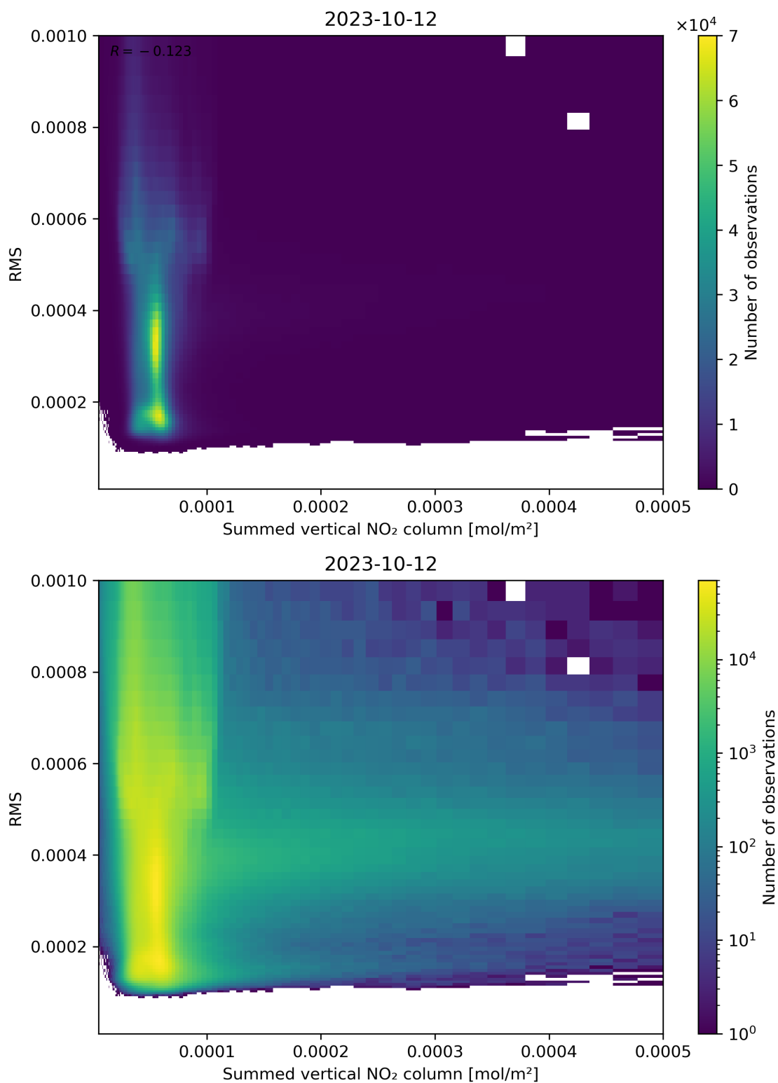
Figure 109: Scatter density plot of “Summed vertical NO 2 column” against “RMS” for 2023-10-12 to 2023-10-13.
