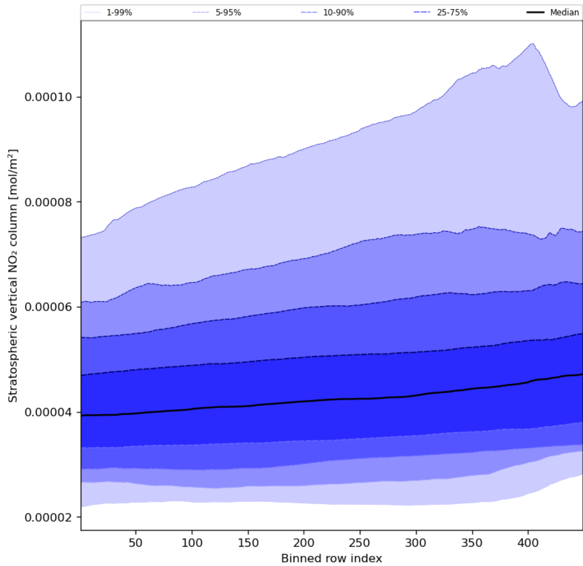
Figure 53: Along track statistics of “Stratospheric vertical NO 2 column” for 2023-10-12 to 2023-10-13
