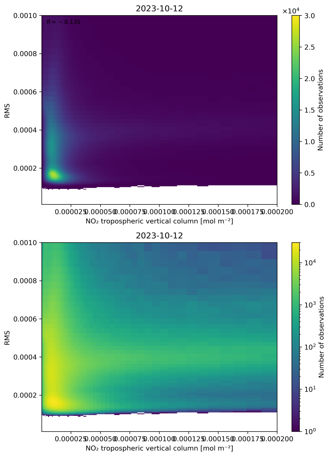
Figure 142: Scatter density plot of “NO 2 tropospheric vertical column” against “RMS” for 2023-10-12 to 2023-10-13.
