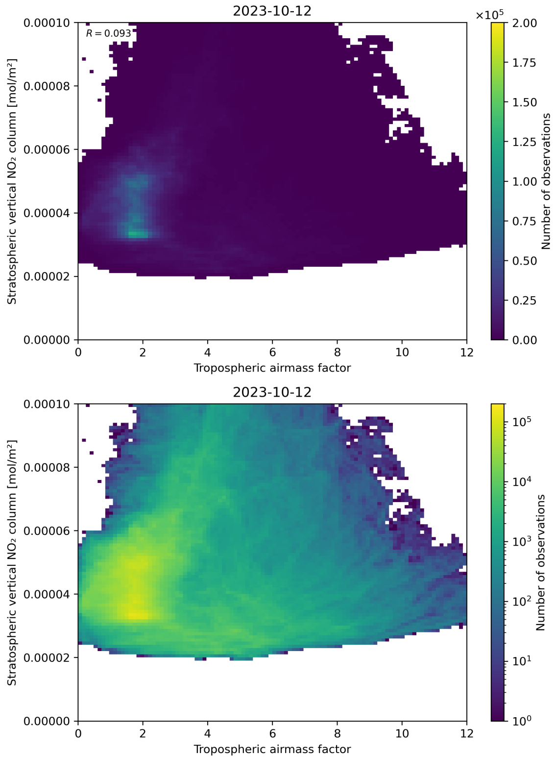
Figure 74: Scatter density plot of “Tropospheric air mass factor” against “Stratospheric vertical NO 2 column” for 2023-10-12 to 2023-10-13.
