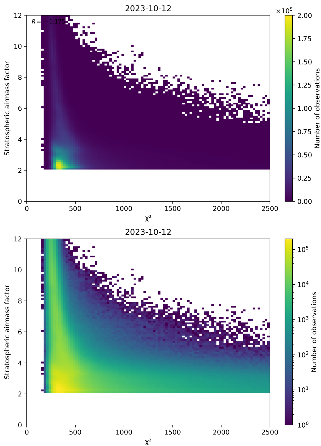
Figure 81: Scatter density plot of “ \chi^2 ” against “Stratospheric airmass factor” for 2023-10-12 to 2023-10-13.
