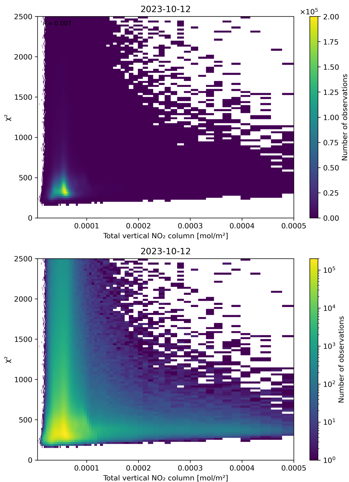
Figure 111: Scatter density plot of “Total vertical NO 2 column” against “ \chi^2 ” for 2023-10-12 to 2023-10-13.
