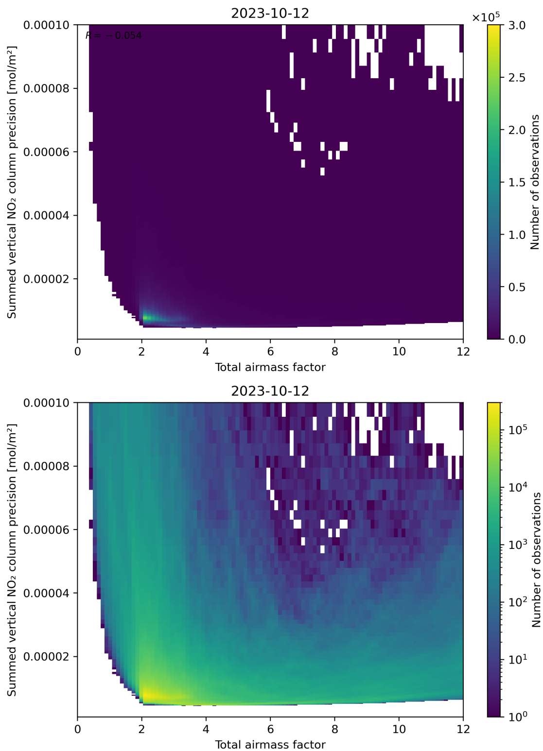
Figure 66: Scatter density plot of “Total airmass factor” against “Summed vertical NO 2 column precision” for 2023-10-12 to 2023-10-13.
