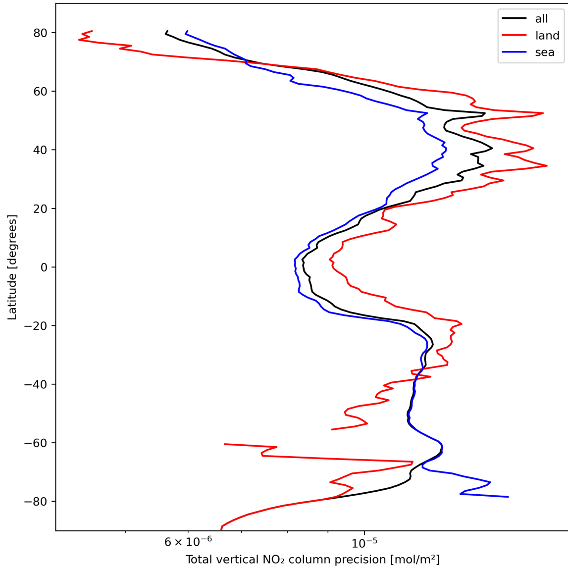
Figure 22: Zonal average of “Total vertical NO 2 column precision” for 2023-10-12 to 2023-10-13.
