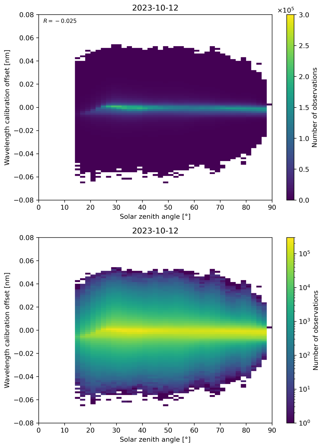
Figure 158: Scatter density plot of “Solar zenith angle” against “Wavelength calibration offset” for 2023-10-12 to 2023-10-13.
