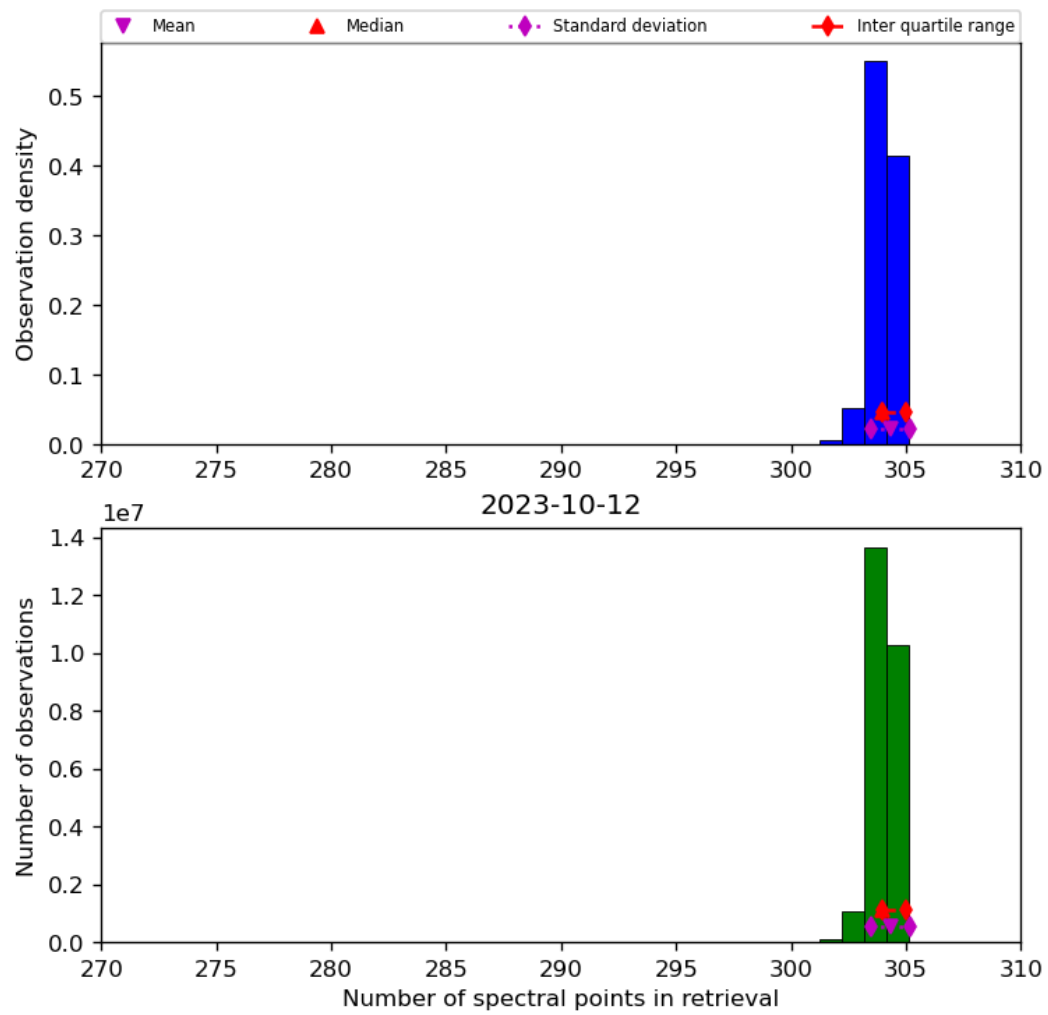
Figure 33: Histogram of “Number of spectral points in retrieval” for 2023-10-12 to 2023-10-13
