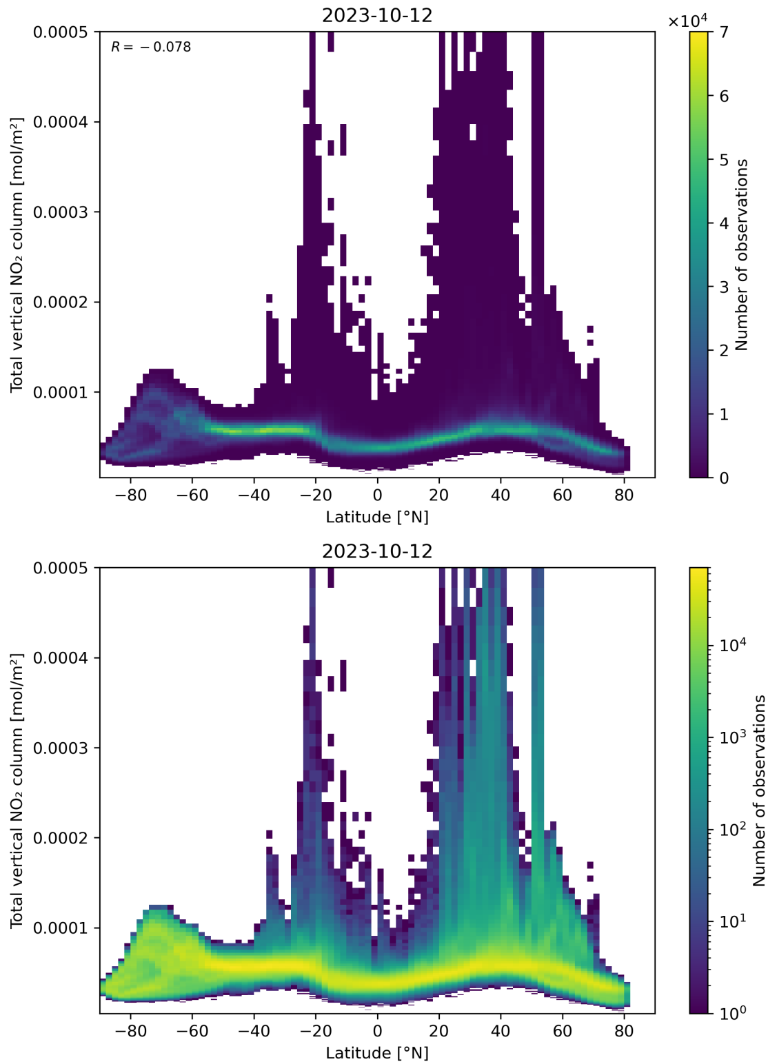
Figure 90: Scatter density plot of “Latitude” against “Total vertical NO 2 column” for 2023-10-12 to 2023-10-13.
