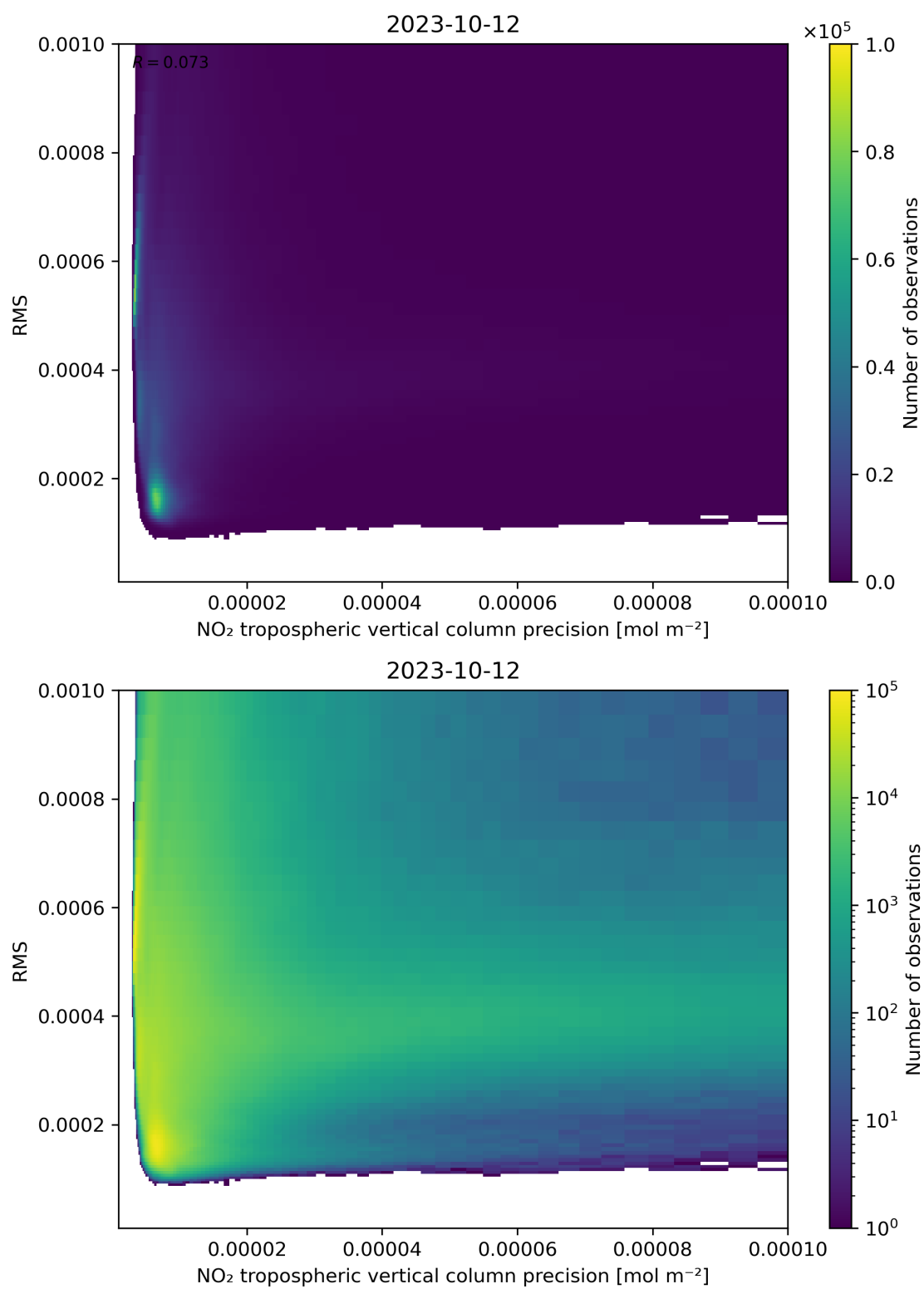
Figure 140: Scatter density plot of “NO 2 tropospheric vertical column precision” against “RMS” for 2023-10-12 to 2023-10-13.
