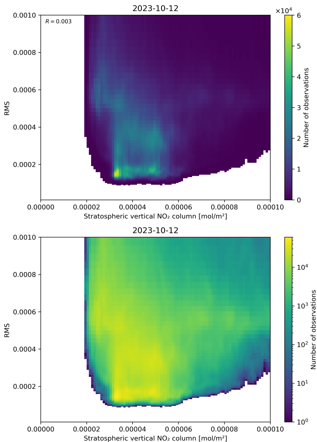
Figure 102: Scatter density plot of “Stratospheric vertical NO 2 column” against “RMS” for 2023-10-12 to 2023-10-13.
