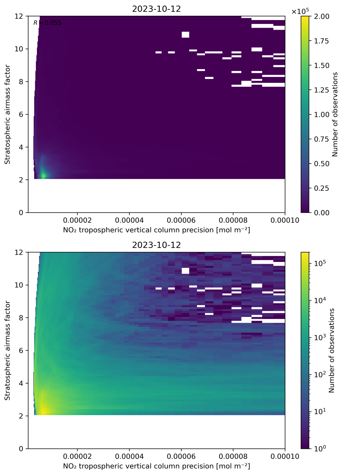
Figure 131: Scatter density plot of “NO 2 tropospheric vertical column precision” against “Stratospheric airmass factor” for 2023-10-12 to 2023-10-13.
