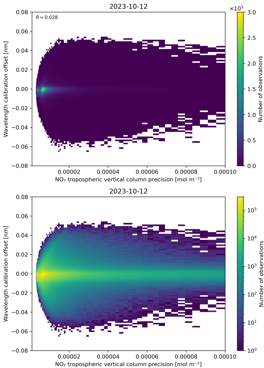
Figure 141: Scatter density plot of “NO 2 tropospheric vertical column precision” against “Wavelength calibration offset” for 2023-10-12 to 2023-10-13.
