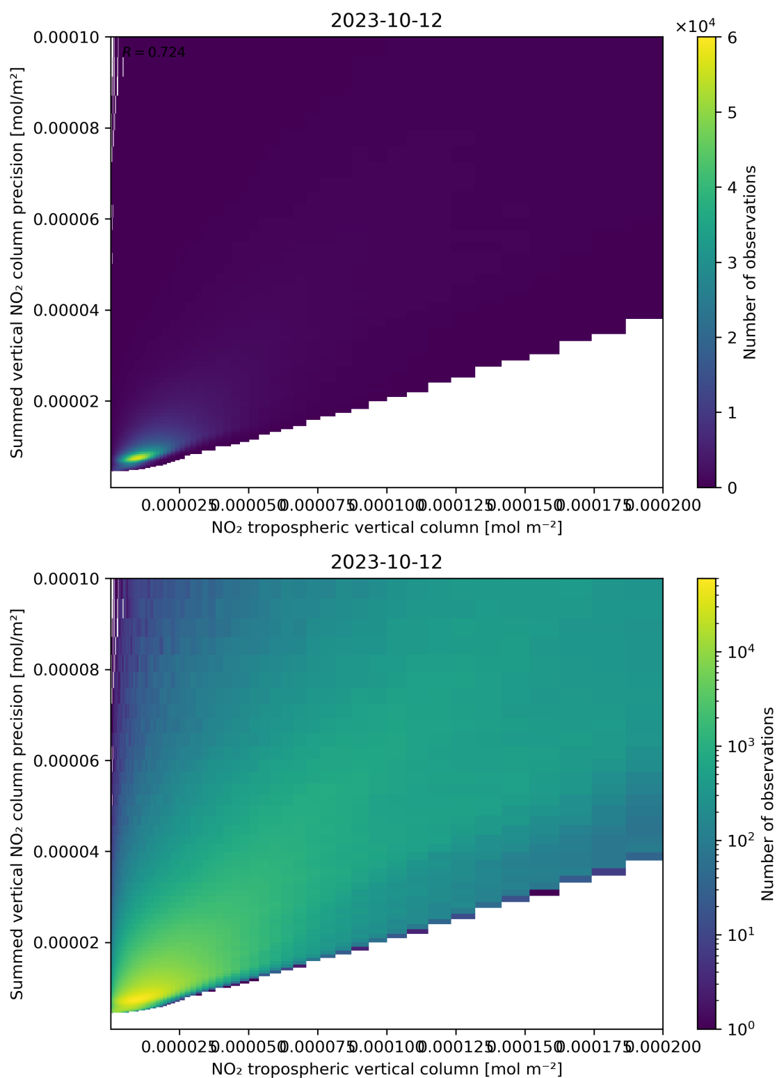
Figure 127: Scatter density plot of “NO 2 tropospheric vertical column” against “Summed vertical NO 2 column precision” for 2023-10-12 to 2023-10-13.
