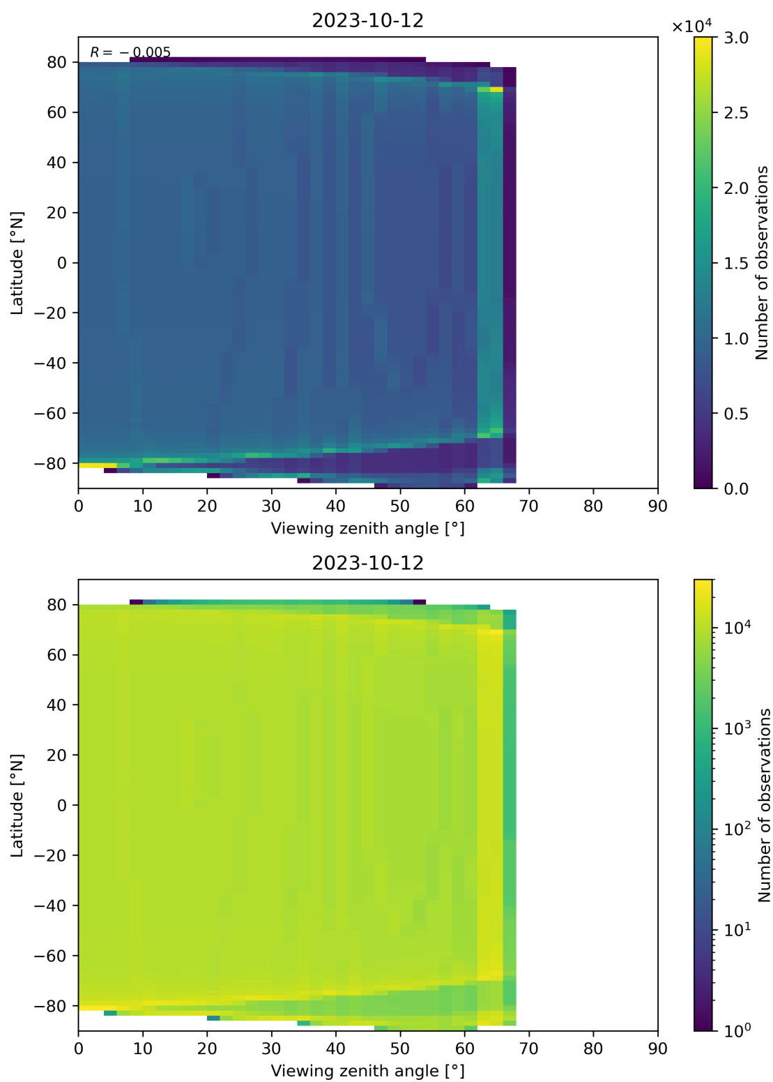
Figure 163: Scatter density plot of “Viewing zenith angle” against “Latitude” for 2023-10-12 to 2023-10-13.
