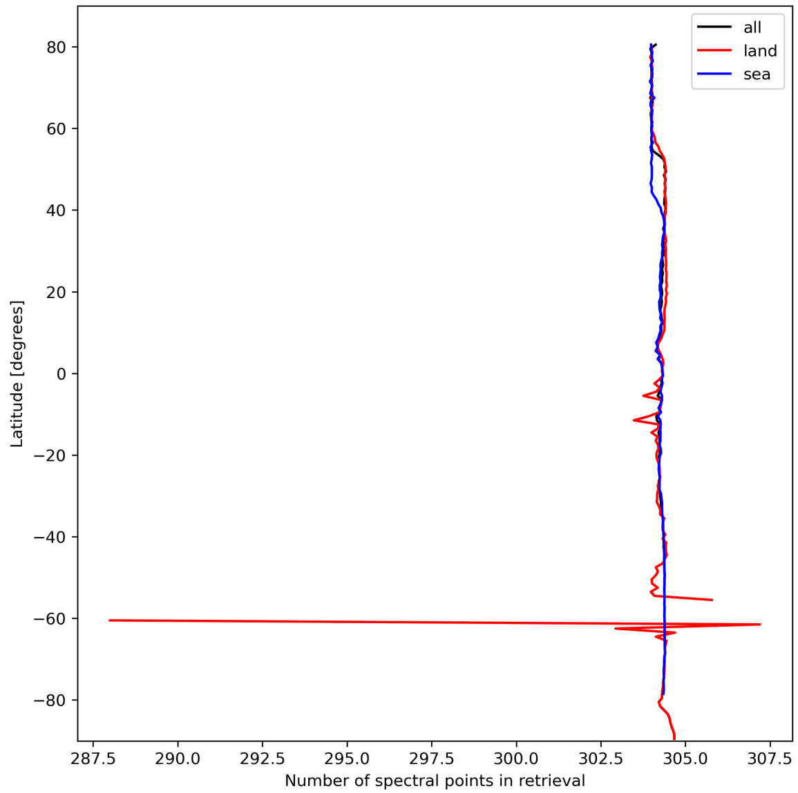
Figure 16: Zonal average of “Number of spectral points in retrieval” for 2023-10-12 to 2023-10-13.
