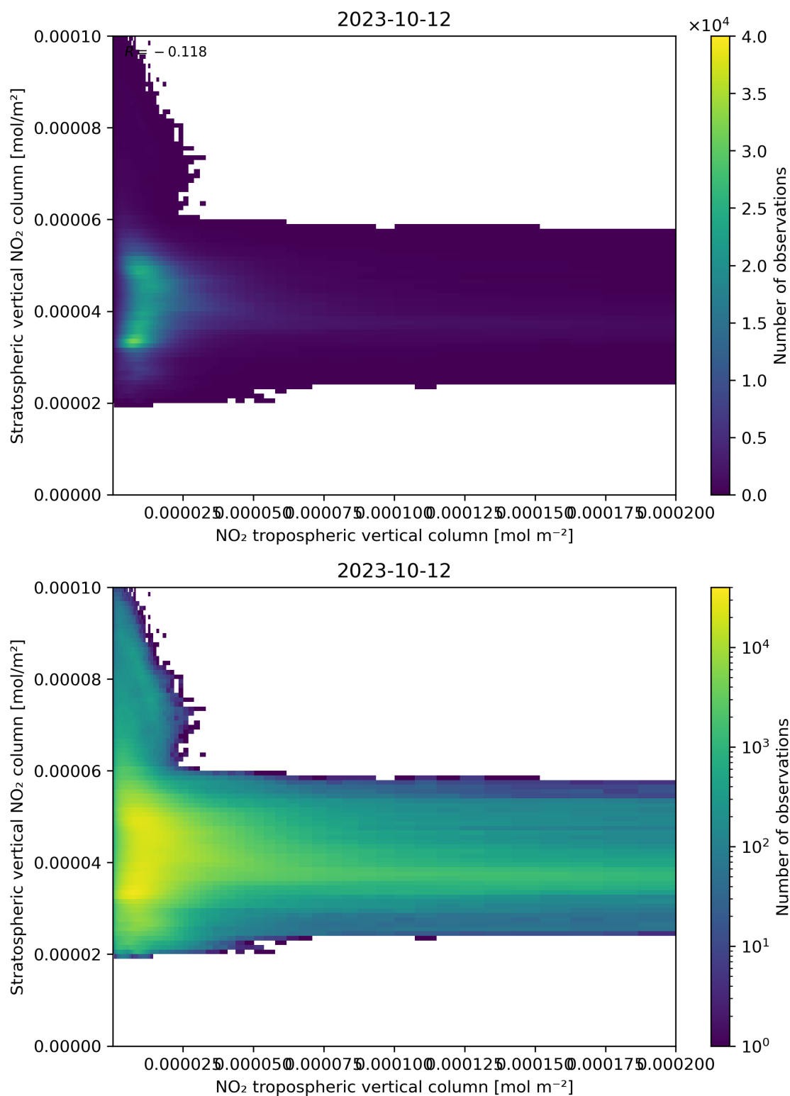
Figure 125: Scatter density plot of “NO 2 tropospheric vertical column” against “Stratospheric vertical NO 2 column” for 2023-10-12 to 2023-10-13.
