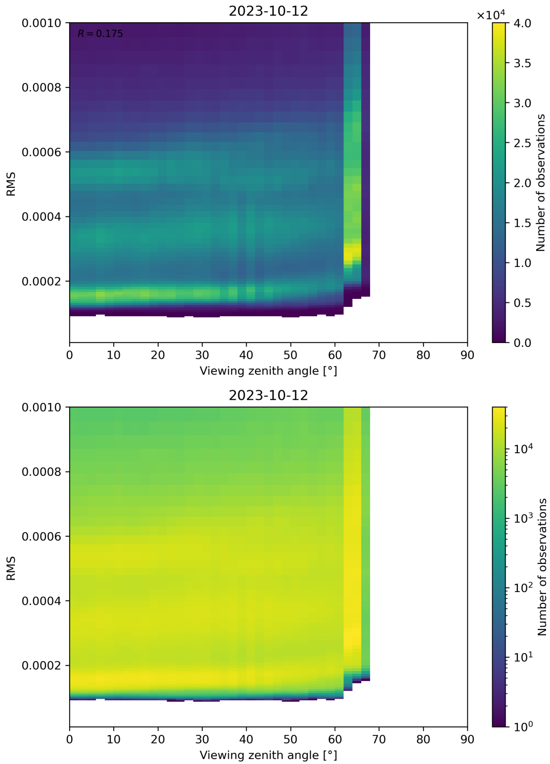
Figure 171: Scatter density plot of “Viewing zenith angle” against “RMS” for 2023-10-12 to 2023-10-13.
