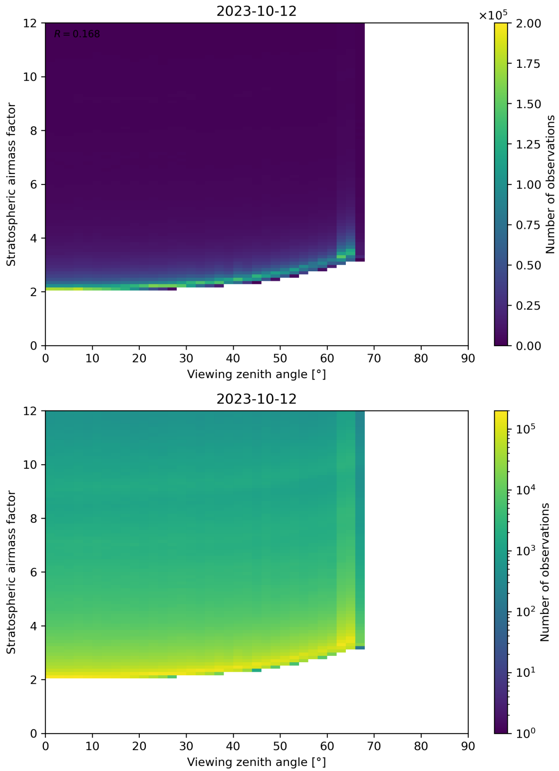
Figure 159: Scatter density plot of “Viewing zenith angle” against “Stratospheric airmass factor” for 2023-10-12 to 2023-10-13.
