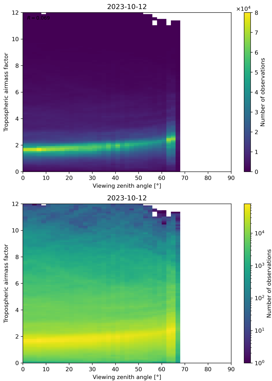
Figure 161: Scatter density plot of “Viewing zenith angle” against “Tropospheric airmass factor” for 2023-10-12 to 2023-10-13.
