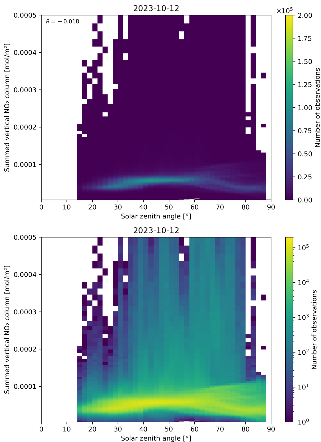
Figure 151: Scatter density plot of “Solar zenith angle” against “Summed vertical NO 2 column” for 2023-10-12 to 2023-10-13.
