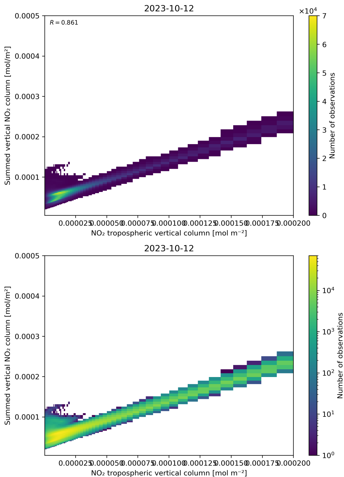
Figure 126: Scatter density plot of “NO 2 tropospheric vertical column” against “Summed vertical NO 2 column” for 2023-10-12 to 2023-10-13.
