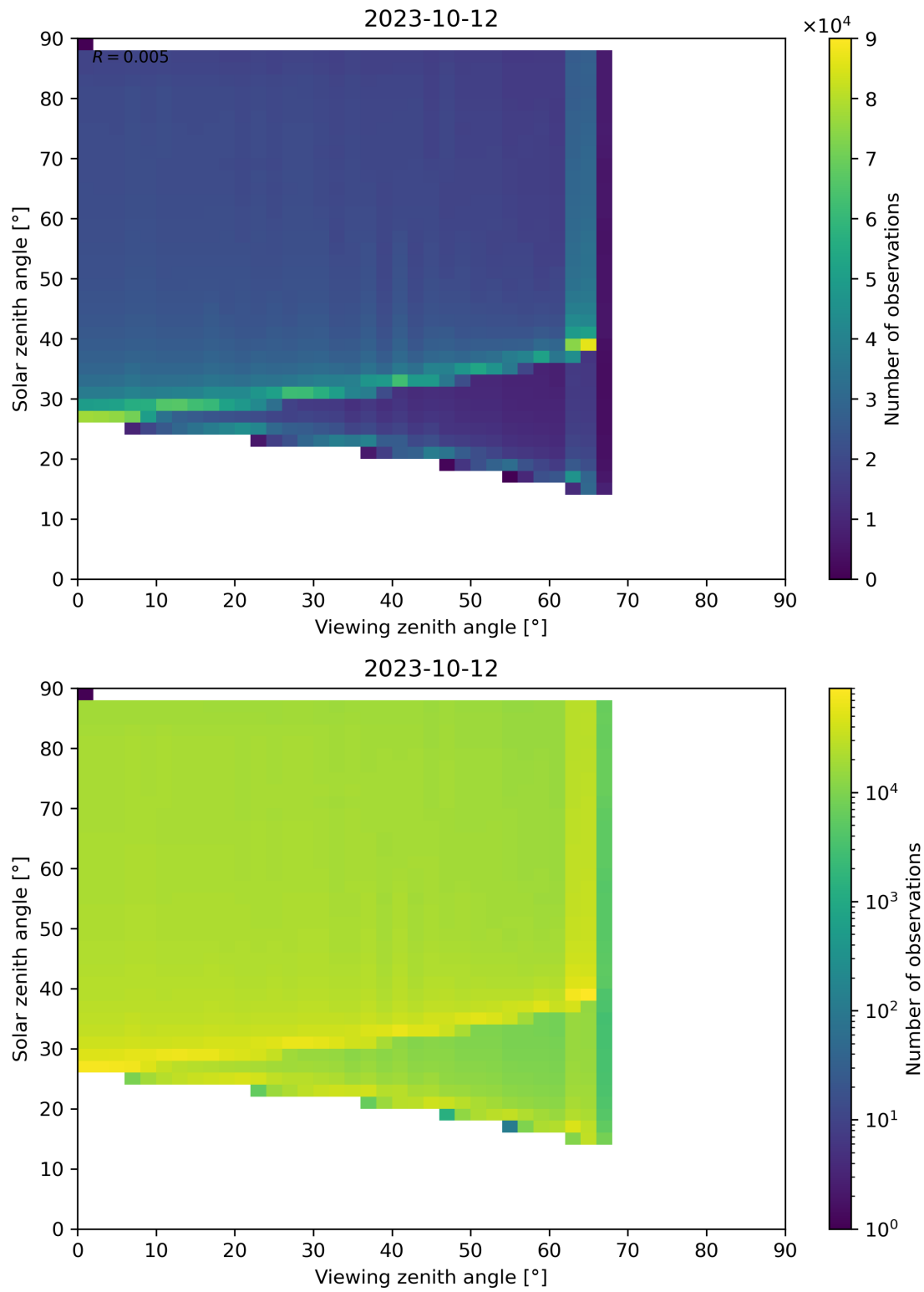
Figure 172: Scatter density plot of “Viewing zenith angle” against “Solar zenith angle” for 2023-10-12 to 2023-10-13.
