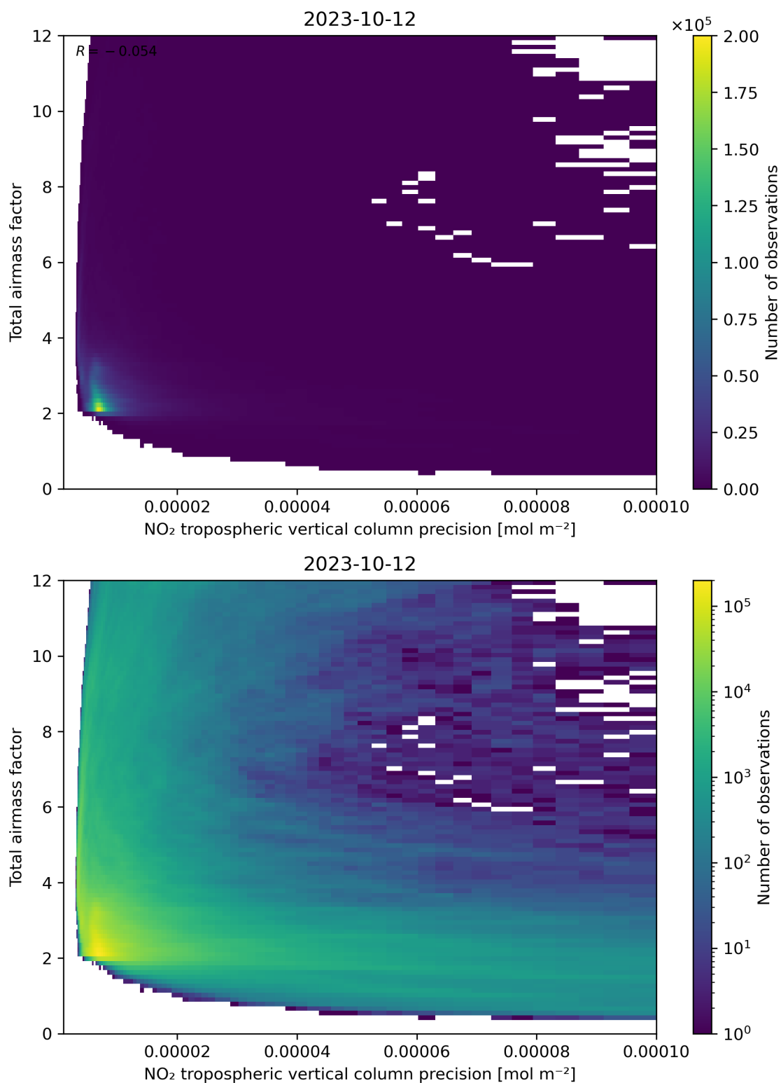
Figure 132: Scatter density plot of “NO 2 tropospheric vertical column precision” against “Total air mass factor” for 2023-10-12 to 2023-10-13.
