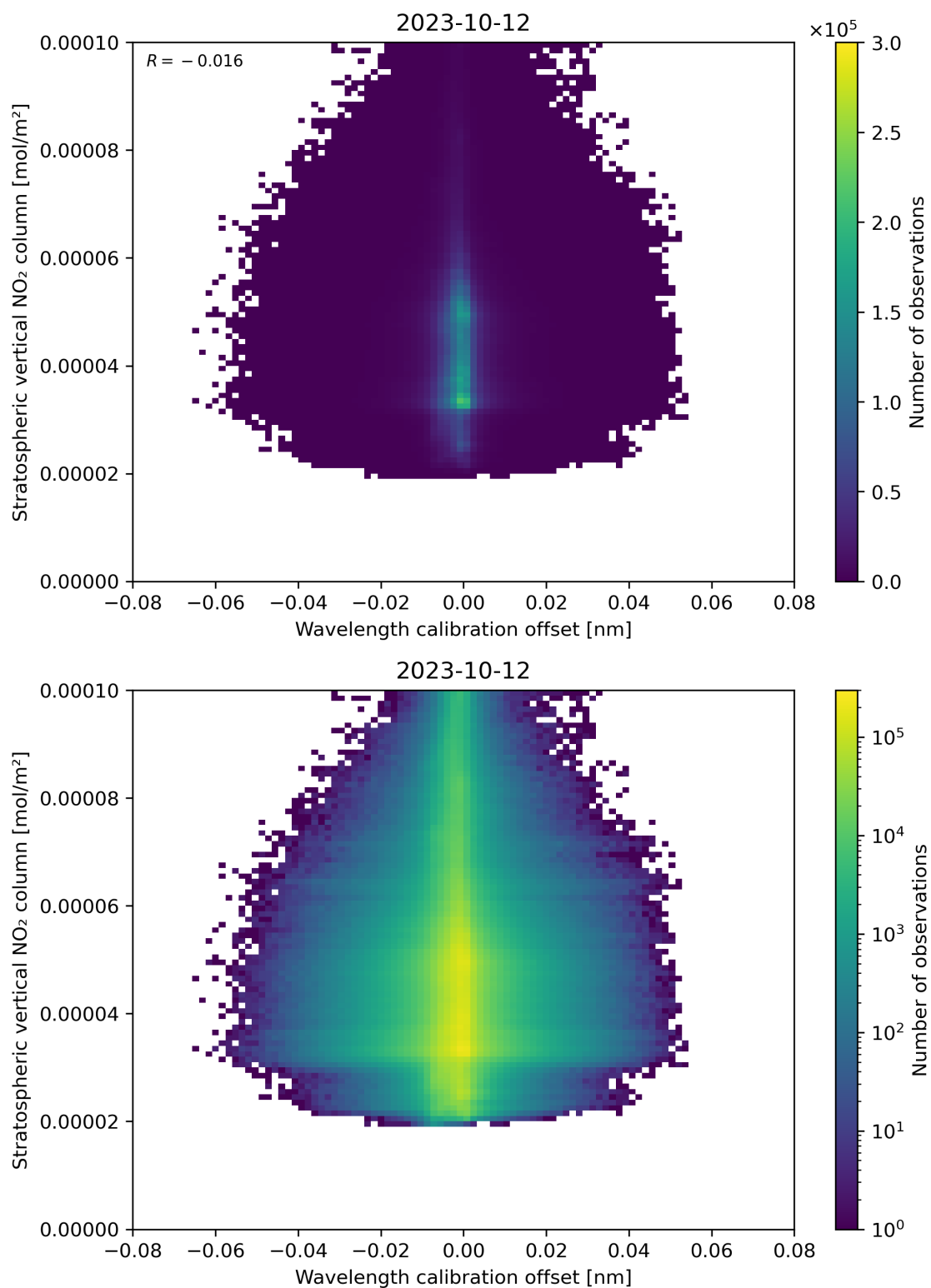
Figure 176: Scatter density plot of “Wavelength calibration offset” against “Stratospheric vertical NO 2 column” for 2023-10-12 to 2023-10-13.
