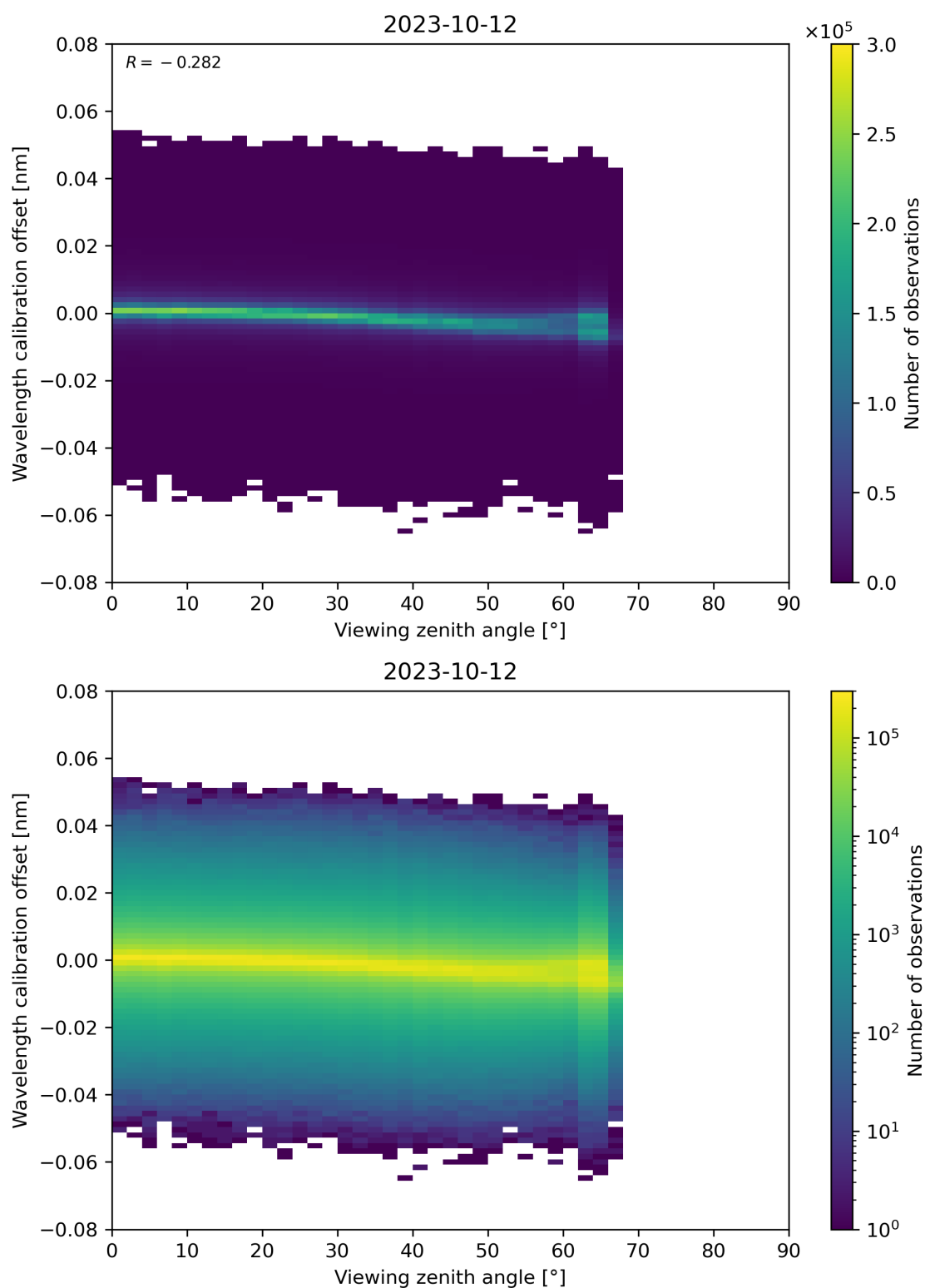
Figure 173: Scatter density plot of “Viewing zenith angle” against “Wavelength calibration offset” for 2023-10-12 to 2023-10-13.
