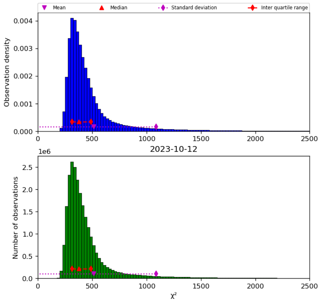
Figure 42: Histogram of “ \chi^2 ” for 2023-10-12 to 2023-10-13
