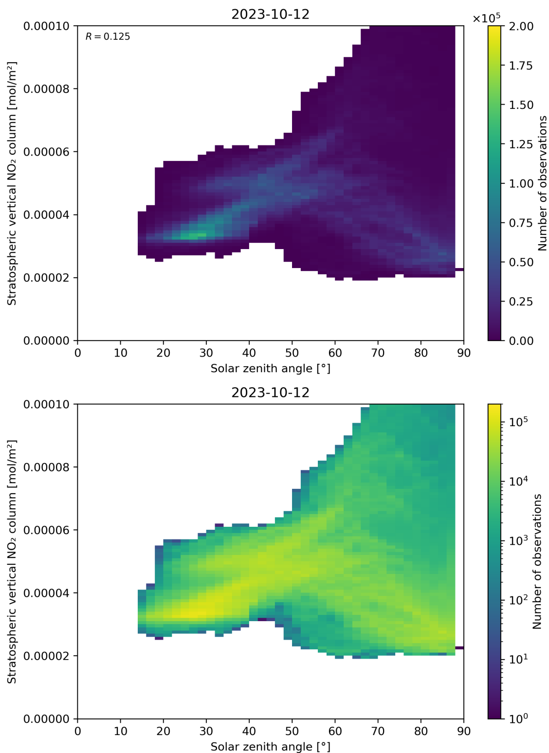
Figure 150: Scatter density plot of “Solar zenith angle” against “Stratospheric vertical NO 2 column” for 2023-10-12 to 2023-10-13.
