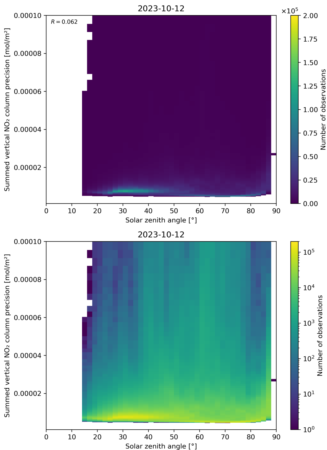
Figure 152: Scatter density plot of “Solar zenith angle” against “Summed vertical NO 2 column precision” for 2023-10-12 to 2023-10-13.
