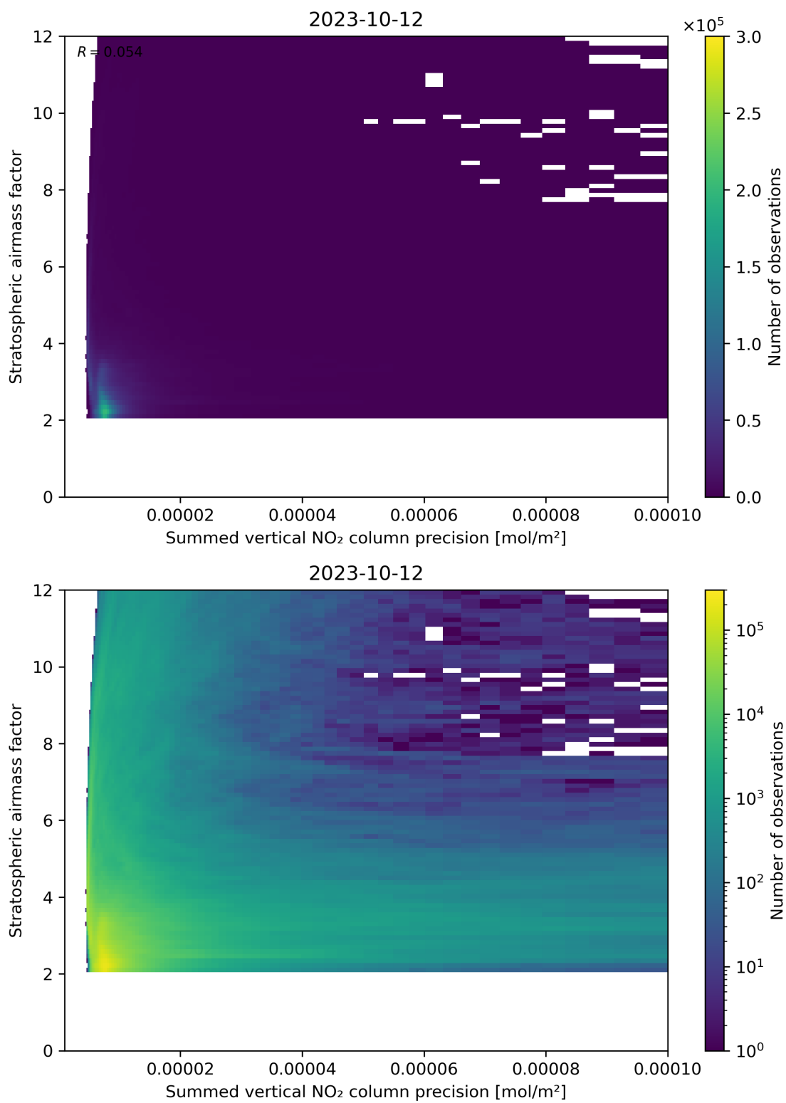
Figure 106: Scatter density plot of “Summed vertical NO 2 column precision” against “Stratospheric airmass factor” for 2023-10-12 to 2023-10-13.
