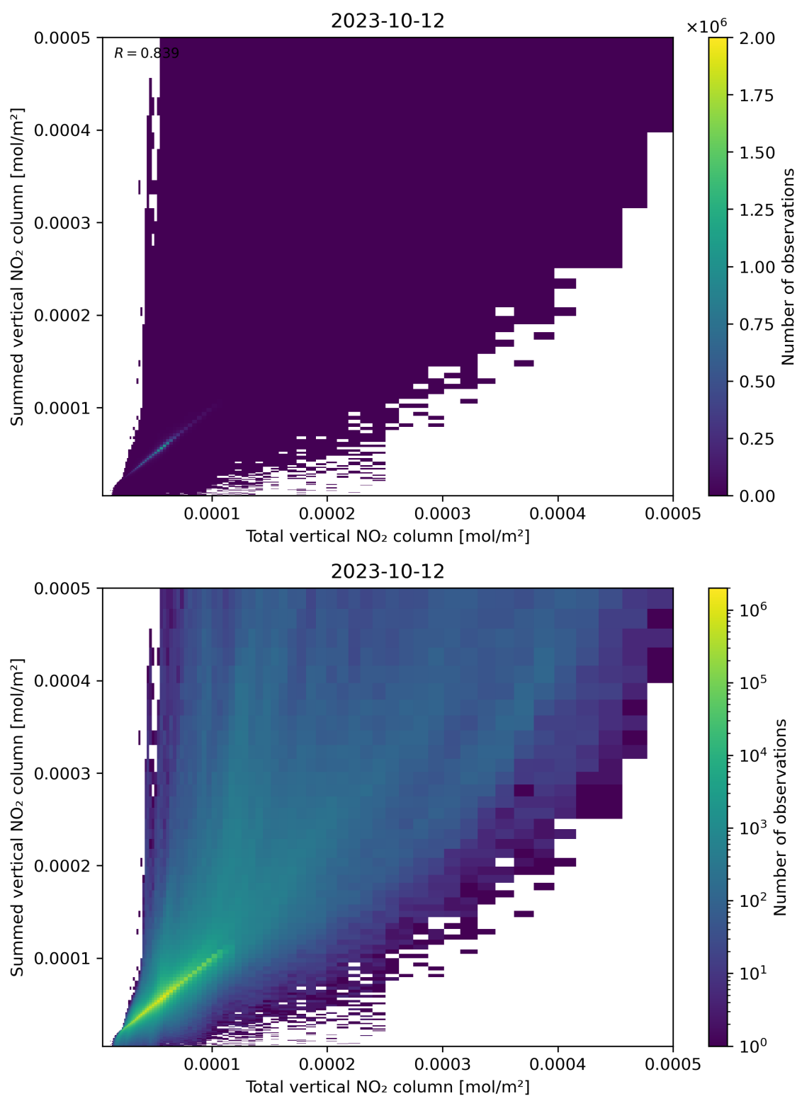
Figure 112: Scatter density plot of “Total vertical NO 2 column” against “Summed vertical NO 2 column” for 2023-10-12 to 2023-10-13.
