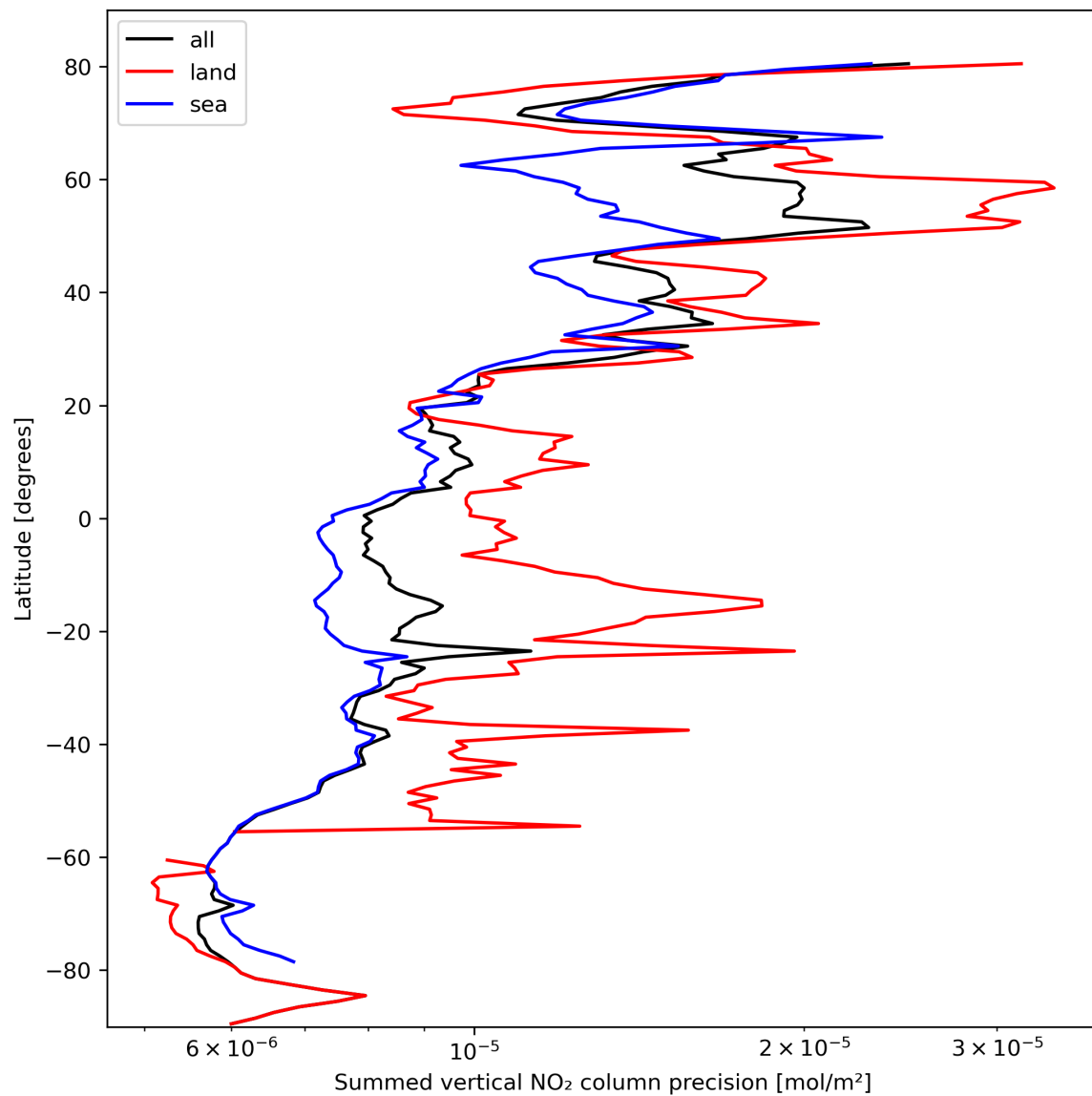
Figure 24: Zonal average of “Summed vertical NO 2 column precision” for 2023-10-12 to 2023-10-13.
