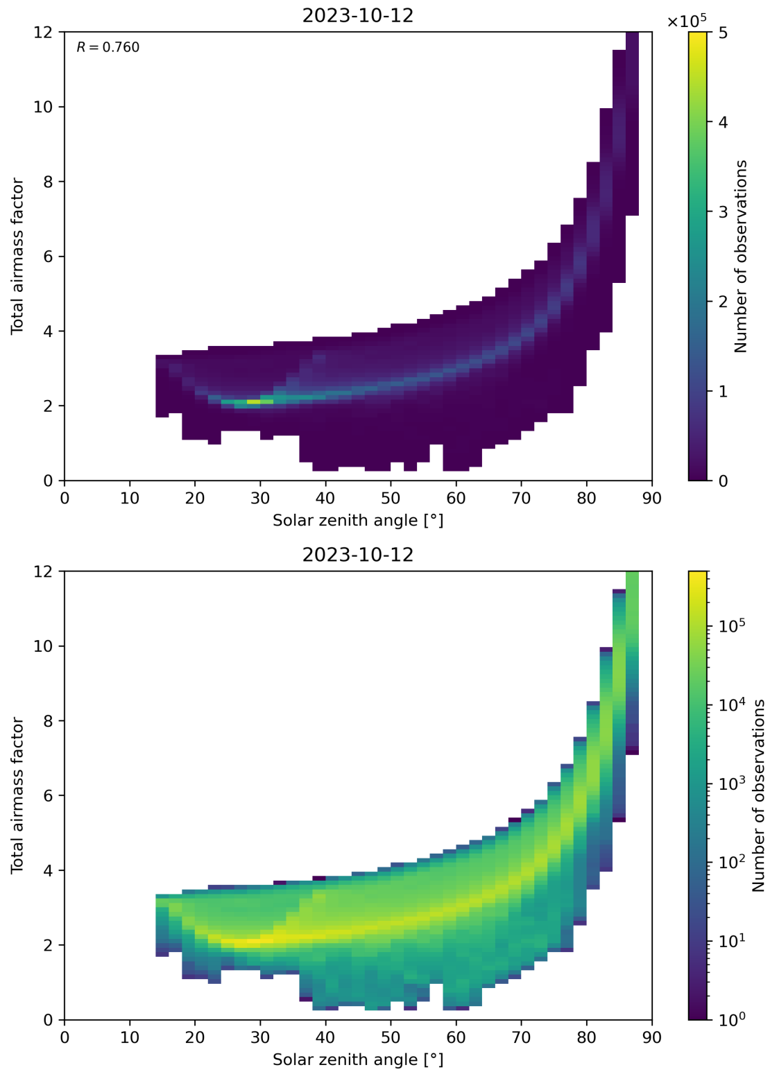
Figure 146: Scatter density plot of “Solar zenith angle” against “Total air mass factor” for 2023-10-12 to 2023-10-13.
