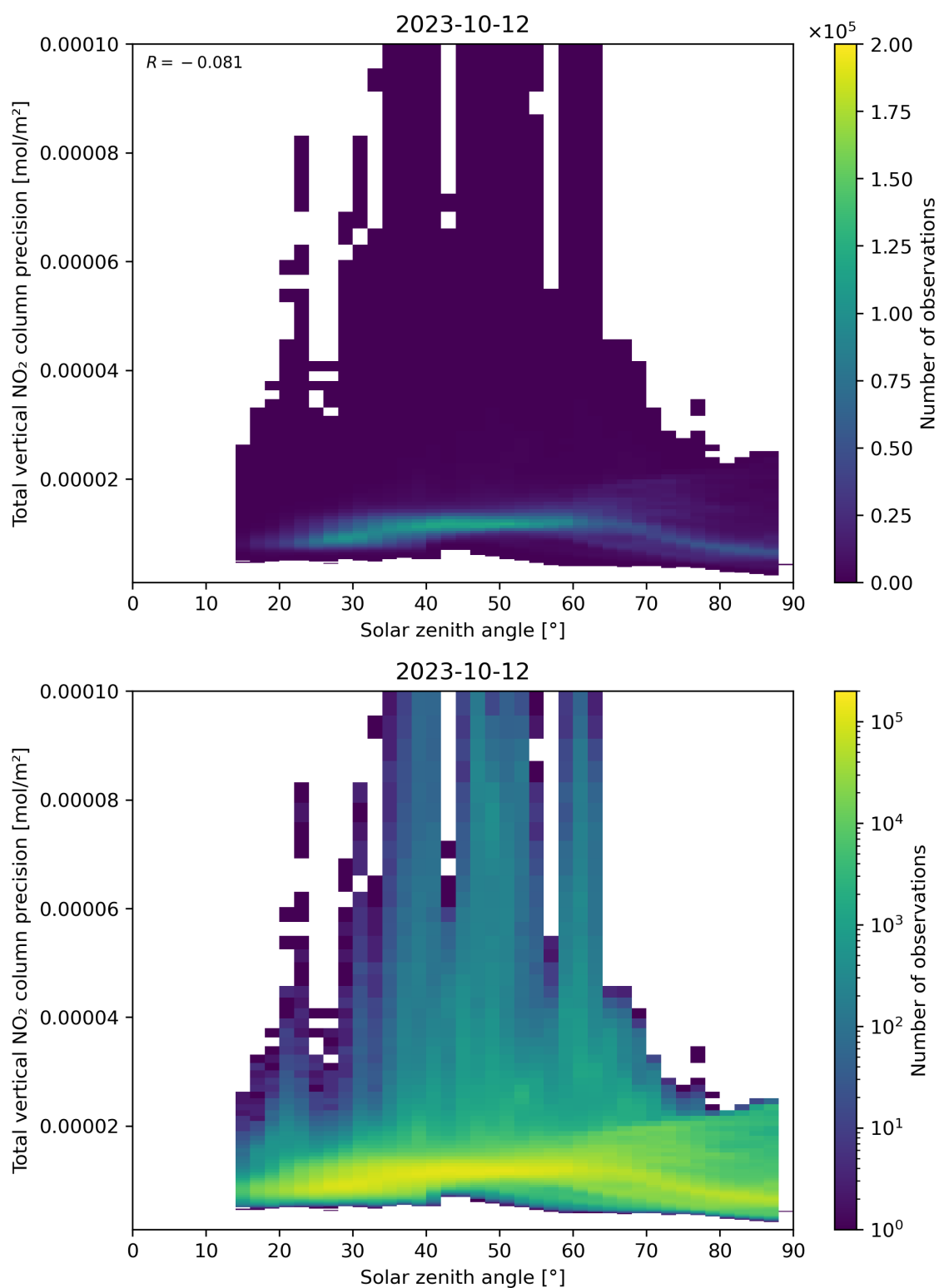
Figure 154: Scatter density plot of “Solar zenith angle” against “Total vertical NO 2 column precision” for 2023-10-12 to 2023-10-13.
