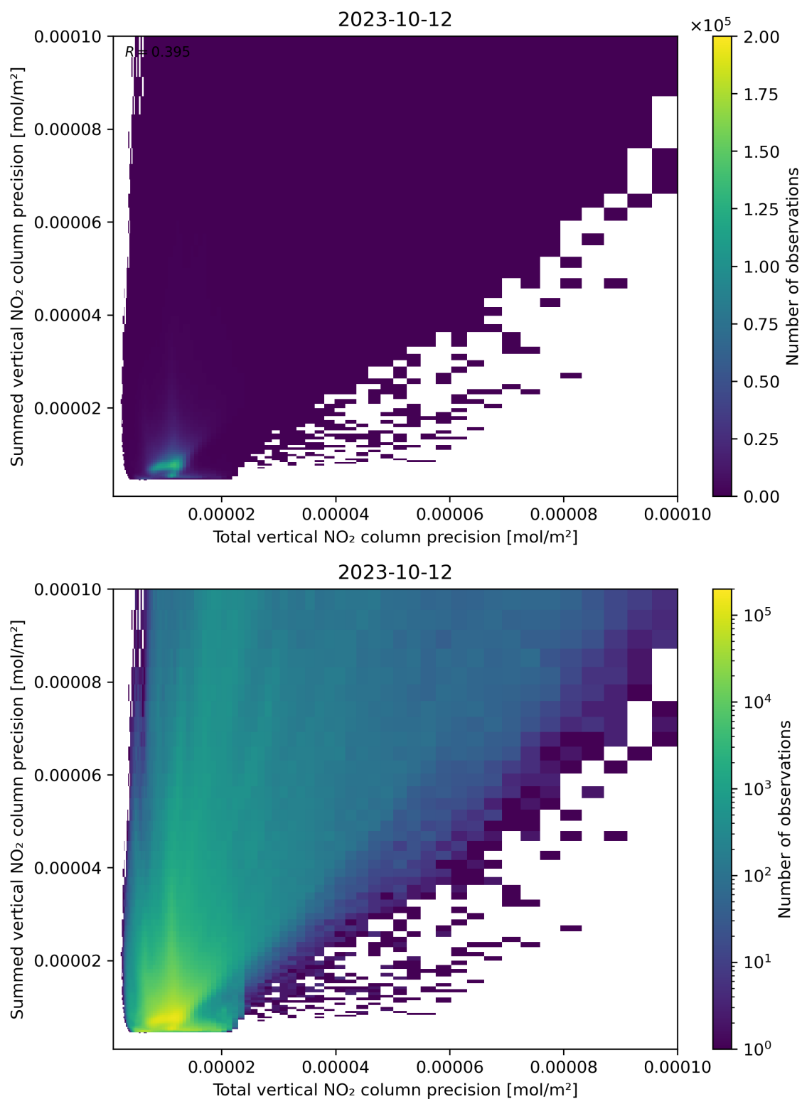
Figure 118: Scatter density plot of “Total vertical NO 2 column precision” against “Summed vertical NO 2 column precision” for 2023-10-12 to 2023-10-13.
