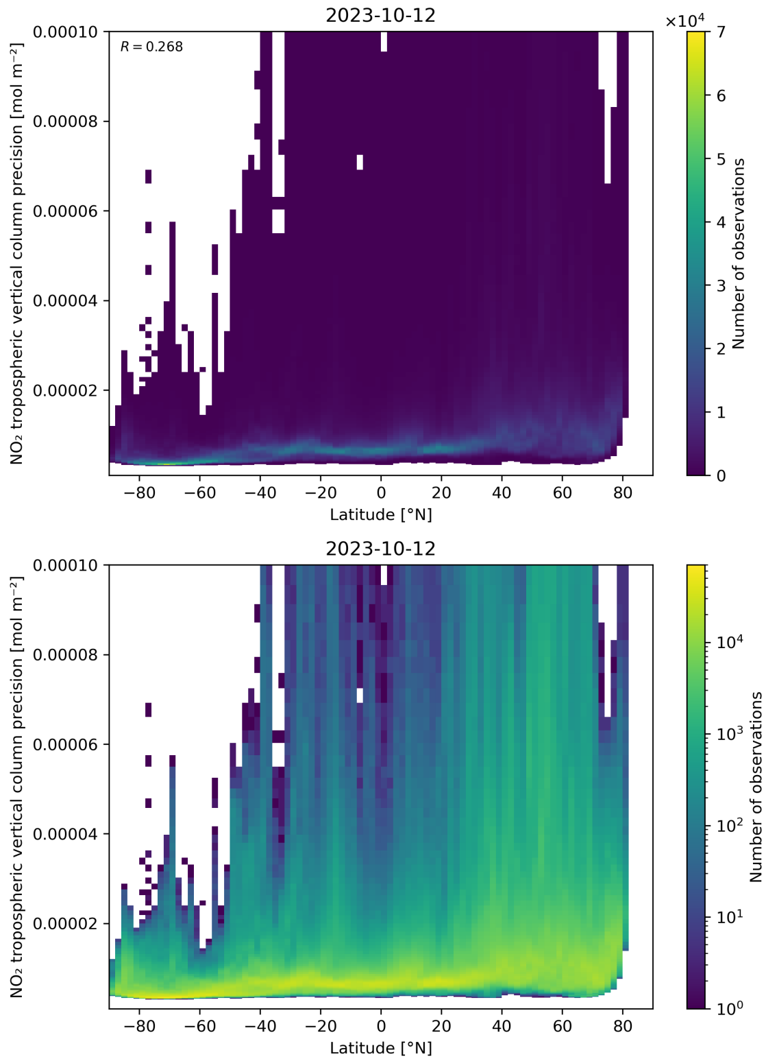
Figure 93: Scatter density plot of “Latitude” against “NO 2 tropospheric vertical column precision” for 2023-10-12 to 2023-10-13.
