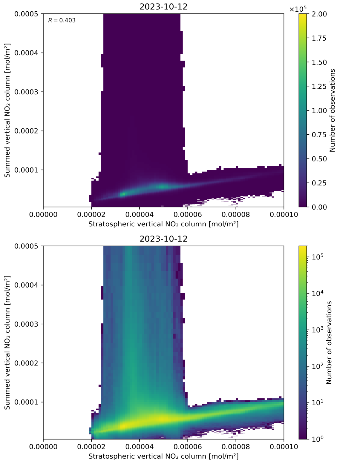
Figure 98: Scatter density plot of “Stratospheric vertical NO 2 column” against “Summed vertical NO 2 column” for 2023-10-12 to 2023-10-13.
