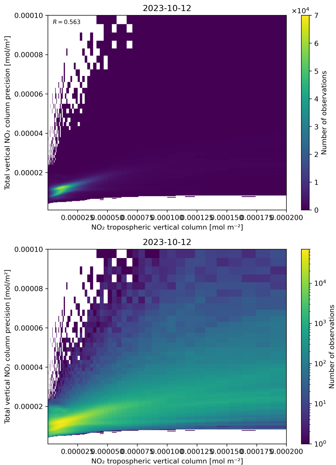
Figure 129: Scatter density plot of “NO 2 tropospheric vertical column” against “Total vertical NO 2 column precision” for 2023-10-12 to 2023-10-13.
