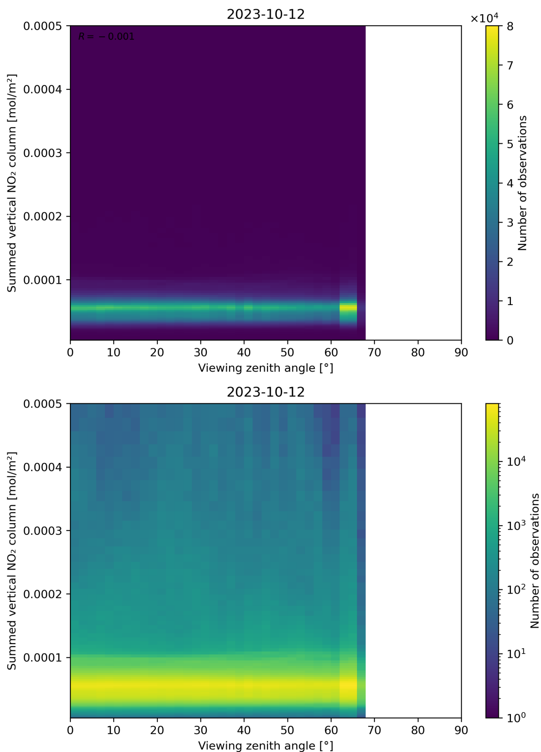
Figure 165: Scatter density plot of “Viewing zenith angle” against “Summed vertical NO 2 column” for 2023-10-12 to 2023-10-13.
