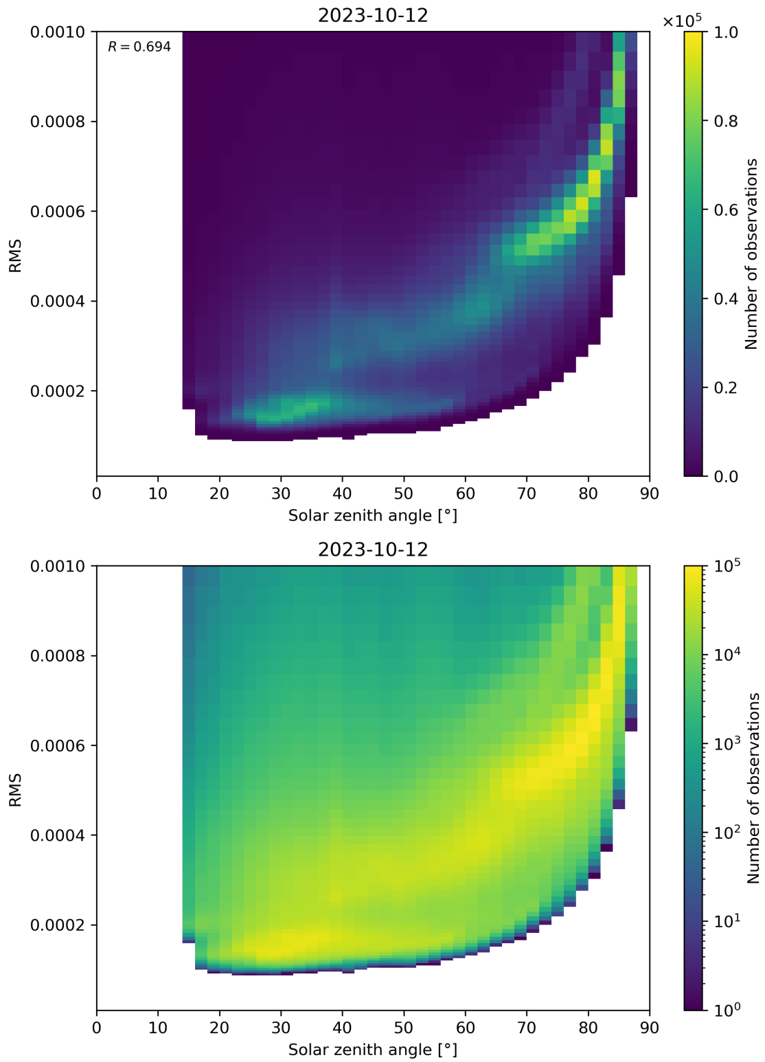
Figure 157: Scatter density plot of “Solar zenith angle” against “RMS” for 2023-10-12 to 2023-10-13.
