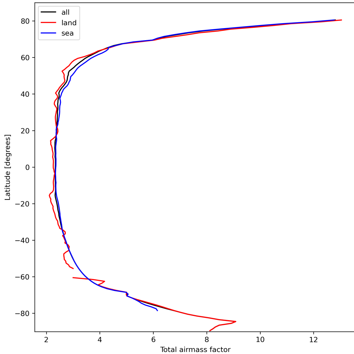
Figure 15: Zonal average of “Total airmass factor” for 2023-10-12 to 2023-10-13.
