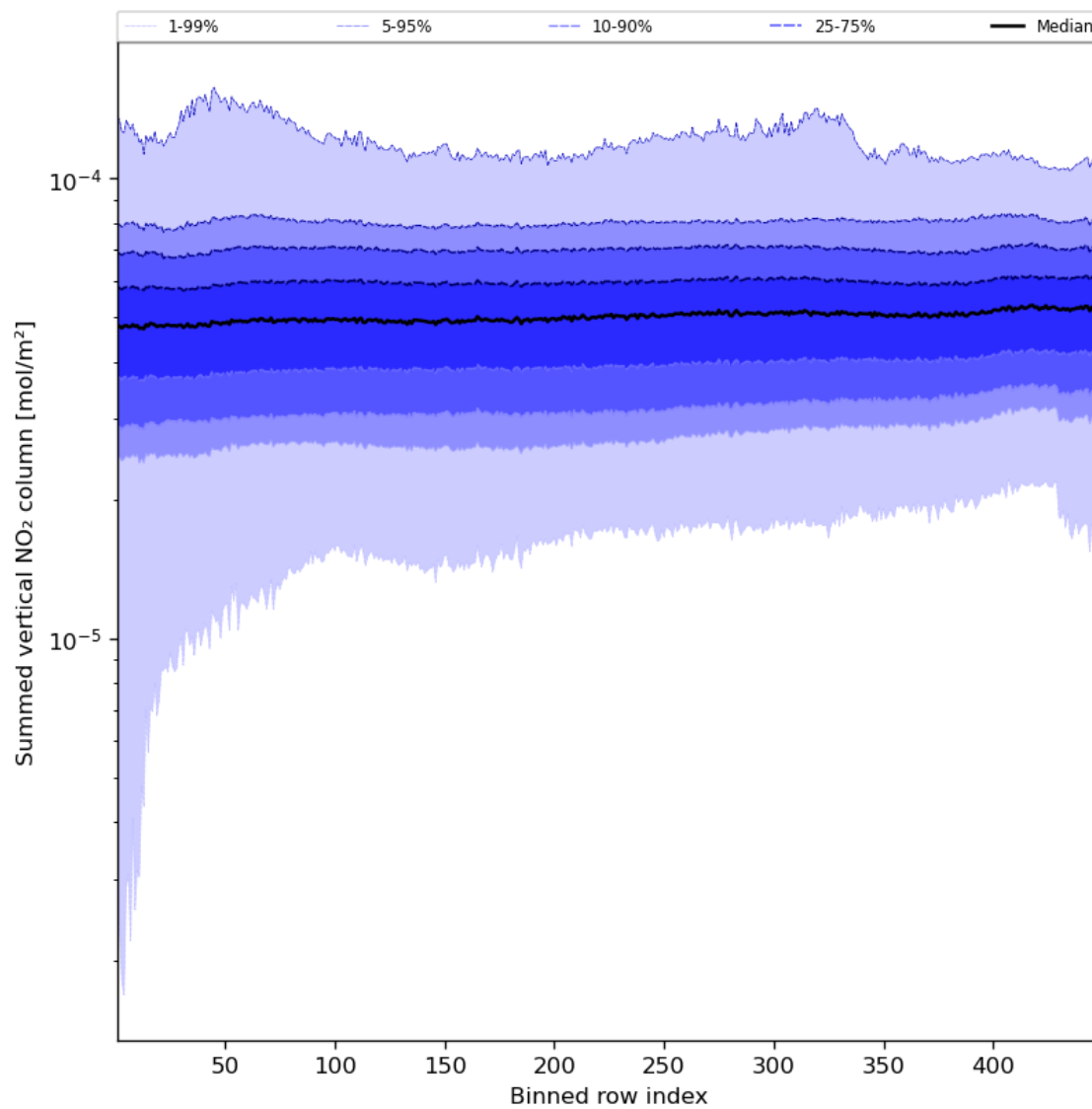
Figure 57: Along track statistics of “Summed vertical NO 2 column” for 2023-10-12 to 2023-10-13
