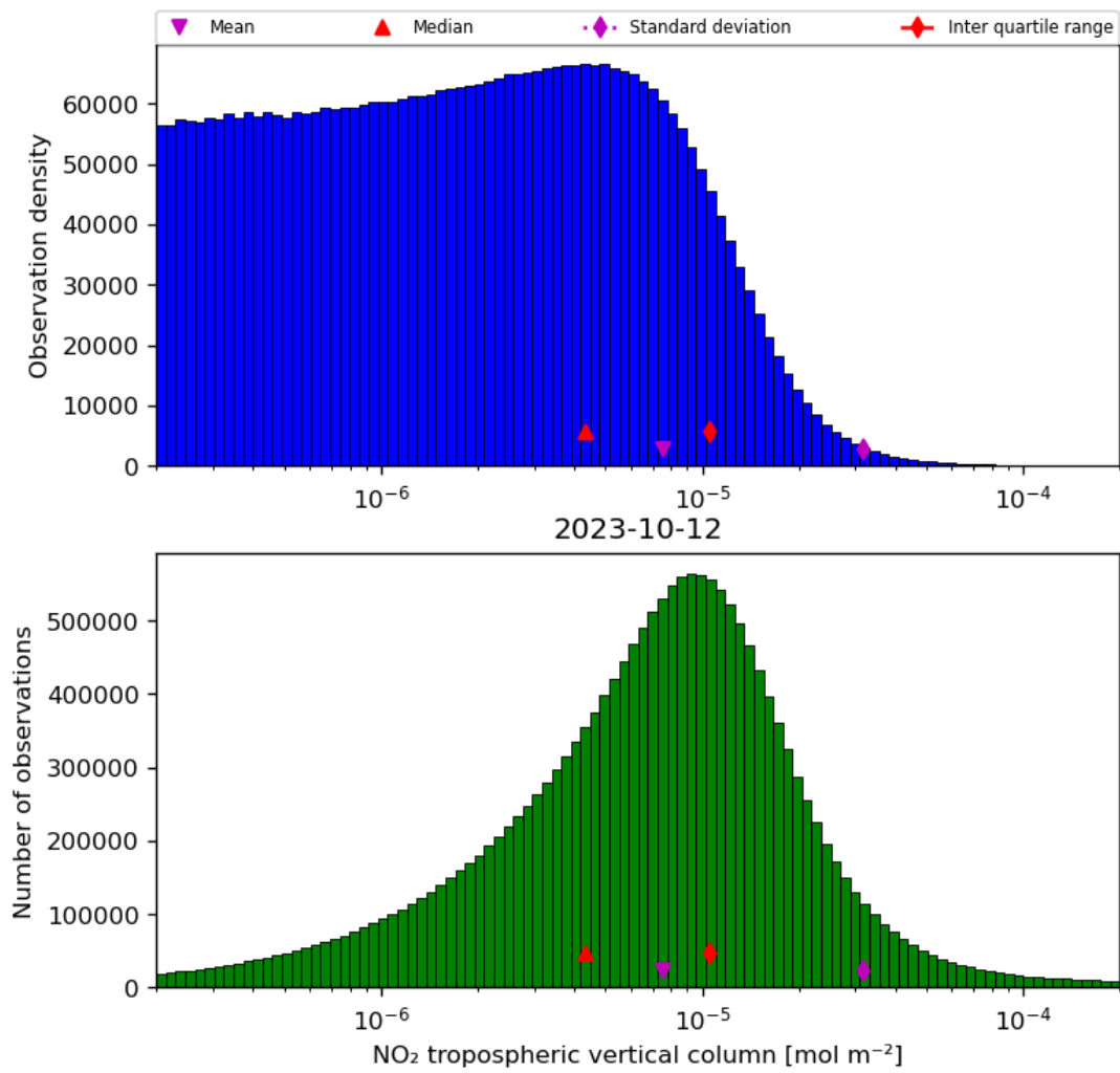
Figure 29: Histogram of “NO 2 tropospheric vertical column” for 2023-10-12 to 2023-10-13
