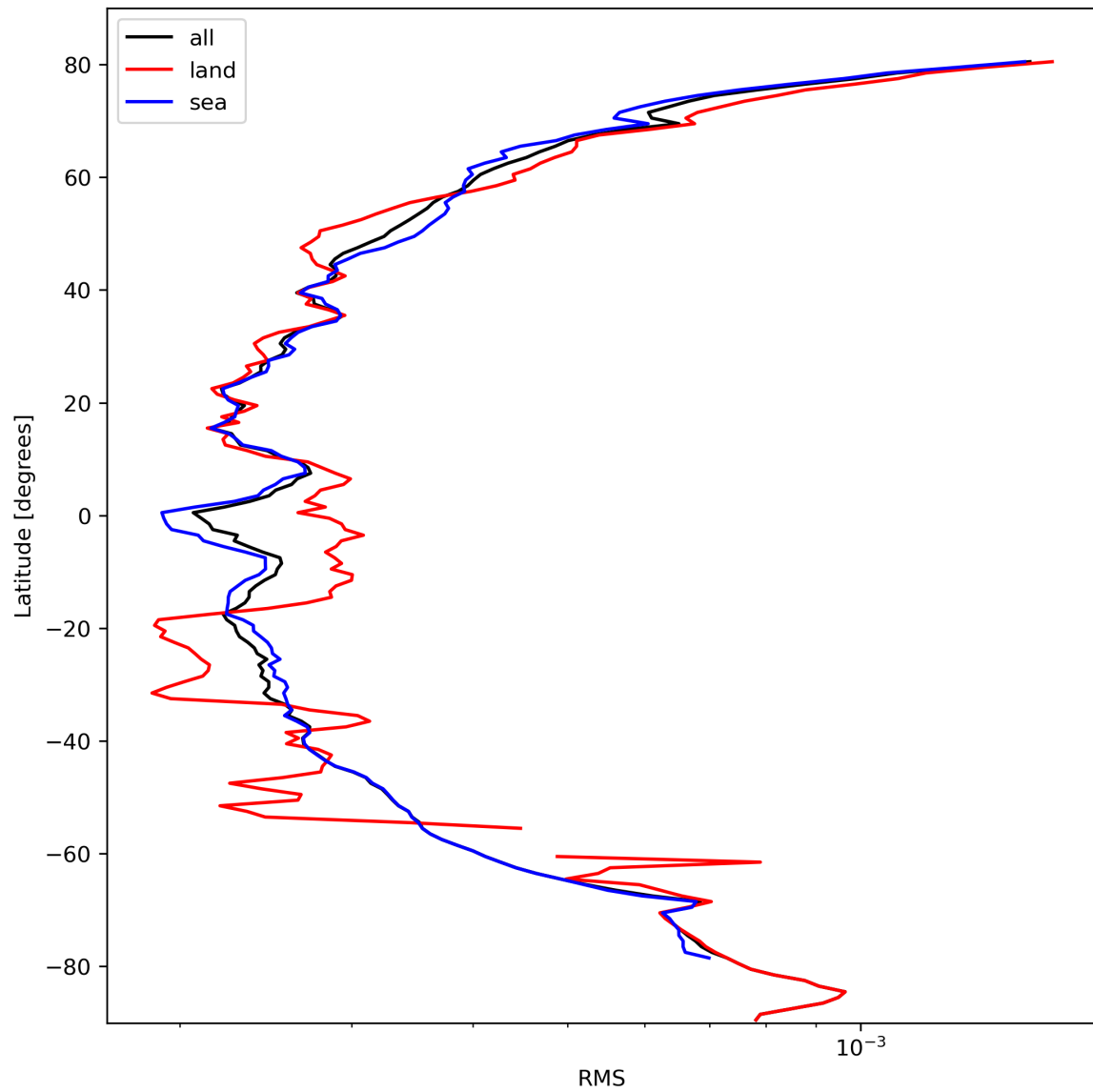
Figure 26: Zonal average of “RMS” for 2023-10-12 to 2023-10-13.
