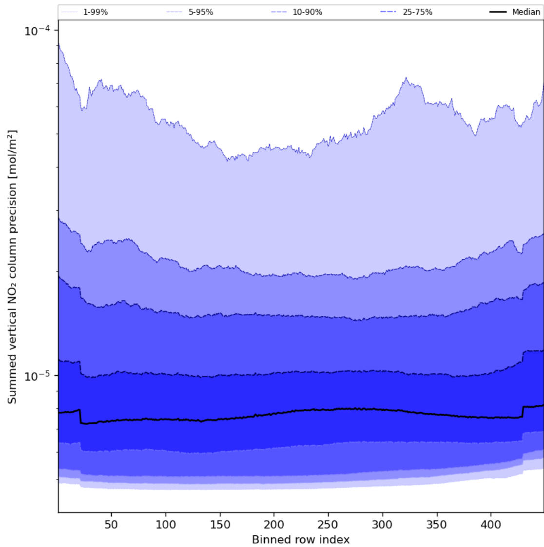
Figure 58: Along track statistics of “Summed vertical NO 2 column precision” for 2023-10-12 to 2023-10-13
