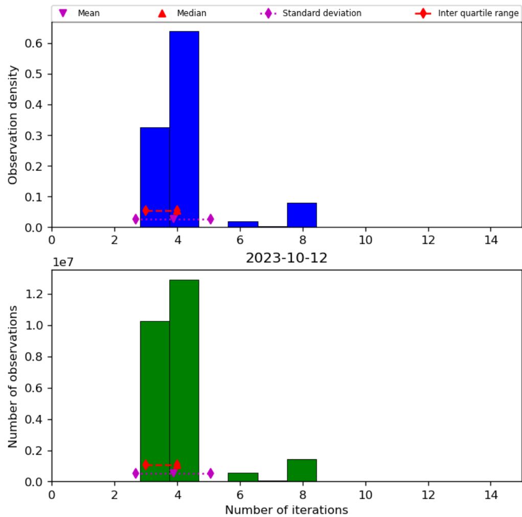
Figure 34: Histogram of “Number of iterations” for 2023-10-12 to 2023-10-13
