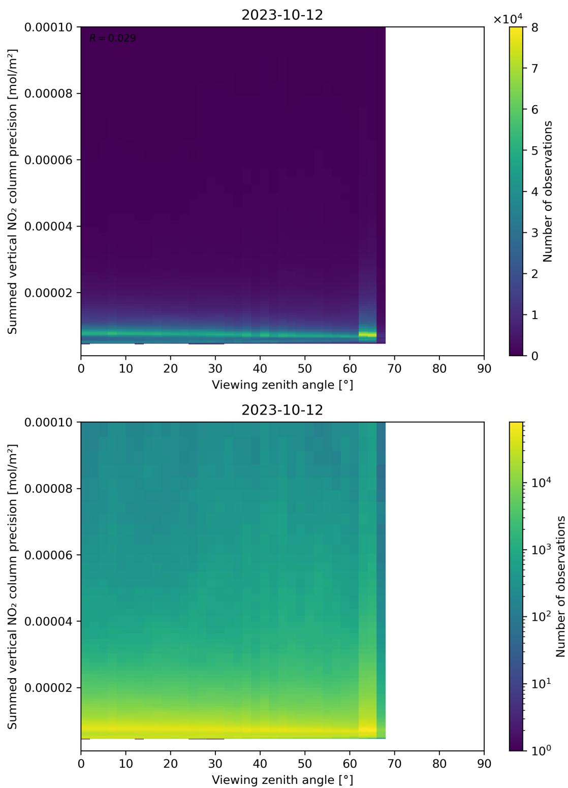
Figure 166: Scatter density plot of “Viewing zenith angle” against “Summed vertical NO 2 column precision” for 2023-10-12 to 2023-10-13.
