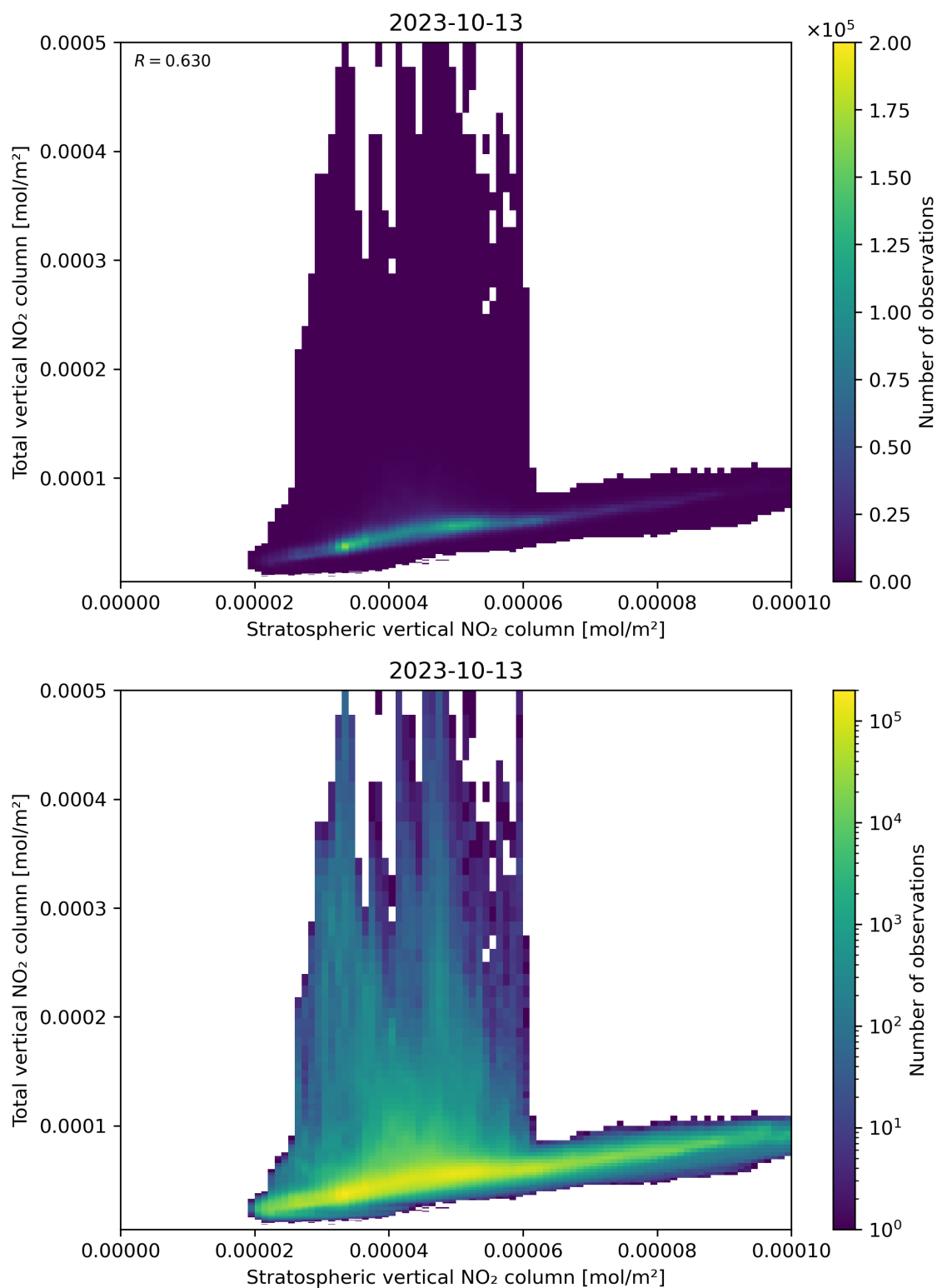
Figure 100: Scatter density plot of “Stratospheric vertical NO 2 column” against “Total vertical NO 2 column” for 2023-10-12 to 2023-10-14.
