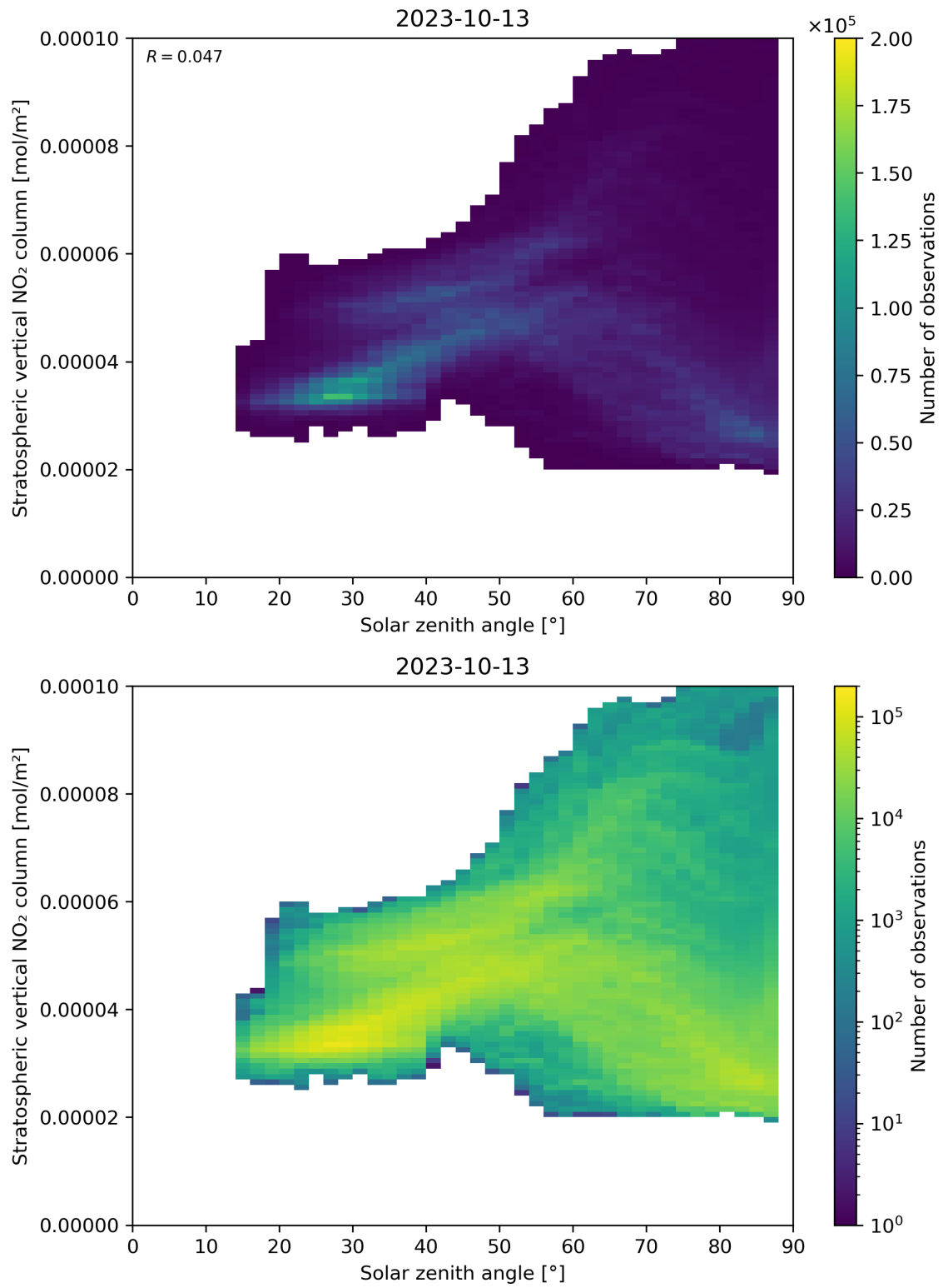
Figure 150: Scatter density plot of “Solar zenith angle” against “Stratospheric vertical NO 2 column” for 2023-10-12 to 2023-10-14.
