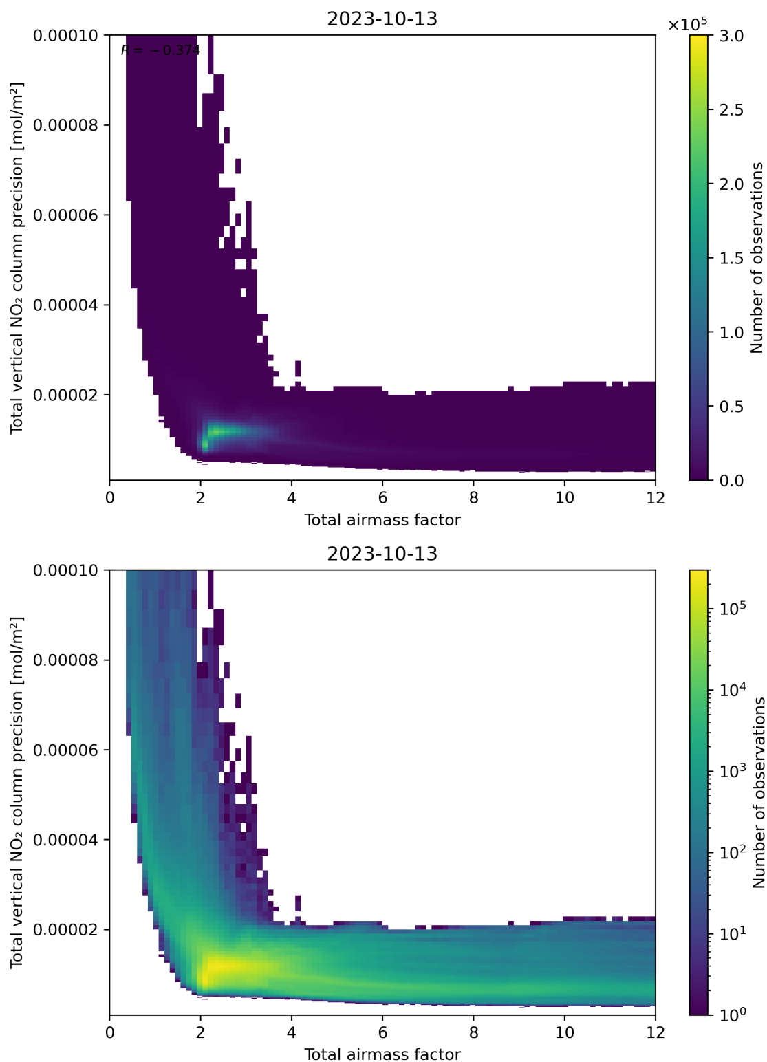
Figure 68: Scatter density plot of “Total airmass factor” against “Total vertical NO 2 column precision” for 2023-10-12 to 2023-10-14.
