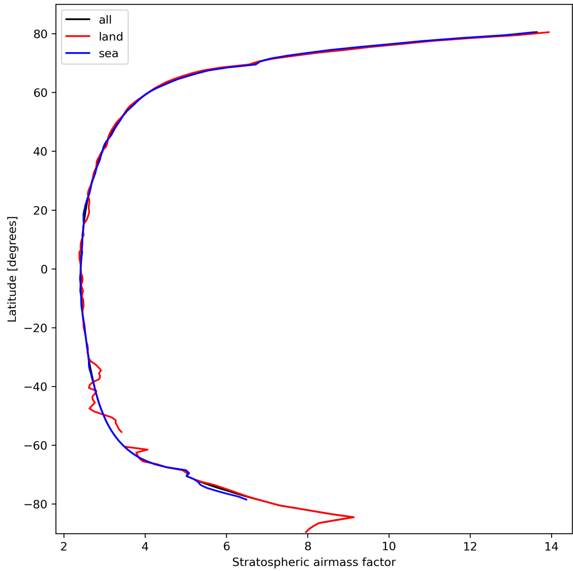
Figure 27: Zonal average of “Stratospheric air mass factor” for 2023-10-12 to 2023-10-14.
