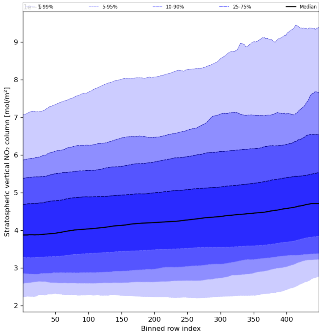
Figure 53: Along track statistics of “Stratospheric vertical NO 2 column” for 2023-10-12 to 2023-10-14
