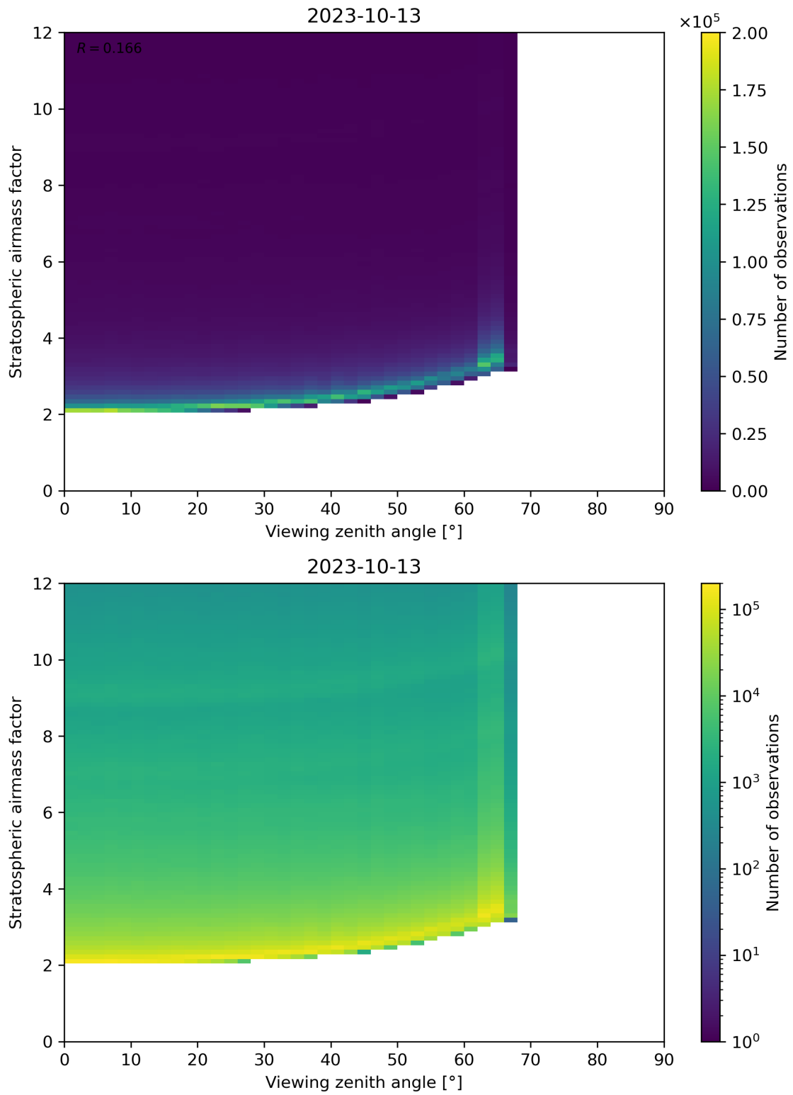
Figure 159: Scatter density plot of “Viewing zenith angle” against “Stratospheric airmass factor” for 2023-10-12 to 2023-10-14.
