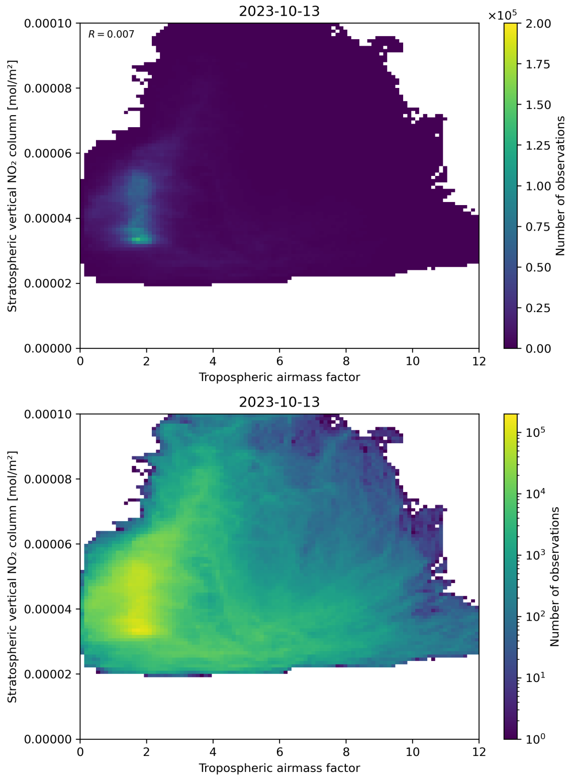
Figure 74: Scatter density plot of “Tropospheric air mass factor” against “Stratospheric vertical NO 2 column” for 2023-10-12 to 2023-10-14.
