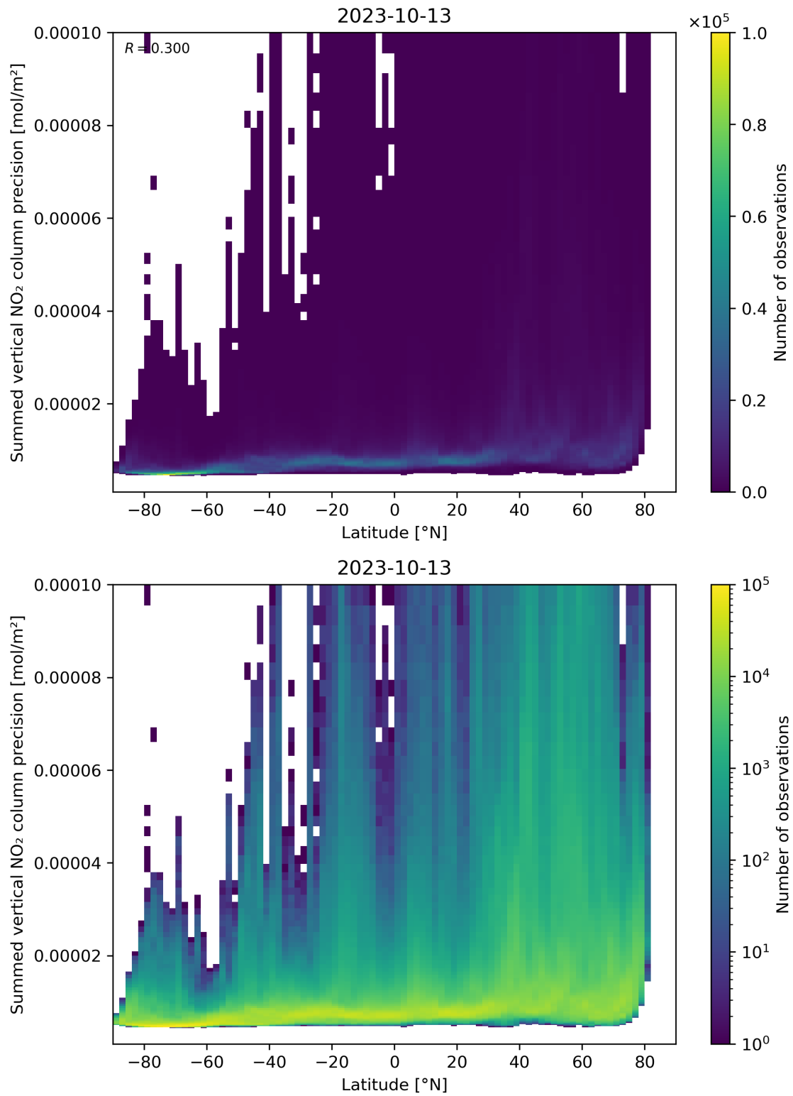
Figure 89: Scatter density plot of “Latitude” against “Summed vertical NO 2 column precision” for 2023-10-12 to 2023-10-14.
