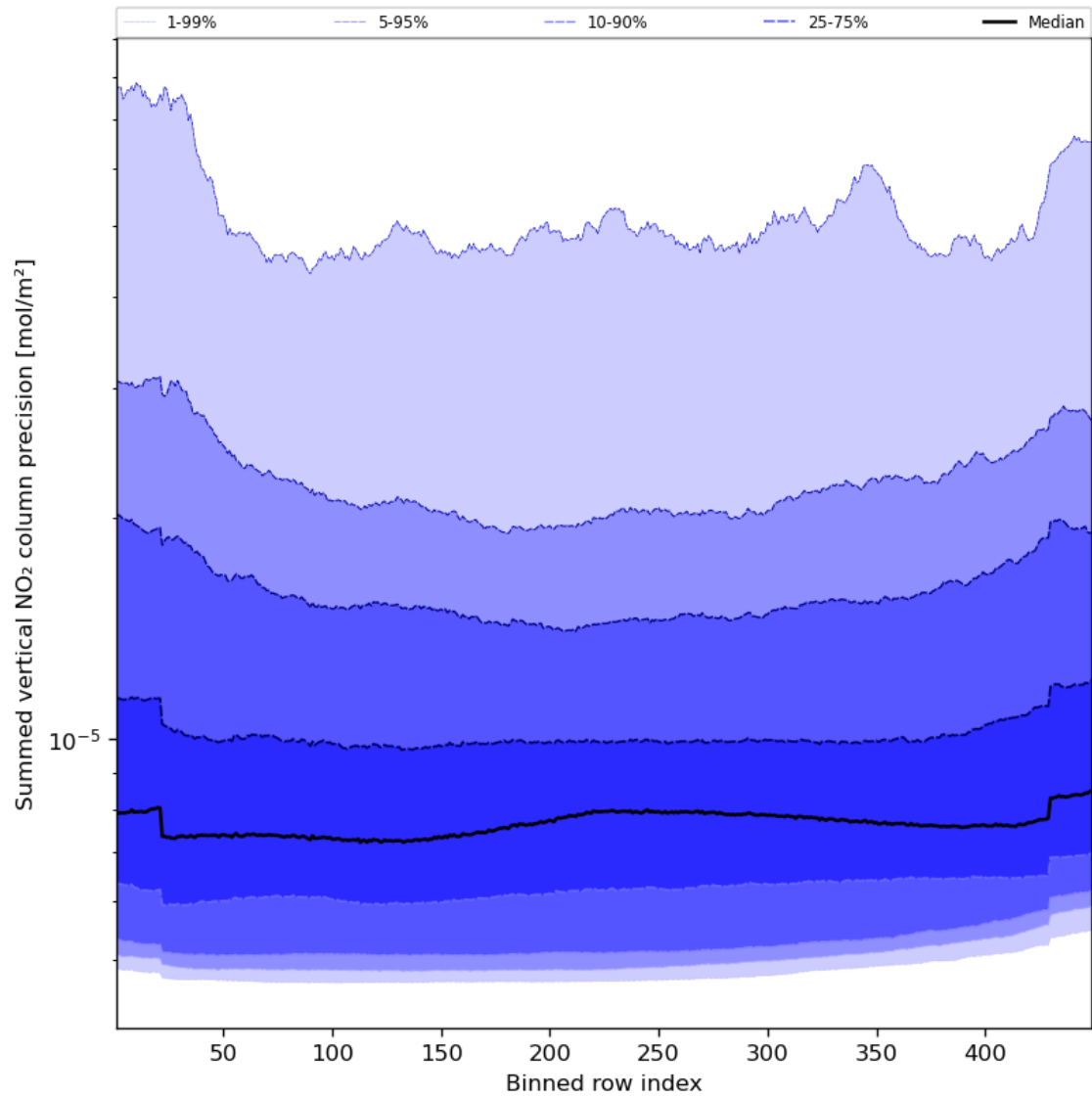
Figure 58: Along track statistics of “Summed vertical NO 2 column precision” for 2023-10-12 to 2023-10-14
