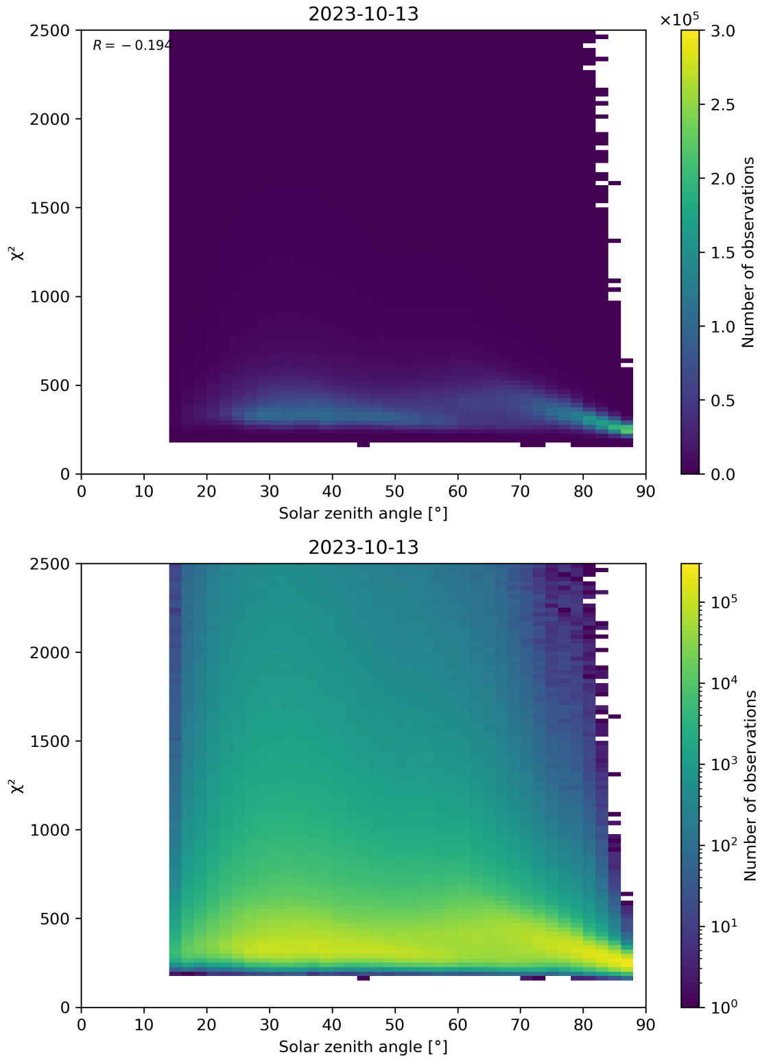
Figure 148: Scatter density plot of “Solar zenith angle” against “ \chi^2 ” for 2023-10-12 to 2023-10-14.
