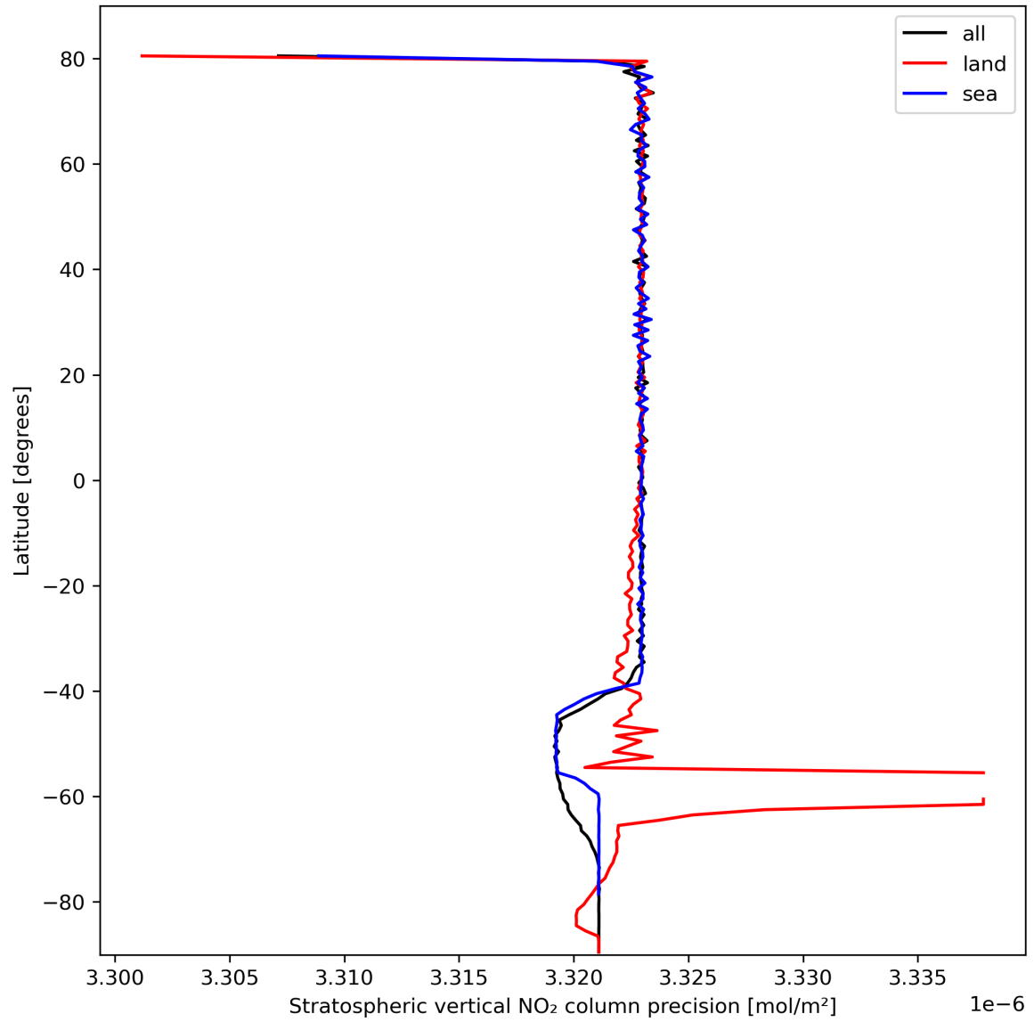
Figure 20: Zonal average of “Stratospheric vertical NO 2 column precision” for 2023-10-12 to 2023-10-14.
