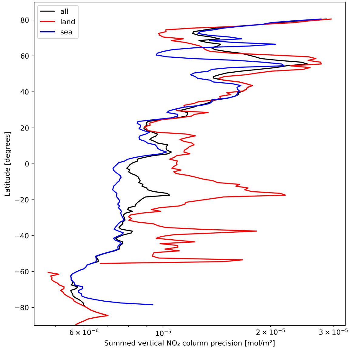
Figure 24: Zonal average of “Summed vertical NO 2 column precision” for 2023-10-12 to 2023-10-14.
