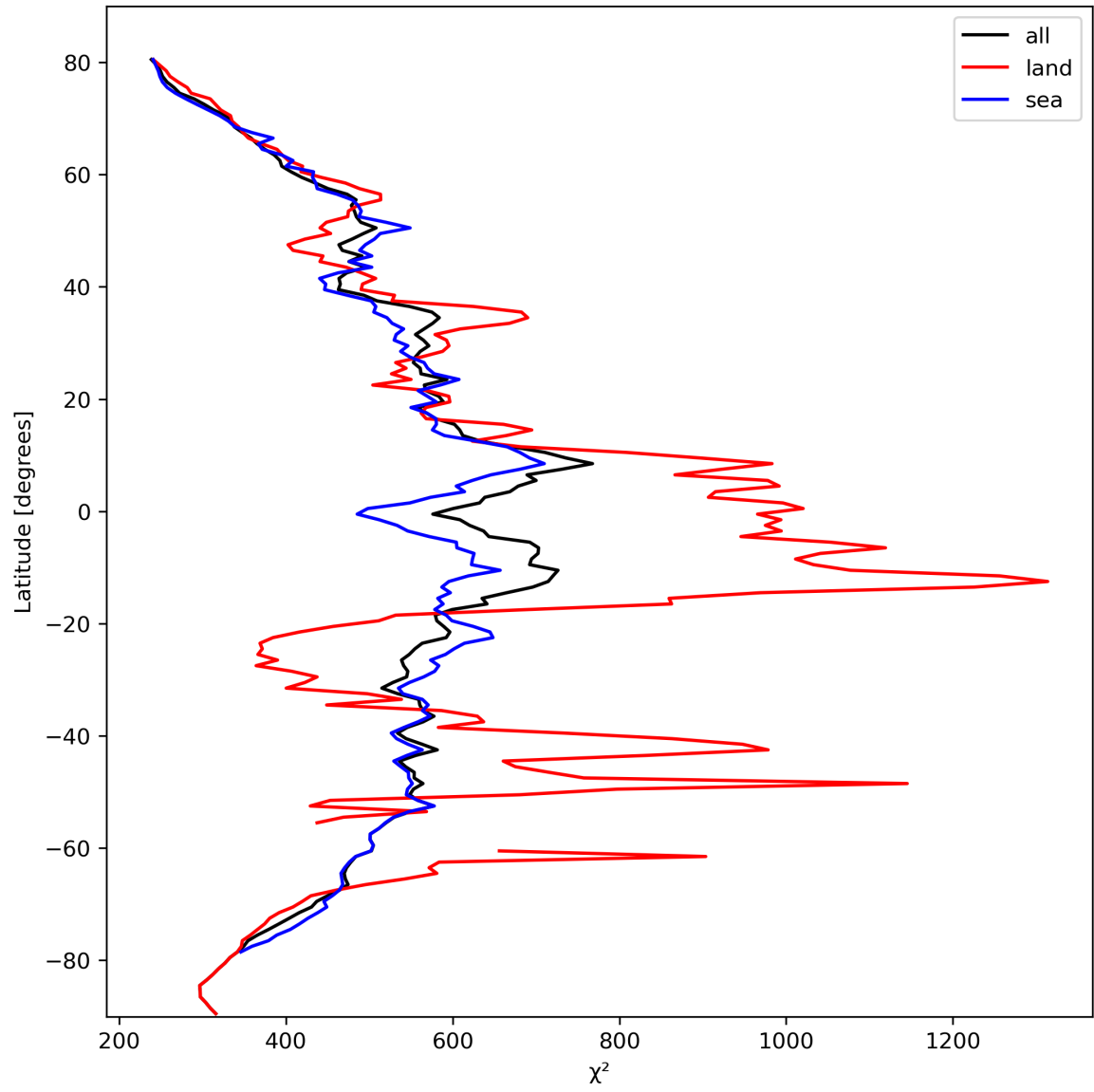
Figure 25: Zonal average of “ \chi^2 ” for 2023-10-12 to 2023-10-14.
