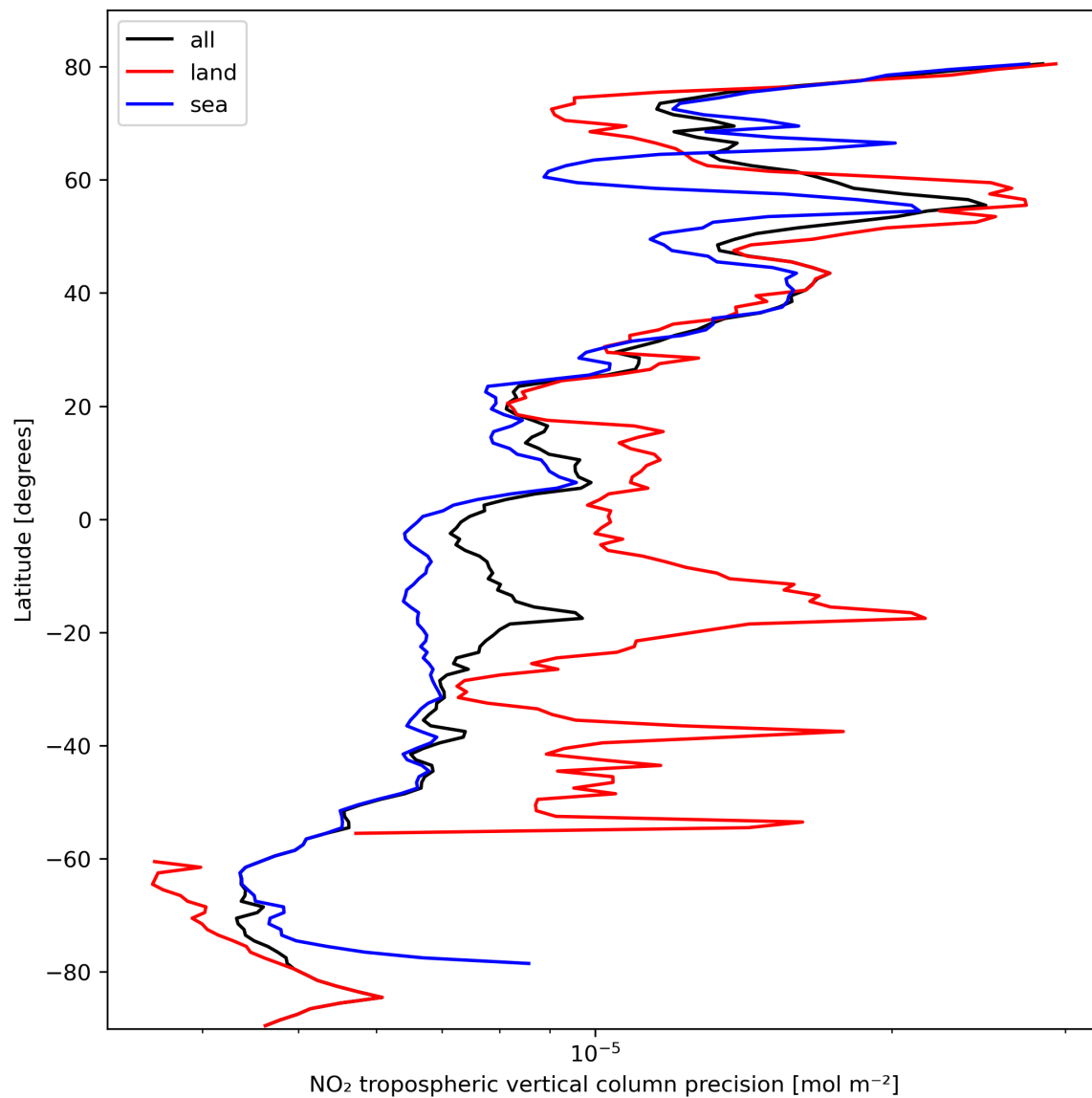
Figure 13: Zonal average of “NO 2 tropospheric vertical column precision” for 2023-10-12 to 2023-10-14.
