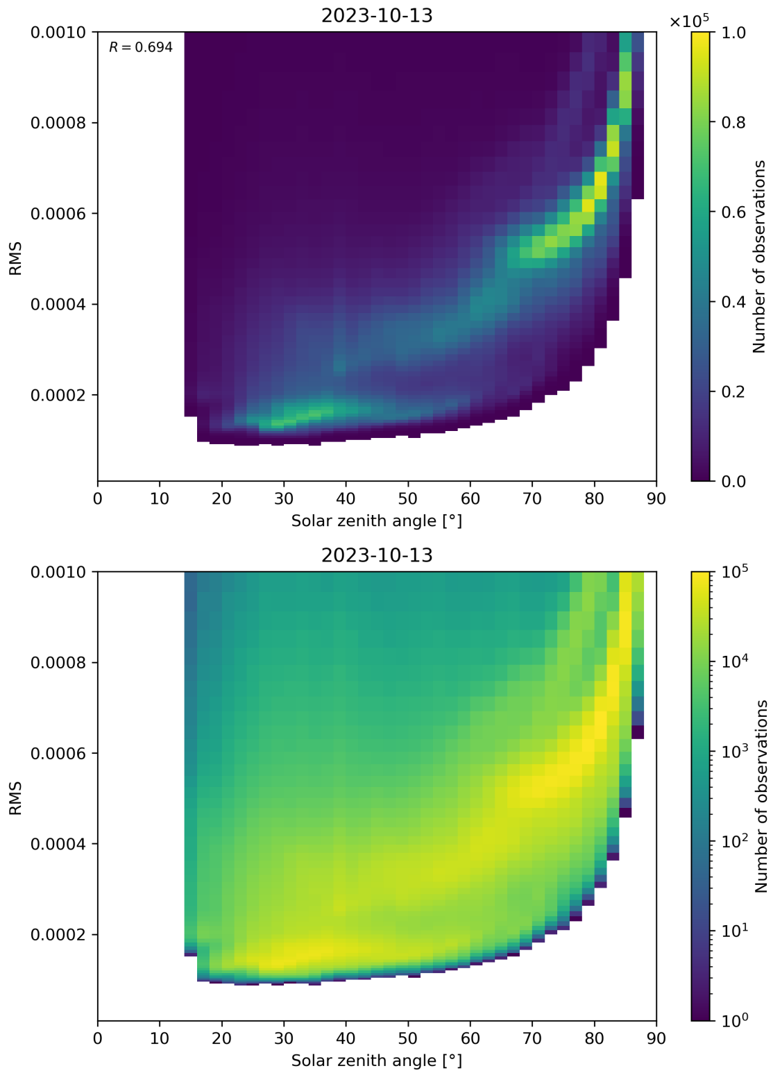
Figure 157: Scatter density plot of “Solar zenith angle” against “RMS” for 2023-10-12 to 2023-10-14.
