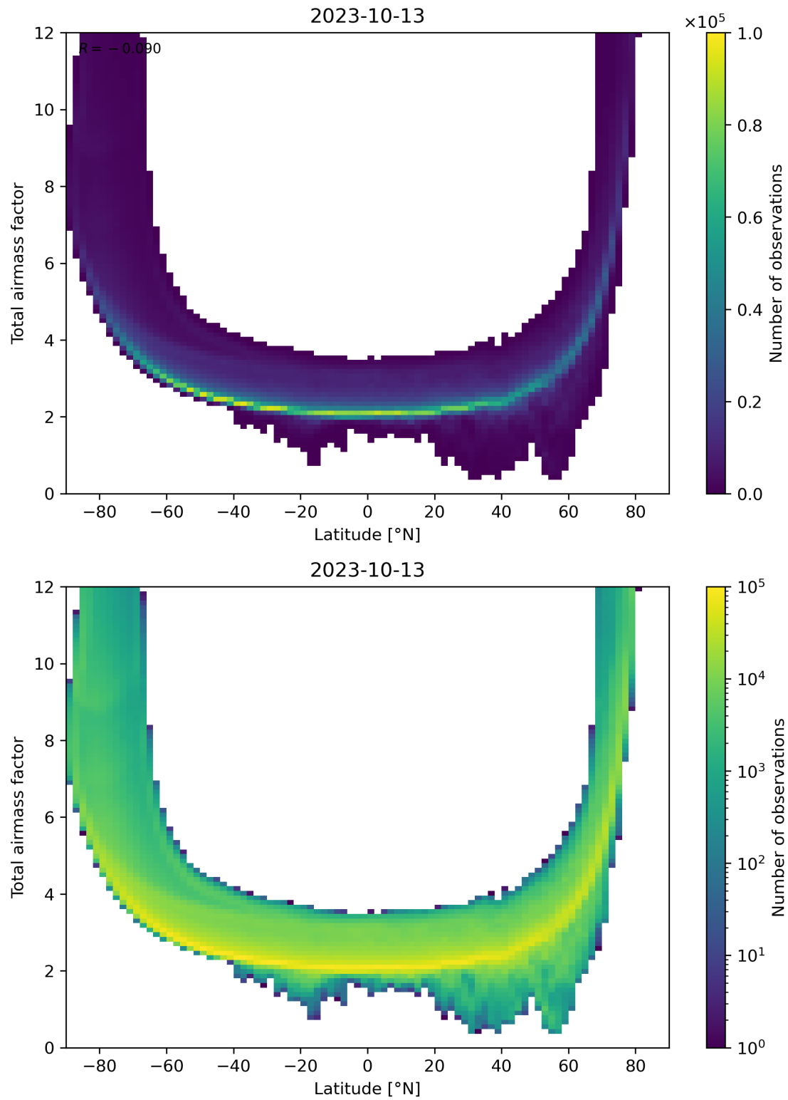
Figure 84: Scatter density plot of “Latitude” against “Total airmass factor” for 2023-10-12 to 2023-10-14.
