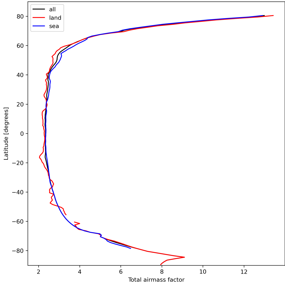
Figure 15: Zonal average of “Total airmass factor” for 2023-10-12 to 2023-10-14.
