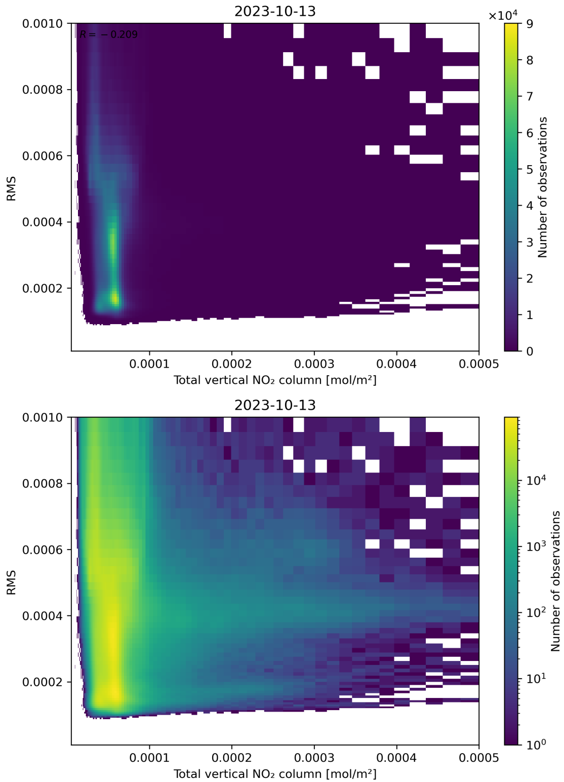
Figure 120: Scatter density plot of “Total vertical NO 2 column” against “RMS” for 2023-10-12 to 2023-10-14.
