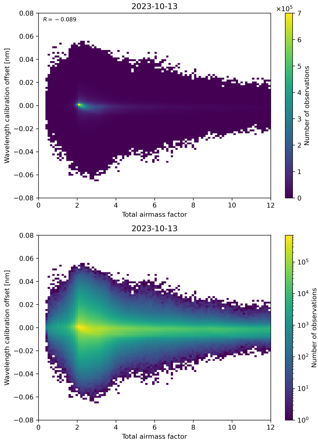
Figure 70: Scatter density plot of “Total airmass factor” against “Wavelength calibration offset” for 2023-10-12 to 2023-10-14.
