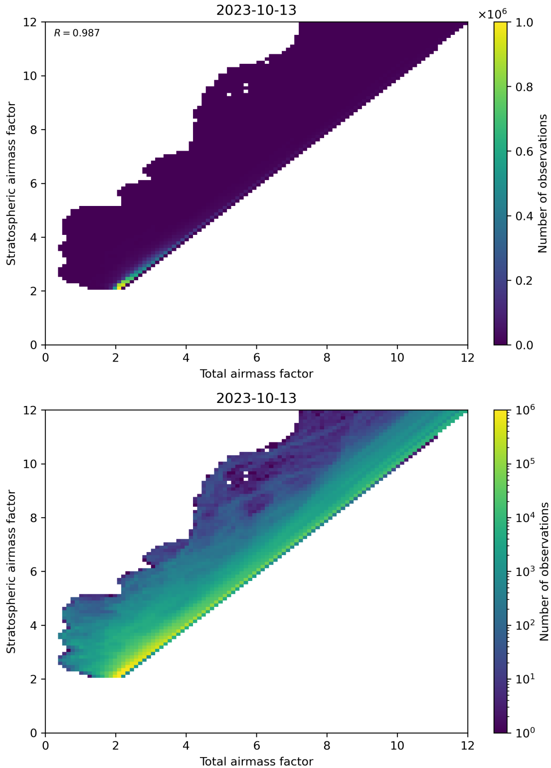
Figure 62: Scatter density plot of “Total airmass factor” against “Stratospheric airmass factor” for 2023-10-12 to 2023-10-14.
