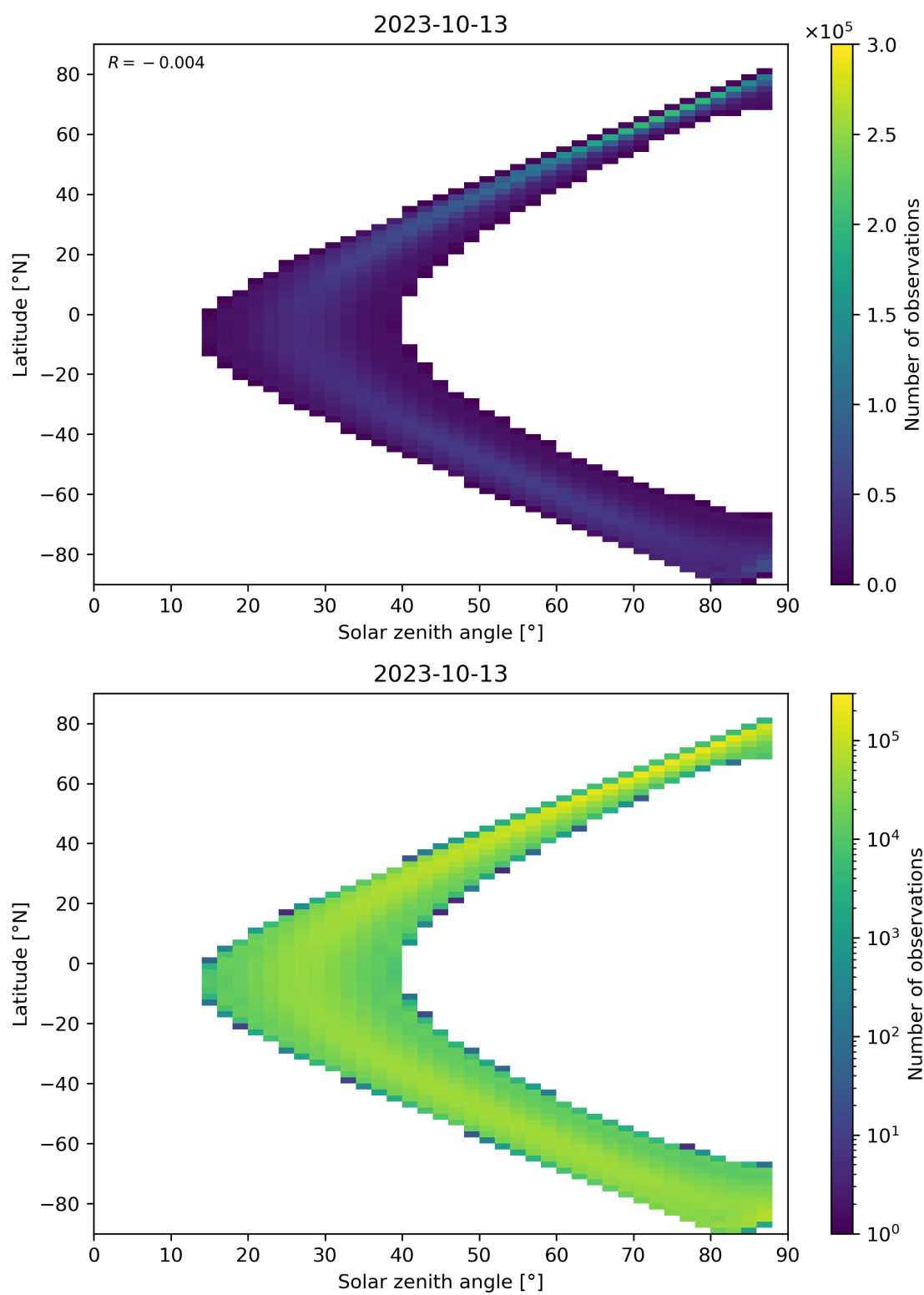
Figure 149: Scatter density plot of “Solar zenith angle” against “Latitude” for 2023-10-12 to 2023-10-14.
