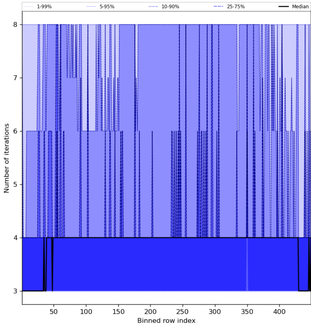
Figure 51: Along track statistics of “Number of iterations” for 2023-10-12 to 2023-10-14
