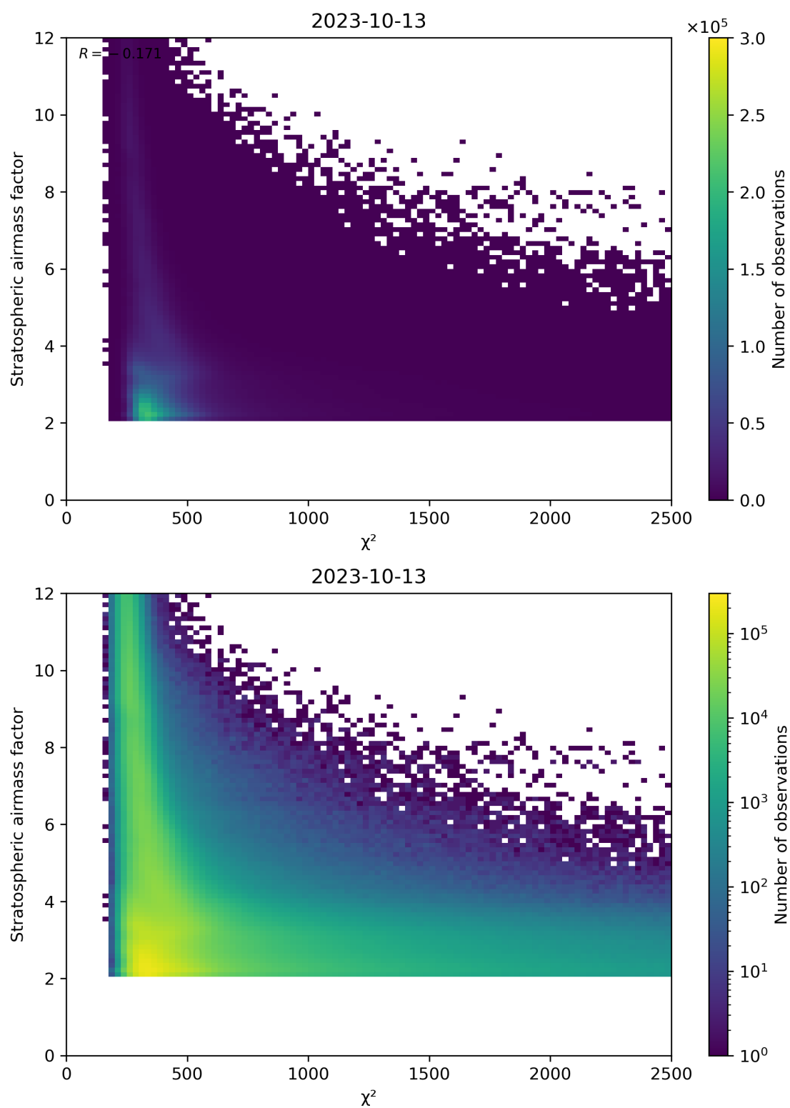
Figure 81: Scatter density plot of “ \chi^2 ” against “Stratospheric airmass factor” for 2023-10-12 to 2023-10-14.
