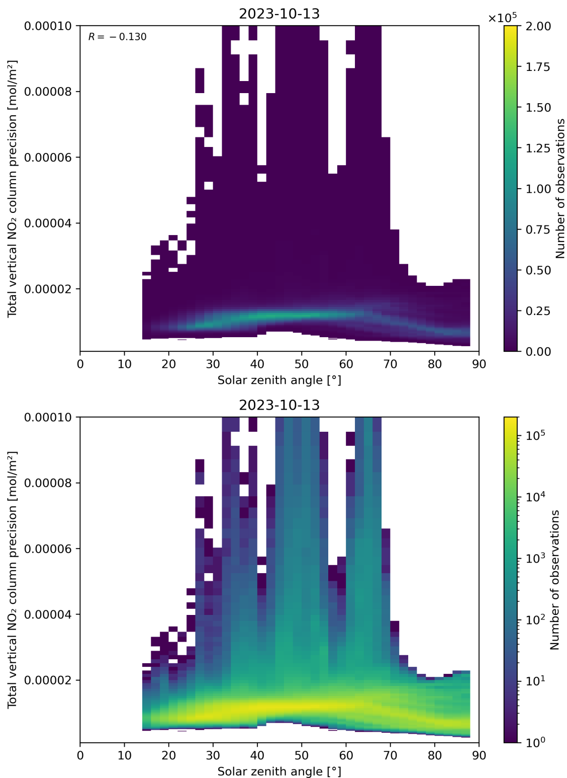
Figure 154: Scatter density plot of “Solar zenith angle” against “Total vertical NO 2 column precision” for 2023-10-12 to 2023-10-14.
