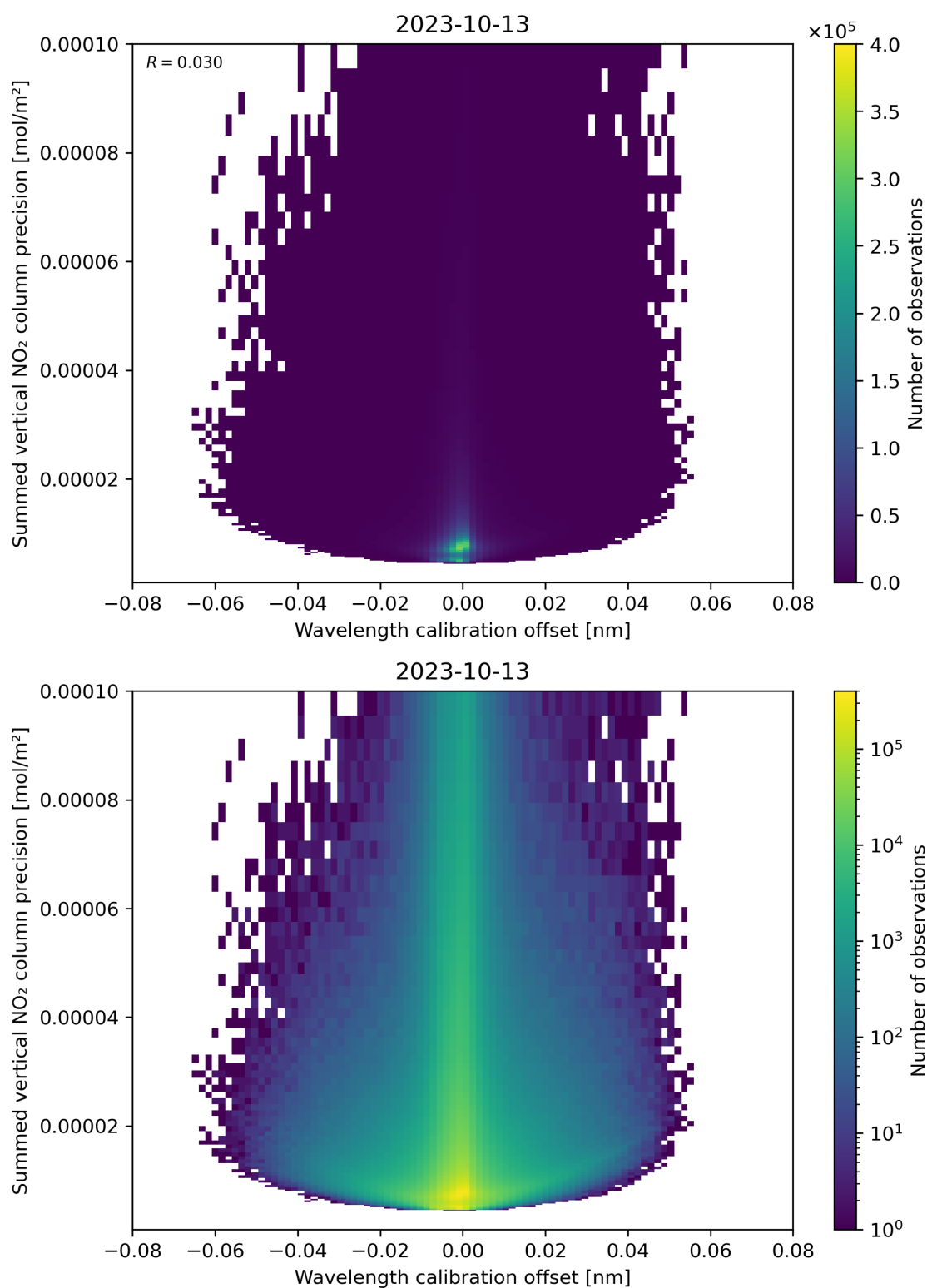
Figure 178: Scatter density plot of “Wavelength calibration offset” against “Summed vertical NO 2 column precision” for 2023-10-12 to 2023-10-14.
