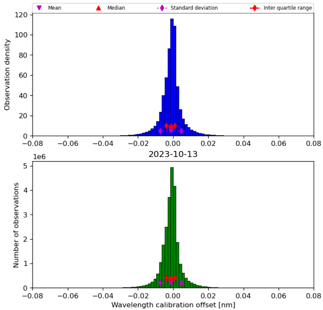
Figure 35: Histogram of “Wavelength calibration offset” for 2023-10-12 to 2023-10-14
