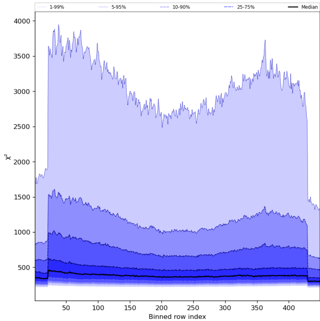
Figure 59: Along track statistics of “ \chi^2 ” for 2023-10-12 to 2023-10-14
