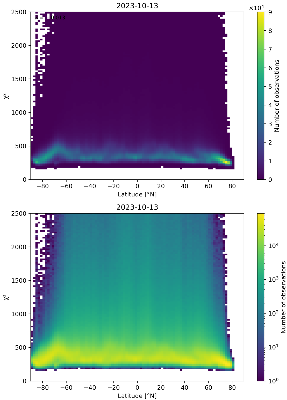
Figure 86: Scatter density plot of “Latitude” against “ \chi^2 ” for 2023-10-12 to 2023-10-14.
