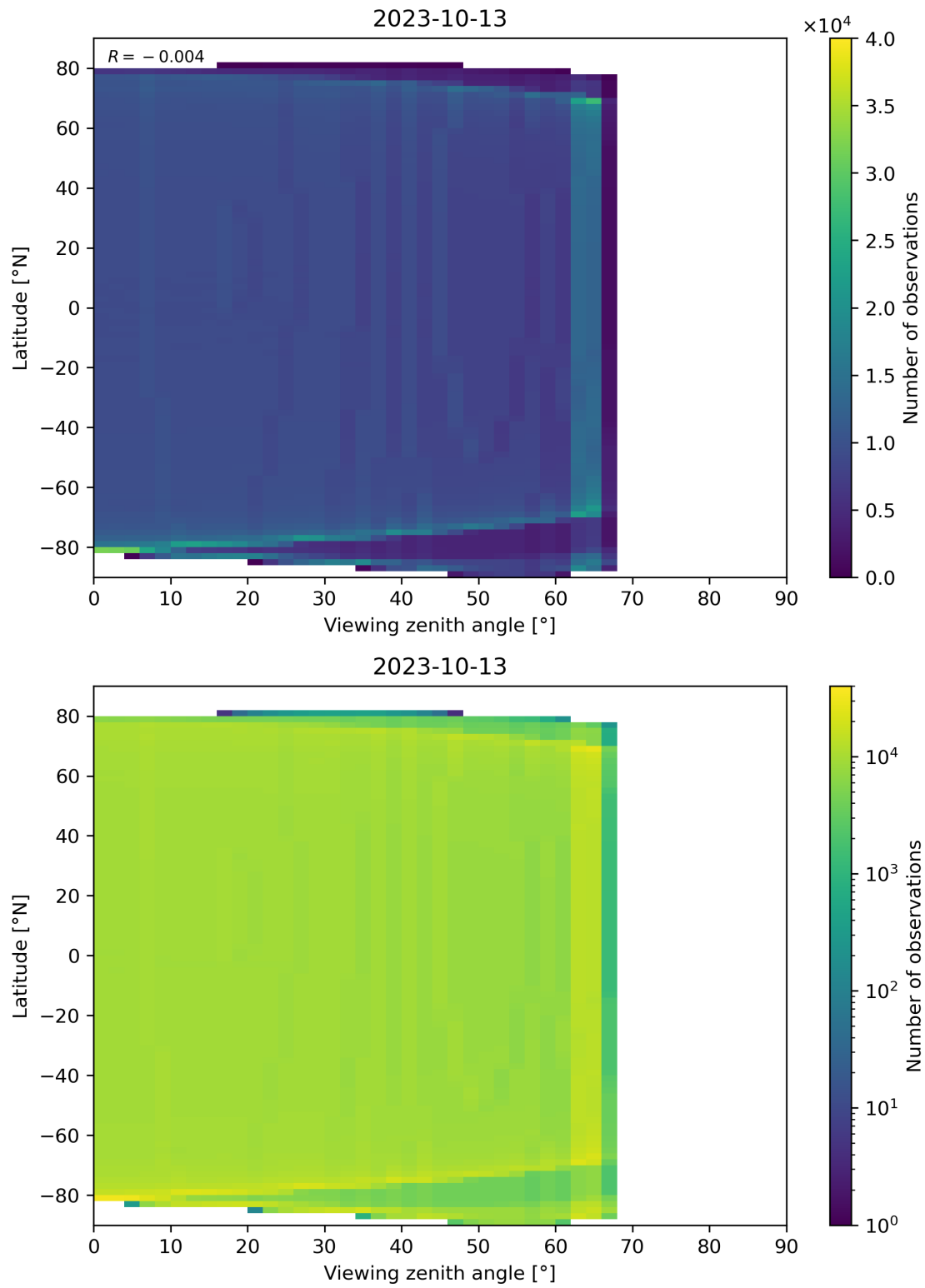
Figure 163: Scatter density plot of “Viewing zenith angle” against “Latitude” for 2023-10-12 to 2023-10-14.
