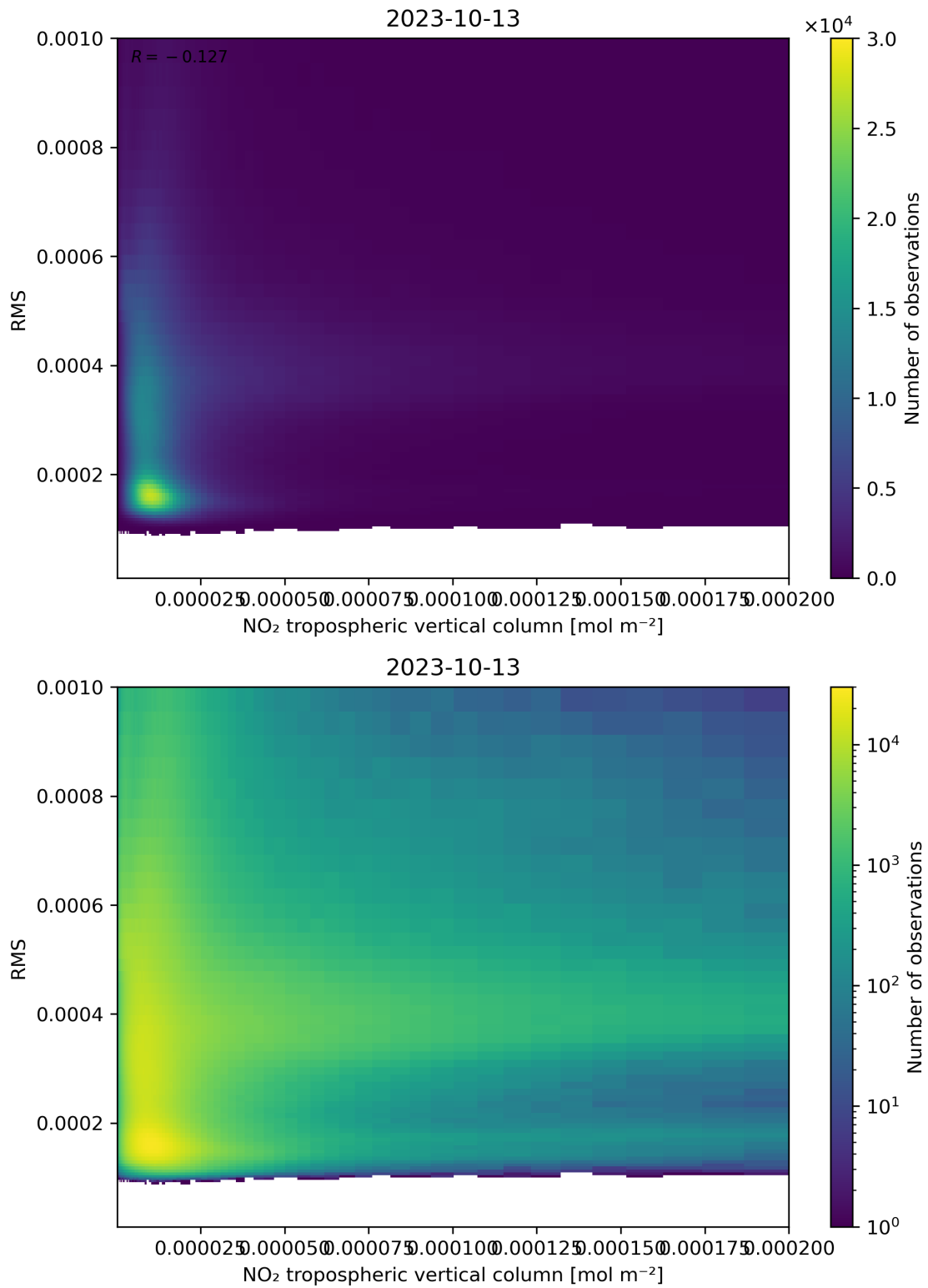
Figure 142: Scatter density plot of “NO 2 tropospheric vertical column” against “RMS” for 2023-10-12 to 2023-10-14.
