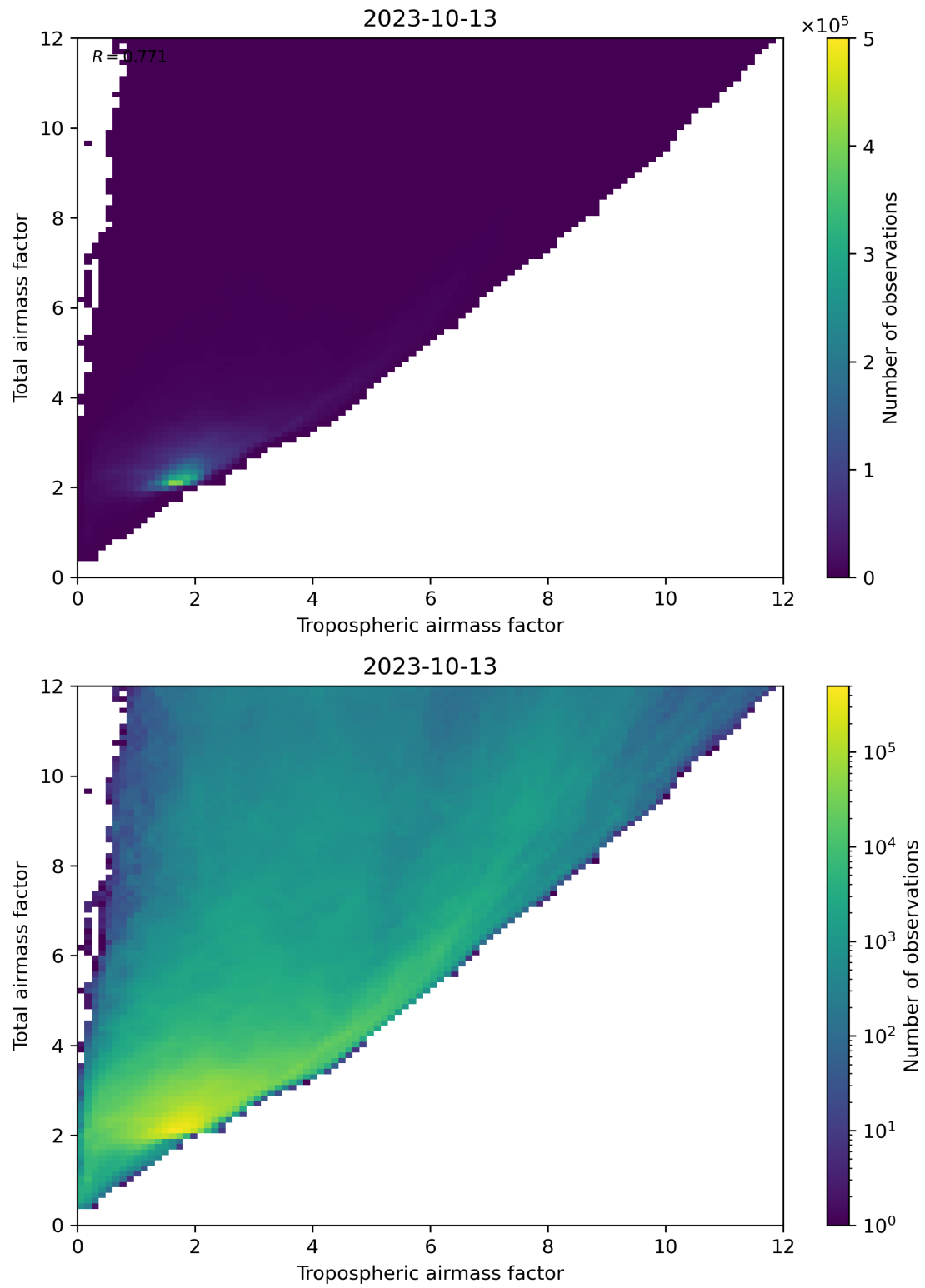
Figure 72: Scatter density plot of “Tropospheric airmass factor” against “Total airmass factor” for 2023-10-12 to 2023-10-14.
