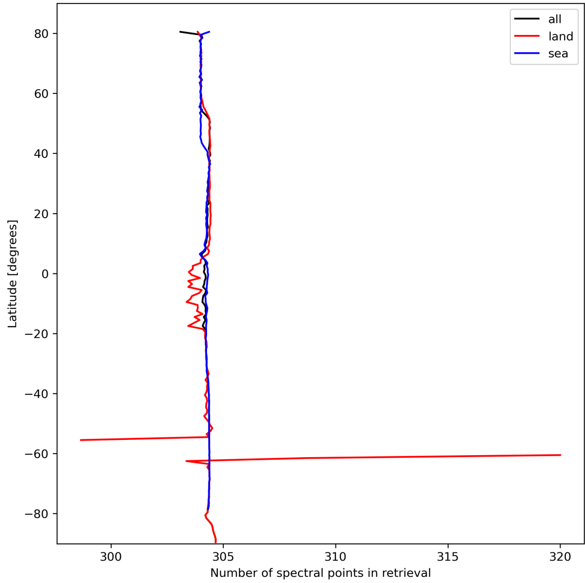
Figure 16: Zonal average of “Number of spectral points in retrieval” for 2023-10-12 to 2023-10-14.
