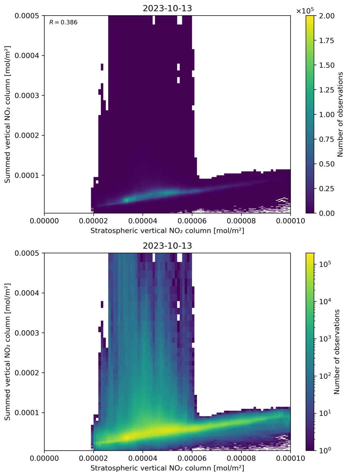
Figure 98: Scatter density plot of “Stratospheric vertical NO 2 column” against “Summed vertical NO 2 column” for 2023-10-12 to 2023-10-14.
