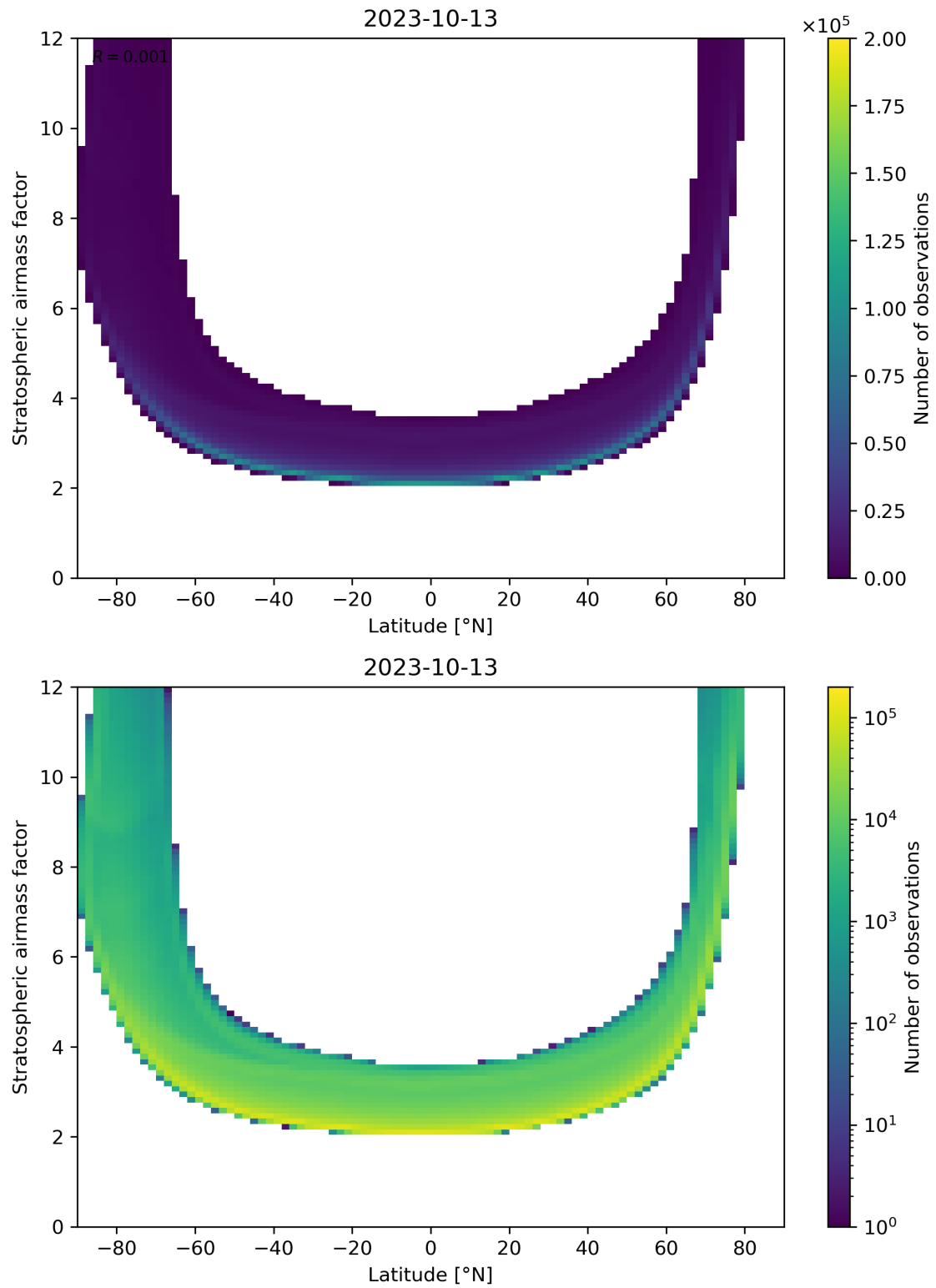
Figure 83: Scatter density plot of “Latitude” against “Stratospheric airmass factor” for 2023-10-12 to 2023-10-14.
