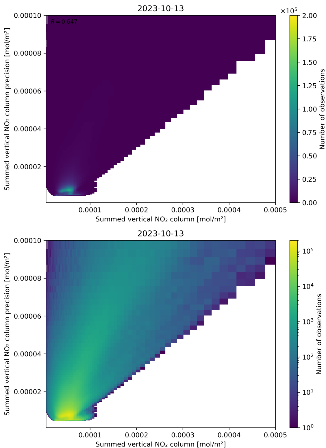
Figure 105: Scatter density plot of “Summed vertical NO 2 column” against “Summed vertical NO 2 column precision” for 2023-10-12 to 2023-10-14.
