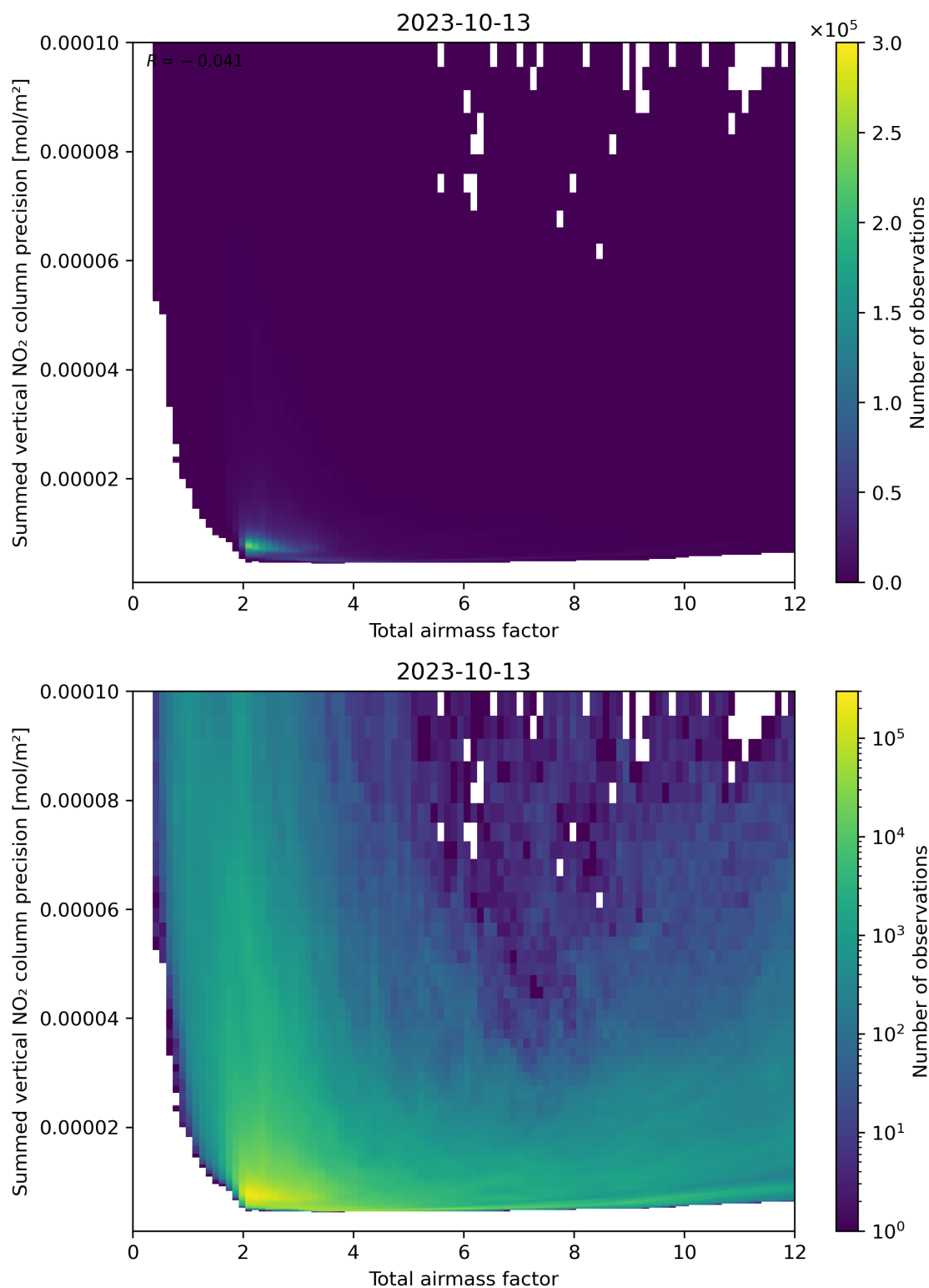
Figure 66: Scatter density plot of “Total airmass factor” against “Summed vertical NO 2 column precision” for 2023-10-12 to 2023-10-14.
