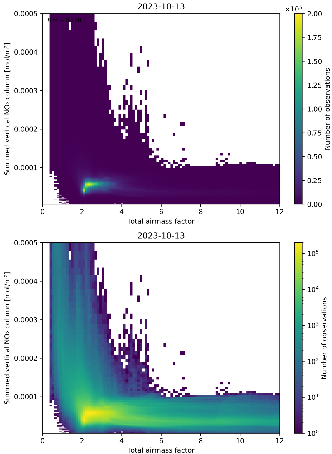
Figure 65: Scatter density plot of “Total airmass factor” against “Summed vertical NO 2 column” for 2023-10-12 to 2023-10-14.
