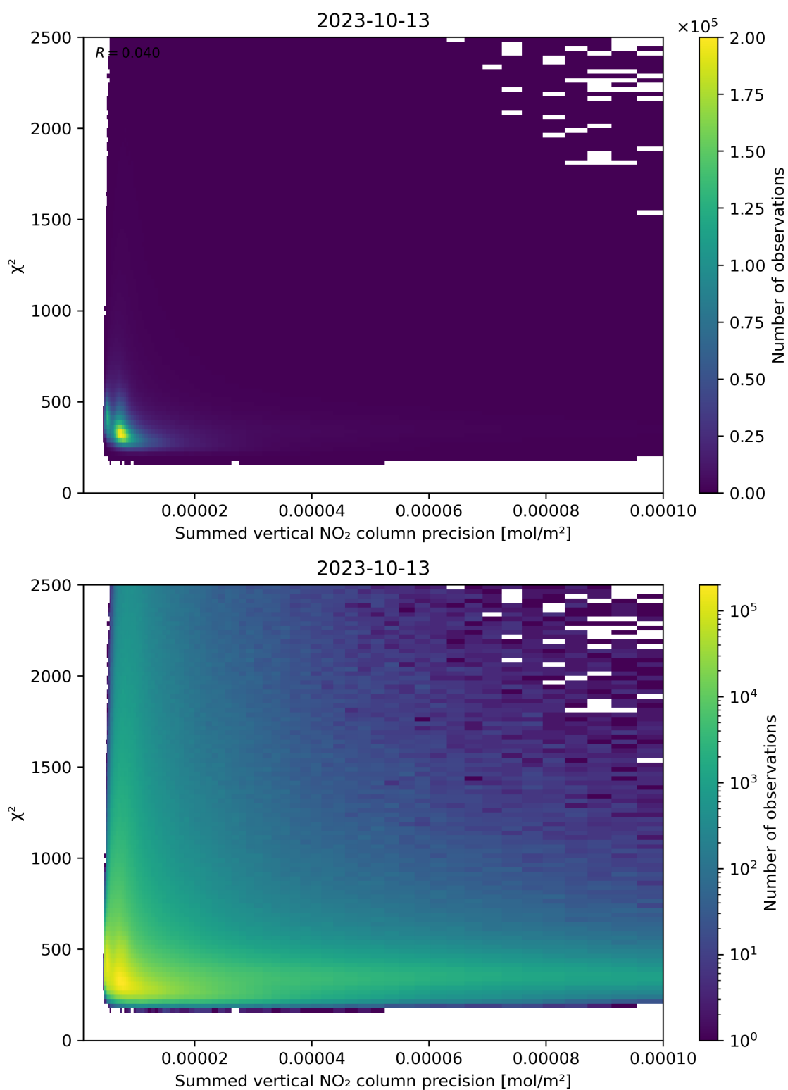
Figure 107: Scatter density plot of “Summed vertical NO 2 column precision” against “ \chi^2 ” for 2023-10-12 to 2023-10-14.
