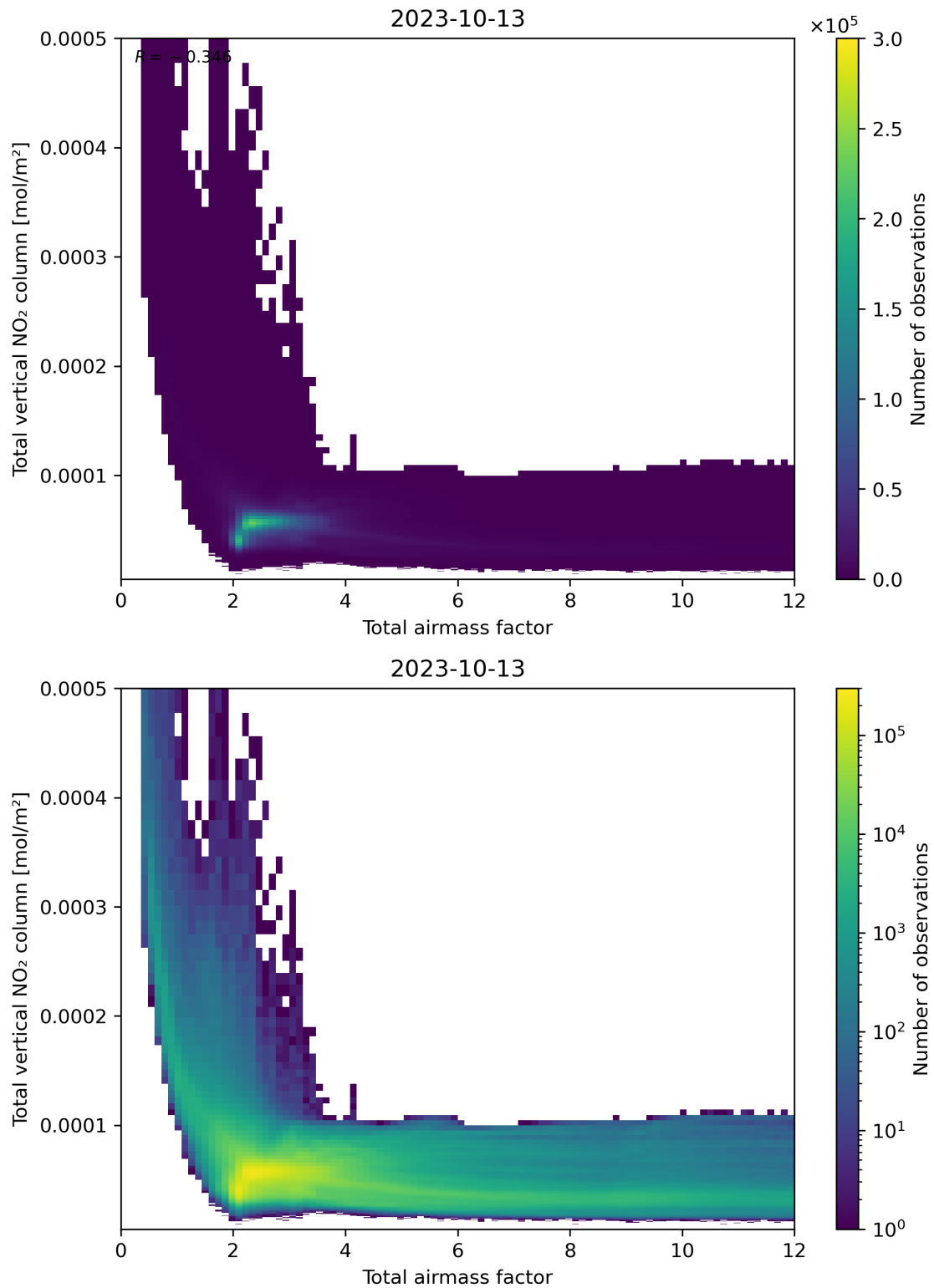
Figure 67: Scatter density plot of “Total airmass factor” against “Total vertical NO 2 column” for 2023-10-12 to 2023-10-14.
