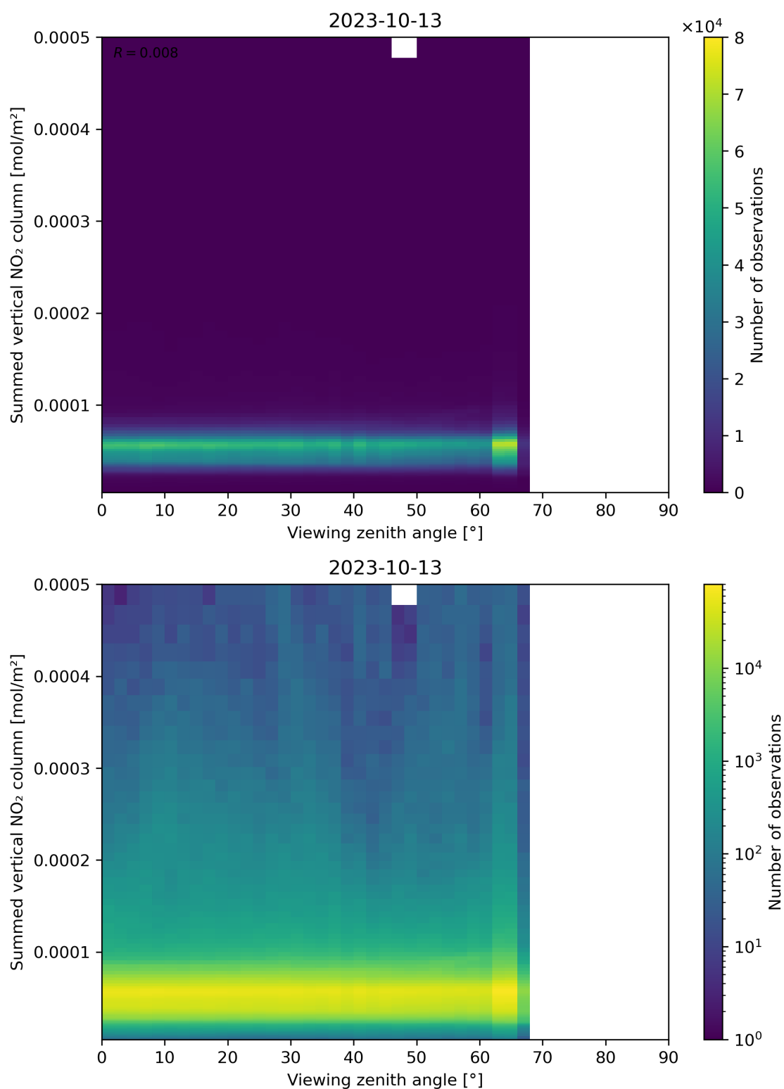
Figure 165: Scatter density plot of “Viewing zenith angle” against “Summed vertical NO 2 column” for 2023-10-12 to 2023-10-14.
