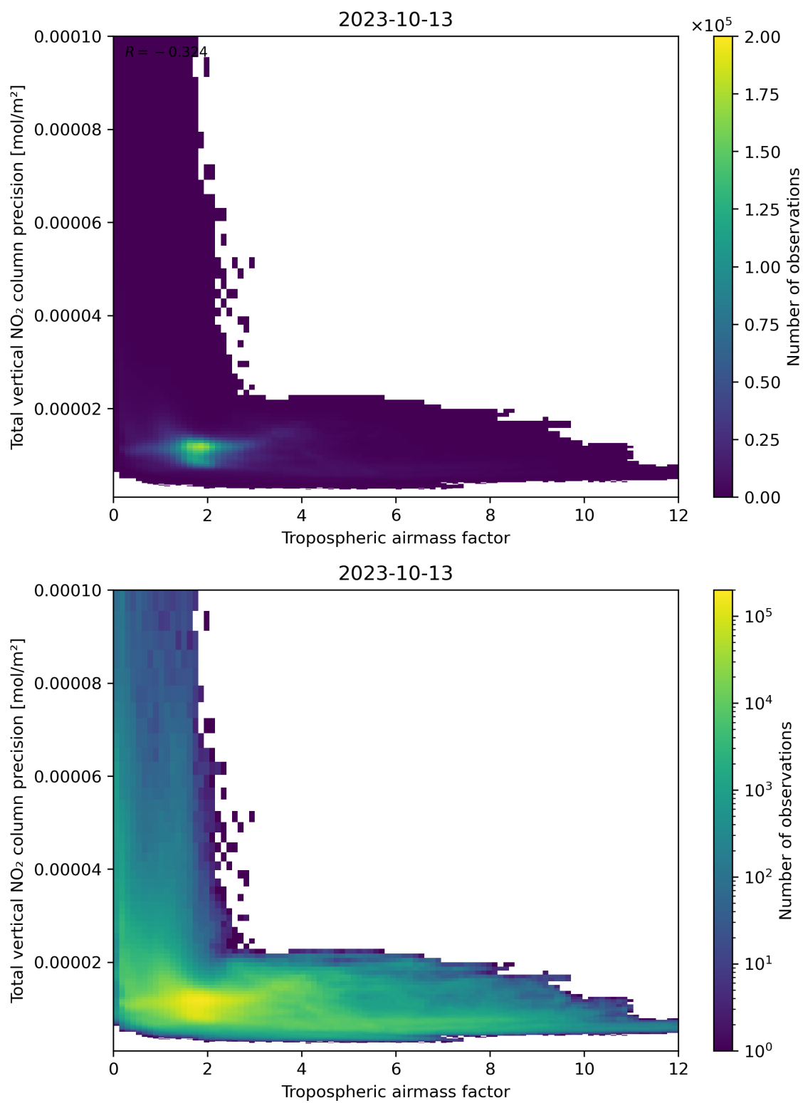
Figure 78: Scatter density plot of “Tropospheric air mass factor” against “Total vertical NO 2 column precision” for 2023-10-12 to 2023-10-14.
