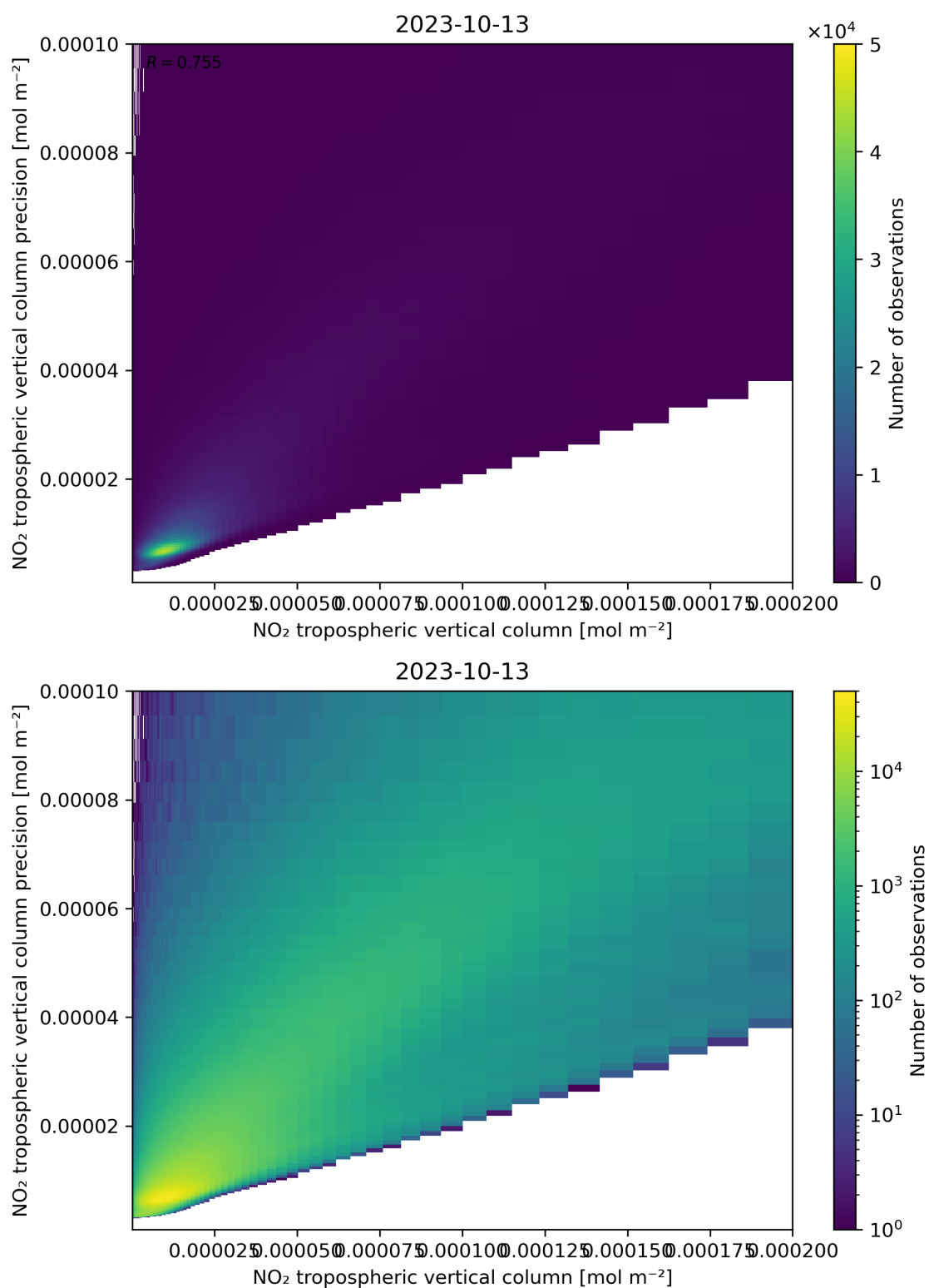
Figure 130: Scatter density plot of “NO 2 tropospheric vertical column” against “NO 2 tropospheric vertical column precision” for 2023-10-12 to 2023-10-14.
