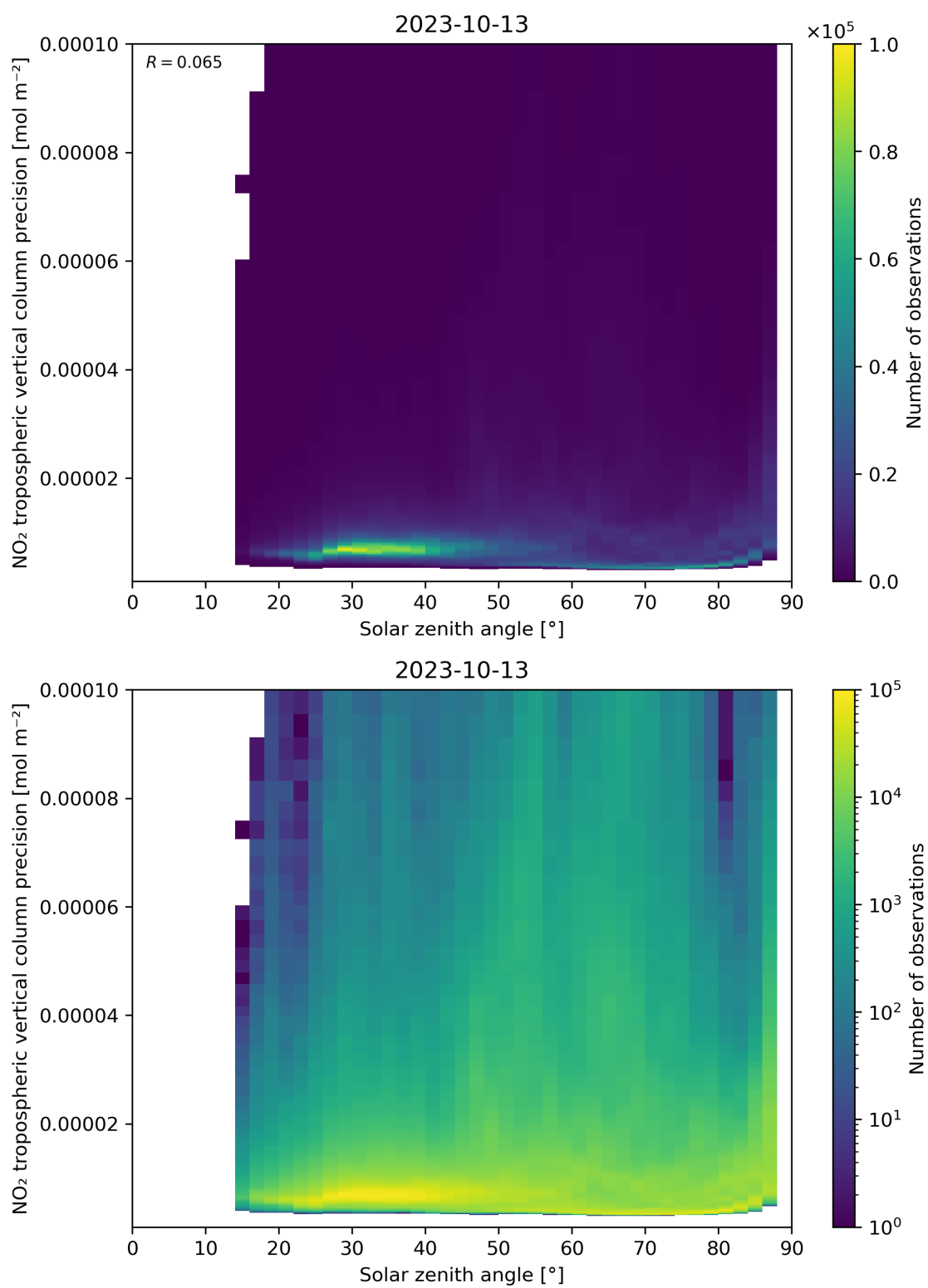
Figure 156: Scatter density plot of “Solar zenith angle” against “NO 2 tropospheric vertical column precision” for 2023-10-12 to 2023-10-14.
