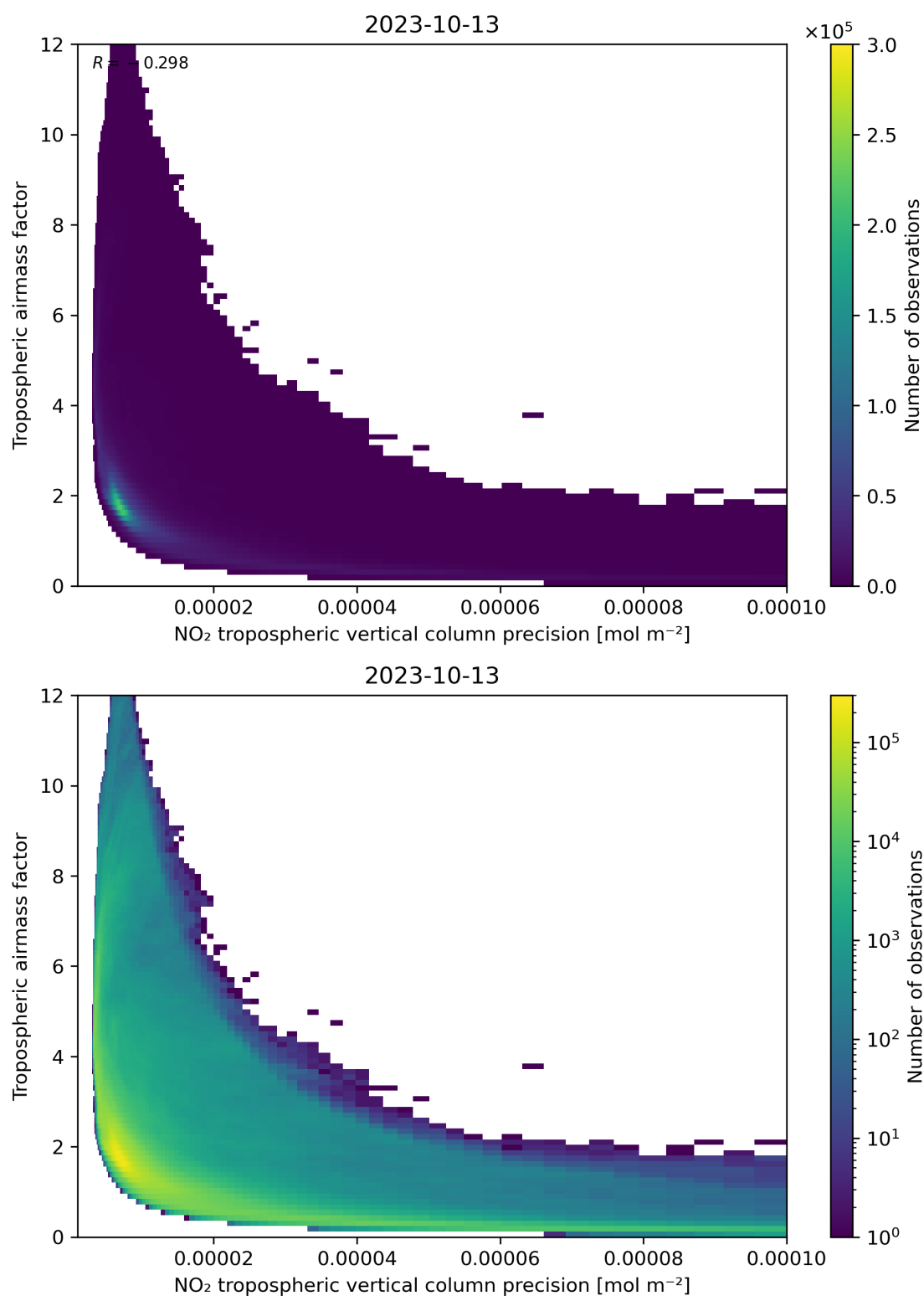
Figure 133: Scatter density plot of “NO 2 tropospheric vertical column precision” against “Tropospheric airmass factor” for 2023-10-12 to 2023-10-14.
