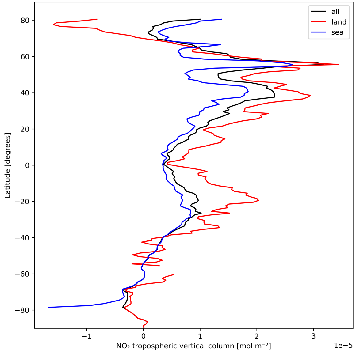
Figure 12: Zonal average of “NO 2 tropospheric vertical column” for 2023-10-12 to 2023-10-14.
