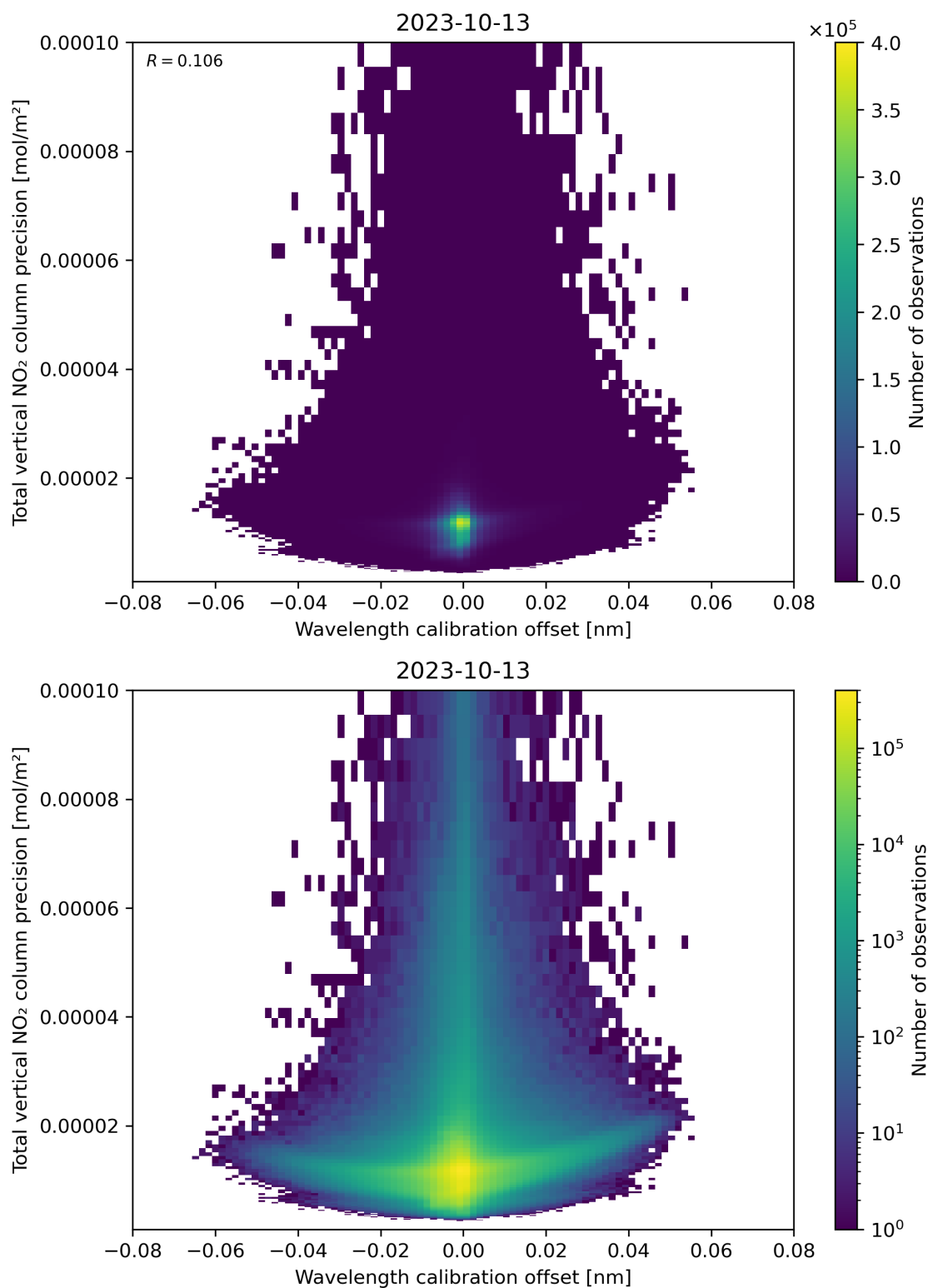
Figure 180: Scatter density plot of “Wavelength calibration offset” against “Total vertical NO 2 column precision” for 2023-10-12 to 2023-10-14.
