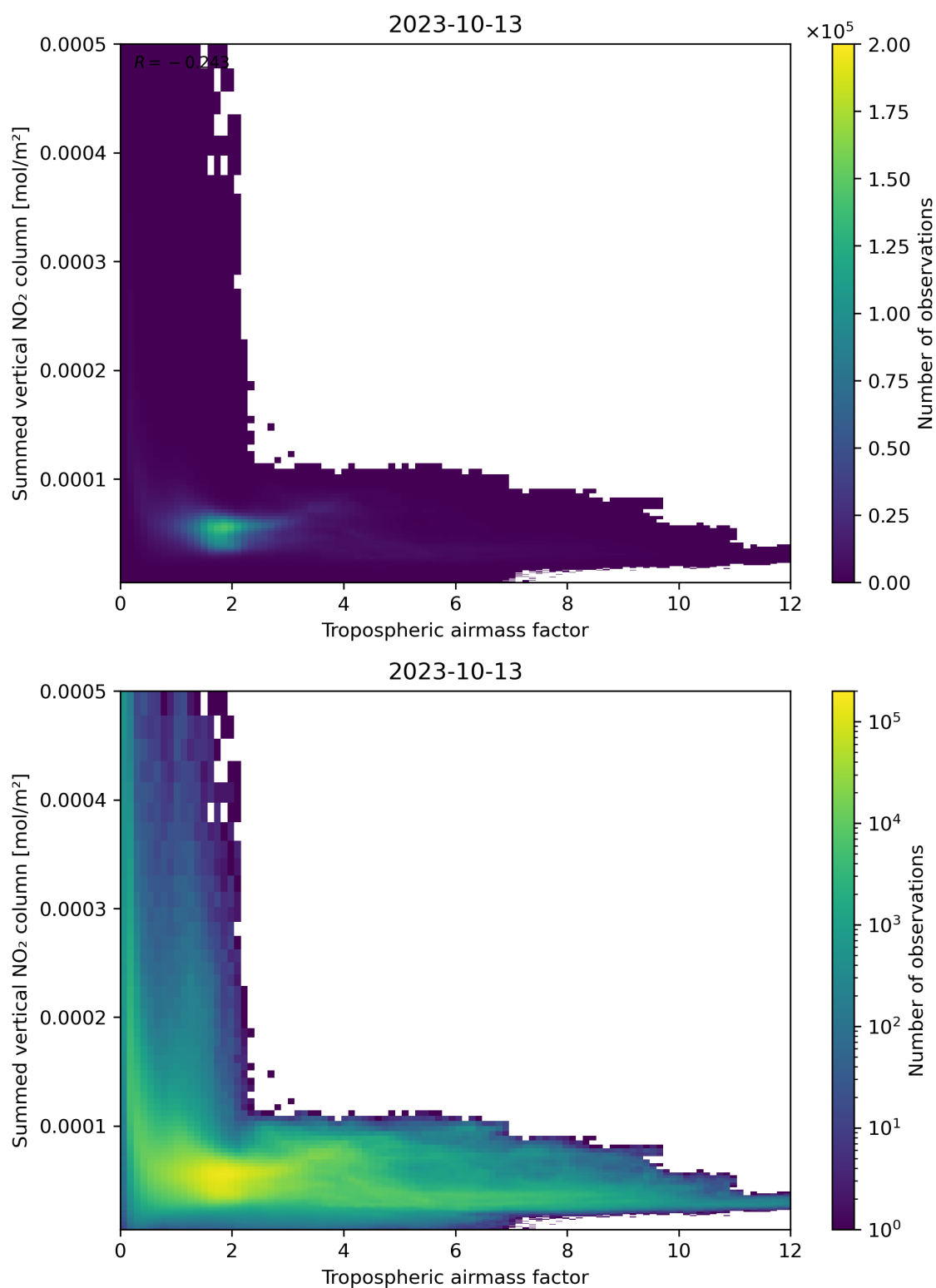
Figure 75: Scatter density plot of “Tropospheric airmass factor” against “Summed vertical NO 2 column” for 2023-10-12 to 2023-10-14.
