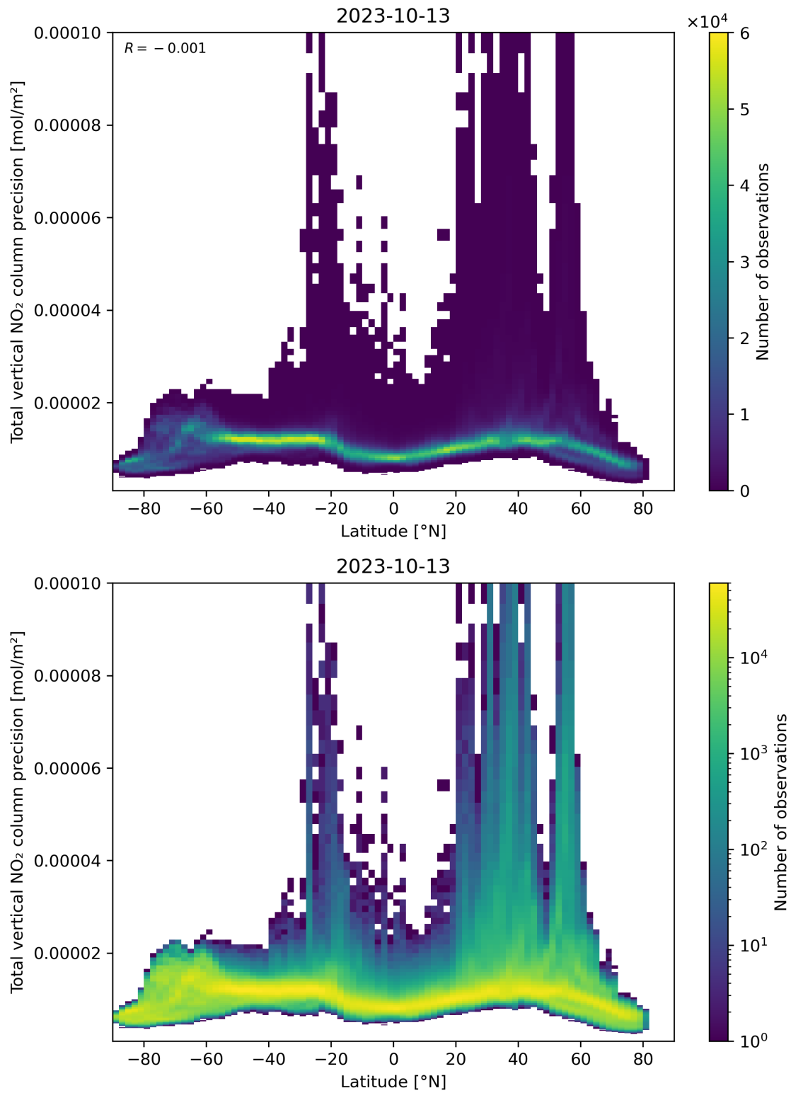
Figure 91: Scatter density plot of “Latitude” against “Total vertical NO 2 column precision” for 2023-10-12 to 2023-10-14.
