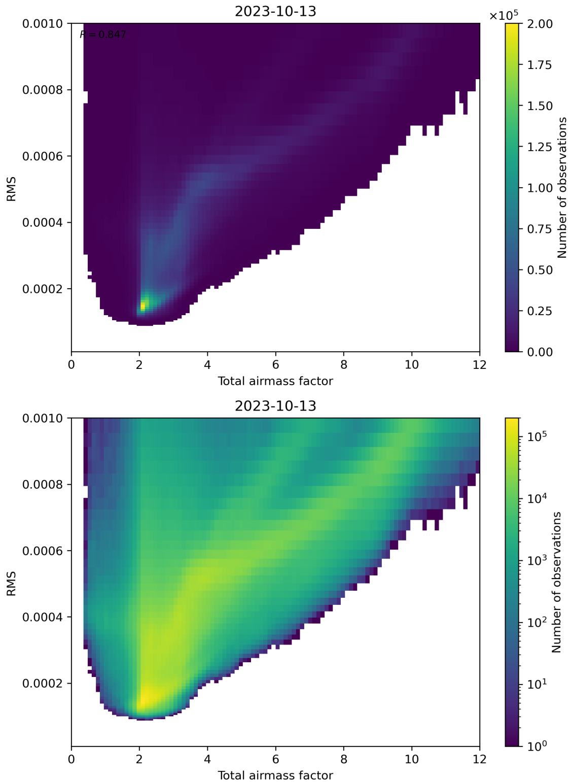
Figure 69: Scatter density plot of “Total airmass factor” against “RMS” for 2023-10-12 to 2023-10-14.
