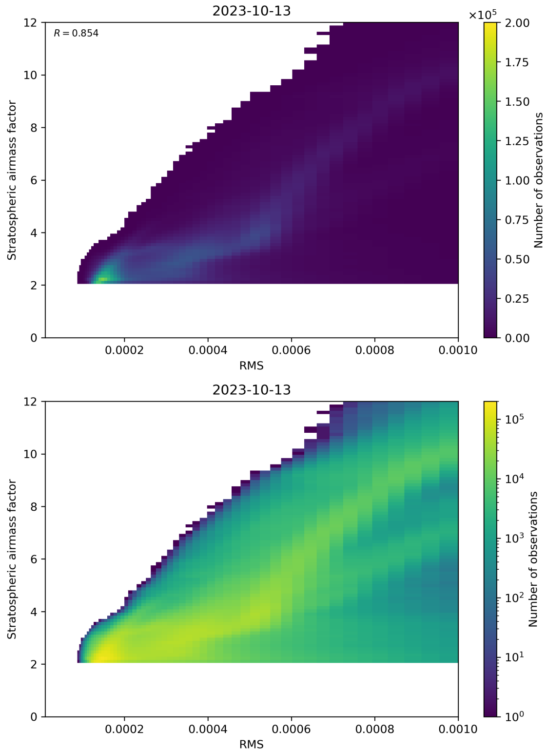
Figure 144: Scatter density plot of “RMS” against “Stratospheric airmass factor” for 2023-10-12 to 2023-10-14.
