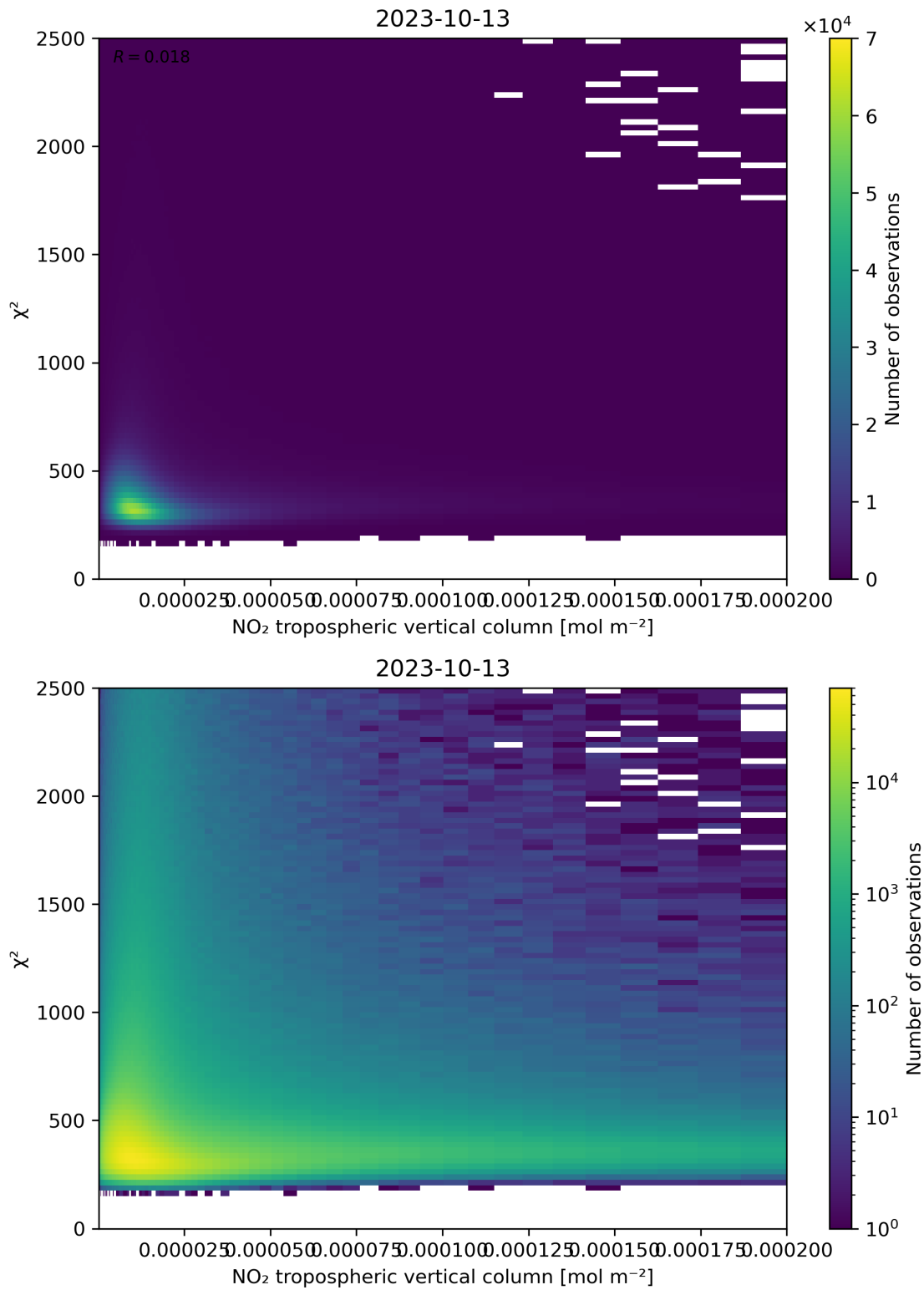
Figure 124: Scatter density plot of “NO 2 tropospheric vertical column” against “ \chi^2 ” for 2023-10-12 to 2023-10-14.
