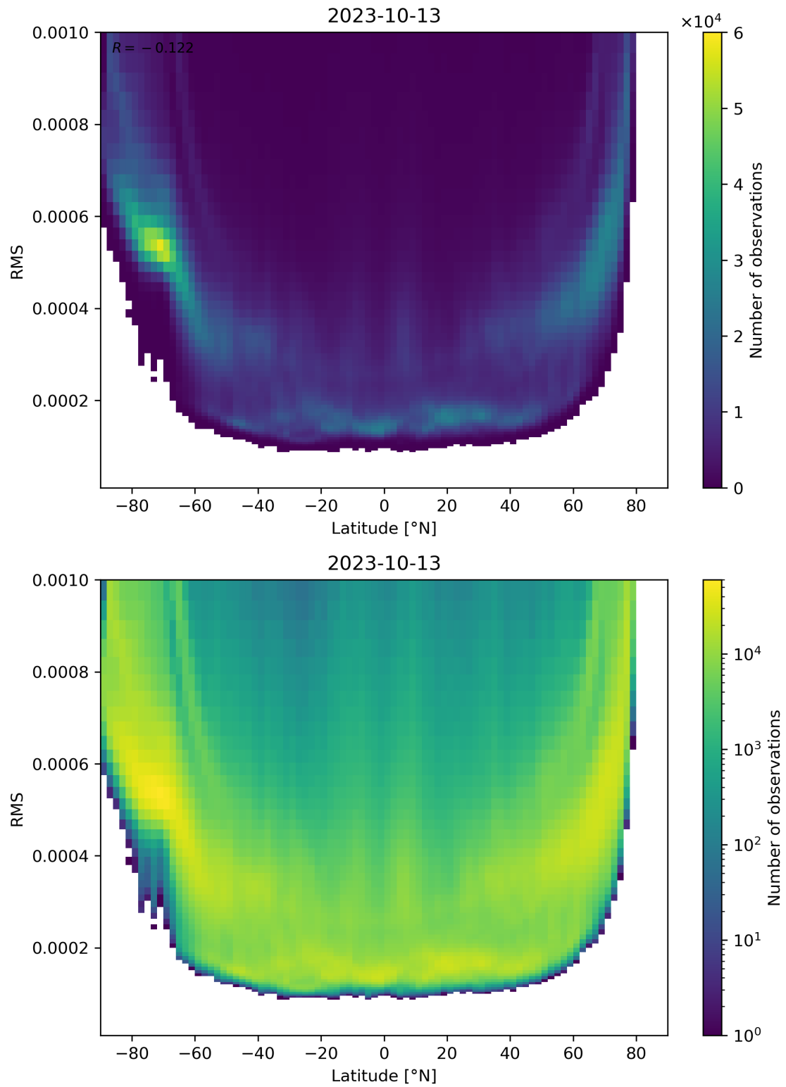
Figure 94: Scatter density plot of “Latitude” against “RMS” for 2023-10-12 to 2023-10-14.
