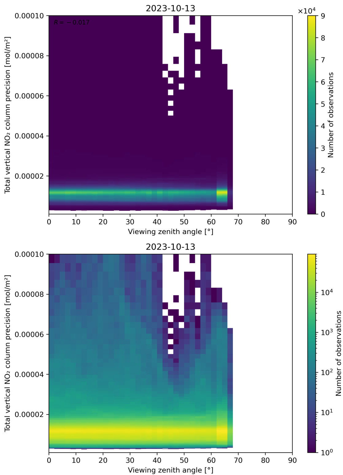
Figure 168: Scatter density plot of “Viewing zenith angle” against “Total vertical NO 2 column precision” for 2023-10-12 to 2023-10-14.
