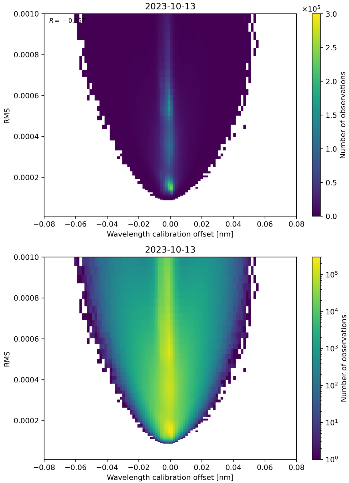
Figure 181: Scatter density plot of “Wavelength calibration offset” against “RMS” for 2023-10-12 to 2023-10-14.
