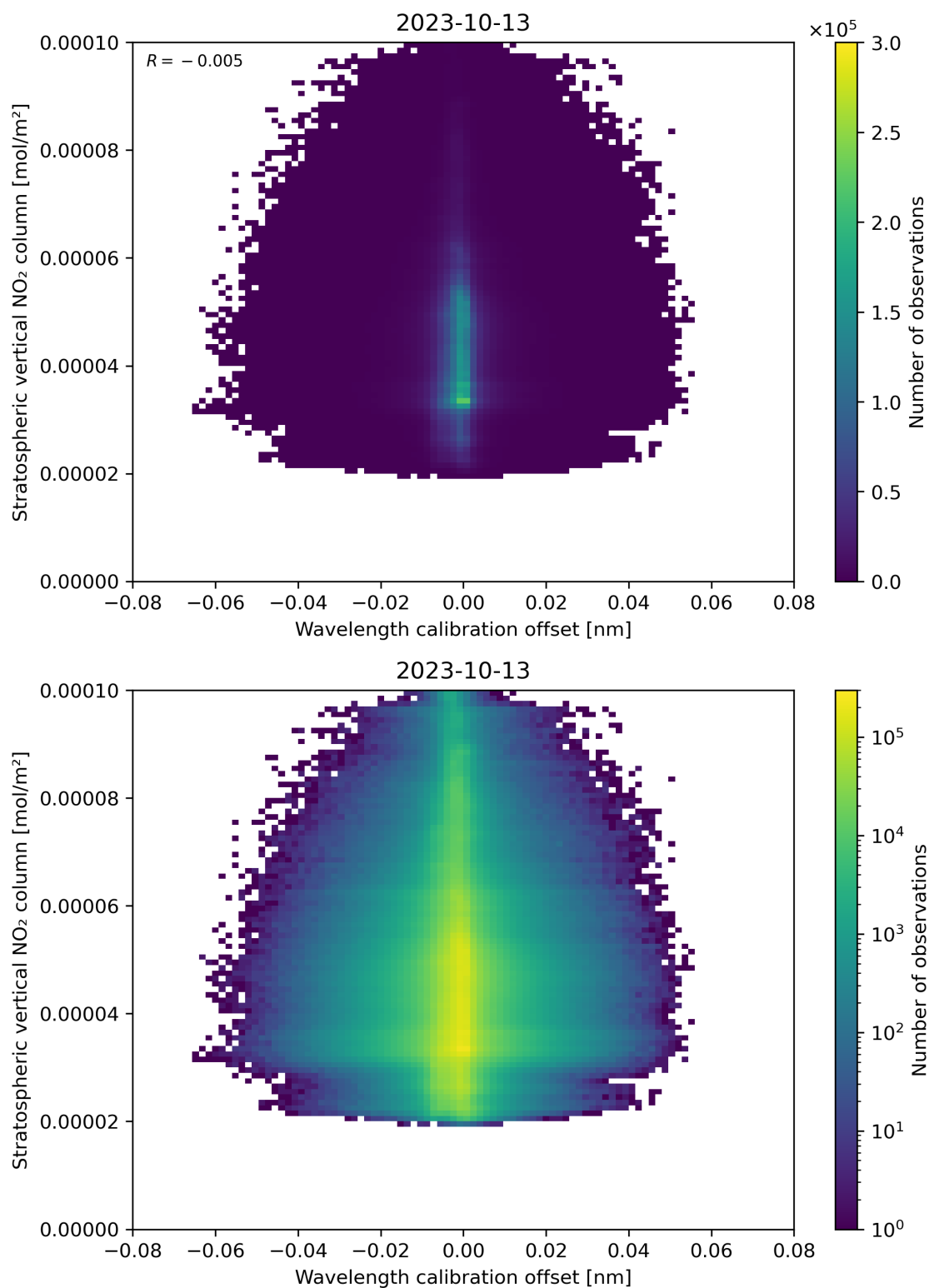
Figure 176: Scatter density plot of “Wavelength calibration offset” against “Stratospheric vertical NO 2 column” for 2023-10-12 to 2023-10-14.
