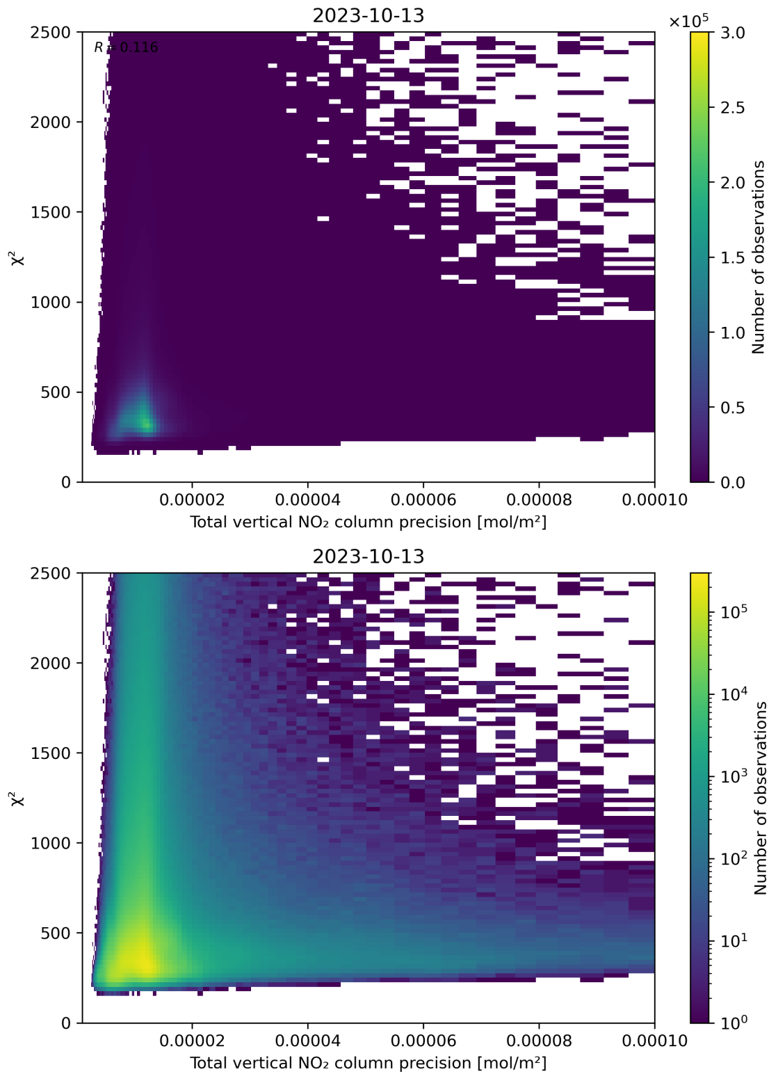
Figure 116: Scatter density plot of “Total vertical NO 2 column precision” against “ \chi^2 ” for 2023-10-12 to 2023-10-14.
