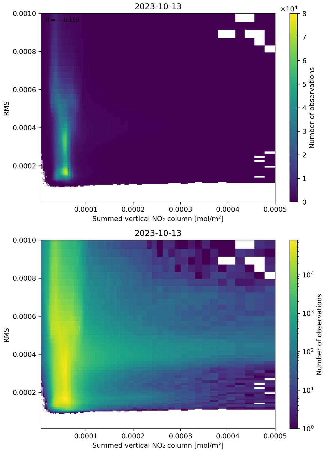
Figure 109: Scatter density plot of “Summed vertical NO 2 column” against “RMS” for 2023-10-12 to 2023-10-14.
