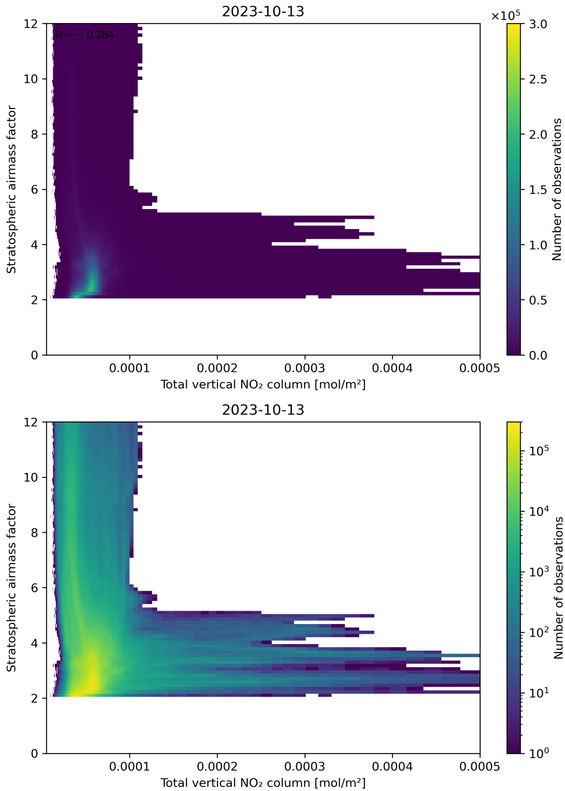
Figure 110: Scatter density plot of “Total vertical NO 2 column” against “Stratospheric airmass factor” for 2023-10-12 to 2023-10-14.
