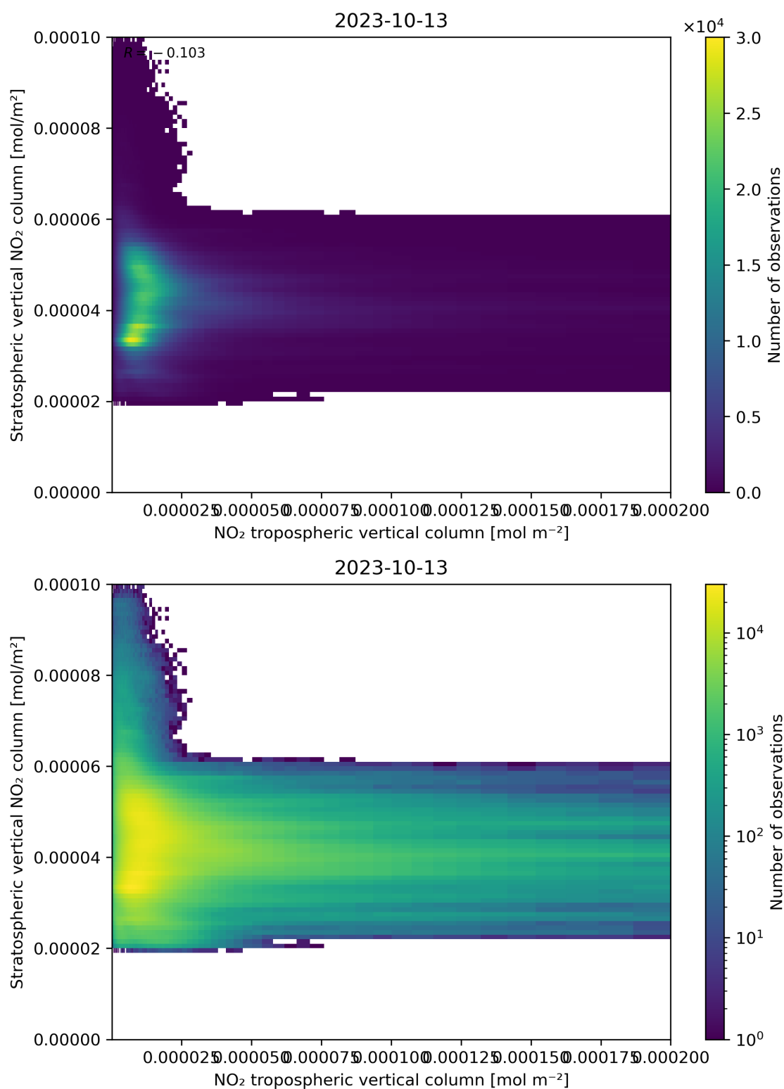
Figure 125: Scatter density plot of “NO 2 tropospheric vertical column” against “Stratospheric vertical NO 2 column” for 2023-10-12 to 2023-10-14.
