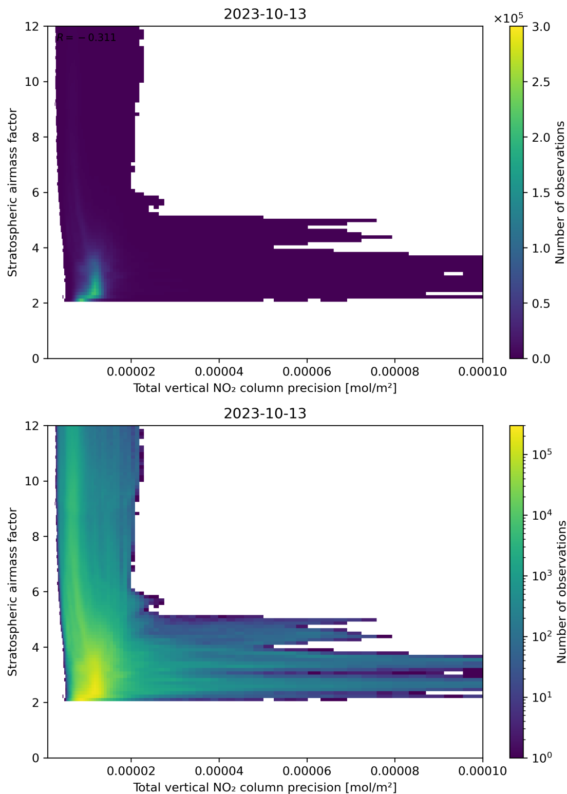
Figure 115: Scatter density plot of “Total vertical NO 2 column precision” against “Stratospheric air mass factor” for 2023-10-12 to 2023-10-14.
