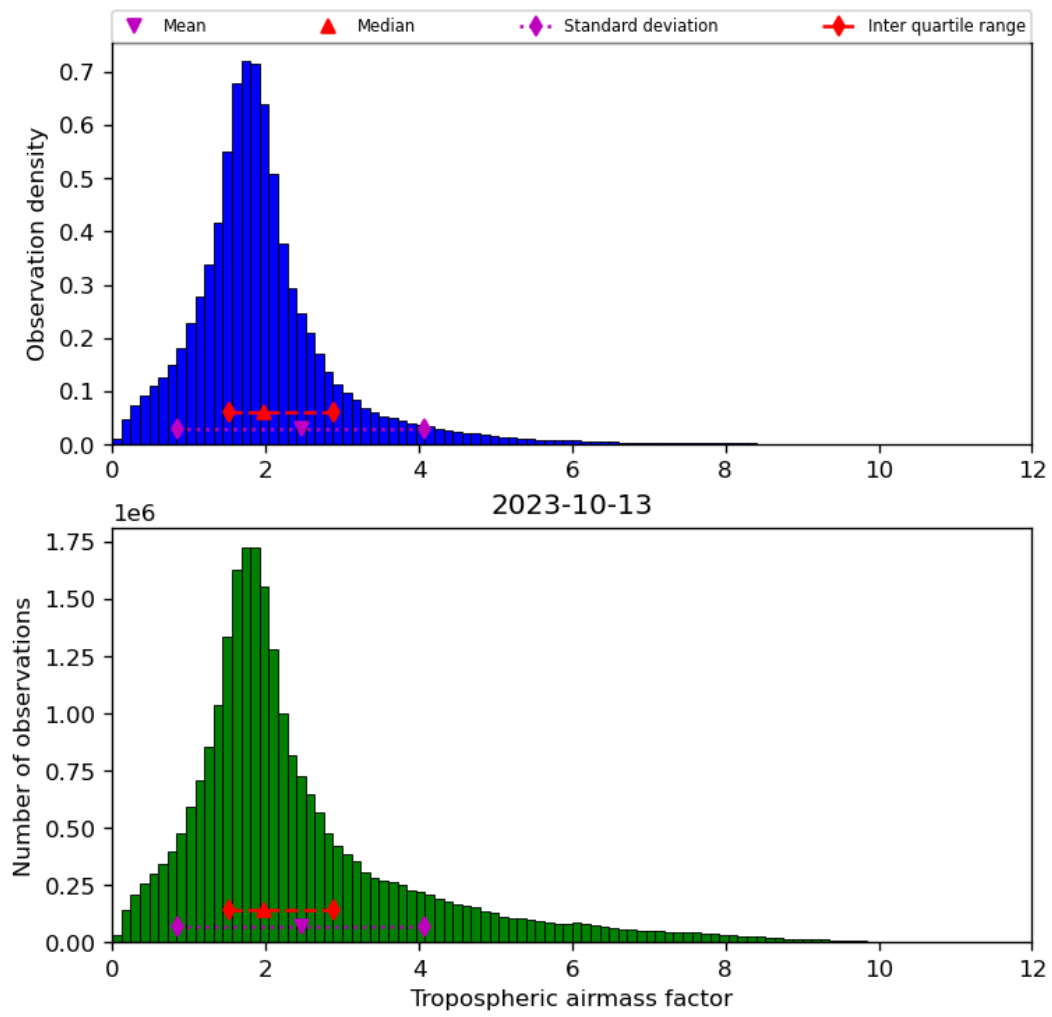
Figure 31: Histogram of “Tropospheric airmass factor” for 2023-10-12 to 2023-10-14
