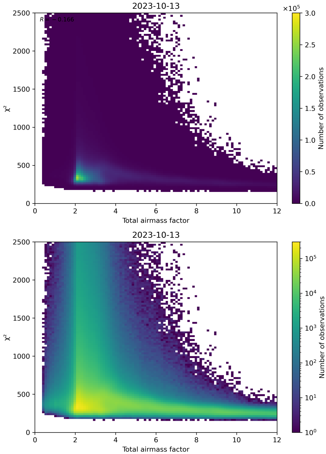
Figure 63: Scatter density plot of “Total airmass factor” against “ \chi^2 ” for 2023-10-12 to 2023-10-14.
