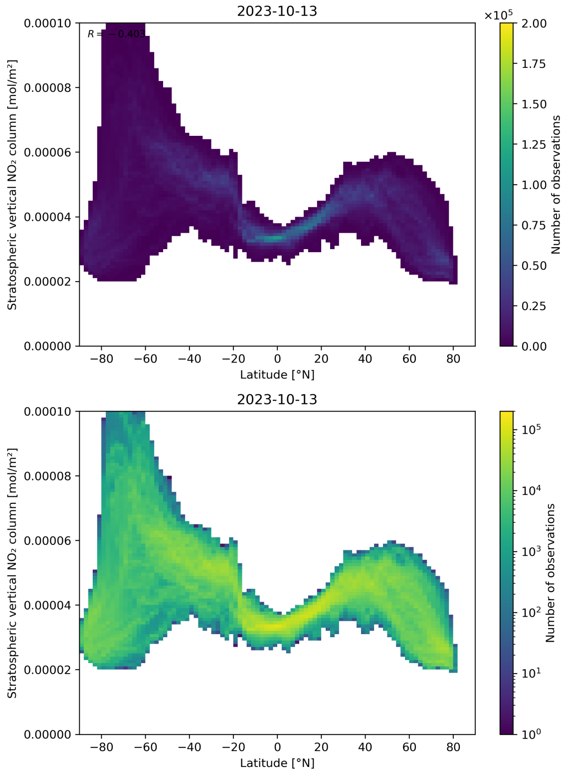
Figure 87: Scatter density plot of “Latitude” against “Stratospheric vertical NO 2 column” for 2023-10-12 to 2023-10-14.
