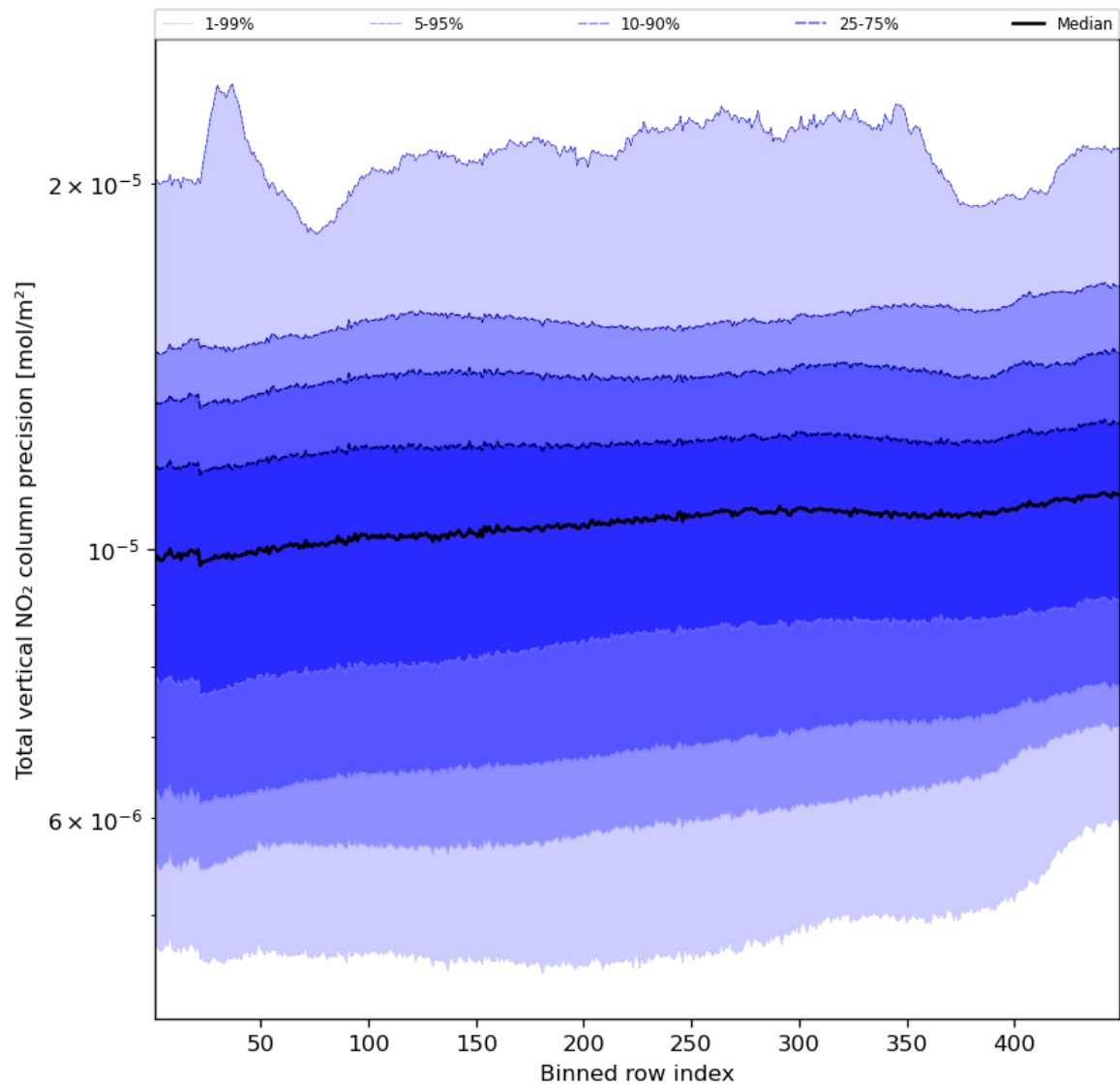
Figure 56: Along track statistics of “Total vertical NO 2 column precision” for 2023-10-12 to 2023-10-14
