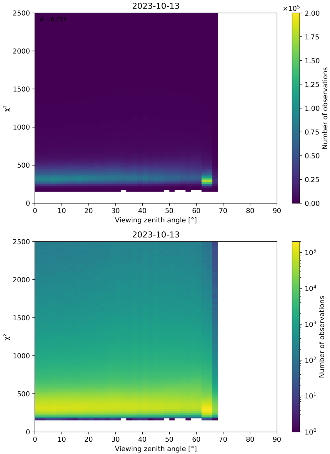
Figure 162: Scatter density plot of “Viewing zenith angle” against “ \chi^2 ” for 2023-10-12 to 2023-10-14.
