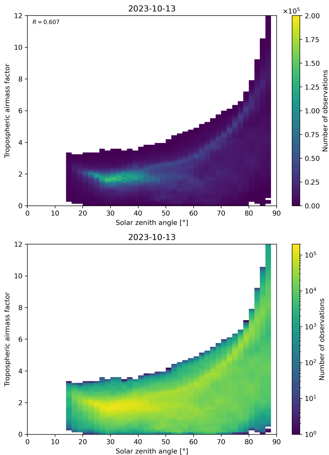
Figure 147: Scatter density plot of “Solar zenith angle” against “Tropospheric airmass factor” for 2023-10-12 to 2023-10-14.
