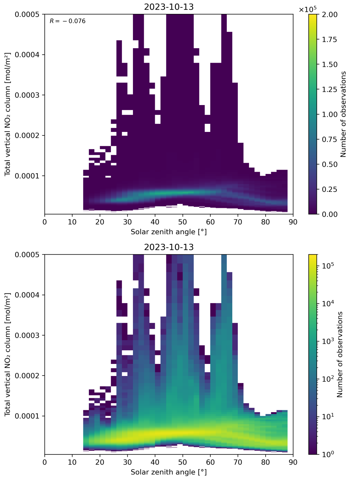
Figure 153: Scatter density plot of “Solar zenith angle” against “Total vertical NO 2 column” for 2023-10-12 to 2023-10-14.
