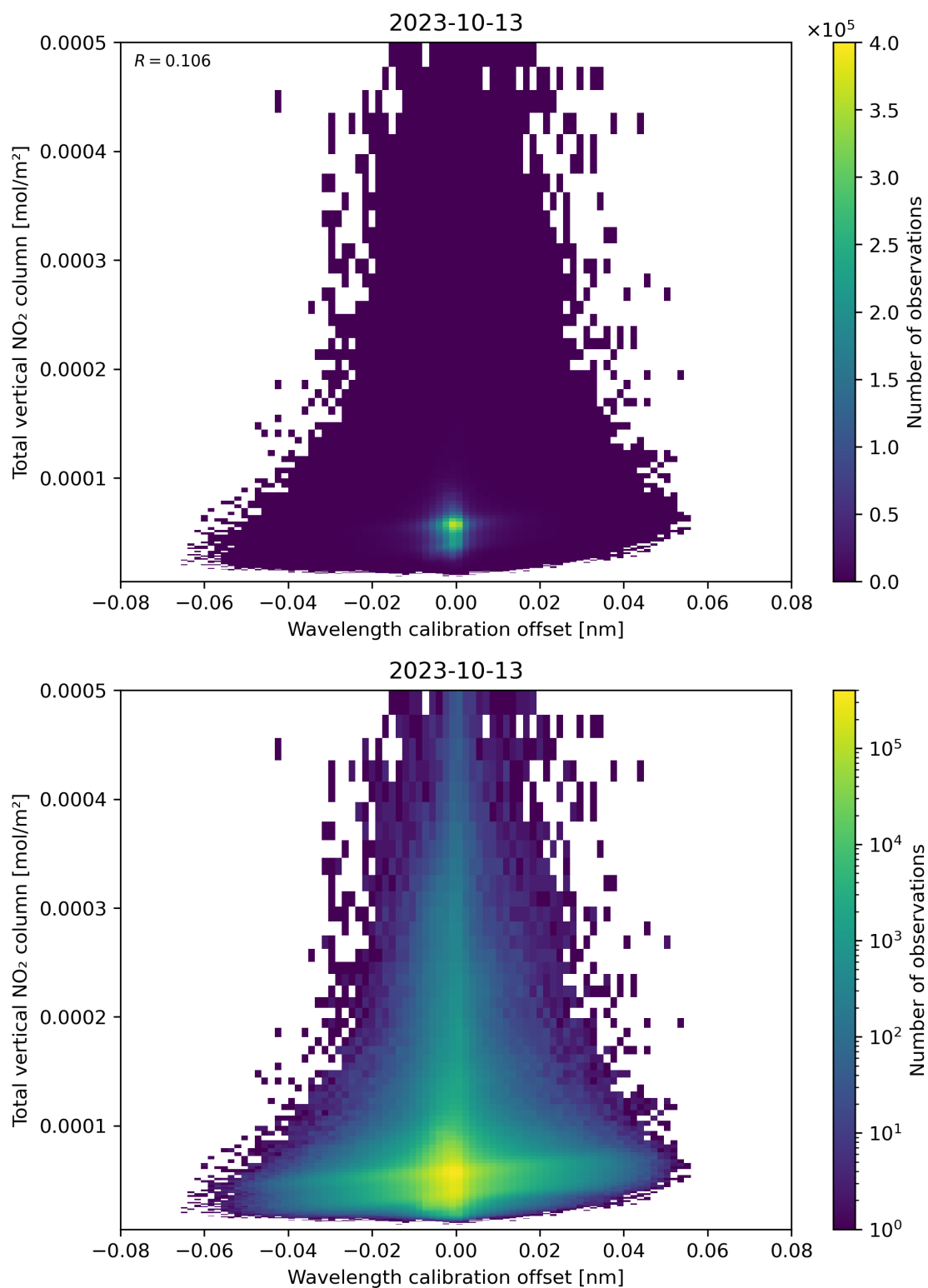
Figure 179: Scatter density plot of “Wavelength calibration offset” against “Total vertical NO 2 column” for 2023-10-12 to 2023-10-14.
