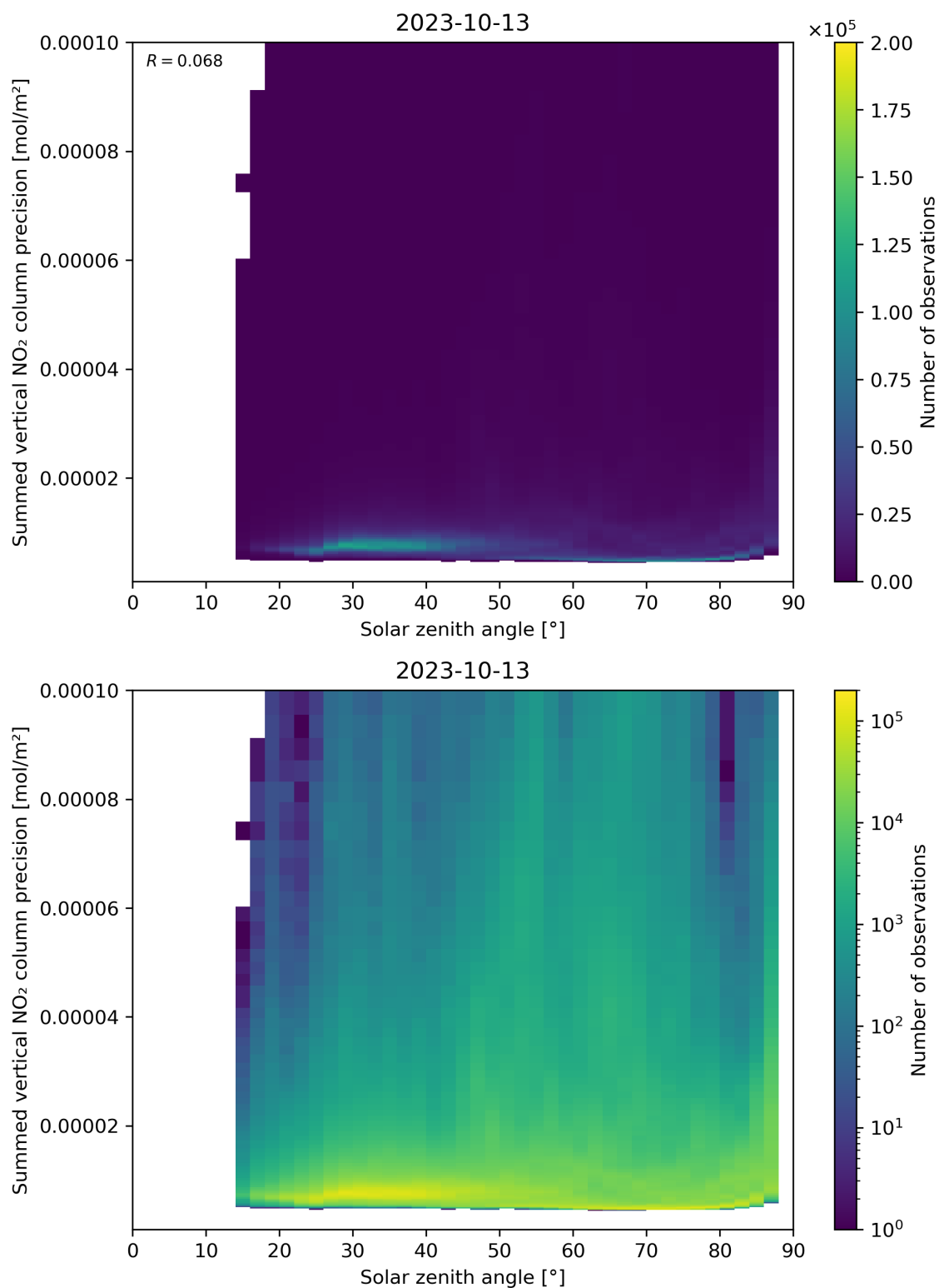
Figure 152: Scatter density plot of “Solar zenith angle” against “Summed vertical NO 2 column precision” for 2023-10-12 to 2023-10-14.
