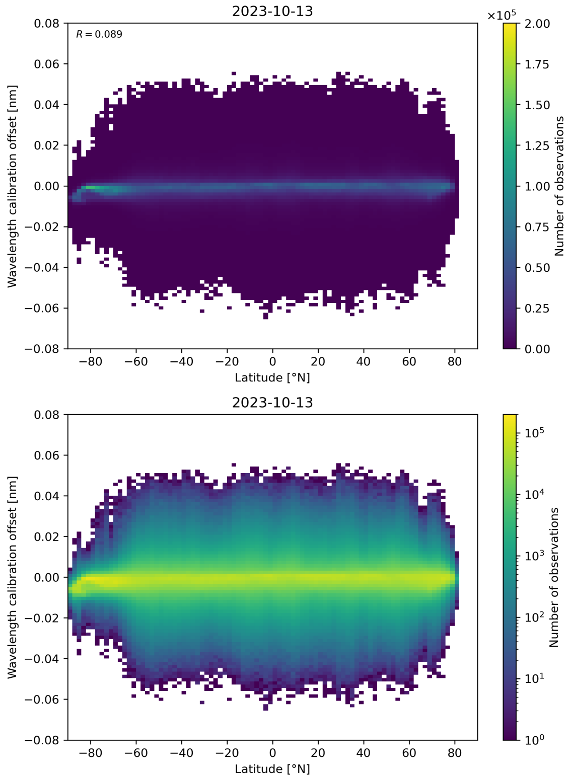
Figure 95: Scatter density plot of “Latitude” against “Wavelength calibration offset” for 2023-10-12 to 2023-10-14.
