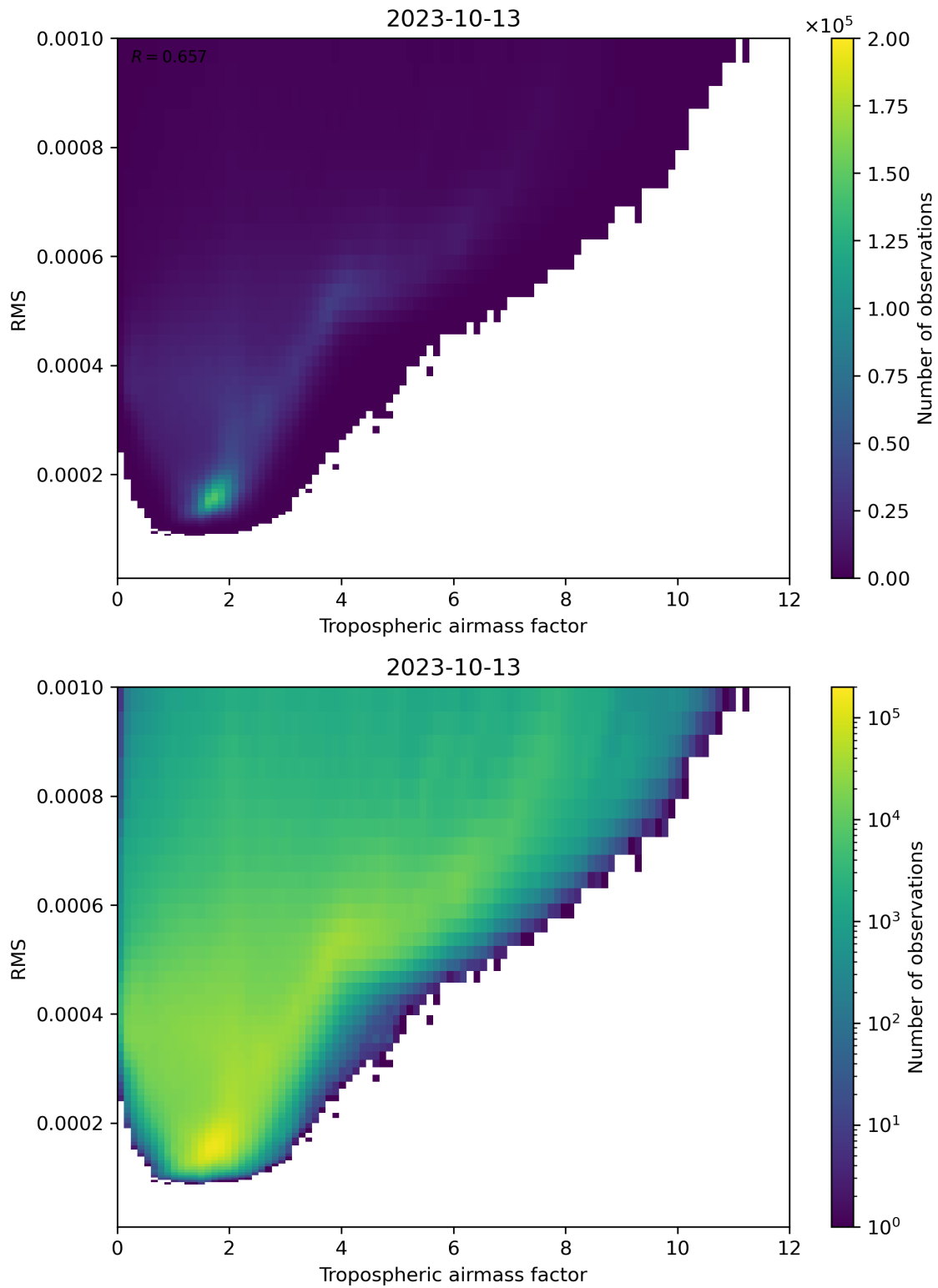
Figure 79: Scatter density plot of “Tropospheric airmass factor” against “RMS” for 2023-10-12 to 2023-10-14.
