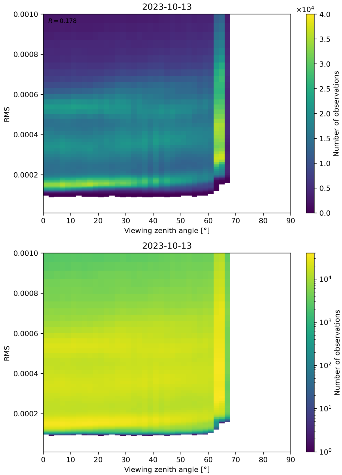
Figure 171: Scatter density plot of “Viewing zenith angle” against “RMS” for 2023-10-12 to 2023-10-14.
