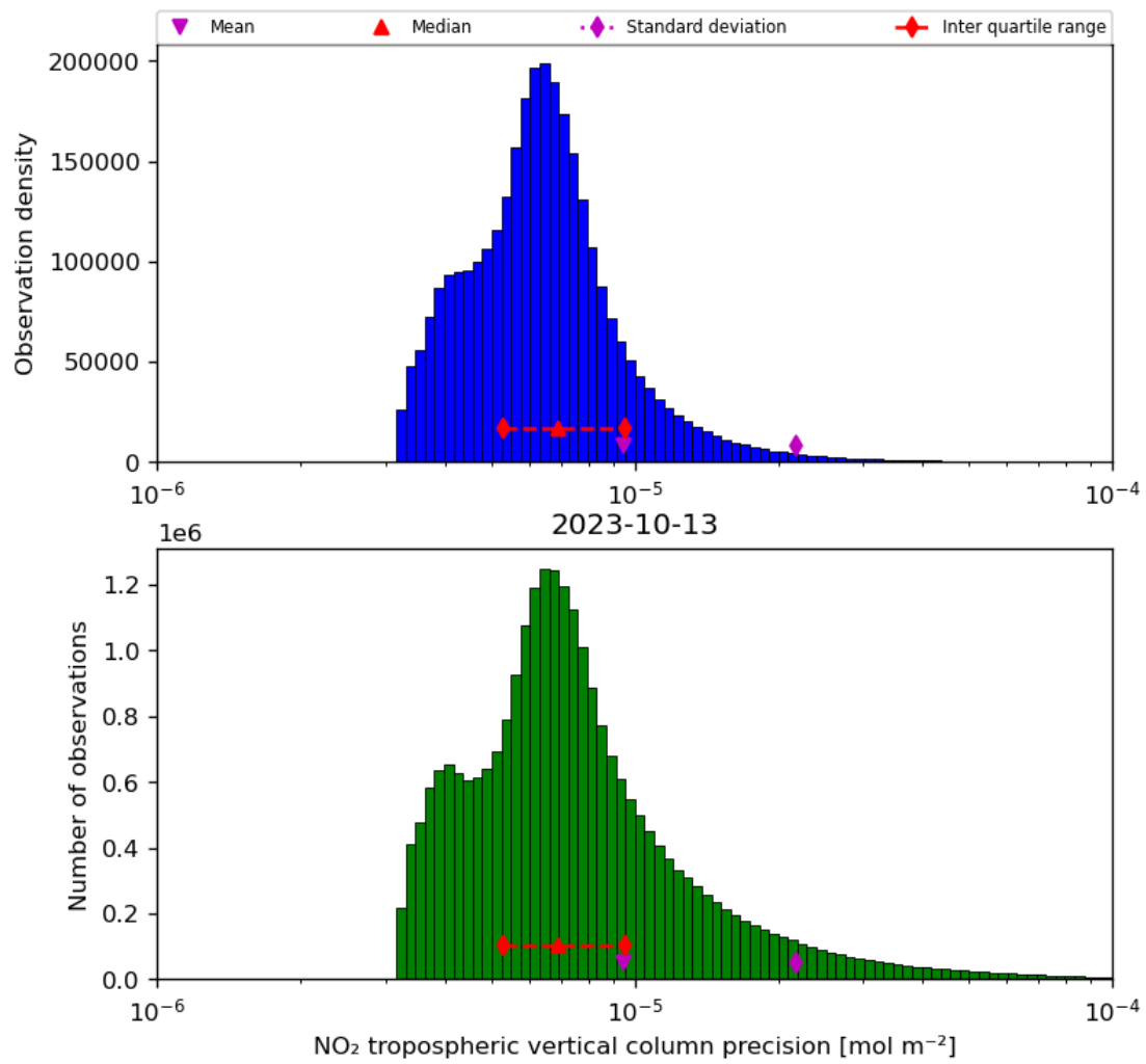
Figure 30: Histogram of “NO 2 tropospheric vertical column precision” for 2023-10-12 to 2023-10-14
