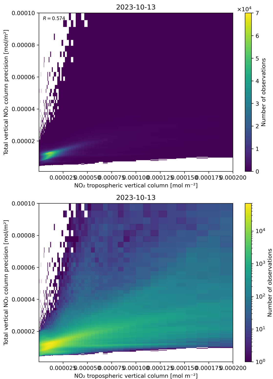
Figure 129: Scatter density plot of “NO 2 tropospheric vertical column” against “Total vertical NO 2 column precision” for 2023-10-12 to 2023-10-14.
