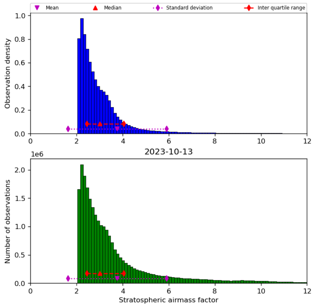
Figure 44: Histogram of “Stratospheric airmass factor” for 2023-10-12 to 2023-10-14
