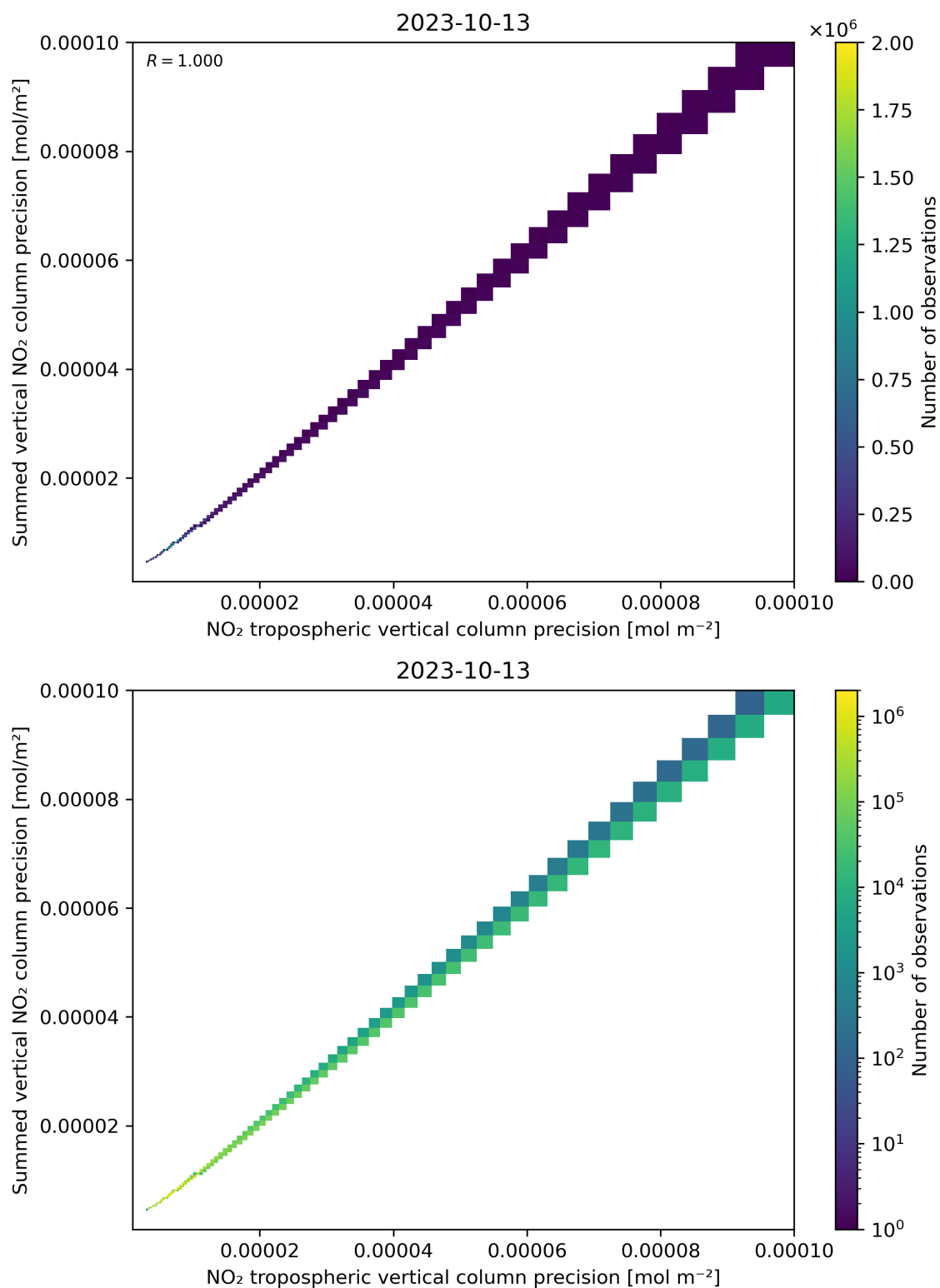
Figure 137: Scatter density plot of “NO 2 tropospheric vertical column precision” against “Summed vertical NO 2 column precision” for 2023-10-12 to 2023-10-14.
