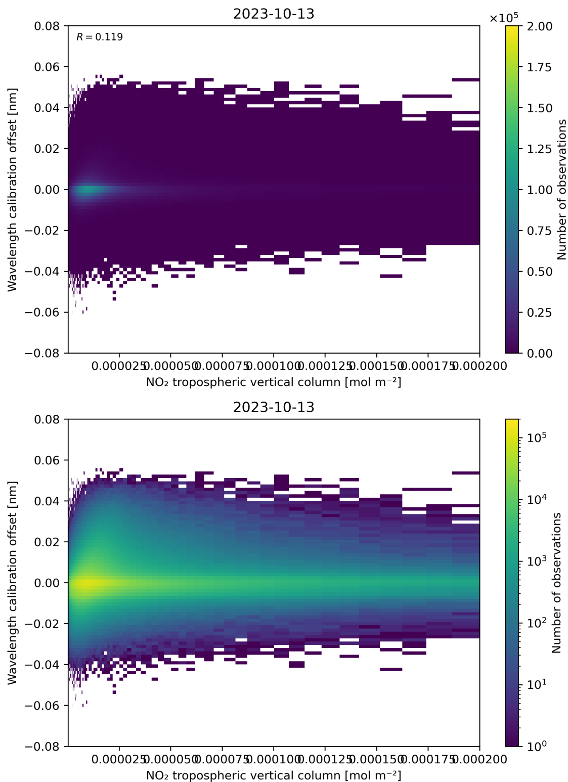
Figure 143: Scatter density plot of “NO 2 tropospheric vertical column” against “Wavelength calibration offset” for 2023-10-12 to 2023-10-14.
