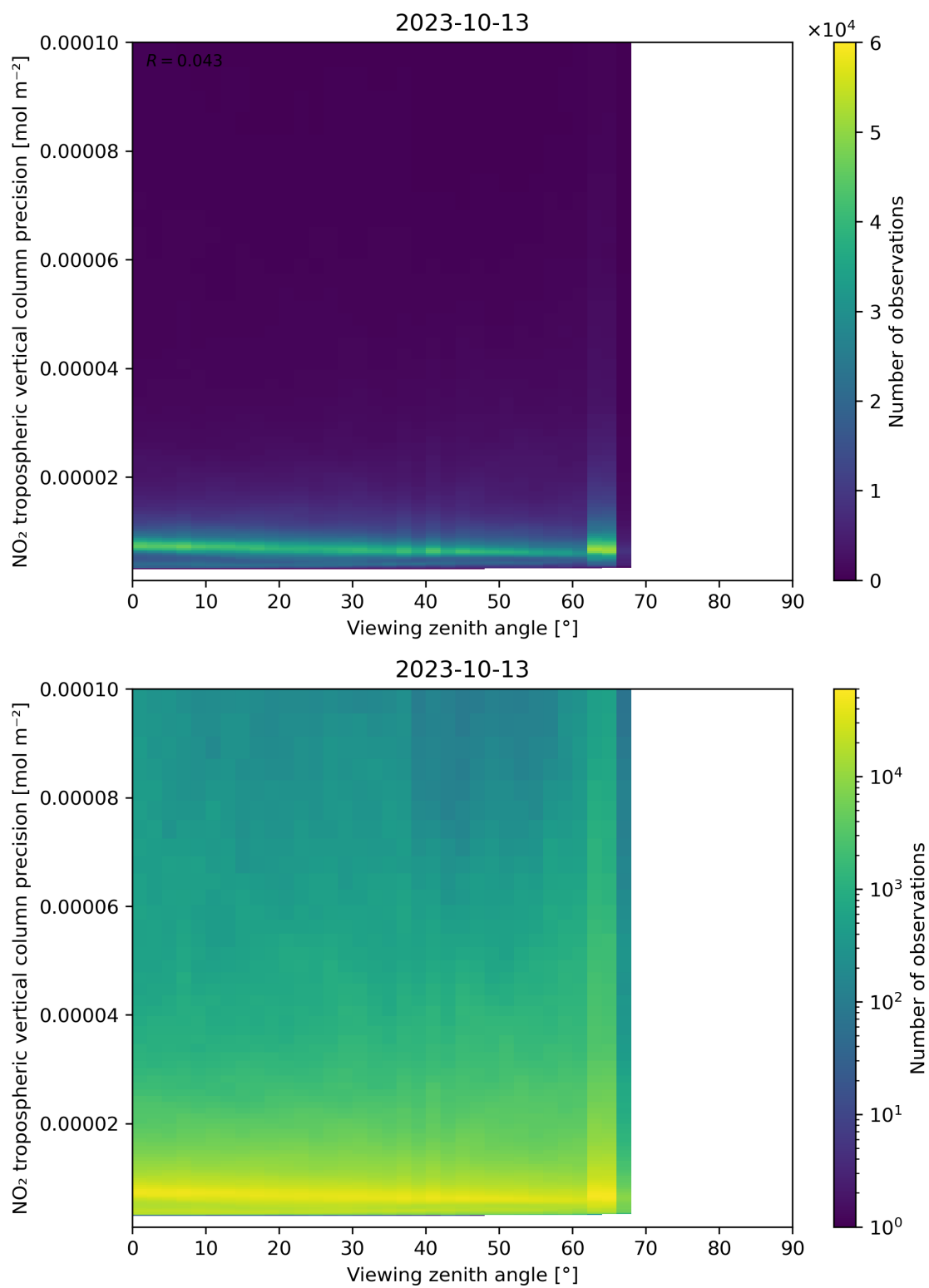
Figure 170: Scatter density plot of “Viewing zenith angle” against “NO 2 tropospheric vertical column precision” for 2023-10-12 to 2023-10-14.
