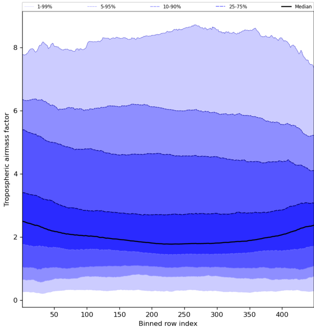
Figure 48: Along track statistics of “Tropospheric airmass factor” for 2023-10-12 to 2023-10-14
