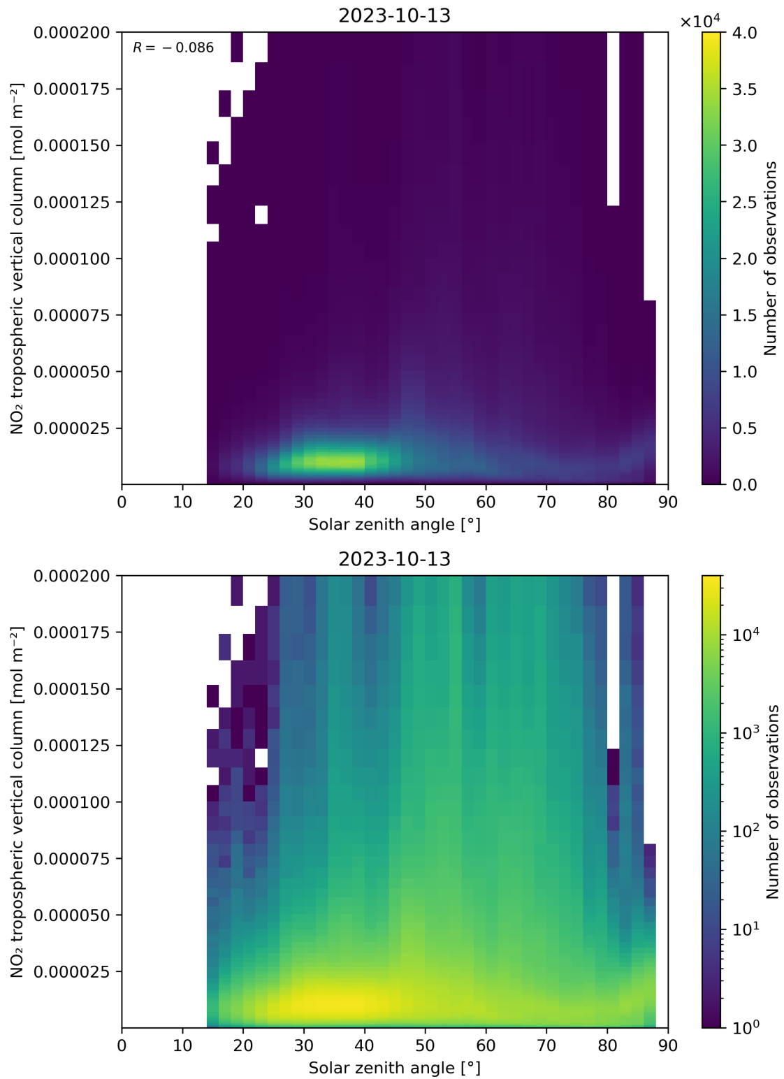
Figure 155: Scatter density plot of “Solar zenith angle” against “NO 2 tropospheric vertical column” for 2023-10-12 to 2023-10-14.
