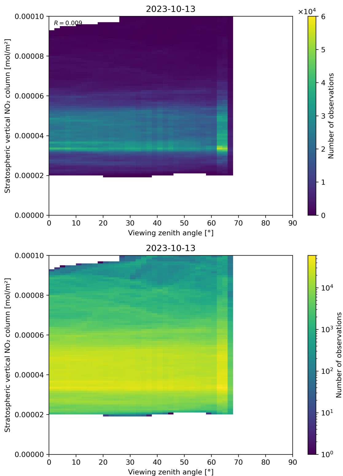
Figure 164: Scatter density plot of “Viewing zenith angle” against “Stratospheric vertical NO 2 column” for 2023-10-12 to 2023-10-14.
