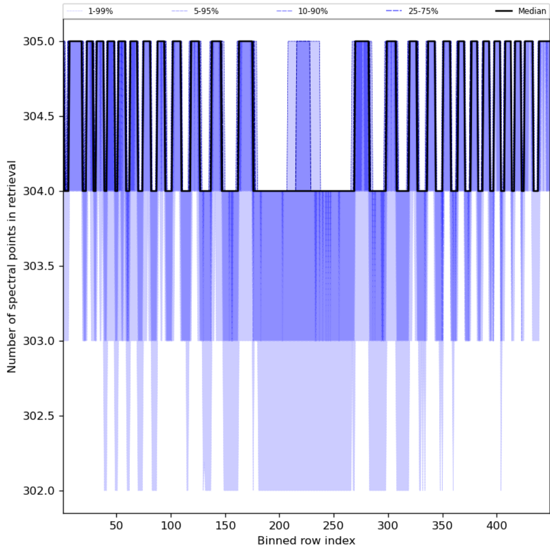
Figure 50: Along track statistics of “Number of spectral points in retrieval” for 2023-10-12 to 2023-10-14
