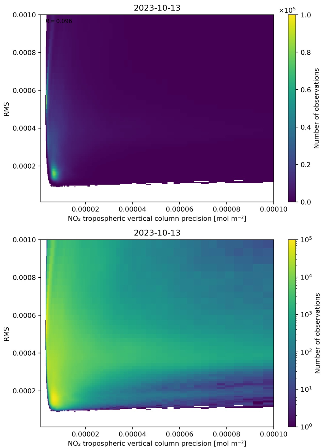
Figure 140: Scatter density plot of “NO 2 tropospheric vertical column precision” against “RMS” for 2023-10-12 to 2023-10-14.
