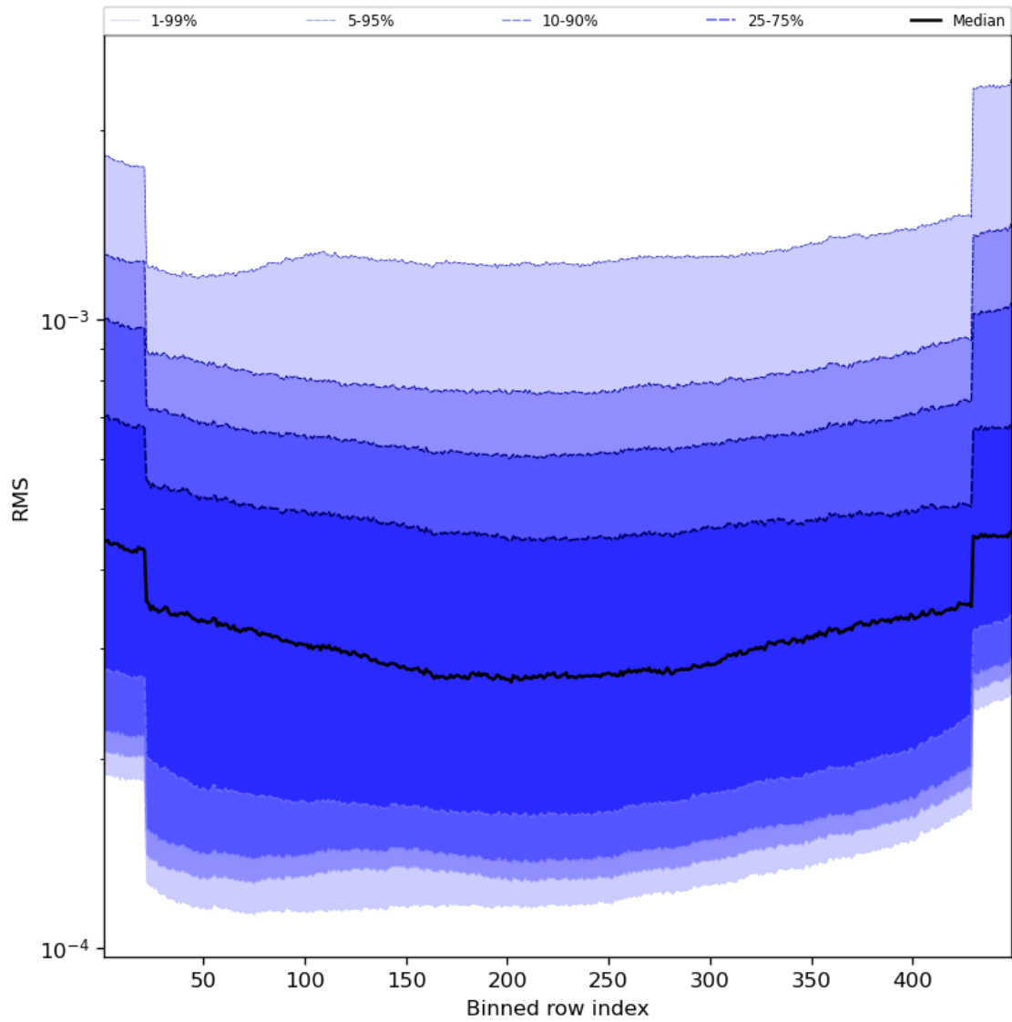
Figure 60: Along track statistics of “RMS” for 2023-10-12 to 2023-10-14
