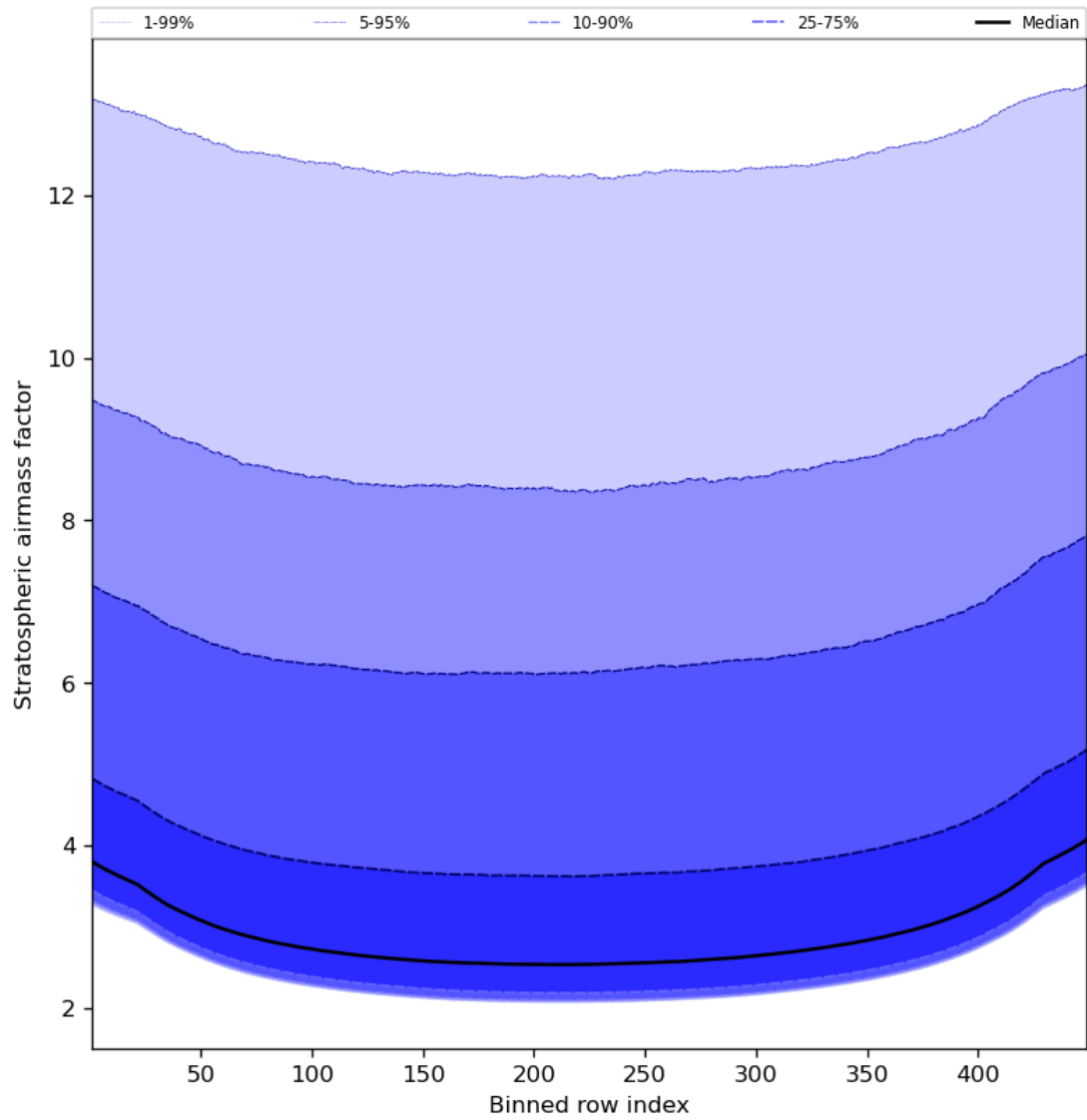
Figure 61: Along track statistics of “Stratospheric airmass factor” for 2023-10-12 to 2023-10-14
