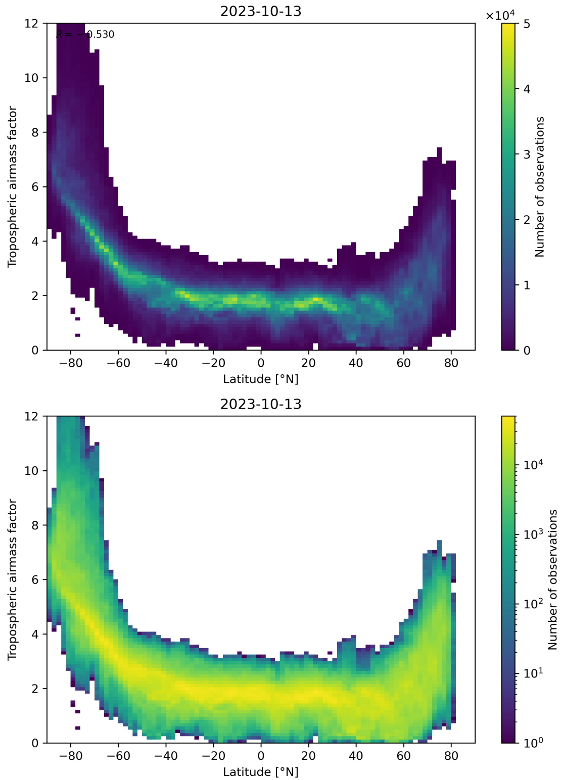
Figure 85: Scatter density plot of “Latitude” against “Tropospheric airmass factor” for 2023-10-12 to 2023-10-14.
