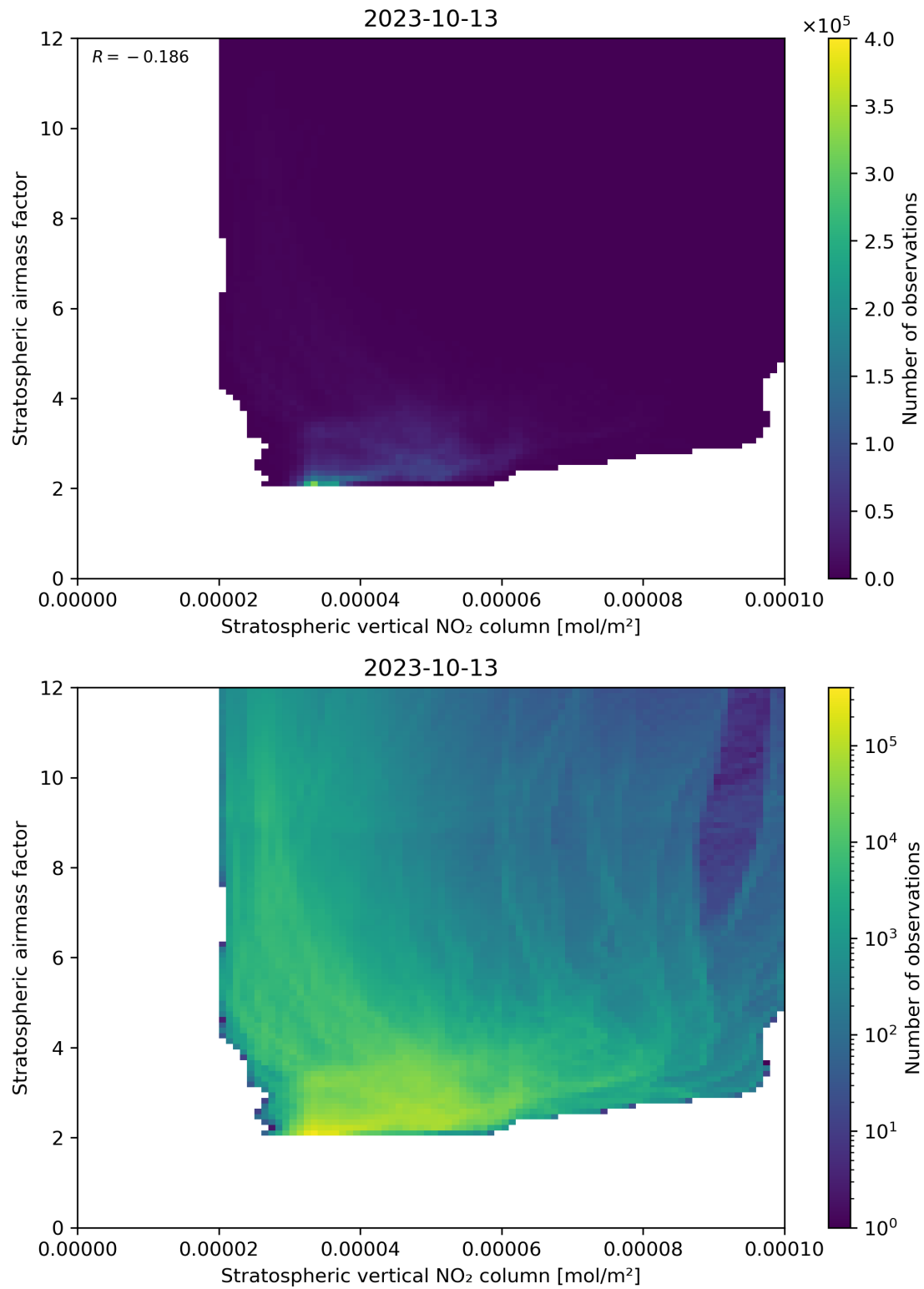
Figure 96: Scatter density plot of “Stratospheric vertical NO 2 column” against “Stratospheric airmass factor” for 2023-10-12 to 2023-10-14.
