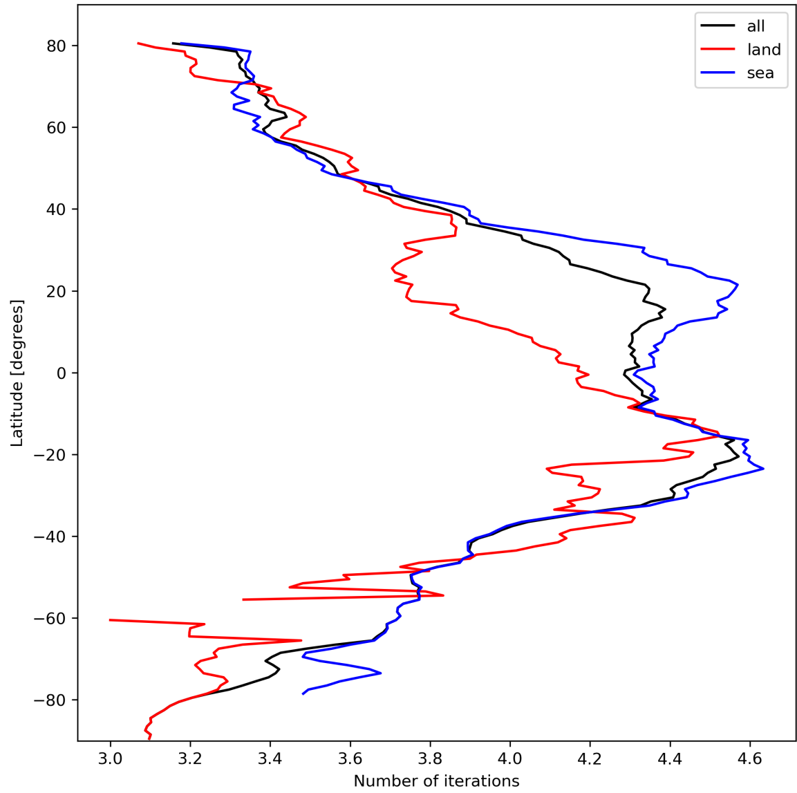
Figure 17: Zonal average of “Number of iterations” for 2023-10-12 to 2023-10-14.
