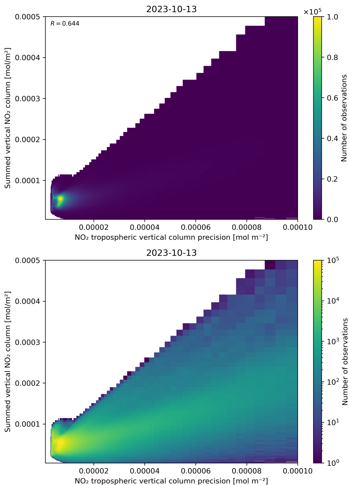
Figure 136: Scatter density plot of “NO 2 tropospheric vertical column precision” against “Summed vertical NO 2 column” for 2023-10-12 to 2023-10-14.
