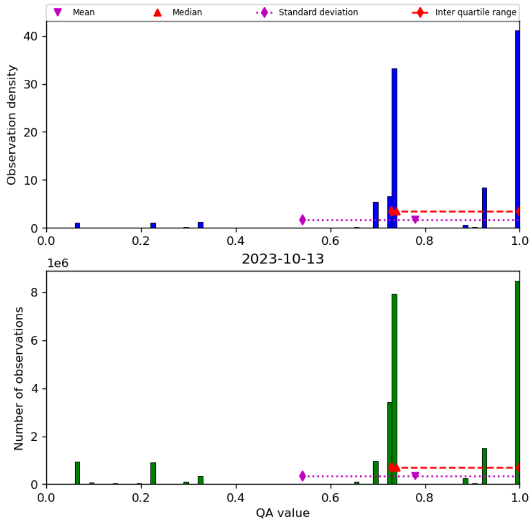
Figure 28: Histogram of “QA value” for 2023-10-12 to 2023-10-14
