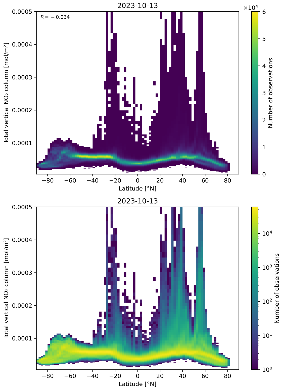
Figure 90: Scatter density plot of “Latitude” against “Total vertical NO 2 column” for 2023-10-12 to 2023-10-14.
