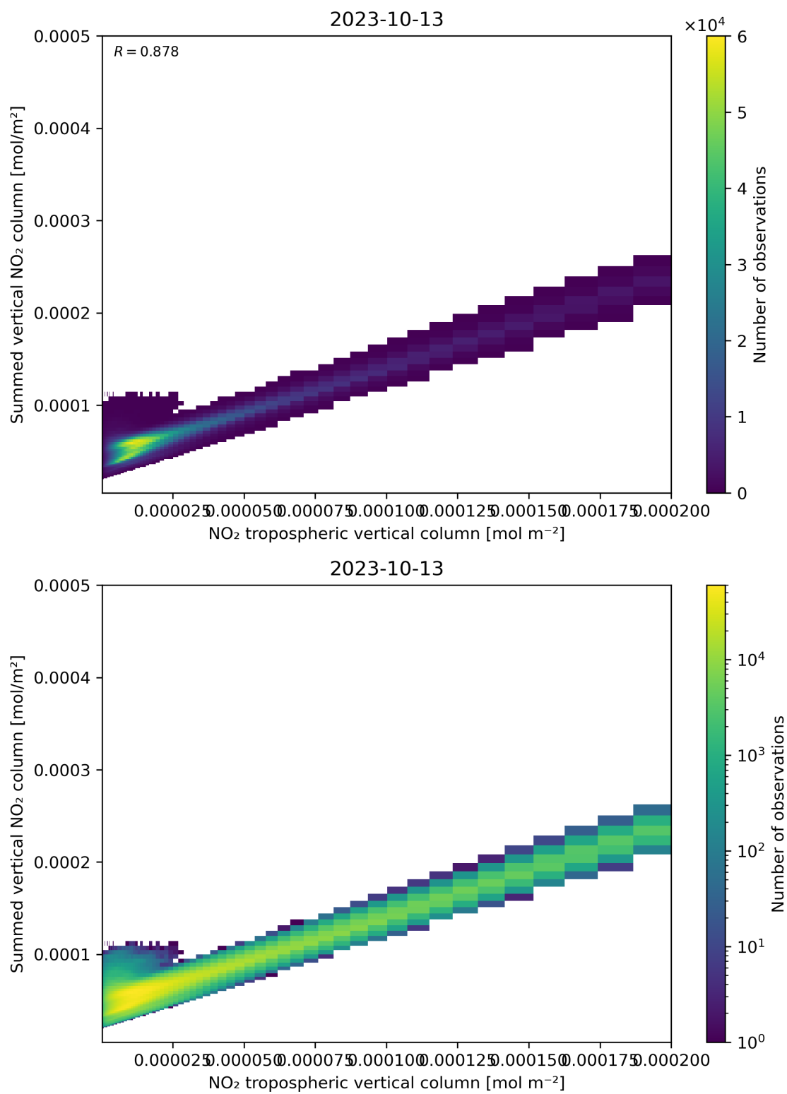
Figure 126: Scatter density plot of “NO 2 tropospheric vertical column” against “Summed vertical NO 2 column” for 2023-10-12 to 2023-10-14.
