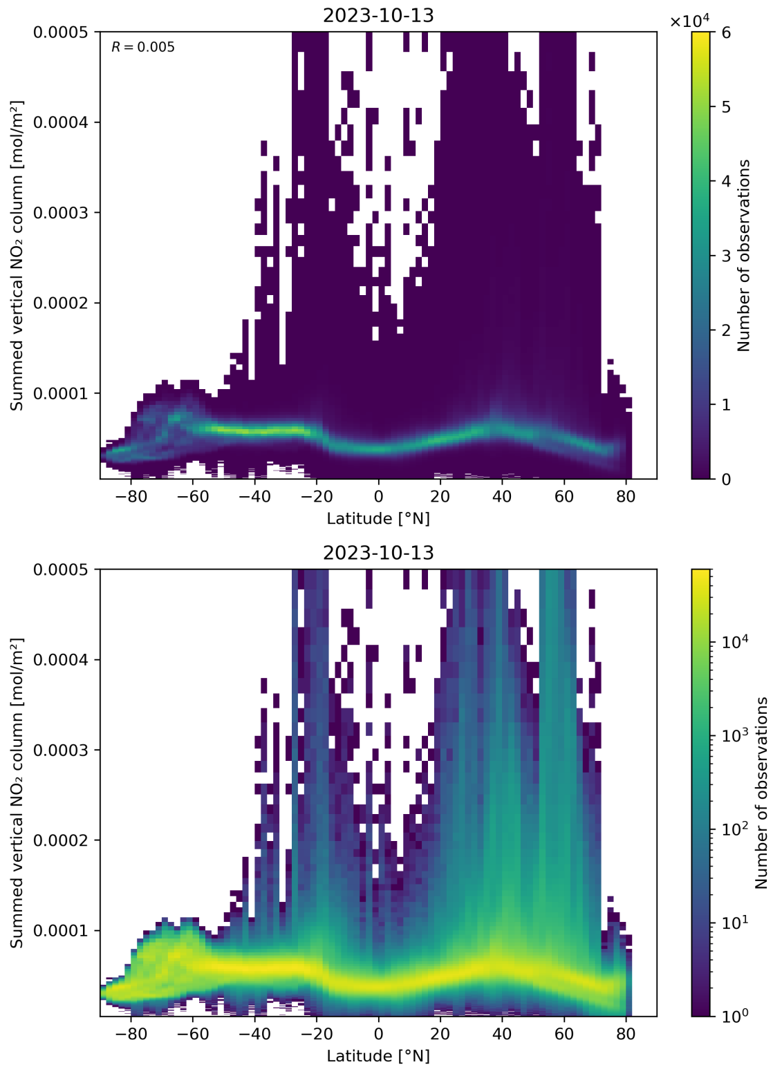
Figure 88: Scatter density plot of “Latitude” against “Summed vertical NO 2 column” for 2023-10-12 to 2023-10-14.
