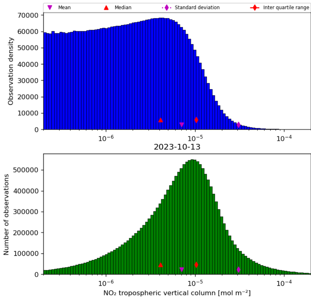
Figure 29: Histogram of “NO 2 tropospheric vertical column” for 2023-10-12 to 2023-10-14
