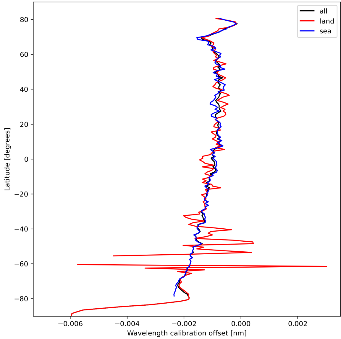
Figure 18: Zonal average of “Wavelength calibration offset” for 2023-10-12 to 2023-10-14.
