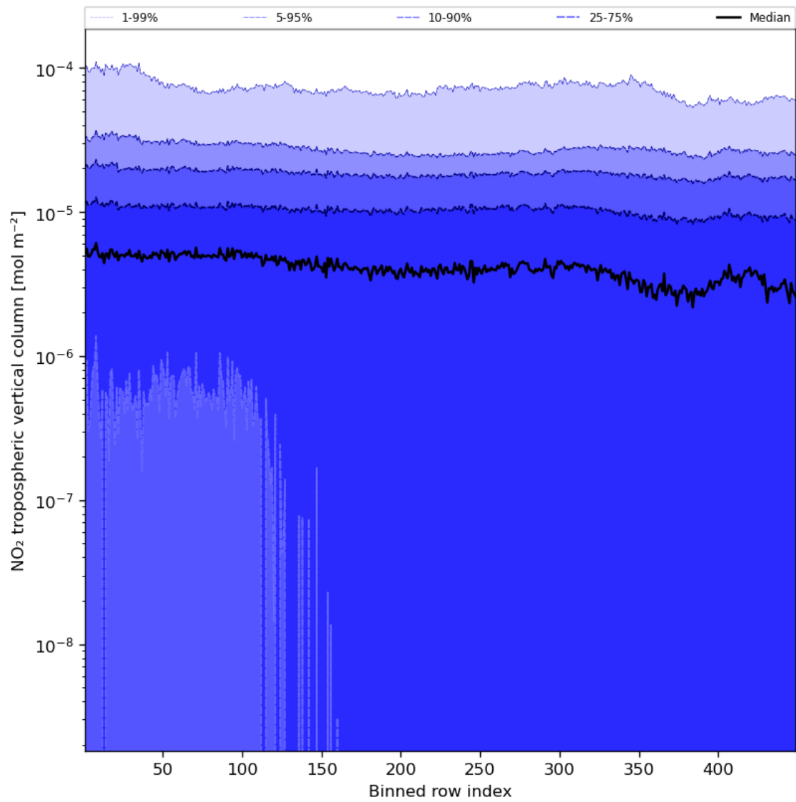
Figure 46: Along track statistics of “NO 2 tropospheric vertical column” for 2023-10-12 to 2023-10-14
