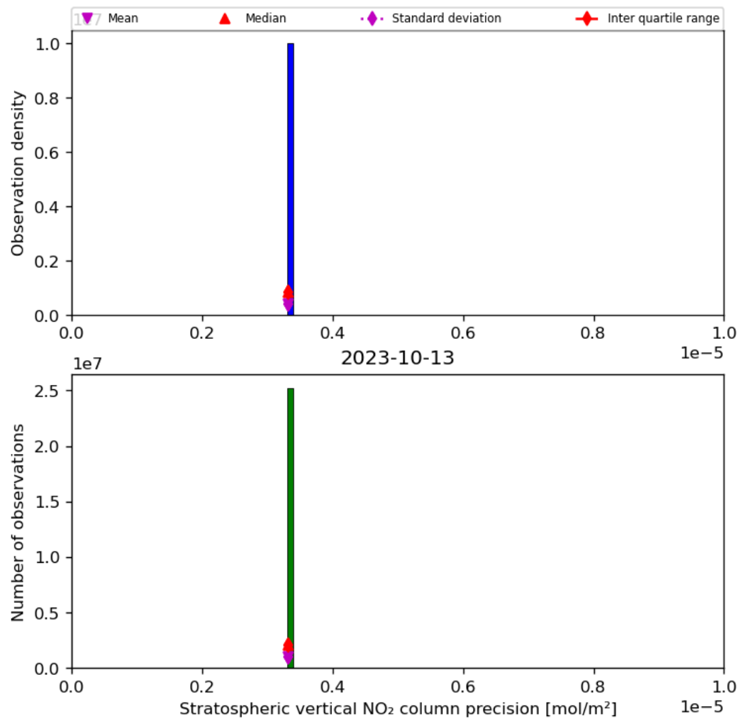
Figure 37: Histogram of “Stratospheric vertical NO 2 column precision” for 2023-10-12 to 2023-10-14
