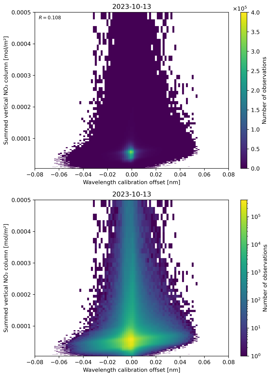
Figure 177: Scatter density plot of “Wavelength calibration offset” against “Summed vertical NO 2 column” for 2023-10-12 to 2023-10-14.
