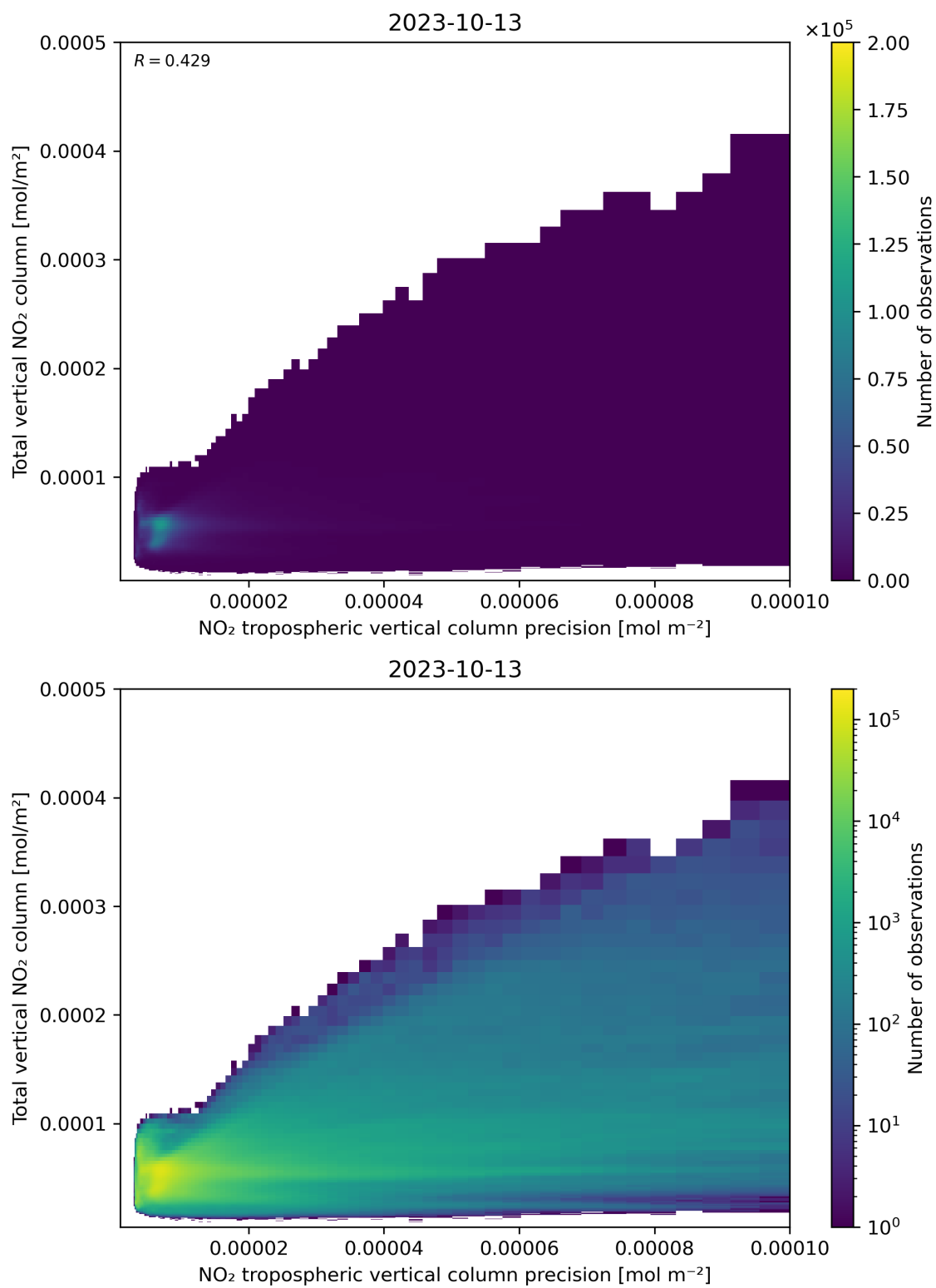
Figure 138: Scatter density plot of “NO 2 tropospheric vertical column precision” against “Total vertical NO 2 column” for 2023-10-12 to 2023-10-14.
