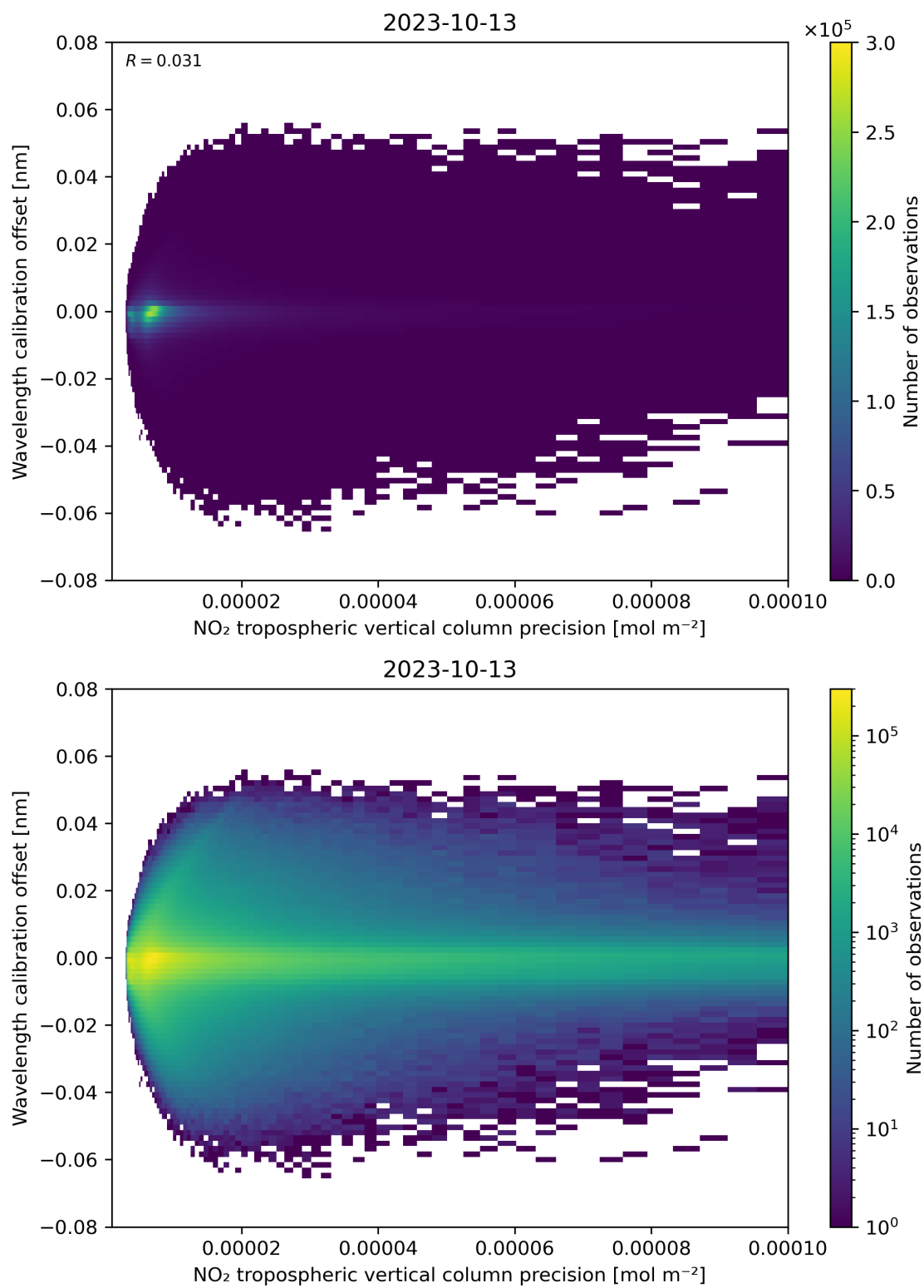
Figure 141: Scatter density plot of “NO 2 tropospheric vertical column precision” against “Wavelength calibration offset” for 2023-10-12 to 2023-10-14.
