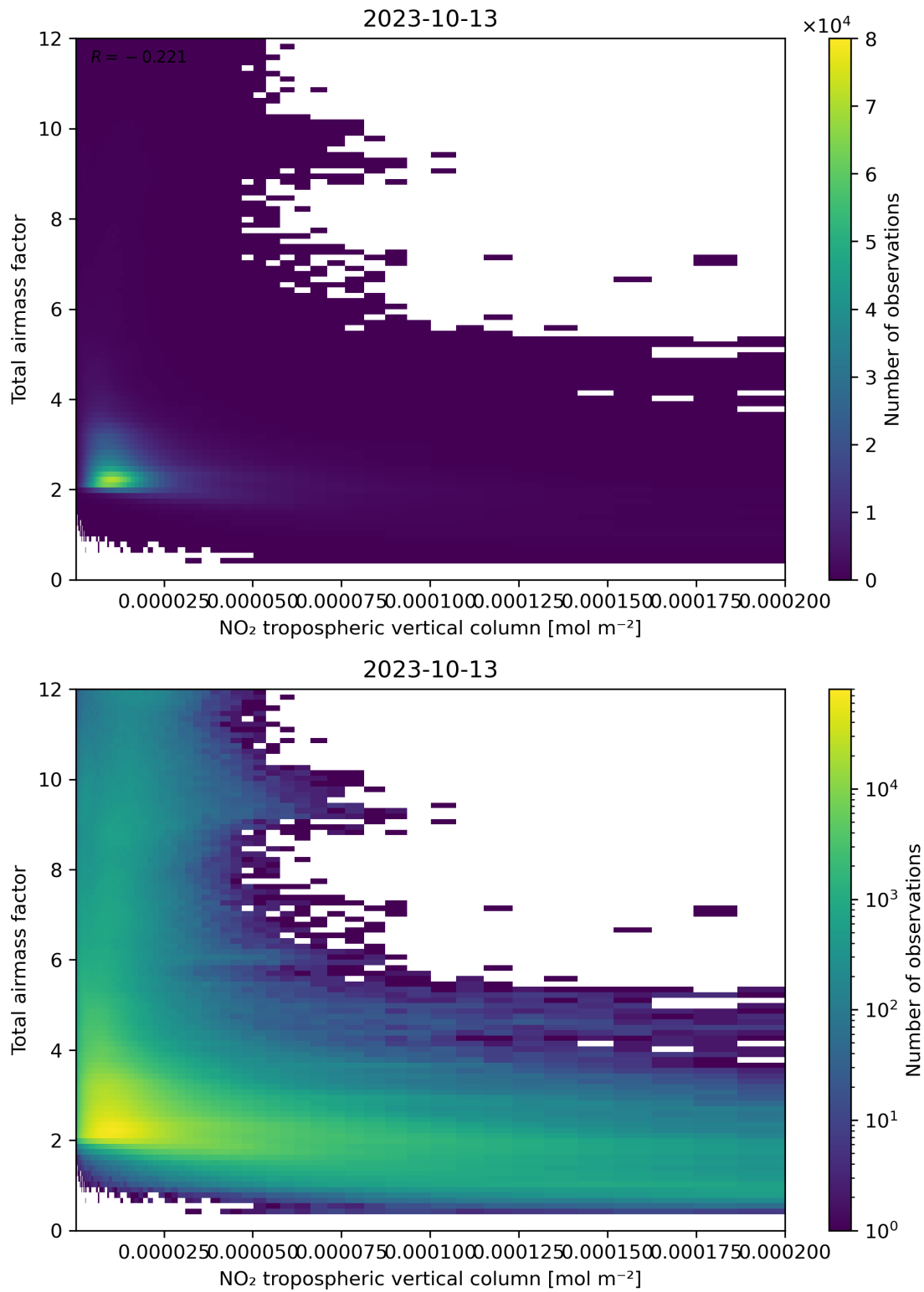
Figure 122: Scatter density plot of “NO 2 tropospheric vertical column” against “Total air mass factor” for 2023-10-12 to 2023-10-14.
