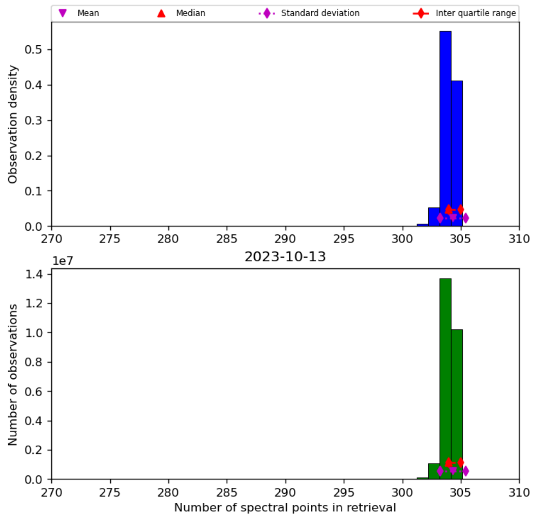
Figure 33: Histogram of “Number of spectral points in retrieval” for 2023-10-12 to 2023-10-14
