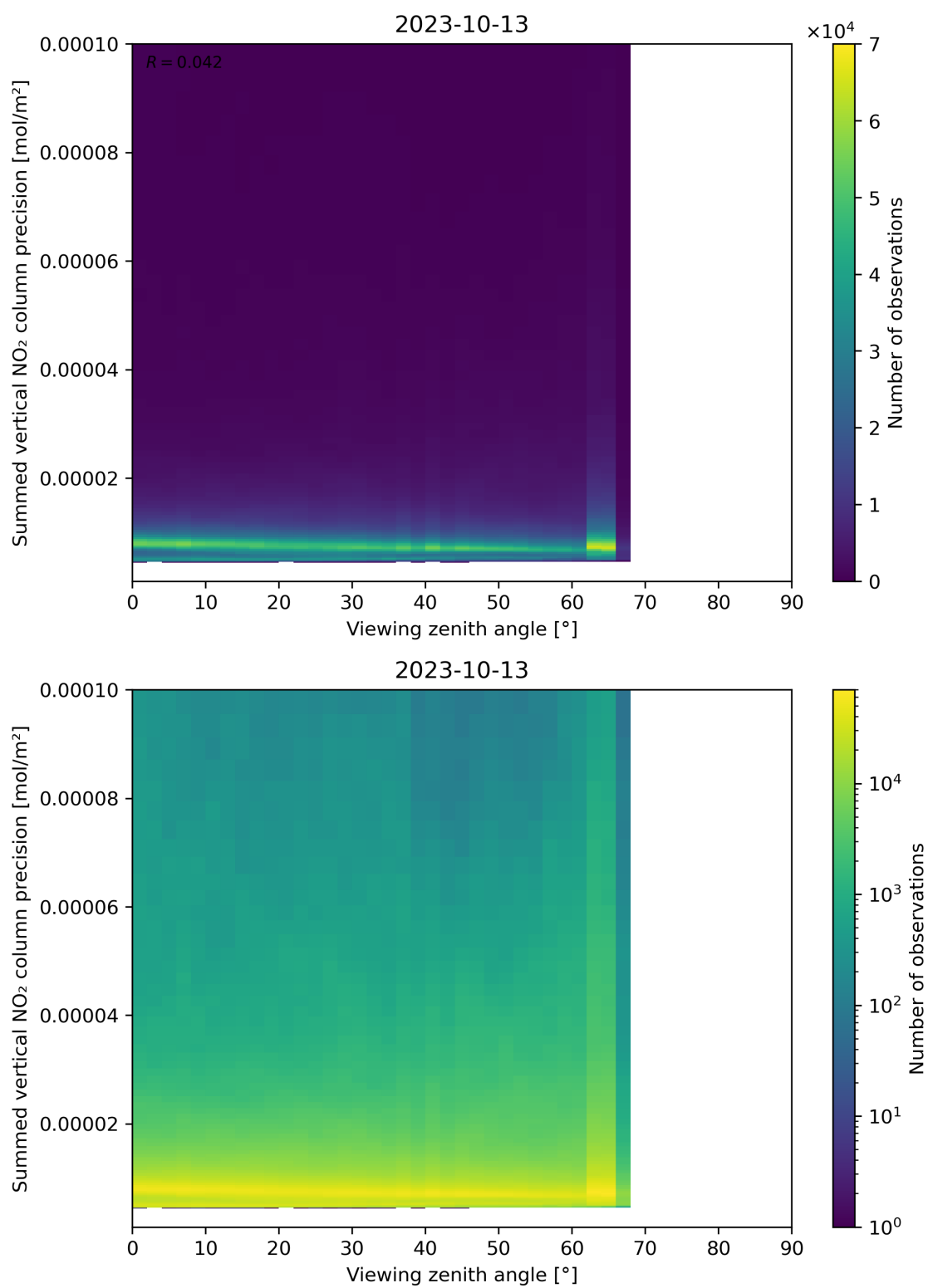
Figure 166: Scatter density plot of “Viewing zenith angle” against “Summed vertical NO 2 column precision” for 2023-10-12 to 2023-10-14.
