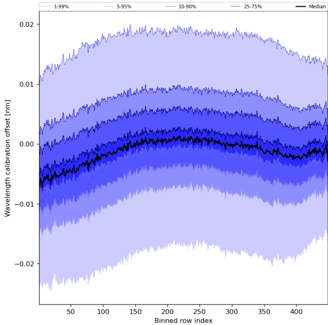
Figure 52: Along track statistics of “Wavelength calibration offset” for 2023-10-12 to 2023-10-14
