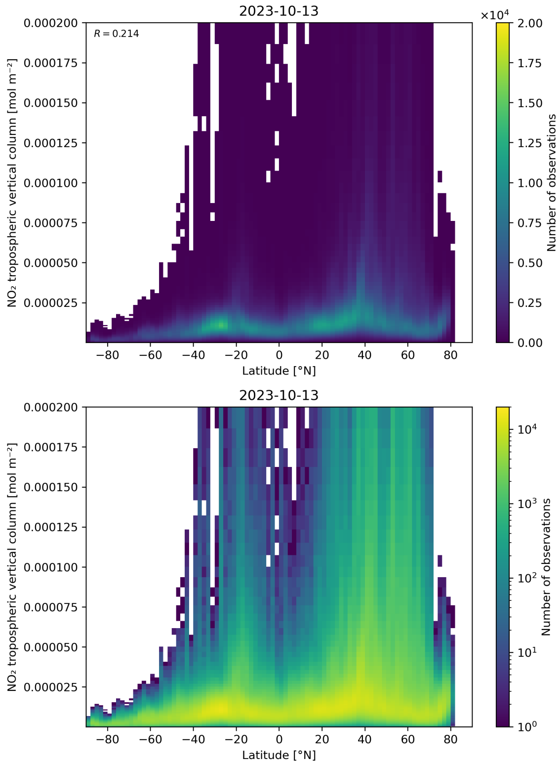
Figure 92: Scatter density plot of “Latitude” against “NO 2 tropospheric vertical column” for 2023-10-12 to 2023-10-14.
