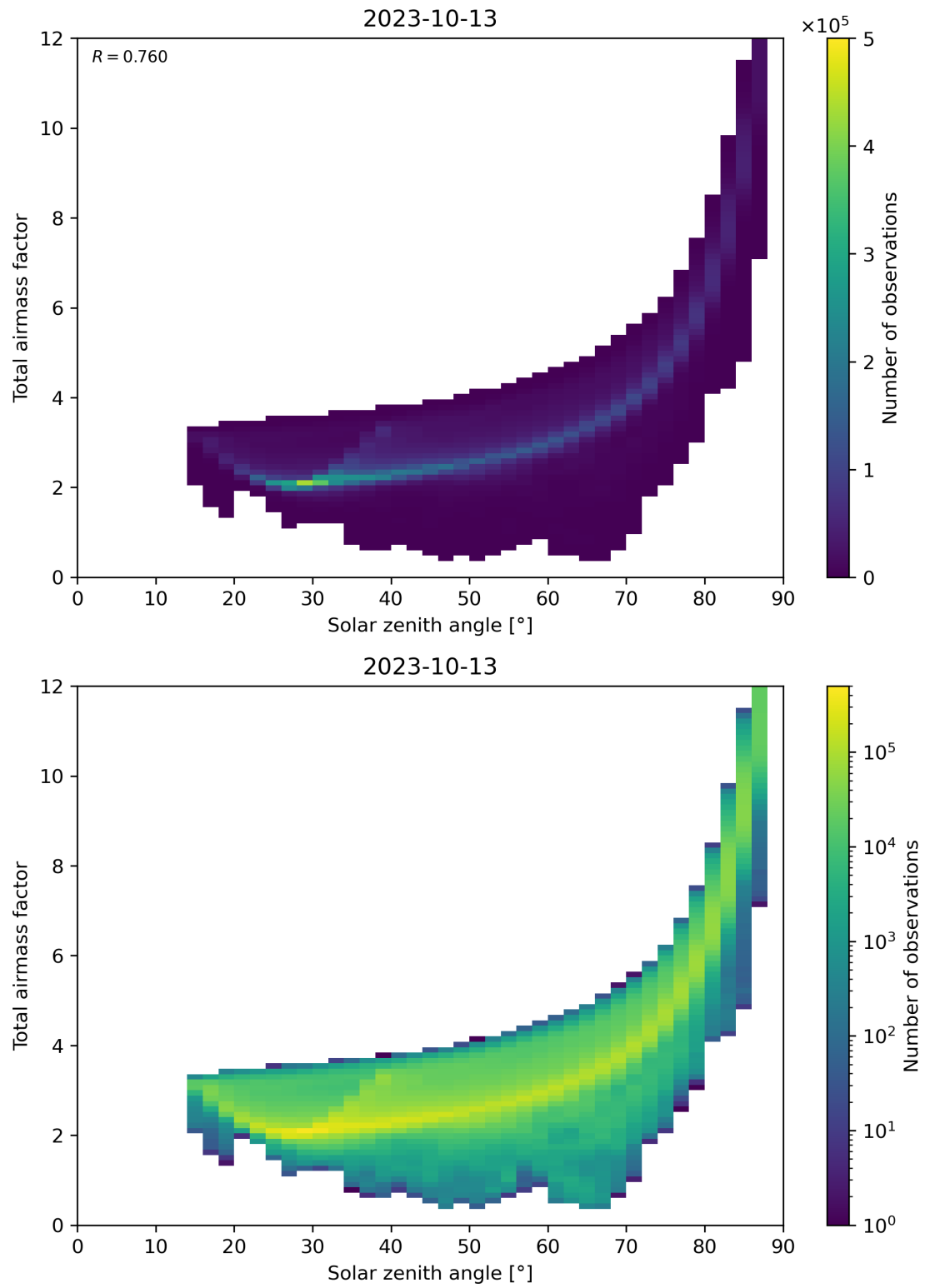
Figure 146: Scatter density plot of “Solar zenith angle” against “Total air mass factor” for 2023-10-12 to 2023-10-14.
