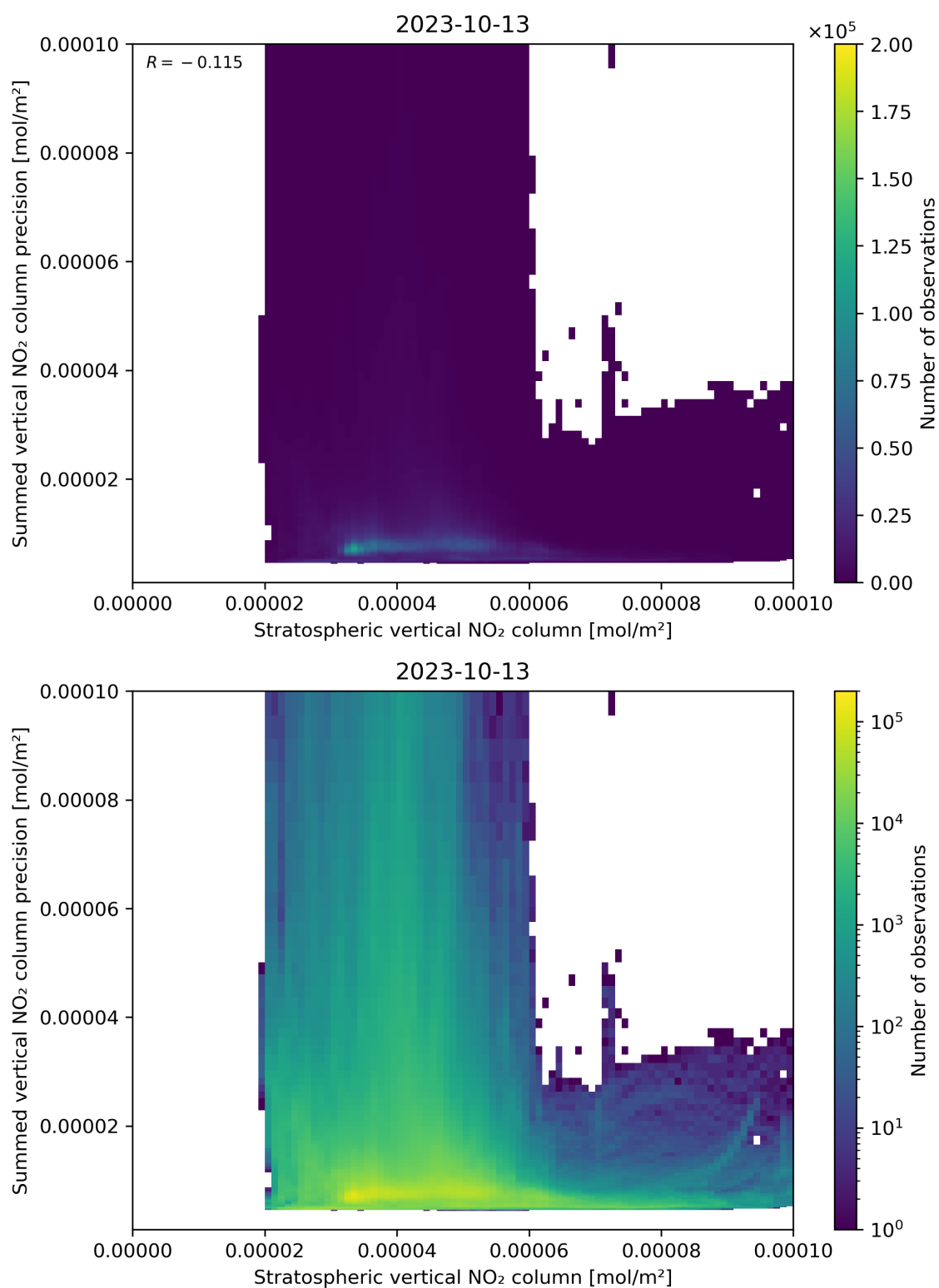
Figure 99: Scatter density plot of “Stratospheric vertical NO 2 column” against “Summed vertical NO 2 column precision” for 2023-10-12 to 2023-10-14.
