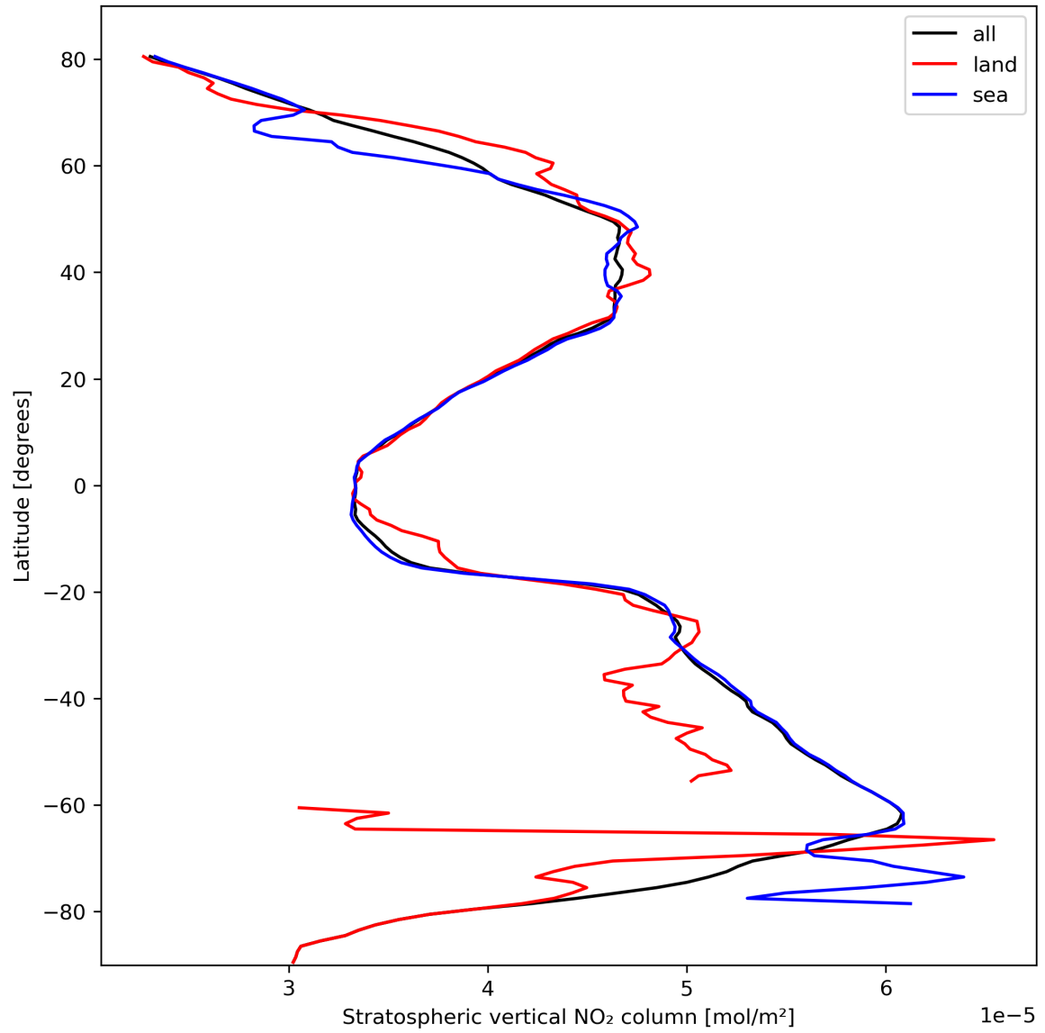
Figure 19: Zonal average of “Stratospheric vertical NO 2 column” for 2023-10-12 to 2023-10-14.
