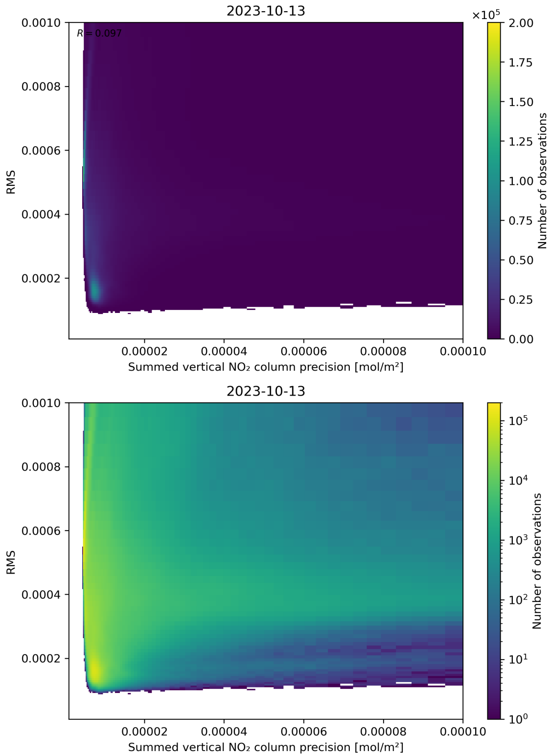
Figure 108: Scatter density plot of “Summed vertical NO 2 column precision” against “RMS” for 2023-10-12 to 2023-10-14.
