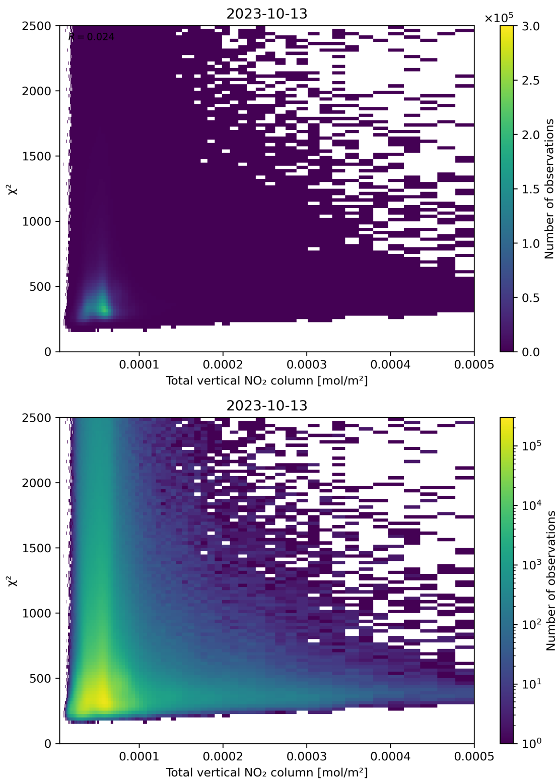
Figure 111: Scatter density plot of “Total vertical NO 2 column” against “ \chi^2 ” for 2023-10-12 to 2023-10-14.
