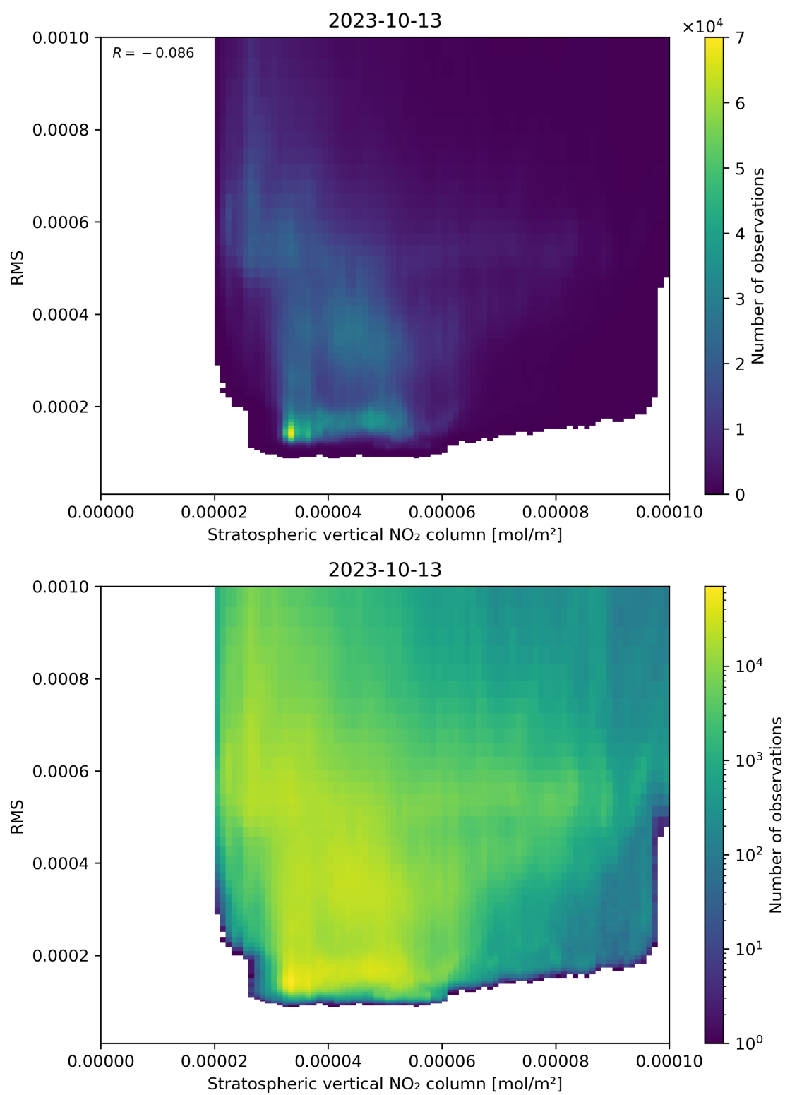
Figure 102: Scatter density plot of “Stratospheric vertical NO 2 column” against “RMS” for 2023-10-12 to 2023-10-14.
