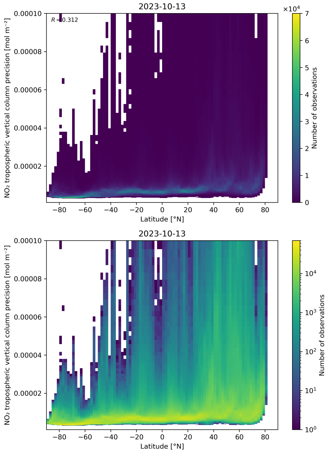
Figure 93: Scatter density plot of “Latitude” against “NO 2 tropospheric vertical column precision” for 2023-10-12 to 2023-10-14.
