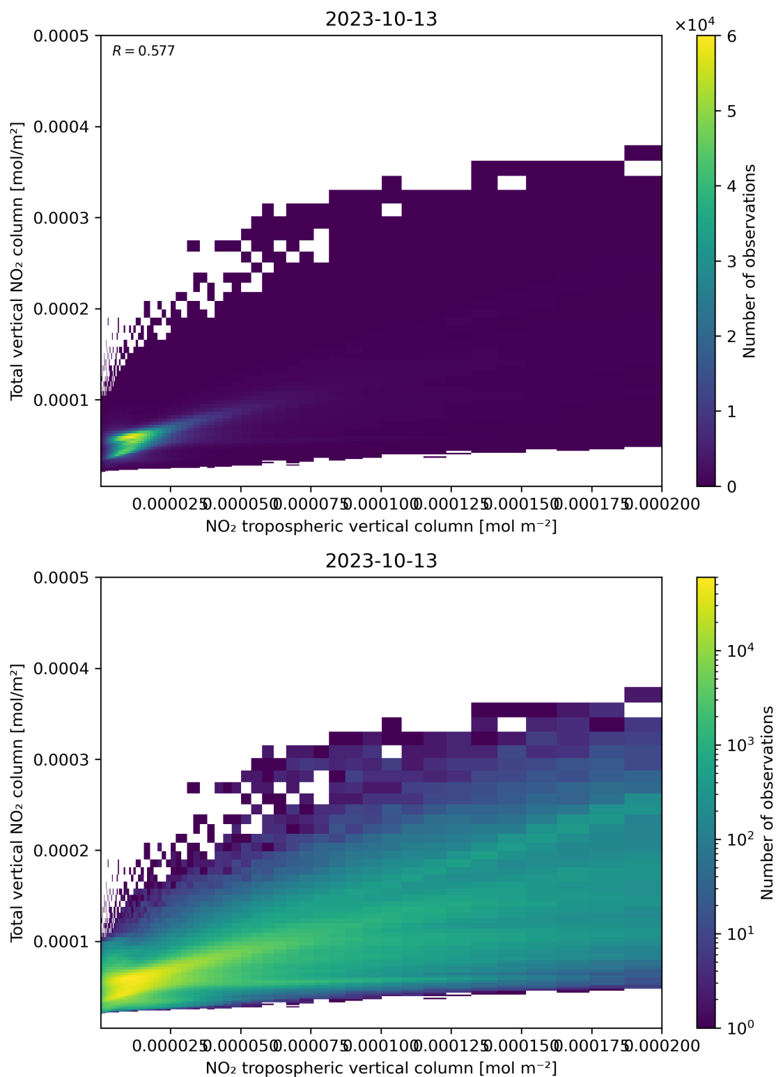
Figure 128: Scatter density plot of “NO 2 tropospheric vertical column” against “Total vertical NO 2 column” for 2023-10-12 to 2023-10-14.
