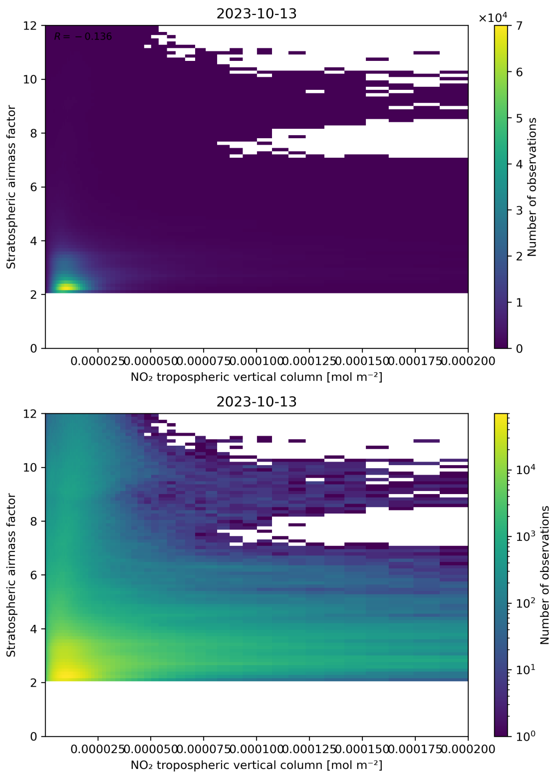
Figure 121: Scatter density plot of “NO 2 tropospheric vertical column” against “Stratospheric air mass factor” for 2023-10-12 to 2023-10-14.
