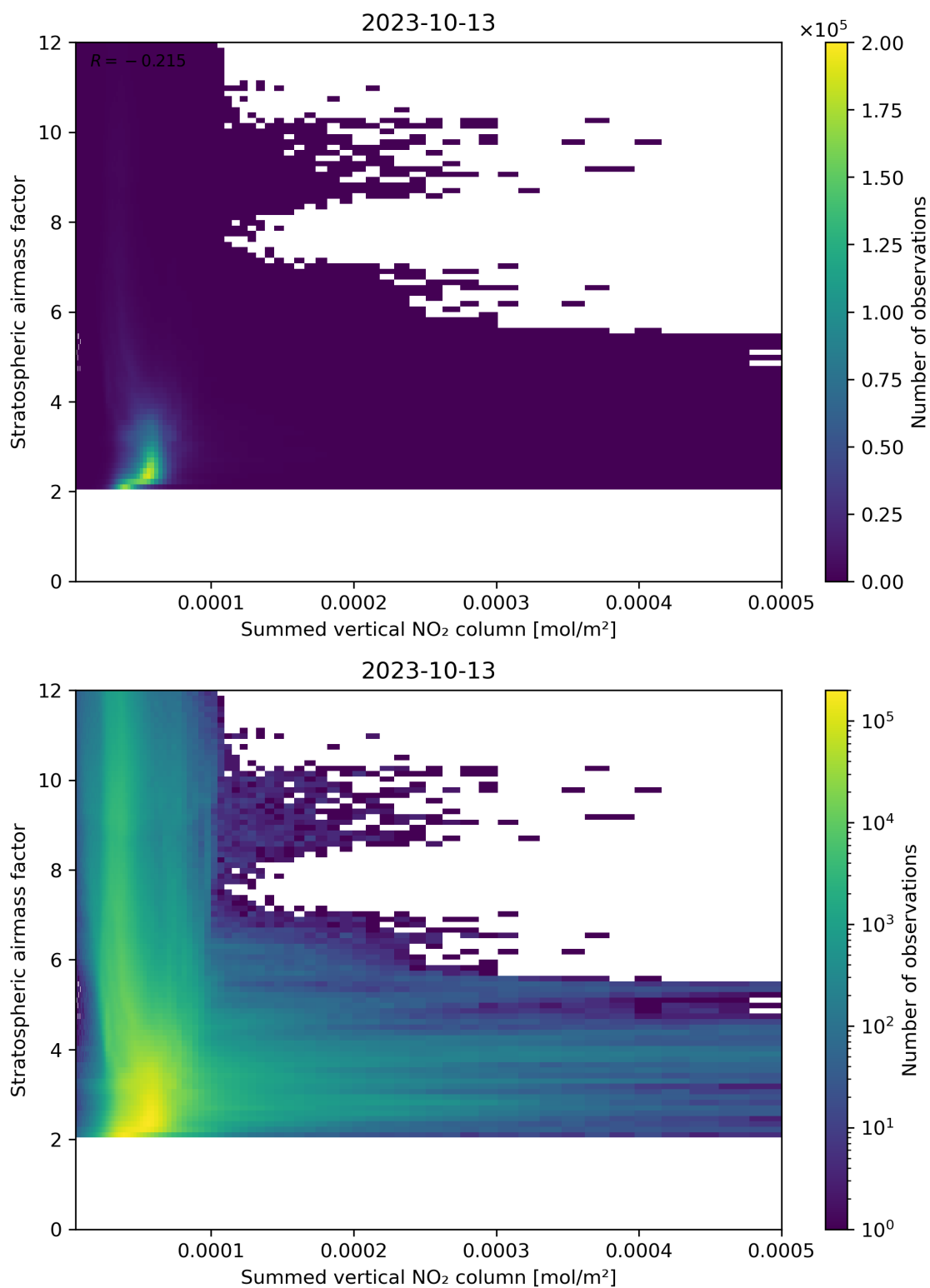
Figure 103: Scatter density plot of “Summed vertical NO 2 column” against “Stratospheric air mass factor” for 2023-10-12 to 2023-10-14.
