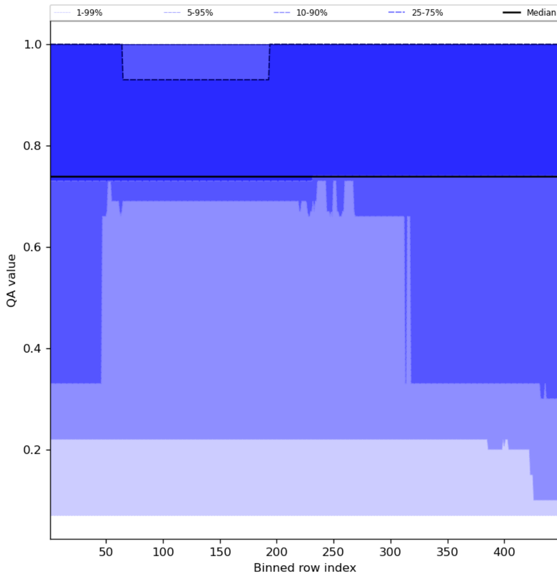
Figure 45: Along track statistics of “QA value” for 2023-10-12 to 2023-10-14
