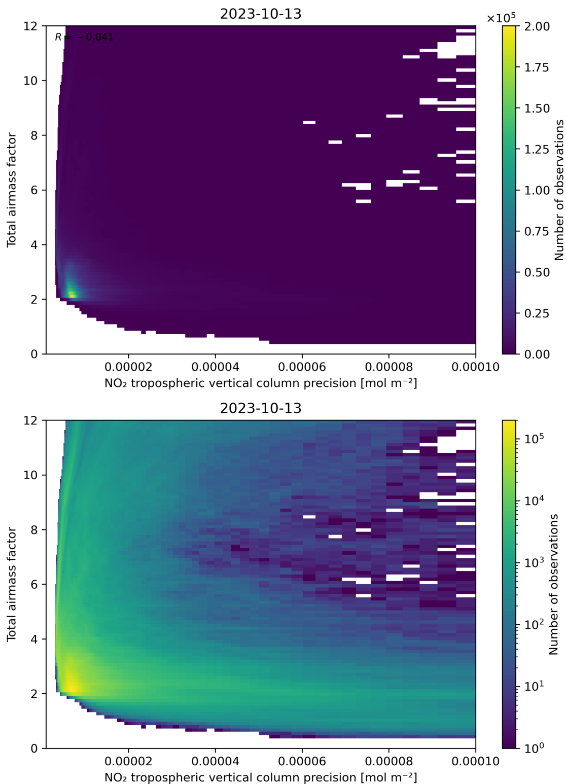
Figure 132: Scatter density plot of “NO 2 tropospheric vertical column precision” against “Total air mass factor” for 2023-10-12 to 2023-10-14.
