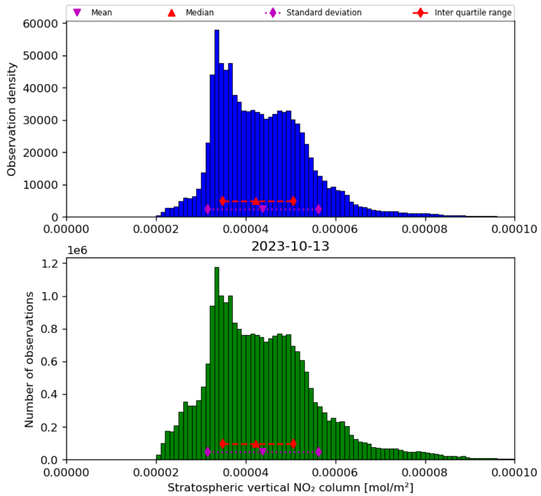
Figure 36: Histogram of “Stratospheric vertical NO 2 column” for 2023-10-12 to 2023-10-14
