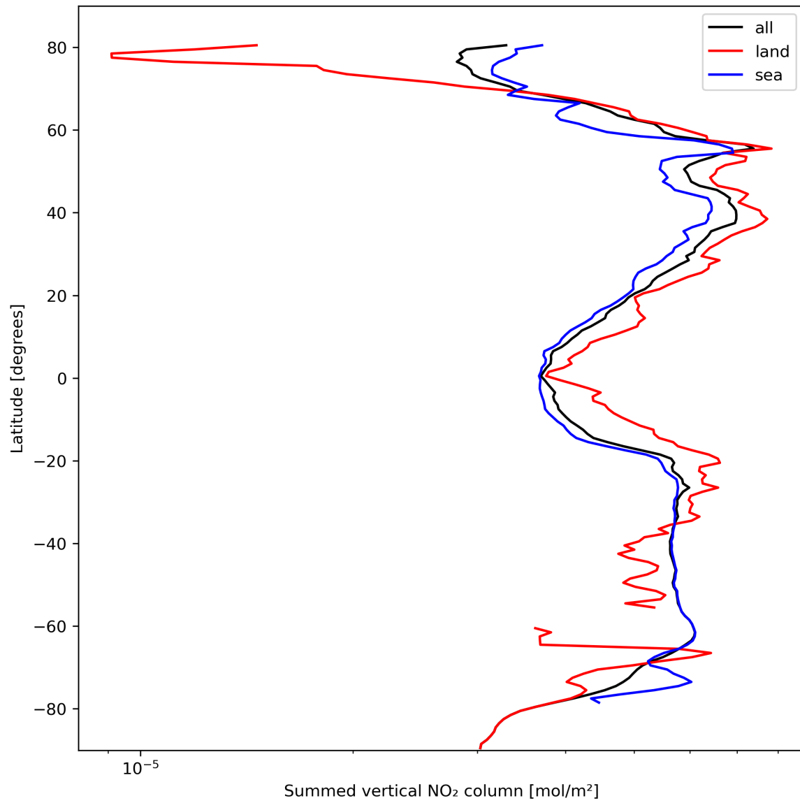
Figure 23: Zonal average of “Summed vertical NO 2 column” for 2023-10-12 to 2023-10-14.
