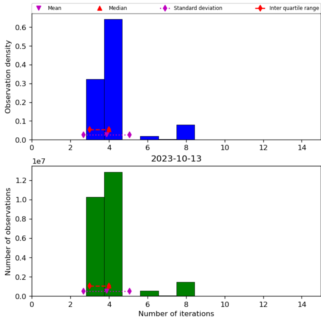
Figure 34: Histogram of “Number of iterations” for 2023-10-12 to 2023-10-14
