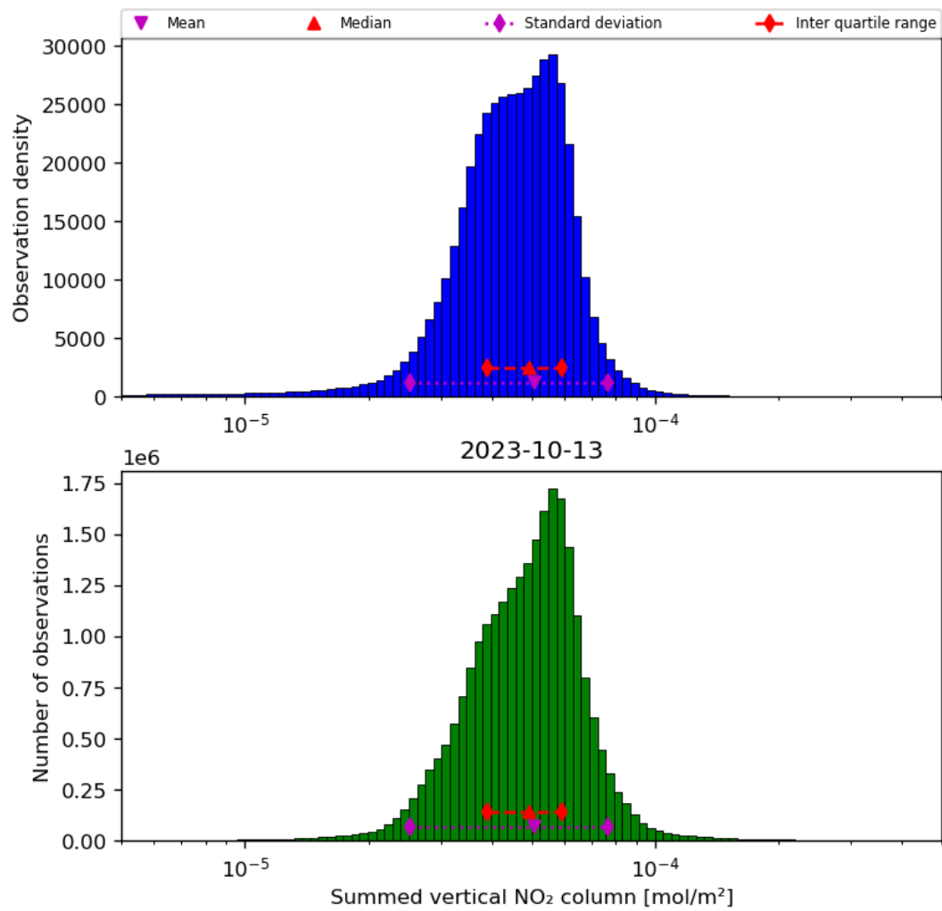
Figure 40: Histogram of “Summed vertical NO 2 column” for 2023-10-12 to 2023-10-14
