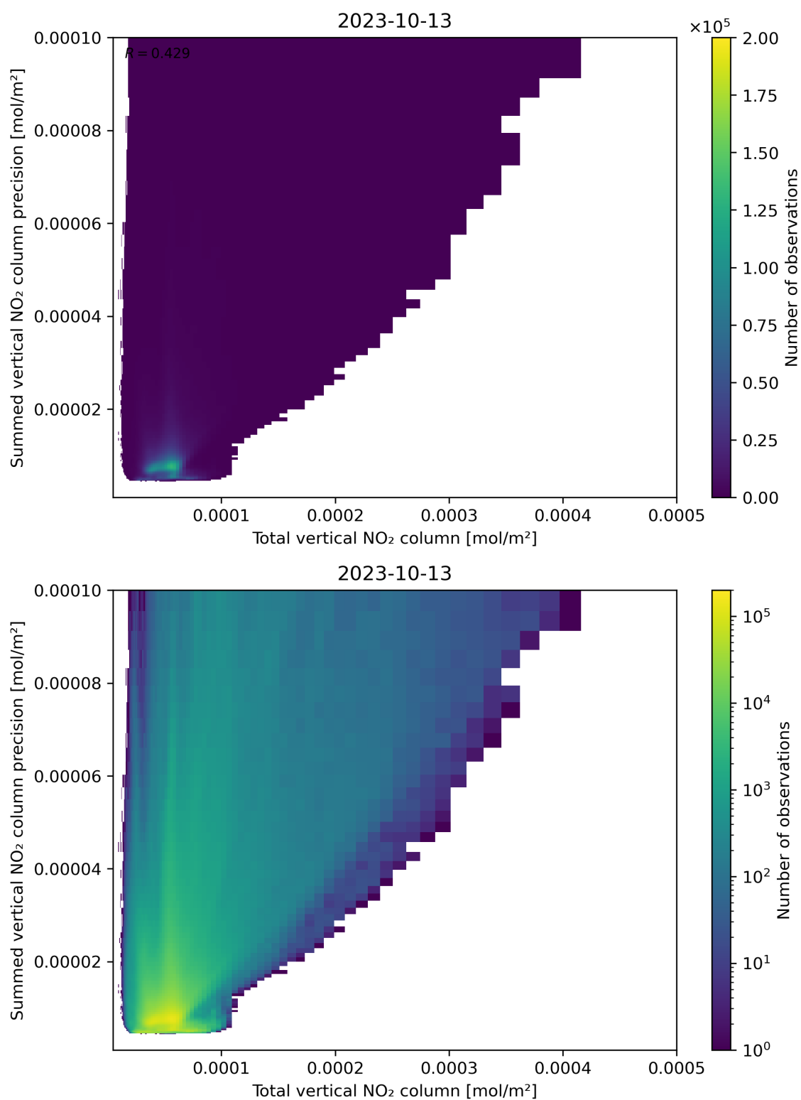
Figure 113: Scatter density plot of “Total vertical NO 2 column” against “Summed vertical NO 2 column precision” for 2023-10-12 to 2023-10-14.
