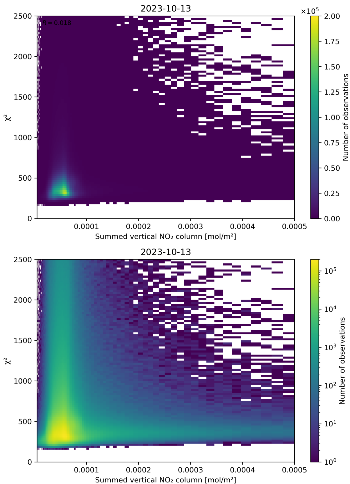
Figure 104: Scatter density plot of “Summed vertical NO 2 column” against “ \chi^2 ” for 2023-10-12 to 2023-10-14.
