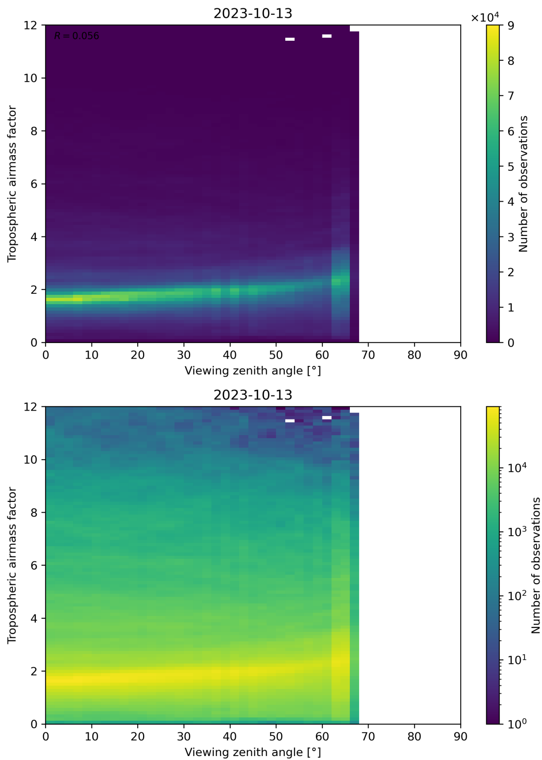
Figure 161: Scatter density plot of “Viewing zenith angle” against “Tropospheric airmass factor” for 2023-10-12 to 2023-10-14.
