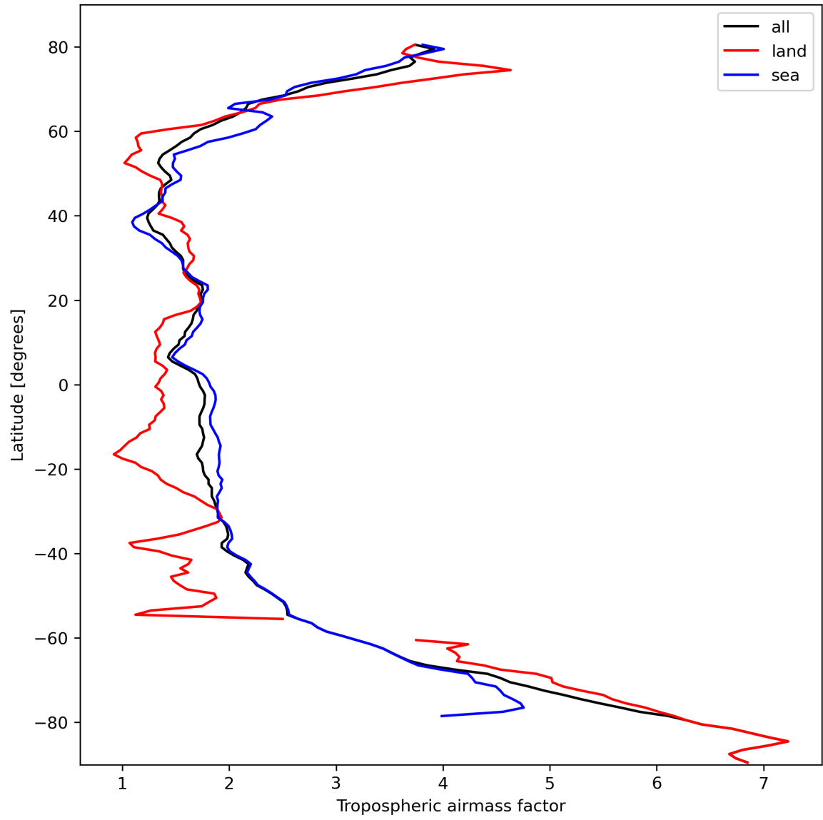
Figure 14: Zonal average of “Tropospheric airmass factor” for 2023-10-12 to 2023-10-14.
