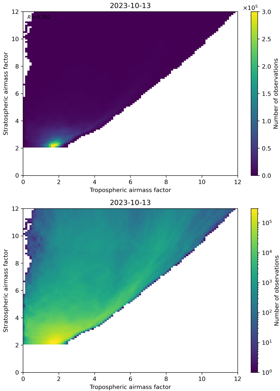
Figure 71: Scatter density plot of “Tropospheric airmass factor” against “Stratospheric airmass factor” for 2023-10-12 to 2023-10-14.
