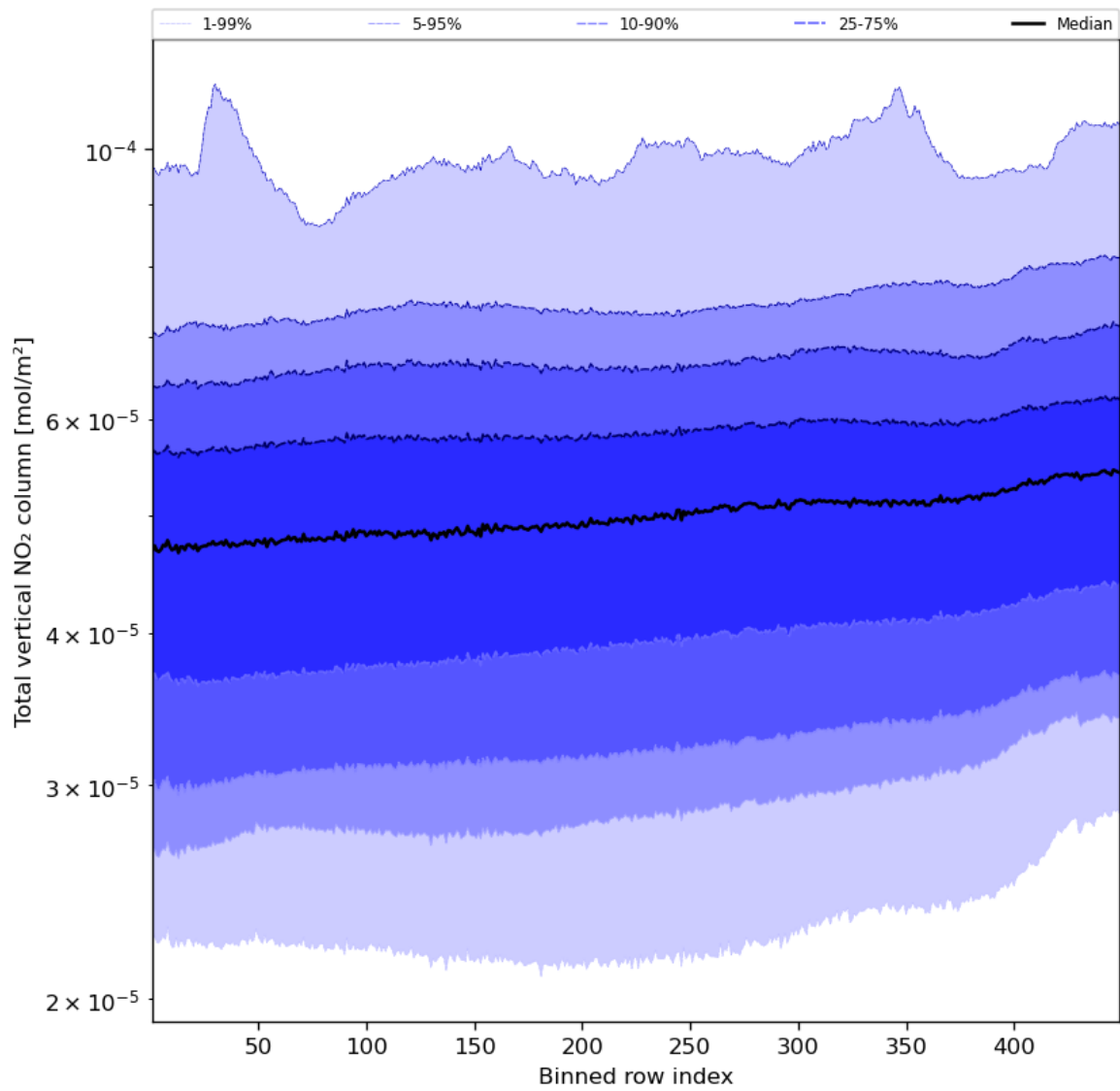
Figure 55: Along track statistics of “Total vertical NO 2 column” for 2023-10-12 to 2023-10-14
