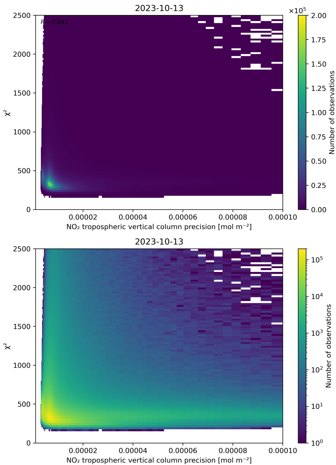
Figure 134: Scatter density plot of “NO 2 tropospheric vertical column precision” against “ \chi^2 ” for 2023-10-12 to 2023-10-14.
