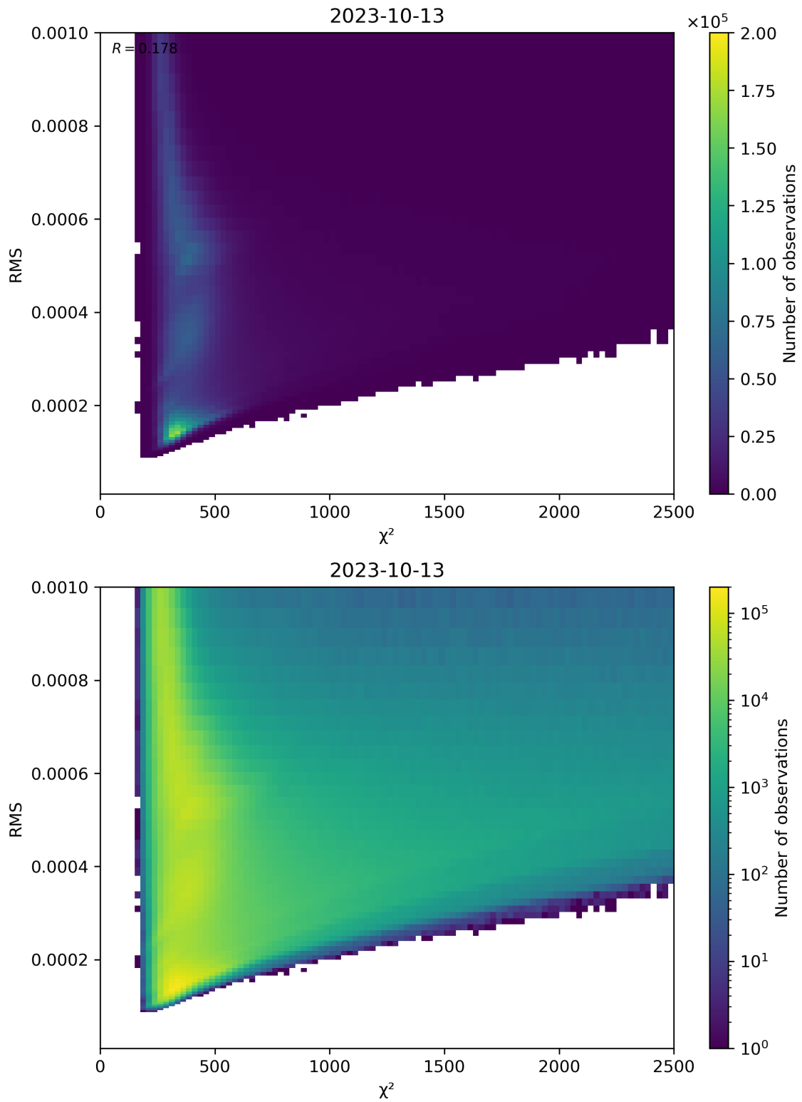
Figure 82: Scatter density plot of “ \chi^2 ” against “RMS” for 2023-10-12 to 2023-10-14.
