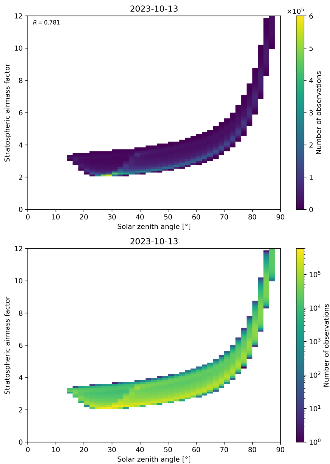
Figure 145: Scatter density plot of “Solar zenith angle” against “Stratospheric airmass factor” for 2023-10-12 to 2023-10-14.
