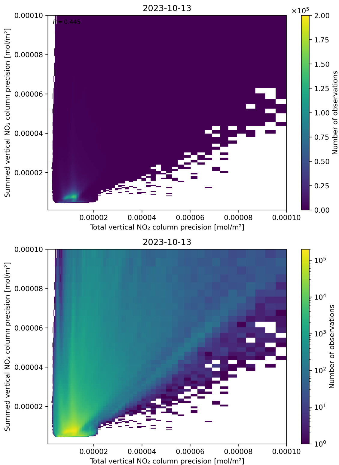
Figure 118: Scatter density plot of “Total vertical NO 2 column precision” against “Summed vertical NO 2 column precision” for 2023-10-12 to 2023-10-14.
