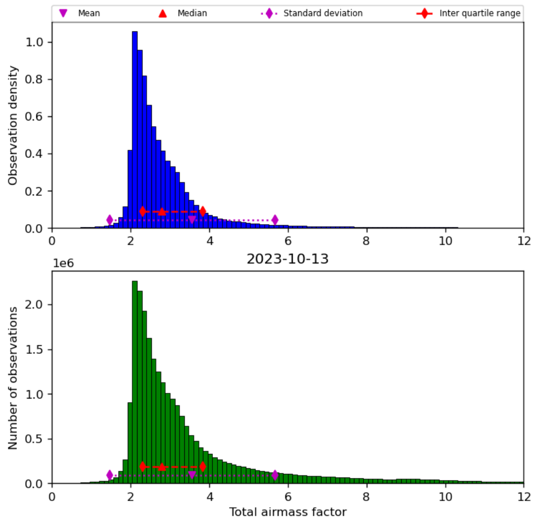
Figure 32: Histogram of “Total airmass factor” for 2023-10-12 to 2023-10-14
