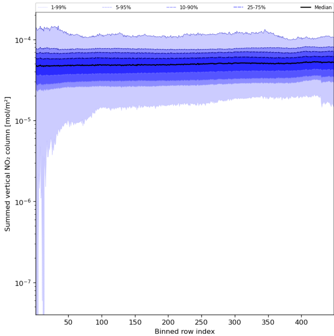
Figure 57: Along track statistics of “Summed vertical NO 2 column” for 2023-10-12 to 2023-10-14
