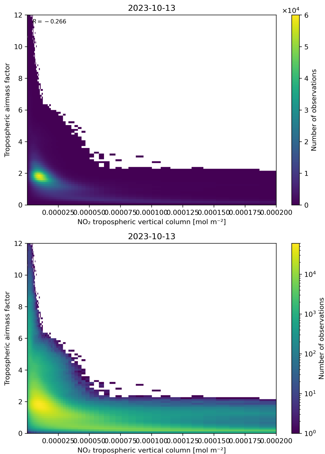
Figure 123: Scatter density plot of “NO 2 tropospheric vertical column” against “Tropospheric air mass factor” for 2023-10-12 to 2023-10-14.
