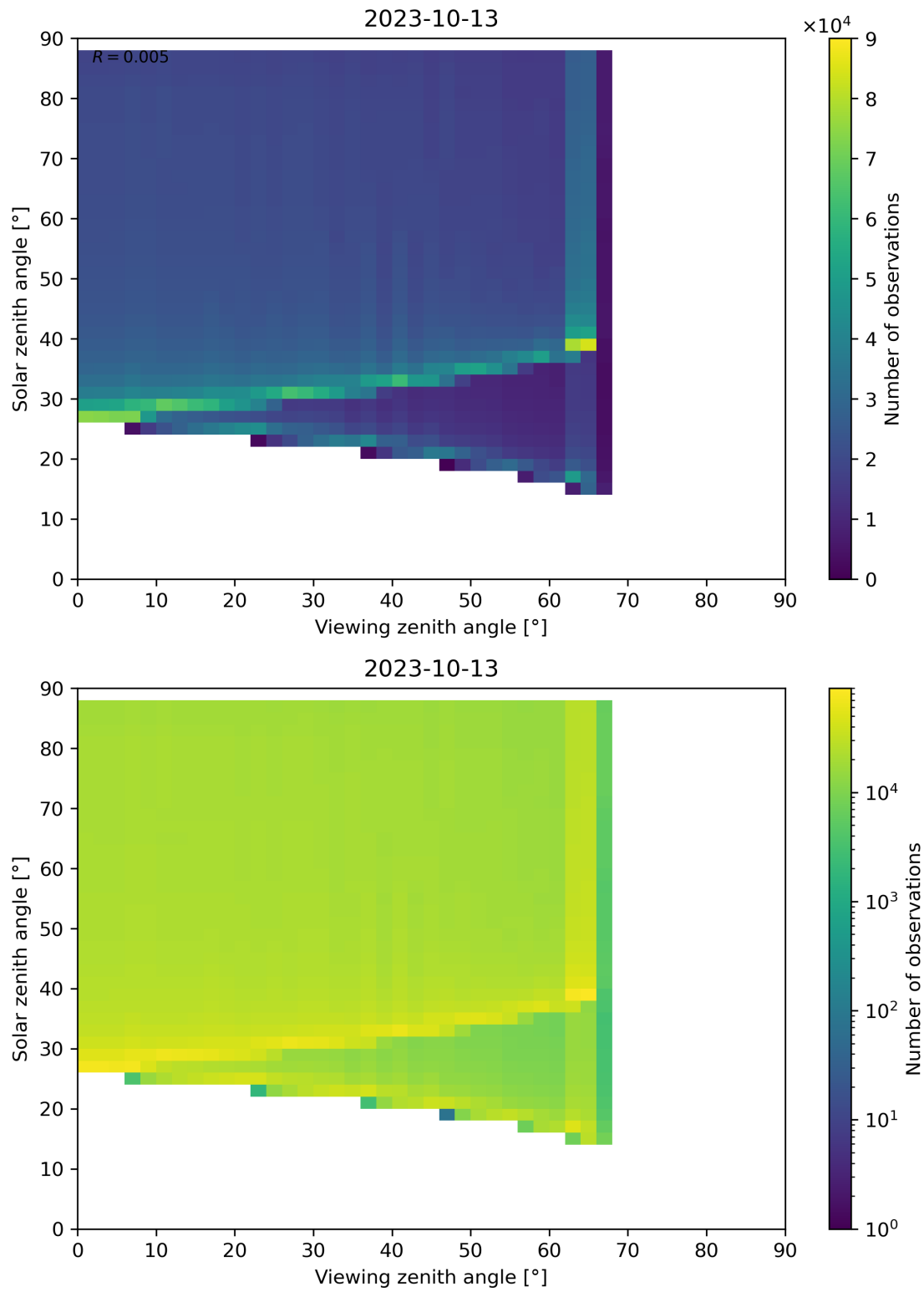
Figure 172: Scatter density plot of “Viewing zenith angle” against “Solar zenith angle” for 2023-10-12 to 2023-10-14.
