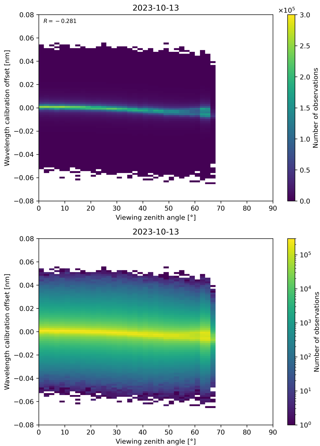
Figure 173: Scatter density plot of “Viewing zenith angle” against “Wavelength calibration offset” for 2023-10-12 to 2023-10-14.
