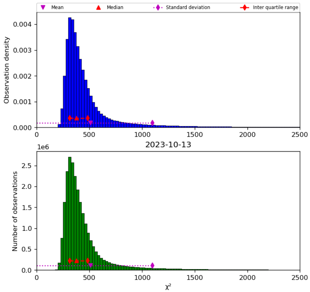
Figure 42: Histogram of “ \chi^2 ” for 2023-10-12 to 2023-10-14
