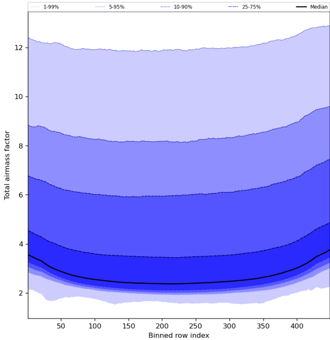
Figure 49: Along track statistics of “Total airmass factor” for 2023-10-12 to 2023-10-14
