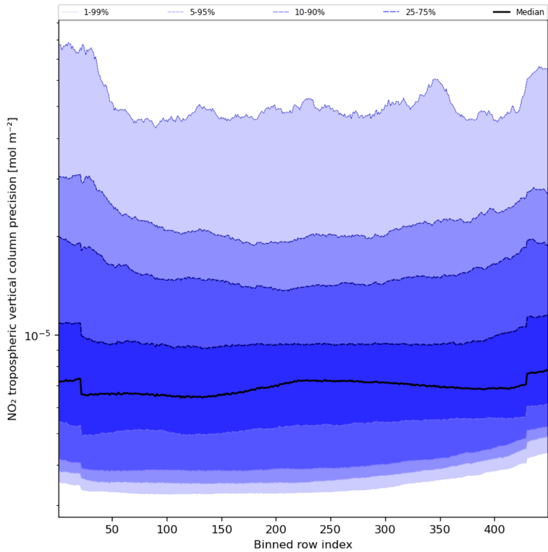
Figure 47: Along track statistics of “NO 2 tropospheric vertical column precision” for 2023-10-12 to 2023-10-14
