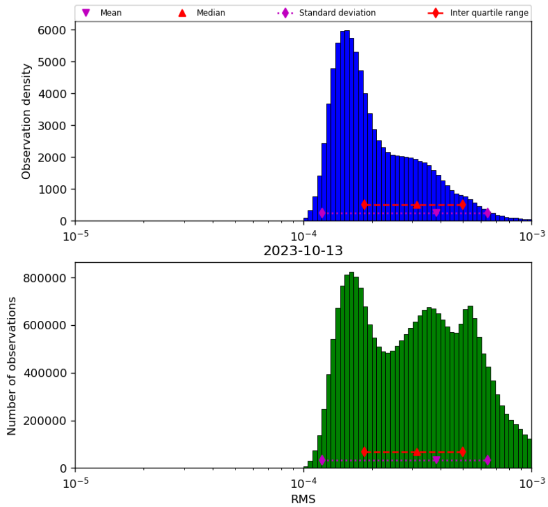
Figure 43: Histogram of “RMS” for 2023-10-12 to 2023-10-14
