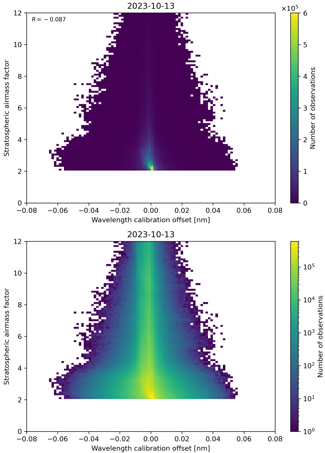
Figure 174: Scatter density plot of “Wavelength calibration offset” against “Stratospheric airmass factor” for 2023-10-12 to 2023-10-14.
