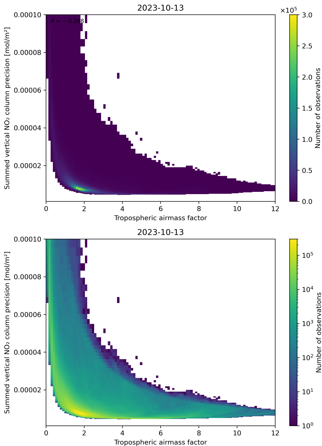
Figure 76: Scatter density plot of “Tropospheric air mass factor” against “Summed vertical NO 2 column precision” for 2023-10-12 to 2023-10-14.
