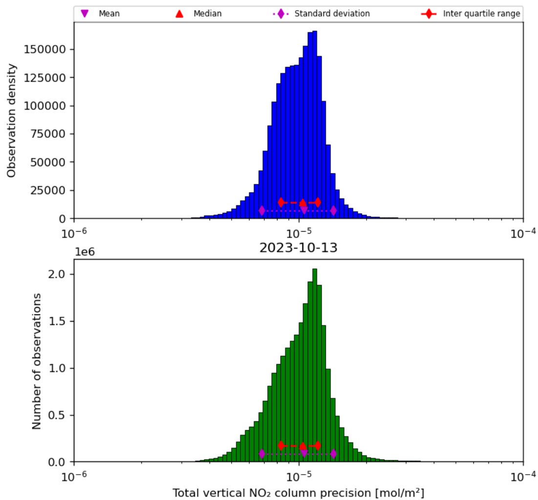
Figure 39: Histogram of “Total vertical NO 2 column precision” for 2023-10-12 to 2023-10-14
