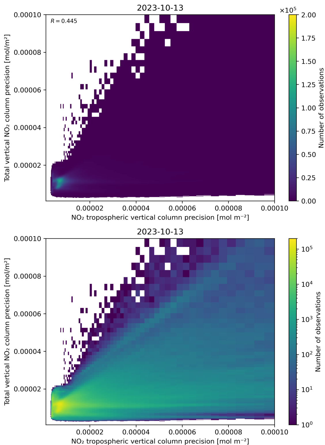
Figure 139: Scatter density plot of “NO 2 tropospheric vertical column precision” against “Total vertical NO 2 column precision” for 2023-10-12 to 2023-10-14.
