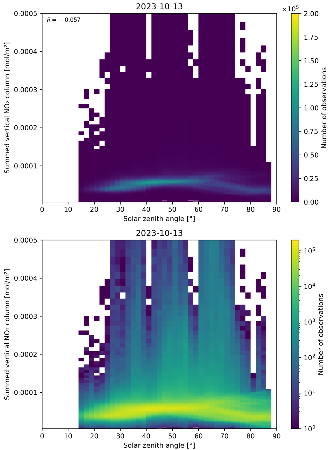
Figure 151: Scatter density plot of “Solar zenith angle” against “Summed vertical NO 2 column” for 2023-10-12 to 2023-10-14.
