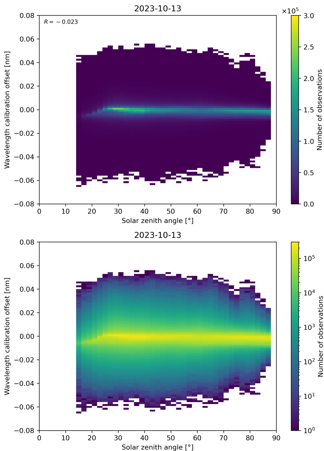
Figure 158: Scatter density plot of “Solar zenith angle” against “Wavelength calibration offset” for 2023-10-12 to 2023-10-14.
