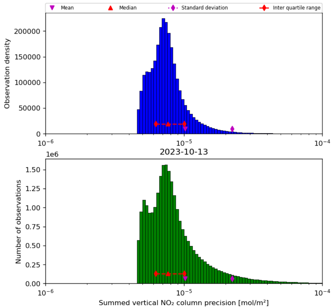
Figure 41: Histogram of "Summed vertical NO 2 column precision" for 2023-10-12 to 2023-10-14
