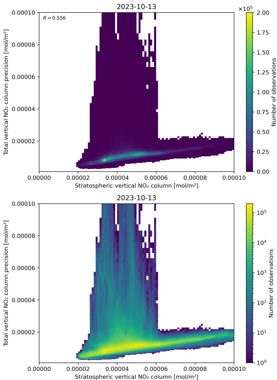
Figure 101: Scatter density plot of “Stratospheric vertical NO 2 column” against “Total vertical NO 2 column precision” for 2023-10-12 to 2023-10-14.
