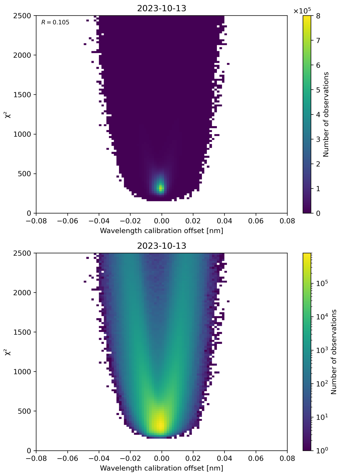
Figure 175: Scatter density plot of “Wavelength calibration offset” against “ \chi^2 ” for 2023-10-12 to 2023-10-14.
