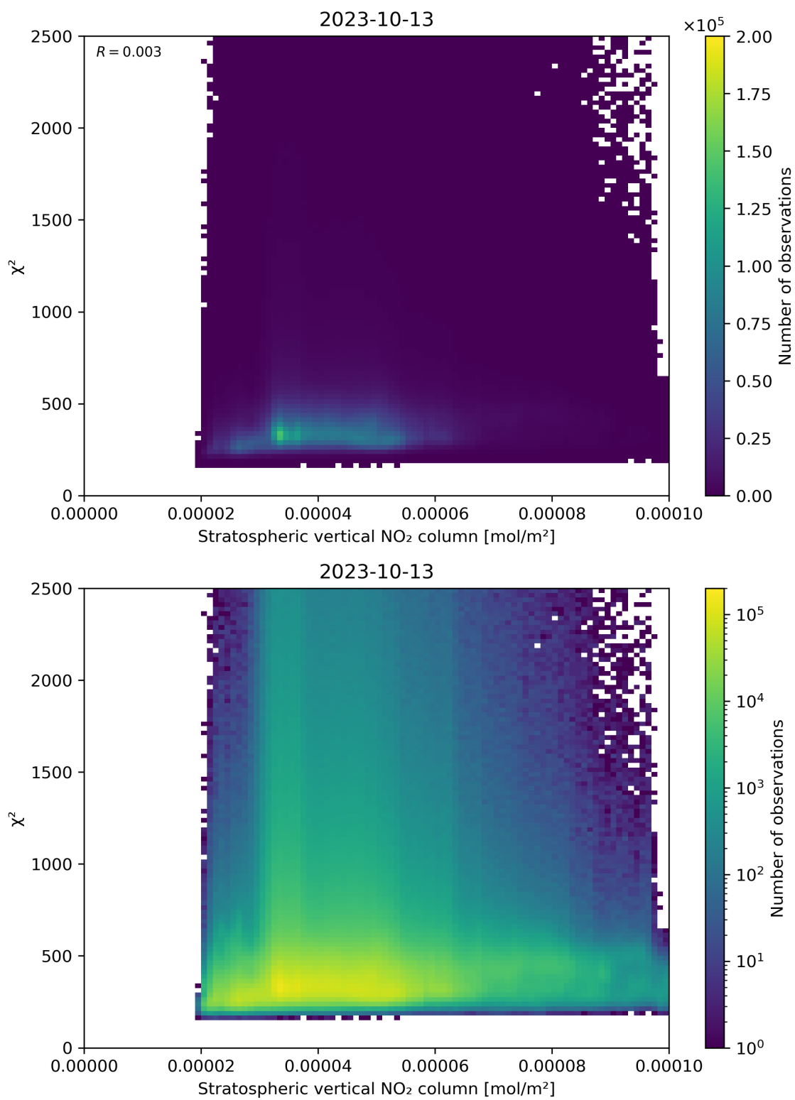
Figure 97: Scatter density plot of “Stratospheric vertical NO 2 column” against “ \chi^2 ” for 2023-10-12 to 2023-10-14.
