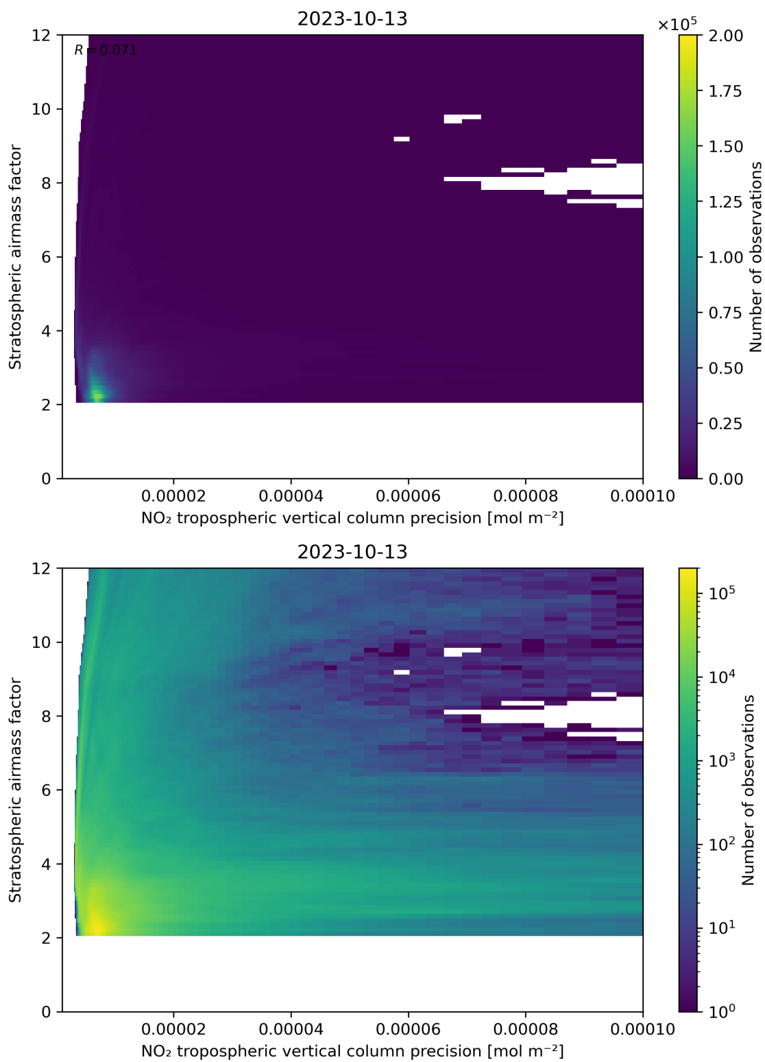
Figure 131: Scatter density plot of “NO 2 tropospheric vertical column precision” against “Stratospheric airmass factor” for 2023-10-12 to 2023-10-14.
