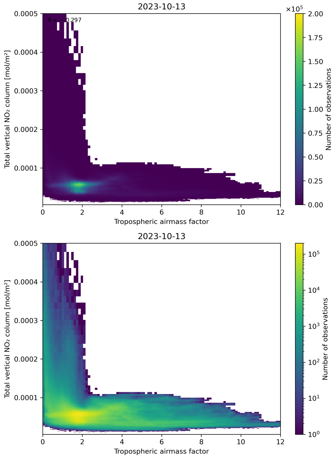
Figure 77: Scatter density plot of “Tropospheric airmass factor” against “Total vertical NO 2 column” for 2023-10-12 to 2023-10-14.
