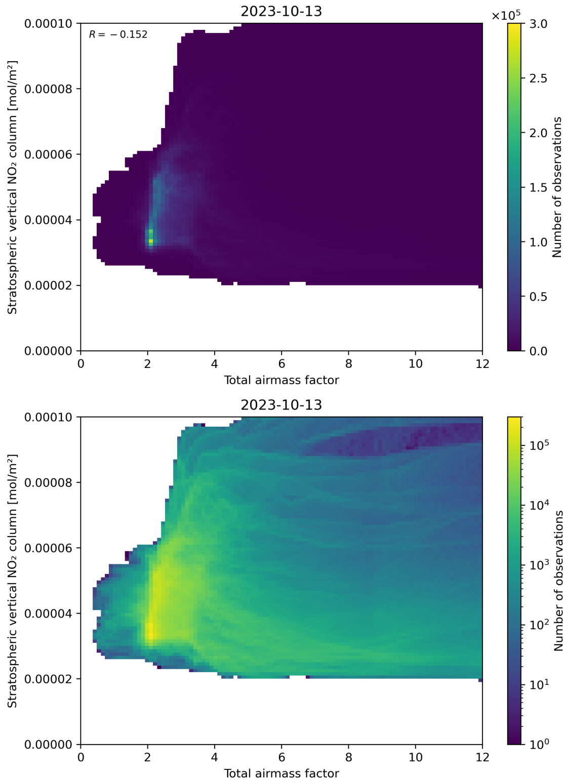
Figure 64: Scatter density plot of “Total airmass factor” against “Stratospheric vertical NO 2 column” for 2023-10-12 to 2023-10-14.
