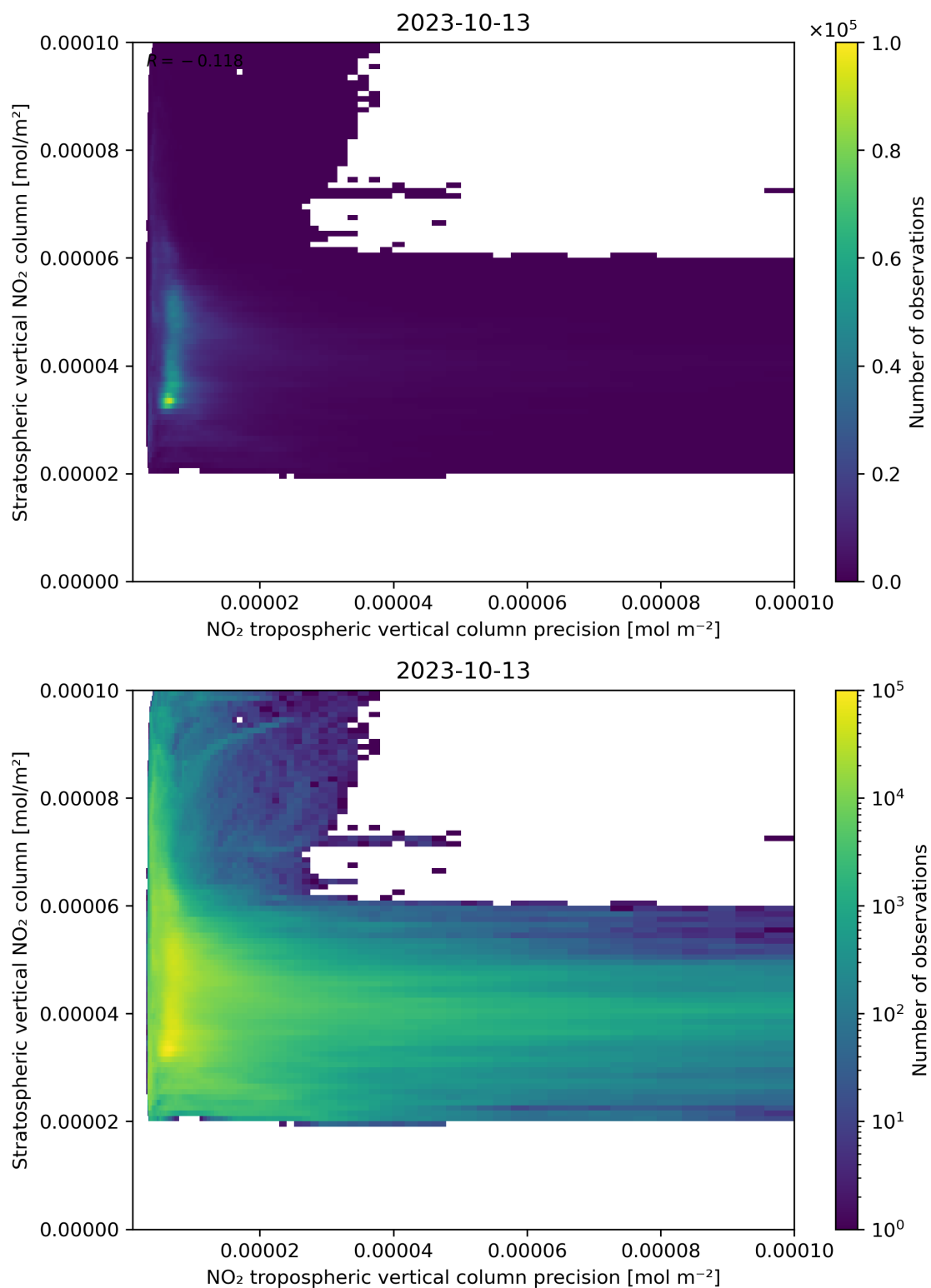
Figure 135: Scatter density plot of “NO 2 tropospheric vertical column precision” against “Stratospheric vertical NO 2 column” for 2023-10-12 to 2023-10-14.
