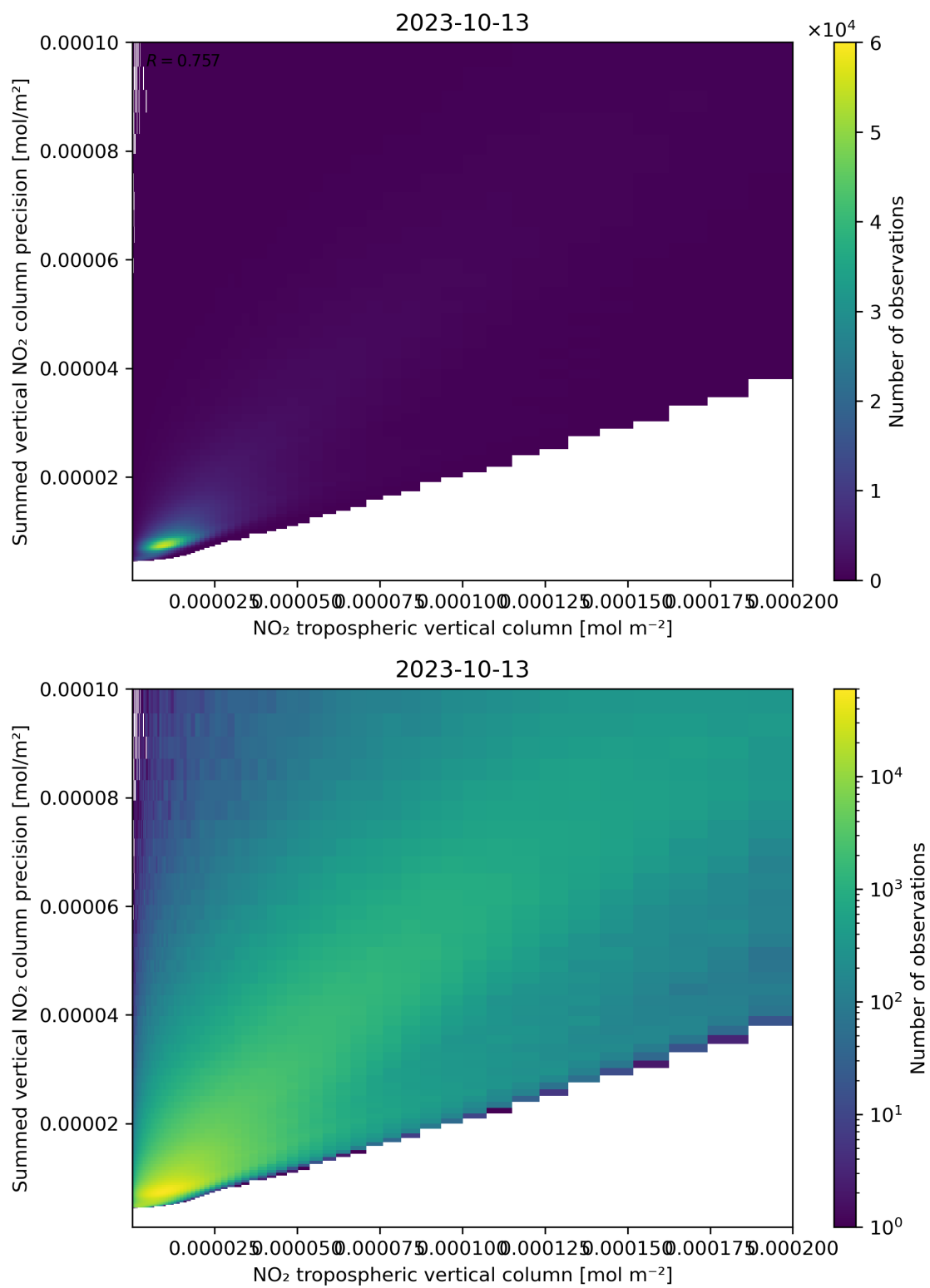
Figure 127: Scatter density plot of “NO 2 tropospheric vertical column” against “Summed vertical NO 2 column precision” for 2023-10-12 to 2023-10-14.
