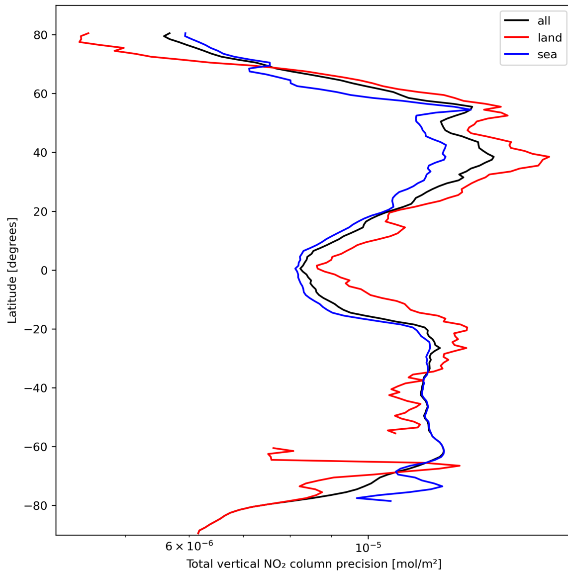
Figure 22: Zonal average of “Total vertical NO 2 column precision” for 2023-10-12 to 2023-10-14.
