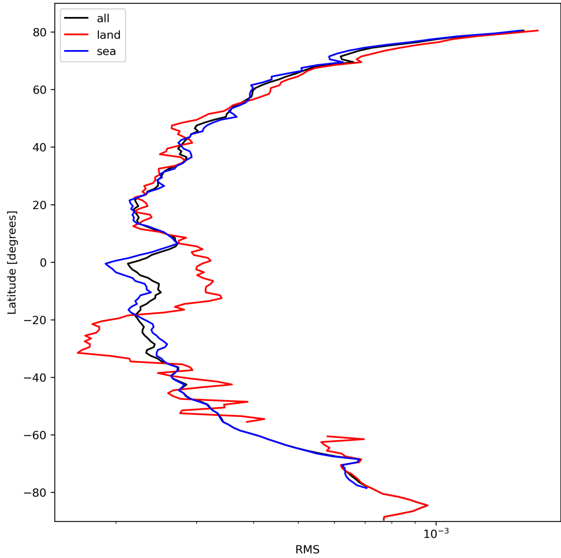
Figure 26: Zonal average of “RMS” for 2023-10-12 to 2023-10-14.
