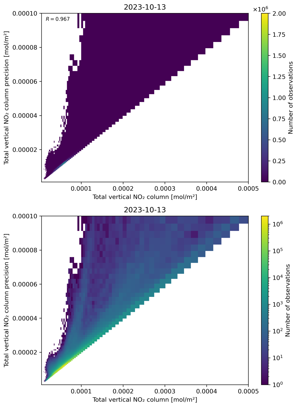
Figure 114: Scatter density plot of “Total vertical NO 2 column” against “Total vertical NO 2 column precision” for 2023-10-12 to 2023-10-14.
