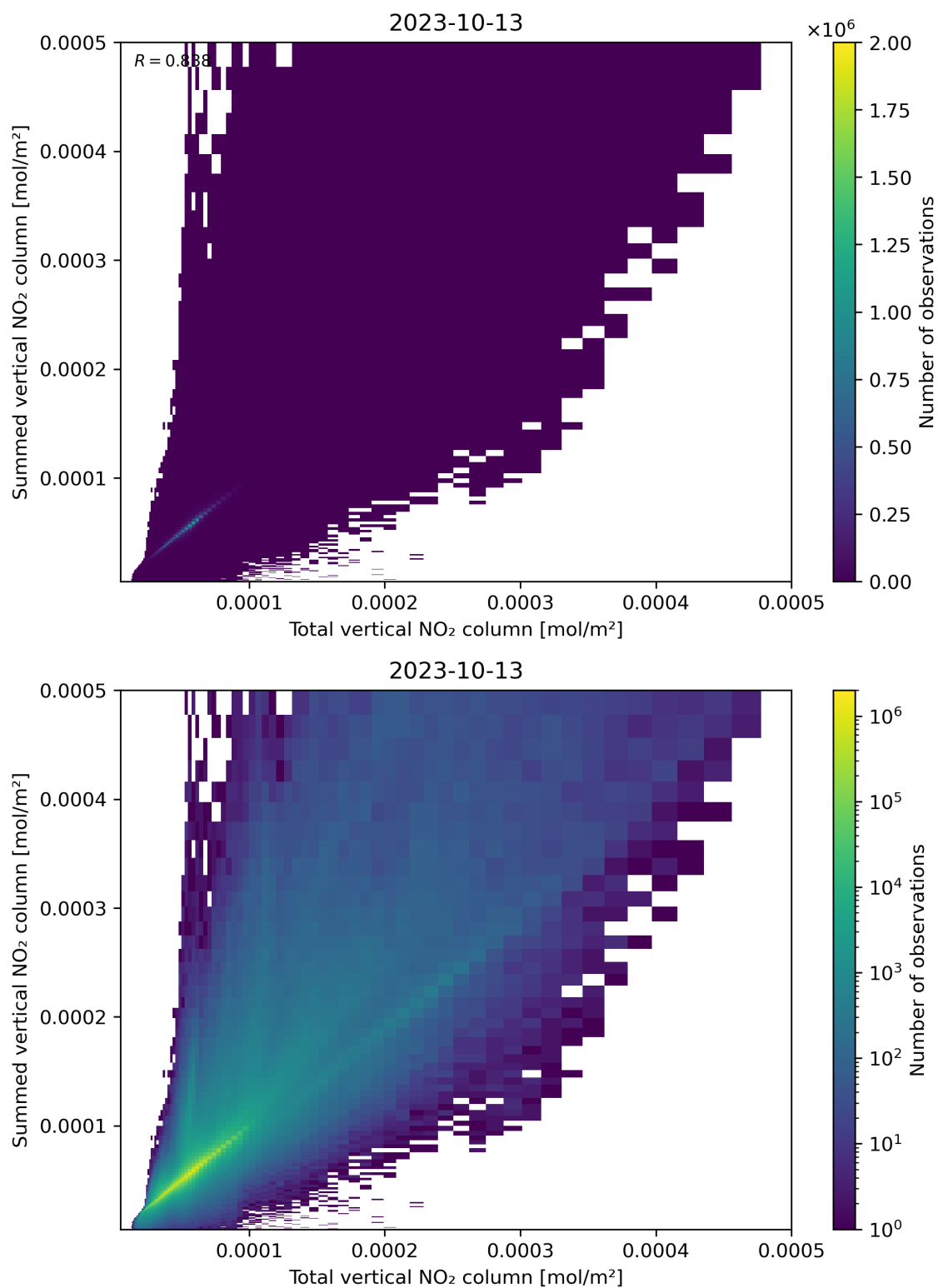
Figure 112: Scatter density plot of “Total vertical NO 2 column” against “Summed vertical NO 2 column” for 2023-10-12 to 2023-10-14.
