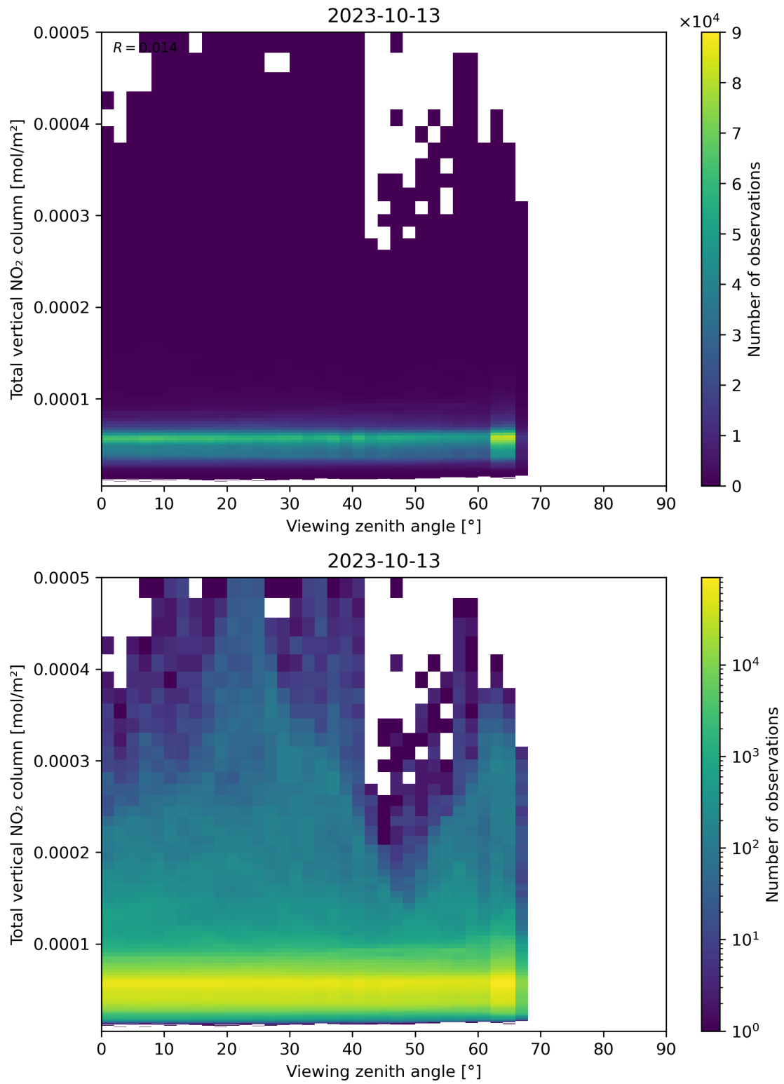
Figure 167: Scatter density plot of “Viewing zenith angle” against “Total vertical NO 2 column” for 2023-10-12 to 2023-10-14.
