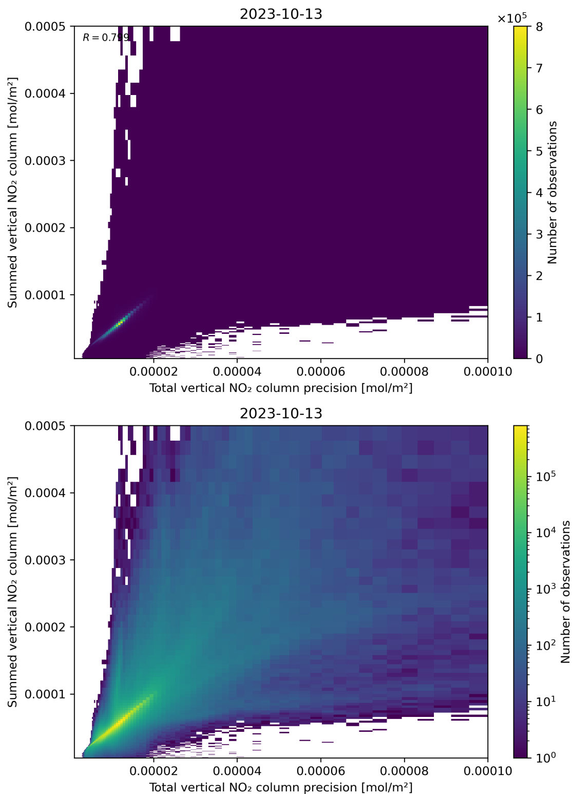
Figure 117: Scatter density plot of “Total vertical NO 2 column precision” against “Summed vertical NO 2 column” for 2023-10-12 to 2023-10-14.
