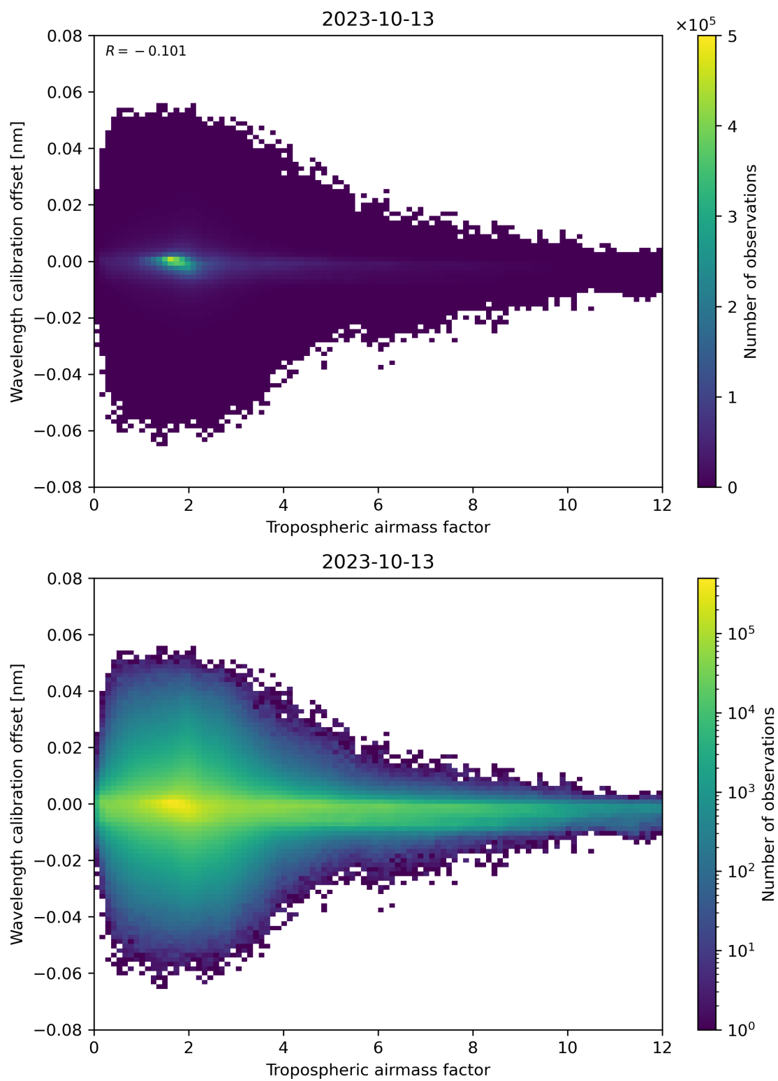
Figure 80: Scatter density plot of “Tropospheric airmass factor” against “Wavelength calibration offset” for 2023-10-12 to 2023-10-14.
