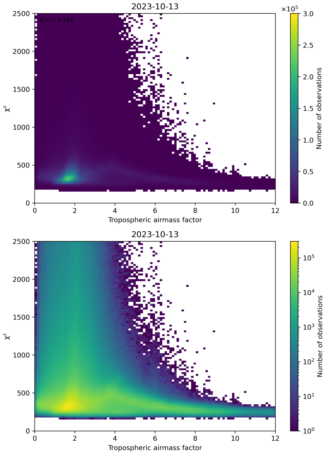
Figure 73: Scatter density plot of “Tropospheric airmass factor” against “ \chi^2 ” for 2023-10-12 to 2023-10-14.
