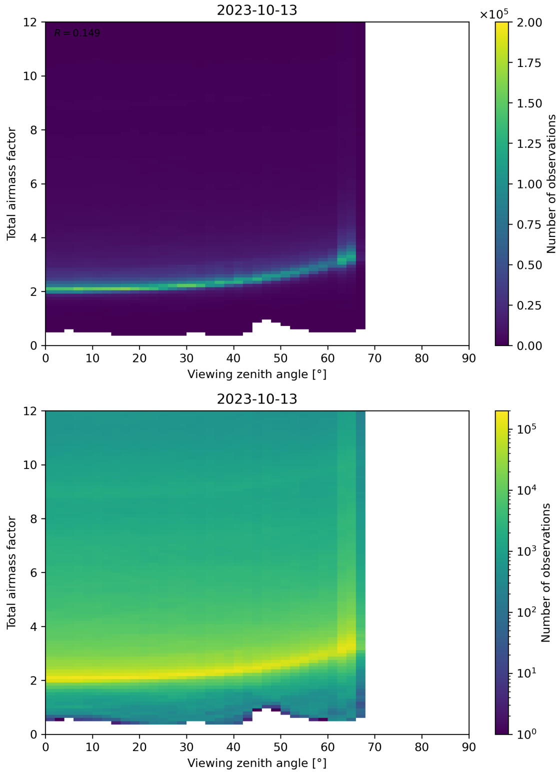
Figure 160: Scatter density plot of “Viewing zenith angle” against “Total airmass factor” for 2023-10-12 to 2023-10-14.
