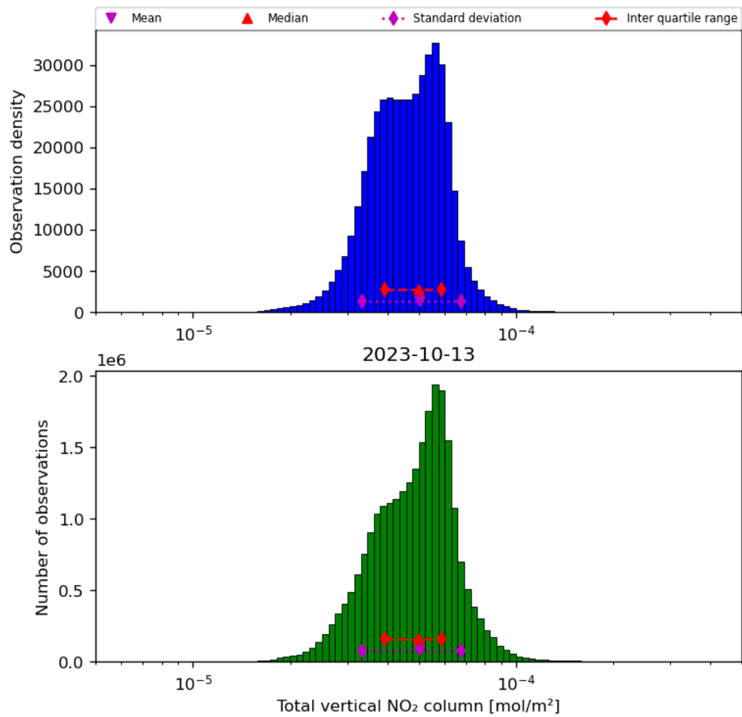
Figure 38: Histogram of “Total vertical NO 2 column” for 2023-10-12 to 2023-10-14
