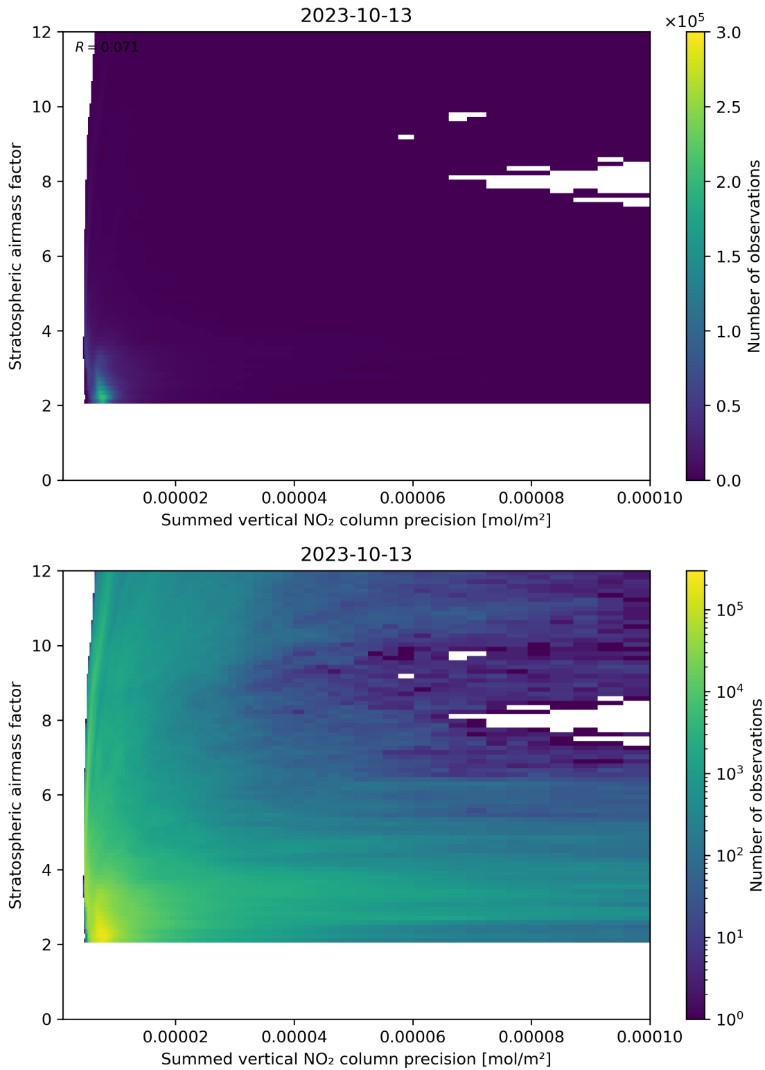
Figure 106: Scatter density plot of “Summed vertical NO 2 column precision” against “Stratospheric airmass factor” for 2023-10-12 to 2023-10-14.
