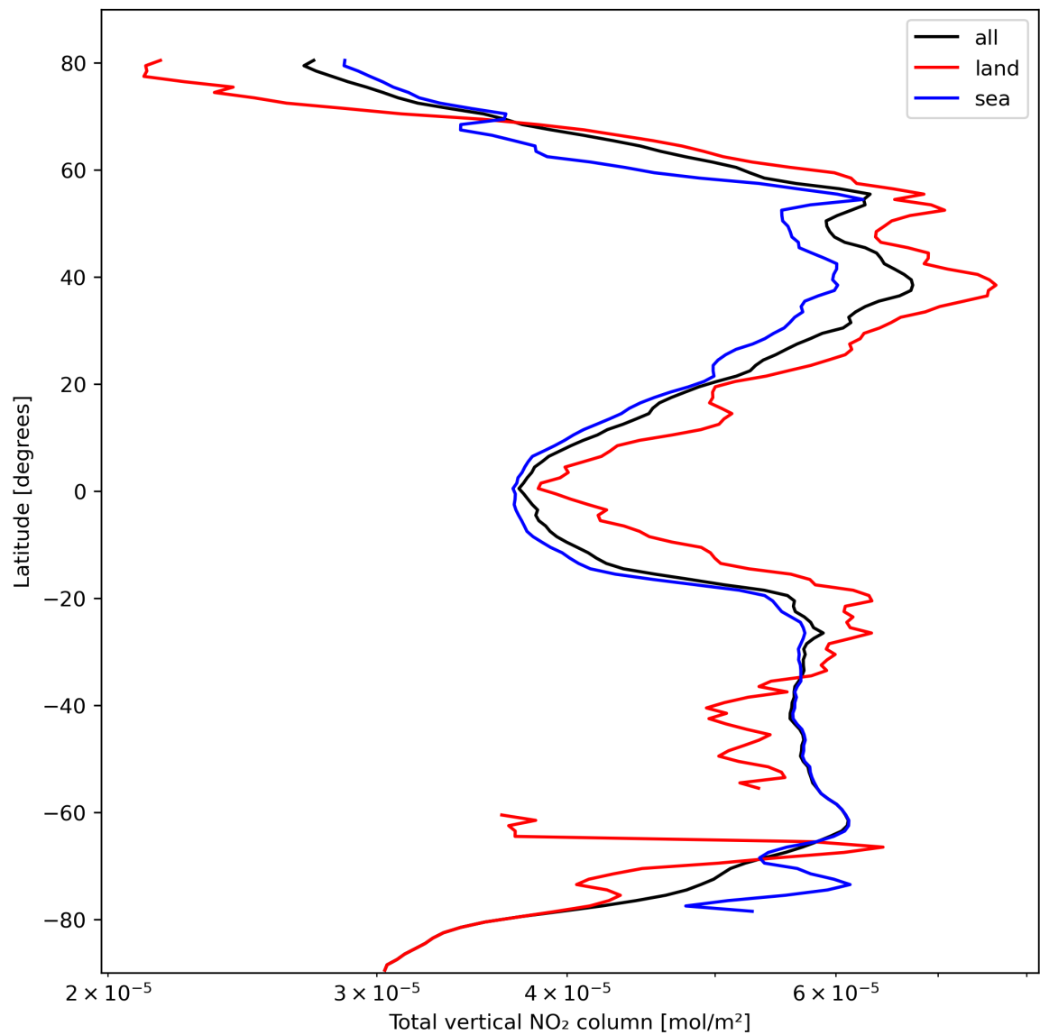
Figure 21: Zonal average of “Total vertical NO 2 column” for 2023-10-12 to 2023-10-14.
