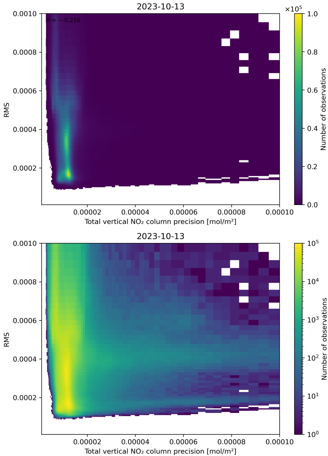
Figure 119: Scatter density plot of “Total vertical NO 2 column precision” against “RMS” for 2023-10-12 to 2023-10-14.
