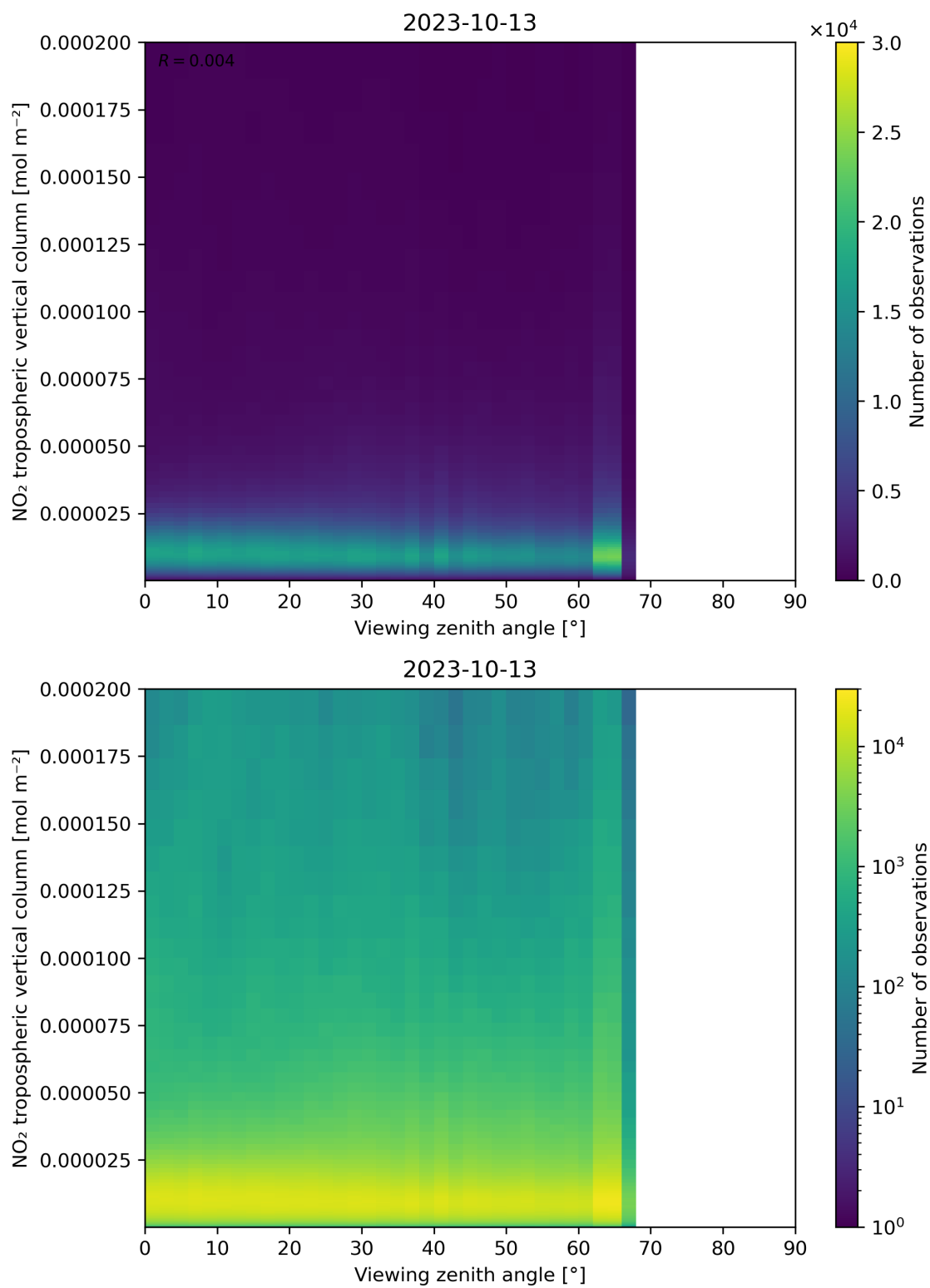
Figure 169: Scatter density plot of “Viewing zenith angle” against “NO 2 tropospheric vertical column” for 2023-10-12 to 2023-10-14.
