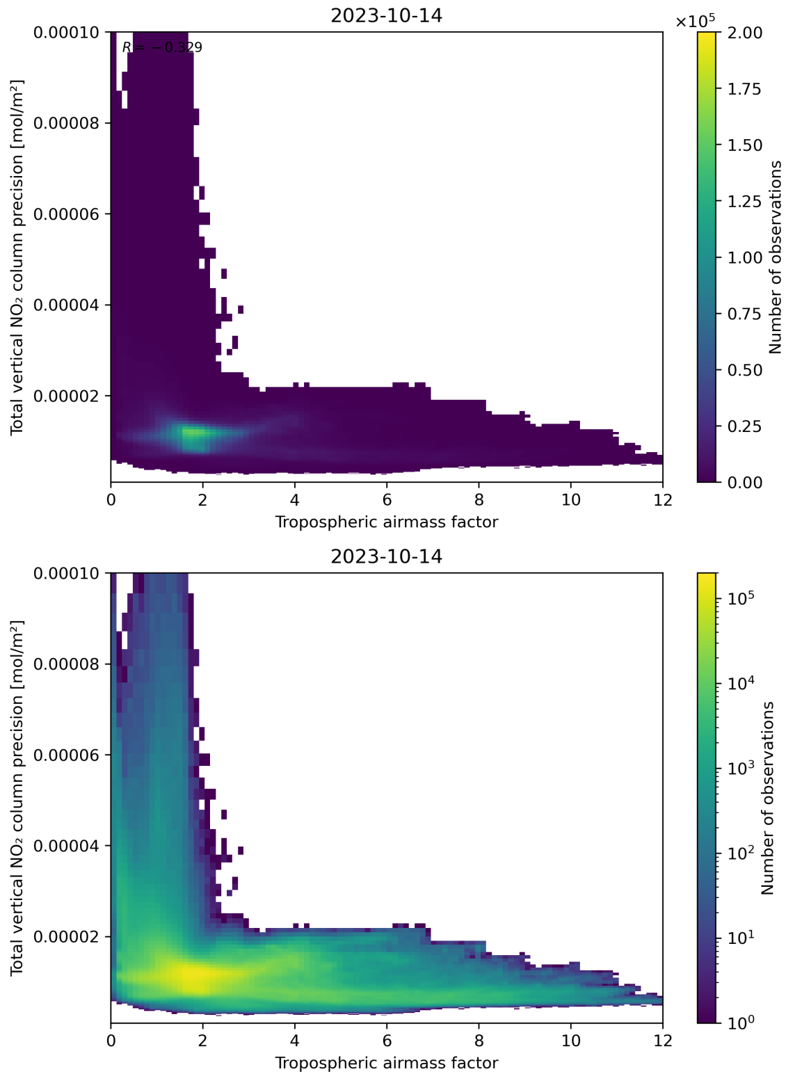
Figure 78: Scatter density plot of “Tropospheric air mass factor” against “Total vertical NO 2 column precision” for 2023-10-13 to 2023-10-15.
