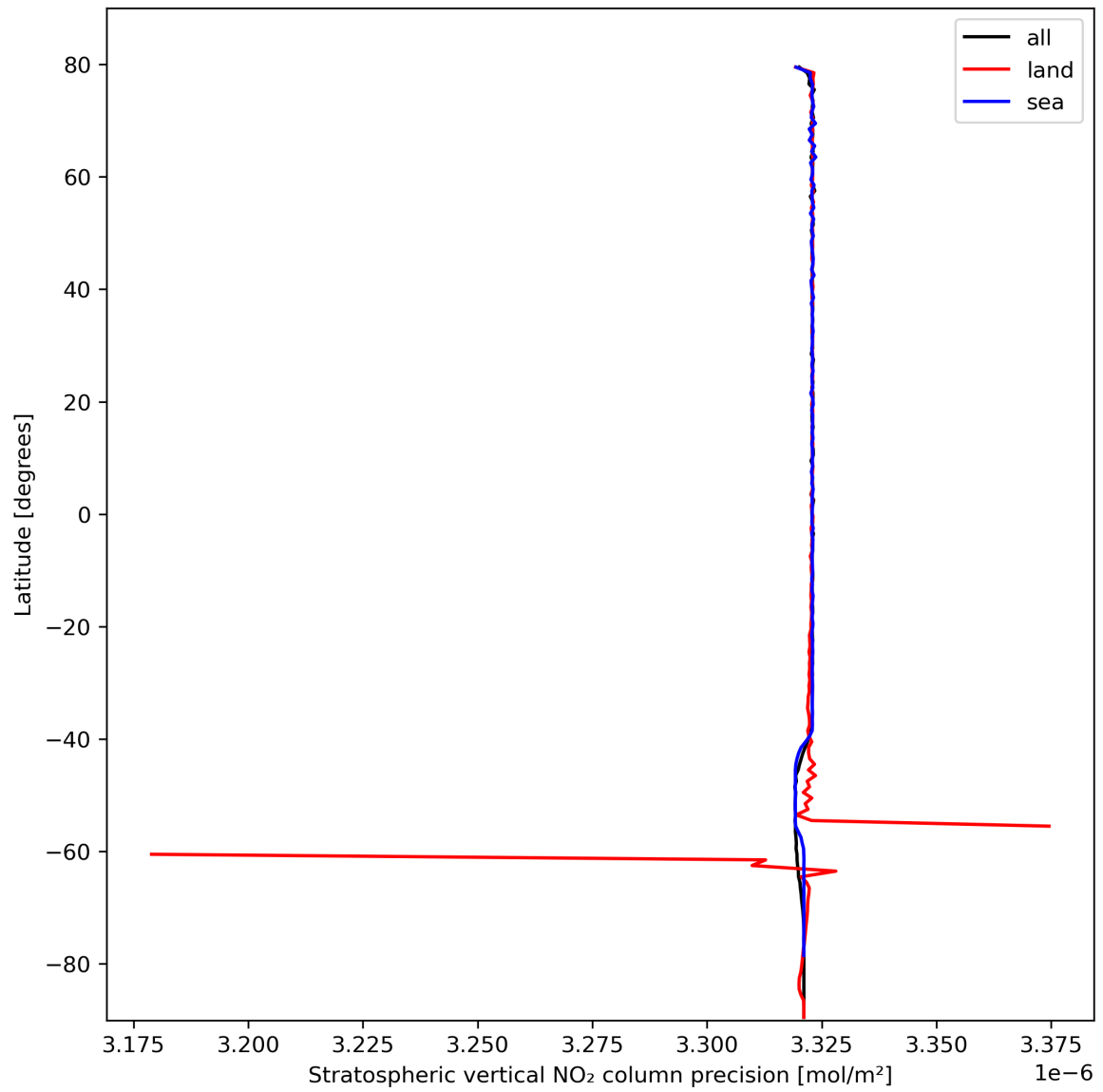
Figure 20: Zonal average of “Stratospheric vertical NO 2 column precision” for 2023-10-13 to 2023-10-15.
