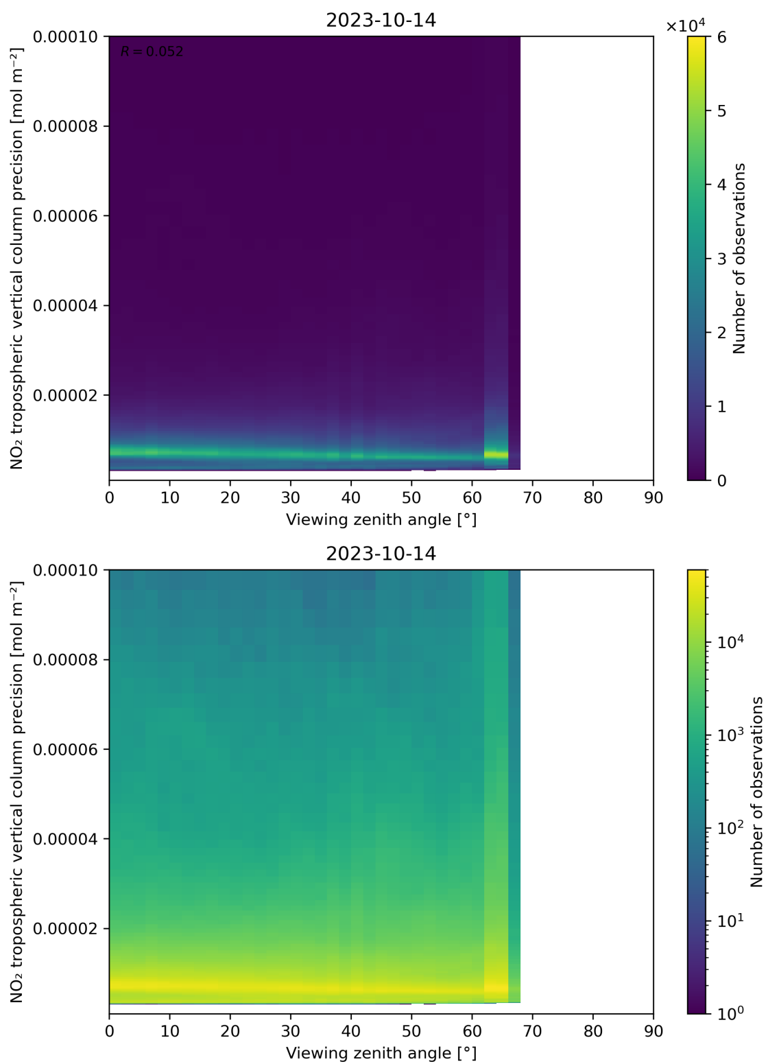
Figure 170: Scatter density plot of “Viewing zenith angle” against “NO 2 tropospheric vertical column precision” for 2023-10-13 to 2023-10-15.
