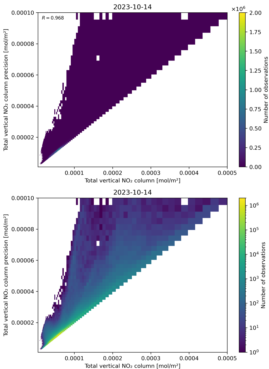
Figure 114: Scatter density plot of “Total vertical NO 2 column” against “Total vertical NO 2 column precision” for 2023-10-13 to 2023-10-15.
