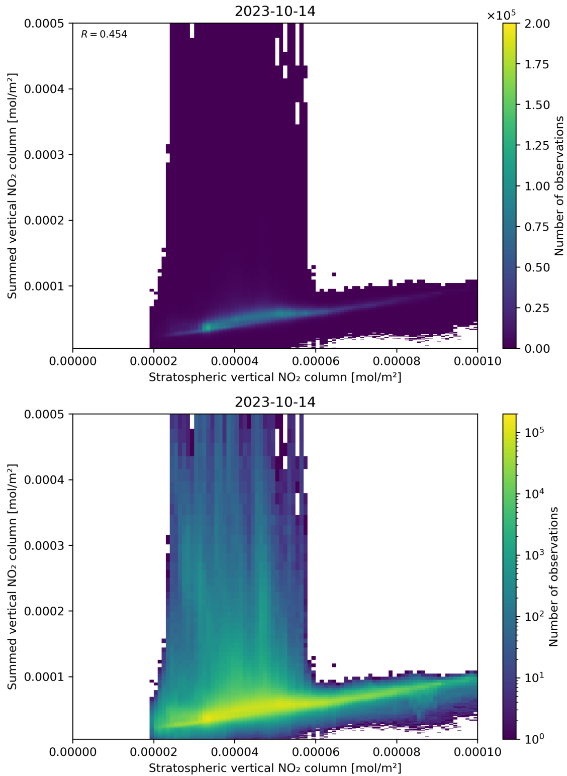
Figure 98: Scatter density plot of “Stratospheric vertical NO 2 column” against “Summed vertical NO 2 column” for 2023-10-13 to 2023-10-15.
