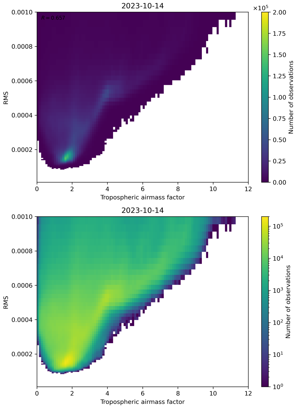
Figure 79: Scatter density plot of “Tropospheric airmass factor” against “RMS” for 2023-10-13 to 2023-10-15.
