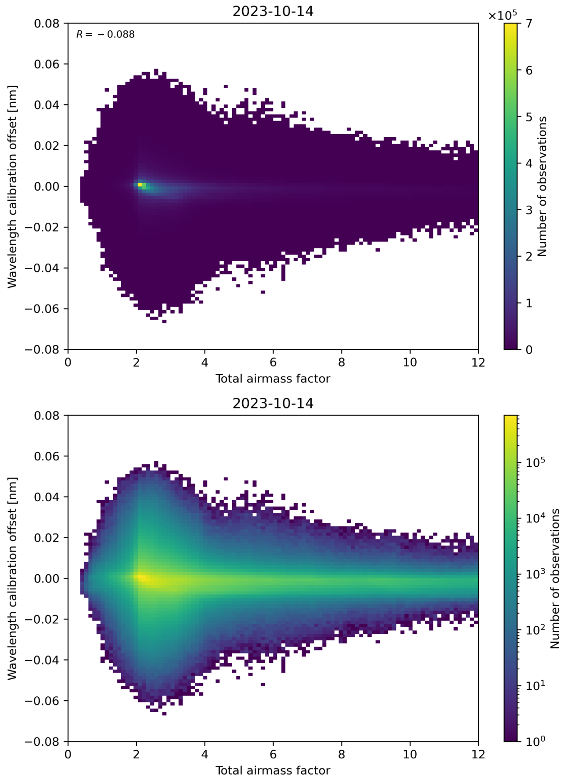
Figure 70: Scatter density plot of “Total airmass factor” against “Wavelength calibration offset” for 2023-10-13 to 2023-10-15.
