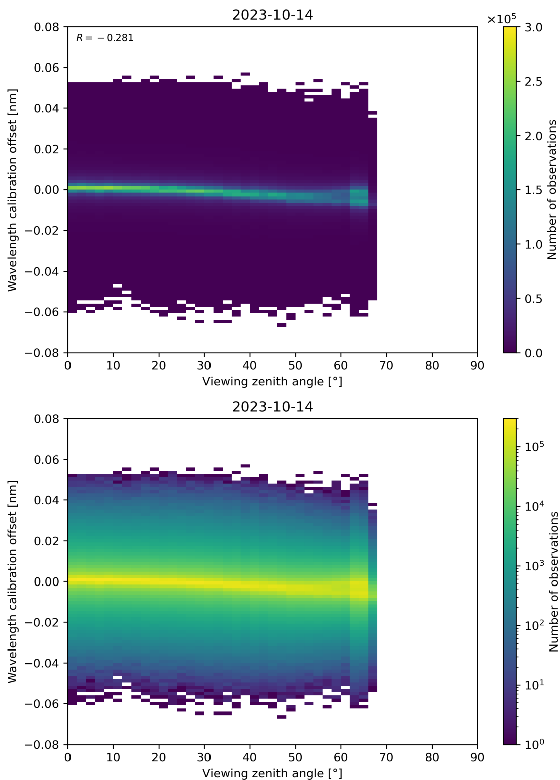
Figure 173: Scatter density plot of “Viewing zenith angle” against “Wavelength calibration offset” for 2023-10-13 to 2023-10-15.
