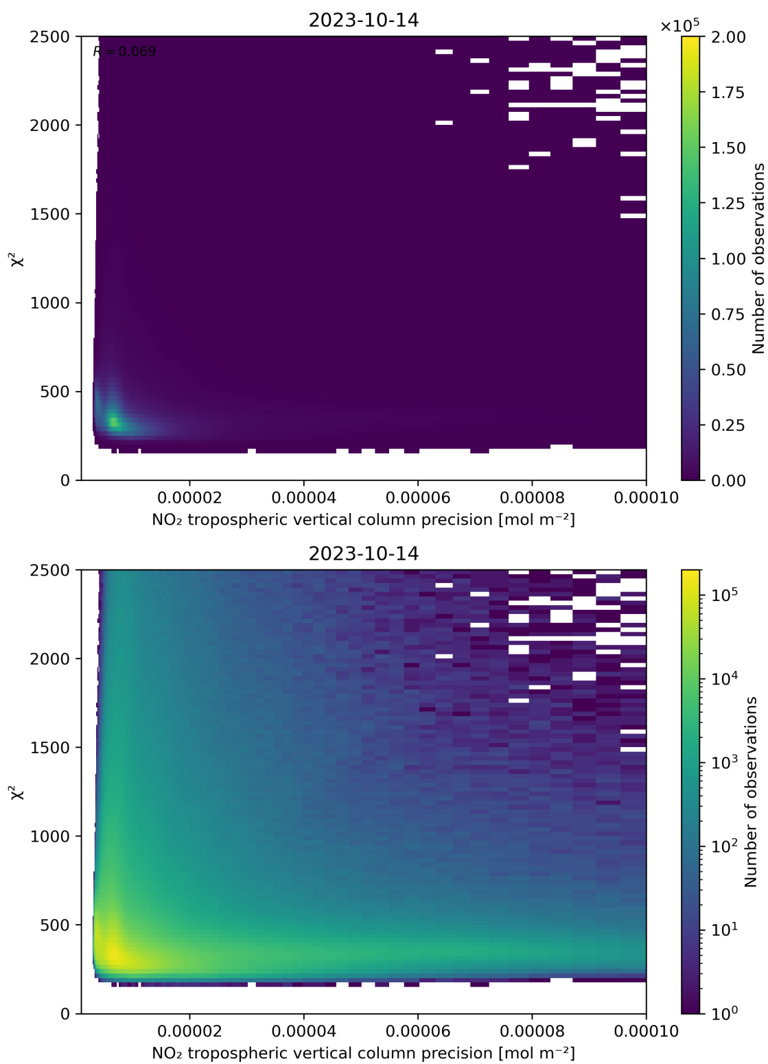
Figure 134: Scatter density plot of “NO 2 tropospheric vertical column precision” against “ \chi^2 ” for 2023-10-13 to 2023-10-15.
