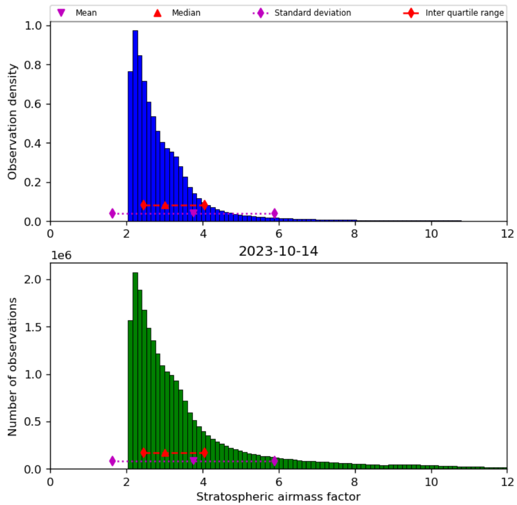
Figure 44: Histogram of “Stratospheric airmass factor” for 2023-10-13 to 2023-10-15
