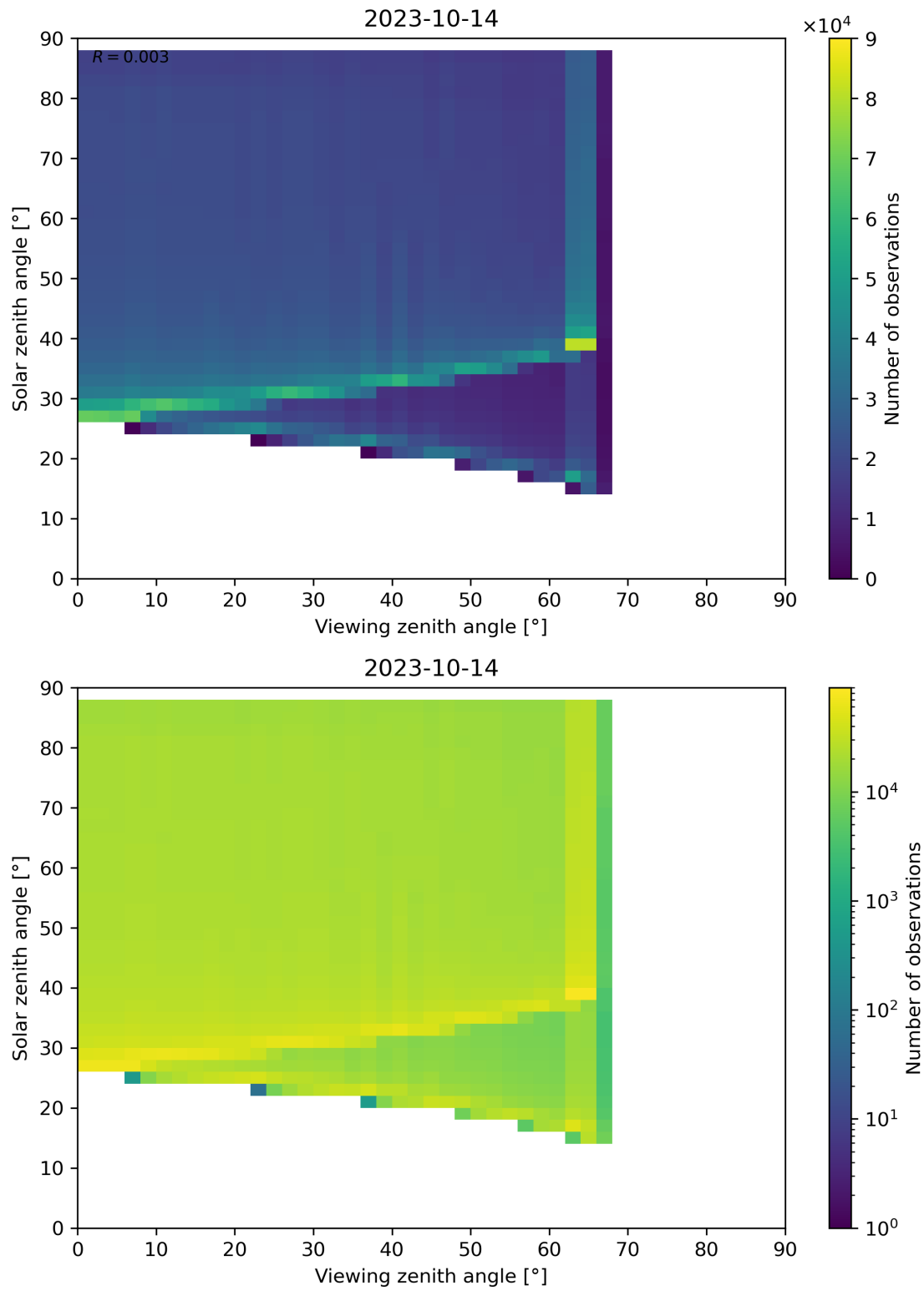
Figure 172: Scatter density plot of “Viewing zenith angle” against “Solar zenith angle” for 2023-10-13 to 2023-10-15.
