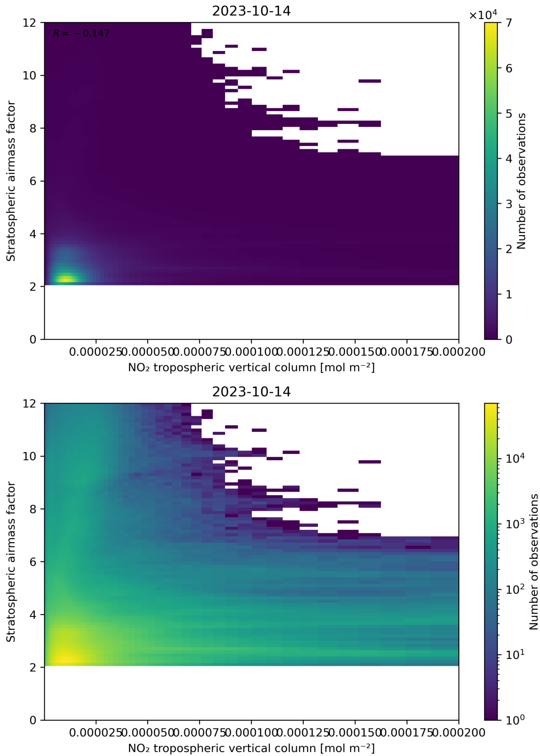
Figure 121: Scatter density plot of “NO 2 tropospheric vertical column” against “Stratospheric air mass factor” for 2023-10-13 to 2023-10-15.
