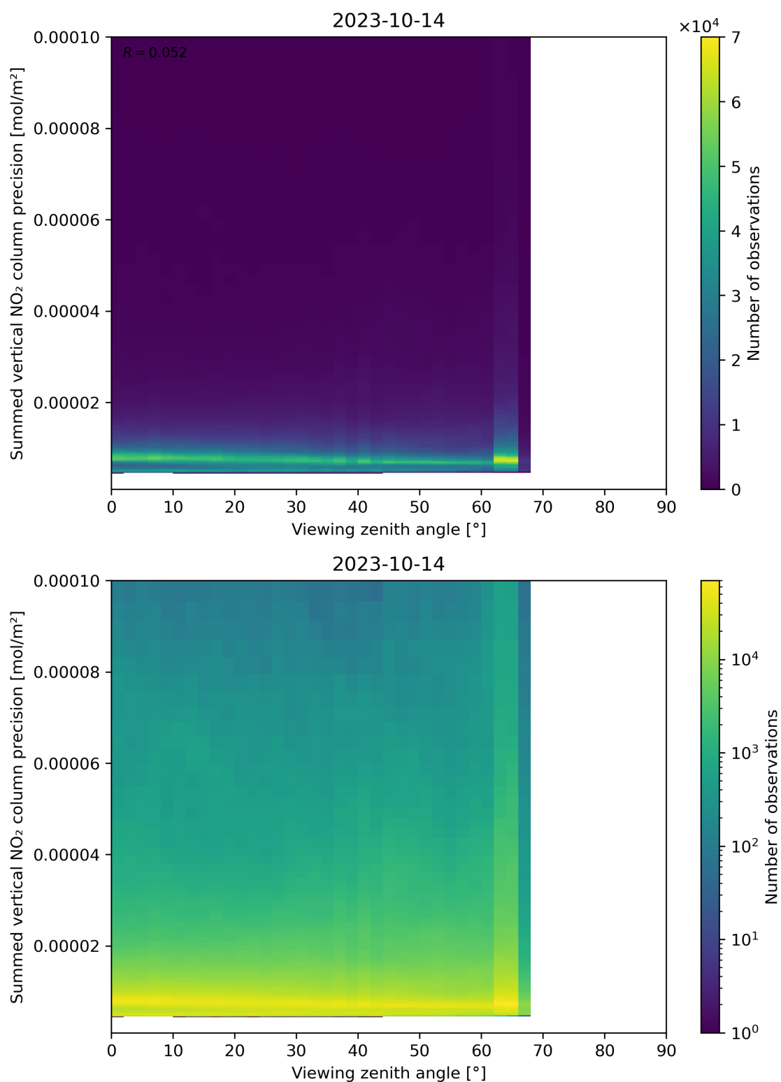
Figure 166: Scatter density plot of “Viewing zenith angle” against “Summed vertical NO 2 column precision” for 2023-10-13 to 2023-10-15.
