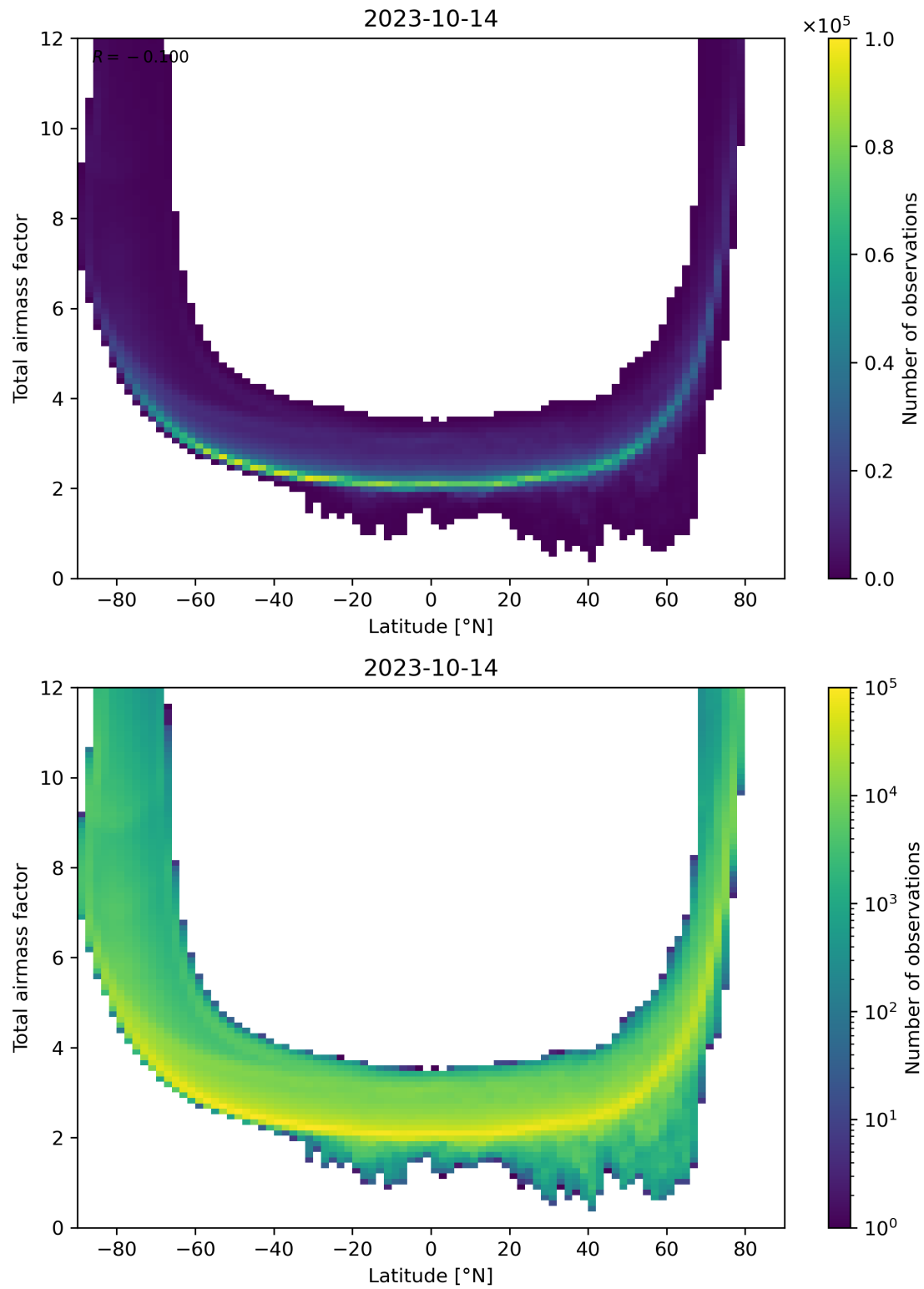
Figure 84: Scatter density plot of “Latitude” against “Total airmass factor” for 2023-10-13 to 2023-10-15.
