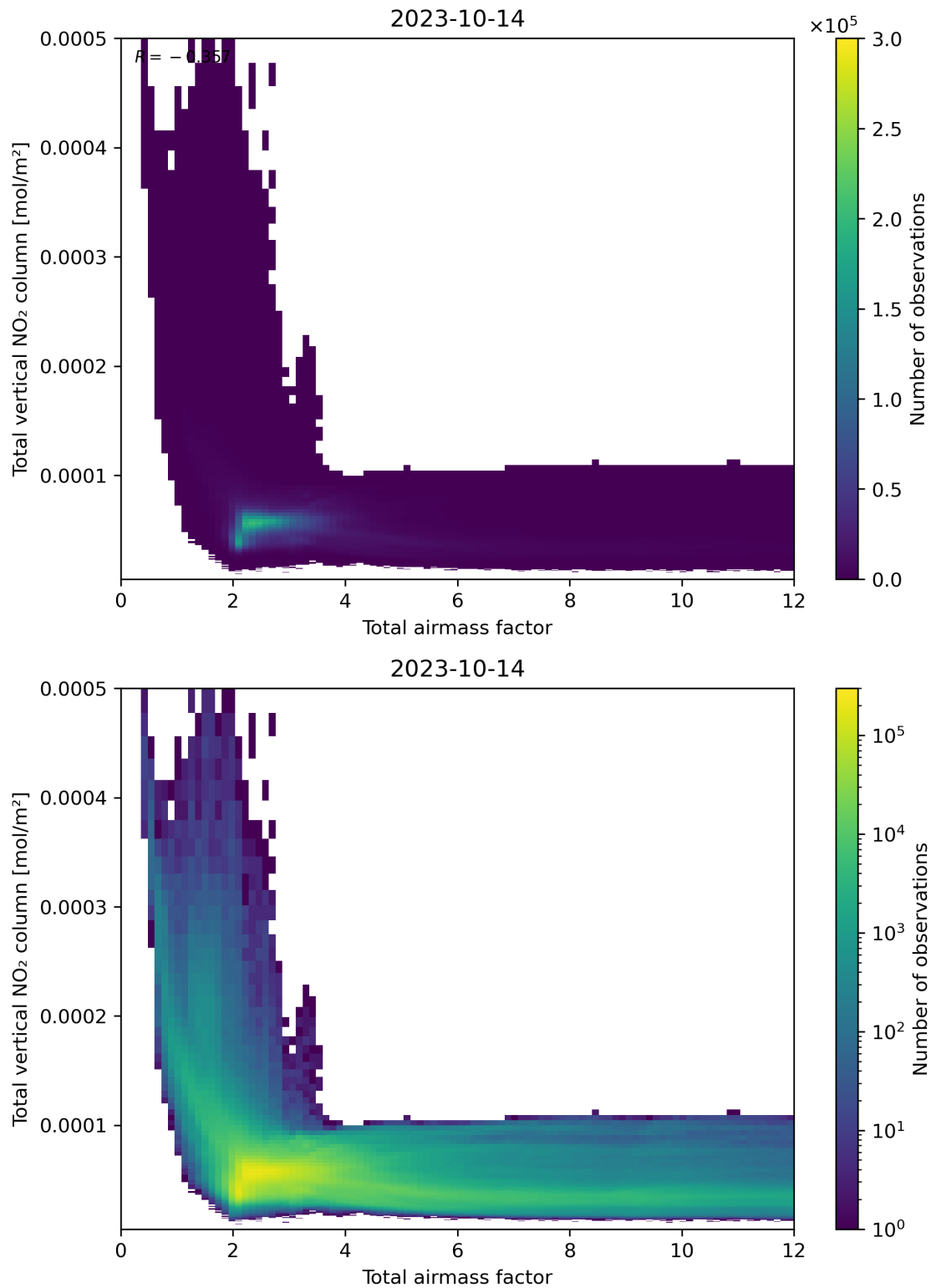
Figure 67: Scatter density plot of “Total airmass factor” against “Total vertical NO 2 column” for 2023-10-13 to 2023-10-15.
