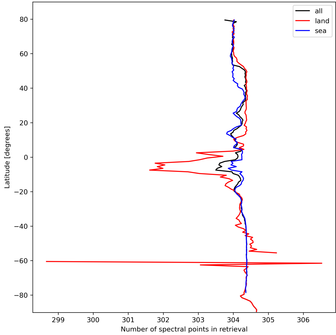
Figure 16: Zonal average of “Number of spectral points in retrieval” for 2023-10-13 to 2023-10-15.
