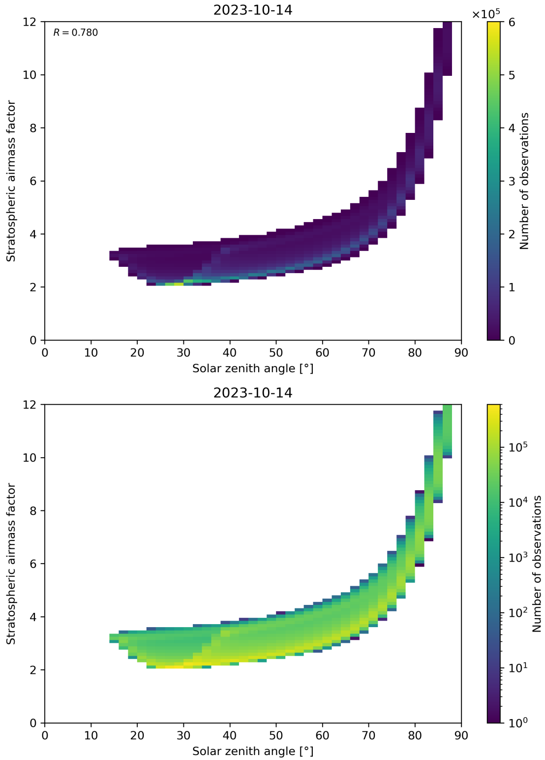
Figure 145: Scatter density plot of “Solar zenith angle” against “Stratospheric airmass factor” for 2023-10-13 to 2023-10-15.
