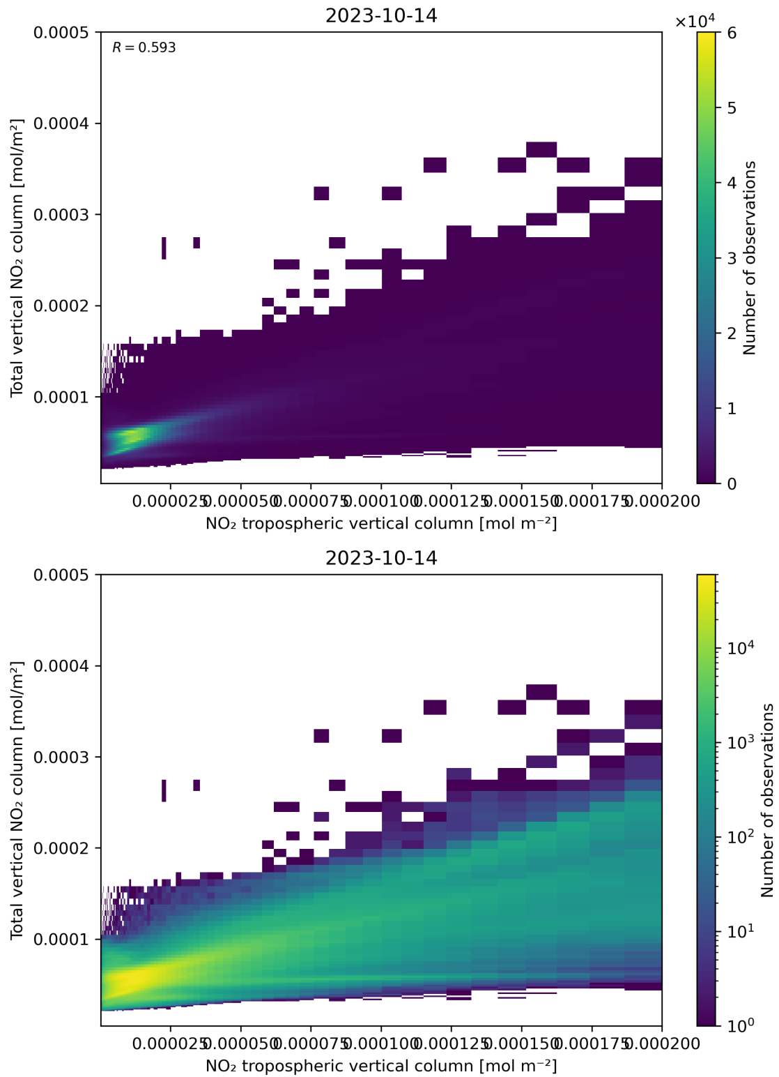
Figure 128: Scatter density plot of “NO 2 tropospheric vertical column” against “Total vertical NO 2 column” for 2023-10-13 to 2023-10-15.
