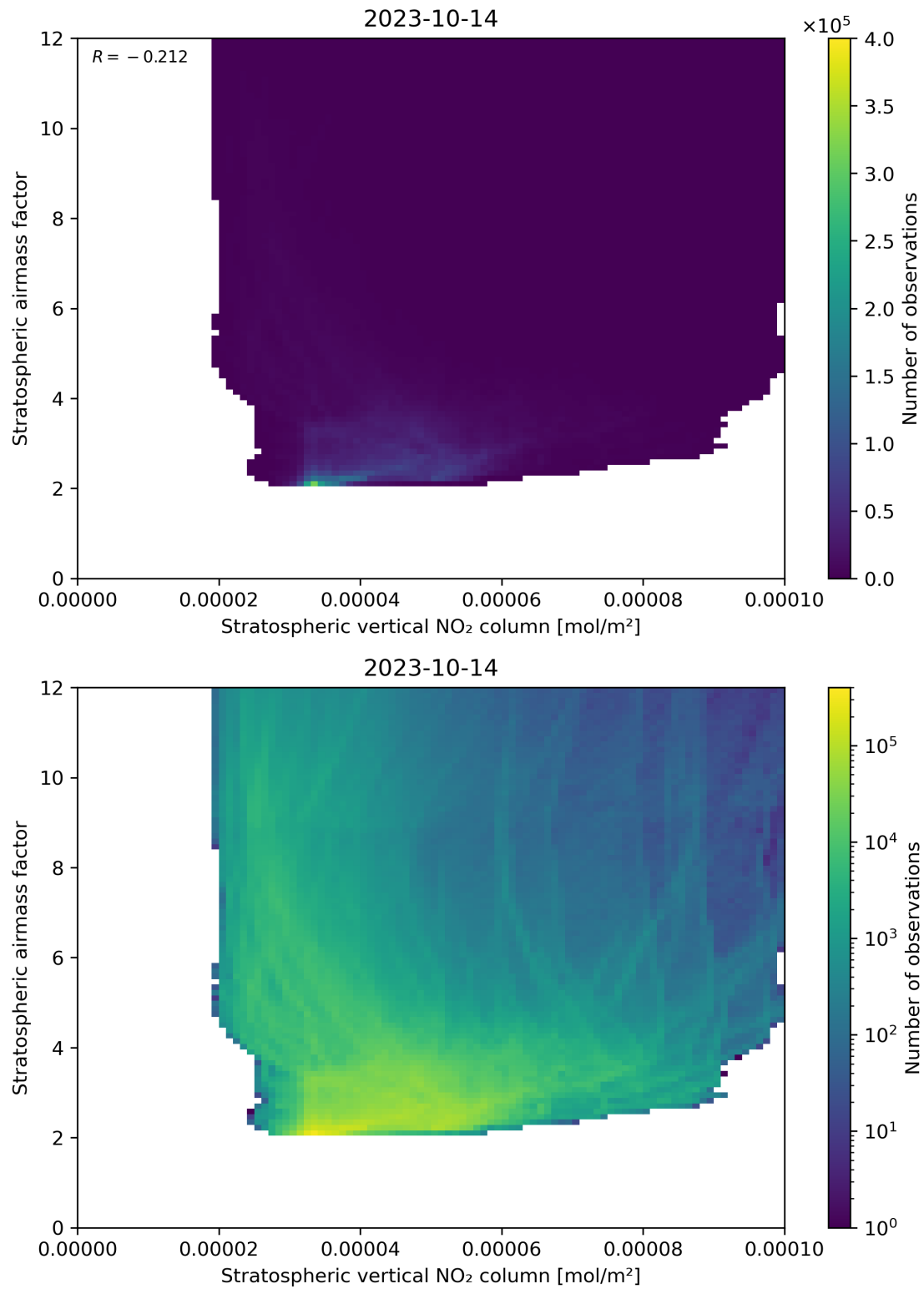
Figure 96: Scatter density plot of “Stratospheric vertical NO 2 column” against “Stratospheric airmass factor” for 2023-10-13 to 2023-10-15.
