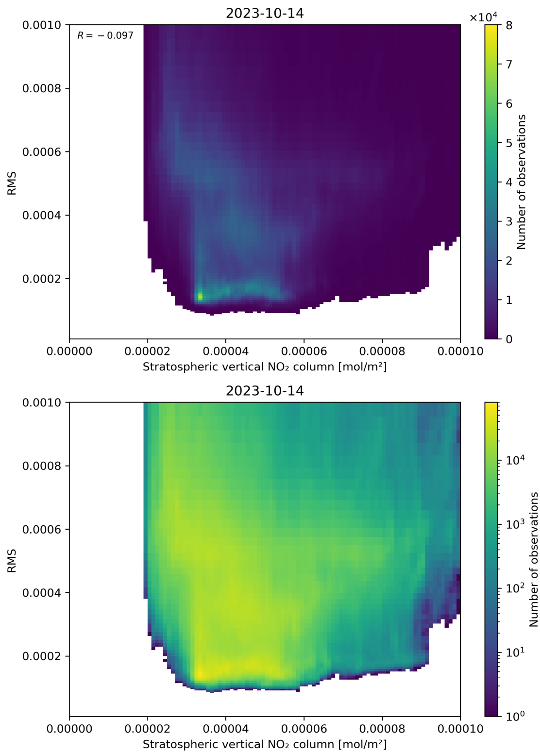
Figure 102: Scatter density plot of “Stratospheric vertical NO 2 column” against “RMS” for 2023-10-13 to 2023-10-15.
