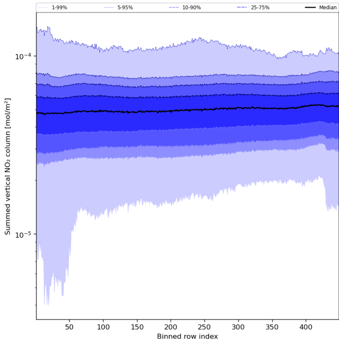
Figure 57: Along track statistics of “Summed vertical NO 2 column” for 2023-10-13 to 2023-10-15
