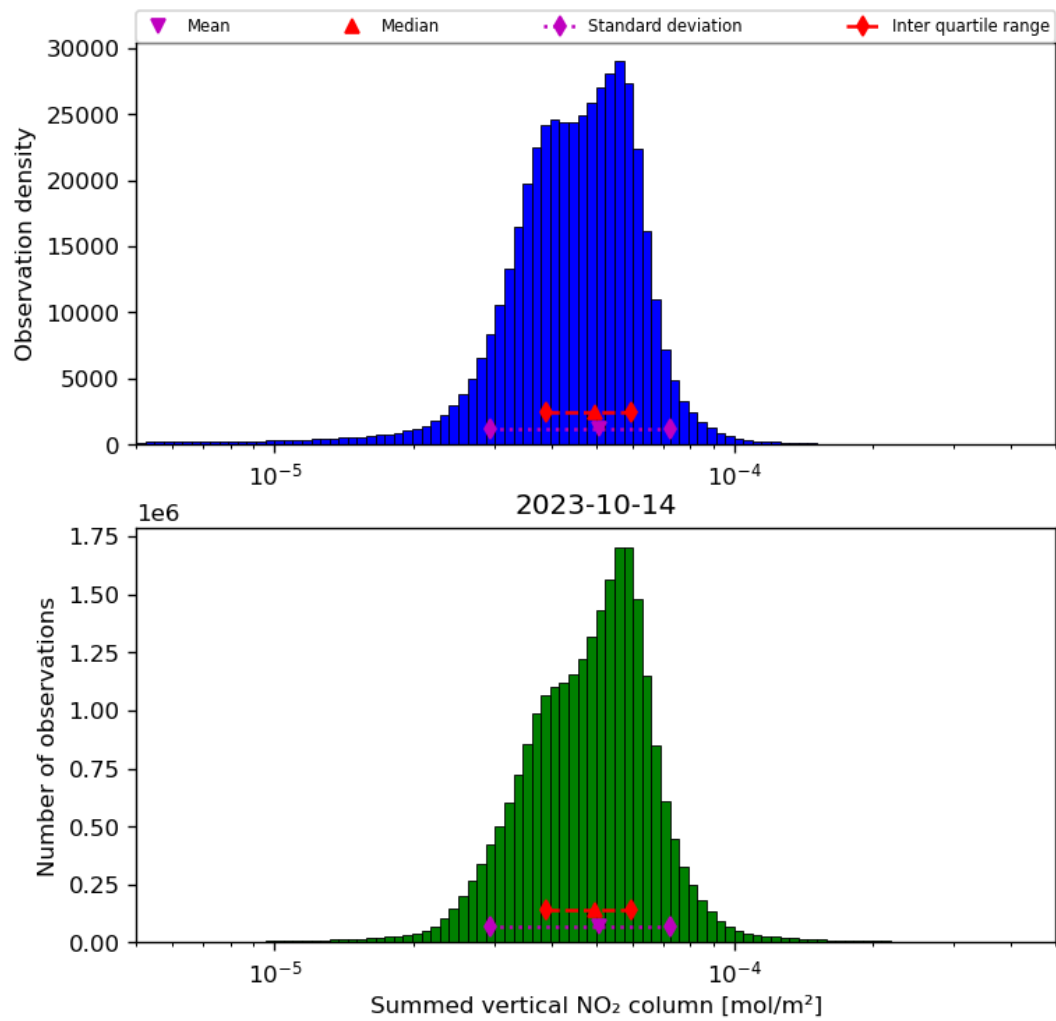
Figure 40: Histogram of “Summed vertical NO 2 column” for 2023-10-13 to 2023-10-15
