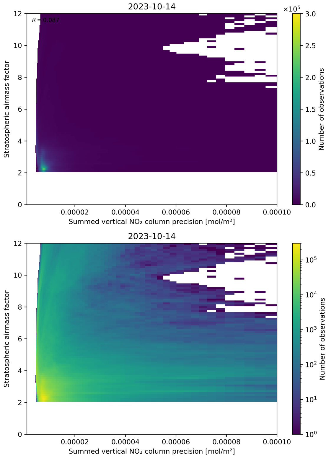
Figure 106: Scatter density plot of “Summed vertical NO 2 column precision” against “Stratospheric airmass factor” for 2023-10-13 to 2023-10-15.
