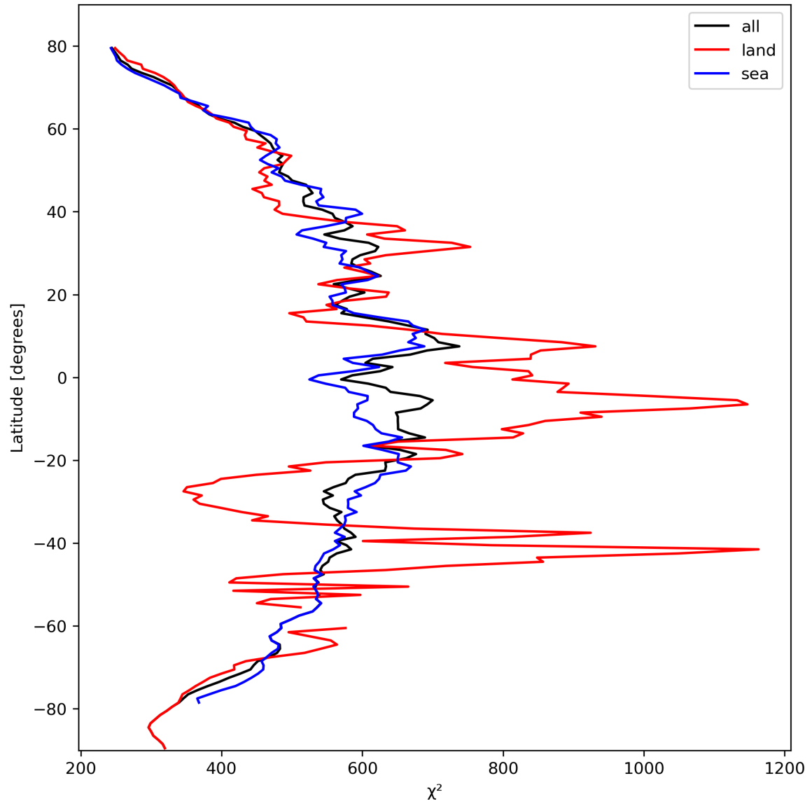
Figure 25: Zonal average of “ \chi^2 ” for 2023-10-13 to 2023-10-15.
