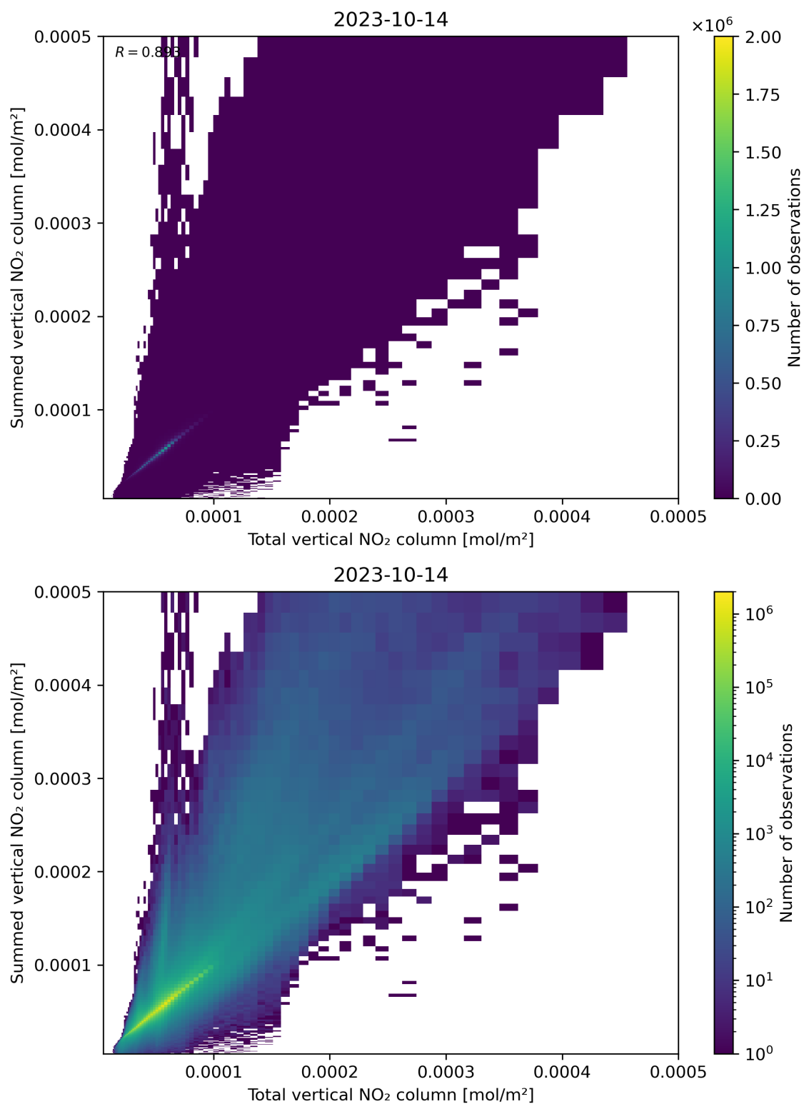
Figure 112: Scatter density plot of “Total vertical NO 2 column” against “Summed vertical NO 2 column” for 2023-10-13 to 2023-10-15.
