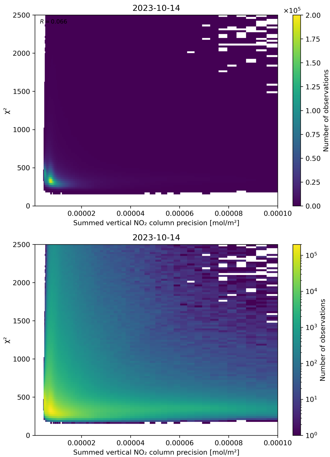
Figure 107: Scatter density plot of “Summed vertical NO 2 column precision” against “ \chi^2 ” for 2023-10-13 to 2023-10-15.
