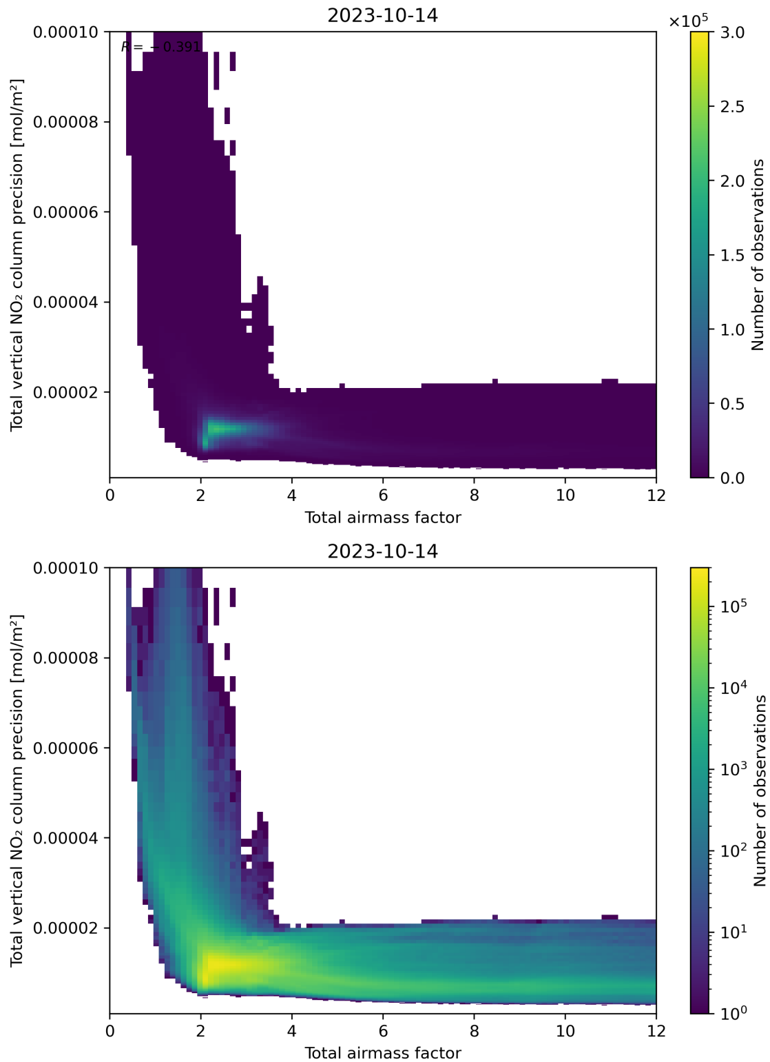
Figure 68: Scatter density plot of “Total airmass factor” against “Total vertical NO 2 column precision” for 2023-10-13 to 2023-10-15.
