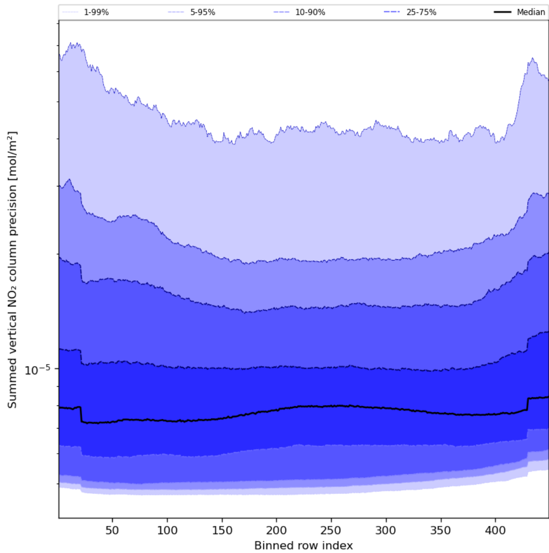
Figure 58: Along track statistics of “Summed vertical NO 2 column precision” for 2023-10-13 to 2023-10-15
