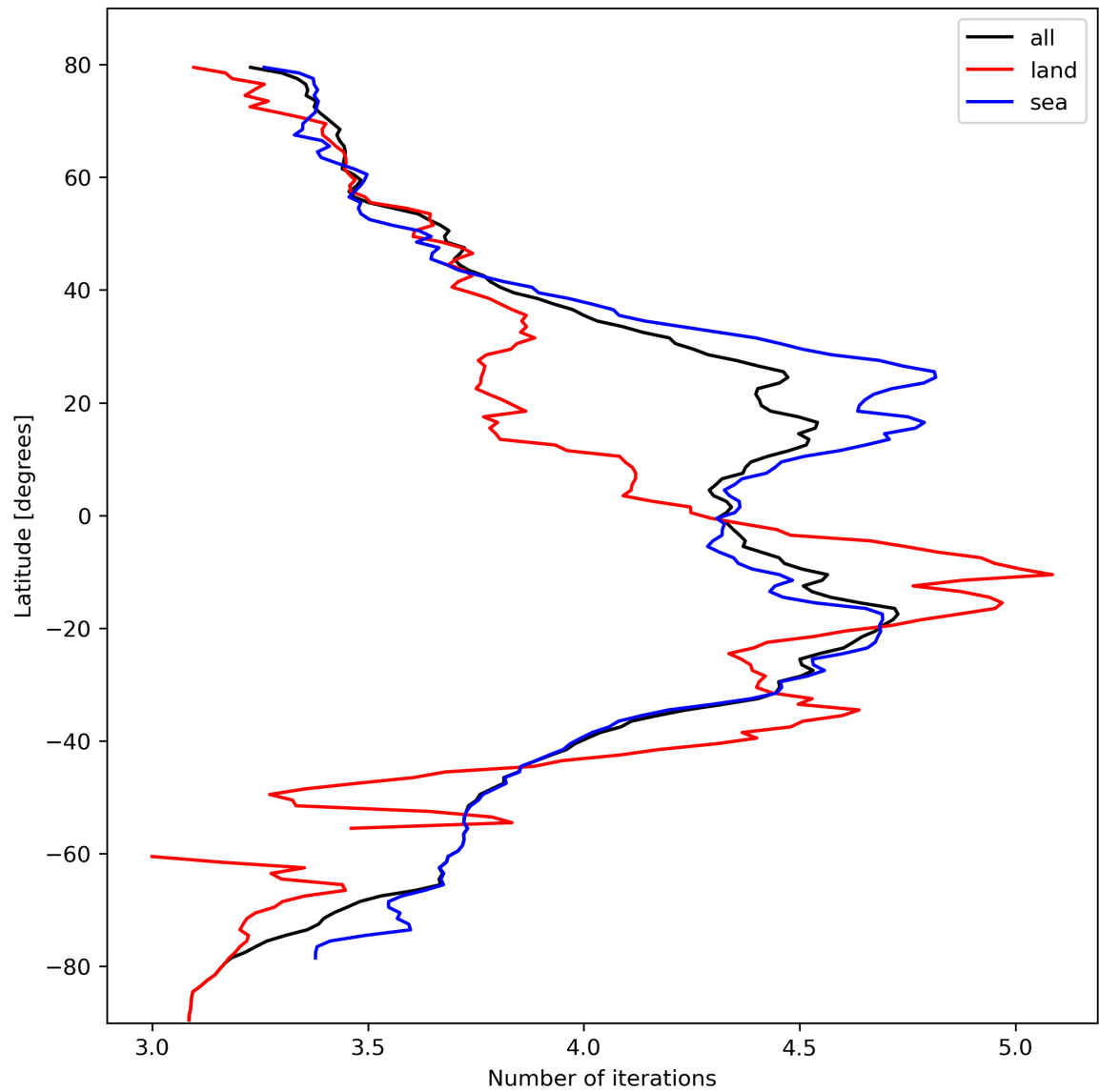
Figure 17: Zonal average of “Number of iterations” for 2023-10-13 to 2023-10-15.
