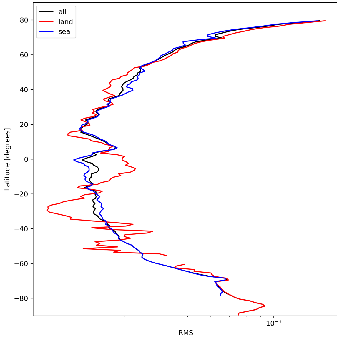
Figure 26: Zonal average of “RMS” for 2023-10-13 to 2023-10-15.
