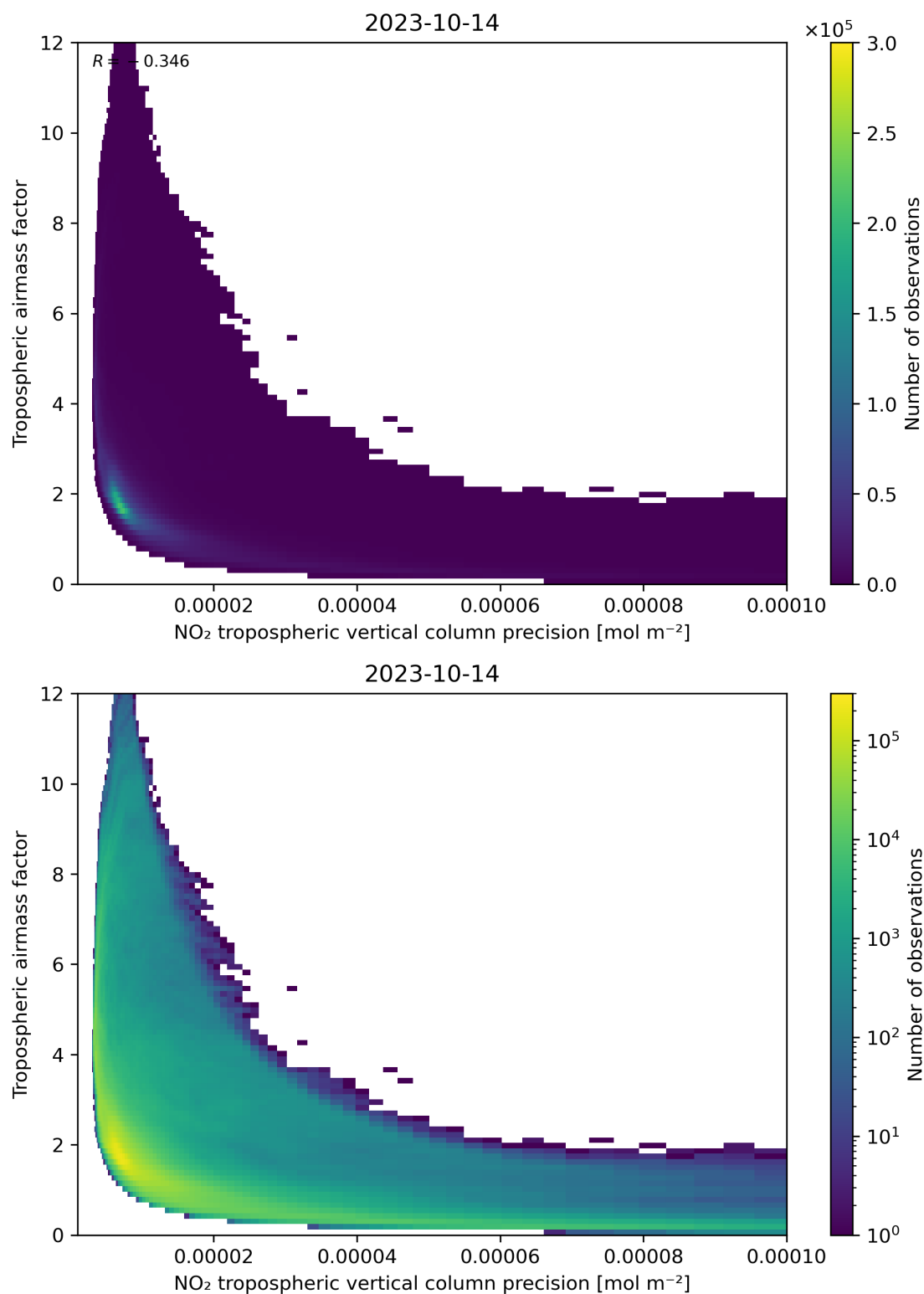
Figure 133: Scatter density plot of “NO 2 tropospheric vertical column precision” against “Tropospheric airmass factor” for 2023-10-13 to 2023-10-15.
