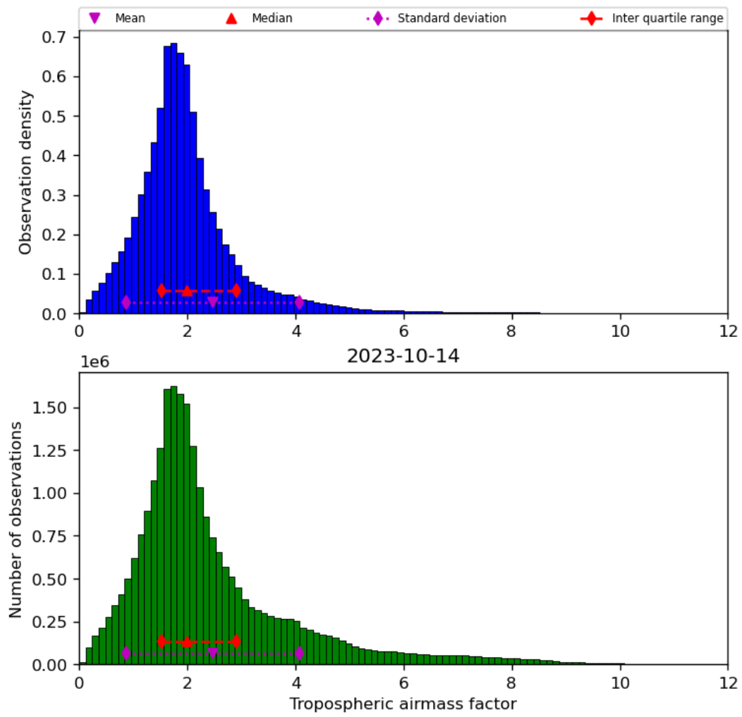
Figure 31: Histogram of “Tropospheric airmass factor” for 2023-10-13 to 2023-10-15
