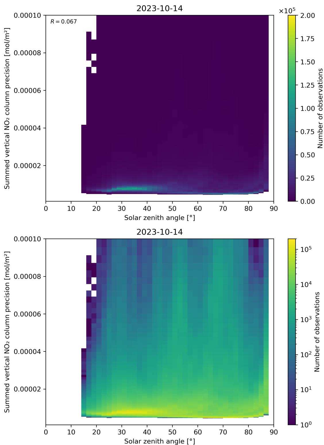
Figure 152: Scatter density plot of “Solar zenith angle” against “Summed vertical NO 2 column precision” for 2023-10-13 to 2023-10-15.
