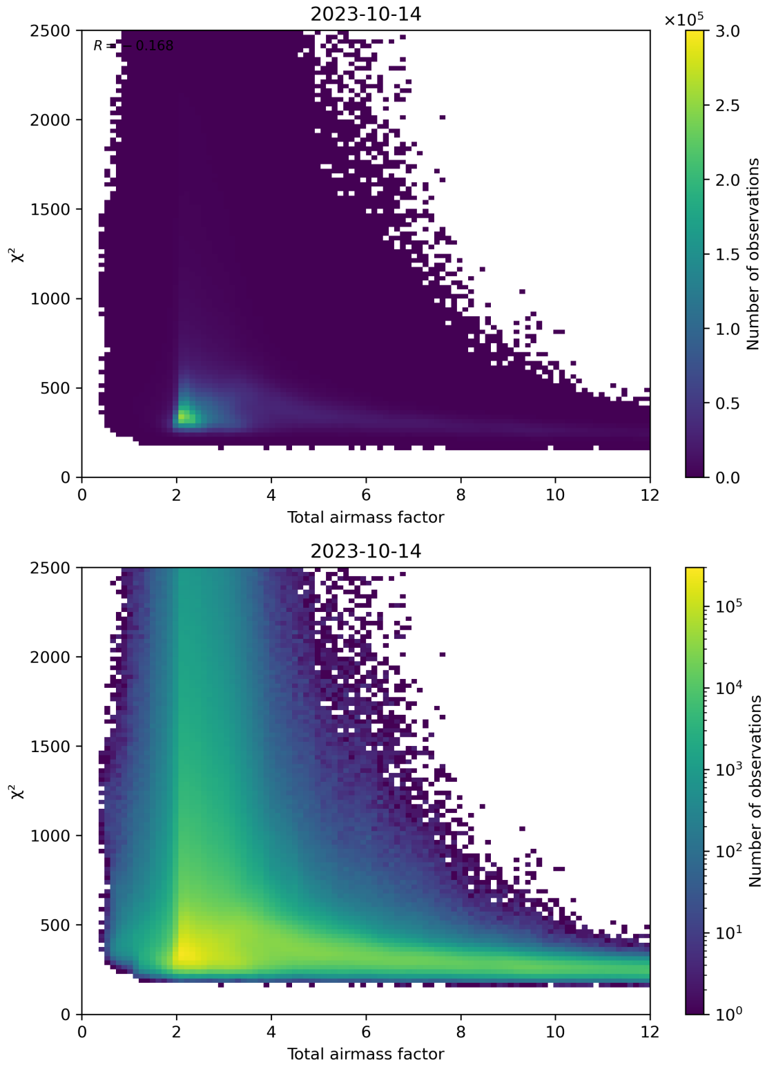
Figure 63: Scatter density plot of “Total airmass factor” against “ \chi^2 ” for 2023-10-13 to 2023-10-15.
