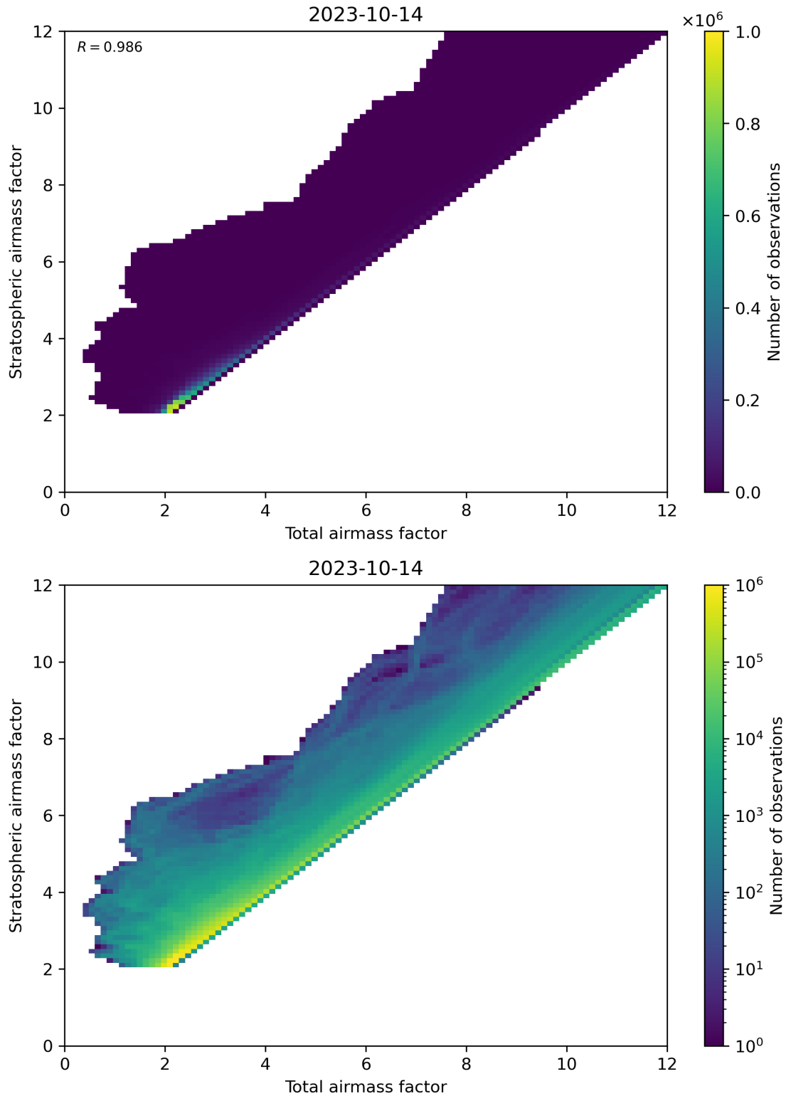
Figure 62: Scatter density plot of “Total airmass factor” against “Stratospheric airmass factor” for 2023-10-13 to 2023-10-15.
