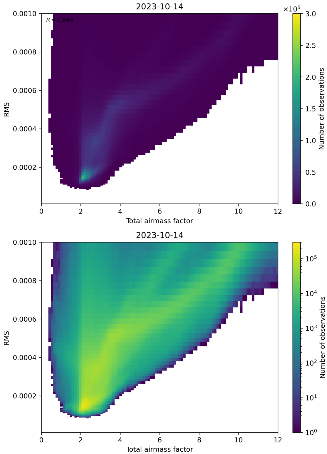
Figure 69: Scatter density plot of “Total airmass factor” against “RMS” for 2023-10-13 to 2023-10-15.
