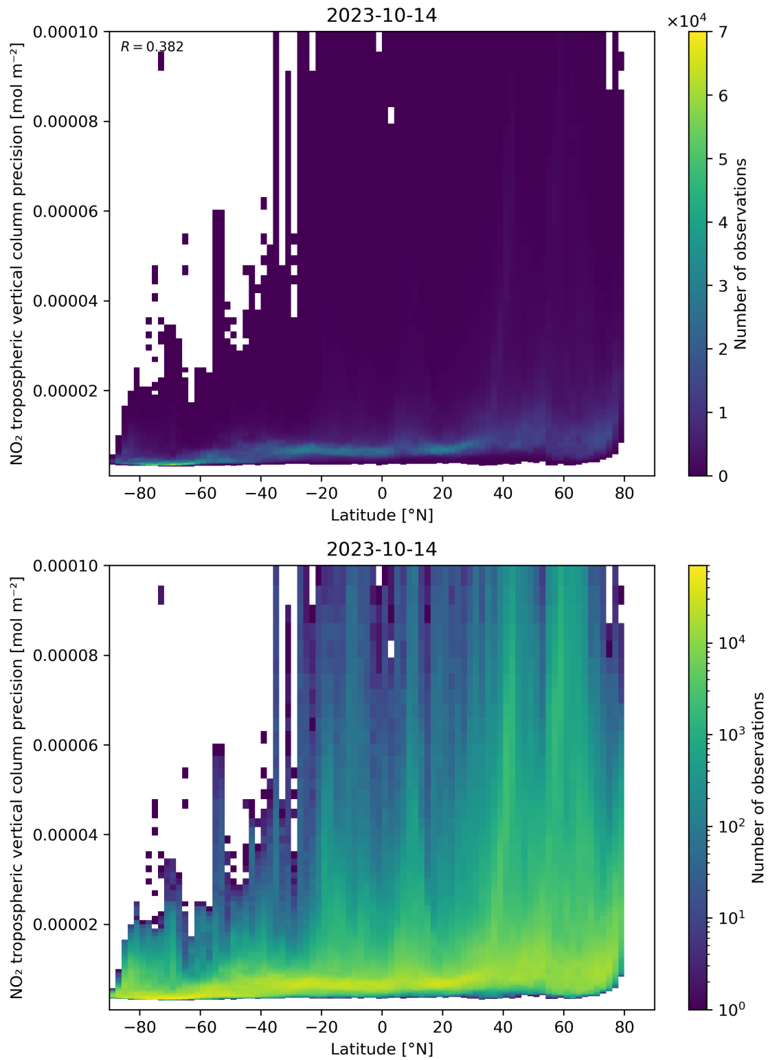
Figure 93: Scatter density plot of “Latitude” against “NO 2 tropospheric vertical column precision” for 2023-10-13 to 2023-10-15.
