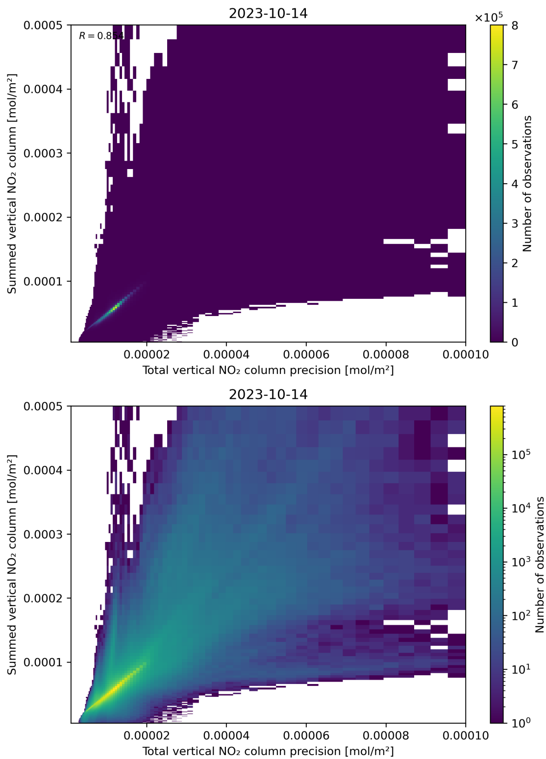
Figure 117: Scatter density plot of “Total vertical NO 2 column precision” against “Summed vertical NO 2 column” for 2023-10-13 to 2023-10-15.
