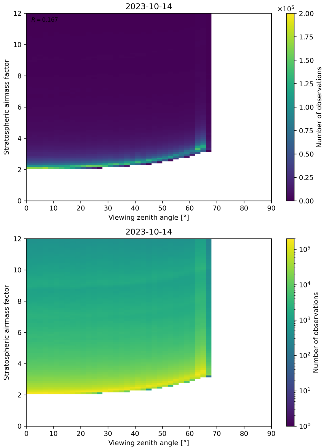
Figure 159: Scatter density plot of “Viewing zenith angle” against “Stratospheric airmass factor” for 2023-10-13 to 2023-10-15.
