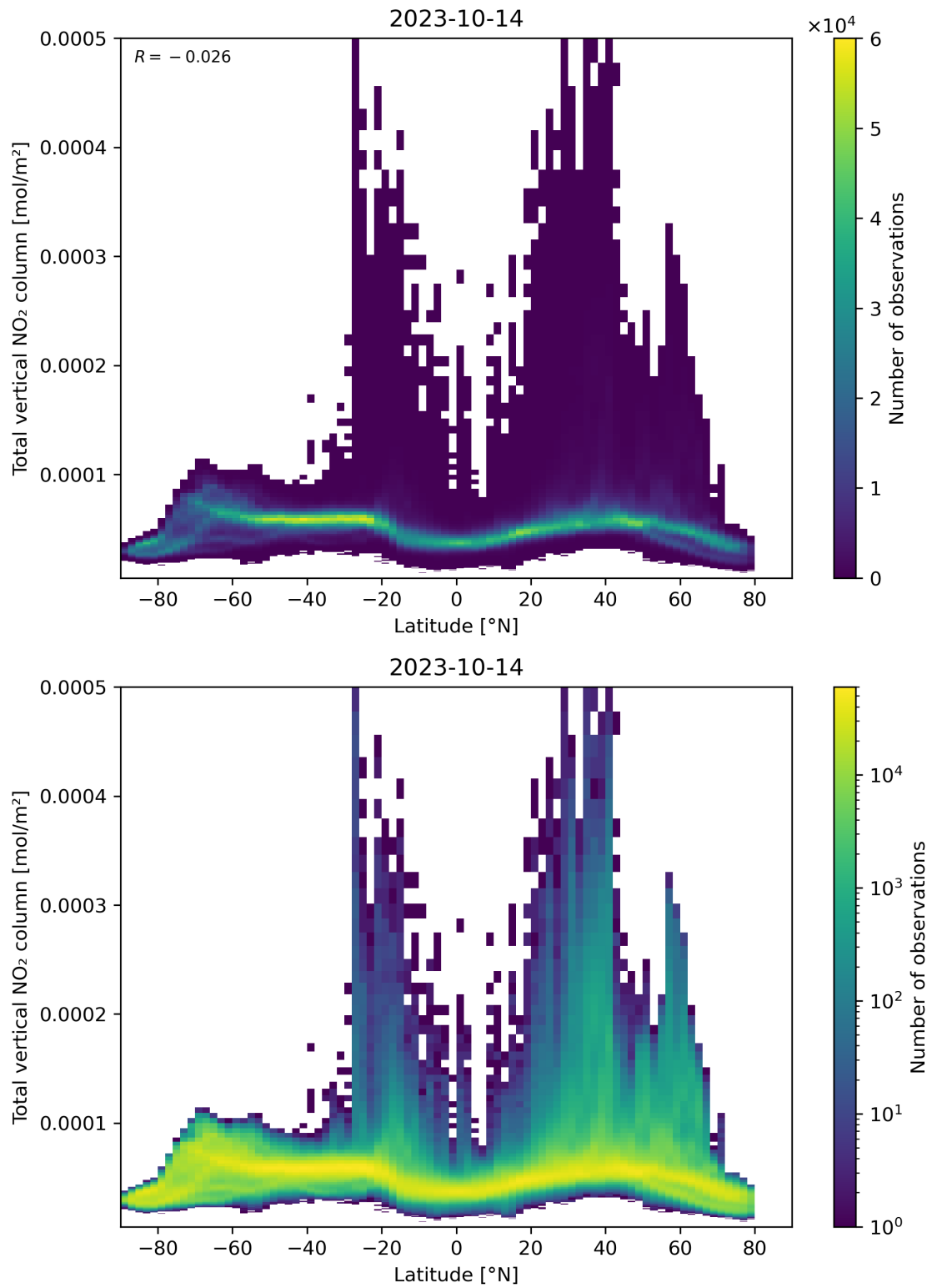
Figure 90: Scatter density plot of “Latitude” against “Total vertical NO 2 column” for 2023-10-13 to 2023-10-15.
