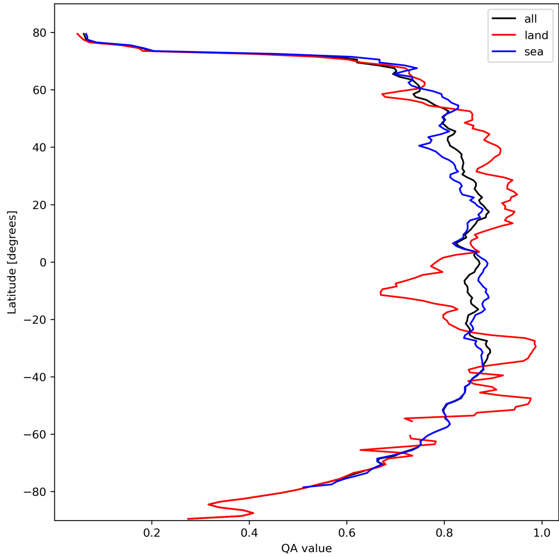
Figure 11: Zonal average of “QA value” for 2023-10-13 to 2023-10-15.
