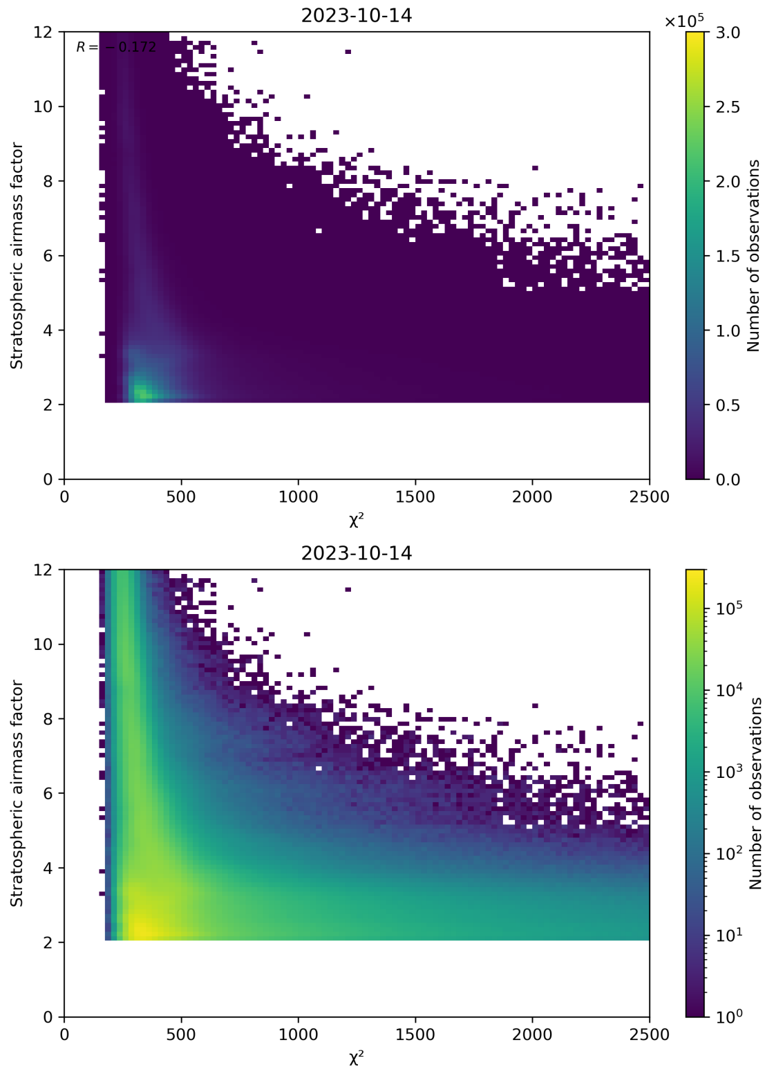
Figure 81: Scatter density plot of “ \chi^2 ” against “Stratospheric airmass factor” for 2023-10-13 to 2023-10-15.
