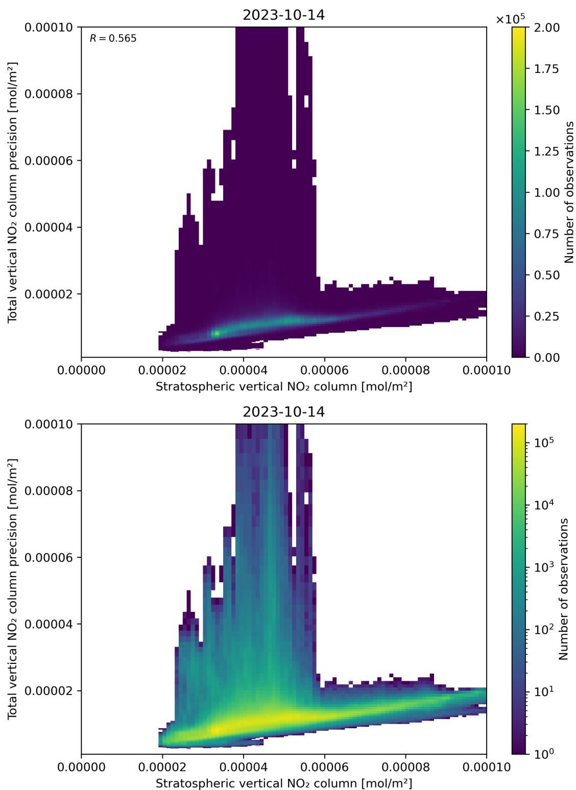
Figure 101: Scatter density plot of “Stratospheric vertical NO 2 column” against “Total vertical NO 2 column precision” for 2023-10-13 to 2023-10-15.
