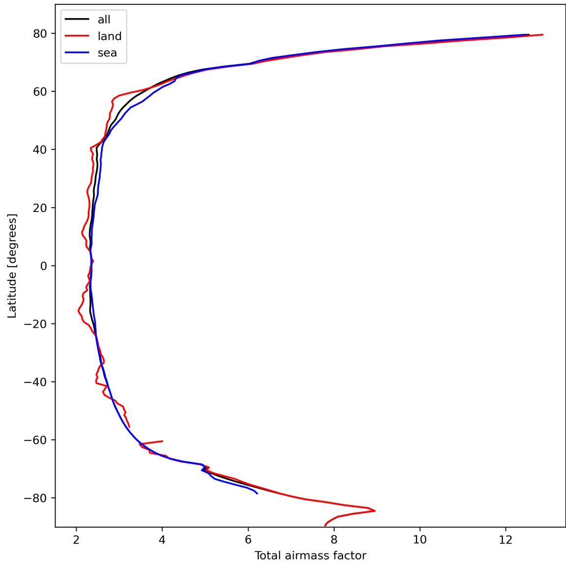
Figure 15: Zonal average of “Total airmass factor” for 2023-10-13 to 2023-10-15.
