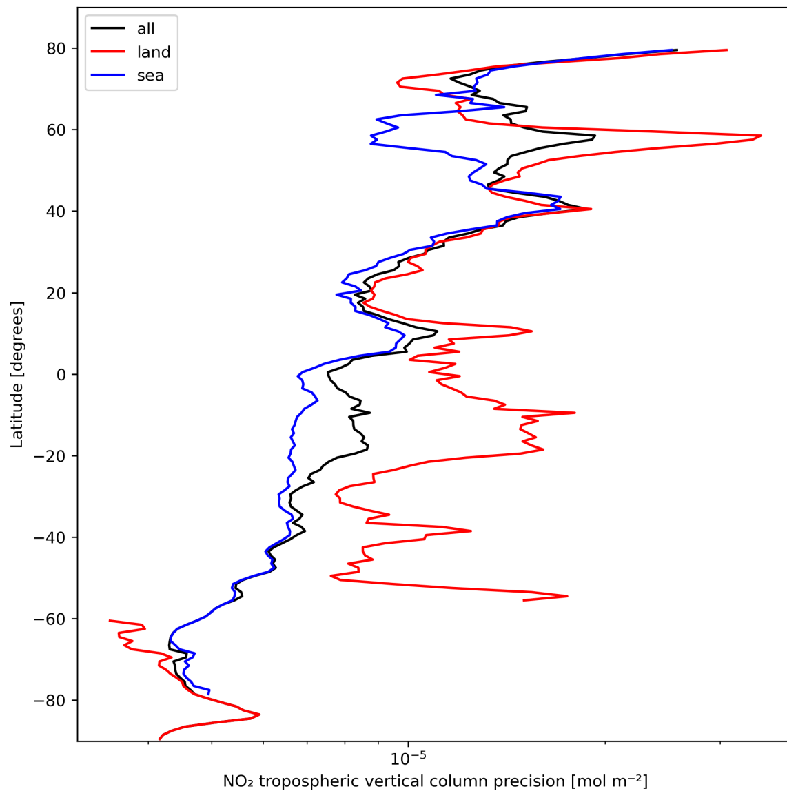
Figure 13: Zonal average of “NO 2 tropospheric vertical column precision” for 2023-10-13 to 2023-10-15.
