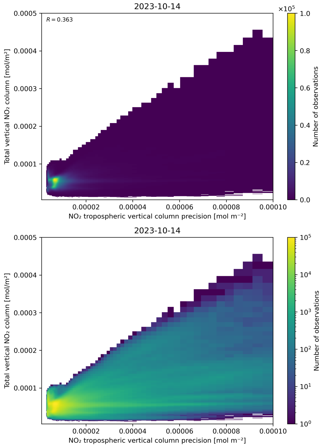
Figure 138: Scatter density plot of “NO 2 tropospheric vertical column precision” against “Total vertical NO 2 column” for 2023-10-13 to 2023-10-15.
