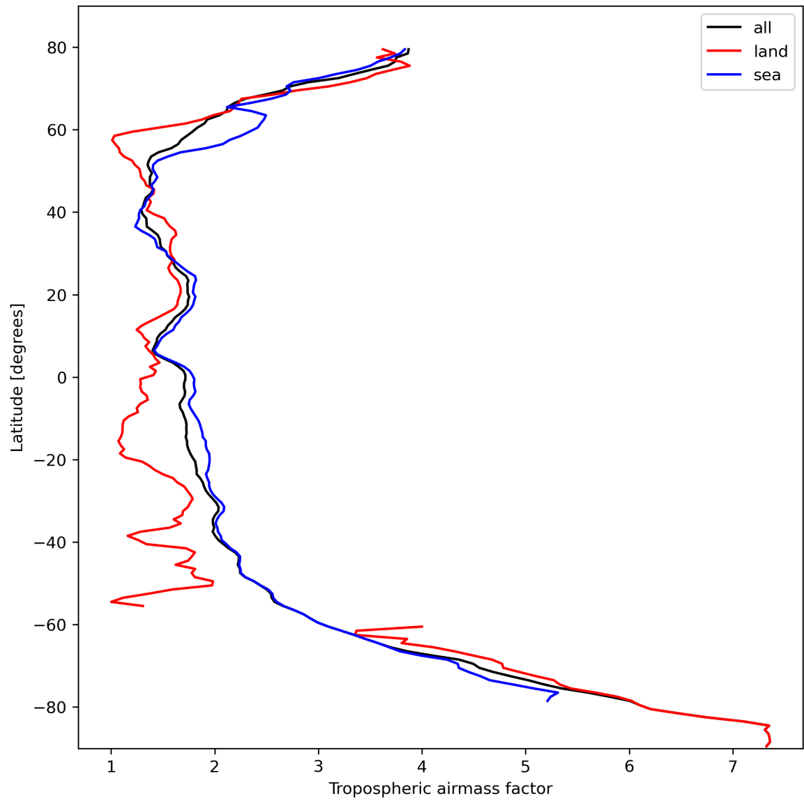
Figure 14: Zonal average of “Tropospheric airmass factor” for 2023-10-13 to 2023-10-15.
