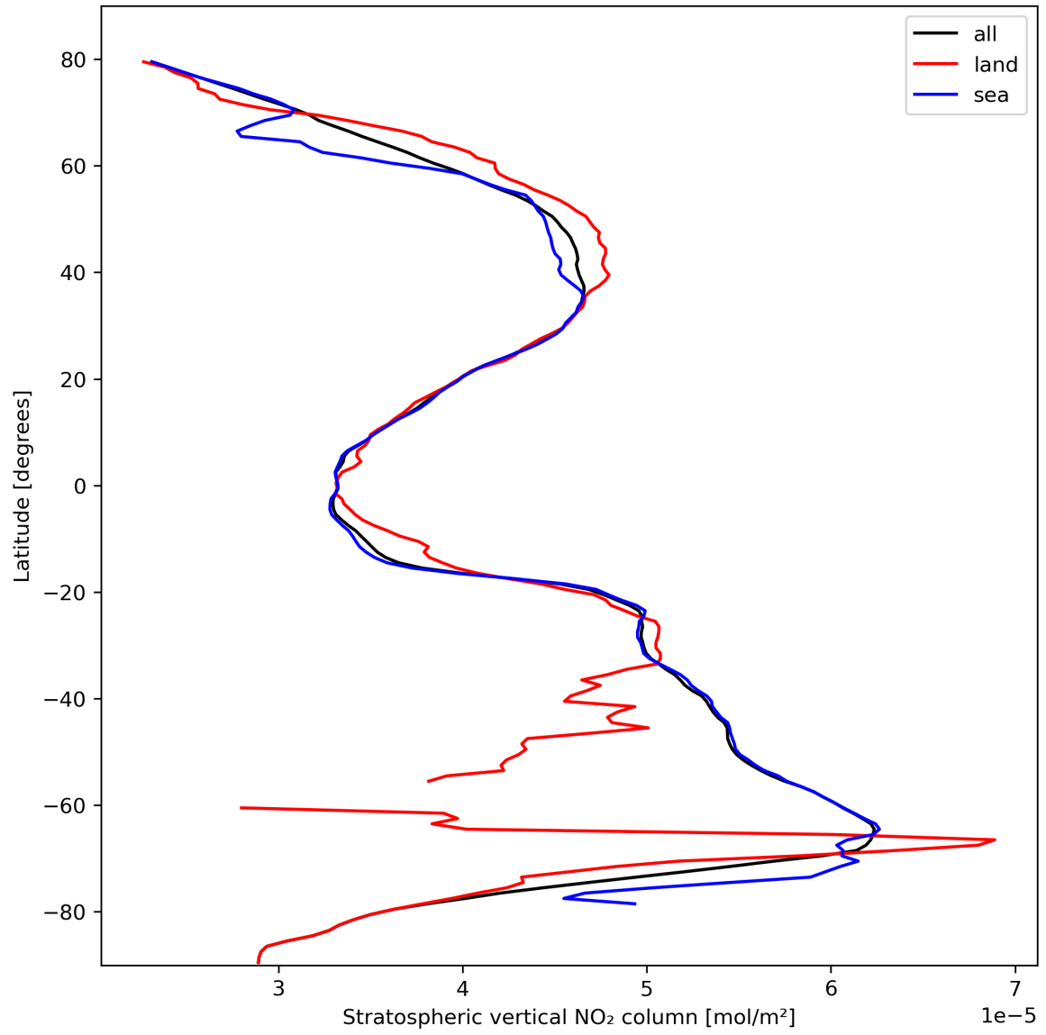
Figure 19: Zonal average of “Stratospheric vertical NO 2 column” for 2023-10-13 to 2023-10-15.
