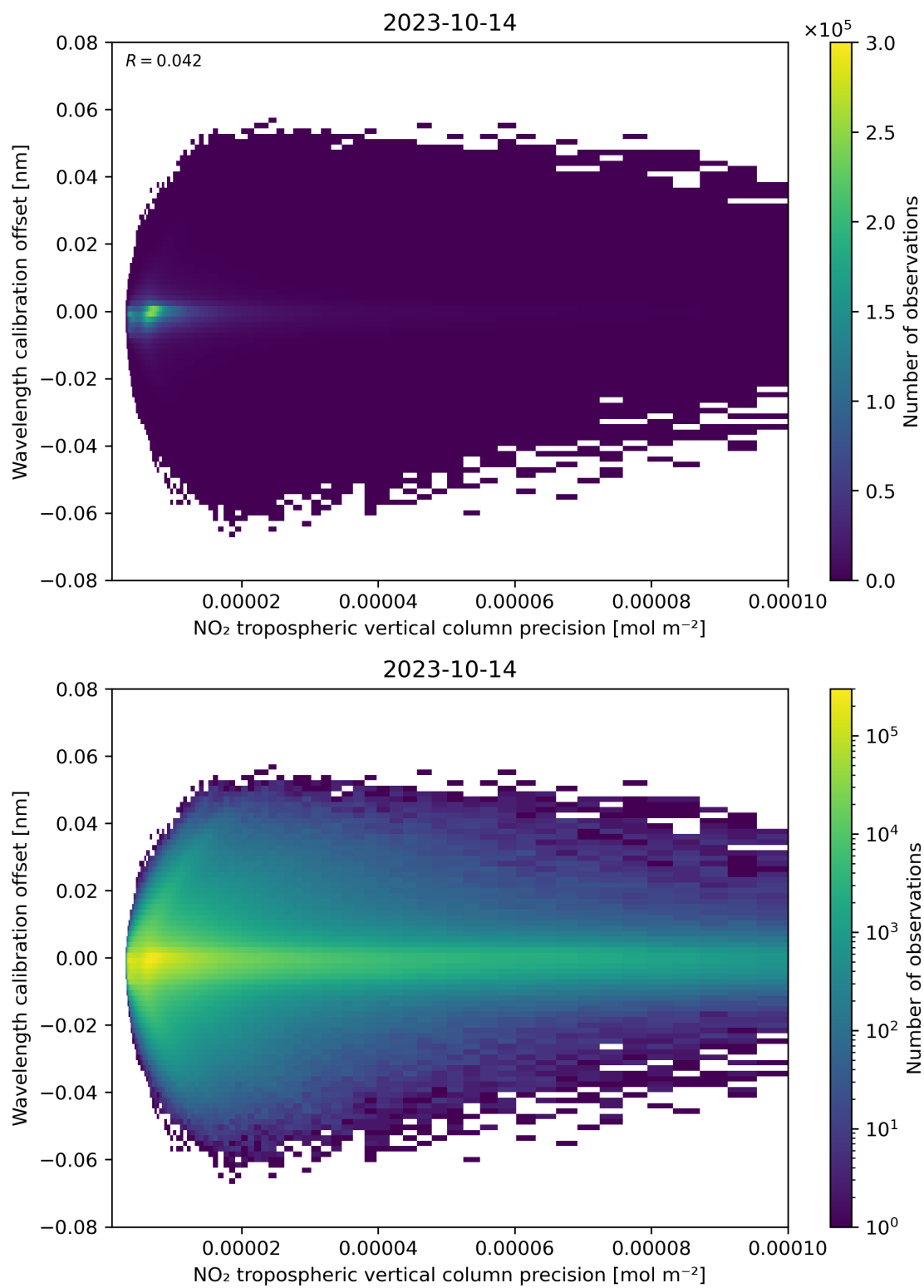
Figure 141: Scatter density plot of “NO 2 tropospheric vertical column precision” against “Wavelength calibration offset” for 2023-10-13 to 2023-10-15.
