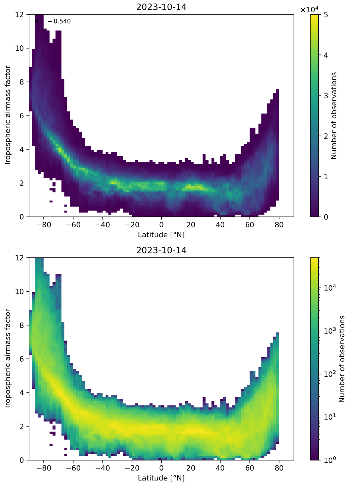
Figure 85: Scatter density plot of “Latitude” against “Tropospheric air mass factor” for 2023-10-13 to 2023-10-15.
