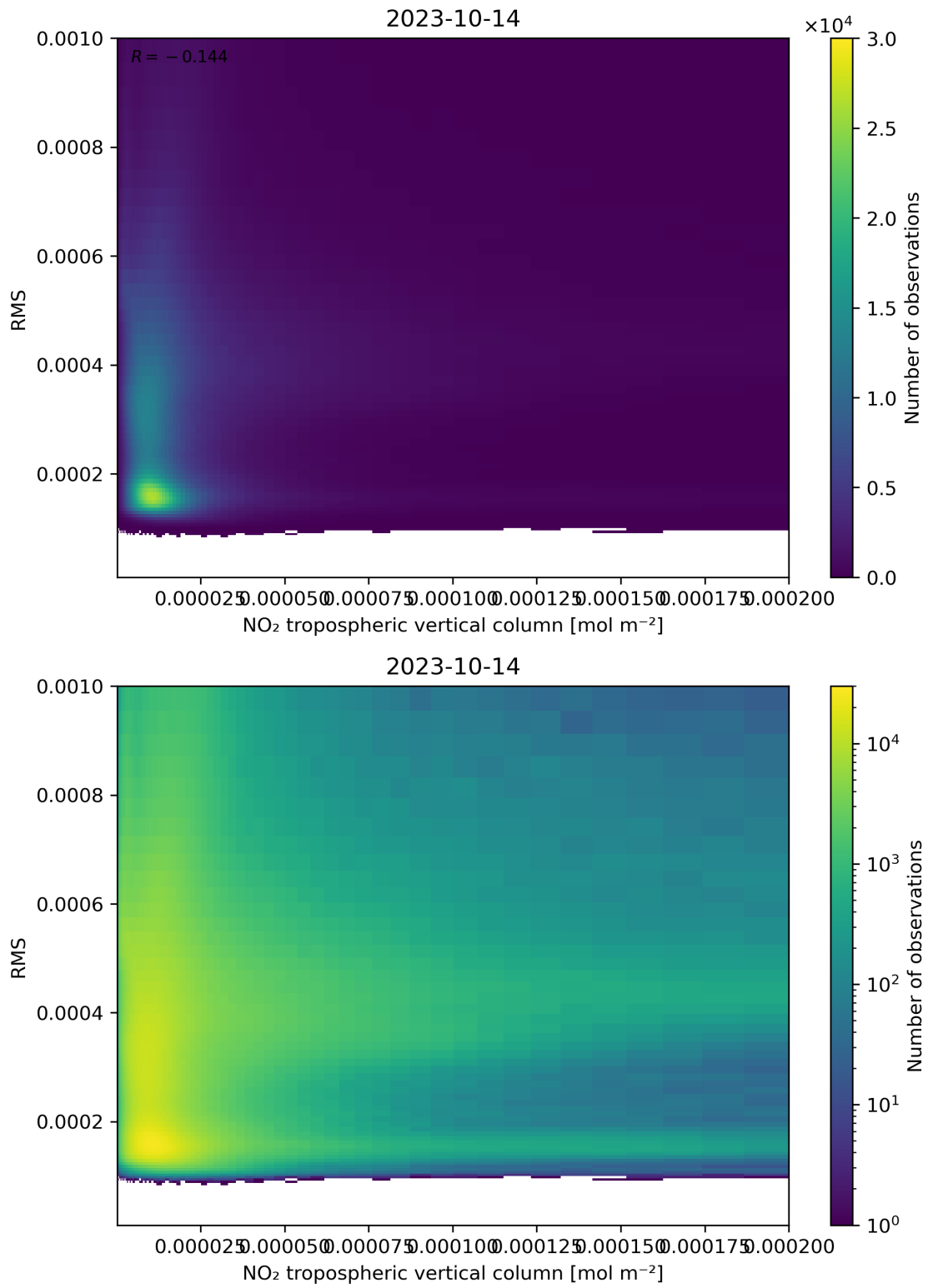
Figure 142: Scatter density plot of “NO 2 tropospheric vertical column” against “RMS” for 2023-10-13 to 2023-10-15.
