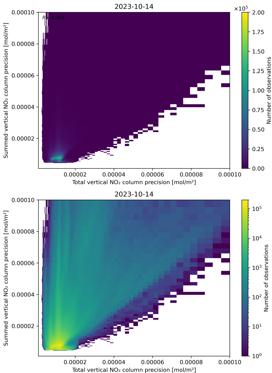
Figure 118: Scatter density plot of “Total vertical NO 2 column precision” against “Summed vertical NO 2 column precision” for 2023-10-13 to 2023-10-15.
