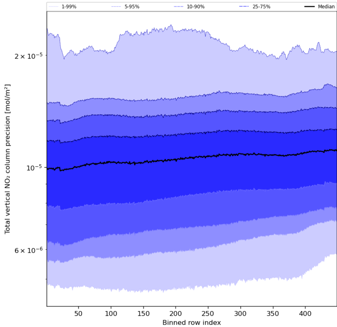
Figure 56: Along track statistics of “Total vertical NO 2 column precision” for 2023-10-13 to 2023-10-15
