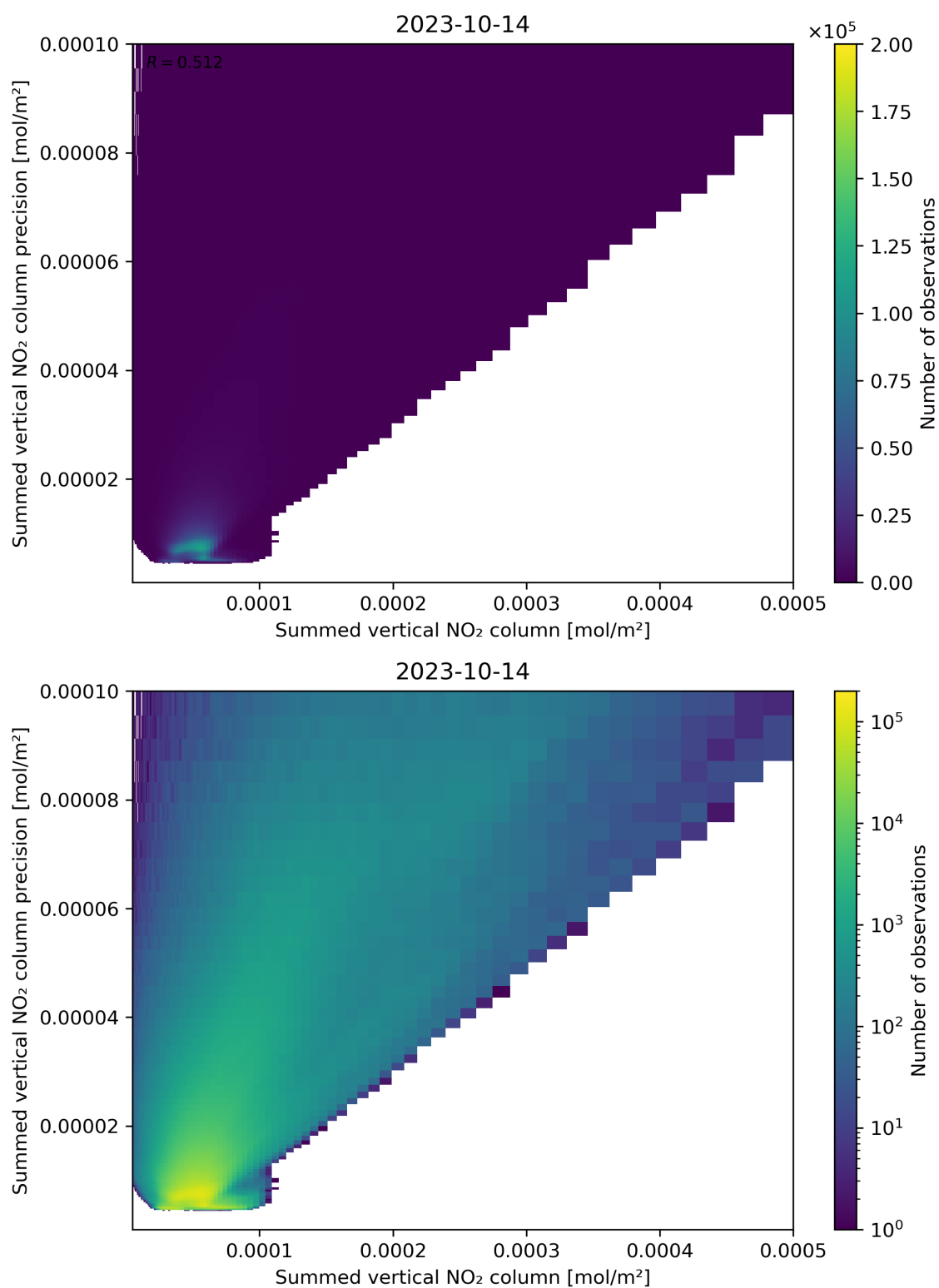
Figure 105: Scatter density plot of “Summed vertical NO 2 column” against “Summed vertical NO 2 column precision” for 2023-10-13 to 2023-10-15.
