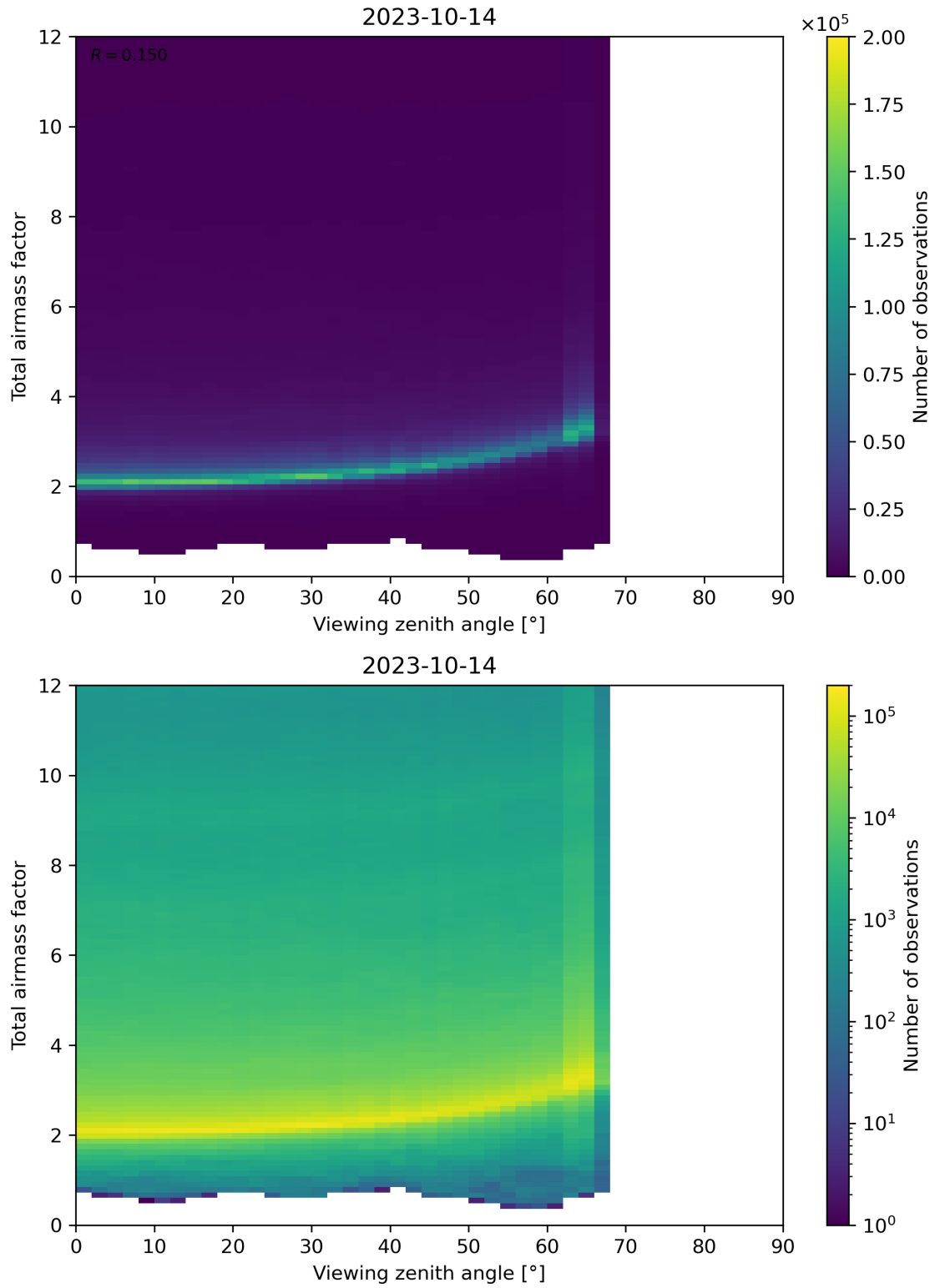
Figure 160: Scatter density plot of “Viewing zenith angle” against “Total airmass factor” for 2023-10-13 to 2023-10-15.
