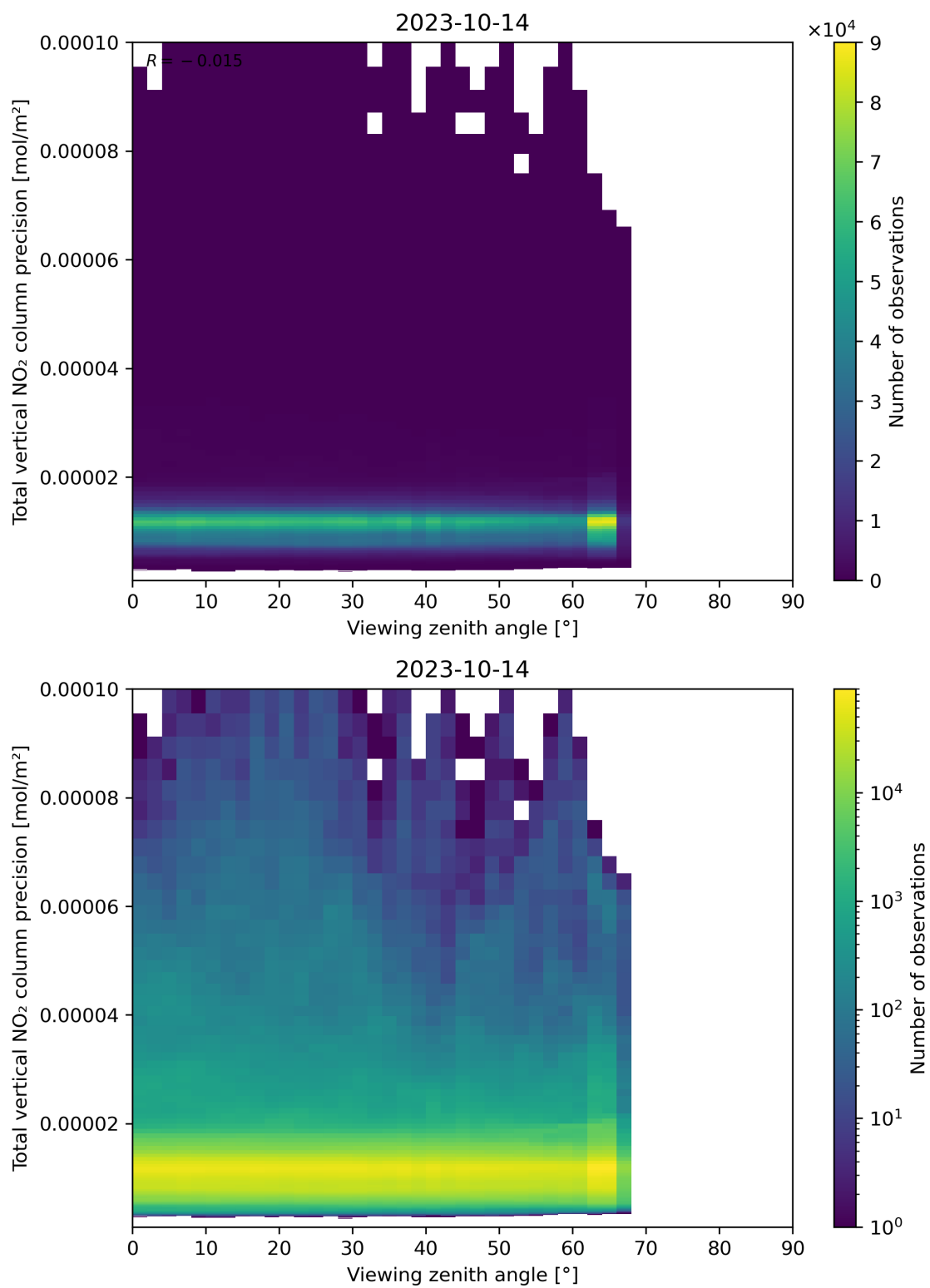
Figure 168: Scatter density plot of “Viewing zenith angle” against “Total vertical NO 2 column precision” for 2023-10-13 to 2023-10-15.
