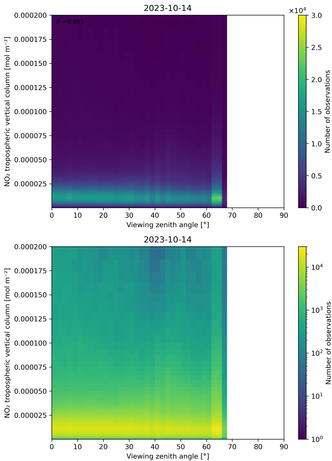
Figure 169: Scatter density plot of “Viewing zenith angle” against “NO 2 tropospheric vertical column” for 2023-10-13 to 2023-10-15.
