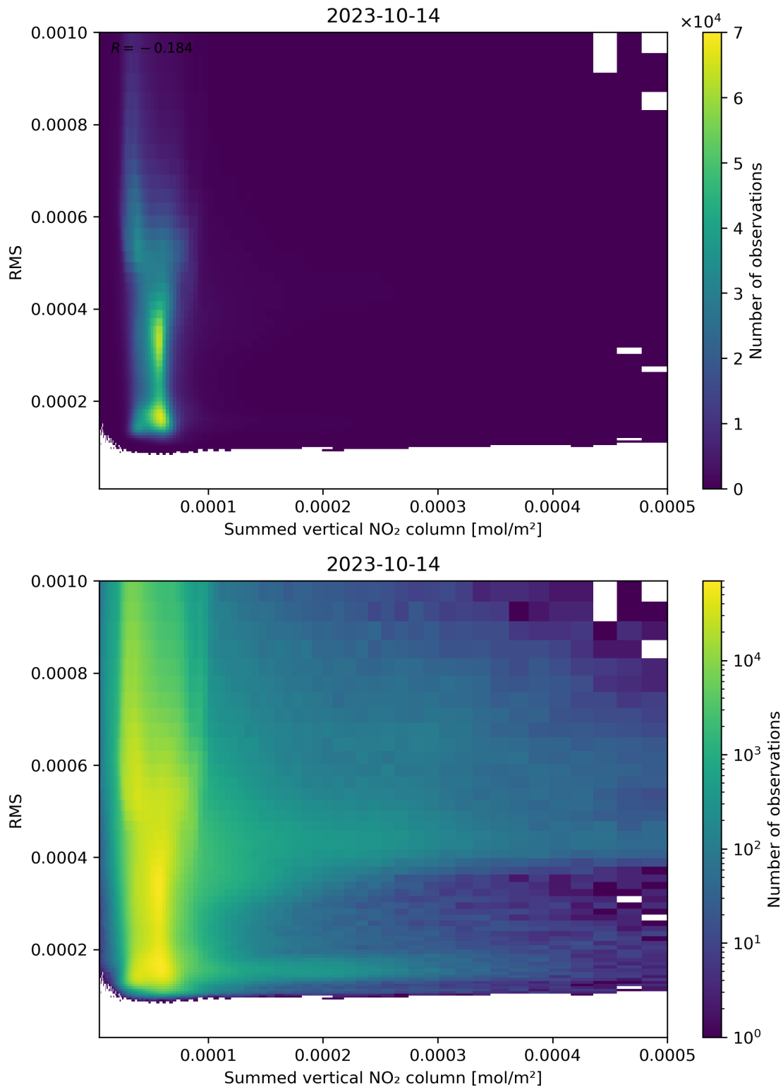
Figure 109: Scatter density plot of “Summed vertical NO 2 column” against “RMS” for 2023-10-13 to 2023-10-15.
