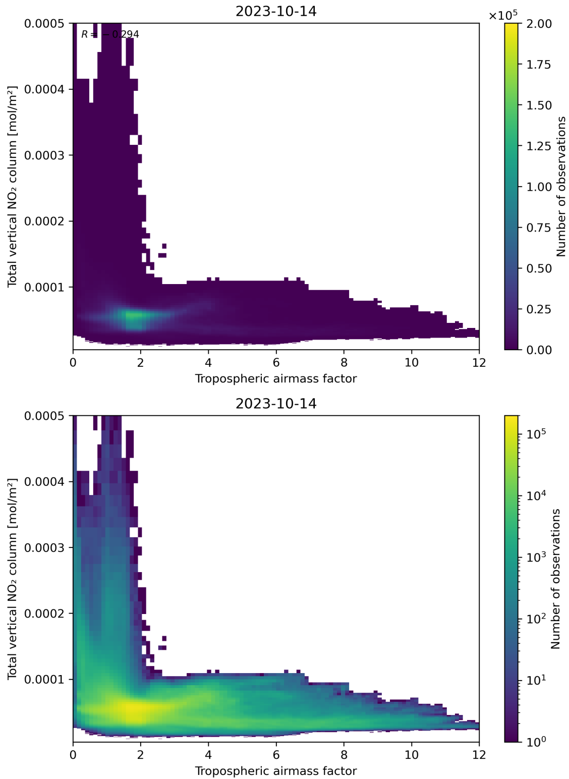
Figure 77: Scatter density plot of “Tropospheric airmass factor” against “Total vertical NO 2 column” for 2023-10-13 to 2023-10-15.
