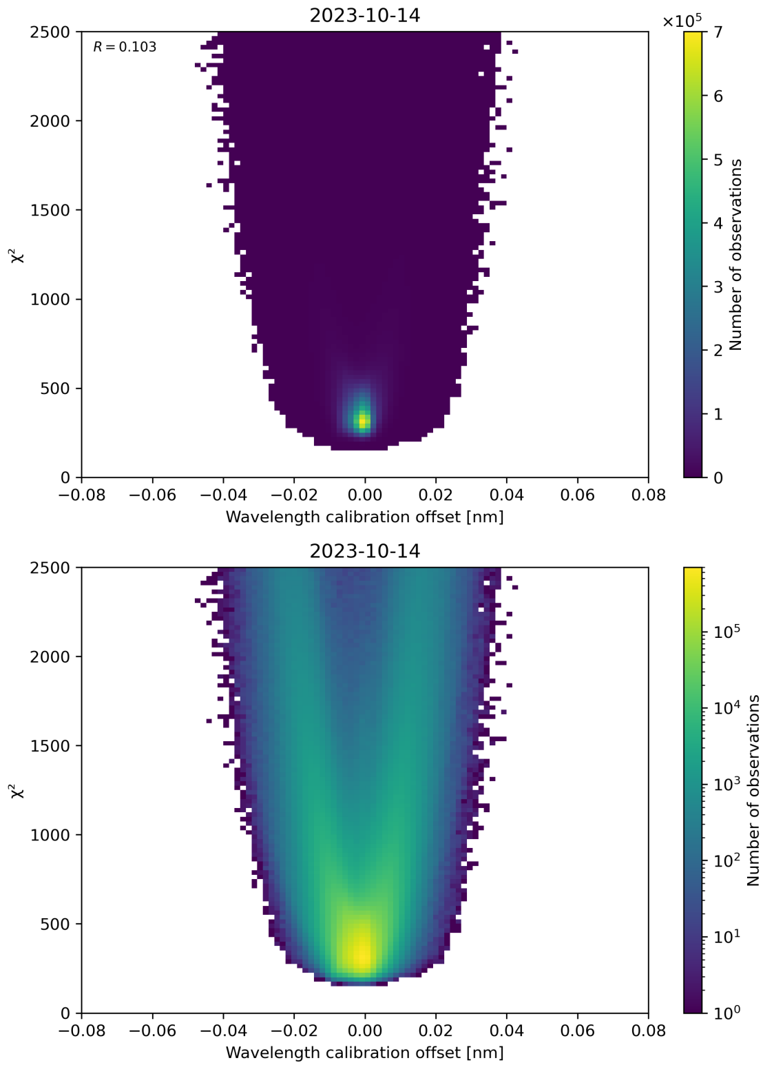
Figure 175: Scatter density plot of “Wavelength calibration offset” against “ \chi^2 ” for 2023-10-13 to 2023-10-15.
