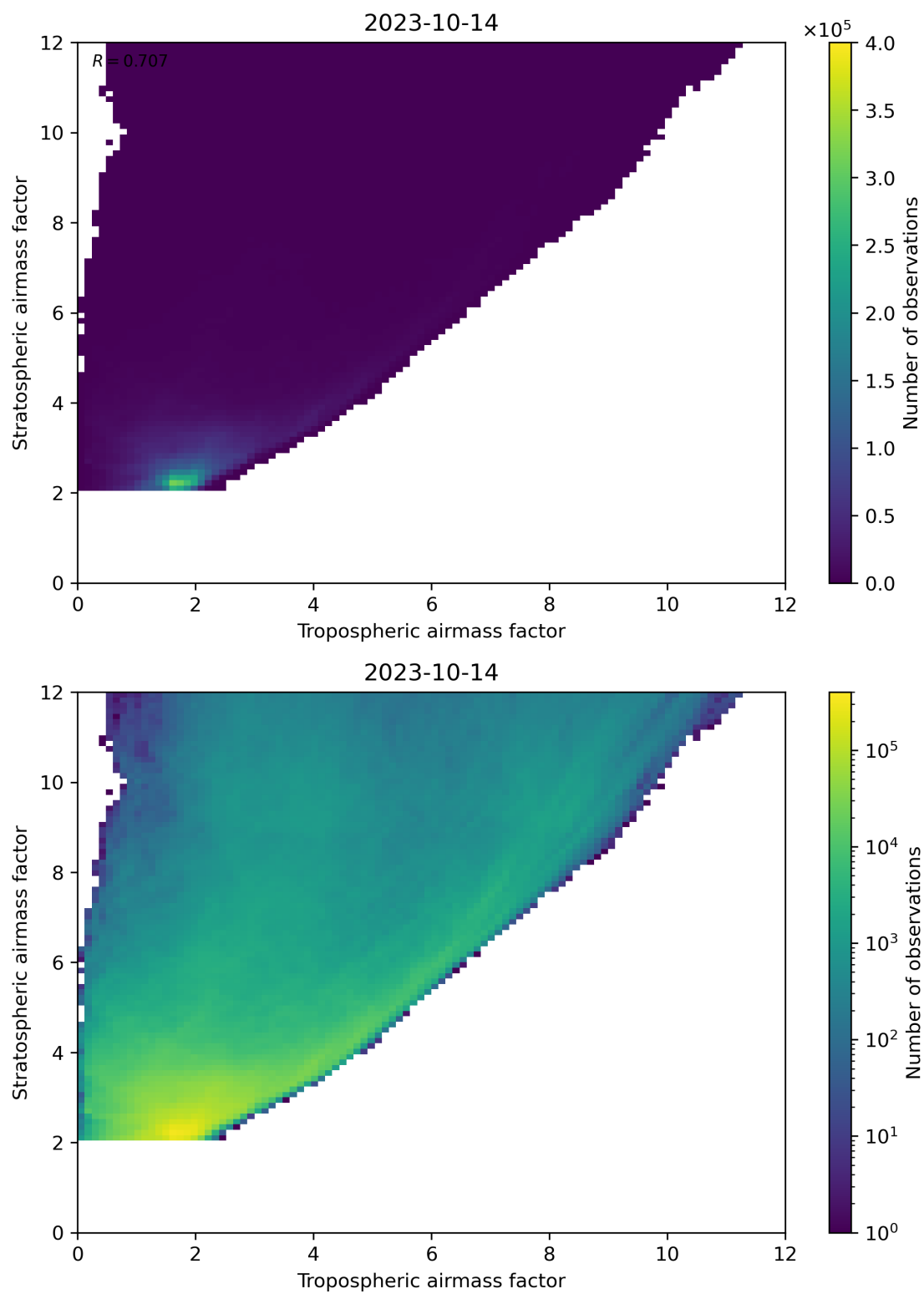
Figure 71: Scatter density plot of “Tropospheric airmass factor” against “Stratospheric airmass factor” for 2023-10-13 to 2023-10-15.
