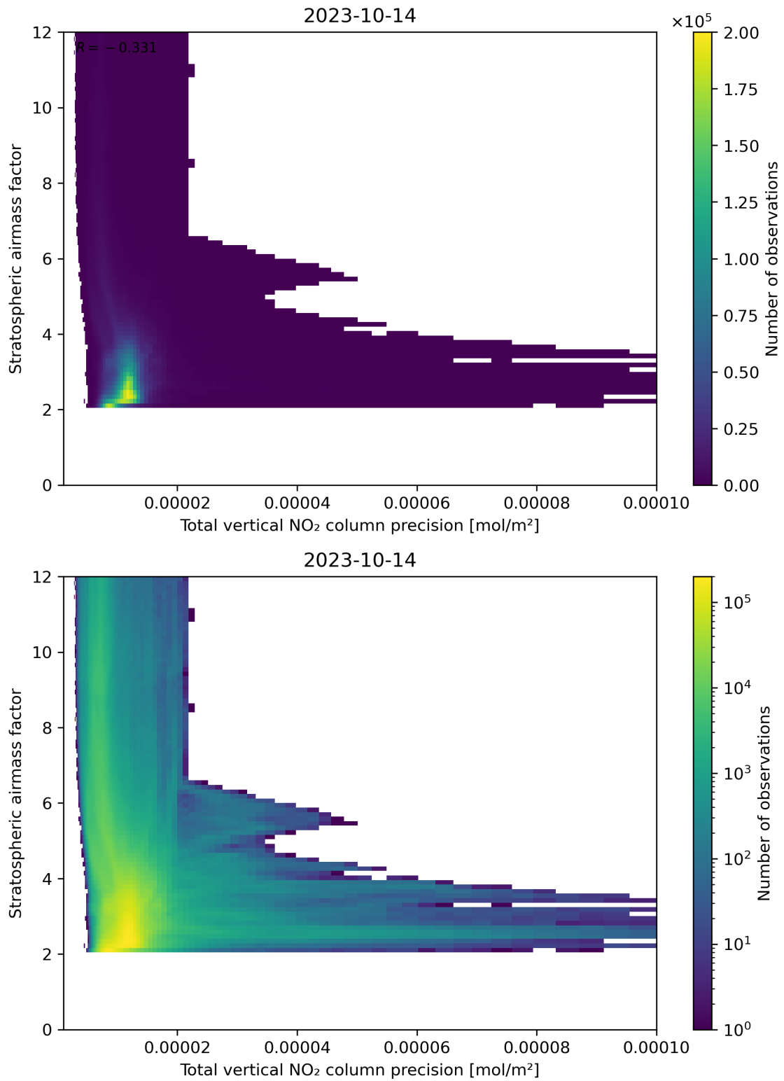
Figure 115: Scatter density plot of “Total vertical NO 2 column precision” against “Stratospheric air mass factor” for 2023-10-13 to 2023-10-15.
