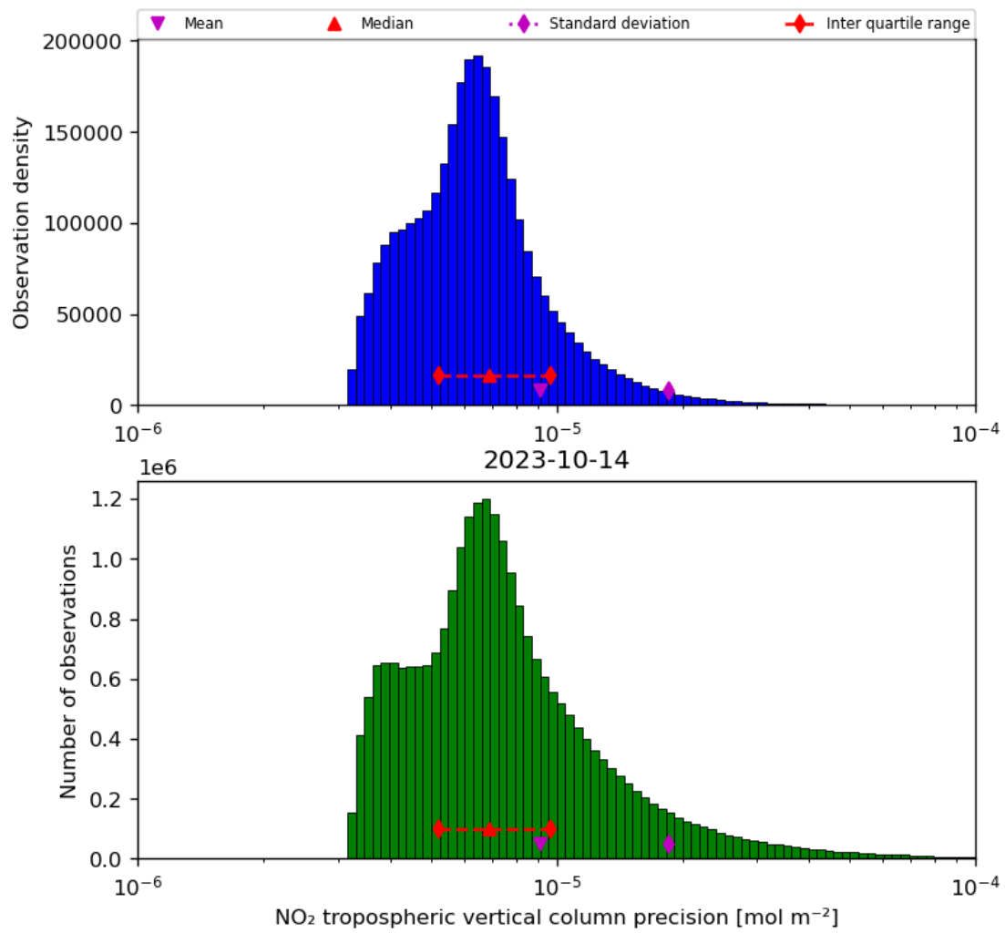
Figure 30: Histogram of “NO 2 tropospheric vertical column precision” for 2023-10-13 to 2023-10-15
