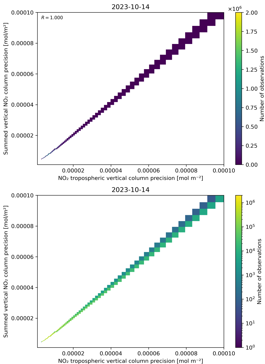
Figure 137: Scatter density plot of “NO 2 tropospheric vertical column precision” against “Summed vertical NO 2 column precision” for 2023-10-13 to 2023-10-15.
