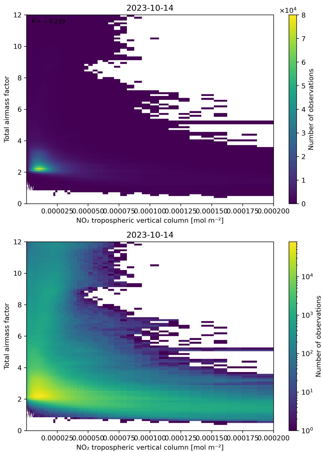
Figure 122: Scatter density plot of “NO 2 tropospheric vertical column” against “Total air mass factor” for 2023-10-13 to 2023-10-15.
