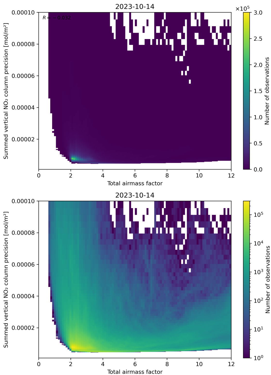
Figure 66: Scatter density plot of “Total airmass factor” against “Summed vertical NO 2 column precision” for 2023-10-13 to 2023-10-15.
