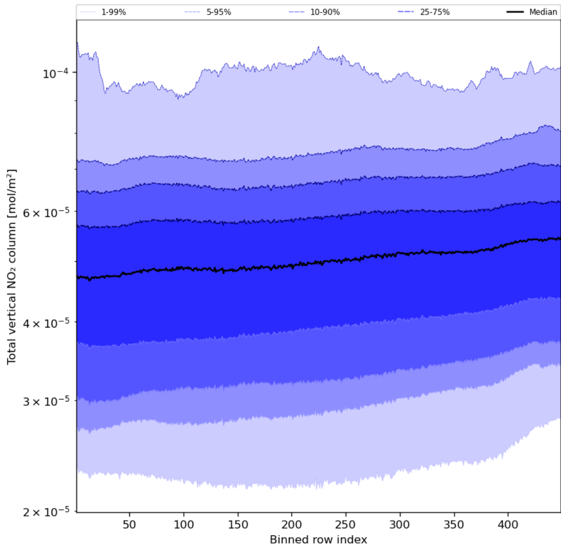
Figure 55: Along track statistics of “Total vertical NO 2 column” for 2023-10-13 to 2023-10-15
