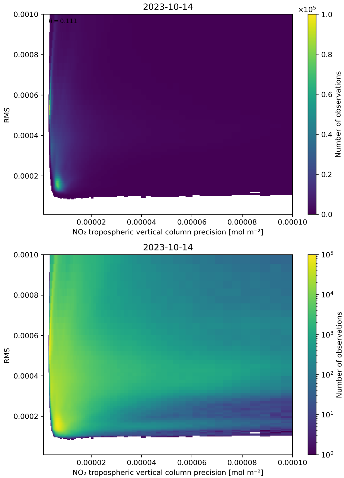
Figure 140: Scatter density plot of “NO 2 tropospheric vertical column precision” against “RMS” for 2023-10-13 to 2023-10-15.
