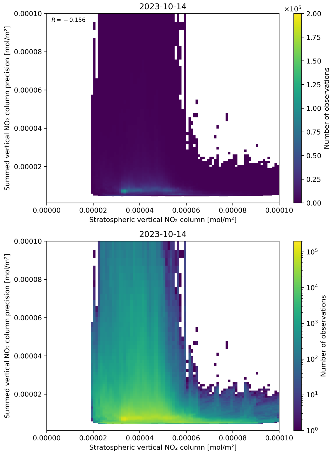
Figure 99: Scatter density plot of “Stratospheric vertical NO 2 column” against “Summed vertical NO 2 column precision” for 2023-10-13 to 2023-10-15.
