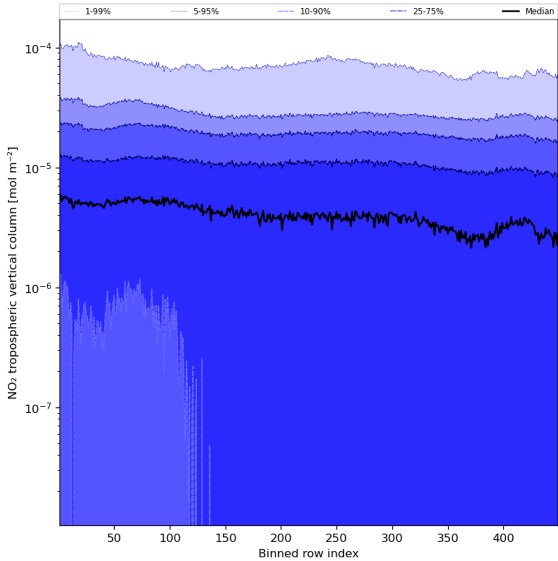
Figure 46: Along track statistics of “NO 2 tropospheric vertical column” for 2023-10-13 to 2023-10-15
