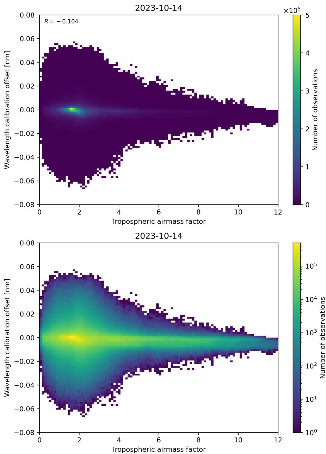
Figure 80: Scatter density plot of “Tropospheric airmass factor” against “Wavelength calibration offset” for 2023-10-13 to 2023-10-15.
