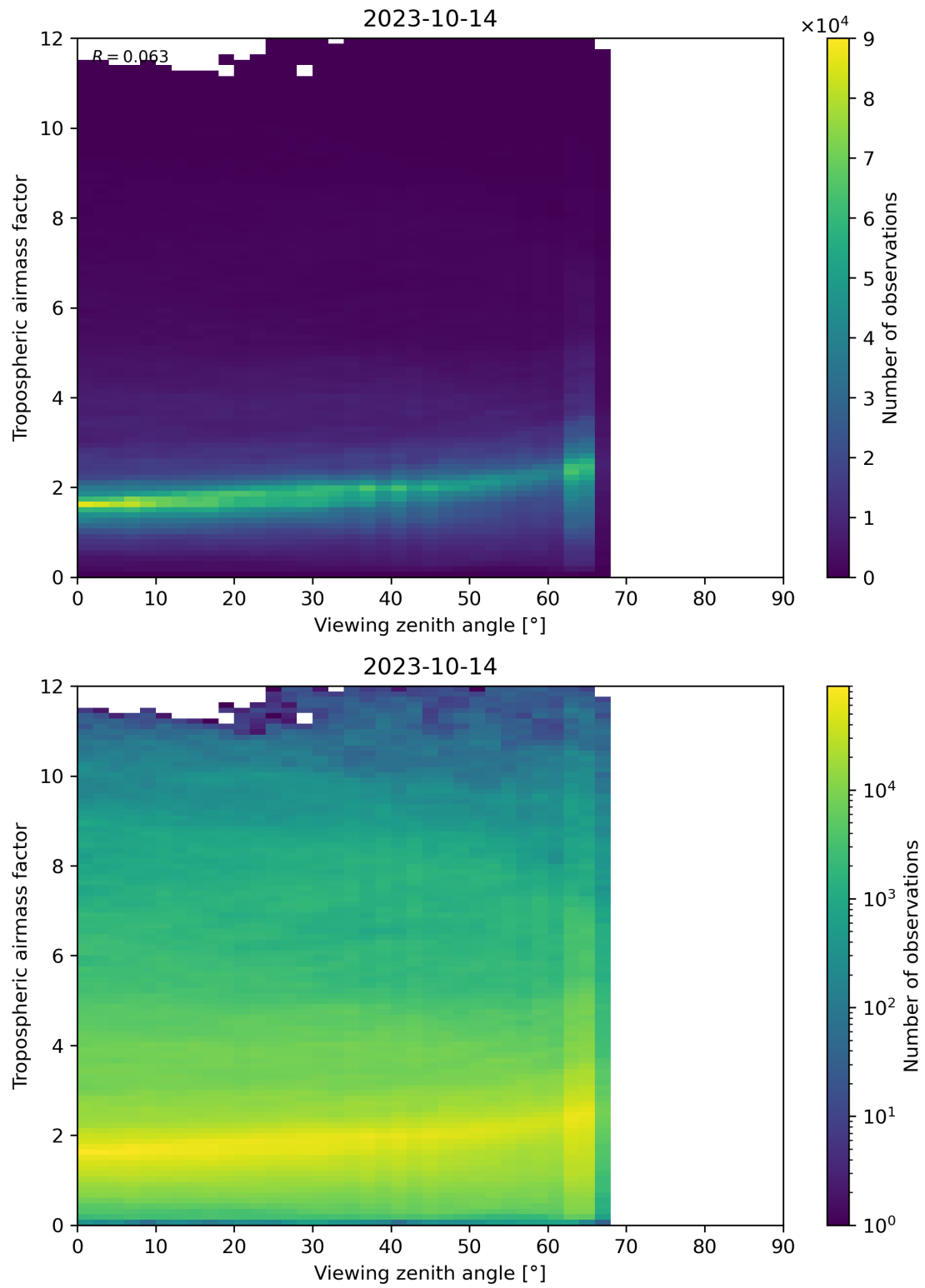
Figure 161: Scatter density plot of “Viewing zenith angle” against “Tropospheric airmass factor” for 2023-10-13 to 2023-10-15.
