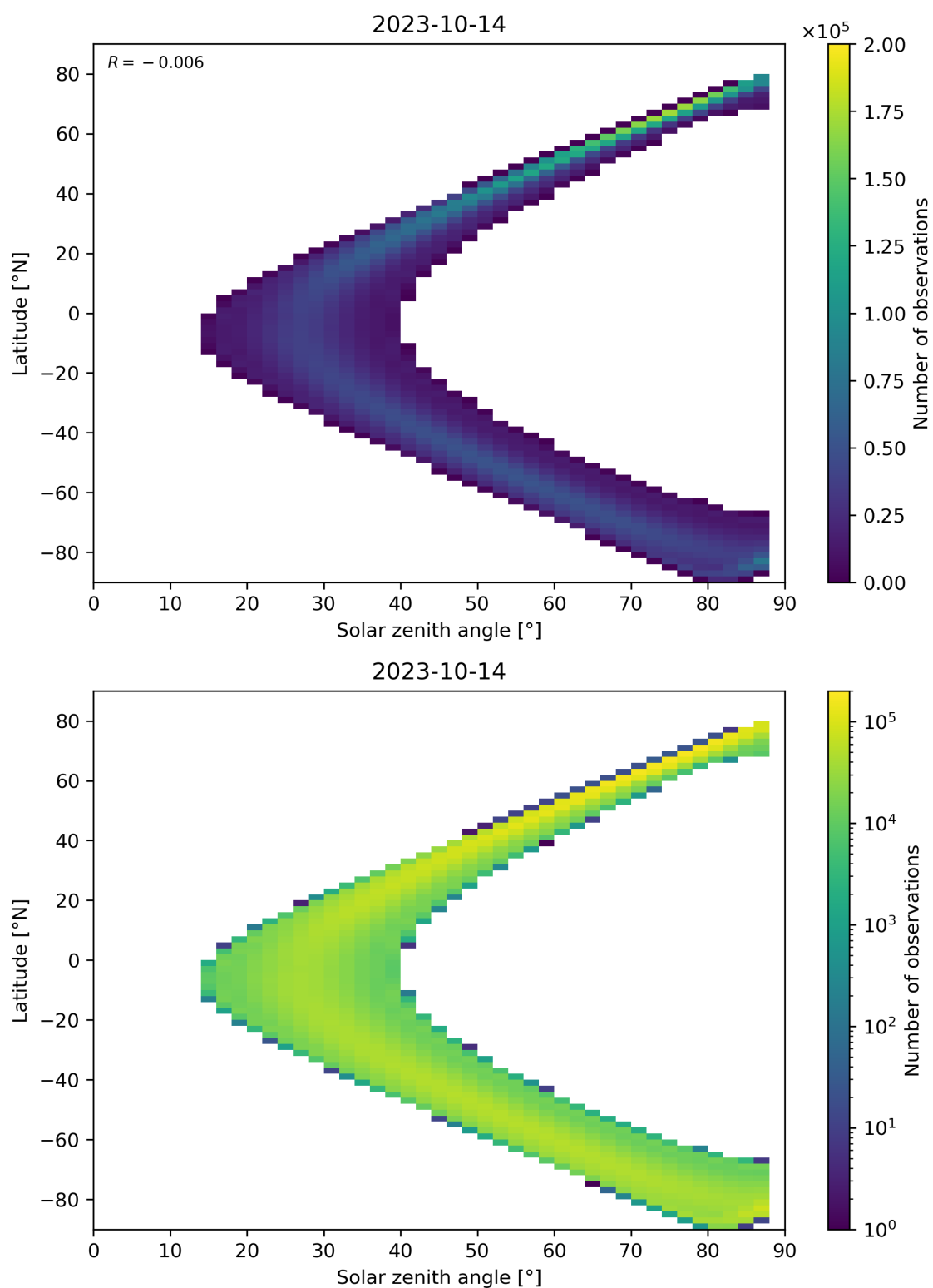
Figure 149: Scatter density plot of “Solar zenith angle” against “Latitude” for 2023-10-13 to 2023-10-15.
