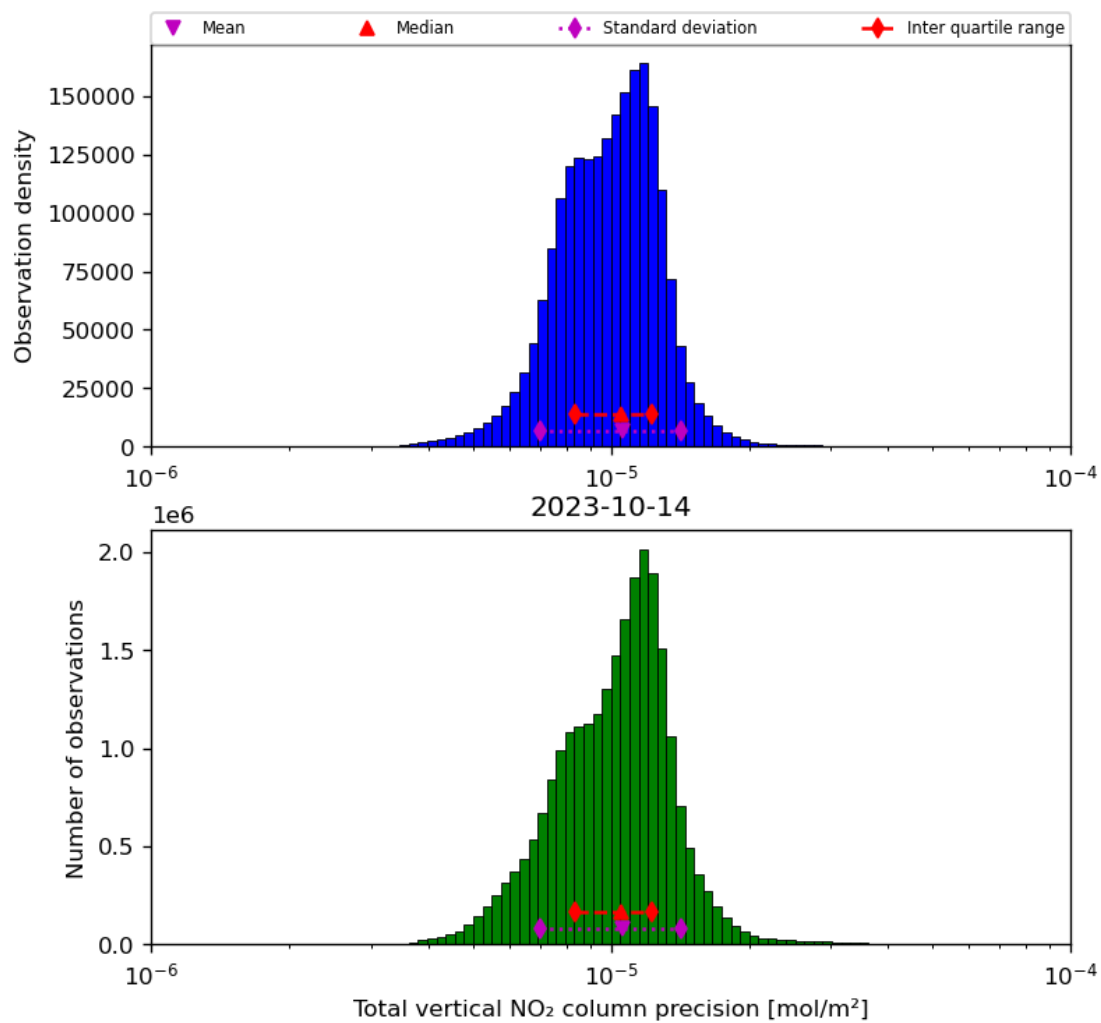
Figure 39: Histogram of “Total vertical NO 2 column precision” for 2023-10-13 to 2023-10-15
