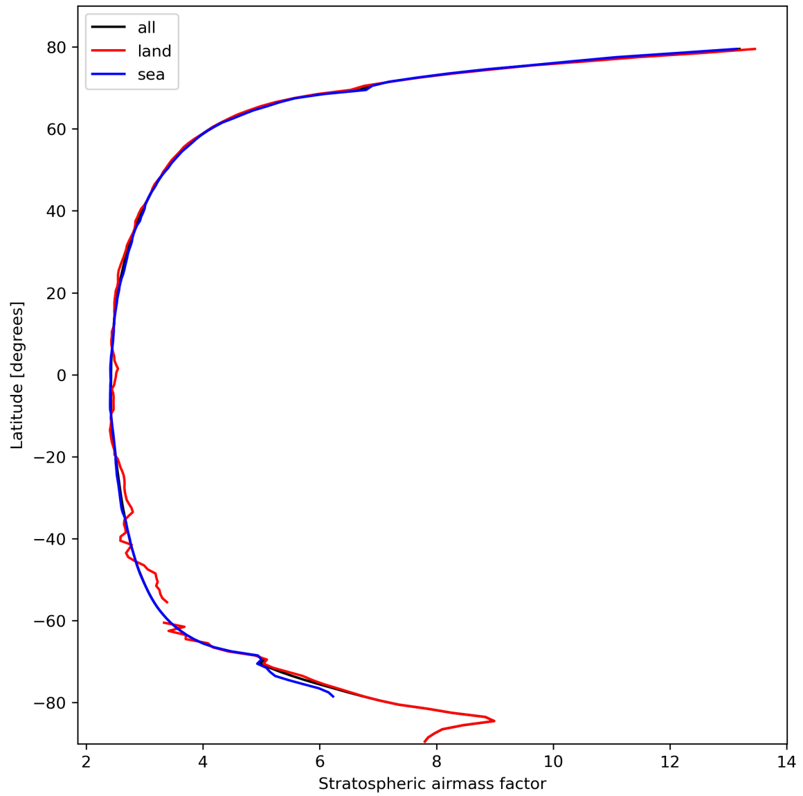
Figure 27: Zonal average of “Stratospheric airmass factor” for 2023-10-13 to 2023-10-15.
