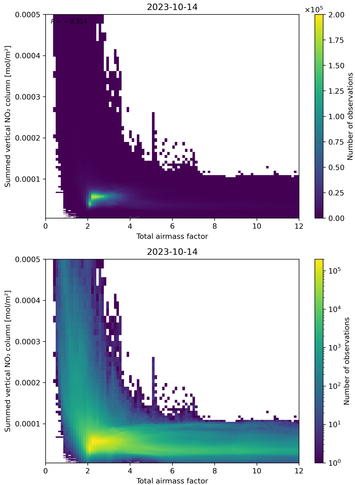
Figure 65: Scatter density plot of “Total airmass factor” against “Summed vertical NO 2 column” for 2023-10-13 to 2023-10-15.
