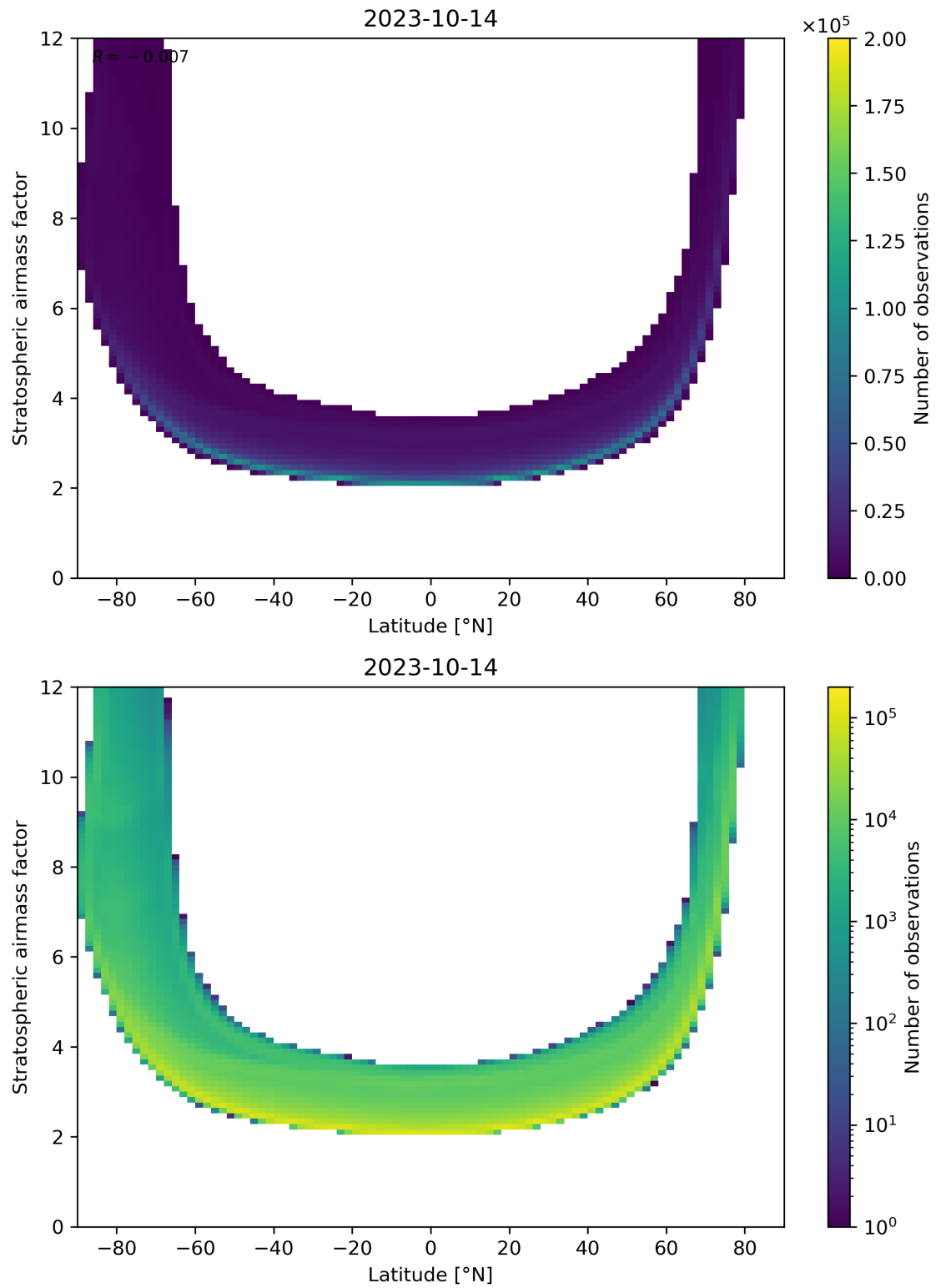
Figure 83: Scatter density plot of “Latitude” against “Stratospheric air mass factor” for 2023-10-13 to 2023-10-15.
