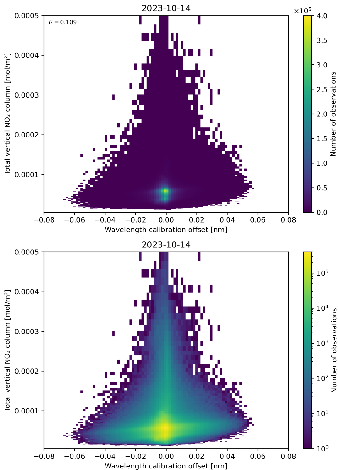
Figure 179: Scatter density plot of “Wavelength calibration offset” against “Total vertical NO 2 column” for 2023-10-13 to 2023-10-15.
