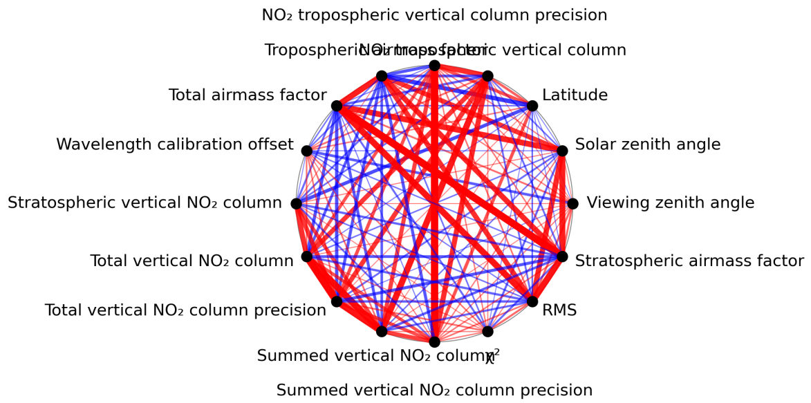
Figure 1: Map of correlation graph for 2023-10-13 to 2023-10-15.
