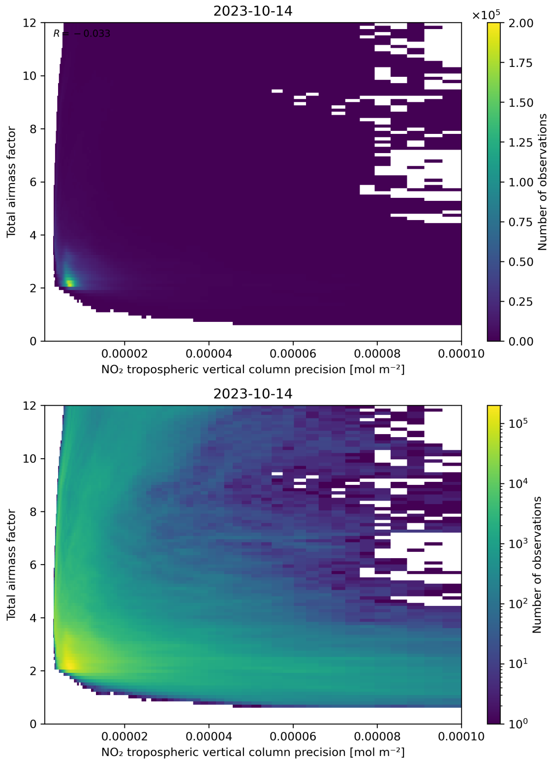
Figure 132: Scatter density plot of “NO 2 tropospheric vertical column precision” against “Total air mass factor” for 2023-10-13 to 2023-10-15.
