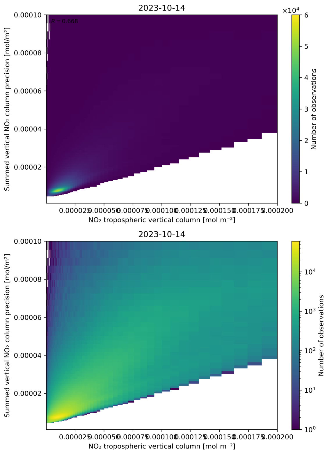
Figure 127: Scatter density plot of “NO 2 tropospheric vertical column” against “Summed vertical NO 2 column precision” for 2023-10-13 to 2023-10-15.
