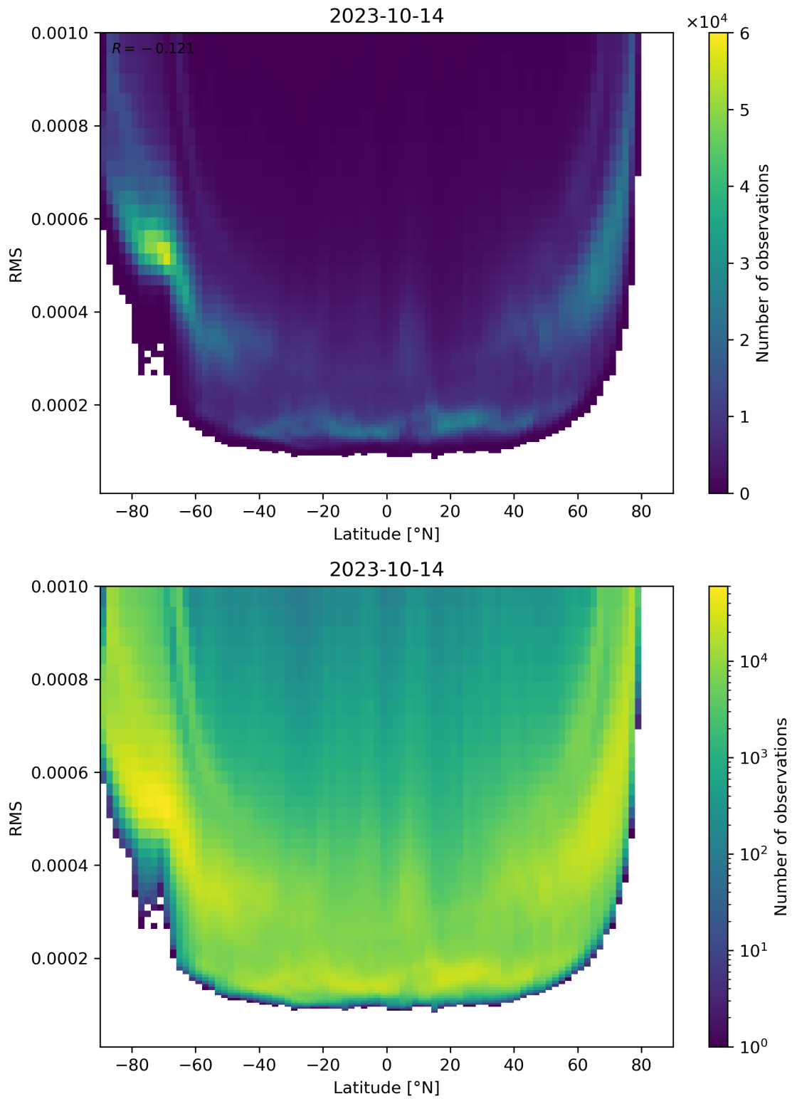
Figure 94: Scatter density plot of “Latitude” against “RMS” for 2023-10-13 to 2023-10-15.
