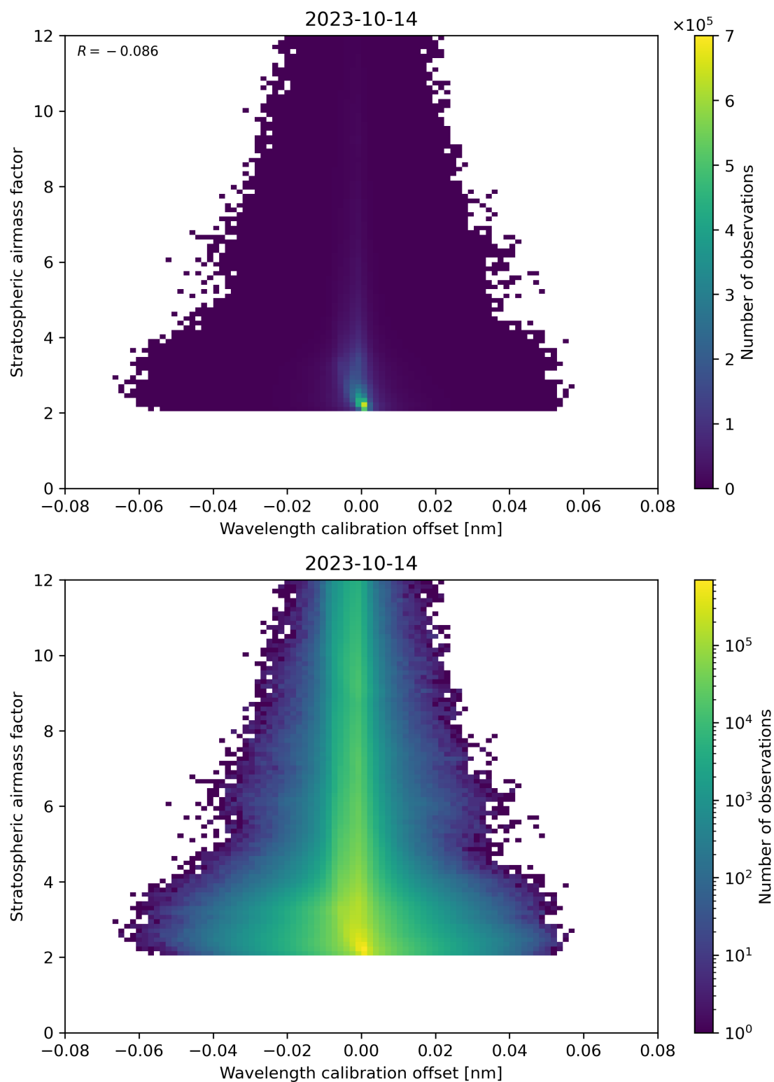
Figure 174: Scatter density plot of “Wavelength calibration offset” against “Stratospheric airmass factor” for 2023-10-13 to 2023-10-15.
