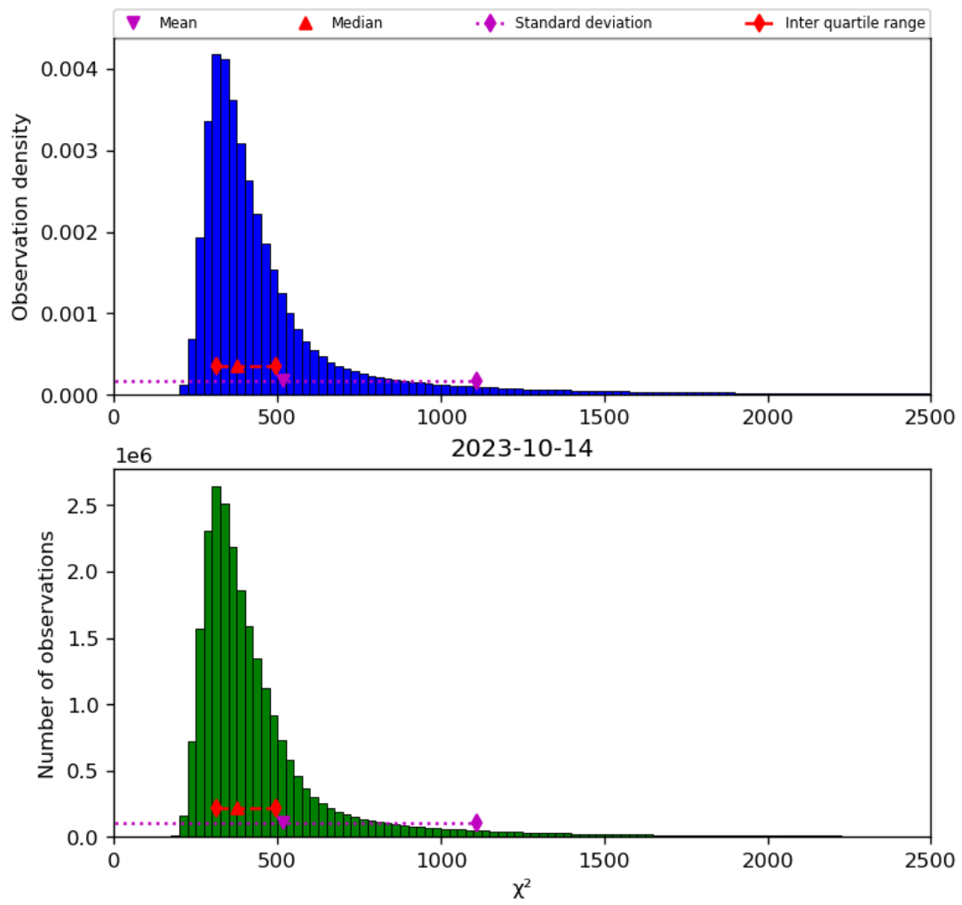
Figure 42: Histogram of “ \chi^2 ” for 2023-10-13 to 2023-10-15
