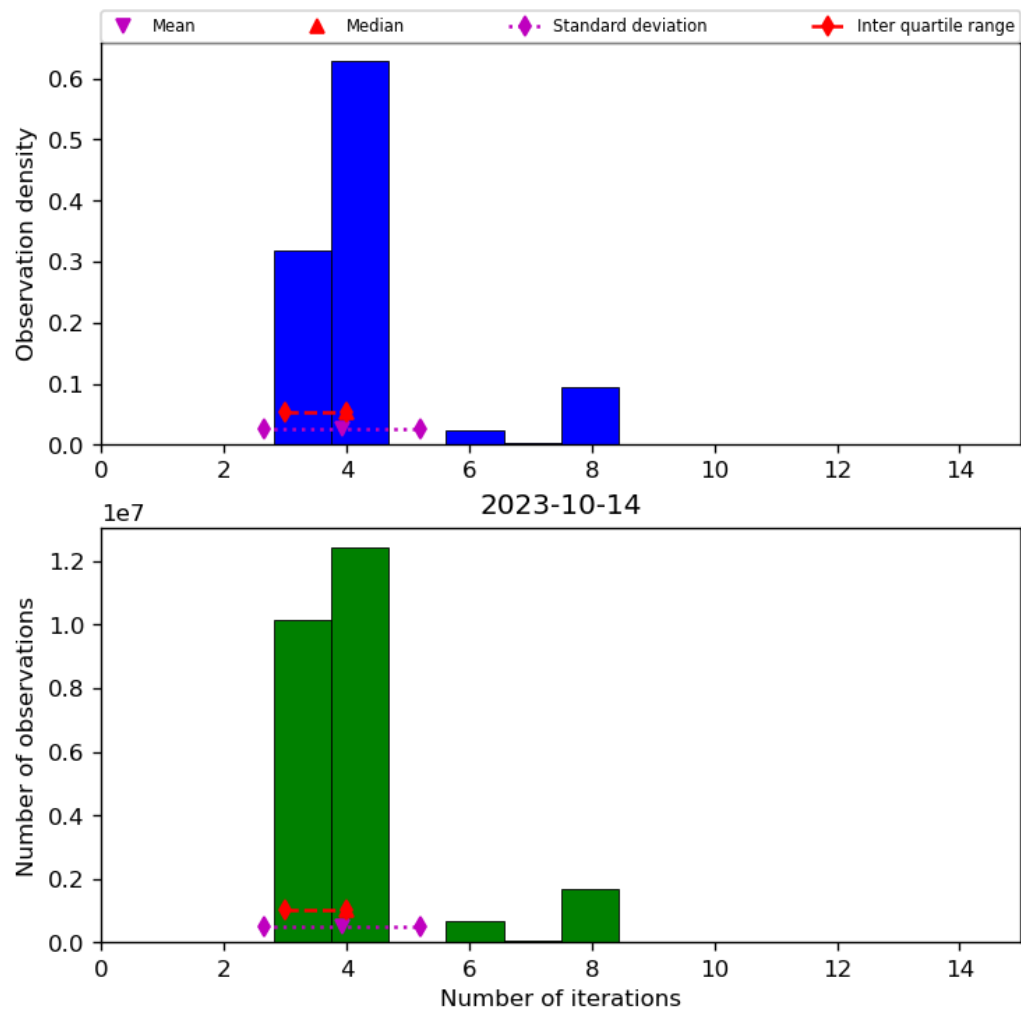
Figure 34: Histogram of “Number of iterations” for 2023-10-13 to 2023-10-15
