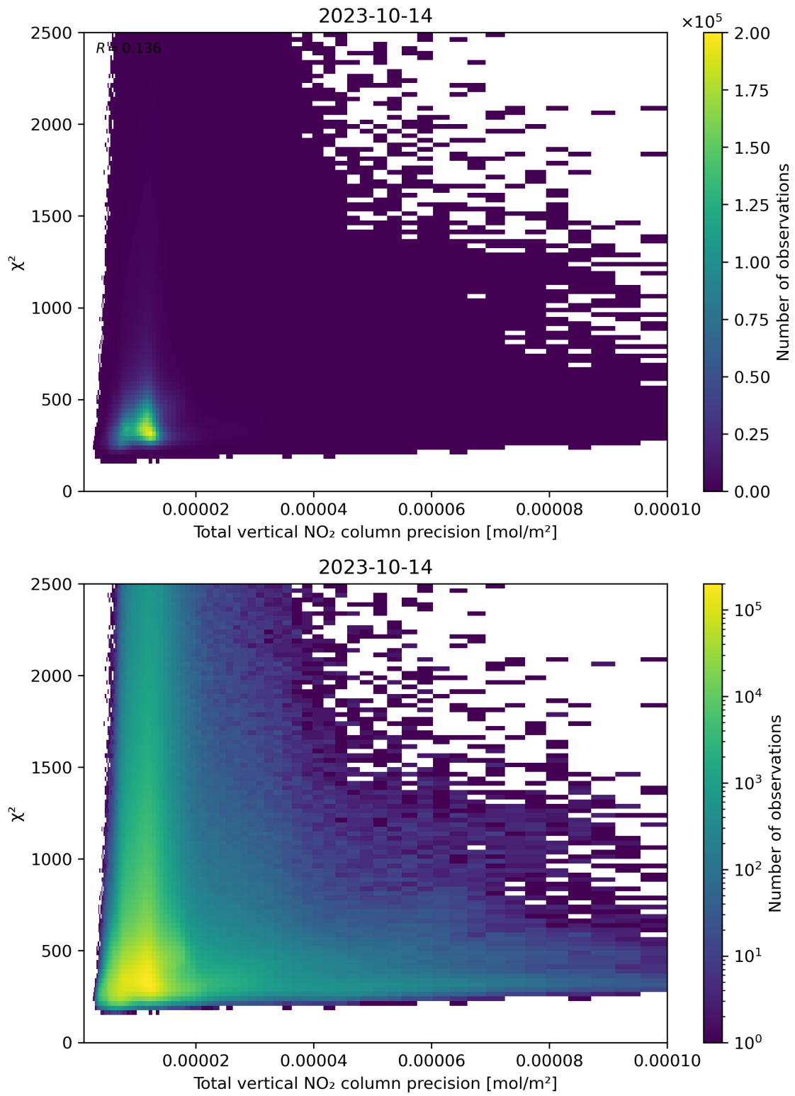
Figure 116: Scatter density plot of “Total vertical NO 2 column precision” against “ \chi^2 ” for 2023-10-13 to 2023-10-15.
