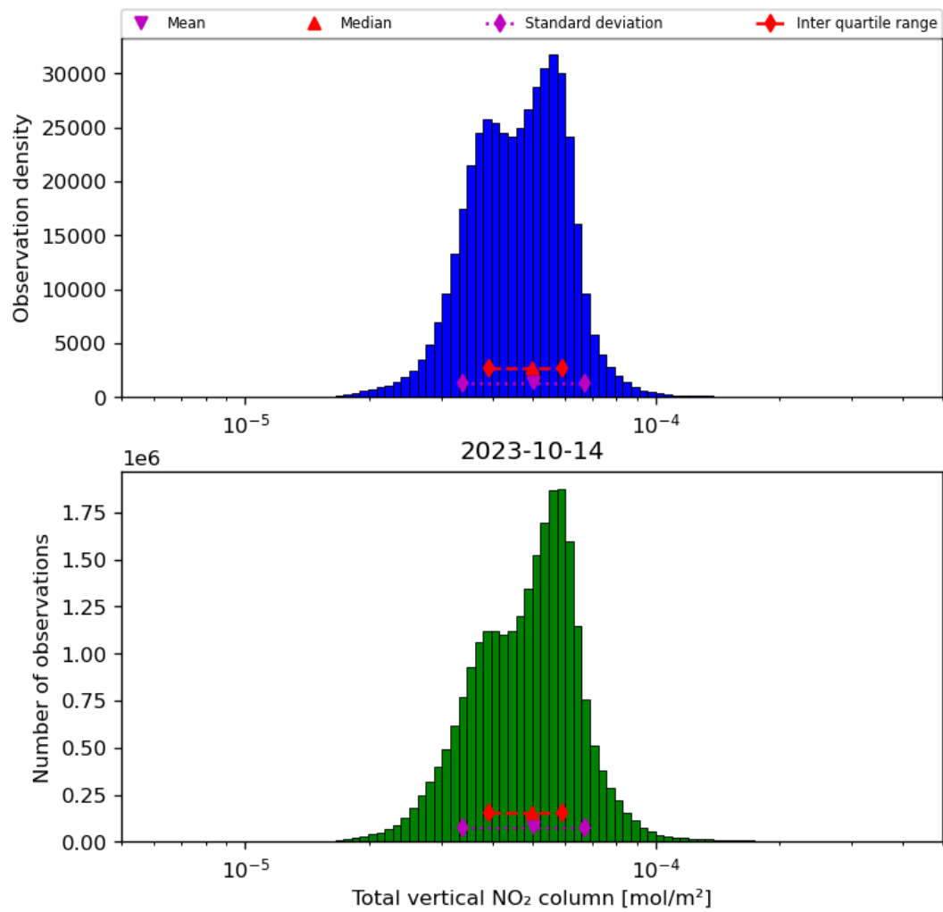
Figure 38: Histogram of “Total vertical NO 2 column” for 2023-10-13 to 2023-10-15
