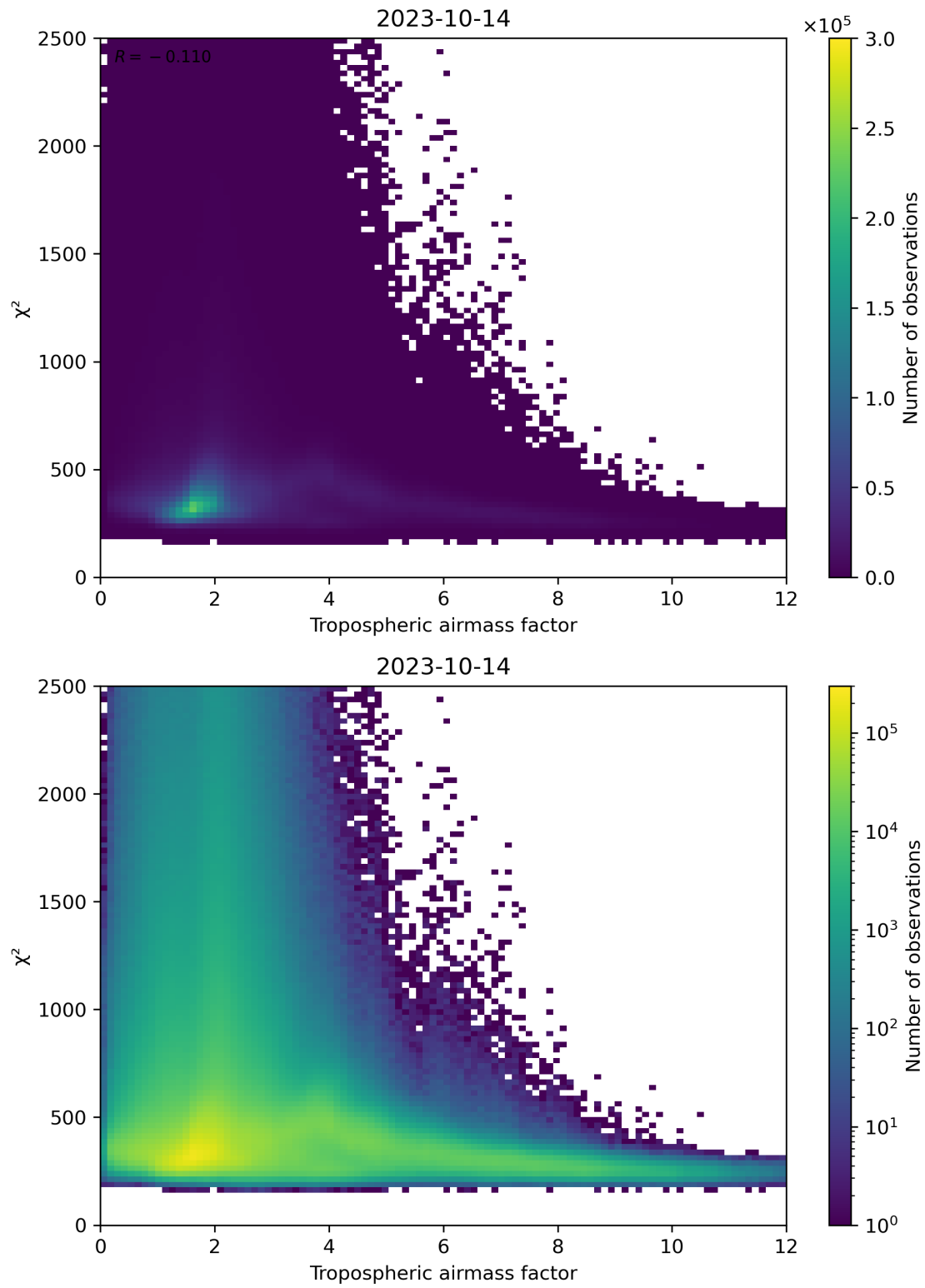
Figure 73: Scatter density plot of “Tropospheric airmass factor” against “ \chi^2 ” for 2023-10-13 to 2023-10-15.
