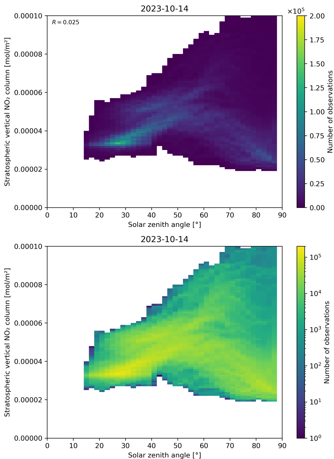
Figure 150: Scatter density plot of “Solar zenith angle” against “Stratospheric vertical NO 2 column” for 2023-10-13 to 2023-10-15.
