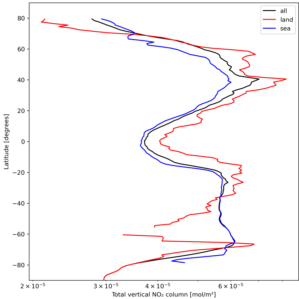
Figure 21: Zonal average of “Total vertical NO 2 column” for 2023-10-13 to 2023-10-15.
