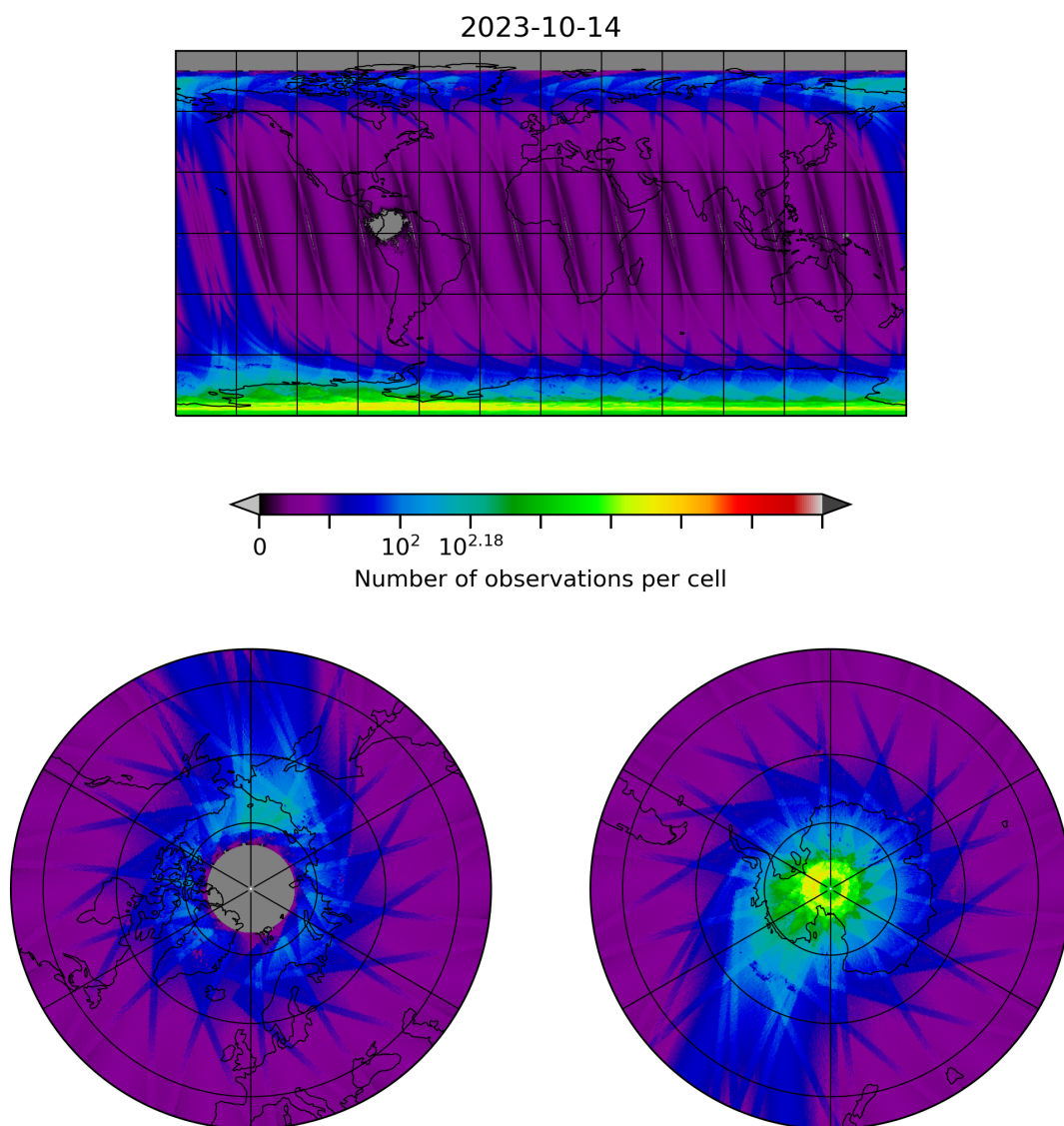
Figure 10: Map of the number of observations for 2023-10-13 to 2023-10-15
