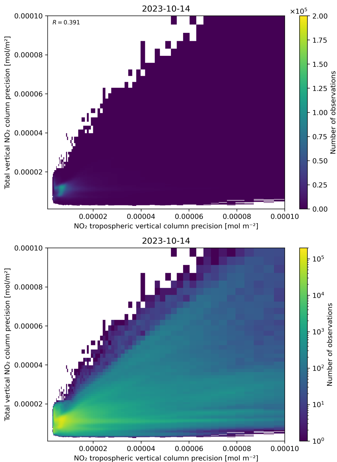
Figure 139: Scatter density plot of “NO 2 tropospheric vertical column precision” against “Total vertical NO 2 column precision” for 2023-10-13 to 2023-10-15.
