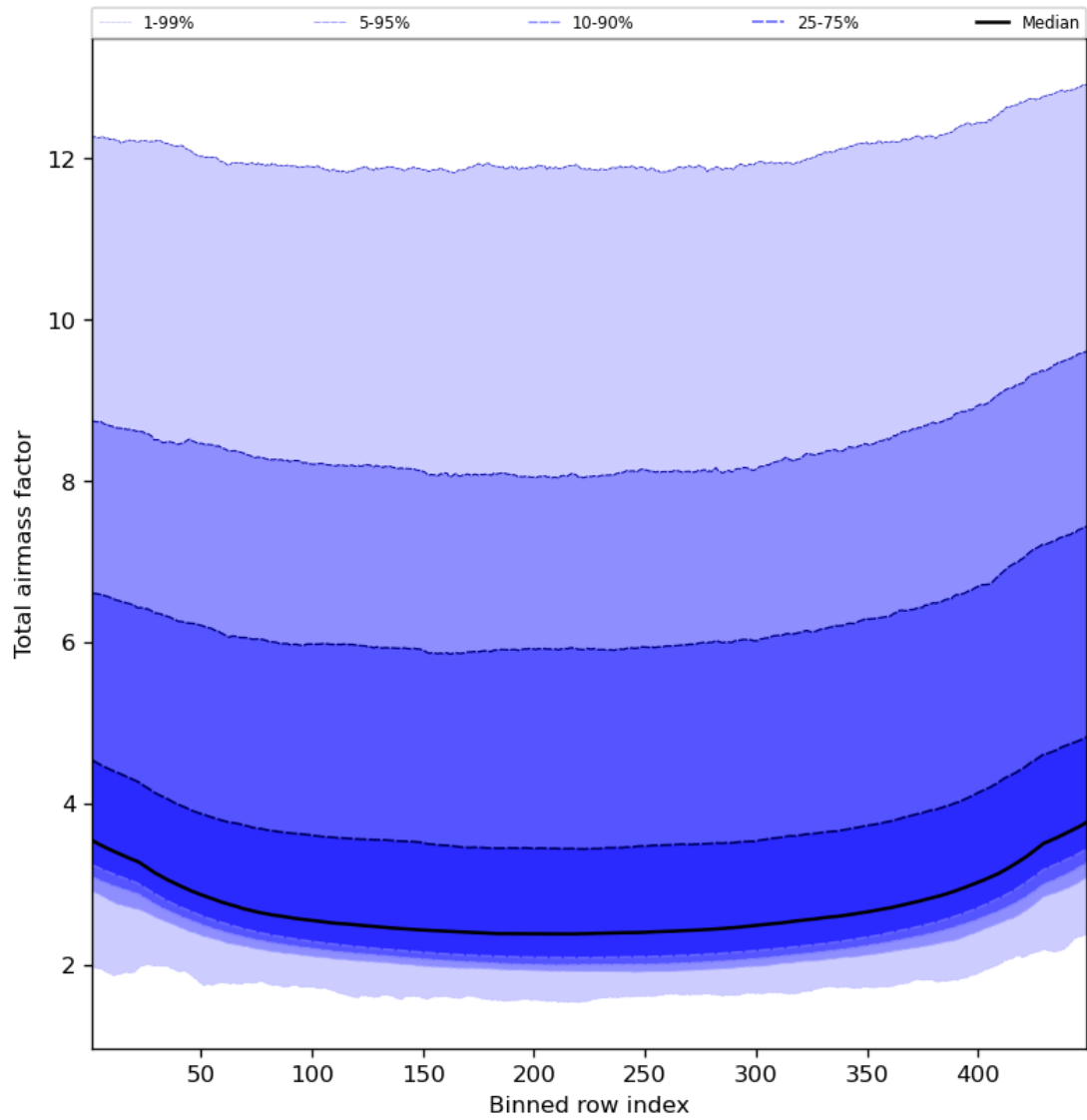
Figure 49: Along track statistics of “Total airmass factor” for 2023-10-13 to 2023-10-15
