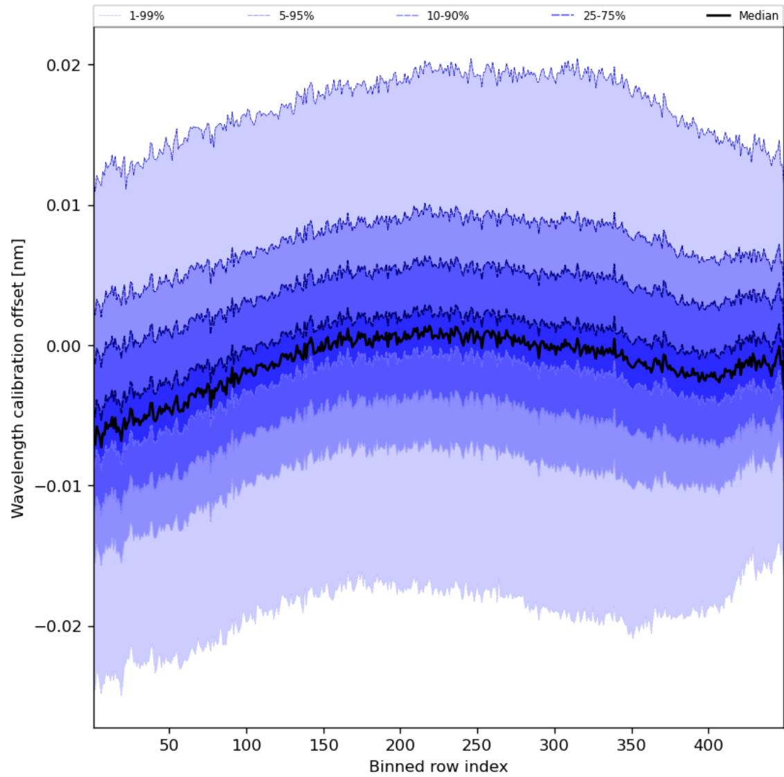
Figure 52: Along track statistics of “Wavelength calibration offset” for 2023-10-13 to 2023-10-15
