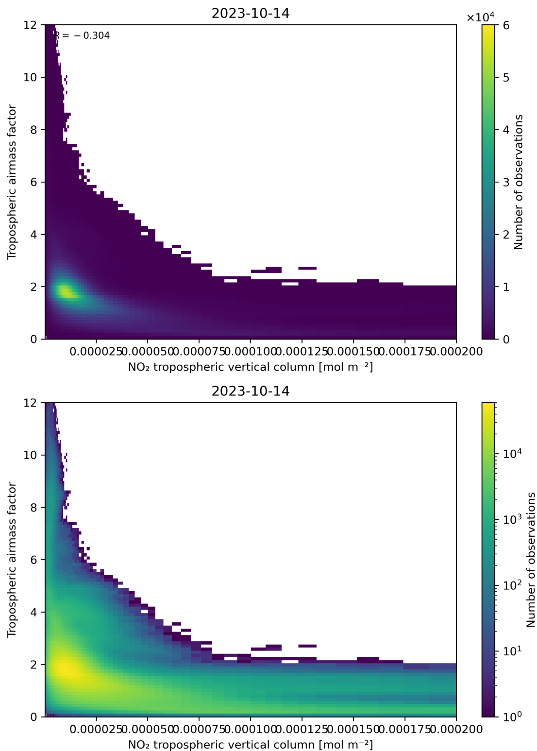
Figure 123: Scatter density plot of “NO 2 tropospheric vertical column” against “Tropospheric air mass factor” for 2023-10-13 to 2023-10-15.
