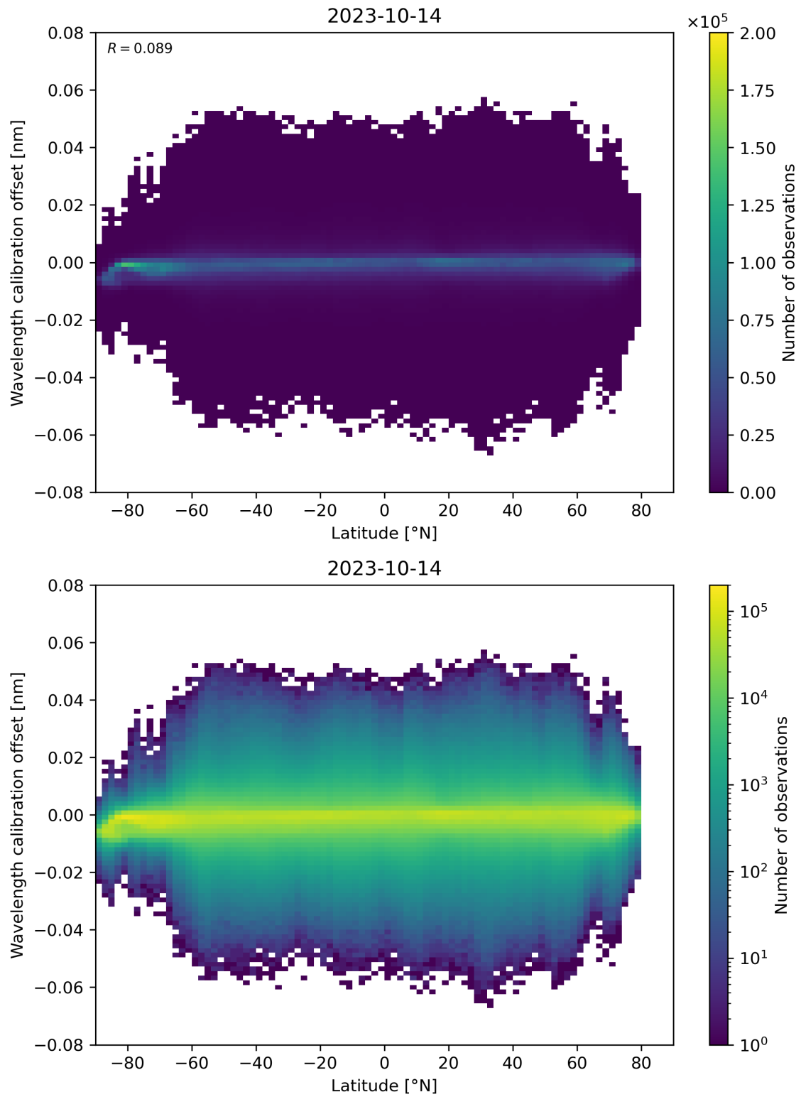
Figure 95: Scatter density plot of “Latitude” against “Wavelength calibration offset” for 2023-10-13 to 2023-10-15.
