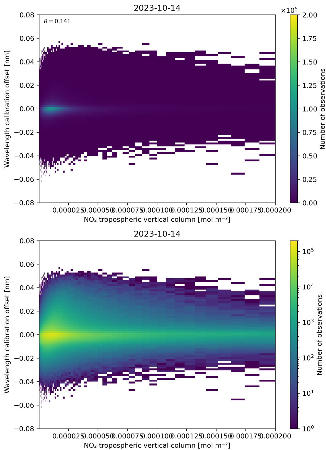
Figure 143: Scatter density plot of “NO 2 tropospheric vertical column” against “Wavelength calibration offset” for 2023-10-13 to 2023-10-15.
