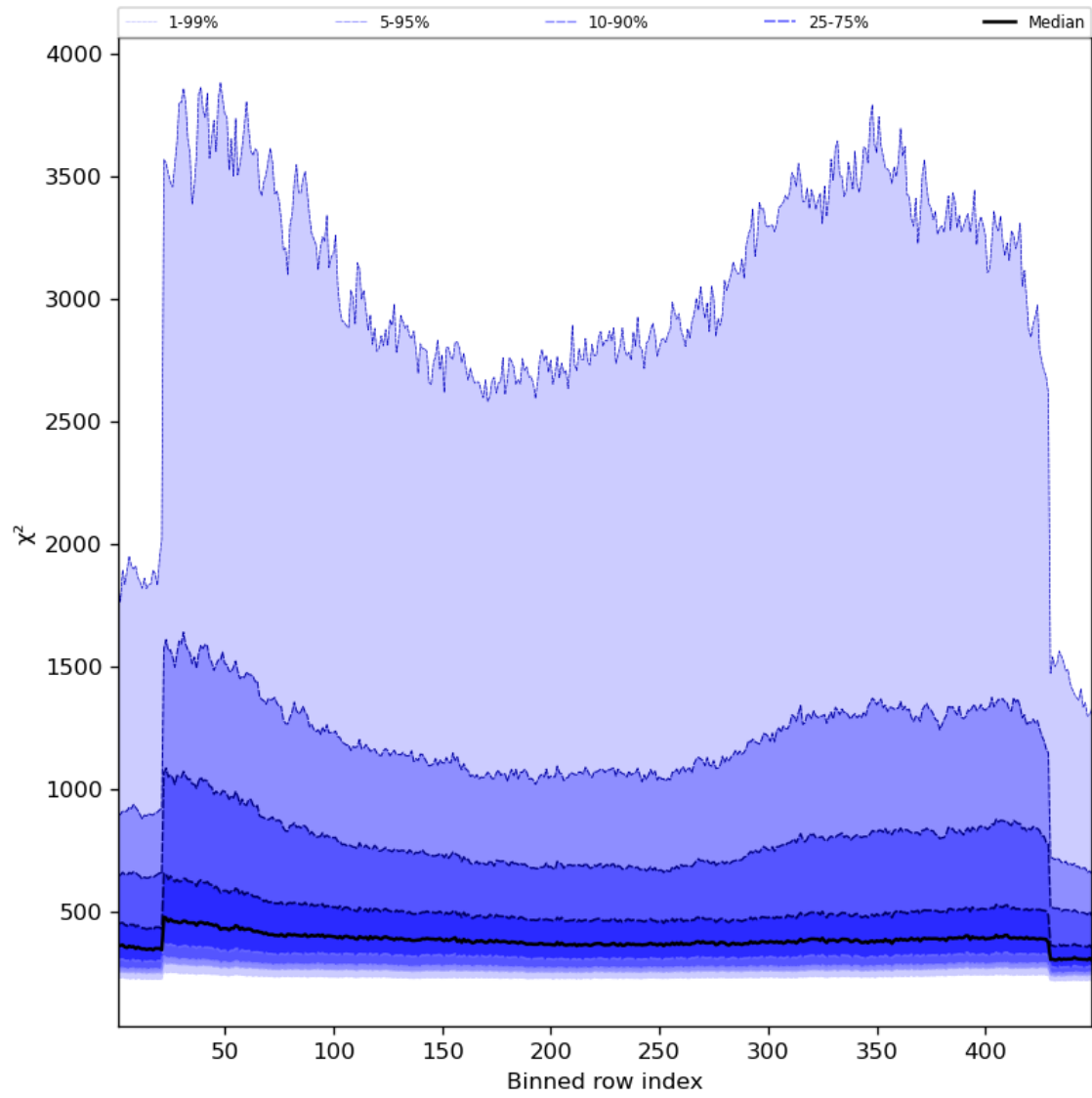
Figure 59: Along track statistics of “ \chi^2 ” for 2023-10-13 to 2023-10-15
