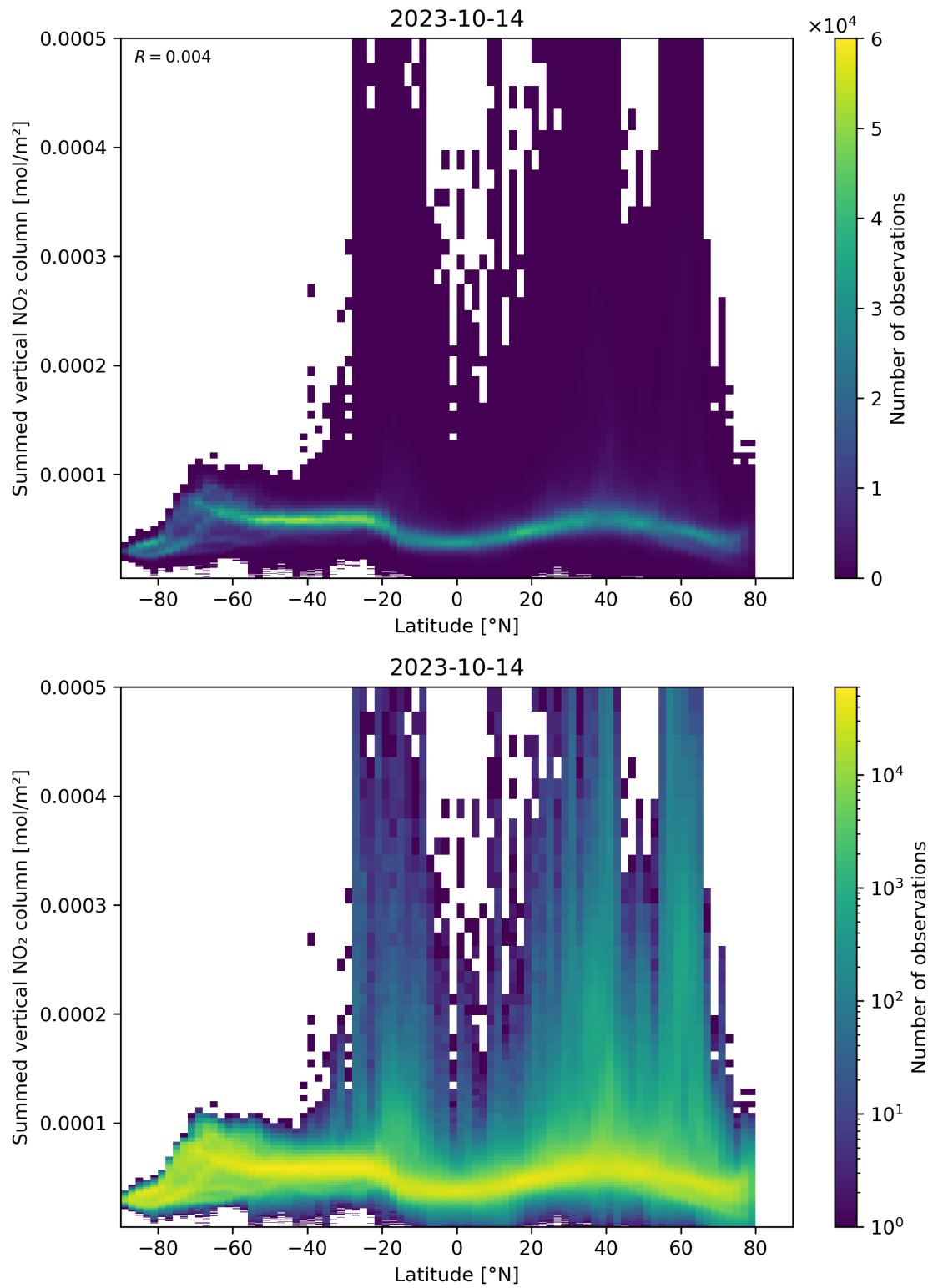
Figure 88: Scatter density plot of “Latitude” against “Summed vertical NO 2 column” for 2023-10-13 to 2023-10-15.
