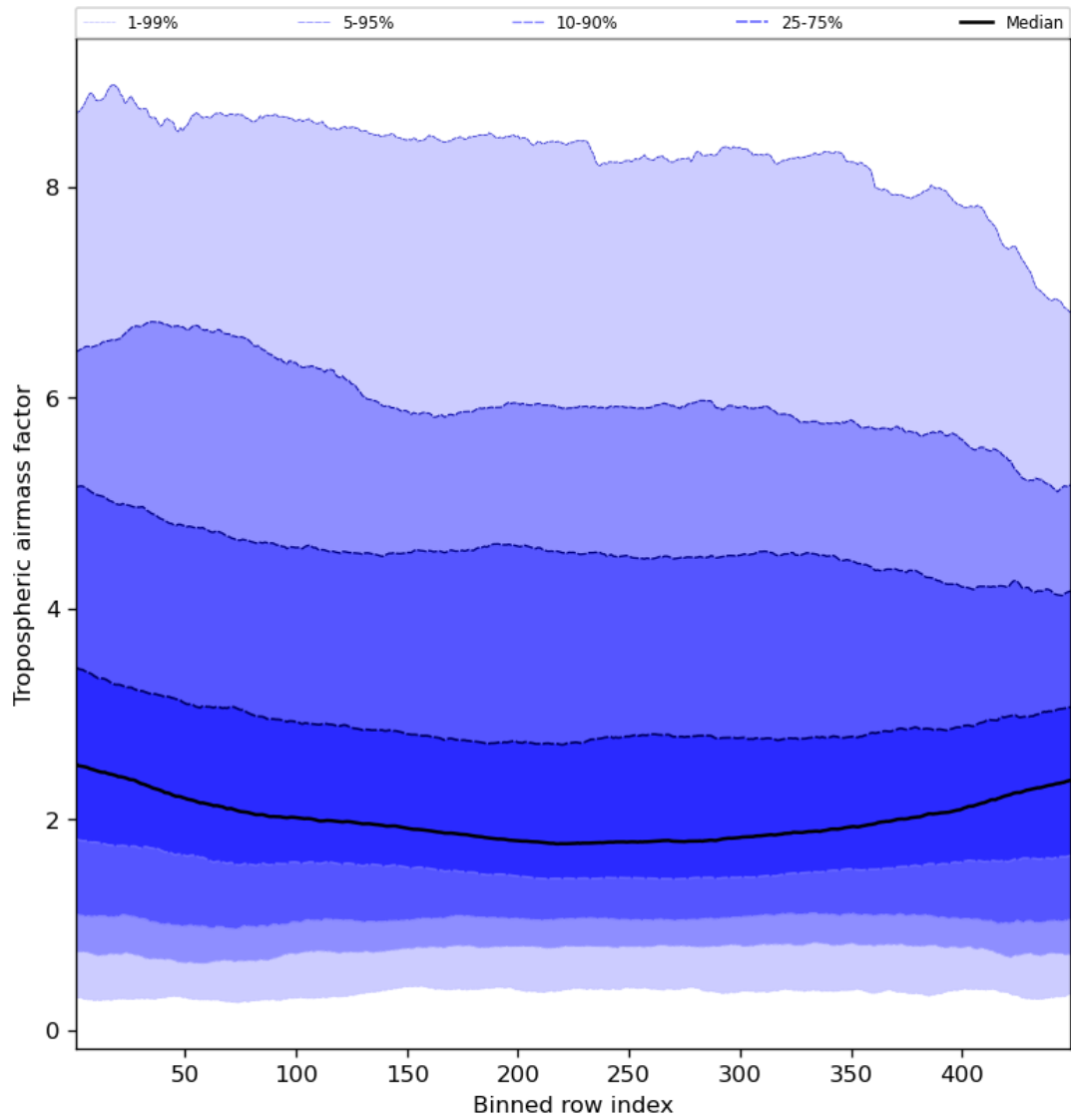
Figure 48: Along track statistics of “Tropospheric air mass factor” for 2023-10-13 to 2023-10-15
