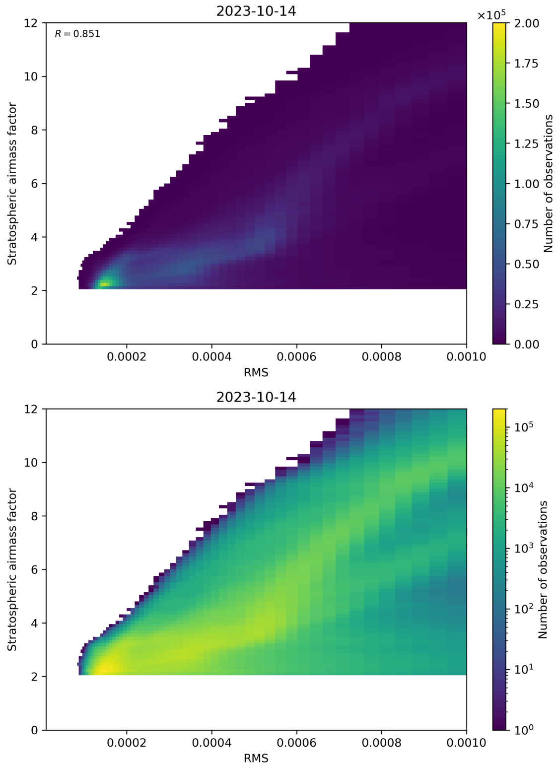
Figure 144: Scatter density plot of “RMS” against “Stratospheric airmass factor” for 2023-10-13 to 2023-10-15.
