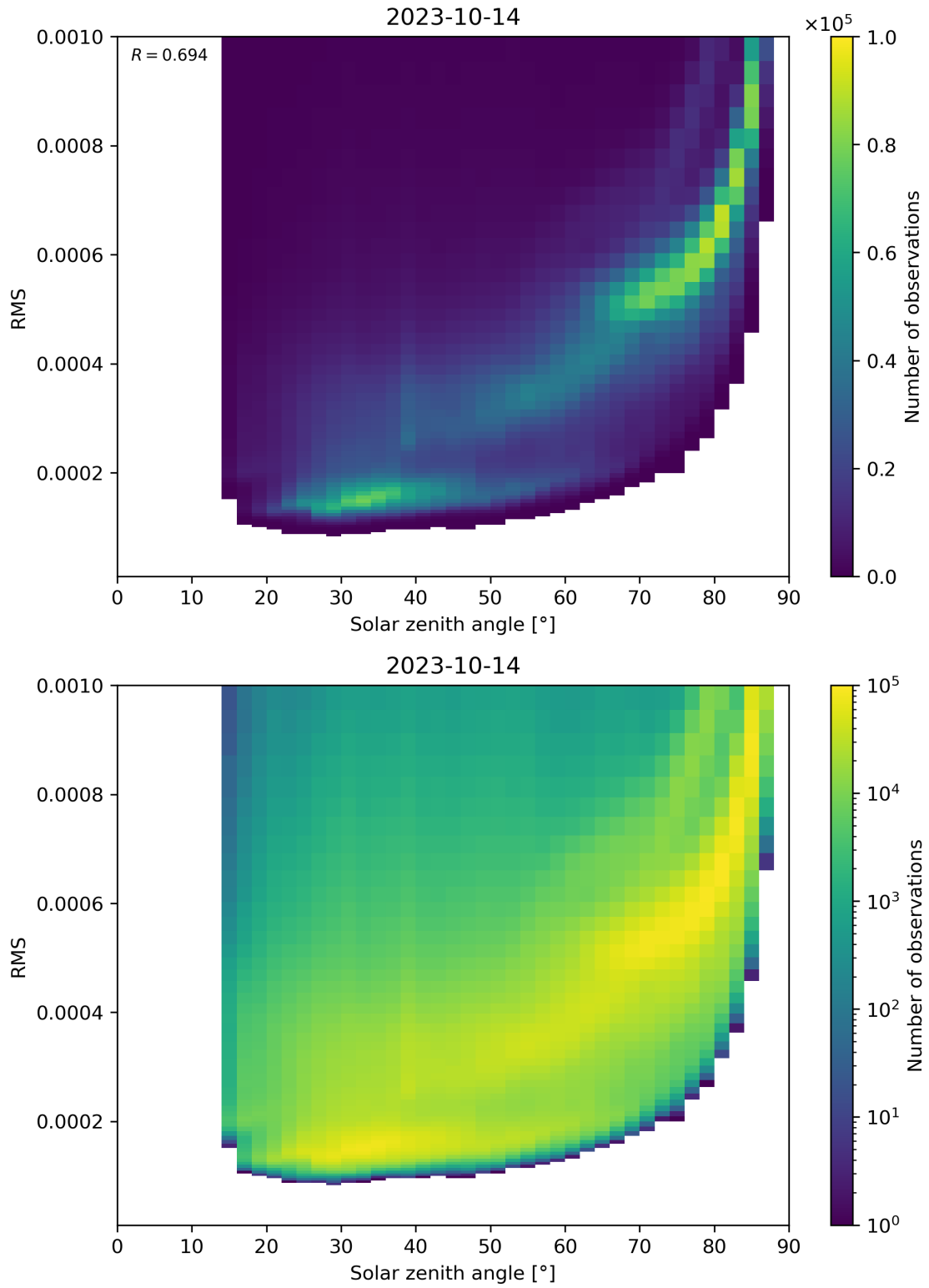
Figure 157: Scatter density plot of “Solar zenith angle” against “RMS” for 2023-10-13 to 2023-10-15.
