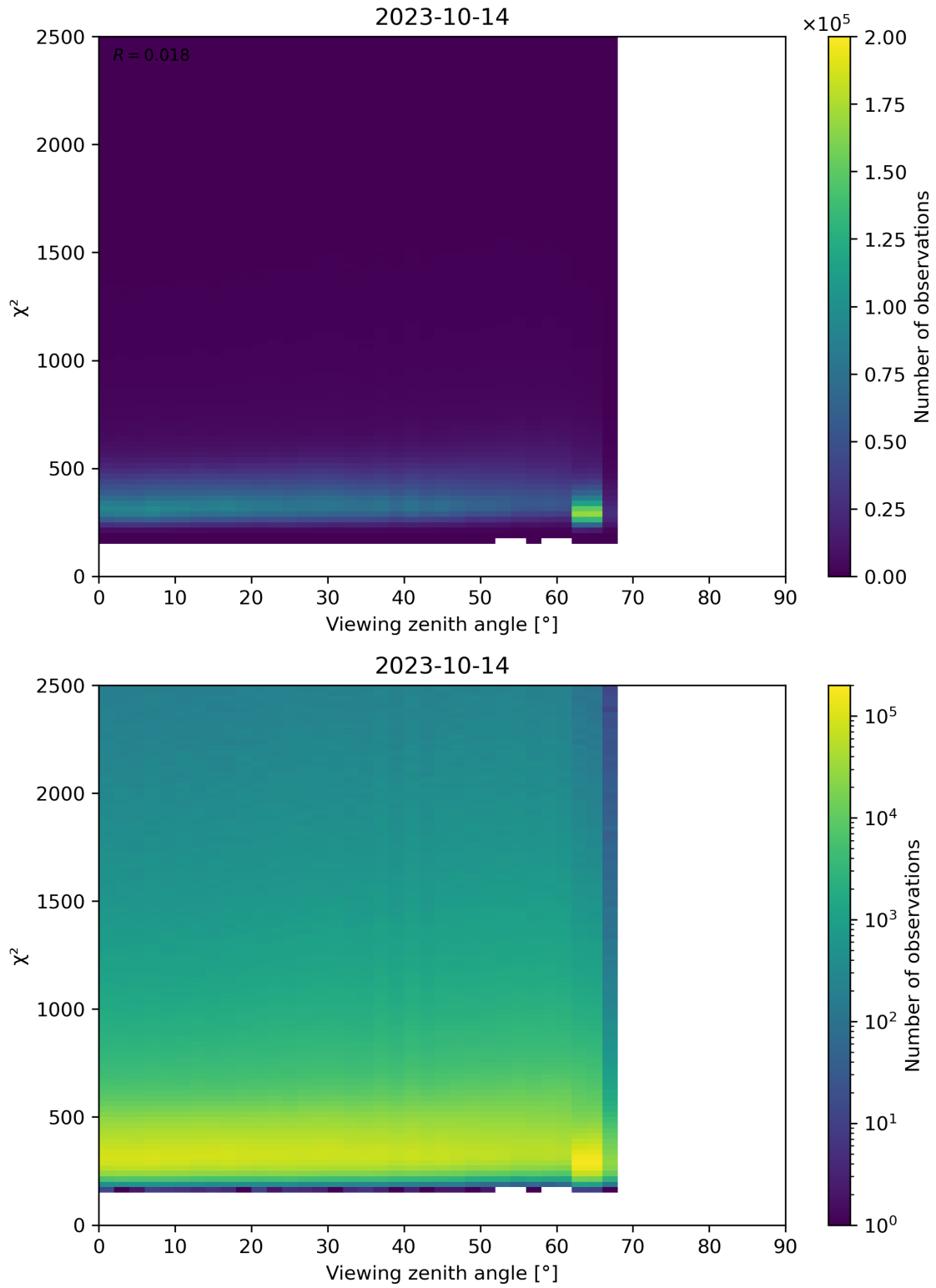
Figure 162: Scatter density plot of “Viewing zenith angle” against “ \chi^2 ” for 2023-10-13 to 2023-10-15.
