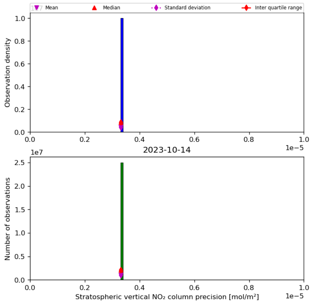
Figure 37: Histogram of “Stratospheric vertical NO 2 column precision” for 2023-10-13 to 2023-10-15
