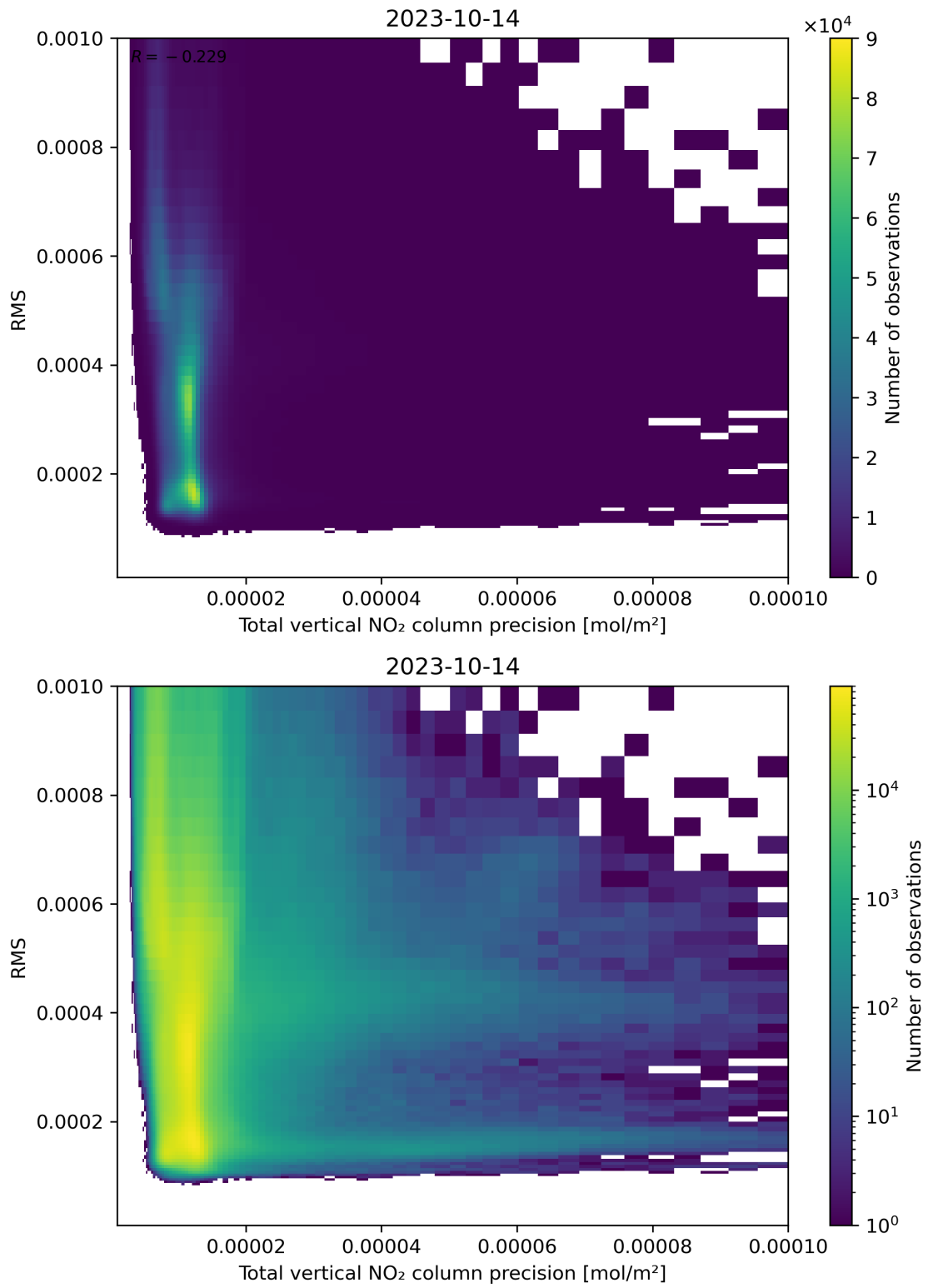
Figure 119: Scatter density plot of “Total vertical NO 2 column precision” against “RMS” for 2023-10-13 to 2023-10-15.
