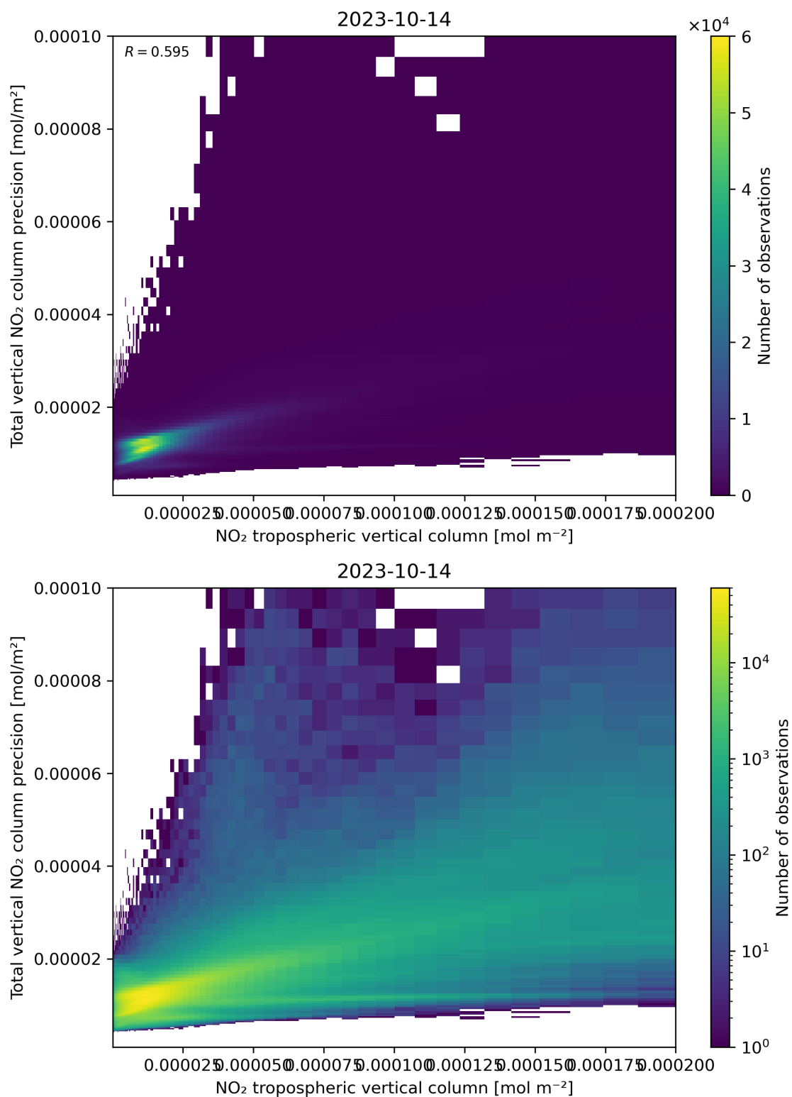
Figure 129: Scatter density plot of “NO 2 tropospheric vertical column” against “Total vertical NO 2 column precision” for 2023-10-13 to 2023-10-15.
