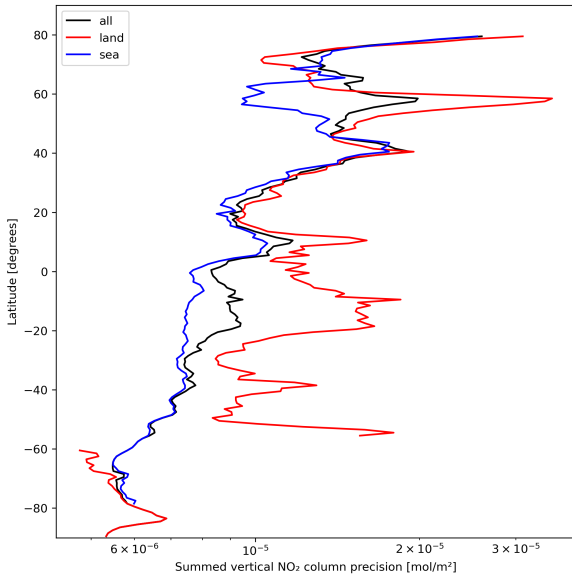
Figure 24: Zonal average of “Summed vertical NO 2 column precision” for 2023-10-13 to 2023-10-15.
