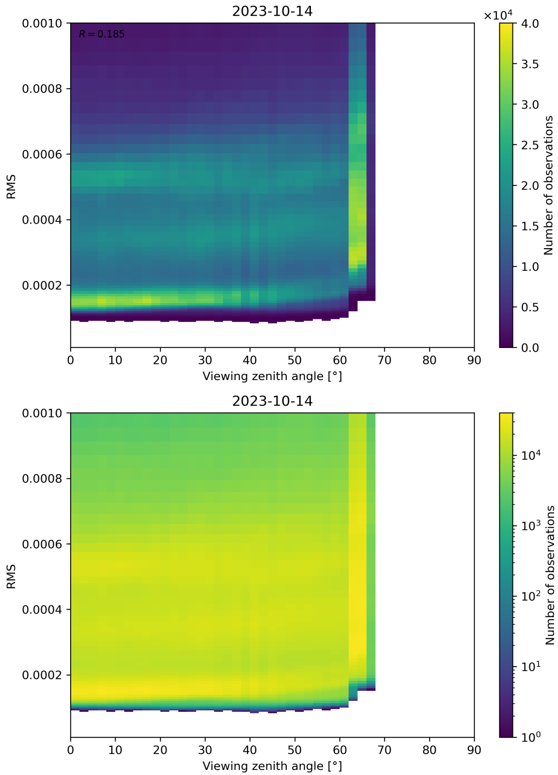
Figure 171: Scatter density plot of “Viewing zenith angle” against “RMS” for 2023-10-13 to 2023-10-15.
