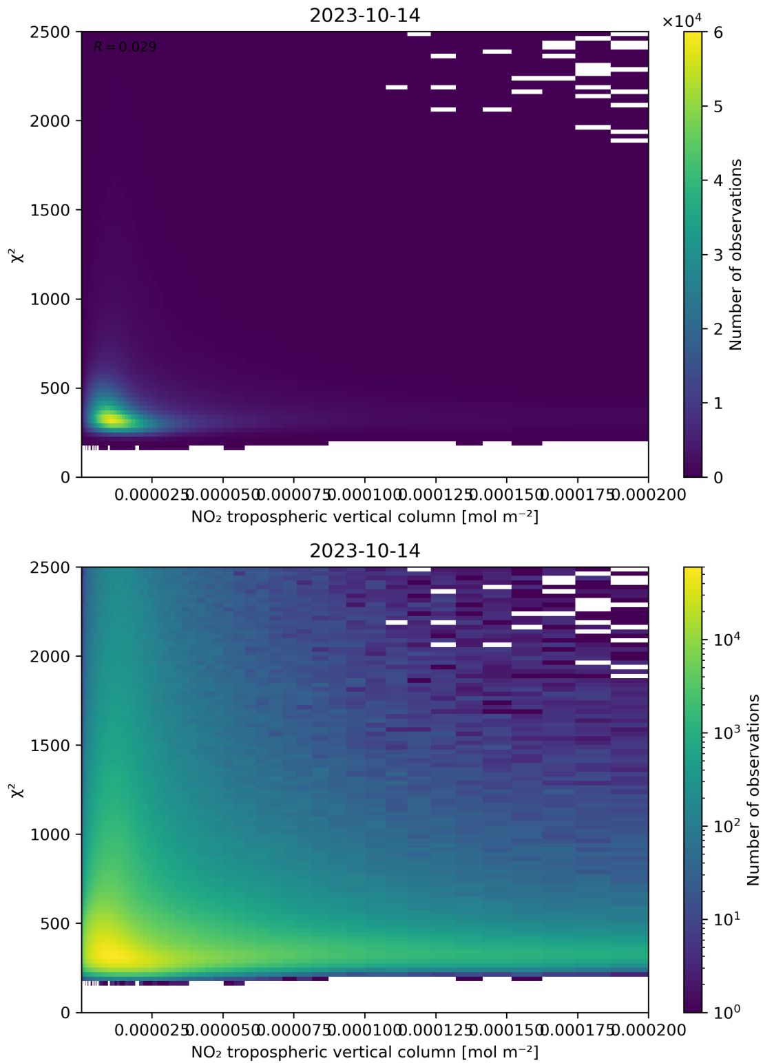
Figure 124: Scatter density plot of “NO 2 tropospheric vertical column” against “ \chi^2 ” for 2023-10-13 to 2023-10-15.
