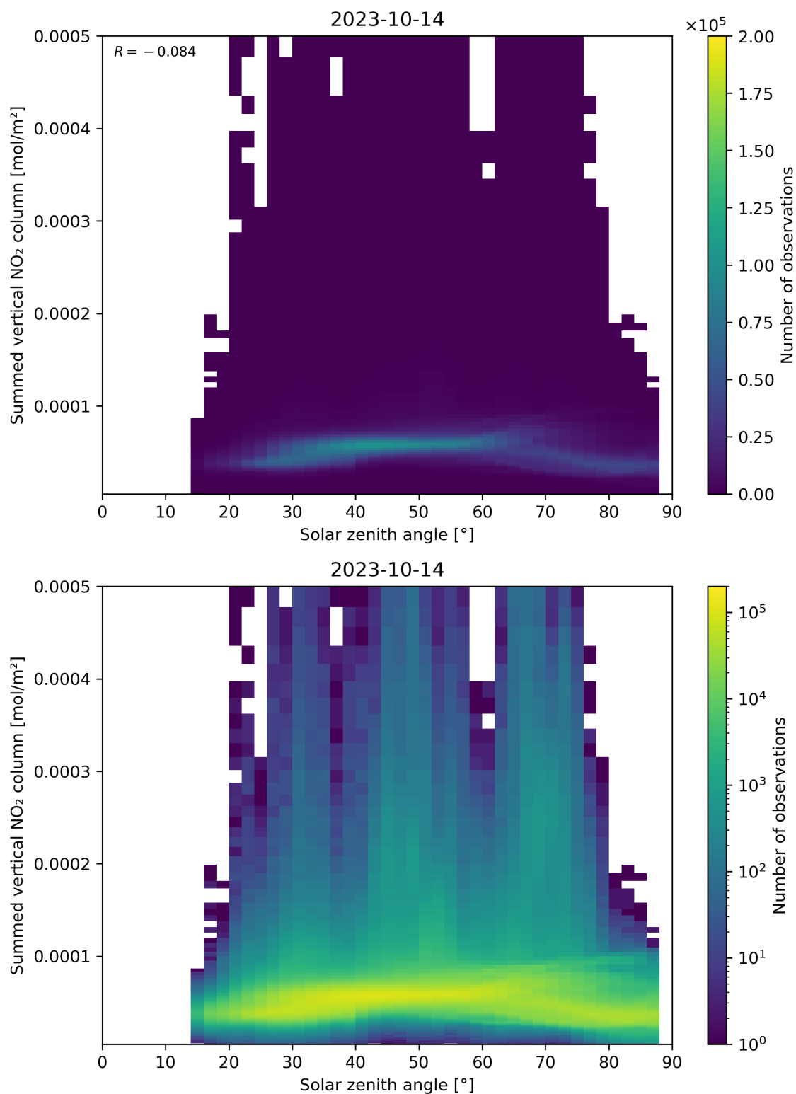
Figure 151: Scatter density plot of “Solar zenith angle” against “Summed vertical NO 2 column” for 2023-10-13 to 2023-10-15.
