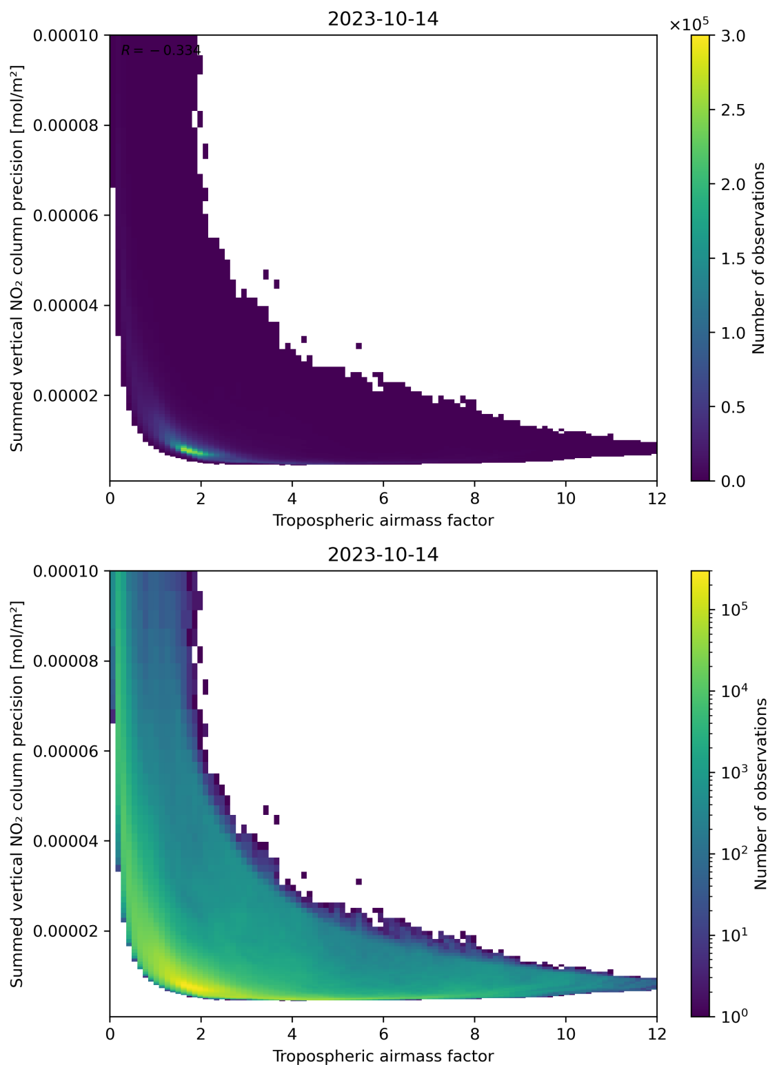
Figure 76: Scatter density plot of “Tropospheric air mass factor” against “Summed vertical NO 2 column precision” for 2023-10-13 to 2023-10-15.
