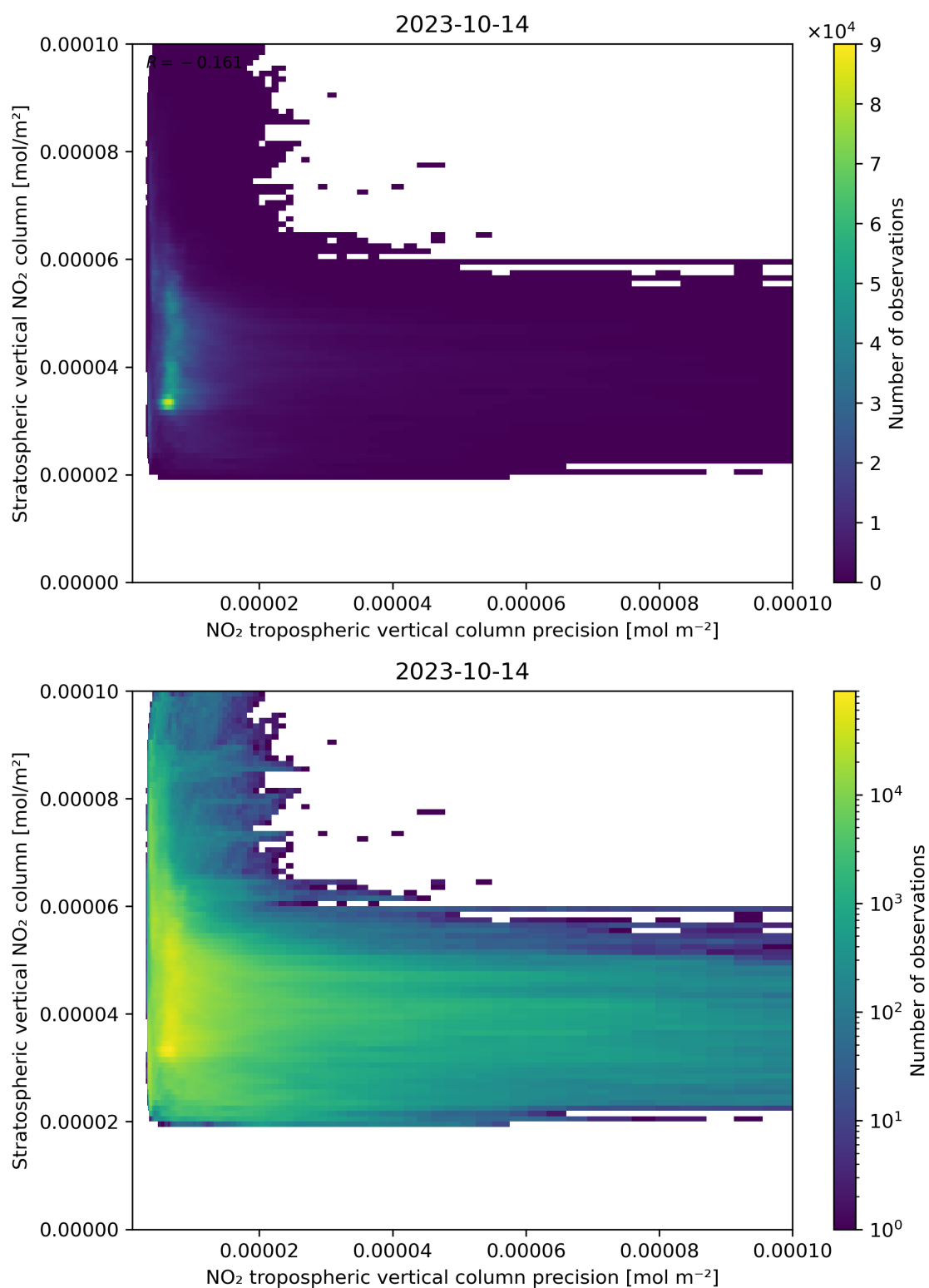
Figure 135: Scatter density plot of “NO 2 tropospheric vertical column precision” against “Stratospheric vertical NO 2 column” for 2023-10-13 to 2023-10-15.
