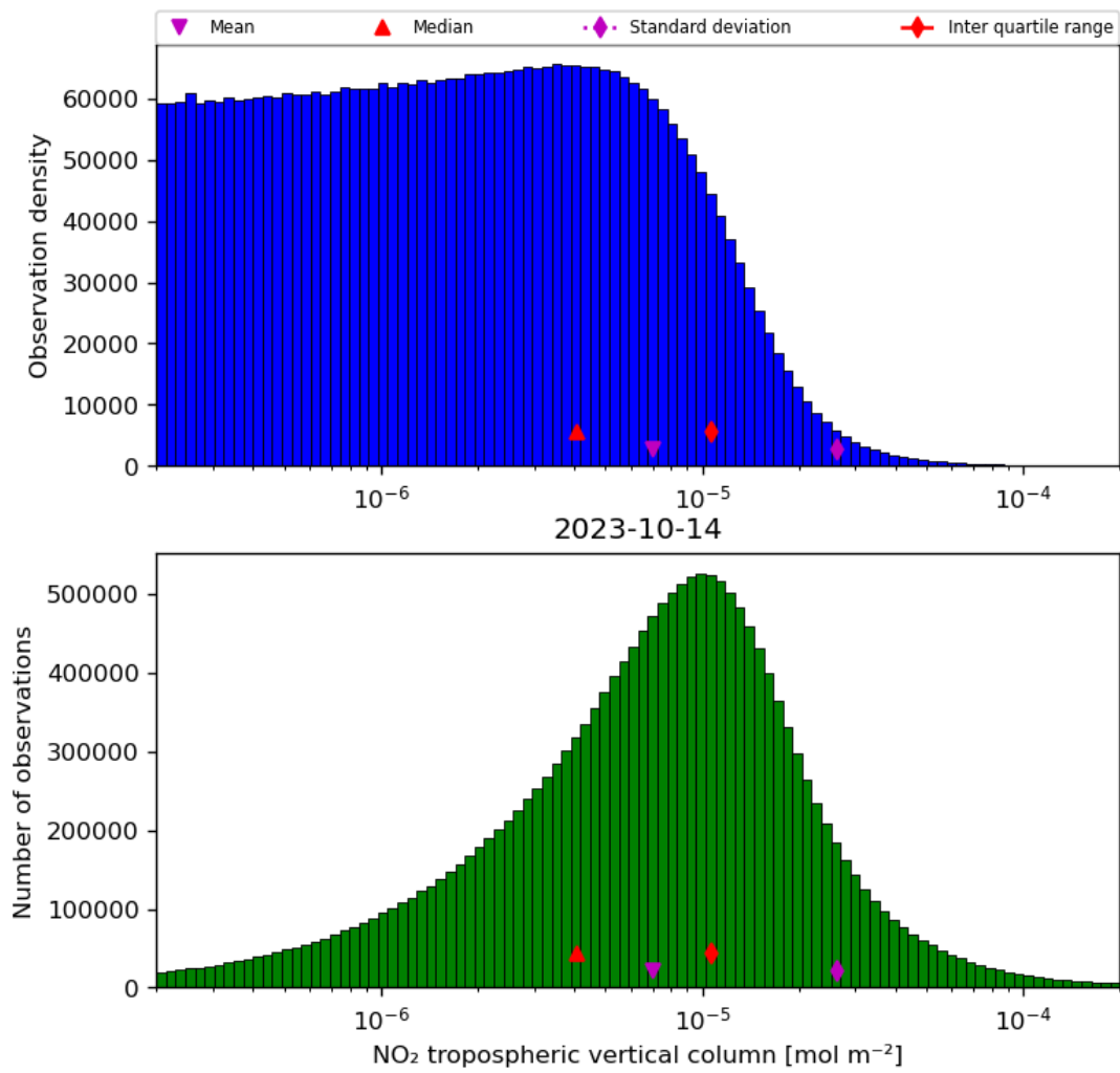
Figure 29: Histogram of “NO 2 tropospheric vertical column” for 2023-10-13 to 2023-10-15
