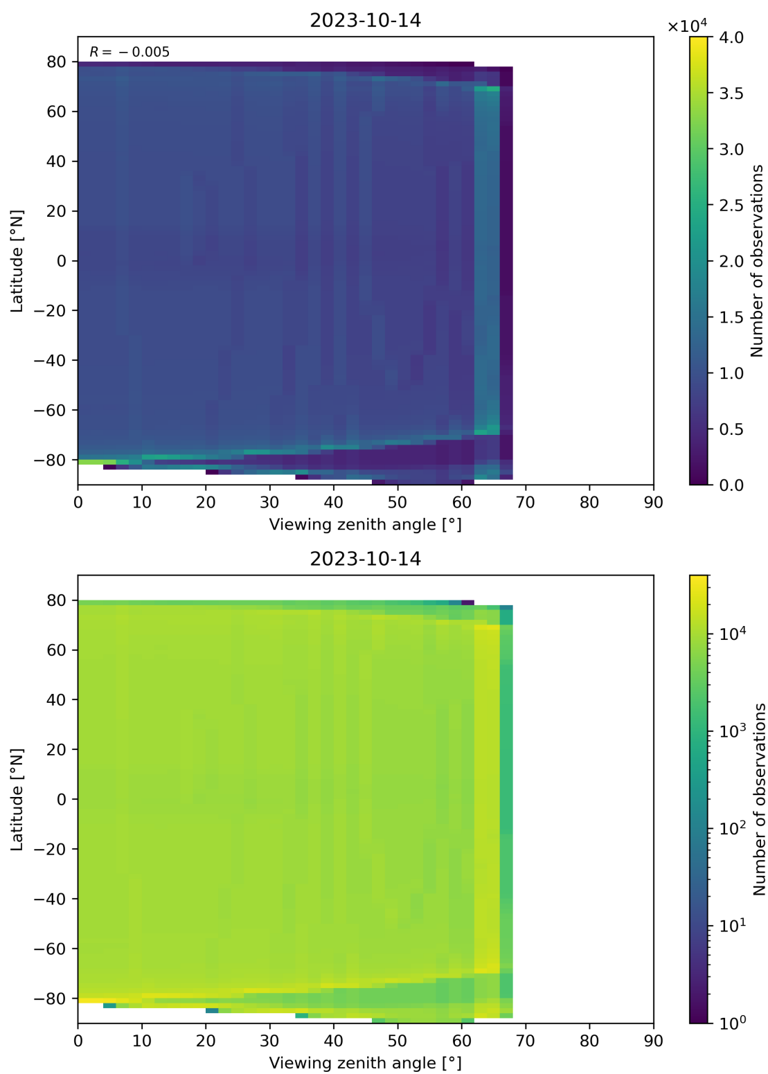
Figure 163: Scatter density plot of “Viewing zenith angle” against “Latitude” for 2023-10-13 to 2023-10-15.
