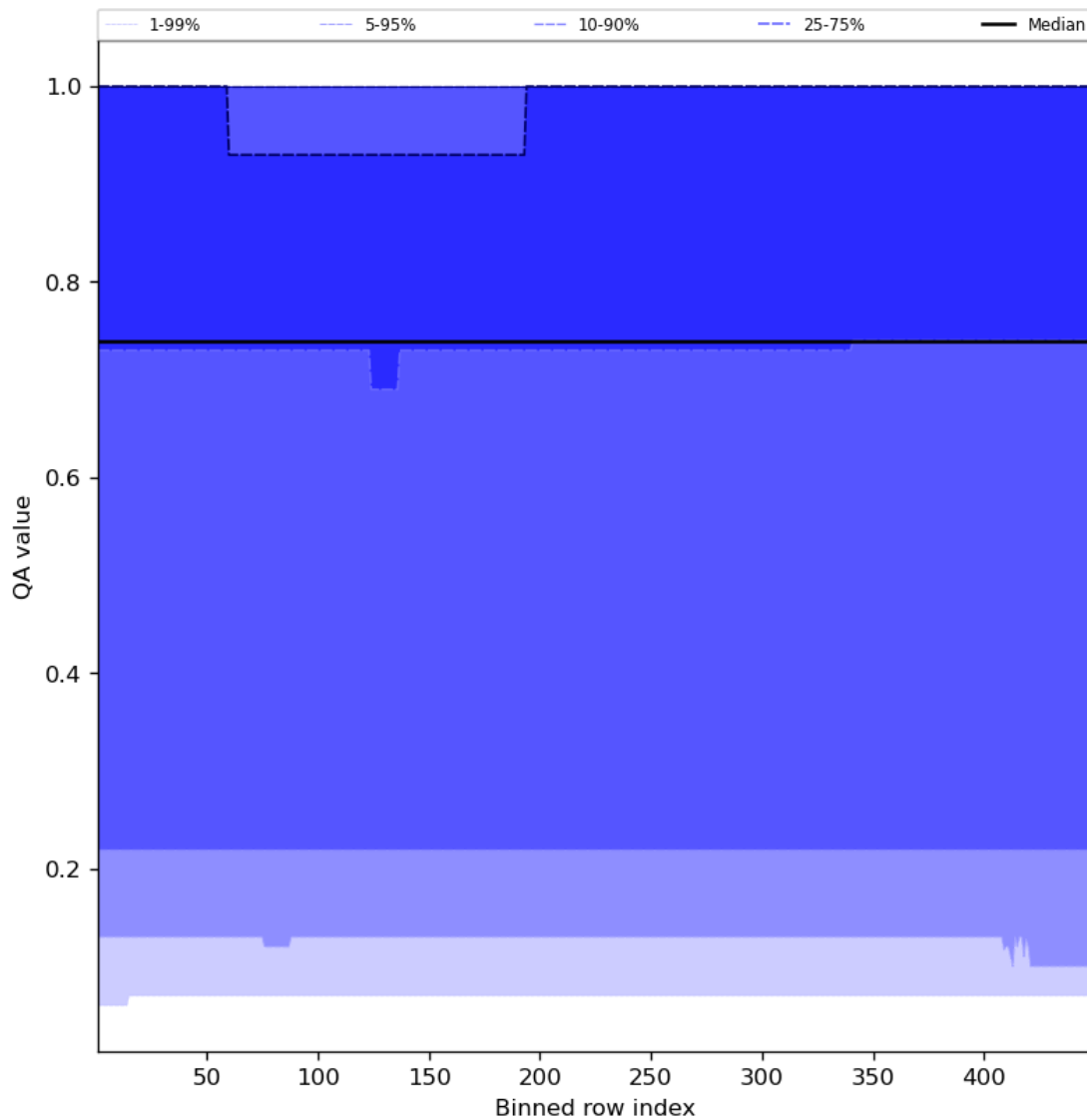
Figure 45: Along track statistics of “QA value” for 2023-10-13 to 2023-10-15
