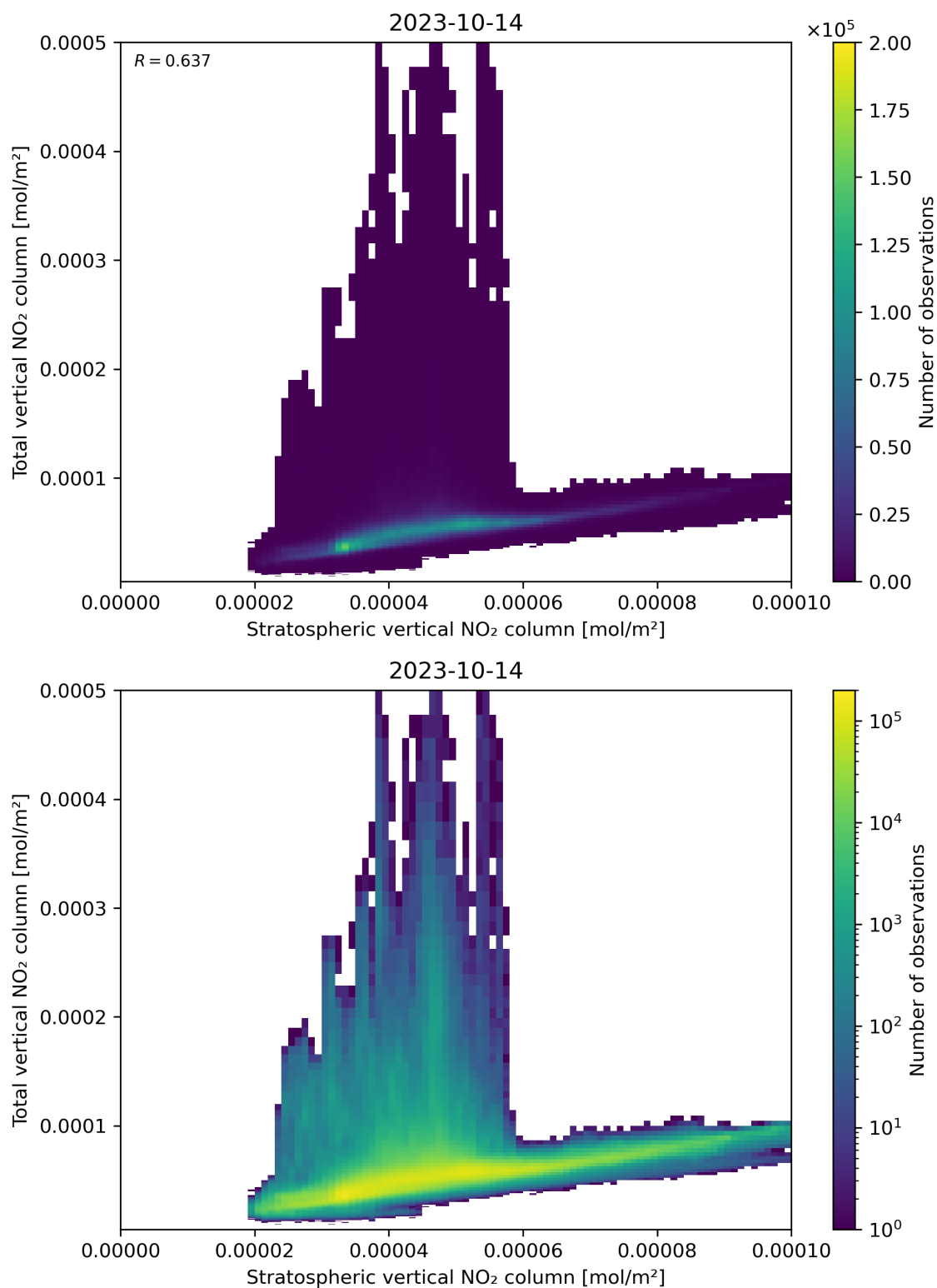
Figure 100: Scatter density plot of “Stratospheric vertical NO 2 column” against “Total vertical NO 2 column” for 2023-10-13 to 2023-10-15.
