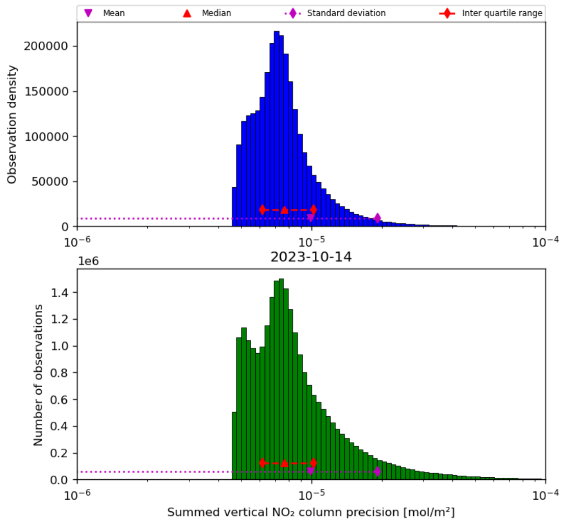
Figure 41: Histogram of “Summed vertical NO 2 column precision” for 2023-10-13 to 2023-10-15
