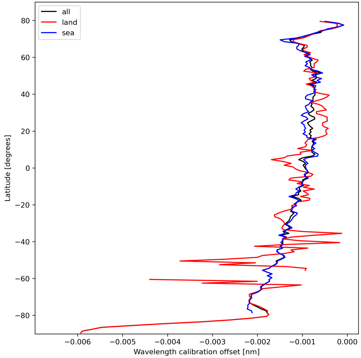
Figure 18: Zonal average of “Wavelength calibration offset” for 2023-10-13 to 2023-10-15.
