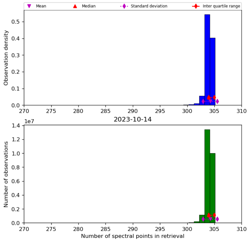
Figure 33: Histogram of “Number of spectral points in retrieval” for 2023-10-13 to 2023-10-15
