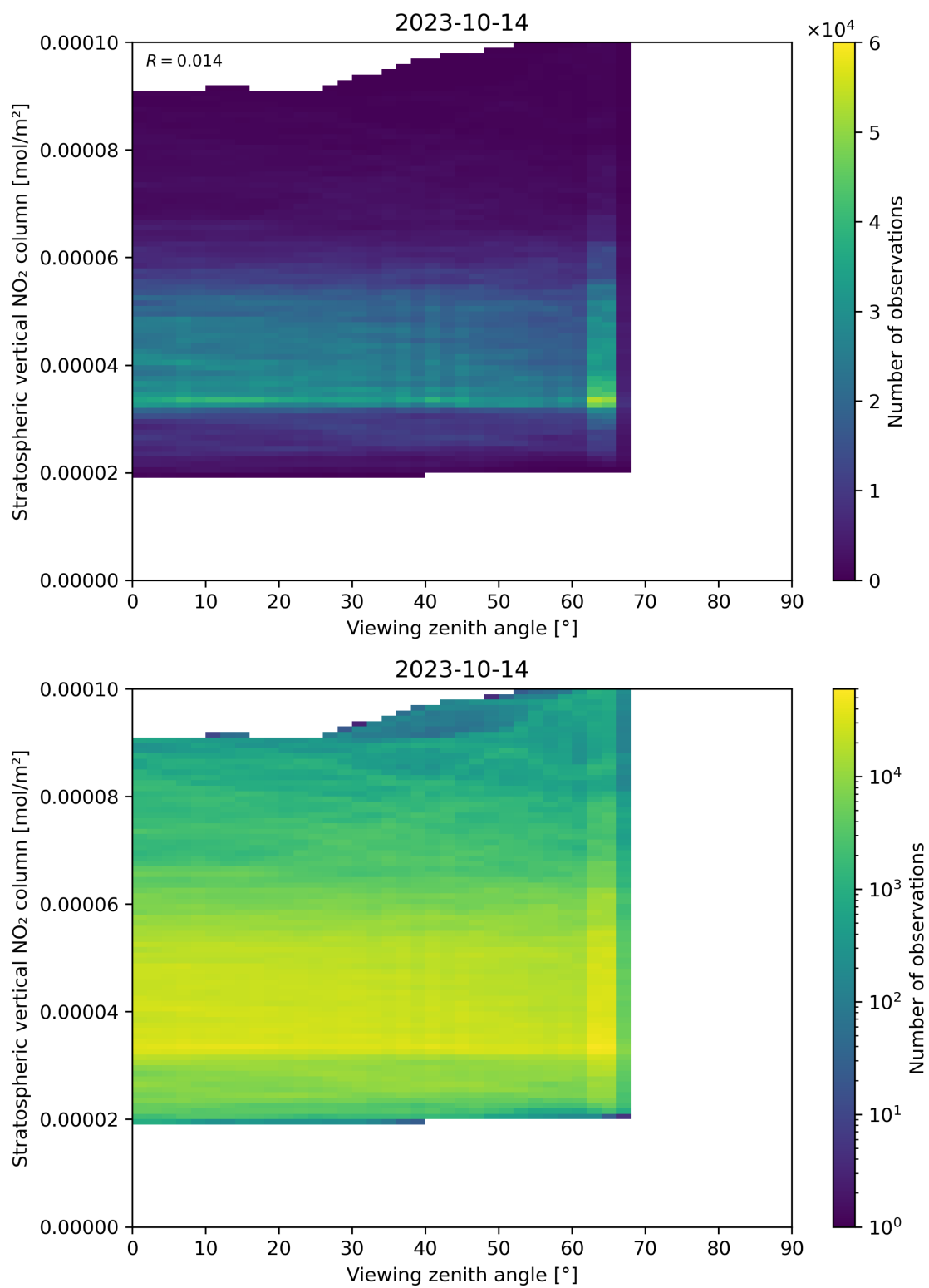
Figure 164: Scatter density plot of “Viewing zenith angle” against “Stratospheric vertical NO 2 column” for 2023-10-13 to 2023-10-15.
