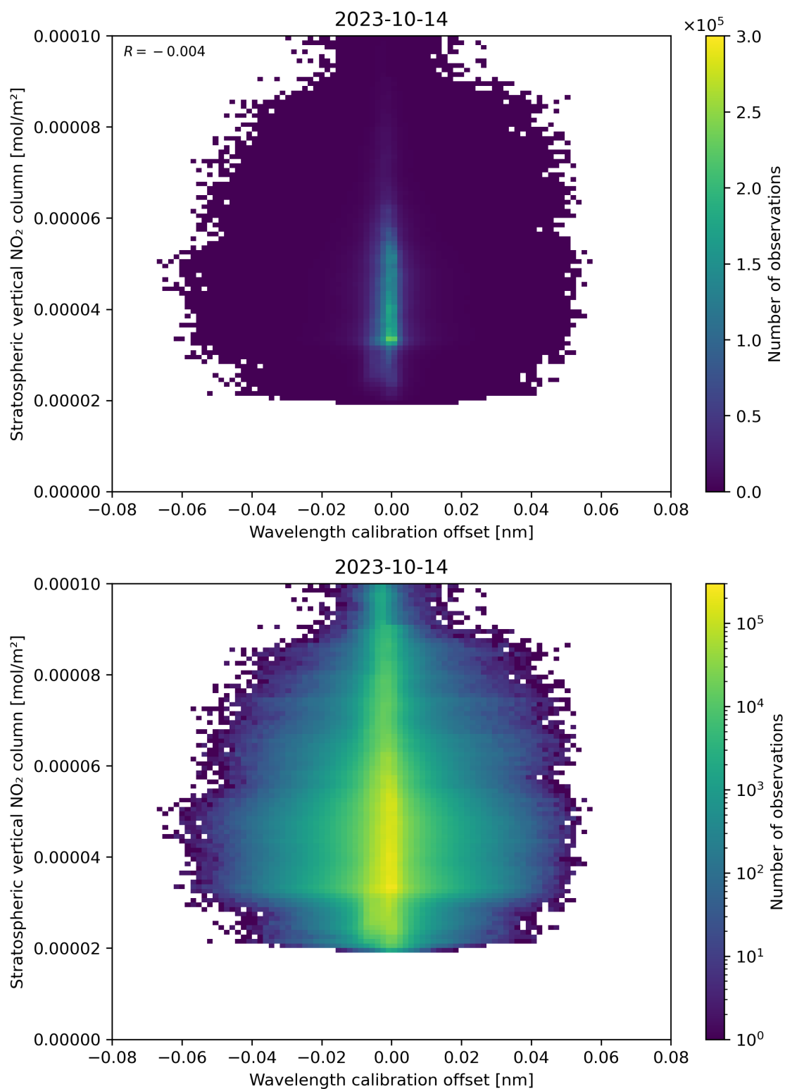
Figure 176: Scatter density plot of “Wavelength calibration offset” against “Stratospheric vertical NO 2 column” for 2023-10-13 to 2023-10-15.
