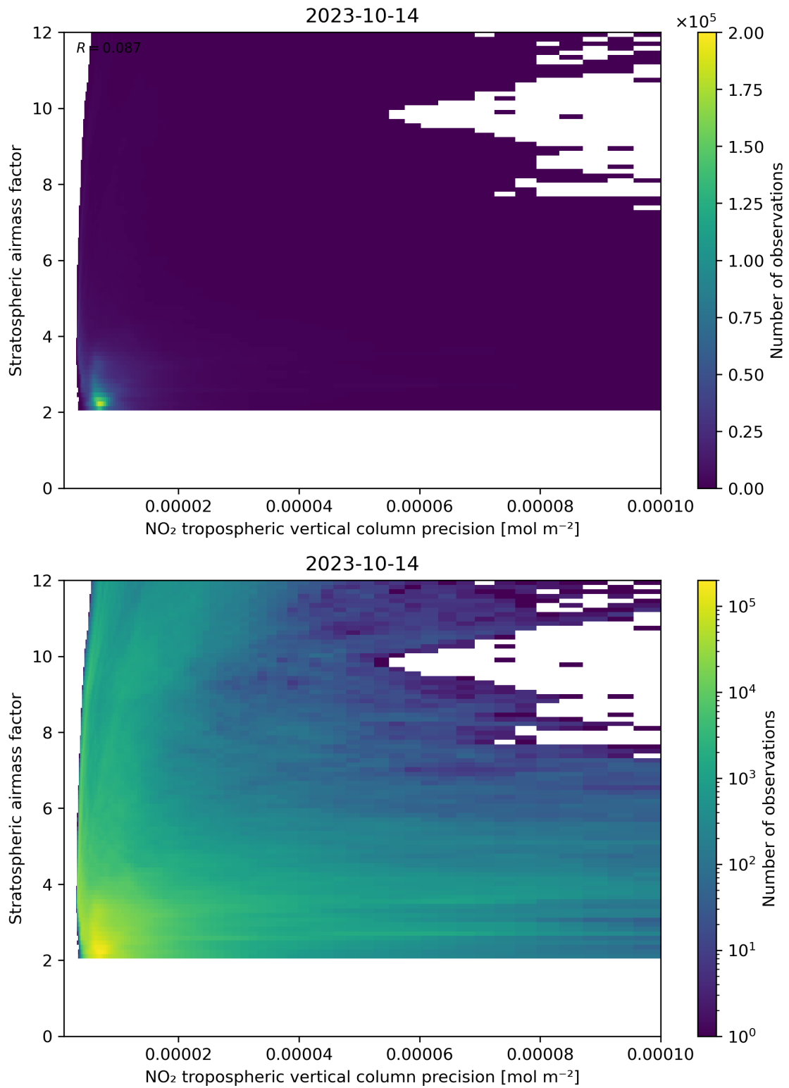
Figure 131: Scatter density plot of “NO 2 tropospheric vertical column precision” against “Stratospheric airmass factor” for 2023-10-13 to 2023-10-15.
