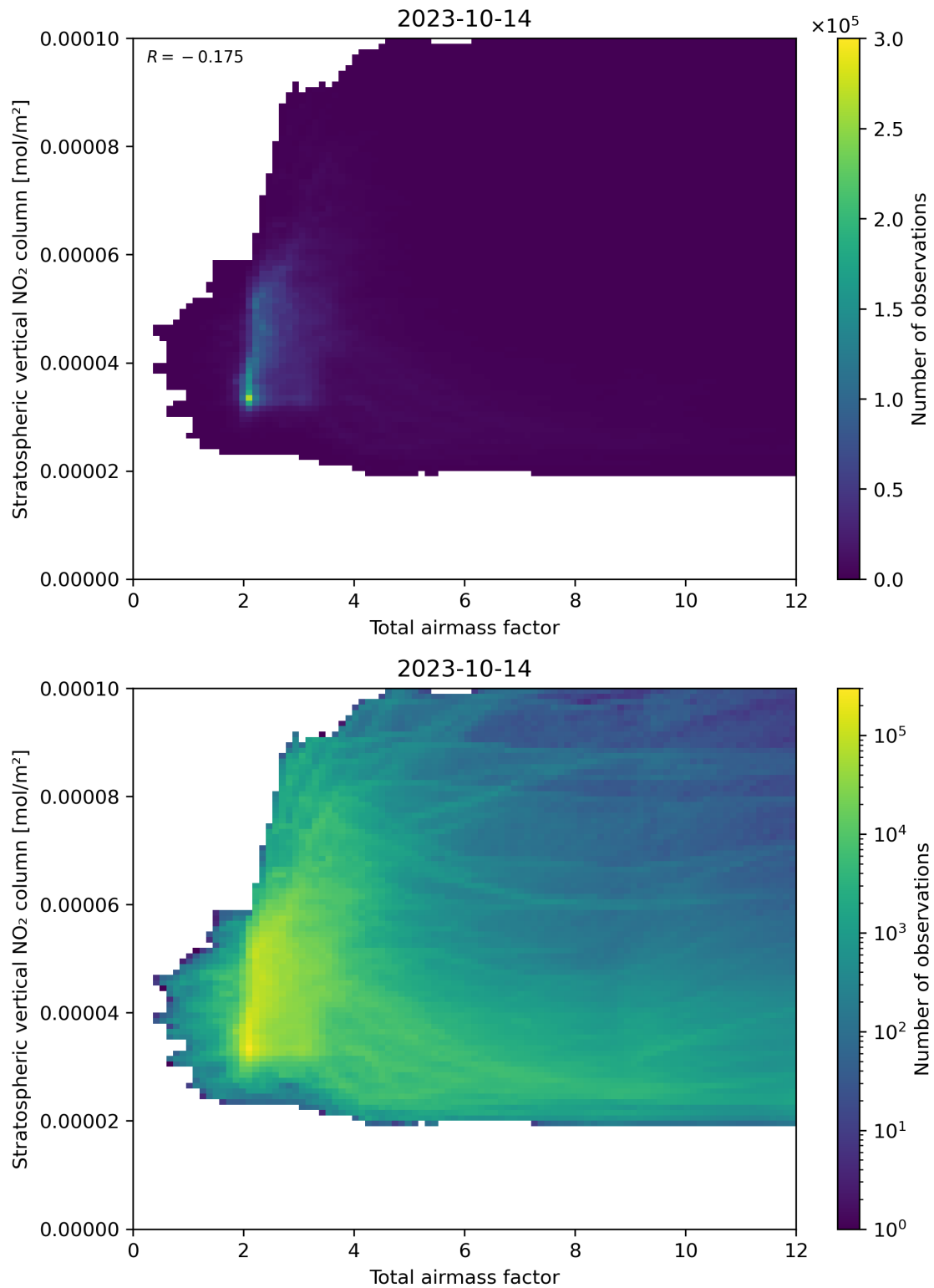
Figure 64: Scatter density plot of “Total airmass factor” against “Stratospheric vertical NO 2 column” for 2023-10-13 to 2023-10-15.
