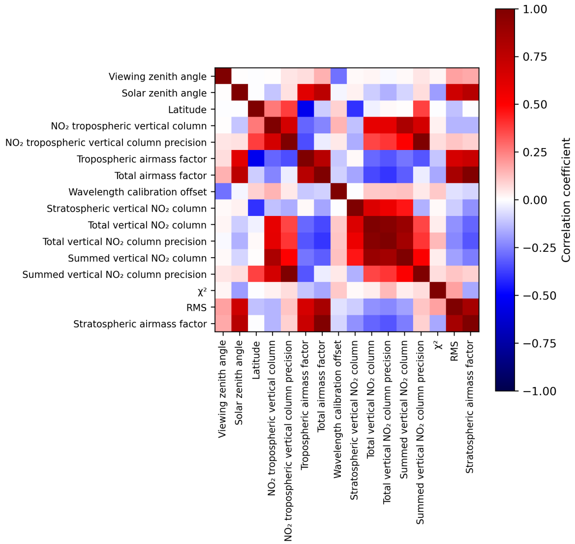
Figure 2: Map of correlation matrix for 2023-10-13 to 2023-10-15.
