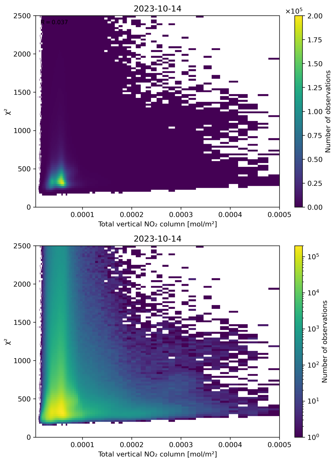
Figure 111: Scatter density plot of “Total vertical NO 2 column” against “ \chi^2 ” for 2023-10-13 to 2023-10-15.
