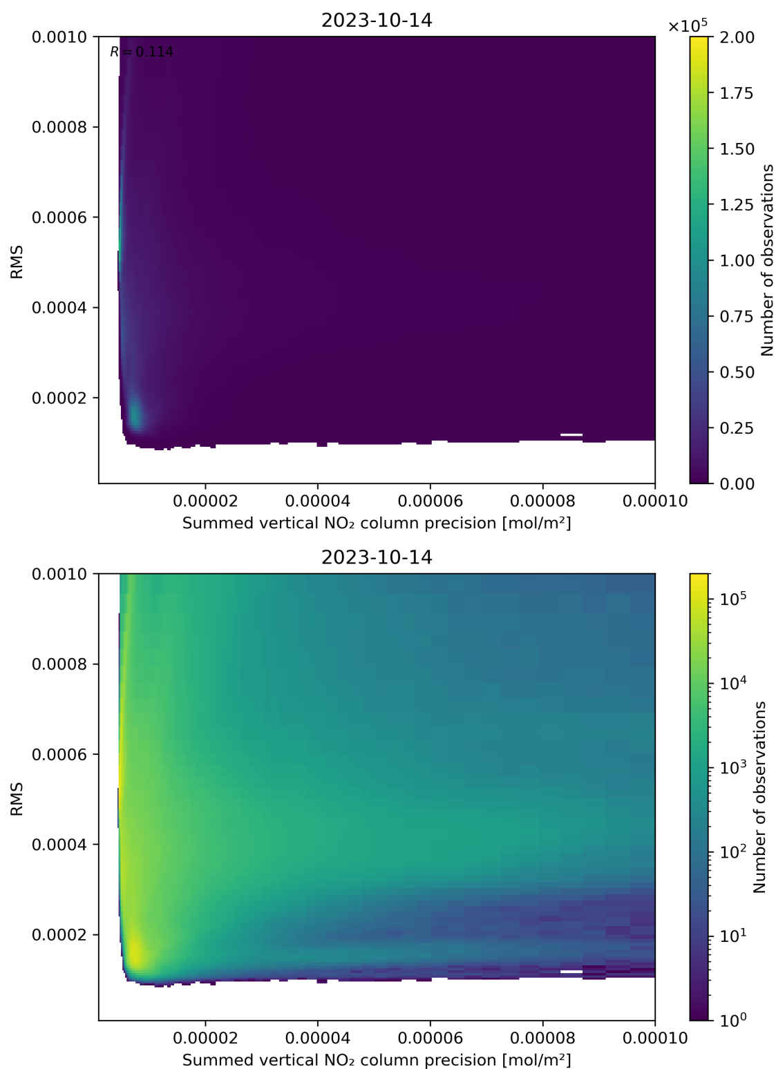
Figure 108: Scatter density plot of “Summed vertical NO 2 column precision” against “RMS” for 2023-10-13 to 2023-10-15.
