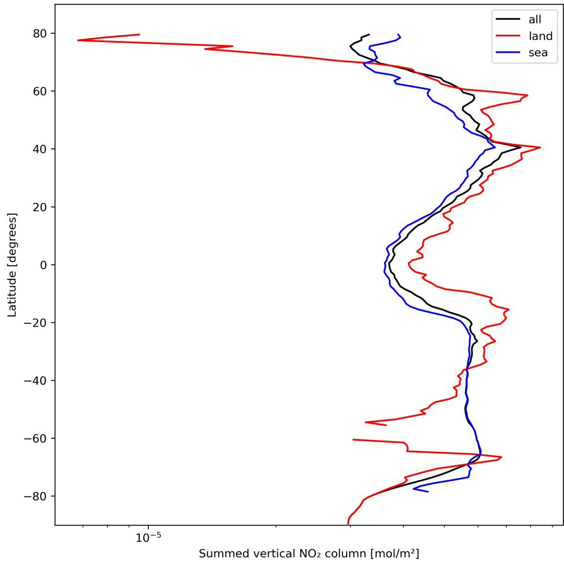
Figure 23: Zonal average of “Summed vertical NO 2 column” for 2023-10-13 to 2023-10-15.
