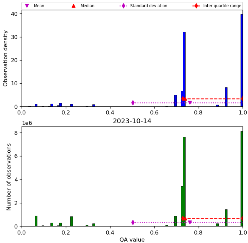
Figure 28: Histogram of “QA value” for 2023-10-13 to 2023-10-15
