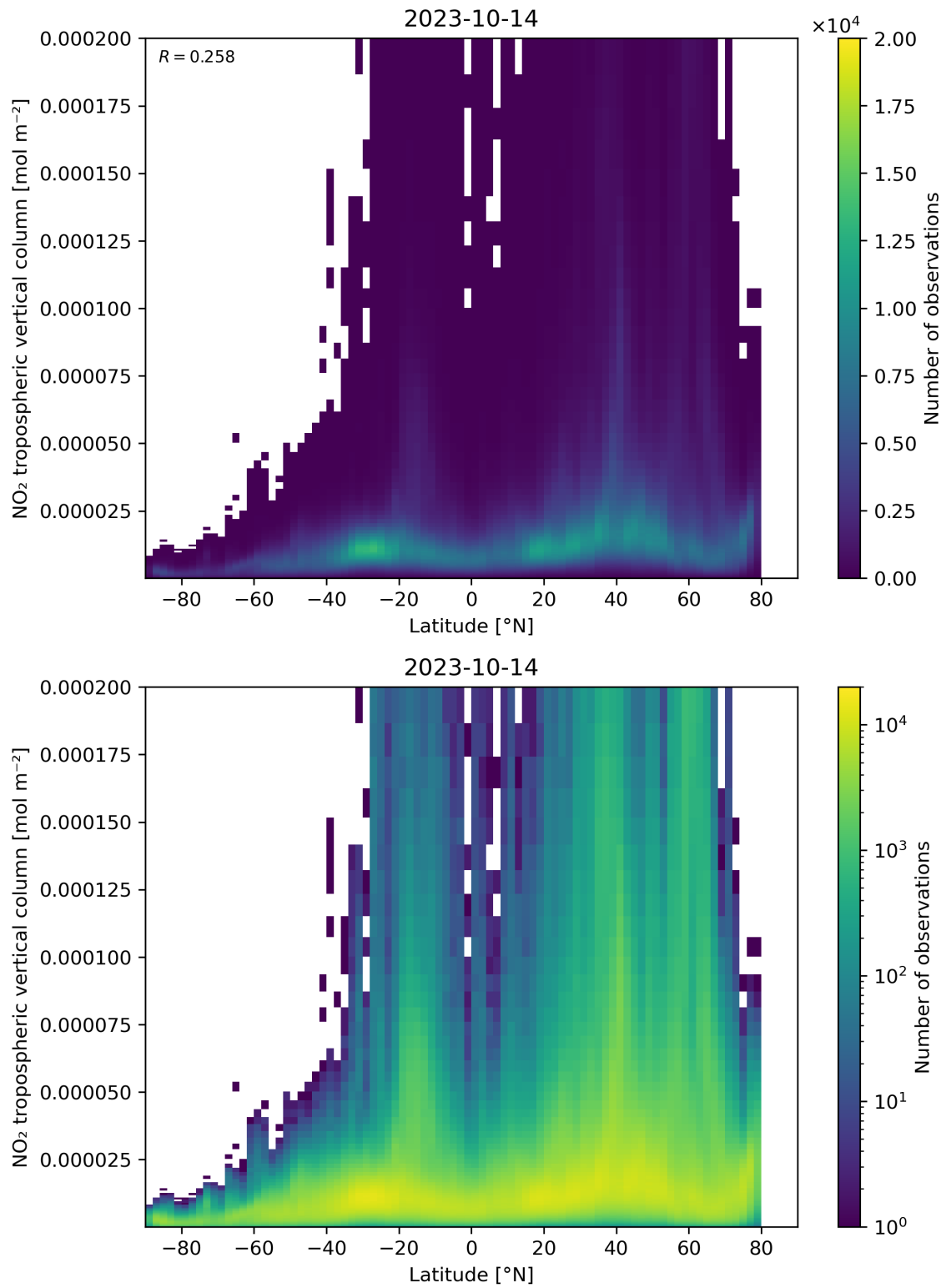
Figure 92: Scatter density plot of “Latitude” against “NO 2 tropospheric vertical column” for 2023-10-13 to 2023-10-15.
