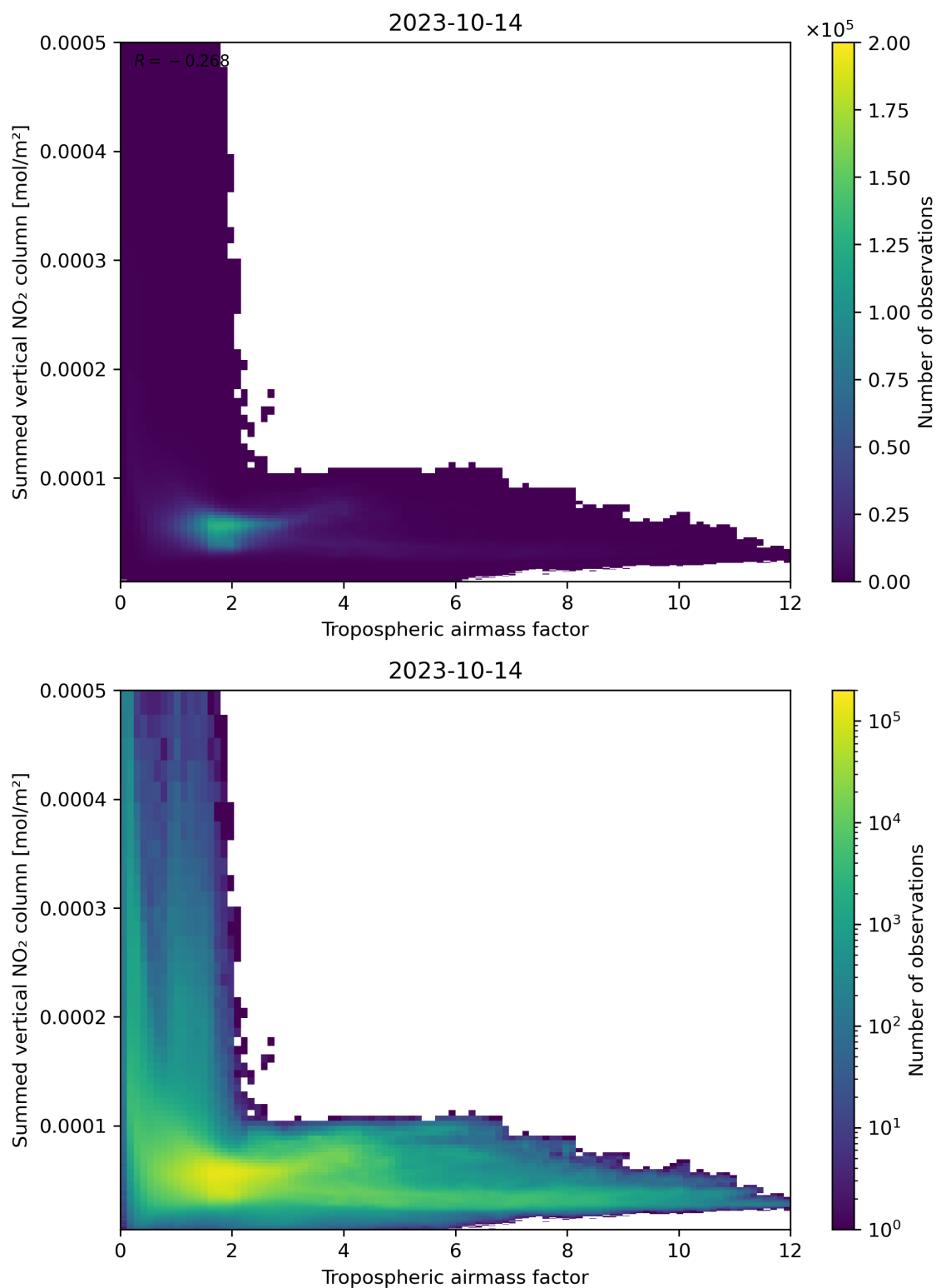
Figure 75: Scatter density plot of “Tropospheric air mass factor” against “Summed vertical NO 2 column” for 2023-10-13 to 2023-10-15.
