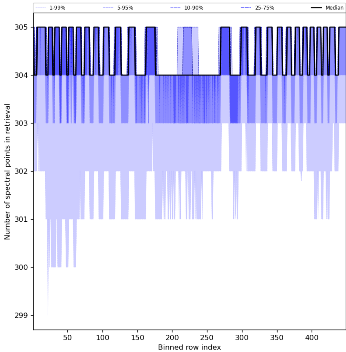
Figure 50: Along track statistics of “Number of spectral points in retrieval” for 2023-10-13 to 2023-10-15
