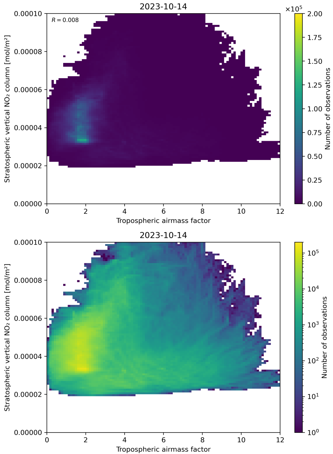
Figure 74: Scatter density plot of “Tropospheric air mass factor” against “Stratospheric vertical NO 2 column” for 2023-10-13 to 2023-10-15.
