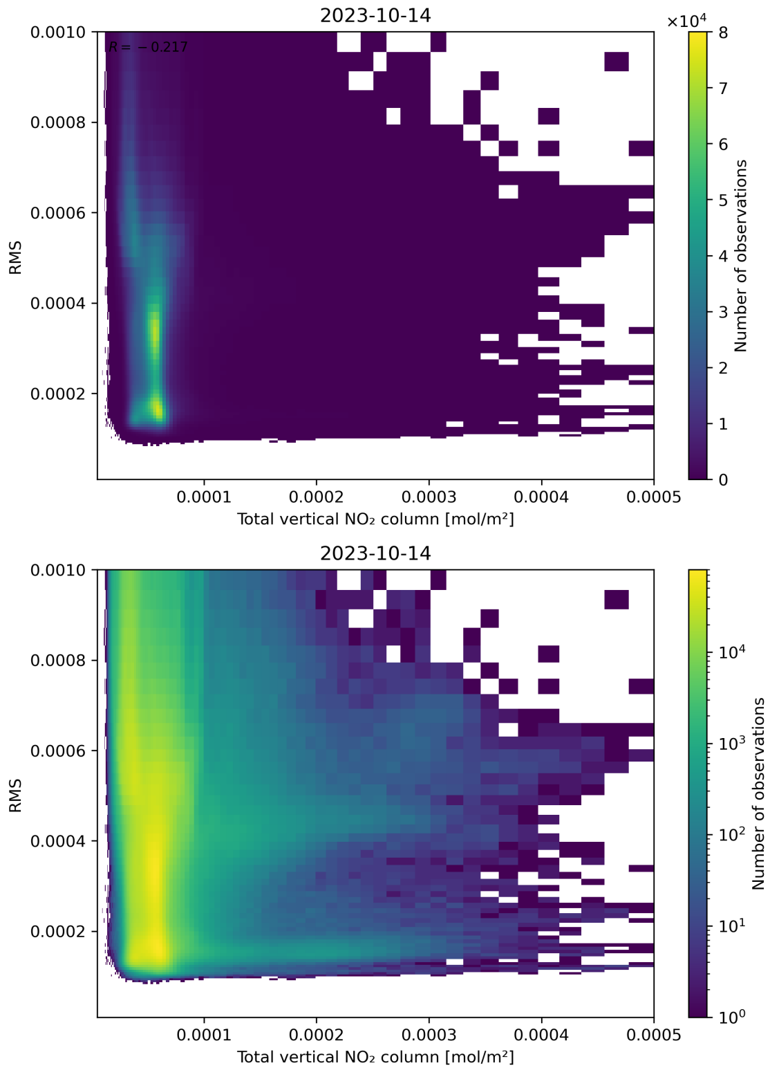
Figure 120: Scatter density plot of “Total vertical NO 2 column” against “RMS” for 2023-10-13 to 2023-10-15.
