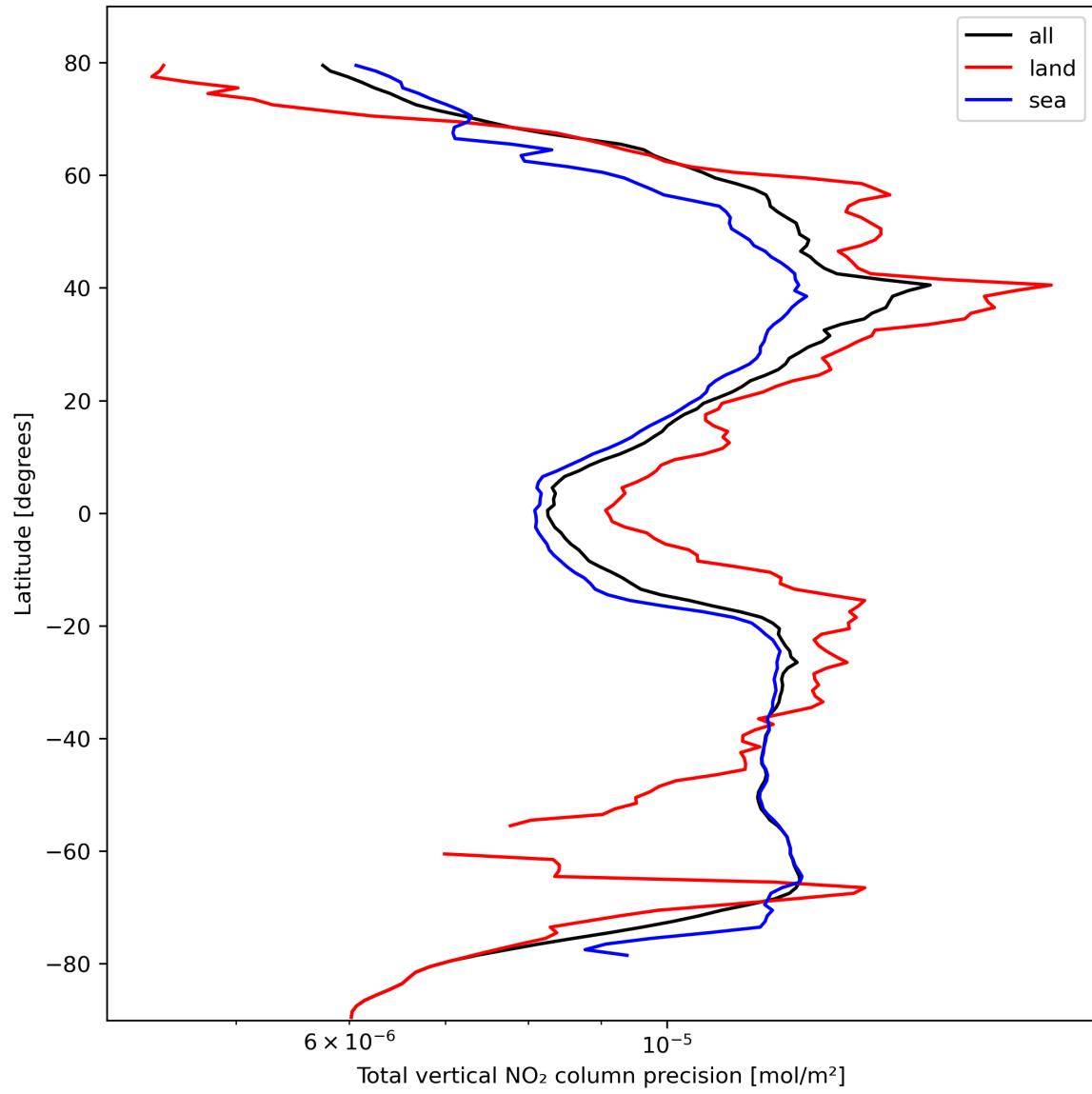
Figure 22: Zonal average of “Total vertical NO 2 column precision” for 2023-10-13 to 2023-10-15.
