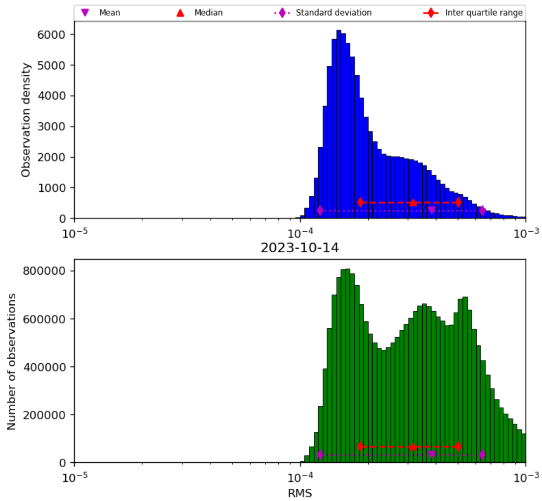
Figure 43: Histogram of “RMS” for 2023-10-13 to 2023-10-15
