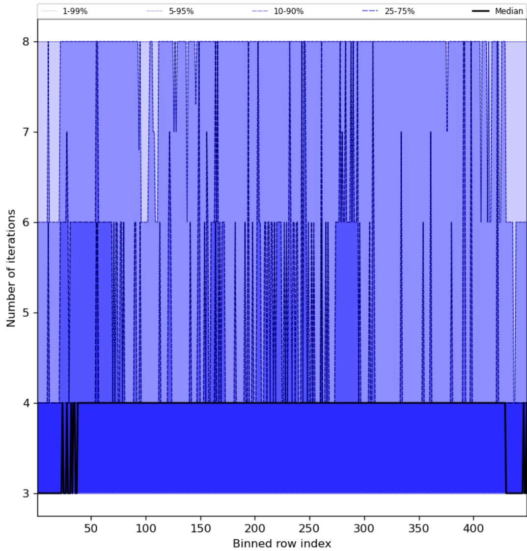
Figure 51: Along track statistics of “Number of iterations” for 2023-10-13 to 2023-10-15
