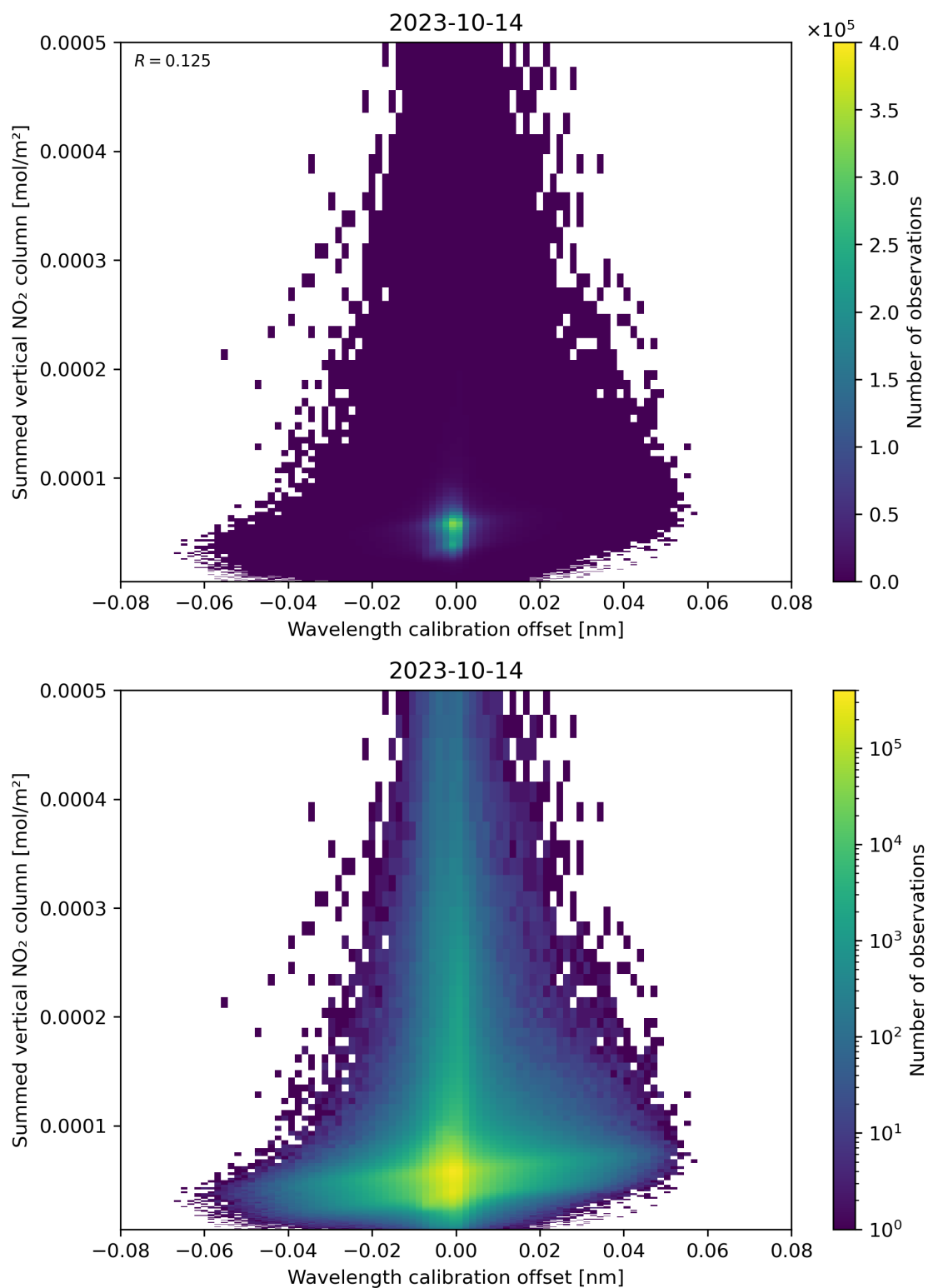
Figure 177: Scatter density plot of “Wavelength calibration offset” against “Summed vertical NO 2 column” for 2023-10-13 to 2023-10-15.
