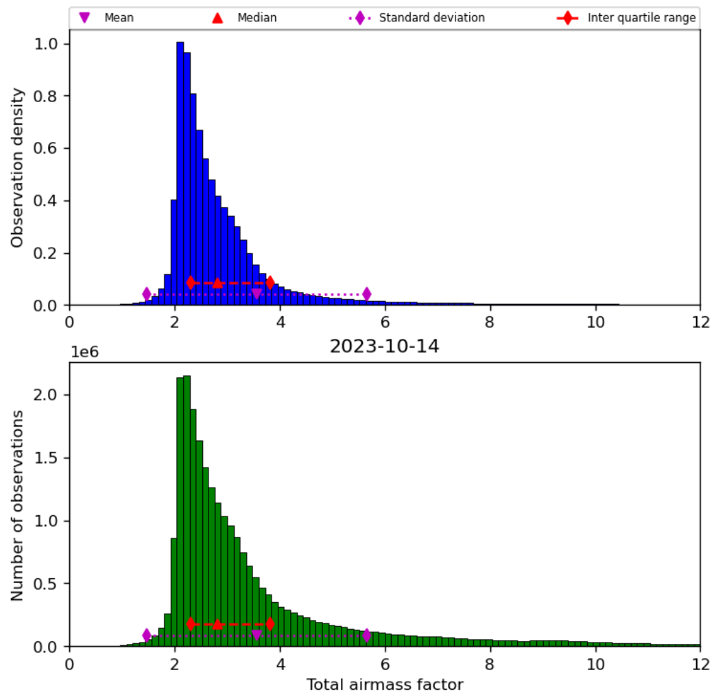
Figure 32: Histogram of “Total airmass factor” for 2023-10-13 to 2023-10-15
