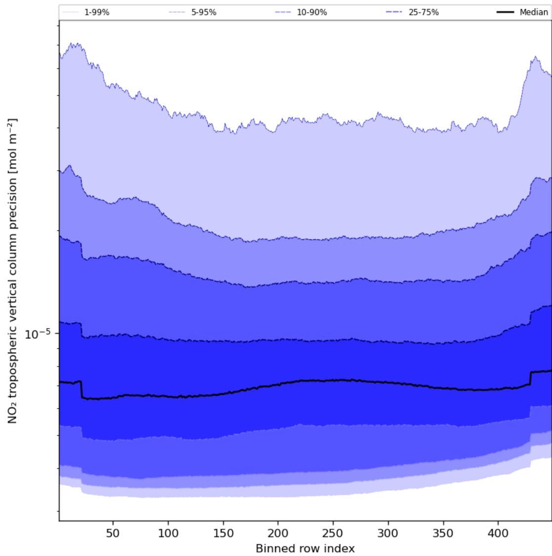
Figure 47: Along track statistics of “NO 2 tropospheric vertical column precision” for 2023-10-13 to 2023-10-15
