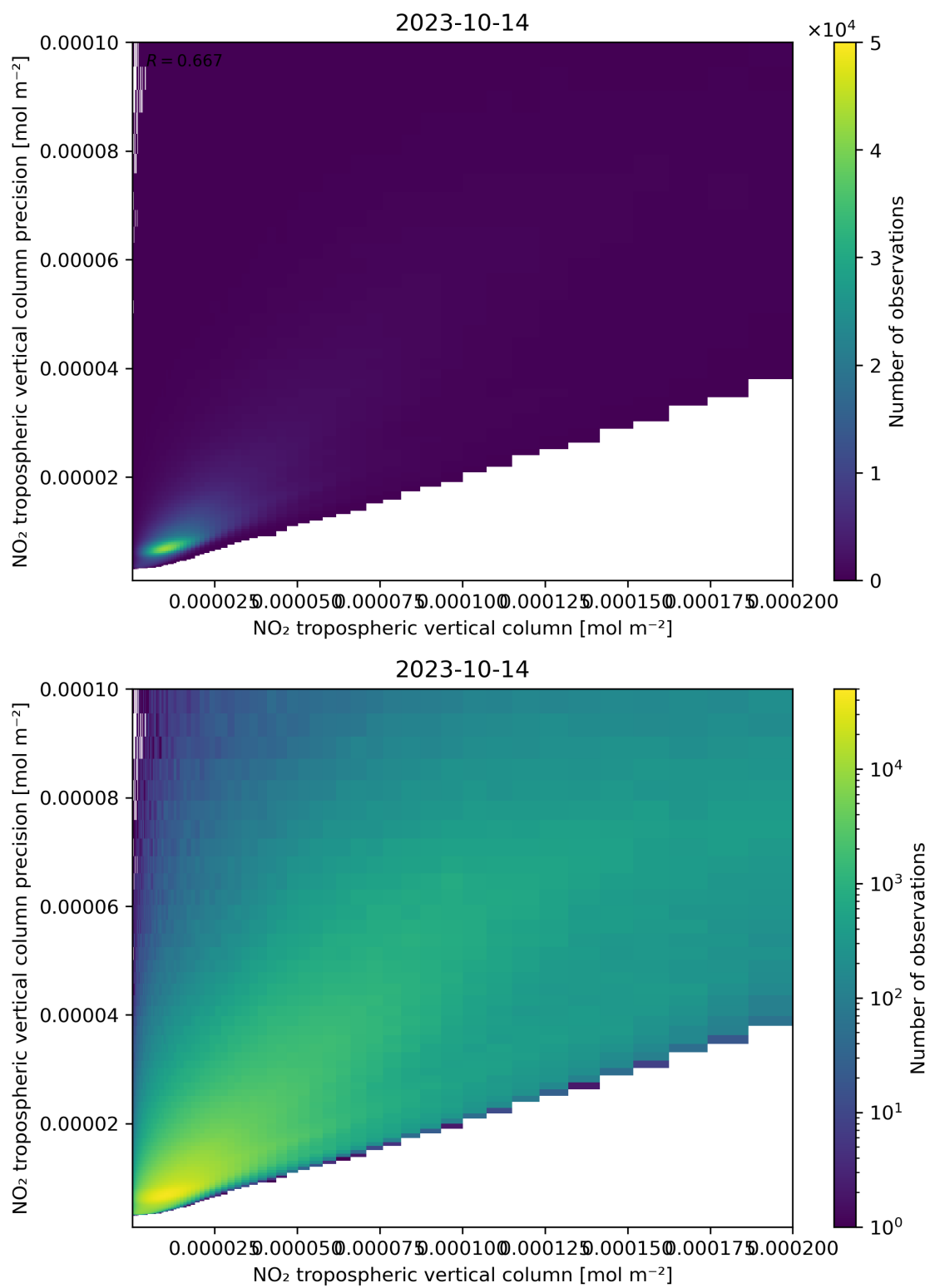
Figure 130: Scatter density plot of “NO 2 tropospheric vertical column” against “NO 2 tropospheric vertical column precision” for 2023-10-13 to 2023-10-15.
