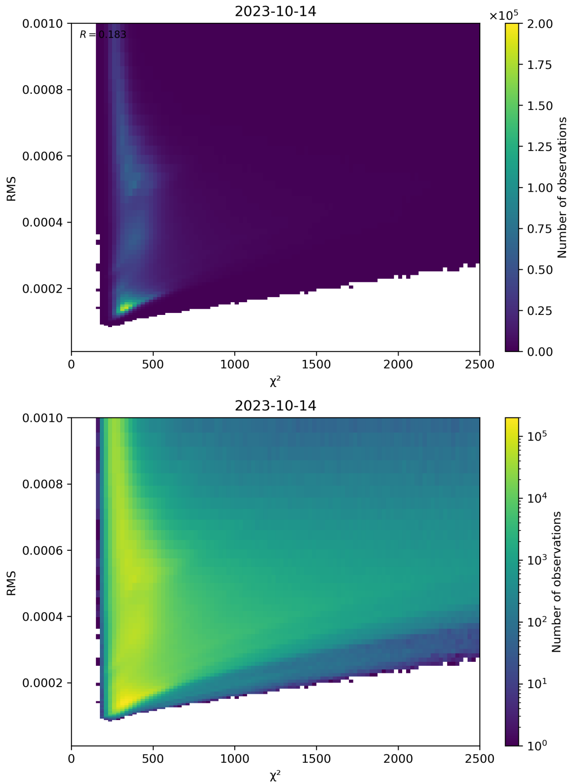
Figure 82: Scatter density plot of “ \chi^2 ” against “RMS” for 2023-10-13 to 2023-10-15.
