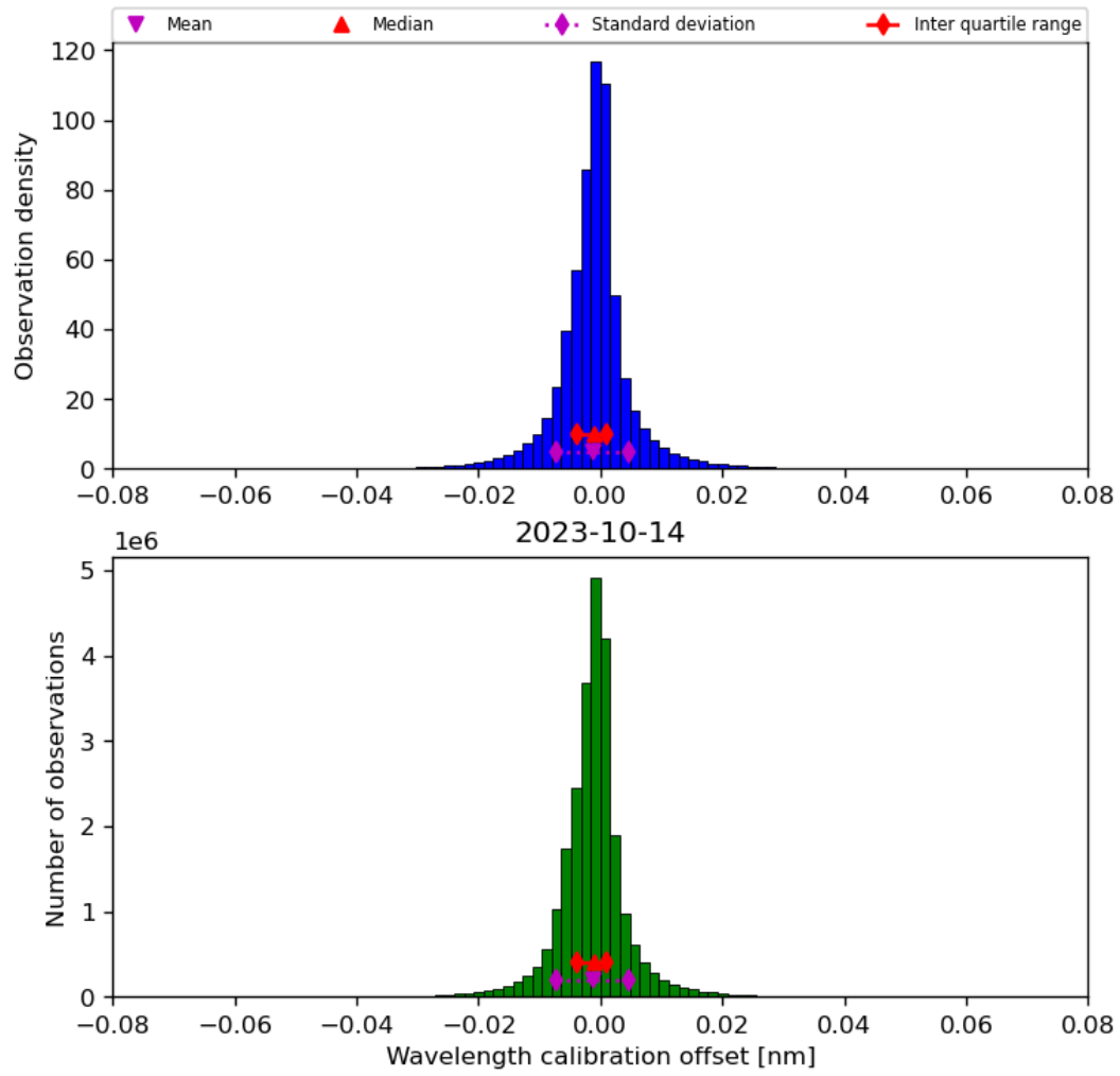
Figure 35: Histogram of “Wavelength calibration offset” for 2023-10-13 to 2023-10-15
