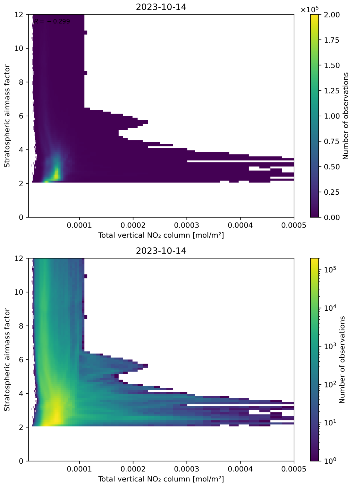
Figure 110: Scatter density plot of “Total vertical NO 2 column” against “Stratospheric airmass factor” for 2023-10-13 to 2023-10-15.
