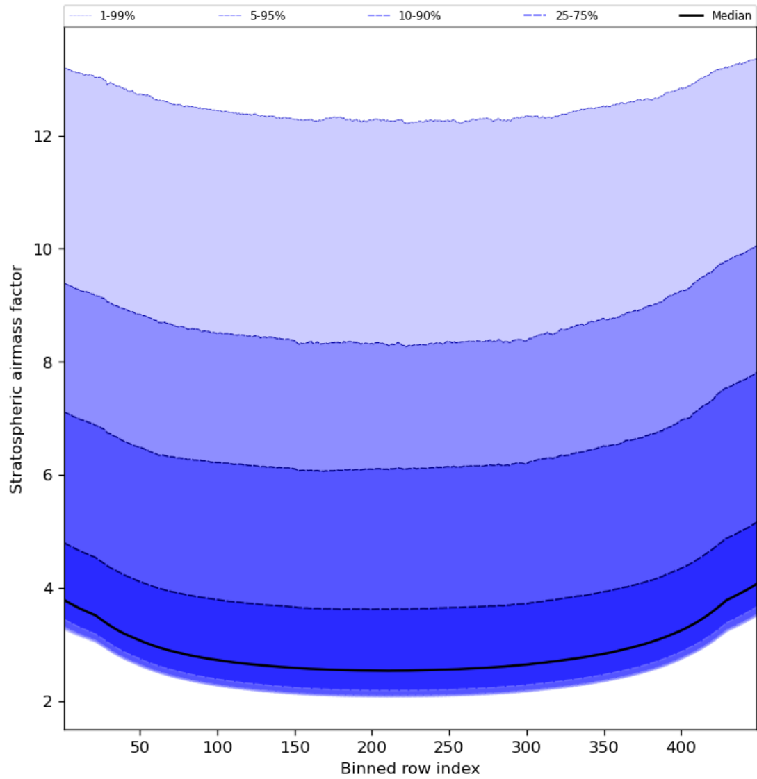
Figure 61: Along track statistics of “Stratospheric airmass factor” for 2023-10-13 to 2023-10-15
