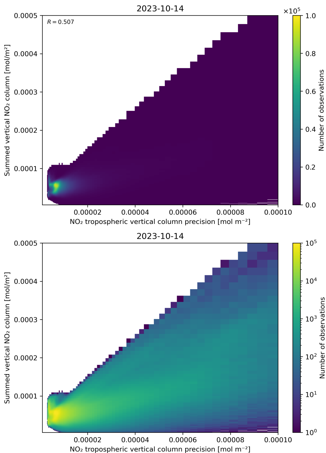
Figure 136: Scatter density plot of “NO 2 tropospheric vertical column precision” against “Summed vertical NO 2 column” for 2023-10-13 to 2023-10-15.
