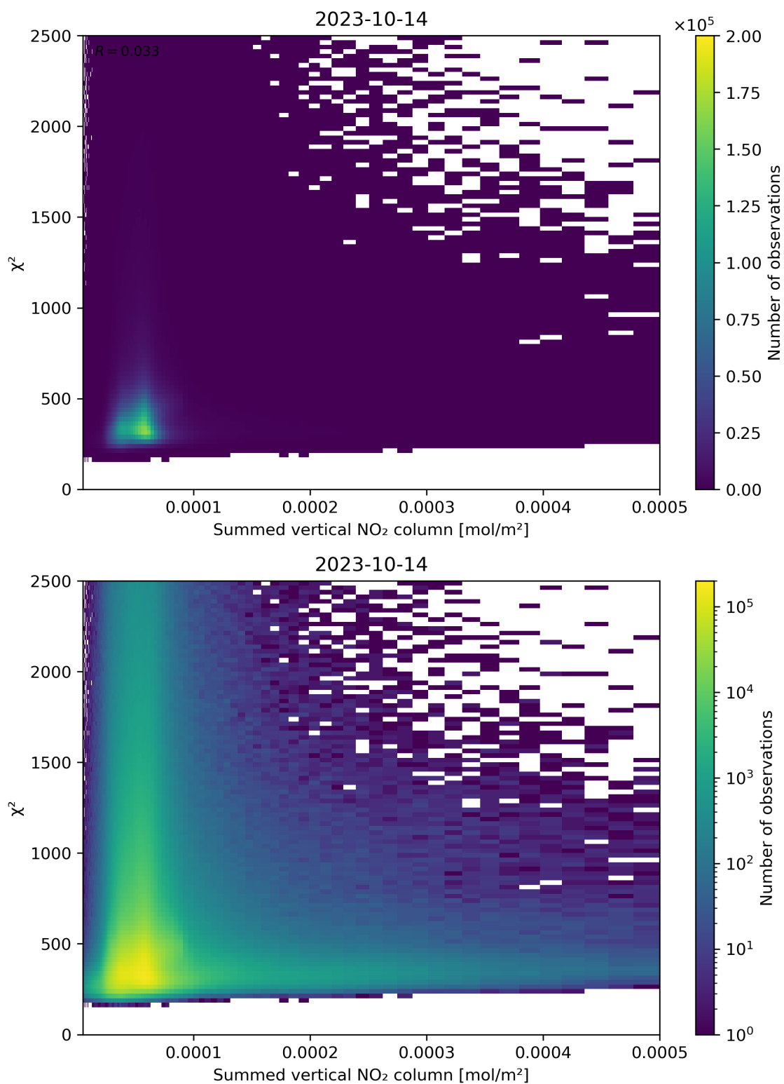
Figure 104: Scatter density plot of “Summed vertical NO 2 column” against “ \chi^2 ” for 2023-10-13 to 2023-10-15.
