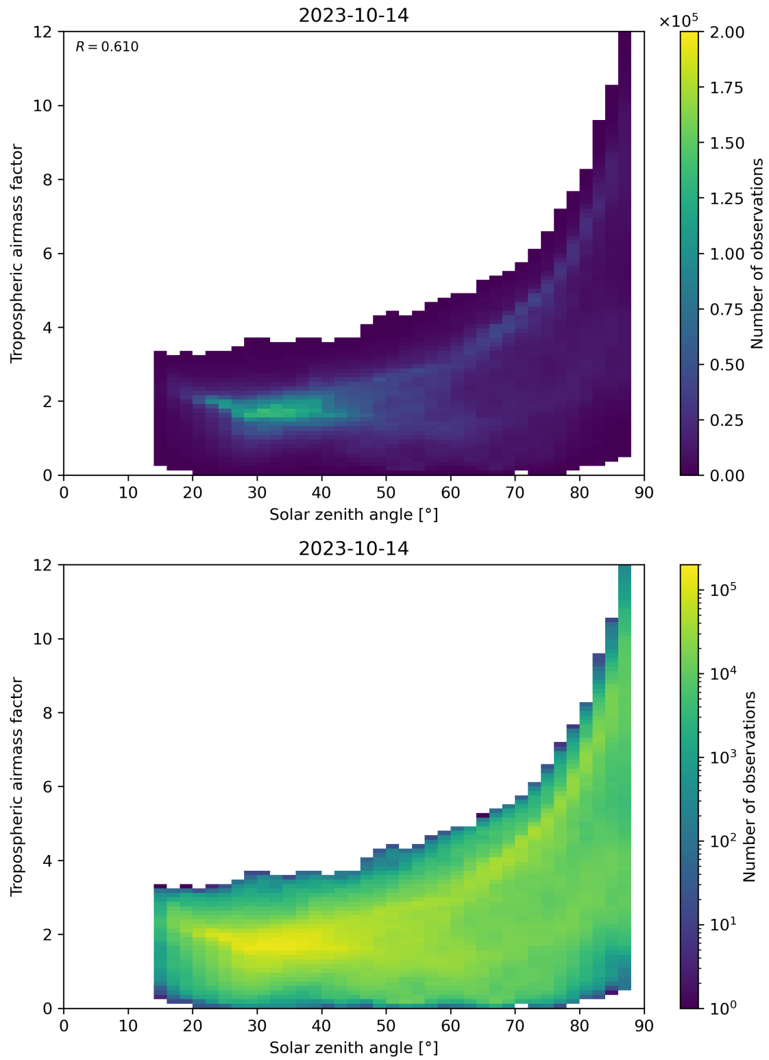
Figure 147: Scatter density plot of “Solar zenith angle” against “Tropospheric airmass factor” for 2023-10-13 to 2023-10-15.
