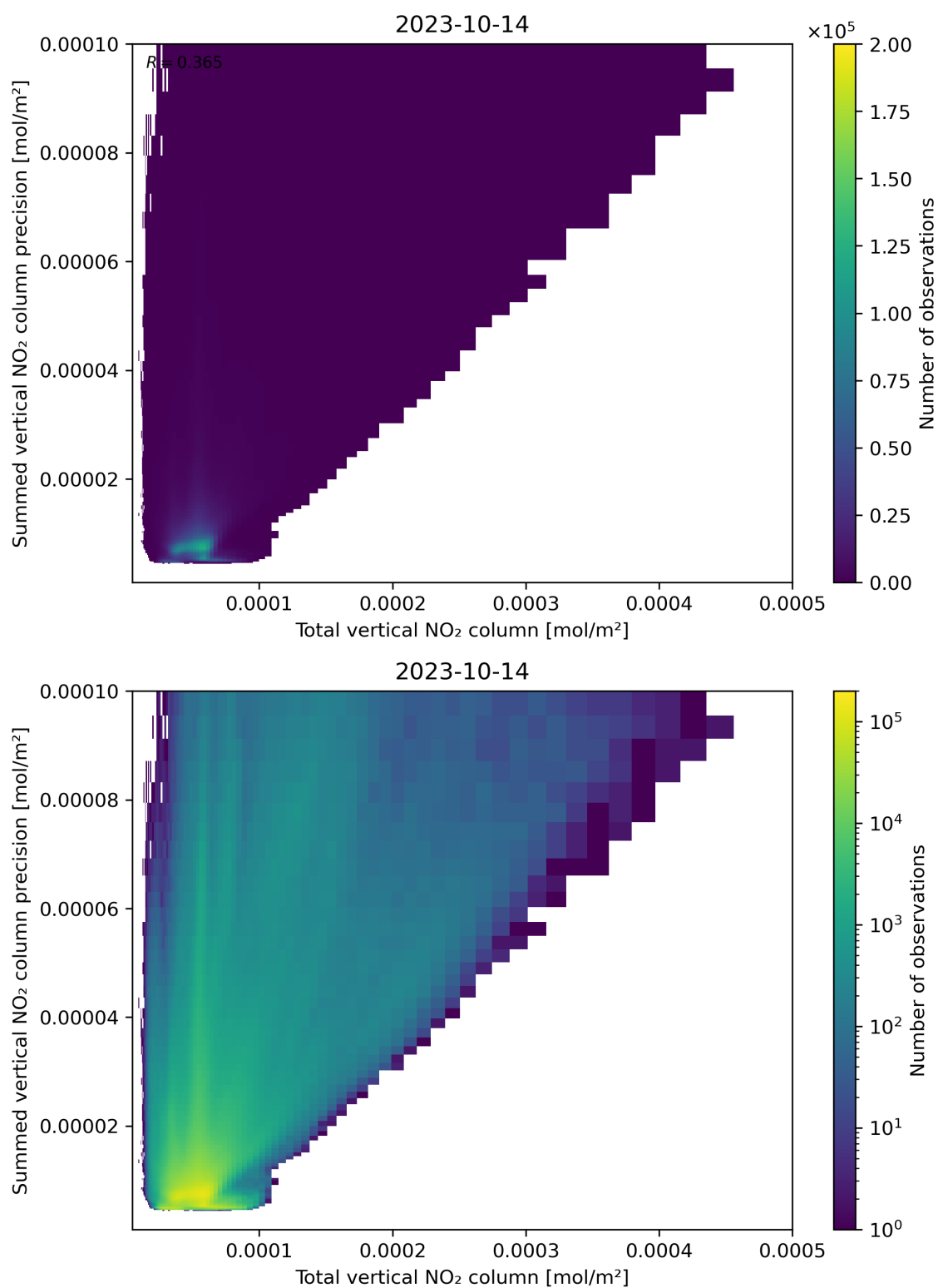
Figure 113: Scatter density plot of “Total vertical NO 2 column” against “Summed vertical NO 2 column precision” for 2023-10-13 to 2023-10-15.
