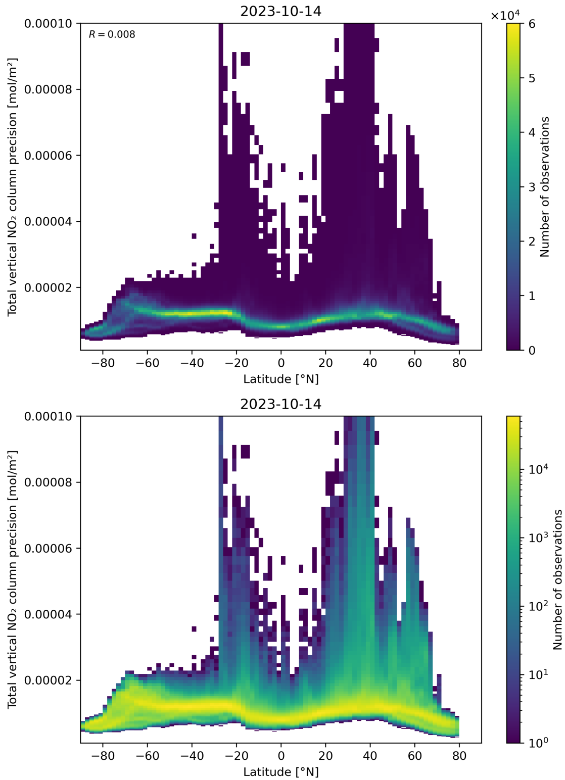
Figure 91: Scatter density plot of “Latitude” against “Total vertical NO 2 column precision” for 2023-10-13 to 2023-10-15.
