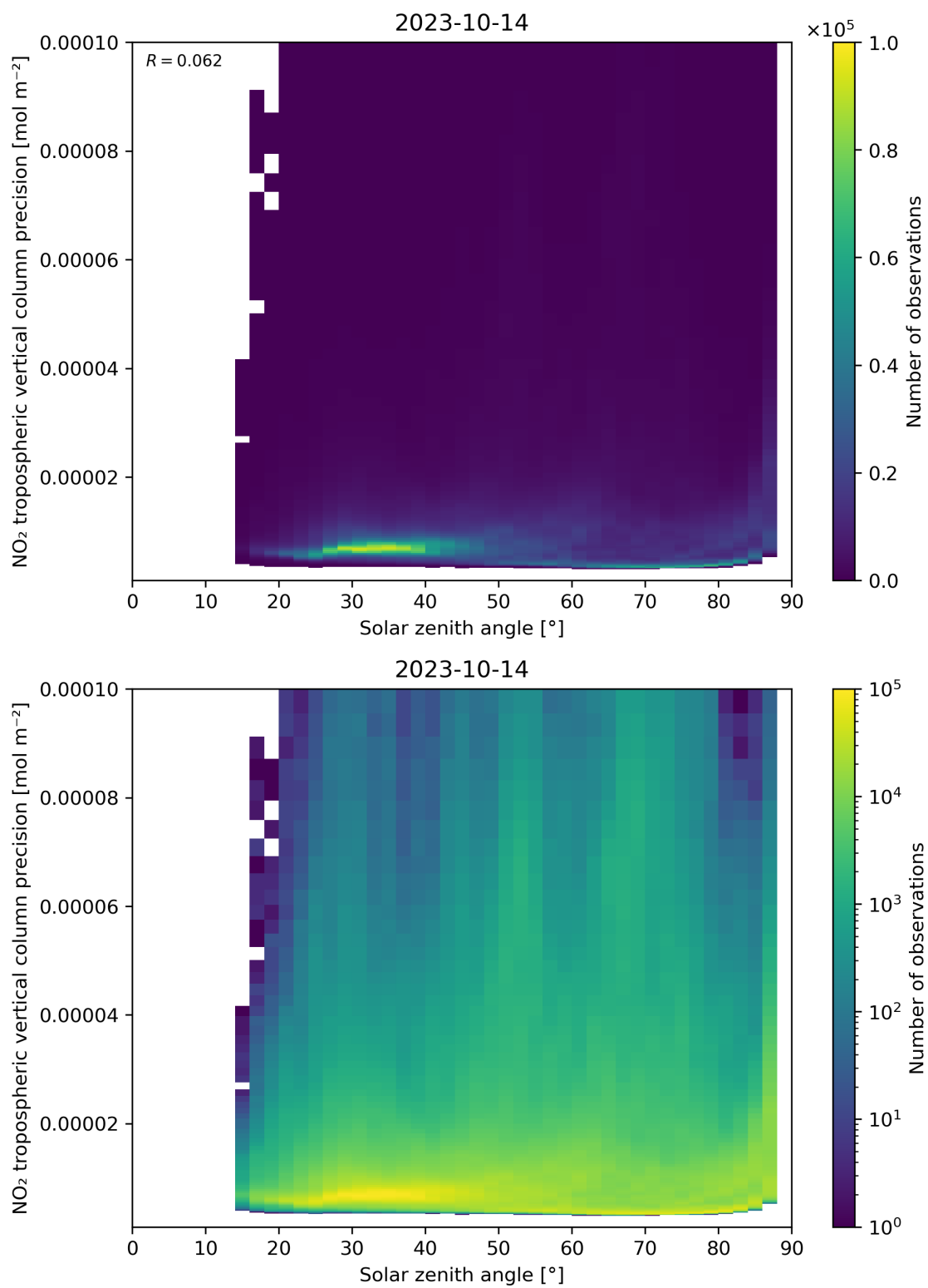
Figure 156: Scatter density plot of “Solar zenith angle” against “NO 2 tropospheric vertical column precision” for 2023-10-13 to 2023-10-15.
