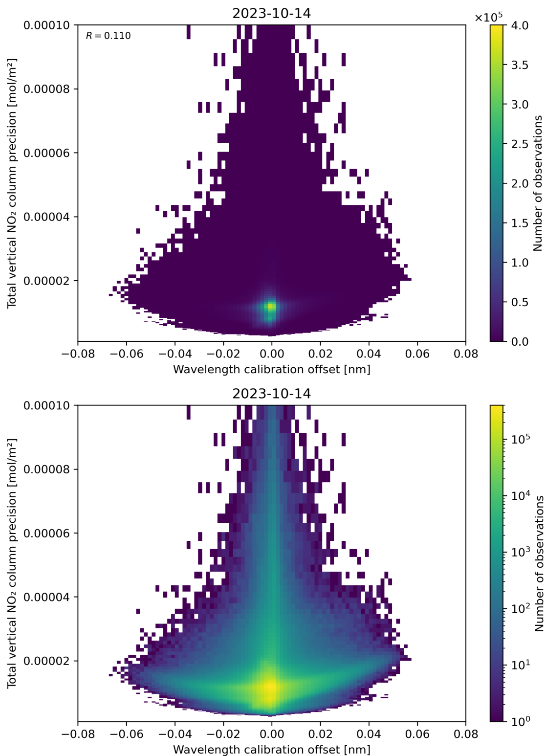
Figure 180: Scatter density plot of “Wavelength calibration offset” against “Total vertical NO 2 column precision” for 2023-10-13 to 2023-10-15.
