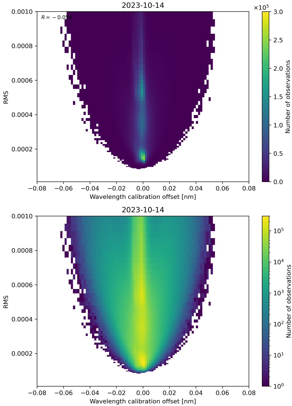
Figure 181: Scatter density plot of “Wavelength calibration offset” against “RMS” for 2023-10-13 to 2023-10-15.
