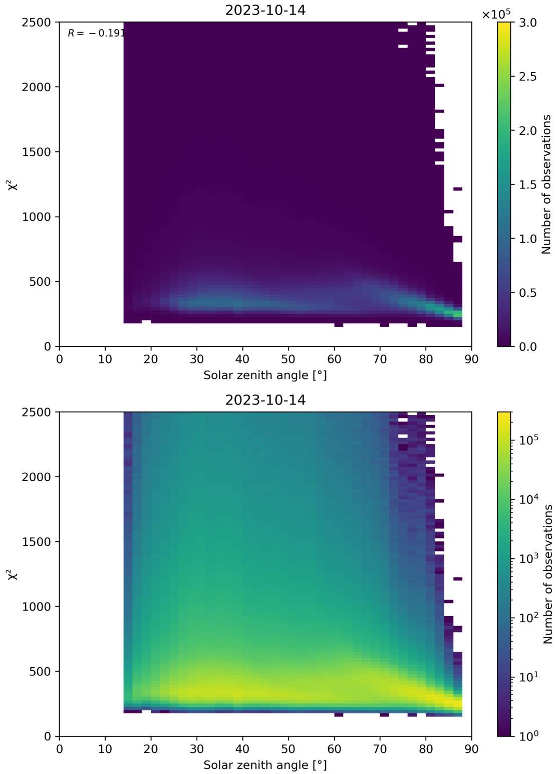
Figure 148: Scatter density plot of “Solar zenith angle” against “ \chi^2 ” for 2023-10-13 to 2023-10-15.
