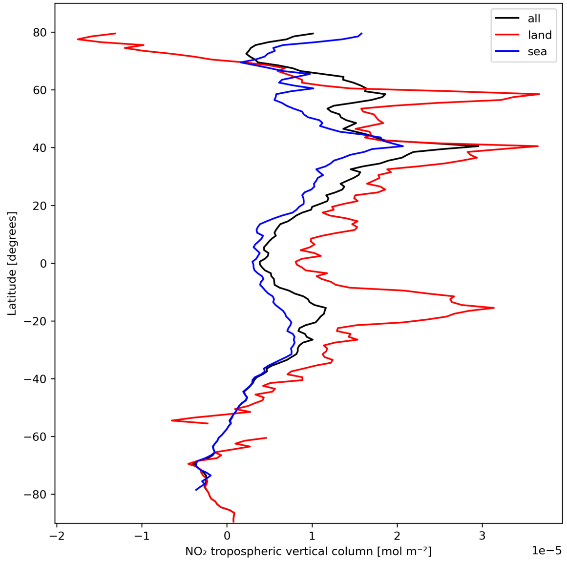
Figure 12: Zonal average of “NO 2 tropospheric vertical column” for 2023-10-13 to 2023-10-15.
