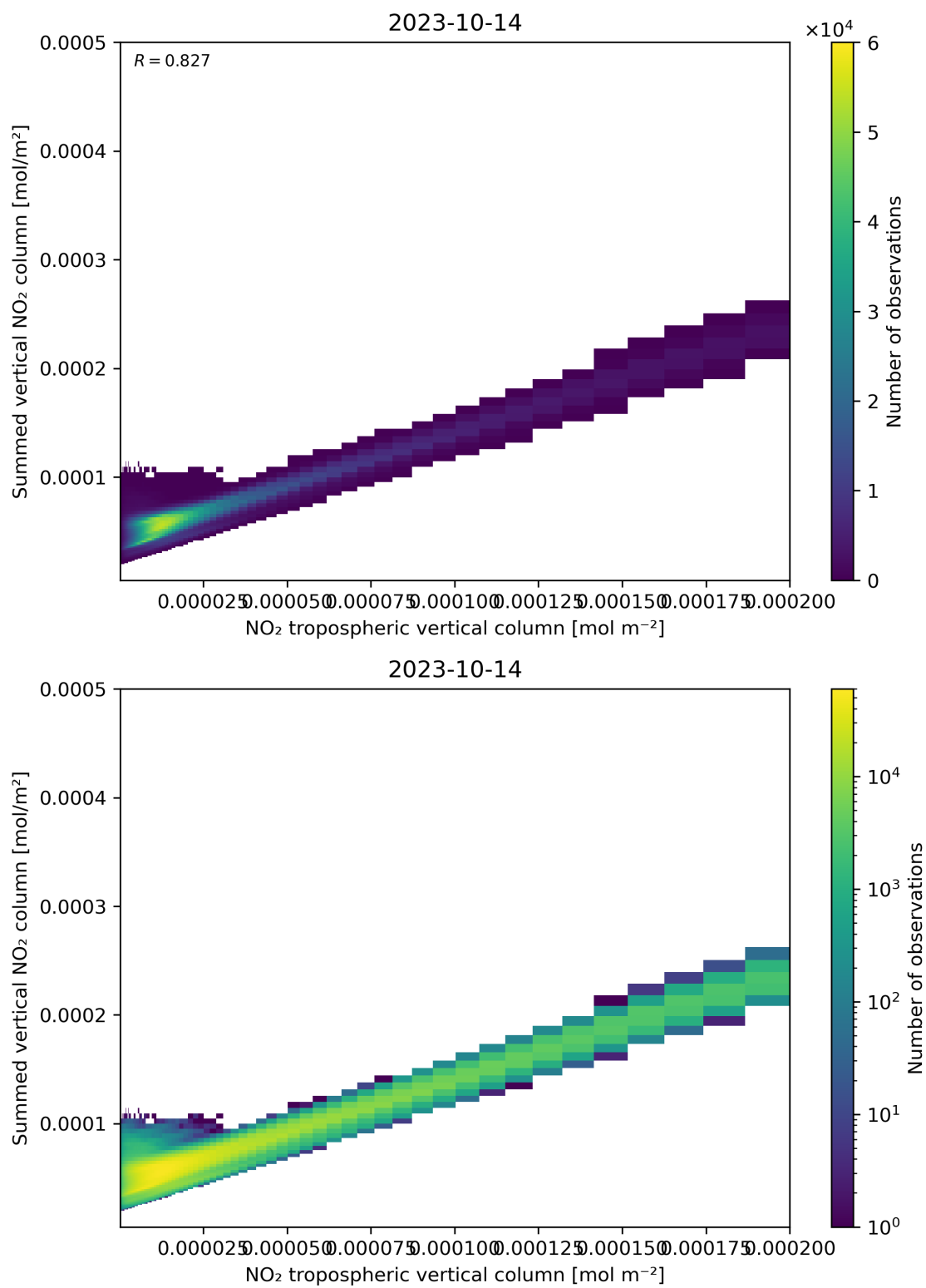
Figure 126: Scatter density plot of “NO 2 tropospheric vertical column” against “Summed vertical NO 2 column” for 2023-10-13 to 2023-10-15.
