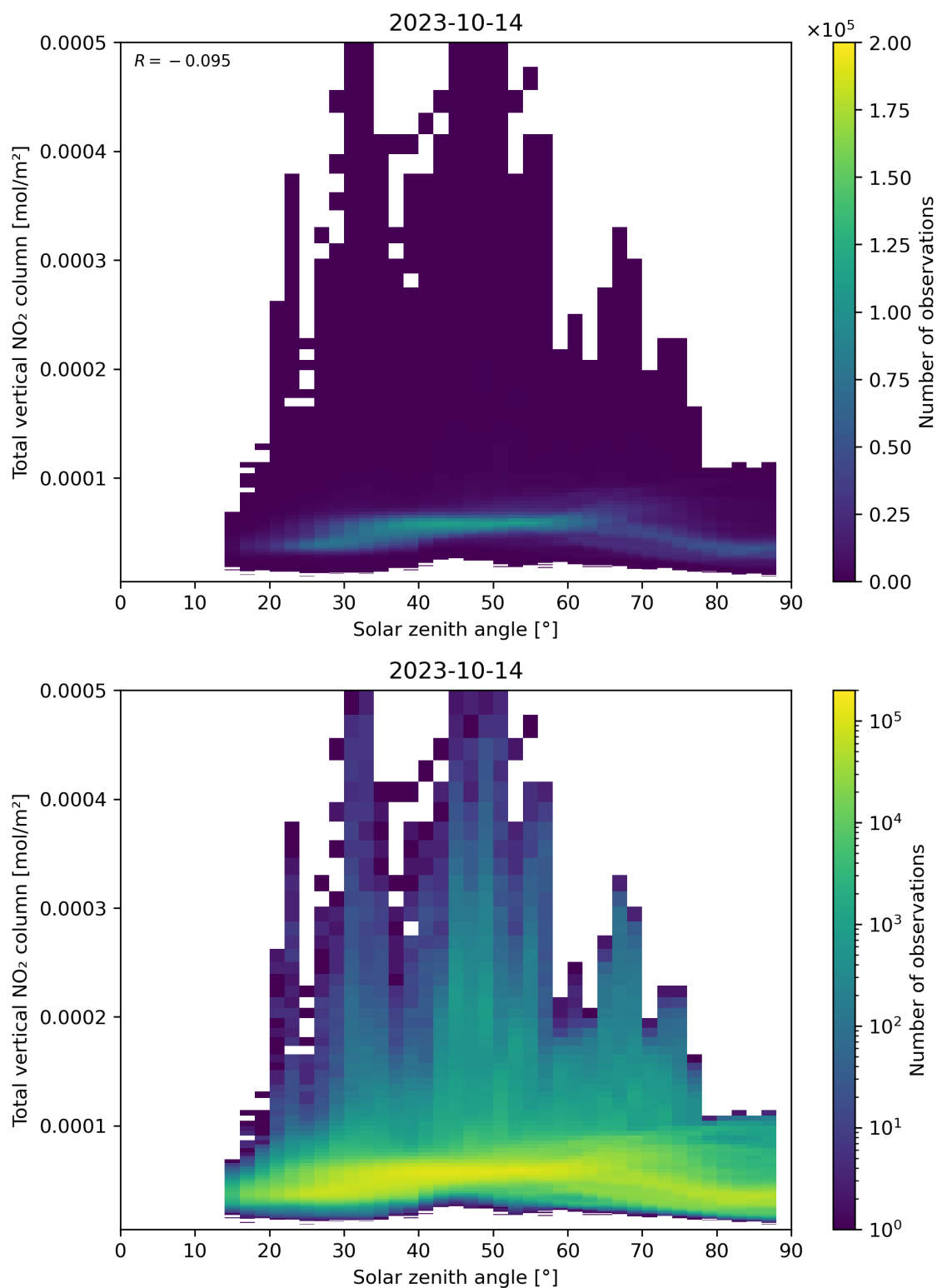
Figure 153: Scatter density plot of “Solar zenith angle” against “Total vertical NO 2 column” for 2023-10-13 to 2023-10-15.
