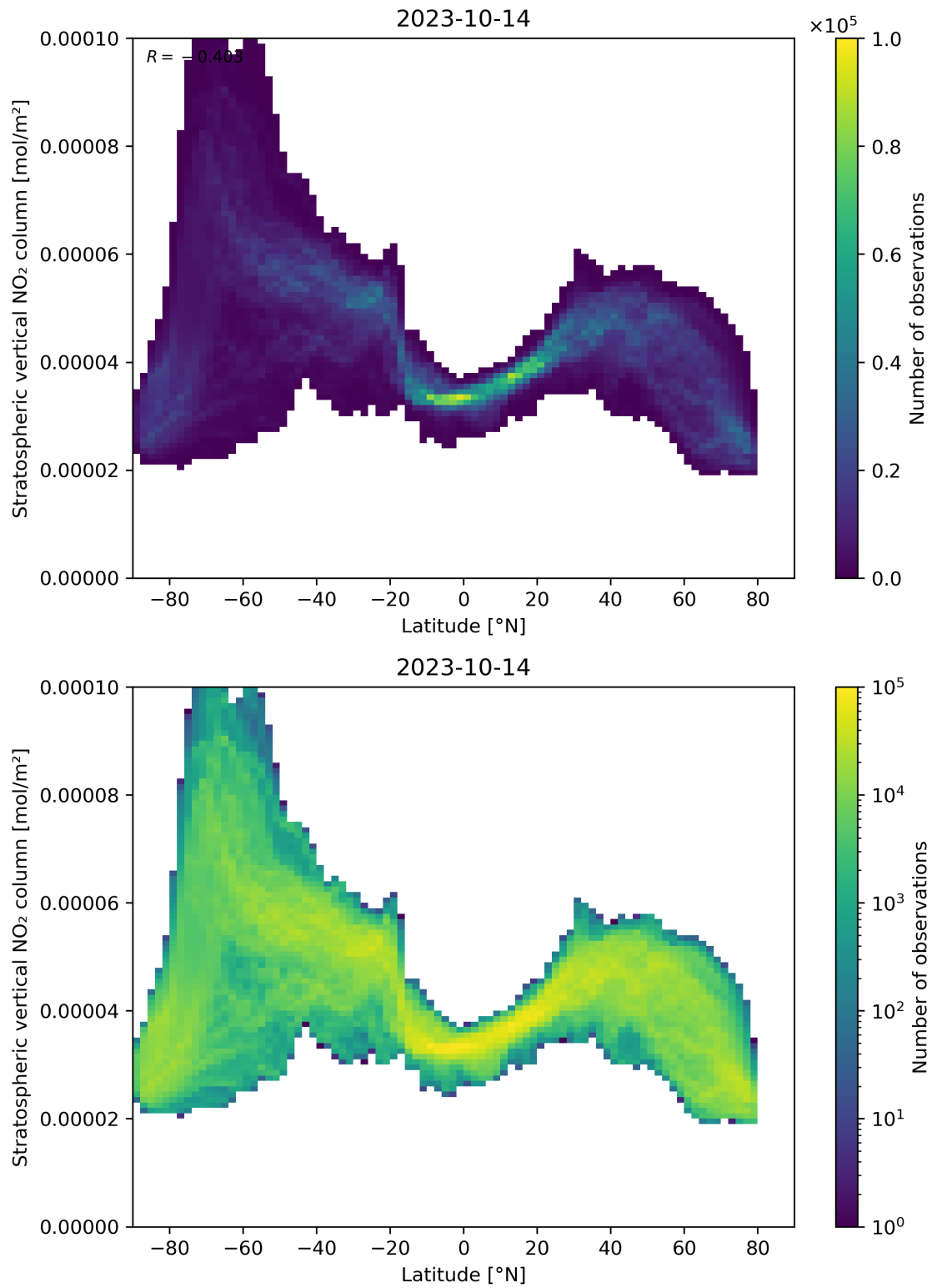
Figure 87: Scatter density plot of “Latitude” against “Stratospheric vertical NO 2 column” for 2023-10-13 to 2023-10-15.
