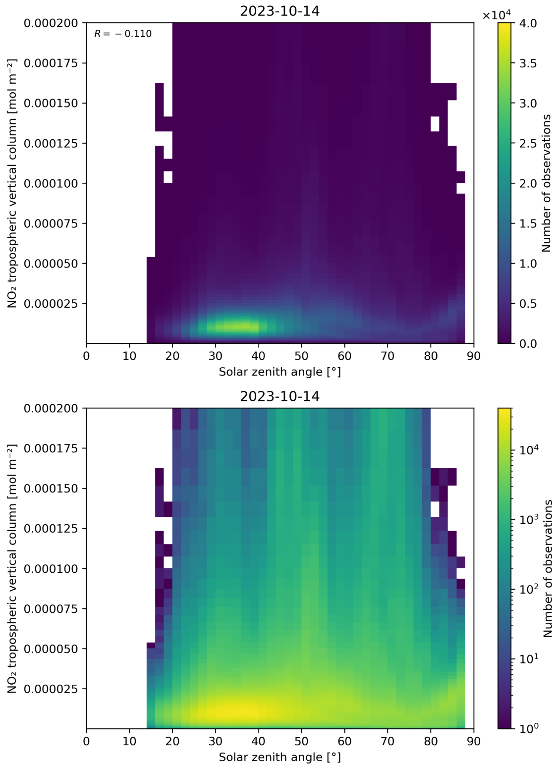
Figure 155: Scatter density plot of “Solar zenith angle” against “NO 2 tropospheric vertical column” for 2023-10-13 to 2023-10-15.
