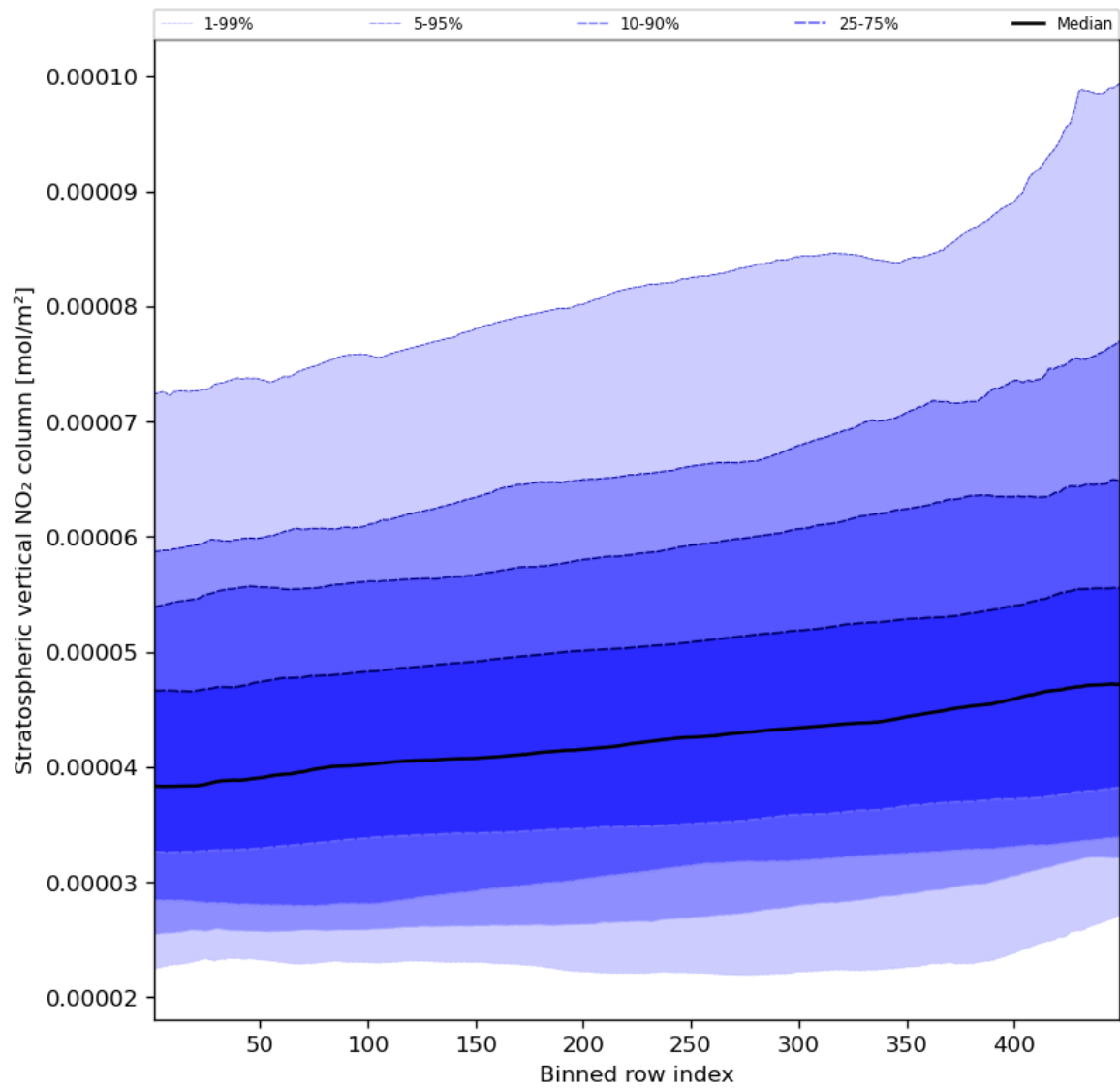
Figure 53: Along track statistics of “Stratospheric vertical NO 2 column” for 2023-10-13 to 2023-10-15
