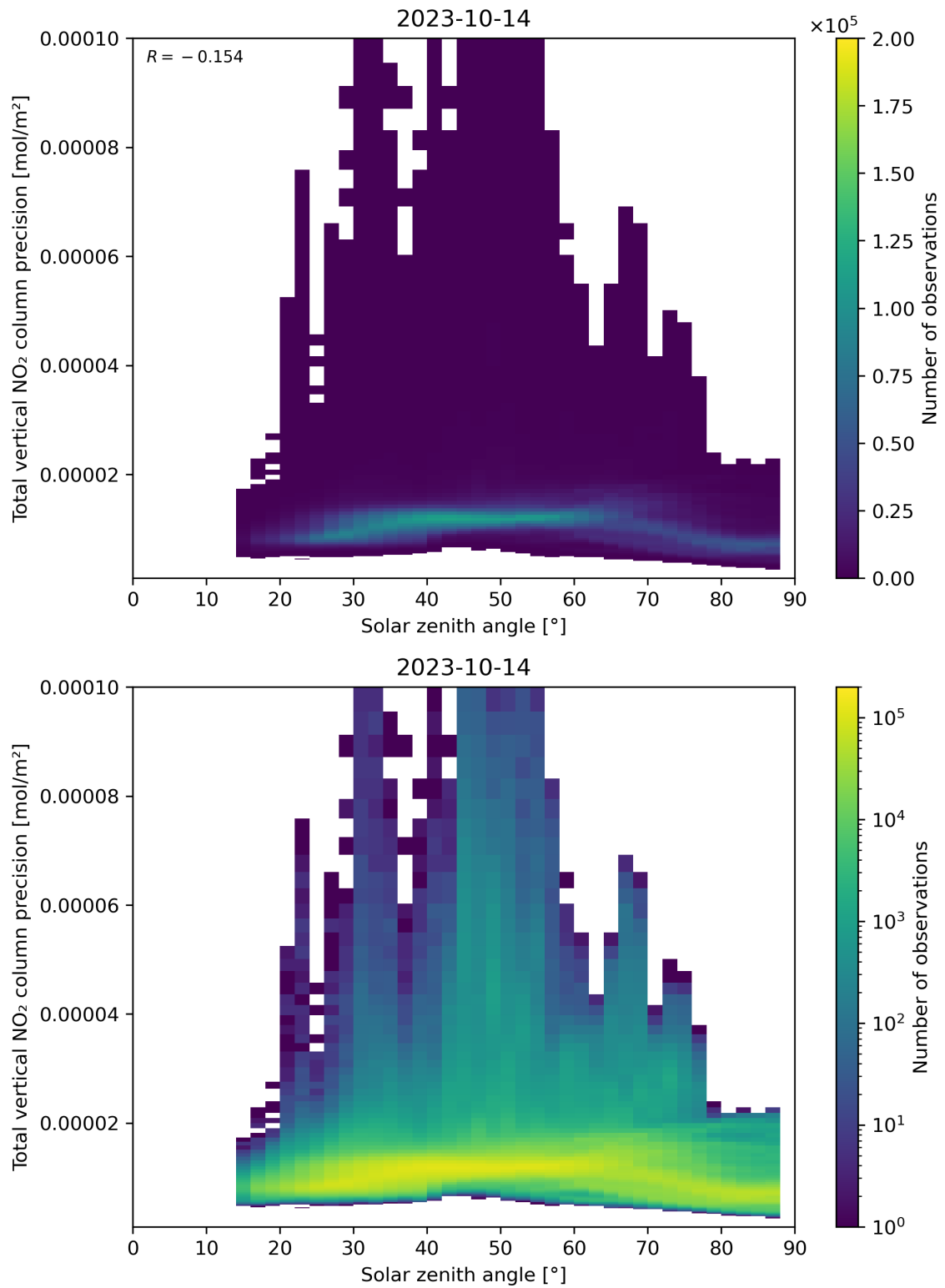
Figure 154: Scatter density plot of “Solar zenith angle” against “Total vertical NO 2 column precision” for 2023-10-13 to 2023-10-15.
