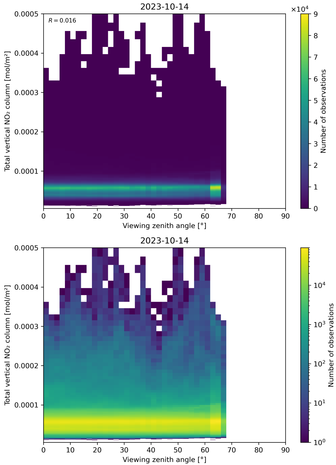
Figure 167: Scatter density plot of “Viewing zenith angle” against “Total vertical NO 2 column” for 2023-10-13 to 2023-10-15.
