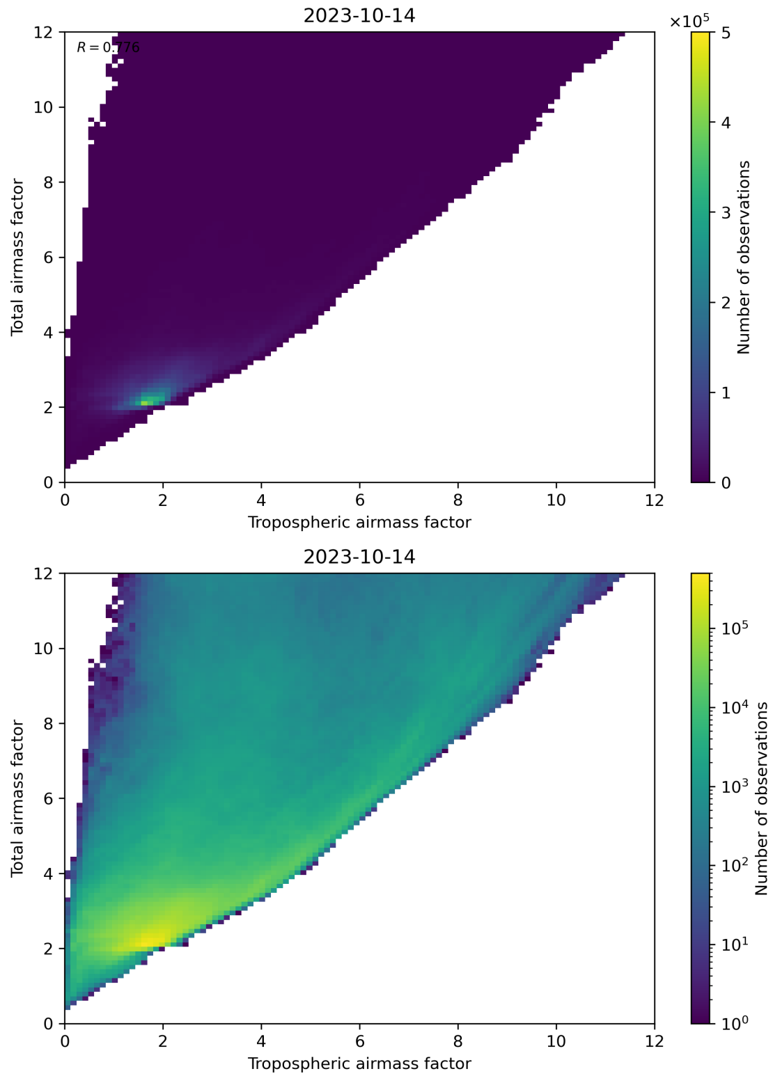
Figure 72: Scatter density plot of “Tropospheric airmass factor” against “Total airmass factor” for 2023-10-13 to 2023-10-15.
