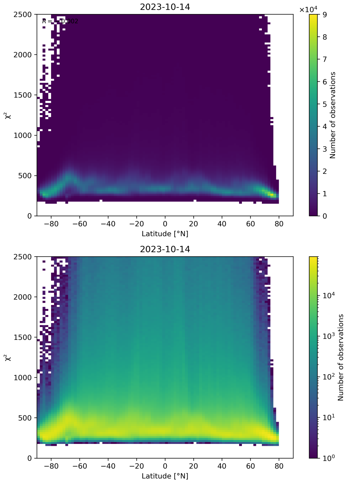
Figure 86: Scatter density plot of “Latitude” against “ \chi^2 ” for 2023-10-13 to 2023-10-15.
