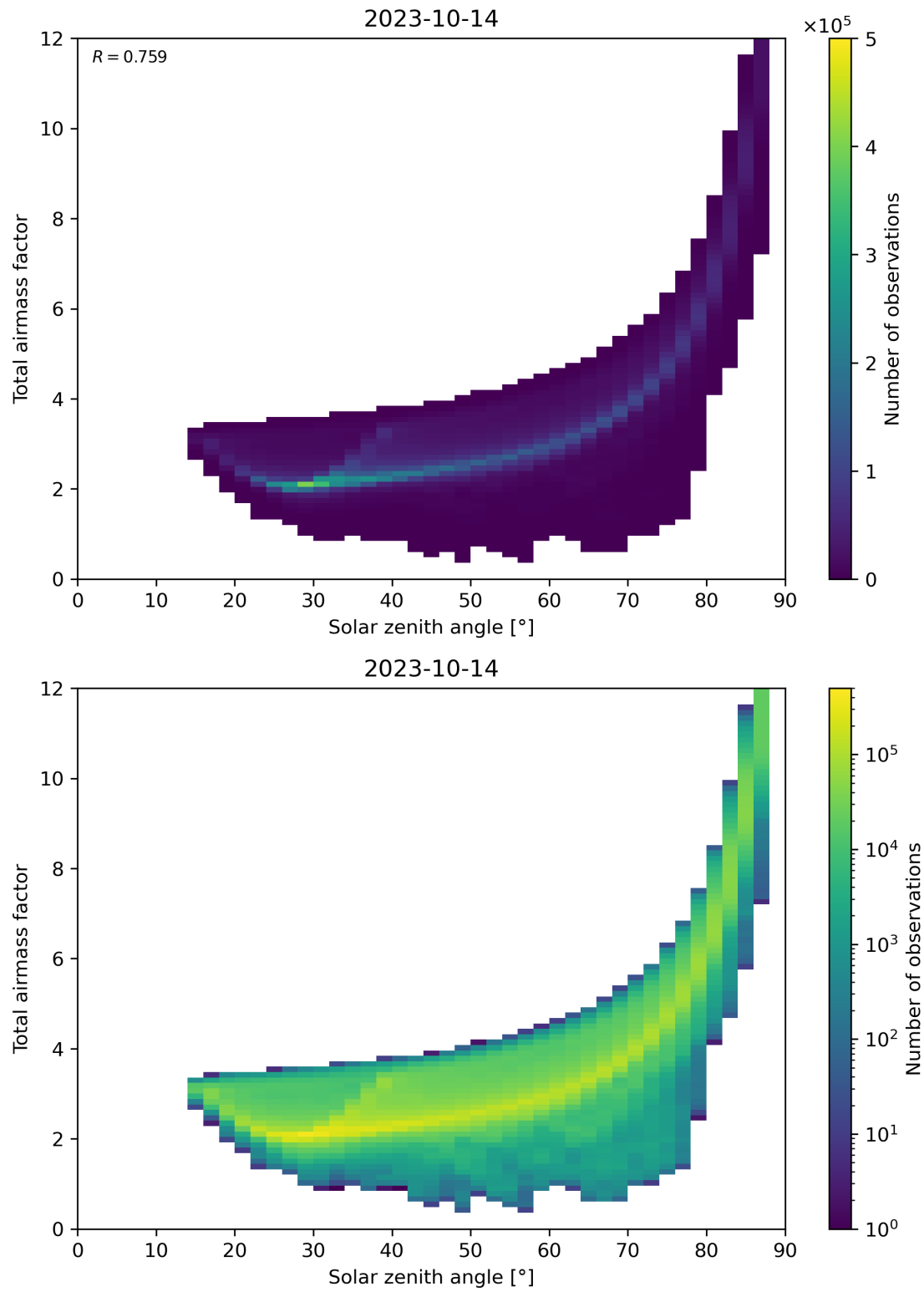
Figure 146: Scatter density plot of “Solar zenith angle” against “Total air mass factor” for 2023-10-13 to 2023-10-15.
