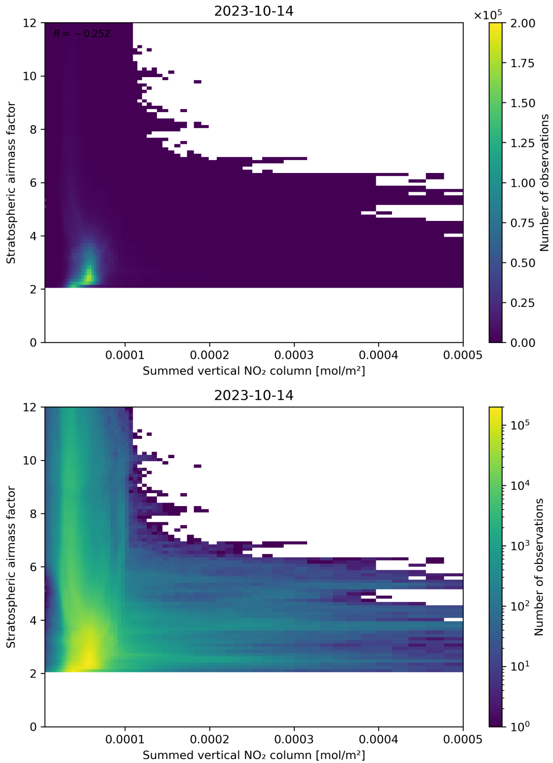
Figure 103: Scatter density plot of “Summed vertical NO 2 column” against “Stratospheric airmass factor” for 2023-10-13 to 2023-10-15.
