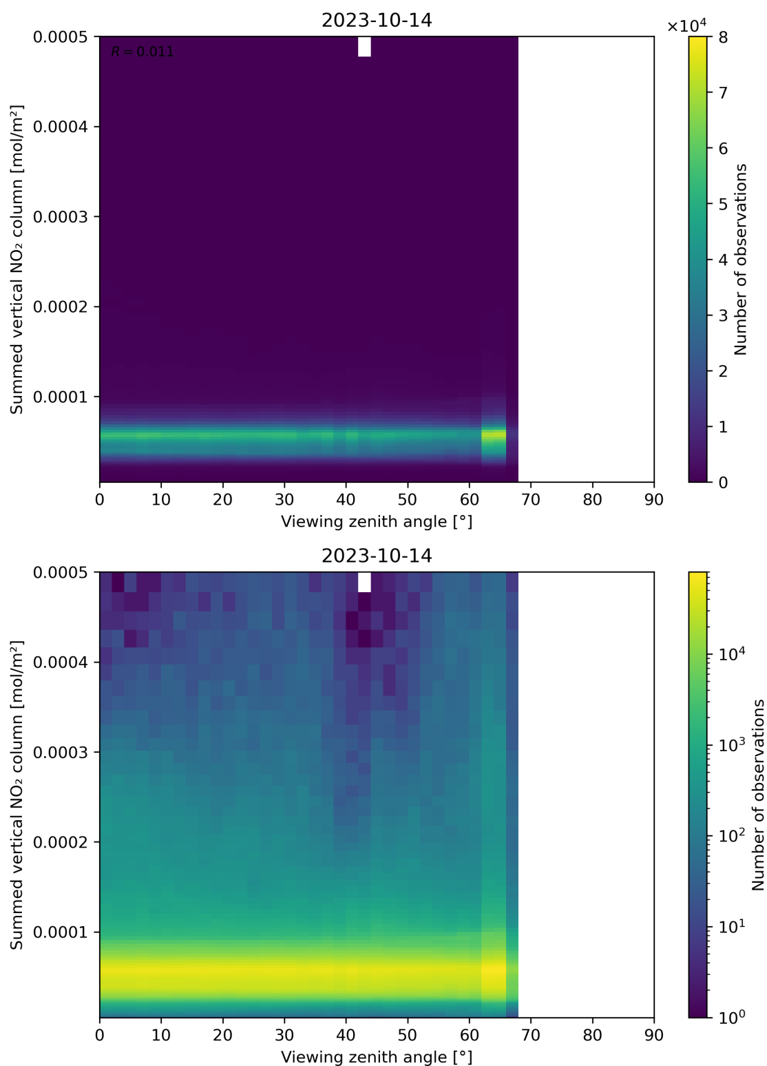
Figure 165: Scatter density plot of “Viewing zenith angle” against “Summed vertical NO 2 column” for 2023-10-13 to 2023-10-15.
