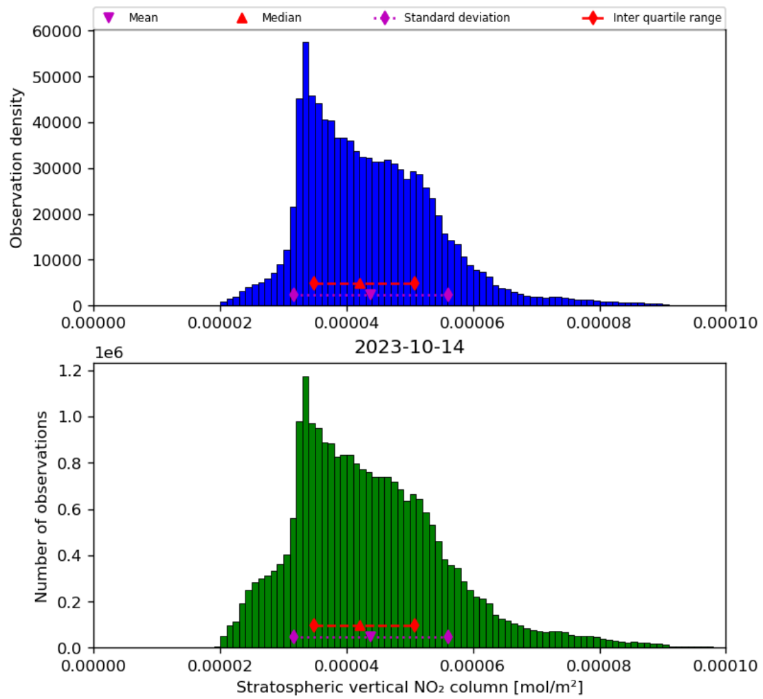
Figure 36: Histogram of “Stratospheric vertical NO 2 column” for 2023-10-13 to 2023-10-15
