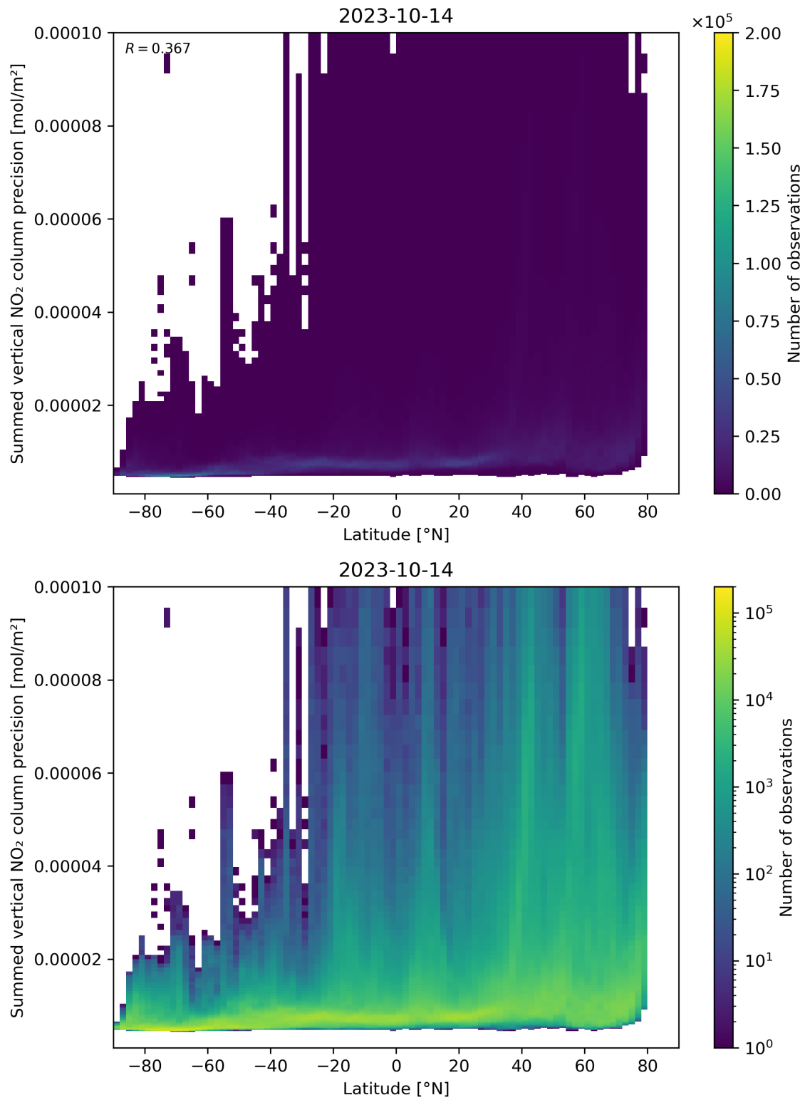
Figure 89: Scatter density plot of “Latitude” against “Summed vertical NO 2 column precision” for 2023-10-13 to 2023-10-15.
