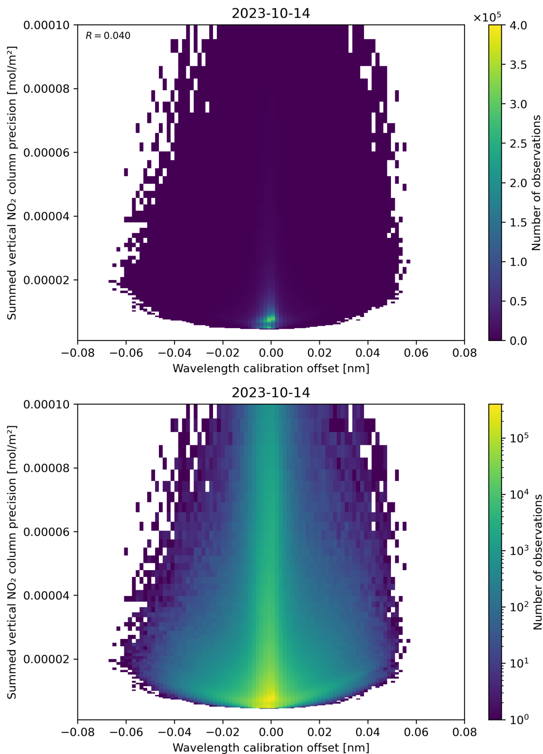
Figure 178: Scatter density plot of “Wavelength calibration offset” against “Summed vertical NO 2 column precision” for 2023-10-13 to 2023-10-15.
