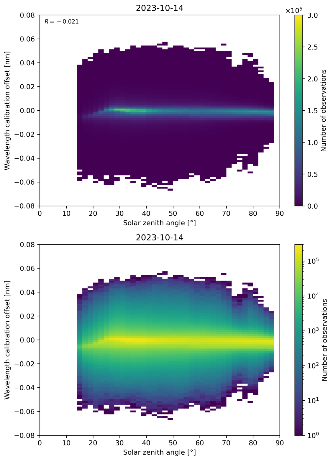
Figure 158: Scatter density plot of “Solar zenith angle” against “Wavelength calibration offset” for 2023-10-13 to 2023-10-15.
