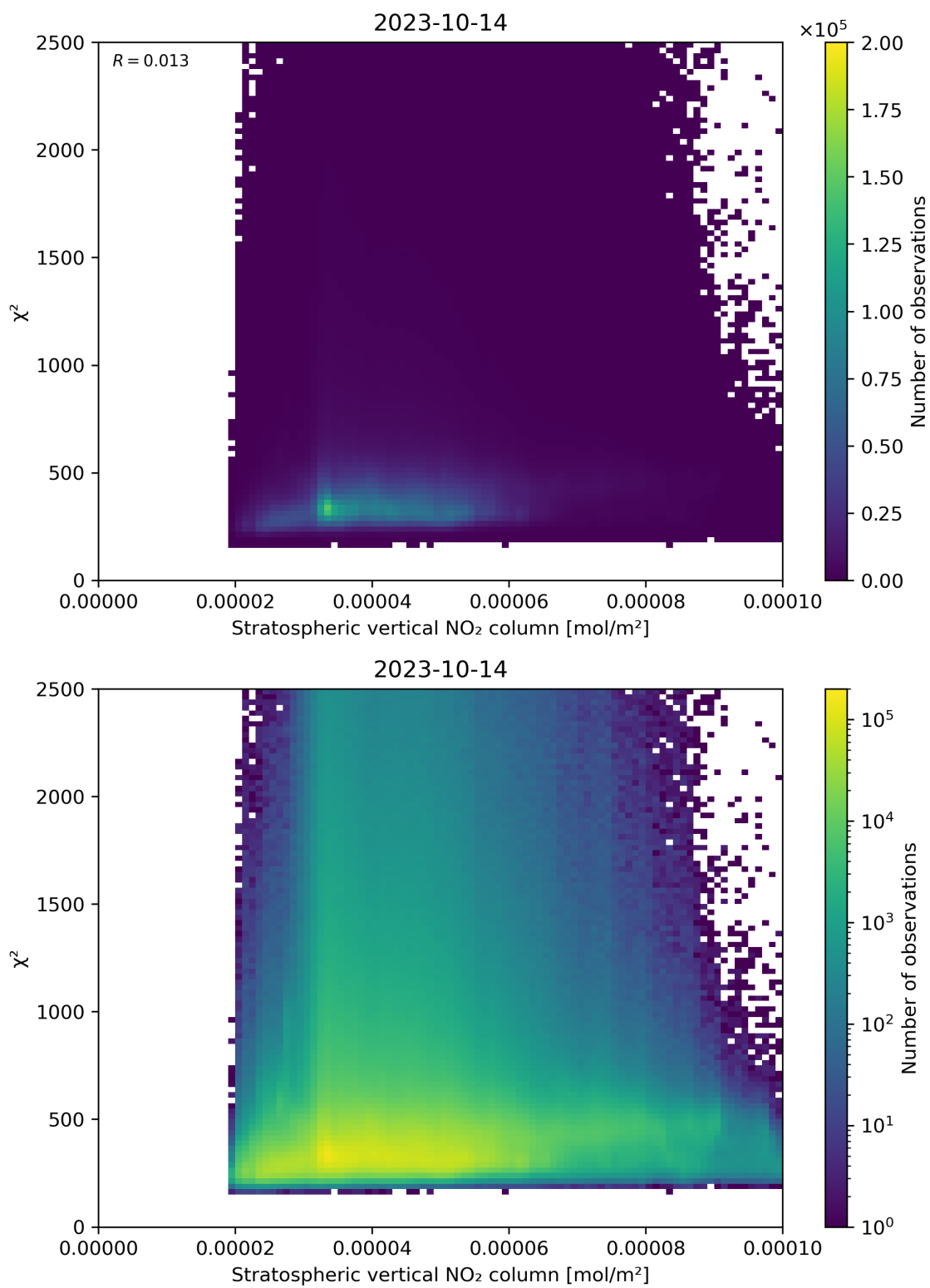
Figure 97: Scatter density plot of “Stratospheric vertical NO 2 column” against “ \chi^2 ” for 2023-10-13 to 2023-10-15.
