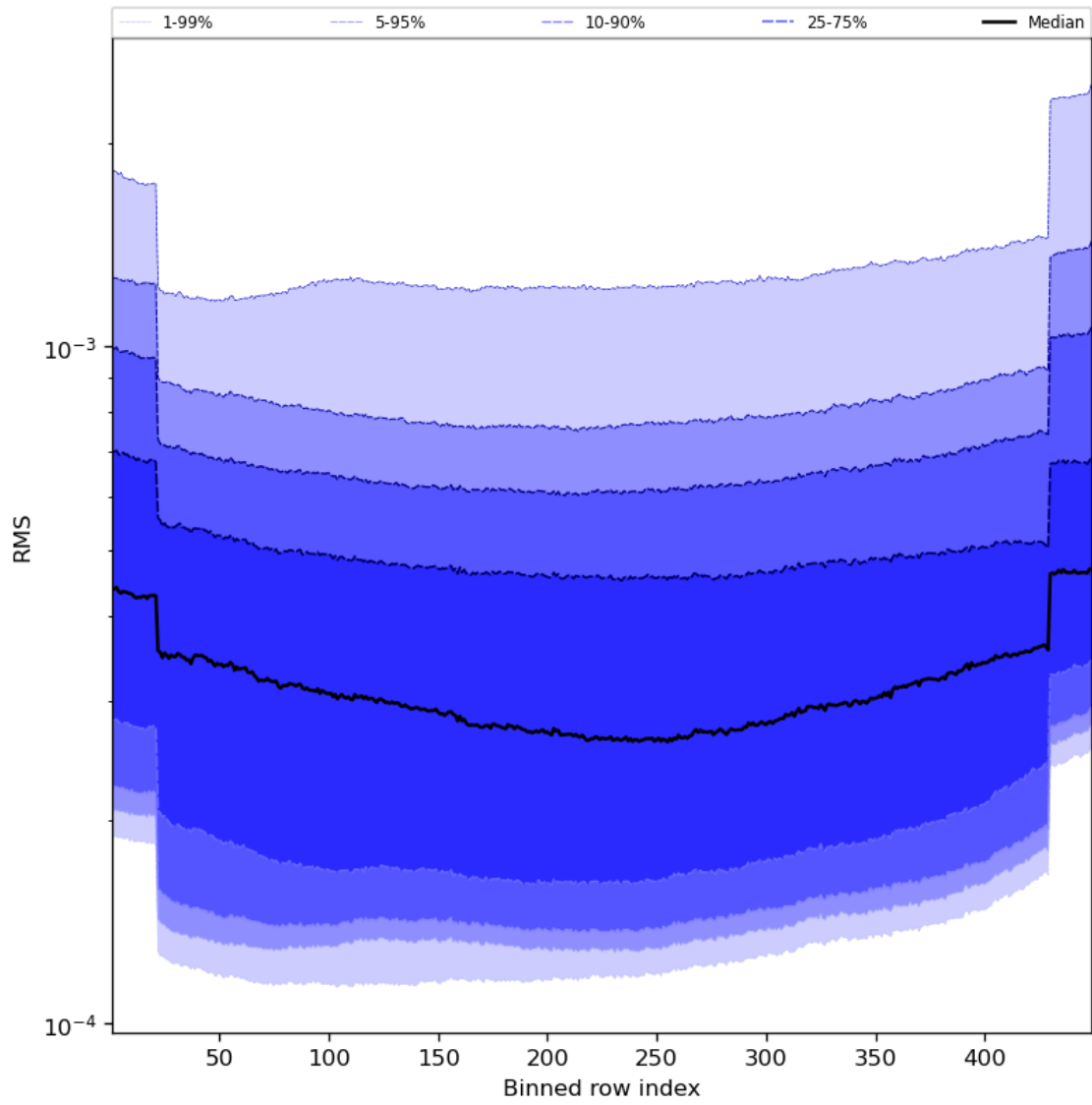
Figure 60: Along track statistics of “RMS” for 2023-10-13 to 2023-10-15
