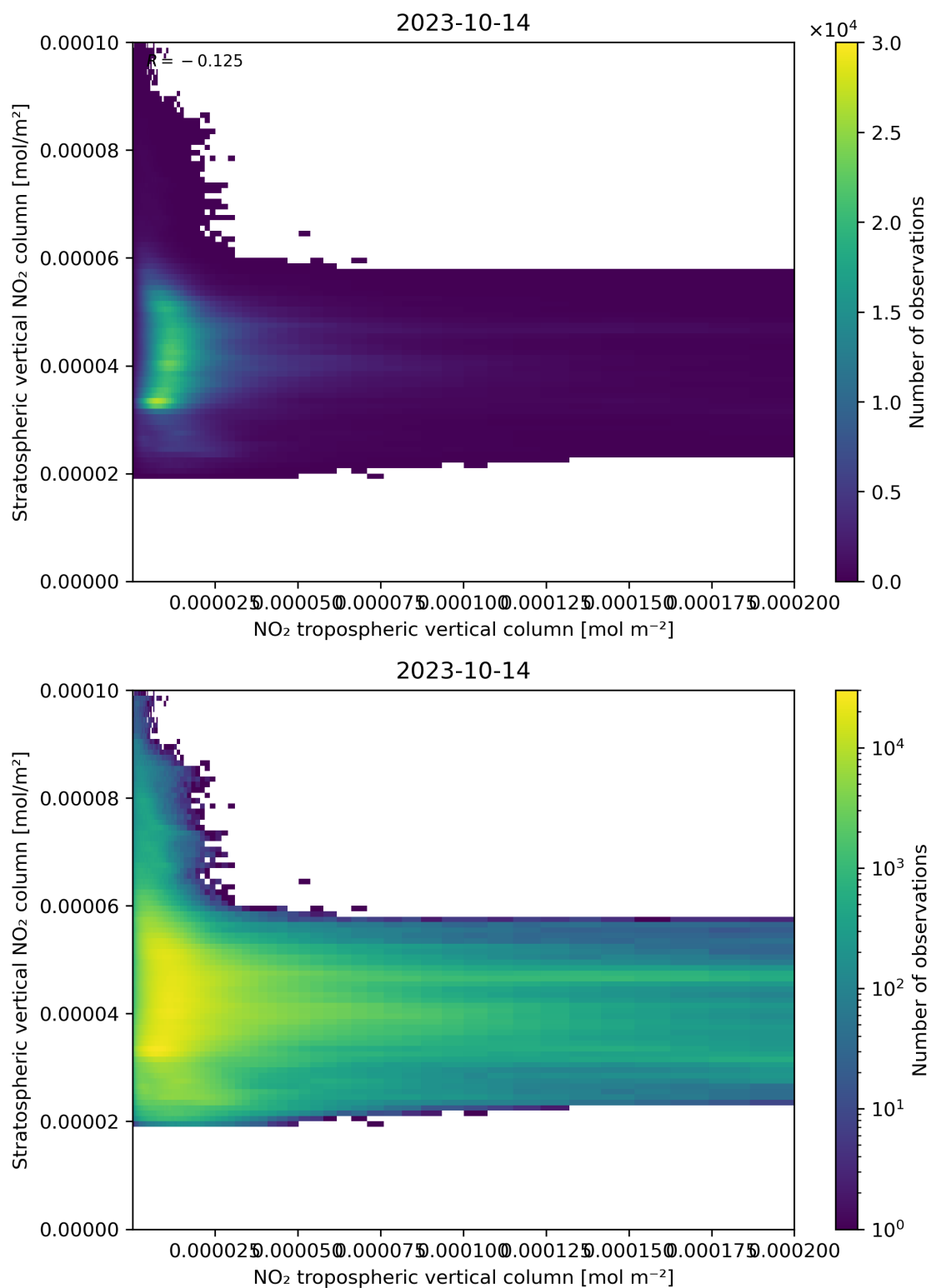
Figure 125: Scatter density plot of “NO 2 tropospheric vertical column” against “Stratospheric vertical NO 2 column” for 2023-10-13 to 2023-10-15.
