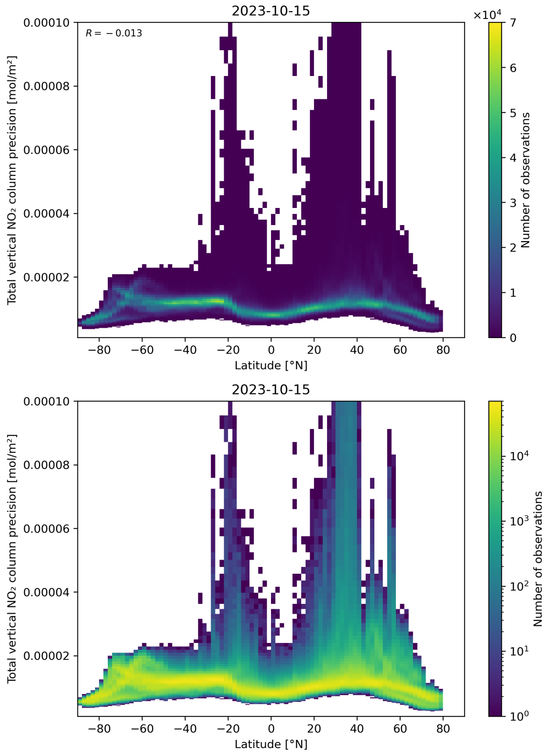
Figure 91: Scatter density plot of “Latitude” against “Total vertical NO 2 column precision” for 2023-10-14 to 2023-10-16.
