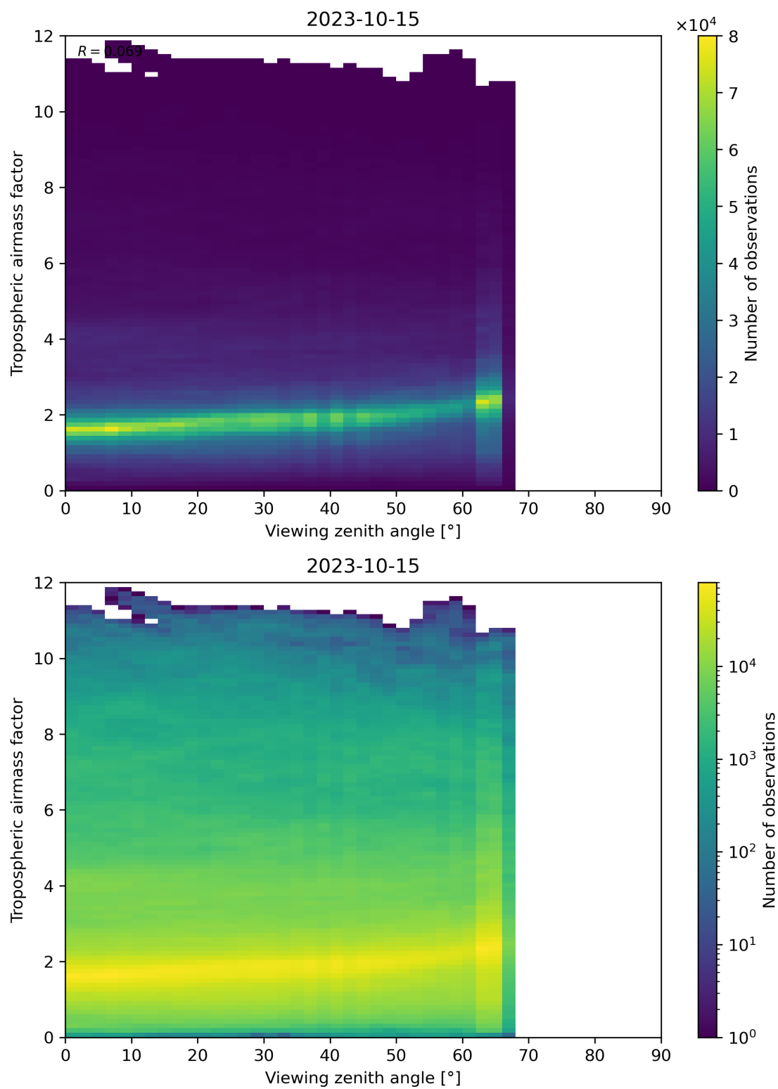
Figure 161: Scatter density plot of “Viewing zenith angle” against “Tropospheric airmass factor” for 2023-10-14 to 2023-10-16.
