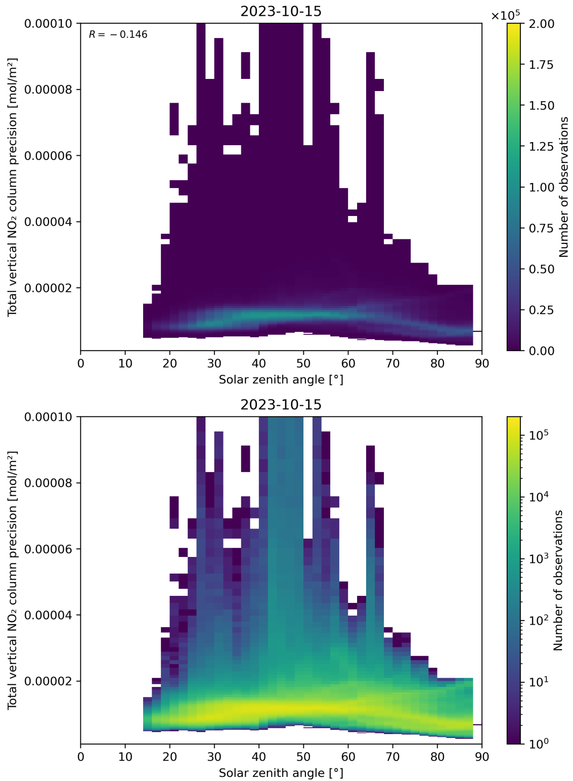
Figure 154: Scatter density plot of “Solar zenith angle” against “Total vertical NO 2 column precision” for 2023-10-14 to 2023-10-16.
