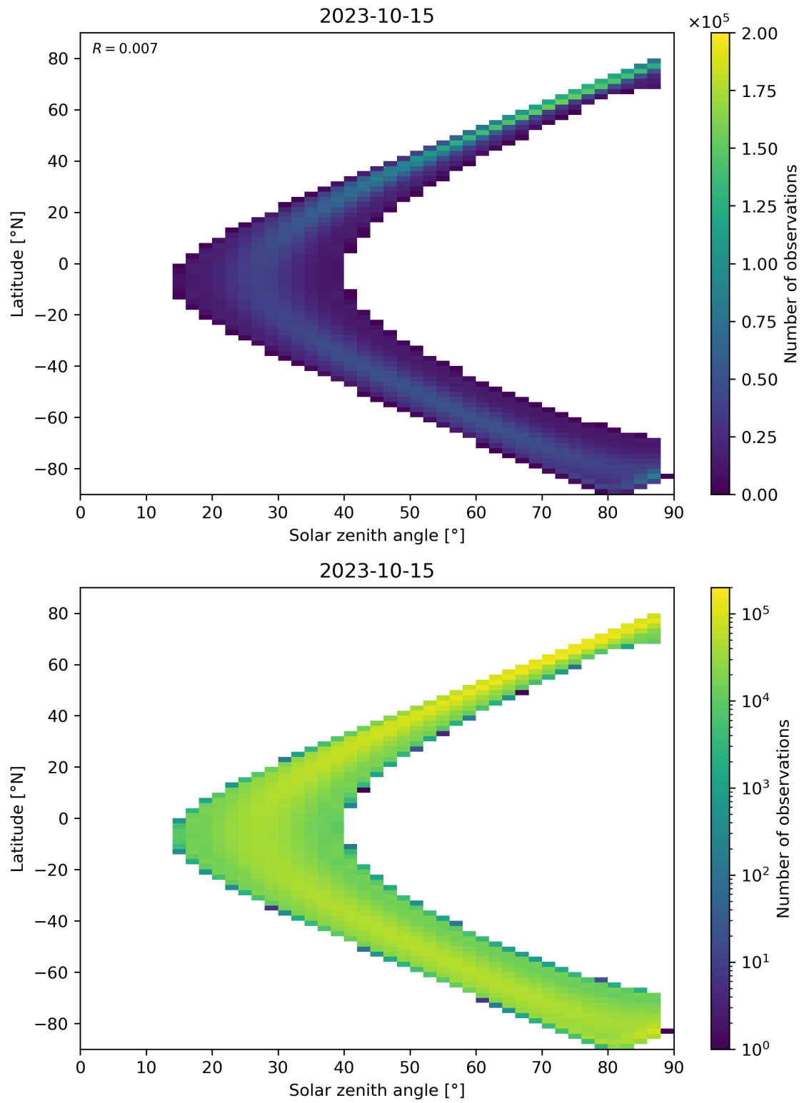
Figure 149: Scatter density plot of “Solar zenith angle” against “Latitude” for 2023-10-14 to 2023-10-16.
