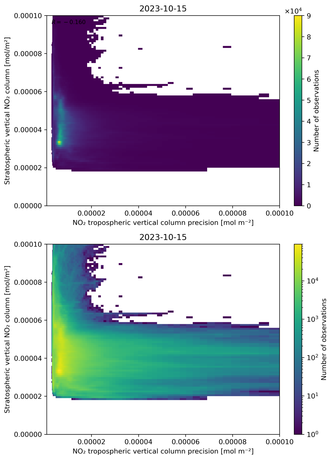
Figure 135: Scatter density plot of “NO 2 tropospheric vertical column precision” against “Stratospheric vertical NO 2 column” for 2023-10-14 to 2023-10-16.
