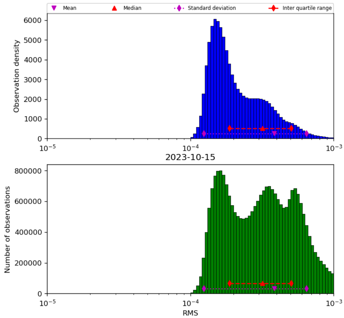
Figure 43: Histogram of “RMS” for 2023-10-14 to 2023-10-16
