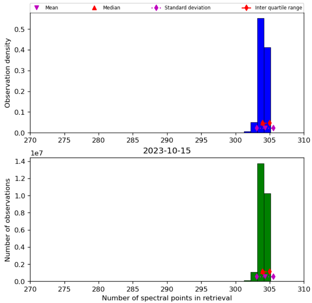
Figure 33: Histogram of “Number of spectral points in retrieval” for 2023-10-14 to 2023-10-16
