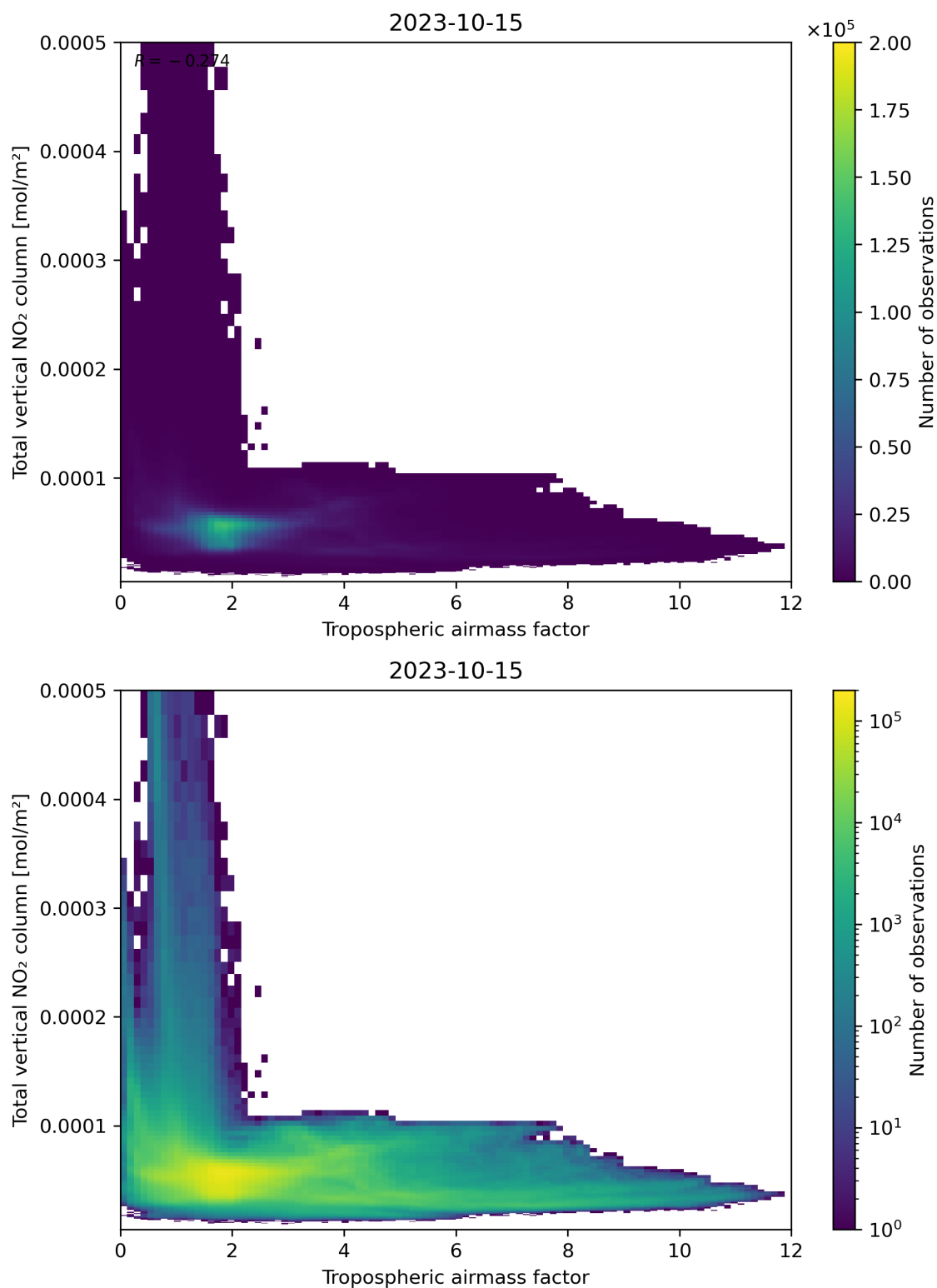
Figure 77: Scatter density plot of “Tropospheric airmass factor” against “Total vertical NO 2 column” for 2023-10-14 to 2023-10-16.
