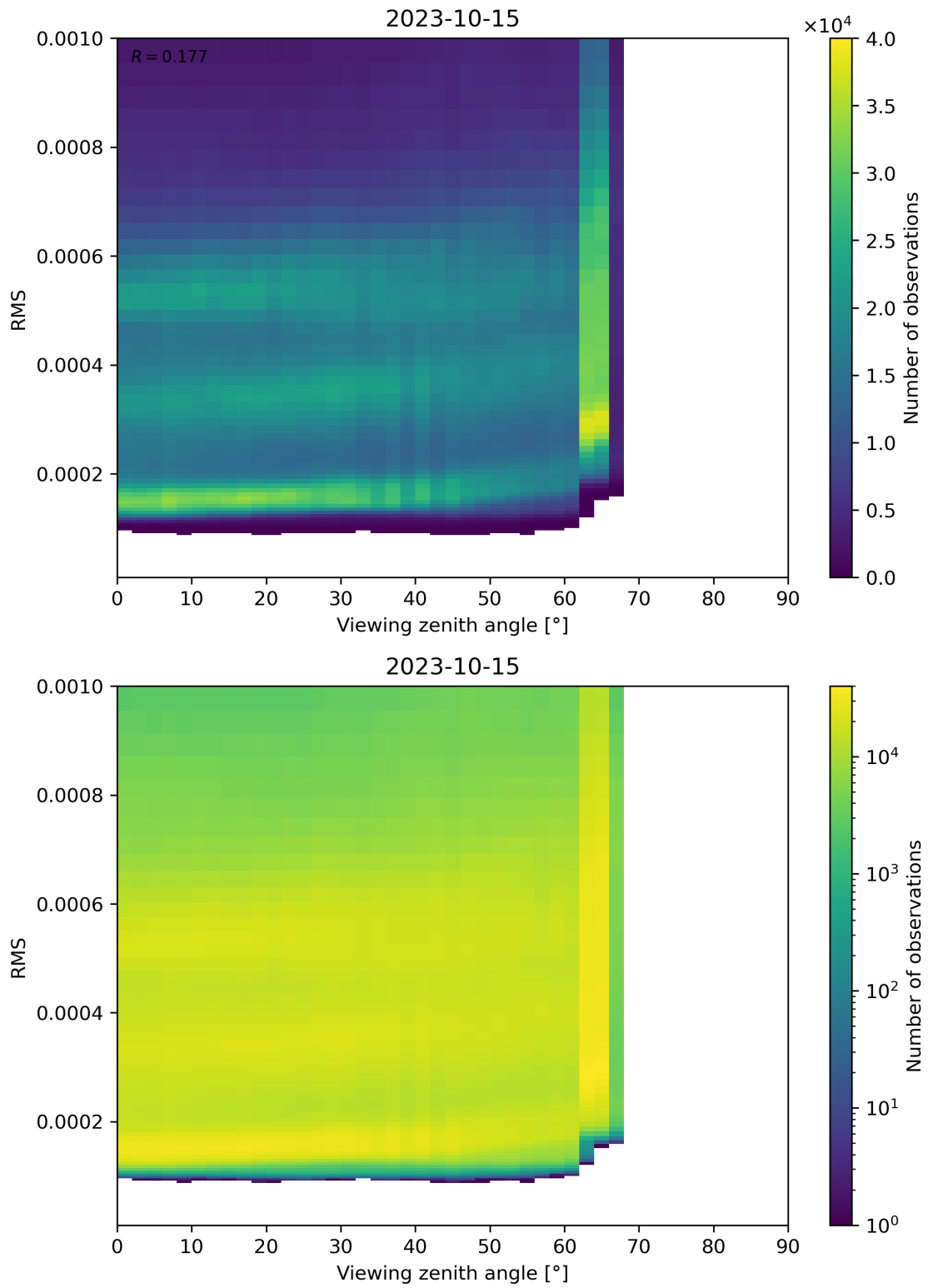
Figure 171: Scatter density plot of “Viewing zenith angle” against “RMS” for 2023-10-14 to 2023-10-16.
