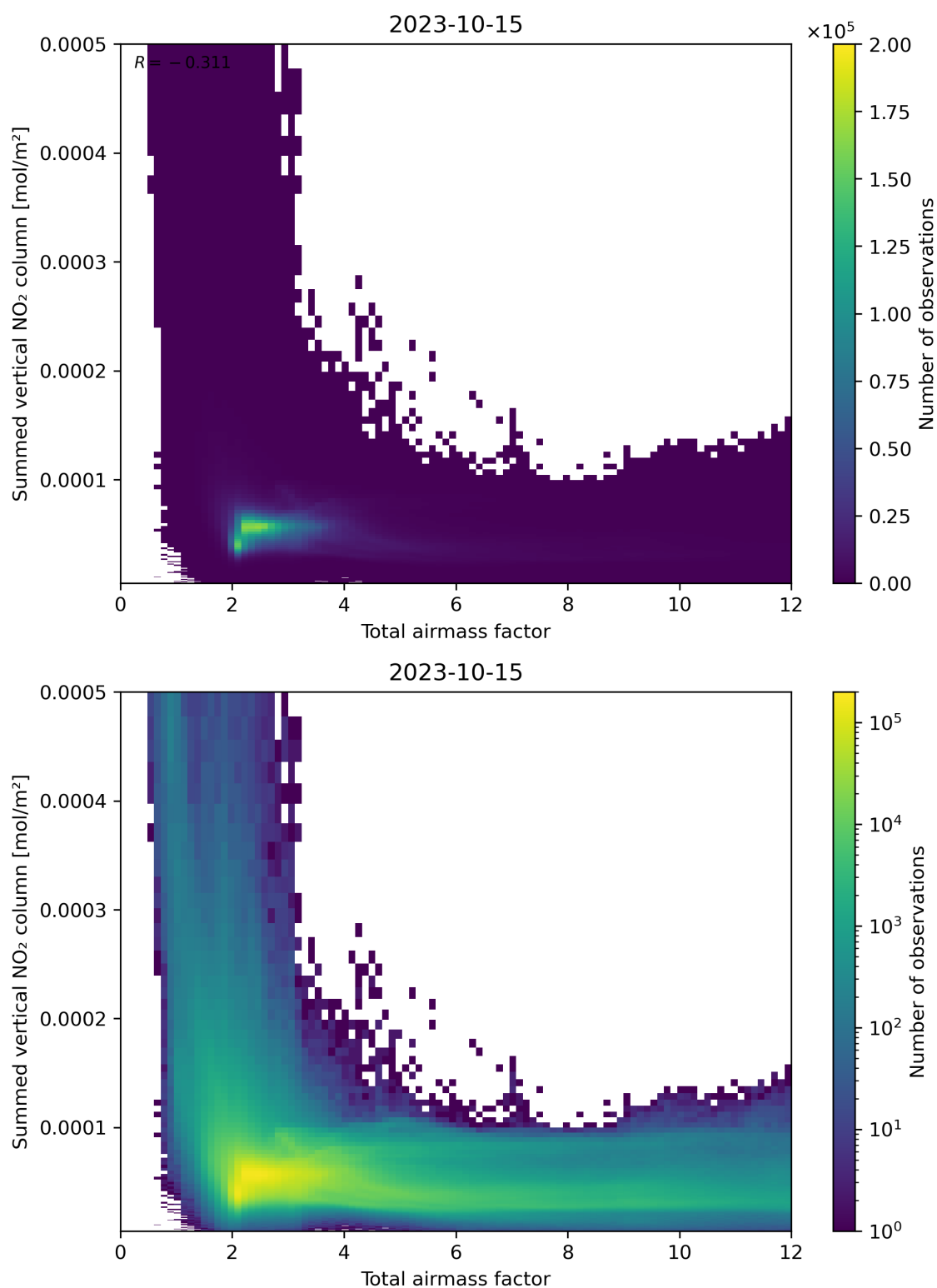
Figure 65: Scatter density plot of “Total airmass factor” against “Summed vertical NO 2 column” for 2023-10-14 to 2023-10-16.
