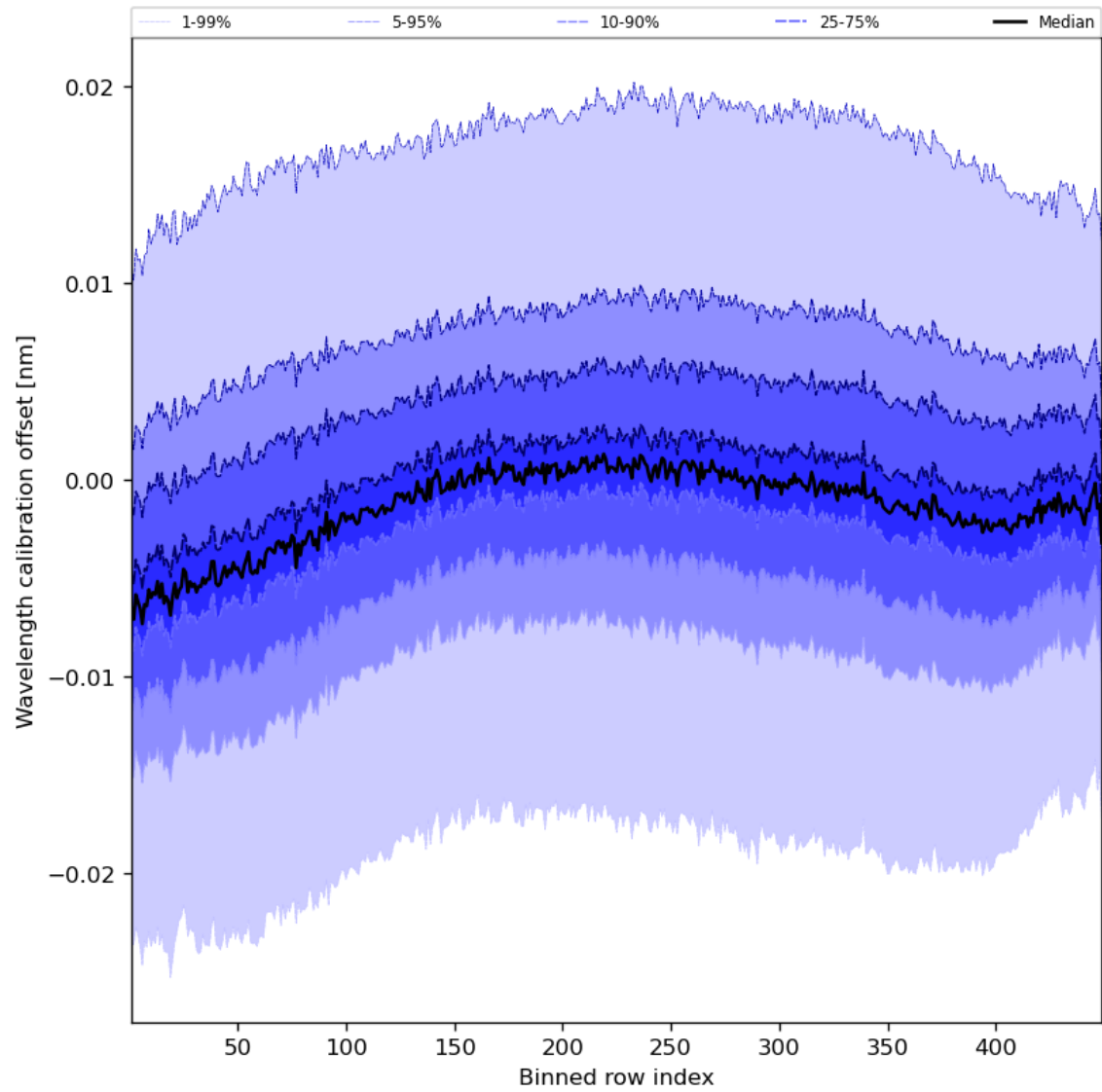
Figure 52: Along track statistics of “Wavelength calibration offset” for 2023-10-14 to 2023-10-16
