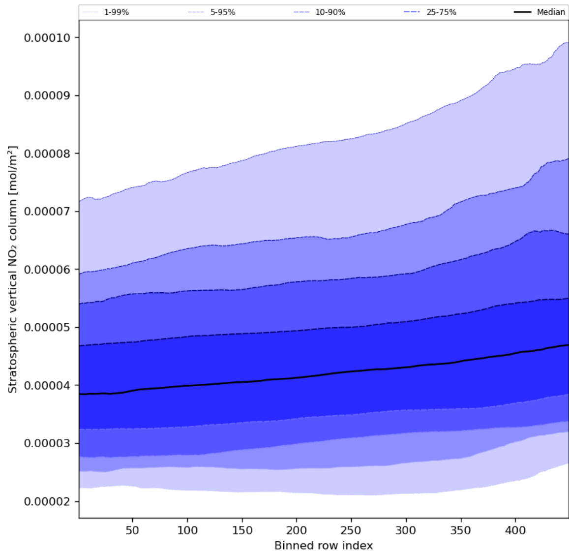
Figure 53: Along track statistics of “Stratospheric vertical NO 2 column” for 2023-10-14 to 2023-10-16
