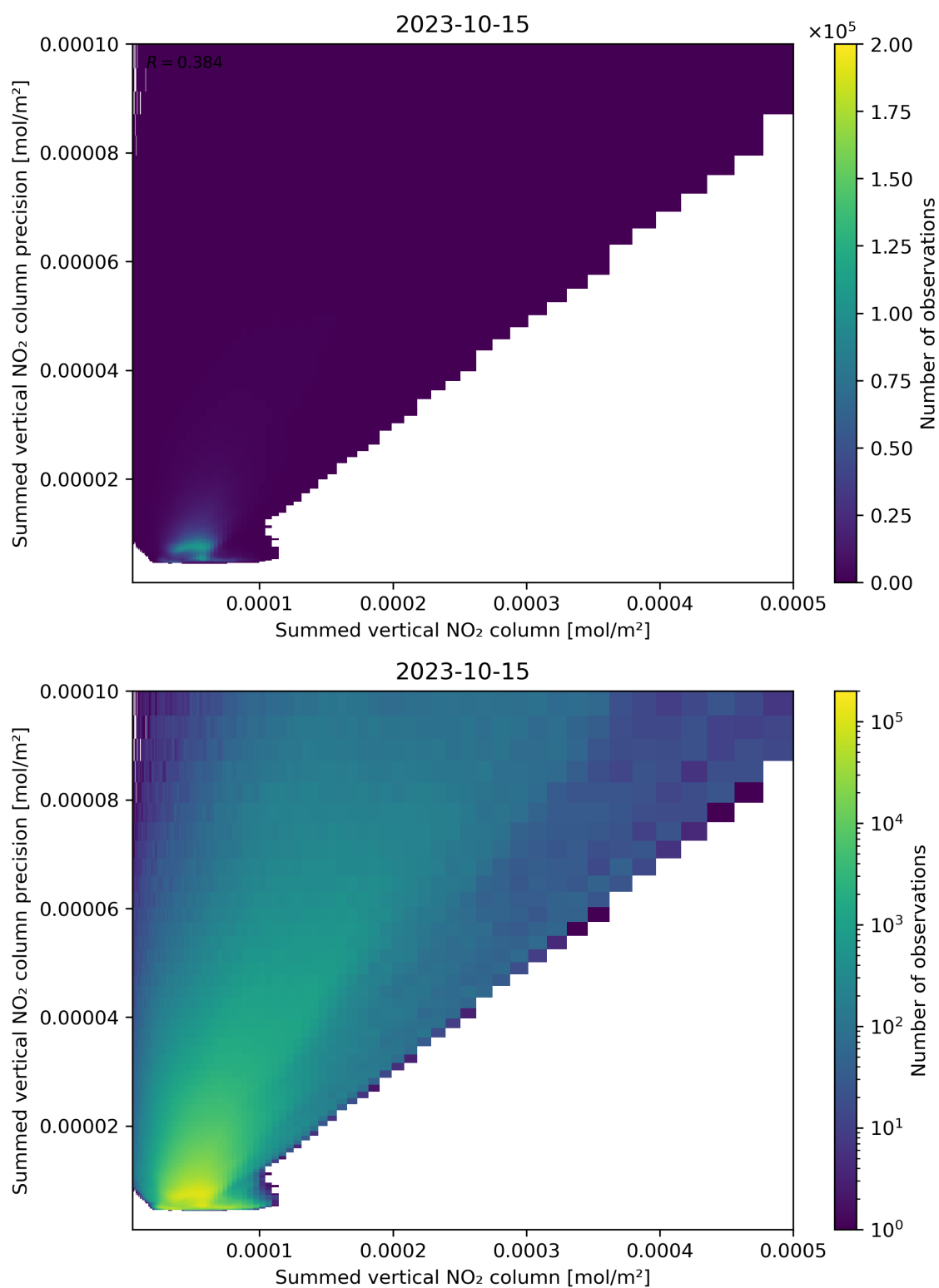
Figure 105: Scatter density plot of “Summed vertical NO 2 column” against “Summed vertical NO 2 column precision” for 2023-10-14 to 2023-10-16.
