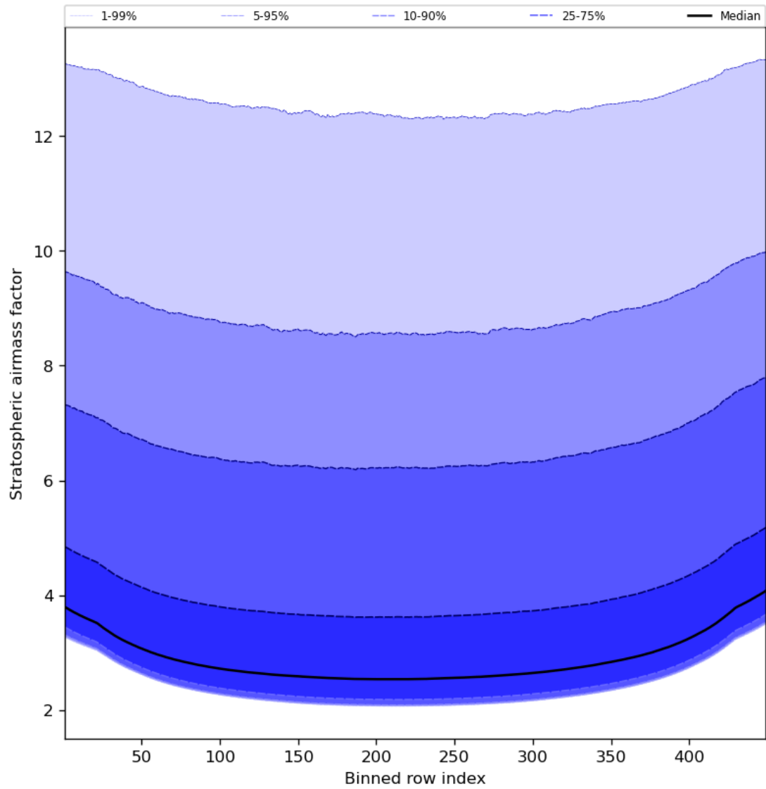
Figure 61: Along track statistics of “Stratospheric airmass factor” for 2023-10-14 to 2023-10-16
