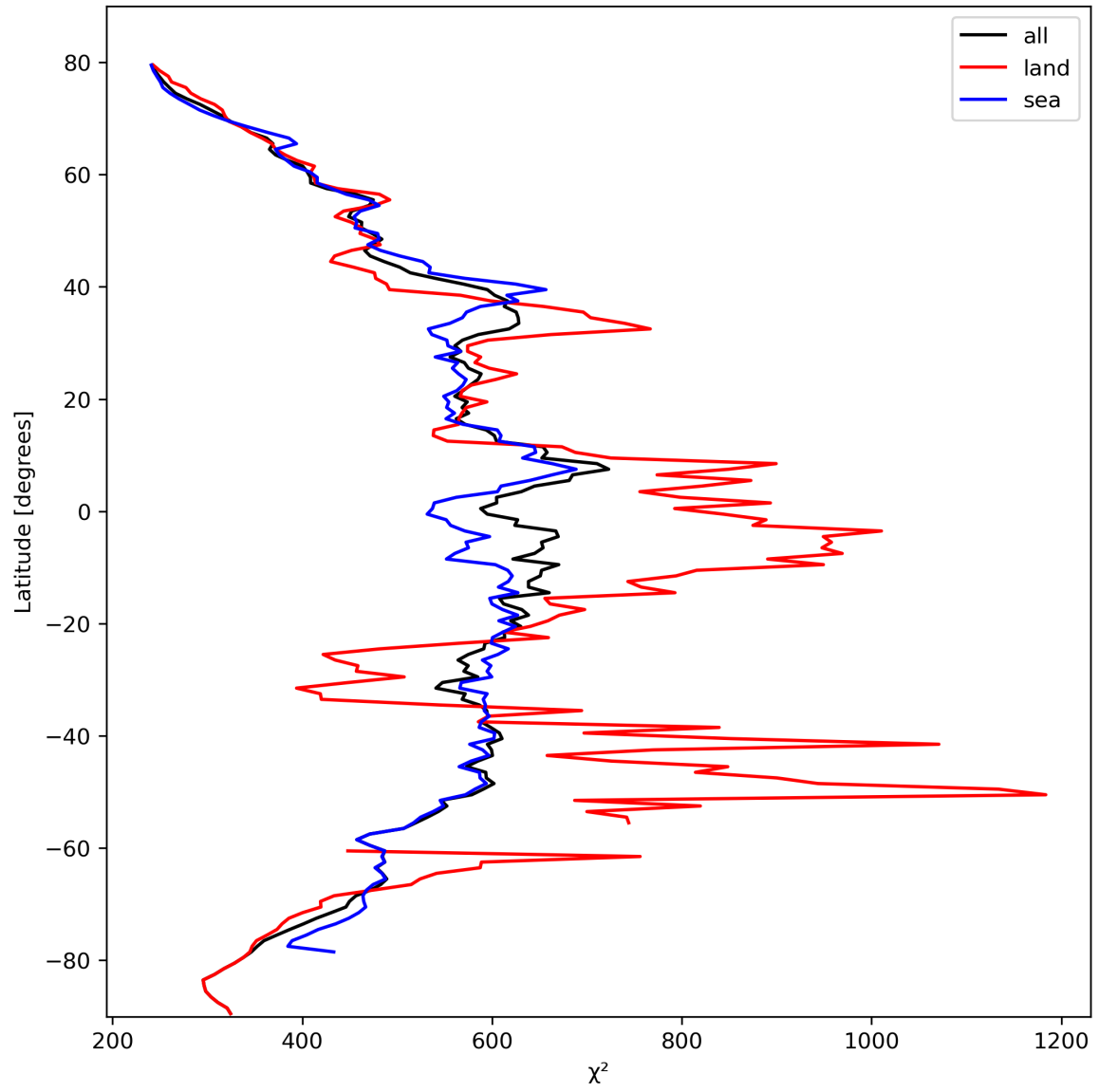
Figure 25: Zonal average of “ \chi^2 ” for 2023-10-14 to 2023-10-16.
