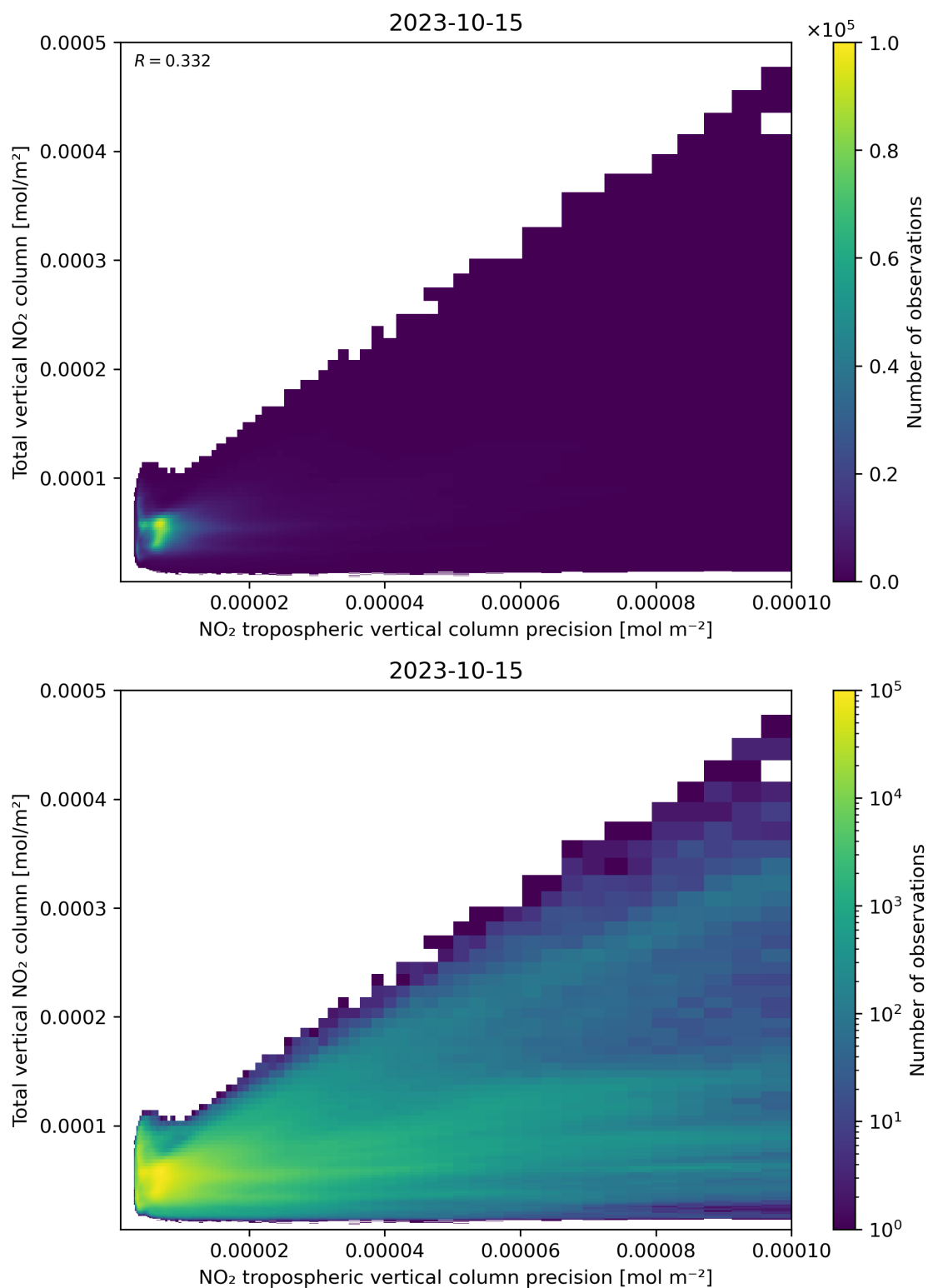
Figure 138: Scatter density plot of “NO 2 tropospheric vertical column precision” against “Total vertical NO 2 column” for 2023-10-14 to 2023-10-16.
