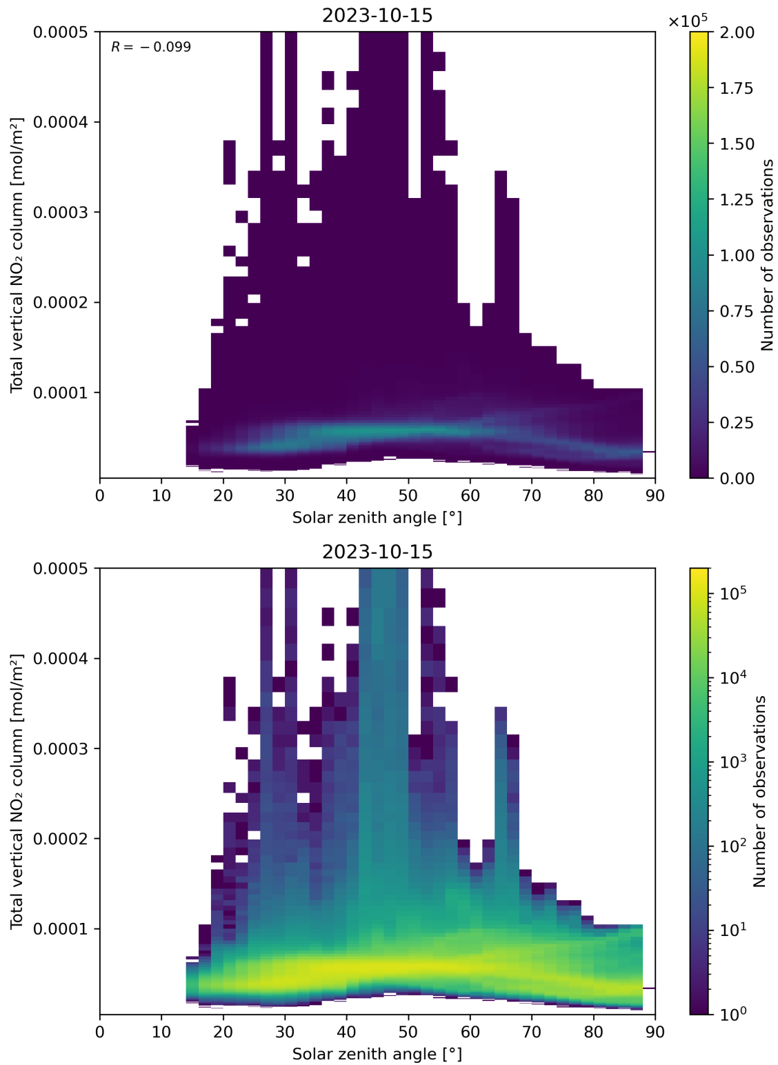
Figure 153: Scatter density plot of “Solar zenith angle” against “Total vertical NO 2 column” for 2023-10-14 to 2023-10-16.
