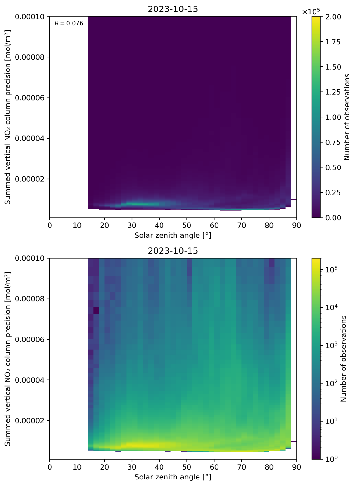
Figure 152: Scatter density plot of “Solar zenith angle” against “Summed vertical NO 2 column precision” for 2023-10-14 to 2023-10-16.
