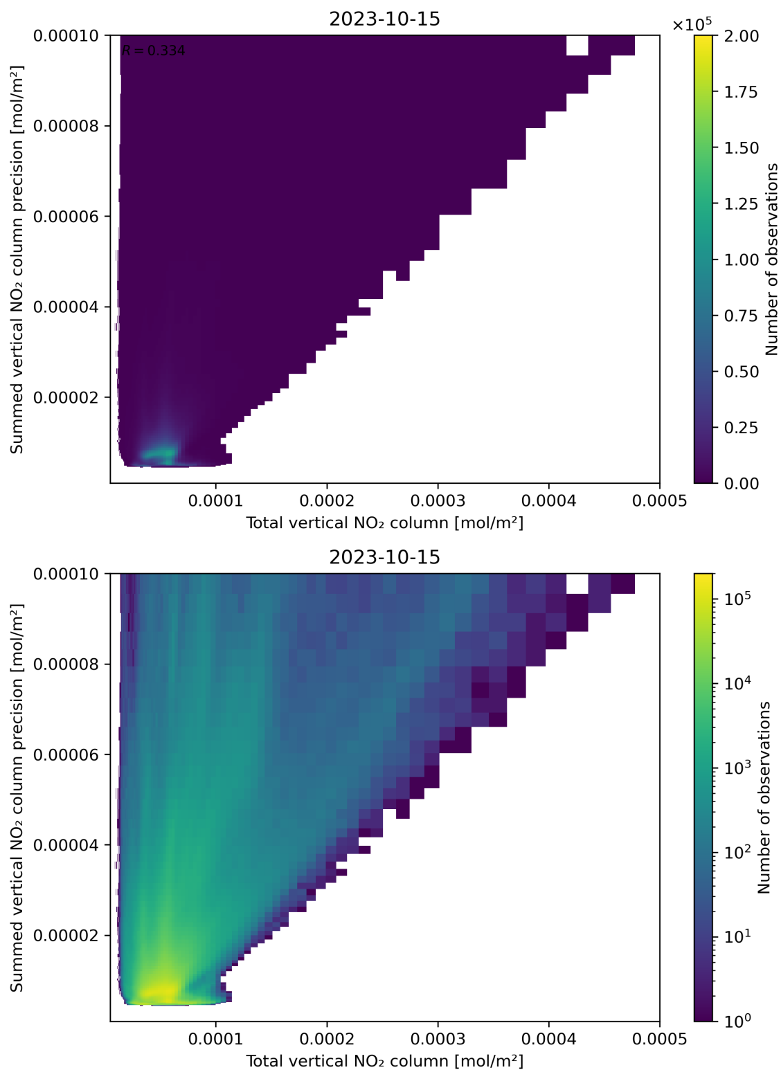
Figure 113: Scatter density plot of “Total vertical NO 2 column” against “Summed vertical NO 2 column precision” for 2023-10-14 to 2023-10-16.
