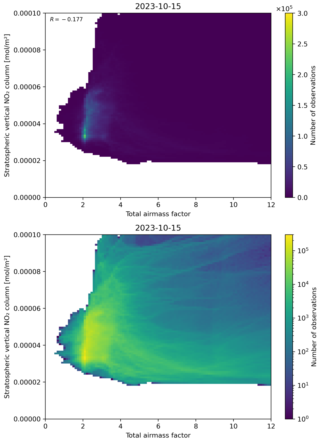
Figure 64: Scatter density plot of “Total airmass factor” against “Stratospheric vertical NO 2 column” for 2023-10-14 to 2023-10-16.
