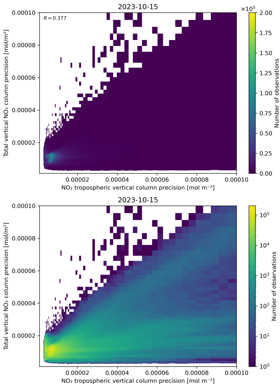
Figure 139: Scatter density plot of “NO 2 tropospheric vertical column precision” against “Total vertical NO 2 column precision” for 2023-10-14 to 2023-10-16.
