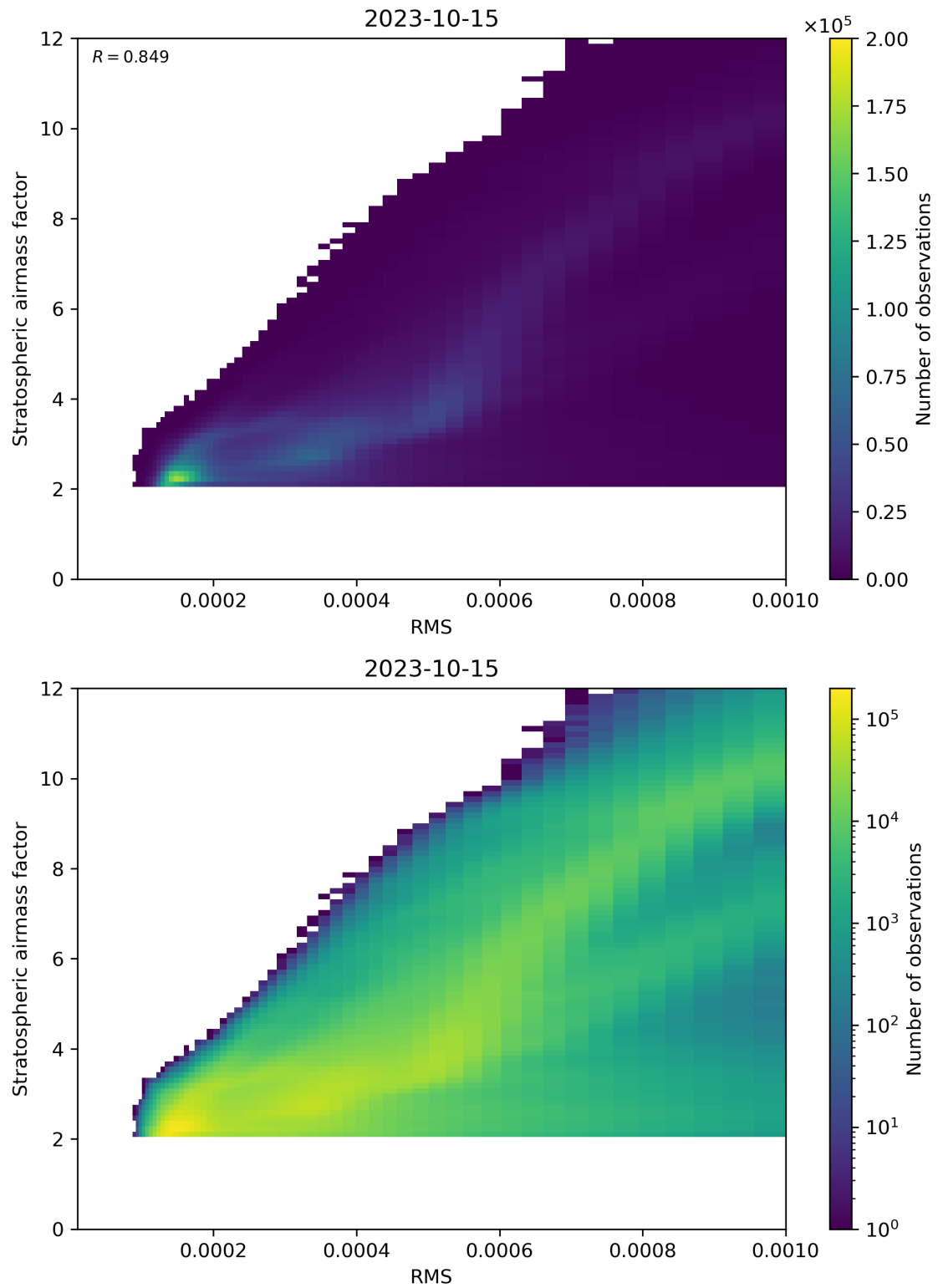
Figure 144: Scatter density plot of “RMS” against “Stratospheric airmass factor” for 2023-10-14 to 2023-10-16.
