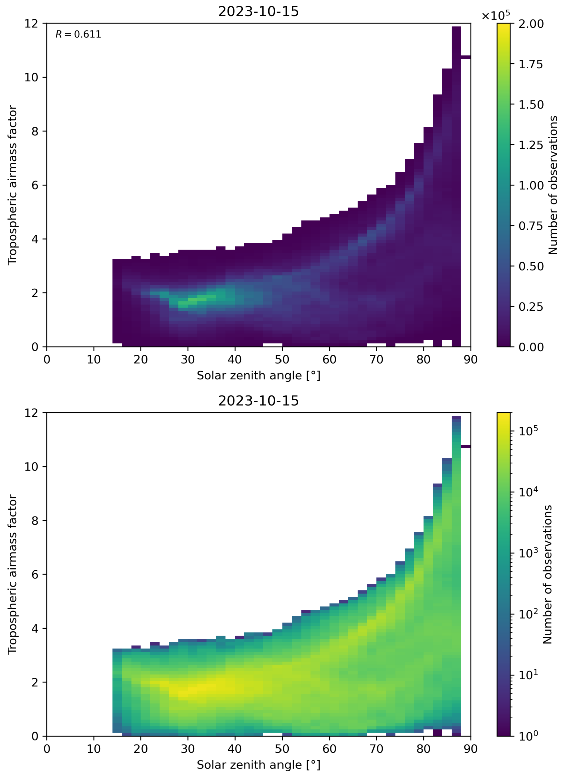
Figure 147: Scatter density plot of “Solar zenith angle” against “Tropospheric airmass factor” for 2023-10-14 to 2023-10-16.
