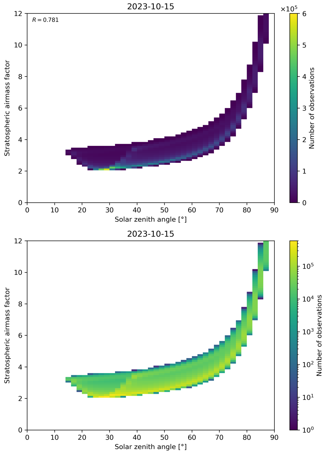
Figure 145: Scatter density plot of “Solar zenith angle” against “Stratospheric airmass factor” for 2023-10-14 to 2023-10-16.
