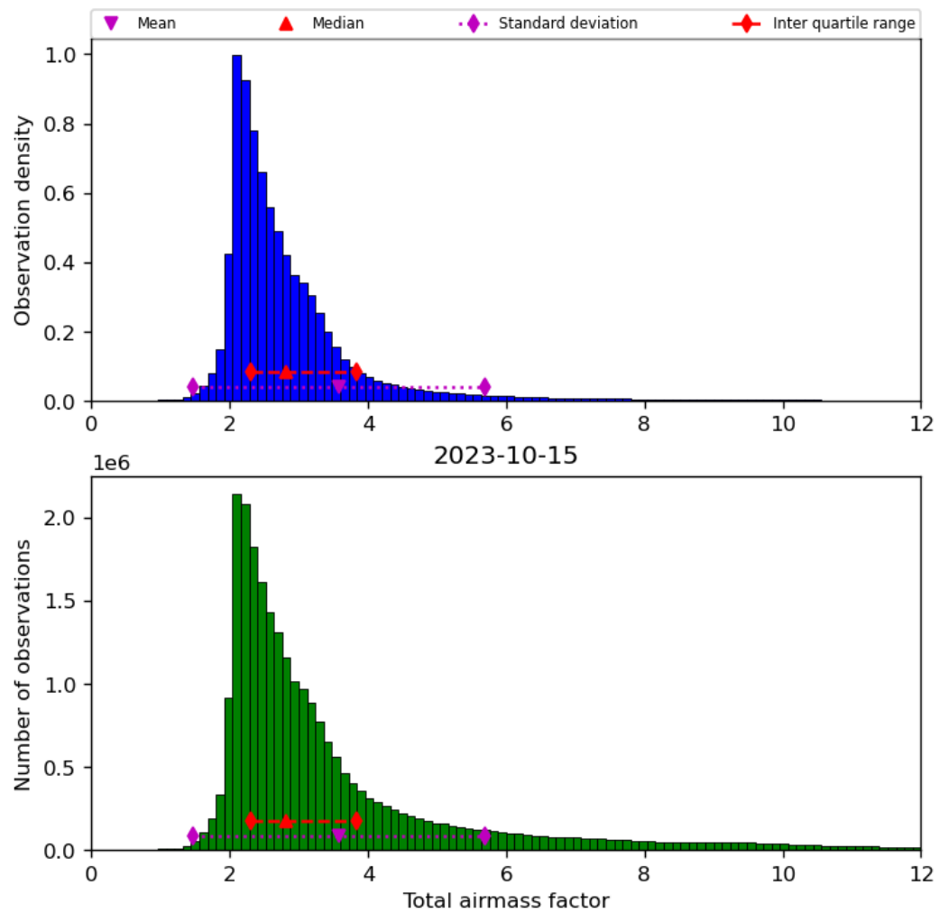
Figure 32: Histogram of “Total airmass factor” for 2023-10-14 to 2023-10-16
