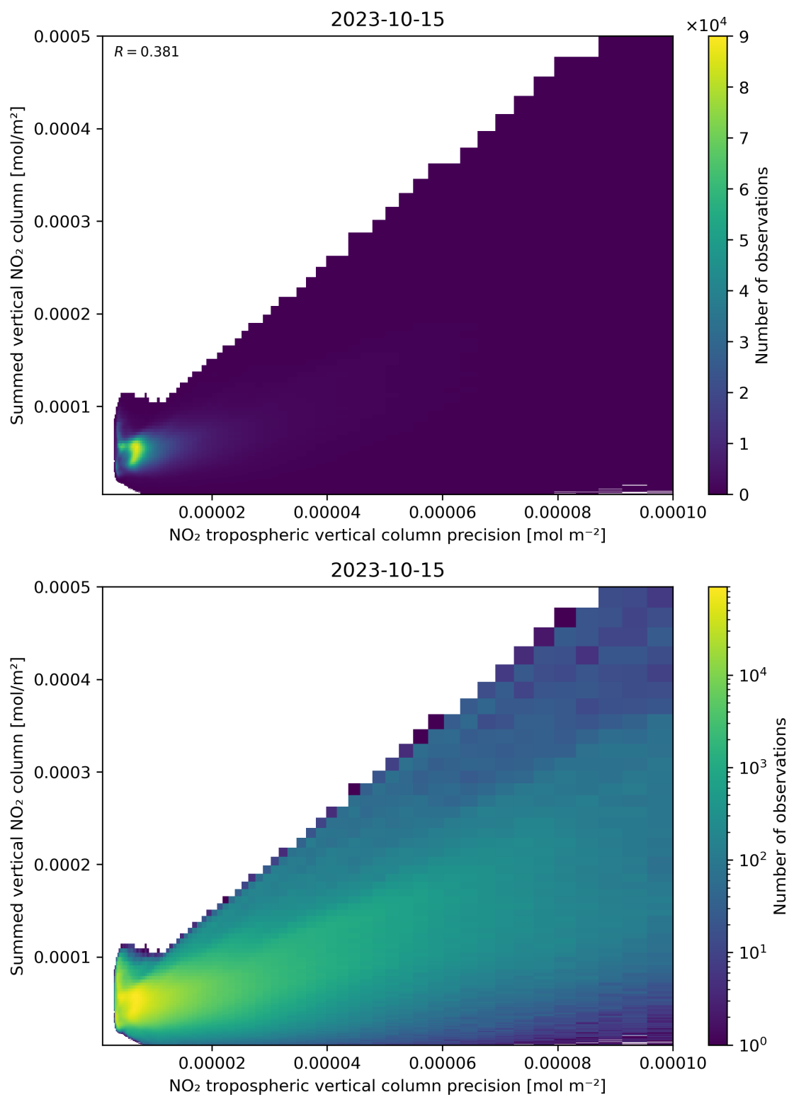
Figure 136: Scatter density plot of “NO 2 tropospheric vertical column precision” against “Summed vertical NO 2 column” for 2023-10-14 to 2023-10-16.
