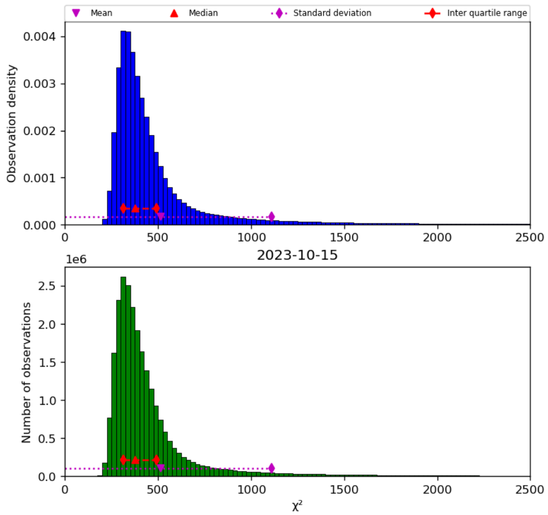
Figure 42: Histogram of “ \chi^2 ” for 2023-10-14 to 2023-10-16
