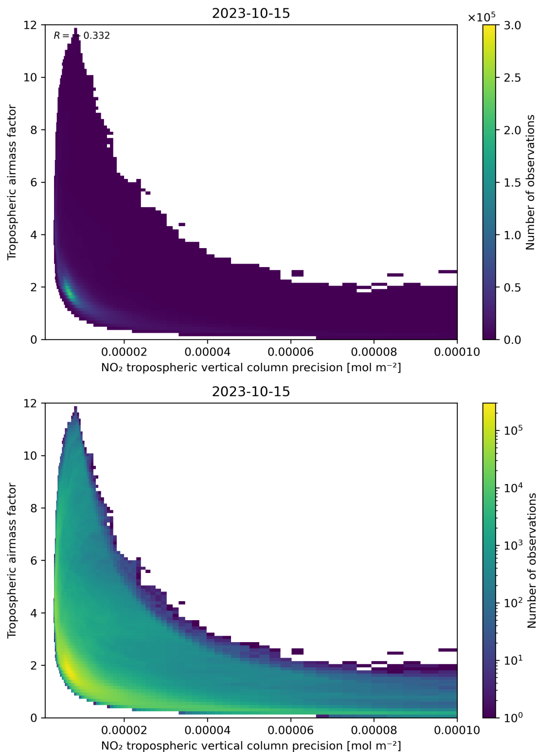
Figure 133: Scatter density plot of “NO 2 tropospheric vertical column precision” against “Tropospheric airmass factor” for 2023-10-14 to 2023-10-16.
