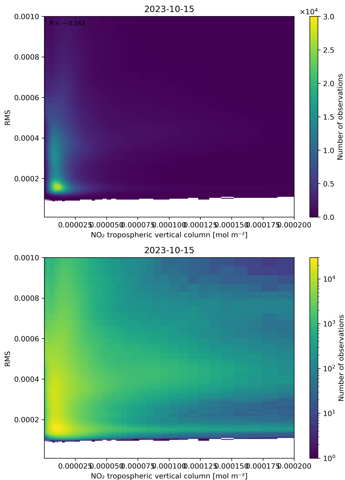
Figure 142: Scatter density plot of “NO 2 tropospheric vertical column” against “RMS” for 2023-10-14 to 2023-10-16.
