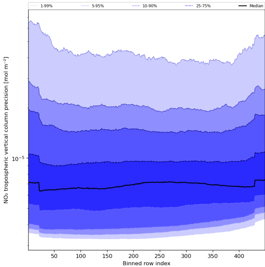
Figure 47: Along track statistics of “NO 2 tropospheric vertical column precision” for 2023-10-14 to 2023-10-16
