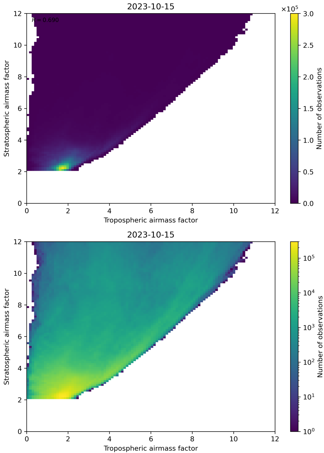
Figure 71: Scatter density plot of “Tropospheric airmass factor” against “Stratospheric airmass factor” for 2023-10-14 to 2023-10-16.
