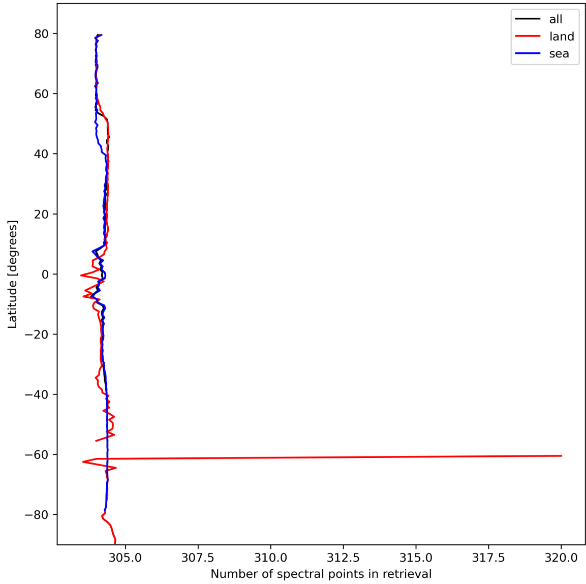
Figure 16: Zonal average of “Number of spectral points in retrieval” for 2023-10-14 to 2023-10-16.
