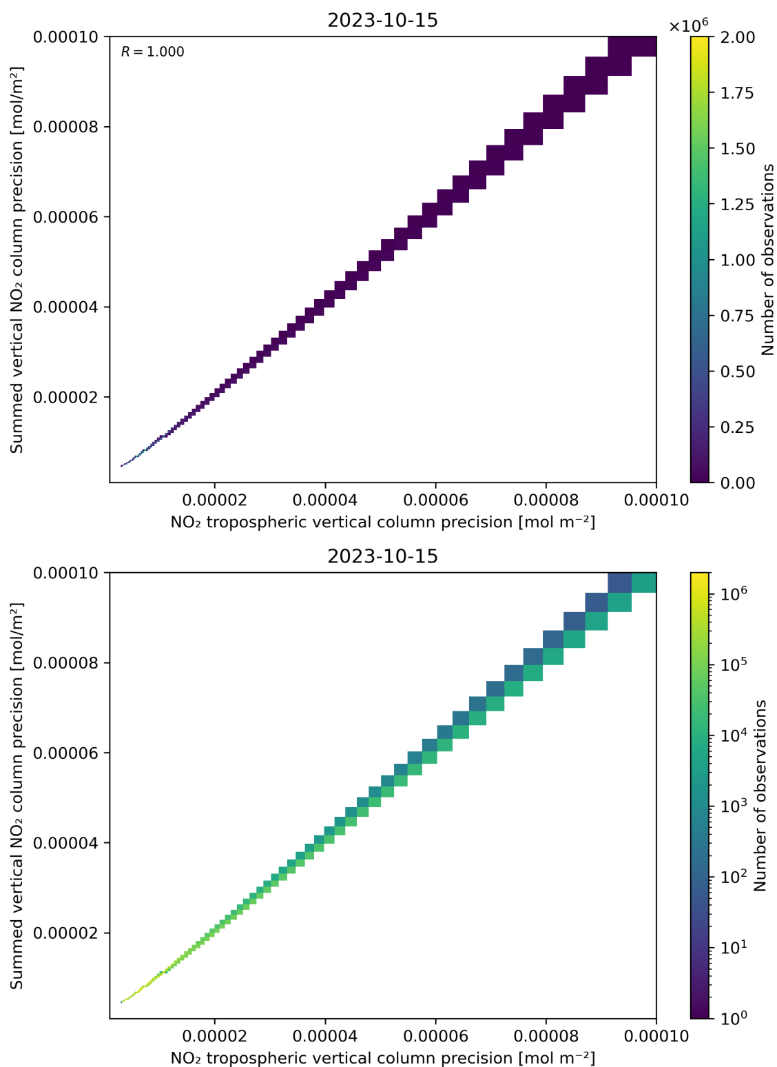
Figure 137: Scatter density plot of “NO 2 tropospheric vertical column precision” against “Summed vertical NO 2 column precision” for 2023-10-14 to 2023-10-16.
