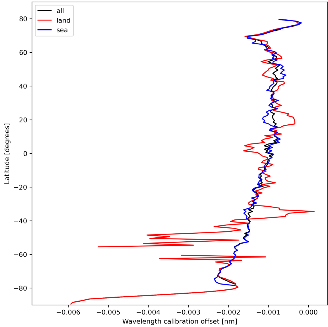
Figure 18: Zonal average of “Wavelength calibration offset” for 2023-10-14 to 2023-10-16.
