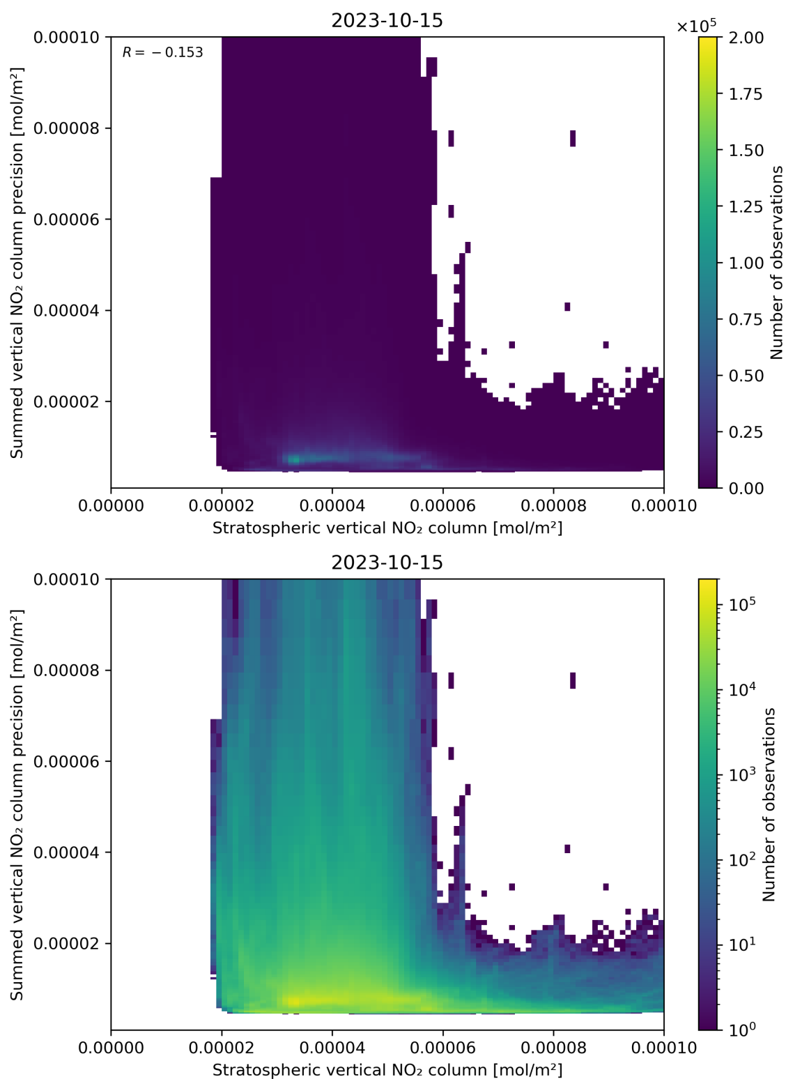
Figure 99: Scatter density plot of “Stratospheric vertical NO 2 column” against “Summed vertical NO 2 column precision” for 2023-10-14 to 2023-10-16.
