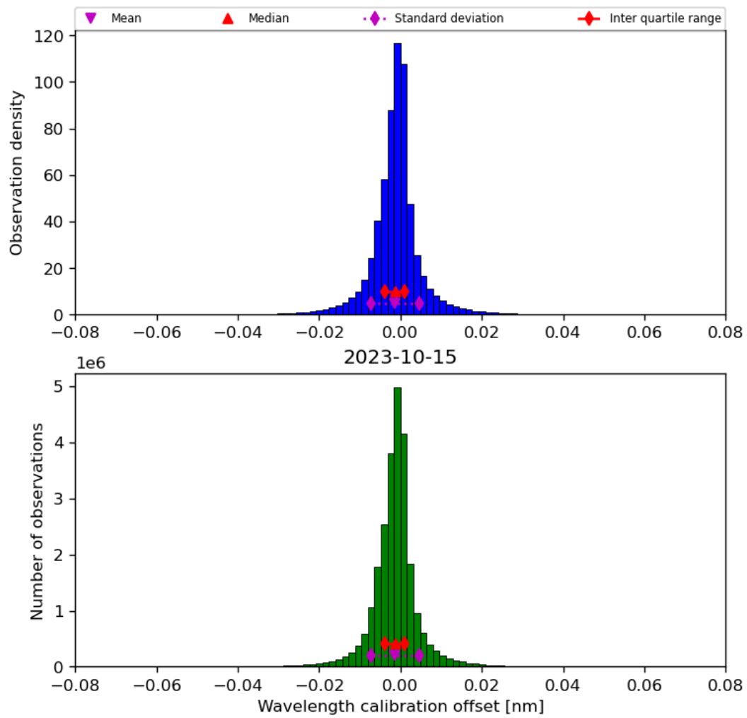
Figure 35: Histogram of “Wavelength calibration offset” for 2023-10-14 to 2023-10-16
