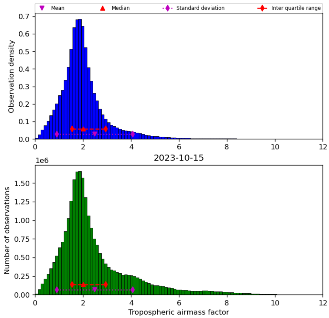
Figure 31: Histogram of “Tropospheric airmass factor” for 2023-10-14 to 2023-10-16
