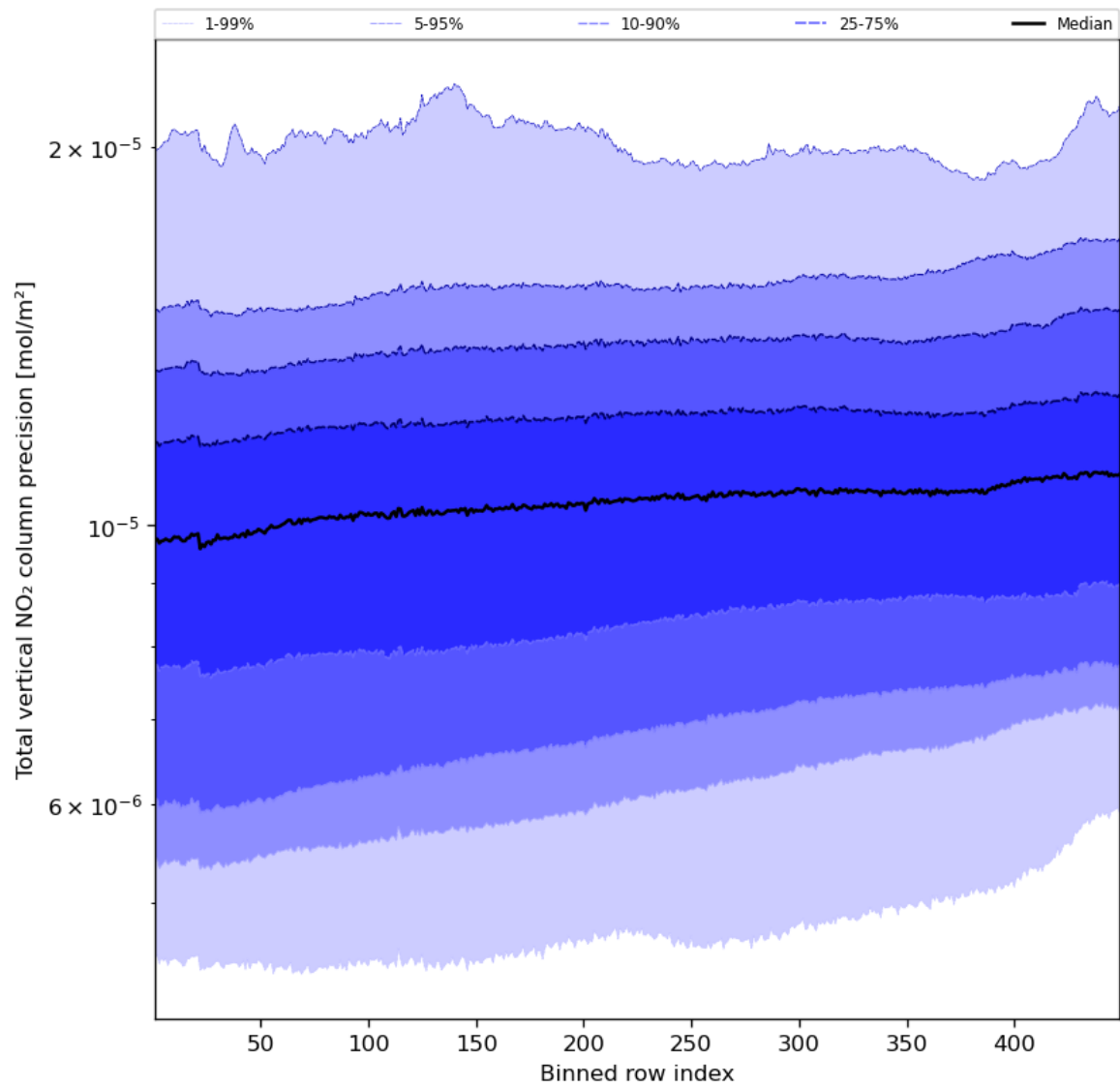
Figure 56: Along track statistics of “Total vertical NO 2 column precision” for 2023-10-14 to 2023-10-16
