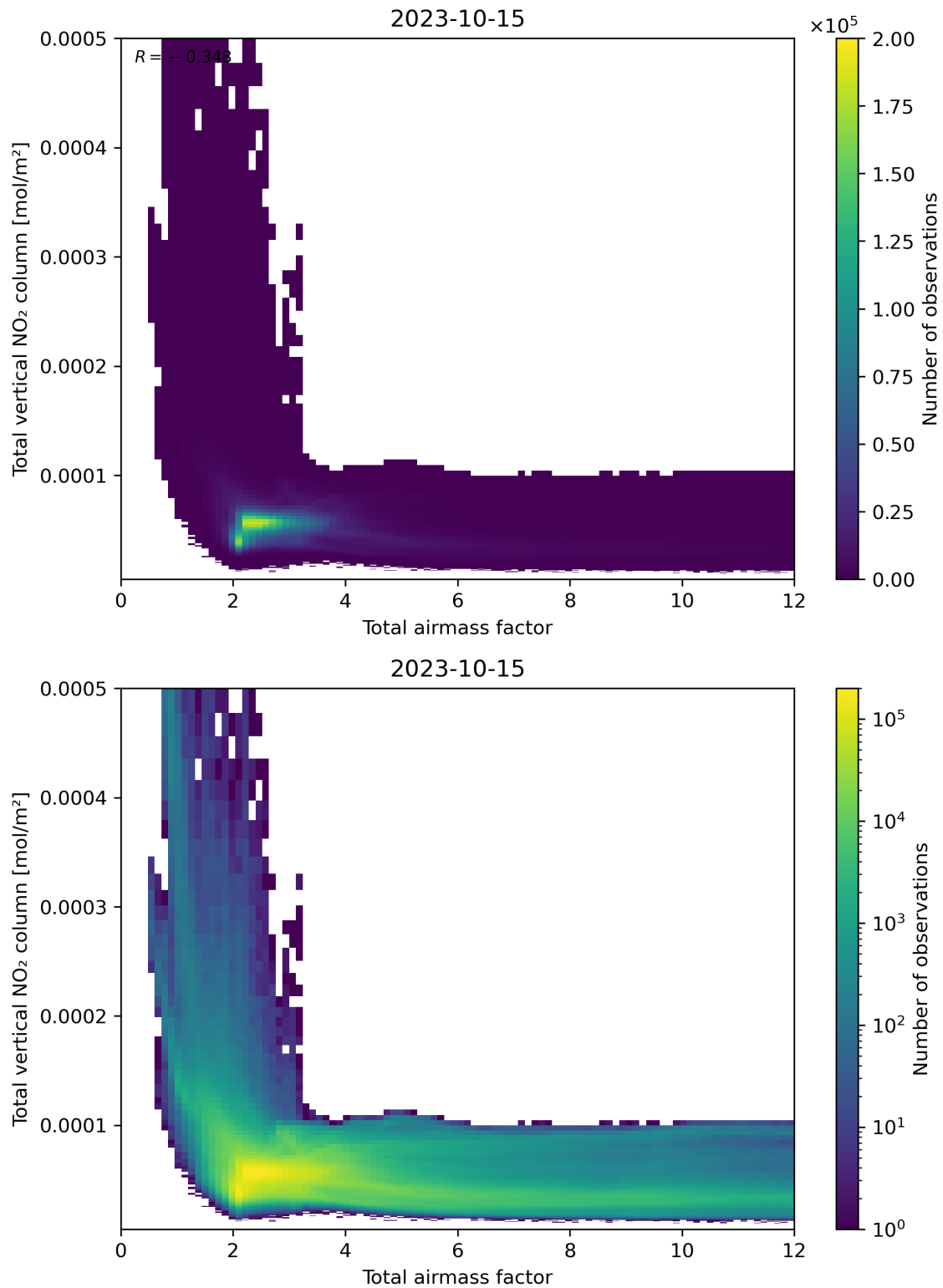
Figure 67: Scatter density plot of “Total airmass factor” against “Total vertical NO 2 column” for 2023-10-14 to 2023-10-16.
