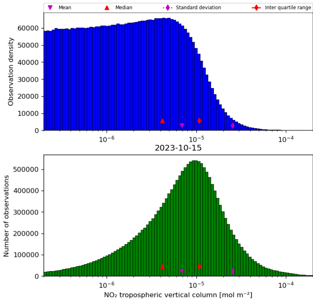
Figure 29: Histogram of “NO 2 tropospheric vertical column” for 2023-10-14 to 2023-10-16
