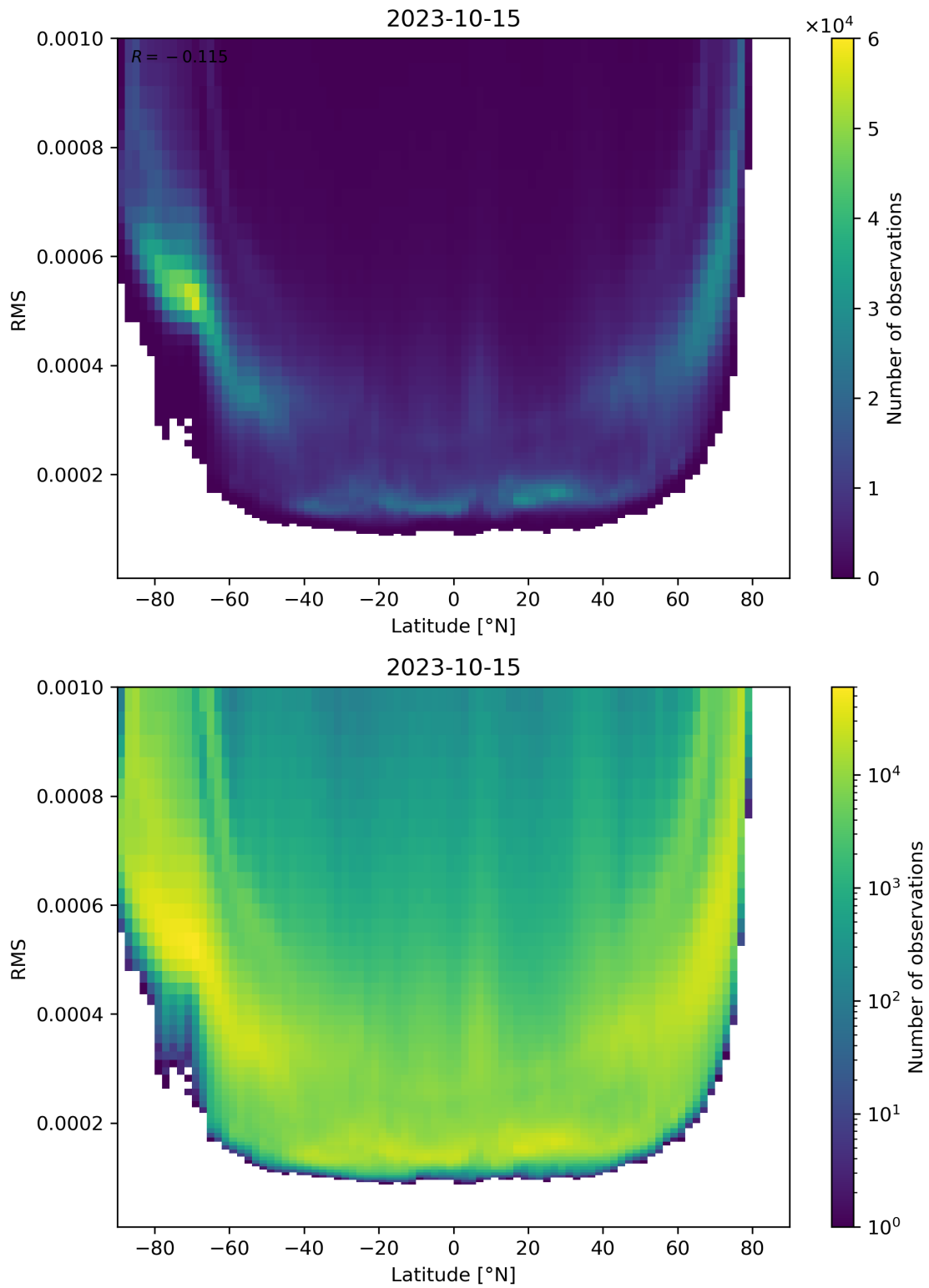
Figure 94: Scatter density plot of “Latitude” against “RMS” for 2023-10-14 to 2023-10-16.
