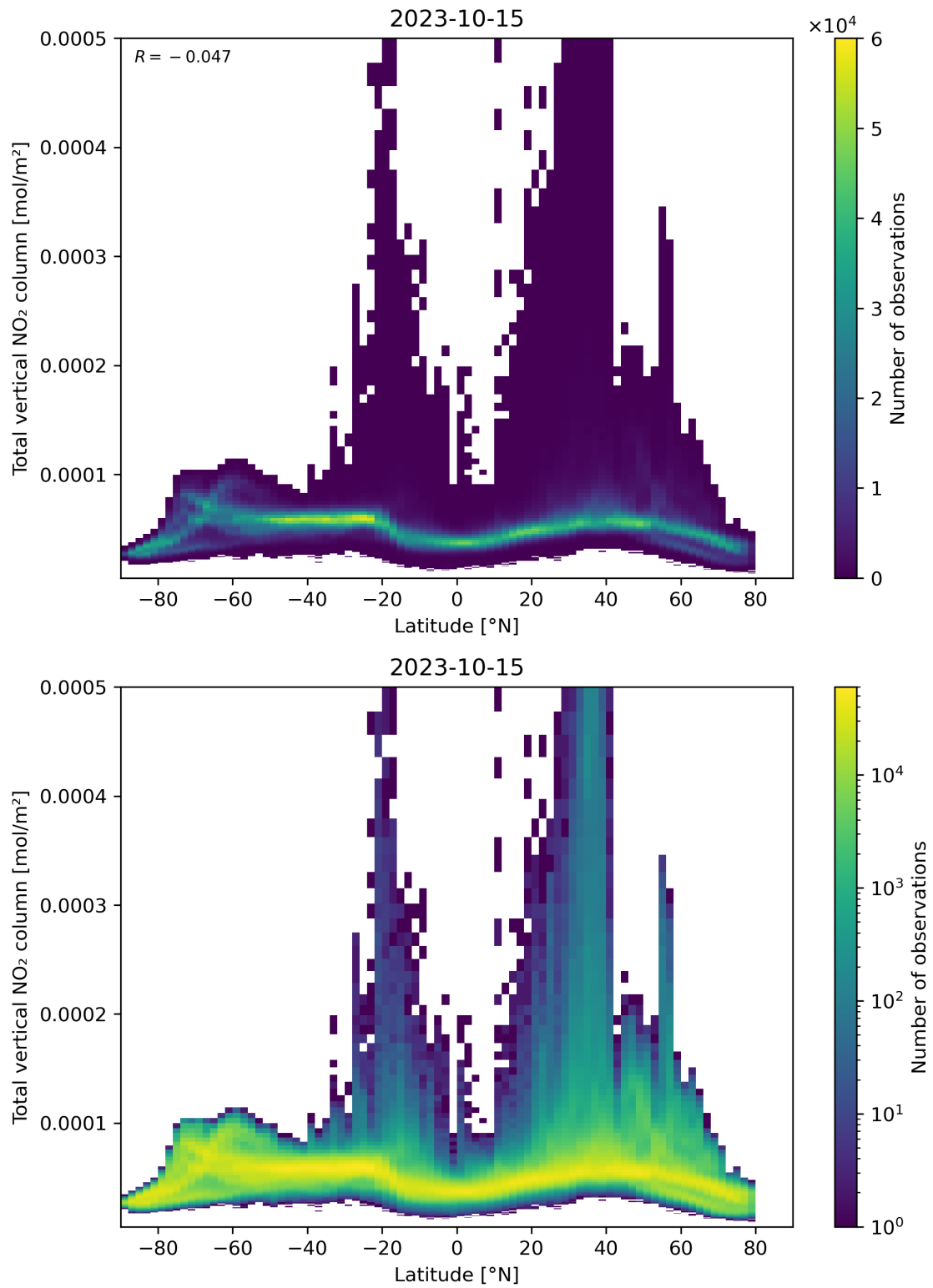
Figure 90: Scatter density plot of “Latitude” against “Total vertical NO 2 column” for 2023-10-14 to 2023-10-16.
