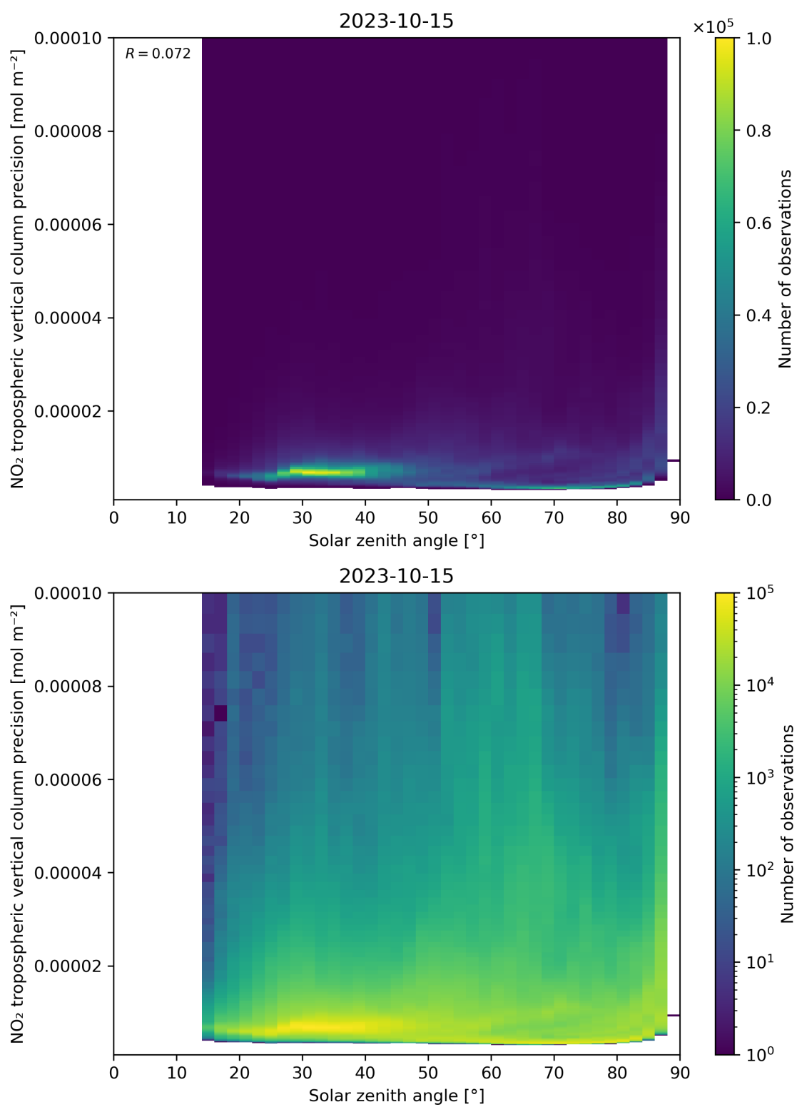
Figure 156: Scatter density plot of “Solar zenith angle” against “NO 2 tropospheric vertical column precision” for 2023-10-14 to 2023-10-16.
