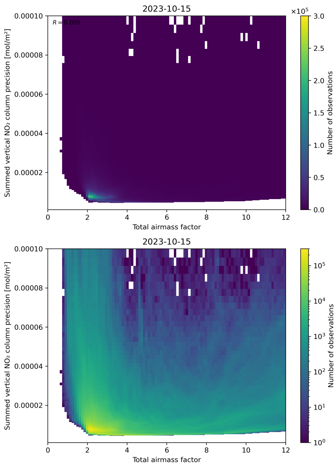
Figure 66: Scatter density plot of “Total airmass factor” against “Summed vertical NO 2 column precision” for 2023-10-14 to 2023-10-16.
