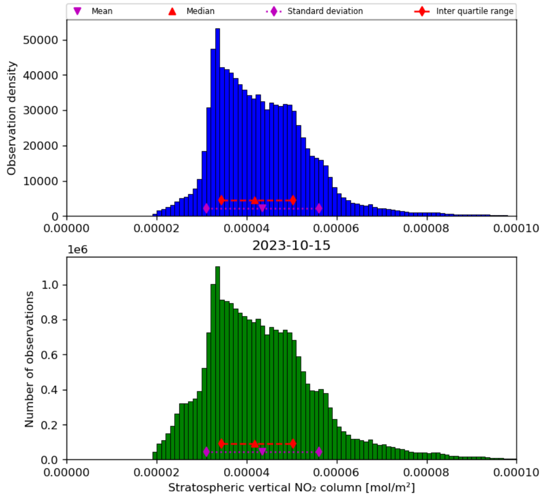
Figure 36: Histogram of “Stratospheric vertical NO 2 column” for 2023-10-14 to 2023-10-16
