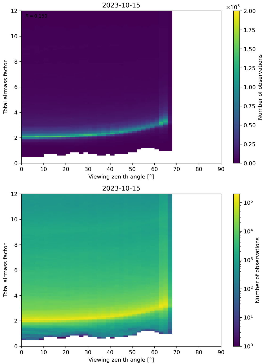
Figure 160: Scatter density plot of “Viewing zenith angle” against “Total airmass factor” for 2023-10-14 to 2023-10-16.
