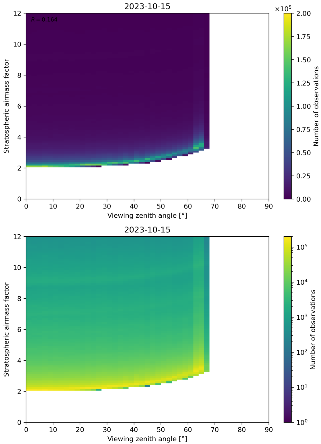
Figure 159: Scatter density plot of “Viewing zenith angle” against “Stratospheric airmass factor” for 2023-10-14 to 2023-10-16.
