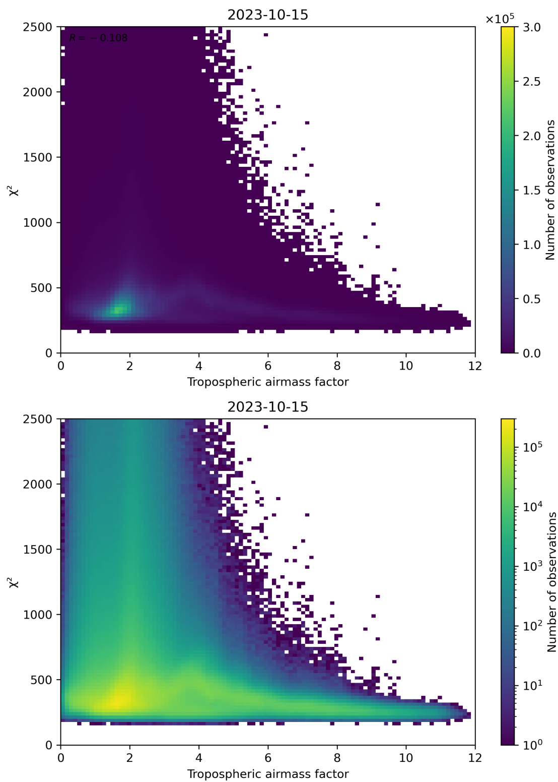
Figure 73: Scatter density plot of “Tropospheric airmass factor” against “ \chi^2 ” for 2023-10-14 to 2023-10-16.
