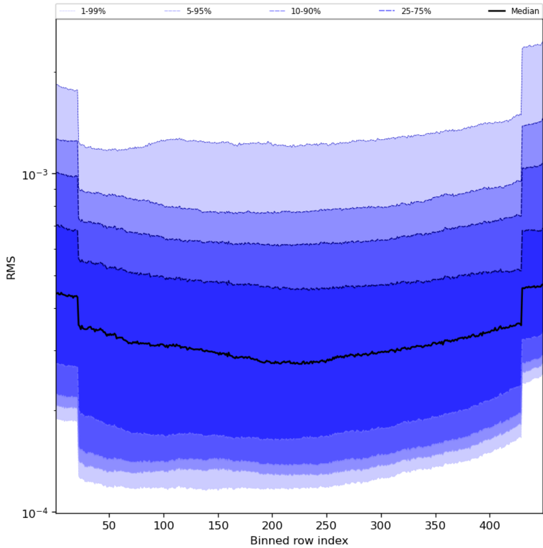
Figure 60: Along track statistics of “RMS” for 2023-10-14 to 2023-10-16
