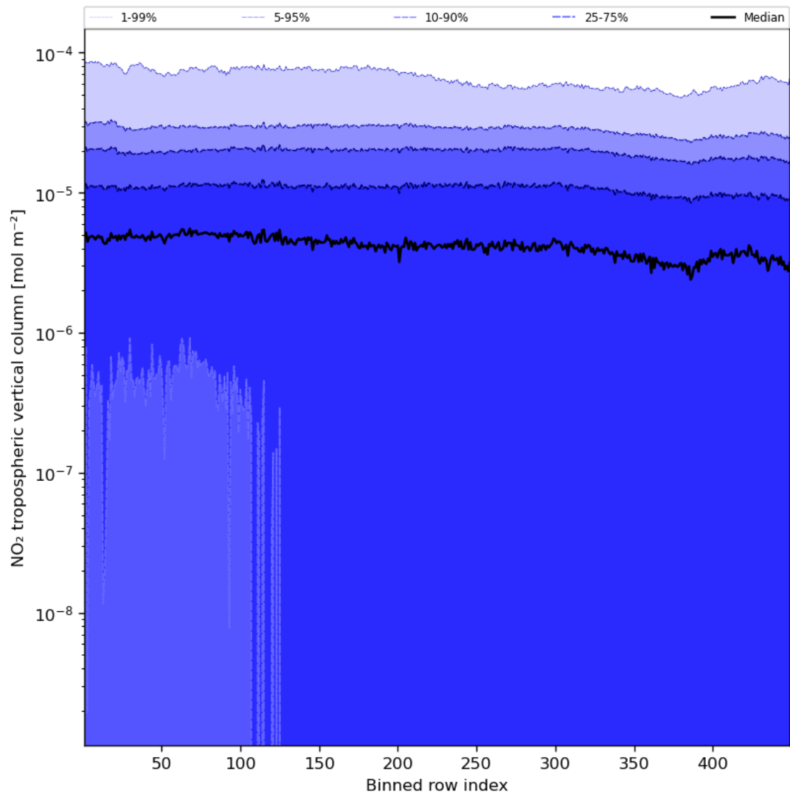
Figure 46: Along track statistics of “NO 2 tropospheric vertical column” for 2023-10-14 to 2023-10-16
