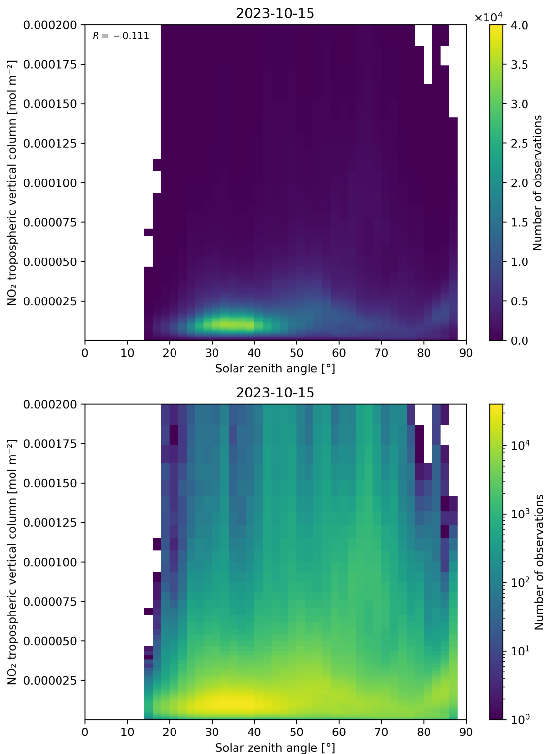
Figure 155: Scatter density plot of “Solar zenith angle” against “NO 2 tropospheric vertical column” for 2023-10-14 to 2023-10-16.
