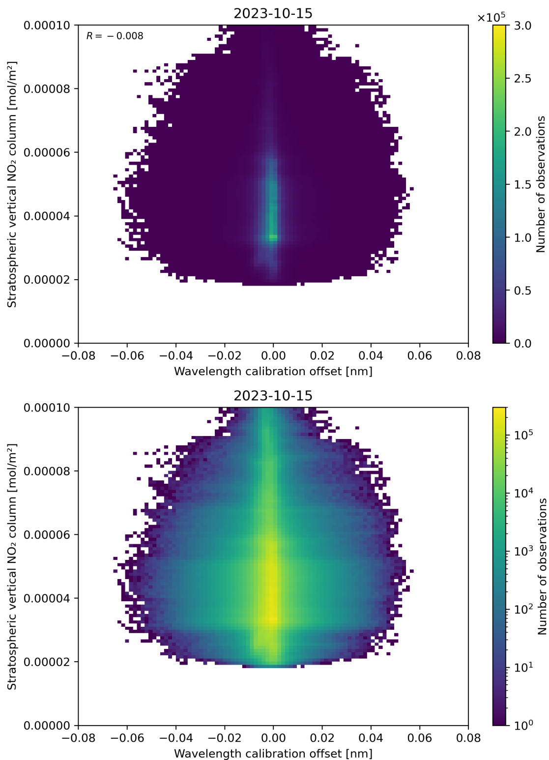
Figure 176: Scatter density plot of “Wavelength calibration offset” against “Stratospheric vertical NO 2 column” for 2023-10-14 to 2023-10-16.
