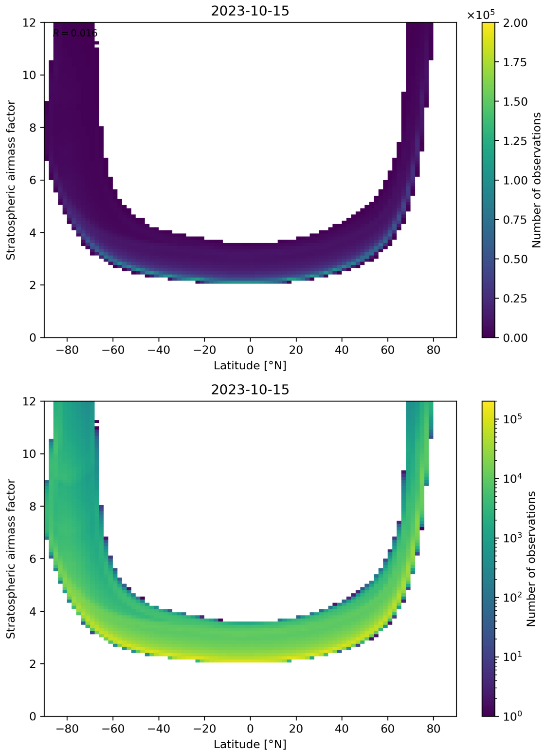
Figure 83: Scatter density plot of “Latitude” against “Stratospheric air mass factor” for 2023-10-14 to 2023-10-16.
