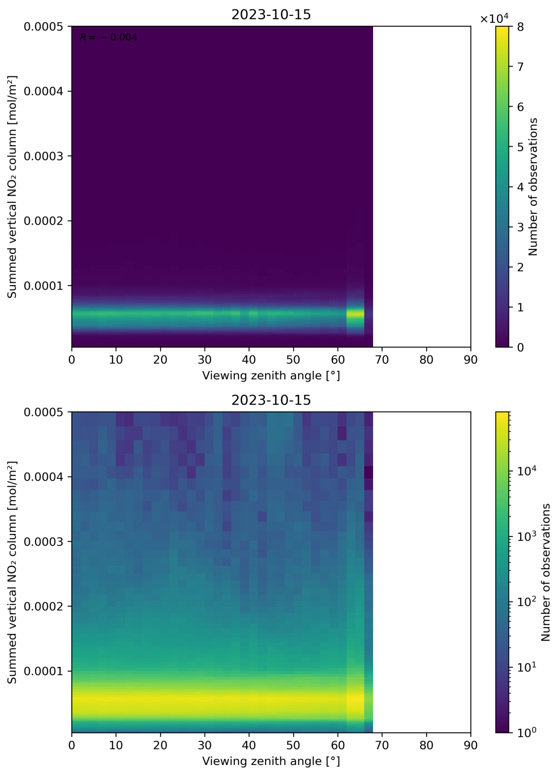
Figure 165: Scatter density plot of “Viewing zenith angle” against “Summed vertical NO 2 column” for 2023-10-14 to 2023-10-16.
