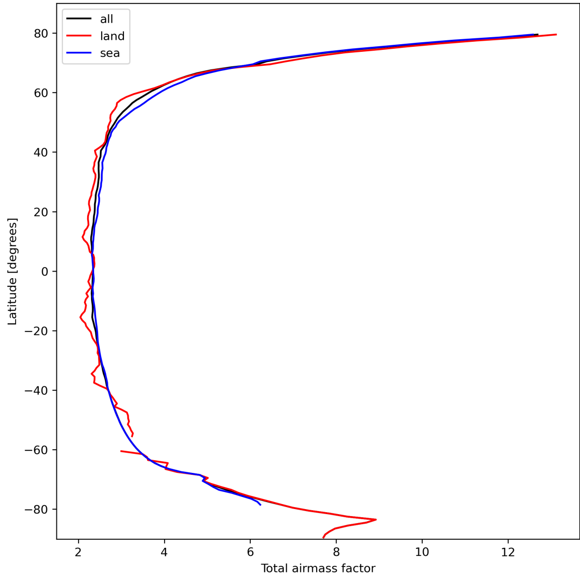
Figure 15: Zonal average of “Total airmass factor” for 2023-10-14 to 2023-10-16.
