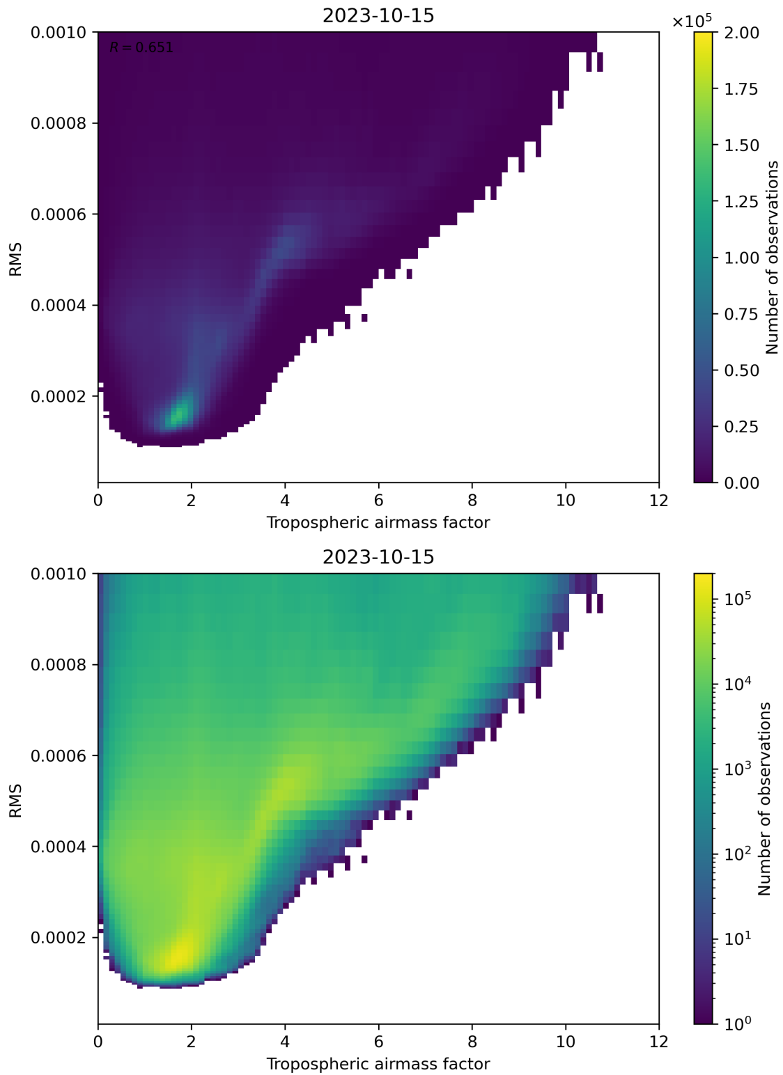
Figure 79: Scatter density plot of “Tropospheric airmass factor” against “RMS” for 2023-10-14 to 2023-10-16.
