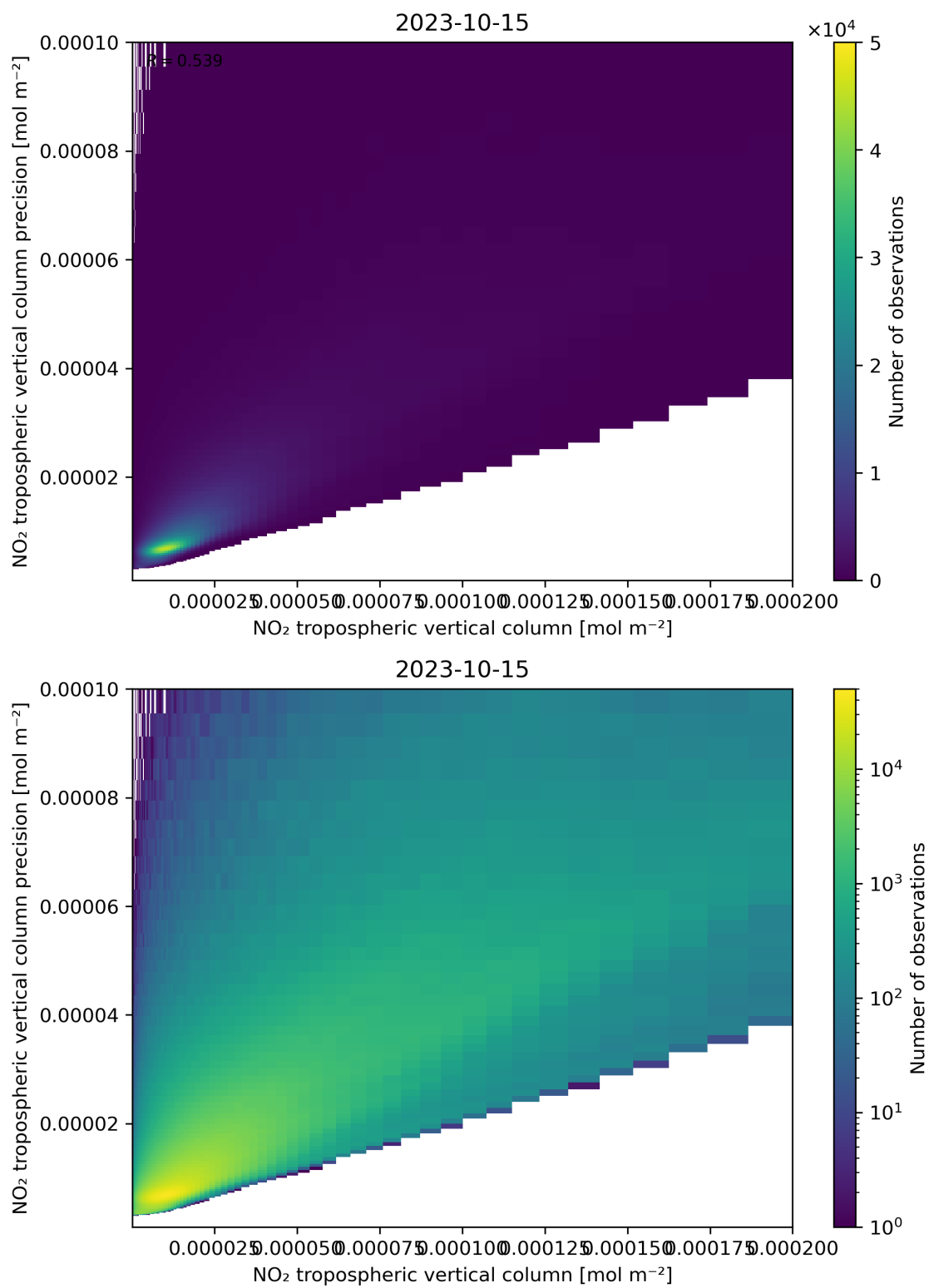
Figure 130: Scatter density plot of “NO 2 tropospheric vertical column” against “NO 2 tropospheric vertical column precision” for 2023-10-14 to 2023-10-16.
