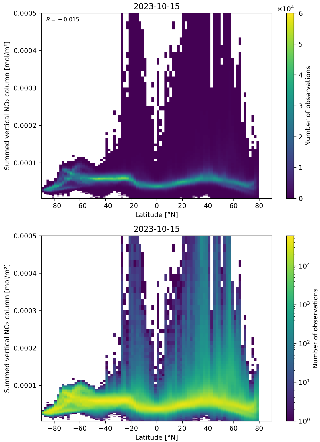
Figure 88: Scatter density plot of “Latitude” against “Summed vertical NO 2 column” for 2023-10-14 to 2023-10-16.
