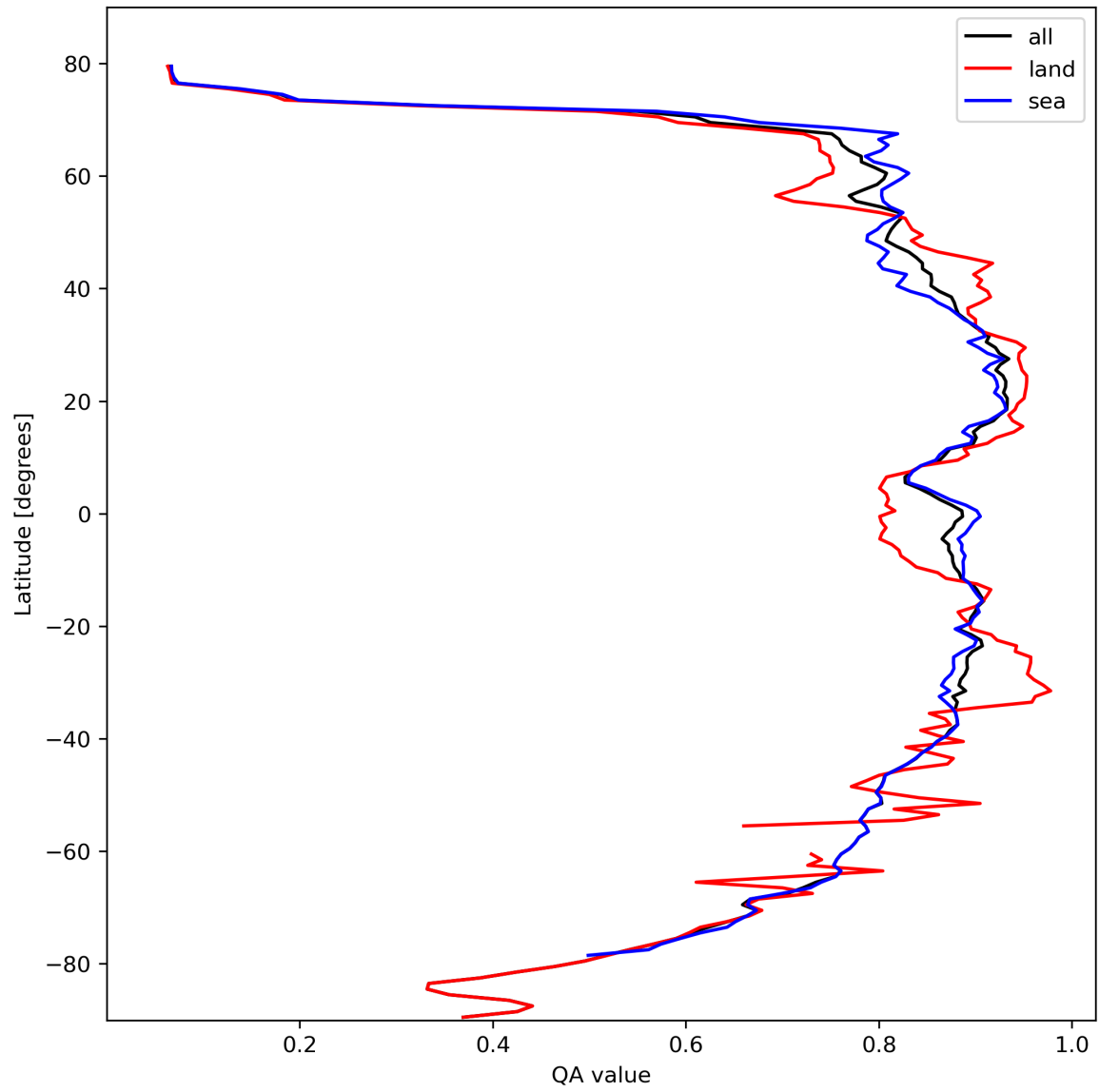
Figure 11: Zonal average of “QA value” for 2023-10-14 to 2023-10-16.
