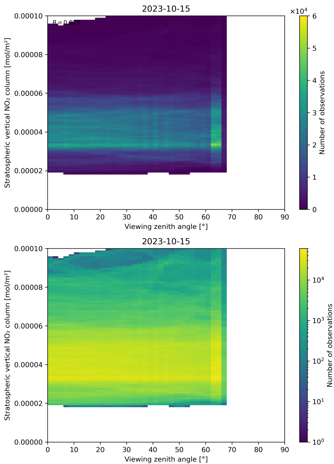
Figure 164: Scatter density plot of “Viewing zenith angle” against “Stratospheric vertical NO 2 column” for 2023-10-14 to 2023-10-16.
