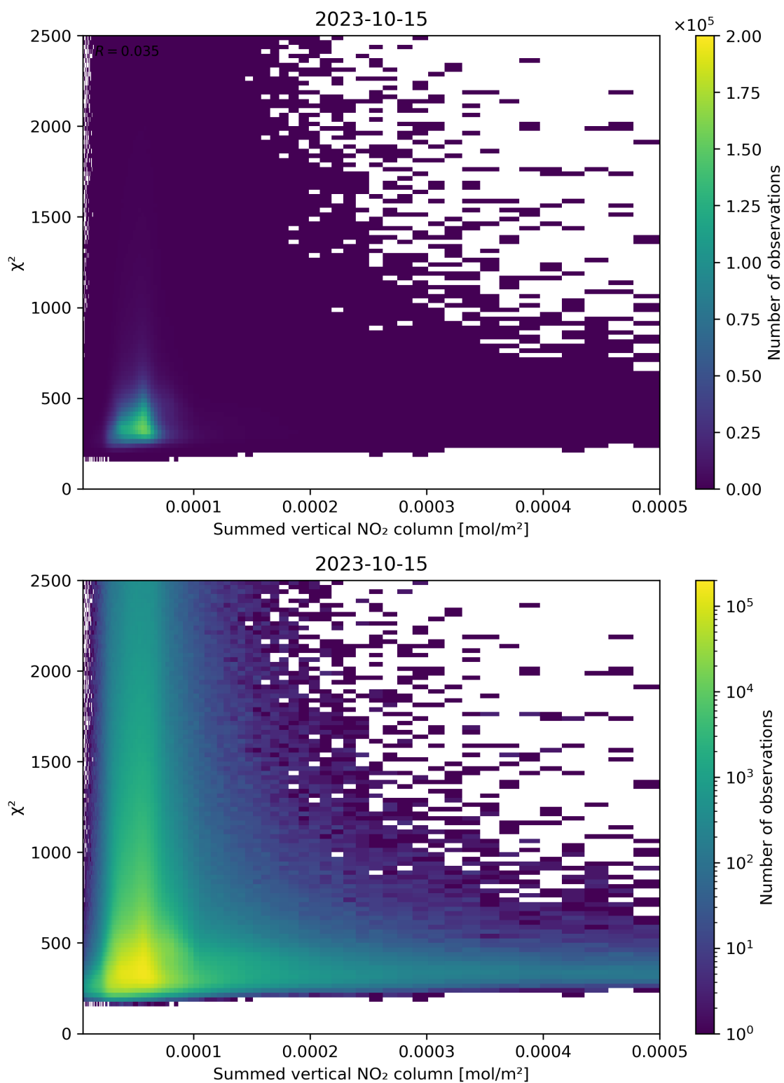
Figure 104: Scatter density plot of “Summed vertical NO 2 column” against “ \chi^2 ” for 2023-10-14 to 2023-10-16.
