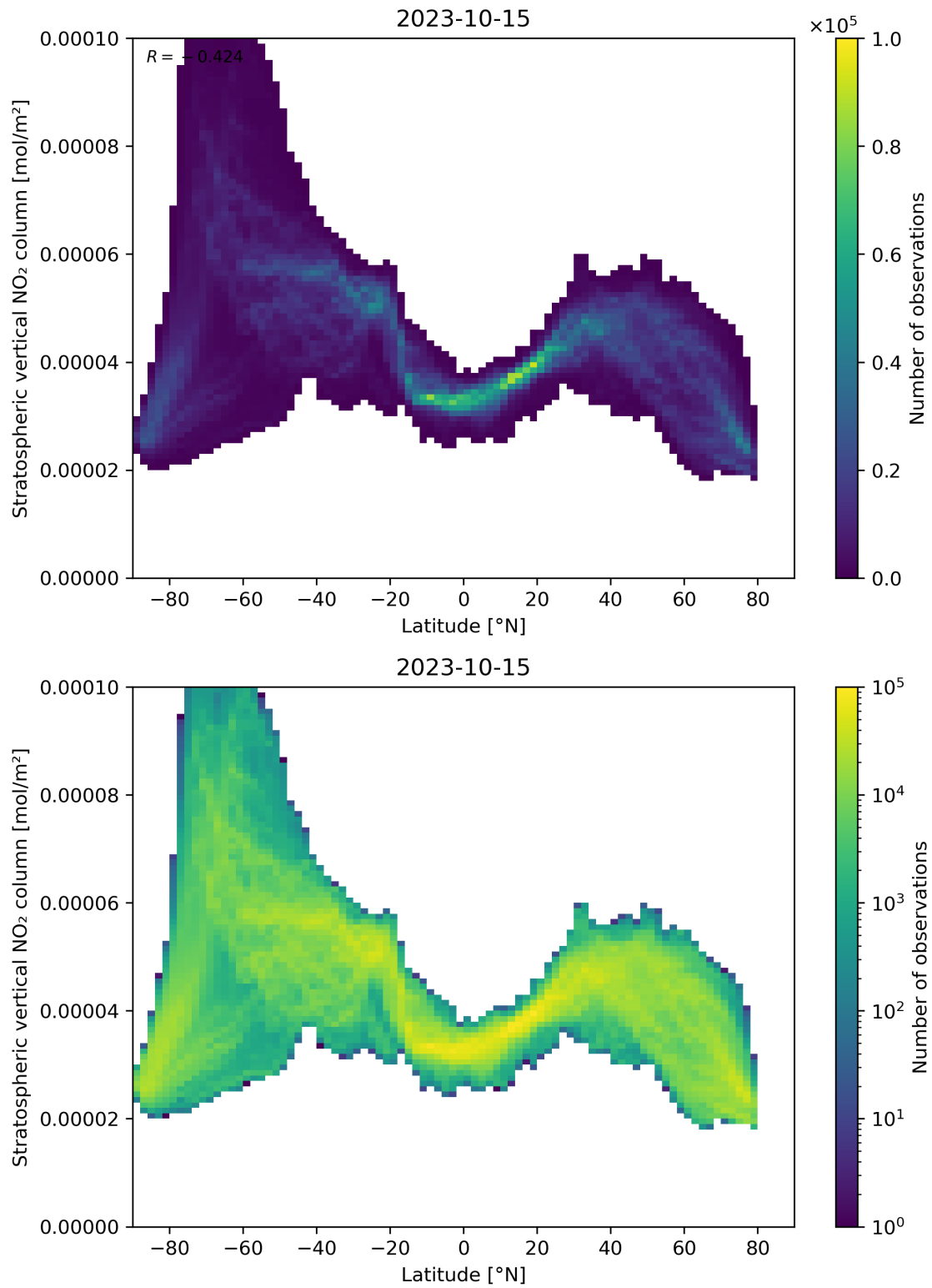
Figure 87: Scatter density plot of “Latitude” against “Stratospheric vertical NO 2 column” for 2023-10-14 to 2023-10-16.
