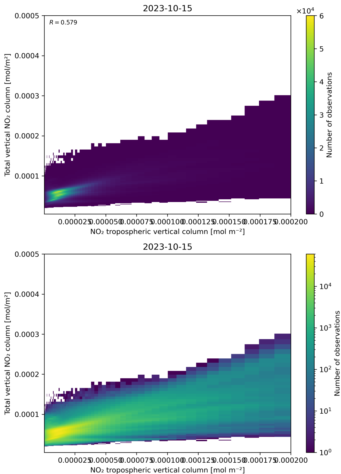
Figure 128: Scatter density plot of “NO 2 tropospheric vertical column” against “Total vertical NO 2 column” for 2023-10-14 to 2023-10-16.
