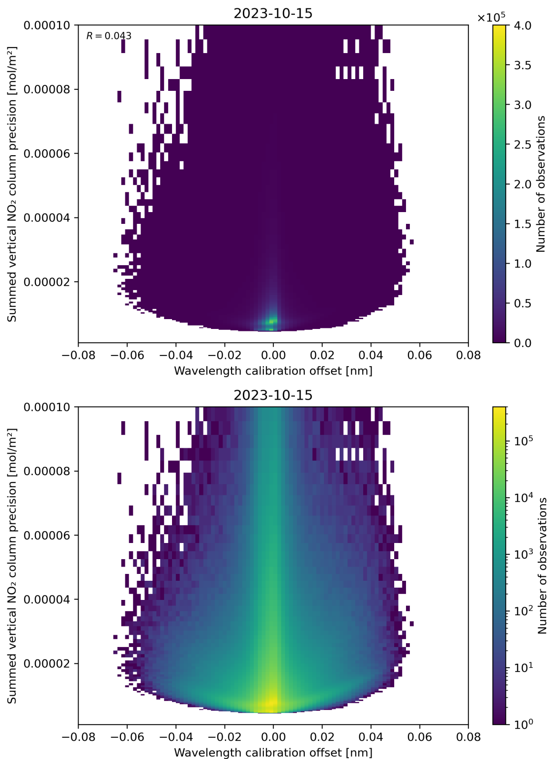
Figure 178: Scatter density plot of “Wavelength calibration offset” against “Summed vertical NO 2 column precision” for 2023-10-14 to 2023-10-16.
