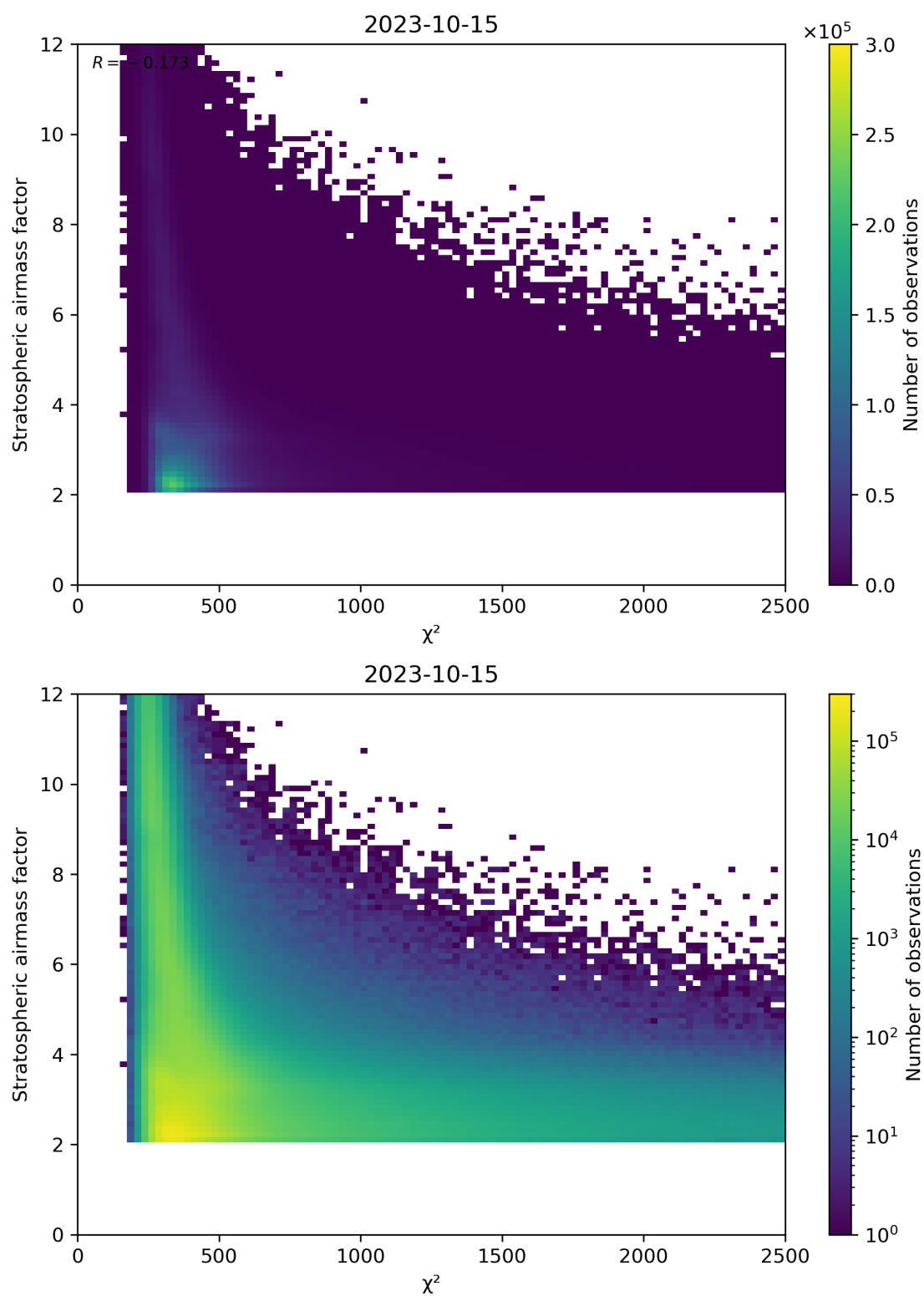
Figure 81: Scatter density plot of “ \chi^2 ” against “Stratospheric airmass factor” for 2023-10-14 to 2023-10-16.
