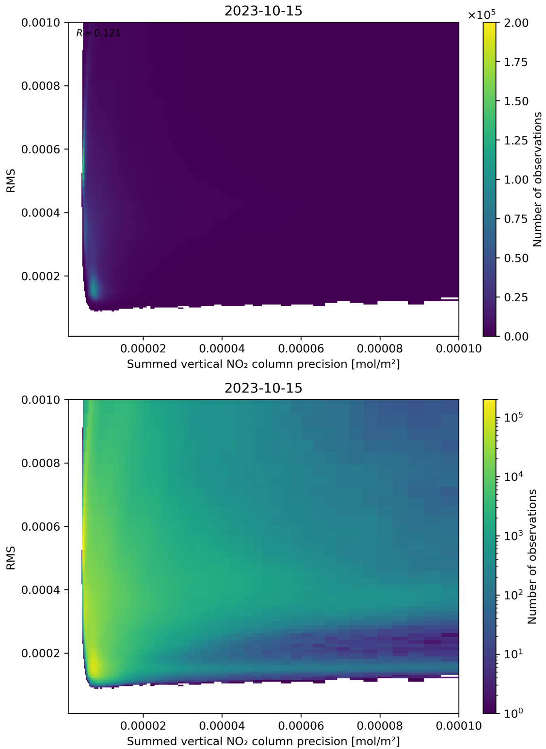
Figure 108: Scatter density plot of “Summed vertical NO 2 column precision” against “RMS” for 2023-10-14 to 2023-10-16.
