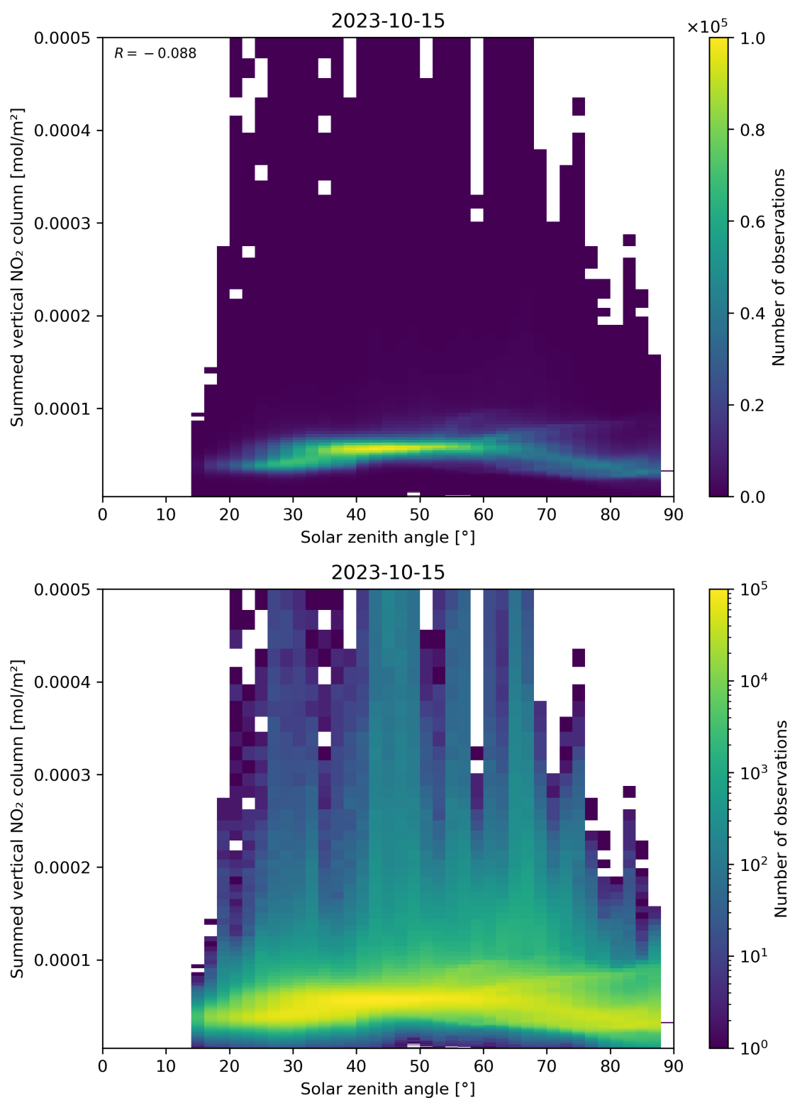
Figure 151: Scatter density plot of “Solar zenith angle” against “Summed vertical NO 2 column” for 2023-10-14 to 2023-10-16.
