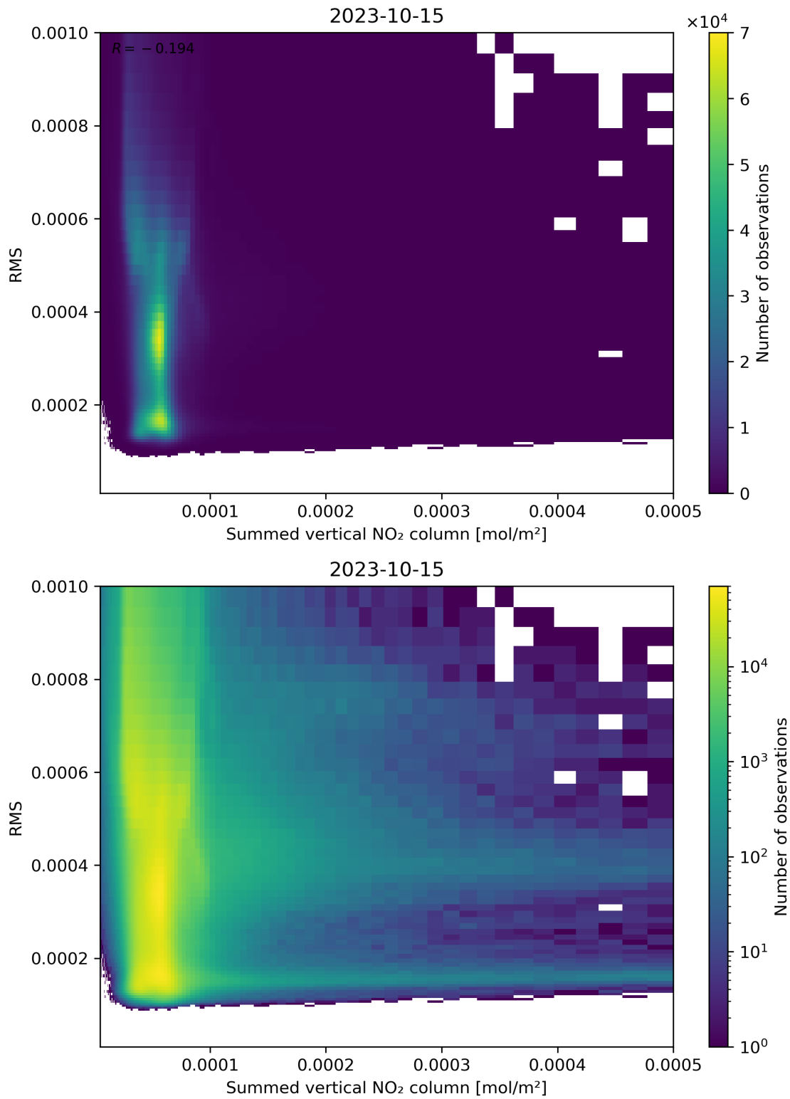
Figure 109: Scatter density plot of “Summed vertical NO 2 column” against “RMS” for 2023-10-14 to 2023-10-16.
