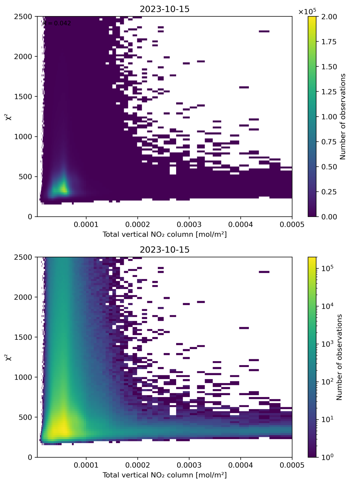
Figure 111: Scatter density plot of “Total vertical NO 2 column” against “ \chi^2 ” for 2023-10-14 to 2023-10-16.
