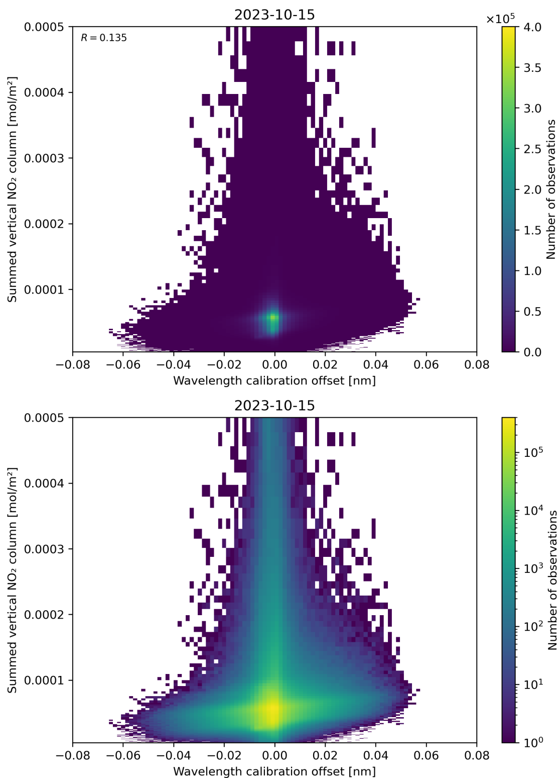
Figure 177: Scatter density plot of “Wavelength calibration offset” against “Summed vertical NO 2 column” for 2023-10-14 to 2023-10-16.
