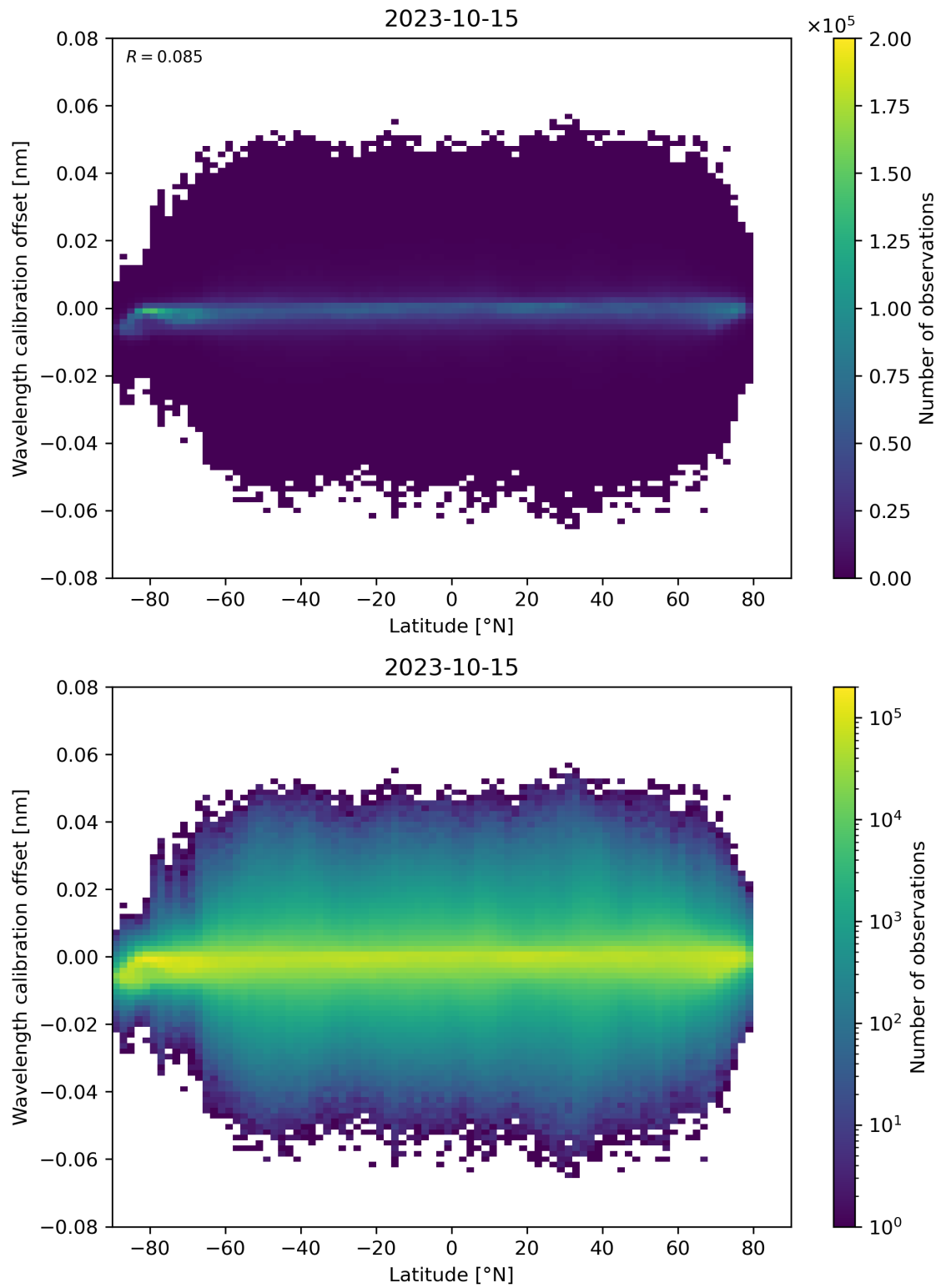
Figure 95: Scatter density plot of “Latitude” against “Wavelength calibration offset” for 2023-10-14 to 2023-10-16.
