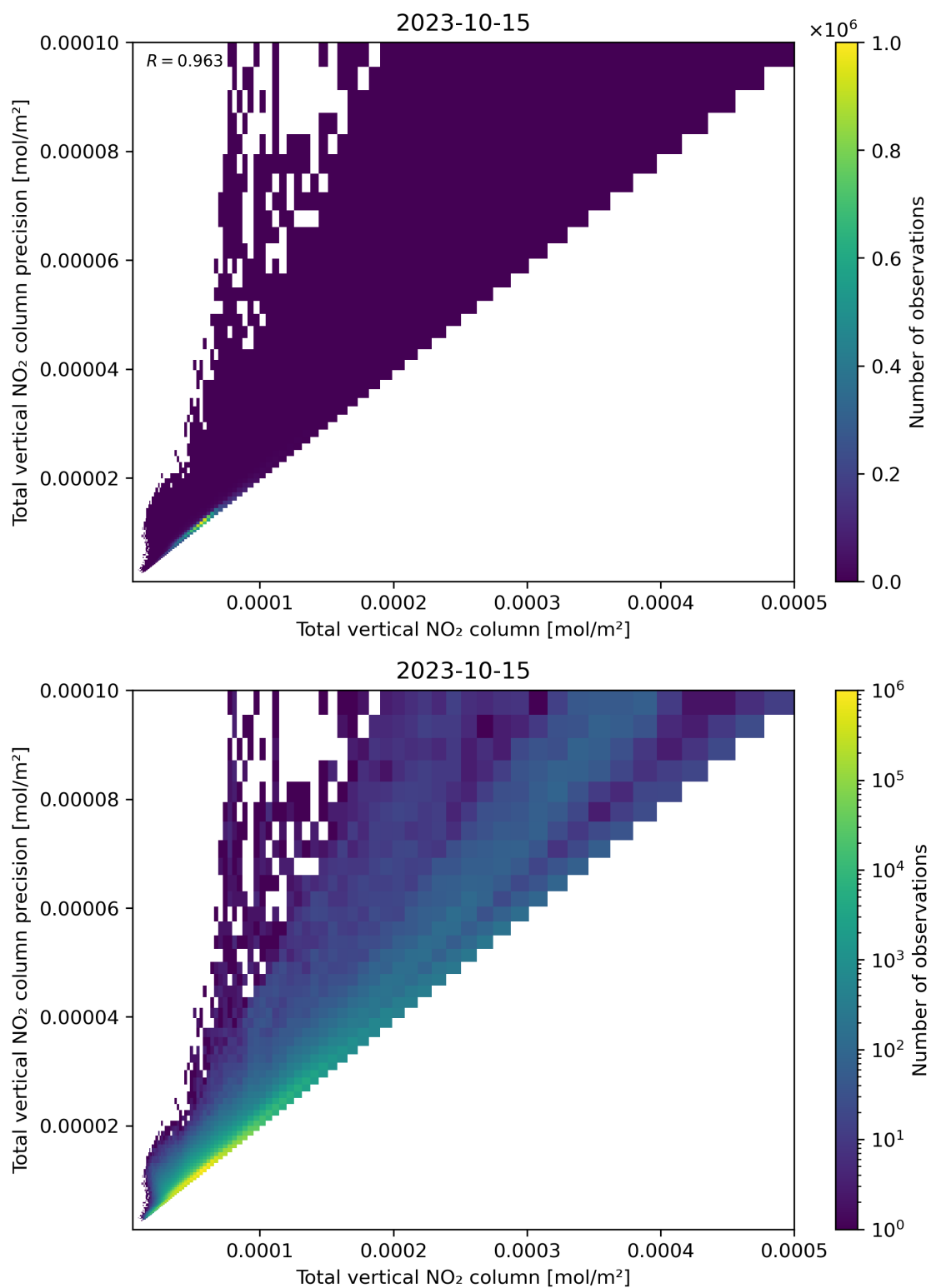
Figure 114: Scatter density plot of “Total vertical NO 2 column” against “Total vertical NO 2 column precision” for 2023-10-14 to 2023-10-16.
