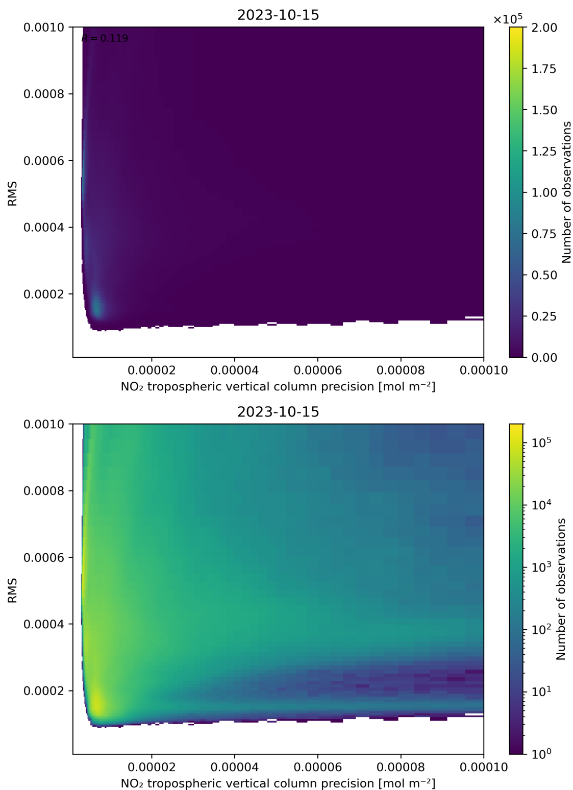
Figure 140: Scatter density plot of “NO 2 tropospheric vertical column precision” against “RMS” for 2023-10-14 to 2023-10-16.
