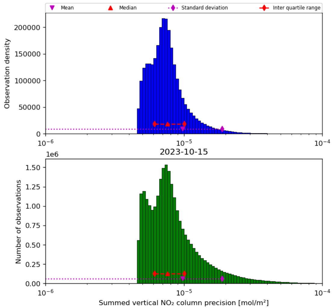
Figure 41: Histogram of “Summed vertical NO 2 column precision” for 2023-10-14 to 2023-10-16
