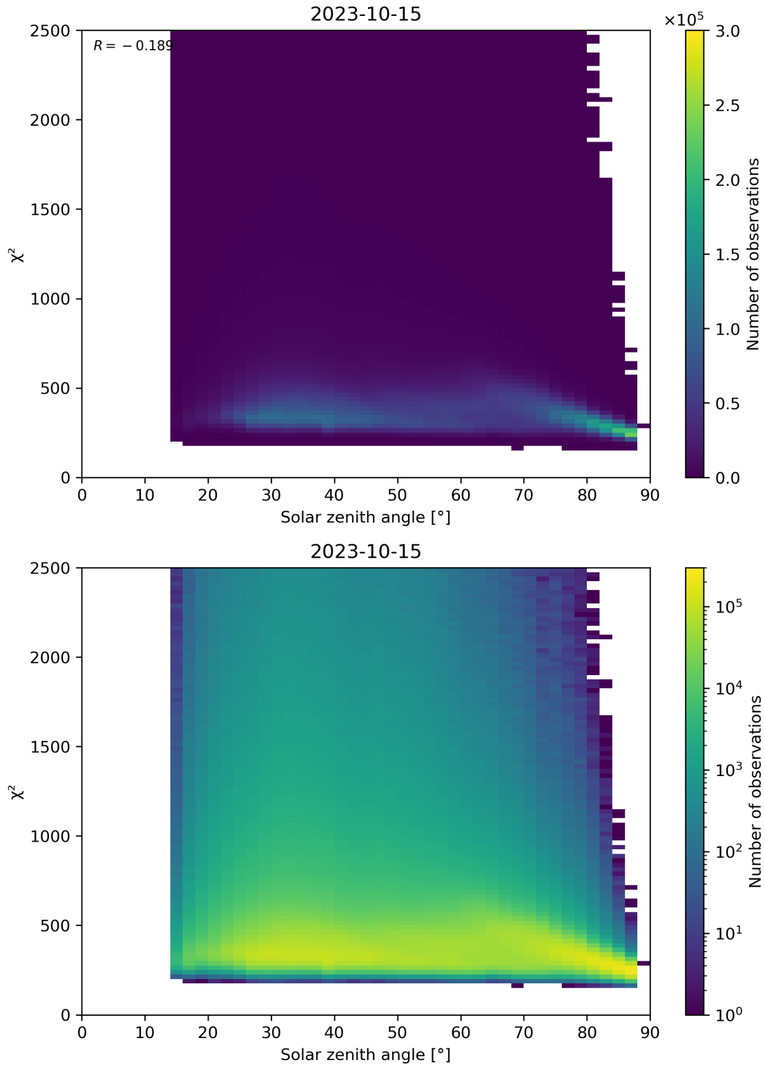
Figure 148: Scatter density plot of “Solar zenith angle” against “ \chi^2 ” for 2023-10-14 to 2023-10-16.
