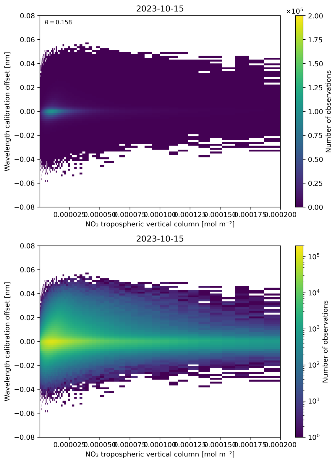
Figure 143: Scatter density plot of “NO 2 tropospheric vertical column” against “Wavelength calibration offset” for 2023-10-14 to 2023-10-16.
