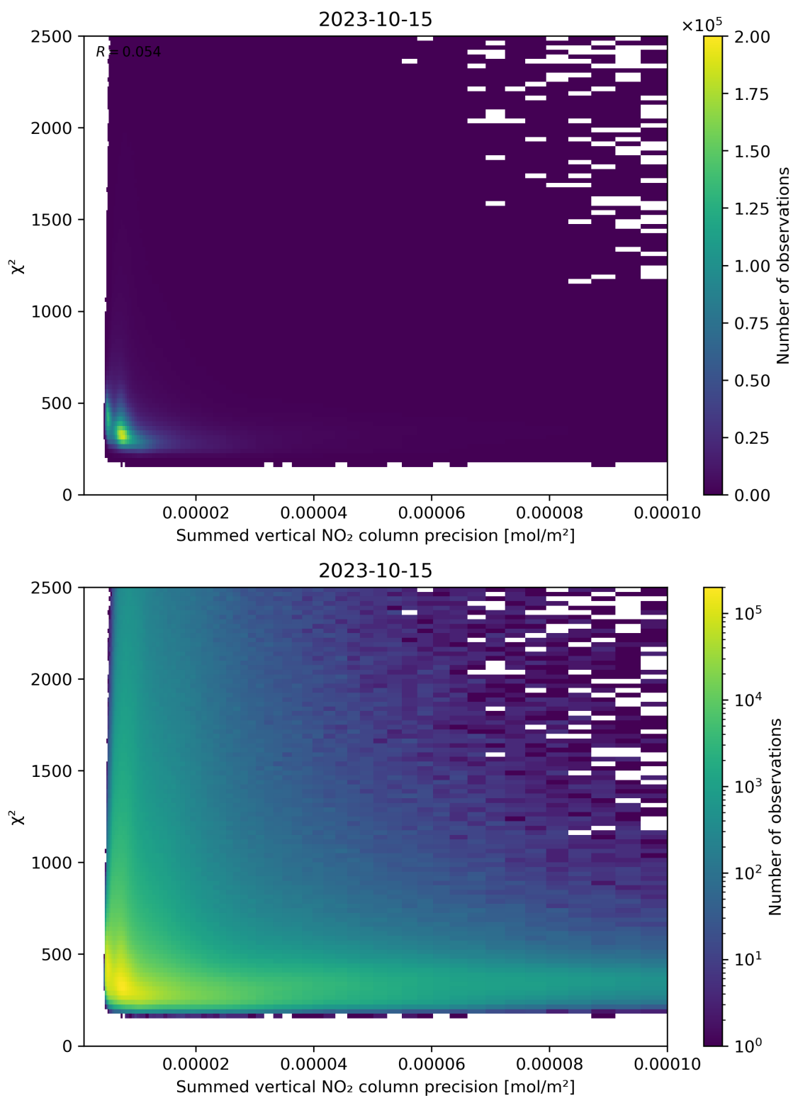
Figure 107: Scatter density plot of “Summed vertical NO 2 column precision” against “ \chi^2 ” for 2023-10-14 to 2023-10-16.
