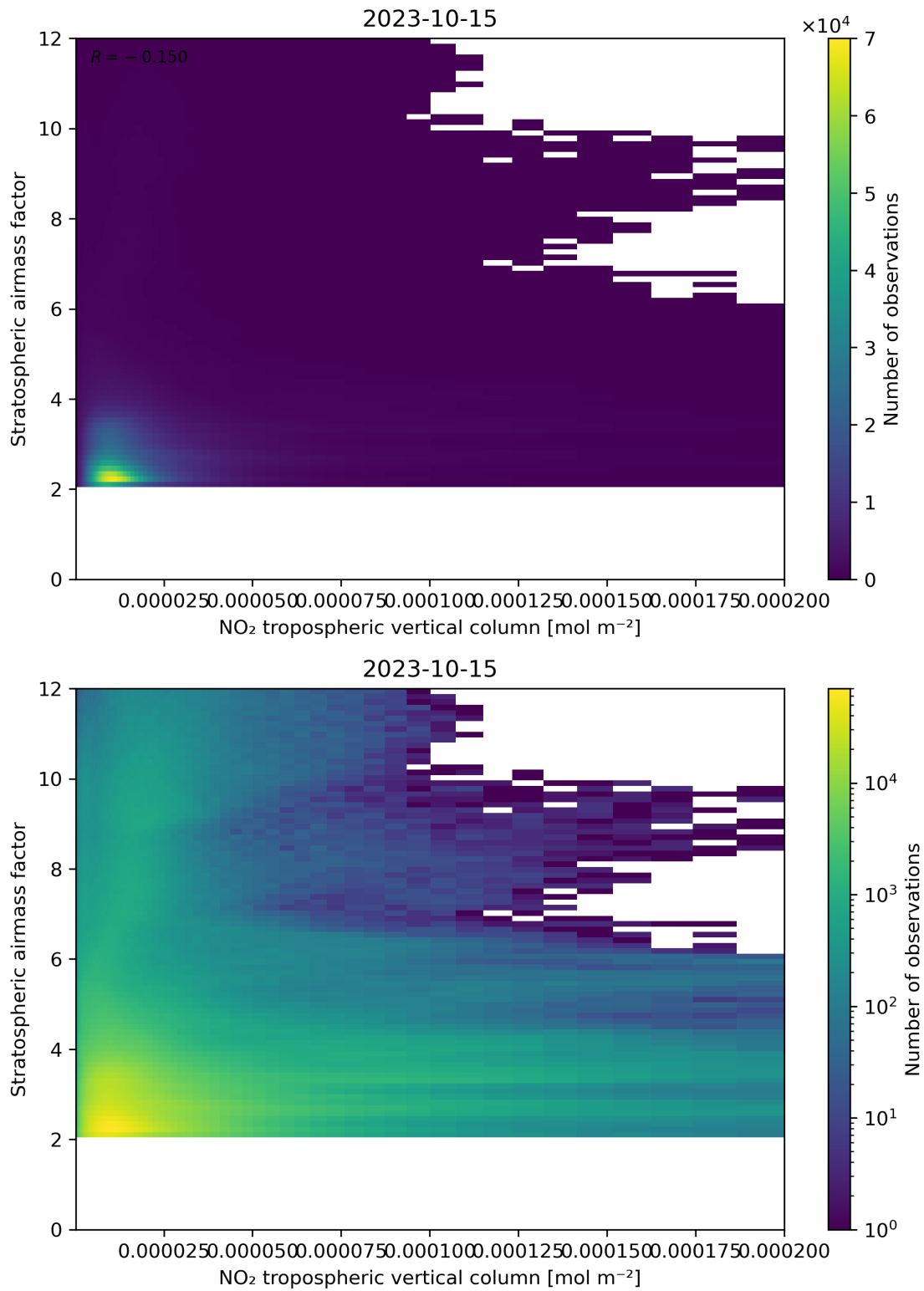
Figure 121: Scatter density plot of “NO 2 tropospheric vertical column” against “Stratospheric air mass factor” for 2023-10-14 to 2023-10-16.
