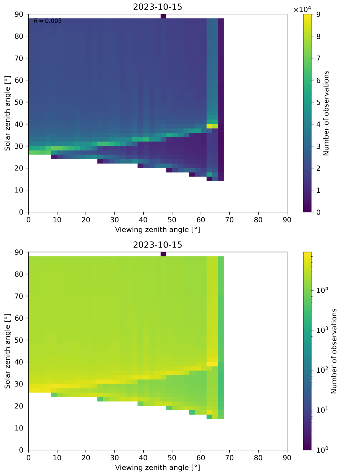
Figure 172: Scatter density plot of “Viewing zenith angle” against “Solar zenith angle” for 2023-10-14 to 2023-10-16.
