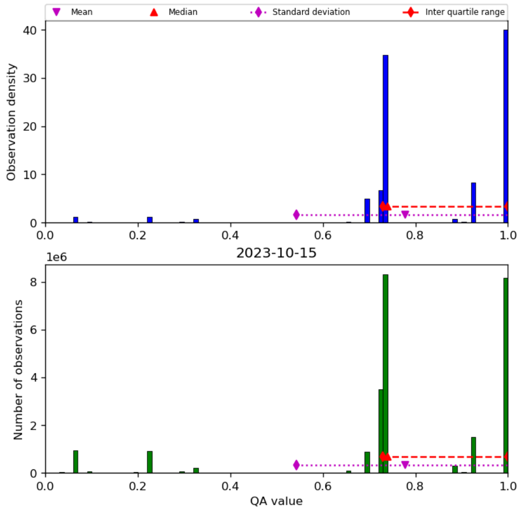
Figure 28: Histogram of “QA value” for 2023-10-14 to 2023-10-16
