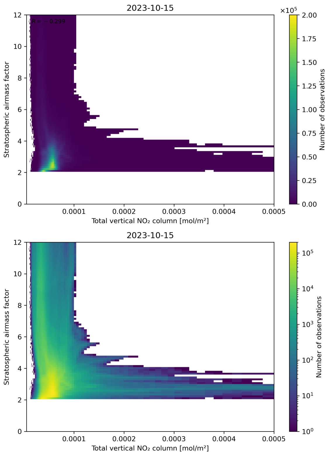
Figure 110: Scatter density plot of “Total vertical NO 2 column” against “Stratospheric airmass factor” for 2023-10-14 to 2023-10-16.
