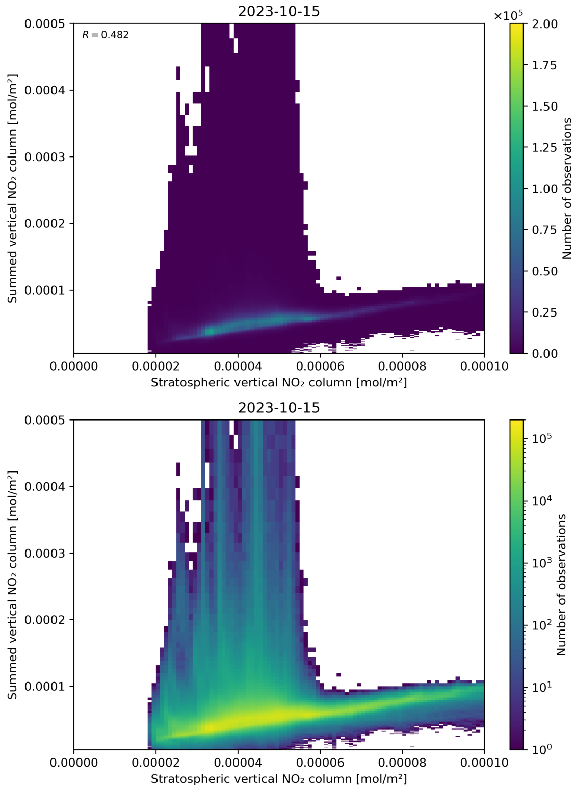
Figure 98: Scatter density plot of “Stratospheric vertical NO 2 column” against “Summed vertical NO 2 column” for 2023-10-14 to 2023-10-16.
