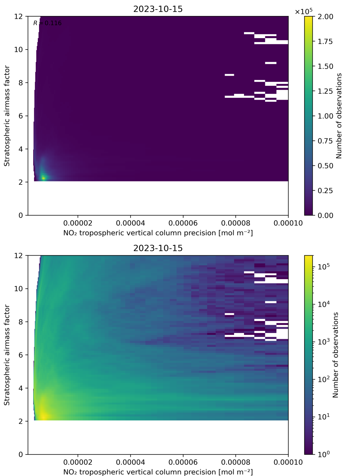
Figure 131: Scatter density plot of “NO 2 tropospheric vertical column precision” against “Stratospheric airmass factor” for 2023-10-14 to 2023-10-16.
