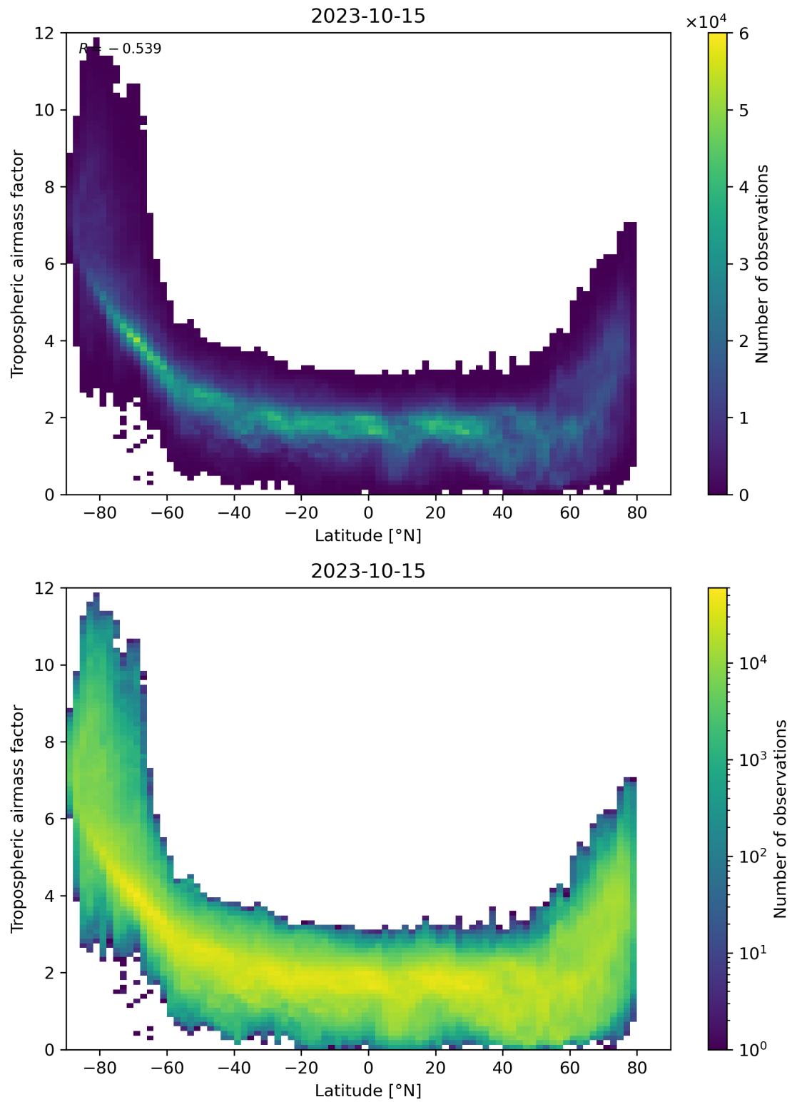
Figure 85: Scatter density plot of “Latitude” against “Tropospheric airmass factor” for 2023-10-14 to 2023-10-16.
