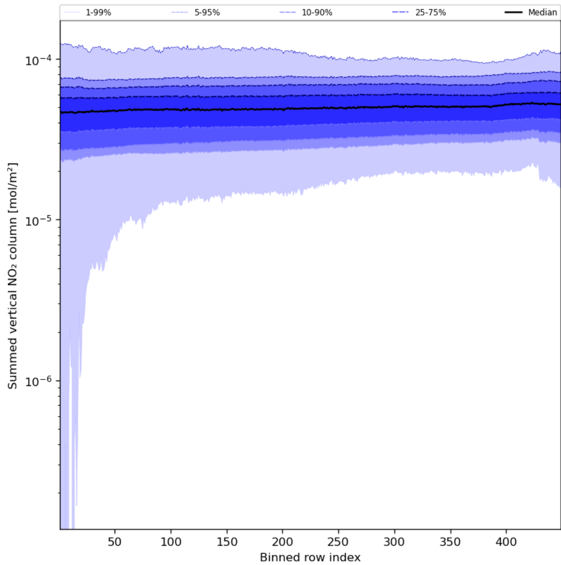
Figure 57: Along track statistics of “Summed vertical NO 2 column” for 2023-10-14 to 2023-10-16
