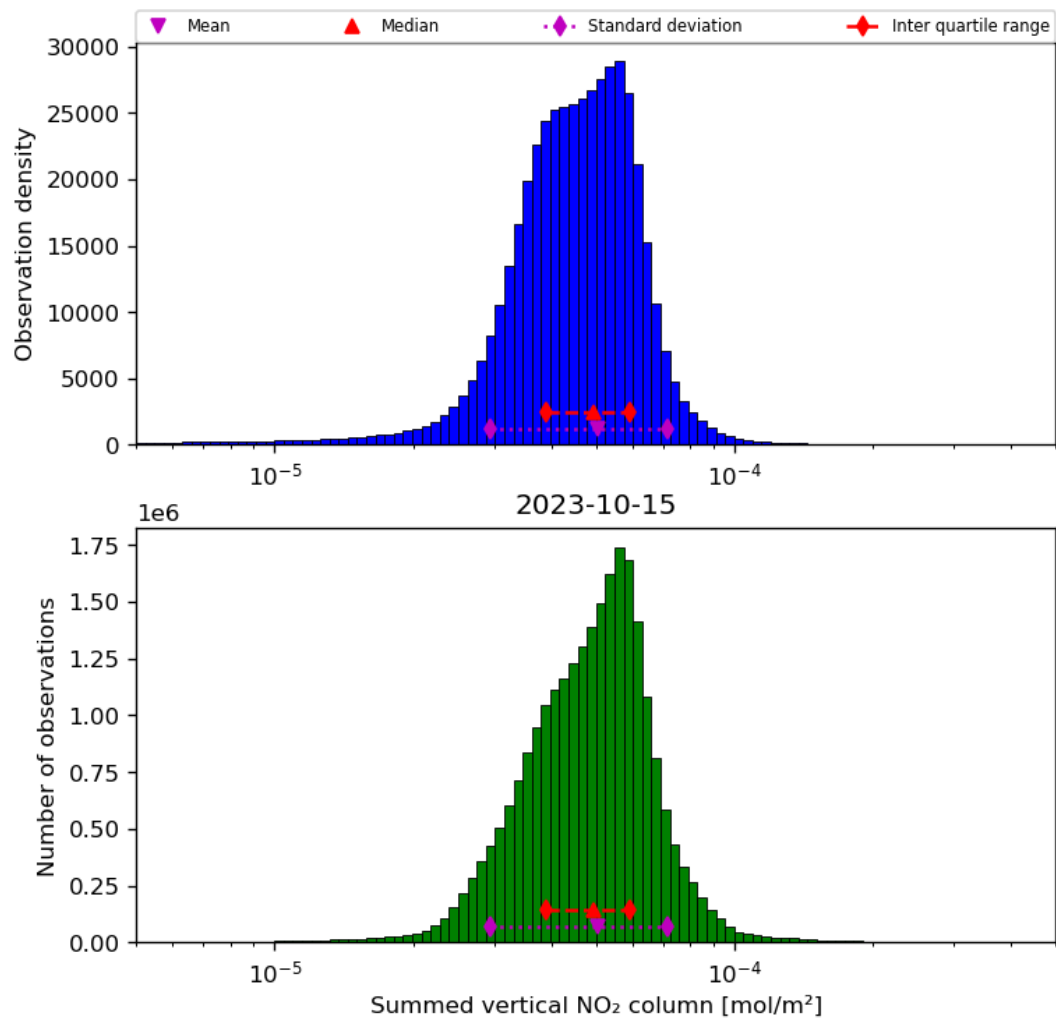
Figure 40: Histogram of “Summed vertical NO 2 column” for 2023-10-14 to 2023-10-16
