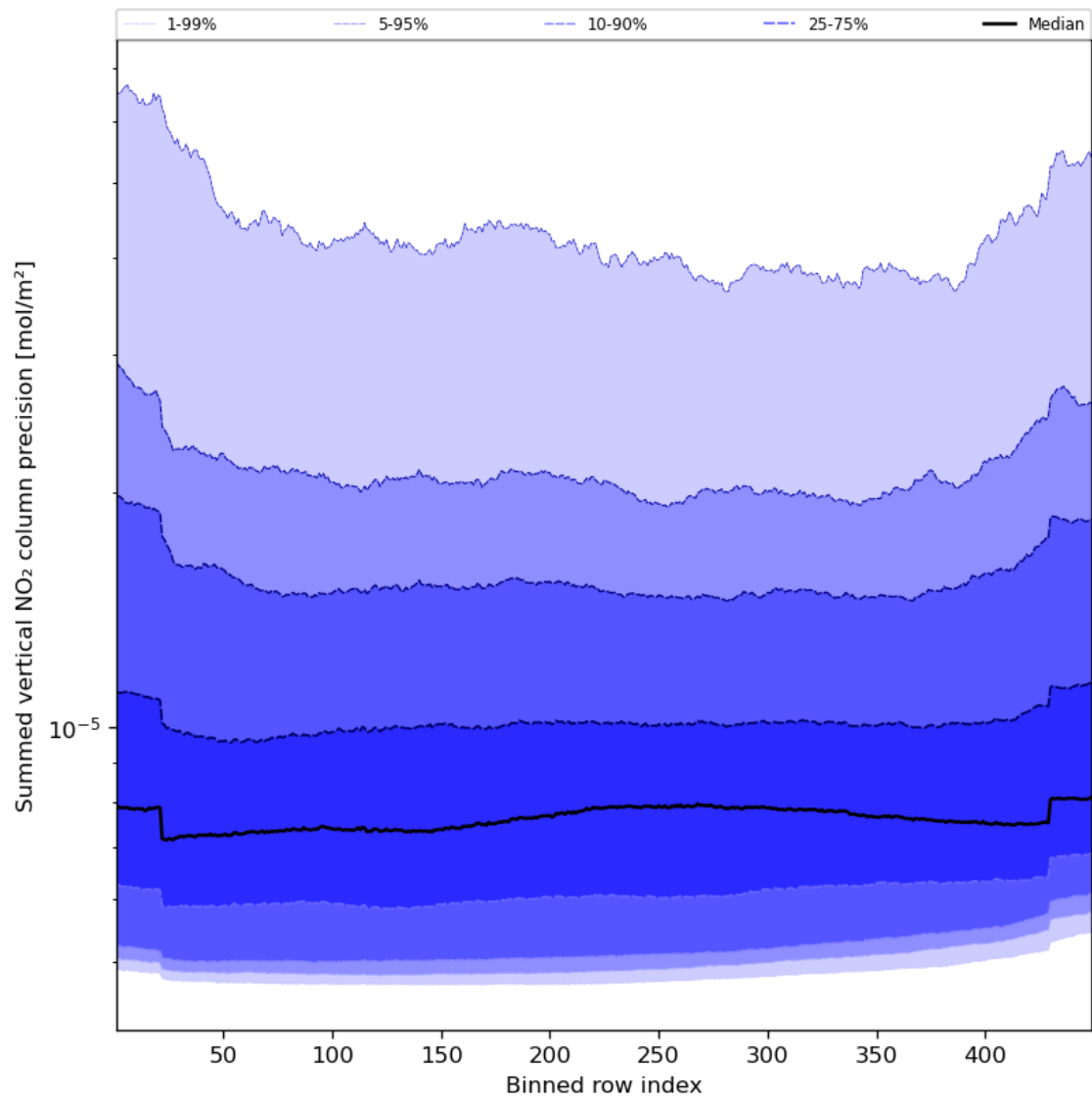
Figure 58: Along track statistics of “Summed vertical NO 2 column precision” for 2023-10-14 to 2023-10-16
