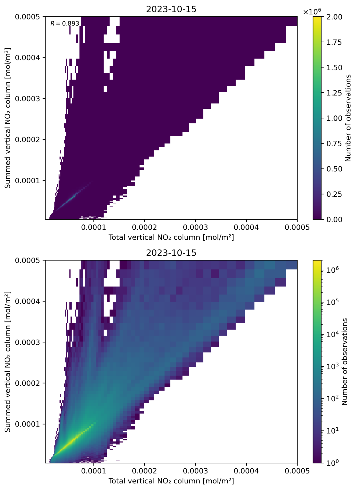
Figure 112: Scatter density plot of “Total vertical NO 2 column” against “Summed vertical NO 2 column” for 2023-10-14 to 2023-10-16.
