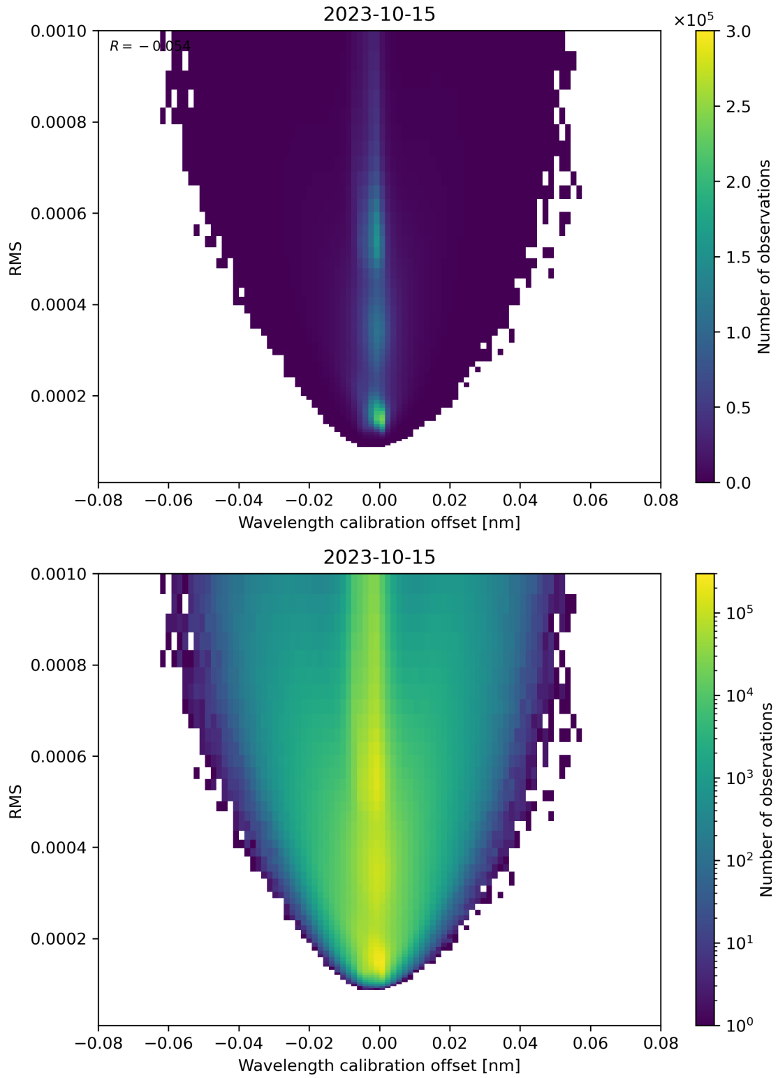
Figure 181: Scatter density plot of “Wavelength calibration offset” against “RMS” for 2023-10-14 to 2023-10-16.
