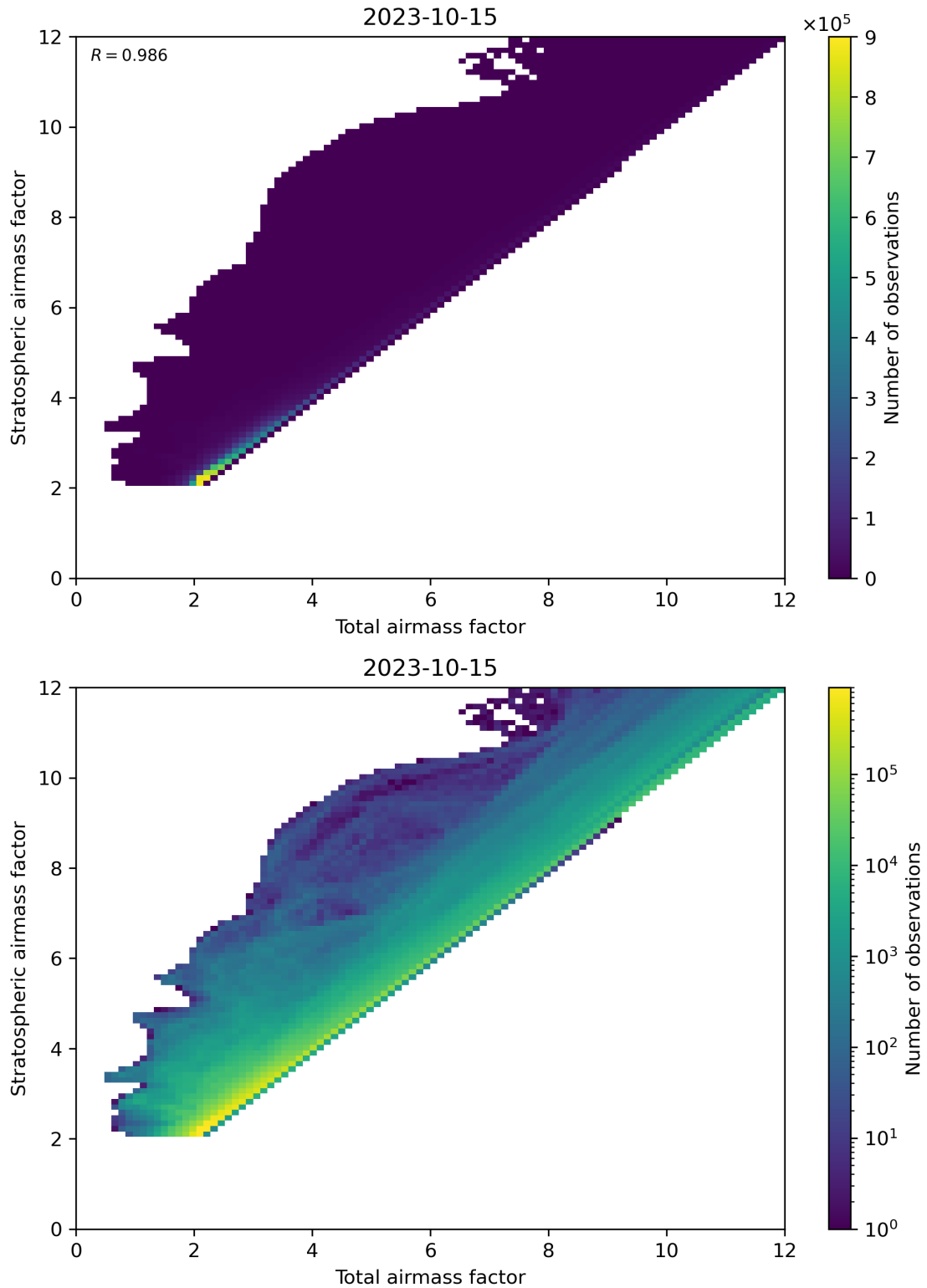
Figure 62: Scatter density plot of “Total airmass factor” against “Stratospheric airmass factor” for 2023-10-14 to 2023-10-16.
