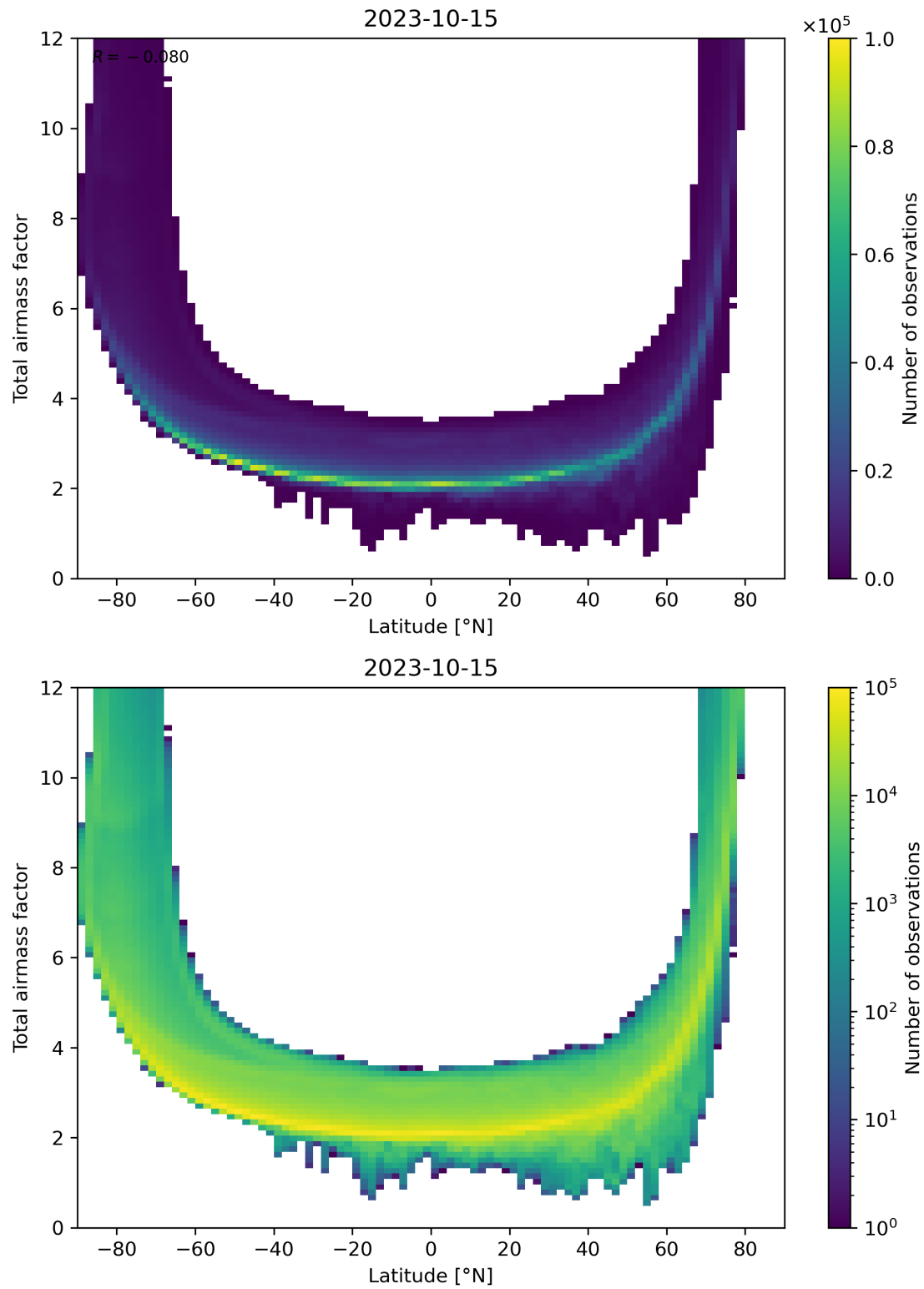
Figure 84: Scatter density plot of “Latitude” against “Total airmass factor” for 2023-10-14 to 2023-10-16.
