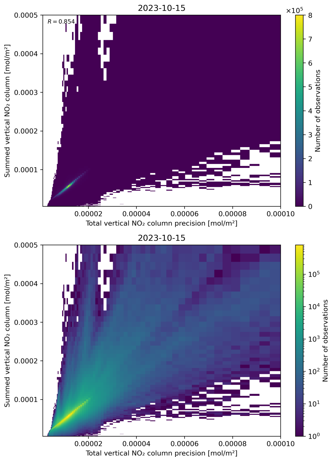
Figure 117: Scatter density plot of “Total vertical NO 2 column precision” against “Summed vertical NO 2 column” for 2023-10-14 to 2023-10-16.
