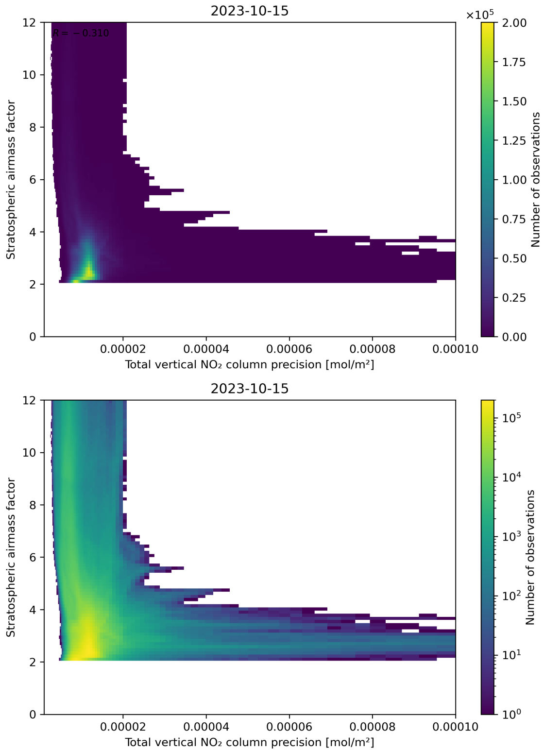
Figure 115: Scatter density plot of “Total vertical NO 2 column precision” against “Stratospheric airmass factor” for 2023-10-14 to 2023-10-16.
