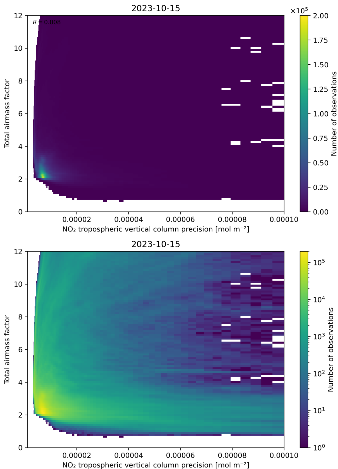
Figure 132: Scatter density plot of “NO 2 tropospheric vertical column precision” against “Total air mass factor” for 2023-10-14 to 2023-10-16.
