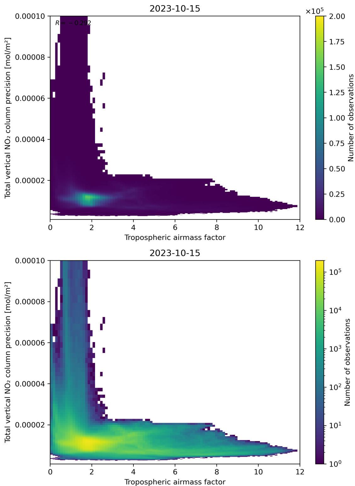
Figure 78: Scatter density plot of “Tropospheric air mass factor” against “Total vertical NO 2 column precision” for 2023-10-14 to 2023-10-16.
