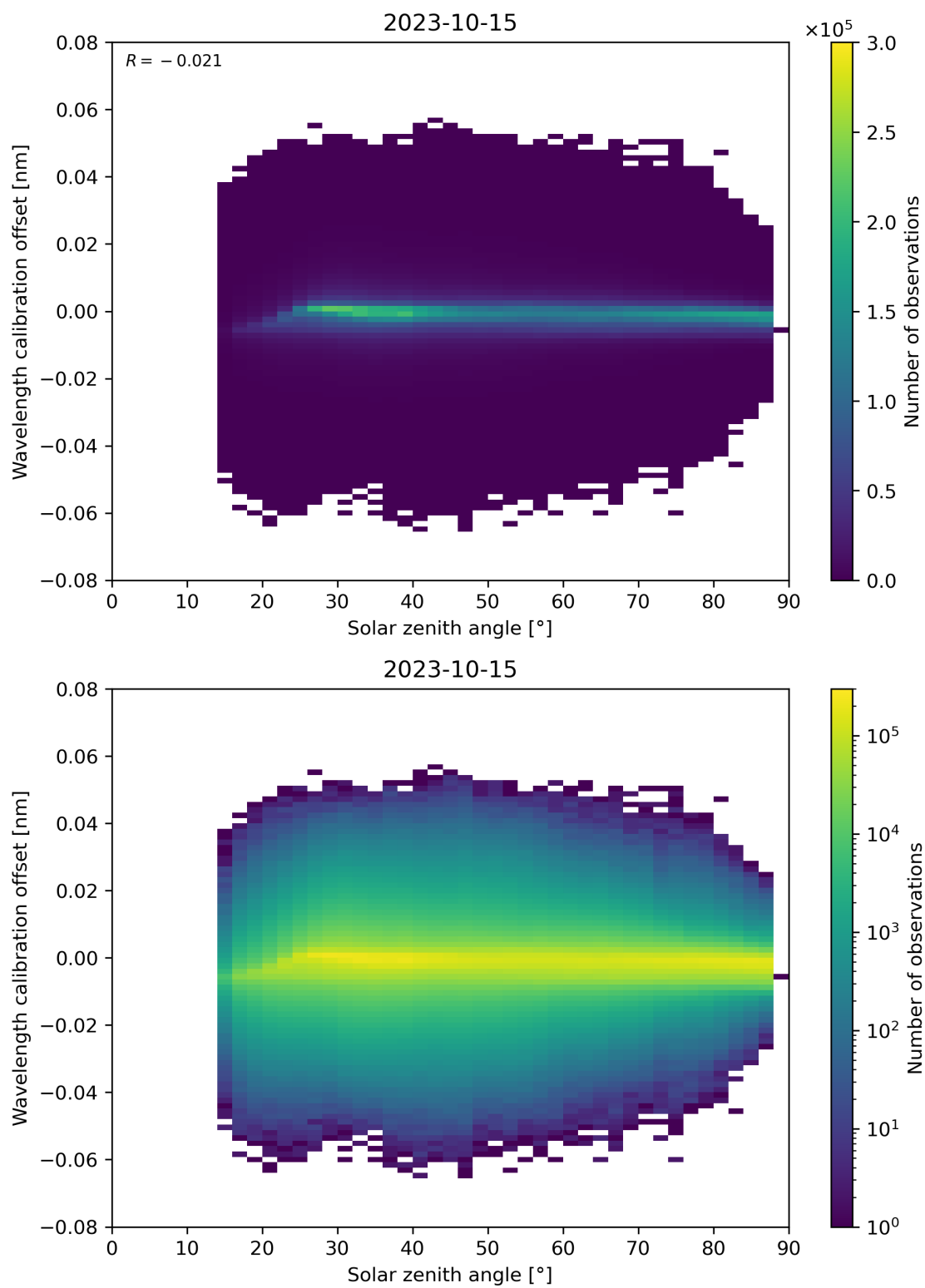
Figure 158: Scatter density plot of “Solar zenith angle” against “Wavelength calibration offset” for 2023-10-14 to 2023-10-16.
