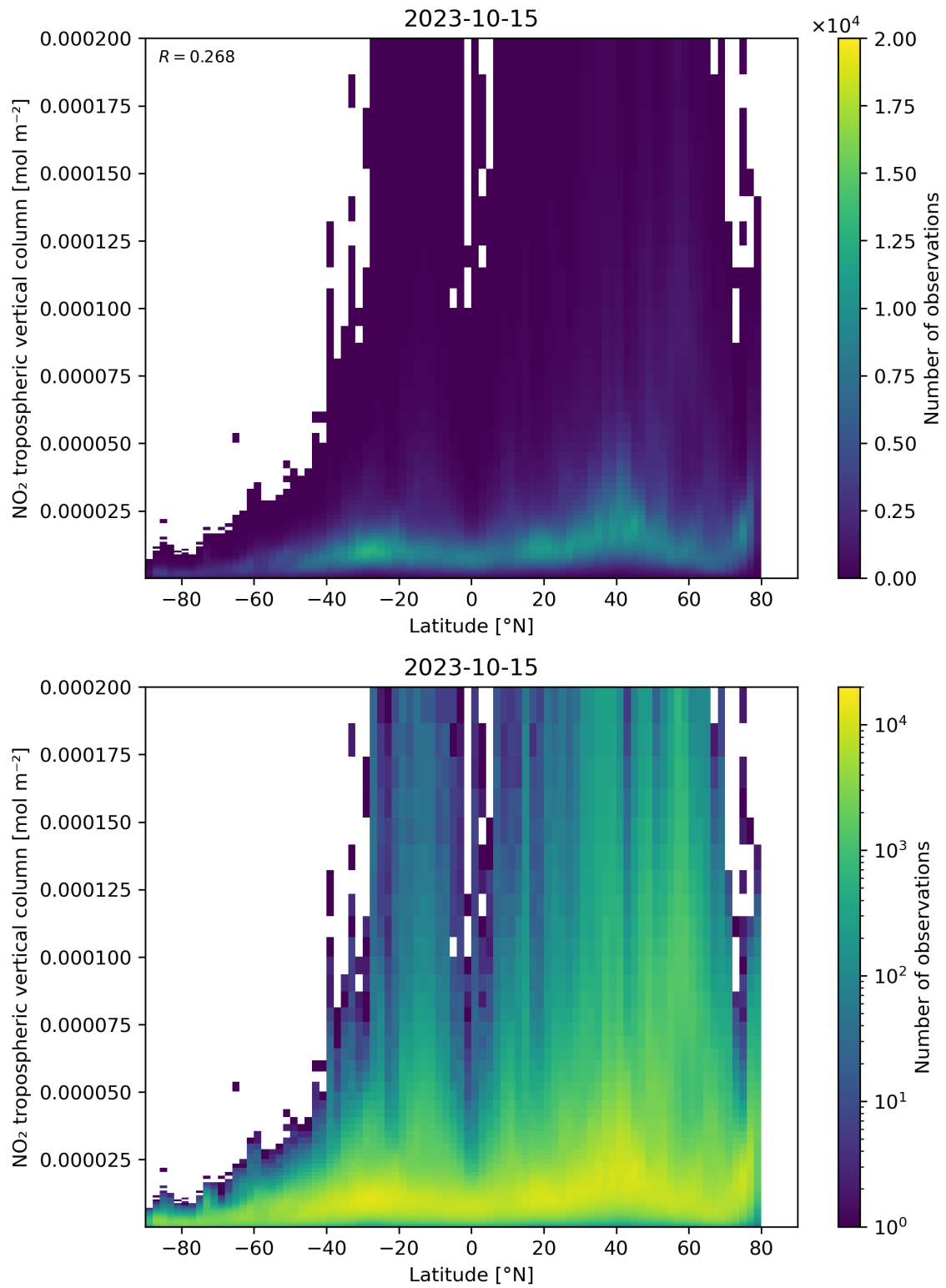
Figure 92: Scatter density plot of “Latitude” against “NO 2 tropospheric vertical column” for 2023-10-14 to 2023-10-16.
