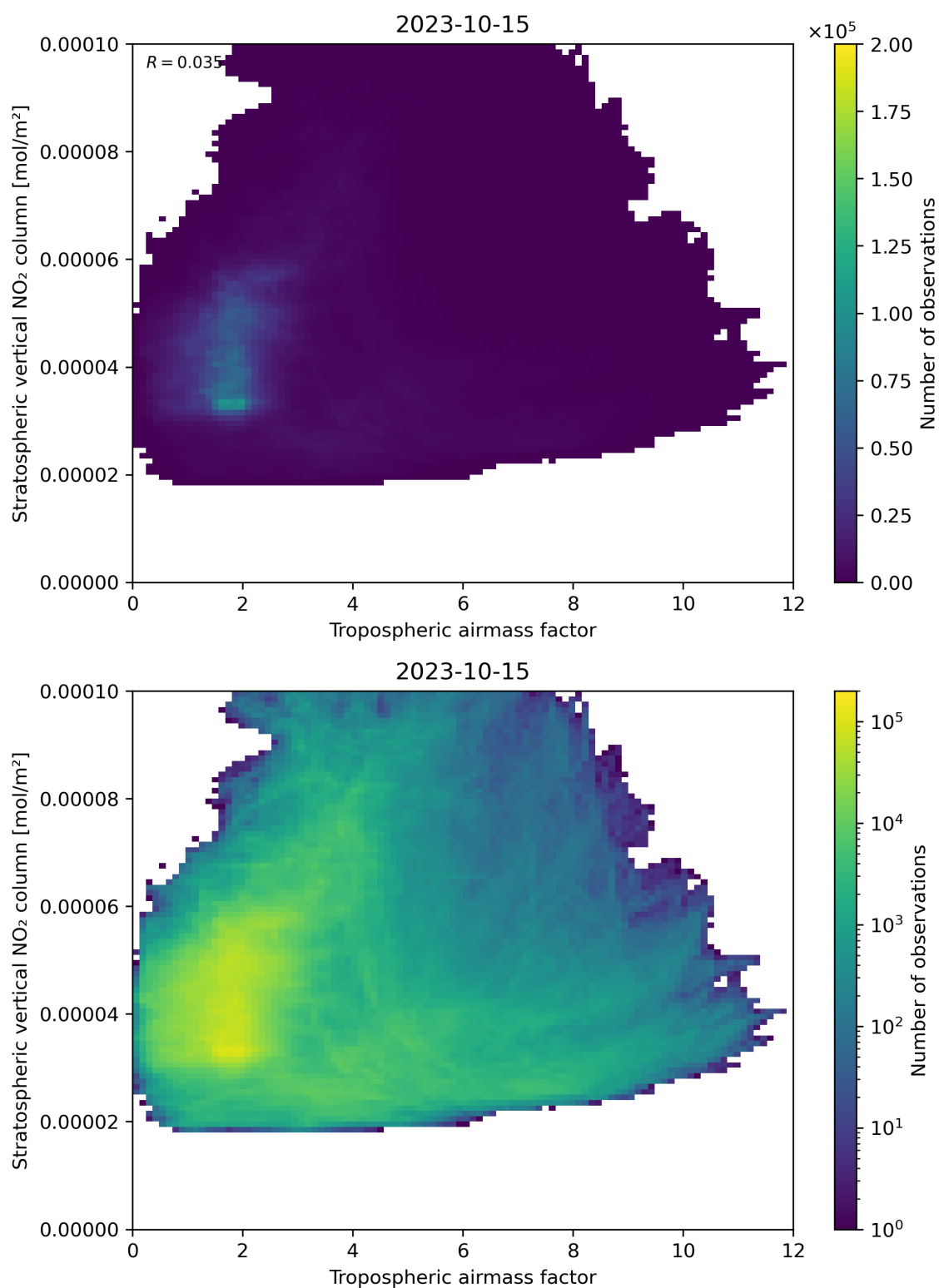
Figure 74: Scatter density plot of “Tropospheric air mass factor” against “Stratospheric vertical NO 2 column” for 2023-10-14 to 2023-10-16.
