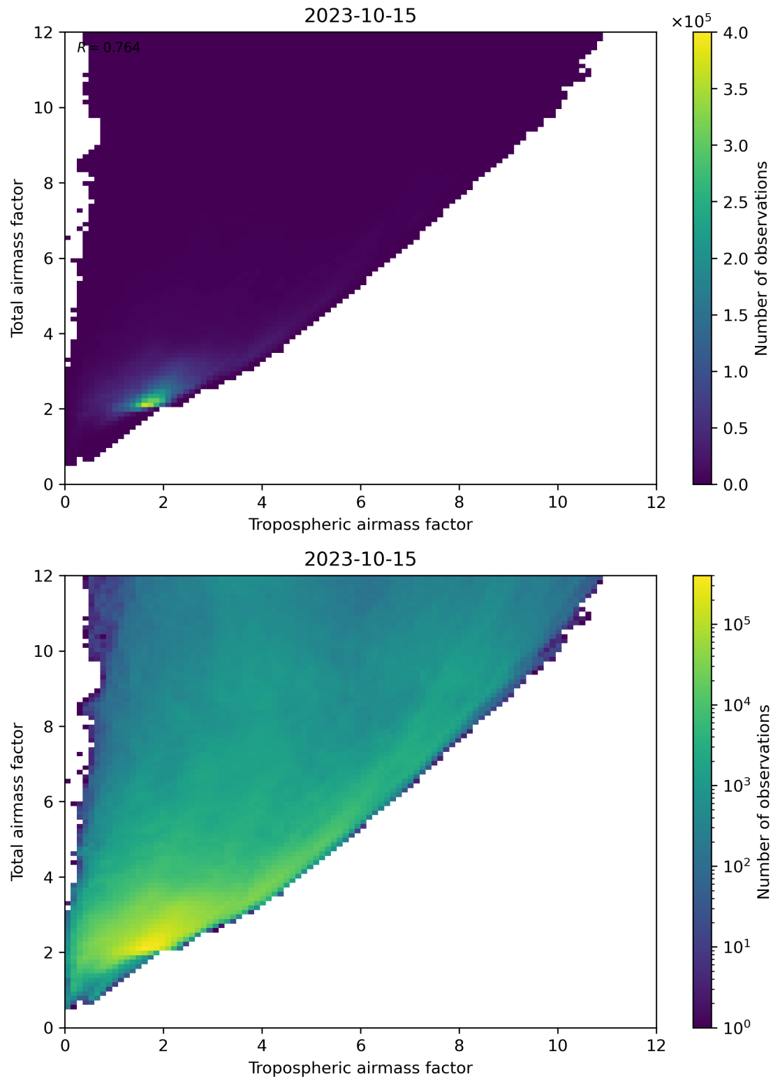
Figure 72: Scatter density plot of “Tropospheric airmass factor” against “Total airmass factor” for 2023-10-14 to 2023-10-16.
