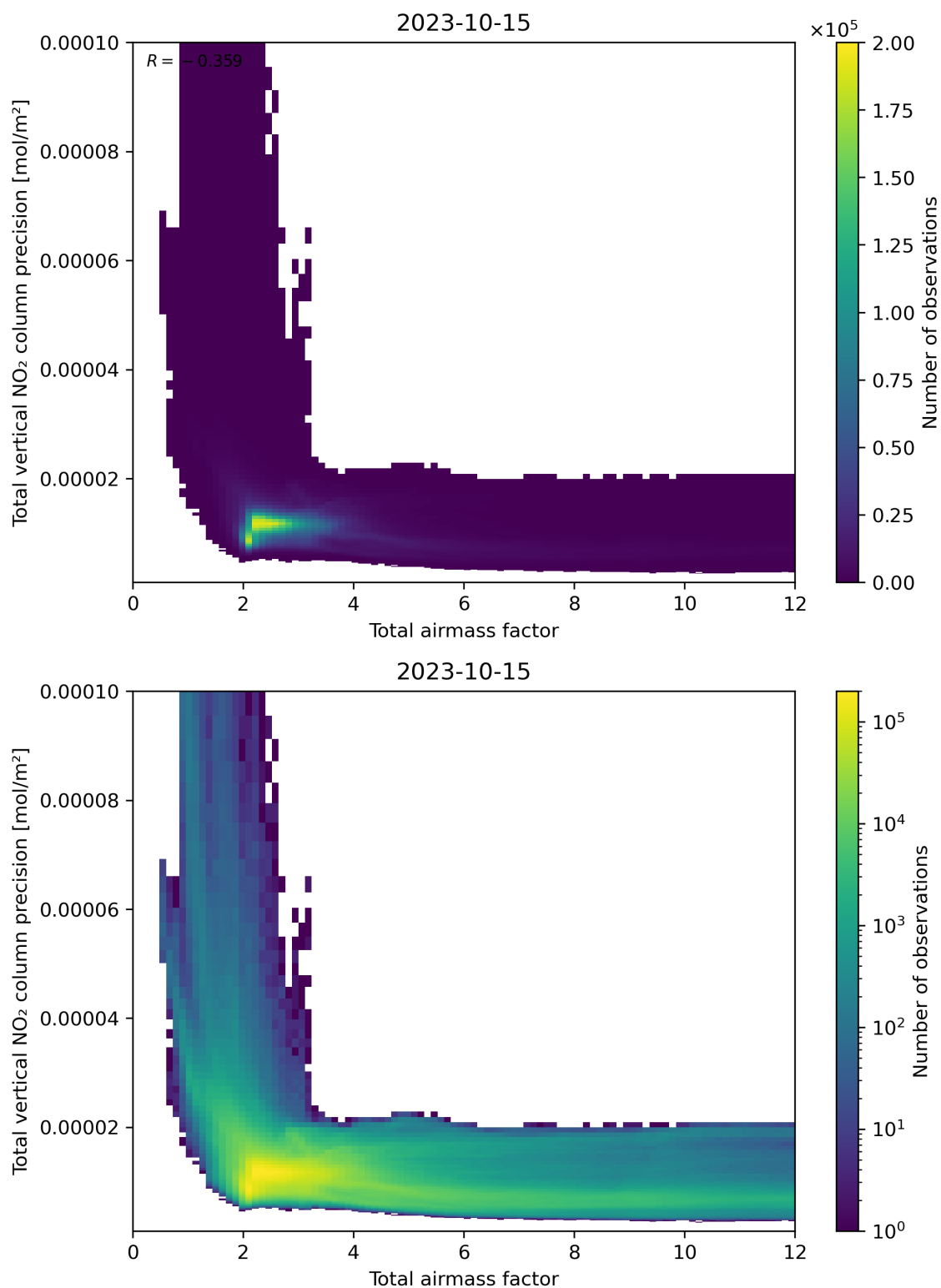
Figure 68: Scatter density plot of “Total airmass factor” against “Total vertical NO 2 column precision” for 2023-10-14 to 2023-10-16.
