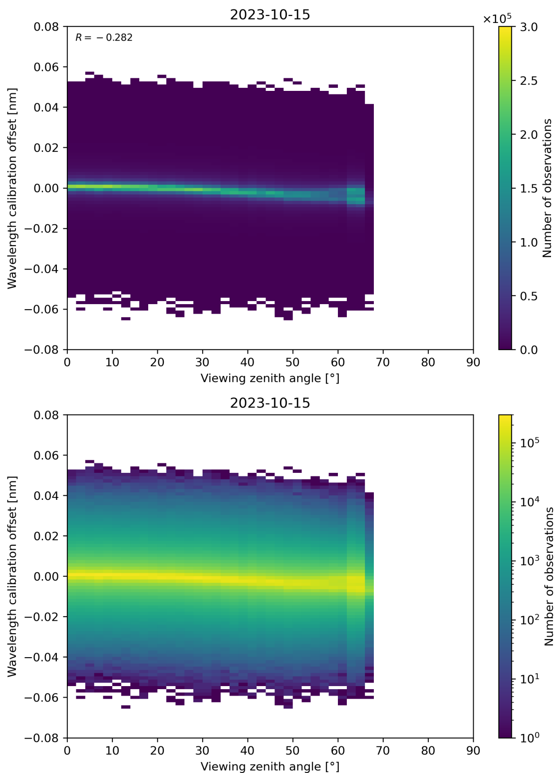
Figure 173: Scatter density plot of “Viewing zenith angle” against “Wavelength calibration offset” for 2023-10-14 to 2023-10-16.
