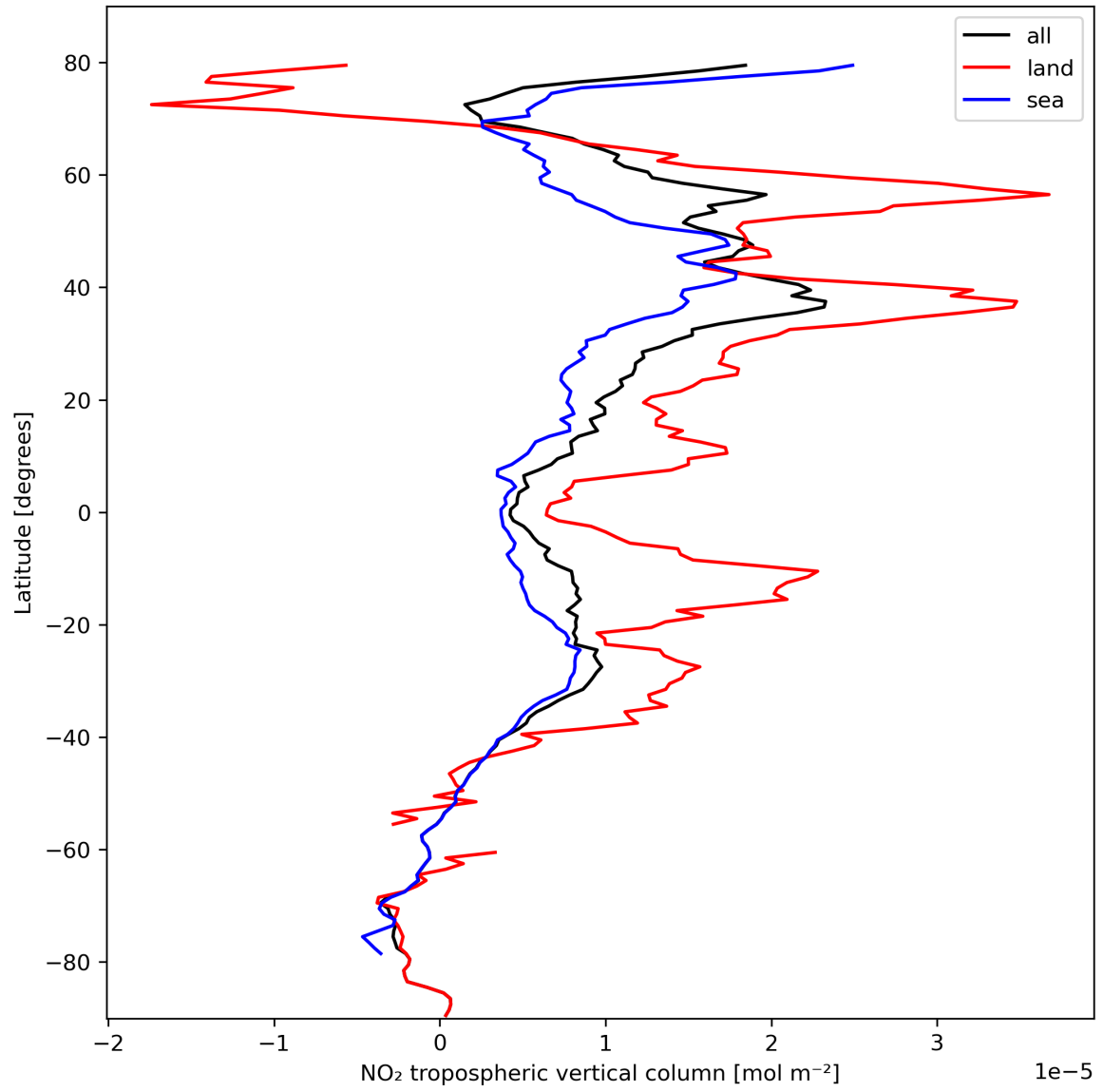
Figure 12: Zonal average of “NO 2 tropospheric vertical column” for 2023-10-14 to 2023-10-16.
