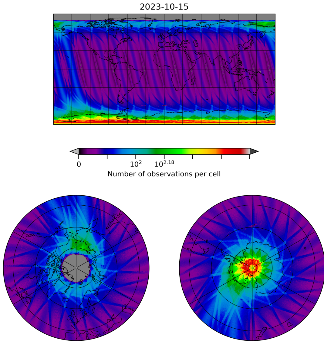
Figure 10: Map of the number of observations for 2023-10-14 to 2023-10-16
