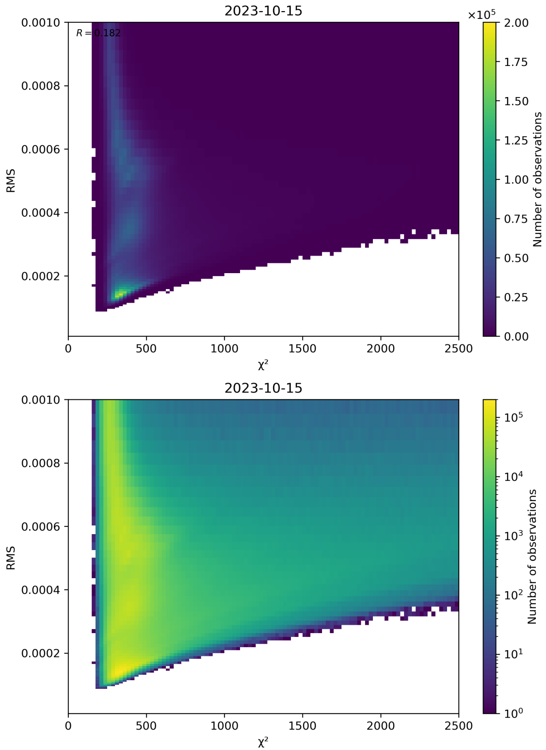
Figure 82: Scatter density plot of “ \chi^2 ” against “RMS” for 2023-10-14 to 2023-10-16.
