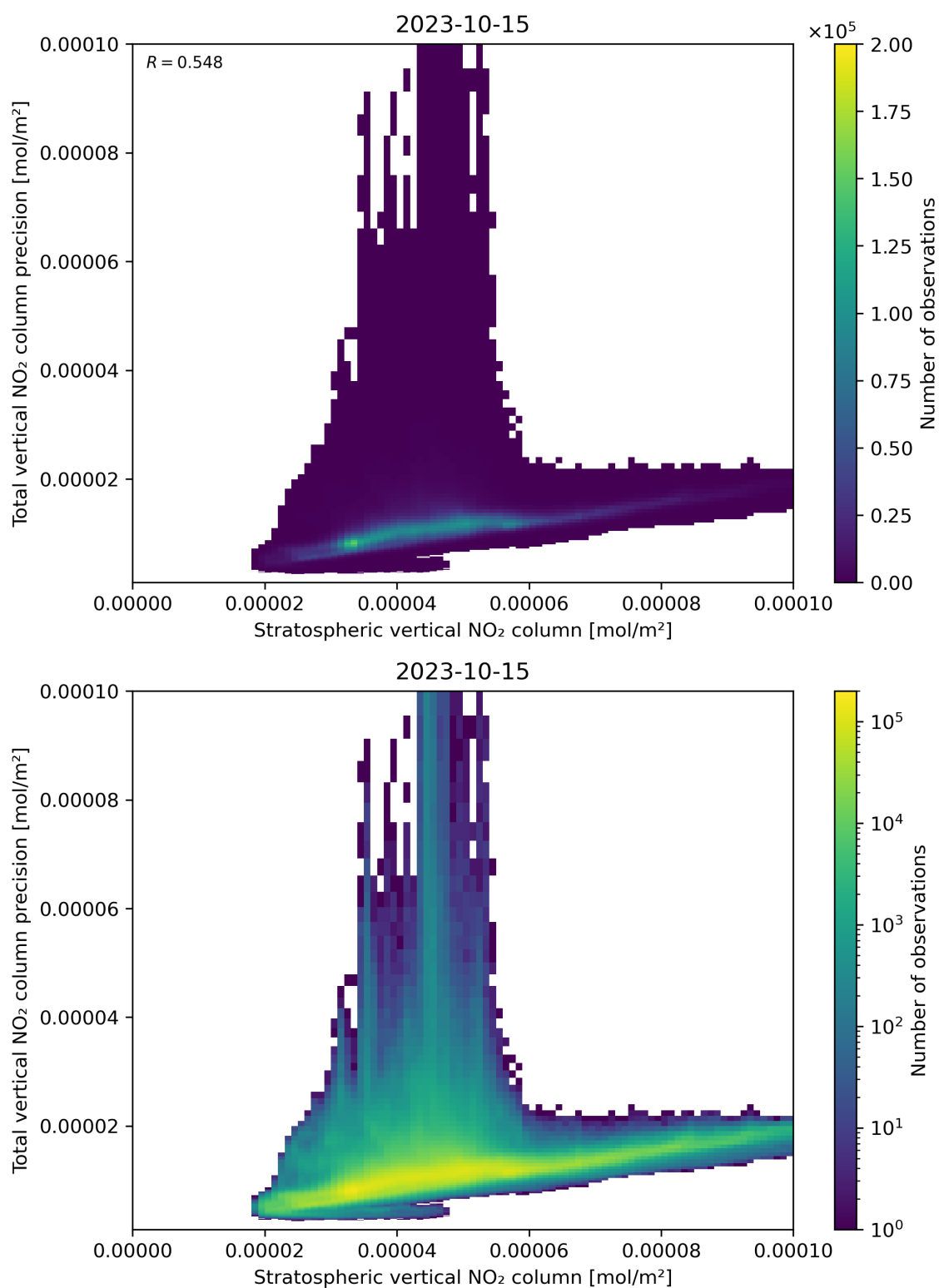
Figure 101: Scatter density plot of “Stratospheric vertical NO 2 column” against “Total vertical NO 2 column precision” for 2023-10-14 to 2023-10-16.
