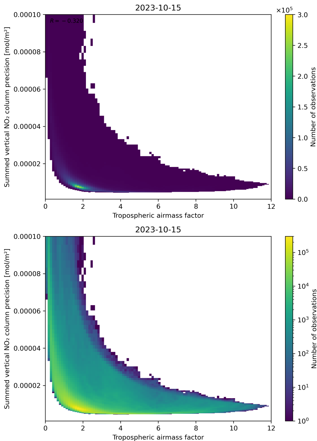
Figure 76: Scatter density plot of “Tropospheric air mass factor” against “Summed vertical NO 2 column precision” for 2023-10-14 to 2023-10-16.
