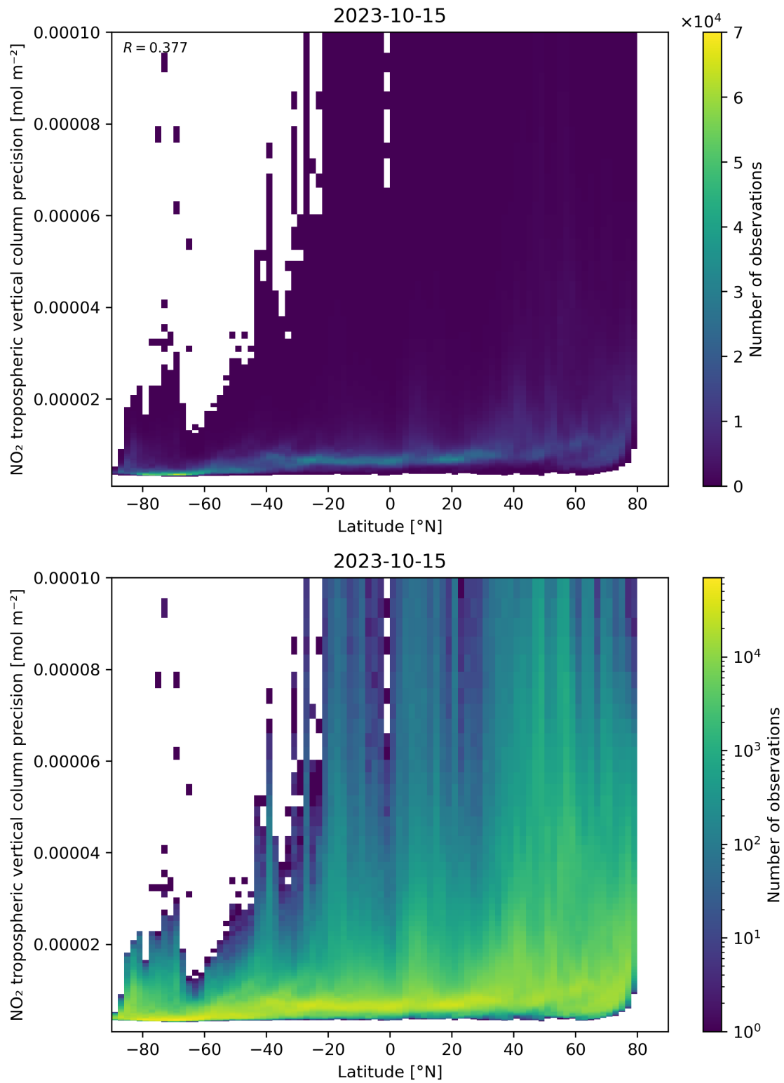
Figure 93: Scatter density plot of “Latitude” against “NO 2 tropospheric vertical column precision” for 2023-10-14 to 2023-10-16.
