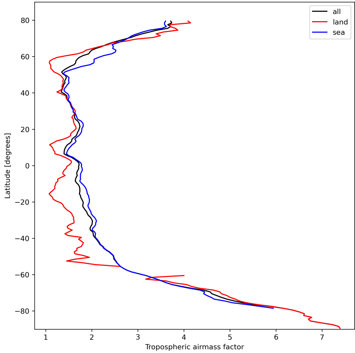
Figure 14: Zonal average of “Tropospheric airmass factor” for 2023-10-14 to 2023-10-16.
