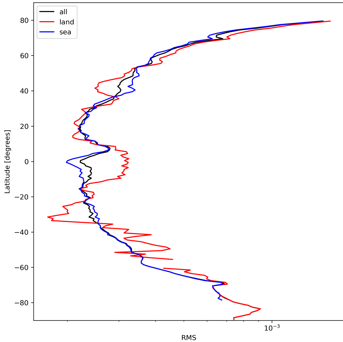
Figure 26: Zonal average of “RMS” for 2023-10-14 to 2023-10-16.
