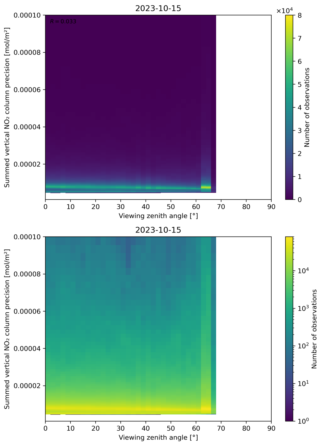
Figure 166: Scatter density plot of “Viewing zenith angle” against “Summed vertical NO 2 column precision” for 2023-10-14 to 2023-10-16.
