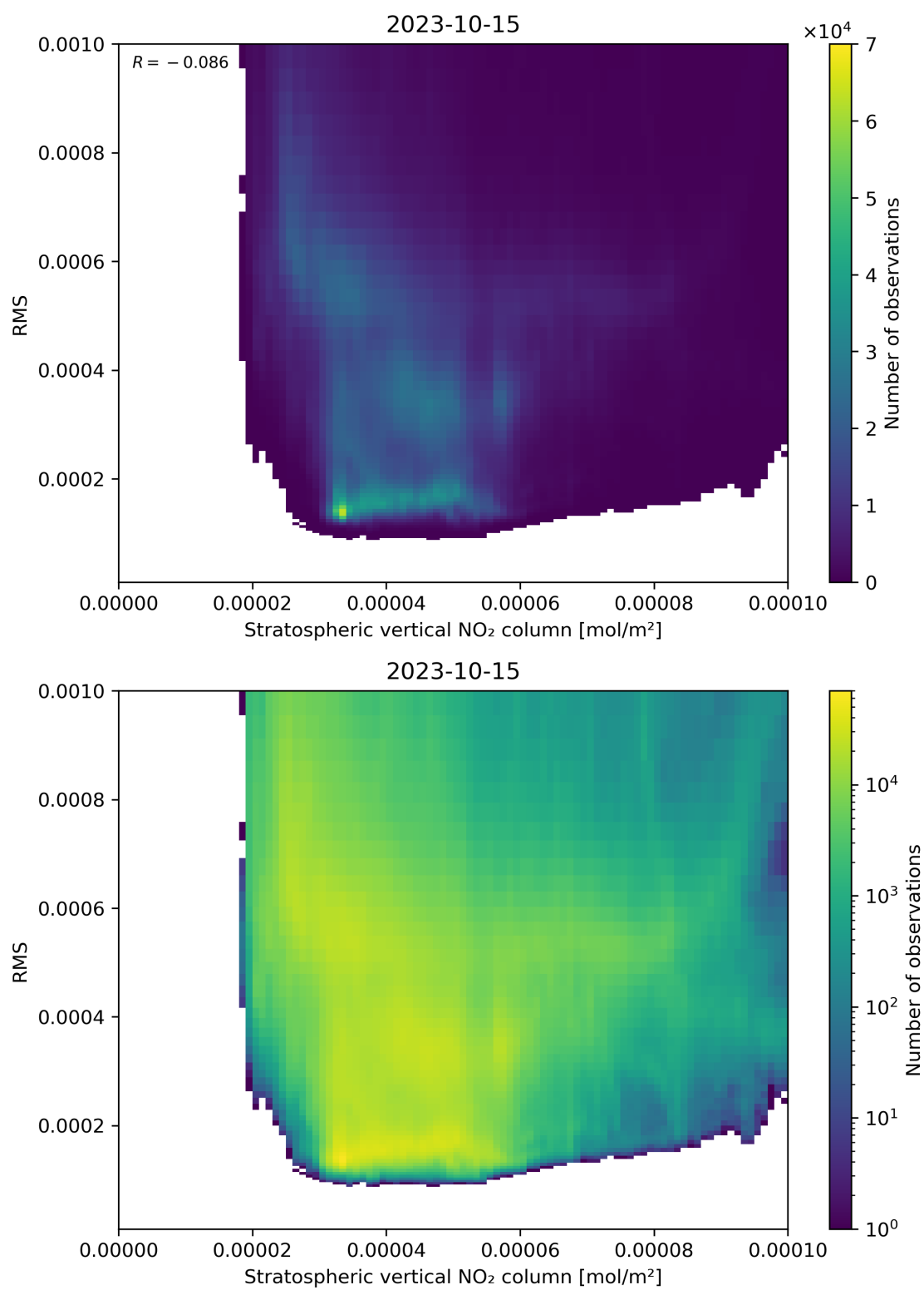
Figure 102: Scatter density plot of “Stratospheric vertical NO 2 column” against “RMS” for 2023-10-14 to 2023-10-16.
