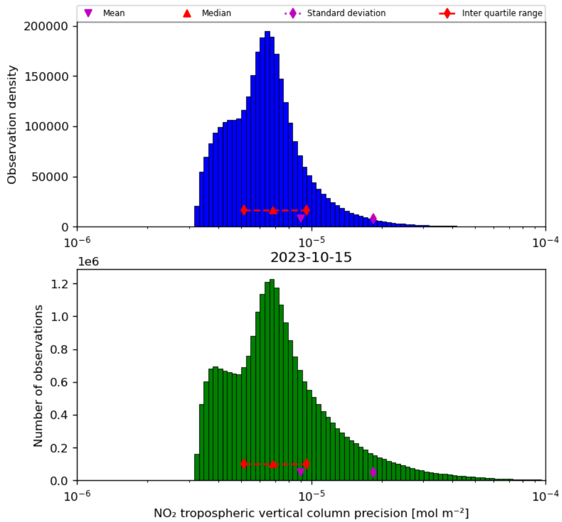
Figure 30: Histogram of “NO 2 tropospheric vertical column precision” for 2023-10-14 to 2023-10-16
