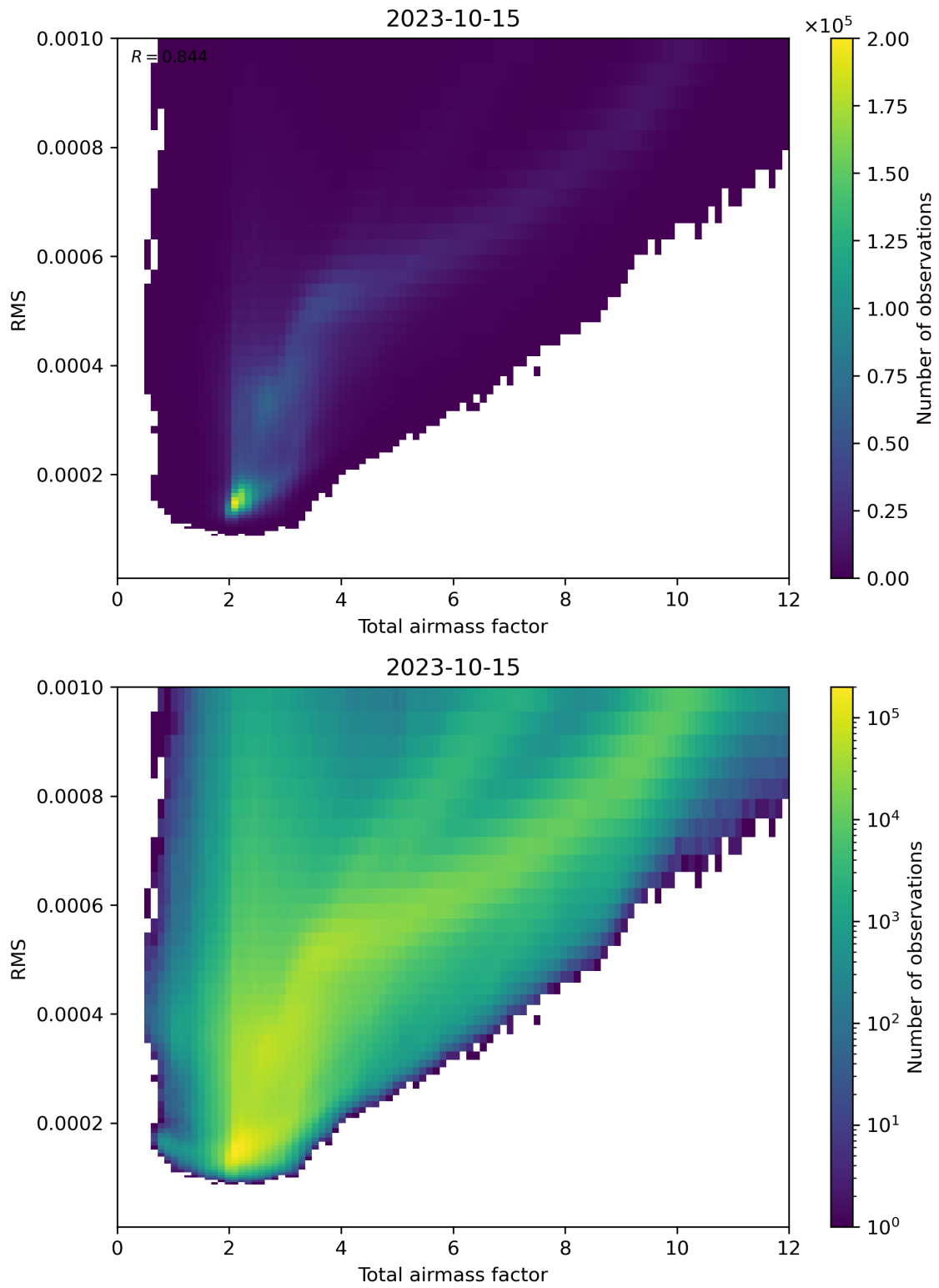
Figure 69: Scatter density plot of “Total airmass factor” against “RMS” for 2023-10-14 to 2023-10-16.
