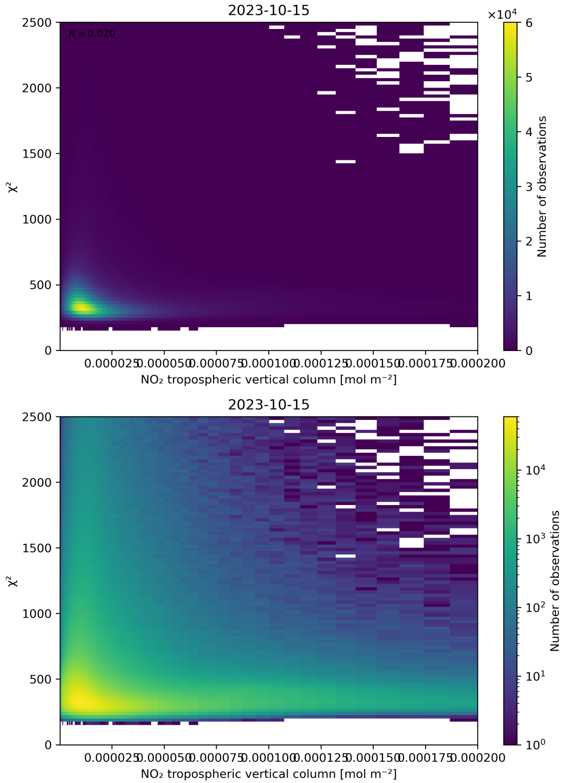
Figure 124: Scatter density plot of “NO 2 tropospheric vertical column” against “ \chi^2 ” for 2023-10-14 to 2023-10-16.
