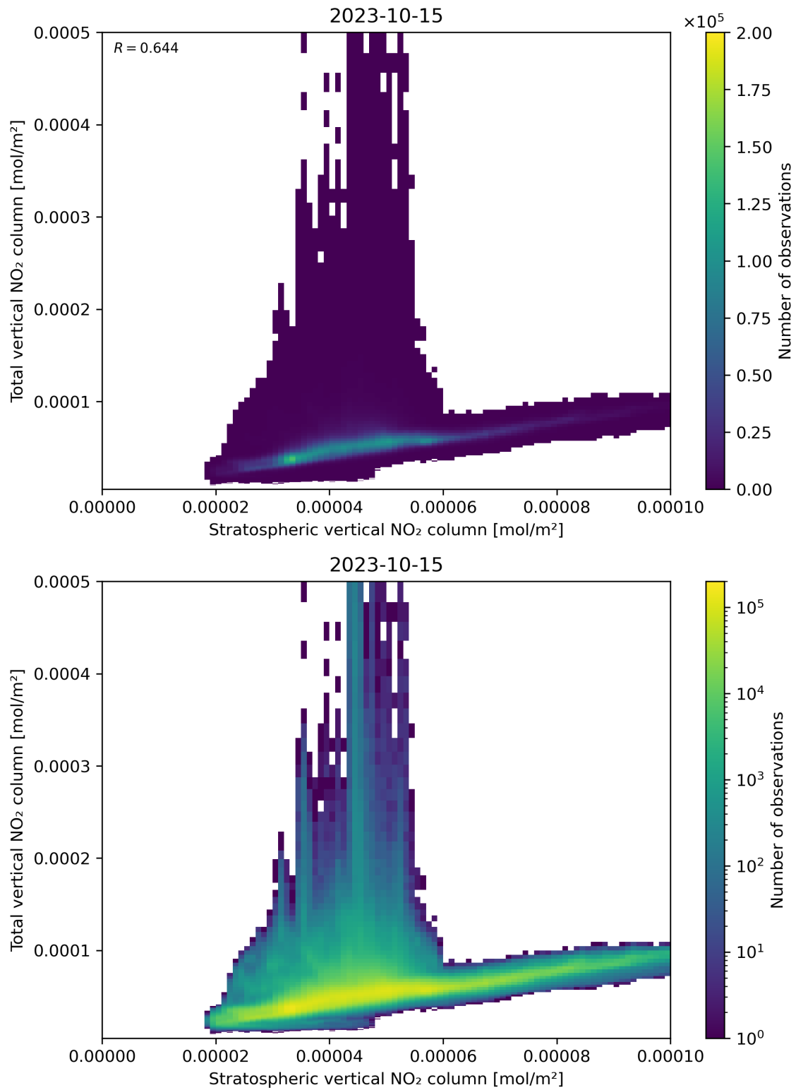
Figure 100: Scatter density plot of “Stratospheric vertical NO 2 column” against “Total vertical NO 2 column” for 2023-10-14 to 2023-10-16.
