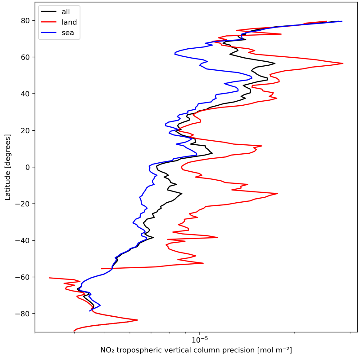
Figure 13: Zonal average of “NO 2 tropospheric vertical column precision” for 2023-10-14 to 2023-10-16.
