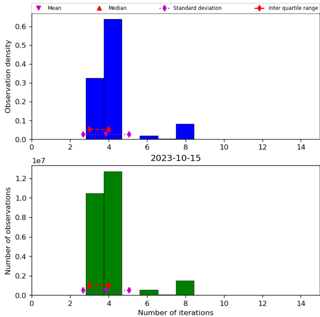
Figure 34: Histogram of “Number of iterations” for 2023-10-14 to 2023-10-16
