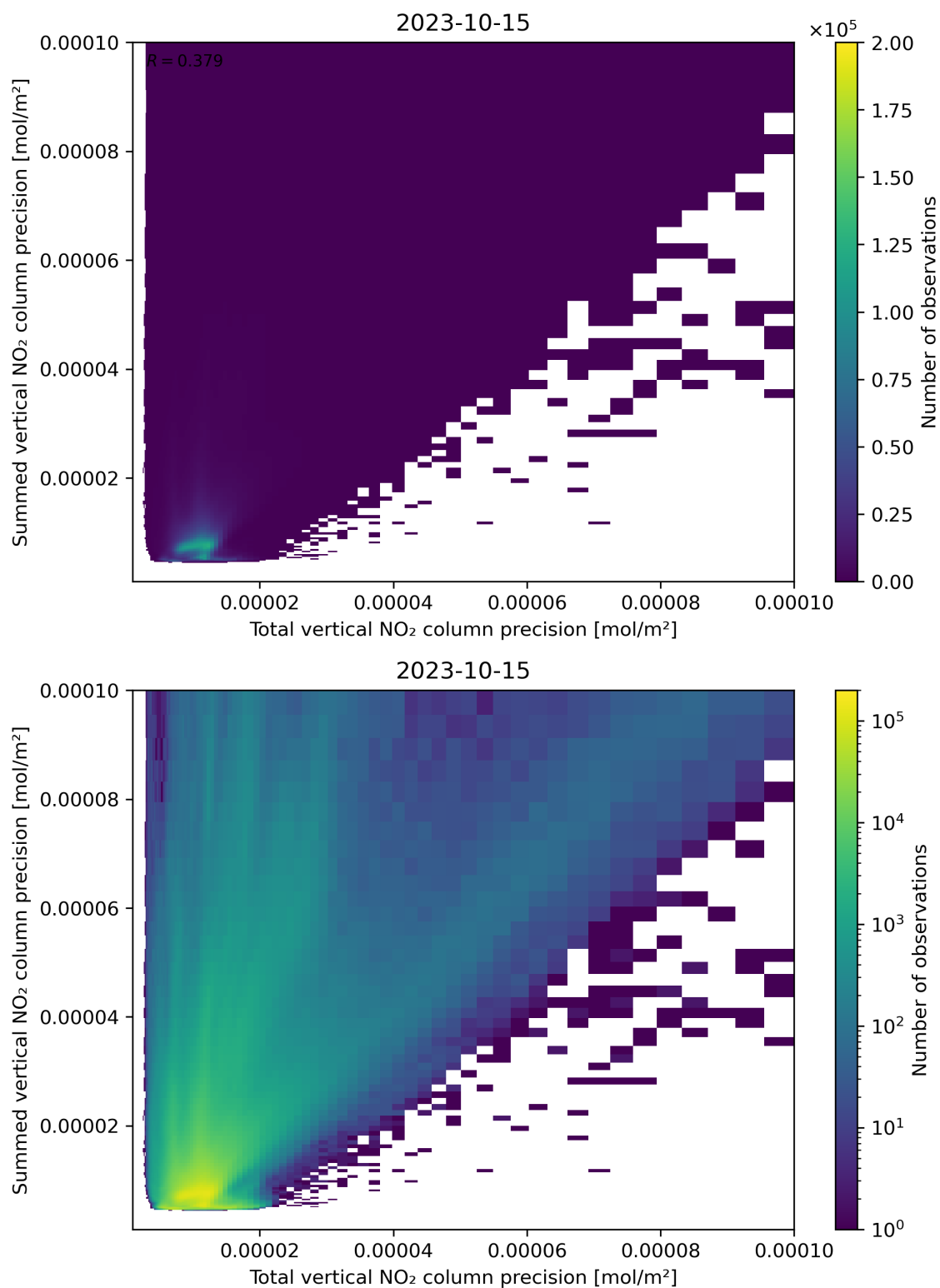
Figure 118: Scatter density plot of “Total vertical NO 2 column precision” against “Summed vertical NO 2 column precision” for 2023-10-14 to 2023-10-16.
