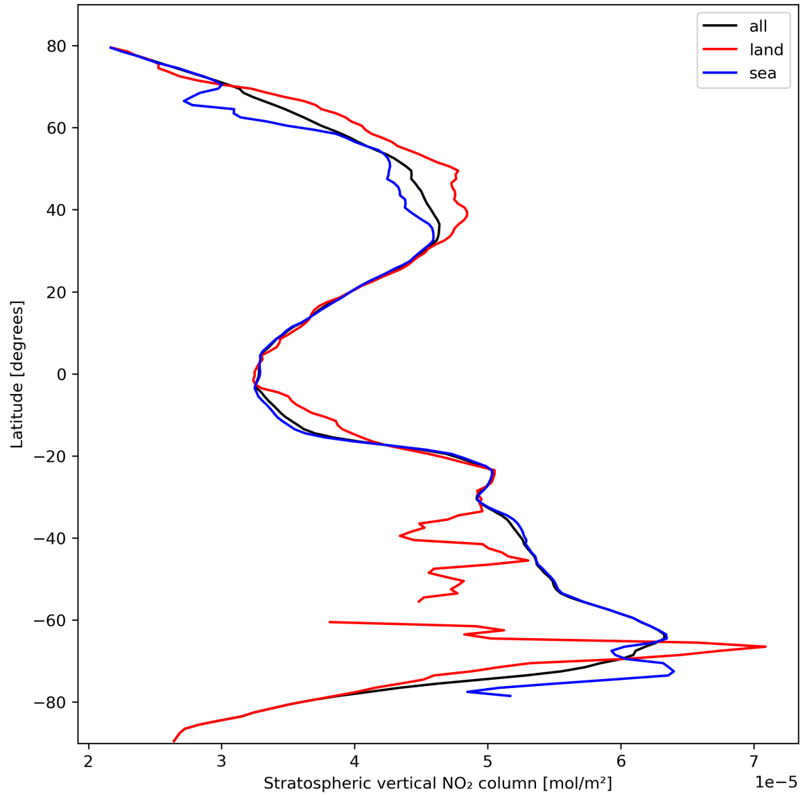
Figure 19: Zonal average of “Stratospheric vertical NO 2 column” for 2023-10-14 to 2023-10-16.
