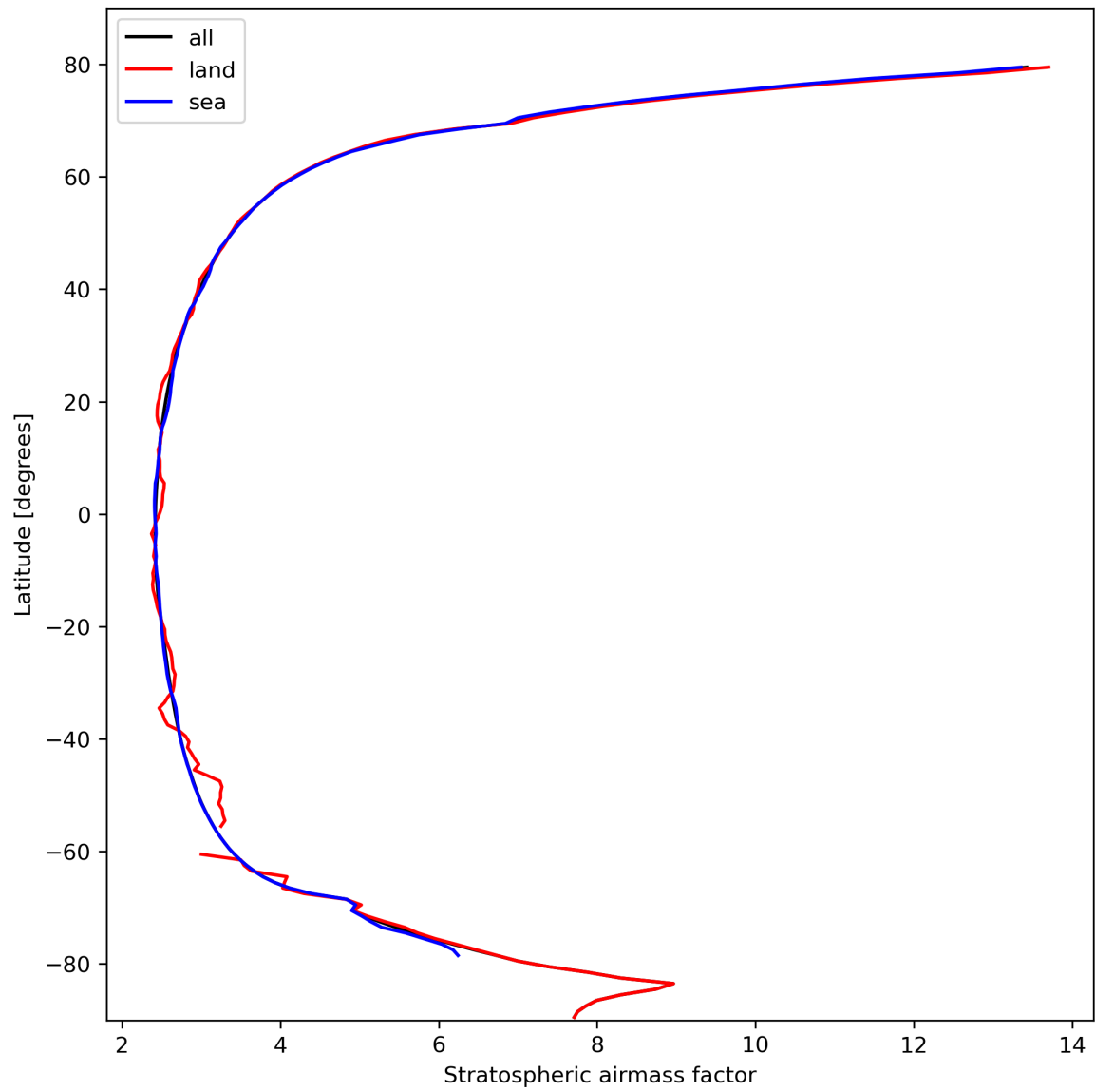
Figure 27: Zonal average of “Stratospheric airmass factor” for 2023-10-14 to 2023-10-16.
