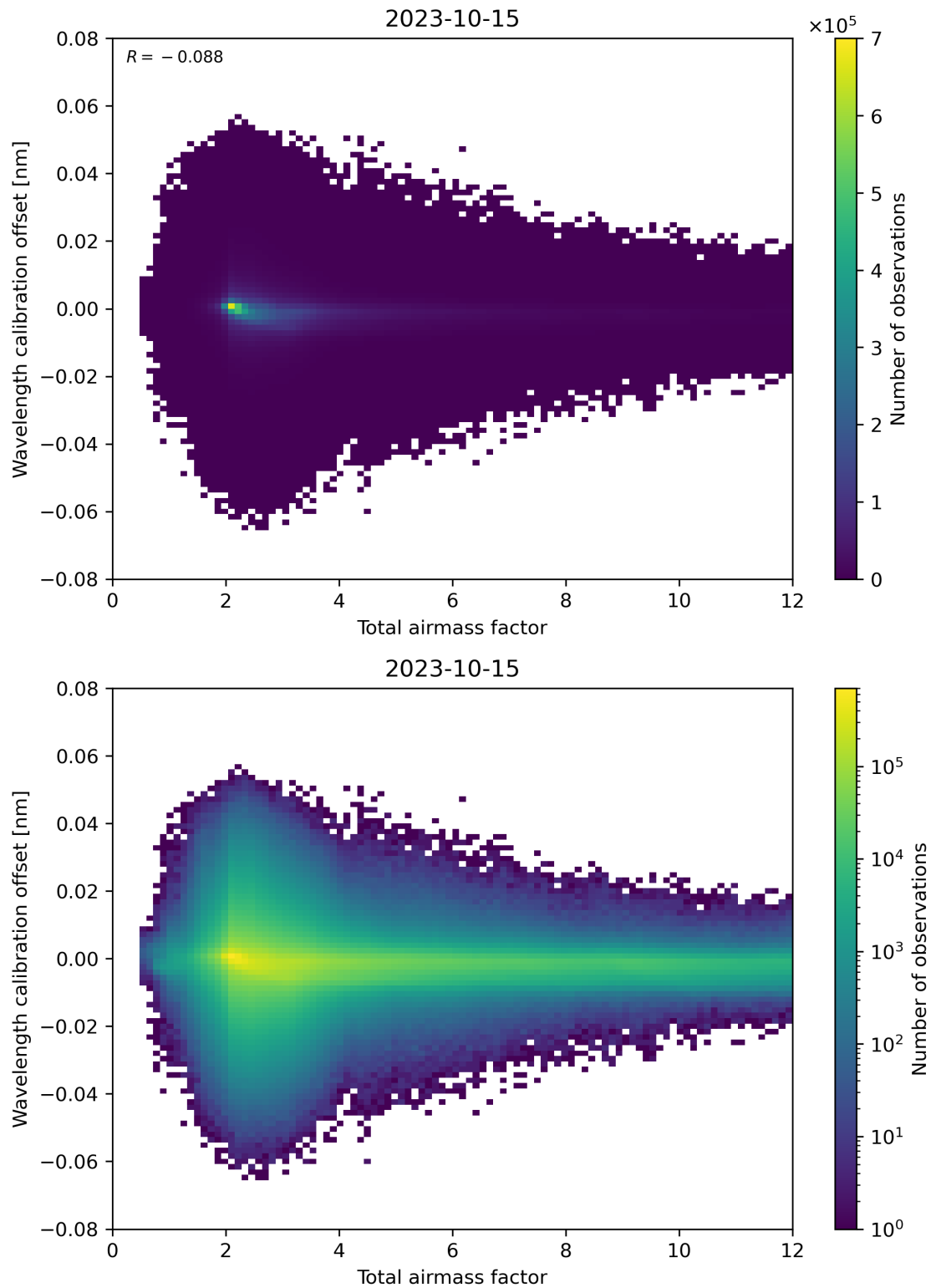
Figure 70: Scatter density plot of “Total airmass factor” against “Wavelength calibration offset” for 2023-10-14 to 2023-10-16.
