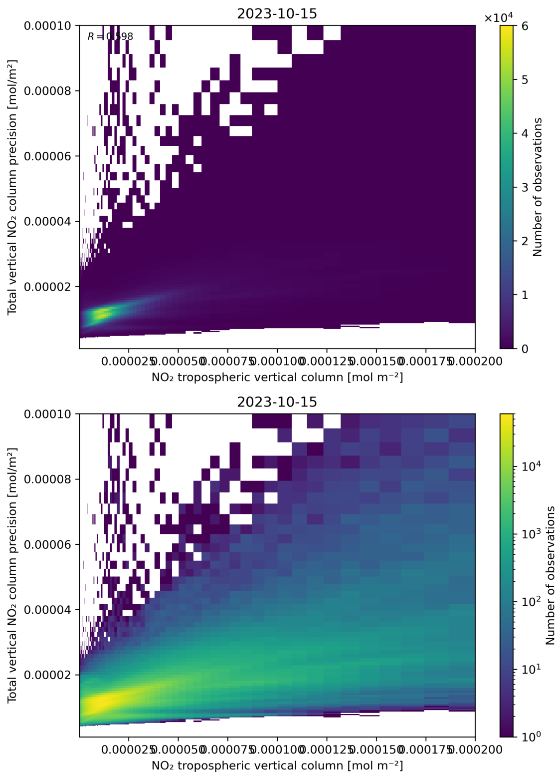
Figure 129: Scatter density plot of “NO 2 tropospheric vertical column” against “Total vertical NO 2 column precision” for 2023-10-14 to 2023-10-16.
