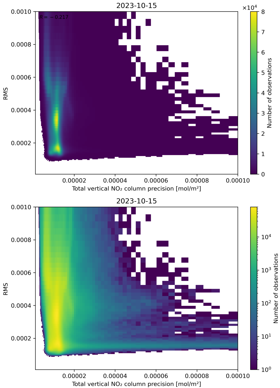
Figure 119: Scatter density plot of “Total vertical NO 2 column precision” against “RMS” for 2023-10-14 to 2023-10-16.
