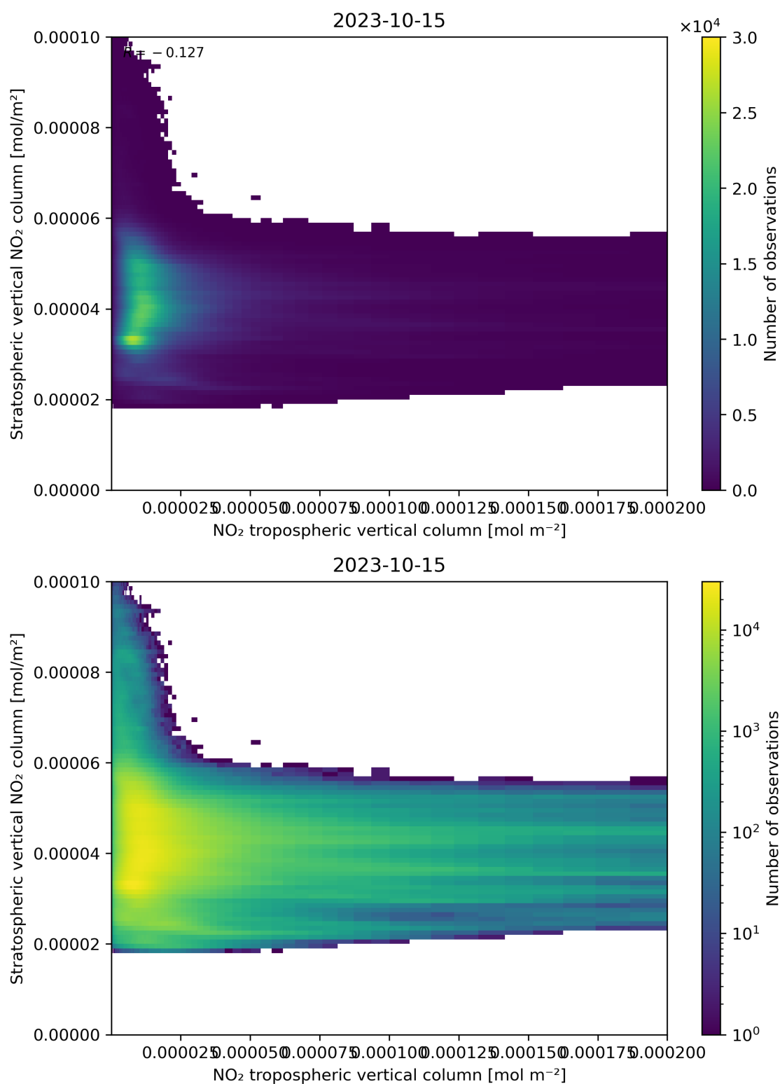
Figure 125: Scatter density plot of “NO 2 tropospheric vertical column” against “Stratospheric vertical NO 2 column” for 2023-10-14 to 2023-10-16.
