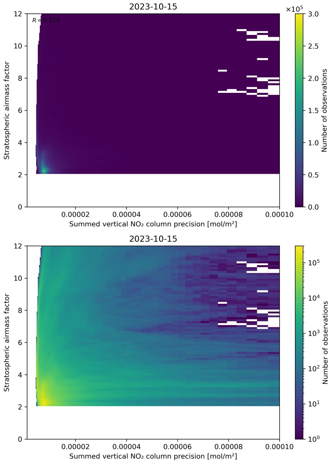
Figure 106: Scatter density plot of “Summed vertical NO 2 column precision” against “Stratospheric airmass factor” for 2023-10-14 to 2023-10-16.
