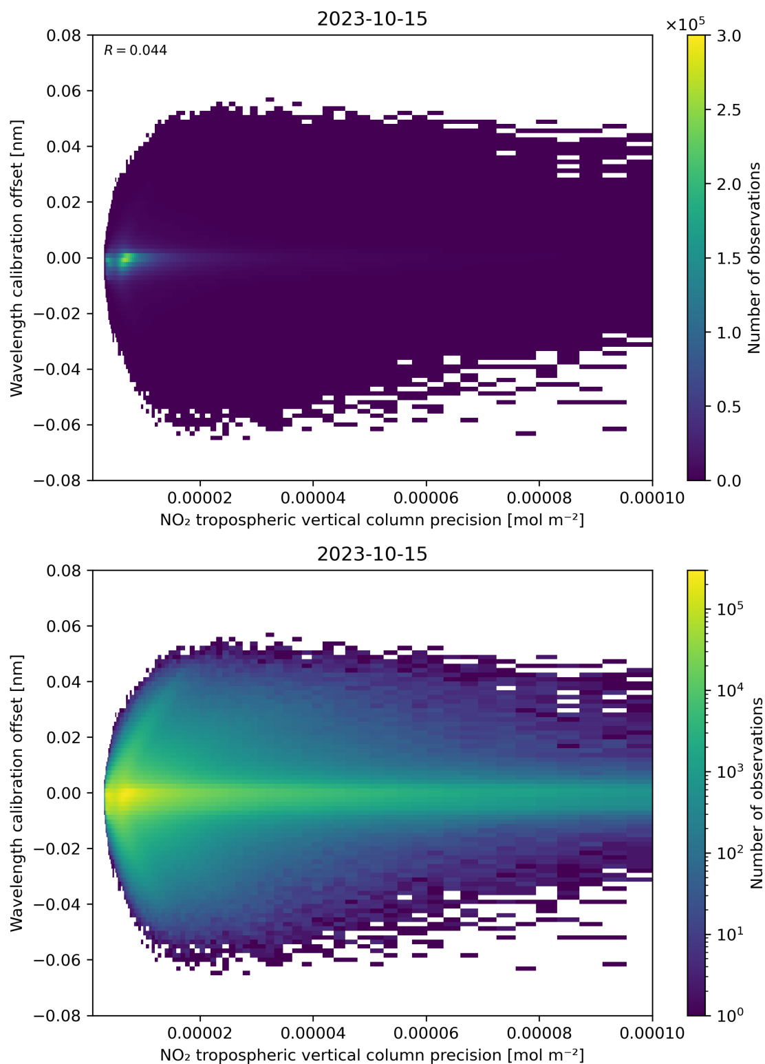
Figure 141: Scatter density plot of “NO 2 tropospheric vertical column precision” against “Wavelength calibration offset” for 2023-10-14 to 2023-10-16.
