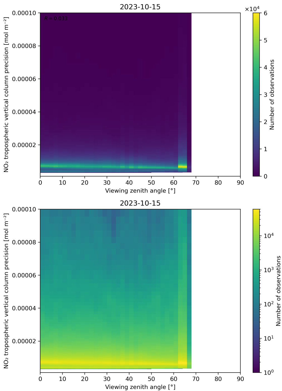
Figure 170: Scatter density plot of “Viewing zenith angle” against “NO 2 tropospheric vertical column precision” for 2023-10-14 to 2023-10-16.
