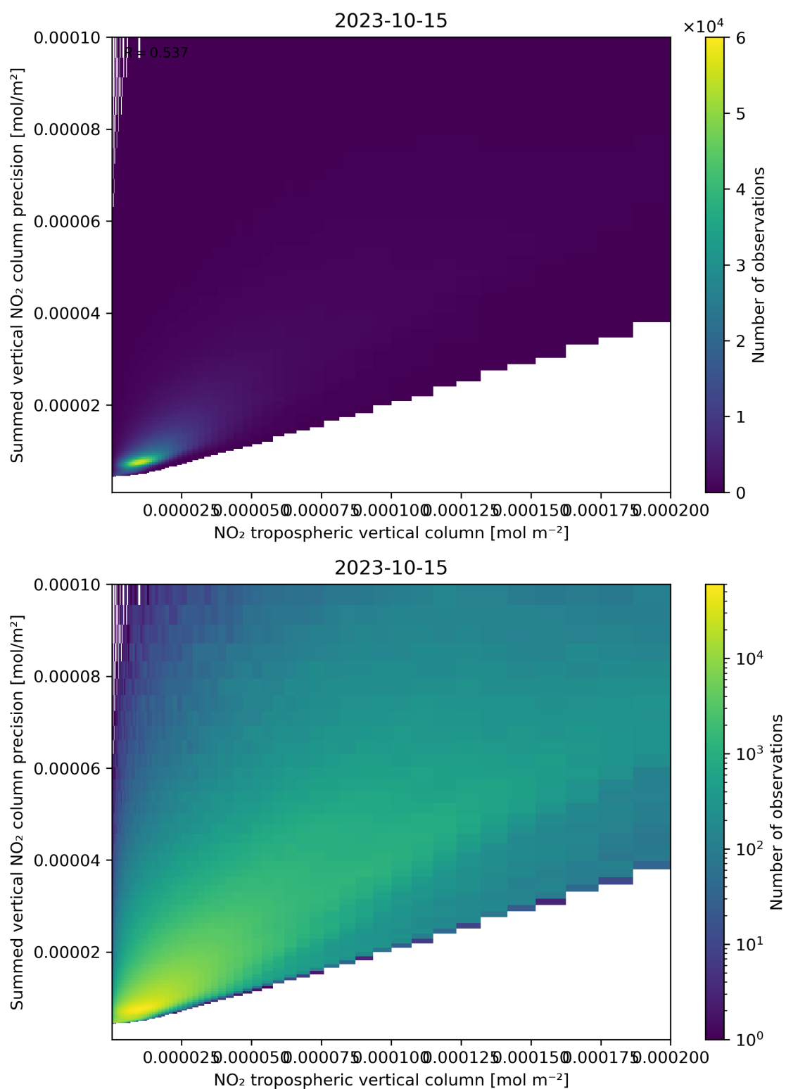
Figure 127: Scatter density plot of “NO 2 tropospheric vertical column” against “Summed vertical NO 2 column precision” for 2023-10-14 to 2023-10-16.
