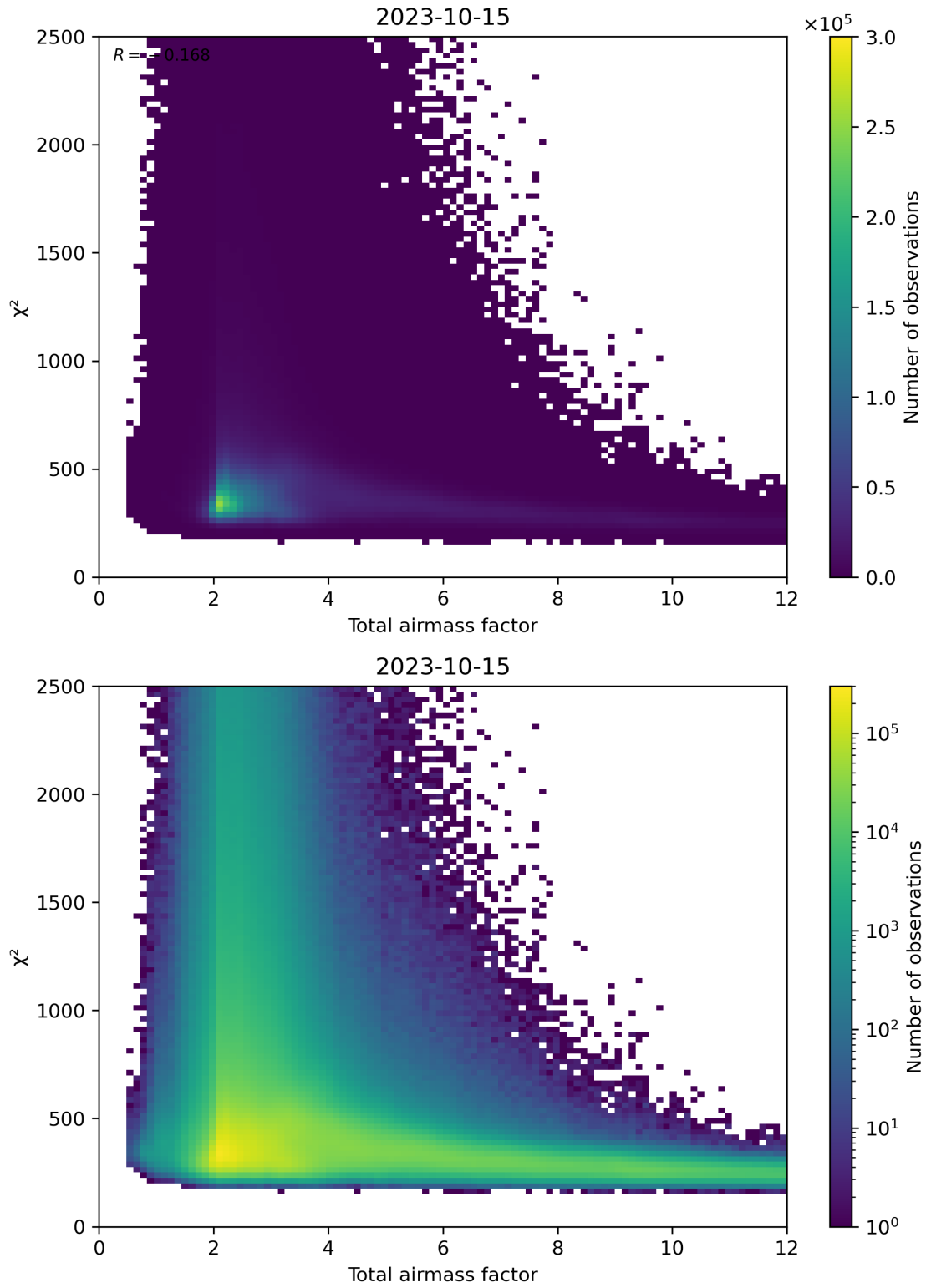
Figure 63: Scatter density plot of “Total airmass factor” against “ \chi^2 ” for 2023-10-14 to 2023-10-16.
