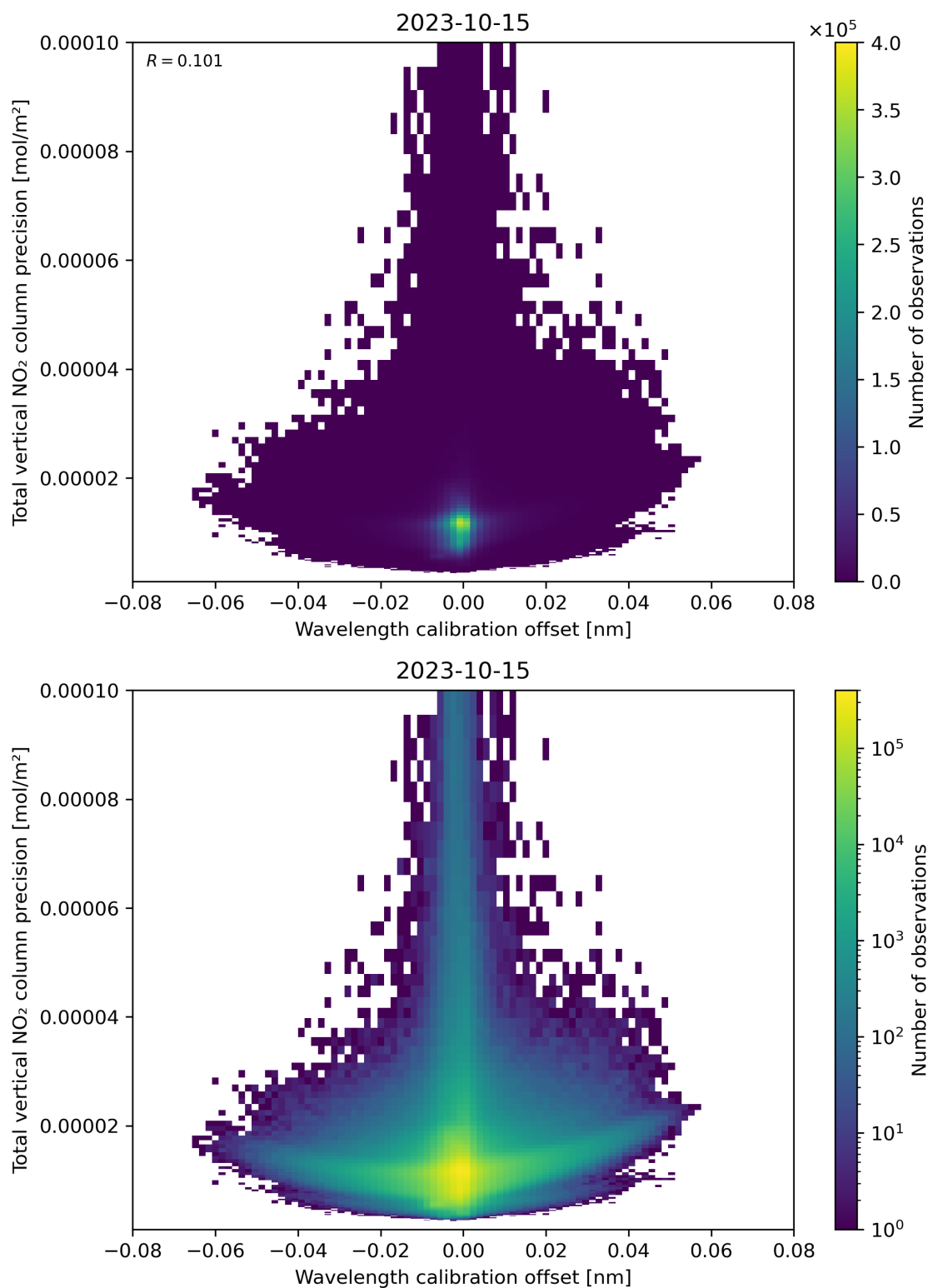
Figure 180: Scatter density plot of “Wavelength calibration offset” against “Total vertical NO 2 column precision” for 2023-10-14 to 2023-10-16.
