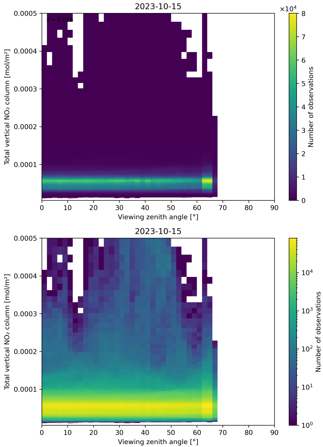
Figure 167: Scatter density plot of “Viewing zenith angle” against “Total vertical NO 2 column” for 2023-10-14 to 2023-10-16.
