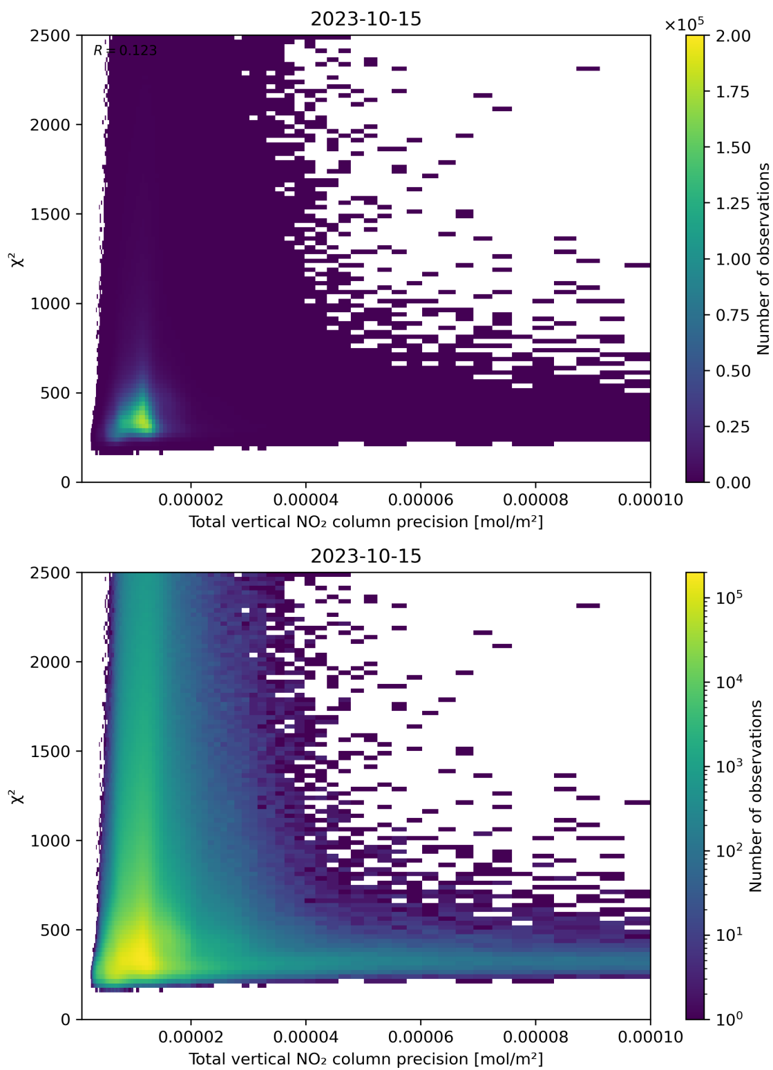
Figure 116: Scatter density plot of “Total vertical NO 2 column precision” against “ \chi^2 ” for 2023-10-14 to 2023-10-16.
