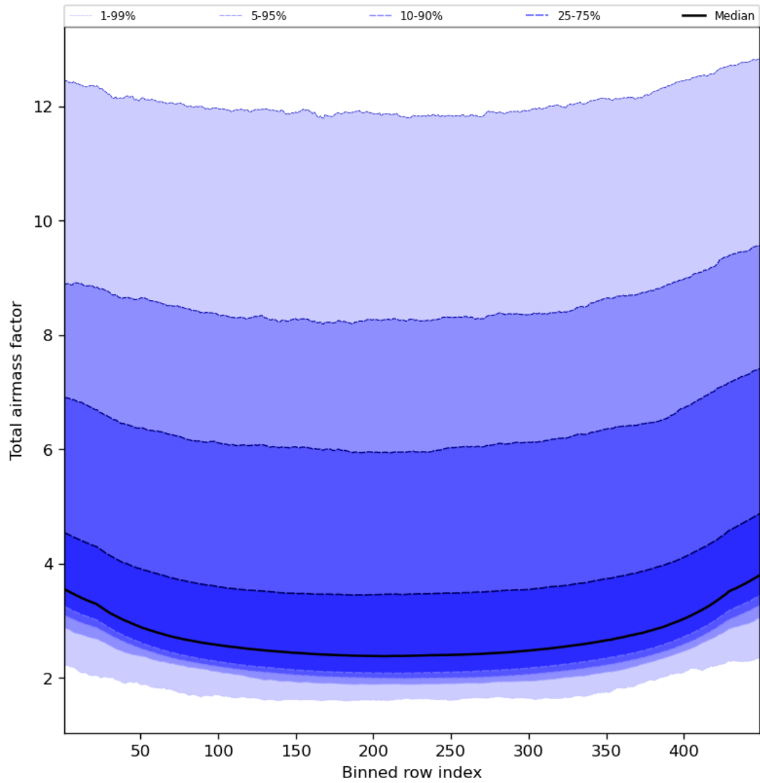
Figure 49: Along track statistics of “Total airmass factor” for 2023-10-14 to 2023-10-16
