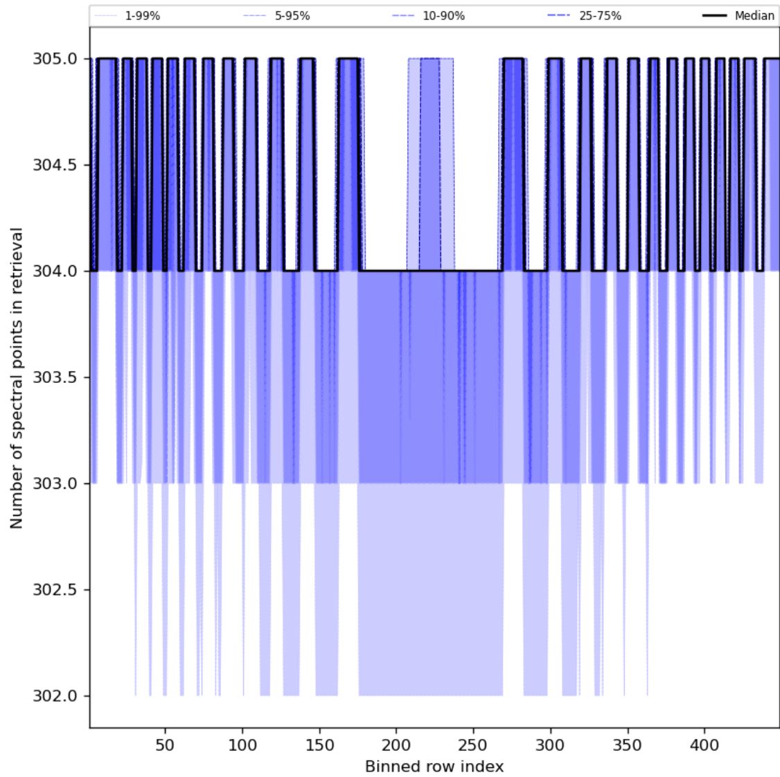
Figure 50: Along track statistics of “Number of spectral points in retrieval” for 2023-10-14 to 2023-10-16
