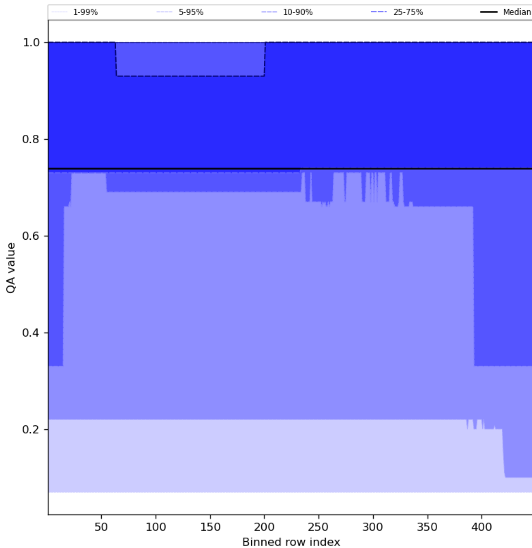
Figure 45: Along track statistics of “QA value” for 2023-10-14 to 2023-10-16
