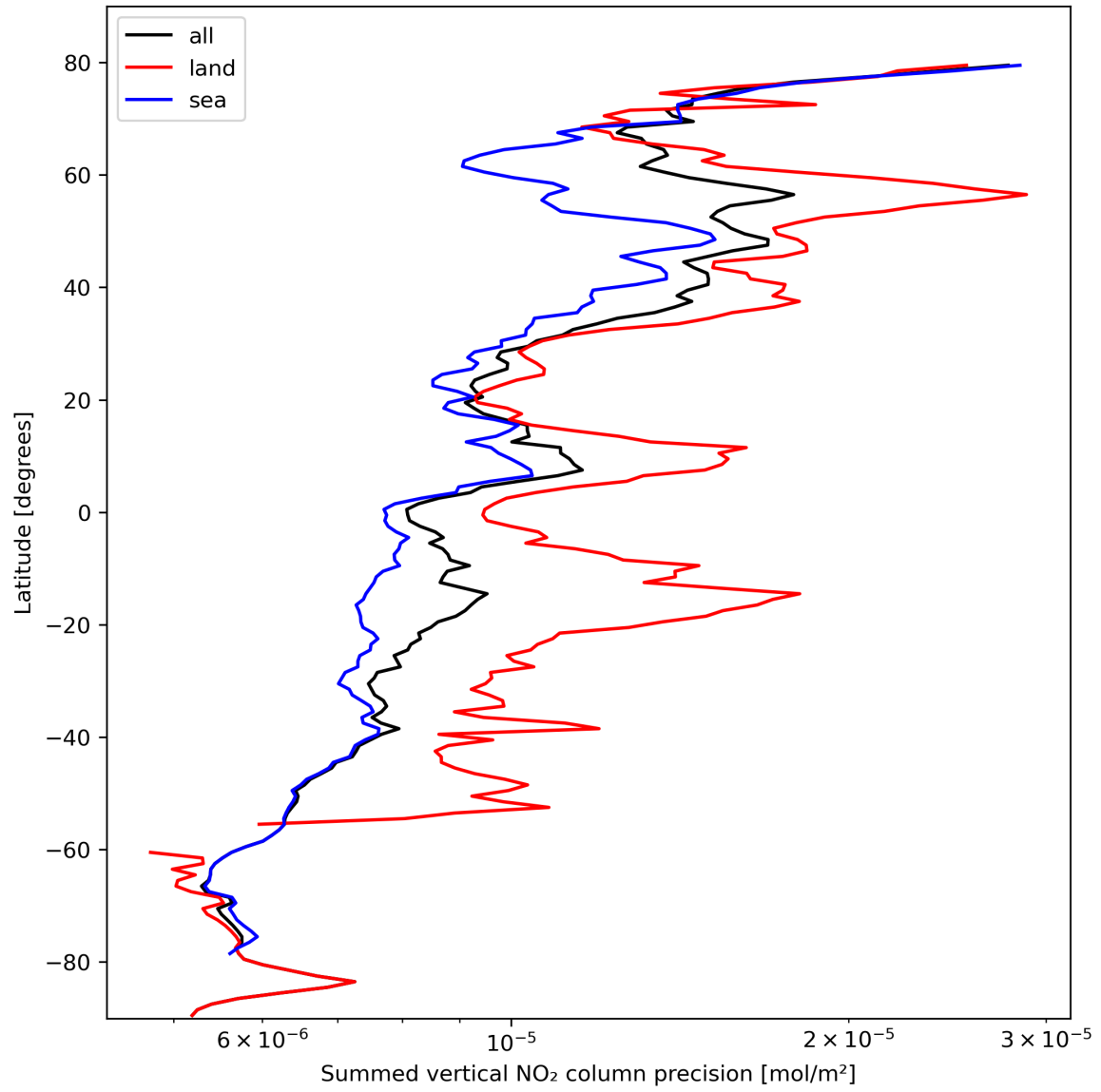
Figure 24: Zonal average of "Summed vertical NO 2 column precision" for 2023-10-14 to 2023-10-16.
