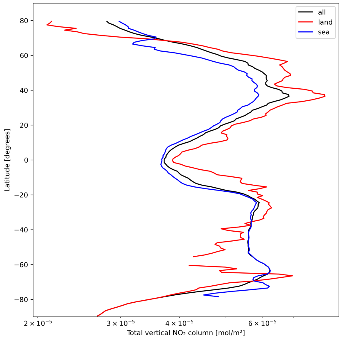
Figure 21: Zonal average of “Total vertical NO 2 column” for 2023-10-14 to 2023-10-16.
