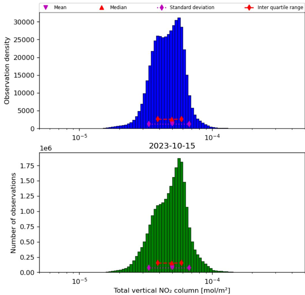
Figure 38: Histogram of “Total vertical NO 2 column” for 2023-10-14 to 2023-10-16
