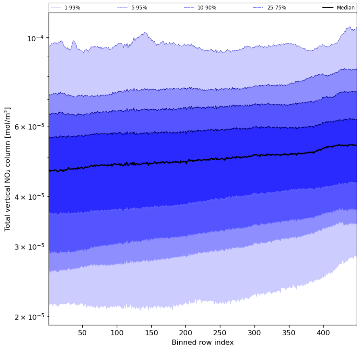
Figure 55: Along track statistics of “Total vertical NO 2 column” for 2023-10-14 to 2023-10-16
