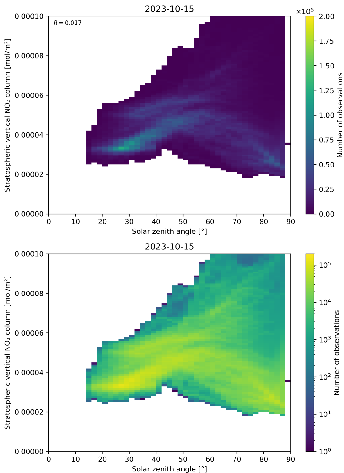
Figure 150: Scatter density plot of “Solar zenith angle” against “Stratospheric vertical NO 2 column” for 2023-10-14 to 2023-10-16.
