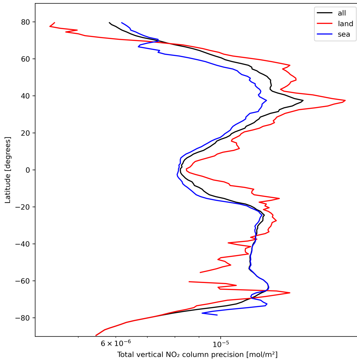
Figure 22: Zonal average of “Total vertical NO 2 column precision” for 2023-10-14 to 2023-10-16.
