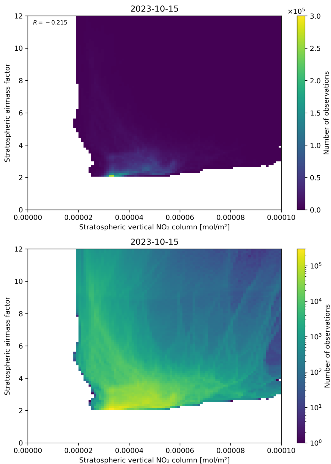
Figure 96: Scatter density plot of “Stratospheric vertical NO 2 column” against “Stratospheric airmass factor” for 2023-10-14 to 2023-10-16.
