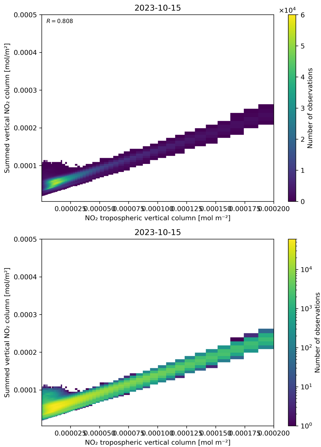
Figure 126: Scatter density plot of “NO 2 tropospheric vertical column” against “Summed vertical NO 2 column” for 2023-10-14 to 2023-10-16.
