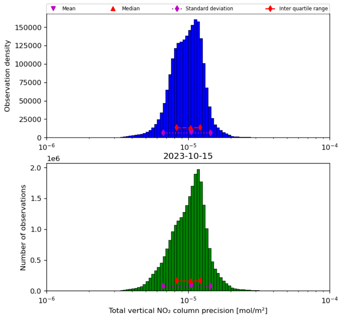
Figure 39: Histogram of "Total vertical NO 2 column precision" for 2023-10-14 to 2023-10-16
