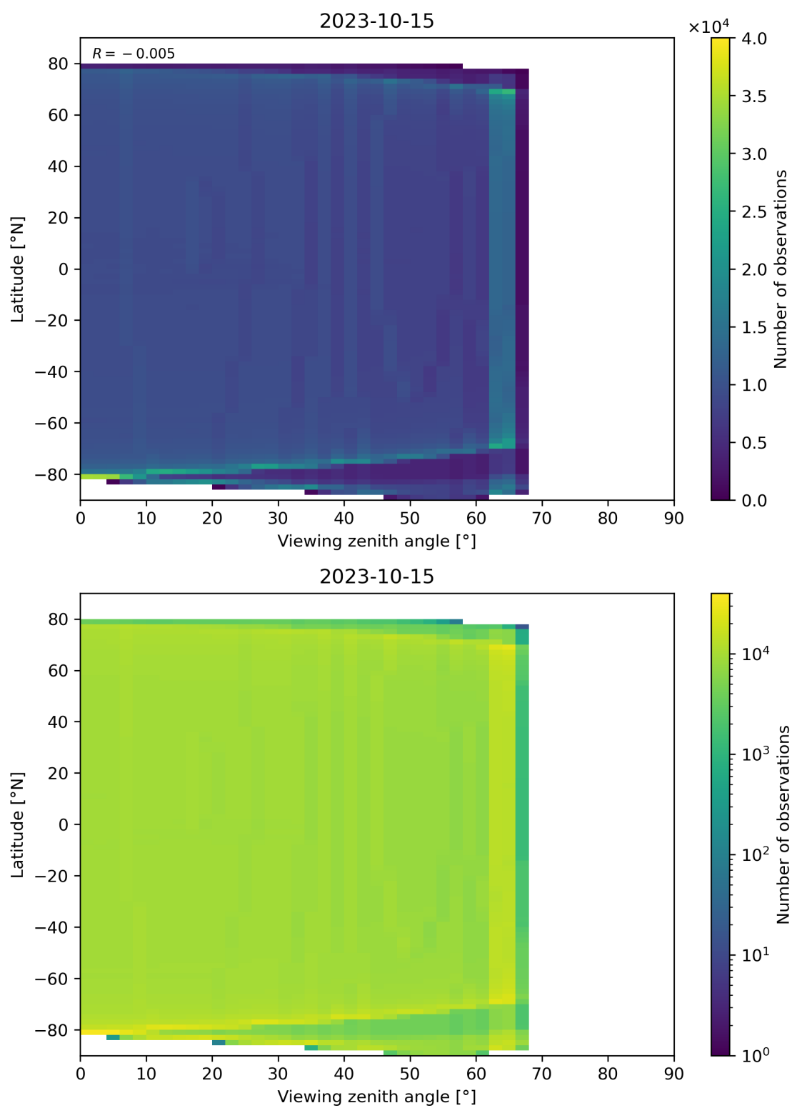
Figure 163: Scatter density plot of “Viewing zenith angle” against “Latitude” for 2023-10-14 to 2023-10-16.
