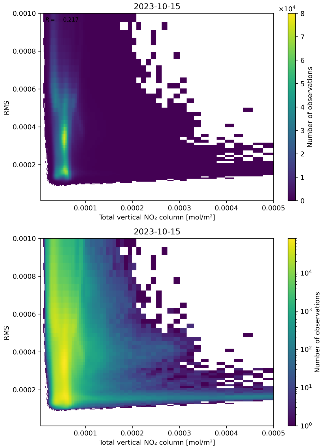
Figure 120: Scatter density plot of “Total vertical NO 2 column” against “RMS” for 2023-10-14 to 2023-10-16.
