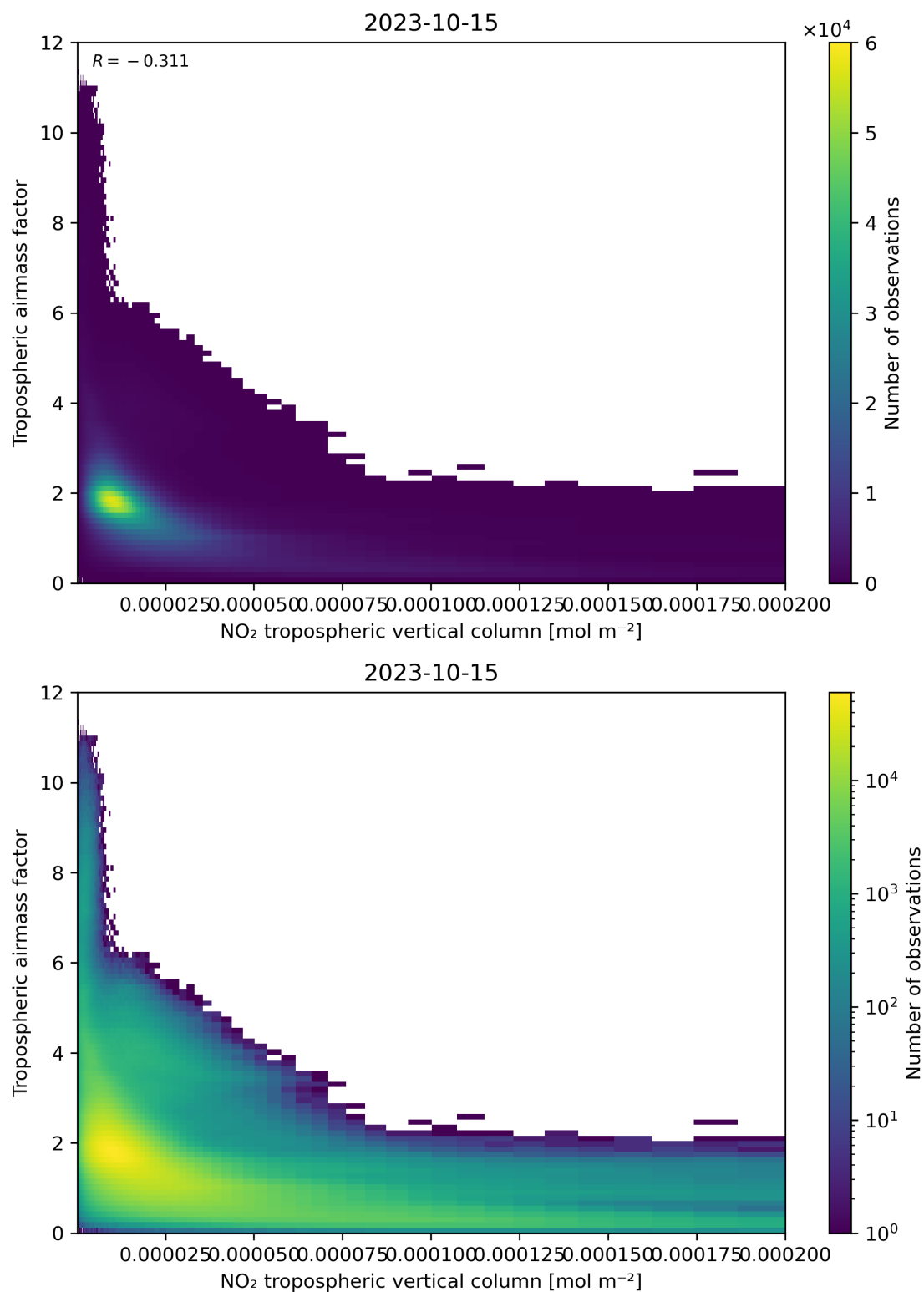
Figure 123: Scatter density plot of “NO 2 tropospheric vertical column” against “Tropospheric air mass factor” for 2023-10-14 to 2023-10-16.
