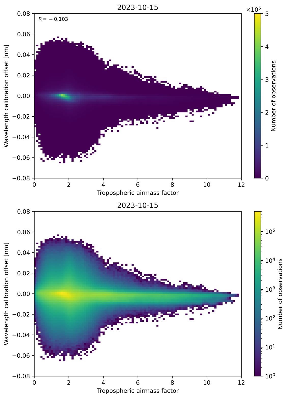
Figure 80: Scatter density plot of “Tropospheric air mass factor” against “Wavelength calibration offset” for 2023-10-14 to 2023-10-16.
