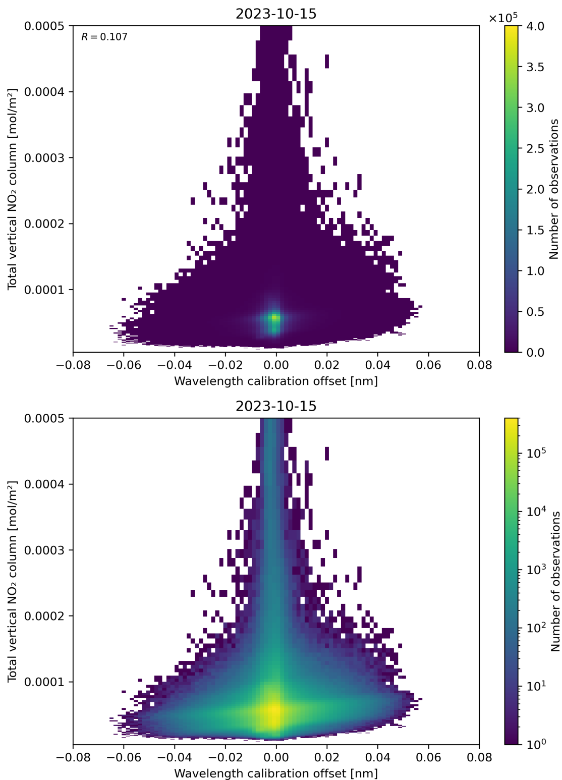
Figure 179: Scatter density plot of “Wavelength calibration offset” against “Total vertical NO 2 column” for 2023-10-14 to 2023-10-16.
