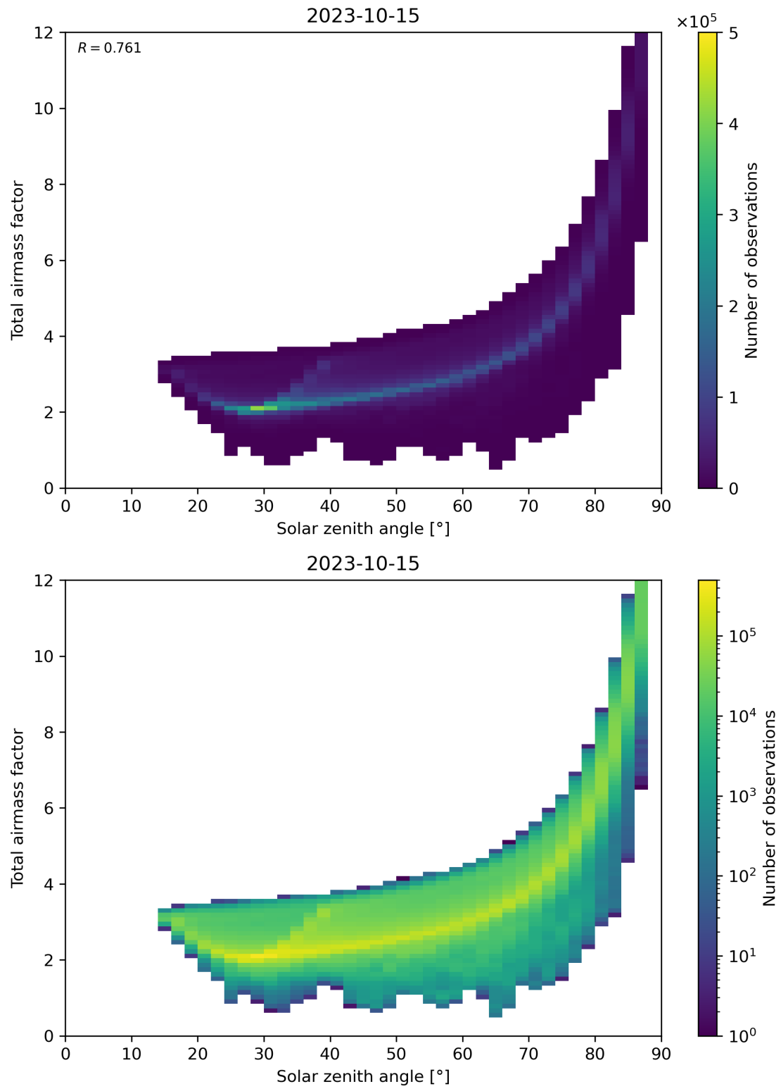
Figure 146: Scatter density plot of “Solar zenith angle” against “Total air mass factor” for 2023-10-14 to 2023-10-16.
