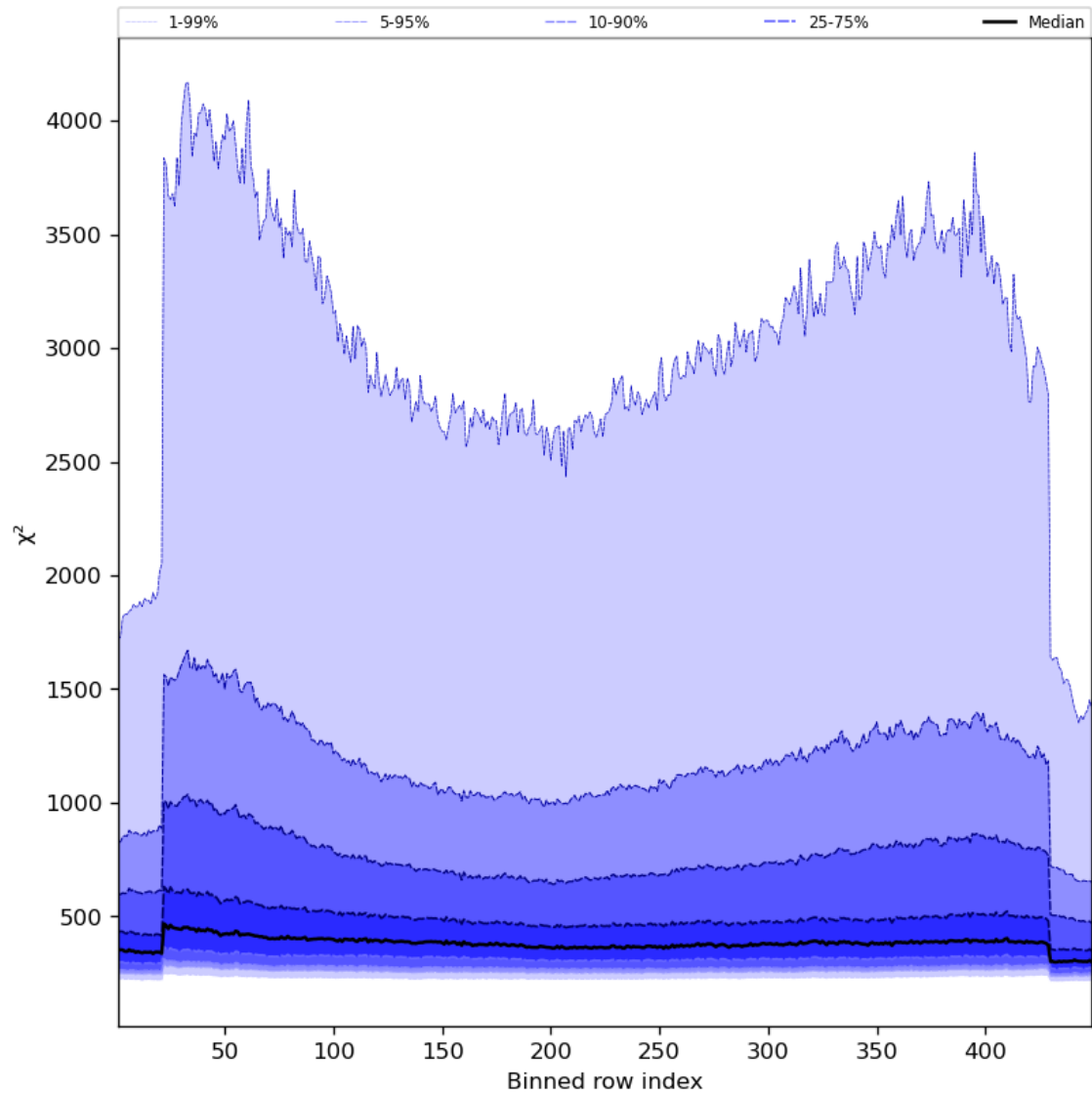
Figure 59: Along track statistics of “ \chi^2 ” for 2023-10-14 to 2023-10-16
