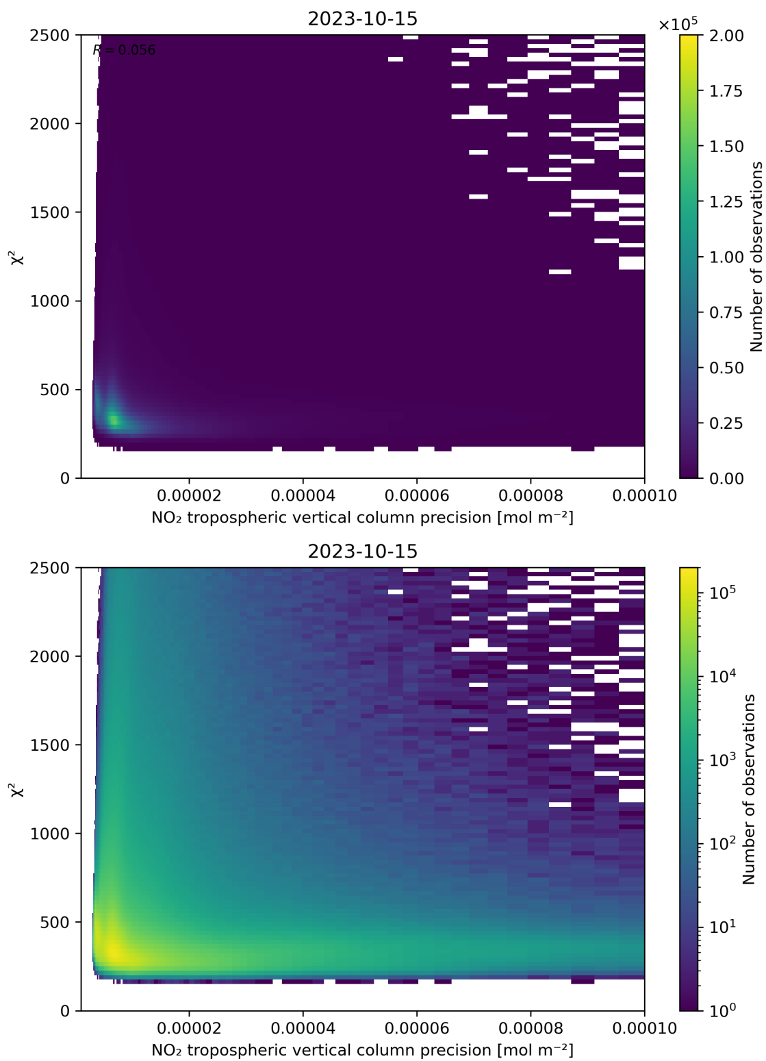
Figure 134: Scatter density plot of “NO 2 tropospheric vertical column precision” against “ \chi^2 ” for 2023-10-14 to 2023-10-16.
