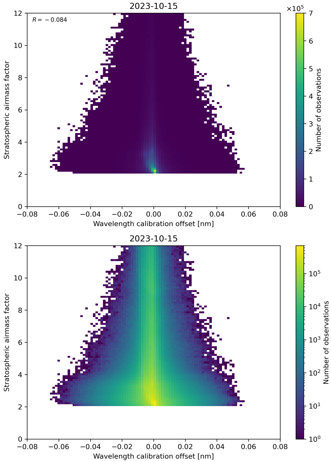
Figure 174: Scatter density plot of “Wavelength calibration offset” against “Stratospheric air mass factor” for 2023-10-14 to 2023-10-16.
