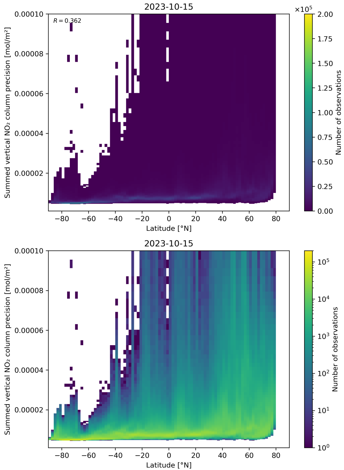
Figure 89: Scatter density plot of “Latitude” against “Summed vertical NO 2 column precision” for 2023-10-14 to 2023-10-16.
