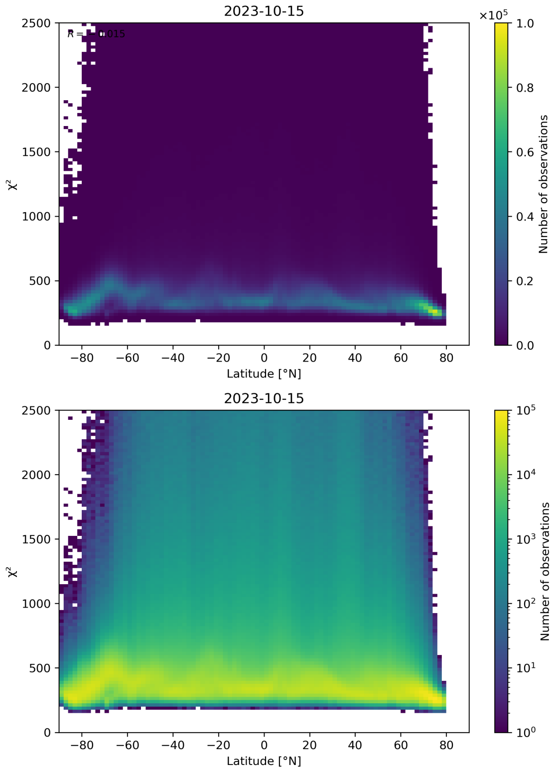
Figure 86: Scatter density plot of “Latitude” against “ \chi^2 ” for 2023-10-14 to 2023-10-16.
