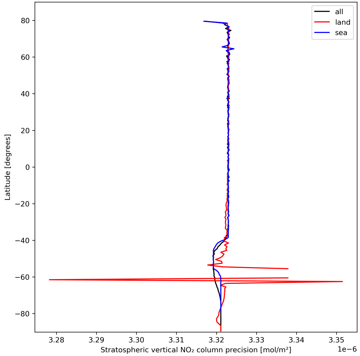
Figure 20: Zonal average of "Stratospheric vertical NO 2 column precision" for 2023-10-14 to 2023-10-16.
