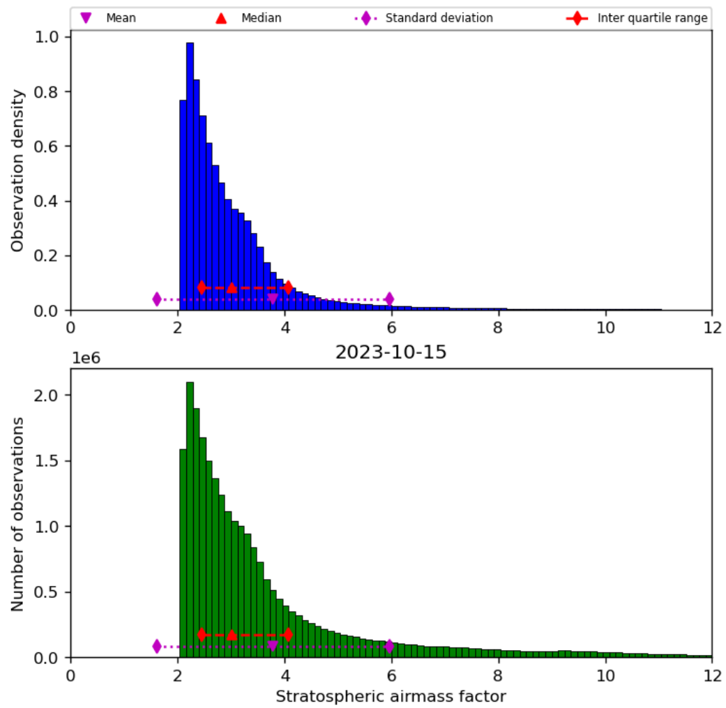
Figure 44: Histogram of “Stratospheric airmass factor” for 2023-10-14 to 2023-10-16
