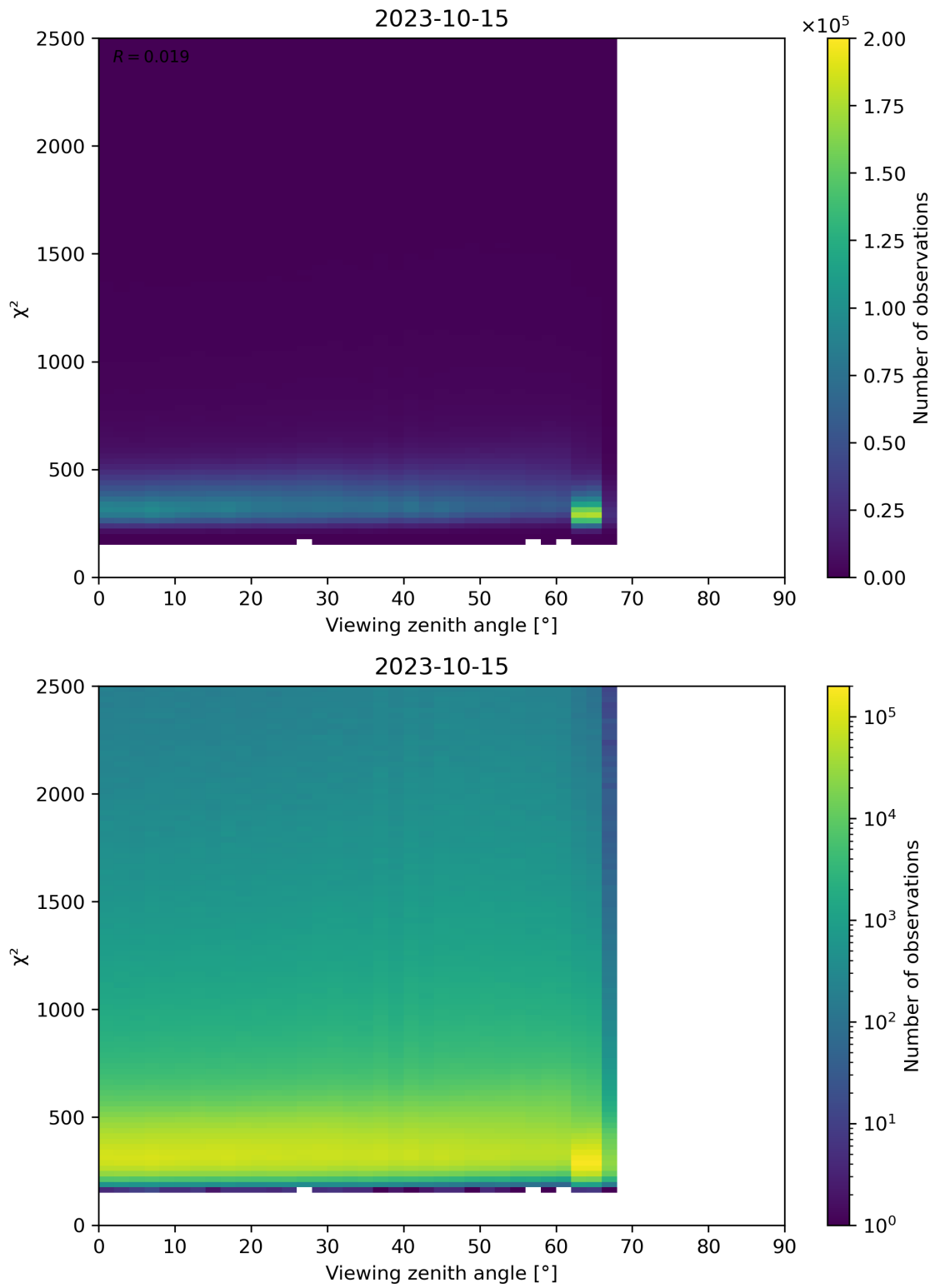
Figure 162: Scatter density plot of “Viewing zenith angle” against “ \chi^2 ” for 2023-10-14 to 2023-10-16.
