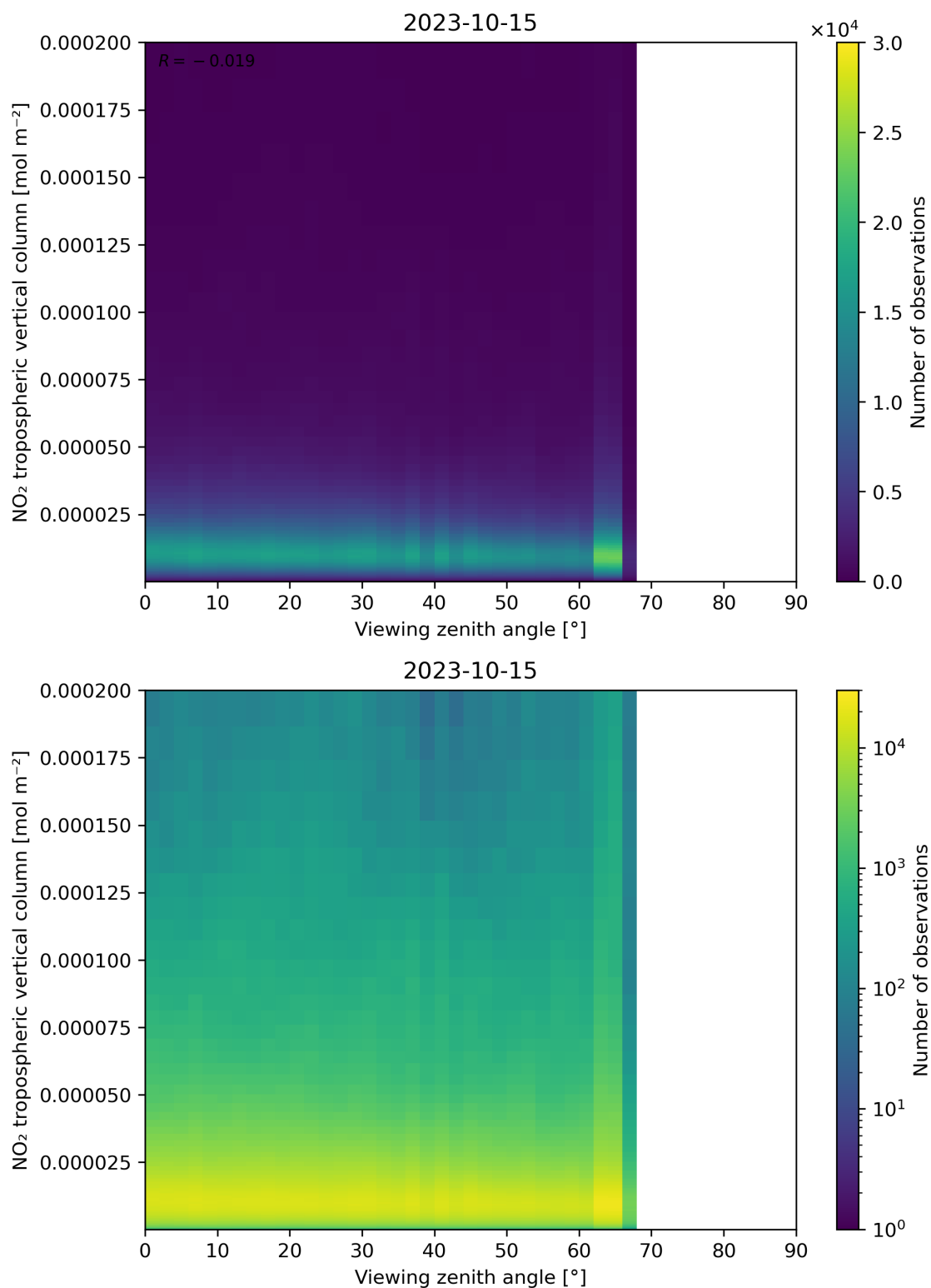
Figure 169: Scatter density plot of “Viewing zenith angle” against “NO 2 tropospheric vertical column” for 2023-10-14 to 2023-10-16.
