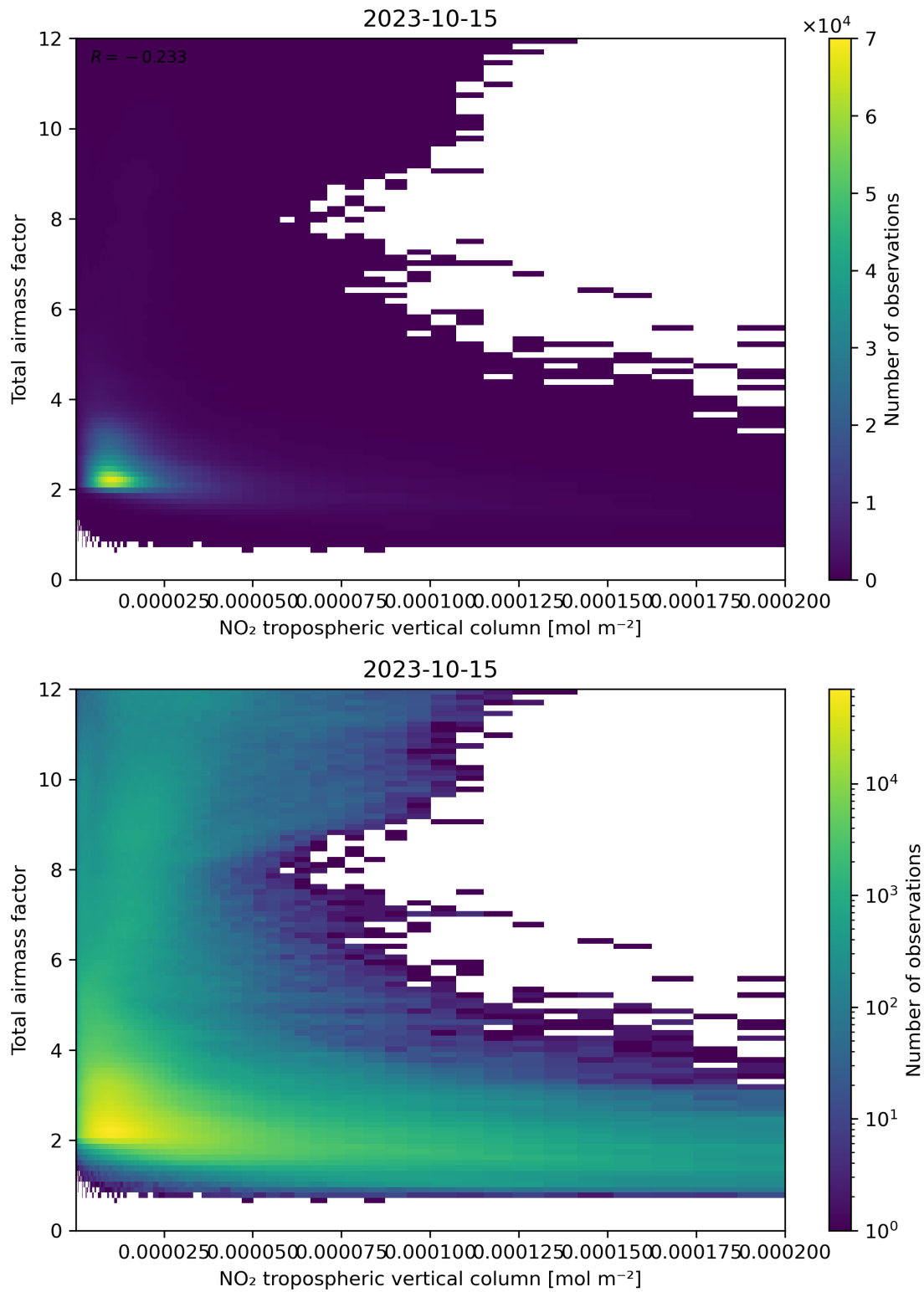
Figure 122: Scatter density plot of “NO 2 tropospheric vertical column” against “Total air mass factor” for 2023-10-14 to 2023-10-16.
