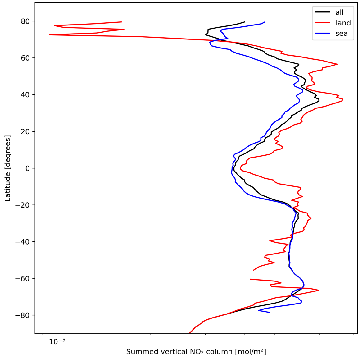
Figure 23: Zonal average of “Summed vertical NO 2 column” for 2023-10-14 to 2023-10-16.
