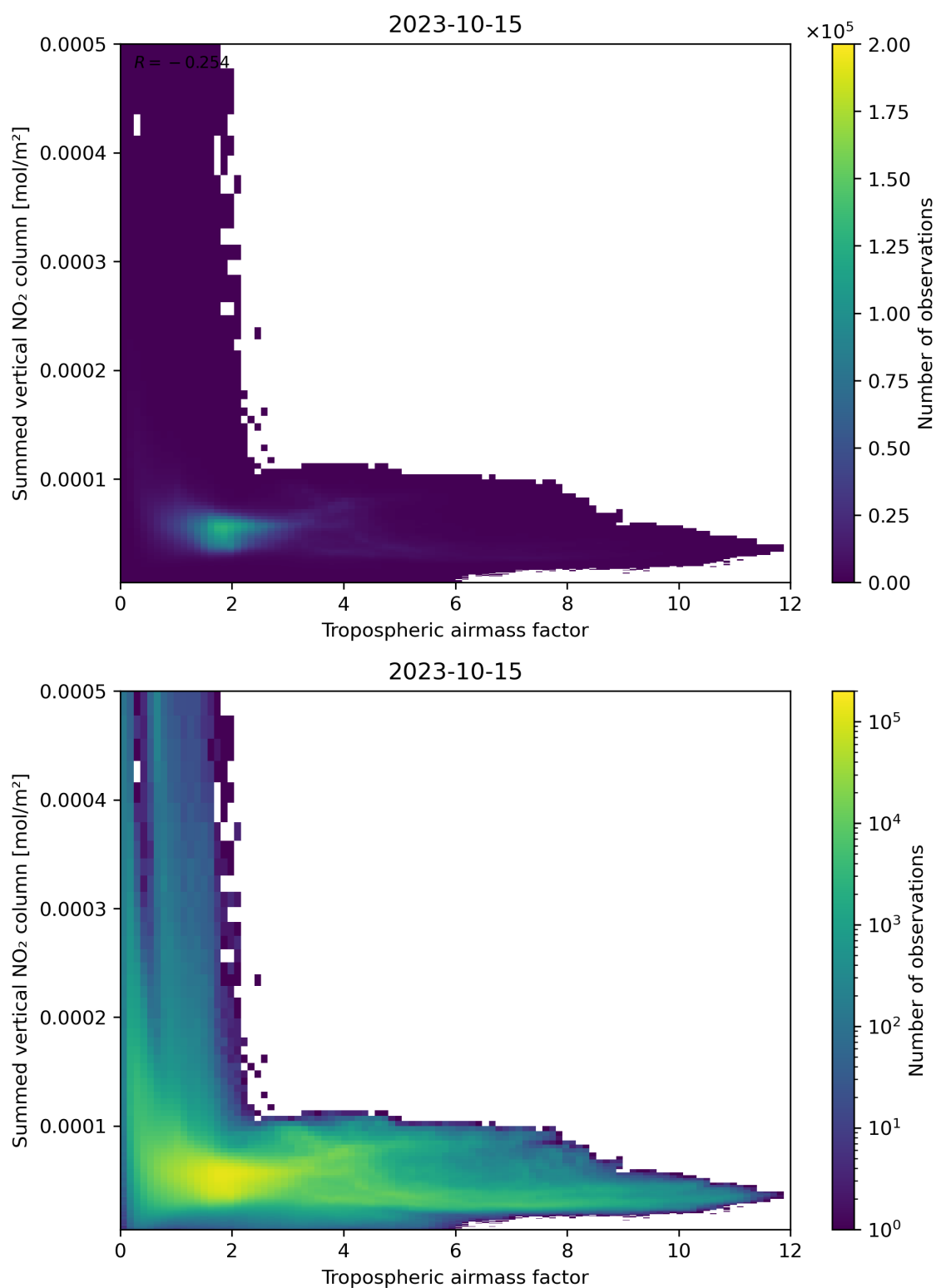
Figure 75: Scatter density plot of “Tropospheric airmass factor” against “Summed vertical NO 2 column” for 2023-10-14 to 2023-10-16.
