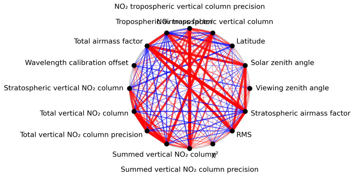
Figure 1: Map of correlation graph for 2023-10-14 to 2023-10-16.
