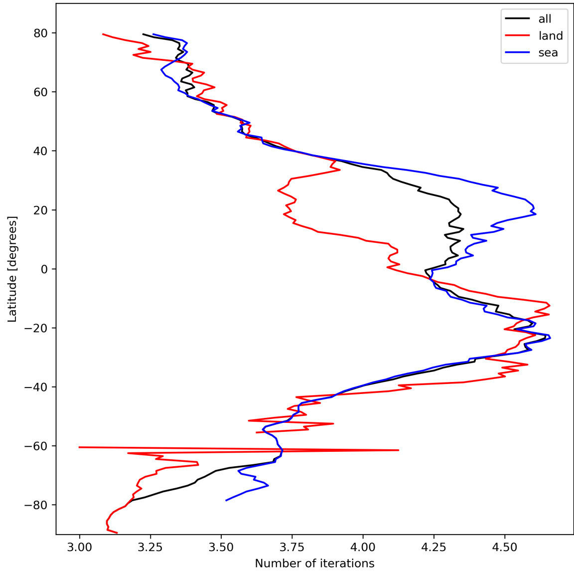
Figure 17: Zonal average of “Number of iterations” for 2023-10-14 to 2023-10-16.
