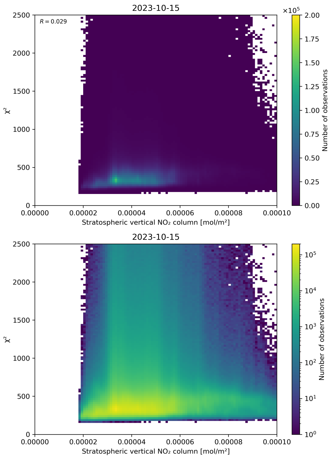
Figure 97: Scatter density plot of “Stratospheric vertical NO 2 column” against “ \chi^2 ” for 2023-10-14 to 2023-10-16.
