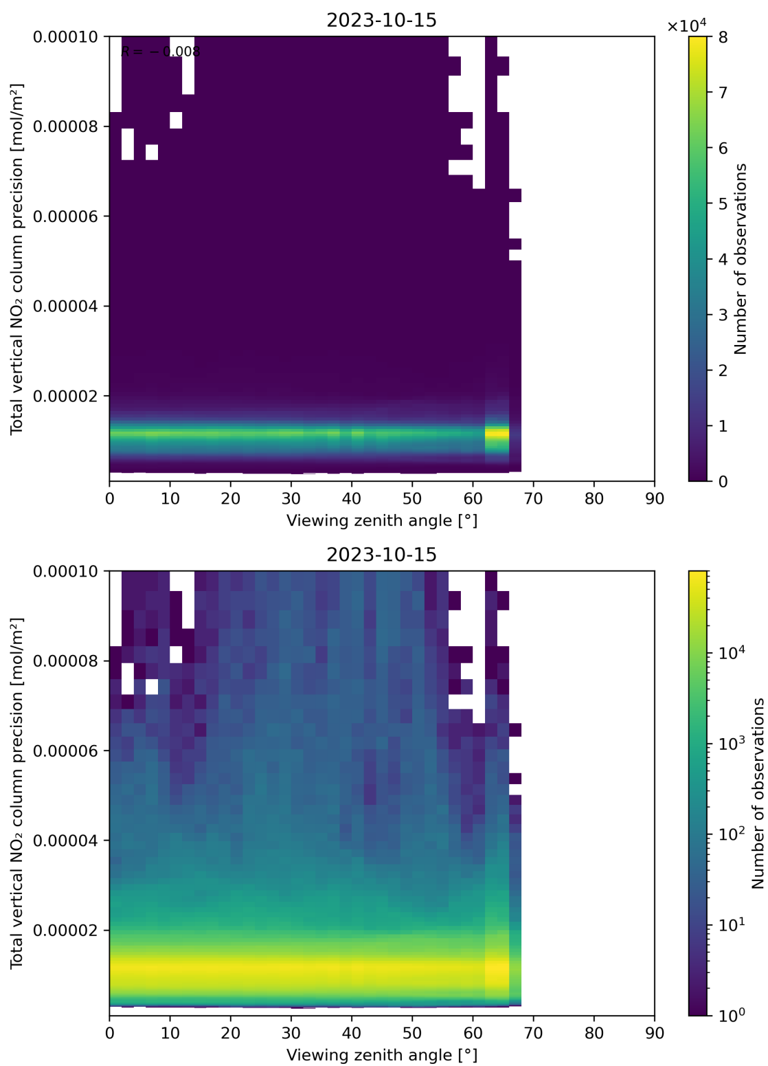
Figure 168: Scatter density plot of “Viewing zenith angle” against “Total vertical NO 2 column precision” for 2023-10-14 to 2023-10-16.
