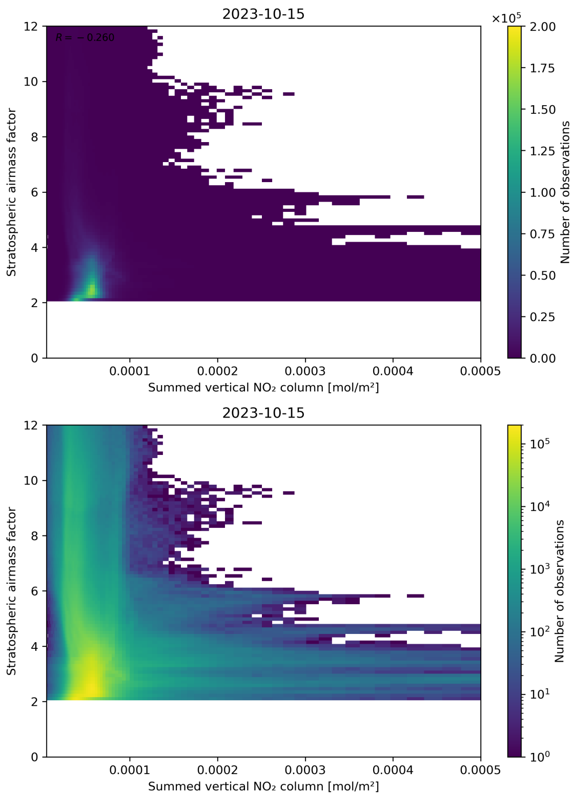
Figure 103: Scatter density plot of “Summed vertical NO 2 column” against “Stratospheric air mass factor” for 2023-10-14 to 2023-10-16.
