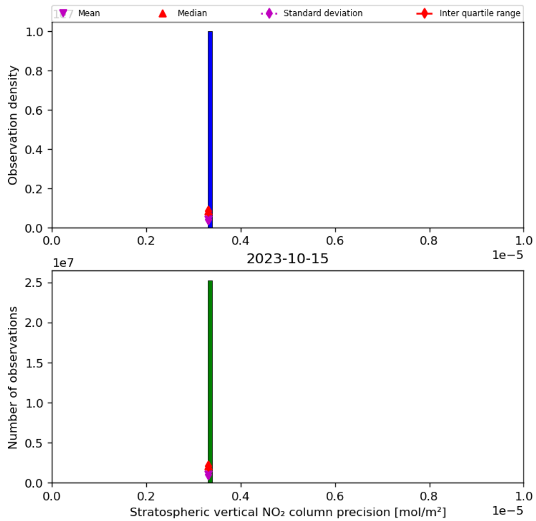
Figure 37: Histogram of “Stratospheric vertical NO 2 column precision” for 2023-10-14 to 2023-10-16
