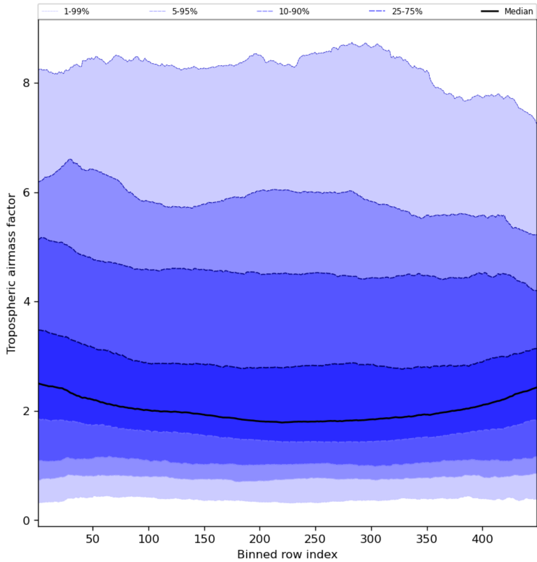
Figure 48: Along track statistics of “Tropospheric airmass factor” for 2023-10-14 to 2023-10-16
