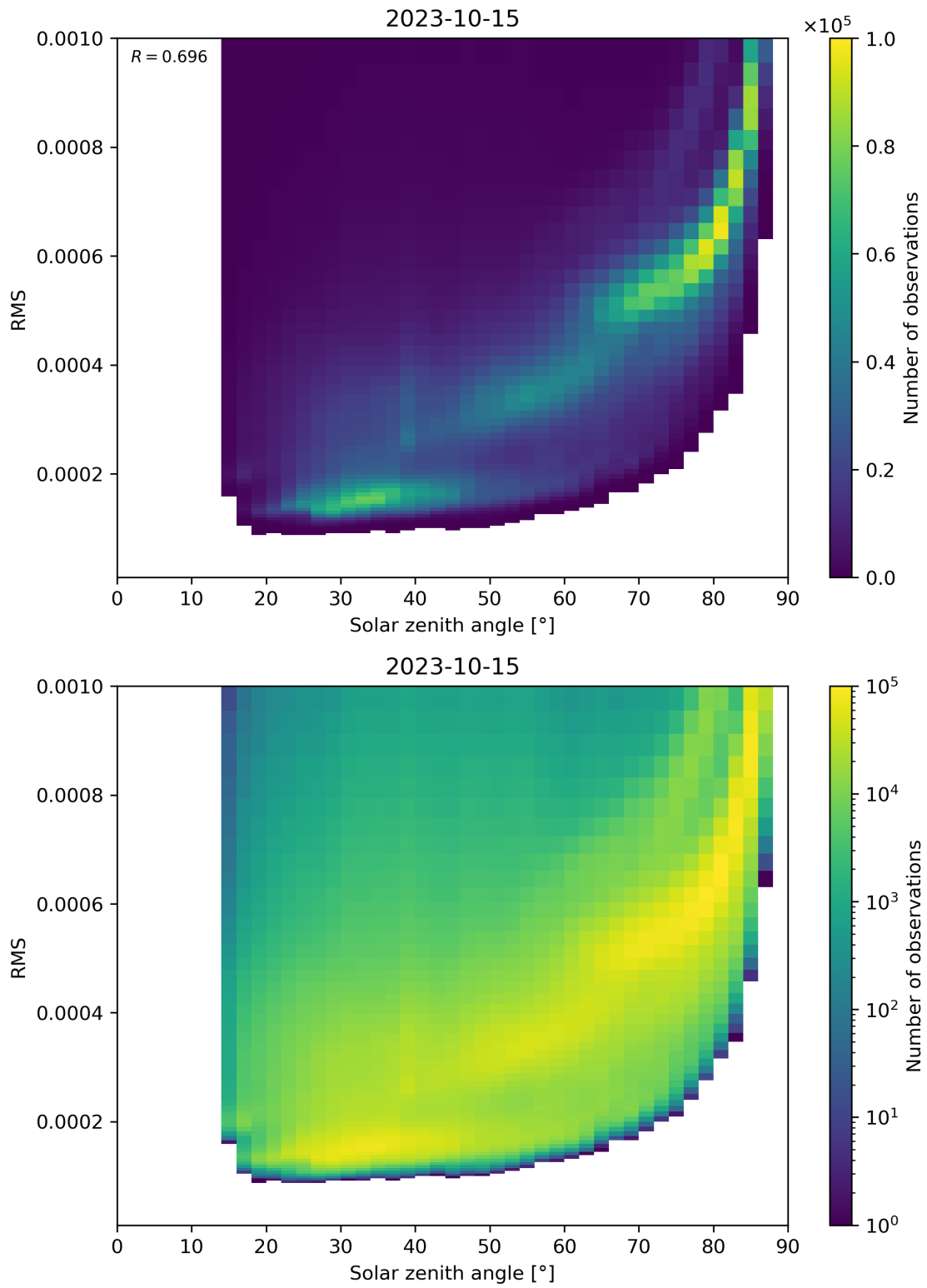
Figure 157: Scatter density plot of “Solar zenith angle” against “RMS” for 2023-10-14 to 2023-10-16.
