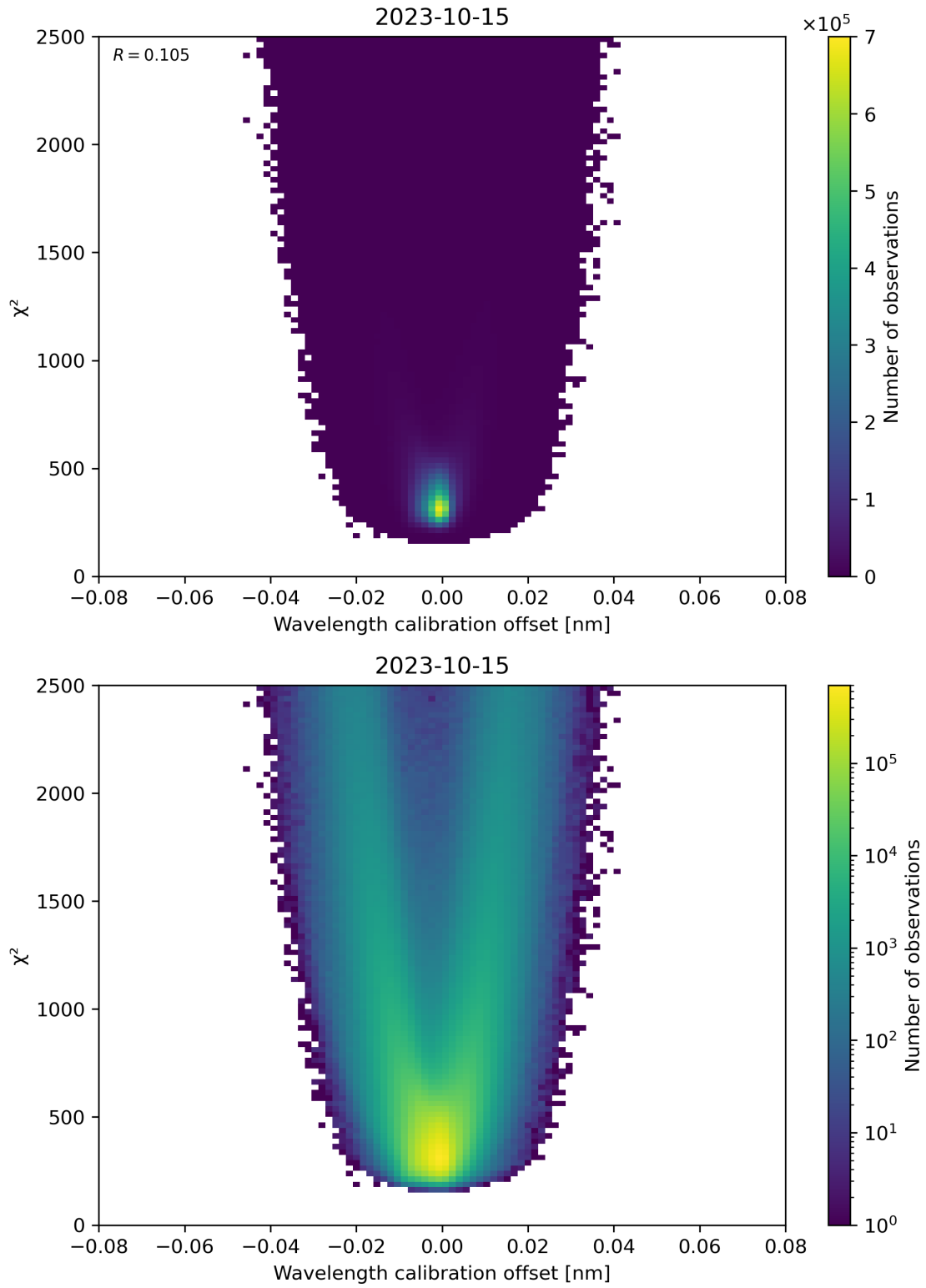
Figure 175: Scatter density plot of “Wavelength calibration offset” against “ \chi^2 ” for 2023-10-14 to 2023-10-16.
