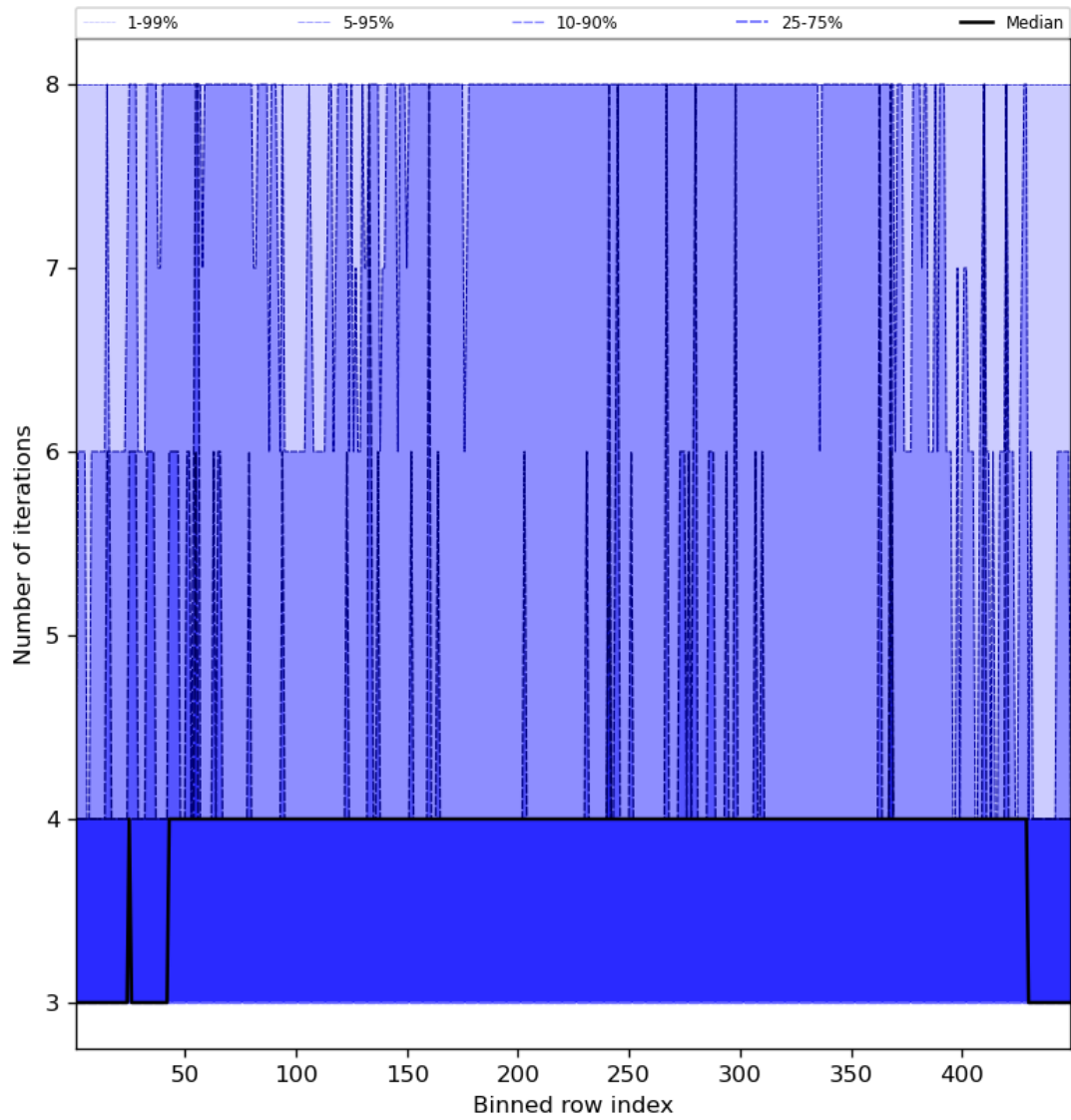
Figure 51: Along track statistics of "Number of iterations" for 2023-10-14 to 2023-10-16
