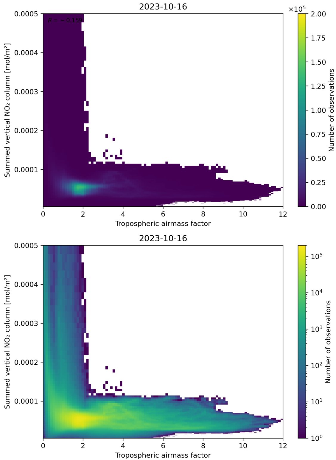
Figure 75: Scatter density plot of “Tropospheric airmass factor” against “Summed vertical NO 2 column” for 2023-10-15 to 2023-10-17.
