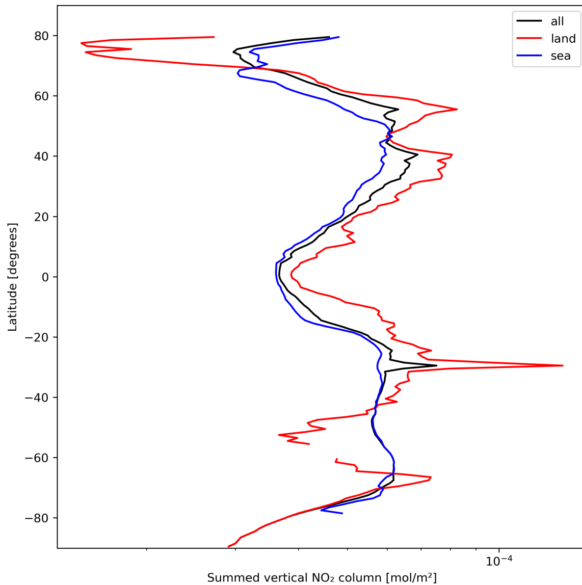
Figure 23: Zonal average of “Summed vertical NO 2 column” for 2023-10-15 to 2023-10-17.
