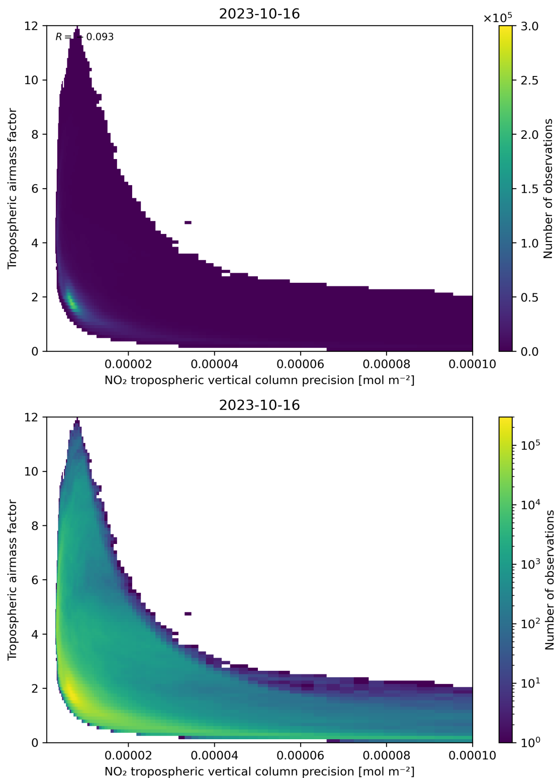
Figure 133: Scatter density plot of “NO 2 tropospheric vertical column precision” against “Tropospheric airmass factor” for 2023-10-15 to 2023-10-17.
