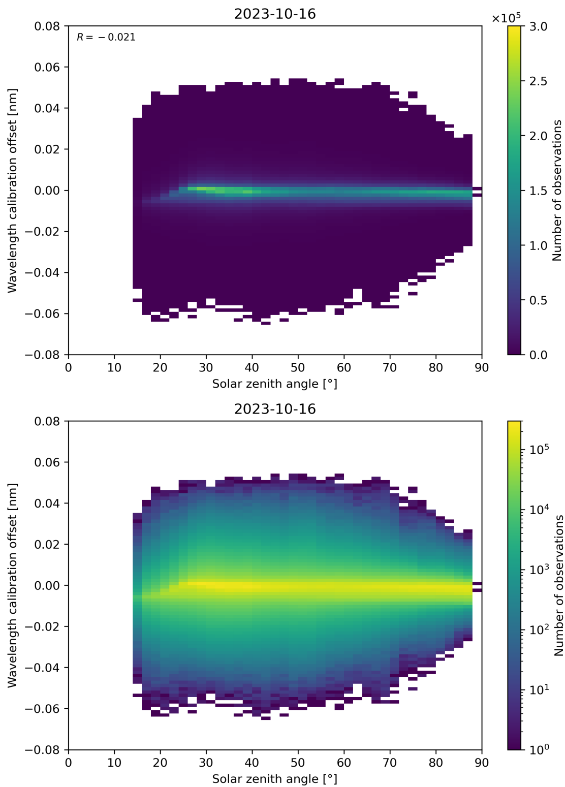
Figure 158: Scatter density plot of “Solar zenith angle” against “Wavelength calibration offset” for 2023-10-15 to 2023-10-17.
