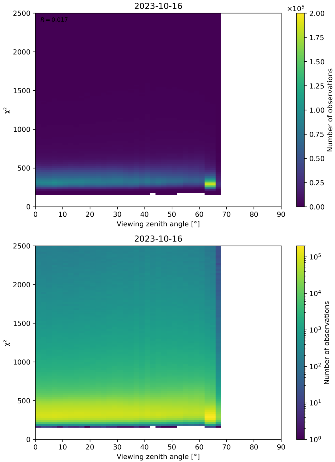
Figure 162: Scatter density plot of “Viewing zenith angle” against “ \chi^2 ” for 2023-10-15 to 2023-10-17.
