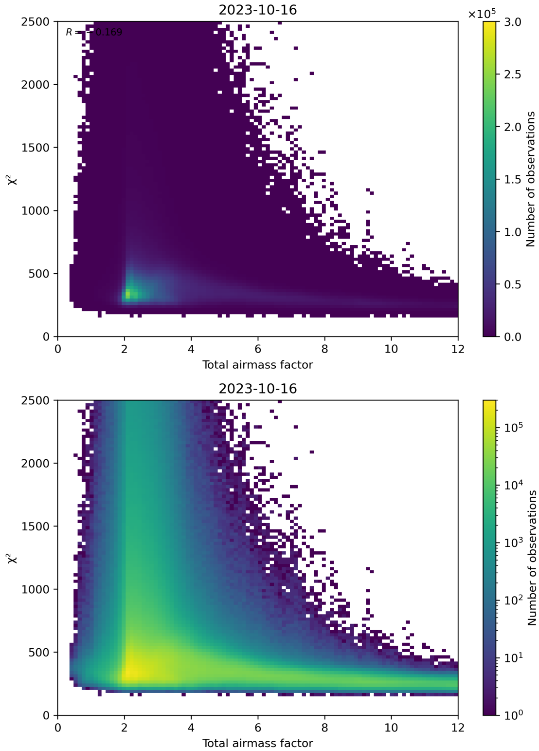
Figure 63: Scatter density plot of “Total airmass factor” against “ \chi^2 ” for 2023-10-15 to 2023-10-17.
