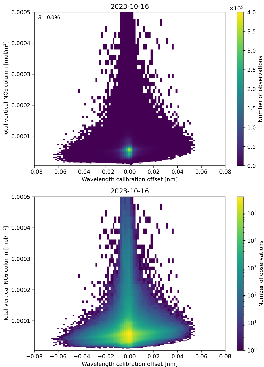
Figure 179: Scatter density plot of “Wavelength calibration offset” against “Total vertical NO 2 column” for 2023-10-15 to 2023-10-17.
