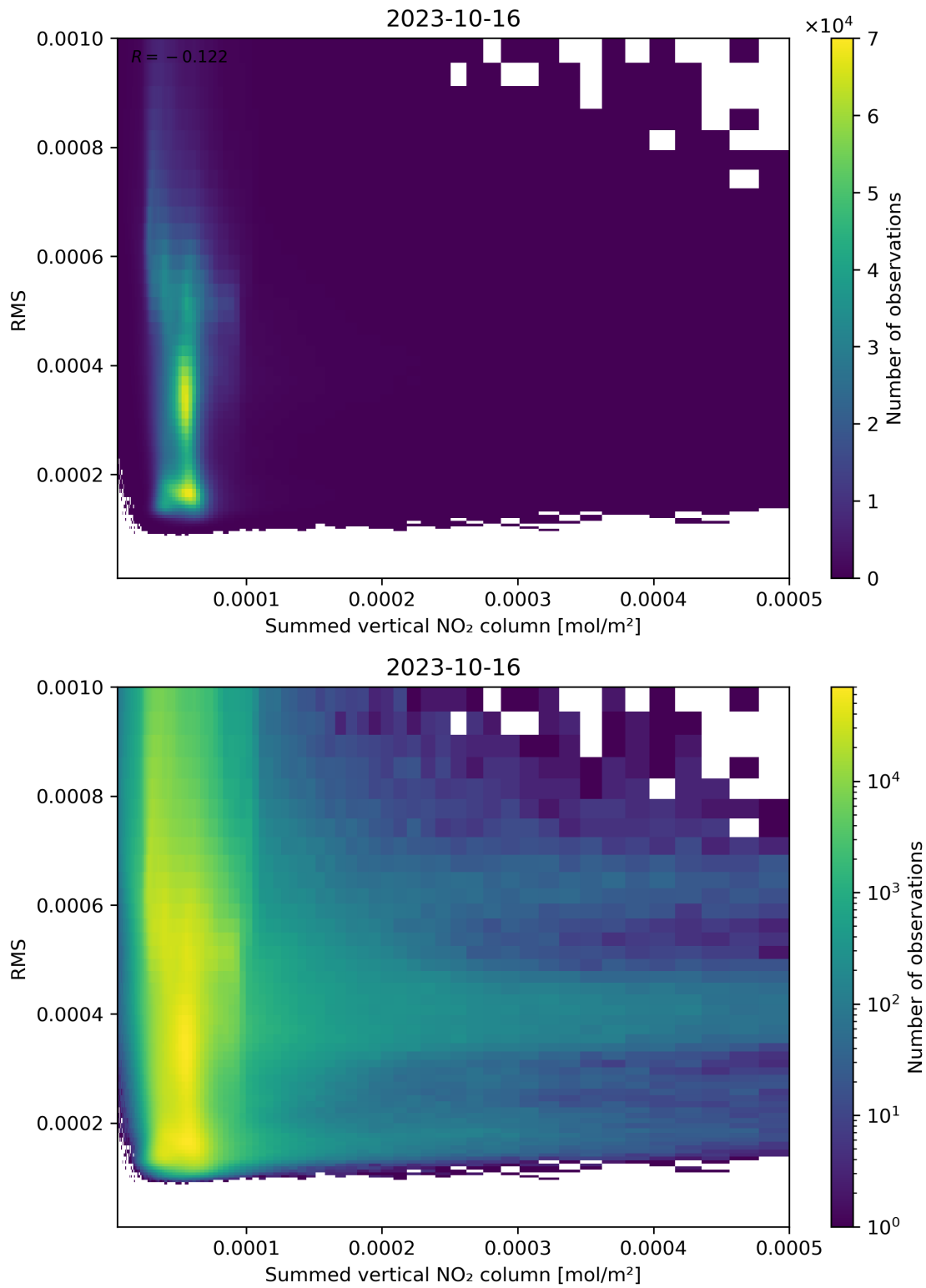
Figure 109: Scatter density plot of “Summed vertical NO 2 column” against “RMS” for 2023-10-15 to 2023-10-17.
