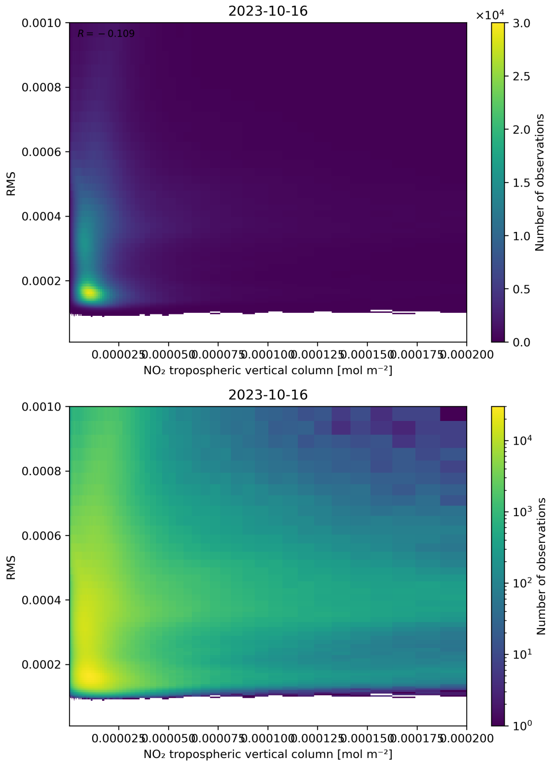
Figure 142: Scatter density plot of “NO 2 tropospheric vertical column” against “RMS” for 2023-10-15 to 2023-10-17.
