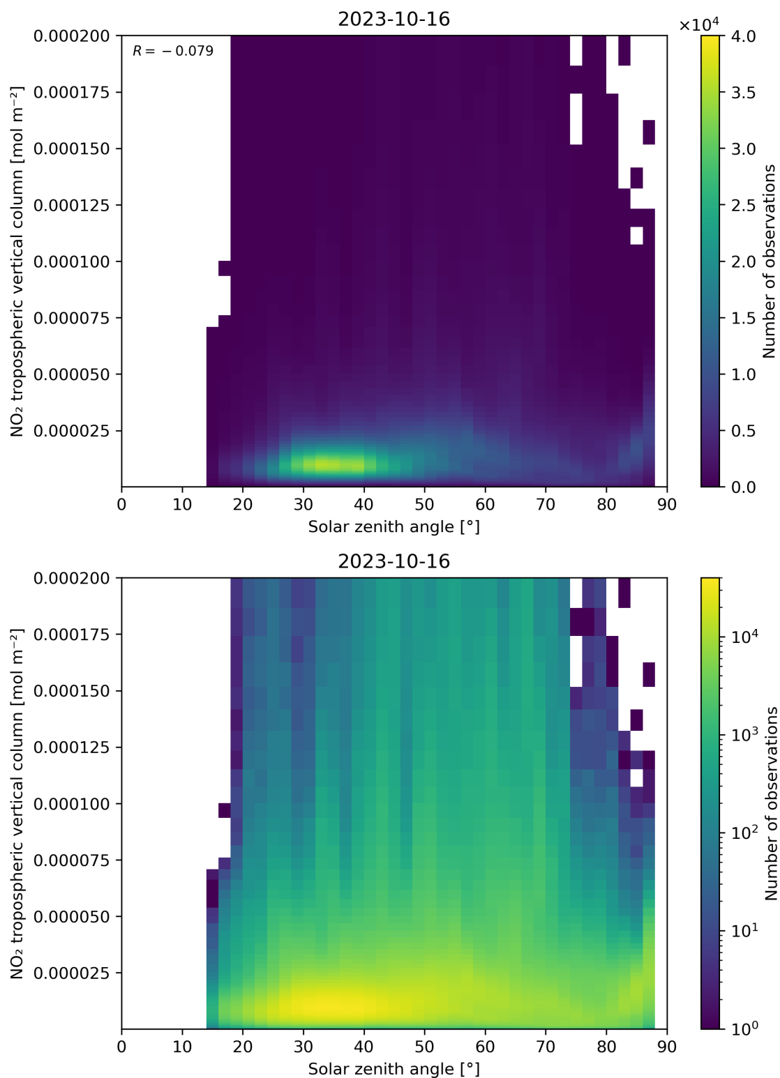
Figure 155: Scatter density plot of “Solar zenith angle” against “NO 2 tropospheric vertical column” for 2023-10-15 to 2023-10-17.
