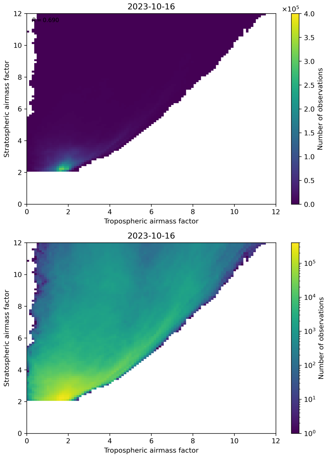
Figure 71: Scatter density plot of “Tropospheric airmass factor” against “Stratospheric airmass factor” for 2023-10-15 to 2023-10-17.
