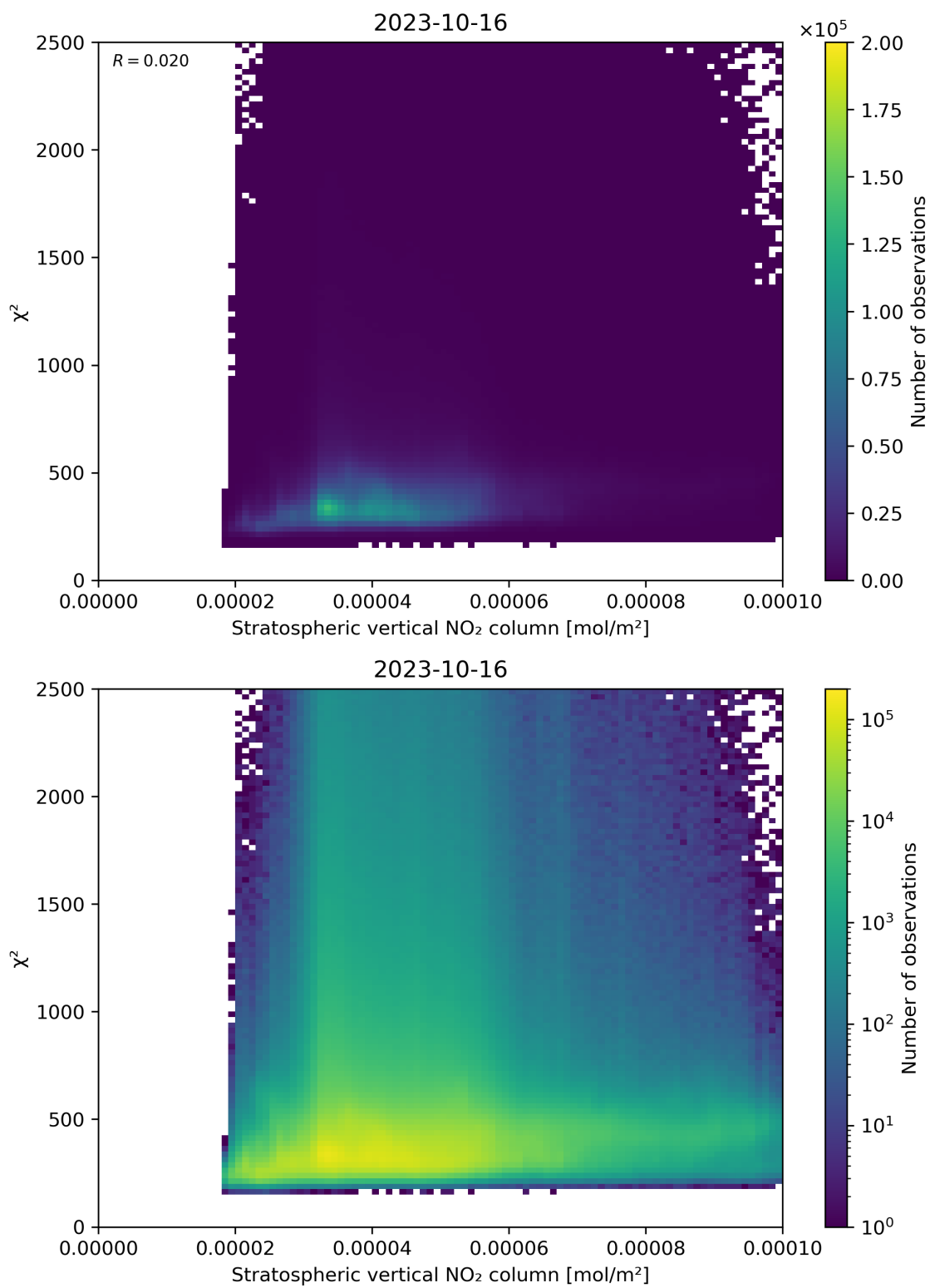
Figure 97: Scatter density plot of “Stratospheric vertical NO 2 column” against “ \chi^2 ” for 2023-10-15 to 2023-10-17.
