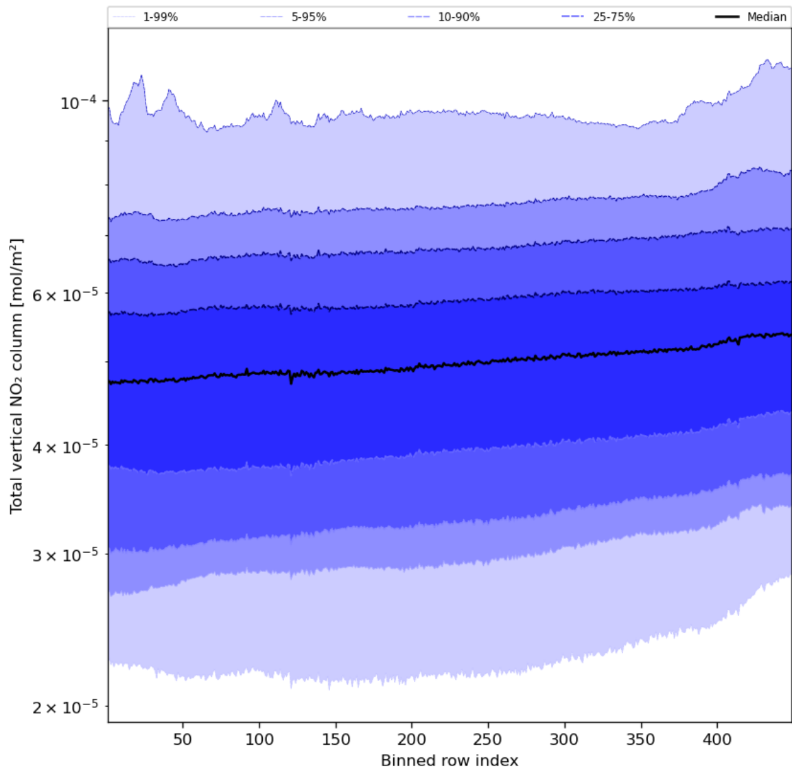
Figure 55: Along track statistics of “Total vertical NO 2 column” for 2023-10-15 to 2023-10-17
