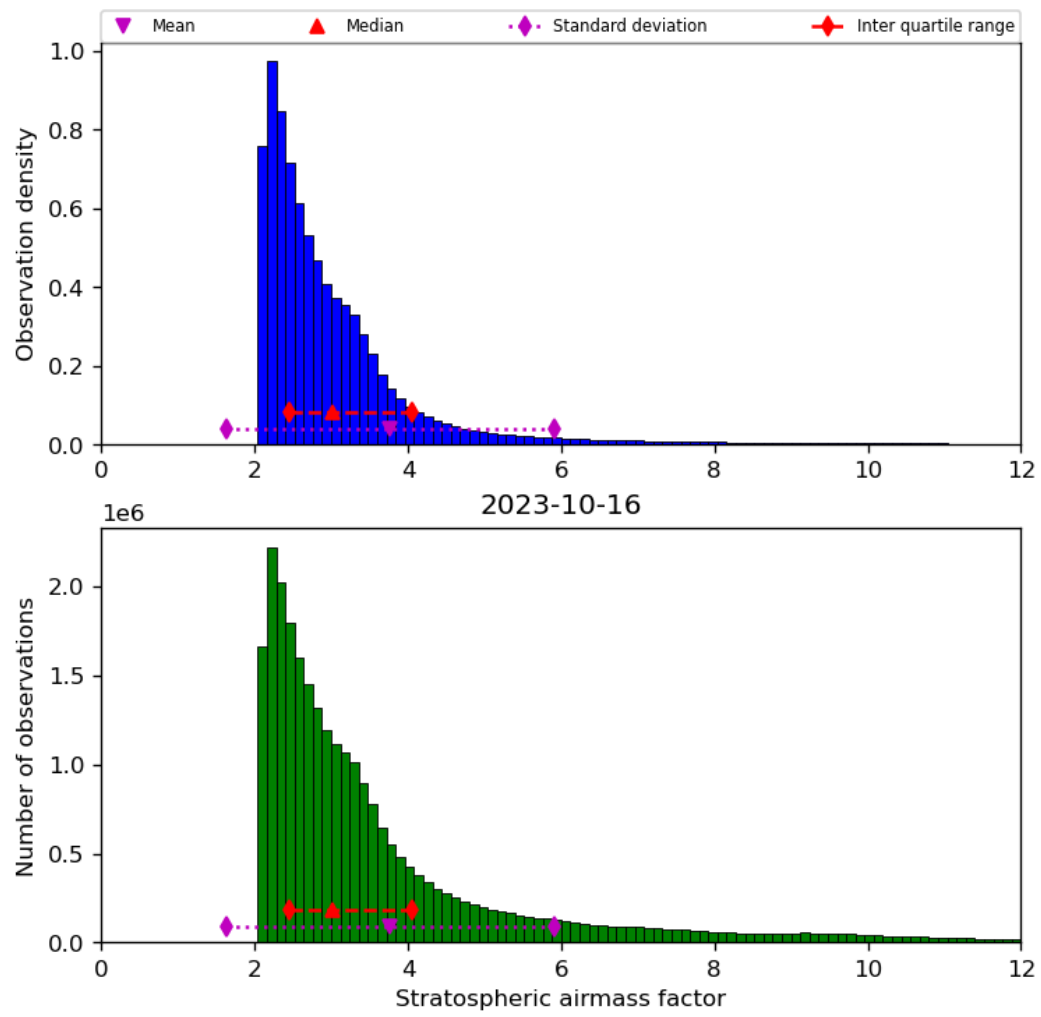
Figure 44: Histogram of “Stratospheric airmass factor” for 2023-10-15 to 2023-10-17
