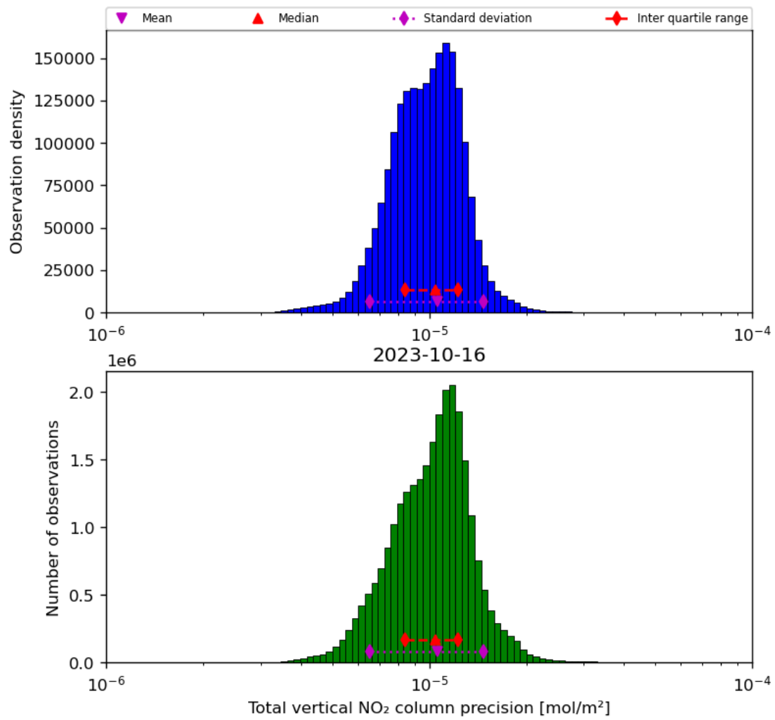
Figure 39: Histogram of “Total vertical NO 2 column precision” for 2023-10-15 to 2023-10-17
