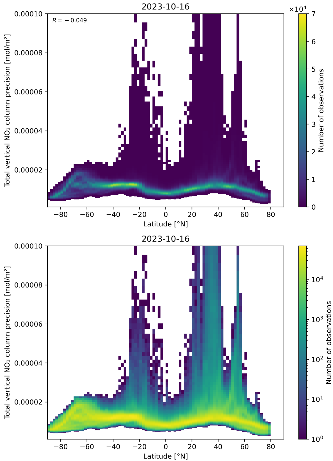
Figure 91: Scatter density plot of “Latitude” against “Total vertical NO 2 column precision” for 2023-10-15 to 2023-10-17.
