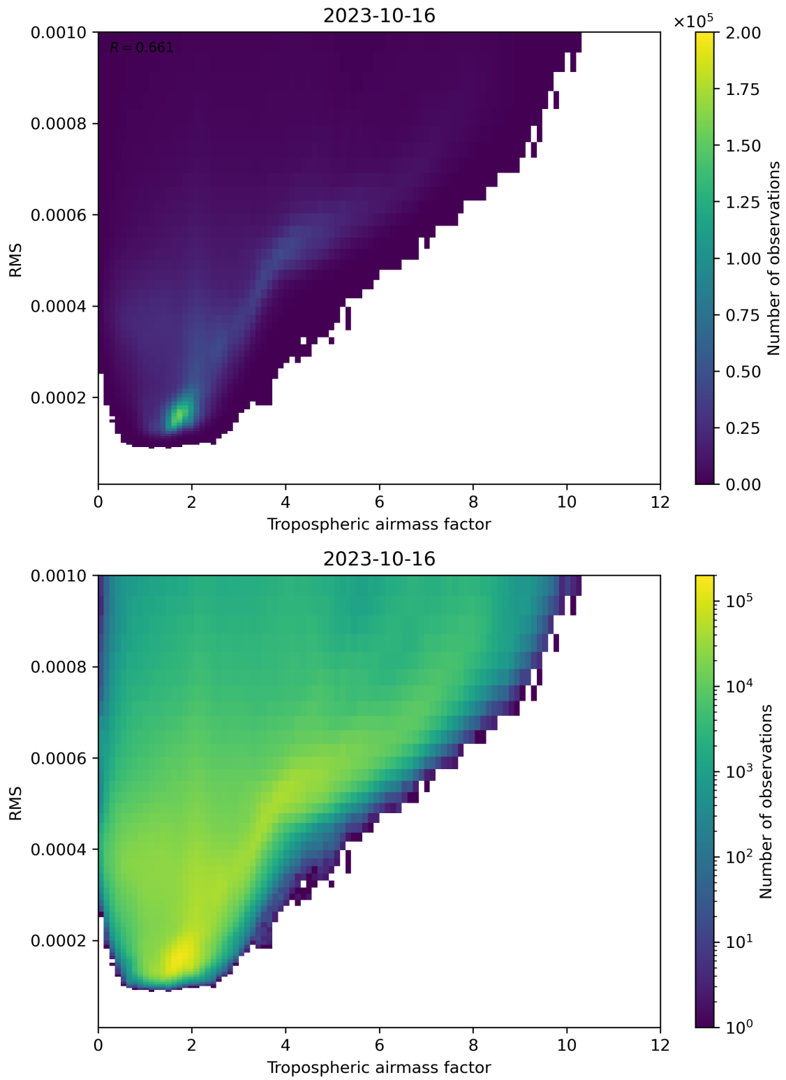
Figure 79: Scatter density plot of “Tropospheric airmass factor” against “RMS” for 2023-10-15 to 2023-10-17.
