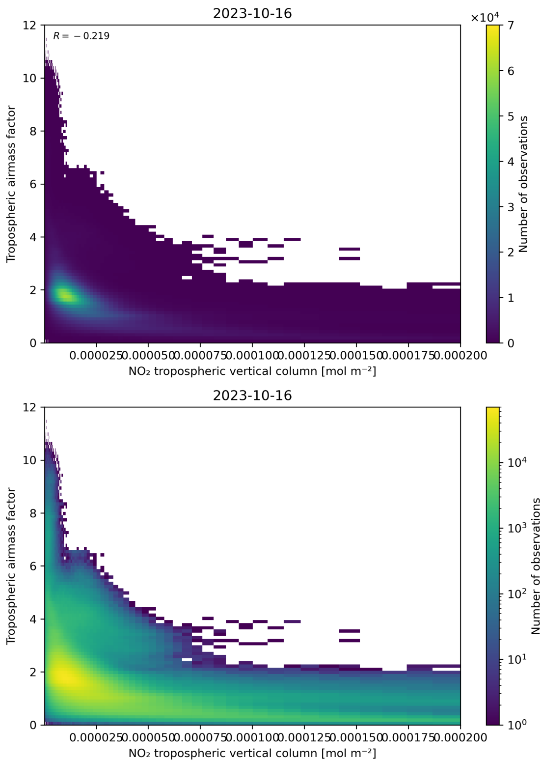
Figure 123: Scatter density plot of “NO 2 tropospheric vertical column” against “Tropospheric air mass factor” for 2023-10-15 to 2023-10-17.
