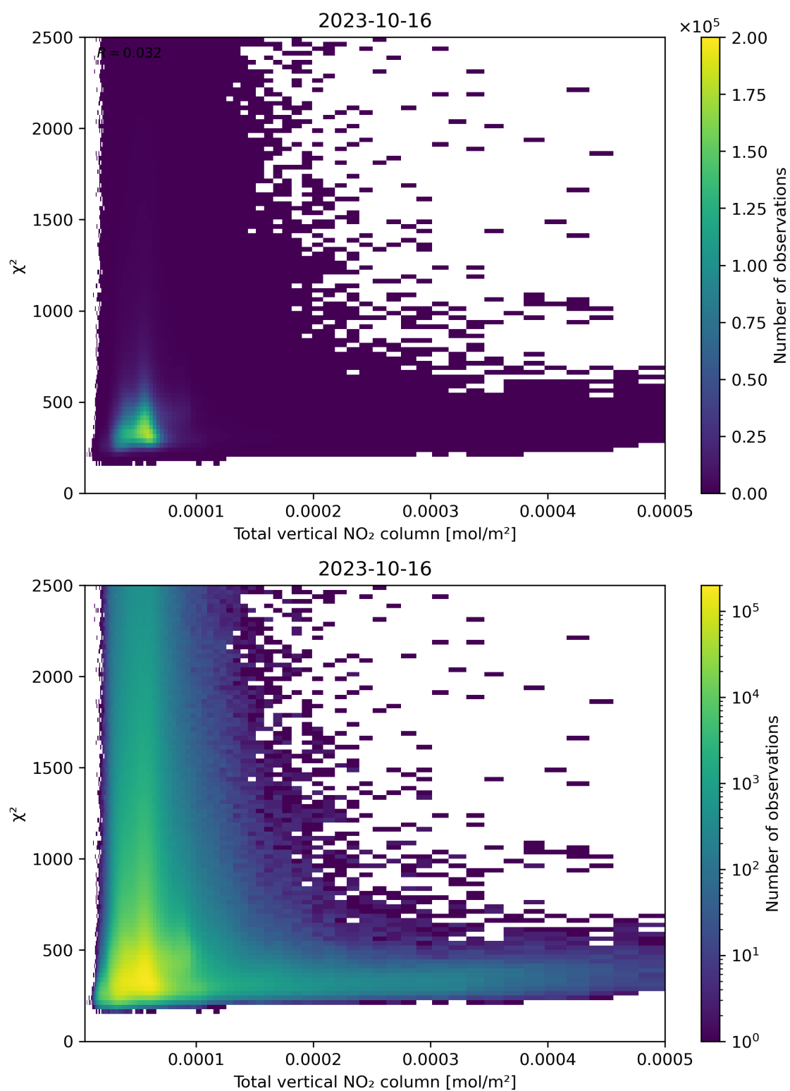
Figure 111: Scatter density plot of “Total vertical NO 2 column” against “ \chi^2 ” for 2023-10-15 to 2023-10-17.
