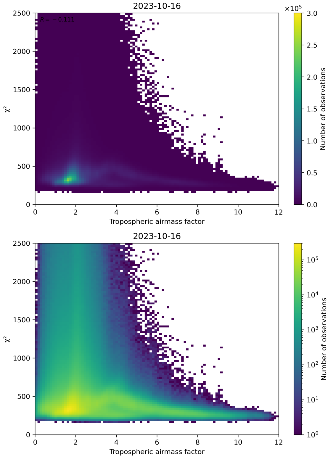
Figure 73: Scatter density plot of “Tropospheric airmass factor” against “ \chi^2 ” for 2023-10-15 to 2023-10-17.
