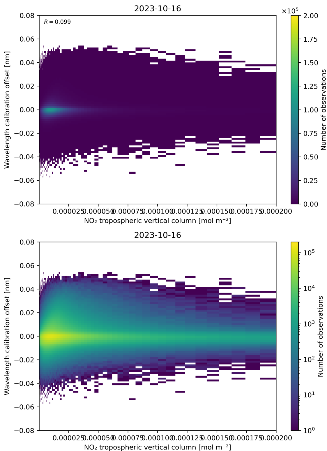
Figure 143: Scatter density plot of “NO 2 tropospheric vertical column” against “Wavelength calibration offset” for 2023-10-15 to 2023-10-17.
