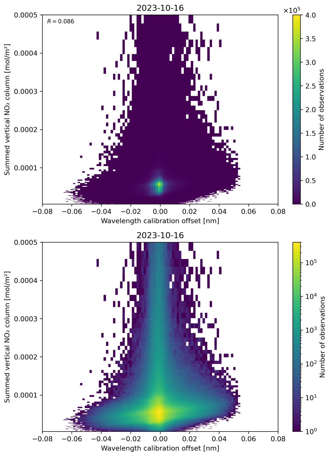
Figure 177: Scatter density plot of “Wavelength calibration offset” against “Summed vertical NO 2 column” for 2023-10-15 to 2023-10-17.
