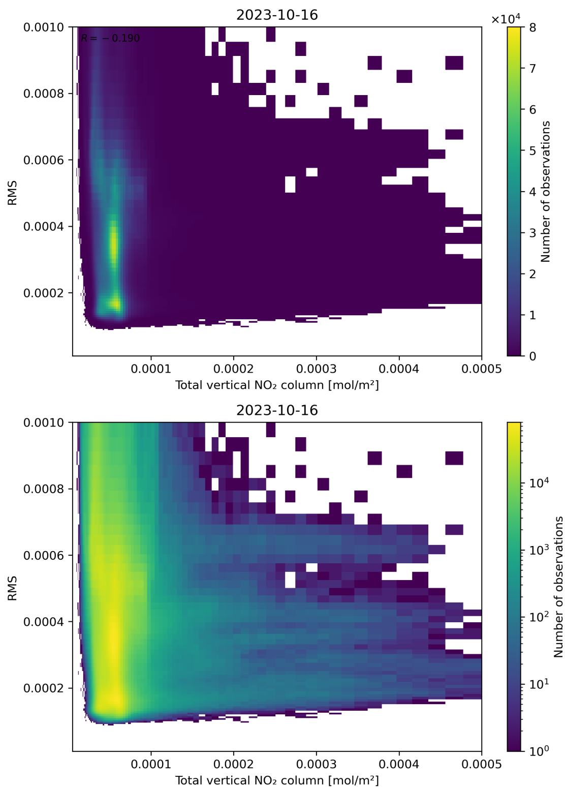
Figure 120: Scatter density plot of “Total vertical NO 2 column” against “RMS” for 2023-10-15 to 2023-10-17.
