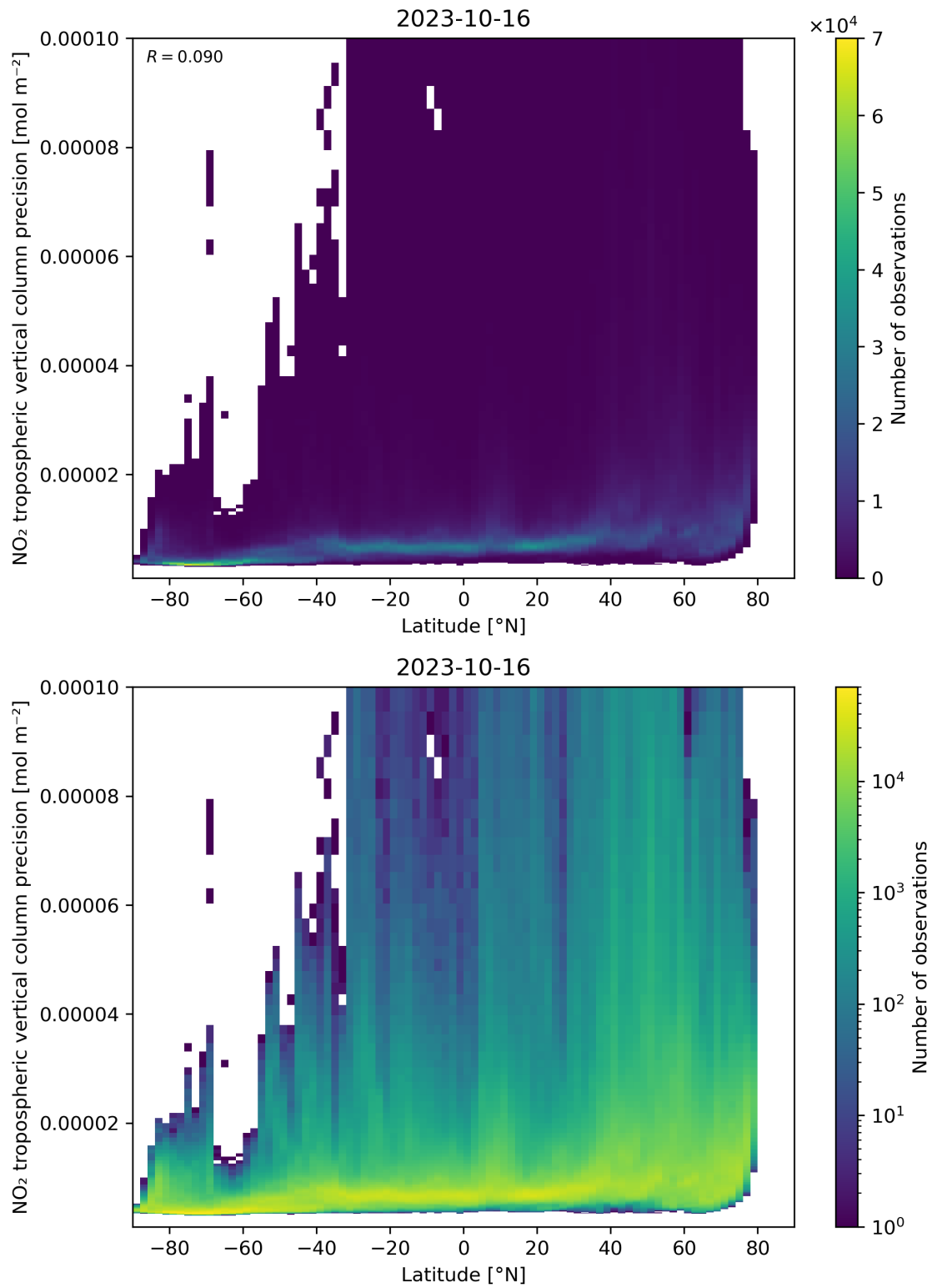
Figure 93: Scatter density plot of “Latitude” against “NO 2 tropospheric vertical column precision” for 2023-10-15 to 2023-10-17.
