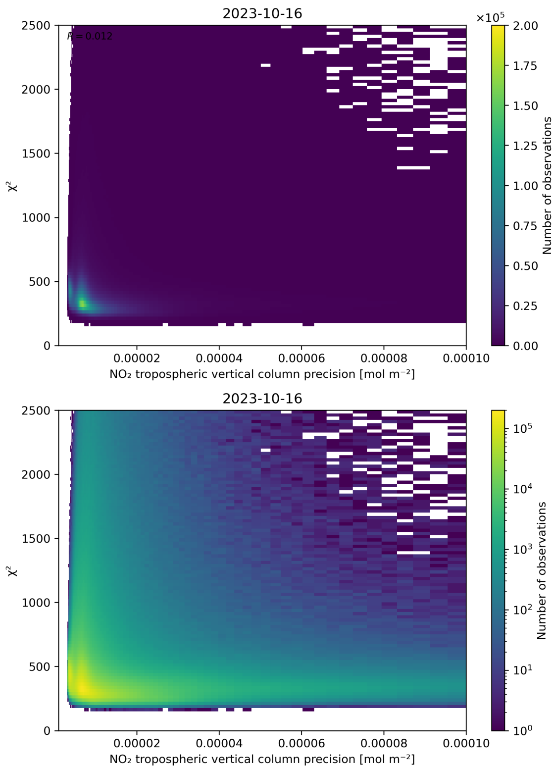
Figure 134: Scatter density plot of “NO 2 tropospheric vertical column precision” against “ \chi^2 ” for 2023-10-15 to 2023-10-17.
