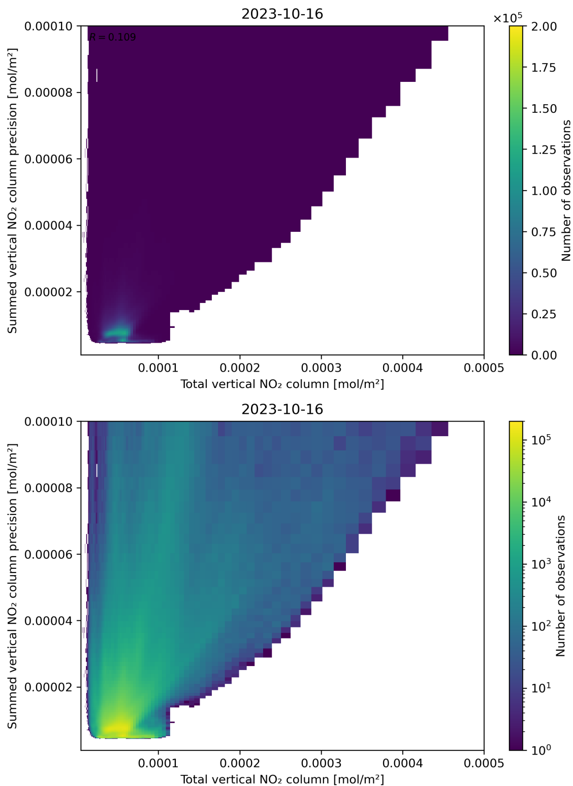
Figure 113: Scatter density plot of “Total vertical NO 2 column” against “Summed vertical NO 2 column precision” for 2023-10-15 to 2023-10-17.
