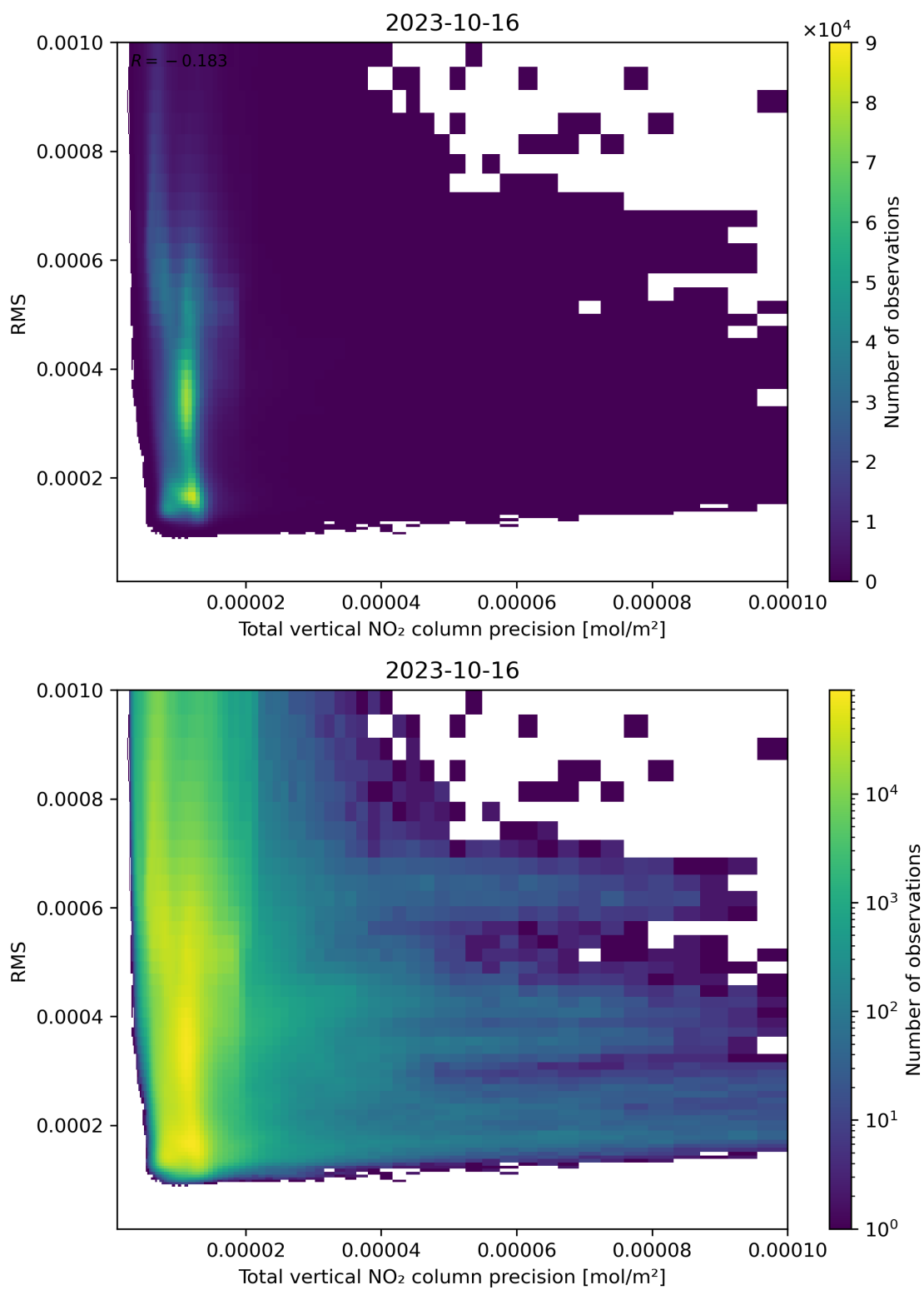
Figure 119: Scatter density plot of “Total vertical NO 2 column precision” against “RMS” for 2023-10-15 to 2023-10-17.
