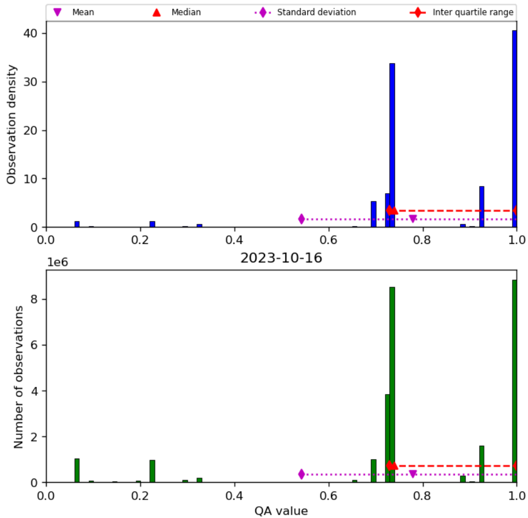
Figure 28: Histogram of “QA value” for 2023-10-15 to 2023-10-17
