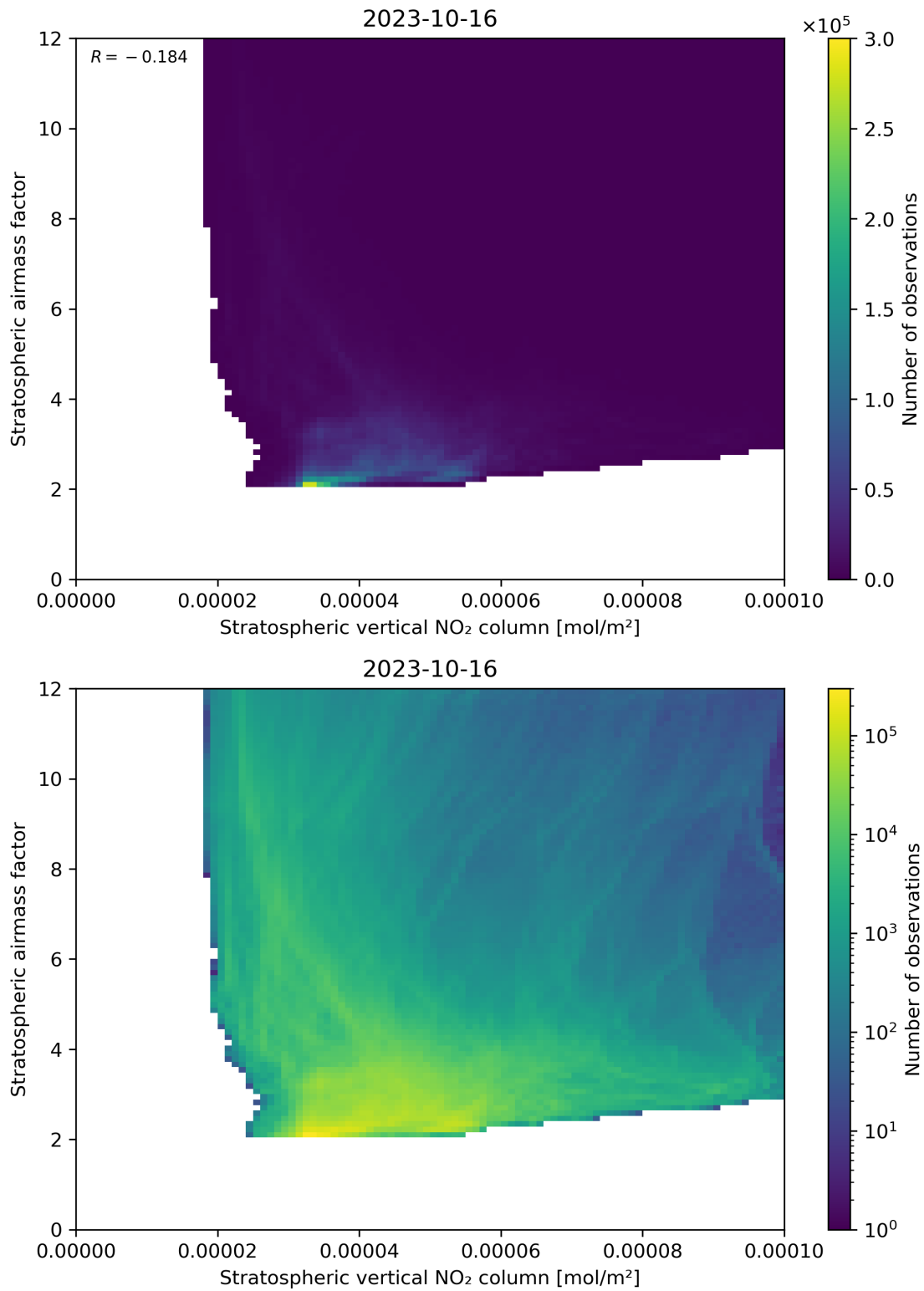
Figure 96: Scatter density plot of “Stratospheric vertical NO 2 column” against “Stratospheric airmass factor” for 2023-10-15 to 2023-10-17.
