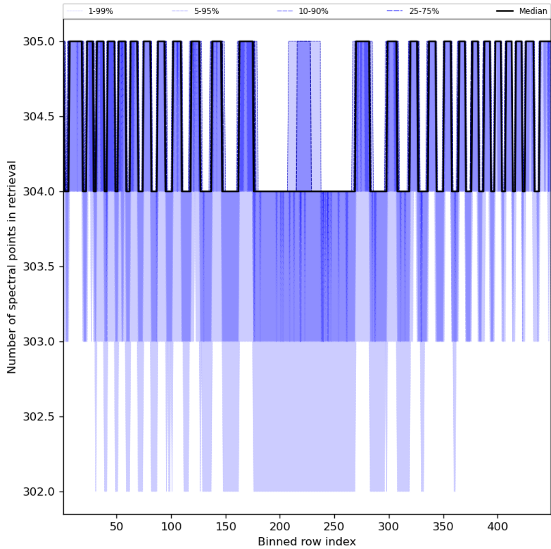
Figure 50: Along track statistics of “Number of spectral points in retrieval” for 2023-10-15 to 2023-10-17
