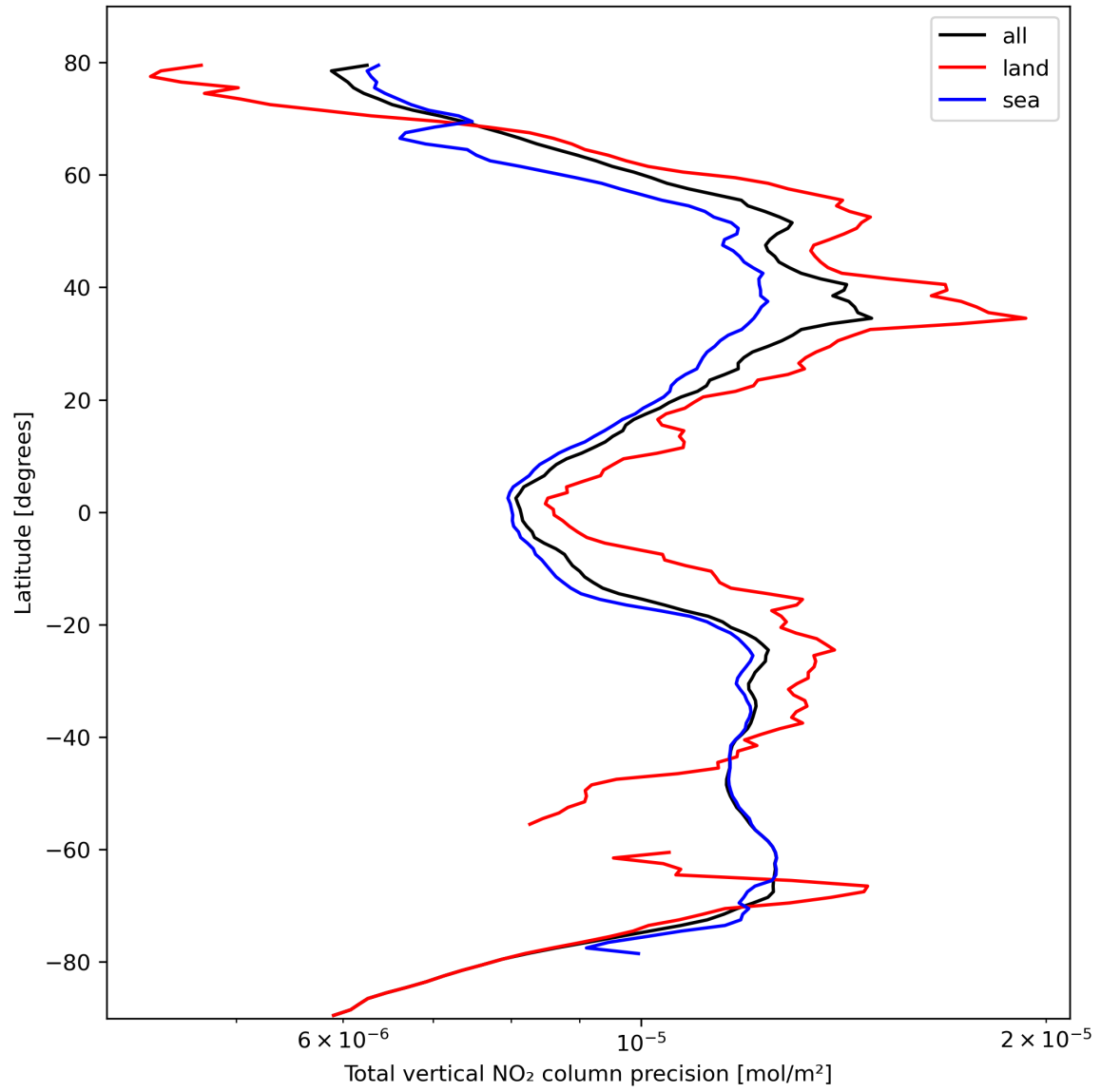
Figure 22: Zonal average of “Total vertical NO 2 column precision” for 2023-10-15 to 2023-10-17.
