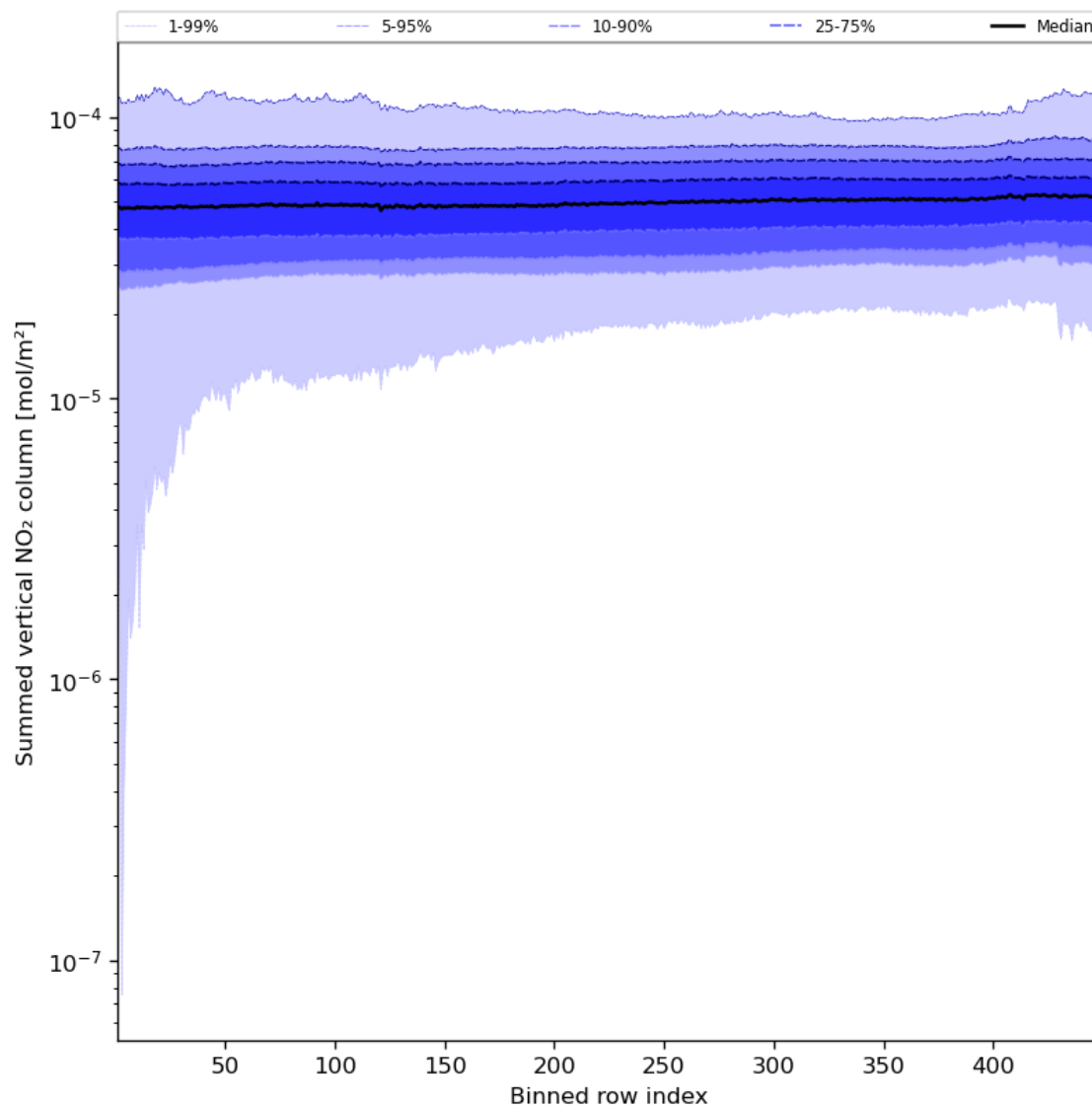
Figure 57: Along track statistics of “Summed vertical NO 2 column” for 2023-10-15 to 2023-10-17
