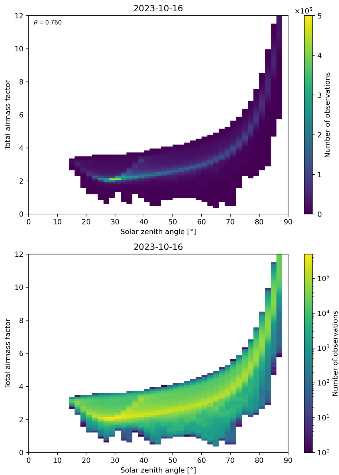
Figure 146: Scatter density plot of “Solar zenith angle” against “Total air mass factor” for 2023-10-15 to 2023-10-17.
