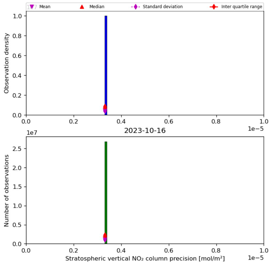
Figure 37: Histogram of “Stratospheric vertical NO 2 column precision” for 2023-10-15 to 2023-10-17
