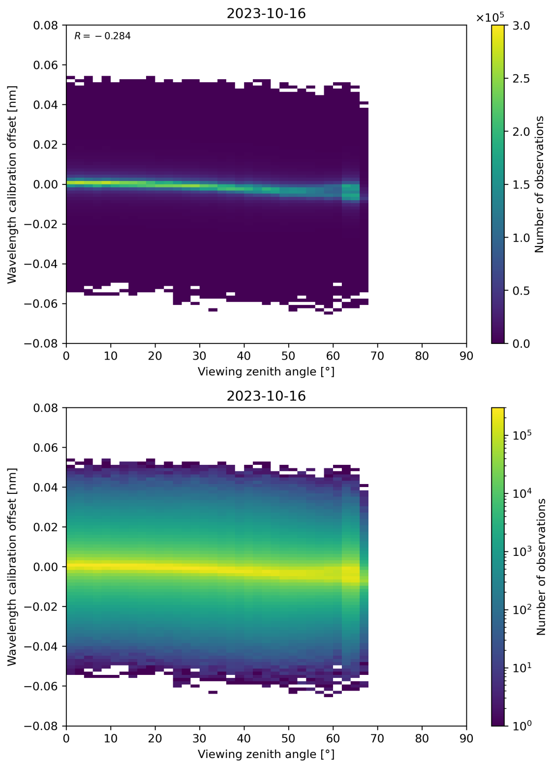
Figure 173: Scatter density plot of “Viewing zenith angle” against “Wavelength calibration offset” for 2023-10-15 to 2023-10-17.
