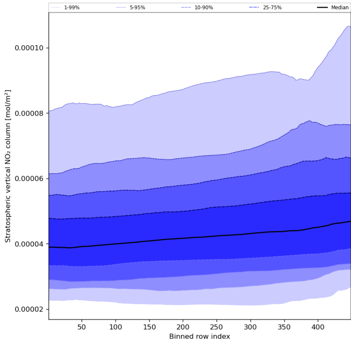
Figure 53: Along track statistics of “Stratospheric vertical NO 2 column” for 2023-10-15 to 2023-10-17
