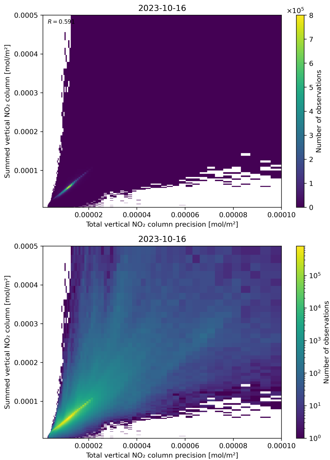
Figure 117: Scatter density plot of “Total vertical NO 2 column precision” against “Summed vertical NO 2 column” for 2023-10-15 to 2023-10-17.
