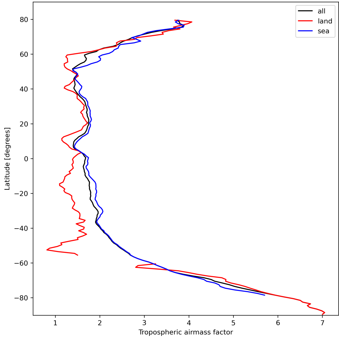
Figure 14: Zonal average of “Tropospheric airmass factor” for 2023-10-15 to 2023-10-17.
