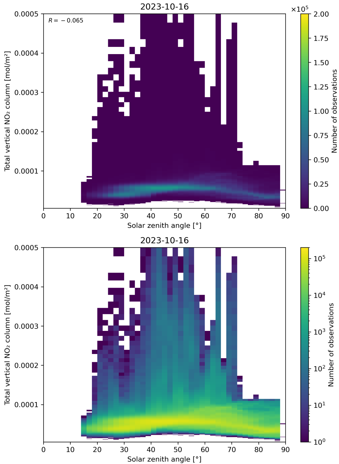
Figure 153: Scatter density plot of “Solar zenith angle” against “Total vertical NO 2 column” for 2023-10-15 to 2023-10-17.
