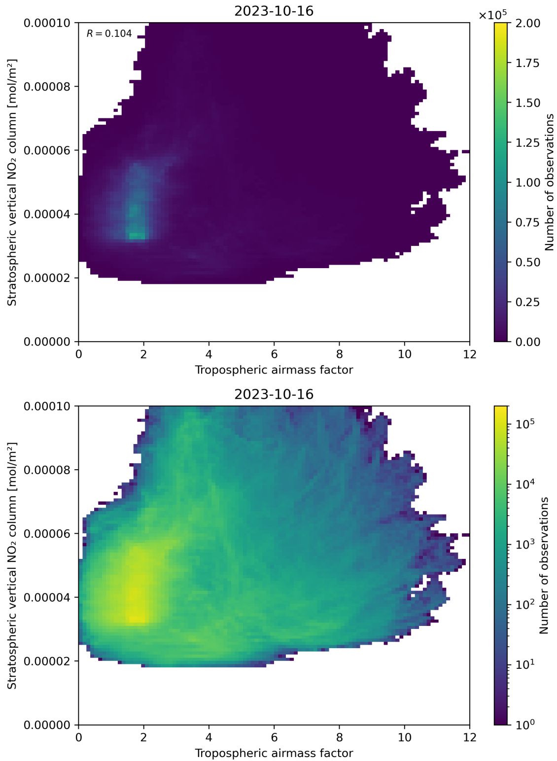
Figure 74: Scatter density plot of “Tropospheric air mass factor” against “Stratospheric vertical NO 2 column” for 2023-10-15 to 2023-10-17.
