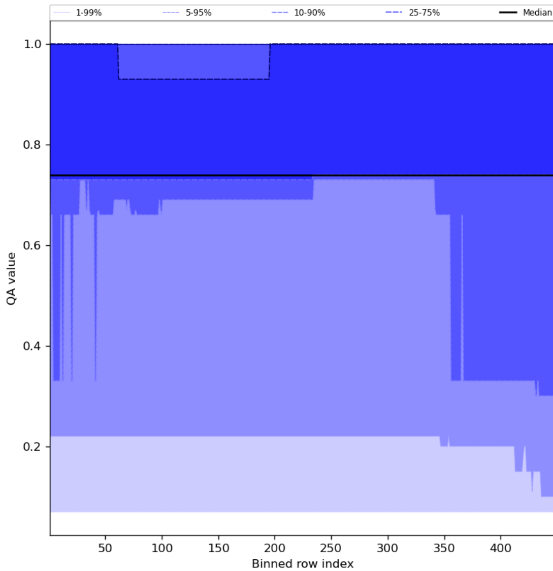
Figure 45: Along track statistics of “QA value” for 2023-10-15 to 2023-10-17
