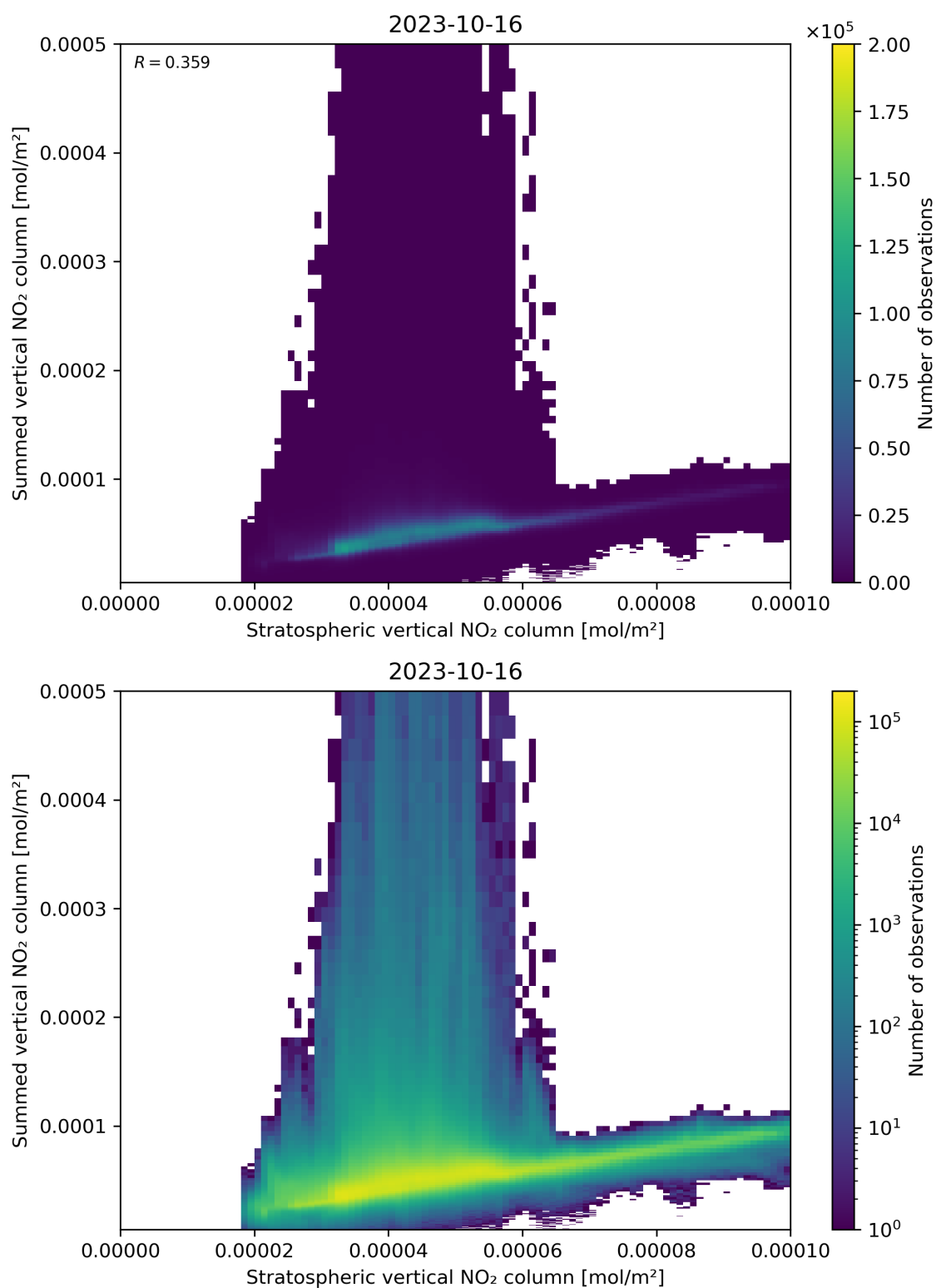
Figure 98: Scatter density plot of “Stratospheric vertical NO 2 column” against “Summed vertical NO 2 column” for 2023-10-15 to 2023-10-17.
