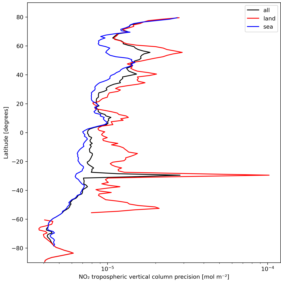
Figure 13: Zonal average of “NO 2 tropospheric vertical column precision” for 2023-10-15 to 2023-10-17.
