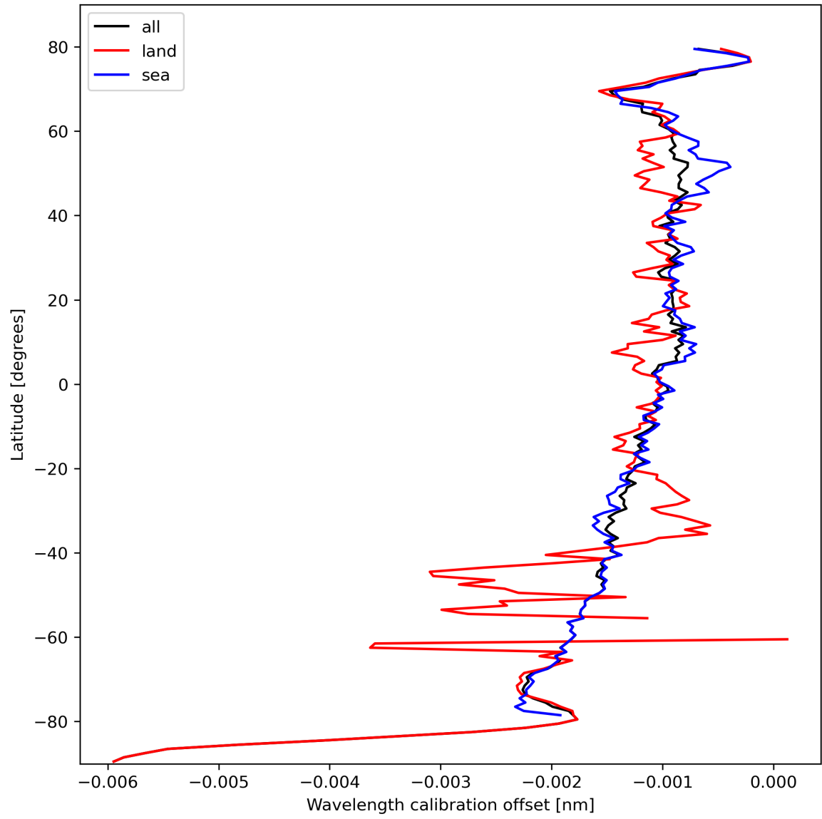
Figure 18: Zonal average of “Wavelength calibration offset” for 2023-10-15 to 2023-10-17.
