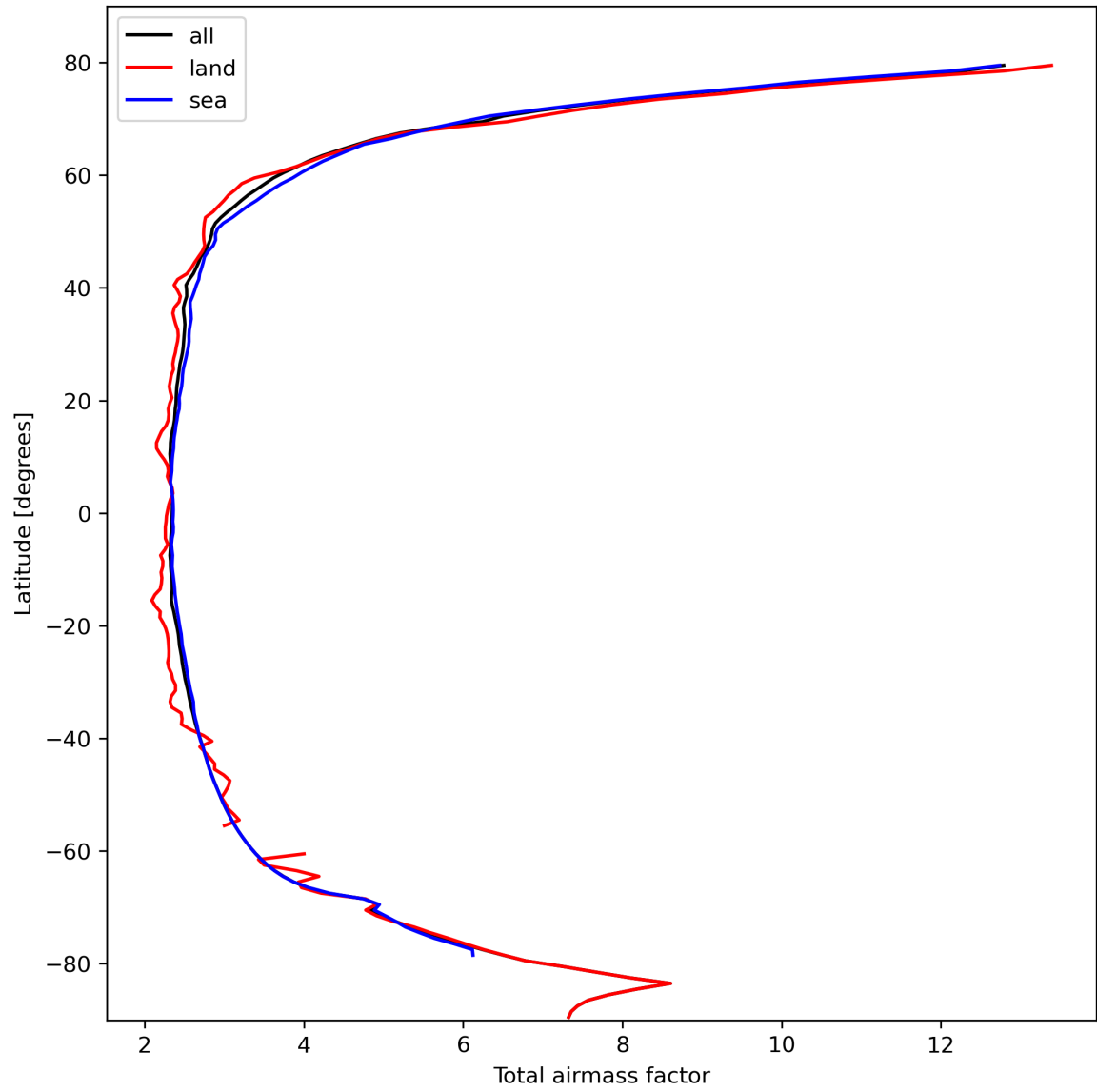
Figure 15: Zonal average of “Total airmass factor” for 2023-10-15 to 2023-10-17.
