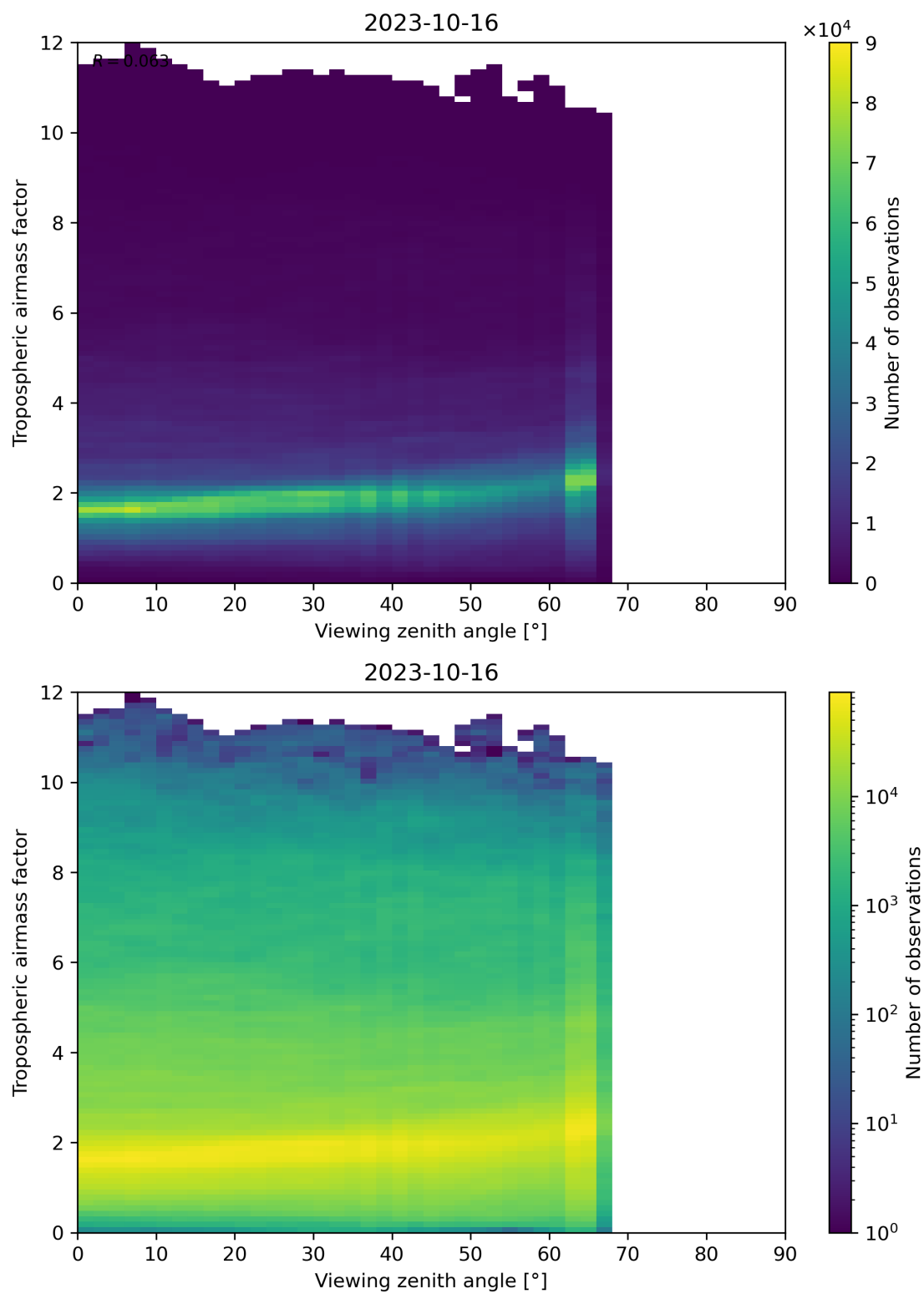
Figure 161: Scatter density plot of “Viewing zenith angle” against “Tropospheric airmass factor” for 2023-10-15 to 2023-10-17.
