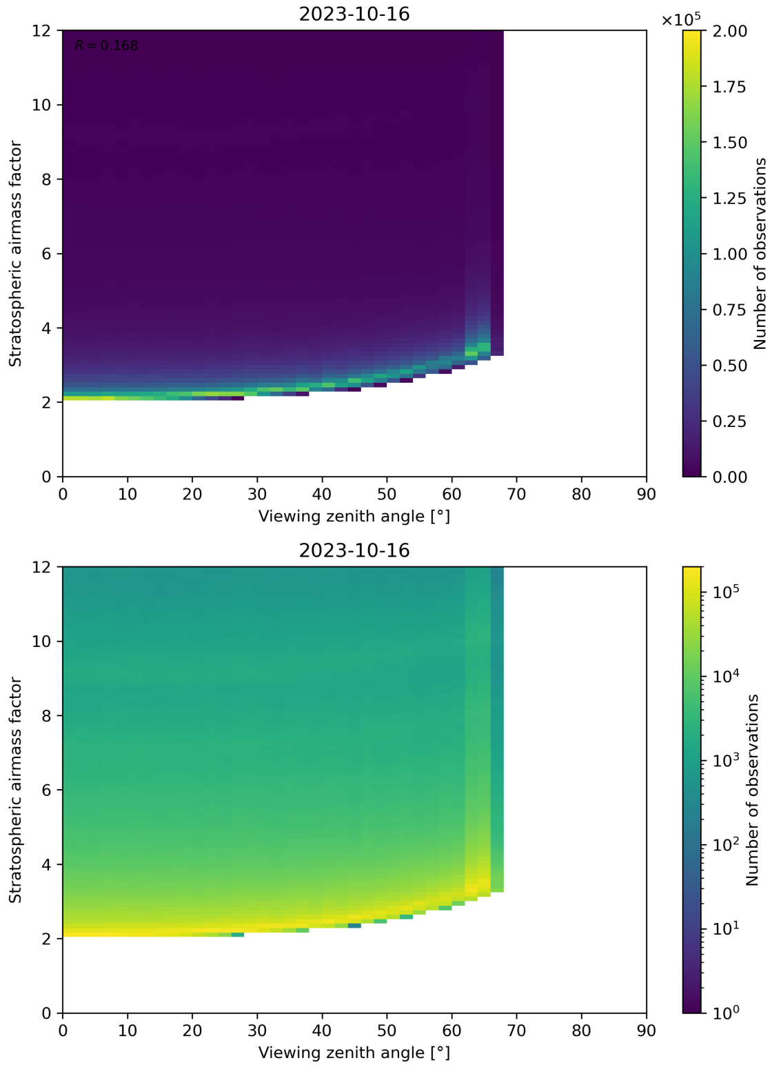
Figure 159: Scatter density plot of “Viewing zenith angle” against “Stratospheric airmass factor” for 2023-10-15 to 2023-10-17.
