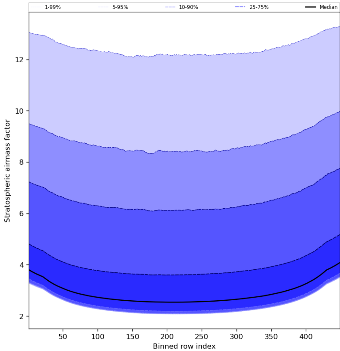
Figure 61: Along track statistics of “Stratospheric airmass factor” for 2023-10-15 to 2023-10-17
