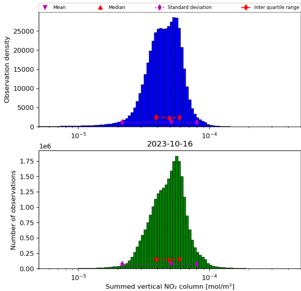
Figure 40: Histogram of “Summed vertical NO 2 column” for 2023-10-15 to 2023-10-17
