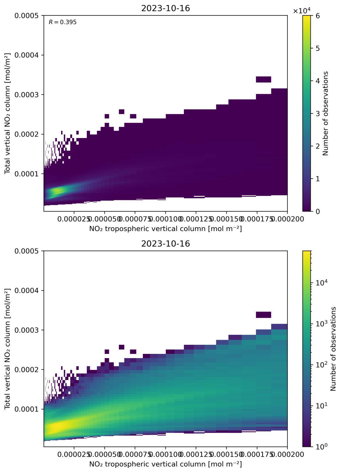
Figure 128: Scatter density plot of “NO 2 tropospheric vertical column” against “Total vertical NO 2 column” for 2023-10-15 to 2023-10-17.
