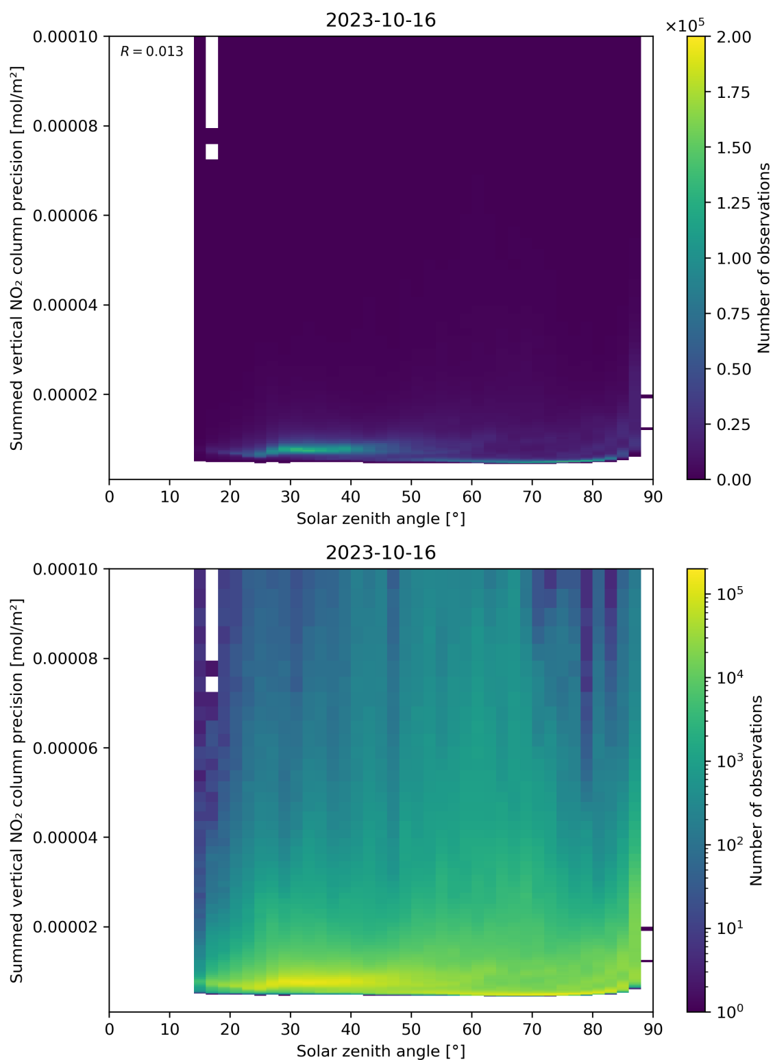
Figure 152: Scatter density plot of “Solar zenith angle” against “Summed vertical NO 2 column precision” for 2023-10-15 to 2023-10-17.
