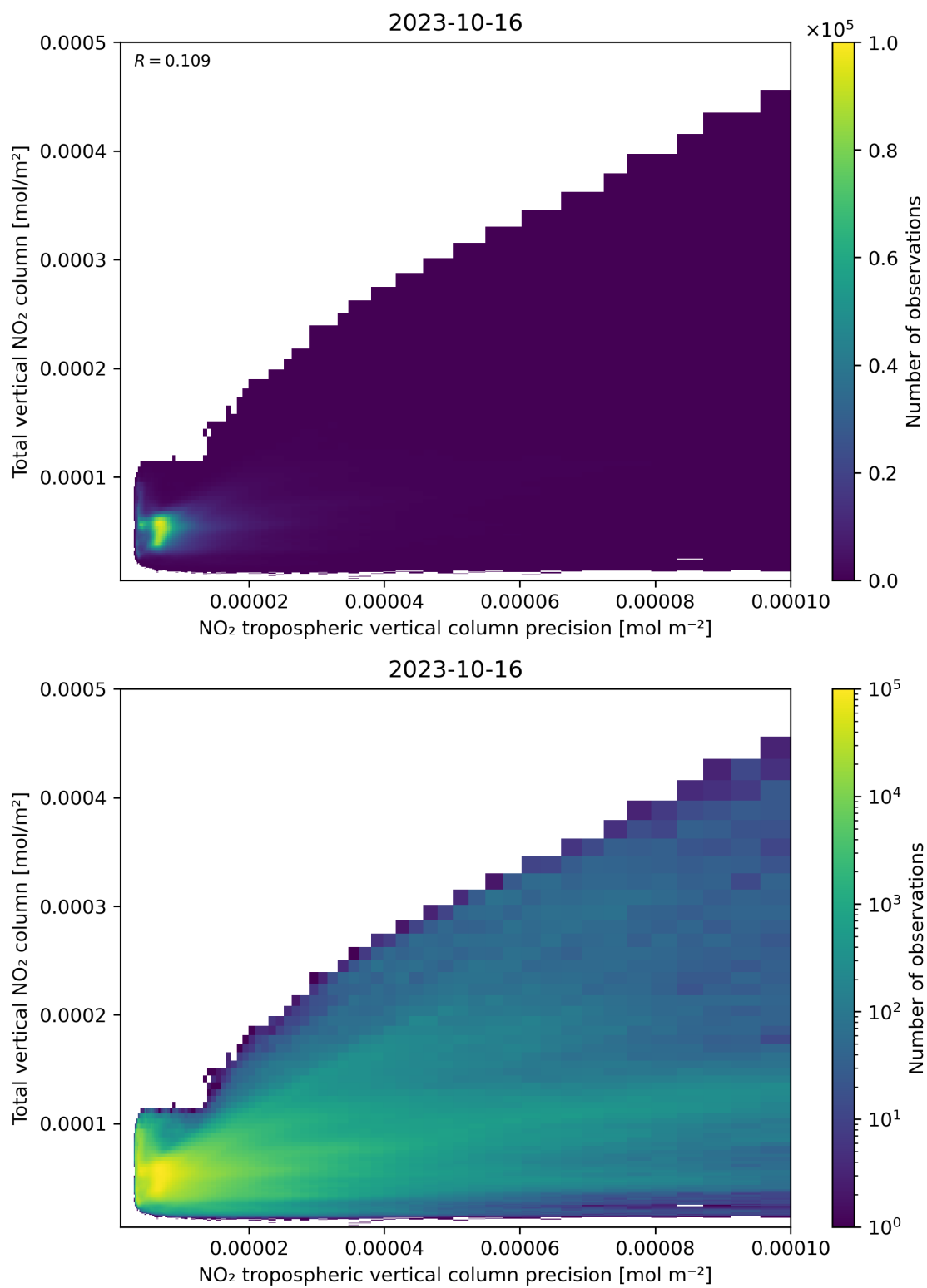
Figure 138: Scatter density plot of “NO 2 tropospheric vertical column precision” against “Total vertical NO 2 column” for 2023-10-15 to 2023-10-17.
