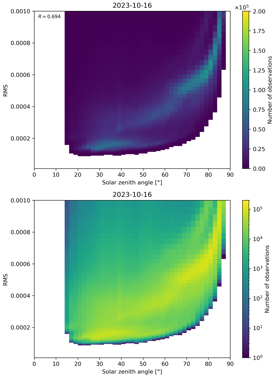
Figure 157: Scatter density plot of “Solar zenith angle” against “RMS” for 2023-10-15 to 2023-10-17.
