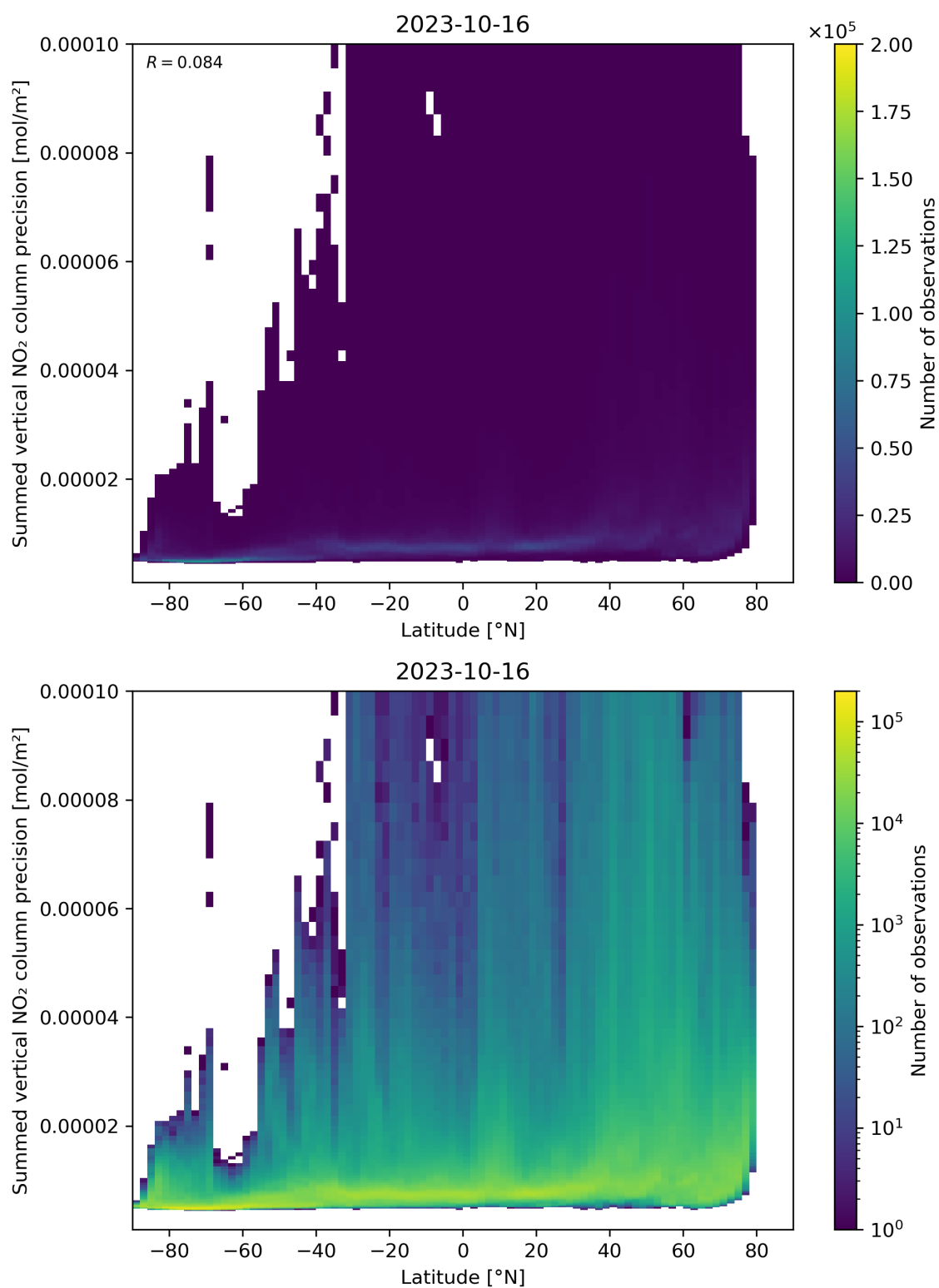
Figure 89: Scatter density plot of “Latitude” against “Summed vertical NO 2 column precision” for 2023-10-15 to 2023-10-17.
