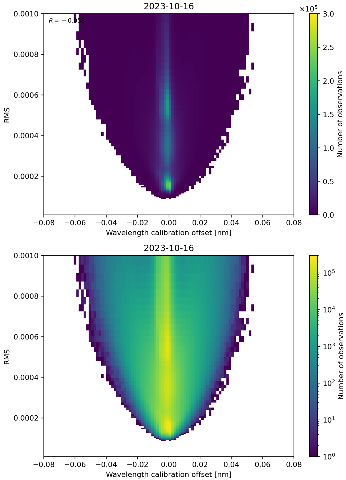
Figure 181: Scatter density plot of “Wavelength calibration offset” against “RMS” for 2023-10-15 to 2023-10-17.
