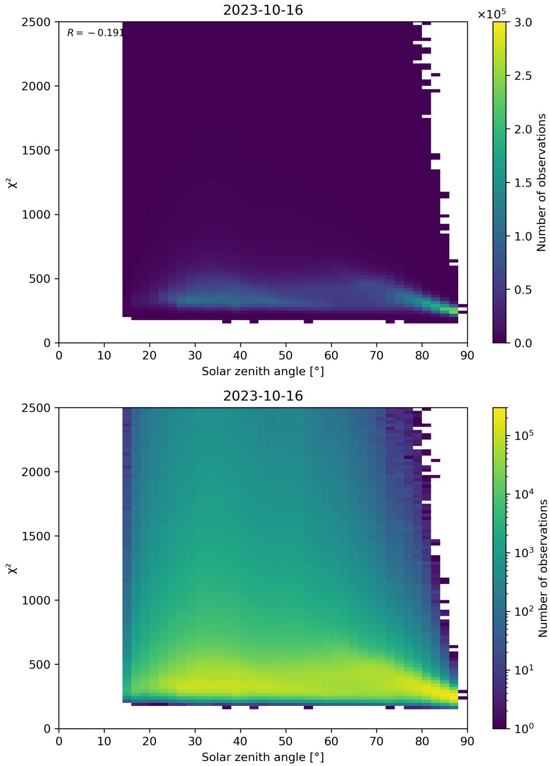
Figure 148: Scatter density plot of “Solar zenith angle” against “ \chi^2 ” for 2023-10-15 to 2023-10-17.
