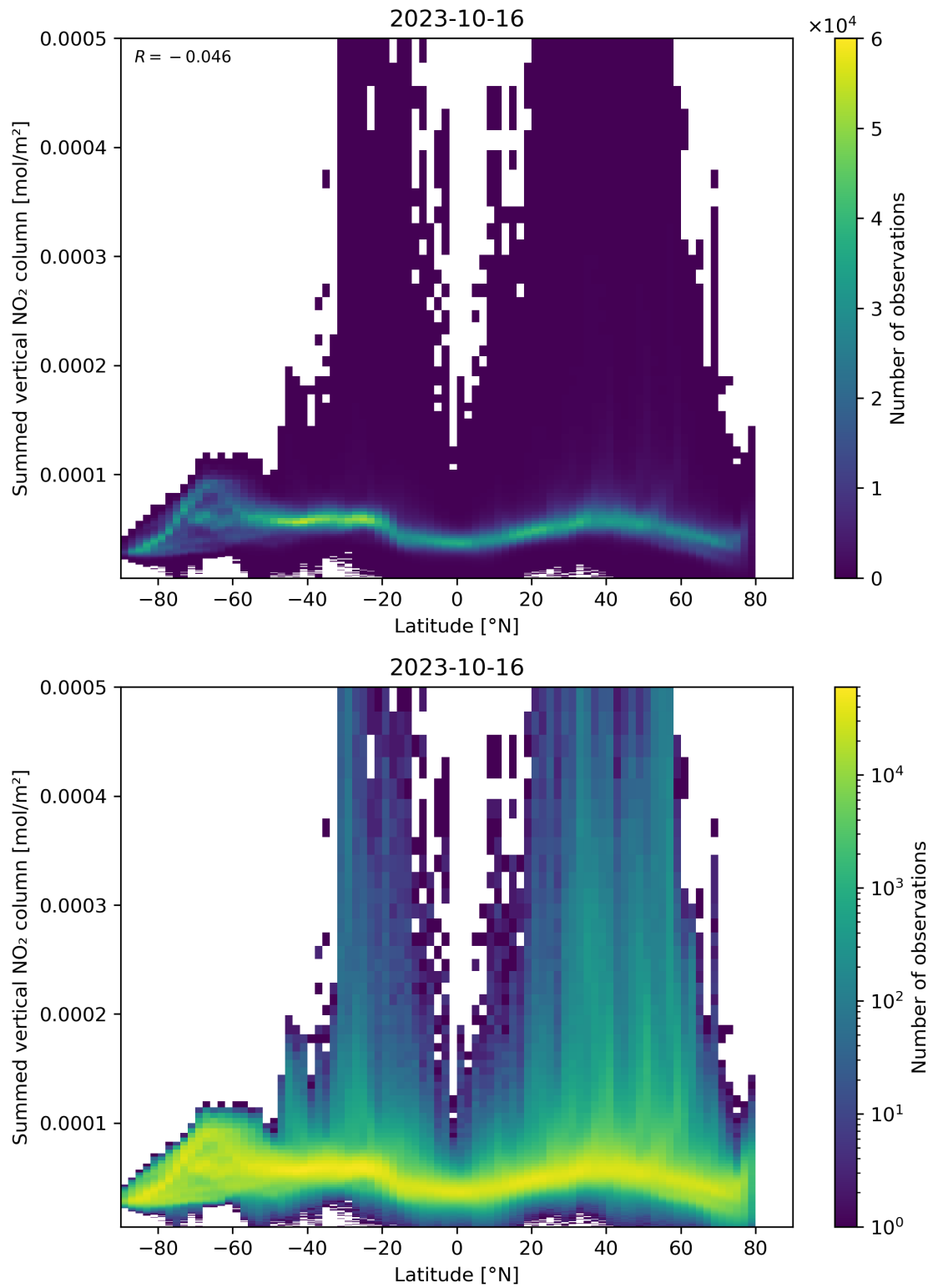
Figure 88: Scatter density plot of “Latitude” against “Summed vertical NO 2 column” for 2023-10-15 to 2023-10-17.
