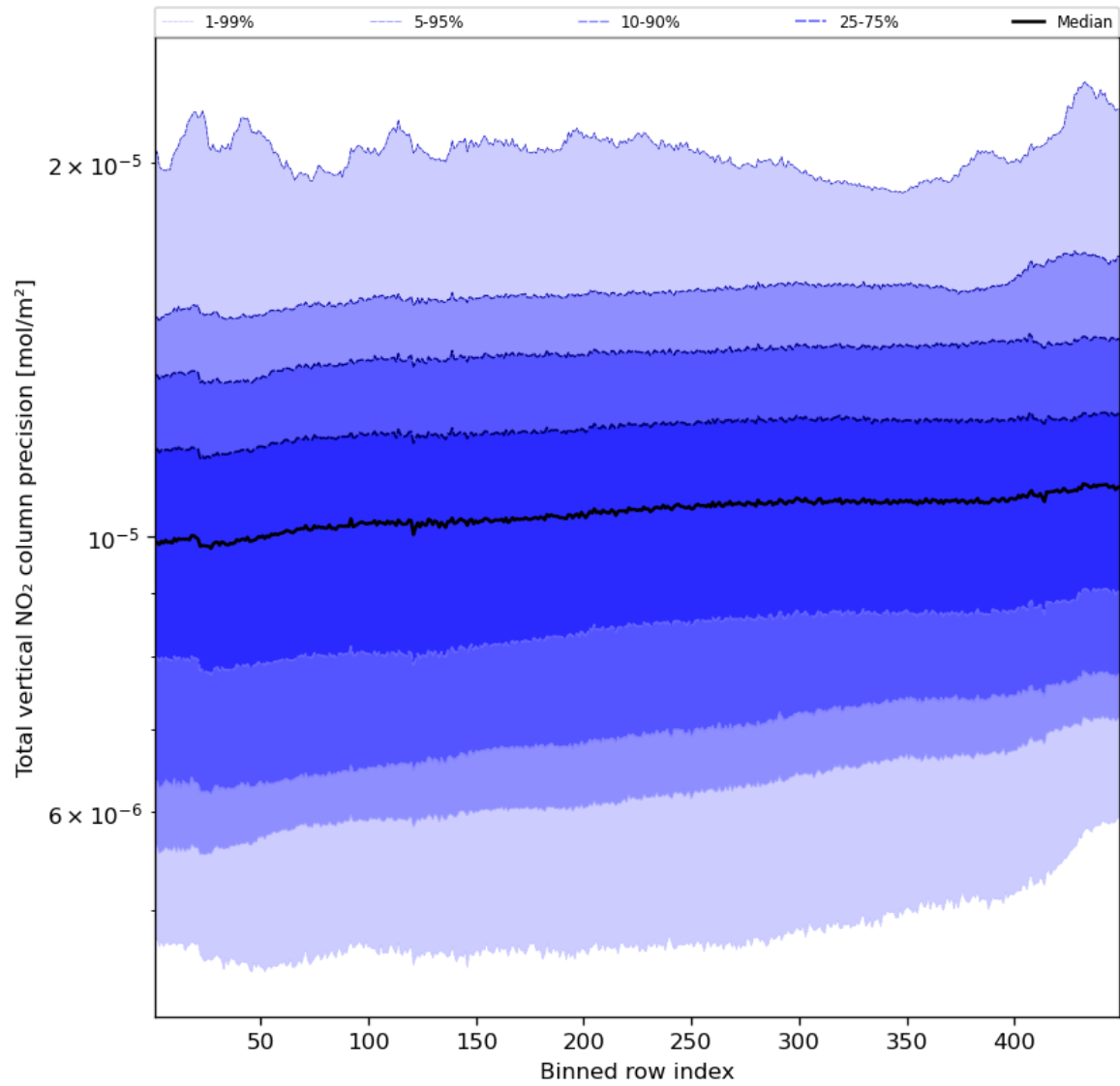
Figure 56: Along track statistics of “Total vertical NO 2 column precision” for 2023-10-15 to 2023-10-17
