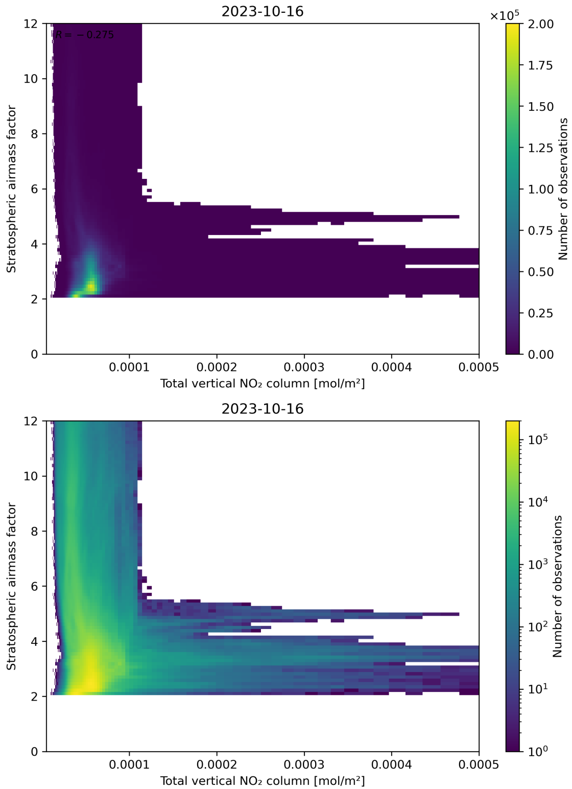
Figure 110: Scatter density plot of “Total vertical NO 2 column” against “Stratospheric airmass factor” for 2023-10-15 to 2023-10-17.
