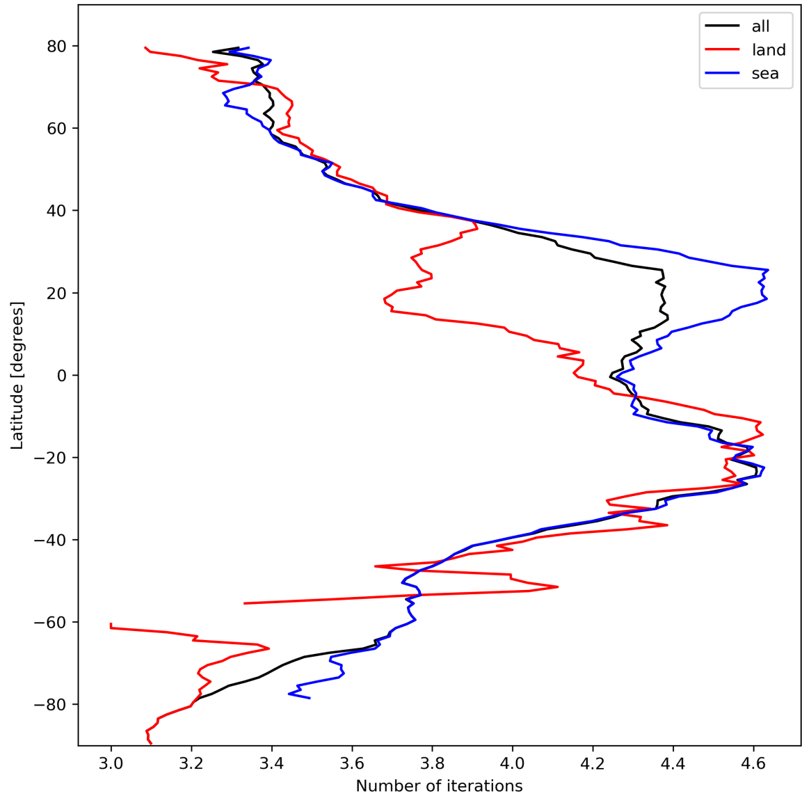
Figure 17: Zonal average of “Number of iterations” for 2023-10-15 to 2023-10-17.
