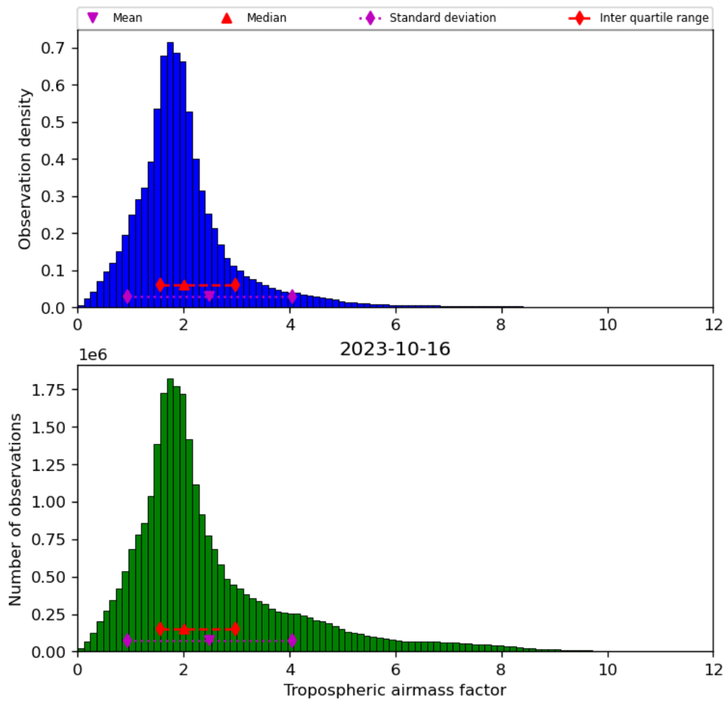
Figure 31: Histogram of “Tropospheric airmass factor” for 2023-10-15 to 2023-10-17
