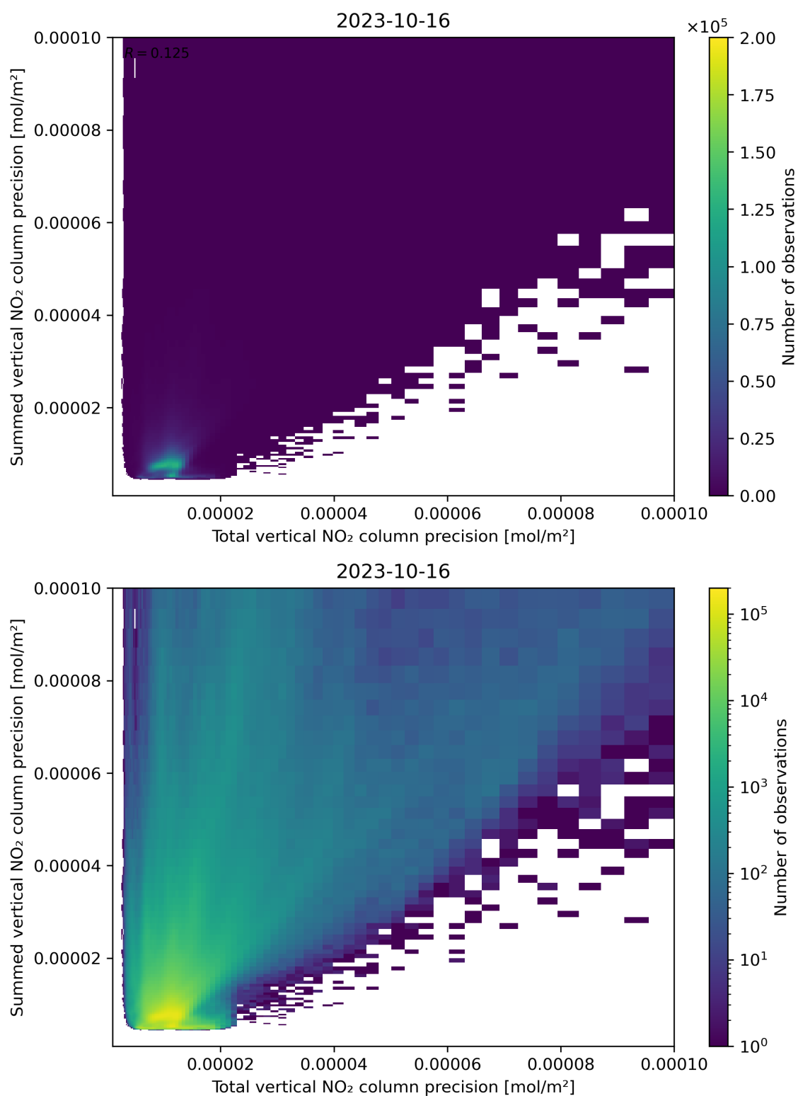
Figure 118: Scatter density plot of “Total vertical NO 2 column precision” against “Summed vertical NO 2 column precision” for 2023-10-15 to 2023-10-17.
