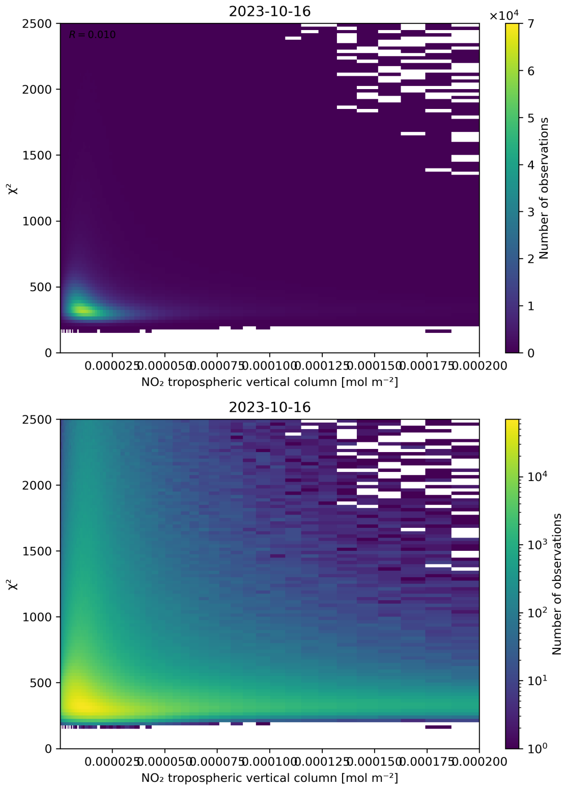
Figure 124: Scatter density plot of “NO 2 tropospheric vertical column” against “ \chi^2 ” for 2023-10-15 to 2023-10-17.
