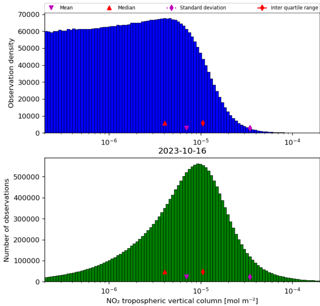
Figure 29: Histogram of “NO 2 tropospheric vertical column” for 2023-10-15 to 2023-10-17
