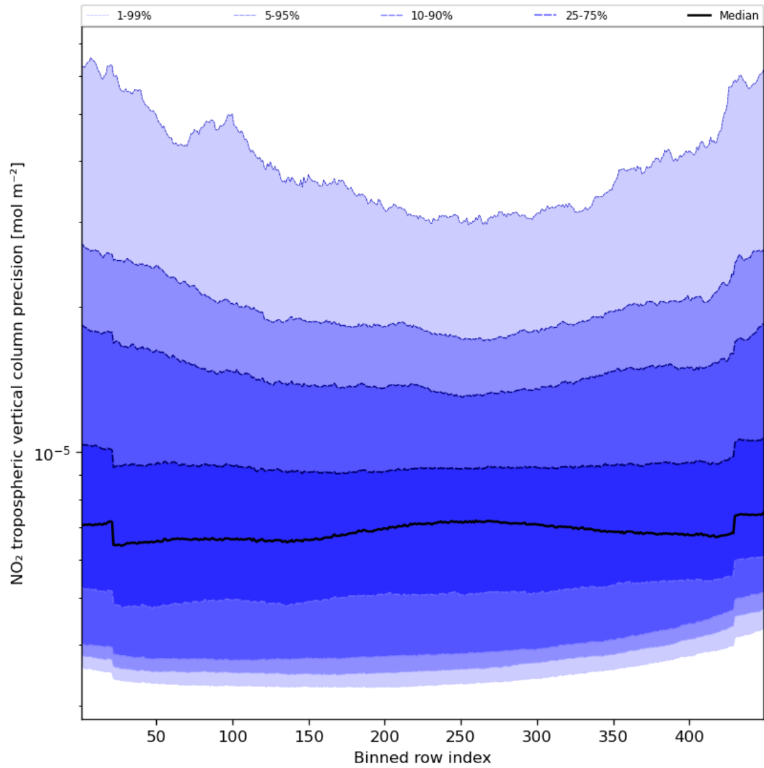
Figure 47: Along track statistics of “NO 2 tropospheric vertical column precision” for 2023-10-15 to 2023-10-17
