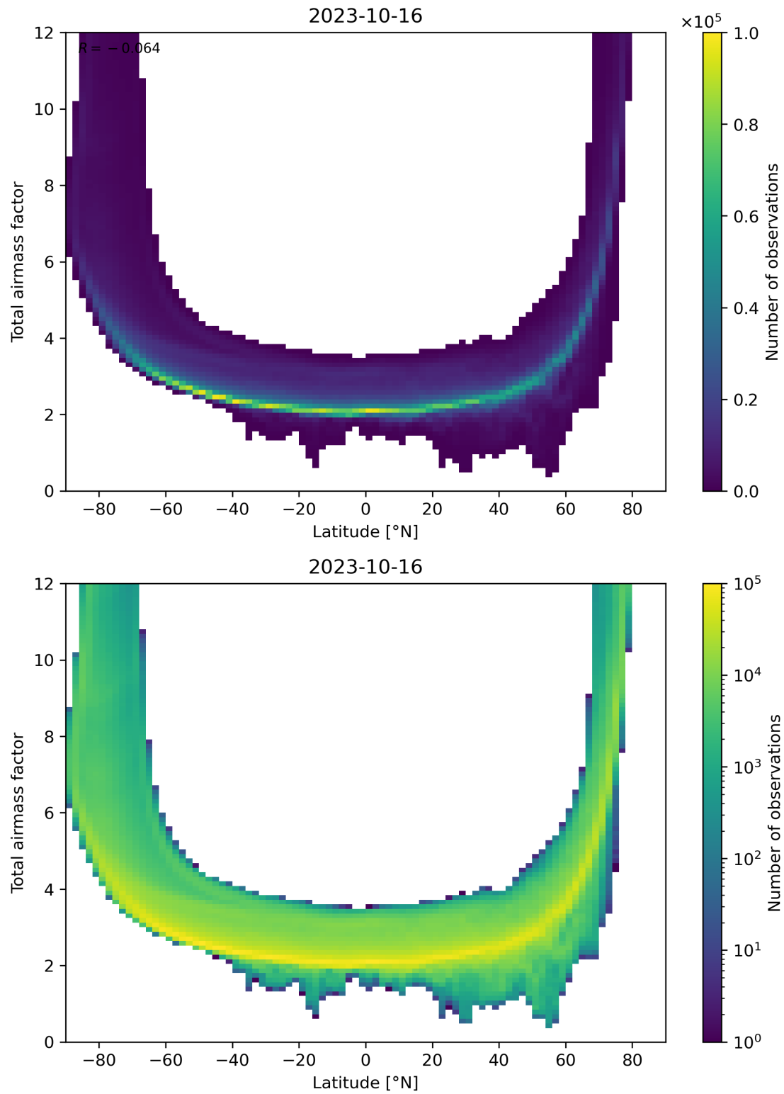
Figure 84: Scatter density plot of “Latitude” against “Total airmass factor” for 2023-10-15 to 2023-10-17.
