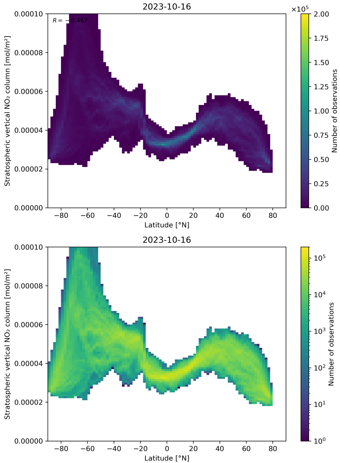
Figure 87: Scatter density plot of “Latitude” against “Stratospheric vertical NO 2 column” for 2023-10-15 to 2023-10-17.
