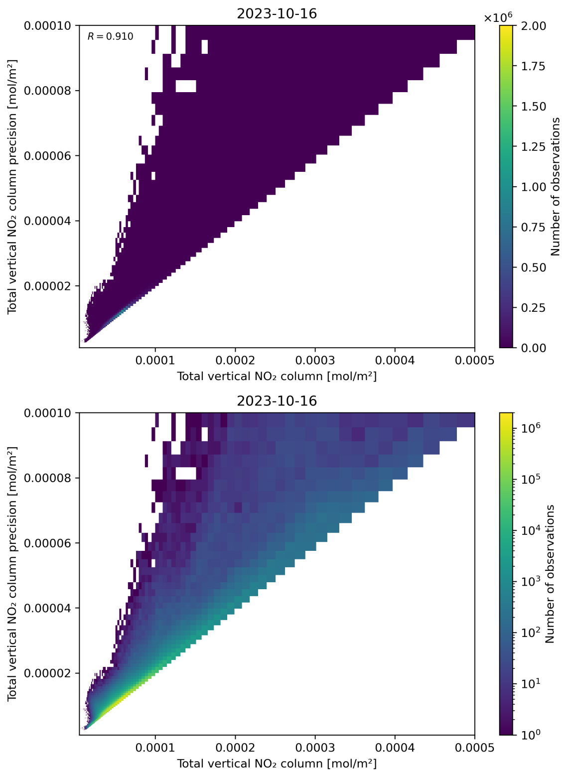
Figure 114: Scatter density plot of “Total vertical NO 2 column” against “Total vertical NO 2 column precision” for 2023-10-15 to 2023-10-17.
