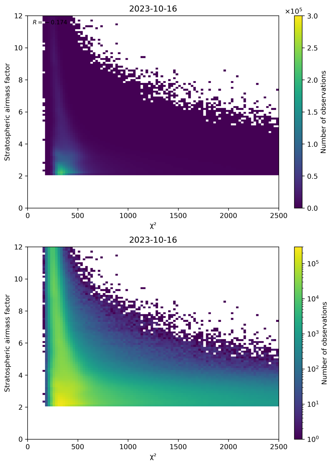
Figure 81: Scatter density plot of “ \chi^2 ” against “Stratospheric airmass factor” for 2023-10-15 to 2023-10-17.
