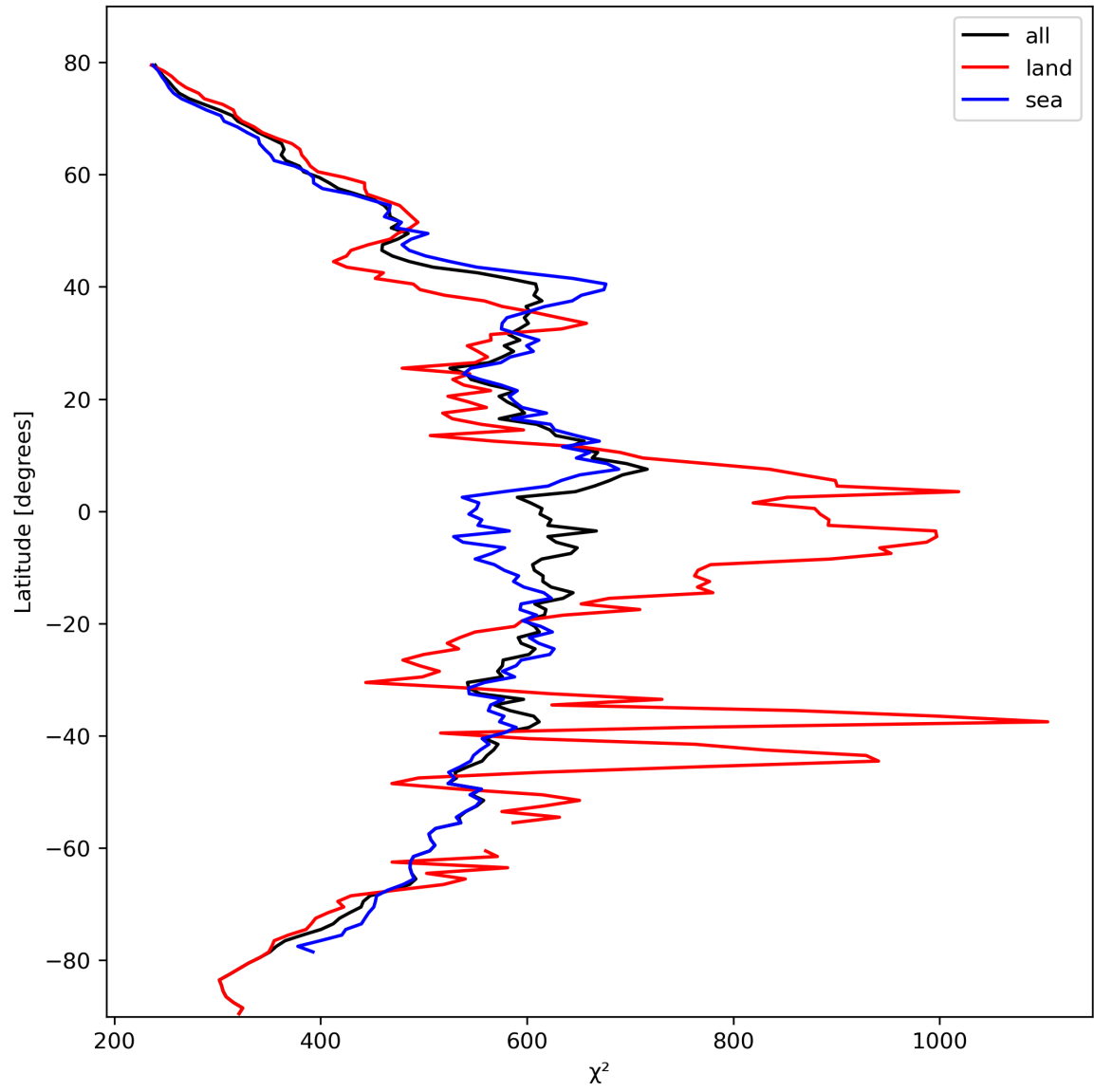
Figure 25: Zonal average of “ \chi^2 ” for 2023-10-15 to 2023-10-17.
