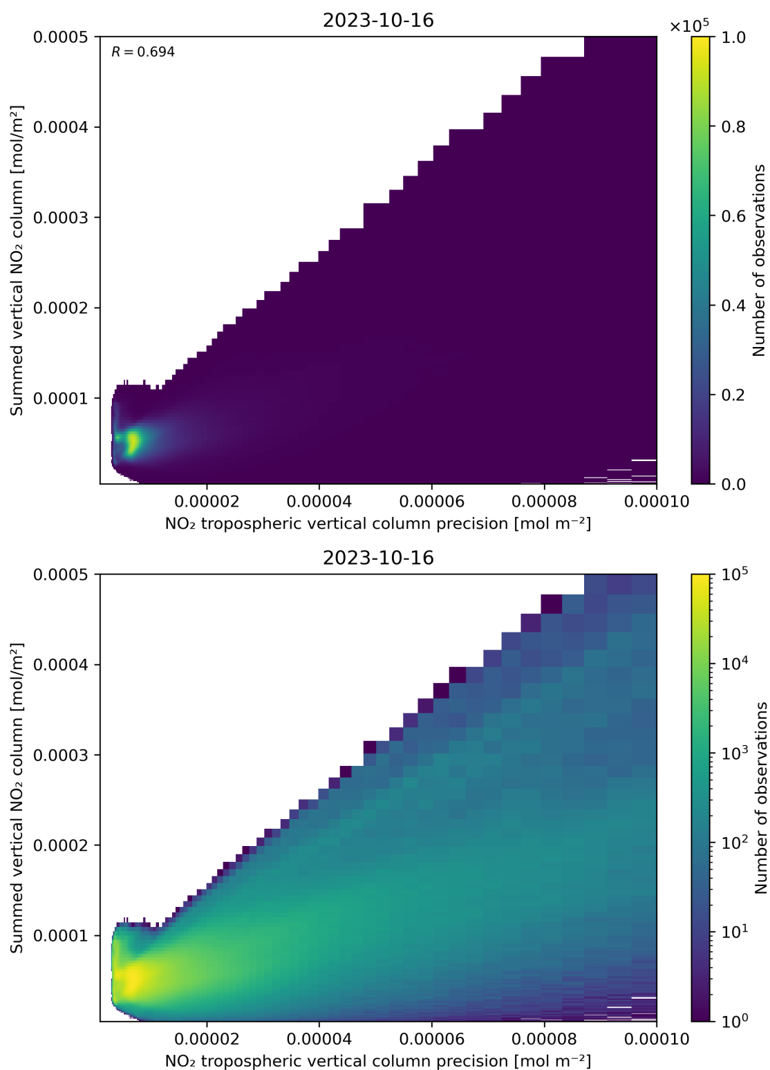
Figure 136: Scatter density plot of “NO 2 tropospheric vertical column precision” against “Summed vertical NO 2 column” for 2023-10-15 to 2023-10-17.
