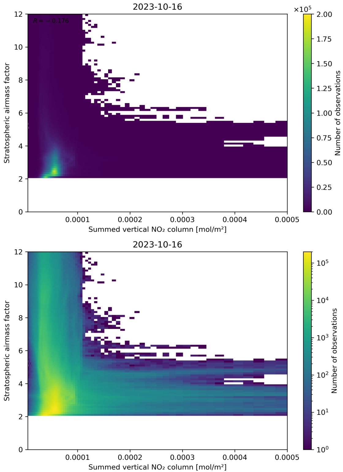
Figure 103: Scatter density plot of “Summed vertical NO 2 column” against “Stratospheric airmass factor” for 2023-10-15 to 2023-10-17.
