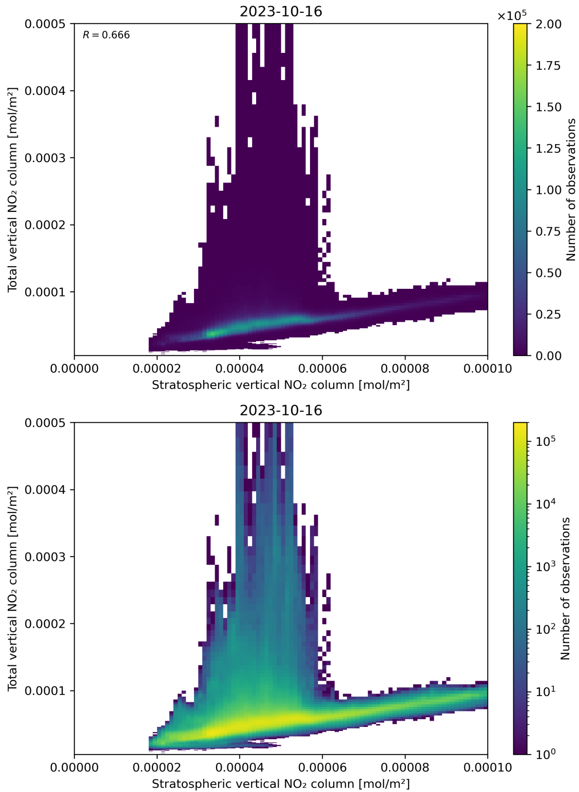
Figure 100: Scatter density plot of “Stratospheric vertical NO 2 column” against “Total vertical NO 2 column” for 2023-10-15 to 2023-10-17.
