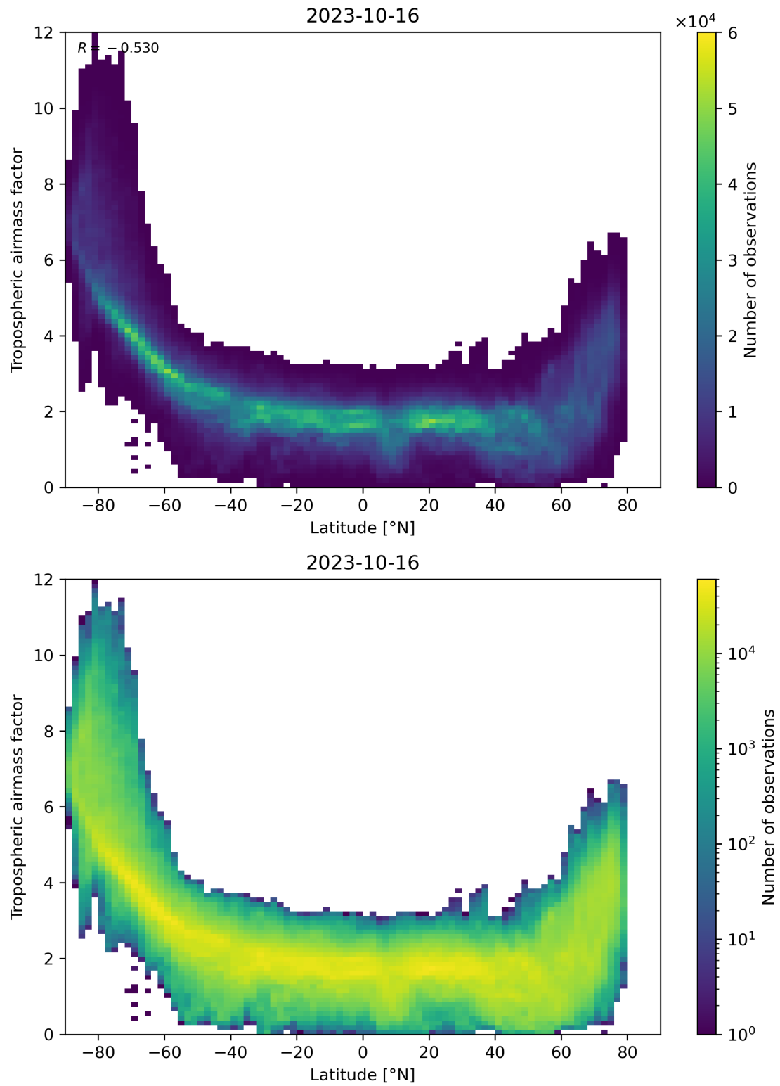
Figure 85: Scatter density plot of “Latitude” against “Tropospheric air mass factor” for 2023-10-15 to 2023-10-17.
