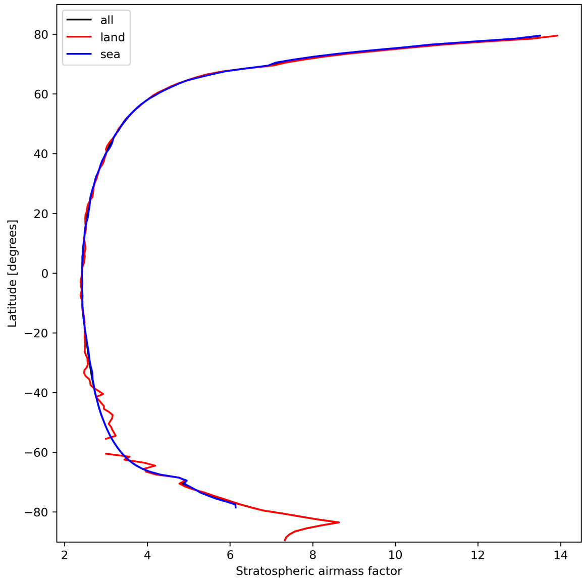
Figure 27: Zonal average of “Stratospheric air mass factor” for 2023-10-15 to 2023-10-17.
