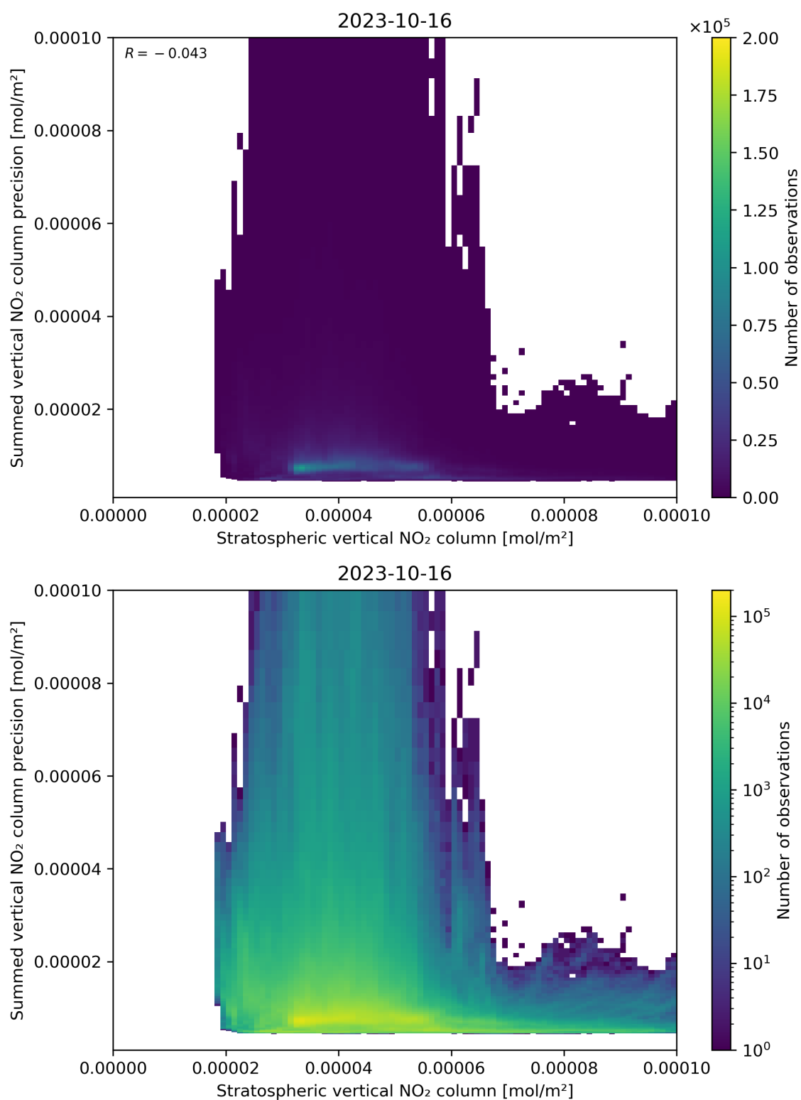
Figure 99: Scatter density plot of “Stratospheric vertical NO 2 column” against “Summed vertical NO 2 column precision” for 2023-10-15 to 2023-10-17.
