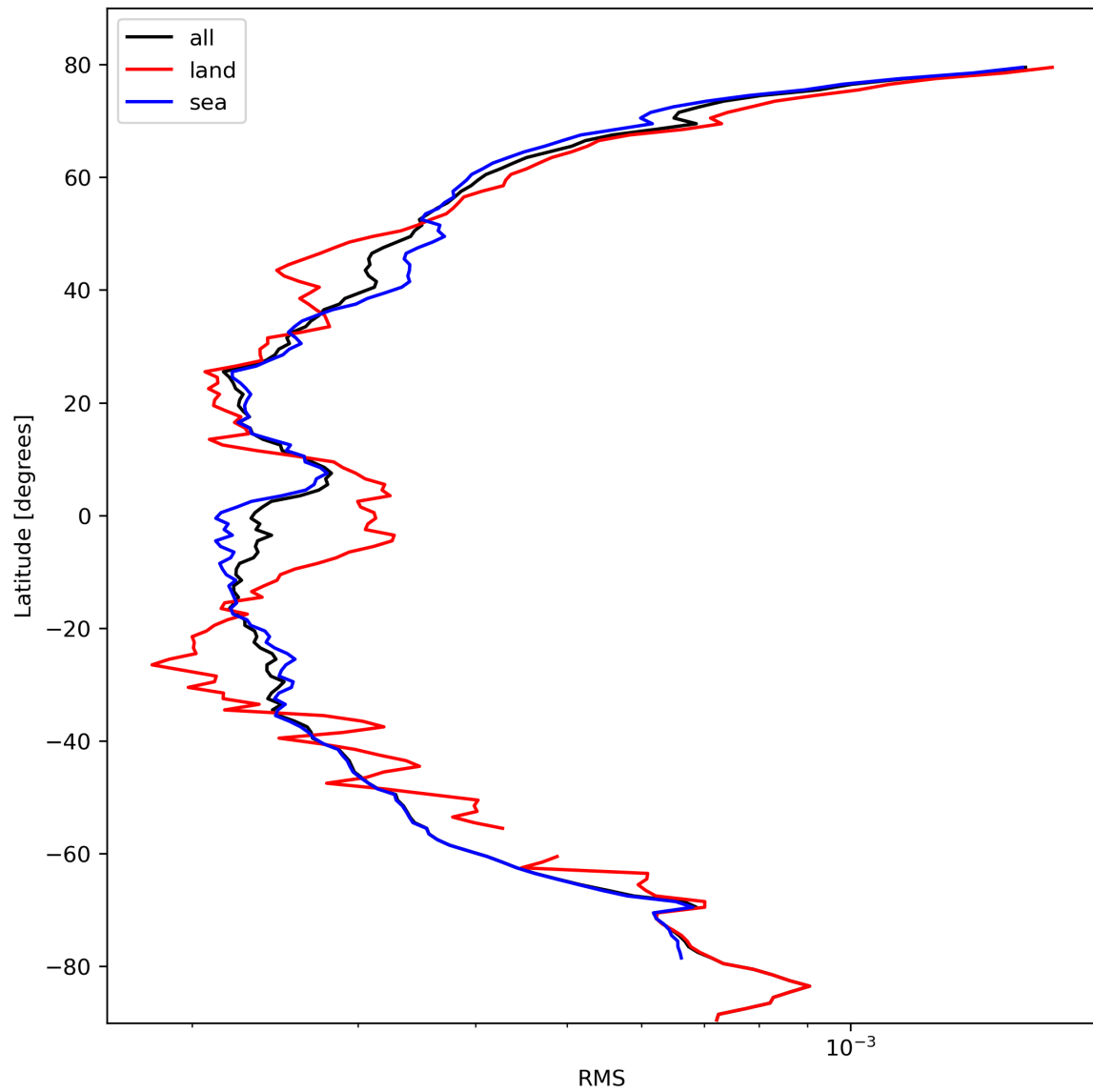
Figure 26: Zonal average of “RMS” for 2023-10-15 to 2023-10-17.
