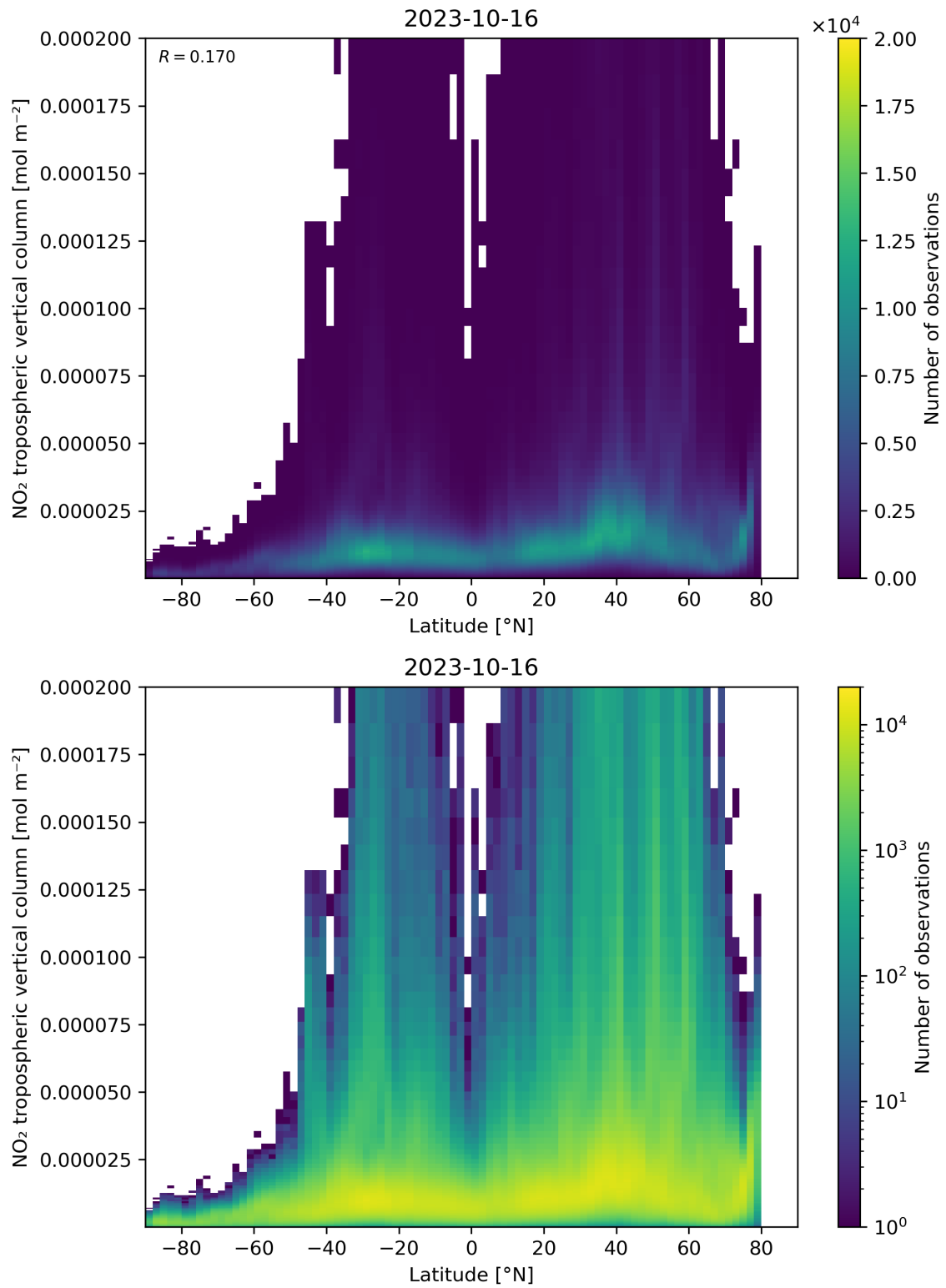
Figure 92: Scatter density plot of “Latitude” against “NO 2 tropospheric vertical column” for 2023-10-15 to 2023-10-17.
