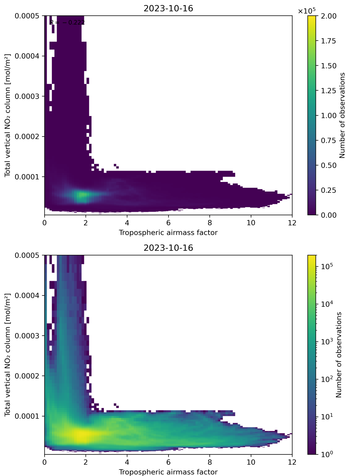
Figure 77: Scatter density plot of “Tropospheric airmass factor” against “Total vertical NO 2 column” for 2023-10-15 to 2023-10-17.
