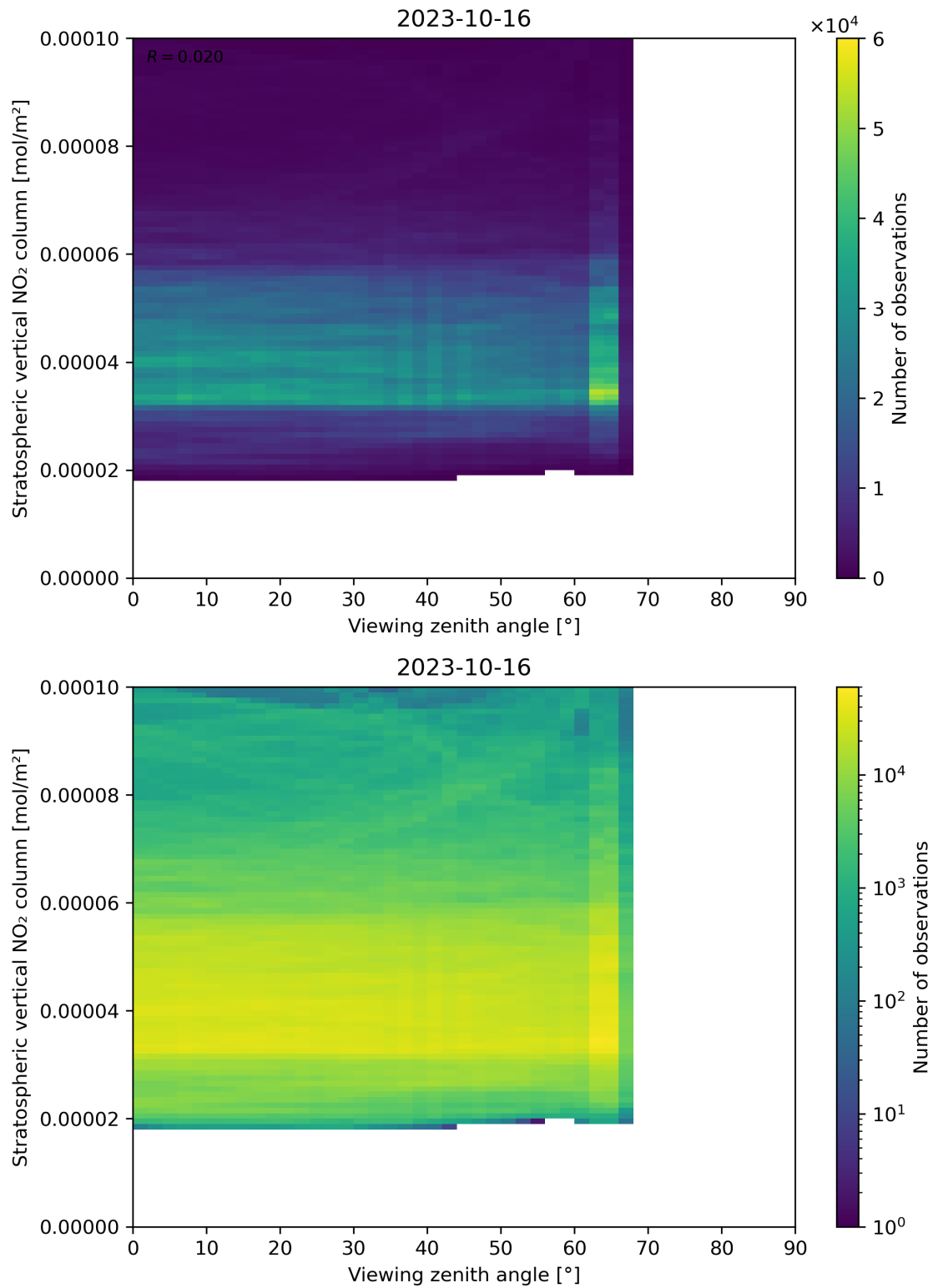
Figure 164: Scatter density plot of “Viewing zenith angle” against “Stratospheric vertical NO 2 column” for 2023-10-15 to 2023-10-17.
