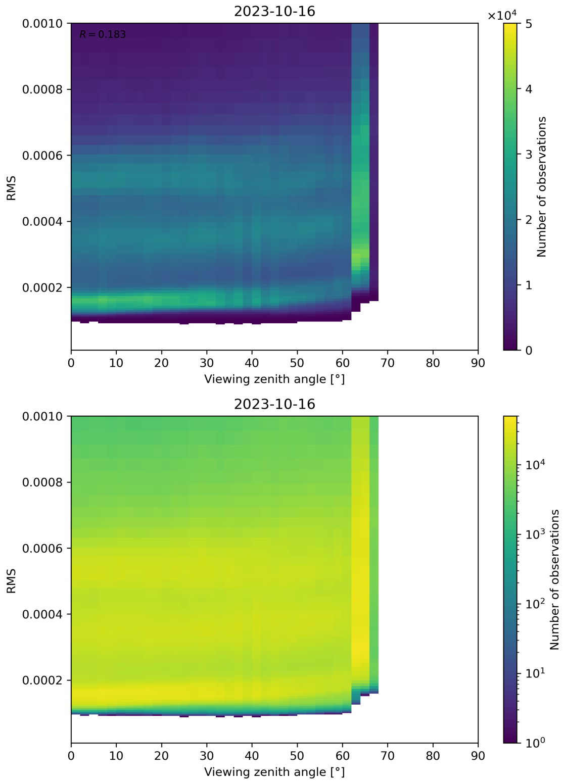
Figure 171: Scatter density plot of “Viewing zenith angle” against “RMS” for 2023-10-15 to 2023-10-17.
