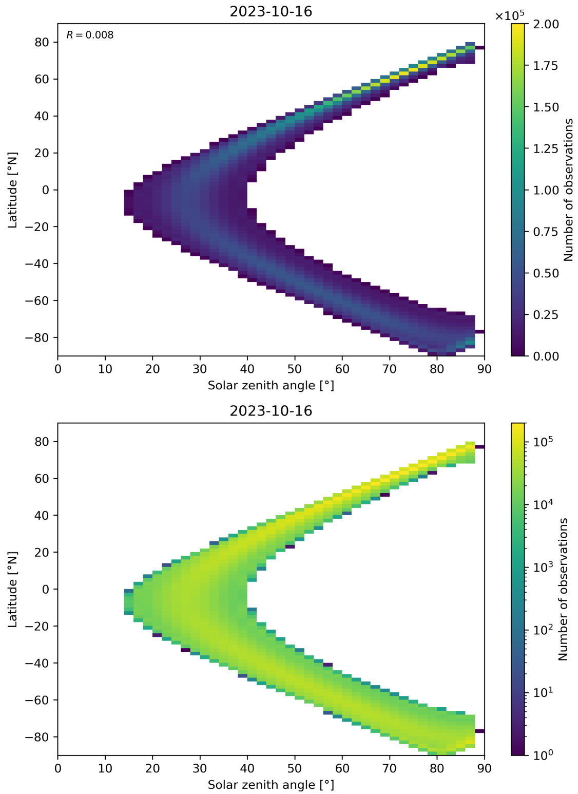
Figure 149: Scatter density plot of “Solar zenith angle” against “Latitude” for 2023-10-15 to 2023-10-17.
