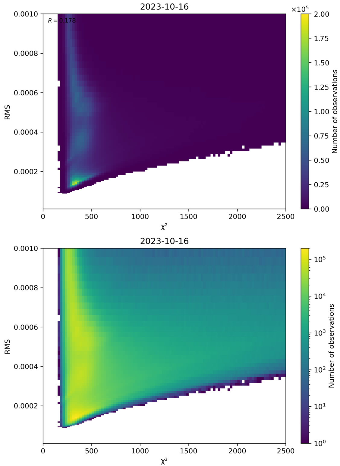
Figure 82: Scatter density plot of “ \chi^2 ” against “RMS” for 2023-10-15 to 2023-10-17.
