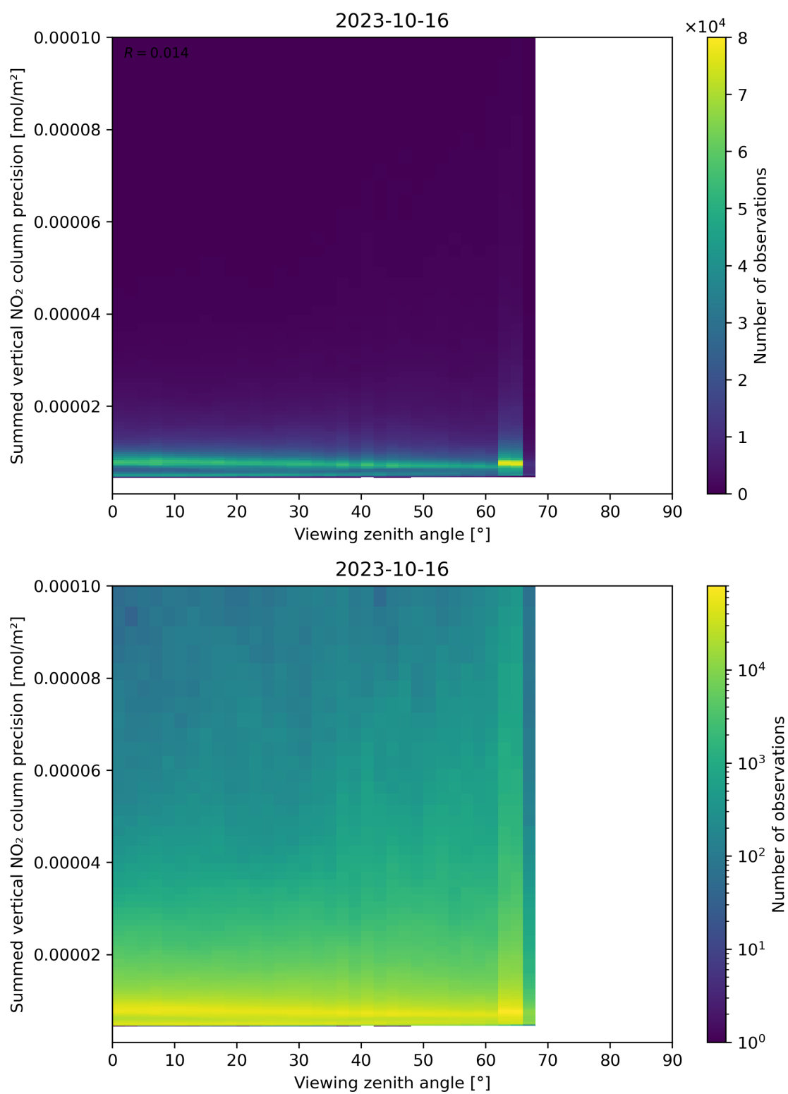
Figure 166: Scatter density plot of “Viewing zenith angle” against “Summed vertical NO 2 column precision” for 2023-10-15 to 2023-10-17.
