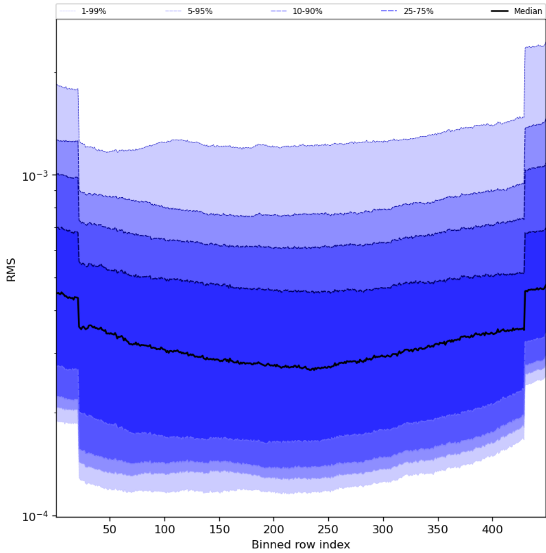
Figure 60: Along track statistics of “RMS” for 2023-10-15 to 2023-10-17
