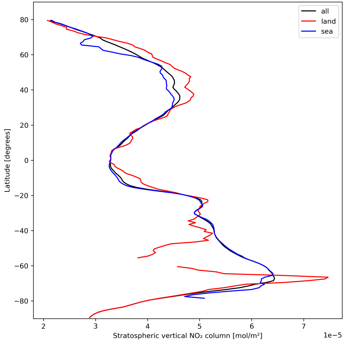
Figure 19: Zonal average of “Stratospheric vertical NO 2 column” for 2023-10-15 to 2023-10-17.
