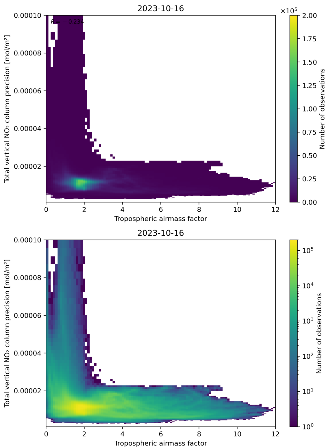
Figure 78: Scatter density plot of “Tropospheric air mass factor” against “Total vertical NO 2 column precision” for 2023-10-15 to 2023-10-17.
