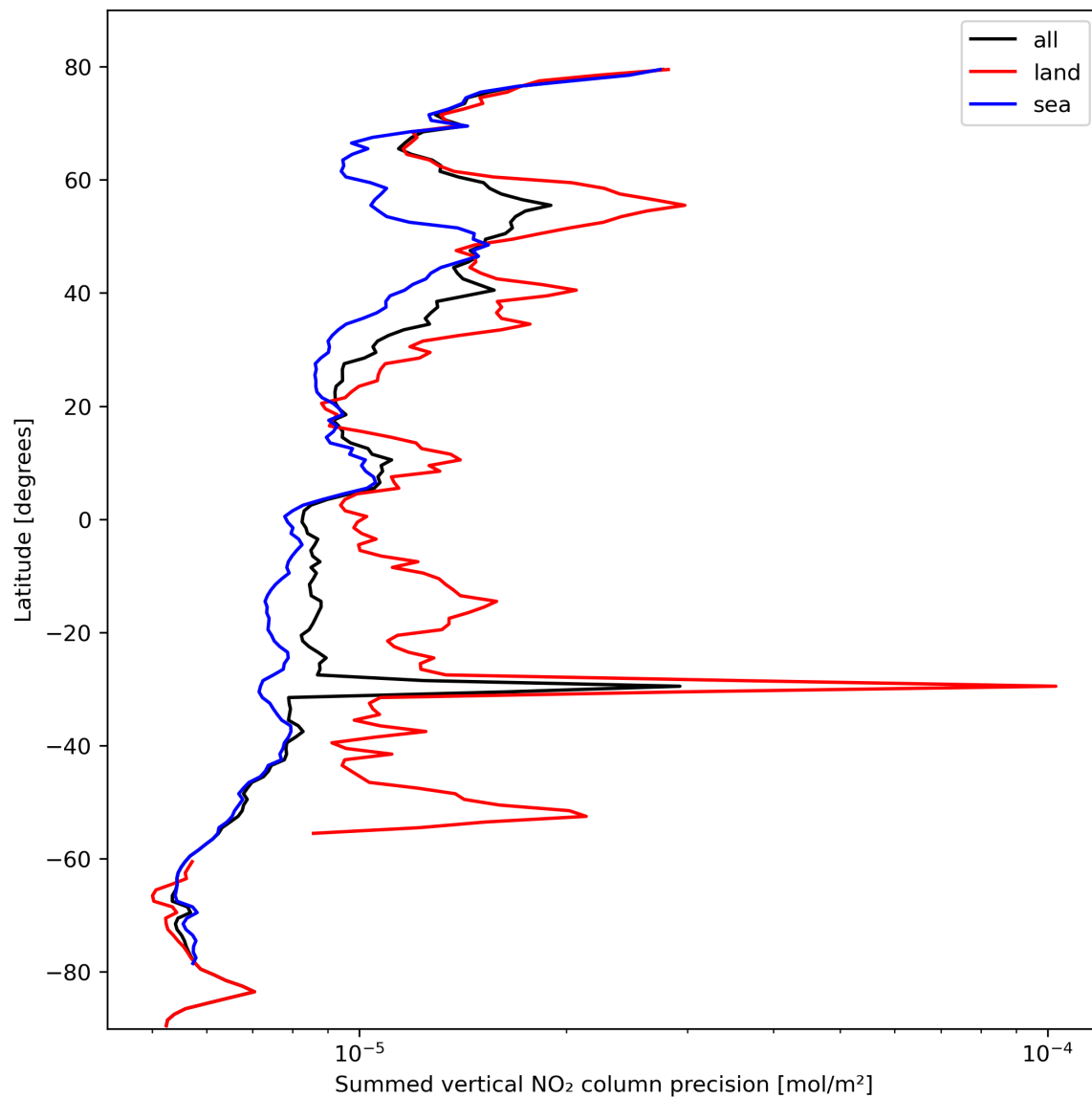
Figure 24: Zonal average of “Summed vertical NO 2 column precision” for 2023-10-15 to 2023-10-17.
