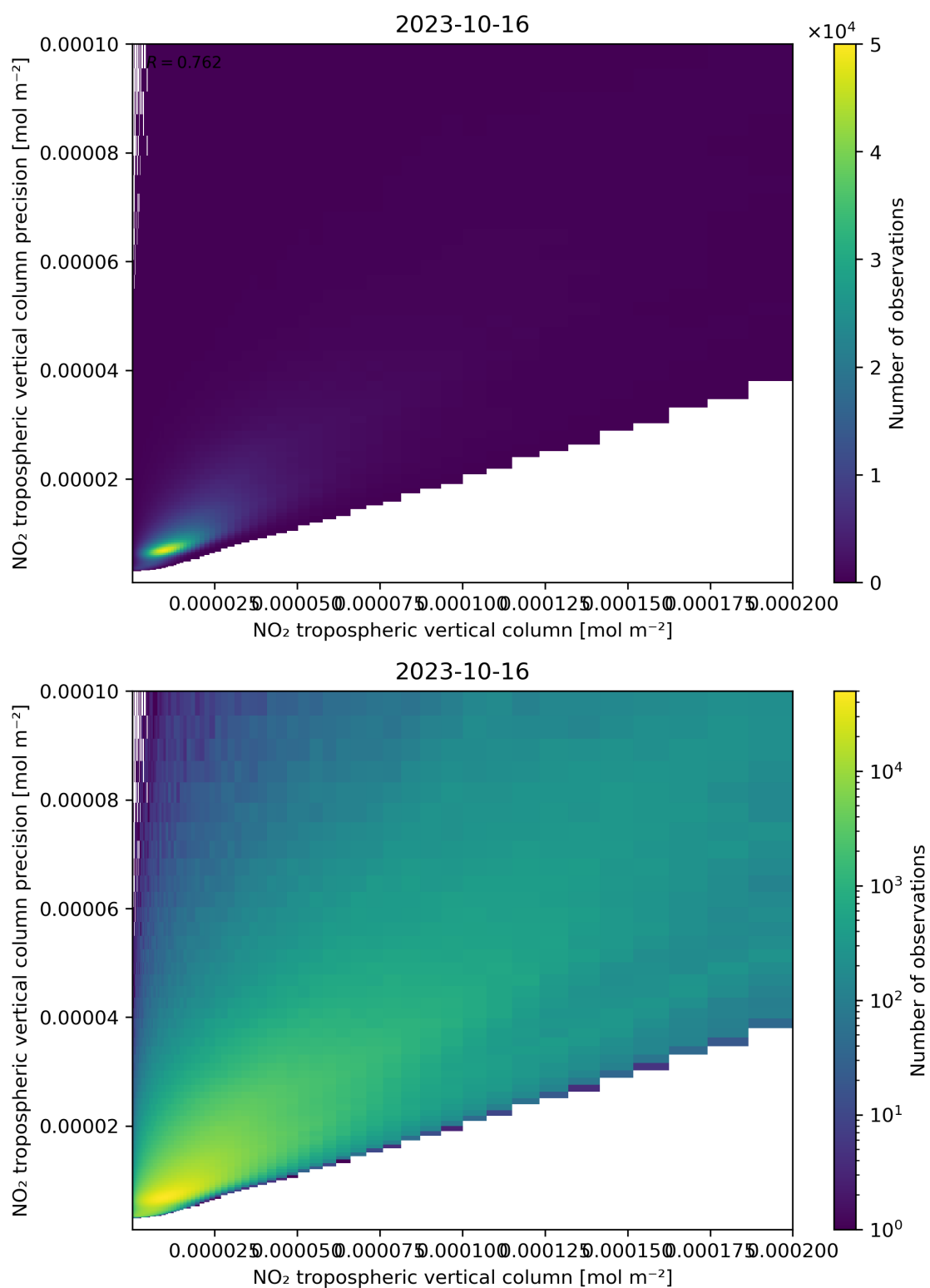
Figure 130: Scatter density plot of “NO 2 tropospheric vertical column” against “NO 2 tropospheric vertical column precision” for 2023-10-15 to 2023-10-17.
