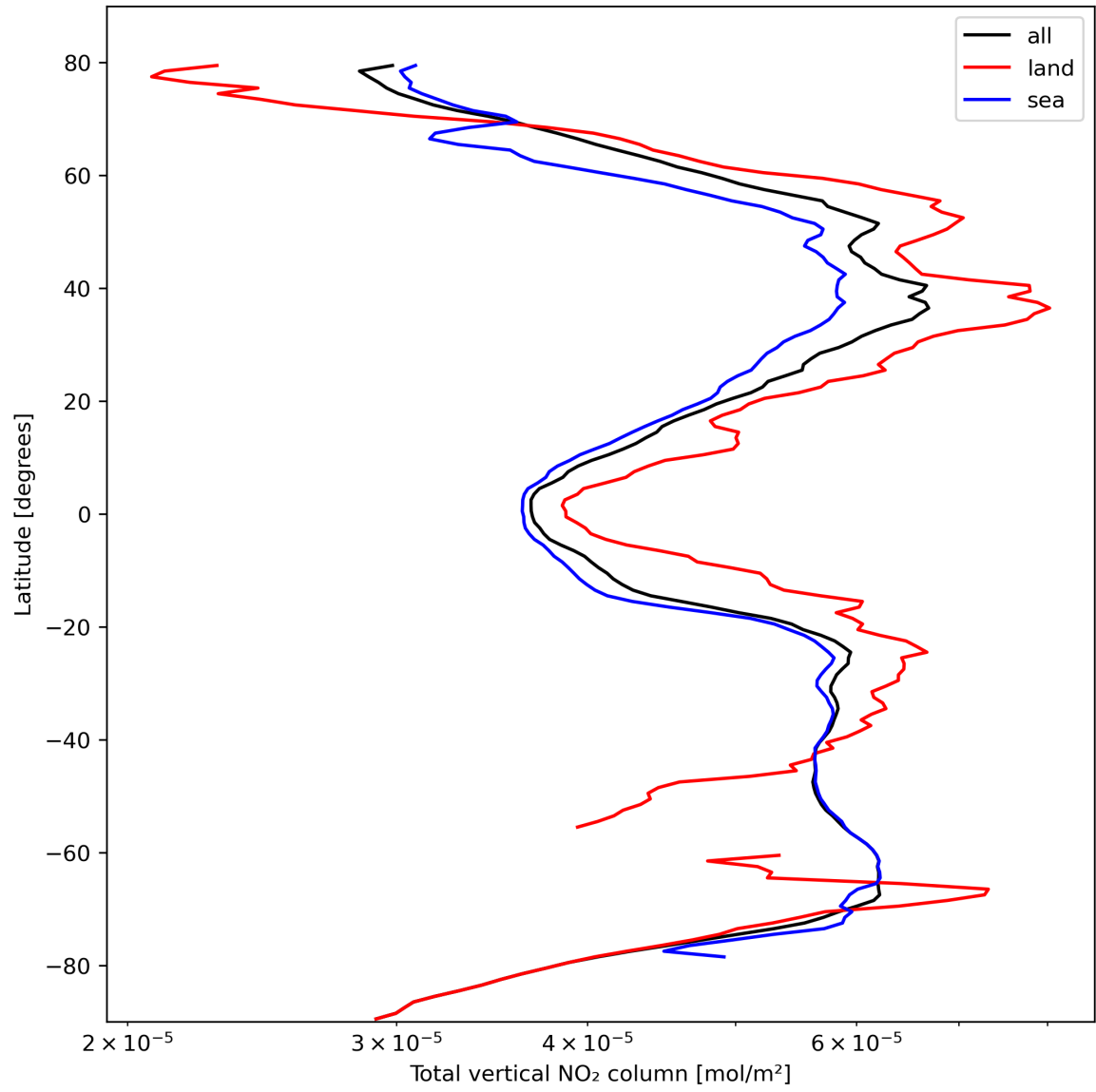
Figure 21: Zonal average of “Total vertical NO 2 column” for 2023-10-15 to 2023-10-17.
