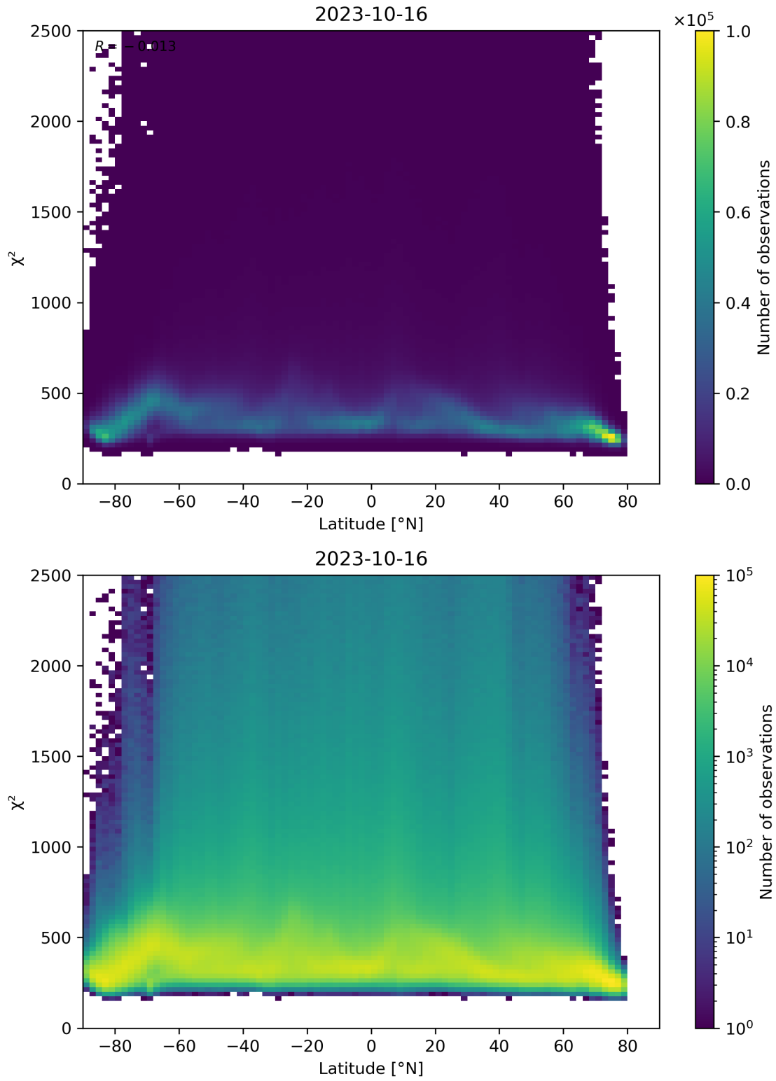
Figure 86: Scatter density plot of “Latitude” against “ \chi^2 ” for 2023-10-15 to 2023-10-17.
