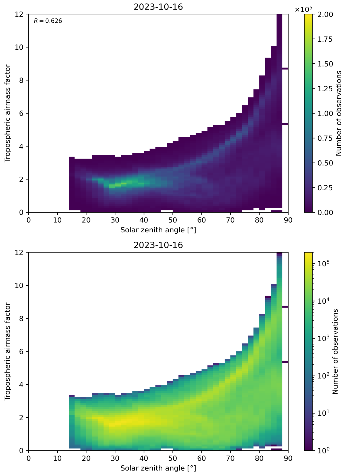
Figure 147: Scatter density plot of “Solar zenith angle” against “Tropospheric airmass factor” for 2023-10-15 to 2023-10-17.
