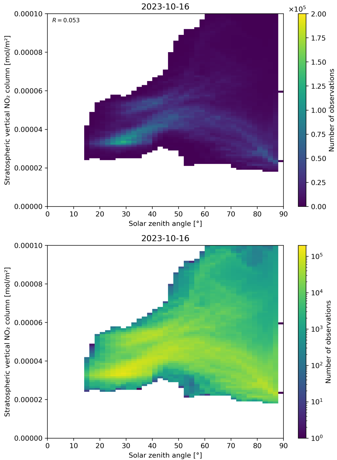
Figure 150: Scatter density plot of “Solar zenith angle” against “Stratospheric vertical NO 2 column” for 2023-10-15 to 2023-10-17.
