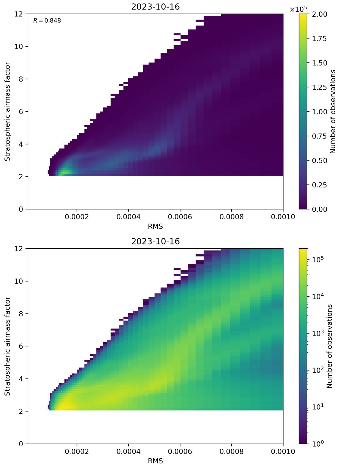
Figure 144: Scatter density plot of “RMS” against “Stratospheric airmass factor” for 2023-10-15 to 2023-10-17.
