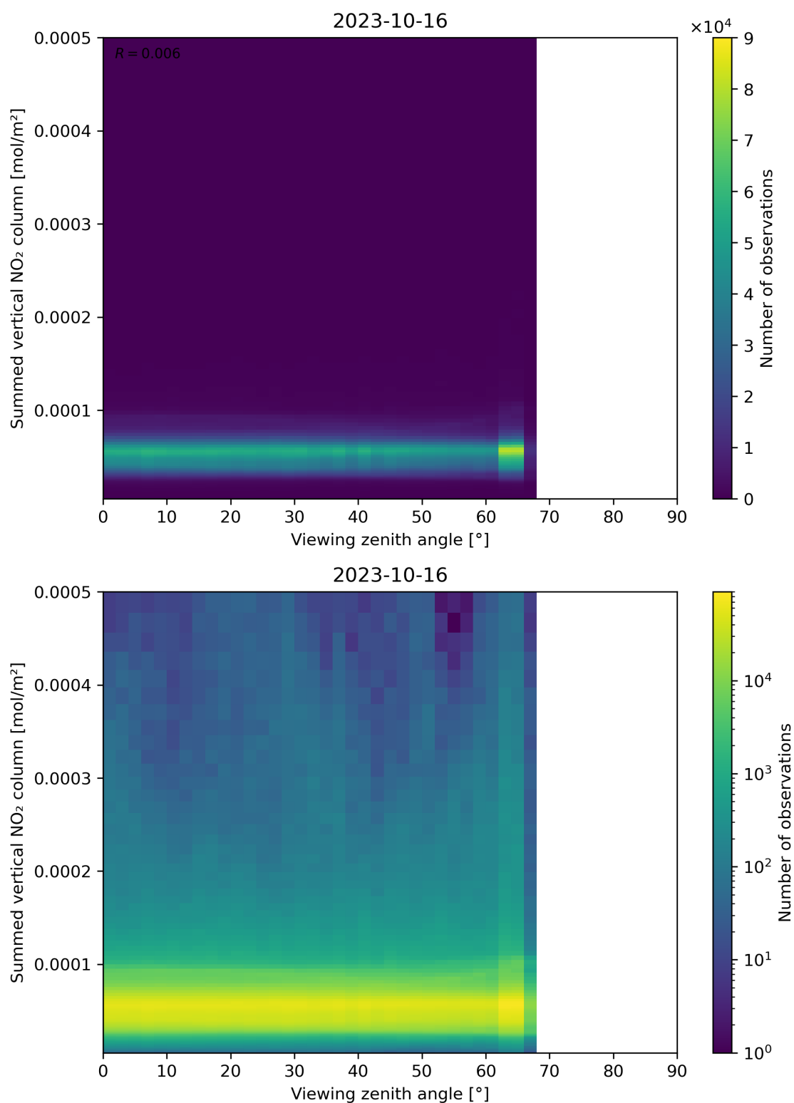
Figure 165: Scatter density plot of “Viewing zenith angle” against “Summed vertical NO 2 column” for 2023-10-15 to 2023-10-17.
