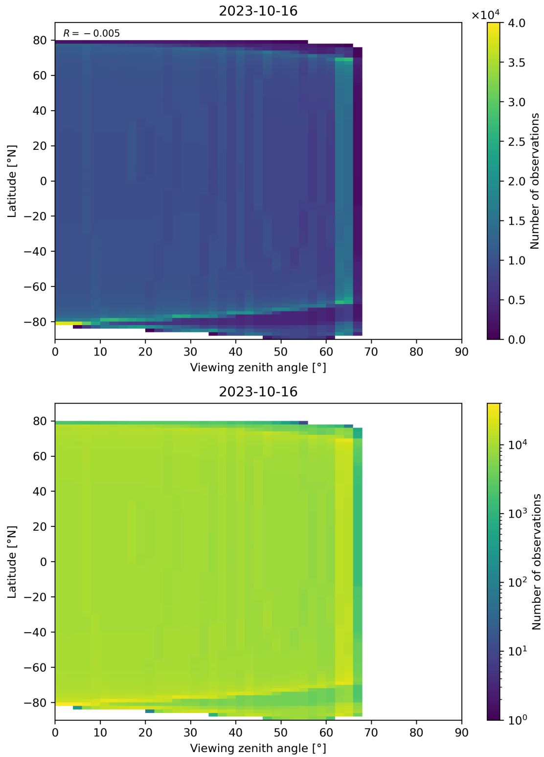
Figure 163: Scatter density plot of “Viewing zenith angle” against “Latitude” for 2023-10-15 to 2023-10-17.
