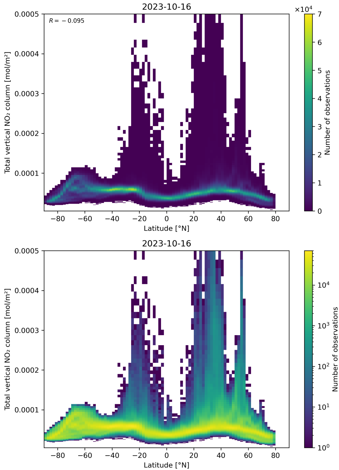
Figure 90: Scatter density plot of “Latitude” against “Total vertical NO 2 column” for 2023-10-15 to 2023-10-17.
