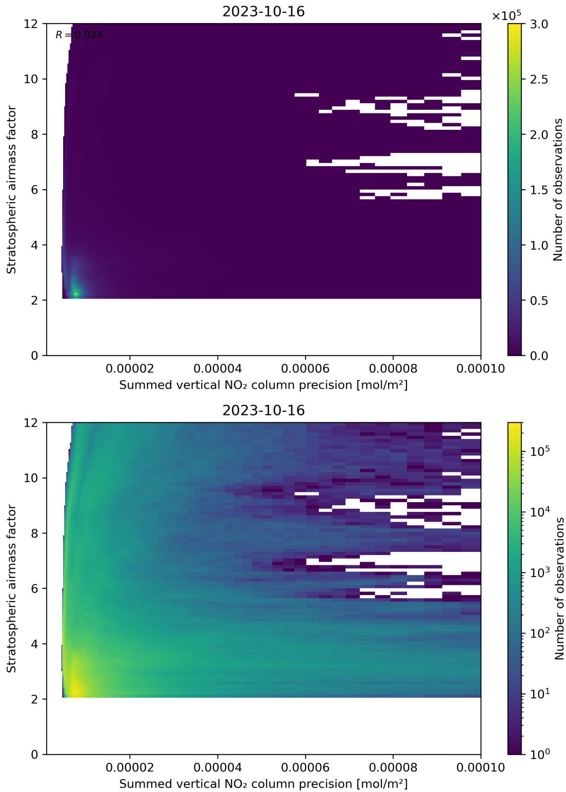
Figure 106: Scatter density plot of “Summed vertical NO 2 column precision” against “Stratospheric airmass factor” for 2023-10-15 to 2023-10-17.
