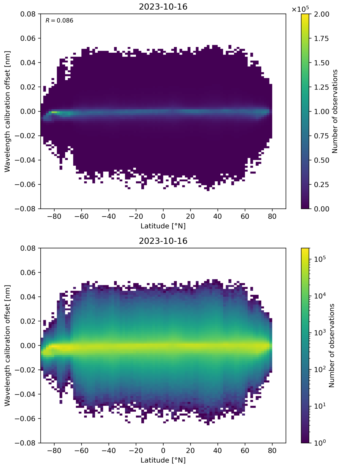
Figure 95: Scatter density plot of “Latitude” against “Wavelength calibration offset” for 2023-10-15 to 2023-10-17.
