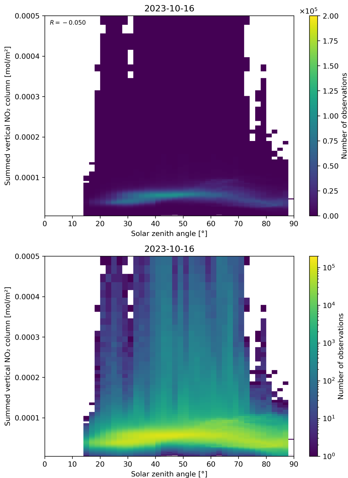
Figure 151: Scatter density plot of “Solar zenith angle” against “Summed vertical NO 2 column” for 2023-10-15 to 2023-10-17.
