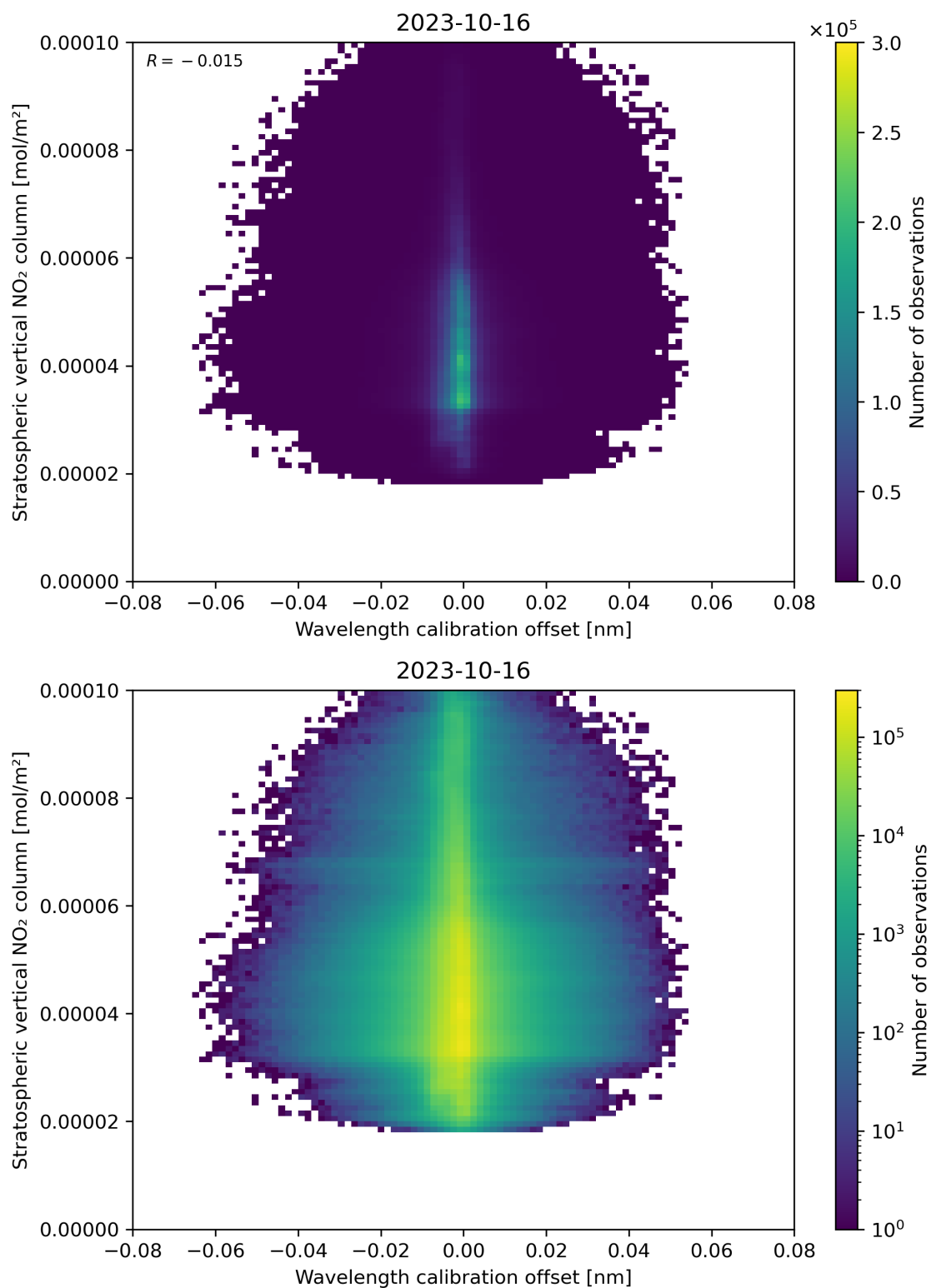
Figure 176: Scatter density plot of “Wavelength calibration offset” against “Stratospheric vertical NO 2 column” for 2023-10-15 to 2023-10-17.
