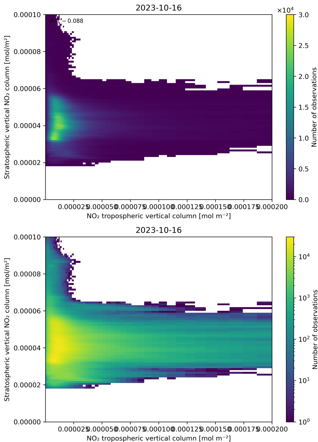
Figure 125: Scatter density plot of “NO 2 tropospheric vertical column” against “Stratospheric vertical NO 2 column” for 2023-10-15 to 2023-10-17.
