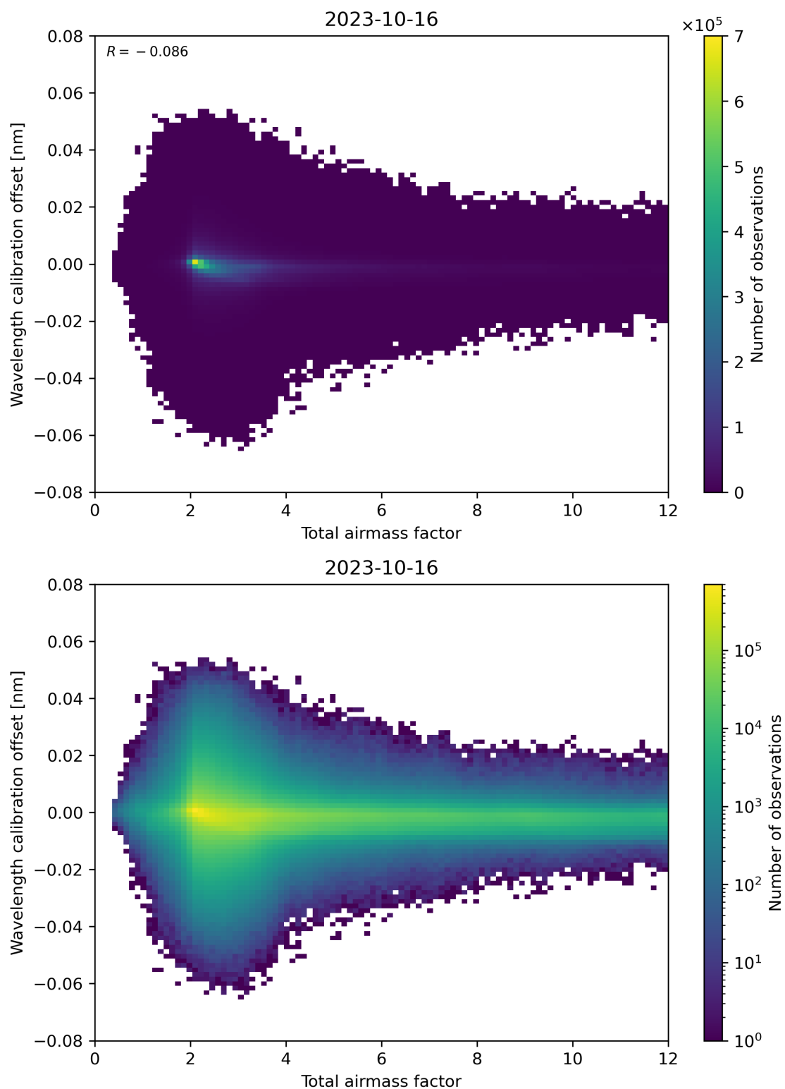
Figure 70: Scatter density plot of “Total airmass factor” against “Wavelength calibration offset” for 2023-10-15 to 2023-10-17.
