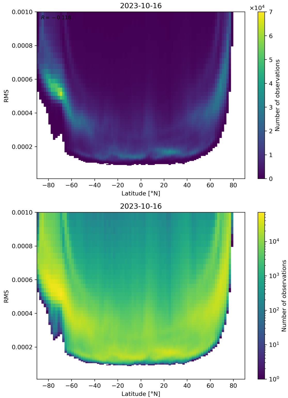
Figure 94: Scatter density plot of “Latitude” against “RMS” for 2023-10-15 to 2023-10-17.
