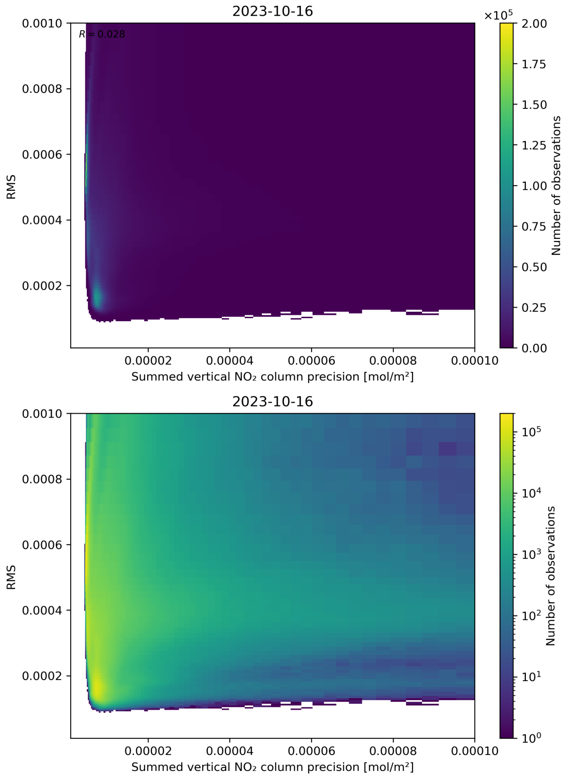
Figure 108: Scatter density plot of “Summed vertical NO 2 column precision” against “RMS” for 2023-10-15 to 2023-10-17.
