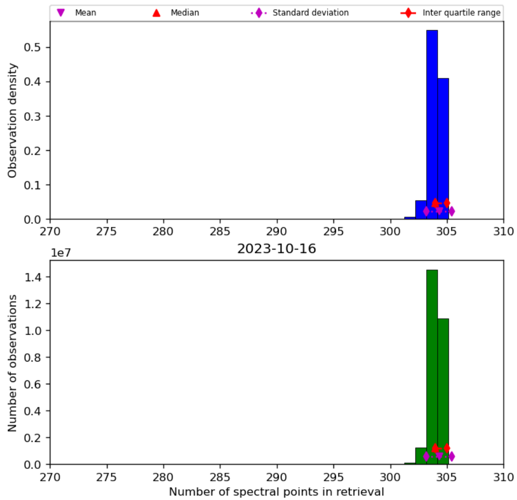
Figure 33: Histogram of “Number of spectral points in retrieval” for 2023-10-15 to 2023-10-17
