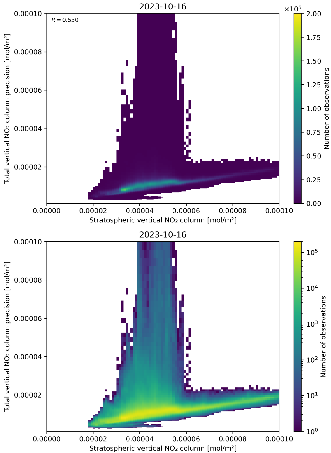
Figure 101: Scatter density plot of “Stratospheric vertical NO 2 column” against “Total vertical NO 2 column precision” for 2023-10-15 to 2023-10-17.
