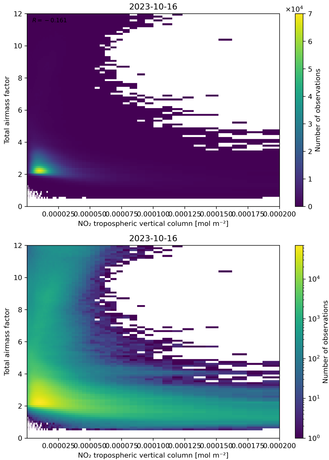
Figure 122: Scatter density plot of “NO 2 tropospheric vertical column” against “Total air mass factor” for 2023-10-15 to 2023-10-17.
