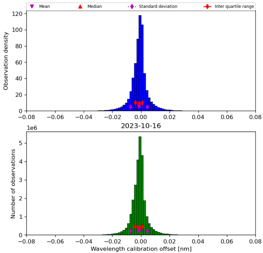
Figure 35: Histogram of “Wavelength calibration offset” for 2023-10-15 to 2023-10-17
