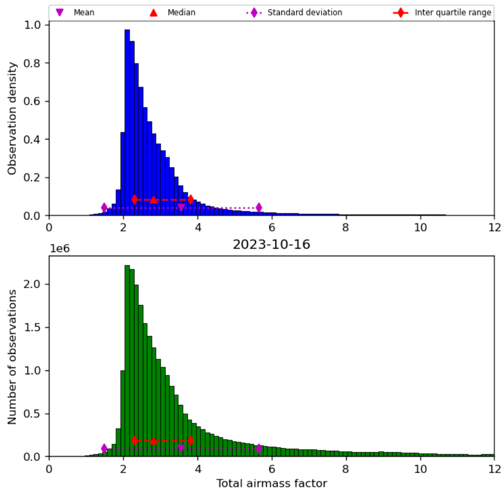
Figure 32: Histogram of “Total airmass factor” for 2023-10-15 to 2023-10-17
