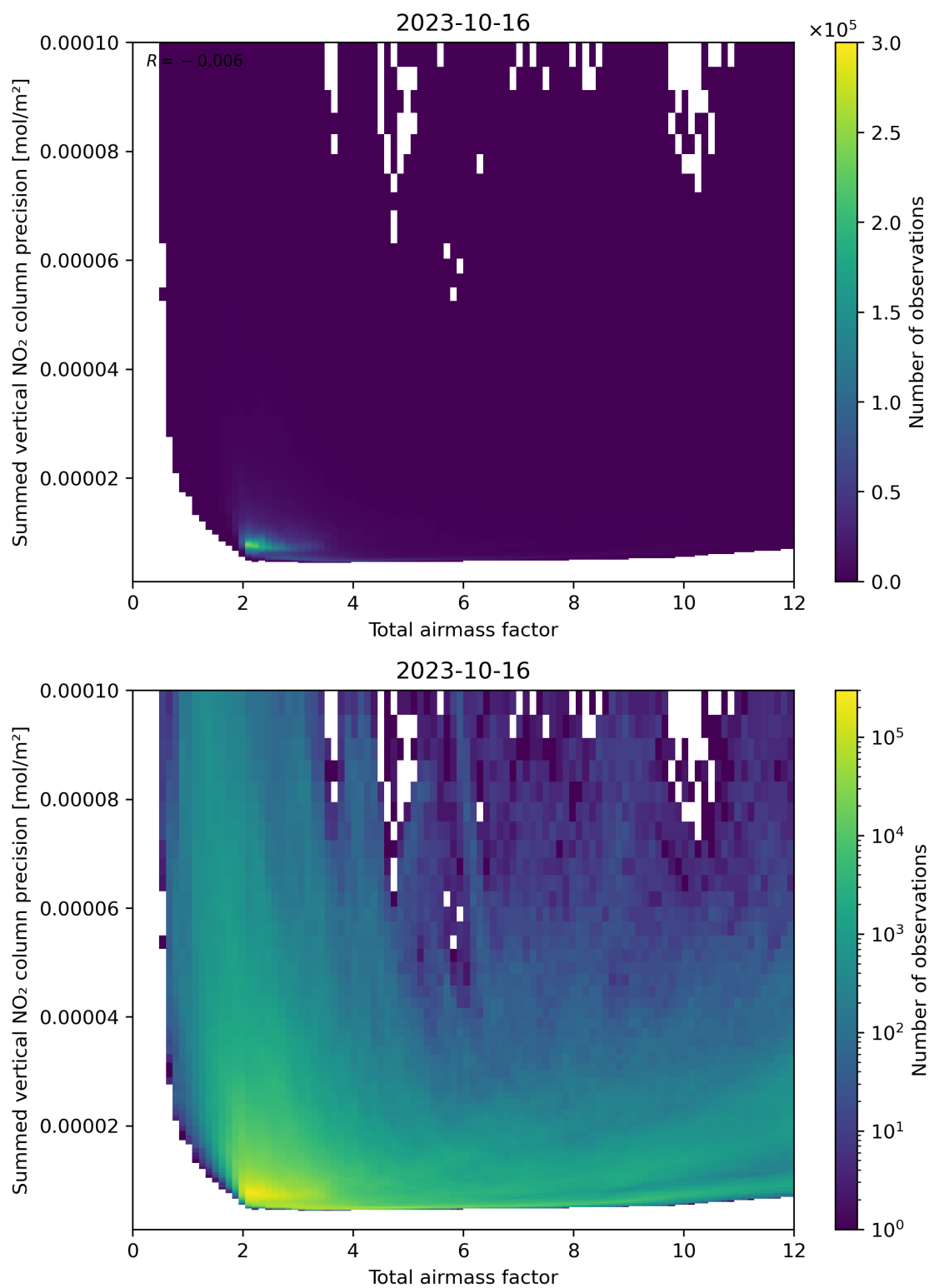
Figure 66: Scatter density plot of “Total airmass factor” against “Summed vertical NO 2 column precision” for 2023-10-15 to 2023-10-17.
