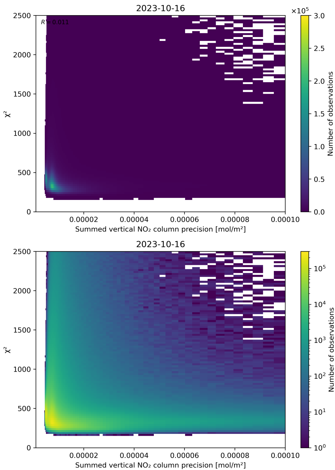
Figure 107: Scatter density plot of “Summed vertical NO 2 column precision” against “ \chi^2 ” for 2023-10-15 to 2023-10-17.
