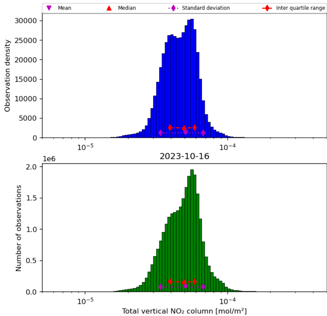
Figure 38: Histogram of "Total vertical NO 2 column" for 2023-10-15 to 2023-10-17
