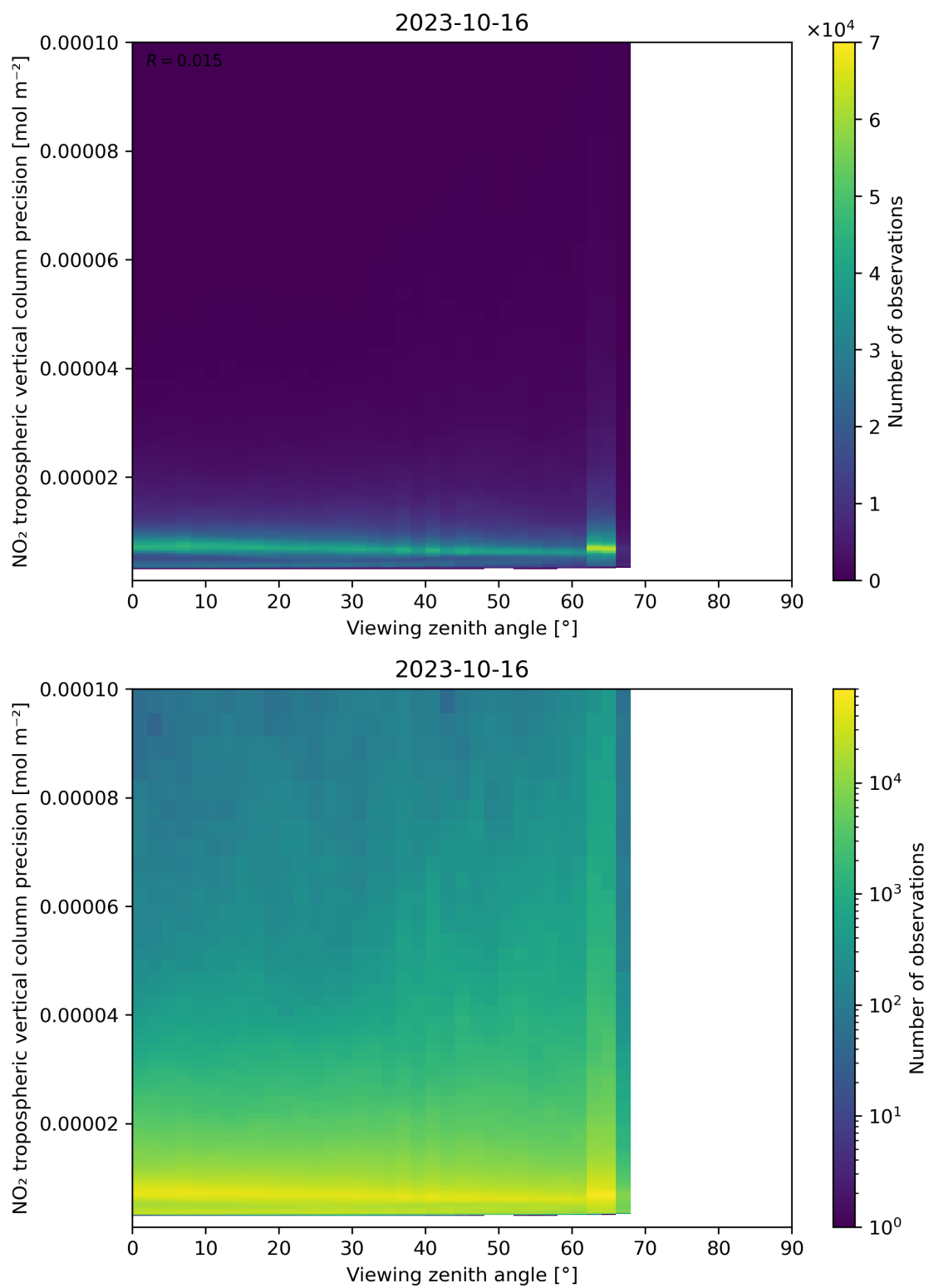
Figure 170: Scatter density plot of “Viewing zenith angle” against “NO 2 tropospheric vertical column precision” for 2023-10-15 to 2023-10-17.
