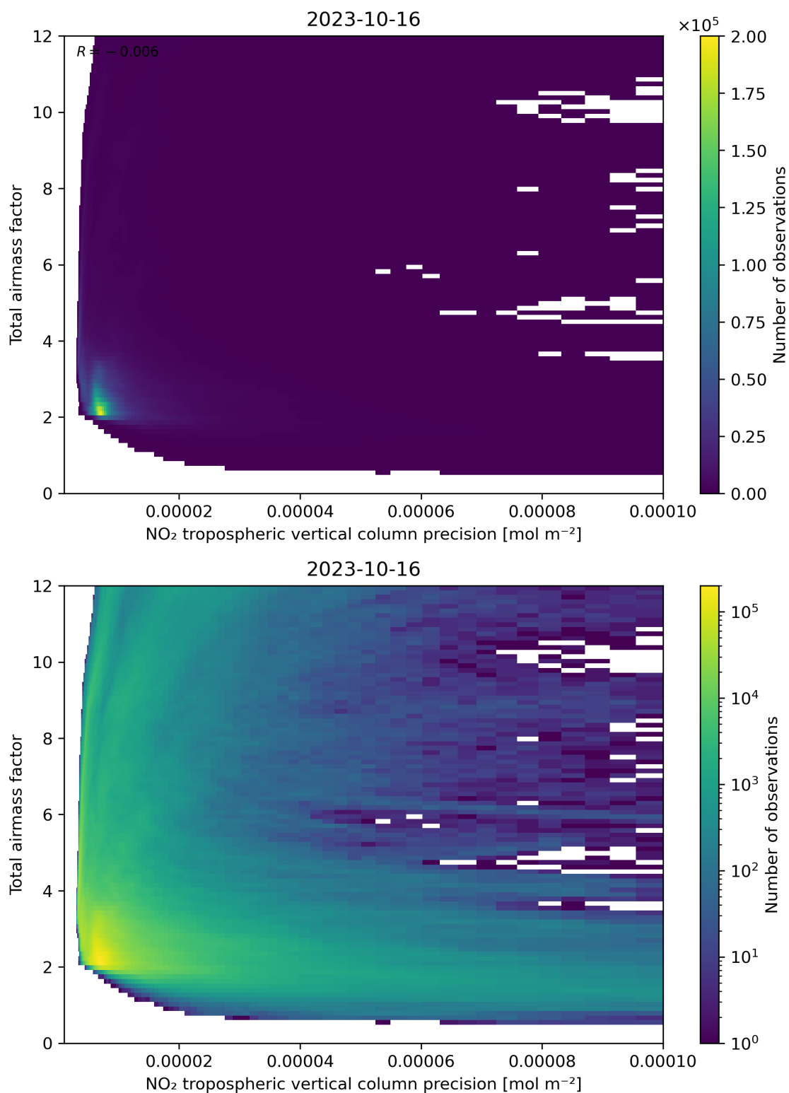
Figure 132: Scatter density plot of “NO 2 tropospheric vertical column precision” against “Total air mass factor” for 2023-10-15 to 2023-10-17.
