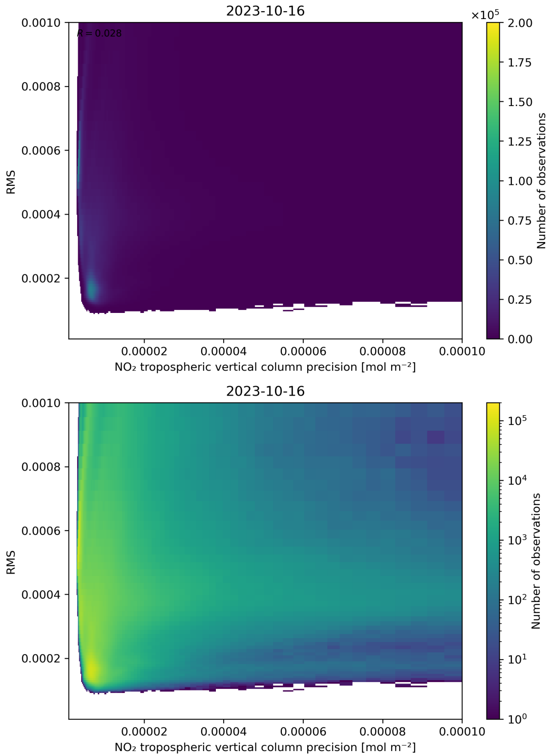
Figure 140: Scatter density plot of “NO 2 tropospheric vertical column precision” against “RMS” for 2023-10-15 to 2023-10-17.
