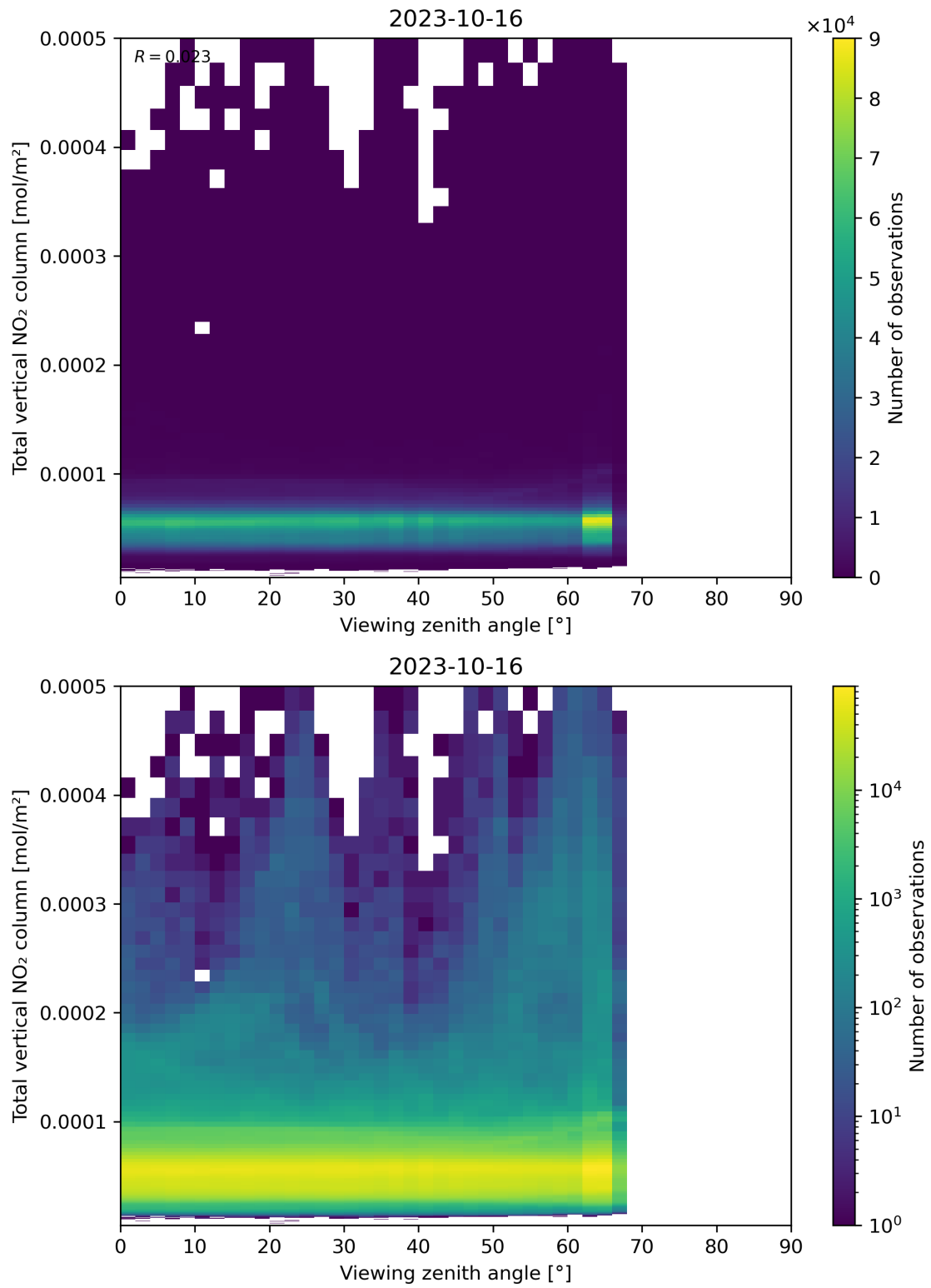
Figure 167: Scatter density plot of “Viewing zenith angle” against “Total vertical NO 2 column” for 2023-10-15 to 2023-10-17.
