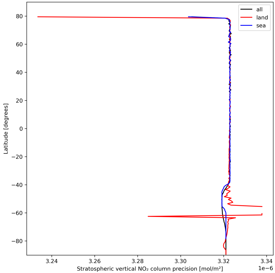
Figure 20: Zonal average of “Stratospheric vertical NO 2 column precision” for 2023-10-15 to 2023-10-17.
