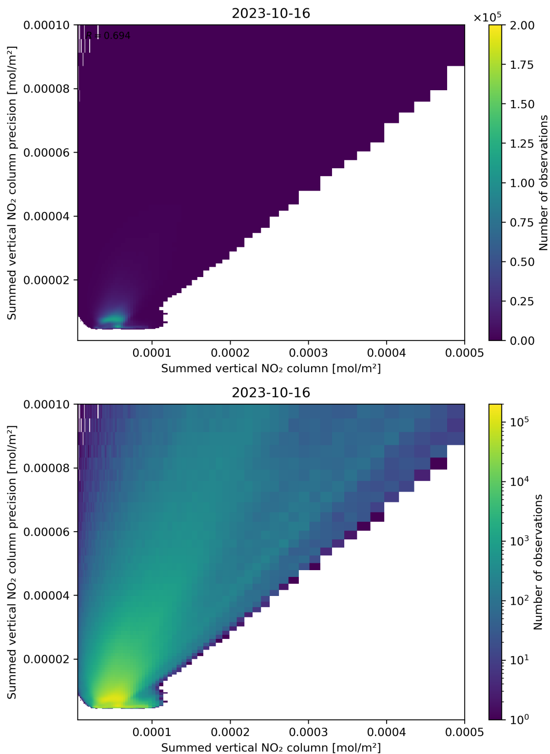
Figure 105: Scatter density plot of “Summed vertical NO 2 column” against “Summed vertical NO 2 column precision” for 2023-10-15 to 2023-10-17.
