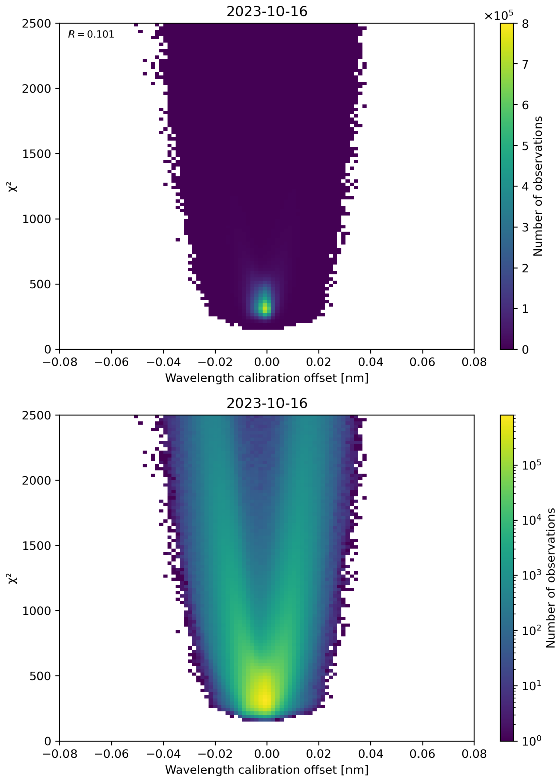
Figure 175: Scatter density plot of “Wavelength calibration offset” against “ \chi^2 ” for 2023-10-15 to 2023-10-17.
