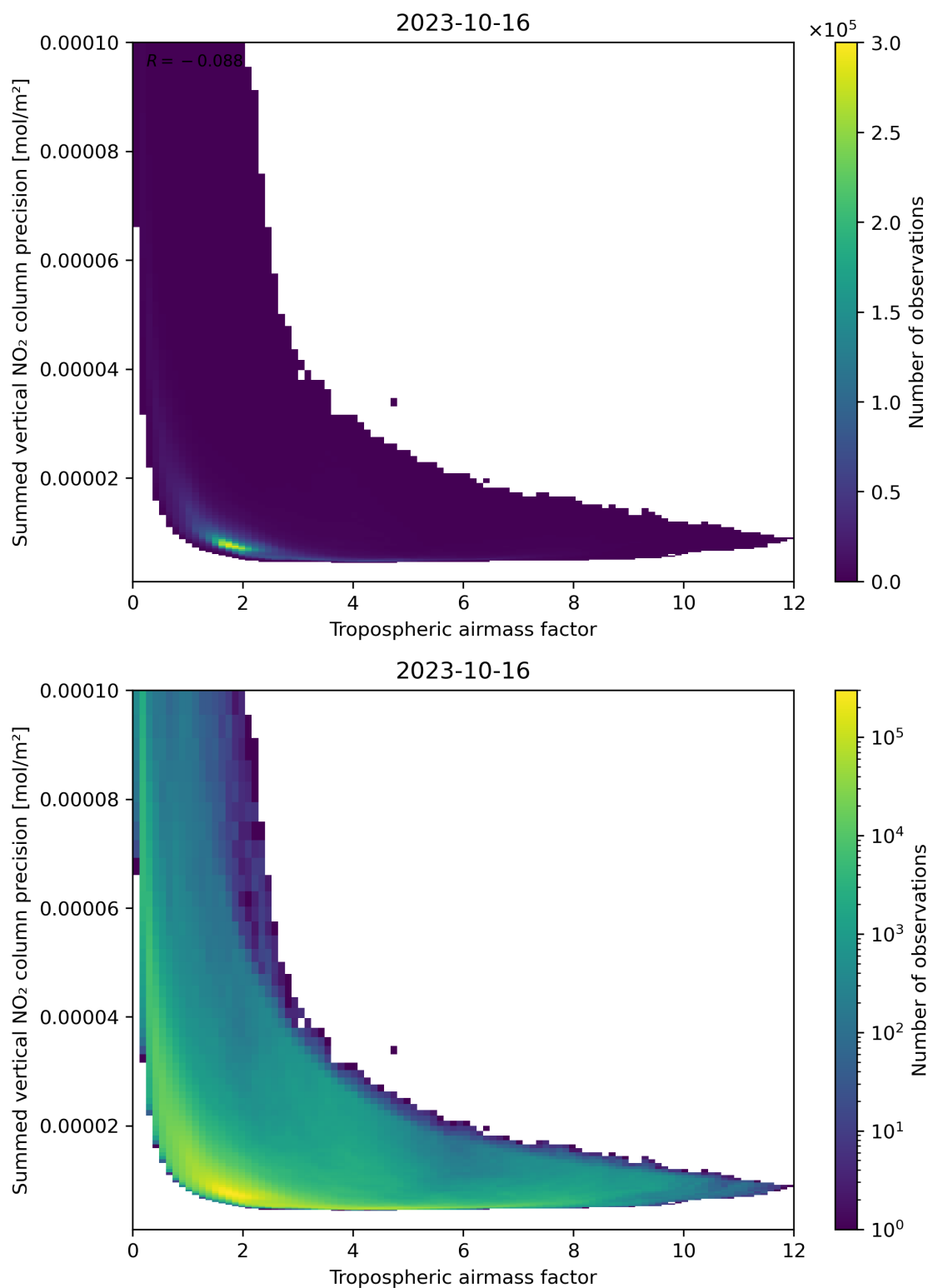
Figure 76: Scatter density plot of “Tropospheric air mass factor” against “Summed vertical NO 2 column precision” for 2023-10-15 to 2023-10-17.
