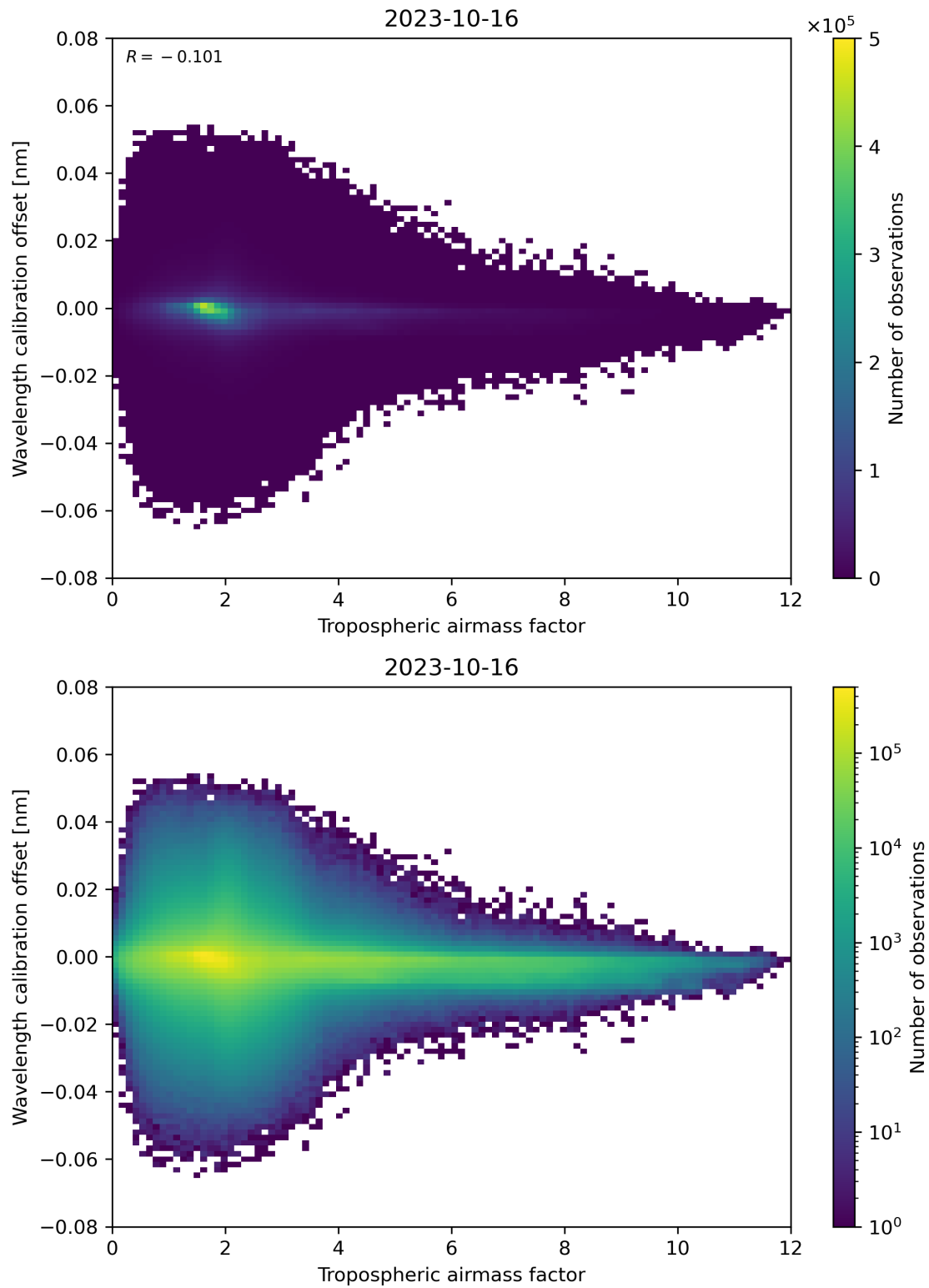
Figure 80: Scatter density plot of “Tropospheric airmass factor” against “Wavelength calibration offset” for 2023-10-15 to 2023-10-17.
