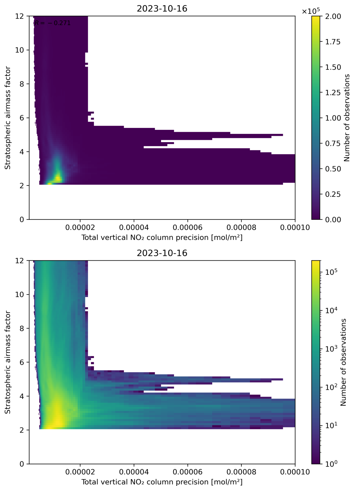
Figure 115: Scatter density plot of “Total vertical NO 2 column precision” against “Stratospheric airmass factor” for 2023-10-15 to 2023-10-17.
