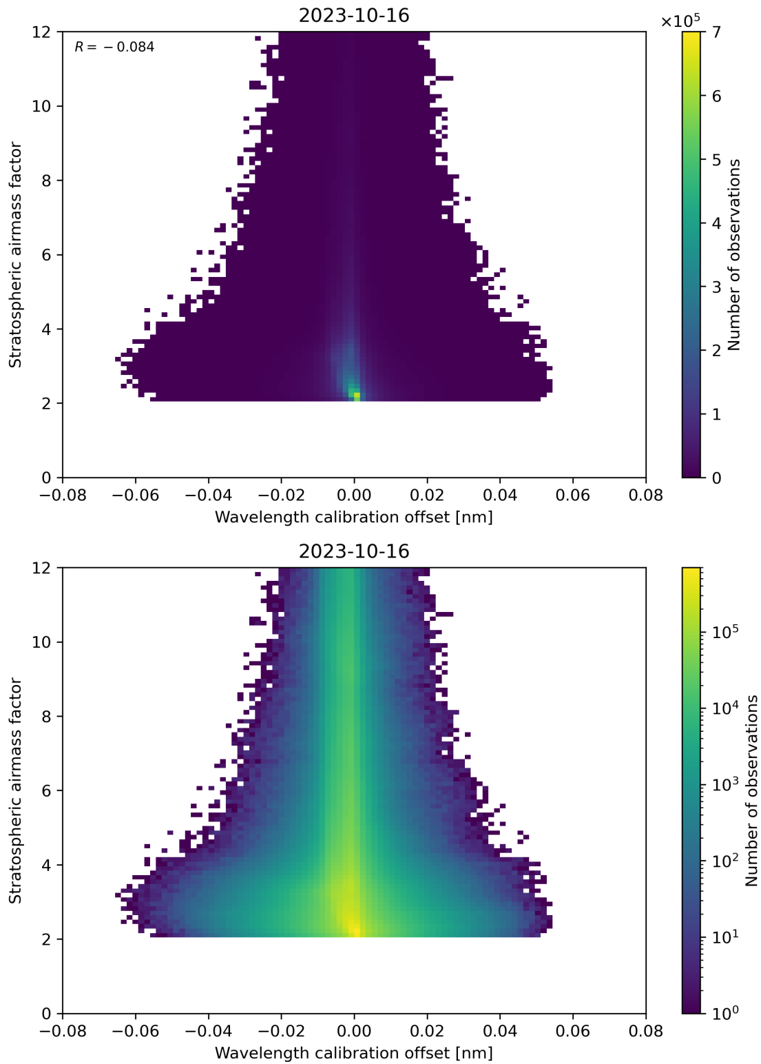
Figure 174: Scatter density plot of “Wavelength calibration offset” against “Stratospheric air mass factor” for 2023-10-15 to 2023-10-17.
