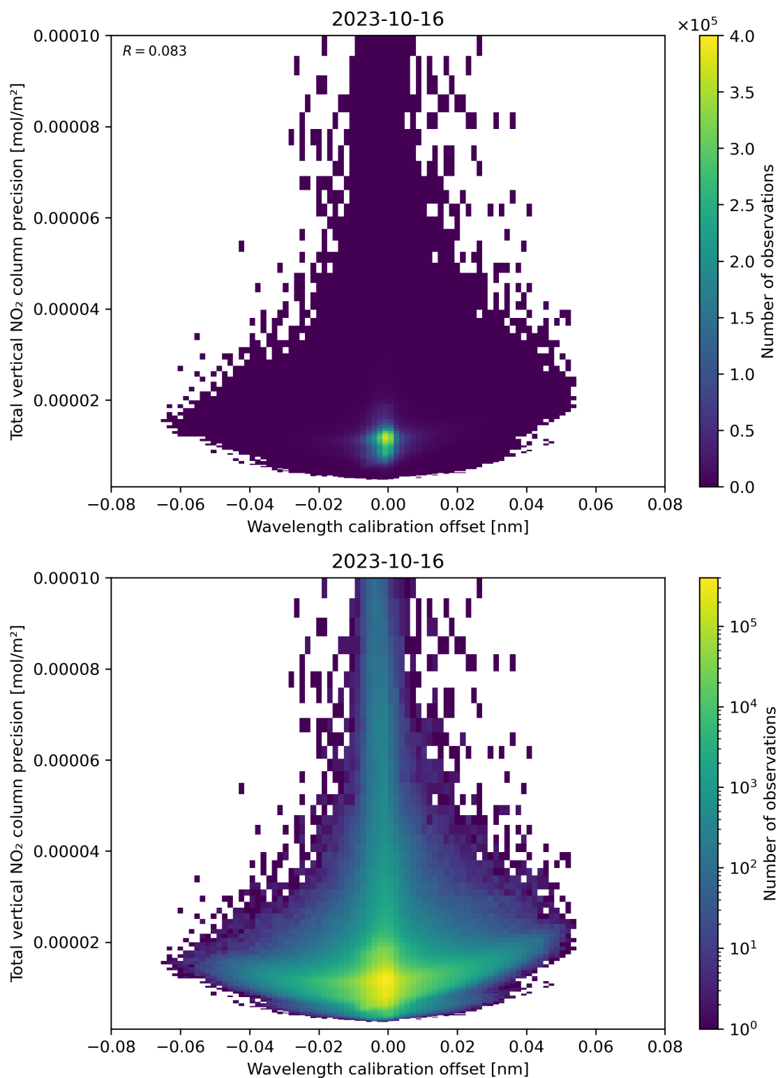
Figure 180: Scatter density plot of “Wavelength calibration offset” against “Total vertical NO 2 column precision” for 2023-10-15 to 2023-10-17.
