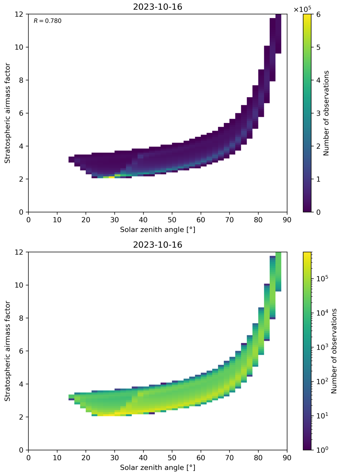
Figure 145: Scatter density plot of “Solar zenith angle” against “Stratospheric airmass factor” for 2023-10-15 to 2023-10-17.
