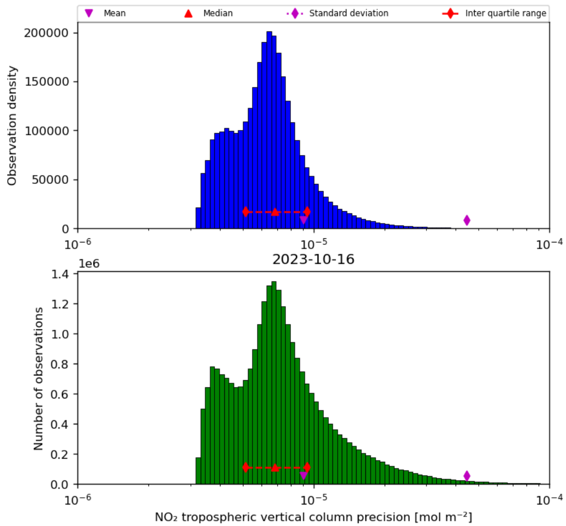
Figure 30: Histogram of “NO 2 tropospheric vertical column precision” for 2023-10-15 to 2023-10-17
