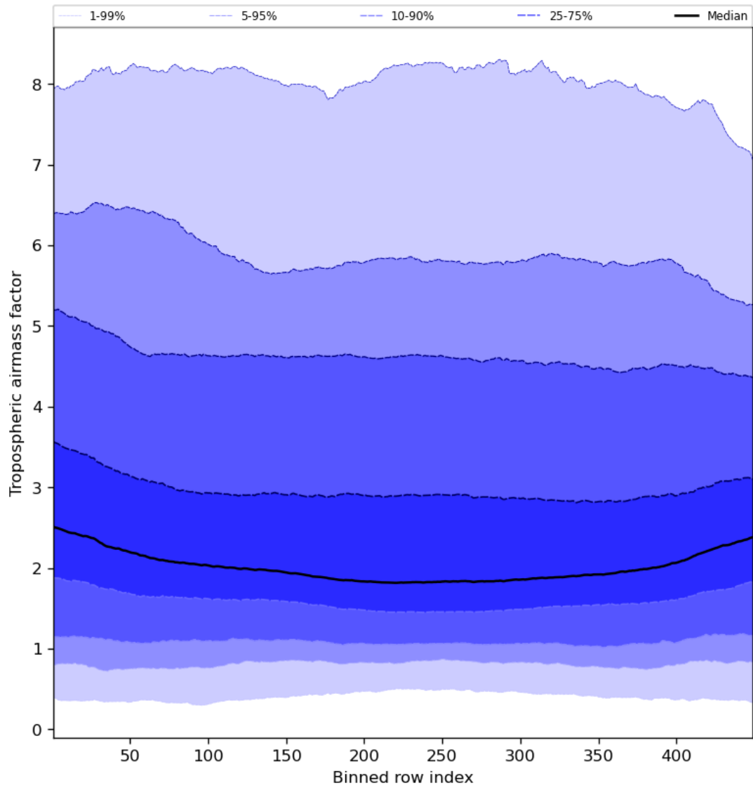
Figure 48: Along track statistics of “Tropospheric air mass factor” for 2023-10-15 to 2023-10-17
