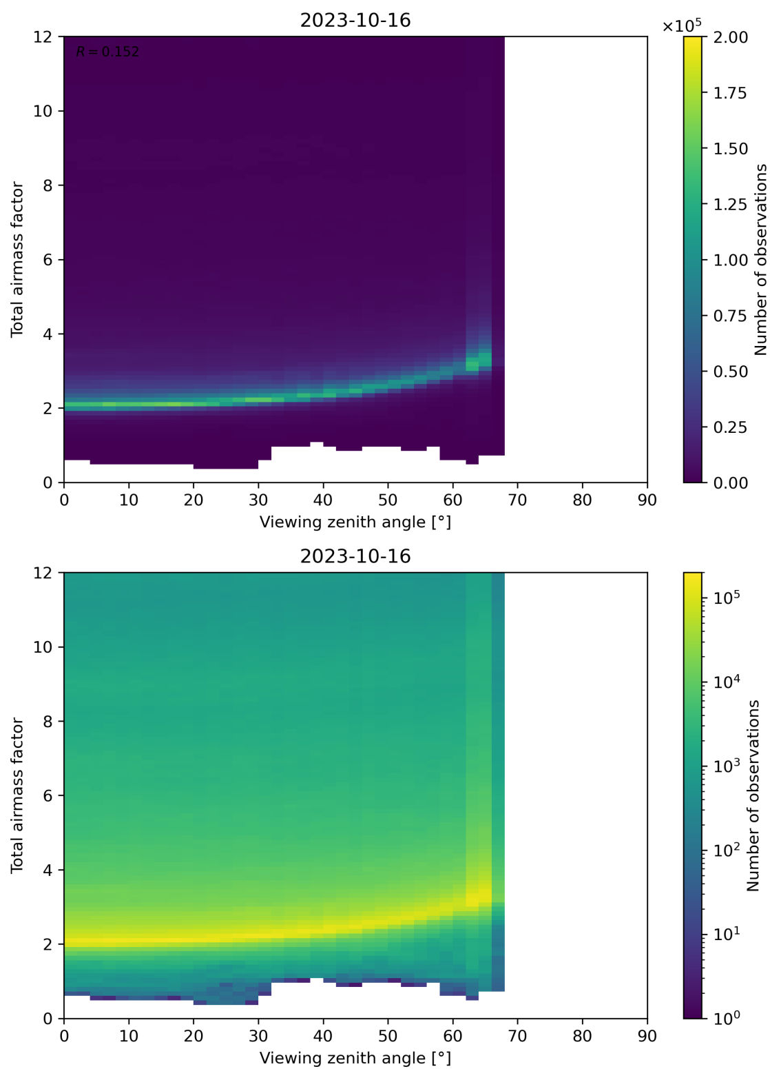
Figure 160: Scatter density plot of “Viewing zenith angle” against “Total airmass factor” for 2023-10-15 to 2023-10-17.
