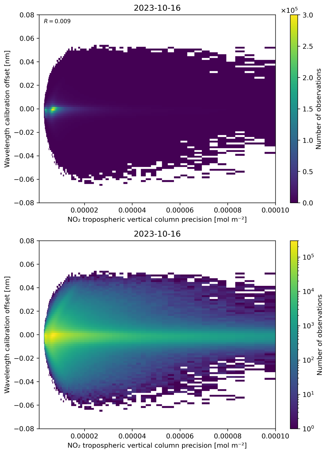
Figure 141: Scatter density plot of “NO 2 tropospheric vertical column precision” against “Wavelength calibration offset” for 2023-10-15 to 2023-10-17.
