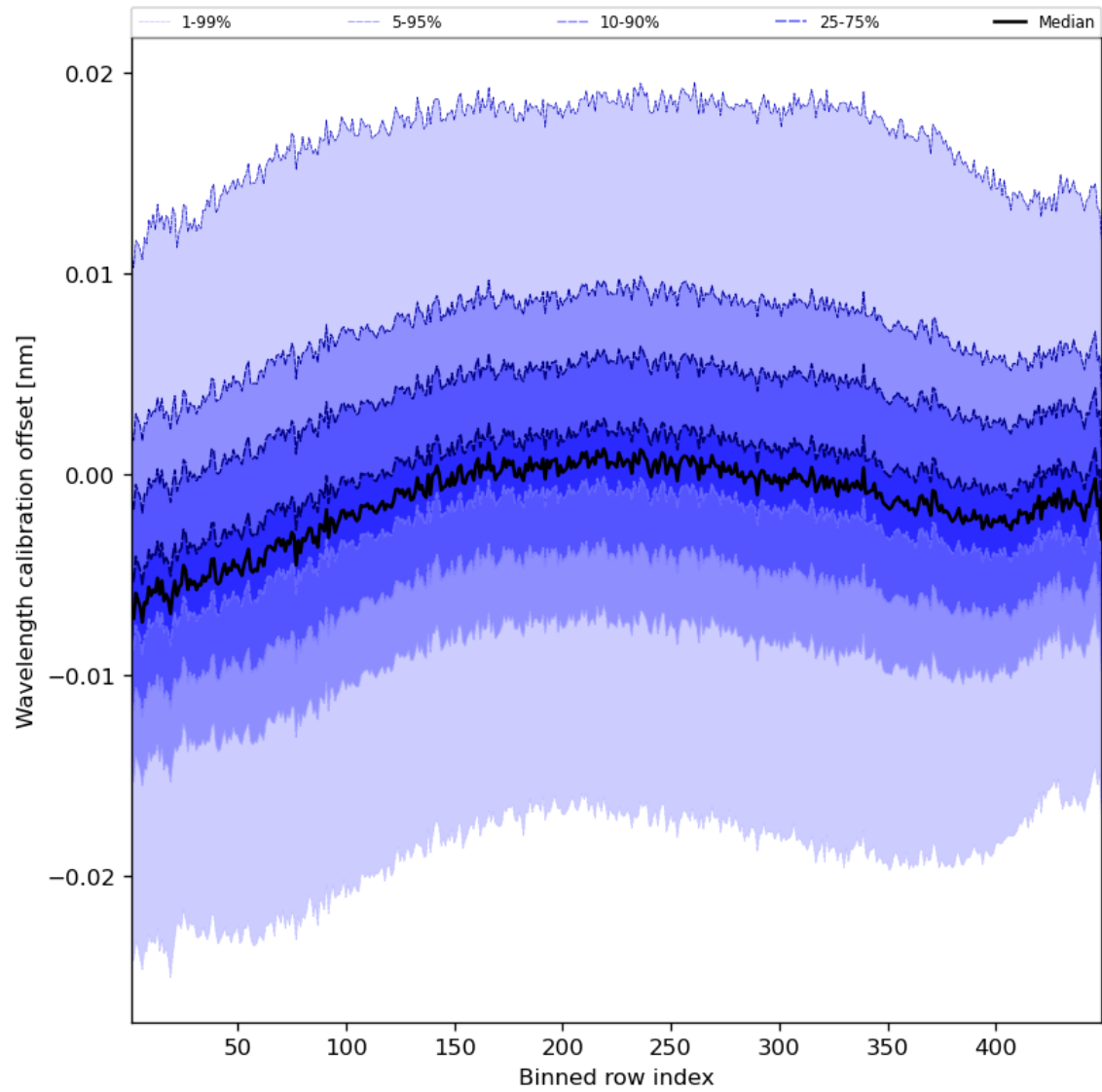
Figure 52: Along track statistics of “Wavelength calibration offset” for 2023-10-15 to 2023-10-17
