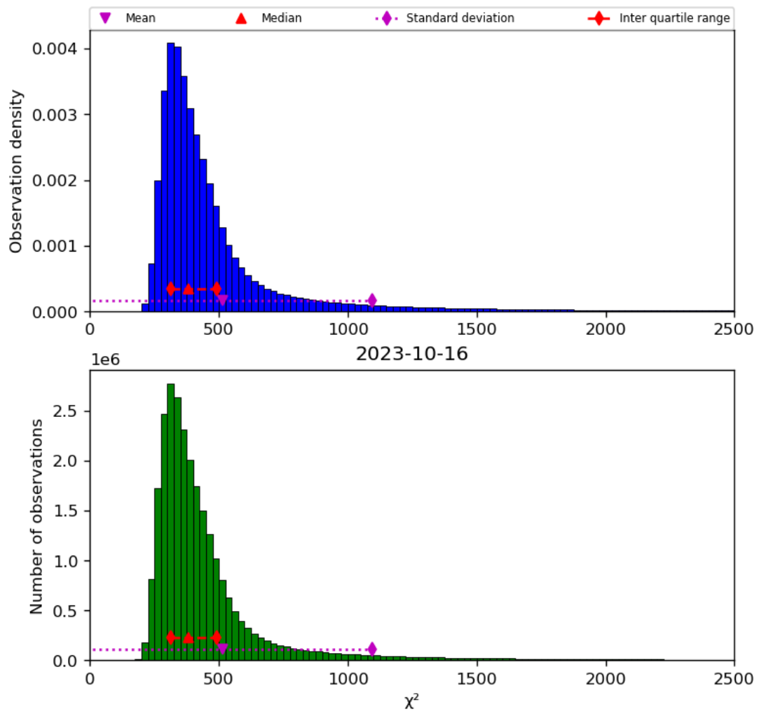
Figure 42: Histogram of “ \chi^2 ” for 2023-10-15 to 2023-10-17
