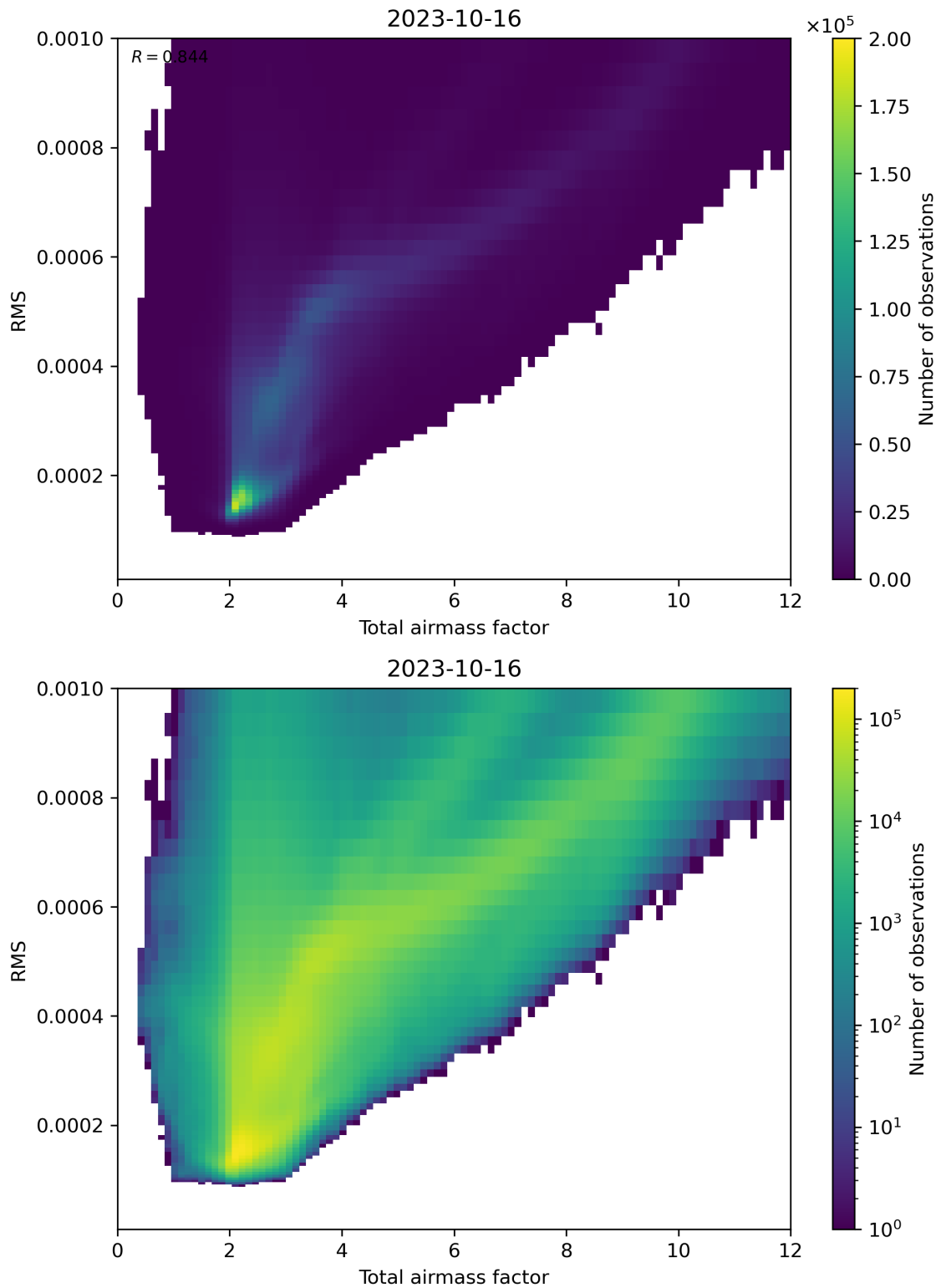
Figure 69: Scatter density plot of “Total airmass factor” against “RMS” for 2023-10-15 to 2023-10-17.
