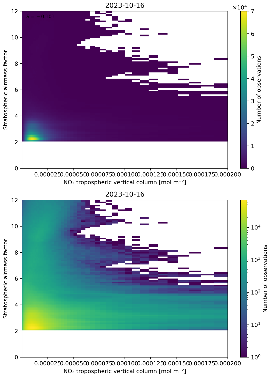
Figure 121: Scatter density plot of “NO 2 tropospheric vertical column” against “Stratospheric air mass factor” for 2023-10-15 to 2023-10-17.
