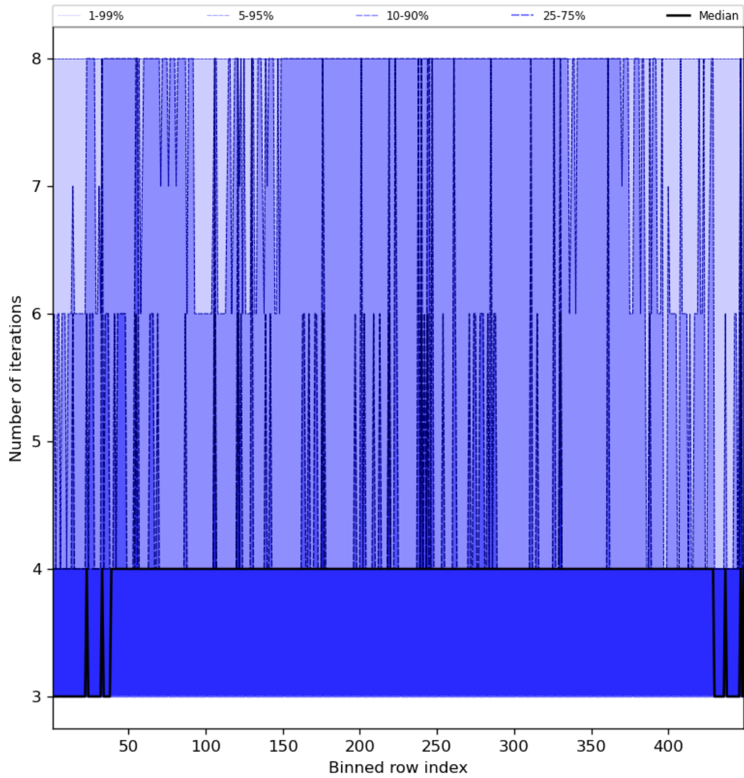
Figure 51: Along track statistics of “Number of iterations” for 2023-10-15 to 2023-10-17
