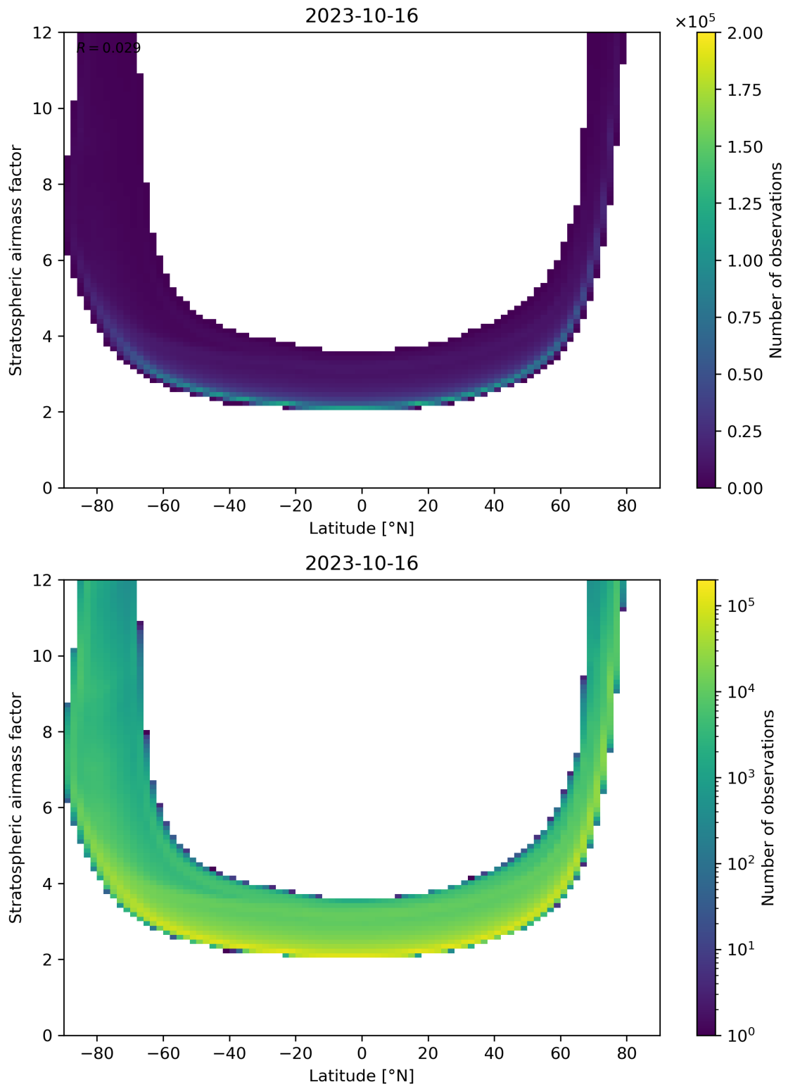
Figure 83: Scatter density plot of “Latitude” against “Stratospheric airmass factor” for 2023-10-15 to 2023-10-17.
