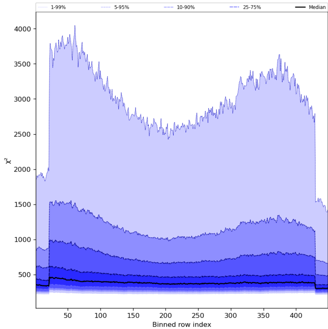
Figure 59: Along track statistics of “ \chi^2 ” for 2023-10-15 to 2023-10-17
