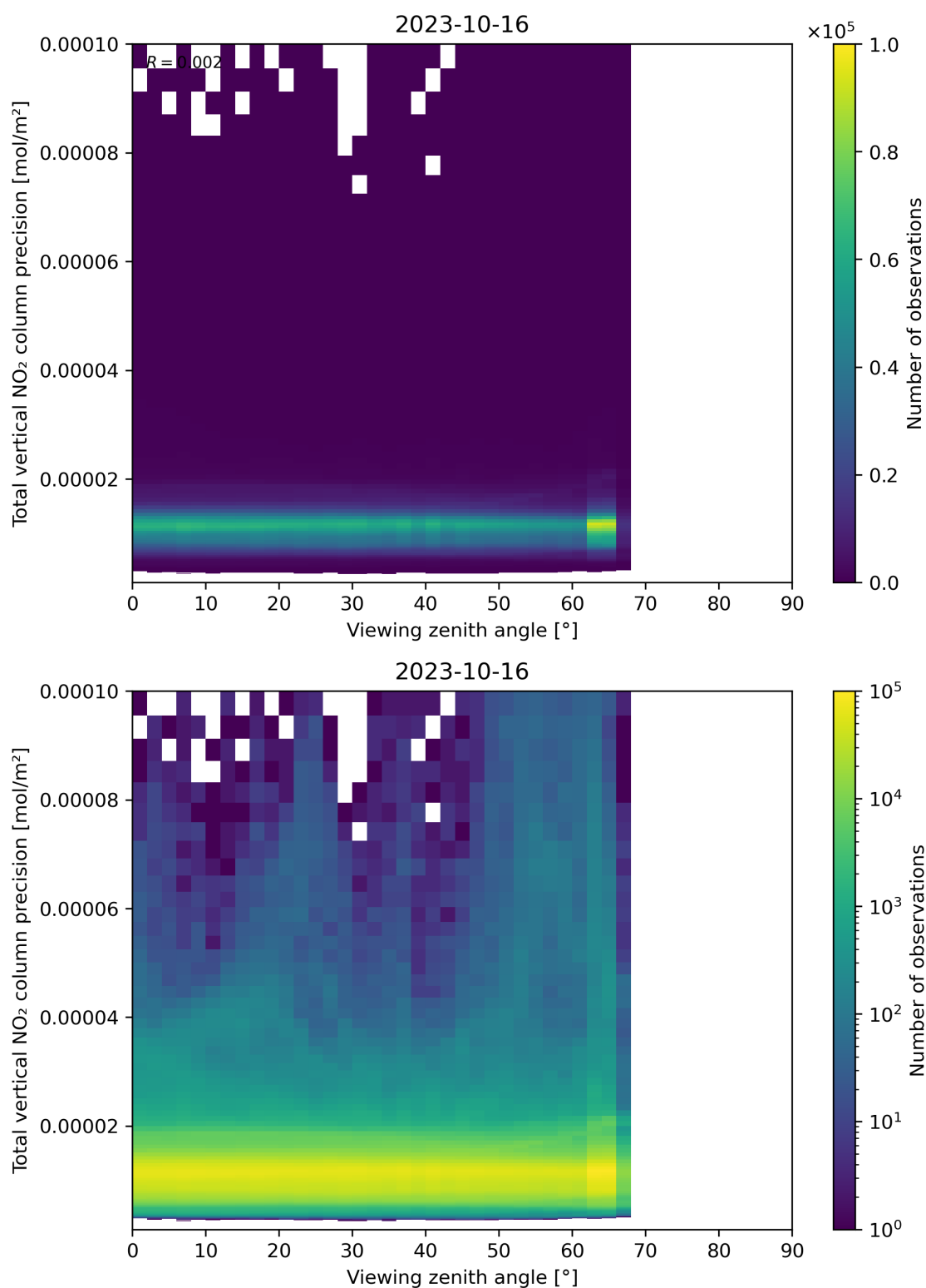
Figure 168: Scatter density plot of “Viewing zenith angle” against “Total vertical NO 2 column precision” for 2023-10-15 to 2023-10-17.
