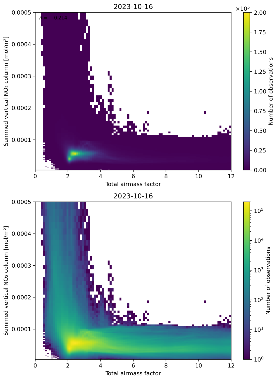
Figure 65: Scatter density plot of “Total airmass factor” against “Summed vertical NO 2 column” for 2023-10-15 to 2023-10-17.
