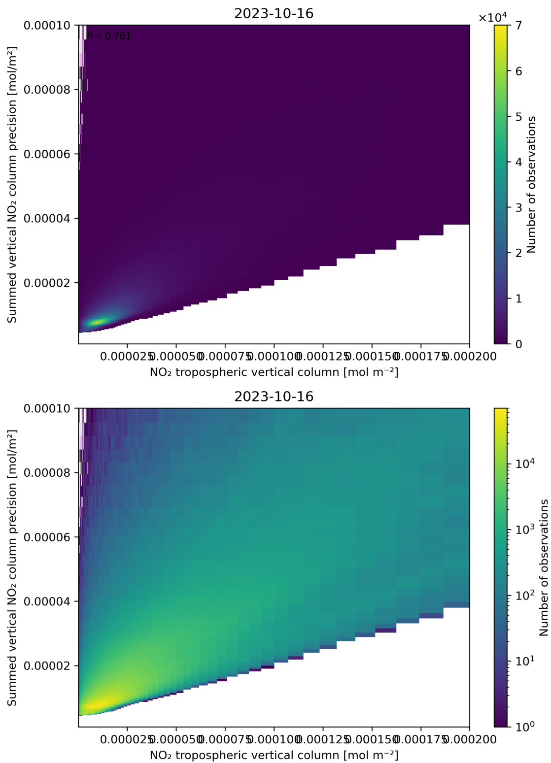
Figure 127: Scatter density plot of “NO 2 tropospheric vertical column” against “Summed vertical NO 2 column precision” for 2023-10-15 to 2023-10-17.
