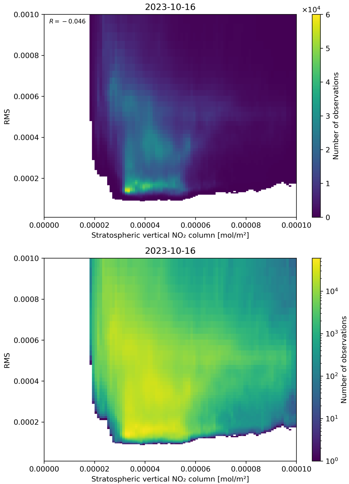
Figure 102: Scatter density plot of “Stratospheric vertical NO 2 column” against “RMS” for 2023-10-15 to 2023-10-17.
