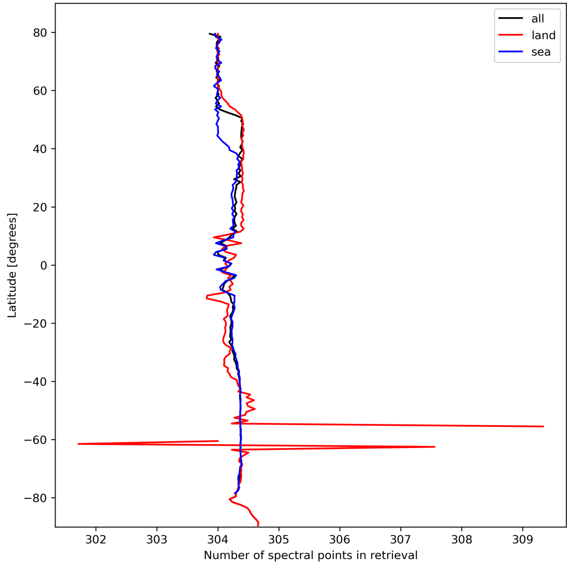
Figure 16: Zonal average of “Number of spectral points in retrieval” for 2023-10-15 to 2023-10-17.
