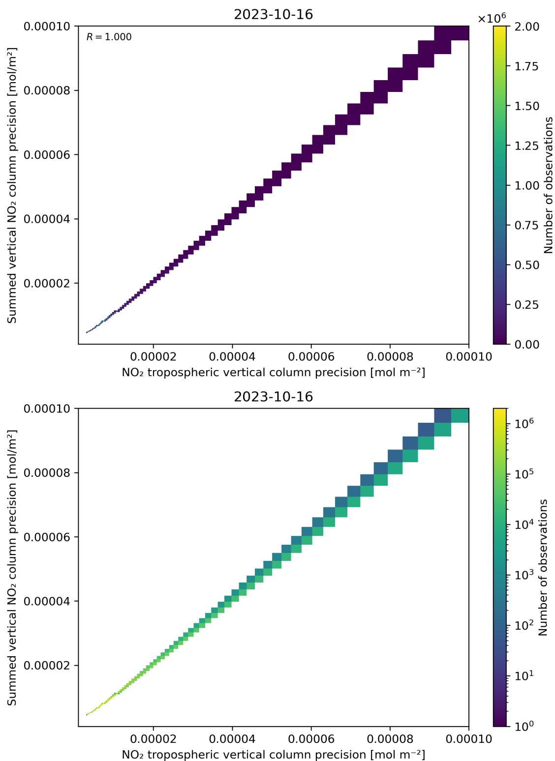
Figure 137: Scatter density plot of “NO 2 tropospheric vertical column precision” against “Summed vertical NO 2 column precision” for 2023-10-15 to 2023-10-17.
