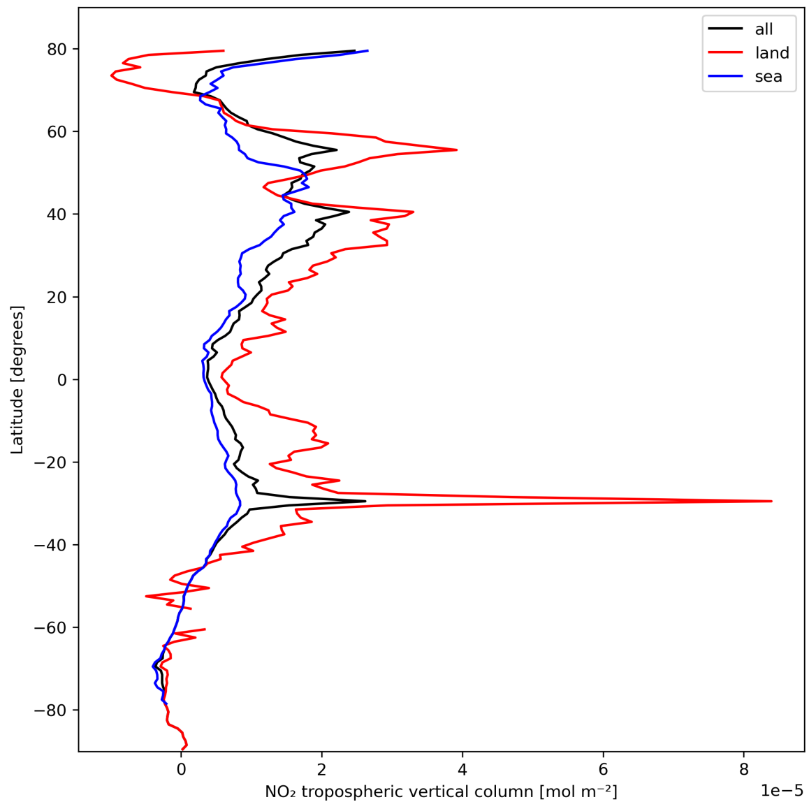
Figure 12: Zonal average of “NO 2 tropospheric vertical column” for 2023-10-15 to 2023-10-17.
