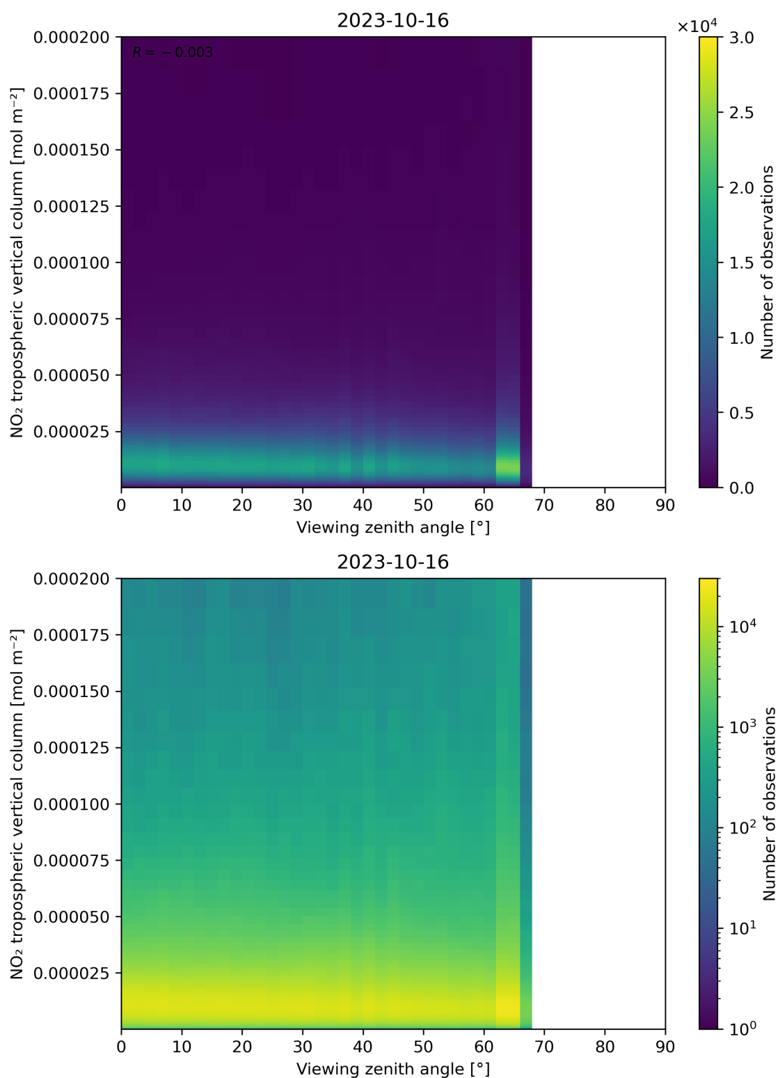
Figure 169: Scatter density plot of “Viewing zenith angle” against “NO 2 tropospheric vertical column” for 2023-10-15 to 2023-10-17.
