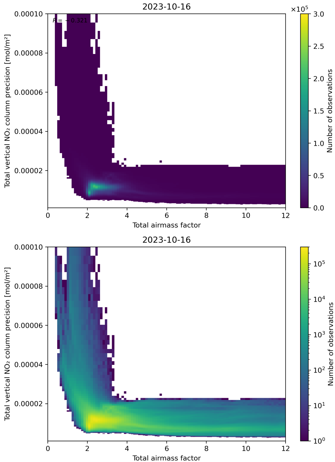
Figure 68: Scatter density plot of “Total airmass factor” against “Total vertical NO 2 column precision” for 2023-10-15 to 2023-10-17.
