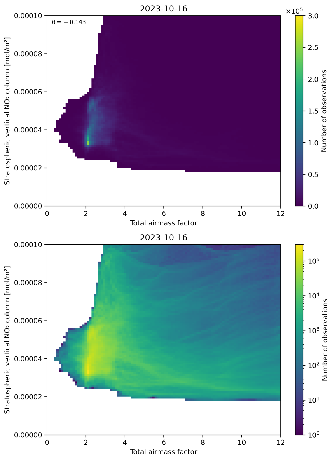
Figure 64: Scatter density plot of “Total airmass factor” against “Stratospheric vertical NO 2 column” for 2023-10-15 to 2023-10-17.
