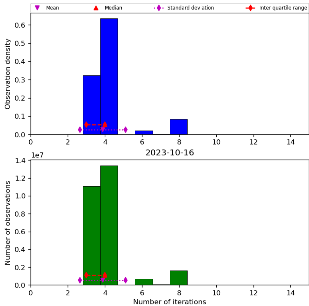
Figure 34: Histogram of “Number of iterations” for 2023-10-15 to 2023-10-17
