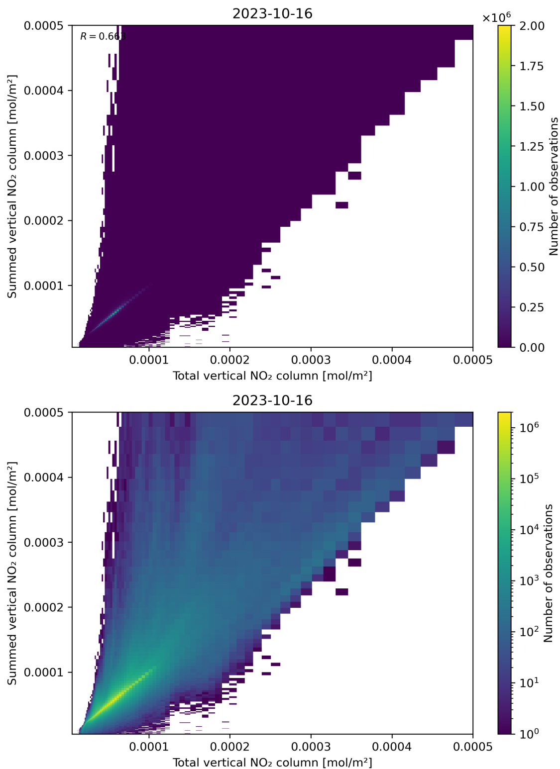
Figure 112: Scatter density plot of “Total vertical NO 2 column” against “Summed vertical NO 2 column” for 2023-10-15 to 2023-10-17.
