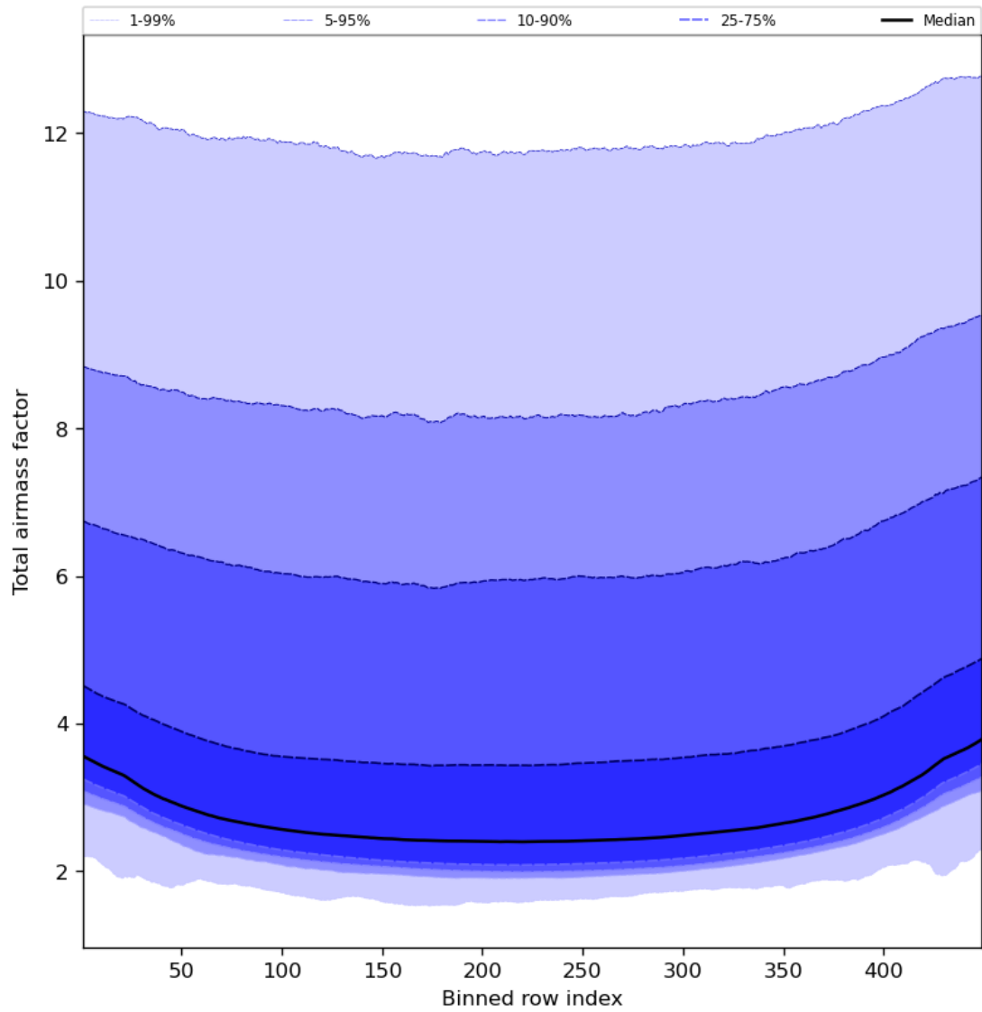
Figure 49: Along track statistics of “Total airmass factor” for 2023-10-15 to 2023-10-17
