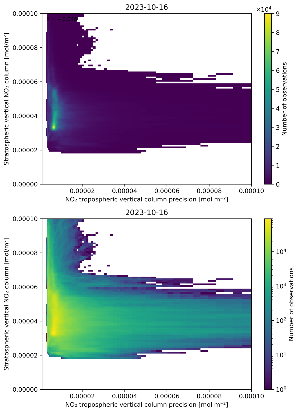
Figure 135: Scatter density plot of “NO 2 tropospheric vertical column precision” against “Stratospheric vertical NO 2 column” for 2023-10-15 to 2023-10-17.
