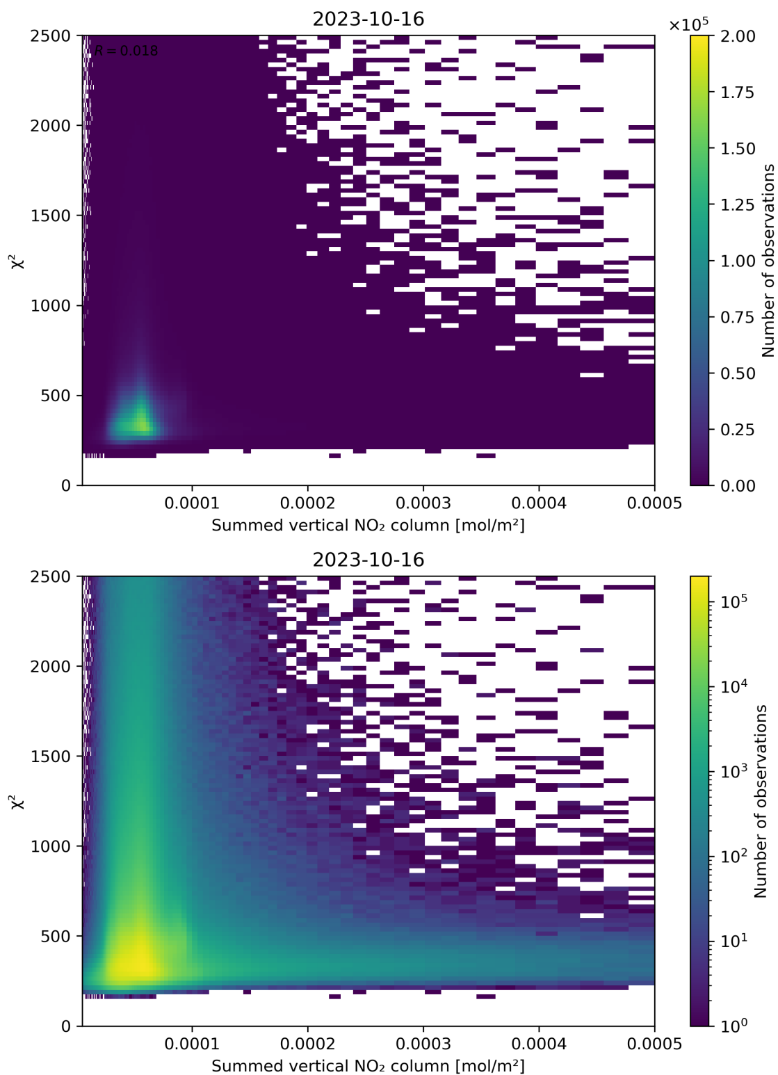
Figure 104: Scatter density plot of “Summed vertical NO 2 column” against “ \chi^2 ” for 2023-10-15 to 2023-10-17.
