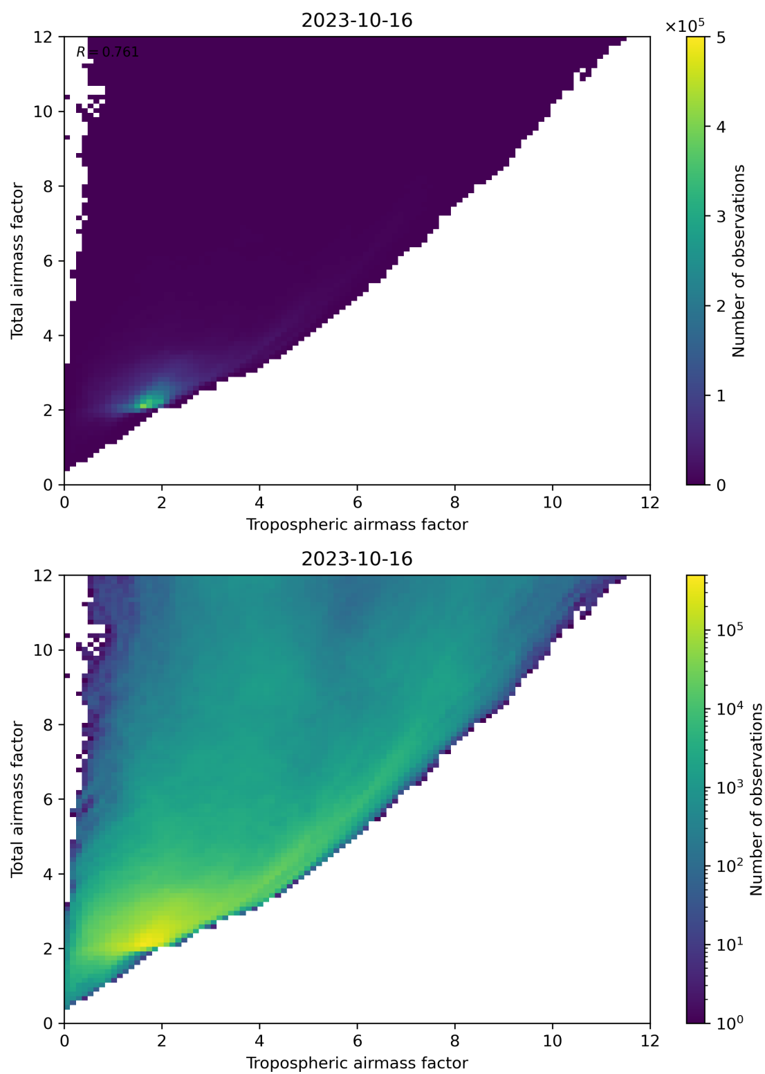
Figure 72: Scatter density plot of “Tropospheric airmass factor” against “Total airmass factor” for 2023-10-15 to 2023-10-17.
