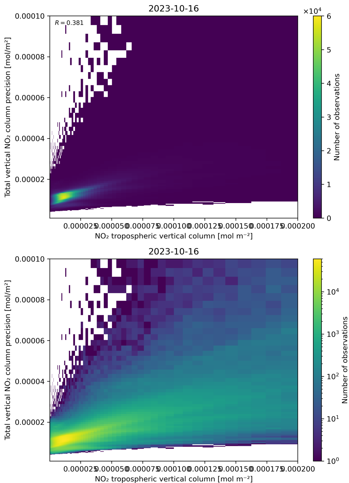
Figure 129: Scatter density plot of “NO 2 tropospheric vertical column” against “Total vertical NO 2 column precision” for 2023-10-15 to 2023-10-17.
