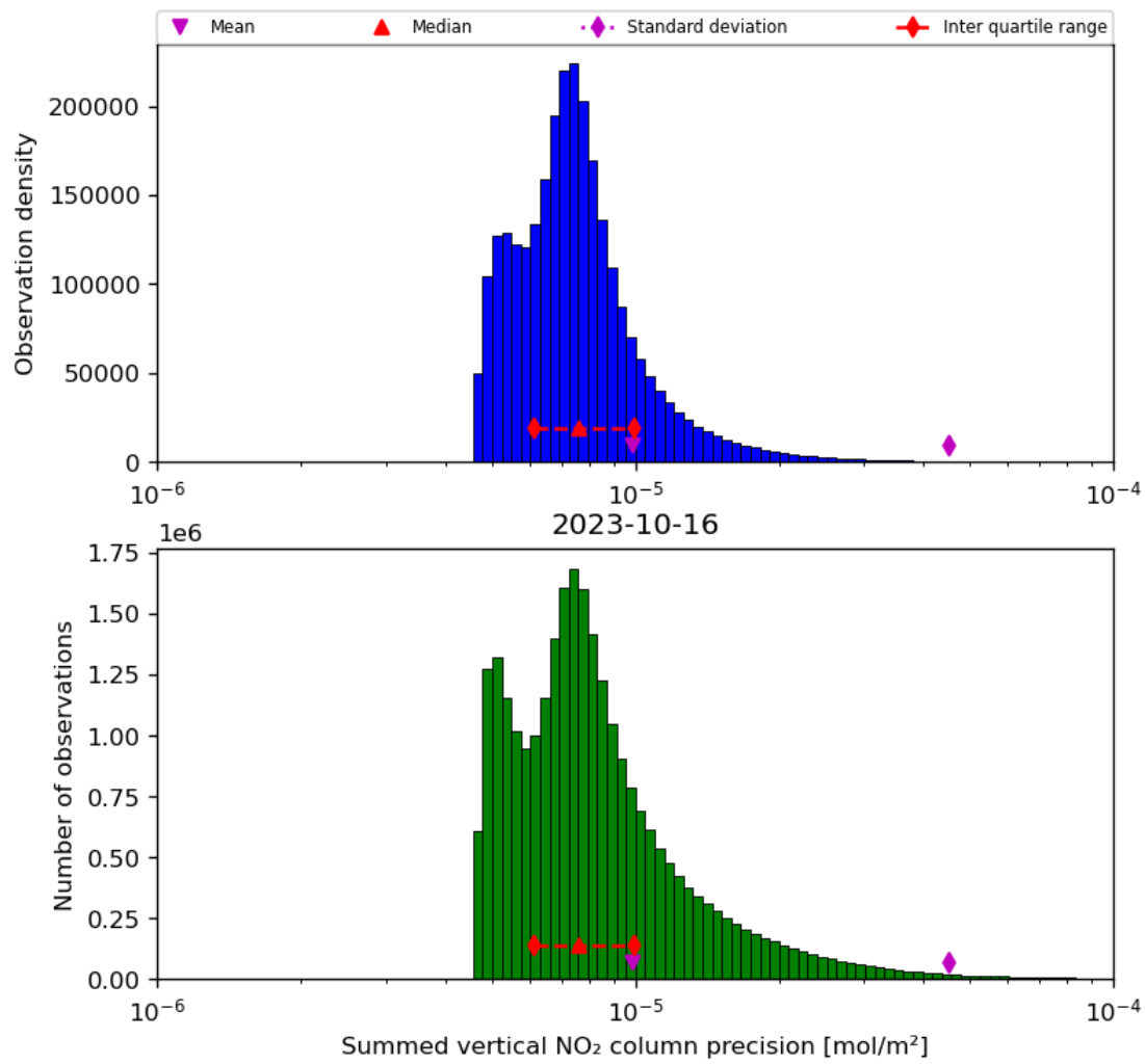
Figure 41: Histogram of "Summed vertical NO 2 column precision" for 2023-10-15 to 2023-10-17
