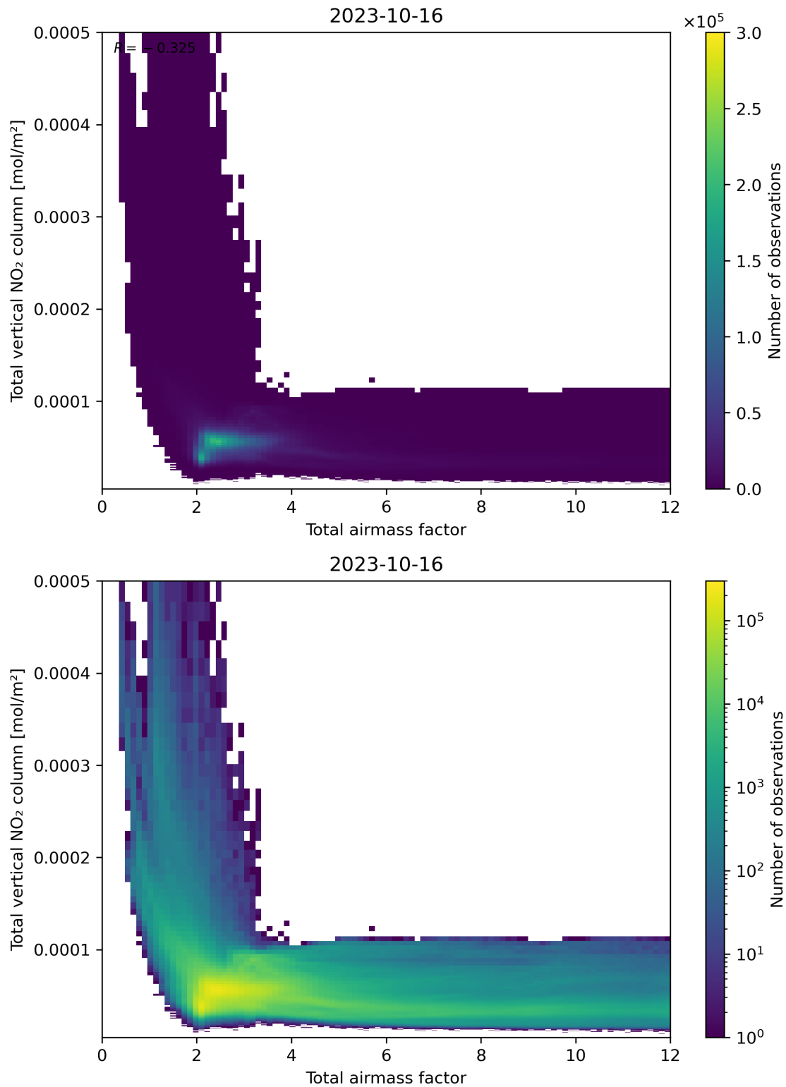
Figure 67: Scatter density plot of “Total airmass factor” against “Total vertical NO 2 column” for 2023-10-15 to 2023-10-17.
