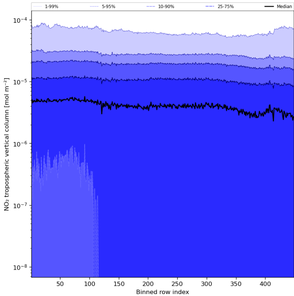
Figure 46: Along track statistics of “NO 2 tropospheric vertical column” for 2023-10-15 to 2023-10-17
