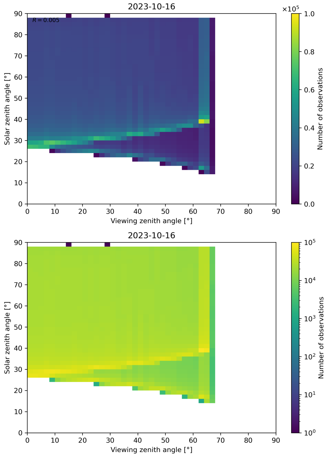
Figure 172: Scatter density plot of “Viewing zenith angle” against “Solar zenith angle” for 2023-10-15 to 2023-10-17.
