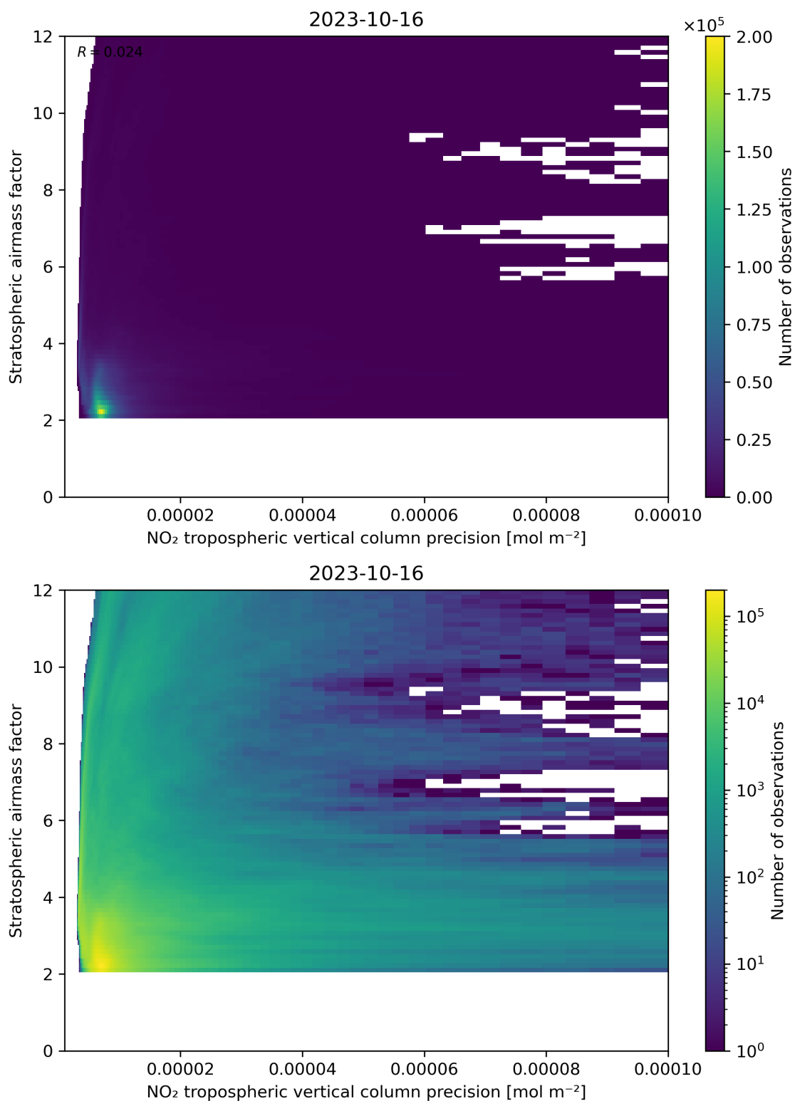
Figure 131: Scatter density plot of “NO 2 tropospheric vertical column precision” against “Stratospheric airmass factor” for 2023-10-15 to 2023-10-17.
