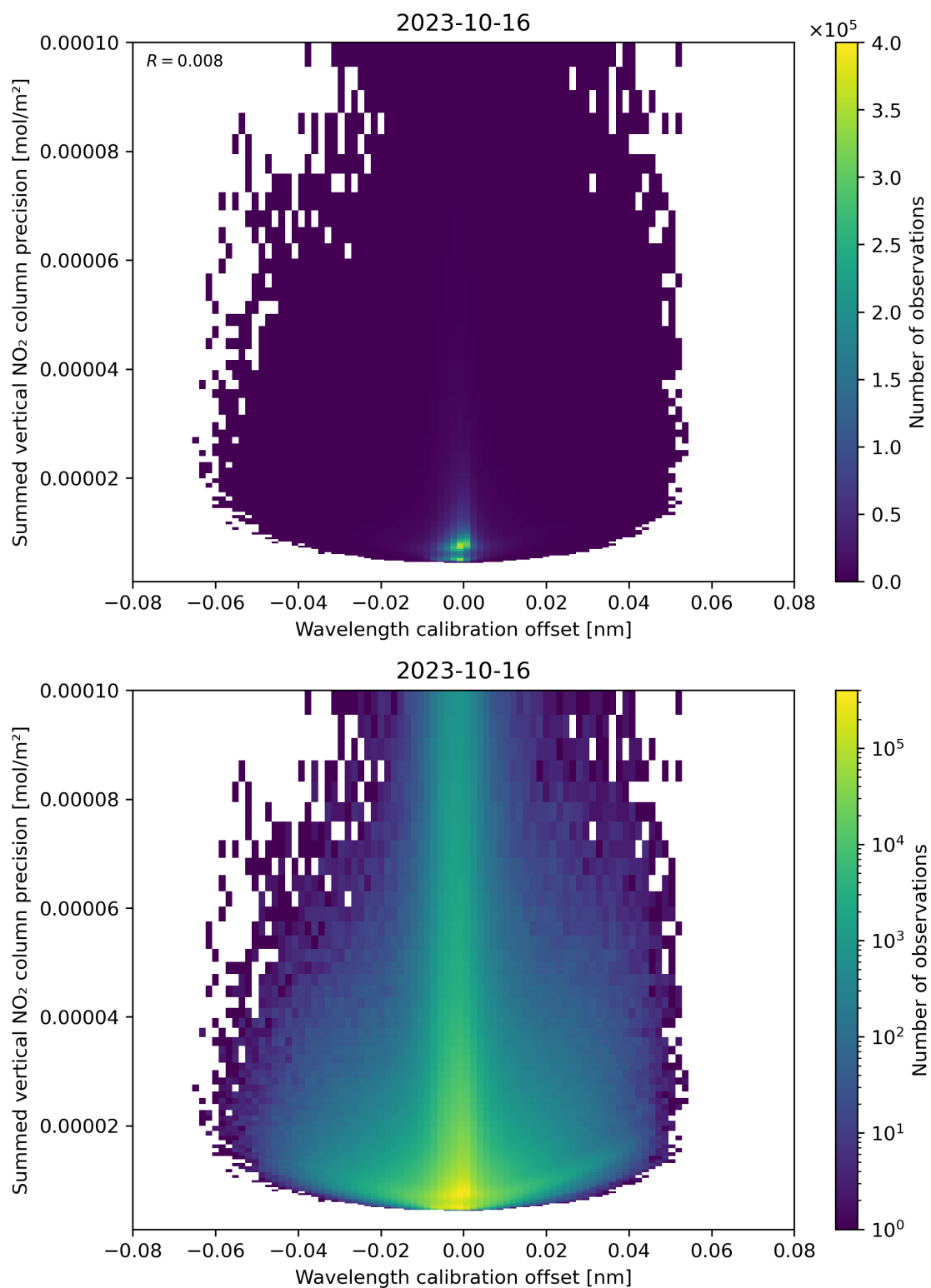
Figure 178: Scatter density plot of “Wavelength calibration offset” against “Summed vertical NO 2 column precision” for 2023-10-15 to 2023-10-17.
