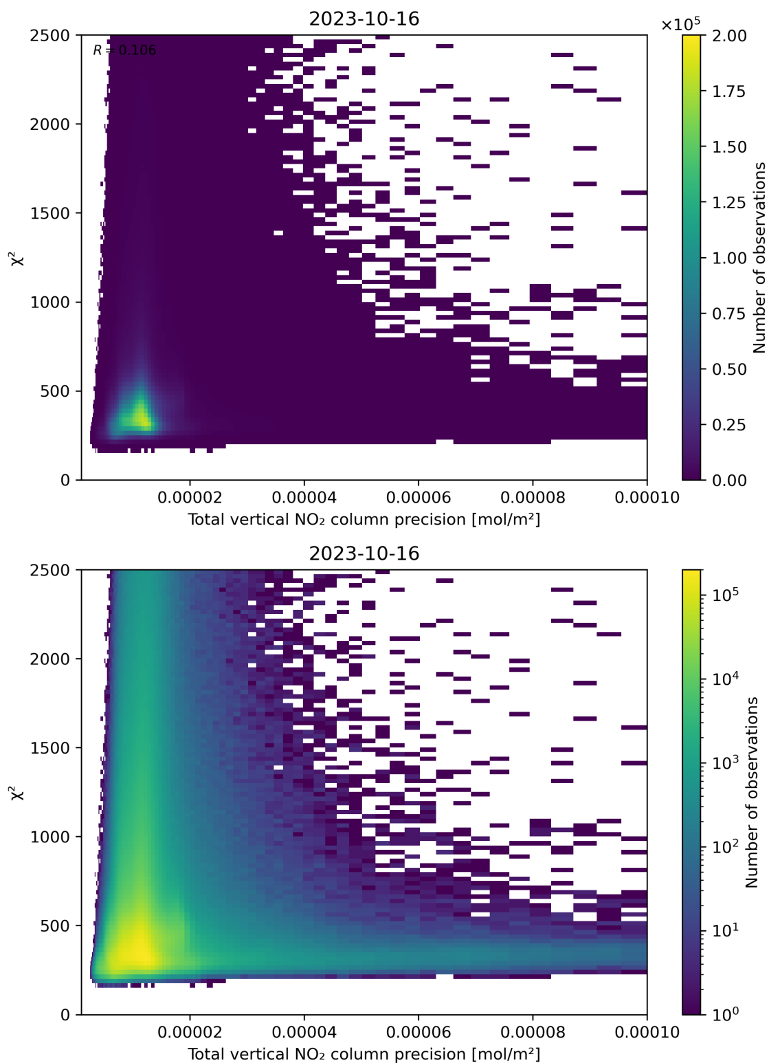
Figure 116: Scatter density plot of “Total vertical NO 2 column precision” against “ \chi^2 ” for 2023-10-15 to 2023-10-17.
