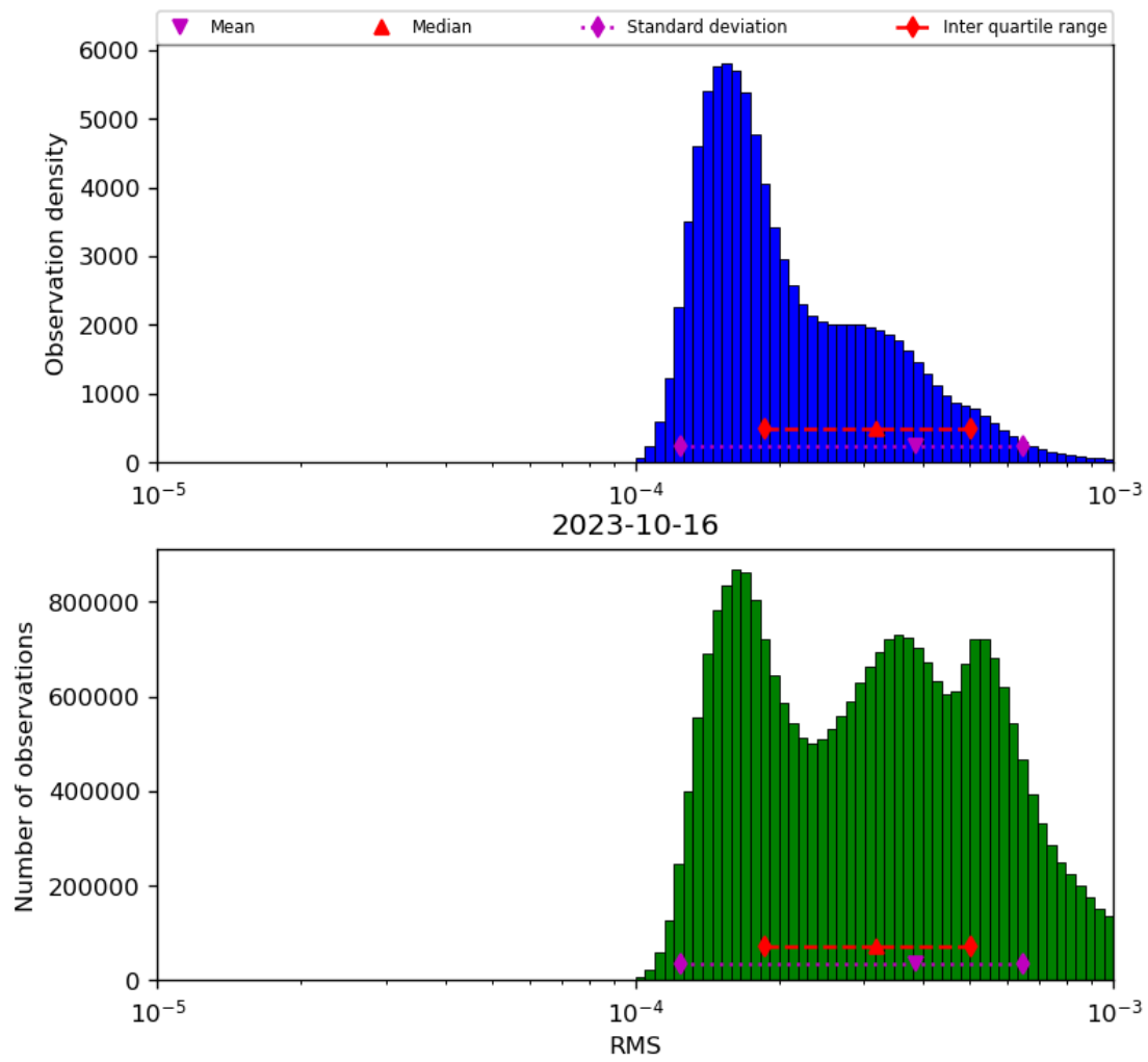
Figure 43: Histogram of “RMS” for 2023-10-15 to 2023-10-17
