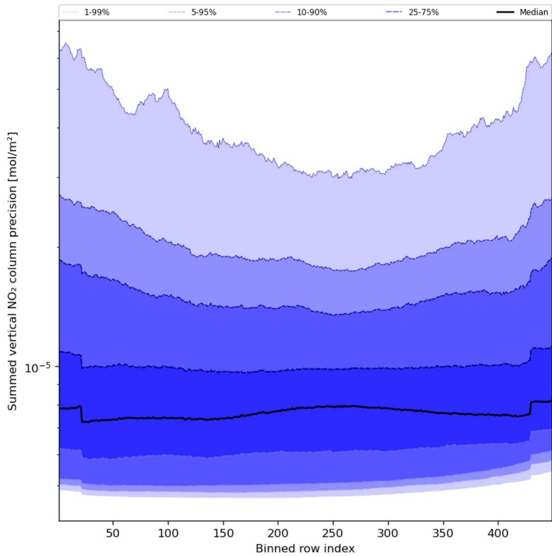
Figure 58: Along track statistics of “Summed vertical NO 2 column precision” for 2023-10-15 to 2023-10-17
