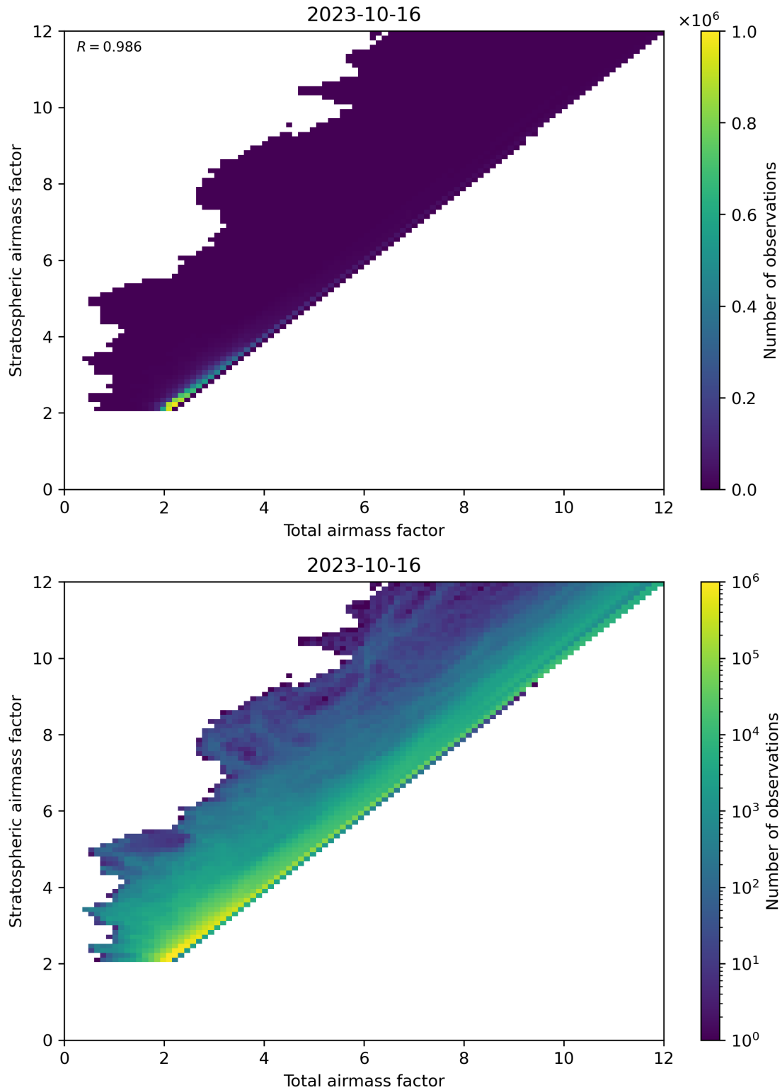
Figure 62: Scatter density plot of “Total airmass factor” against “Stratospheric airmass factor” for 2023-10-15 to 2023-10-17.
