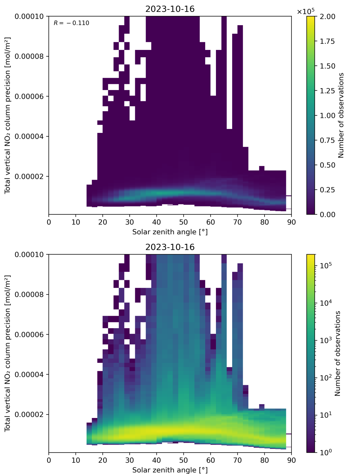
Figure 154: Scatter density plot of “Solar zenith angle” against “Total vertical NO 2 column precision” for 2023-10-15 to 2023-10-17.
