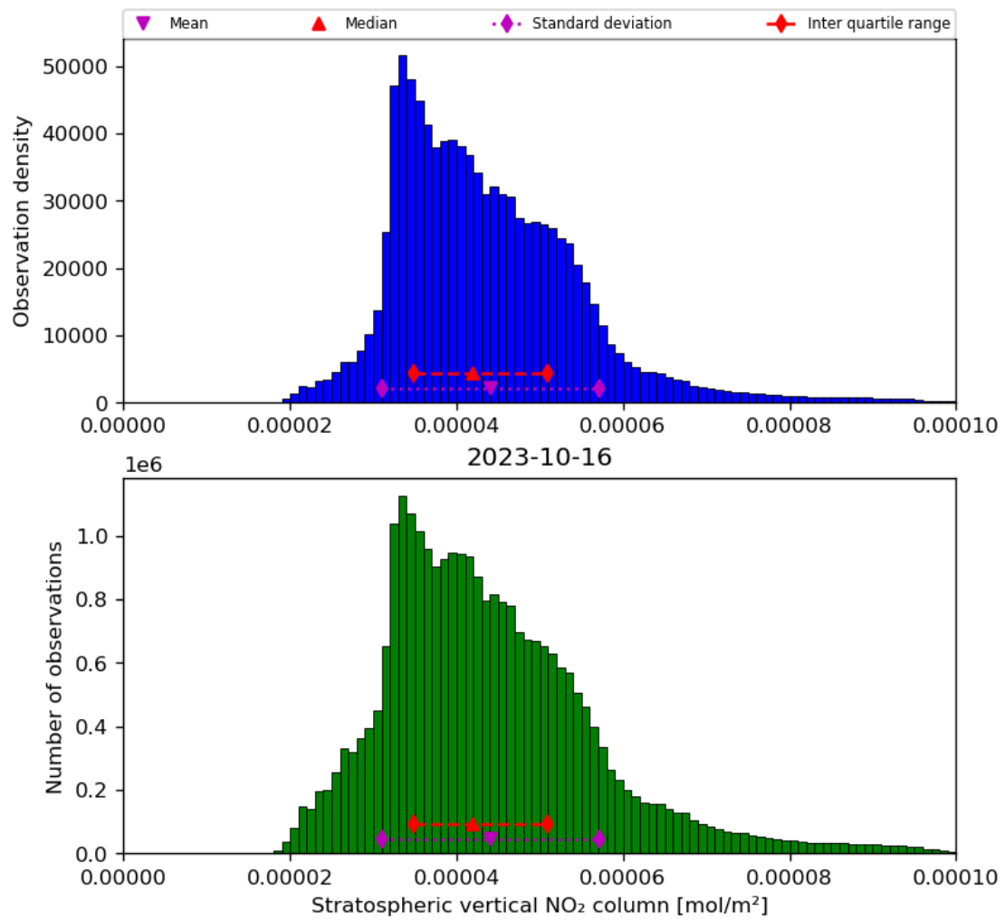
Figure 36: Histogram of “Stratospheric vertical NO 2 column” for 2023-10-15 to 2023-10-17
