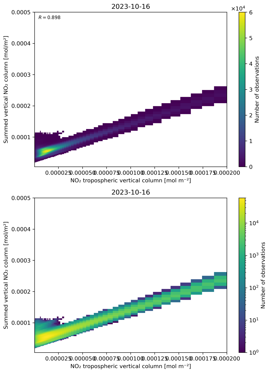
Figure 126: Scatter density plot of “NO 2 tropospheric vertical column” against “Summed vertical NO 2 column” for 2023-10-15 to 2023-10-17.
