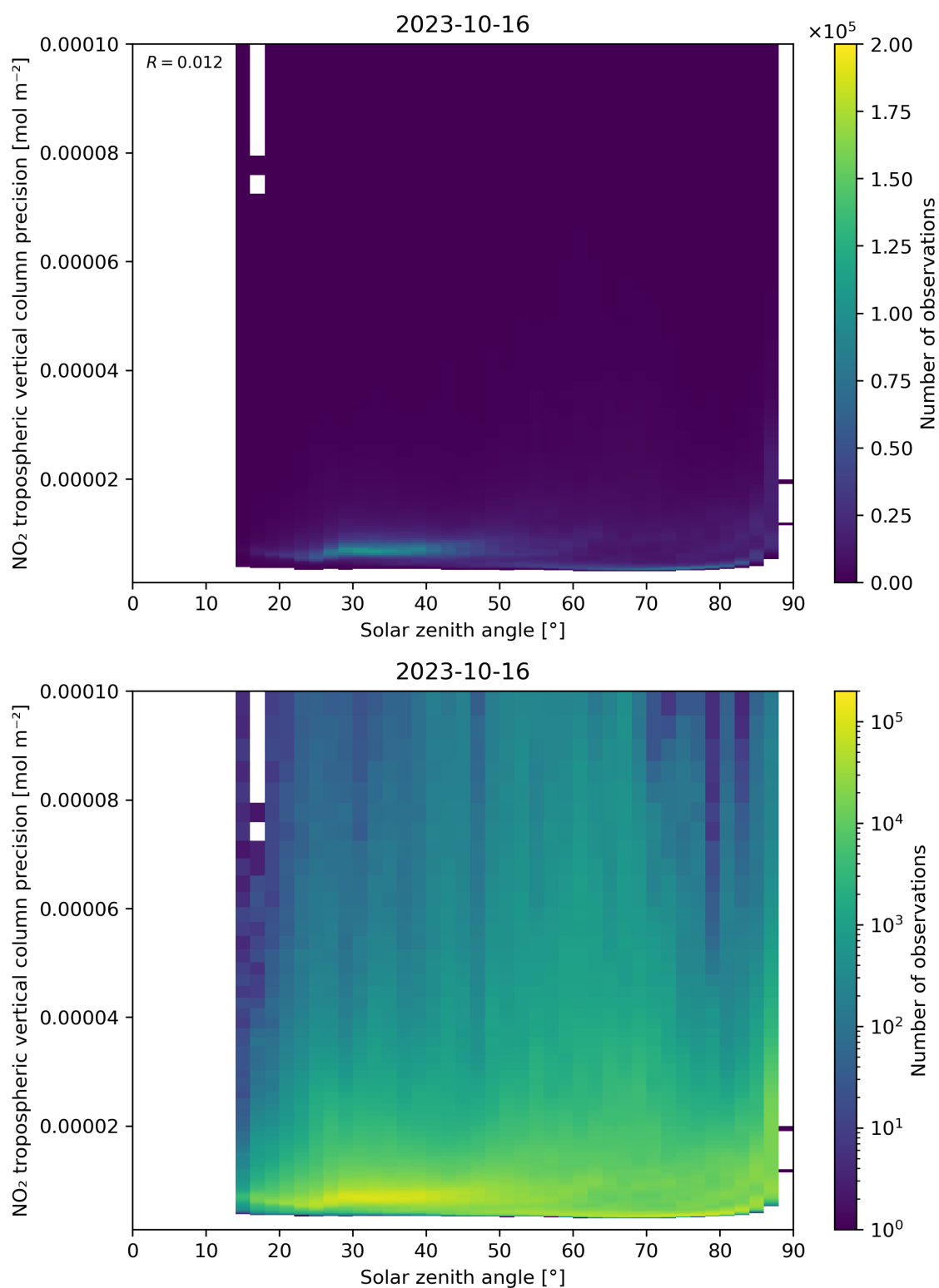
Figure 156: Scatter density plot of “Solar zenith angle” against “NO 2 tropospheric vertical column precision” for 2023-10-15 to 2023-10-17.
