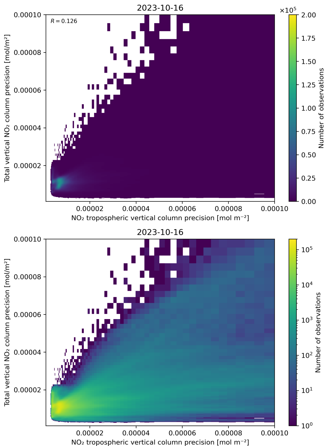
Figure 139: Scatter density plot of “NO 2 tropospheric vertical column precision” against “Total vertical NO 2 column precision” for 2023-10-15 to 2023-10-17.
