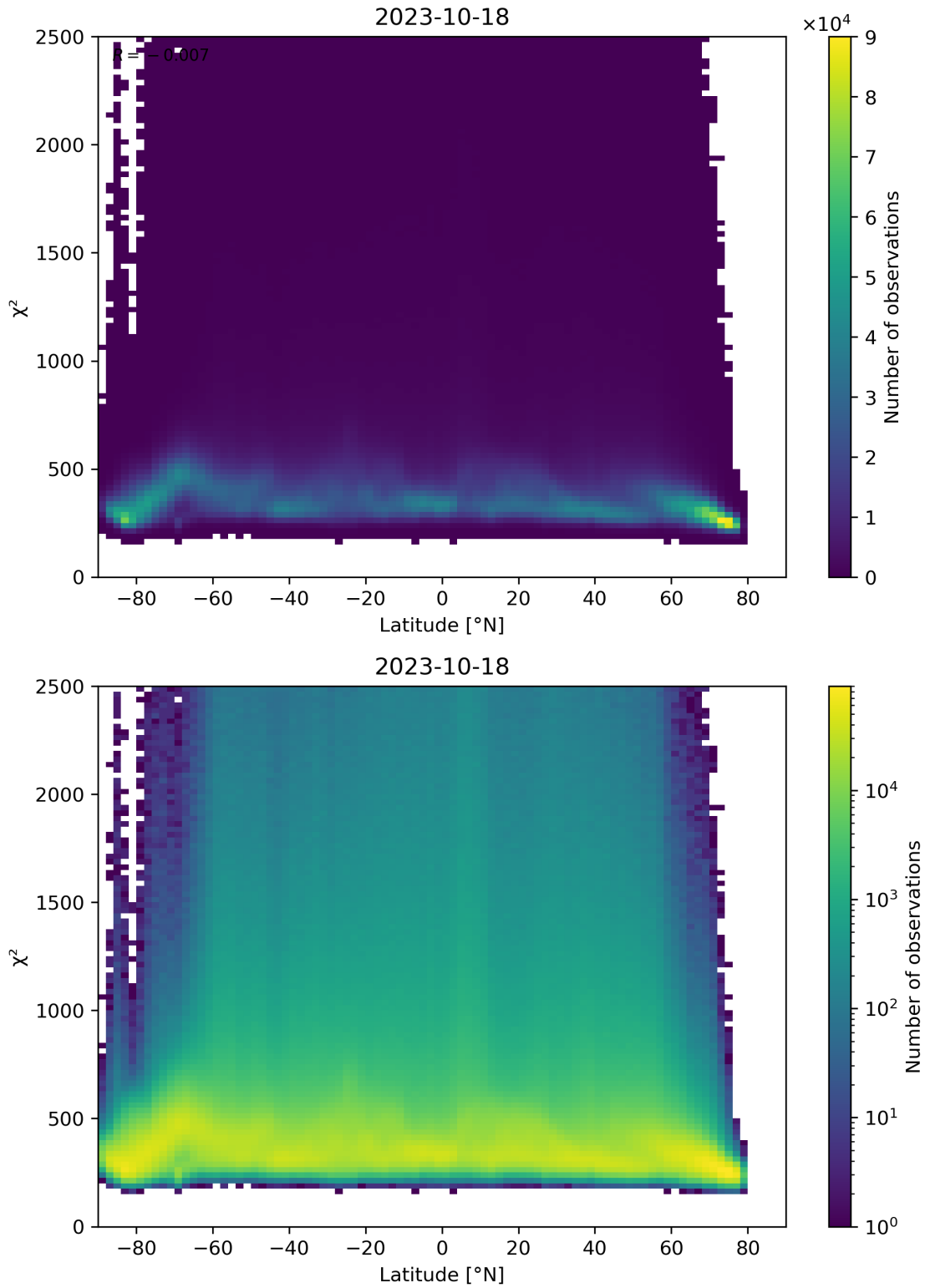
Figure 86: Scatter density plot of “Latitude” against “ \chi^2 ” for 2023-10-17 to 2023-10-19.
