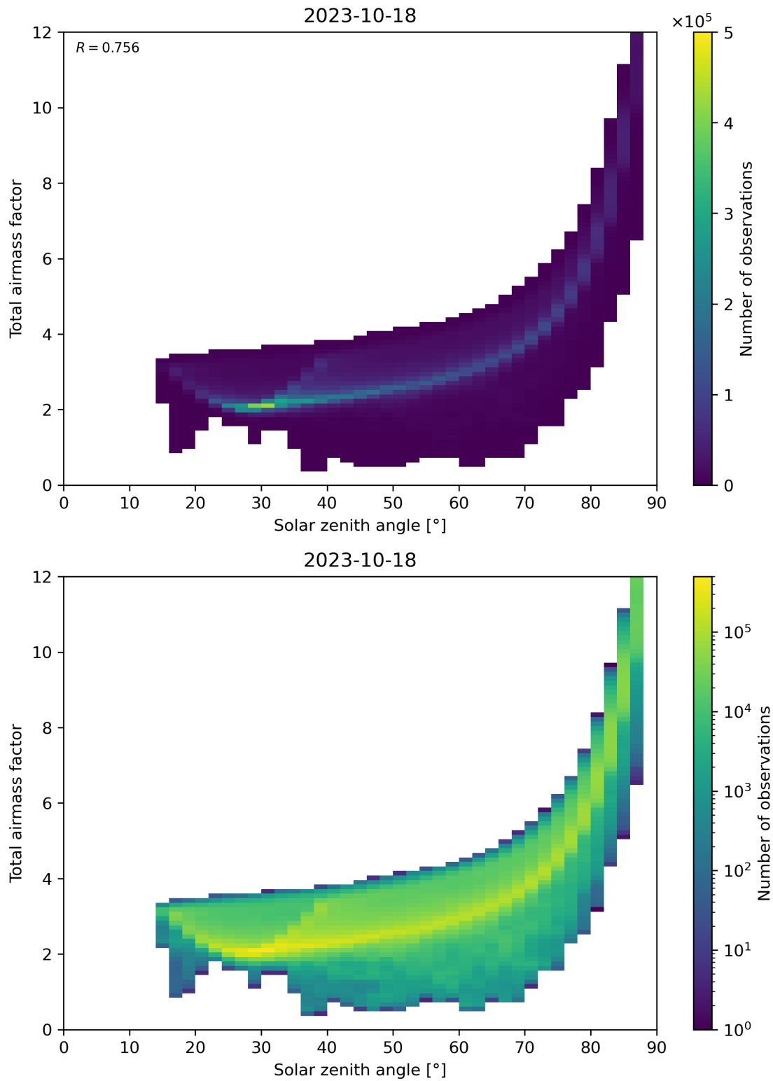
Figure 146: Scatter density plot of “Solar zenith angle” against “Total airmass factor” for 2023-10-17 to 2023-10-19.
