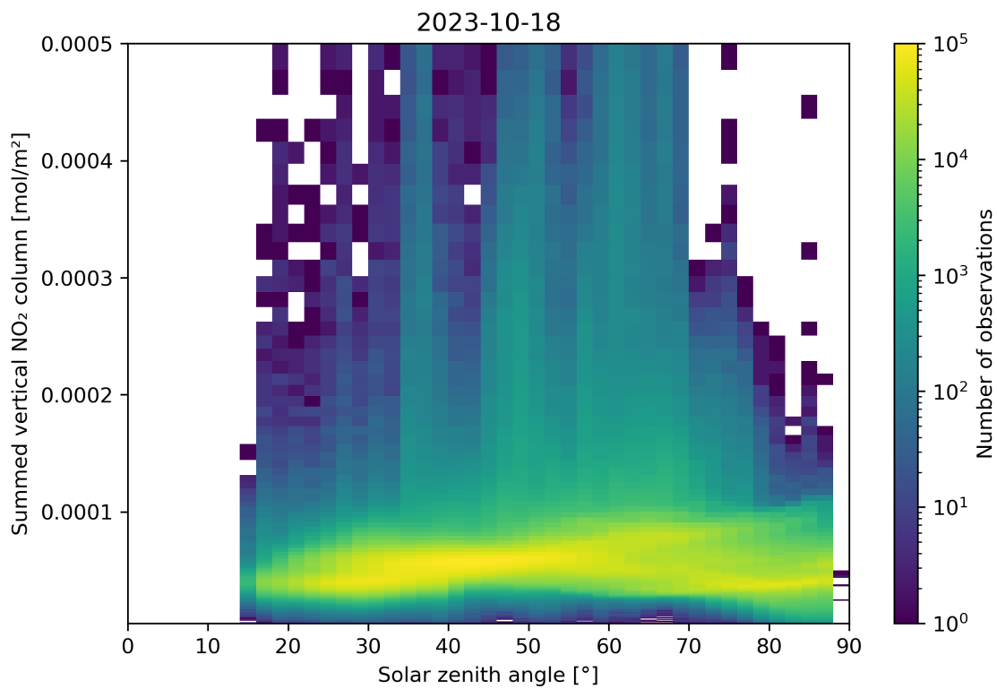
Figure 151: Scatter density plot of “Solar zenith angle” against “Summed vertical NO 2 column” for 2023-10-17 to 2023-10-19.
