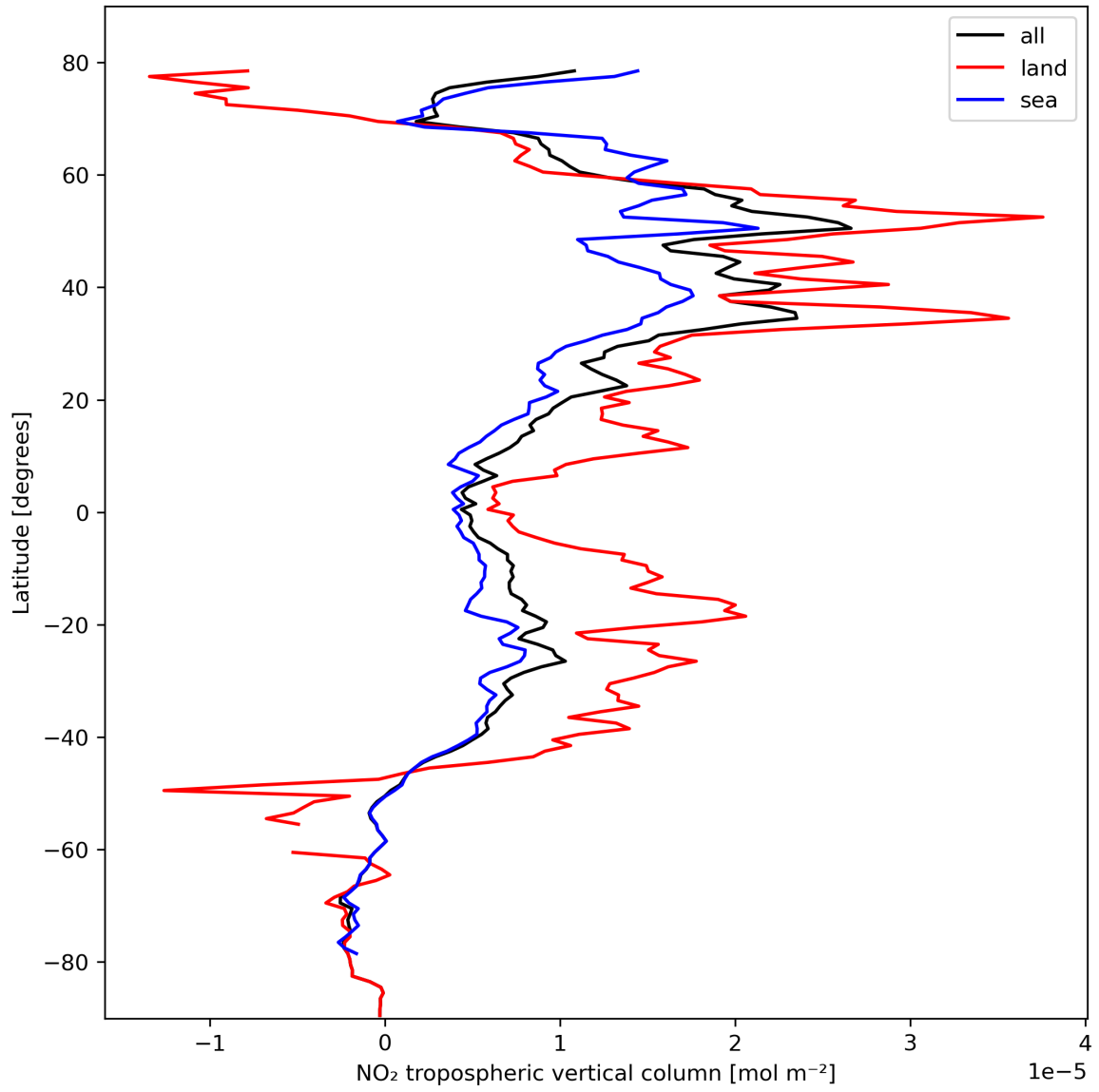
Figure 12: Zonal average of “NO 2 tropospheric vertical column” for 2023-10-17 to 2023-10-19.
