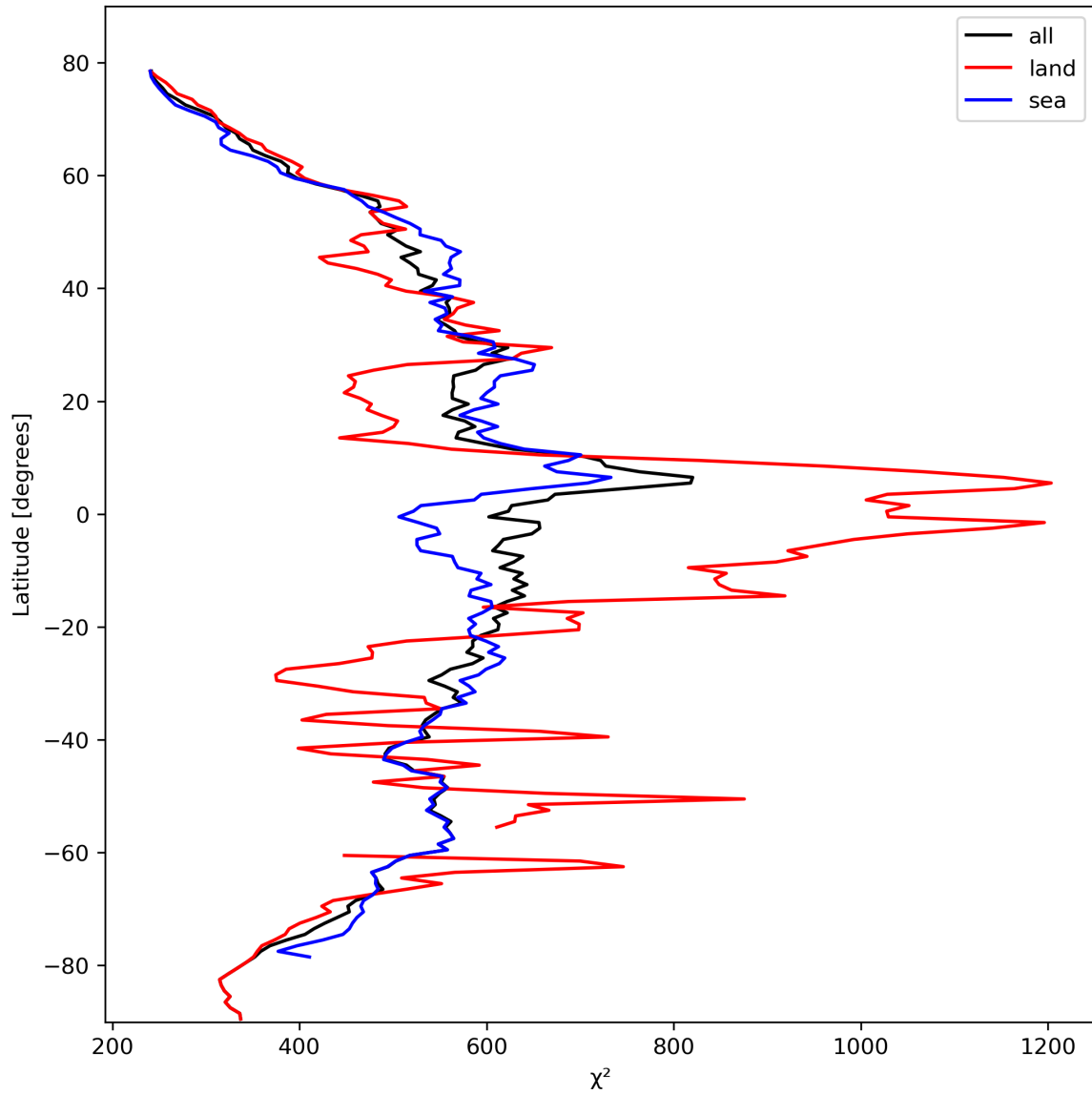
Figure 25: Zonal average of " \chi^2 " for 2023-10-17 to 2023-10-19.
