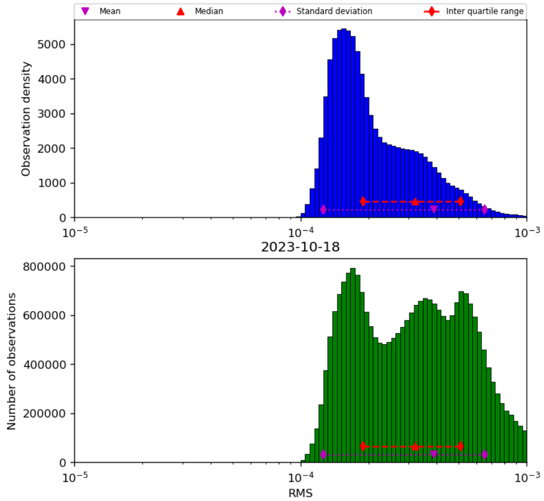
Figure 43: Histogram of “RMS” for 2023-10-17 to 2023-10-19
