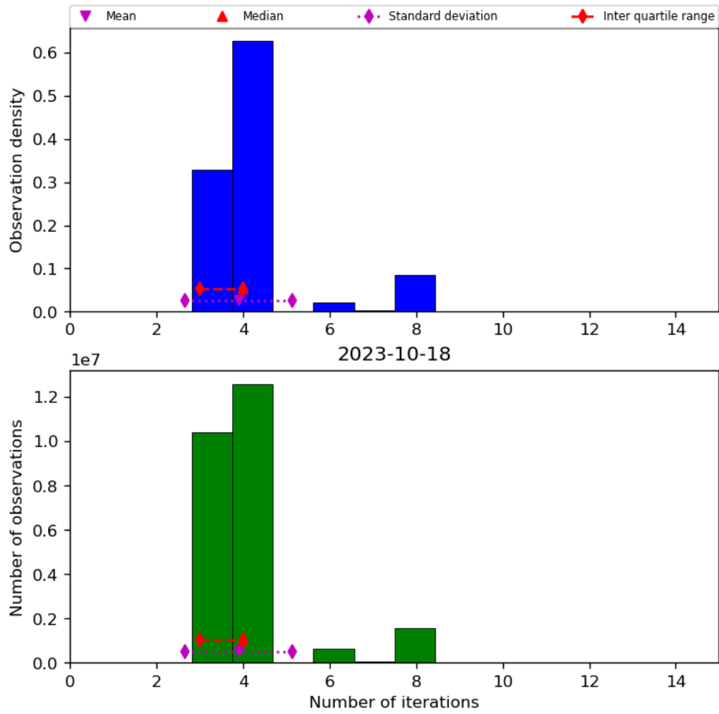
Figure 34: Histogram of “Number of iterations” for 2023-10-17 to 2023-10-19
