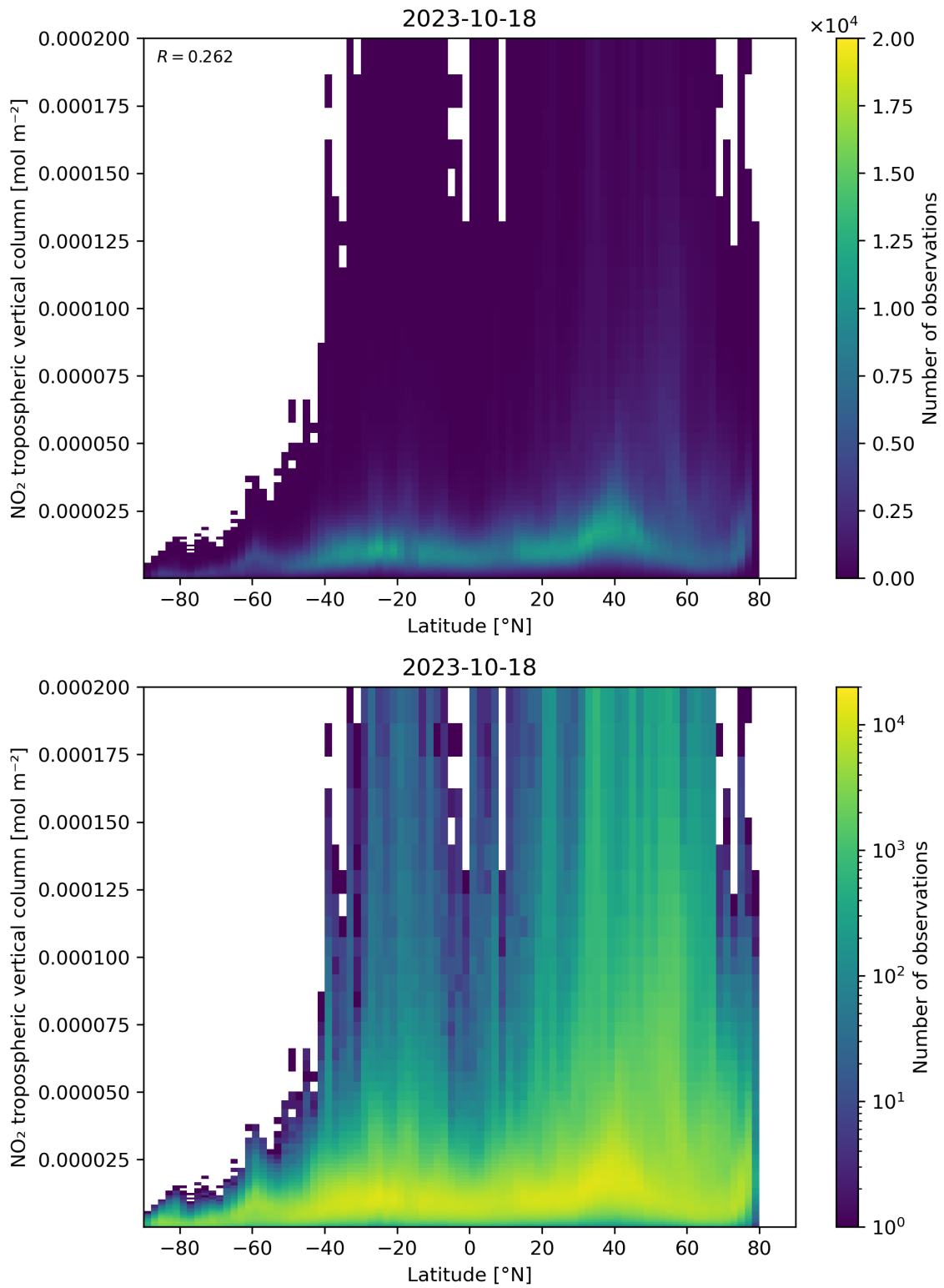
Figure 92: Scatter density plot of “Latitude” against “NO 2 tropospheric vertical column” for 2023-10-17 to 2023-10-19.
