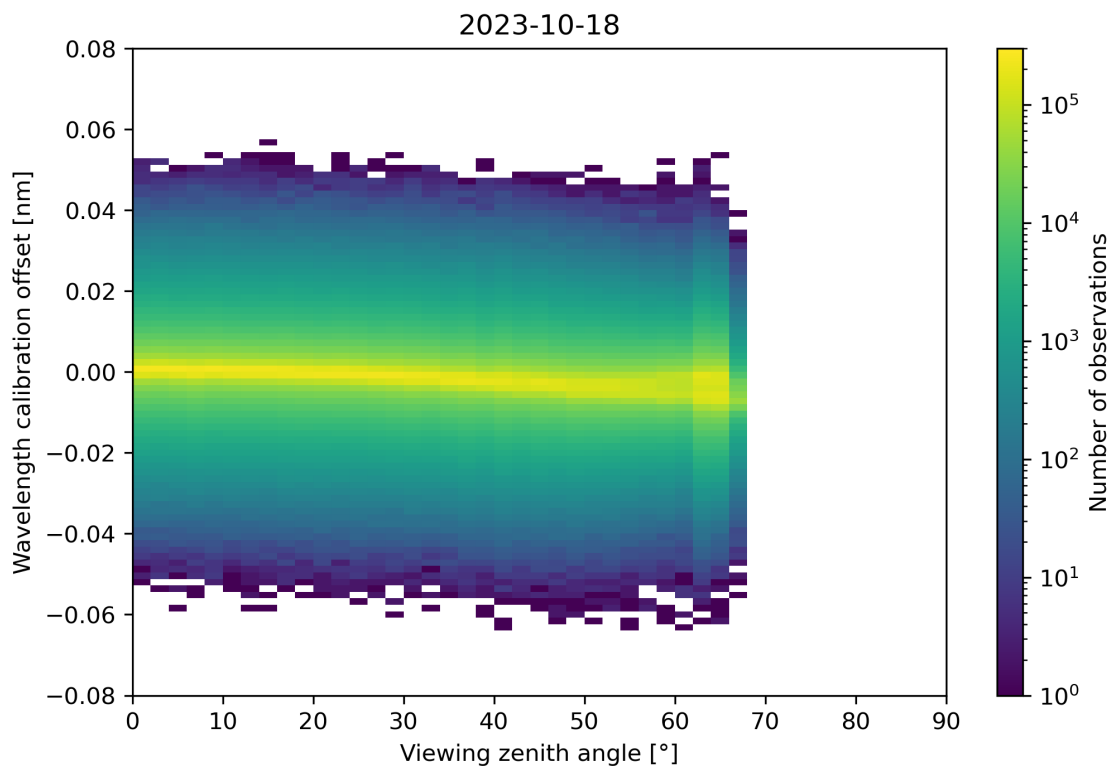
Figure 173: Scatter density plot of “Viewing zenith angle” against “Wavelength calibration offset” for 2023-10-17 to 2023-10-19.
