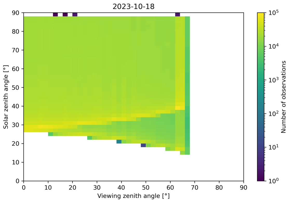
Figure 172: Scatter density plot of “Viewing zenith angle” against “Solar zenith angle” for 2023-10-17 to 2023-10-19.
