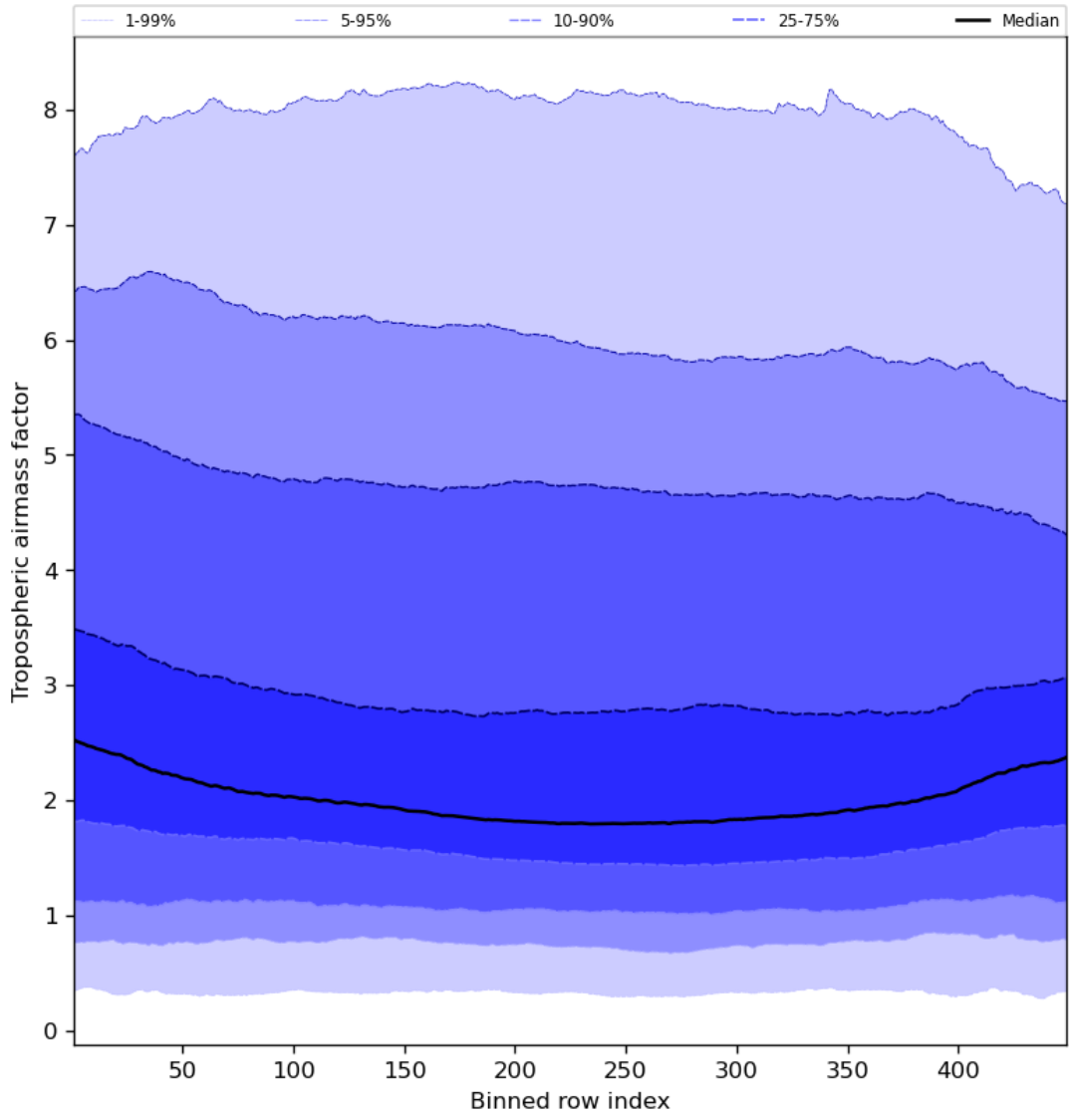
Figure 48: Along track statistics of “Tropospheric airmass factor” for 2023-10-17 to 2023-10-19
