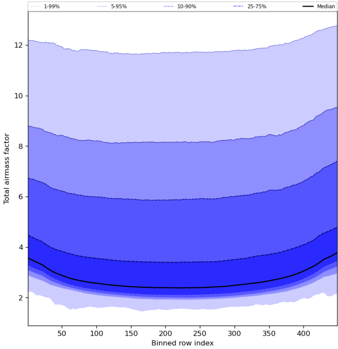
Figure 49: Along track statistics of “Total airmass factor” for 2023-10-17 to 2023-10-19
