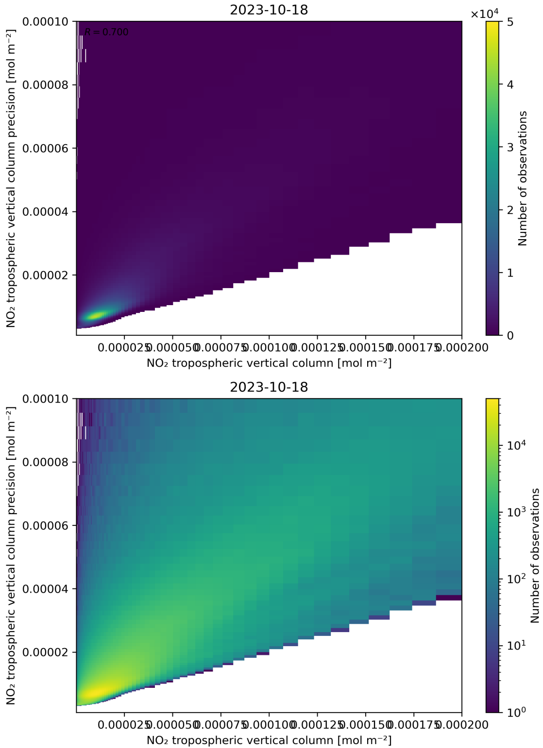
Figure 130: Scatter density plot of “NO 2 tropospheric vertical column” against “NO 2 tropospheric vertical column precision” for 2023-10-17 to 2023-10-19.
