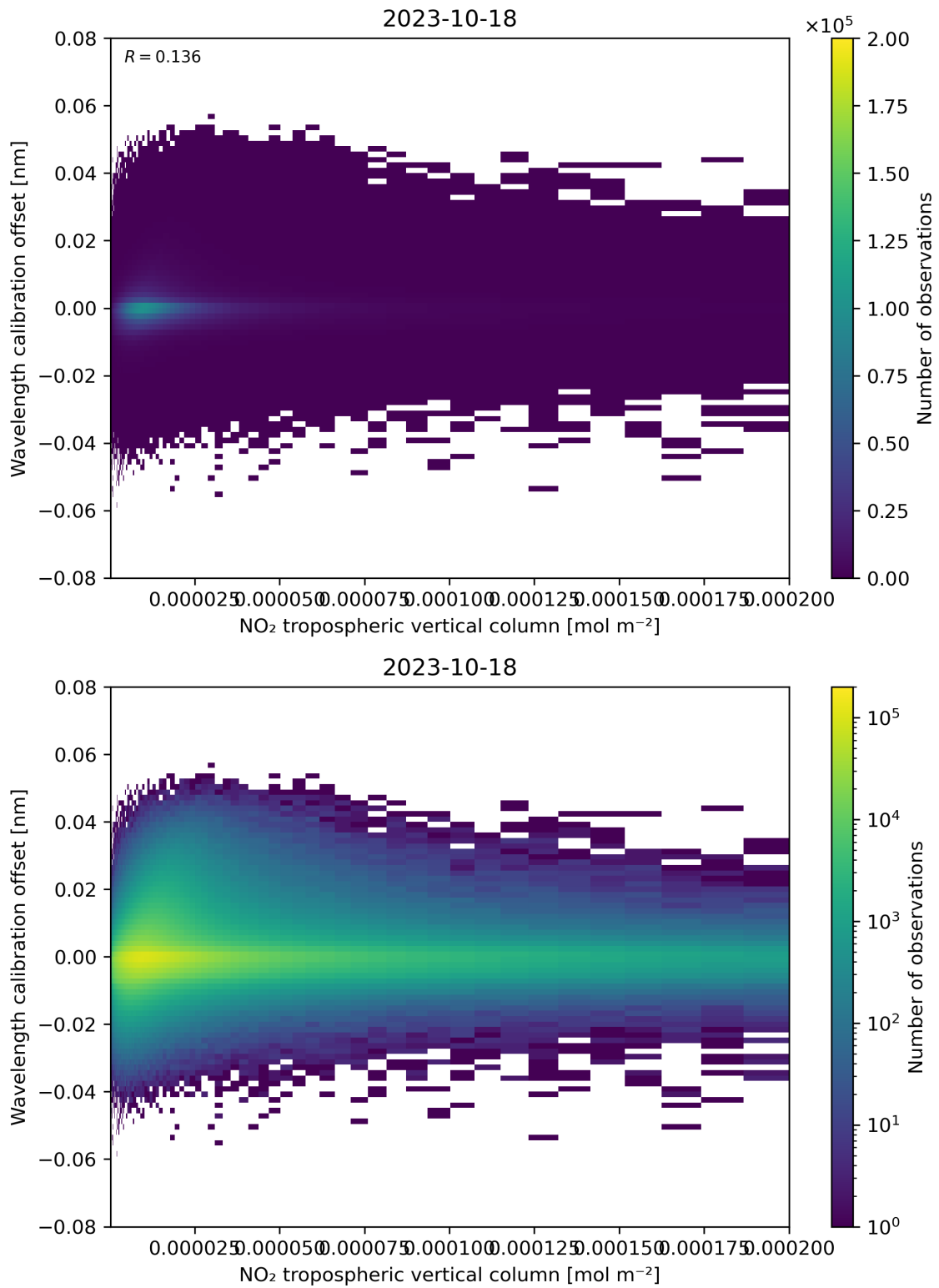
Figure 143: Scatter density plot of “NO 2 tropospheric vertical column” against “Wavelength calibration offset” for 2023-10-17 to 2023-10-19.
