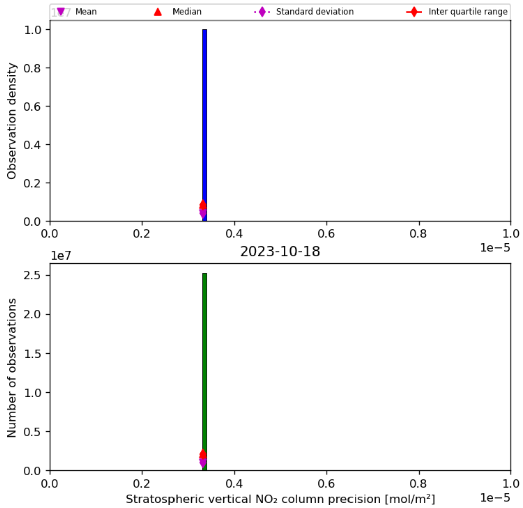
Figure 37: Histogram of “Stratospheric vertical NO 2 column precision” for 2023-10-17 to 2023-10-19
