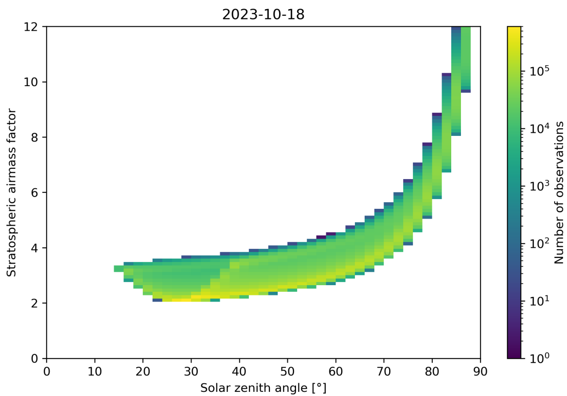
Figure 145: Scatter density plot of “Solar zenith angle” against “Stratospheric airmass factor” for 2023-10-17 to 2023-10-19.
