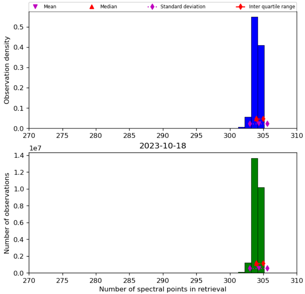
Figure 33: Histogram of “Number of spectral points in retrieval” for 2023-10-17 to 2023-10-19
