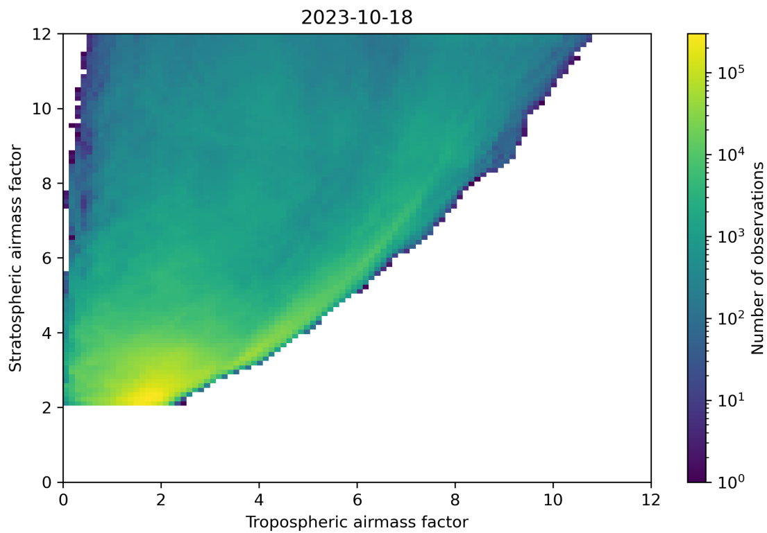
Figure 71: Scatter density plot of “Tropospheric airmass factor” against “Stratospheric airmass factor” for 2023-10-17 to 2023-10-19.
