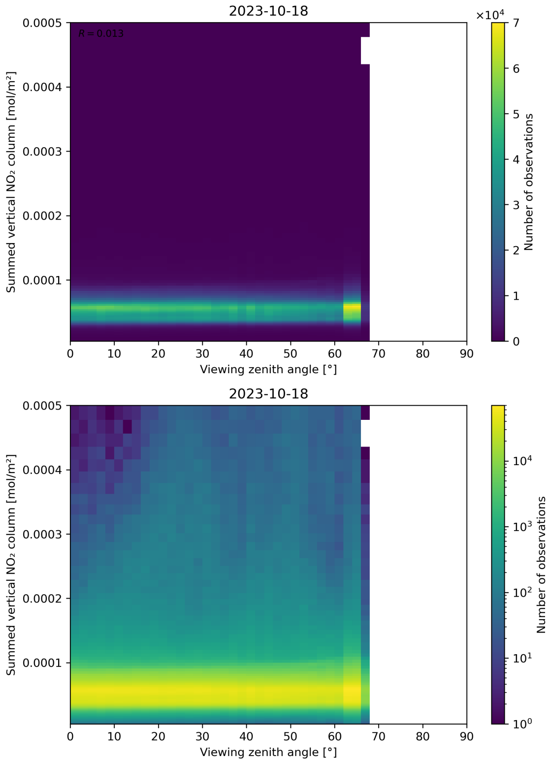
Figure 165: Scatter density plot of “Viewing zenith angle” against “Summed vertical NO 2 column” for 2023-10-17 to 2023-10-19.
