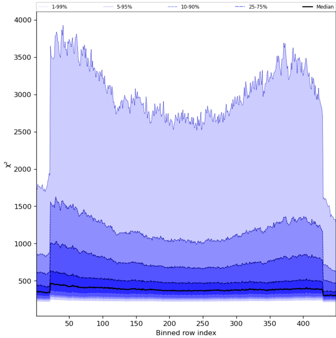
Figure 59: Along track statistics of “ \chi^2 ” for 2023-10-17 to 2023-10-19
