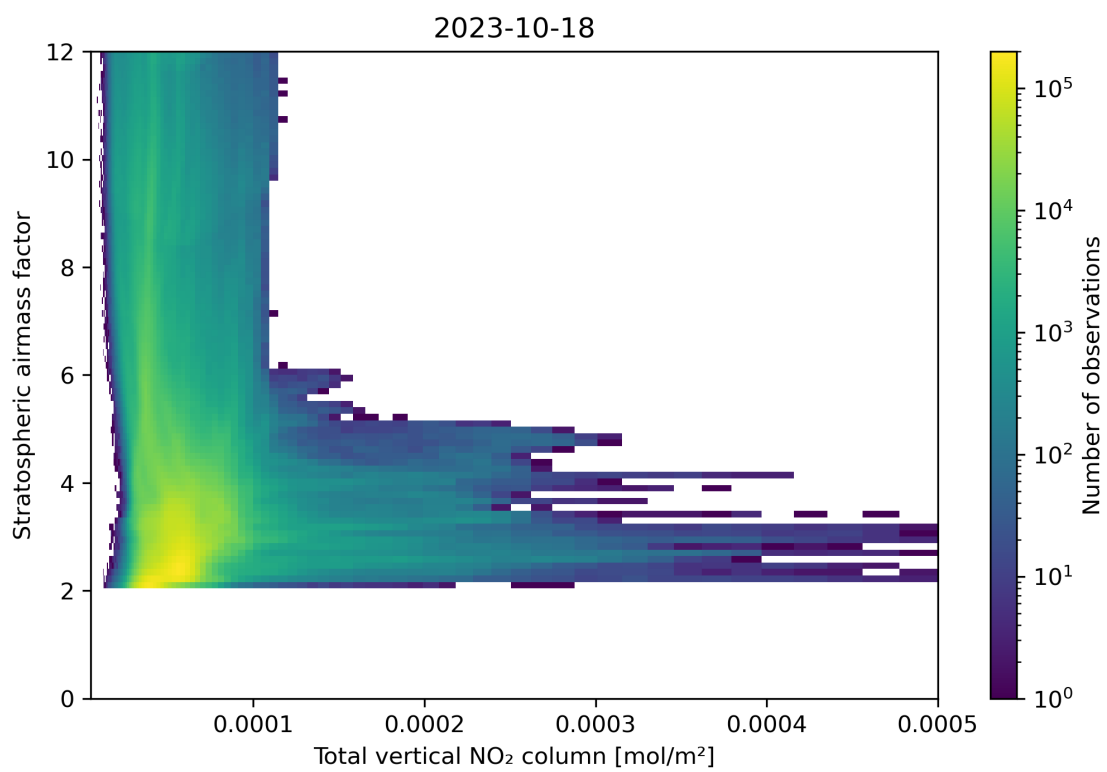
Figure 110: Scatter density plot of “Total vertical NO 2 column” against “Stratospheric airmass factor” for 2023-10-17 to 2023-10-19.
