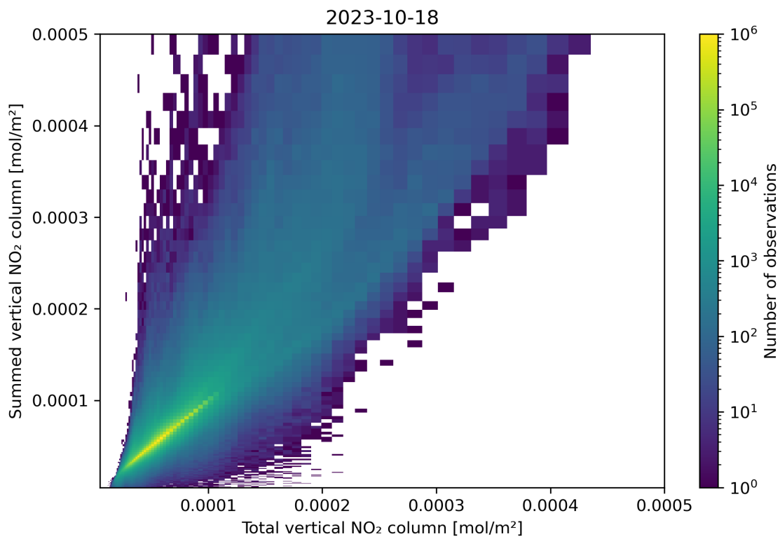
Figure 112: Scatter density plot of “Total vertical NO 2 column” against “Summed vertical NO 2 column” for 2023-10-17 to 2023-10-19.
