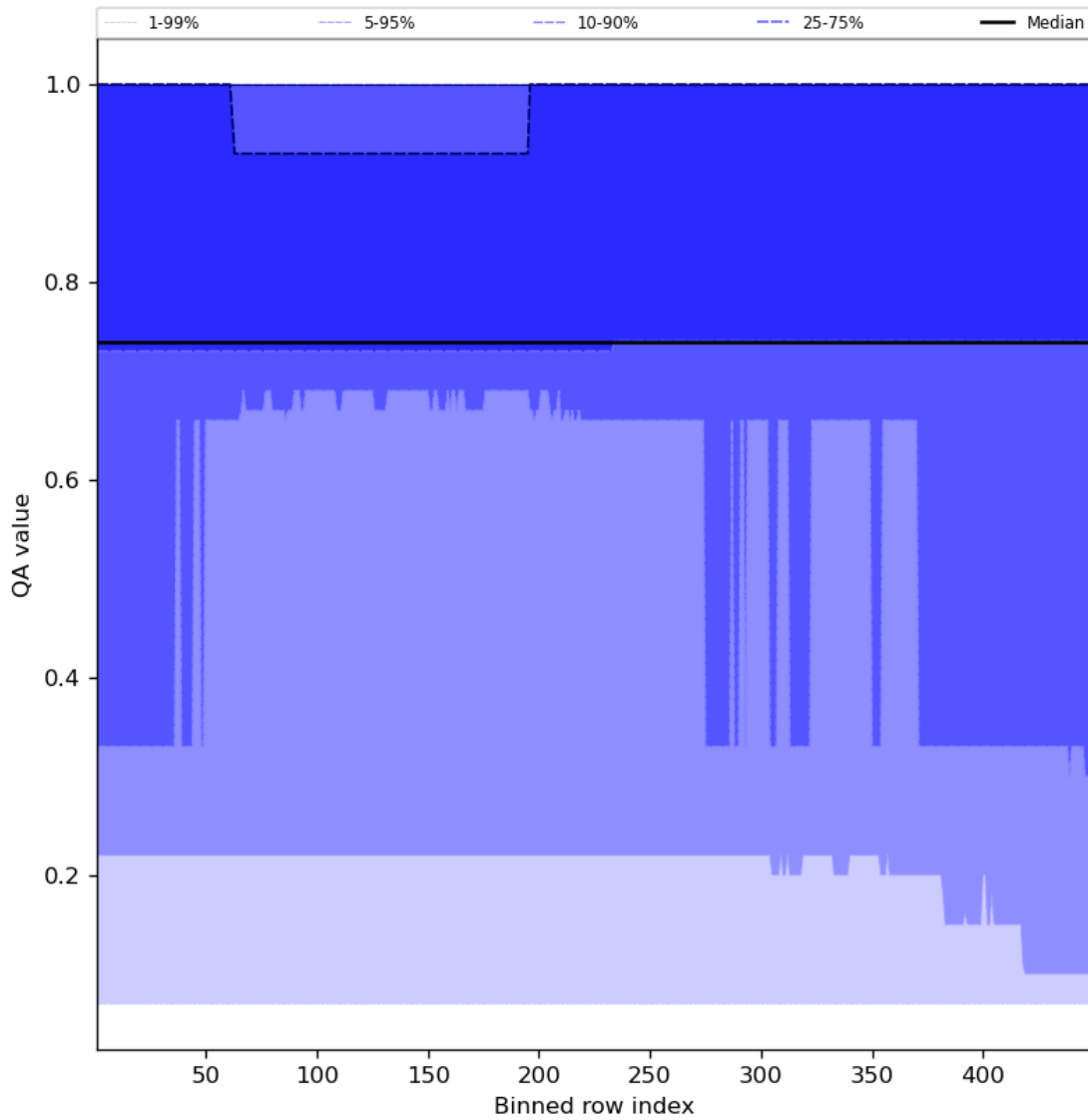
Figure 45: Along track statistics of “QA value” for 2023-10-17 to 2023-10-19
