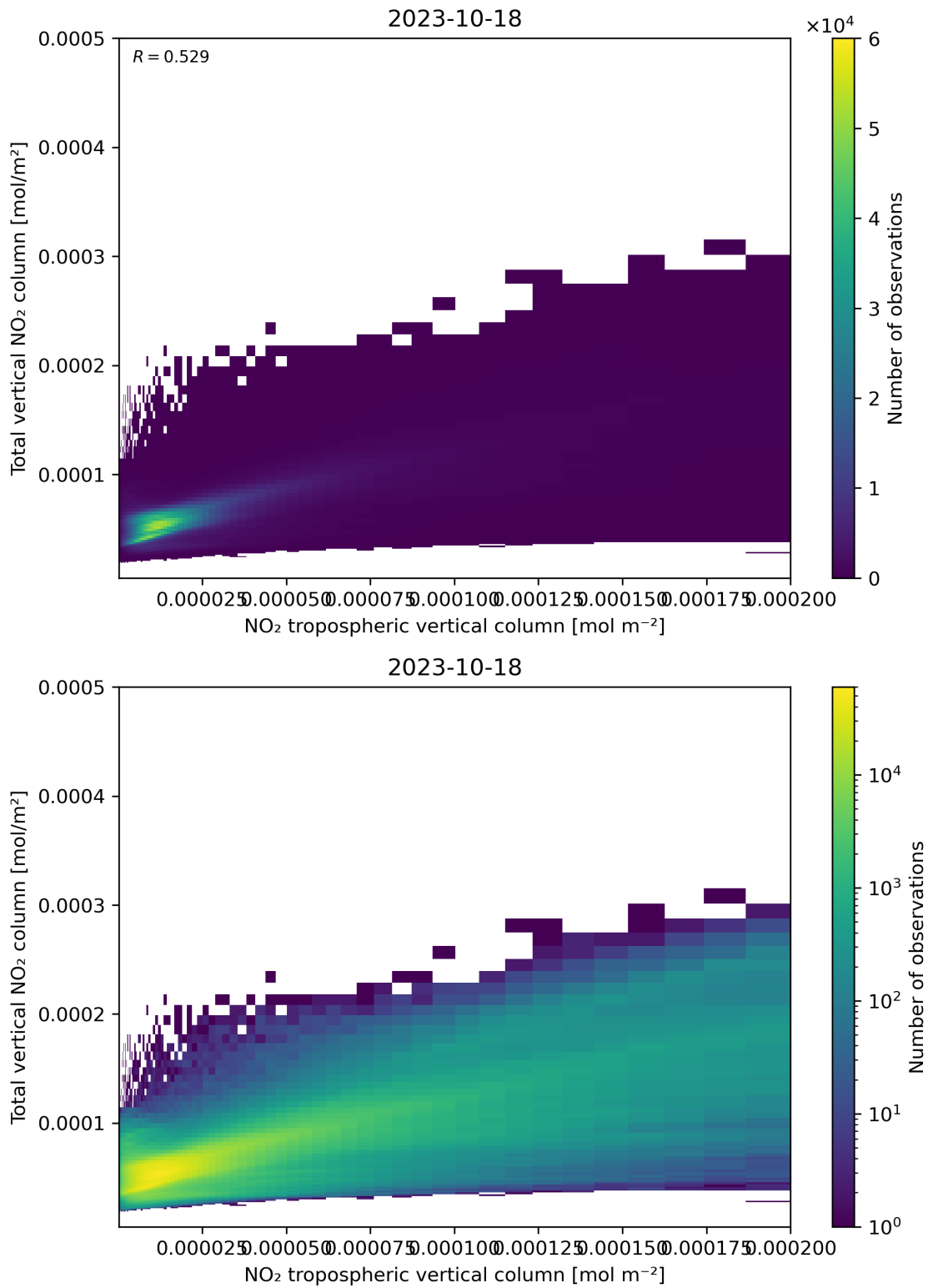
Figure 128: Scatter density plot of “NO 2 tropospheric vertical column” against “Total vertical NO 2 column” for 2023-10-17 to 2023-10-19.
