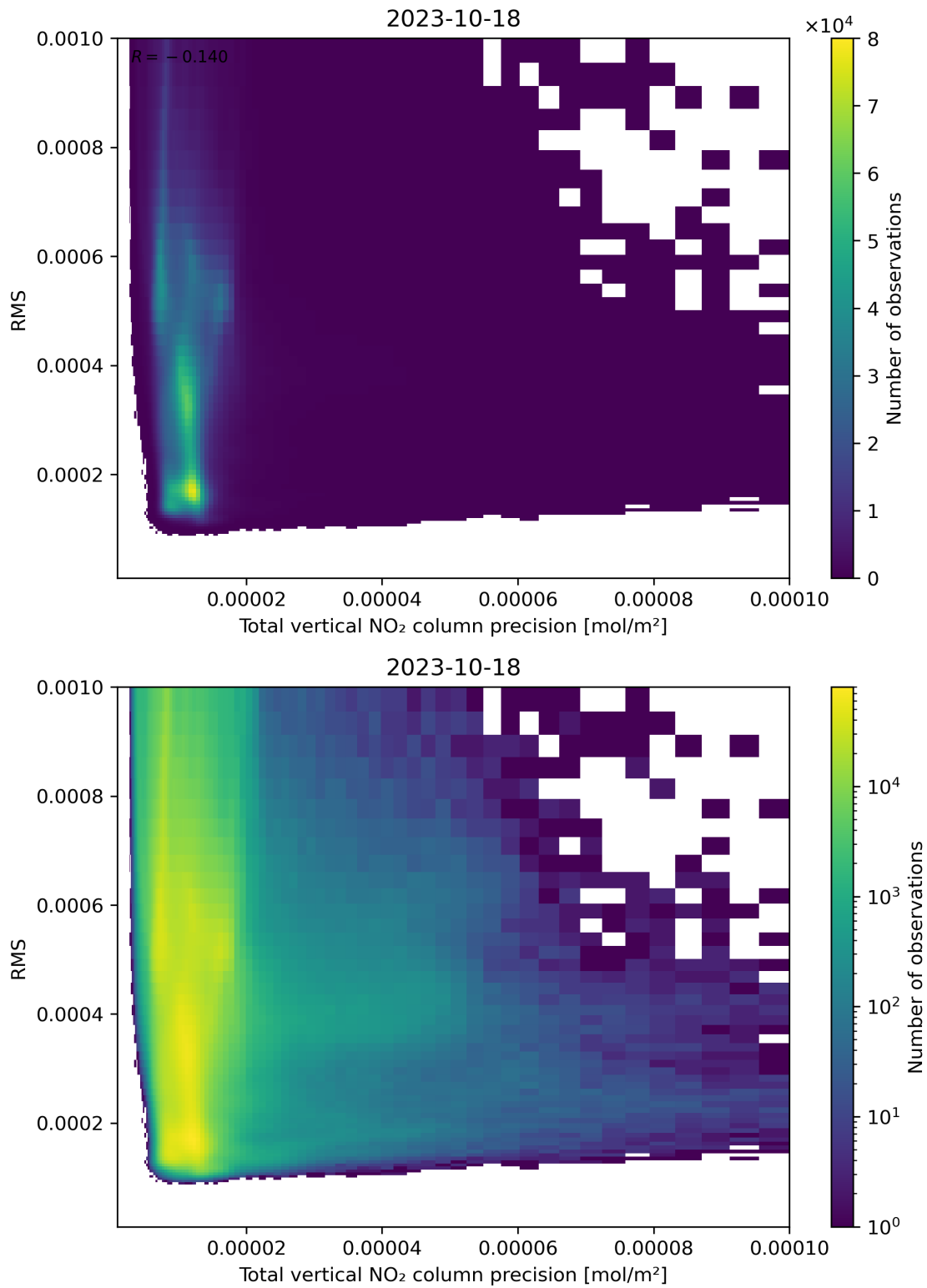
Figure 119: Scatter density plot of “Total vertical NO 2 column precision” against “RMS” for 2023-10-17 to 2023-10-19.
