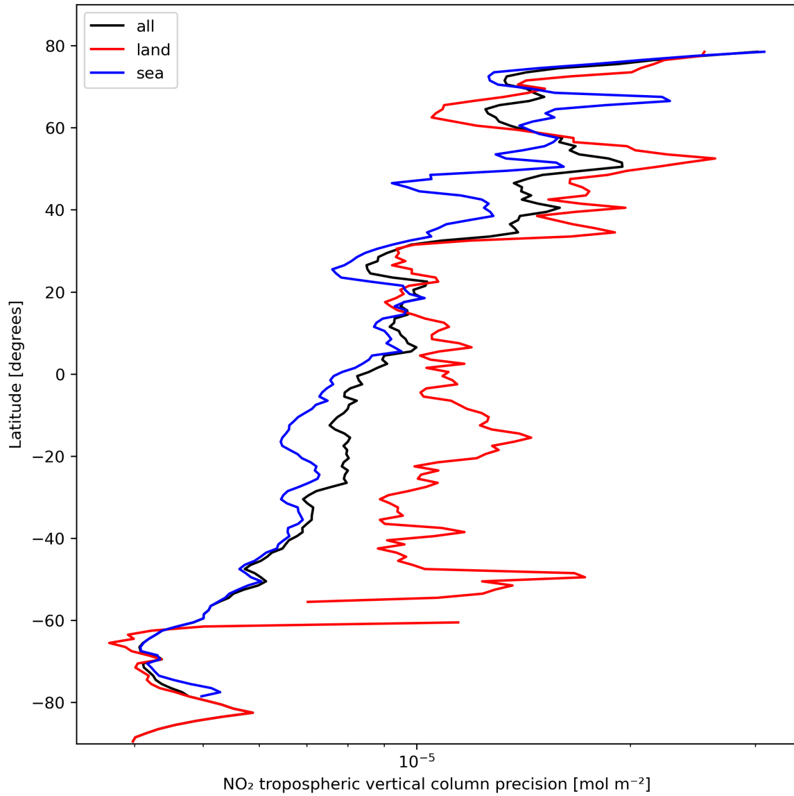
Figure 13: Zonal average of “NO 2 tropospheric vertical column precision” for 2023-10-17 to 2023-10-19.
