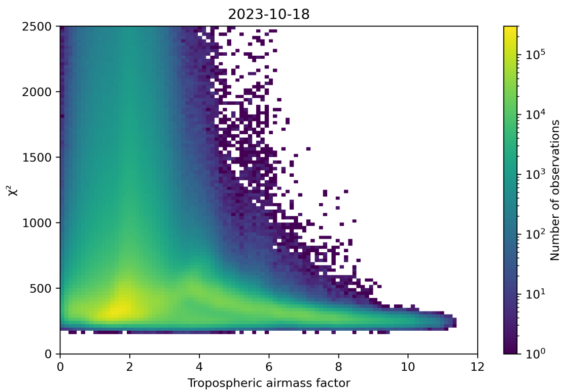
Figure 73: Scatter density plot of “Tropospheric airmass factor” against “ \chi^2 ” for 2023-10-17 to 2023-10-19.
