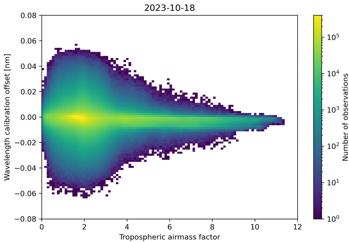
Figure 80: Scatter density plot of “Tropospheric airmass factor” against “Wavelength calibration offset” for 2023-10-17 to 2023-10-19.
