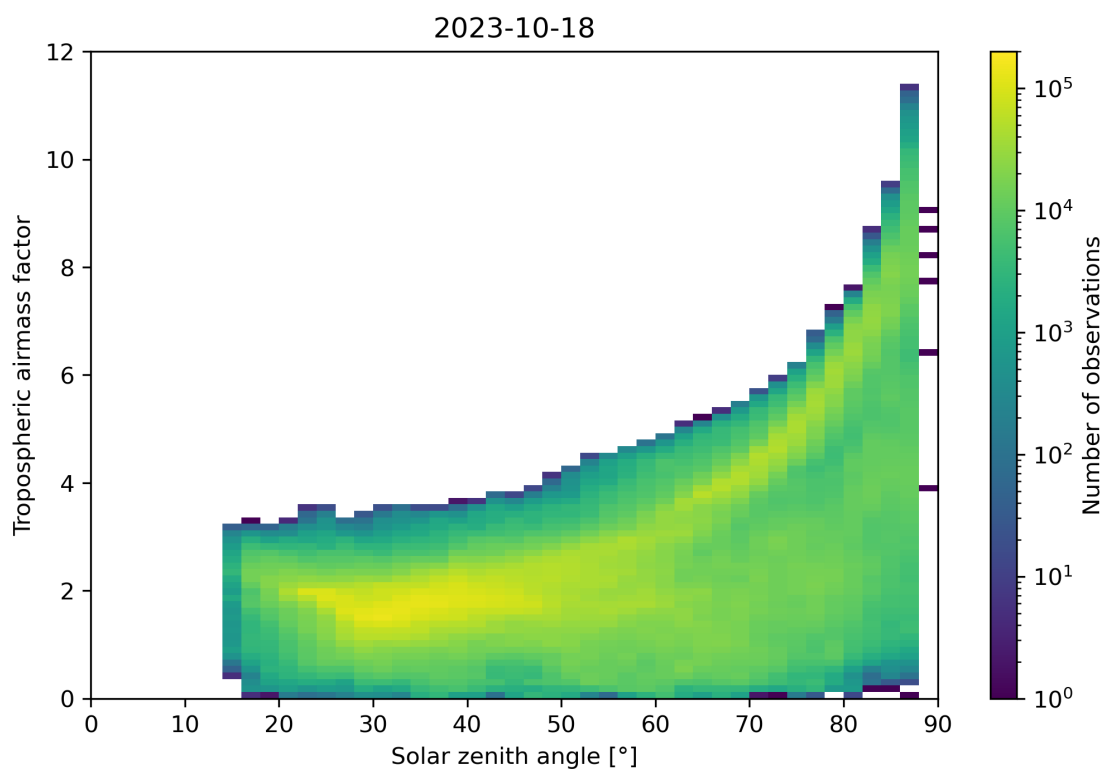
Figure 147: Scatter density plot of “Solar zenith angle” against “Tropospheric airmass factor” for 2023-10-17 to 2023-10-19.
