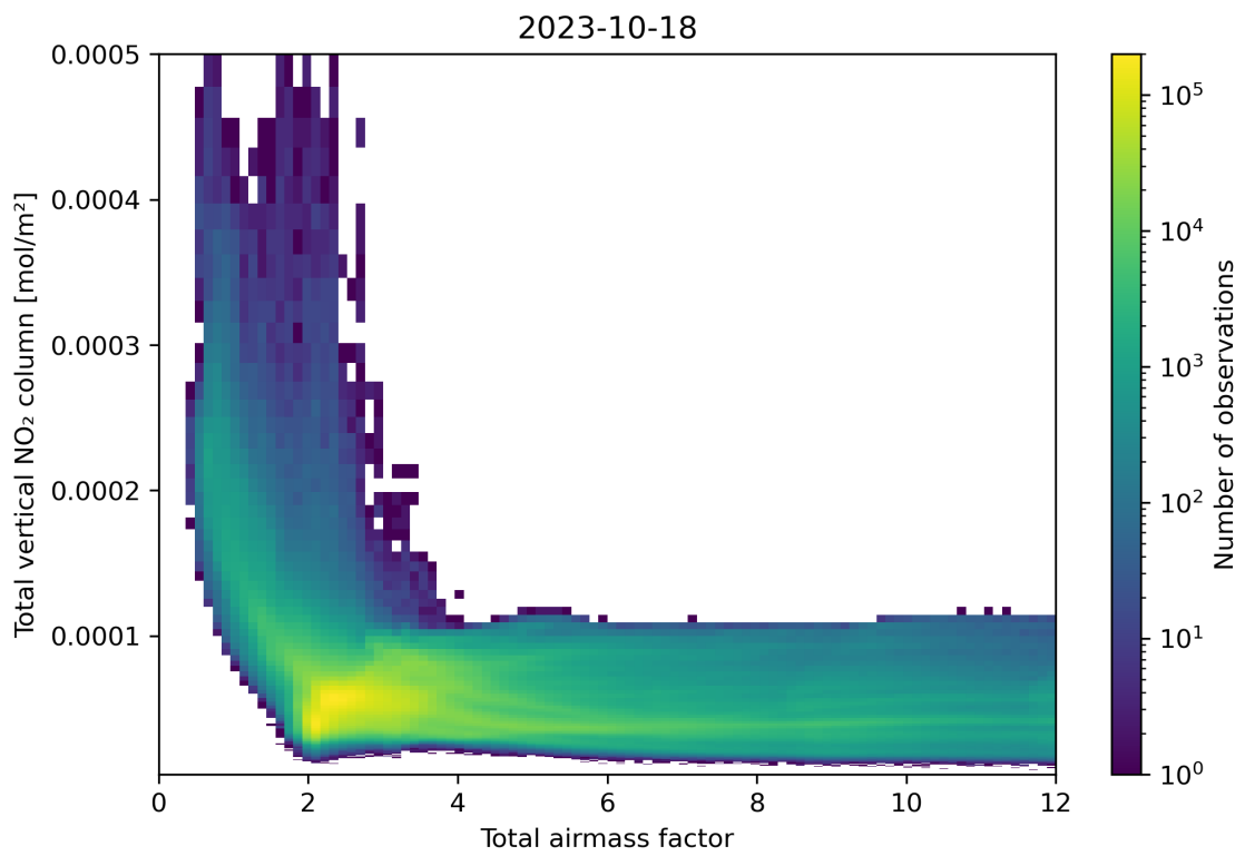
Figure 67: Scatter density plot of “Total airmass factor” against “Total vertical NO 2 column” for 2023-10-17 to 2023-10-19.
