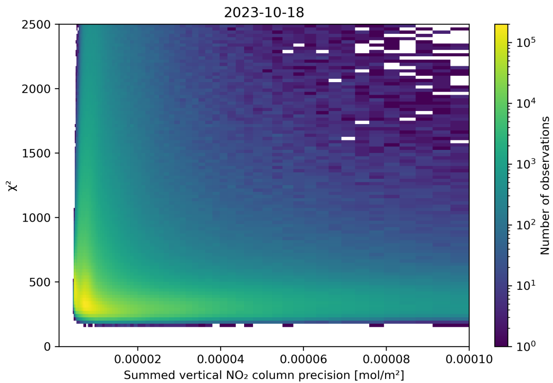
Figure 107: Scatter density plot of “Summed vertical NO 2 column precision” against “ \chi^2 ” for 2023-10-17 to 2023-10-19.
