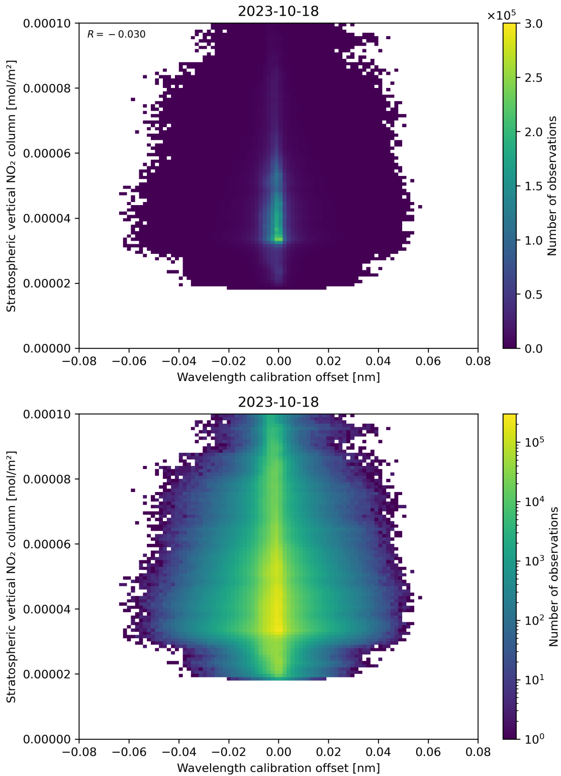
Figure 176: Scatter density plot of “Wavelength calibration offset” against “Stratospheric vertical NO 2 column” for 2023-10-17 to 2023-10-19.
