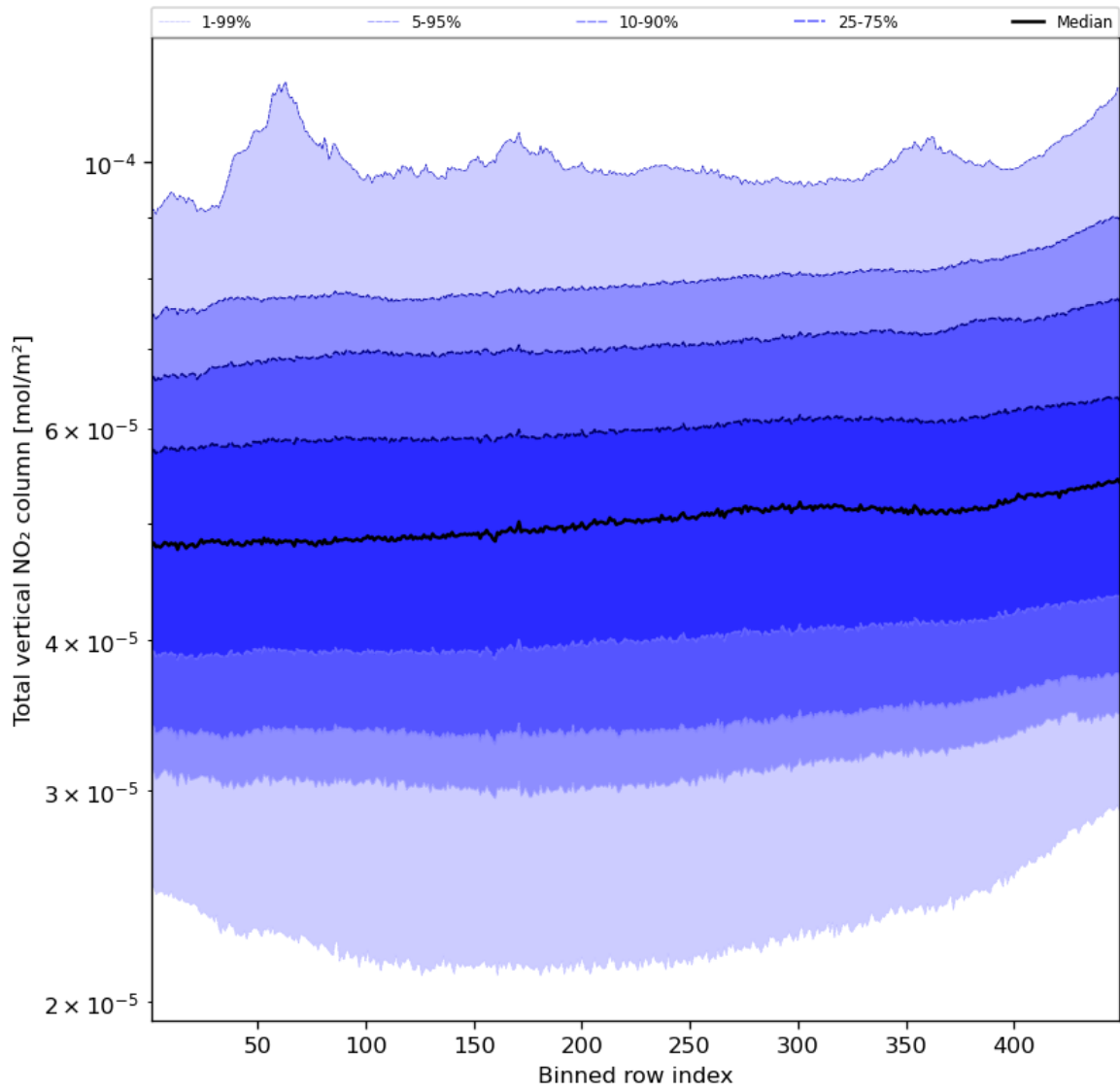
Figure 55: Along track statistics of “Total vertical NO 2 column” for 2023-10-17 to 2023-10-19
