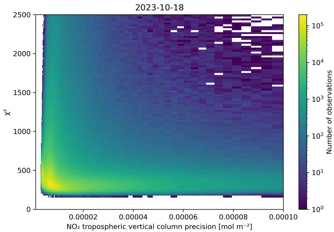
Figure 134: Scatter density plot of “NO 2 tropospheric vertical column precision” against “ \chi^2 ” for 2023-10-17 to 2023-10-19.
