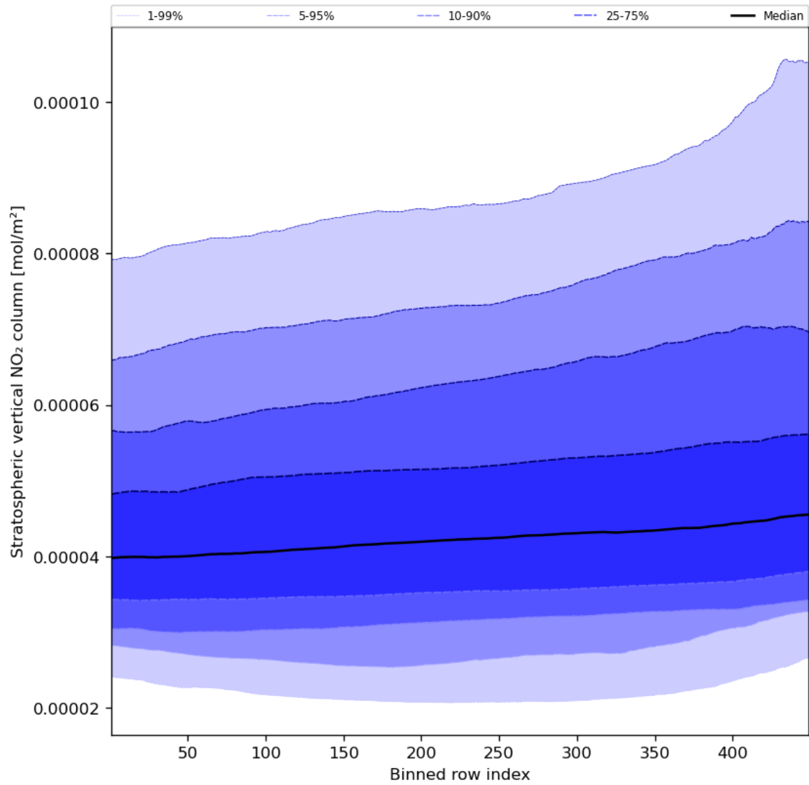
Figure 53: Along track statistics of “Stratospheric vertical NO 2 column” for 2023-10-17 to 2023-10-19
