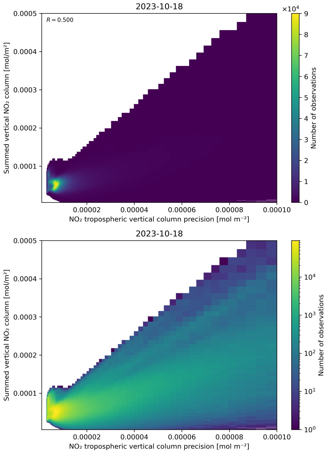
Figure 136: Scatter density plot of “NO 2 tropospheric vertical column precision” against “Summed vertical NO 2 column” for 2023-10-17 to 2023-10-19.
