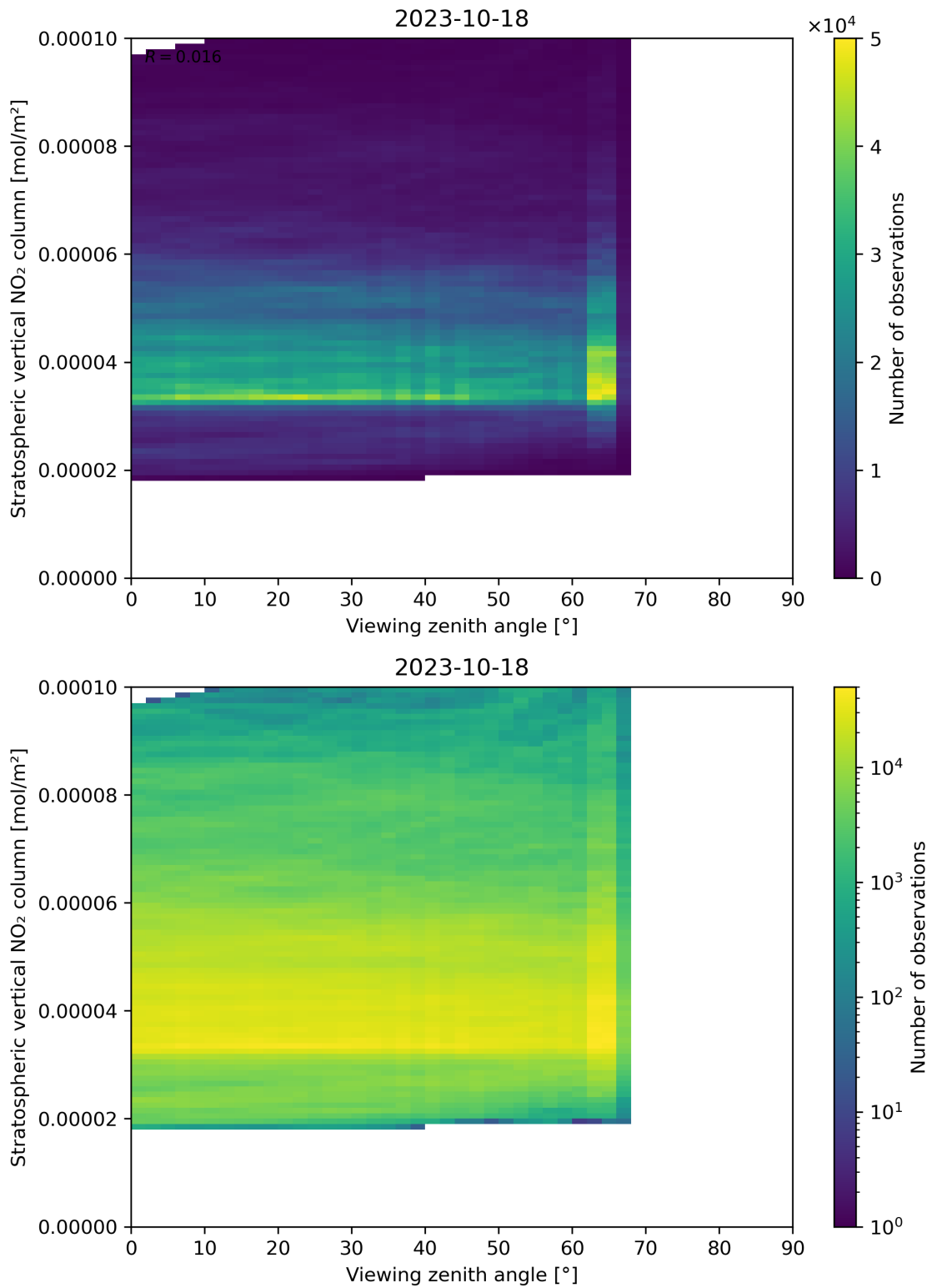
Figure 164: Scatter density plot of “Viewing zenith angle” against “Stratospheric vertical NO 2 column” for 2023-10-17 to 2023-10-19.
