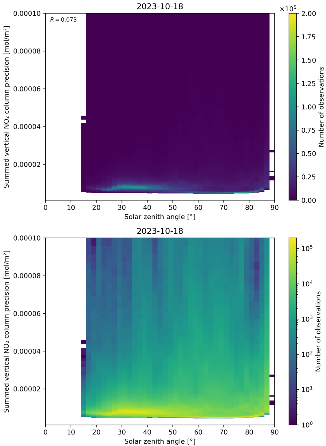
Figure 152: Scatter density plot of “Solar zenith angle” against “Summed vertical NO 2 column precision” for 2023-10-17 to 2023-10-19.
