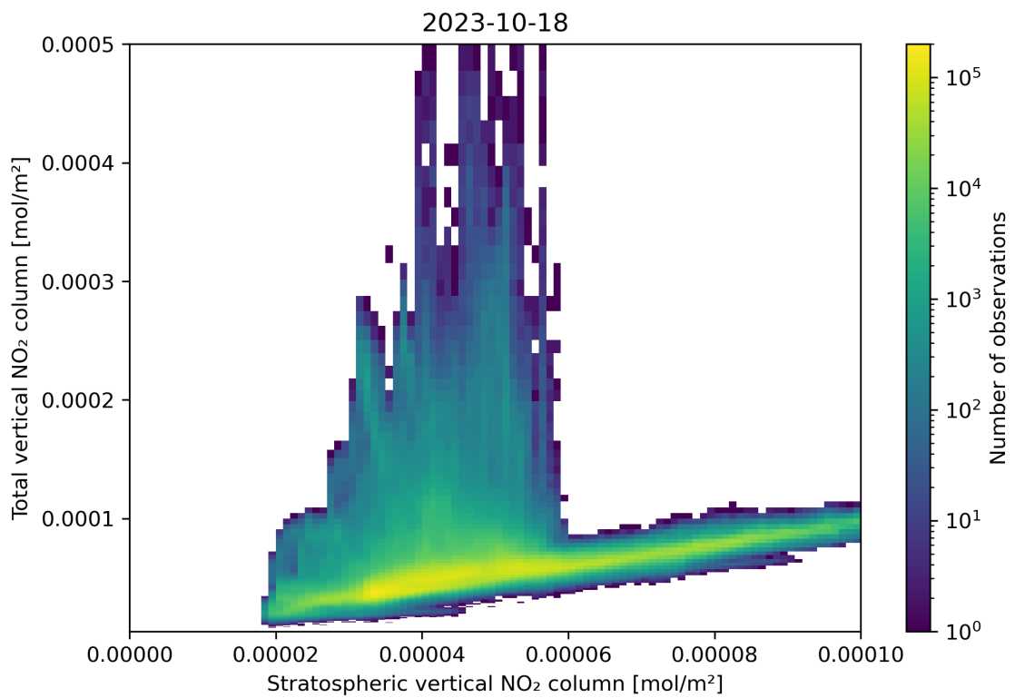
Figure 100: Scatter density plot of “Stratospheric vertical NO 2 column” against “Total vertical NO 2 column” for 2023-10-17 to 2023-10-19.
