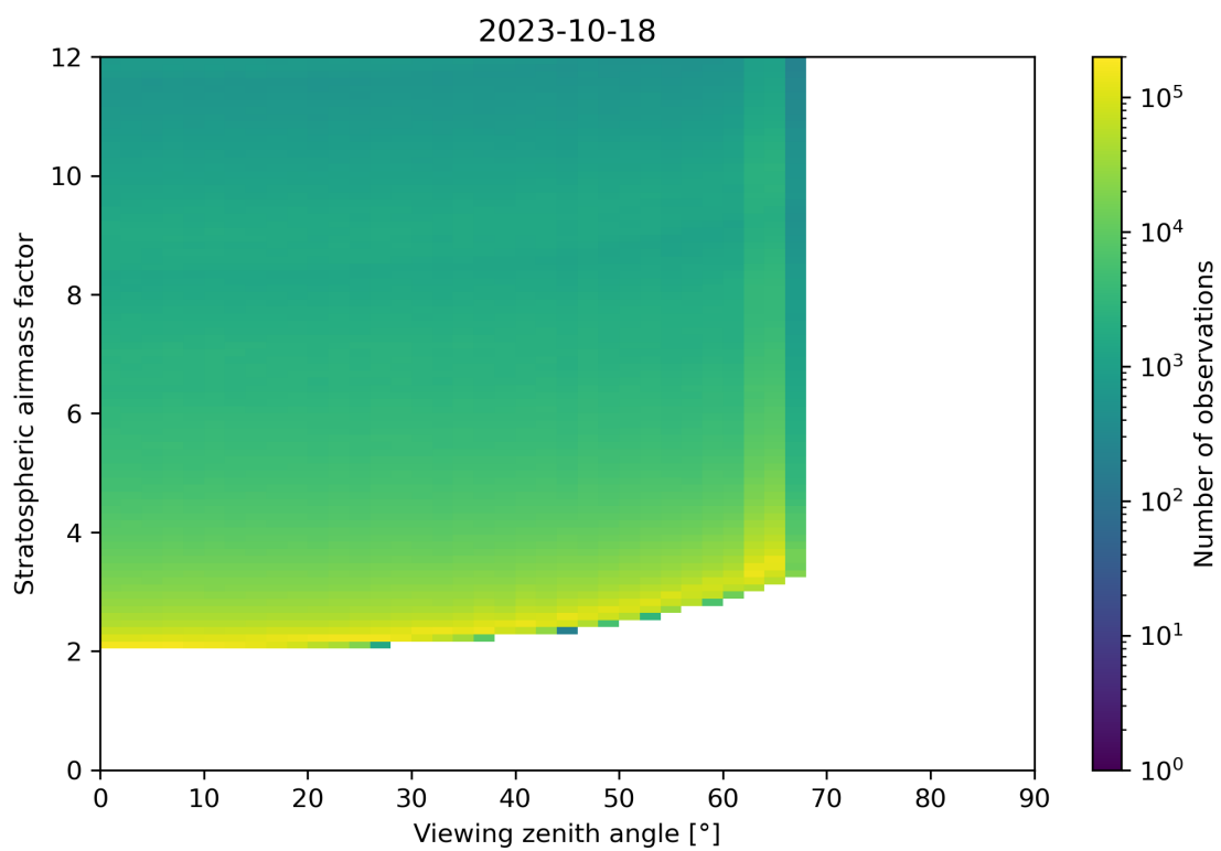
Figure 159: Scatter density plot of “Viewing zenith angle” against “Stratospheric airmass factor” for 2023-10-17 to 2023-10-19.
