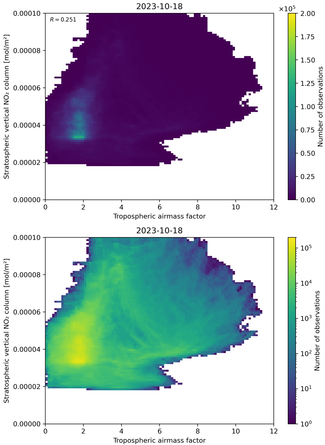
Figure 74: Scatter density plot of “Tropospheric airmass factor” against “Stratospheric vertical NO 2 column” for 2023-10-17 to 2023-10-19.
