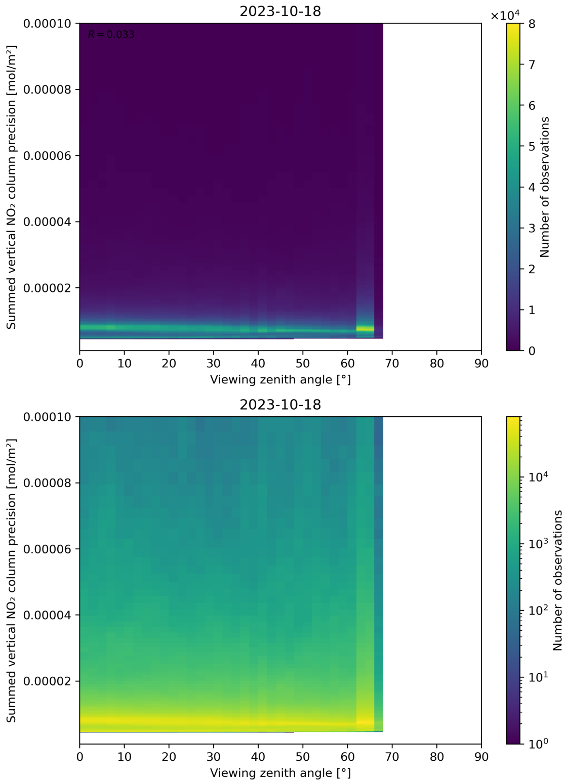
Figure 166: Scatter density plot of “Viewing zenith angle” against “Summed vertical NO 2 column precision” for 2023-10-17 to 2023-10-19.
