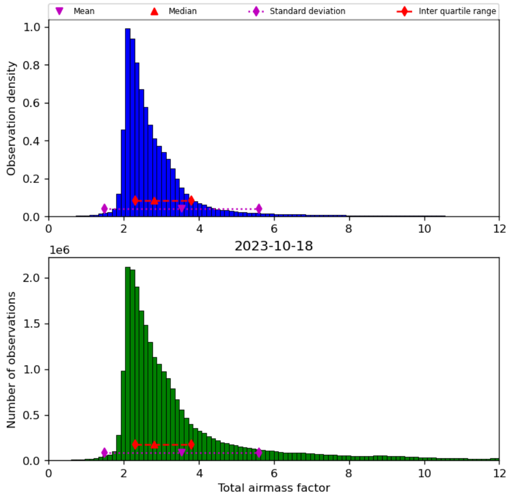
Figure 32: Histogram of “Total air mass factor” for 2023-10-17 to 2023-10-19
