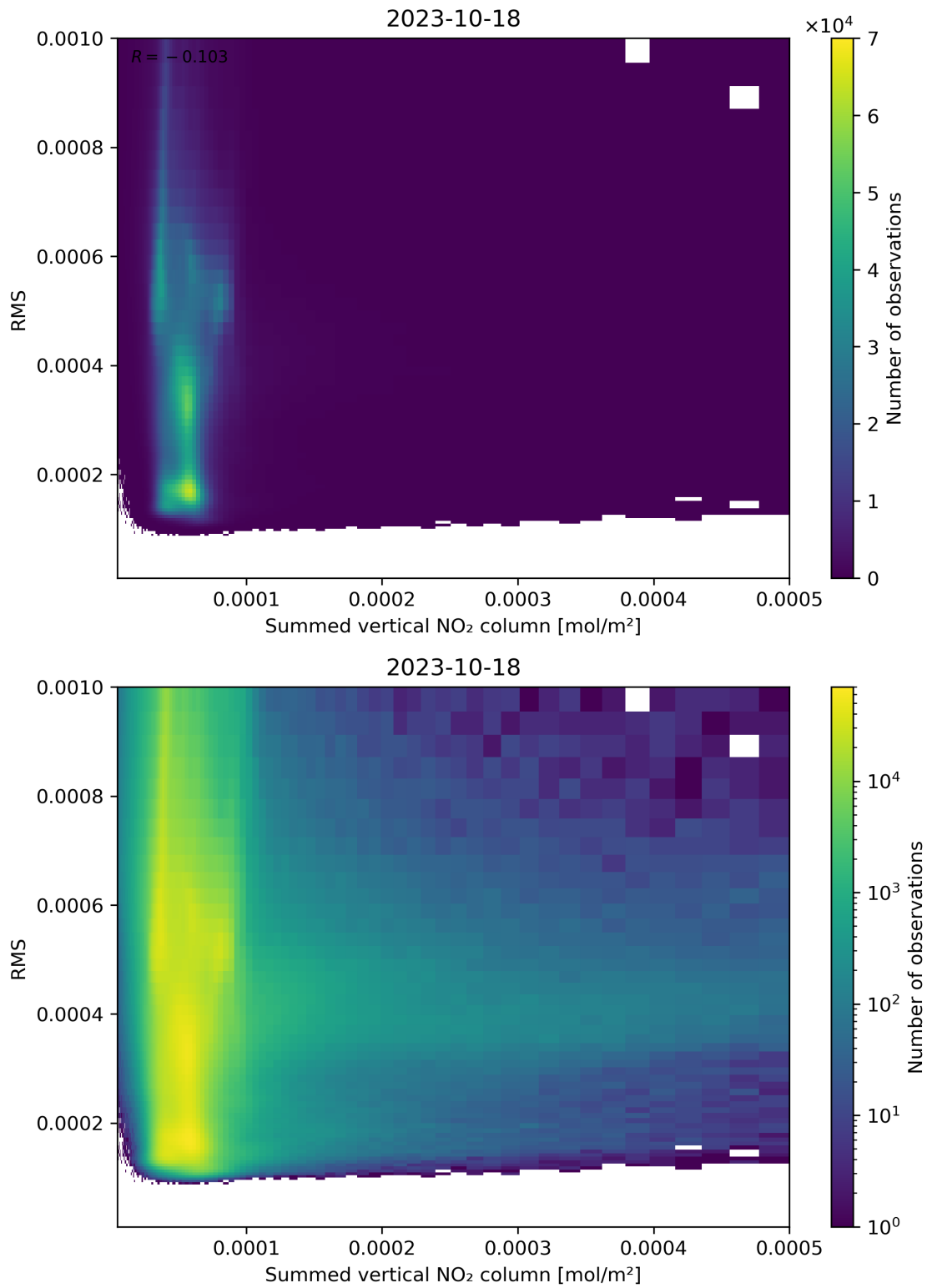
Figure 109: Scatter density plot of “Summed vertical NO 2 column” against “RMS” for 2023-10-17 to 2023-10-19.
