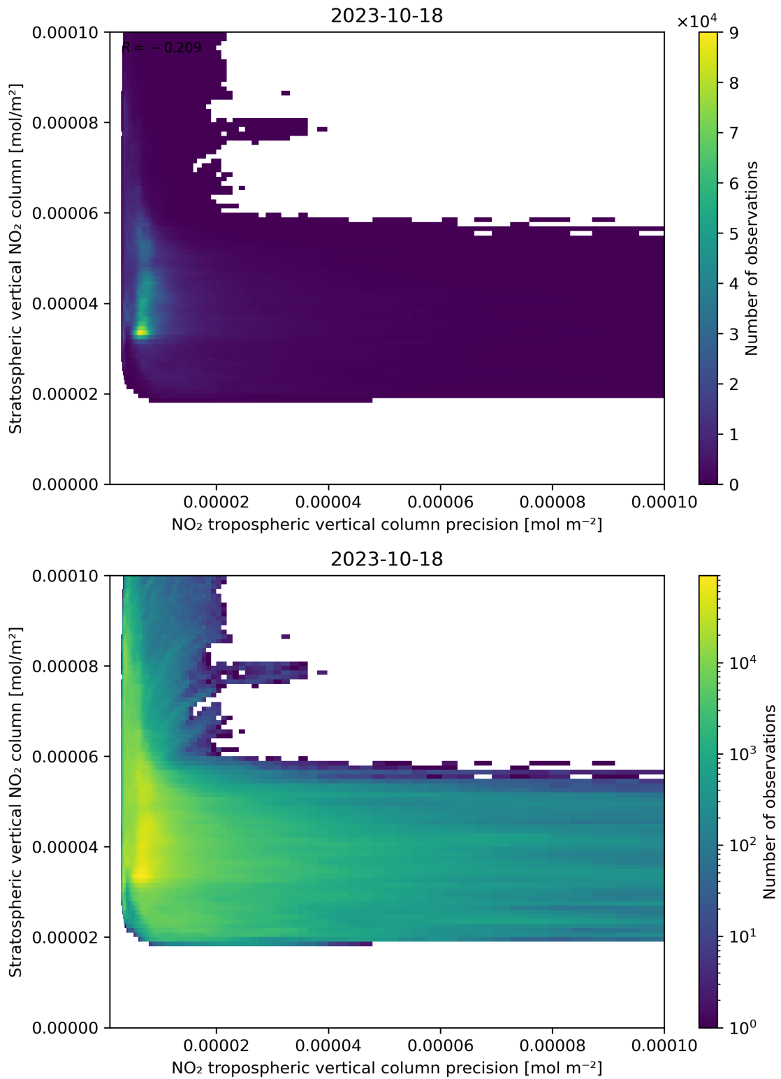
Figure 135: Scatter density plot of “NO 2 tropospheric vertical column precision” against “Stratospheric vertical NO 2 column” for 2023-10-17 to 2023-10-19.
