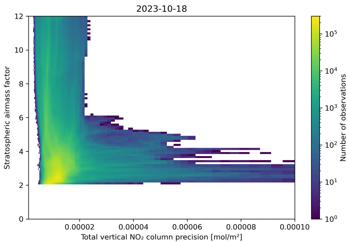
Figure 115: Scatter density plot of “Total vertical NO 2 column precision” against “Stratospheric airmass factor” for 2023-10-17 to 2023-10-19.
