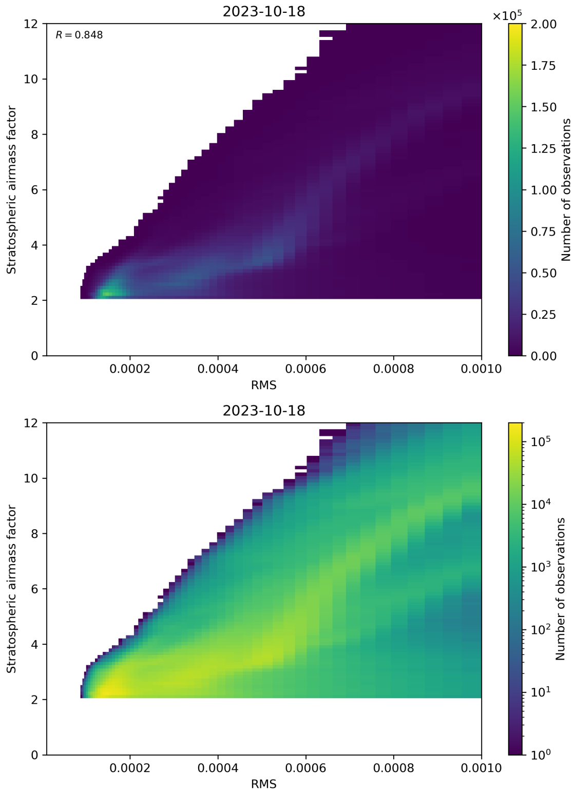
Figure 144: Scatter density plot of “RMS” against “Stratospheric airmass factor” for 2023-10-17 to 2023-10-19.
