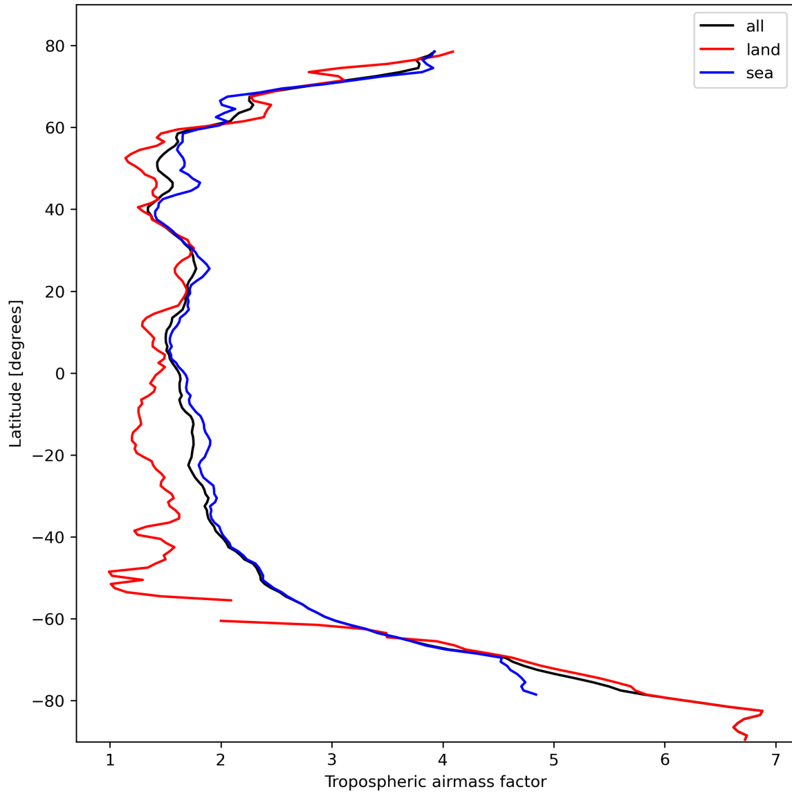
Figure 14: Zonal average of “Tropospheric airmass factor” for 2023-10-17 to 2023-10-19.
