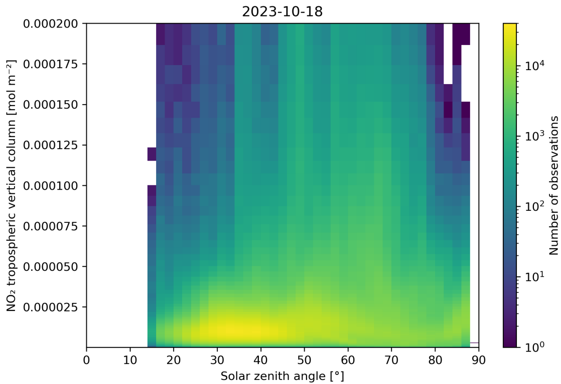
Figure 155: Scatter density plot of “Solar zenith angle” against “NO 2 tropospheric vertical column” for 2023-10-17 to 2023-10-19.
