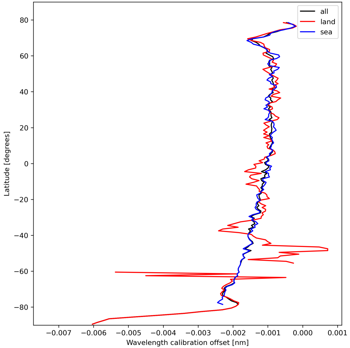
Figure 18: Zonal average of “Wavelength calibration offset” for 2023-10-17 to 2023-10-19.
