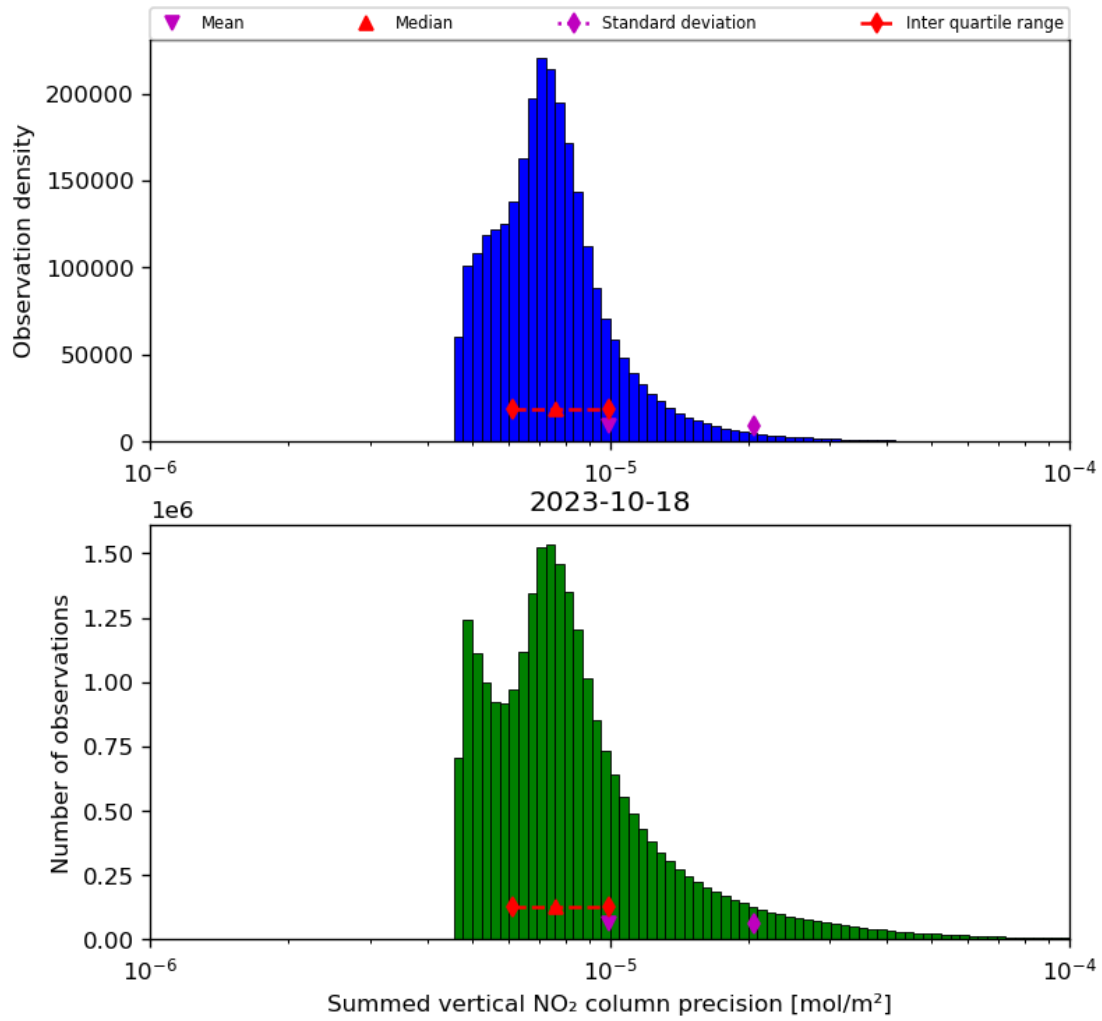
Figure 41: Histogram of “Summed vertical NO 2 column precision” for 2023-10-17 to 2023-10-19
