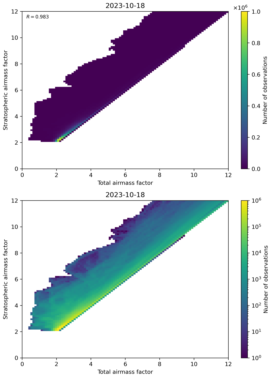
Figure 62: Scatter density plot of “Total airmass factor” against “Stratospheric airmass factor” for 2023-10-17 to 2023-10-19.
