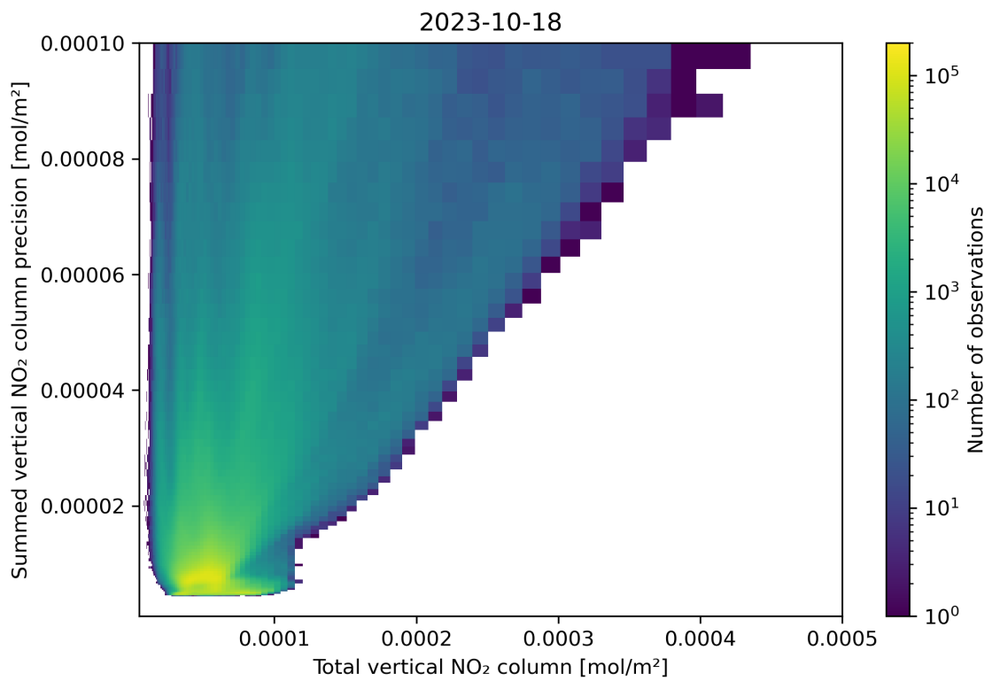
Figure 113: Scatter density plot of “Total vertical NO 2 column” against “Summed vertical NO 2 column precision” for 2023-10-17 to 2023-10-19.
