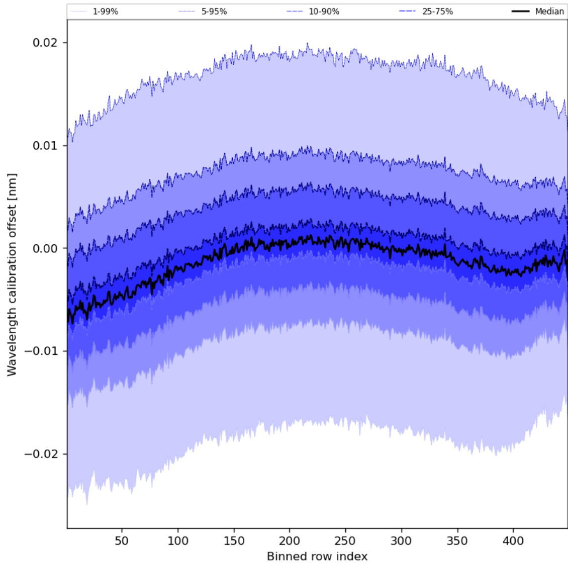
Figure 52: Along track statistics of “Wavelength calibration offset” for 2023-10-17 to 2023-10-19
