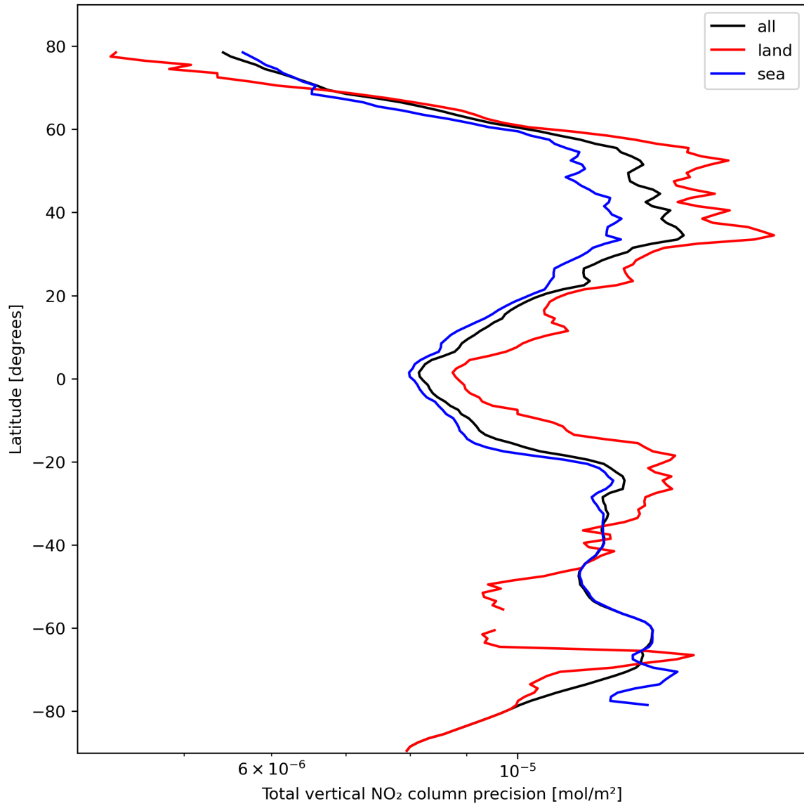
Figure 22: Zonal average of “Total vertical NO 2 column precision” for 2023-10-17 to 2023-10-19.
