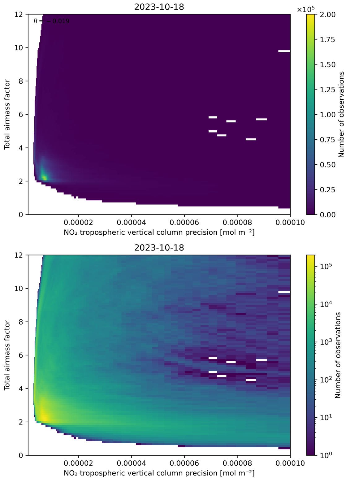
Figure 132: Scatter density plot of “NO 2 tropospheric vertical column precision” against “Total airmass factor” for 2023-10-17 to 2023-10-19.
