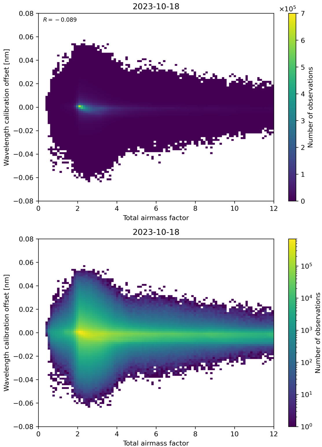
Figure 70: Scatter density plot of “Total airmass factor” against “Wavelength calibration offset” for 2023-10-17 to 2023-10-19.
