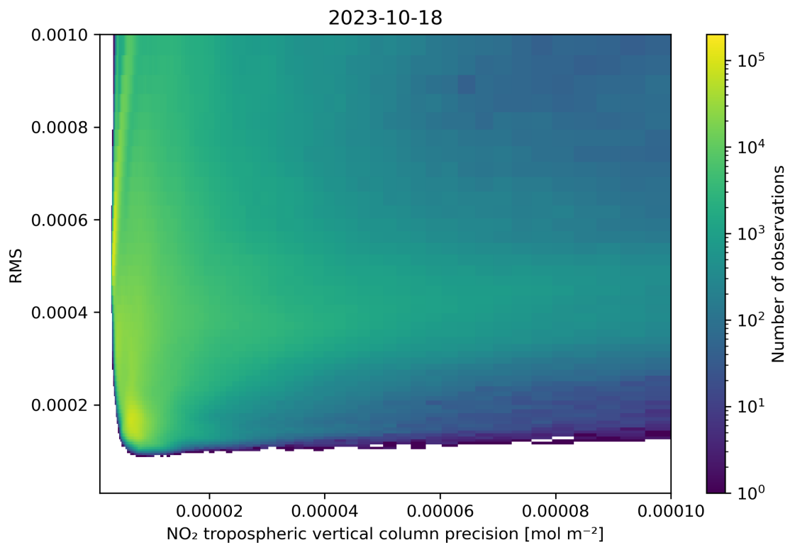
Figure 140: Scatter density plot of “NO 2 tropospheric vertical column precision” against “RMS” for 2023-10-17 to 2023-10-19.
