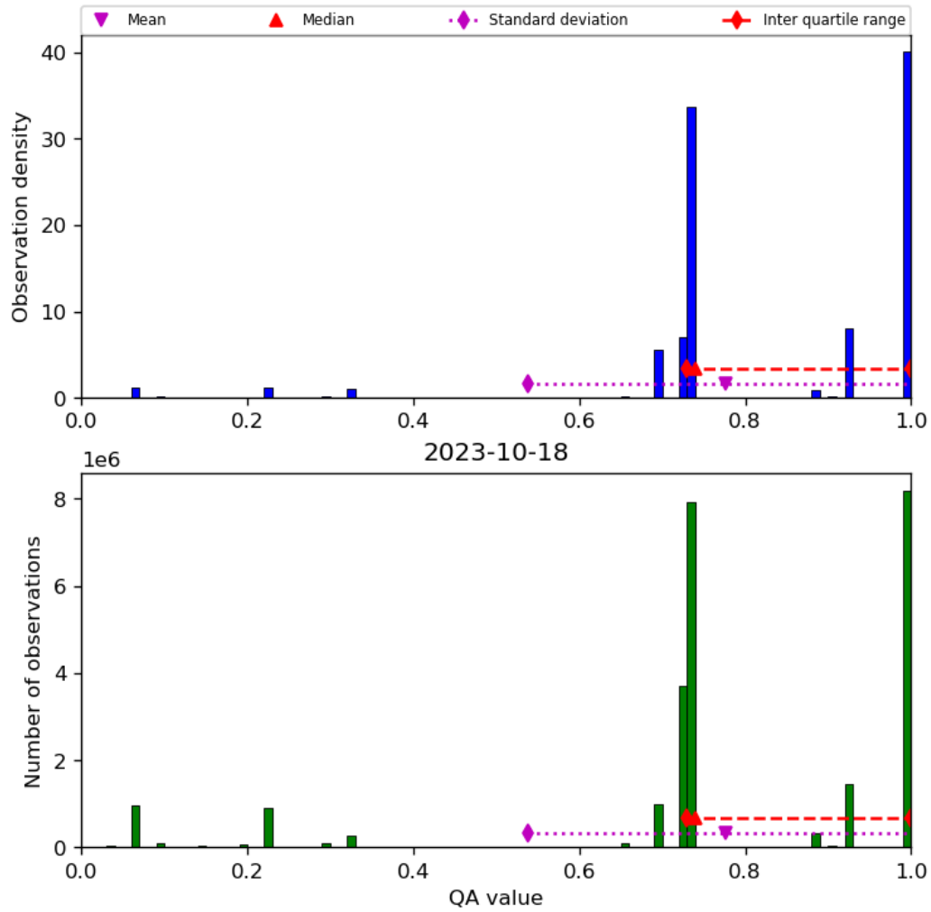
Figure 28: Histogram of “QA value” for 2023-10-17 to 2023-10-19
