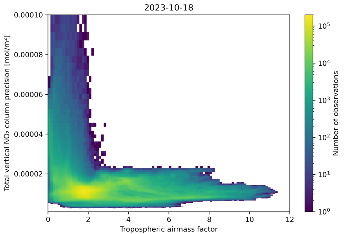
Figure 78: Scatter density plot of “Tropospheric airmass factor” against “Total vertical NO 2 column precision” for 2023-10-17 to 2023-10-19.
