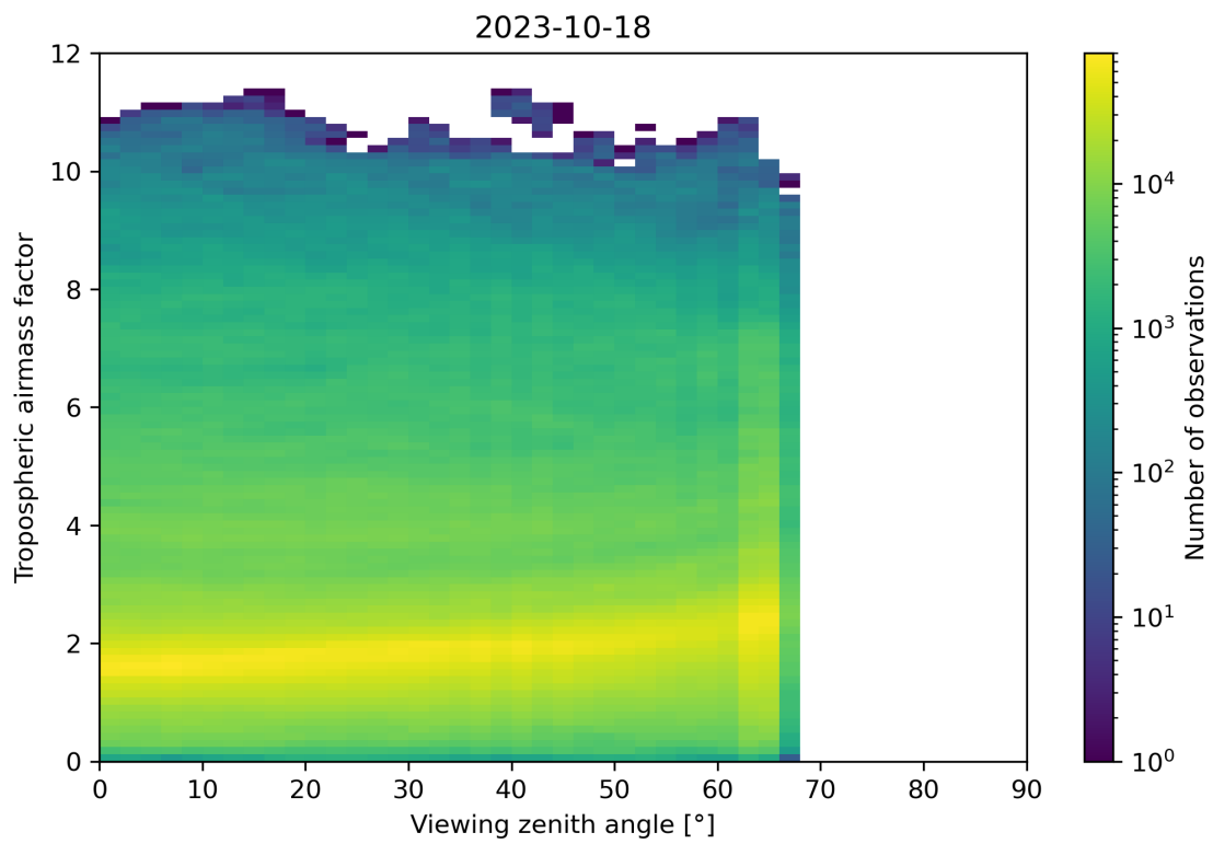
Figure 161: Scatter density plot of “Viewing zenith angle” against “Tropospheric airmass factor” for 2023-10-17 to 2023-10-19.
