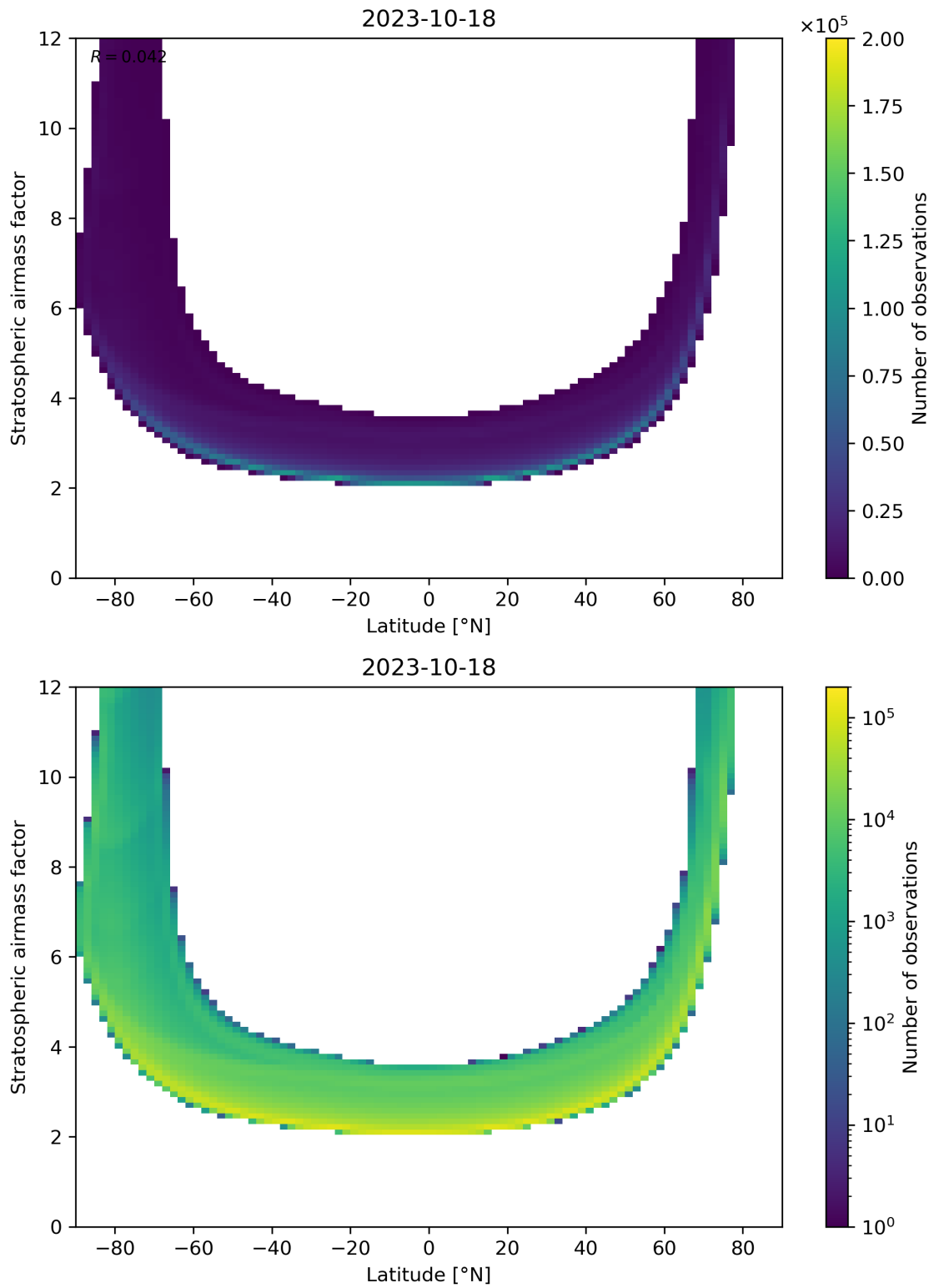
Figure 83: Scatter density plot of “Latitude” against “Stratospheric airmass factor” for 2023-10-17 to 2023-10-19.
