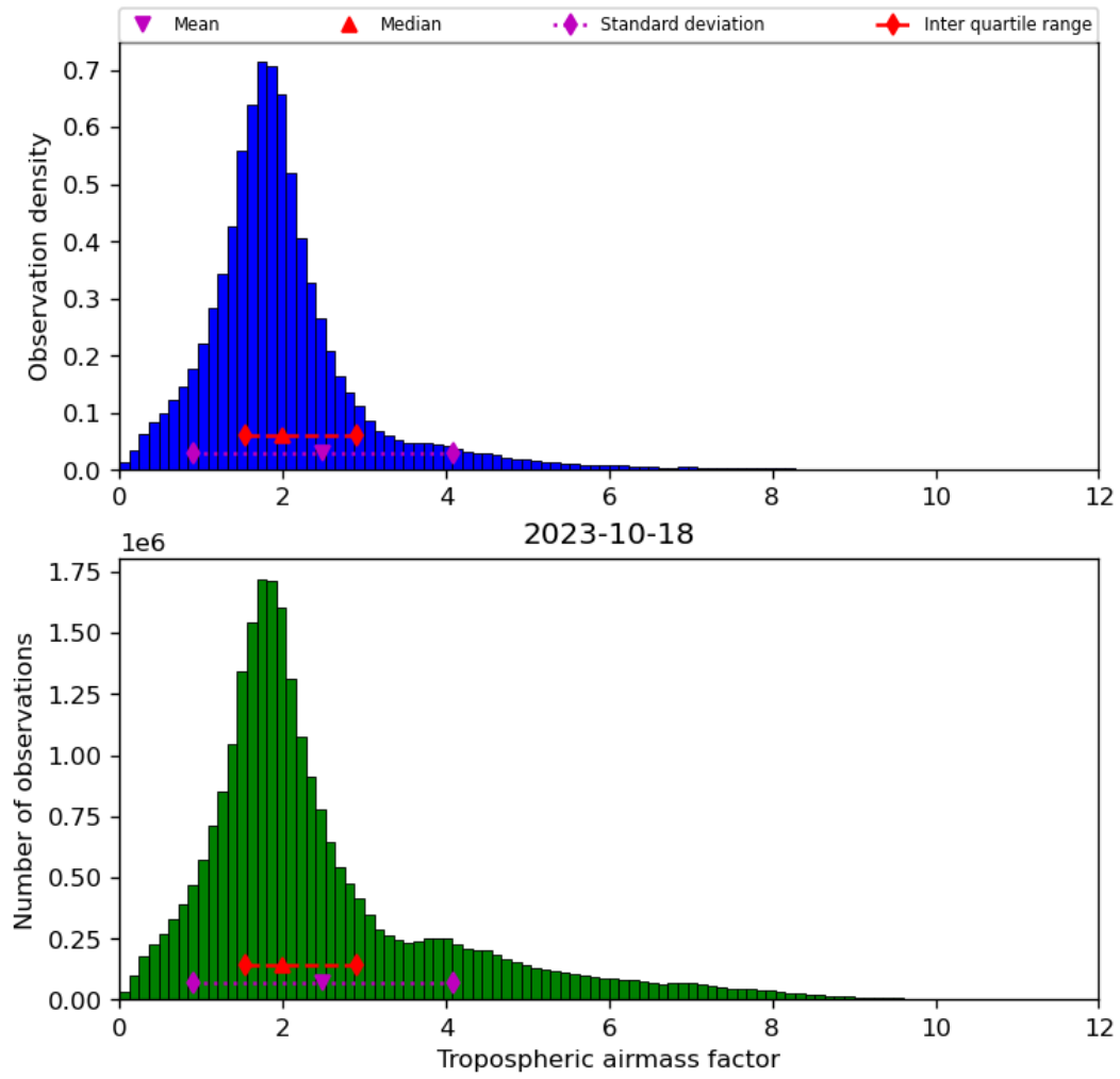
Figure 31: Histogram of “Tropospheric airmass factor” for 2023-10-17 to 2023-10-19
