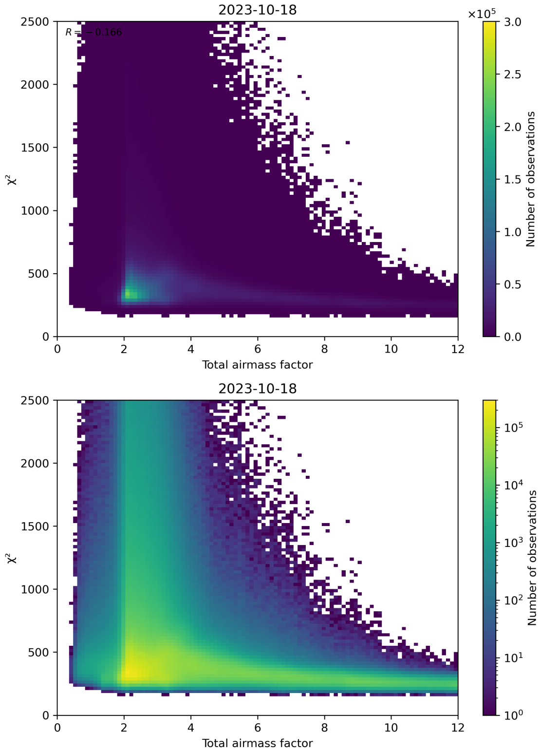
Figure 63: Scatter density plot of “Total airmass factor” against “ \chi^2 ” for 2023-10-17 to 2023-10-19.
