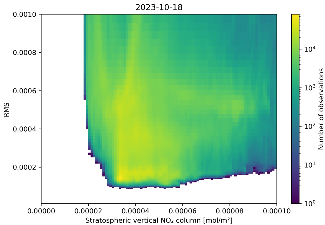
Figure 102: Scatter density plot of “Stratospheric vertical NO 2 column” against “RMS” for 2023-10-17 to 2023-10-19.
