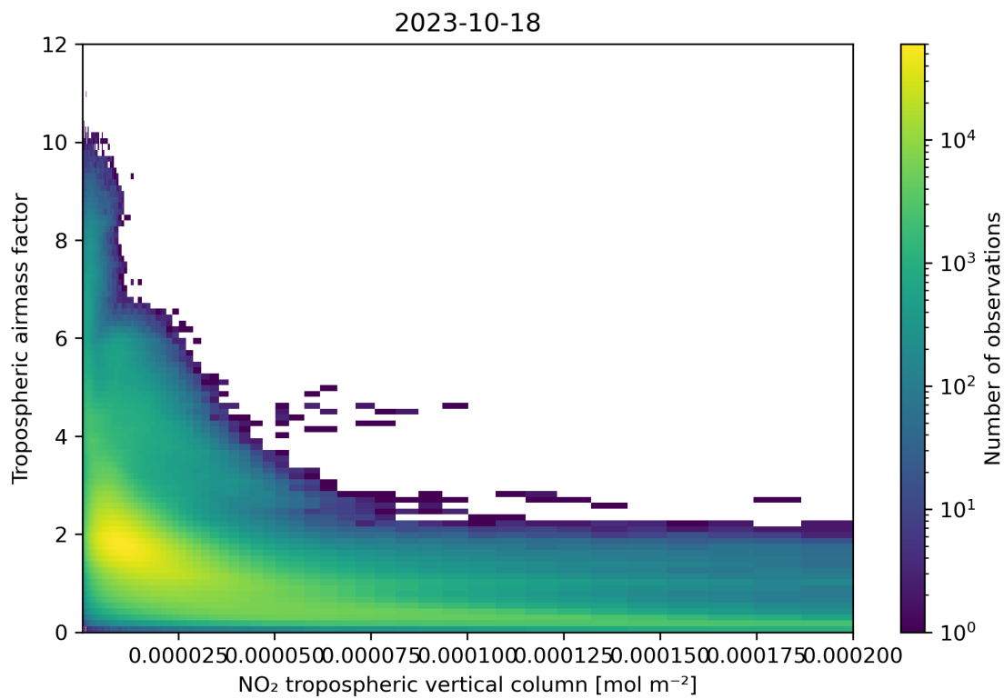
Figure 123: Scatter density plot of “NO 2 tropospheric vertical column” against “Tropospheric air mass factor” for 2023-10-17 to 2023-10-19.
