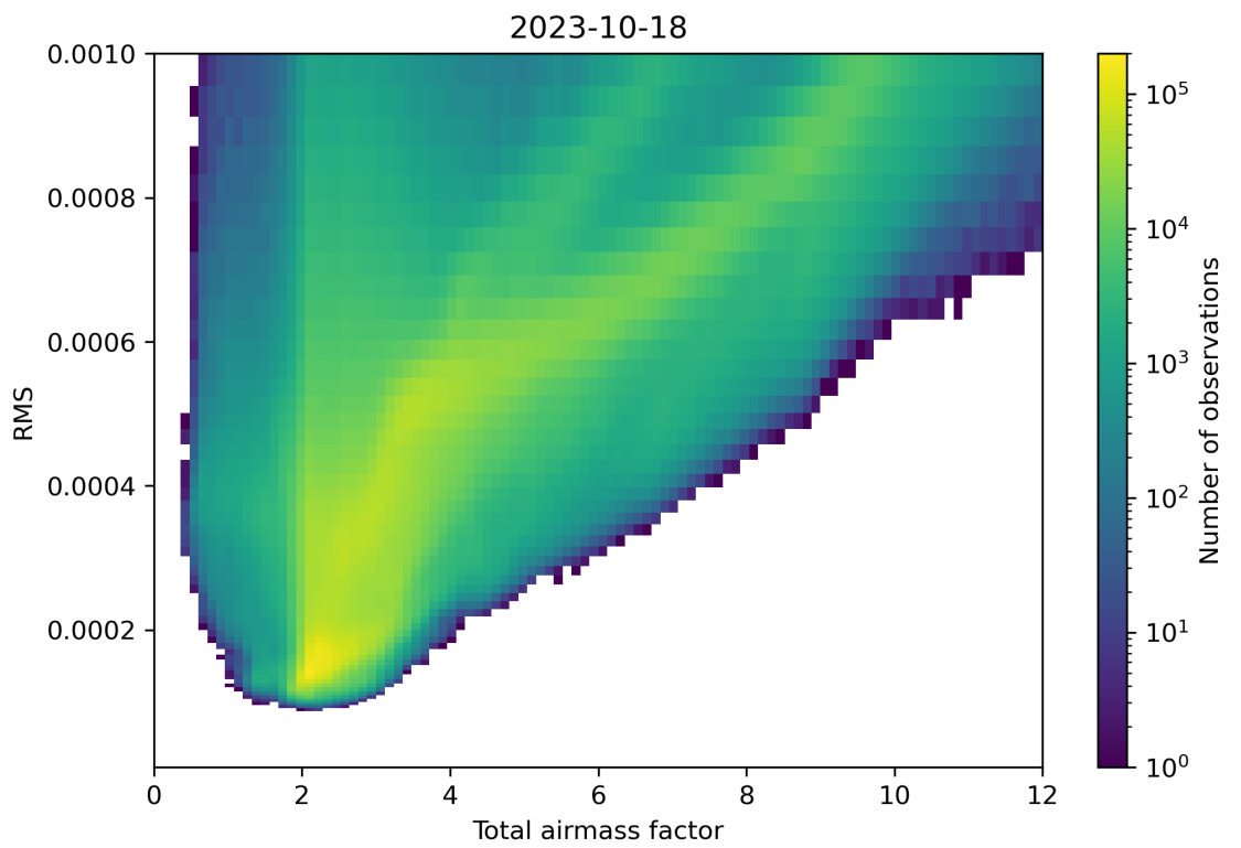
Figure 69: Scatter density plot of “Total airmass factor” against “RMS” for 2023-10-17 to 2023-10-19.
