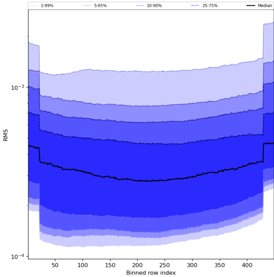
Figure 60: Along track statistics of “RMS” for 2023-10-17 to 2023-10-19
