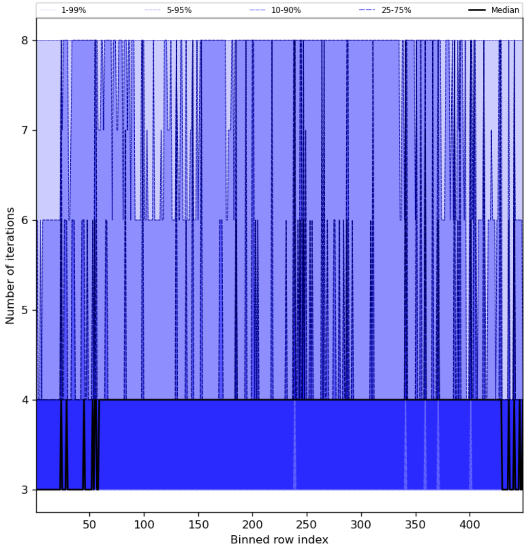
Figure 51: Along track statistics of “Number of iterations” for 2023-10-17 to 2023-10-19
