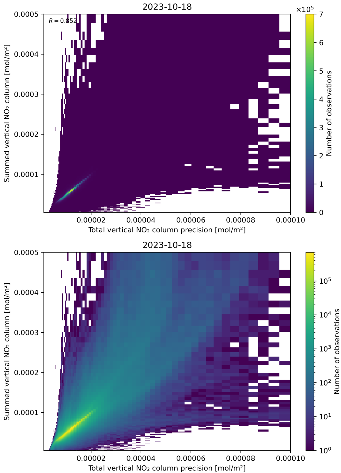
Figure 117: Scatter density plot of “Total vertical NO 2 column precision” against “Summed vertical NO 2 column” for 2023-10-17 to 2023-10-19.
