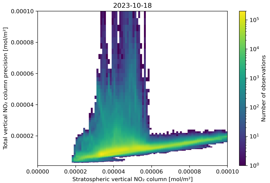
Figure 101: Scatter density plot of “Stratospheric vertical NO 2 column” against “Total vertical NO 2 column precision” for 2023-10-17 to 2023-10-19.
