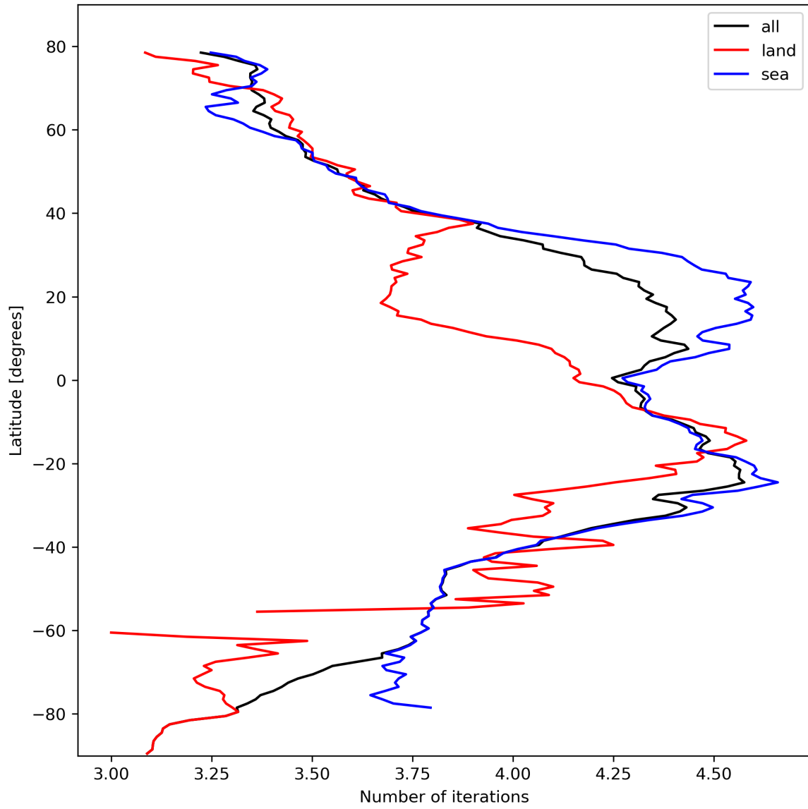
Figure 17: Zonal average of “Number of iterations” for 2023-10-17 to 2023-10-19.
