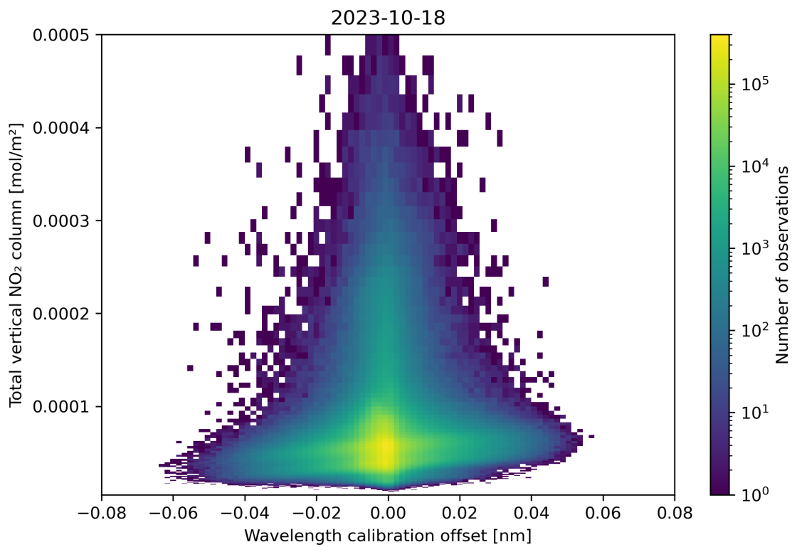
Figure 179: Scatter density plot of “Wavelength calibration offset” against “Total vertical NO 2 column” for 2023-10-17 to 2023-10-19.
