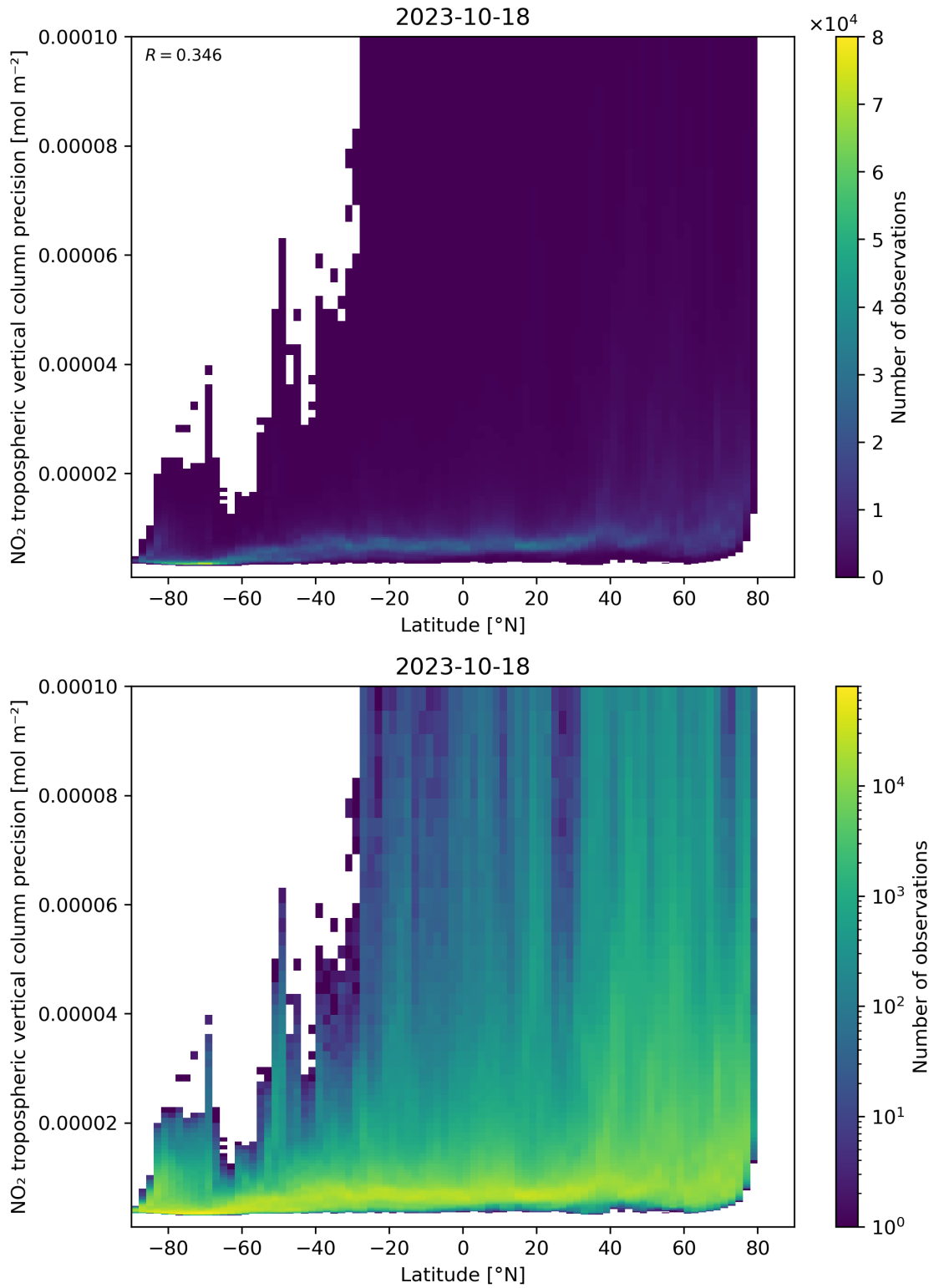
Figure 93: Scatter density plot of “Latitude” against “NO 2 tropospheric vertical column precision” for 2023-10-17 to 2023-10-19.
