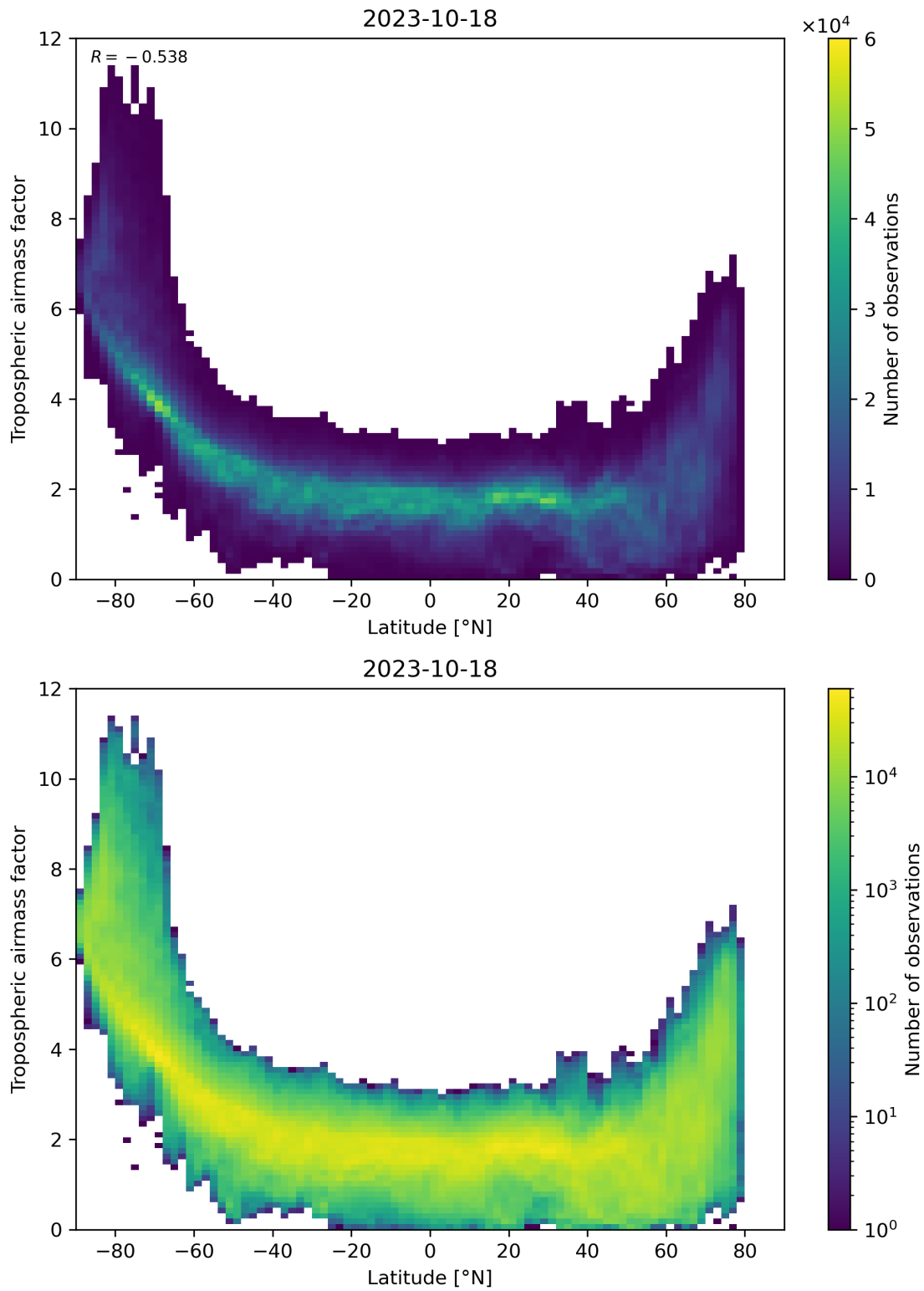
Figure 85: Scatter density plot of “Latitude” against “Tropospheric airmass factor” for 2023-10-17 to 2023-10-19.
