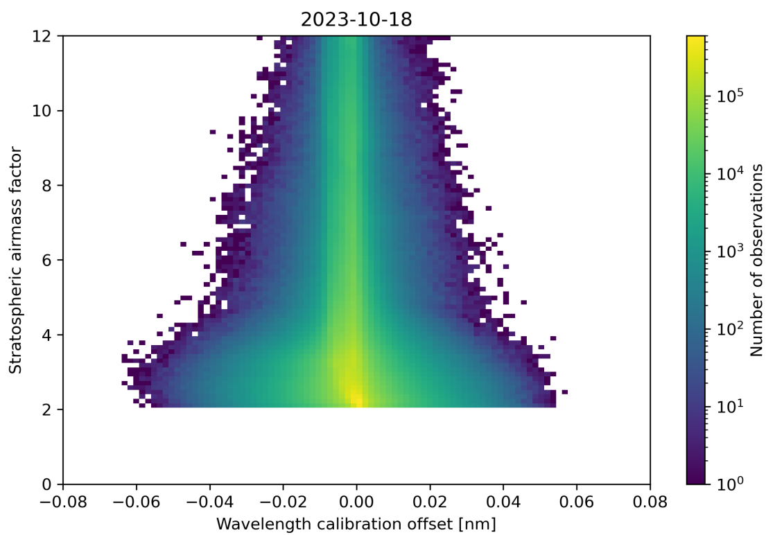
Figure 174: Scatter density plot of “Wavelength calibration offset” against “Stratospheric airmass factor” for 2023-10-17 to 2023-10-19.
