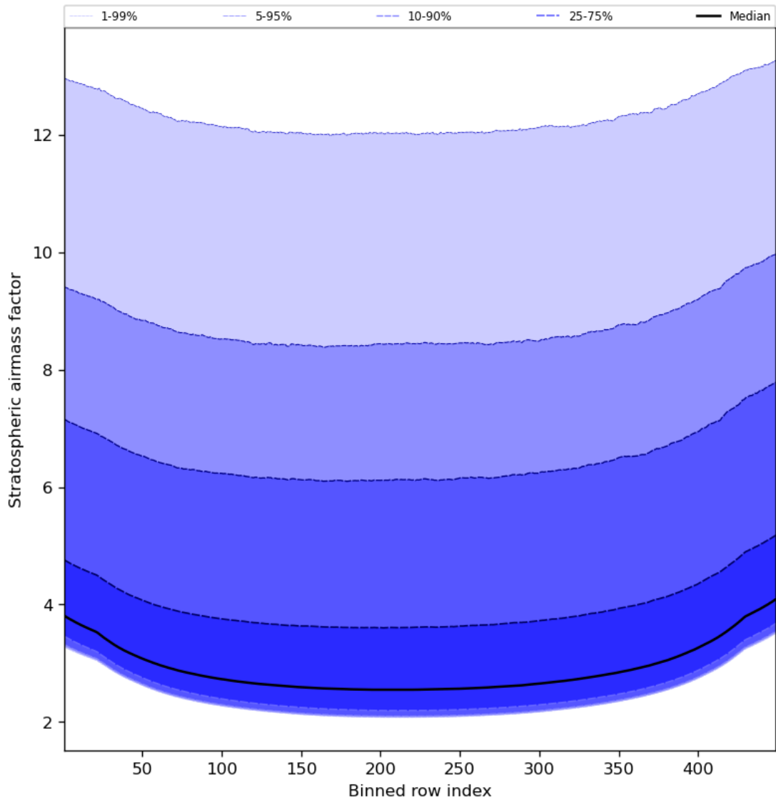
Figure 61: Along track statistics of “Stratospheric airmass factor” for 2023-10-17 to 2023-10-19
