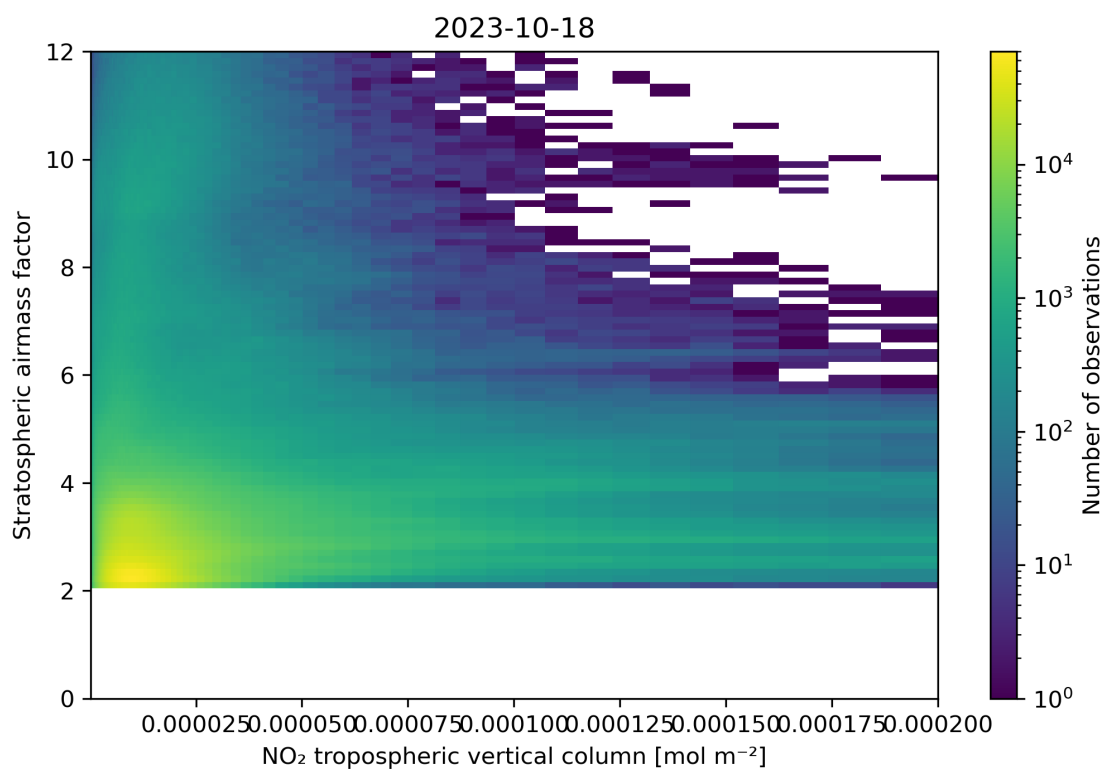
Figure 121: Scatter density plot of “NO 2 tropospheric vertical column” against “Stratospheric airmass factor” for 2023-10-17 to 2023-10-19.
