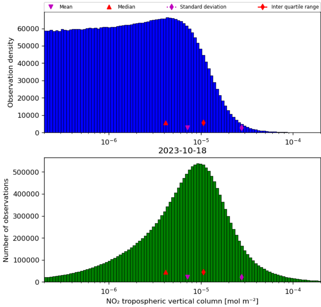
Figure 29: Histogram of “NO 2 tropospheric vertical column” for 2023-10-17 to 2023-10-19
