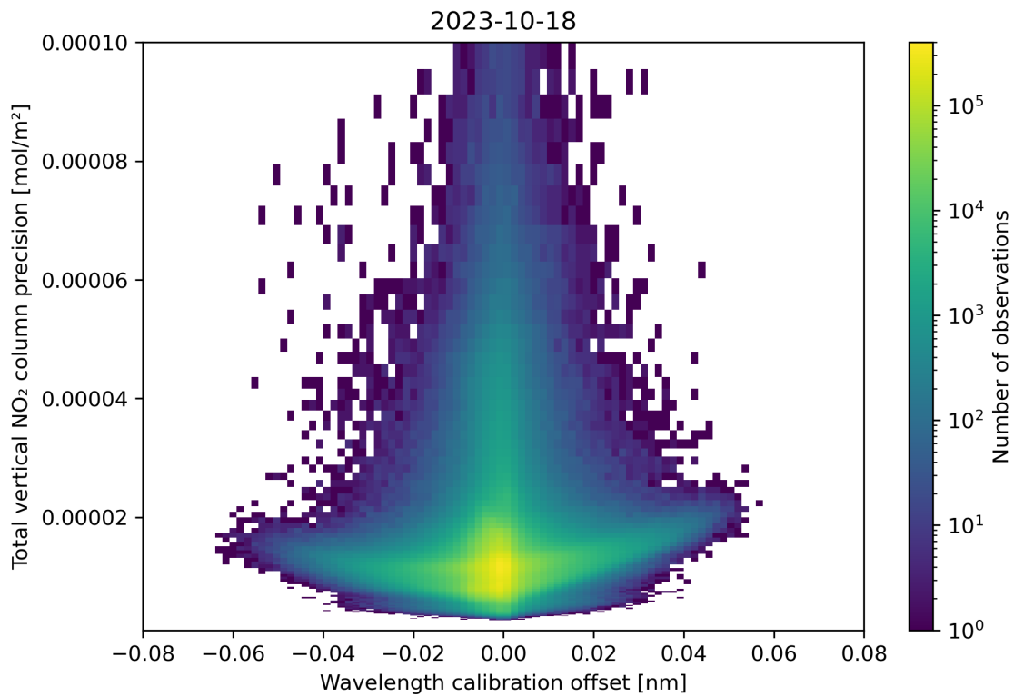
Figure 180: Scatter density plot of “Wavelength calibration offset” against “Total vertical NO 2 column precision” for 2023-10-17 to 2023-10-19.
