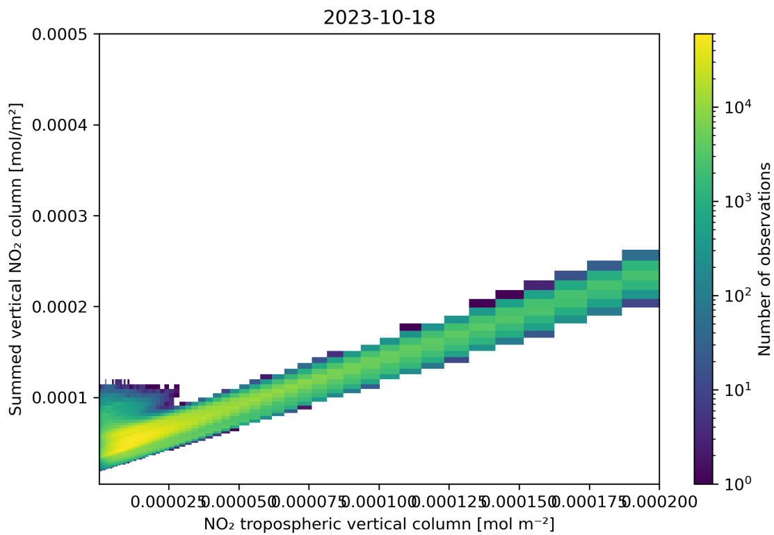
Figure 126: Scatter density plot of “NO 2 tropospheric vertical column” against “Summed vertical NO 2 column” for 2023-10-17 to 2023-10-19.
