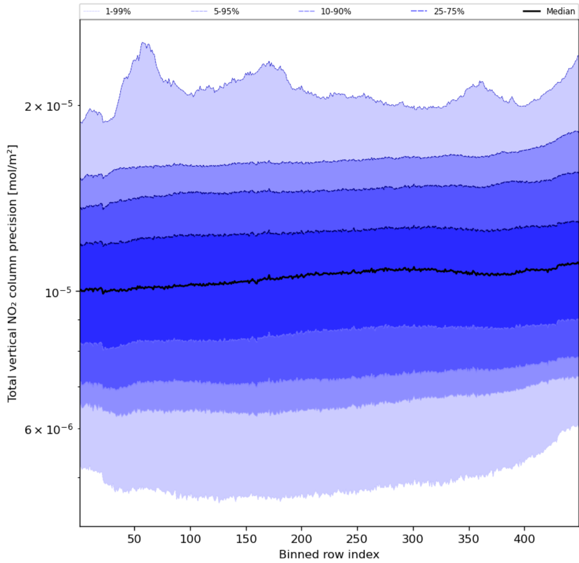
Figure 56: Along track statistics of “Total vertical NO 2 column precision” for 2023-10-17 to 2023-10-19
