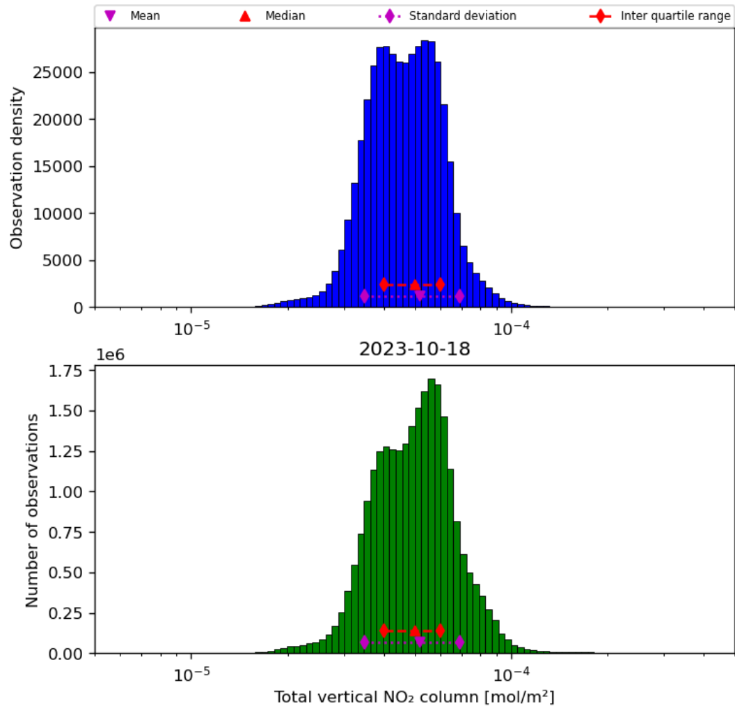
Figure 38: Histogram of “Total vertical NO 2 column” for 2023-10-17 to 2023-10-19
