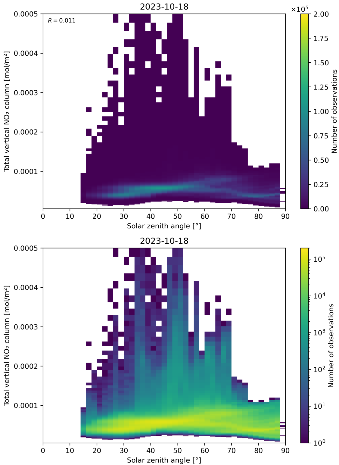
Figure 153: Scatter density plot of “Solar zenith angle” against “Total vertical NO 2 column” for 2023-10-17 to 2023-10-19.
