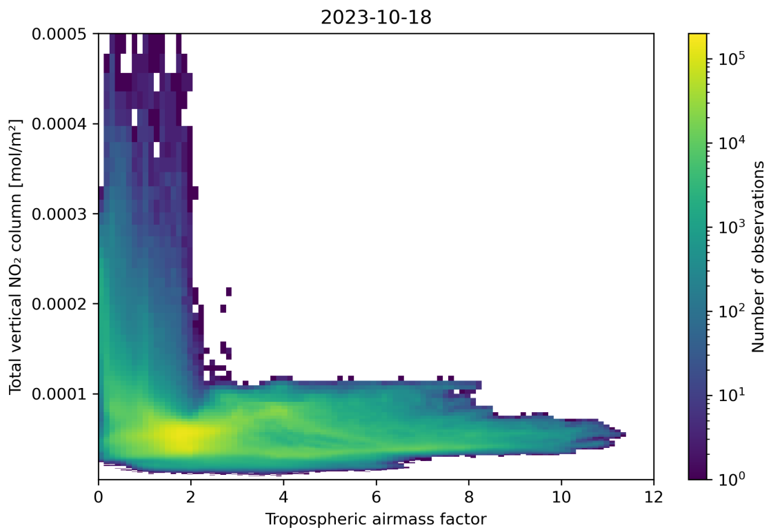
Figure 77: Scatter density plot of “Tropospheric airmass factor” against “Total vertical NO 2 column” for 2023-10-17 to 2023-10-19.
