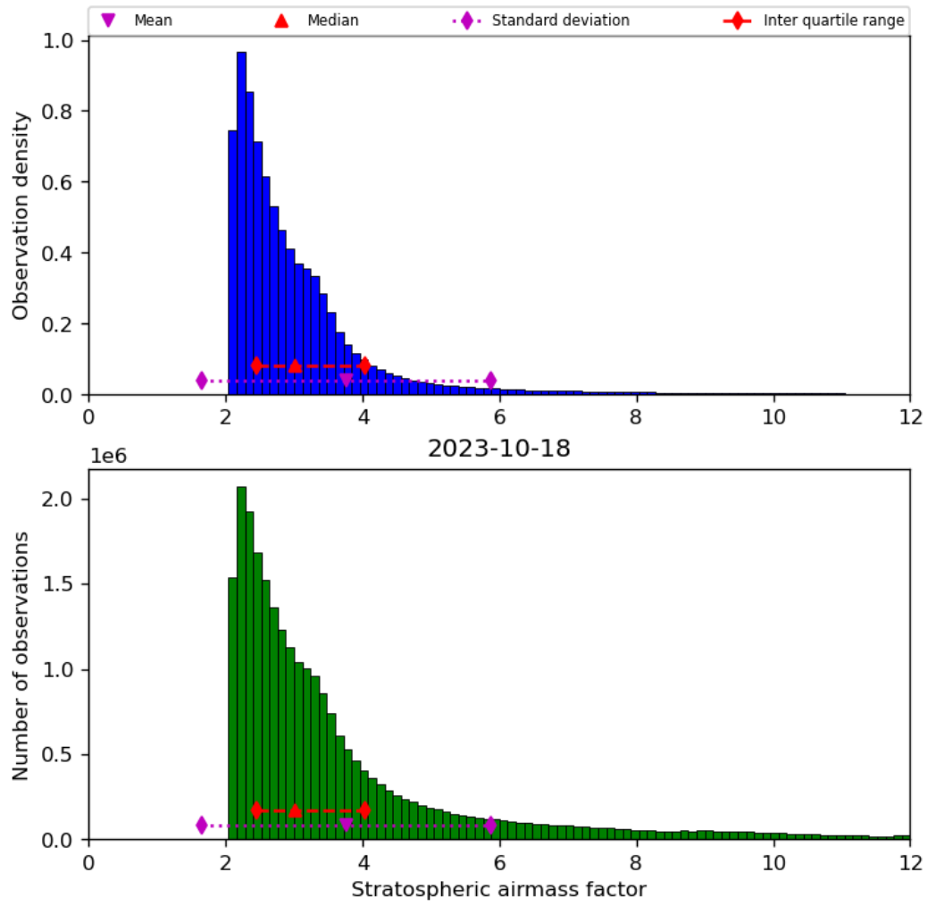
Figure 44: Histogram of “Stratospheric airmass factor” for 2023-10-17 to 2023-10-19
