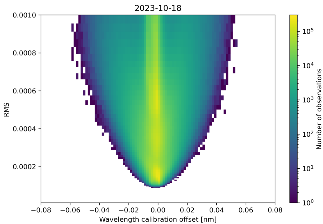
Figure 181: Scatter density plot of “Wavelength calibration offset” against “RMS” for 2023-10-17 to 2023-10-19.
