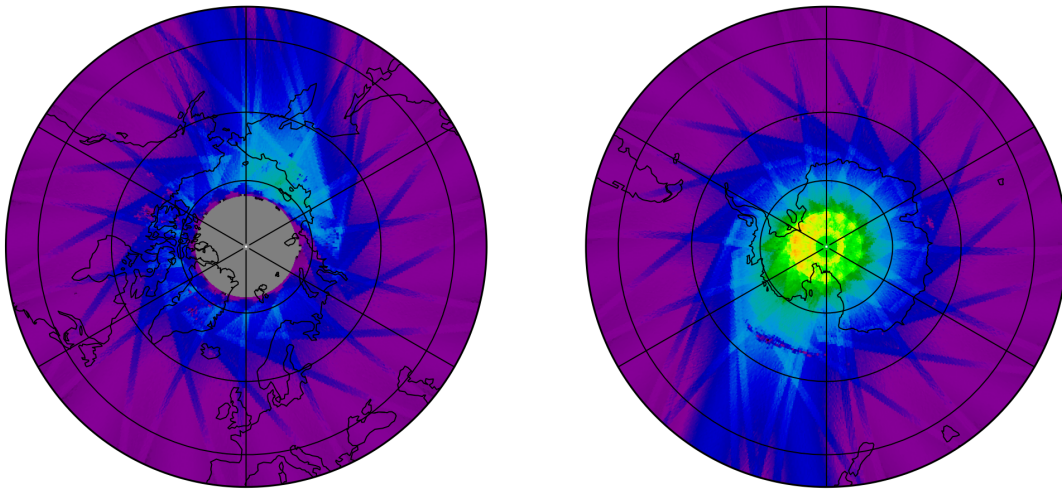
Figure 10: Map of the number of observations for 2023-10-17 to 2023-10-19
