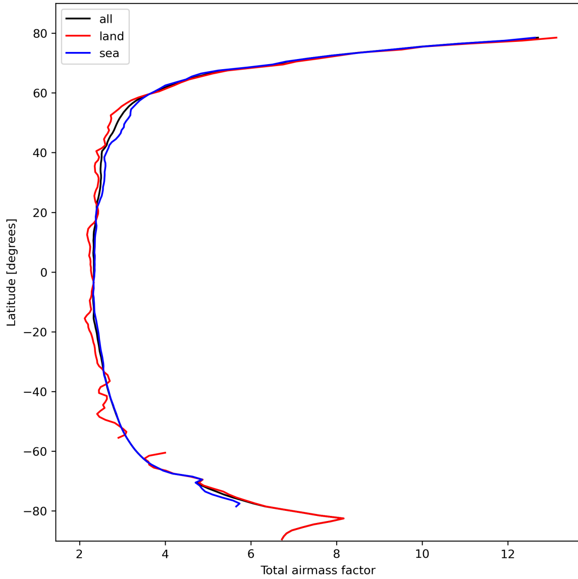
Figure 15: Zonal average of “Total airmass factor” for 2023-10-17 to 2023-10-19.
