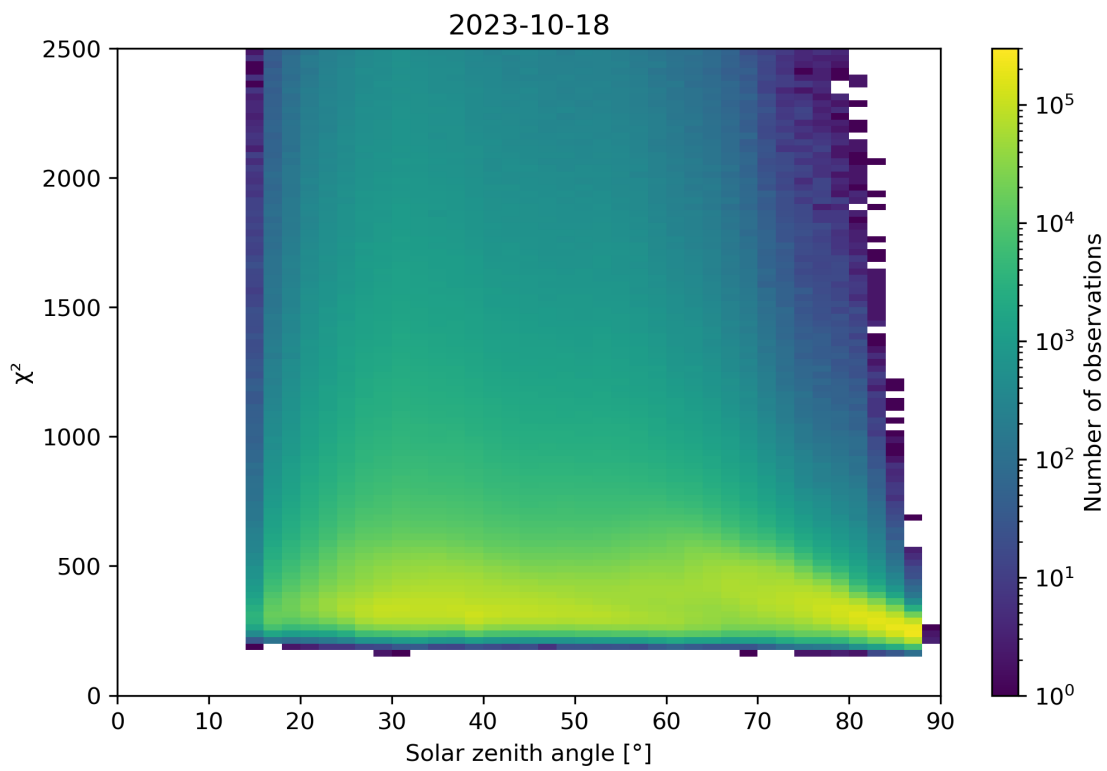
Figure 148: Scatter density plot of “Solar zenith angle” against “ \chi^2 ” for 2023-10-17 to 2023-10-19.
