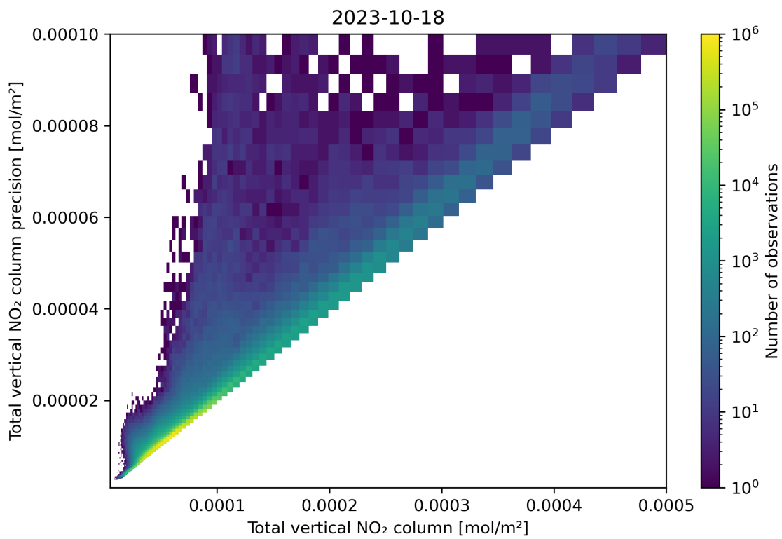
Figure 114: Scatter density plot of “Total vertical NO 2 column” against “Total vertical NO 2 column precision” for 2023-10-17 to 2023-10-19.
