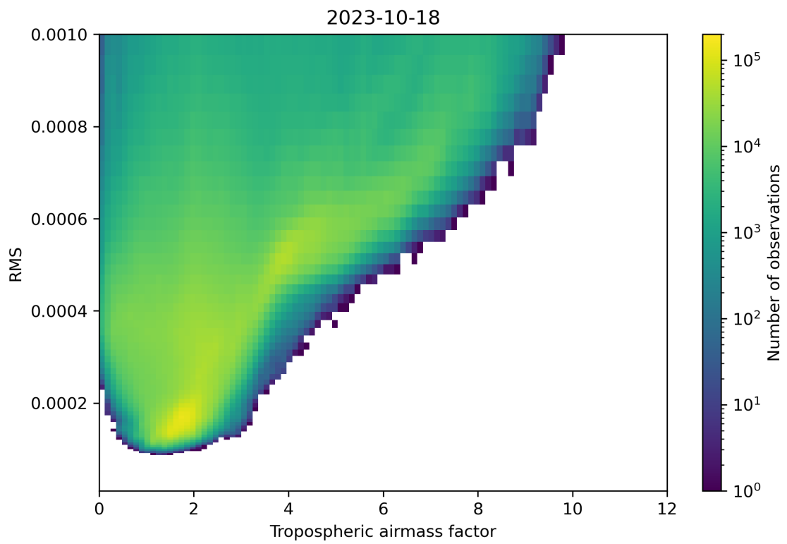
Figure 79: Scatter density plot of “Tropospheric airmass factor” against “RMS” for 2023-10-17 to 2023-10-19.
