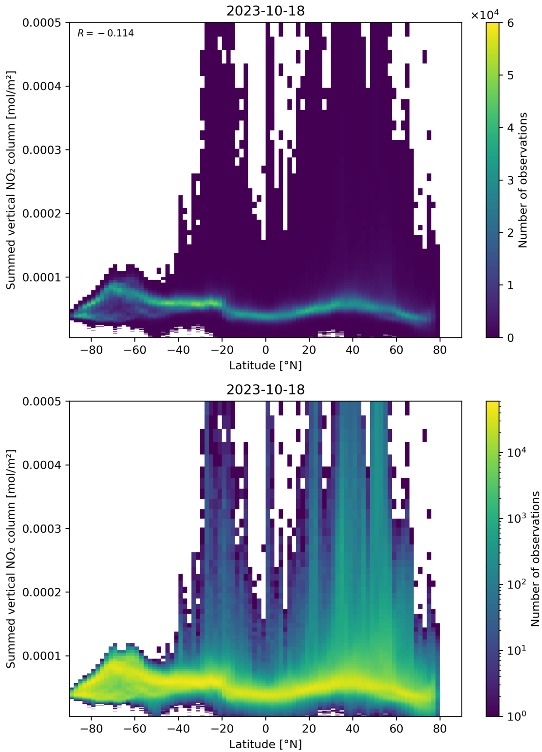
Figure 88: Scatter density plot of “Latitude” against “Summed vertical NO 2 column” for 2023-10-17 to 2023-10-19.
