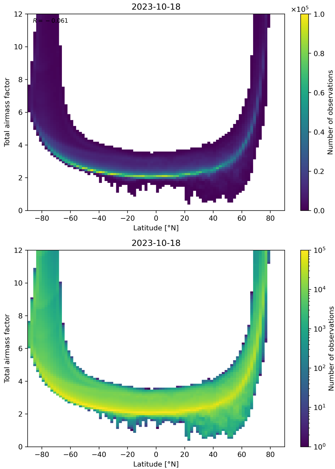
Figure 84: Scatter density plot of “Latitude” against “Total airmass factor” for 2023-10-17 to 2023-10-19.
