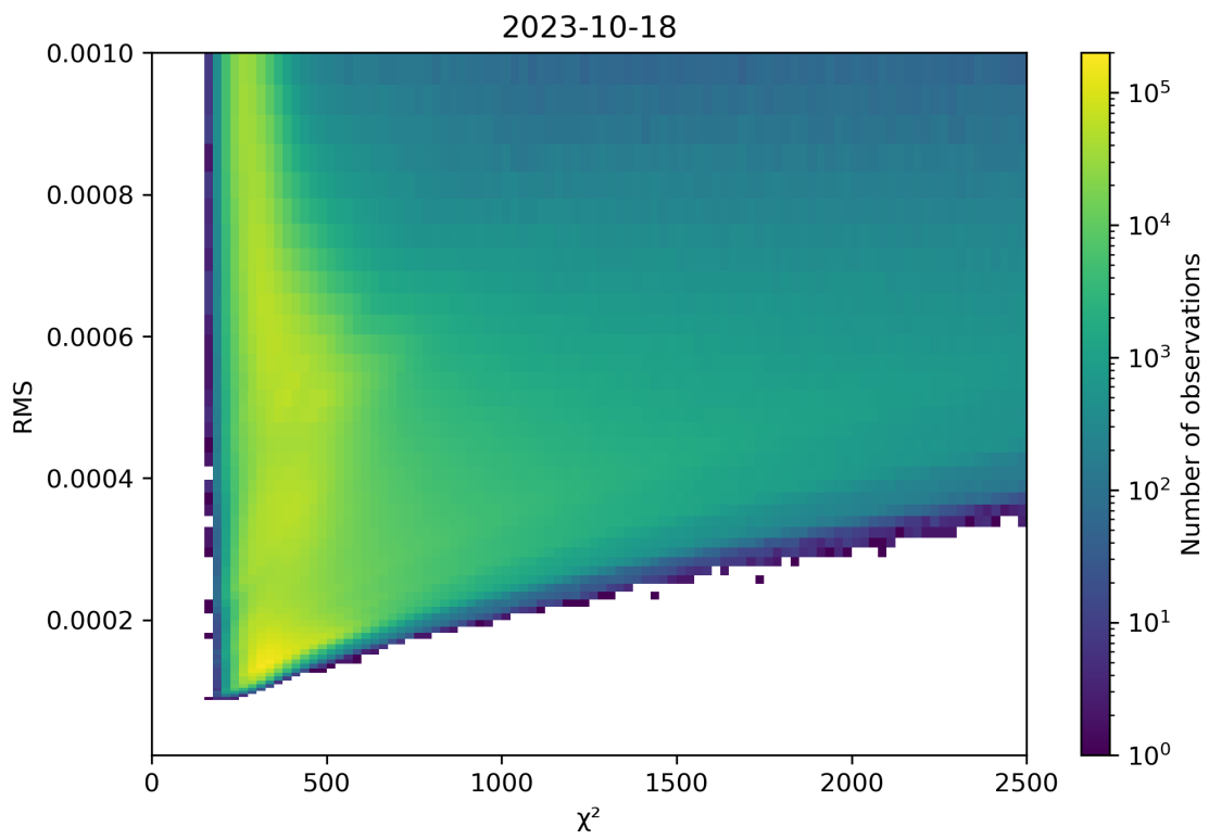
Figure 82: Scatter density plot of " \chi^2 " against "RMS" for 2023-10-17 to 2023-10-19.
