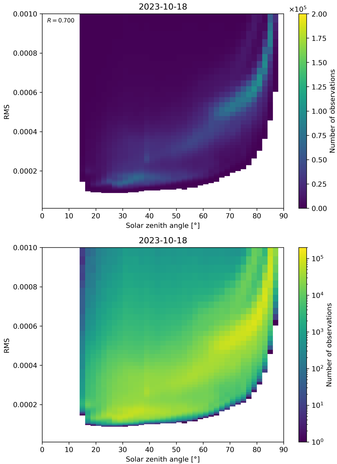
Figure 157: Scatter density plot of “Solar zenith angle” against “RMS” for 2023-10-17 to 2023-10-19.
