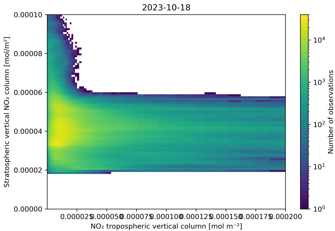
Figure 125: Scatter density plot of “NO 2 tropospheric vertical column” against “Stratospheric vertical NO 2 column” for 2023-10-17 to 2023-10-19.
