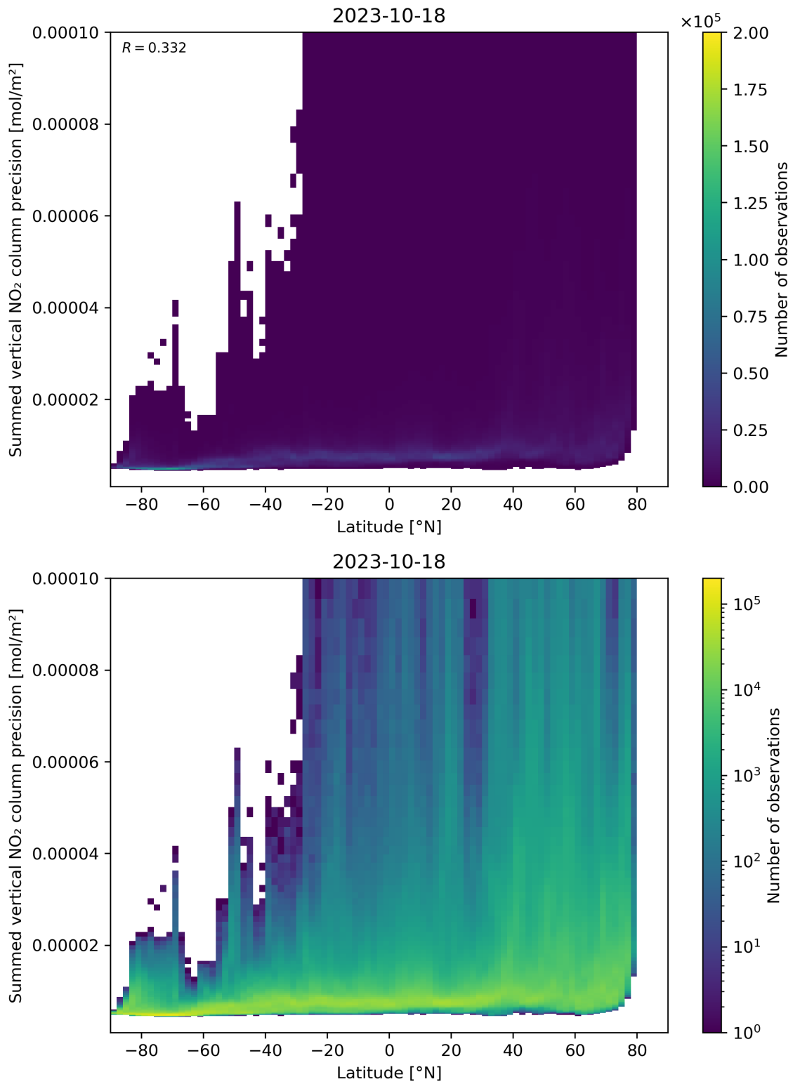
Figure 89: Scatter density plot of “Latitude” against “Summed vertical NO 2 column precision” for 2023-10-17 to 2023-10-19.
