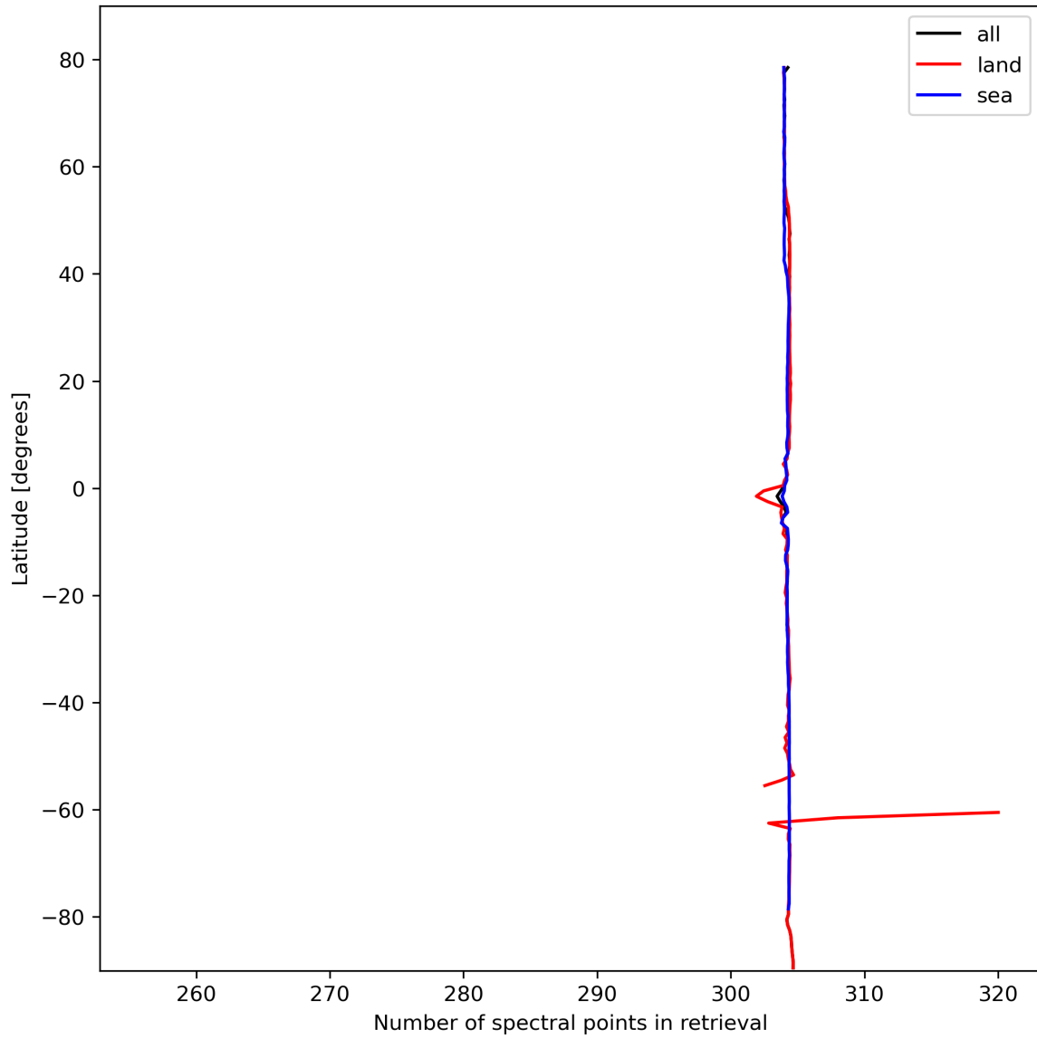
Figure 16: Zonal average of “Number of spectral points in retrieval” for 2023-10-17 to 2023-10-19.
