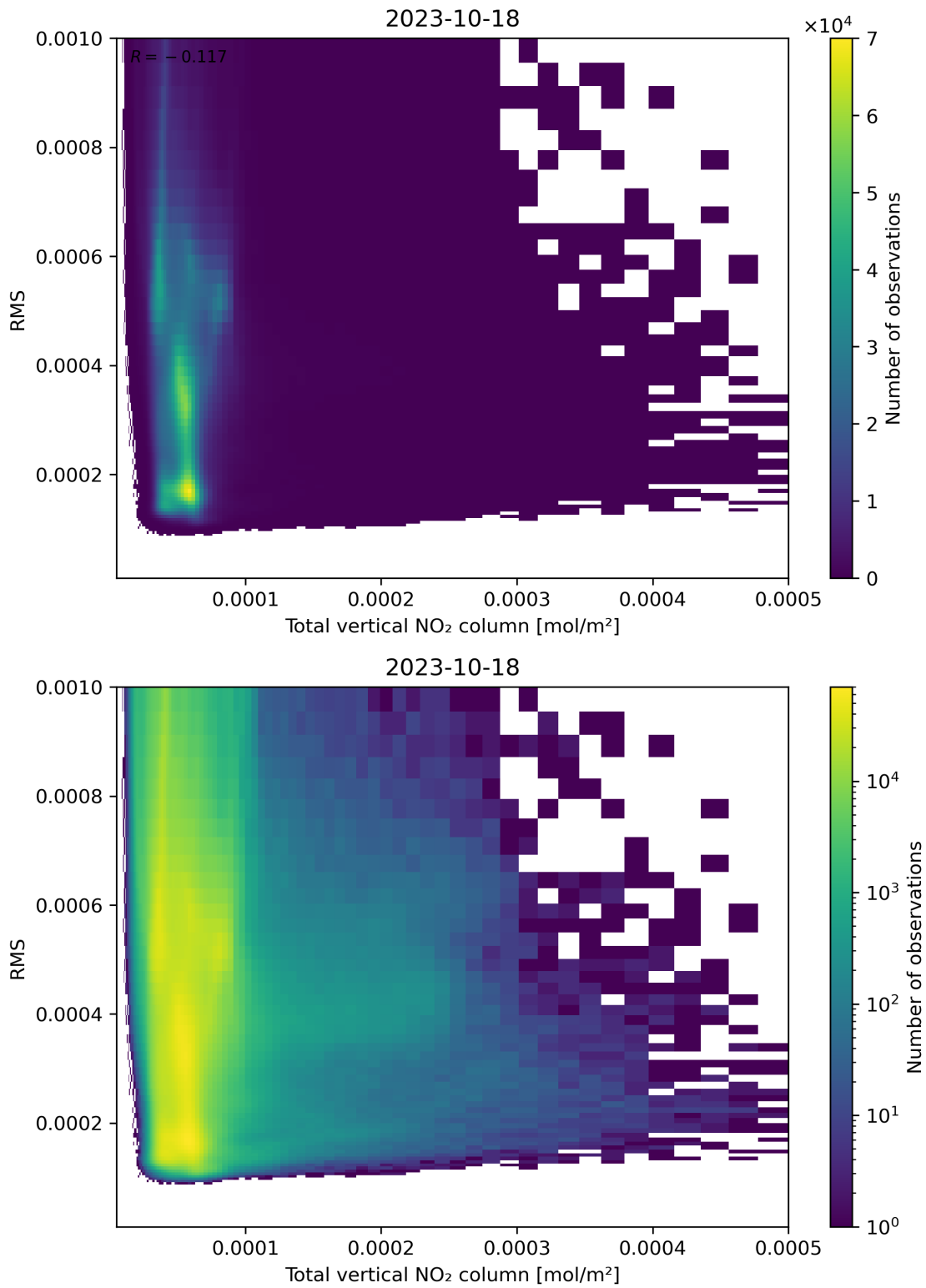
Figure 120: Scatter density plot of “Total vertical NO 2 column” against “RMS” for 2023-10-17 to 2023-10-19.
