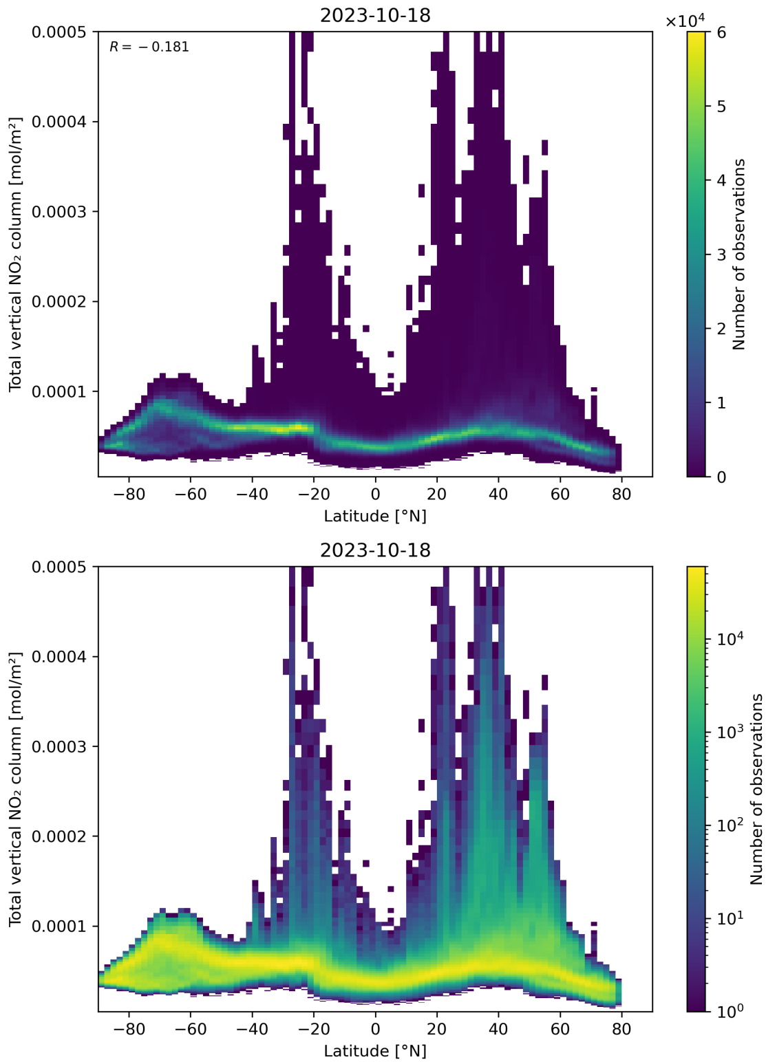
Figure 90: Scatter density plot of “Latitude” against “Total vertical NO 2 column” for 2023-10-17 to 2023-10-19.
