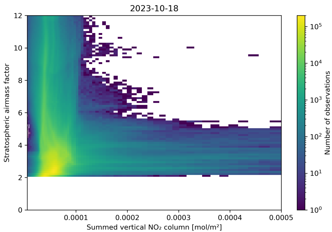
Figure 103: Scatter density plot of “Summed vertical NO 2 column” against “Stratospheric airmass factor” for 2023-10-17 to 2023-10-19.
