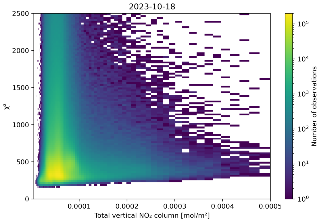
Figure 111: Scatter density plot of “Total vertical NO 2 column” against “ \chi^2 ” for 2023-10-17 to 2023-10-19.
