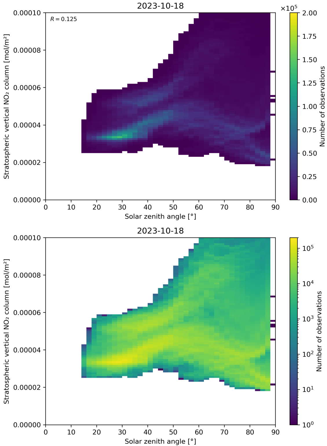
Figure 150: Scatter density plot of “Solar zenith angle” against “Stratospheric vertical NO 2 column” for 2023-10-17 to 2023-10-19.
