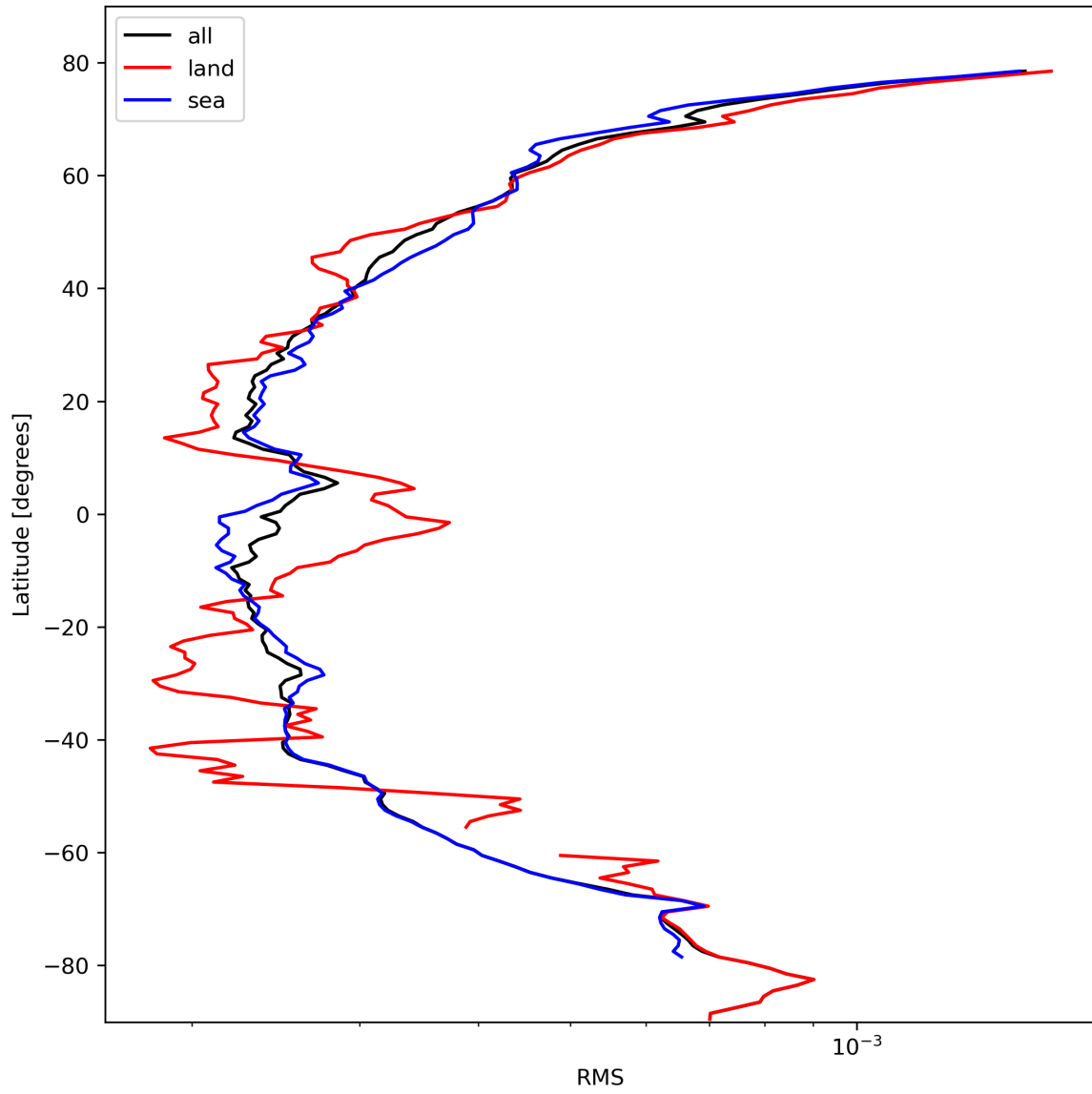
Figure 26: Zonal average of “RMS” for 2023-10-17 to 2023-10-19.
