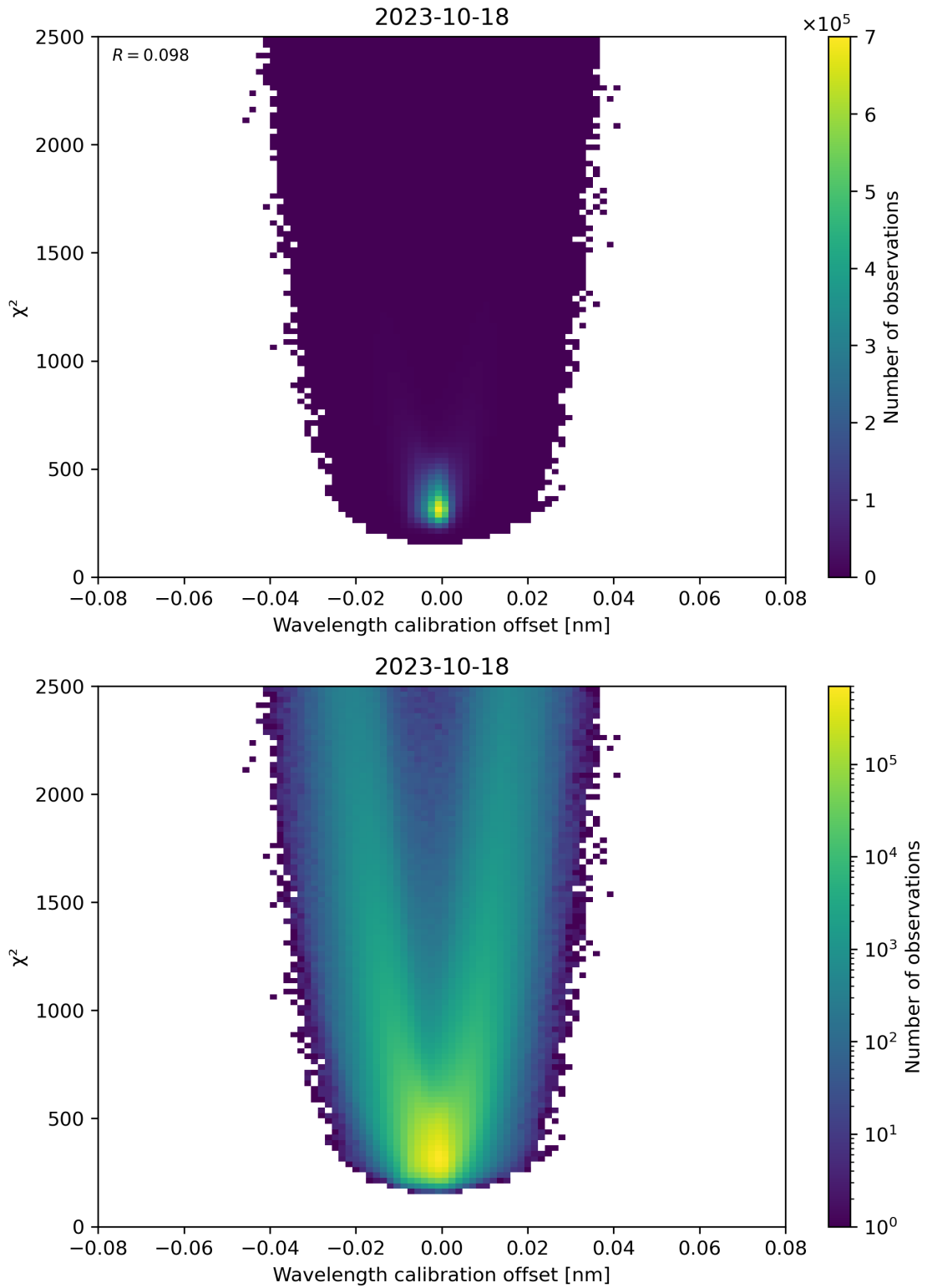
Figure 175: Scatter density plot of “Wavelength calibration offset” against “ \chi^2 ” for 2023-10-17 to 2023-10-19.
