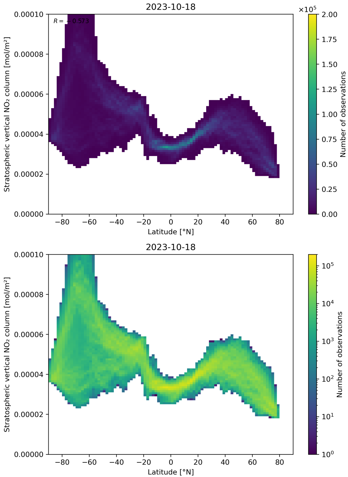
Figure 87: Scatter density plot of “Latitude” against “Stratospheric vertical NO 2 column” for 2023-10-17 to 2023-10-19.
