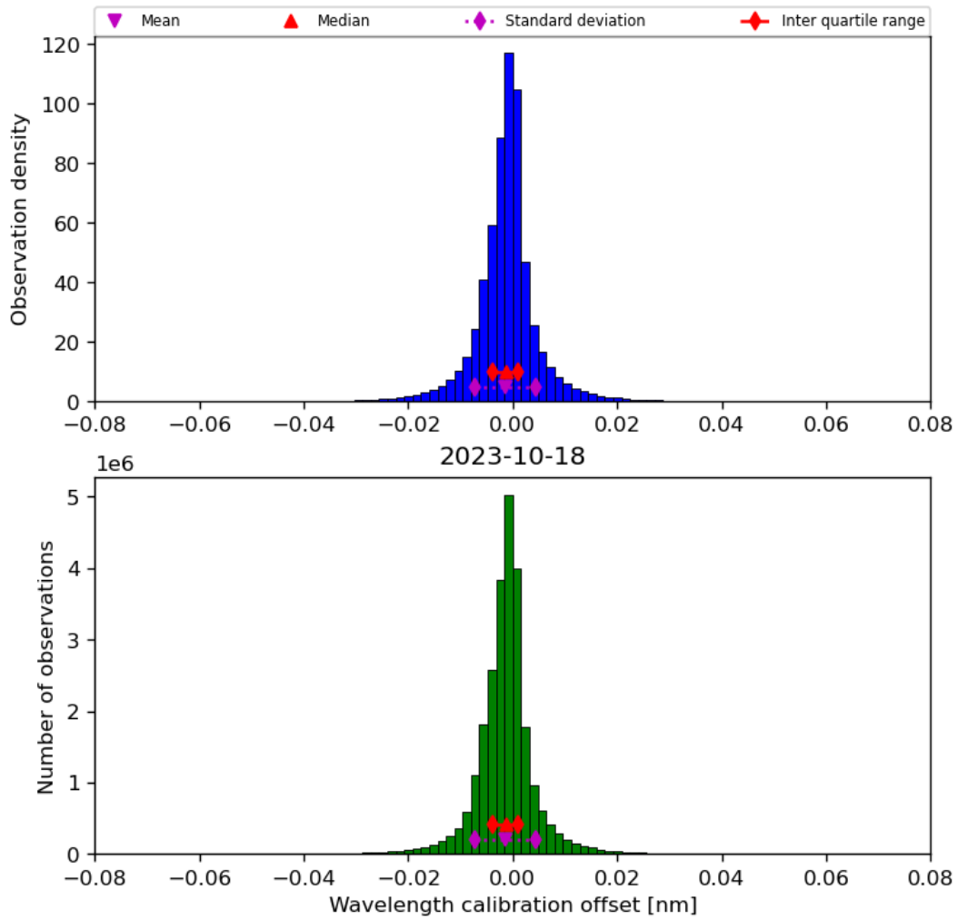
Figure 35: Histogram of “Wavelength calibration offset” for 2023-10-17 to 2023-10-19
