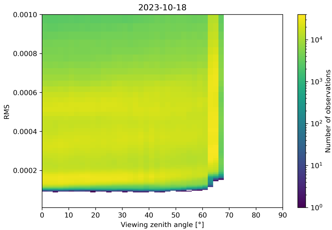
Figure 171: Scatter density plot of “Viewing zenith angle” against “RMS” for 2023-10-17 to 2023-10-19.
