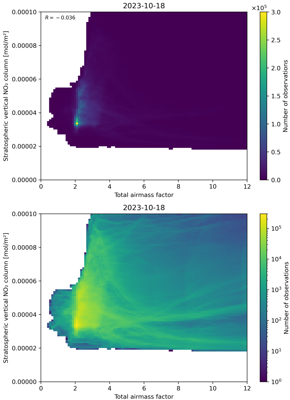
Figure 64: Scatter density plot of “Total airmass factor” against “Stratospheric vertical NO 2 column” for 2023-10-17 to 2023-10-19.
