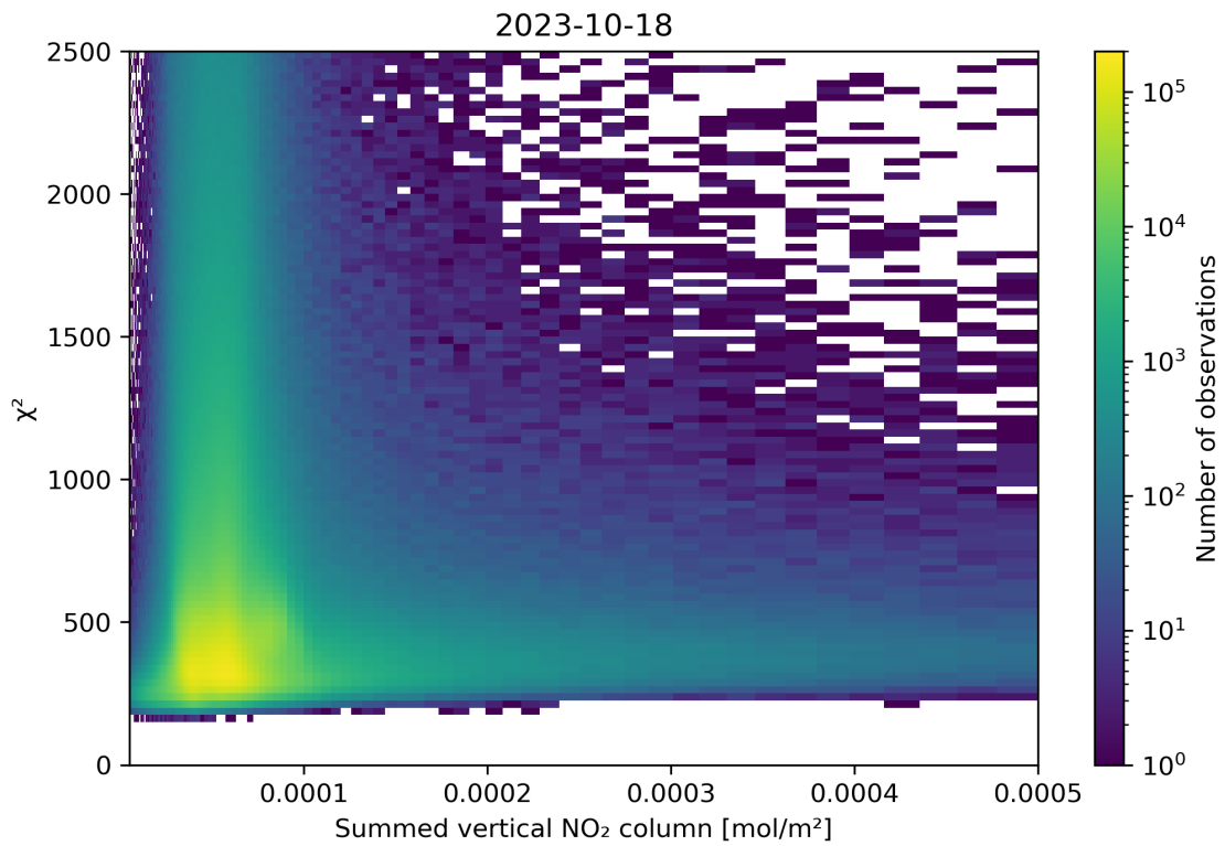
Figure 104: Scatter density plot of “Summed vertical NO 2 column” against “ \chi^2 ” for 2023-10-17 to 2023-10-19.
