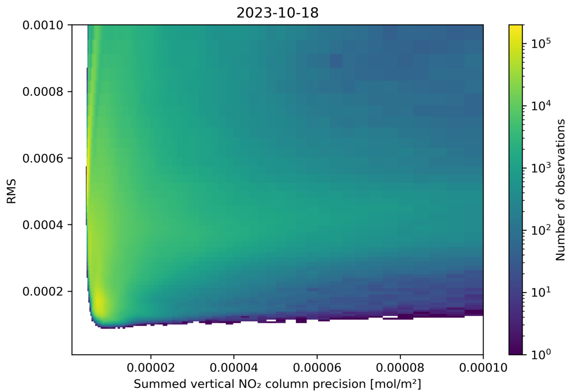
Figure 108: Scatter density plot of “Summed vertical NO 2 column precision” against “RMS” for 2023-10-17 to 2023-10-19.
