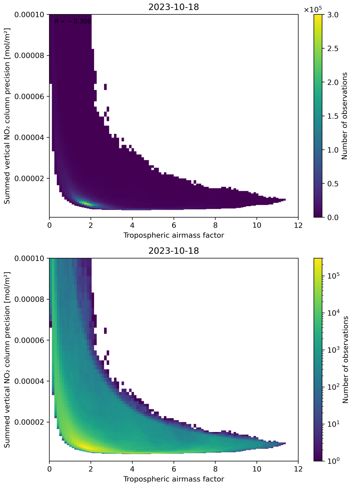
Figure 76: Scatter density plot of “Tropospheric airmass factor” against “Summed vertical NO 2 column precision” for 2023-10-17 to 2023-10-19.
