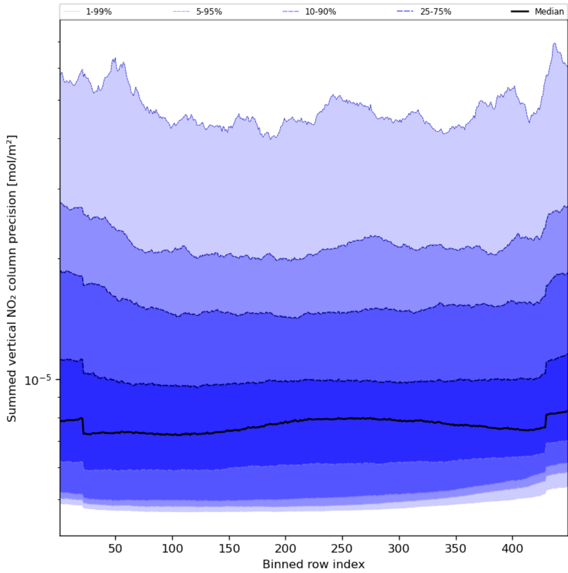
Figure 58: Along track statistics of “Summed vertical NO 2 column precision” for 2023-10-17 to 2023-10-19
