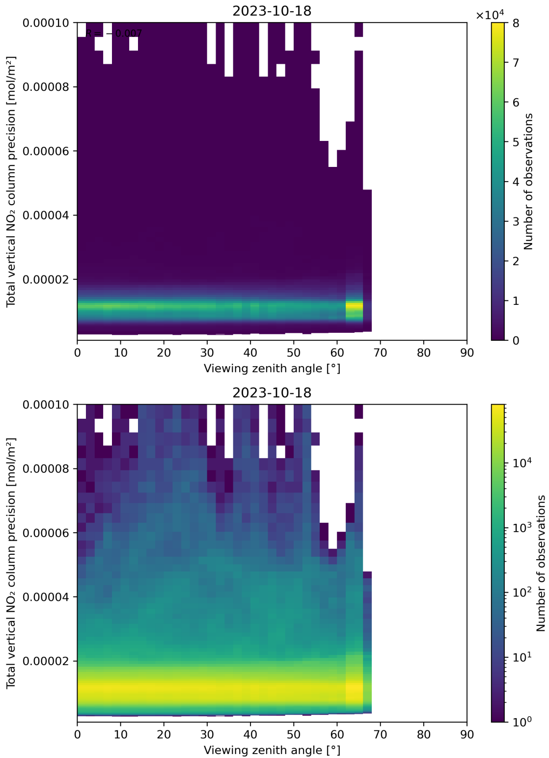
Figure 168: Scatter density plot of “Viewing zenith angle” against “Total vertical NO 2 column precision” for 2023-10-17 to 2023-10-19.
