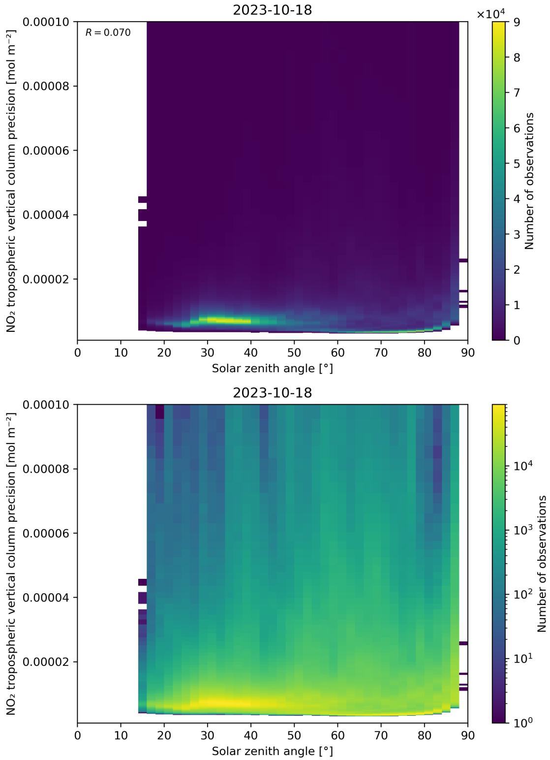
Figure 156: Scatter density plot of “Solar zenith angle” against “NO 2 tropospheric vertical column precision” for 2023-10-17 to 2023-10-19.
