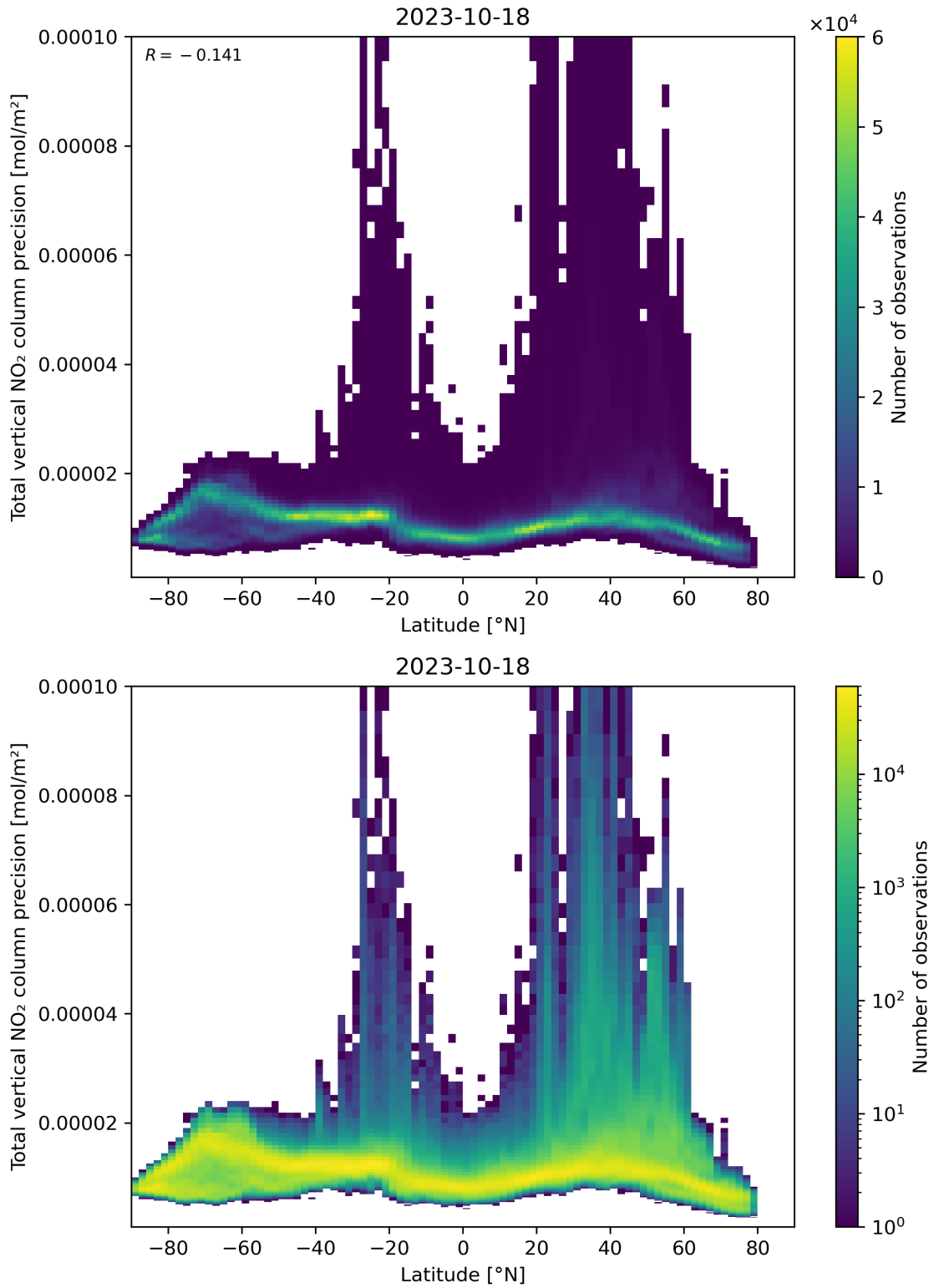
Figure 91: Scatter density plot of “Latitude” against “Total vertical NO 2 column precision” for 2023-10-17 to 2023-10-19.
