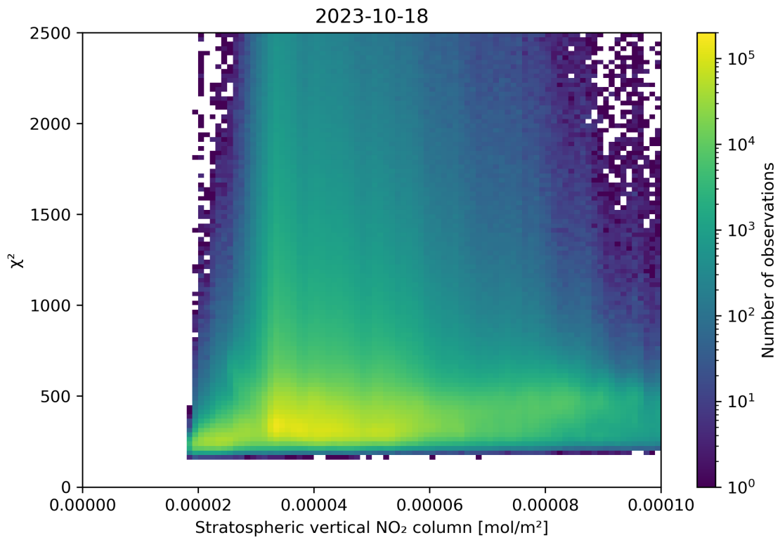
Figure 97: Scatter density plot of “Stratospheric vertical NO 2 column” against “ \chi^2 ” for 2023-10-17 to 2023-10-19.
