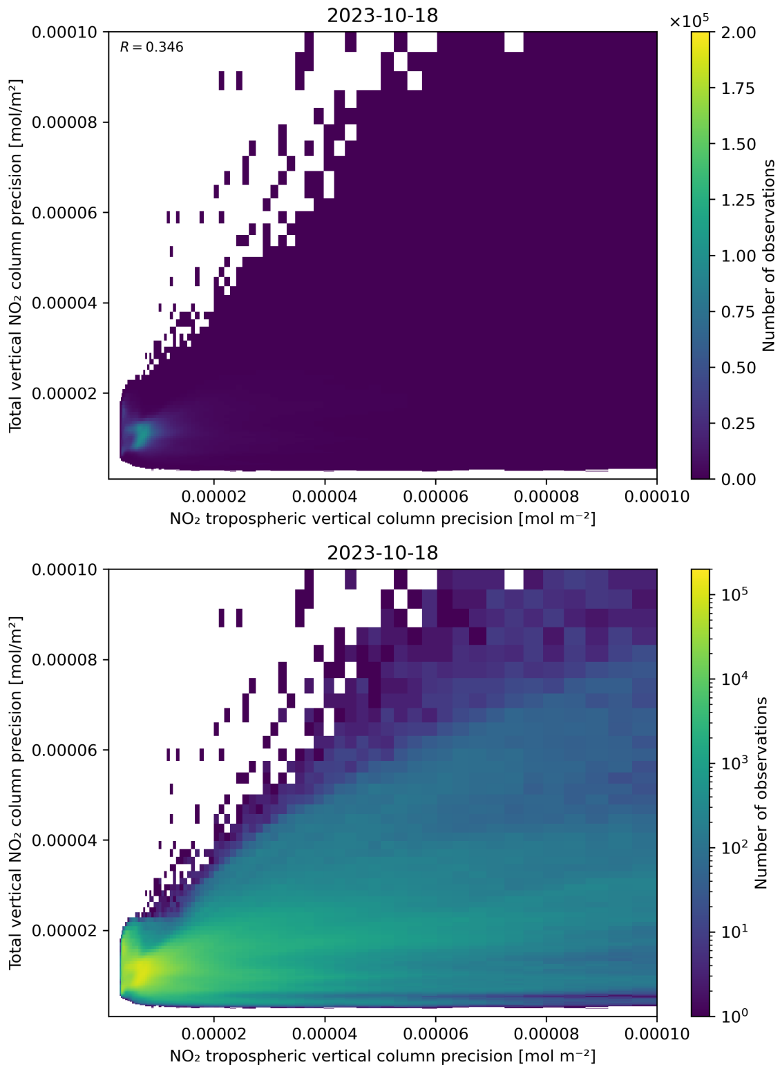
Figure 139: Scatter density plot of “NO 2 tropospheric vertical column precision” against “Total vertical NO 2 column precision” for 2023-10-17 to 2023-10-19.
