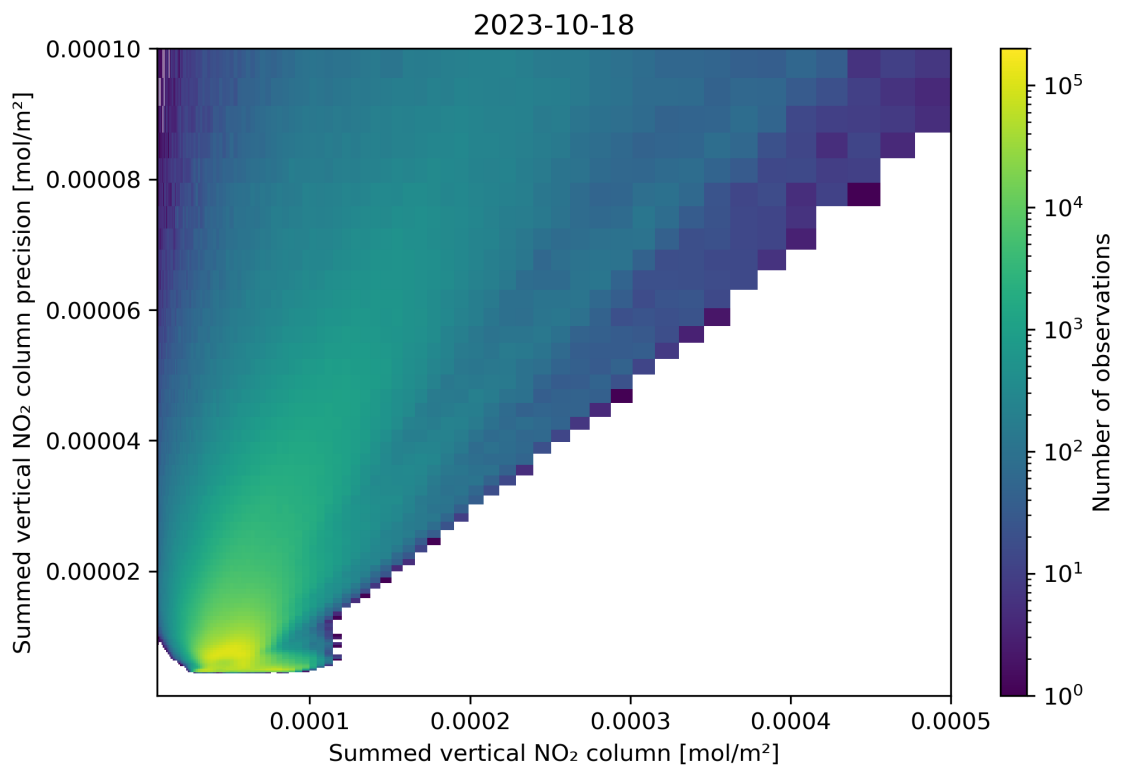
Figure 105: Scatter density plot of “Summed vertical NO 2 column” against “Summed vertical NO 2 column precision” for 2023-10-17 to 2023-10-19.
