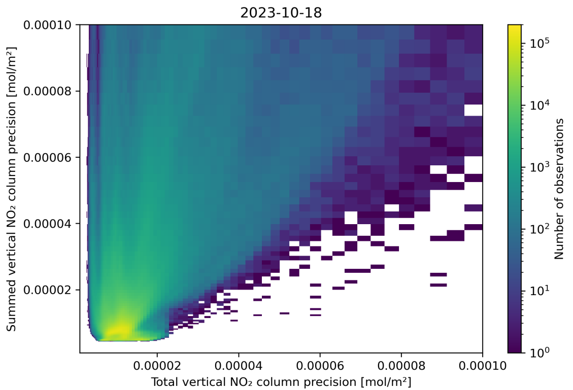
Figure 118: Scatter density plot of “Total vertical NO 2 column precision” against “Summed vertical NO 2 column precision” for 2023-10-17 to 2023-10-19.
