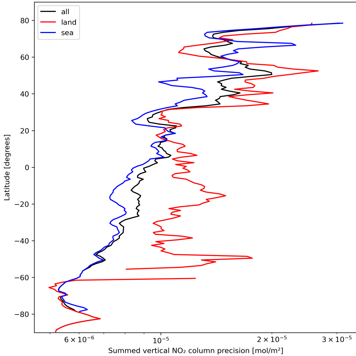
Figure 24: Zonal average of “Summed vertical NO 2 column precision” for 2023-10-17 to 2023-10-19.
