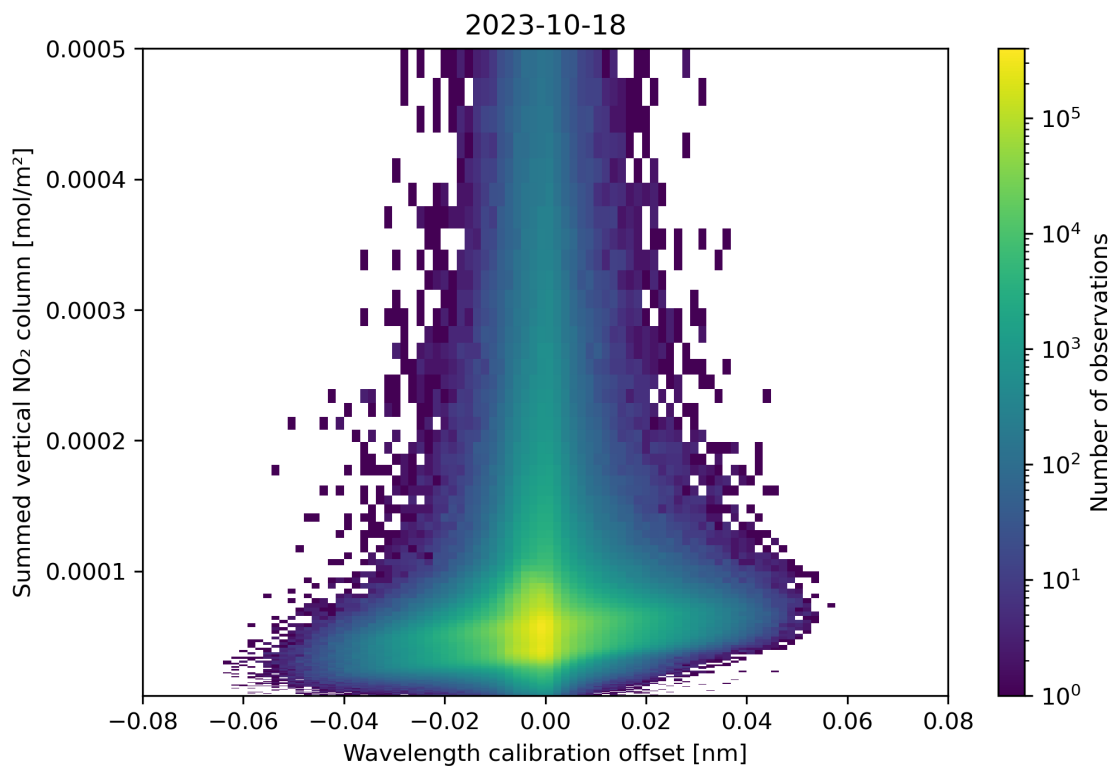
Figure 177: Scatter density plot of “Wavelength calibration offset” against “Summed vertical NO 2 column” for 2023-10-17 to 2023-10-19.
