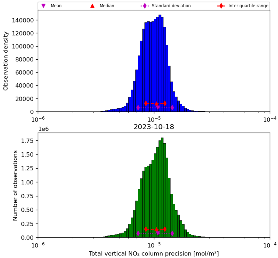
Figure 39: Histogram of “Total vertical NO 2 column precision” for 2023-10-17 to 2023-10-19
