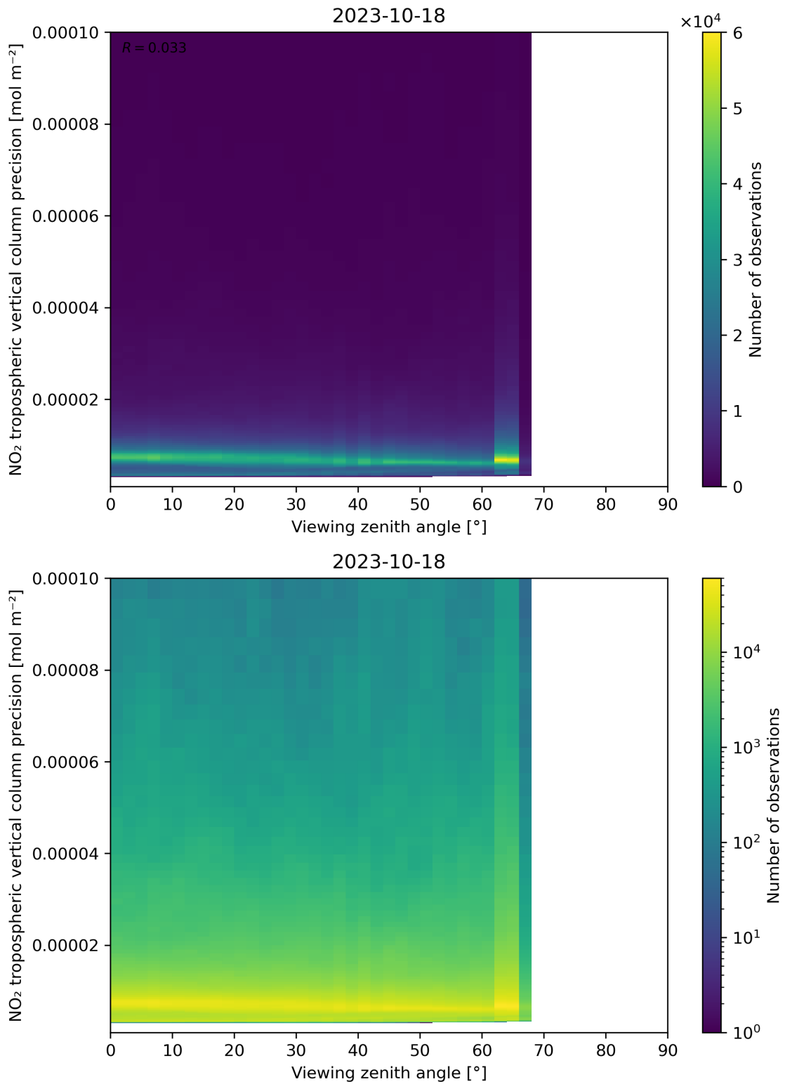
Figure 170: Scatter density plot of “Viewing zenith angle” against “NO 2 tropospheric vertical column precision” for 2023-10-17 to 2023-10-19.
