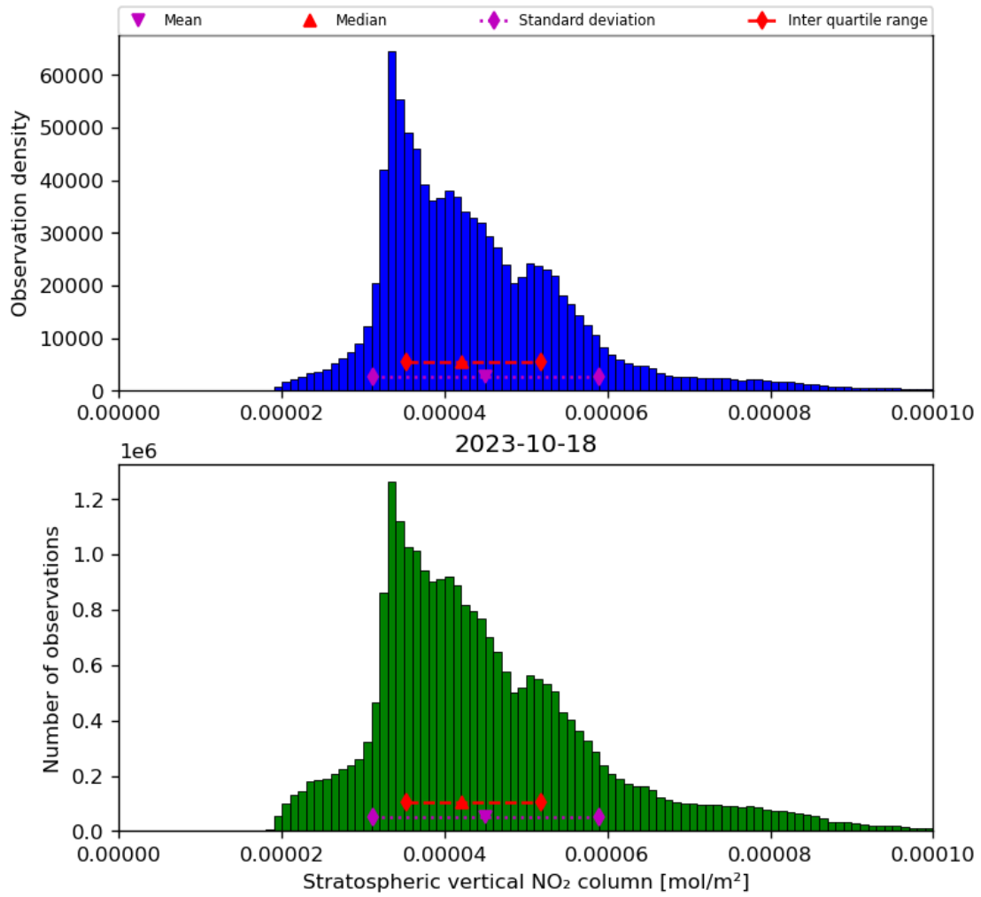
Figure 36: Histogram of “Stratospheric vertical NO 2 column” for 2023-10-17 to 2023-10-19
