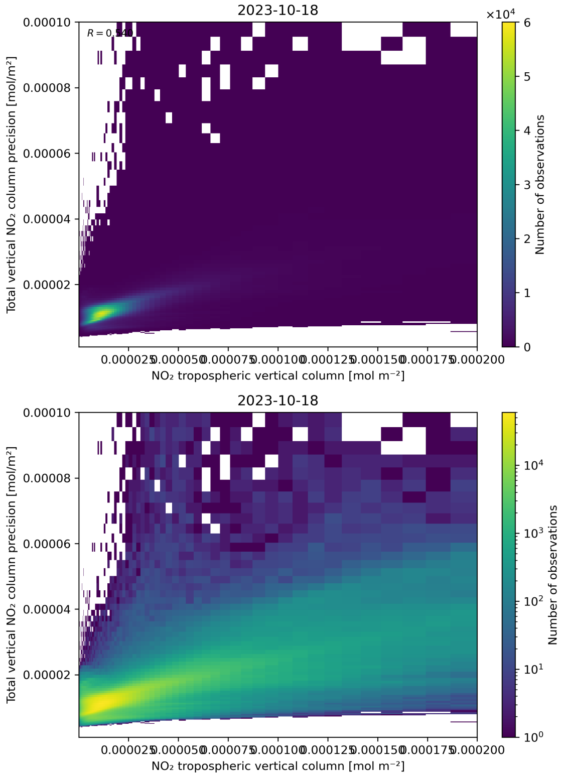
Figure 129: Scatter density plot of “NO 2 tropospheric vertical column” against “Total vertical NO 2 column precision” for 2023-10-17 to 2023-10-19.
