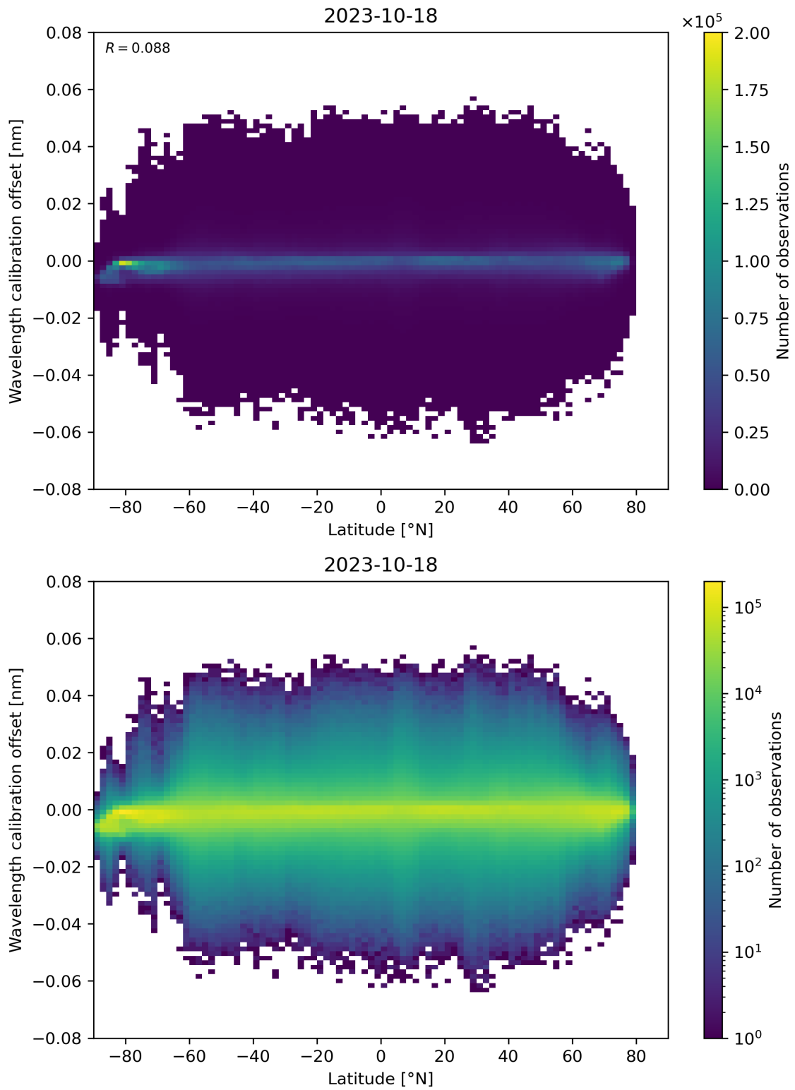
Figure 95: Scatter density plot of “Latitude” against “Wavelength calibration offset” for 2023-10-17 to 2023-10-19.
