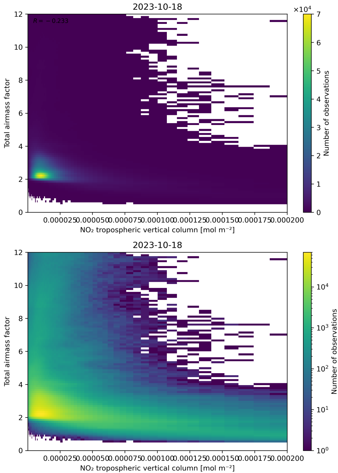
Figure 122: Scatter density plot of “NO 2 tropospheric vertical column” against “Total air mass factor” for 2023-10-17 to 2023-10-19.
