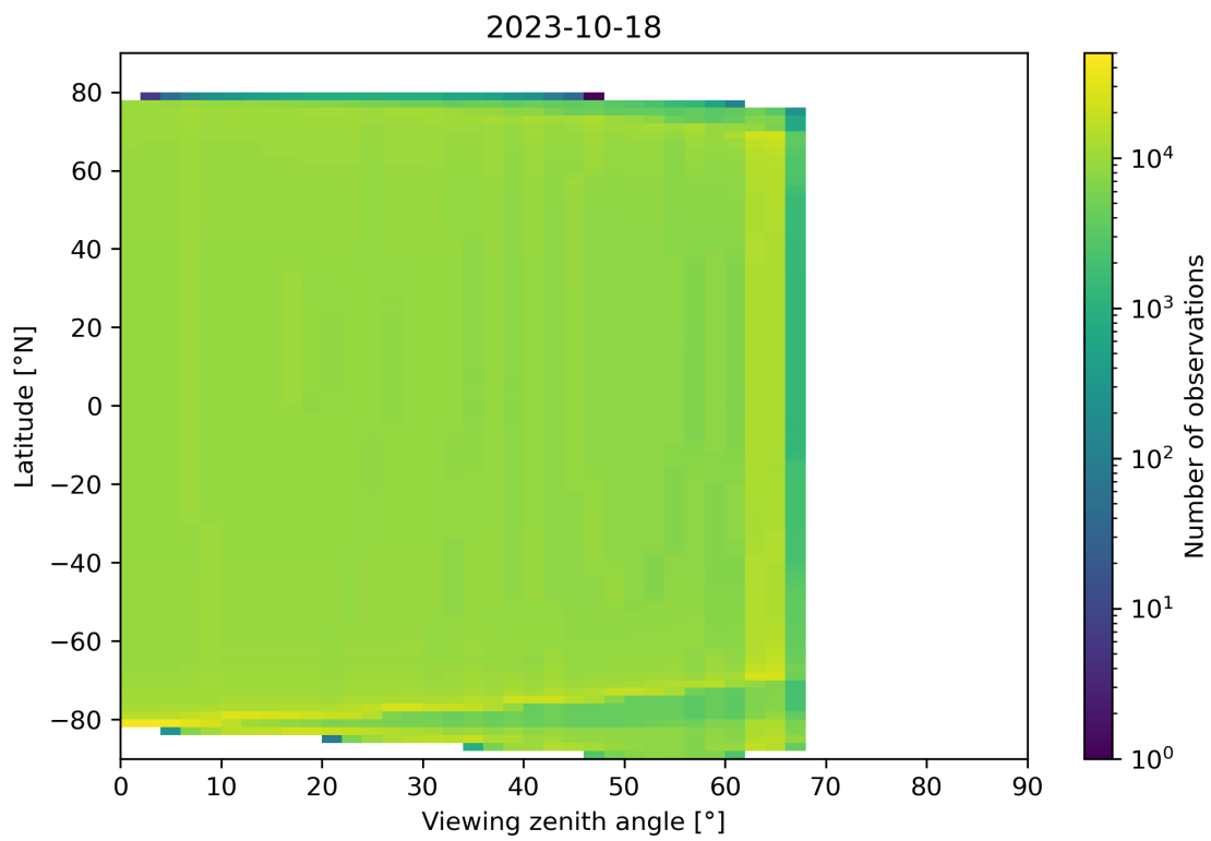
Figure 163: Scatter density plot of “Viewing zenith angle” against “Latitude” for 2023-10-17 to 2023-10-19.
