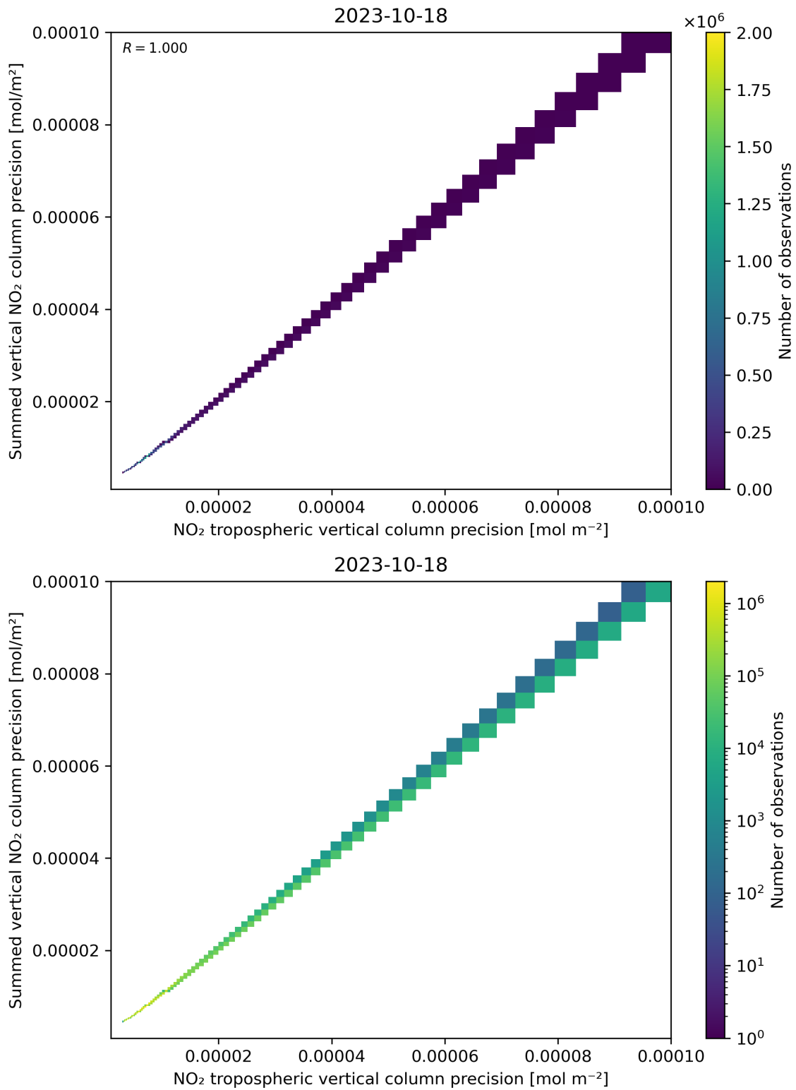
Figure 137: Scatter density plot of “NO 2 tropospheric vertical column precision” against “Summed vertical NO 2 column precision” for 2023-10-17 to 2023-10-19.
