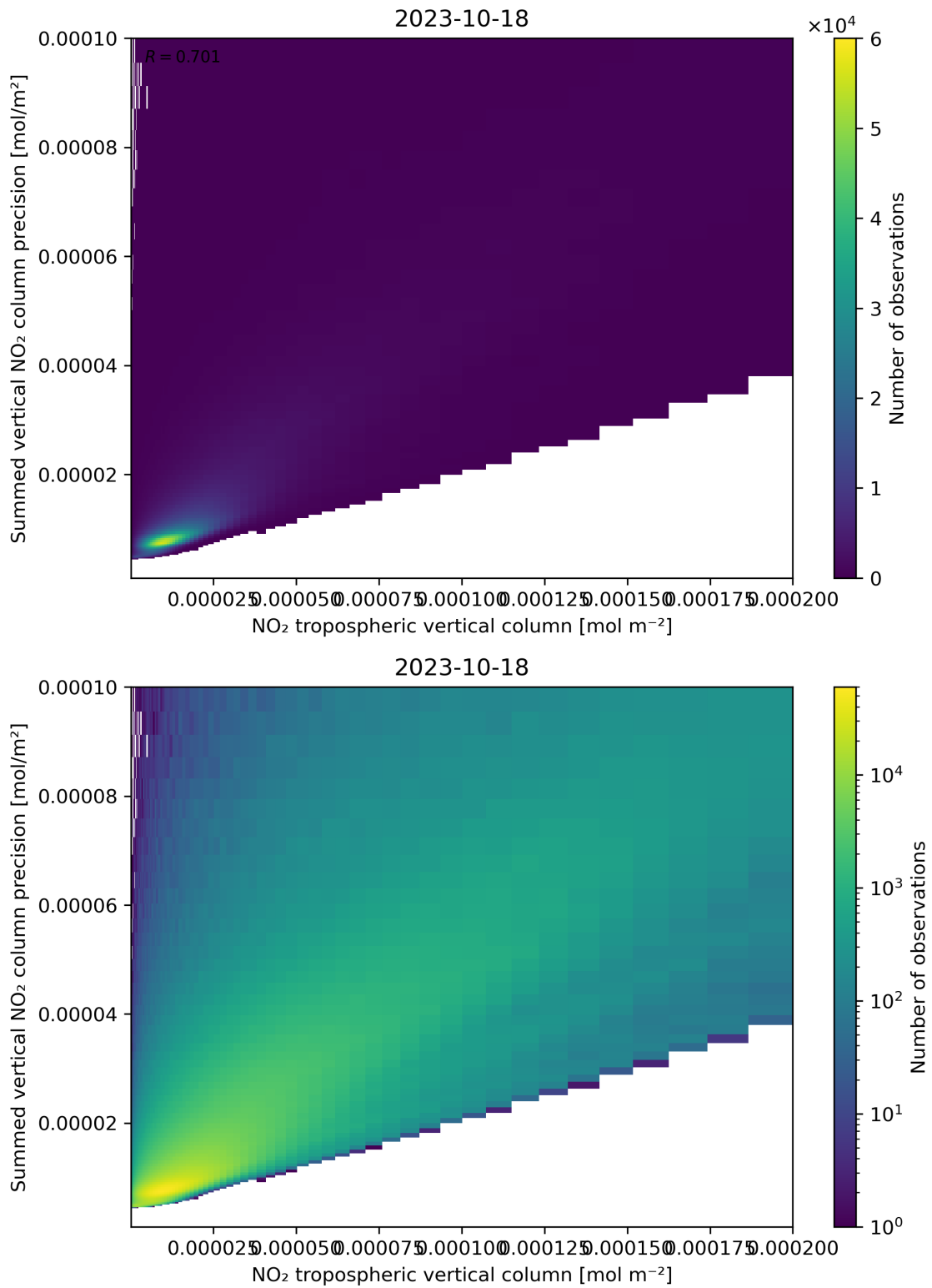
Figure 127: Scatter density plot of “NO 2 tropospheric vertical column” against “Summed vertical NO 2 column precision” for 2023-10-17 to 2023-10-19.
