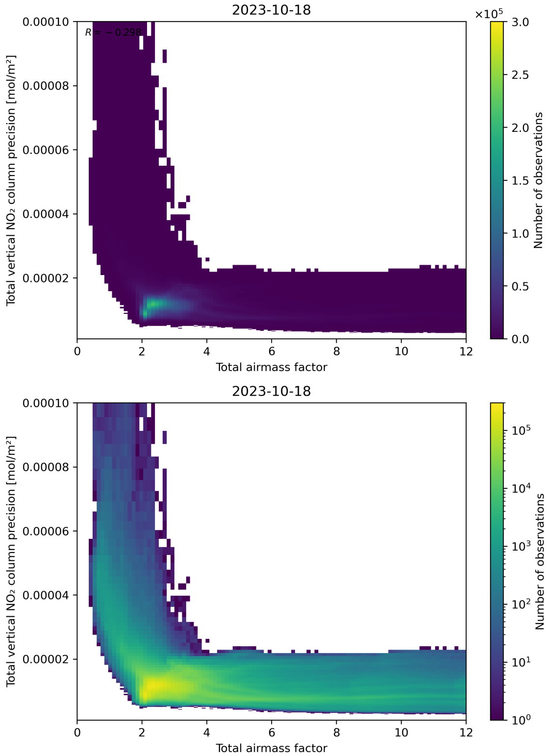
Figure 68: Scatter density plot of “Total airmass factor” against “Total vertical NO 2 column precision” for 2023-10-17 to 2023-10-19.
