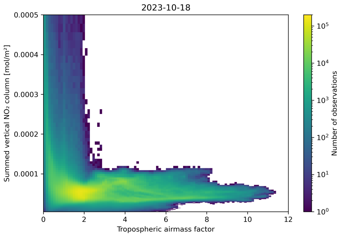
Figure 75: Scatter density plot of “Tropospheric airmass factor” against “Summed vertical NO 2 column” for 2023-10-17 to 2023-10-19.
