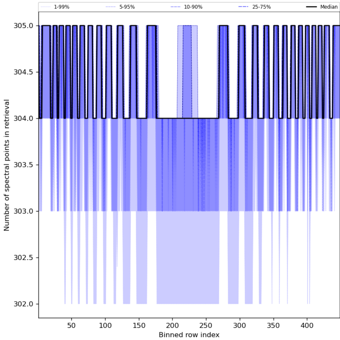
Figure 50: Along track statistics of “Number of spectral points in retrieval” for 2023-10-17 to 2023-10-19
