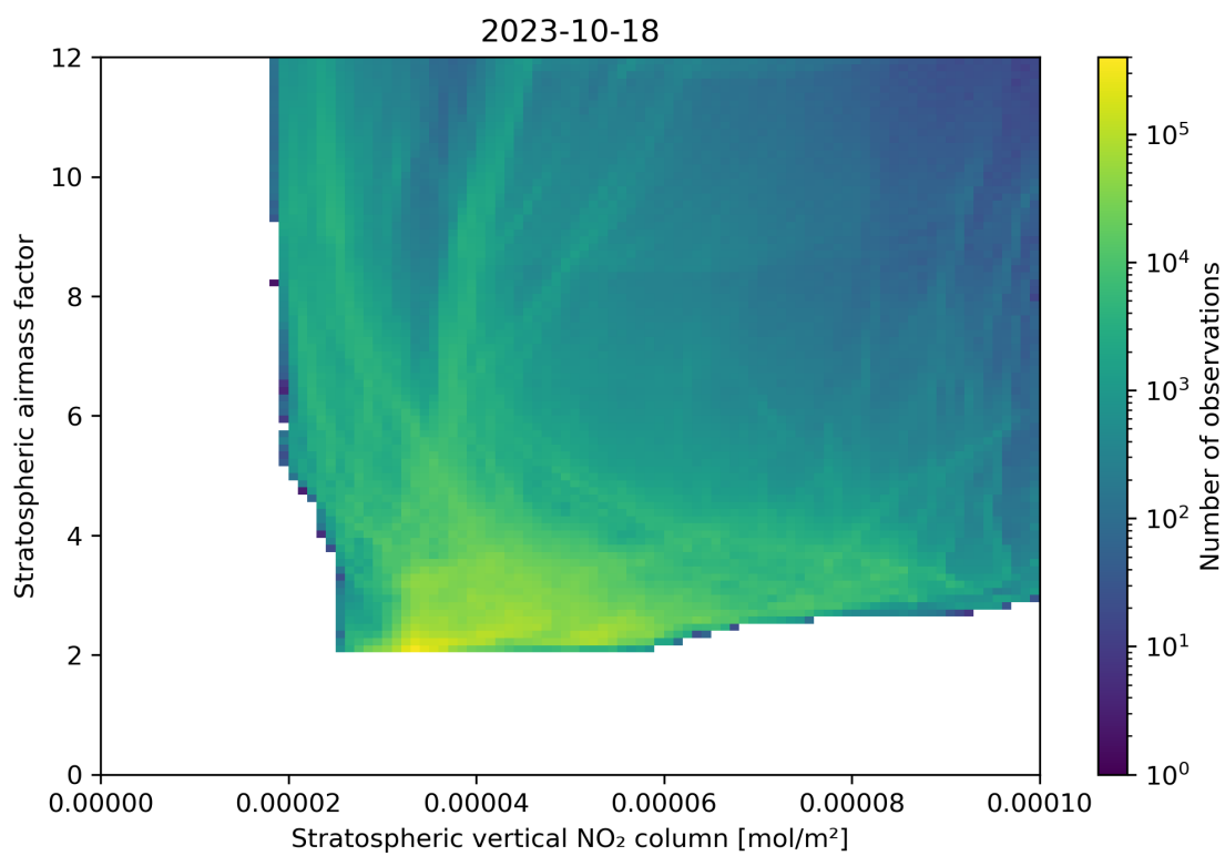
Figure 96: Scatter density plot of “Stratospheric vertical NO 2 column” against “Stratospheric airmass factor” for 2023-10-17 to 2023-10-19.
