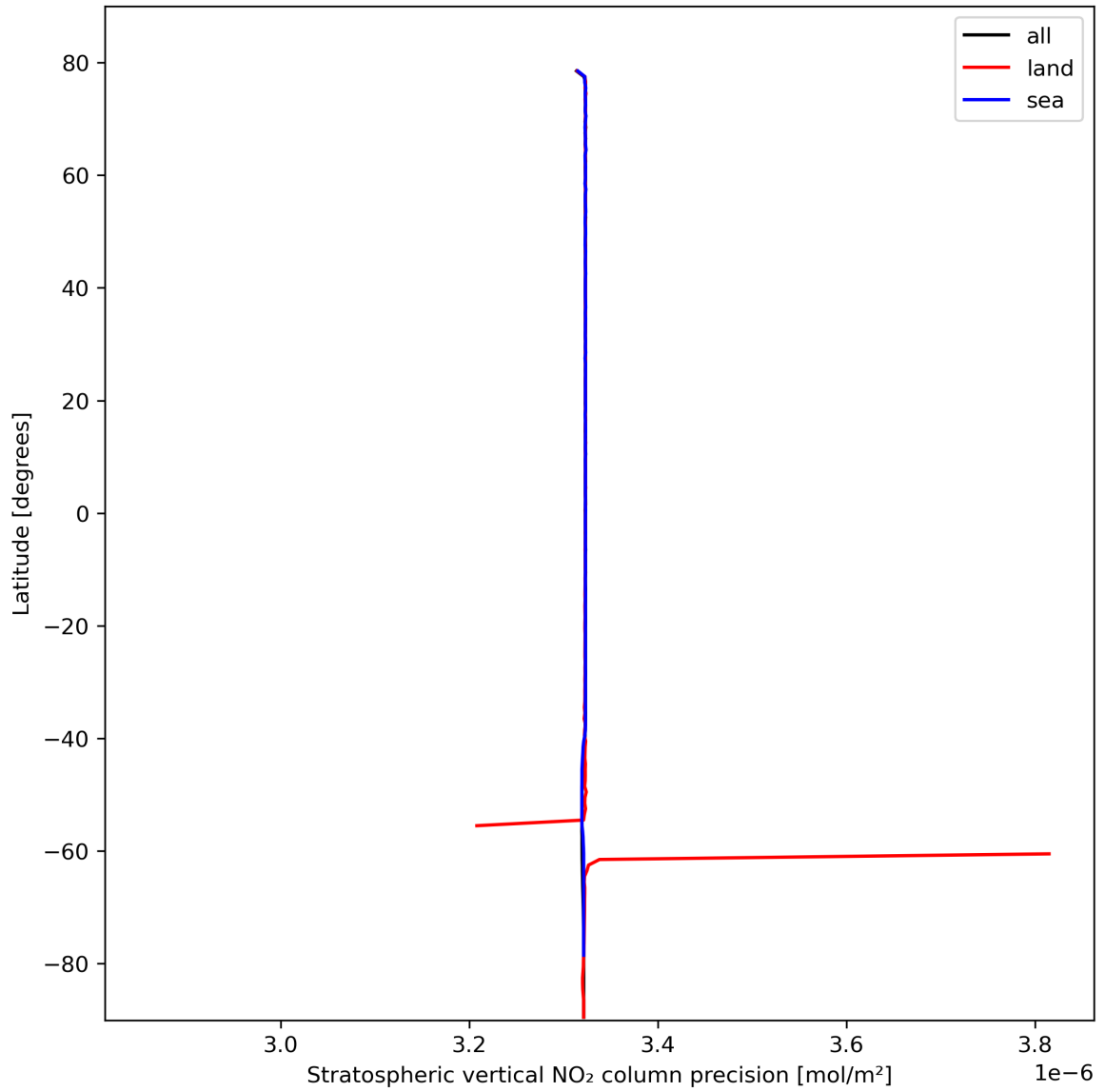
Figure 20: Zonal average of “Stratospheric vertical NO 2 column precision” for 2023-10-17 to 2023-10-19.
