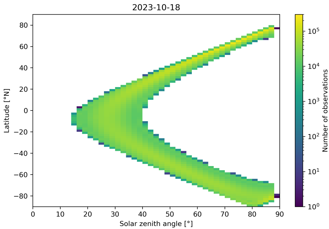
Figure 149: Scatter density plot of “Solar zenith angle” against “Latitude” for 2023-10-17 to 2023-10-19.
