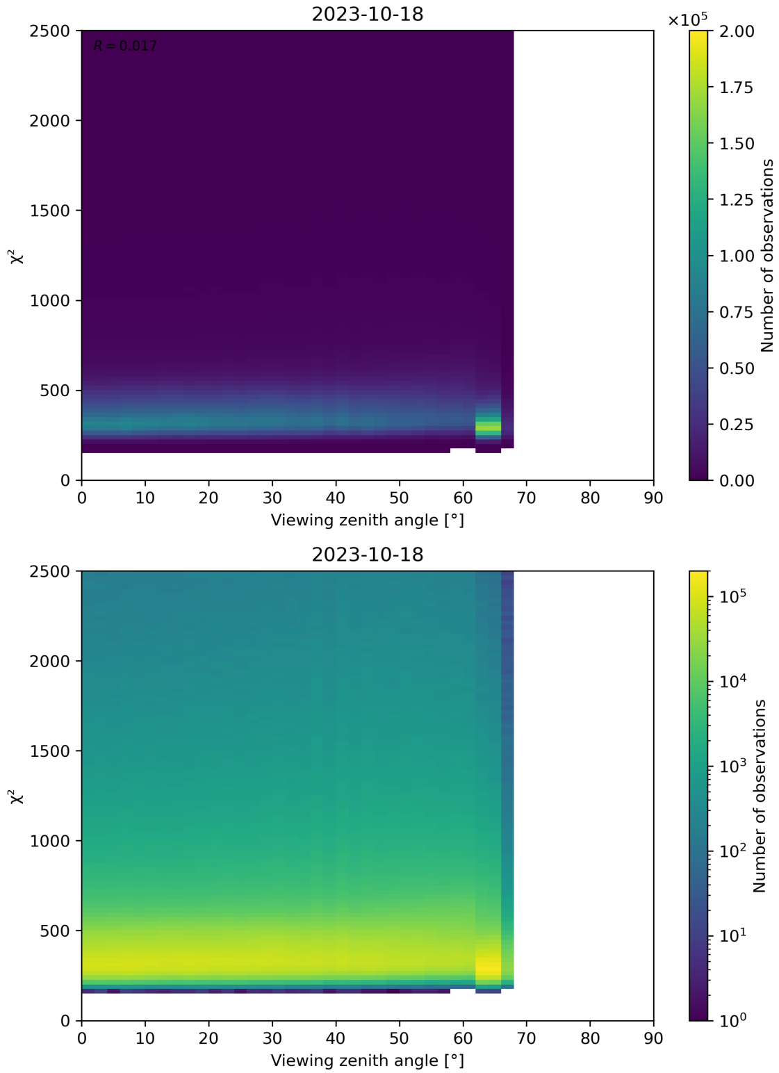
Figure 162: Scatter density plot of “Viewing zenith angle” against “ \chi^2 ” for 2023-10-17 to 2023-10-19.
