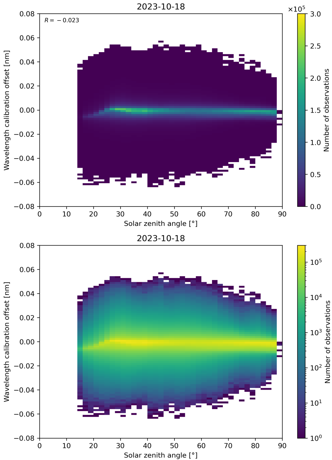
Figure 158: Scatter density plot of “Solar zenith angle” against “Wavelength calibration offset” for 2023-10-17 to 2023-10-19.
