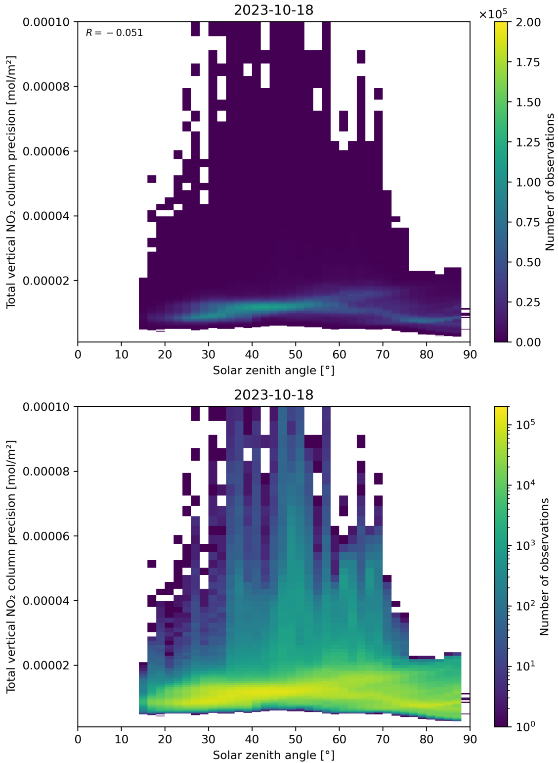
Figure 154: Scatter density plot of “Solar zenith angle” against “Total vertical NO 2 column precision” for 2023-10-17 to 2023-10-19.
