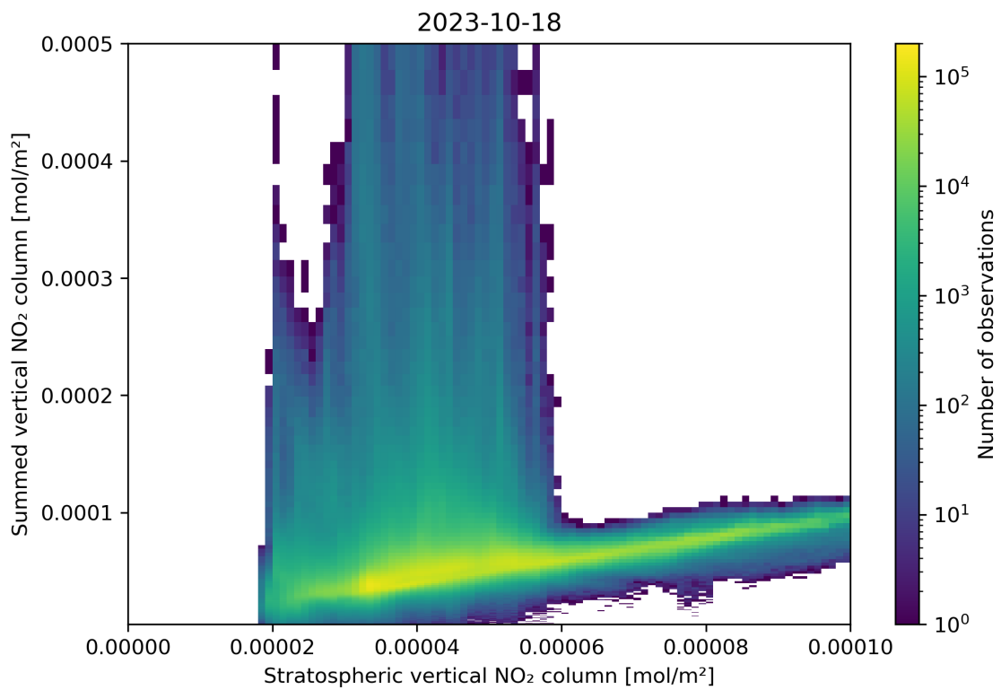
Figure 98: Scatter density plot of “Stratospheric vertical NO 2 column” against “Summed vertical NO 2 column” for 2023-10-17 to 2023-10-19.
