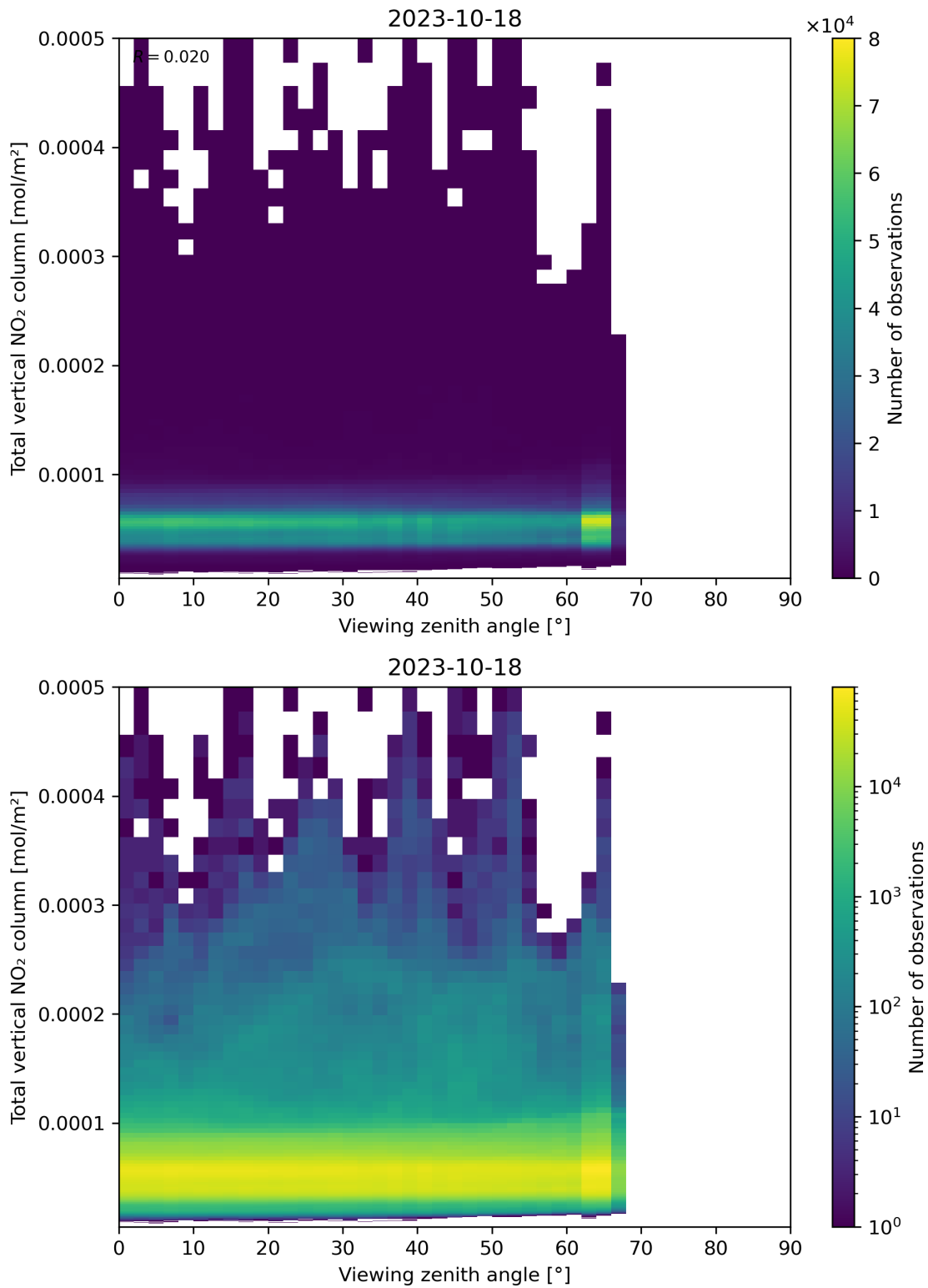
Figure 167: Scatter density plot of “Viewing zenith angle” against “Total vertical NO 2 column” for 2023-10-17 to 2023-10-19.
