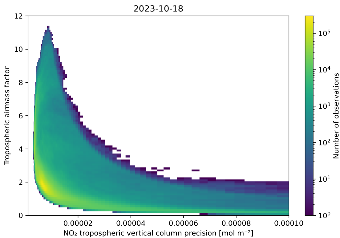
Figure 133: Scatter density plot of “NO 2 tropospheric vertical column precision” against “Tropospheric airmass factor” for 2023-10-17 to 2023-10-19.
