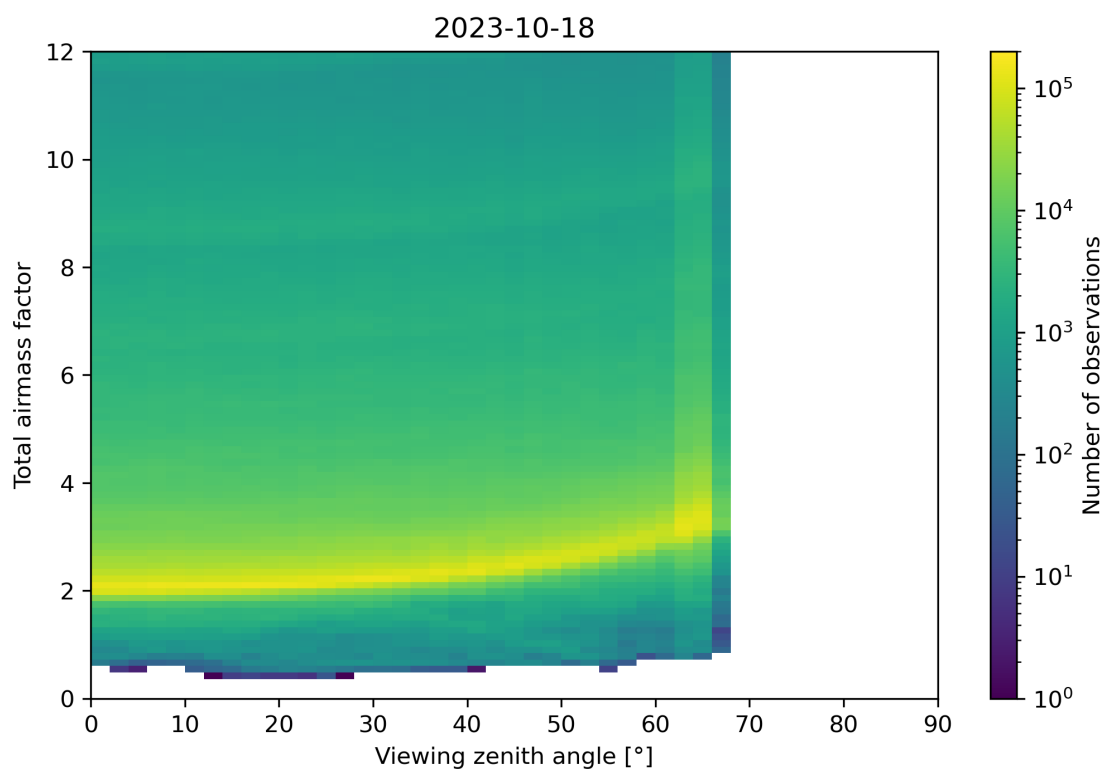
Figure 160: Scatter density plot of “Viewing zenith angle” against “Total airmass factor” for 2023-10-17 to 2023-10-19.
