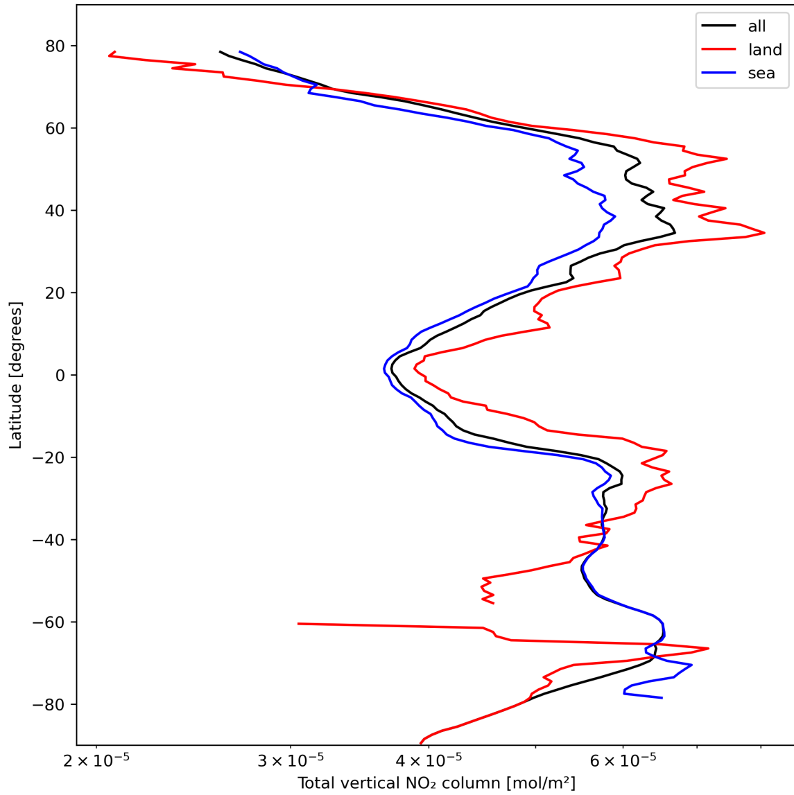
Figure 21: Zonal average of “Total vertical NO 2 column” for 2023-10-17 to 2023-10-19.
