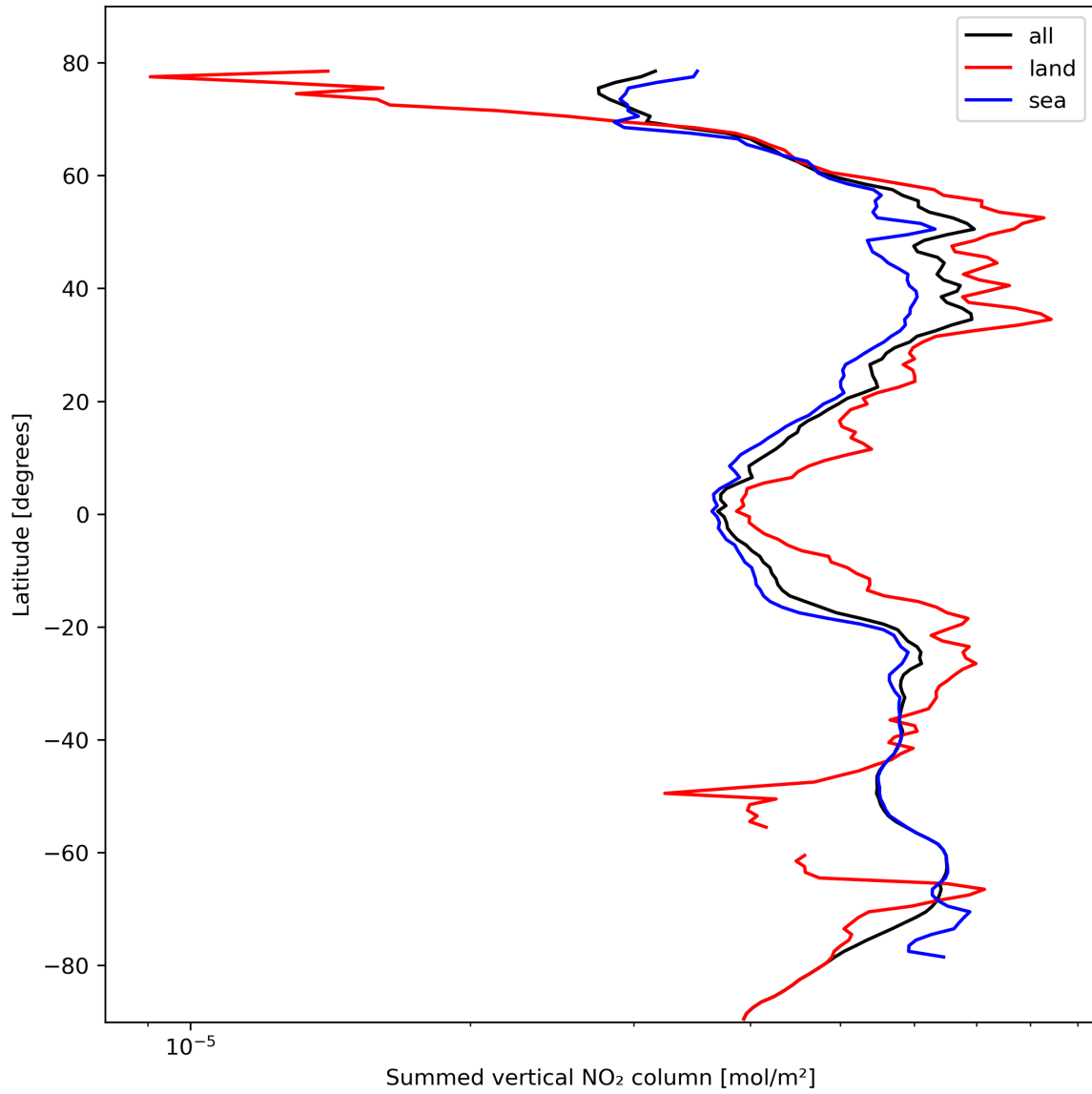
Figure 23: Zonal average of “Summed vertical NO 2 column” for 2023-10-17 to 2023-10-19.
