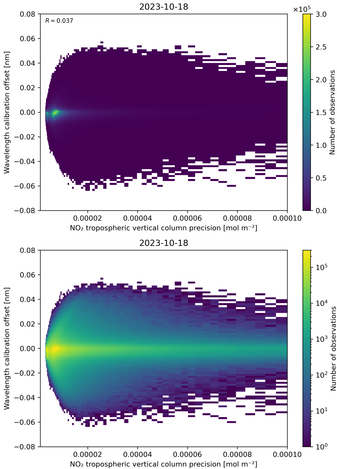
Figure 141: Scatter density plot of “NO 2 tropospheric vertical column precision” against “Wavelength calibration offset” for 2023-10-17 to 2023-10-19.
