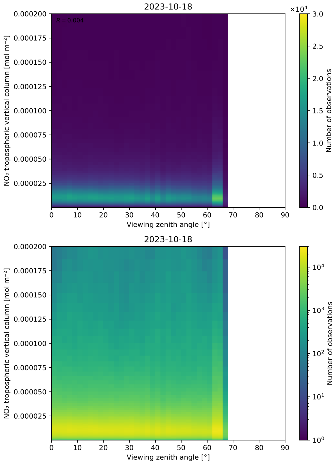
Figure 169: Scatter density plot of “Viewing zenith angle” against “NO 2 tropospheric vertical column” for 2023-10-17 to 2023-10-19.
