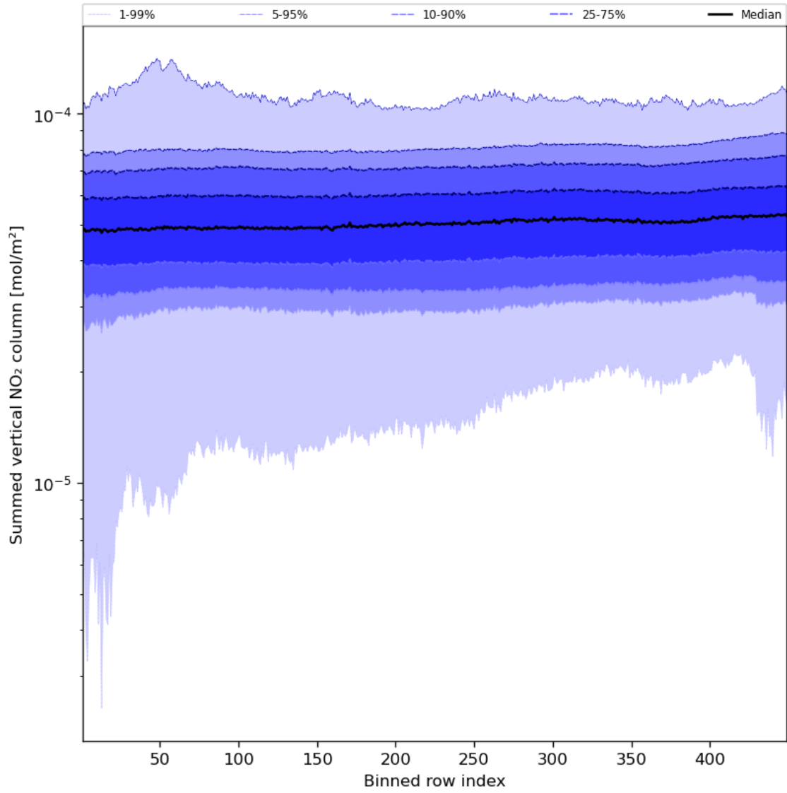
Figure 57: Along track statistics of “Summed vertical NO 2 column” for 2023-10-17 to 2023-10-19
