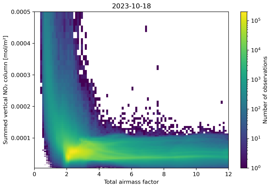
Figure 65: Scatter density plot of “Total airmass factor” against “Summed vertical NO 2 column” for 2023-10-17 to 2023-10-19.
