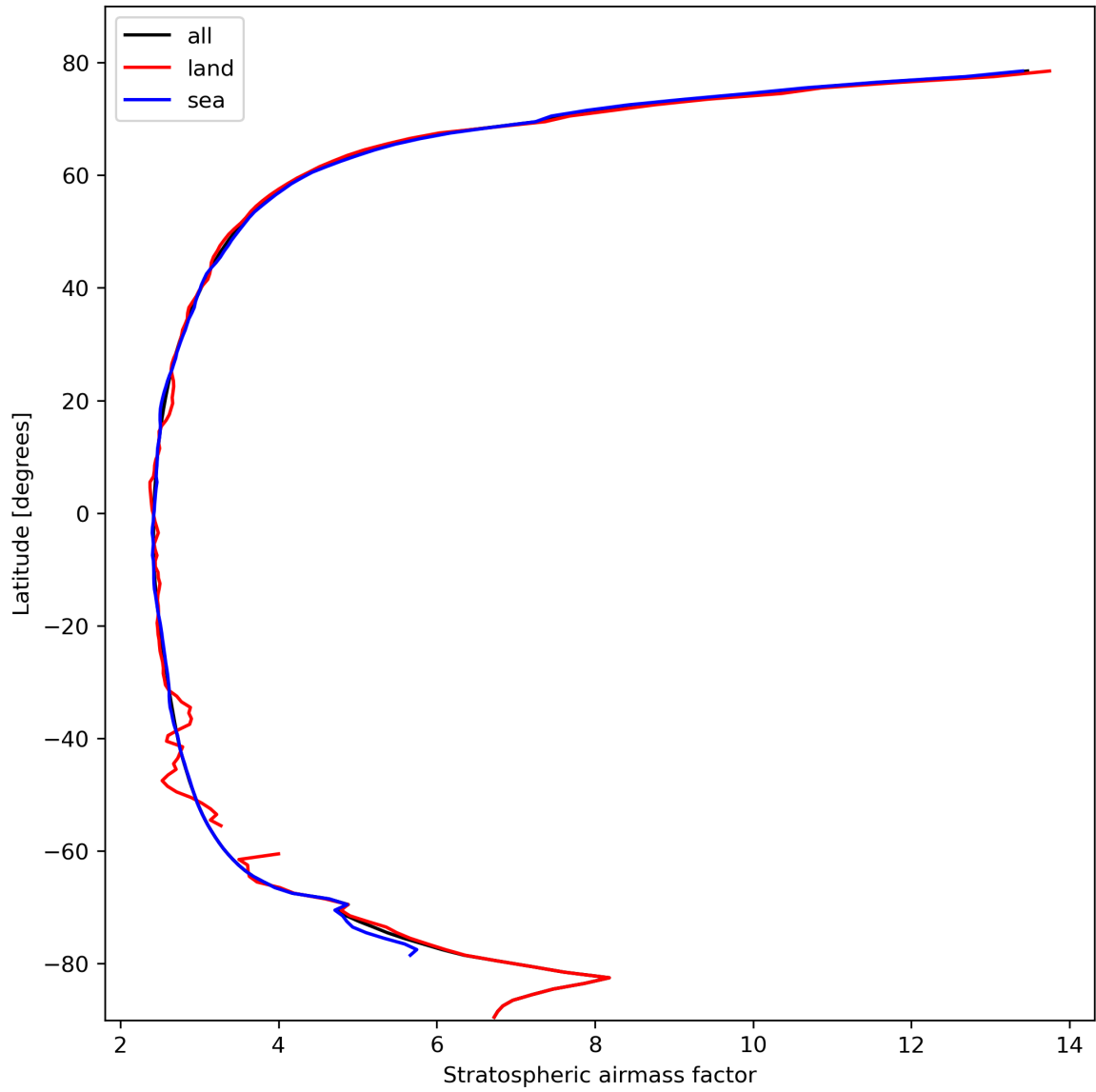
Figure 27: Zonal average of “Stratospheric air mass factor” for 2023-10-17 to 2023-10-19.
