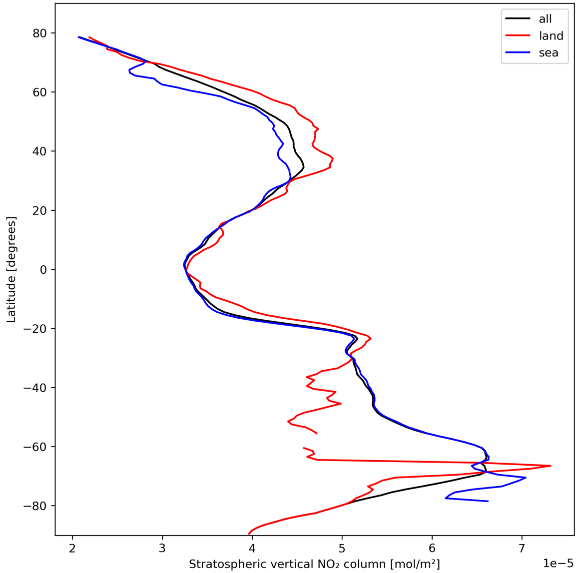
Figure 19: Zonal average of “Stratospheric vertical NO 2 column” for 2023-10-17 to 2023-10-19.
