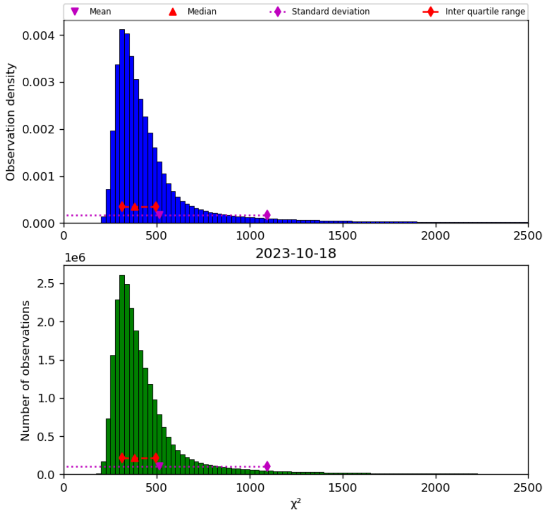
Figure 42: Histogram of “ \chi^2 ” for 2023-10-17 to 2023-10-19
