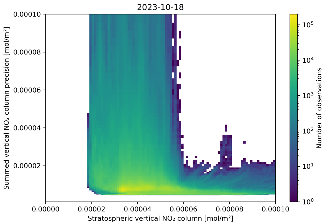
Figure 99: Scatter density plot of “Stratospheric vertical NO 2 column” against “Summed vertical NO 2 column precision” for 2023-10-17 to 2023-10-19.
