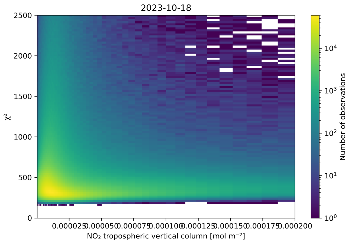
Figure 124: Scatter density plot of “NO 2 tropospheric vertical column” against “ \chi^2 ” for 2023-10-17 to 2023-10-19.
