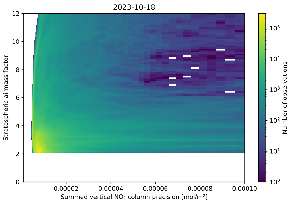
Figure 106: Scatter density plot of “Summed vertical NO 2 column precision” against “Stratospheric airmass factor” for 2023-10-17 to 2023-10-19.
