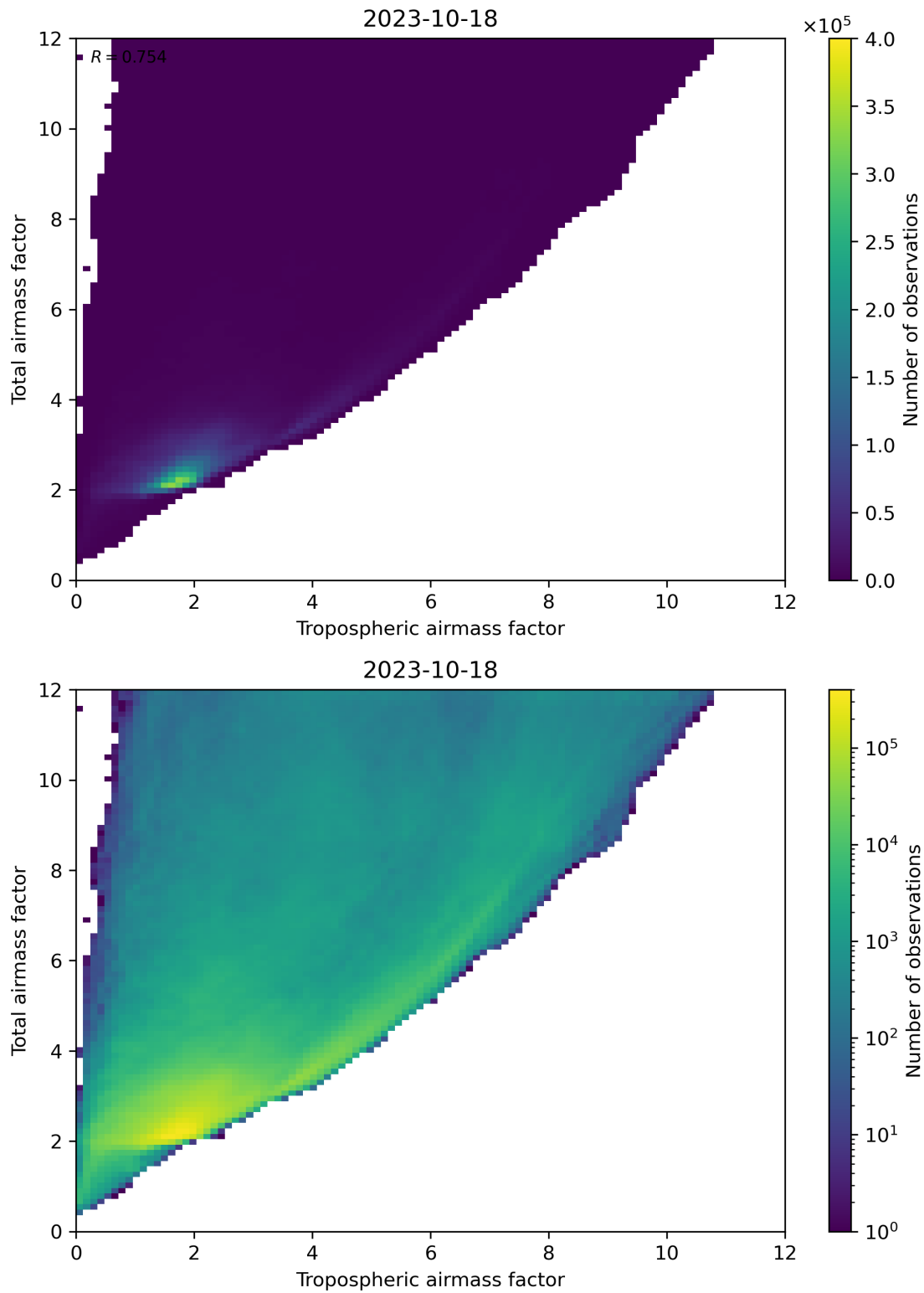
Figure 72: Scatter density plot of “Tropospheric airmass factor” against “Total airmass factor” for 2023-10-17 to 2023-10-19.
