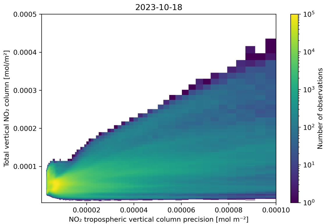
Figure 138: Scatter density plot of “NO 2 tropospheric vertical column precision” against “Total vertical NO 2 column” for 2023-10-17 to 2023-10-19.
