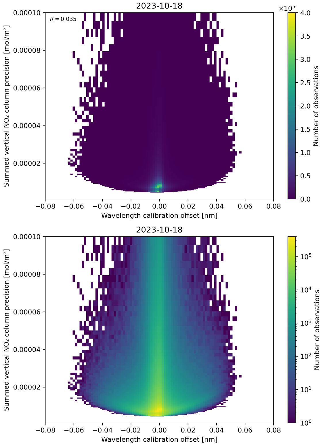
Figure 178: Scatter density plot of “Wavelength calibration offset” against “Summed vertical NO 2 column precision” for 2023-10-17 to 2023-10-19.
