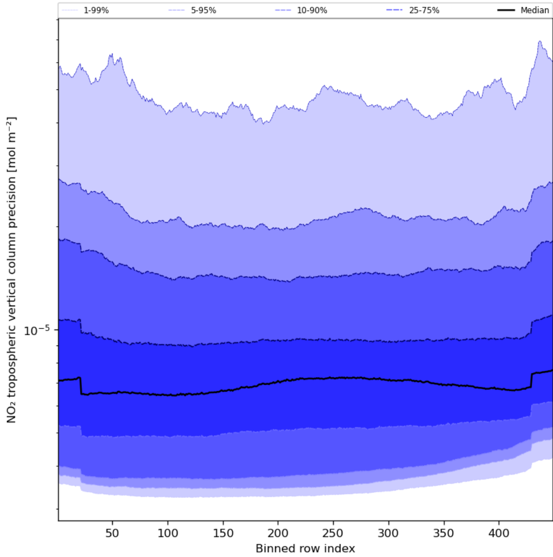
Figure 47: Along track statistics of “NO 2 tropospheric vertical column precision” for 2023-10-17 to 2023-10-19
