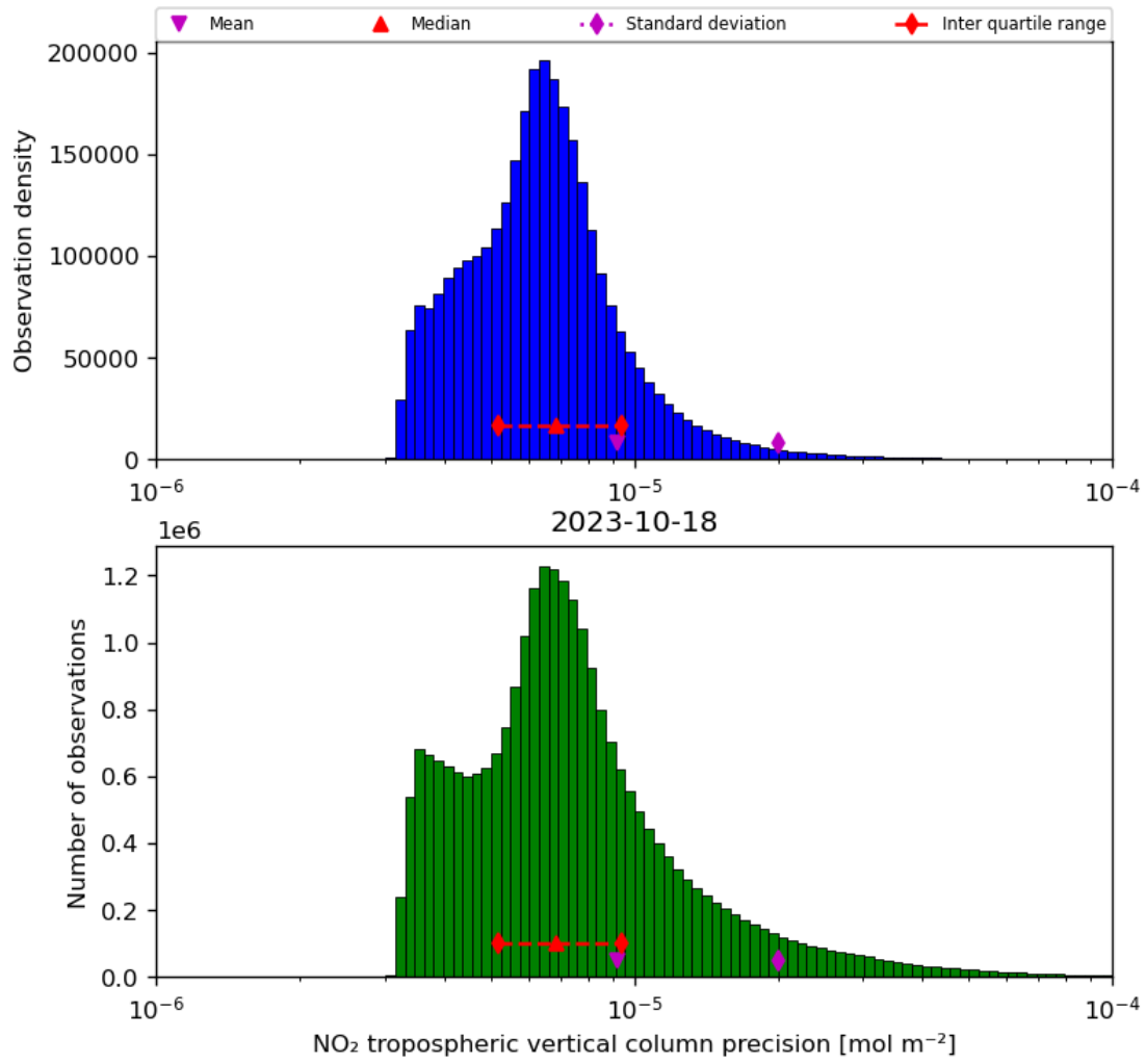
Figure 30: Histogram of “NO 2 tropospheric vertical column precision” for 2023-10-17 to 2023-10-19
