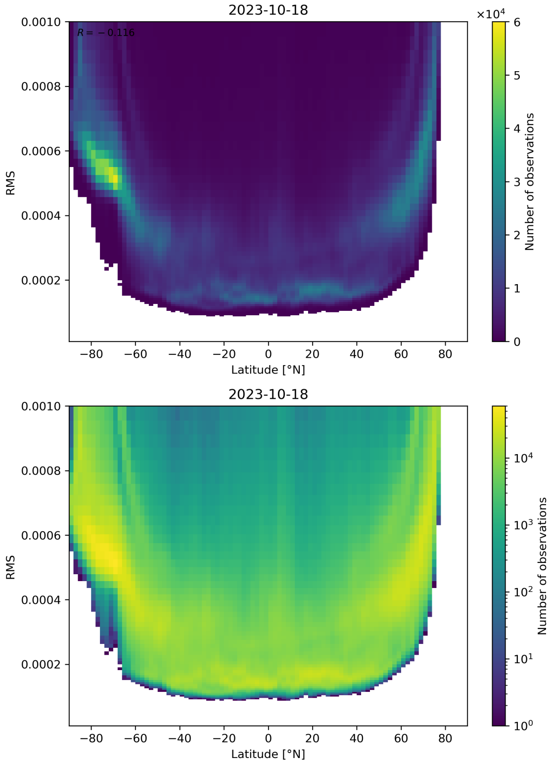
Figure 94: Scatter density plot of “Latitude” against “RMS” for 2023-10-17 to 2023-10-19.
