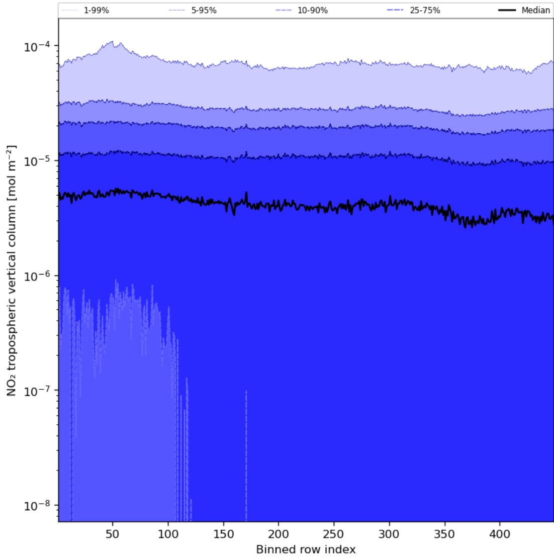
Figure 46: Along track statistics of “NO 2 tropospheric vertical column” for 2023-10-17 to 2023-10-19
