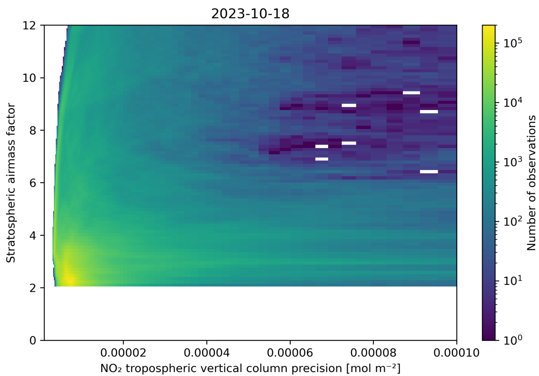
Figure 131: Scatter density plot of “NO 2 tropospheric vertical column precision” against “Stratospheric airmass factor” for 2023-10-17 to 2023-10-19.
