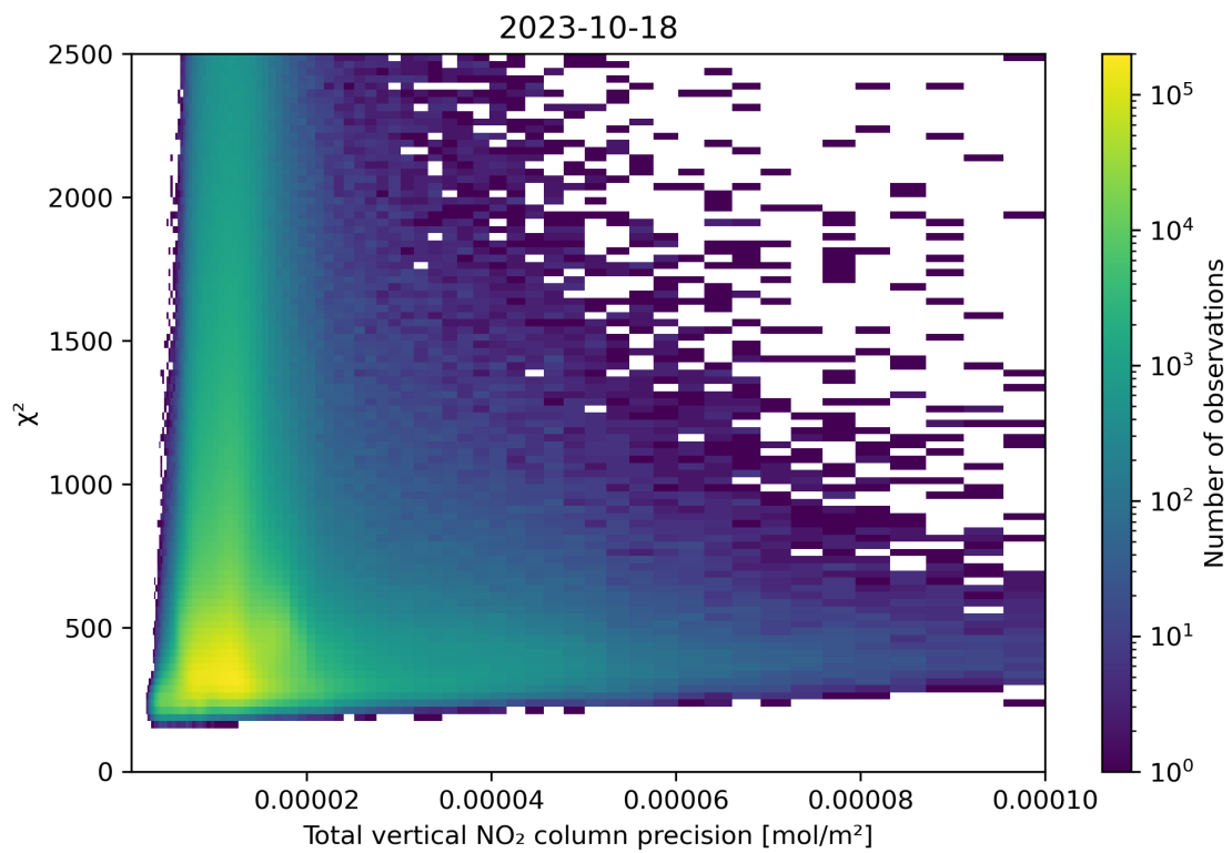
Figure 116: Scatter density plot of “Total vertical NO 2 column precision” against “ \chi^2 ” for 2023-10-17 to 2023-10-19.
