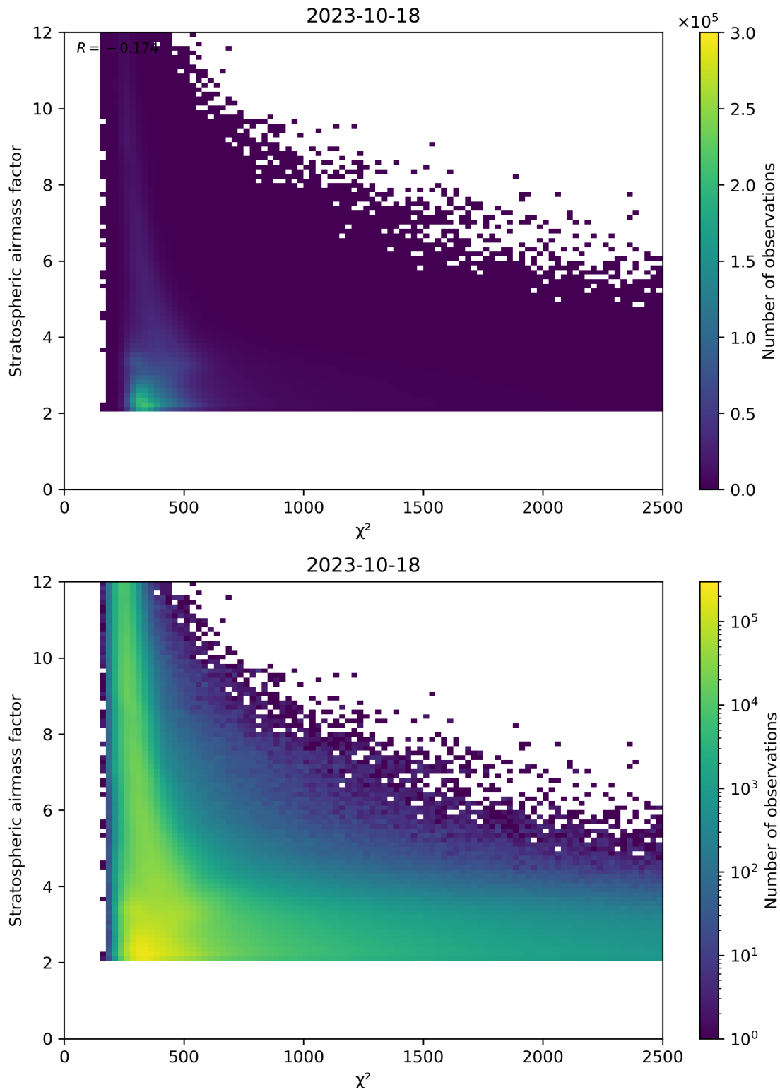
Figure 81: Scatter density plot of “ \chi^2 ” against “Stratospheric airmass factor” for 2023-10-17 to 2023-10-19.
