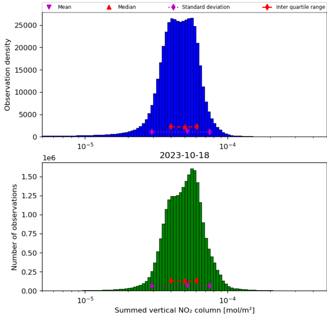
Figure 40: Histogram of “Summed vertical NO 2 column” for 2023-10-17 to 2023-10-19
