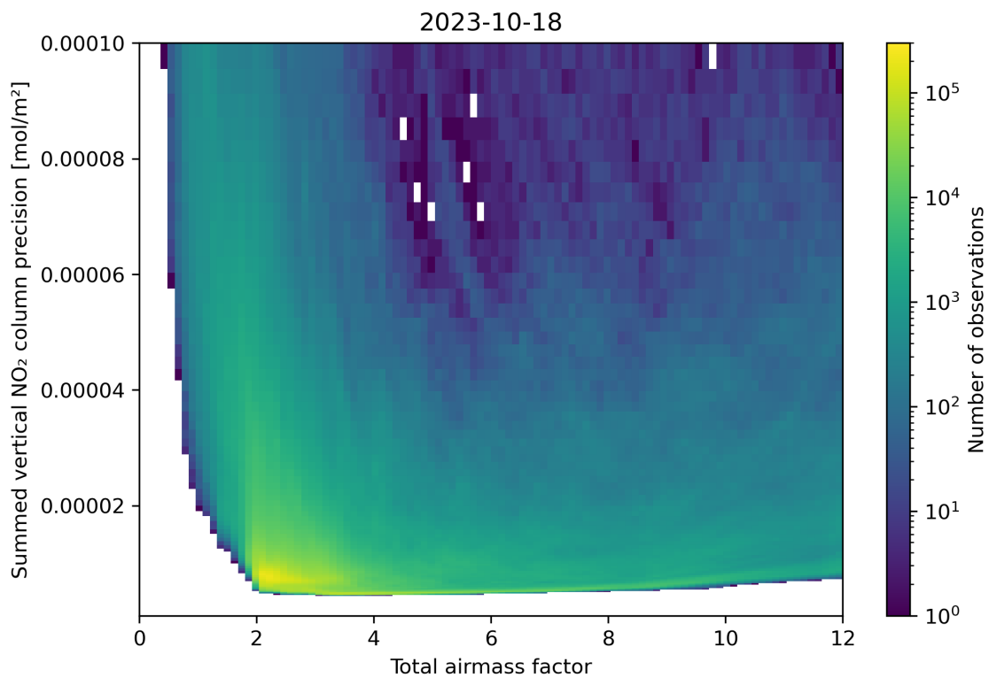
Figure 66: Scatter density plot of “Total airmass factor” against “Summed vertical NO 2 column precision” for 2023-10-17 to 2023-10-19.
