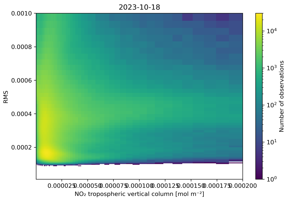
Figure 142: Scatter density plot of “NO 2 tropospheric vertical column” against “RMS” for 2023-10-17 to 2023-10-19.
