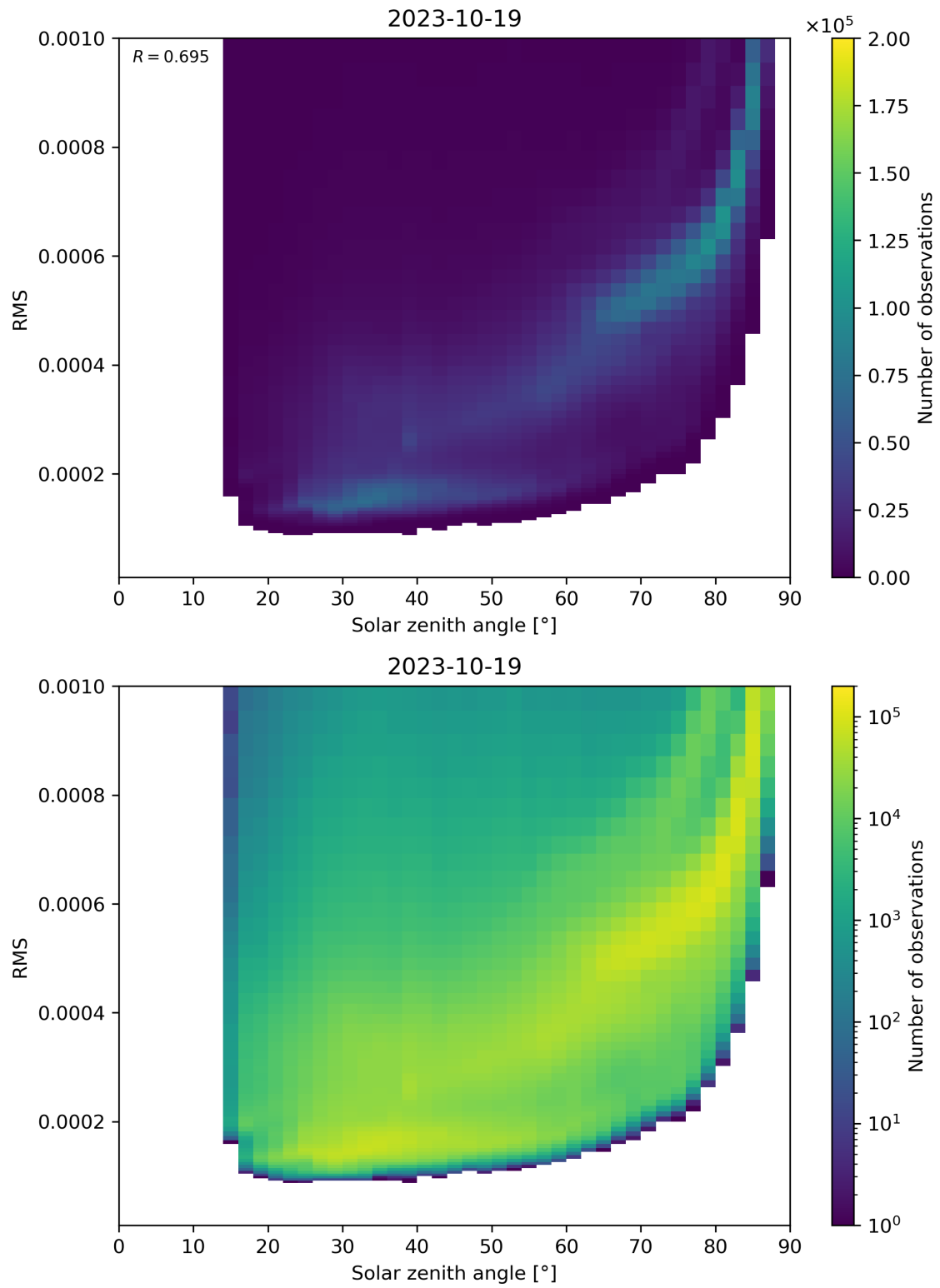
Figure 157: Scatter density plot of “Solar zenith angle” against “RMS” for 2023-10-18 to 2023-10-20.
