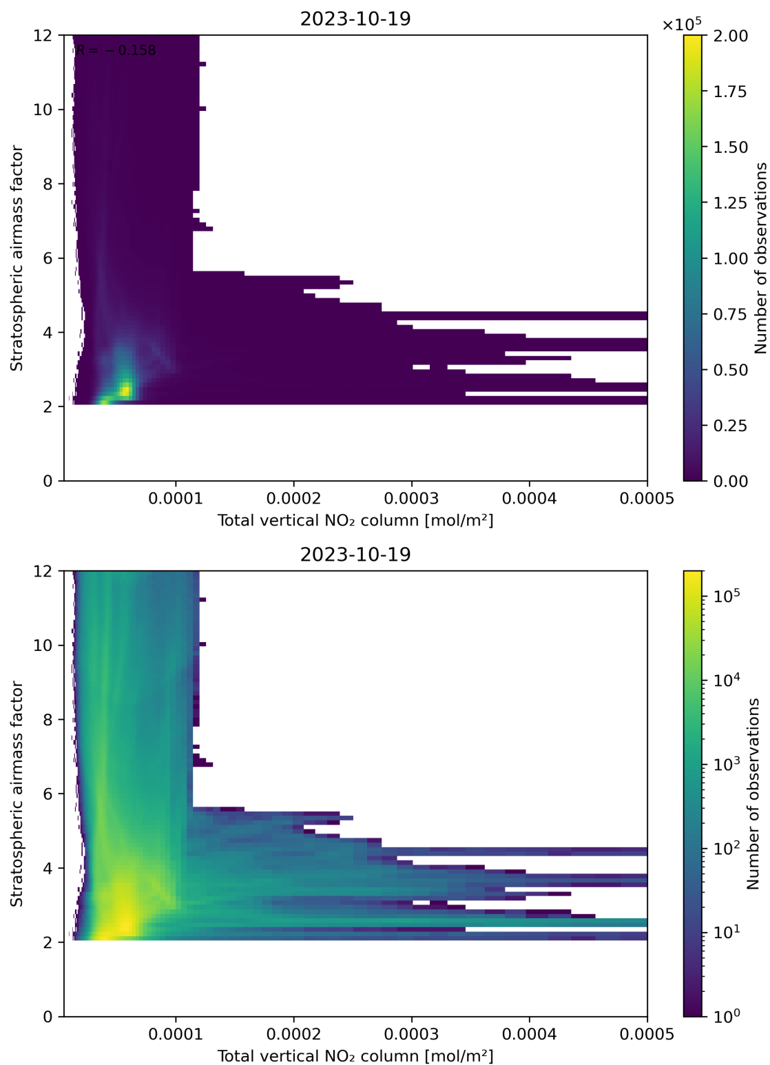
Figure 110: Scatter density plot of “Total vertical NO 2 column” against “Stratospheric airmass factor” for 2023-10-18 to 2023-10-20.
