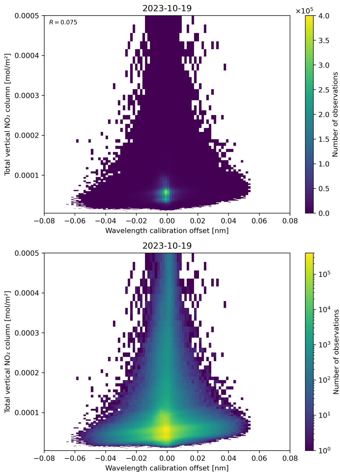
Figure 179: Scatter density plot of “Wavelength calibration offset” against “Total vertical NO 2 column” for 2023-10-18 to 2023-10-20.
