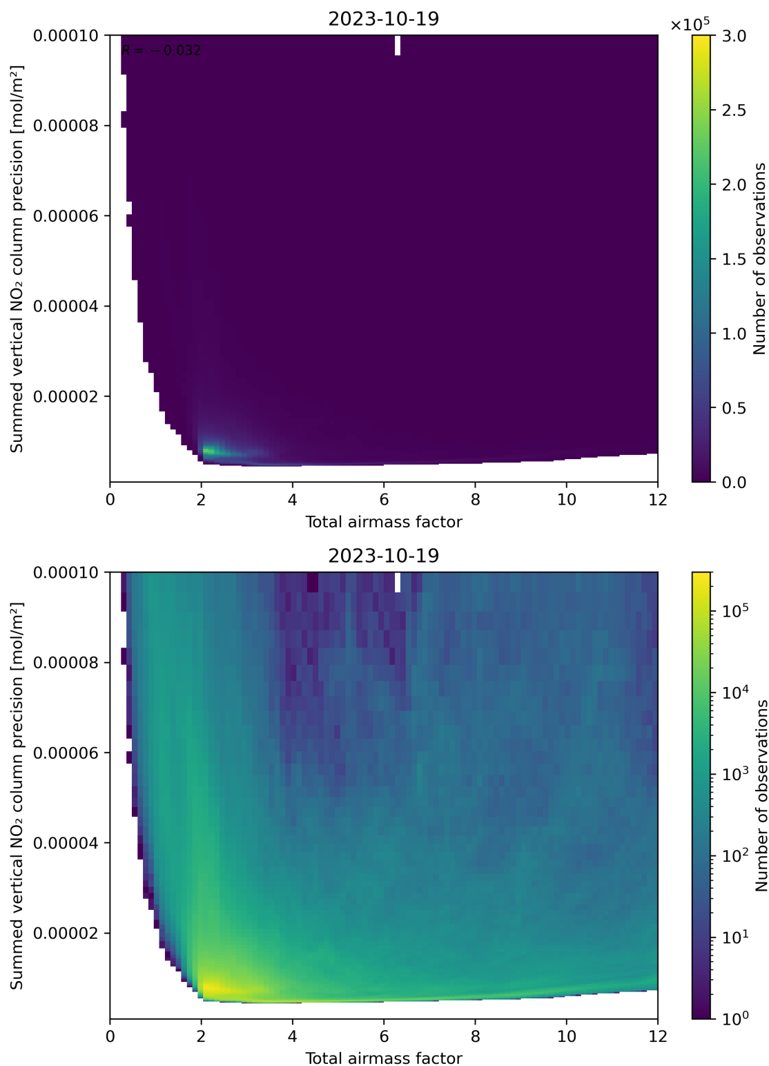
Figure 66: Scatter density plot of “Total airmass factor” against “Summed vertical NO 2 column precision” for 2023-10-18 to 2023-10-20.
