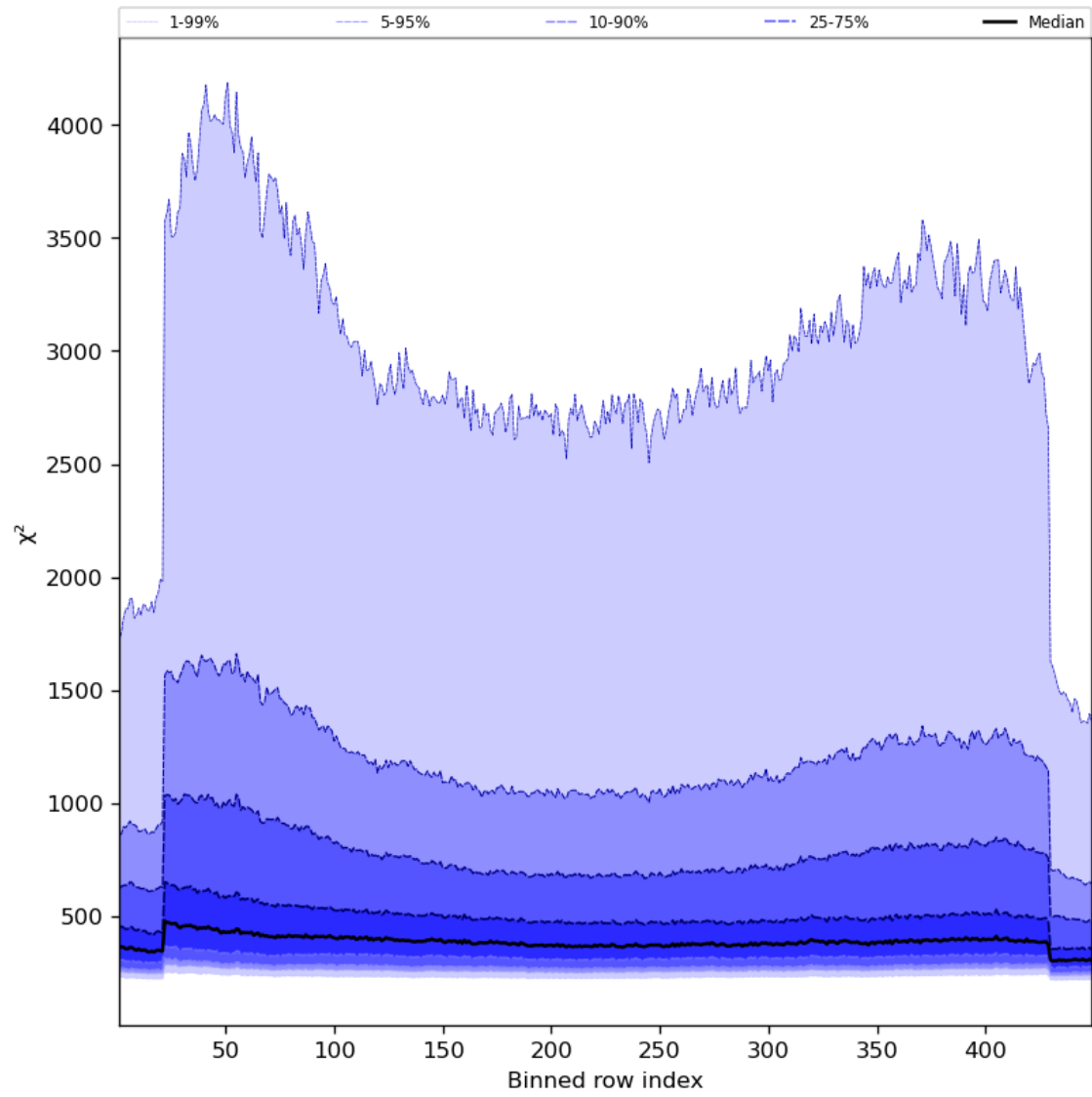
Figure 59: Along track statistics of “ \chi^2 ” for 2023-10-18 to 2023-10-20
