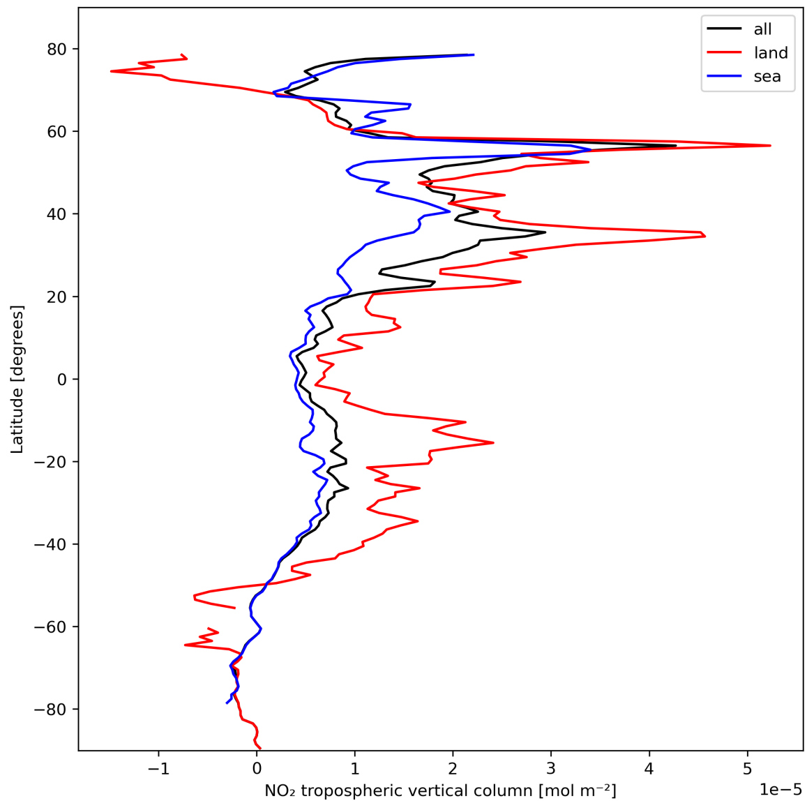
Figure 12: Zonal average of “NO 2 tropospheric vertical column” for 2023-10-18 to 2023-10-20.
