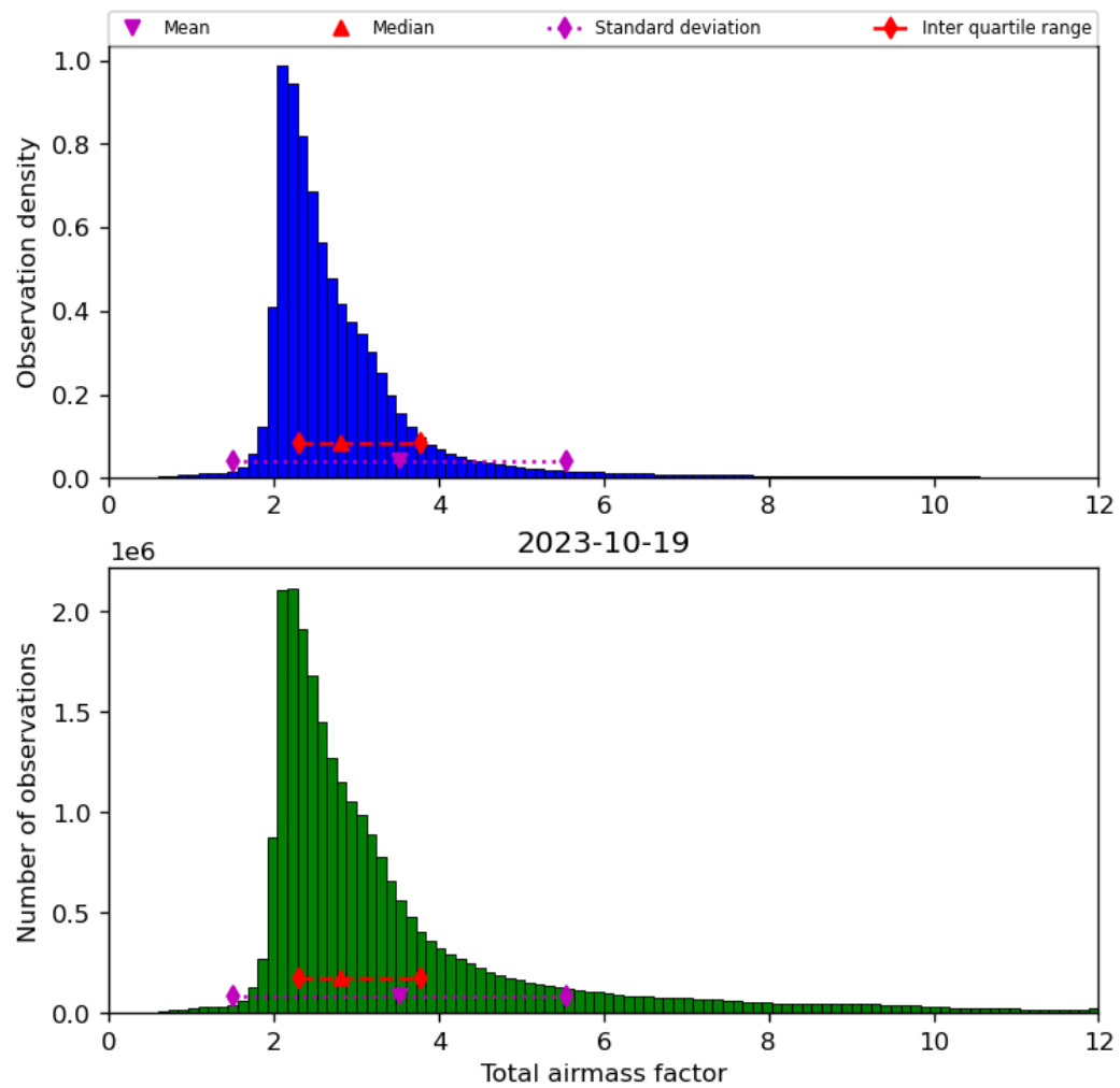
Figure 32: Histogram of “Total airmass factor” for 2023-10-18 to 2023-10-20
