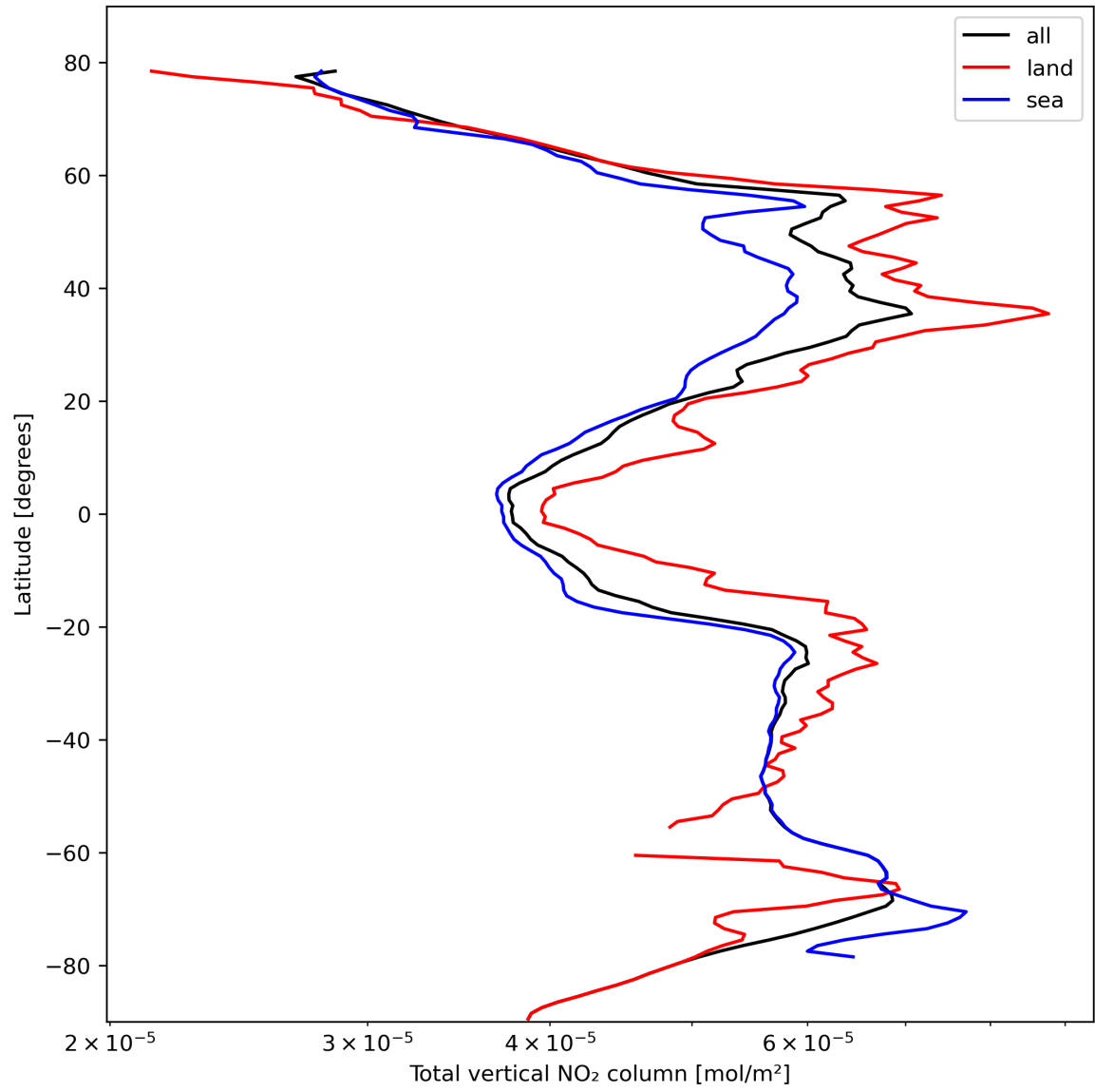
Figure 21: Zonal average of “Total vertical NO 2 column” for 2023-10-18 to 2023-10-20.
