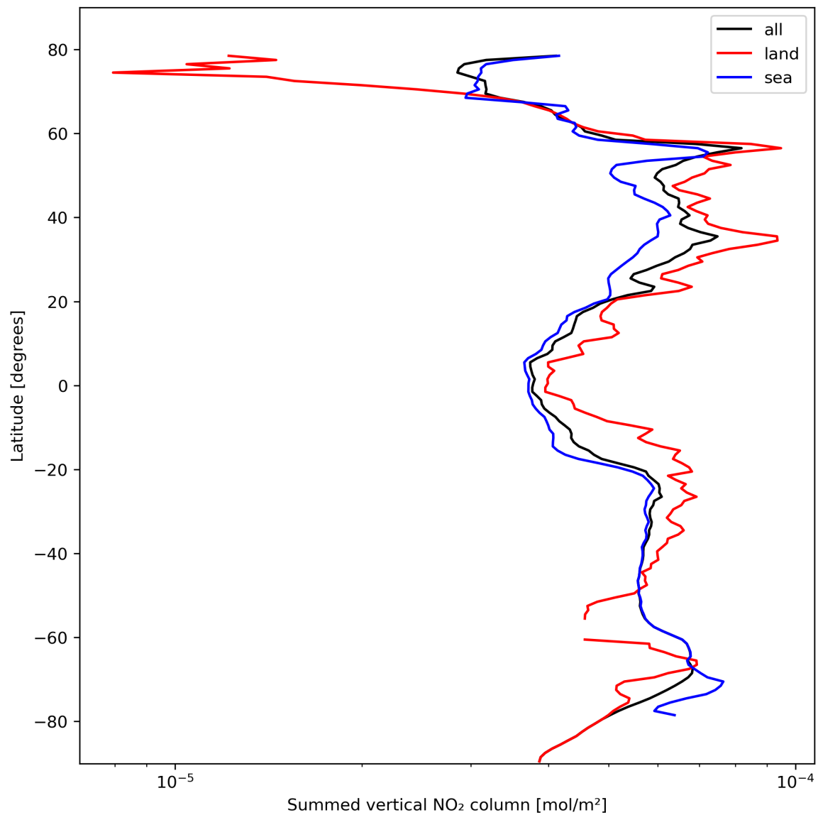
Figure 23: Zonal average of “Summed vertical NO 2 column” for 2023-10-18 to 2023-10-20.
