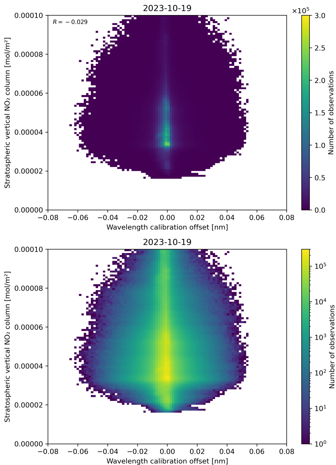
Figure 176: Scatter density plot of “Wavelength calibration offset” against “Stratospheric vertical NO 2 column” for 2023-10-18 to 2023-10-20.
