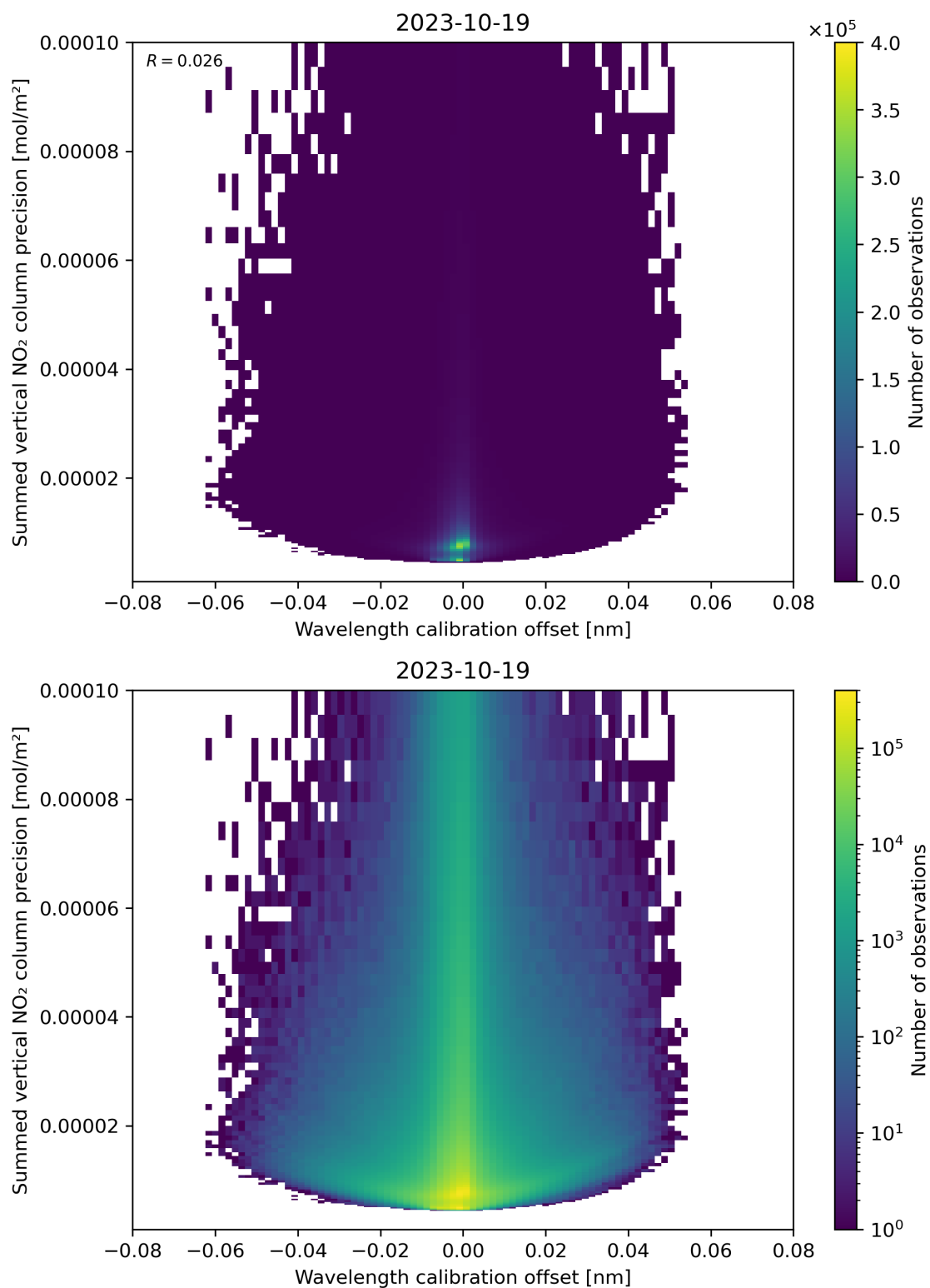
Figure 178: Scatter density plot of “Wavelength calibration offset” against “Summed vertical NO 2 column precision” for 2023-10-18 to 2023-10-20.
