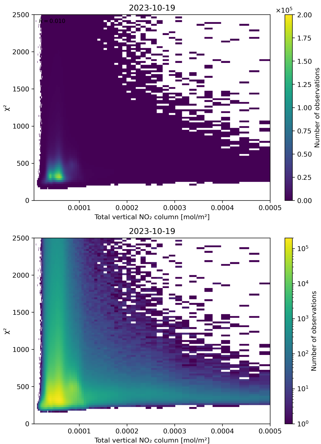
Figure 111: Scatter density plot of “Total vertical NO 2 column” against “ \chi^2 ” for 2023-10-18 to 2023-10-20.
