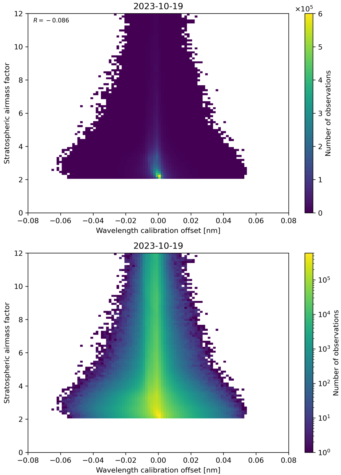
Figure 174: Scatter density plot of “Wavelength calibration offset” against “Stratospheric air mass factor” for 2023-10-18 to 2023-10-20.
