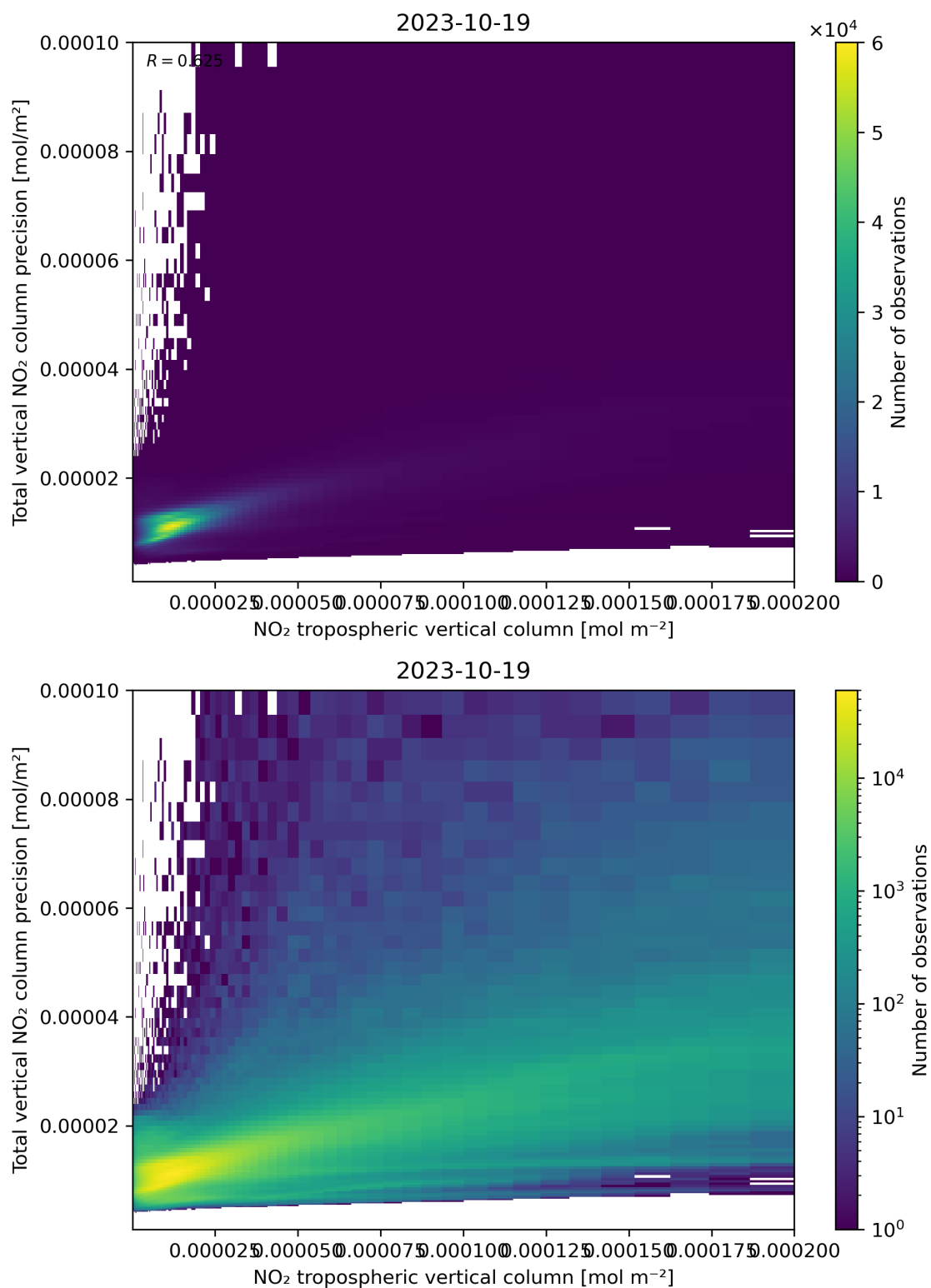
Figure 129: Scatter density plot of “NO 2 tropospheric vertical column” against “Total vertical NO 2 column precision” for 2023-10-18 to 2023-10-20.
