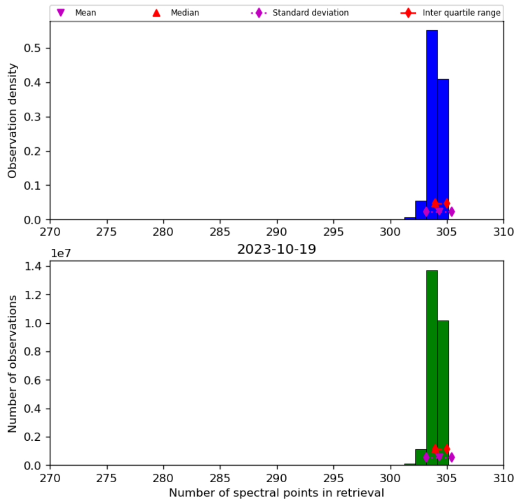
Figure 33: Histogram of “Number of spectral points in retrieval” for 2023-10-18 to 2023-10-20
