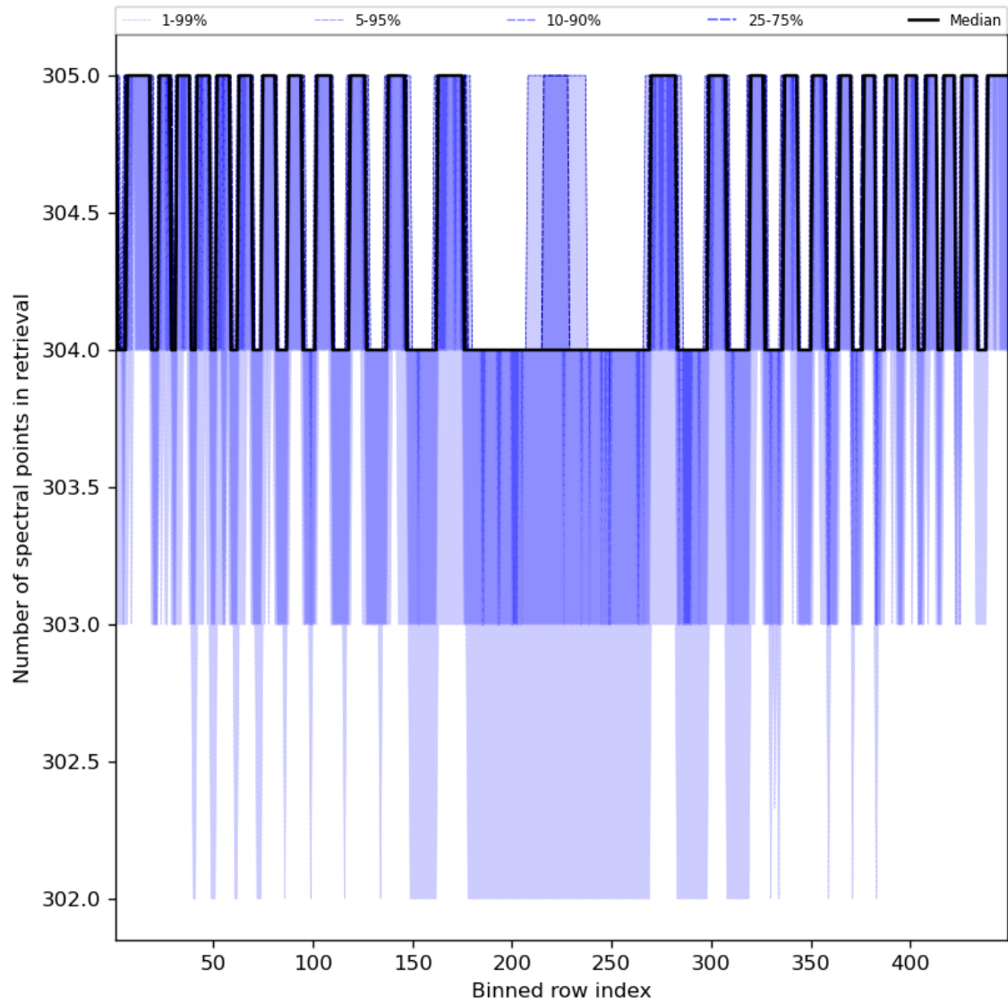
Figure 50: Along track statistics of “Number of spectral points in retrieval” for 2023-10-18 to 2023-10-20
