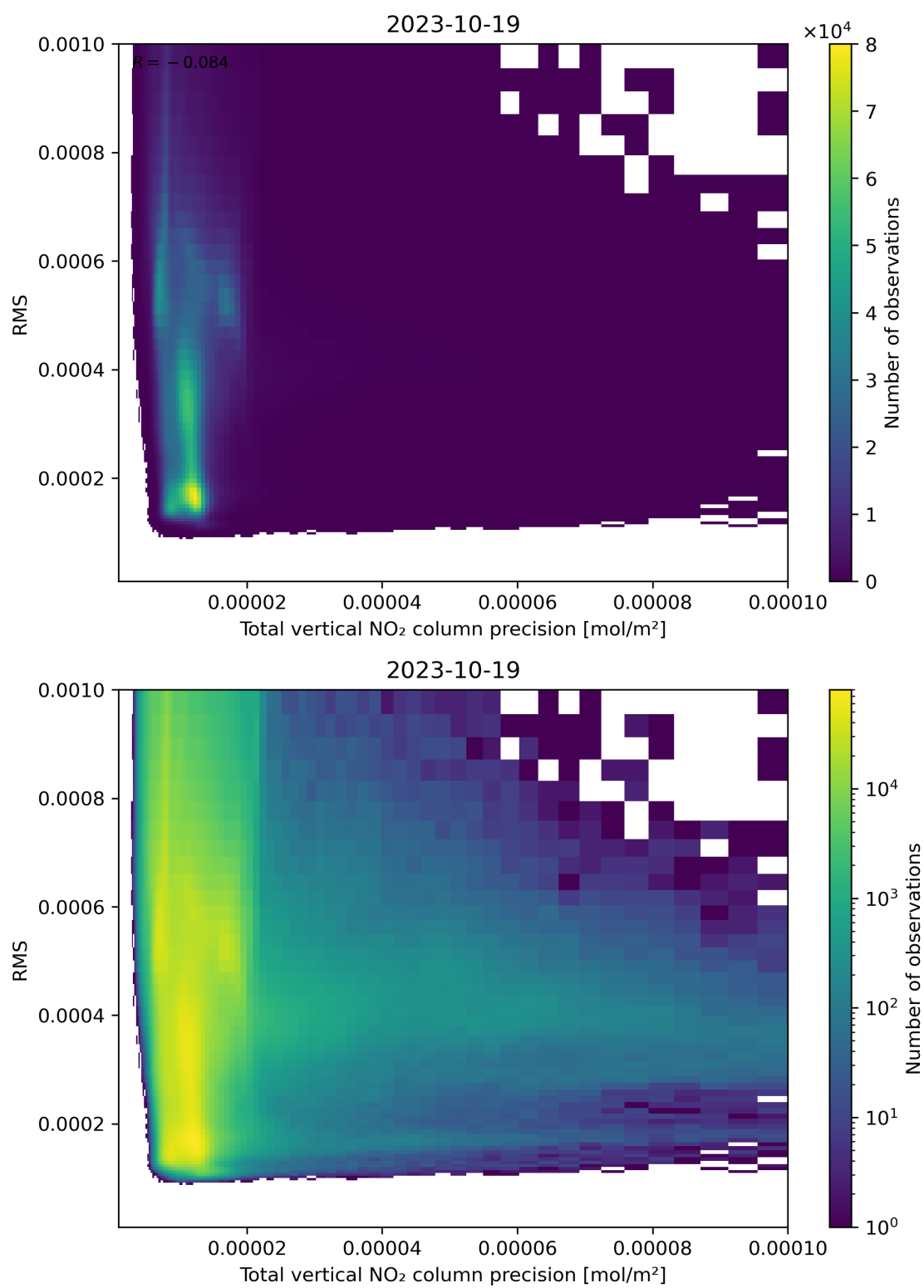
Figure 119: Scatter density plot of “Total vertical NO 2 column precision” against “RMS” for 2023-10-18 to 2023-10-20.
