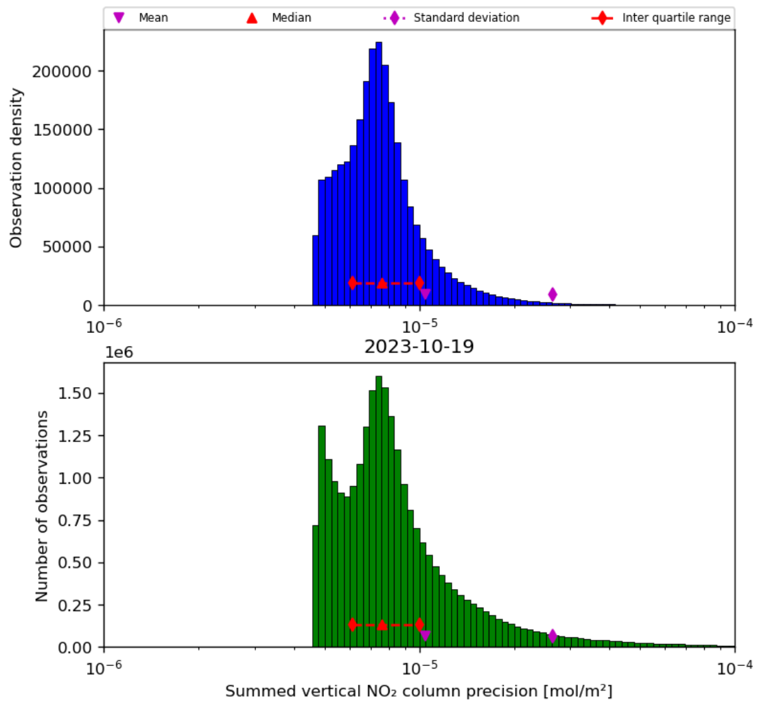
Figure 41: Histogram of "Summed vertical NO 2 column precision" for 2023-10-18 to 2023-10-20
