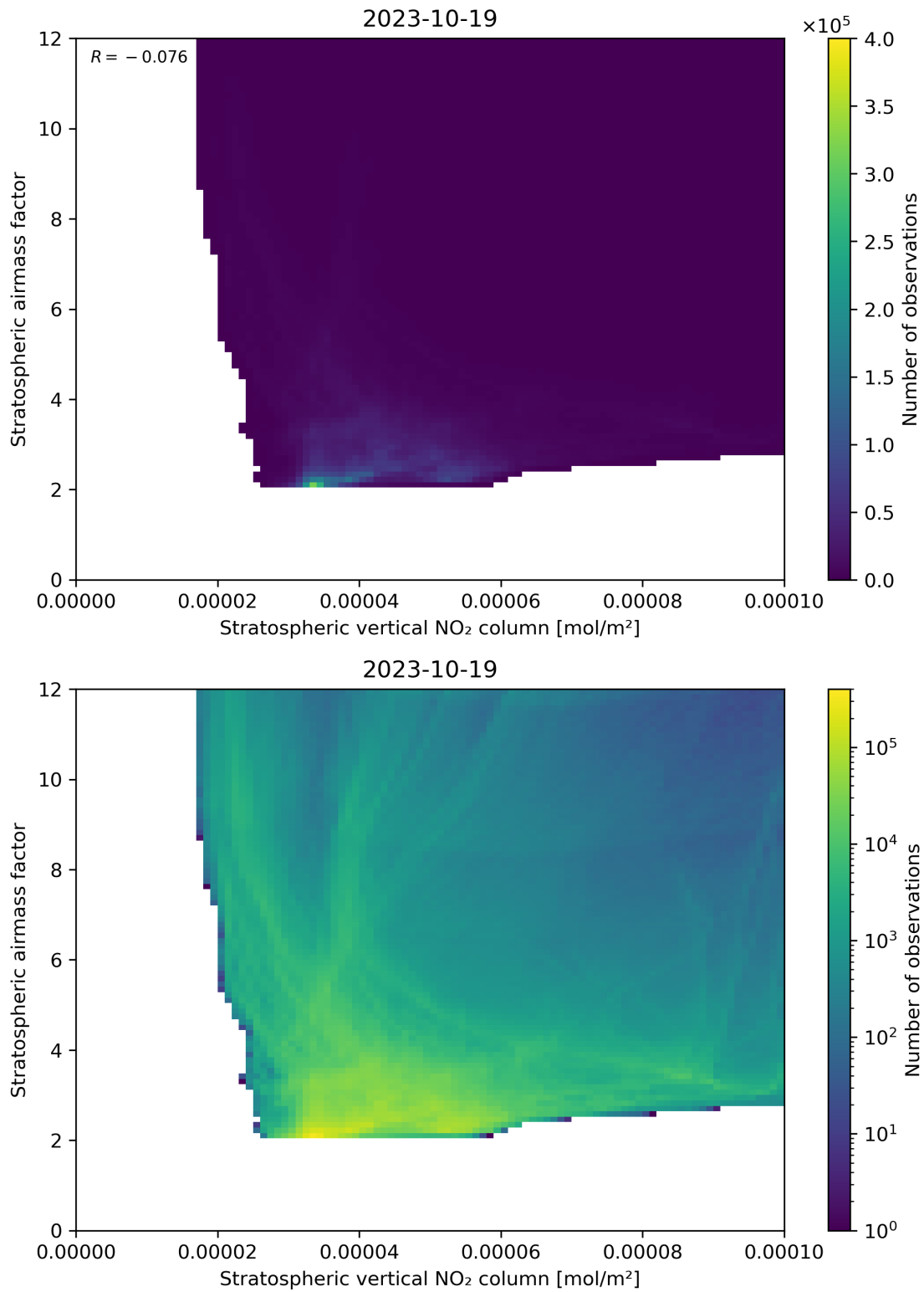
Figure 96: Scatter density plot of “Stratospheric vertical NO 2 column” against “Stratospheric airmass factor” for 2023-10-18 to 2023-10-20.
