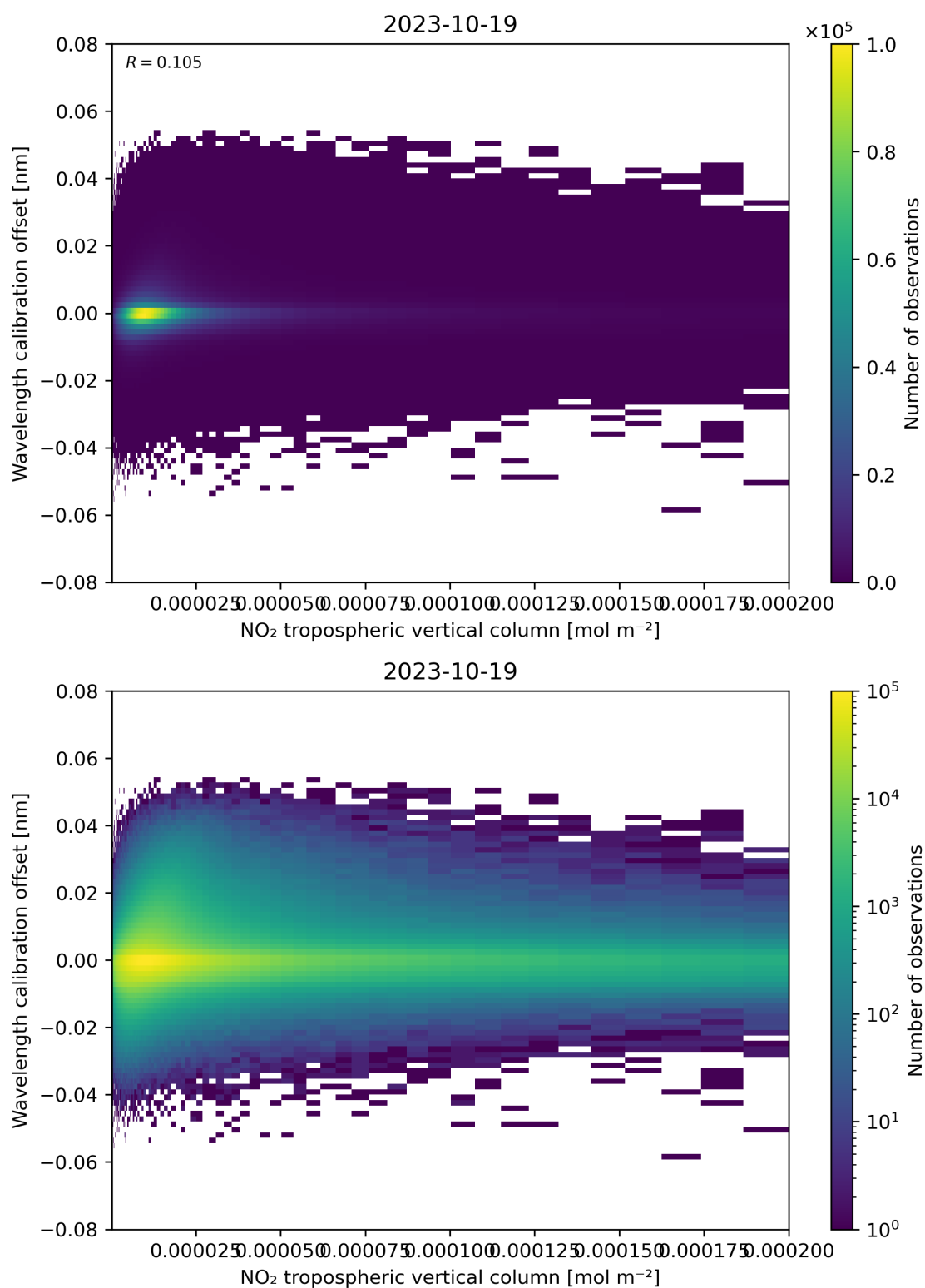
Figure 143: Scatter density plot of “NO 2 tropospheric vertical column” against “Wavelength calibration offset” for 2023-10-18 to 2023-10-20.
