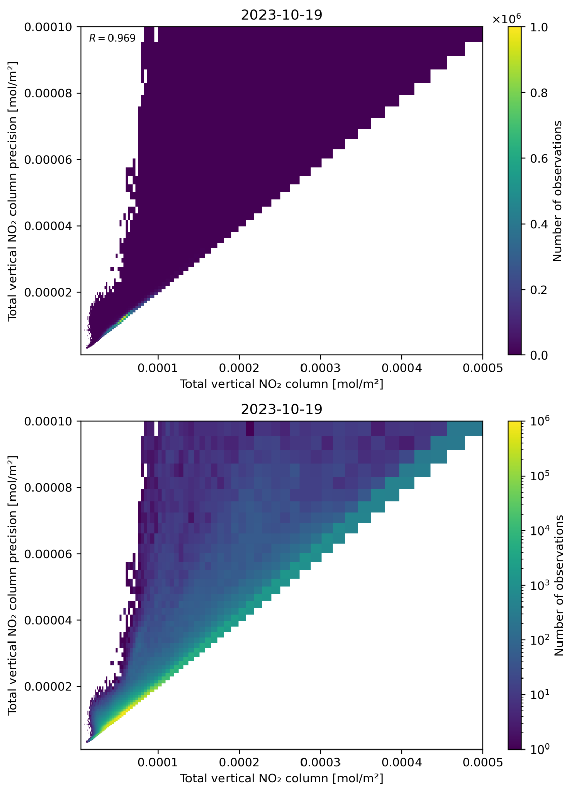
Figure 114: Scatter density plot of “Total vertical NO 2 column” against “Total vertical NO 2 column precision” for 2023-10-18 to 2023-10-20.
