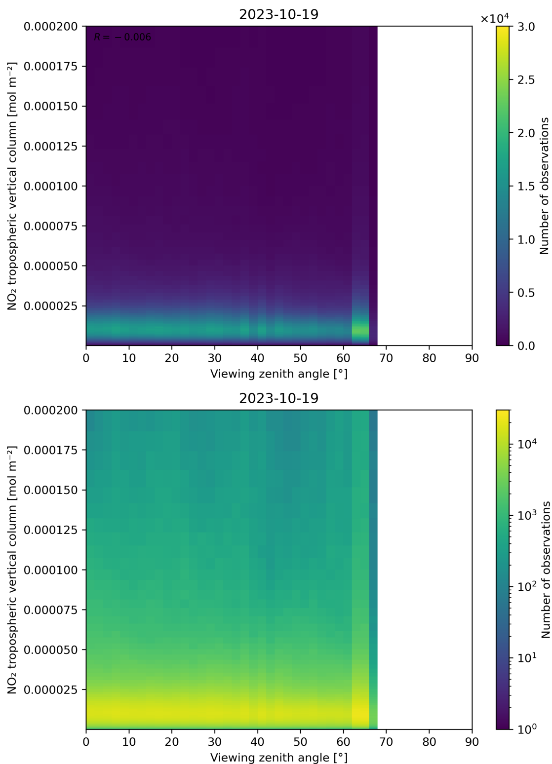
Figure 169: Scatter density plot of “Viewing zenith angle” against “NO 2 tropospheric vertical column” for 2023-10-18 to 2023-10-20.
