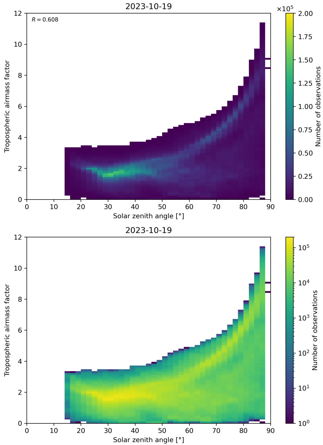
Figure 147: Scatter density plot of “Solar zenith angle” against “Tropospheric airmass factor” for 2023-10-18 to 2023-10-20.
