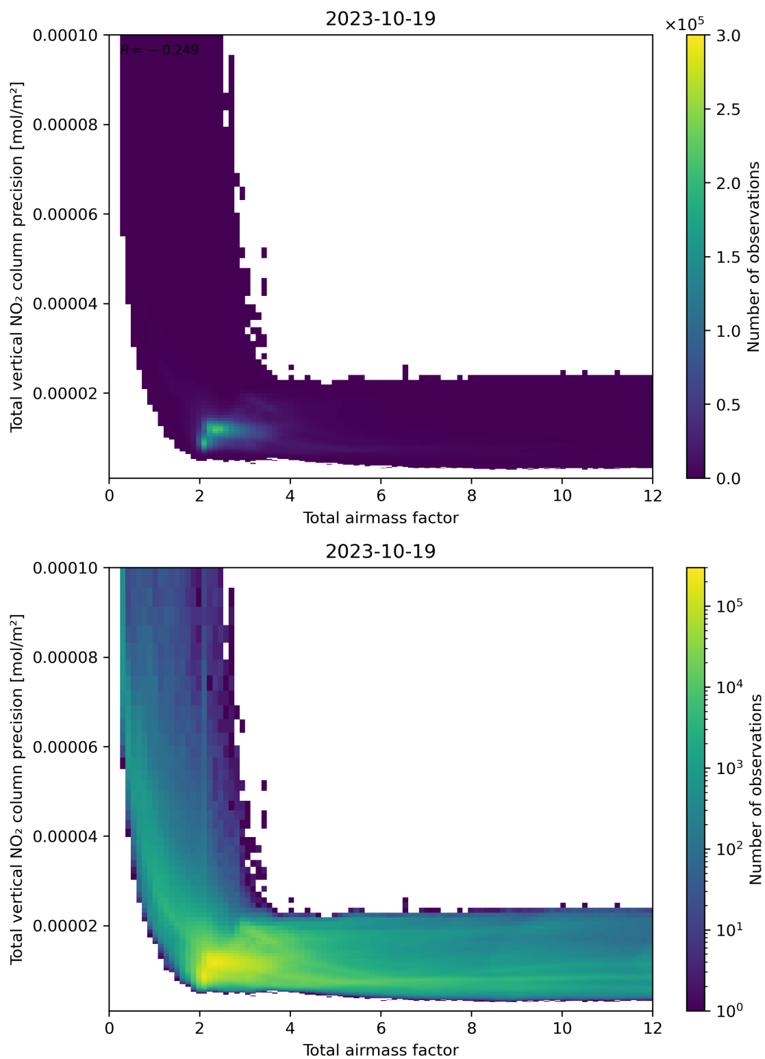
Figure 68: Scatter density plot of “Total airmass factor” against “Total vertical NO 2 column precision” for 2023-10-18 to 2023-10-20.
