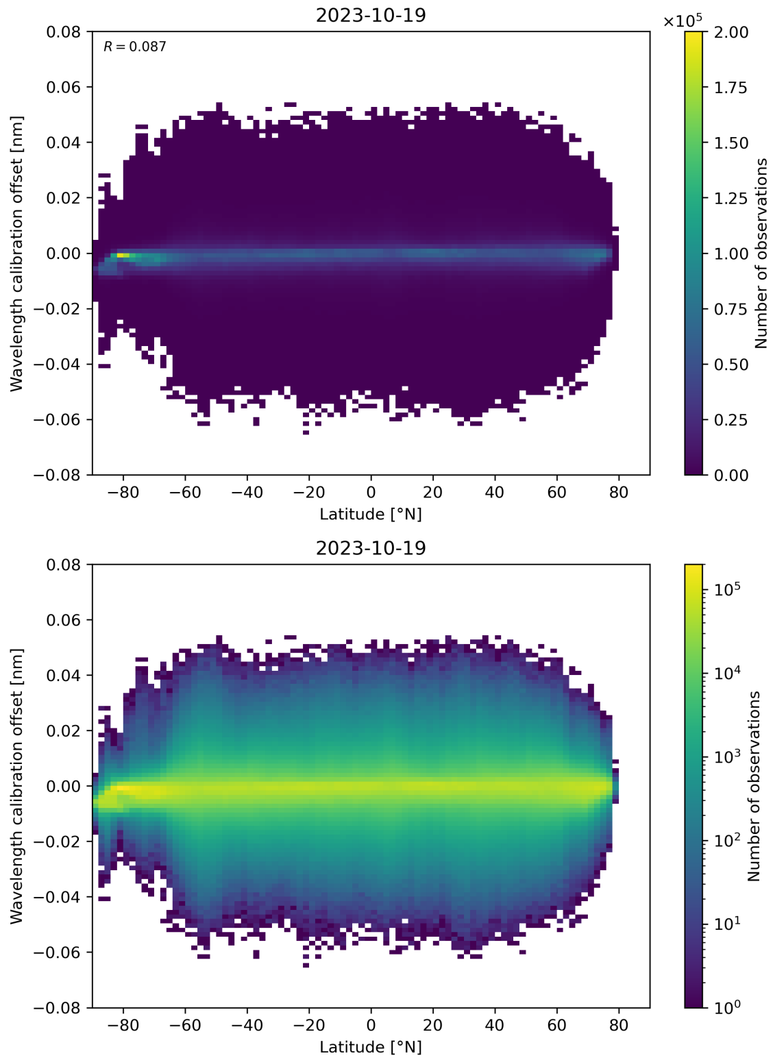
Figure 95: Scatter density plot of “Latitude” against “Wavelength calibration offset” for 2023-10-18 to 2023-10-20.
