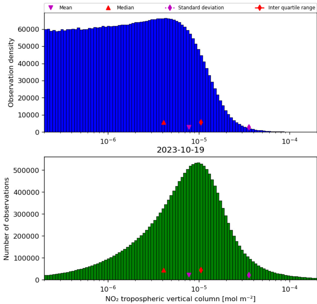
Figure 29: Histogram of “NO 2 tropospheric vertical column” for 2023-10-18 to 2023-10-20
