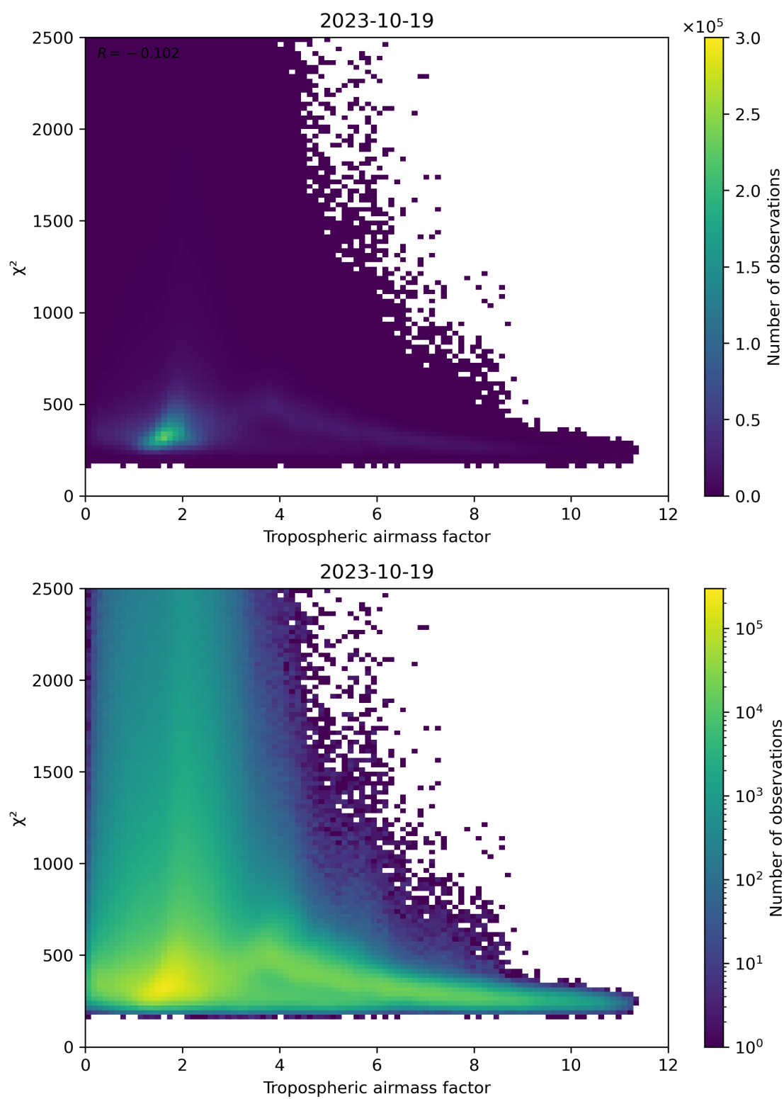
Figure 73: Scatter density plot of “Tropospheric airmass factor” against “ \chi^2 ” for 2023-10-18 to 2023-10-20.
