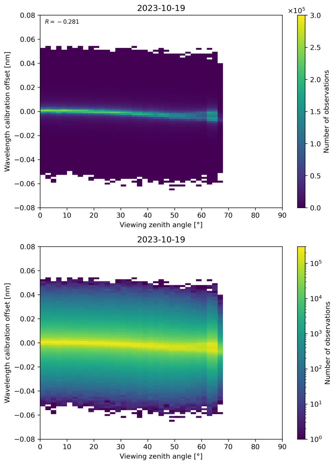
Figure 173: Scatter density plot of “Viewing zenith angle” against “Wavelength calibration offset” for 2023-10-18 to 2023-10-20.
