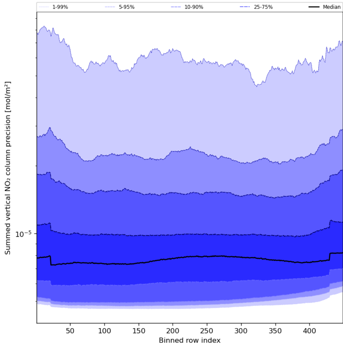
Figure 58: Along track statistics of “Summed vertical NO 2 column precision” for 2023-10-18 to 2023-10-20
