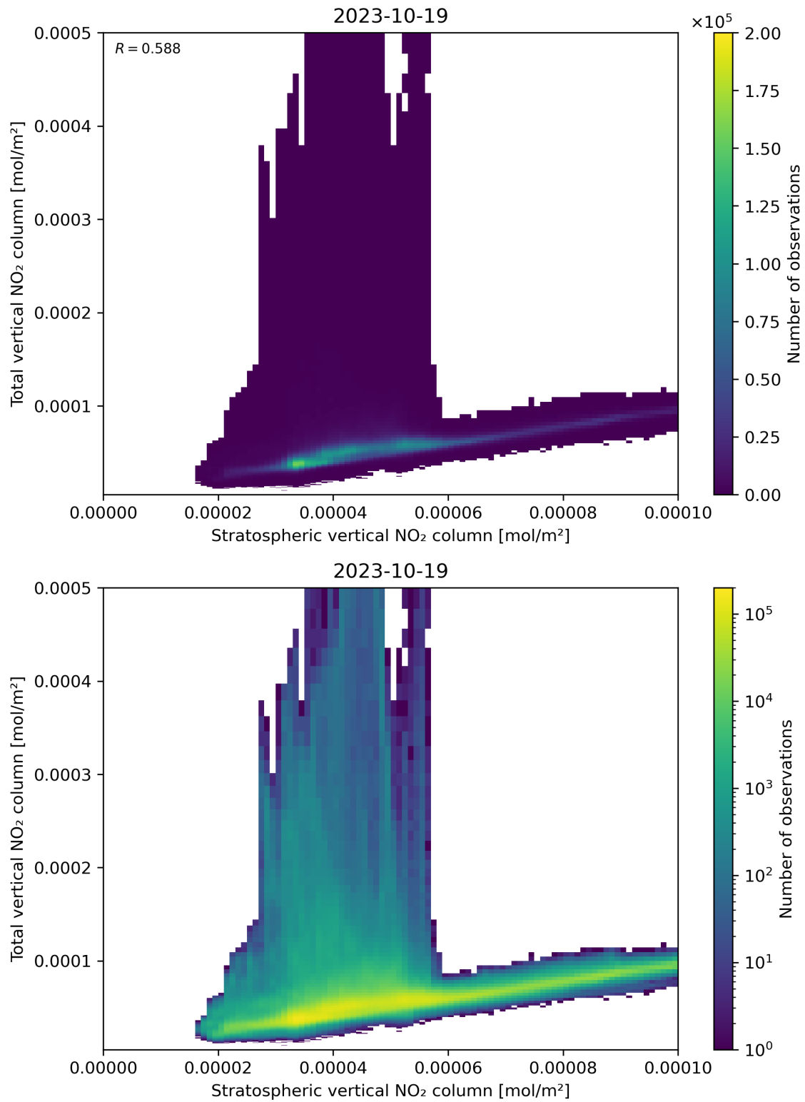
Figure 100: Scatter density plot of “Stratospheric vertical NO 2 column” against “Total vertical NO 2 column” for 2023-10-18 to 2023-10-20.
