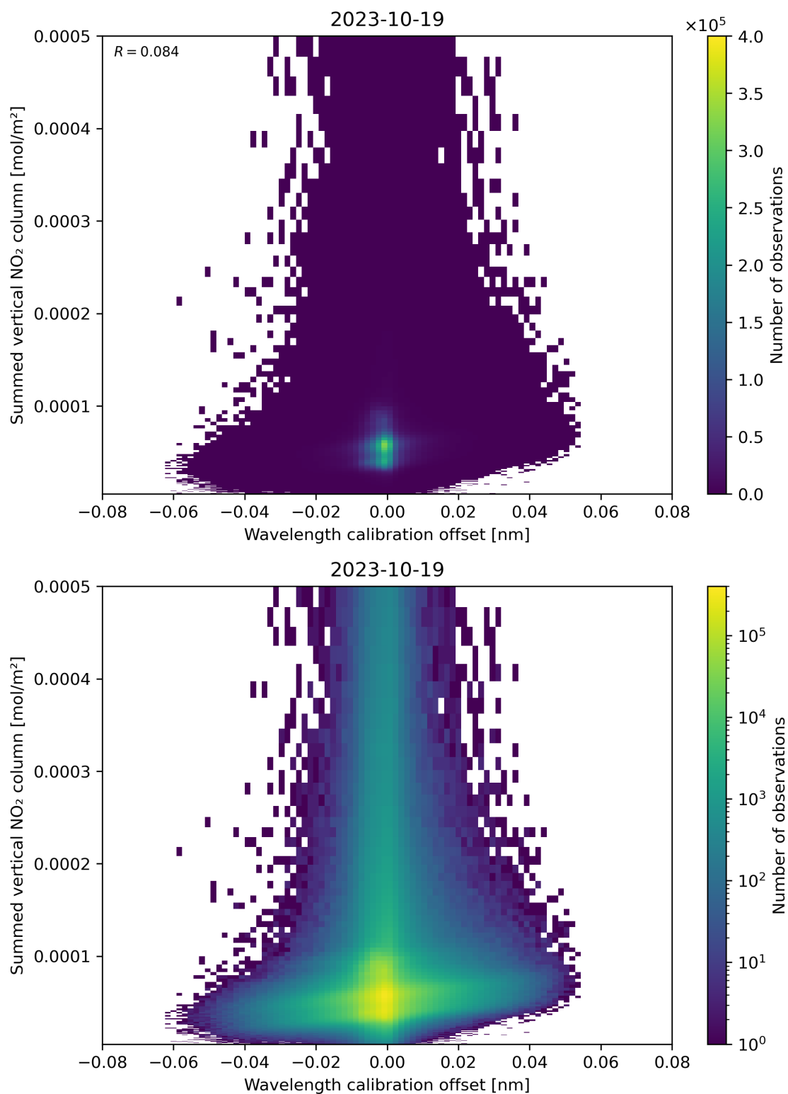
Figure 177: Scatter density plot of “Wavelength calibration offset” against “Summed vertical NO 2 column” for 2023-10-18 to 2023-10-20.
