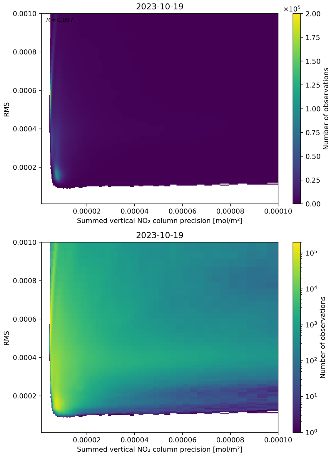
Figure 108: Scatter density plot of “Summed vertical NO 2 column precision” against “RMS” for 2023-10-18 to 2023-10-20.
