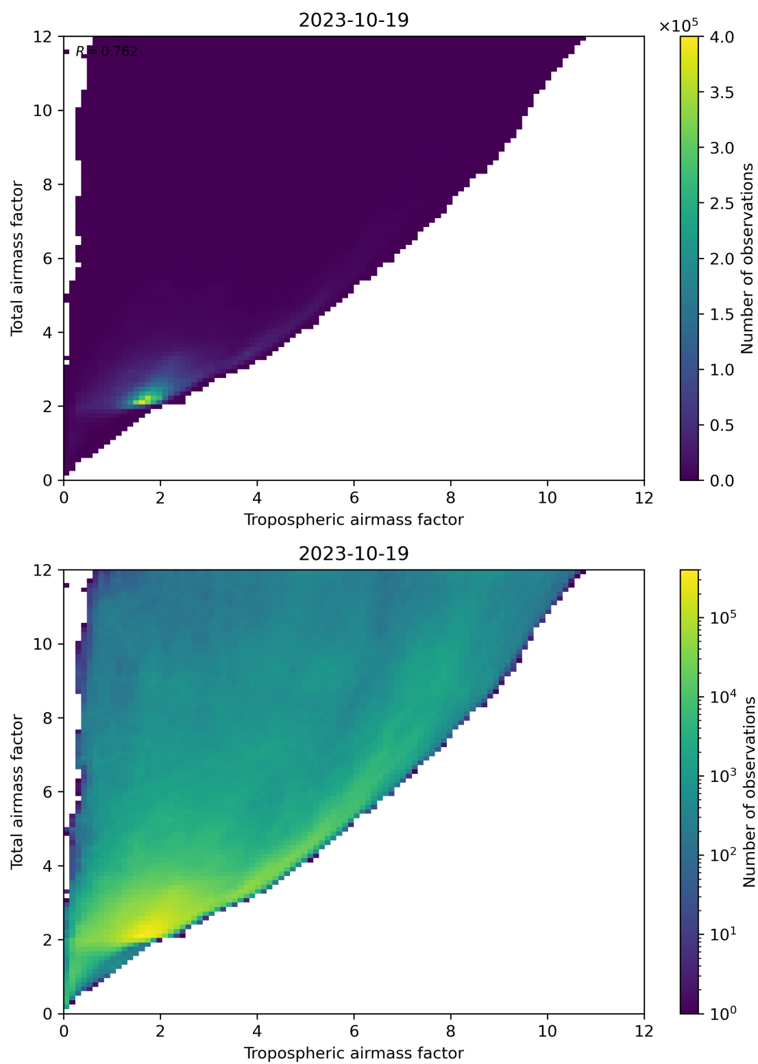
Figure 72: Scatter density plot of “Tropospheric airmass factor” against “Total airmass factor” for 2023-10-18 to 2023-10-20.
