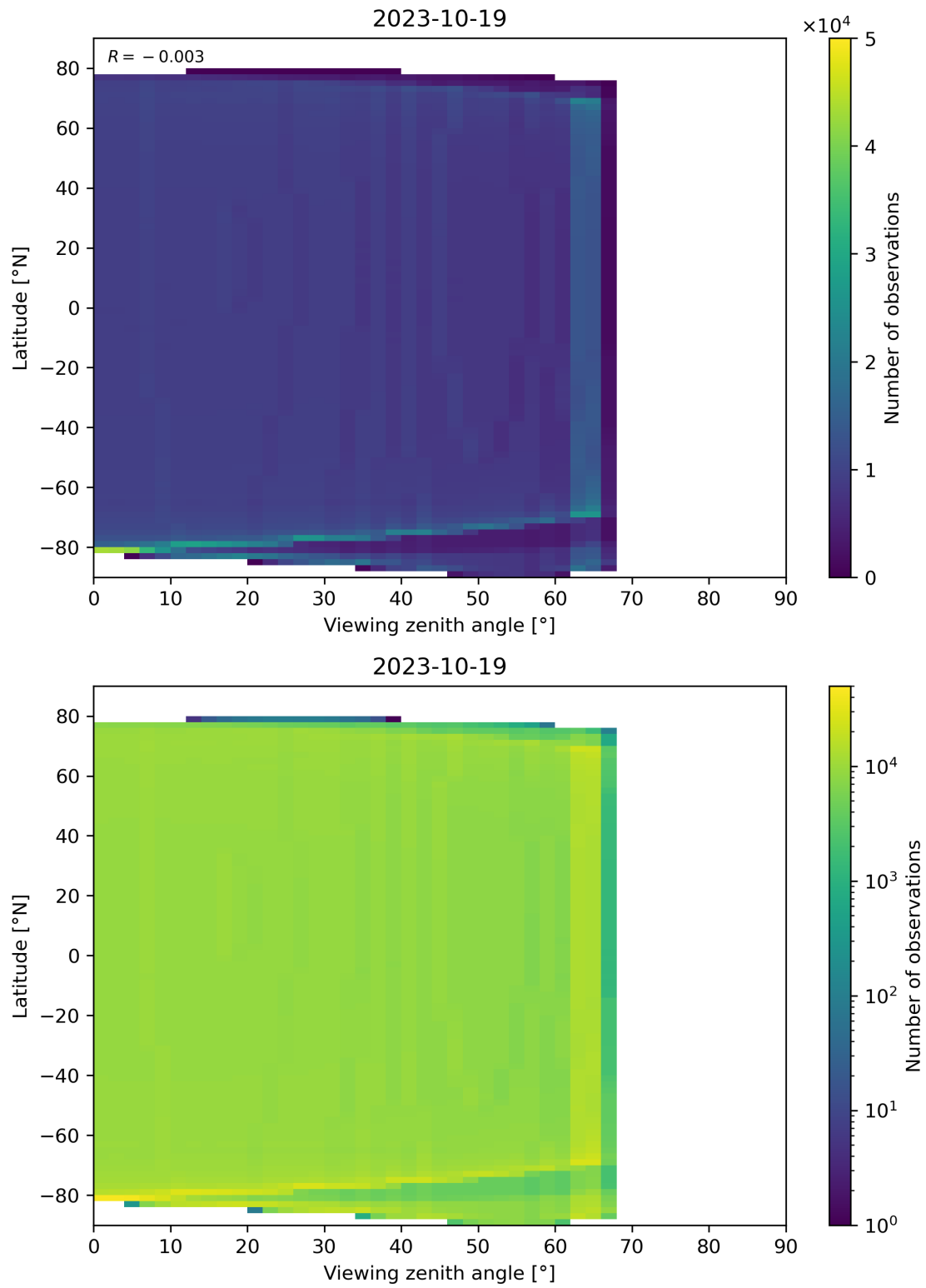
Figure 163: Scatter density plot of “Viewing zenith angle” against “Latitude” for 2023-10-18 to 2023-10-20.
