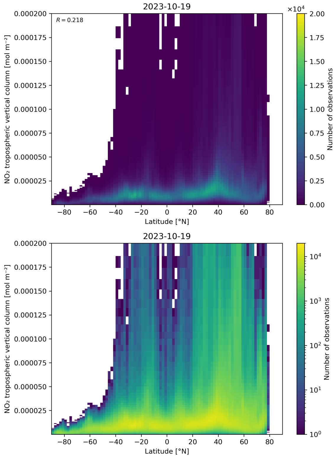
Figure 92: Scatter density plot of “Latitude” against “NO 2 tropospheric vertical column” for 2023-10-18 to 2023-10-20.
