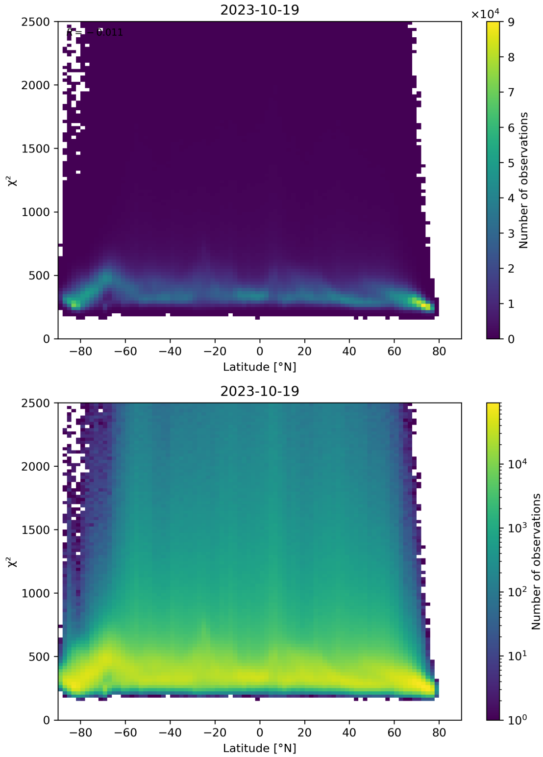
Figure 86: Scatter density plot of “Latitude” against “ \chi^2 ” for 2023-10-18 to 2023-10-20.
