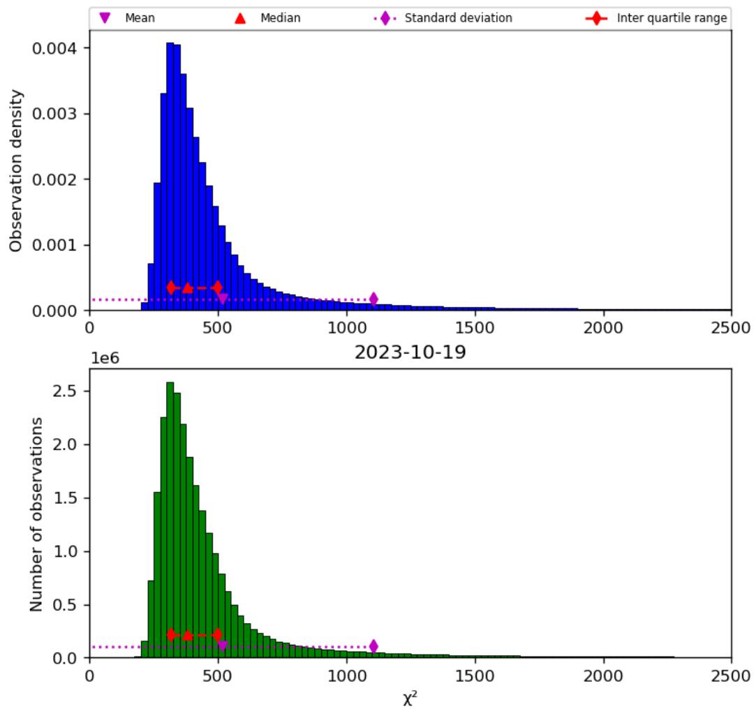
Figure 42: Histogram of “ \chi^2 ” for 2023-10-18 to 2023-10-20
