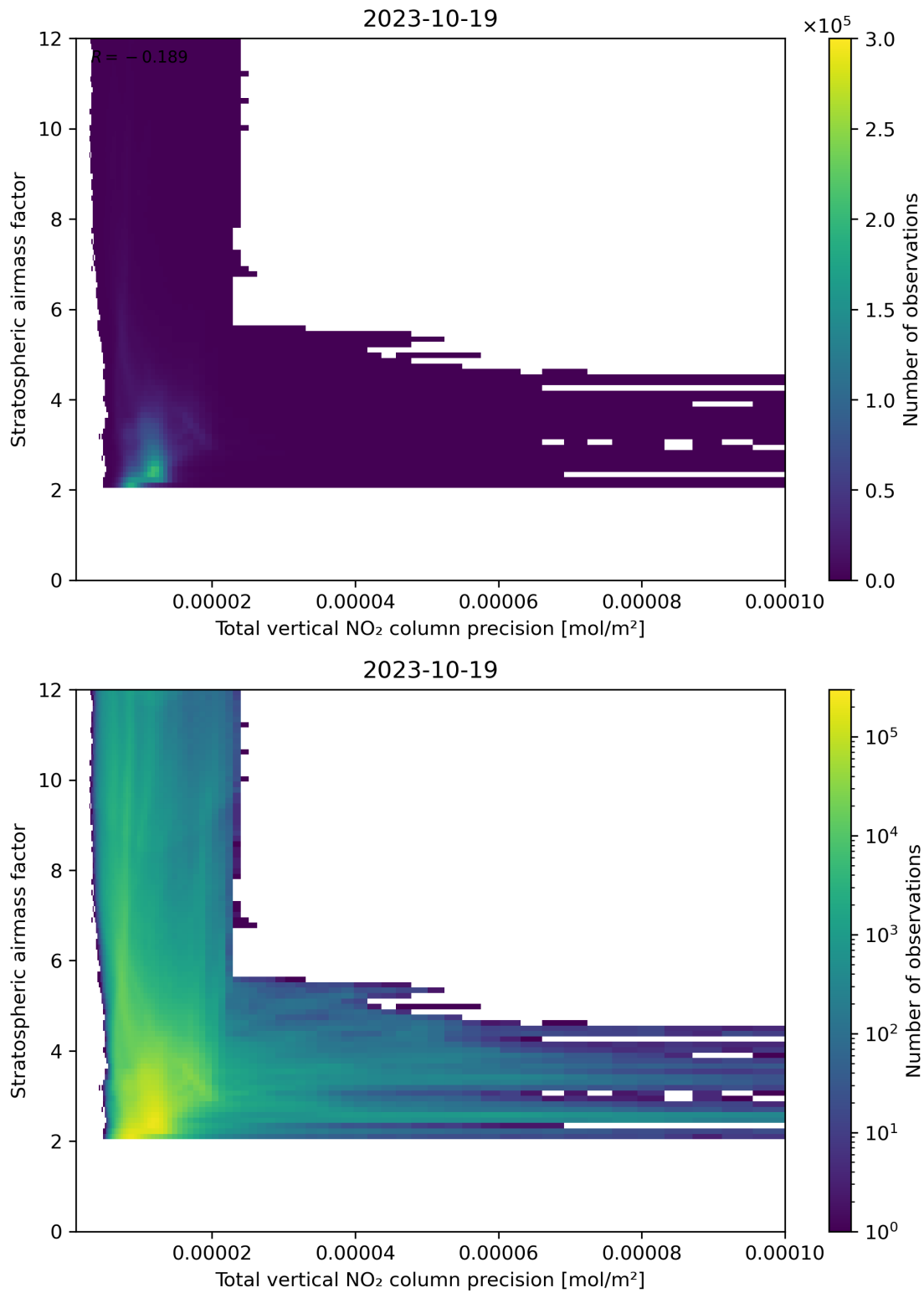
Figure 115: Scatter density plot of “Total vertical NO 2 column precision” against “Stratospheric air mass factor” for 2023-10-18 to 2023-10-20.
