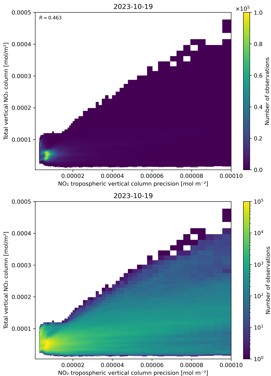
Figure 138: Scatter density plot of “NO 2 tropospheric vertical column precision” against “Total vertical NO 2 column” for 2023-10-18 to 2023-10-20.
