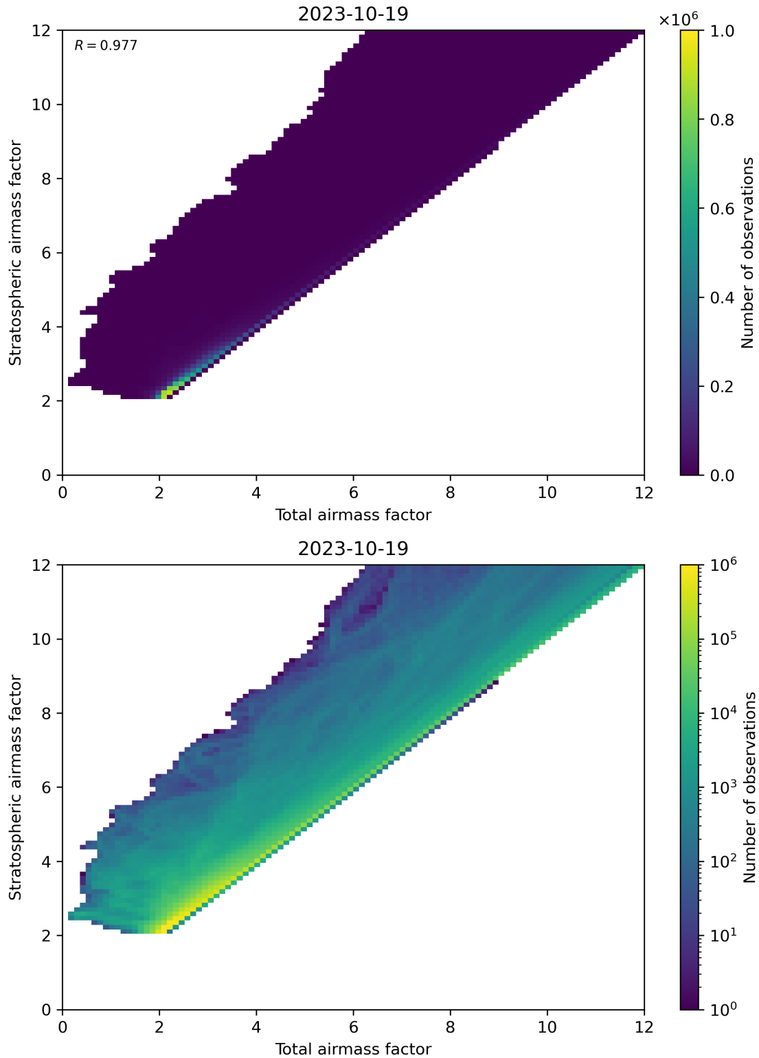
Figure 62: Scatter density plot of “Total airmass factor” against “Stratospheric airmass factor” for 2023-10-18 to 2023-10-20.
