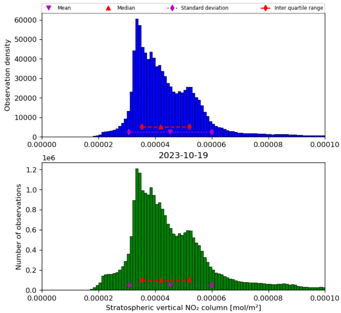
Figure 36: Histogram of “Stratospheric vertical NO 2 column” for 2023-10-18 to 2023-10-20
