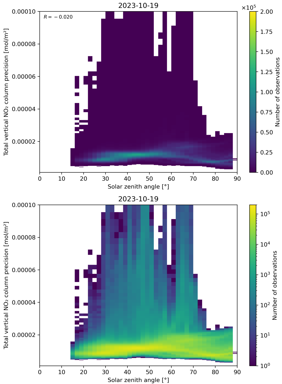
Figure 154: Scatter density plot of “Solar zenith angle” against “Total vertical NO 2 column precision” for 2023-10-18 to 2023-10-20.
