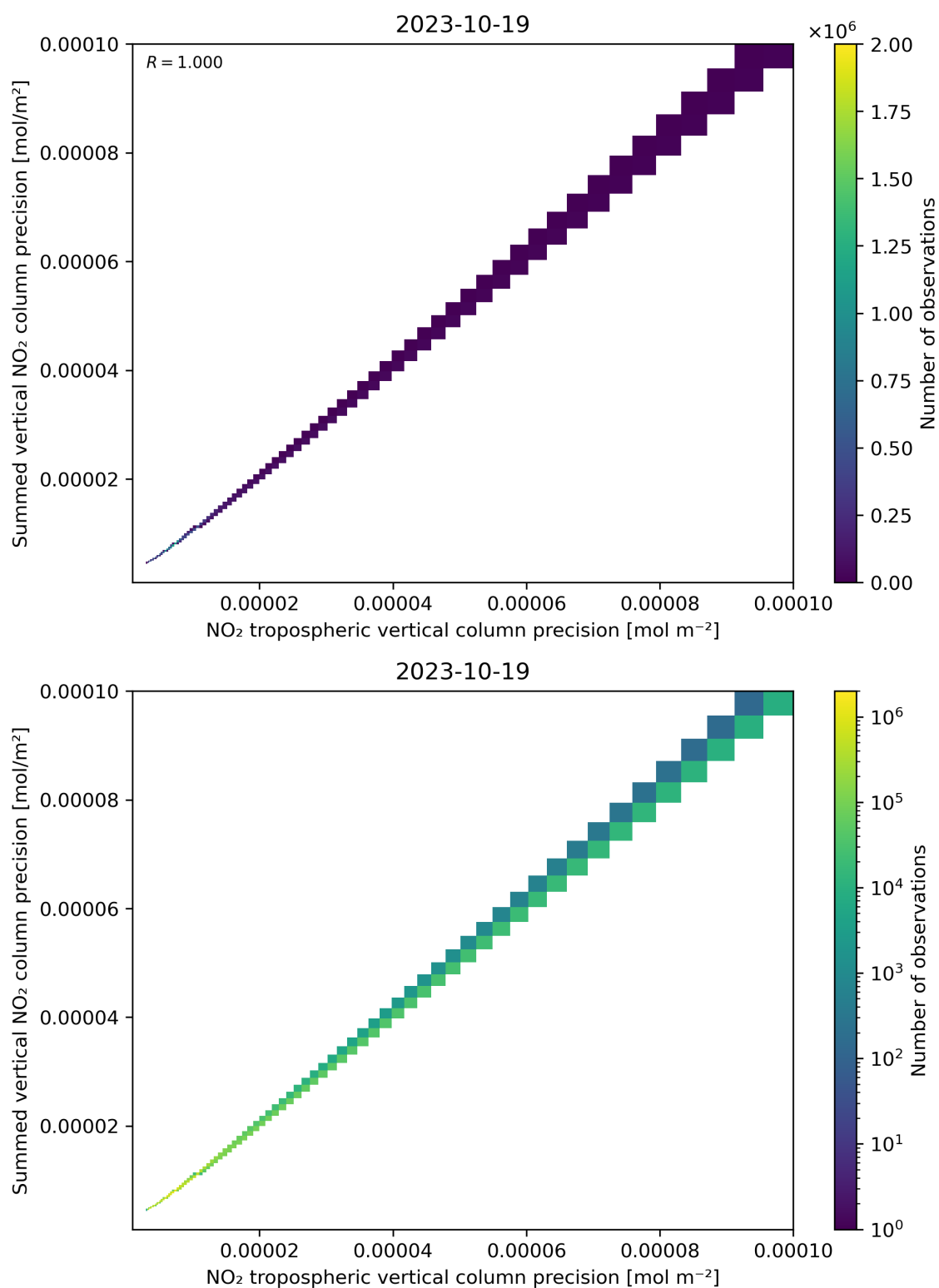
Figure 137: Scatter density plot of “NO 2 tropospheric vertical column precision” against “Summed vertical NO 2 column precision” for 2023-10-18 to 2023-10-20.
