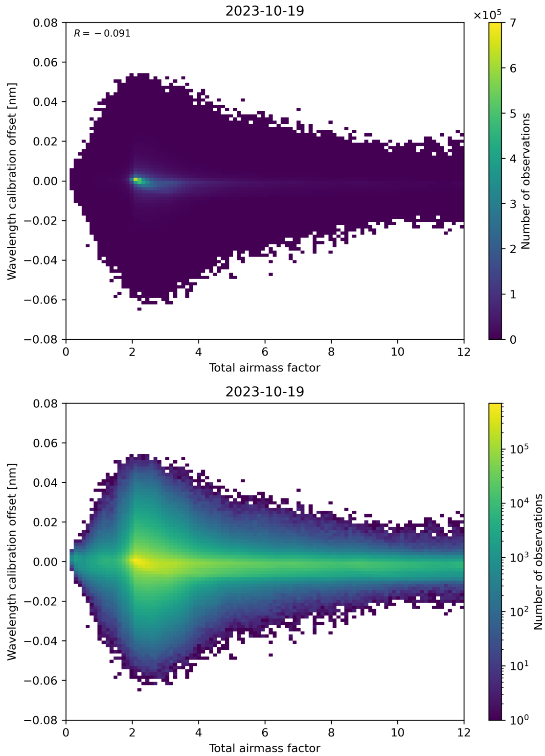
Figure 70: Scatter density plot of “Total airmass factor” against “Wavelength calibration offset” for 2023-10-18 to 2023-10-20.
