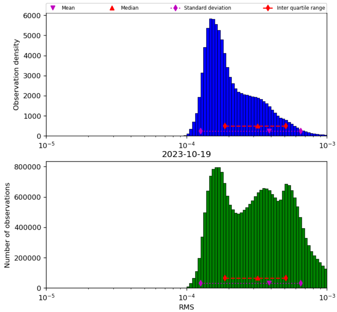
Figure 43: Histogram of “RMS” for 2023-10-18 to 2023-10-20
