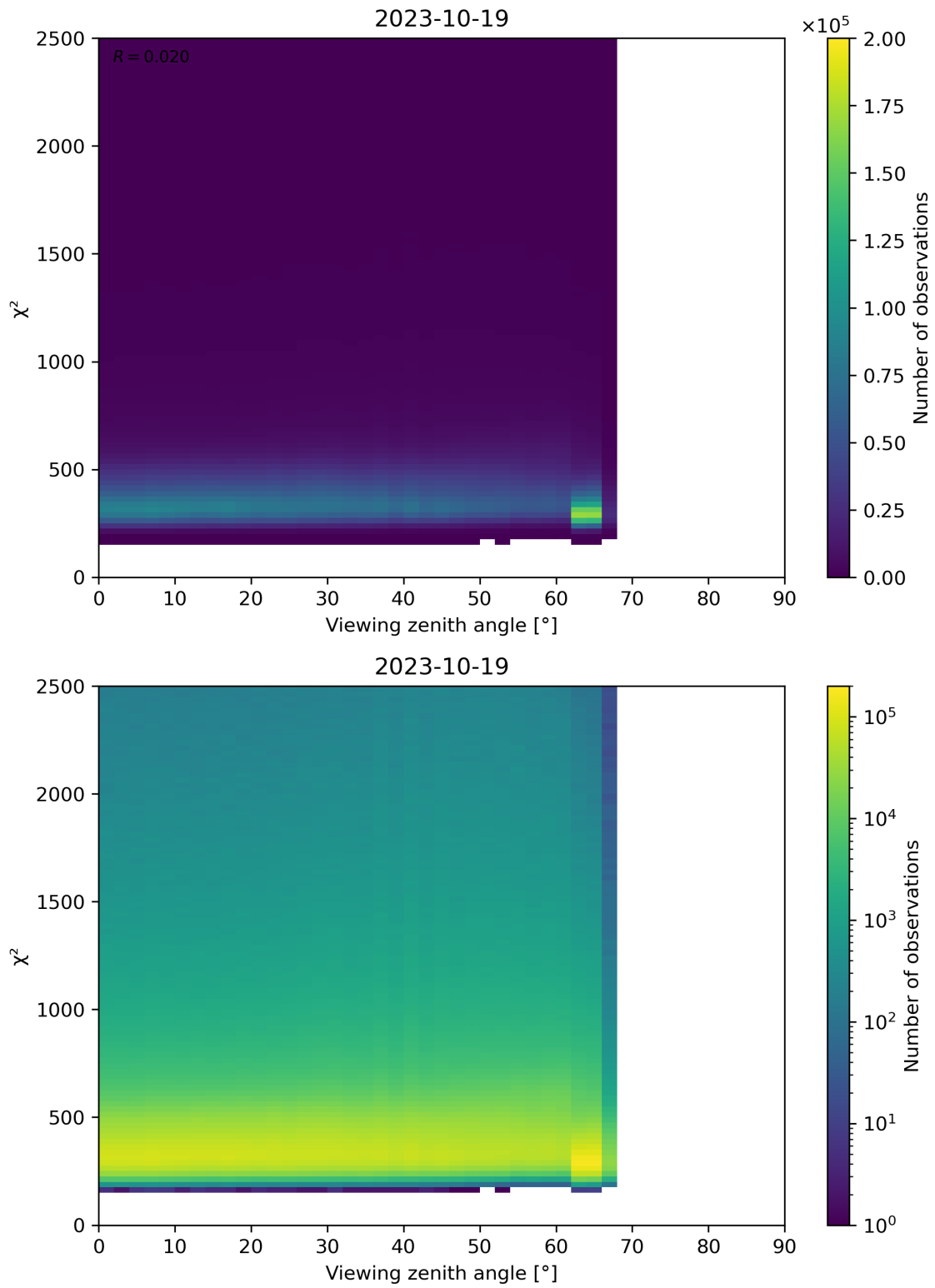
Figure 162: Scatter density plot of “Viewing zenith angle” against “ \chi^2 ” for 2023-10-18 to 2023-10-20.
