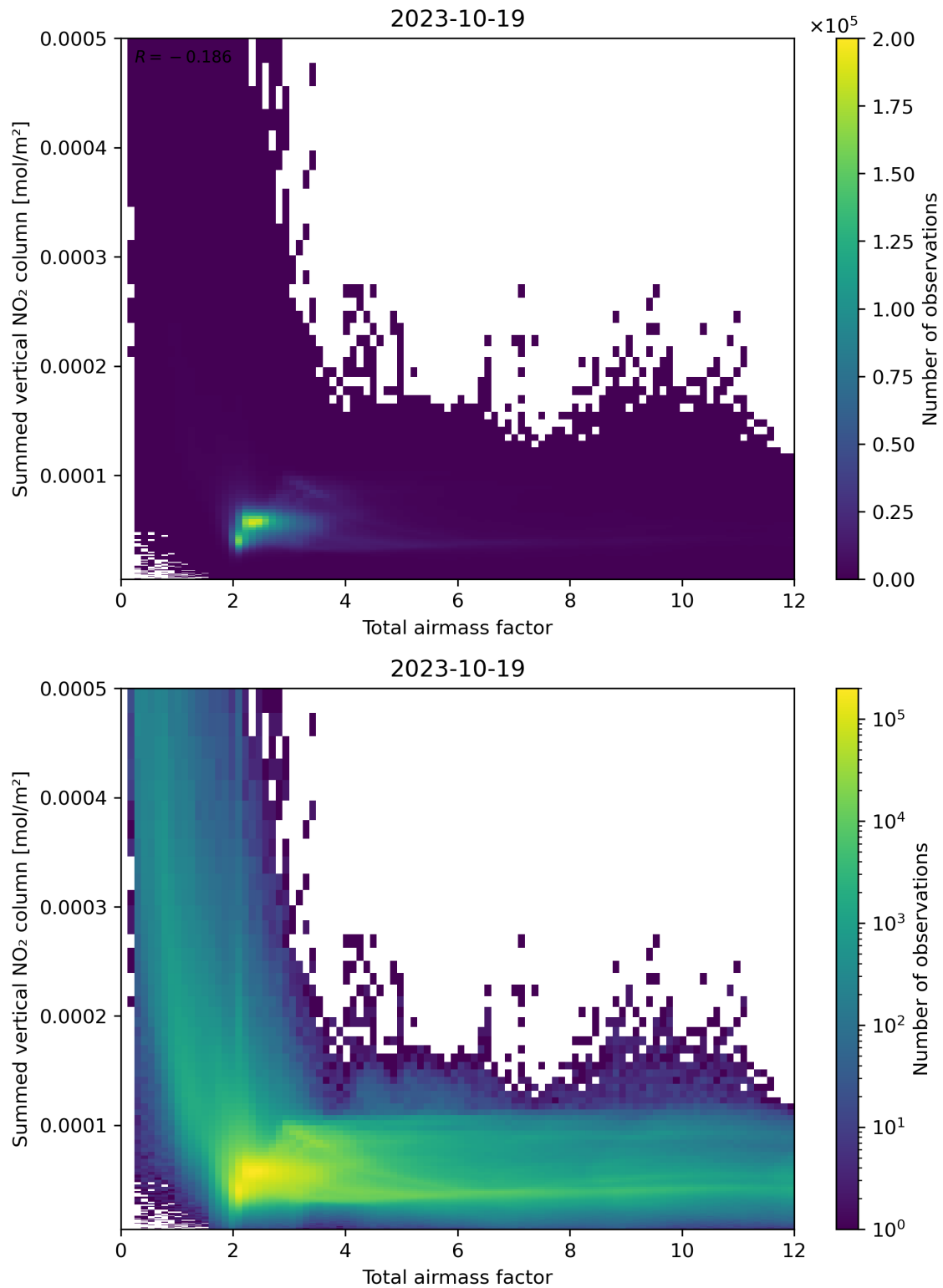
Figure 65: Scatter density plot of “Total airmass factor” against “Summed vertical NO 2 column” for 2023-10-18 to 2023-10-20.
