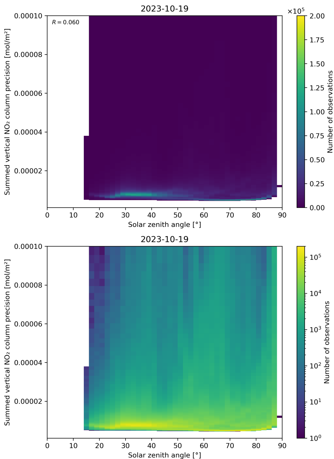
Figure 152: Scatter density plot of “Solar zenith angle” against “Summed vertical NO 2 column precision” for 2023-10-18 to 2023-10-20.
