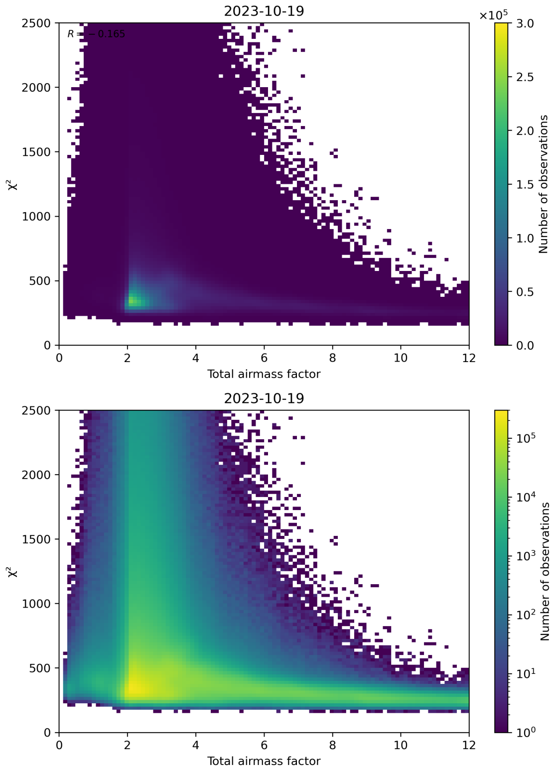
Figure 63: Scatter density plot of “Total airmass factor” against “ \chi^2 ” for 2023-10-18 to 2023-10-20.
