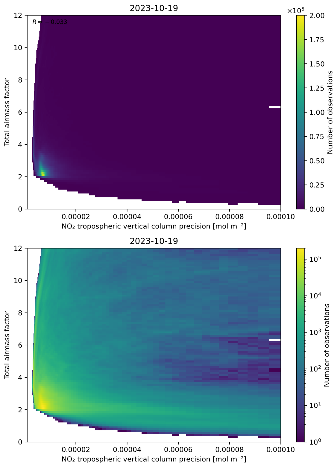
Figure 132: Scatter density plot of “NO 2 tropospheric vertical column precision” against “Total air mass factor” for 2023-10-18 to 2023-10-20.
