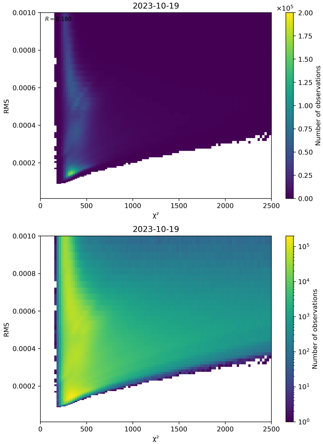
Figure 82: Scatter density plot of “ \chi^2 ” against “RMS” for 2023-10-18 to 2023-10-20.
