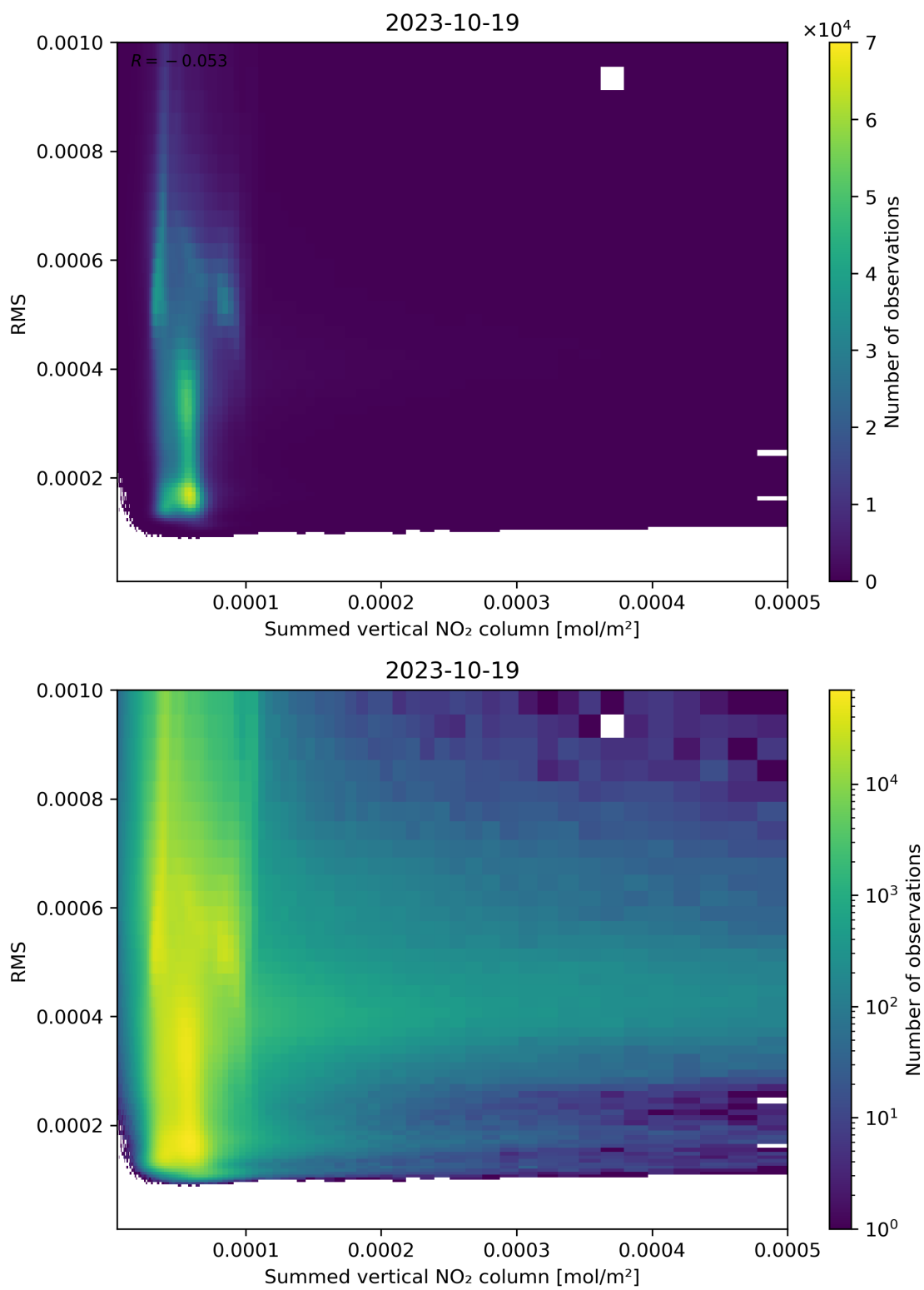
Figure 109: Scatter density plot of “Summed vertical NO 2 column” against “RMS” for 2023-10-18 to 2023-10-20.
