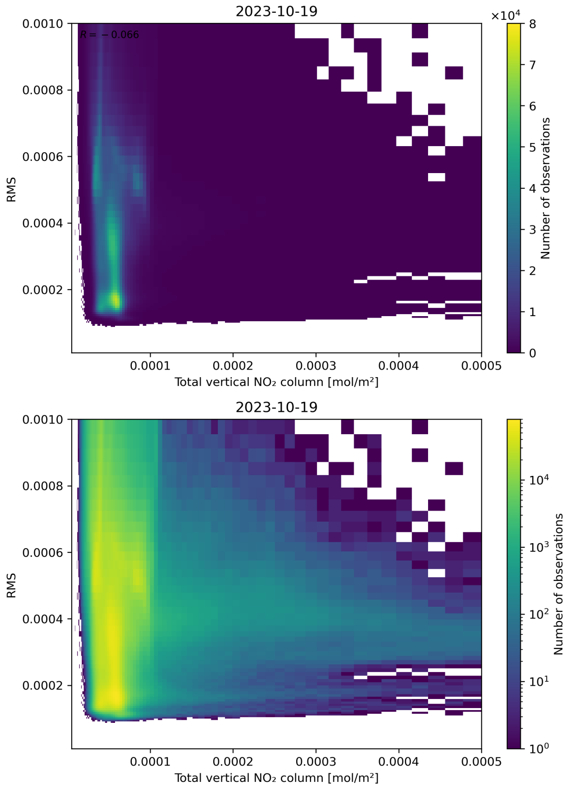
Figure 120: Scatter density plot of “Total vertical NO 2 column” against “RMS” for 2023-10-18 to 2023-10-20.
