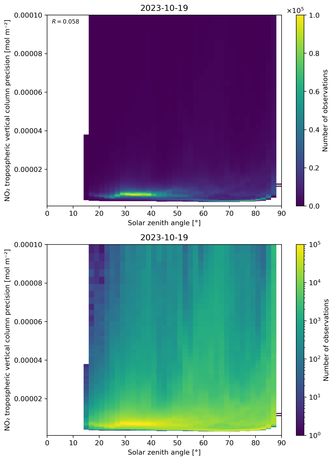
Figure 156: Scatter density plot of “Solar zenith angle” against “NO 2 tropospheric vertical column precision” for 2023-10-18 to 2023-10-20.
