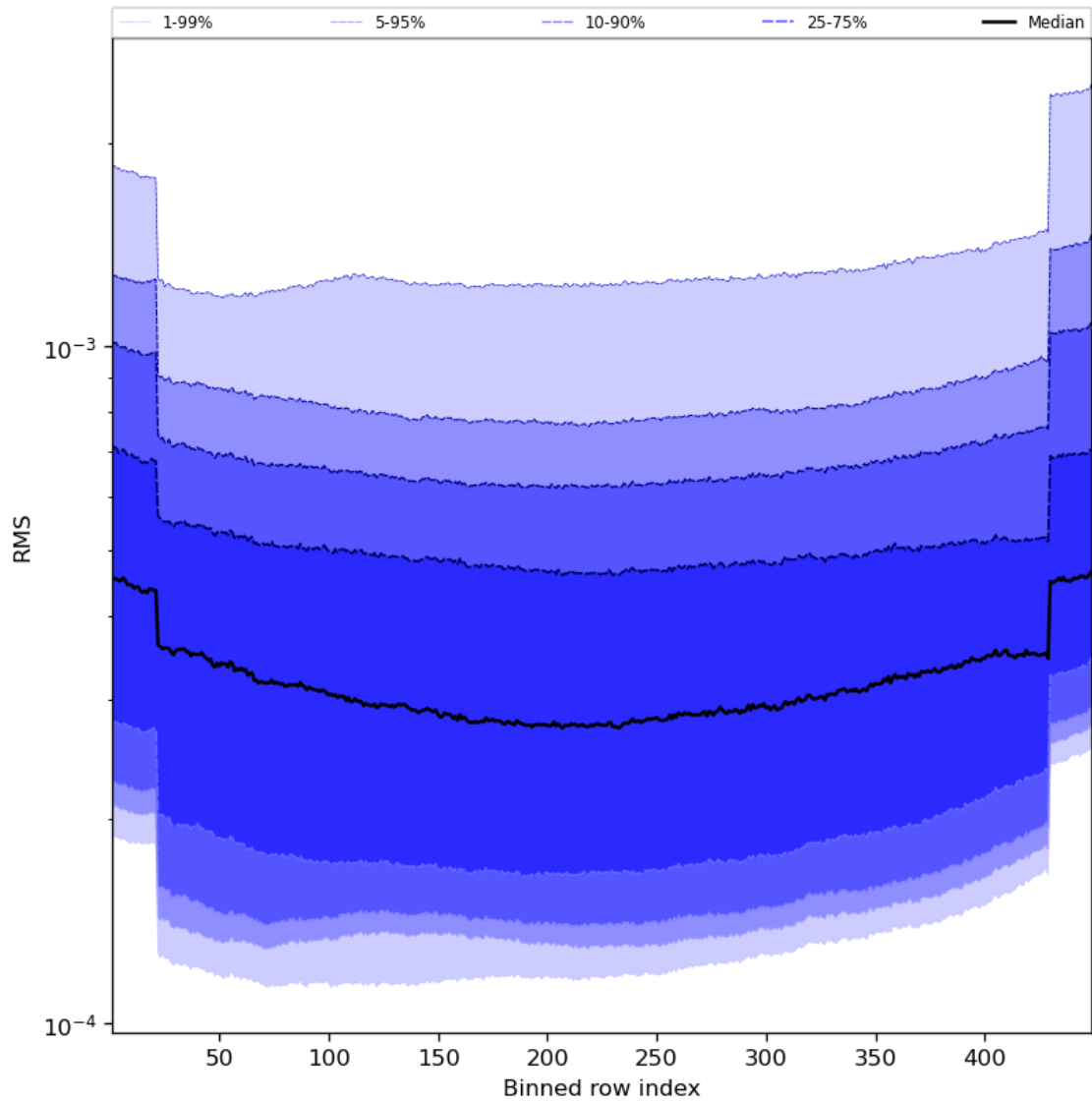
Figure 60: Along track statistics of “RMS” for 2023-10-18 to 2023-10-20
