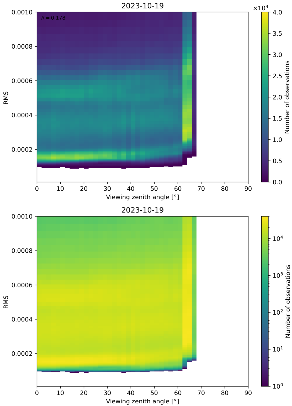
Figure 171: Scatter density plot of “Viewing zenith angle” against “RMS” for 2023-10-18 to 2023-10-20.
