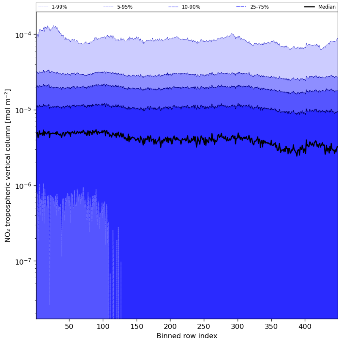
Figure 46: Along track statistics of “NO 2 tropospheric vertical column” for 2023-10-18 to 2023-10-20
