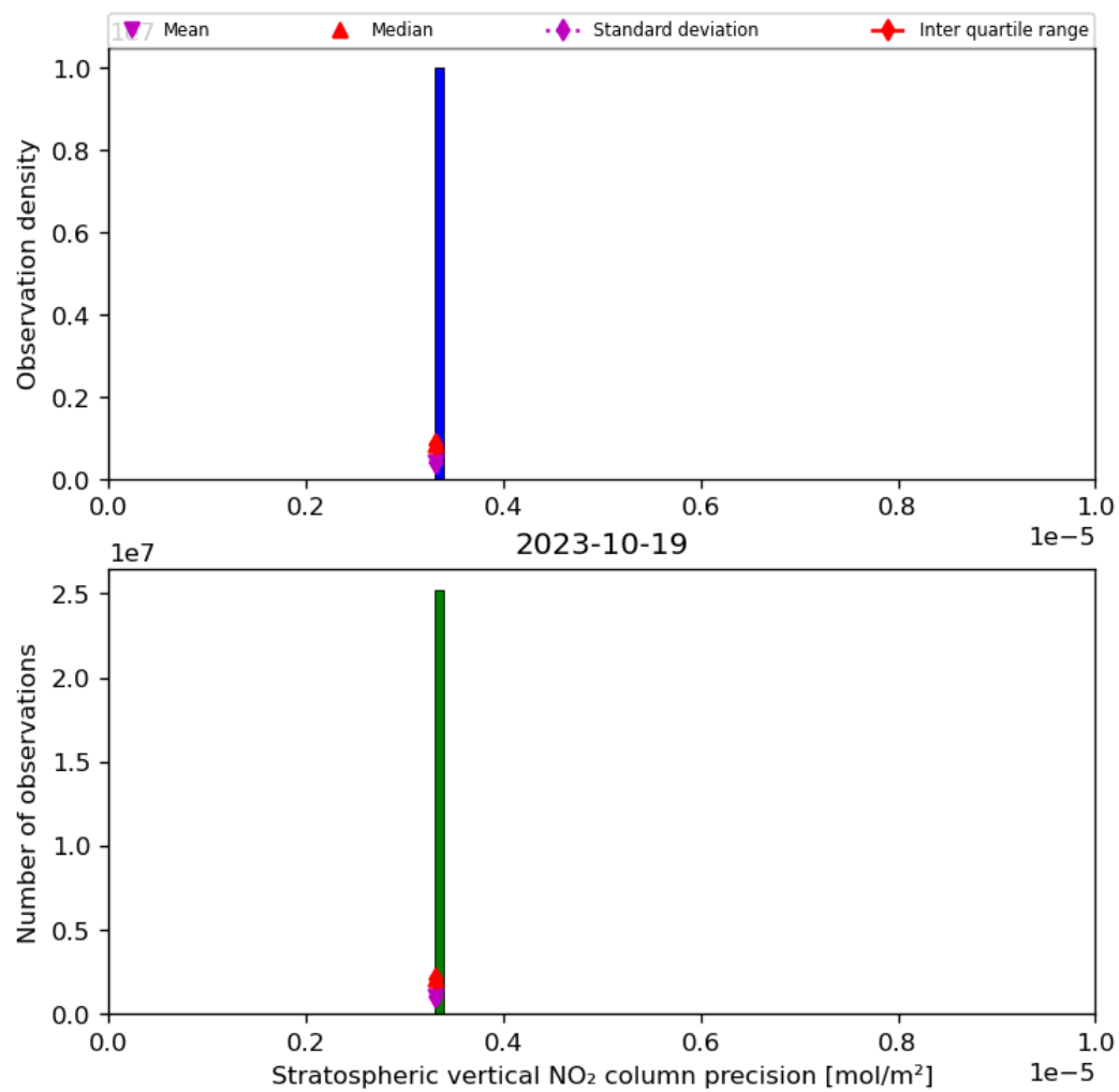
Figure 37: Histogram of “Stratospheric vertical NO 2 column precision” for 2023-10-18 to 2023-10-20
