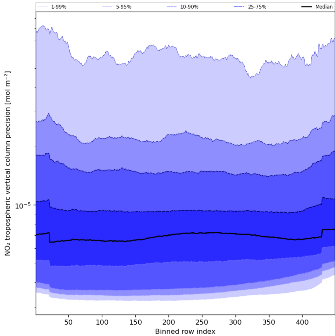
Figure 47: Along track statistics of “NO 2 tropospheric vertical column precision” for 2023-10-18 to 2023-10-20
