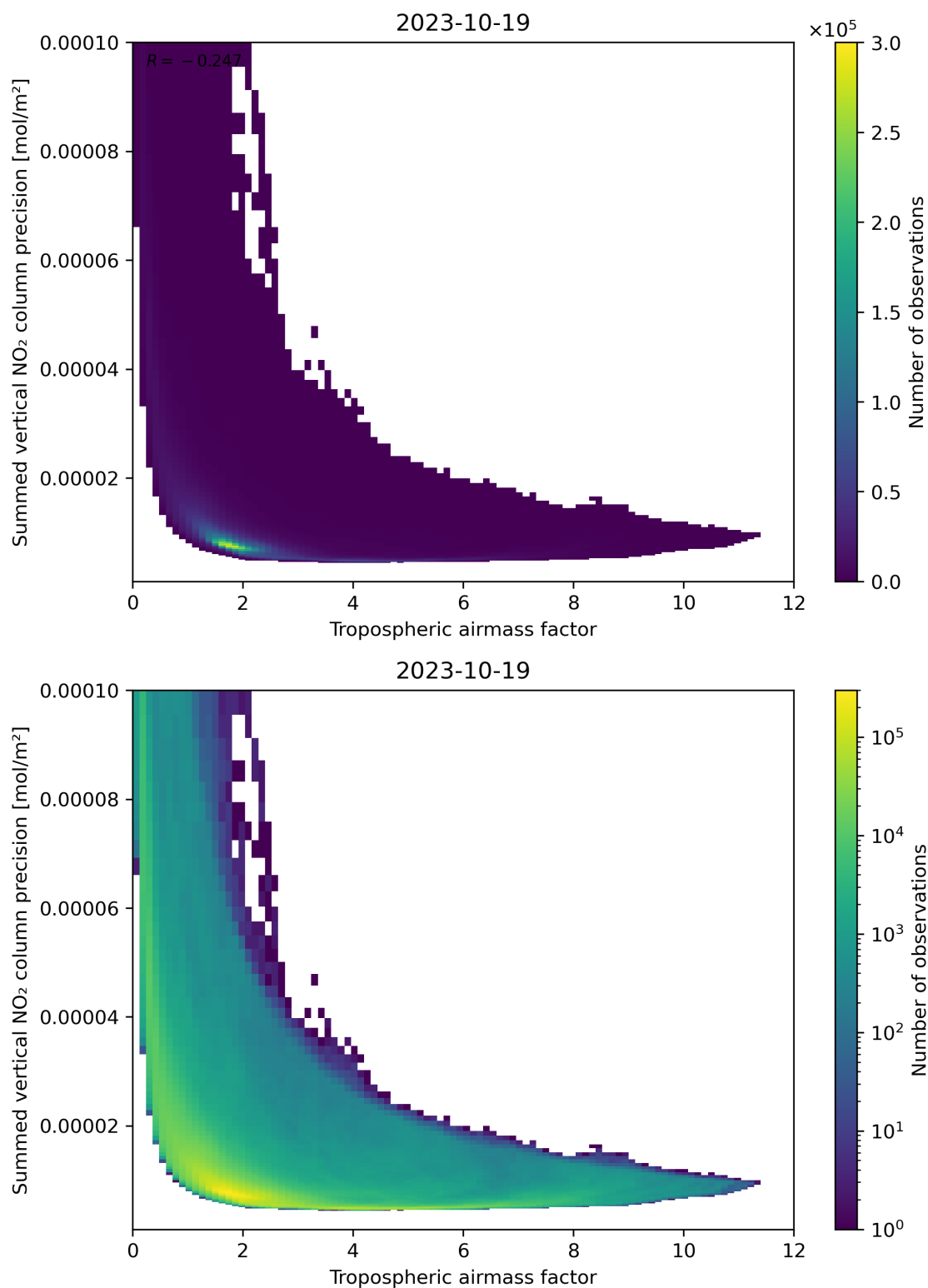
Figure 76: Scatter density plot of “Tropospheric air mass factor” against “Summed vertical NO 2 column precision” for 2023-10-18 to 2023-10-20.
