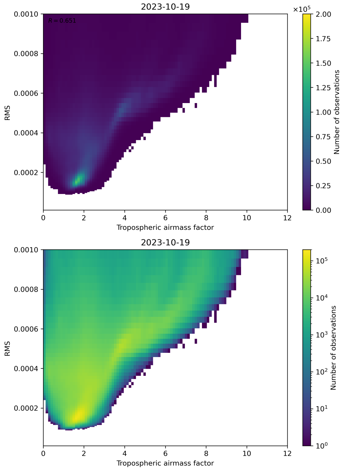
Figure 79: Scatter density plot of “Tropospheric airmass factor” against “RMS” for 2023-10-18 to 2023-10-20.
