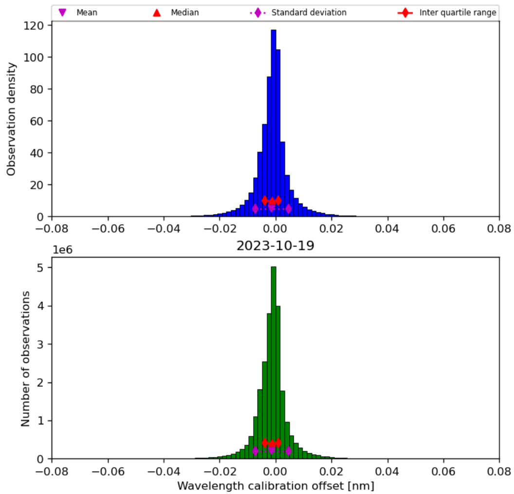
Figure 35: Histogram of “Wavelength calibration offset” for 2023-10-18 to 2023-10-20
