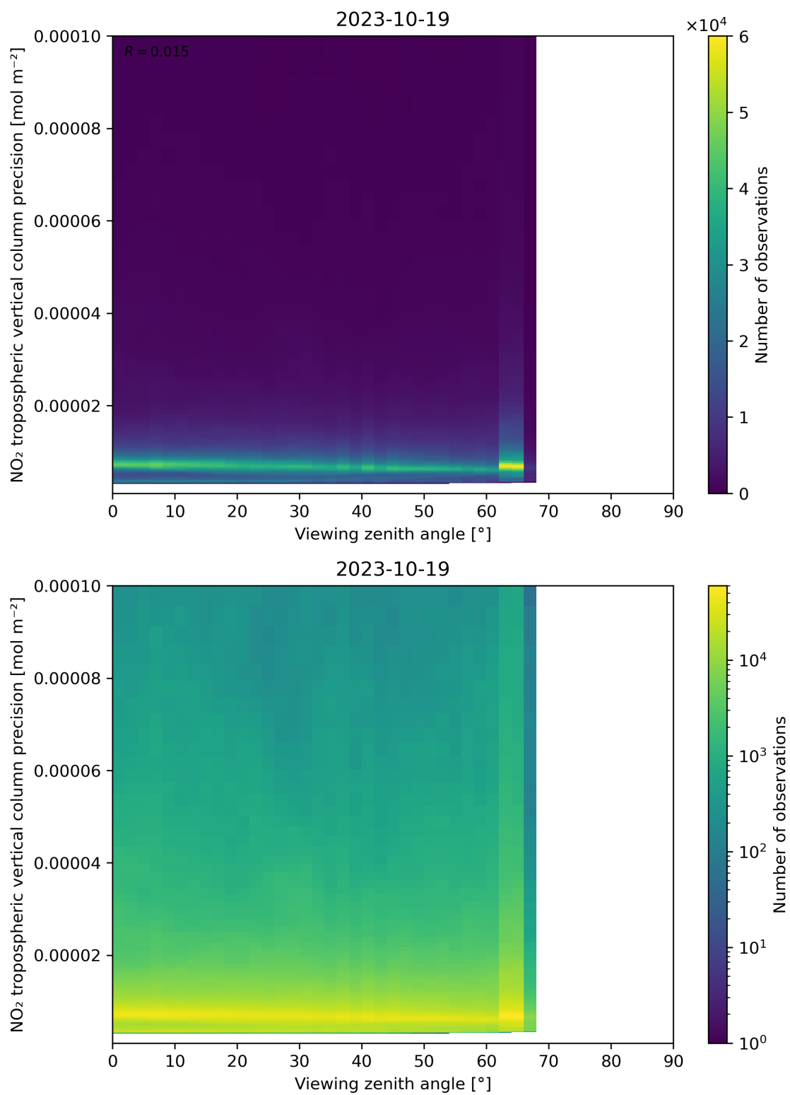
Figure 170: Scatter density plot of “Viewing zenith angle” against “NO 2 tropospheric vertical column precision” for 2023-10-18 to 2023-10-20.
