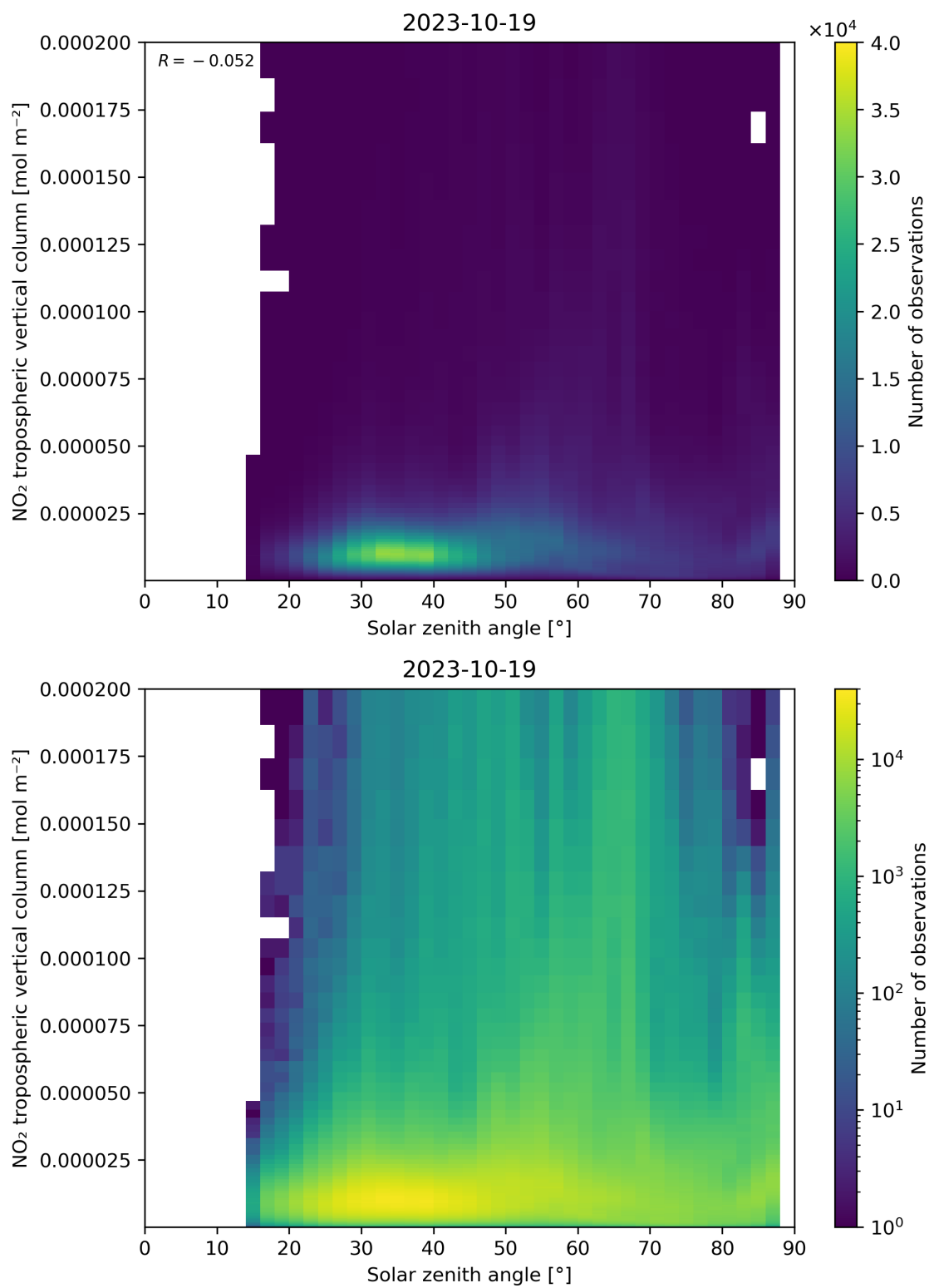
Figure 155: Scatter density plot of “Solar zenith angle” against “NO 2 tropospheric vertical column” for 2023-10-18 to 2023-10-20.
