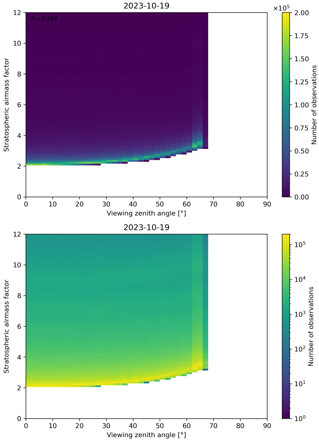
Figure 159: Scatter density plot of “Viewing zenith angle” against “Stratospheric airmass factor” for 2023-10-18 to 2023-10-20.
