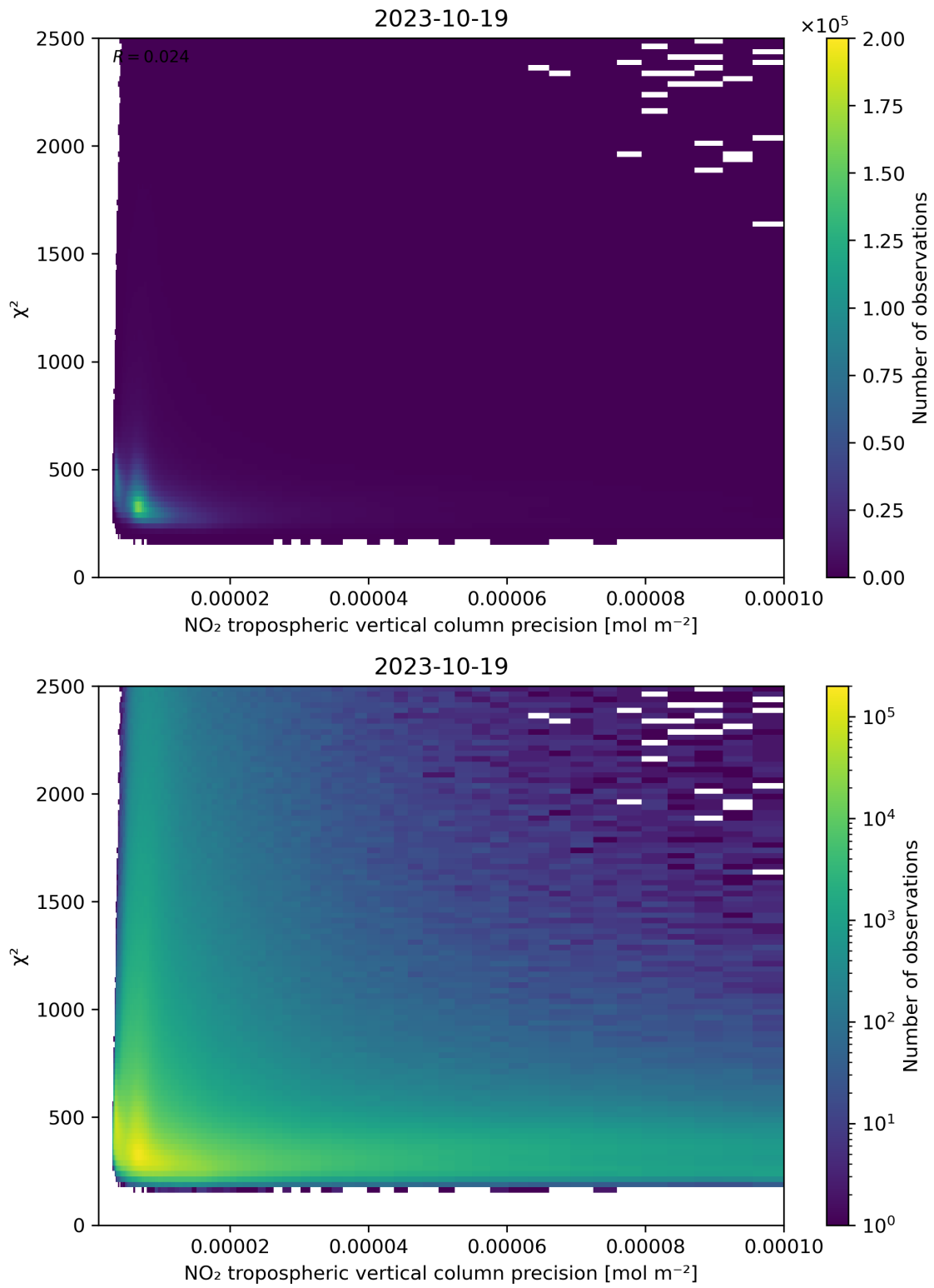
Figure 134: Scatter density plot of “NO 2 tropospheric vertical column precision” against “ \chi^2 ” for 2023-10-18 to 2023-10-20.
