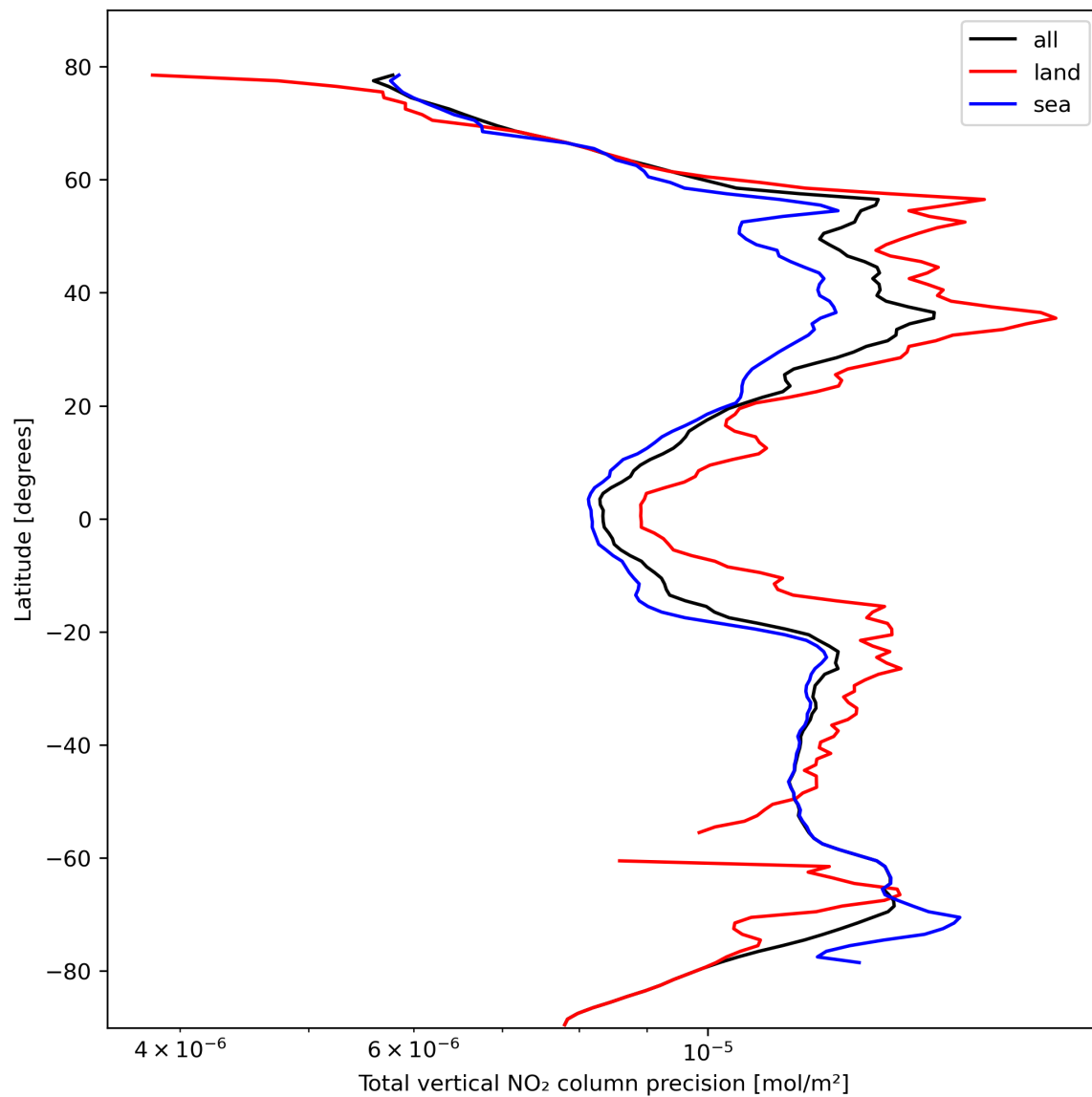
Figure 22: Zonal average of “Total vertical NO 2 column precision” for 2023-10-18 to 2023-10-20.
