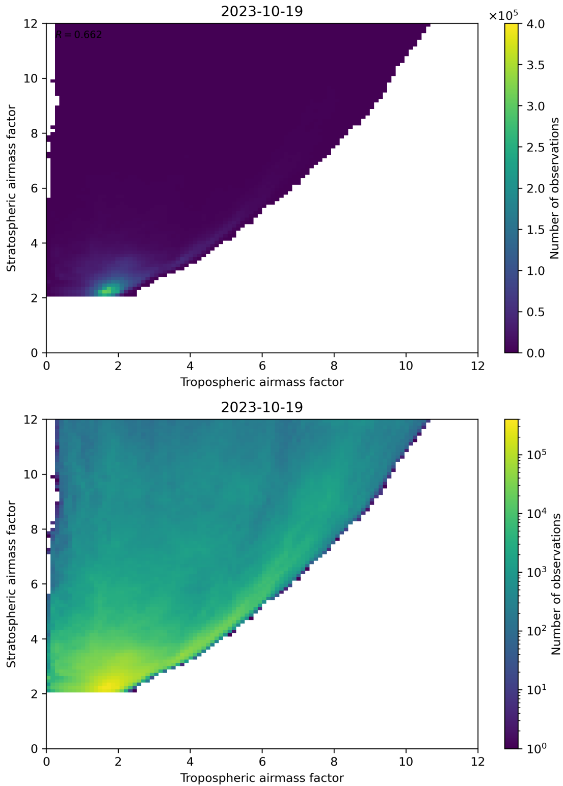
Figure 71: Scatter density plot of “Tropospheric airmass factor” against “Stratospheric airmass factor” for 2023-10-18 to 2023-10-20.
