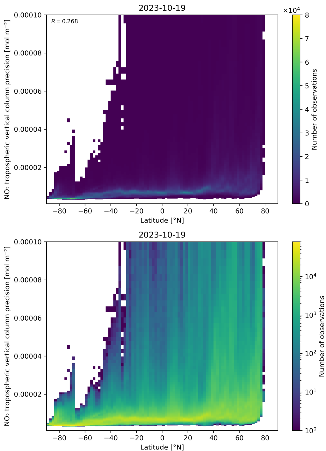
Figure 93: Scatter density plot of “Latitude” against “NO 2 tropospheric vertical column precision” for 2023-10-18 to 2023-10-20.
