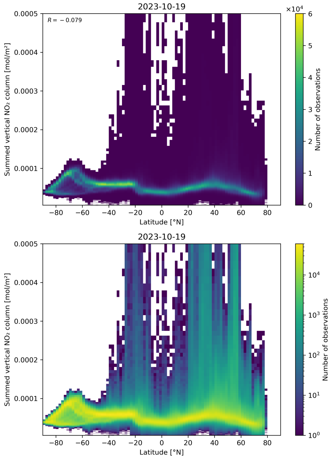
Figure 88: Scatter density plot of “Latitude” against “Summed vertical NO 2 column” for 2023-10-18 to 2023-10-20.
