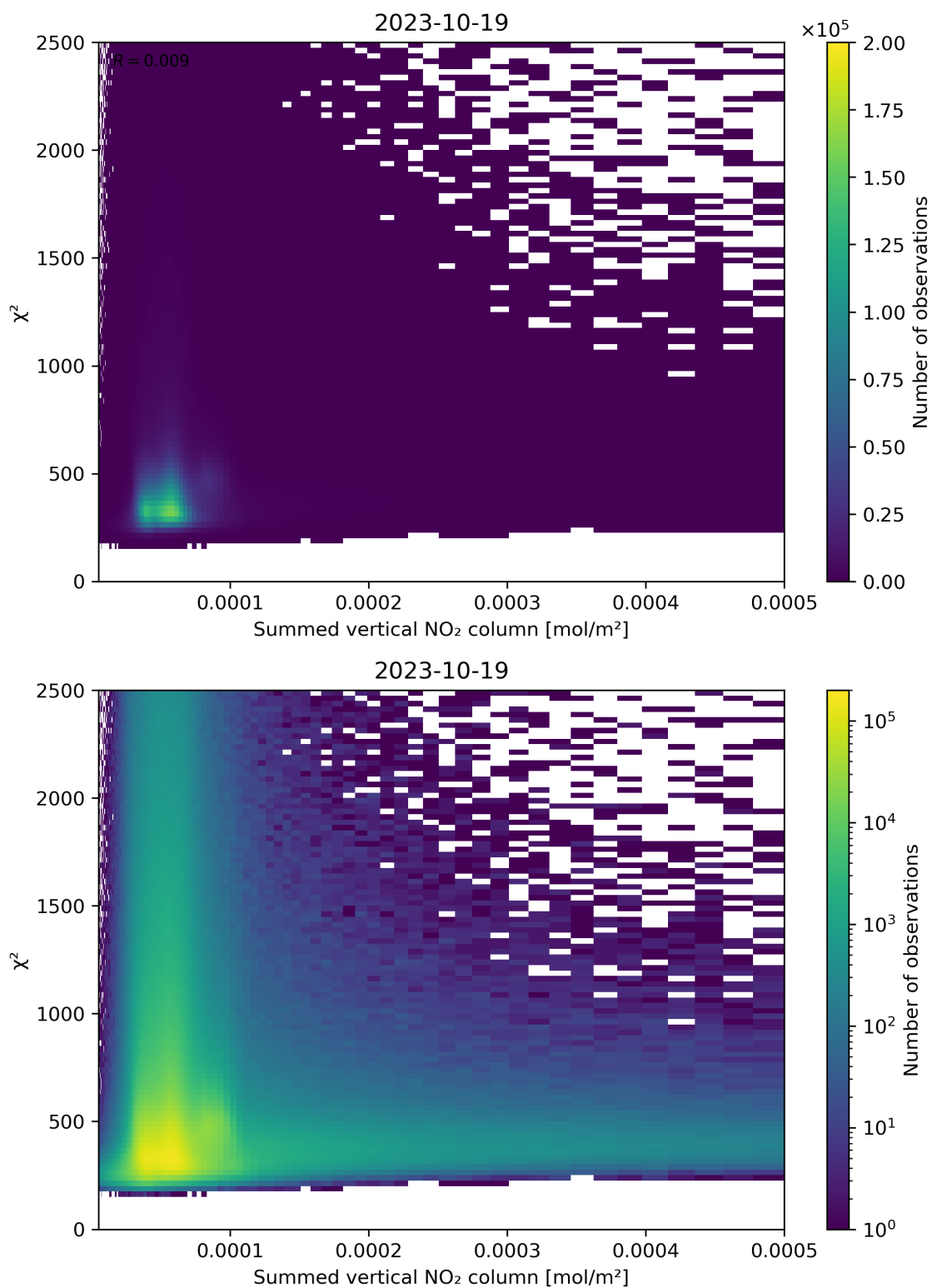
Figure 104: Scatter density plot of “Summed vertical NO 2 column” against “ \chi^2 ” for 2023-10-18 to 2023-10-20.
