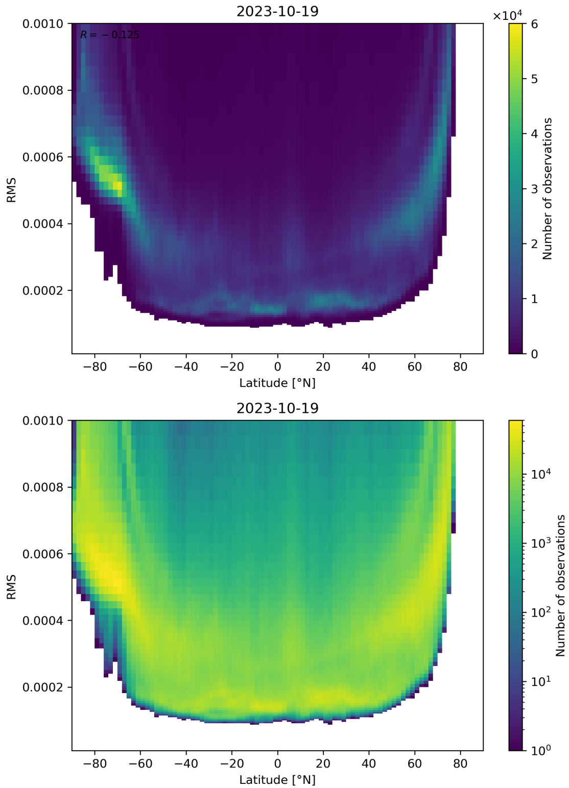
Figure 94: Scatter density plot of “Latitude” against “RMS” for 2023-10-18 to 2023-10-20.
