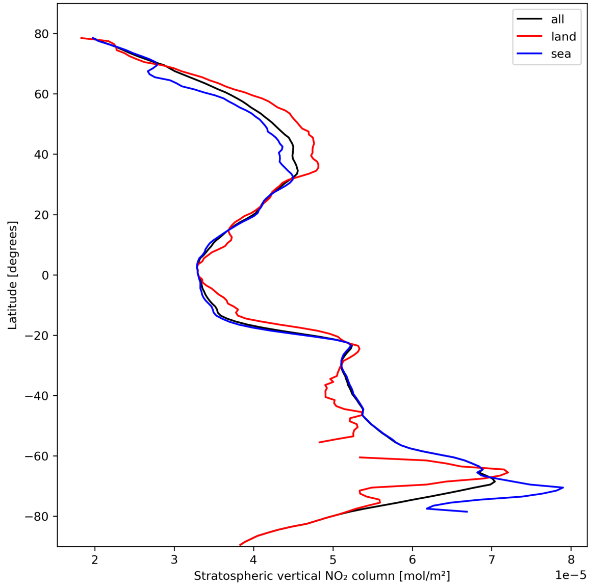
Figure 19: Zonal average of “Stratospheric vertical NO 2 column” for 2023-10-18 to 2023-10-20.
