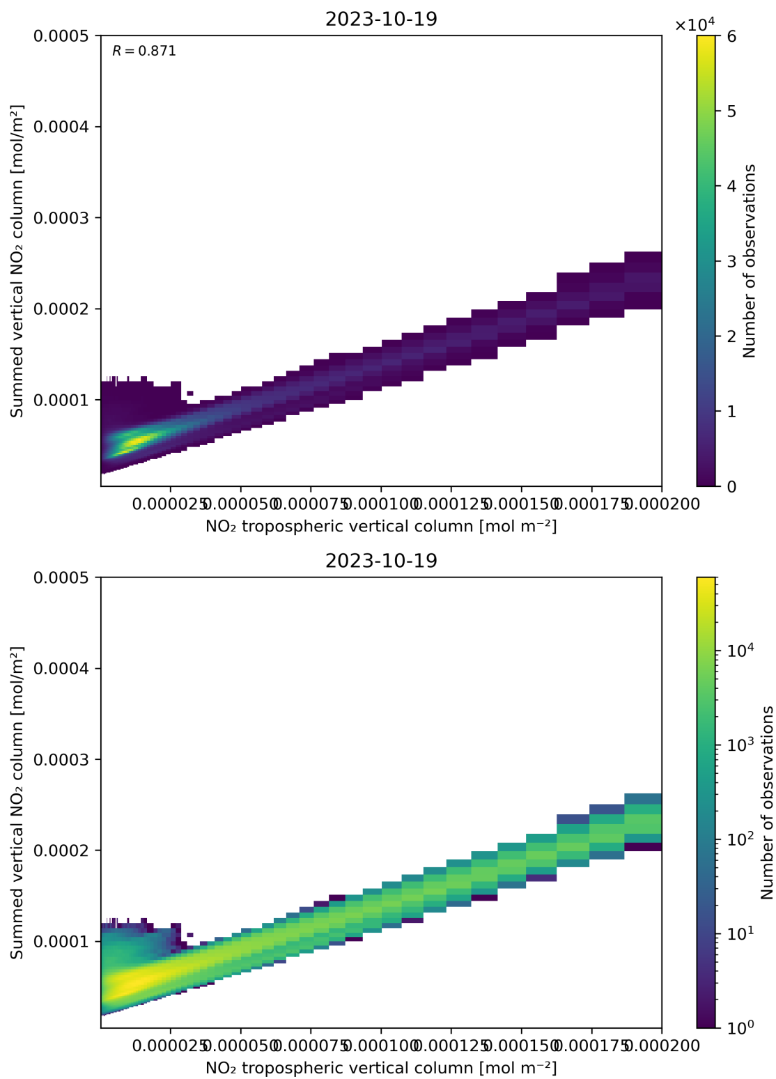
Figure 126: Scatter density plot of “NO 2 tropospheric vertical column” against “Summed vertical NO 2 column” for 2023-10-18 to 2023-10-20.
