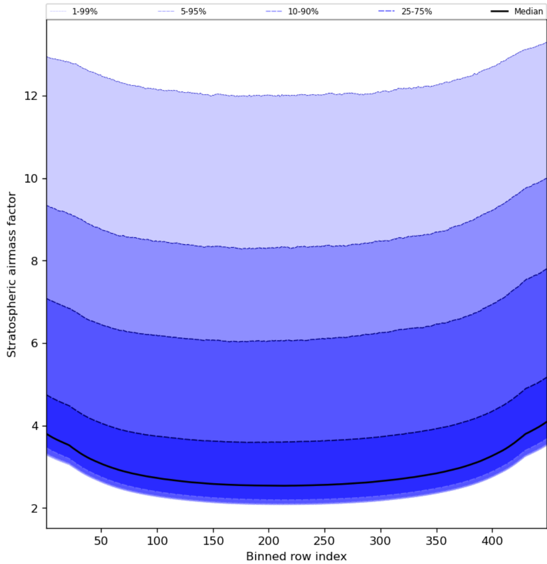
Figure 61: Along track statistics of “Stratospheric airmass factor” for 2023-10-18 to 2023-10-20
