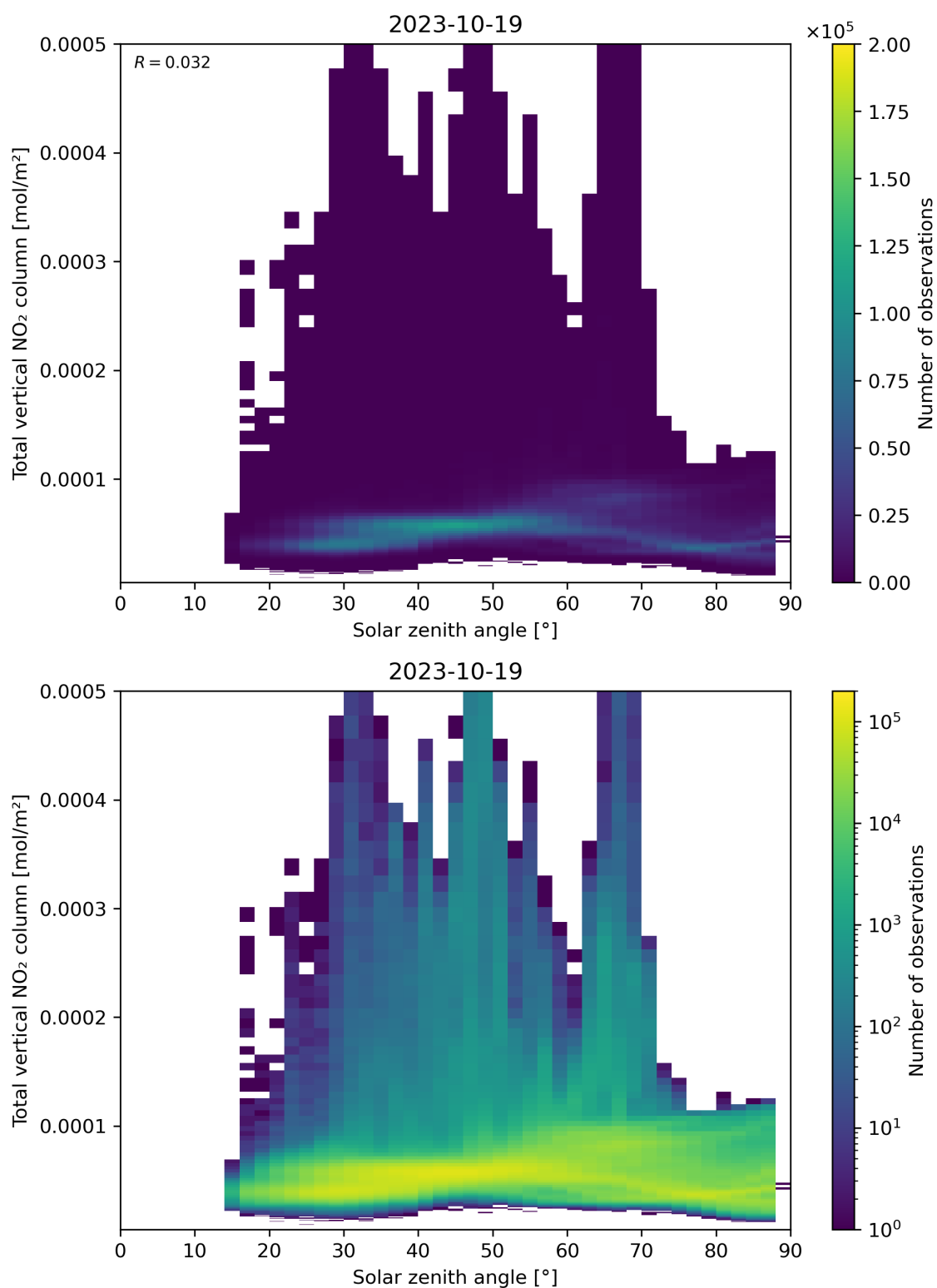
Figure 153: Scatter density plot of “Solar zenith angle” against “Total vertical NO 2 column” for 2023-10-18 to 2023-10-20.
