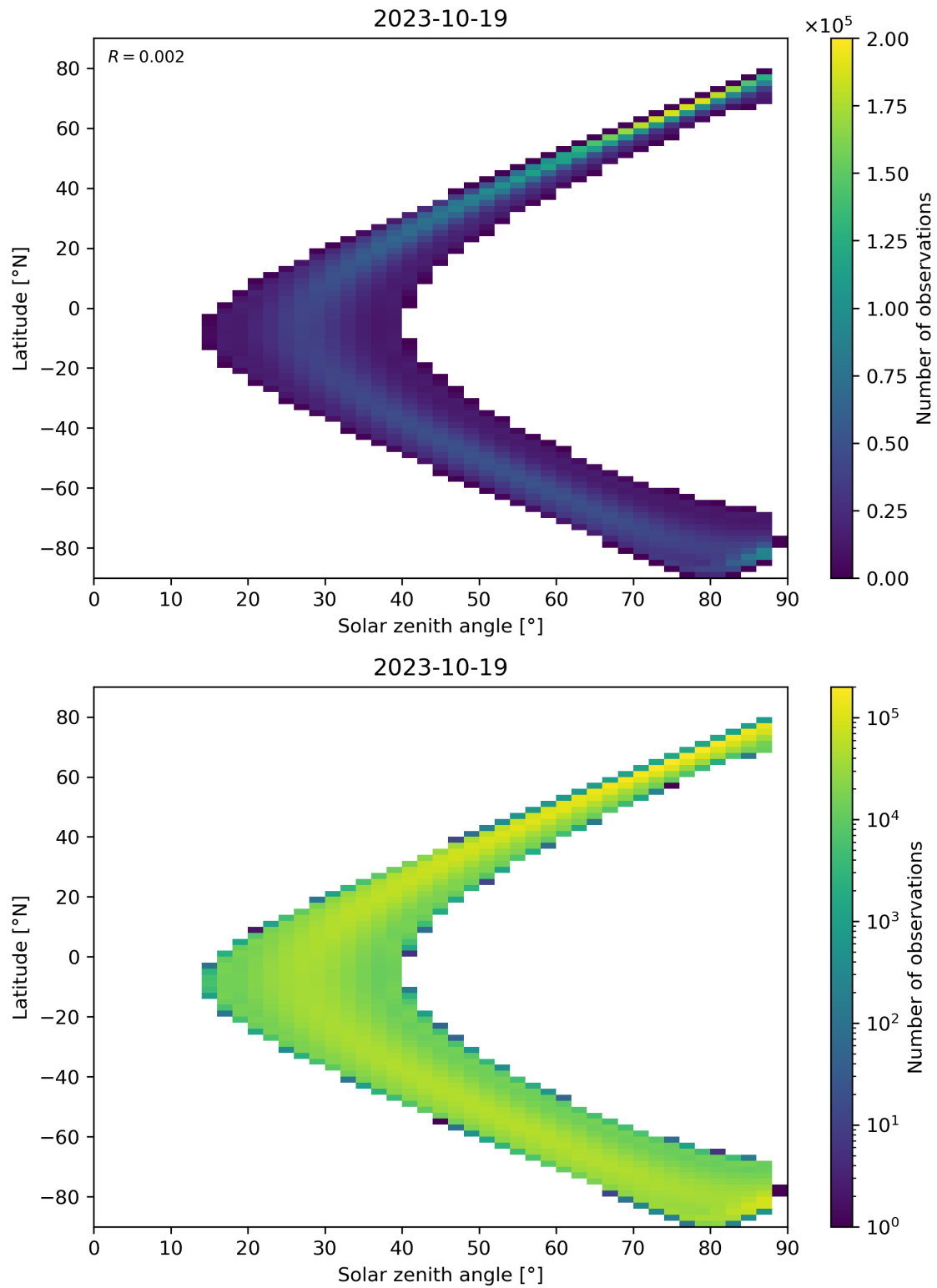
Figure 149: Scatter density plot of “Solar zenith angle” against “Latitude” for 2023-10-18 to 2023-10-20.
