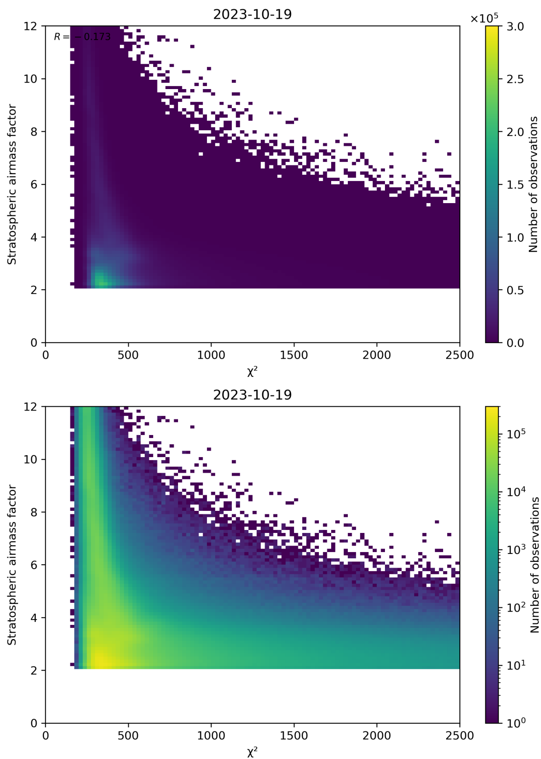
Figure 81: Scatter density plot of “ \chi^2 ” against “Stratospheric airmass factor” for 2023-10-18 to 2023-10-20.
