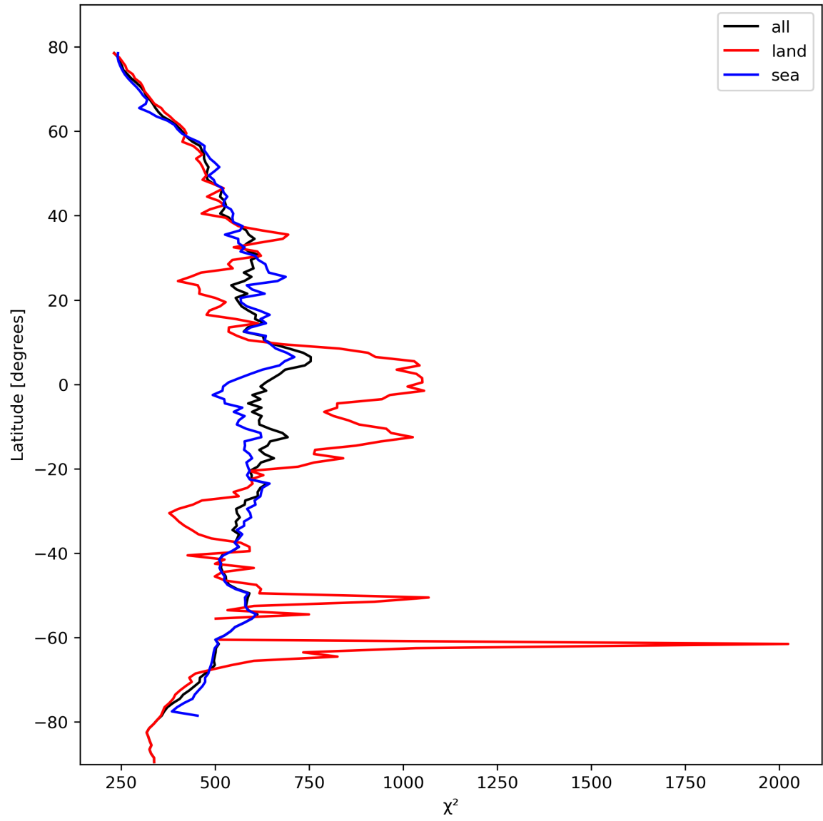
Figure 25: Zonal average of “ \chi^2 ” for 2023-10-18 to 2023-10-20.
