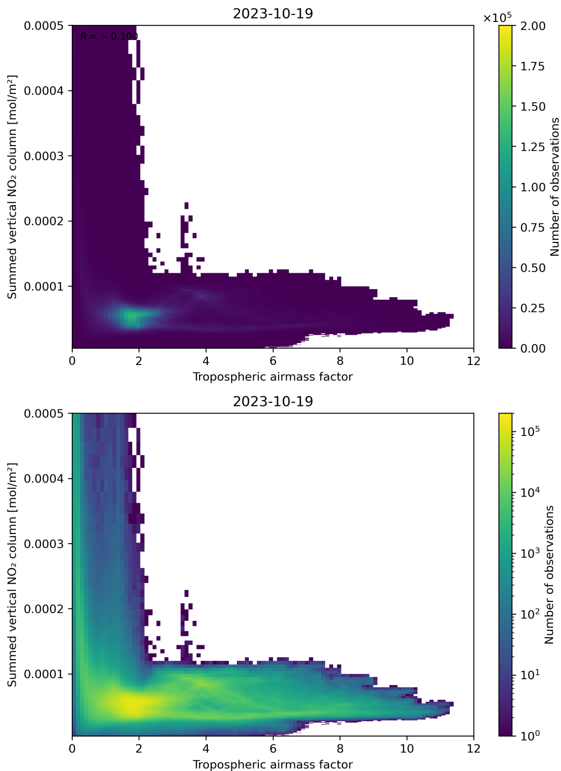
Figure 75: Scatter density plot of “Tropospheric air mass factor” against “Summed vertical NO 2 column” for 2023-10-18 to 2023-10-20.
