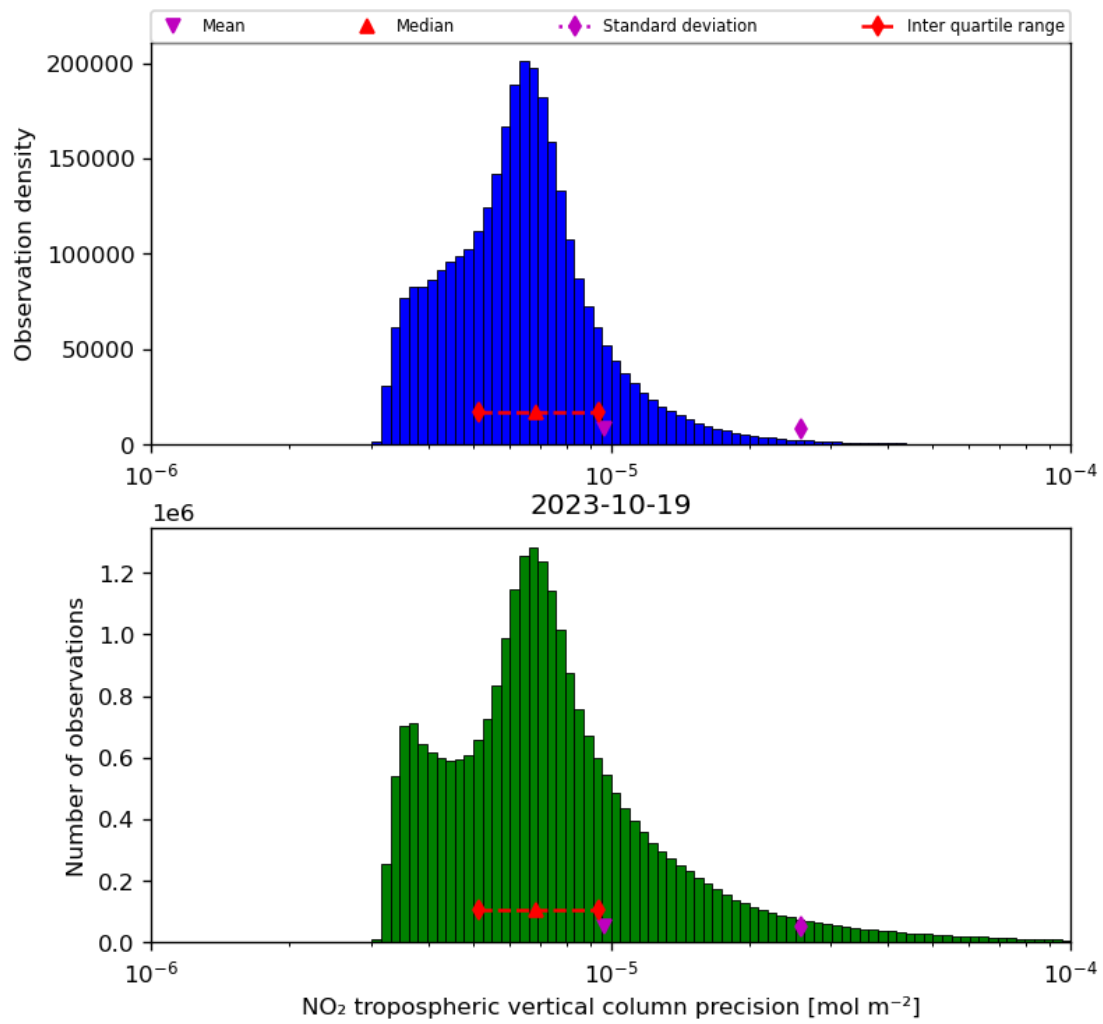
Figure 30: Histogram of “NO 2 tropospheric vertical column precision” for 2023-10-18 to 2023-10-20
