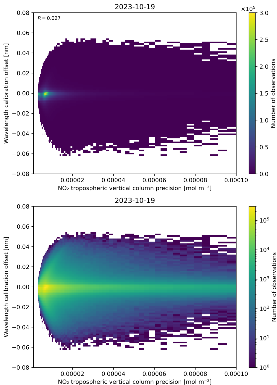
Figure 141: Scatter density plot of “NO 2 tropospheric vertical column precision” against “Wavelength calibration offset” for 2023-10-18 to 2023-10-20.
