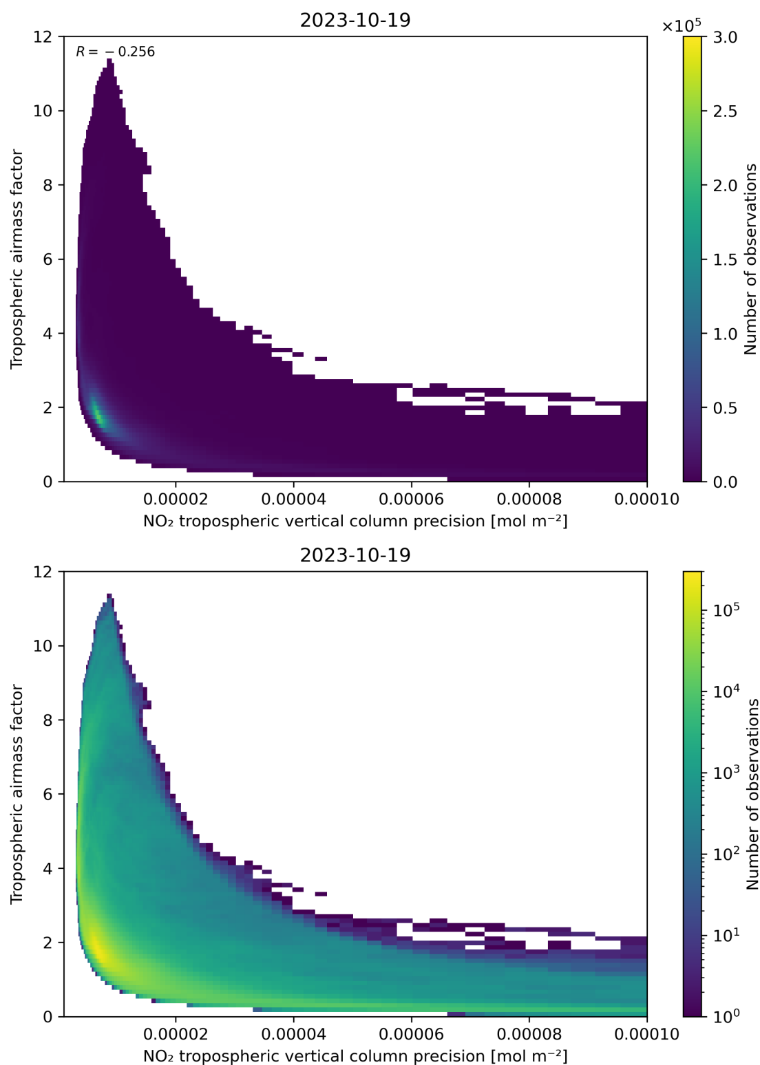
Figure 133: Scatter density plot of “NO 2 tropospheric vertical column precision” against “Tropospheric airmass factor” for 2023-10-18 to 2023-10-20.
