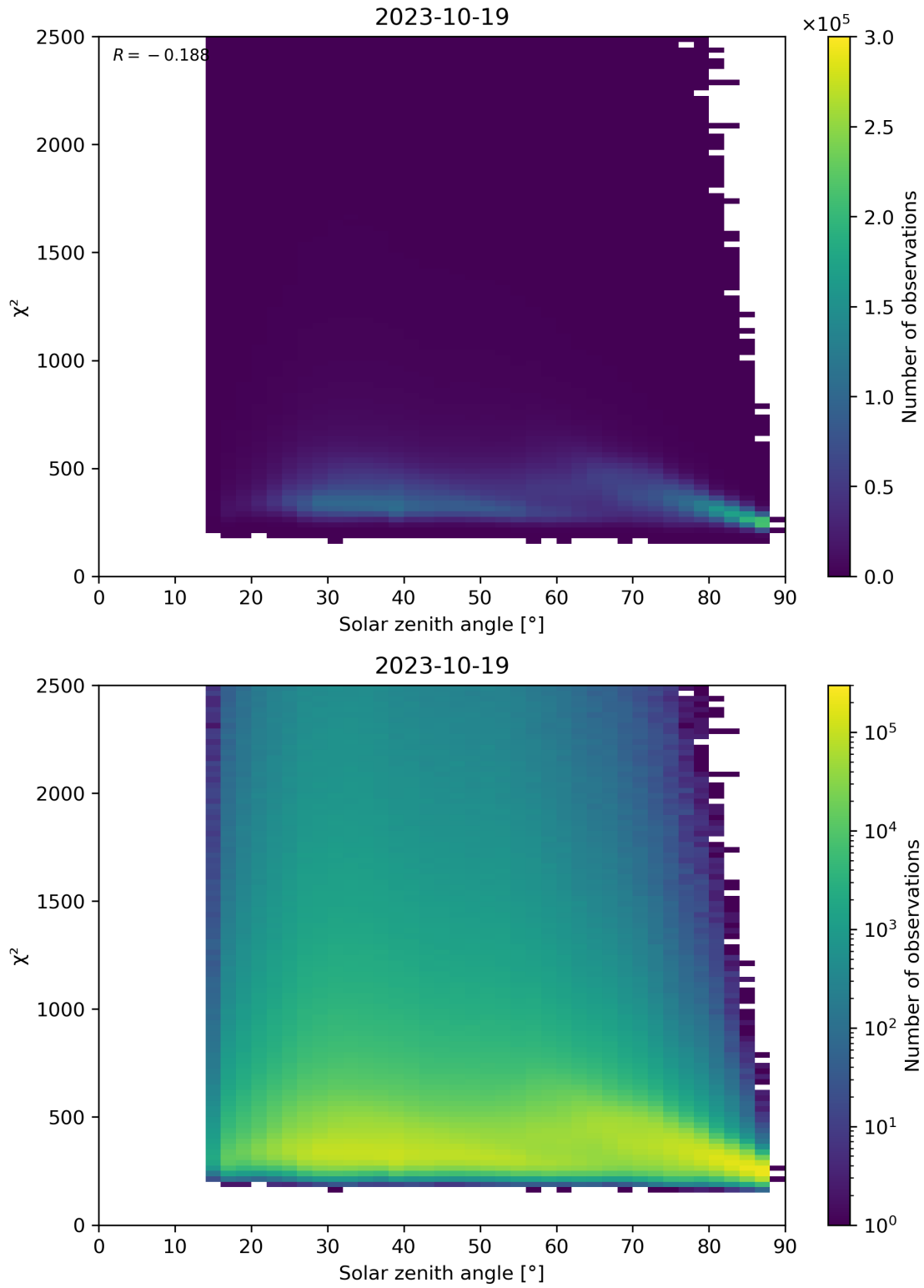
Figure 148: Scatter density plot of “Solar zenith angle” against “ \chi^2 ” for 2023-10-18 to 2023-10-20.
