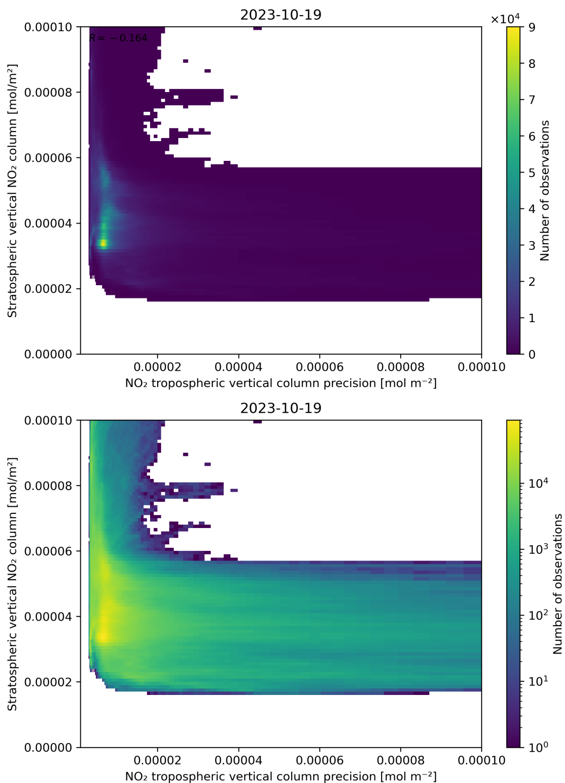
Figure 135: Scatter density plot of “NO 2 tropospheric vertical column precision” against “Stratospheric vertical NO 2 column” for 2023-10-18 to 2023-10-20.
