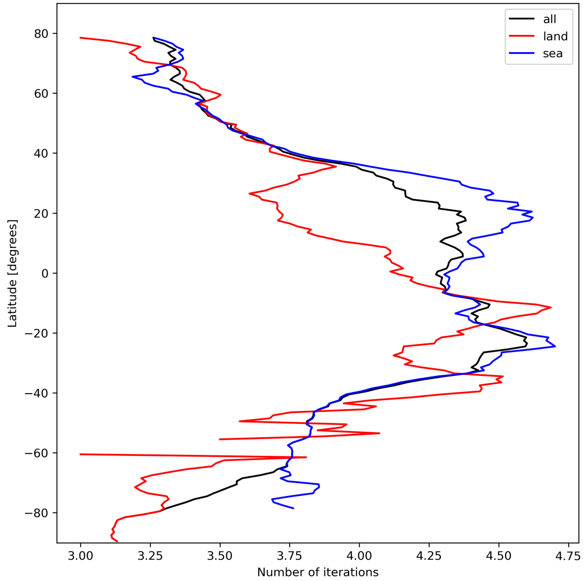
Figure 17: Zonal average of “Number of iterations” for 2023-10-18 to 2023-10-20.
