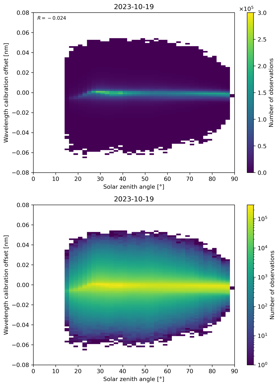
Figure 158: Scatter density plot of “Solar zenith angle” against “Wavelength calibration offset” for 2023-10-18 to 2023-10-20.
