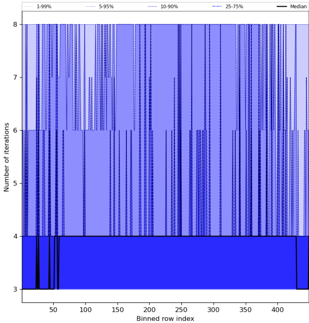
Figure 51: Along track statistics of “Number of iterations” for 2023-10-18 to 2023-10-20
