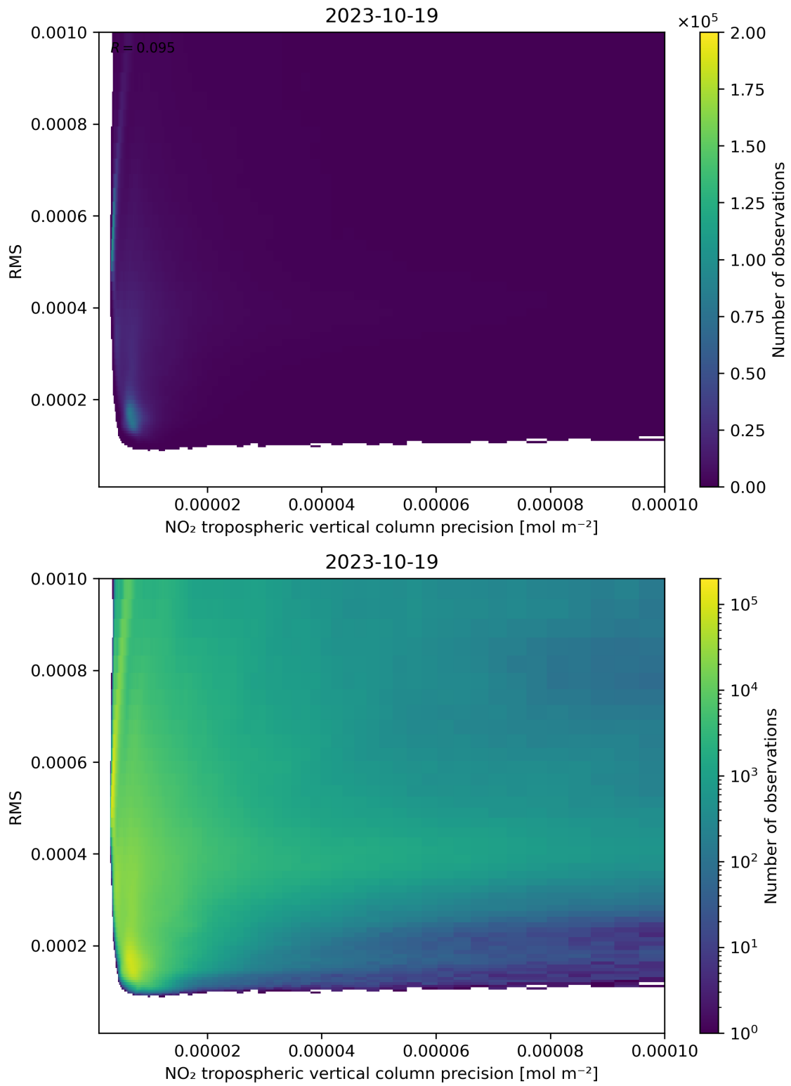
Figure 140: Scatter density plot of “NO 2 tropospheric vertical column precision” against “RMS” for 2023-10-18 to 2023-10-20.
