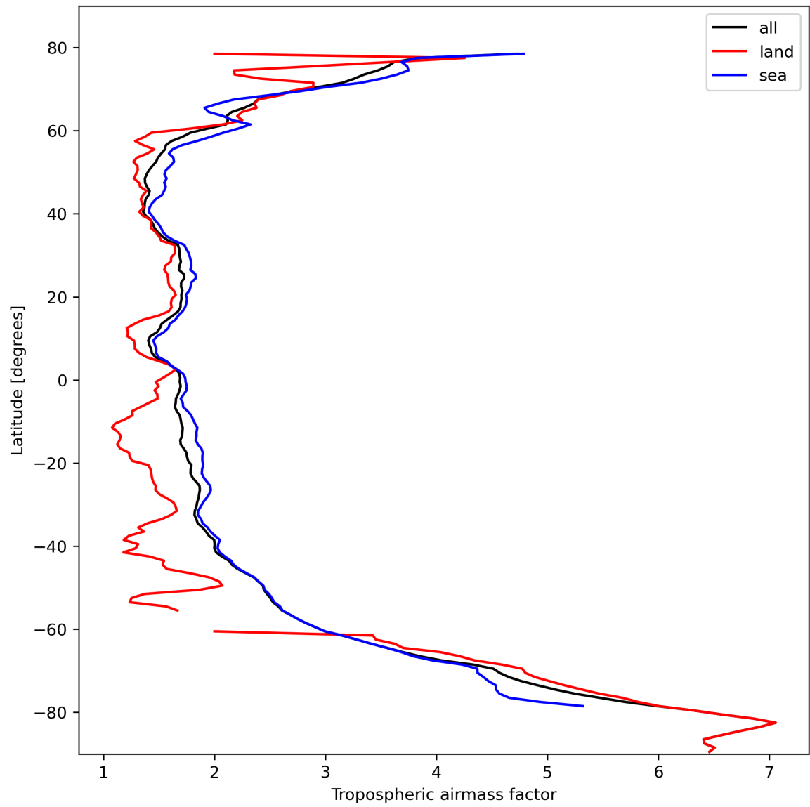
Figure 14: Zonal average of “Tropospheric airmass factor” for 2023-10-18 to 2023-10-20.
