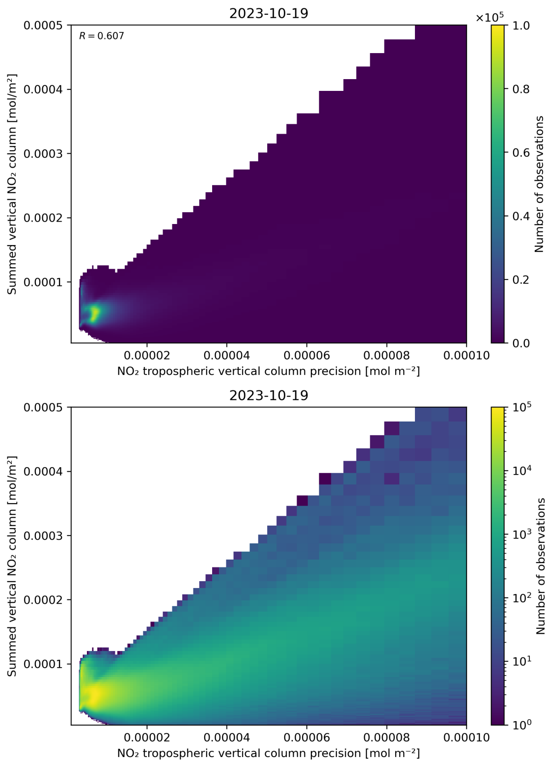
Figure 136: Scatter density plot of “NO 2 tropospheric vertical column precision” against “Summed vertical NO 2 column” for 2023-10-18 to 2023-10-20.
