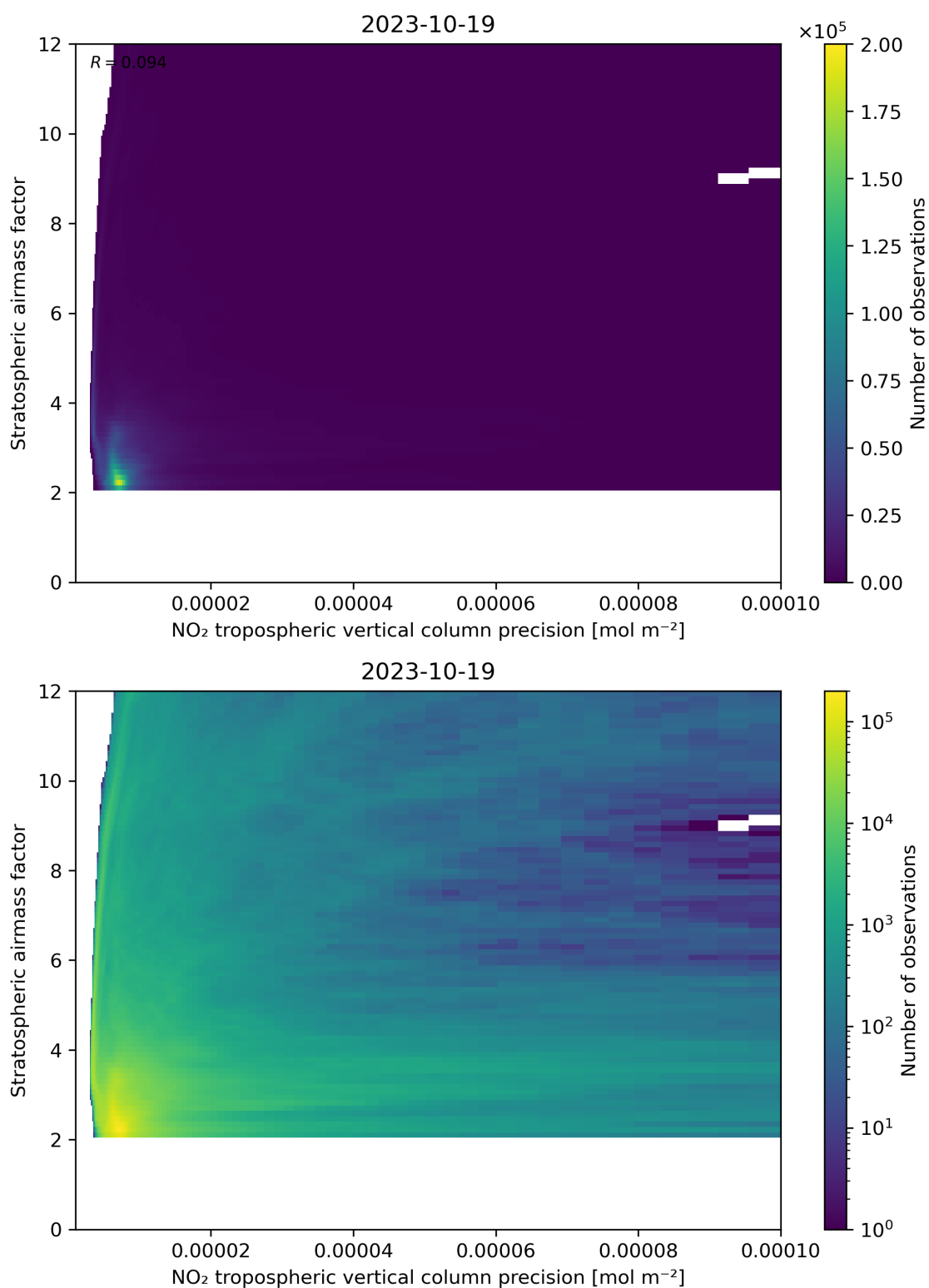
Figure 131: Scatter density plot of “NO 2 tropospheric vertical column precision” against “Stratospheric airmass factor” for 2023-10-18 to 2023-10-20.
