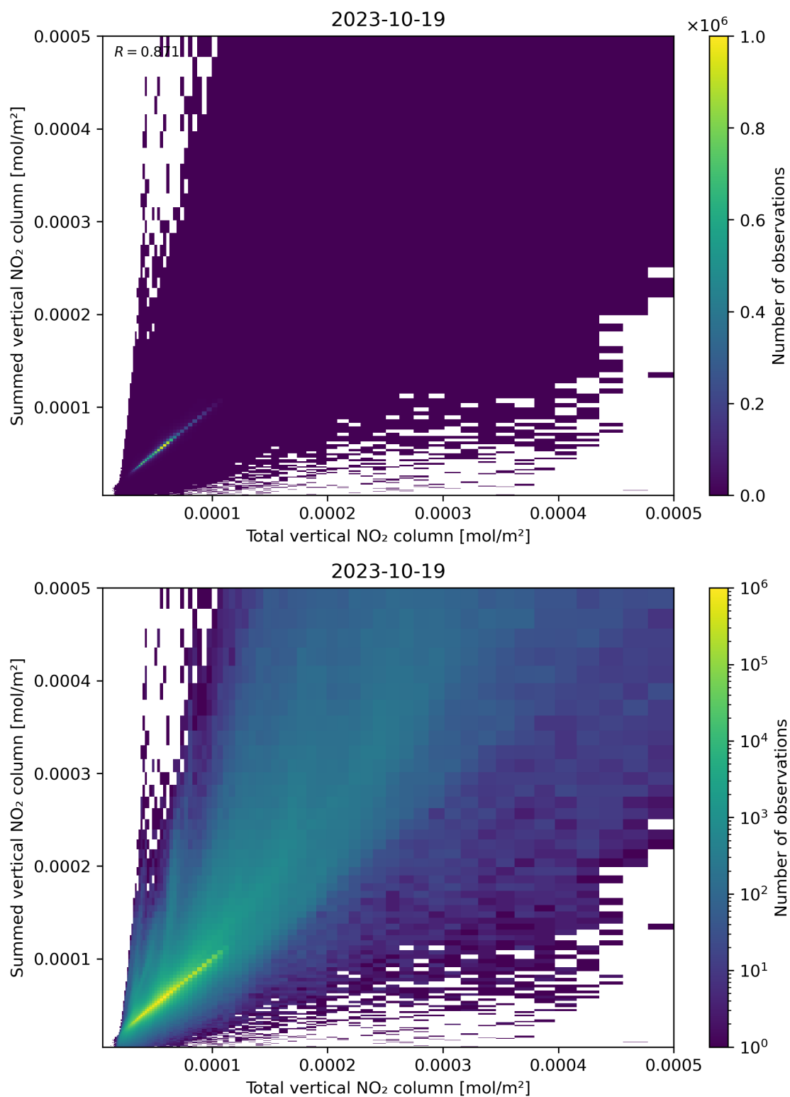
Figure 112: Scatter density plot of “Total vertical NO 2 column” against “Summed vertical NO 2 column” for 2023-10-18 to 2023-10-20.
