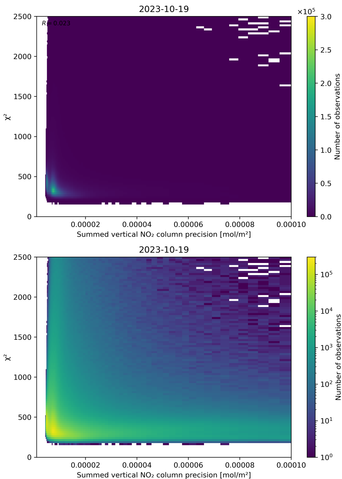
Figure 107: Scatter density plot of “Summed vertical NO 2 column precision” against “ \chi^2 ” for 2023-10-18 to 2023-10-20.
