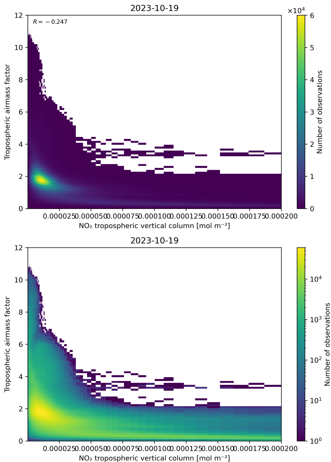
Figure 123: Scatter density plot of “NO 2 tropospheric vertical column” against “Tropospheric air mass factor” for 2023-10-18 to 2023-10-20.
