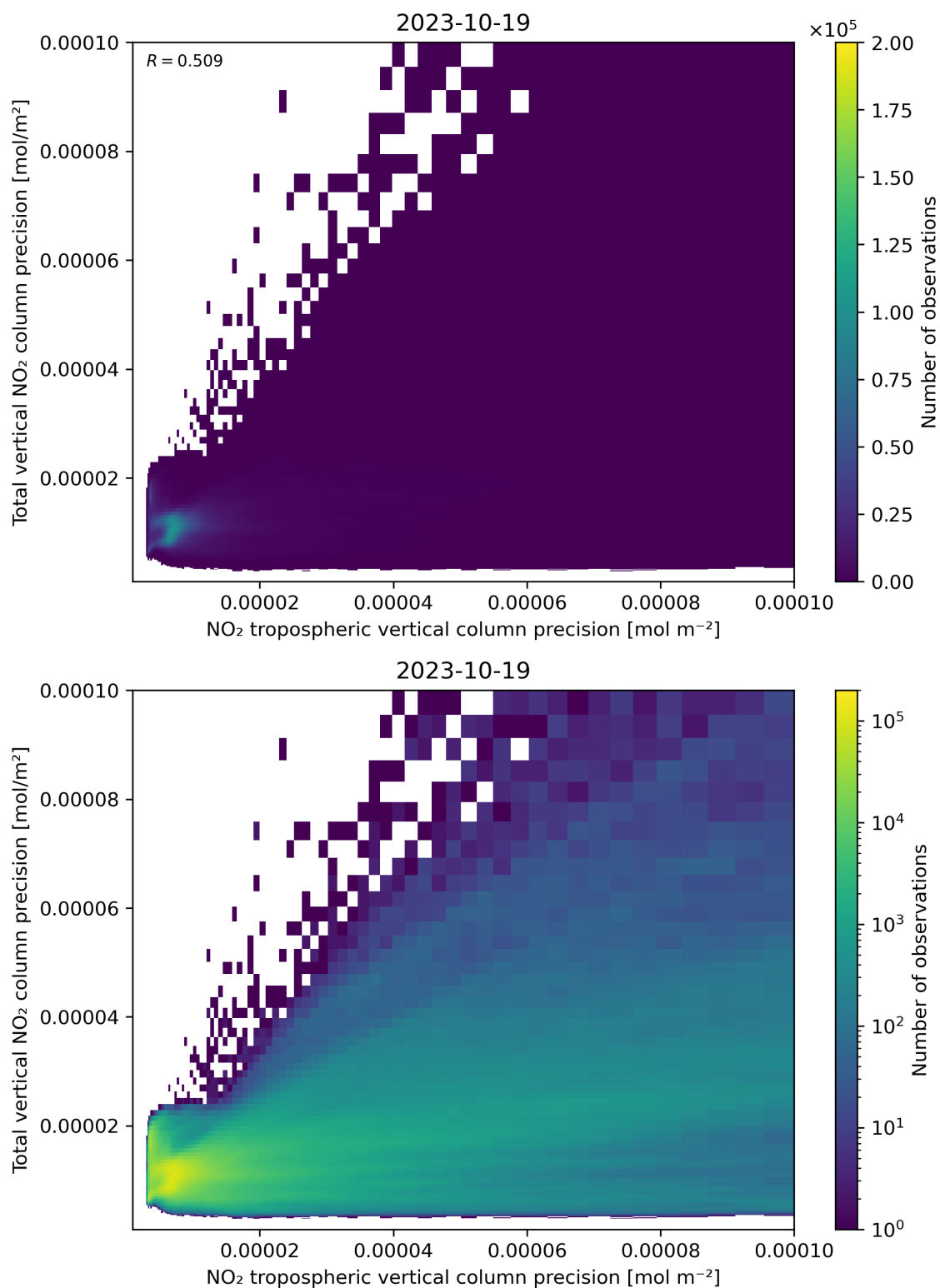
Figure 139: Scatter density plot of “NO 2 tropospheric vertical column precision” against “Total vertical NO 2 column precision” for 2023-10-18 to 2023-10-20.
