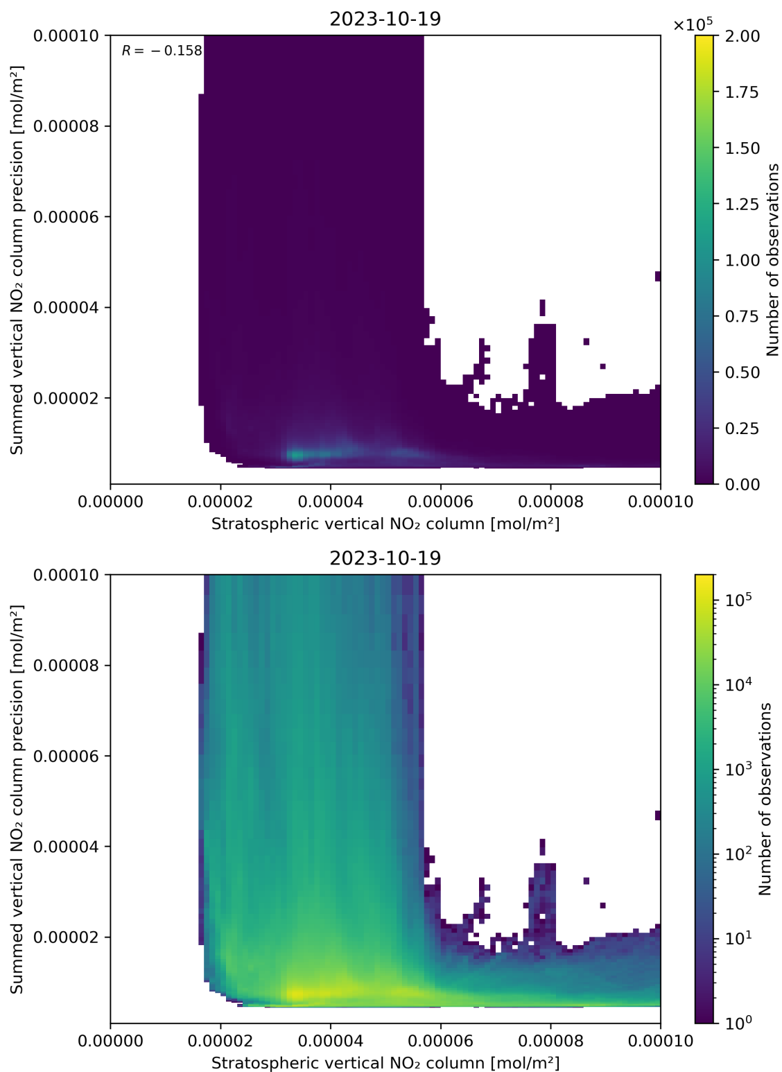
Figure 99: Scatter density plot of “Stratospheric vertical NO 2 column” against “Summed vertical NO 2 column precision” for 2023-10-18 to 2023-10-20.
