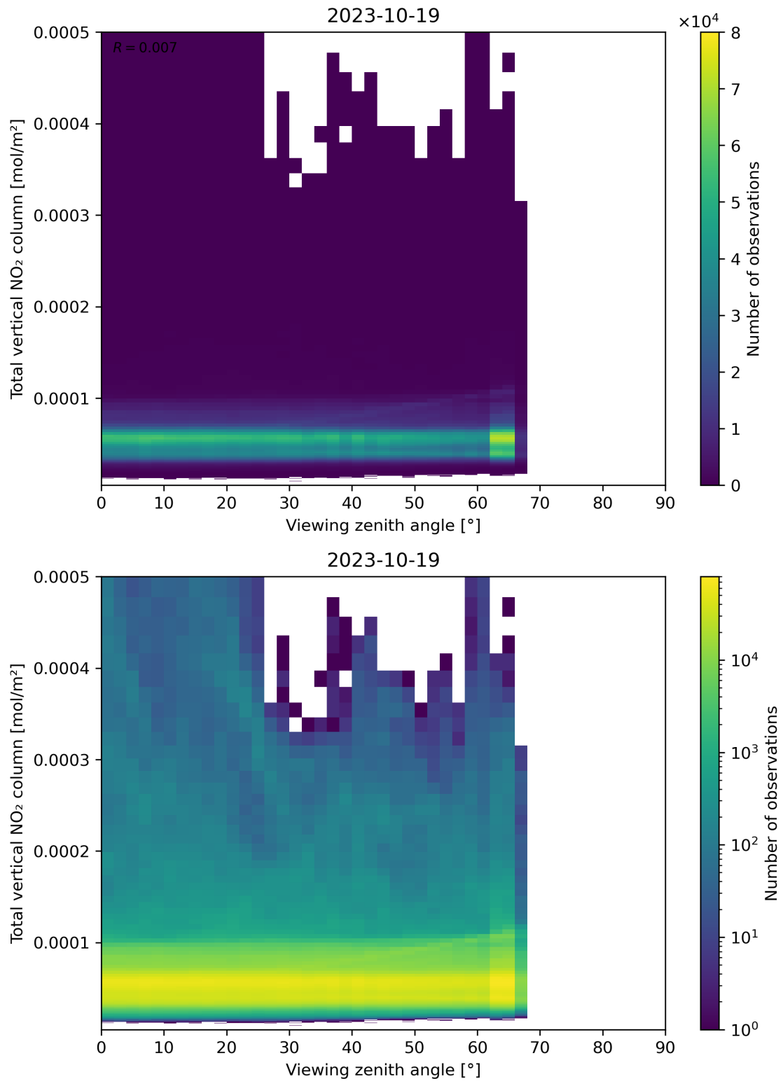
Figure 167: Scatter density plot of “Viewing zenith angle” against “Total vertical NO 2 column” for 2023-10-18 to 2023-10-20.
