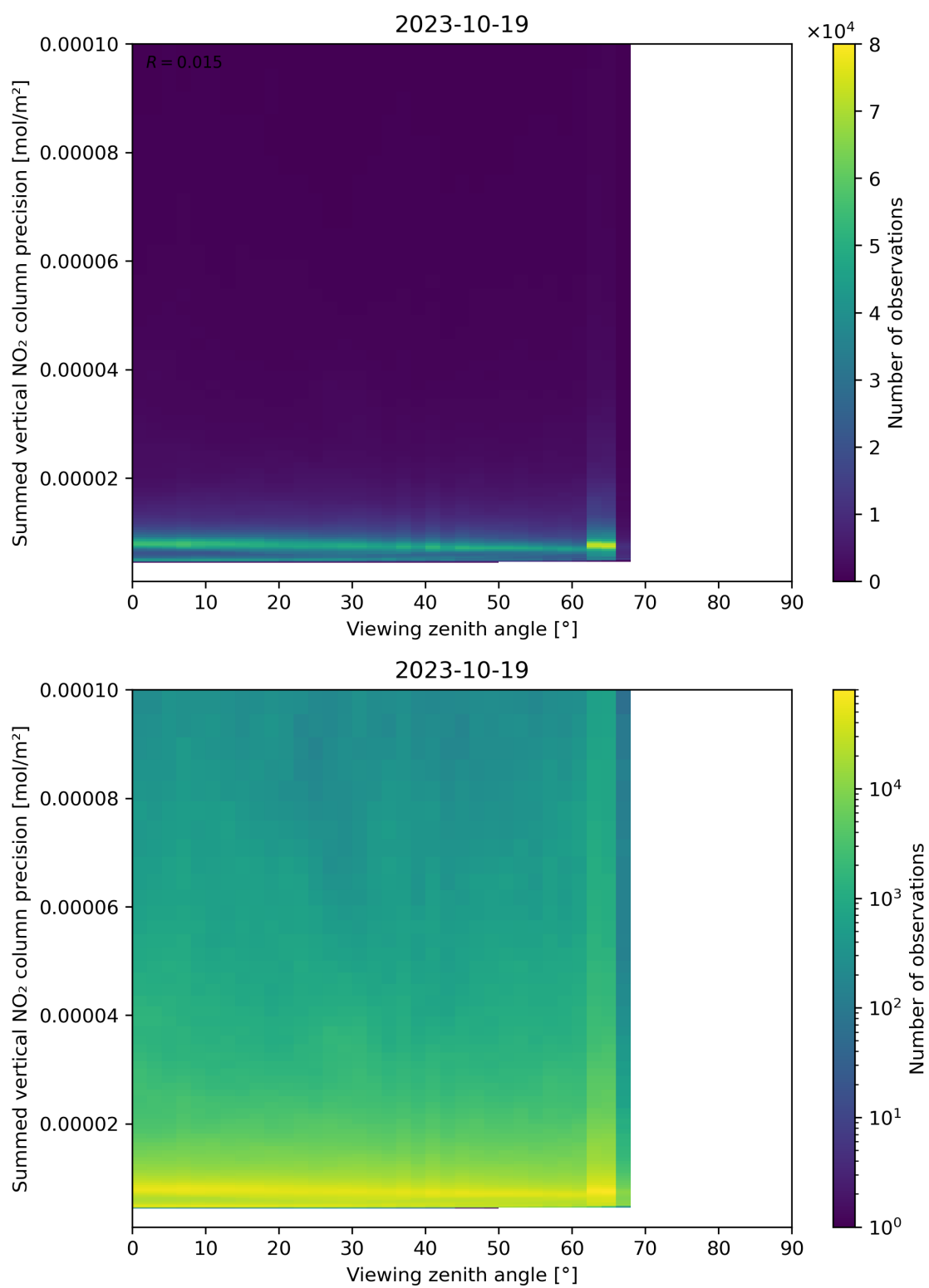
Figure 166: Scatter density plot of “Viewing zenith angle” against “Summed vertical NO 2 column precision” for 2023-10-18 to 2023-10-20.
