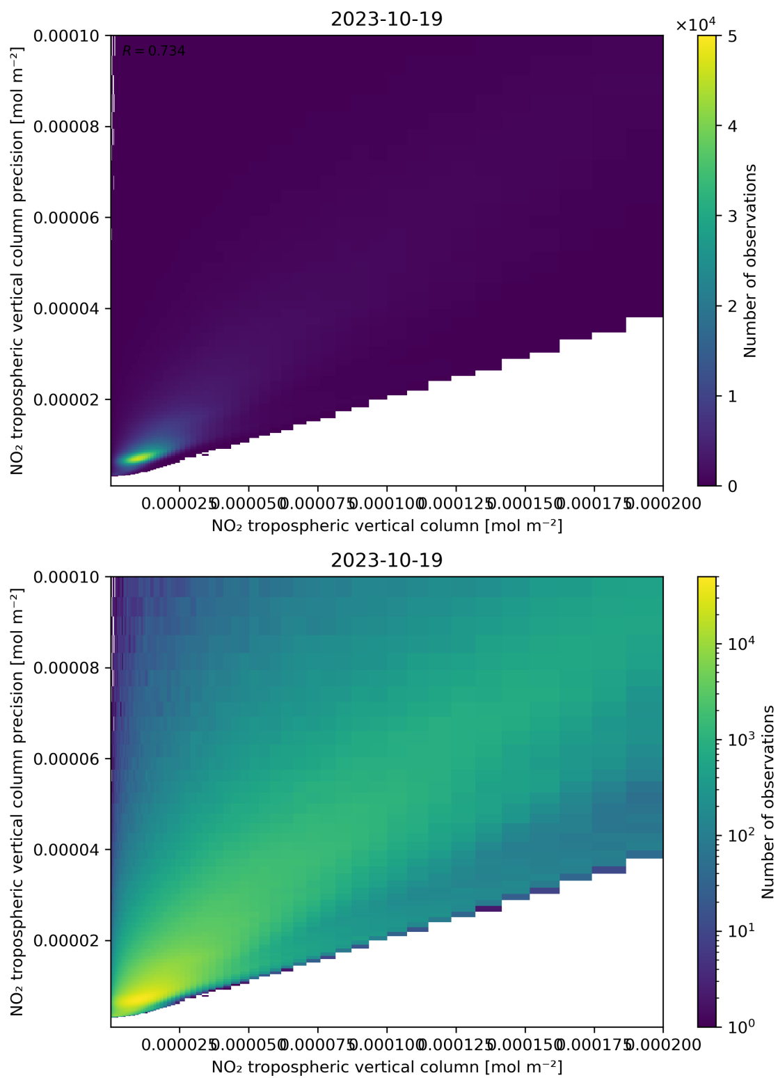
Figure 130: Scatter density plot of “NO 2 tropospheric vertical column” against “NO 2 tropospheric vertical column precision” for 2023-10-18 to 2023-10-20.
