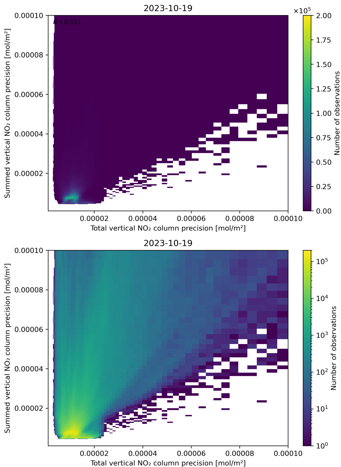
Figure 118: Scatter density plot of “Total vertical NO 2 column precision” against “Summed vertical NO 2 column precision” for 2023-10-18 to 2023-10-20.
