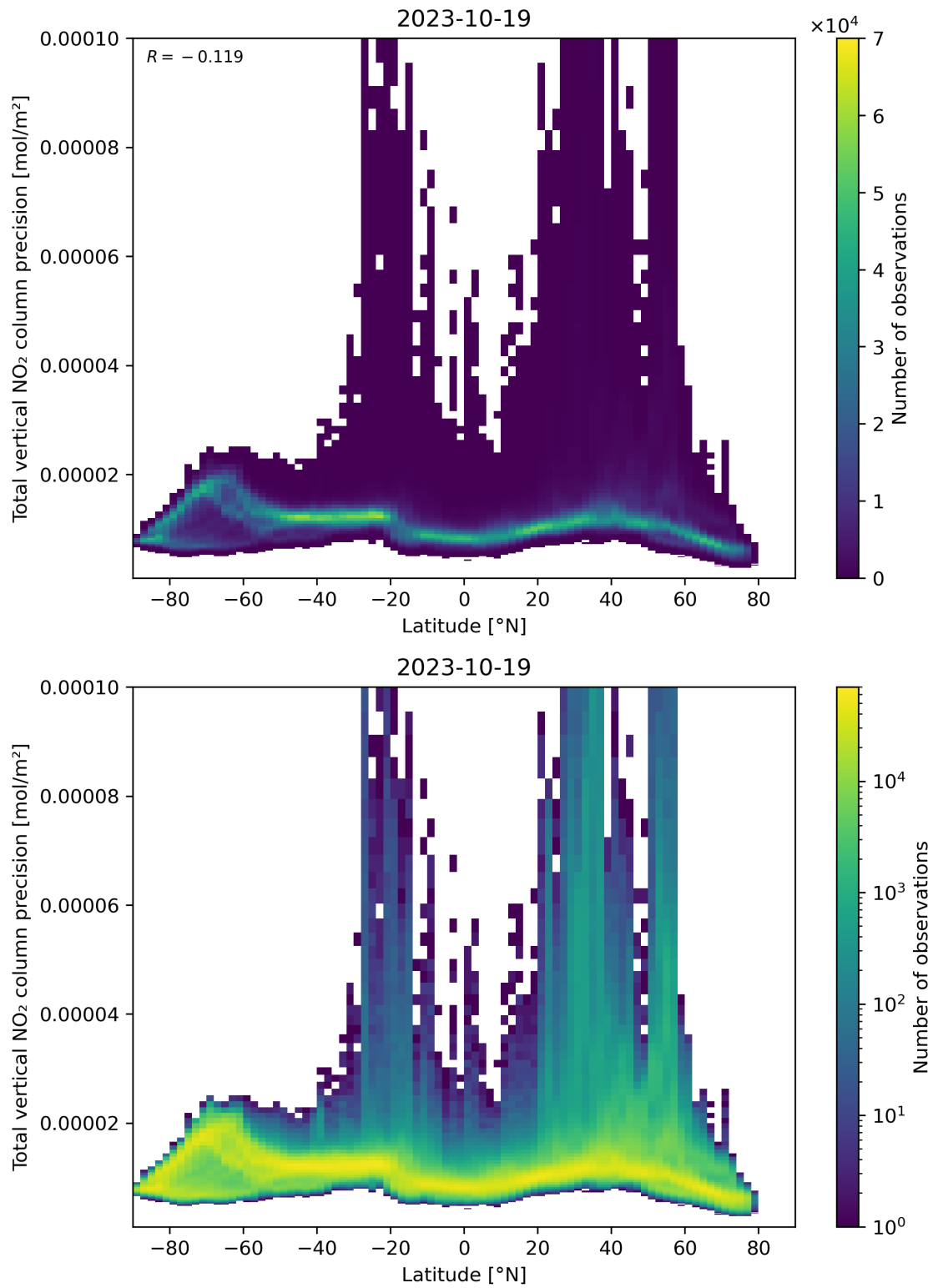
Figure 91: Scatter density plot of “Latitude” against “Total vertical NO 2 column precision” for 2023-10-18 to 2023-10-20.
