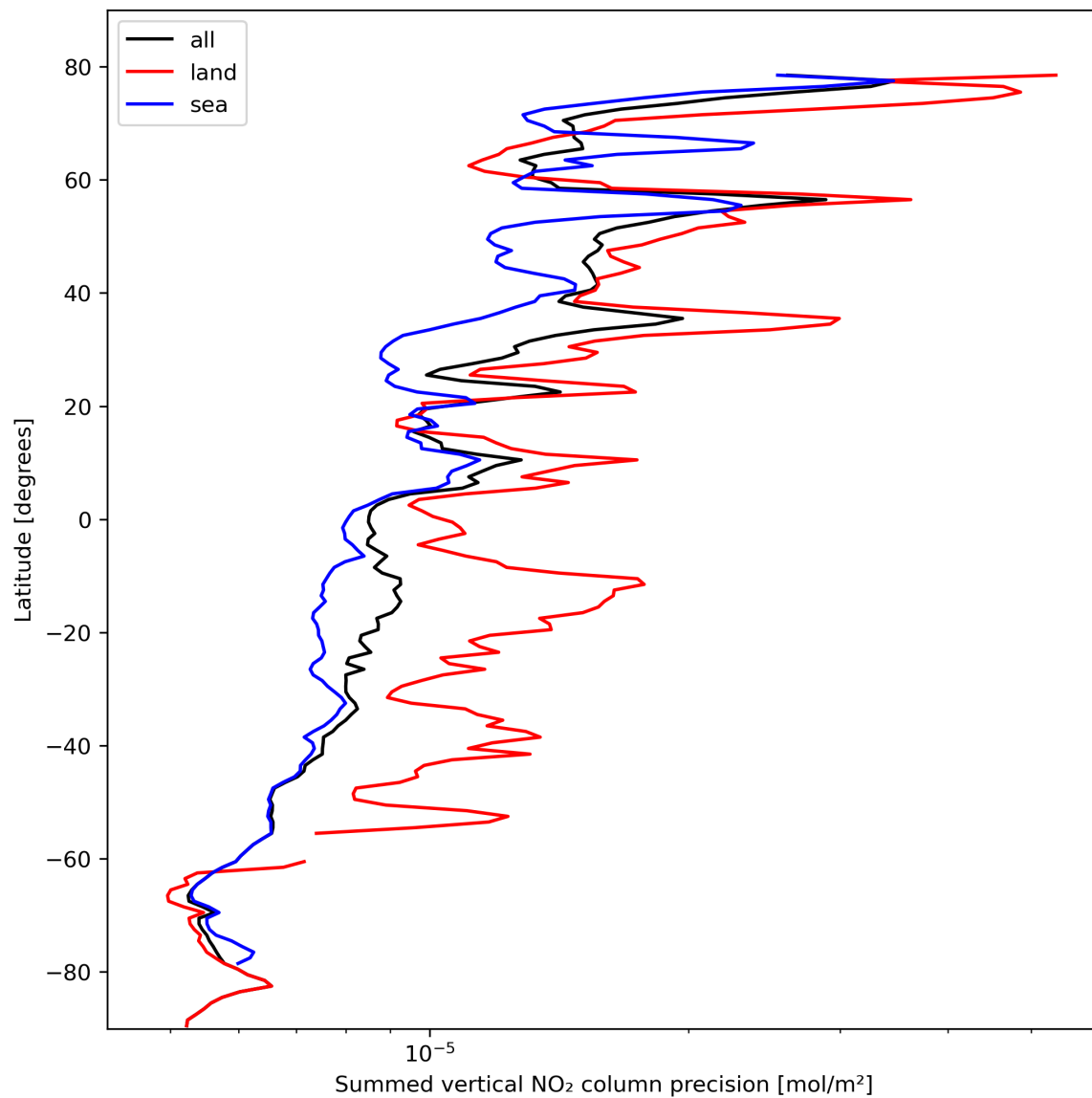
Figure 24: Zonal average of “Summed vertical NO 2 column precision” for 2023-10-18 to 2023-10-20.
