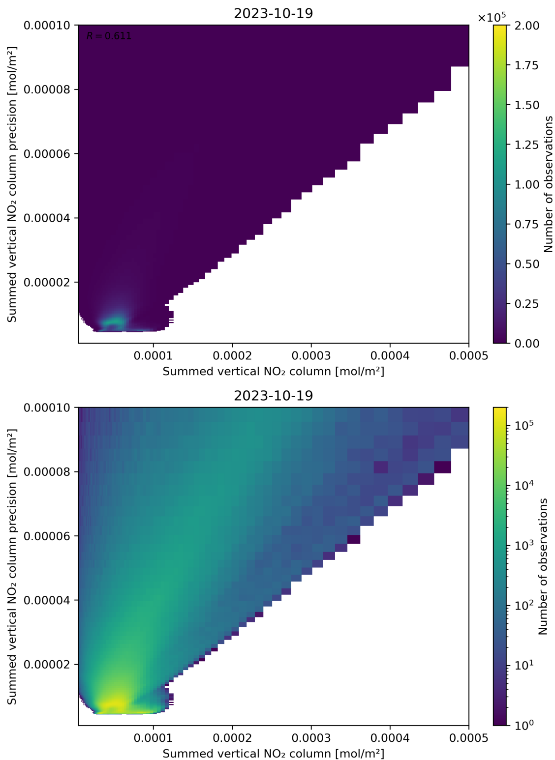
Figure 105: Scatter density plot of “Summed vertical NO 2 column” against “Summed vertical NO 2 column precision” for 2023-10-18 to 2023-10-20.
