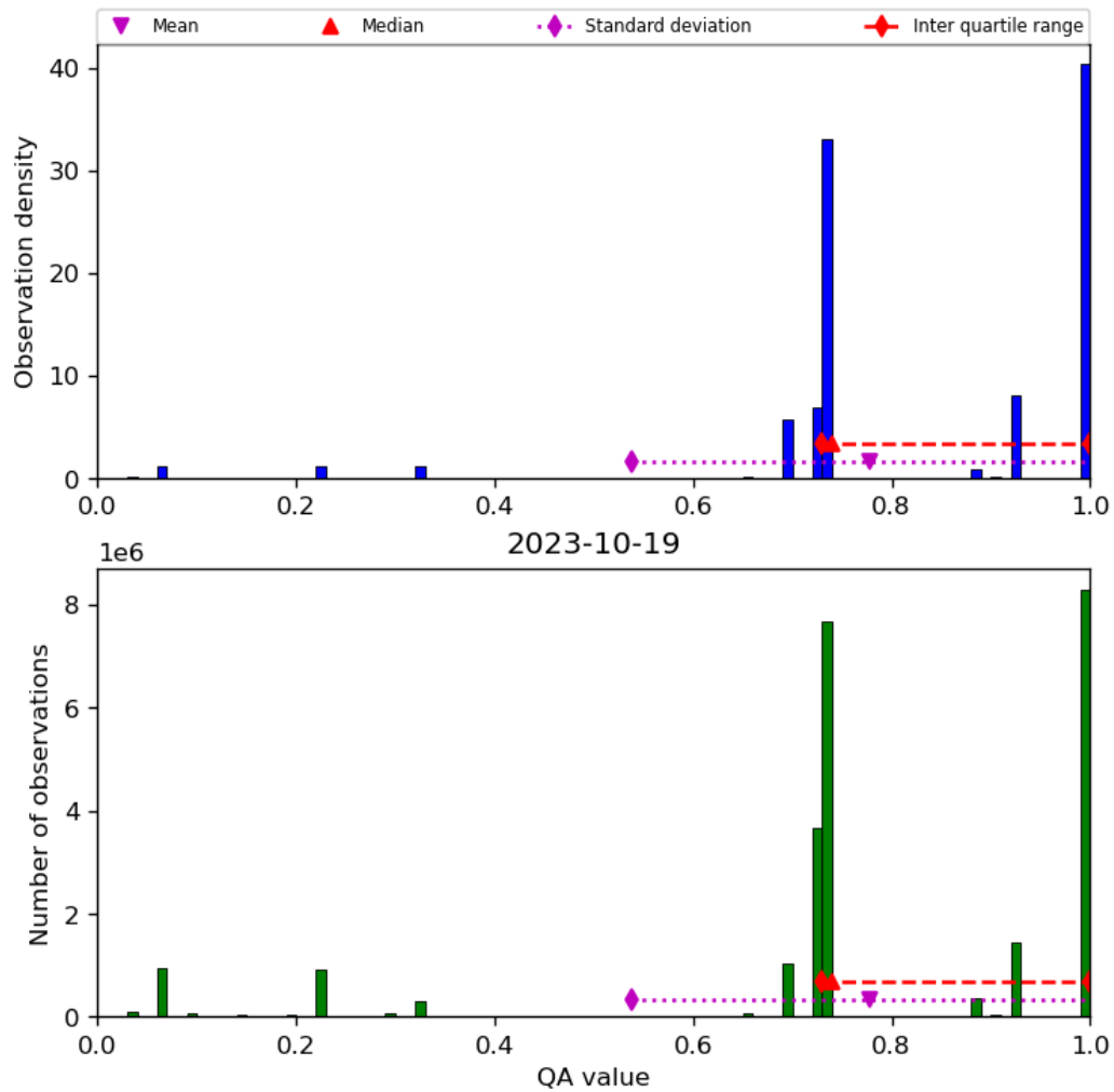
Figure 28: Histogram of “QA value” for 2023-10-18 to 2023-10-20
