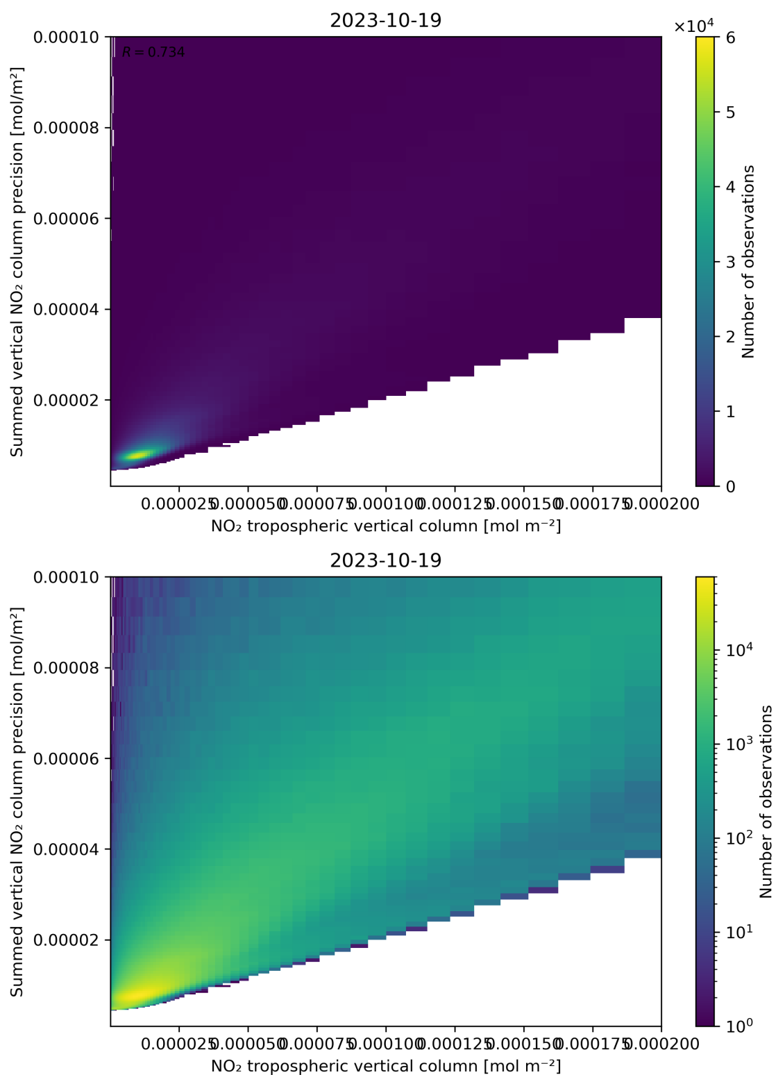
Figure 127: Scatter density plot of “NO 2 tropospheric vertical column” against “Summed vertical NO 2 column precision” for 2023-10-18 to 2023-10-20.
