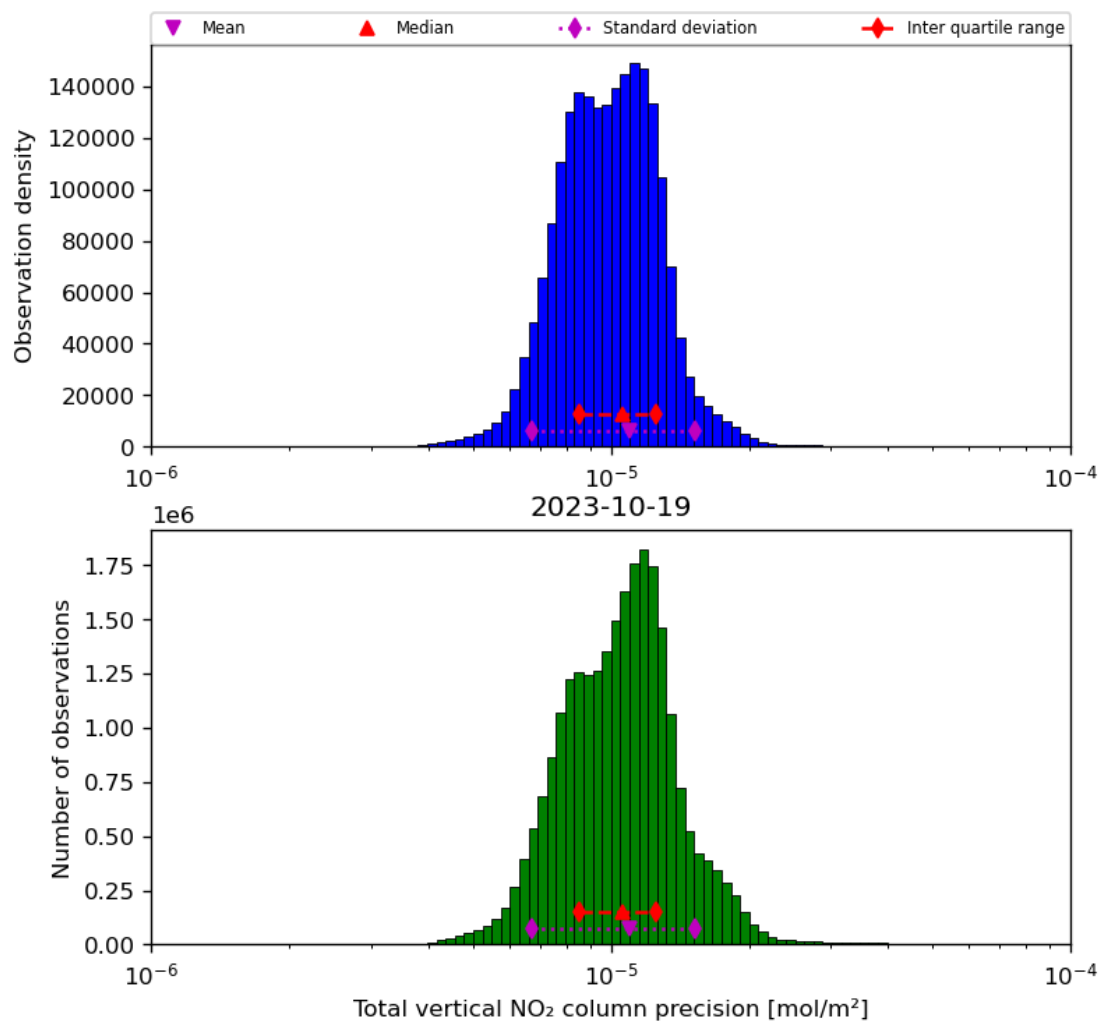
Figure 39: Histogram of “Total vertical NO 2 column precision” for 2023-10-18 to 2023-10-20
