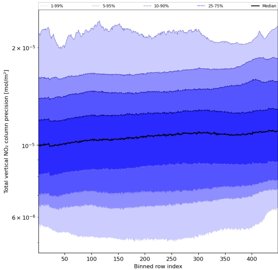
Figure 56: Along track statistics of “Total vertical NO 2 column precision” for 2023-10-18 to 2023-10-20
