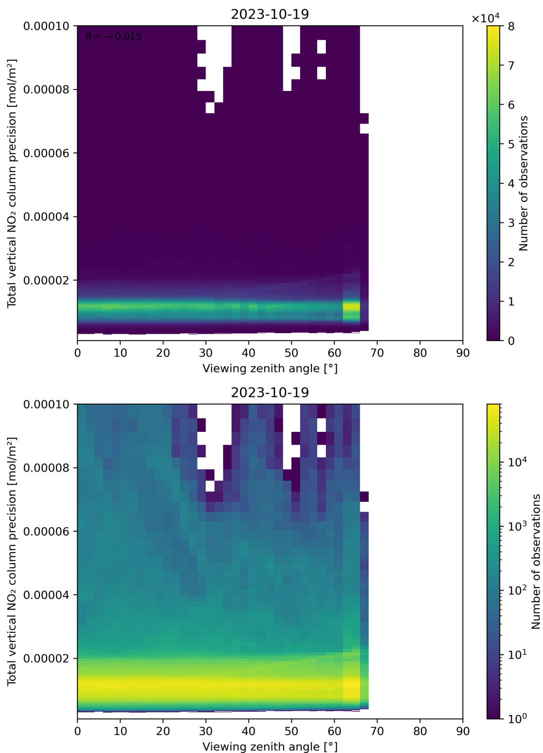
Figure 168: Scatter density plot of “Viewing zenith angle” against “Total vertical NO 2 column precision” for 2023-10-18 to 2023-10-20.
