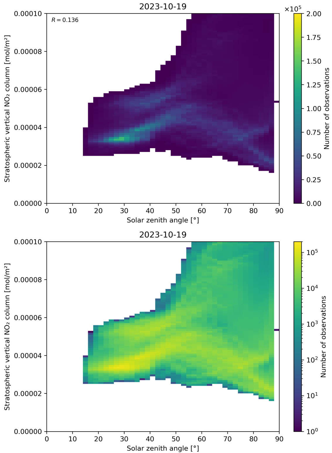
Figure 150: Scatter density plot of “Solar zenith angle” against “Stratospheric vertical NO 2 column” for 2023-10-18 to 2023-10-20.
