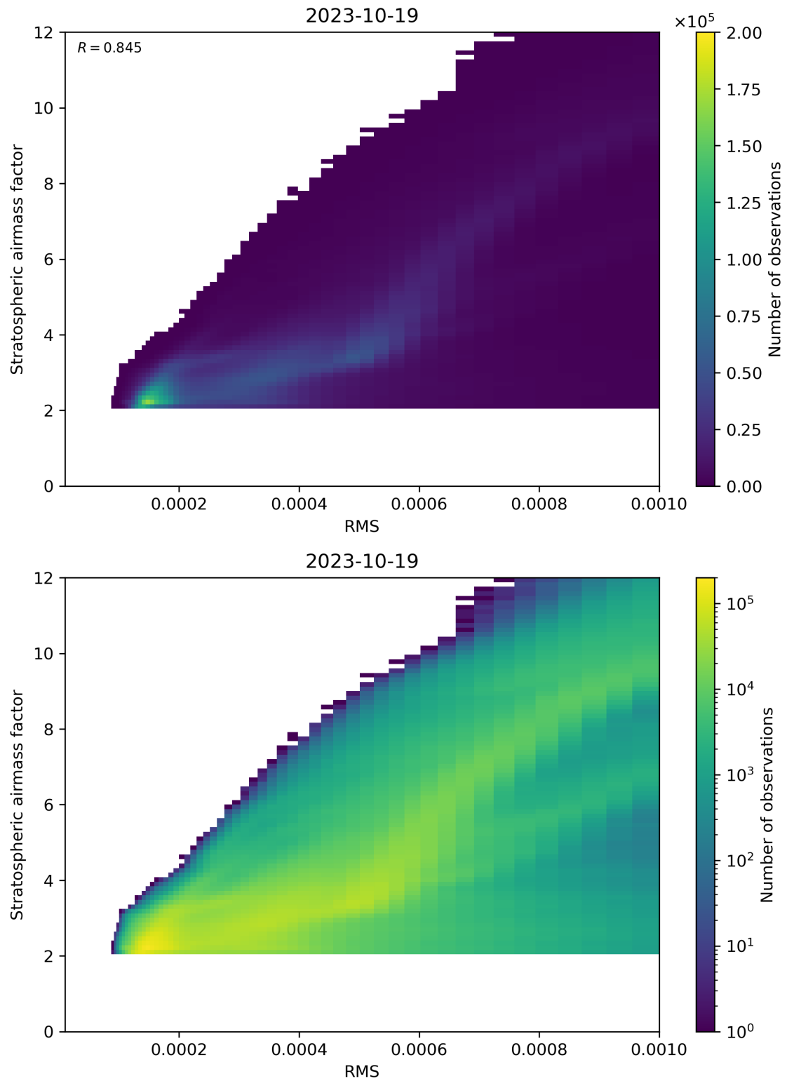
Figure 144: Scatter density plot of “RMS” against “Stratospheric airmass factor” for 2023-10-18 to 2023-10-20.
