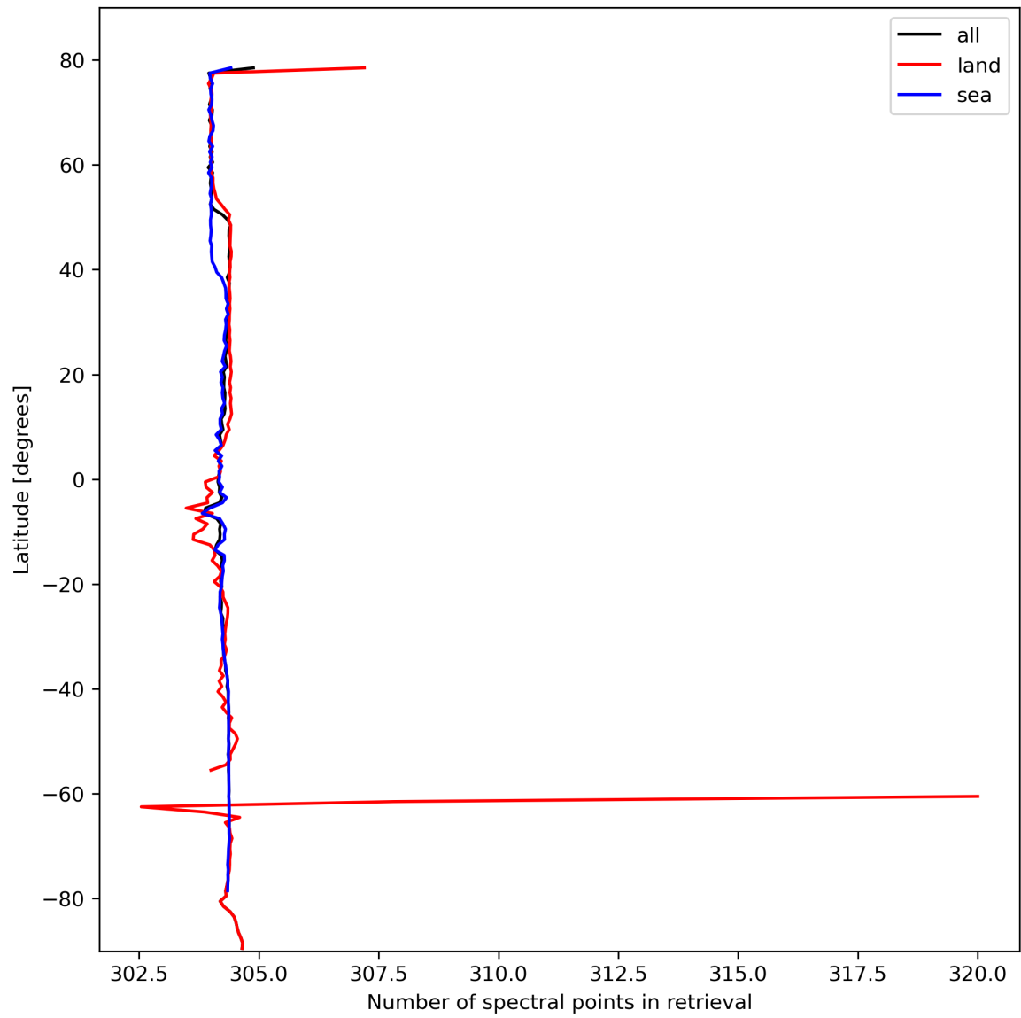
Figure 16: Zonal average of “Number of spectral points in retrieval” for 2023-10-18 to 2023-10-20.
