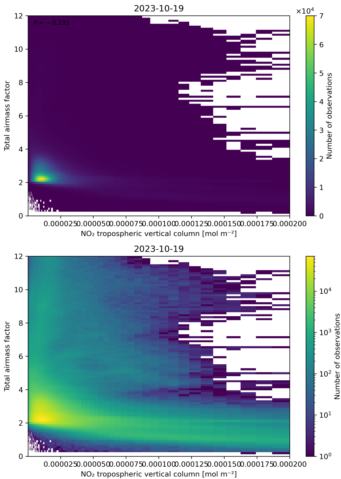
Figure 122: Scatter density plot of “NO 2 tropospheric vertical column” against “Total air mass factor” for 2023-10-18 to 2023-10-20.
