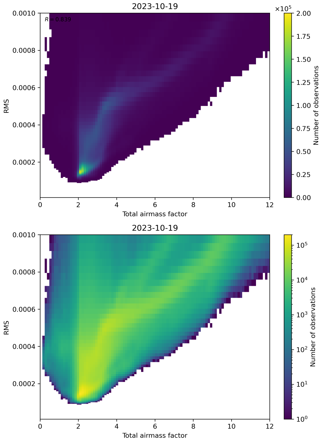
Figure 69: Scatter density plot of “Total airmass factor” against “RMS” for 2023-10-18 to 2023-10-20.
