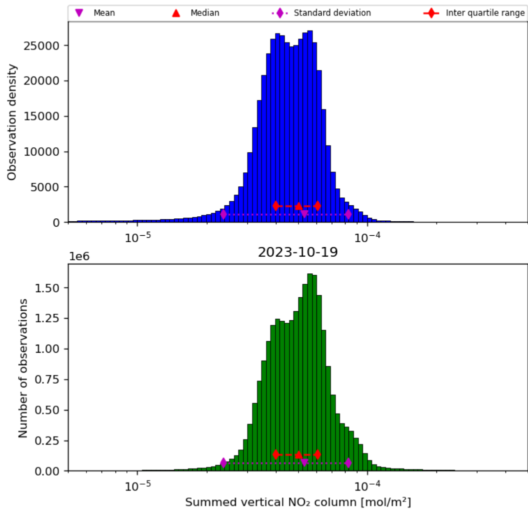
Figure 40: Histogram of “Summed vertical NO 2 column” for 2023-10-18 to 2023-10-20
