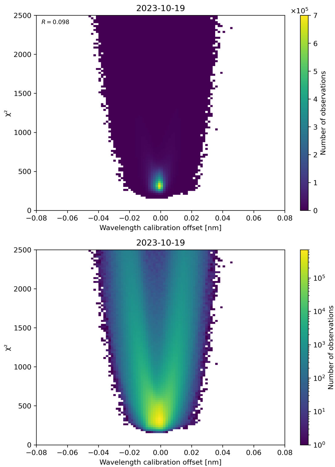
Figure 175: Scatter density plot of “Wavelength calibration offset” against “ \chi^2 ” for 2023-10-18 to 2023-10-20.
