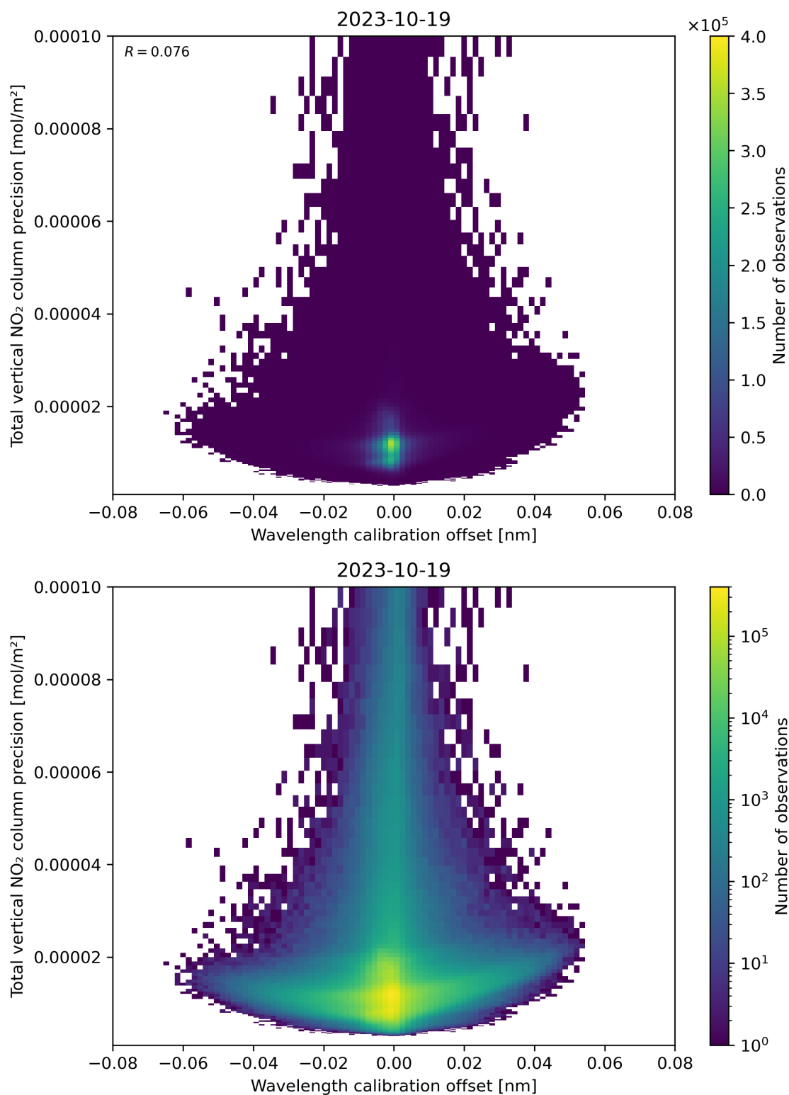
Figure 180: Scatter density plot of “Wavelength calibration offset” against “Total vertical NO 2 column precision” for 2023-10-18 to 2023-10-20.
