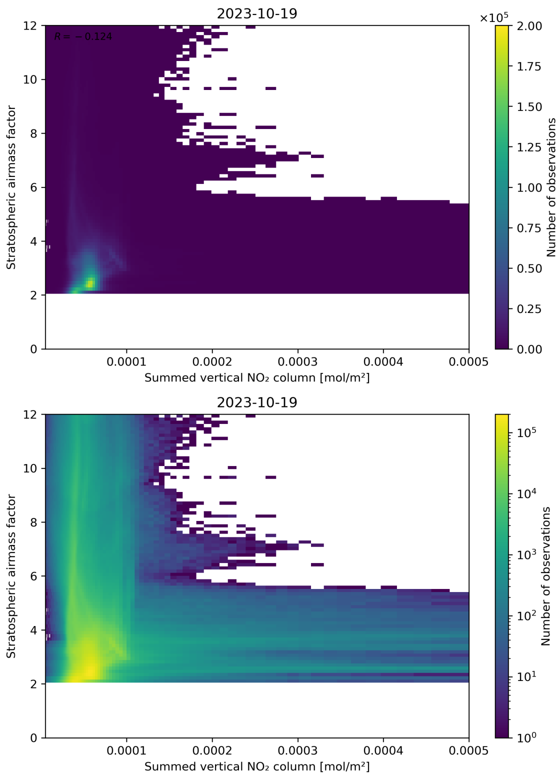
Figure 103: Scatter density plot of “Summed vertical NO 2 column” against “Stratospheric air mass factor” for 2023-10-18 to 2023-10-20.
