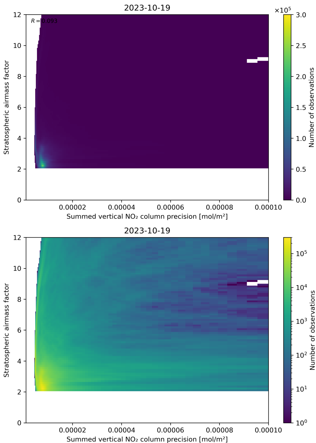
Figure 106: Scatter density plot of “Summed vertical NO 2 column precision” against “Stratospheric airmass factor” for 2023-10-18 to 2023-10-20.
