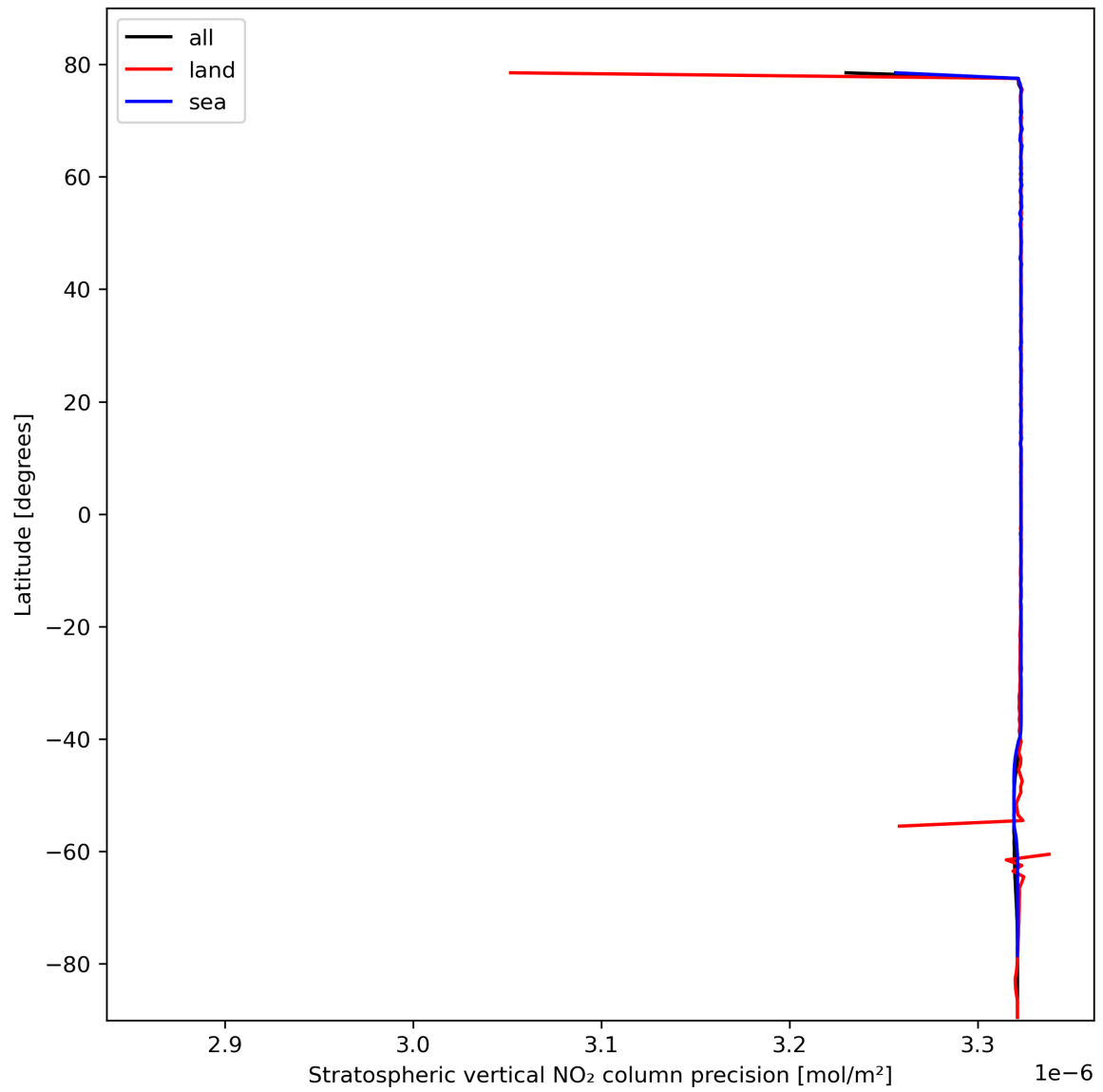
Figure 20: Zonal average of “Stratospheric vertical NO 2 column precision” for 2023-10-18 to 2023-10-20.
