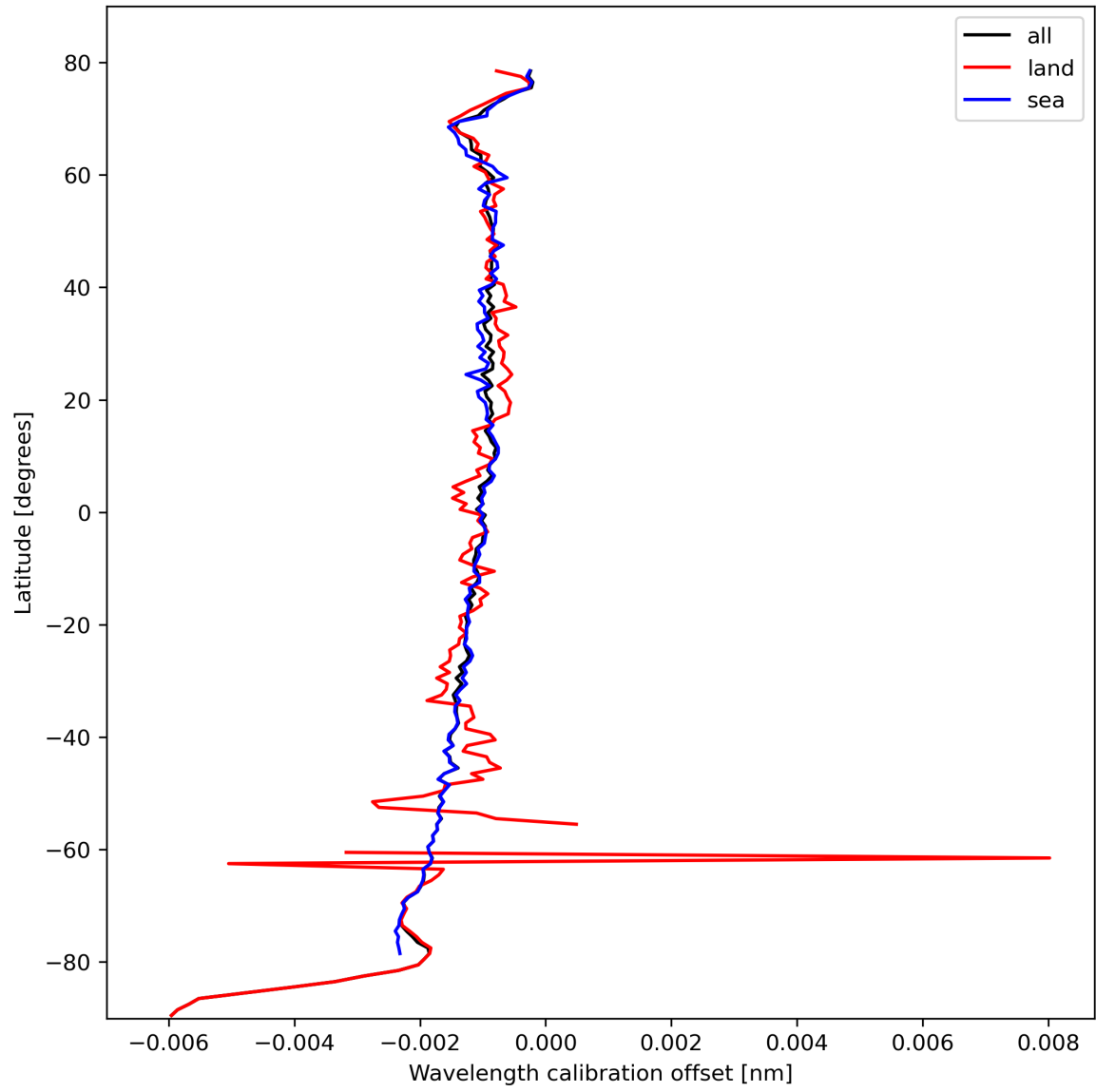
Figure 18: Zonal average of “Wavelength calibration offset” for 2023-10-18 to 2023-10-20.
