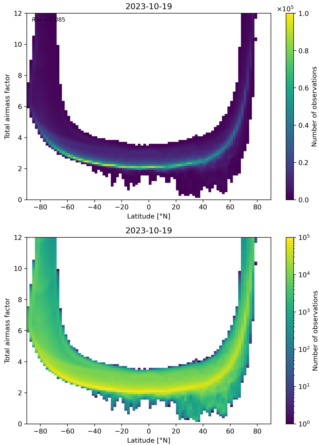
Figure 84: Scatter density plot of “Latitude” against “Total airmass factor” for 2023-10-18 to 2023-10-20.
