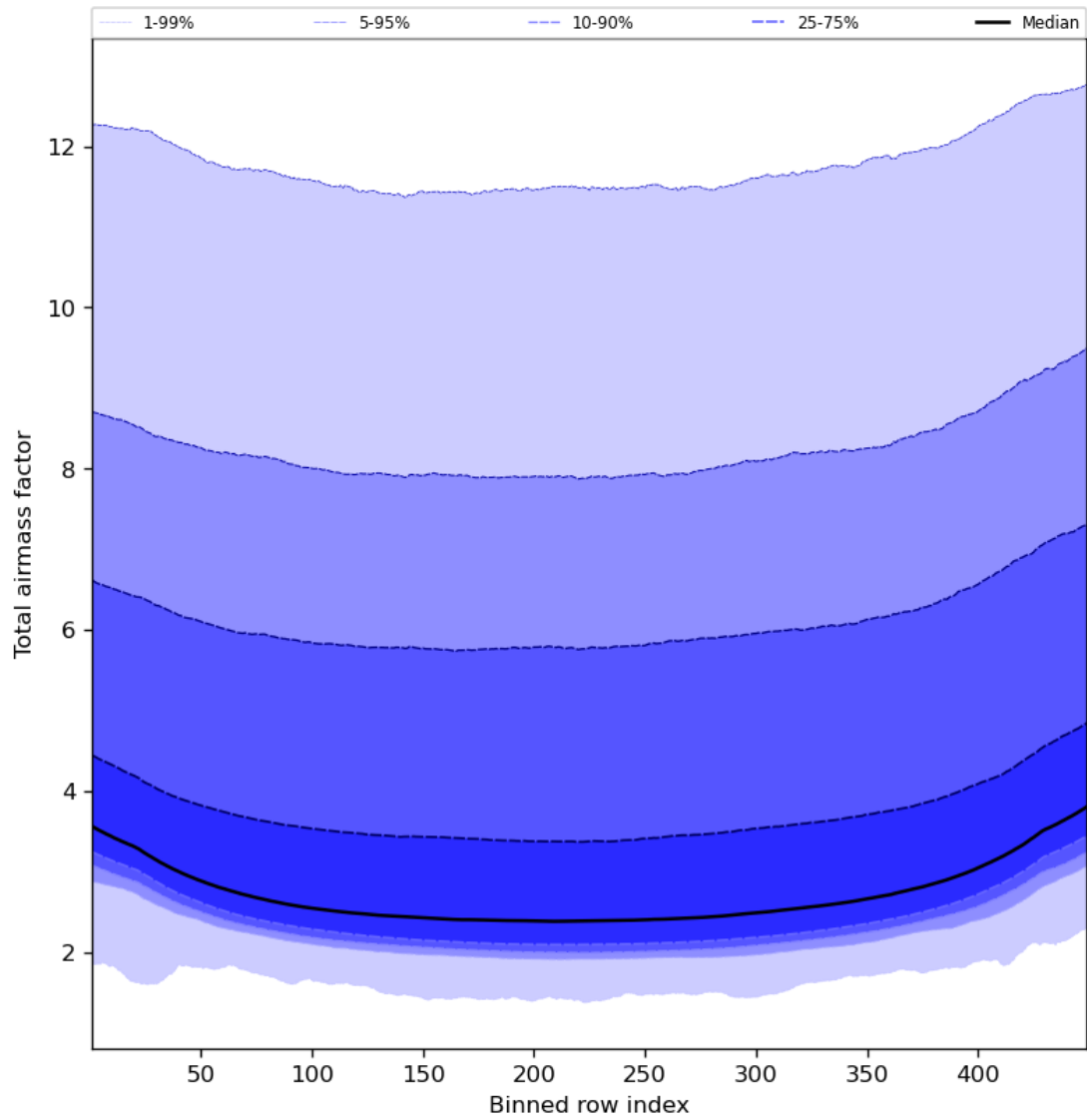
Figure 49: Along track statistics of “Total airmass factor” for 2023-10-18 to 2023-10-20
