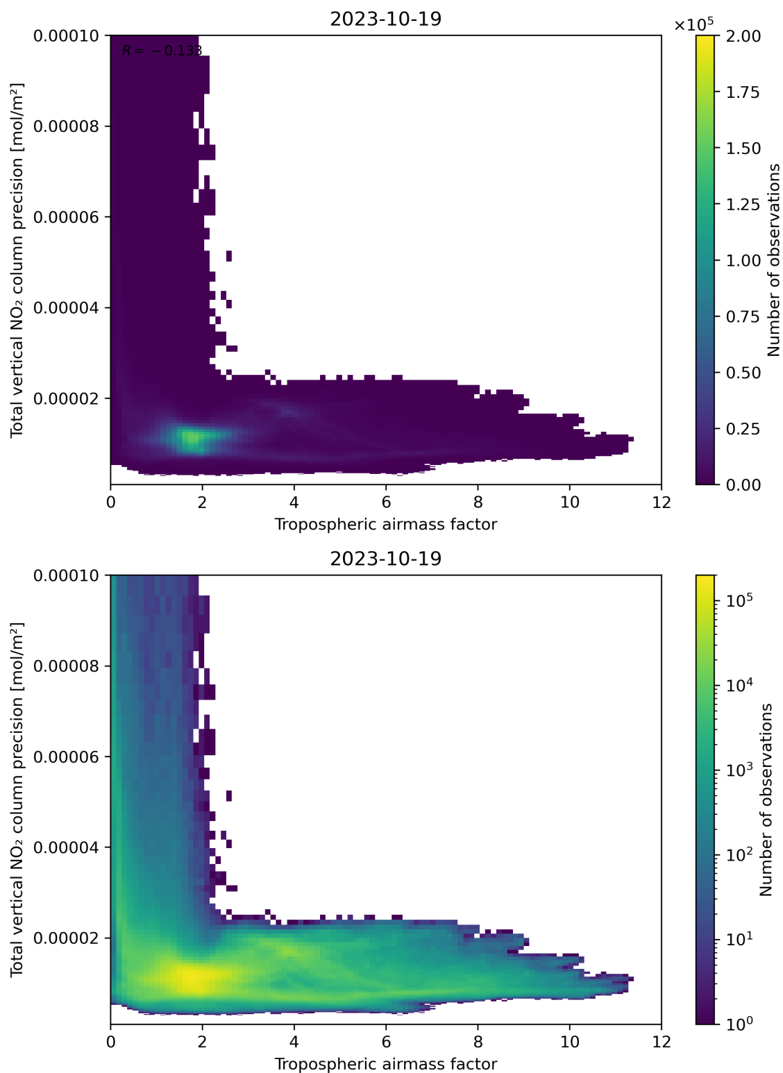
Figure 78: Scatter density plot of “Tropospheric air mass factor” against “Total vertical NO 2 column precision” for 2023-10-18 to 2023-10-20.
