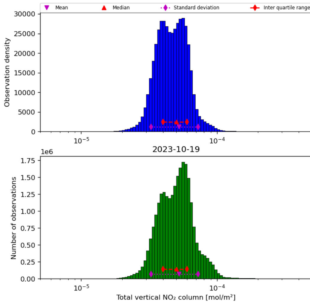
Figure 38: Histogram of “Total vertical NO 2 column” for 2023-10-18 to 2023-10-20
