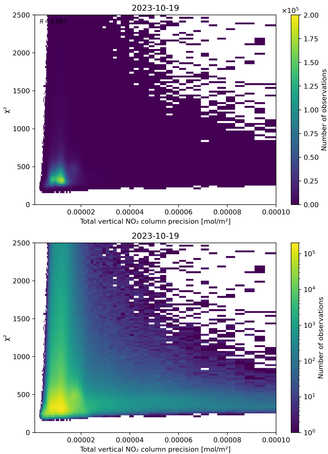
Figure 116: Scatter density plot of “Total vertical NO 2 column precision” against “ \chi^2 ” for 2023-10-18 to 2023-10-20.
