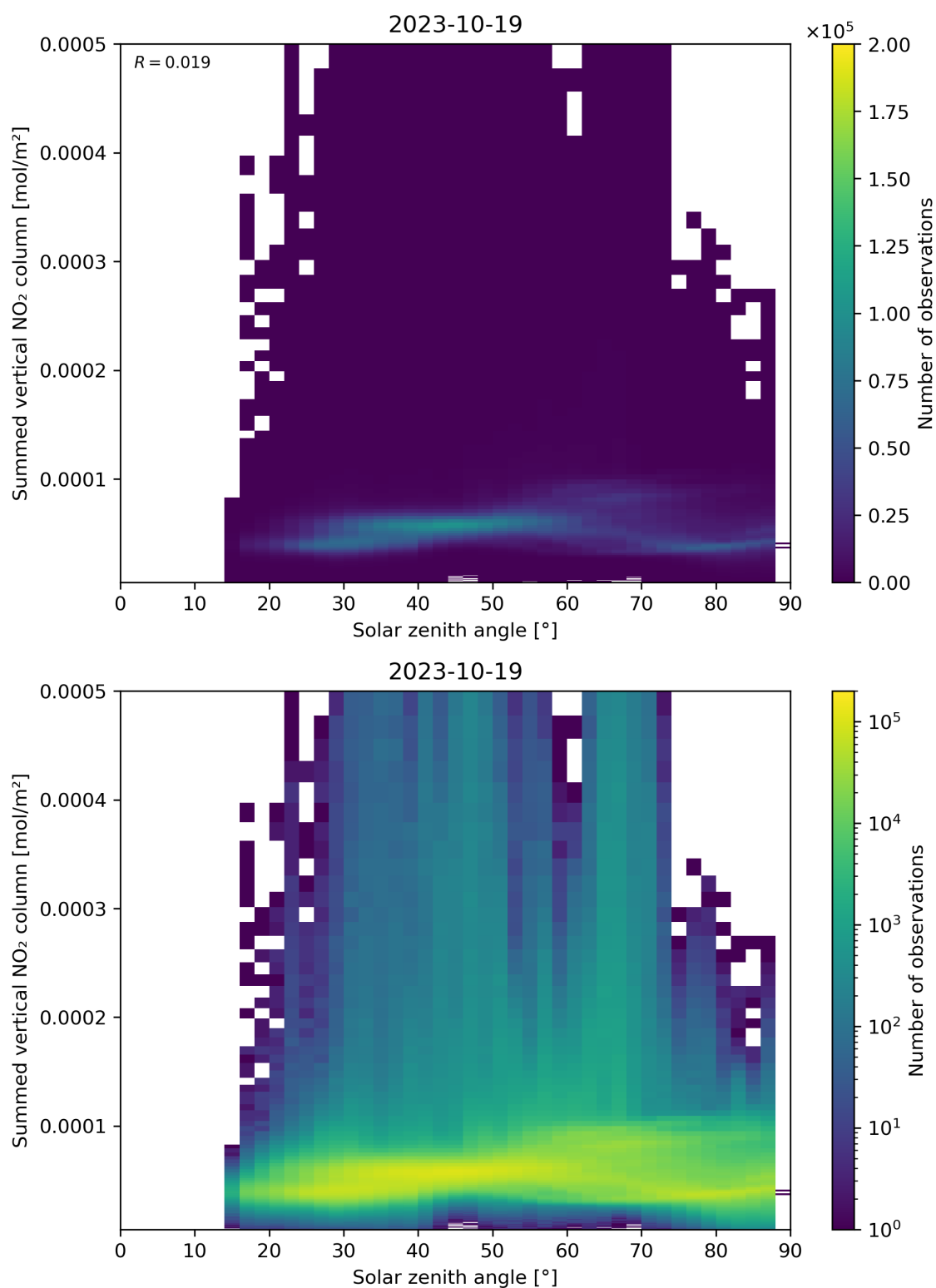
Figure 151: Scatter density plot of “Solar zenith angle” against “Summed vertical NO 2 column” for 2023-10-18 to 2023-10-20.
