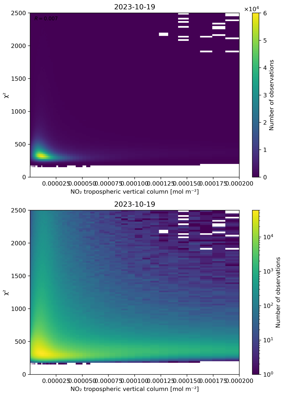
Figure 124: Scatter density plot of “NO 2 tropospheric vertical column” against “ \chi^2 ” for 2023-10-18 to 2023-10-20.
