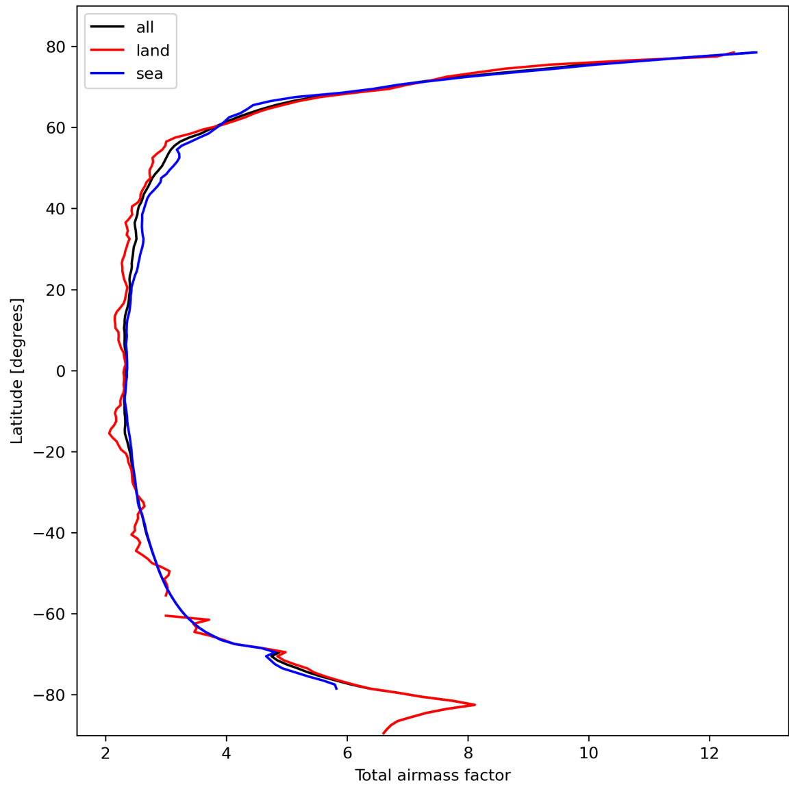
Figure 15: Zonal average of “Total airmass factor” for 2023-10-18 to 2023-10-20.
