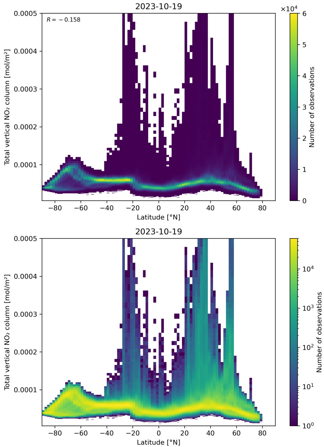
Figure 90: Scatter density plot of “Latitude” against “Total vertical NO 2 column” for 2023-10-18 to 2023-10-20.
