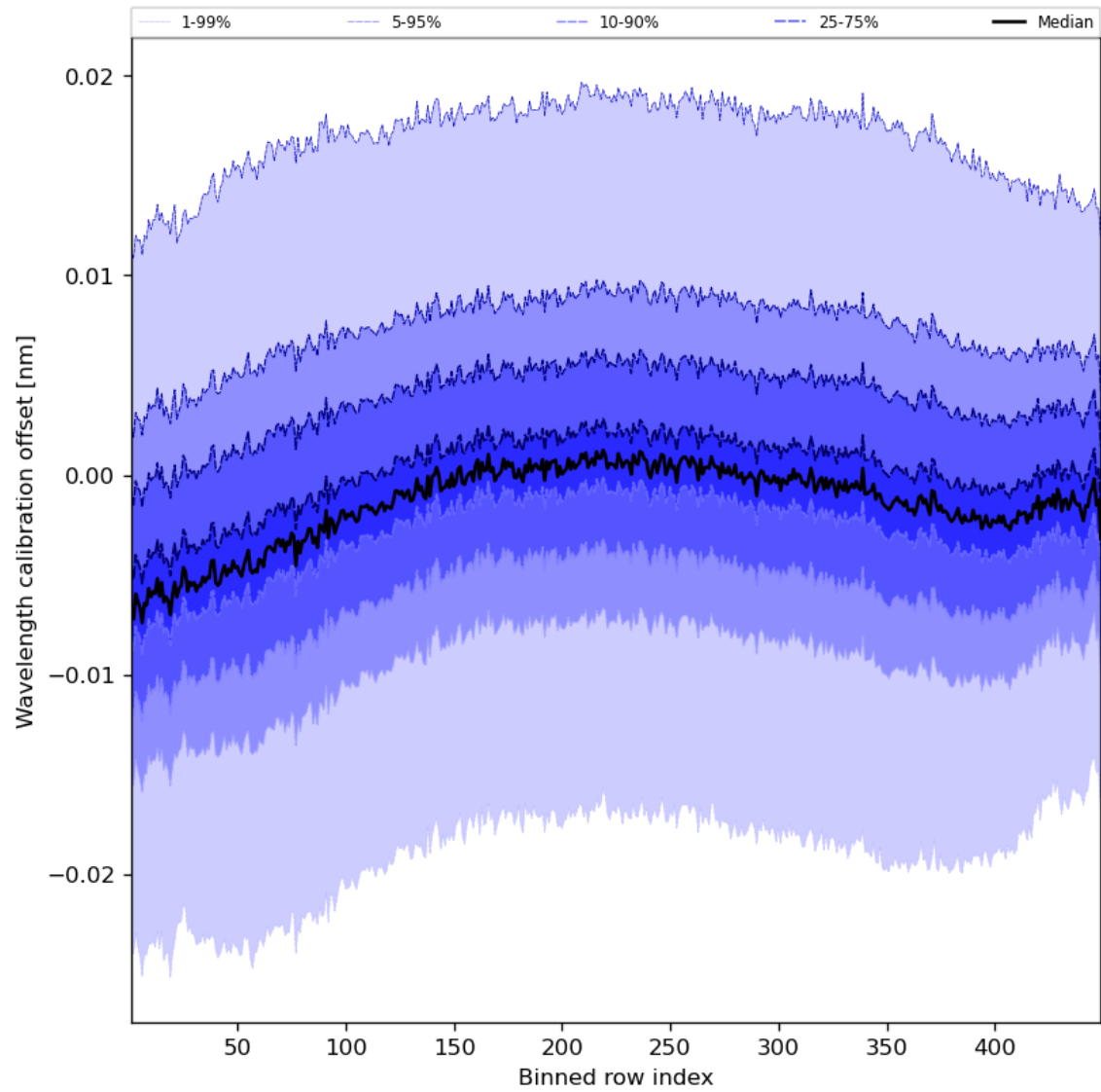
Figure 52: Along track statistics of “Wavelength calibration offset” for 2023-10-18 to 2023-10-20
