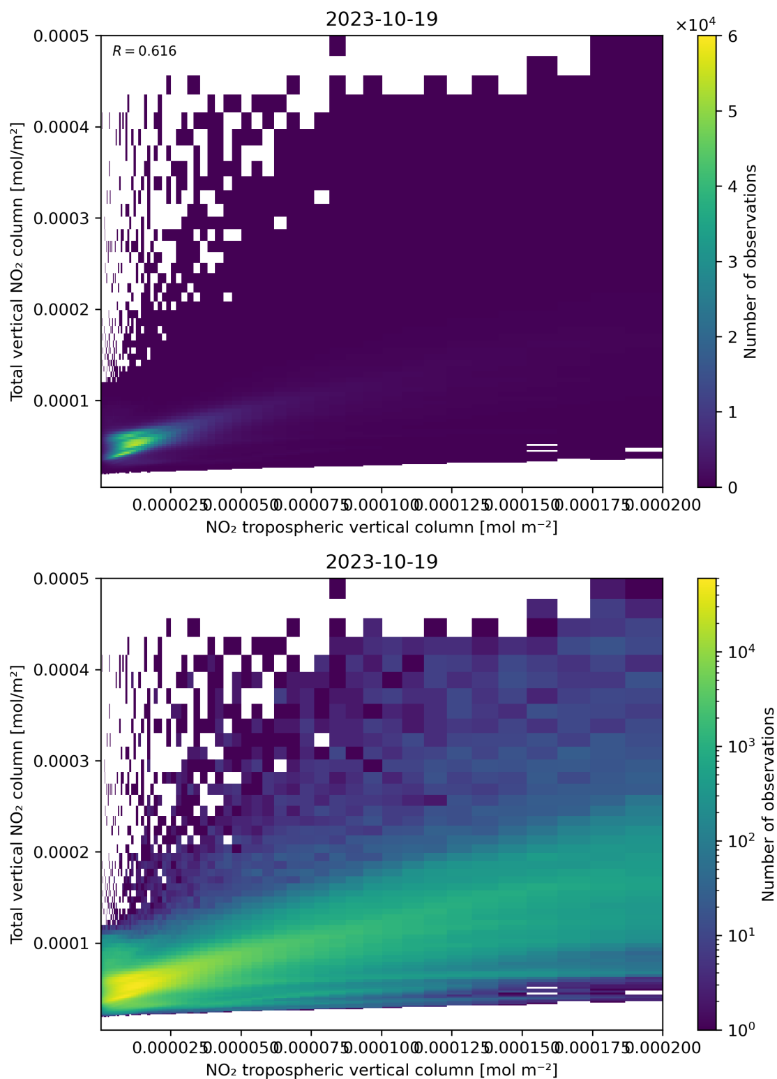
Figure 128: Scatter density plot of “NO 2 tropospheric vertical column” against “Total vertical NO 2 column” for 2023-10-18 to 2023-10-20.
