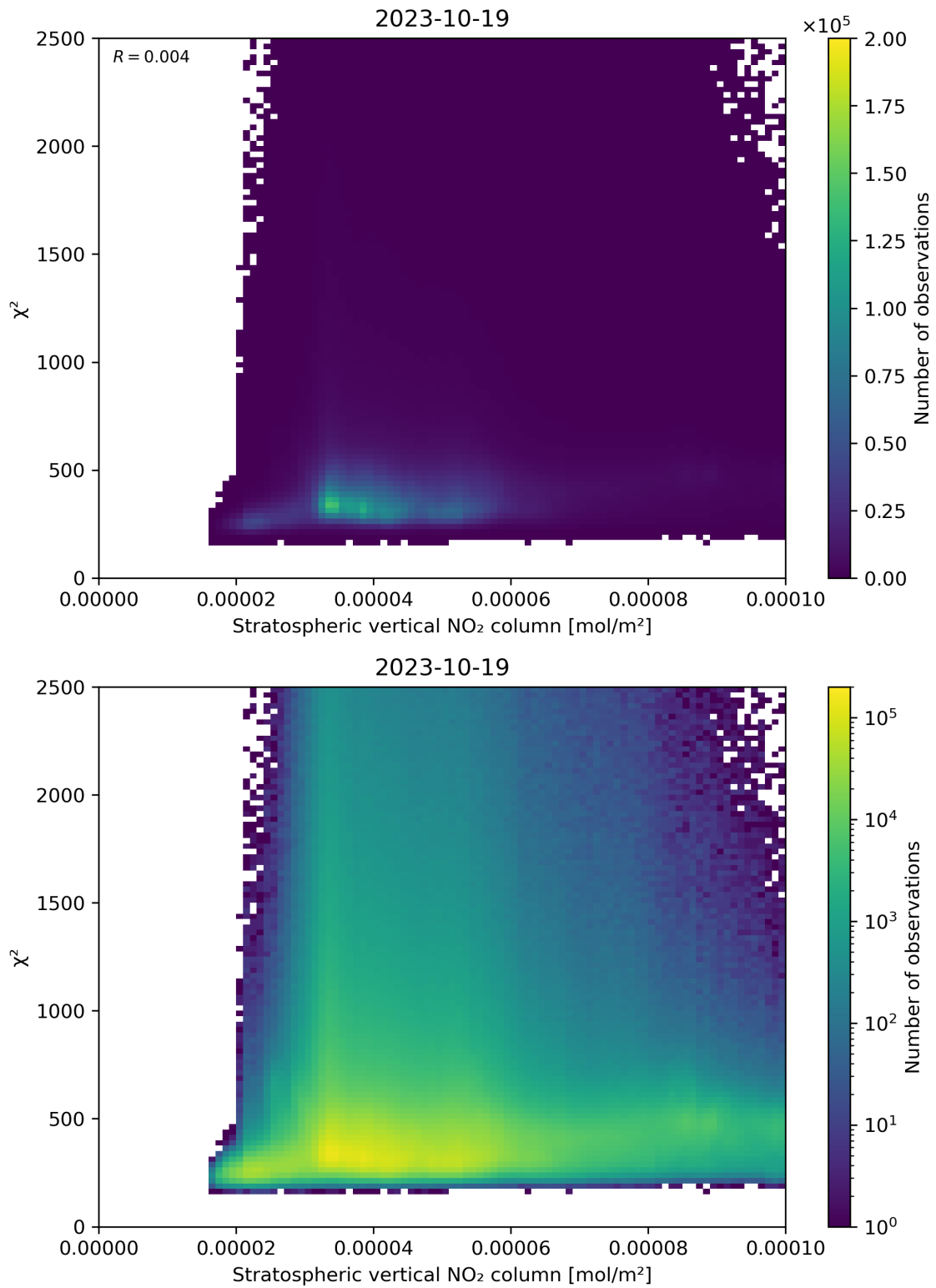
Figure 97: Scatter density plot of “Stratospheric vertical NO 2 column” against “ \chi^2 ” for 2023-10-18 to 2023-10-20.
