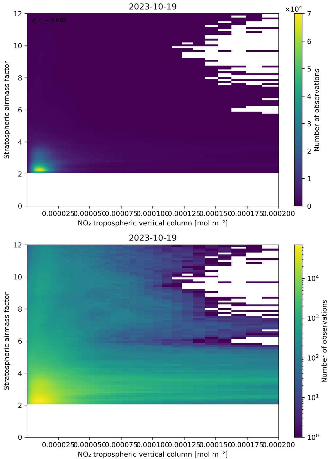
Figure 121: Scatter density plot of “NO 2 tropospheric vertical column” against “Stratospheric air mass factor” for 2023-10-18 to 2023-10-20.
