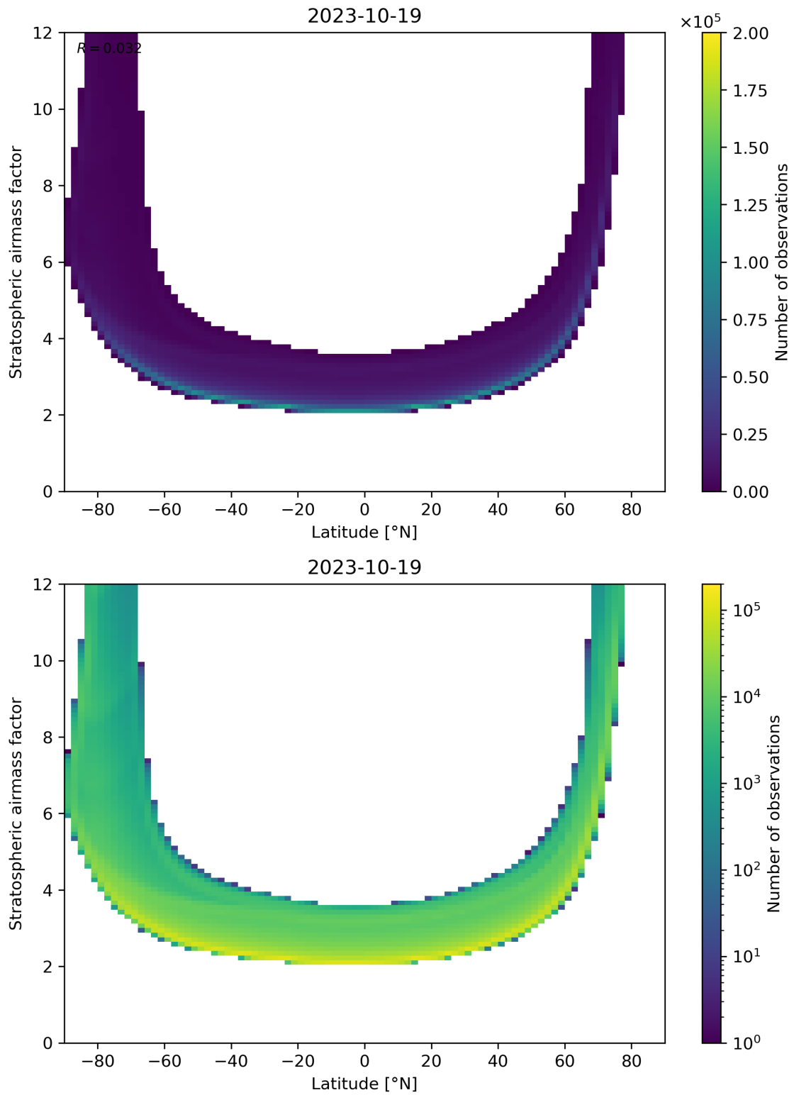
Figure 83: Scatter density plot of “Latitude” against “Stratospheric airmass factor” for 2023-10-18 to 2023-10-20.
