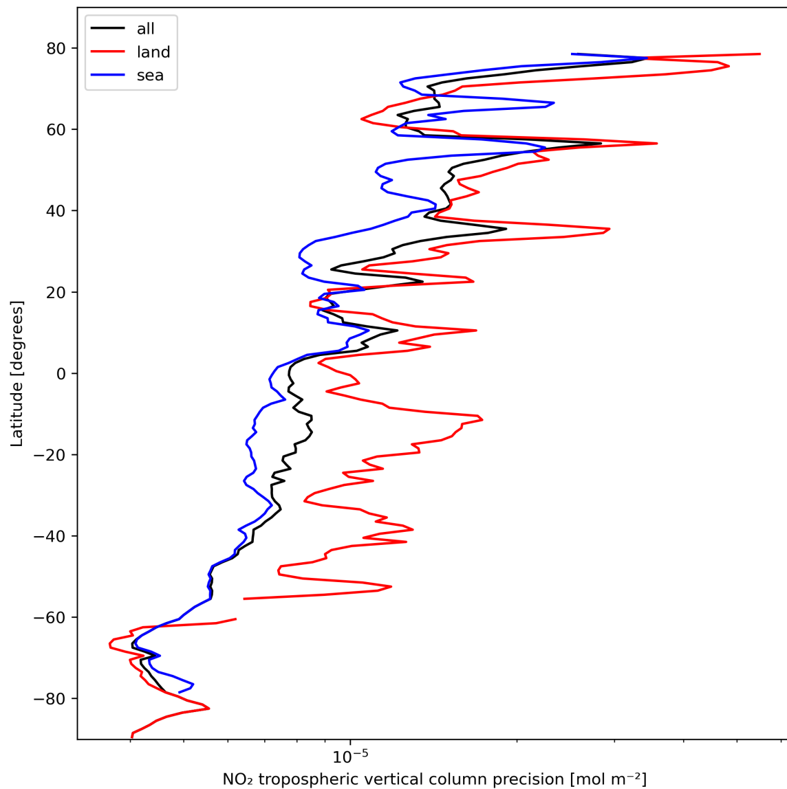
Figure 13: Zonal average of “NO 2 tropospheric vertical column precision” for 2023-10-18 to 2023-10-20.
