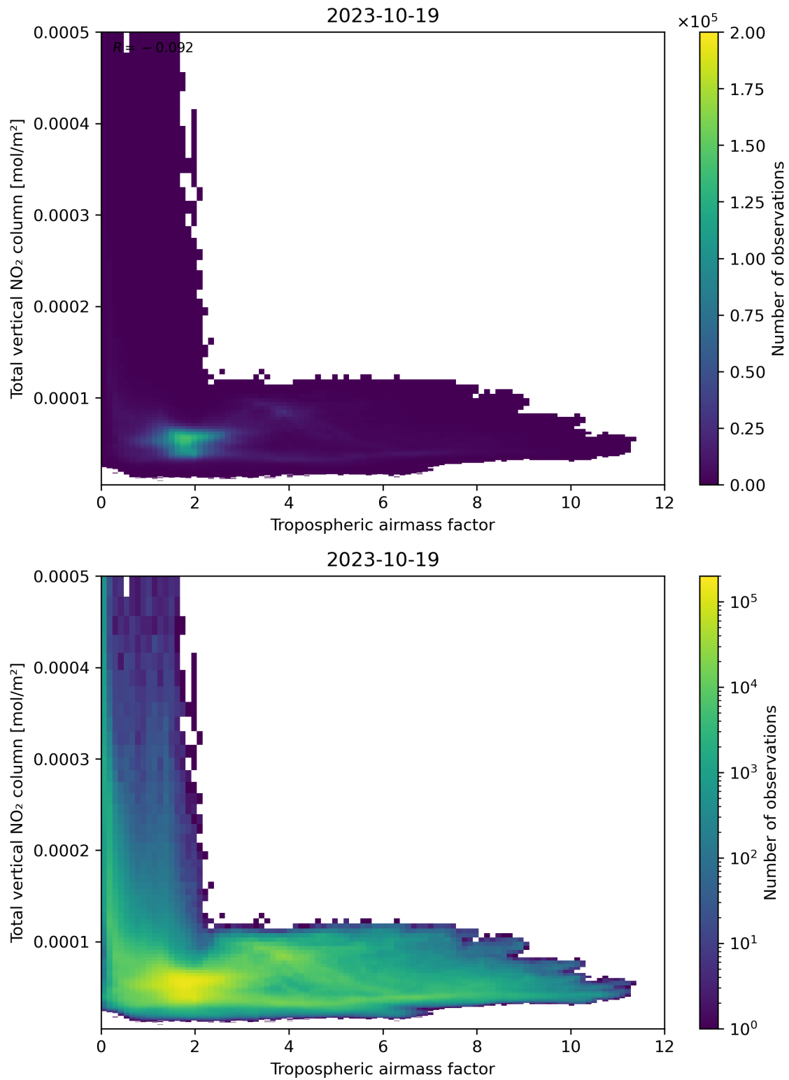
Figure 77: Scatter density plot of “Tropospheric airmass factor” against “Total vertical NO 2 column” for 2023-10-18 to 2023-10-20.
