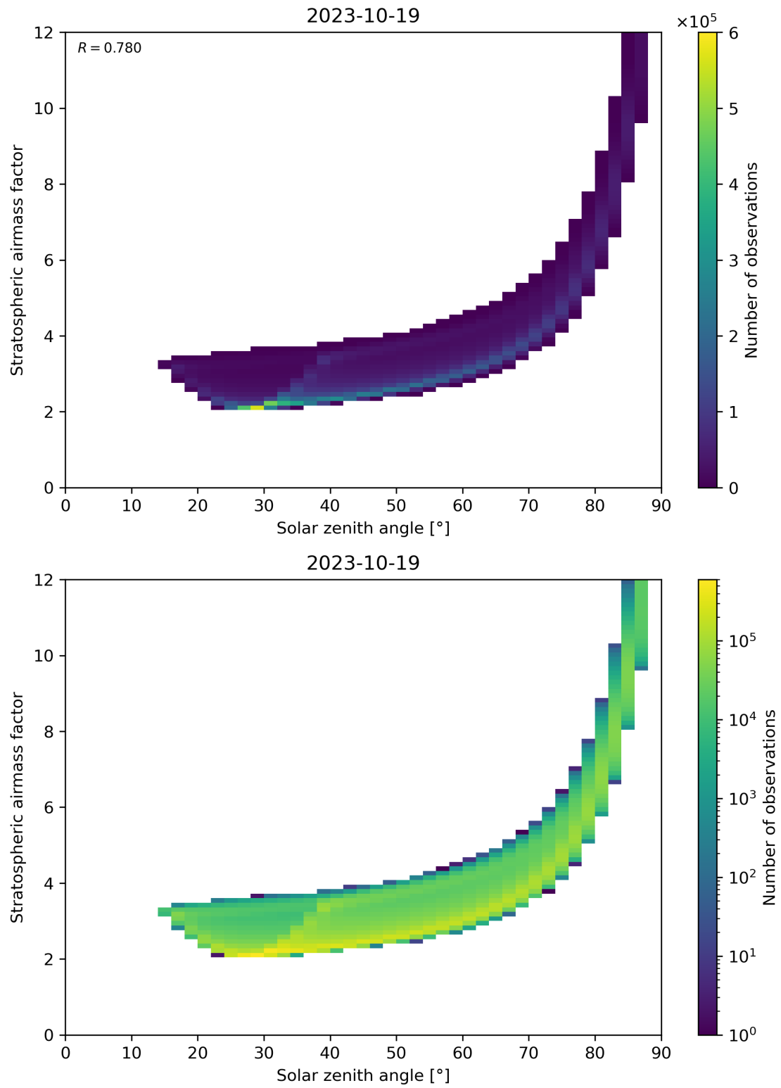
Figure 145: Scatter density plot of “Solar zenith angle” against “Stratospheric airmass factor” for 2023-10-18 to 2023-10-20.
