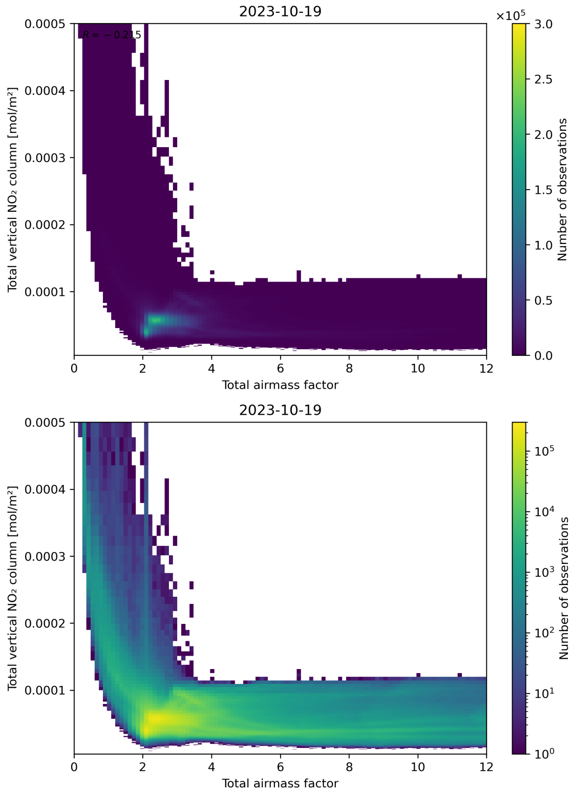
Figure 67: Scatter density plot of “Total airmass factor” against “Total vertical NO 2 column” for 2023-10-18 to 2023-10-20.
