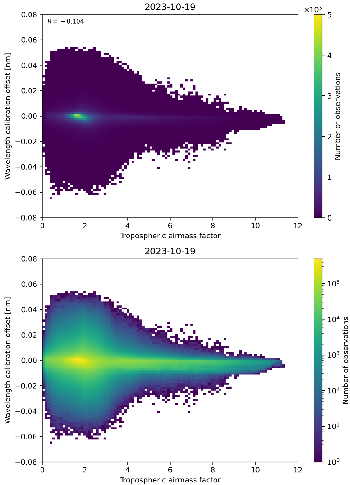
Figure 80: Scatter density plot of “Tropospheric airmass factor” against “Wavelength calibration offset” for 2023-10-18 to 2023-10-20.
