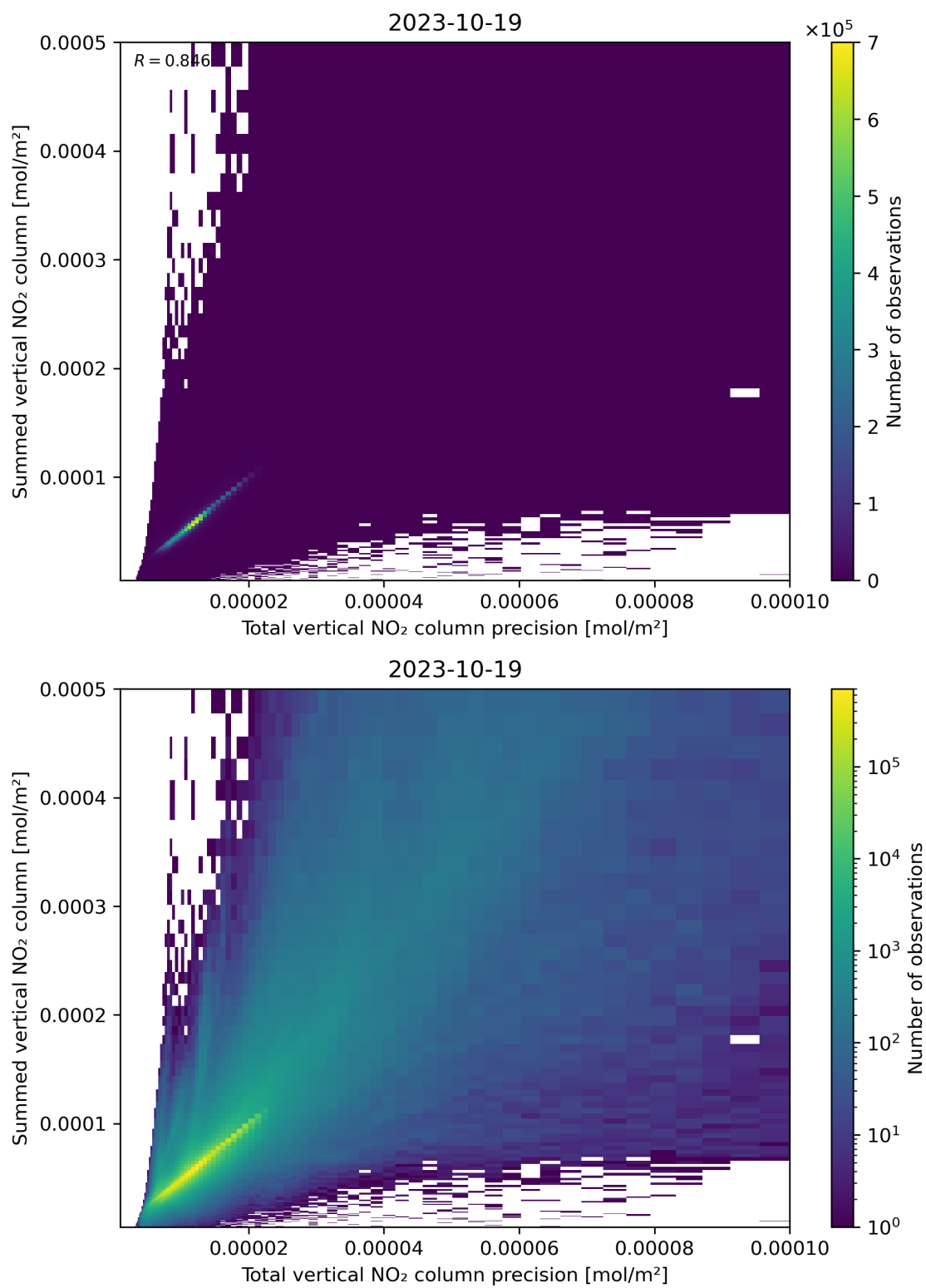
Figure 117: Scatter density plot of “Total vertical NO 2 column precision” against “Summed vertical NO 2 column” for 2023-10-18 to 2023-10-20.
