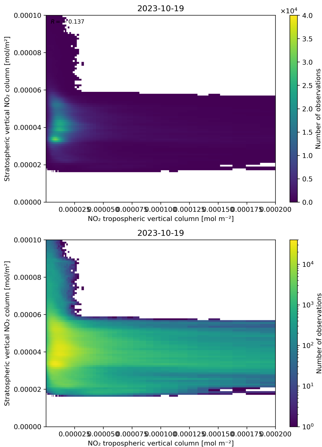
Figure 125: Scatter density plot of “NO 2 tropospheric vertical column” against “Stratospheric vertical NO 2 column” for 2023-10-18 to 2023-10-20.
