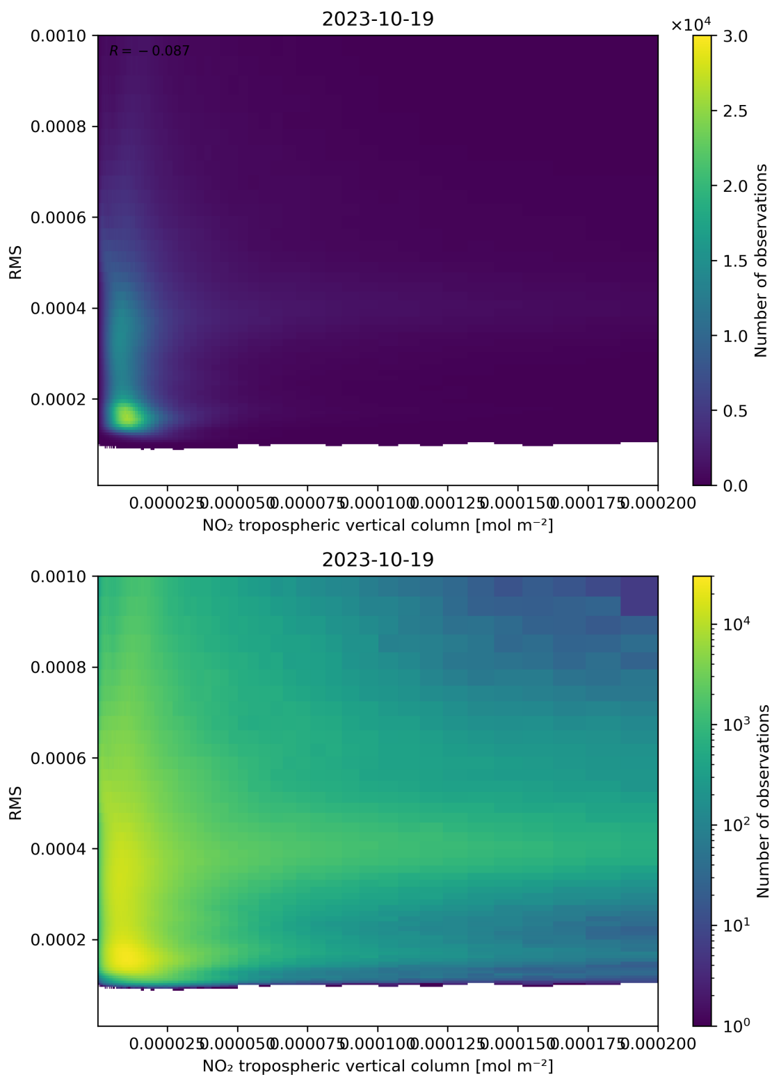
Figure 142: Scatter density plot of “NO 2 tropospheric vertical column” against “RMS” for 2023-10-18 to 2023-10-20.
