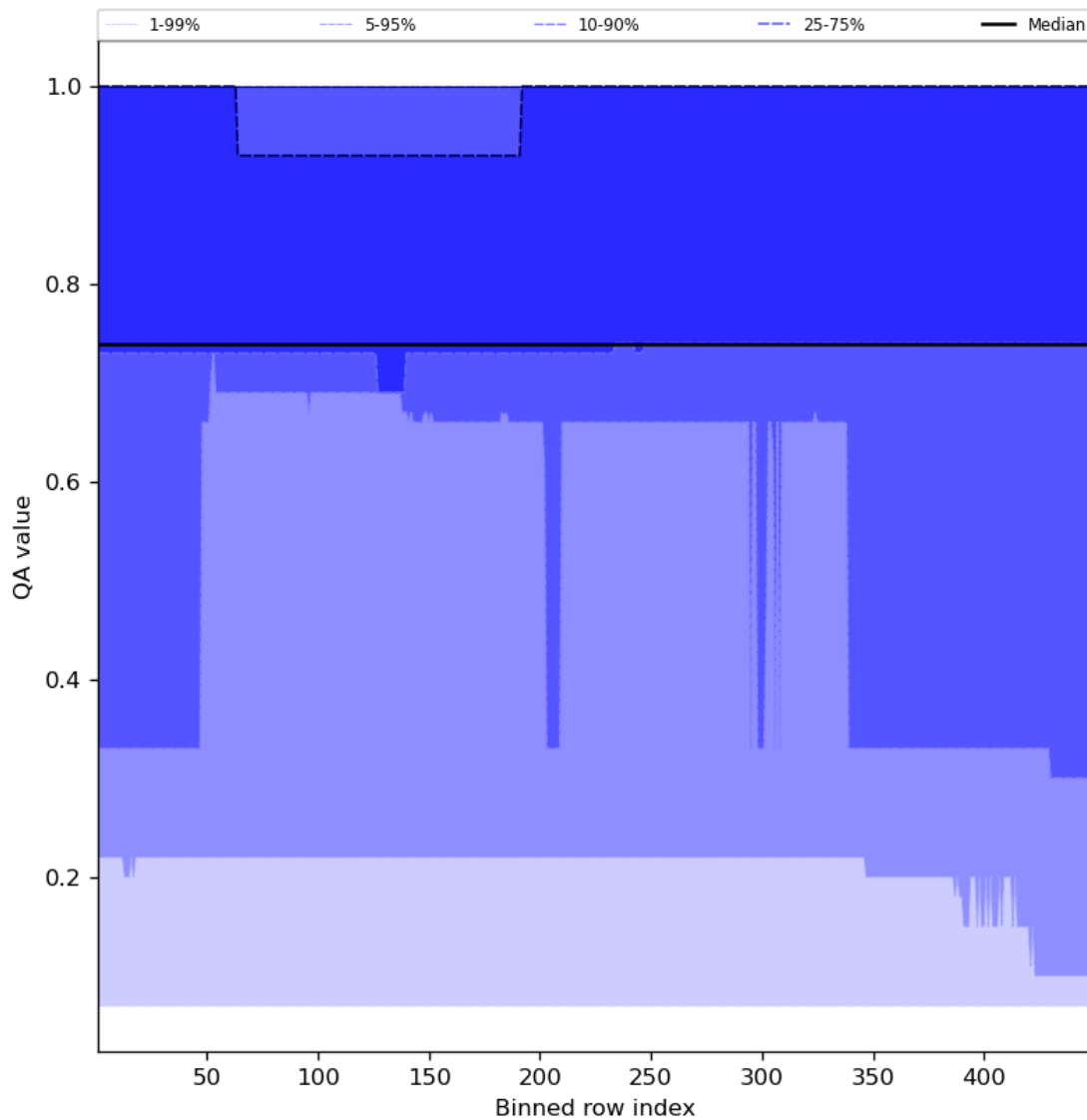
Figure 45: Along track statistics of “QA value” for 2023-10-18 to 2023-10-20
