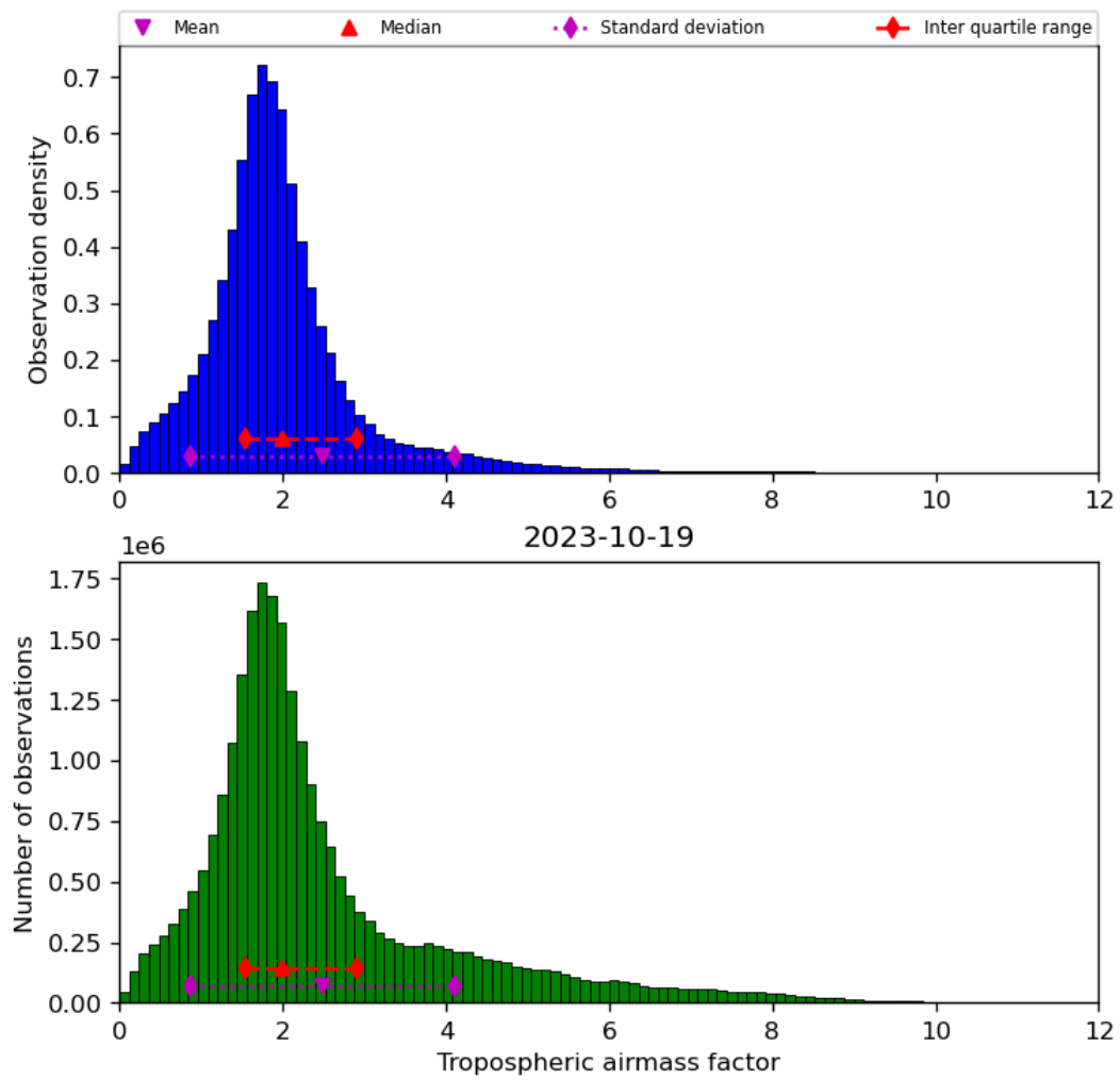
Figure 31: Histogram of “Tropospheric airmass factor” for 2023-10-18 to 2023-10-20
