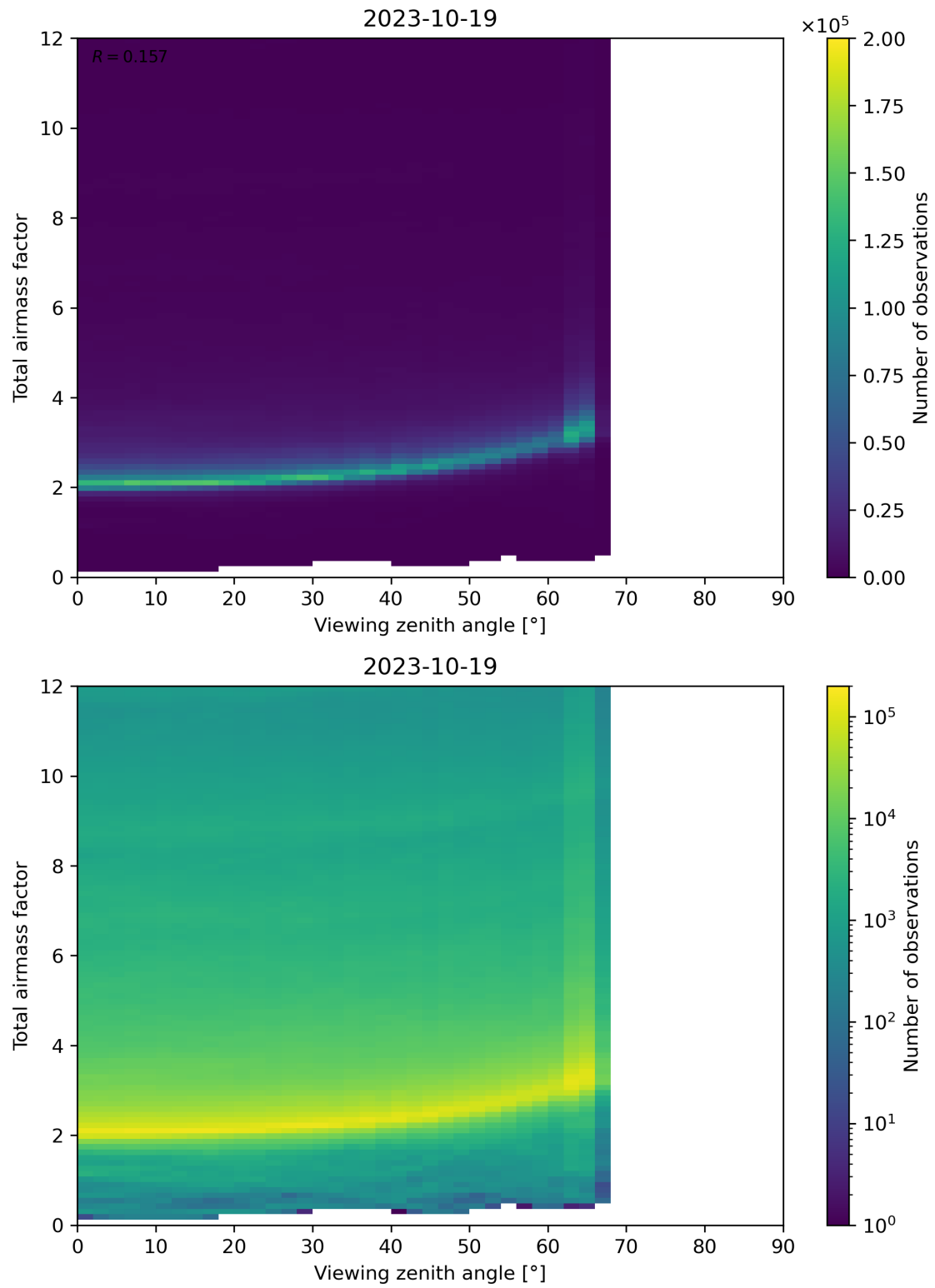
Figure 160: Scatter density plot of “Viewing zenith angle” against “Total airmass factor” for 2023-10-18 to 2023-10-20.
