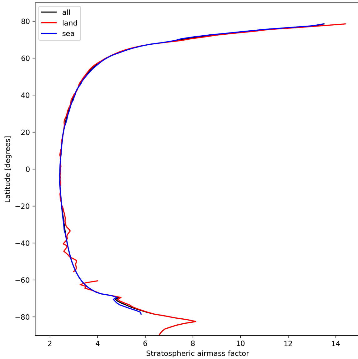
Figure 27: Zonal average of “Stratospheric airmass factor” for 2023-10-18 to 2023-10-20.
