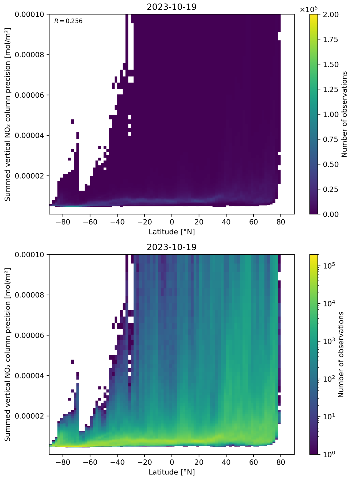
Figure 89: Scatter density plot of “Latitude” against “Summed vertical NO 2 column precision” for 2023-10-18 to 2023-10-20.
