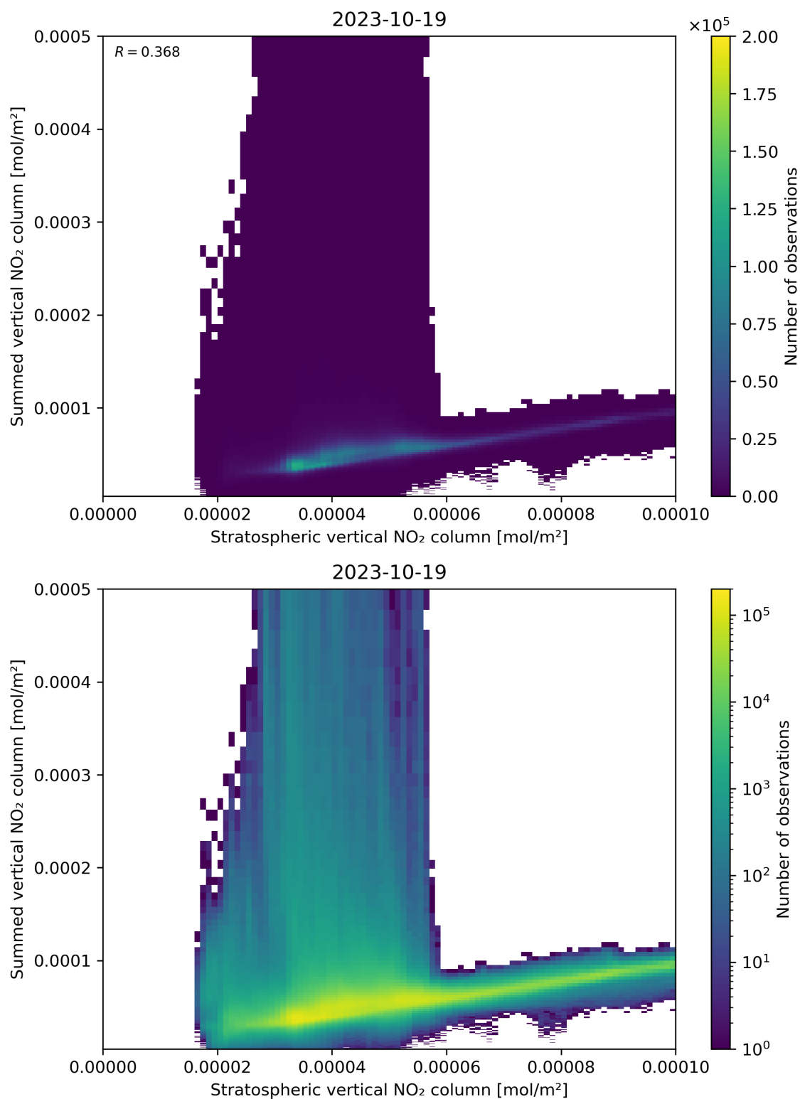
Figure 98: Scatter density plot of “Stratospheric vertical NO 2 column” against “Summed vertical NO 2 column” for 2023-10-18 to 2023-10-20.
