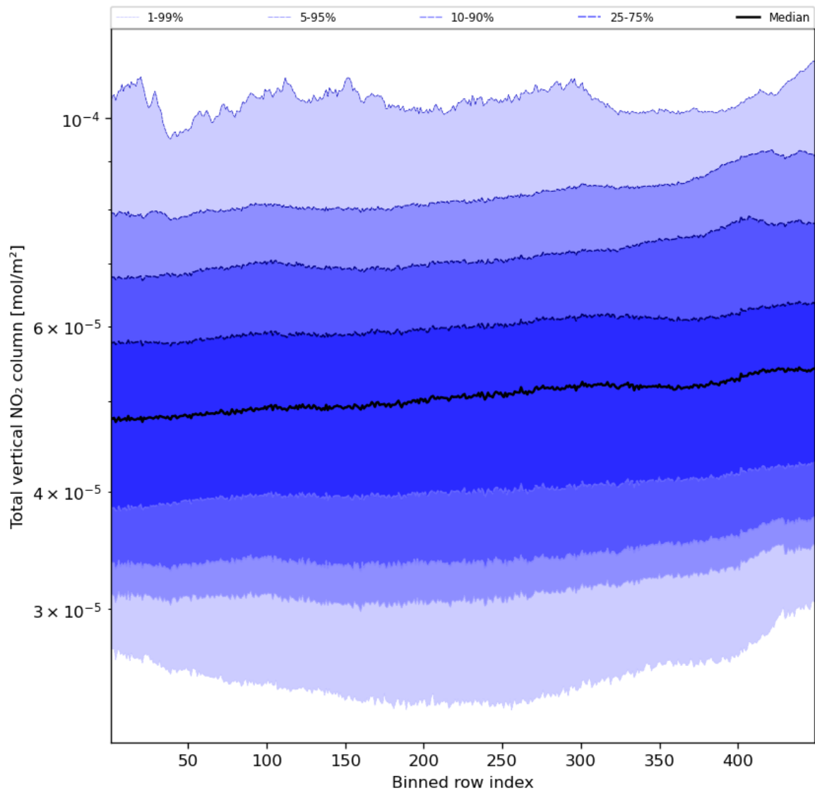
Figure 55: Along track statistics of “Total vertical NO 2 column” for 2023-10-18 to 2023-10-20
