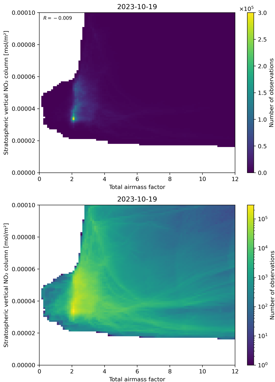
Figure 64: Scatter density plot of “Total airmass factor” against “Stratospheric vertical NO 2 column” for 2023-10-18 to 2023-10-20.
