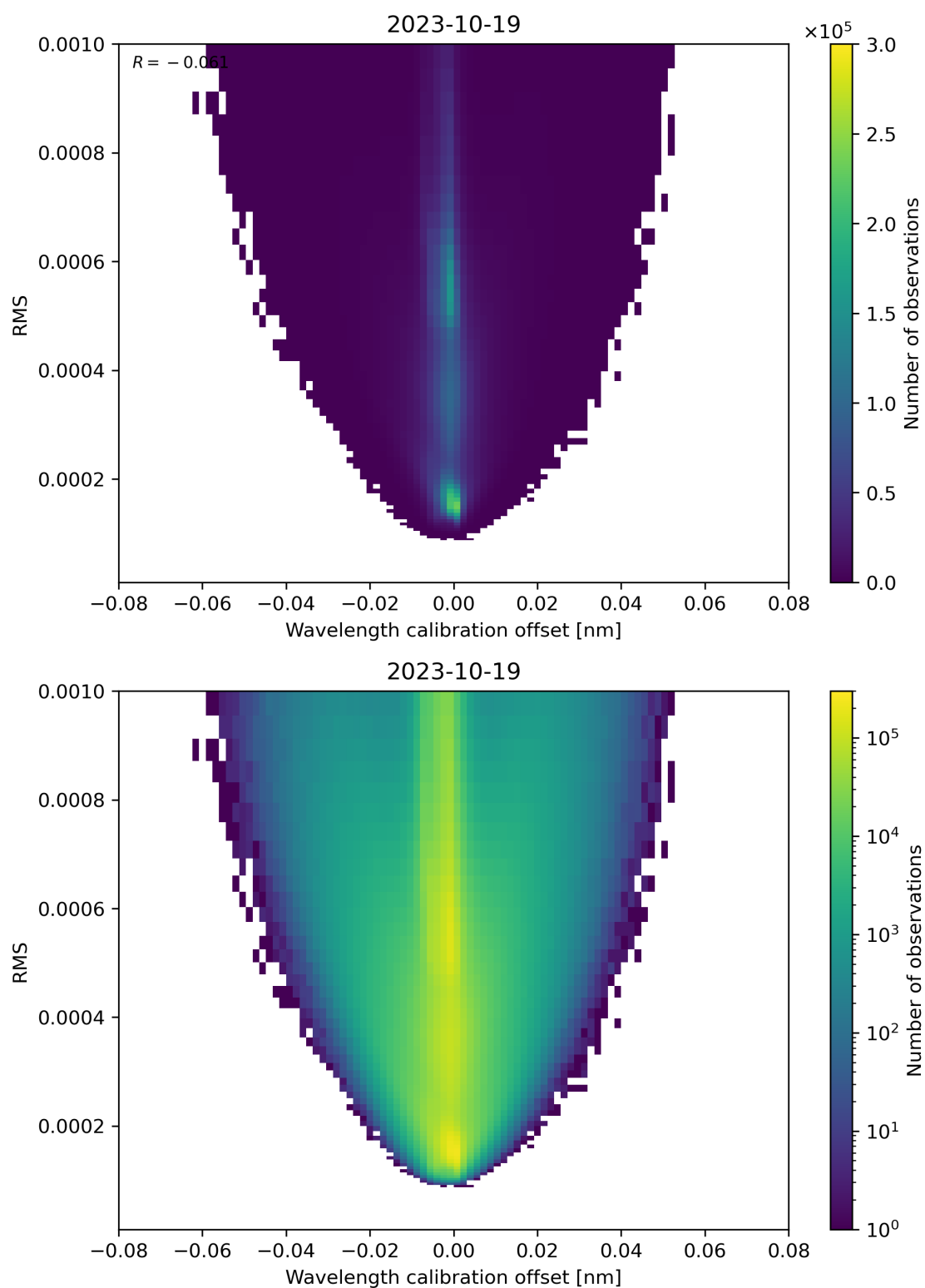
Figure 181: Scatter density plot of “Wavelength calibration offset” against “RMS” for 2023-10-18 to 2023-10-20.
