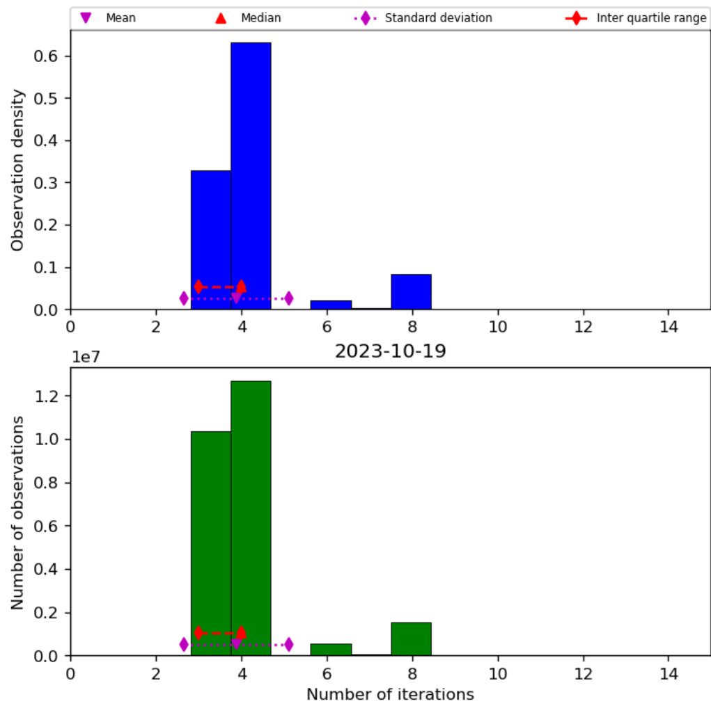
Figure 34: Histogram of “Number of iterations” for 2023-10-18 to 2023-10-20
