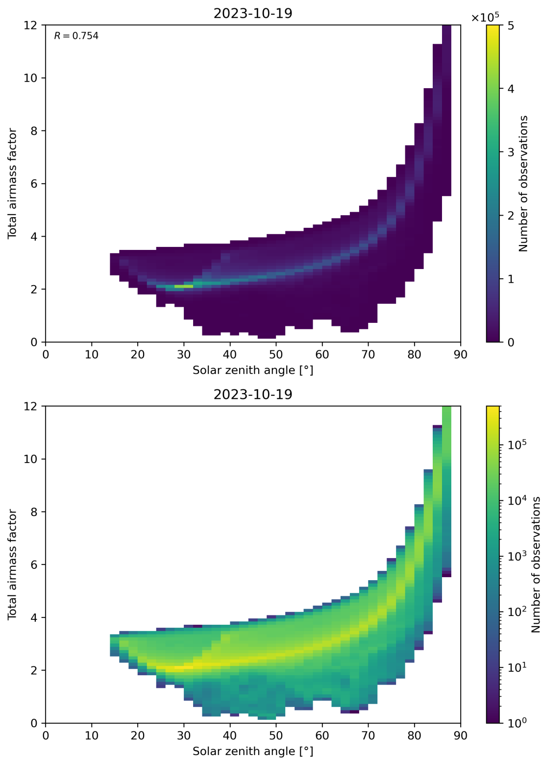
Figure 146: Scatter density plot of “Solar zenith angle” against “Total airmass factor” for 2023-10-18 to 2023-10-20.
