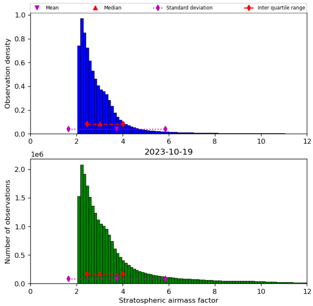
Figure 44: Histogram of “Stratospheric airmass factor” for 2023-10-18 to 2023-10-20
