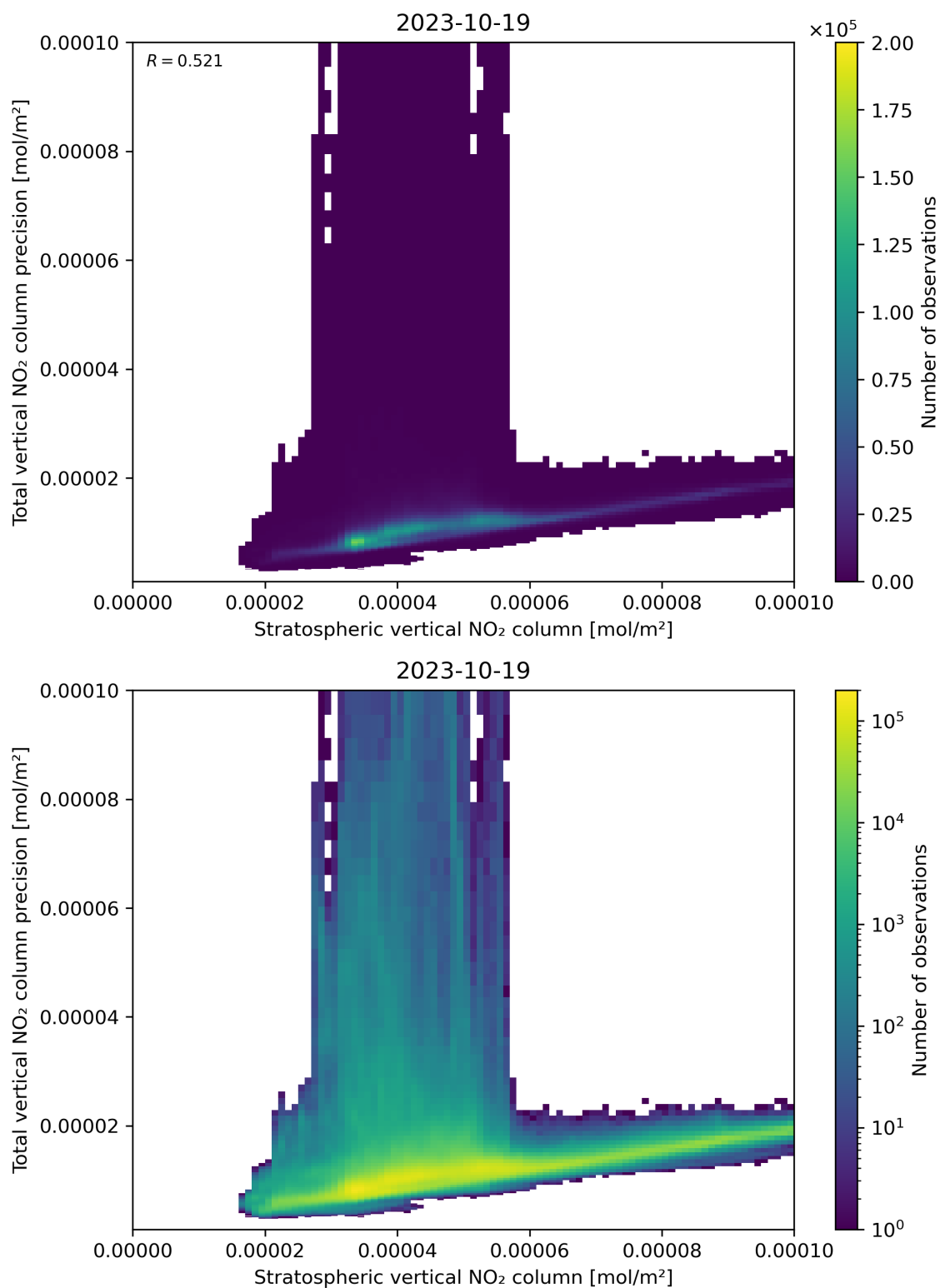
Figure 101: Scatter density plot of “Stratospheric vertical NO 2 column” against “Total vertical NO 2 column precision” for 2023-10-18 to 2023-10-20.
