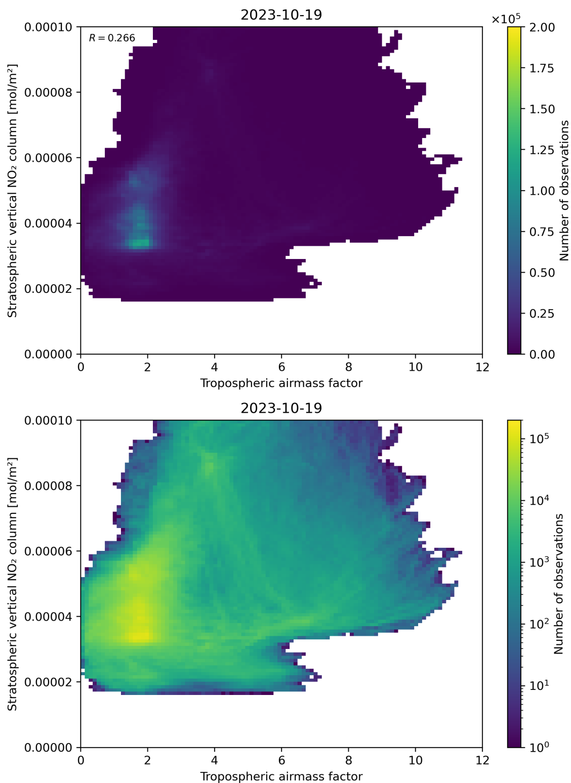
Figure 74: Scatter density plot of “Tropospheric air mass factor” against “Stratospheric vertical NO 2 column” for 2023-10-18 to 2023-10-20.
