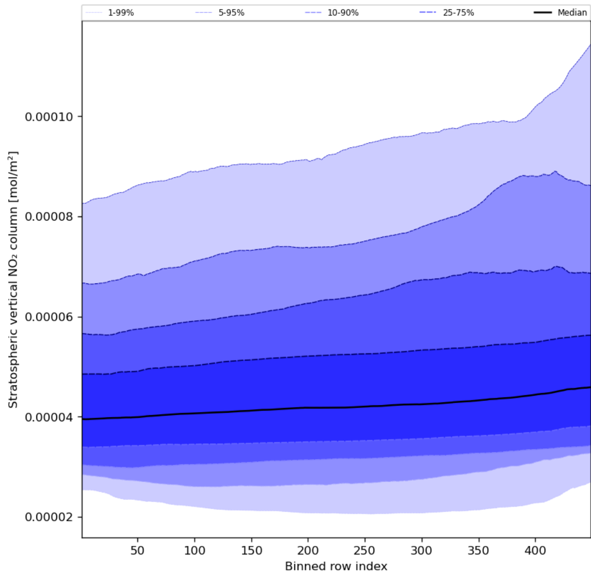
Figure 53: Along track statistics of “Stratospheric vertical NO 2 column” for 2023-10-18 to 2023-10-20
