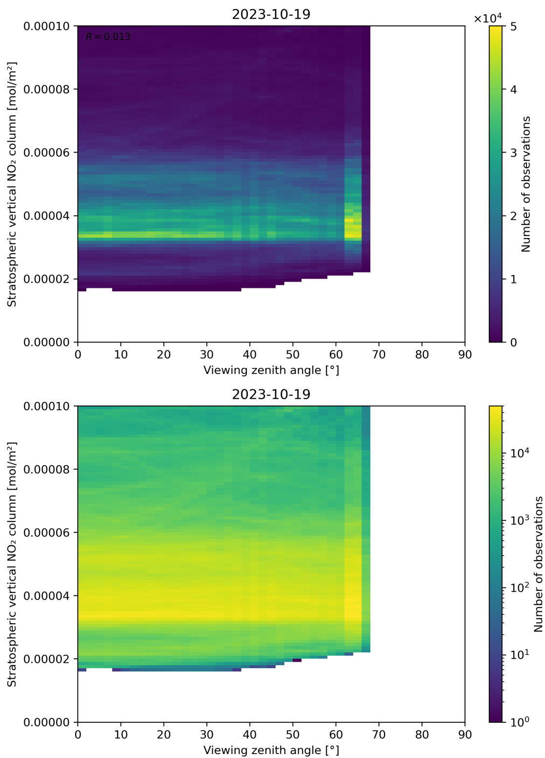
Figure 164: Scatter density plot of “Viewing zenith angle” against “Stratospheric vertical NO 2 column” for 2023-10-18 to 2023-10-20.
