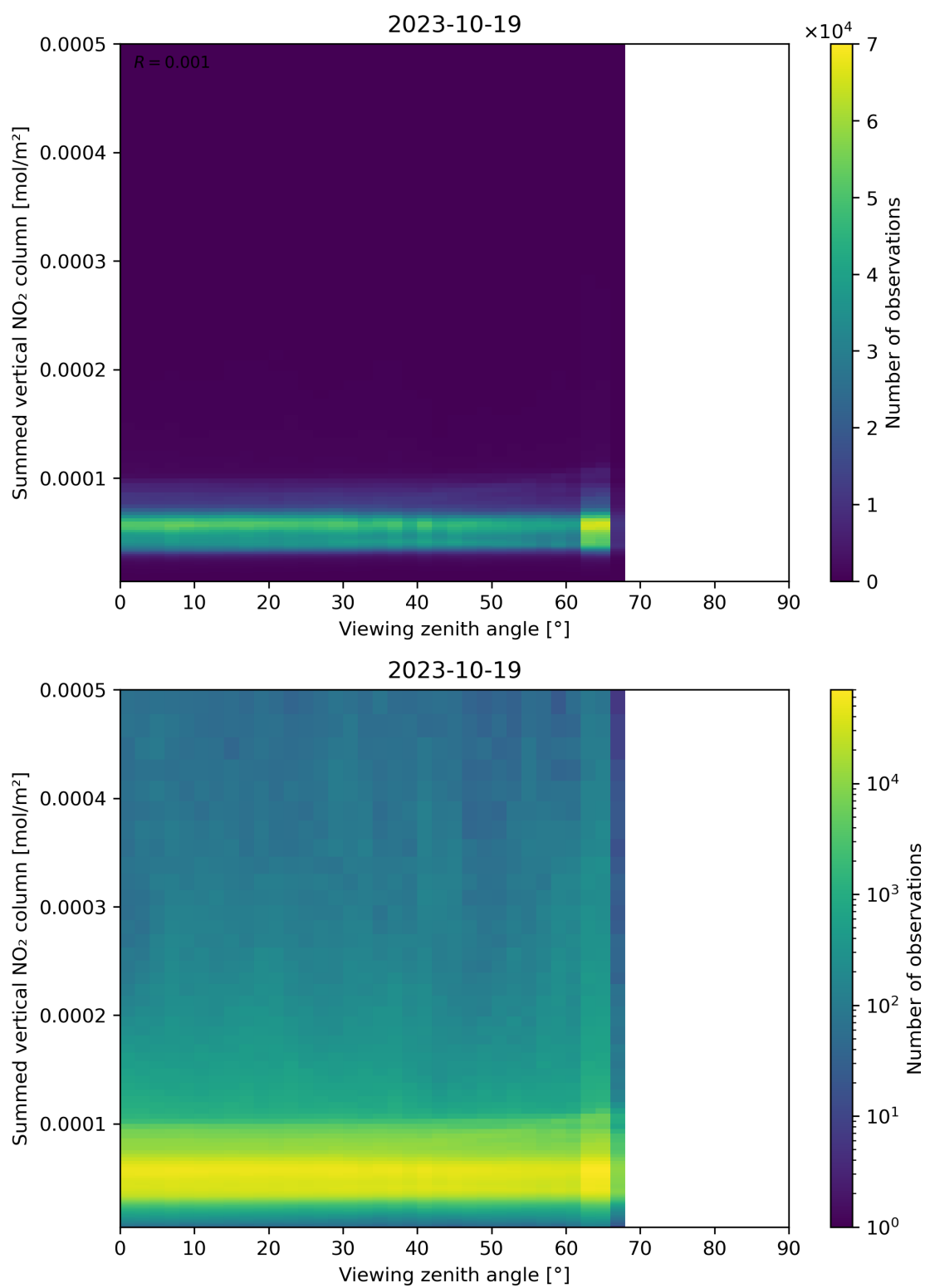
Figure 165: Scatter density plot of “Viewing zenith angle” against “Summed vertical NO 2 column” for 2023-10-18 to 2023-10-20.
