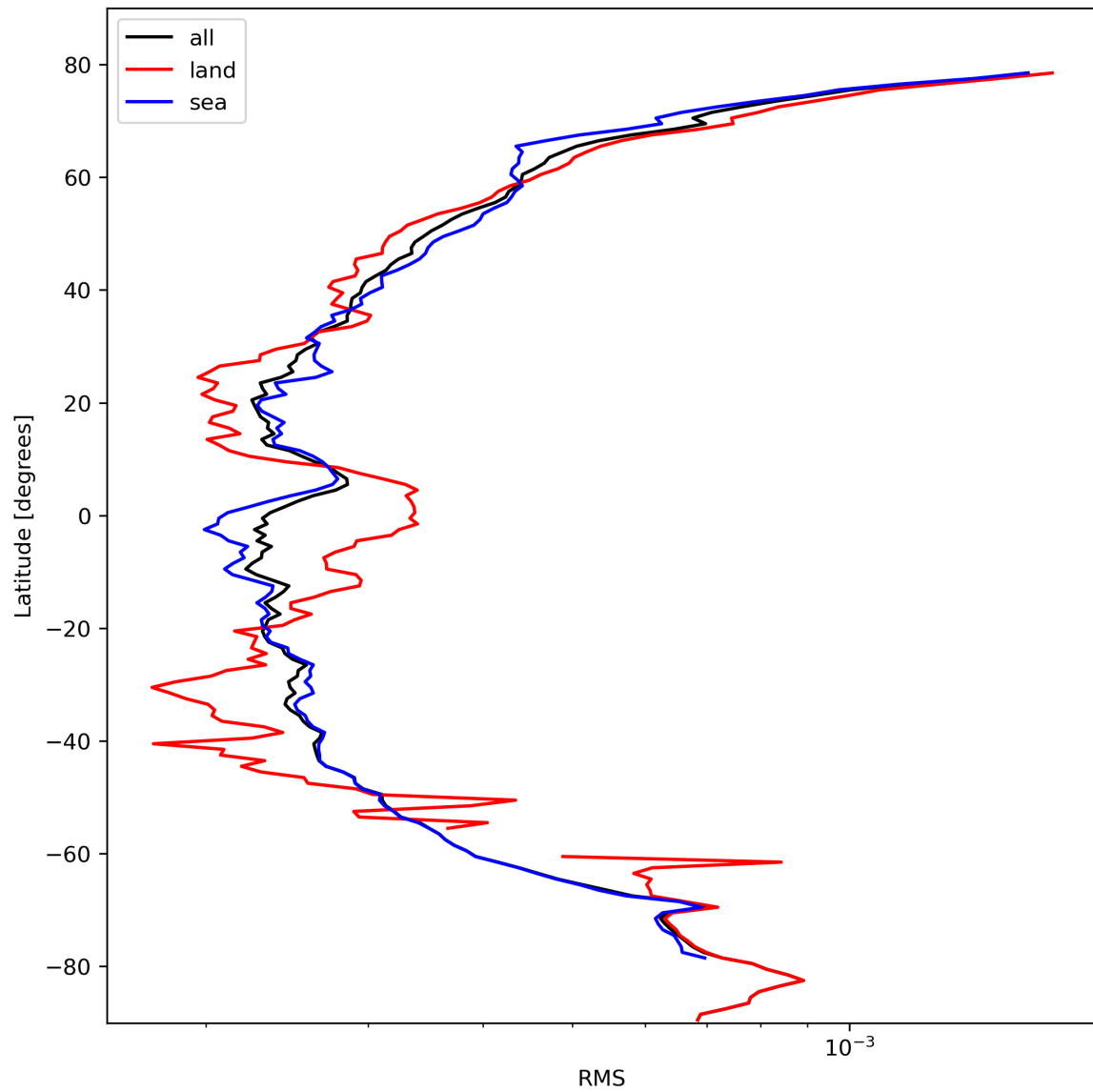
Figure 26: Zonal average of “RMS” for 2023-10-18 to 2023-10-20.
