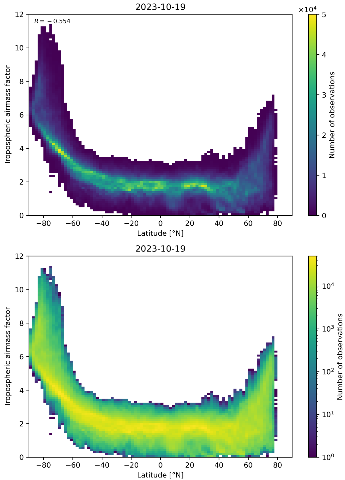
Figure 85: Scatter density plot of “Latitude” against “Tropospheric airmass factor” for 2023-10-18 to 2023-10-20.
