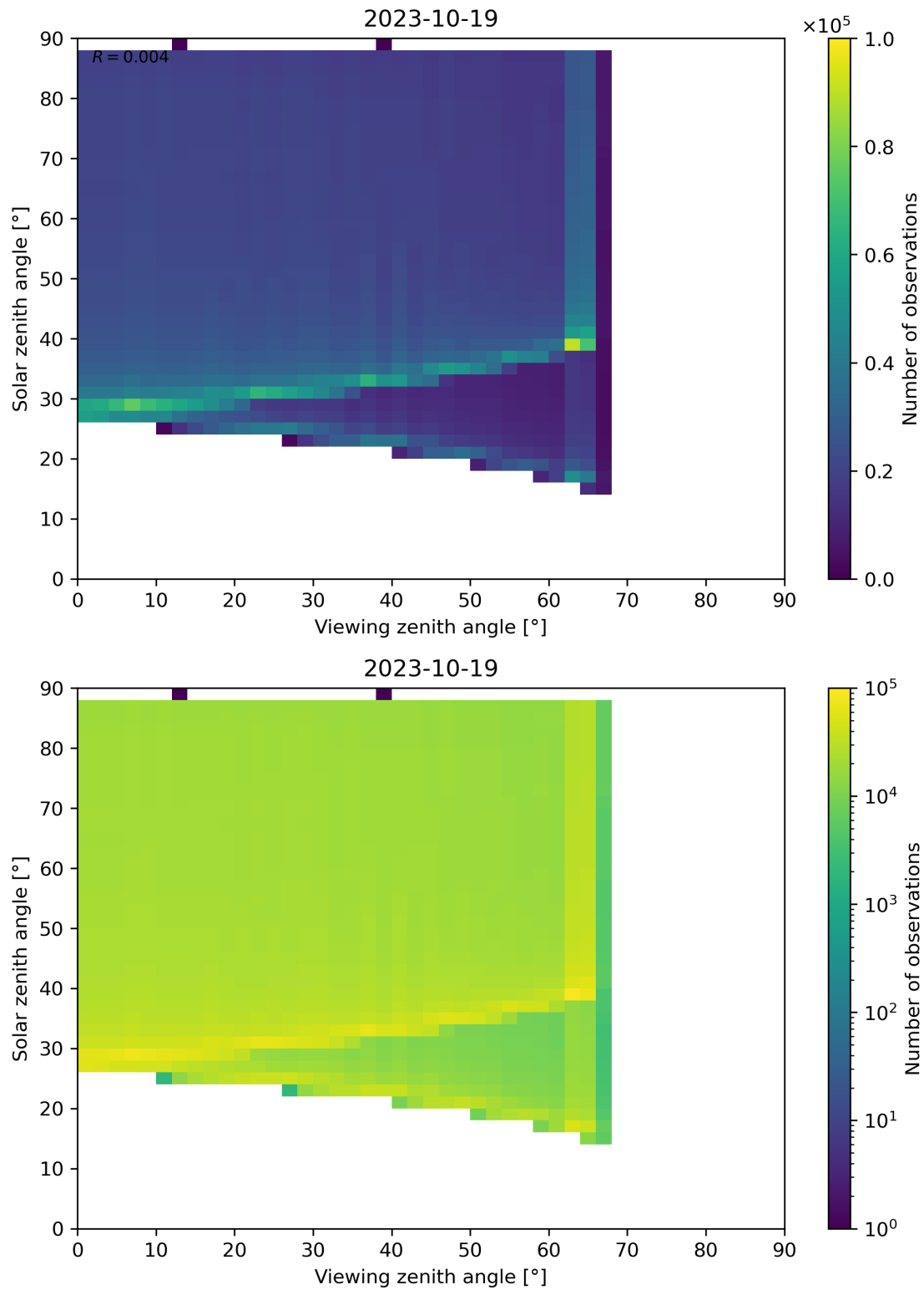
Figure 172: Scatter density plot of “Viewing zenith angle” against “Solar zenith angle” for 2023-10-18 to 2023-10-20.
