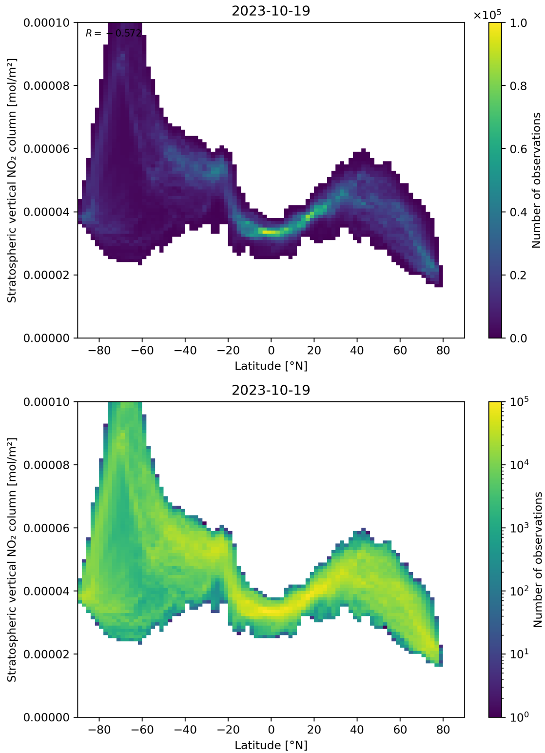
Figure 87: Scatter density plot of “Latitude” against “Stratospheric vertical NO 2 column” for 2023-10-18 to 2023-10-20.
