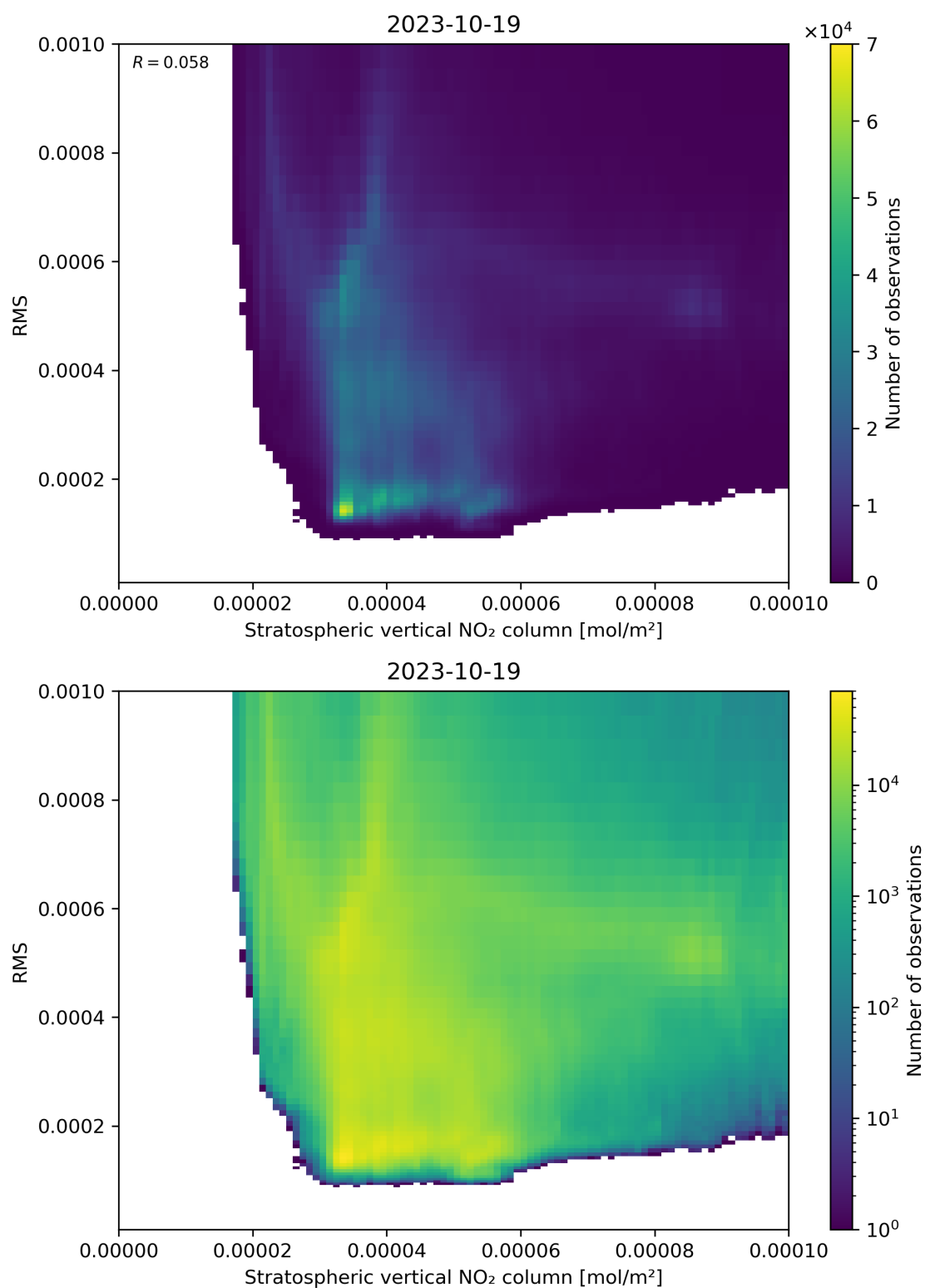
Figure 102: Scatter density plot of “Stratospheric vertical NO 2 column” against “RMS” for 2023-10-18 to 2023-10-20.
