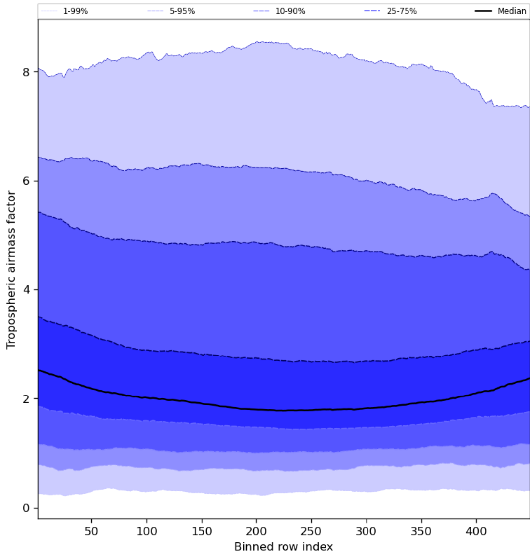
Figure 48: Along track statistics of “Tropospheric air mass factor” for 2023-10-18 to 2023-10-20
