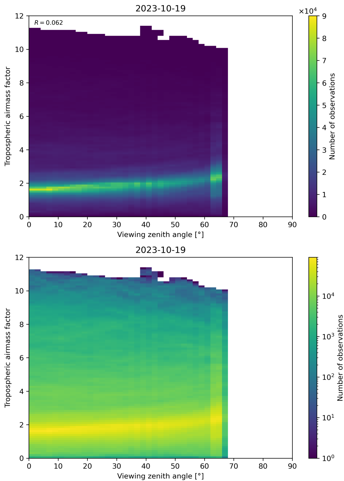
Figure 161: Scatter density plot of “Viewing zenith angle” against “Tropospheric airmass factor” for 2023-10-18 to 2023-10-20.
