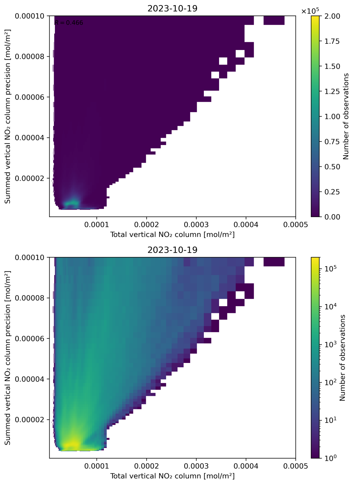
Figure 113: Scatter density plot of “Total vertical NO 2 column” against “Summed vertical NO 2 column precision” for 2023-10-18 to 2023-10-20.
