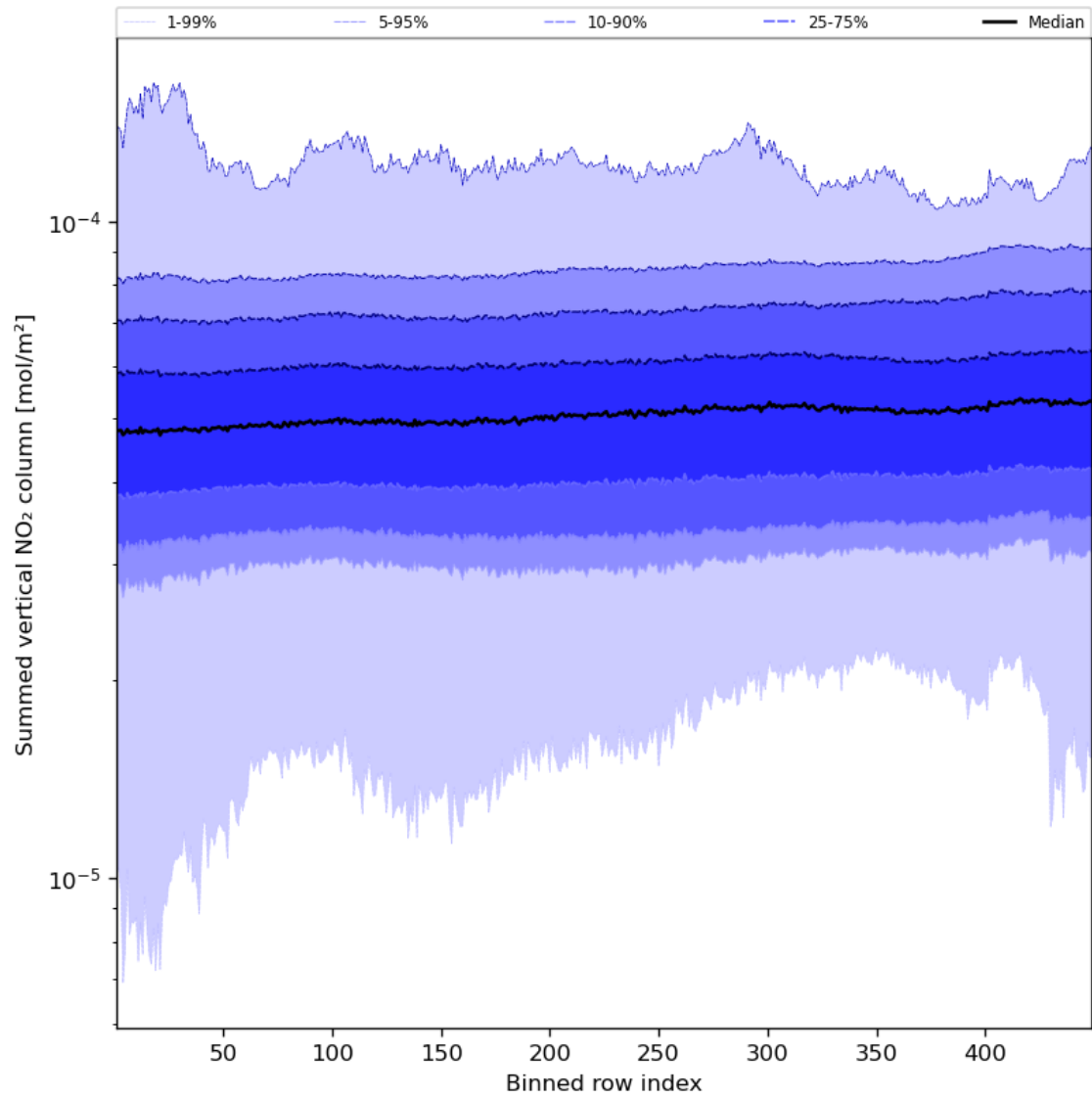
Figure 57: Along track statistics of “Summed vertical NO 2 column” for 2023-10-18 to 2023-10-20
