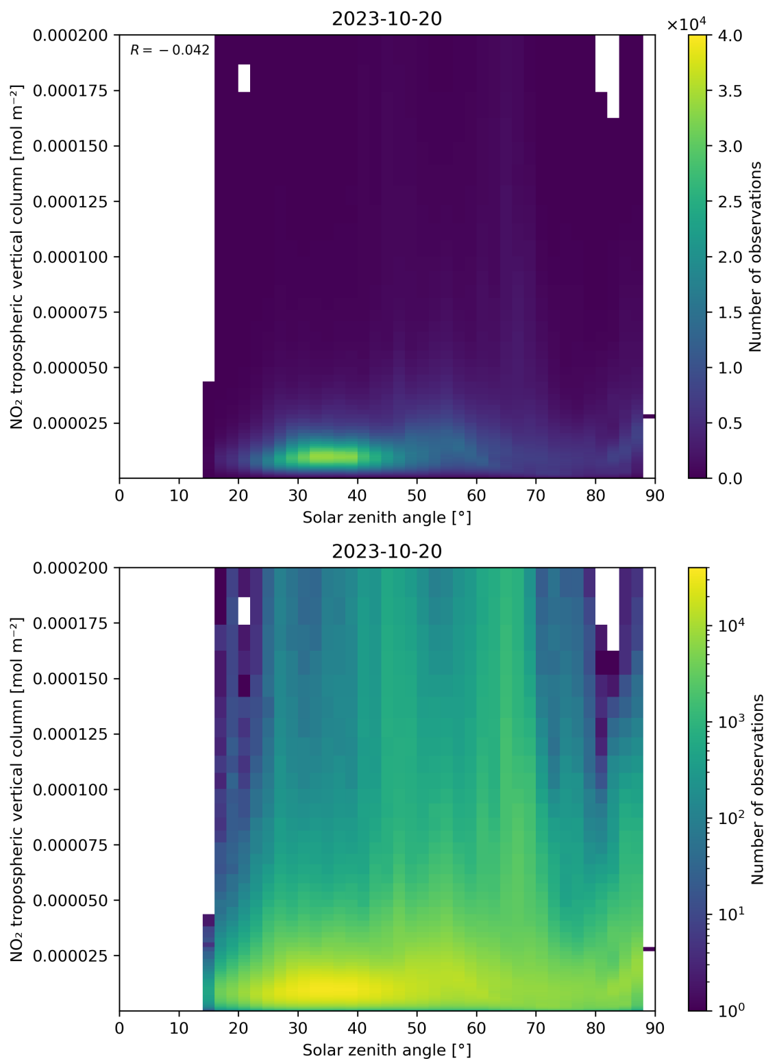
Figure 155: Scatter density plot of “Solar zenith angle” against “NO 2 tropospheric vertical column” for 2023-10-19 to 2023-10-21.
