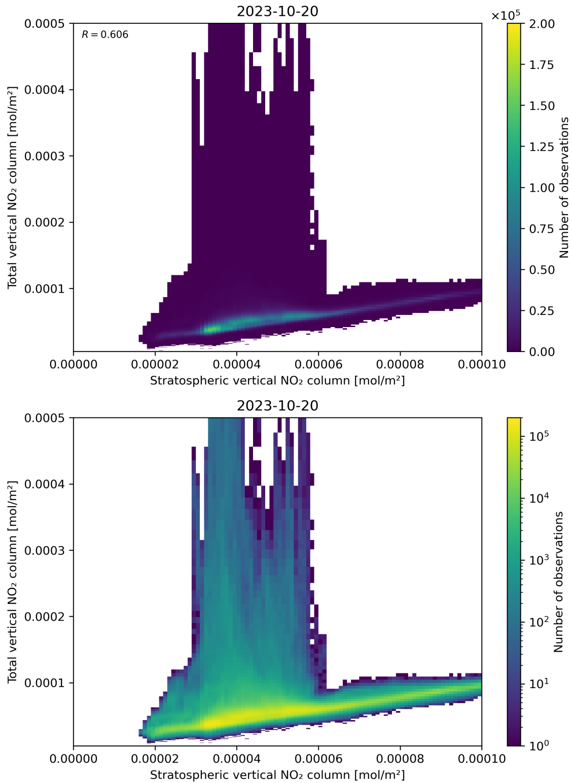
Figure 100: Scatter density plot of “Stratospheric vertical NO 2 column” against “Total vertical NO 2 column” for 2023-10-19 to 2023-10-21.
