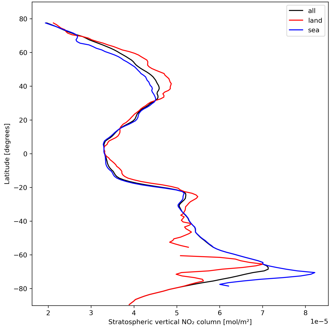
Figure 19: Zonal average of “Stratospheric vertical NO 2 column” for 2023-10-19 to 2023-10-21.
