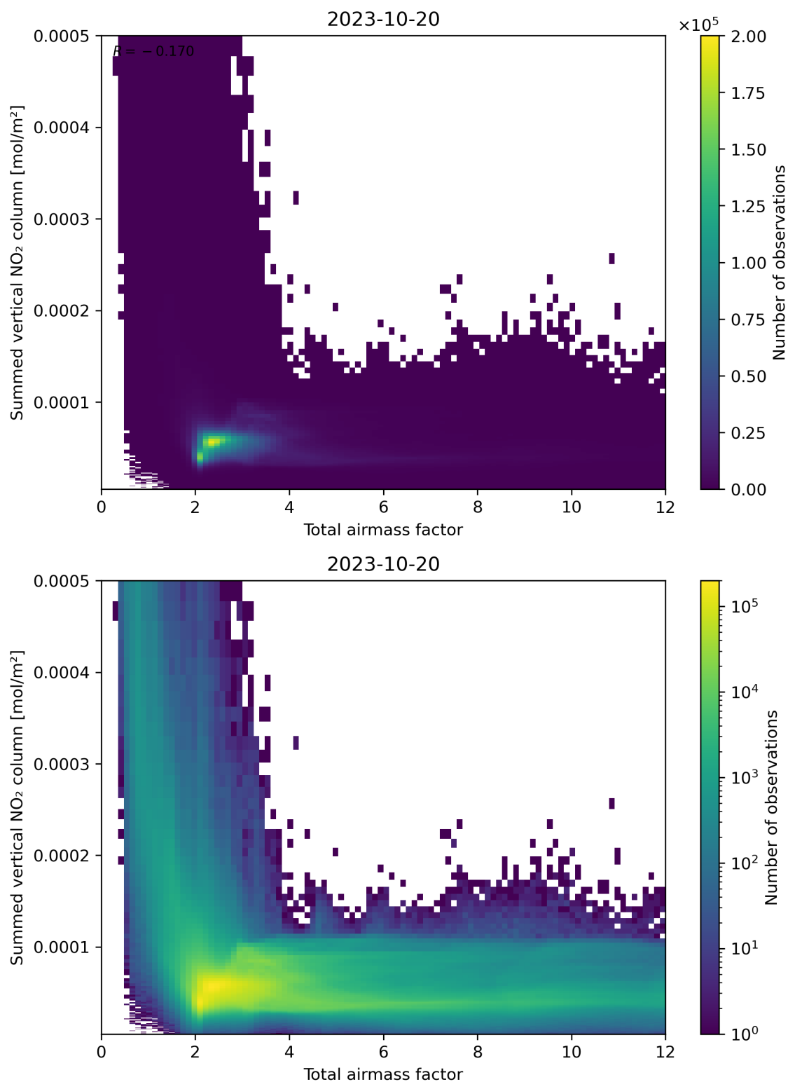
Figure 65: Scatter density plot of “Total airmass factor” against “Summed vertical NO 2 column” for 2023-10-19 to 2023-10-21.
