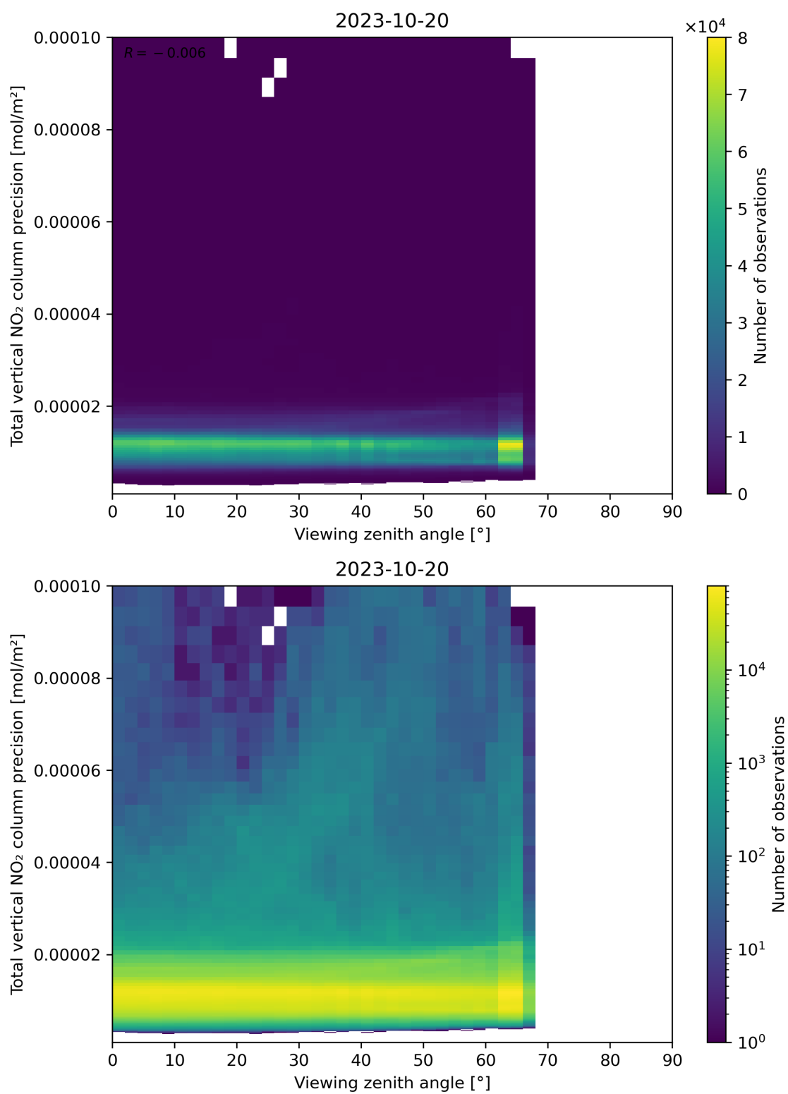
Figure 168: Scatter density plot of “Viewing zenith angle” against “Total vertical NO 2 column precision” for 2023-10-19 to 2023-10-21.
