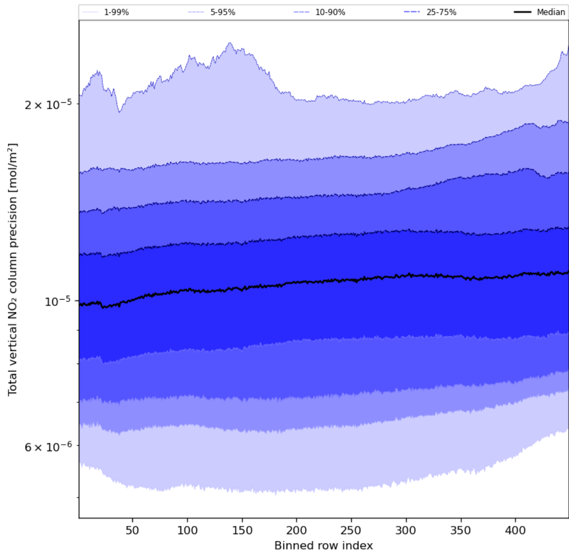
Figure 56: Along track statistics of “Total vertical NO 2 column precision” for 2023-10-19 to 2023-10-21
