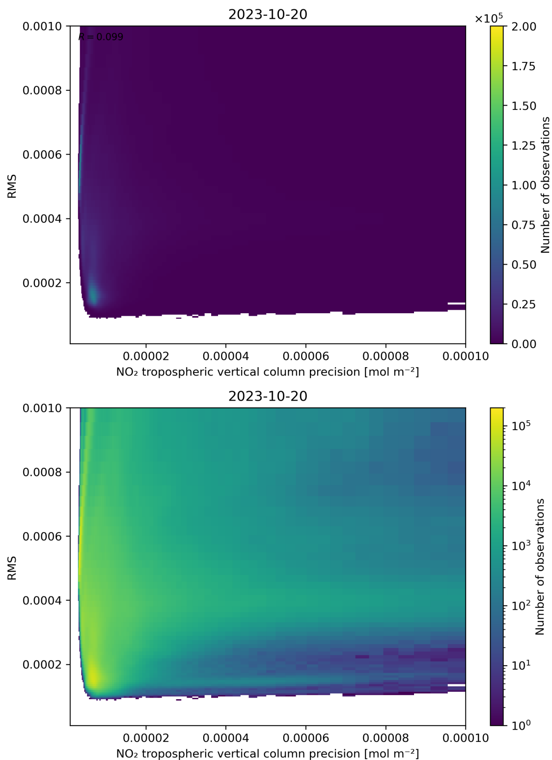
Figure 140: Scatter density plot of “NO 2 tropospheric vertical column precision” against “RMS” for 2023-10-19 to 2023-10-21.
