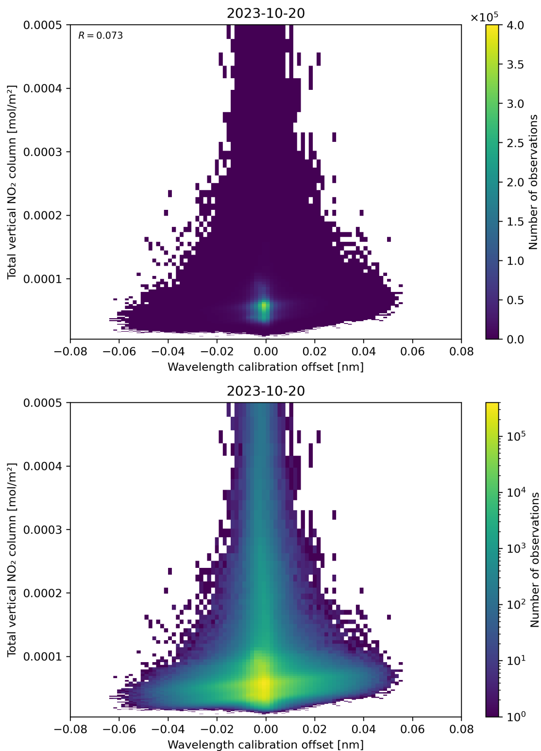
Figure 179: Scatter density plot of “Wavelength calibration offset” against “Total vertical NO 2 column” for 2023-10-19 to 2023-10-21.
