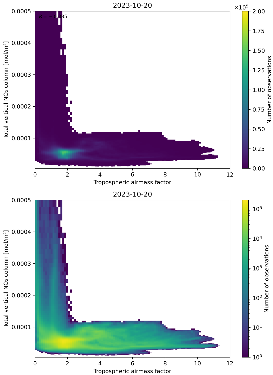
Figure 77: Scatter density plot of “Tropospheric airmass factor” against “Total vertical NO 2 column” for 2023-10-19 to 2023-10-21.
