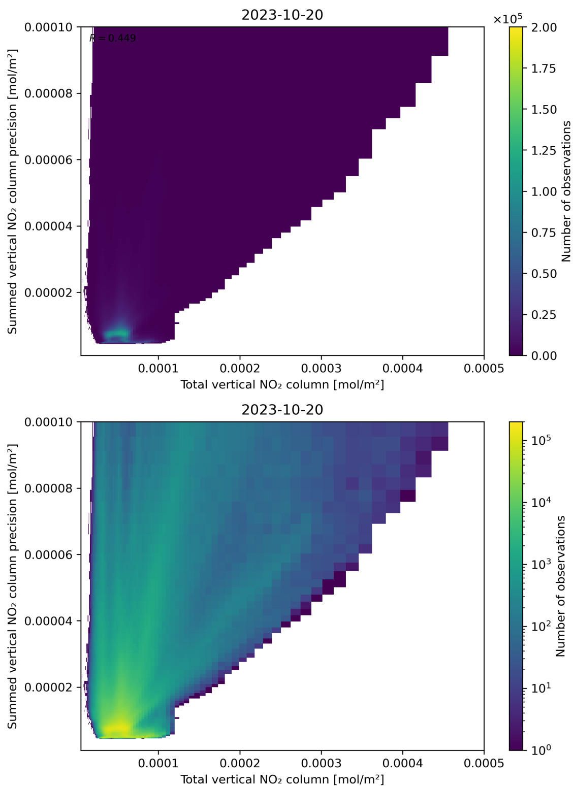
Figure 113: Scatter density plot of “Total vertical NO 2 column” against “Summed vertical NO 2 column precision” for 2023-10-19 to 2023-10-21.
