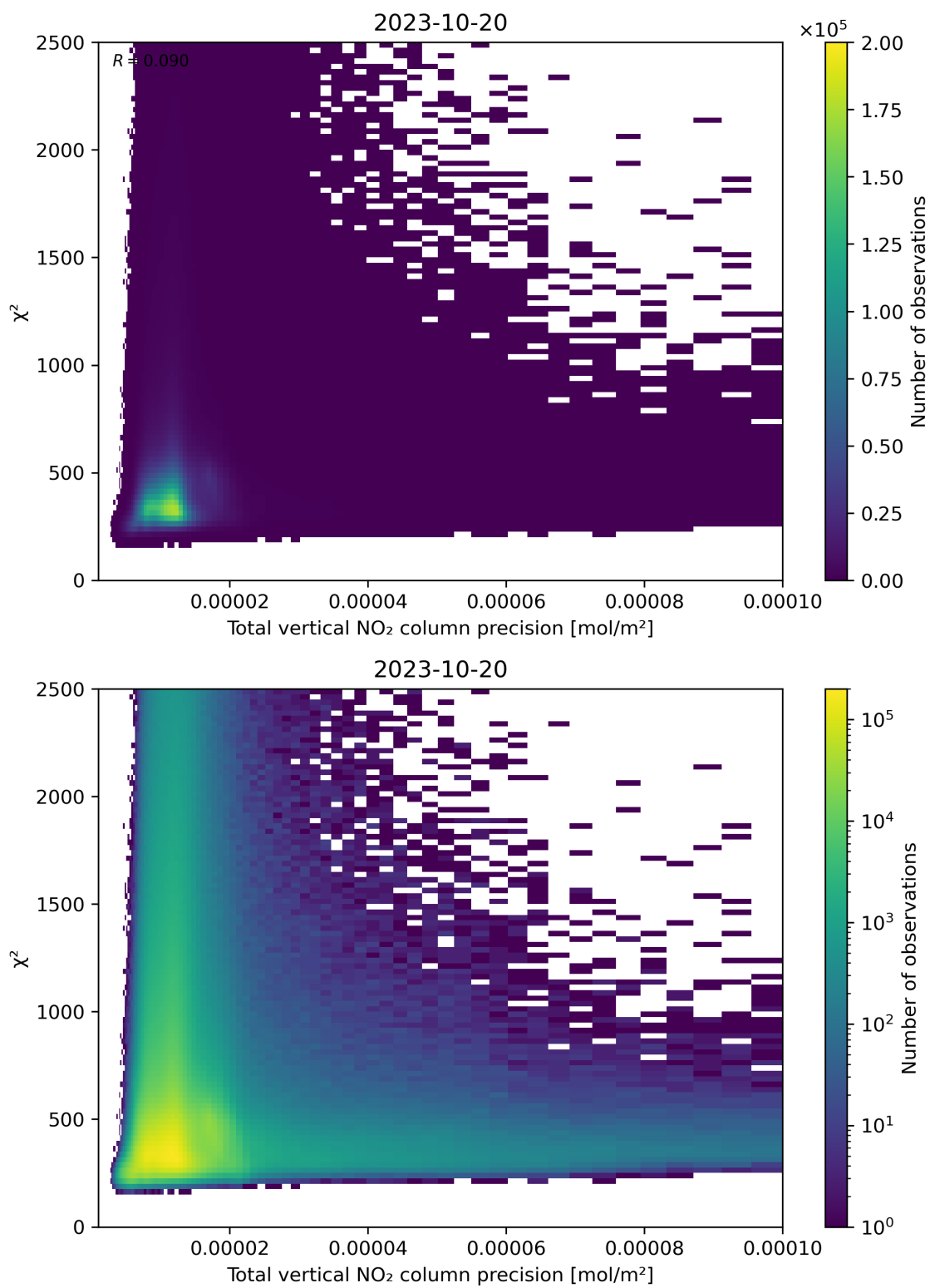
Figure 116: Scatter density plot of “Total vertical NO 2 column precision” against “ \chi^2 ” for 2023-10-19 to 2023-10-21.
