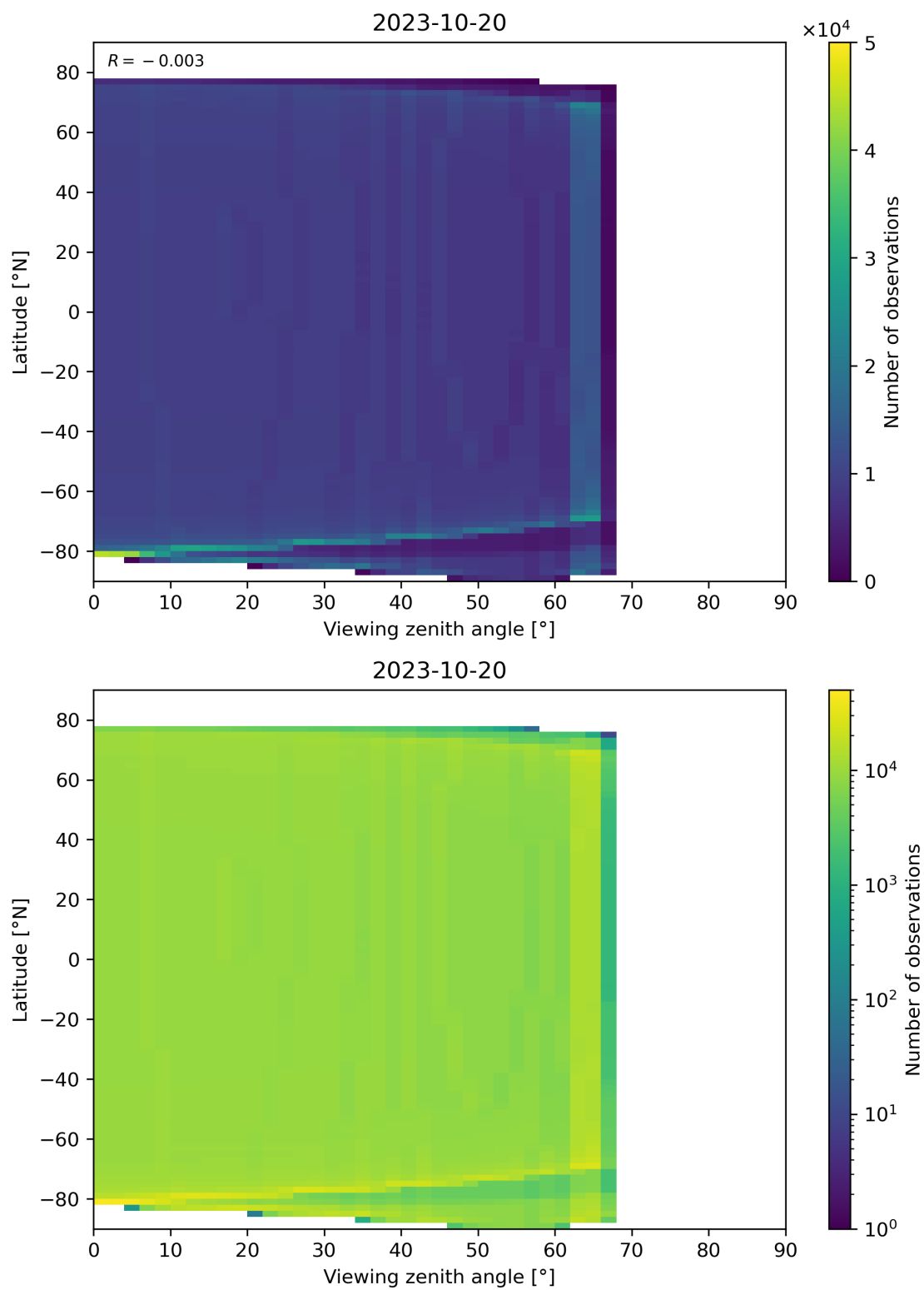
Figure 163: Scatter density plot of “Viewing zenith angle” against “Latitude” for 2023-10-19 to 2023-10-21.
