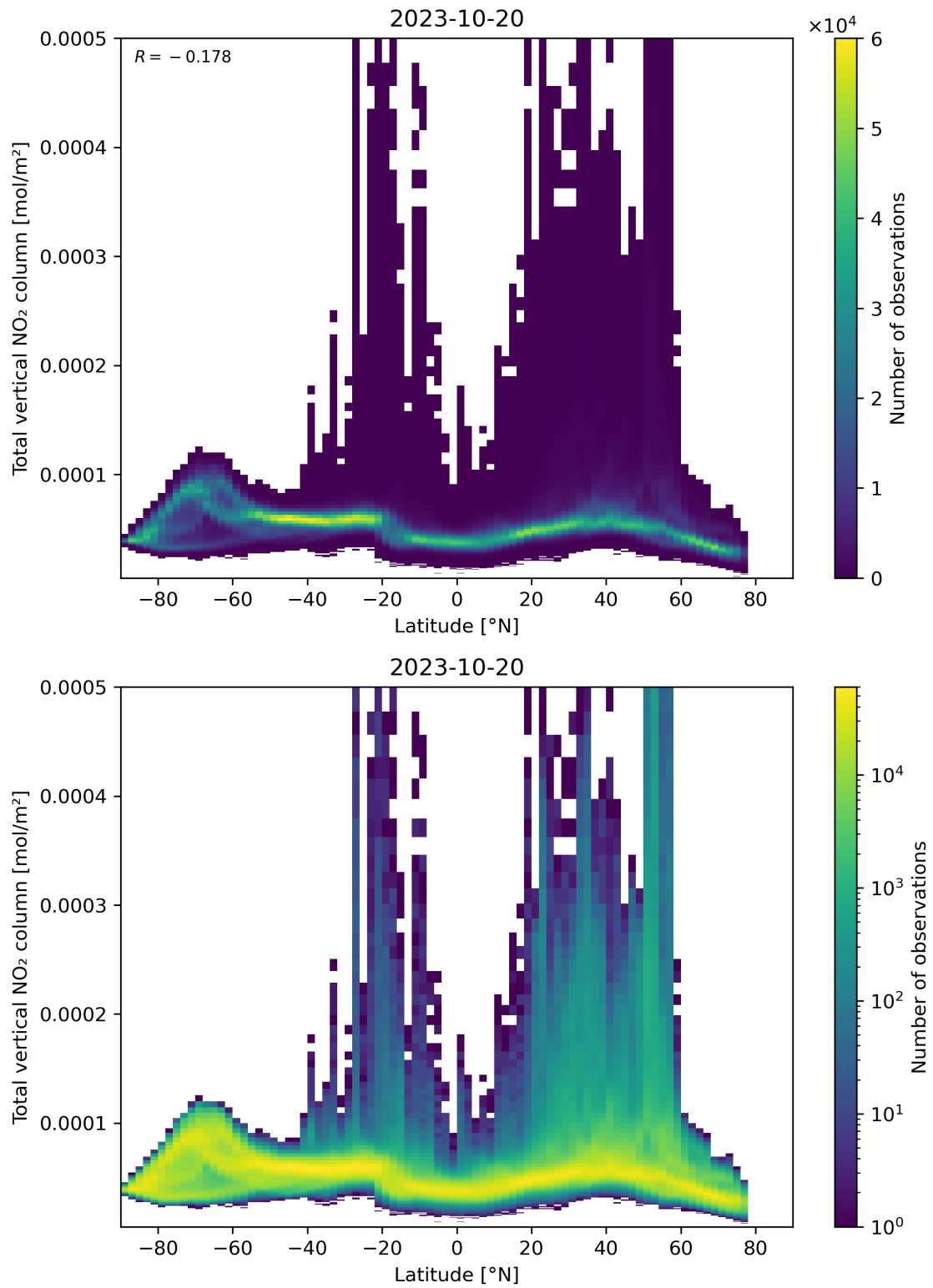
Figure 90: Scatter density plot of “Latitude” against “Total vertical NO 2 column” for 2023-10-19 to 2023-10-21.
