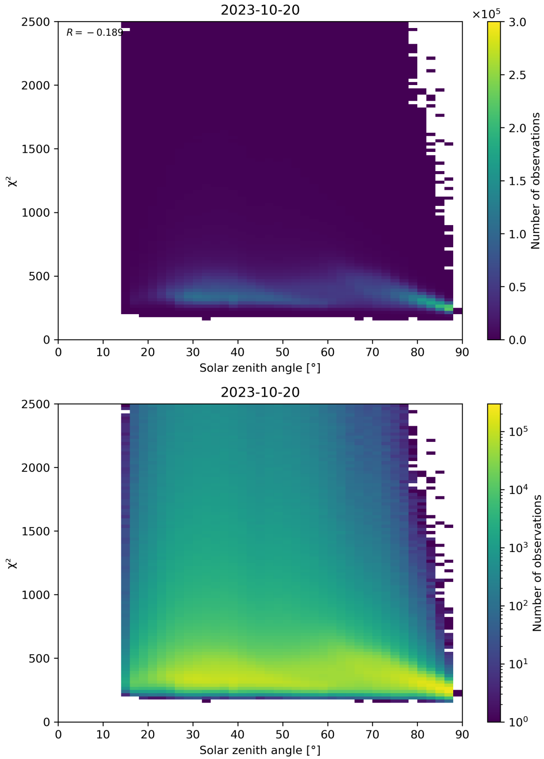
Figure 148: Scatter density plot of “Solar zenith angle” against “ \chi^2 ” for 2023-10-19 to 2023-10-21.
