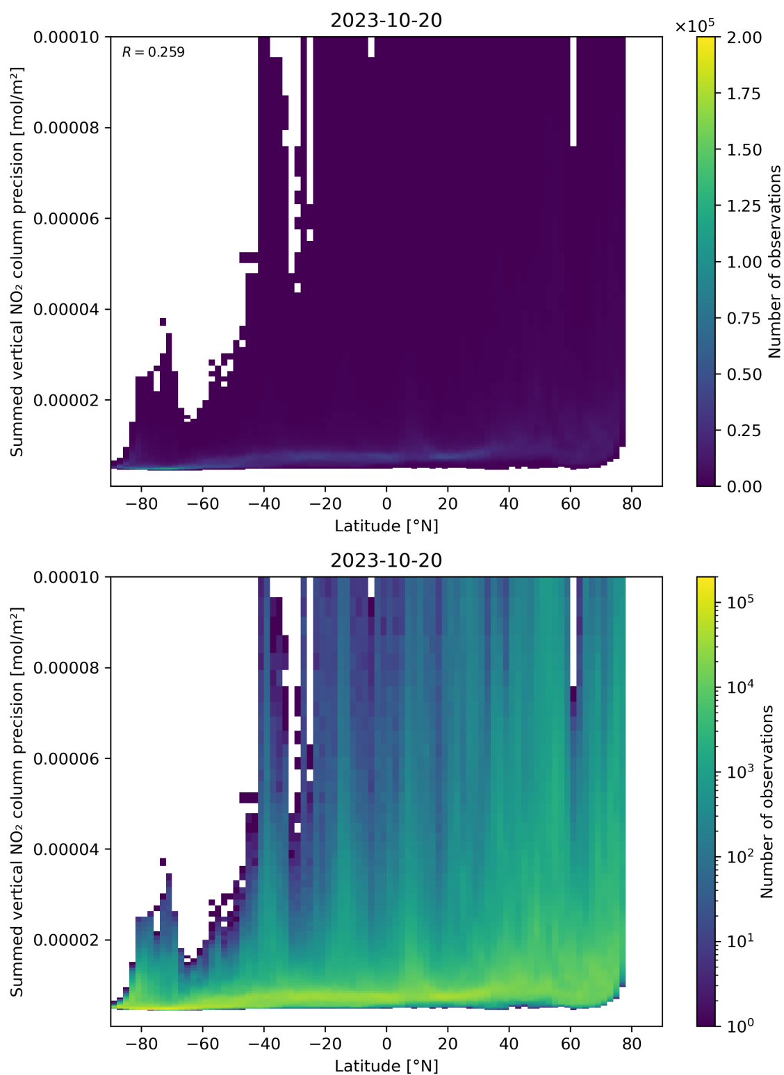
Figure 89: Scatter density plot of “Latitude” against “Summed vertical NO 2 column precision” for 2023-10-19 to 2023-10-21.
