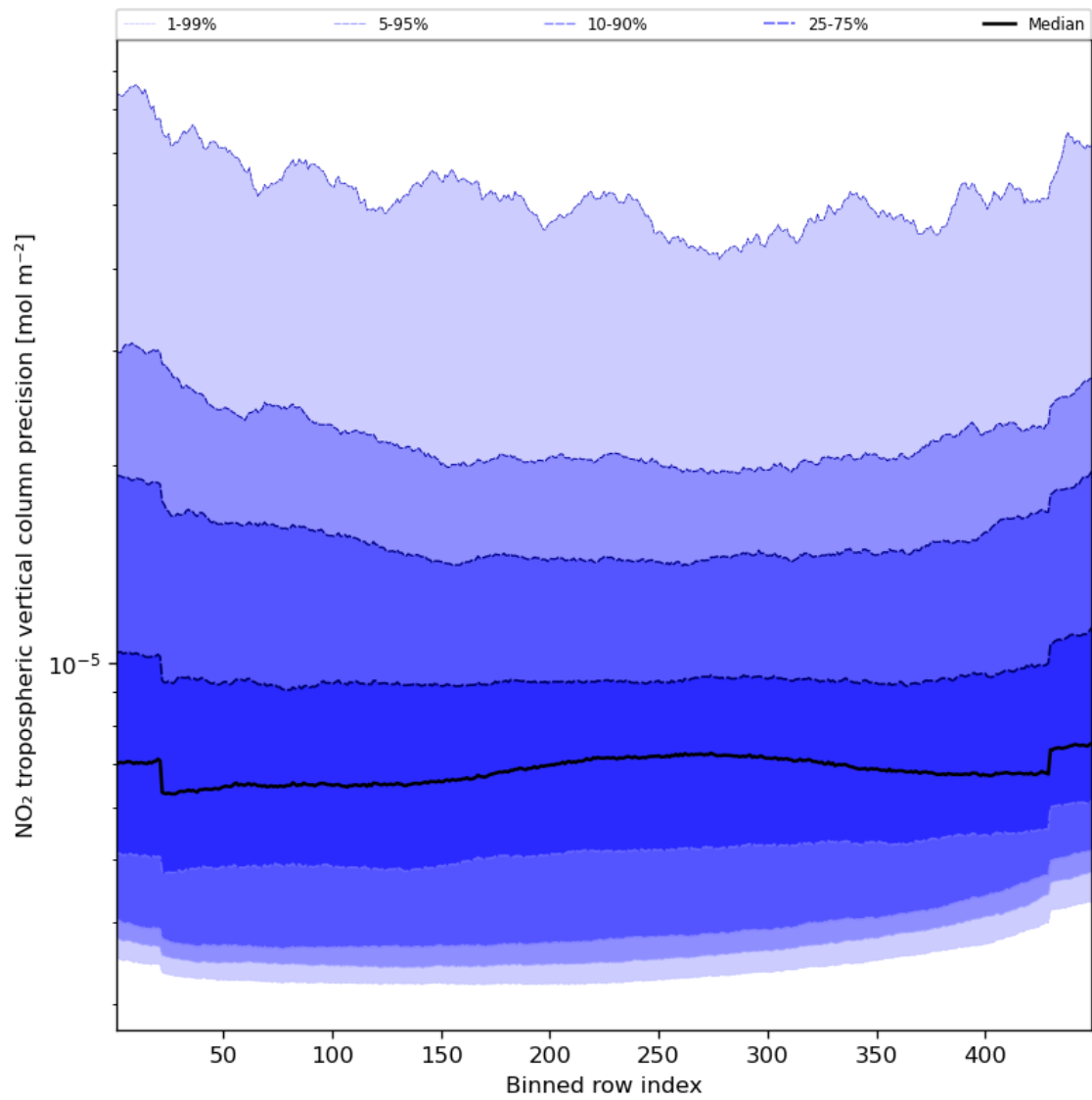
Figure 47: Along track statistics of “NO 2 tropospheric vertical column precision” for 2023-10-19 to 2023-10-21
