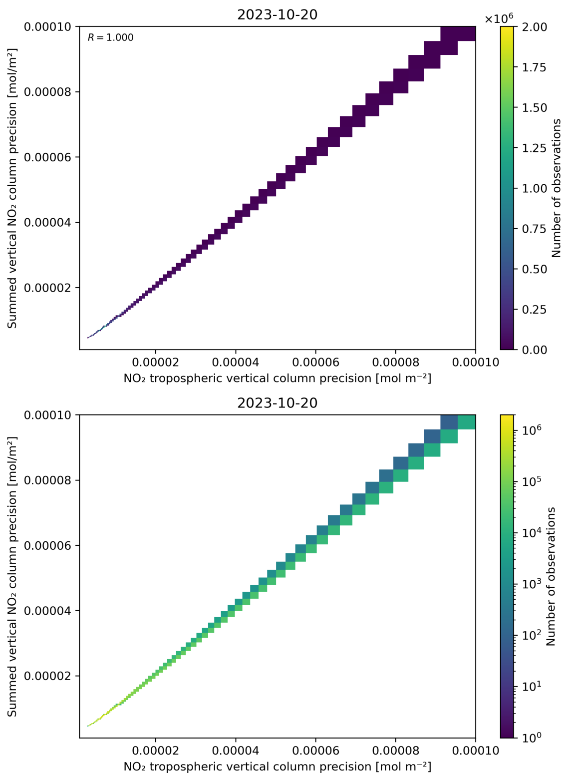
Figure 137: Scatter density plot of “NO 2 tropospheric vertical column precision” against “Summed vertical NO 2 column precision” for 2023-10-19 to 2023-10-21.
