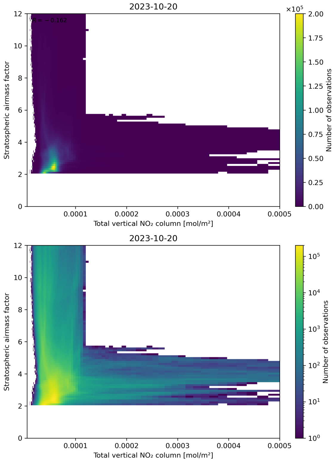
Figure 110: Scatter density plot of “Total vertical NO 2 column” against “Stratospheric airmass factor” for 2023-10-19 to 2023-10-21.
