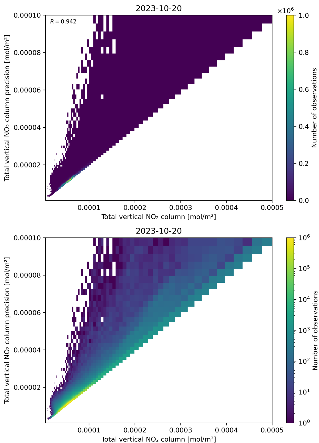
Figure 114: Scatter density plot of “Total vertical NO 2 column” against “Total vertical NO 2 column precision” for 2023-10-19 to 2023-10-21.
