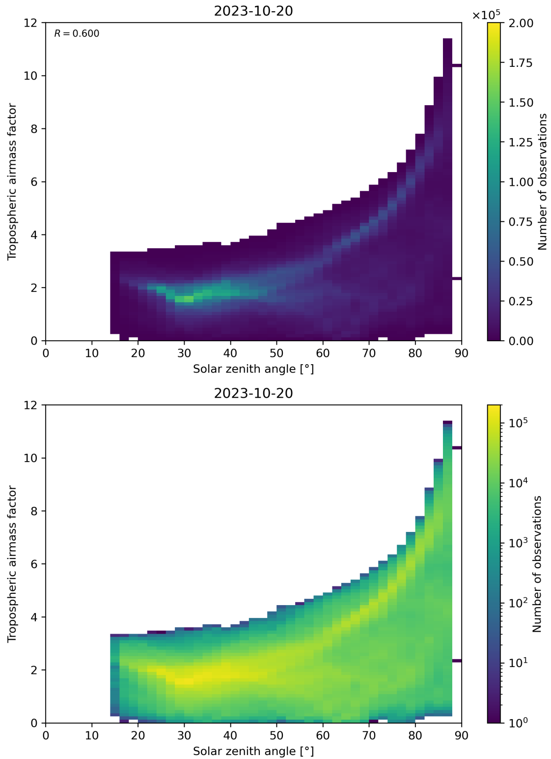
Figure 147: Scatter density plot of “Solar zenith angle” against “Tropospheric airmass factor” for 2023-10-19 to 2023-10-21.
