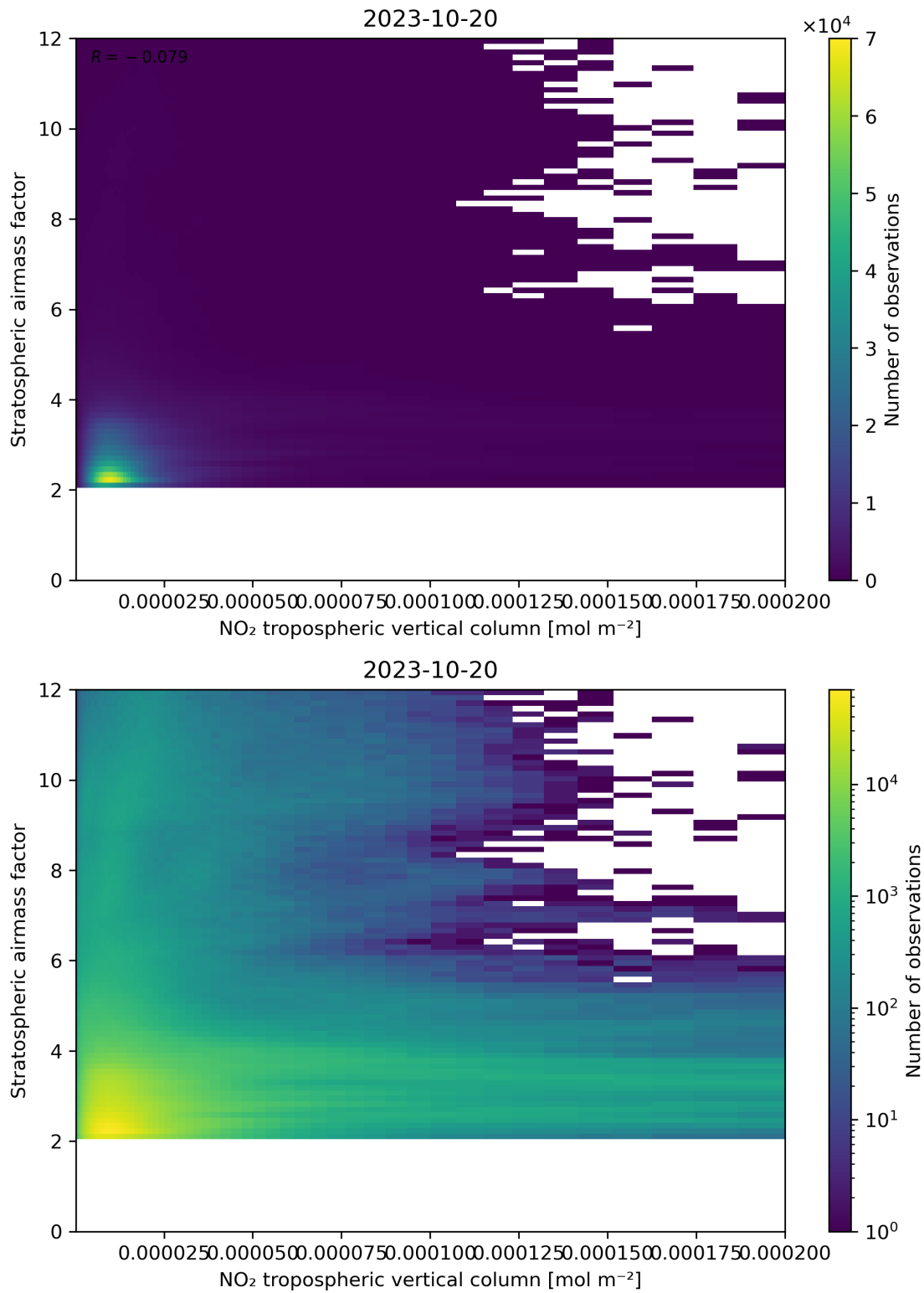
Figure 121: Scatter density plot of “NO 2 tropospheric vertical column” against “Stratospheric air mass factor” for 2023-10-19 to 2023-10-21.
