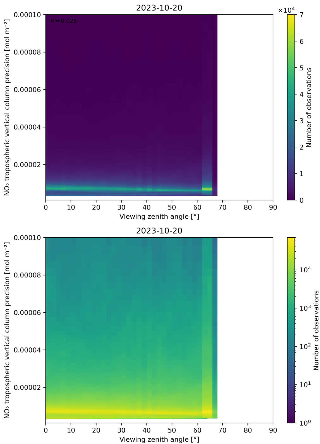
Figure 170: Scatter density plot of “Viewing zenith angle” against “NO 2 tropospheric vertical column precision” for 2023-10-19 to 2023-10-21.
