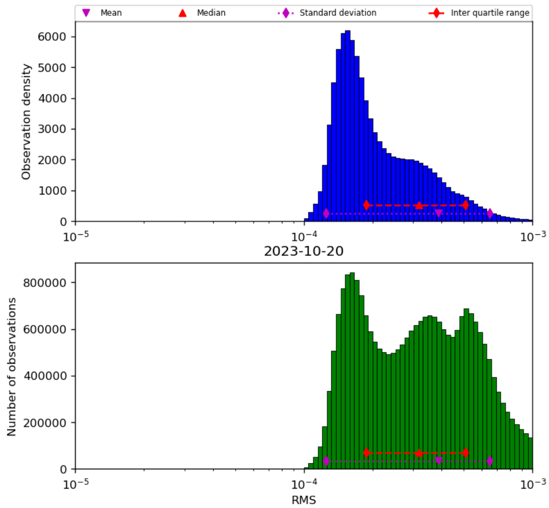
Figure 43: Histogram of “RMS” for 2023-10-19 to 2023-10-21
