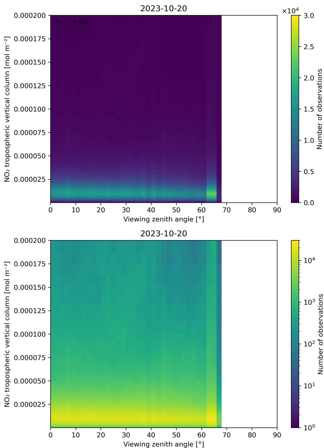
Figure 169: Scatter density plot of “Viewing zenith angle” against “NO 2 tropospheric vertical column” for 2023-10-19 to 2023-10-21.
