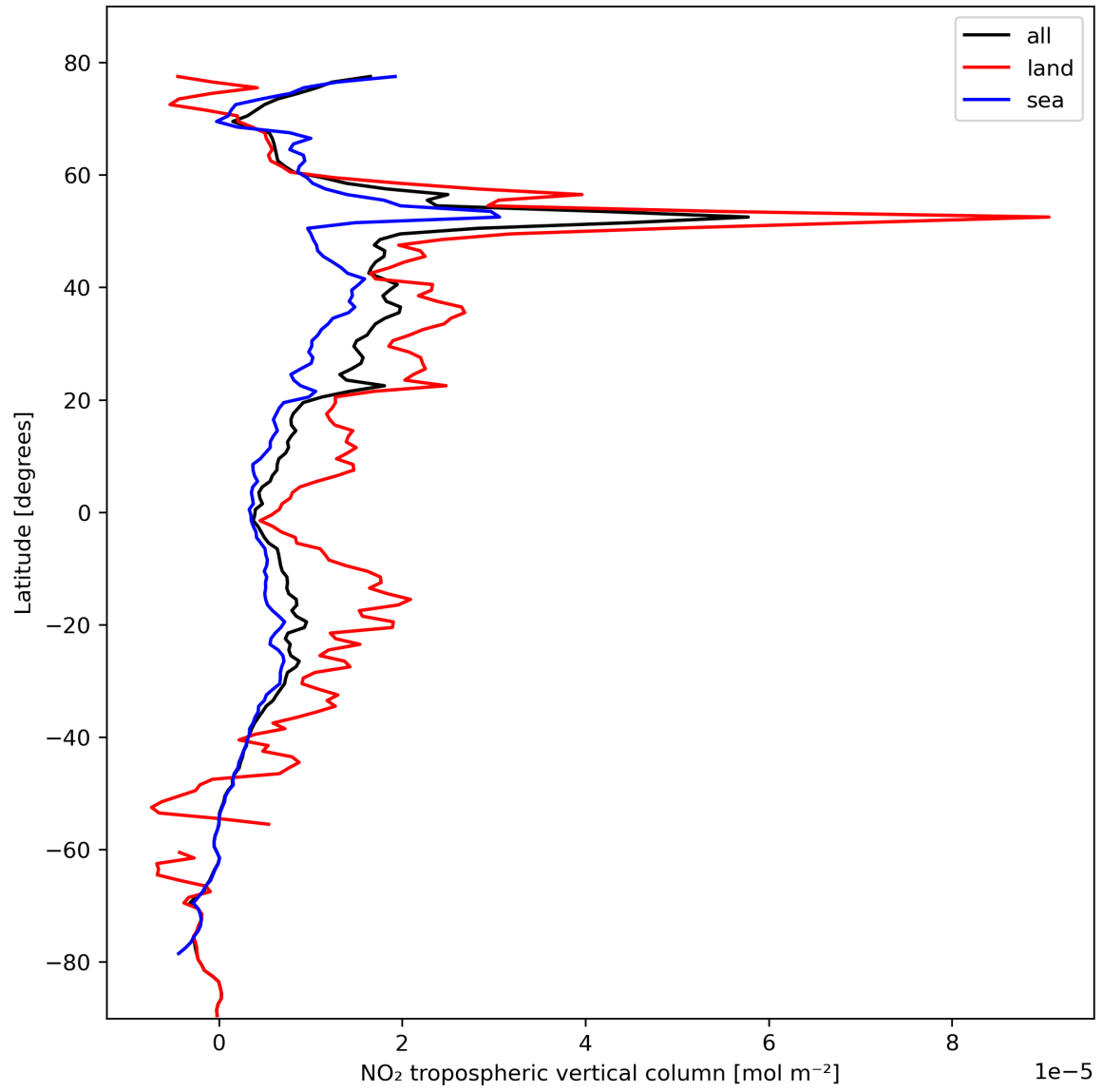
Figure 12: Zonal average of “NO 2 tropospheric vertical column” for 2023-10-19 to 2023-10-21.
