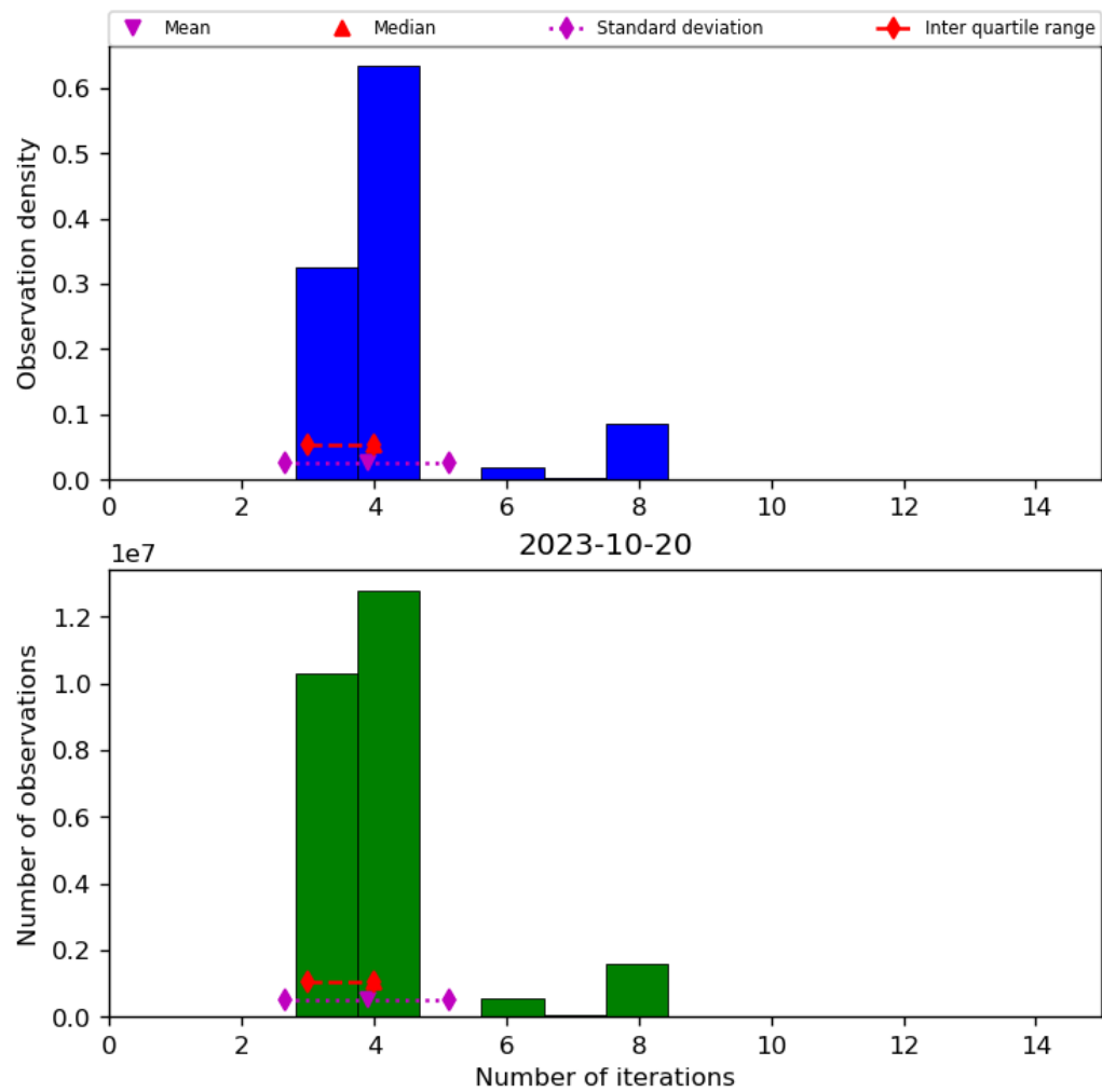
Figure 34: Histogram of “Number of iterations” for 2023-10-19 to 2023-10-21
