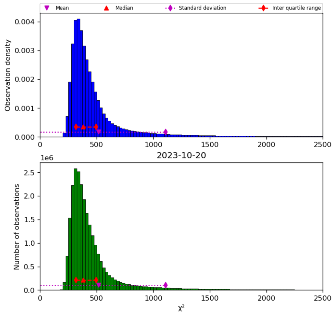
Figure 42: Histogram of “ \chi^2 ” for 2023-10-19 to 2023-10-21
