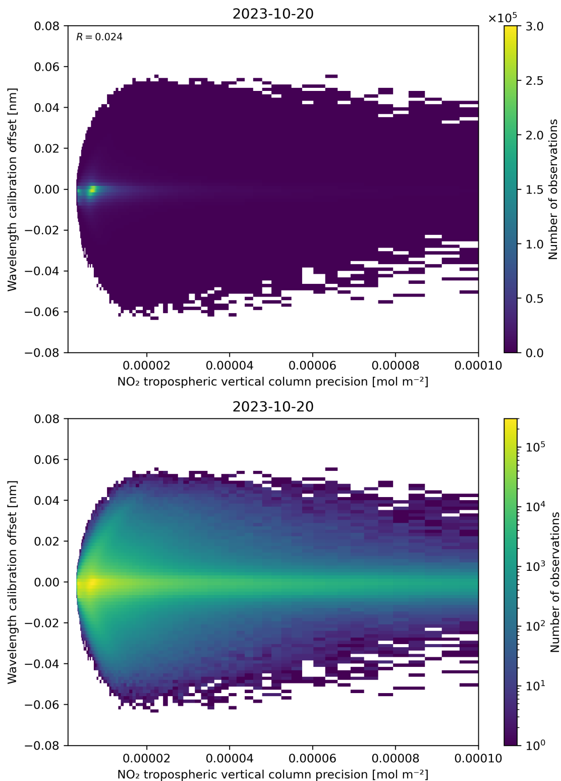
Figure 141: Scatter density plot of “NO 2 tropospheric vertical column precision” against “Wavelength calibration offset” for 2023-10-19 to 2023-10-21.
