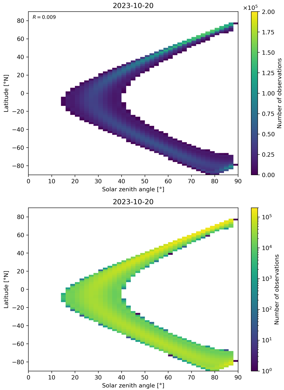
Figure 149: Scatter density plot of “Solar zenith angle” against “Latitude” for 2023-10-19 to 2023-10-21.
