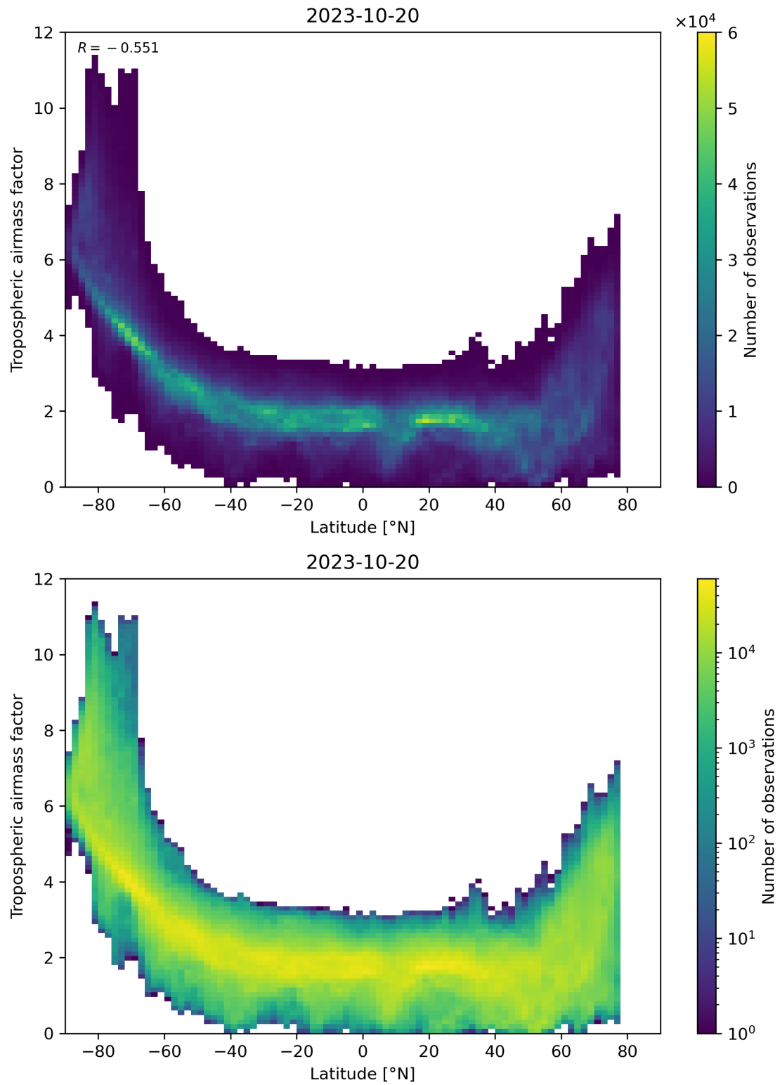
Figure 85: Scatter density plot of “Latitude” against “Tropospheric air mass factor” for 2023-10-19 to 2023-10-21.
