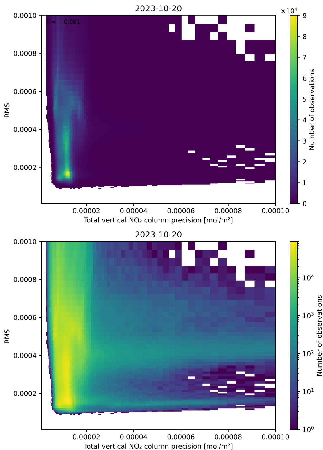
Figure 119: Scatter density plot of “Total vertical NO 2 column precision” against “RMS” for 2023-10-19 to 2023-10-21.
