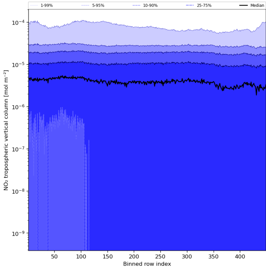
Figure 46: Along track statistics of “NO 2 tropospheric vertical column” for 2023-10-19 to 2023-10-21
