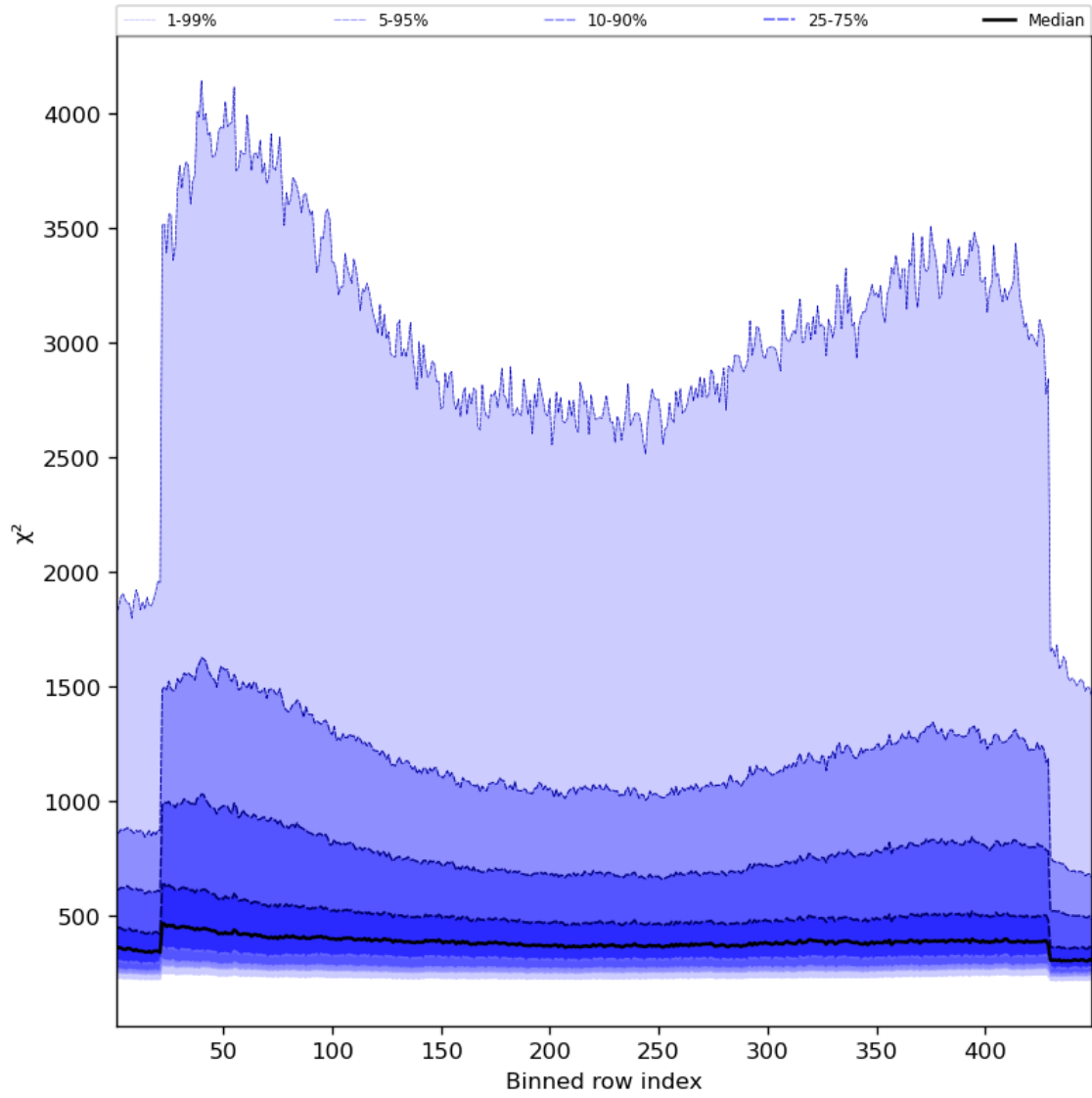
Figure 59: Along track statistics of “ \chi^2 ” for 2023-10-19 to 2023-10-21
