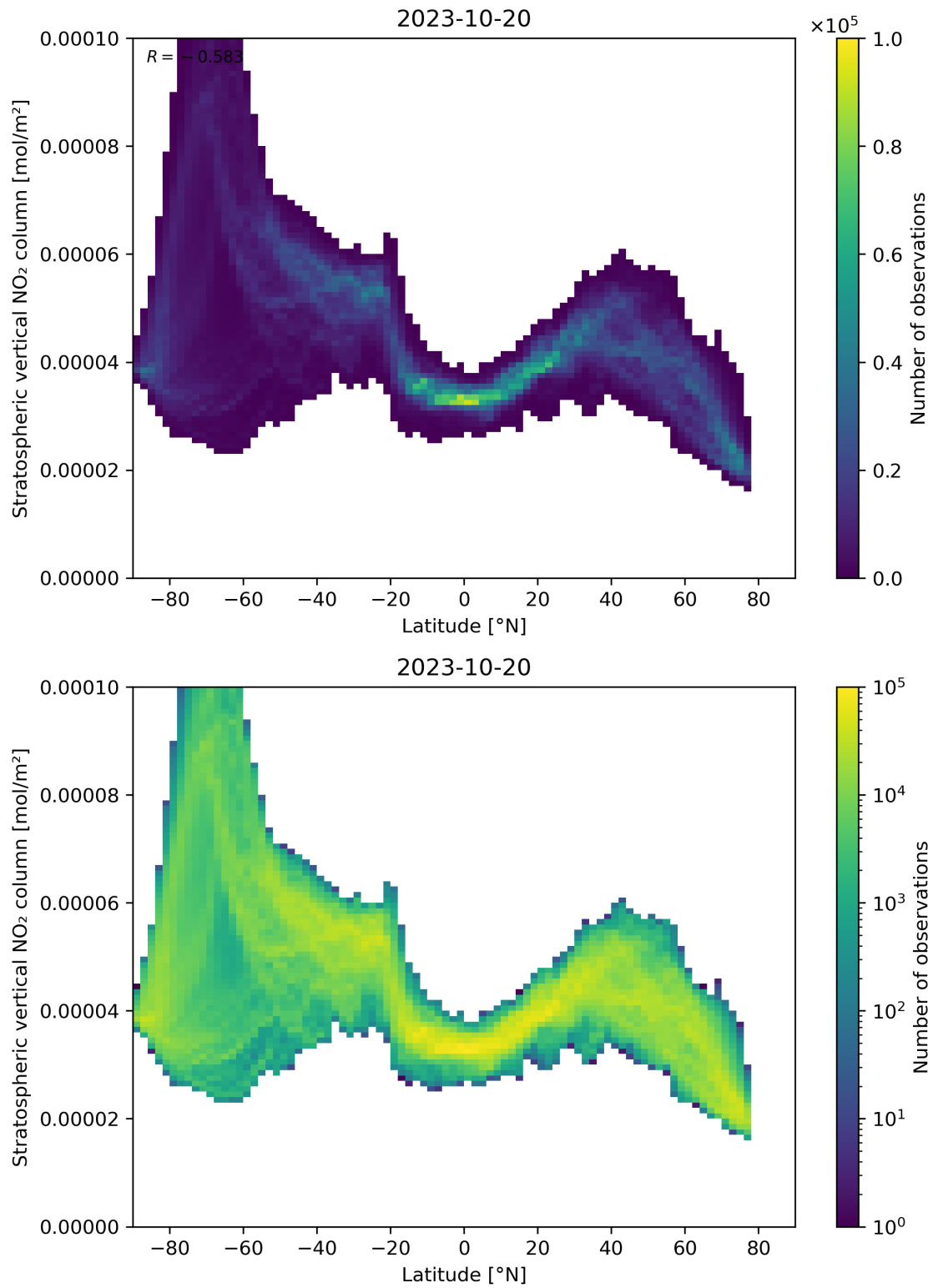
Figure 87: Scatter density plot of “Latitude” against “Stratospheric vertical NO 2 column” for 2023-10-19 to 2023-10-21.
