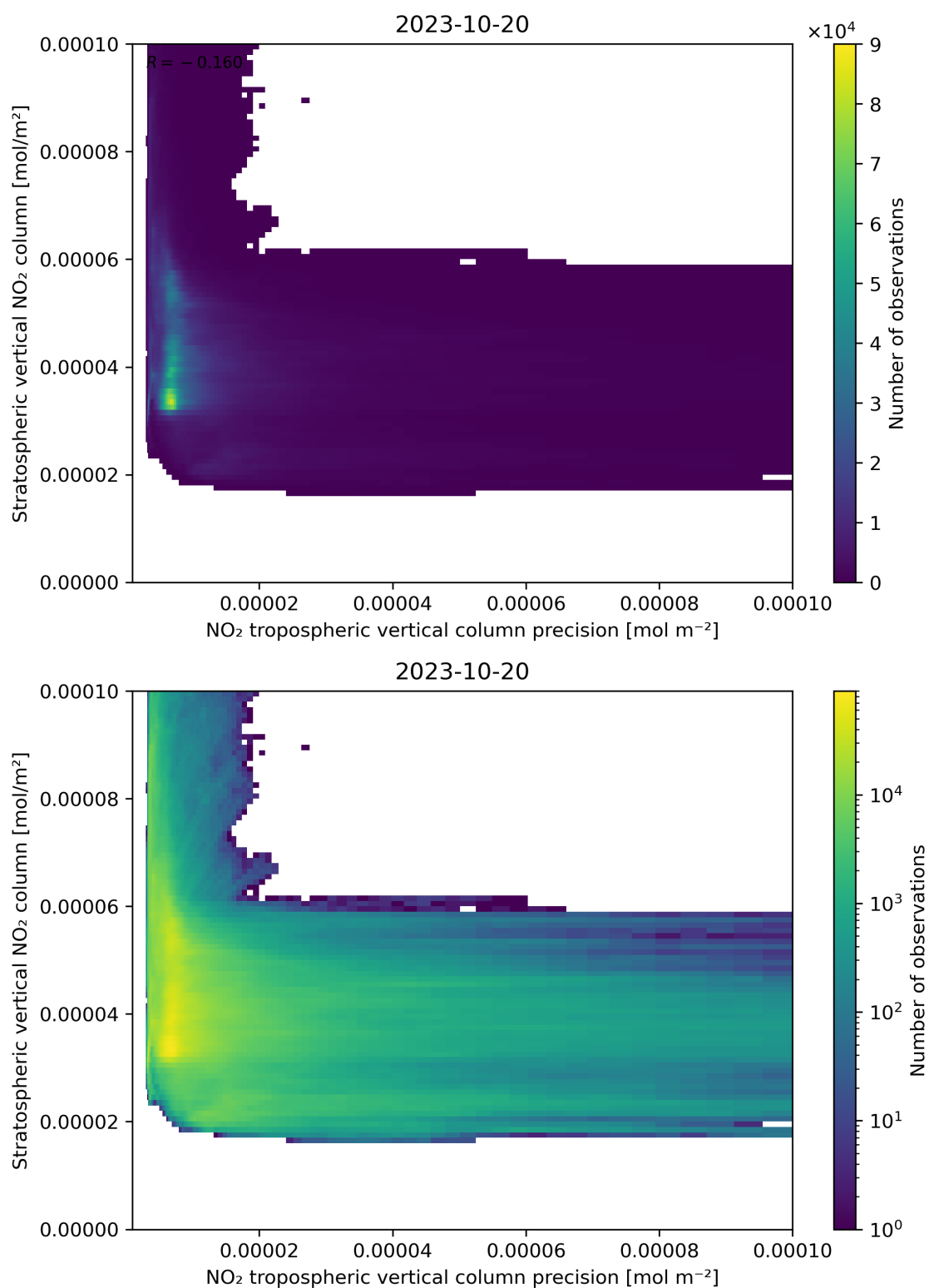
Figure 135: Scatter density plot of “NO 2 tropospheric vertical column precision” against “Stratospheric vertical NO 2 column” for 2023-10-19 to 2023-10-21.
