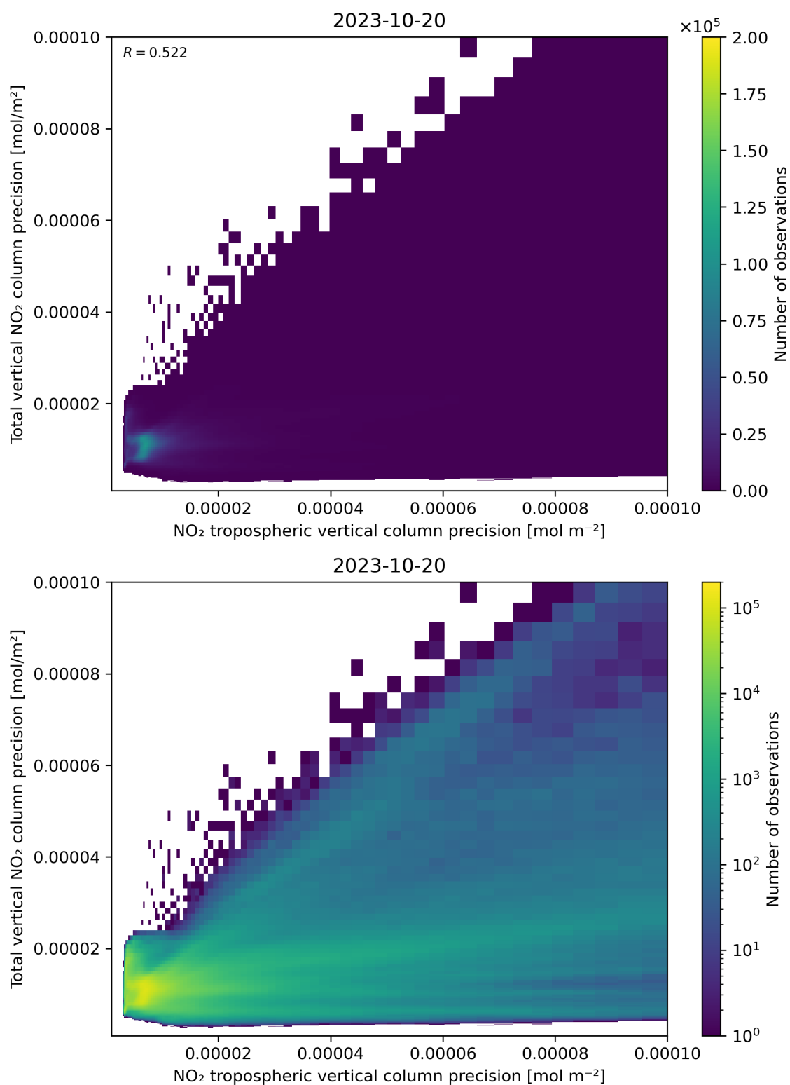
Figure 139: Scatter density plot of “NO 2 tropospheric vertical column precision” against “Total vertical NO 2 column precision” for 2023-10-19 to 2023-10-21.
