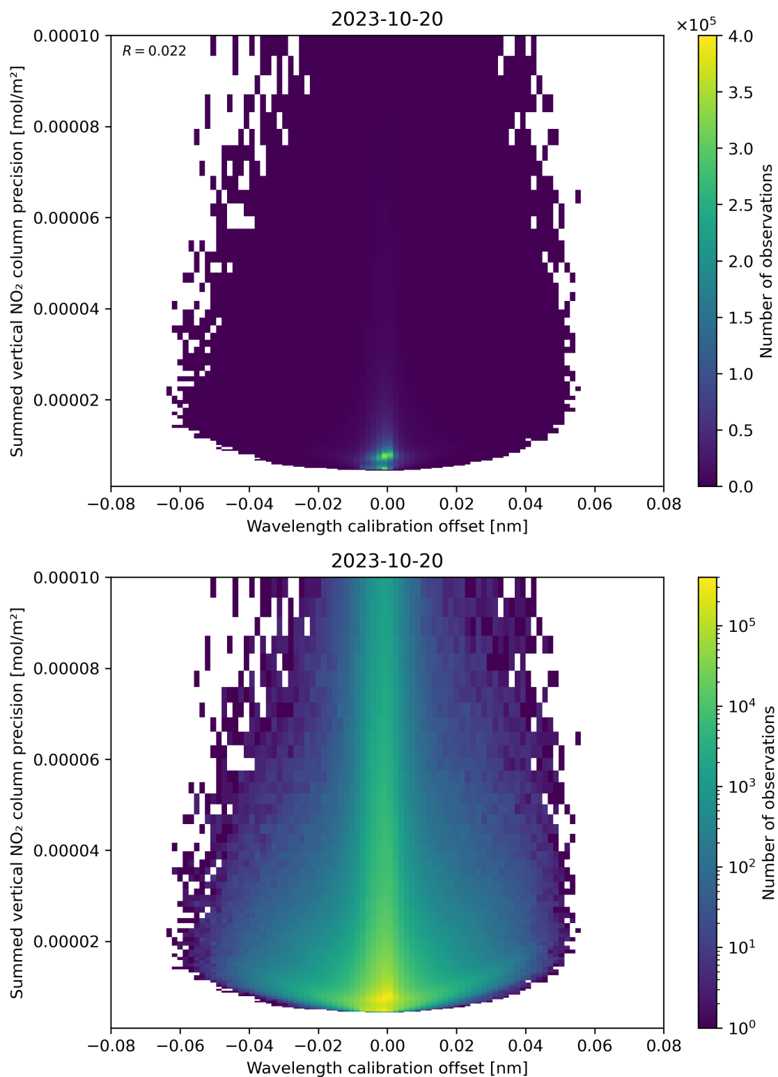
Figure 178: Scatter density plot of “Wavelength calibration offset” against “Summed vertical NO 2 column precision” for 2023-10-19 to 2023-10-21.
