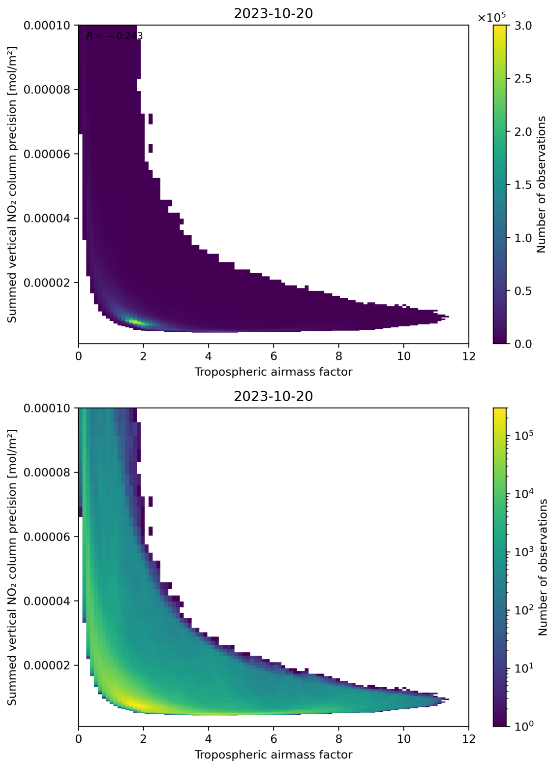
Figure 76: Scatter density plot of “Tropospheric air mass factor” against “Summed vertical NO 2 column precision” for 2023-10-19 to 2023-10-21.
