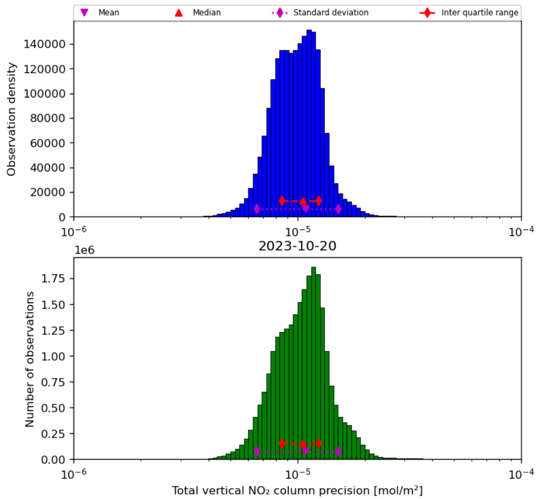
Figure 39: Histogram of "Total vertical NO 2 column precision" for 2023-10-19 to 2023-10-21
