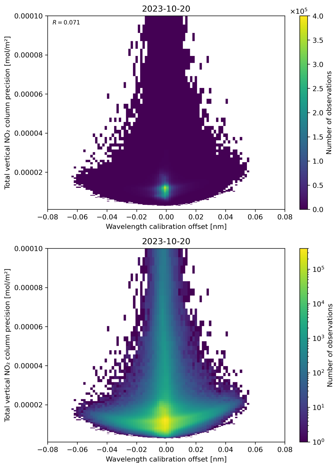
Figure 180: Scatter density plot of “Wavelength calibration offset” against “Total vertical NO 2 column precision” for 2023-10-19 to 2023-10-21.
