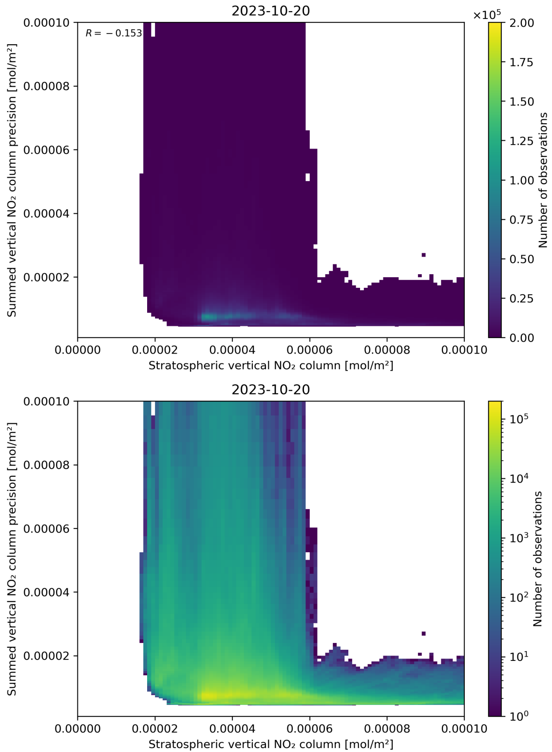
Figure 99: Scatter density plot of “Stratospheric vertical NO 2 column” against “Summed vertical NO 2 column precision” for 2023-10-19 to 2023-10-21.
