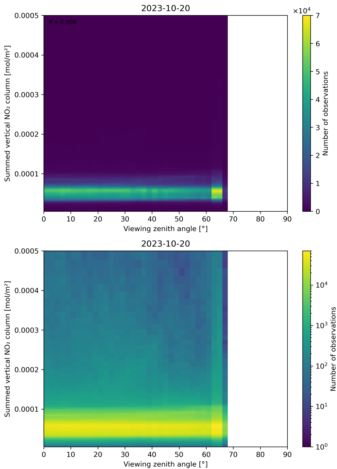
Figure 165: Scatter density plot of “Viewing zenith angle” against “Summed vertical NO 2 column” for 2023-10-19 to 2023-10-21.
