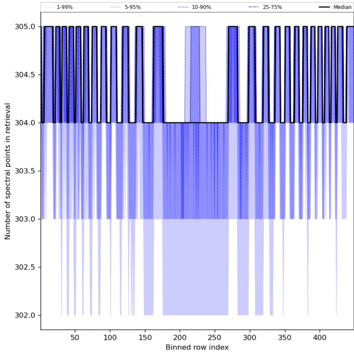
Figure 50: Along track statistics of “Number of spectral points in retrieval” for 2023-10-19 to 2023-10-21
