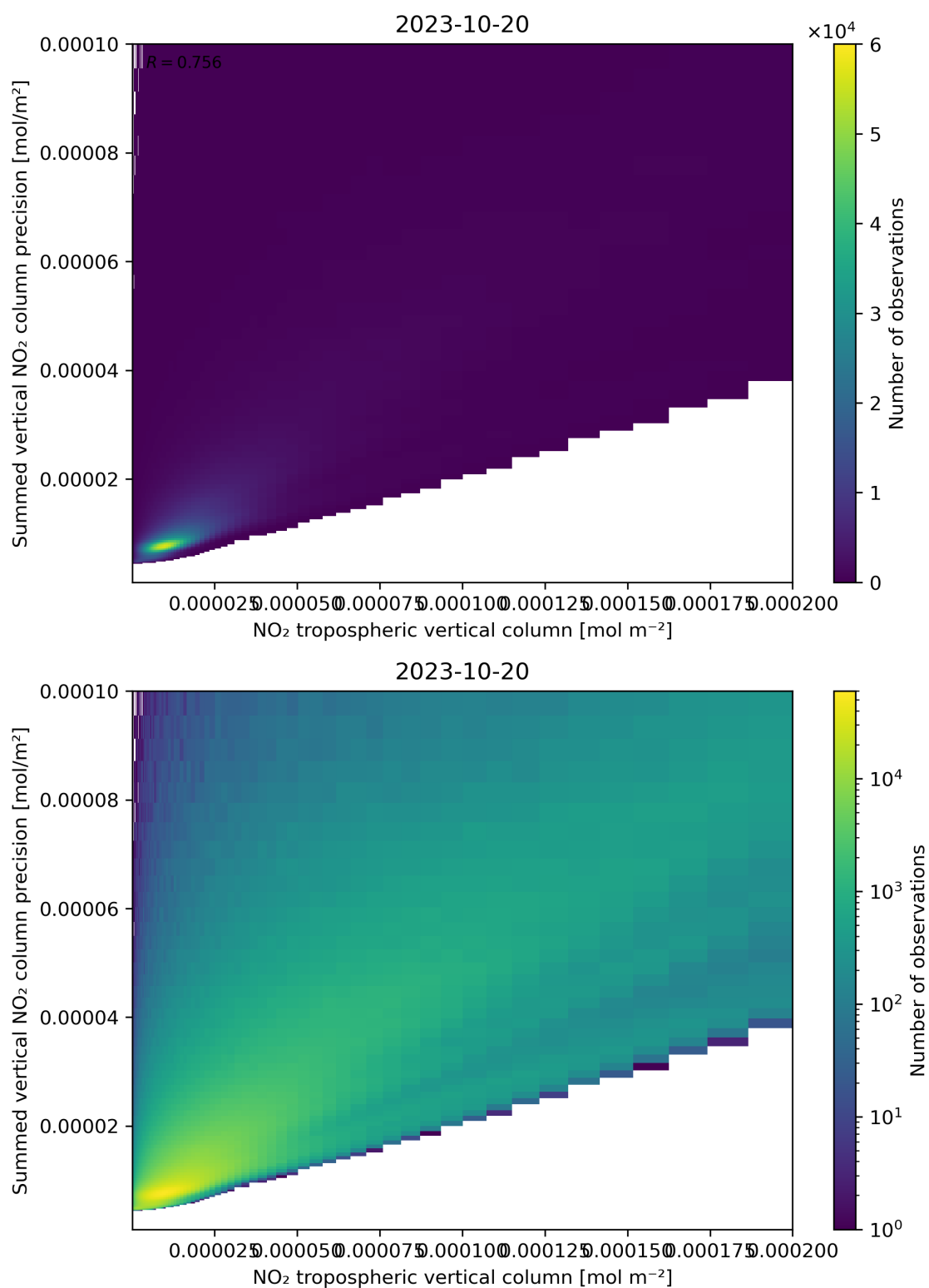
Figure 127: Scatter density plot of “NO 2 tropospheric vertical column” against “Summed vertical NO 2 column precision” for 2023-10-19 to 2023-10-21.
