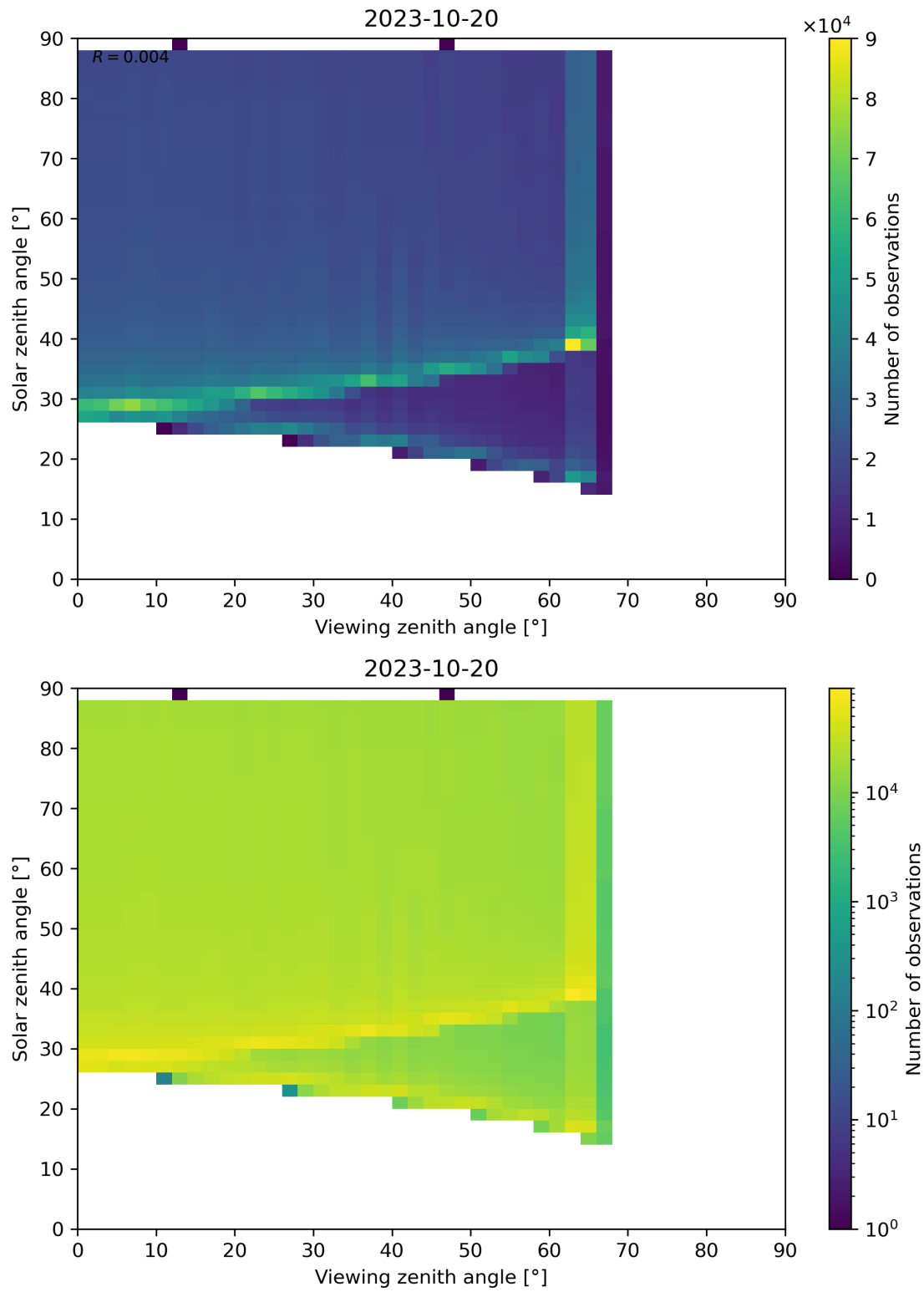
Figure 172: Scatter density plot of “Viewing zenith angle” against “Solar zenith angle” for 2023-10-19 to 2023-10-21.
