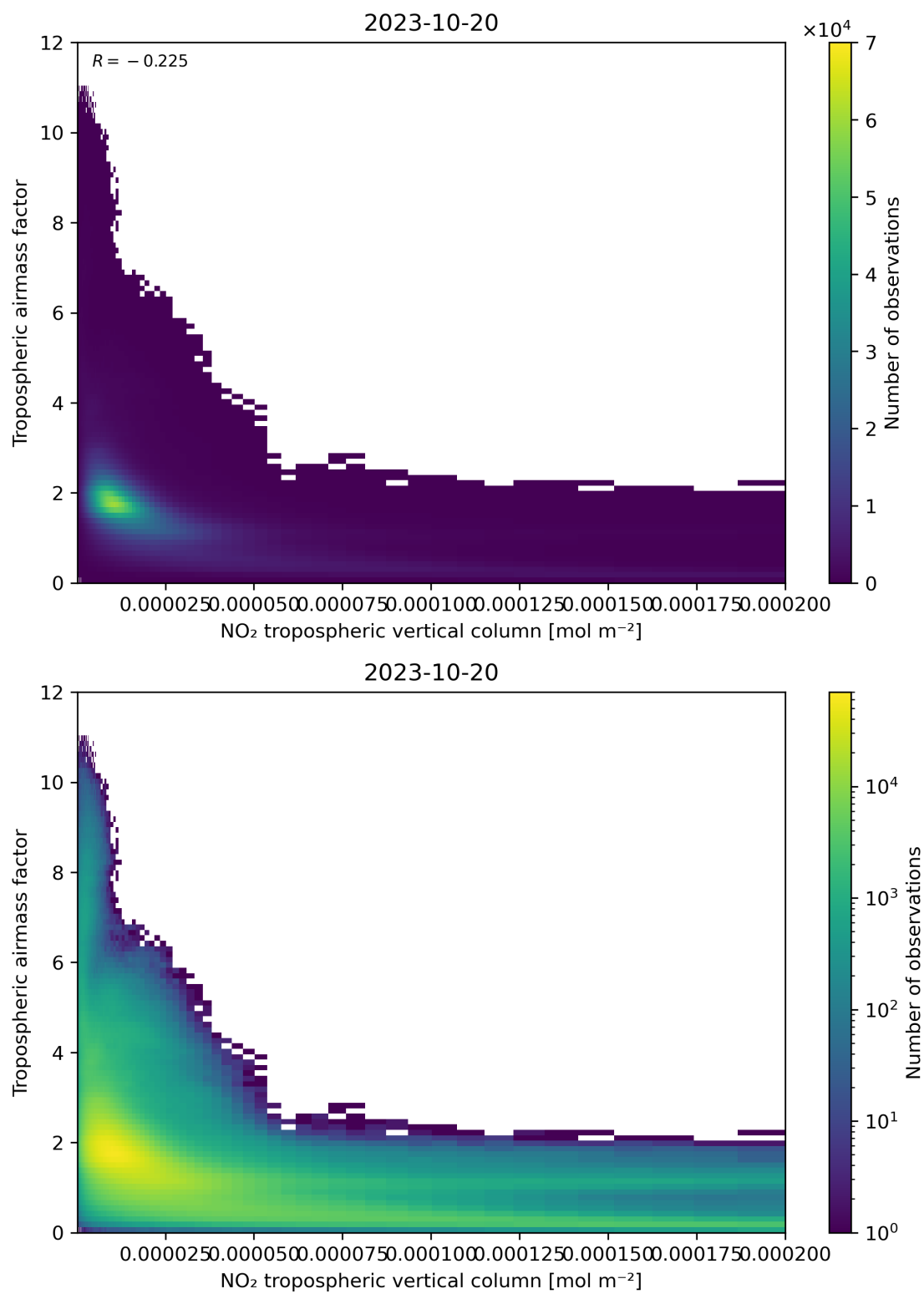
Figure 123: Scatter density plot of “NO 2 tropospheric vertical column” against “Tropospheric air mass factor” for 2023-10-19 to 2023-10-21.
