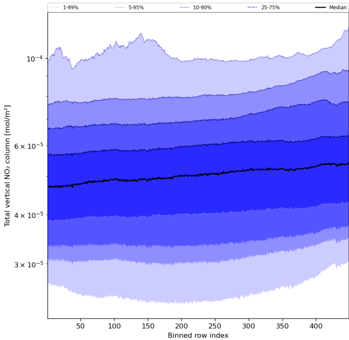
Figure 55: Along track statistics of “Total vertical NO 2 column” for 2023-10-19 to 2023-10-21
