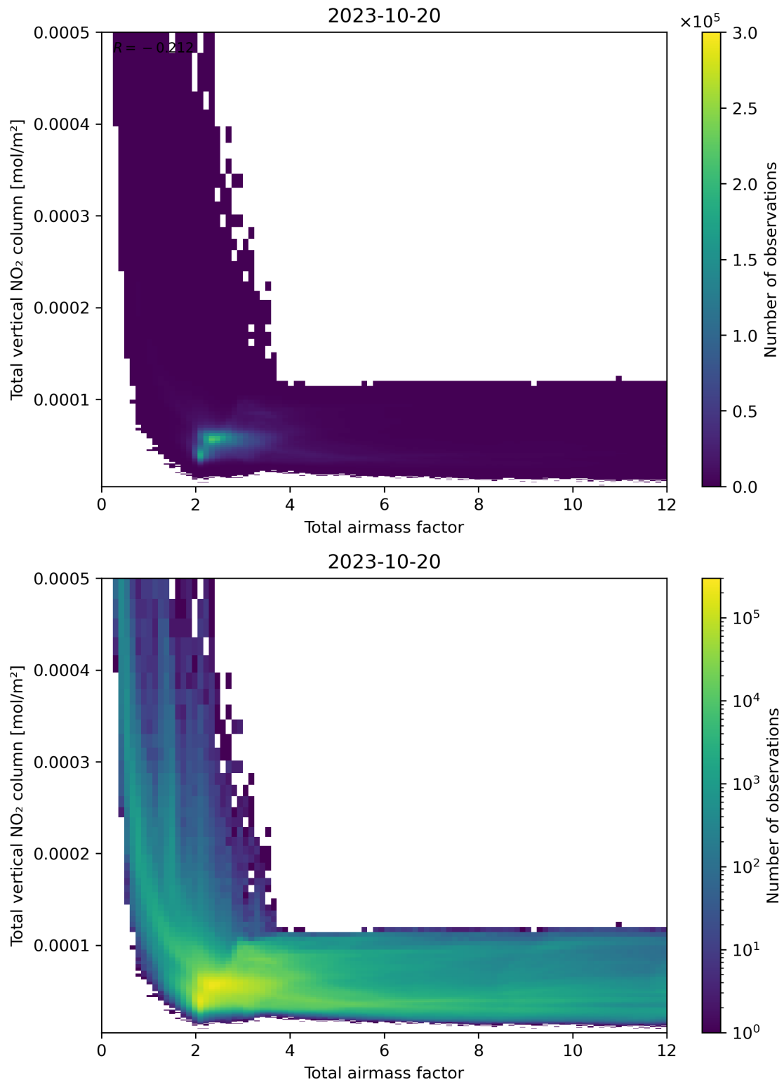
Figure 67: Scatter density plot of “Total airmass factor” against “Total vertical NO 2 column” for 2023-10-19 to 2023-10-21.
