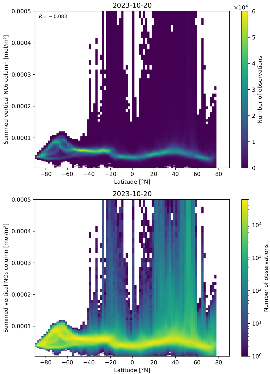
Figure 88: Scatter density plot of “Latitude” against “Summed vertical NO 2 column” for 2023-10-19 to 2023-10-21.
