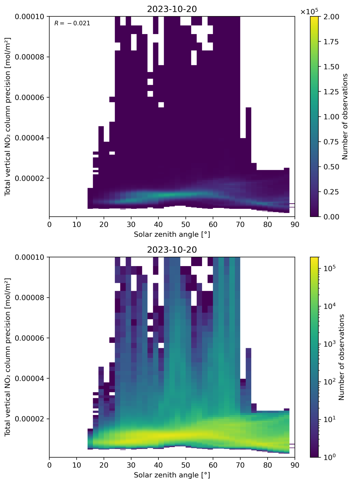
Figure 154: Scatter density plot of “Solar zenith angle” against “Total vertical NO 2 column precision” for 2023-10-19 to 2023-10-21.
