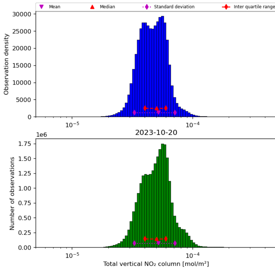
Figure 38: Histogram of "Total vertical NO 2 column" for 2023-10-19 to 2023-10-21
