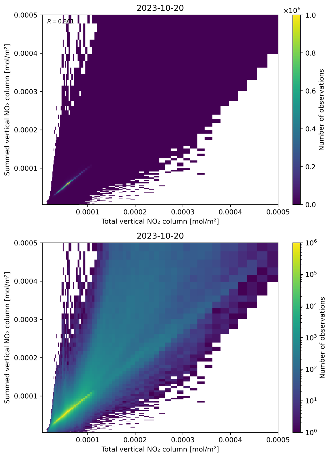
Figure 112: Scatter density plot of “Total vertical NO 2 column” against “Summed vertical NO 2 column” for 2023-10-19 to 2023-10-21.
