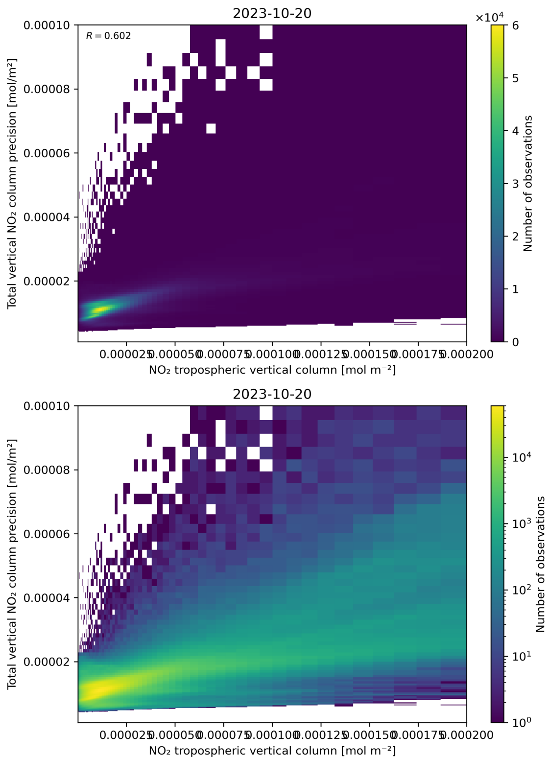
Figure 129: Scatter density plot of “NO 2 tropospheric vertical column” against “Total vertical NO 2 column precision” for 2023-10-19 to 2023-10-21.
