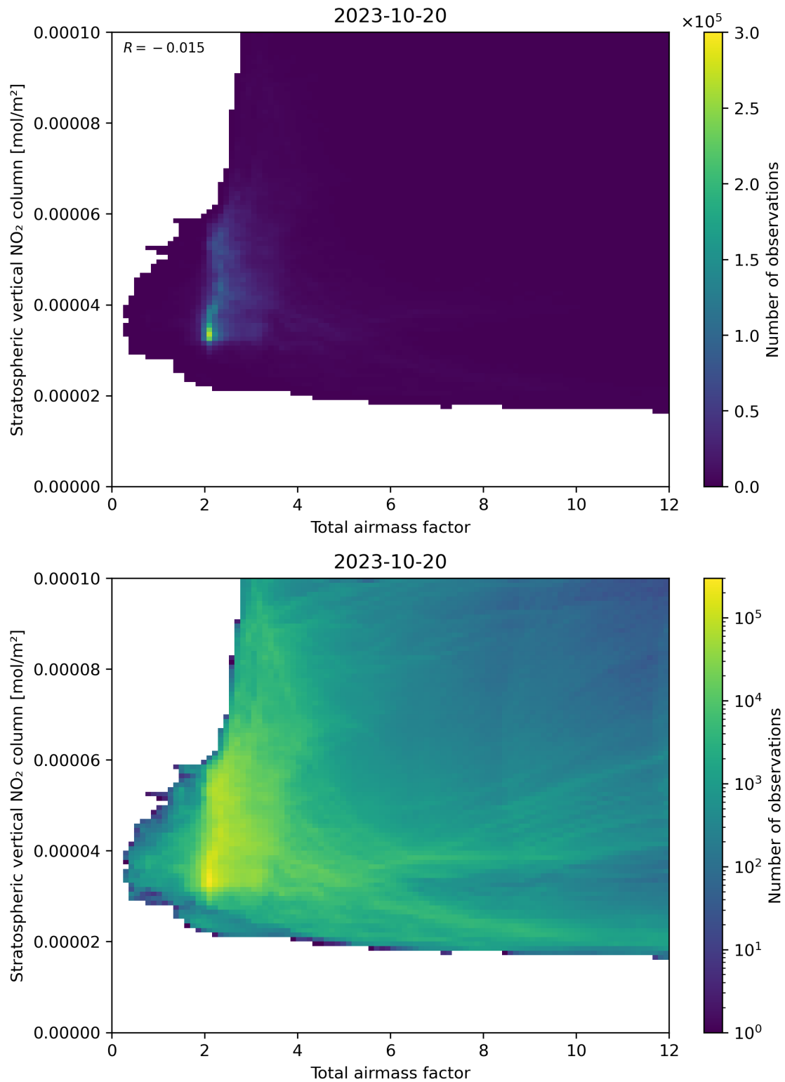
Figure 64: Scatter density plot of “Total airmass factor” against “Stratospheric vertical NO 2 column” for 2023-10-19 to 2023-10-21.
