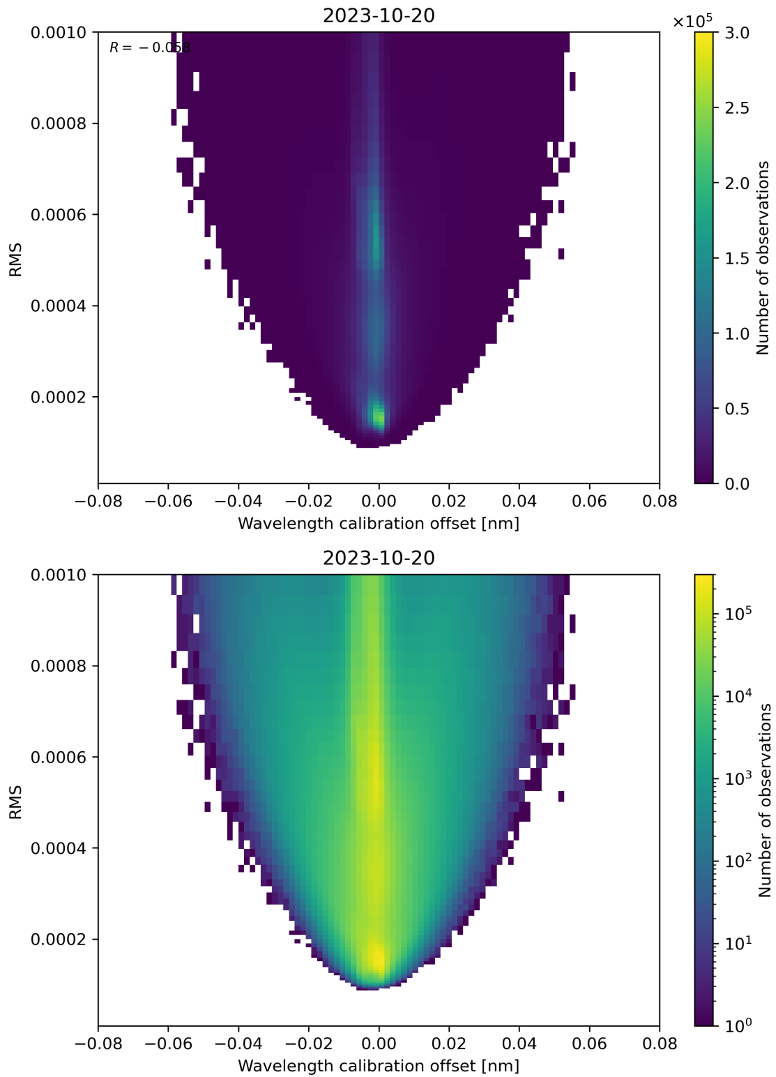
Figure 181: Scatter density plot of “Wavelength calibration offset” against “RMS” for 2023-10-19 to 2023-10-21.
