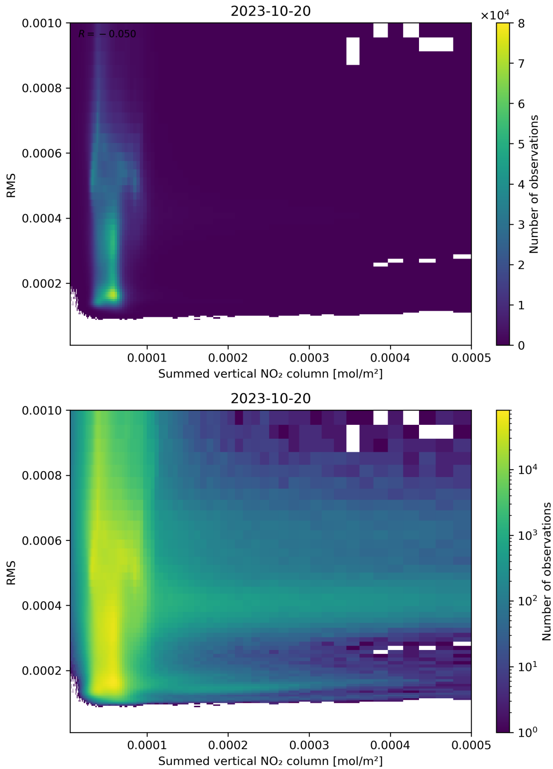
Figure 109: Scatter density plot of “Summed vertical NO 2 column” against “RMS” for 2023-10-19 to 2023-10-21.
