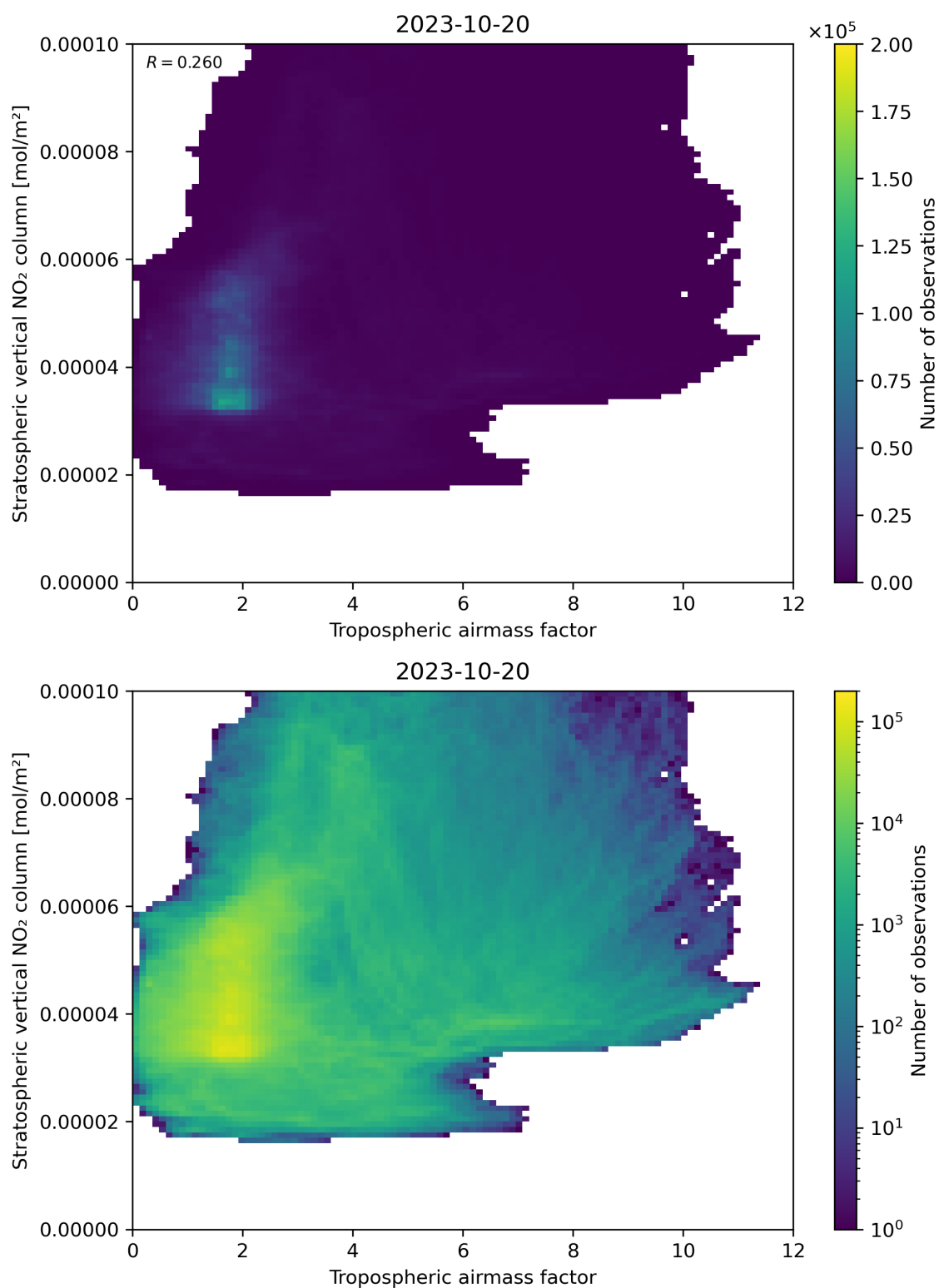
Figure 74: Scatter density plot of “Tropospheric air mass factor” against “Stratospheric vertical NO 2 column” for 2023-10-19 to 2023-10-21.
