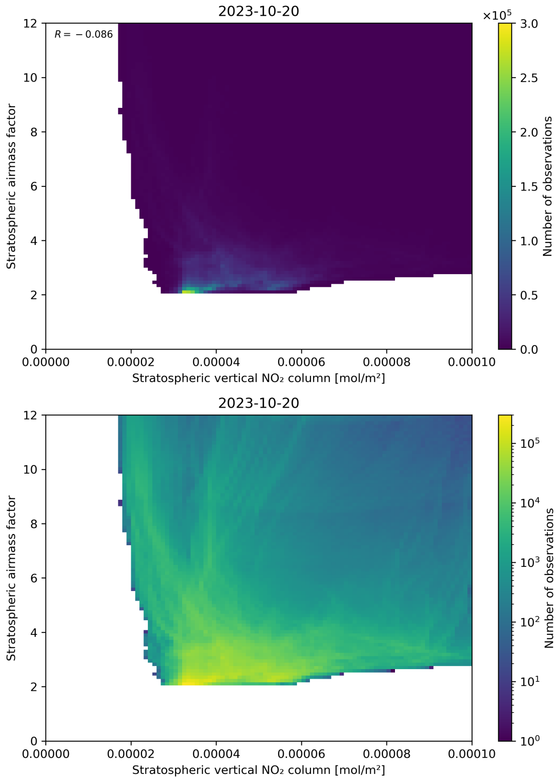
Figure 96: Scatter density plot of “Stratospheric vertical NO 2 column” against “Stratospheric airmass factor” for 2023-10-19 to 2023-10-21.
