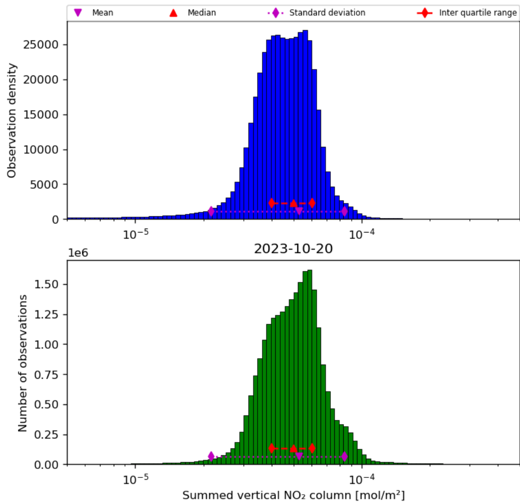
Figure 40: Histogram of “Summed vertical NO 2 column” for 2023-10-19 to 2023-10-21
