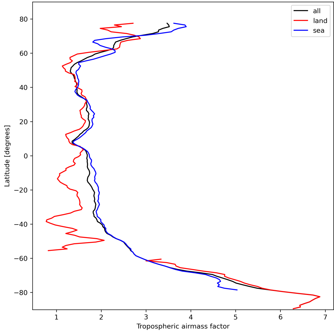
Figure 14: Zonal average of “Tropospheric airmass factor” for 2023-10-19 to 2023-10-21.
