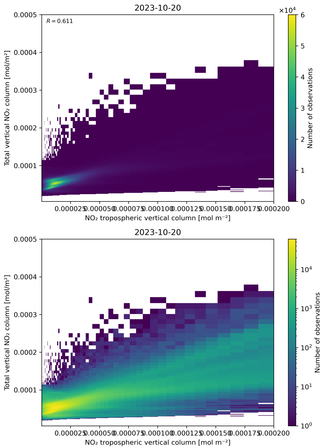
Figure 128: Scatter density plot of “NO 2 tropospheric vertical column” against “Total vertical NO 2 column” for 2023-10-19 to 2023-10-21.
