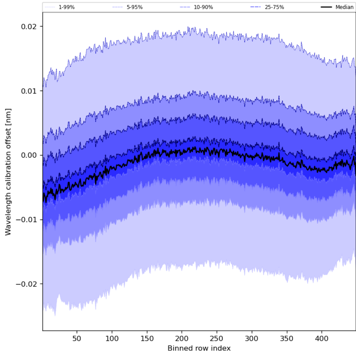
Figure 52: Along track statistics of “Wavelength calibration offset” for 2023-10-19 to 2023-10-21
