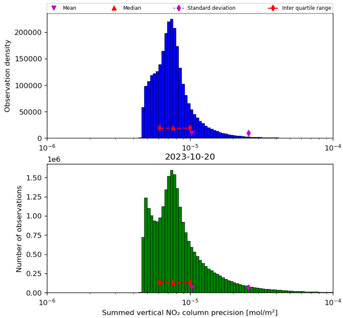
Figure 41: Histogram of "Summed vertical NO 2 column precision" for 2023-10-19 to 2023-10-21
