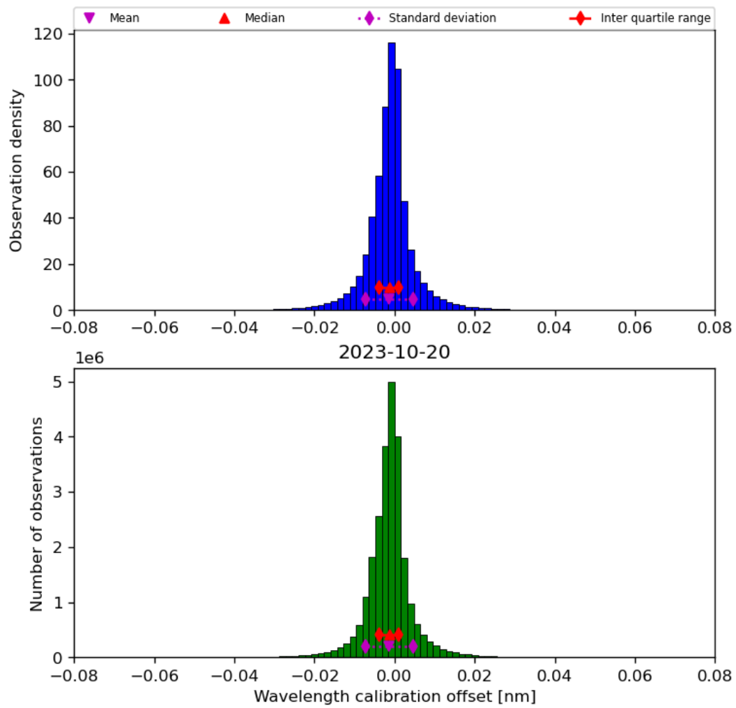
Figure 35: Histogram of “Wavelength calibration offset” for 2023-10-19 to 2023-10-21
