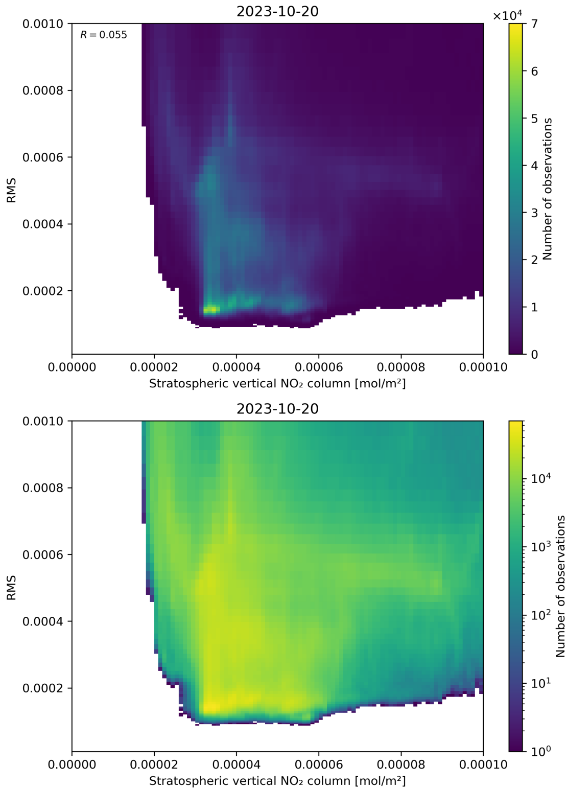
Figure 102: Scatter density plot of “Stratospheric vertical NO 2 column” against “RMS” for 2023-10-19 to 2023-10-21.
