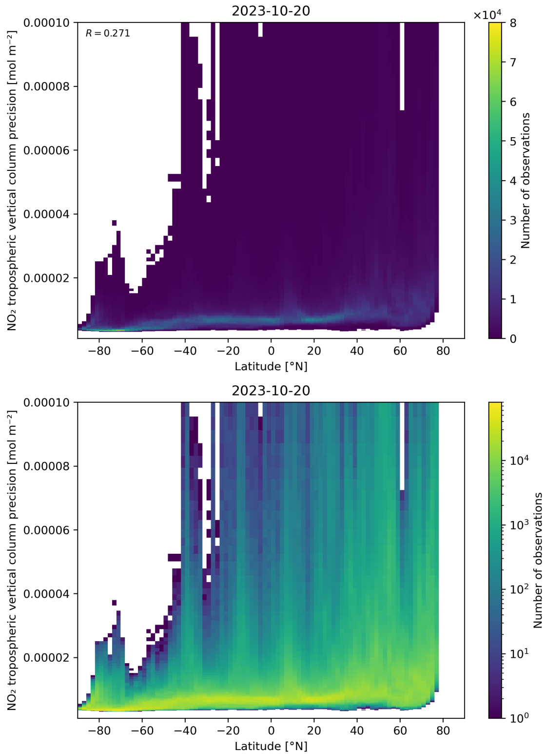
Figure 93: Scatter density plot of “Latitude” against “NO 2 tropospheric vertical column precision” for 2023-10-19 to 2023-10-21.
