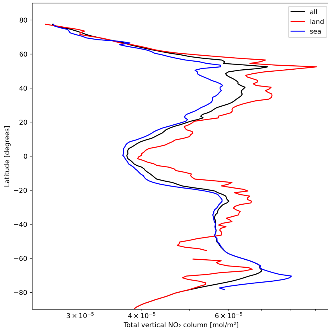
Figure 21: Zonal average of “Total vertical NO 2 column” for 2023-10-19 to 2023-10-21.
