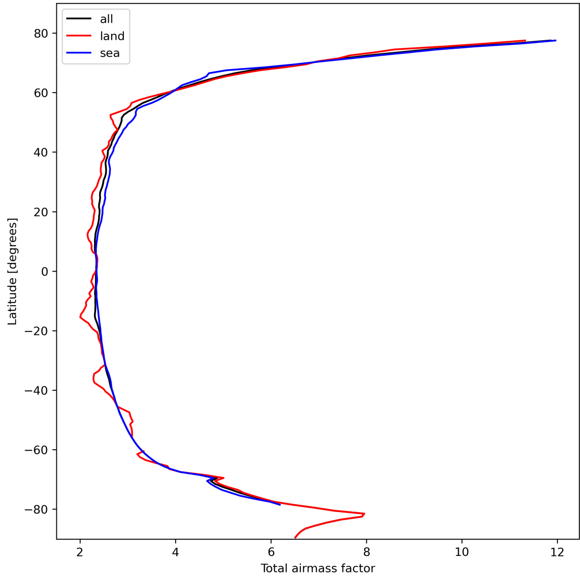
Figure 15: Zonal average of “Total airmass factor” for 2023-10-19 to 2023-10-21.
