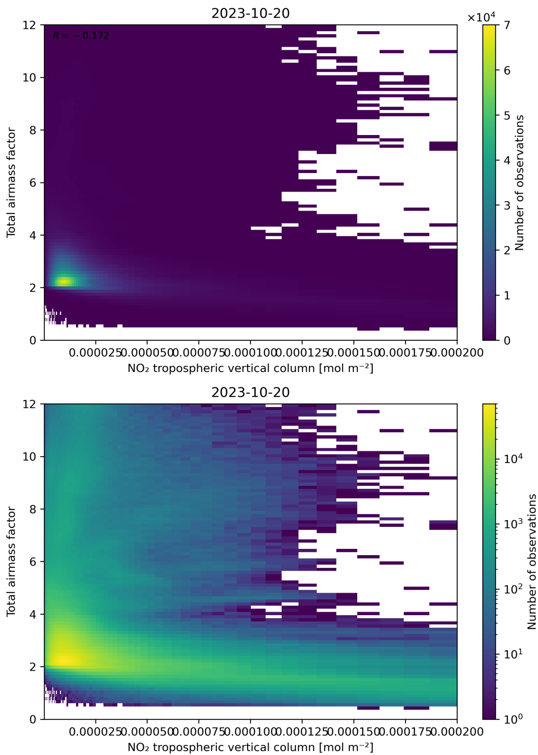
Figure 122: Scatter density plot of “NO 2 tropospheric vertical column” against “Total air mass factor” for 2023-10-19 to 2023-10-21.
