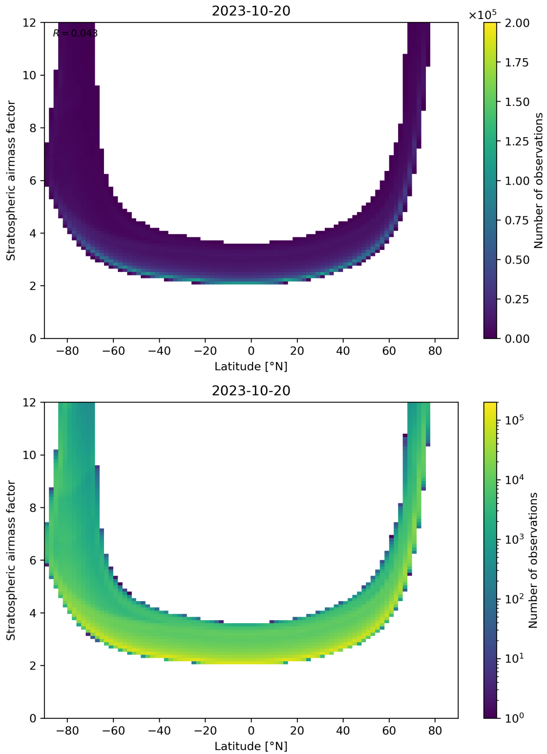
Figure 83: Scatter density plot of “Latitude” against “Stratospheric air mass factor” for 2023-10-19 to 2023-10-21.
