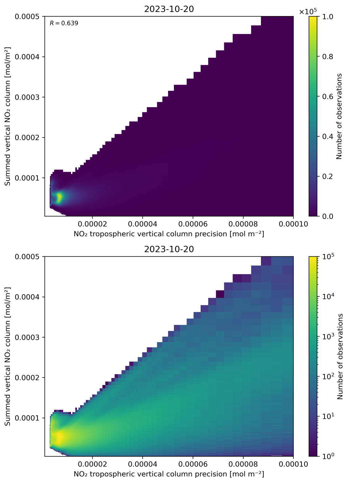
Figure 136: Scatter density plot of “NO 2 tropospheric vertical column precision” against “Summed vertical NO 2 column” for 2023-10-19 to 2023-10-21.
