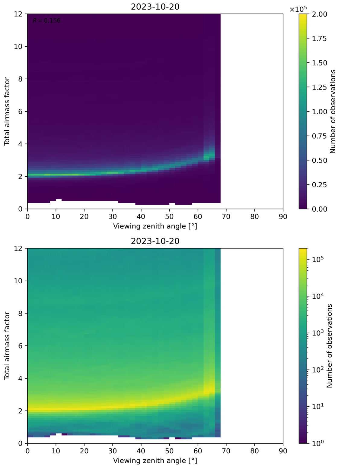
Figure 160: Scatter density plot of “Viewing zenith angle” against “Total airmass factor” for 2023-10-19 to 2023-10-21.
