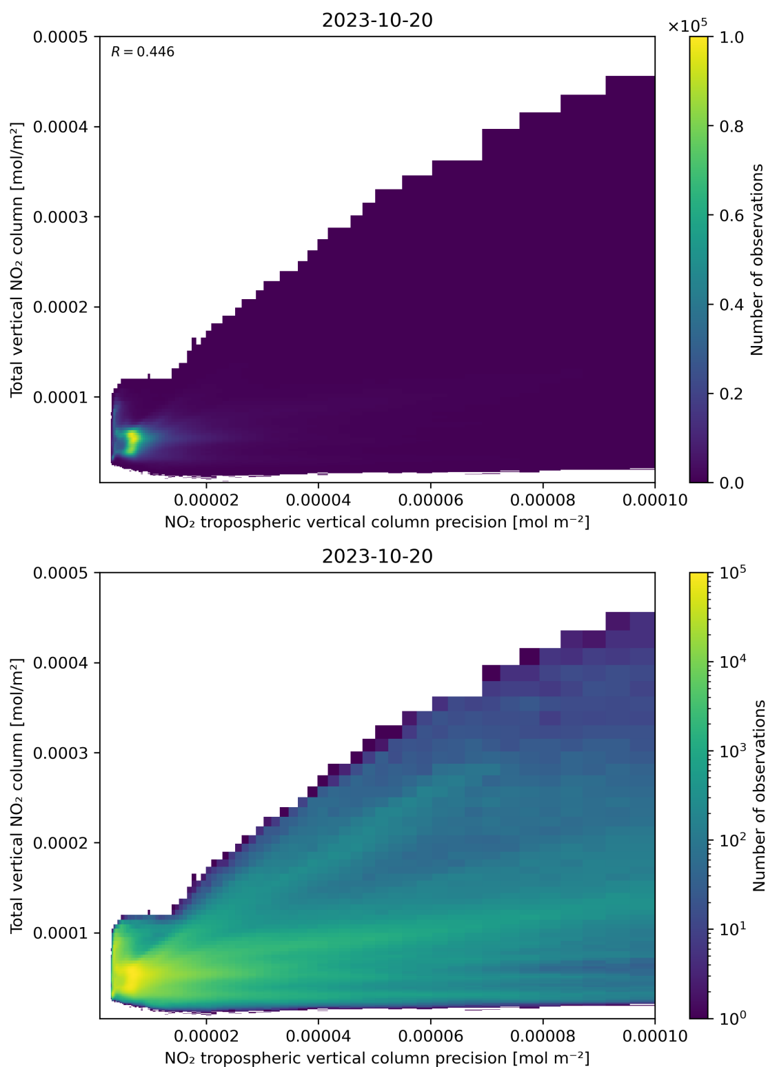
Figure 138: Scatter density plot of “NO 2 tropospheric vertical column precision” against “Total vertical NO 2 column” for 2023-10-19 to 2023-10-21.
