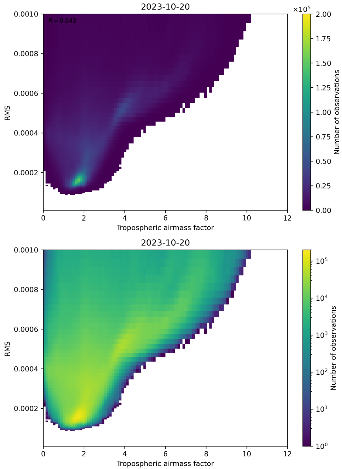
Figure 79: Scatter density plot of “Tropospheric airmass factor” against “RMS” for 2023-10-19 to 2023-10-21.
