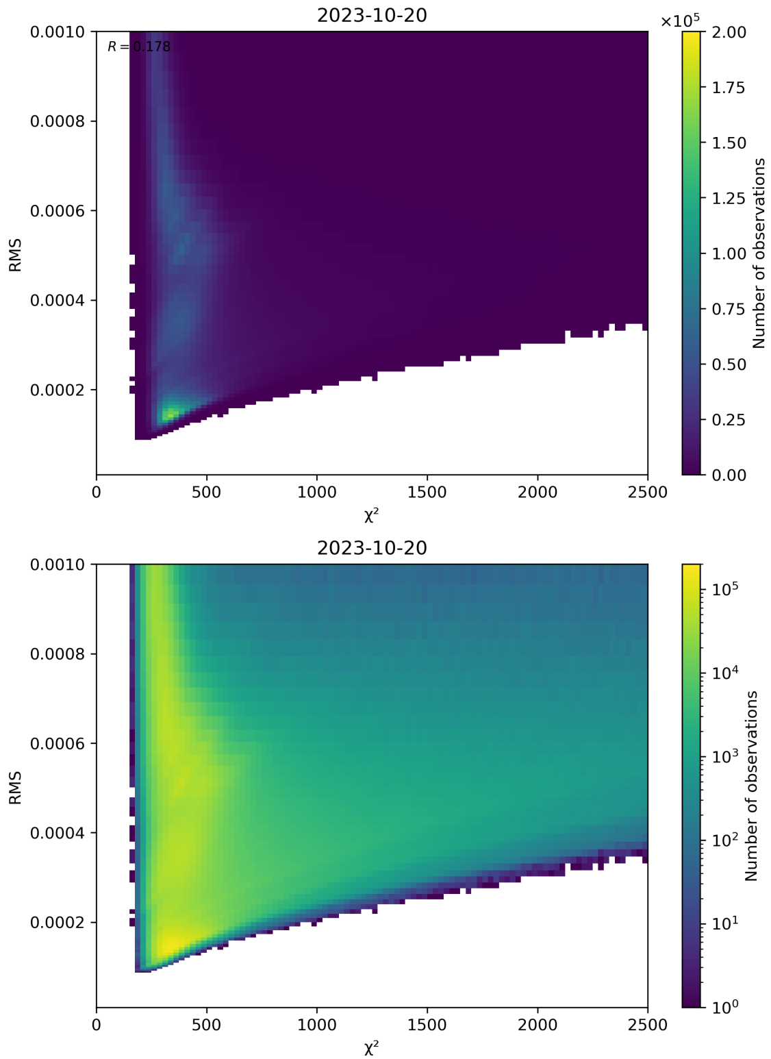
Figure 82: Scatter density plot of “ \chi^2 ” against “RMS” for 2023-10-19 to 2023-10-21.
