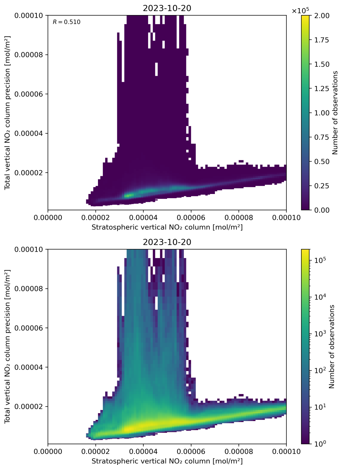
Figure 101: Scatter density plot of “Stratospheric vertical NO 2 column” against “Total vertical NO 2 column precision” for 2023-10-19 to 2023-10-21.
