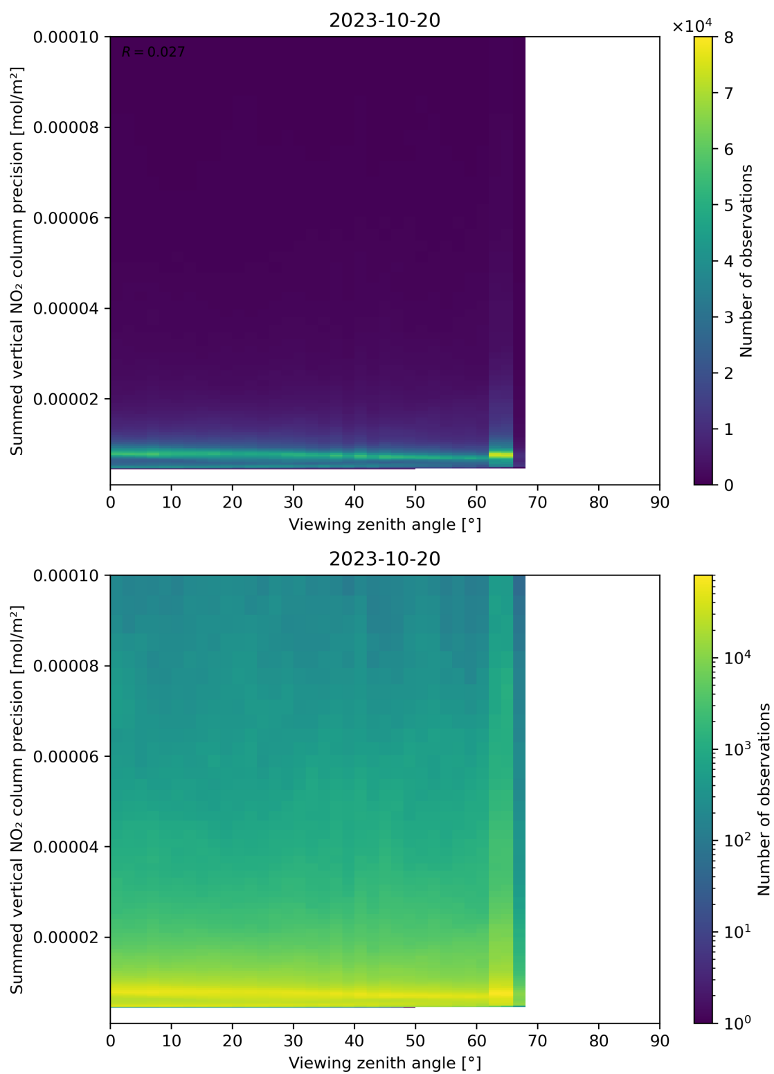
Figure 166: Scatter density plot of “Viewing zenith angle” against “Summed vertical NO 2 column precision” for 2023-10-19 to 2023-10-21.
