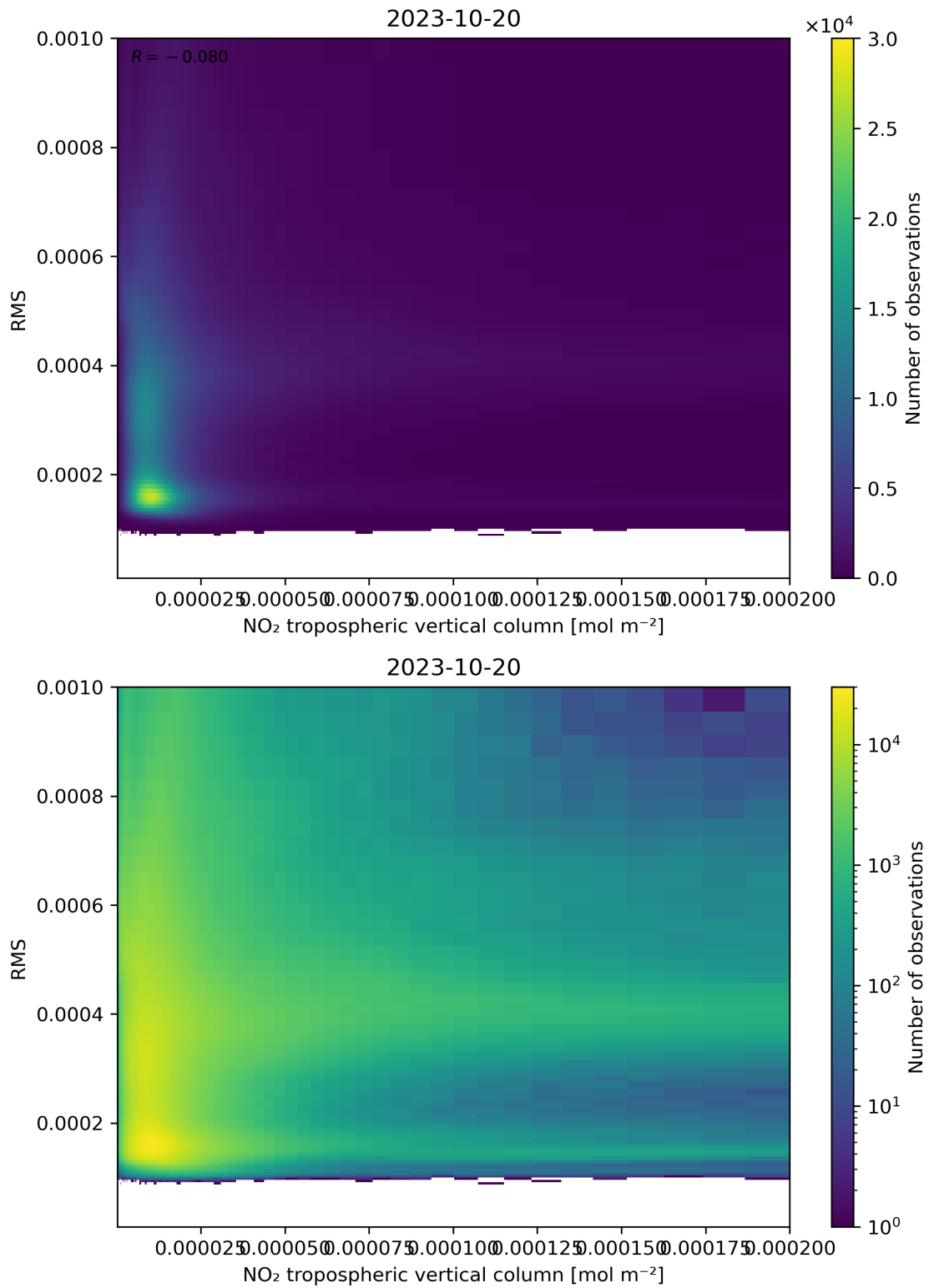
Figure 142: Scatter density plot of “NO 2 tropospheric vertical column” against “RMS” for 2023-10-19 to 2023-10-21.
