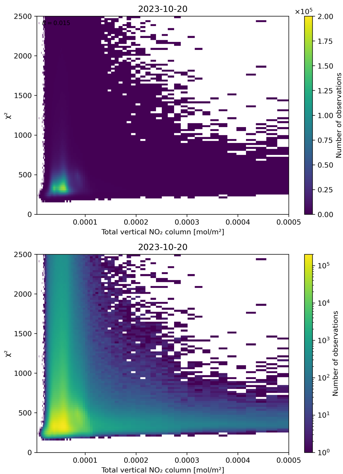
Figure 111: Scatter density plot of “Total vertical NO 2 column” against “ \chi^2 ” for 2023-10-19 to 2023-10-21.
