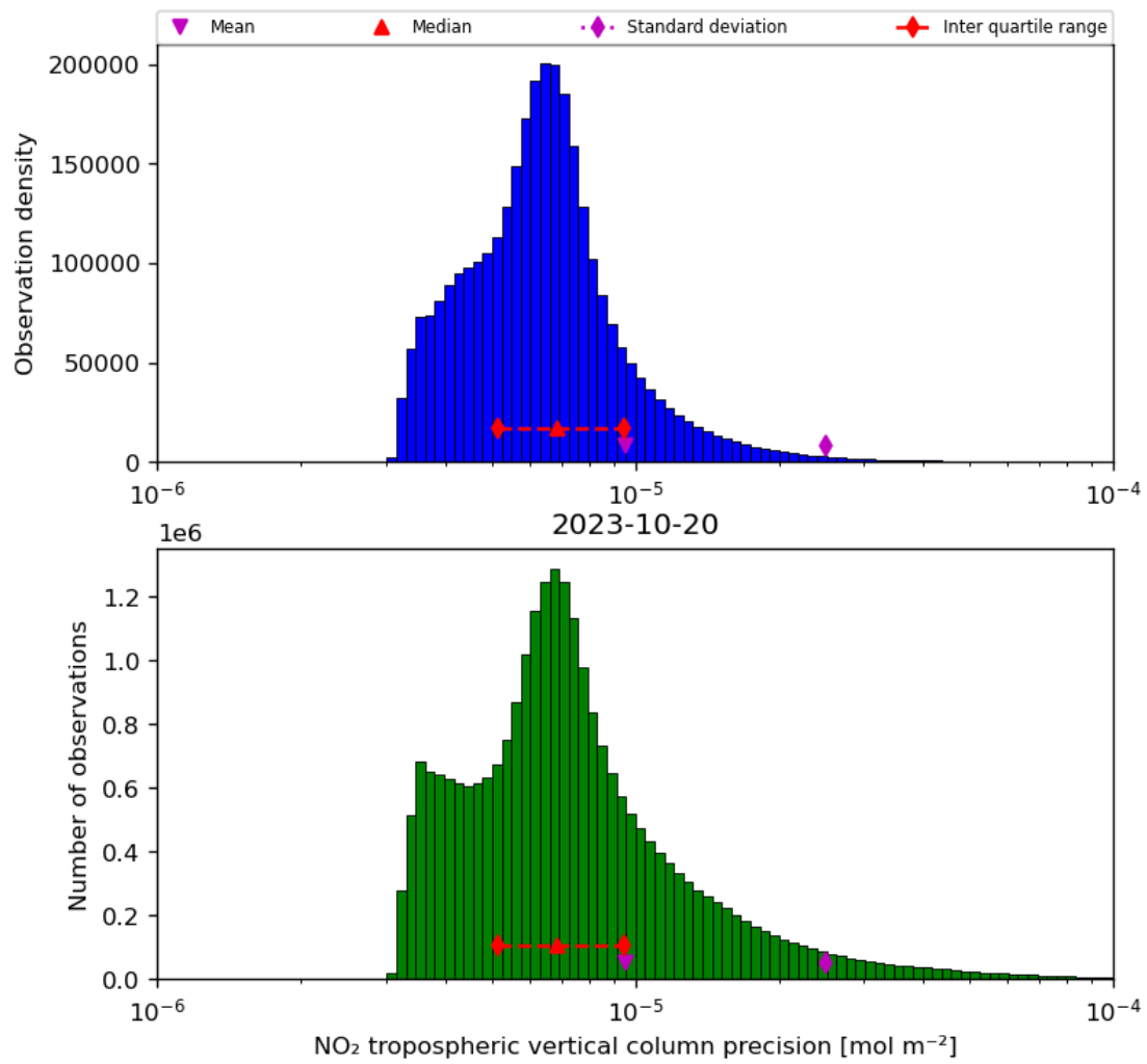
Figure 30: Histogram of “NO 2 tropospheric vertical column precision” for 2023-10-19 to 2023-10-21
