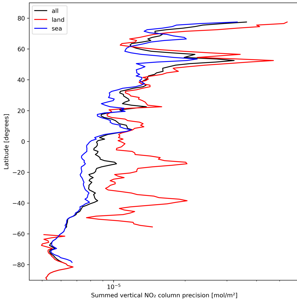
Figure 24: Zonal average of “Summed vertical NO 2 column precision” for 2023-10-19 to 2023-10-21.
