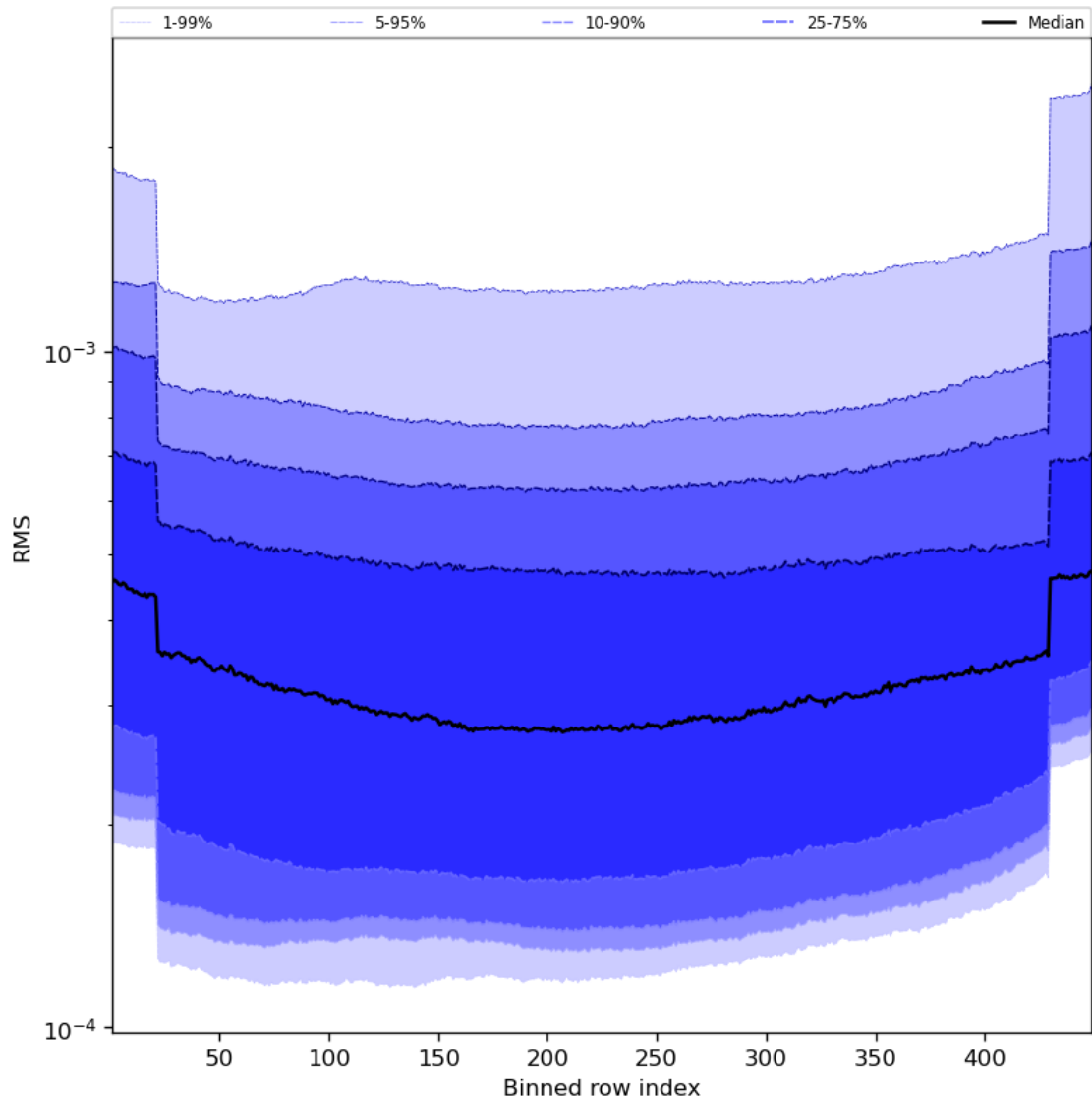
Figure 60: Along track statistics of “RMS” for 2023-10-19 to 2023-10-21
