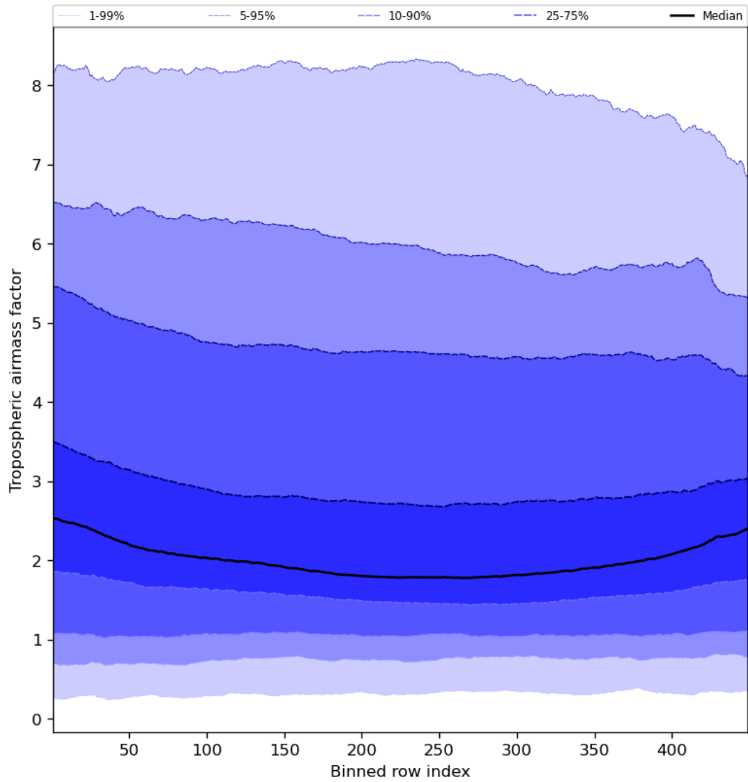
Figure 48: Along track statistics of “Tropospheric air mass factor” for 2023-10-19 to 2023-10-21
