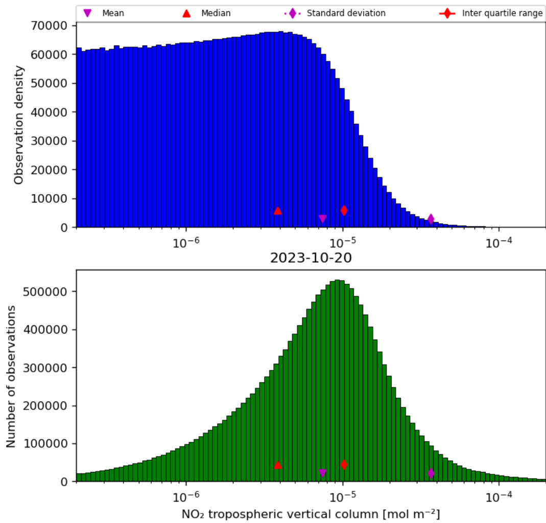
Figure 29: Histogram of “NO 2 tropospheric vertical column” for 2023-10-19 to 2023-10-21
