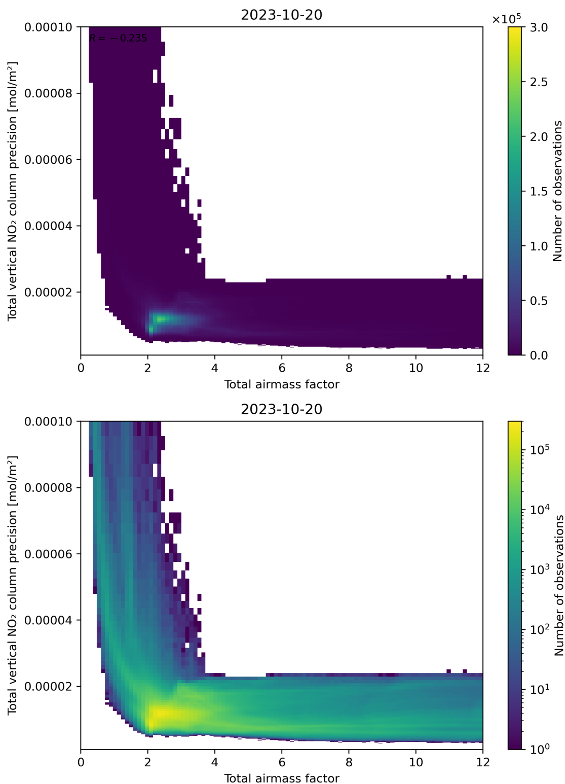
Figure 68: Scatter density plot of “Total airmass factor” against “Total vertical NO 2 column precision” for 2023-10-19 to 2023-10-21.
