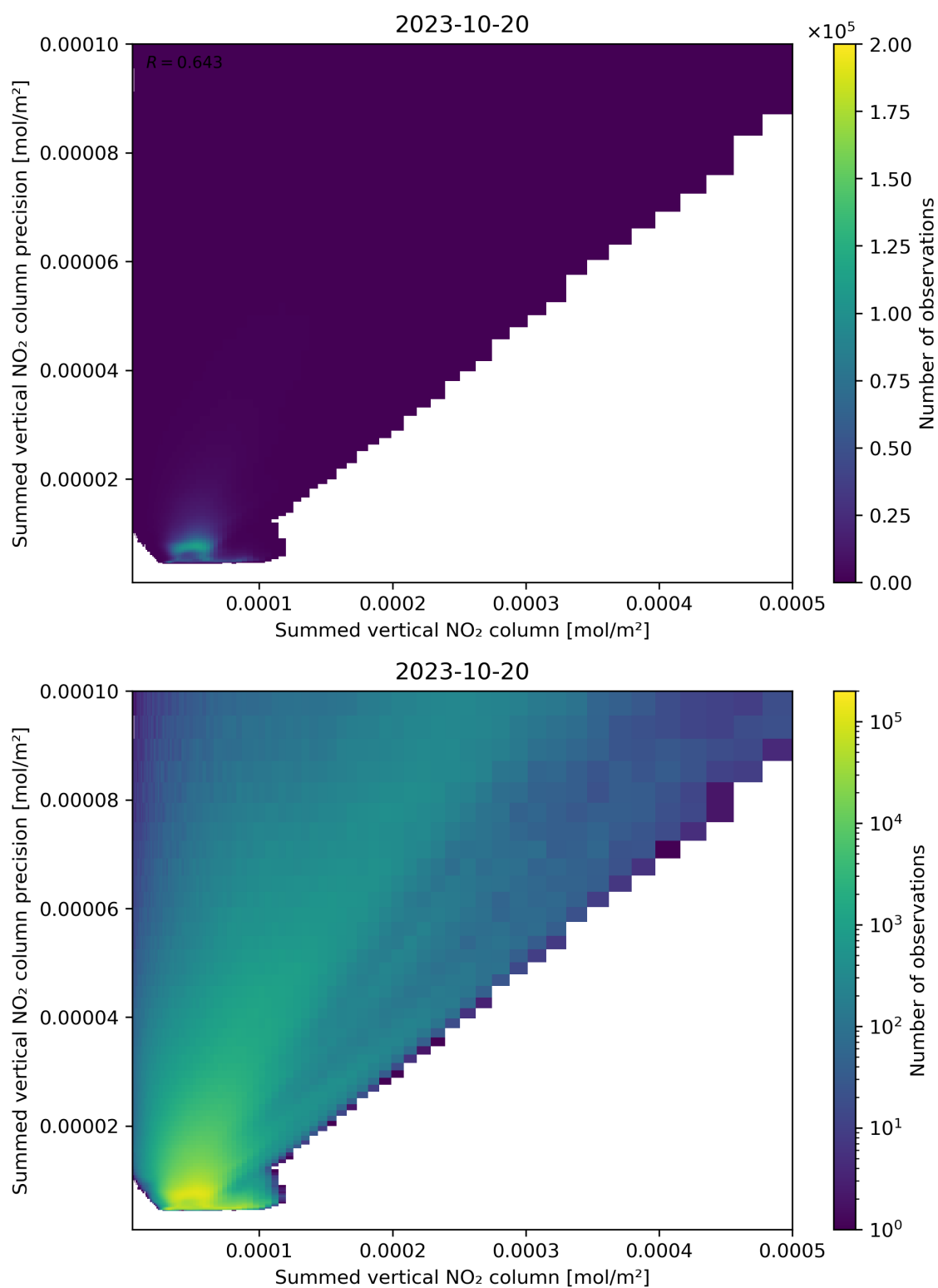
Figure 105: Scatter density plot of “Summed vertical NO 2 column” against “Summed vertical NO 2 column precision” for 2023-10-19 to 2023-10-21.
