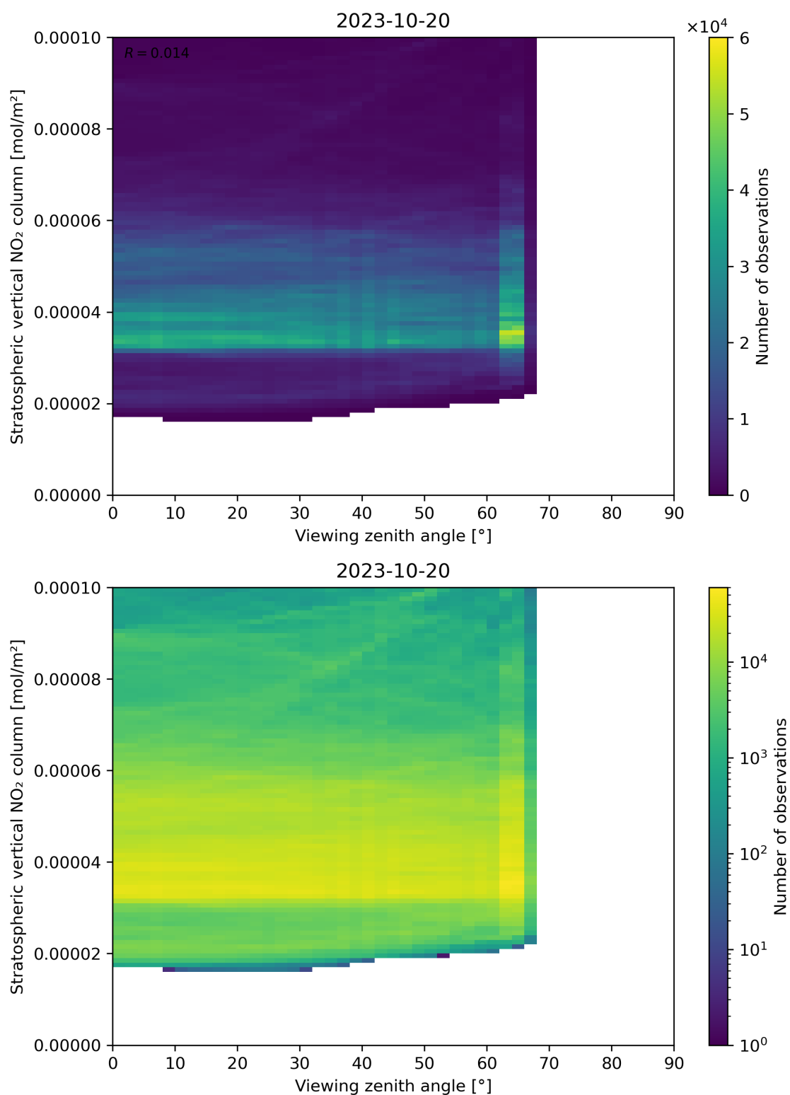
Figure 164: Scatter density plot of “Viewing zenith angle” against “Stratospheric vertical NO 2 column” for 2023-10-19 to 2023-10-21.
