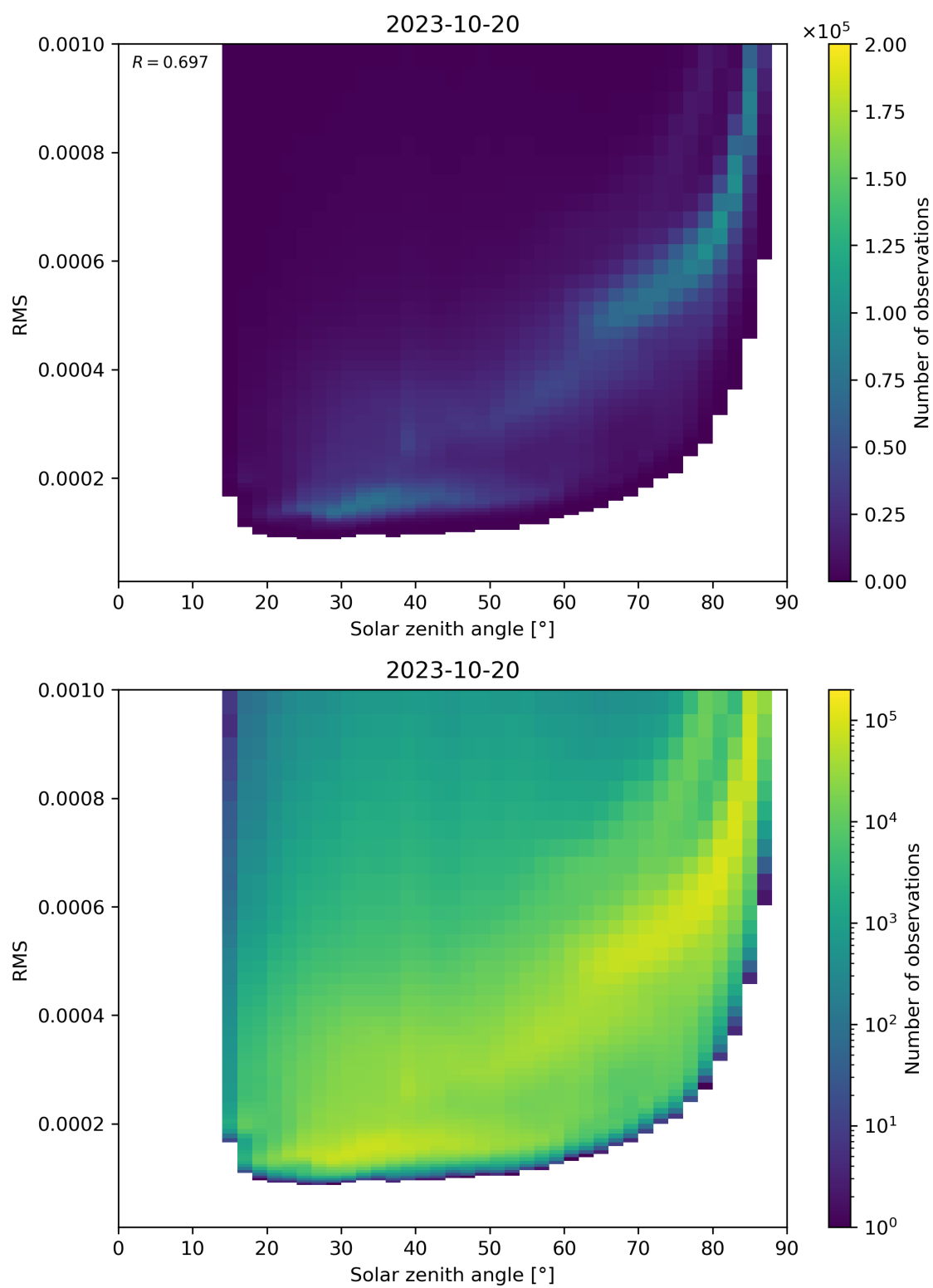
Figure 157: Scatter density plot of “Solar zenith angle” against “RMS” for 2023-10-19 to 2023-10-21.
