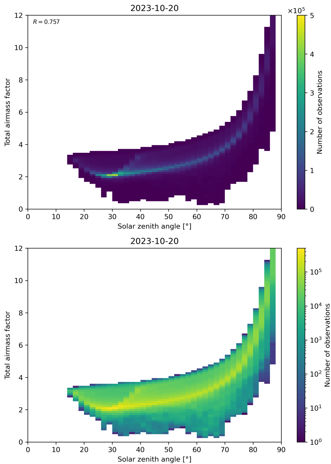
Figure 146: Scatter density plot of “Solar zenith angle” against “Total air mass factor” for 2023-10-19 to 2023-10-21.
