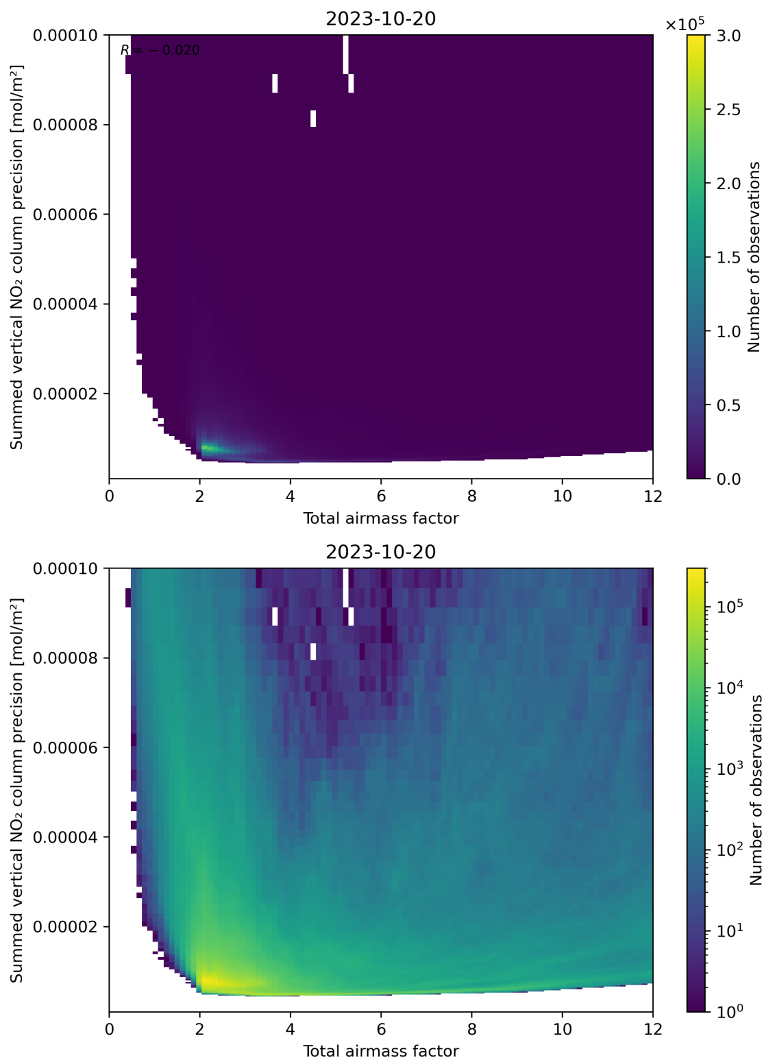
Figure 66: Scatter density plot of “Total airmass factor” against “Summed vertical NO 2 column precision” for 2023-10-19 to 2023-10-21.
