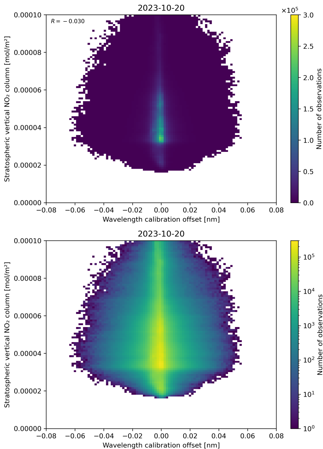
Figure 176: Scatter density plot of “Wavelength calibration offset” against “Stratospheric vertical NO 2 column” for 2023-10-19 to 2023-10-21.
