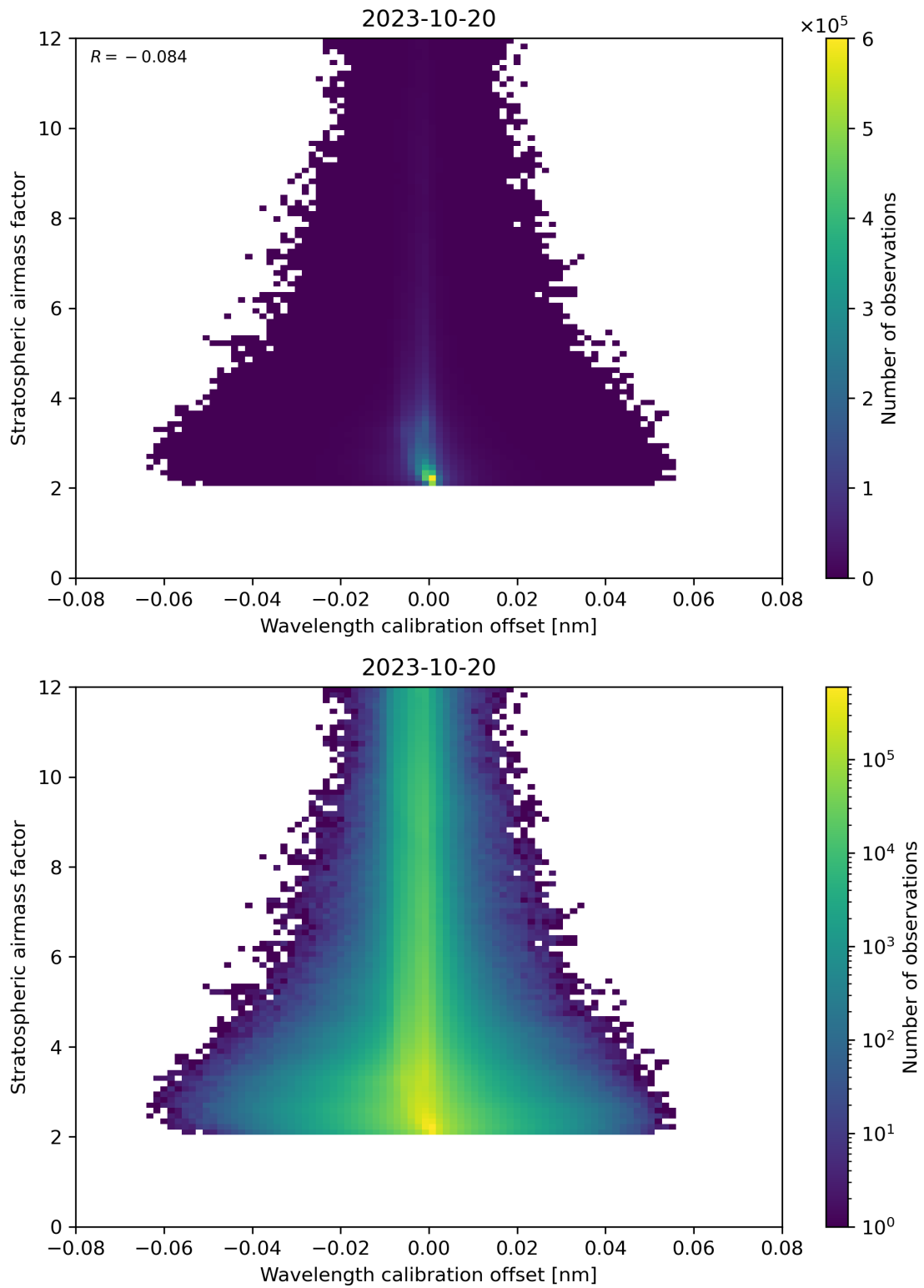
Figure 174: Scatter density plot of “Wavelength calibration offset” against “Stratospheric airmass factor” for 2023-10-19 to 2023-10-21.
