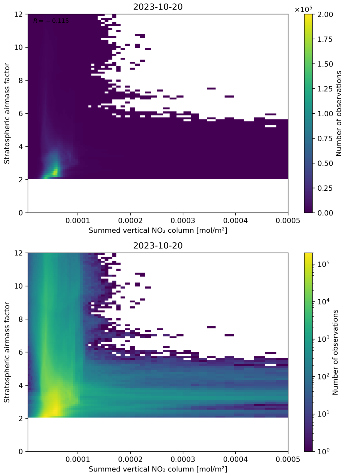
Figure 103: Scatter density plot of “Summed vertical NO 2 column” against “Stratospheric air mass factor” for 2023-10-19 to 2023-10-21.
