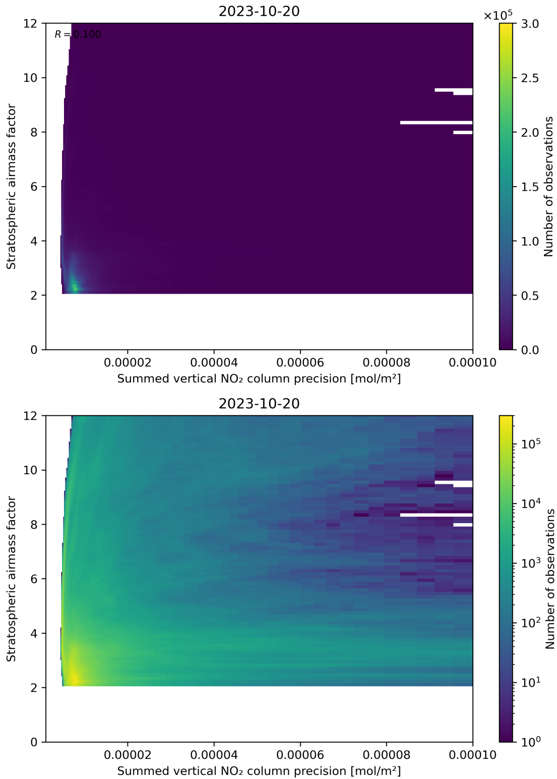
Figure 106: Scatter density plot of “Summed vertical NO 2 column precision” against “Stratospheric airmass factor” for 2023-10-19 to 2023-10-21.
