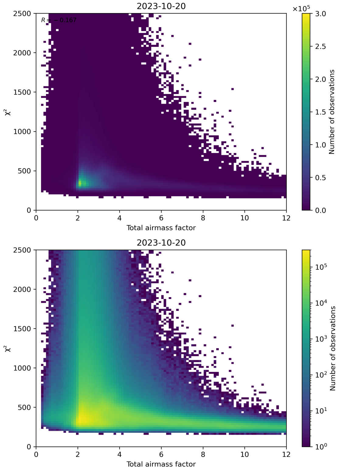
Figure 63: Scatter density plot of “Total airmass factor” against “ \chi^2 ” for 2023-10-19 to 2023-10-21.
