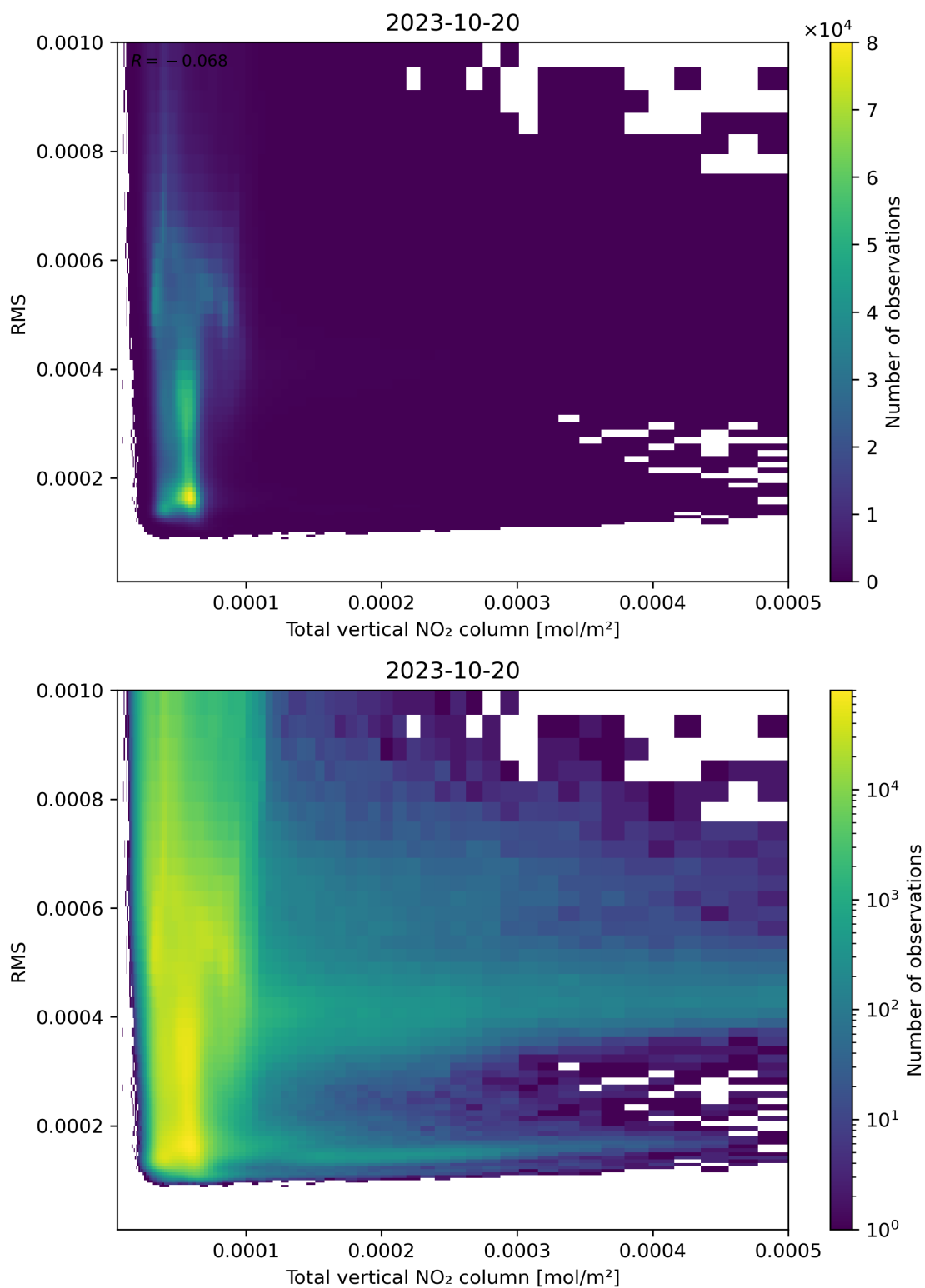
Figure 120: Scatter density plot of “Total vertical NO 2 column” against “RMS” for 2023-10-19 to 2023-10-21.
