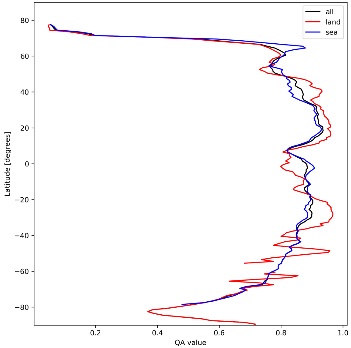
Figure 11: Zonal average of “QA value” for 2023-10-19 to 2023-10-21.
