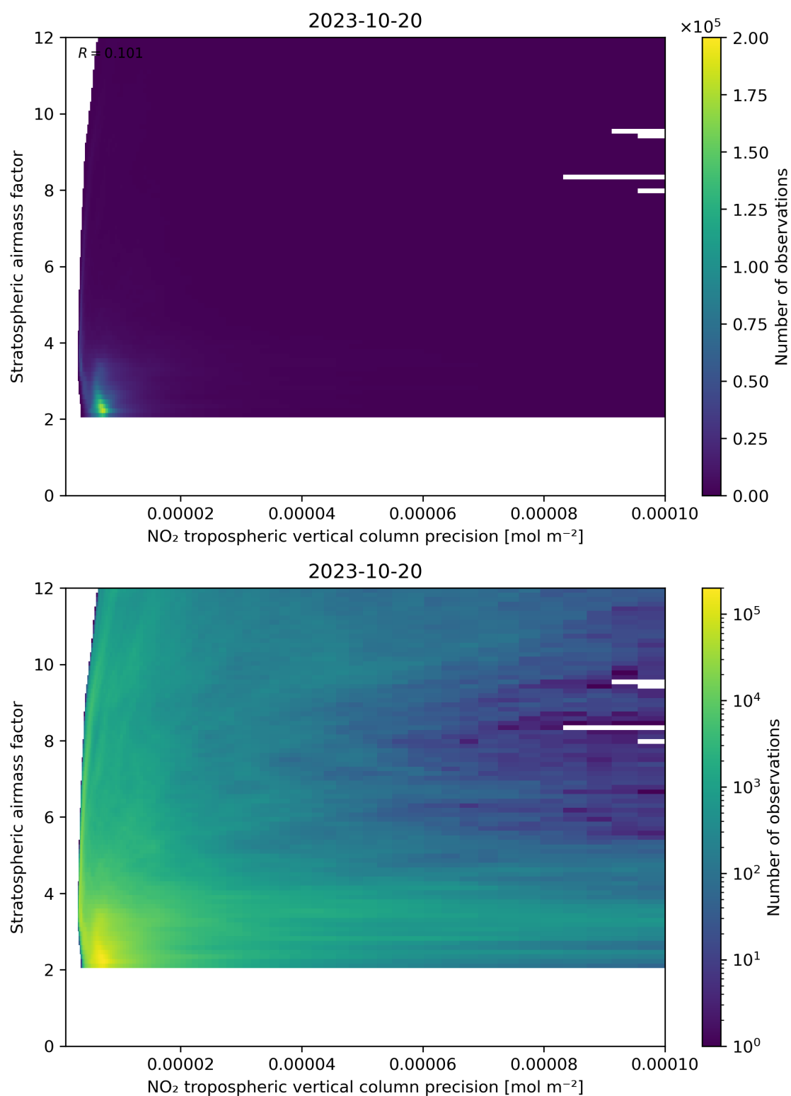
Figure 131: Scatter density plot of “NO 2 tropospheric vertical column precision” against “Stratospheric airmass factor” for 2023-10-19 to 2023-10-21.
