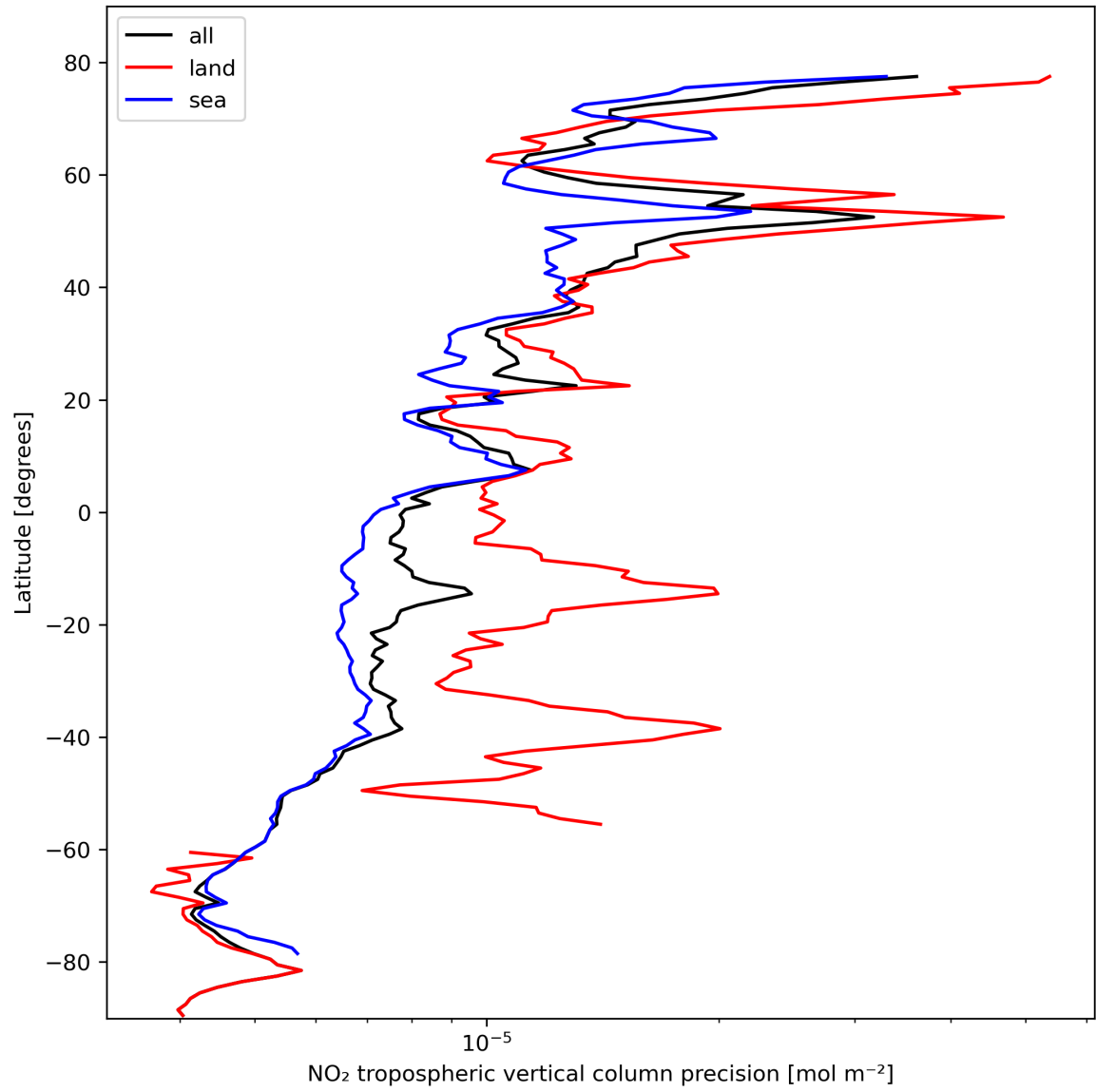
Figure 13: Zonal average of “NO 2 tropospheric vertical column precision” for 2023-10-19 to 2023-10-21.
