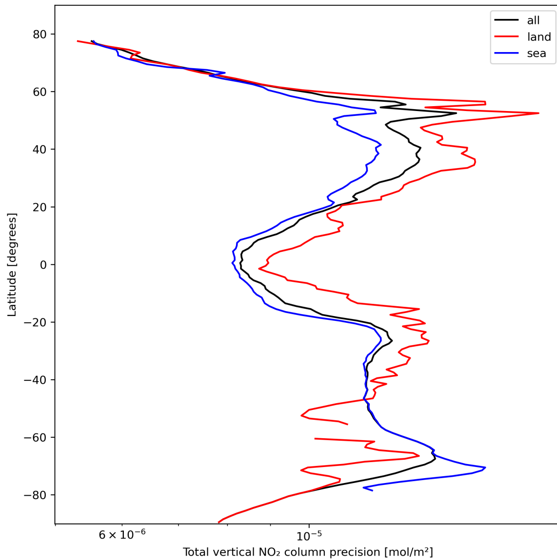
Figure 22: Zonal average of “Total vertical NO 2 column precision” for 2023-10-19 to 2023-10-21.
