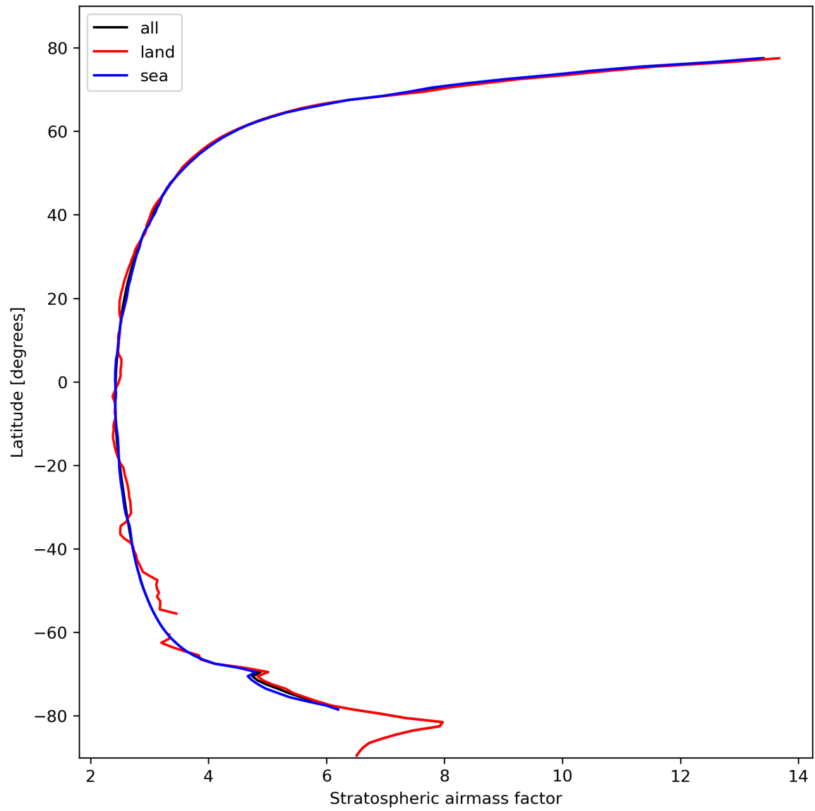
Figure 27: Zonal average of “Stratospheric air mass factor” for 2023-10-19 to 2023-10-21.
