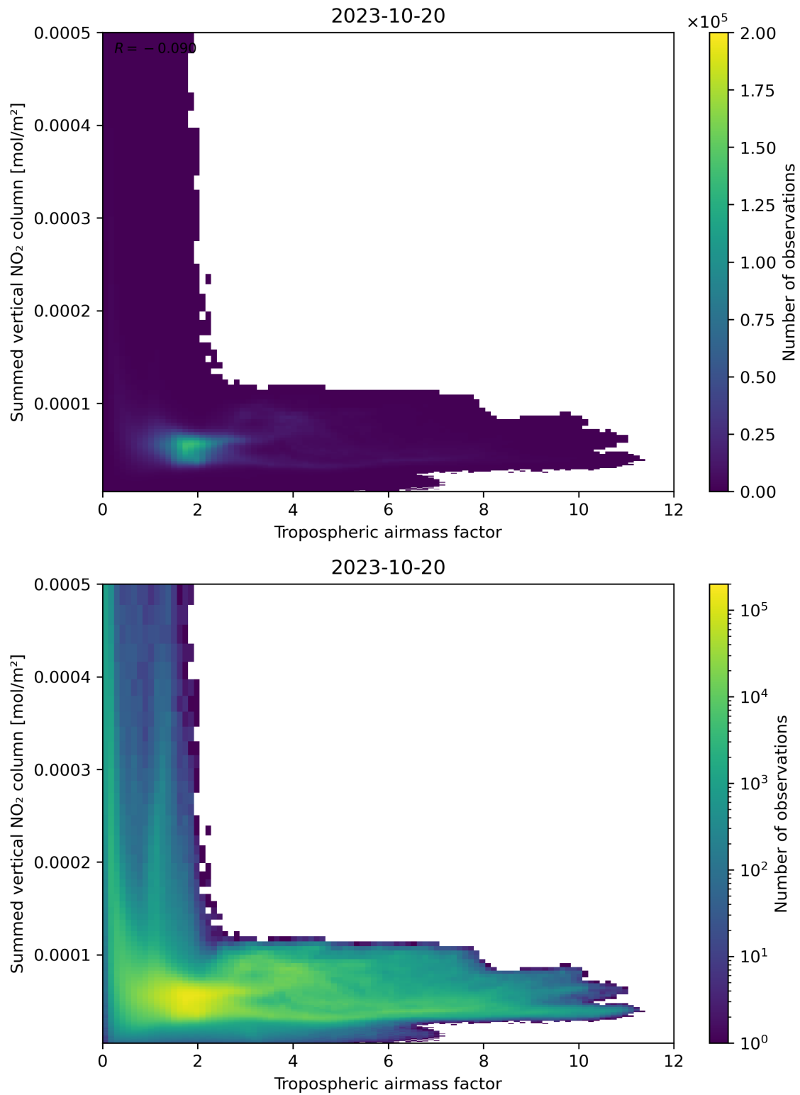
Figure 75: Scatter density plot of “Tropospheric air mass factor” against “Summed vertical NO 2 column” for 2023-10-19 to 2023-10-21.
