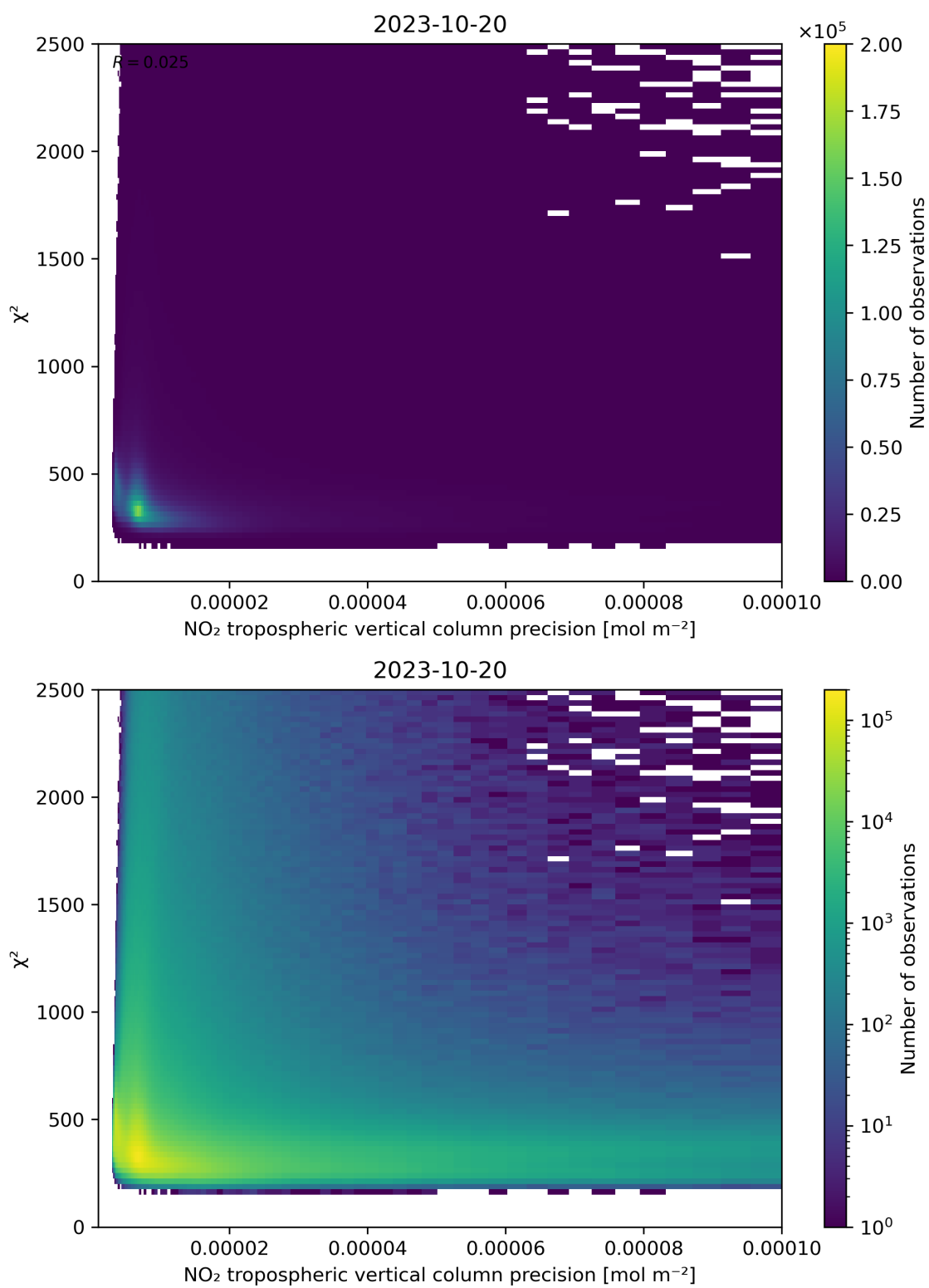
Figure 134: Scatter density plot of “NO 2 tropospheric vertical column precision” against “ \chi^2 ” for 2023-10-19 to 2023-10-21.
