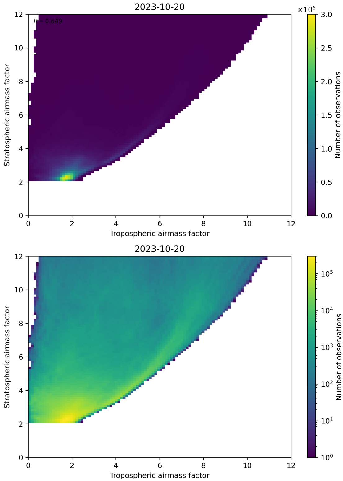
Figure 71: Scatter density plot of “Tropospheric airmass factor” against “Stratospheric airmass factor” for 2023-10-19 to 2023-10-21.
