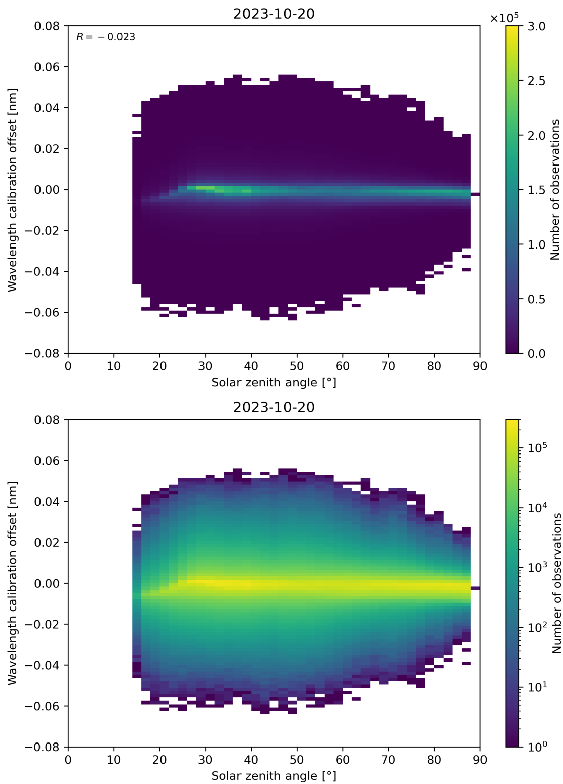
Figure 158: Scatter density plot of “Solar zenith angle” against “Wavelength calibration offset” for 2023-10-19 to 2023-10-21.
