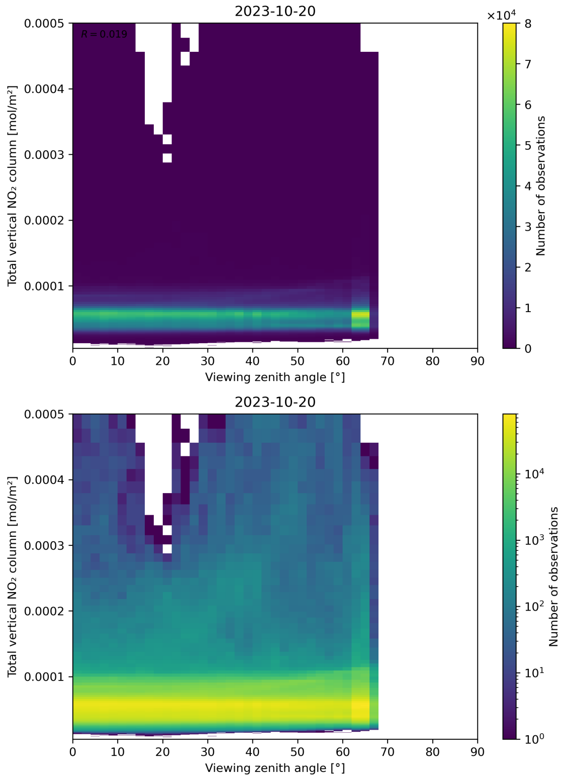
Figure 167: Scatter density plot of “Viewing zenith angle” against “Total vertical NO 2 column” for 2023-10-19 to 2023-10-21.
