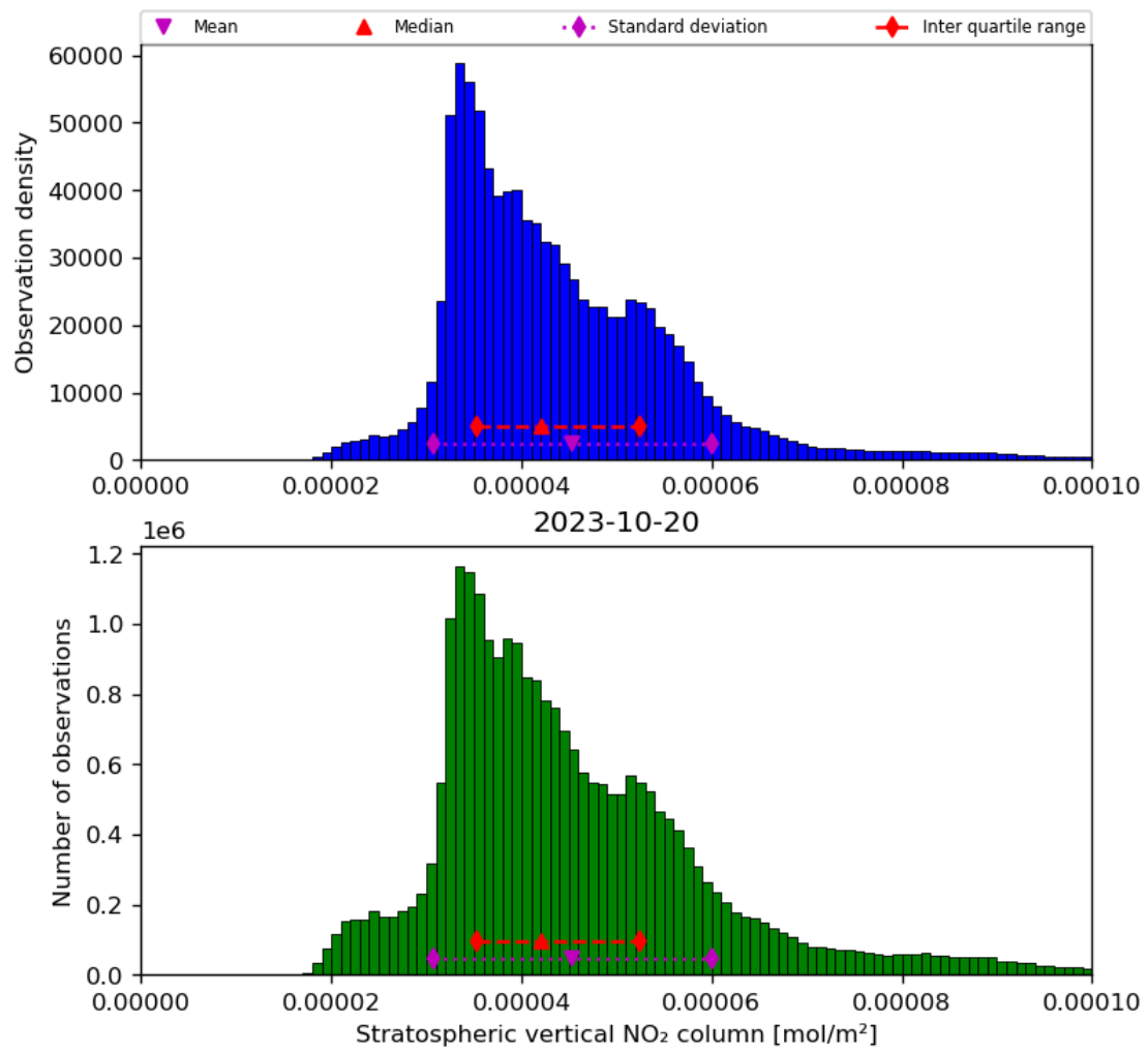
Figure 36: Histogram of “Stratospheric vertical NO 2 column” for 2023-10-19 to 2023-10-21
