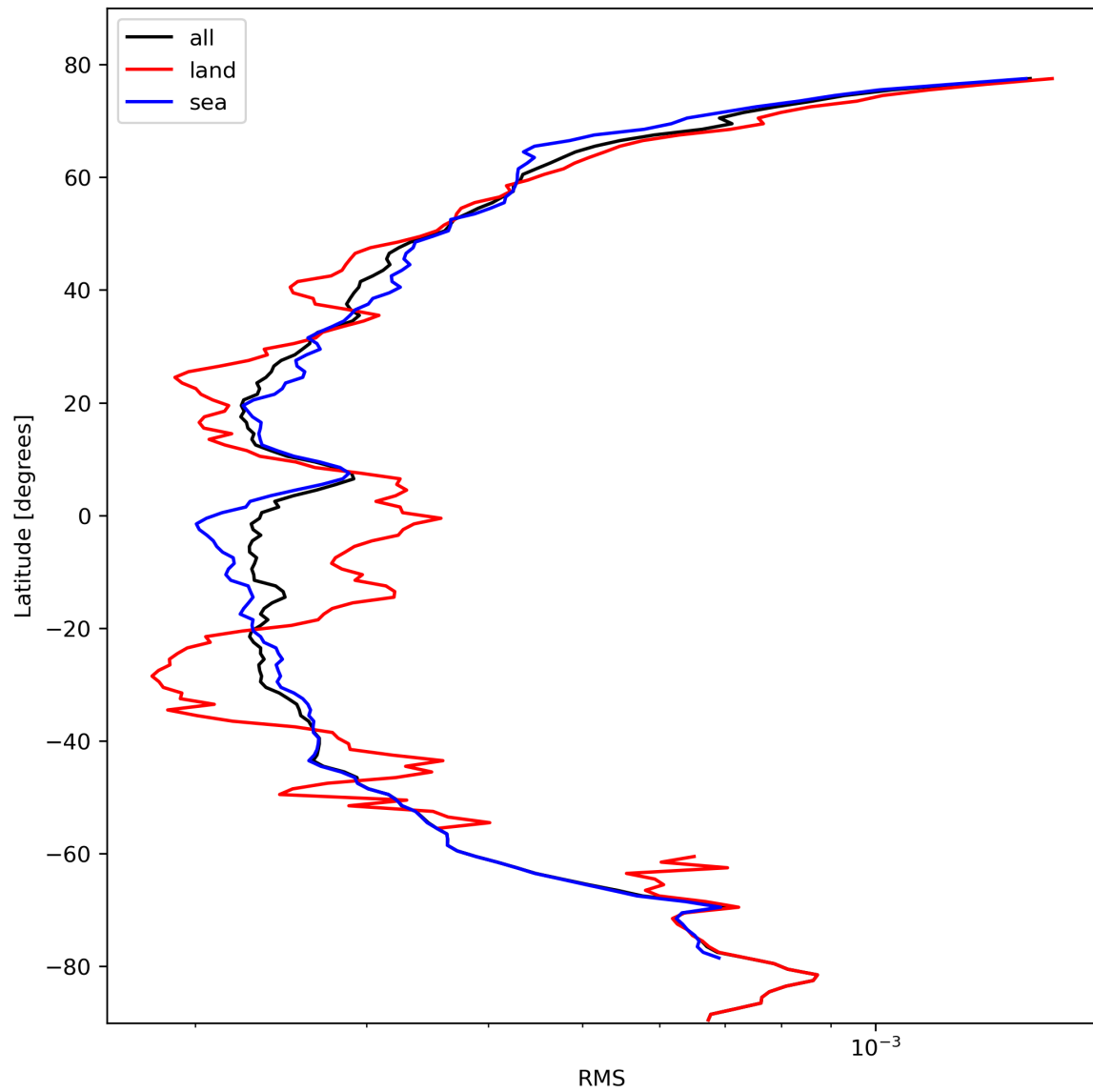
Figure 26: Zonal average of “RMS” for 2023-10-19 to 2023-10-21.
