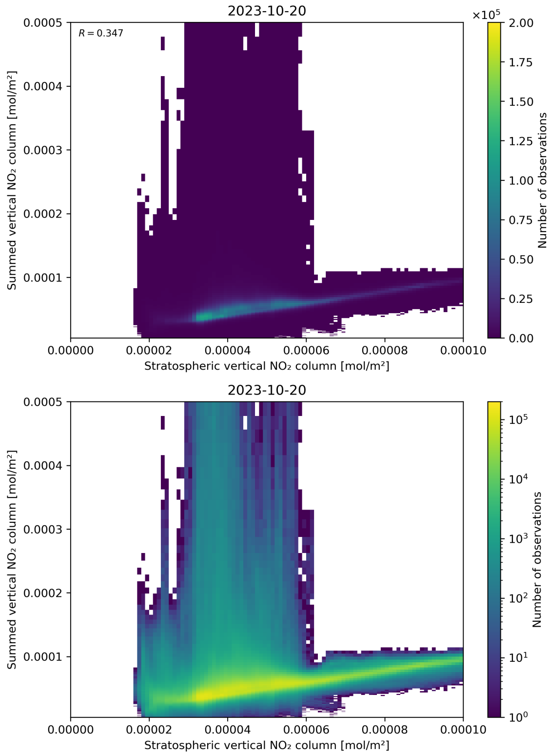
Figure 98: Scatter density plot of “Stratospheric vertical NO 2 column” against “Summed vertical NO 2 column” for 2023-10-19 to 2023-10-21.
