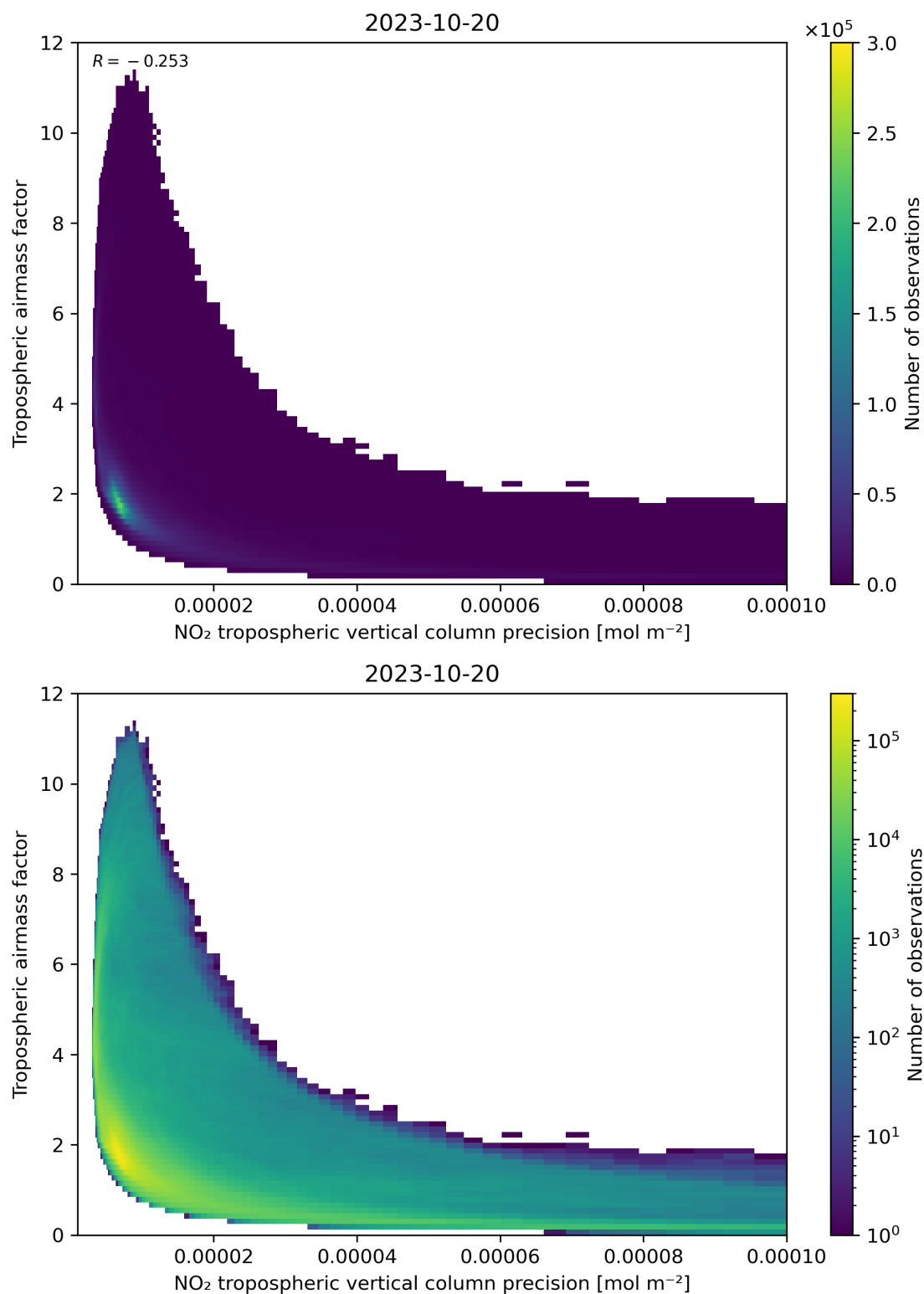
Figure 133: Scatter density plot of “NO 2 tropospheric vertical column precision” against “Tropospheric air mass factor” for 2023-10-19 to 2023-10-21.
