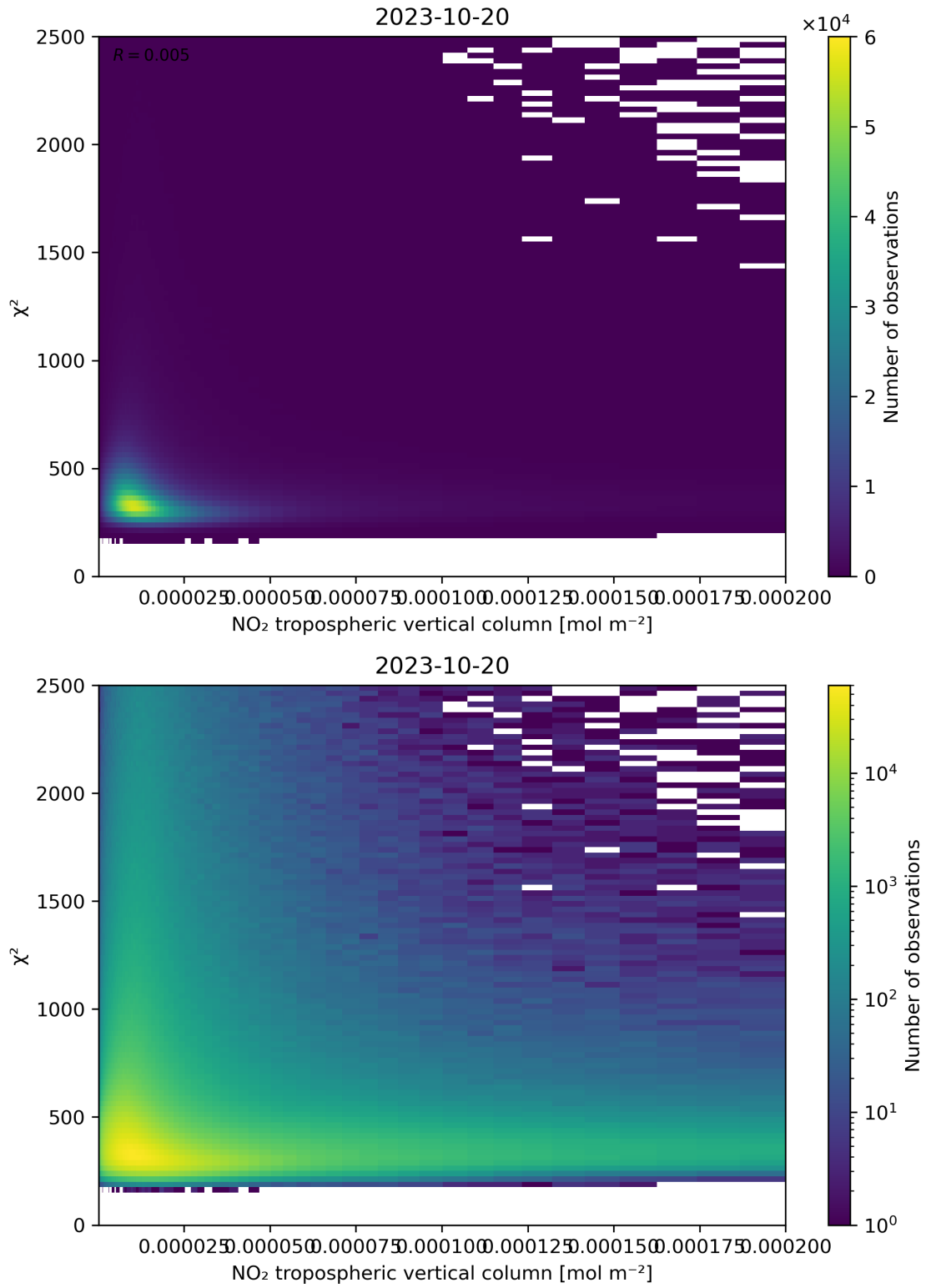
Figure 124: Scatter density plot of “NO 2 tropospheric vertical column” against “ \chi^2 ” for 2023-10-19 to 2023-10-21.
