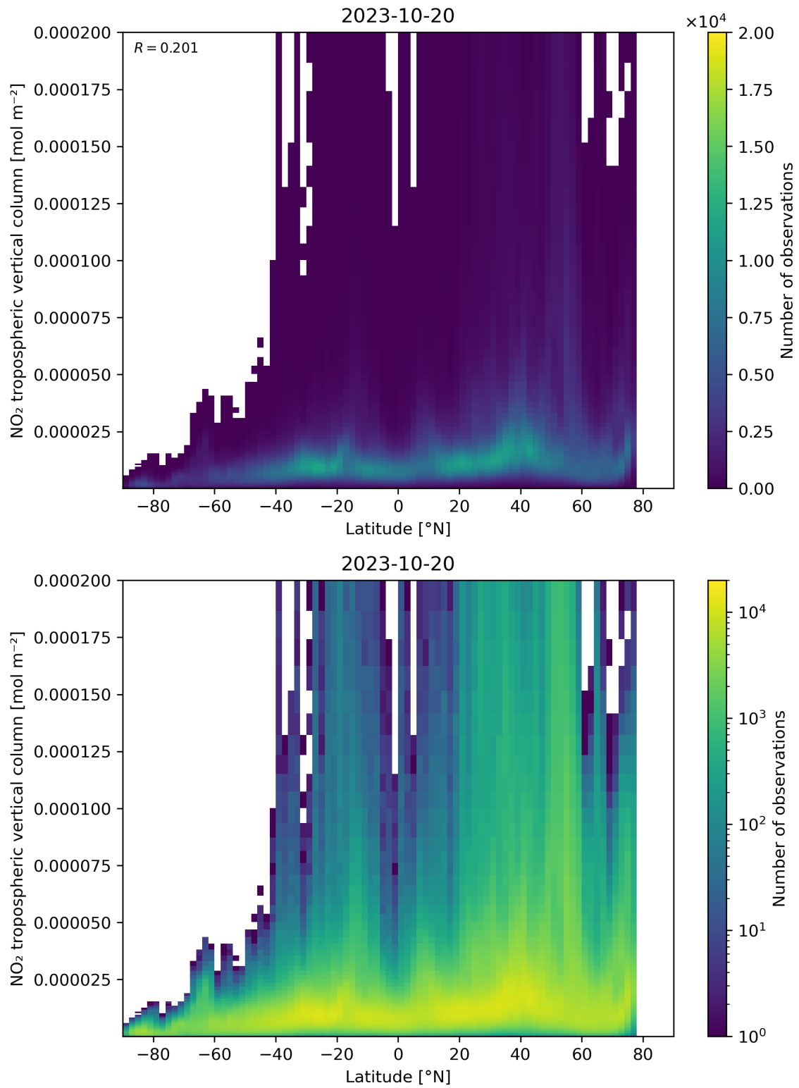
Figure 92: Scatter density plot of “Latitude” against “NO 2 tropospheric vertical column” for 2023-10-19 to 2023-10-21.
