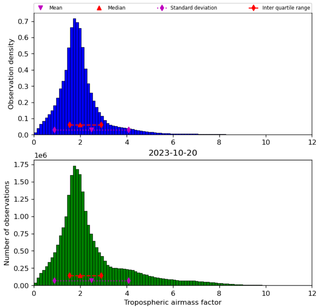
Figure 31: Histogram of “Tropospheric airmass factor” for 2023-10-19 to 2023-10-21
