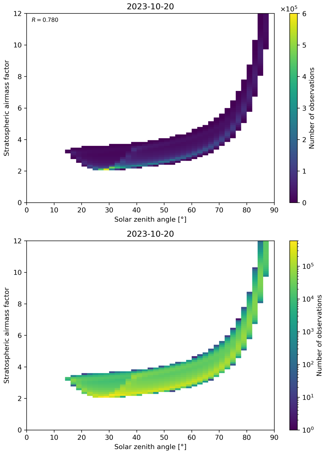
Figure 145: Scatter density plot of “Solar zenith angle” against “Stratospheric airmass factor” for 2023-10-19 to 2023-10-21.
