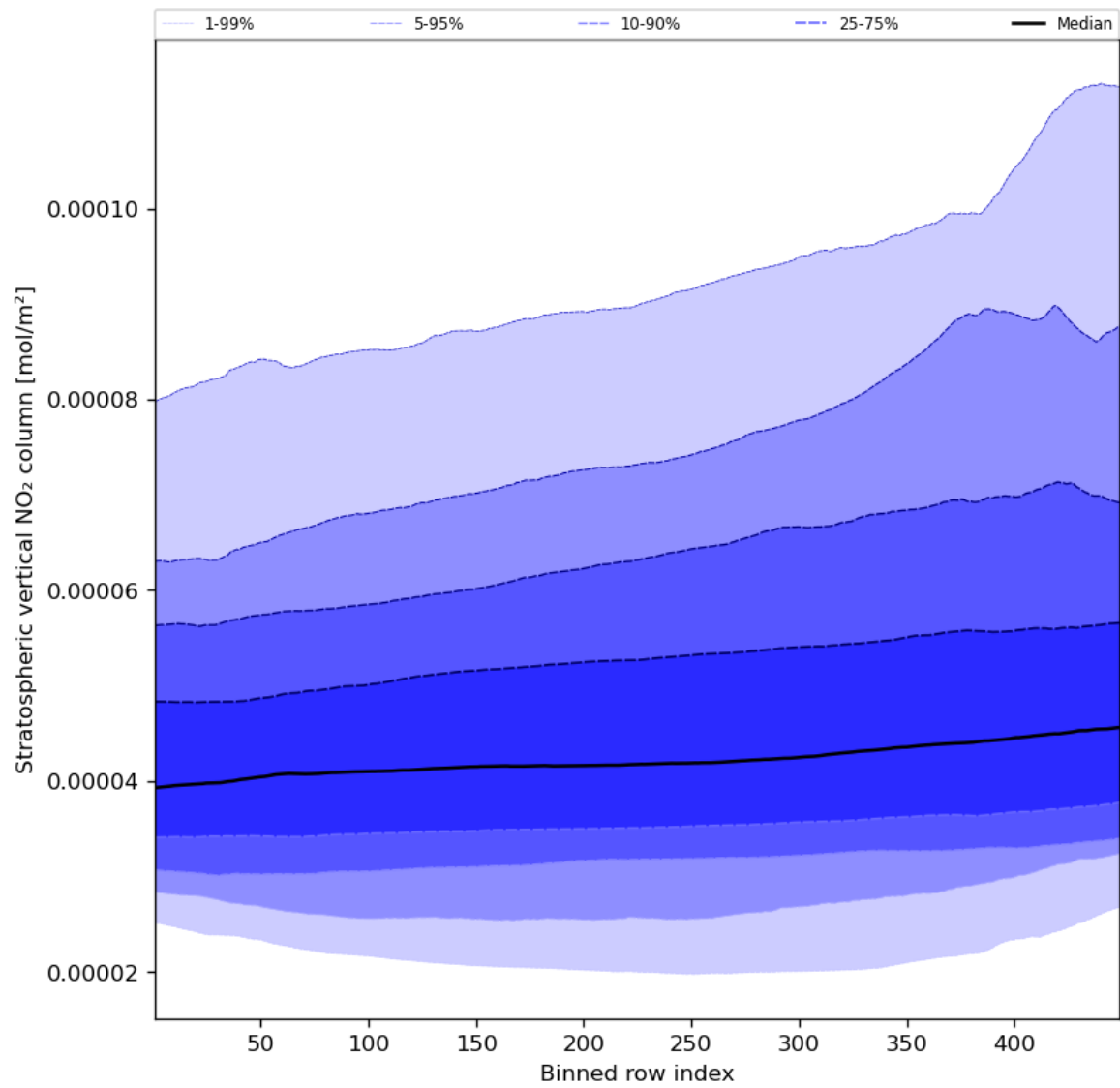
Figure 53: Along track statistics of “Stratospheric vertical NO 2 column” for 2023-10-19 to 2023-10-21
