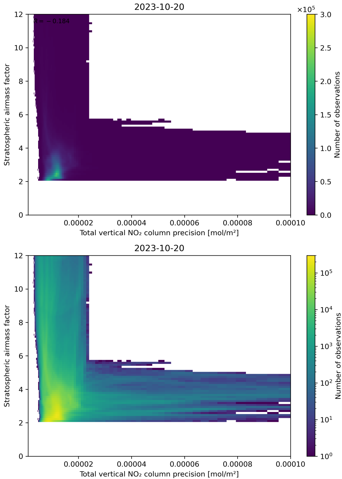
Figure 115: Scatter density plot of “Total vertical NO 2 column precision” against “Stratospheric airmass factor” for 2023-10-19 to 2023-10-21.
