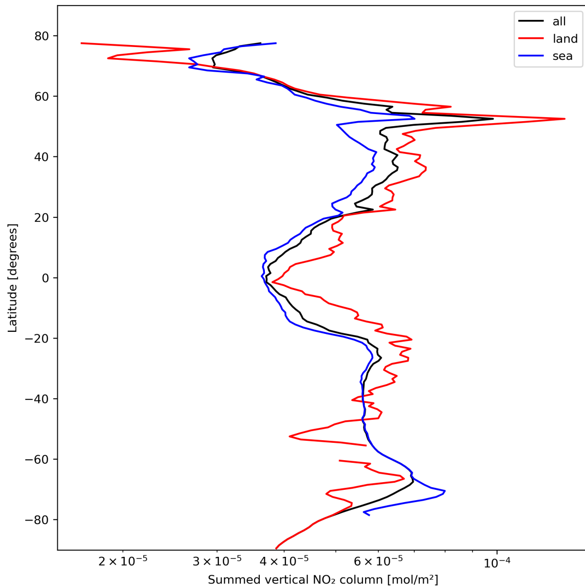
Figure 23: Zonal average of “Summed vertical NO 2 column” for 2023-10-19 to 2023-10-21.
