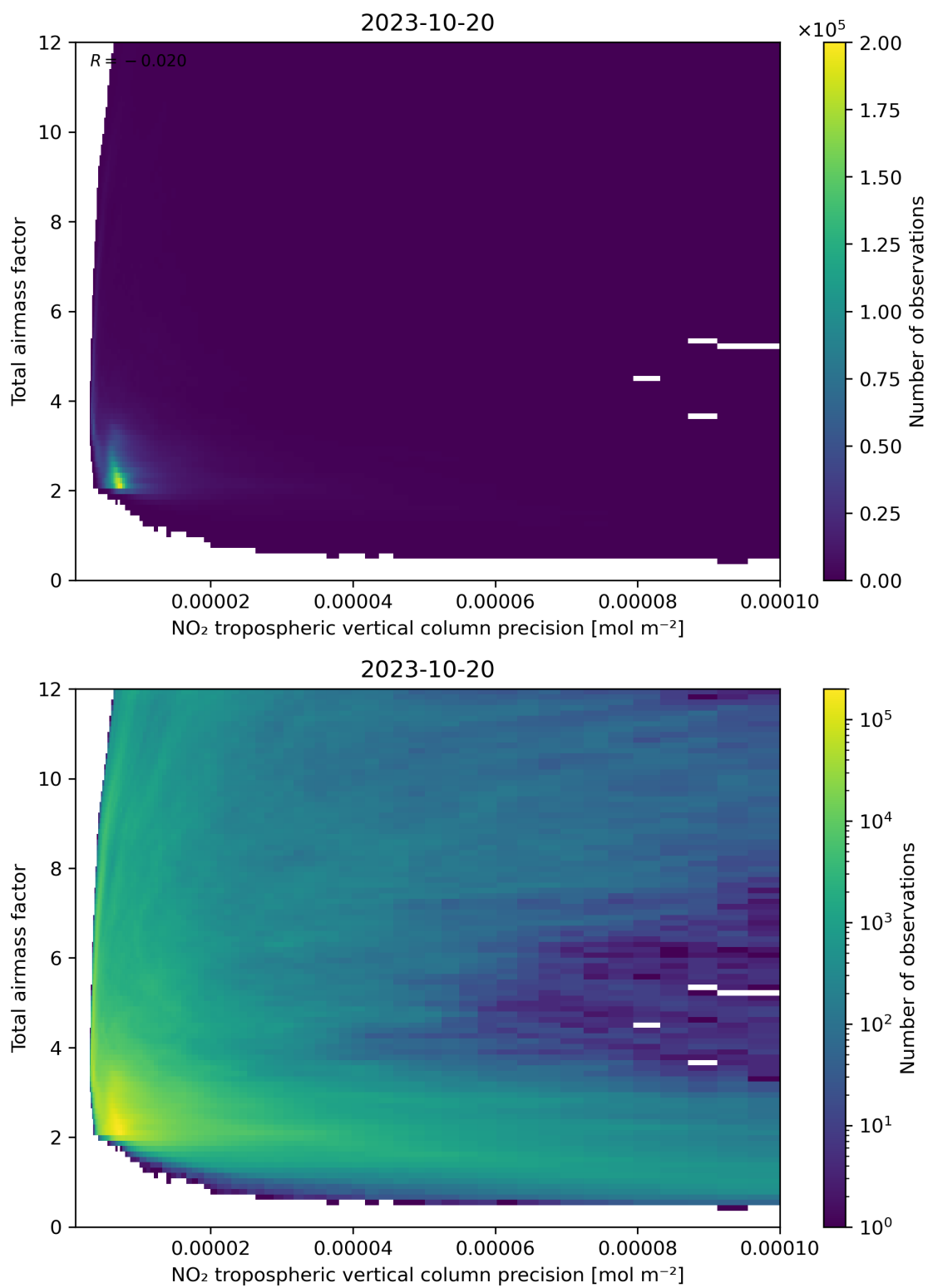
Figure 132: Scatter density plot of “NO 2 tropospheric vertical column precision” against “Total air mass factor” for 2023-10-19 to 2023-10-21.
