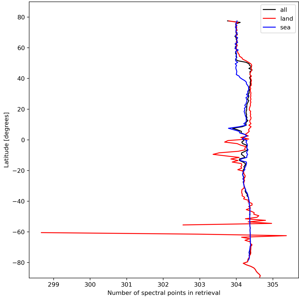
Figure 16: Zonal average of “Number of spectral points in retrieval” for 2023-10-19 to 2023-10-21.
