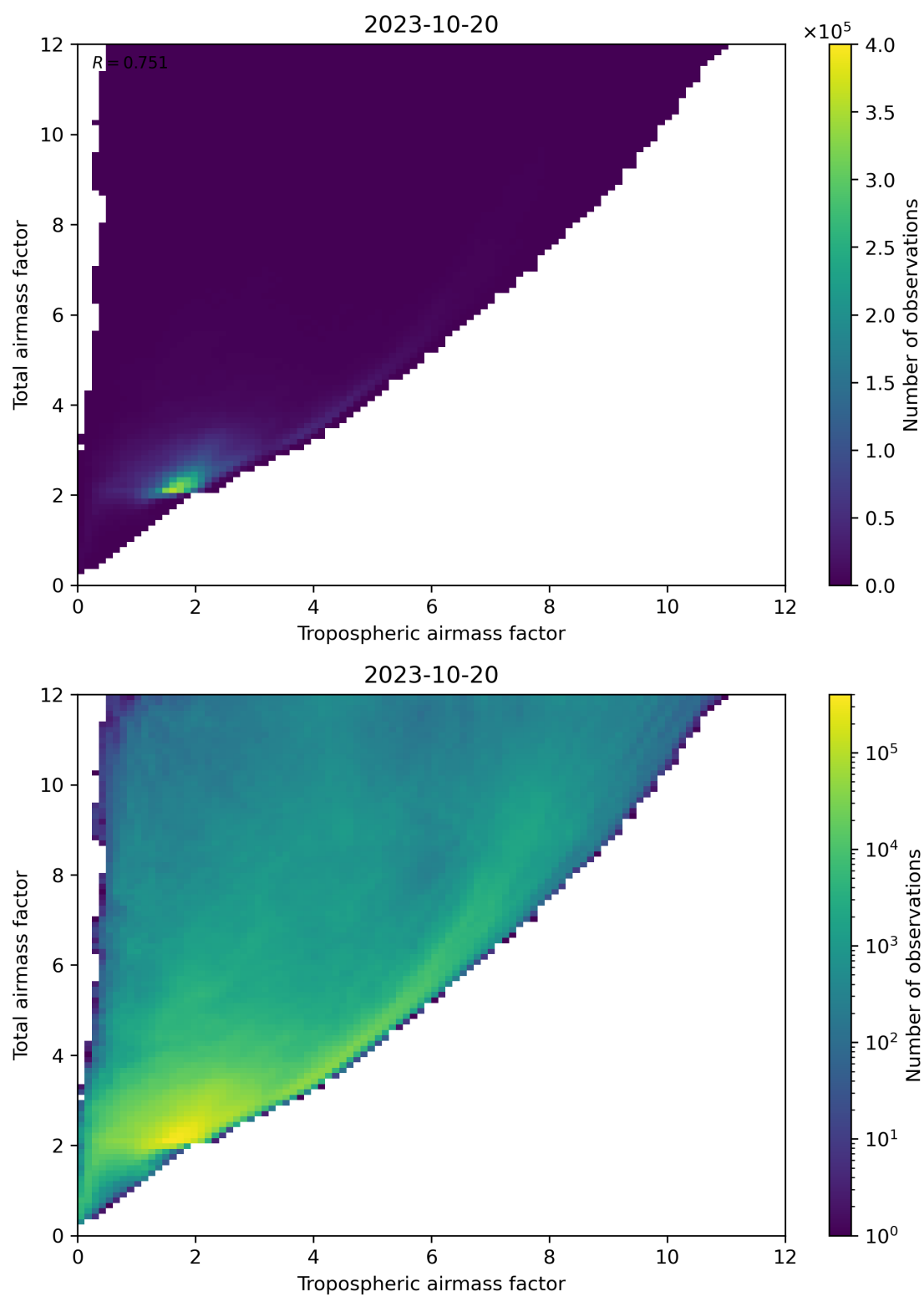
Figure 72: Scatter density plot of “Tropospheric airmass factor” against “Total airmass factor” for 2023-10-19 to 2023-10-21.
