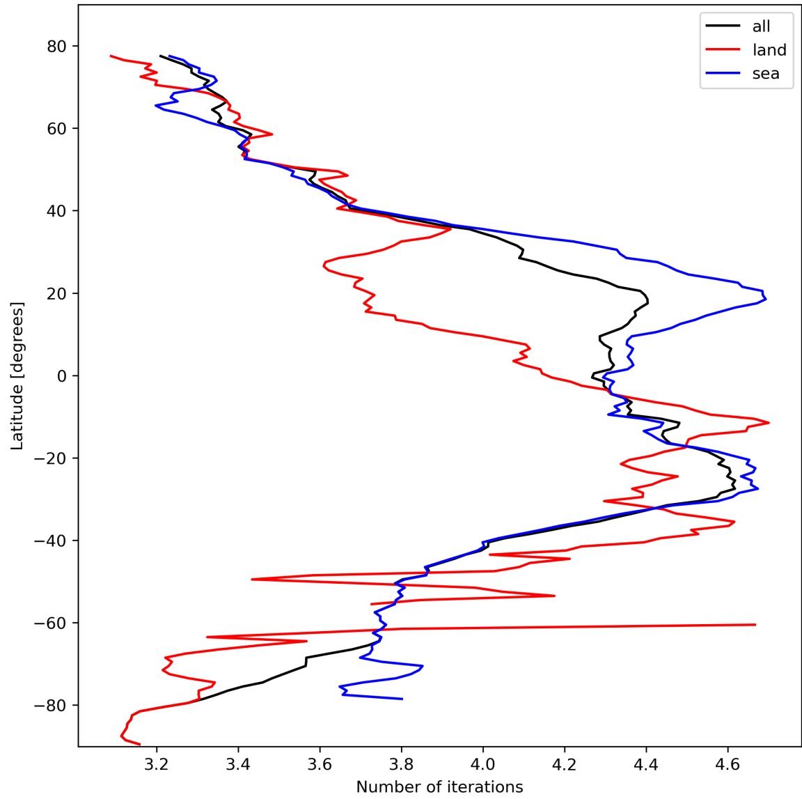
Figure 17: Zonal average of “Number of iterations” for 2023-10-19 to 2023-10-21.
