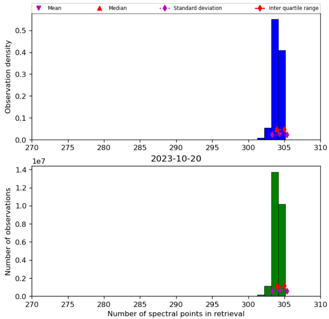
Figure 33: Histogram of “Number of spectral points in retrieval” for 2023-10-19 to 2023-10-21
