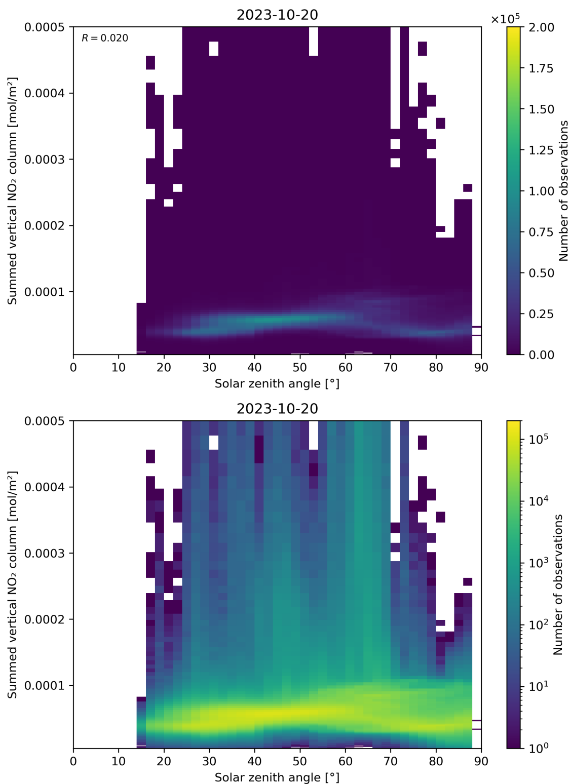
Figure 151: Scatter density plot of “Solar zenith angle” against “Summed vertical NO 2 column” for 2023-10-19 to 2023-10-21.
