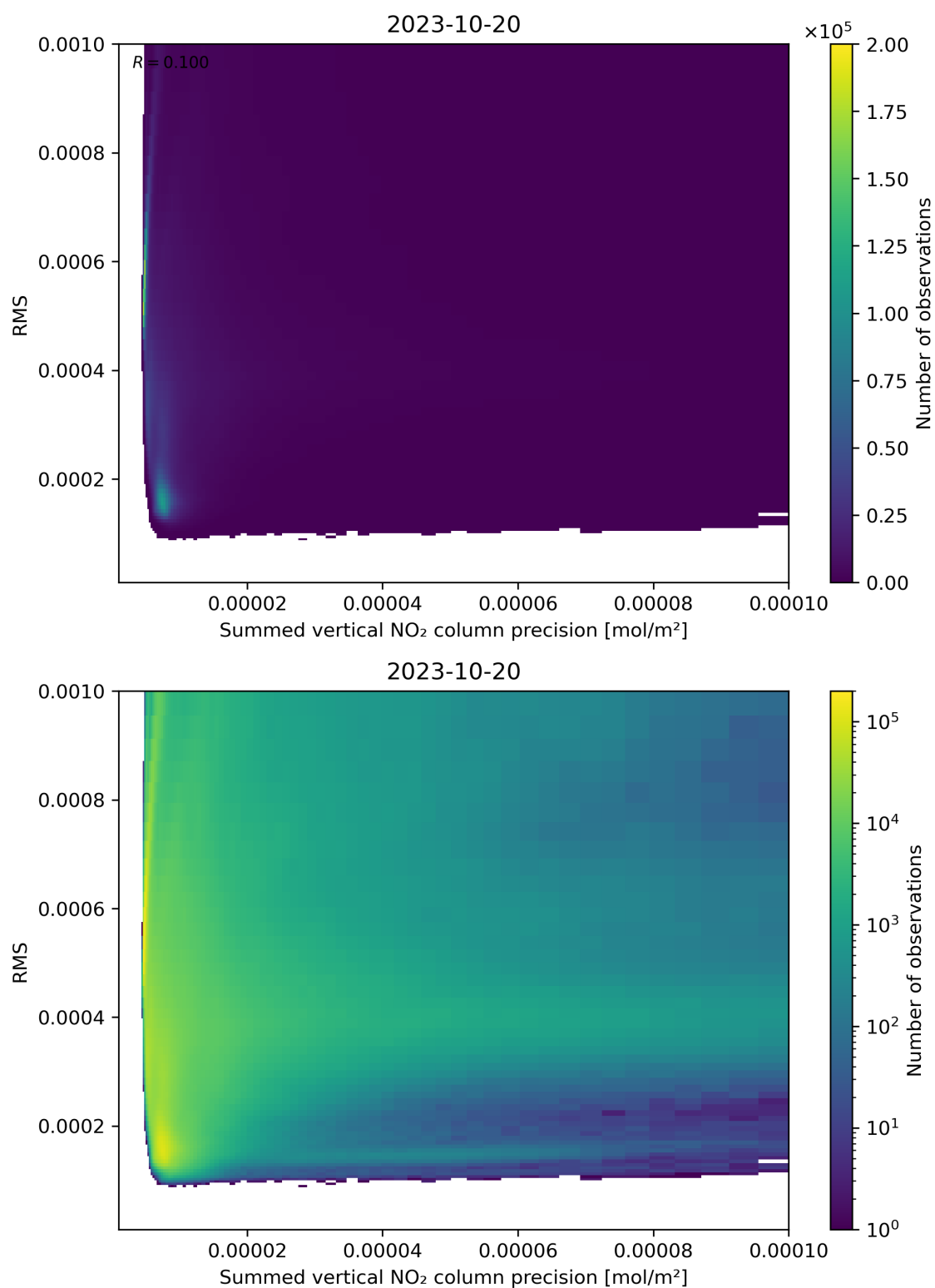
Figure 108: Scatter density plot of “Summed vertical NO 2 column precision” against “RMS” for 2023-10-19 to 2023-10-21.
