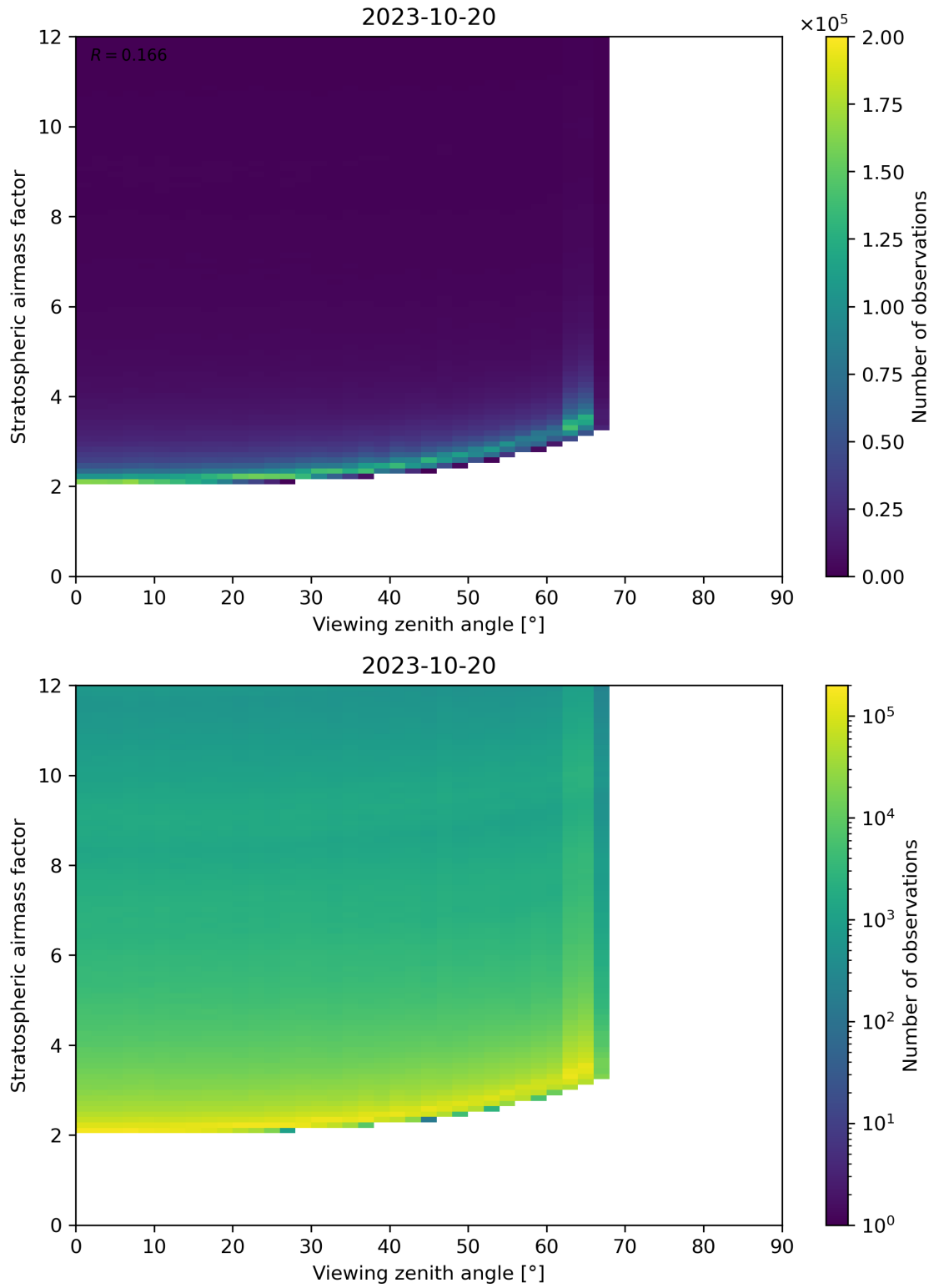
Figure 159: Scatter density plot of “Viewing zenith angle” against “Stratospheric airmass factor” for 2023-10-19 to 2023-10-21.
