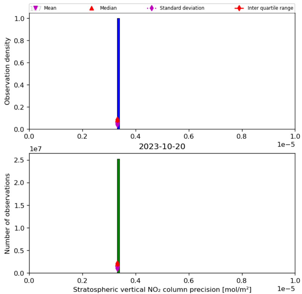
Figure 37: Histogram of “Stratospheric vertical NO 2 column precision” for 2023-10-19 to 2023-10-21
