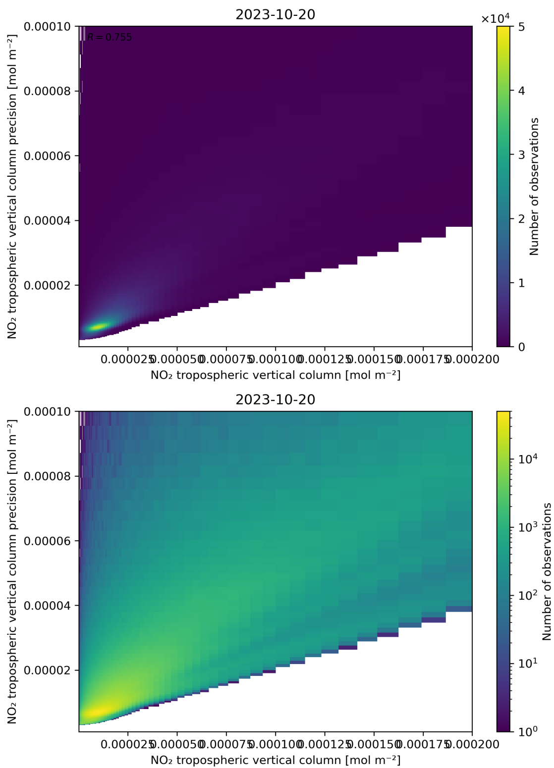
Figure 130: Scatter density plot of “NO 2 tropospheric vertical column” against “NO 2 tropospheric vertical column precision” for 2023-10-19 to 2023-10-21.
