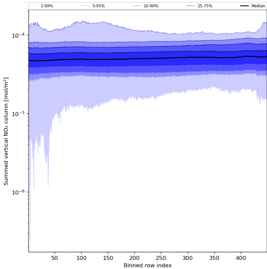
Figure 57: Along track statistics of “Summed vertical NO 2 column” for 2023-10-19 to 2023-10-21
