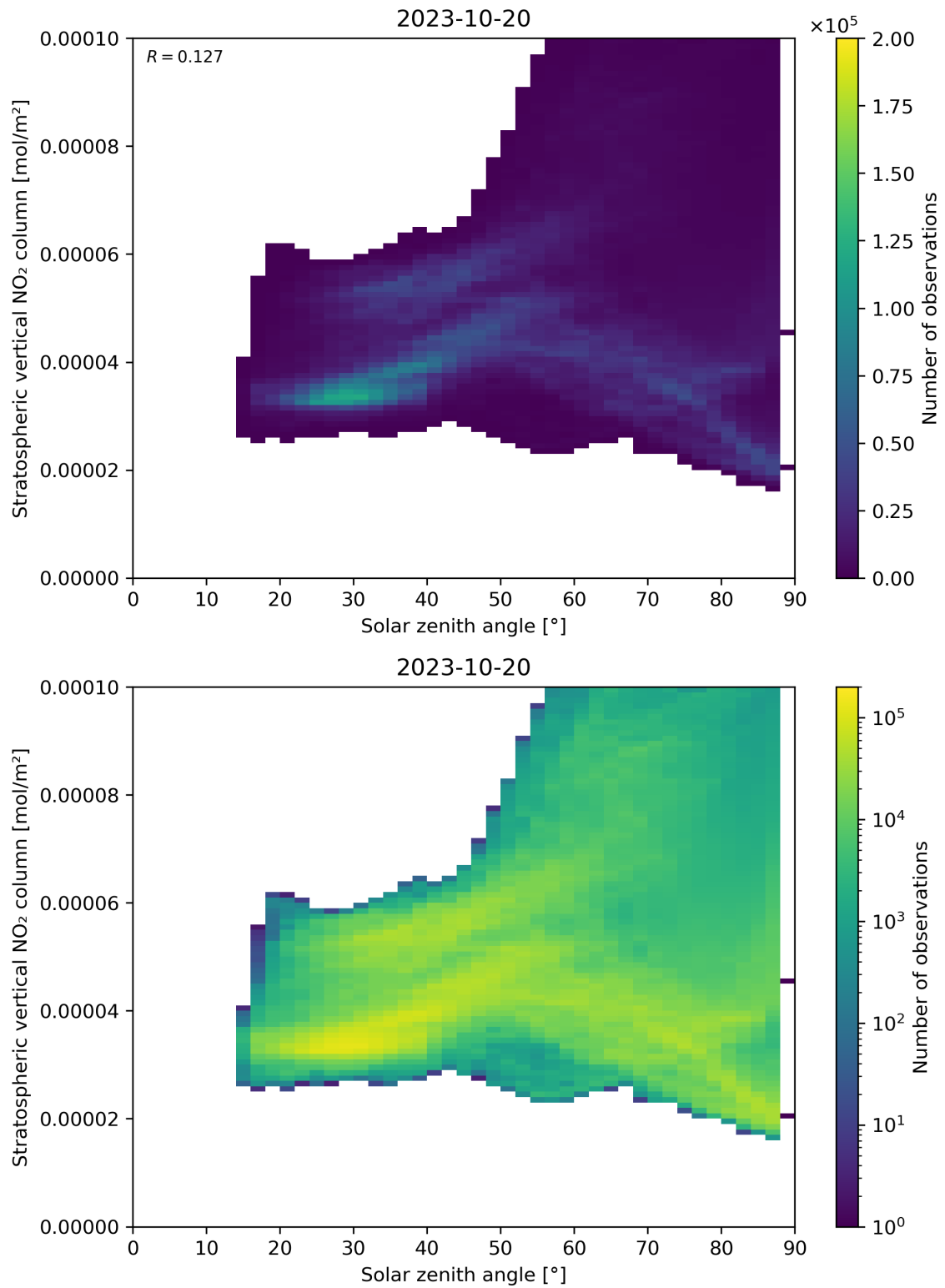
Figure 150: Scatter density plot of “Solar zenith angle” against “Stratospheric vertical \text{NO}_2 column” for 2023-10-19 to 2023-10-21.
