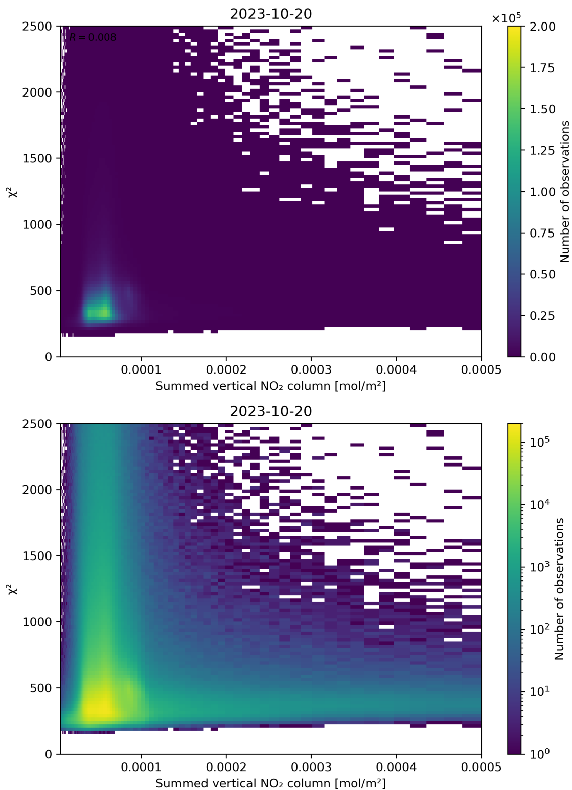
Figure 104: Scatter density plot of “Summed vertical NO 2 column” against “ \chi^2 ” for 2023-10-19 to 2023-10-21.
