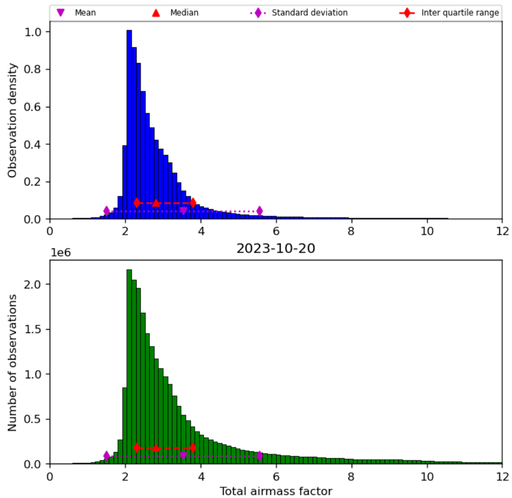
Figure 32: Histogram of “Total airmass factor” for 2023-10-19 to 2023-10-21
