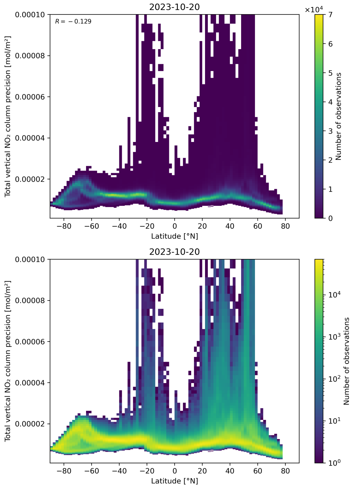
Figure 91: Scatter density plot of “Latitude” against “Total vertical NO 2 column precision” for 2023-10-19 to 2023-10-21.
