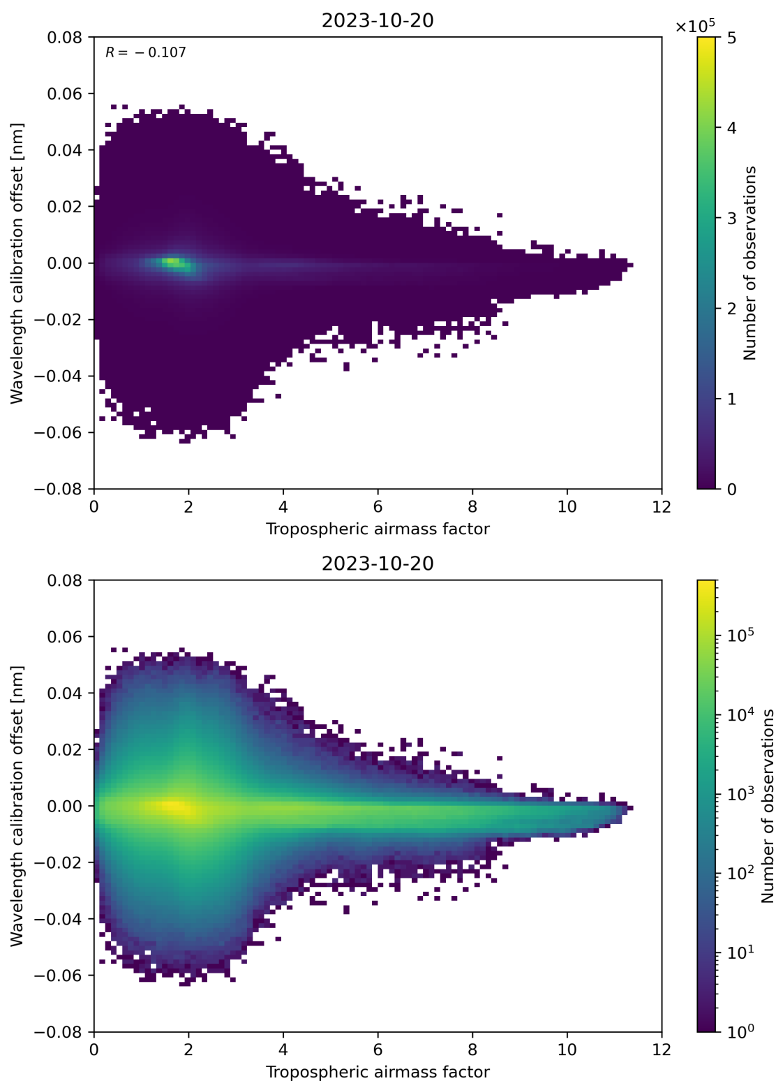
Figure 80: Scatter density plot of “Tropospheric air mass factor” against “Wavelength calibration offset” for 2023-10-19 to 2023-10-21.
