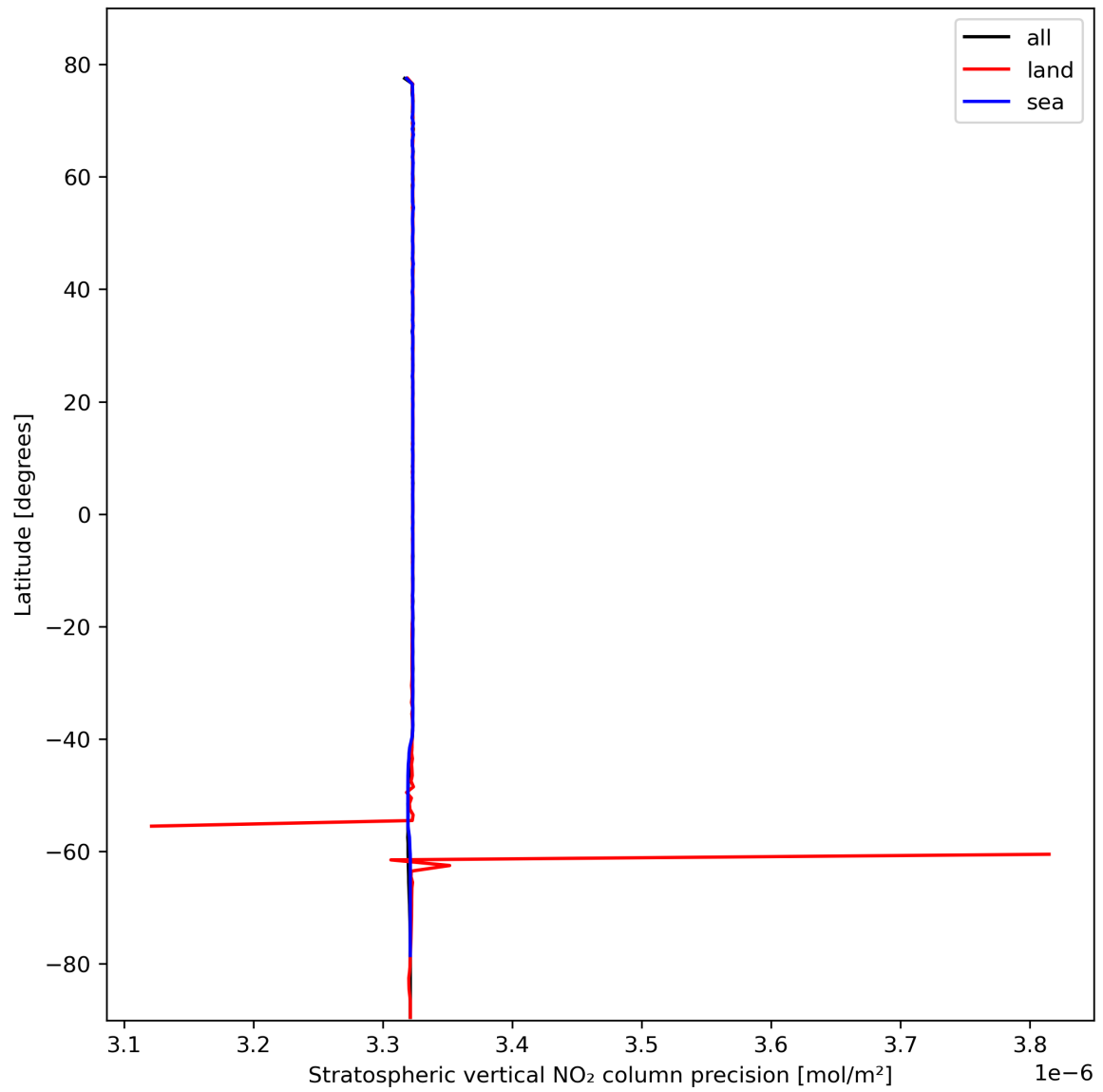
Figure 20: Zonal average of “Stratospheric vertical NO 2 column precision” for 2023-10-19 to 2023-10-21.
