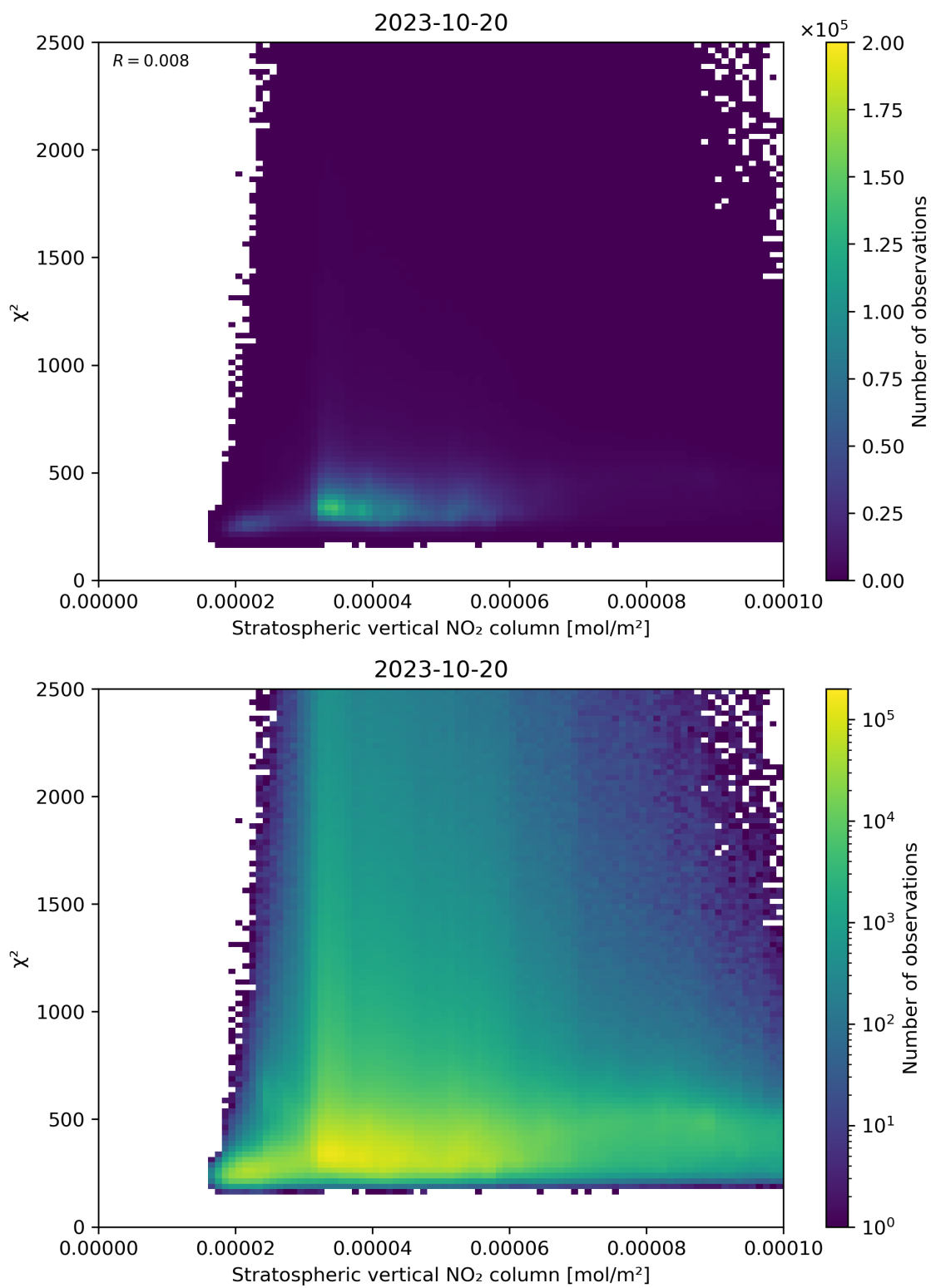
Figure 97: Scatter density plot of “Stratospheric vertical NO 2 column” against “ \chi^2 ” for 2023-10-19 to 2023-10-21.
