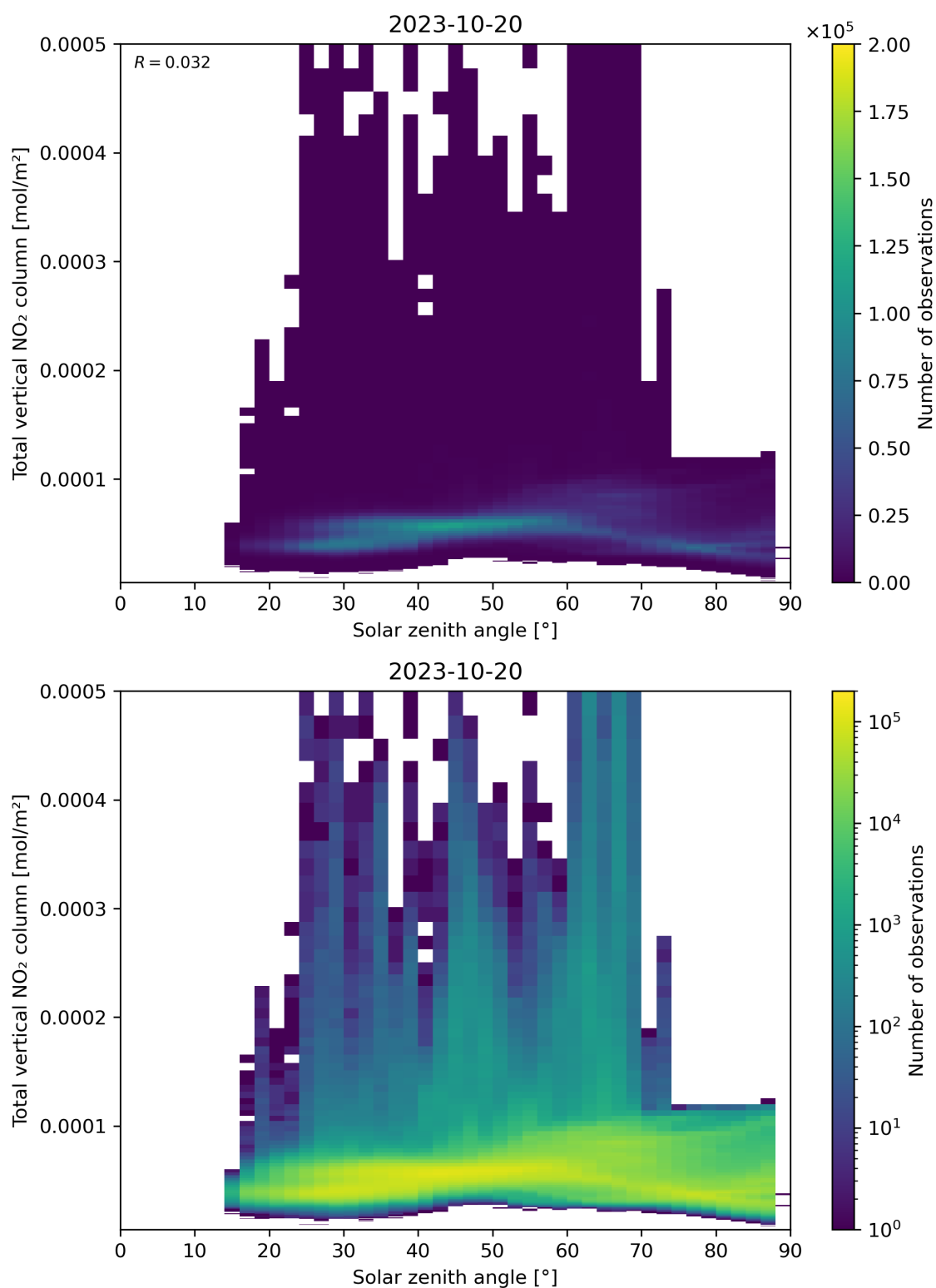
Figure 153: Scatter density plot of “Solar zenith angle” against “Total vertical NO 2 column” for 2023-10-19 to 2023-10-21.
