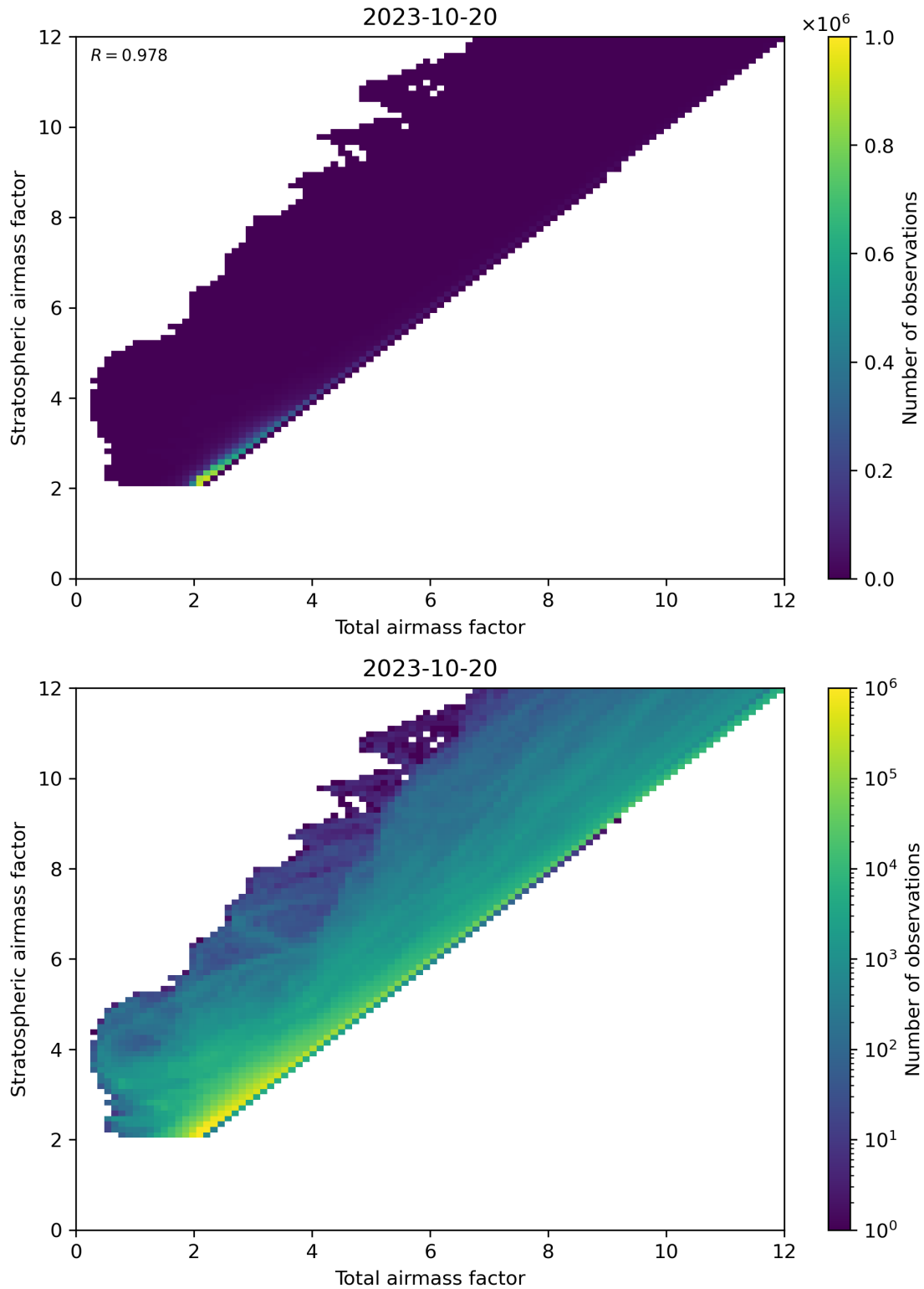
Figure 62: Scatter density plot of “Total airmass factor” against “Stratospheric airmass factor” for 2023-10-19 to 2023-10-21.
