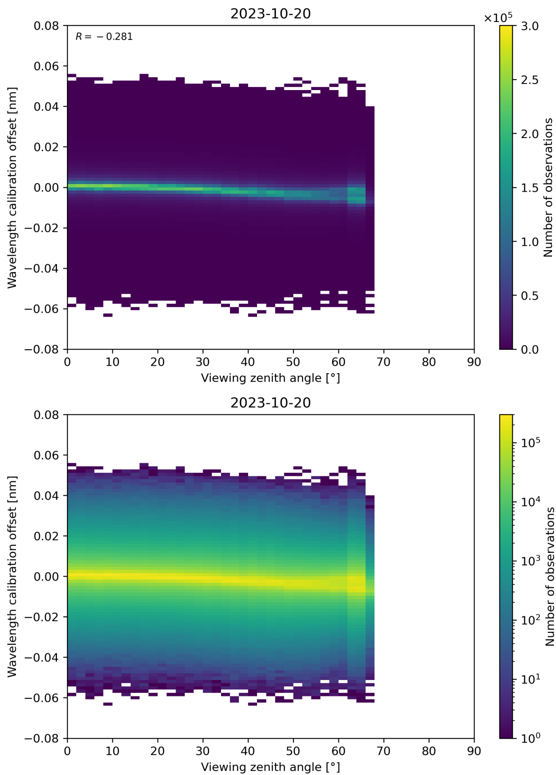
Figure 173: Scatter density plot of “Viewing zenith angle” against “Wavelength calibration offset” for 2023-10-19 to 2023-10-21.
