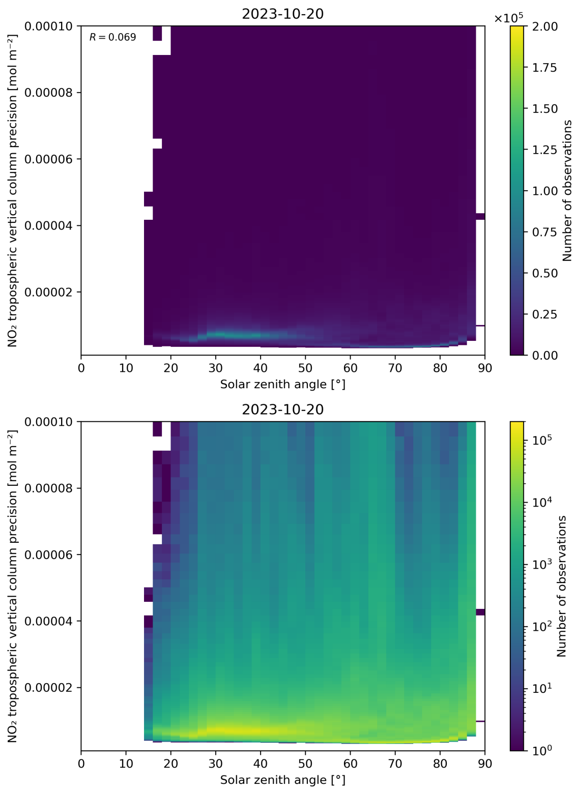
Figure 156: Scatter density plot of “Solar zenith angle” against “NO 2 tropospheric vertical column precision” for 2023-10-19 to 2023-10-21.
