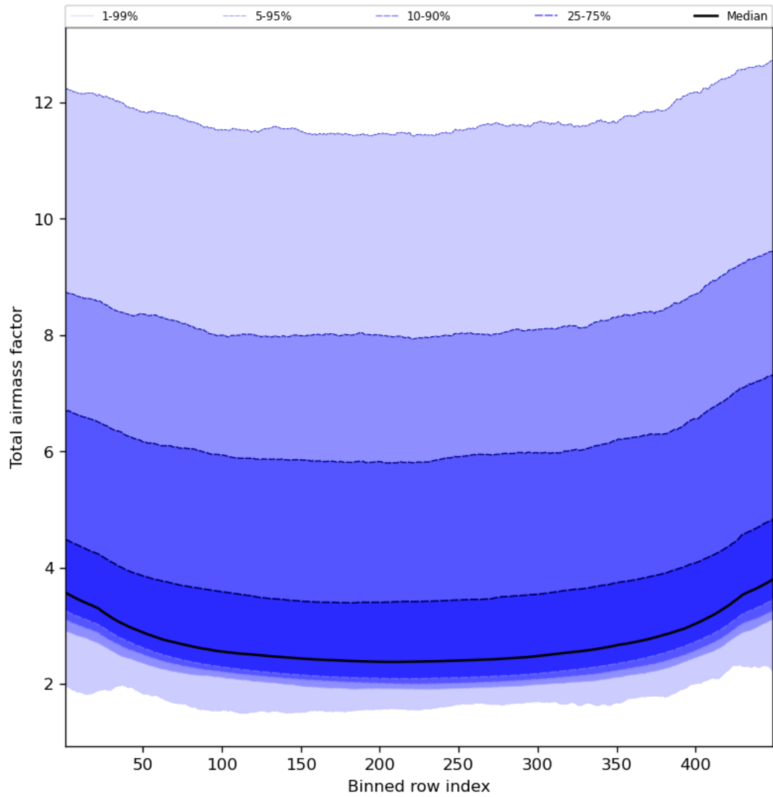
Figure 49: Along track statistics of “Total airmass factor” for 2023-10-19 to 2023-10-21
