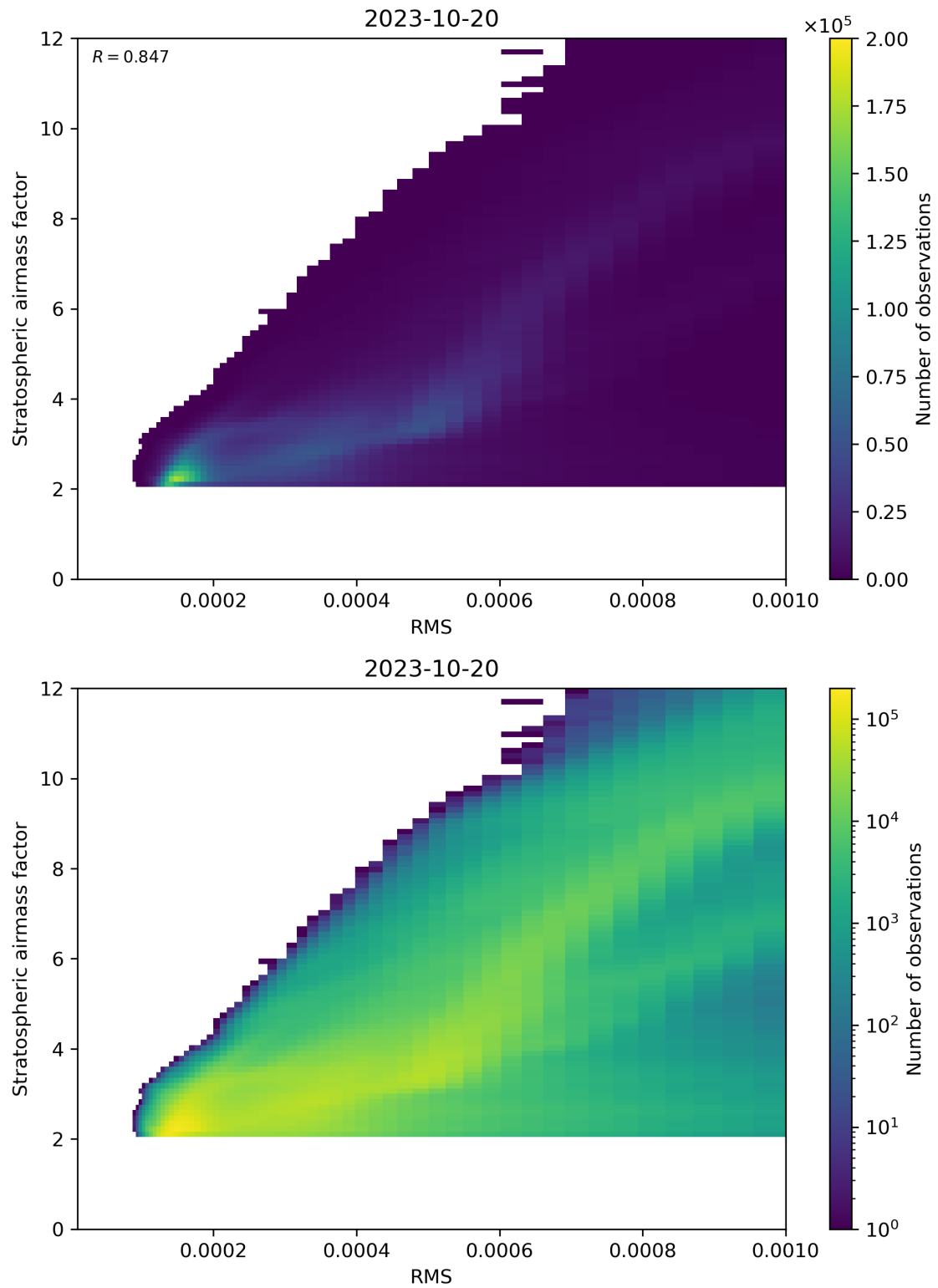
Figure 144: Scatter density plot of “RMS” against “Stratospheric airmass factor” for 2023-10-19 to 2023-10-21.
