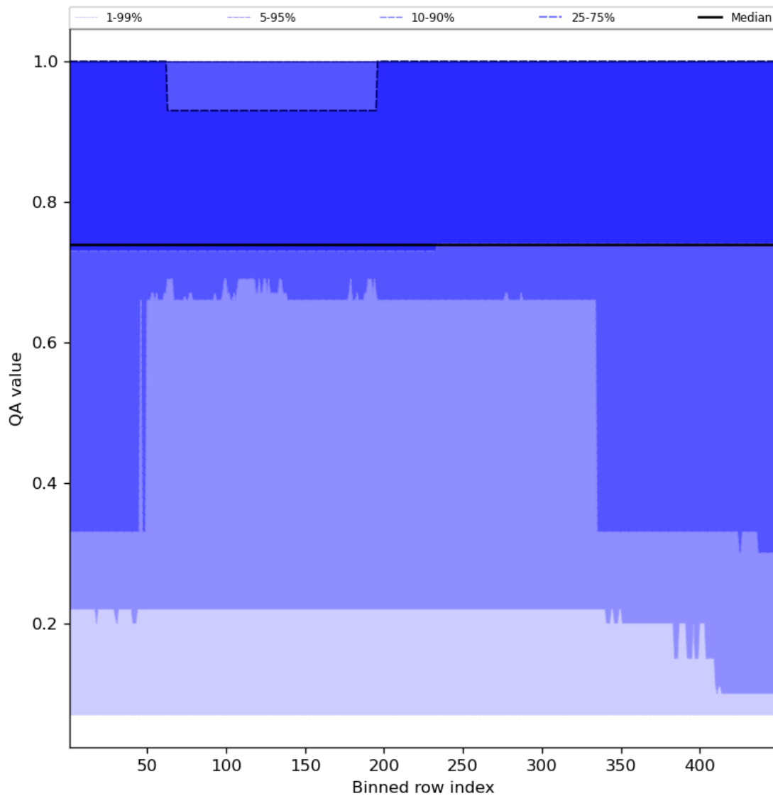
Figure 45: Along track statistics of “QA value” for 2023-10-19 to 2023-10-21
