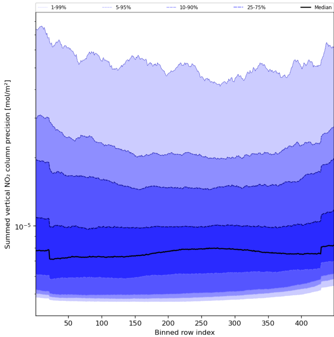
Figure 58: Along track statistics of “Summed vertical NO 2 column precision” for 2023-10-19 to 2023-10-21
