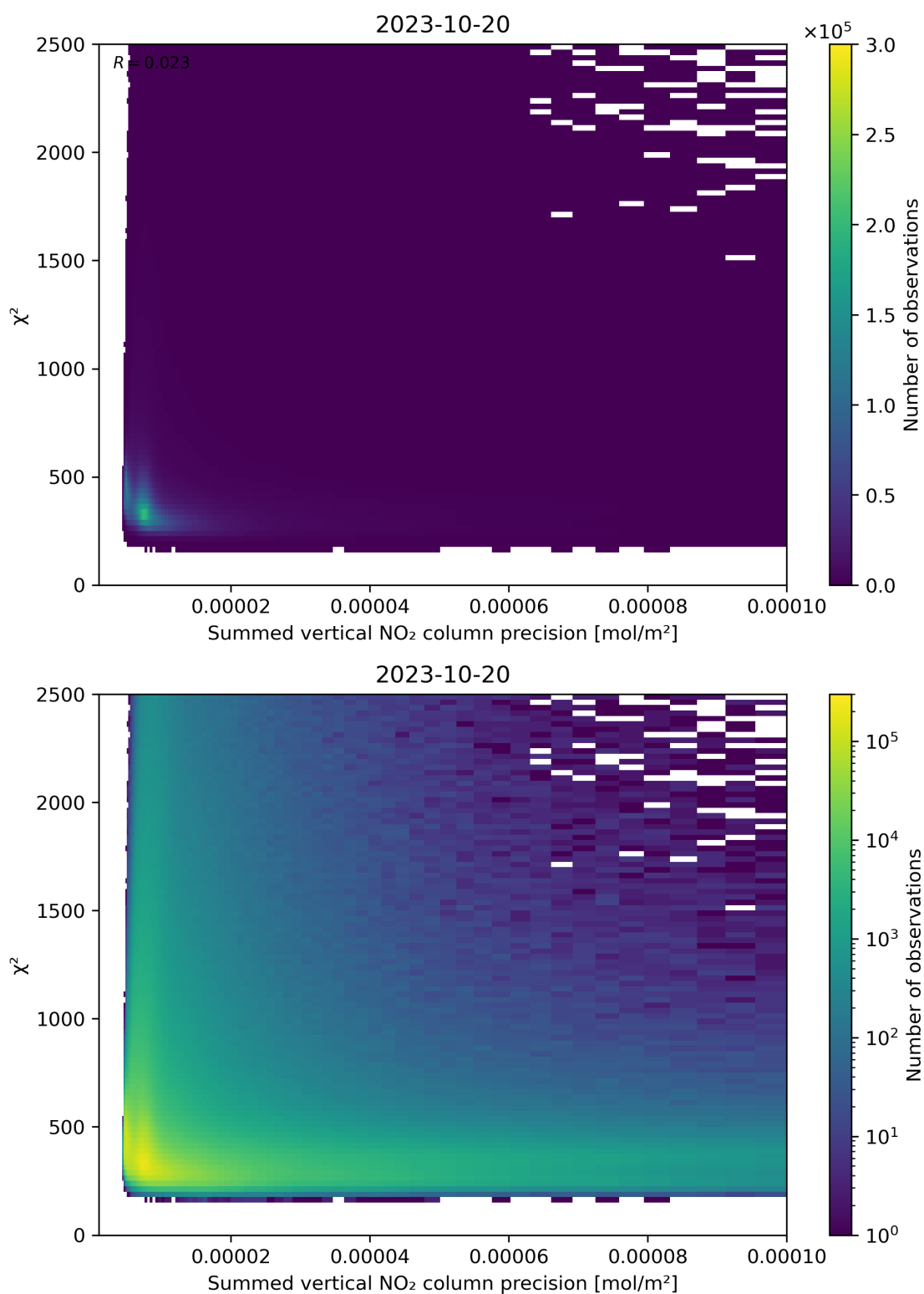
Figure 107: Scatter density plot of “Summed vertical NO 2 column precision” against “ \chi^2 ” for 2023-10-19 to 2023-10-21.
