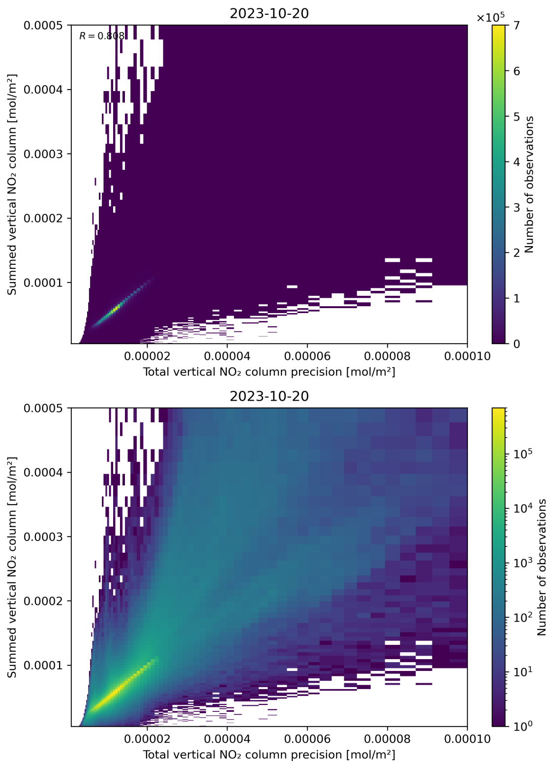
Figure 117: Scatter density plot of “Total vertical NO 2 column precision” against “Summed vertical NO 2 column” for 2023-10-19 to 2023-10-21.
