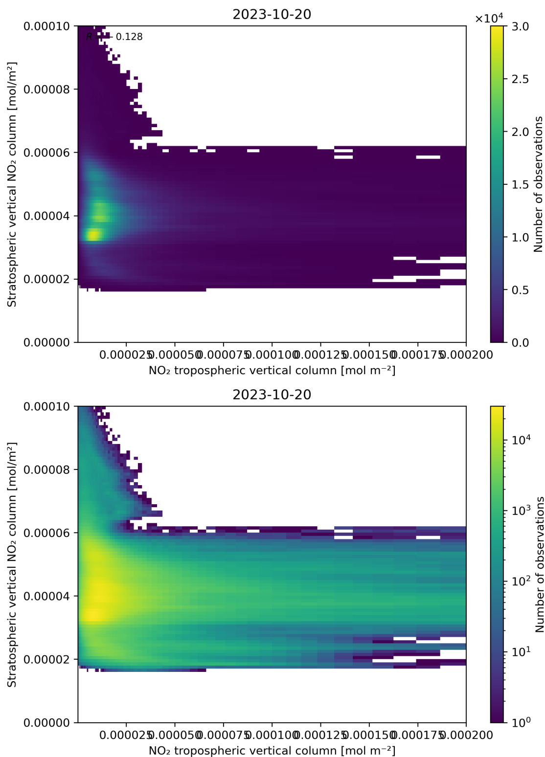
Figure 125: Scatter density plot of “NO 2 tropospheric vertical column” against “Stratospheric vertical NO 2 column” for 2023-10-19 to 2023-10-21.
