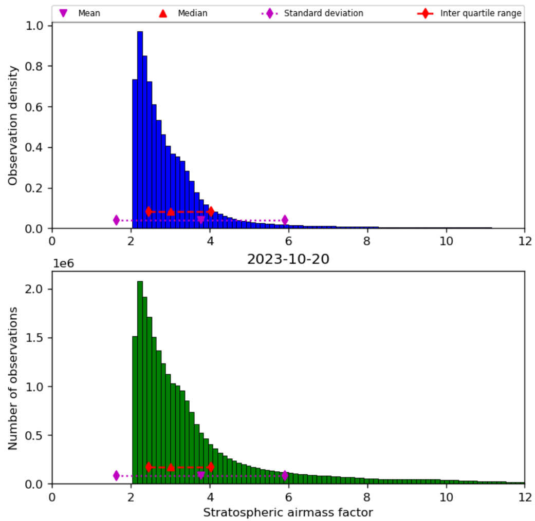
Figure 44: Histogram of “Stratospheric airmass factor” for 2023-10-19 to 2023-10-21
