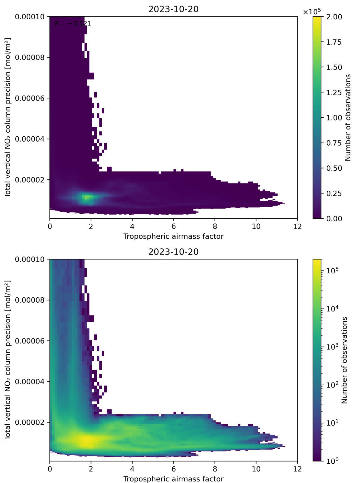
Figure 78: Scatter density plot of “Tropospheric air mass factor” against “Total vertical NO 2 column precision” for 2023-10-19 to 2023-10-21.
