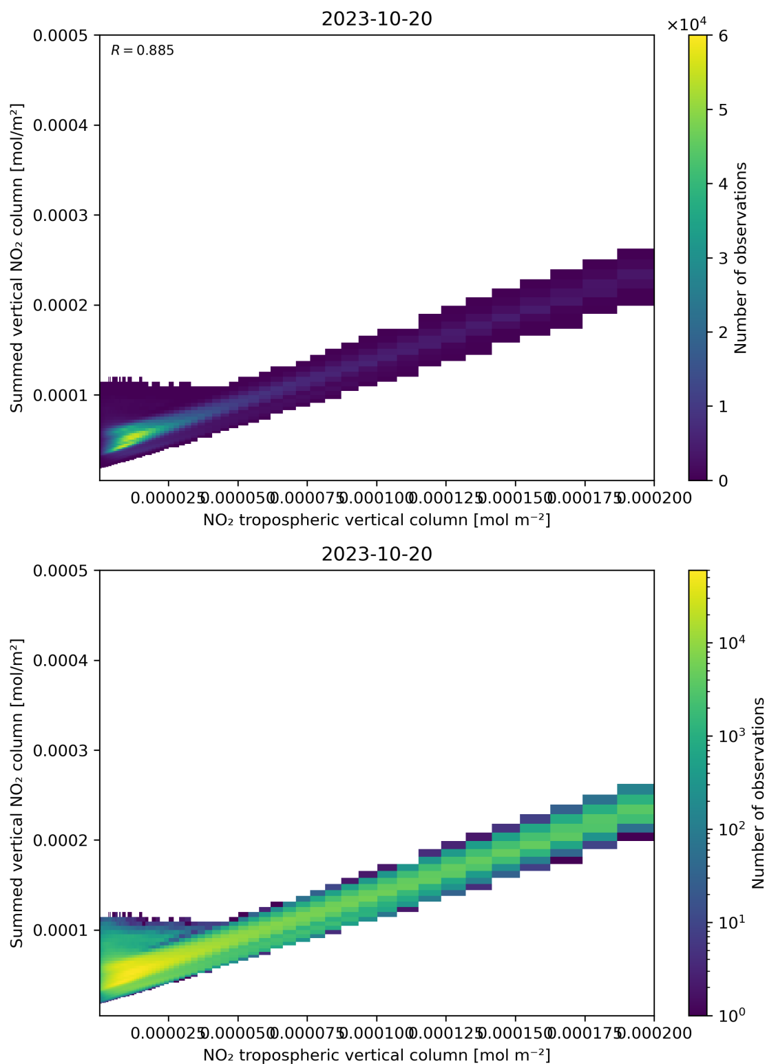
Figure 126: Scatter density plot of “NO 2 tropospheric vertical column” against “Summed vertical NO 2 column” for 2023-10-19 to 2023-10-21.
