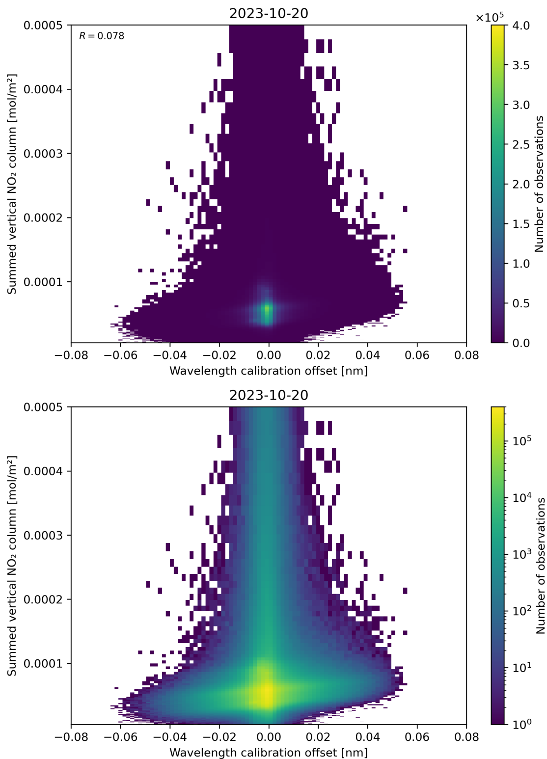
Figure 177: Scatter density plot of “Wavelength calibration offset” against “Summed vertical NO 2 column” for 2023-10-19 to 2023-10-21.
