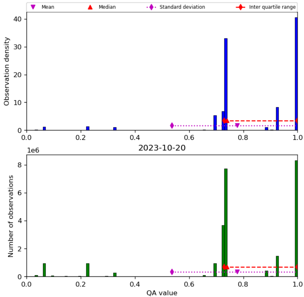
Figure 28: Histogram of “QA value” for 2023-10-19 to 2023-10-21
