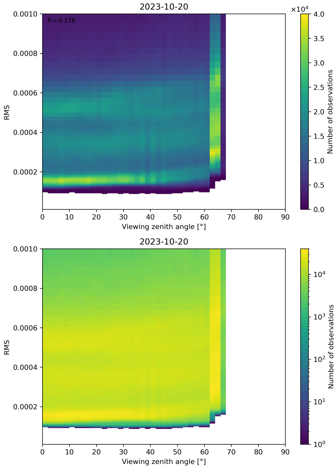
Figure 171: Scatter density plot of “Viewing zenith angle” against “RMS” for 2023-10-19 to 2023-10-21.
