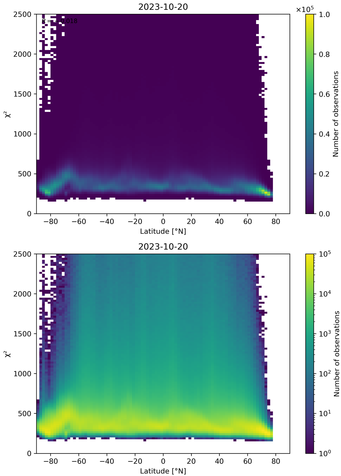
Figure 86: Scatter density plot of “Latitude” against “ \chi^2 ” for 2023-10-19 to 2023-10-21.
