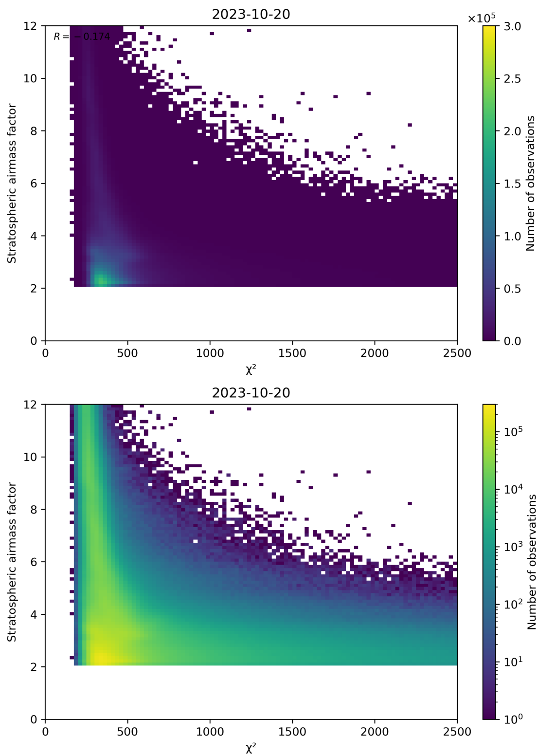
Figure 81: Scatter density plot of “ \chi^2 ” against “Stratospheric airmass factor” for 2023-10-19 to 2023-10-21.
