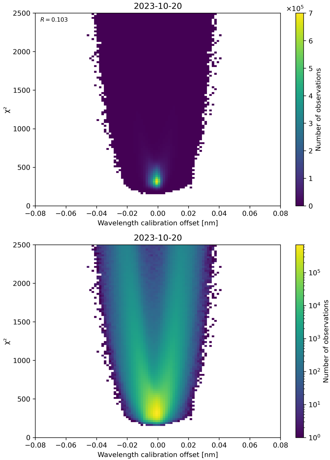
Figure 175: Scatter density plot of “Wavelength calibration offset” against “ \chi^2 ” for 2023-10-19 to 2023-10-21.
