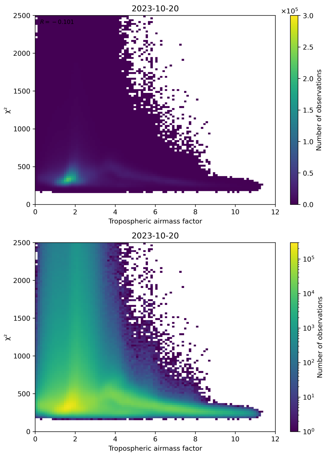
Figure 73: Scatter density plot of “Tropospheric airmass factor” against “ \chi^2 ” for 2023-10-19 to 2023-10-21.
