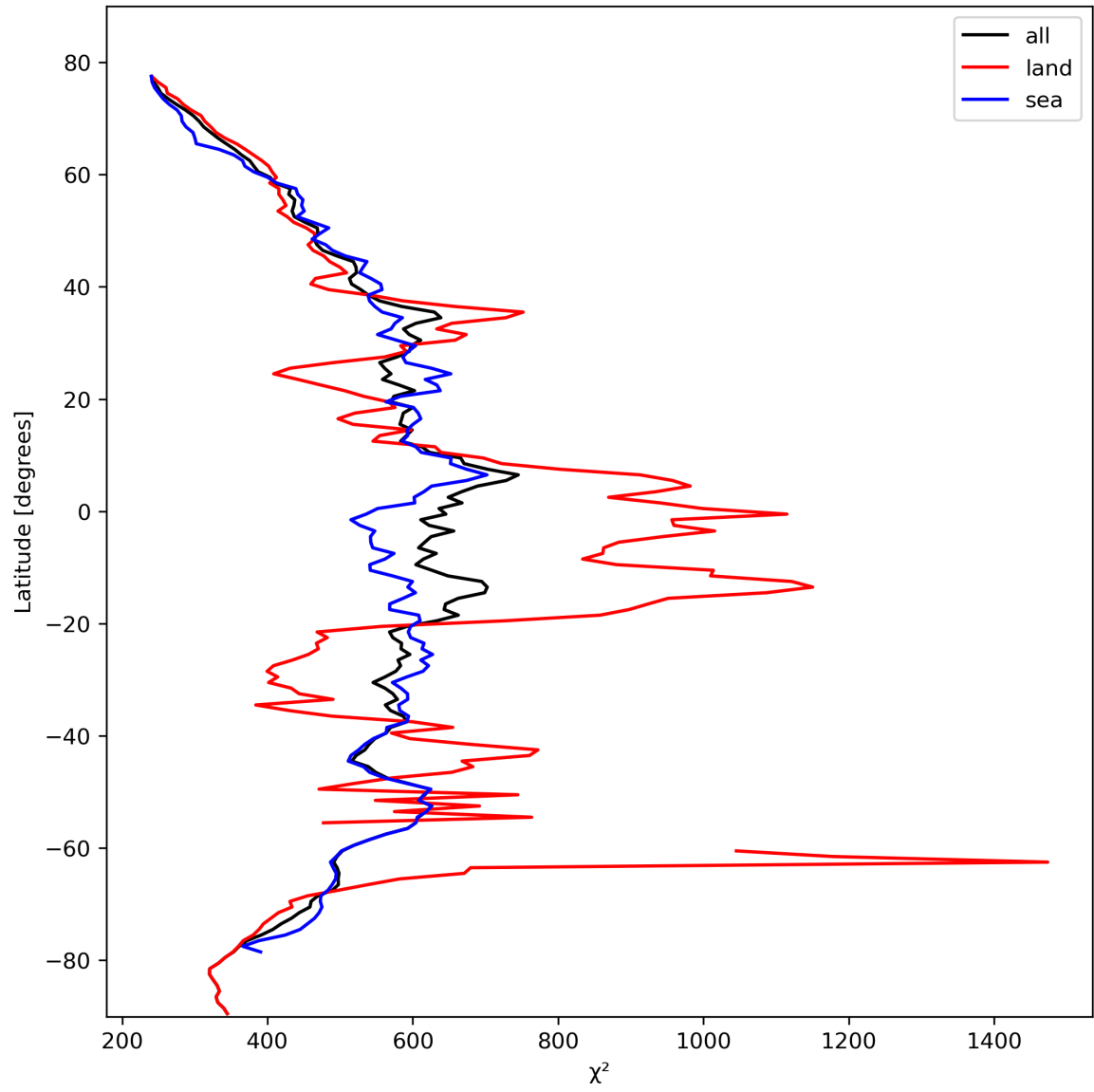
Figure 25: Zonal average of “ \chi^2 ” for 2023-10-19 to 2023-10-21.
