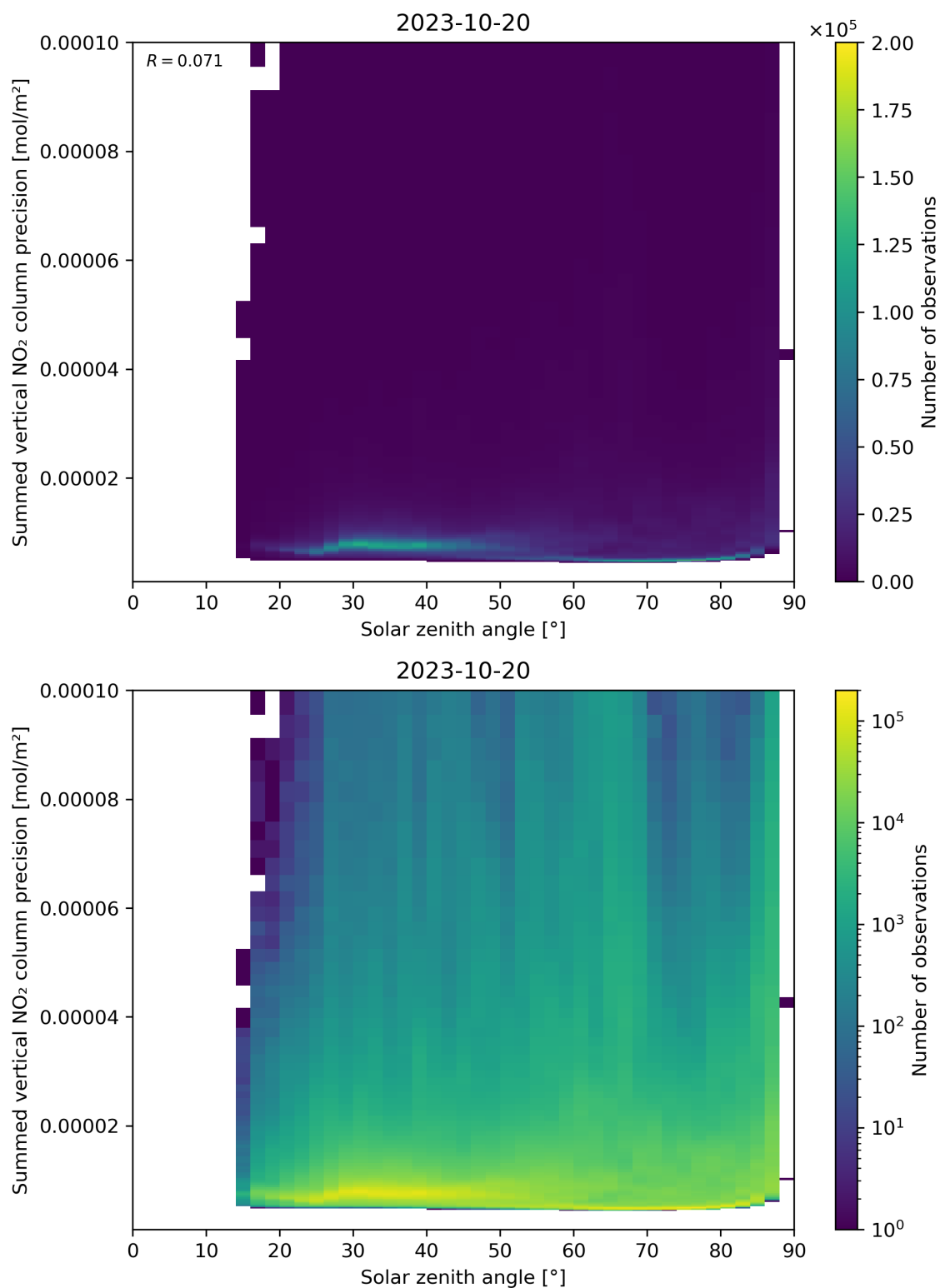
Figure 152: Scatter density plot of “Solar zenith angle” against “Summed vertical NO 2 column precision” for 2023-10-19 to 2023-10-21.
