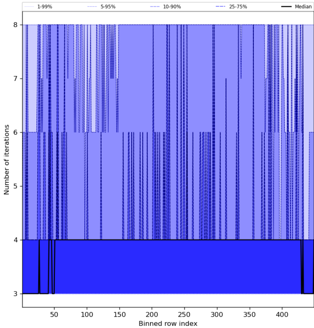
Figure 51: Along track statistics of “Number of iterations” for 2023-10-19 to 2023-10-21
