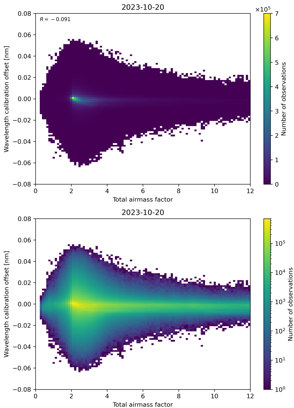
Figure 70: Scatter density plot of “Total airmass factor” against “Wavelength calibration offset” for 2023-10-19 to 2023-10-21.
