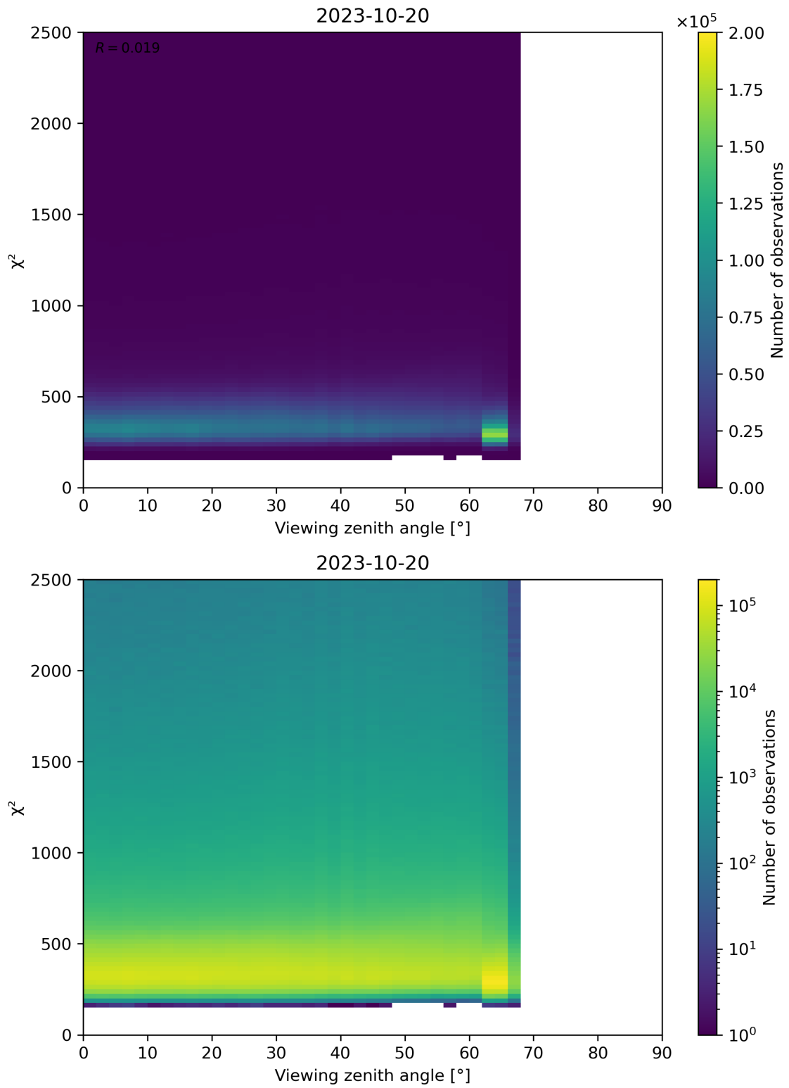
Figure 162: Scatter density plot of “Viewing zenith angle” against “ \chi^2 ” for 2023-10-19 to 2023-10-21.
