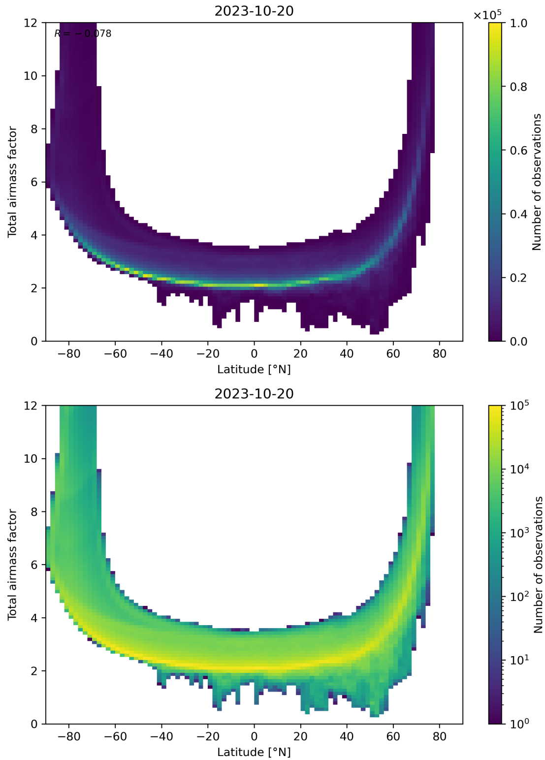
Figure 84: Scatter density plot of “Latitude” against “Total airmass factor” for 2023-10-19 to 2023-10-21.
