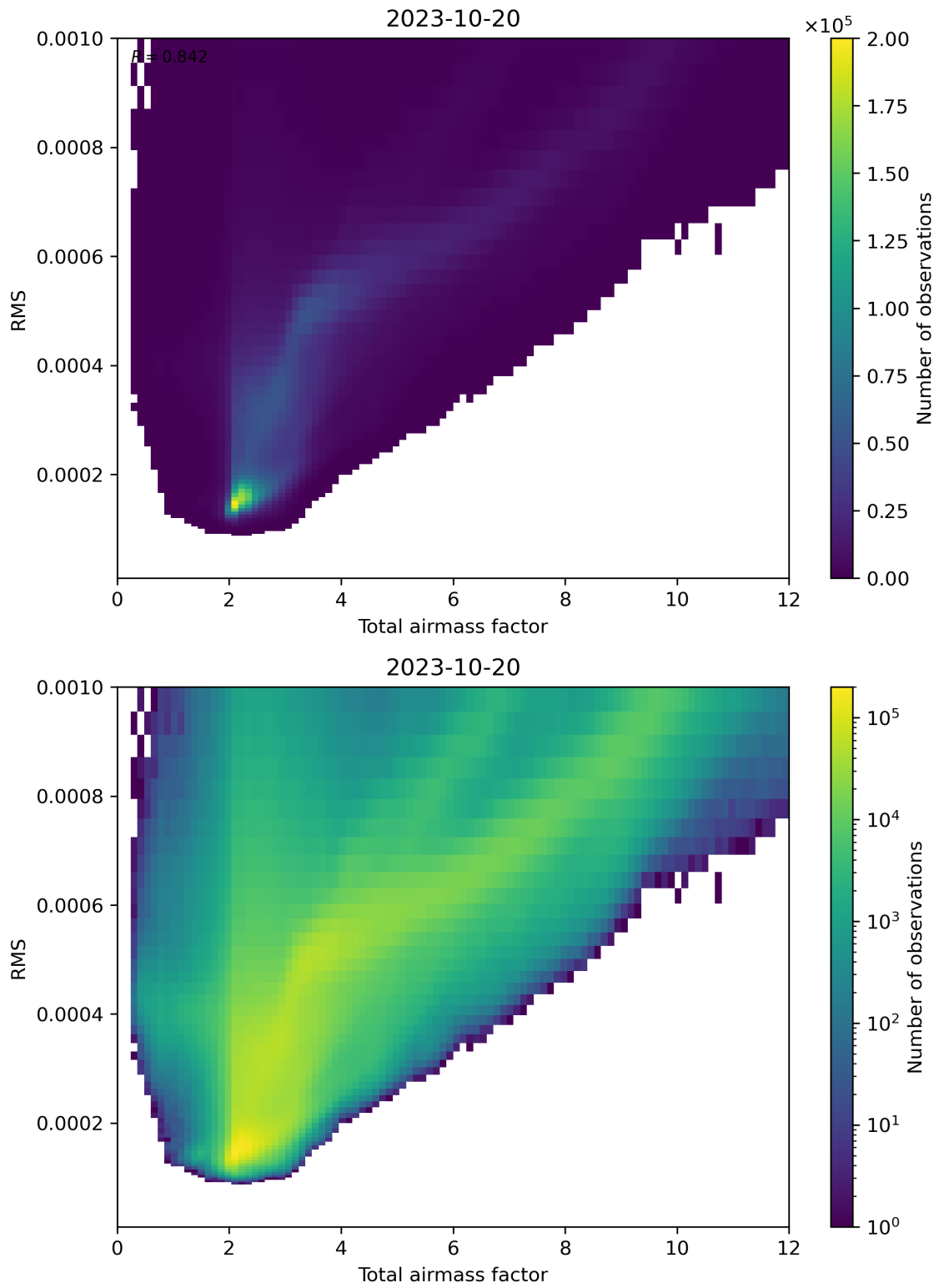
Figure 69: Scatter density plot of “Total airmass factor” against “RMS” for 2023-10-19 to 2023-10-21.
