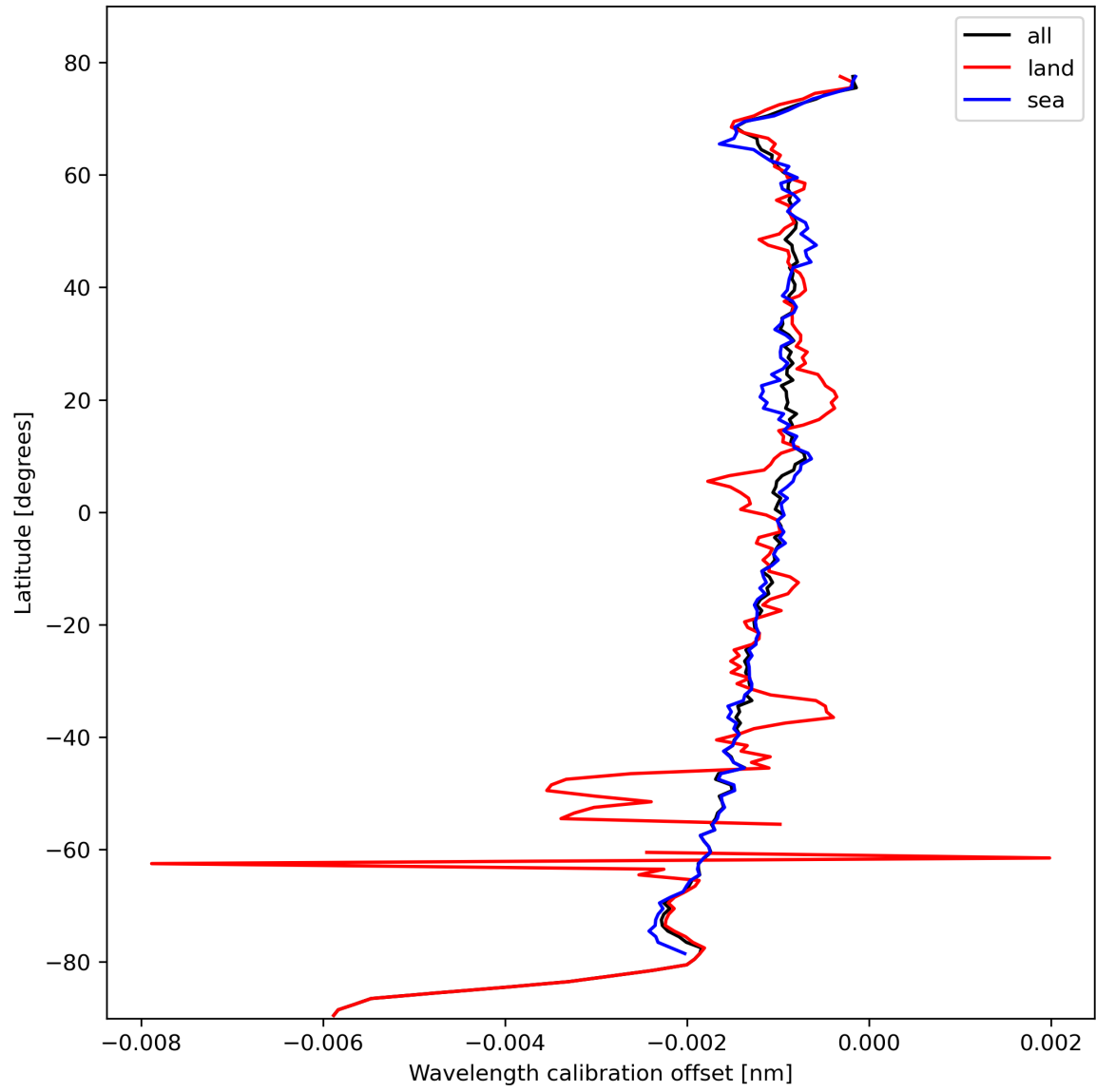
Figure 18: Zonal average of “Wavelength calibration offset” for 2023-10-19 to 2023-10-21.
