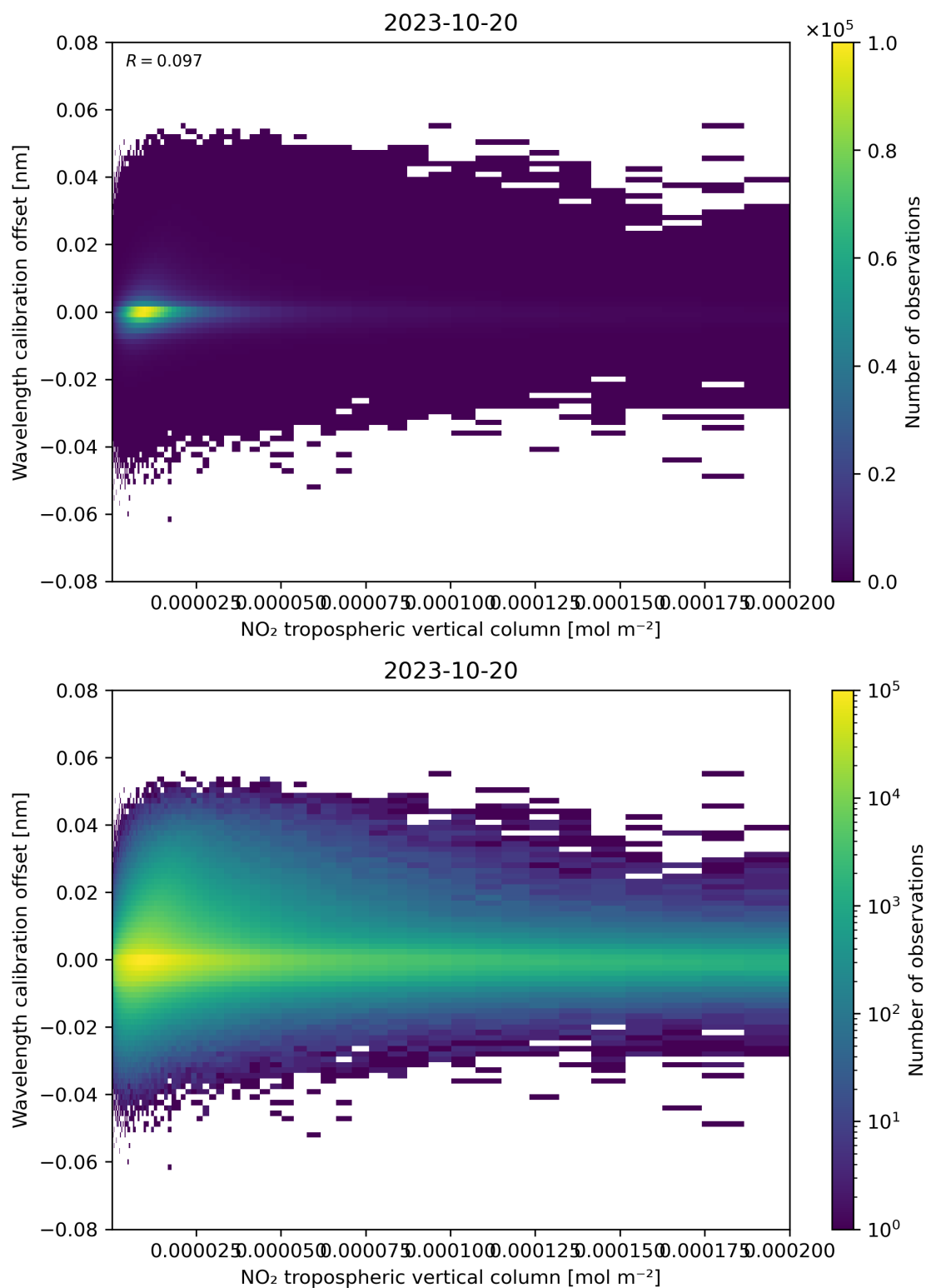
Figure 143: Scatter density plot of “NO 2 tropospheric vertical column” against “Wavelength calibration offset” for 2023-10-19 to 2023-10-21.
