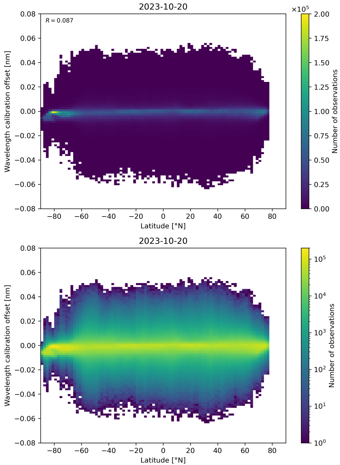
Figure 95: Scatter density plot of “Latitude” against “Wavelength calibration offset” for 2023-10-19 to 2023-10-21.
