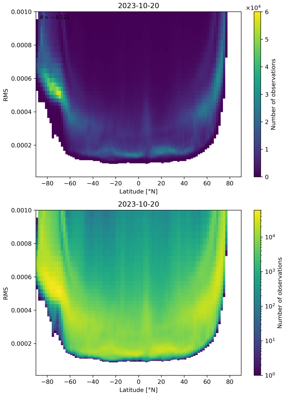
Figure 94: Scatter density plot of “Latitude” against “RMS” for 2023-10-19 to 2023-10-21.
