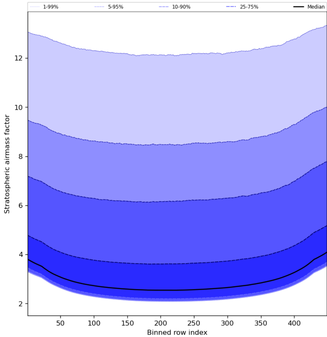
Figure 61: Along track statistics of “Stratospheric air mass factor” for 2023-10-19 to 2023-10-21
