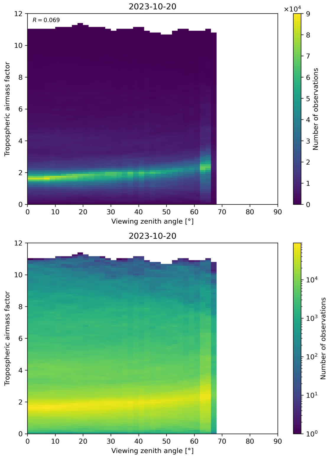
Figure 161: Scatter density plot of “Viewing zenith angle” against “Tropospheric airmass factor” for 2023-10-19 to 2023-10-21.
