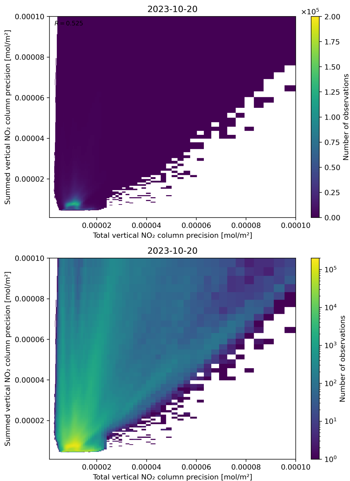
Figure 118: Scatter density plot of “Total vertical NO 2 column precision” against “Summed vertical NO 2 column precision” for 2023-10-19 to 2023-10-21.
