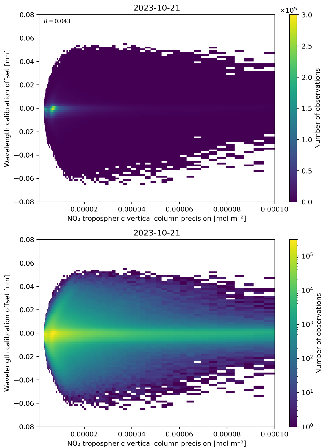
Figure 141: Scatter density plot of “NO 2 tropospheric vertical column precision” against “Wavelength calibration offset” for 2023-10-20 to 2023-10-22.
