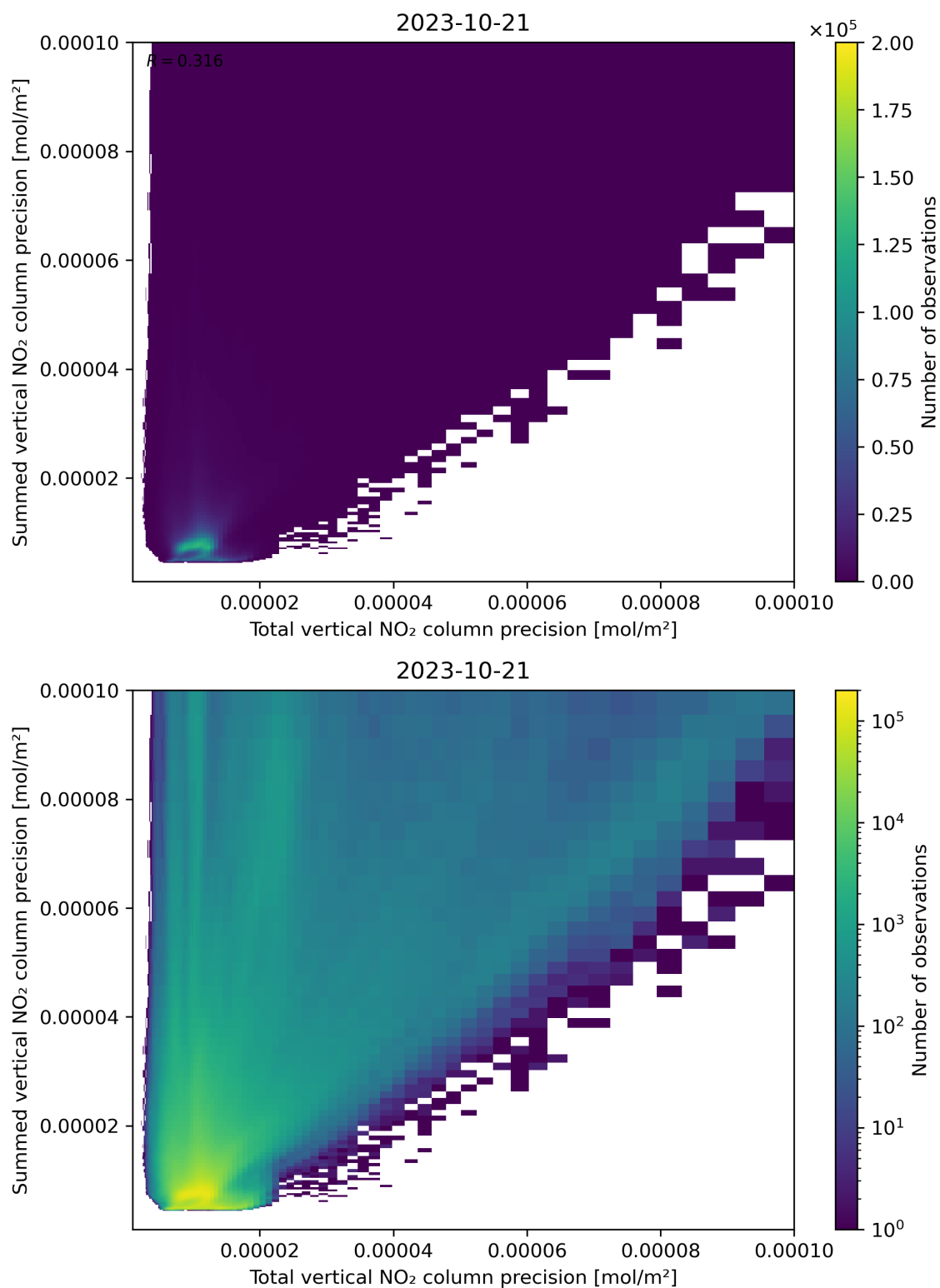
Figure 118: Scatter density plot of “Total vertical NO 2 column precision” against “Summed vertical NO 2 column precision” for 2023-10-20 to 2023-10-22.
