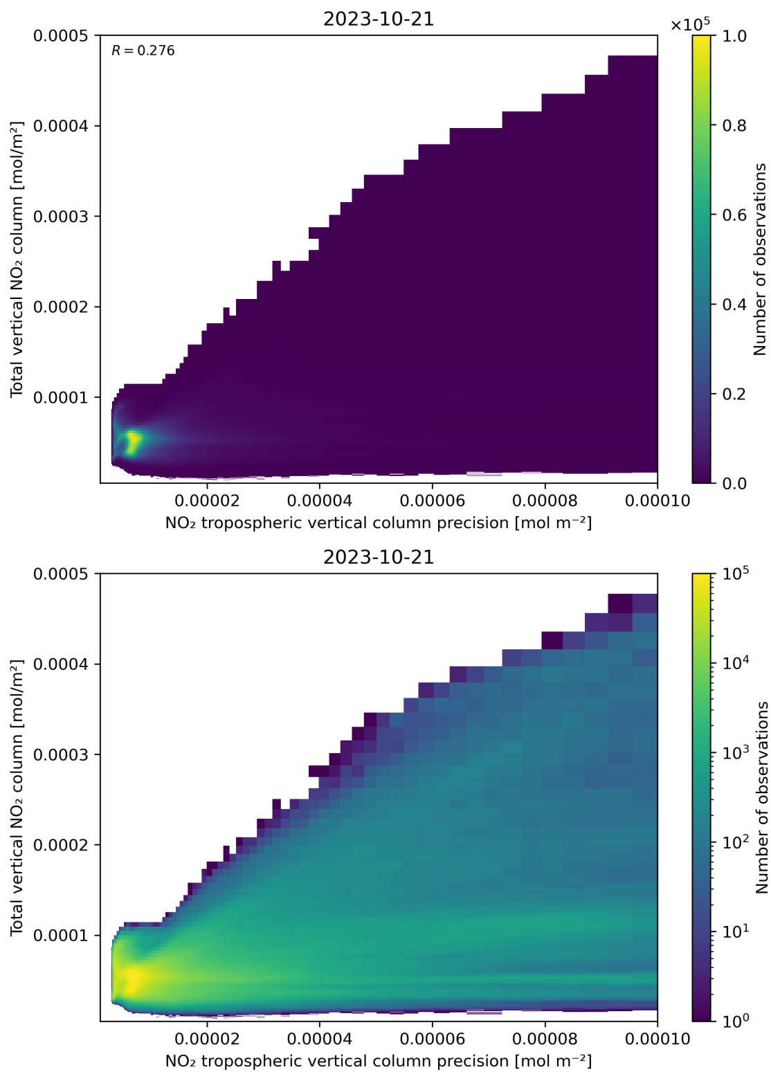
Figure 138: Scatter density plot of “NO 2 tropospheric vertical column precision” against “Total vertical NO 2 column” for 2023-10-20 to 2023-10-22.
