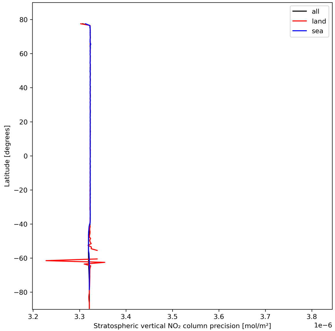
Figure 20: Zonal average of “Stratospheric vertical NO 2 column precision” for 2023-10-20 to 2023-10-22.
