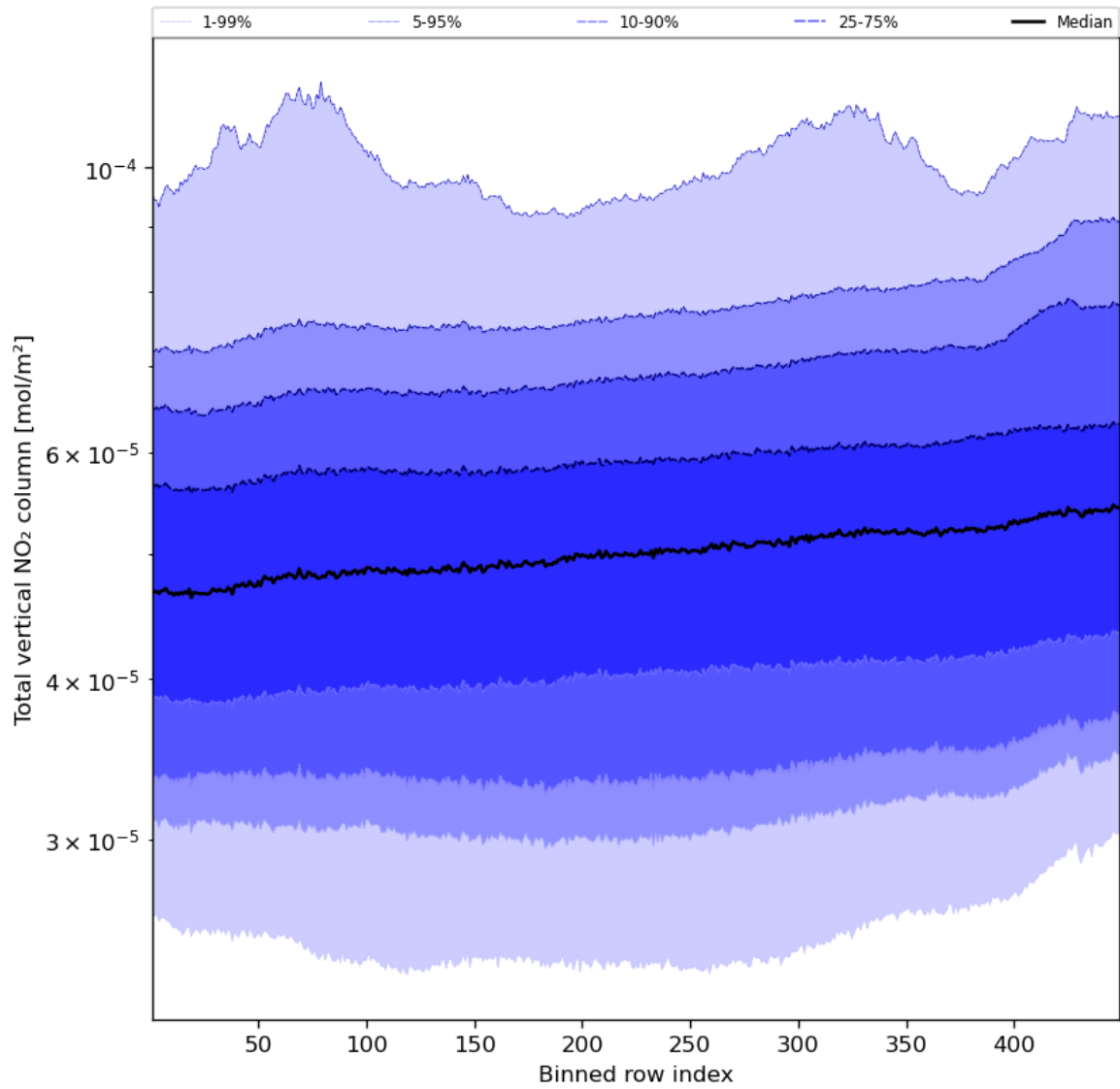
Figure 55: Along track statistics of “Total vertical NO 2 column” for 2023-10-20 to 2023-10-22
