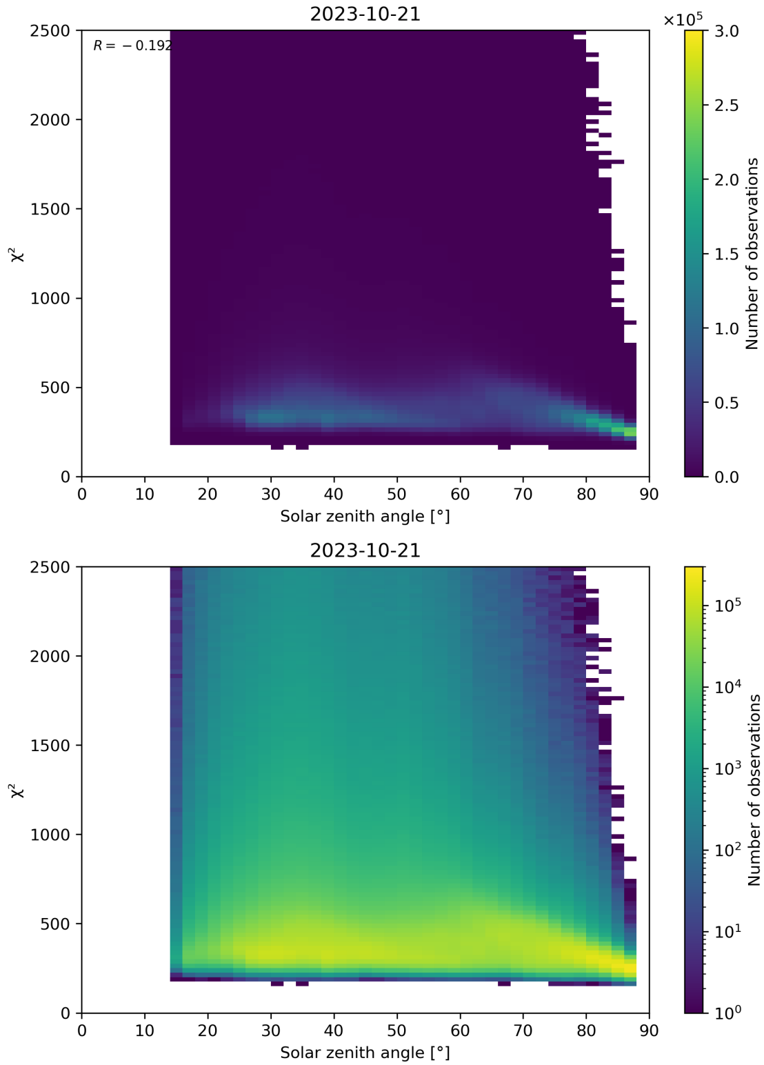
Figure 148: Scatter density plot of “Solar zenith angle” against “ \chi^2 ” for 2023-10-20 to 2023-10-22.
