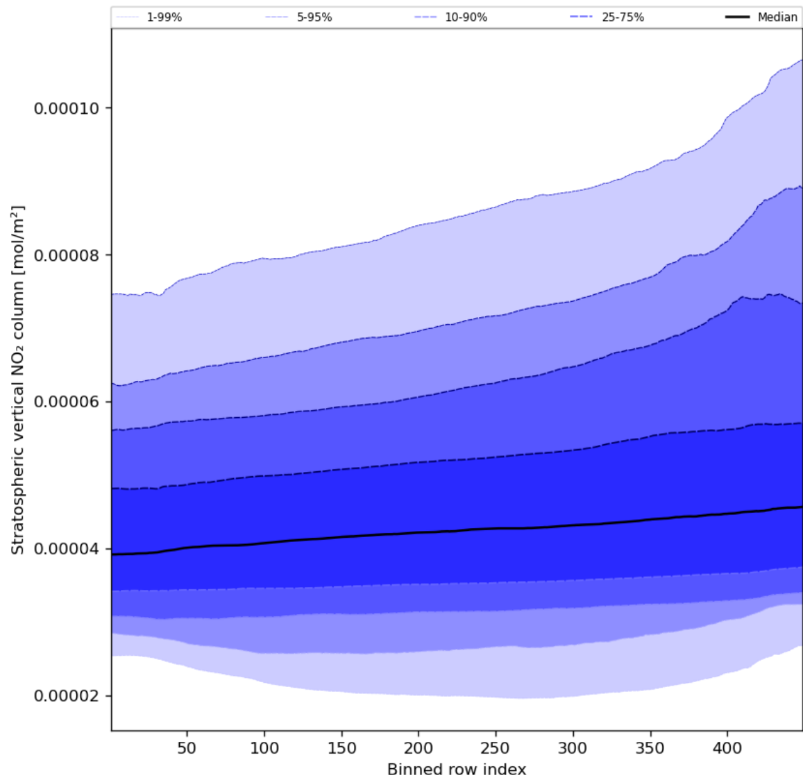
Figure 53: Along track statistics of “Stratospheric vertical NO 2 column” for 2023-10-20 to 2023-10-22
