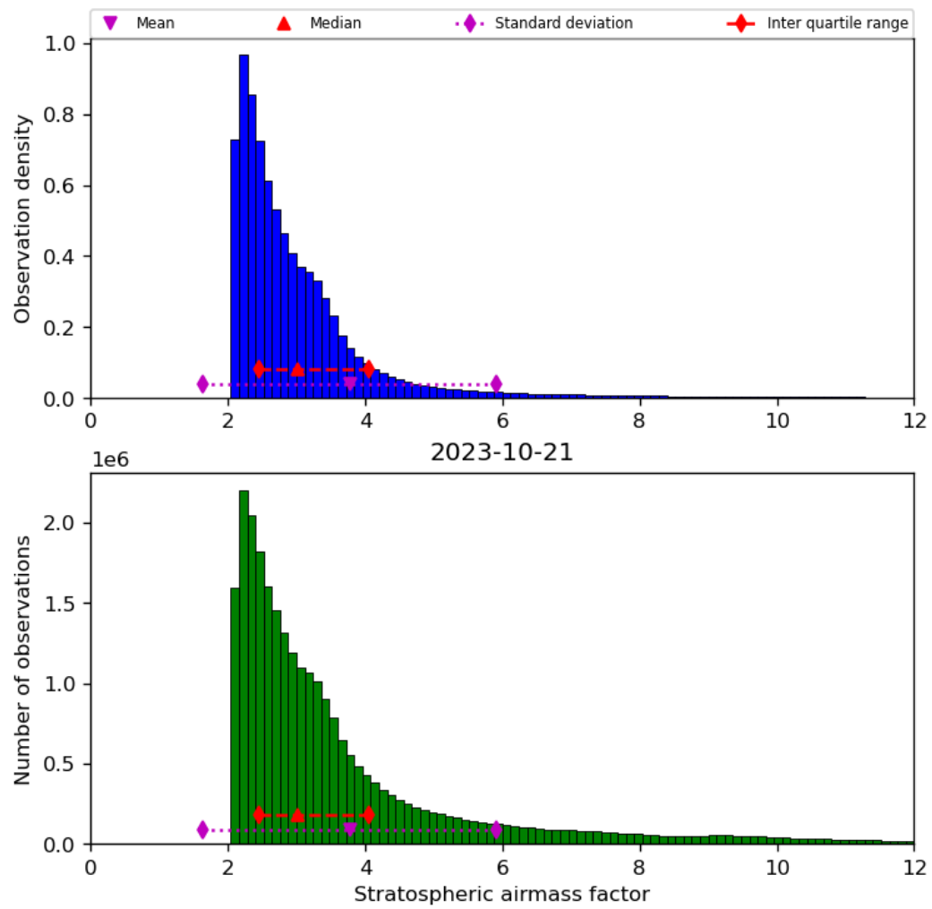
Figure 44: Histogram of “Stratospheric airmass factor” for 2023-10-20 to 2023-10-22
