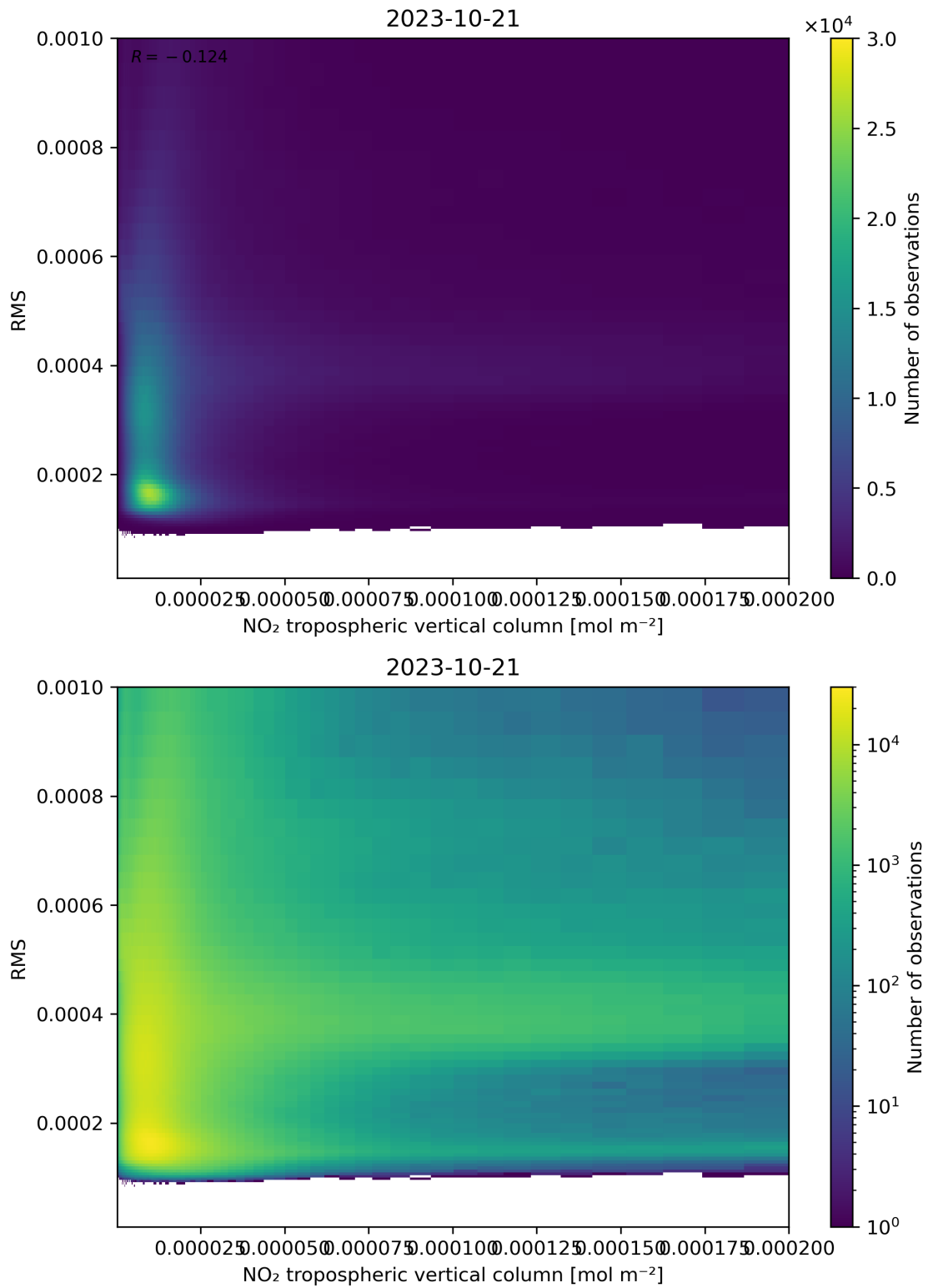
Figure 142: Scatter density plot of “NO 2 tropospheric vertical column” against “RMS” for 2023-10-20 to 2023-10-22.
