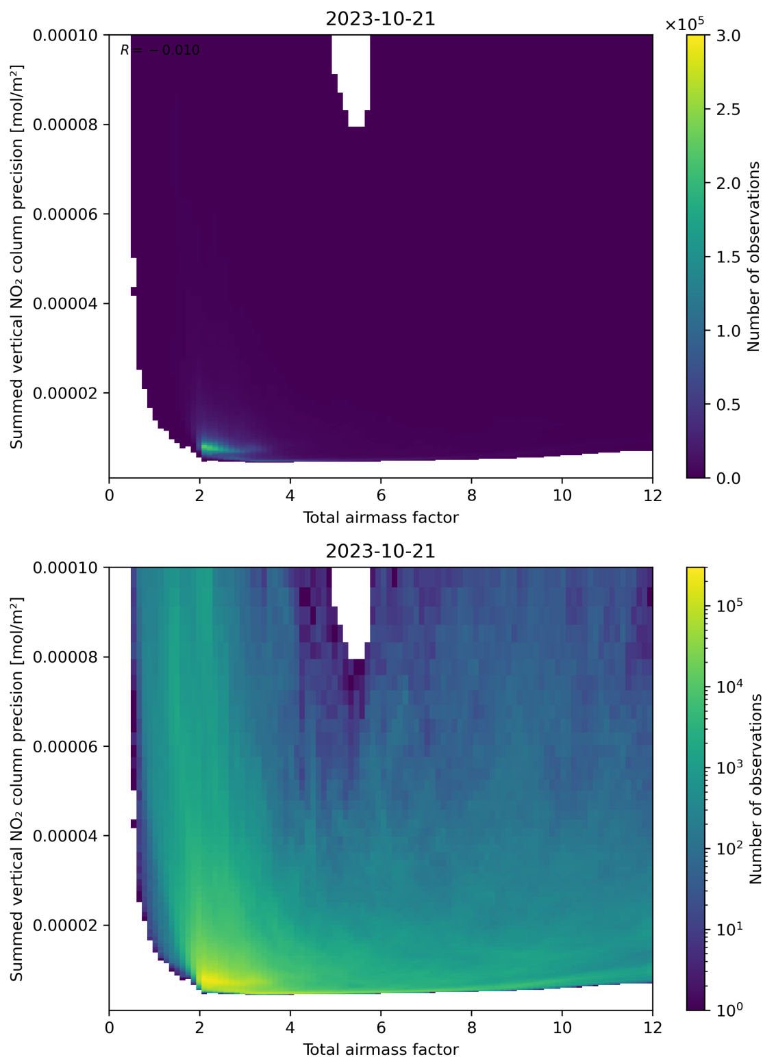
Figure 66: Scatter density plot of “Total airmass factor” against “Summed vertical NO 2 column precision” for 2023-10-20 to 2023-10-22.
