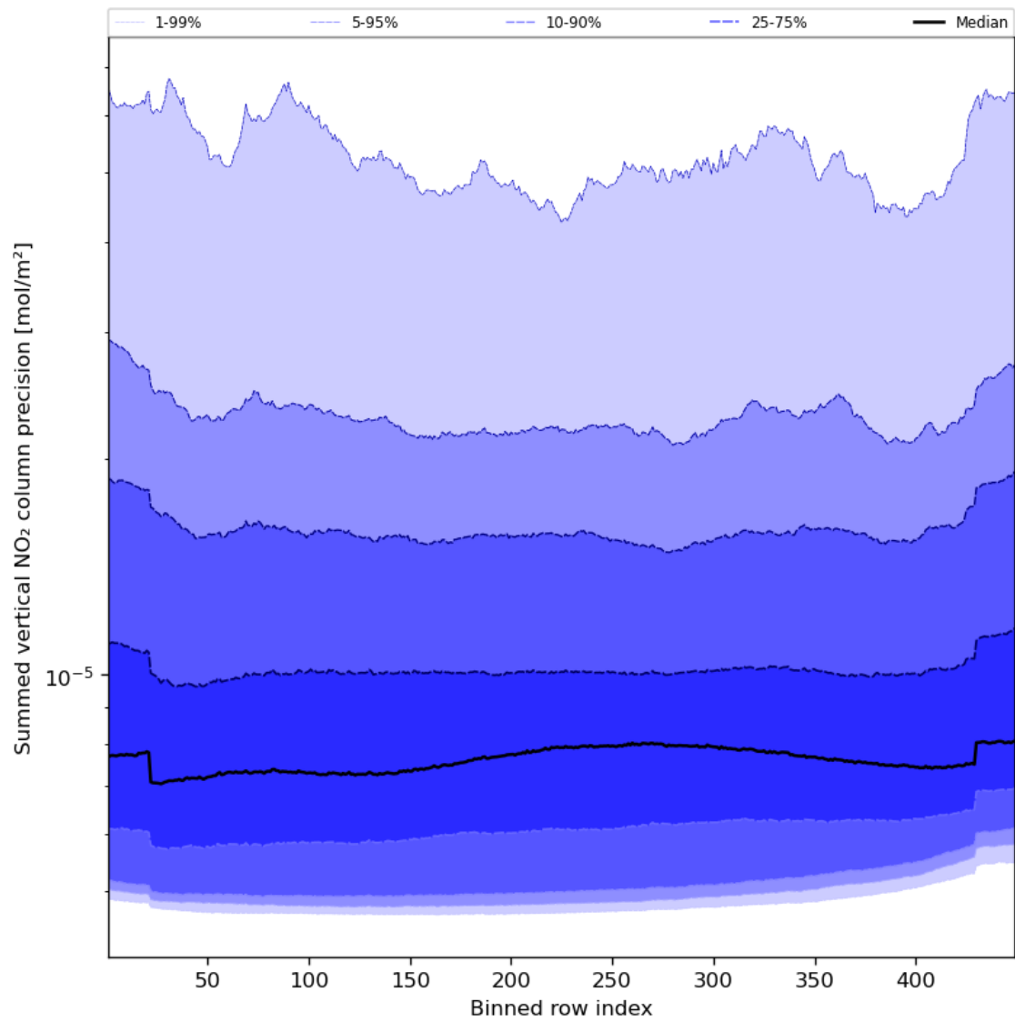
Figure 58: Along track statistics of “Summed vertical NO 2 column precision” for 2023-10-20 to 2023-10-22
