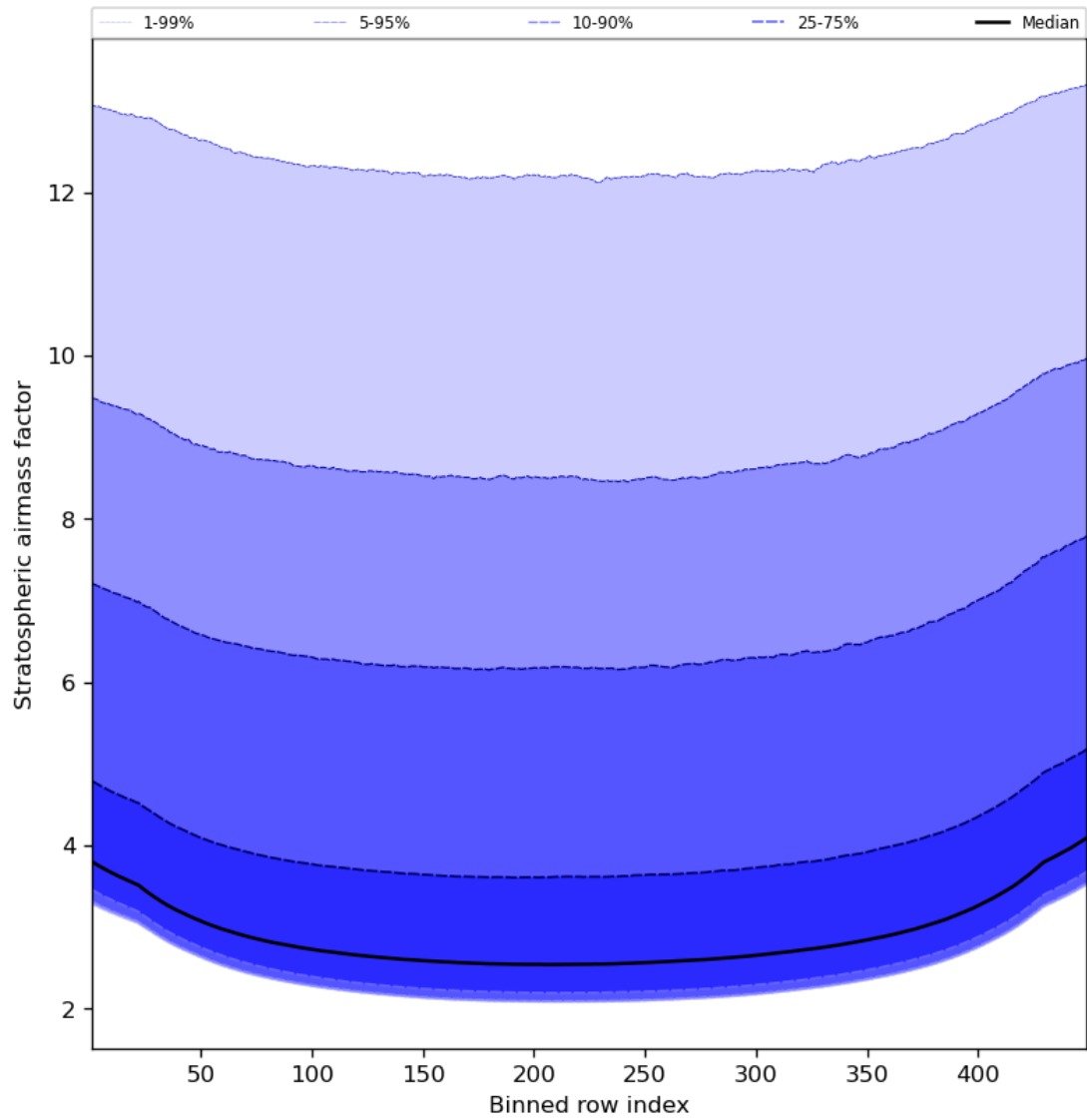
Figure 61: Along track statistics of “Stratospheric airmass factor” for 2023-10-20 to 2023-10-22
