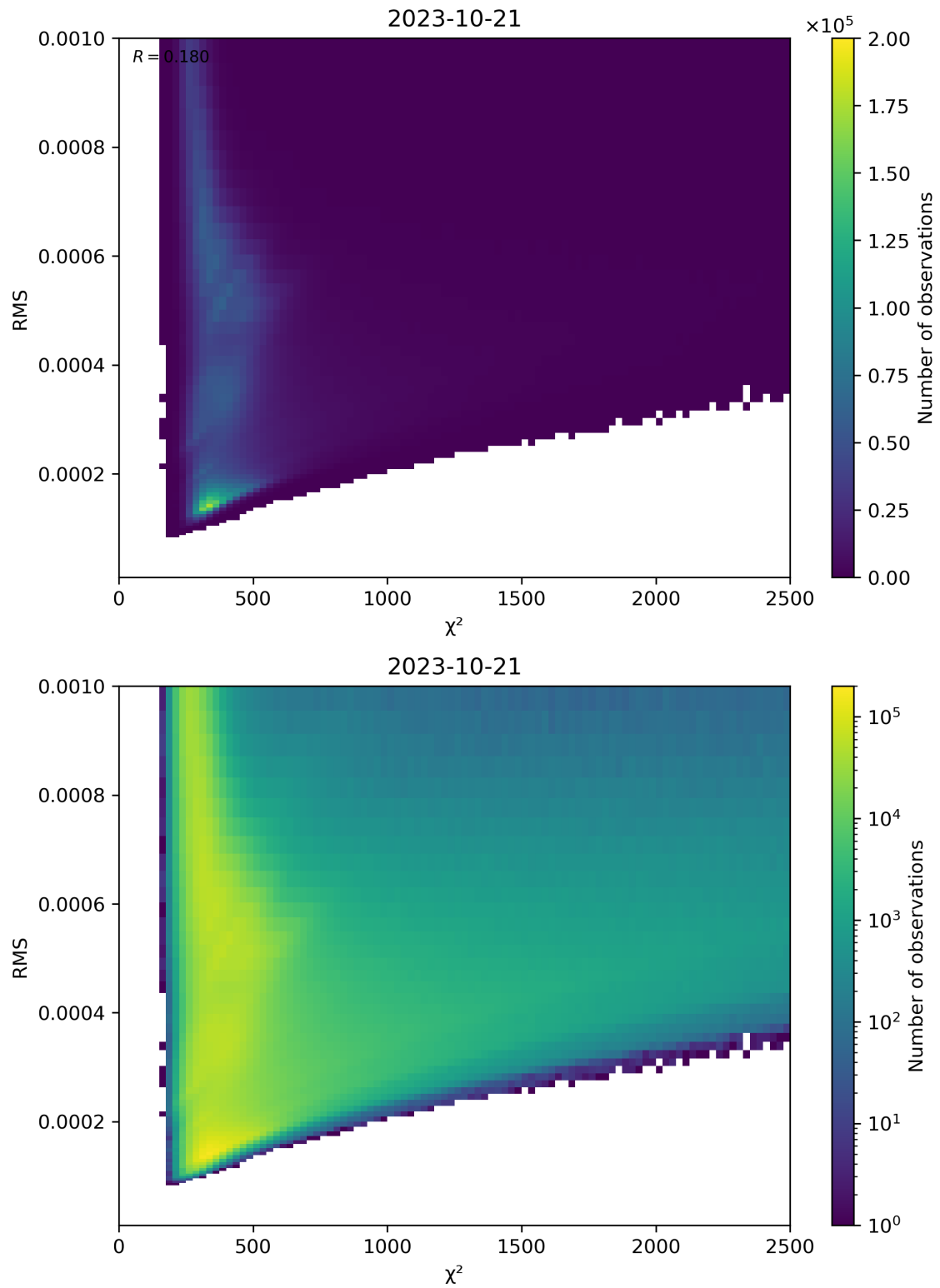
Figure 82: Scatter density plot of “ \chi^2 ” against “RMS” for 2023-10-20 to 2023-10-22.
