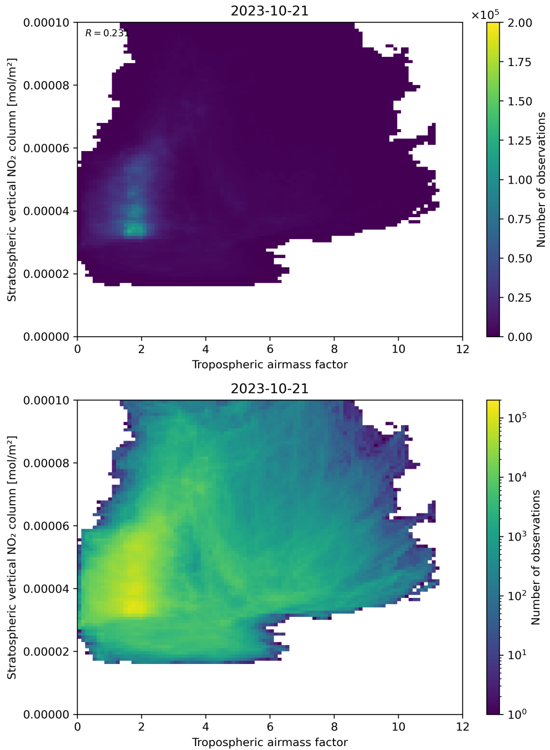
Figure 74: Scatter density plot of “Tropospheric air mass factor” against “Stratospheric vertical NO 2 column” for 2023-10-20 to 2023-10-22.
