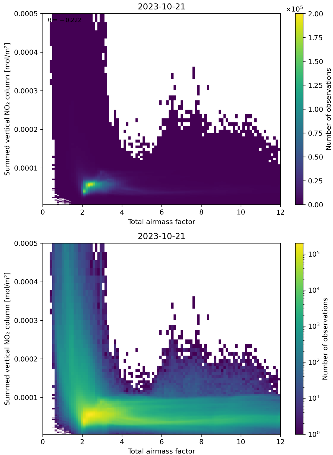
Figure 65: Scatter density plot of “Total airmass factor” against “Summed vertical NO 2 column” for 2023-10-20 to 2023-10-22.
