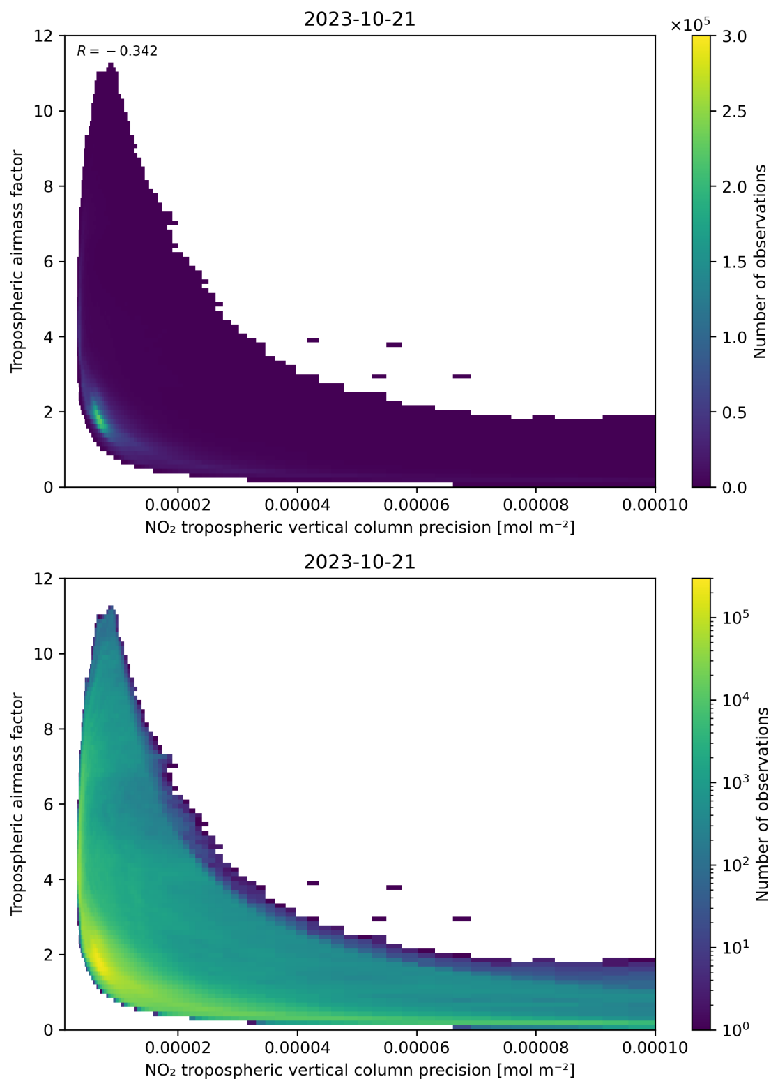
Figure 133: Scatter density plot of “NO 2 tropospheric vertical column precision” against “Tropospheric airmass factor” for 2023-10-20 to 2023-10-22.
