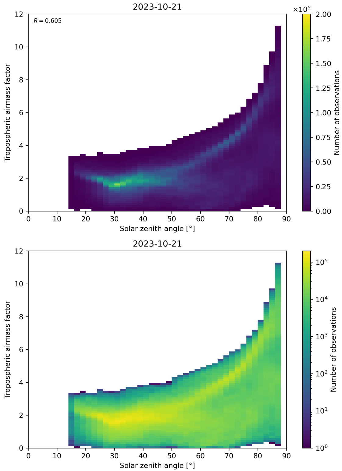
Figure 147: Scatter density plot of “Solar zenith angle” against “Tropospheric airmass factor” for 2023-10-20 to 2023-10-22.
