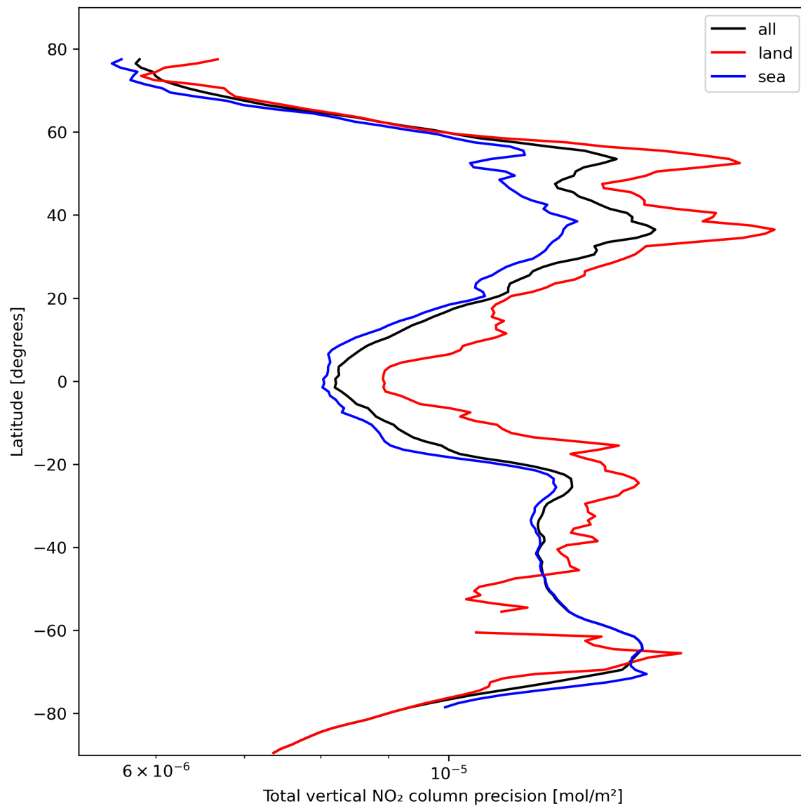
Figure 22: Zonal average of “Total vertical NO 2 column precision” for 2023-10-20 to 2023-10-22.
