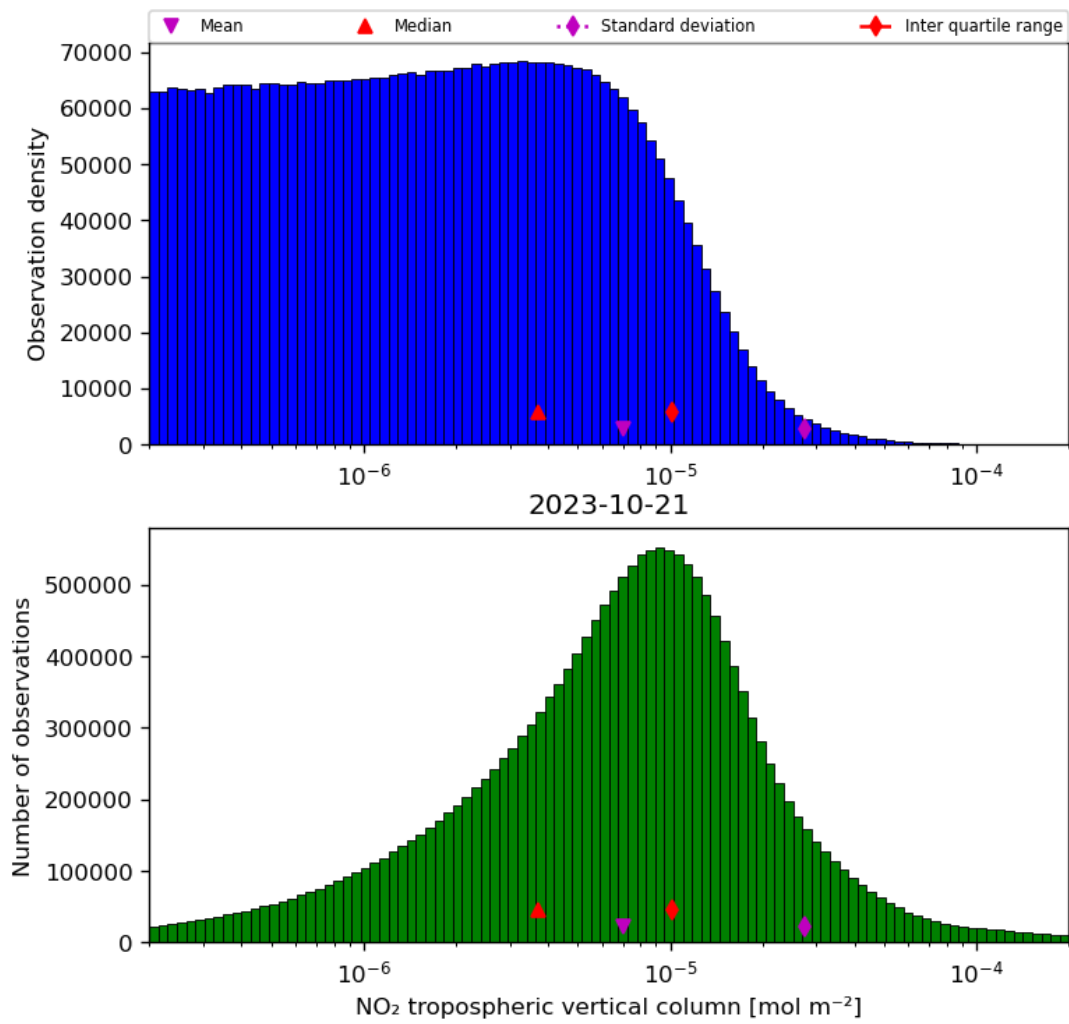
Figure 29: Histogram of “NO 2 tropospheric vertical column” for 2023-10-20 to 2023-10-22
