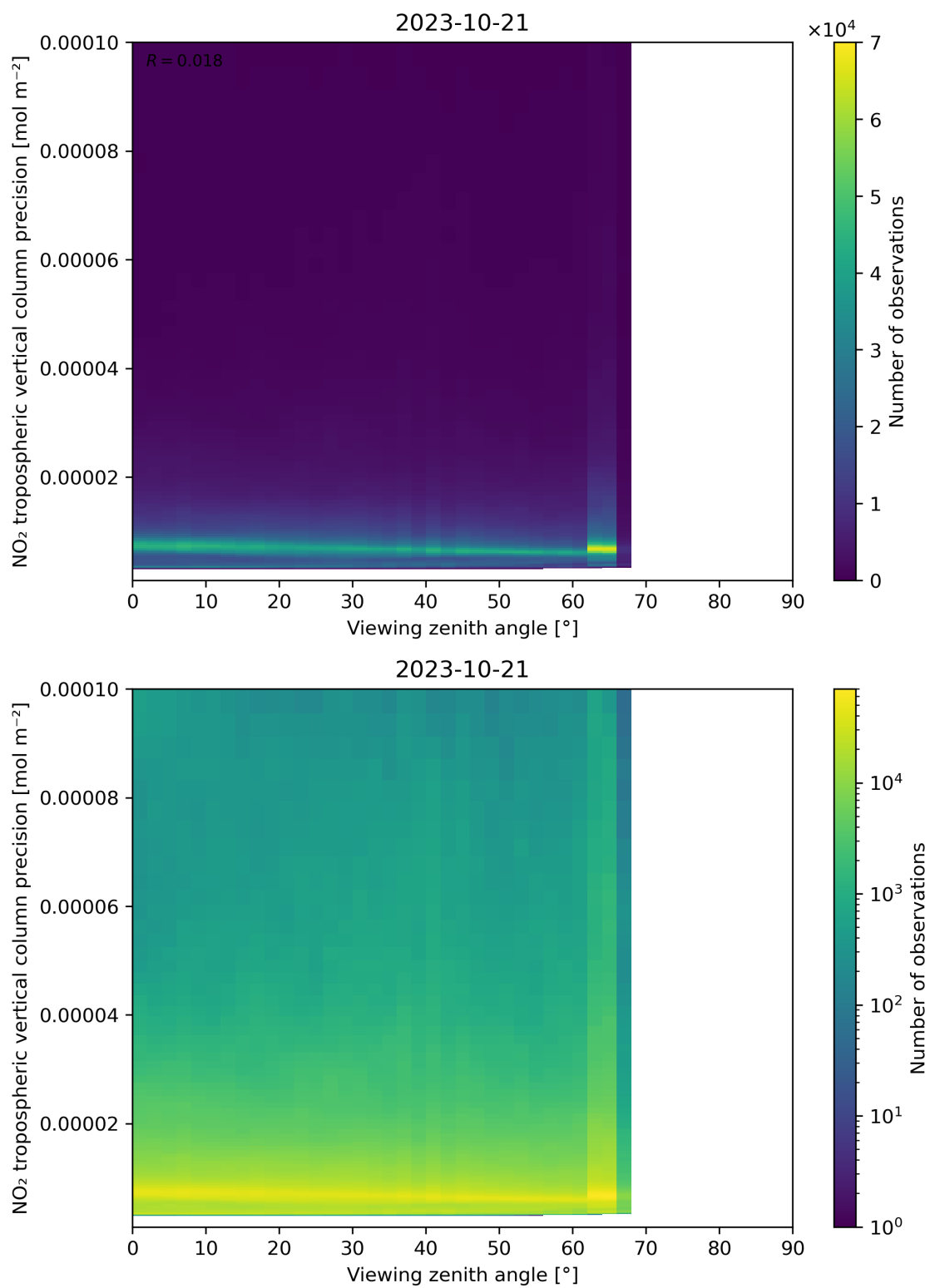
Figure 170: Scatter density plot of “Viewing zenith angle” against “NO 2 tropospheric vertical column precision” for 2023-10-20 to 2023-10-22.
