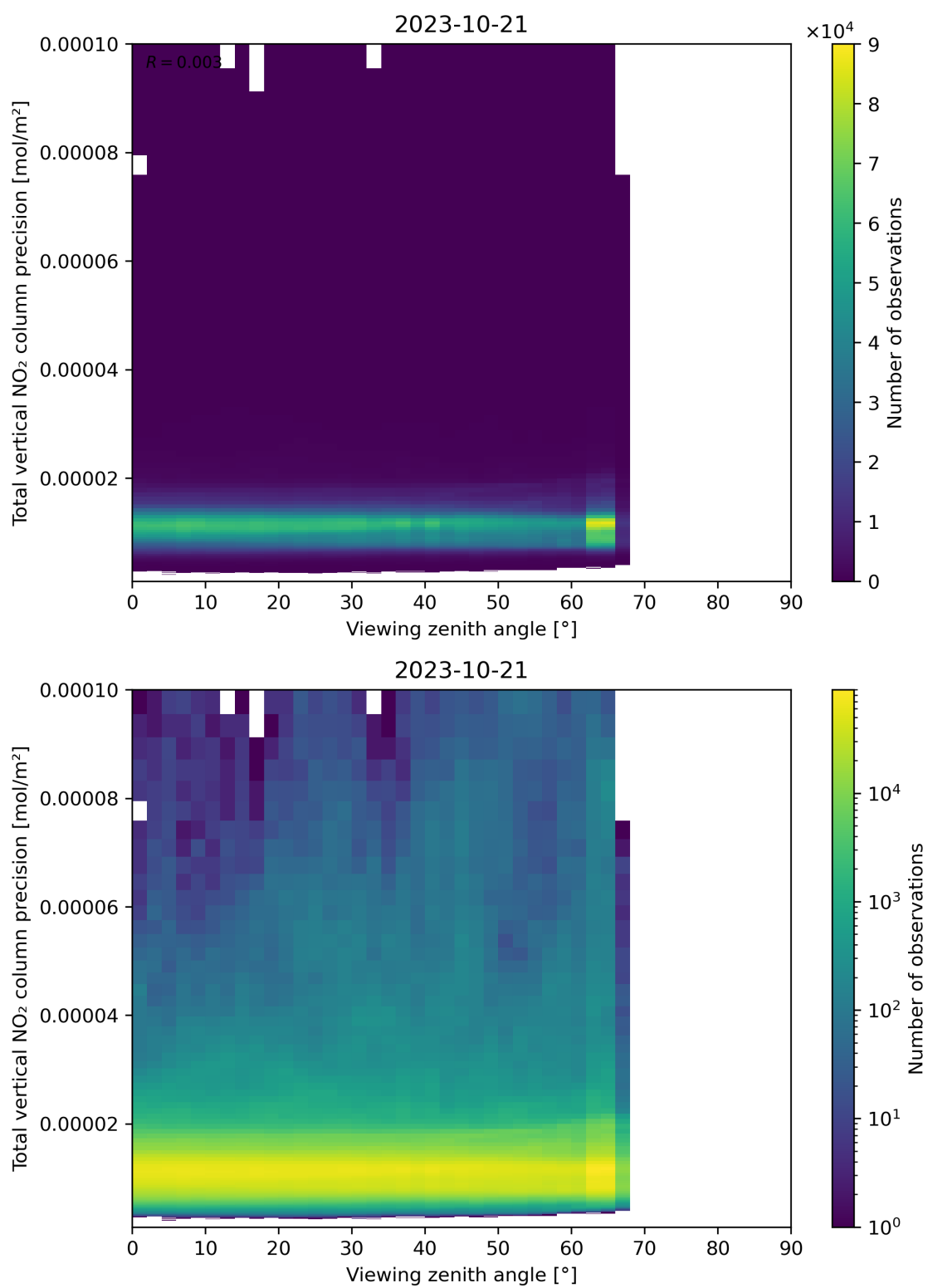
Figure 168: Scatter density plot of “Viewing zenith angle” against “Total vertical NO 2 column precision” for 2023-10-20 to 2023-10-22.
