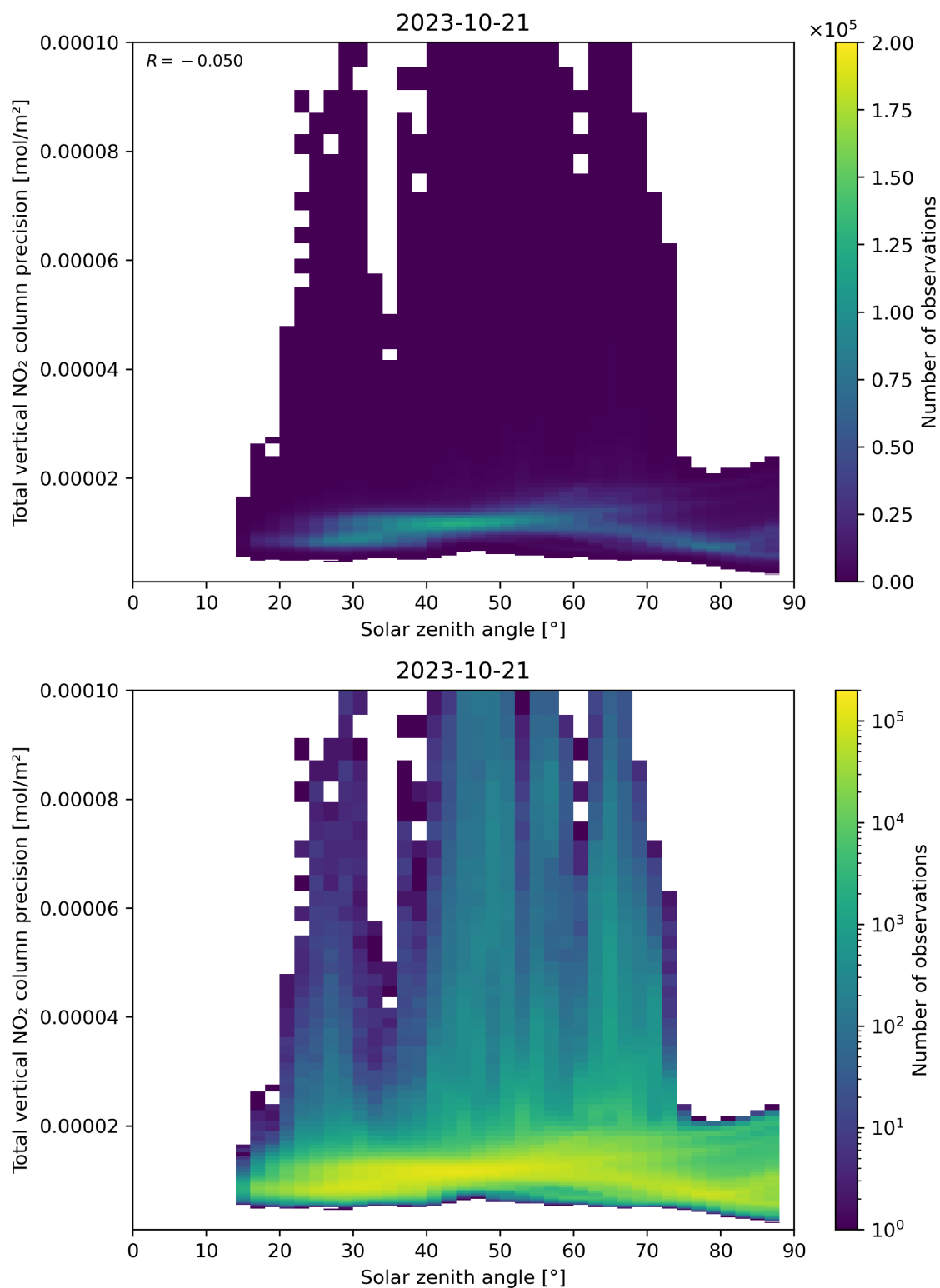
Figure 154: Scatter density plot of “Solar zenith angle” against “Total vertical NO 2 column precision” for 2023-10-20 to 2023-10-22.
