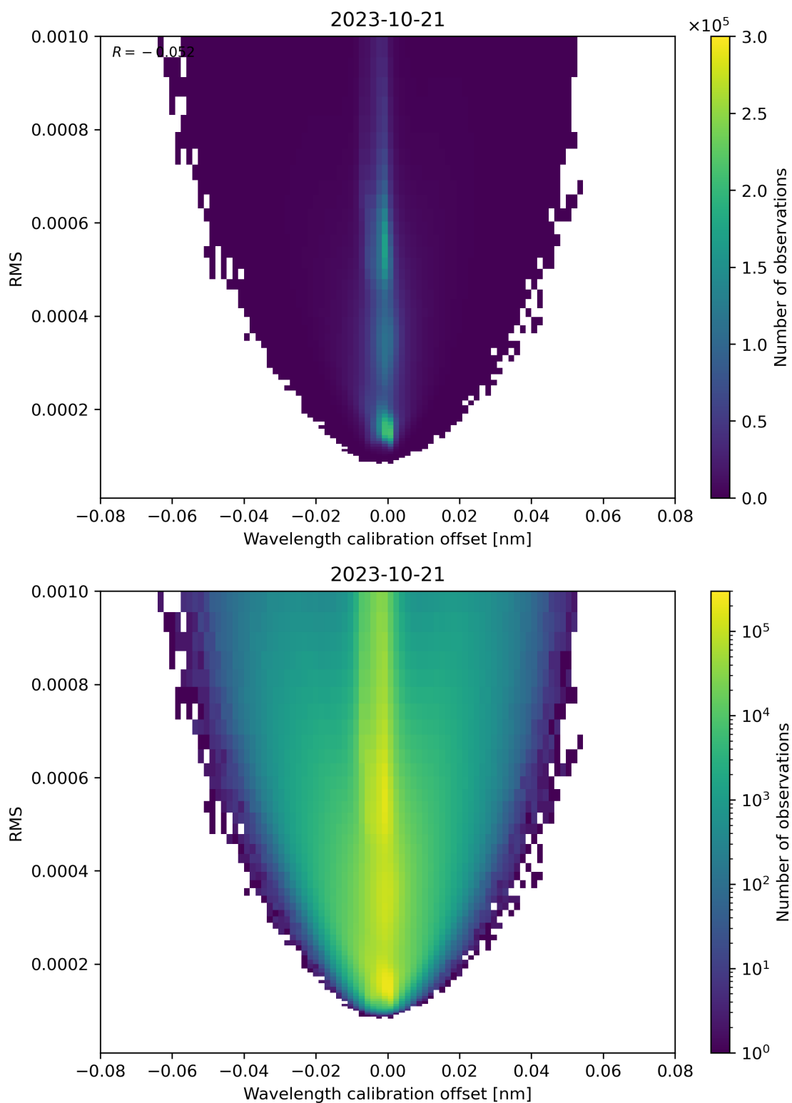
Figure 181: Scatter density plot of “Wavelength calibration offset” against “RMS” for 2023-10-20 to 2023-10-22.
