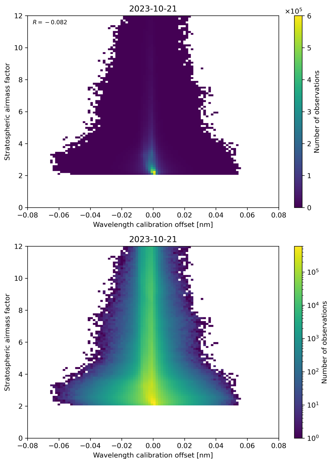
Figure 174: Scatter density plot of “Wavelength calibration offset” against “Stratospheric airmass factor” for 2023-10-20 to 2023-10-22.
