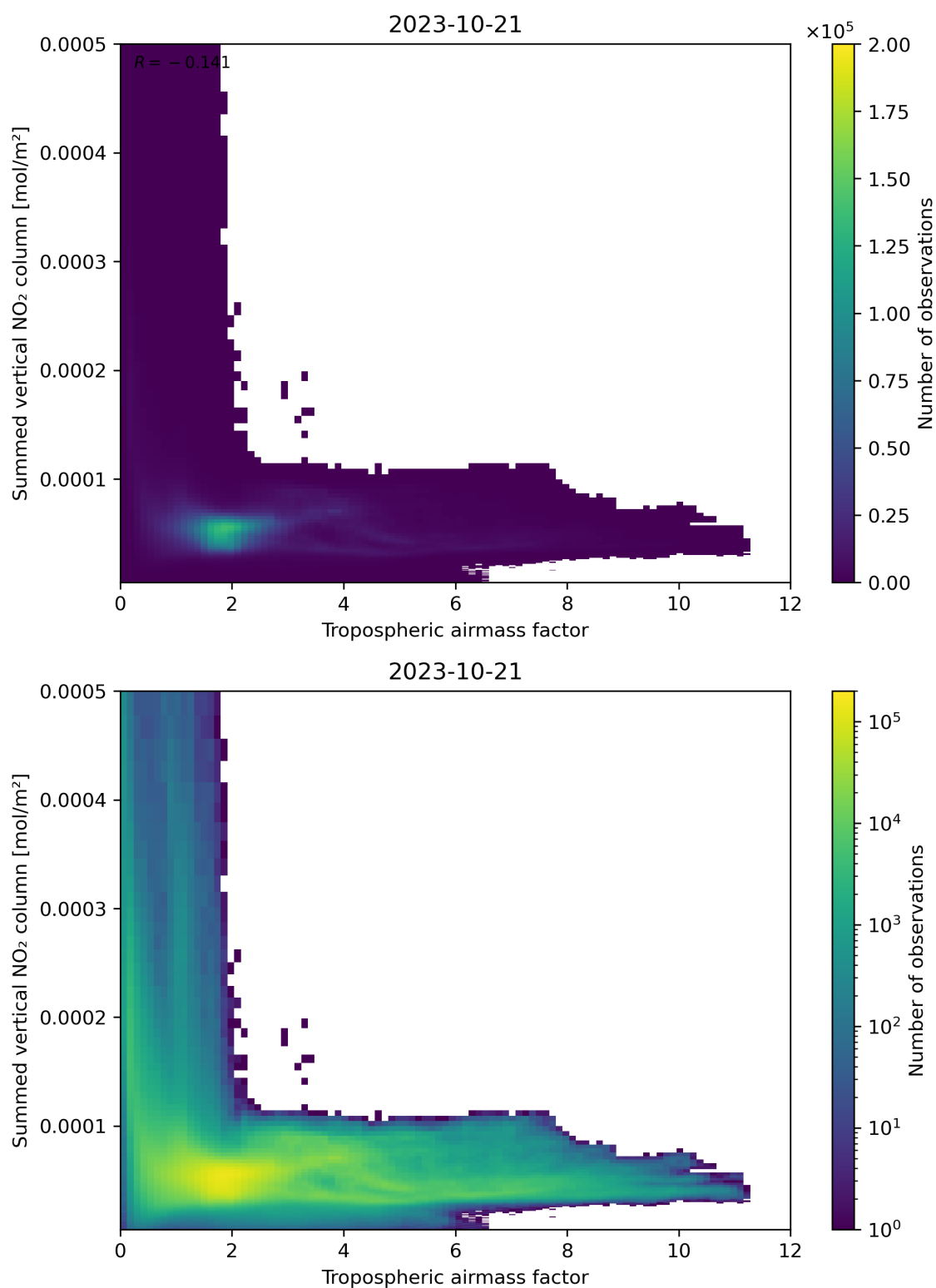
Figure 75: Scatter density plot of “Tropospheric airmass factor” against “Summed vertical NO 2 column” for 2023-10-20 to 2023-10-22.
