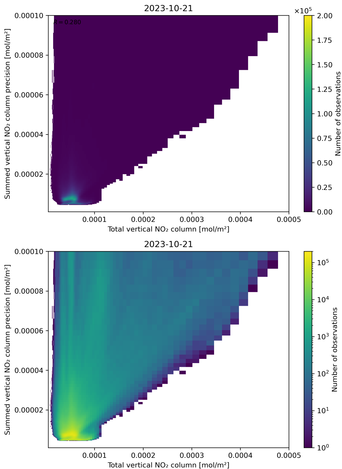
Figure 113: Scatter density plot of “Total vertical NO 2 column” against “Summed vertical NO 2 column precision” for 2023-10-20 to 2023-10-22.
