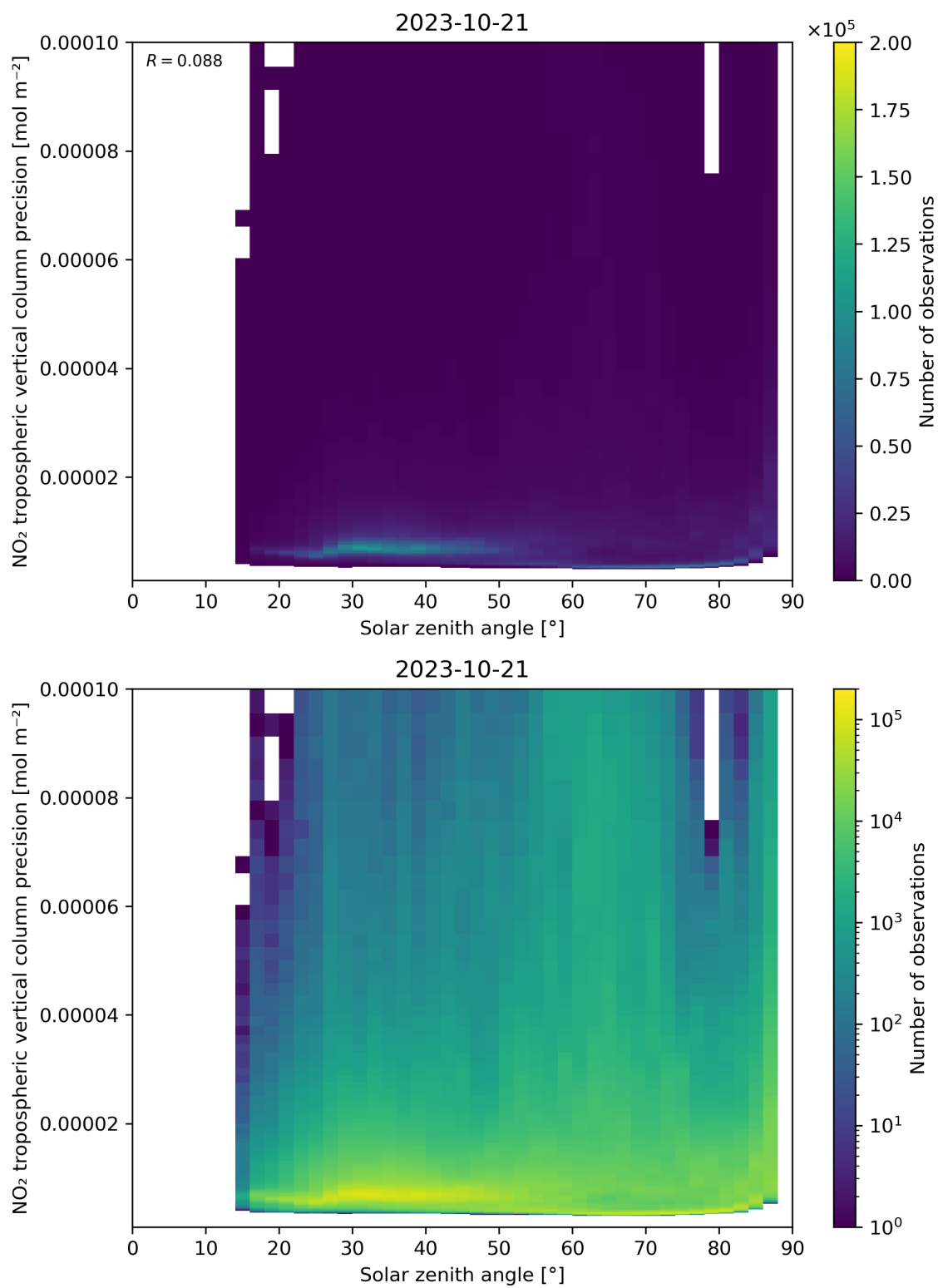
Figure 156: Scatter density plot of “Solar zenith angle” against “NO 2 tropospheric vertical column precision” for 2023-10-20 to 2023-10-22.
