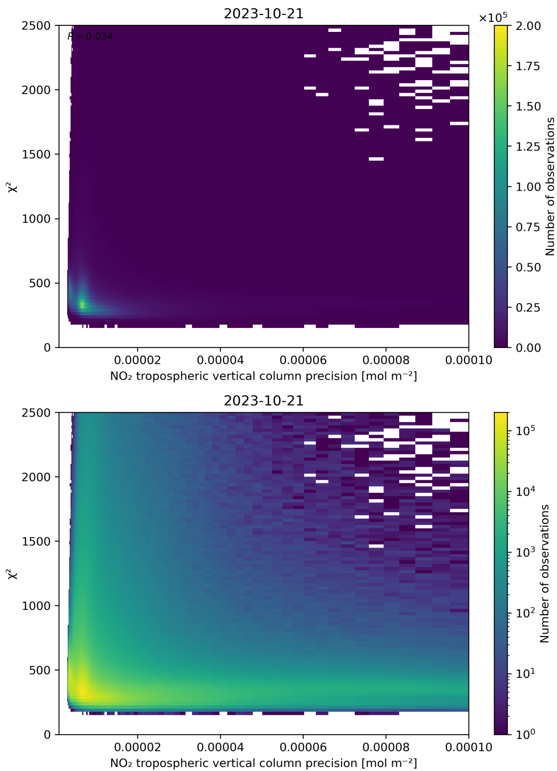
Figure 134: Scatter density plot of “NO 2 tropospheric vertical column precision” against “ \chi^2 ” for 2023-10-20 to 2023-10-22.
