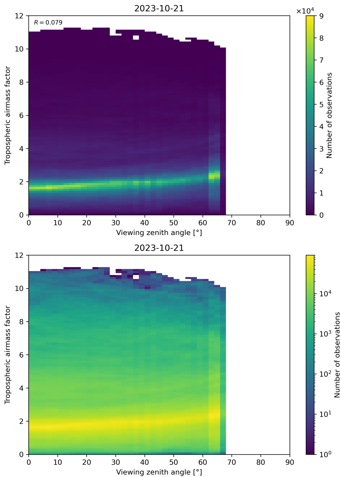
Figure 161: Scatter density plot of “Viewing zenith angle” against “Tropospheric airmass factor” for 2023-10-20 to 2023-10-22.
