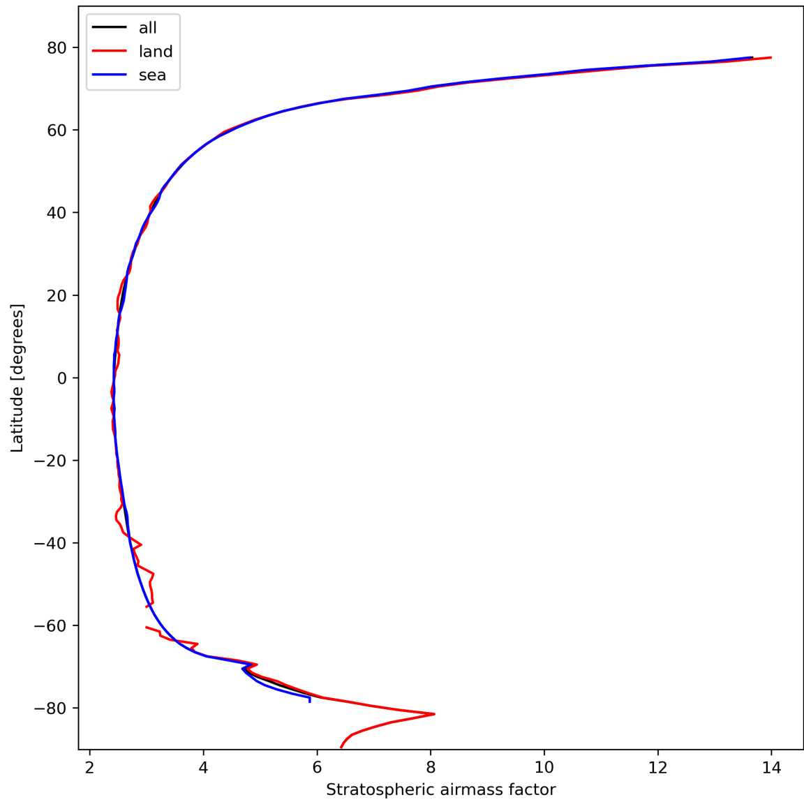
Figure 27: Zonal average of “Stratospheric airmass factor” for 2023-10-20 to 2023-10-22.
