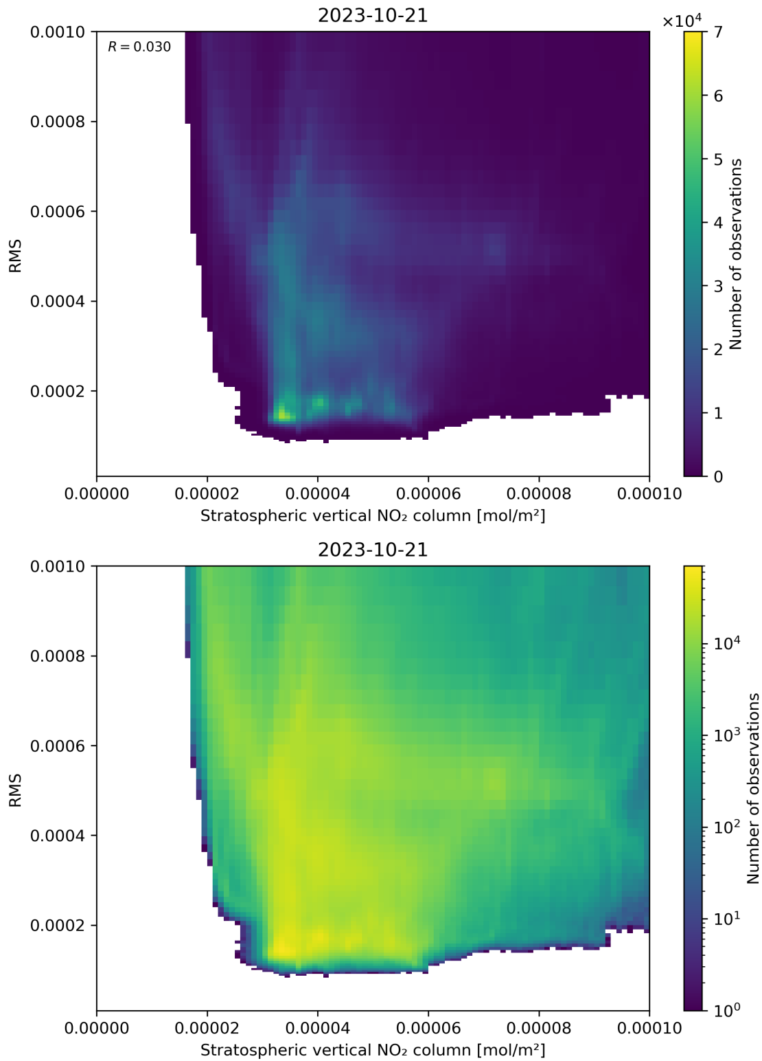
Figure 102: Scatter density plot of “Stratospheric vertical NO 2 column” against “RMS” for 2023-10-20 to 2023-10-22.
