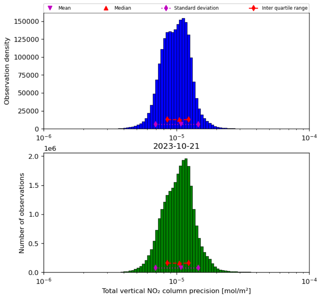
Figure 39: Histogram of “Total vertical NO 2 column precision” for 2023-10-20 to 2023-10-22
