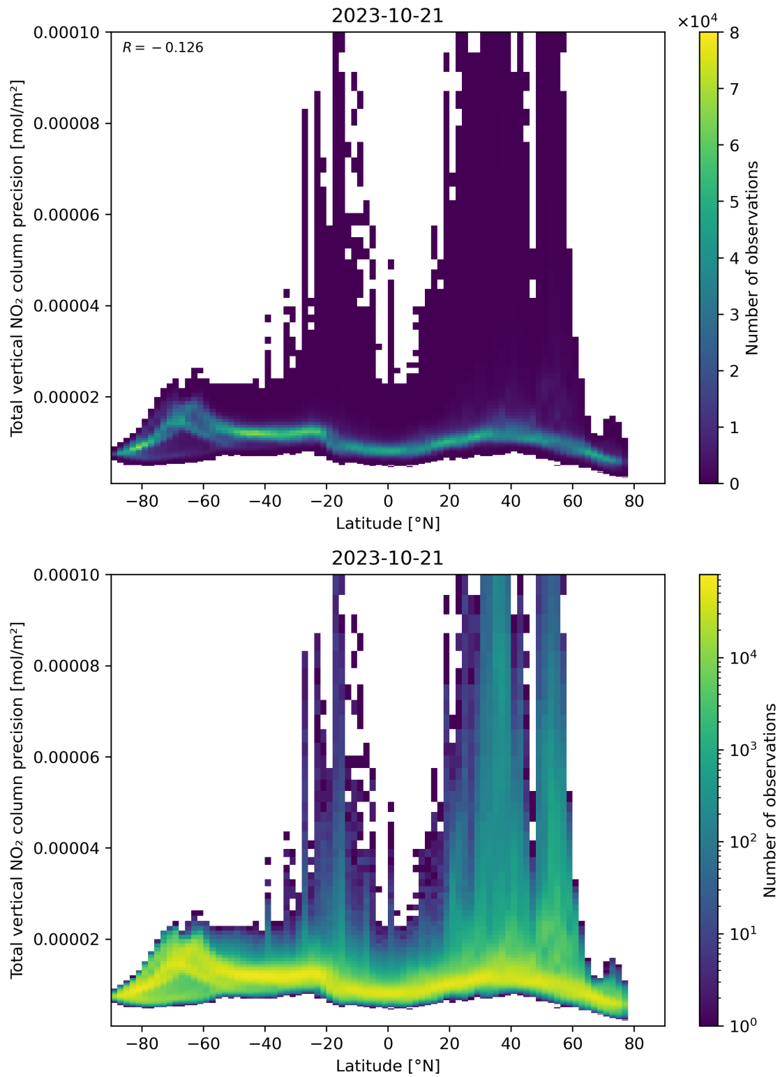
Figure 91: Scatter density plot of “Latitude” against “Total vertical NO 2 column precision” for 2023-10-20 to 2023-10-22.
