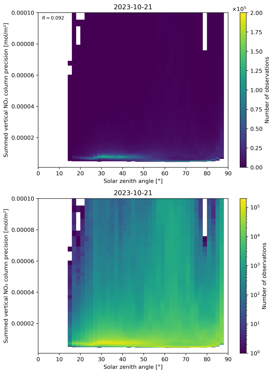
Figure 152: Scatter density plot of “Solar zenith angle” against “Summed vertical NO 2 column precision” for 2023-10-20 to 2023-10-22.
