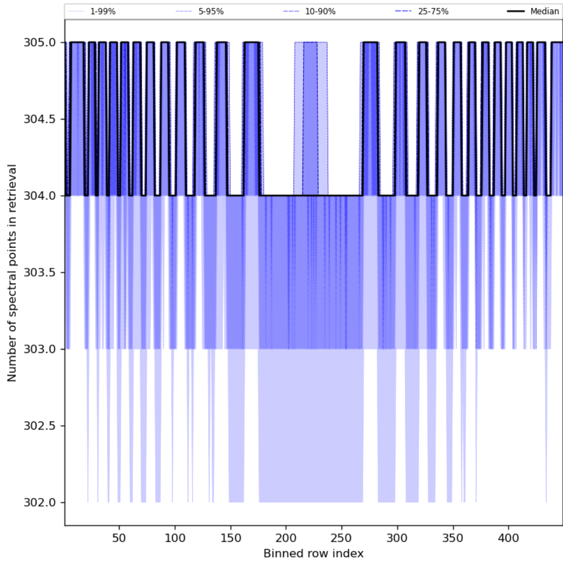
Figure 50: Along track statistics of “Number of spectral points in retrieval” for 2023-10-20 to 2023-10-22
