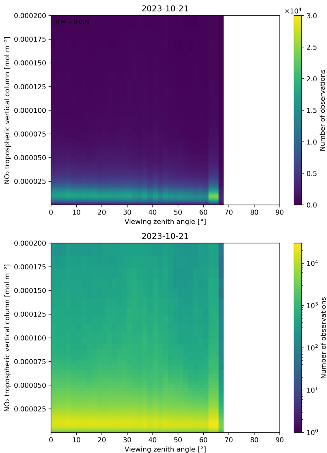
Figure 169: Scatter density plot of “Viewing zenith angle” against “NO 2 tropospheric vertical column” for 2023-10-20 to 2023-10-22.
