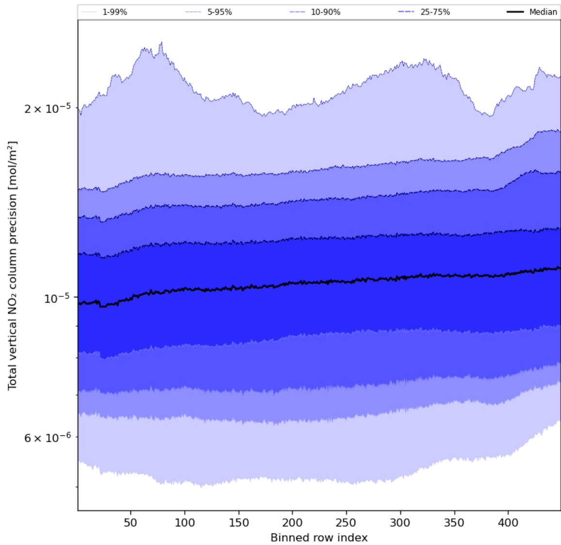
Figure 56: Along track statistics of “Total vertical NO 2 column precision” for 2023-10-20 to 2023-10-22
