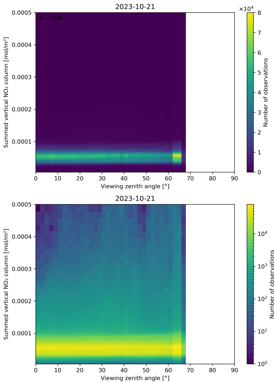
Figure 165: Scatter density plot of “Viewing zenith angle” against “Summed vertical NO 2 column” for 2023-10-20 to 2023-10-22.
