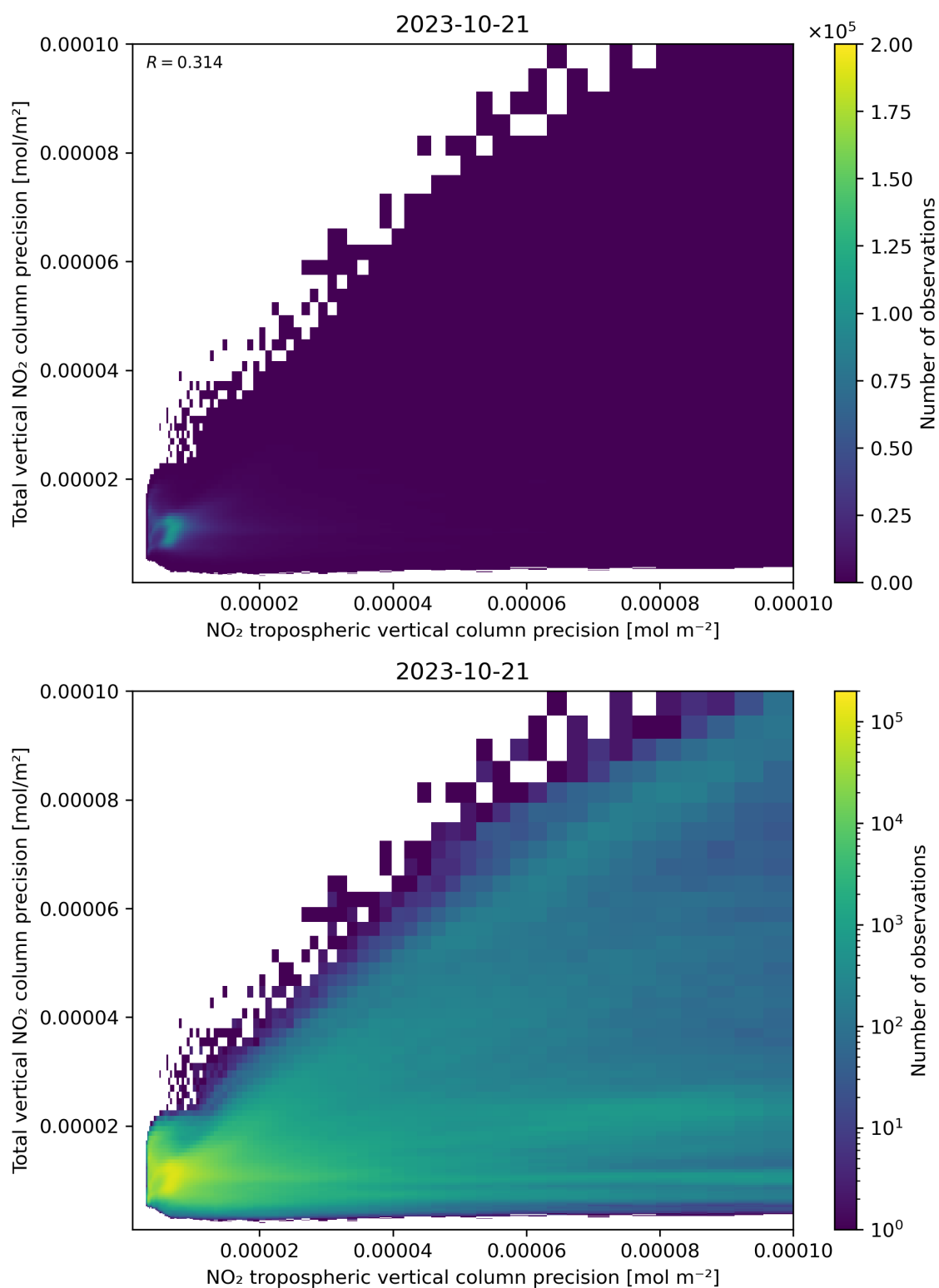
Figure 139: Scatter density plot of “NO 2 tropospheric vertical column precision” against “Total vertical NO 2 column precision” for 2023-10-20 to 2023-10-22.
