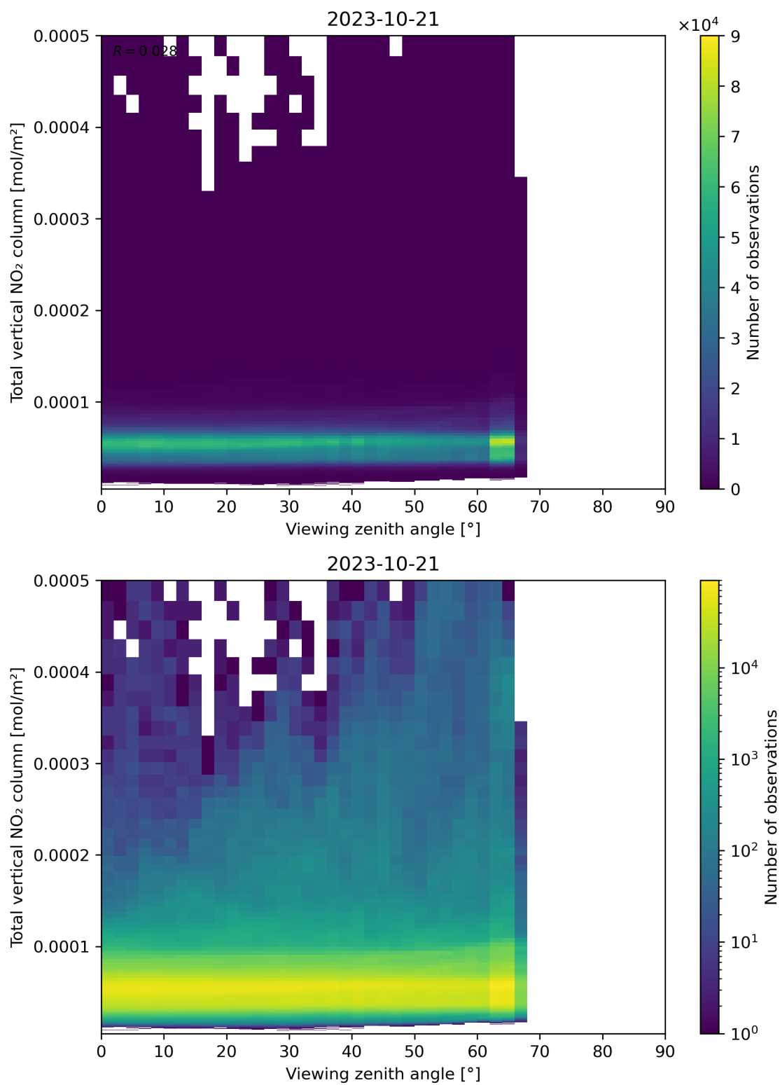
Figure 167: Scatter density plot of “Viewing zenith angle” against “Total vertical NO 2 column” for 2023-10-20 to 2023-10-22.
