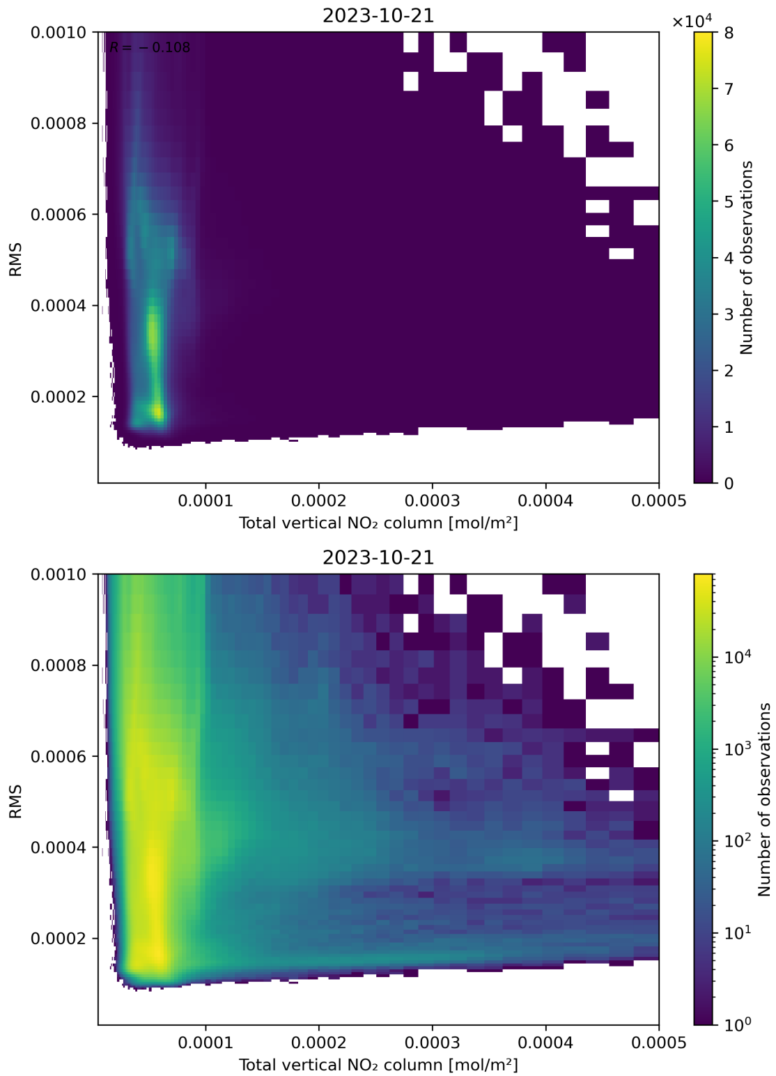
Figure 120: Scatter density plot of “Total vertical NO 2 column” against “RMS” for 2023-10-20 to 2023-10-22.
