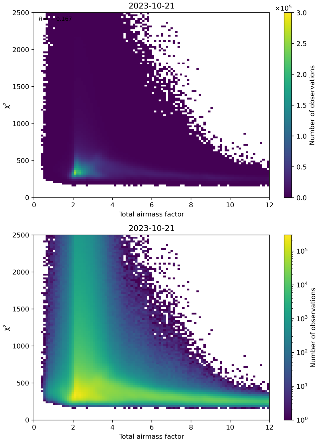
Figure 63: Scatter density plot of “Total airmass factor” against “ \chi^2 ” for 2023-10-20 to 2023-10-22.
