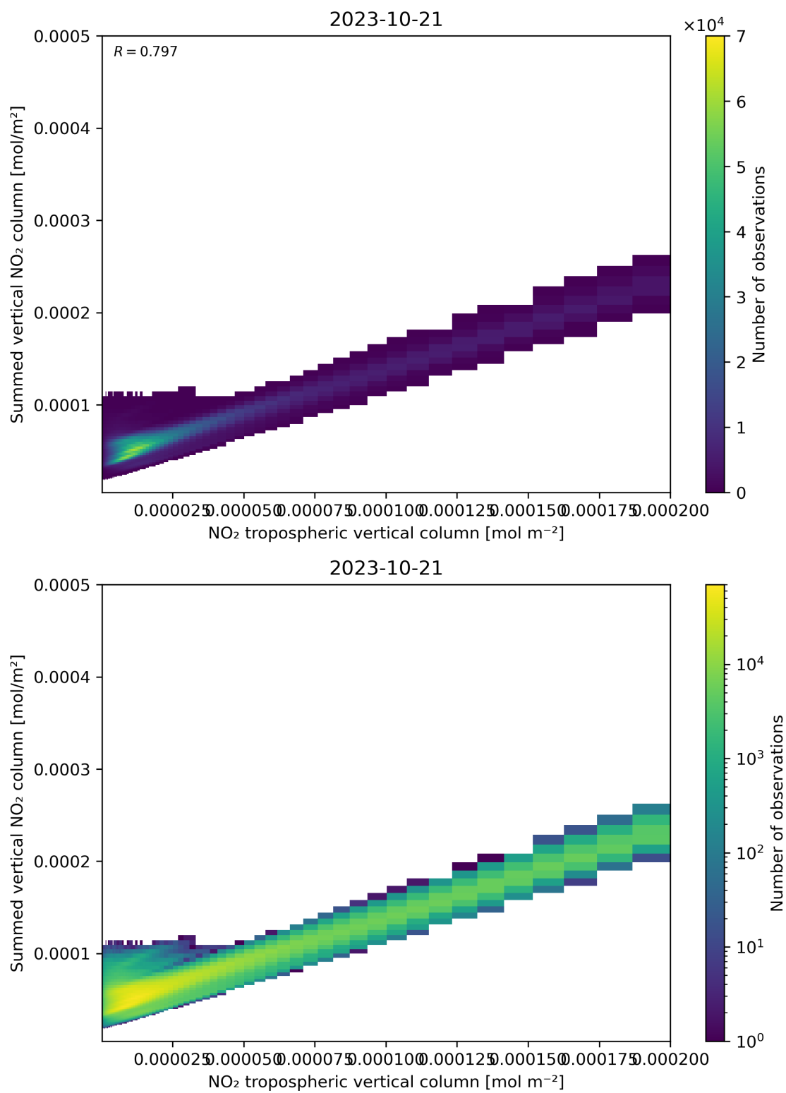
Figure 126: Scatter density plot of “NO 2 tropospheric vertical column” against “Summed vertical NO 2 column” for 2023-10-20 to 2023-10-22.
