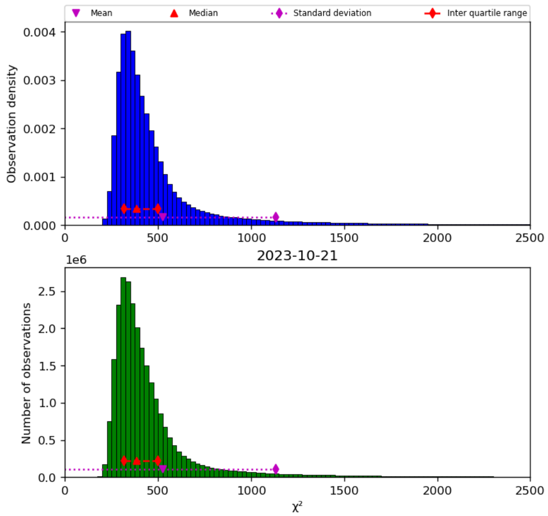
Figure 42: Histogram of “ \chi^2 ” for 2023-10-20 to 2023-10-22
