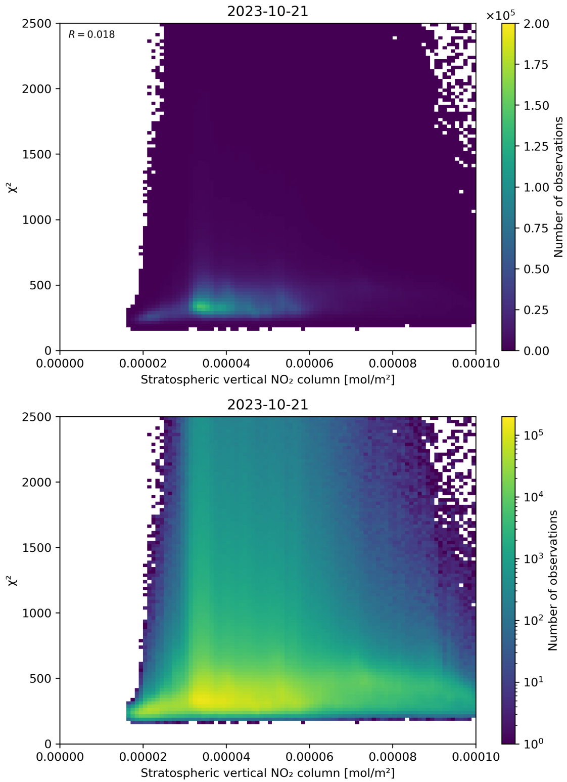
Figure 97: Scatter density plot of “Stratospheric vertical NO 2 column” against “ \chi^2 ” for 2023-10-20 to 2023-10-22.
