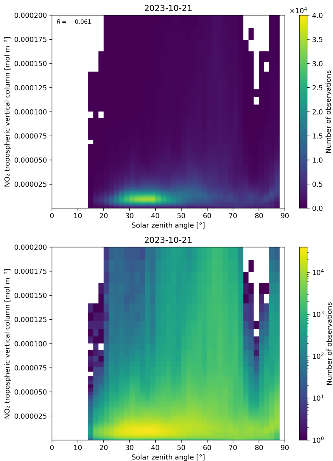
Figure 155: Scatter density plot of “Solar zenith angle” against “NO 2 tropospheric vertical column” for 2023-10-20 to 2023-10-22.
