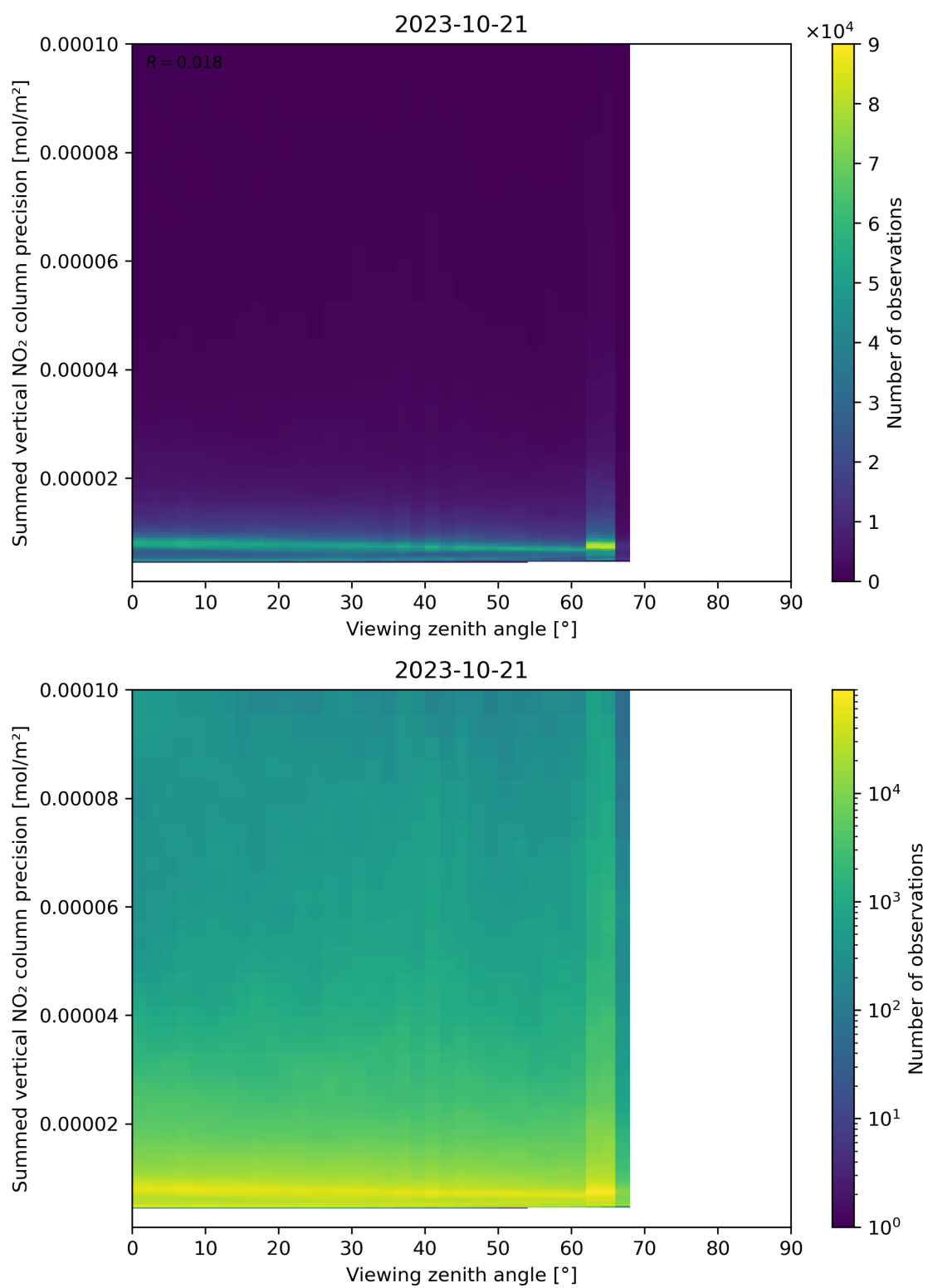
Figure 166: Scatter density plot of “Viewing zenith angle” against “Summed vertical NO 2 column precision” for 2023-10-20 to 2023-10-22.
