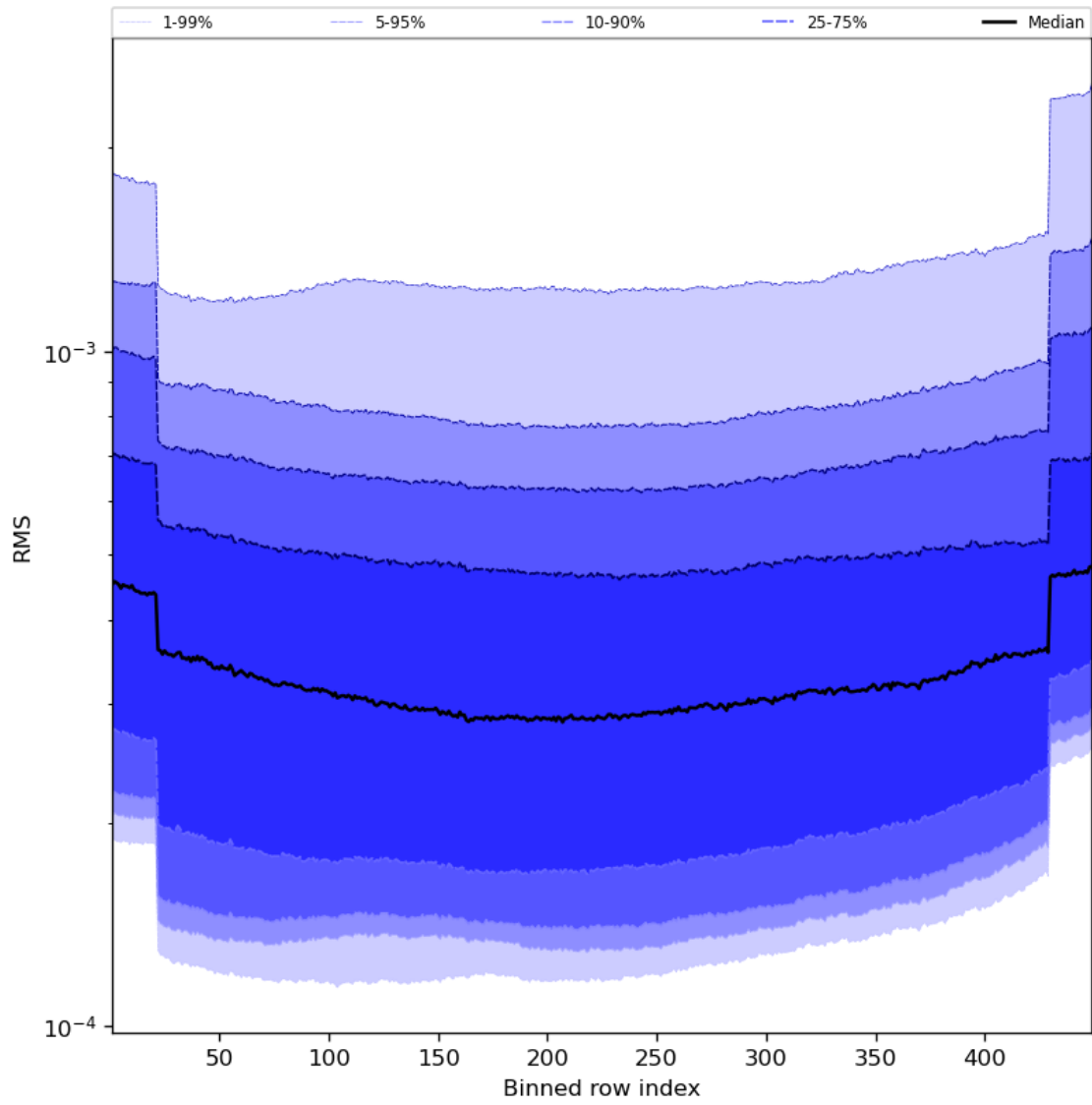
Figure 60: Along track statistics of “RMS” for 2023-10-20 to 2023-10-22
