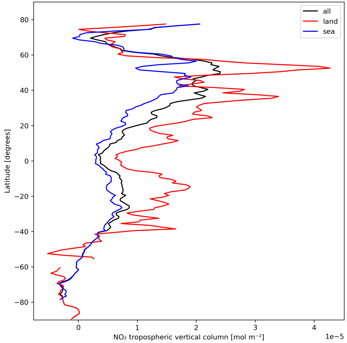
Figure 12: Zonal average of “NO 2 tropospheric vertical column” for 2023-10-20 to 2023-10-22.
