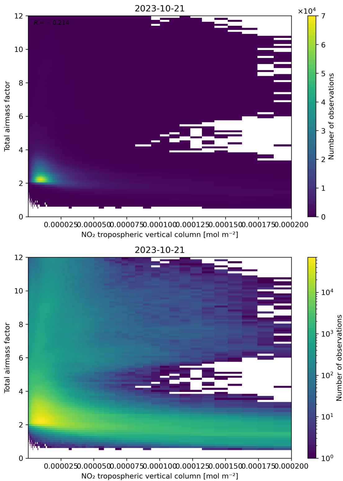
Figure 122: Scatter density plot of “NO 2 tropospheric vertical column” against “Total air mass factor” for 2023-10-20 to 2023-10-22.
