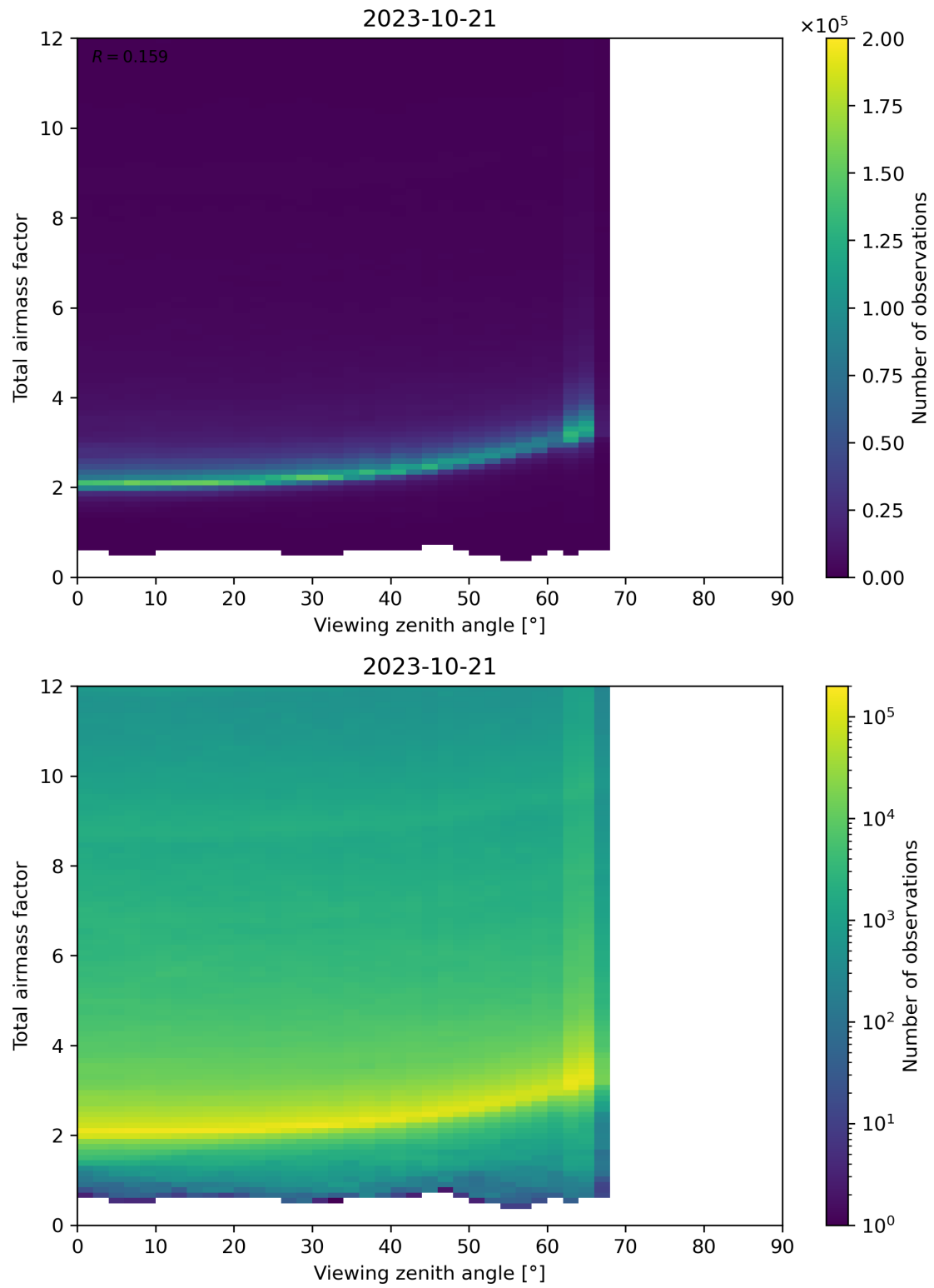
Figure 160: Scatter density plot of “Viewing zenith angle” against “Total airmass factor” for 2023-10-20 to 2023-10-22.
