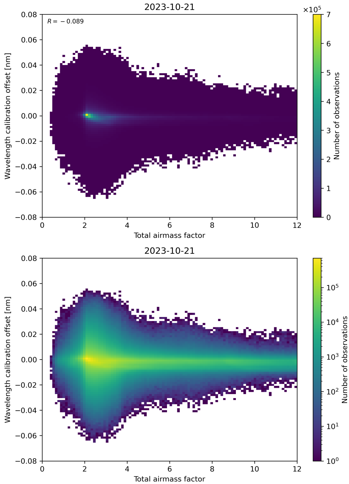
Figure 70: Scatter density plot of “Total airmass factor” against “Wavelength calibration offset” for 2023-10-20 to 2023-10-22.
