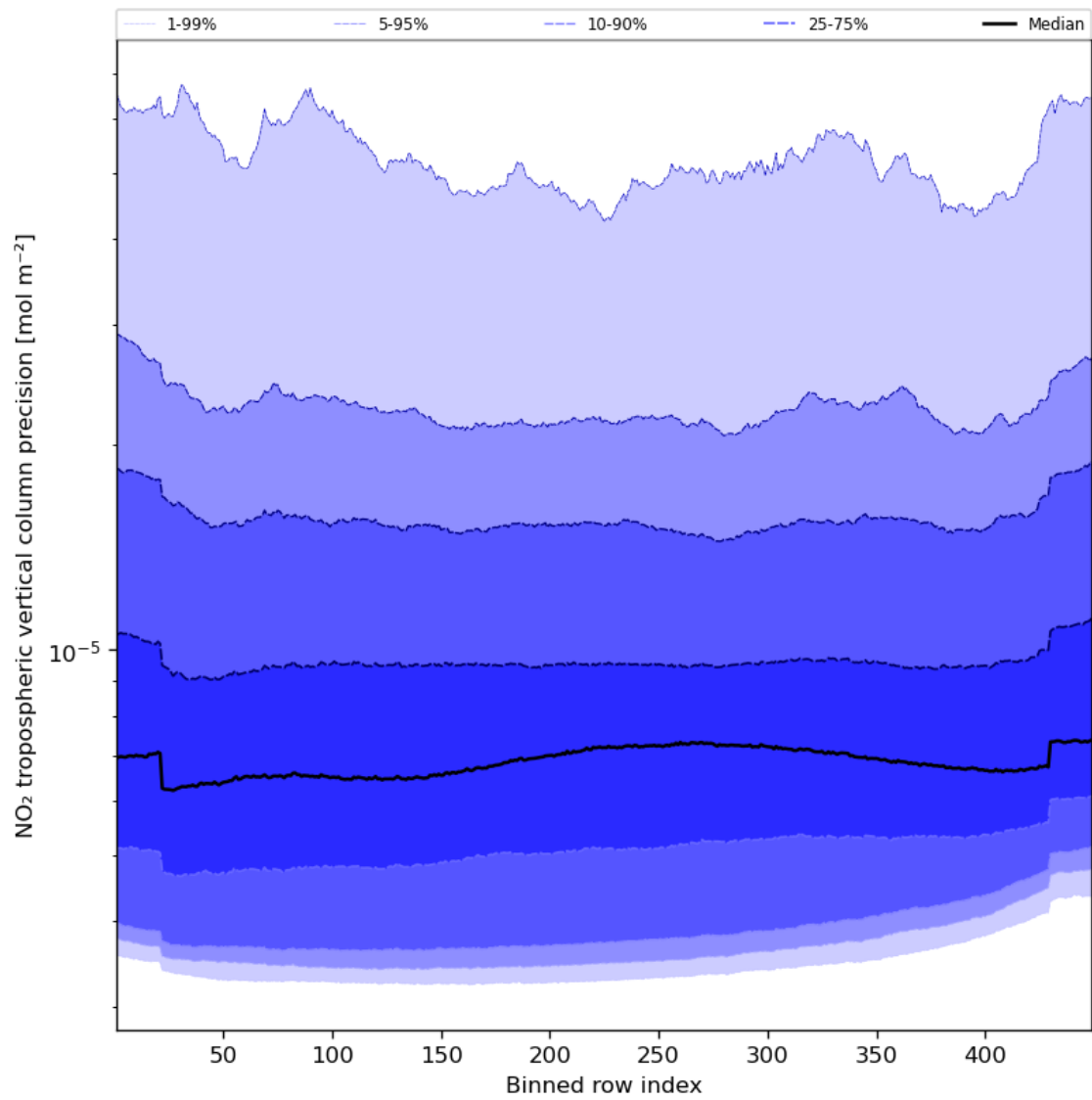
Figure 47: Along track statistics of “NO 2 tropospheric vertical column precision” for 2023-10-20 to 2023-10-22
