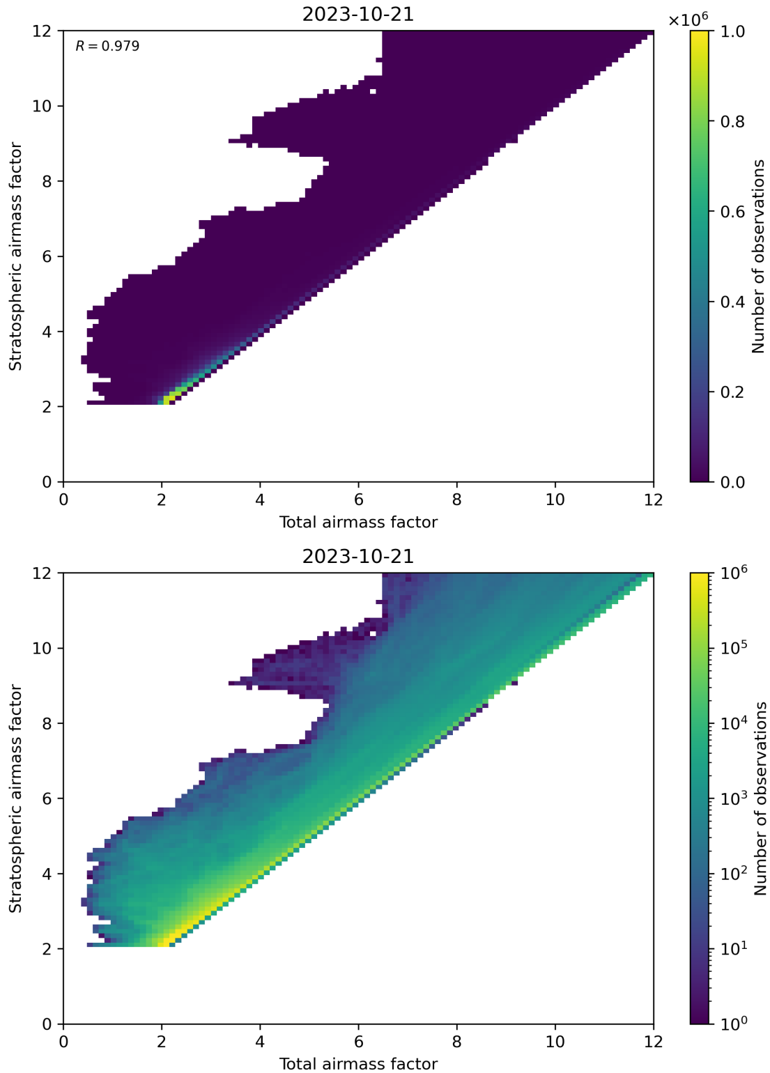
Figure 62: Scatter density plot of “Total airmass factor” against “Stratospheric airmass factor” for 2023-10-20 to 2023-10-22.
