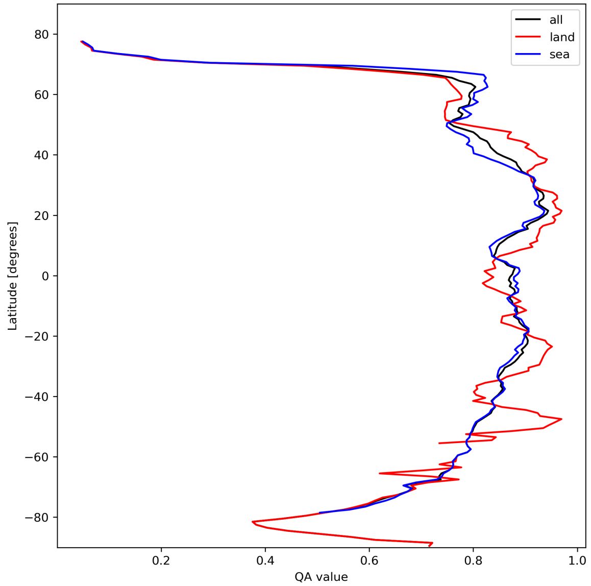
Figure 11: Zonal average of “QA value” for 2023-10-20 to 2023-10-22.
