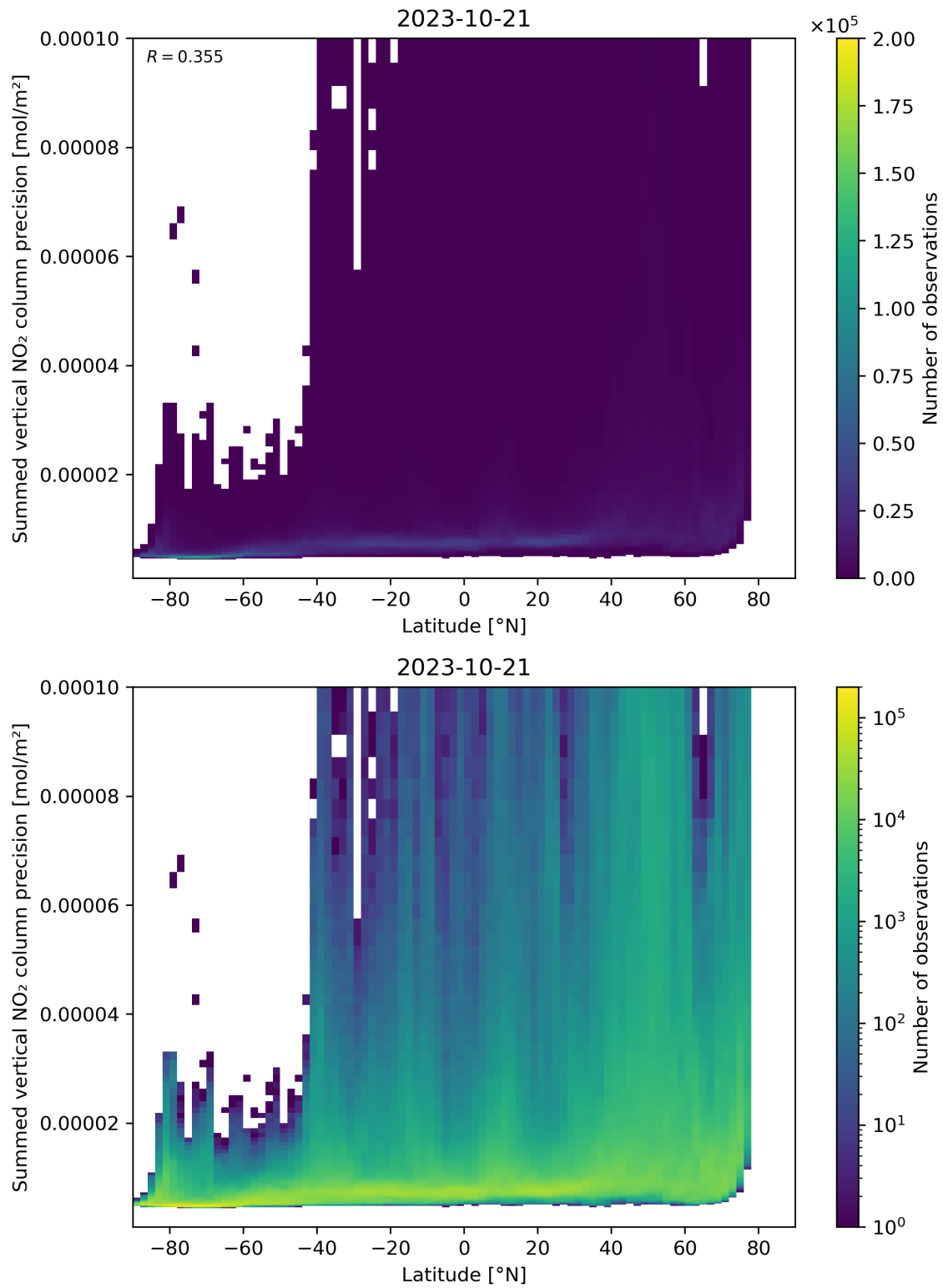
Figure 89: Scatter density plot of “Latitude” against “Summed vertical NO 2 column precision” for 2023-10-20 to 2023-10-22.
