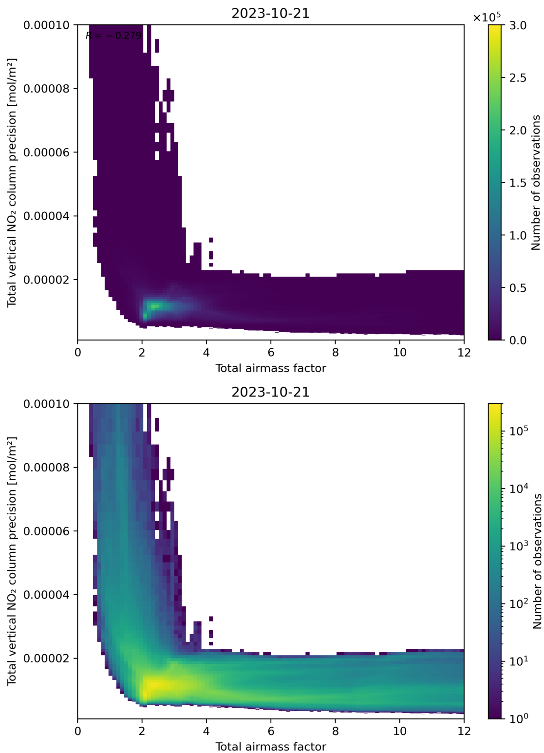
Figure 68: Scatter density plot of “Total airmass factor” against “Total vertical NO 2 column precision” for 2023-10-20 to 2023-10-22.
