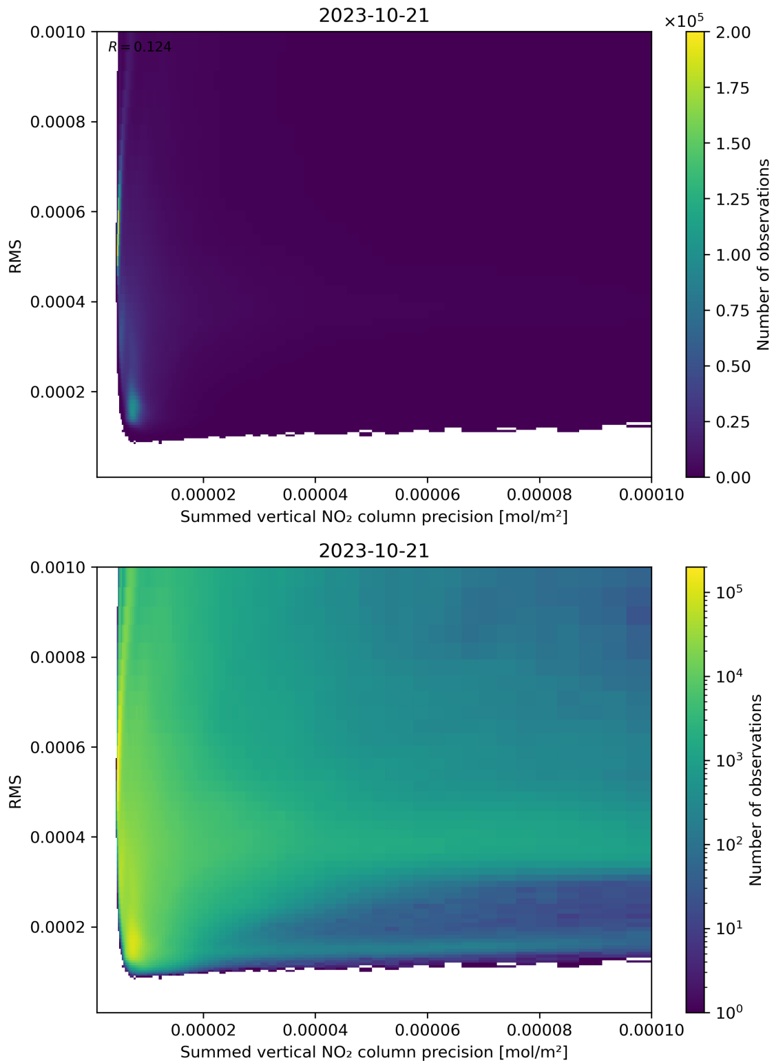
Figure 108: Scatter density plot of “Summed vertical NO 2 column precision” against “RMS” for 2023-10-20 to 2023-10-22.
