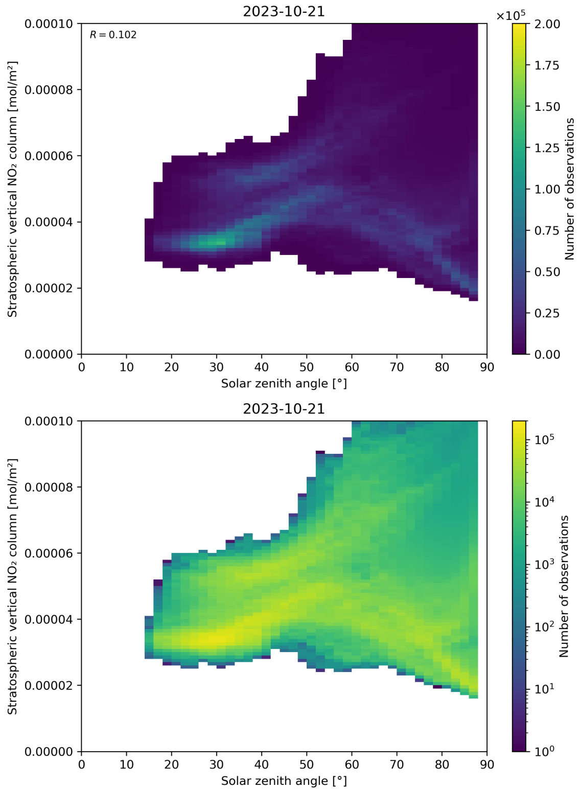
Figure 150: Scatter density plot of “Solar zenith angle” against “Stratospheric vertical NO 2 column” for 2023-10-20 to 2023-10-22.
