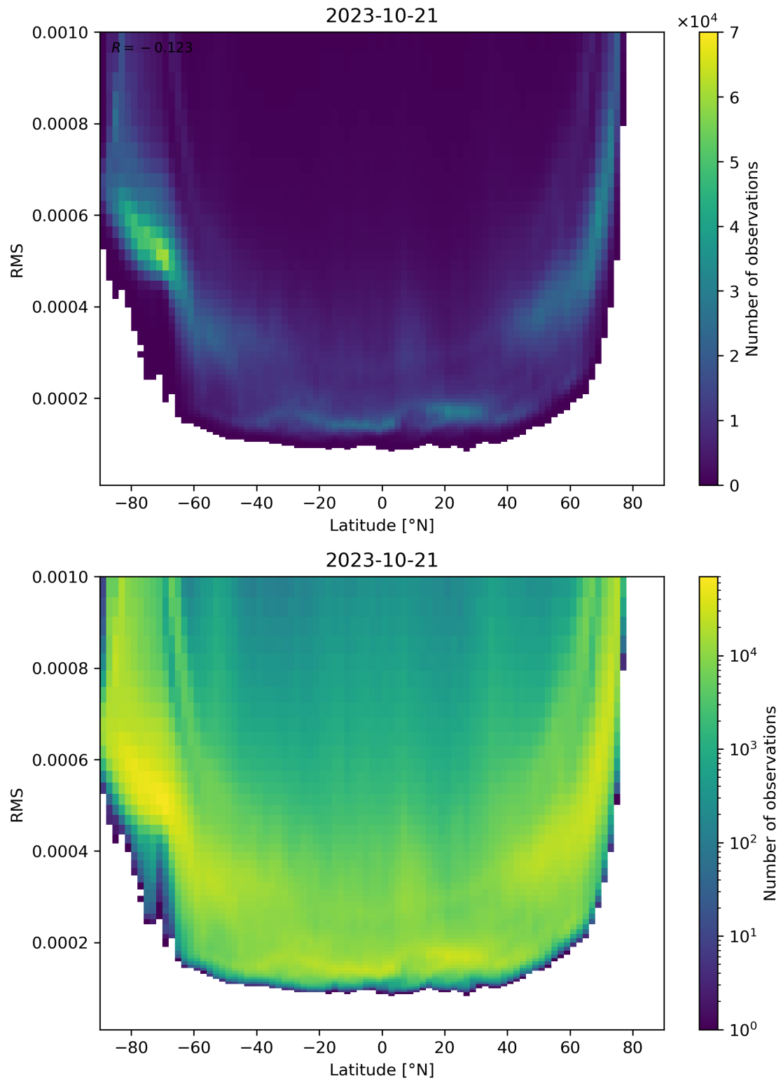
Figure 94: Scatter density plot of “Latitude” against “RMS” for 2023-10-20 to 2023-10-22.
