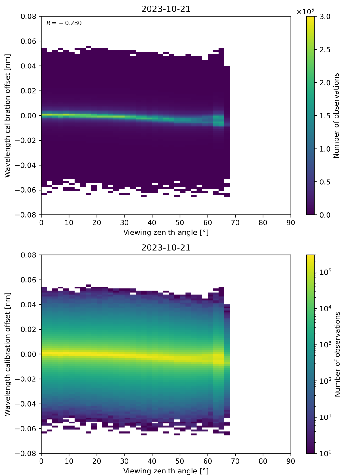
Figure 173: Scatter density plot of “Viewing zenith angle” against “Wavelength calibration offset” for 2023-10-20 to 2023-10-22.
