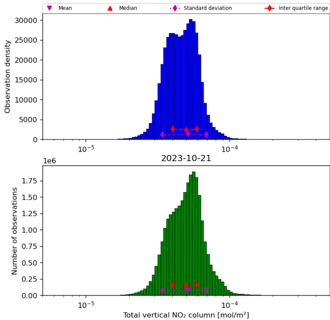
Figure 38: Histogram of “Total vertical NO 2 column” for 2023-10-20 to 2023-10-22
