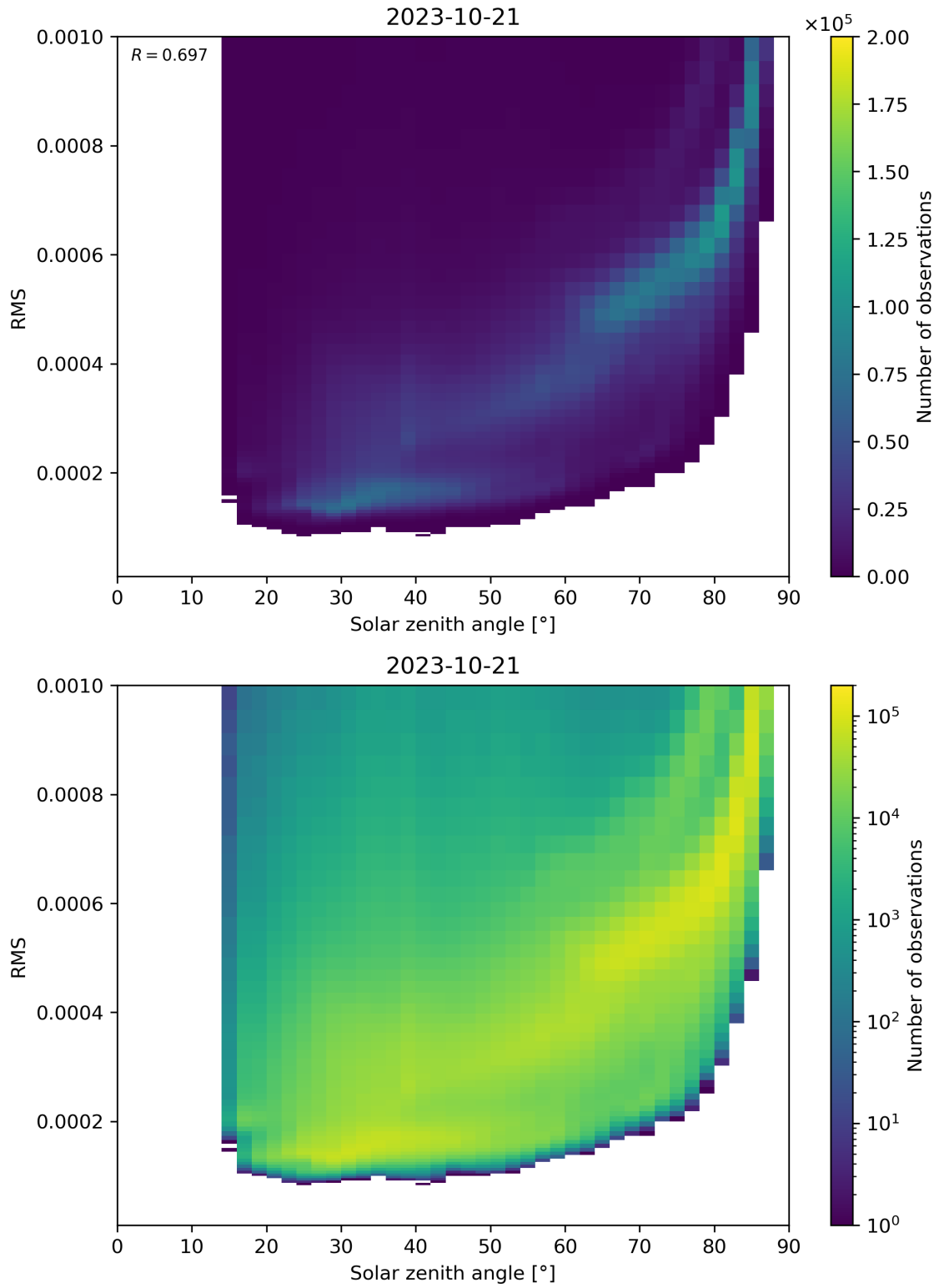
Figure 157: Scatter density plot of “Solar zenith angle” against “RMS” for 2023-10-20 to 2023-10-22.
