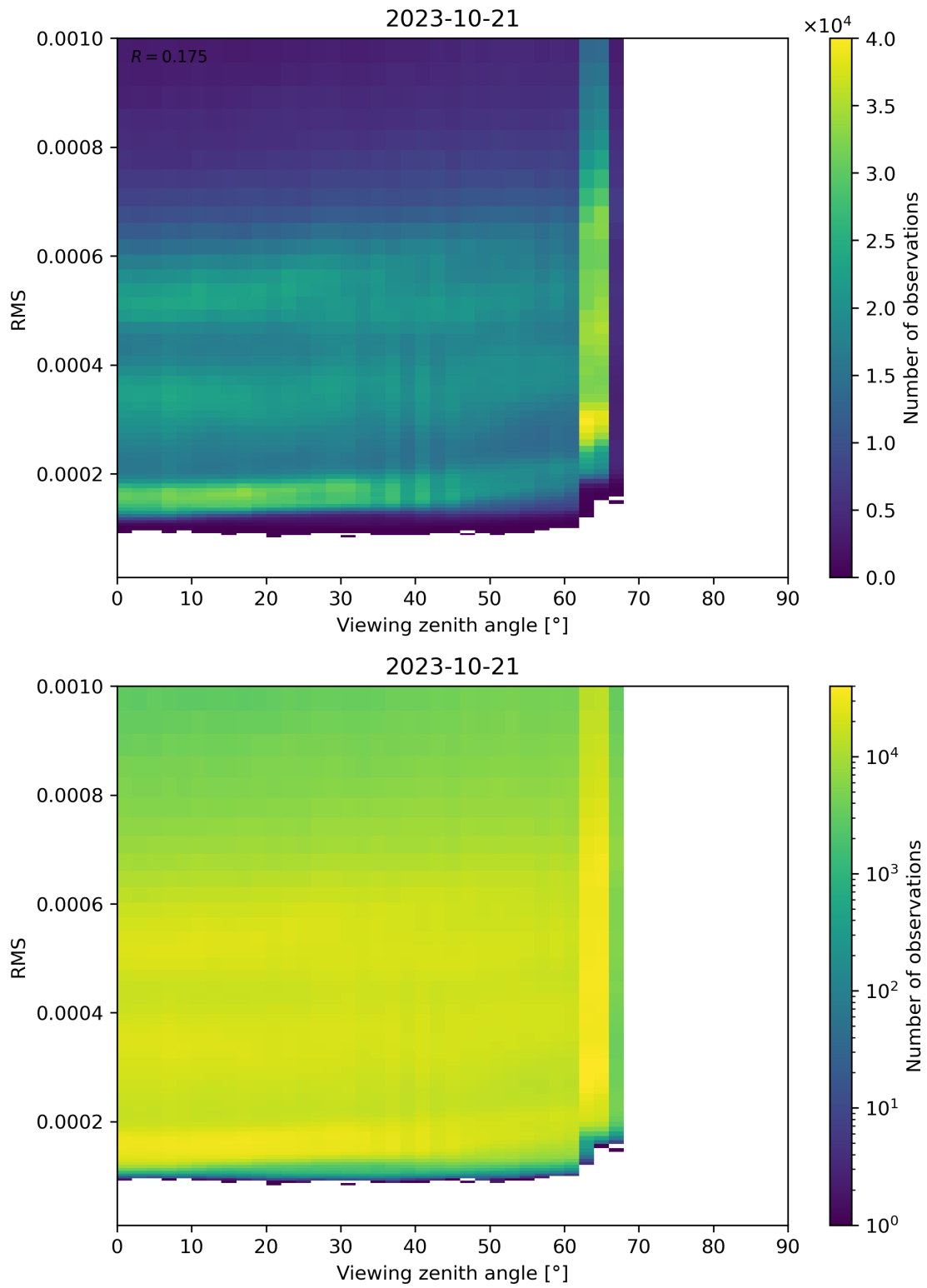
Figure 171: Scatter density plot of “Viewing zenith angle” against “RMS” for 2023-10-20 to 2023-10-22.
