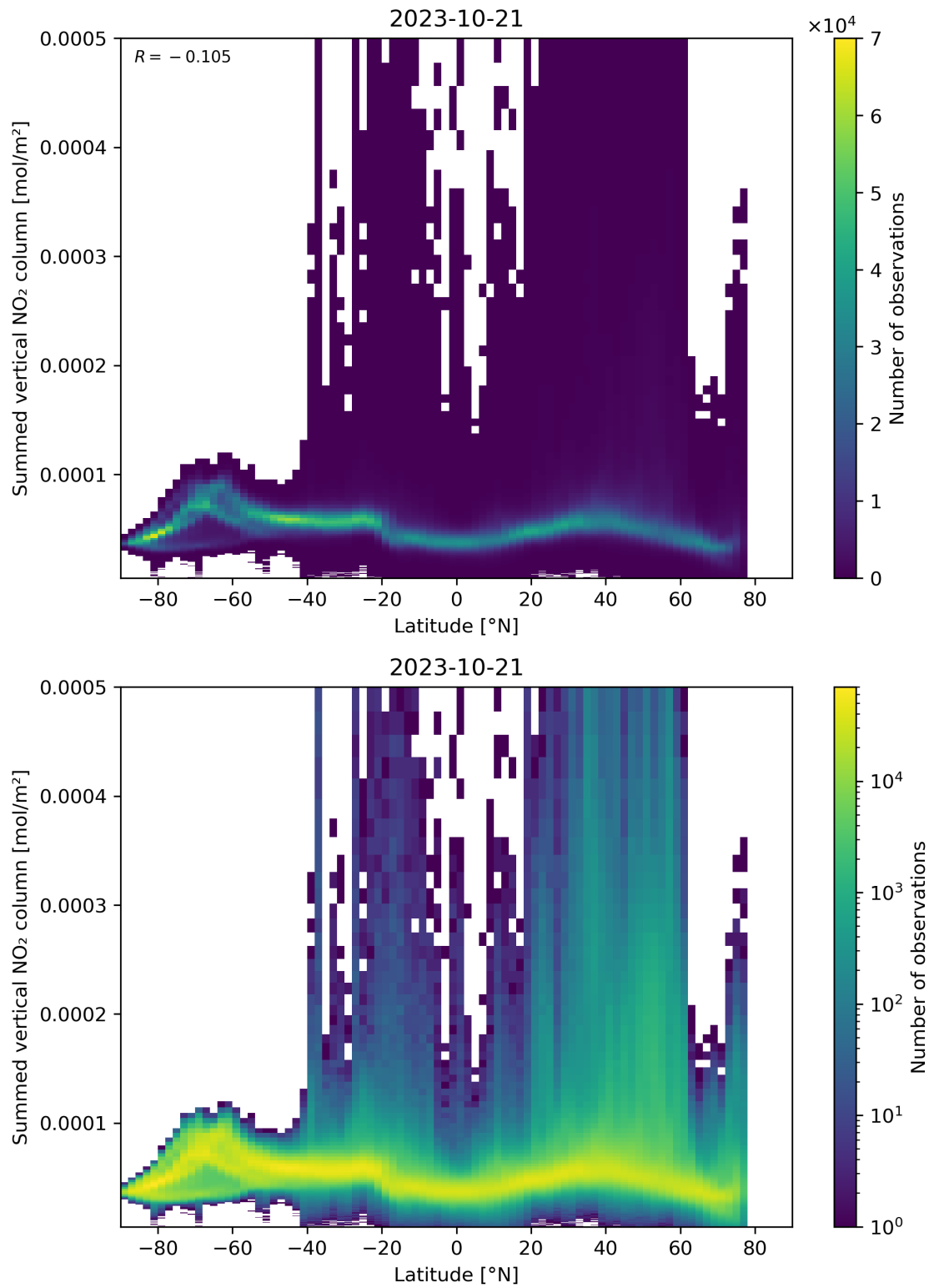
Figure 88: Scatter density plot of “Latitude” against “Summed vertical NO 2 column” for 2023-10-20 to 2023-10-22.
