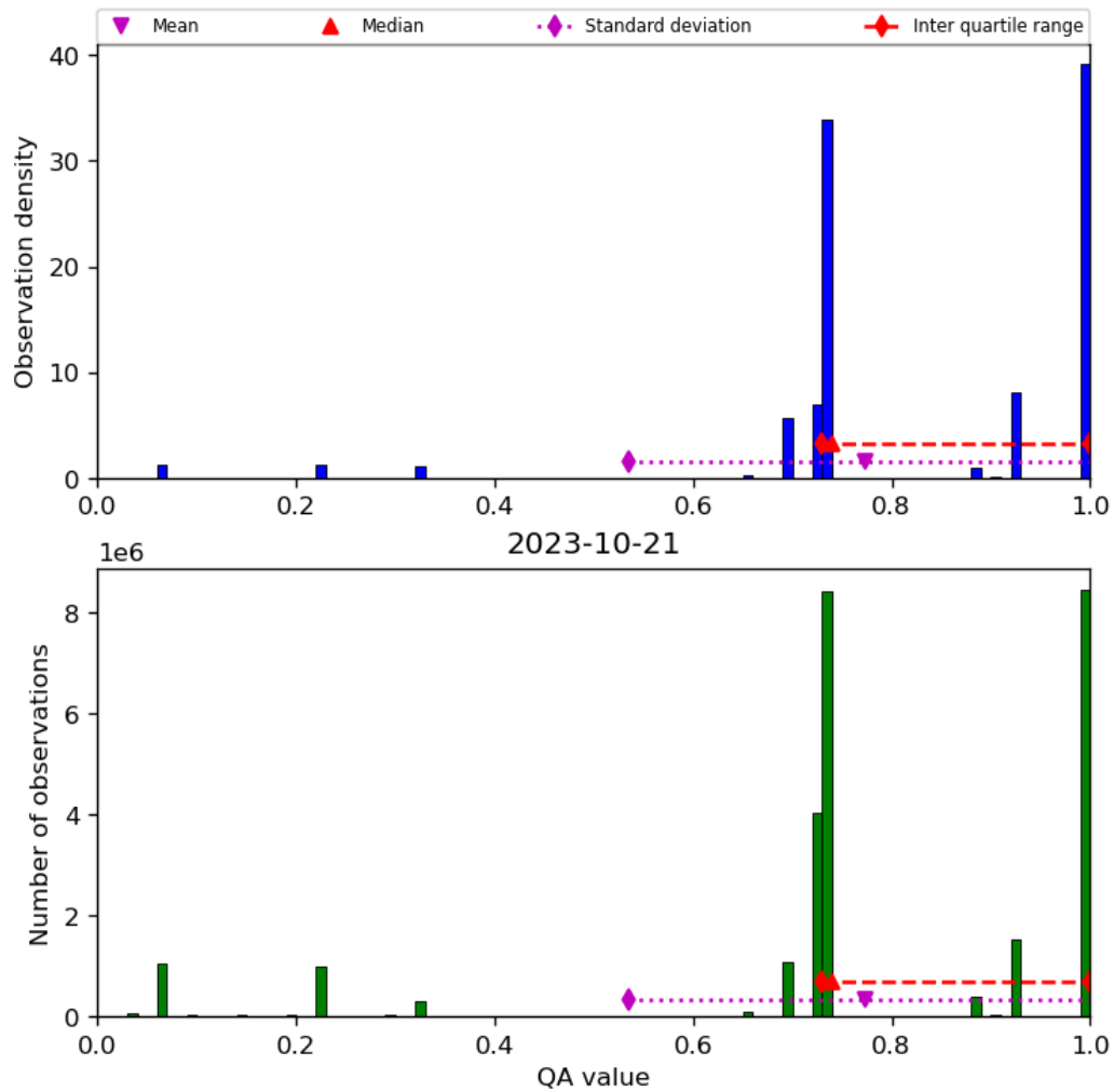
Figure 28: Histogram of “QA value” for 2023-10-20 to 2023-10-22
