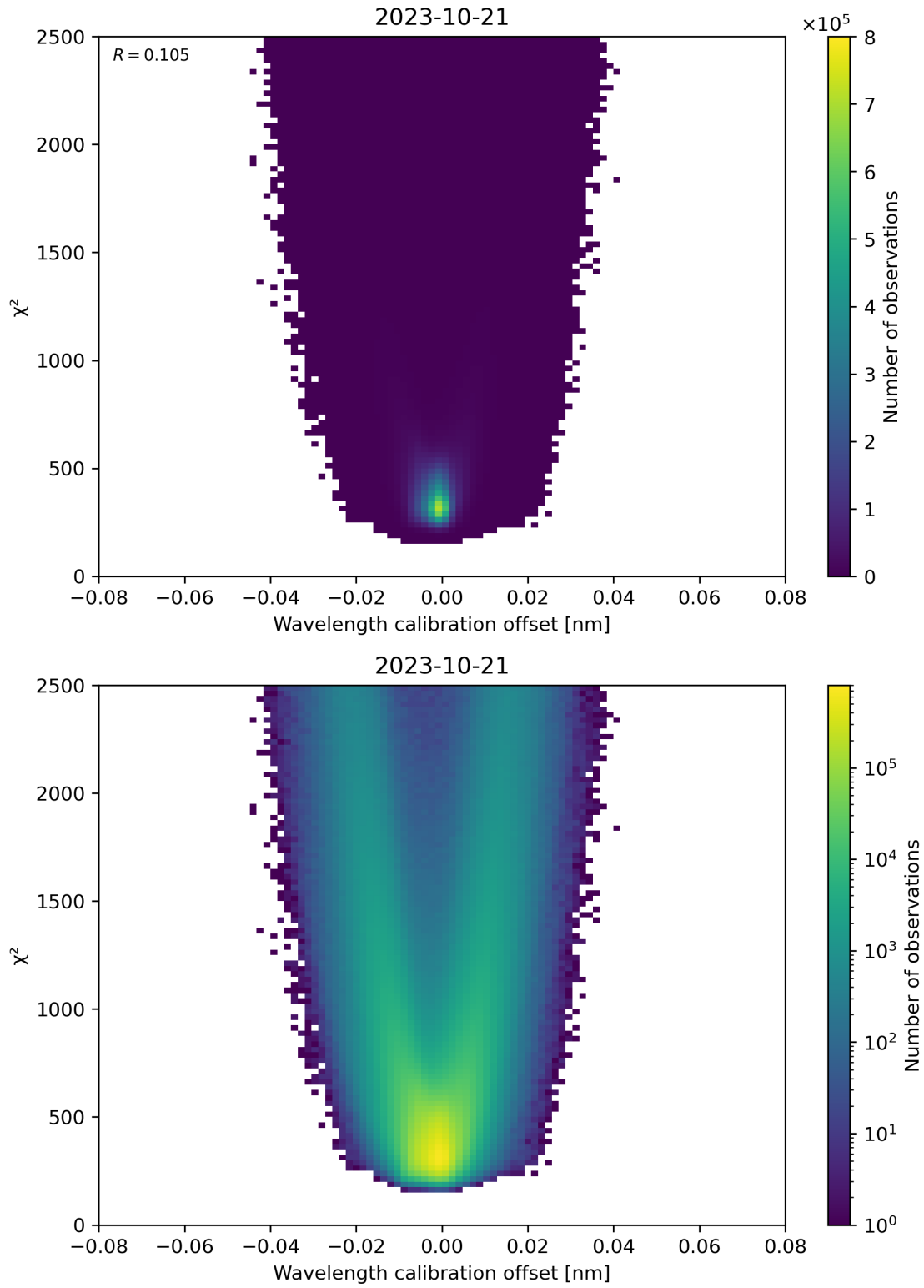
Figure 175: Scatter density plot of “Wavelength calibration offset” against “ \chi^2 ” for 2023-10-20 to 2023-10-22.
