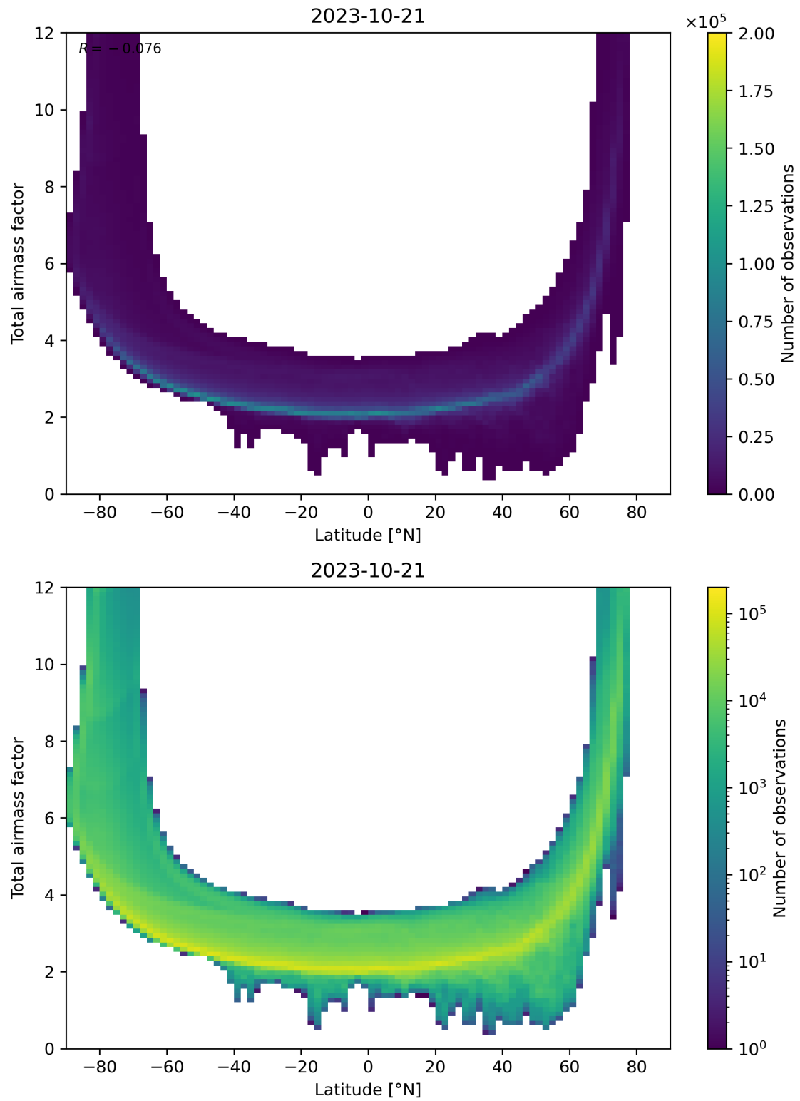
Figure 84: Scatter density plot of “Latitude” against “Total airmass factor” for 2023-10-20 to 2023-10-22.
