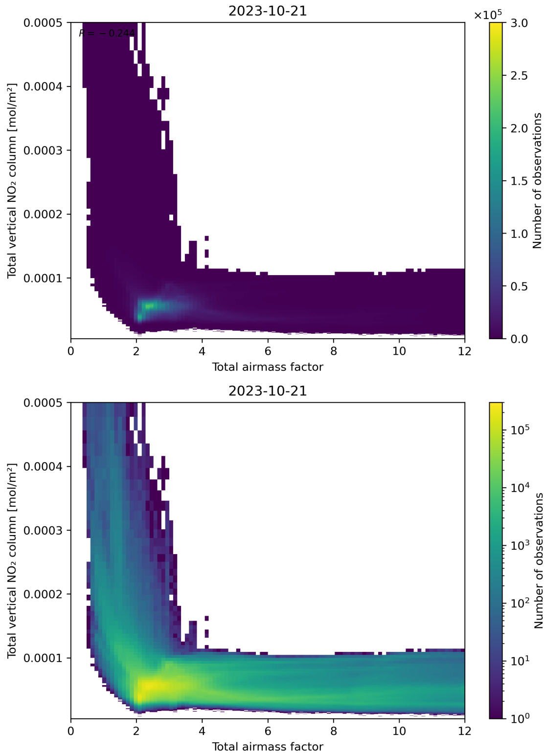
Figure 67: Scatter density plot of “Total airmass factor” against “Total vertical NO 2 column” for 2023-10-20 to 2023-10-22.
