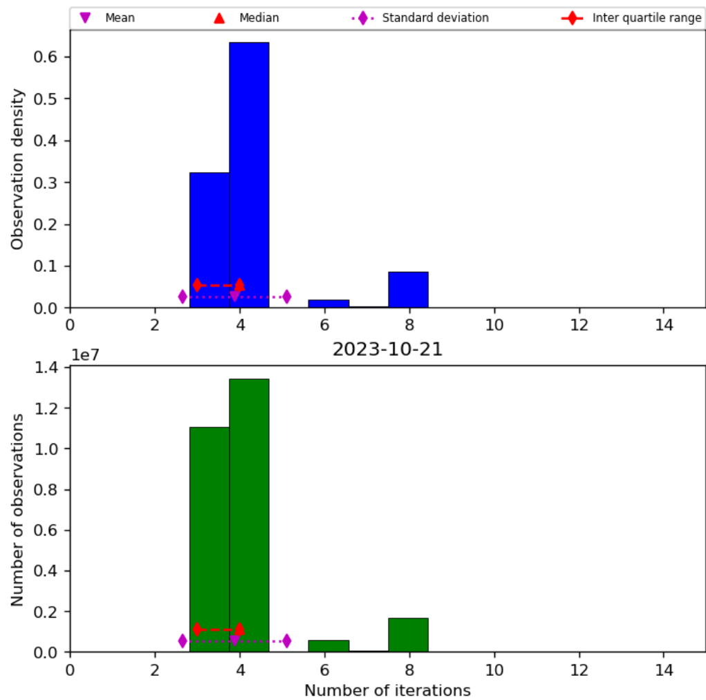
Figure 34: Histogram of “Number of iterations” for 2023-10-20 to 2023-10-22
