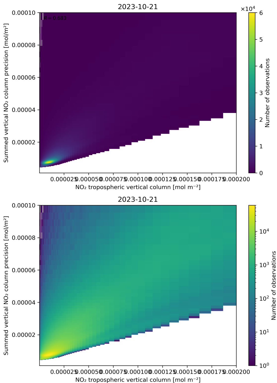
Figure 127: Scatter density plot of “NO 2 tropospheric vertical column” against “Summed vertical NO 2 column precision” for 2023-10-20 to 2023-10-22.
