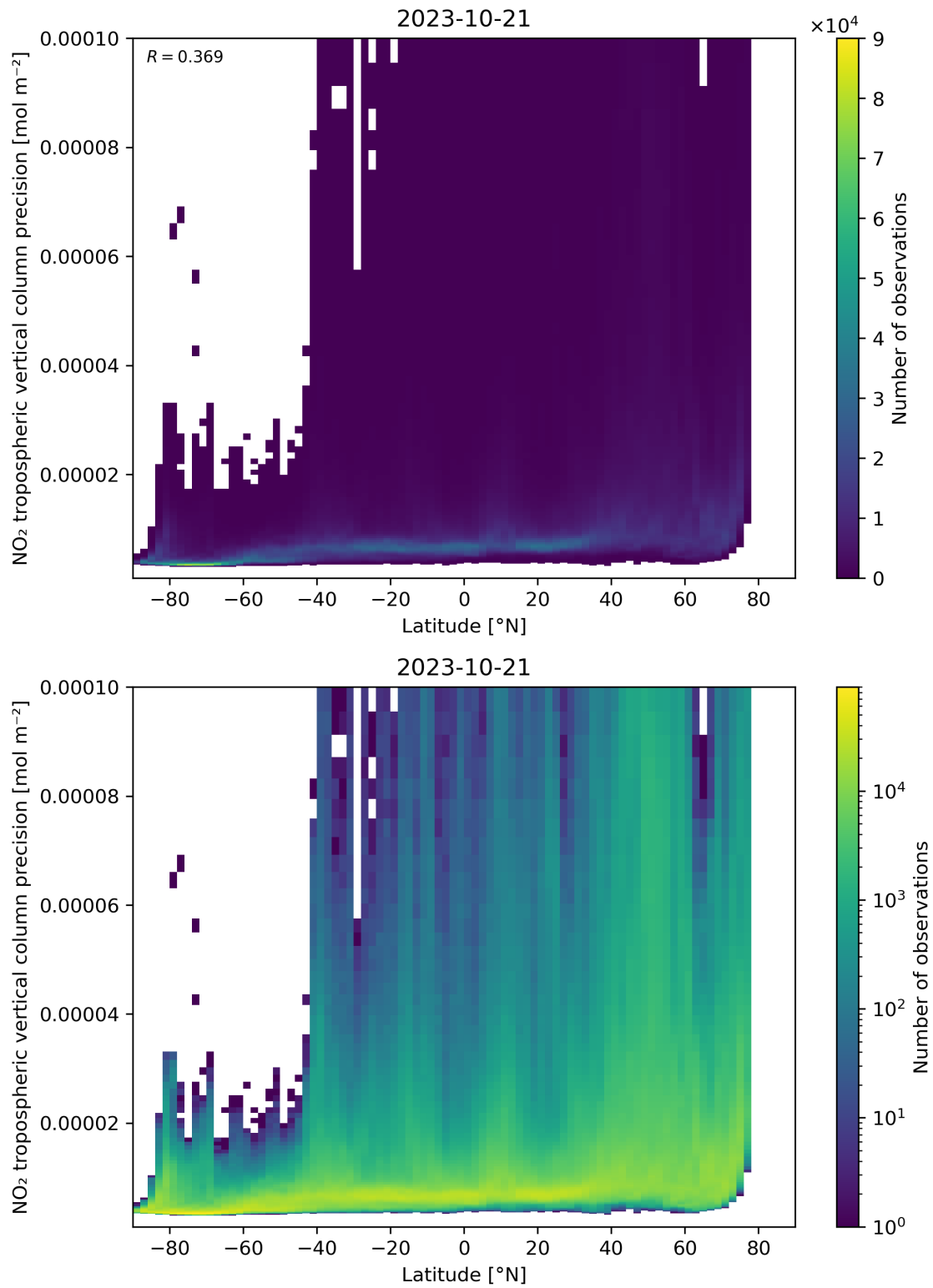
Figure 93: Scatter density plot of “Latitude” against “NO 2 tropospheric vertical column precision” for 2023-10-20 to 2023-10-22.
