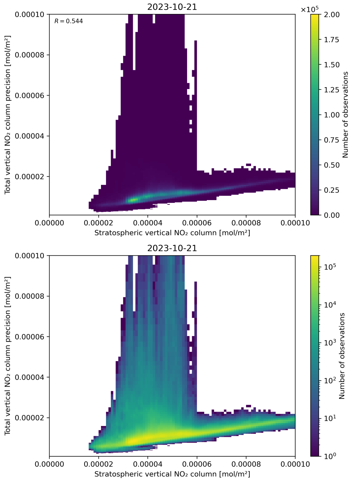
Figure 101: Scatter density plot of “Stratospheric vertical NO 2 column” against “Total vertical NO 2 column precision” for 2023-10-20 to 2023-10-22.
