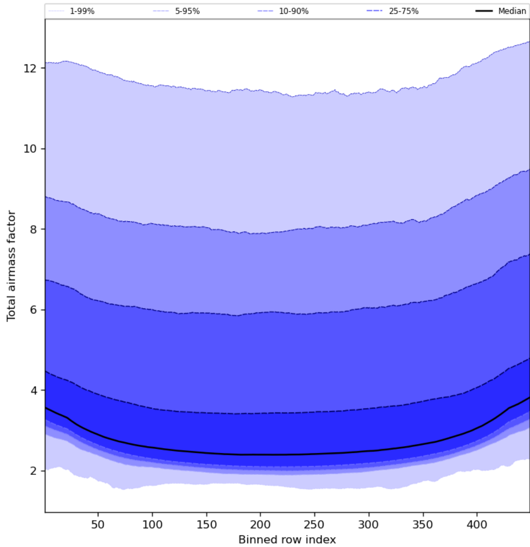
Figure 49: Along track statistics of “Total airmass factor” for 2023-10-20 to 2023-10-22
