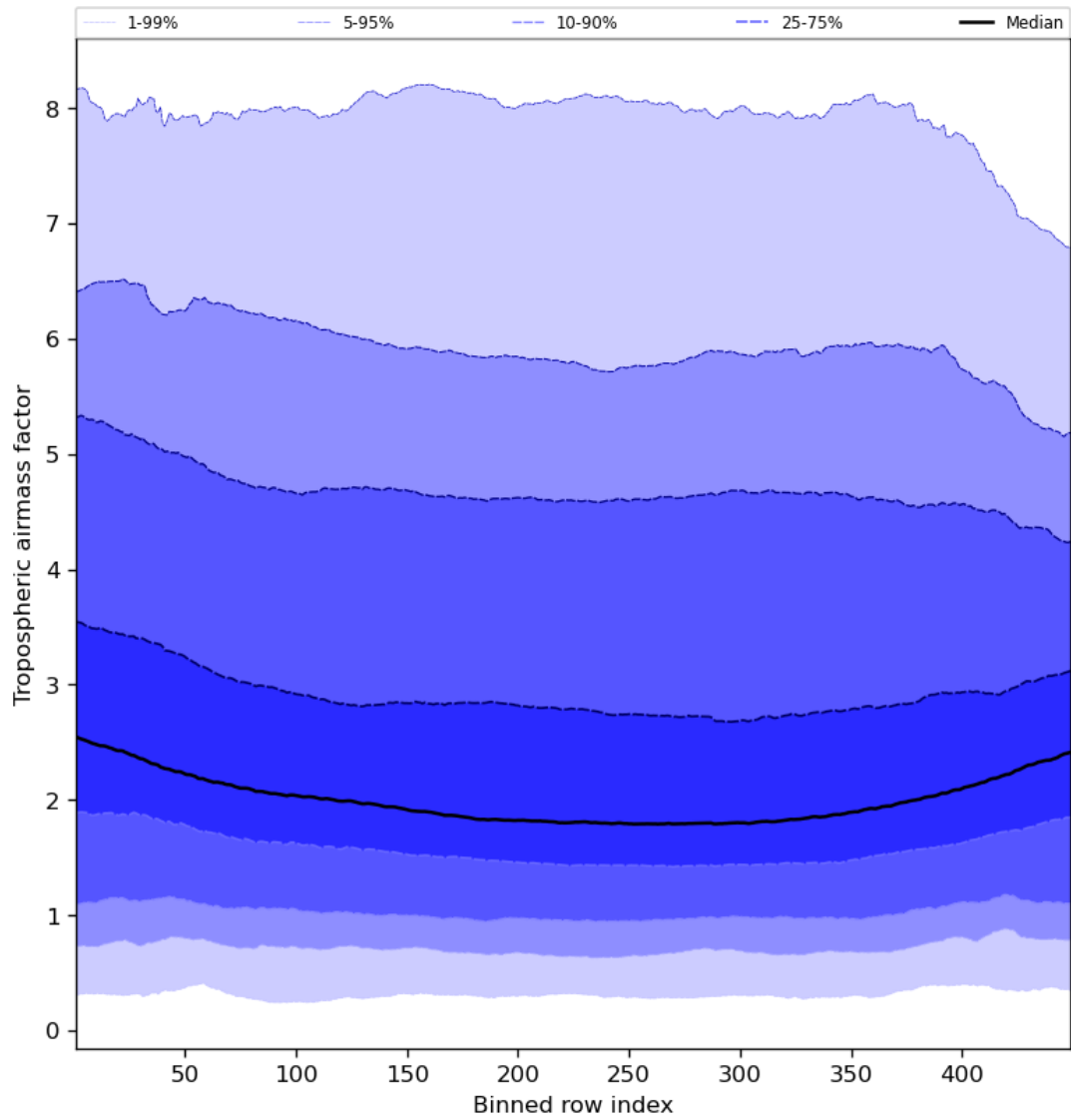
Figure 48: Along track statistics of “Tropospheric air mass factor” for 2023-10-20 to 2023-10-22
