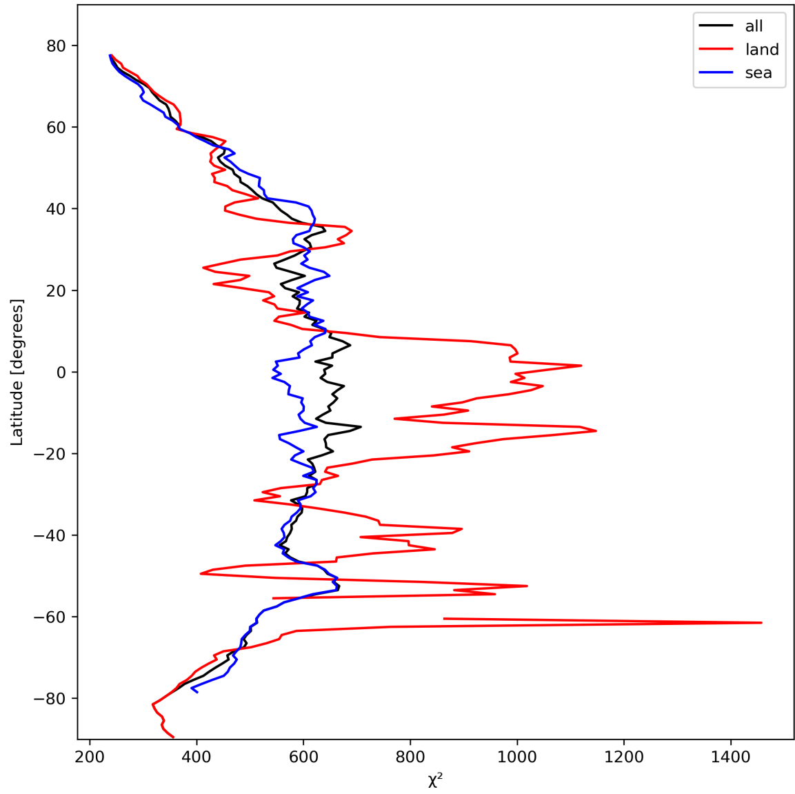
Figure 25: Zonal average of “ \chi^2 ” for 2023-10-20 to 2023-10-22.
