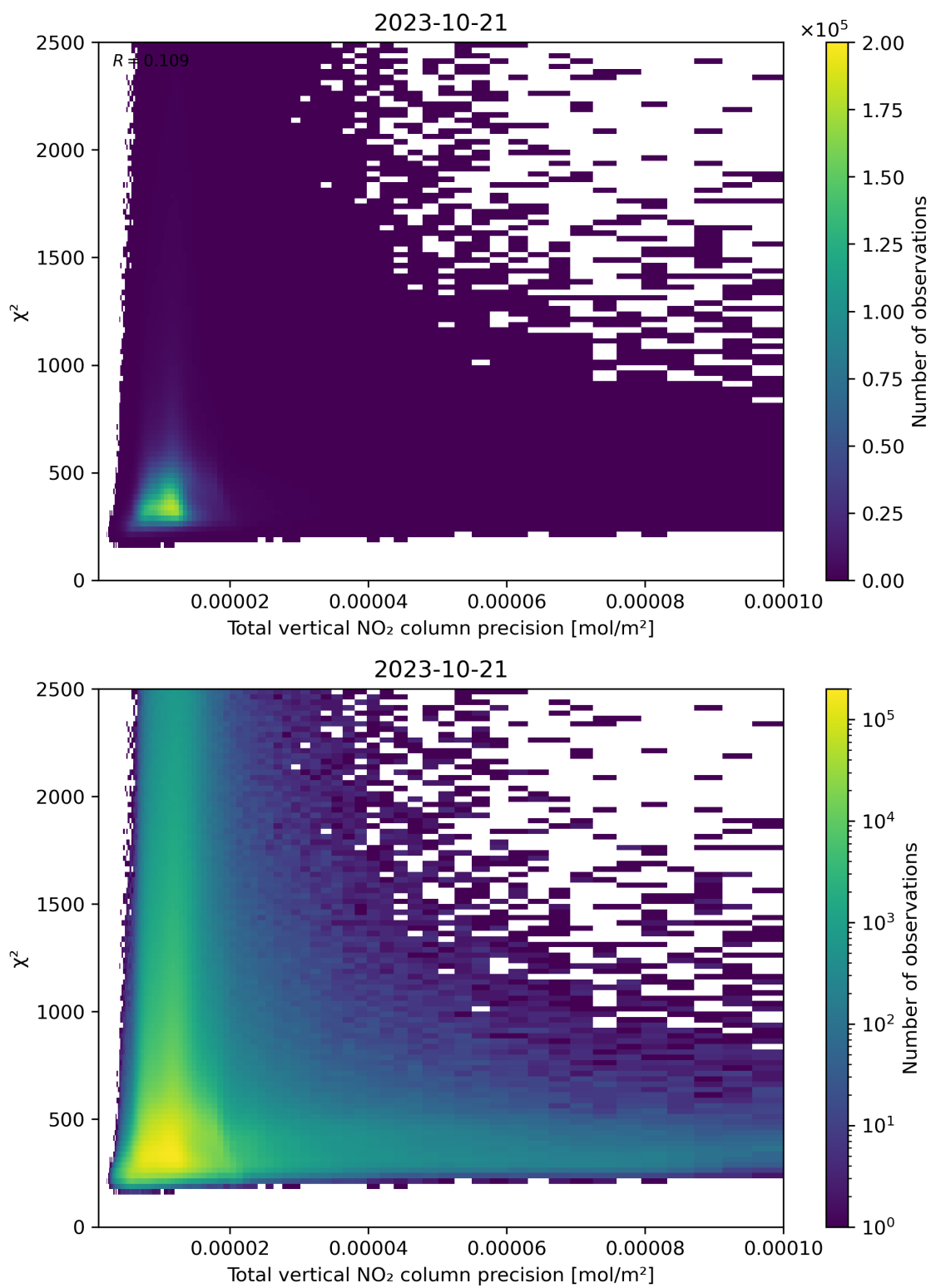
Figure 116: Scatter density plot of “Total vertical NO 2 column precision” against “ \chi^2 ” for 2023-10-20 to 2023-10-22.
