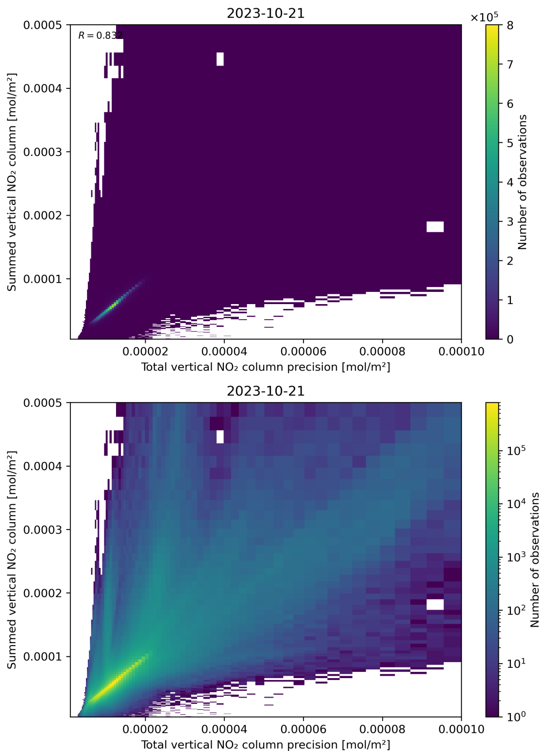
Figure 117: Scatter density plot of “Total vertical NO 2 column precision” against “Summed vertical NO 2 column” for 2023-10-20 to 2023-10-22.
