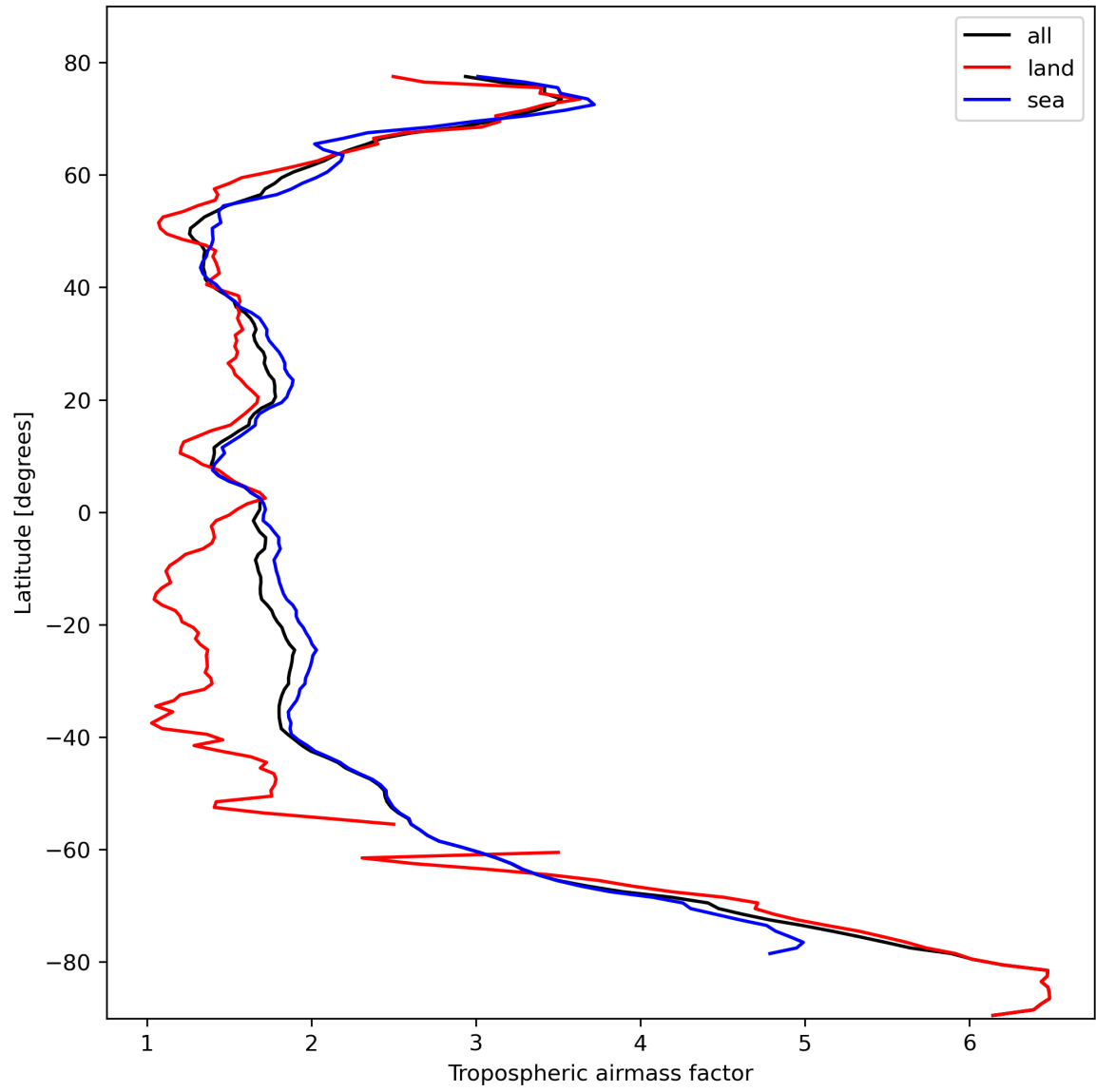
Figure 14: Zonal average of “Tropospheric airmass factor” for 2023-10-20 to 2023-10-22.
