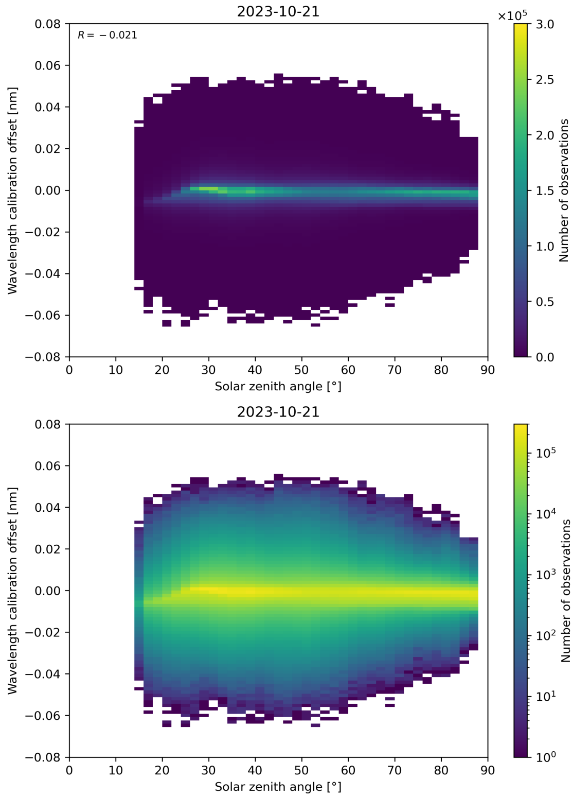
Figure 158: Scatter density plot of “Solar zenith angle” against “Wavelength calibration offset” for 2023-10-20 to 2023-10-22.
