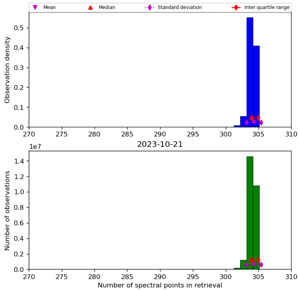
Figure 33: Histogram of “Number of spectral points in retrieval” for 2023-10-20 to 2023-10-22
