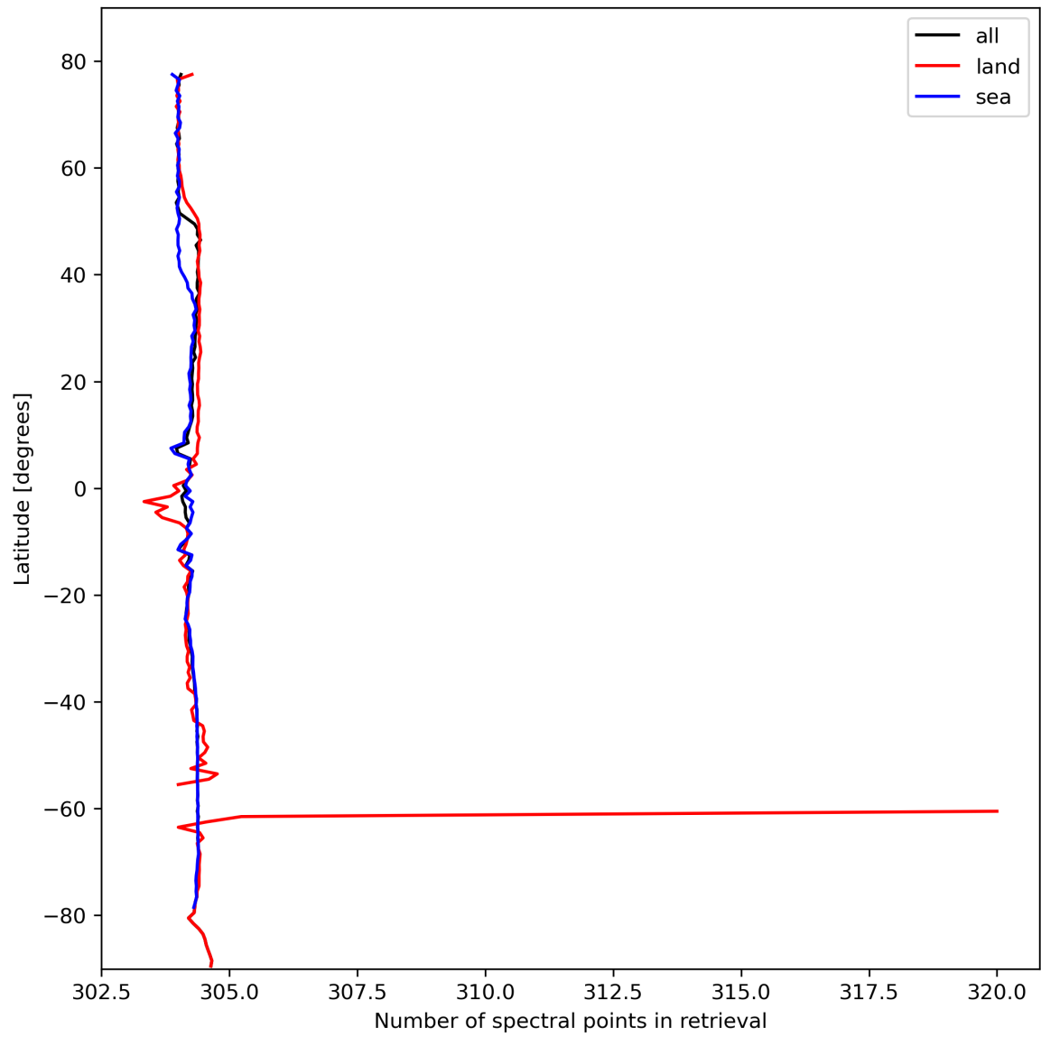
Figure 16: Zonal average of “Number of spectral points in retrieval” for 2023-10-20 to 2023-10-22.
