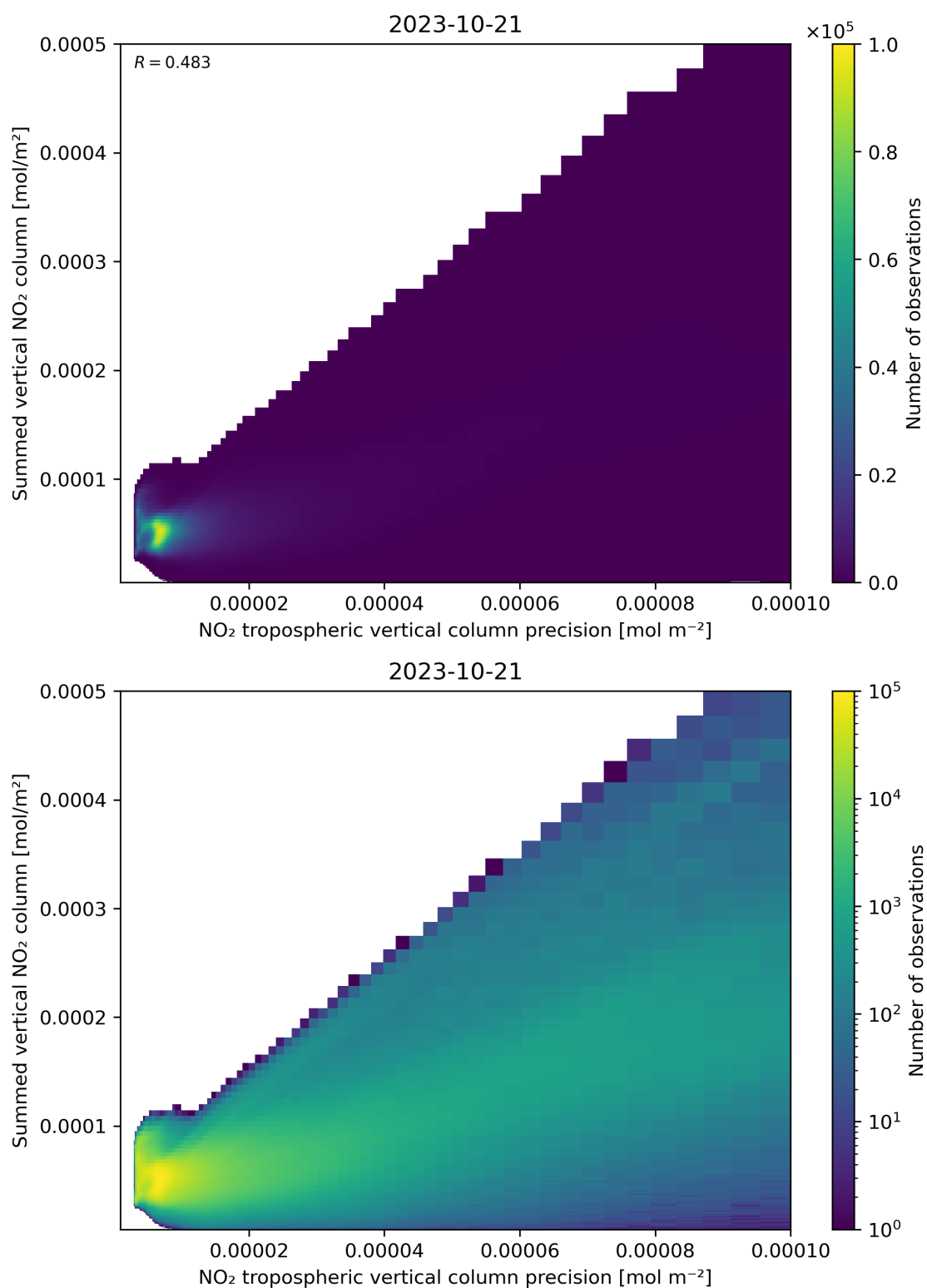
Figure 136: Scatter density plot of “NO 2 tropospheric vertical column precision” against “Summed vertical NO 2 column” for 2023-10-20 to 2023-10-22.
