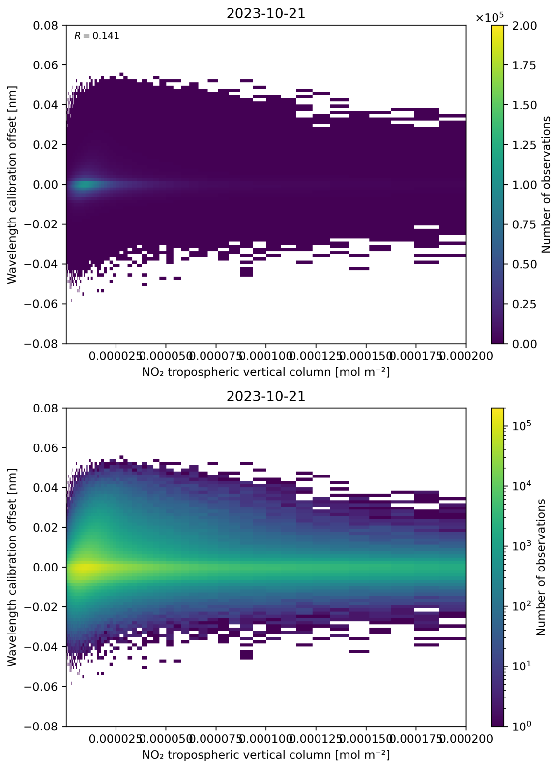
Figure 143: Scatter density plot of “NO 2 tropospheric vertical column” against “Wavelength calibration offset” for 2023-10-20 to 2023-10-22.
