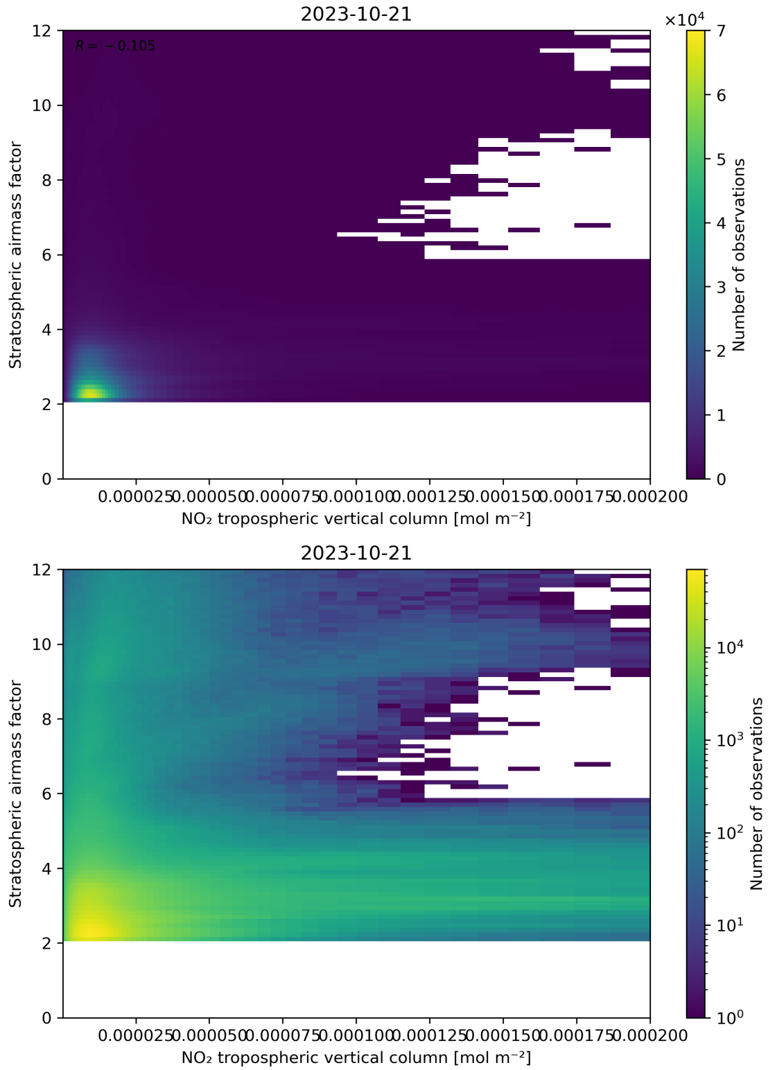
Figure 121: Scatter density plot of “NO 2 tropospheric vertical column” against “Stratospheric air mass factor” for 2023-10-20 to 2023-10-22.
