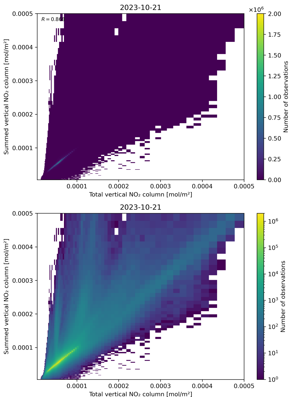
Figure 112: Scatter density plot of “Total vertical NO 2 column” against “Summed vertical NO 2 column” for 2023-10-20 to 2023-10-22.
