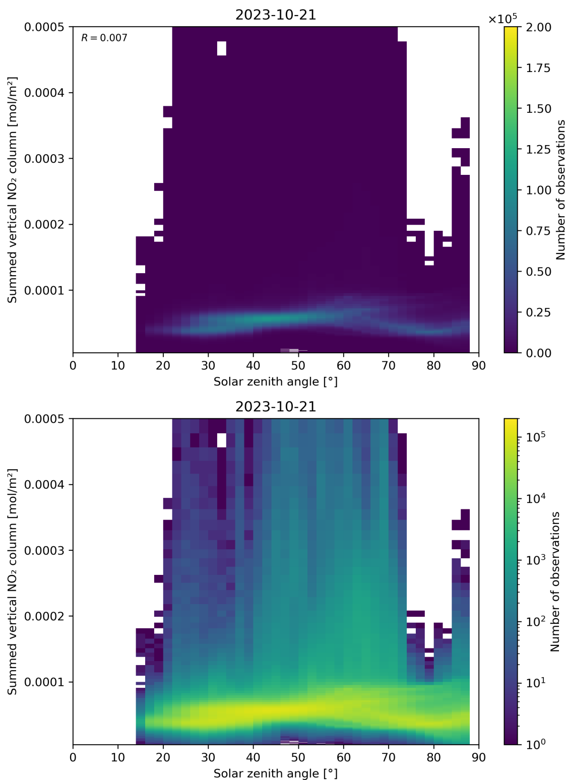
Figure 151: Scatter density plot of “Solar zenith angle” against “Summed vertical NO 2 column” for 2023-10-20 to 2023-10-22.
