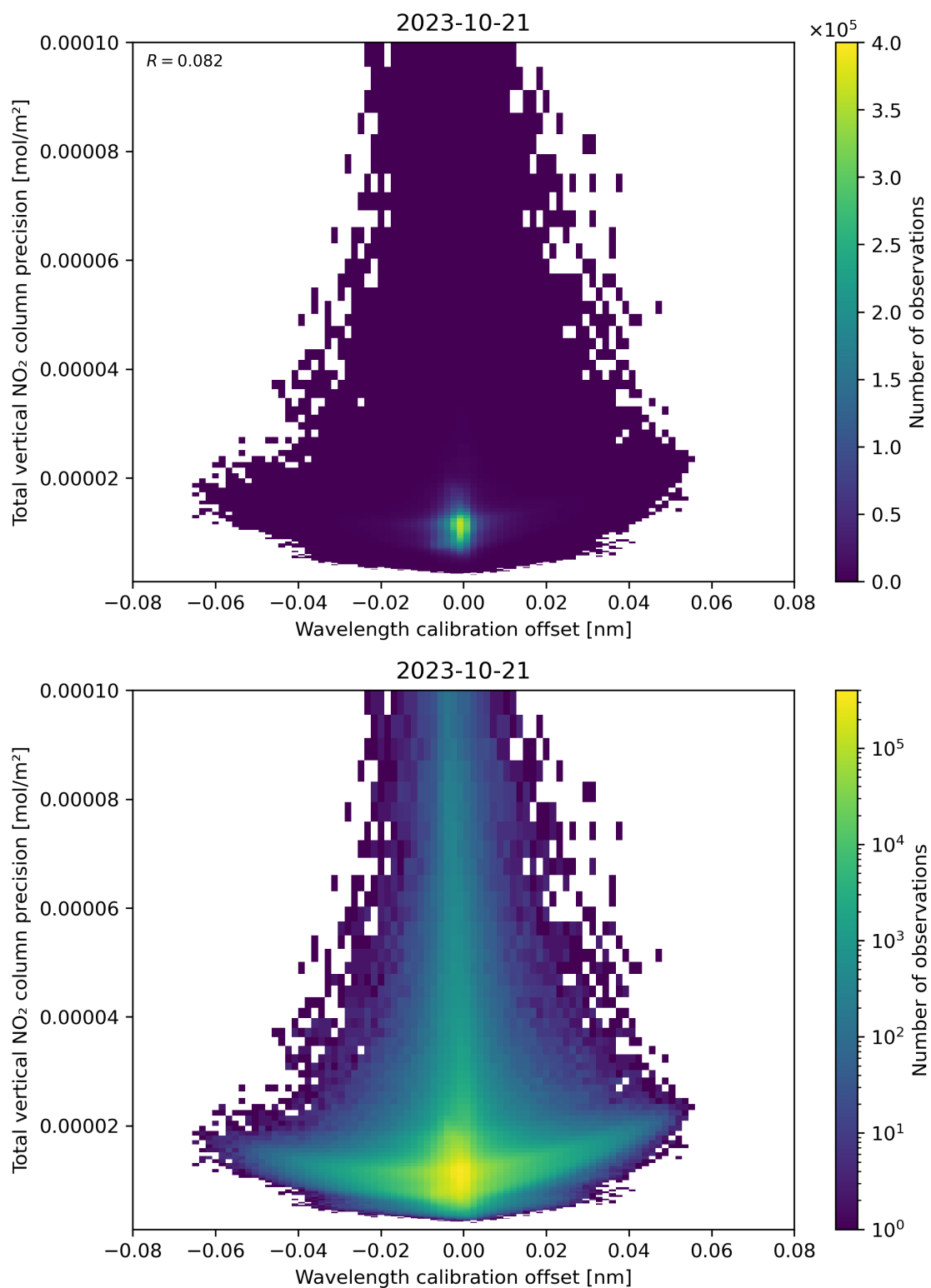
Figure 180: Scatter density plot of “Wavelength calibration offset” against “Total vertical NO 2 column precision” for 2023-10-20 to 2023-10-22.
