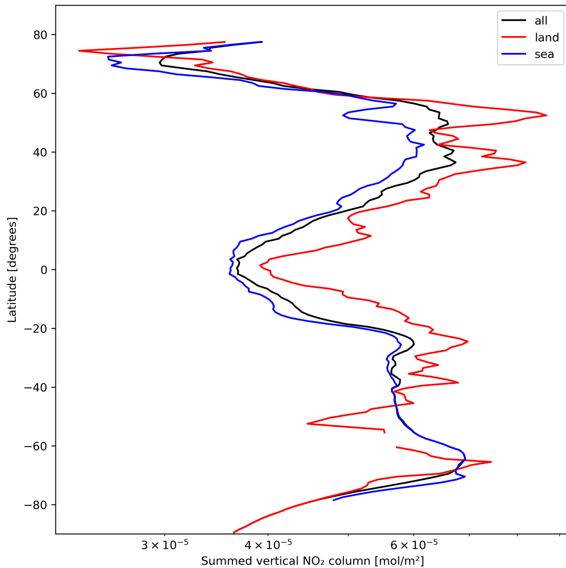
Figure 23: Zonal average of “Summed vertical NO 2 column” for 2023-10-20 to 2023-10-22.
