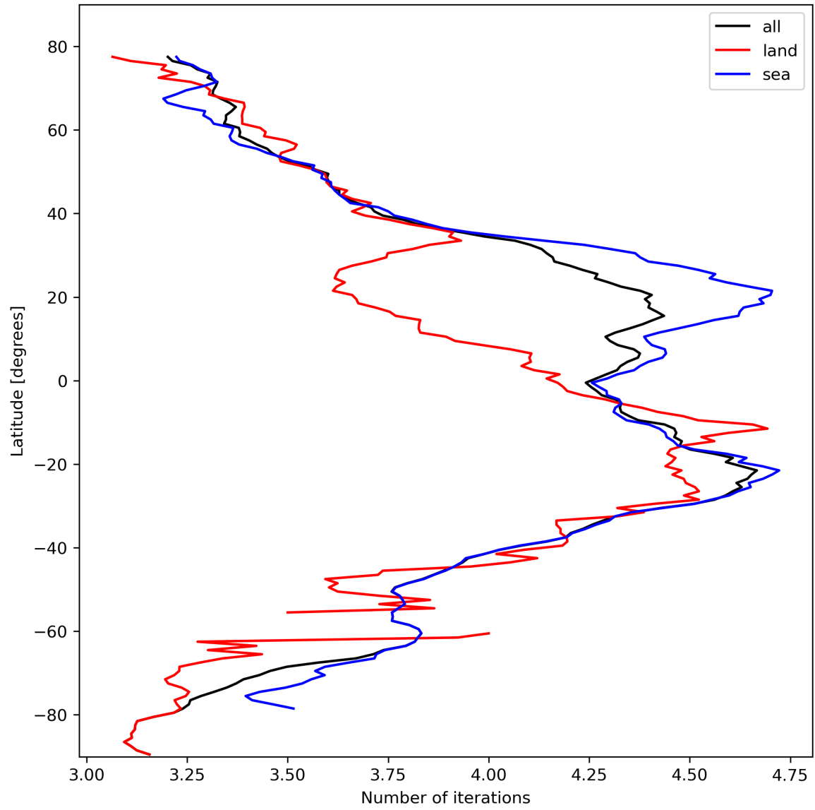
Figure 17: Zonal average of “Number of iterations” for 2023-10-20 to 2023-10-22.
