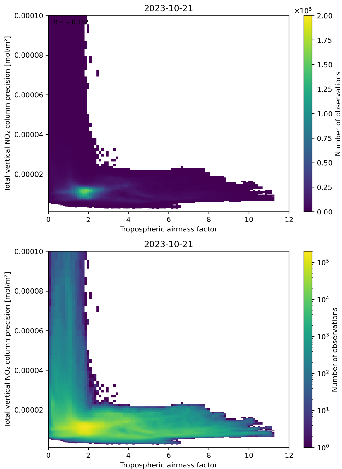
Figure 78: Scatter density plot of “Tropospheric air mass factor” against “Total vertical NO 2 column precision” for 2023-10-20 to 2023-10-22.
