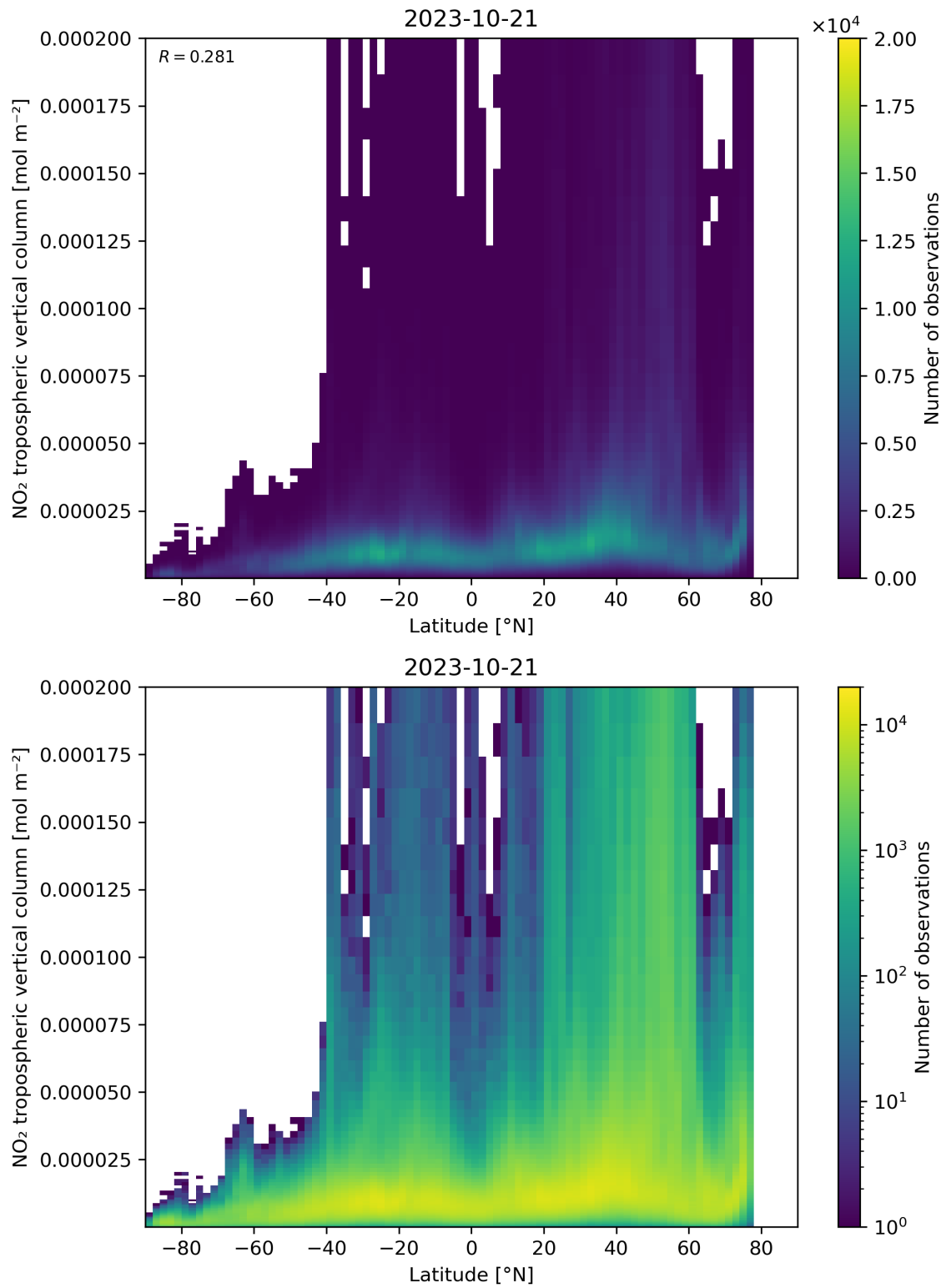
Figure 92: Scatter density plot of “Latitude” against “NO 2 tropospheric vertical column” for 2023-10-20 to 2023-10-22.
