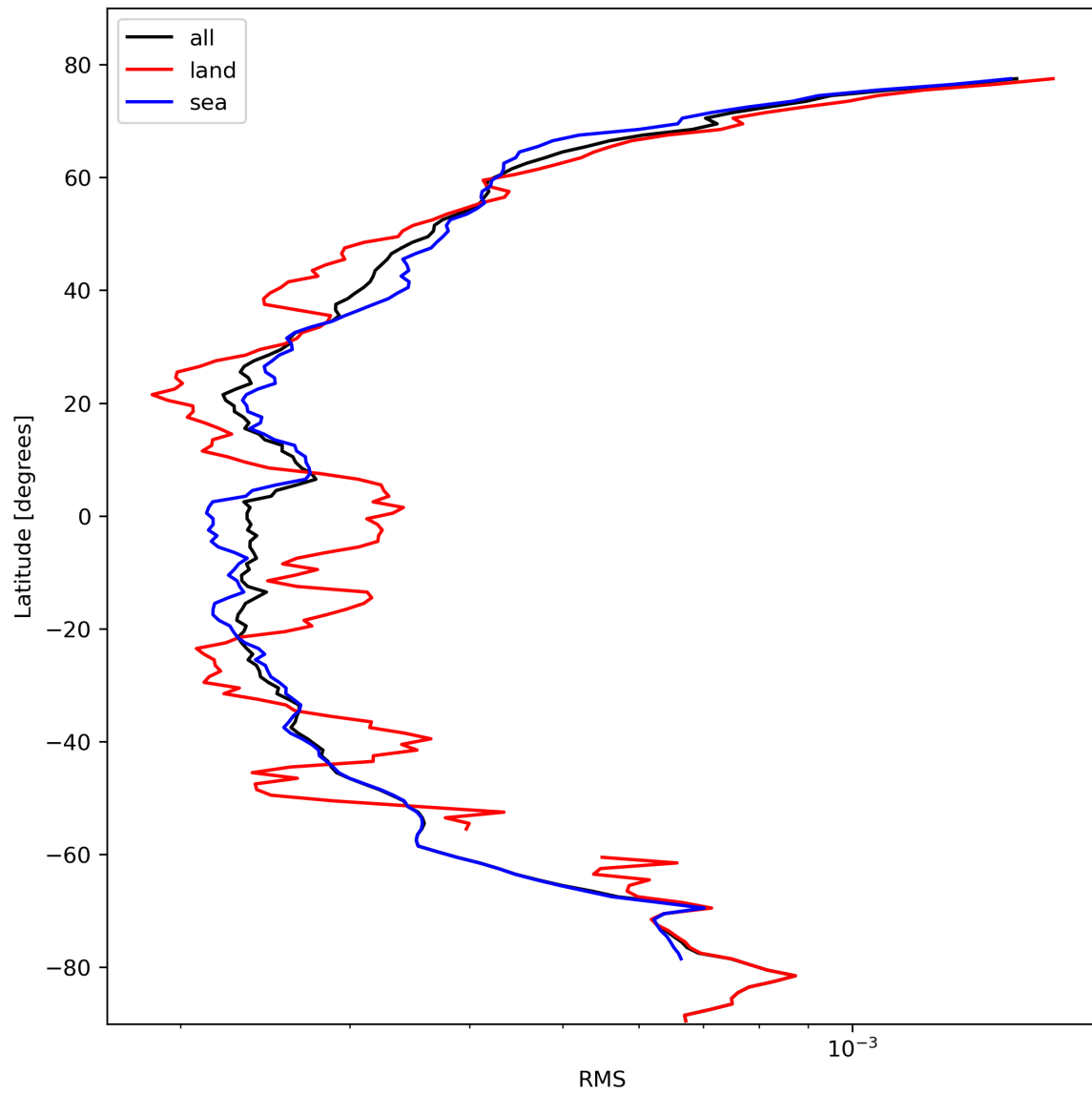
Figure 26: Zonal average of “RMS” for 2023-10-20 to 2023-10-22.
