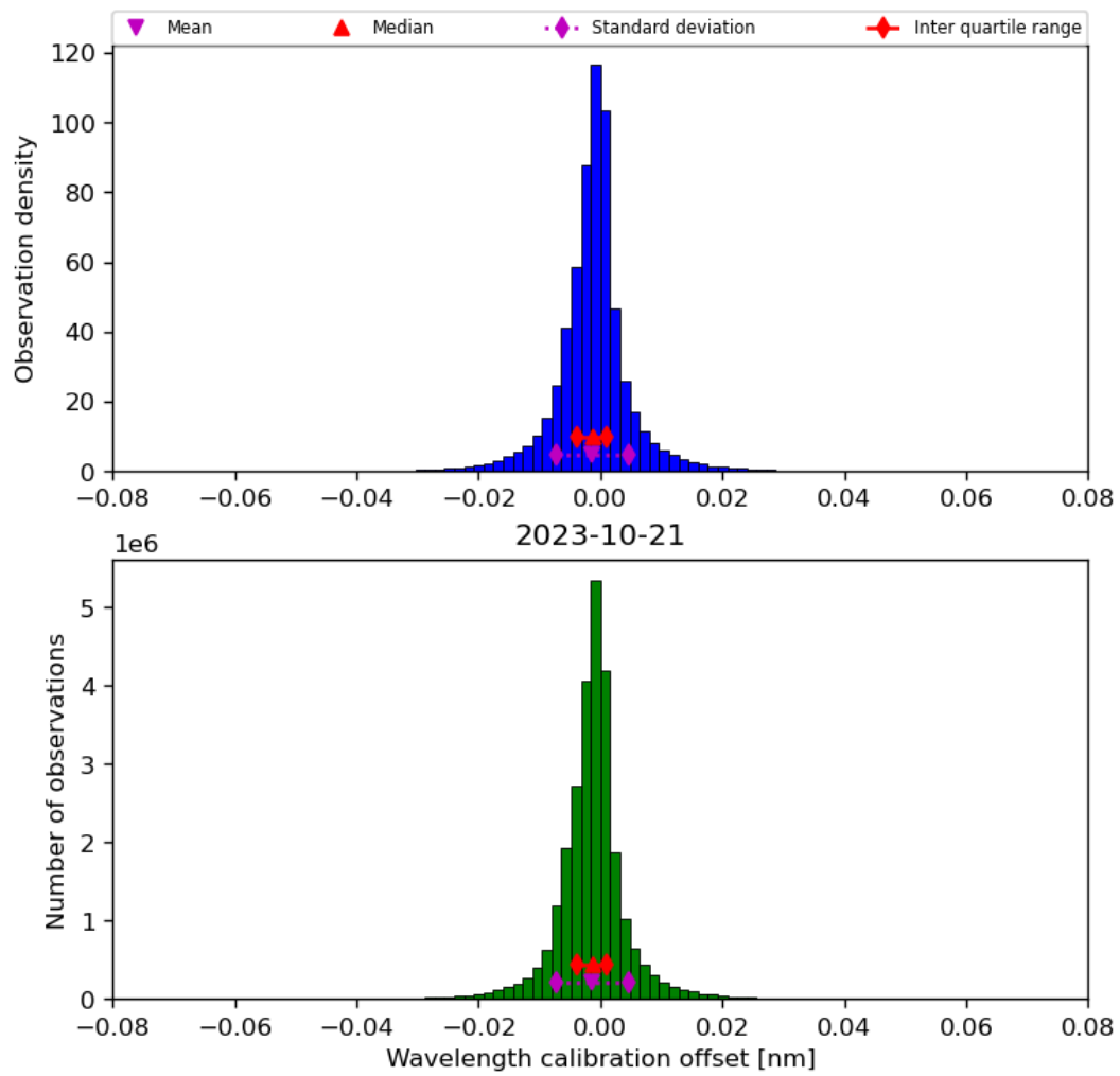
Figure 35: Histogram of “Wavelength calibration offset” for 2023-10-20 to 2023-10-22
