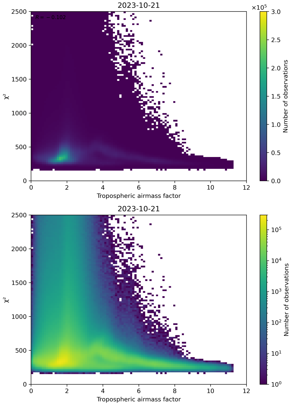
Figure 73: Scatter density plot of “Tropospheric airmass factor” against “ \chi^2 ” for 2023-10-20 to 2023-10-22.
