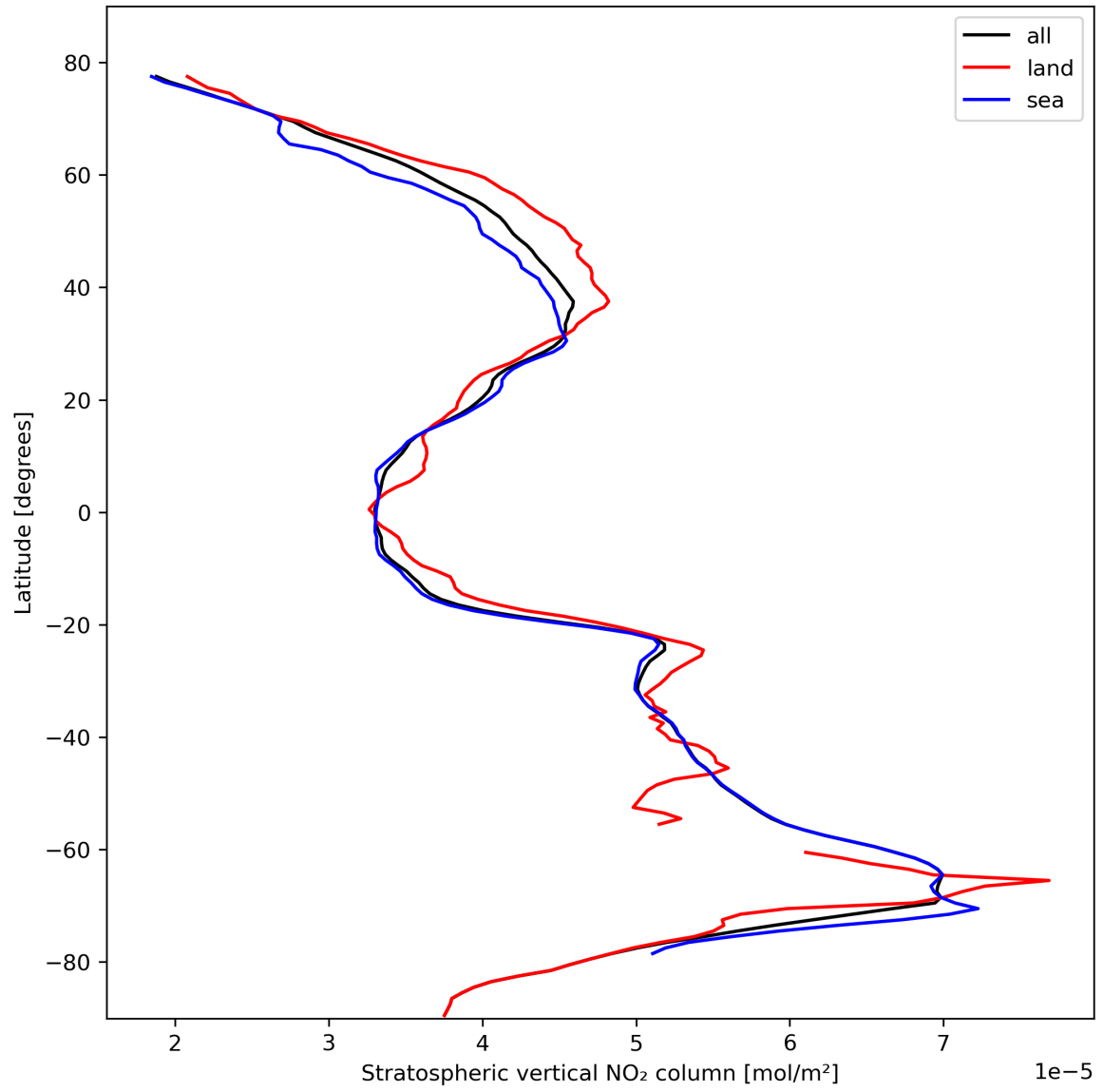
Figure 19: Zonal average of “Stratospheric vertical NO 2 column” for 2023-10-20 to 2023-10-22.
