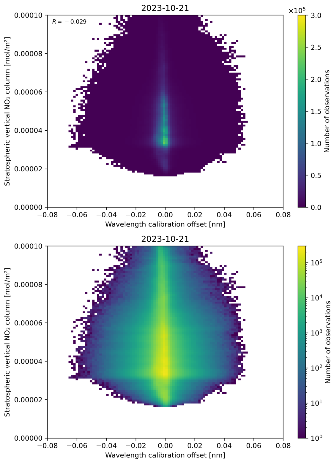
Figure 176: Scatter density plot of “Wavelength calibration offset” against “Stratospheric vertical NO 2 column” for 2023-10-20 to 2023-10-22.
