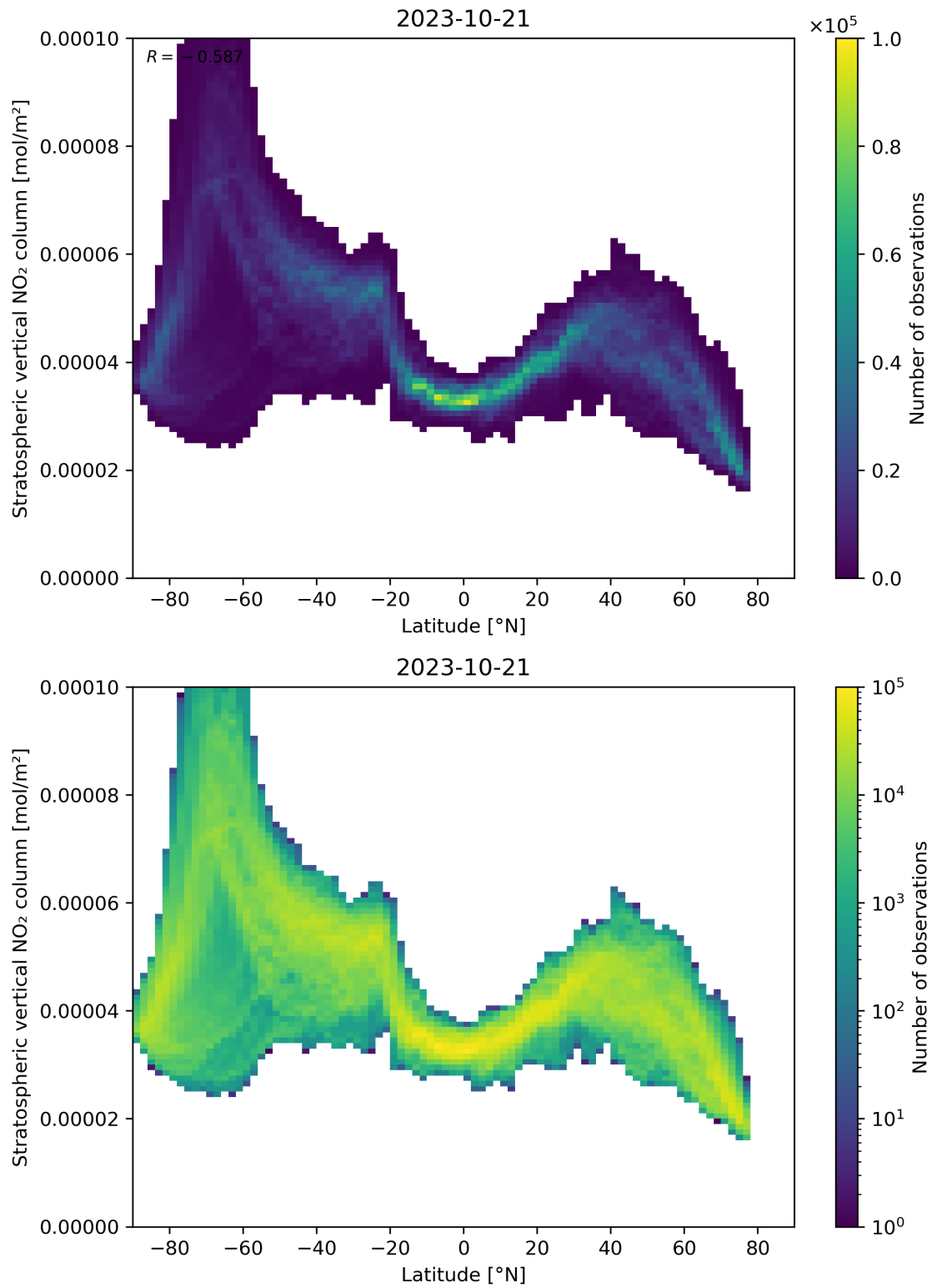
Figure 87: Scatter density plot of “Latitude” against “Stratospheric vertical NO 2 column” for 2023-10-20 to 2023-10-22.
