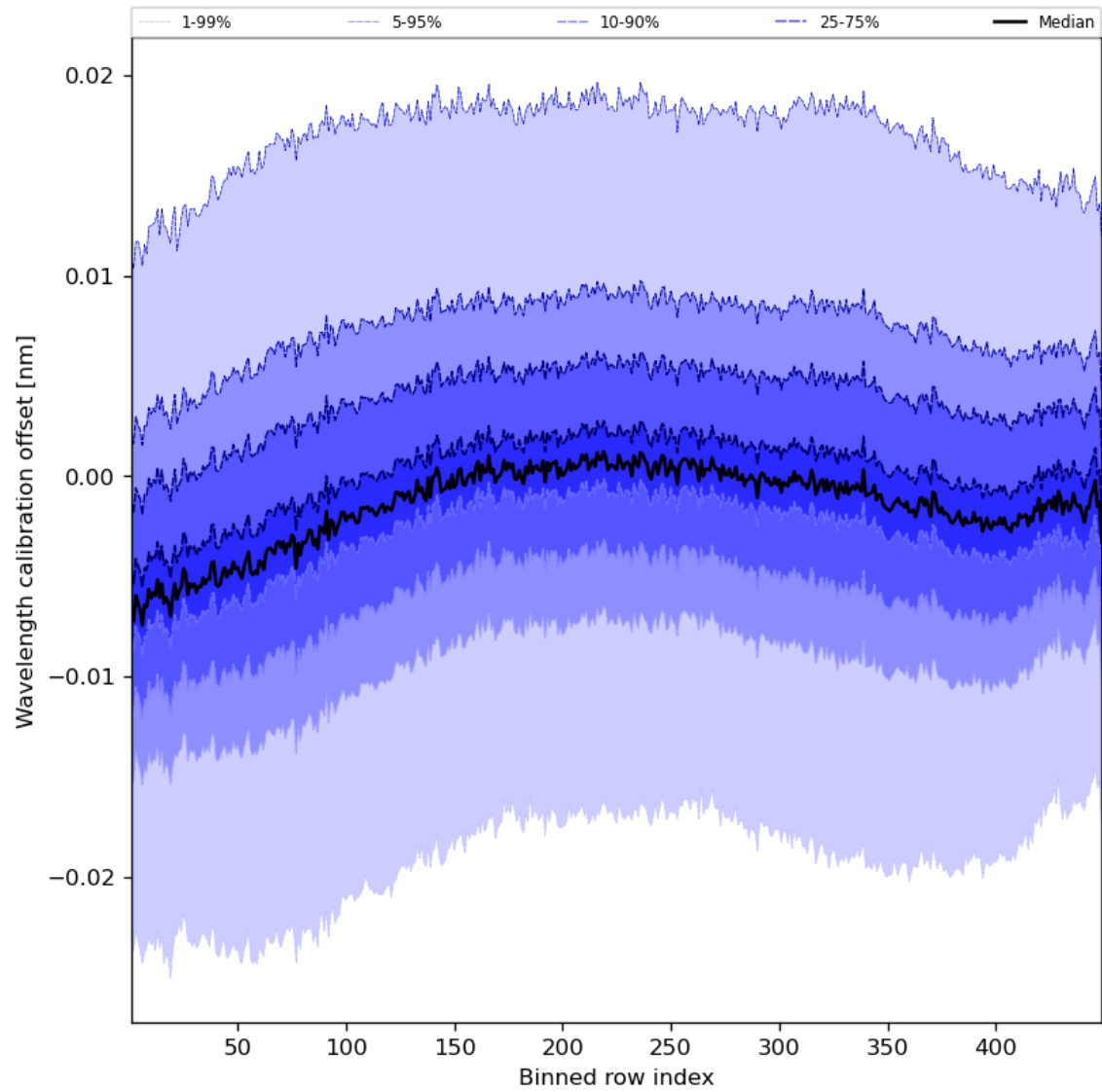
Figure 52: Along track statistics of “Wavelength calibration offset” for 2023-10-20 to 2023-10-22
