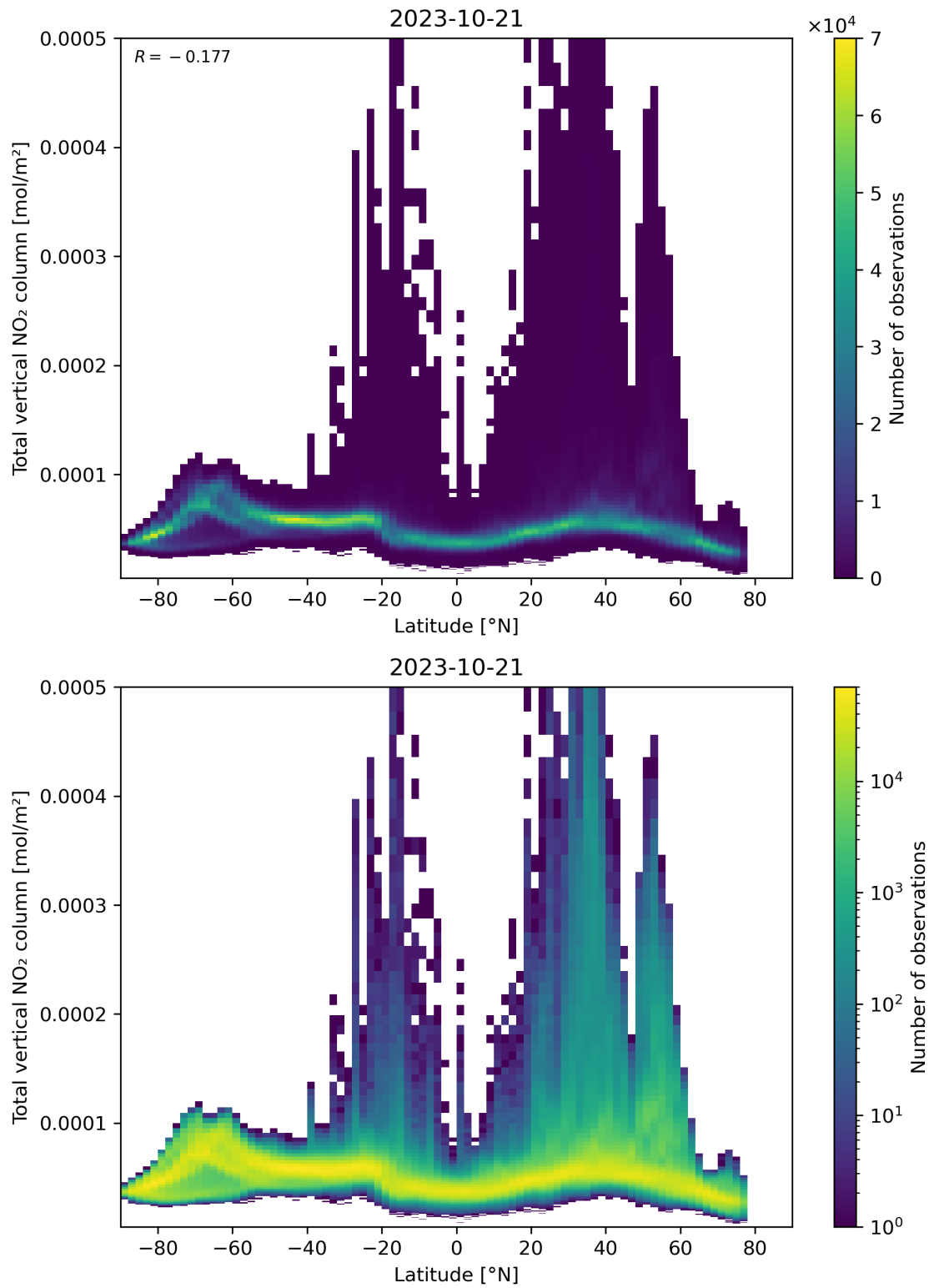
Figure 90: Scatter density plot of “Latitude” against “Total vertical NO 2 column” for 2023-10-20 to 2023-10-22.
