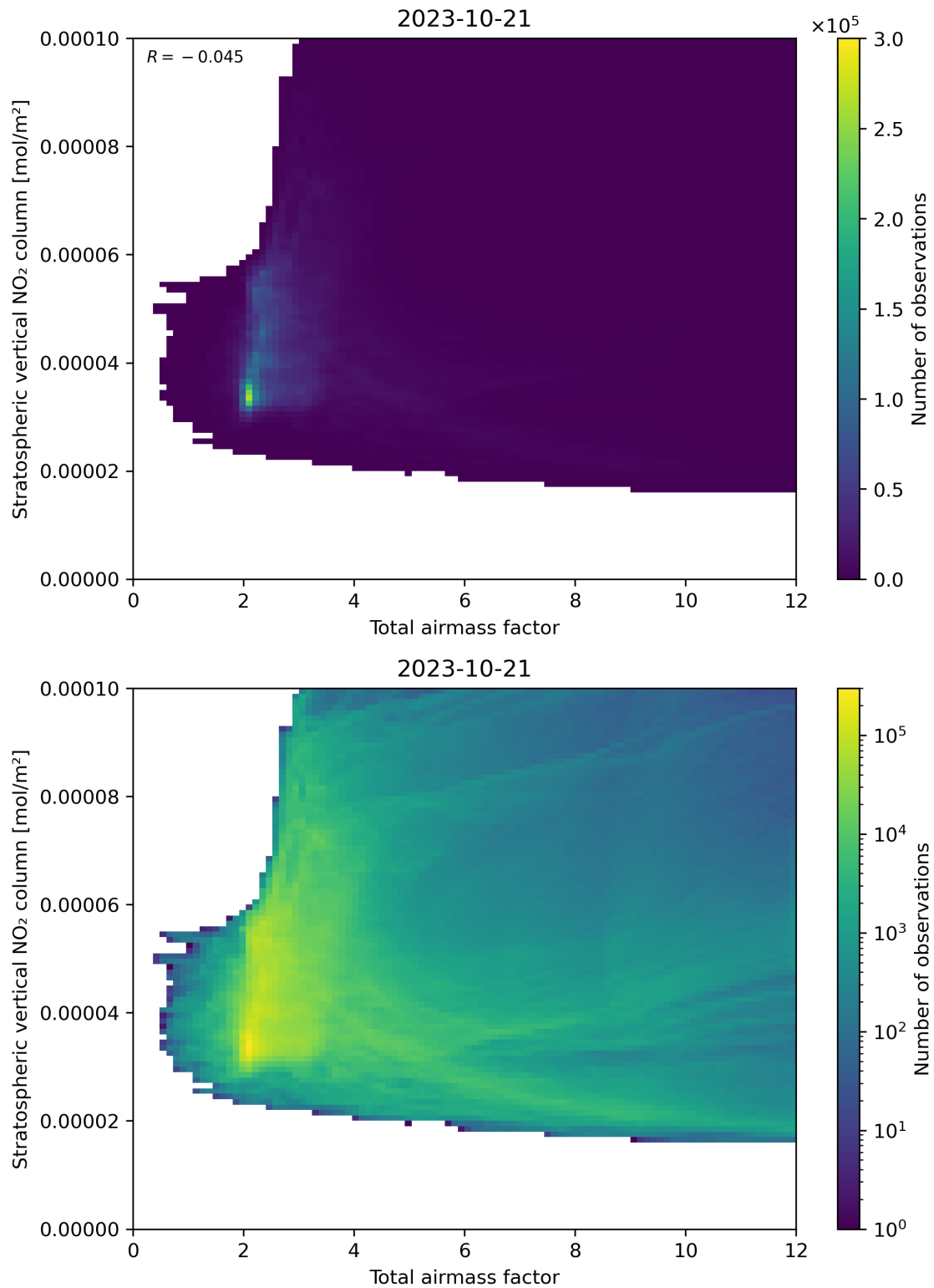
Figure 64: Scatter density plot of “Total airmass factor” against “Stratospheric vertical NO 2 column” for 2023-10-20 to 2023-10-22.
