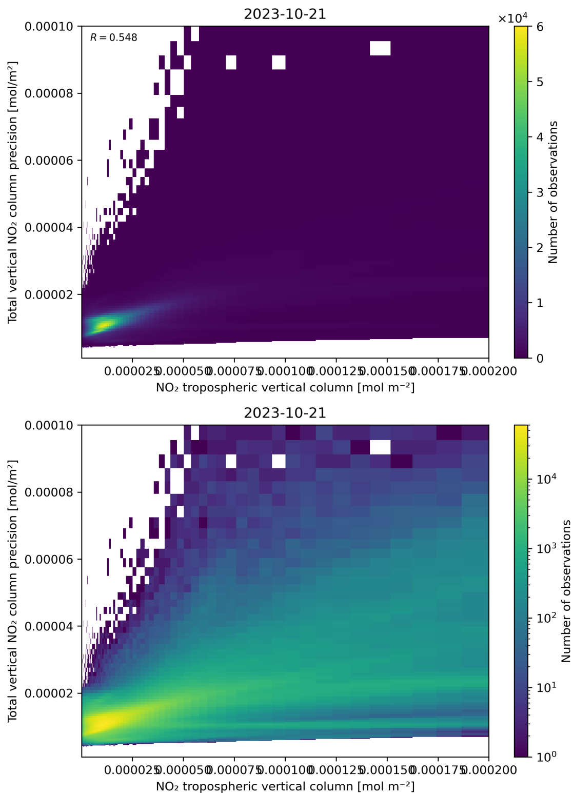
Figure 129: Scatter density plot of “NO 2 tropospheric vertical column” against “Total vertical NO 2 column precision” for 2023-10-20 to 2023-10-22.
