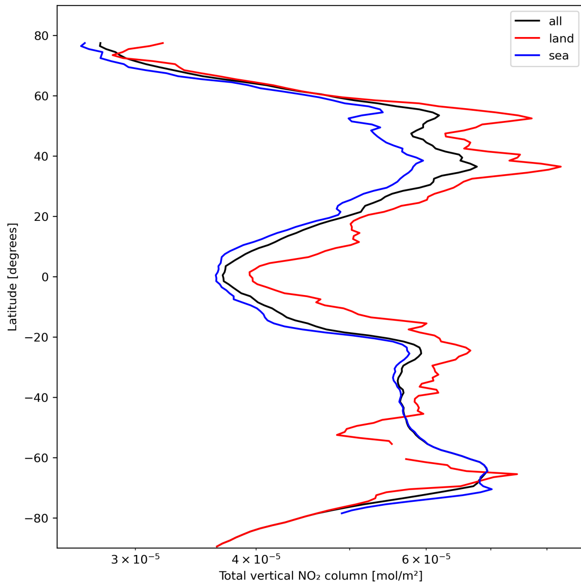
Figure 21: Zonal average of “Total vertical NO 2 column” for 2023-10-20 to 2023-10-22.
