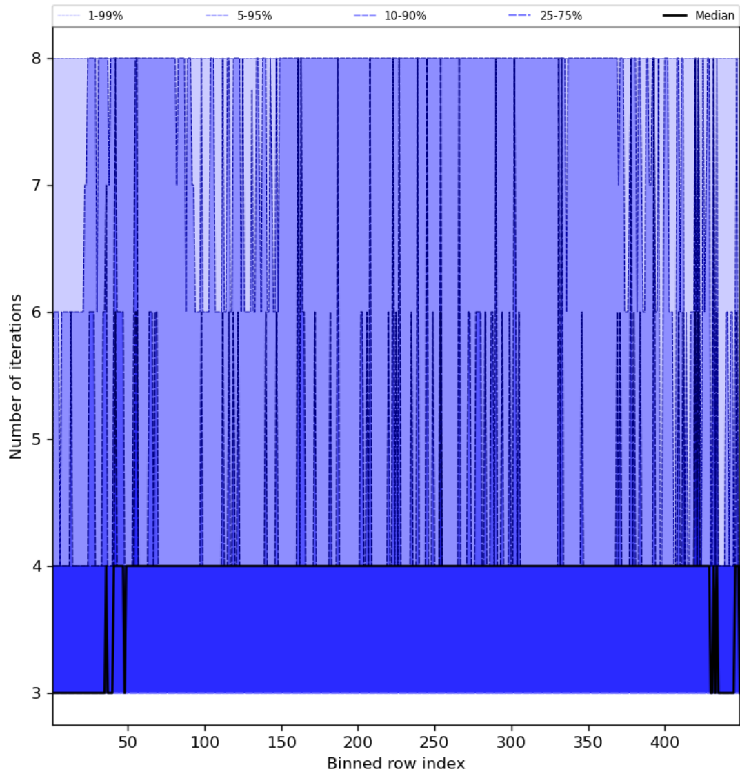
Figure 51: Along track statistics of “Number of iterations” for 2023-10-20 to 2023-10-22
