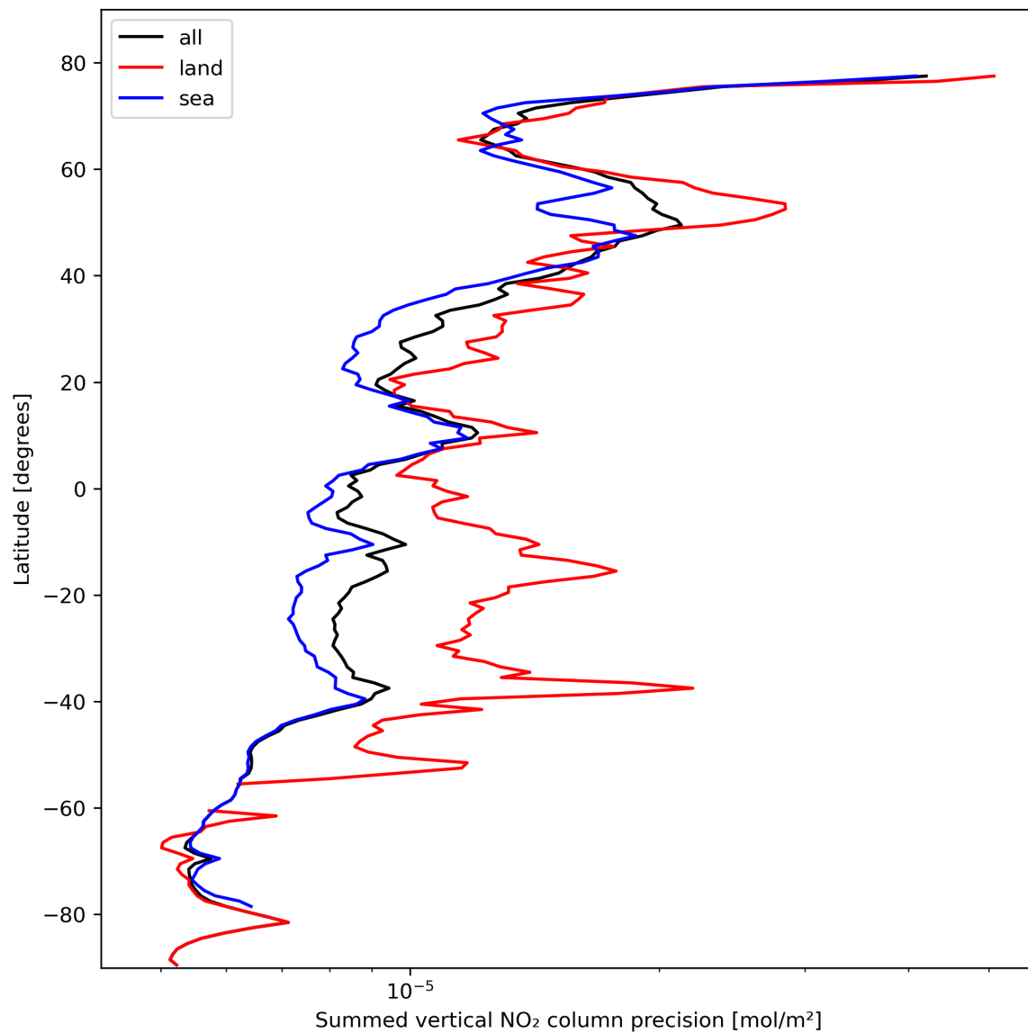
Figure 24: Zonal average of “Summed vertical NO 2 column precision” for 2023-10-20 to 2023-10-22.
