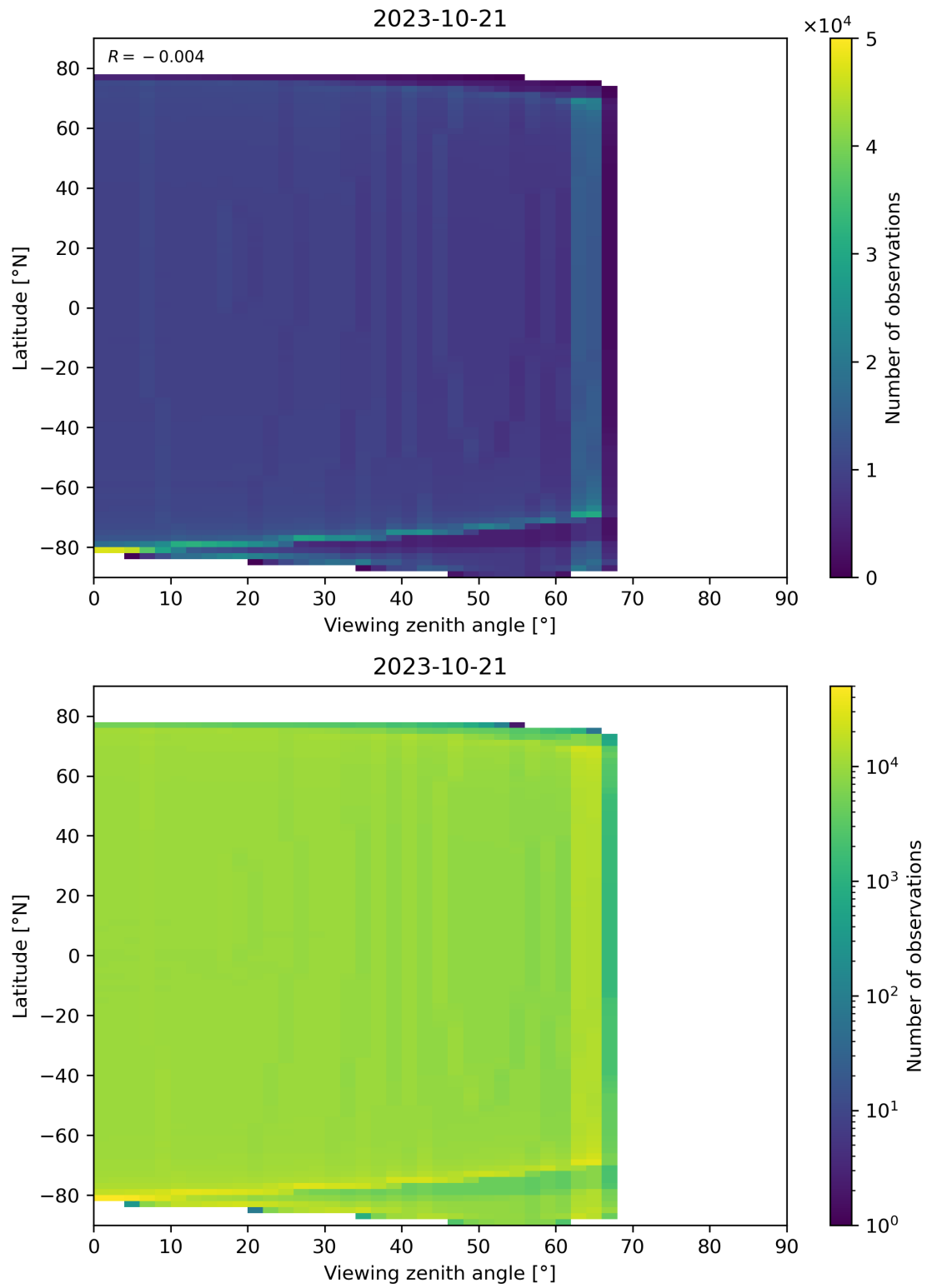
Figure 163: Scatter density plot of “Viewing zenith angle” against “Latitude” for 2023-10-20 to 2023-10-22.
