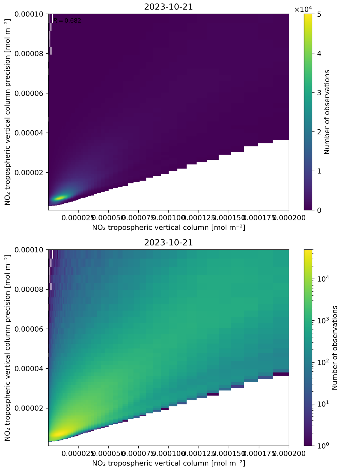
Figure 130: Scatter density plot of “NO 2 tropospheric vertical column” against “NO 2 tropospheric vertical column precision” for 2023-10-20 to 2023-10-22.
