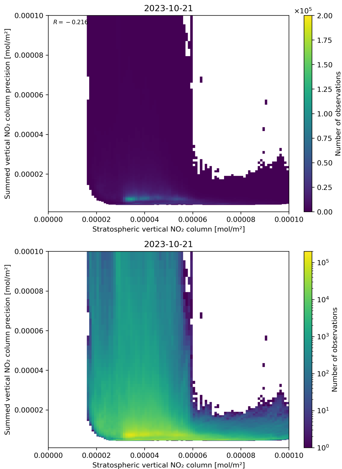
Figure 99: Scatter density plot of “Stratospheric vertical NO 2 column” against “Summed vertical NO 2 column precision” for 2023-10-20 to 2023-10-22.
