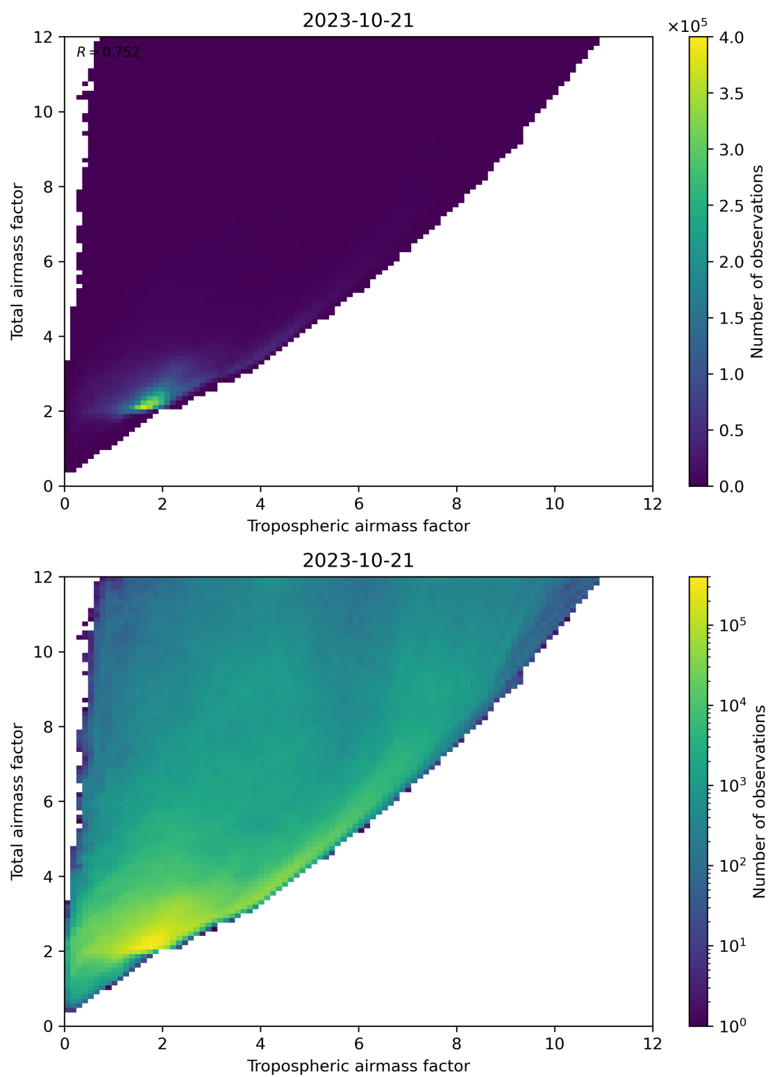
Figure 72: Scatter density plot of “Tropospheric airmass factor” against “Total airmass factor” for 2023-10-20 to 2023-10-22.
