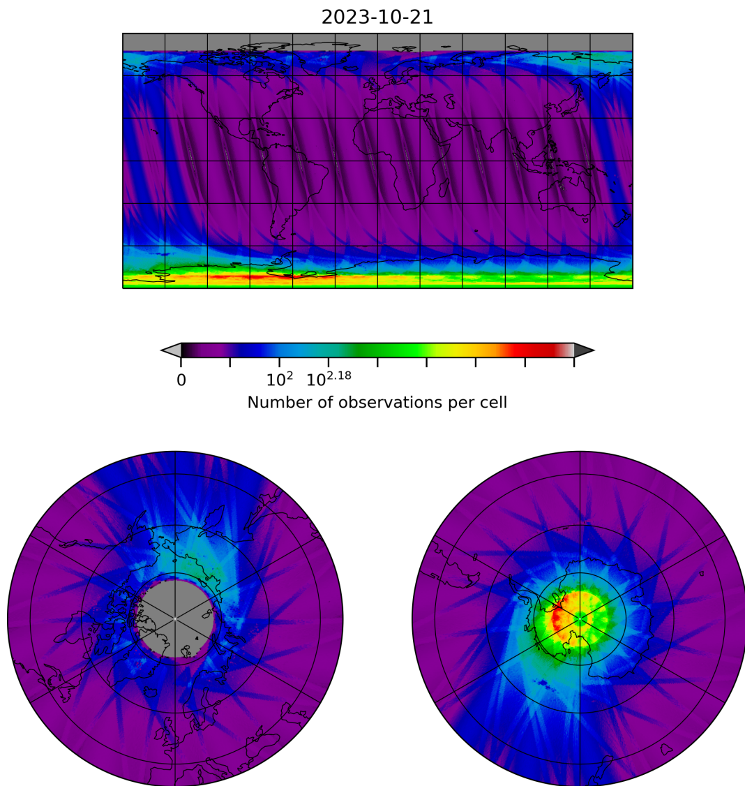
Figure 10: Map of the number of observations for 2023-10-20 to 2023-10-22
