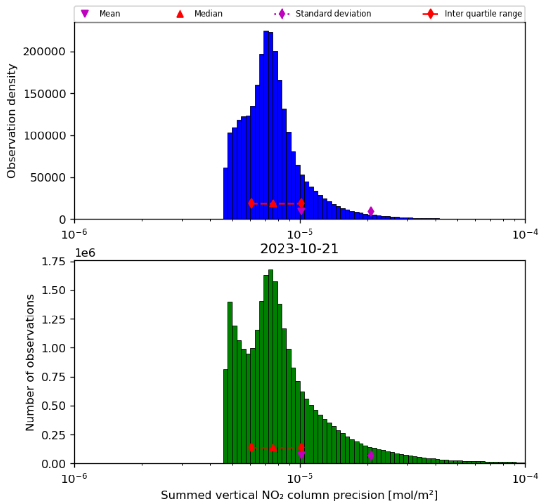
Figure 41: Histogram of “Summed vertical NO 2 column precision” for 2023-10-20 to 2023-10-22
