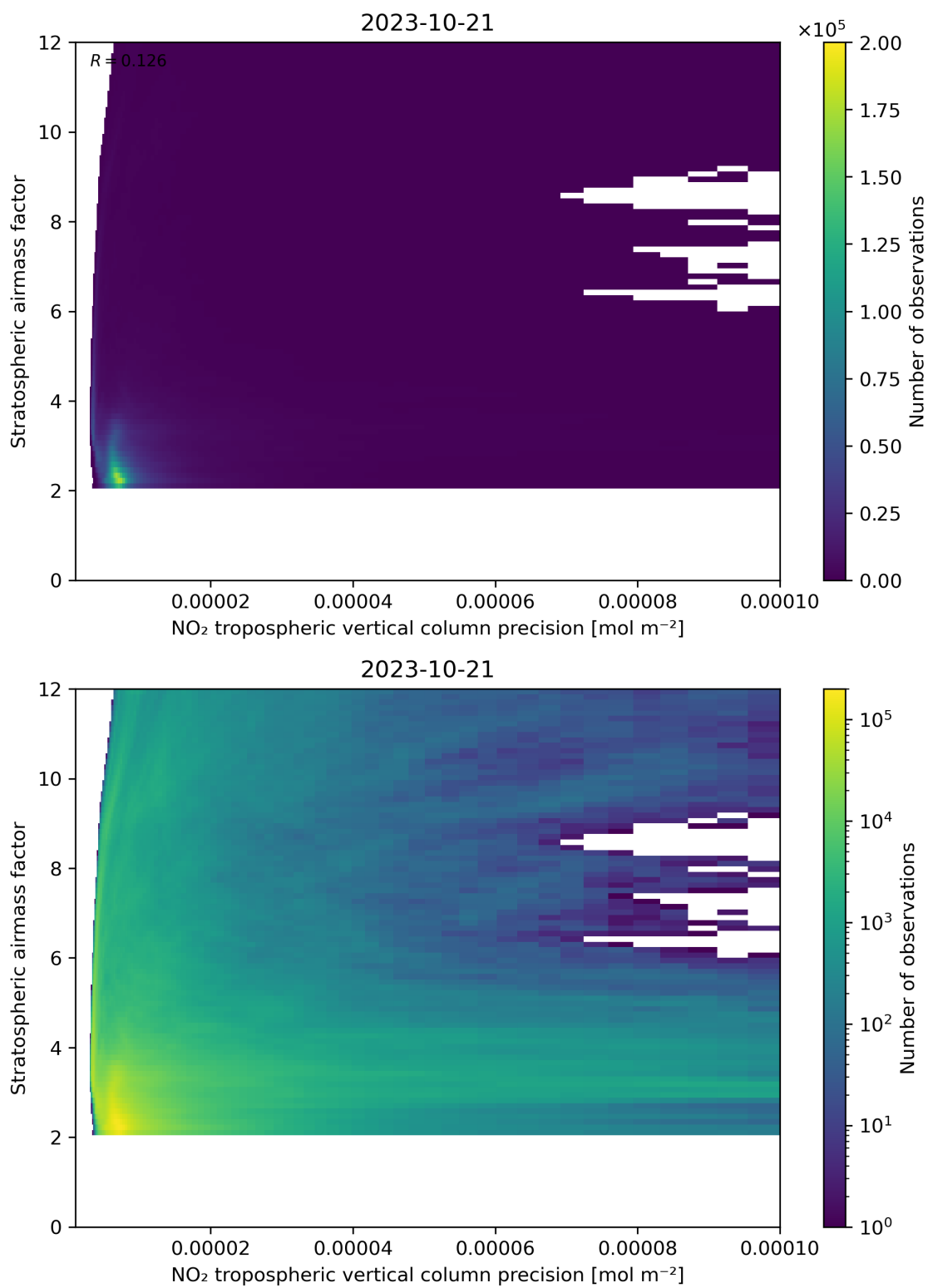
Figure 131: Scatter density plot of “NO 2 tropospheric vertical column precision” against “Stratospheric airmass factor” for 2023-10-20 to 2023-10-22.
