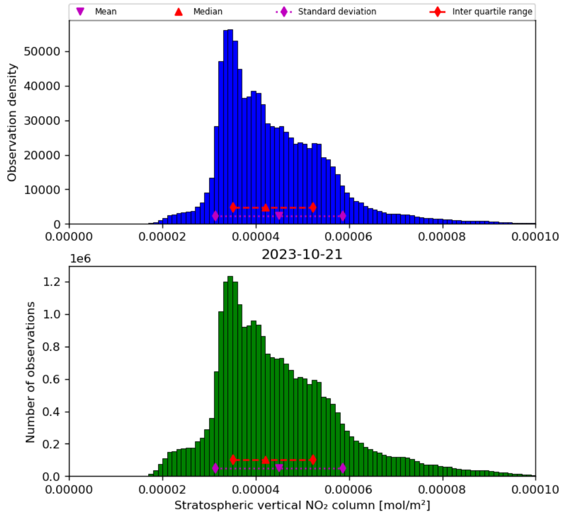
Figure 36: Histogram of “Stratospheric vertical NO 2 column” for 2023-10-20 to 2023-10-22
