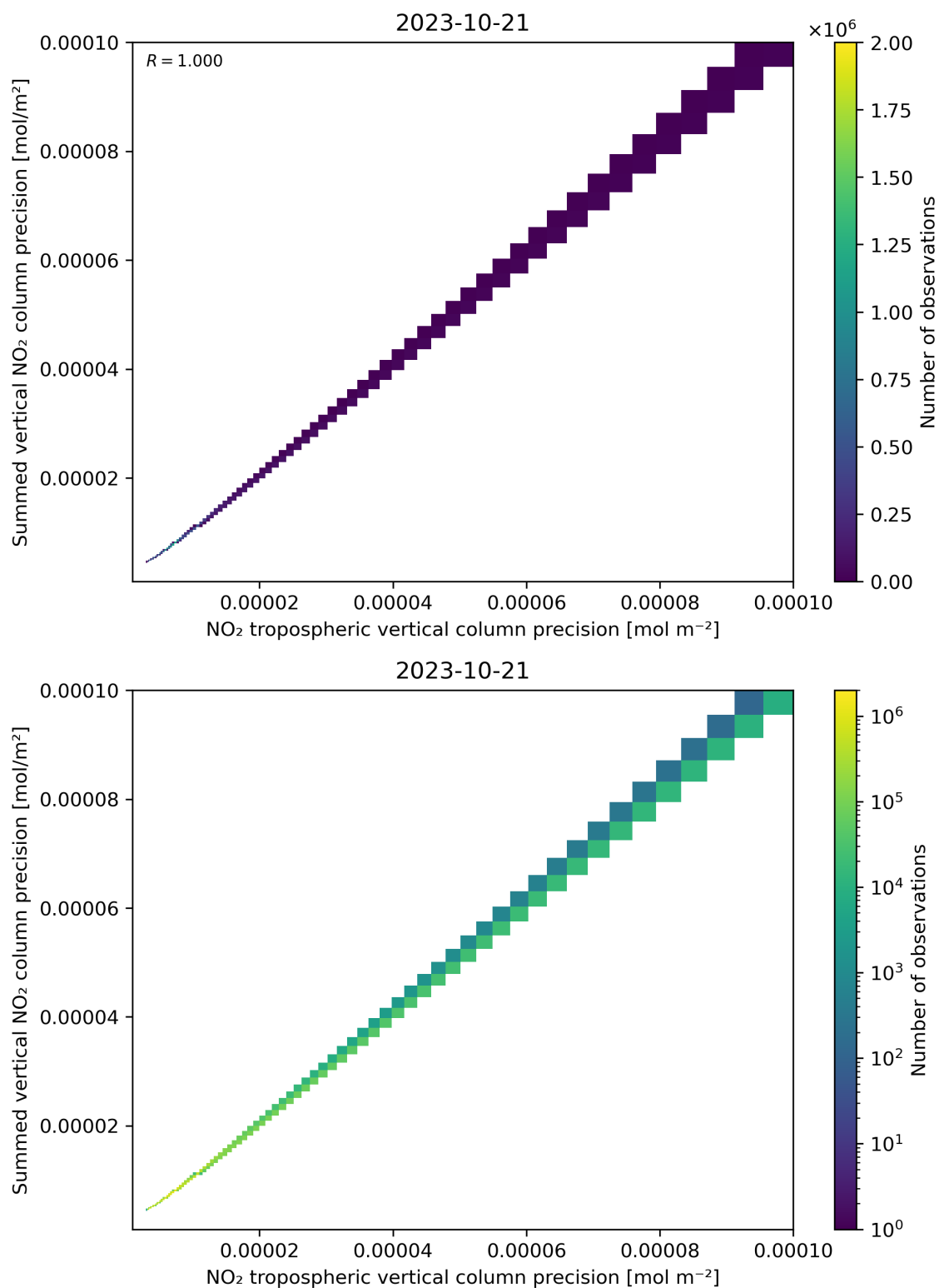
Figure 137: Scatter density plot of “NO 2 tropospheric vertical column precision” against “Summed vertical NO 2 column precision” for 2023-10-20 to 2023-10-22.
