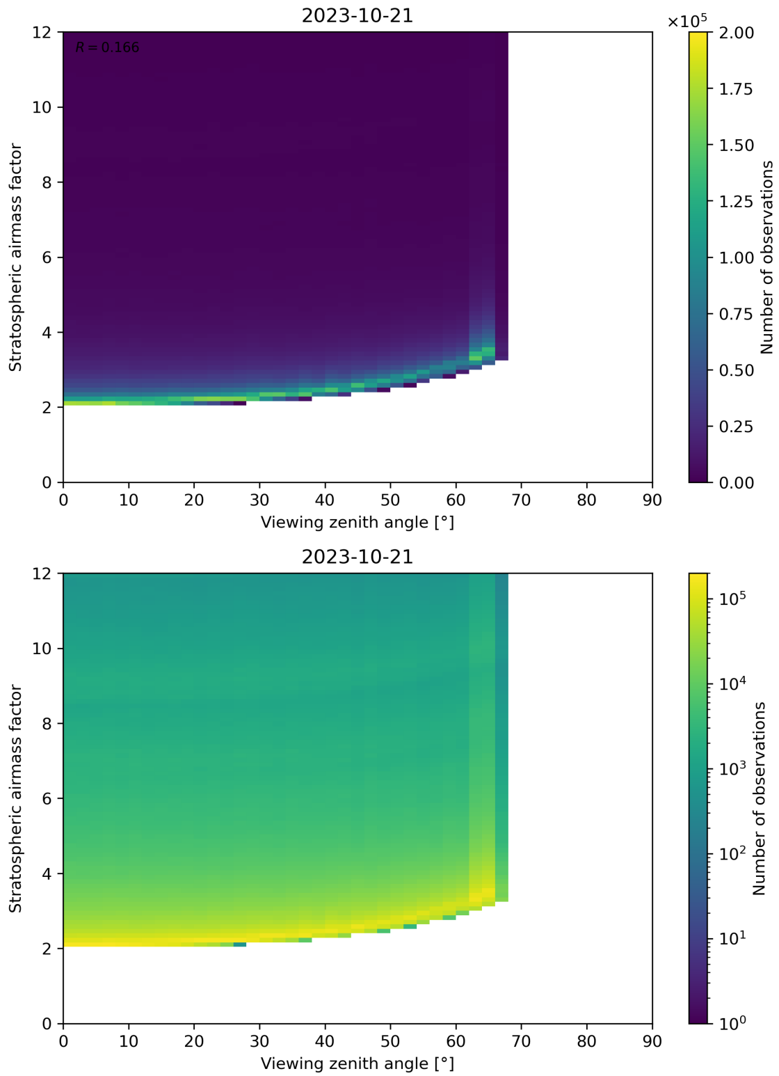
Figure 159: Scatter density plot of “Viewing zenith angle” against “Stratospheric airmass factor” for 2023-10-20 to 2023-10-22.
