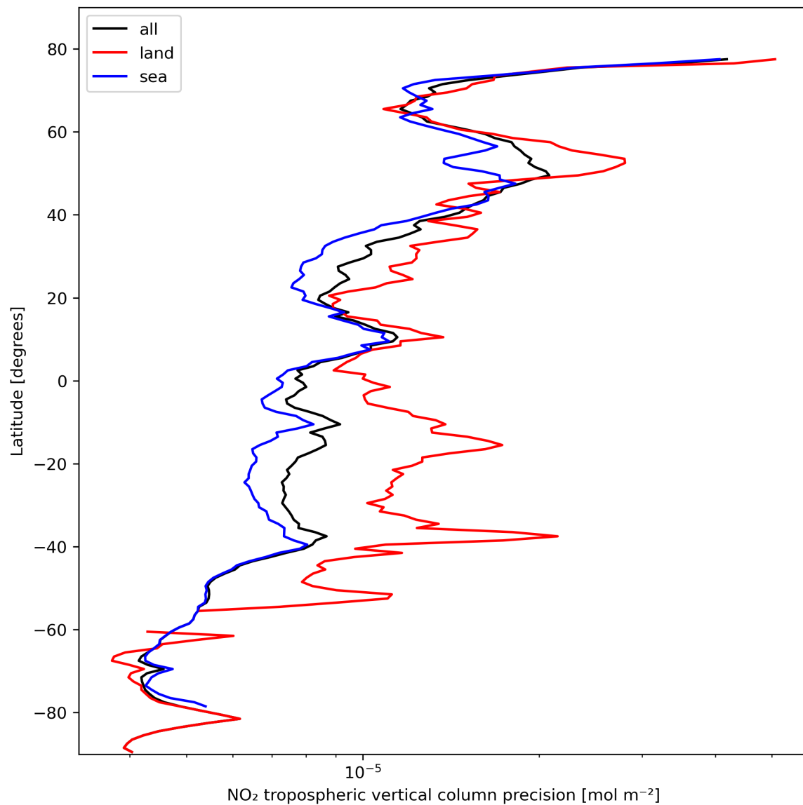
Figure 13: Zonal average of “NO 2 tropospheric vertical column precision” for 2023-10-20 to 2023-10-22.
