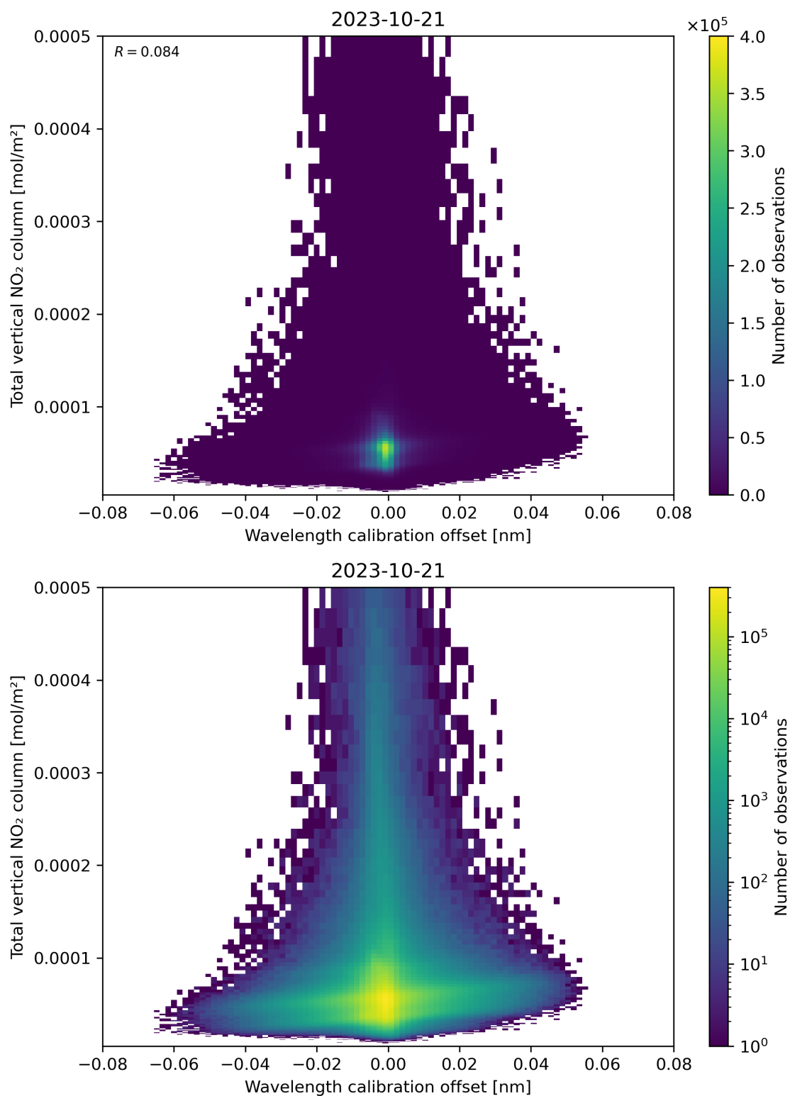
Figure 179: Scatter density plot of “Wavelength calibration offset” against “Total vertical NO 2 column” for 2023-10-20 to 2023-10-22.
