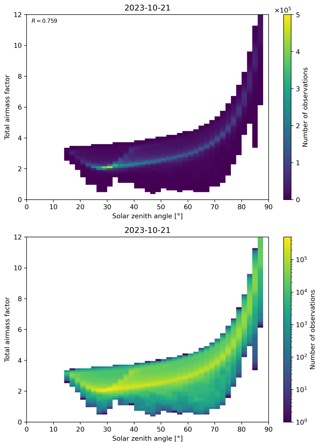
Figure 146: Scatter density plot of “Solar zenith angle” against “Total airmass factor” for 2023-10-20 to 2023-10-22.
