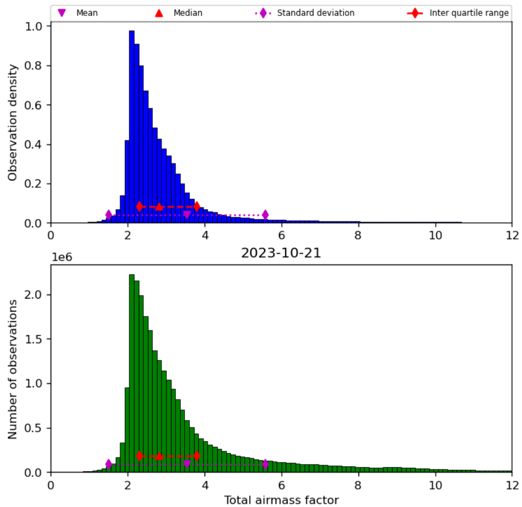
Figure 32: Histogram of “Total airmass factor” for 2023-10-20 to 2023-10-22
