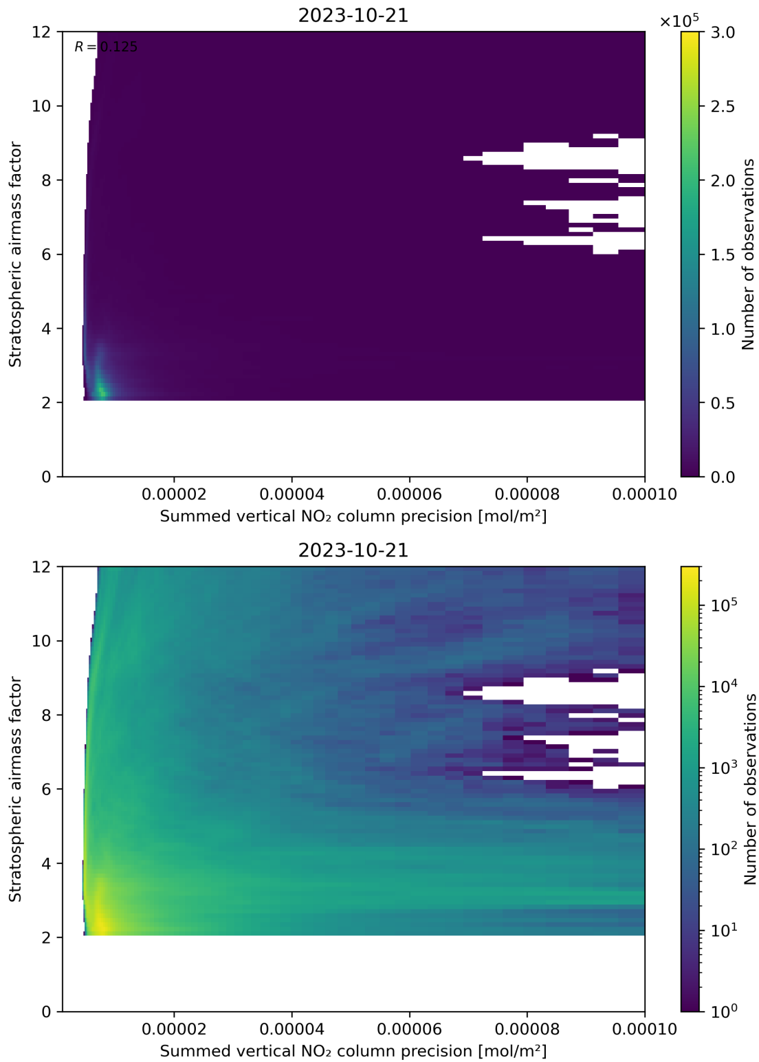
Figure 106: Scatter density plot of “Summed vertical NO 2 column precision” against “Stratospheric airmass factor” for 2023-10-20 to 2023-10-22.
