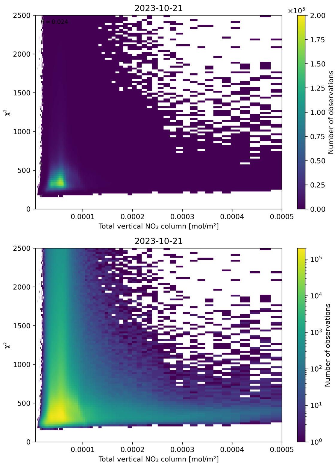
Figure 111: Scatter density plot of “Total vertical NO 2 column” against “ \chi^2 ” for 2023-10-20 to 2023-10-22.
