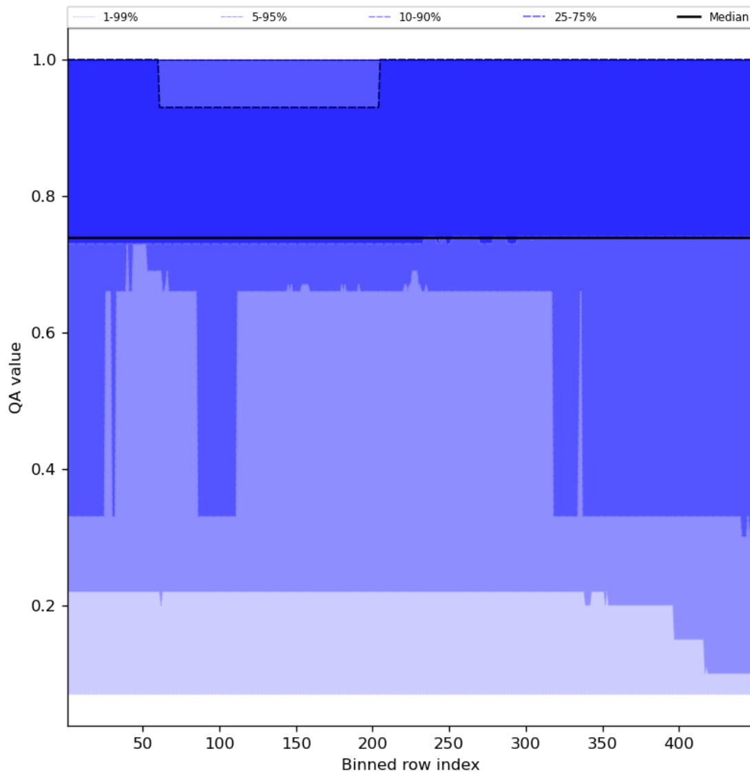
Figure 45: Along track statistics of “QA value” for 2023-10-20 to 2023-10-22
