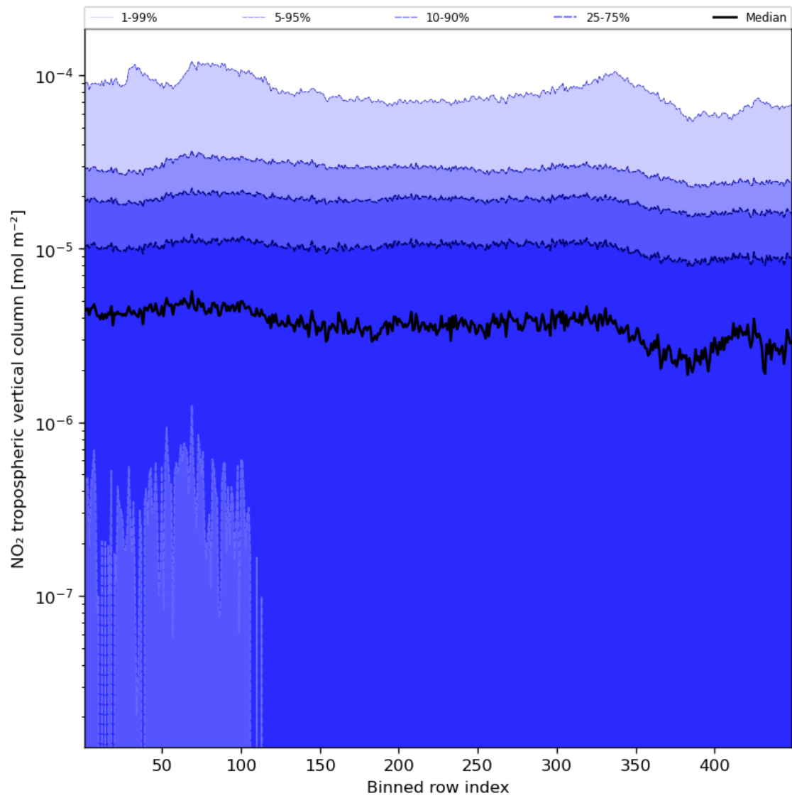
Figure 46: Along track statistics of “NO 2 tropospheric vertical column” for 2023-10-20 to 2023-10-22
