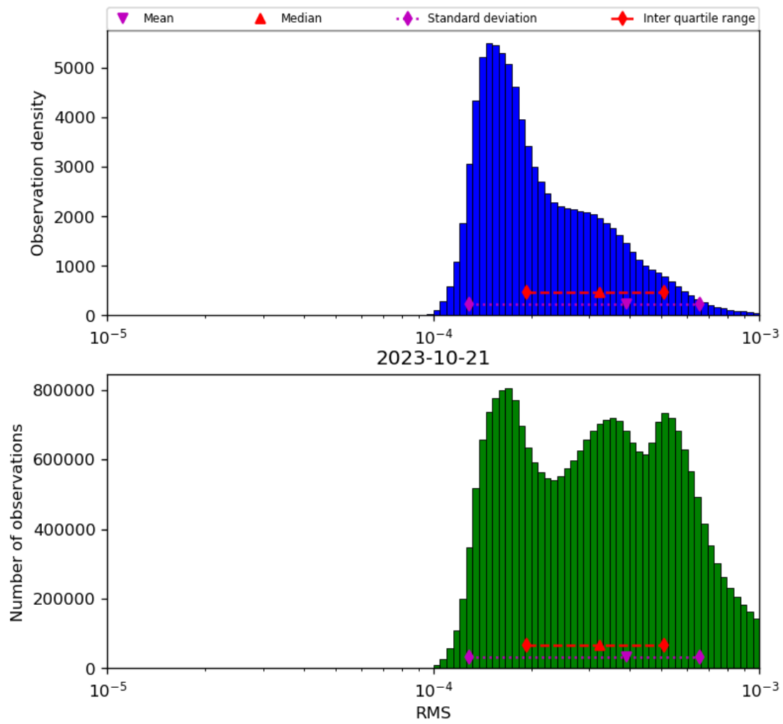
Figure 43: Histogram of “RMS” for 2023-10-20 to 2023-10-22
