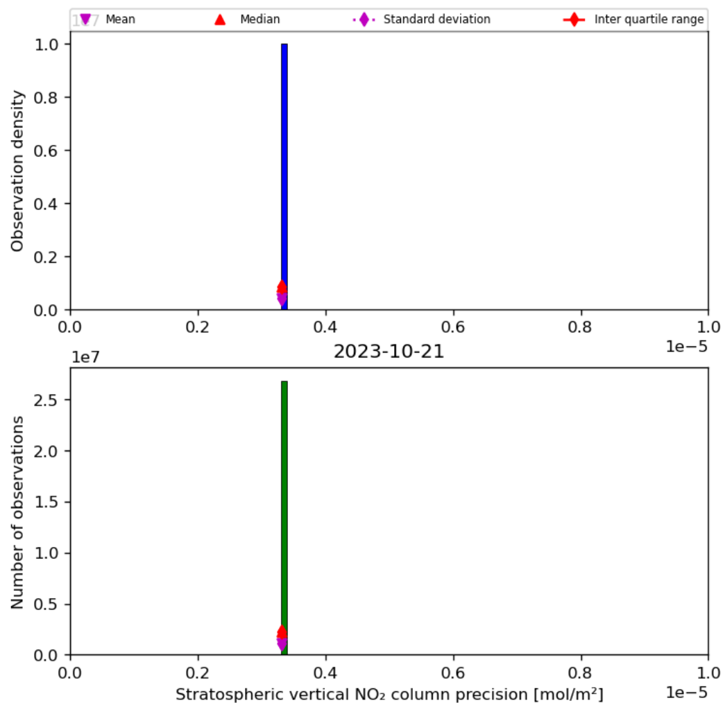
Figure 37: Histogram of “Stratospheric vertical NO 2 column precision” for 2023-10-20 to 2023-10-22
