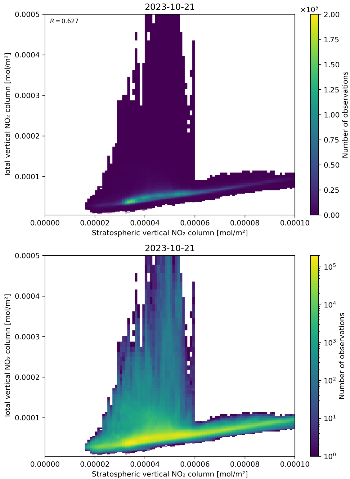
Figure 100: Scatter density plot of “Stratospheric vertical NO 2 column” against “Total vertical NO 2 column” for 2023-10-20 to 2023-10-22.
