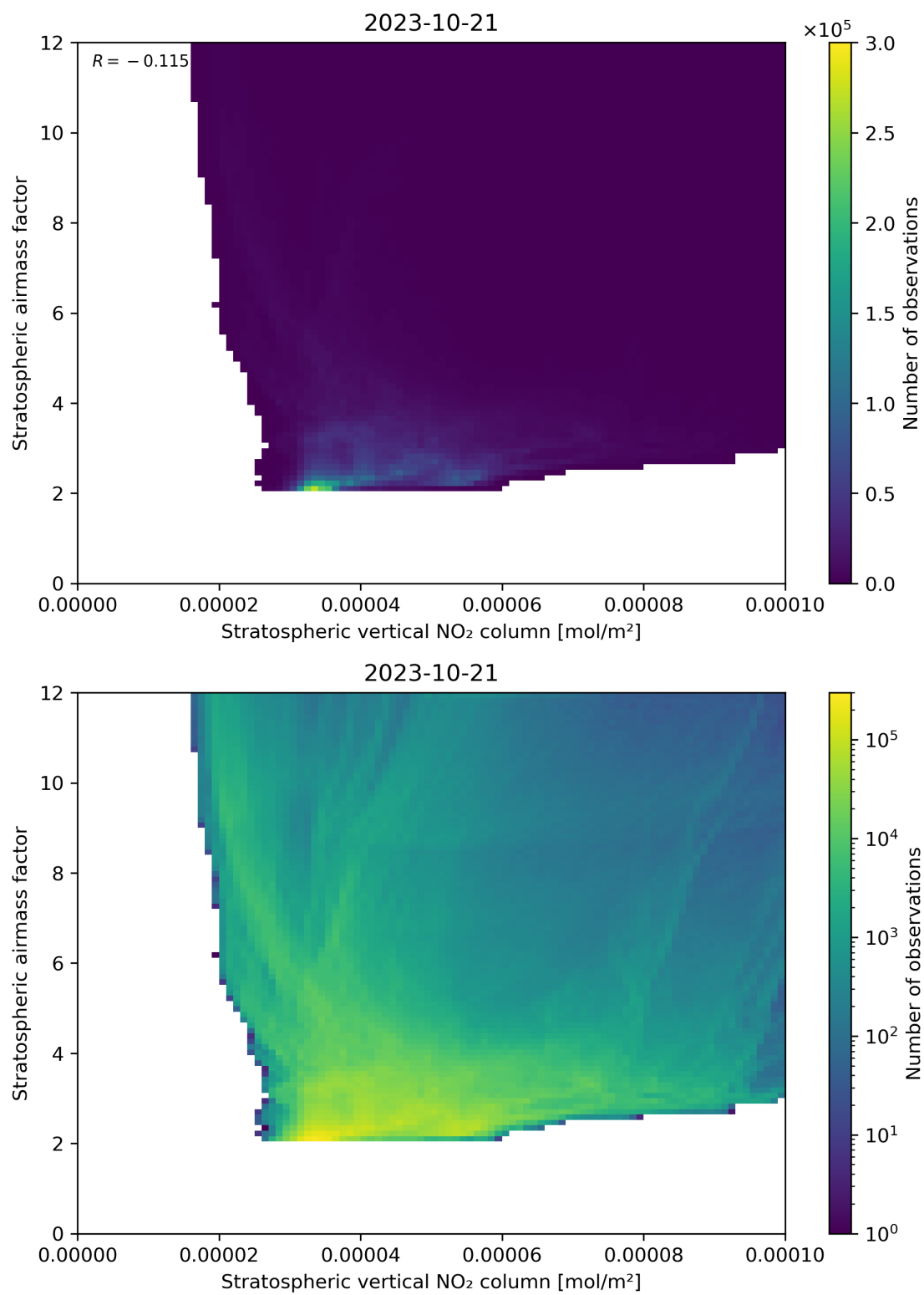
Figure 96: Scatter density plot of “Stratospheric vertical NO 2 column” against “Stratospheric airmass factor” for 2023-10-20 to 2023-10-22.
