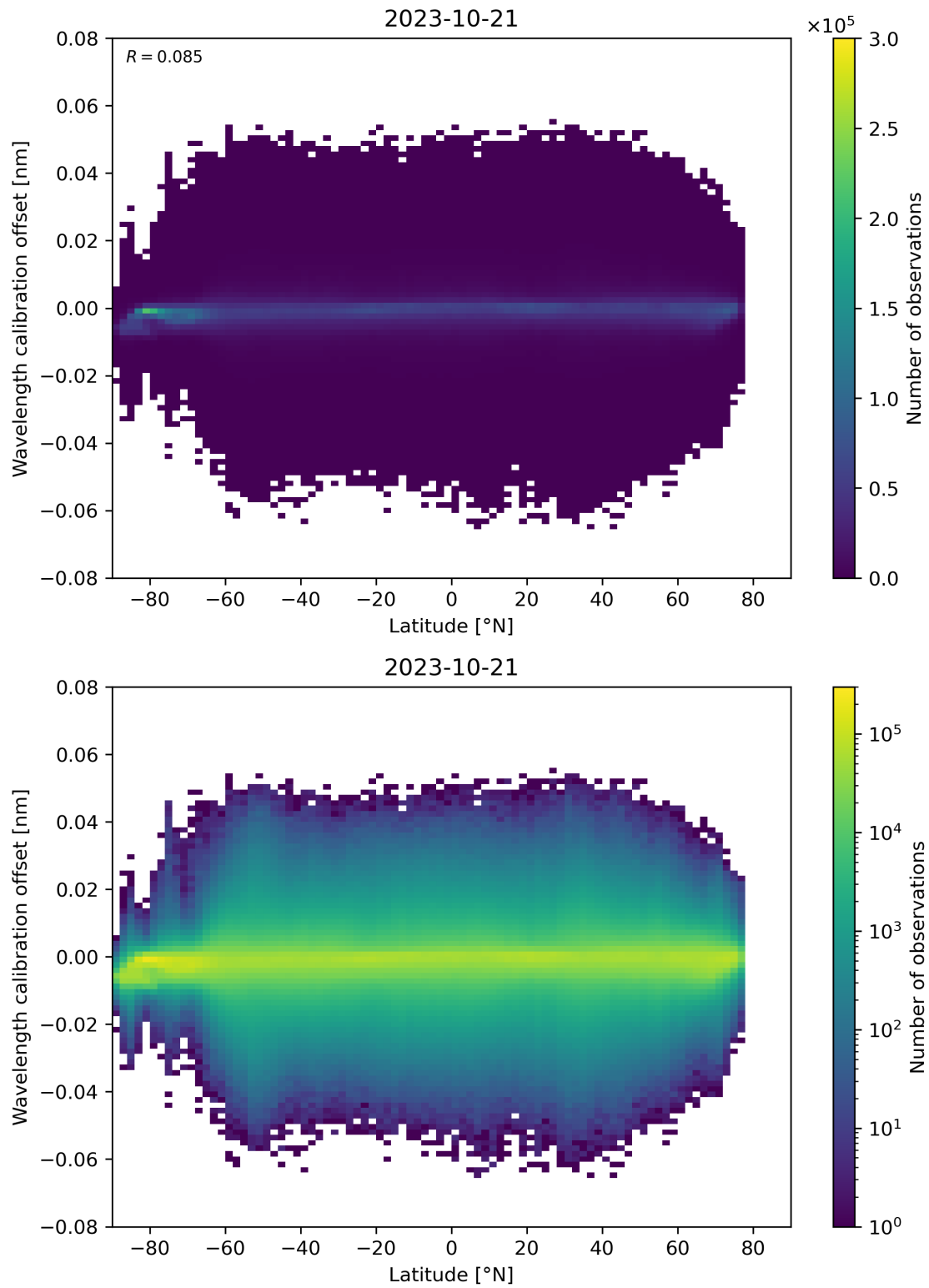
Figure 95: Scatter density plot of “Latitude” against “Wavelength calibration offset” for 2023-10-20 to 2023-10-22.
