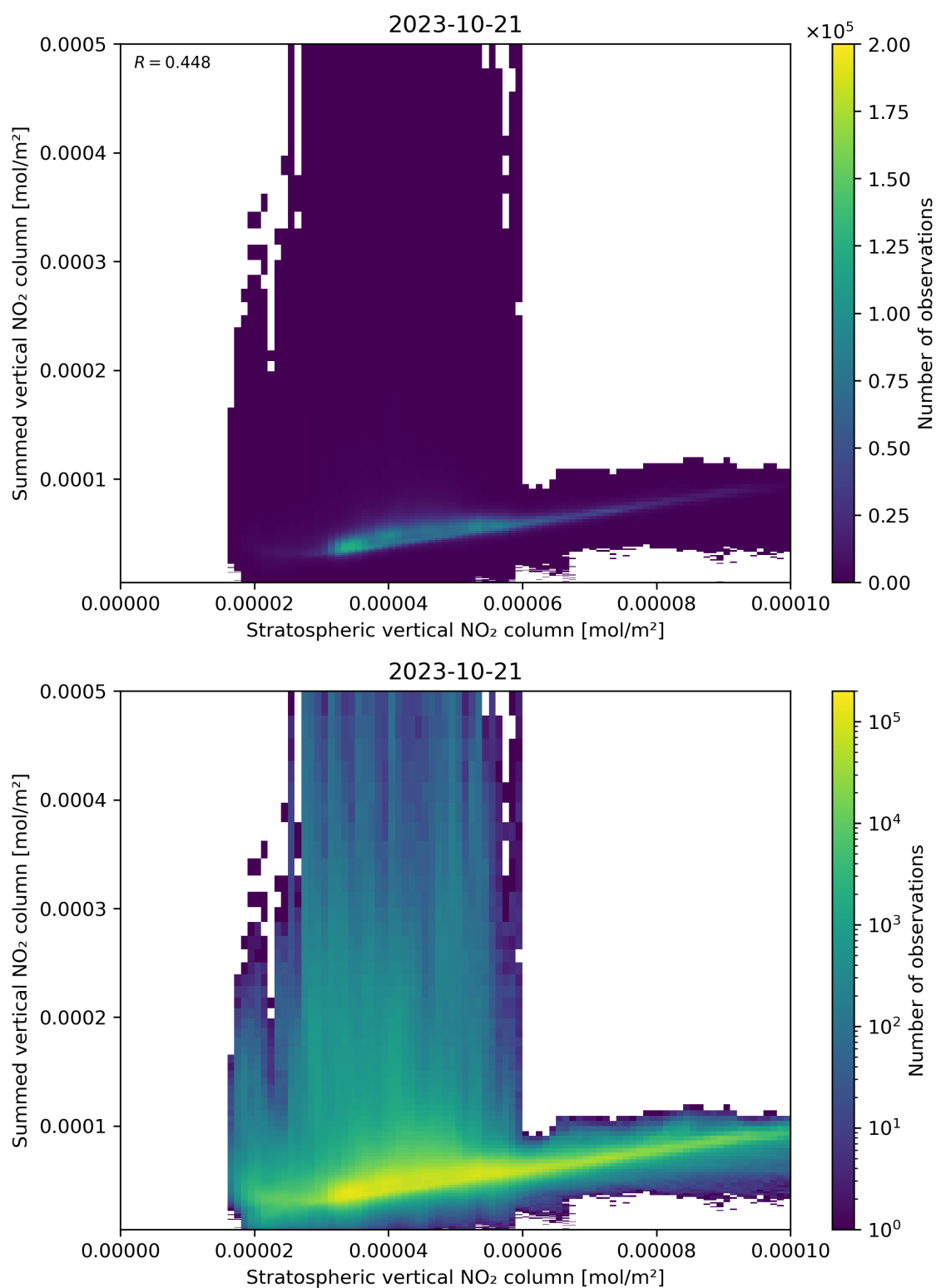
Figure 98: Scatter density plot of “Stratospheric vertical NO 2 column” against “Summed vertical NO 2 column” for 2023-10-20 to 2023-10-22.
