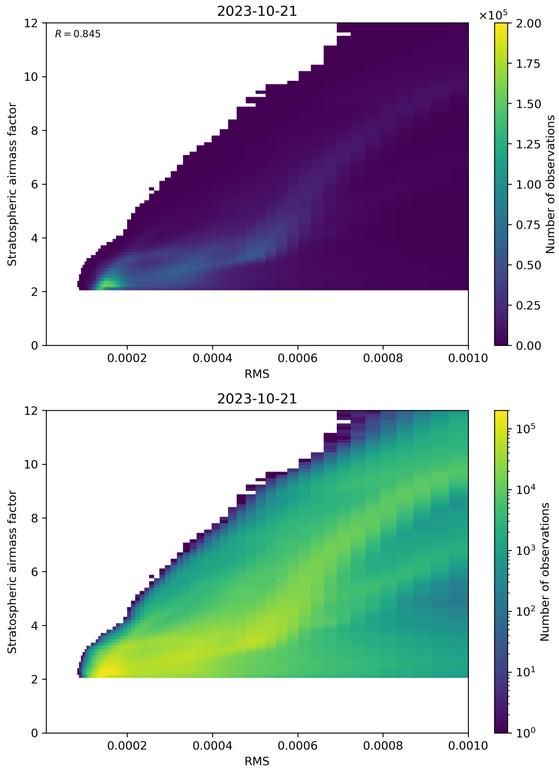
Figure 144: Scatter density plot of “RMS” against “Stratospheric airmass factor” for 2023-10-20 to 2023-10-22.
