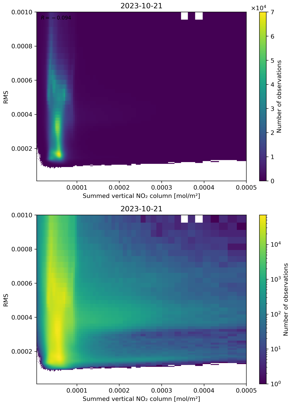
Figure 109: Scatter density plot of “Summed vertical NO 2 column” against “RMS” for 2023-10-20 to 2023-10-22.
