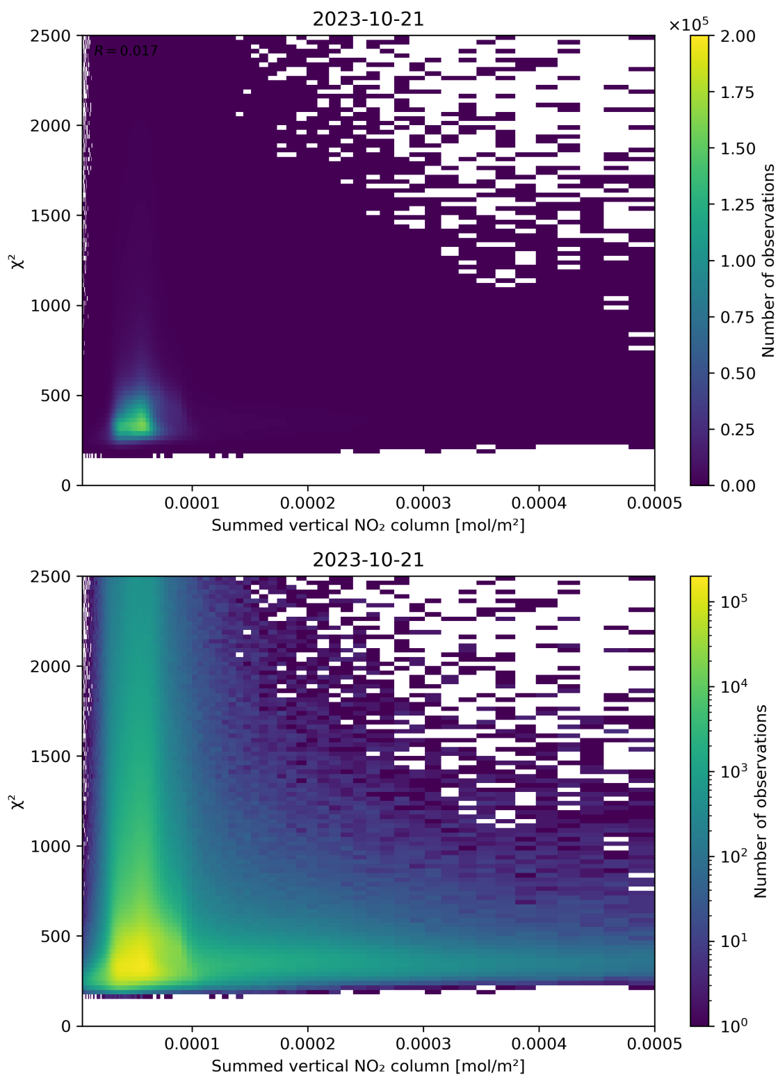
Figure 104: Scatter density plot of “Summed vertical NO 2 column” against “ \chi^2 ” for 2023-10-20 to 2023-10-22.
