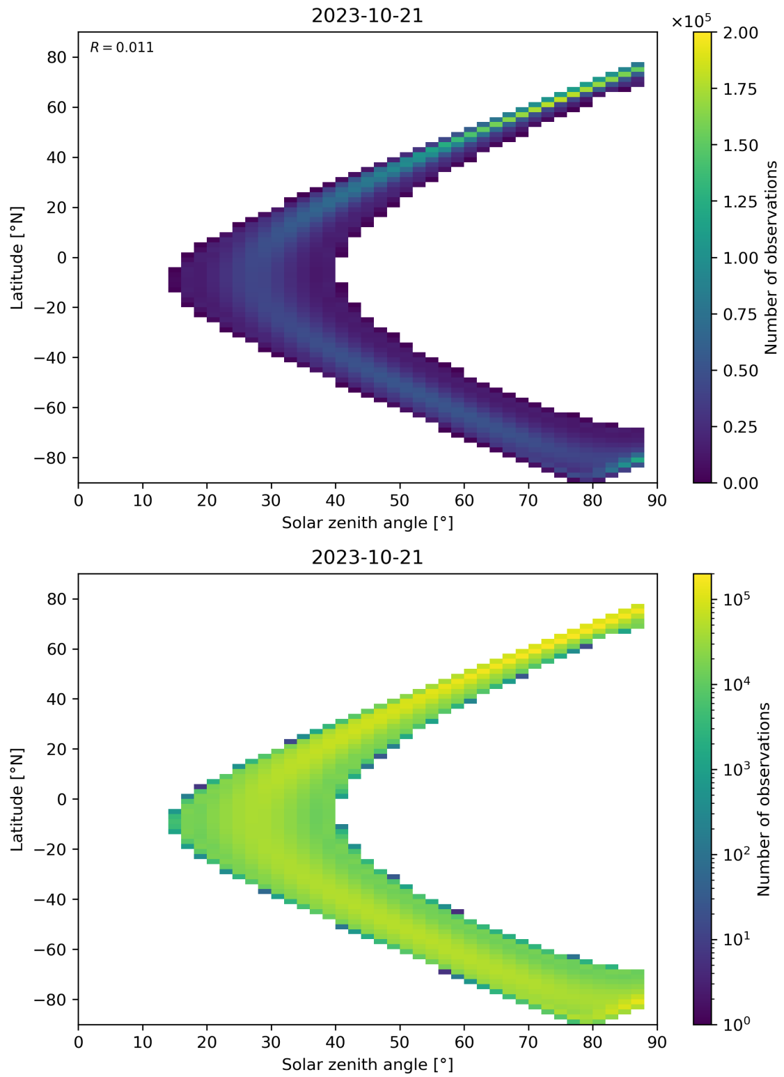
Figure 149: Scatter density plot of “Solar zenith angle” against “Latitude” for 2023-10-20 to 2023-10-22.
