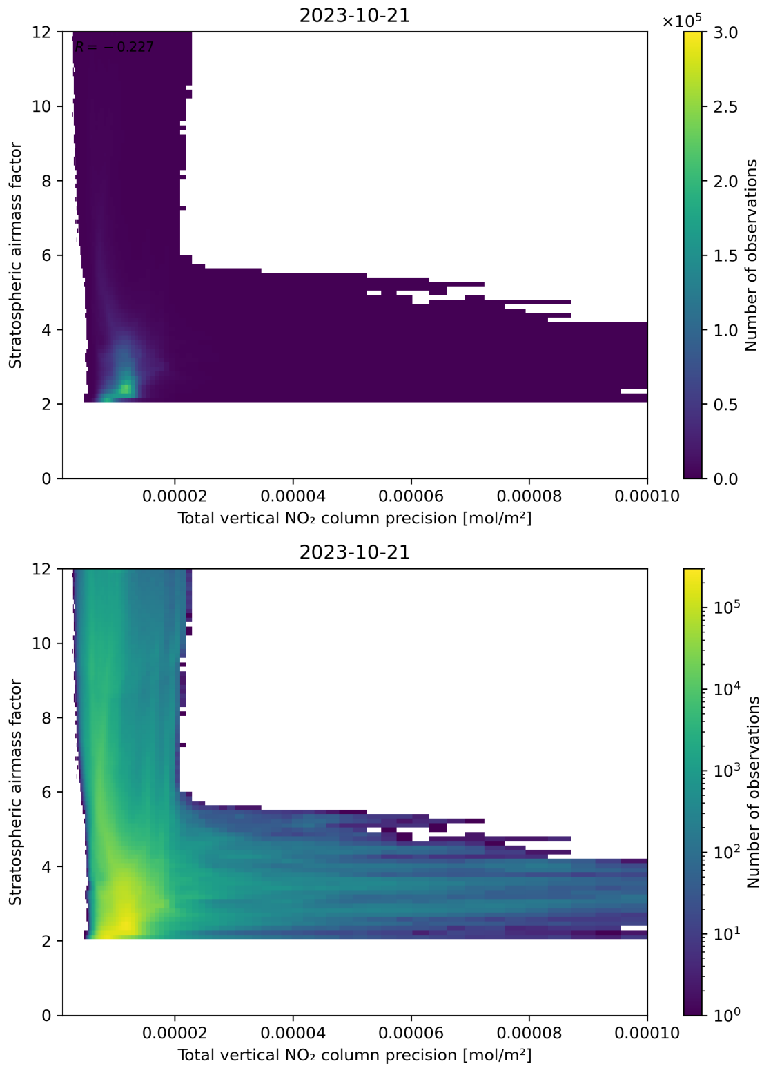
Figure 115: Scatter density plot of “Total vertical NO 2 column precision” against “Stratospheric airmass factor” for 2023-10-20 to 2023-10-22.
