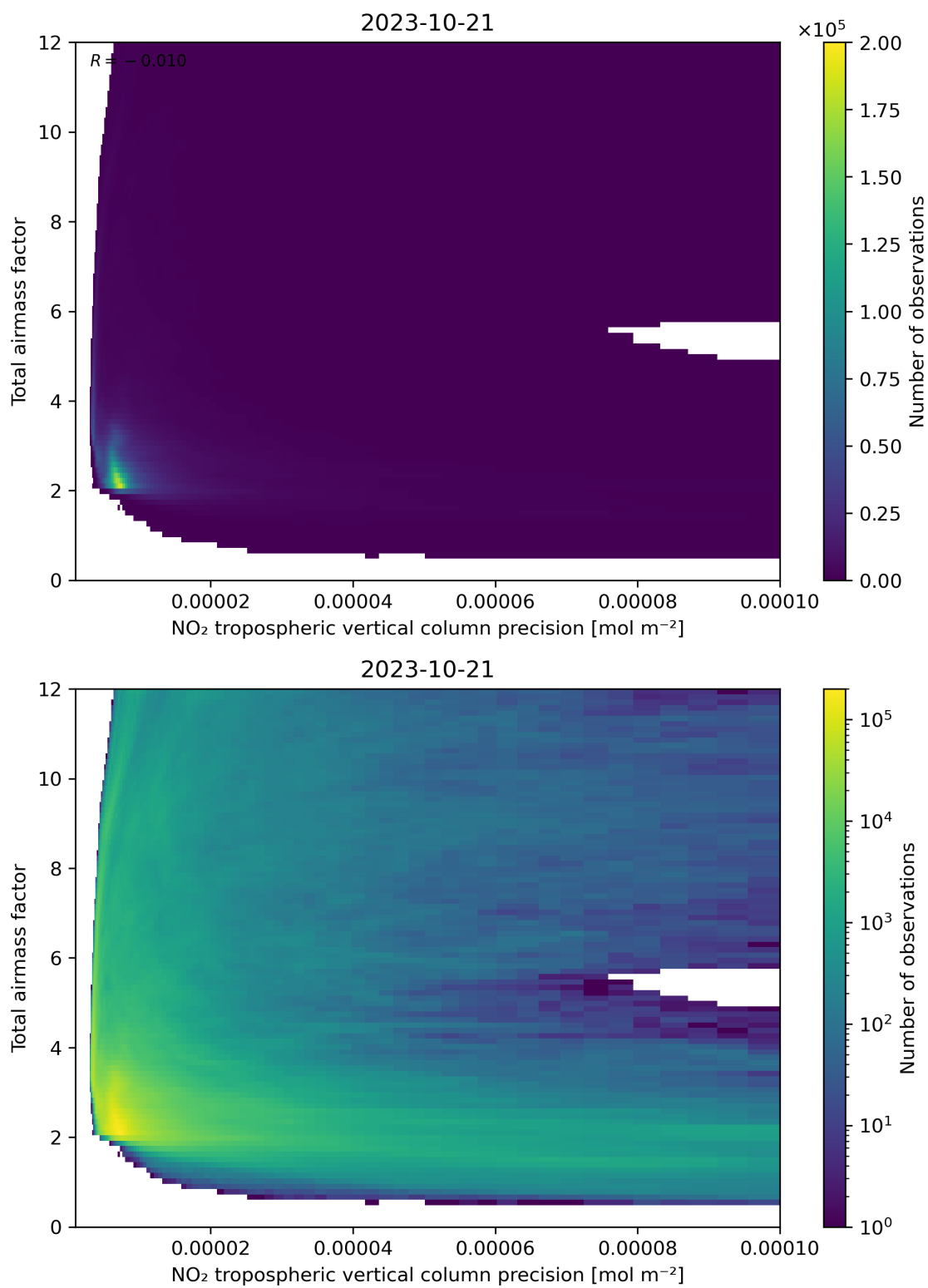
Figure 132: Scatter density plot of “NO 2 tropospheric vertical column precision” against “Total air mass factor” for 2023-10-20 to 2023-10-22.
