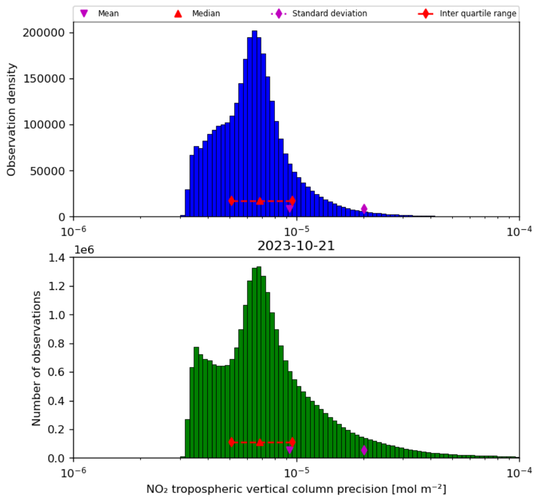
Figure 30: Histogram of “NO 2 tropospheric vertical column precision” for 2023-10-20 to 2023-10-22
