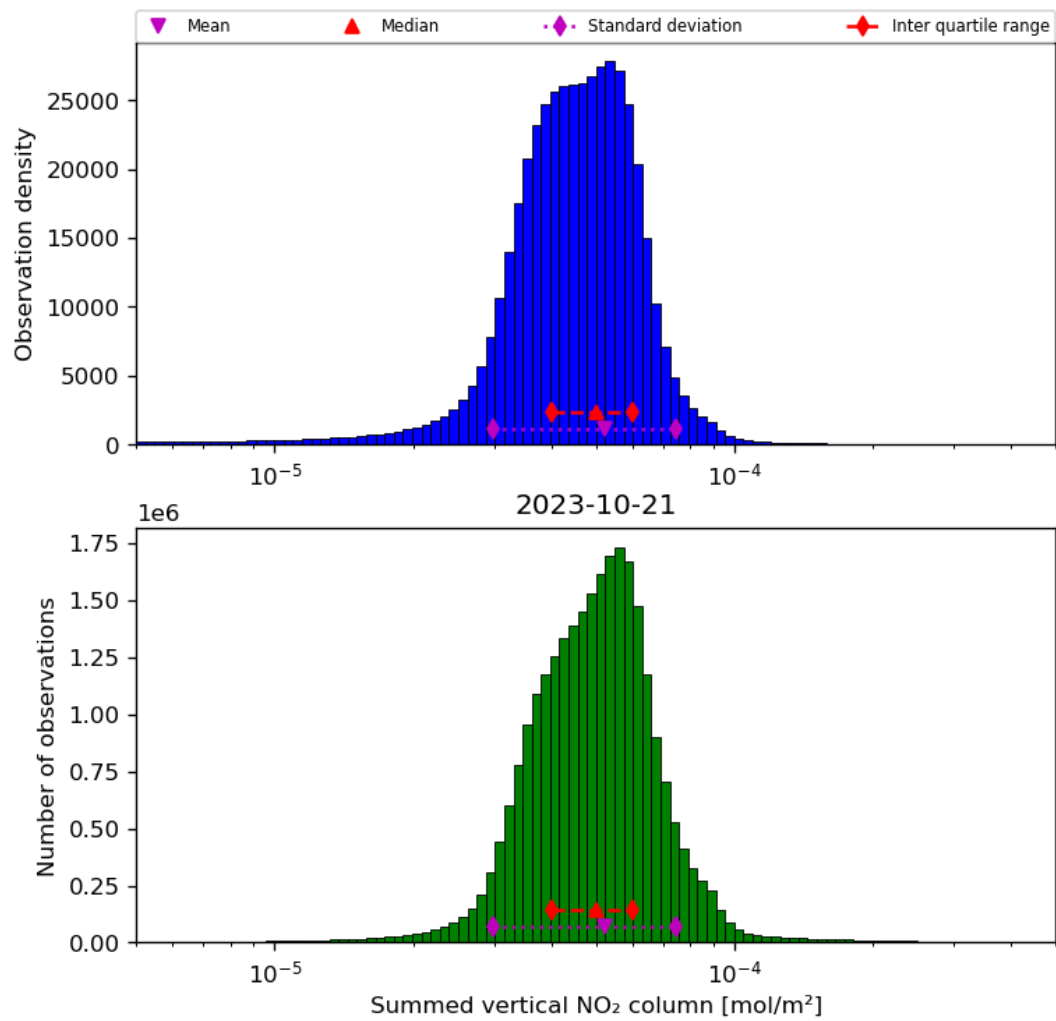
Figure 40: Histogram of "Summed vertical NO 2 column" for 2023-10-20 to 2023-10-22
