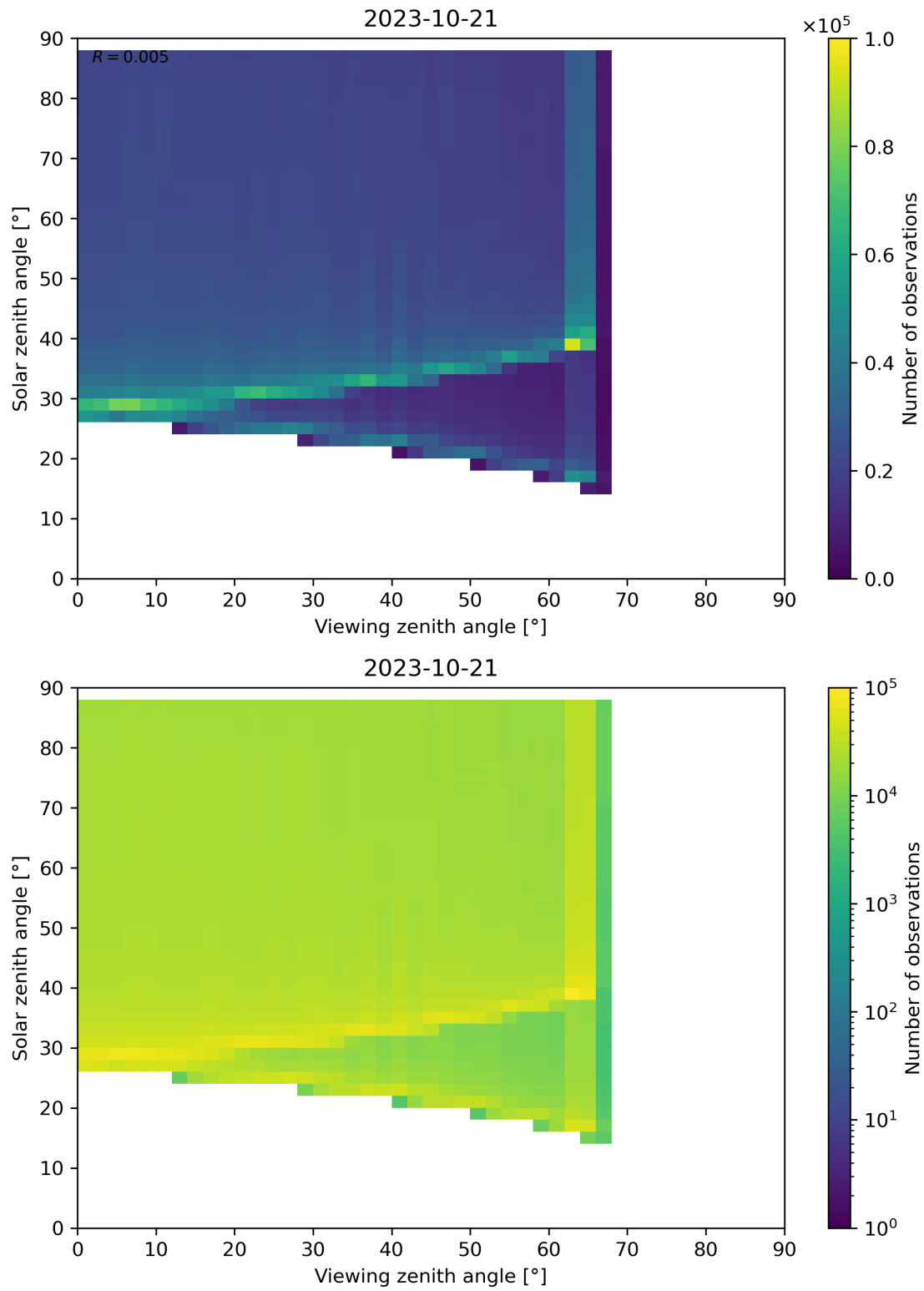
Figure 172: Scatter density plot of “Viewing zenith angle” against “Solar zenith angle” for 2023-10-20 to 2023-10-22.
