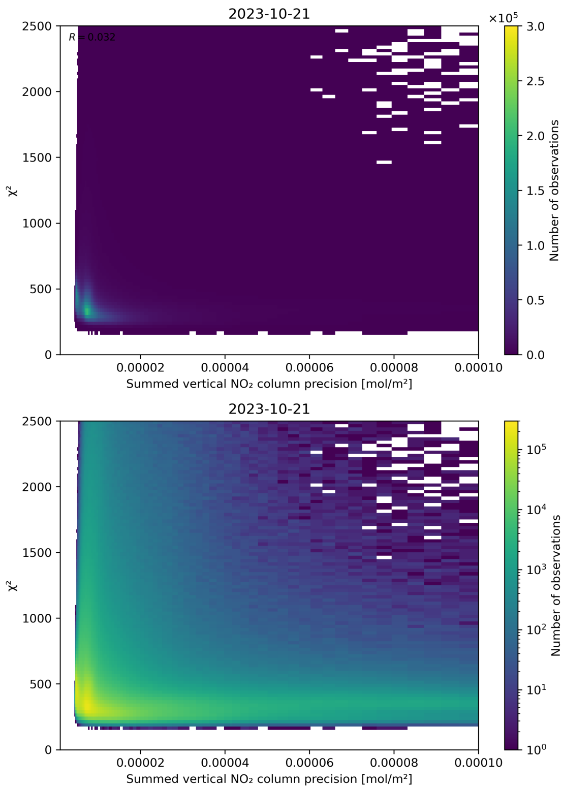
Figure 107: Scatter density plot of “Summed vertical NO 2 column precision” against “ \chi^2 ” for 2023-10-20 to 2023-10-22.
