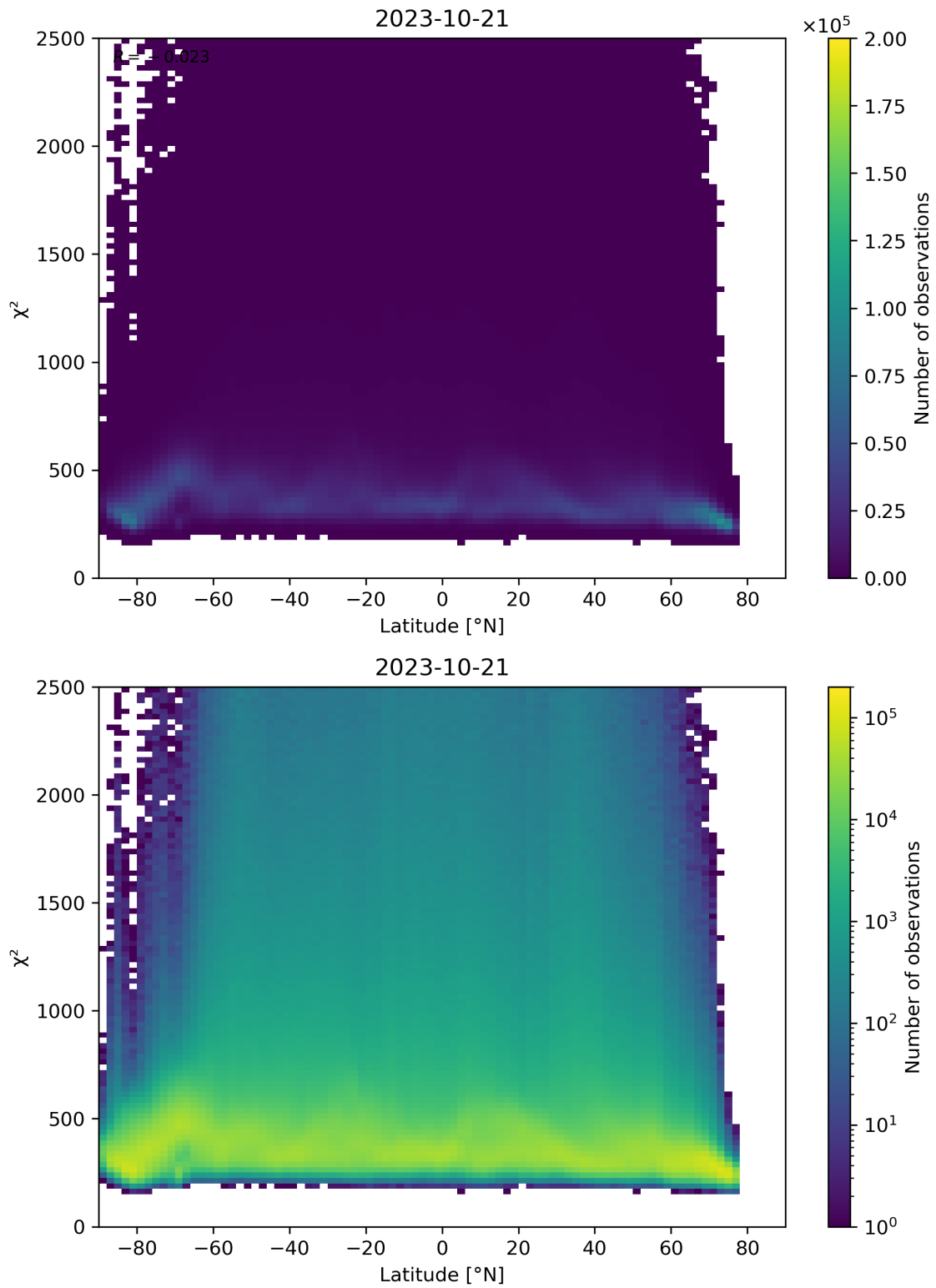
Figure 86: Scatter density plot of “Latitude” against “ \chi^2 ” for 2023-10-20 to 2023-10-22.
