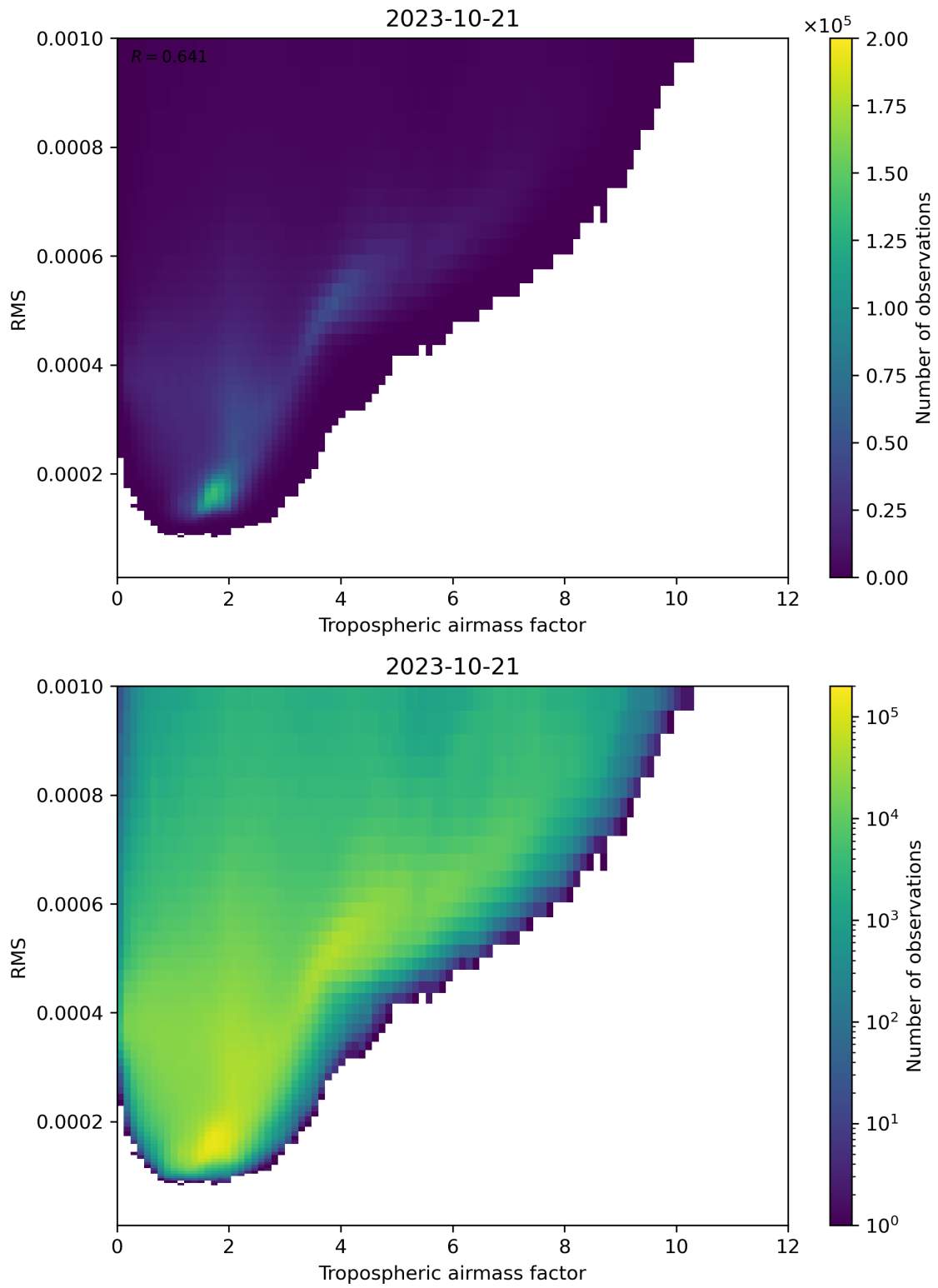
Figure 79: Scatter density plot of “Tropospheric airmass factor” against “RMS” for 2023-10-20 to 2023-10-22.
