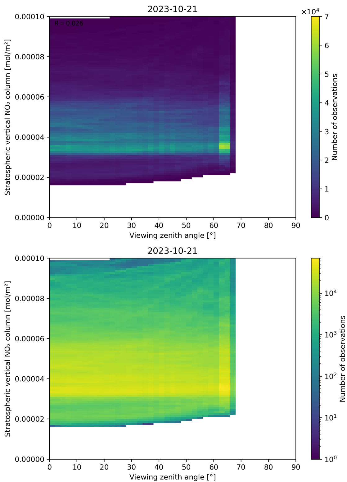
Figure 164: Scatter density plot of “Viewing zenith angle” against “Stratospheric vertical NO 2 column” for 2023-10-20 to 2023-10-22.
