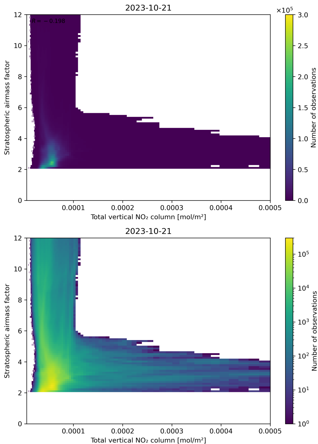
Figure 110: Scatter density plot of “Total vertical NO 2 column” against “Stratospheric air mass factor” for 2023-10-20 to 2023-10-22.
