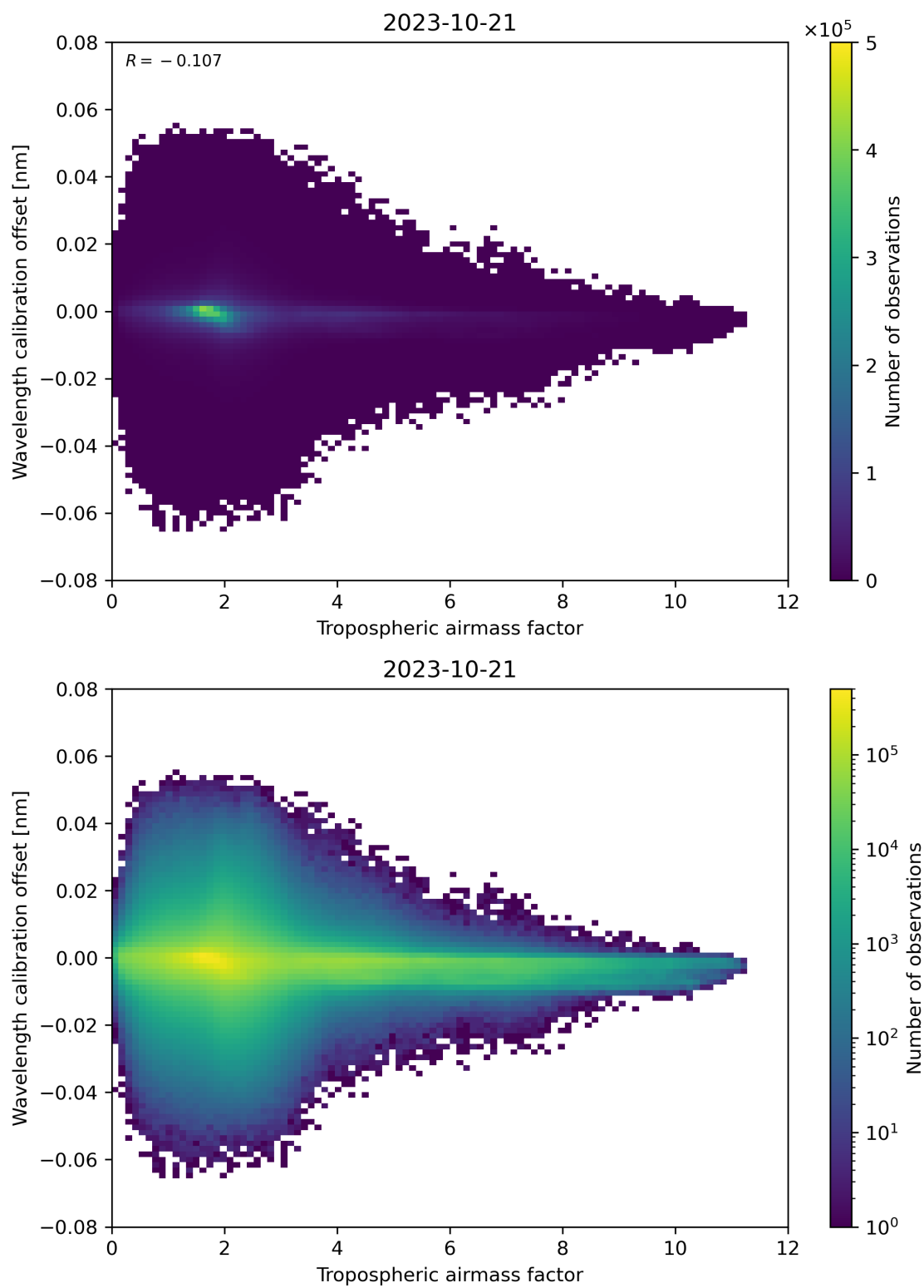
Figure 80: Scatter density plot of “Tropospheric airmass factor” against “Wavelength calibration offset” for 2023-10-20 to 2023-10-22.
