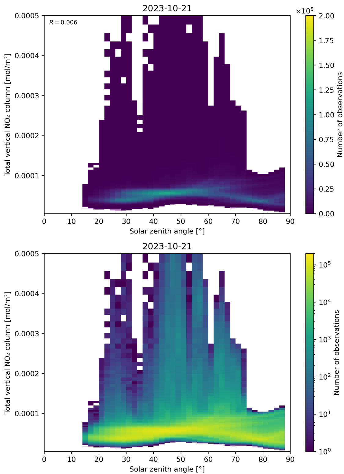
Figure 153: Scatter density plot of “Solar zenith angle” against “Total vertical NO 2 column” for 2023-10-20 to 2023-10-22.
