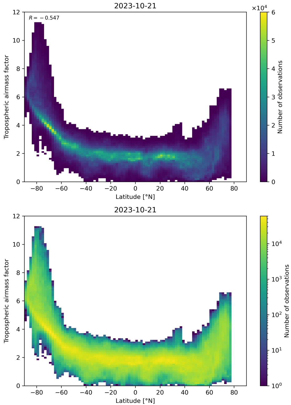
Figure 85: Scatter density plot of “Latitude” against “Tropospheric airmass factor” for 2023-10-20 to 2023-10-22.
