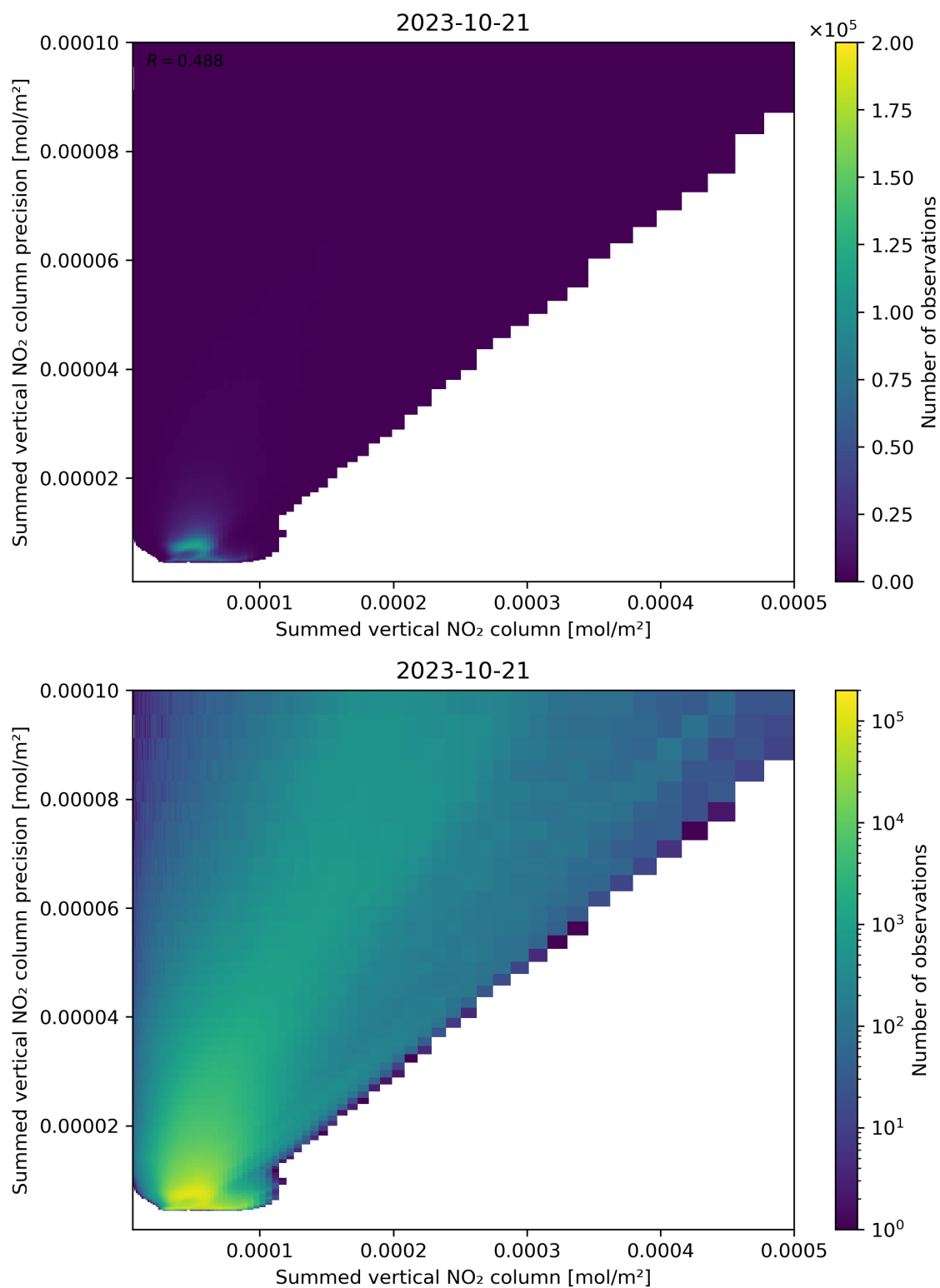
Figure 105: Scatter density plot of “Summed vertical NO 2 column” against “Summed vertical NO 2 column precision” for 2023-10-20 to 2023-10-22.
