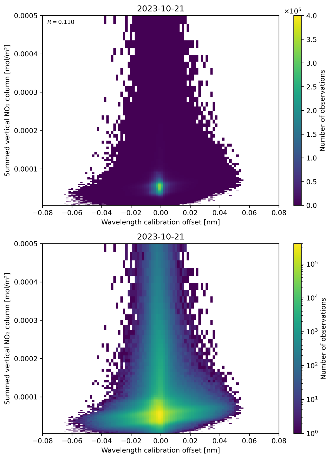
Figure 177: Scatter density plot of “Wavelength calibration offset” against “Summed vertical NO 2 column” for 2023-10-20 to 2023-10-22.
