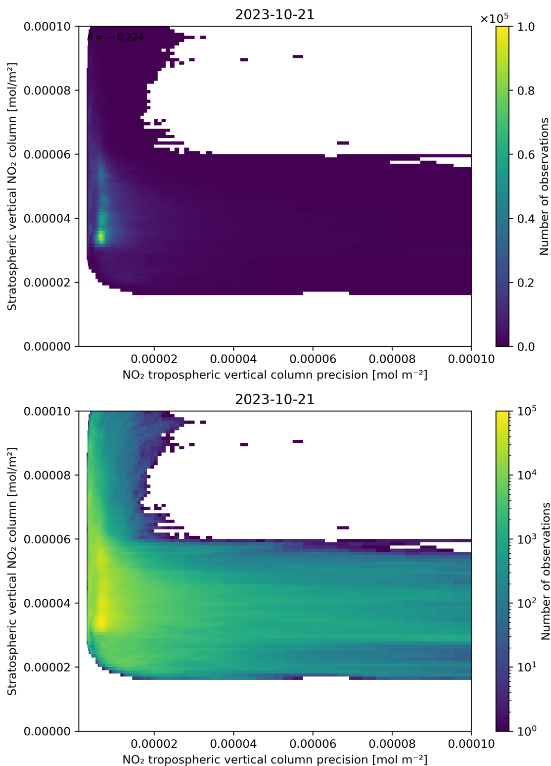
Figure 135: Scatter density plot of “NO 2 tropospheric vertical column precision” against “Stratospheric vertical NO 2 column” for 2023-10-20 to 2023-10-22.
