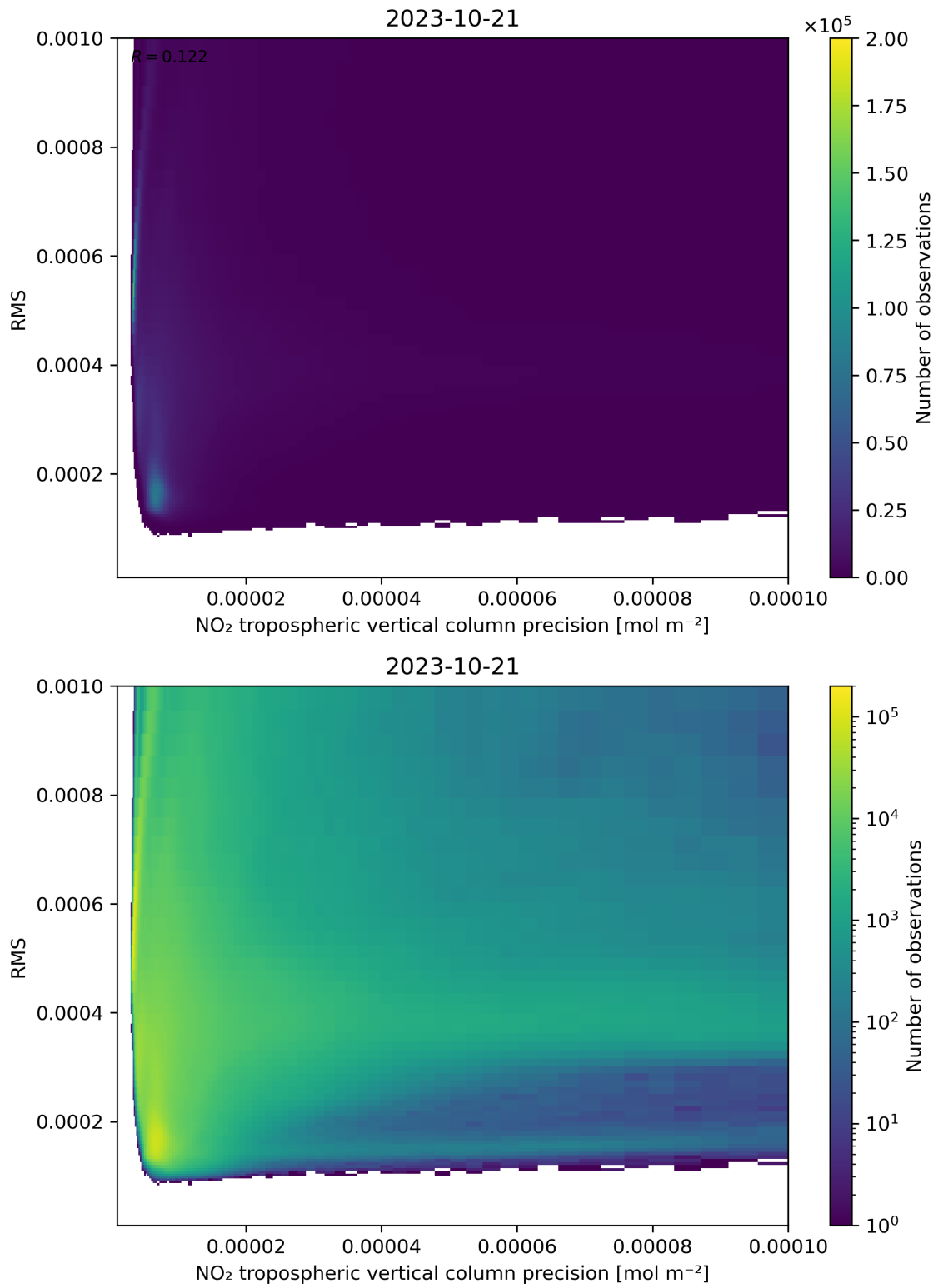
Figure 140: Scatter density plot of “NO 2 tropospheric vertical column precision” against “RMS” for 2023-10-20 to 2023-10-22.
