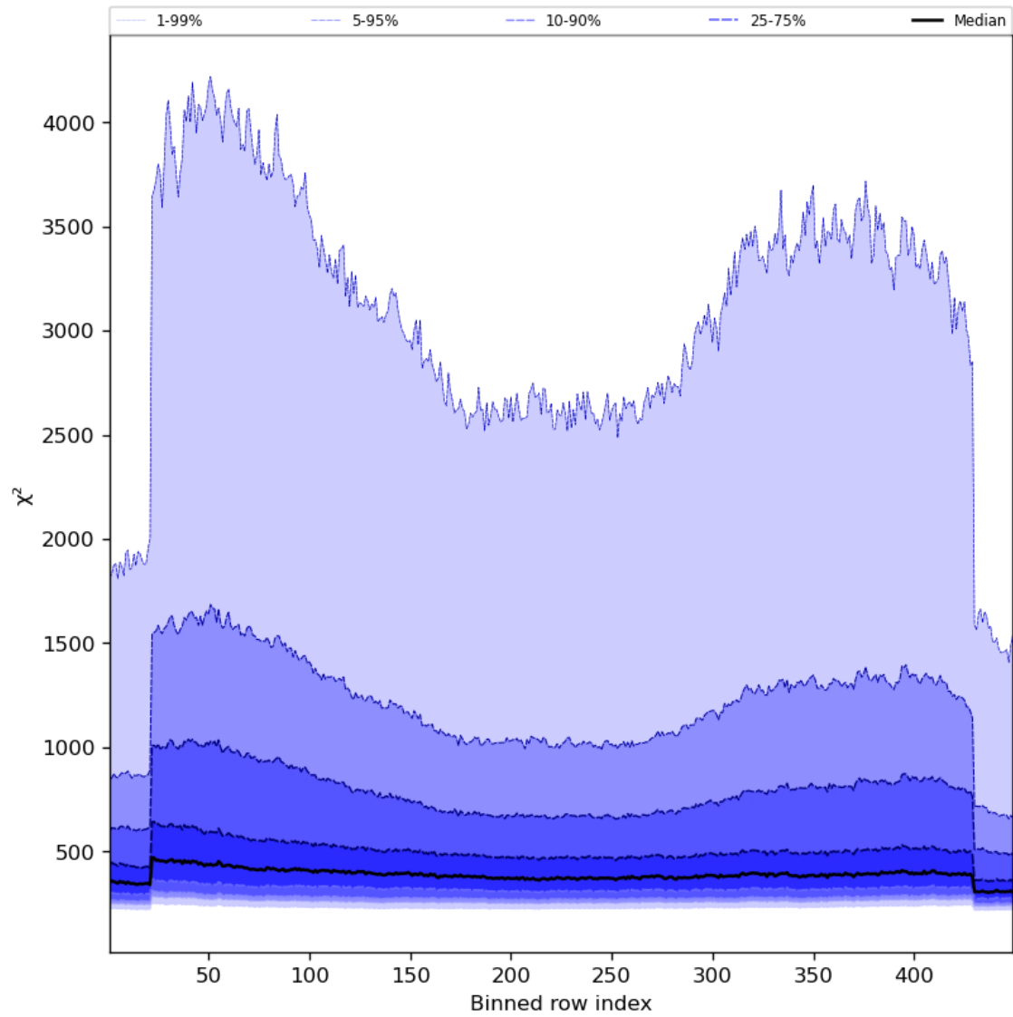
Figure 59: Along track statistics of “ \chi^2 ” for 2023-10-20 to 2023-10-22
