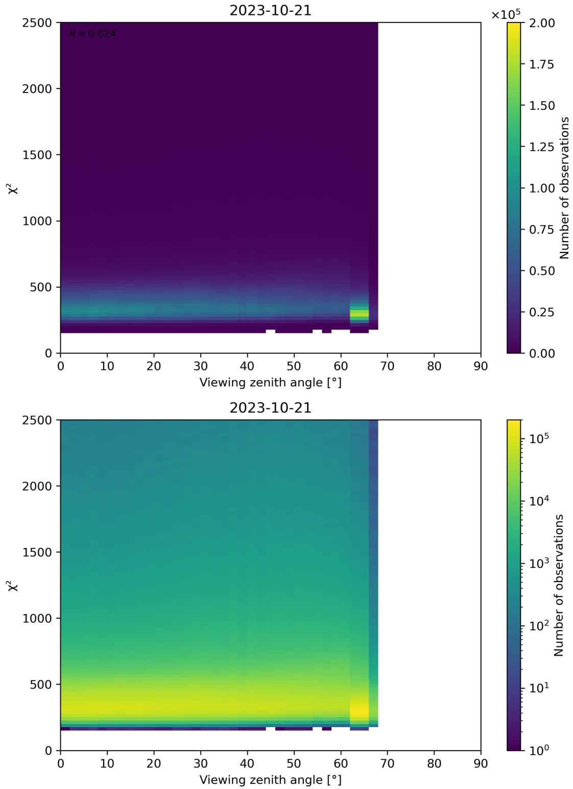
Figure 162: Scatter density plot of “Viewing zenith angle” against “ \chi^2 ” for 2023-10-20 to 2023-10-22.
