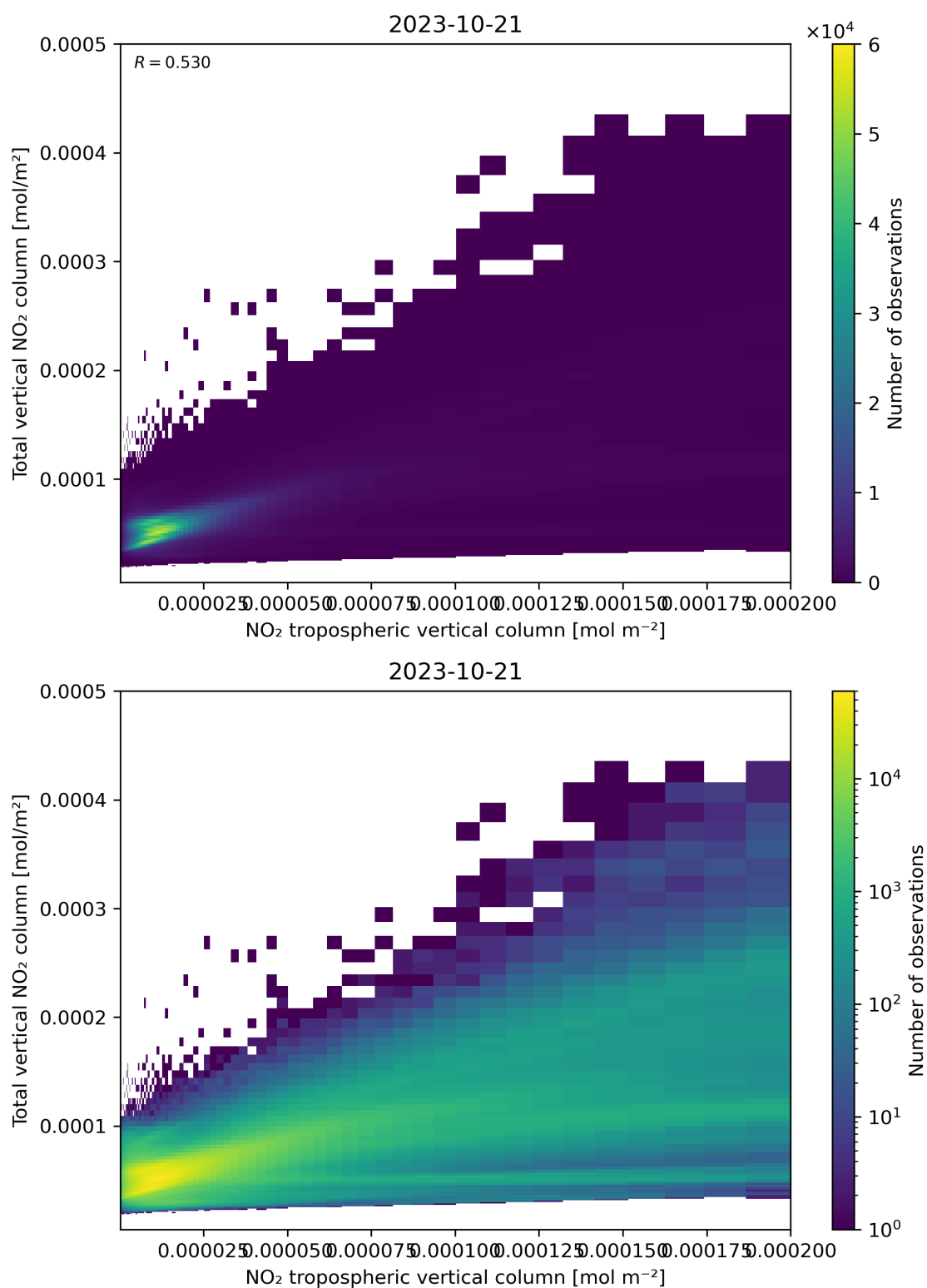
Figure 128: Scatter density plot of “NO 2 tropospheric vertical column” against “Total vertical NO 2 column” for 2023-10-20 to 2023-10-22.
