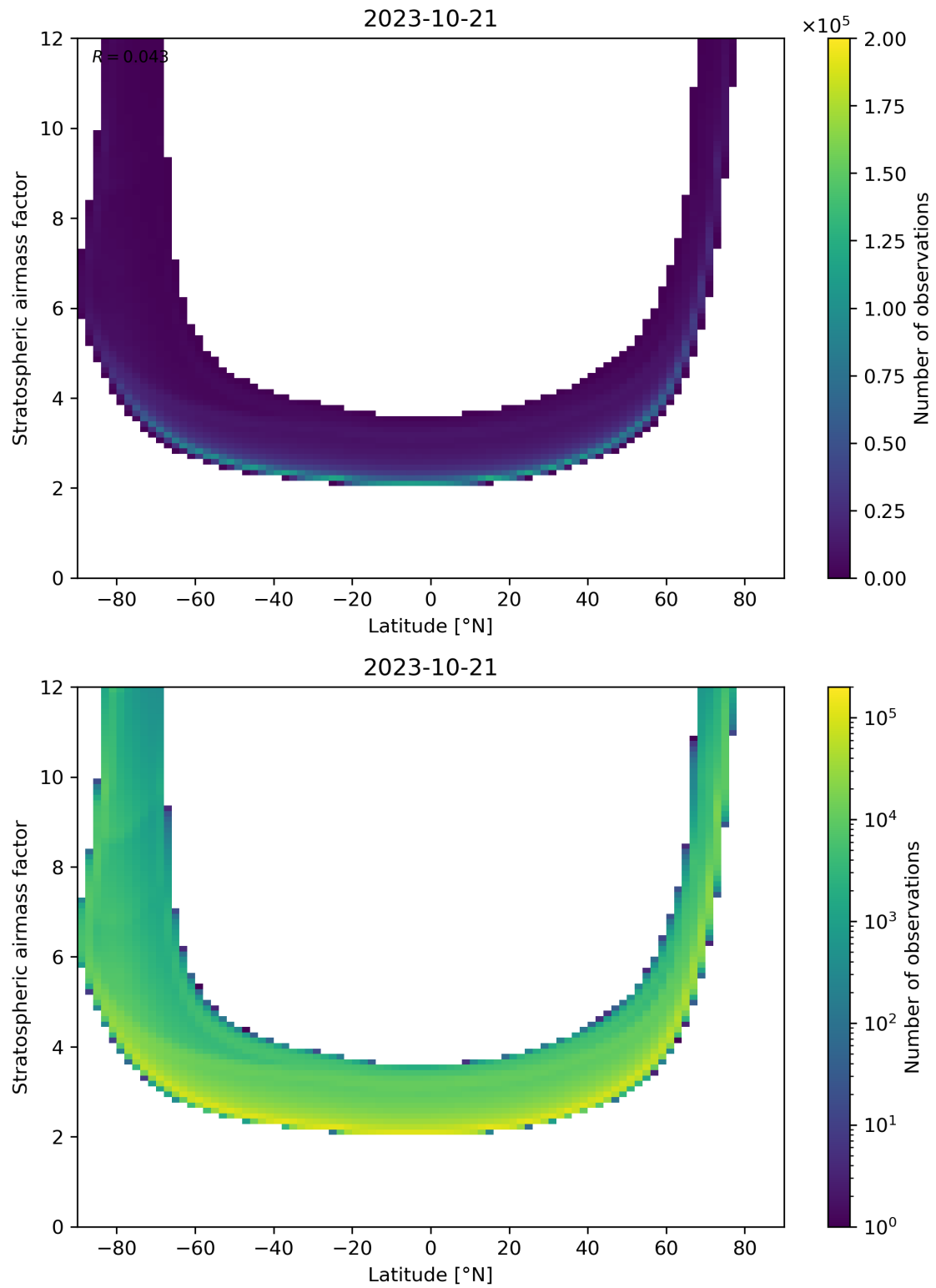
Figure 83: Scatter density plot of “Latitude” against “Stratospheric airmass factor” for 2023-10-20 to 2023-10-22.
