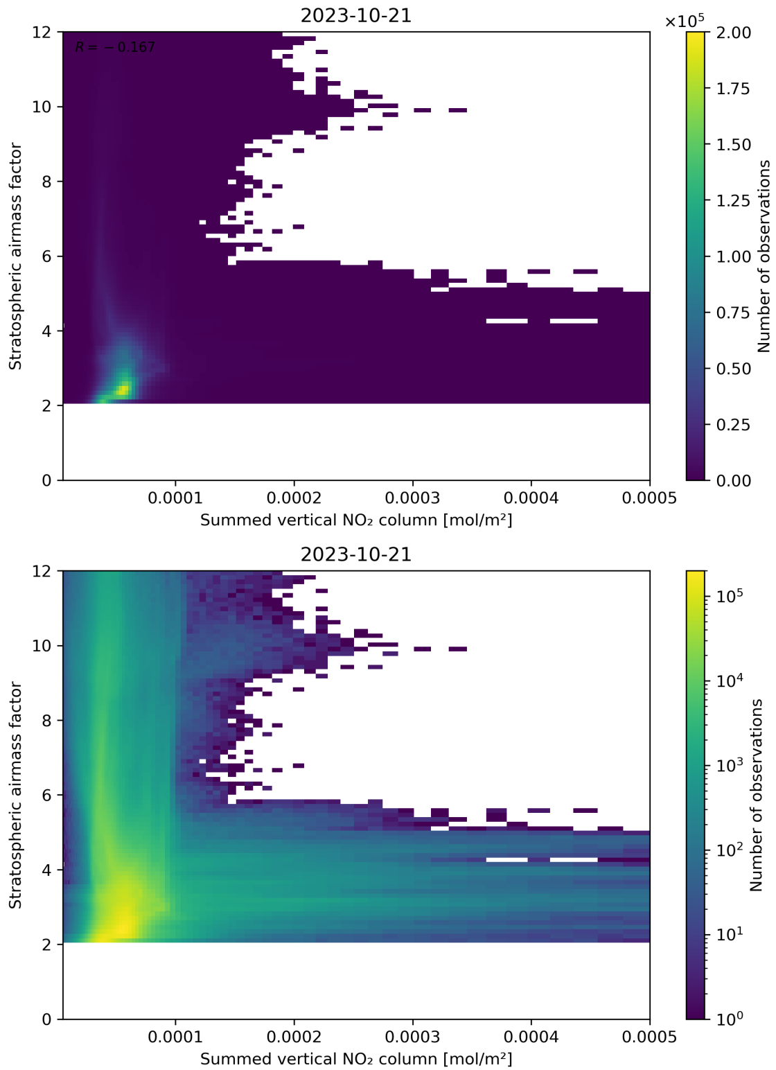
Figure 103: Scatter density plot of “Summed vertical NO 2 column” against “Stratospheric air mass factor” for 2023-10-20 to 2023-10-22.
