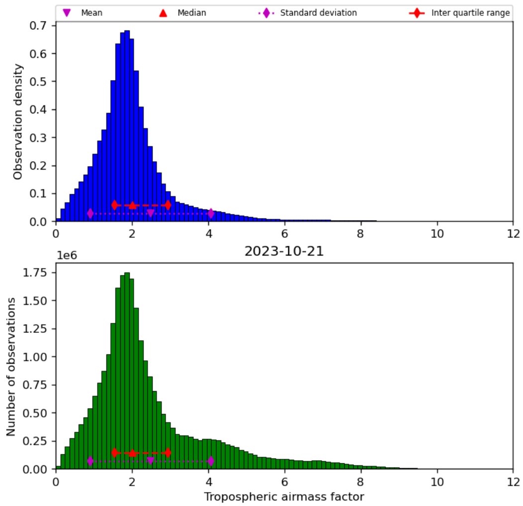
Figure 31: Histogram of “Tropospheric airmass factor” for 2023-10-20 to 2023-10-22
