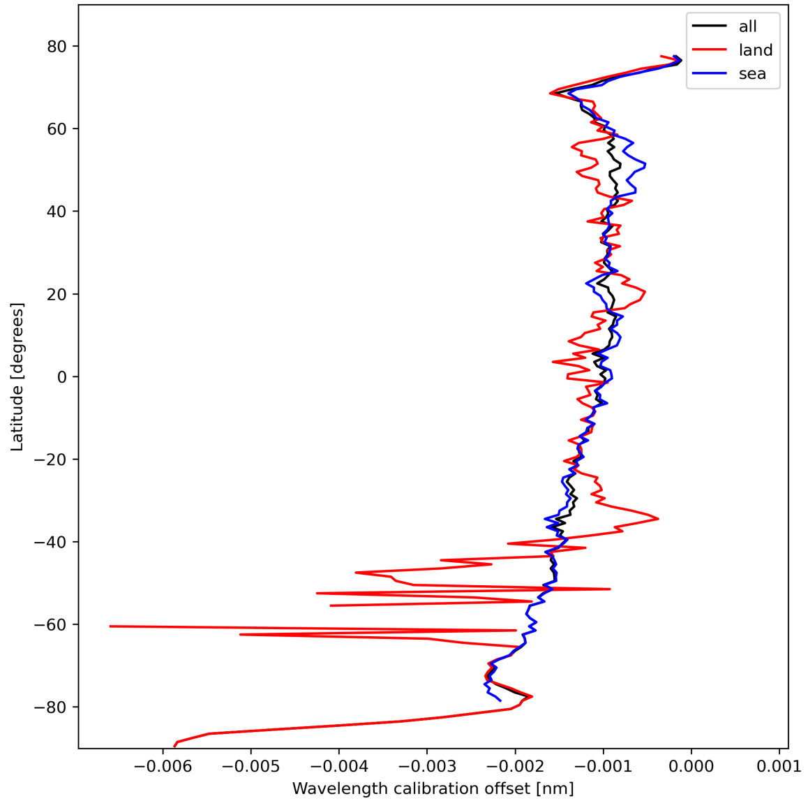
Figure 18: Zonal average of “Wavelength calibration offset” for 2023-10-20 to 2023-10-22.
