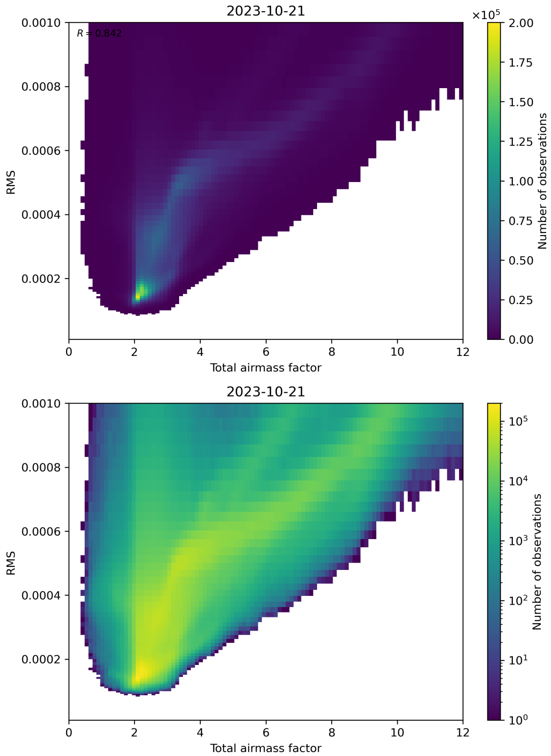
Figure 69: Scatter density plot of “Total airmass factor” against “RMS” for 2023-10-20 to 2023-10-22.
