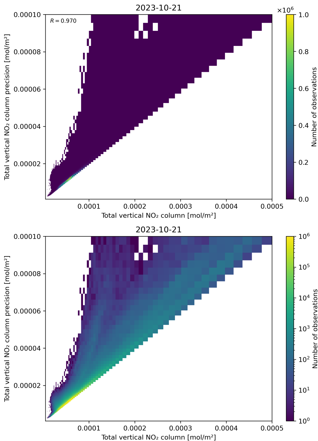
Figure 114: Scatter density plot of “Total vertical NO 2 column” against “Total vertical NO 2 column precision” for 2023-10-20 to 2023-10-22.
