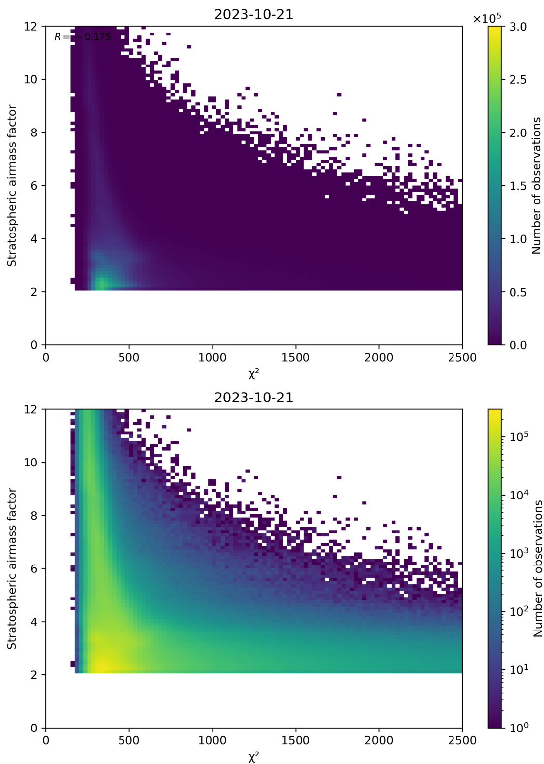
Figure 81: Scatter density plot of “ \chi^2 ” against “Stratospheric airmass factor” for 2023-10-20 to 2023-10-22.
