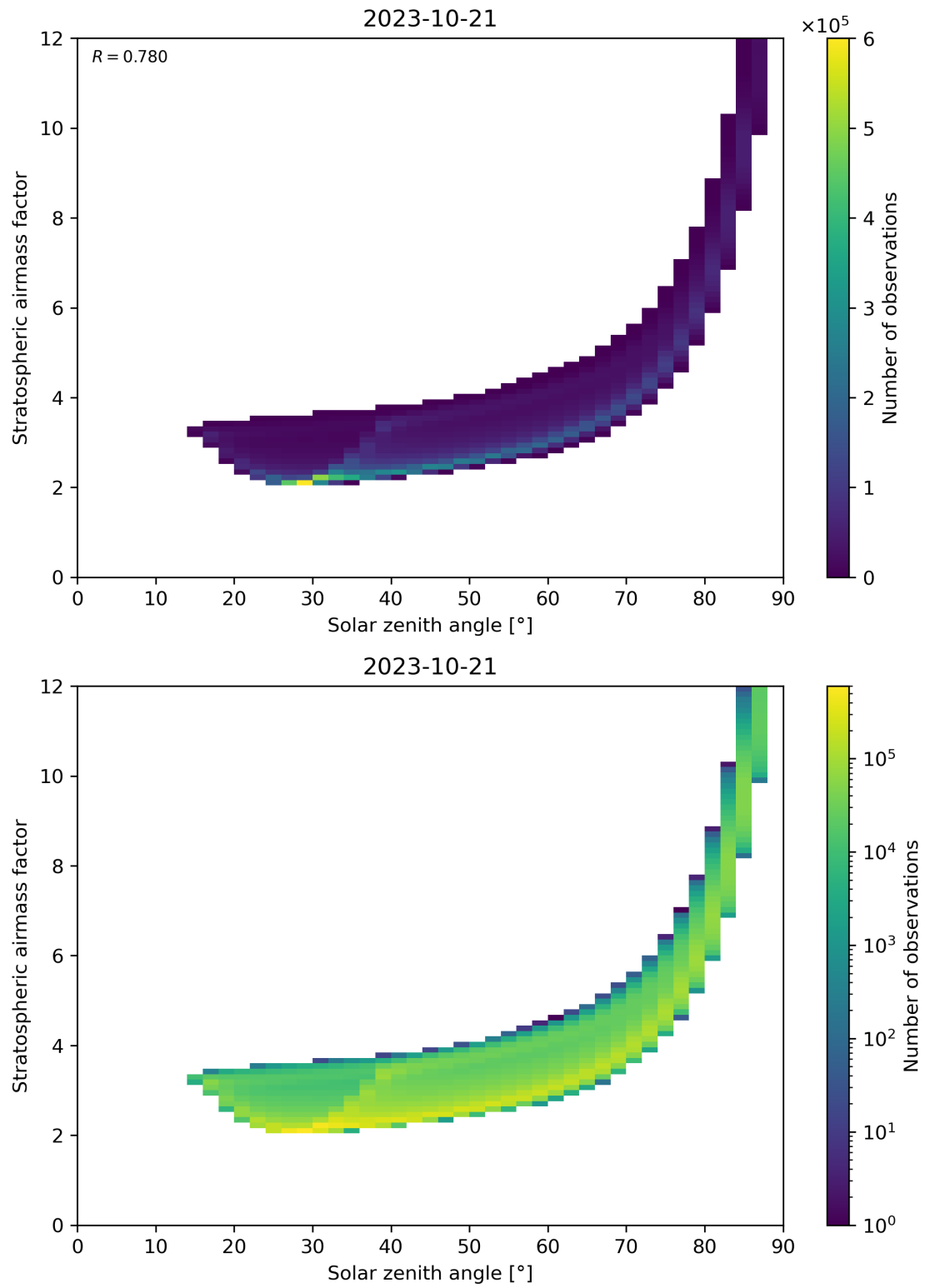
Figure 145: Scatter density plot of “Solar zenith angle” against “Stratospheric airmass factor” for 2023-10-20 to 2023-10-22.
