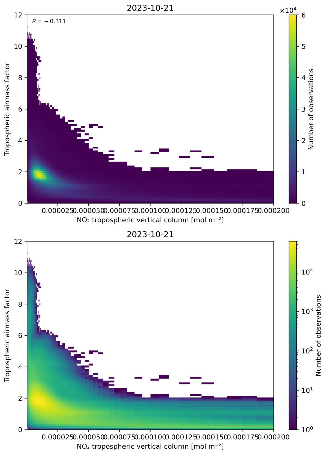
Figure 123: Scatter density plot of “NO 2 tropospheric vertical column” against “Tropospheric airmass factor” for 2023-10-20 to 2023-10-22.
