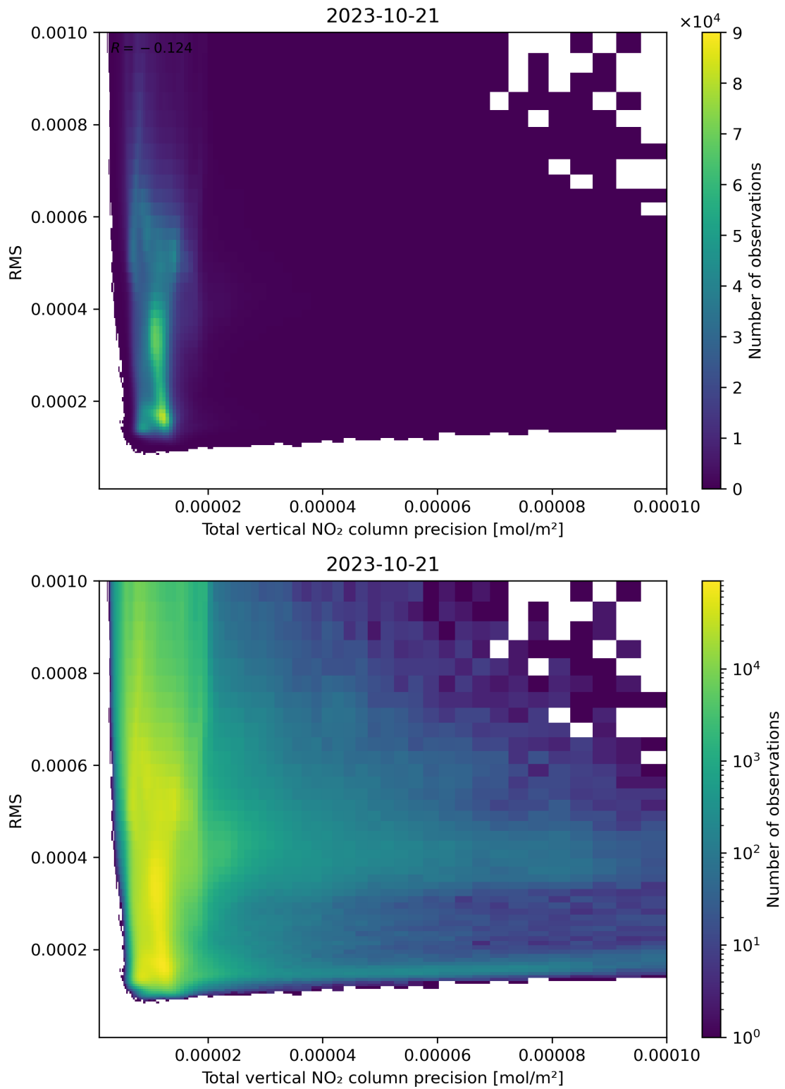
Figure 119: Scatter density plot of “Total vertical NO 2 column precision” against “RMS” for 2023-10-20 to 2023-10-22.
