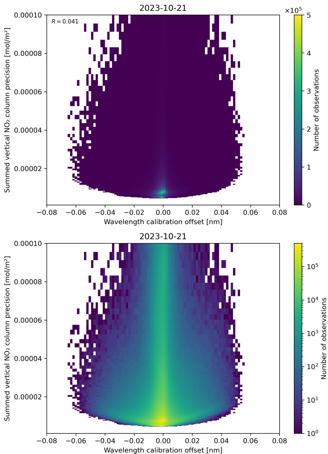
Figure 178: Scatter density plot of “Wavelength calibration offset” against “Summed vertical NO 2 column precision” for 2023-10-20 to 2023-10-22.
