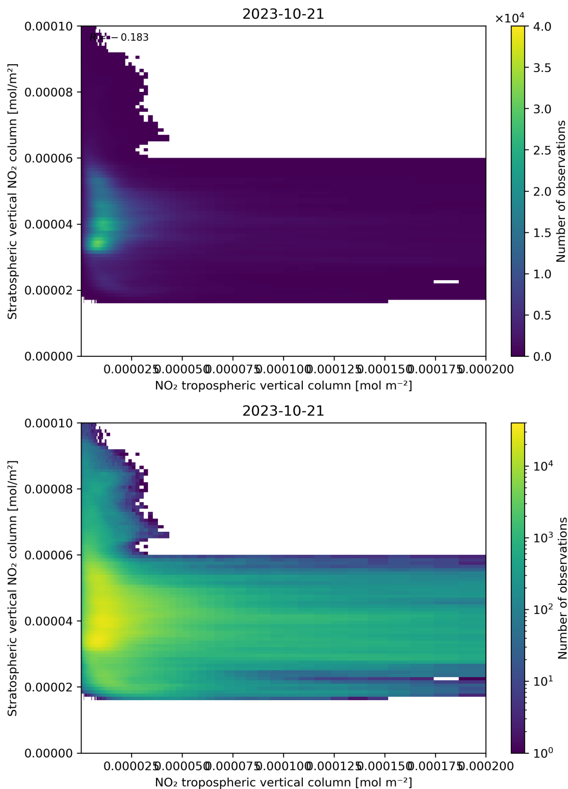
Figure 125: Scatter density plot of “NO 2 tropospheric vertical column” against “Stratospheric vertical NO 2 column” for 2023-10-20 to 2023-10-22.
