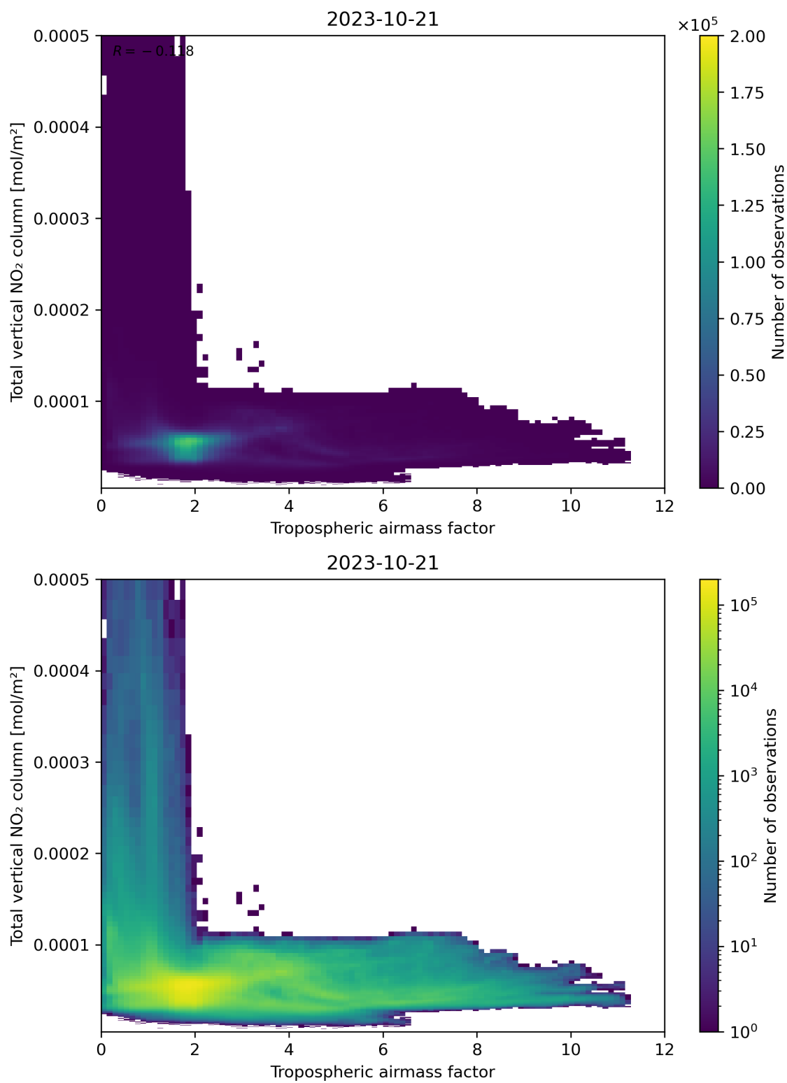
Figure 77: Scatter density plot of “Tropospheric airmass factor” against “Total vertical NO 2 column” for 2023-10-20 to 2023-10-22.
