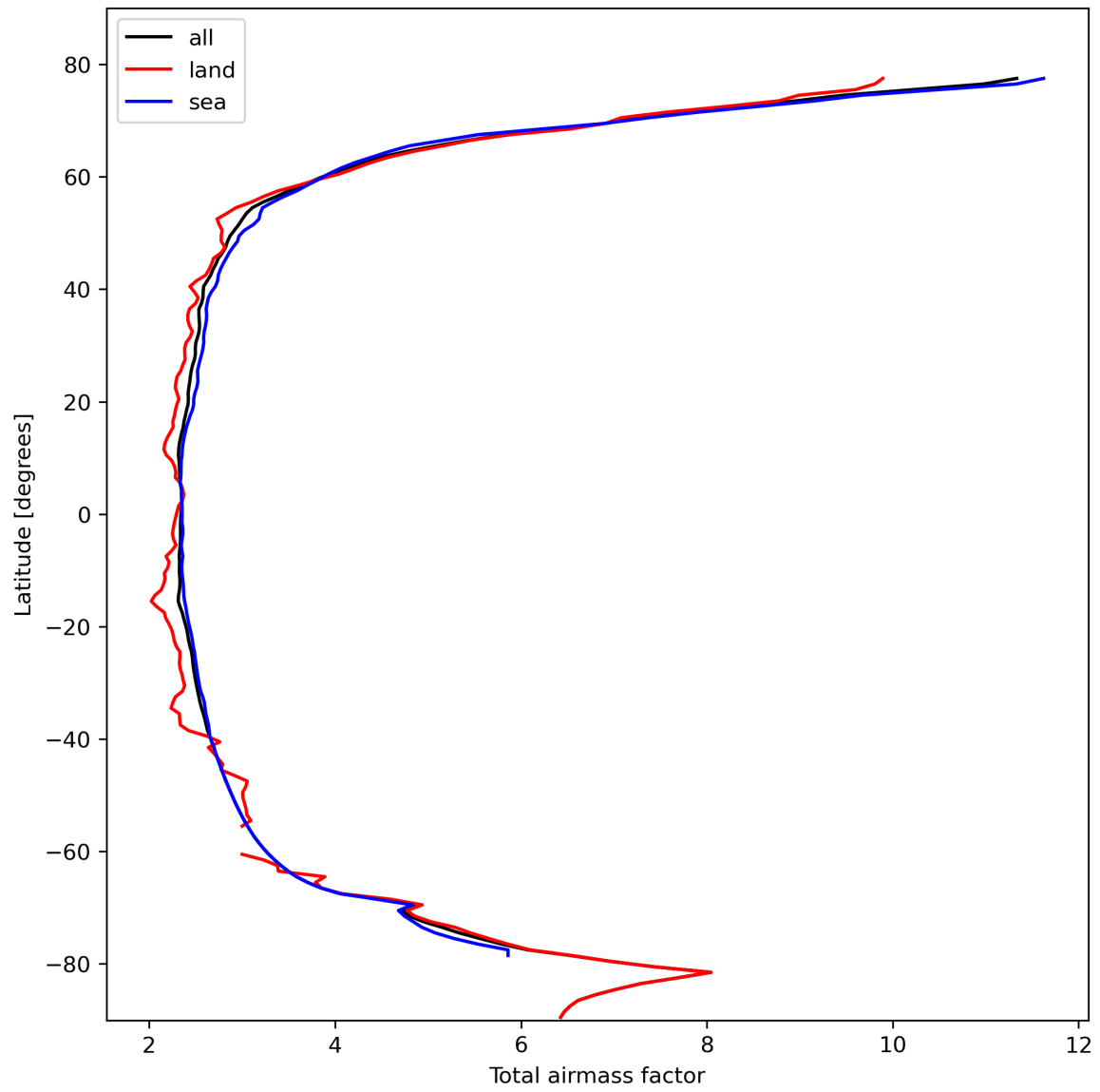
Figure 15: Zonal average of “Total airmass factor” for 2023-10-20 to 2023-10-22.
