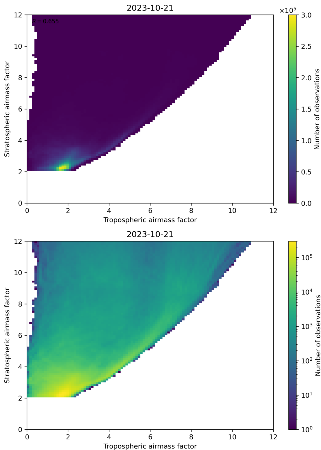
Figure 71: Scatter density plot of “Tropospheric airmass factor” against “Stratospheric airmass factor” for 2023-10-20 to 2023-10-22.
