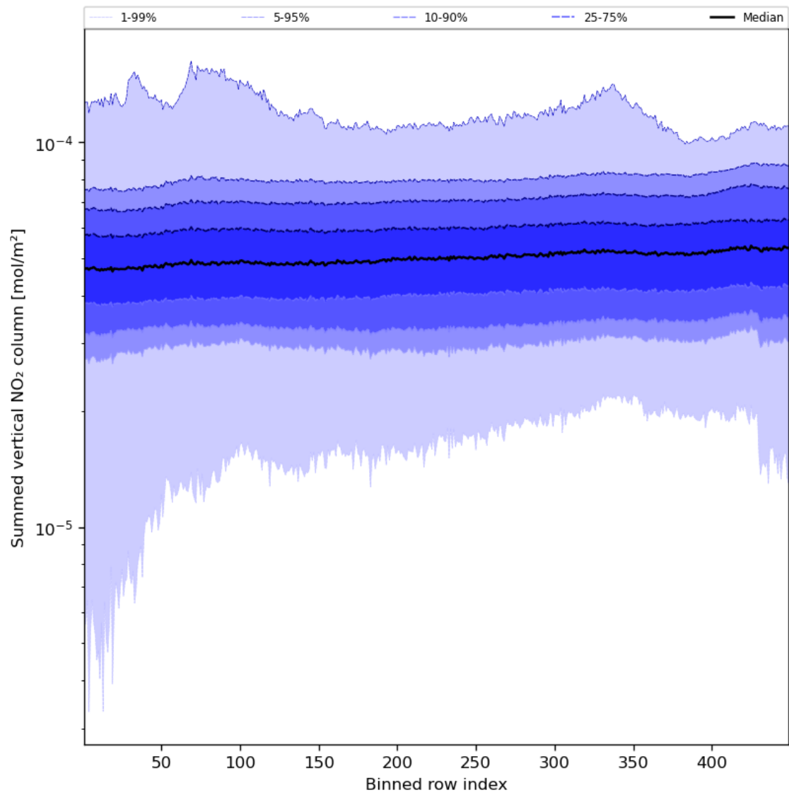
Figure 57: Along track statistics of “Summed vertical NO 2 column” for 2023-10-20 to 2023-10-22
