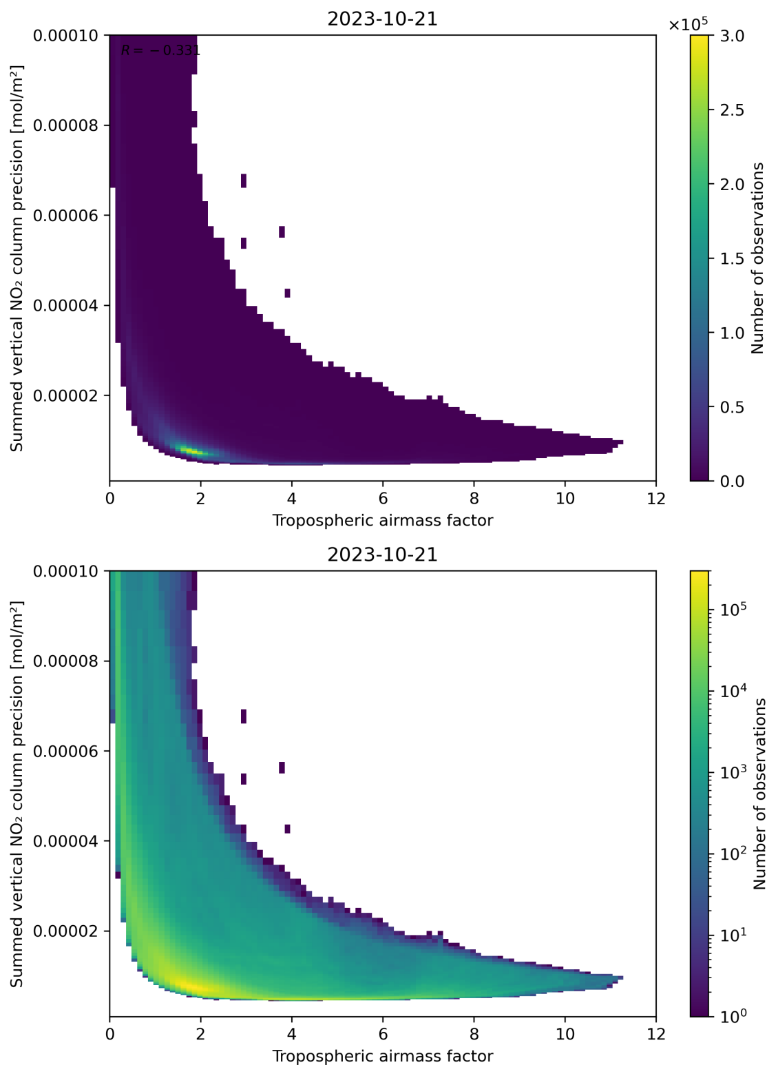
Figure 76: Scatter density plot of “Tropospheric air mass factor” against “Summed vertical NO 2 column precision” for 2023-10-20 to 2023-10-22.
