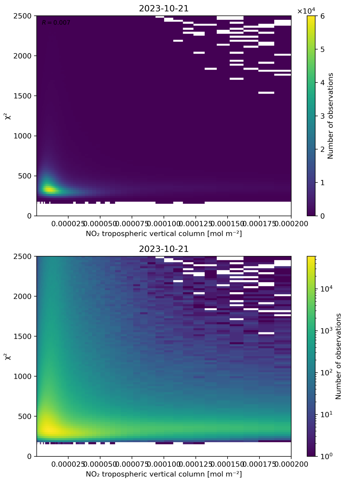
Figure 124: Scatter density plot of “NO 2 tropospheric vertical column” against “ \chi^2 ” for 2023-10-20 to 2023-10-22.
