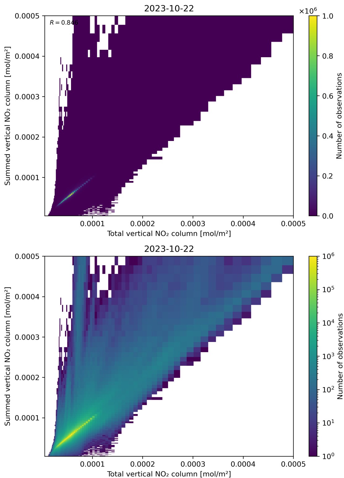
Figure 112: Scatter density plot of “Total vertical NO 2 column” against “Summed vertical NO 2 column” for 2023-10-22 to 2023-10-23.
