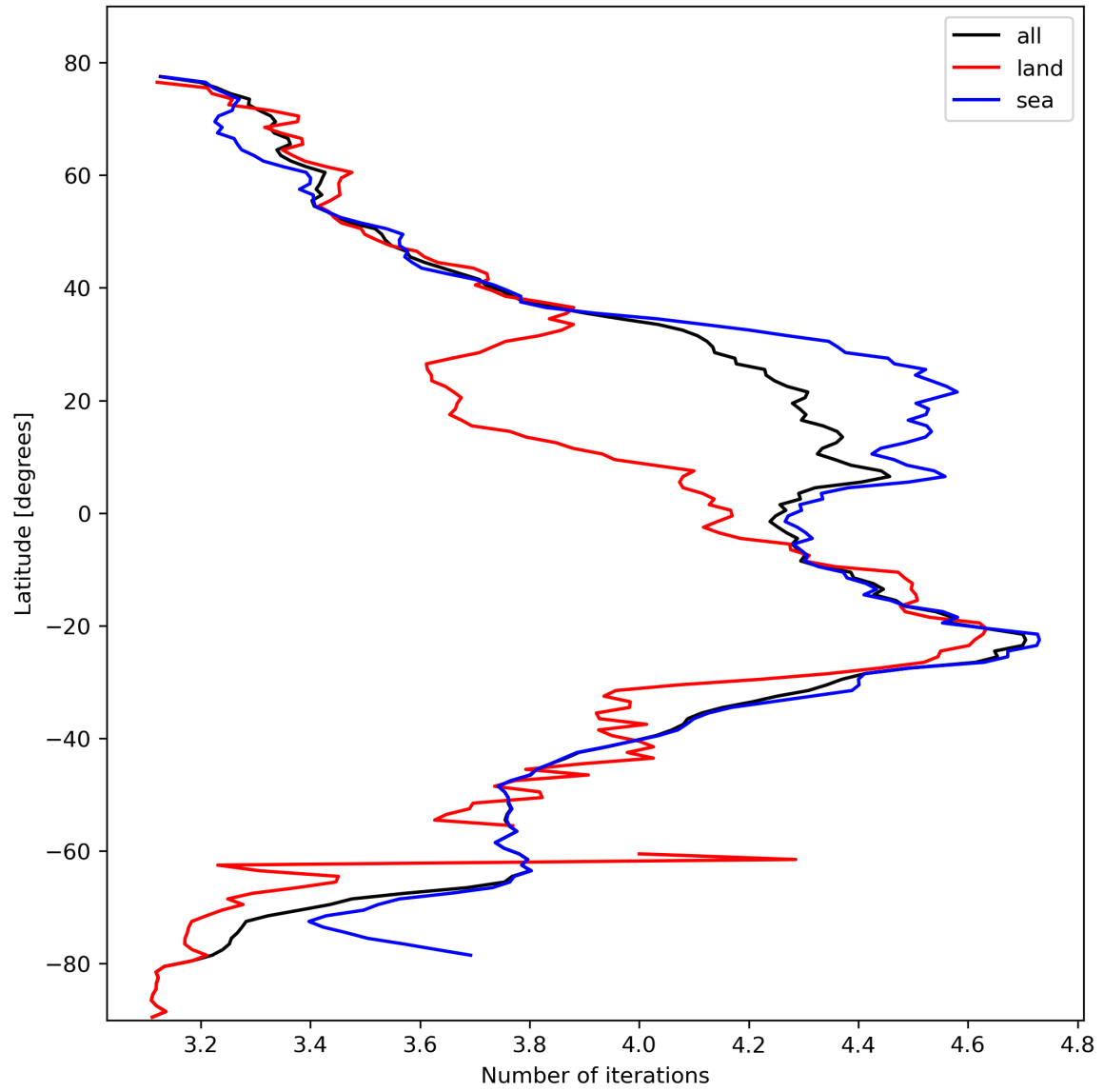
Figure 17: Zonal average of “Number of iterations” for 2023-10-22 to 2023-10-23.
