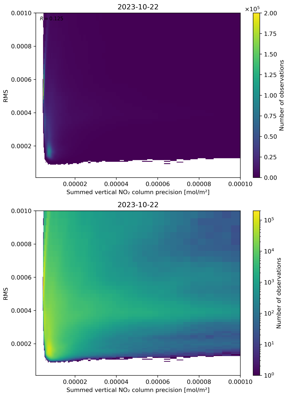
Figure 108: Scatter density plot of “Summed vertical NO 2 column precision” against “RMS” for 2023-10-22 to 2023-10-23.
