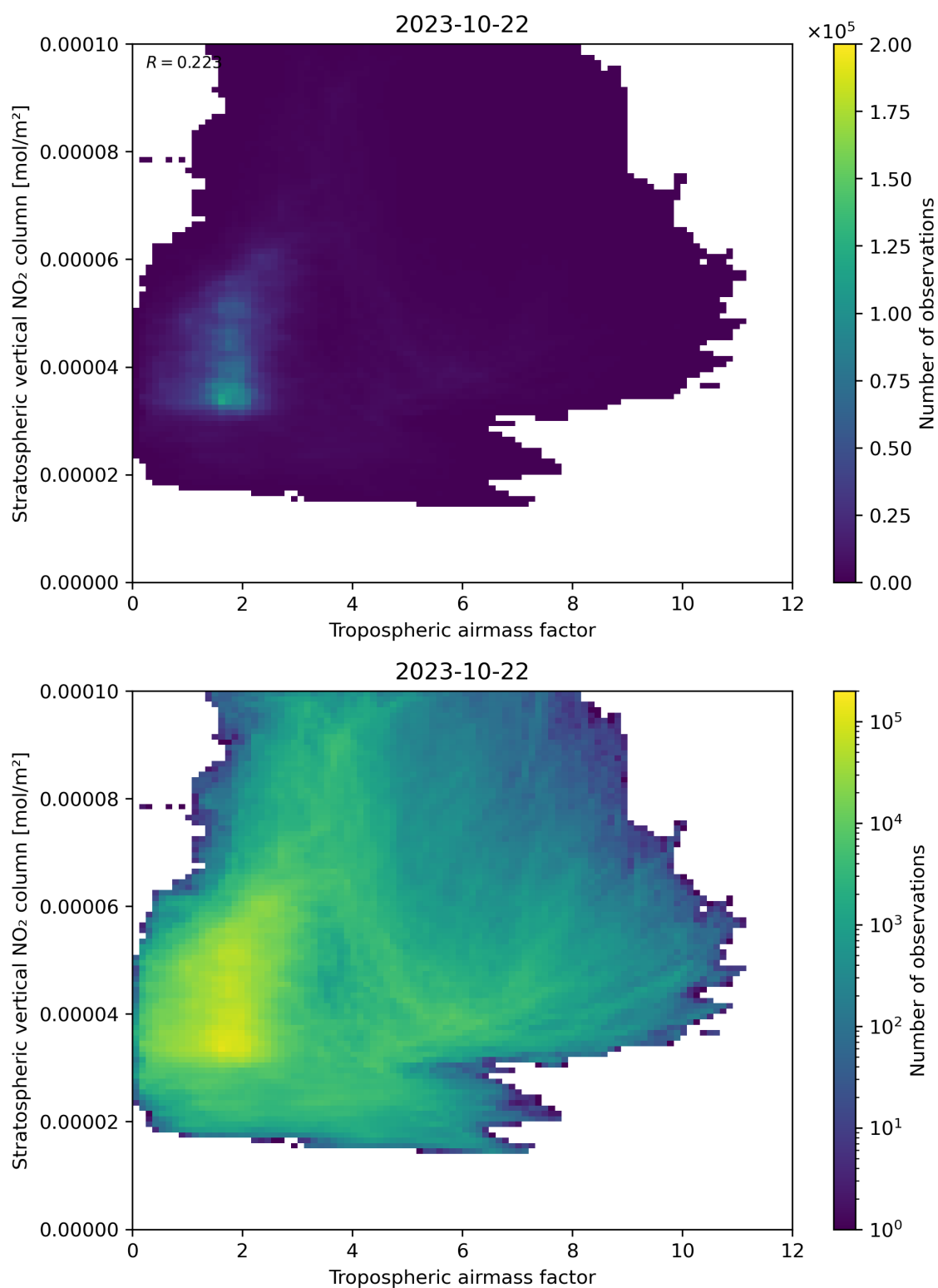
Figure 74: Scatter density plot of “Tropospheric air mass factor” against “Stratospheric vertical NO 2 column” for 2023-10-22 to 2023-10-23.
