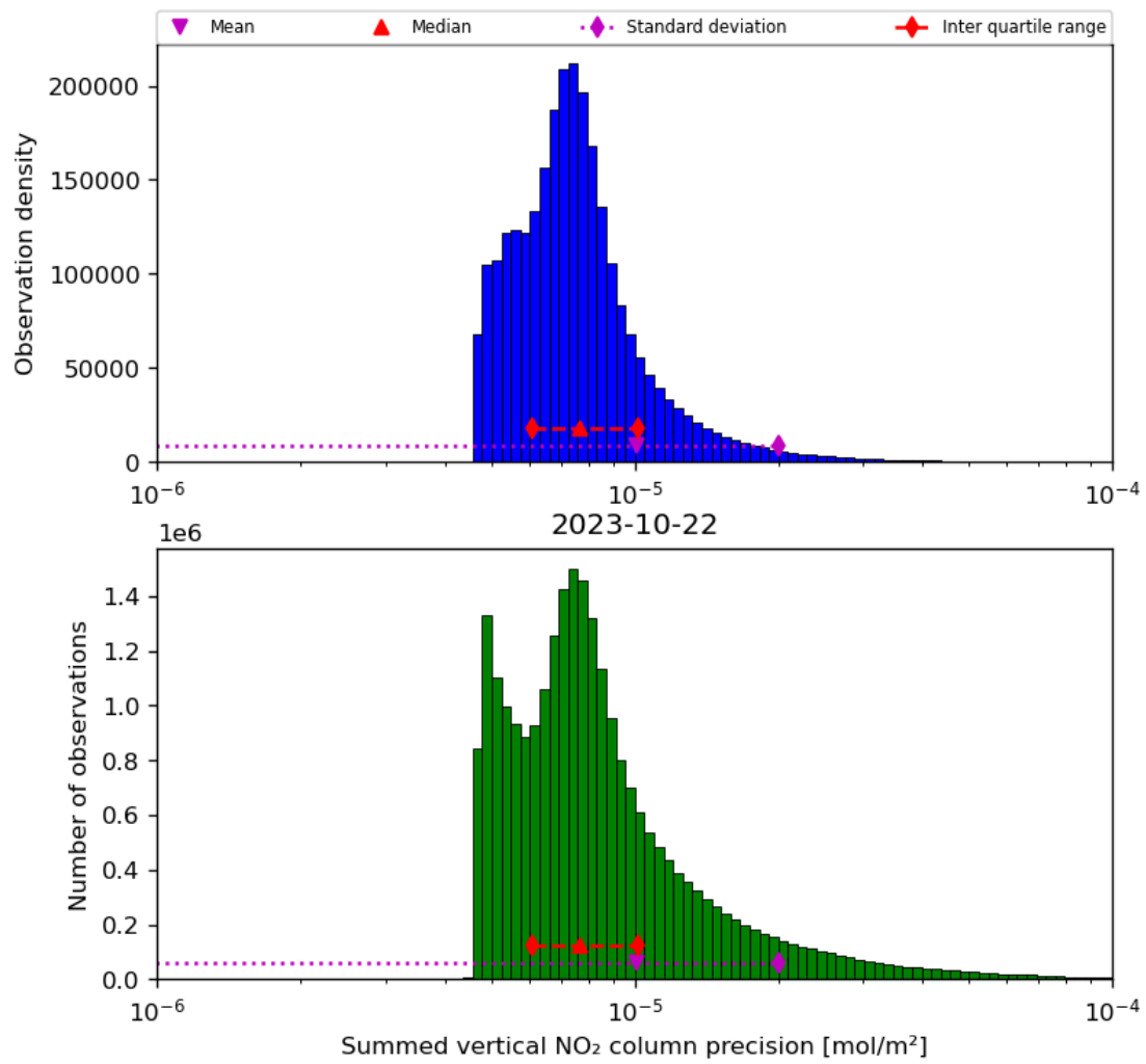
Figure 41: Histogram of “Summed vertical NO 2 column precision” for 2023-10-22 to 2023-10-23
