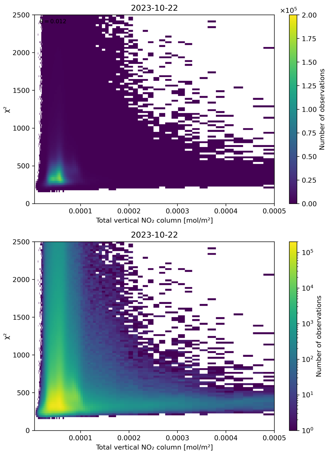
Figure 111: Scatter density plot of “Total vertical NO 2 column” against “ \chi^2 ” for 2023-10-22 to 2023-10-23.
