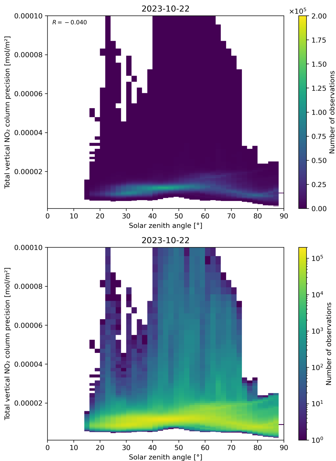
Figure 154: Scatter density plot of “Solar zenith angle” against “Total vertical NO 2 column precision” for 2023-10-22 to 2023-10-23.
