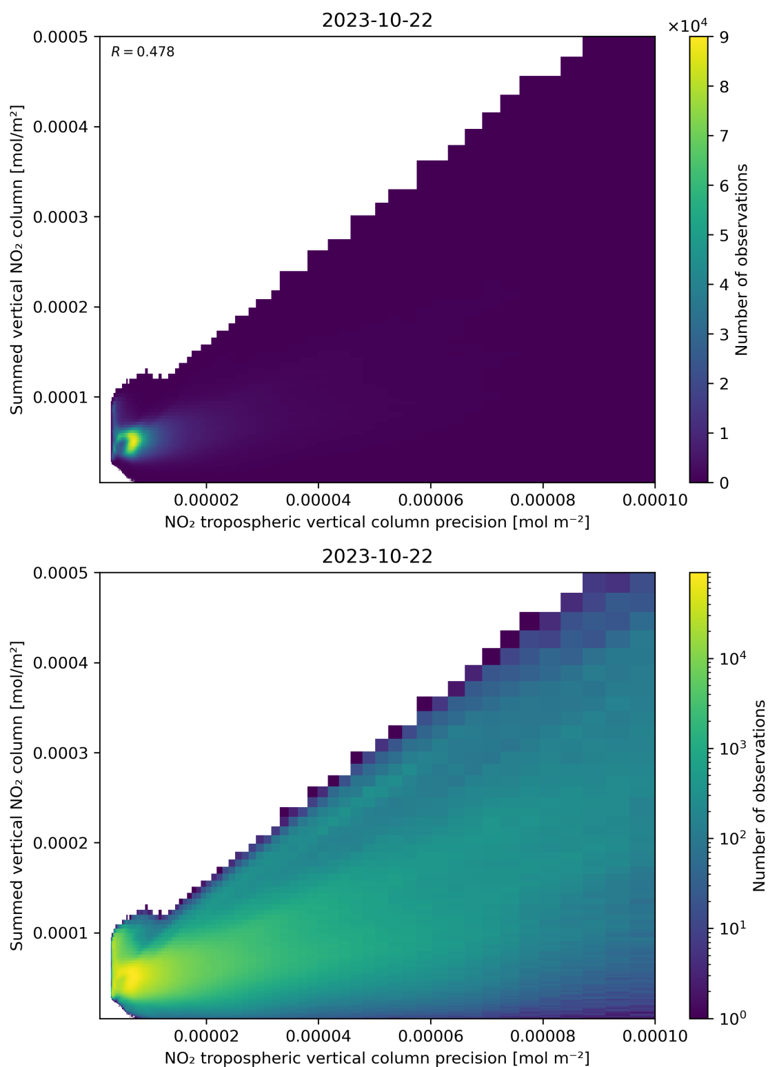
Figure 136: Scatter density plot of “NO 2 tropospheric vertical column precision” against “Summed vertical NO 2 column” for 2023-10-22 to 2023-10-23.
