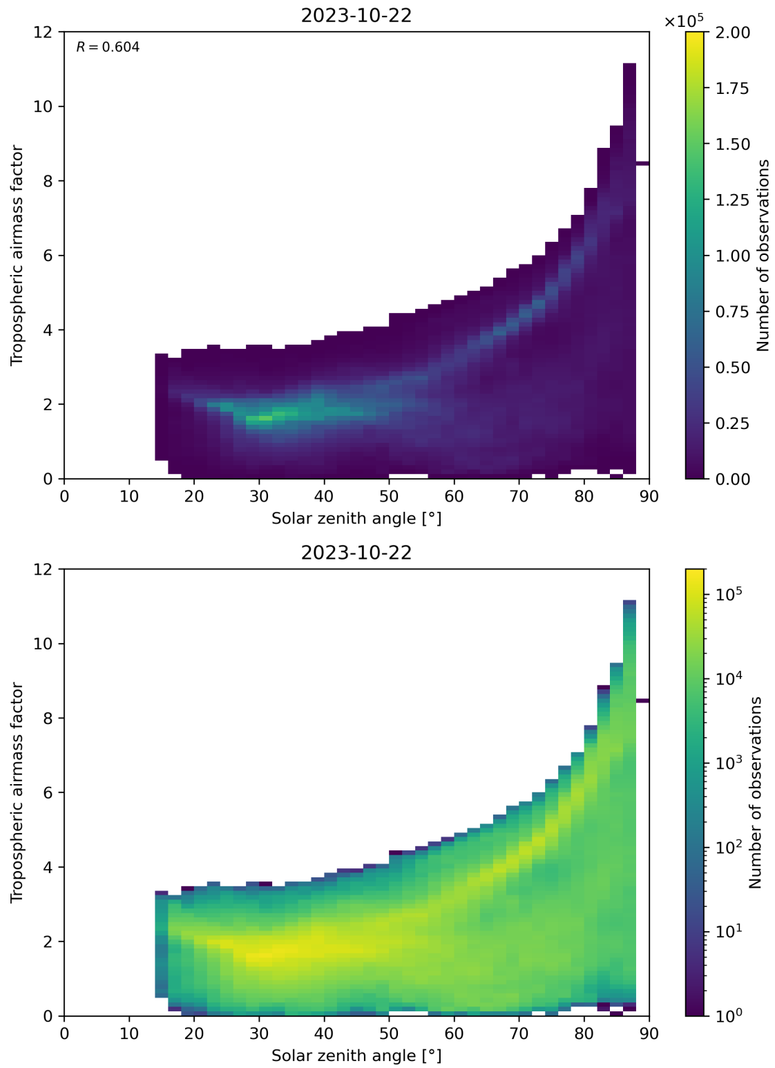
Figure 147: Scatter density plot of “Solar zenith angle” against “Tropospheric airmass factor” for 2023-10-22 to 2023-10-23.
