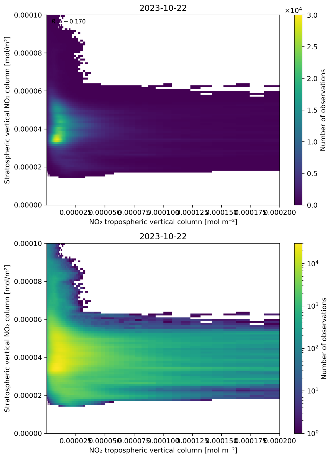
Figure 125: Scatter density plot of “NO 2 tropospheric vertical column” against “Stratospheric vertical NO 2 column” for 2023-10-22 to 2023-10-23.
