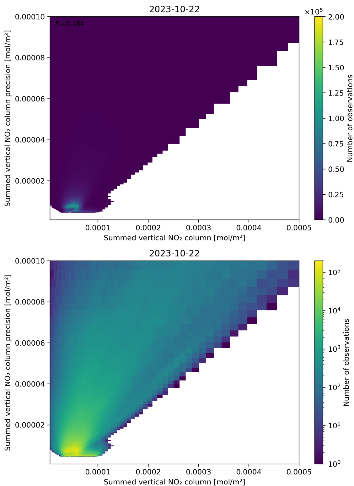
Figure 105: Scatter density plot of “Summed vertical NO 2 column” against “Summed vertical NO 2 column precision” for 2023-10-22 to 2023-10-23.
