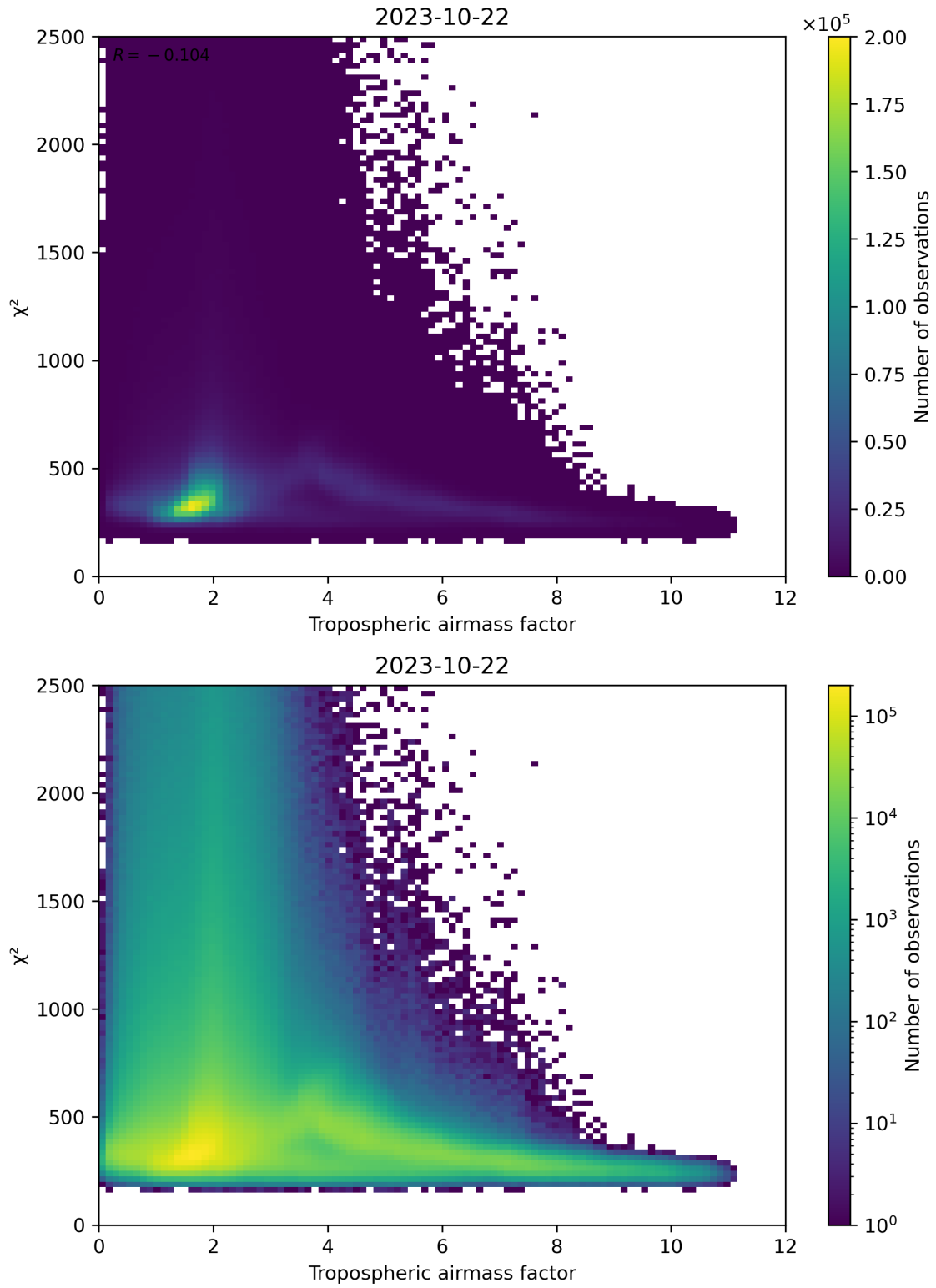
Figure 73: Scatter density plot of “Tropospheric airmass factor” against “ \chi^2 ” for 2023-10-22 to 2023-10-23.
