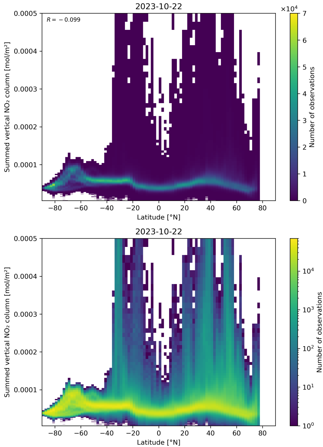
Figure 88: Scatter density plot of “Latitude” against “Summed vertical NO 2 column” for 2023-10-22 to 2023-10-23.
