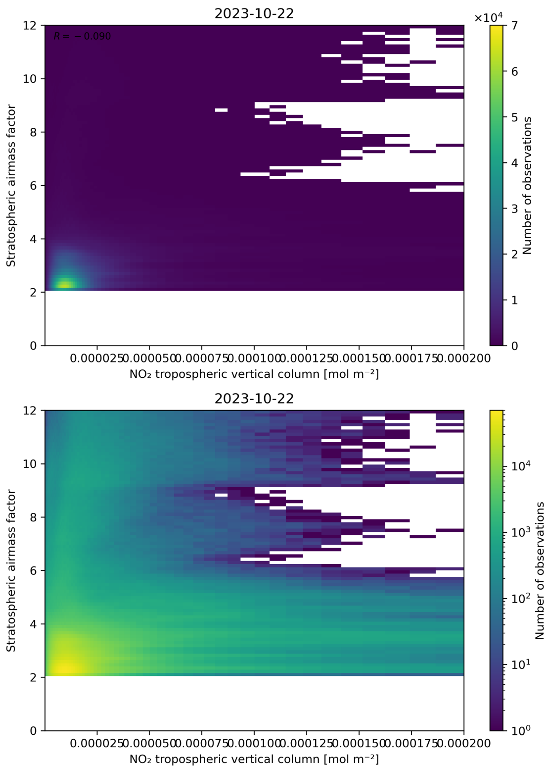
Figure 121: Scatter density plot of “NO 2 tropospheric vertical column” against “Stratospheric air mass factor” for 2023-10-22 to 2023-10-23.
