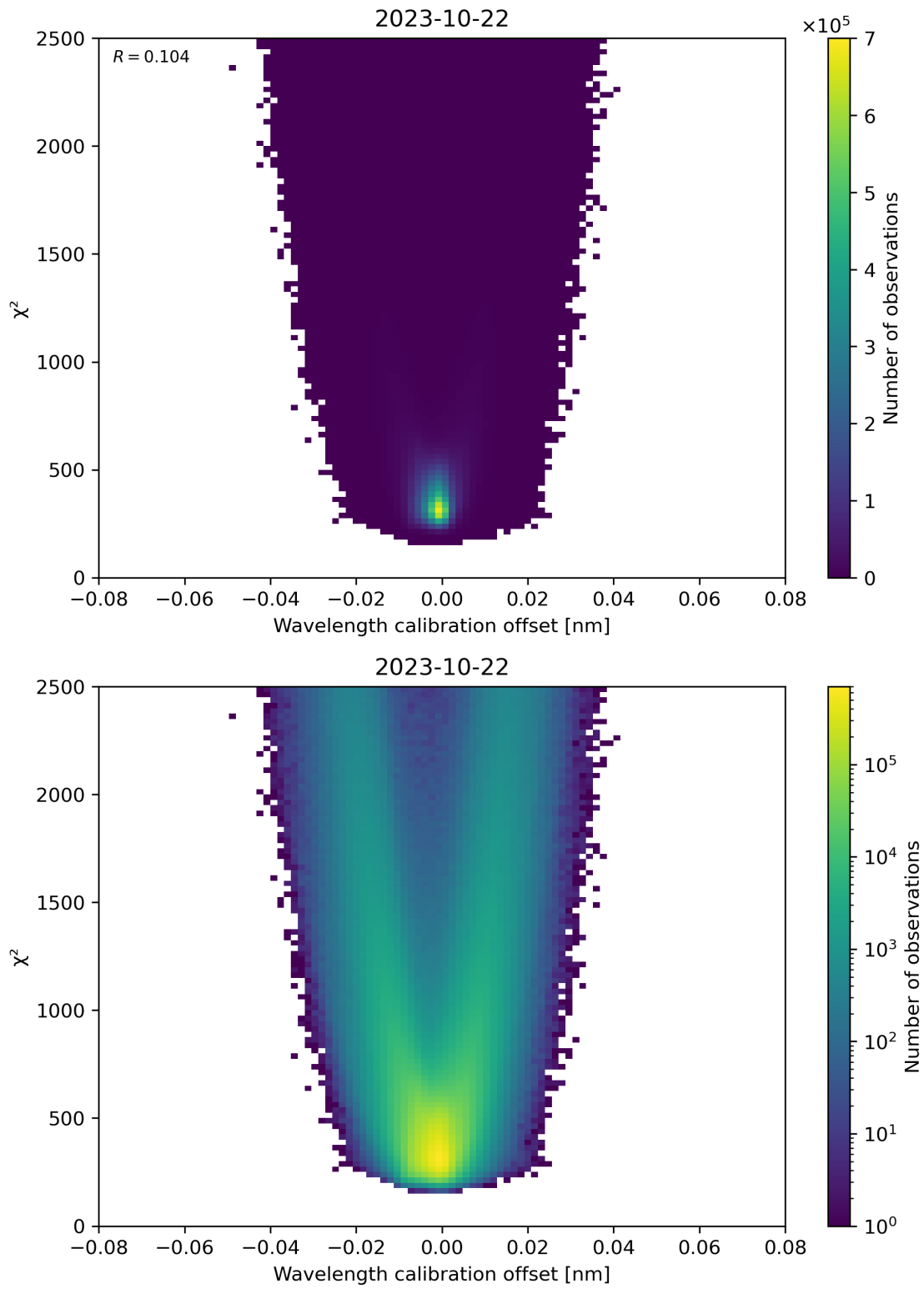
Figure 175: Scatter density plot of “Wavelength calibration offset” against “ \chi^2 ” for 2023-10-22 to 2023-10-23.
