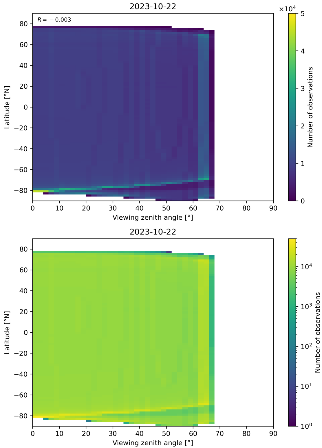
Figure 163: Scatter density plot of “Viewing zenith angle” against “Latitude” for 2023-10-22 to 2023-10-23.
