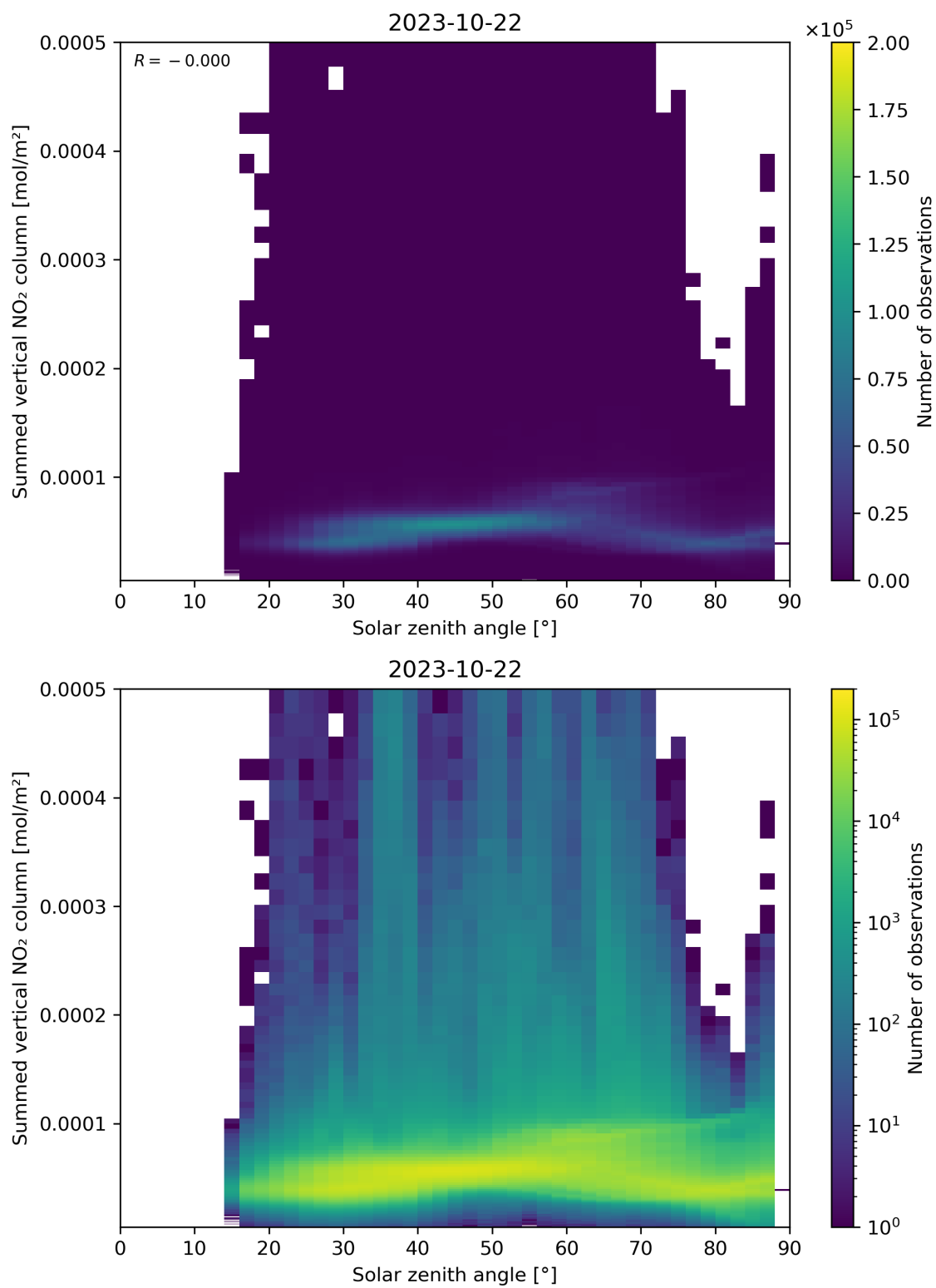
Figure 151: Scatter density plot of “Solar zenith angle” against “Summed vertical NO 2 column” for 2023-10-22 to 2023-10-23.
