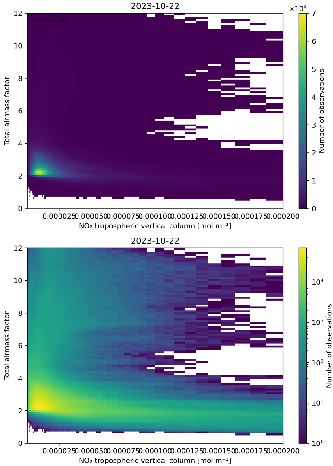
Figure 122: Scatter density plot of “NO 2 tropospheric vertical column” against “Total air mass factor” for 2023-10-22 to 2023-10-23.
