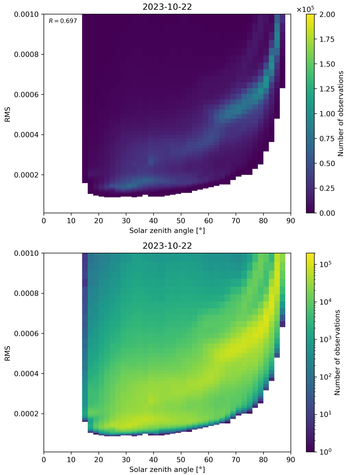
Figure 157: Scatter density plot of “Solar zenith angle” against “RMS” for 2023-10-22 to 2023-10-23.
