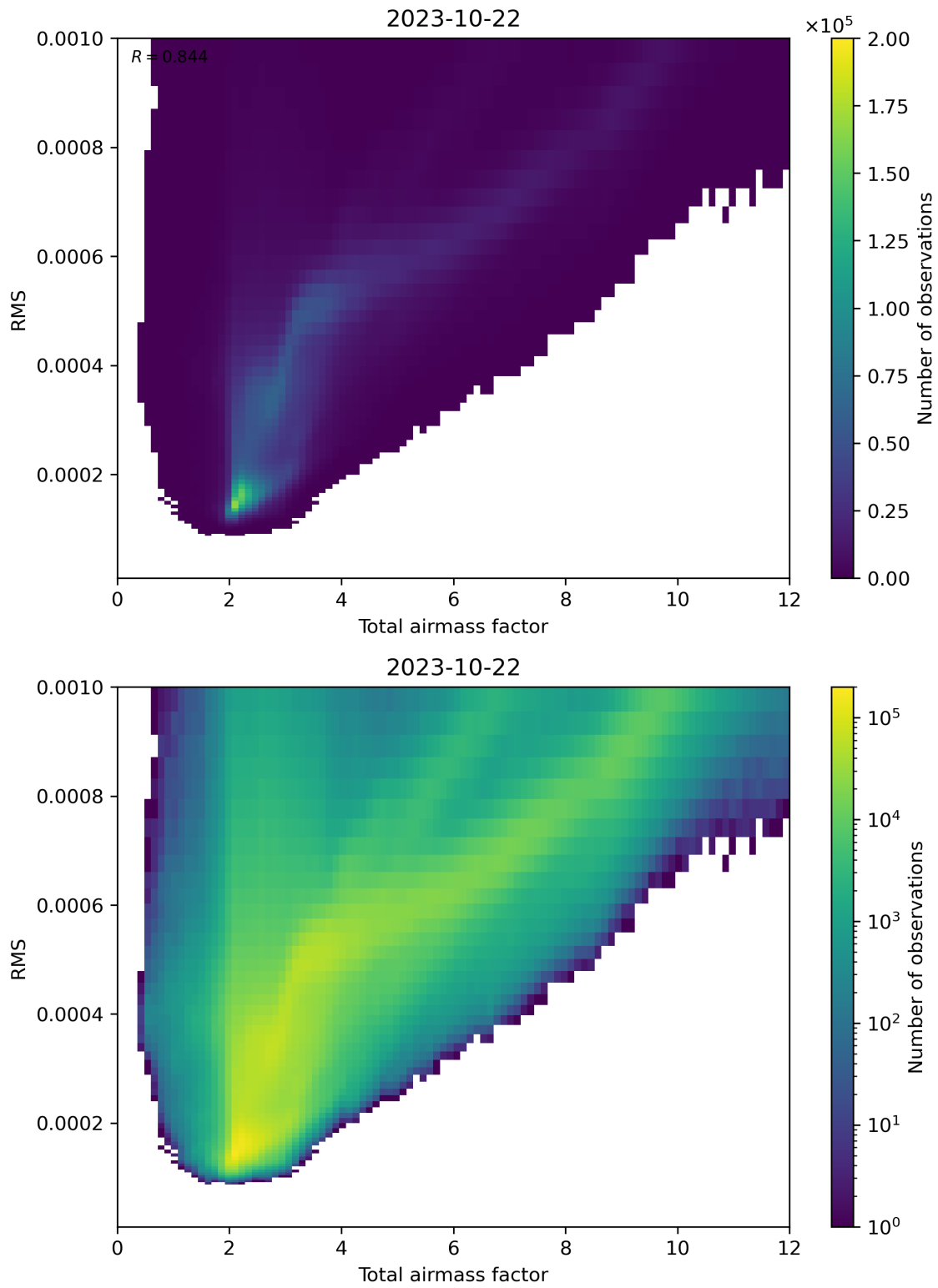
Figure 69: Scatter density plot of “Total airmass factor” against “RMS” for 2023-10-22 to 2023-10-23.
