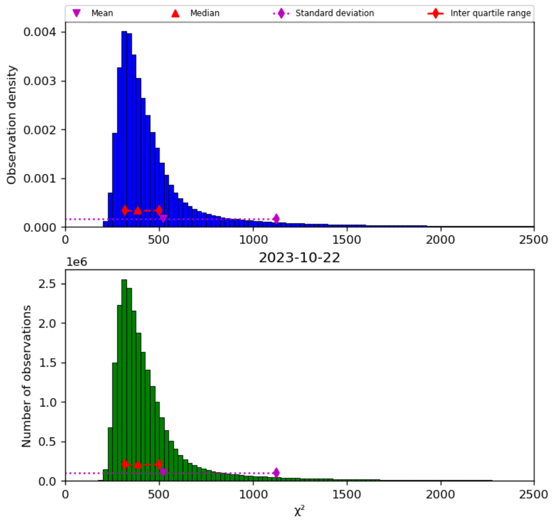
Figure 42: Histogram of “ \chi^2 ” for 2023-10-22 to 2023-10-23
