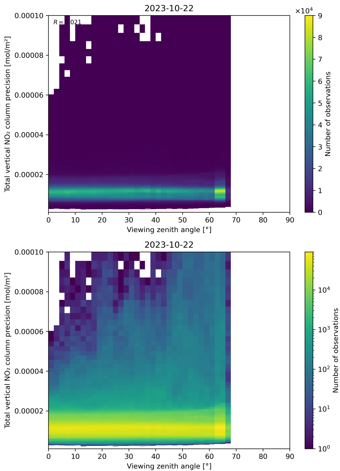
Figure 168: Scatter density plot of “Viewing zenith angle” against “Total vertical NO 2 column precision” for 2023-10-22 to 2023-10-23.
