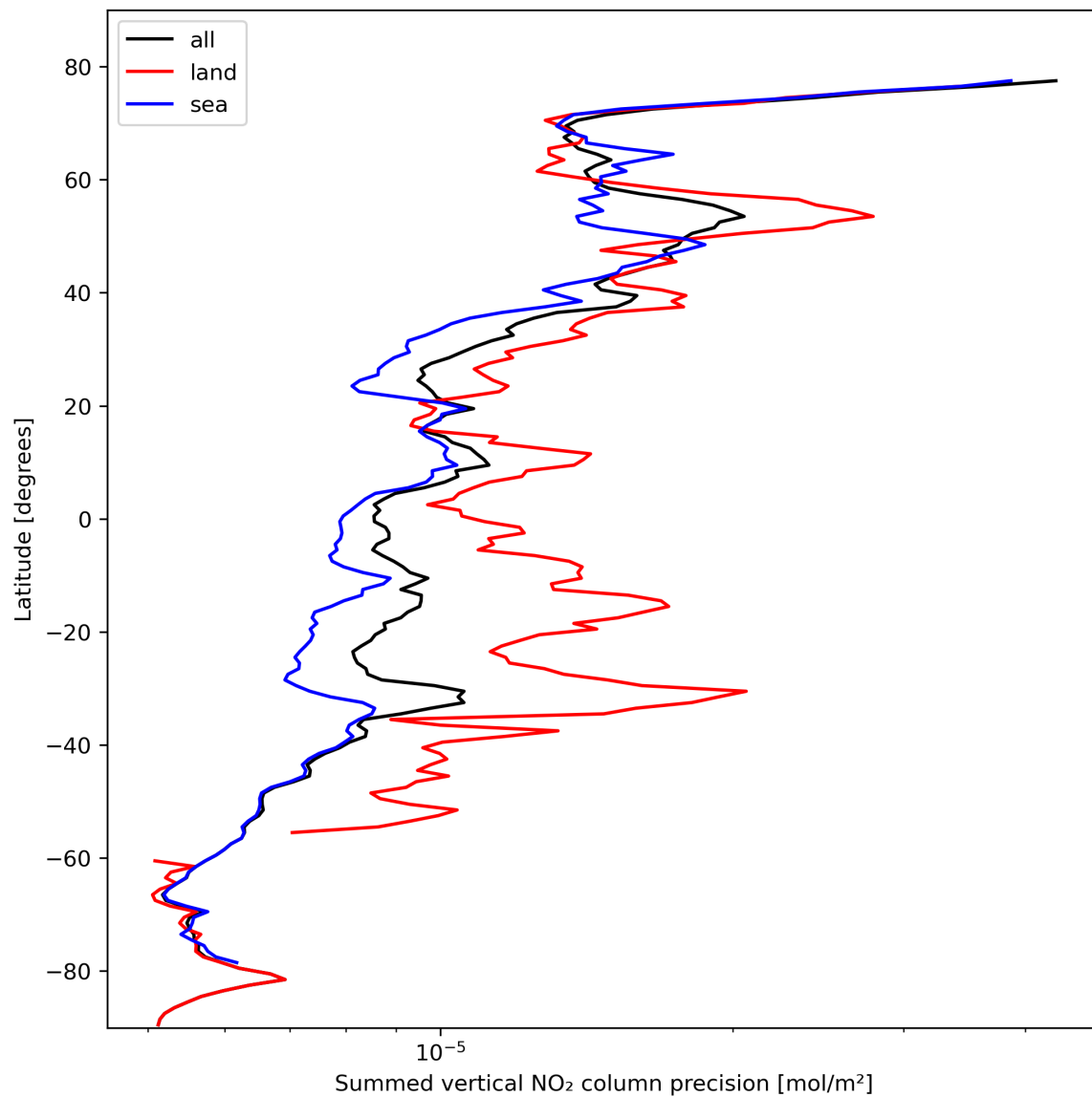
Figure 24: Zonal average of “Summed vertical NO 2 column precision” for 2023-10-22 to 2023-10-23.
