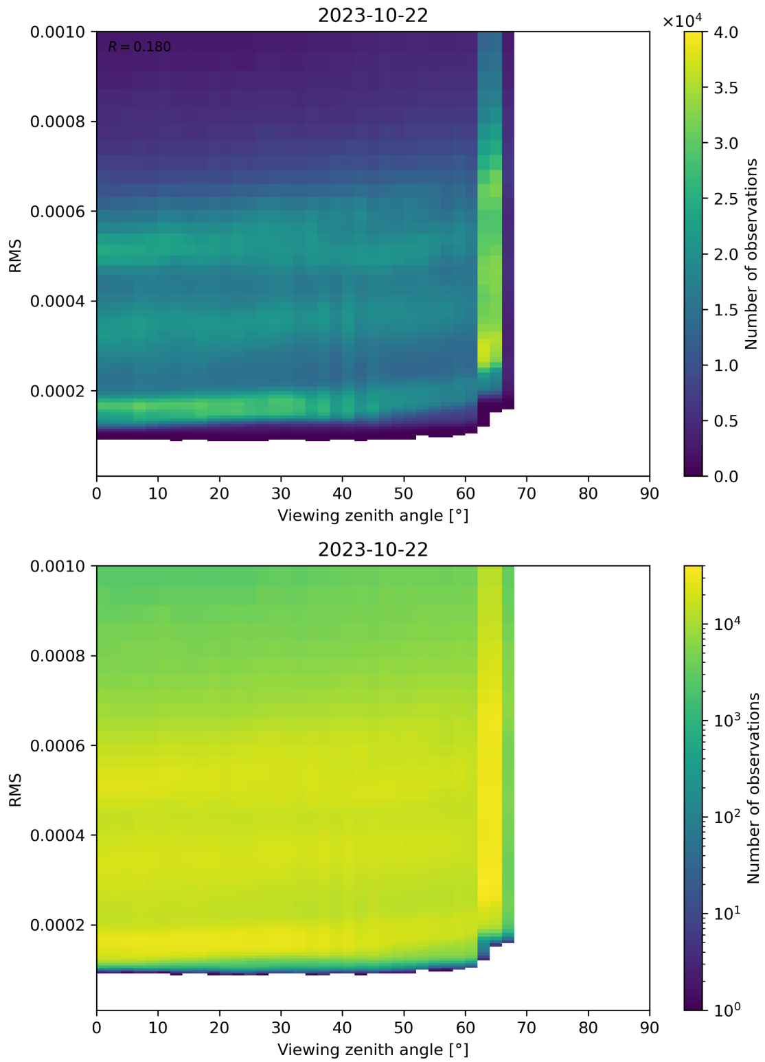
Figure 171: Scatter density plot of “Viewing zenith angle” against “RMS” for 2023-10-22 to 2023-10-23.
