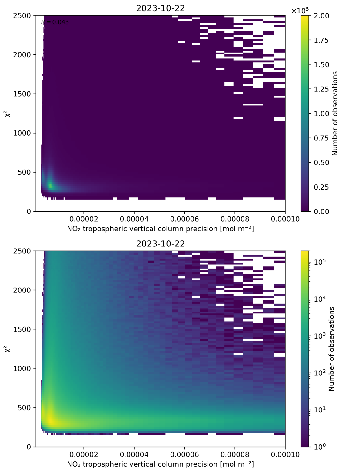
Figure 134: Scatter density plot of “NO 2 tropospheric vertical column precision” against “ \chi^2 ” for 2023-10-22 to 2023-10-23.
