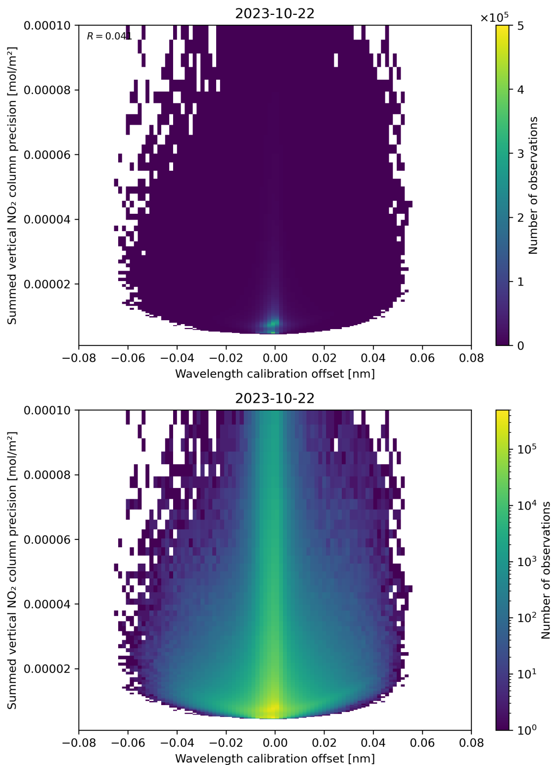
Figure 178: Scatter density plot of “Wavelength calibration offset” against “Summed vertical NO 2 column precision” for 2023-10-22 to 2023-10-23.
