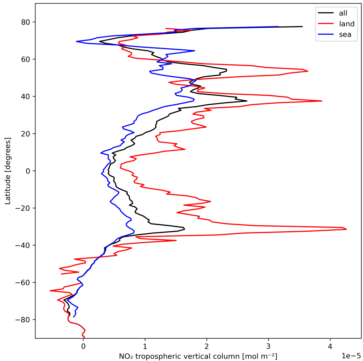
Figure 12: Zonal average of “NO 2 tropospheric vertical column” for 2023-10-22 to 2023-10-23.
