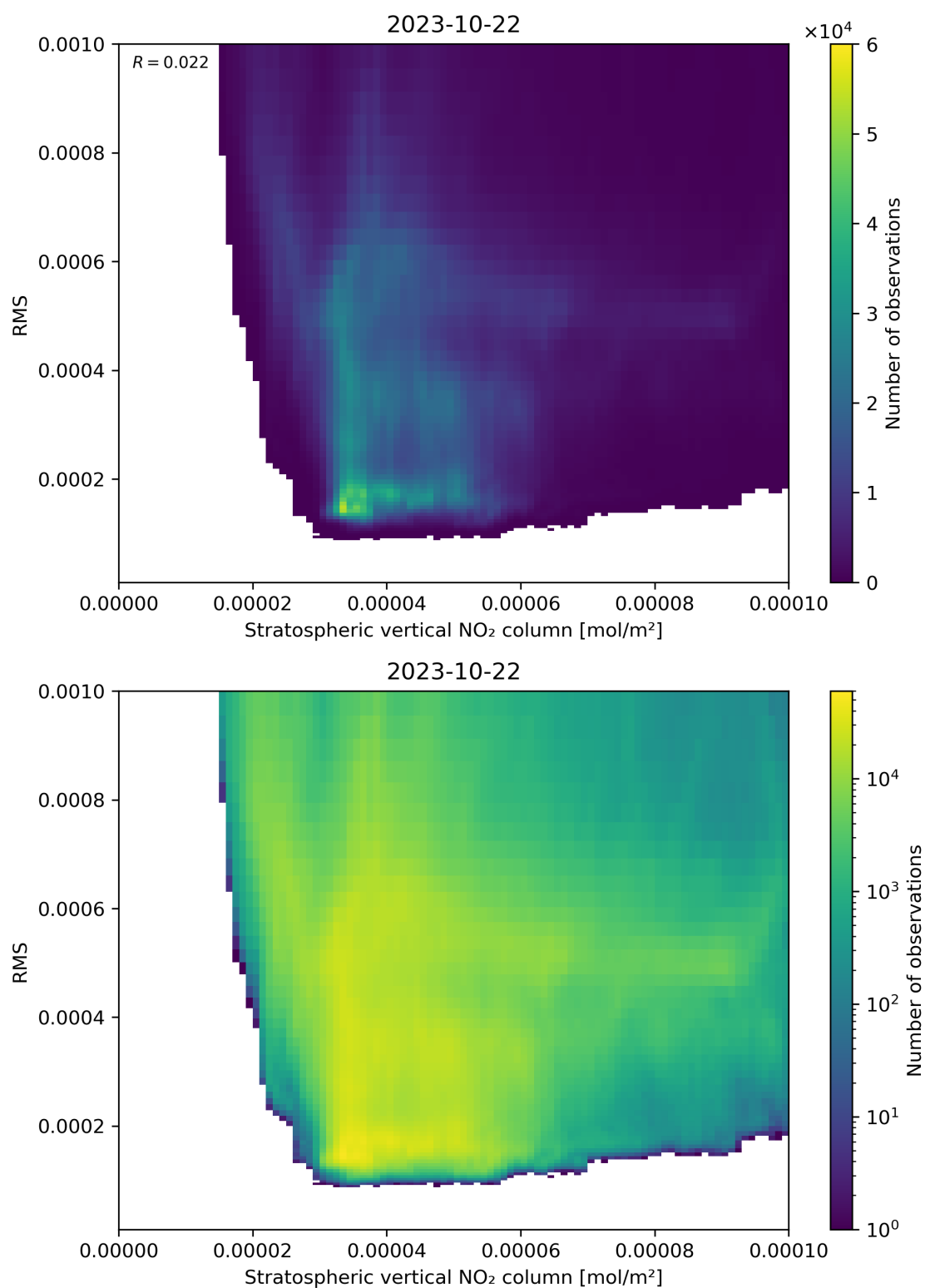
Figure 102: Scatter density plot of “Stratospheric vertical NO 2 column” against “RMS” for 2023-10-22 to 2023-10-23.
