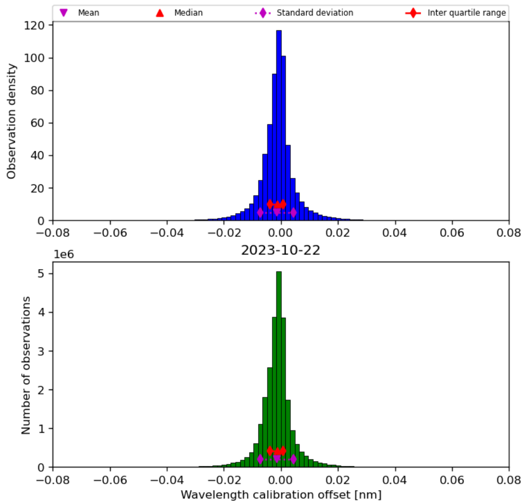
Figure 35: Histogram of “Wavelength calibration offset” for 2023-10-22 to 2023-10-23
