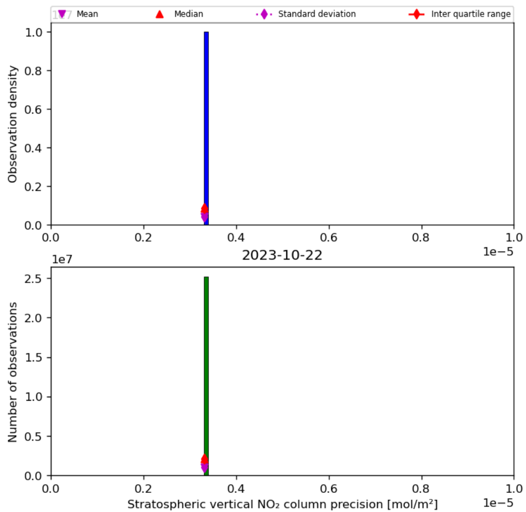
Figure 37: Histogram of “Stratospheric vertical NO 2 column precision” for 2023-10-22 to 2023-10-23
