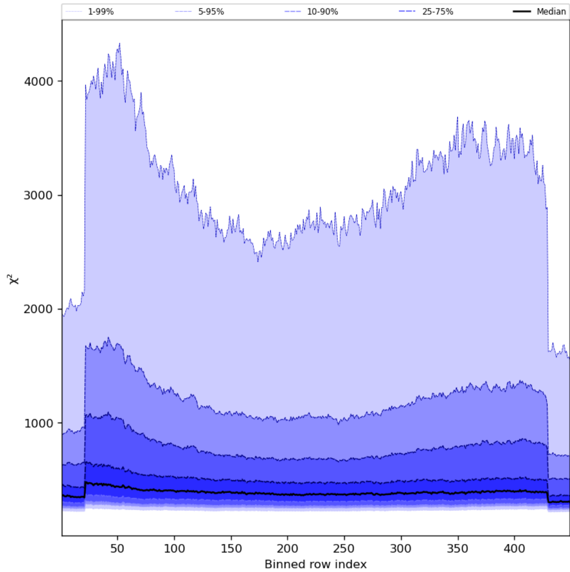
Figure 59: Along track statistics of “ \chi^2 ” for 2023-10-22 to 2023-10-23
