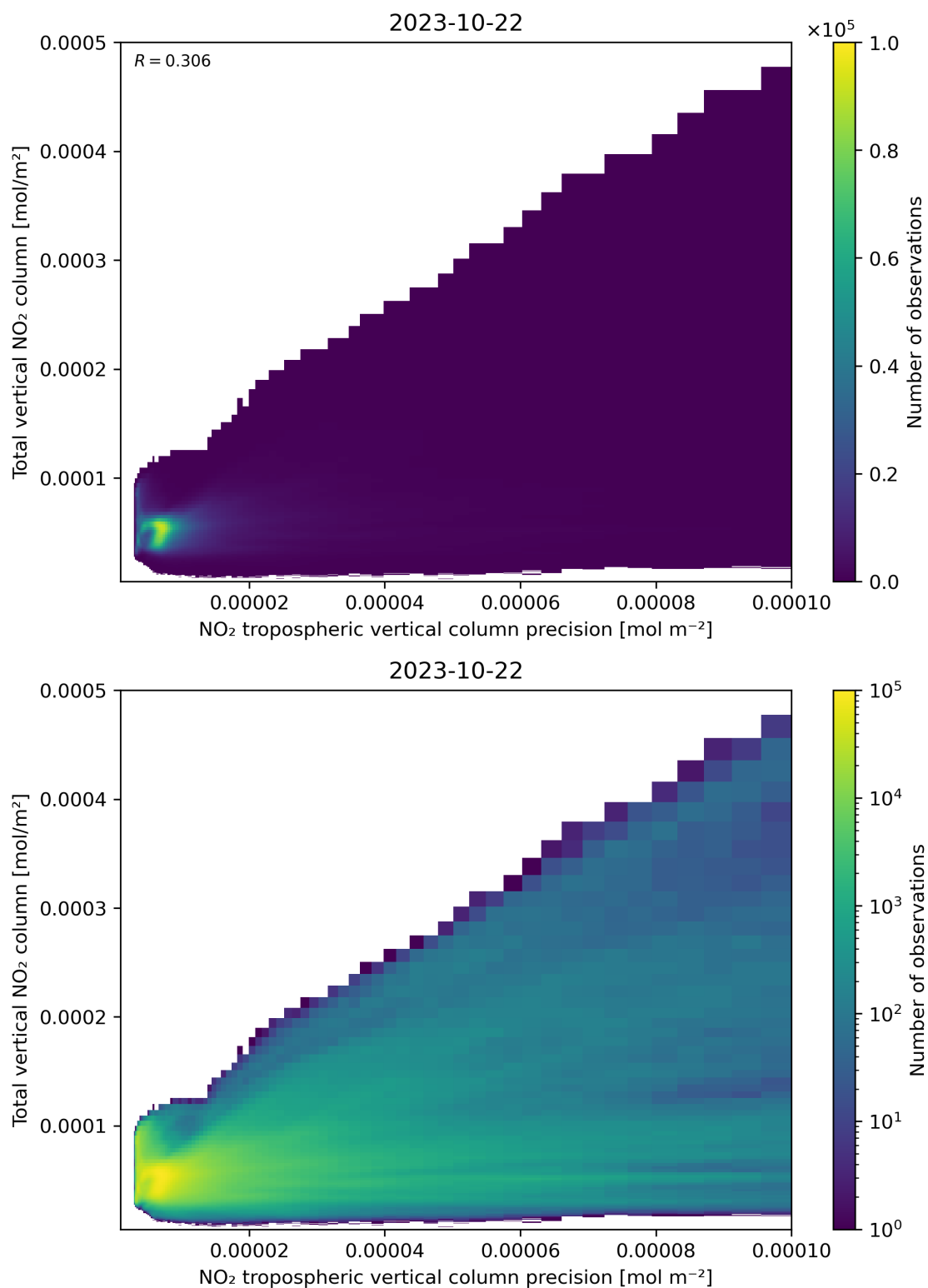
Figure 138: Scatter density plot of “NO 2 tropospheric vertical column precision” against “Total vertical NO 2 column” for 2023-10-22 to 2023-10-23.
