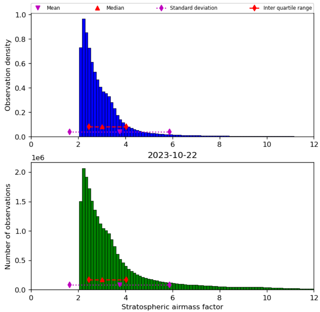
Figure 44: Histogram of “Stratospheric airmass factor” for 2023-10-22 to 2023-10-23
