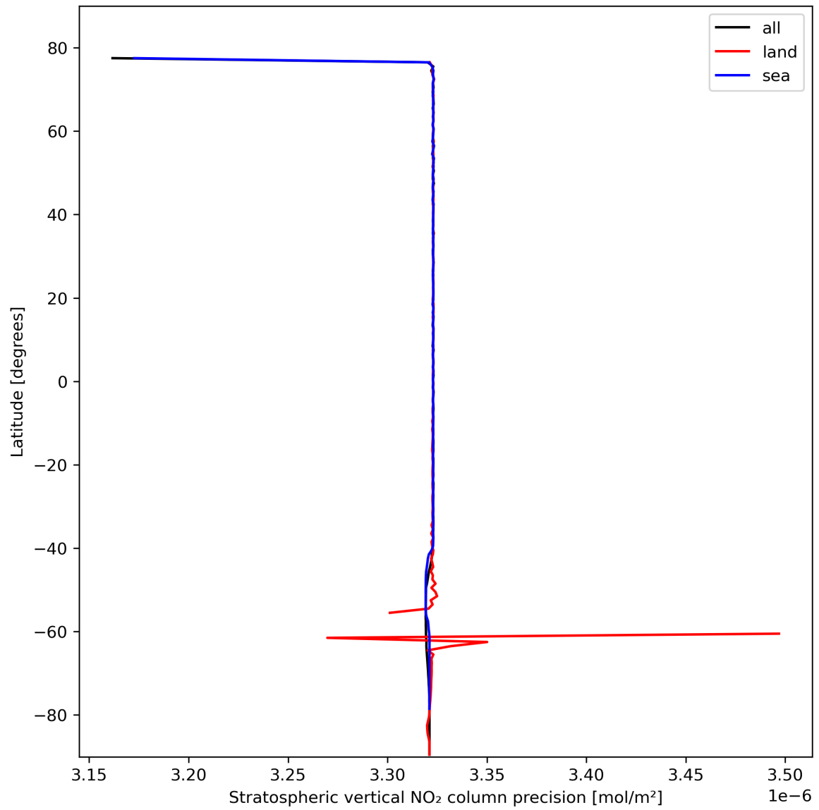
Figure 20: Zonal average of “Stratospheric vertical NO 2 column precision” for 2023-10-22 to 2023-10-23.
