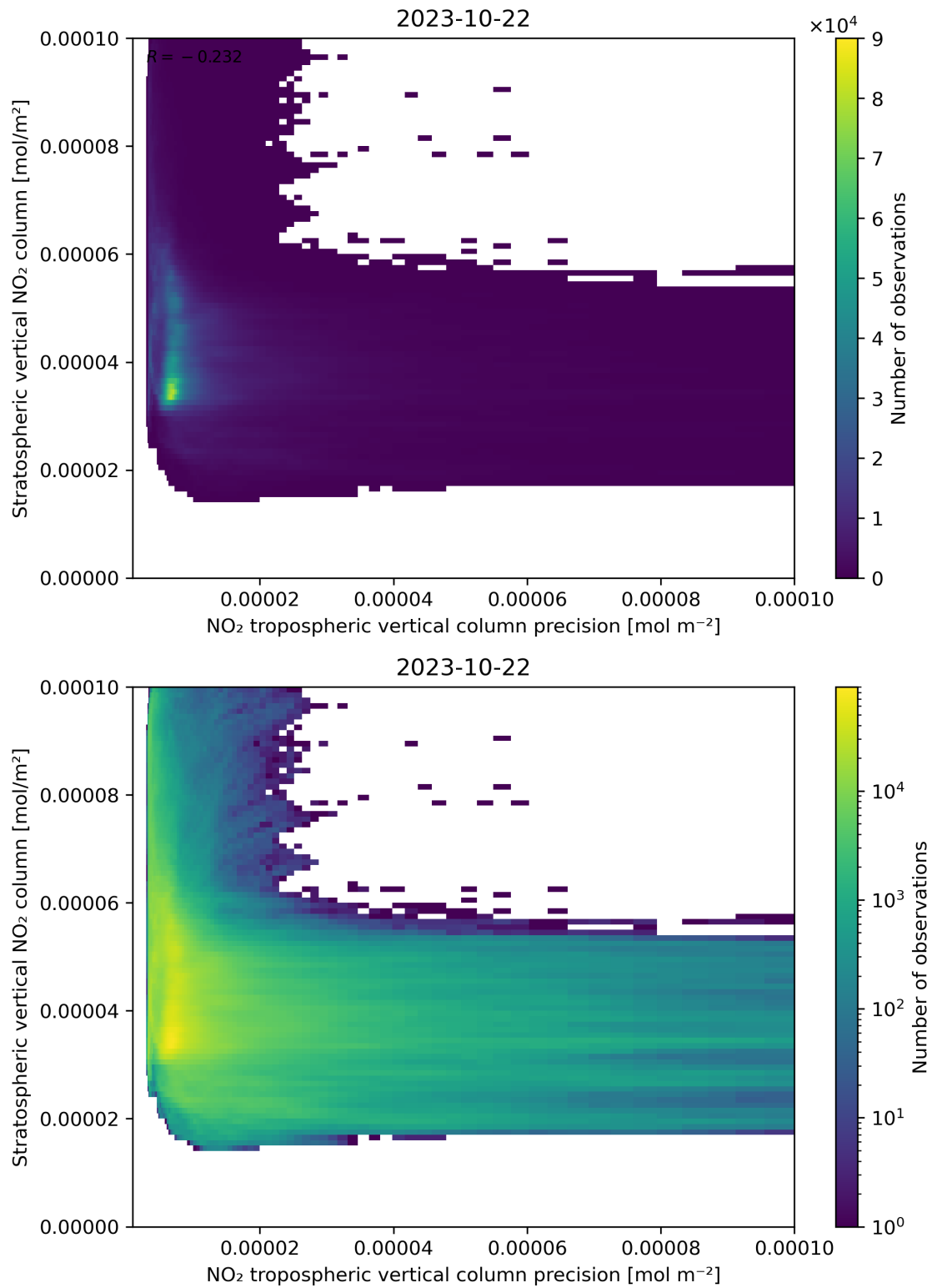
Figure 135: Scatter density plot of “NO 2 tropospheric vertical column precision” against “Stratospheric vertical NO 2 column” for 2023-10-22 to 2023-10-23.
