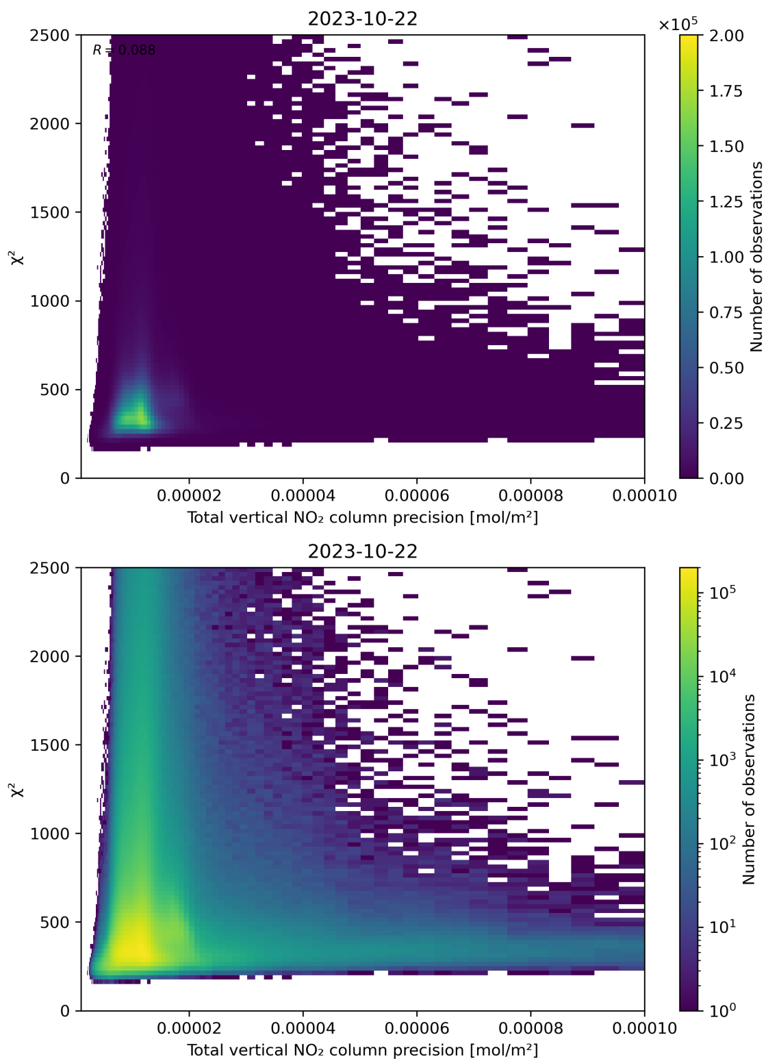
Figure 116: Scatter density plot of “Total vertical NO 2 column precision” against “ \chi^2 ” for 2023-10-22 to 2023-10-23.
