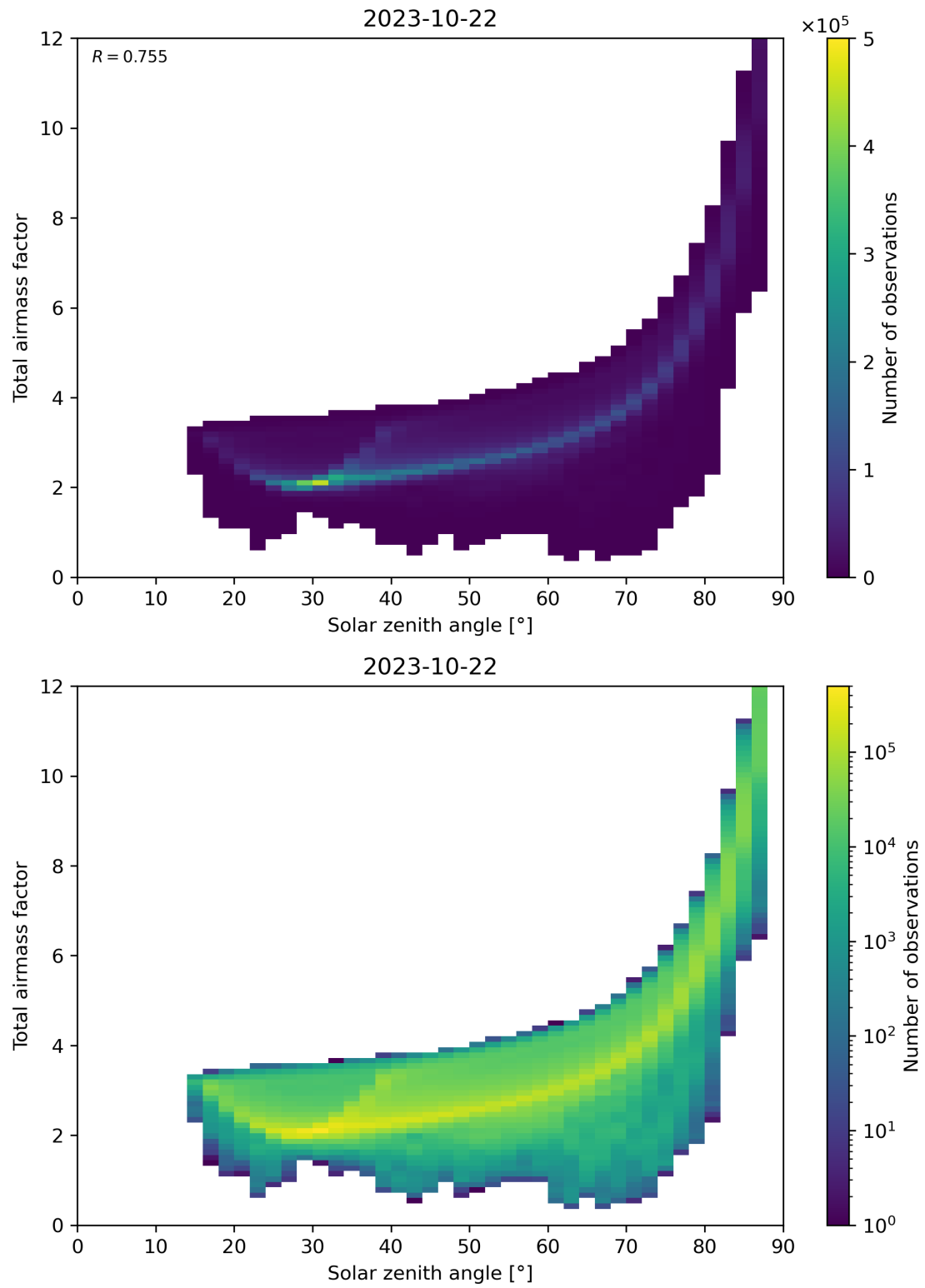
Figure 146: Scatter density plot of “Solar zenith angle” against “Total airmass factor” for 2023-10-22 to 2023-10-23.
