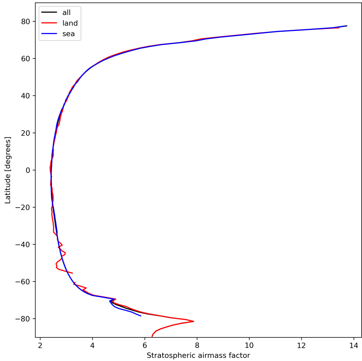
Figure 27: Zonal average of “Stratospheric air mass factor” for 2023-10-22 to 2023-10-23.
