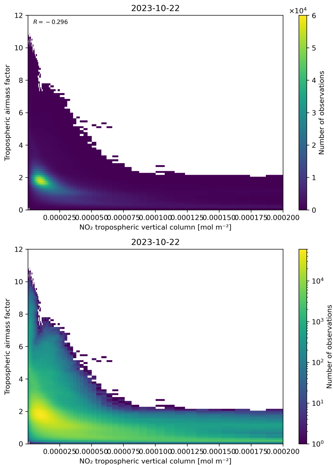
Figure 123: Scatter density plot of “NO 2 tropospheric vertical column” against “Tropospheric air mass factor” for 2023-10-22 to 2023-10-23.
