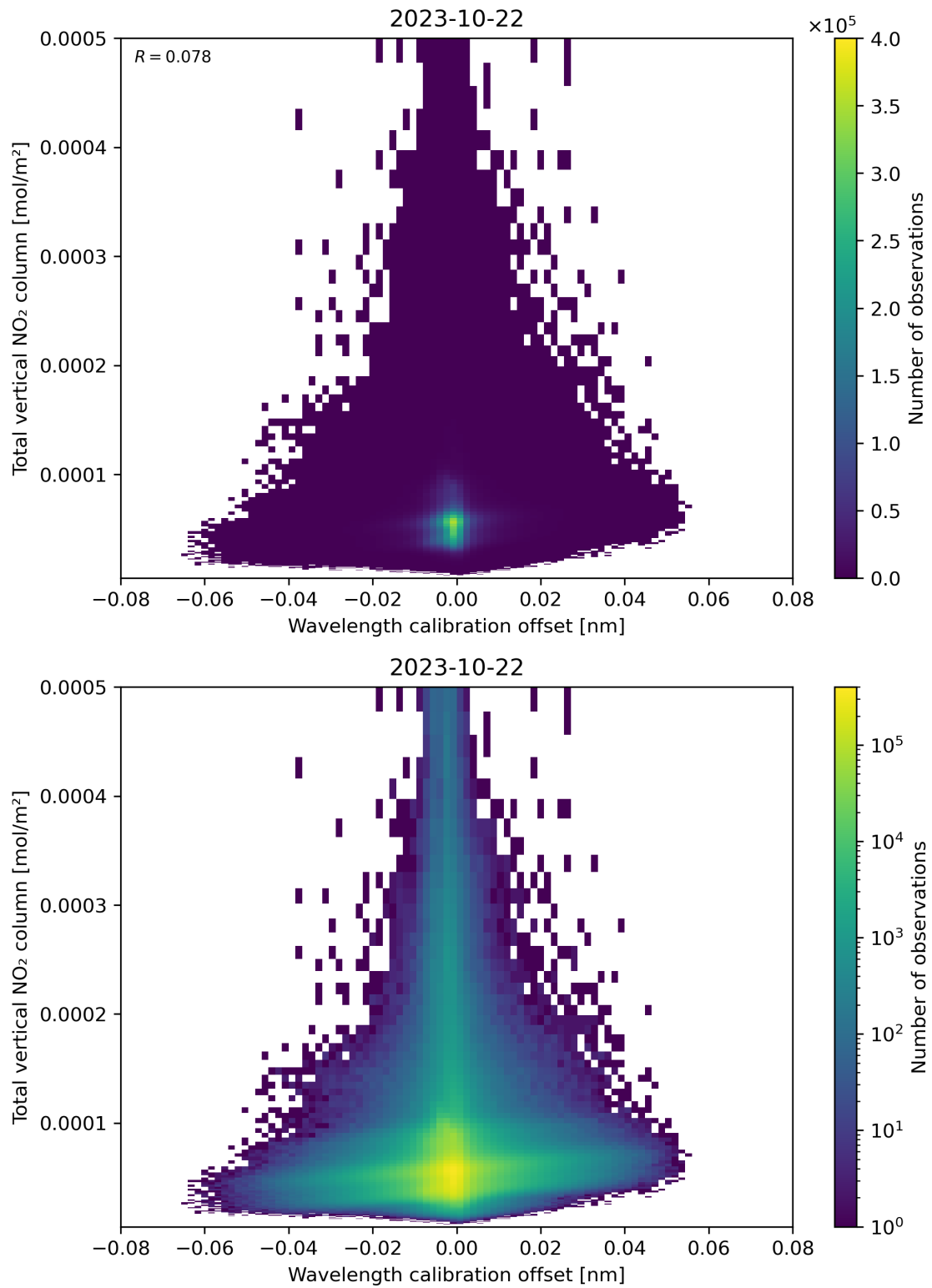
Figure 179: Scatter density plot of “Wavelength calibration offset” against “Total vertical NO 2 column” for 2023-10-22 to 2023-10-23.
