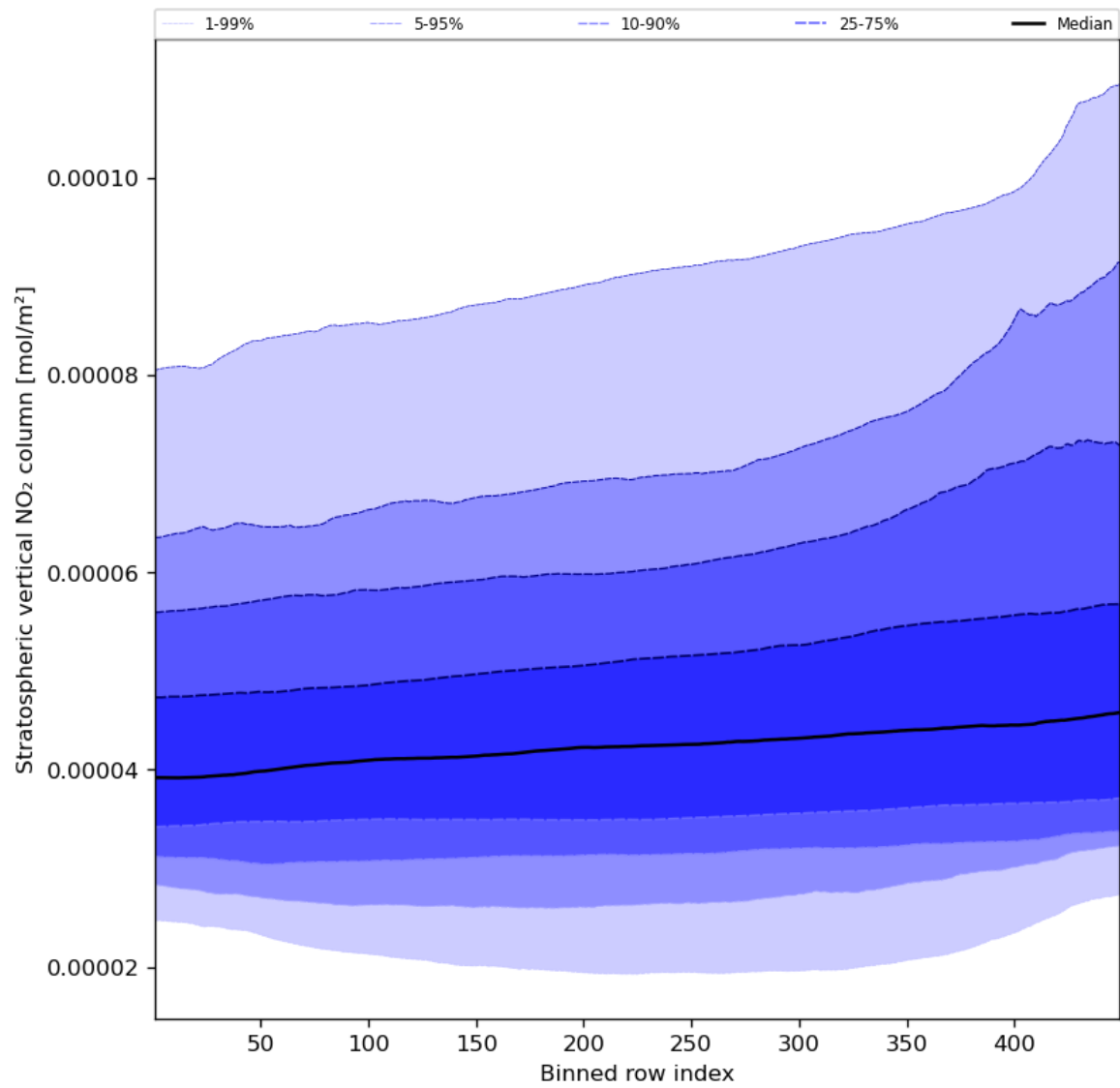
Figure 53: Along track statistics of “Stratospheric vertical NO 2 column” for 2023-10-22 to 2023-10-23
