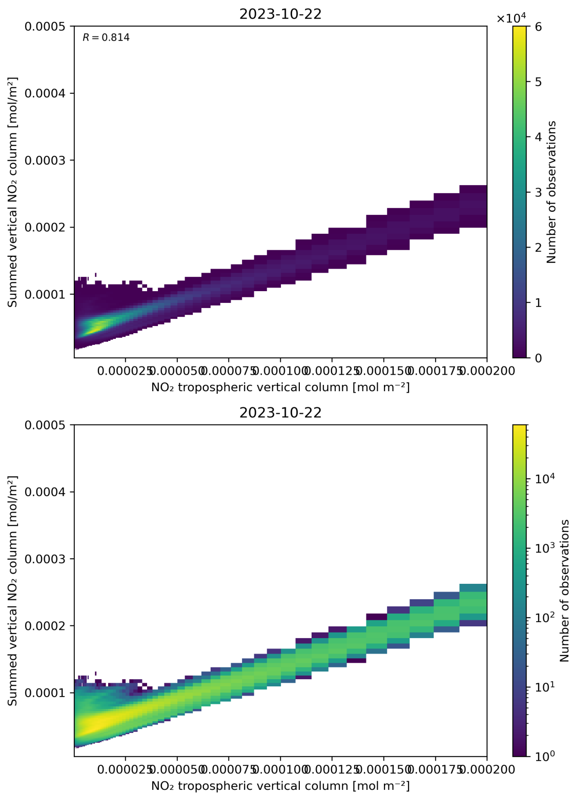
Figure 126: Scatter density plot of “NO 2 tropospheric vertical column” against “Summed vertical NO 2 column” for 2023-10-22 to 2023-10-23.
