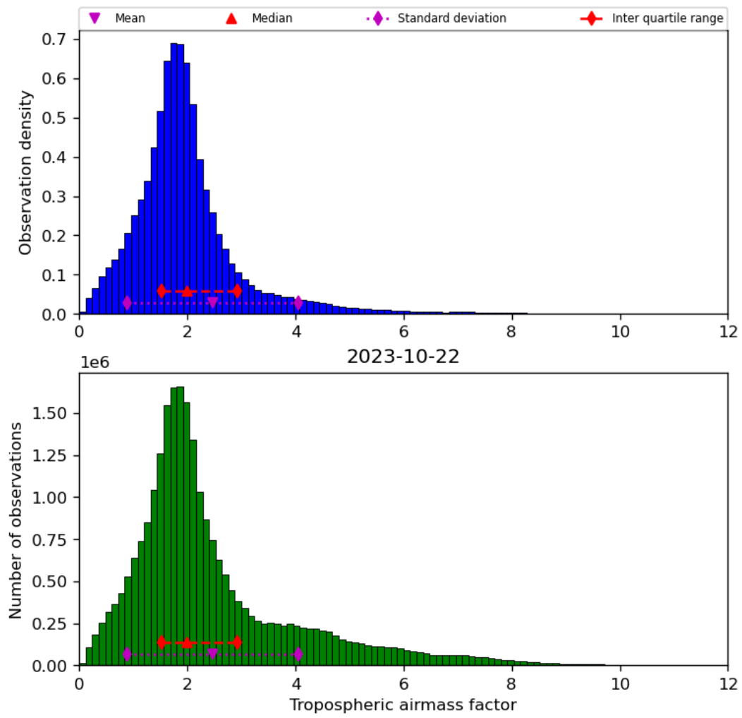
Figure 31: Histogram of “Tropospheric airmass factor” for 2023-10-22 to 2023-10-23
