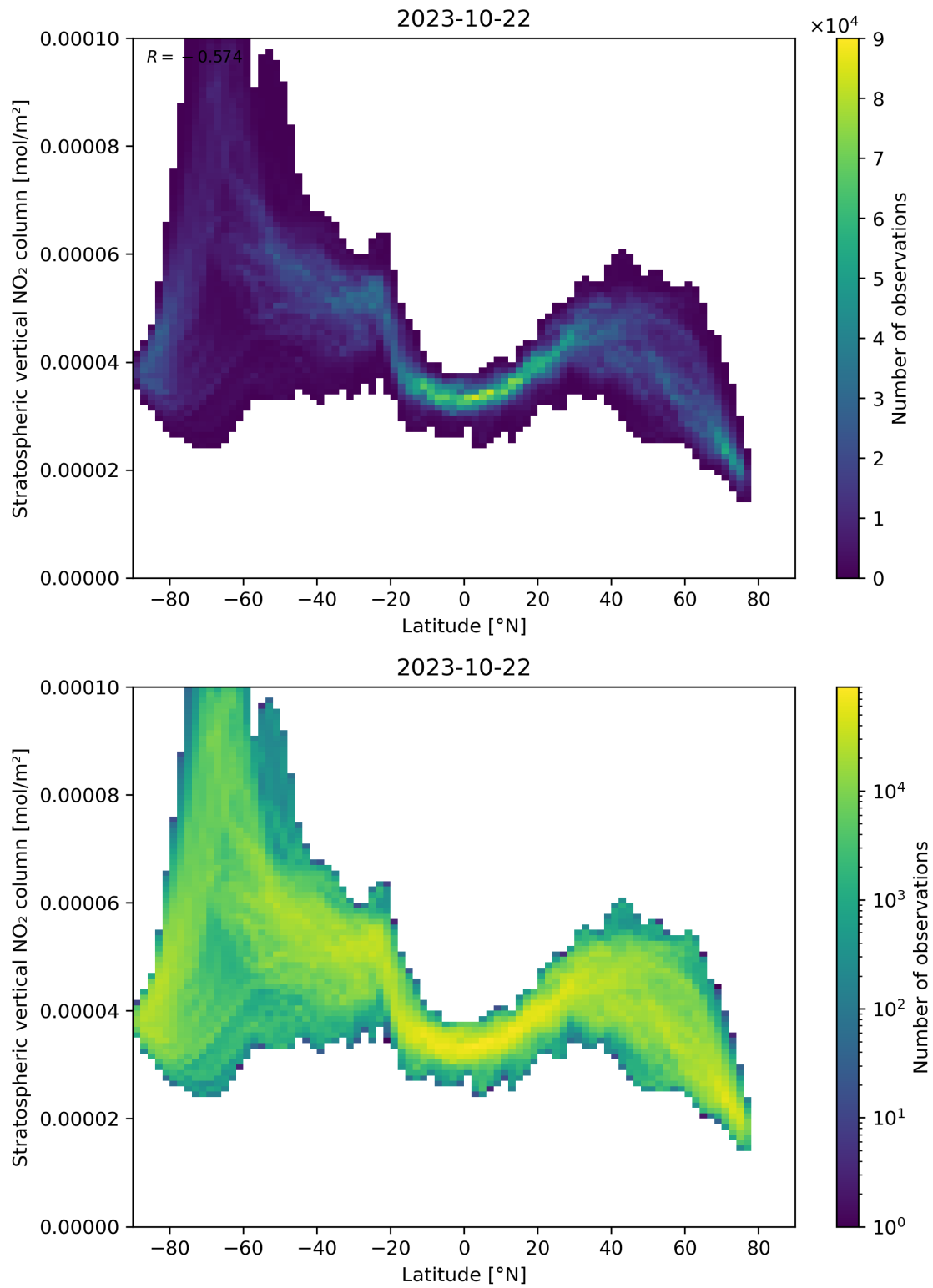
Figure 87: Scatter density plot of “Latitude” against “Stratospheric vertical NO 2 column” for 2023-10-22 to 2023-10-23.
