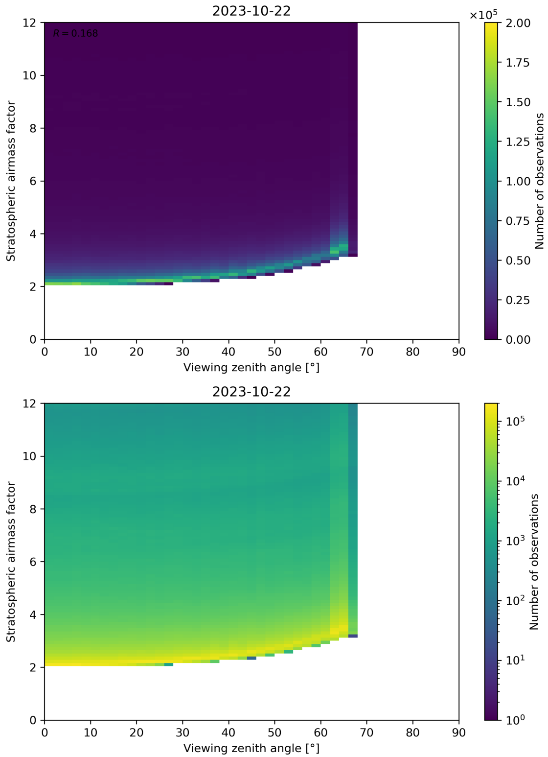
Figure 159: Scatter density plot of “Viewing zenith angle” against “Stratospheric airmass factor” for 2023-10-22 to 2023-10-23.
