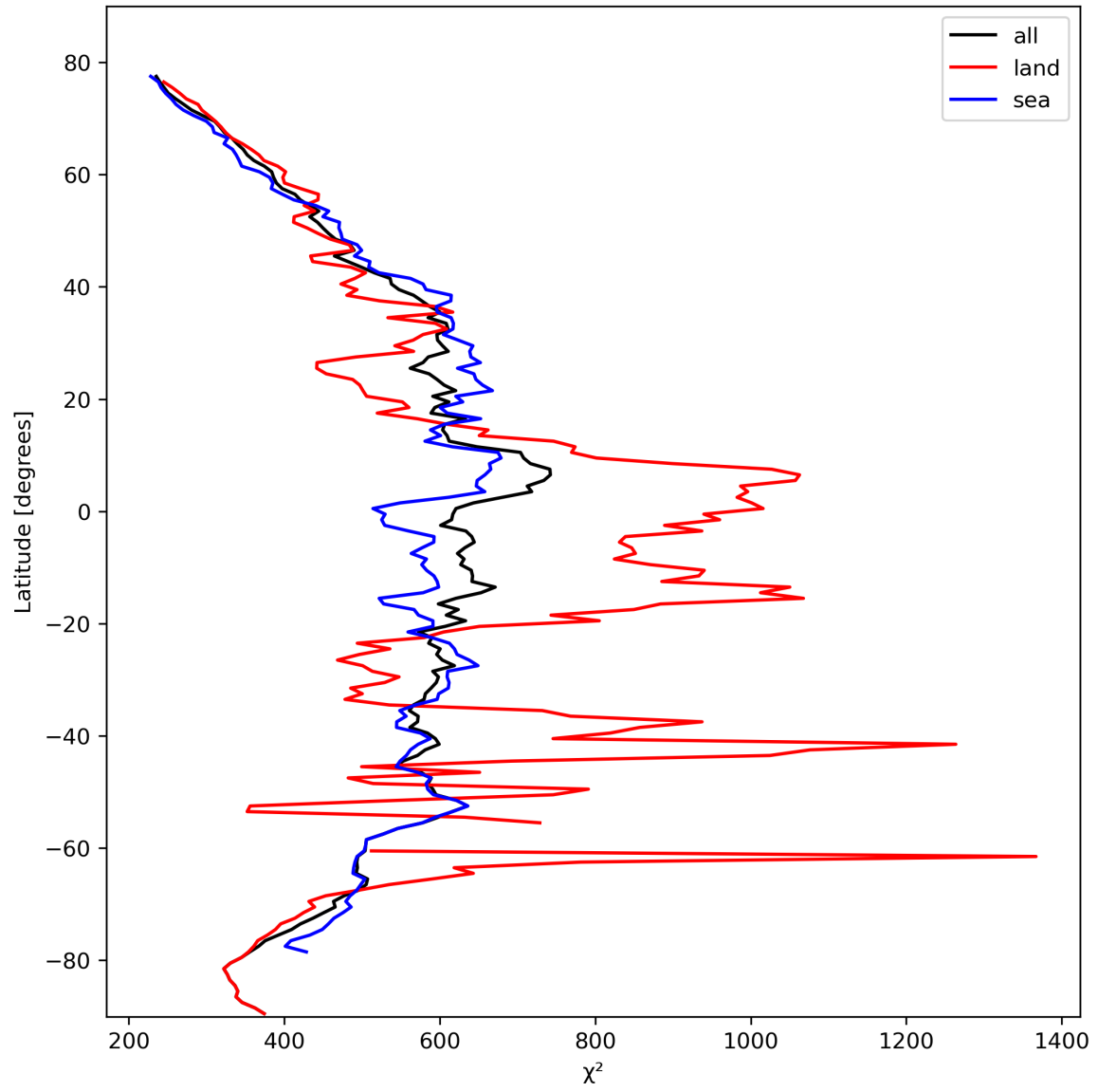
Figure 25: Zonal average of “ \chi^2 ” for 2023-10-22 to 2023-10-23.
