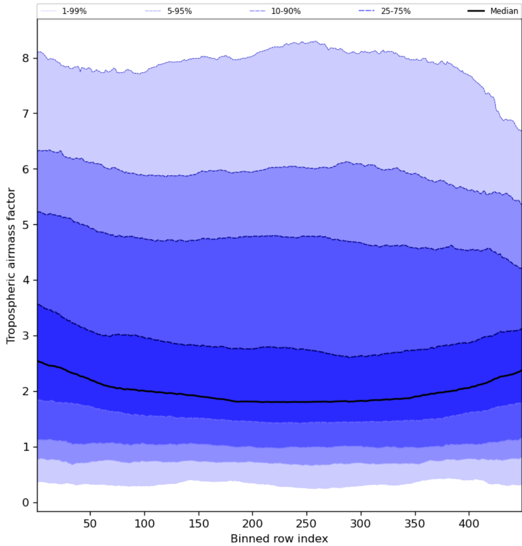
Figure 48: Along track statistics of “Tropospheric air mass factor” for 2023-10-22 to 2023-10-23
