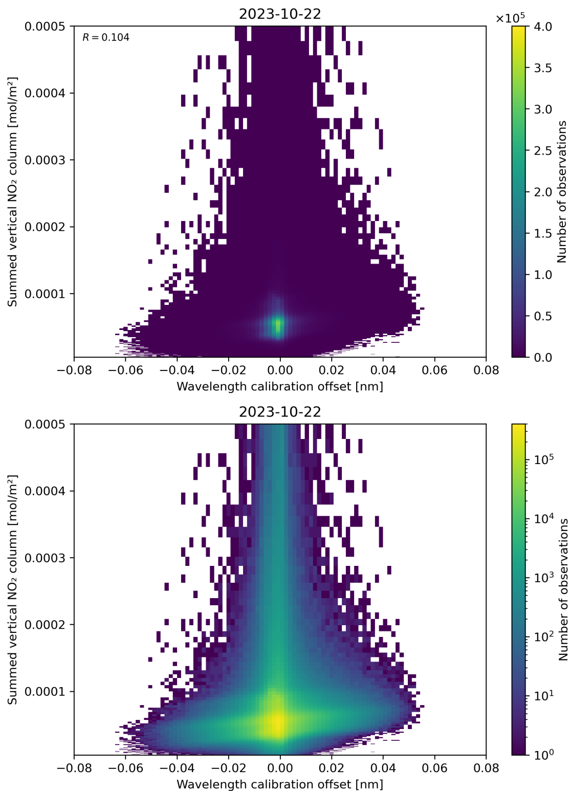
Figure 177: Scatter density plot of “Wavelength calibration offset” against “Summed vertical NO 2 column” for 2023-10-22 to 2023-10-23.
