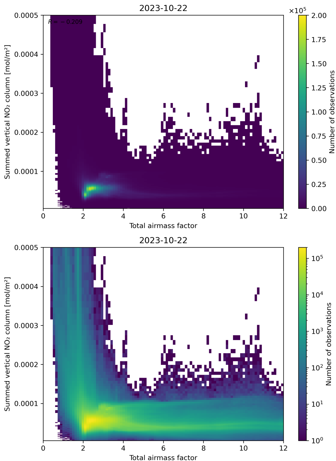
Figure 65: Scatter density plot of “Total airmass factor” against “Summed vertical NO 2 column” for 2023-10-22 to 2023-10-23.
