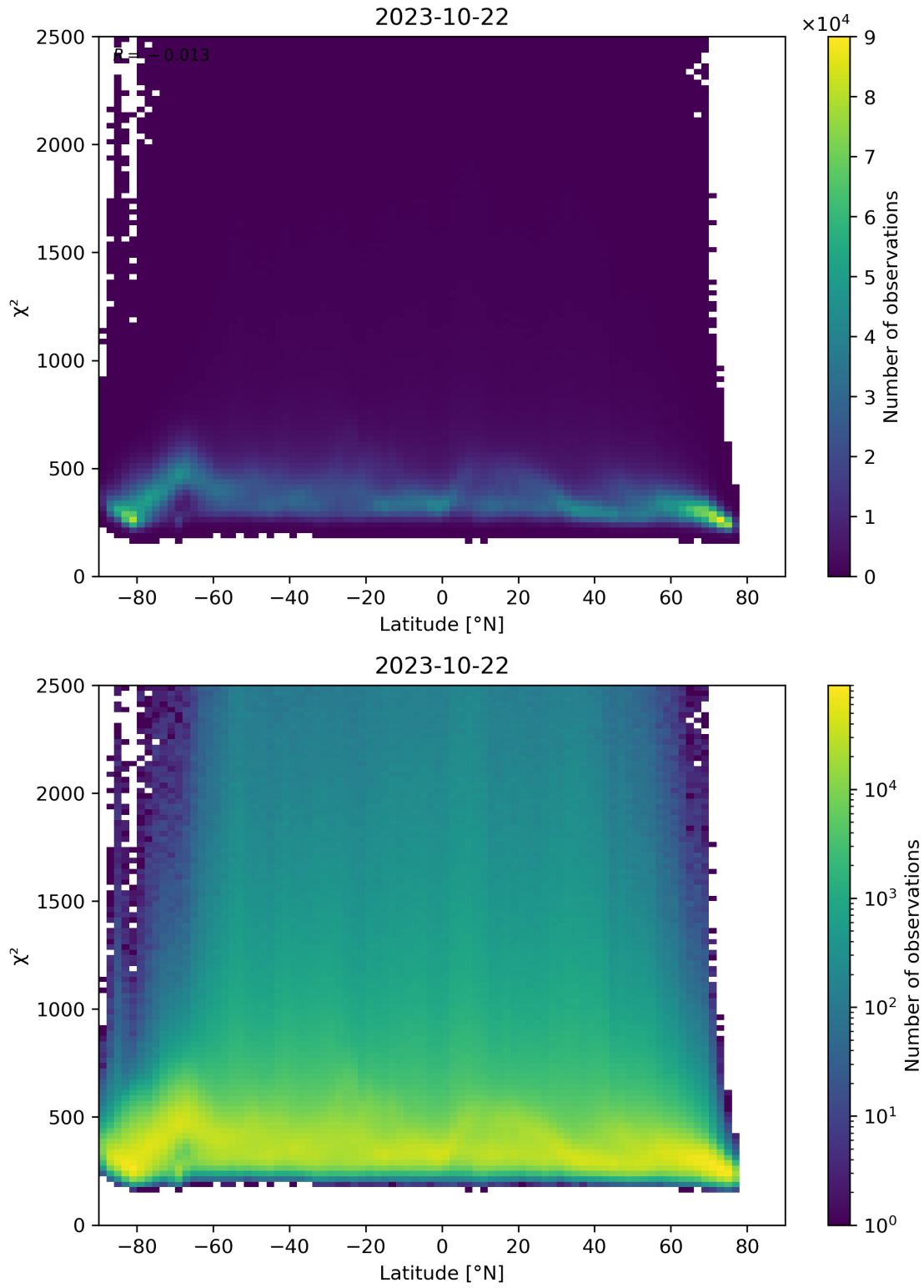
Figure 86: Scatter density plot of “Latitude” against “ \chi^2 ” for 2023-10-22 to 2023-10-23.
