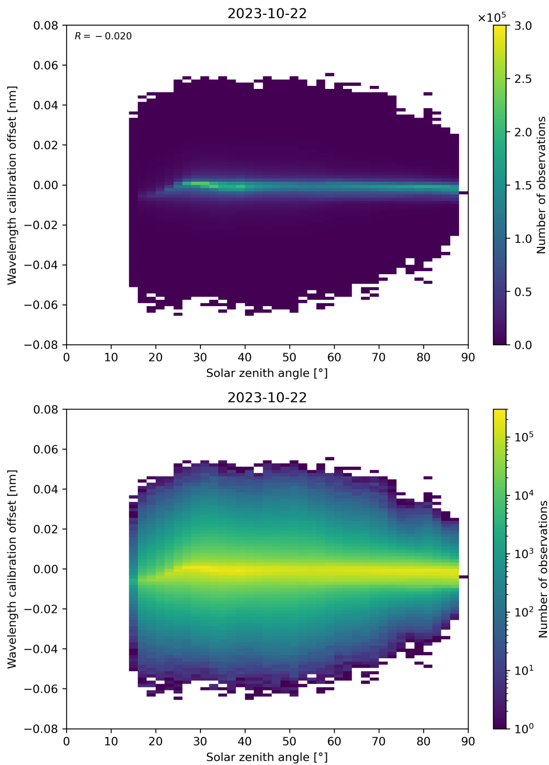
Figure 158: Scatter density plot of “Solar zenith angle” against “Wavelength calibration offset” for 2023-10-22 to 2023-10-23.
