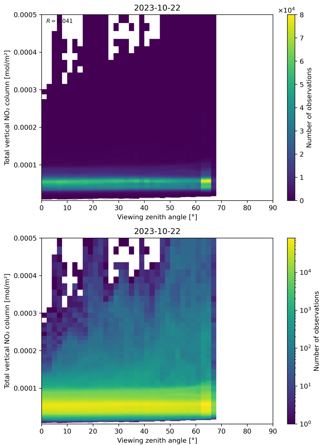
Figure 167: Scatter density plot of “Viewing zenith angle” against “Total vertical NO 2 column” for 2023-10-22 to 2023-10-23.
