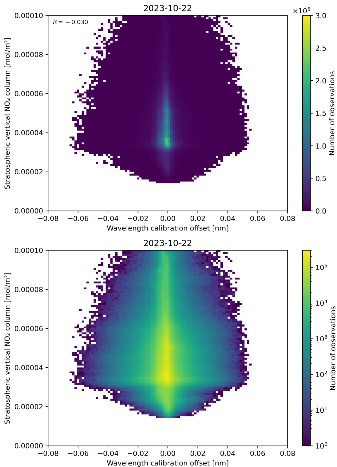
Figure 176: Scatter density plot of “Wavelength calibration offset” against “Stratospheric vertical NO 2 column” for 2023-10-22 to 2023-10-23.
