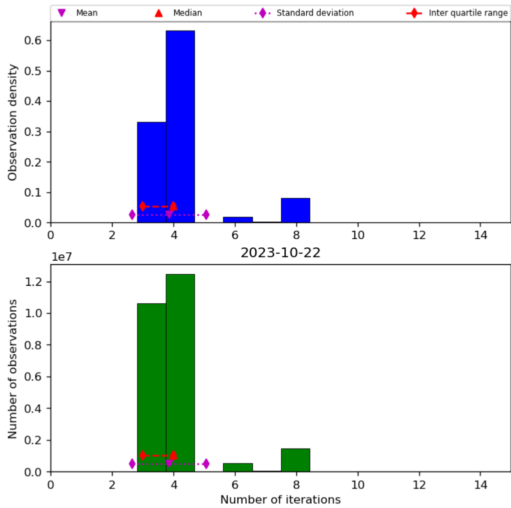
Figure 34: Histogram of “Number of iterations” for 2023-10-22 to 2023-10-23
