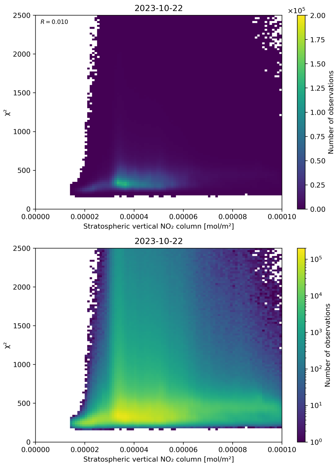
Figure 97: Scatter density plot of “Stratospheric vertical NO 2 column” against “ \chi^2 ” for 2023-10-22 to 2023-10-23.
