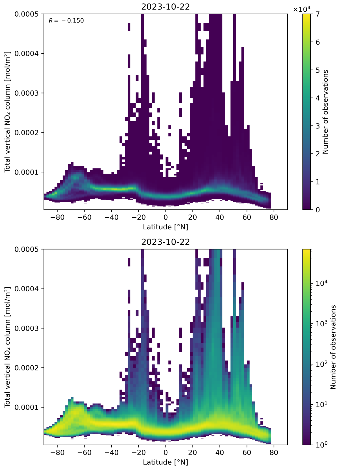
Figure 90: Scatter density plot of “Latitude” against “Total vertical NO 2 column” for 2023-10-22 to 2023-10-23.
