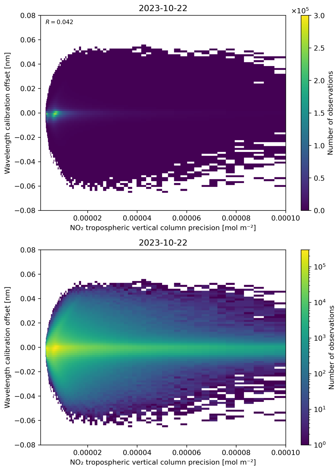
Figure 141: Scatter density plot of “NO 2 tropospheric vertical column precision” against “Wavelength calibration offset” for 2023-10-22 to 2023-10-23.
