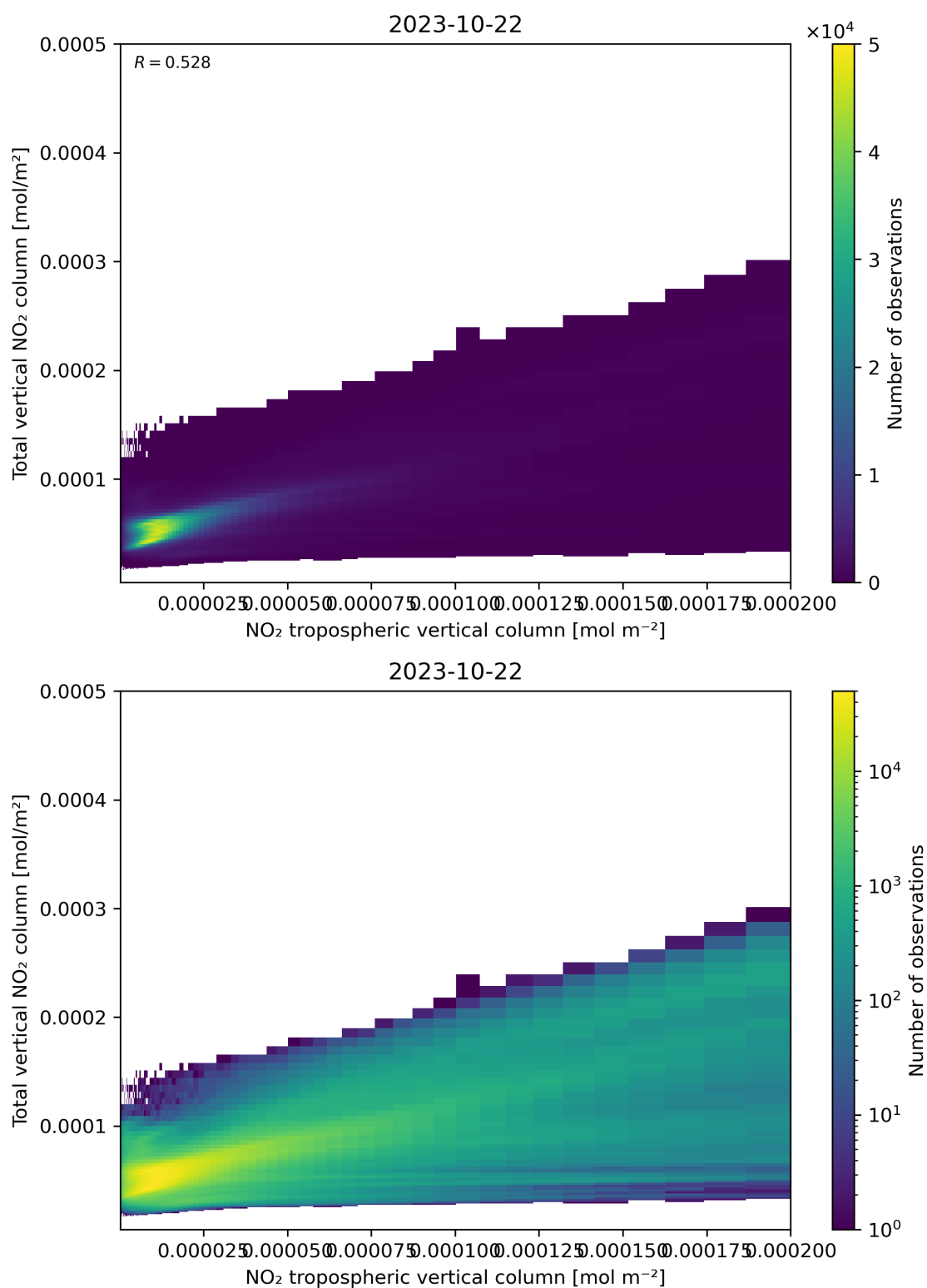
Figure 128: Scatter density plot of “NO 2 tropospheric vertical column” against “Total vertical NO 2 column” for 2023-10-22 to 2023-10-23.
