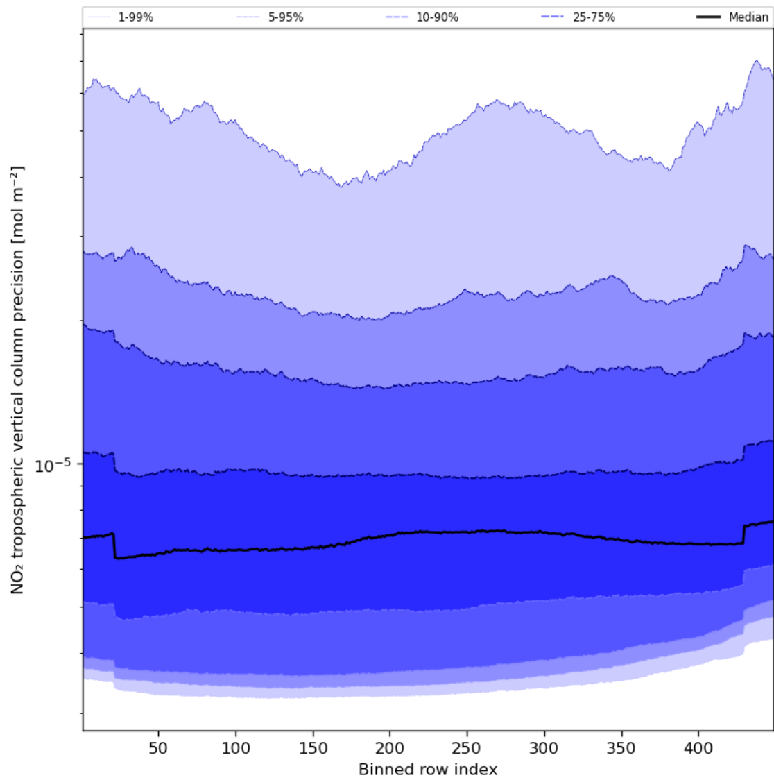
Figure 47: Along track statistics of “NO 2 tropospheric vertical column precision” for 2023-10-22 to 2023-10-23
