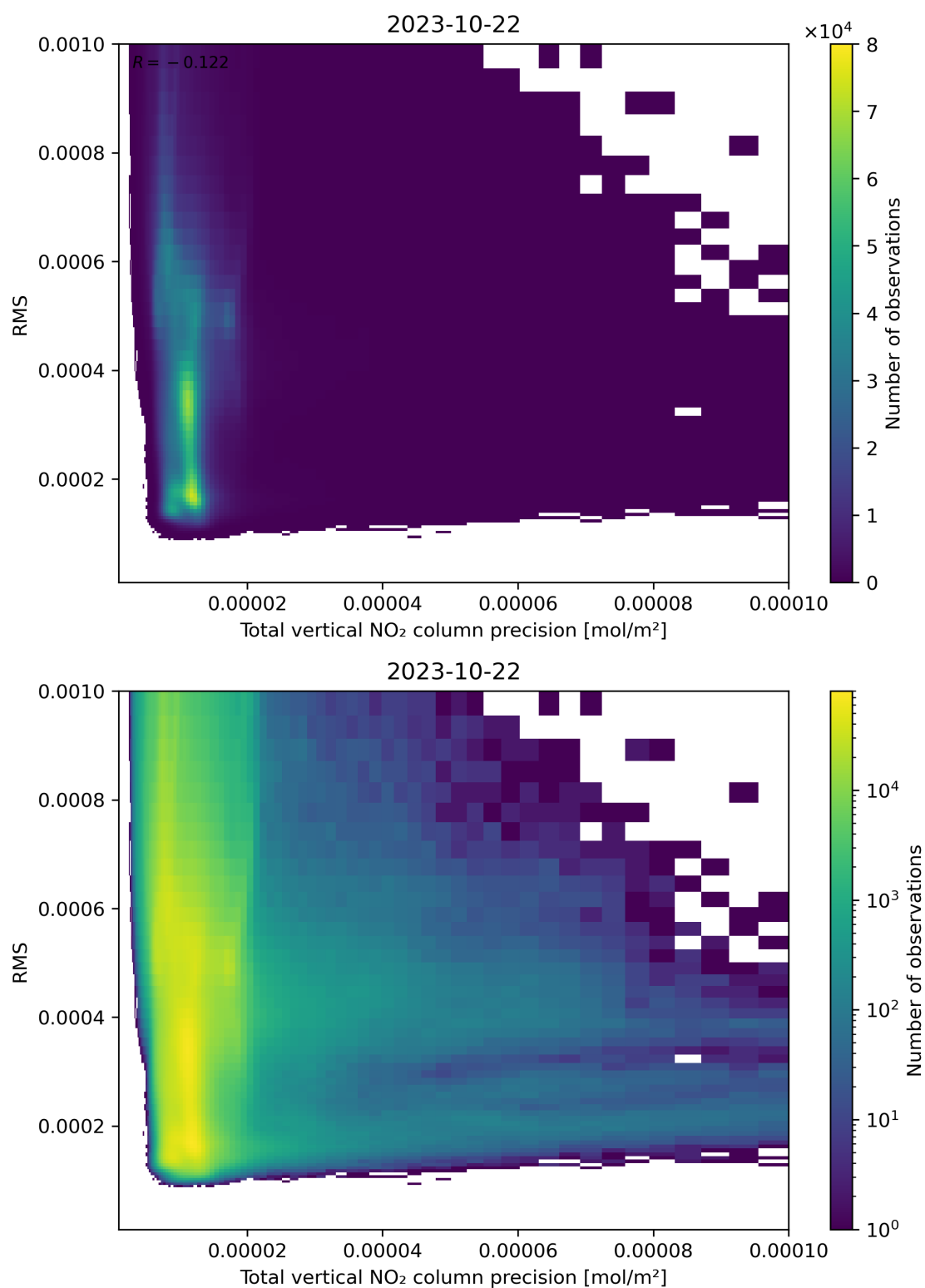
Figure 119: Scatter density plot of “Total vertical NO 2 column precision” against “RMS” for 2023-10-22 to 2023-10-23.
