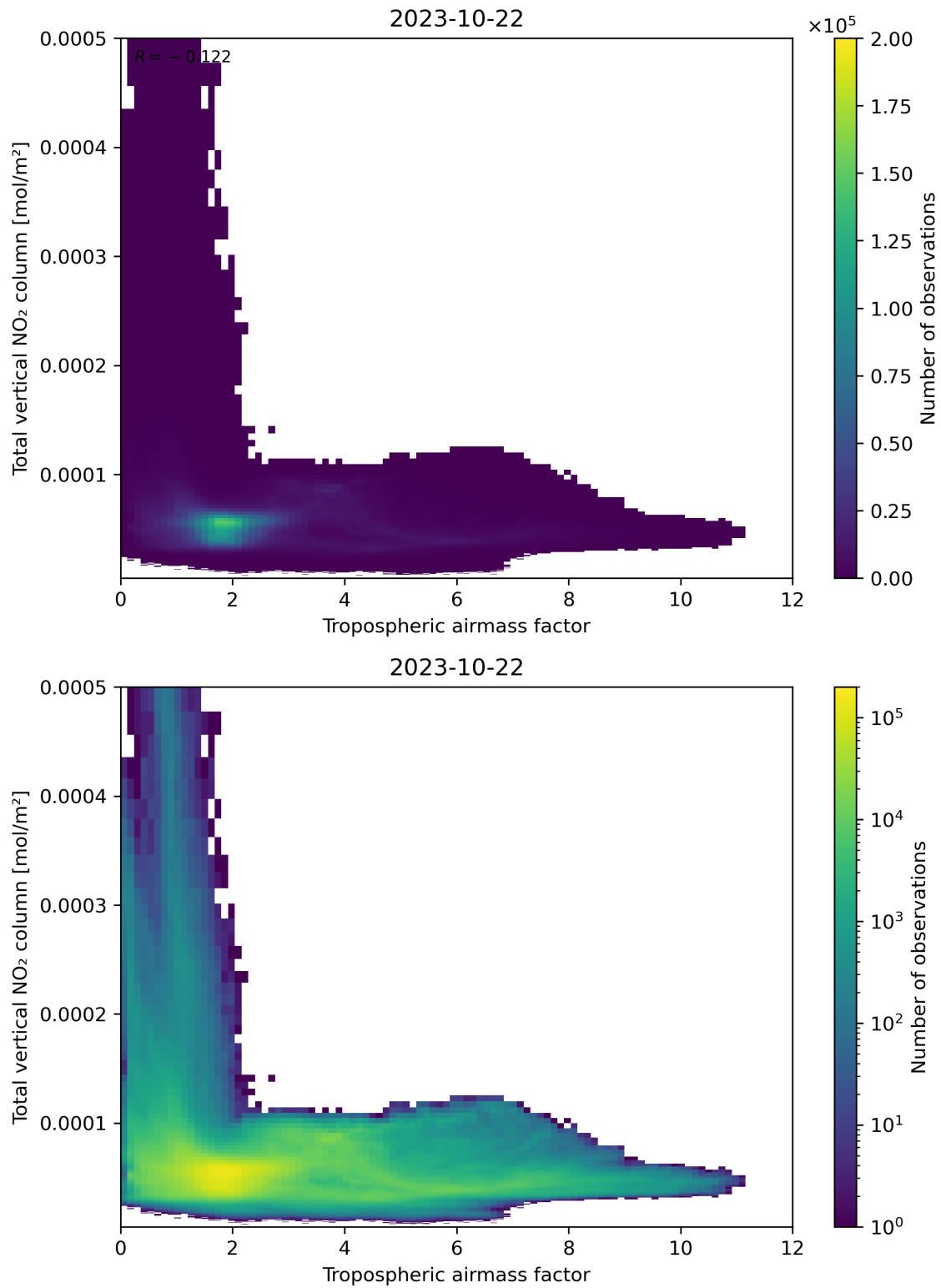
Figure 77: Scatter density plot of “Tropospheric airmass factor” against “Total vertical NO 2 column” for 2023-10-22 to 2023-10-23.
