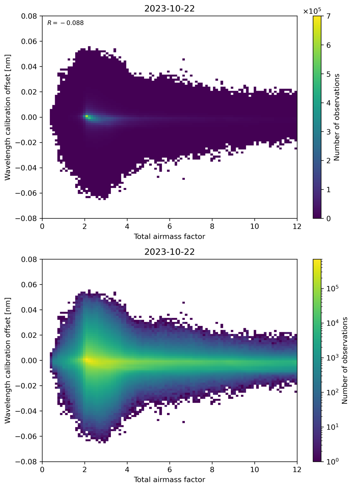
Figure 70: Scatter density plot of “Total airmass factor” against “Wavelength calibration offset” for 2023-10-22 to 2023-10-23.
