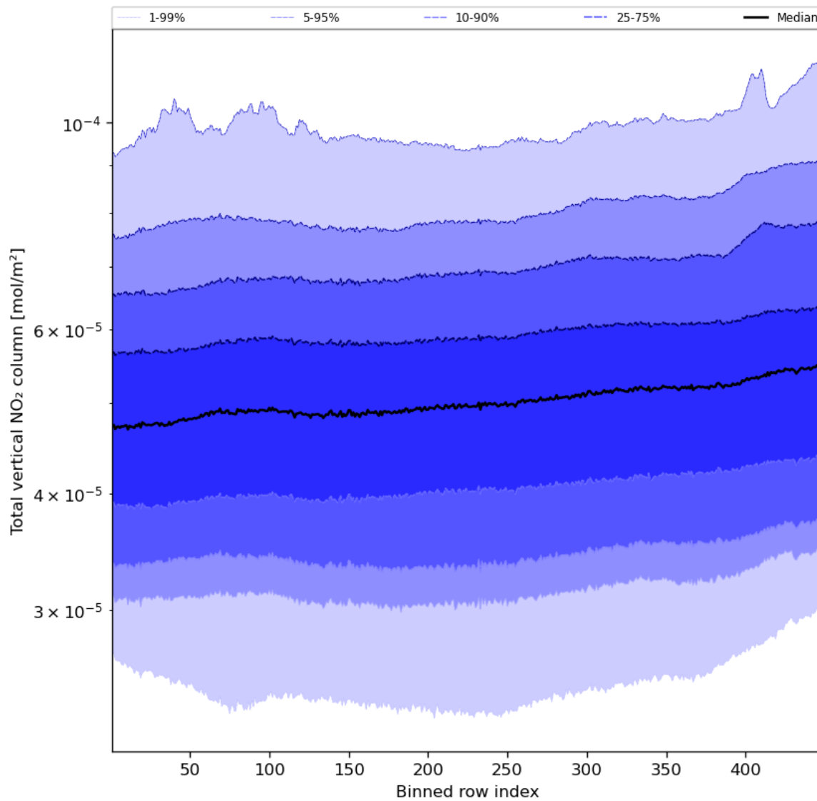
Figure 55: Along track statistics of “Total vertical NO 2 column” for 2023-10-22 to 2023-10-23
