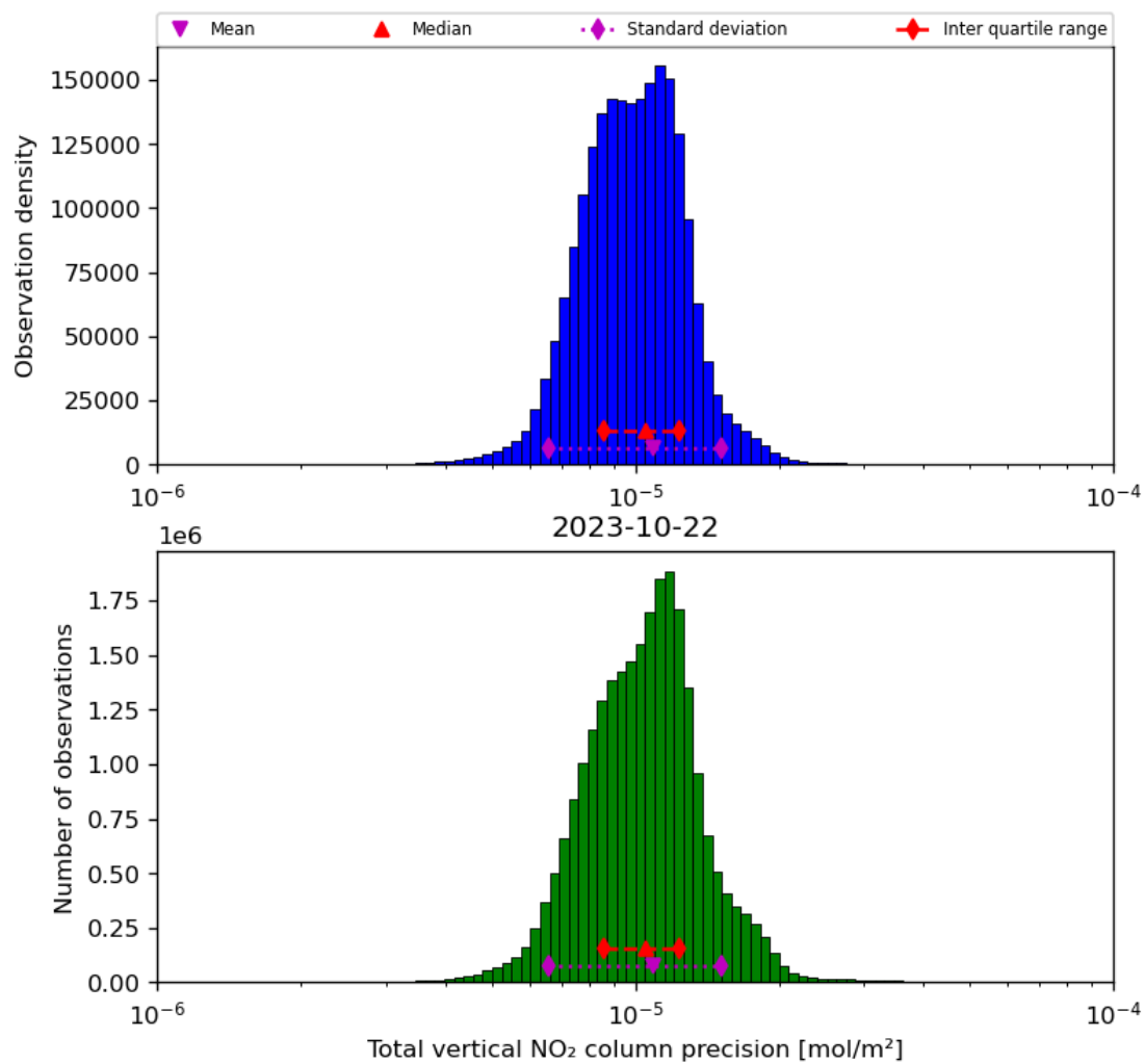
Figure 39: Histogram of “Total vertical NO 2 column precision” for 2023-10-22 to 2023-10-23
