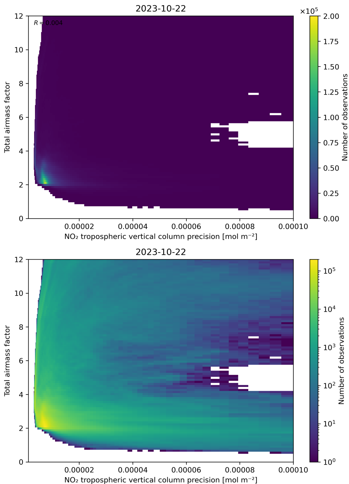
Figure 132: Scatter density plot of “NO 2 tropospheric vertical column precision” against “Total air mass factor” for 2023-10-22 to 2023-10-23.
