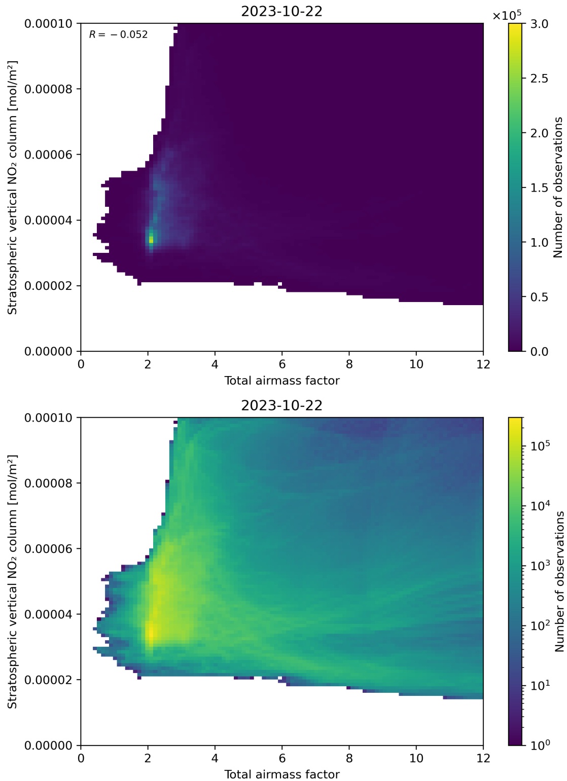
Figure 64: Scatter density plot of “Total airmass factor” against “Stratospheric vertical NO 2 column” for 2023-10-22 to 2023-10-23.
