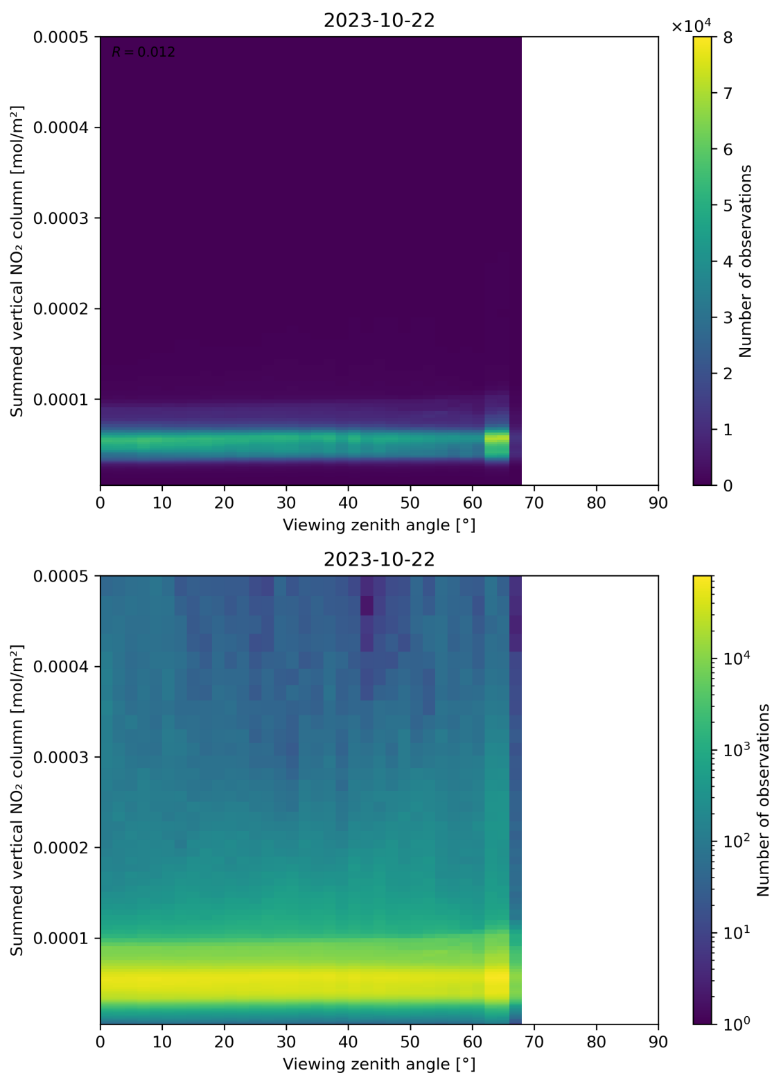
Figure 165: Scatter density plot of “Viewing zenith angle” against “Summed vertical NO 2 column” for 2023-10-22 to 2023-10-23.
