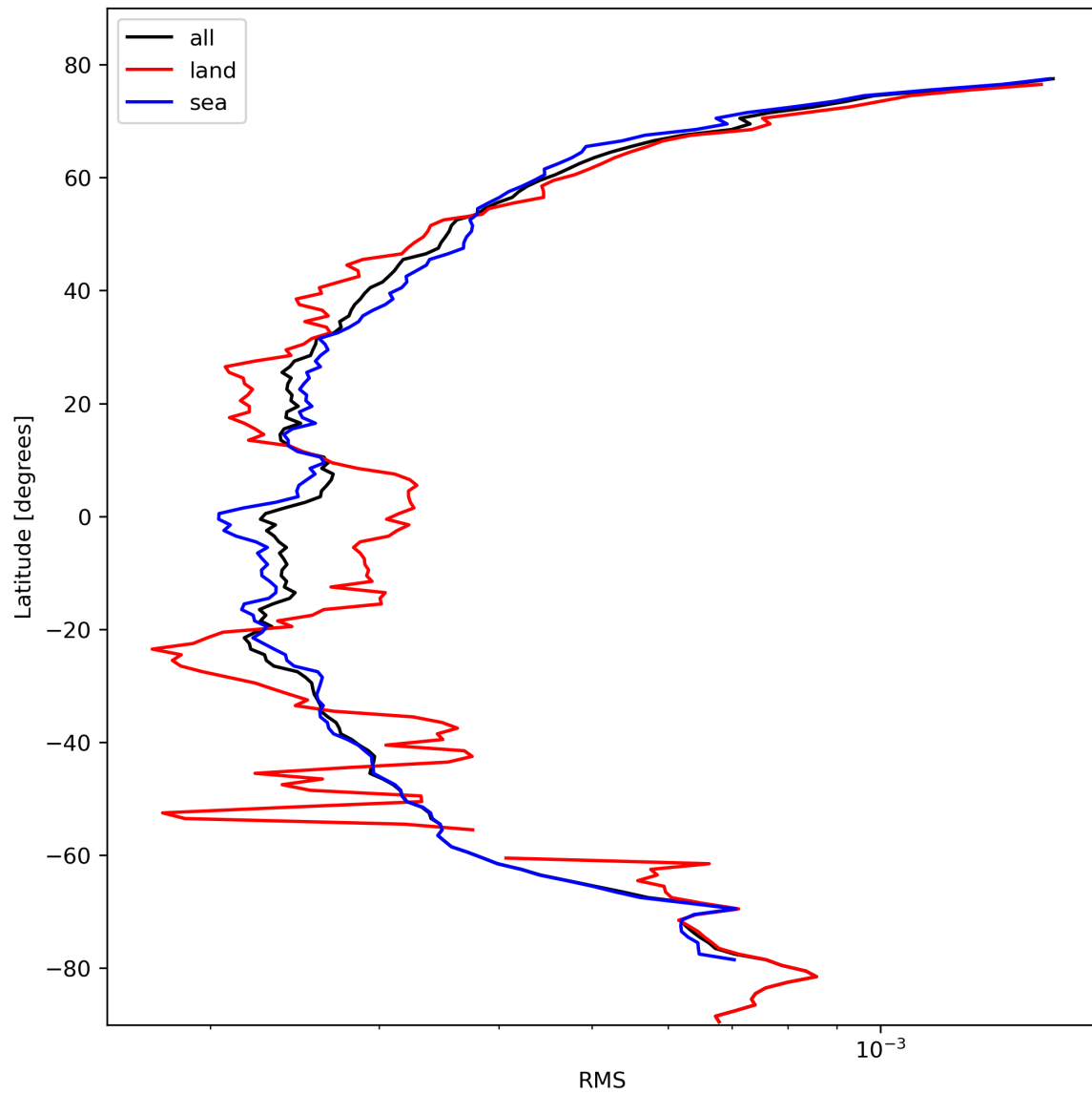
Figure 26: Zonal average of “RMS” for 2023-10-22 to 2023-10-23.
