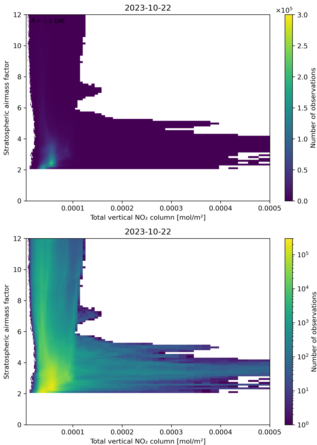
Figure 110: Scatter density plot of “Total vertical NO 2 column” against “Stratospheric airmass factor” for 2023-10-22 to 2023-10-23.
