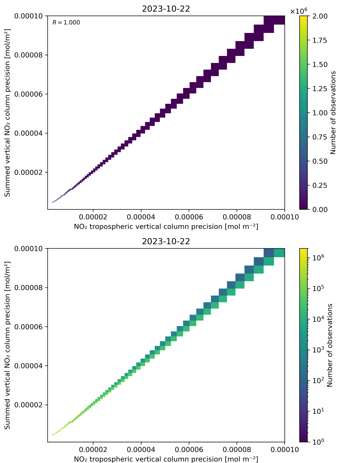
Figure 137: Scatter density plot of “NO 2 tropospheric vertical column precision” against “Summed vertical NO 2 column precision” for 2023-10-22 to 2023-10-23.
