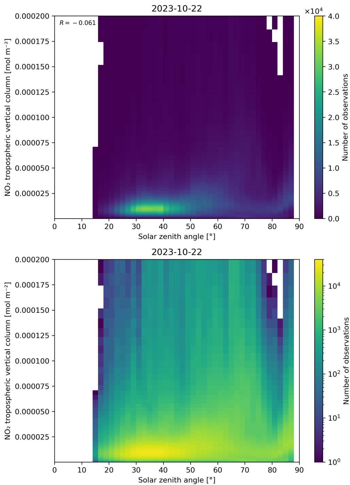
Figure 155: Scatter density plot of “Solar zenith angle” against “NO 2 tropospheric vertical column” for 2023-10-22 to 2023-10-23.
