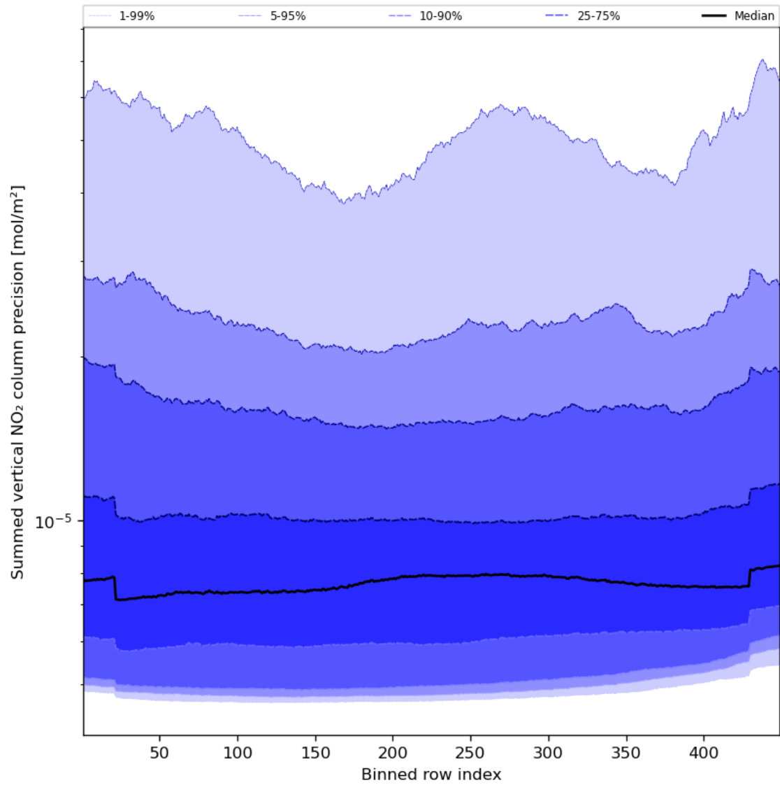
Figure 58: Along track statistics of “Summed vertical NO 2 column precision” for 2023-10-22 to 2023-10-23
