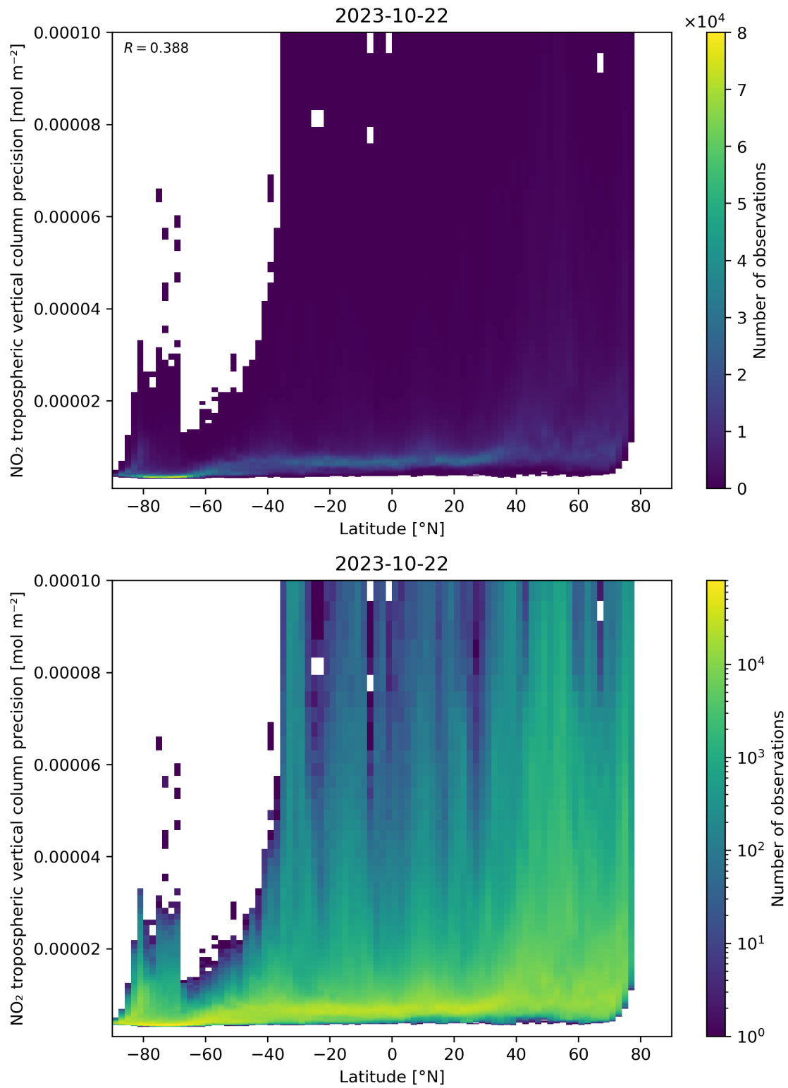
Figure 93: Scatter density plot of “Latitude” against “NO 2 tropospheric vertical column precision” for 2023-10-22 to 2023-10-23.
