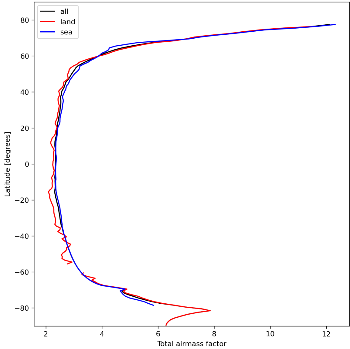
Figure 15: Zonal average of “Total airmass factor” for 2023-10-22 to 2023-10-23.
