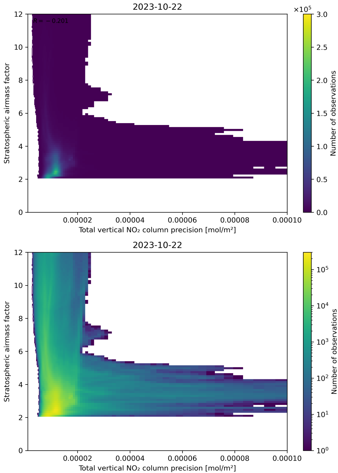
Figure 115: Scatter density plot of “Total vertical NO 2 column precision” against “Stratospheric airmass factor” for 2023-10-22 to 2023-10-23.
