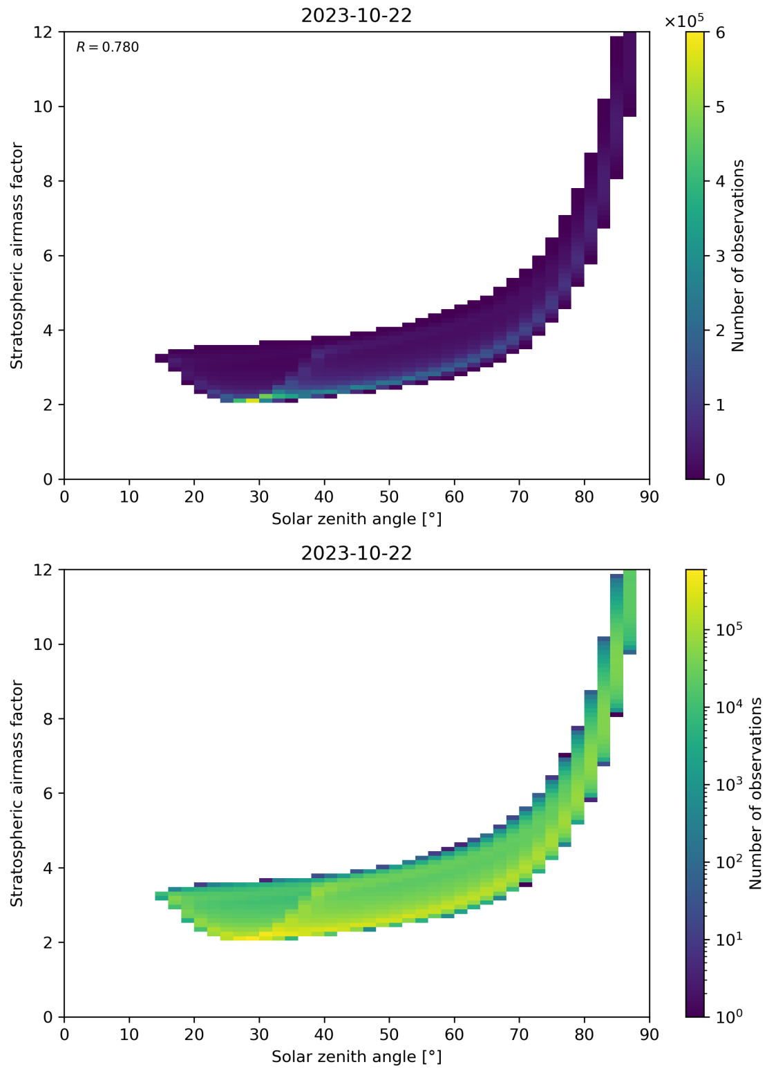
Figure 145: Scatter density plot of “Solar zenith angle” against “Stratospheric airmass factor” for 2023-10-22 to 2023-10-23.
