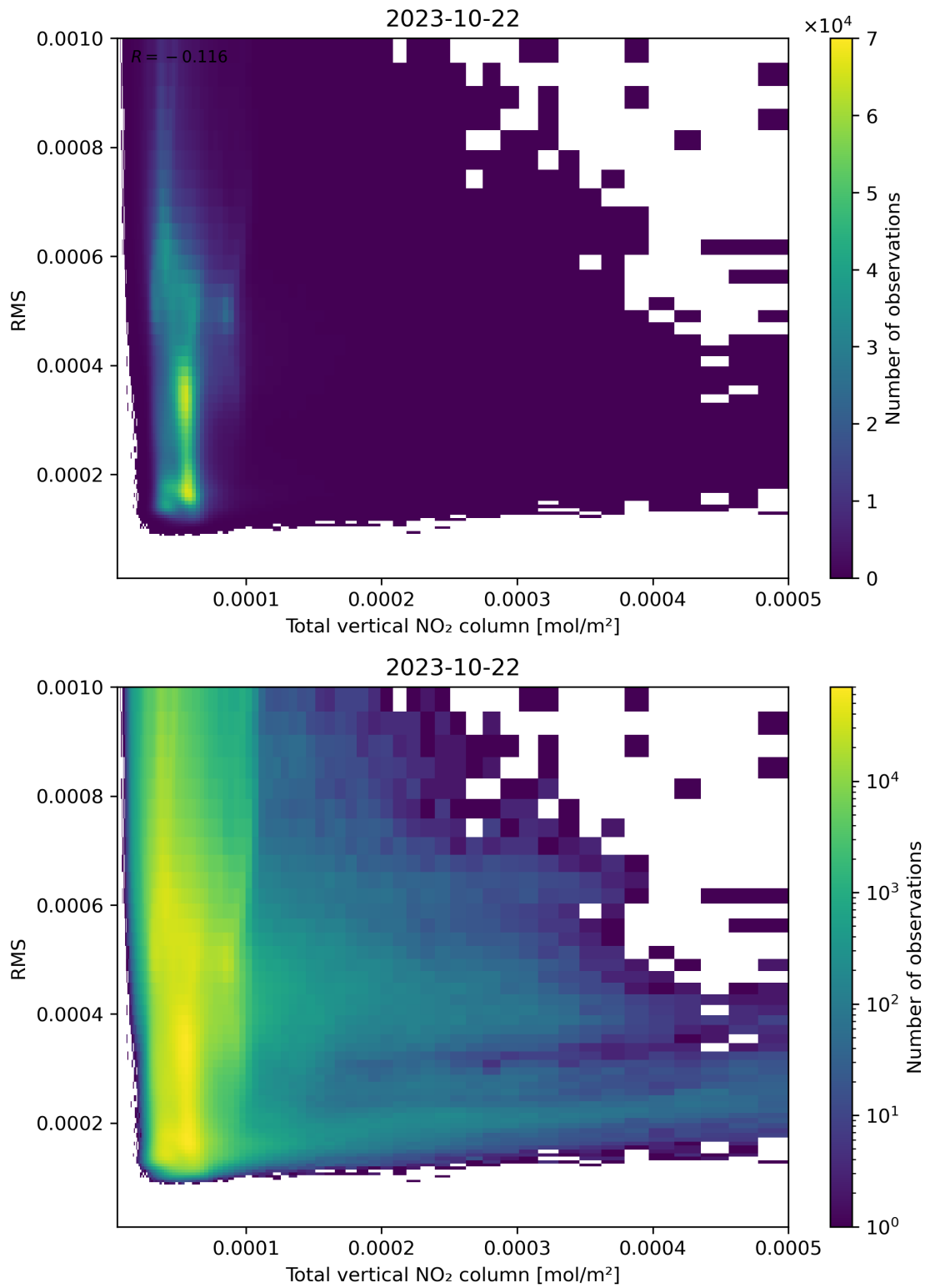
Figure 120: Scatter density plot of “Total vertical NO 2 column” against “RMS” for 2023-10-22 to 2023-10-23.
