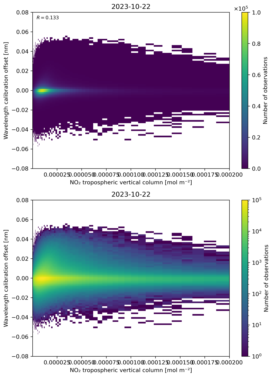
Figure 143: Scatter density plot of “NO 2 tropospheric vertical column” against “Wavelength calibration offset” for 2023-10-22 to 2023-10-23.
