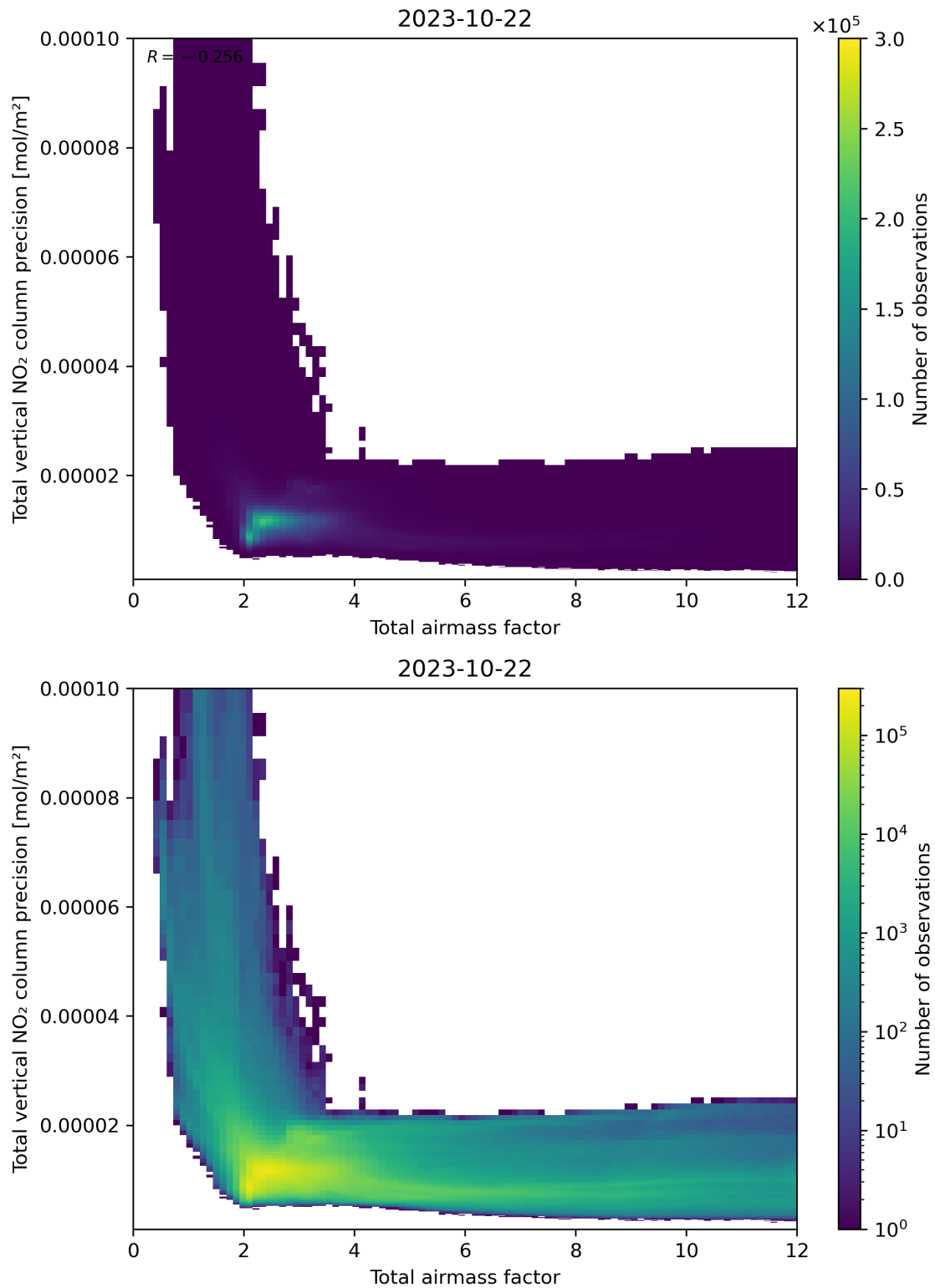
Figure 68: Scatter density plot of “Total airmass factor” against “Total vertical NO 2 column precision” for 2023-10-22 to 2023-10-23.
