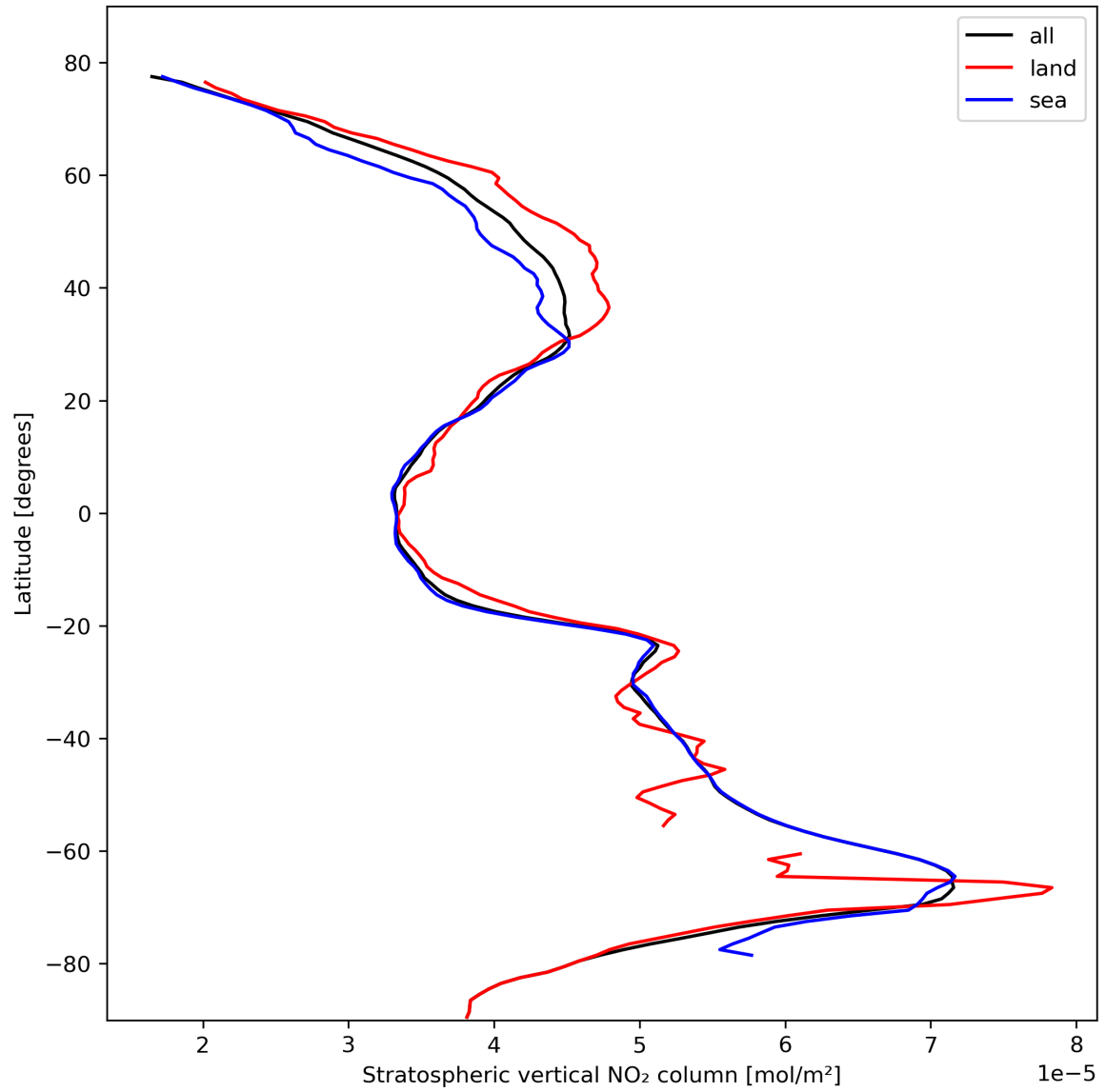
Figure 19: Zonal average of “Stratospheric vertical NO 2 column” for 2023-10-22 to 2023-10-23.
