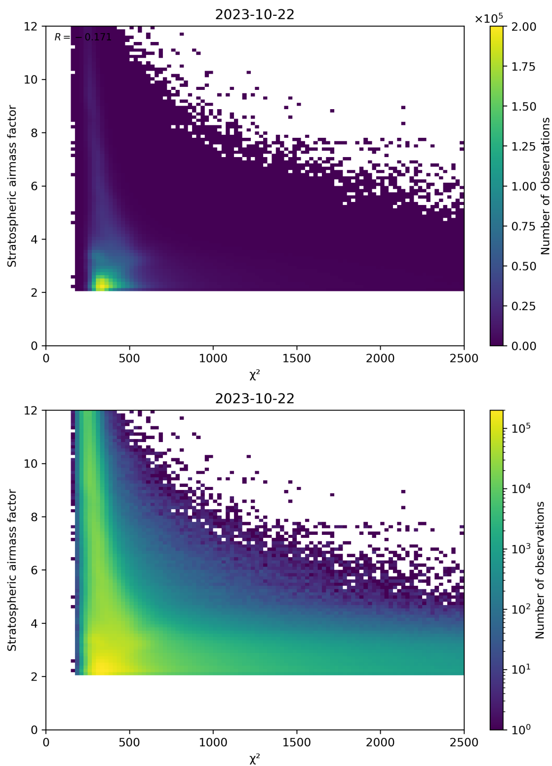
Figure 81: Scatter density plot of " \chi^2 " against "Stratospheric airmass factor" for 2023-10-22 to 2023-10-23.
