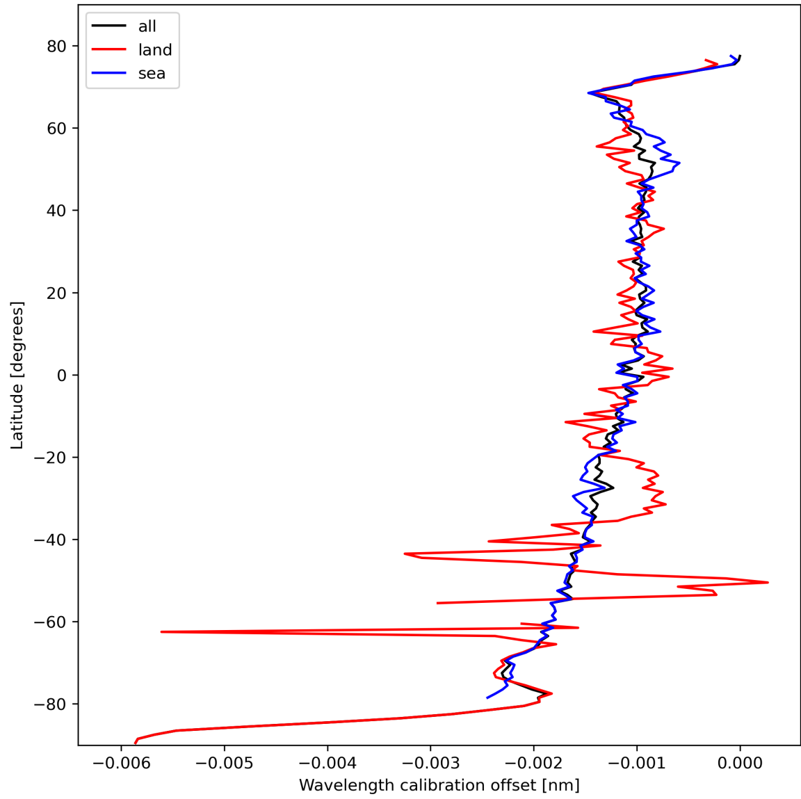
Figure 18: Zonal average of “Wavelength calibration offset” for 2023-10-22 to 2023-10-23.
