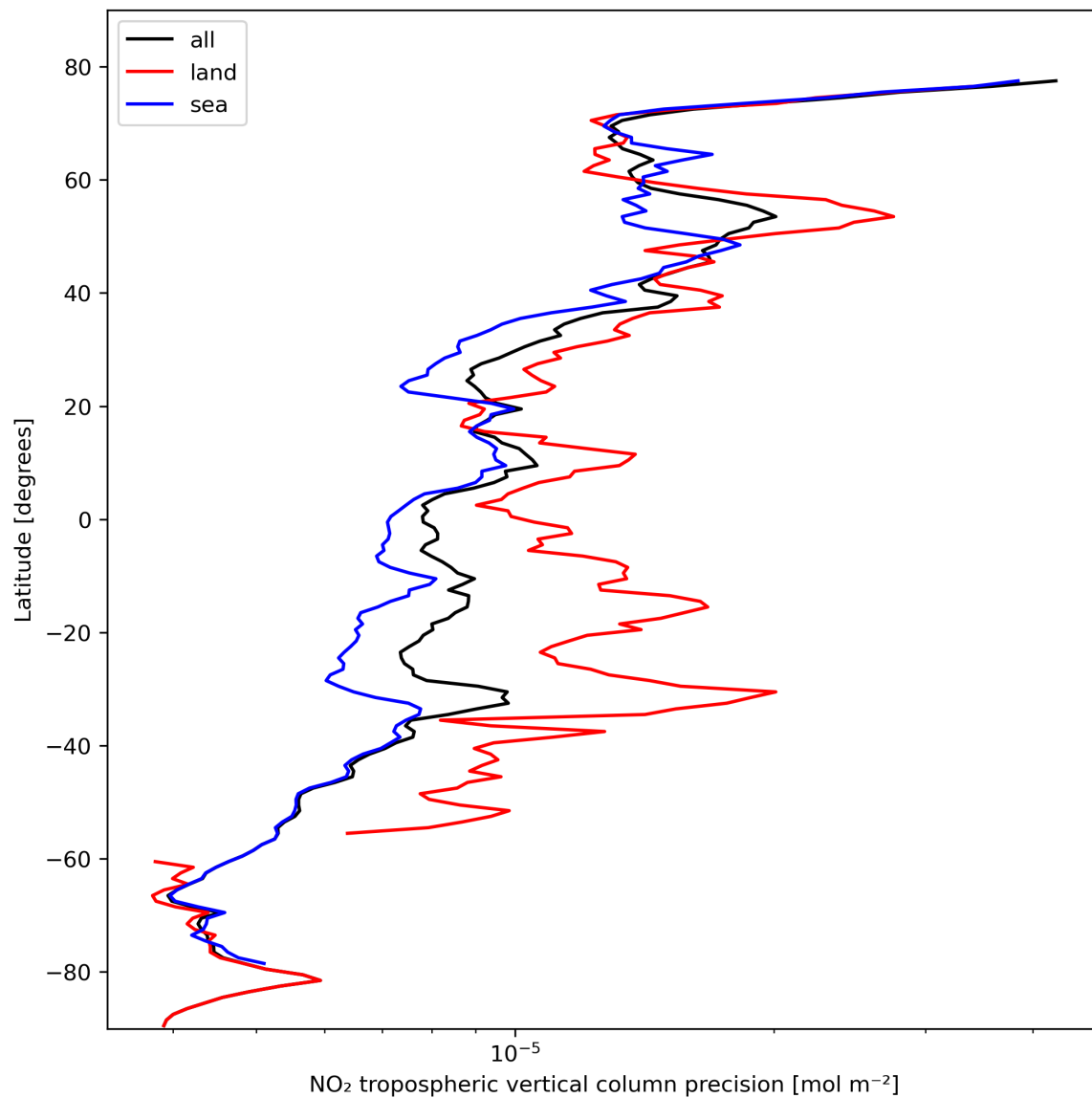
Figure 13: Zonal average of “NO 2 tropospheric vertical column precision” for 2023-10-22 to 2023-10-23.
