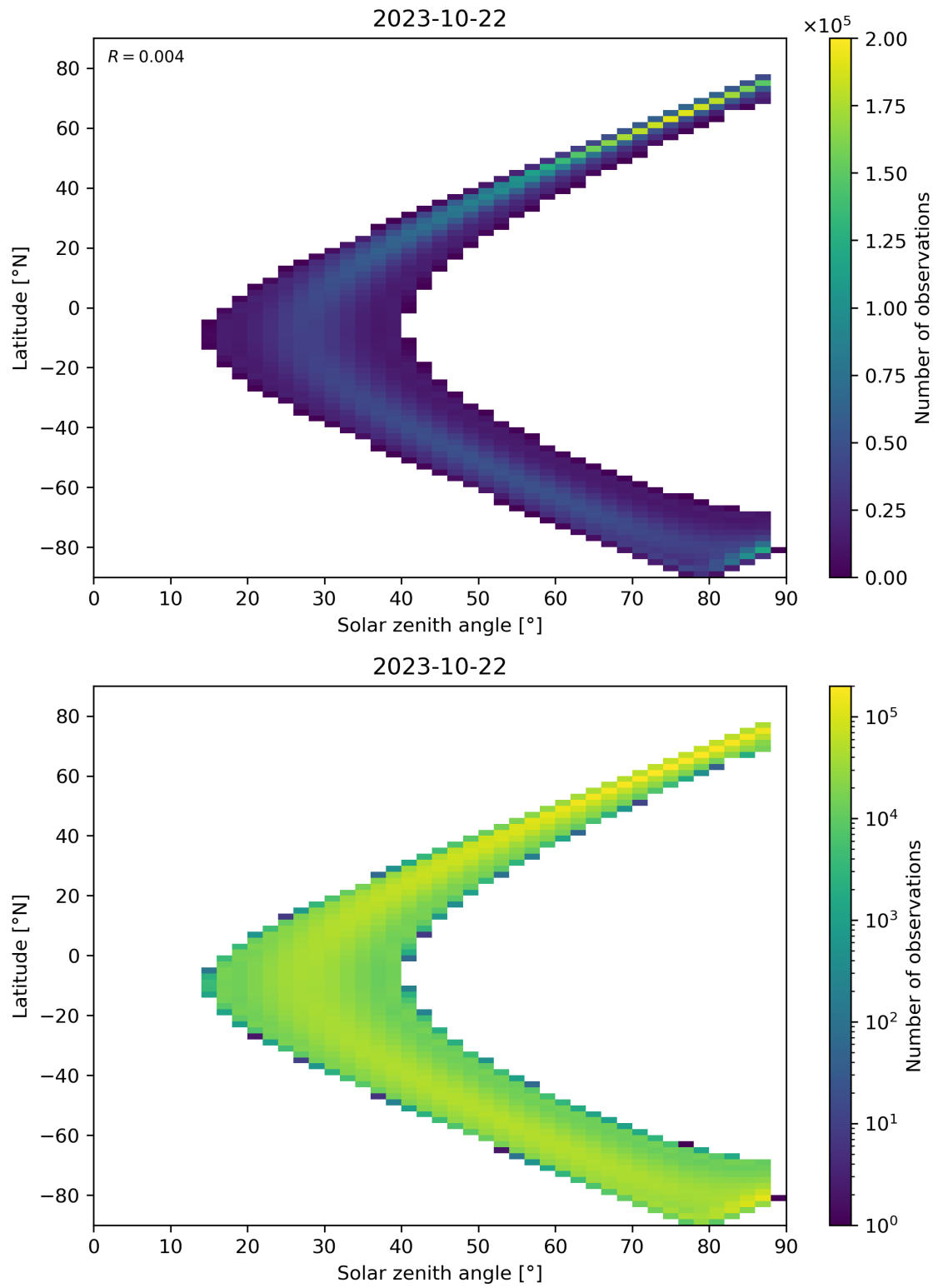
Figure 149: Scatter density plot of “Solar zenith angle” against “Latitude” for 2023-10-22 to 2023-10-23.
