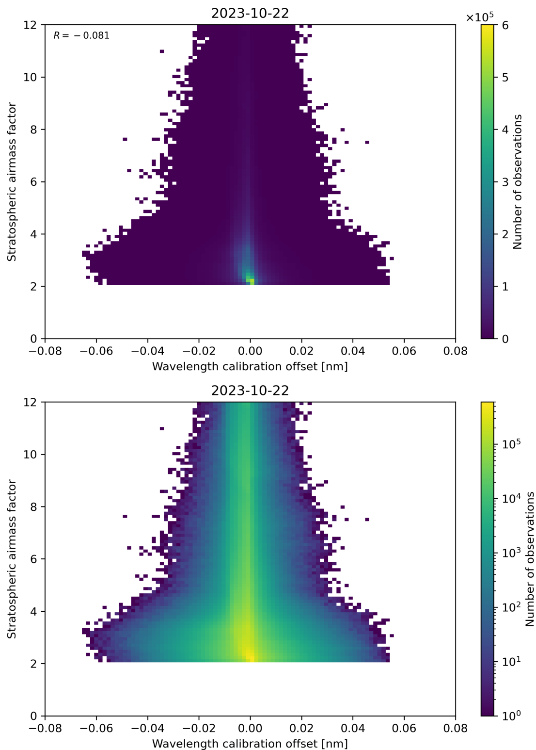
Figure 174: Scatter density plot of “Wavelength calibration offset” against “Stratospheric airmass factor” for 2023-10-22 to 2023-10-23.
