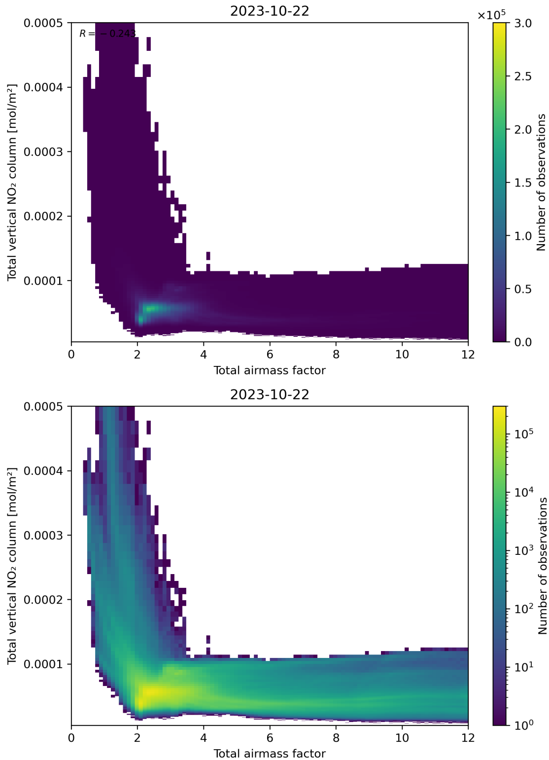
Figure 67: Scatter density plot of “Total airmass factor” against “Total vertical NO 2 column” for 2023-10-22 to 2023-10-23.
