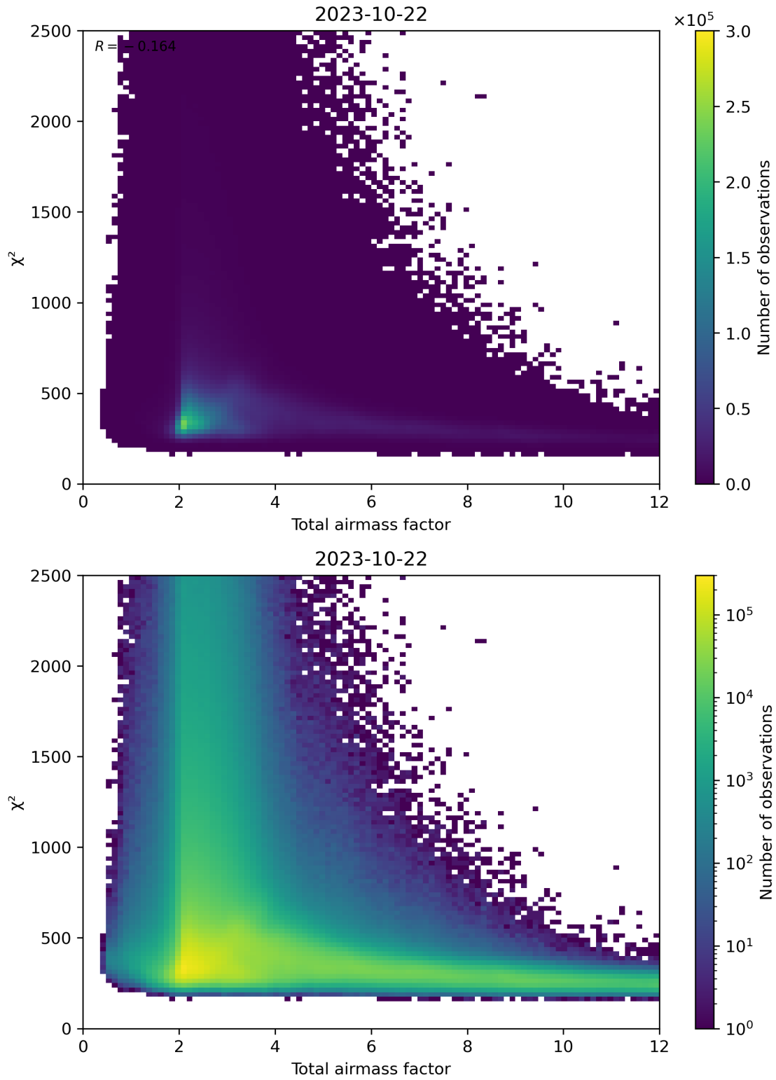
Figure 63: Scatter density plot of “Total airmass factor” against “ \chi^2 ” for 2023-10-22 to 2023-10-23.
