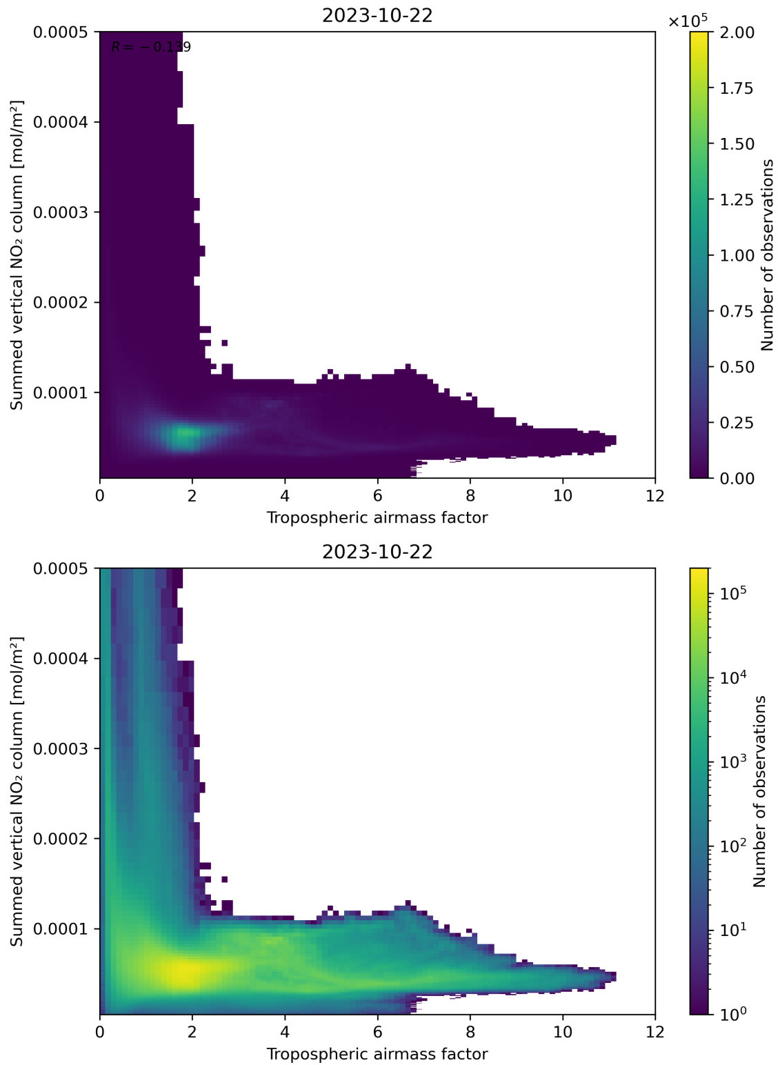
Figure 75: Scatter density plot of “Tropospheric airmass factor” against “Summed vertical NO 2 column” for 2023-10-22 to 2023-10-23.
