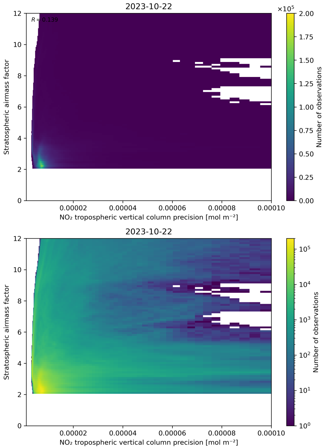
Figure 131: Scatter density plot of “NO 2 tropospheric vertical column precision” against “Stratospheric airmass factor” for 2023-10-22 to 2023-10-23.
