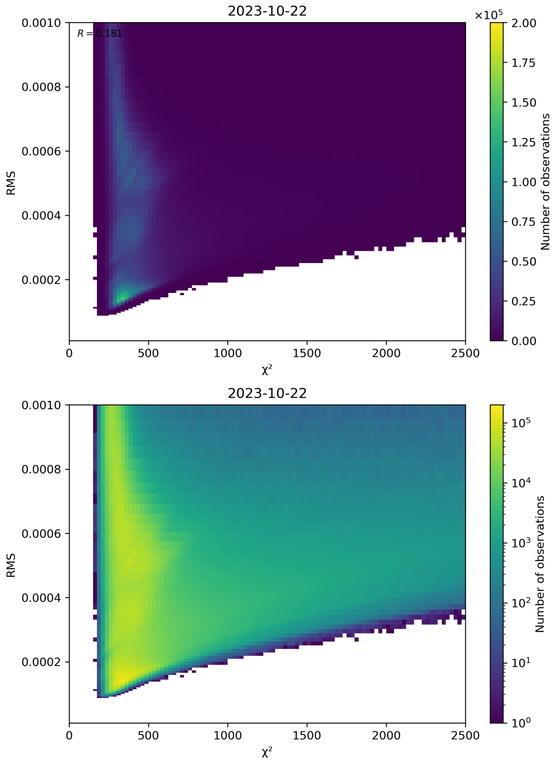
Figure 82: Scatter density plot of “ \chi^2 ” against “RMS” for 2023-10-22 to 2023-10-23.
