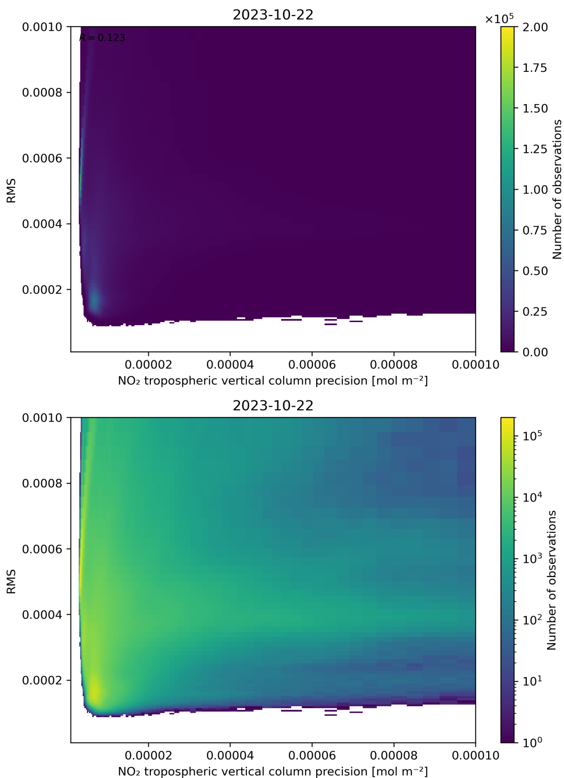
Figure 140: Scatter density plot of “NO 2 tropospheric vertical column precision” against “RMS” for 2023-10-22 to 2023-10-23.
