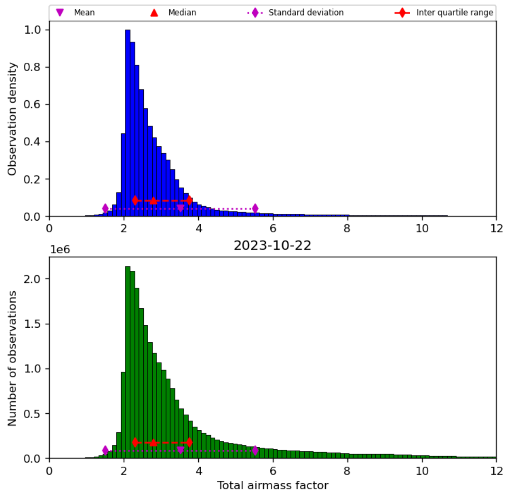
Figure 32: Histogram of “Total airmass factor” for 2023-10-22 to 2023-10-23
