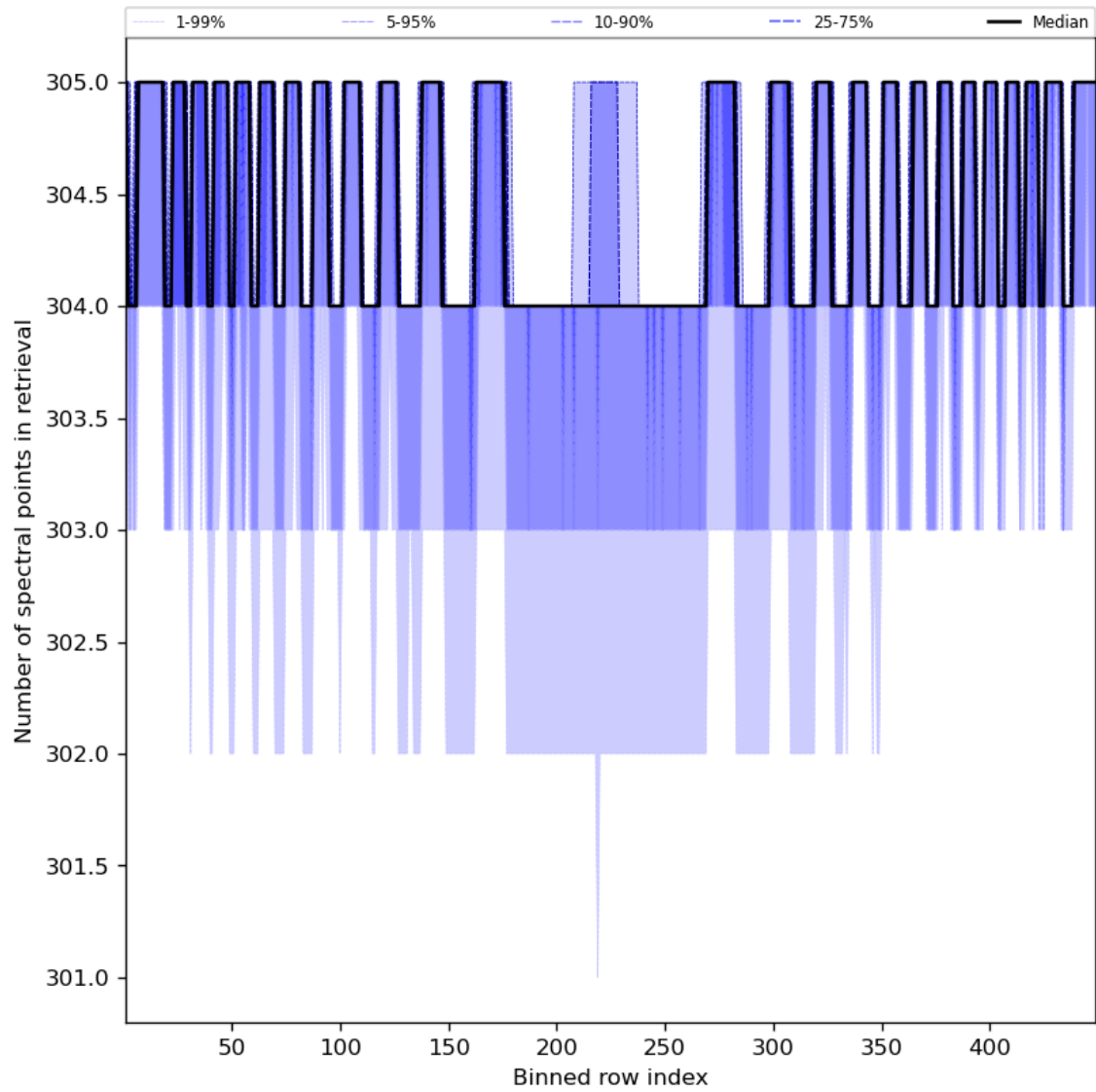
Figure 50: Along track statistics of “Number of spectral points in retrieval” for 2023-10-22 to 2023-10-23
