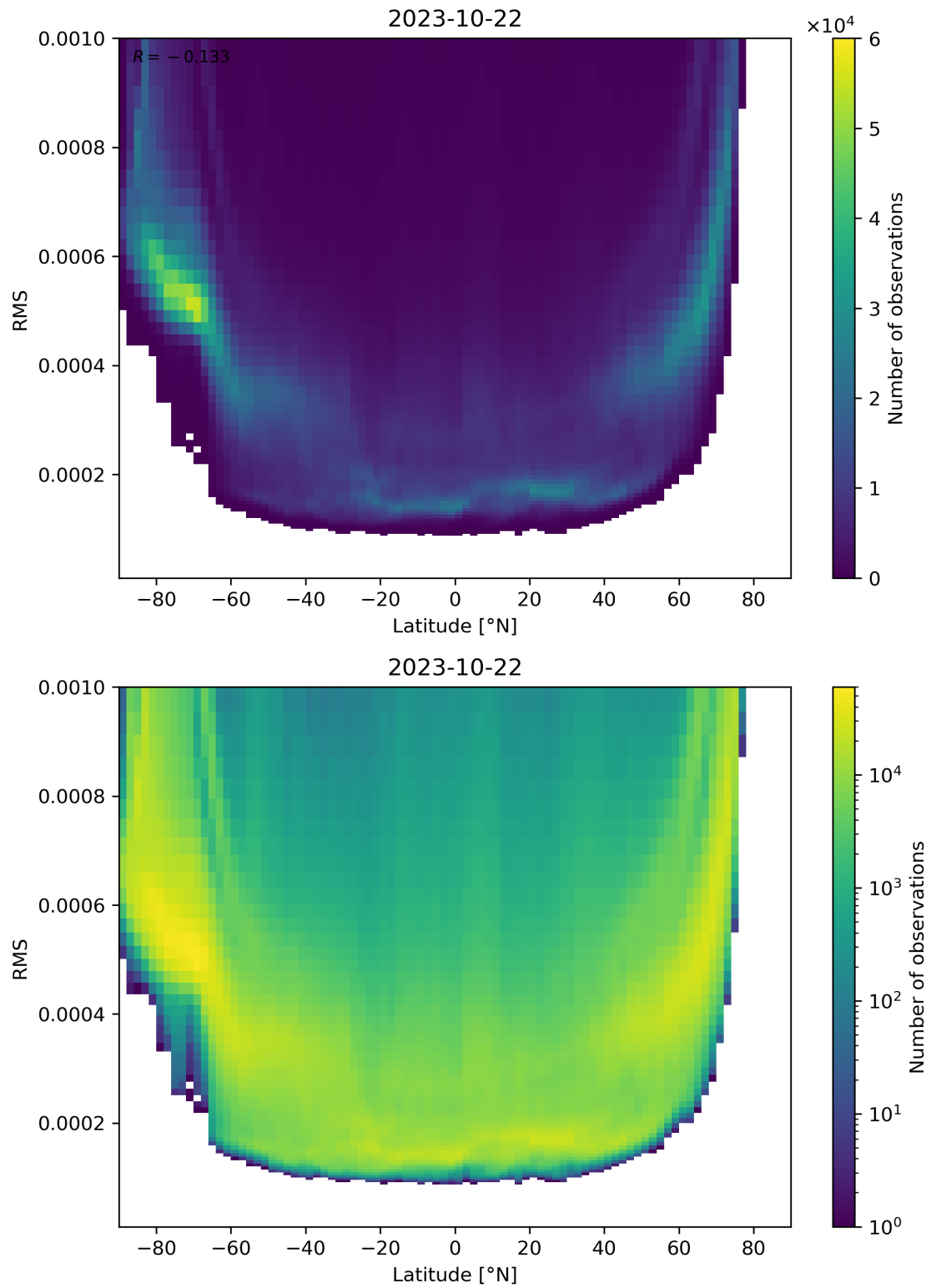
Figure 94: Scatter density plot of “Latitude” against “RMS” for 2023-10-22 to 2023-10-23.
