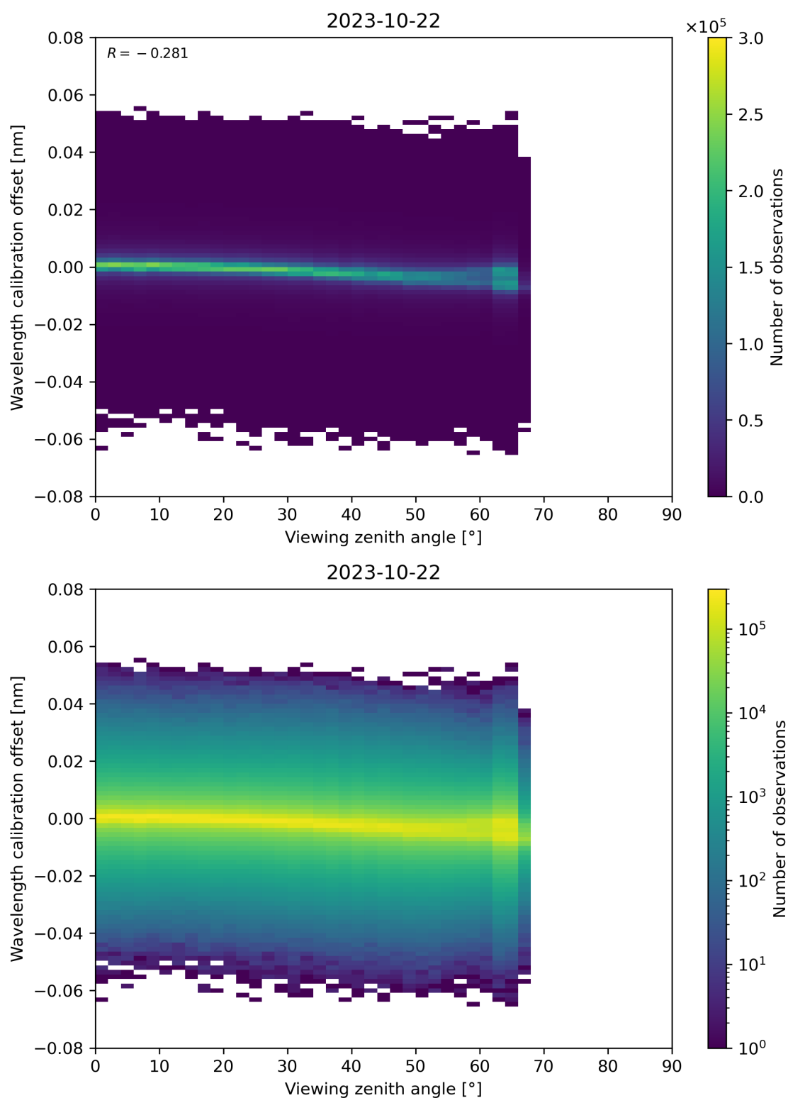
Figure 173: Scatter density plot of “Viewing zenith angle” against “Wavelength calibration offset” for 2023-10-22 to 2023-10-23.
