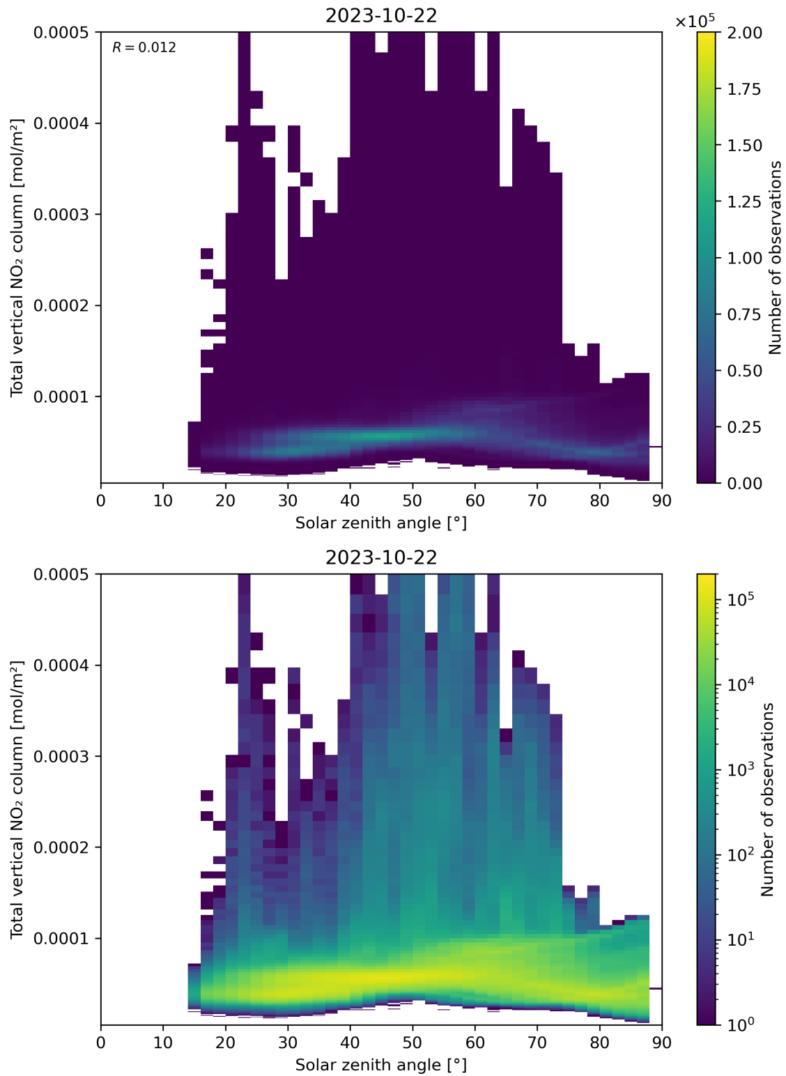
Figure 153: Scatter density plot of “Solar zenith angle” against “Total vertical NO 2 column” for 2023-10-22 to 2023-10-23.
