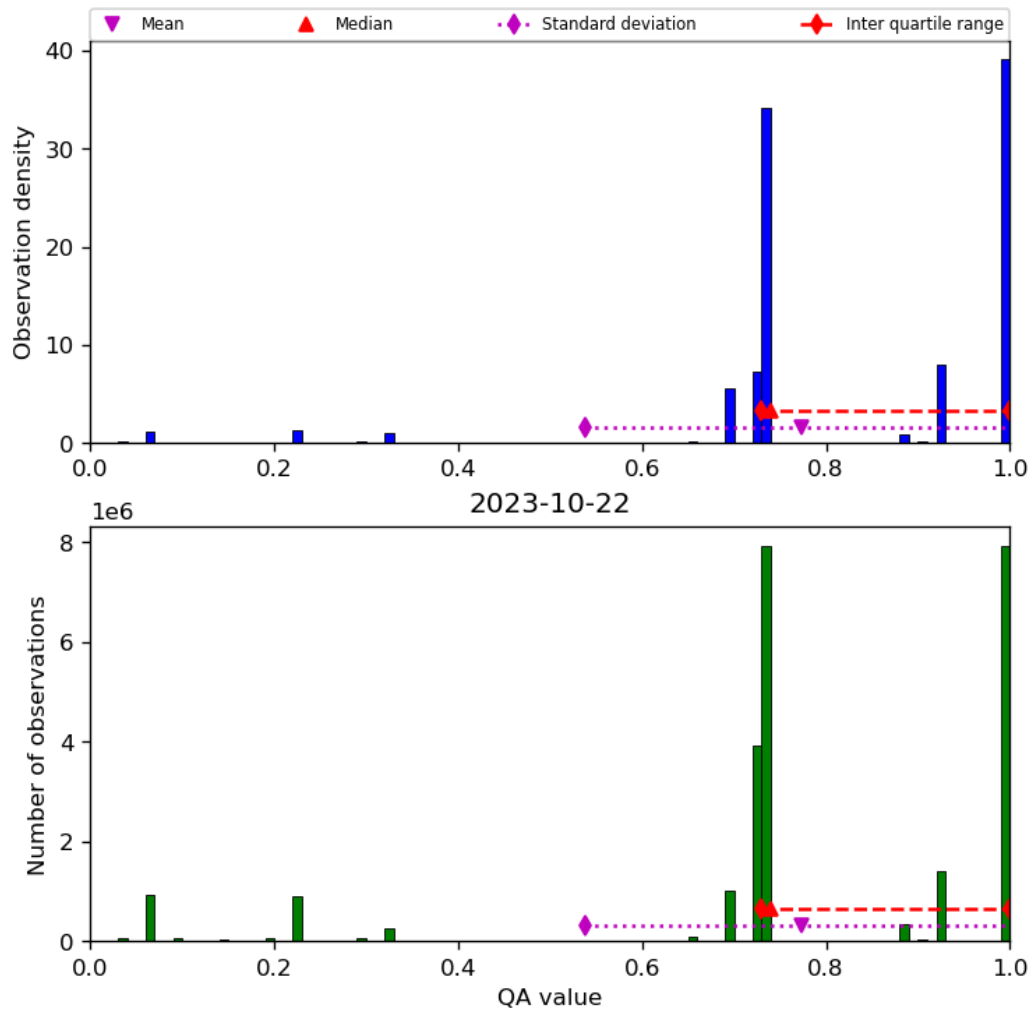
Figure 28: Histogram of “QA value” for 2023-10-22 to 2023-10-23
