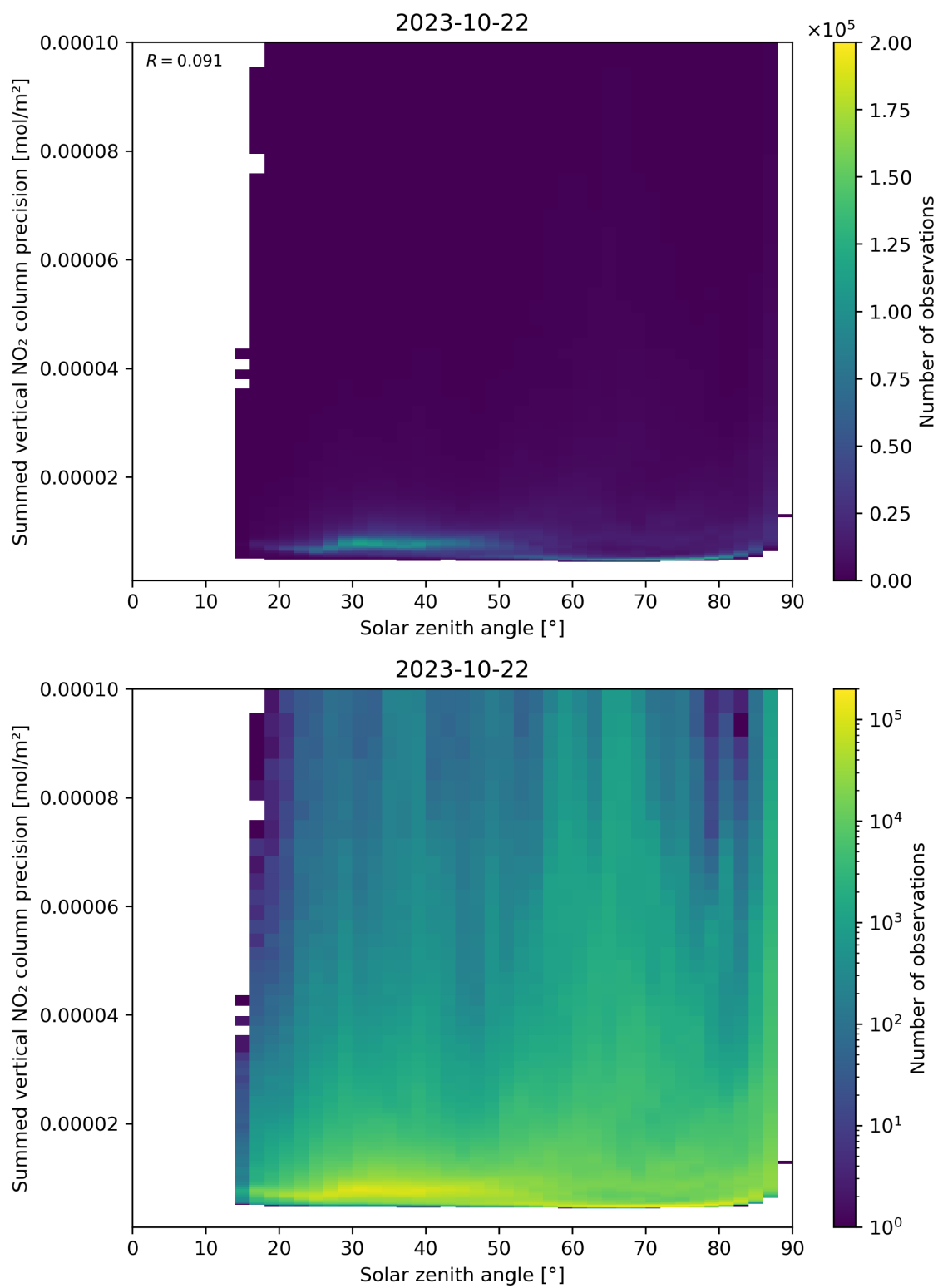
Figure 152: Scatter density plot of “Solar zenith angle” against “Summed vertical NO 2 column precision” for 2023-10-22 to 2023-10-23.
