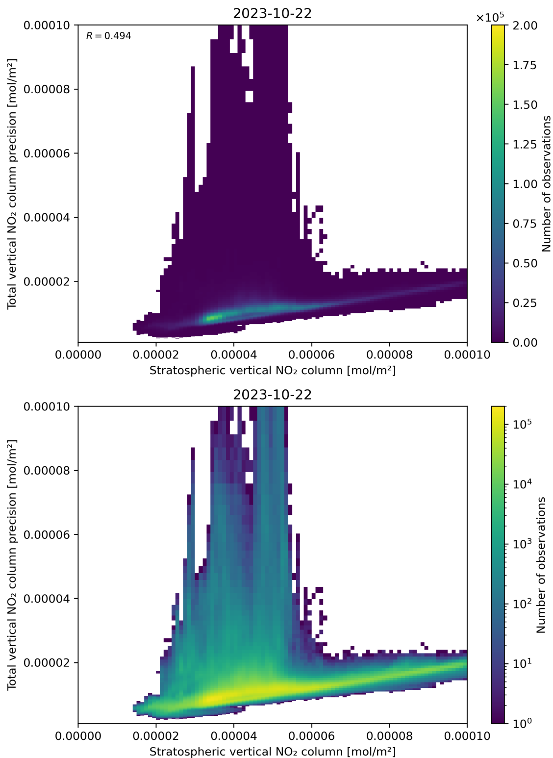
Figure 101: Scatter density plot of “Stratospheric vertical NO 2 column” against “Total vertical NO 2 column precision” for 2023-10-22 to 2023-10-23.
