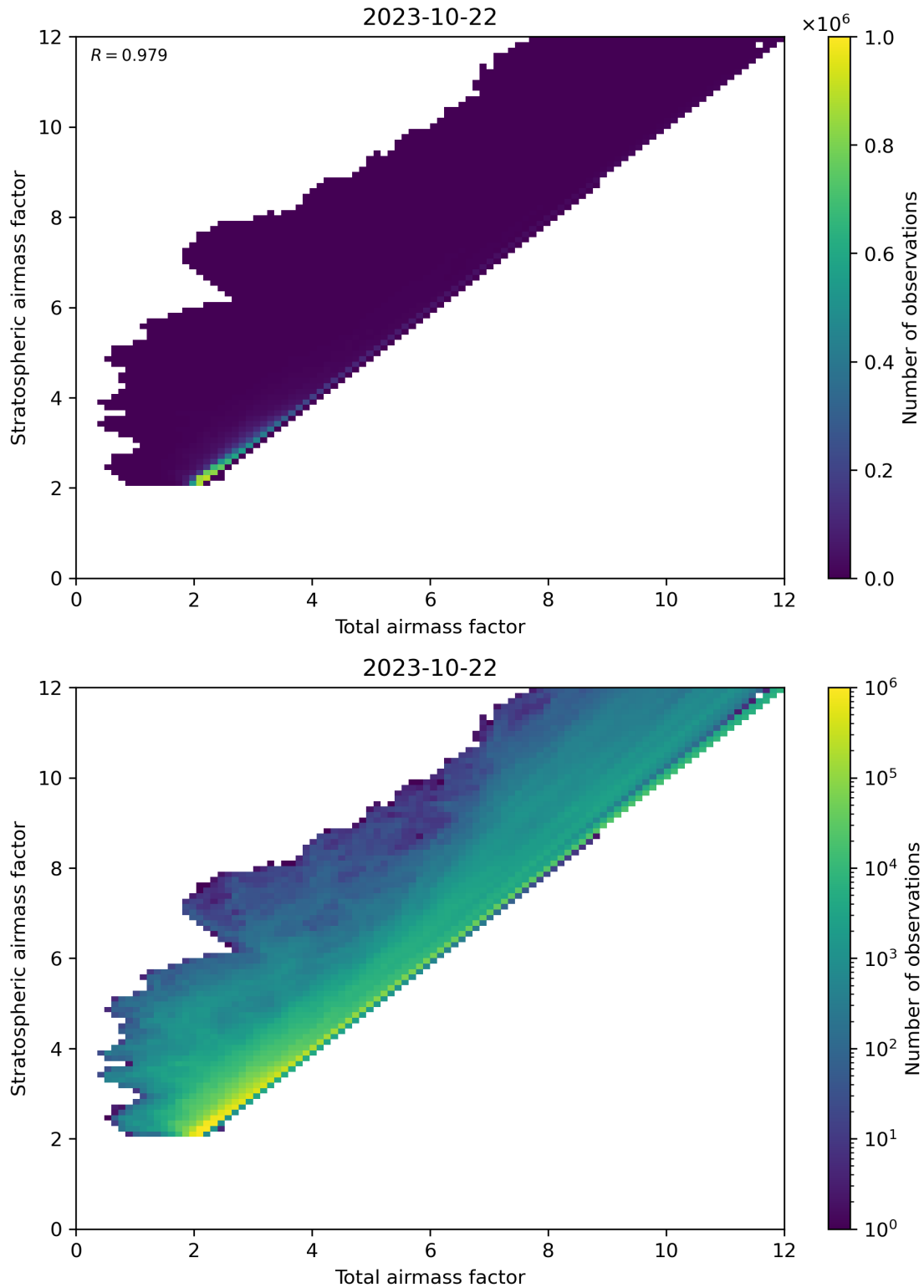
Figure 62: Scatter density plot of “Total airmass factor” against “Stratospheric airmass factor” for 2023-10-22 to 2023-10-23.
