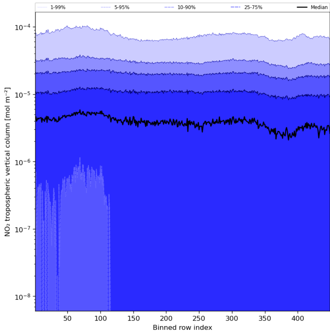
Figure 46: Along track statistics of “NO 2 tropospheric vertical column” for 2023-10-22 to 2023-10-23
