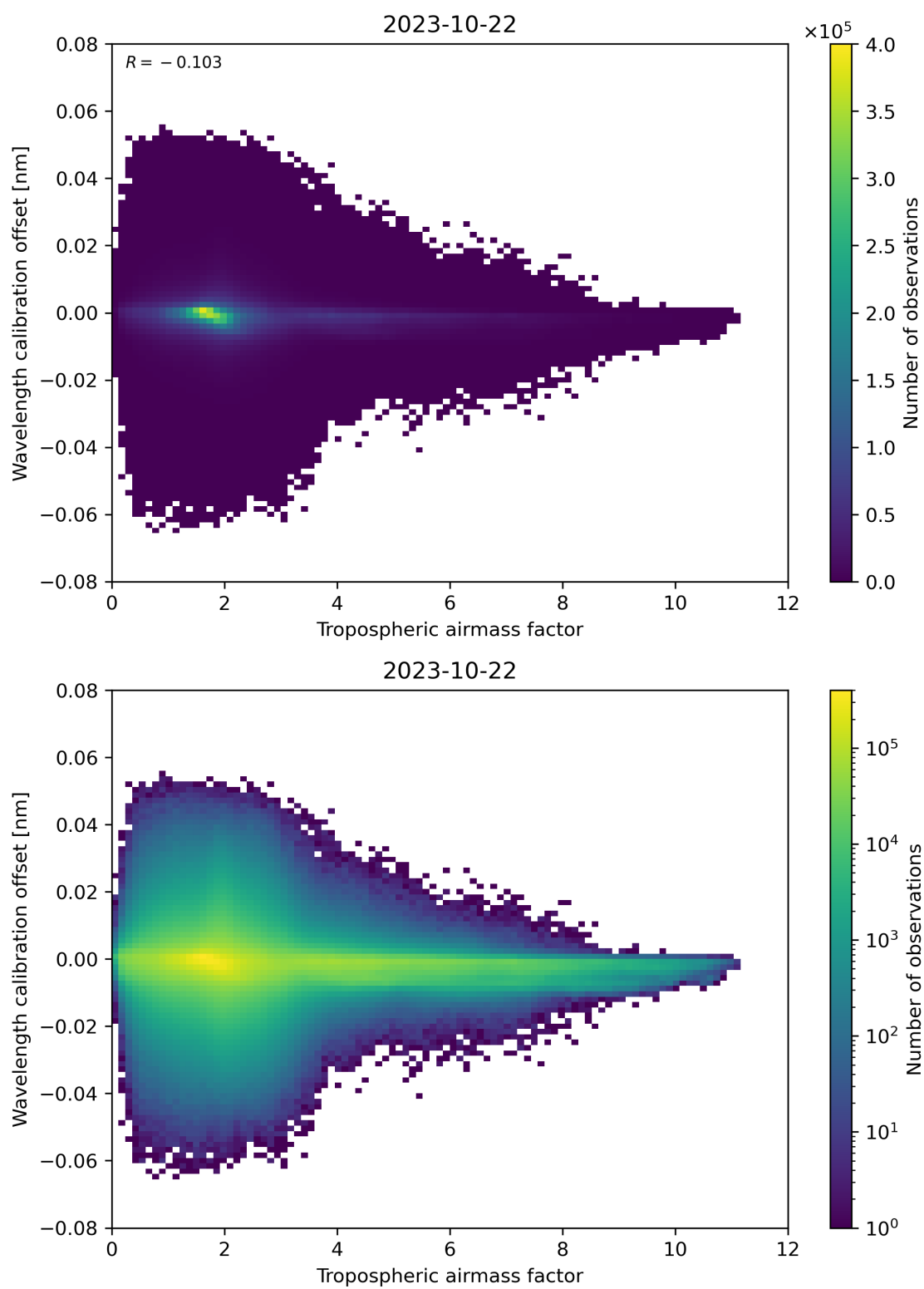
Figure 80: Scatter density plot of “Tropospheric airmass factor” against “Wavelength calibration offset” for 2023-10-22 to 2023-10-23.
