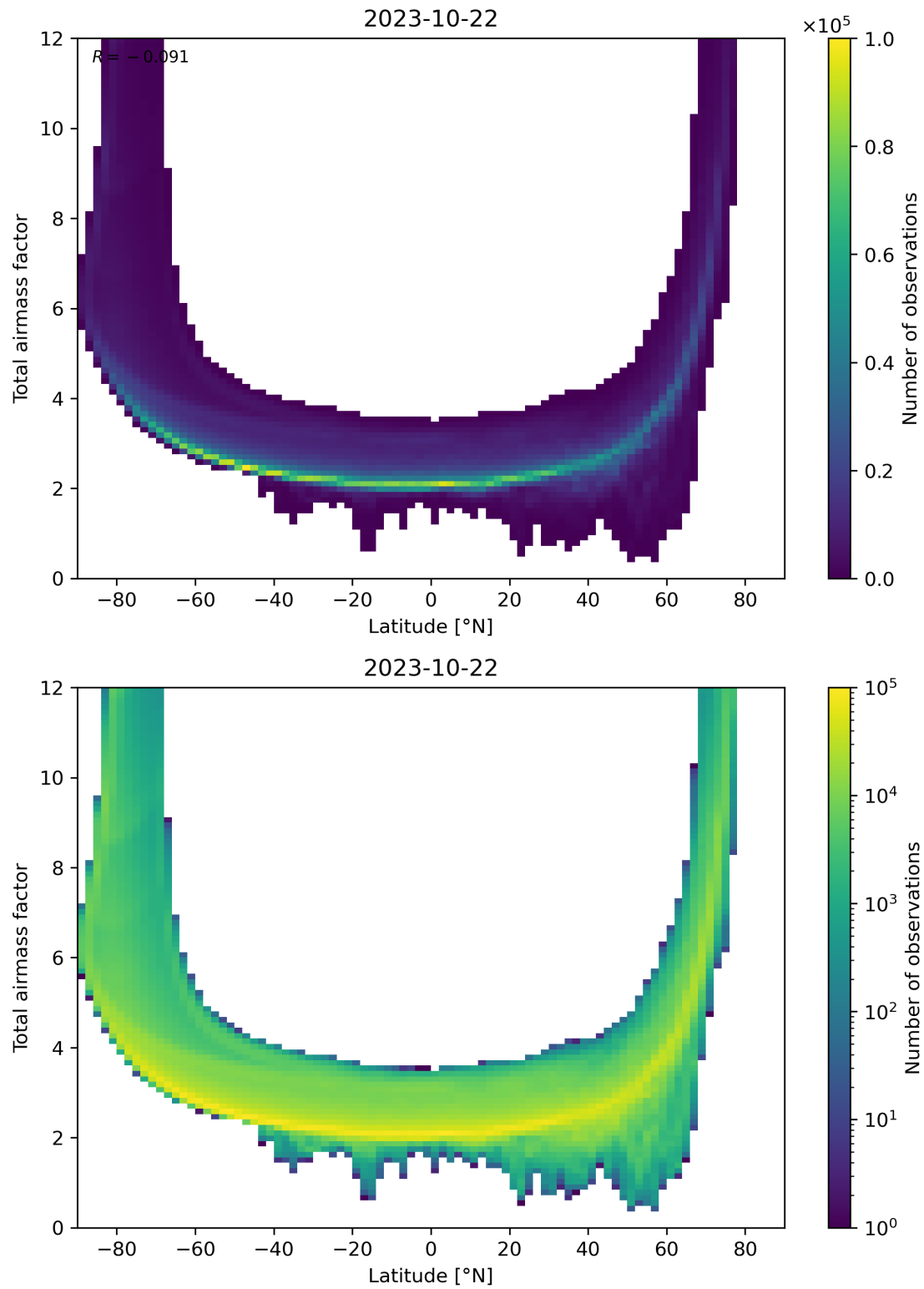
Figure 84: Scatter density plot of “Latitude” against “Total airmass factor” for 2023-10-22 to 2023-10-23.
