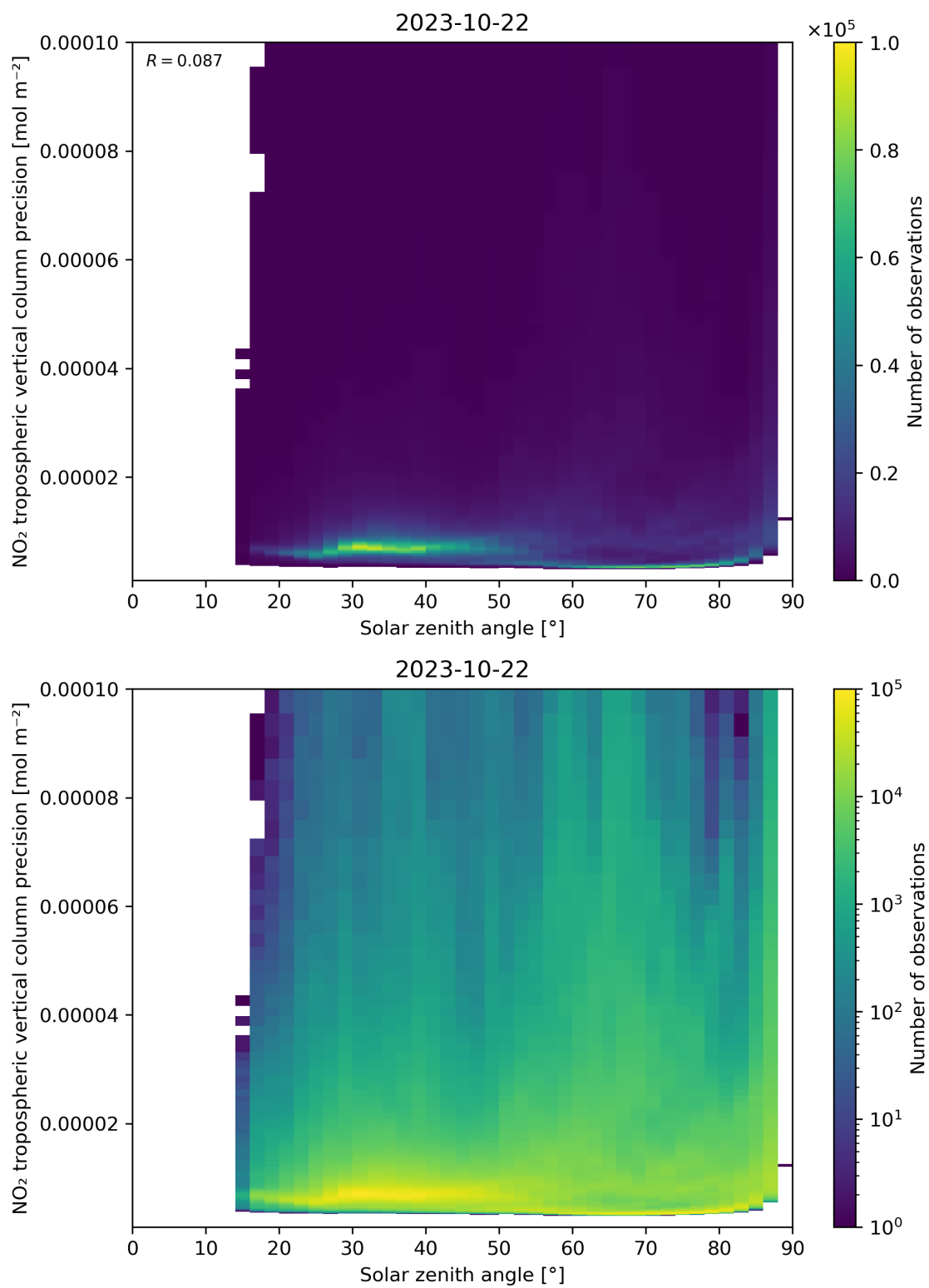
Figure 156: Scatter density plot of “Solar zenith angle” against “NO 2 tropospheric vertical column precision” for 2023-10-22 to 2023-10-23.
