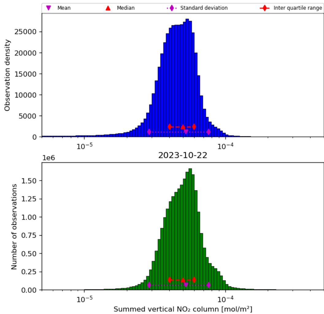
Figure 40: Histogram of “Summed vertical NO 2 column” for 2023-10-22 to 2023-10-23
