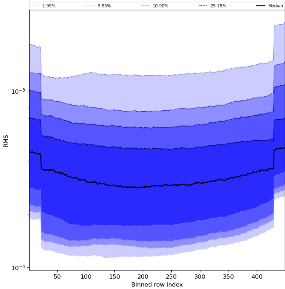
Figure 60: Along track statistics of “RMS” for 2023-10-22 to 2023-10-23
