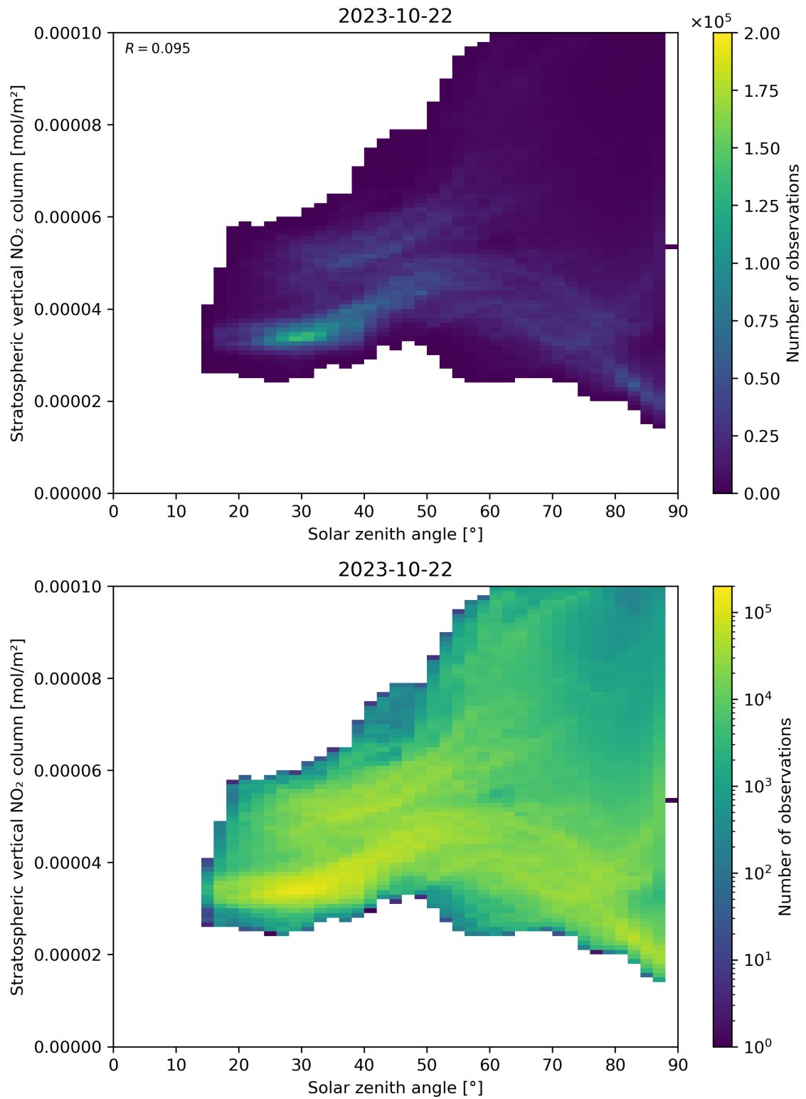
Figure 150: Scatter density plot of “Solar zenith angle” against “Stratospheric vertical NO 2 column” for 2023-10-22 to 2023-10-23.
