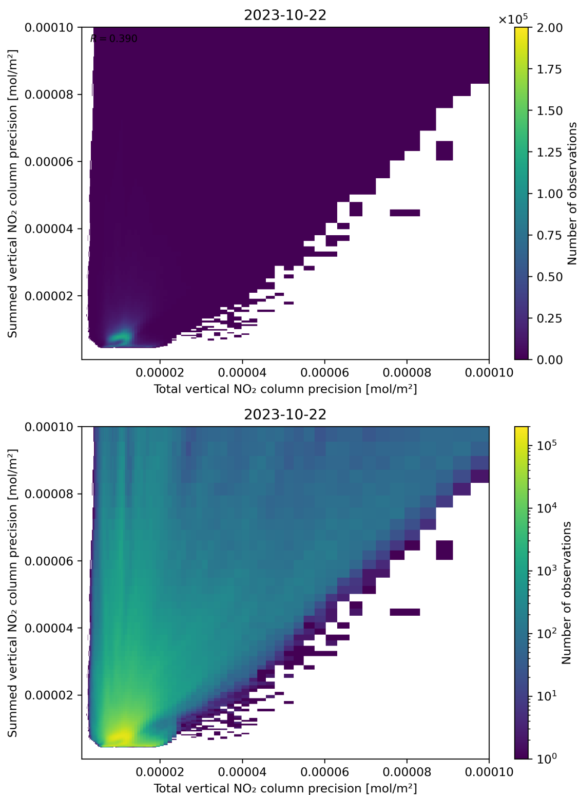
Figure 118: Scatter density plot of “Total vertical NO 2 column precision” against “Summed vertical NO 2 column precision” for 2023-10-22 to 2023-10-23.
