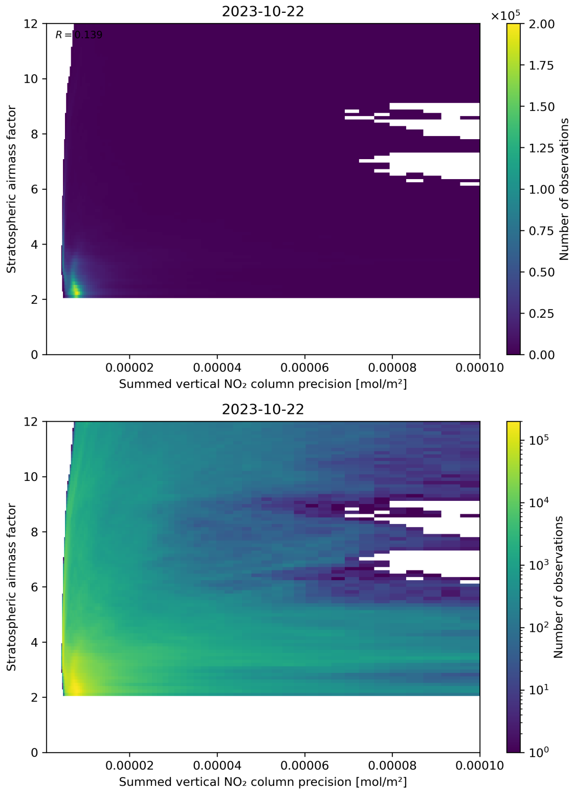
Figure 106: Scatter density plot of “Summed vertical NO 2 column precision” against “Stratospheric airmass factor” for 2023-10-22 to 2023-10-23.
