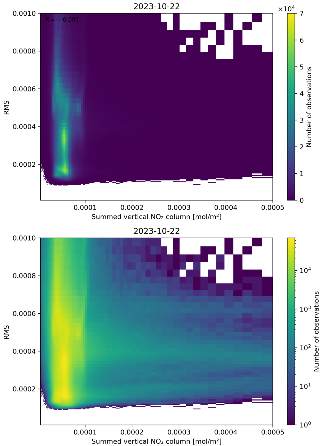
Figure 109: Scatter density plot of “Summed vertical NO 2 column” against “RMS” for 2023-10-22 to 2023-10-23.
