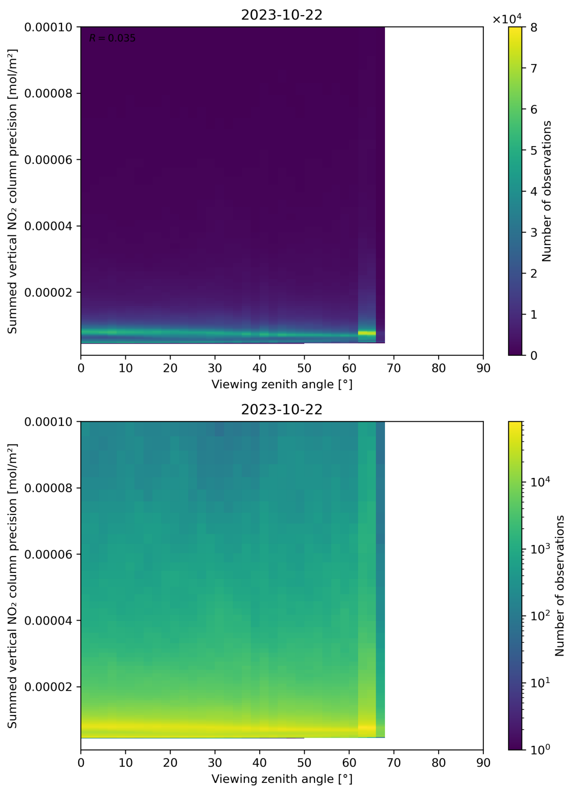
Figure 166: Scatter density plot of “Viewing zenith angle” against “Summed vertical NO 2 column precision” for 2023-10-22 to 2023-10-23.
