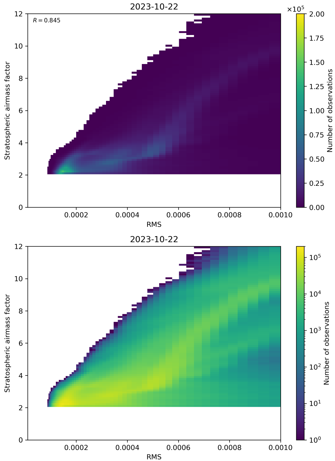
Figure 144: Scatter density plot of “RMS” against “Stratospheric airmass factor” for 2023-10-22 to 2023-10-23.
