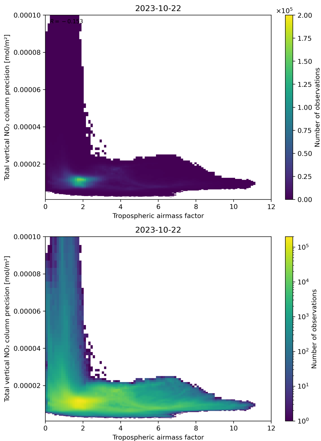
Figure 78: Scatter density plot of “Tropospheric air mass factor” against “Total vertical NO 2 column precision” for 2023-10-22 to 2023-10-23.
