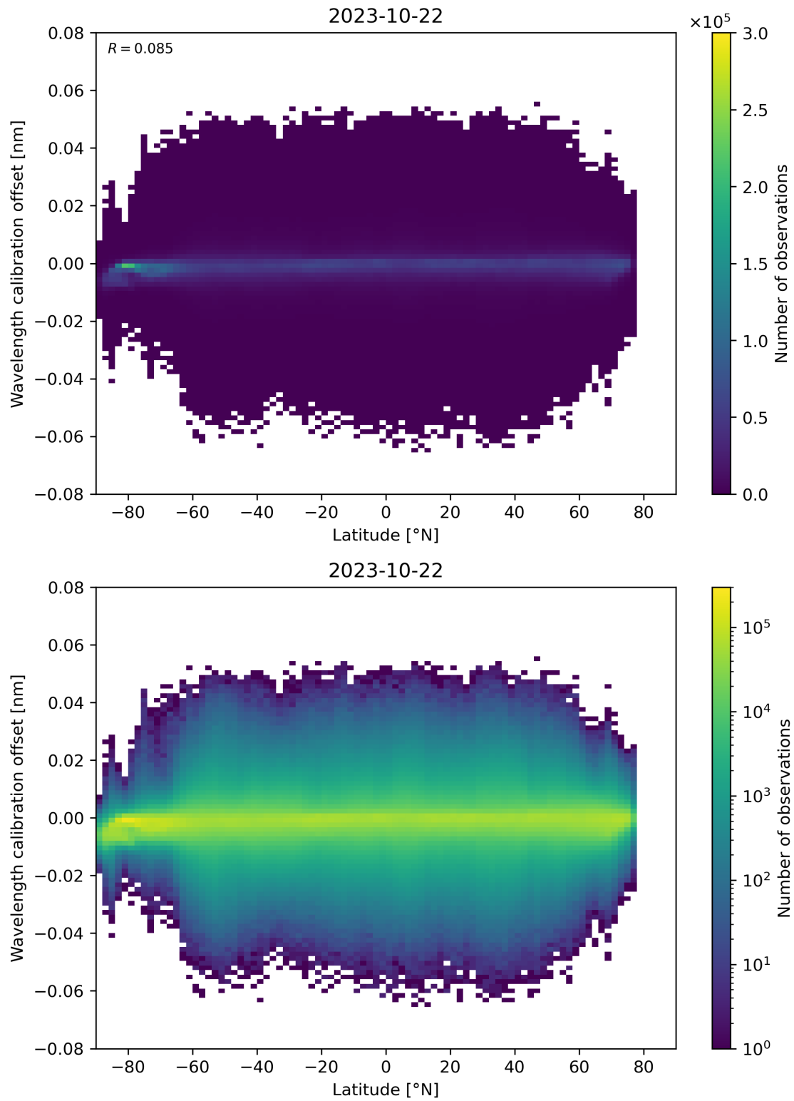
Figure 95: Scatter density plot of “Latitude” against “Wavelength calibration offset” for 2023-10-22 to 2023-10-23.
