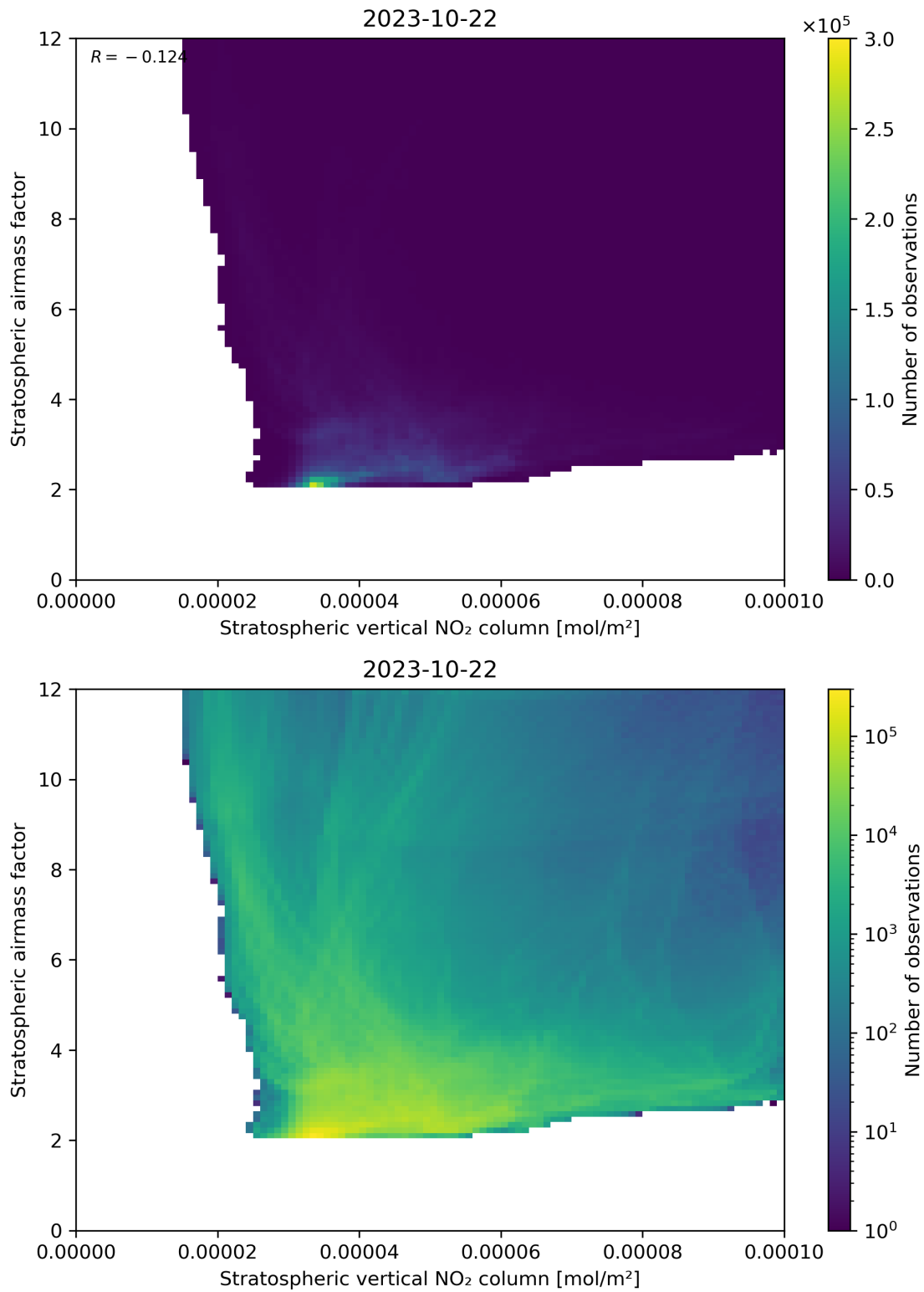
Figure 96: Scatter density plot of “Stratospheric vertical NO 2 column” against “Stratospheric airmass factor” for 2023-10-22 to 2023-10-23.
