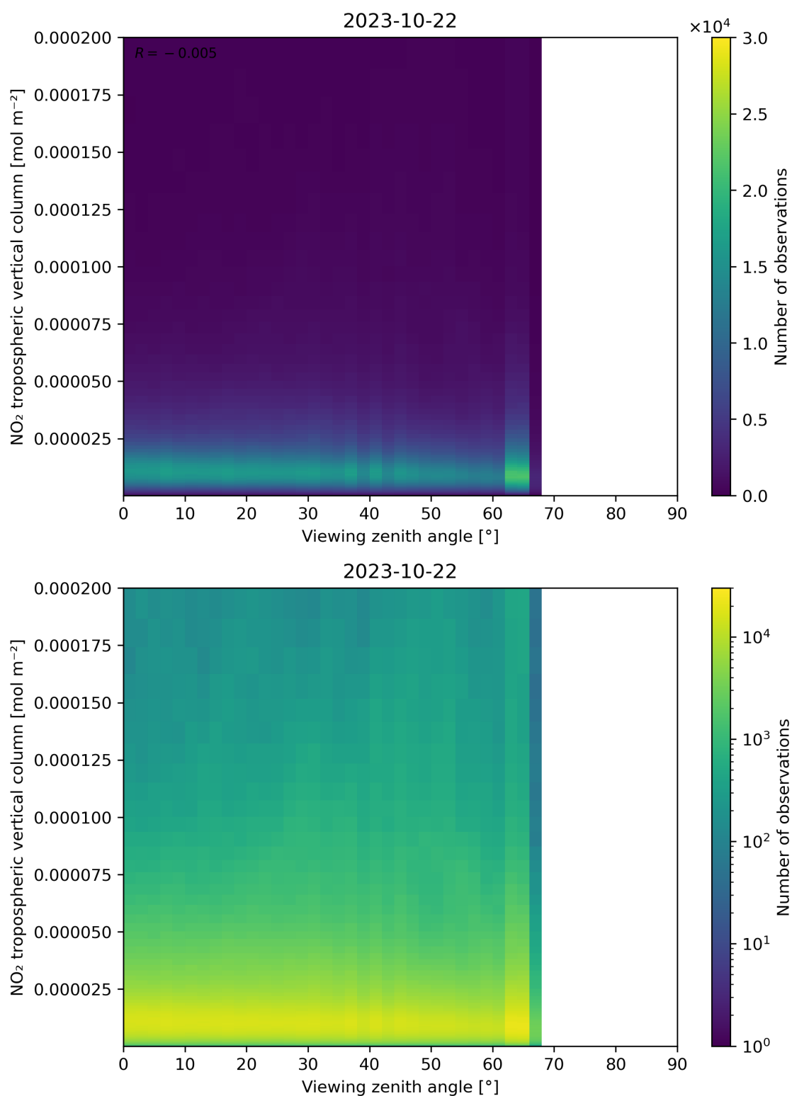
Figure 169: Scatter density plot of “Viewing zenith angle” against “NO 2 tropospheric vertical column” for 2023-10-22 to 2023-10-23.
