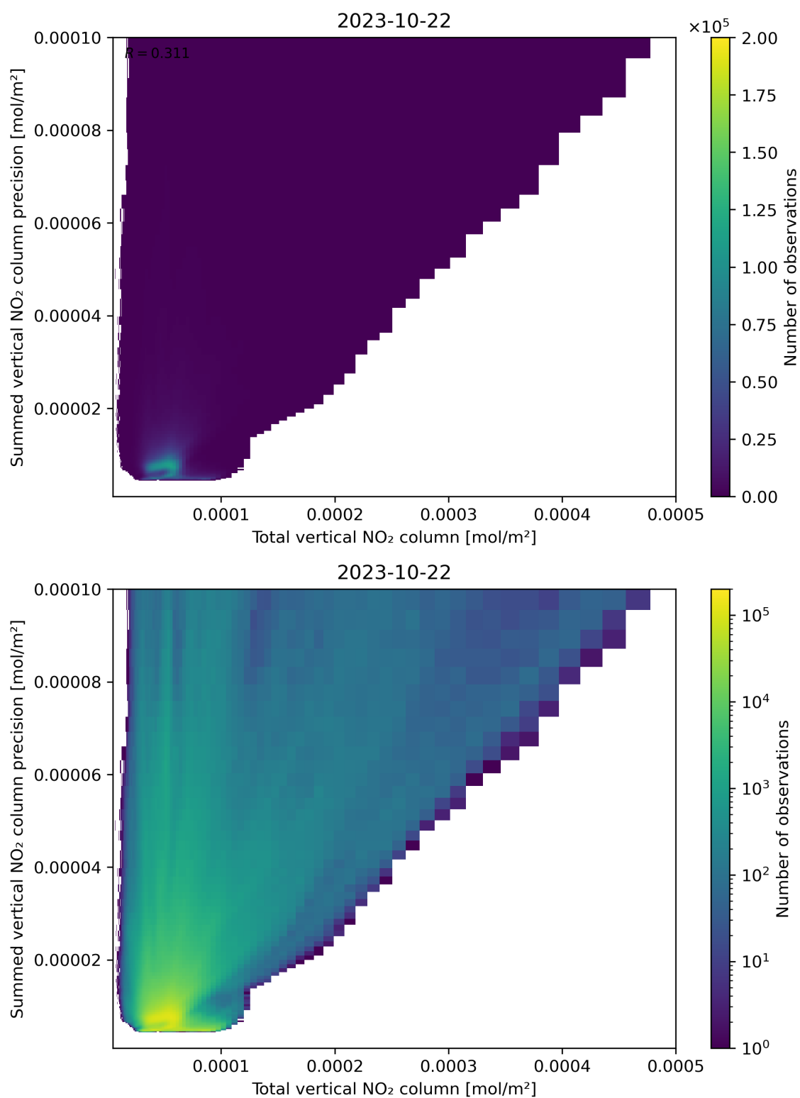
Figure 113: Scatter density plot of “Total vertical NO 2 column” against “Summed vertical NO 2 column precision” for 2023-10-22 to 2023-10-23.
