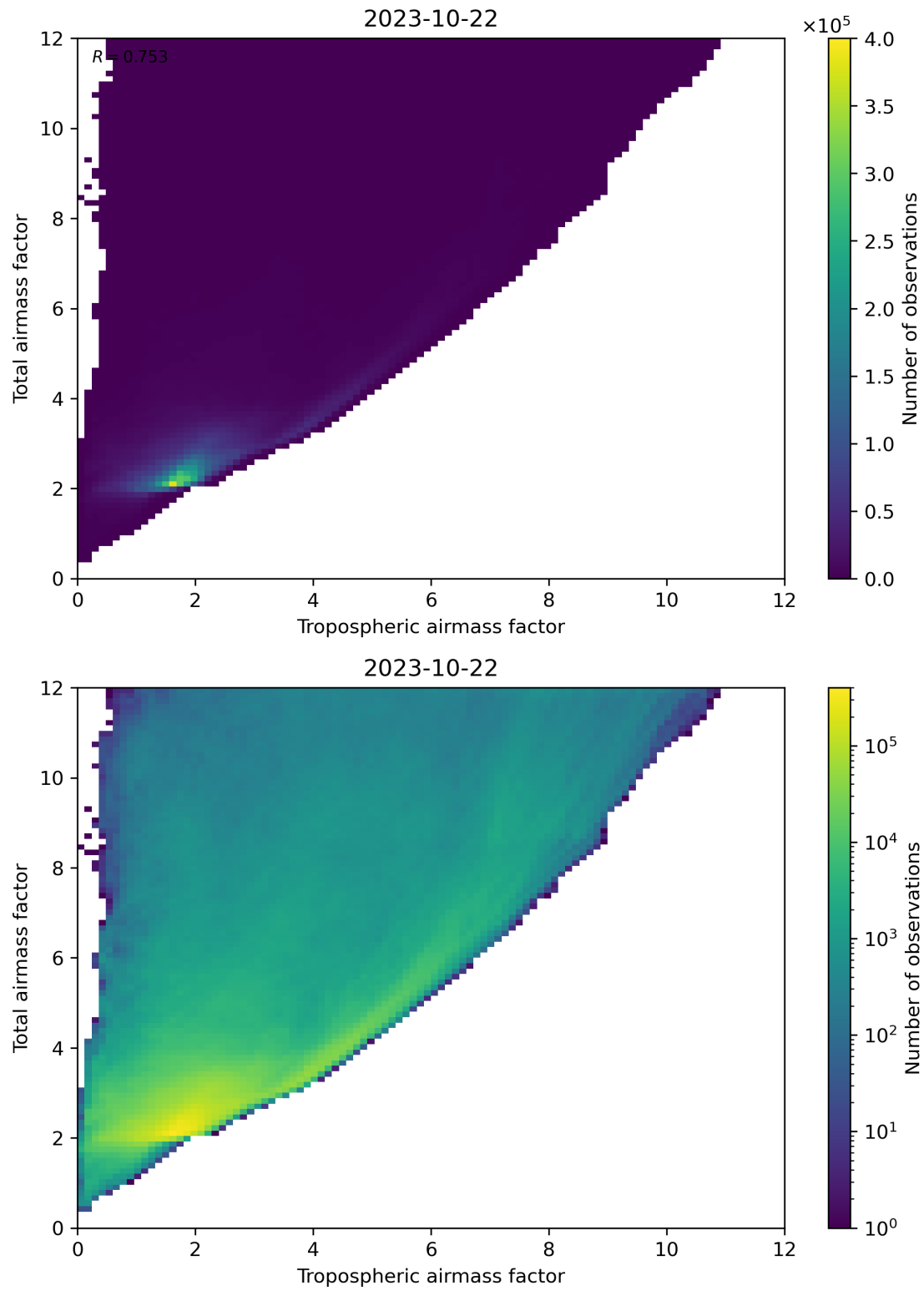
Figure 72: Scatter density plot of “Tropospheric airmass factor” against “Total airmass factor” for 2023-10-22 to 2023-10-23.
