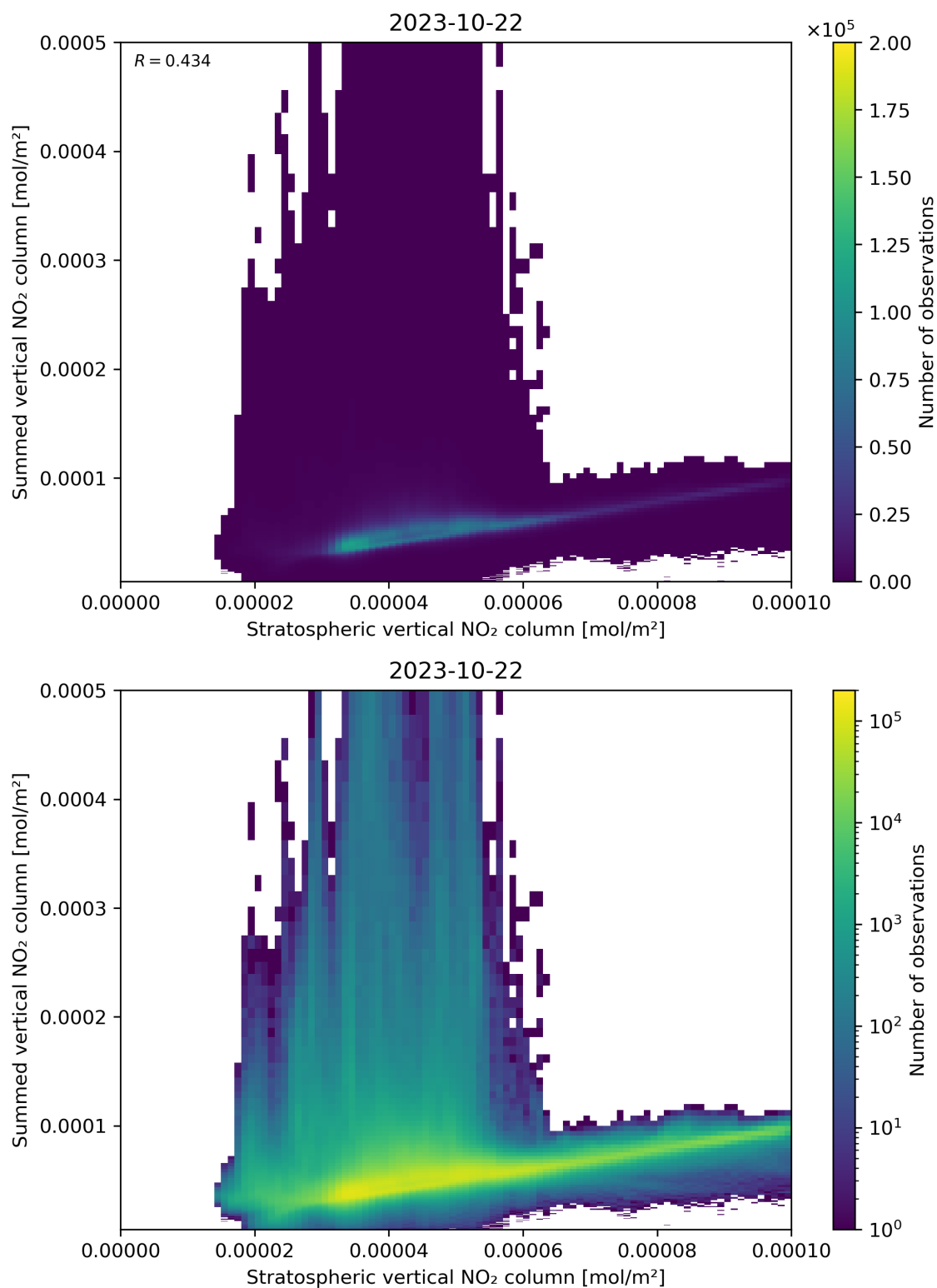
Figure 98: Scatter density plot of “Stratospheric vertical NO 2 column” against “Summed vertical NO 2 column” for 2023-10-22 to 2023-10-23.
