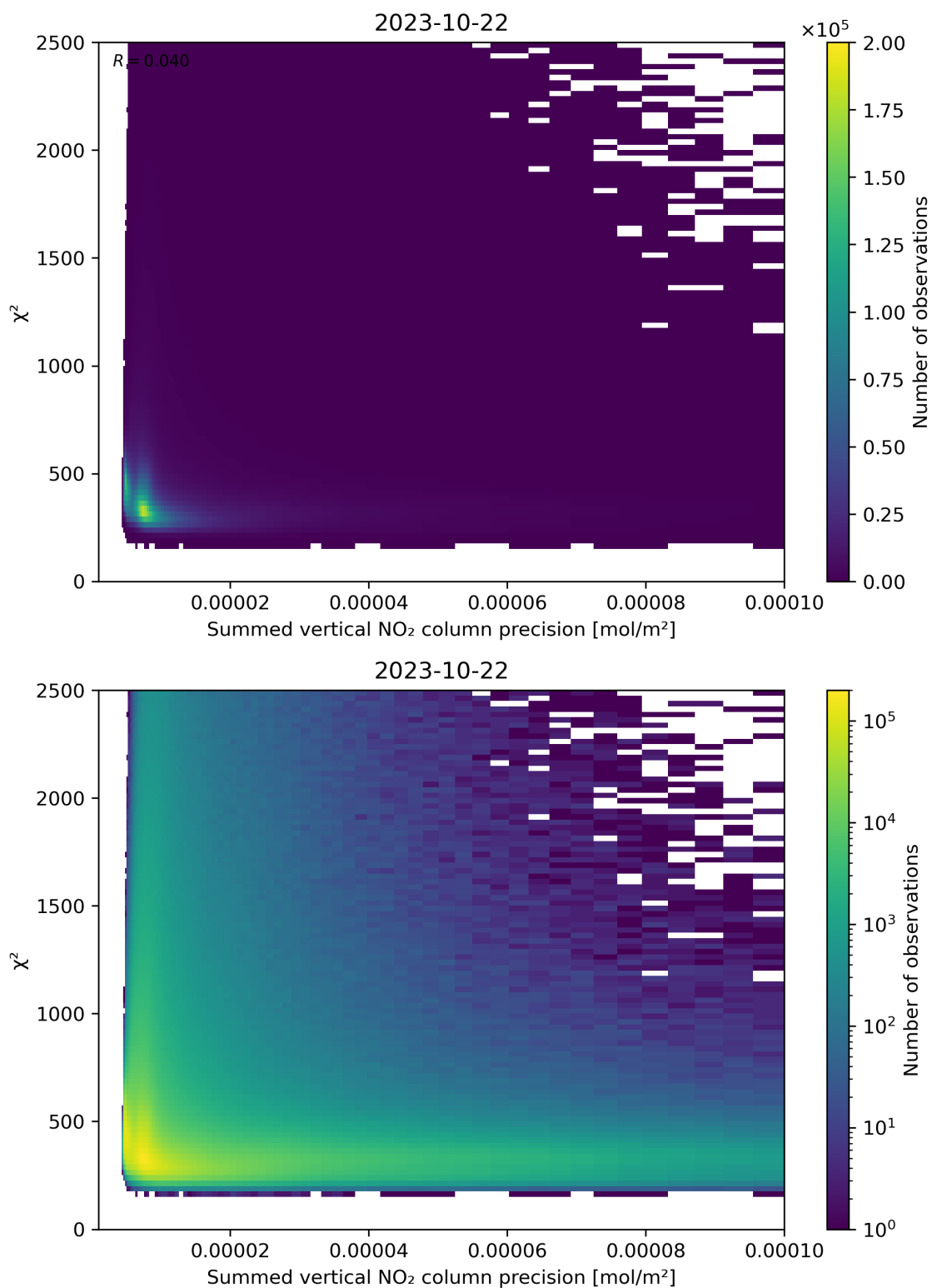
Figure 107: Scatter density plot of “Summed vertical NO 2 column precision” against “ \chi^2 ” for 2023-10-22 to 2023-10-23.
