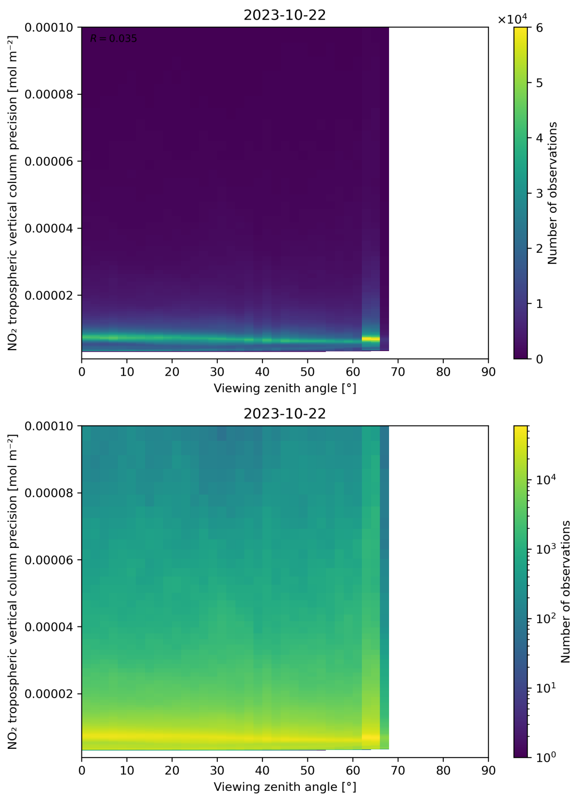
Figure 170: Scatter density plot of “Viewing zenith angle” against “NO 2 tropospheric vertical column precision” for 2023-10-22 to 2023-10-23.
