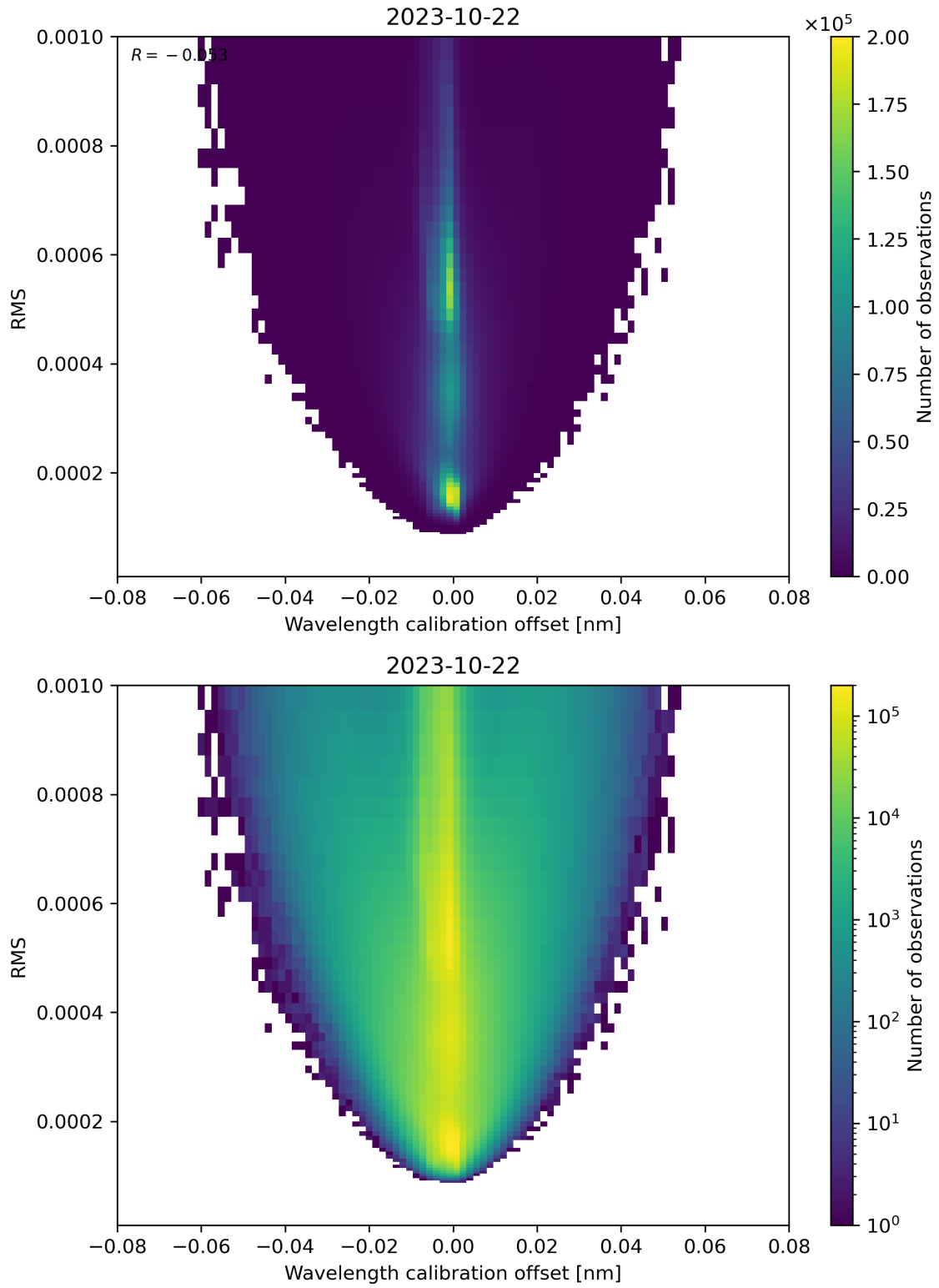
Figure 181: Scatter density plot of “Wavelength calibration offset” against “RMS” for 2023-10-22 to 2023-10-23.
