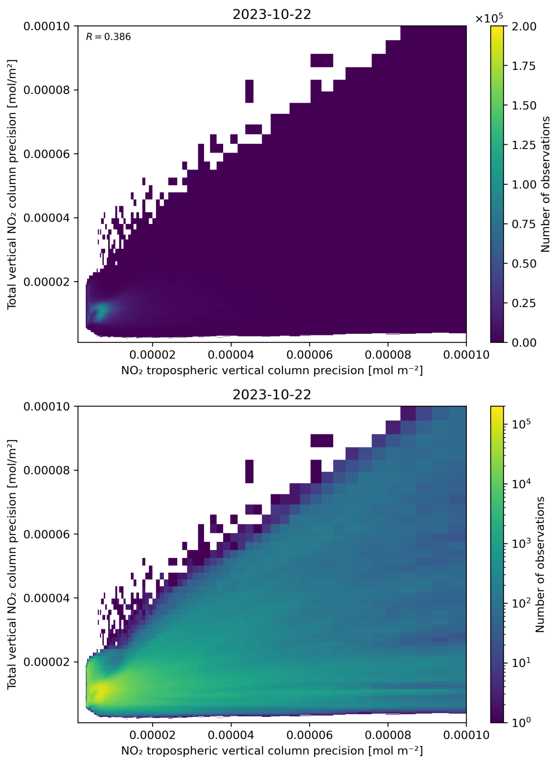
Figure 139: Scatter density plot of “NO 2 tropospheric vertical column precision” against “Total vertical NO 2 column precision” for 2023-10-22 to 2023-10-23.
