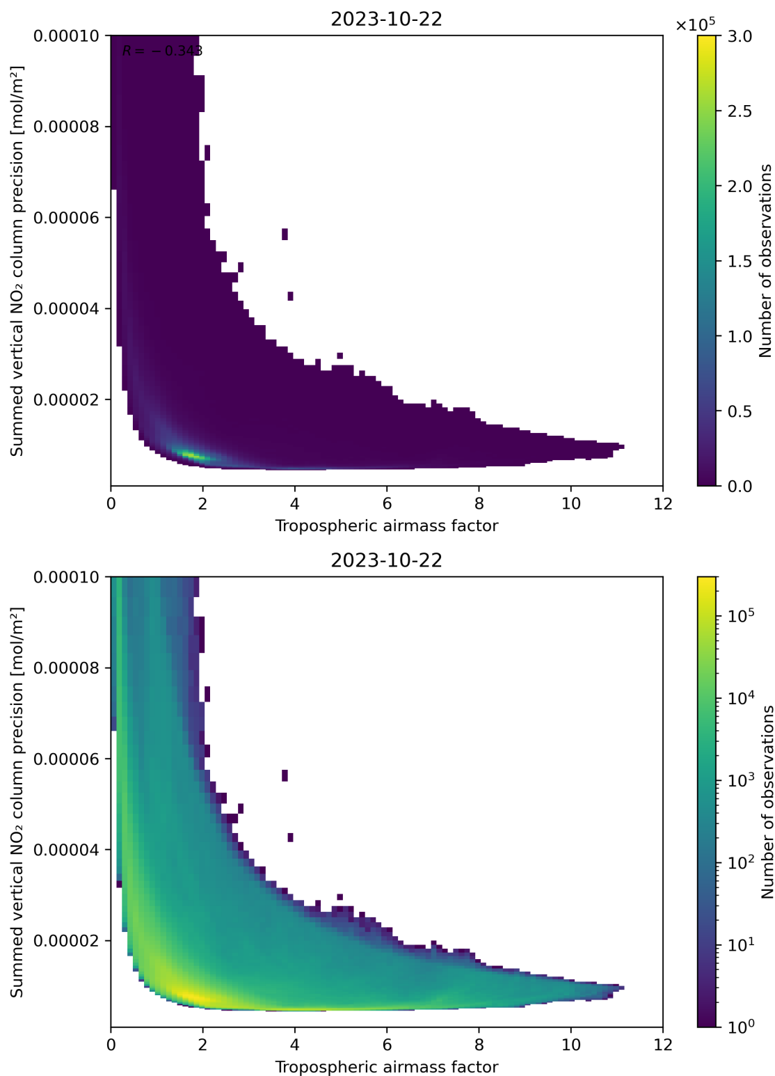
Figure 76: Scatter density plot of “Tropospheric air mass factor” against “Summed vertical NO 2 column precision” for 2023-10-22 to 2023-10-23.
