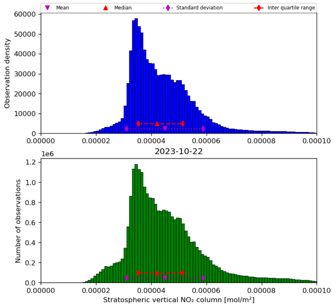
Figure 36: Histogram of “Stratospheric vertical NO 2 column” for 2023-10-22 to 2023-10-23
