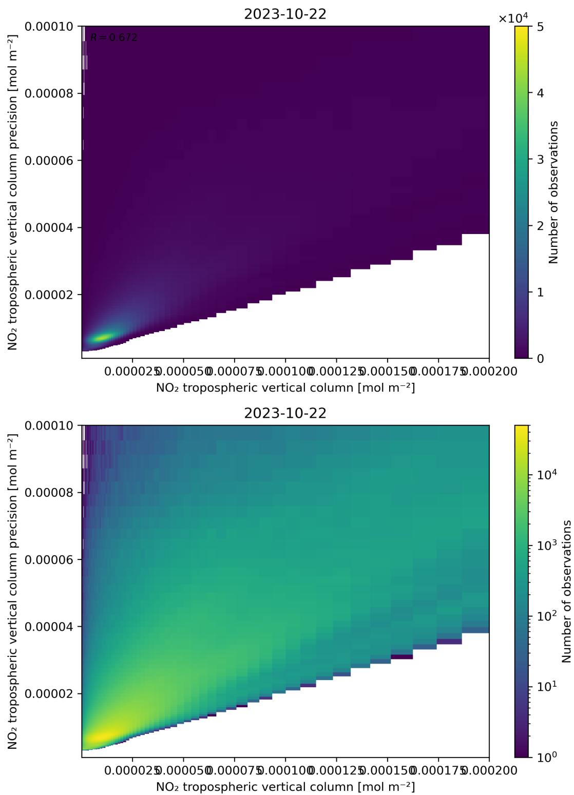
Figure 130: Scatter density plot of “NO 2 tropospheric vertical column” against “NO 2 tropospheric vertical column precision” for 2023-10-22 to 2023-10-23.
