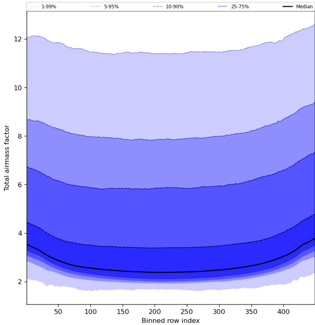
Figure 49: Along track statistics of “Total airmass factor” for 2023-10-22 to 2023-10-23
