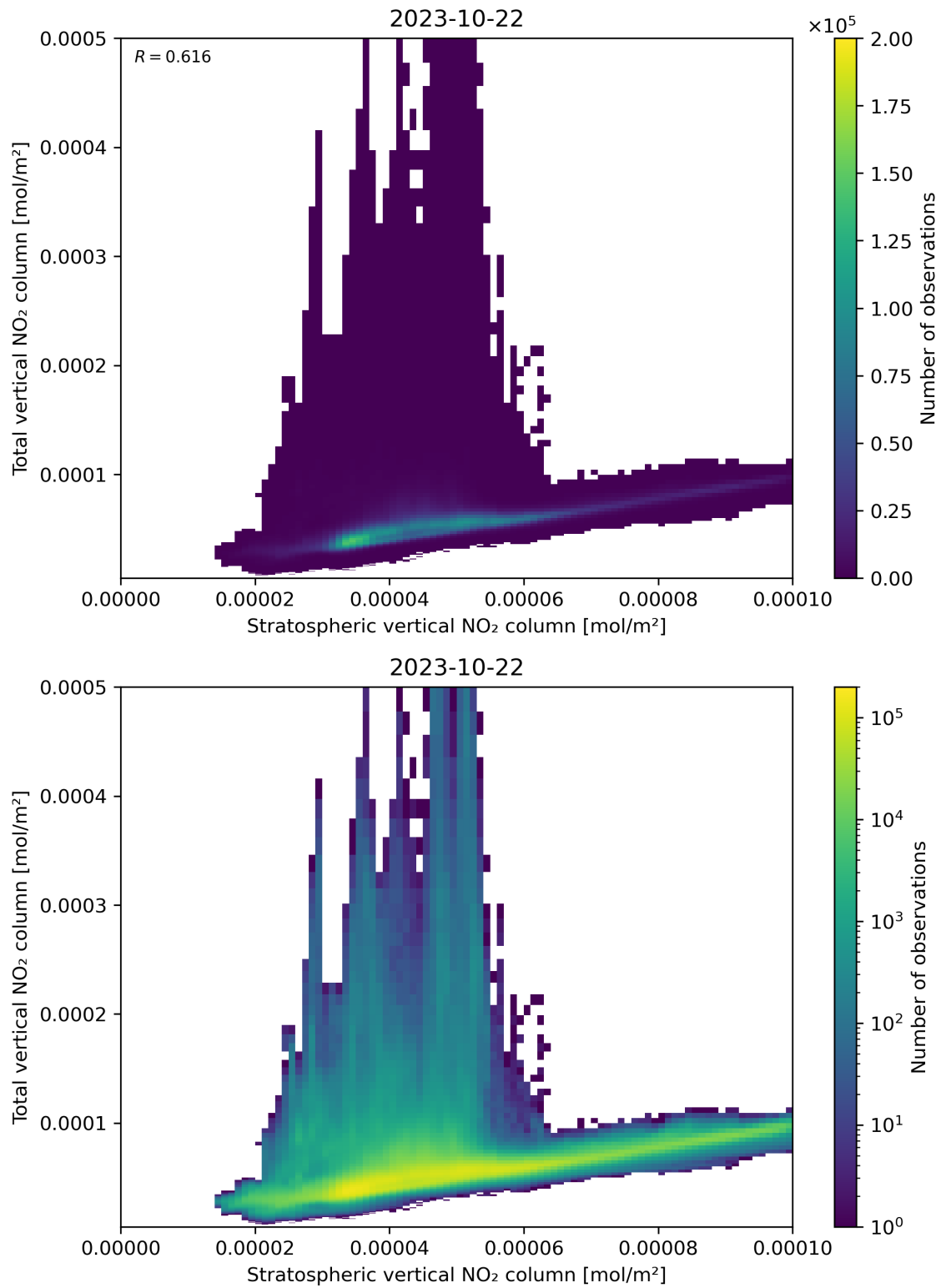
Figure 100: Scatter density plot of “Stratospheric vertical NO 2 column” against “Total vertical NO 2 column” for 2023-10-22 to 2023-10-23.
