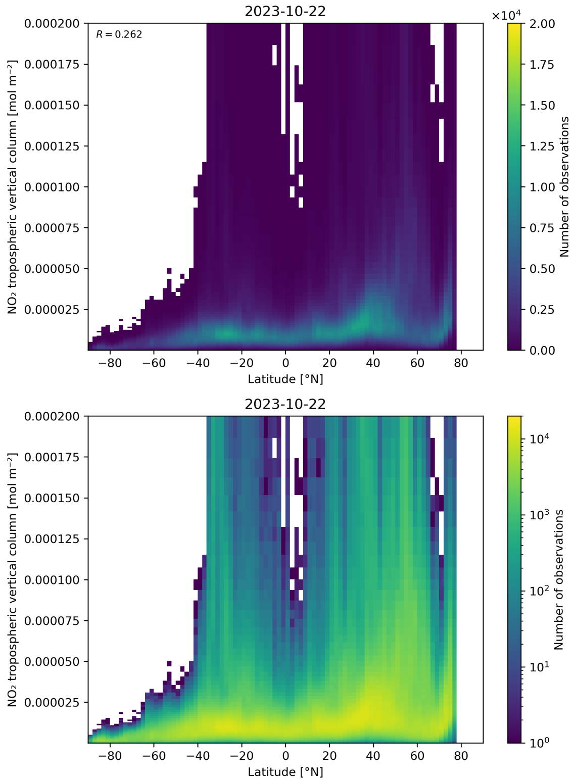
Figure 92: Scatter density plot of “Latitude” against “NO 2 tropospheric vertical column” for 2023-10-22 to 2023-10-23.
