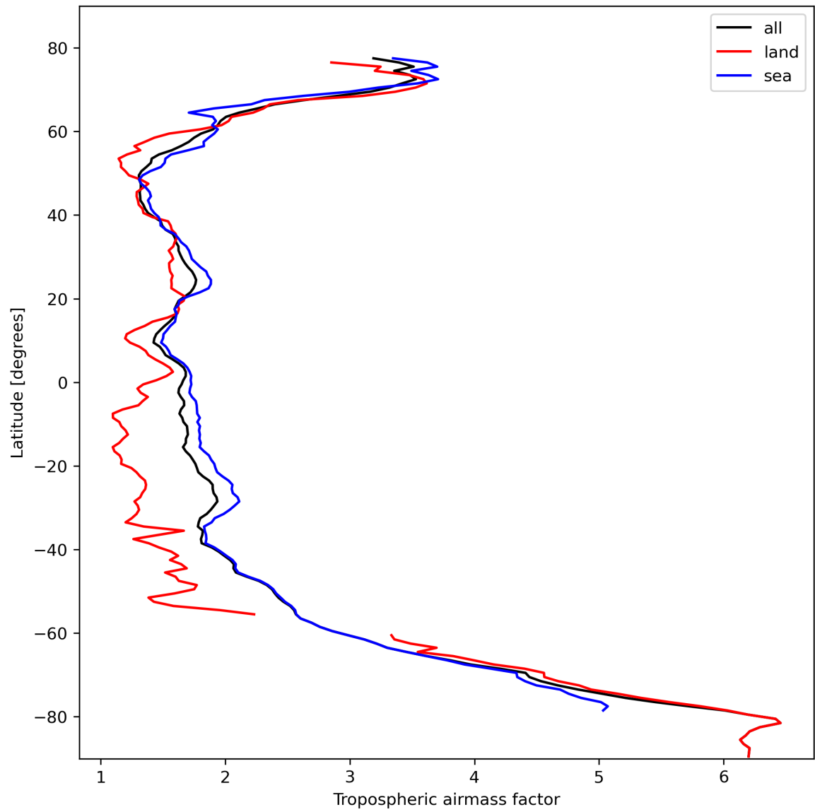
Figure 14: Zonal average of “Tropospheric airmass factor” for 2023-10-22 to 2023-10-23.
