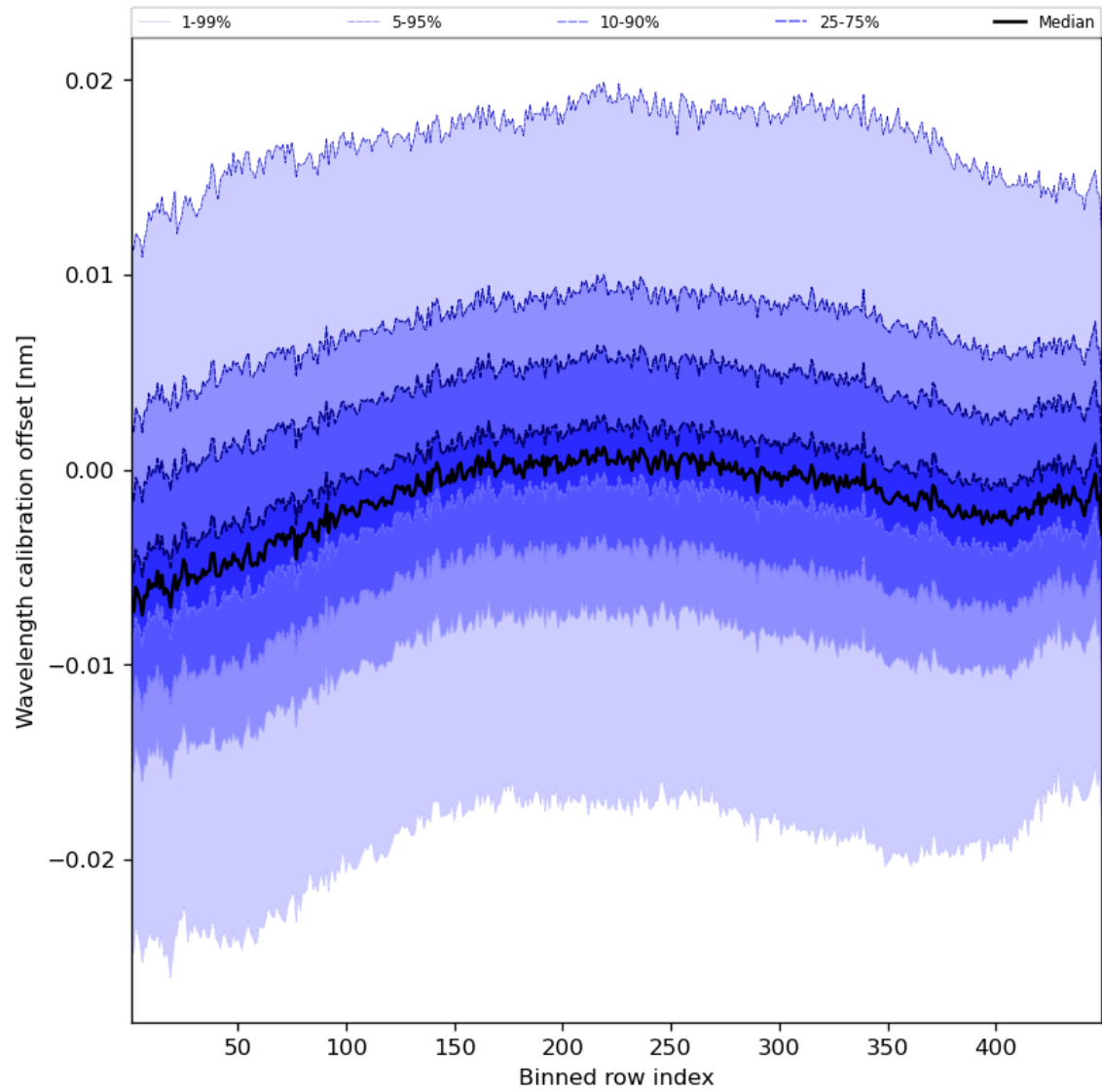
Figure 52: Along track statistics of “Wavelength calibration offset” for 2023-10-22 to 2023-10-23
