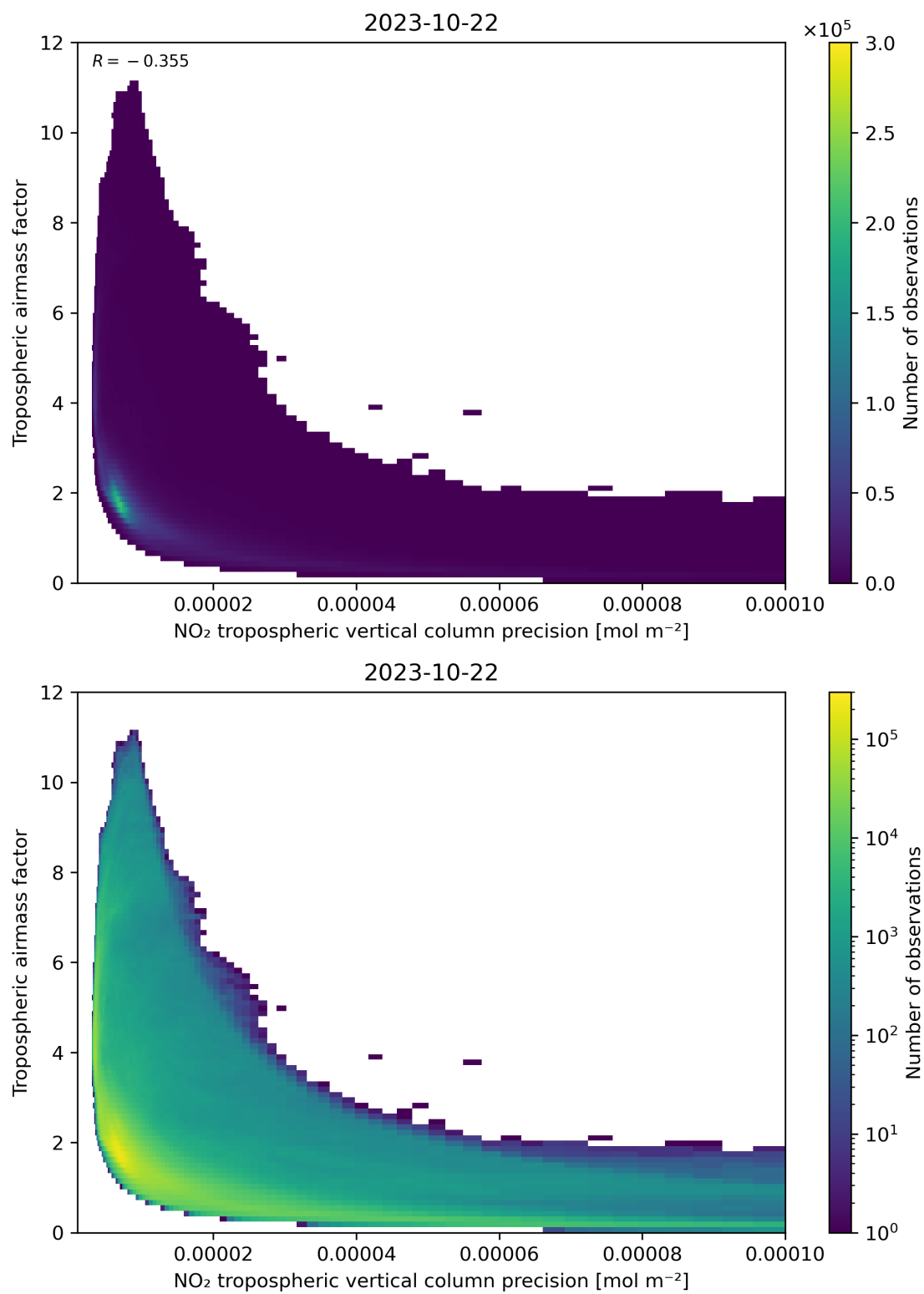
Figure 133: Scatter density plot of “NO 2 tropospheric vertical column precision” against “Tropospheric airmass factor” for 2023-10-22 to 2023-10-23.
