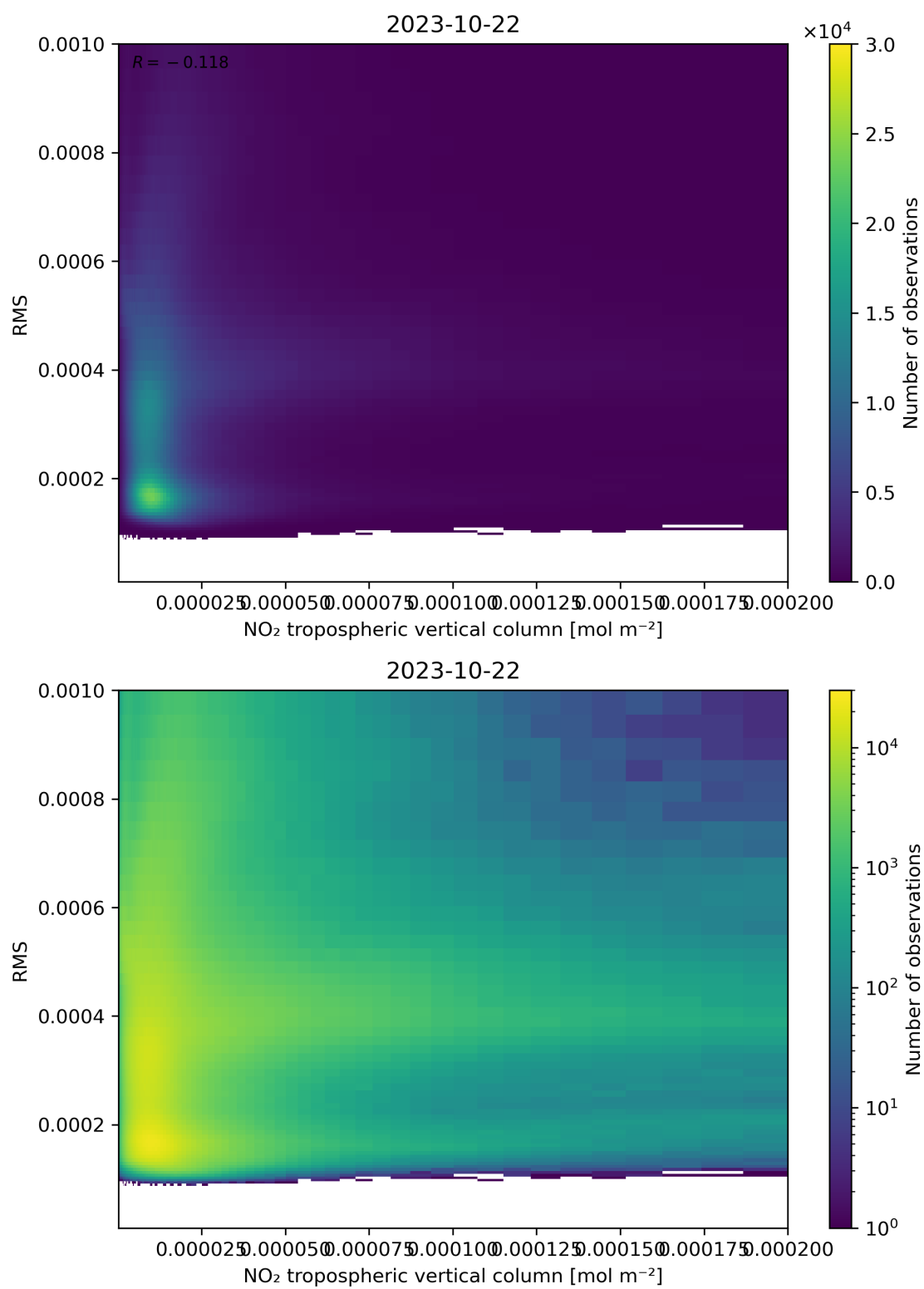
Figure 142: Scatter density plot of “NO 2 tropospheric vertical column” against “RMS” for 2023-10-22 to 2023-10-23.
