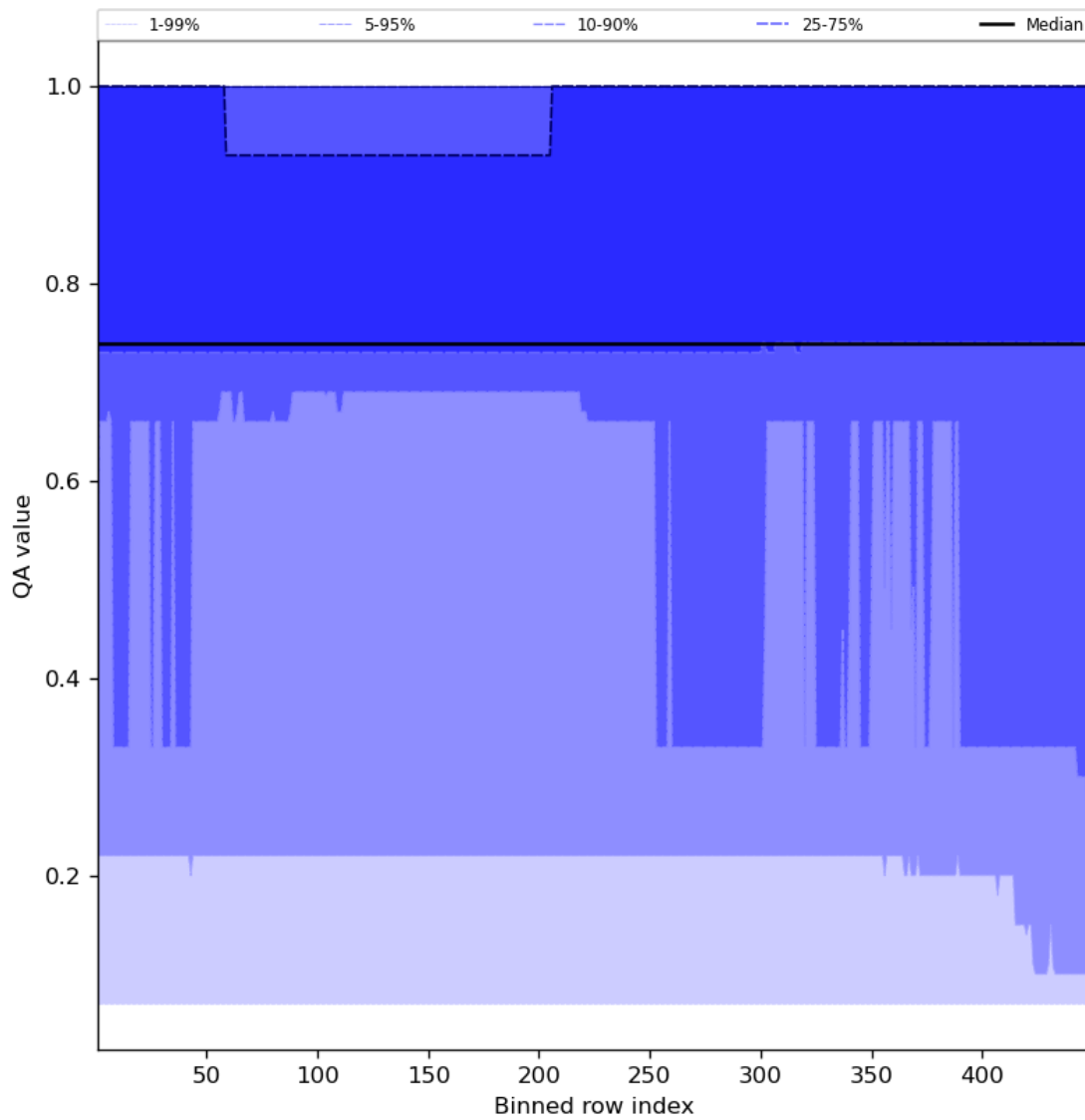
Figure 45: Along track statistics of “QA value” for 2023-10-22 to 2023-10-23
