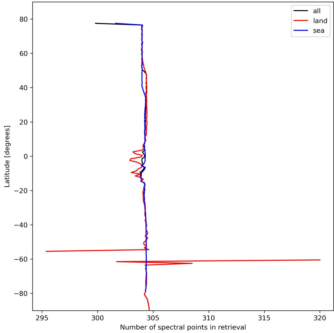
Figure 16: Zonal average of “Number of spectral points in retrieval” for 2023-10-22 to 2023-10-23.
