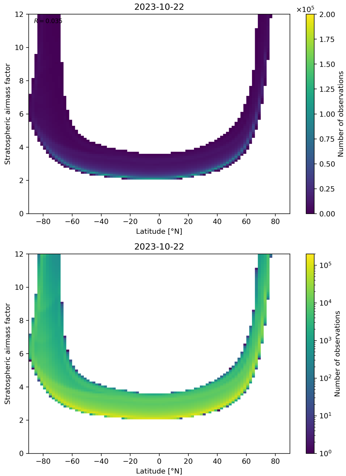
Figure 83: Scatter density plot of “Latitude” against “Stratospheric air mass factor” for 2023-10-22 to 2023-10-23.
