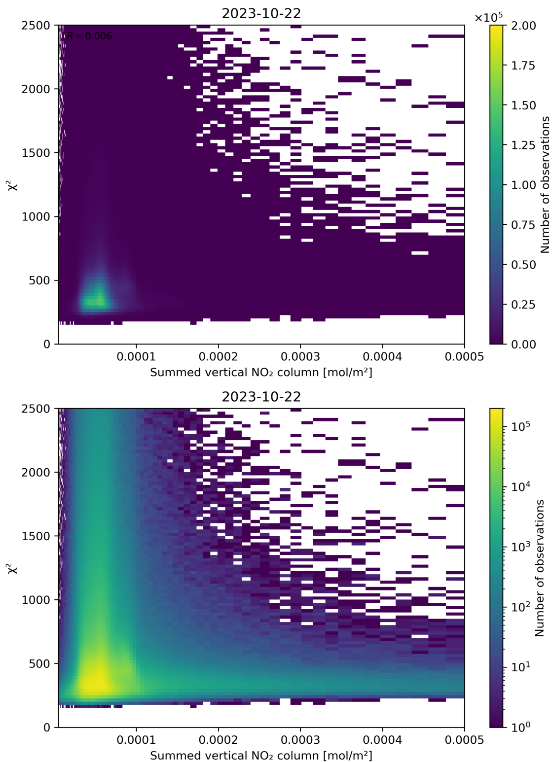
Figure 104: Scatter density plot of “Summed vertical NO 2 column” against “ \chi^2 ” for 2023-10-22 to 2023-10-23.
