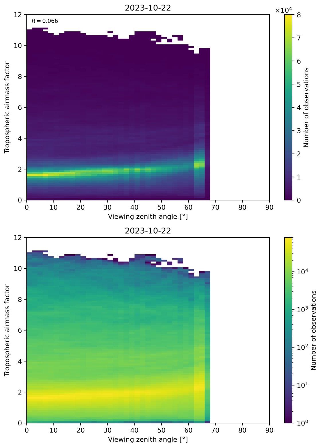
Figure 161: Scatter density plot of “Viewing zenith angle” against “Tropospheric airmass factor” for 2023-10-22 to 2023-10-23.
