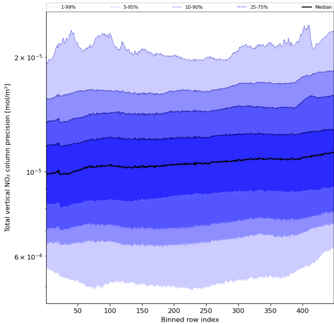
Figure 56: Along track statistics of “Total vertical NO 2 column precision” for 2023-10-22 to 2023-10-23
