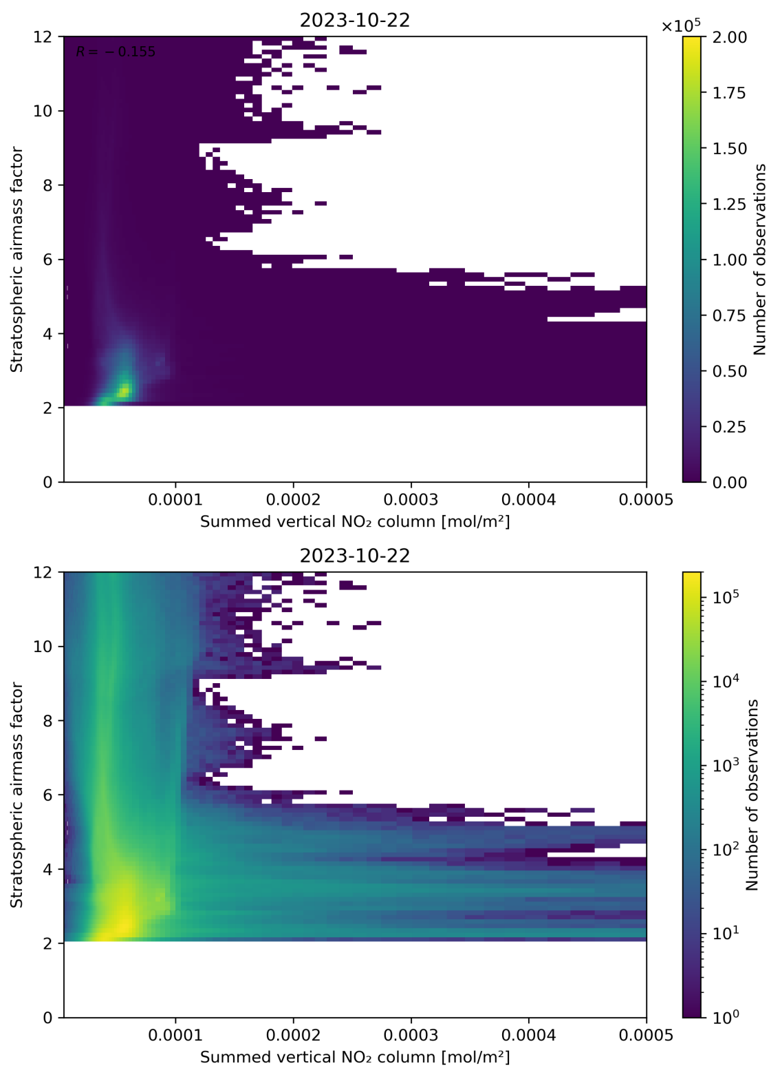
Figure 103: Scatter density plot of “Summed vertical NO 2 column” against “Stratospheric air mass factor” for 2023-10-22 to 2023-10-23.
