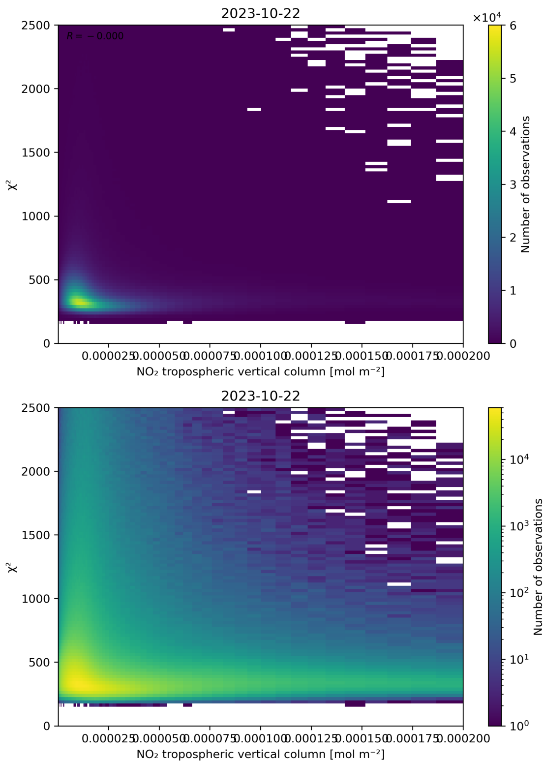
Figure 124: Scatter density plot of “NO 2 tropospheric vertical column” against “ \chi^2 ” for 2023-10-22 to 2023-10-23.
