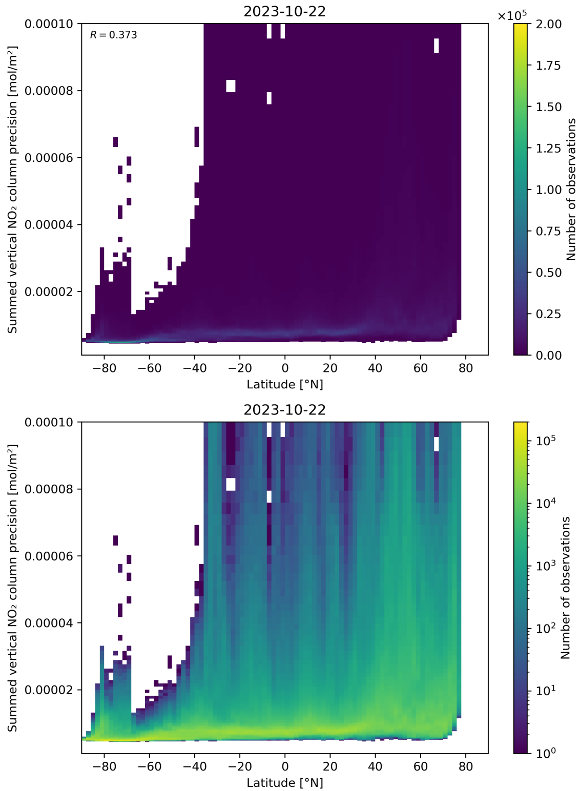
Figure 89: Scatter density plot of “Latitude” against “Summed vertical NO 2 column precision” for 2023-10-22 to 2023-10-23.
