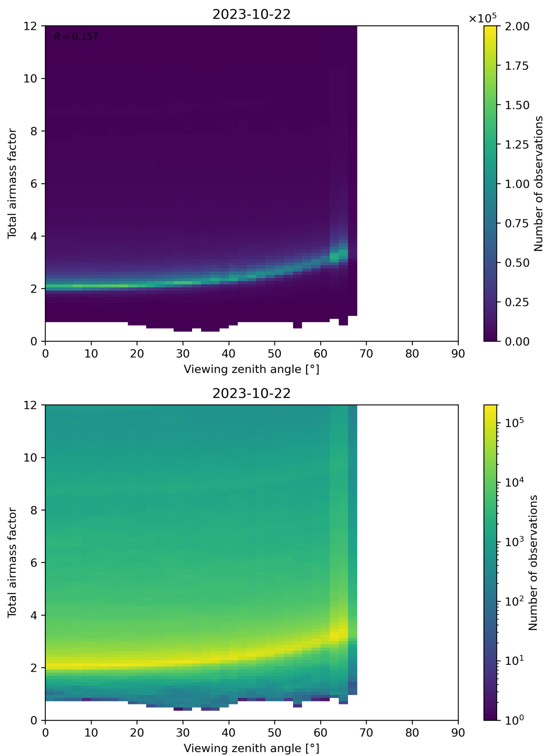
Figure 160: Scatter density plot of “Viewing zenith angle” against “Total airmass factor” for 2023-10-22 to 2023-10-23.
