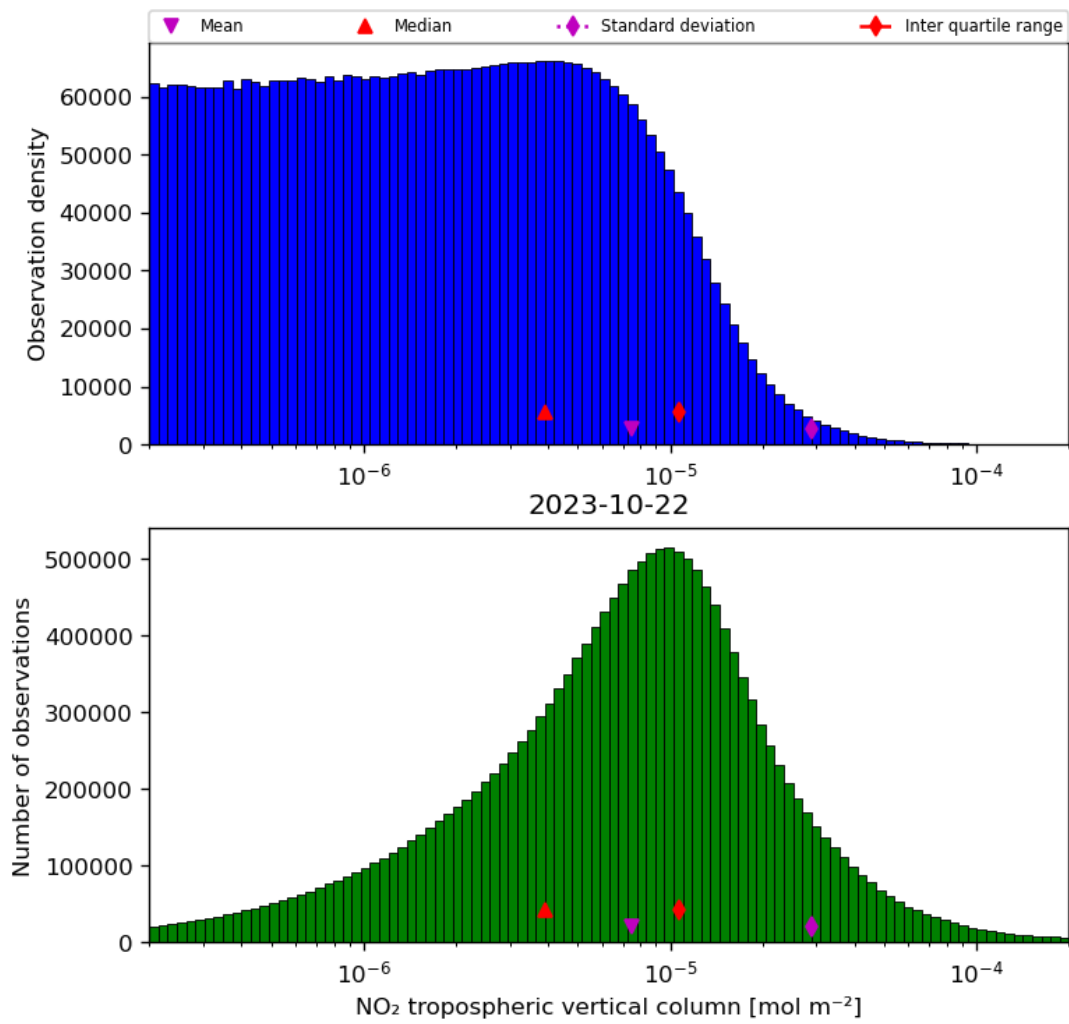
Figure 29: Histogram of “NO 2 tropospheric vertical column” for 2023-10-22 to 2023-10-23
