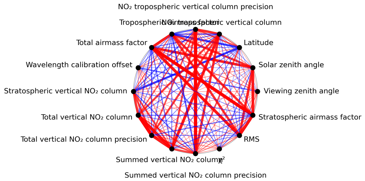
Figure 1: Map of correlation graph for 2023-10-22 to 2023-10-23.
