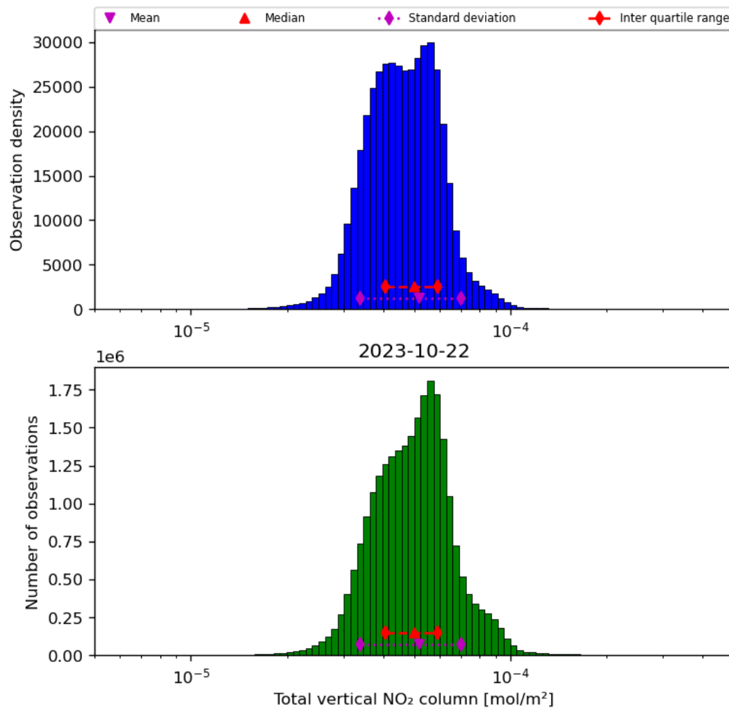
Figure 38: Histogram of “Total vertical NO 2 column” for 2023-10-22 to 2023-10-23
