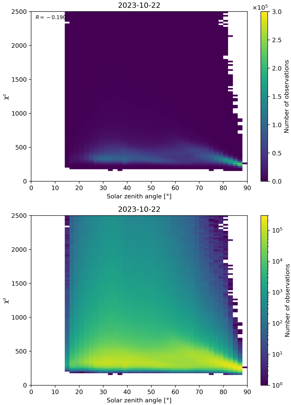
Figure 148: Scatter density plot of “Solar zenith angle” against “ \chi^2 ” for 2023-10-22 to 2023-10-23.
