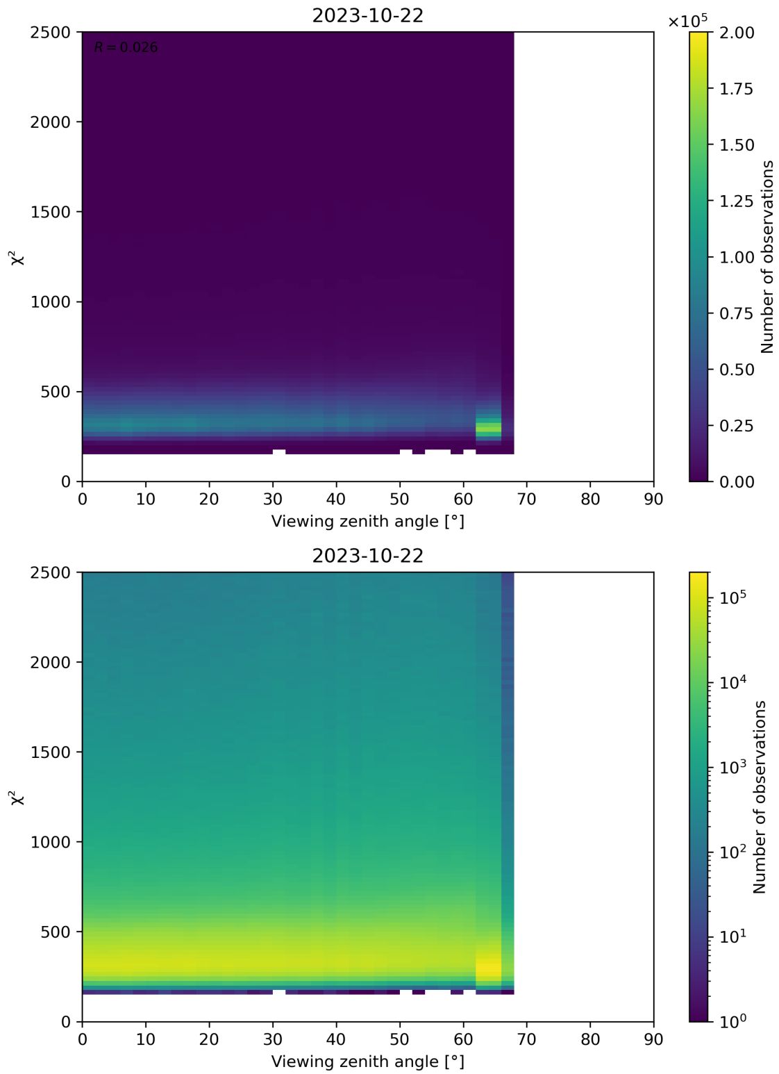
Figure 162: Scatter density plot of “Viewing zenith angle” against “ \chi^2 ” for 2023-10-22 to 2023-10-23.
