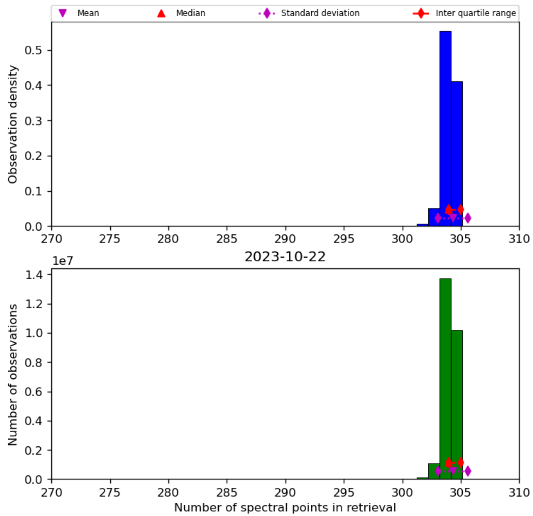
Figure 33: Histogram of “Number of spectral points in retrieval” for 2023-10-22 to 2023-10-23
