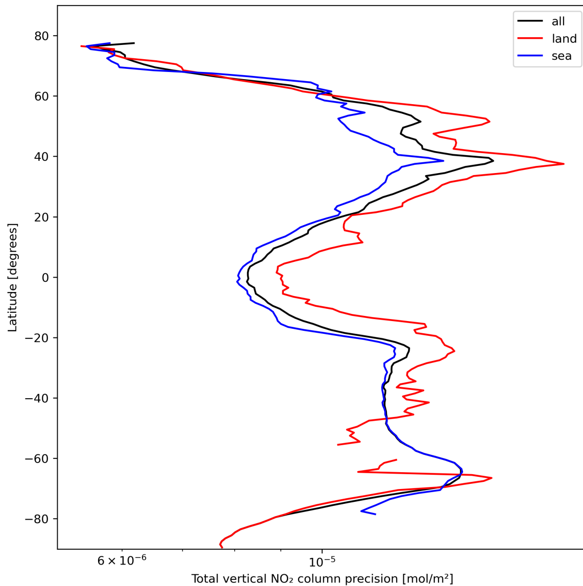
Figure 22: Zonal average of “Total vertical NO 2 column precision” for 2023-10-22 to 2023-10-23.
