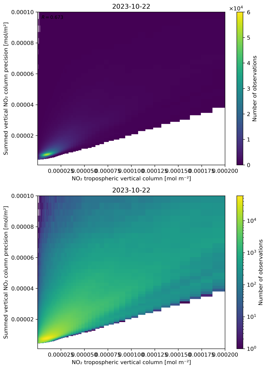
Figure 127: Scatter density plot of “NO 2 tropospheric vertical column” against “Summed vertical NO 2 column precision” for 2023-10-22 to 2023-10-23.
