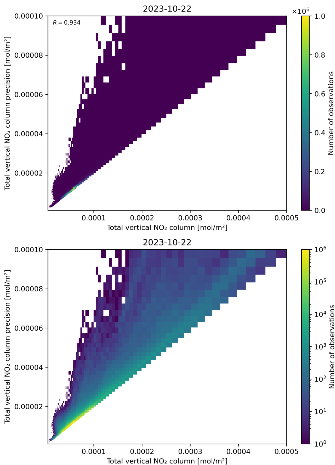
Figure 114: Scatter density plot of “Total vertical NO 2 column” against “Total vertical NO 2 column precision” for 2023-10-22 to 2023-10-23.
