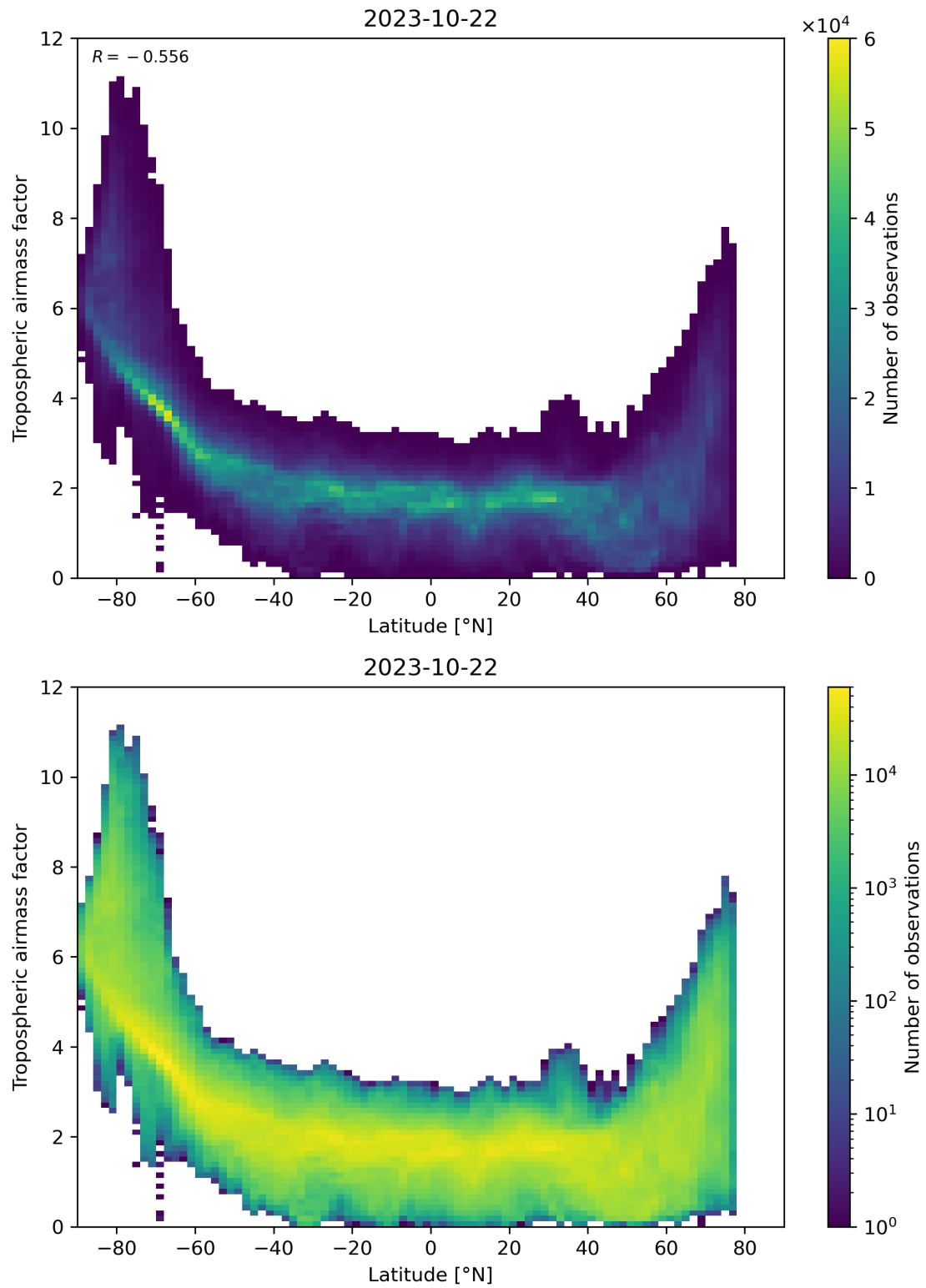
Figure 85: Scatter density plot of “Latitude” against “Tropospheric airmass factor” for 2023-10-22 to 2023-10-23.
