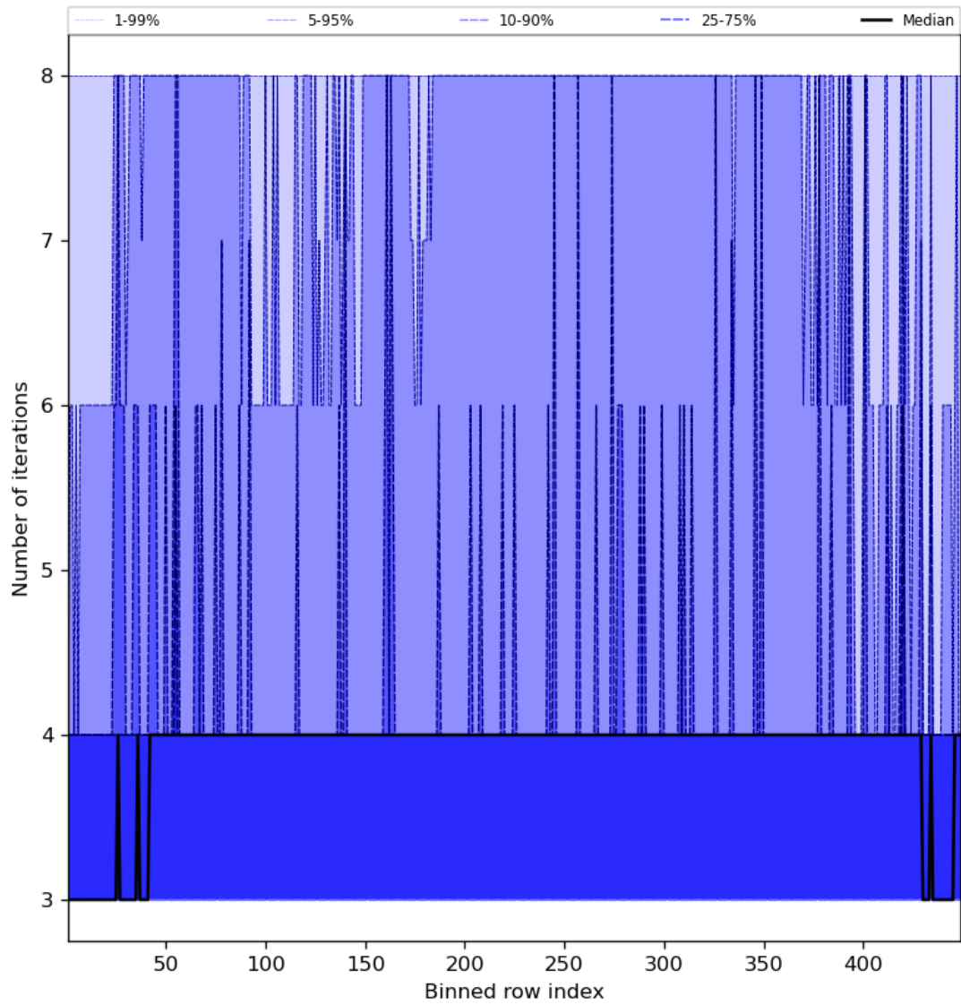
Figure 51: Along track statistics of “Number of iterations” for 2023-10-22 to 2023-10-23
