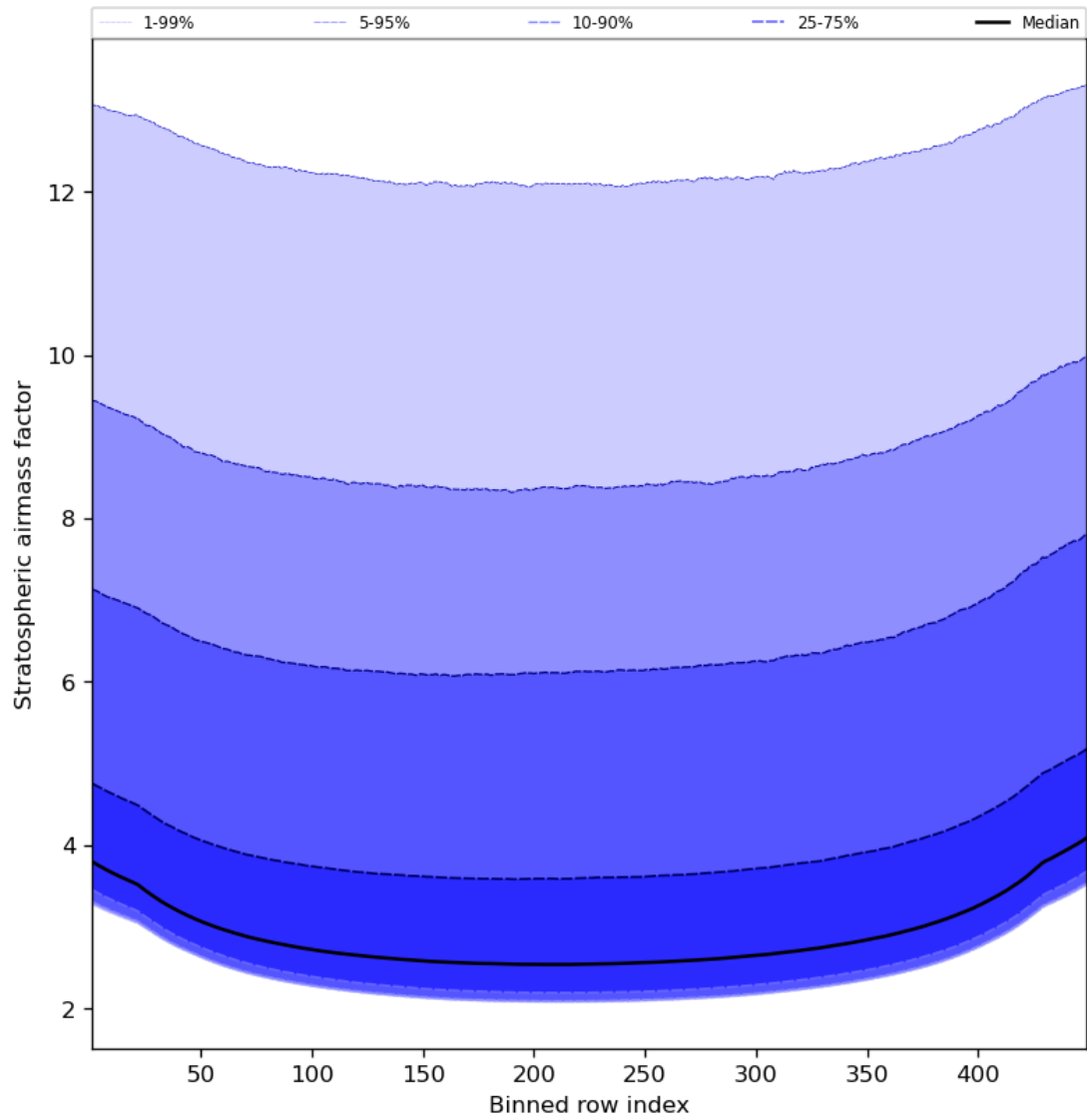
Figure 61: Along track statistics of “Stratospheric airmass factor” for 2023-10-22 to 2023-10-23
