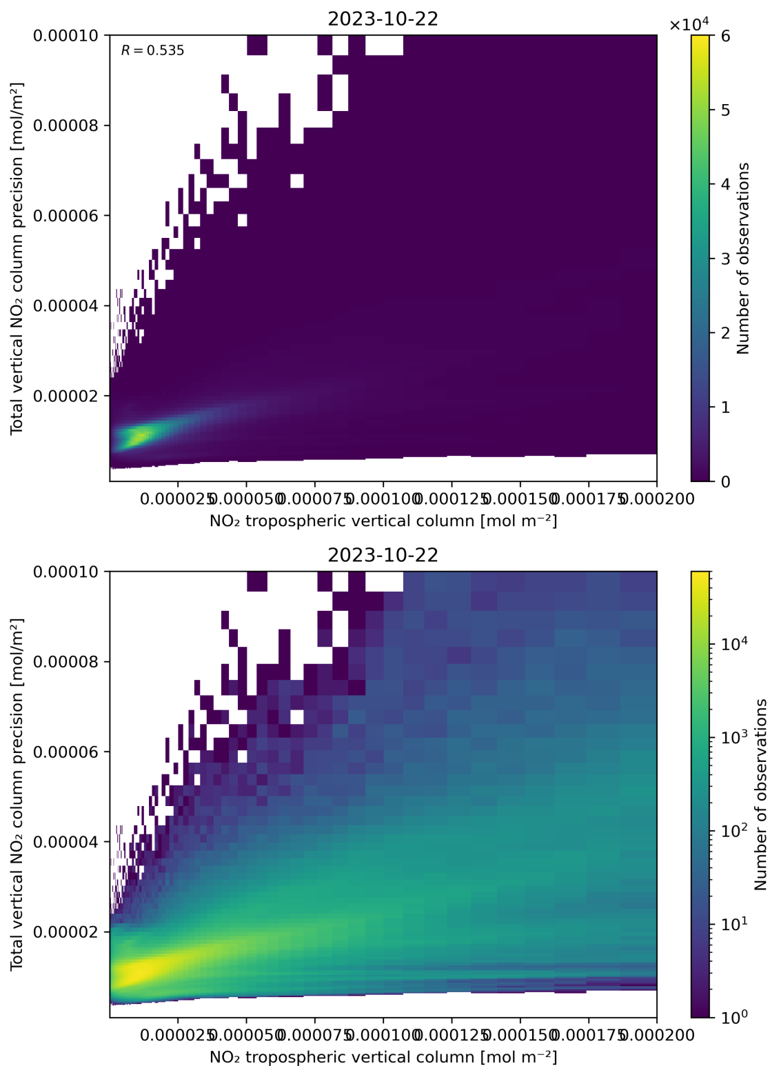
Figure 129: Scatter density plot of “NO 2 tropospheric vertical column” against “Total vertical NO 2 column precision” for 2023-10-22 to 2023-10-23.
