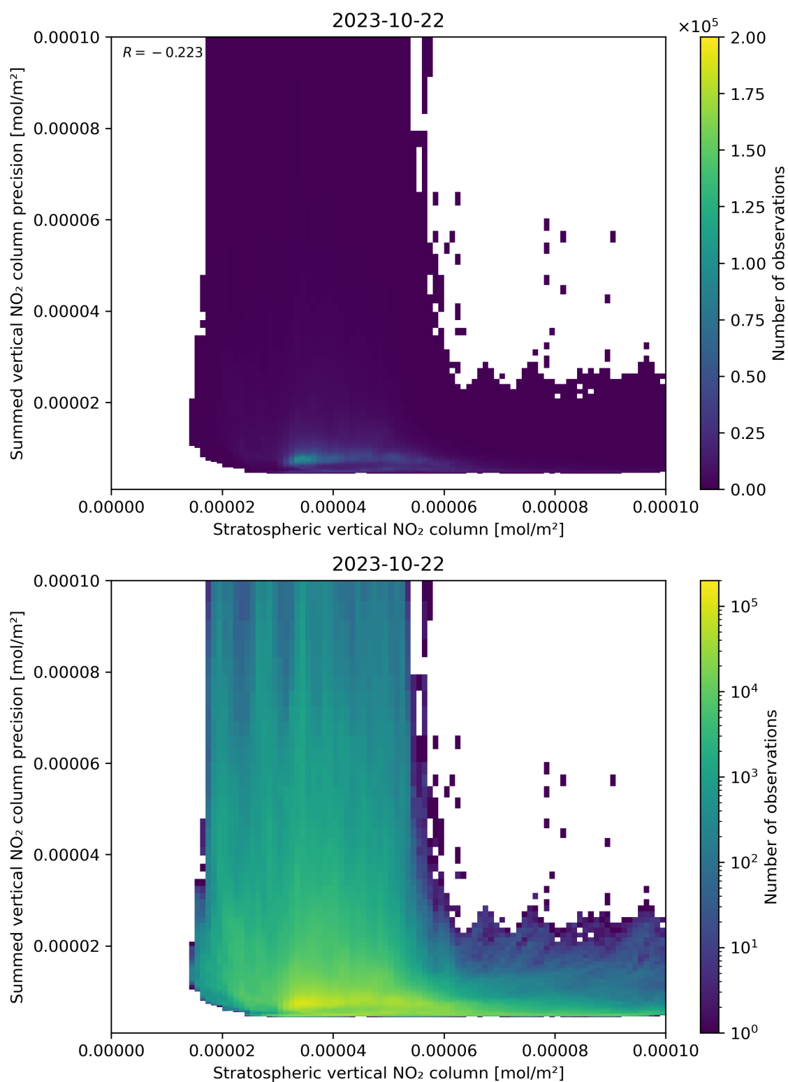
Figure 99: Scatter density plot of “Stratospheric vertical NO 2 column” against “Summed vertical NO 2 column precision” for 2023-10-22 to 2023-10-23.
