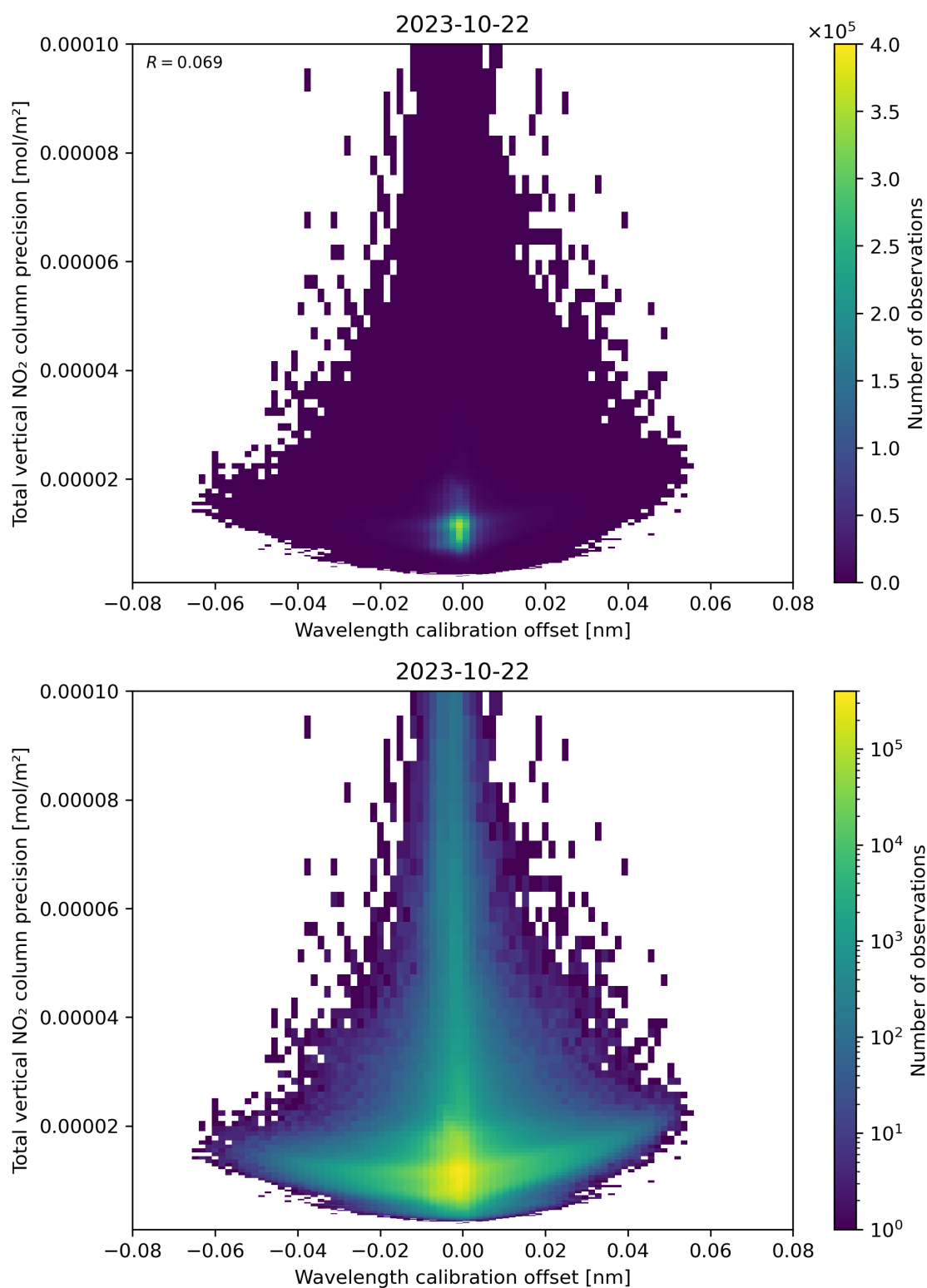
Figure 180: Scatter density plot of “Wavelength calibration offset” against “Total vertical NO 2 column precision” for 2023-10-22 to 2023-10-23.
