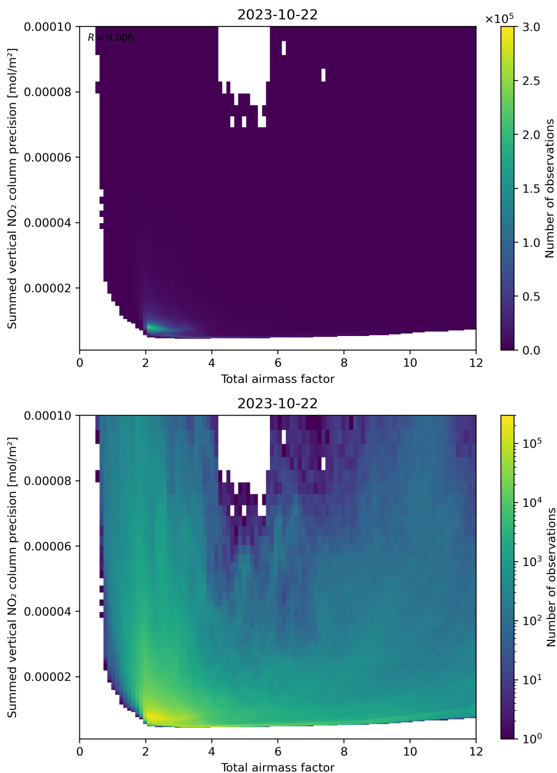
Figure 66: Scatter density plot of “Total airmass factor” against “Summed vertical NO 2 column precision” for 2023-10-22 to 2023-10-23.
