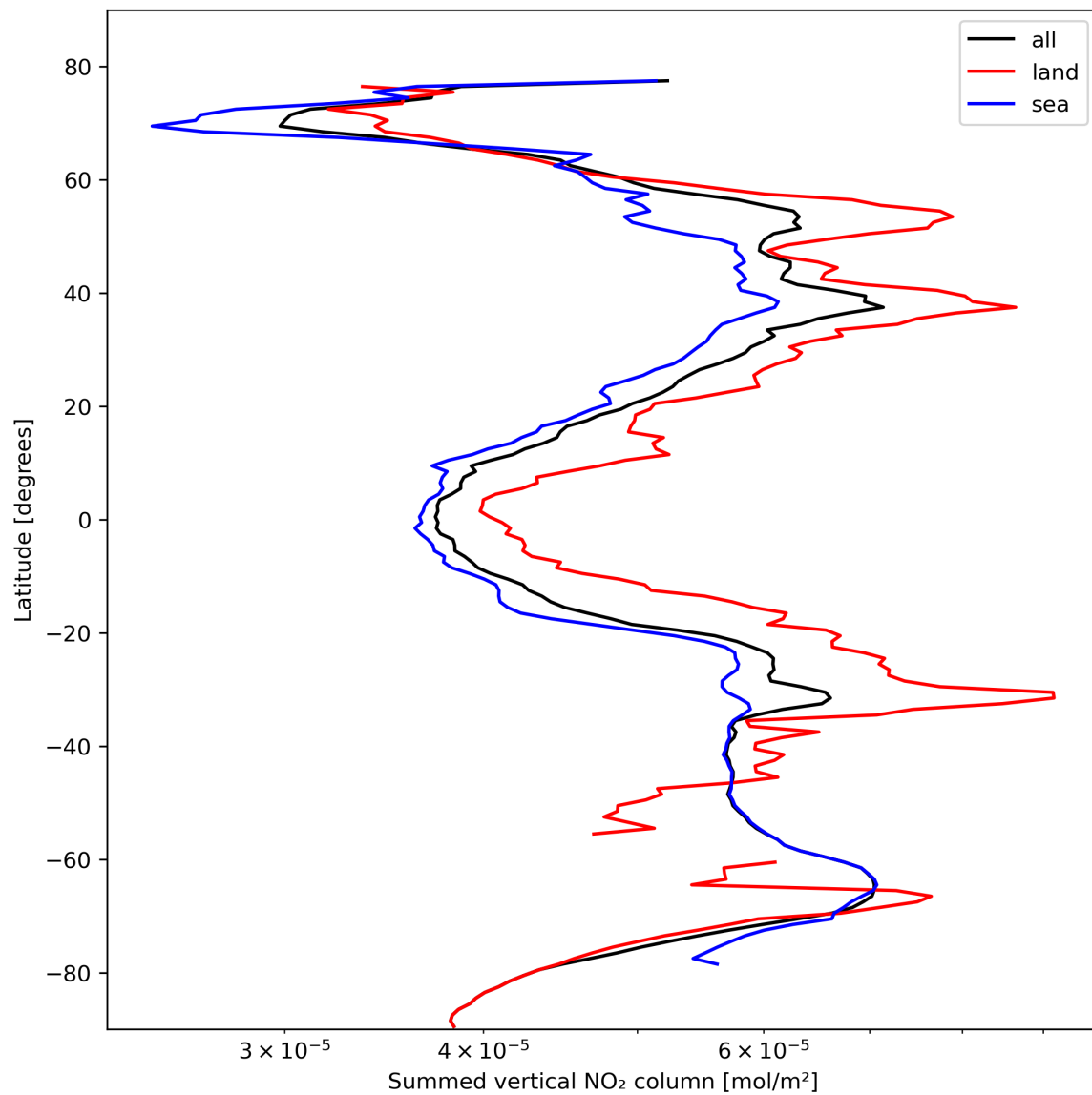
Figure 23: Zonal average of “Summed vertical NO 2 column” for 2023-10-22 to 2023-10-23.
