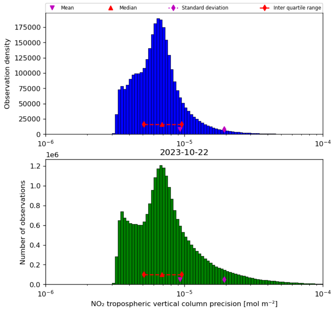
Figure 30: Histogram of “NO 2 tropospheric vertical column precision” for 2023-10-22 to 2023-10-23
