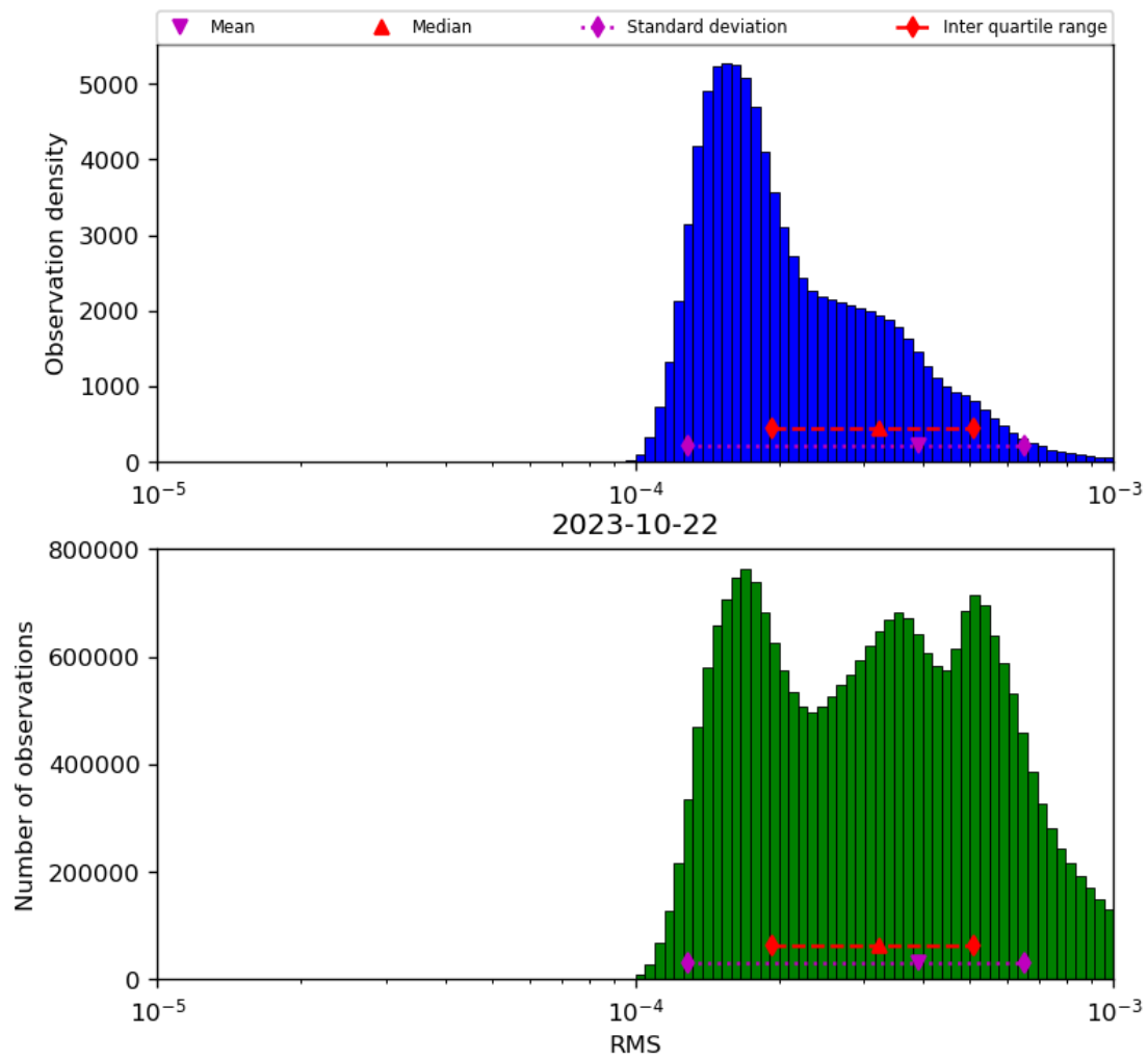
Figure 43: Histogram of “RMS” for 2023-10-22 to 2023-10-23
