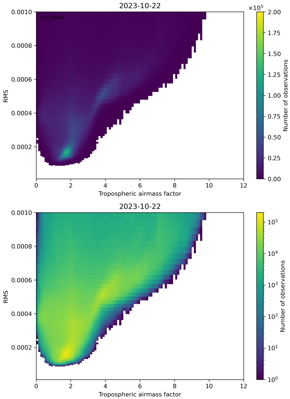
Figure 79: Scatter density plot of “Tropospheric airmass factor” against “RMS” for 2023-10-22 to 2023-10-23.
