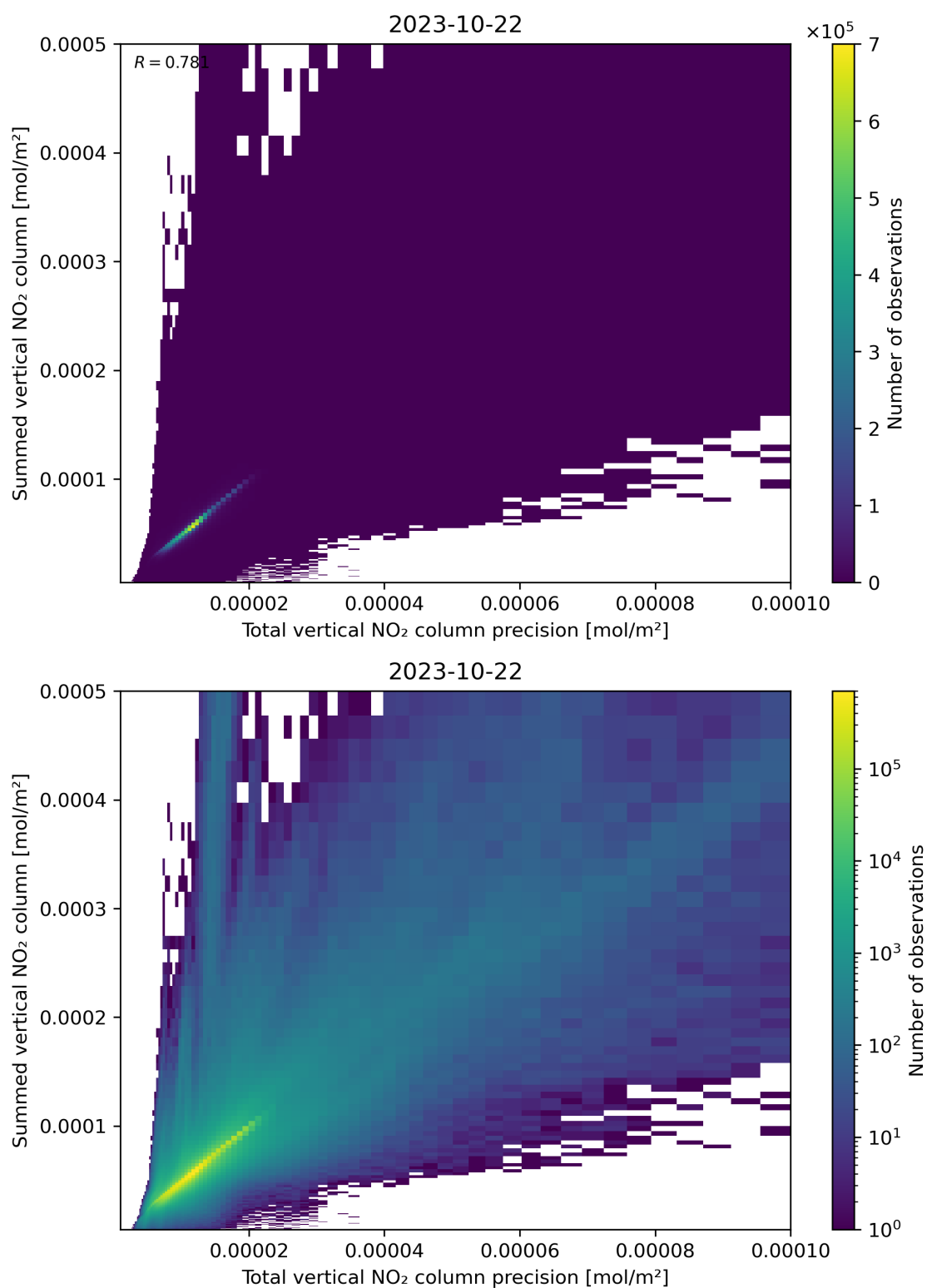
Figure 117: Scatter density plot of “Total vertical NO 2 column precision” against “Summed vertical NO 2 column” for 2023-10-22 to 2023-10-23.
