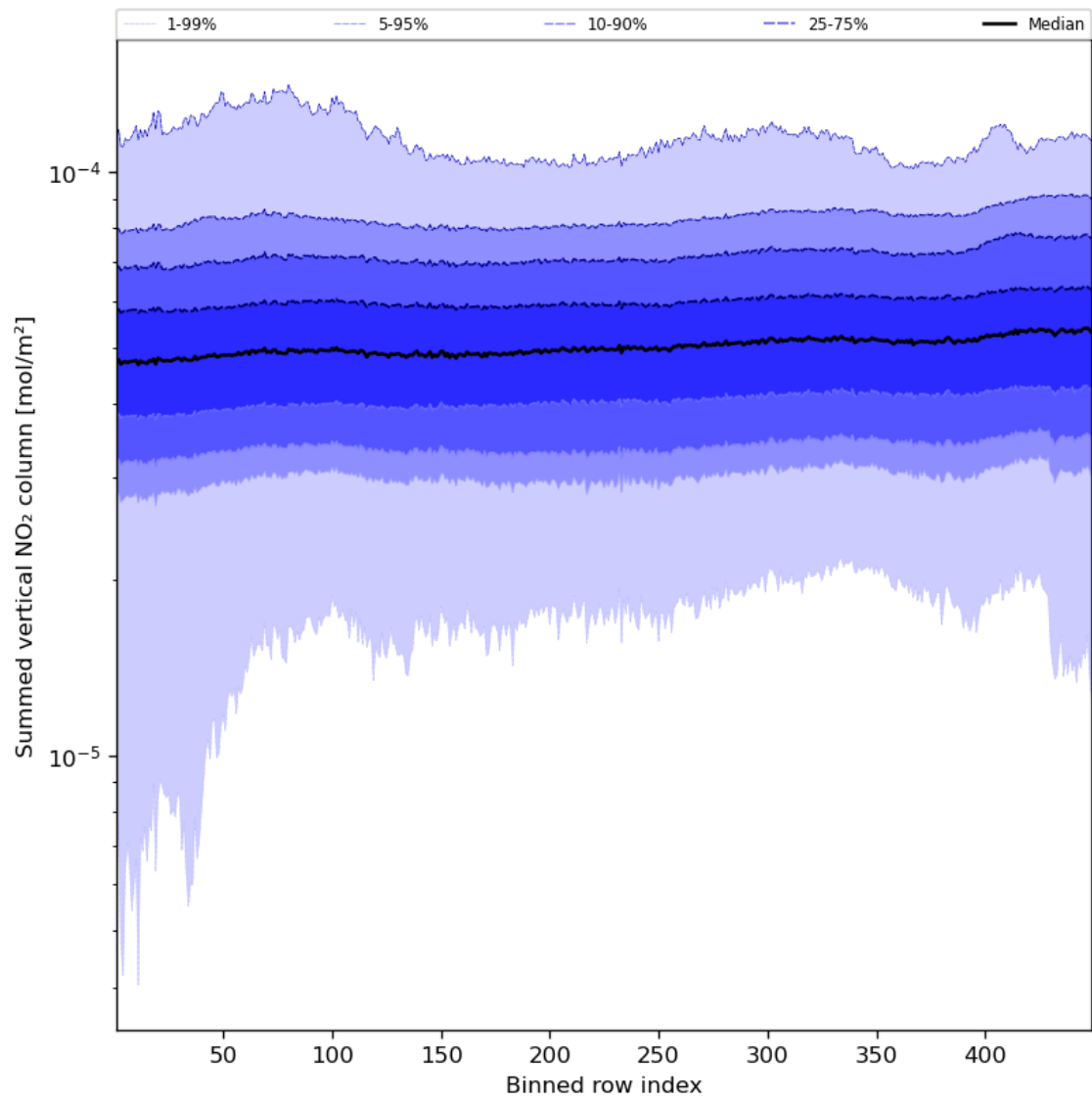
Figure 57: Along track statistics of “Summed vertical NO 2 column” for 2023-10-22 to 2023-10-23
