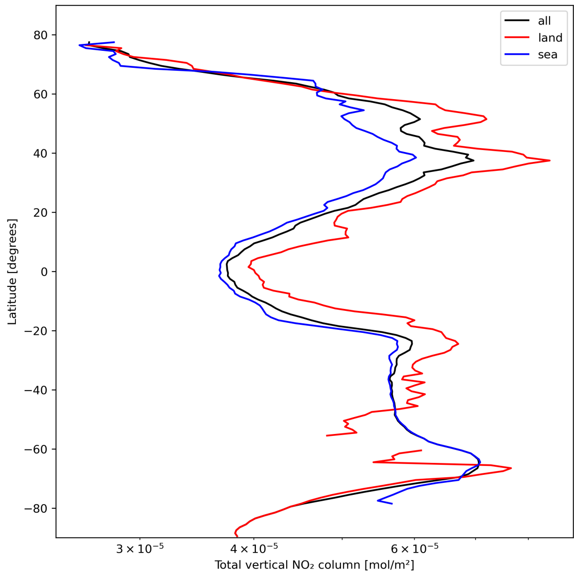
Figure 21: Zonal average of “Total vertical NO 2 column” for 2023-10-22 to 2023-10-23.
