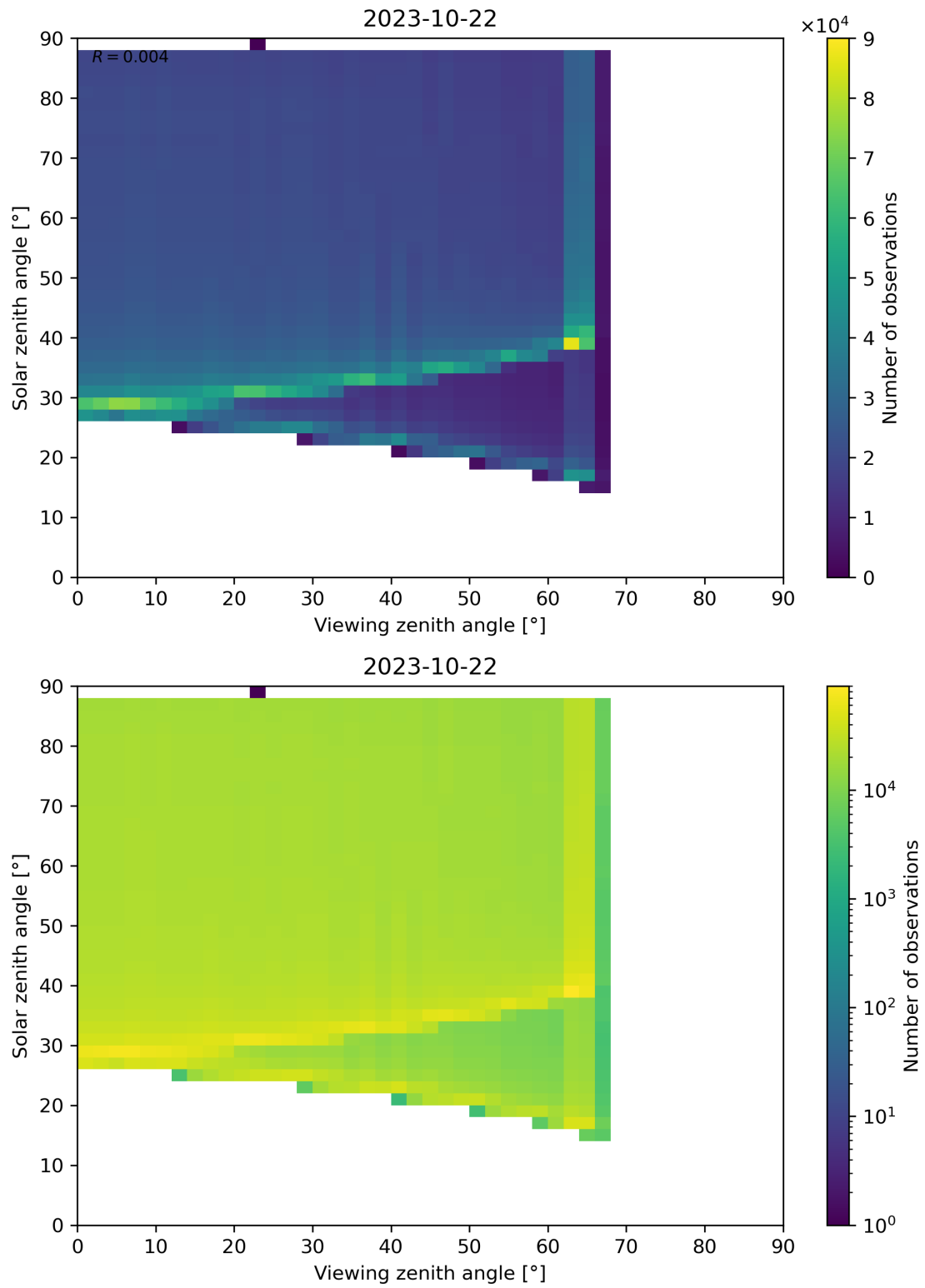
Figure 172: Scatter density plot of “Viewing zenith angle” against “Solar zenith angle” for 2023-10-22 to 2023-10-23.
