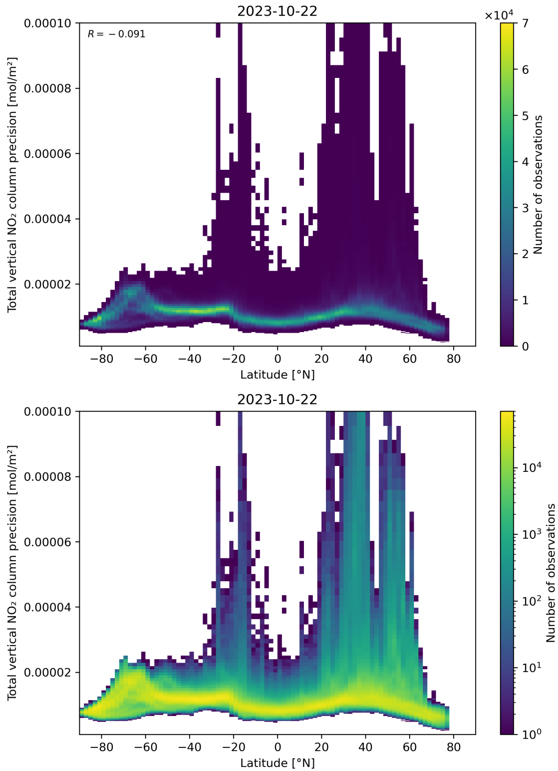
Figure 91: Scatter density plot of “Latitude” against “Total vertical NO 2 column precision” for 2023-10-22 to 2023-10-23.
