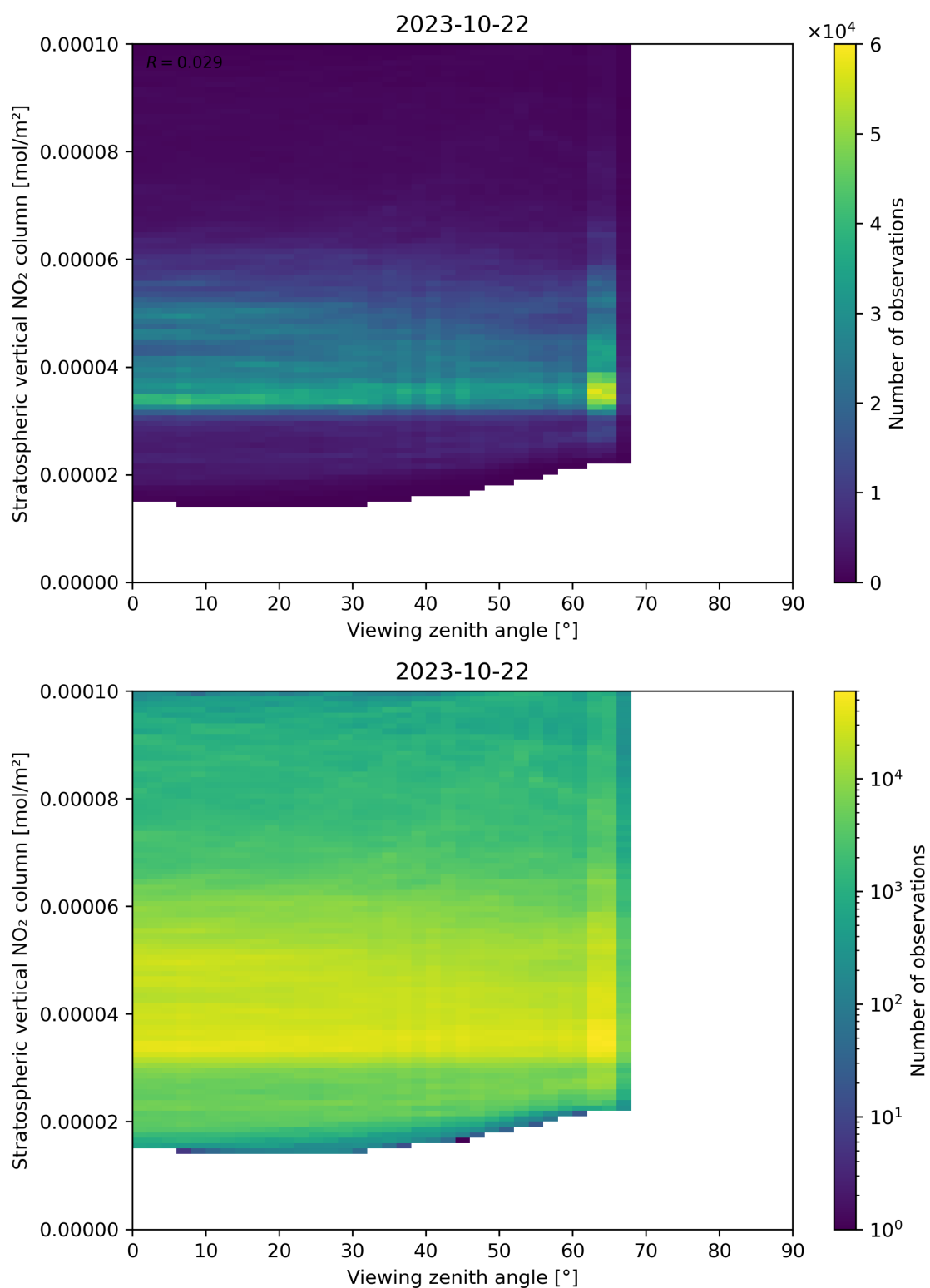
Figure 164: Scatter density plot of “Viewing zenith angle” against “Stratospheric vertical NO 2 column” for 2023-10-22 to 2023-10-23.
