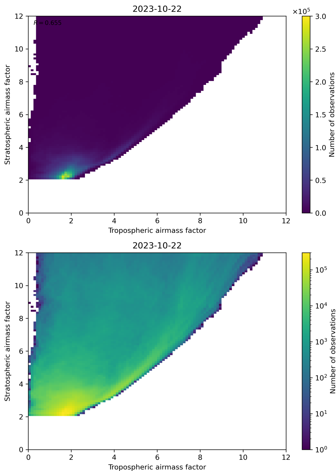
Figure 71: Scatter density plot of “Tropospheric airmass factor” against “Stratospheric airmass factor” for 2023-10-22 to 2023-10-23.
