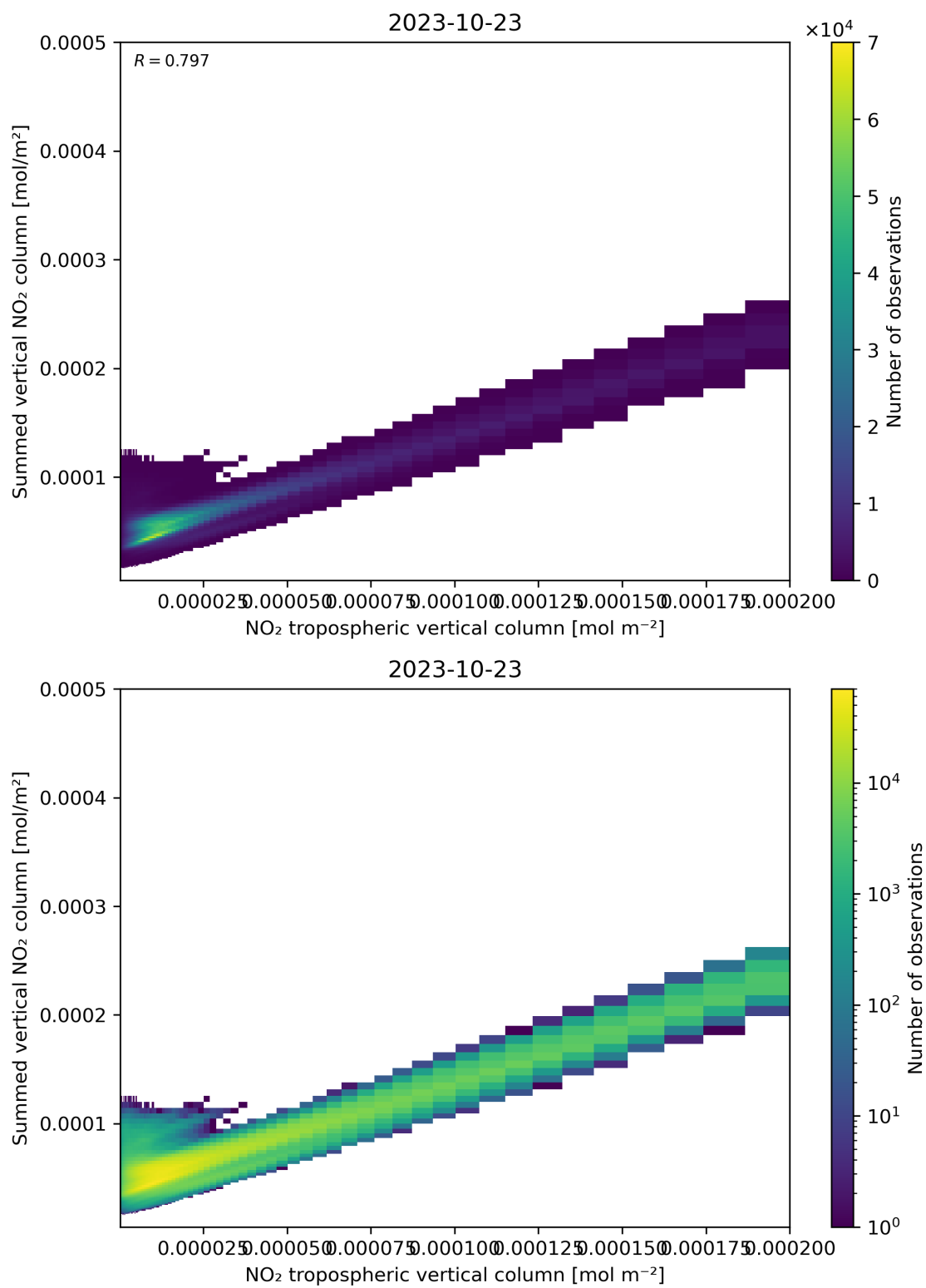
Figure 126: Scatter density plot of “NO 2 tropospheric vertical column” against “Summed vertical NO 2 column” for 2023-10-22 to 2023-10-24.
