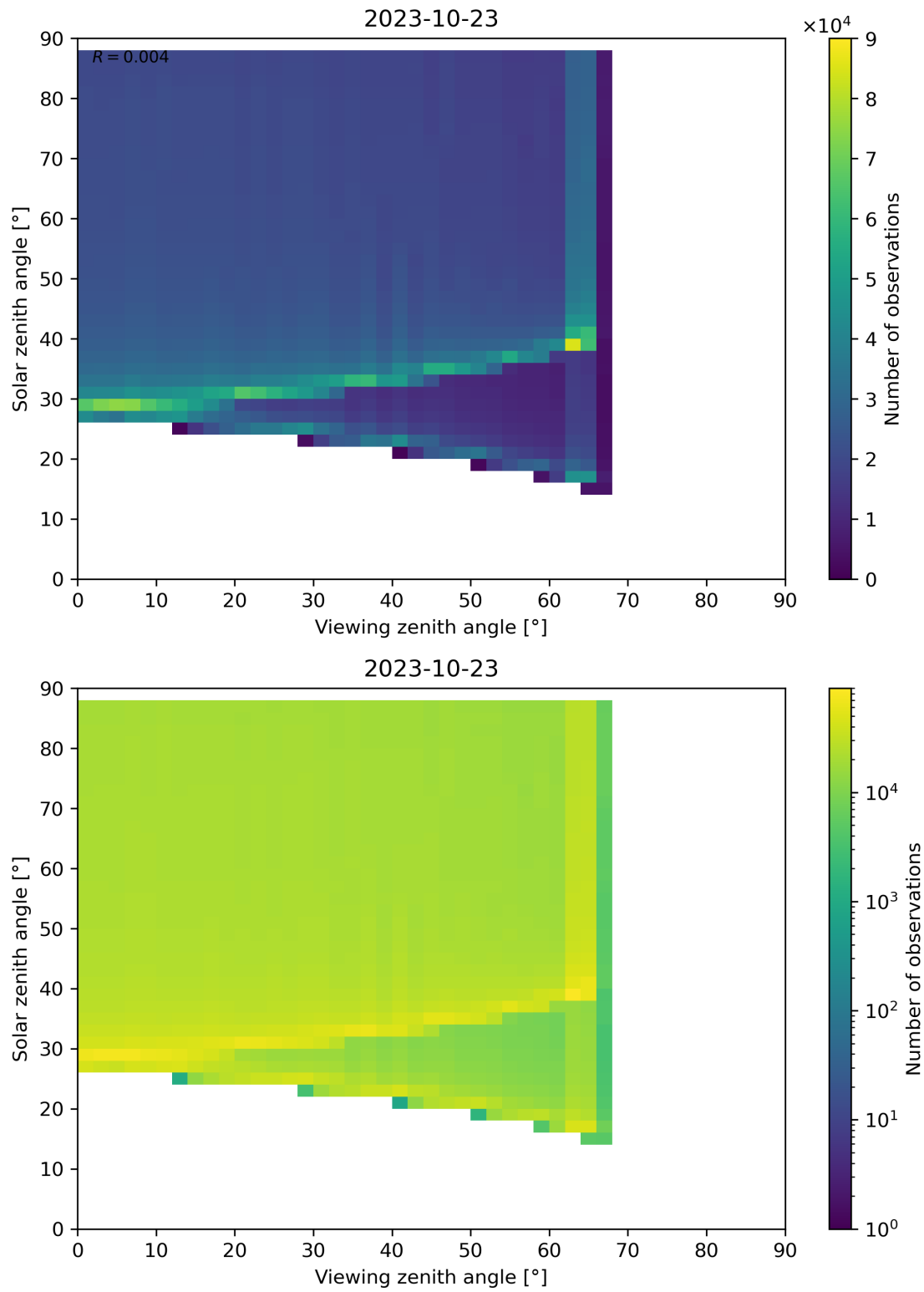
Figure 172: Scatter density plot of “Viewing zenith angle” against “Solar zenith angle” for 2023-10-22 to 2023-10-24.
