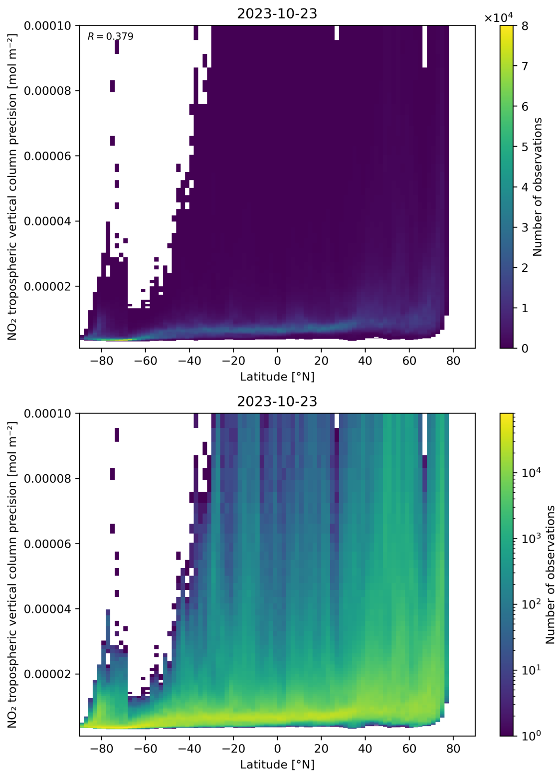
Figure 93: Scatter density plot of “Latitude” against “NO 2 tropospheric vertical column precision” for 2023-10-22 to 2023-10-24.
