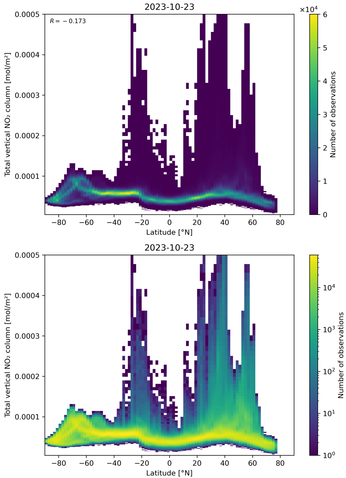
Figure 90: Scatter density plot of “Latitude” against “Total vertical NO 2 column” for 2023-10-22 to 2023-10-24.
