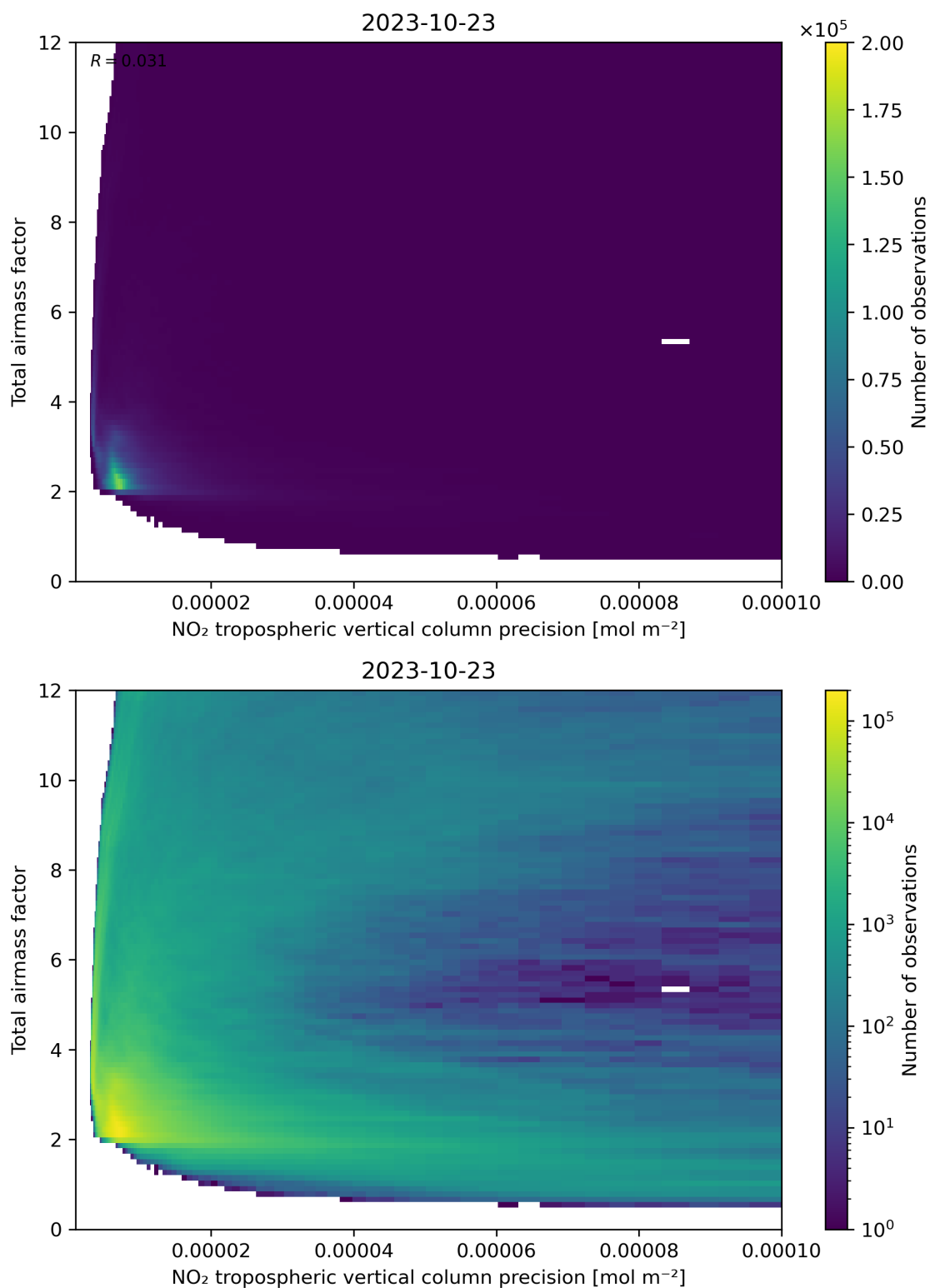
Figure 132: Scatter density plot of “NO 2 tropospheric vertical column precision” against “Total air mass factor” for 2023-10-22 to 2023-10-24.
