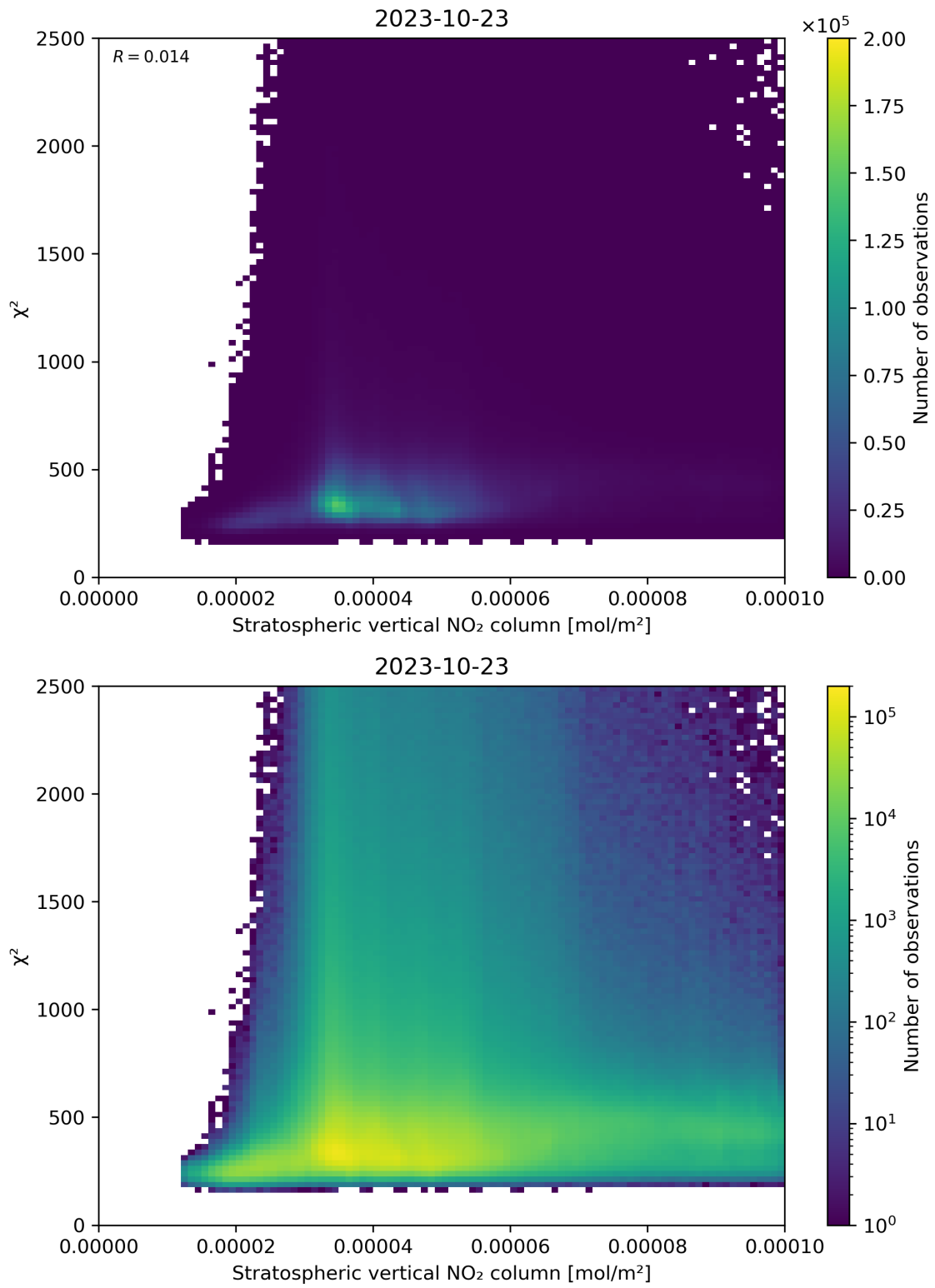
Figure 97: Scatter density plot of “Stratospheric vertical NO 2 column” against “ \chi^2 ” for 2023-10-22 to 2023-10-24.
