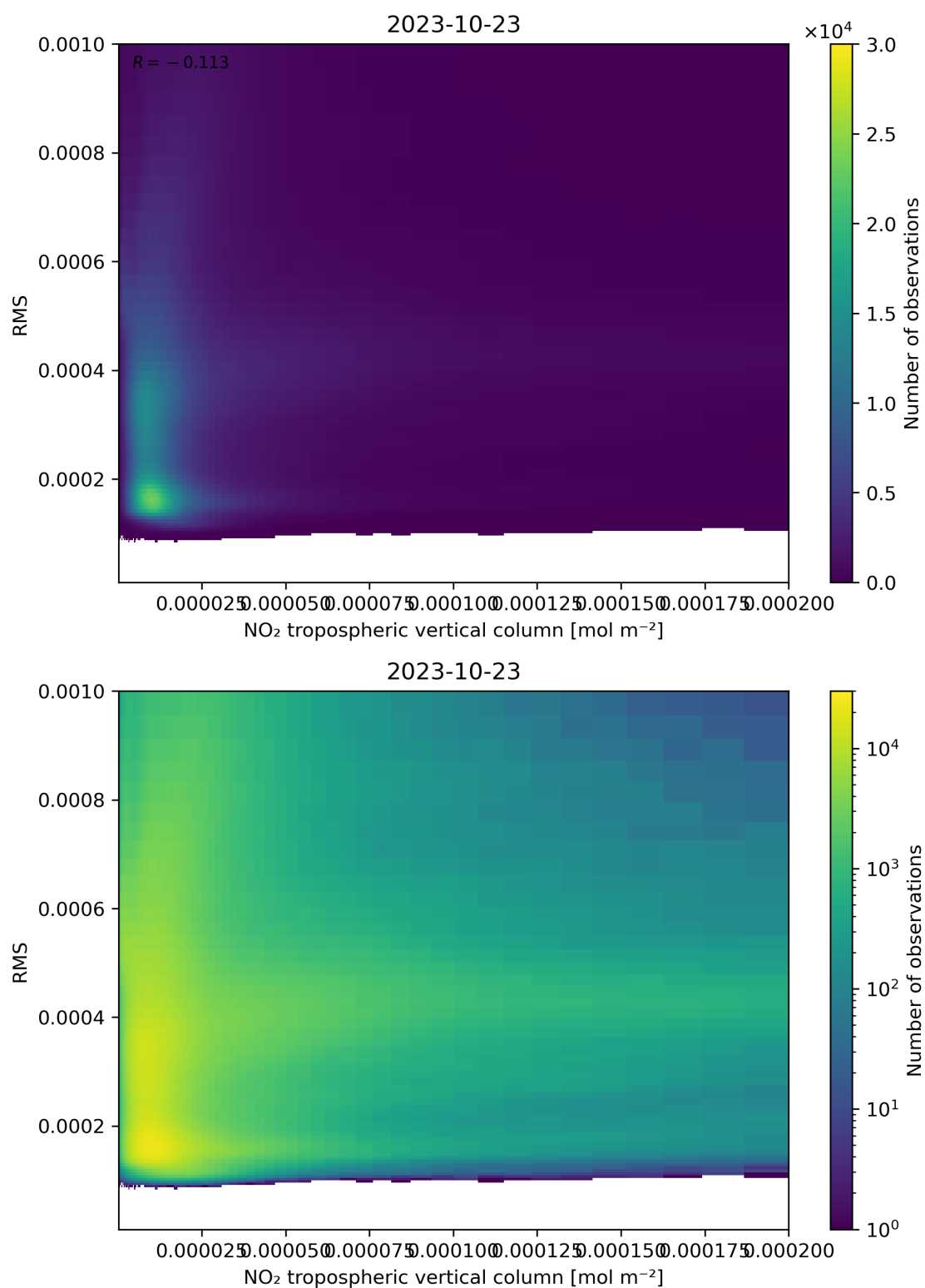
Figure 142: Scatter density plot of “NO 2 tropospheric vertical column” against “RMS” for 2023-10-22 to 2023-10-24.
