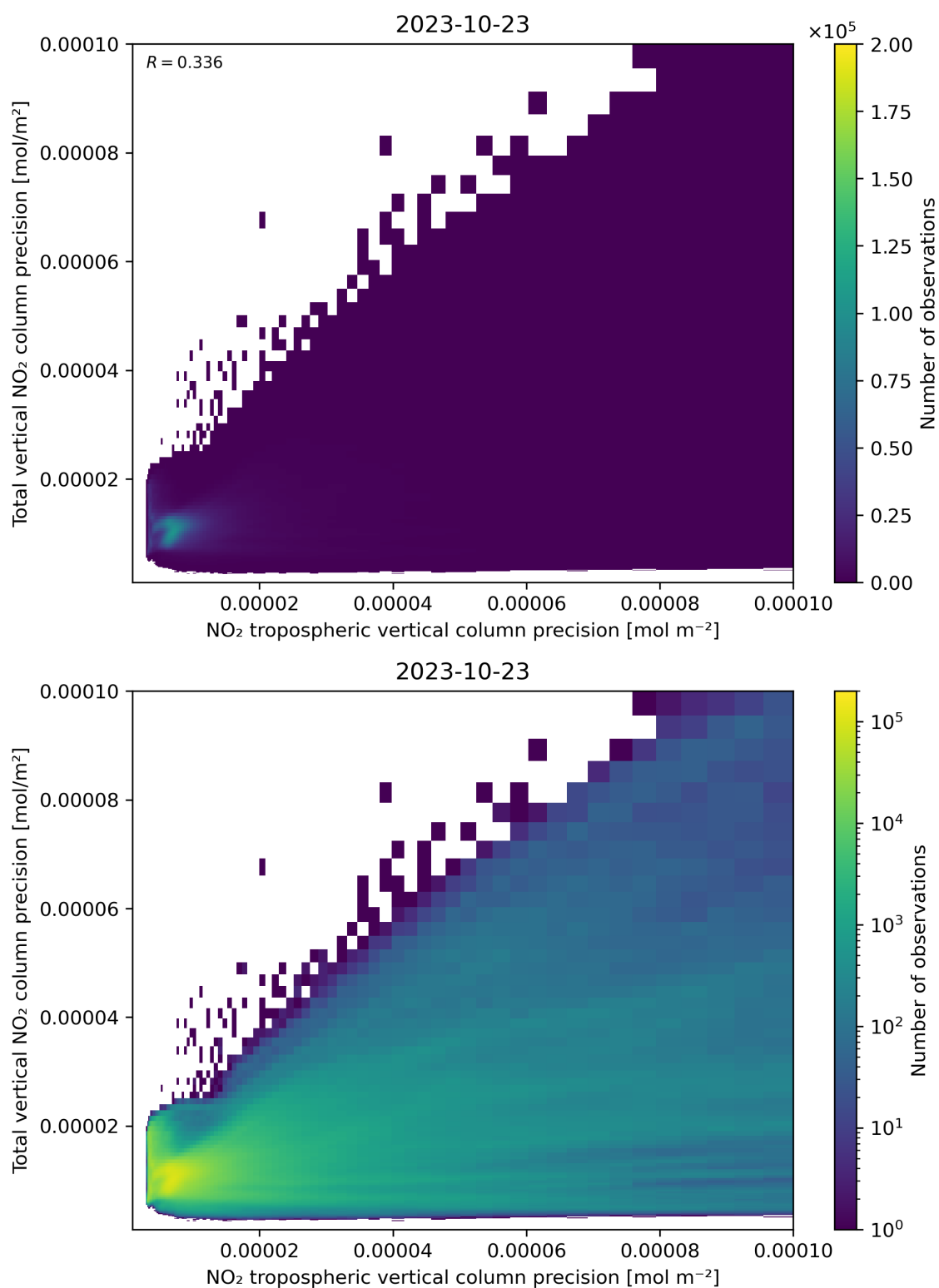
Figure 139: Scatter density plot of “NO 2 tropospheric vertical column precision” against “Total vertical NO 2 column precision” for 2023-10-22 to 2023-10-24.
