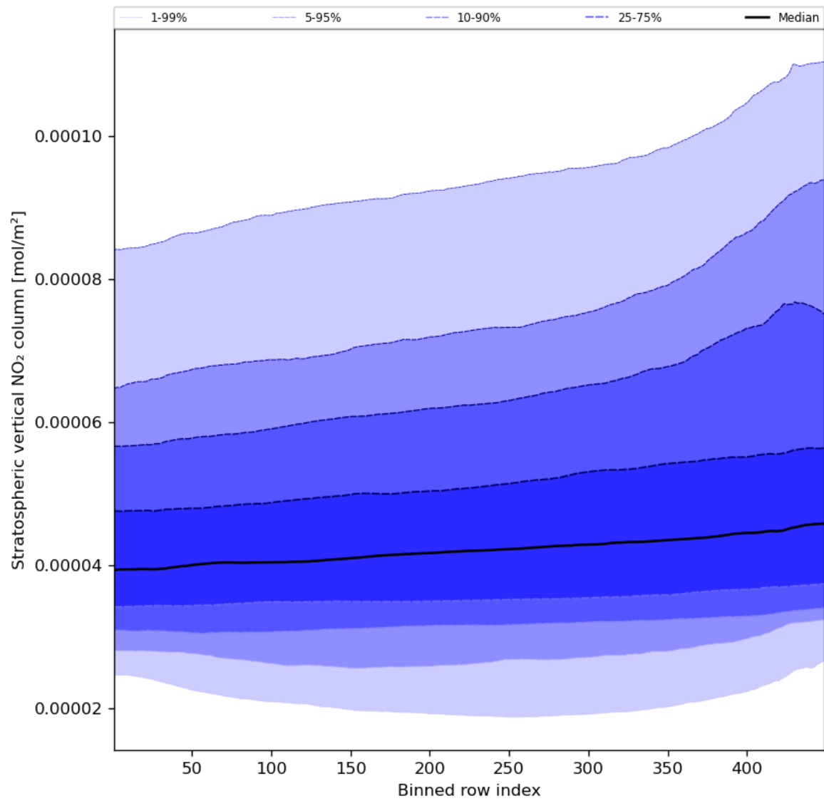
Figure 53: Along track statistics of “Stratospheric vertical NO 2 column” for 2023-10-22 to 2023-10-24
