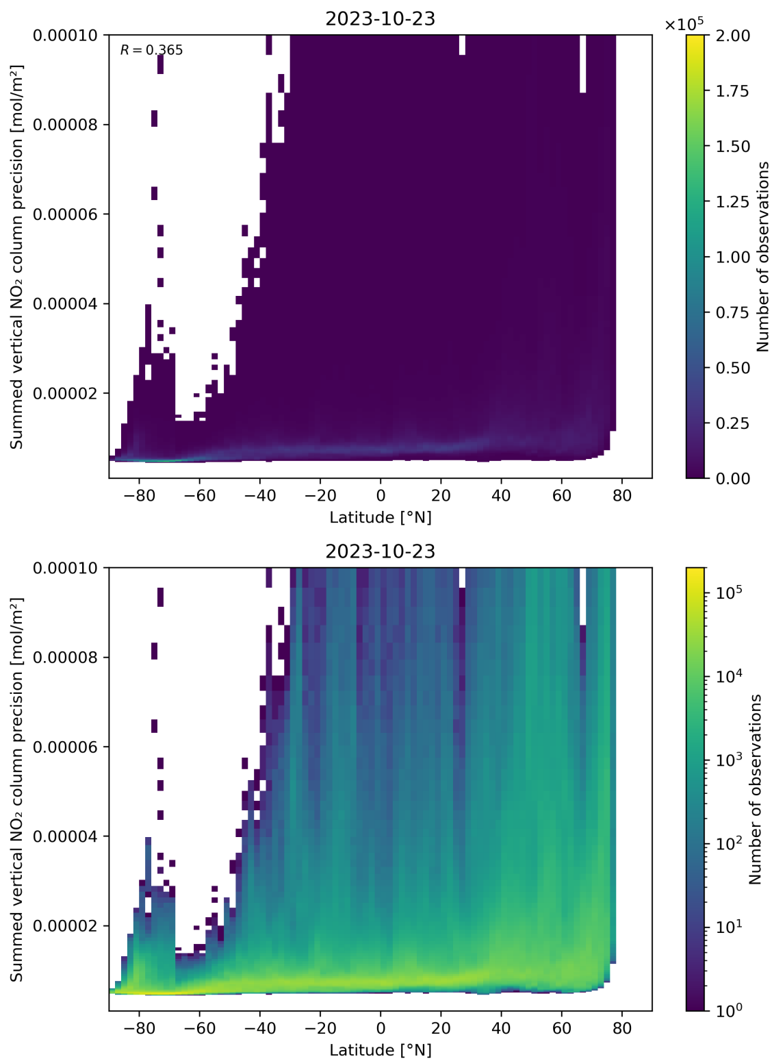
Figure 89: Scatter density plot of “Latitude” against “Summed vertical NO 2 column precision” for 2023-10-22 to 2023-10-24.
