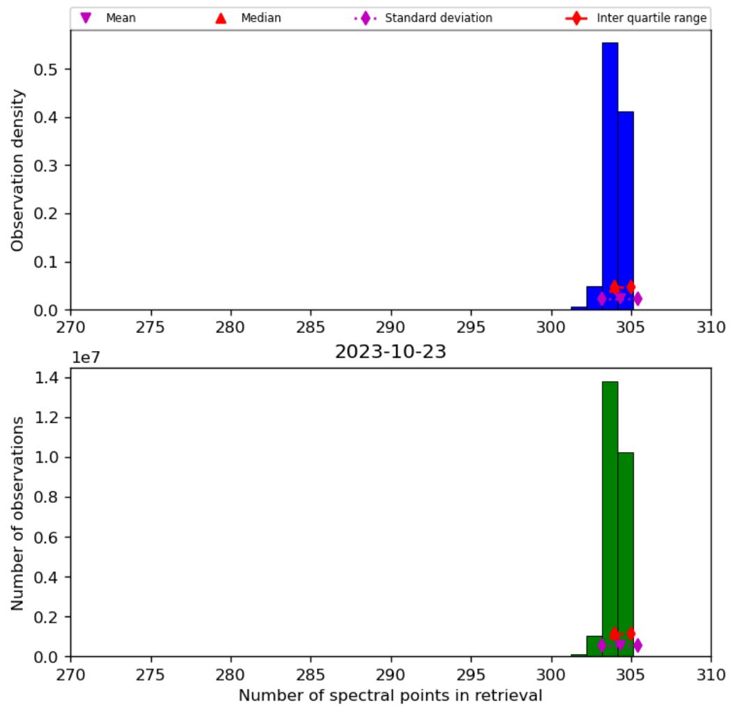
Figure 33: Histogram of “Number of spectral points in retrieval” for 2023-10-22 to 2023-10-24
