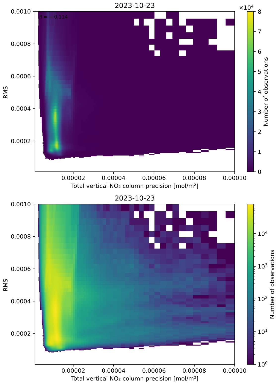
Figure 119: Scatter density plot of “Total vertical NO 2 column precision” against “RMS” for 2023-10-22 to 2023-10-24.
