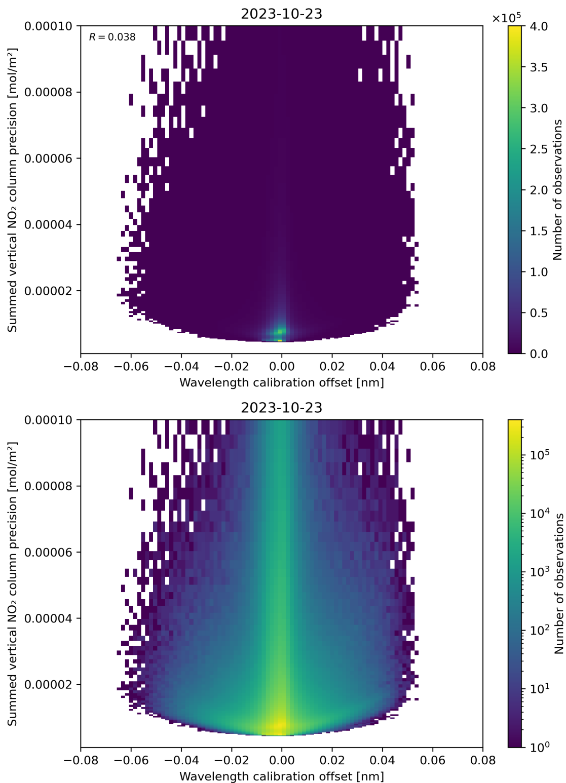
Figure 178: Scatter density plot of “Wavelength calibration offset” against “Summed vertical NO 2 column precision” for 2023-10-22 to 2023-10-24.
