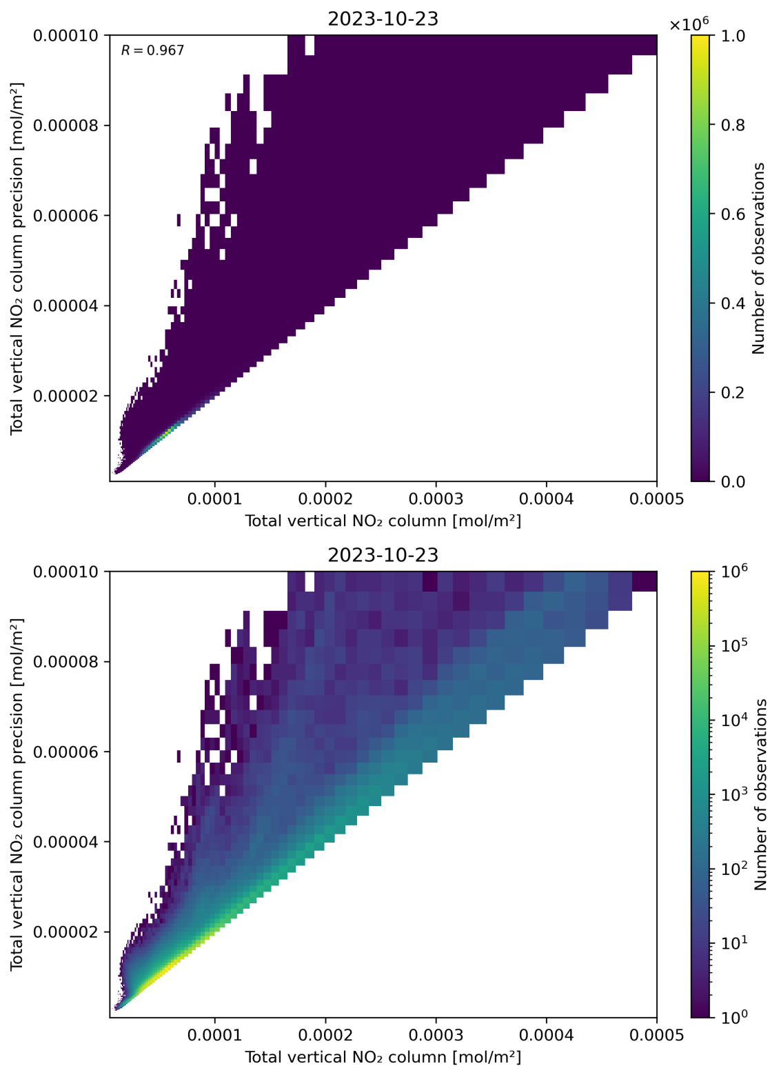
Figure 114: Scatter density plot of “Total vertical NO 2 column” against “Total vertical NO 2 column precision” for 2023-10-22 to 2023-10-24.
