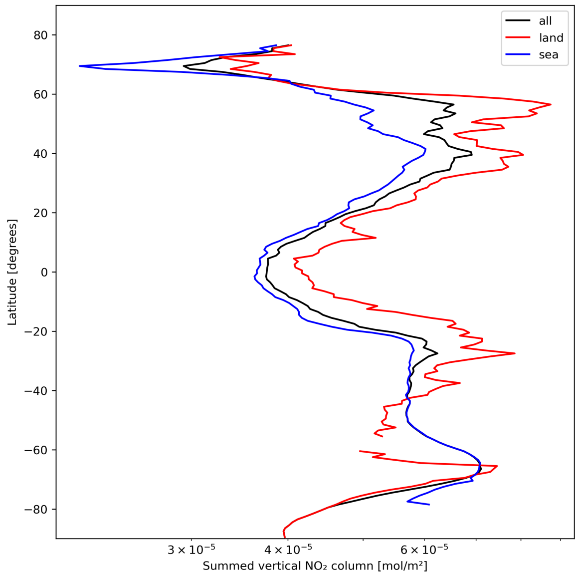
Figure 23: Zonal average of “Summed vertical NO 2 column” for 2023-10-22 to 2023-10-24.
