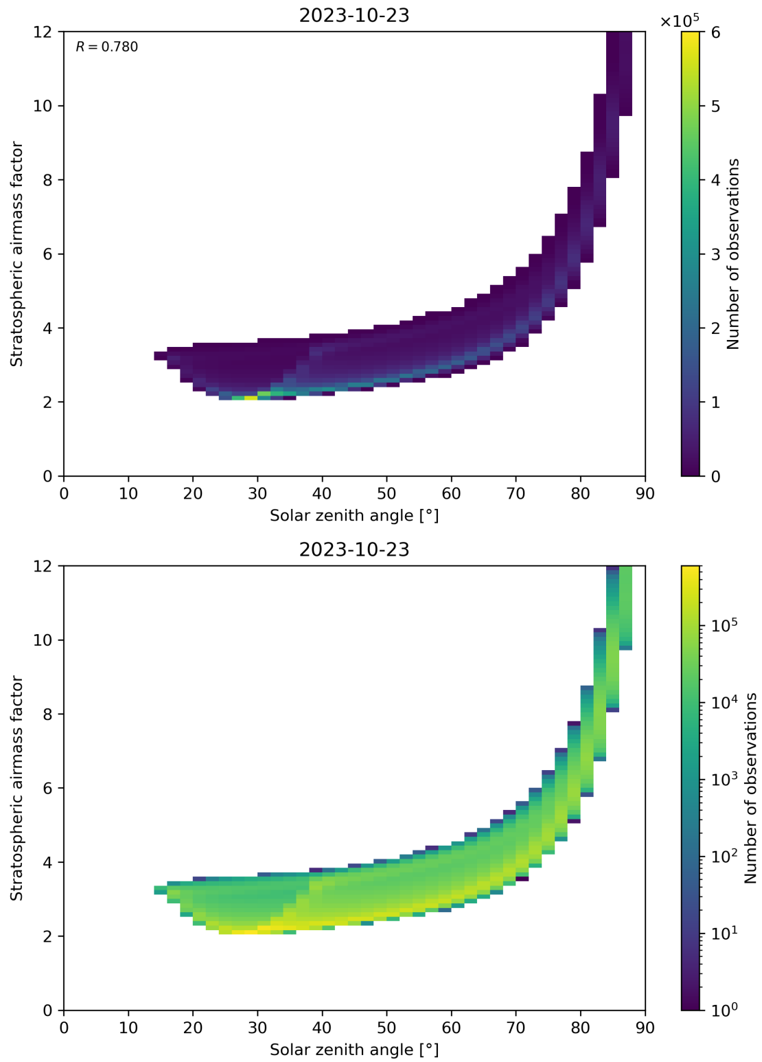
Figure 145: Scatter density plot of “Solar zenith angle” against “Stratospheric airmass factor” for 2023-10-22 to 2023-10-24.
