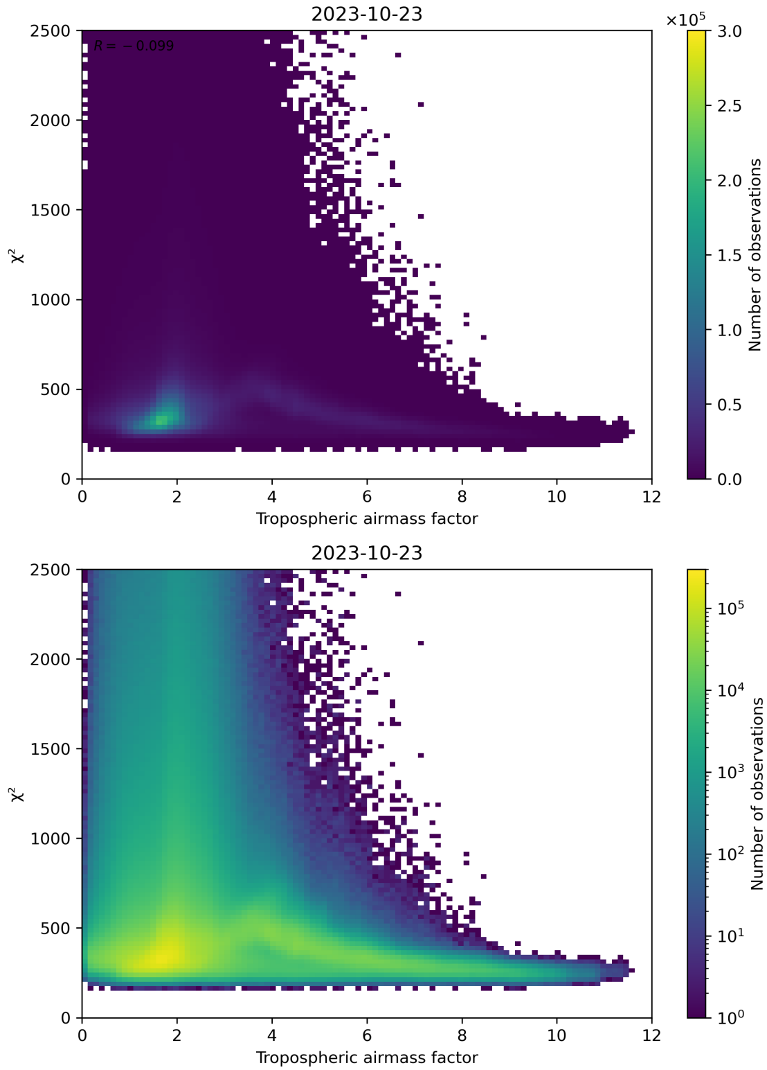
Figure 73: Scatter density plot of “Tropospheric airmass factor” against “ \chi^2 ” for 2023-10-22 to 2023-10-24.
