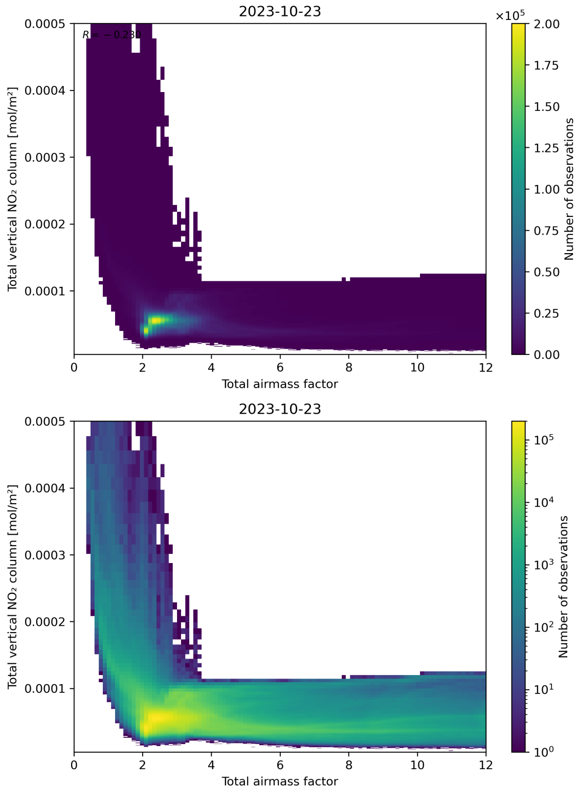
Figure 67: Scatter density plot of “Total airmass factor” against “Total vertical NO 2 column” for 2023-10-22 to 2023-10-24.
