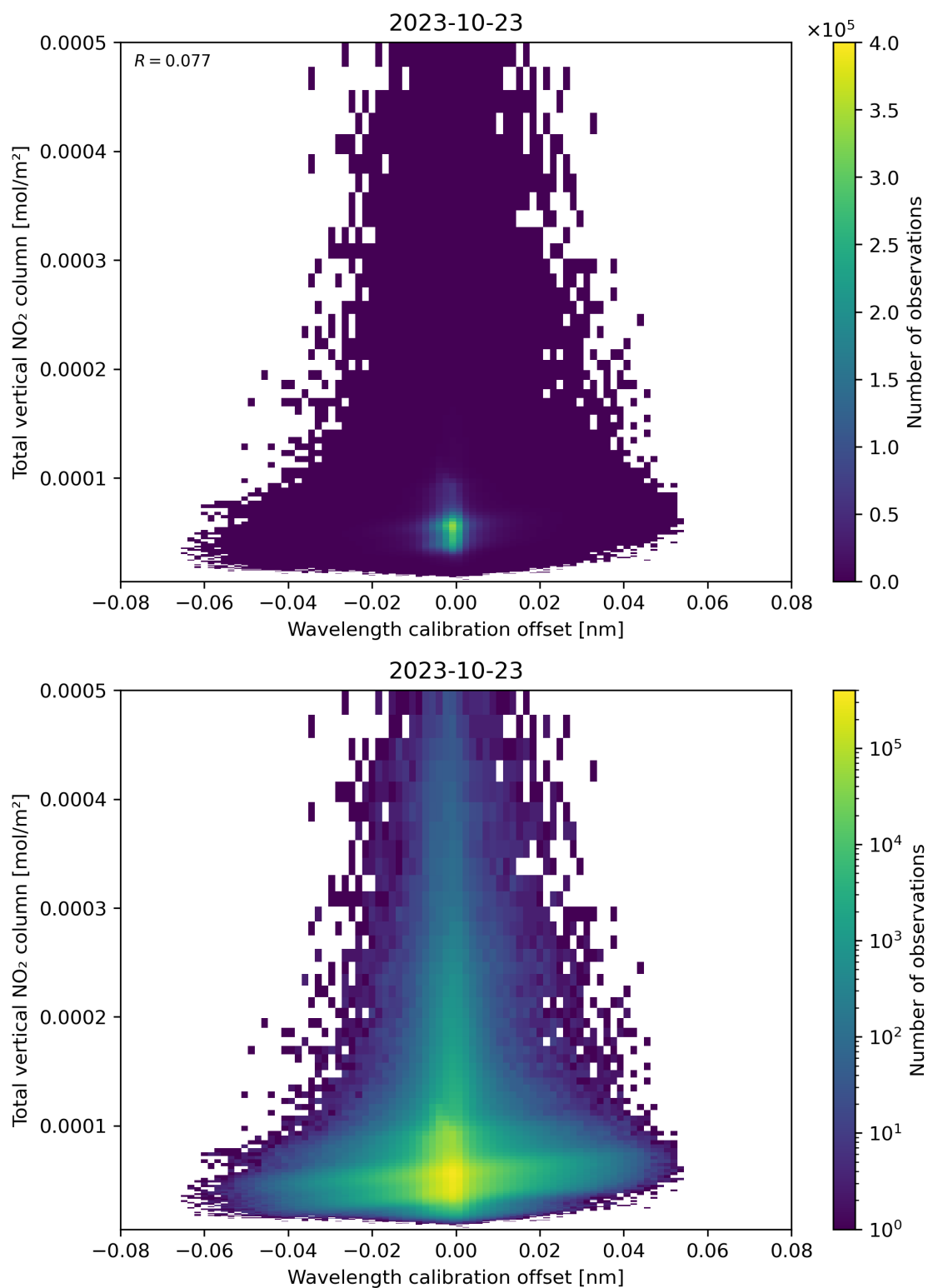
Figure 179: Scatter density plot of “Wavelength calibration offset” against “Total vertical NO 2 column” for 2023-10-22 to 2023-10-24.
