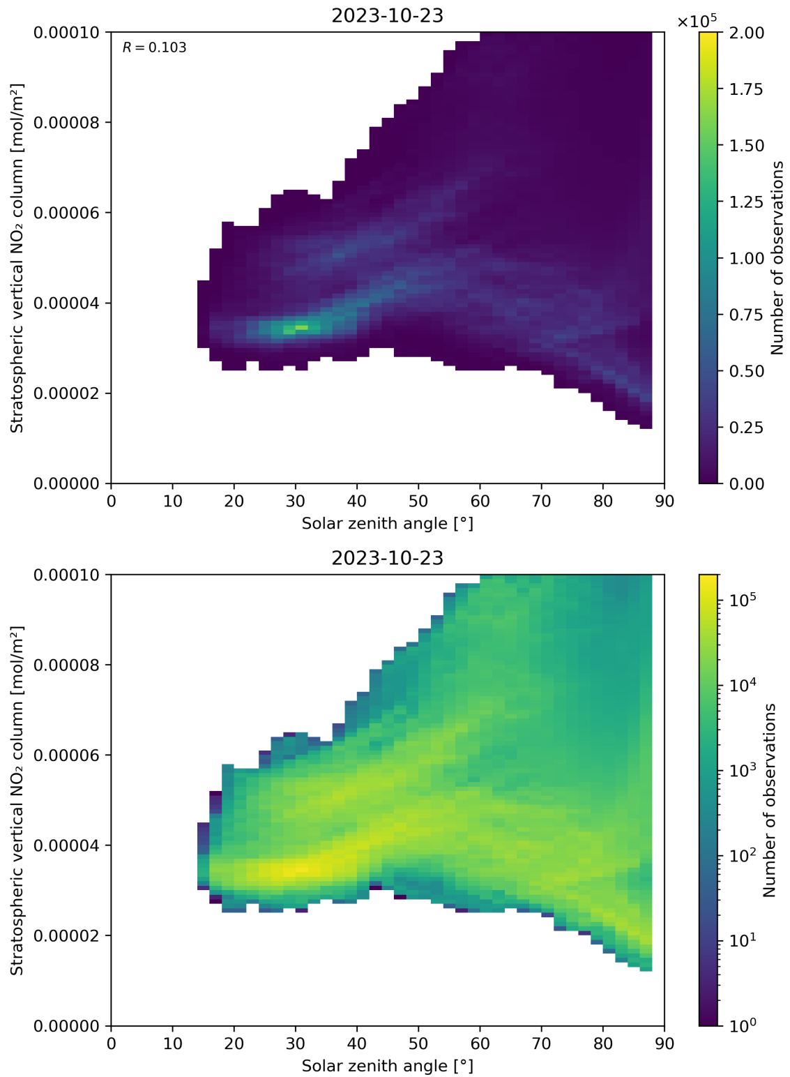
Figure 150: Scatter density plot of “Solar zenith angle” against “Stratospheric vertical NO 2 column” for 2023-10-22 to 2023-10-24.
