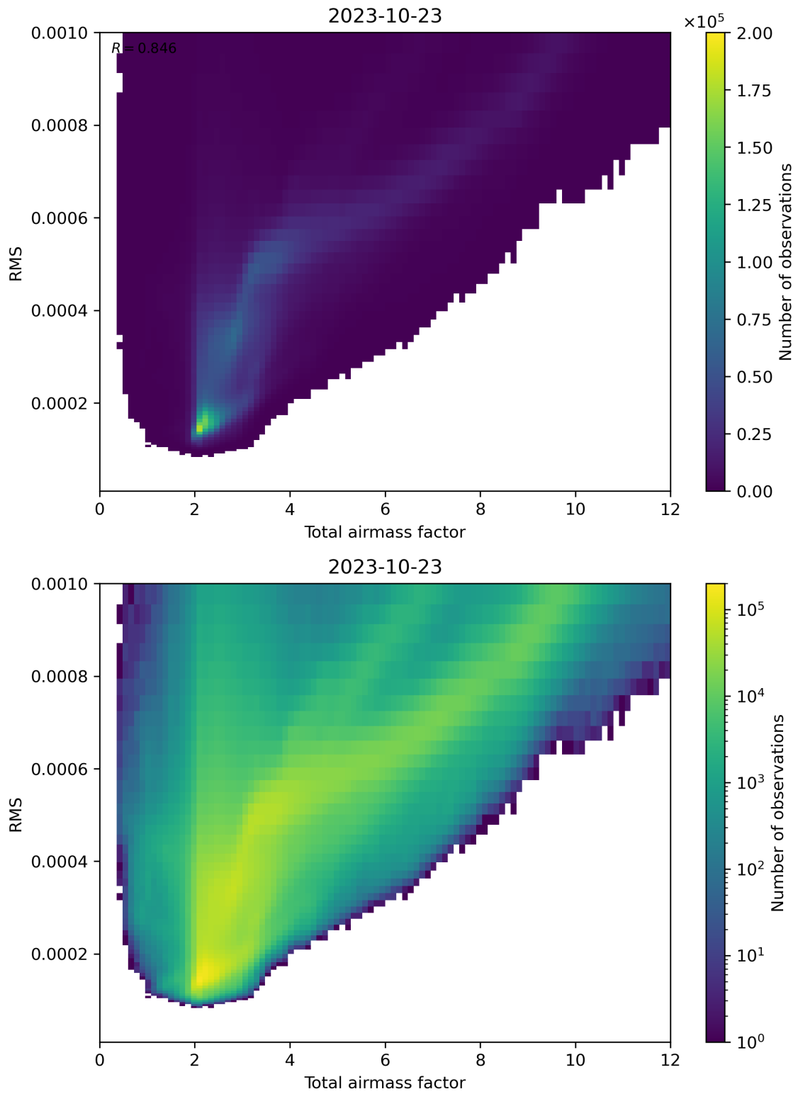
Figure 69: Scatter density plot of “Total airmass factor” against “RMS” for 2023-10-22 to 2023-10-24.
