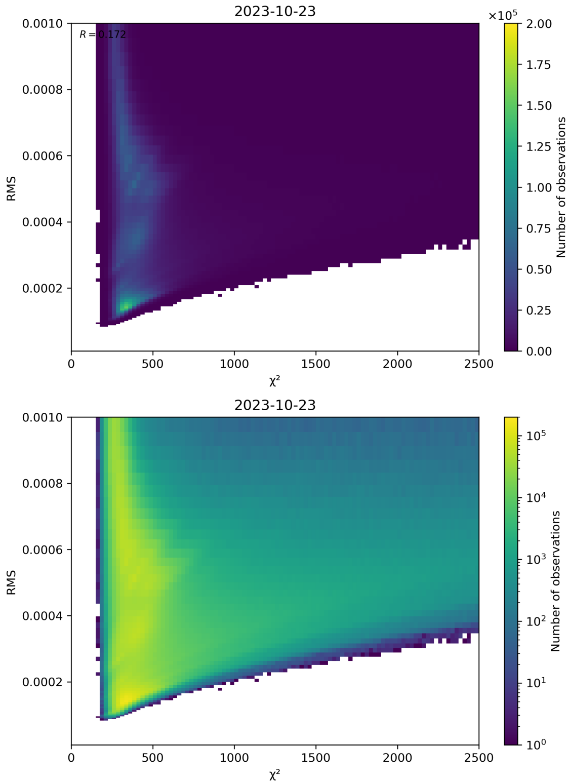
Figure 82: Scatter density plot of “ \chi^2 ” against “RMS” for 2023-10-22 to 2023-10-24.
