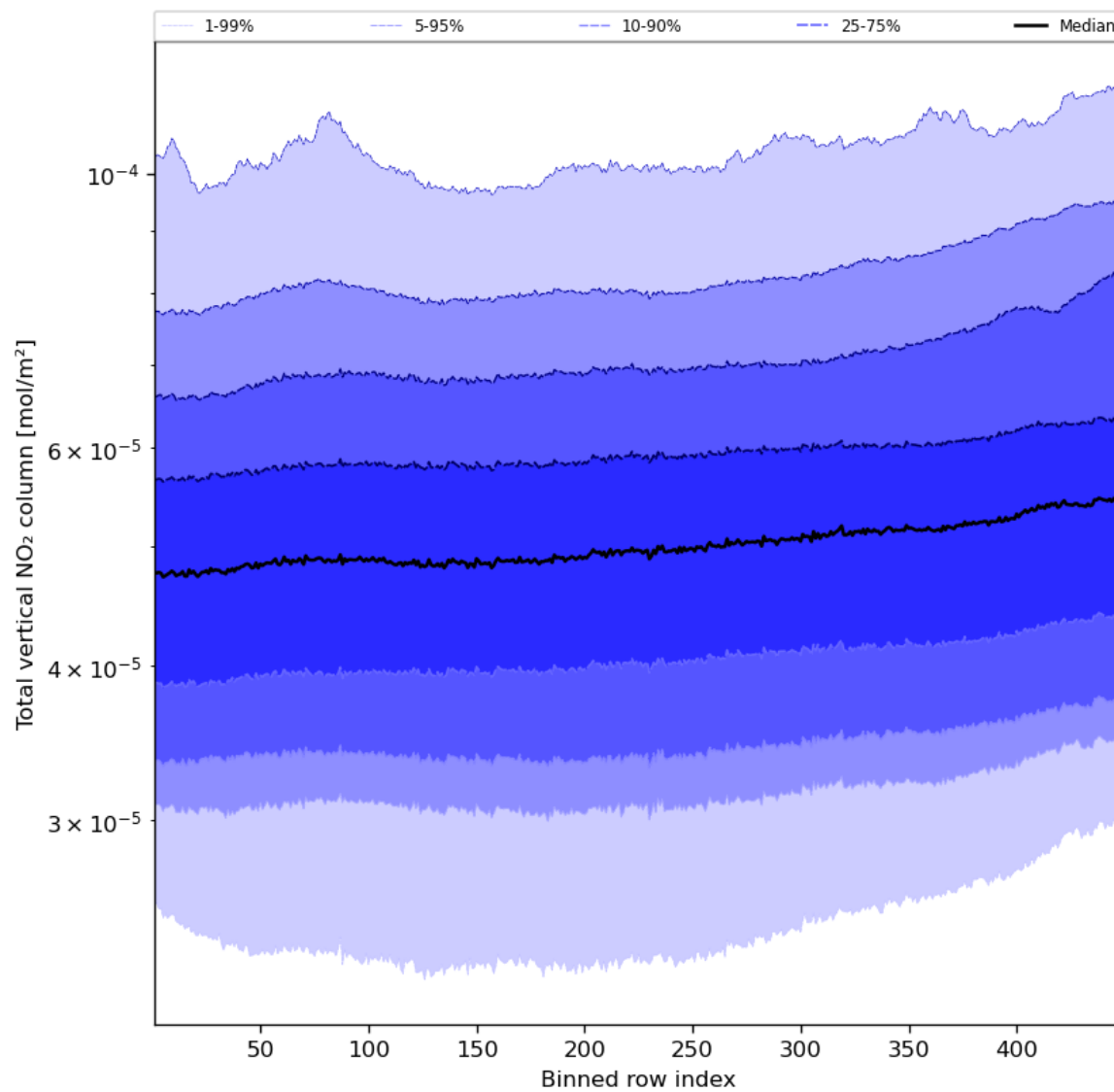
Figure 55: Along track statistics of “Total vertical NO 2 column” for 2023-10-22 to 2023-10-24
