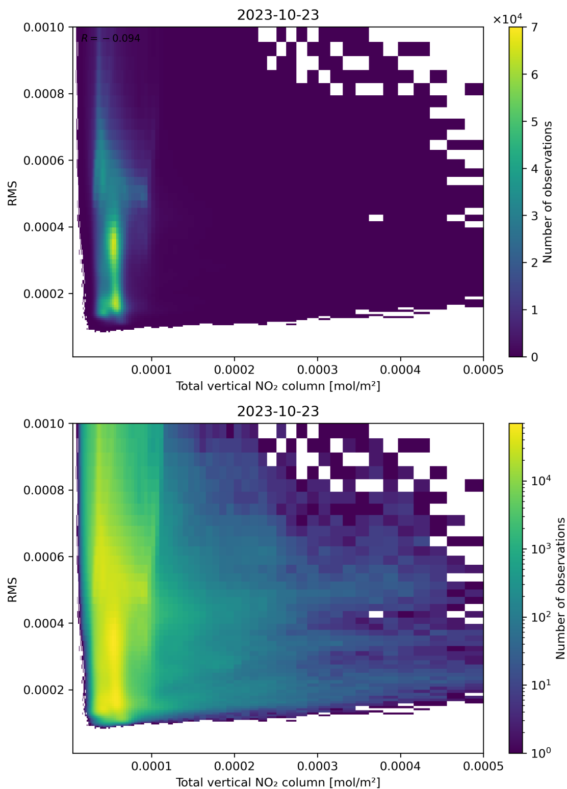
Figure 120: Scatter density plot of “Total vertical NO 2 column” against “RMS” for 2023-10-22 to 2023-10-24.
