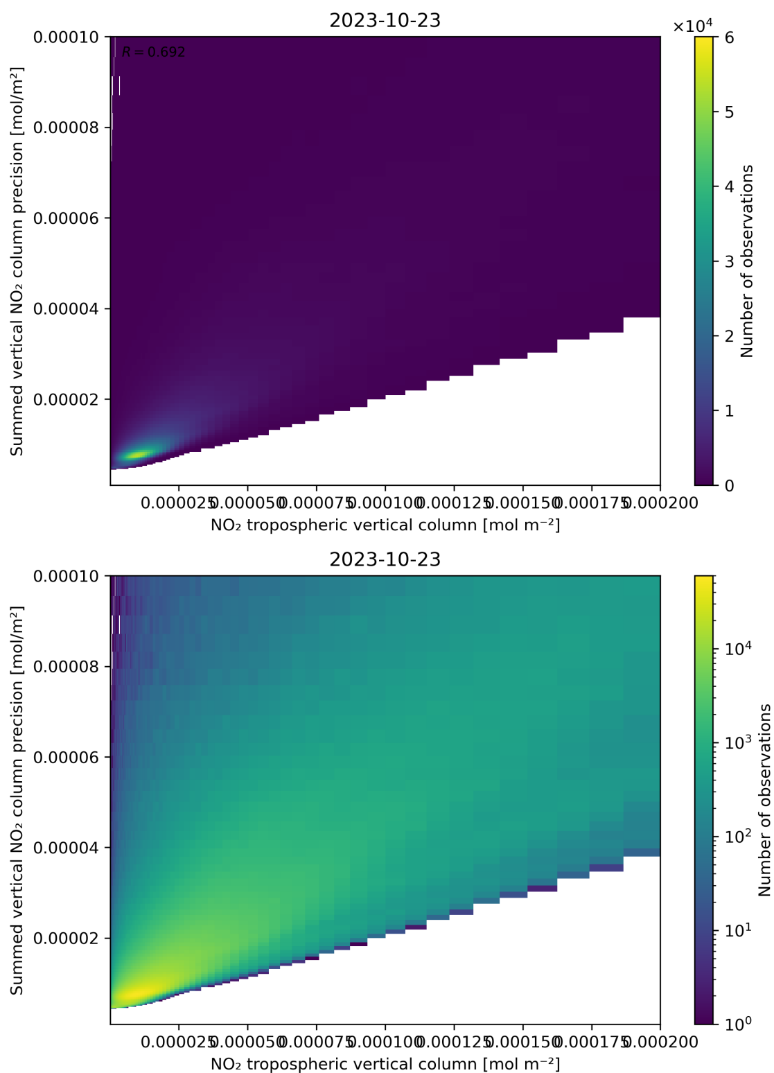
Figure 127: Scatter density plot of “NO 2 tropospheric vertical column” against “Summed vertical NO 2 column precision” for 2023-10-22 to 2023-10-24.
