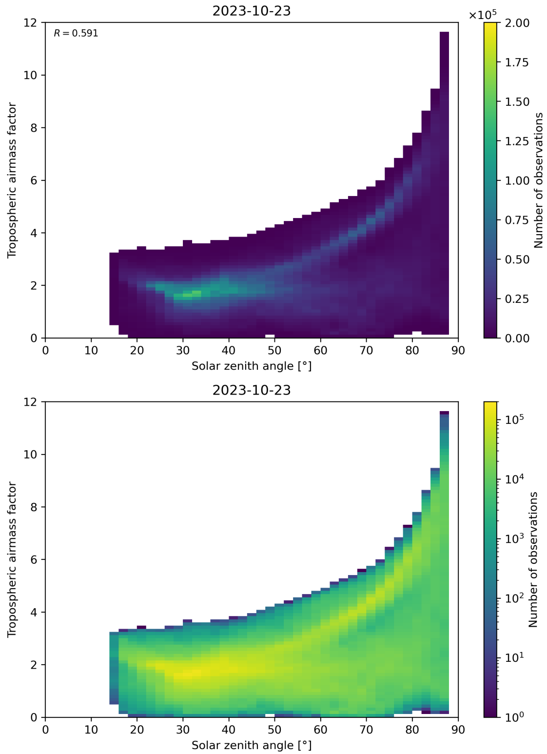
Figure 147: Scatter density plot of “Solar zenith angle” against “Tropospheric airmass factor” for 2023-10-22 to 2023-10-24.
