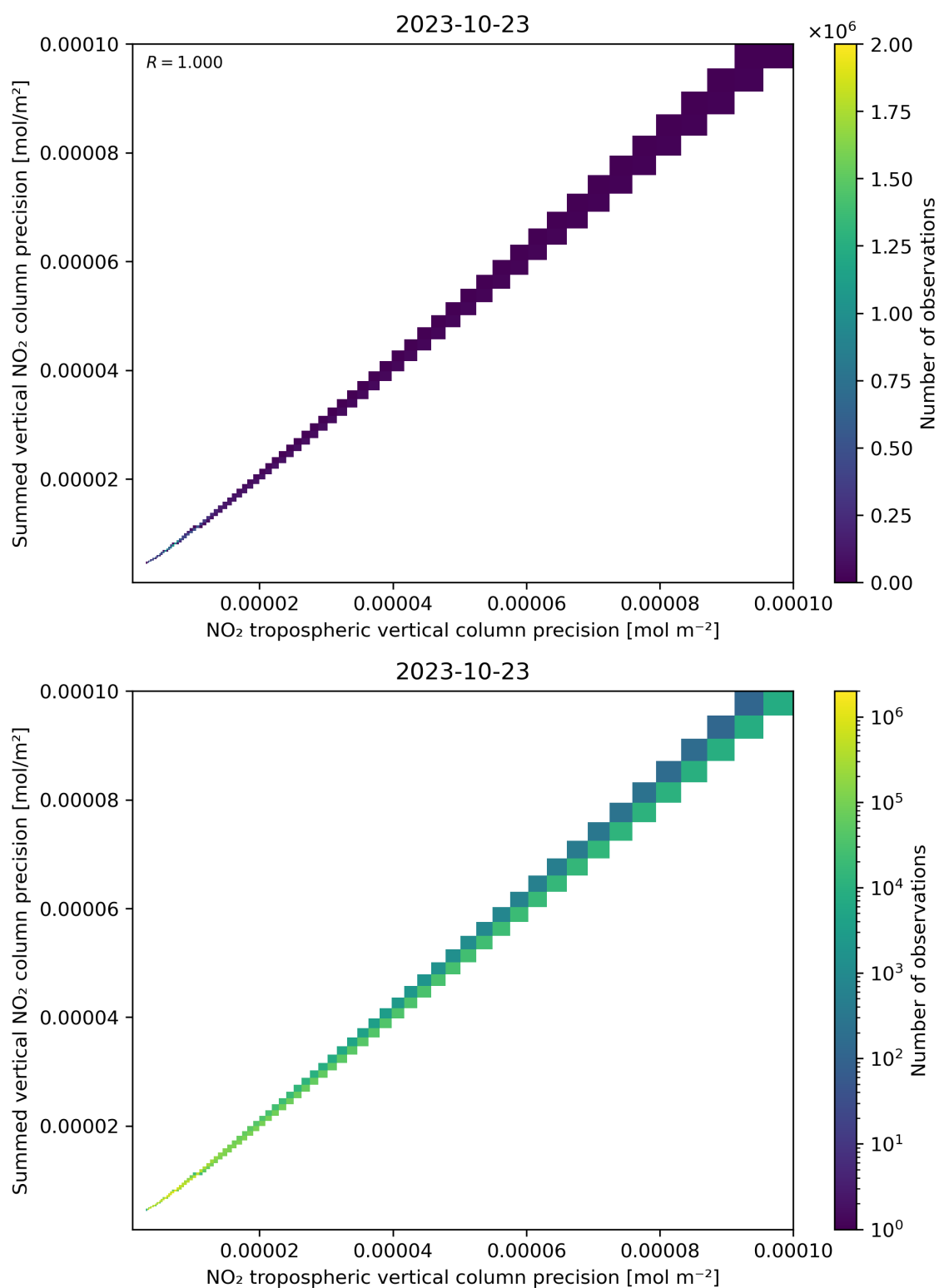
Figure 137: Scatter density plot of “NO 2 tropospheric vertical column precision” against “Summed vertical NO 2 column precision” for 2023-10-22 to 2023-10-24.
