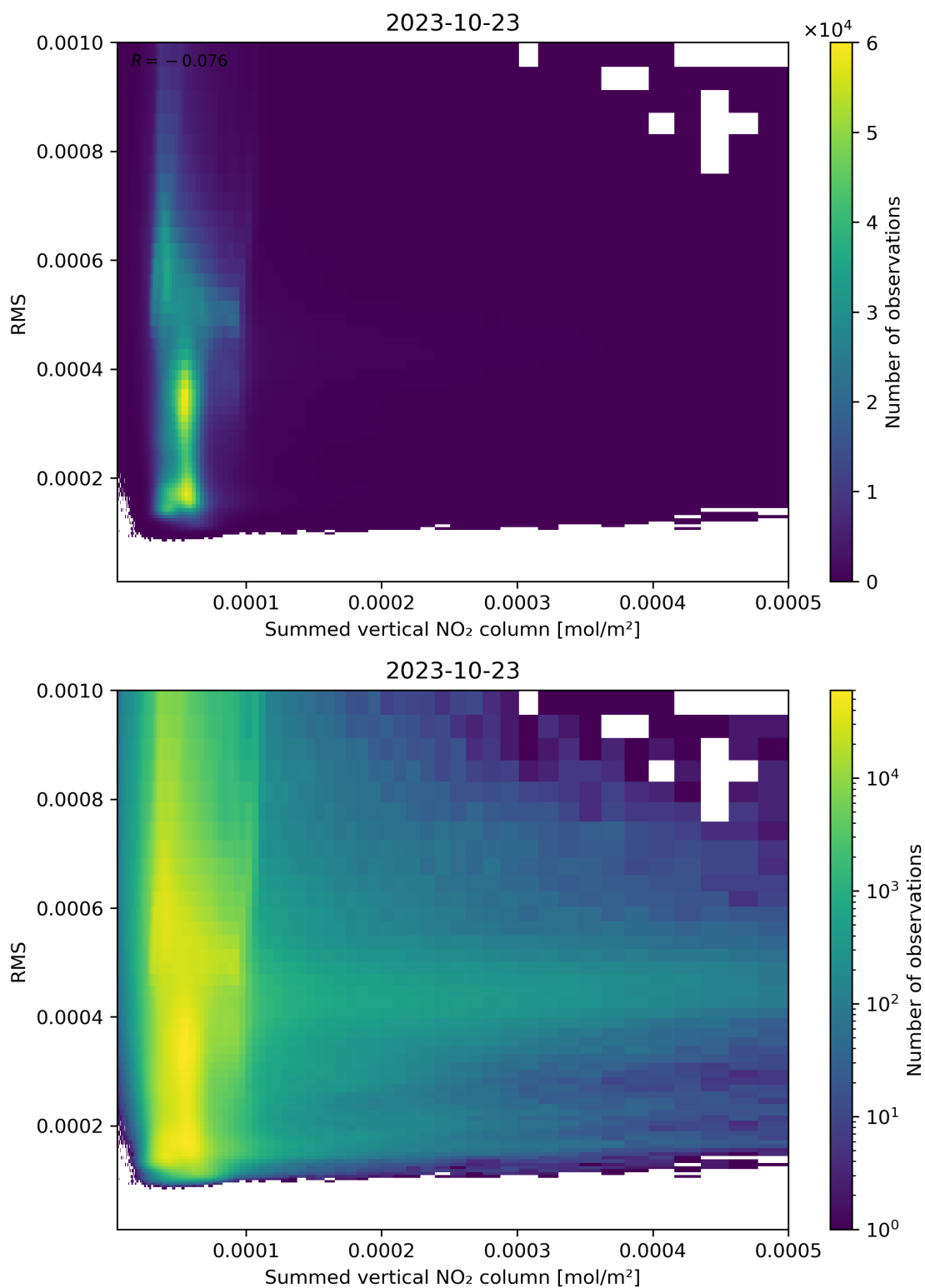
Figure 109: Scatter density plot of “Summed vertical NO 2 column” against “RMS” for 2023-10-22 to 2023-10-24.
