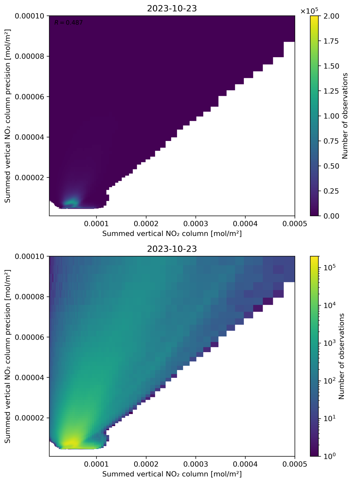
Figure 105: Scatter density plot of “Summed vertical NO 2 column” against “Summed vertical NO 2 column precision” for 2023-10-22 to 2023-10-24.
