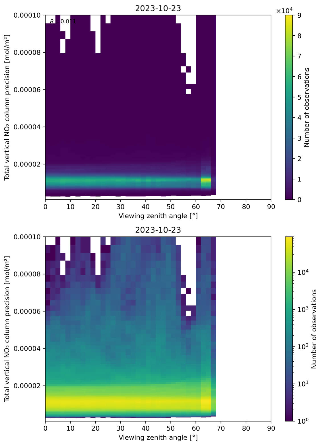
Figure 168: Scatter density plot of “Viewing zenith angle” against “Total vertical NO 2 column precision” for 2023-10-22 to 2023-10-24.
