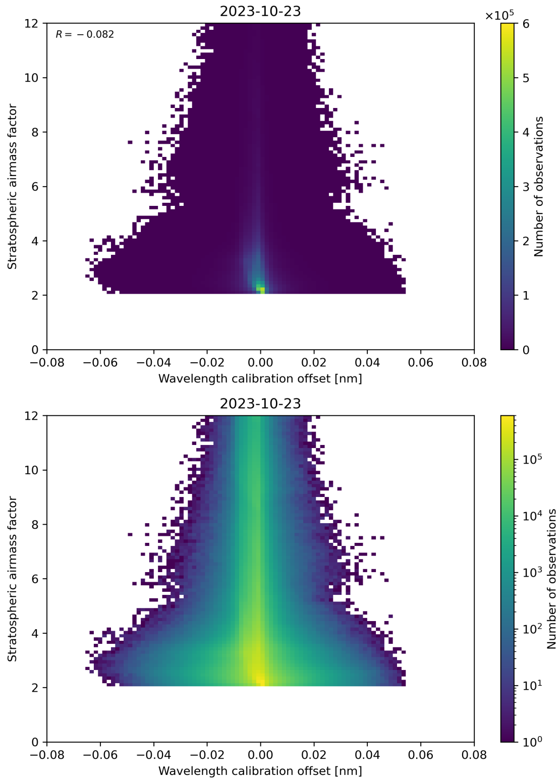
Figure 174: Scatter density plot of “Wavelength calibration offset” against “Stratospheric airmass factor” for 2023-10-22 to 2023-10-24.
