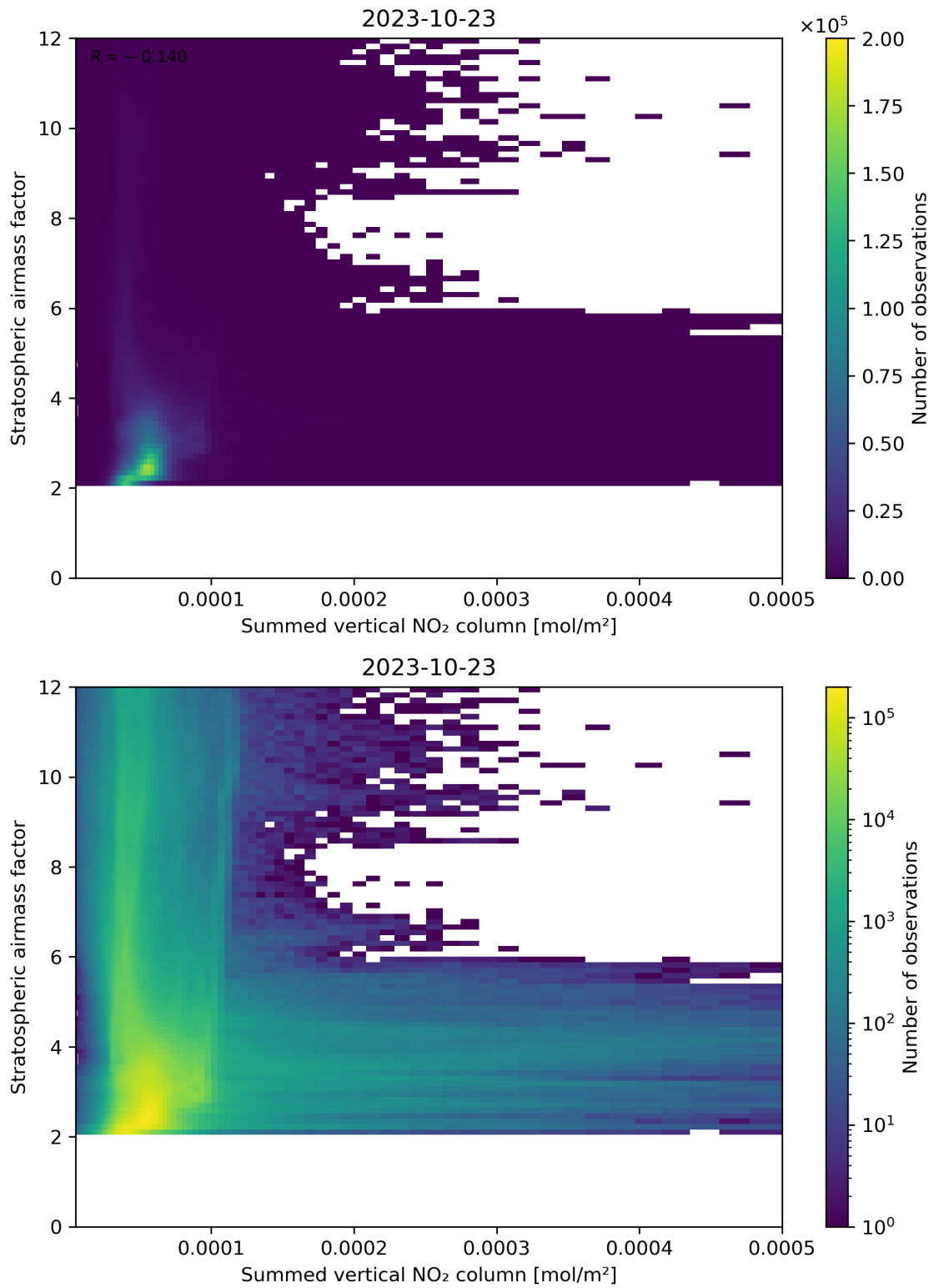
Figure 103: Scatter density plot of “Summed vertical NO 2 column” against “Stratospheric air mass factor” for 2023-10-22 to 2023-10-24.
