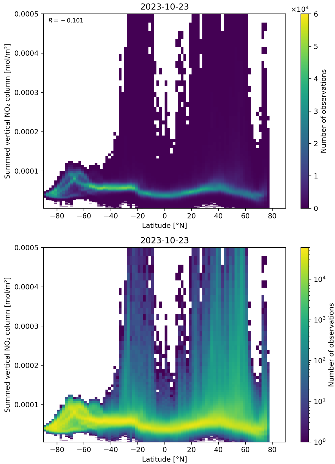
Figure 88: Scatter density plot of “Latitude” against “Summed vertical NO 2 column” for 2023-10-22 to 2023-10-24.
