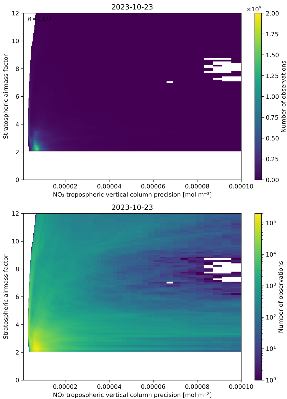
Figure 131: Scatter density plot of “NO 2 tropospheric vertical column precision” against “Stratospheric airmass factor” for 2023-10-22 to 2023-10-24.
