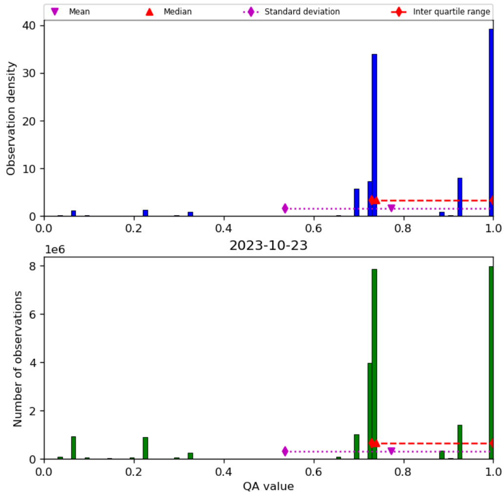
Figure 28: Histogram of “QA value” for 2023-10-22 to 2023-10-24
