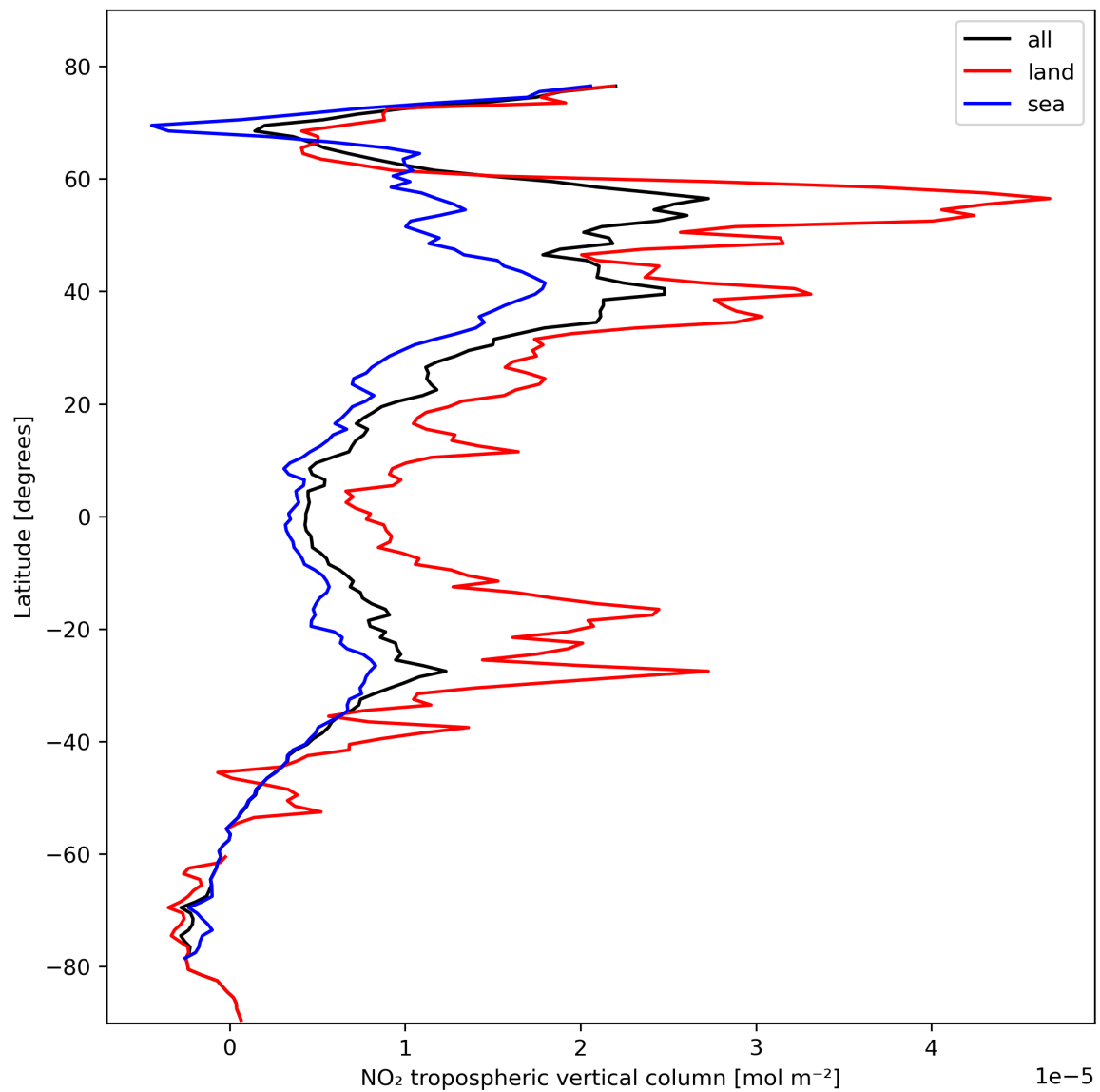
Figure 12: Zonal average of “NO 2 tropospheric vertical column” for 2023-10-22 to 2023-10-24.
