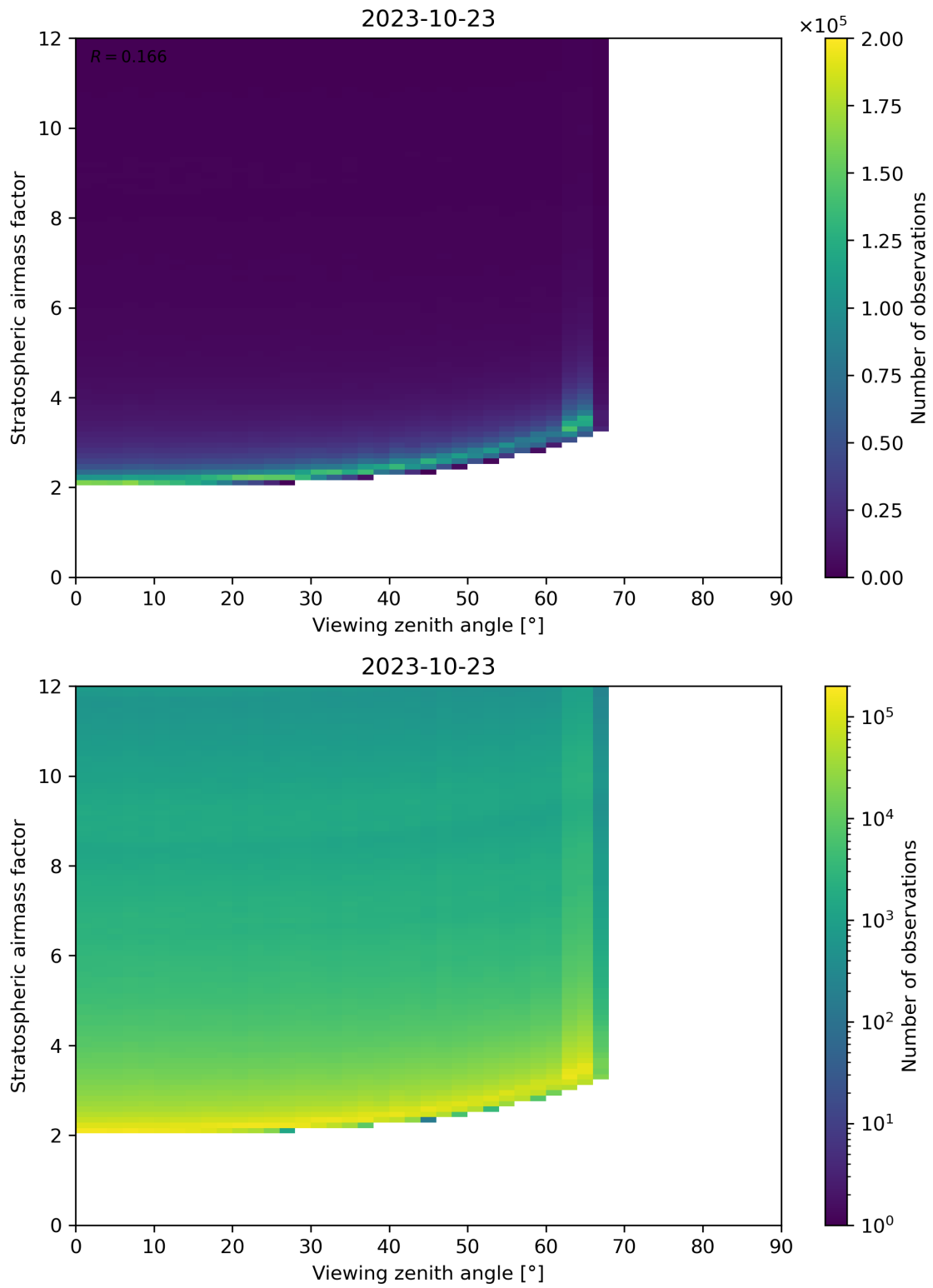
Figure 159: Scatter density plot of “Viewing zenith angle” against “Stratospheric airmass factor” for 2023-10-22 to 2023-10-24.
