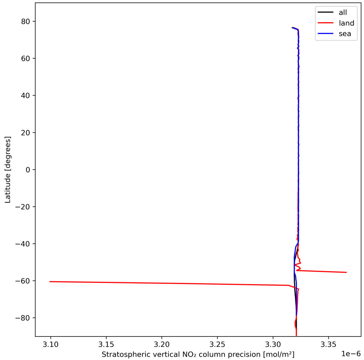
Figure 20: Zonal average of “Stratospheric vertical NO 2 column precision” for 2023-10-22 to 2023-10-24.
