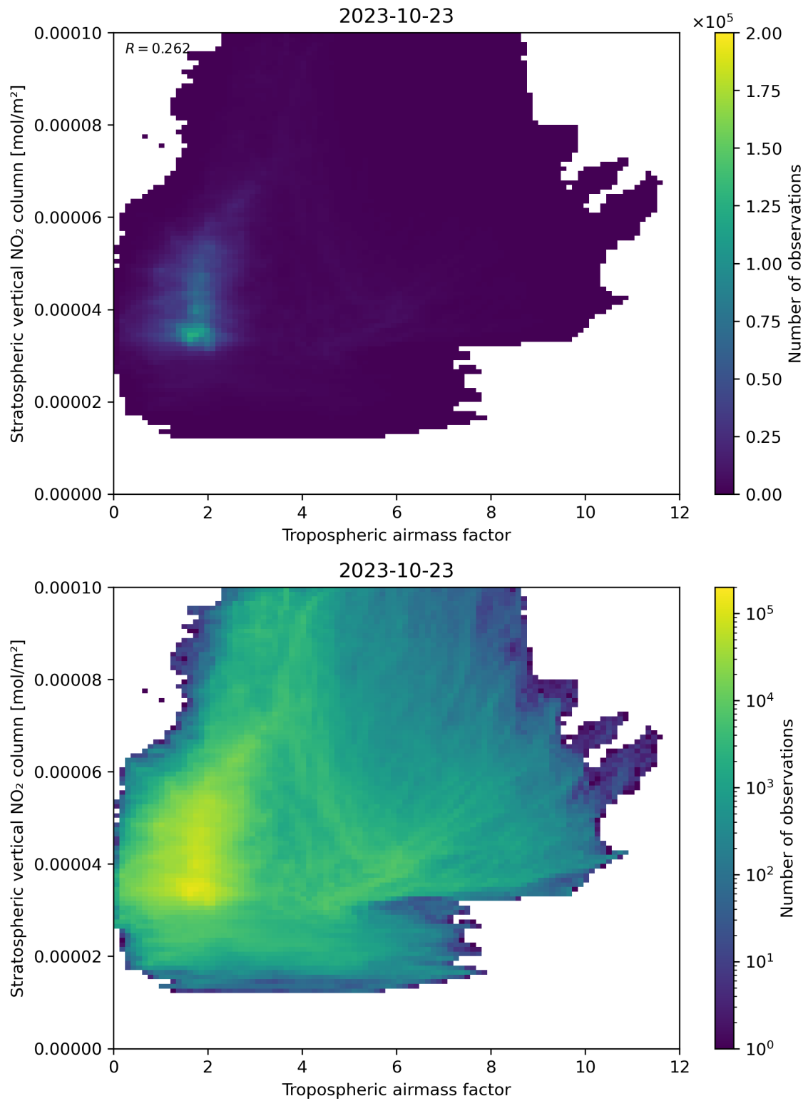
Figure 74: Scatter density plot of “Tropospheric air mass factor” against “Stratospheric vertical NO 2 column” for 2023-10-22 to 2023-10-24.
