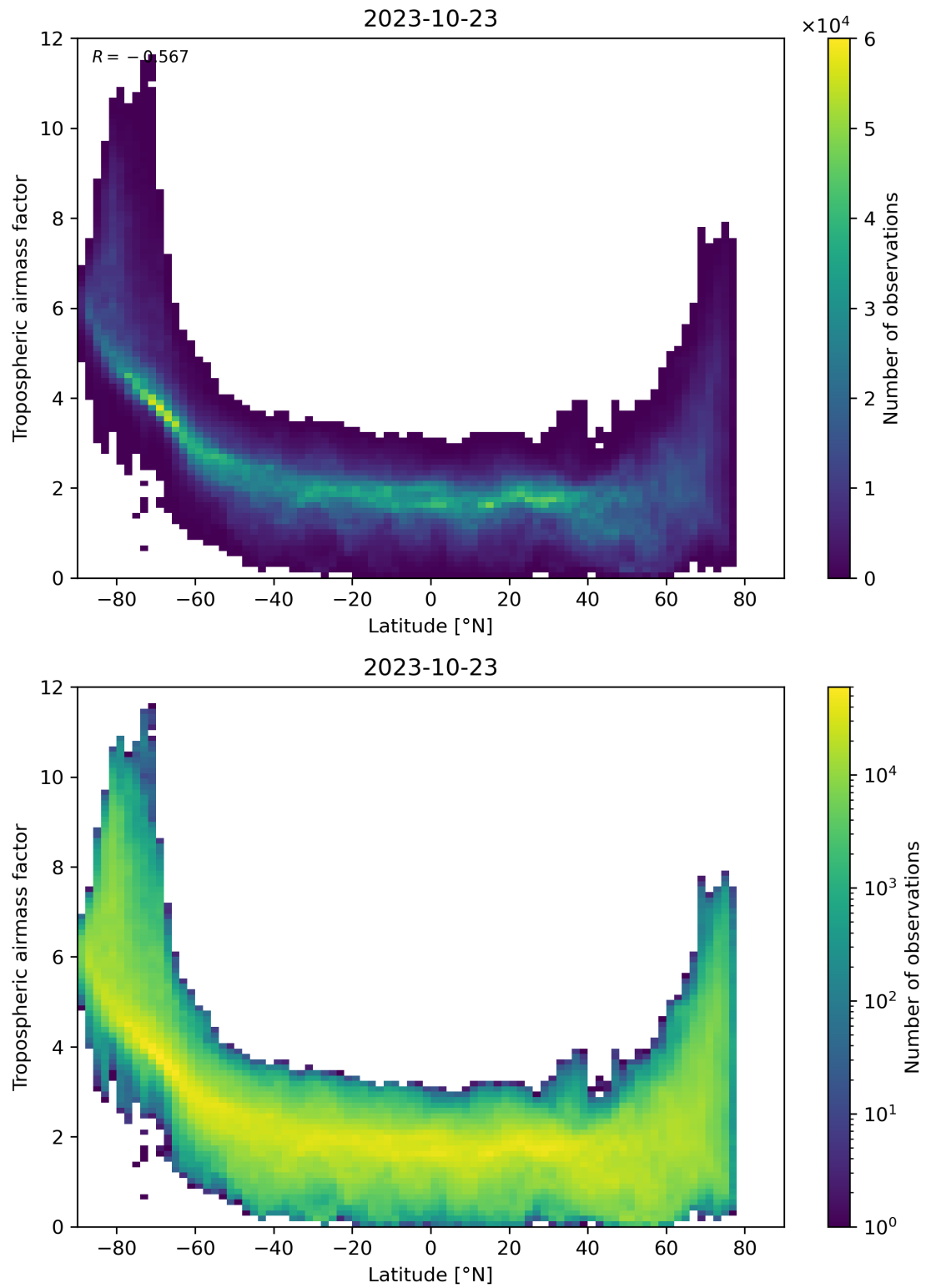
Figure 85: Scatter density plot of “Latitude” against “Tropospheric airmass factor” for 2023-10-22 to 2023-10-24.
