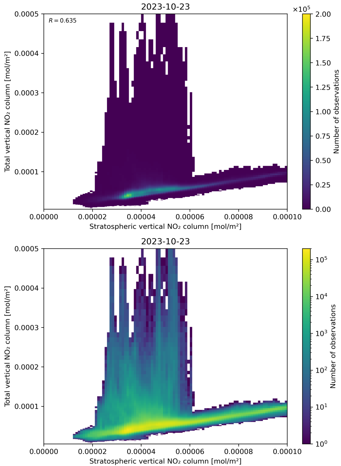
Figure 100: Scatter density plot of “Stratospheric vertical NO 2 column” against “Total vertical NO 2 column” for 2023-10-22 to 2023-10-24.
