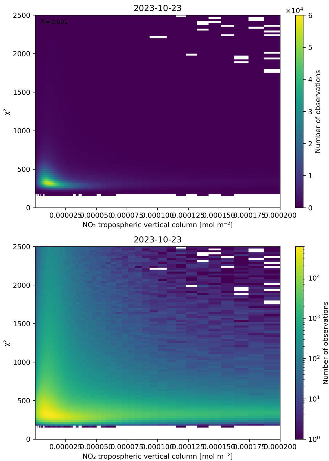
Figure 124: Scatter density plot of “NO 2 tropospheric vertical column” against “ \chi^2 ” for 2023-10-22 to 2023-10-24.
