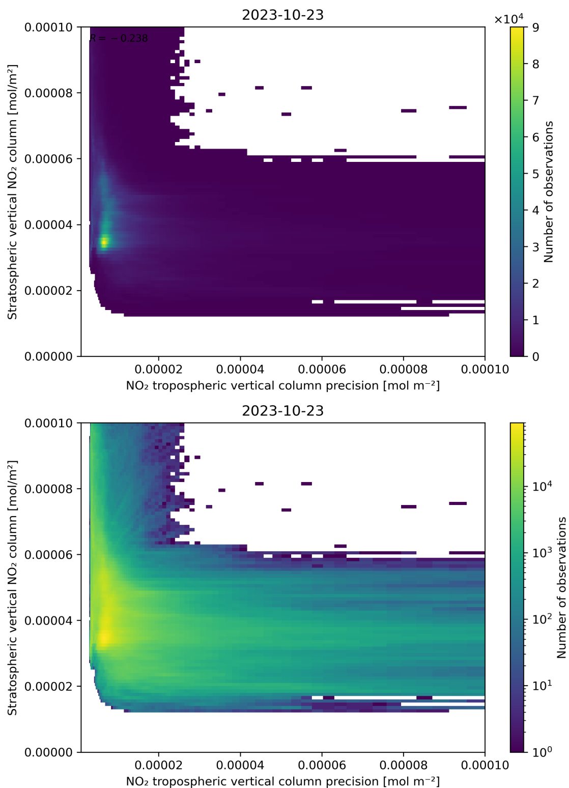
Figure 135: Scatter density plot of “NO 2 tropospheric vertical column precision” against “Stratospheric vertical NO 2 column” for 2023-10-22 to 2023-10-24.
