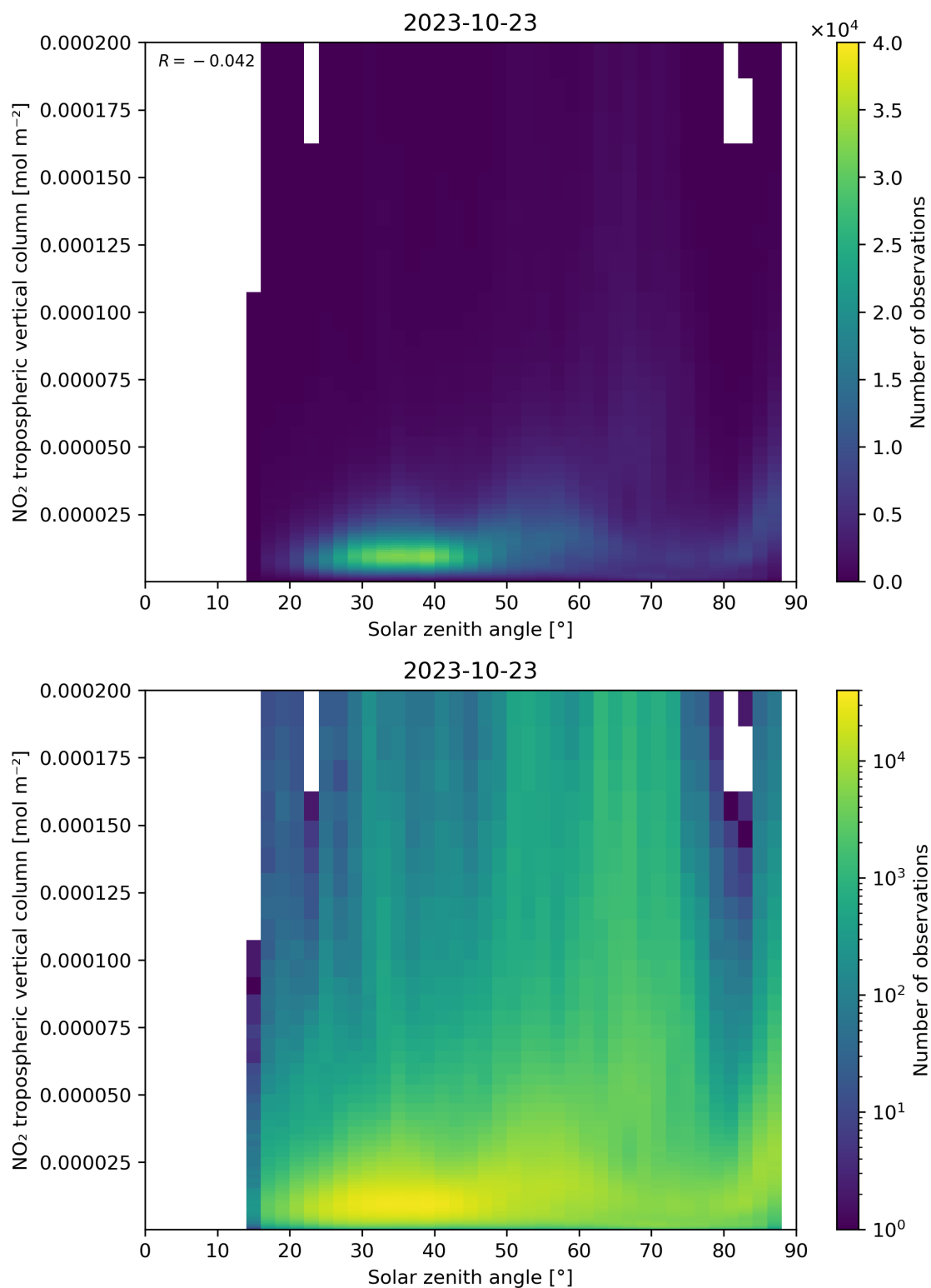
Figure 155: Scatter density plot of “Solar zenith angle” against “NO 2 tropospheric vertical column” for 2023-10-22 to 2023-10-24.
