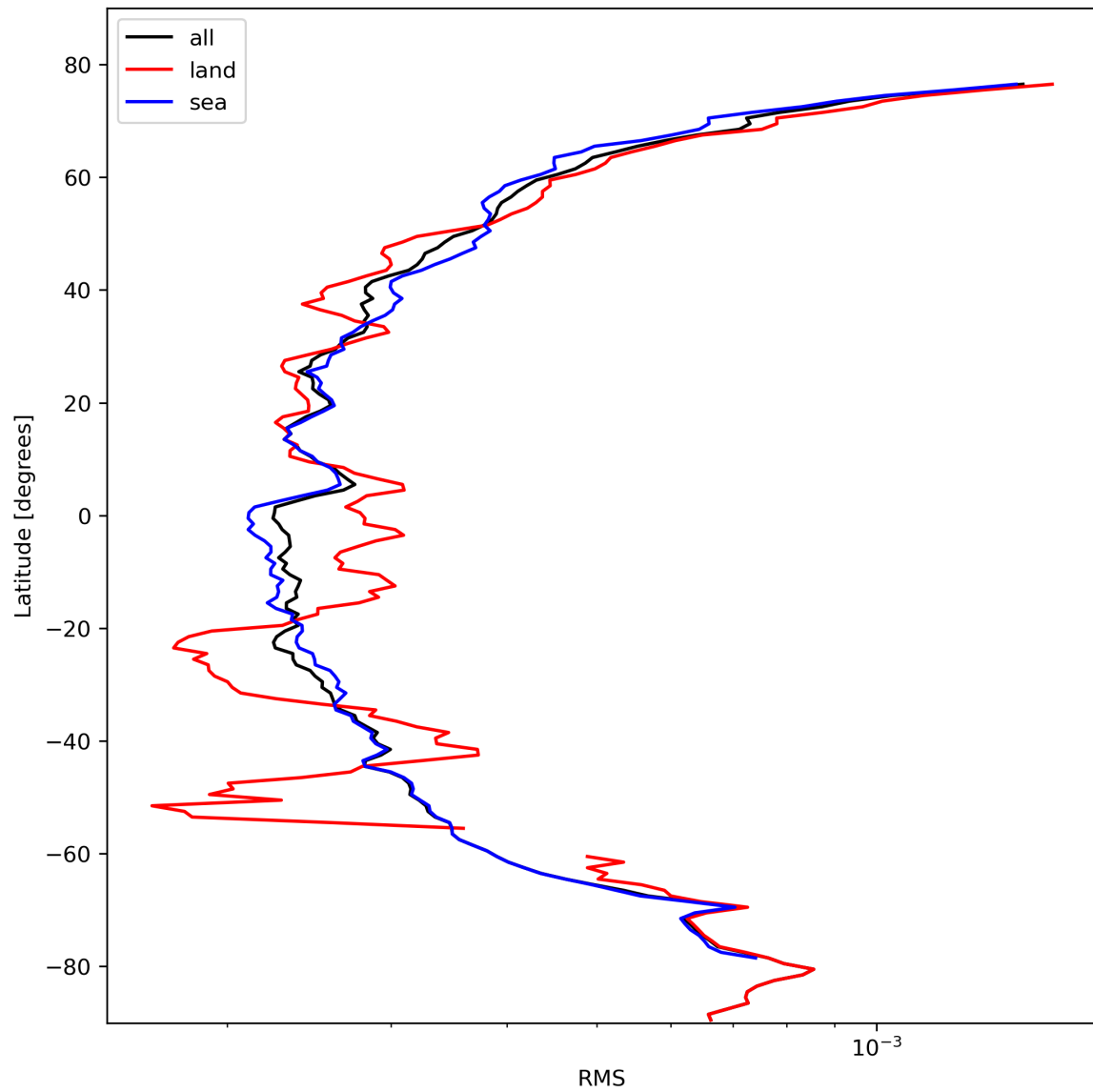
Figure 26: Zonal average of “RMS” for 2023-10-22 to 2023-10-24.
