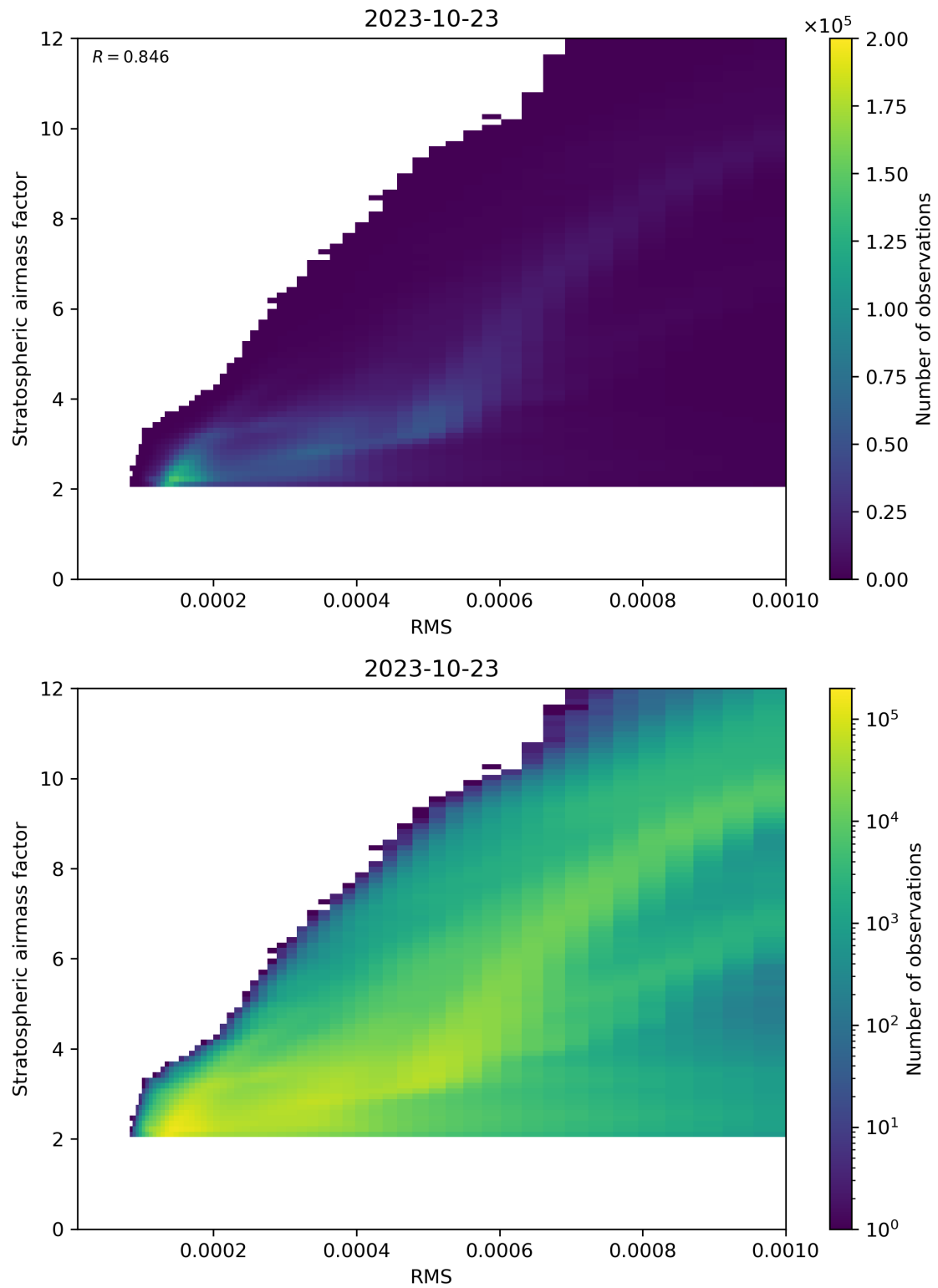
Figure 144: Scatter density plot of “RMS” against “Stratospheric airmass factor” for 2023-10-22 to 2023-10-24.
