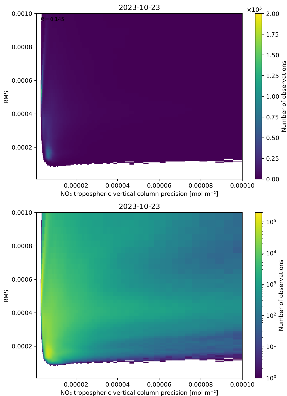
Figure 140: Scatter density plot of “NO 2 tropospheric vertical column precision” against “RMS” for 2023-10-22 to 2023-10-24.
