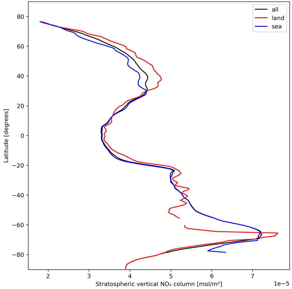
Figure 19: Zonal average of “Stratospheric vertical NO 2 column” for 2023-10-22 to 2023-10-24.
