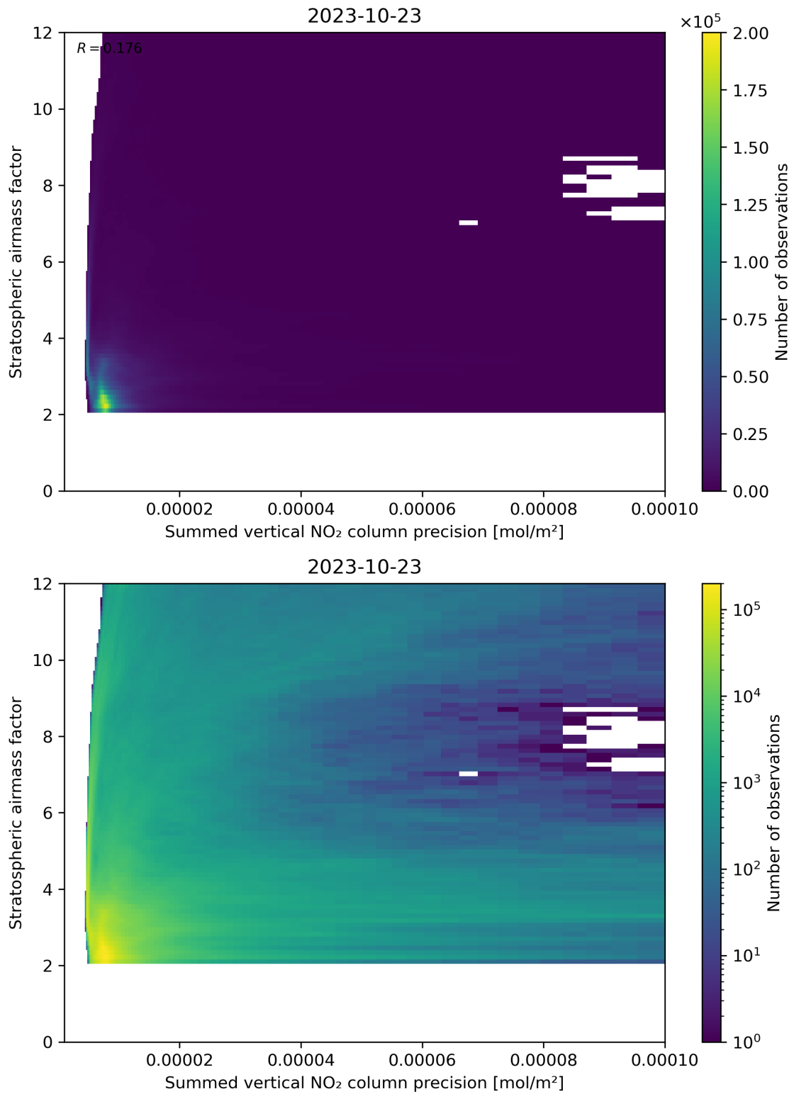
Figure 106: Scatter density plot of “Summed vertical NO 2 column precision” against “Stratospheric airmass factor” for 2023-10-22 to 2023-10-24.
