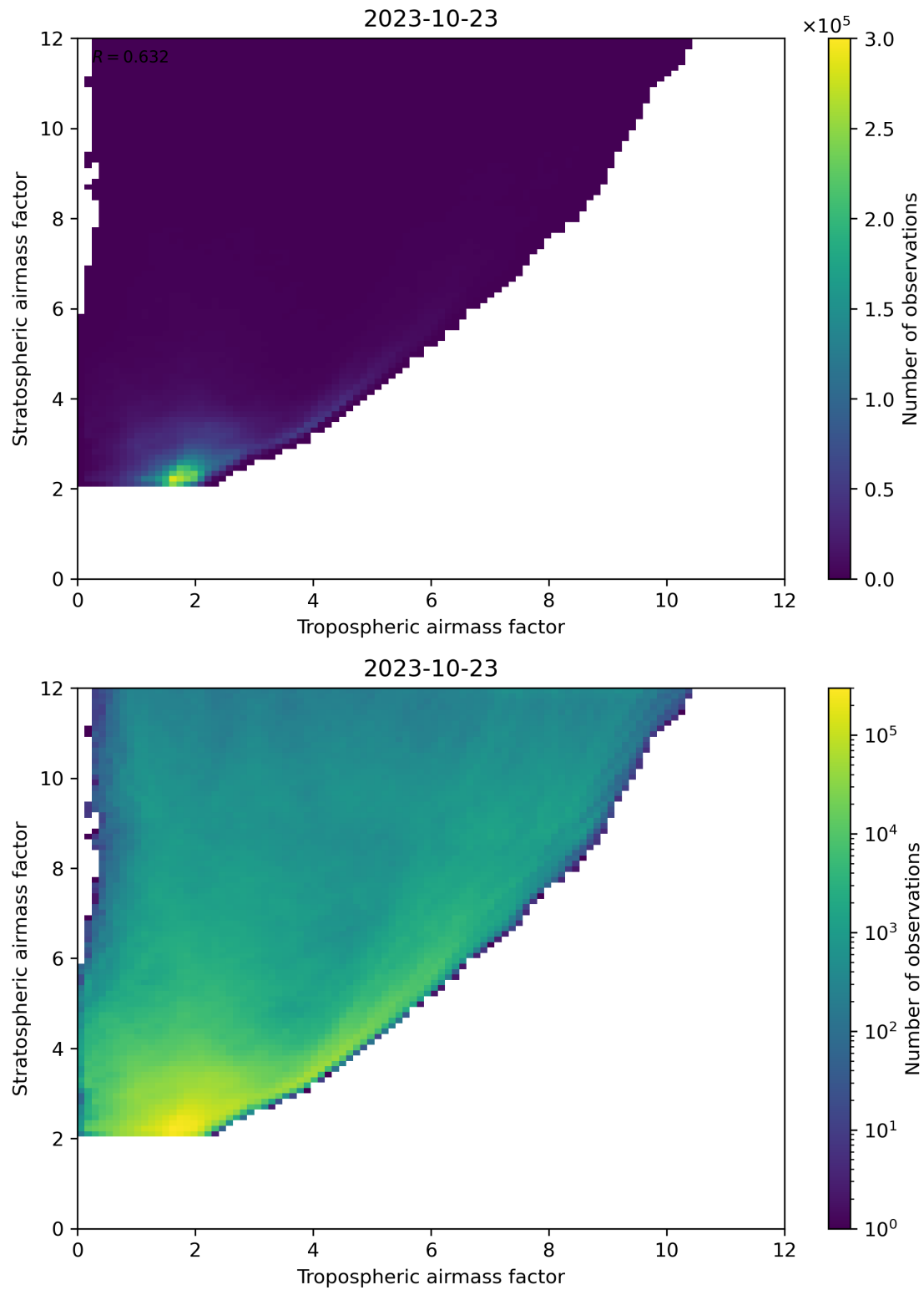
Figure 71: Scatter density plot of “Tropospheric airmass factor” against “Stratospheric airmass factor” for 2023-10-22 to 2023-10-24.
