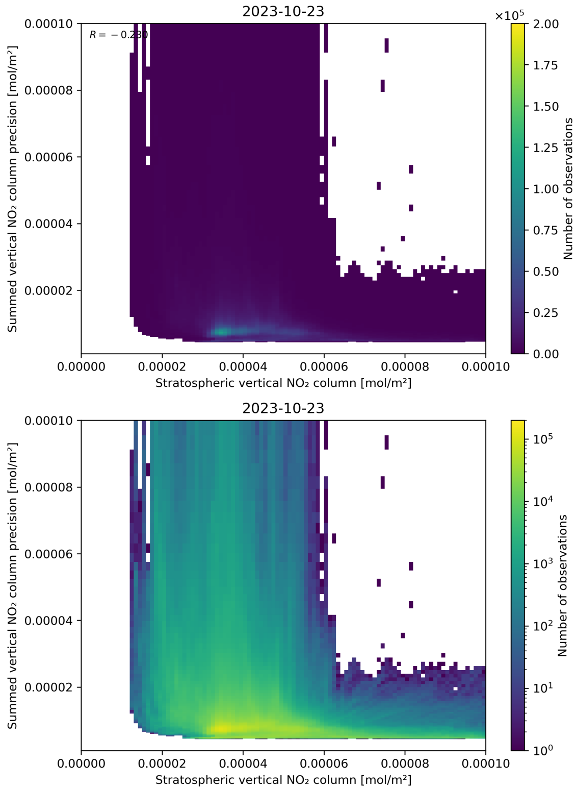
Figure 99: Scatter density plot of “Stratospheric vertical NO 2 column” against “Summed vertical NO 2 column precision” for 2023-10-22 to 2023-10-24.
