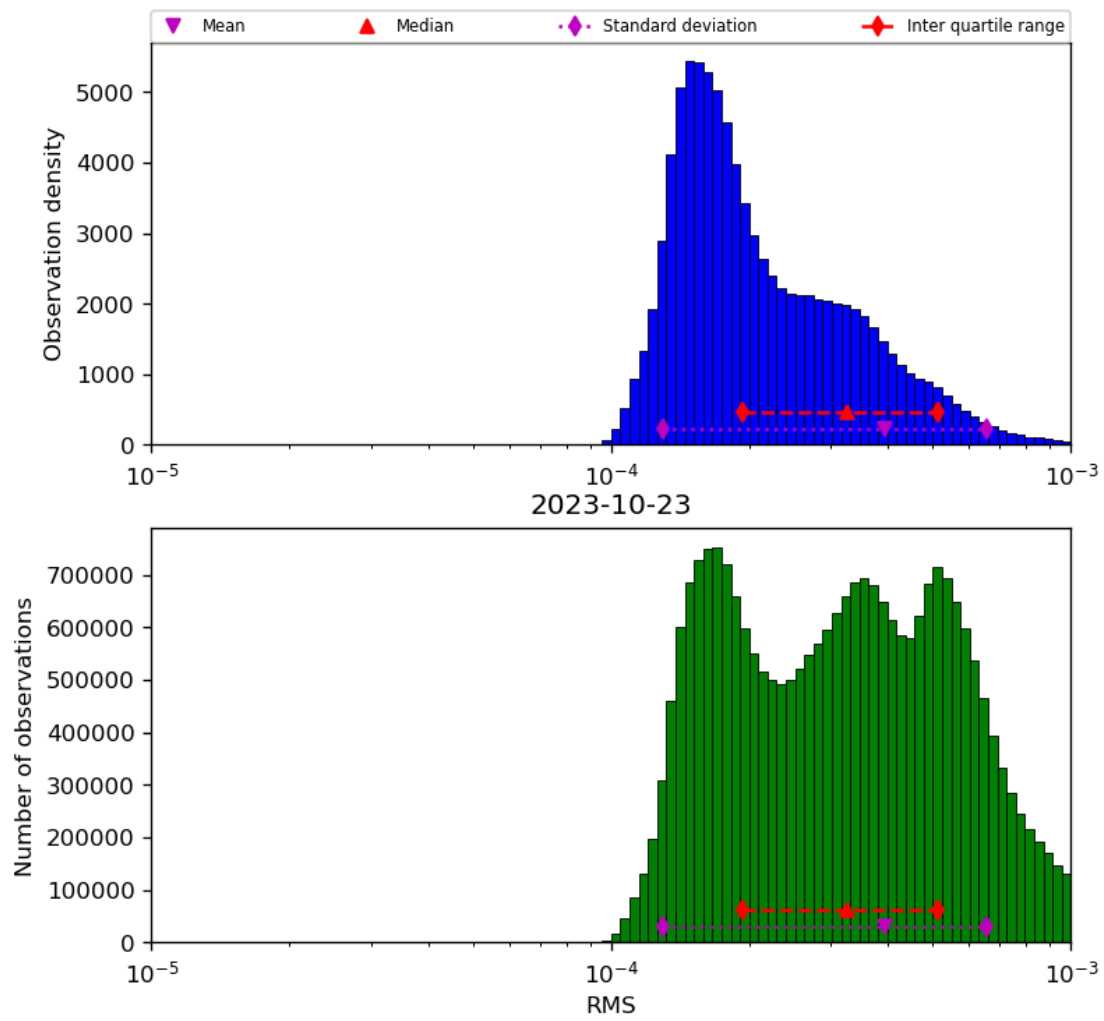
Figure 43: Histogram of “RMS” for 2023-10-22 to 2023-10-24
