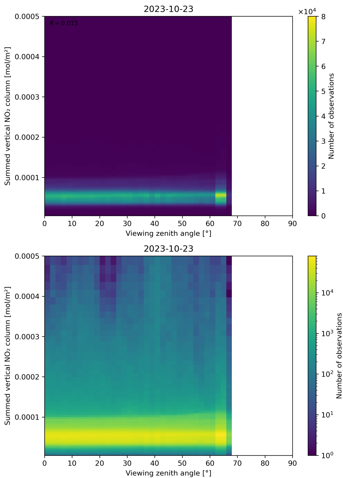
Figure 165: Scatter density plot of “Viewing zenith angle” against “Summed vertical NO 2 column” for 2023-10-22 to 2023-10-24.
