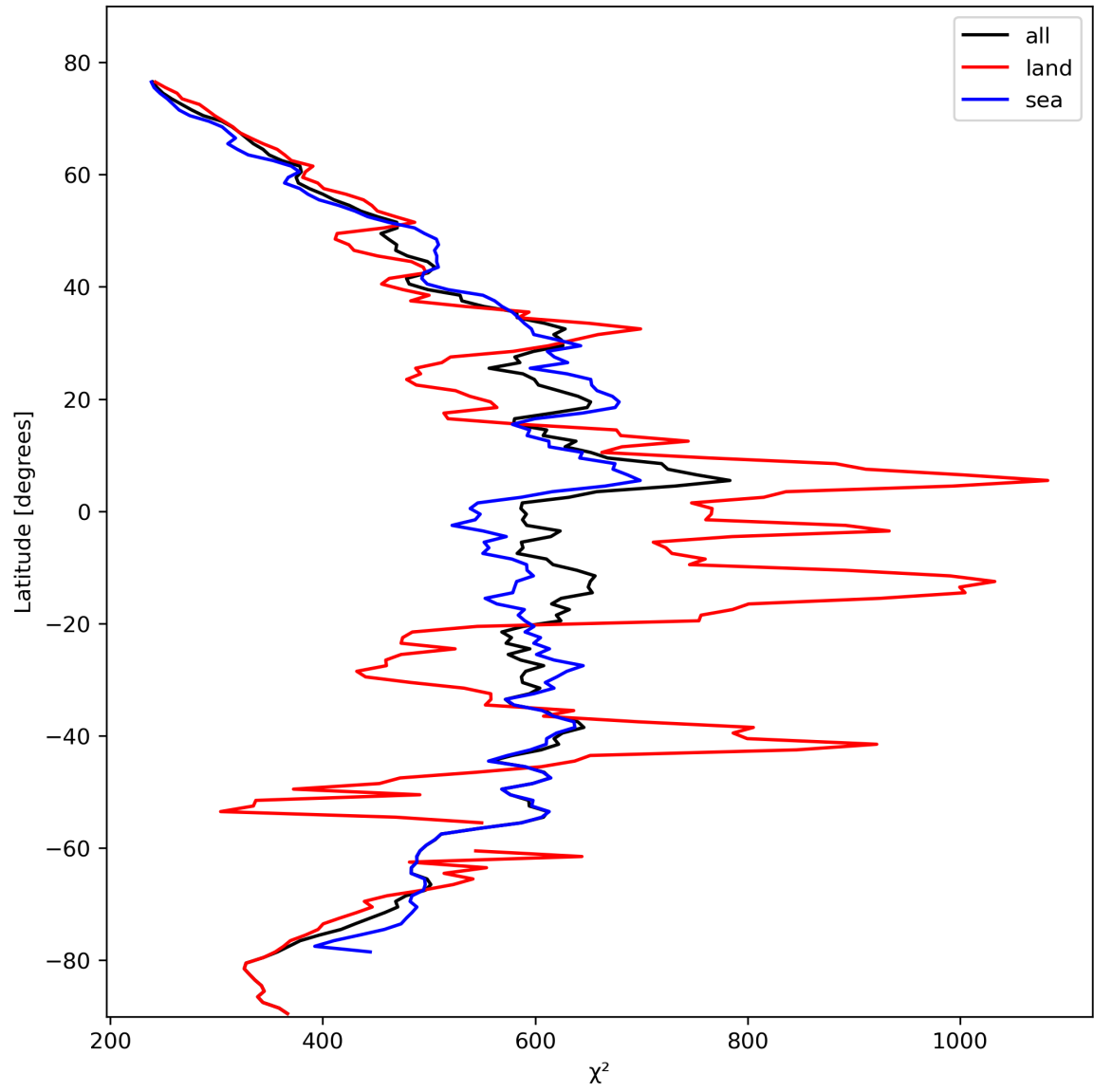
Figure 25: Zonal average of “ \chi^2 ” for 2023-10-22 to 2023-10-24.
