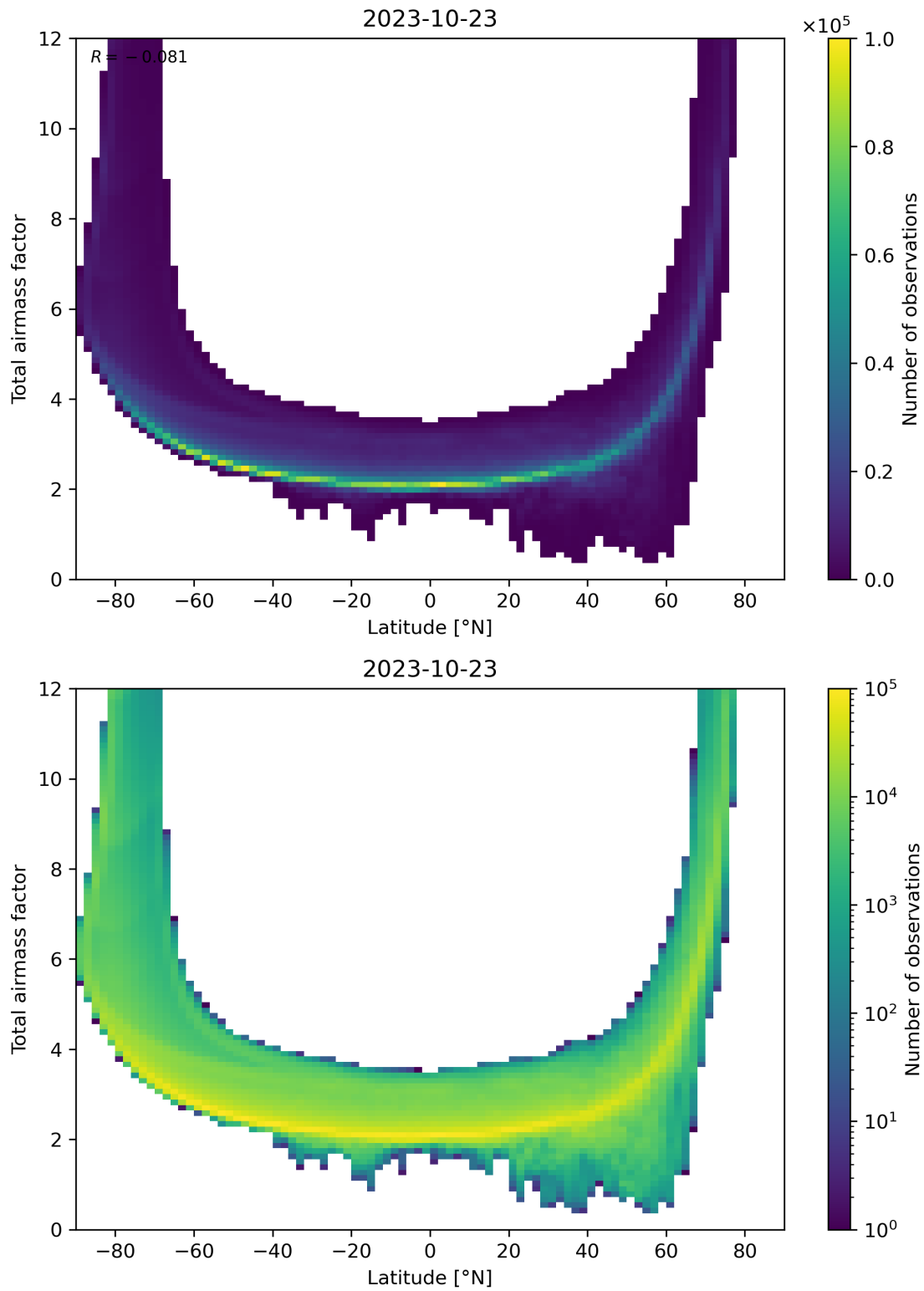
Figure 84: Scatter density plot of “Latitude” against “Total airmass factor” for 2023-10-22 to 2023-10-24.
