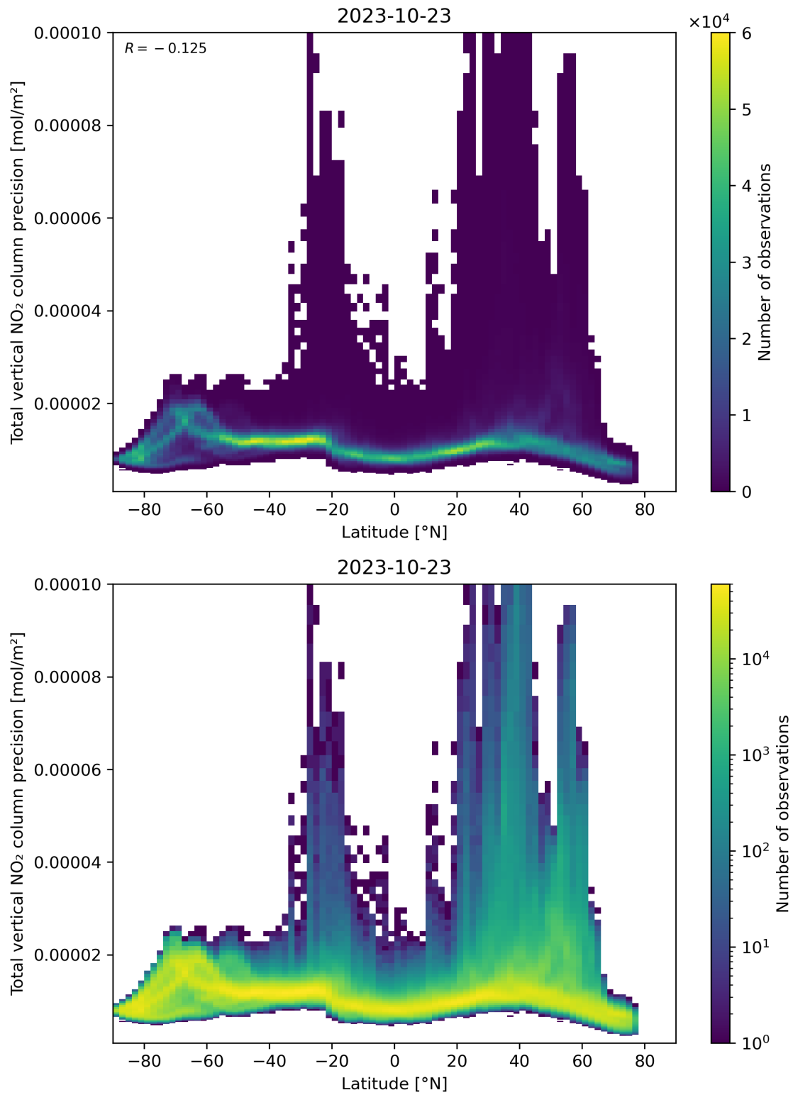
Figure 91: Scatter density plot of “Latitude” against “Total vertical NO 2 column precision” for 2023-10-22 to 2023-10-24.
