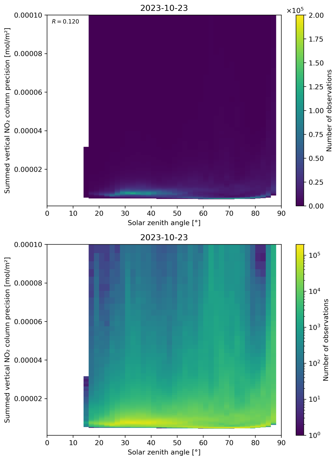
Figure 152: Scatter density plot of “Solar zenith angle” against “Summed vertical NO 2 column precision” for 2023-10-22 to 2023-10-24.
