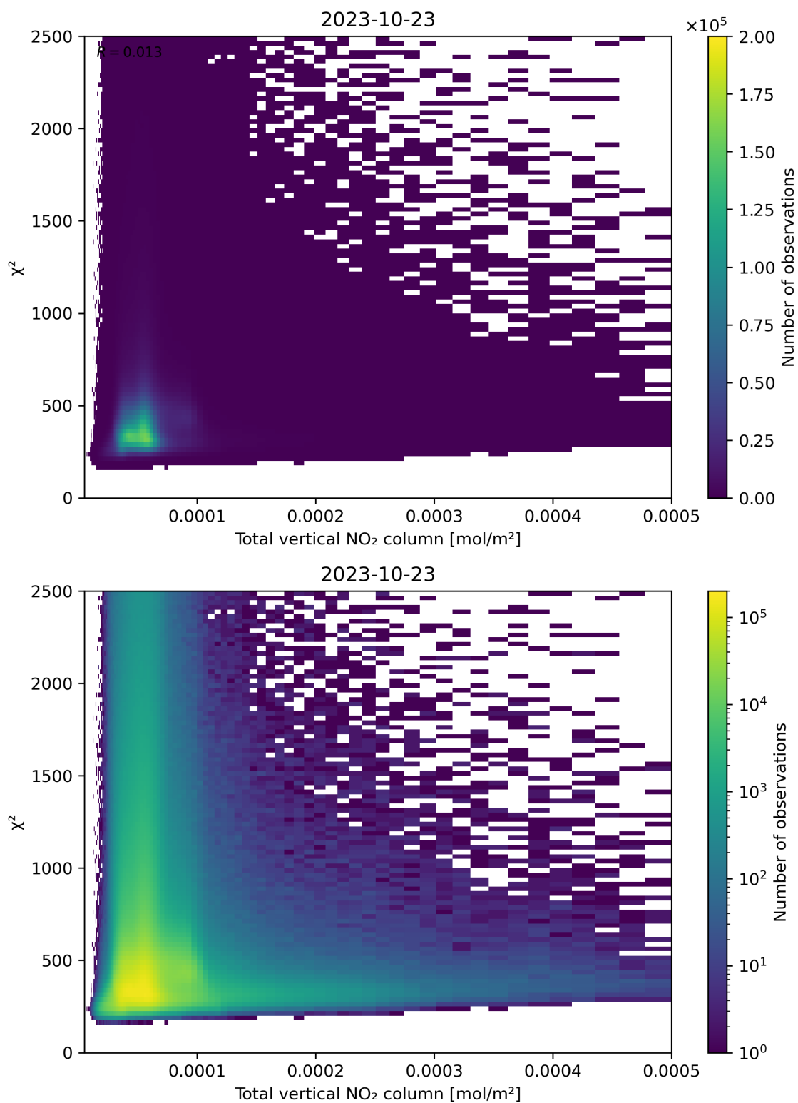
Figure 111: Scatter density plot of “Total vertical NO 2 column” against “ \chi^2 ” for 2023-10-22 to 2023-10-24.
