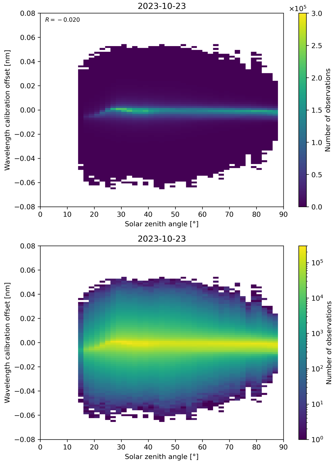
Figure 158: Scatter density plot of “Solar zenith angle” against “Wavelength calibration offset” for 2023-10-22 to 2023-10-24.
