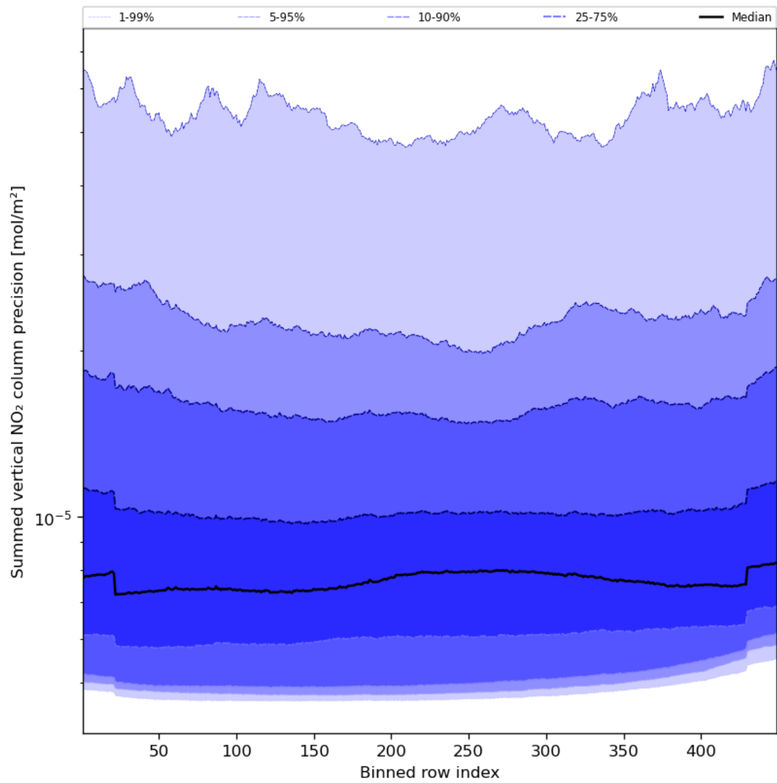
Figure 58: Along track statistics of “Summed vertical NO 2 column precision” for 2023-10-22 to 2023-10-24
