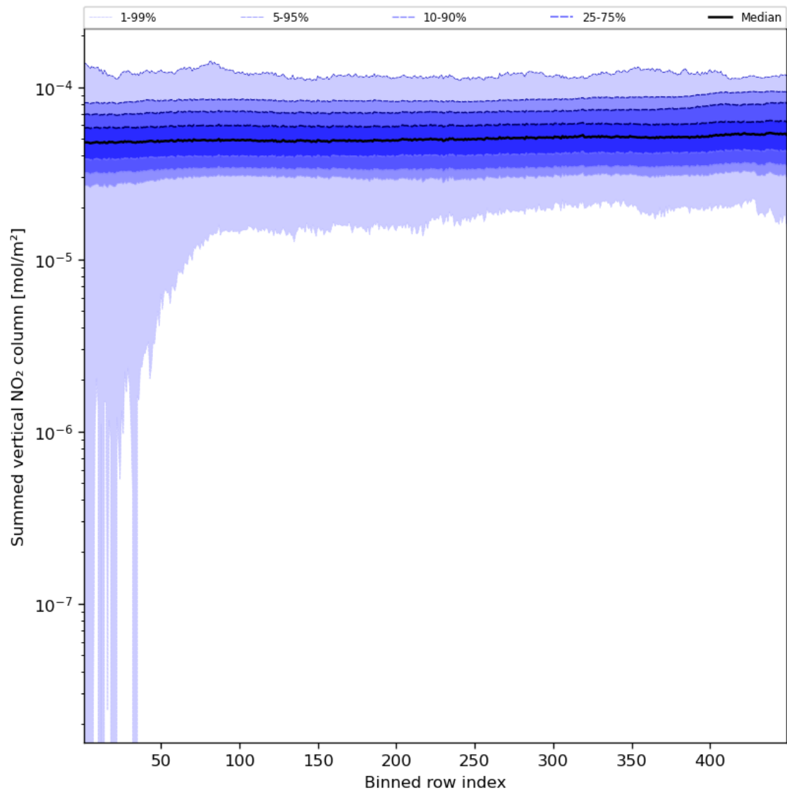
Figure 57: Along track statistics of “Summed vertical NO 2 column” for 2023-10-22 to 2023-10-24
