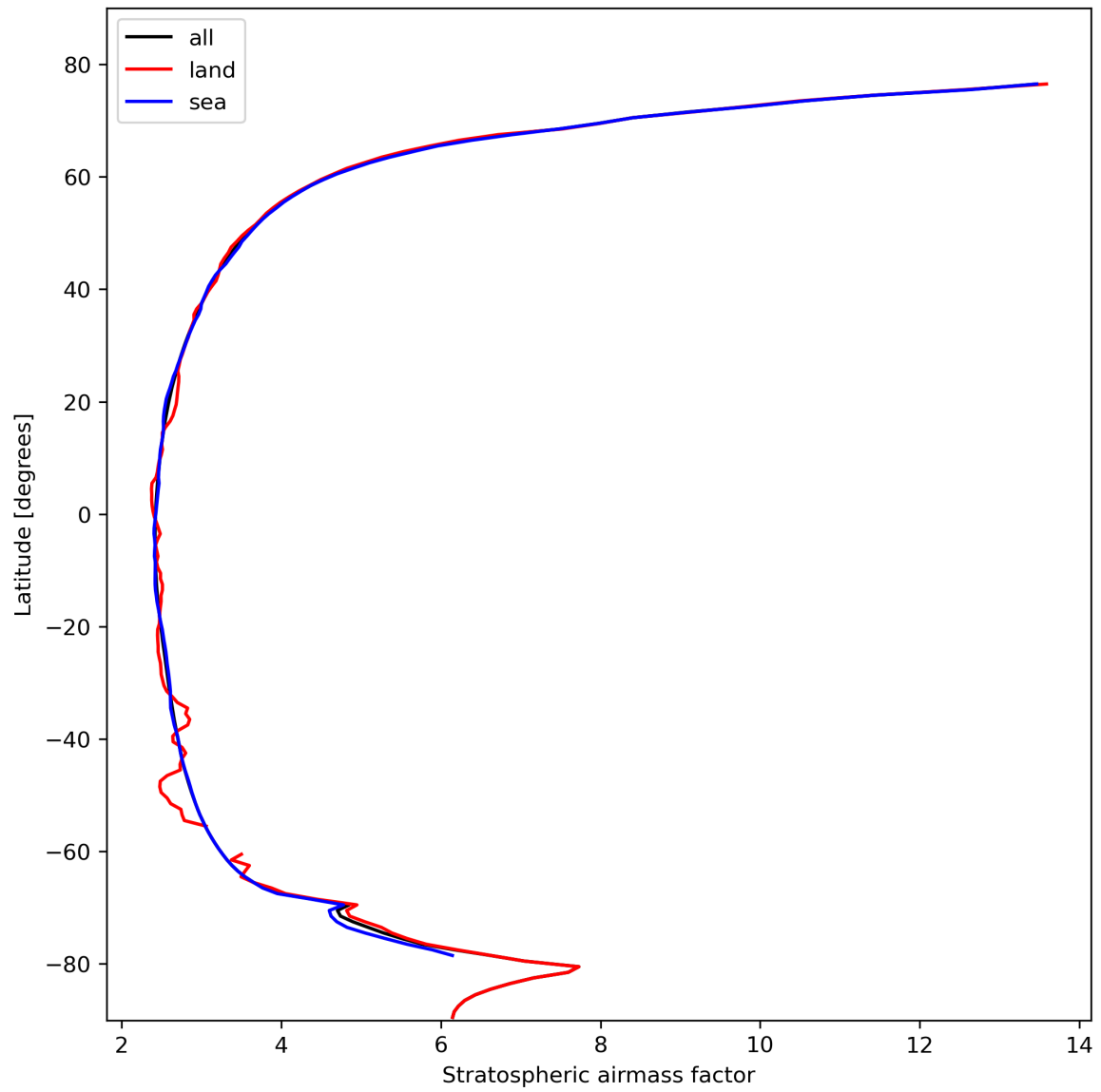
Figure 27: Zonal average of “Stratospheric airmass factor” for 2023-10-22 to 2023-10-24.
