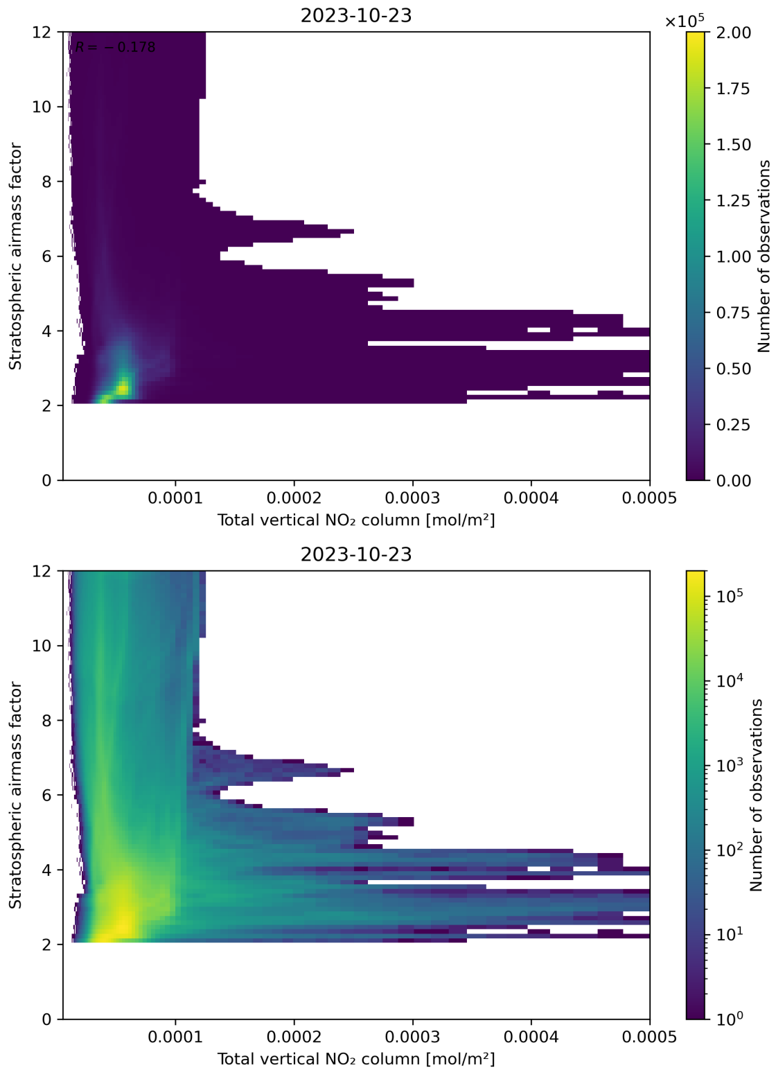
Figure 110: Scatter density plot of “Total vertical NO 2 column” against “Stratospheric airmass factor” for 2023-10-22 to 2023-10-24.
