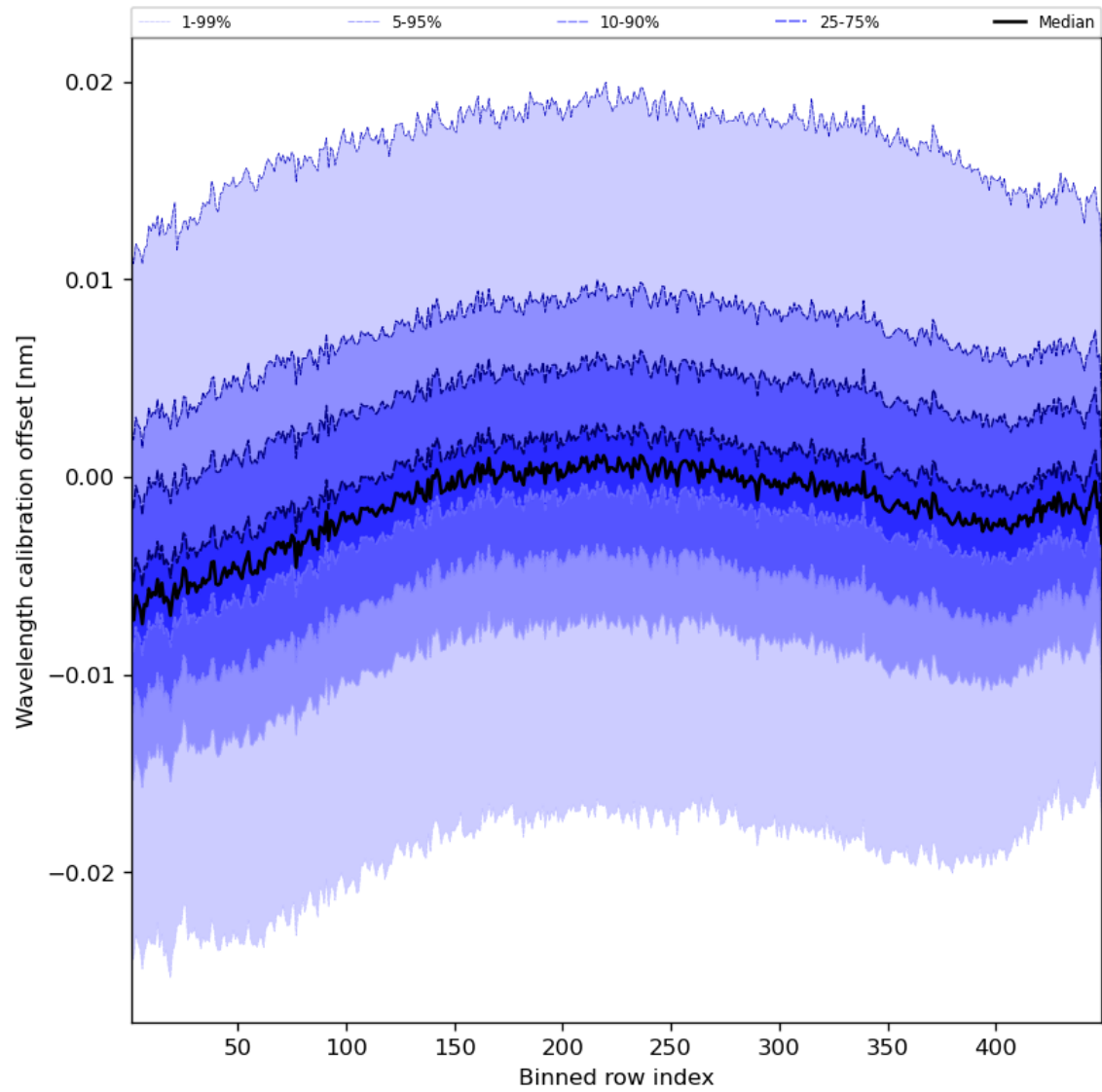
Figure 52: Along track statistics of “Wavelength calibration offset” for 2023-10-22 to 2023-10-24
