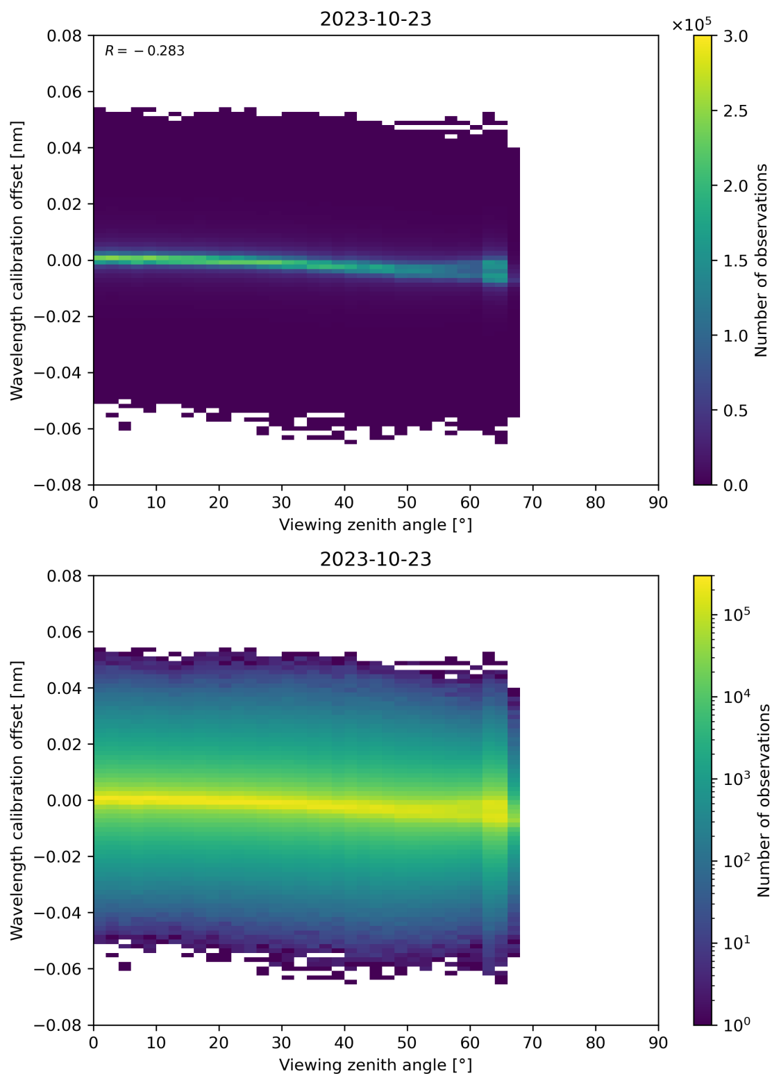
Figure 173: Scatter density plot of “Viewing zenith angle” against “Wavelength calibration offset” for 2023-10-22 to 2023-10-24.
