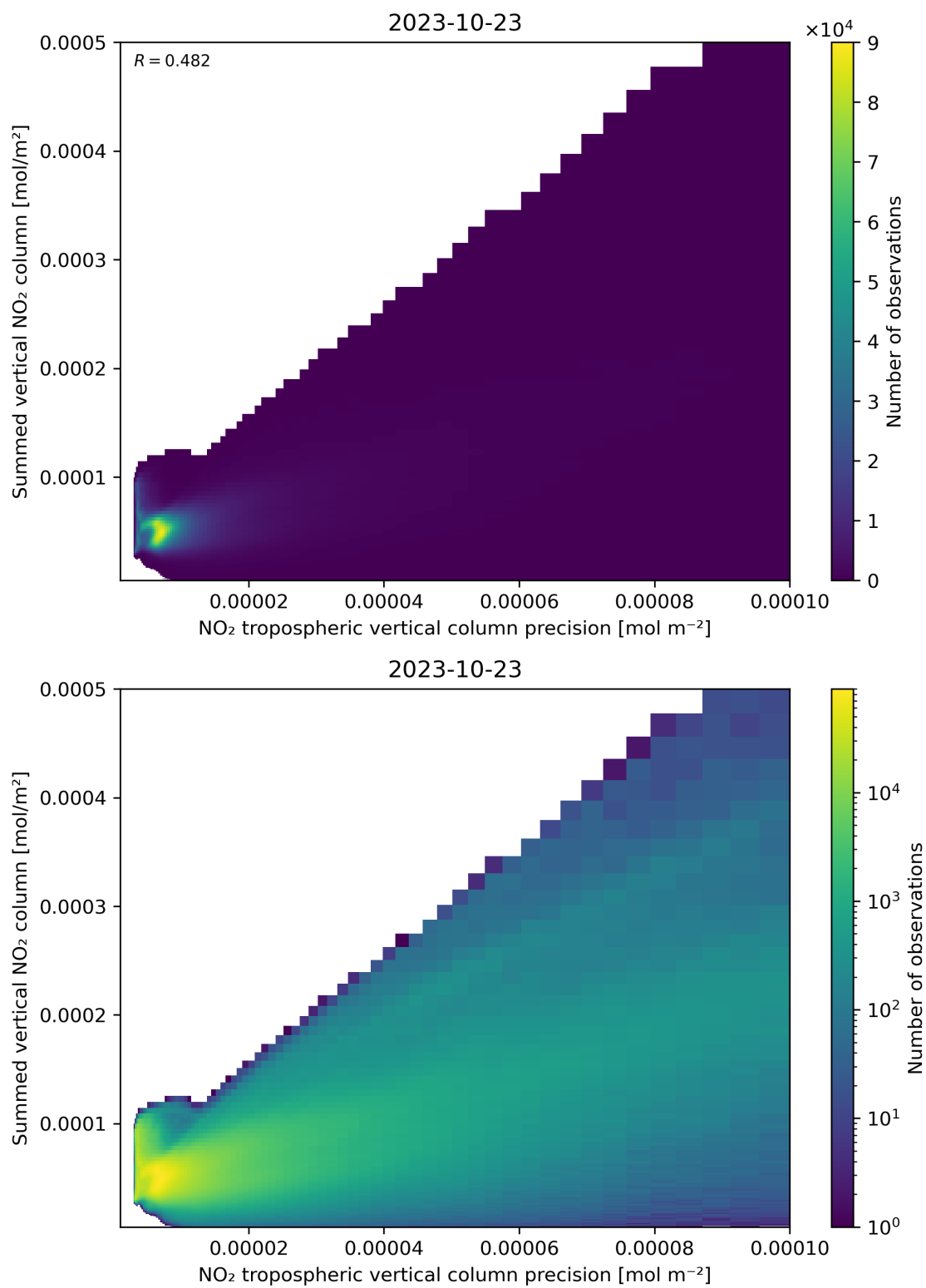
Figure 136: Scatter density plot of “NO 2 tropospheric vertical column precision” against “Summed vertical NO 2 column” for 2023-10-22 to 2023-10-24.
