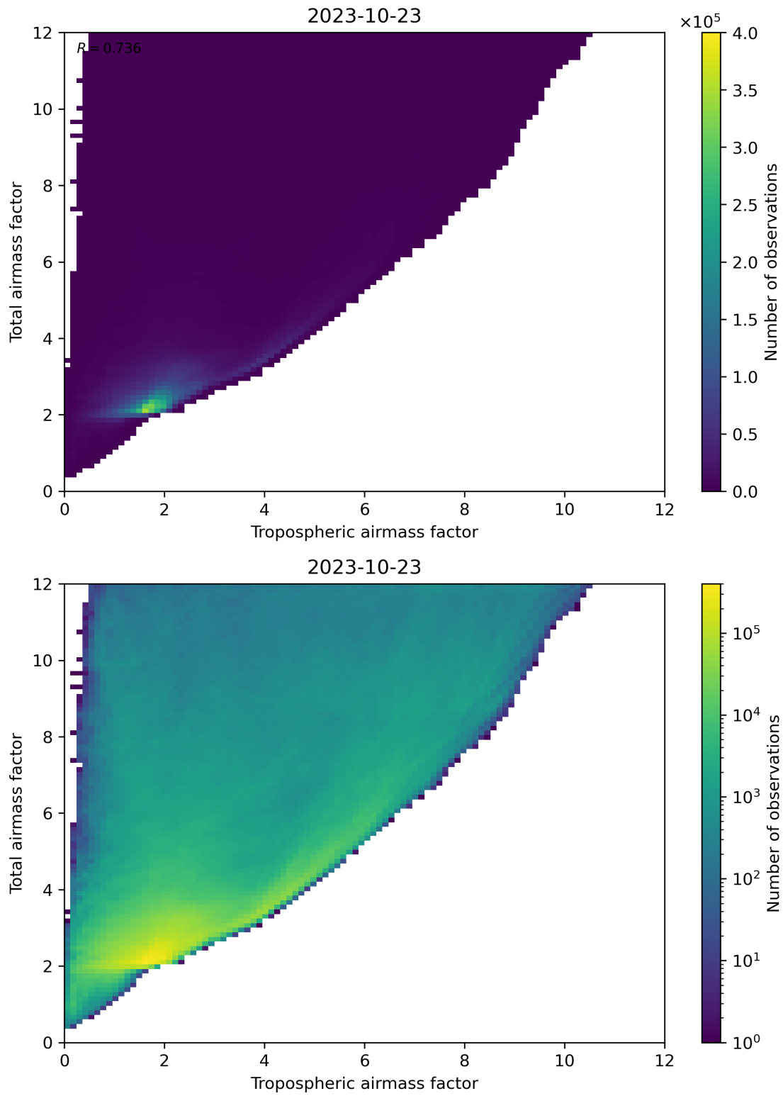
Figure 72: Scatter density plot of “Tropospheric airmass factor” against “Total airmass factor” for 2023-10-22 to 2023-10-24.
