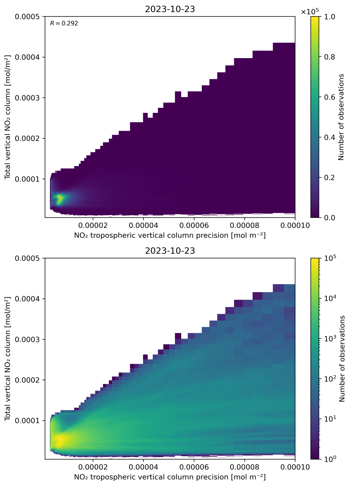
Figure 138: Scatter density plot of “NO 2 tropospheric vertical column precision” against “Total vertical NO 2 column” for 2023-10-22 to 2023-10-24.
