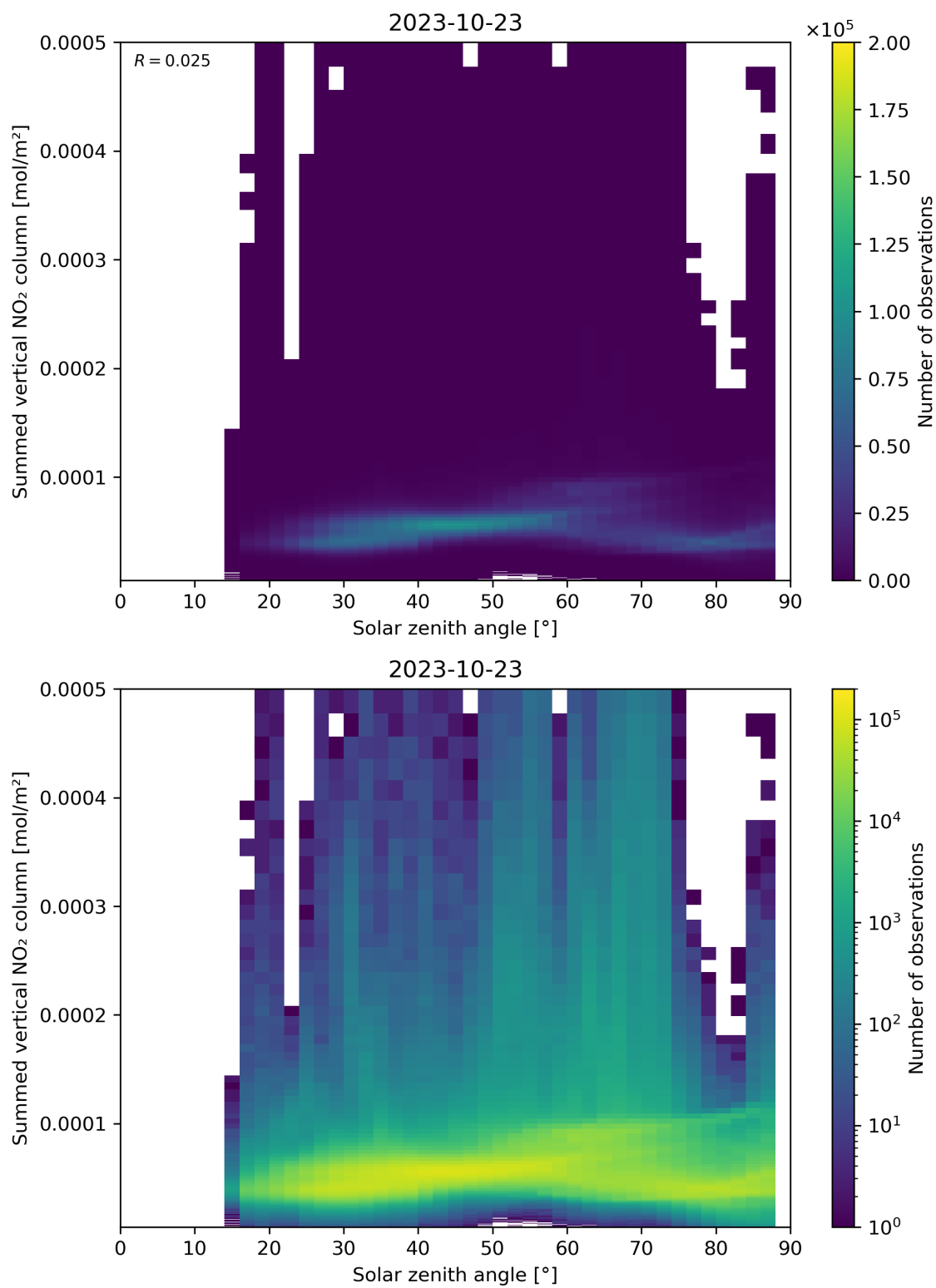
Figure 151: Scatter density plot of “Solar zenith angle” against “Summed vertical NO 2 column” for 2023-10-22 to 2023-10-24.
