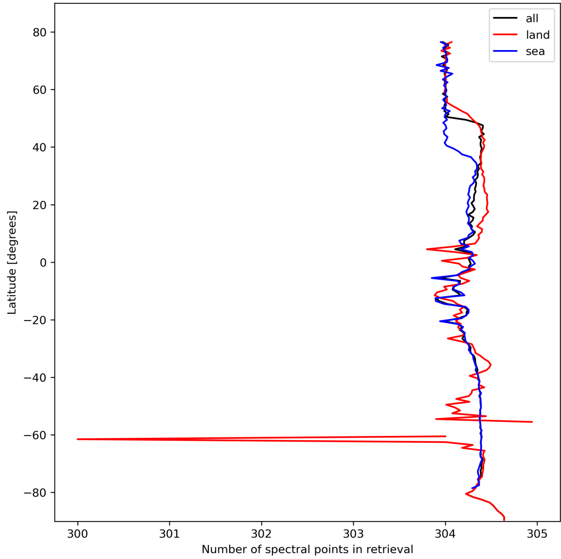
Figure 16: Zonal average of “Number of spectral points in retrieval” for 2023-10-22 to 2023-10-24.
