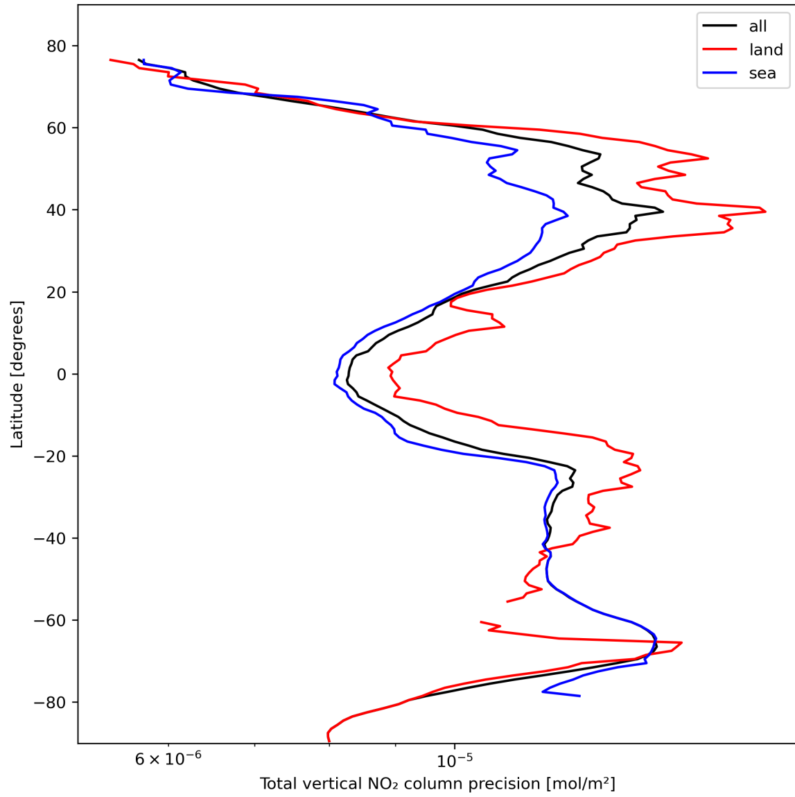
Figure 22: Zonal average of “Total vertical NO 2 column precision” for 2023-10-22 to 2023-10-24.
