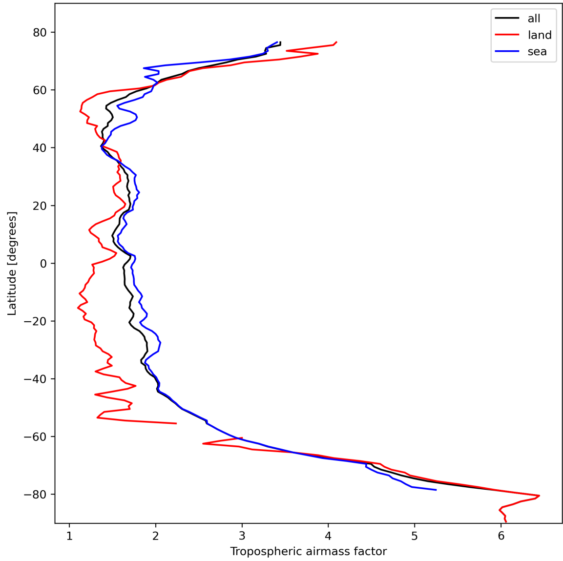
Figure 14: Zonal average of “Tropospheric airmass factor” for 2023-10-22 to 2023-10-24.
