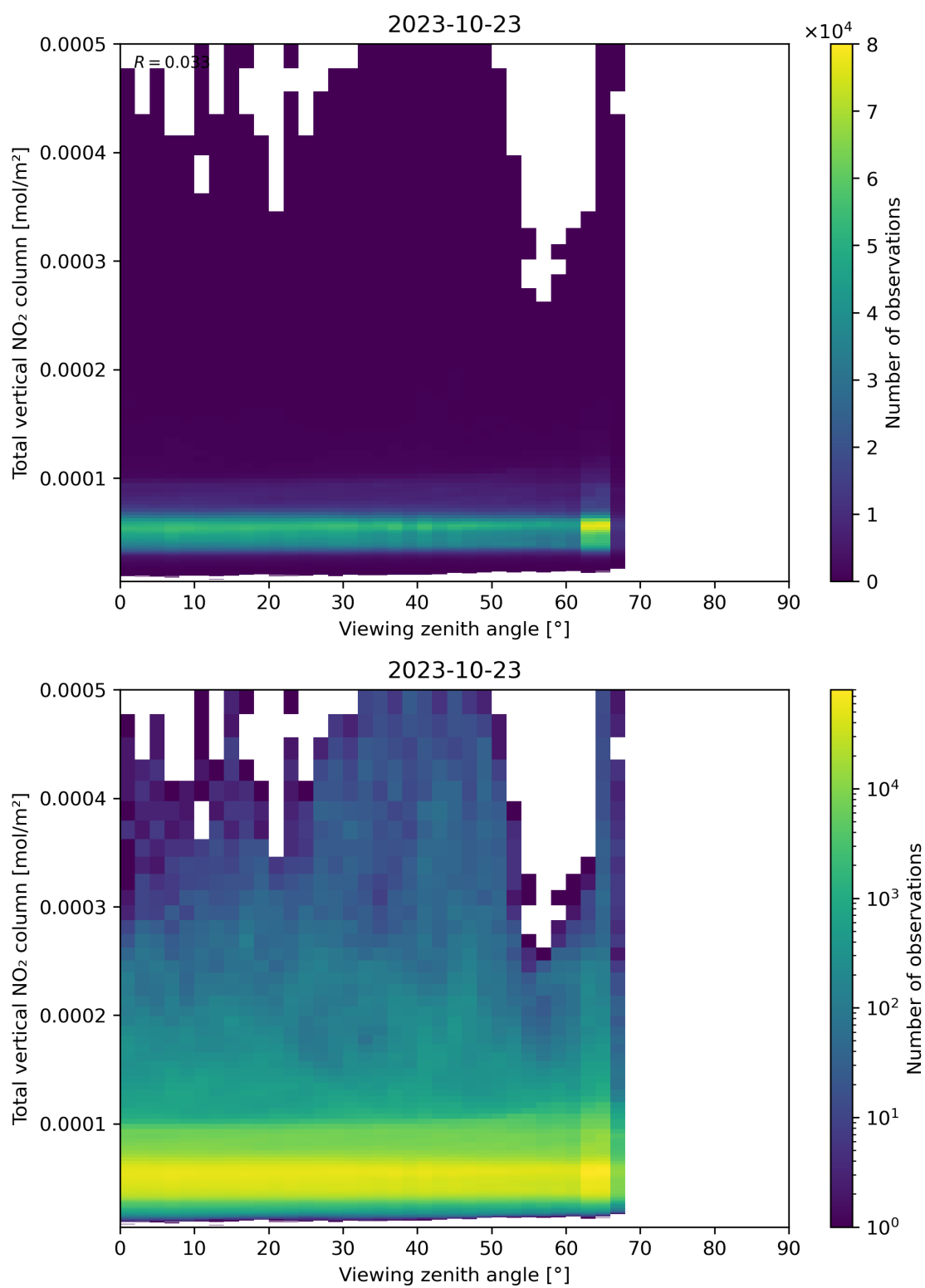
Figure 167: Scatter density plot of “Viewing zenith angle” against “Total vertical NO 2 column” for 2023-10-22 to 2023-10-24.
