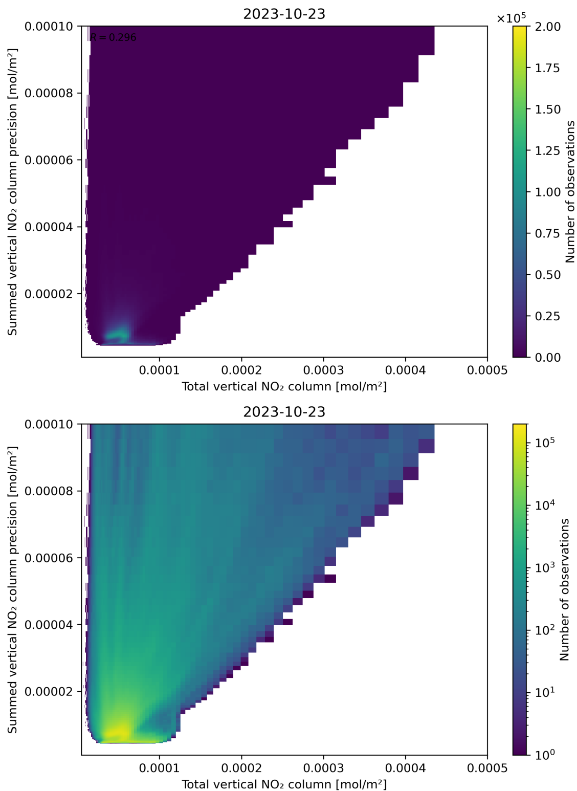
Figure 113: Scatter density plot of “Total vertical NO 2 column” against “Summed vertical NO 2 column precision” for 2023-10-22 to 2023-10-24.
