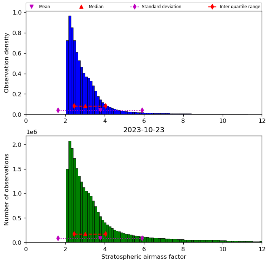
Figure 44: Histogram of “Stratospheric airmass factor” for 2023-10-22 to 2023-10-24
