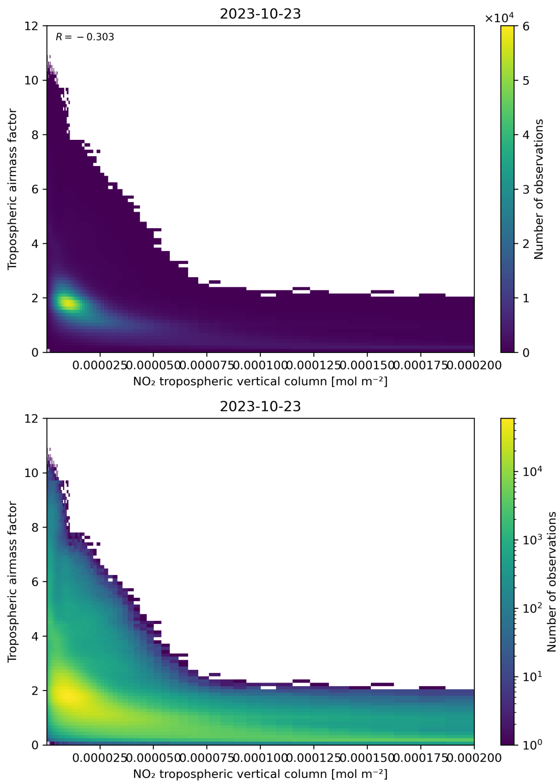
Figure 123: Scatter density plot of “NO 2 tropospheric vertical column” against “Tropospheric airmass factor” for 2023-10-22 to 2023-10-24.
