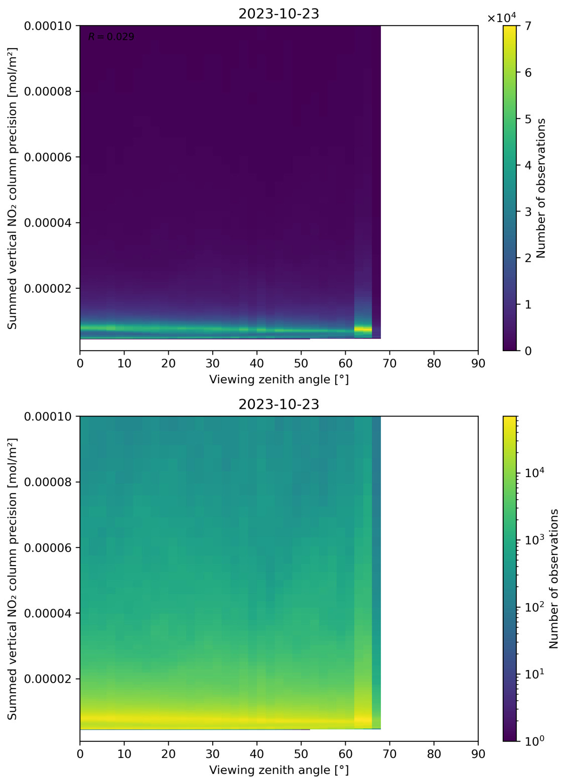
Figure 166: Scatter density plot of “Viewing zenith angle” against “Summed vertical NO 2 column precision” for 2023-10-22 to 2023-10-24.
