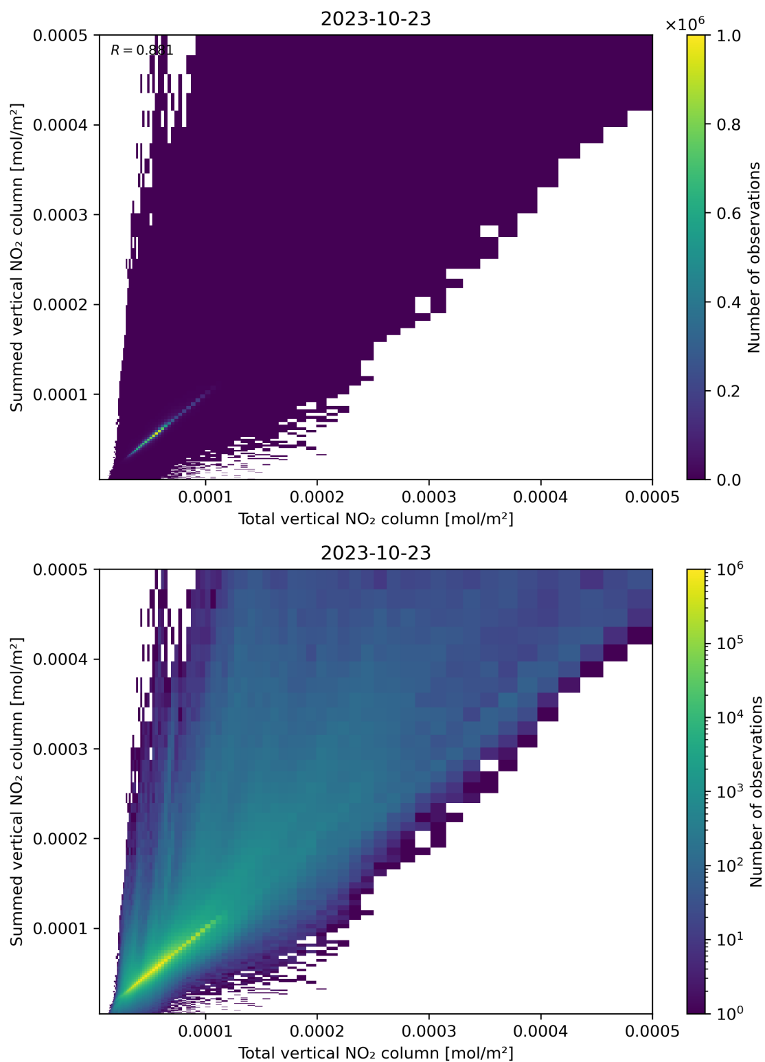
Figure 112: Scatter density plot of “Total vertical NO 2 column” against “Summed vertical NO 2 column” for 2023-10-22 to 2023-10-24.
