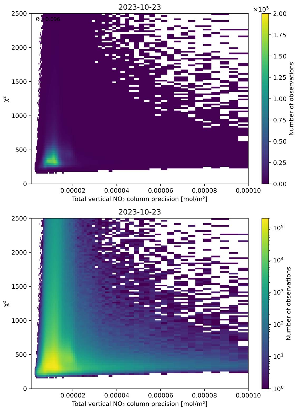
Figure 116: Scatter density plot of “Total vertical NO 2 column precision” against “ \chi^2 ” for 2023-10-22 to 2023-10-24.
