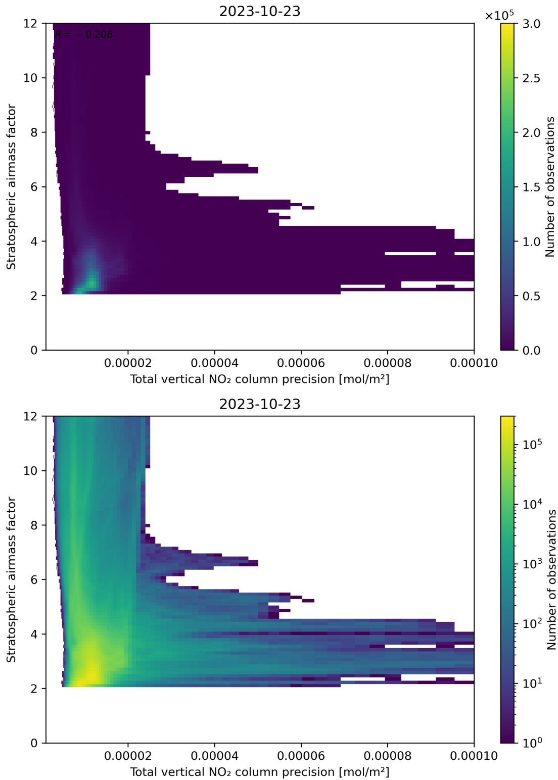
Figure 115: Scatter density plot of “Total vertical NO 2 column precision” against “Stratospheric air mass factor” for 2023-10-22 to 2023-10-24.
