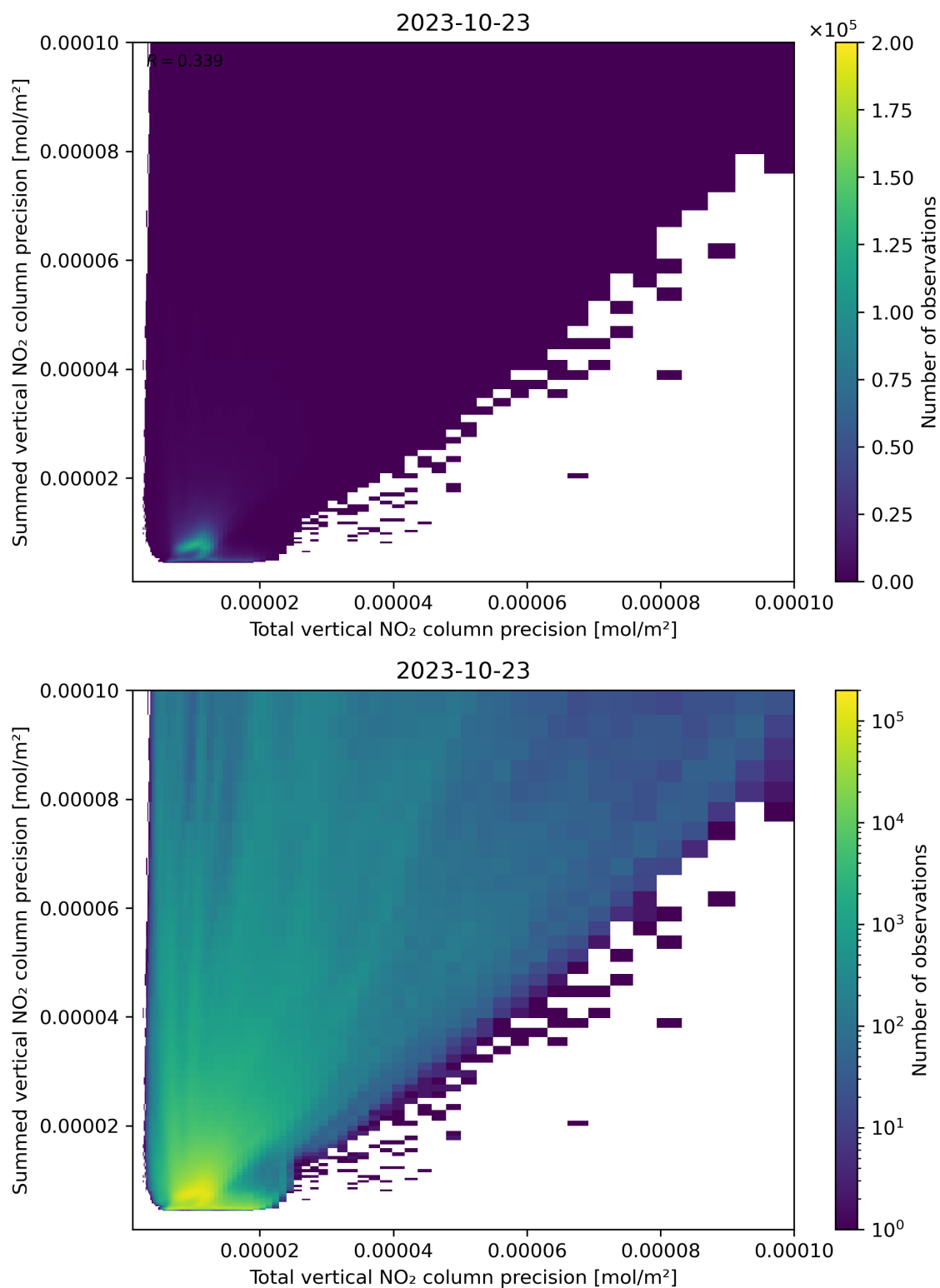
Figure 118: Scatter density plot of “Total vertical NO 2 column precision” against “Summed vertical NO 2 column precision” for 2023-10-22 to 2023-10-24.
