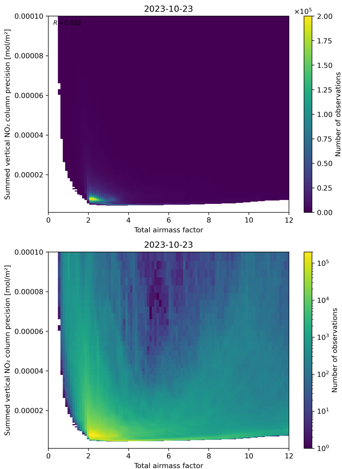
Figure 66: Scatter density plot of “Total airmass factor” against “Summed vertical NO 2 column precision” for 2023-10-22 to 2023-10-24.
