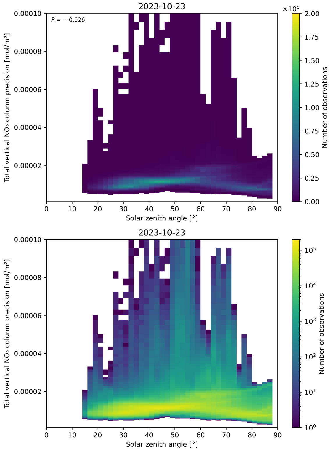
Figure 154: Scatter density plot of “Solar zenith angle” against “Total vertical NO 2 column precision” for 2023-10-22 to 2023-10-24.
