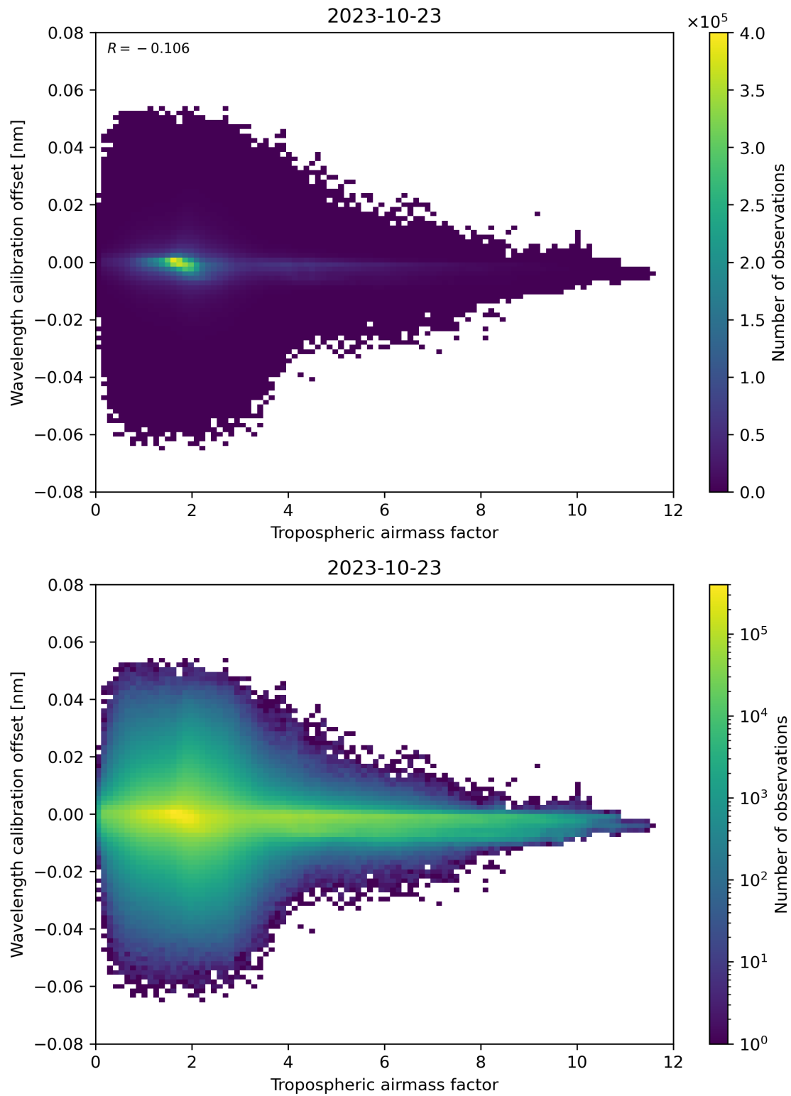
Figure 80: Scatter density plot of “Tropospheric airmass factor” against “Wavelength calibration offset” for 2023-10-22 to 2023-10-24.
