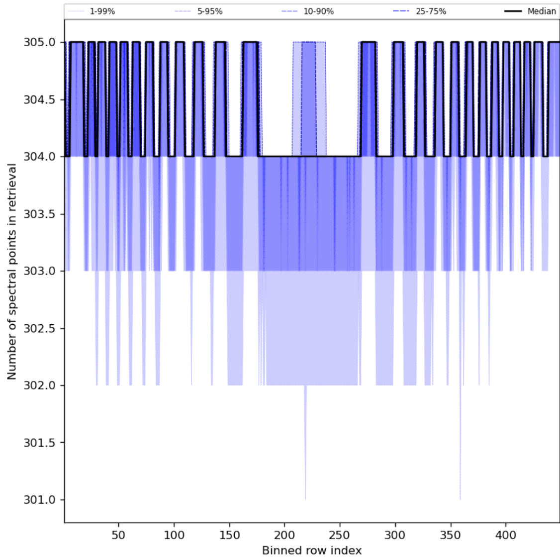
Figure 50: Along track statistics of “Number of spectral points in retrieval” for 2023-10-22 to 2023-10-24
