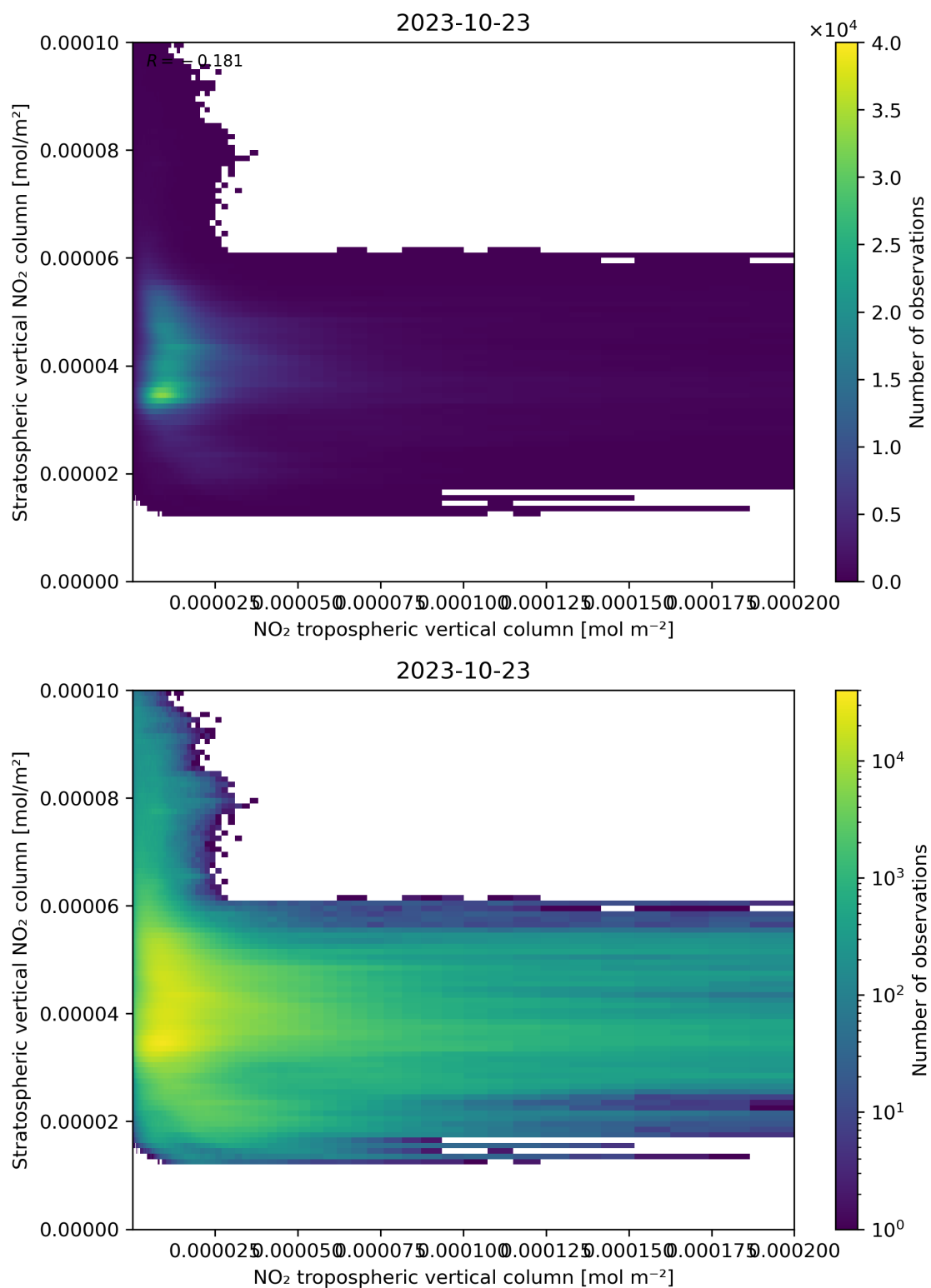
Figure 125: Scatter density plot of “NO 2 tropospheric vertical column” against “Stratospheric vertical NO 2 column” for 2023-10-22 to 2023-10-24.
