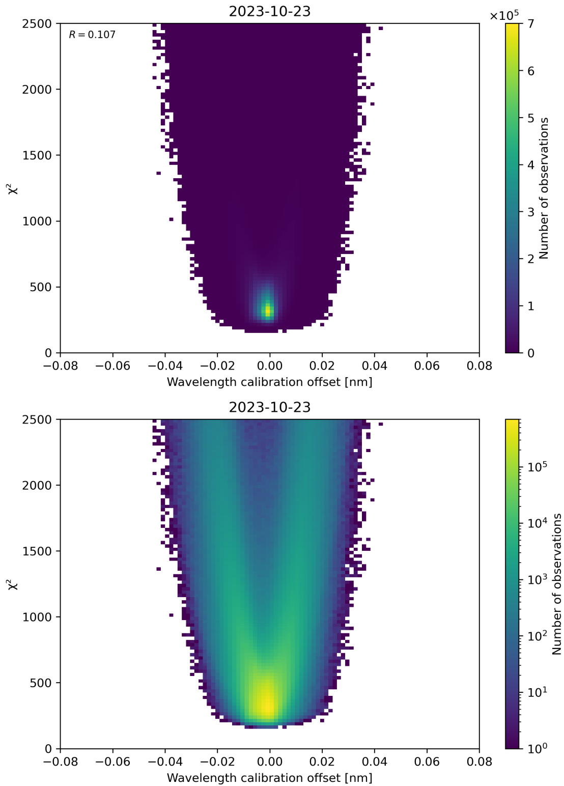
Figure 175: Scatter density plot of “Wavelength calibration offset” against “ \chi^2 ” for 2023-10-22 to 2023-10-24.
