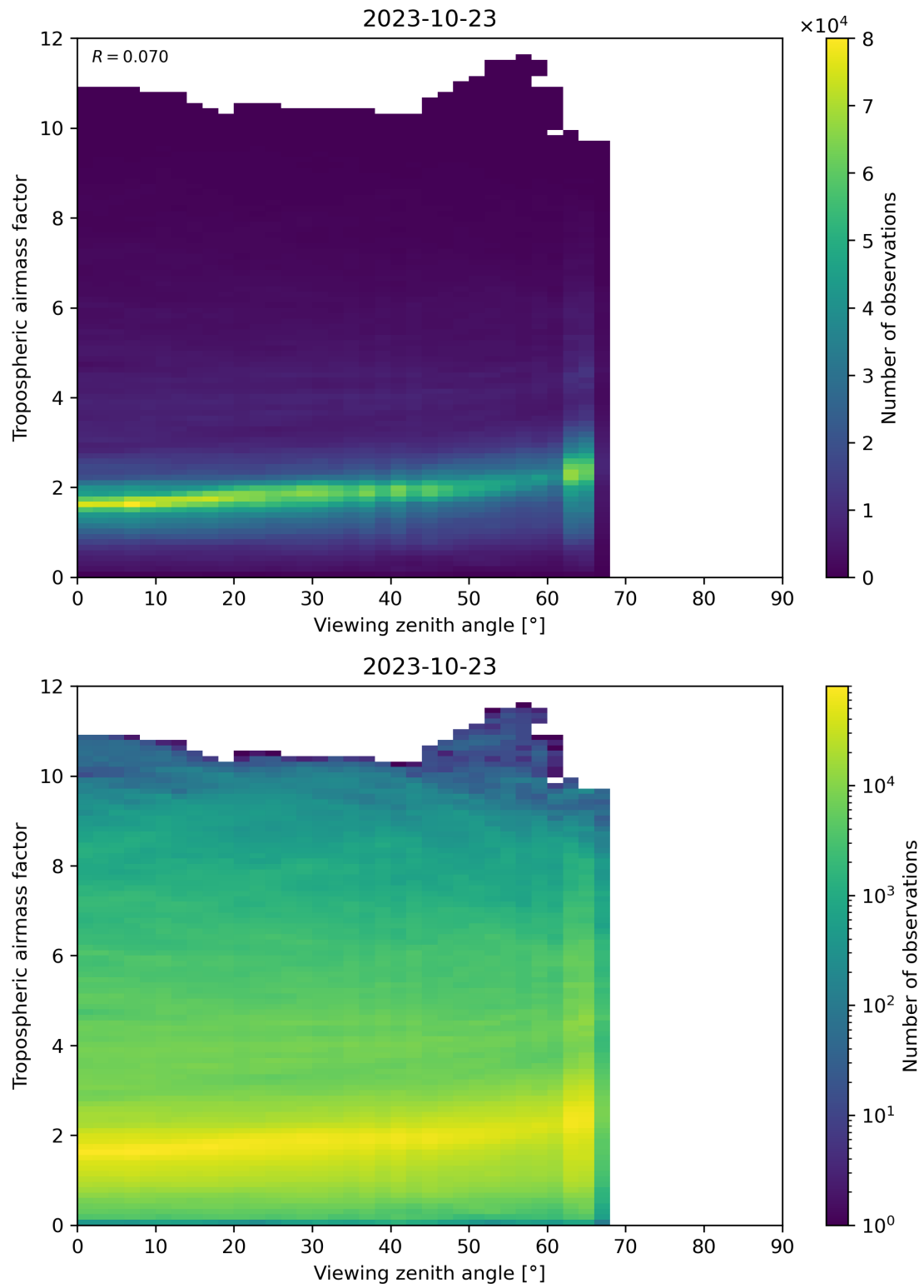
Figure 161: Scatter density plot of “Viewing zenith angle” against “Tropospheric airmass factor” for 2023-10-22 to 2023-10-24.
