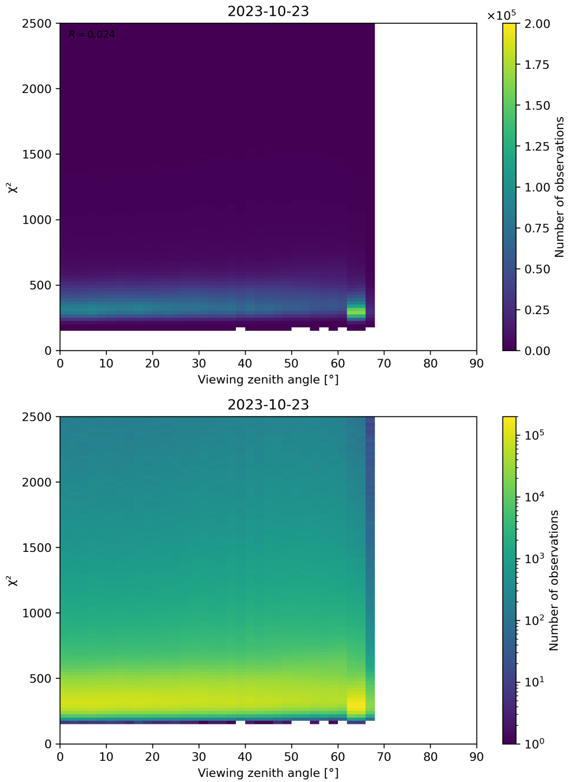
Figure 162: Scatter density plot of “Viewing zenith angle” against “ \chi^2 ” for 2023-10-22 to 2023-10-24.
