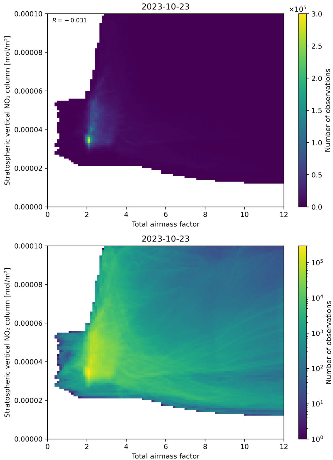
Figure 64: Scatter density plot of “Total airmass factor” against “Stratospheric vertical NO 2 column” for 2023-10-22 to 2023-10-24.
