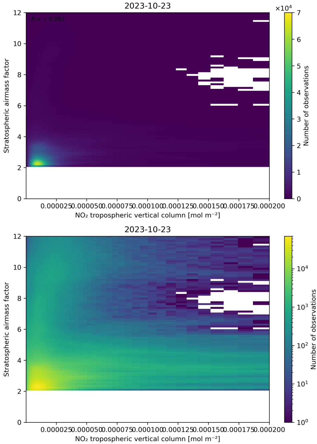
Figure 121: Scatter density plot of “NO 2 tropospheric vertical column” against “Stratospheric air mass factor” for 2023-10-22 to 2023-10-24.
