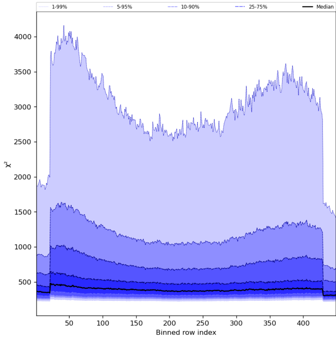
Figure 59: Along track statistics of “ \chi^2 ” for 2023-10-22 to 2023-10-24
