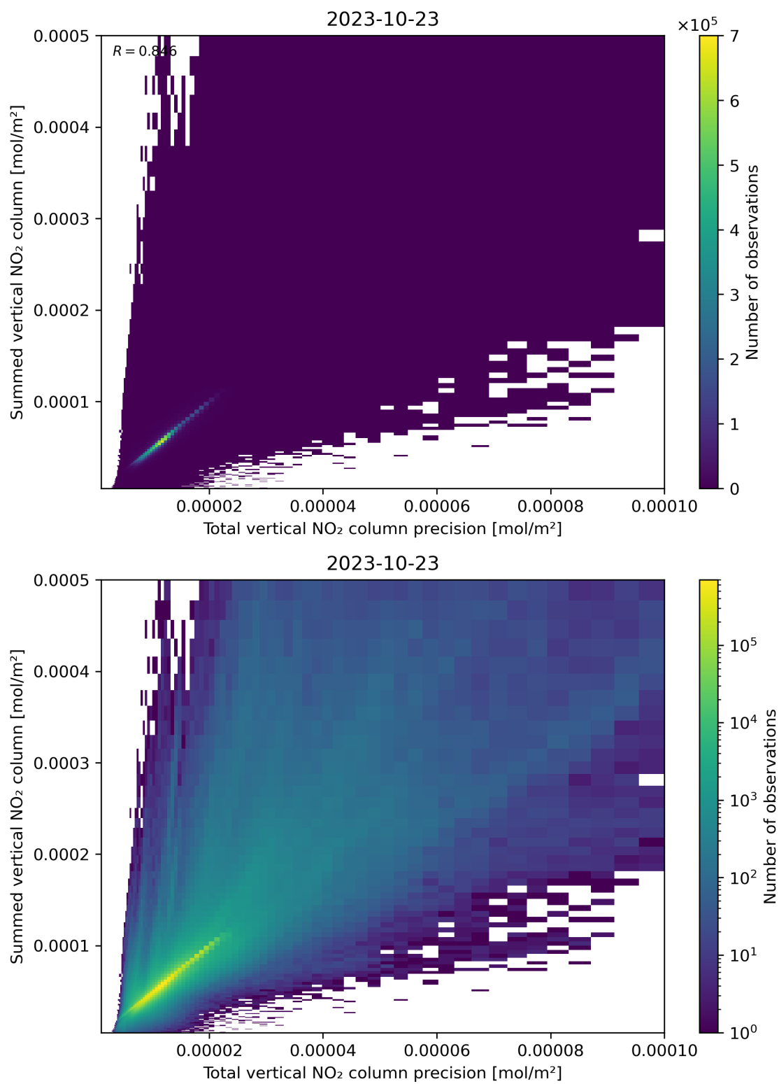
Figure 117: Scatter density plot of “Total vertical NO 2 column precision” against “Summed vertical NO 2 column” for 2023-10-22 to 2023-10-24.
