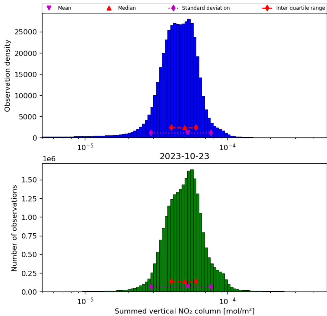
Figure 40: Histogram of “Summed vertical NO 2 column” for 2023-10-22 to 2023-10-24
