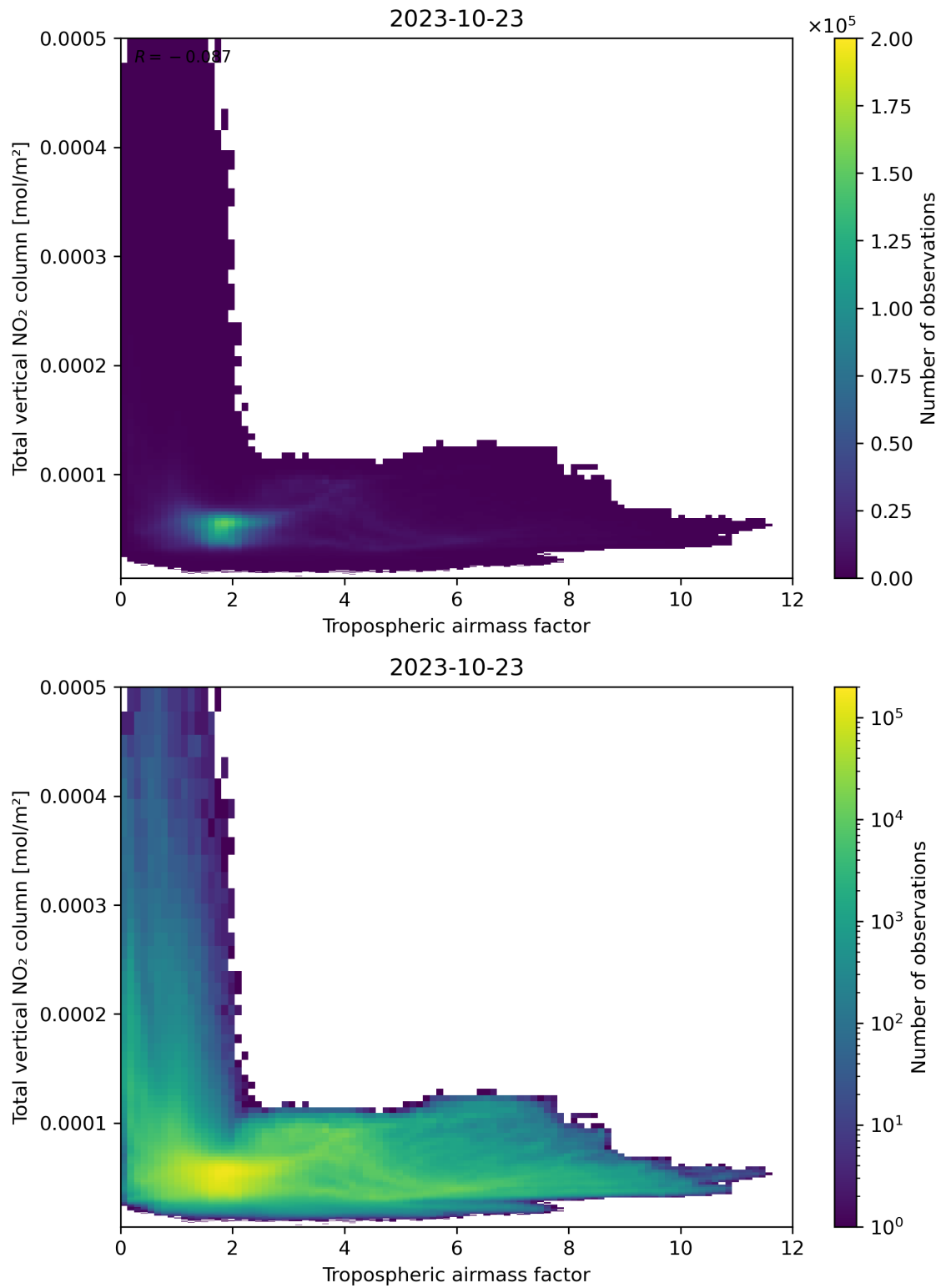
Figure 77: Scatter density plot of “Tropospheric airmass factor” against “Total vertical NO 2 column” for 2023-10-22 to 2023-10-24.
