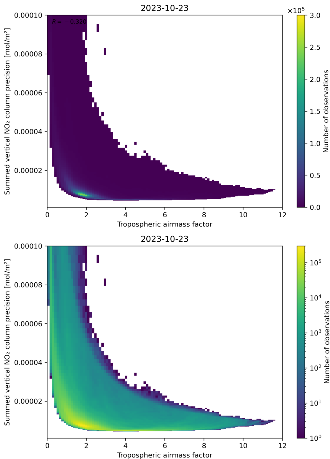
Figure 76: Scatter density plot of “Tropospheric air mass factor” against “Summed vertical NO 2 column precision” for 2023-10-22 to 2023-10-24.
