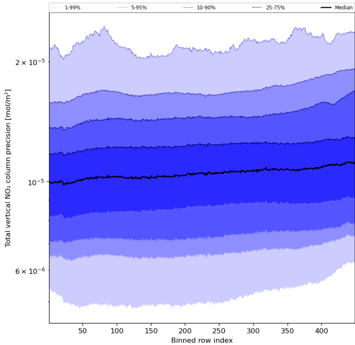
Figure 56: Along track statistics of “Total vertical NO 2 column precision” for 2023-10-22 to 2023-10-24
