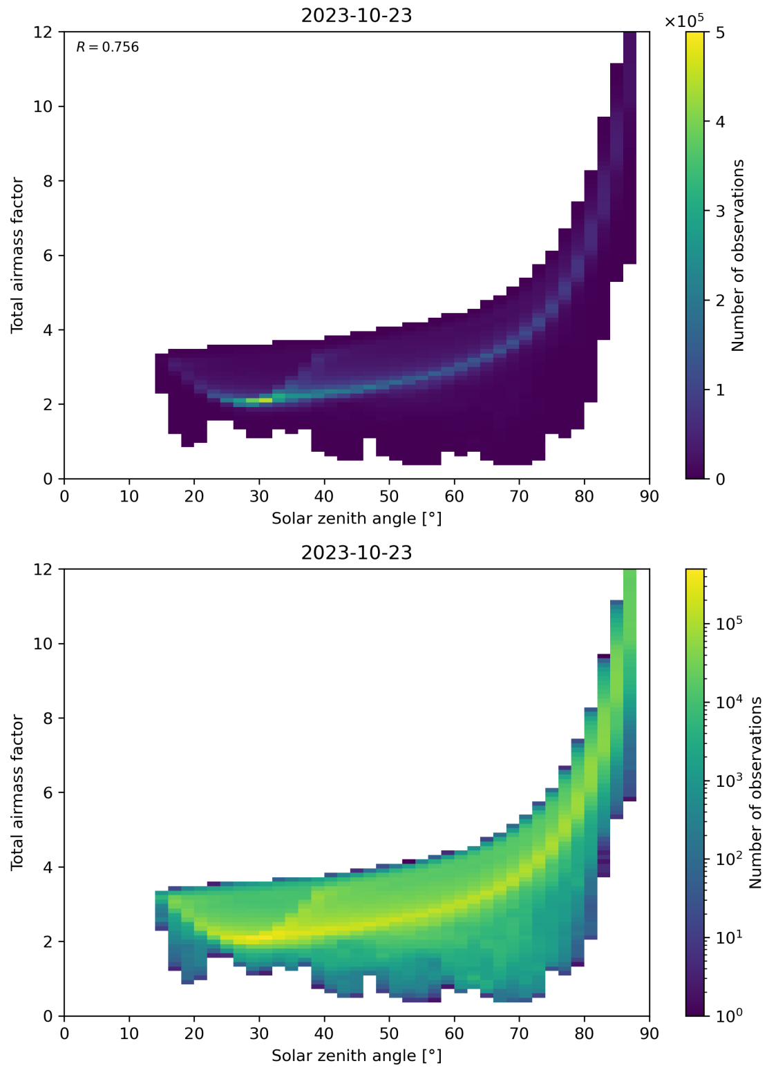
Figure 146: Scatter density plot of “Solar zenith angle” against “Total air mass factor” for 2023-10-22 to 2023-10-24.
