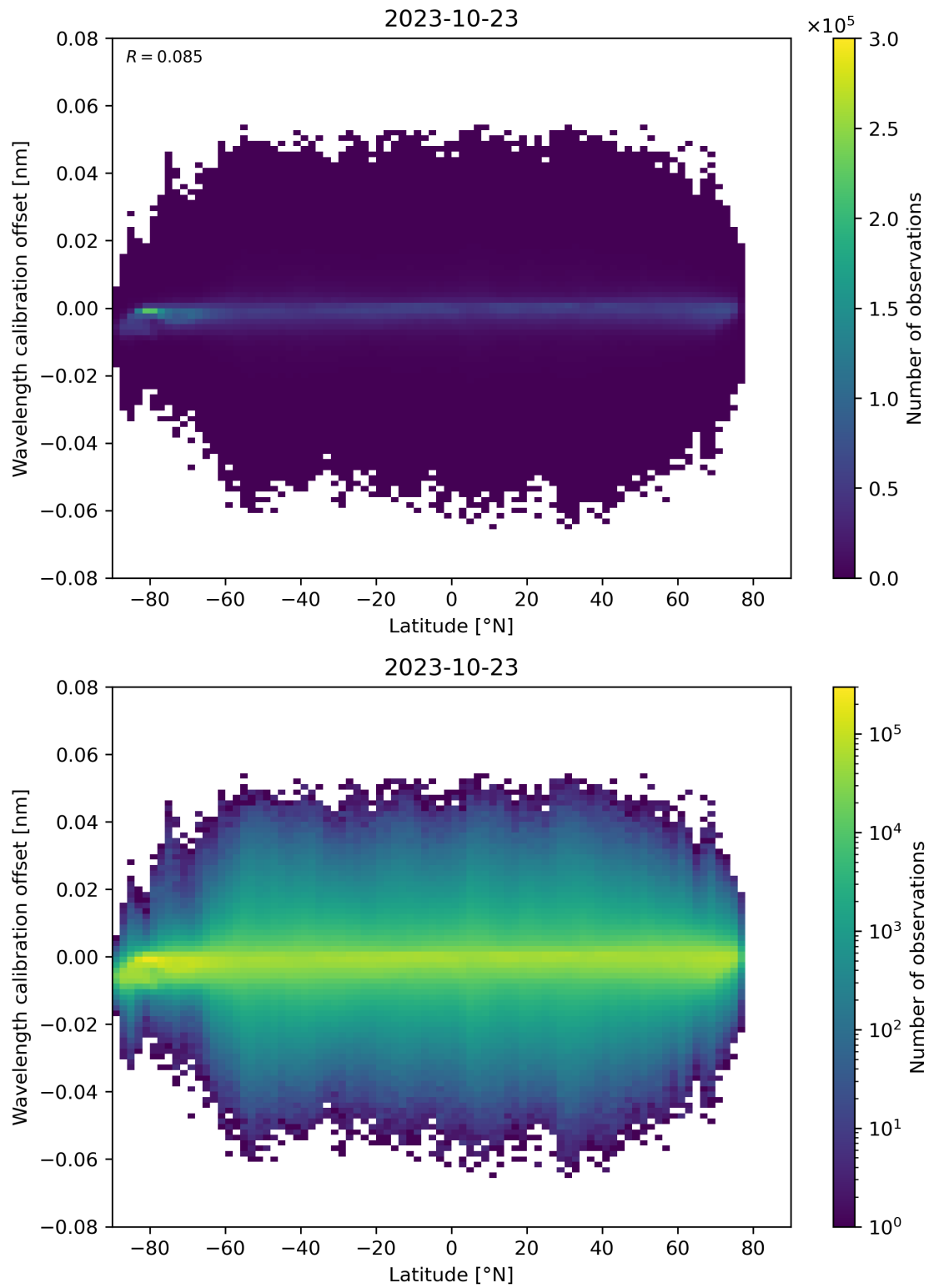
Figure 95: Scatter density plot of “Latitude” against “Wavelength calibration offset” for 2023-10-22 to 2023-10-24.
