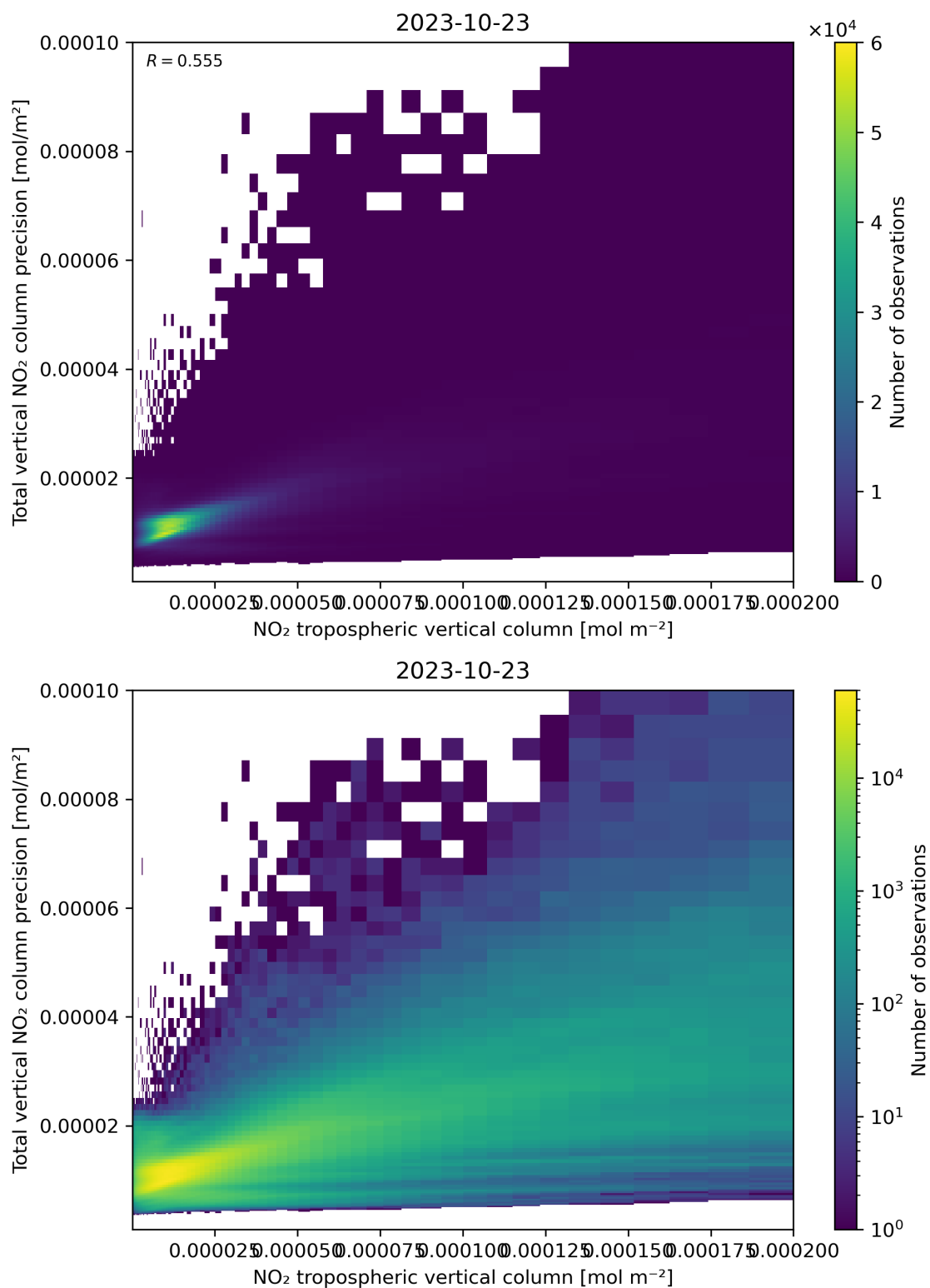
Figure 129: Scatter density plot of “NO 2 tropospheric vertical column” against “Total vertical NO 2 column precision” for 2023-10-22 to 2023-10-24.
