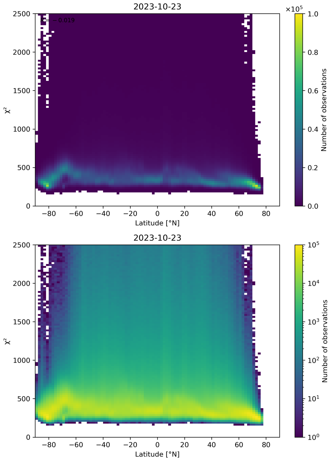
Figure 86: Scatter density plot of “Latitude” against “ \chi^2 ” for 2023-10-22 to 2023-10-24.
