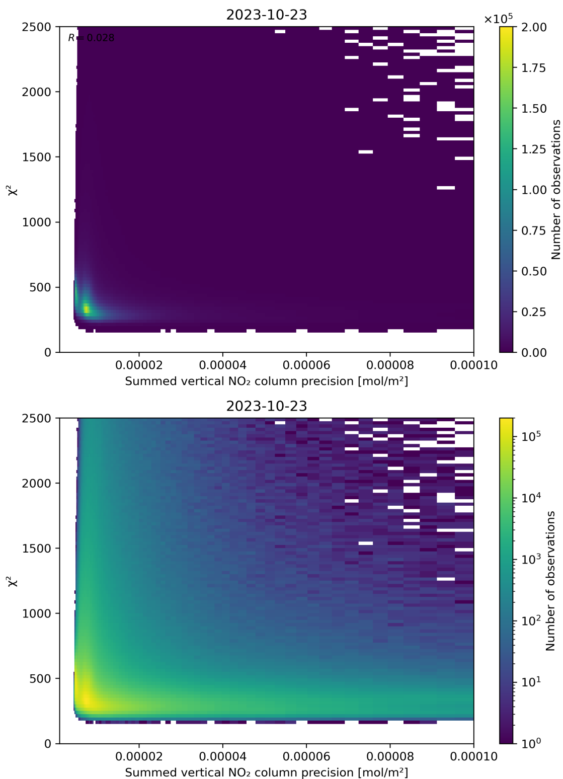
Figure 107: Scatter density plot of “Summed vertical NO 2 column precision” against “ \chi^2 ” for 2023-10-22 to 2023-10-24.
