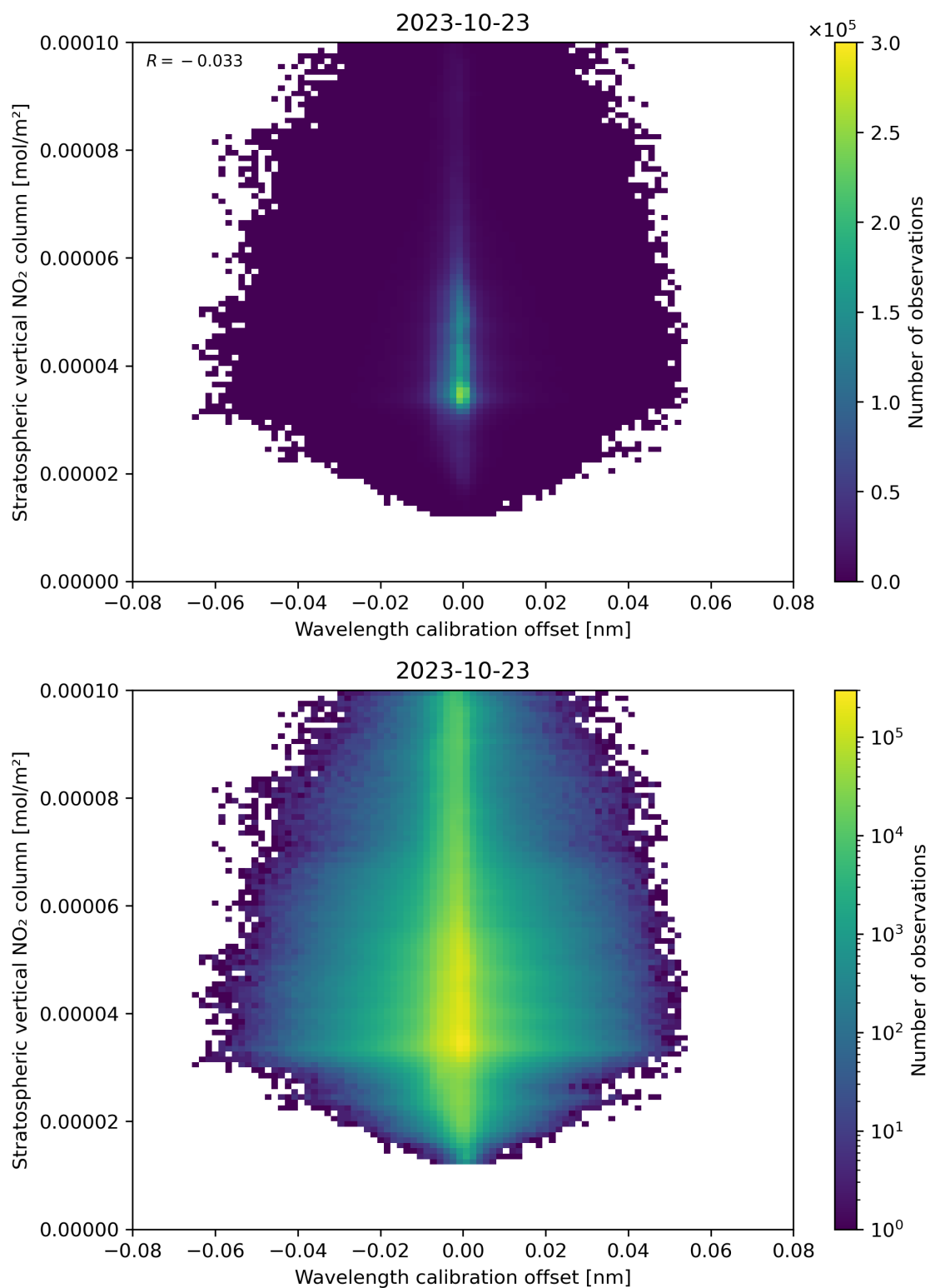
Figure 176: Scatter density plot of “Wavelength calibration offset” against “Stratospheric vertical NO 2 column” for 2023-10-22 to 2023-10-24.
