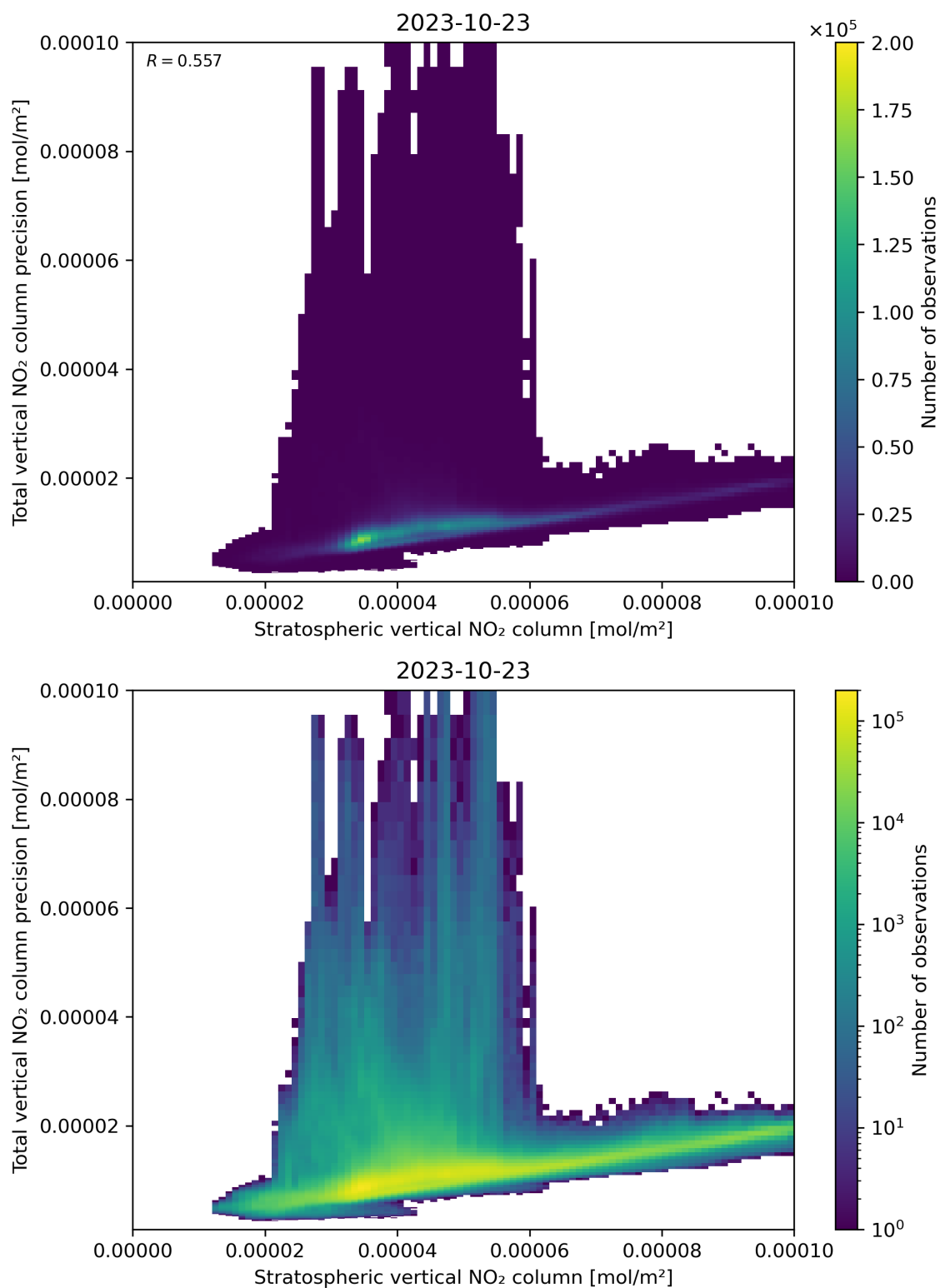
Figure 101: Scatter density plot of “Stratospheric vertical NO 2 column” against “Total vertical NO 2 column precision” for 2023-10-22 to 2023-10-24.
