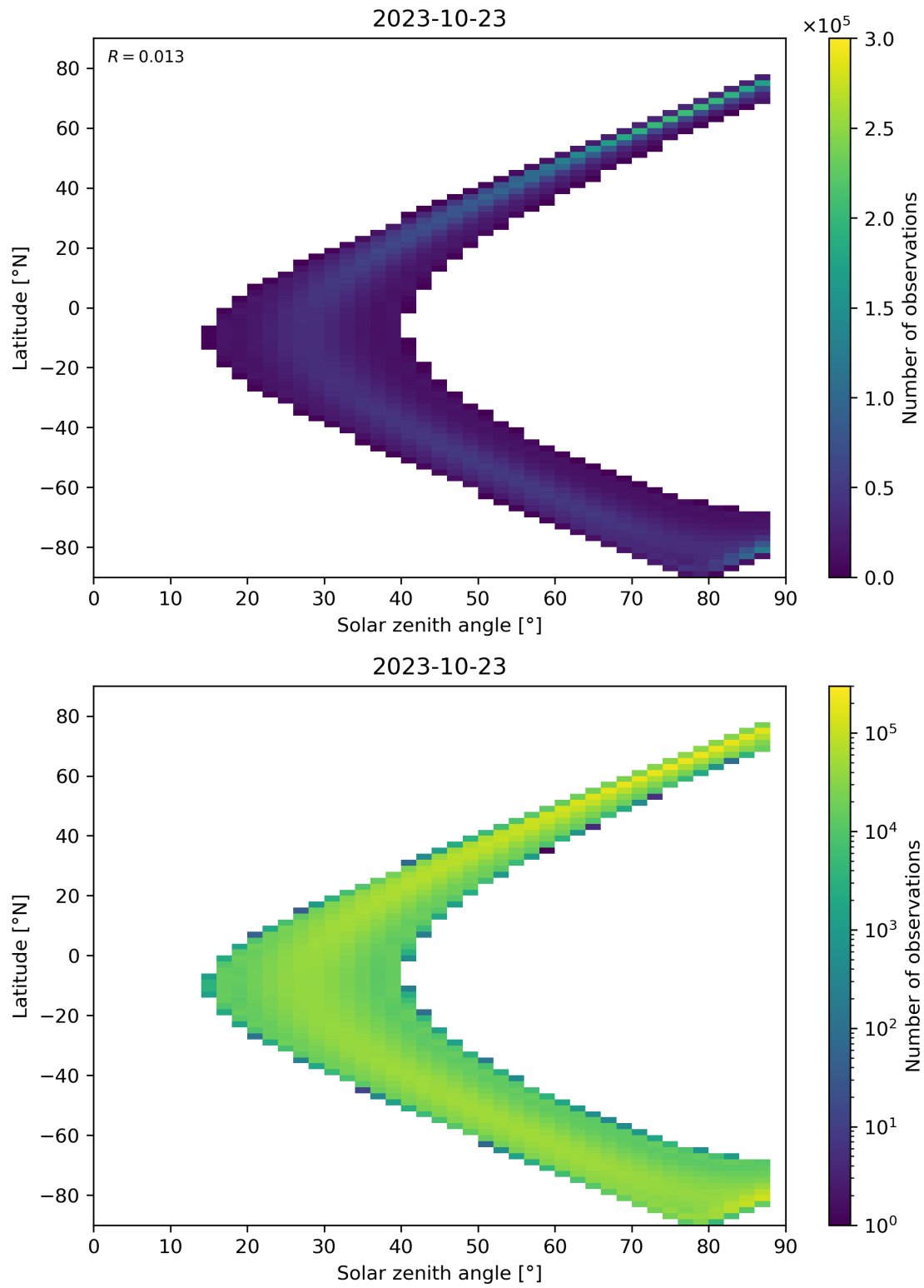
Figure 149: Scatter density plot of “Solar zenith angle” against “Latitude” for 2023-10-22 to 2023-10-24.
