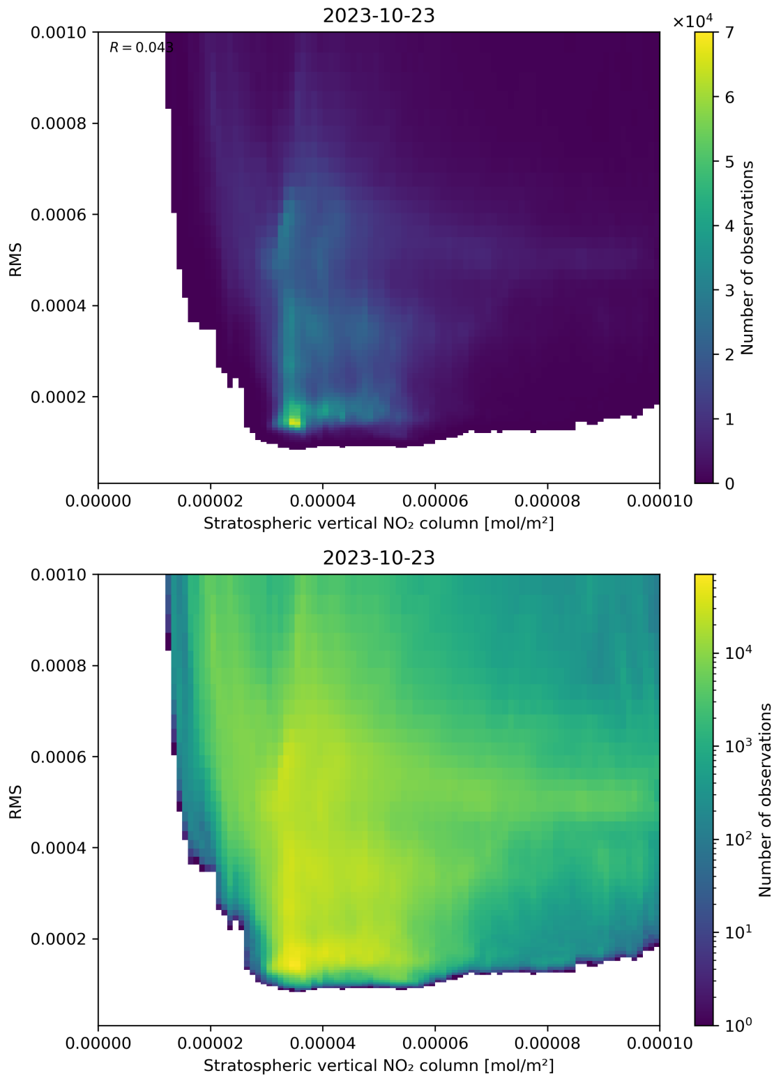
Figure 102: Scatter density plot of “Stratospheric vertical NO 2 column” against “RMS” for 2023-10-22 to 2023-10-24.
