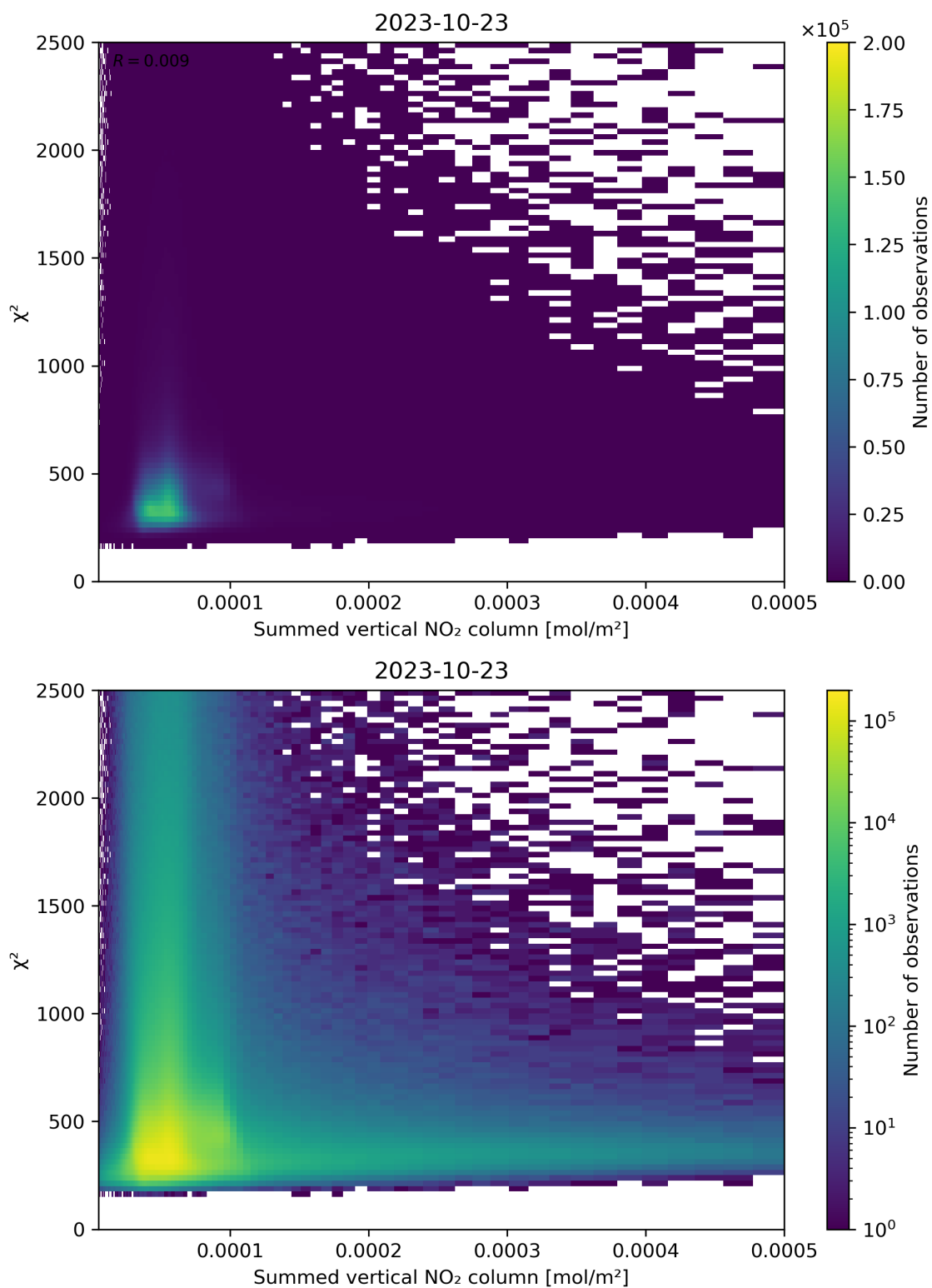
Figure 104: Scatter density plot of “Summed vertical NO 2 column” against “ \chi^2 ” for 2023-10-22 to 2023-10-24.
