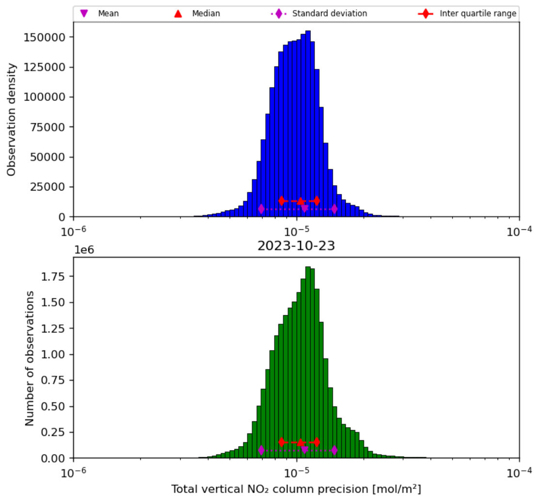
Figure 39: Histogram of "Total vertical NO 2 column precision" for 2023-10-22 to 2023-10-24
