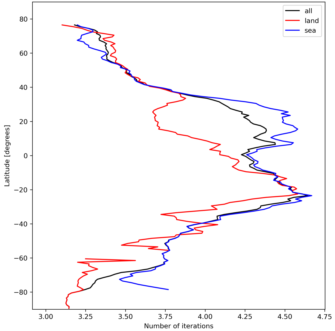
Figure 17: Zonal average of “Number of iterations” for 2023-10-22 to 2023-10-24.
