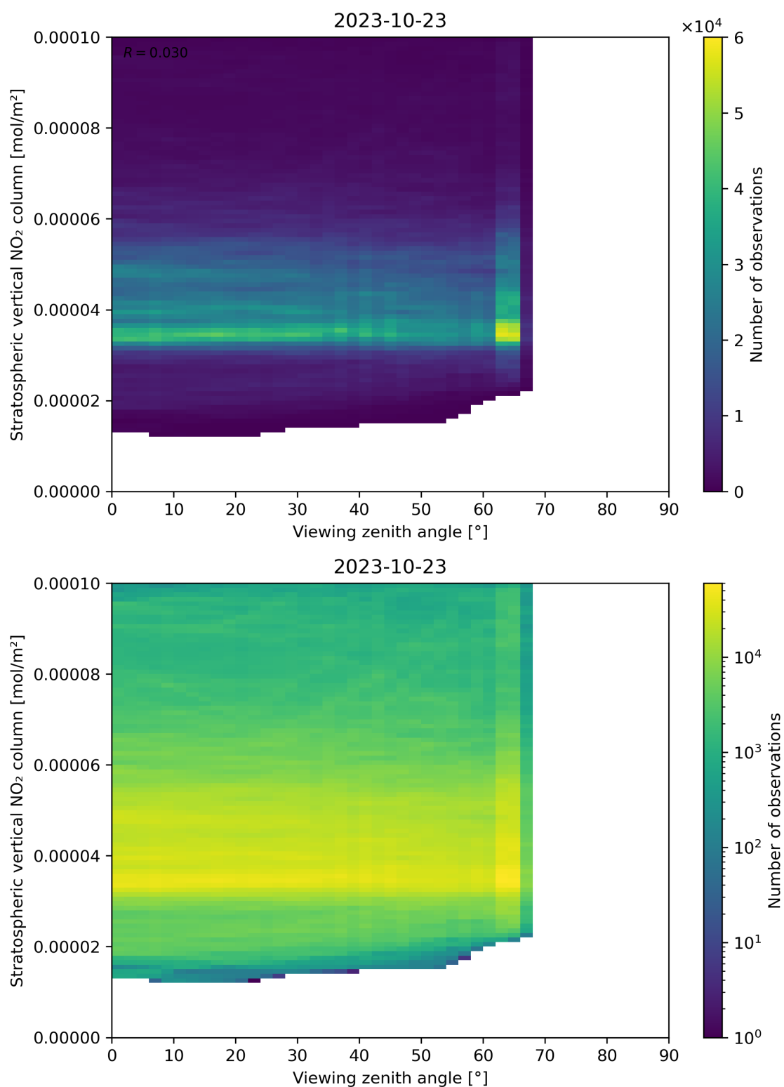
Figure 164: Scatter density plot of “Viewing zenith angle” against “Stratospheric vertical NO 2 column” for 2023-10-22 to 2023-10-24.
