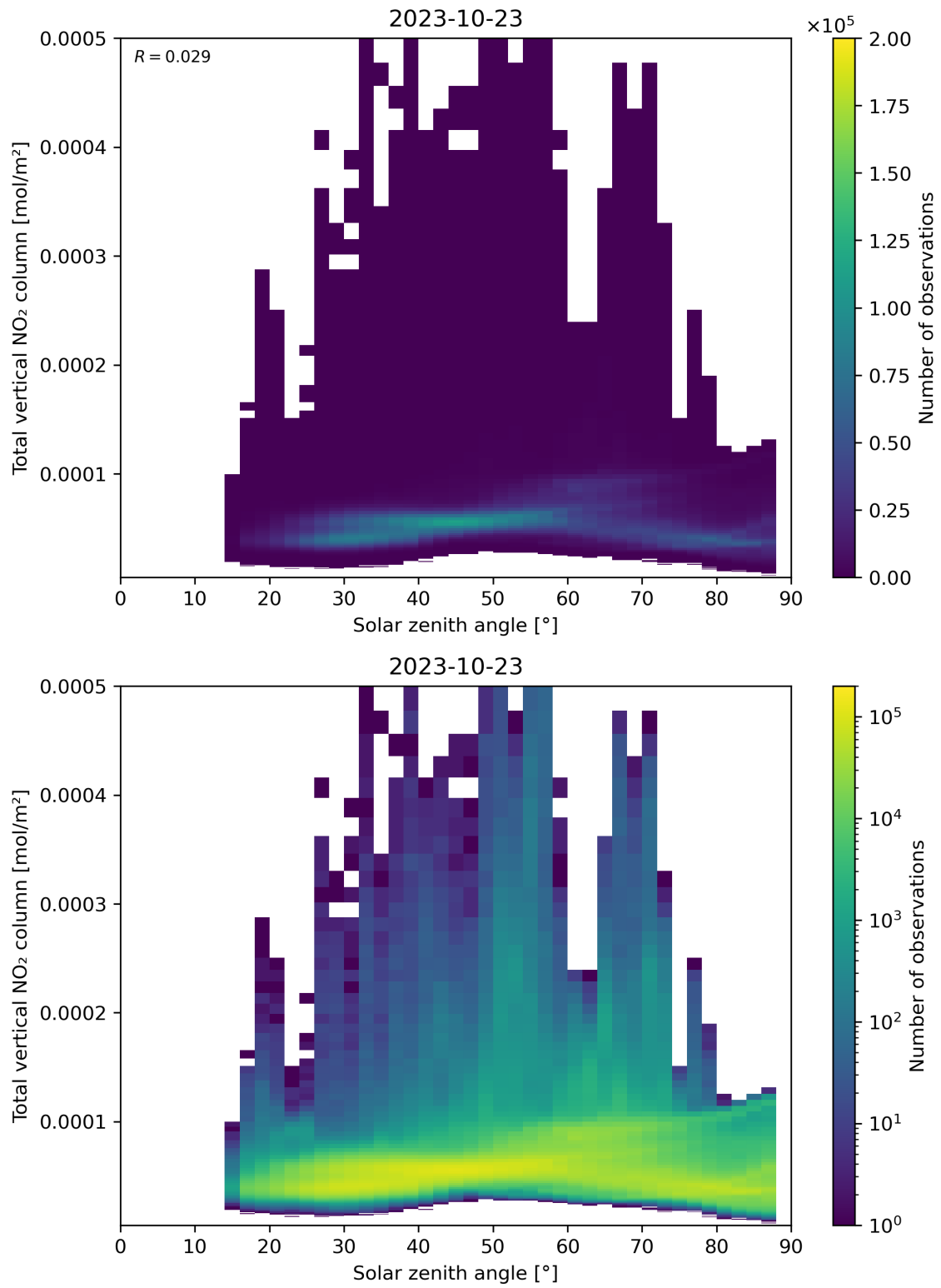
Figure 153: Scatter density plot of “Solar zenith angle” against “Total vertical NO 2 column” for 2023-10-22 to 2023-10-24.
