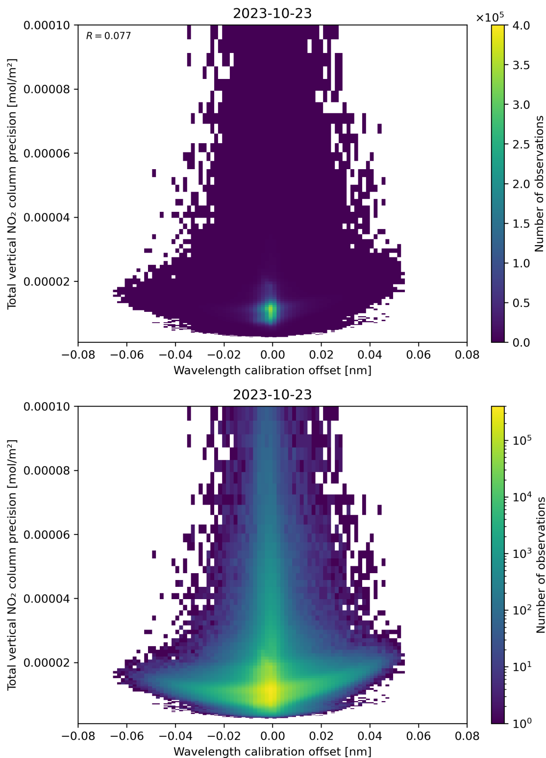
Figure 180: Scatter density plot of “Wavelength calibration offset” against “Total vertical NO 2 column precision” for 2023-10-22 to 2023-10-24.
