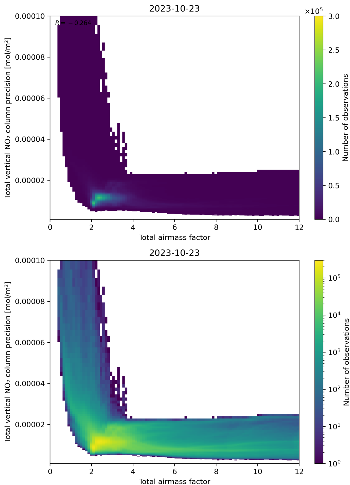
Figure 68: Scatter density plot of “Total airmass factor” against “Total vertical NO 2 column precision” for 2023-10-22 to 2023-10-24.
