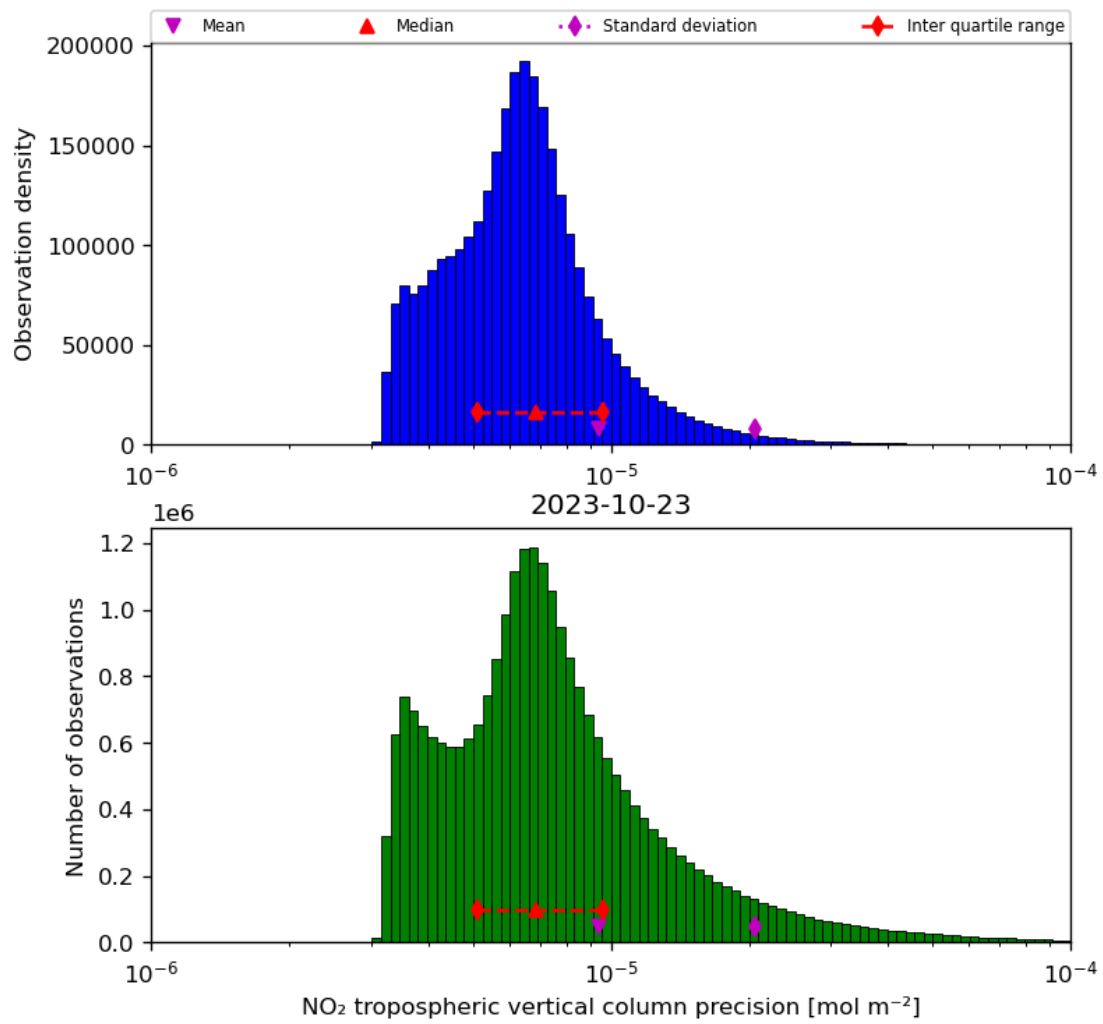
Figure 30: Histogram of “NO 2 tropospheric vertical column precision” for 2023-10-22 to 2023-10-24
