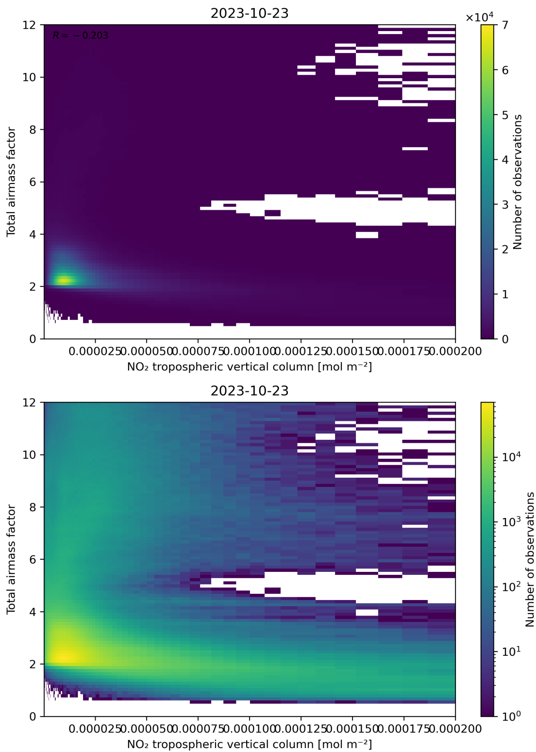
Figure 122: Scatter density plot of “NO 2 tropospheric vertical column” against “Total airmass factor” for 2023-10-22 to 2023-10-24.
