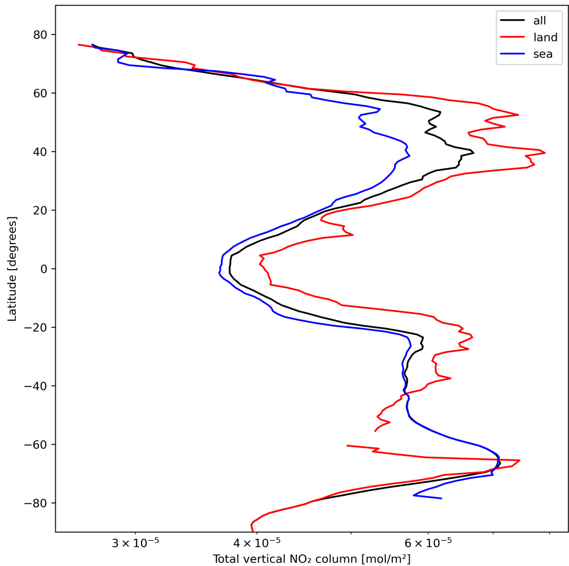
Figure 21: Zonal average of “Total vertical NO 2 column” for 2023-10-22 to 2023-10-24.
