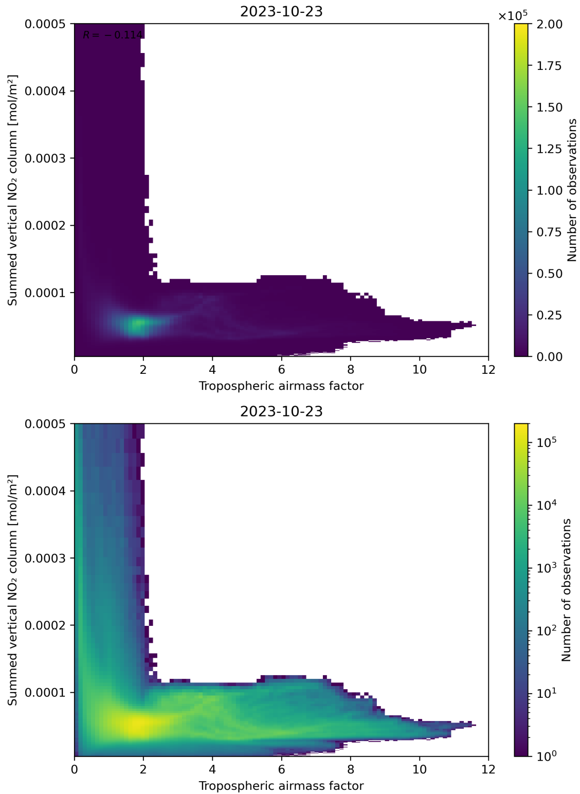
Figure 75: Scatter density plot of “Tropospheric airmass factor” against “Summed vertical NO 2 column” for 2023-10-22 to 2023-10-24.
