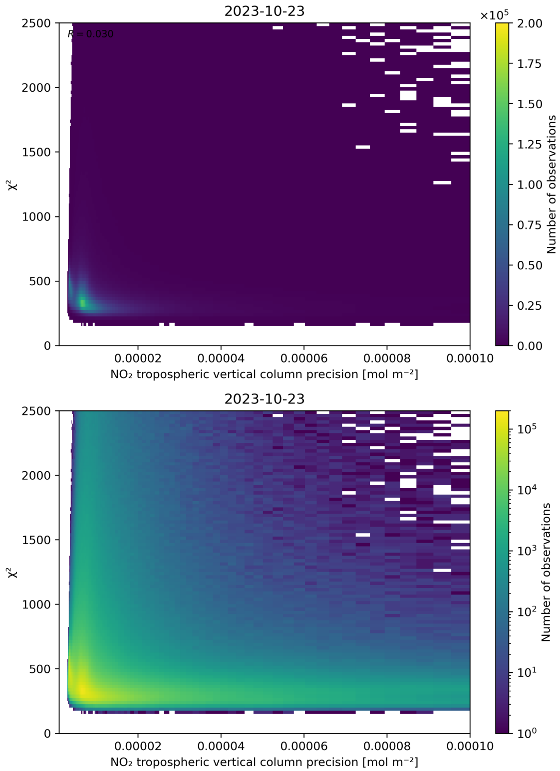
Figure 134: Scatter density plot of “NO 2 tropospheric vertical column precision” against “ \chi^2 ” for 2023-10-22 to 2023-10-24.
