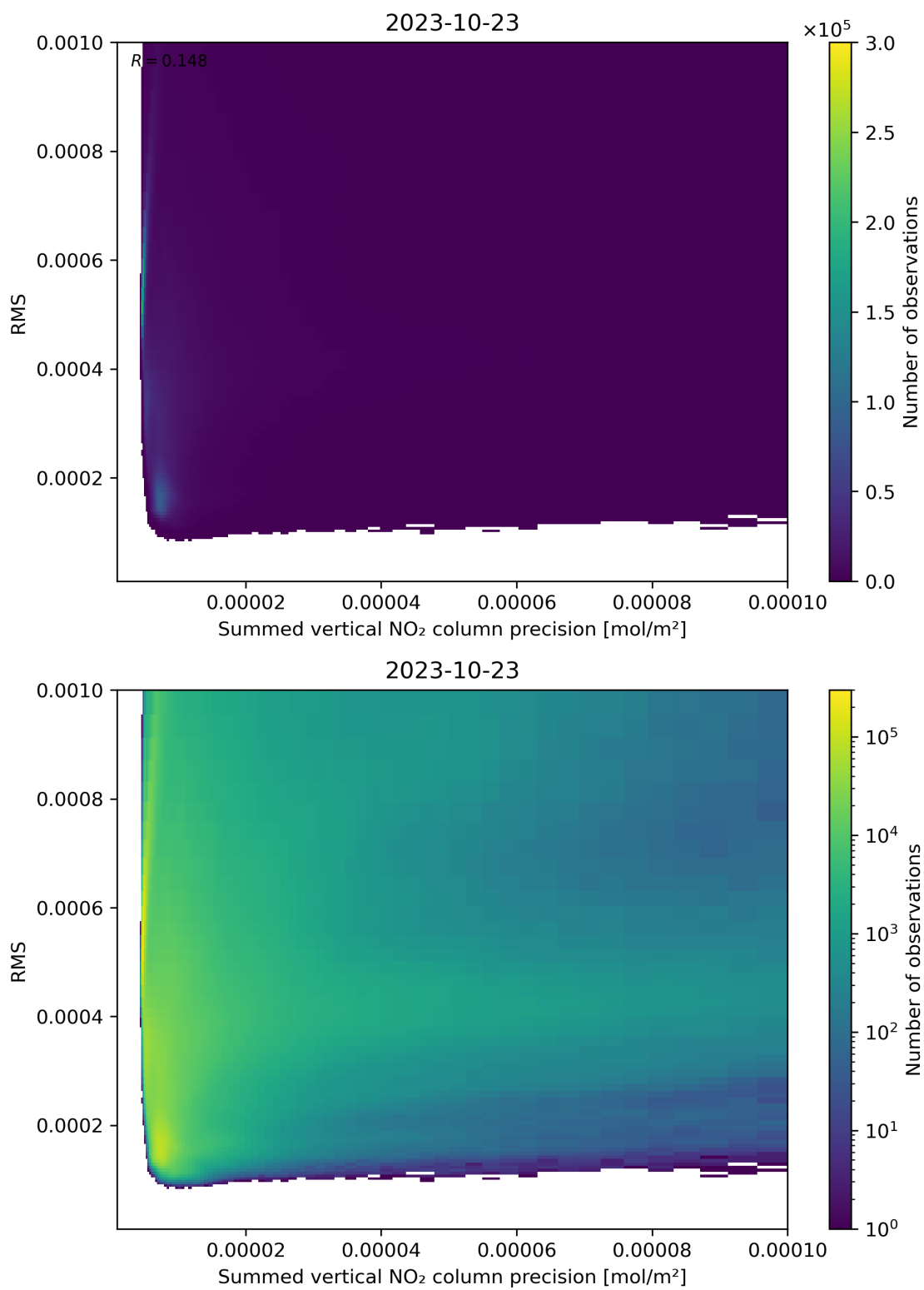
Figure 108: Scatter density plot of “Summed vertical NO 2 column precision” against “RMS” for 2023-10-22 to 2023-10-24.
