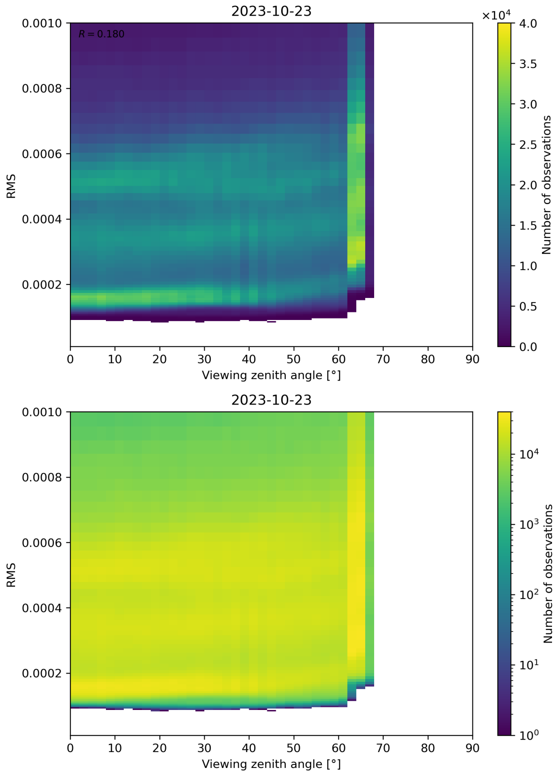
Figure 171: Scatter density plot of “Viewing zenith angle” against “RMS” for 2023-10-22 to 2023-10-24.
