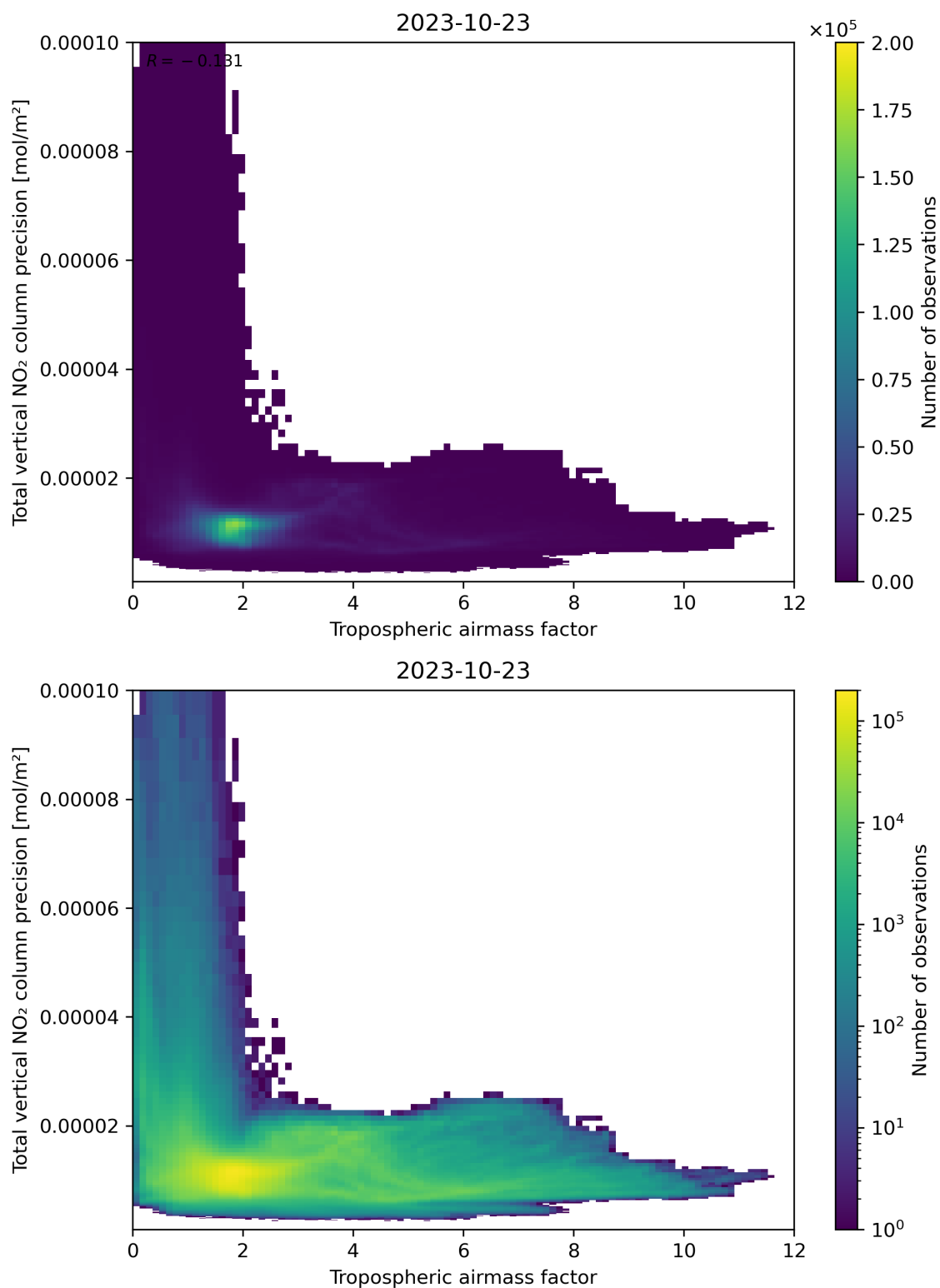
Figure 78: Scatter density plot of “Tropospheric air mass factor” against “Total vertical NO 2 column precision” for 2023-10-22 to 2023-10-24.
