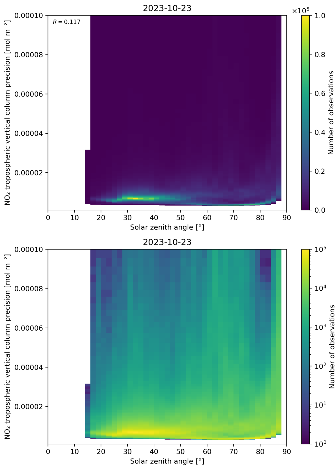
Figure 156: Scatter density plot of “Solar zenith angle” against “NO 2 tropospheric vertical column precision” for 2023-10-22 to 2023-10-24.
