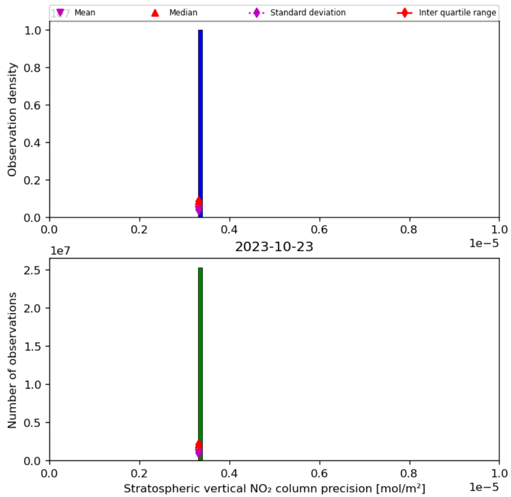
Figure 37: Histogram of “Stratospheric vertical NO 2 column precision” for 2023-10-22 to 2023-10-24
