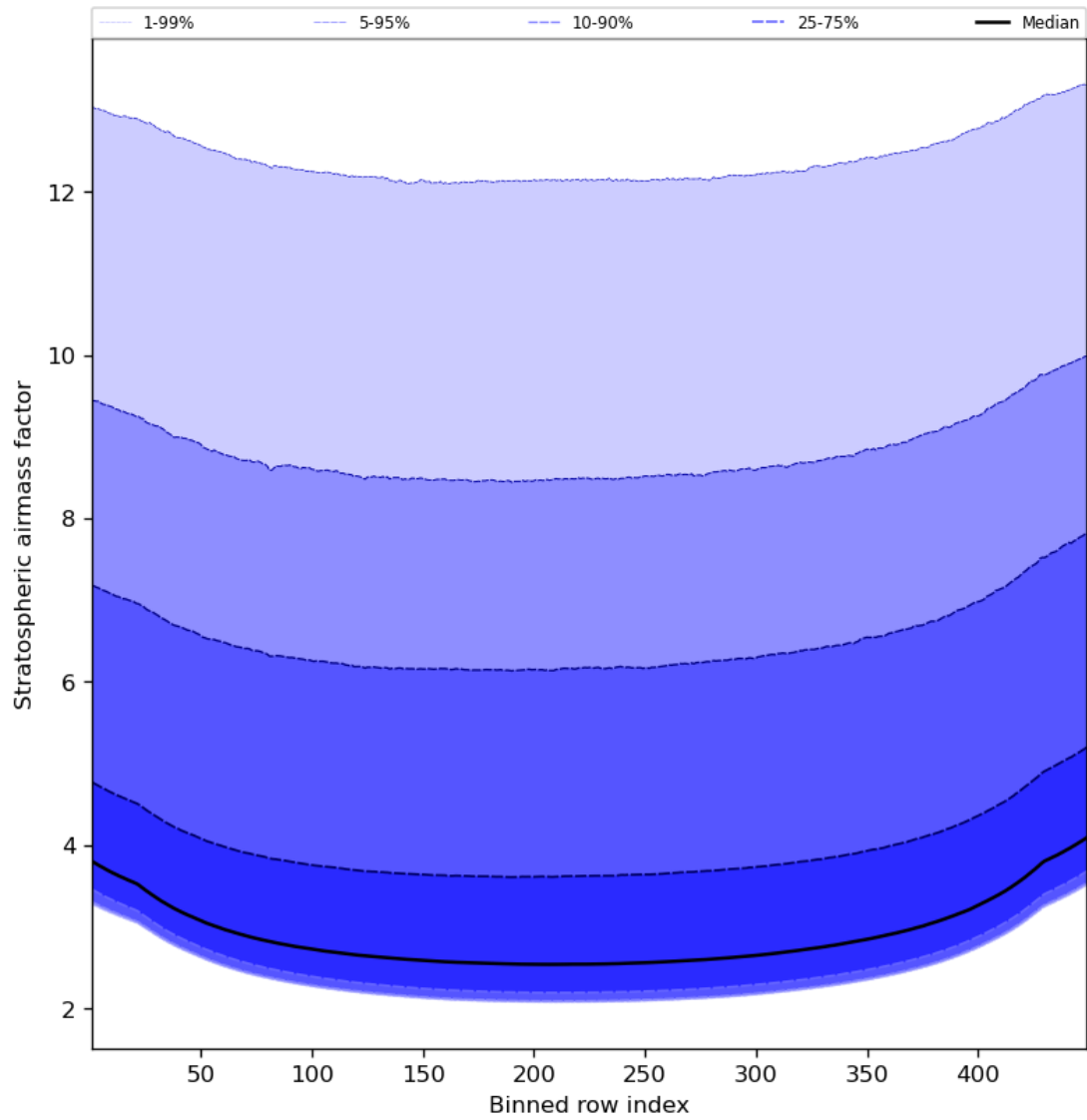
Figure 61: Along track statistics of “Stratospheric airmass factor” for 2023-10-22 to 2023-10-24
