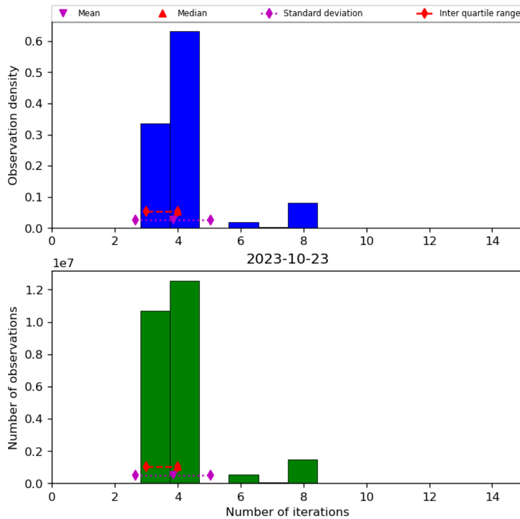
Figure 34: Histogram of “Number of iterations” for 2023-10-22 to 2023-10-24
