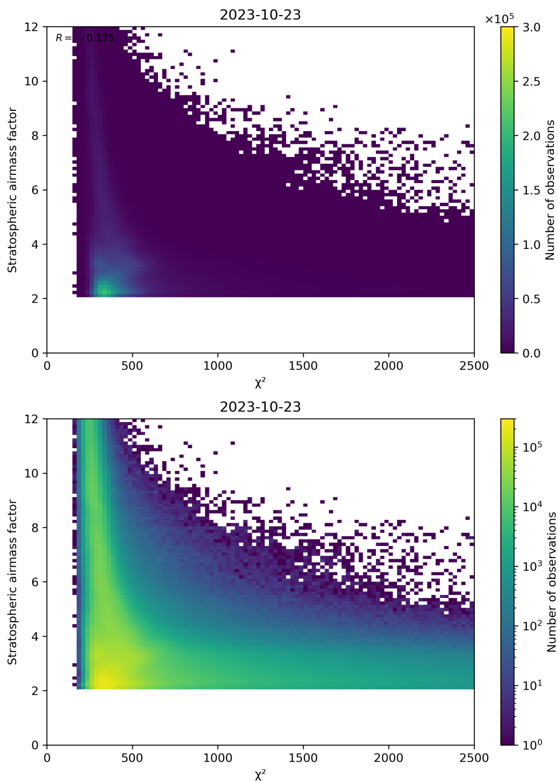
Figure 81: Scatter density plot of “ \chi^2 ” against “Stratospheric airmass factor” for 2023-10-22 to 2023-10-24.
