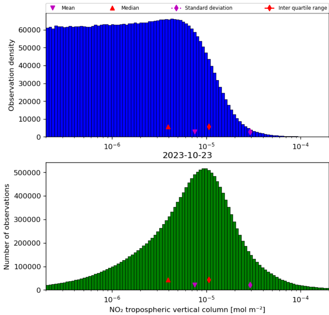
Figure 29: Histogram of “NO 2 tropospheric vertical column” for 2023-10-22 to 2023-10-24
