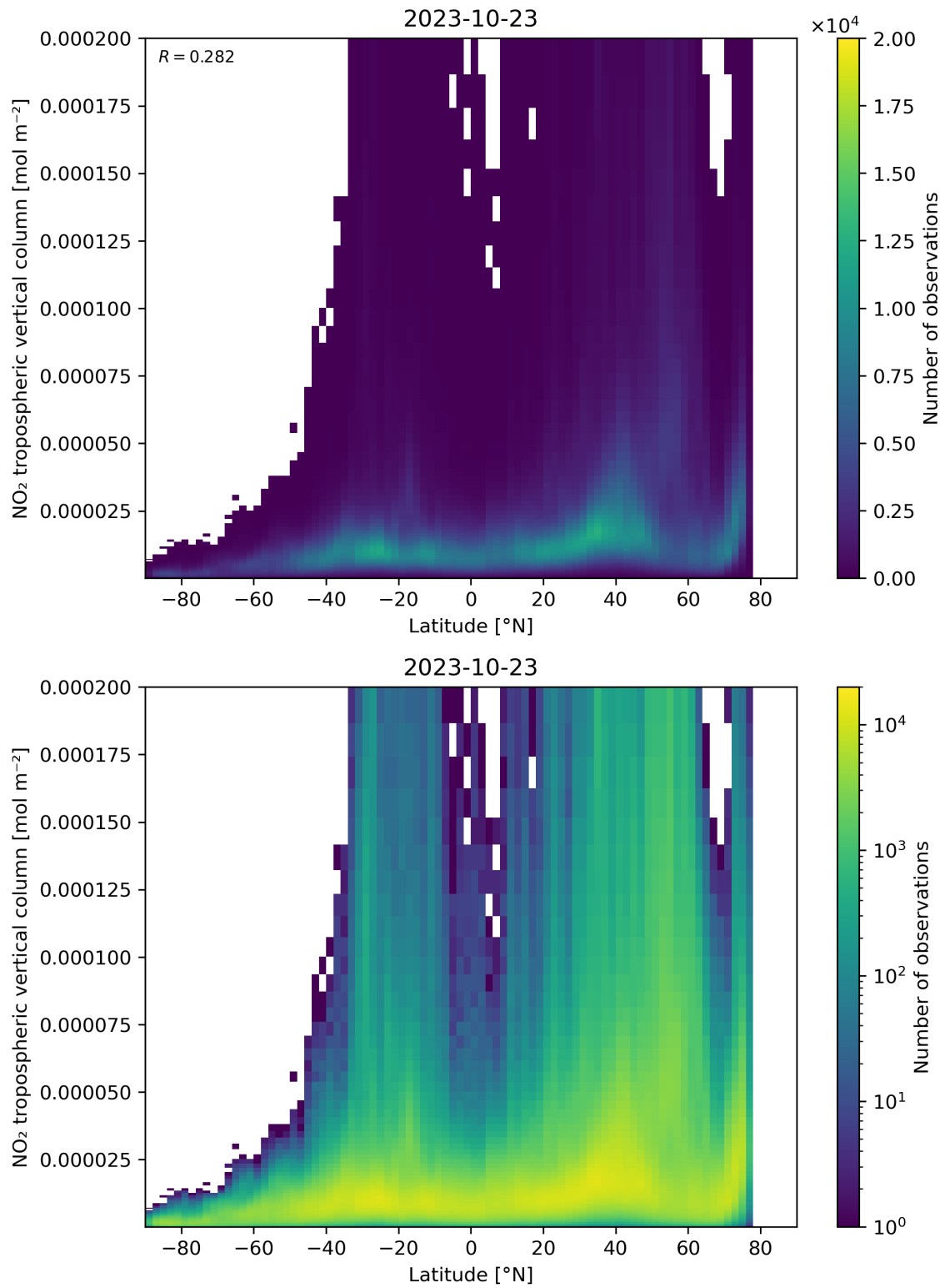
Figure 92: Scatter density plot of “Latitude” against “NO 2 tropospheric vertical column” for 2023-10-22 to 2023-10-24.
