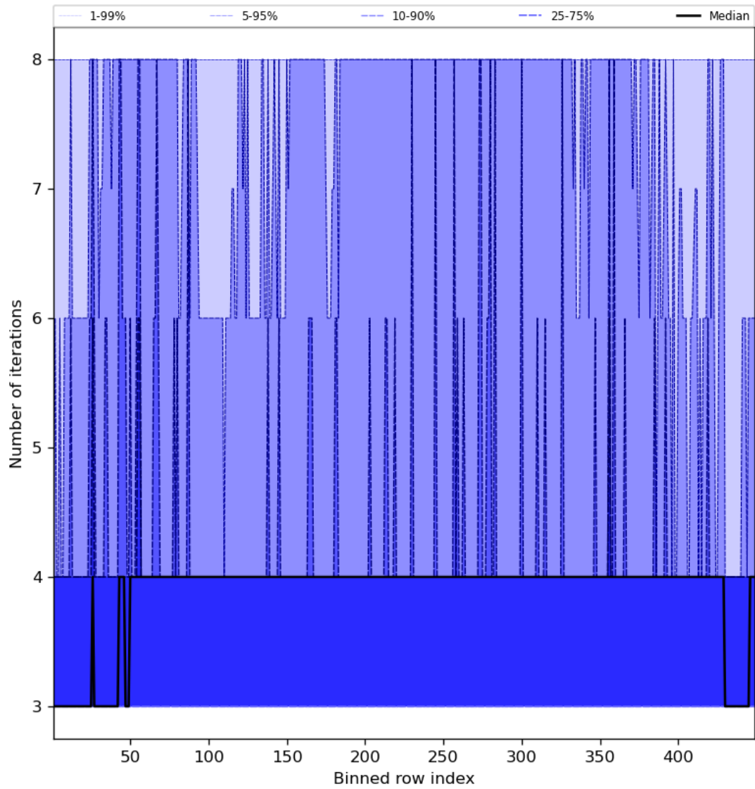
Figure 51: Along track statistics of “Number of iterations” for 2023-10-22 to 2023-10-24
