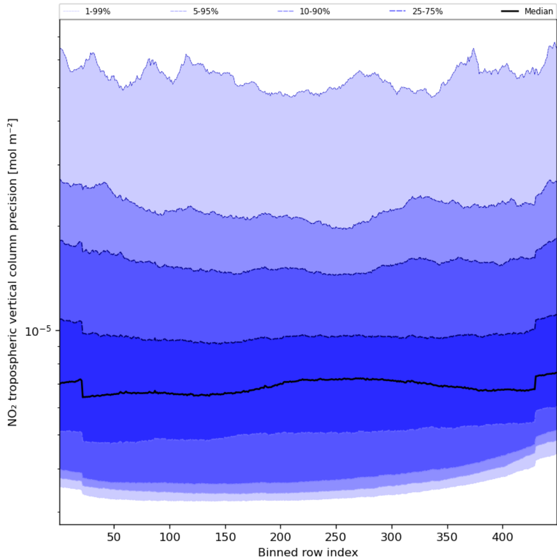
Figure 47: Along track statistics of “NO 2 tropospheric vertical column precision” for 2023-10-22 to 2023-10-24
