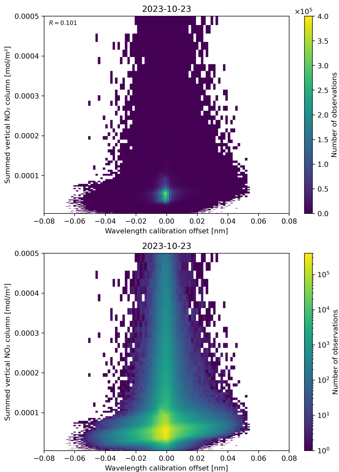
Figure 177: Scatter density plot of “Wavelength calibration offset” against “Summed vertical NO 2 column” for 2023-10-22 to 2023-10-24.
