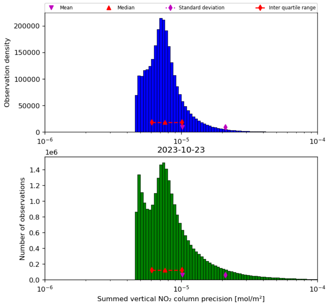
Figure 41: Histogram of "Summed vertical NO 2 column precision" for 2023-10-22 to 2023-10-24
