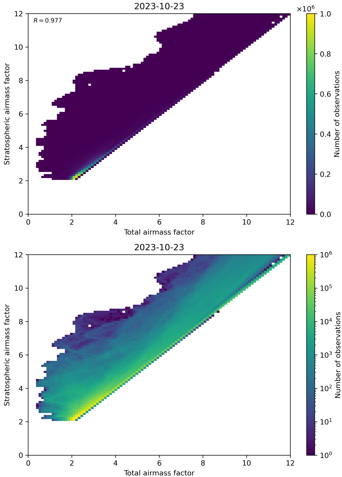
Figure 62: Scatter density plot of “Total airmass factor” against “Stratospheric airmass factor” for 2023-10-22 to 2023-10-24.
