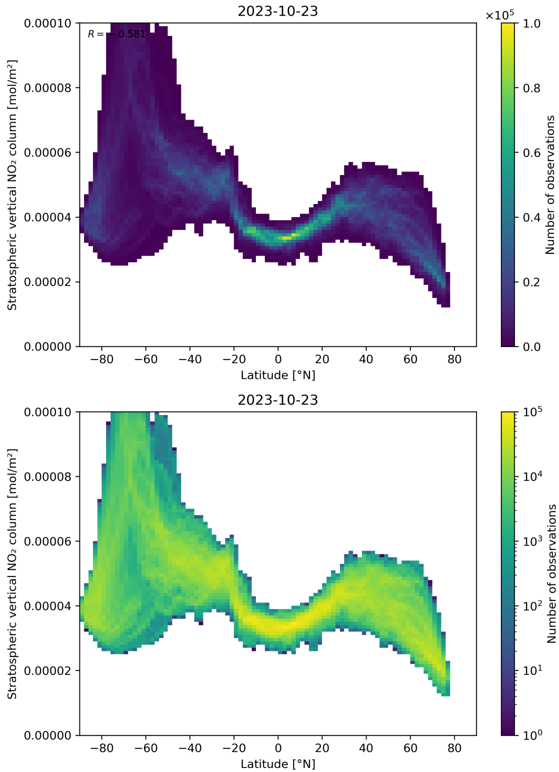
Figure 87: Scatter density plot of “Latitude” against “Stratospheric vertical NO 2 column” for 2023-10-22 to 2023-10-24.
