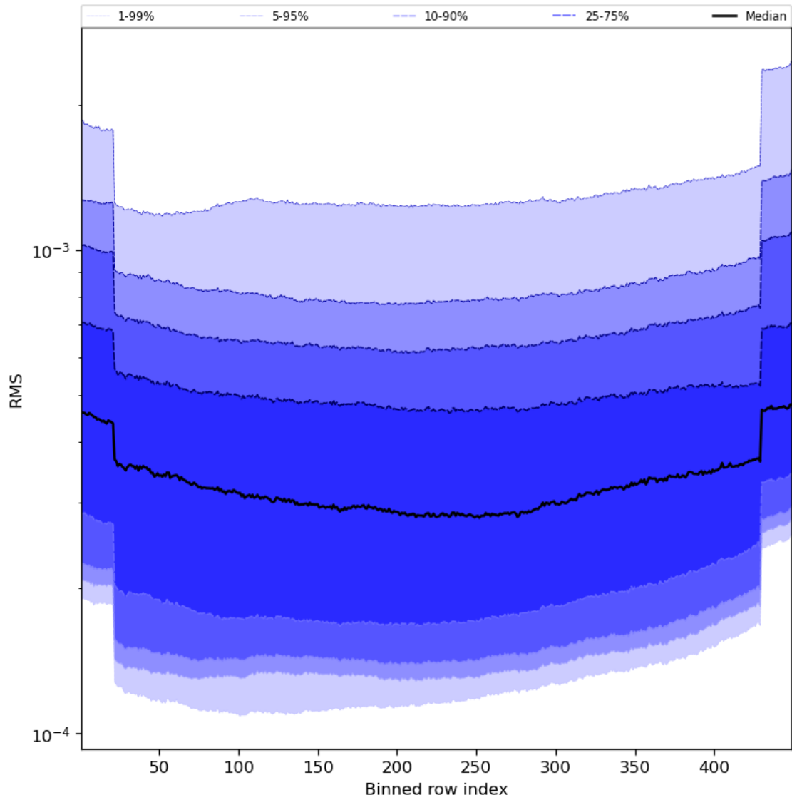
Figure 60: Along track statistics of “RMS” for 2023-10-22 to 2023-10-24
