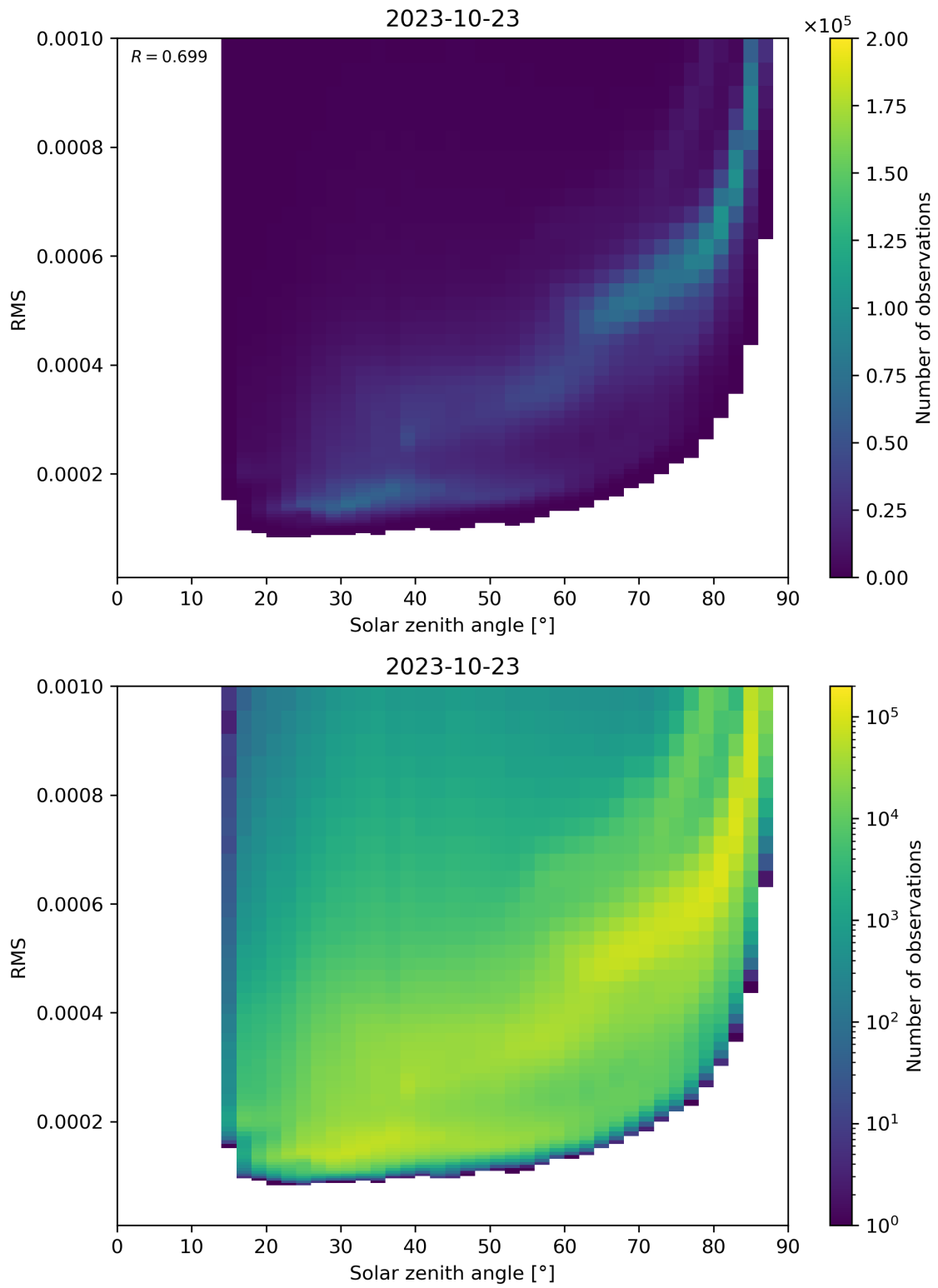
Figure 157: Scatter density plot of “Solar zenith angle” against “RMS” for 2023-10-22 to 2023-10-24.
