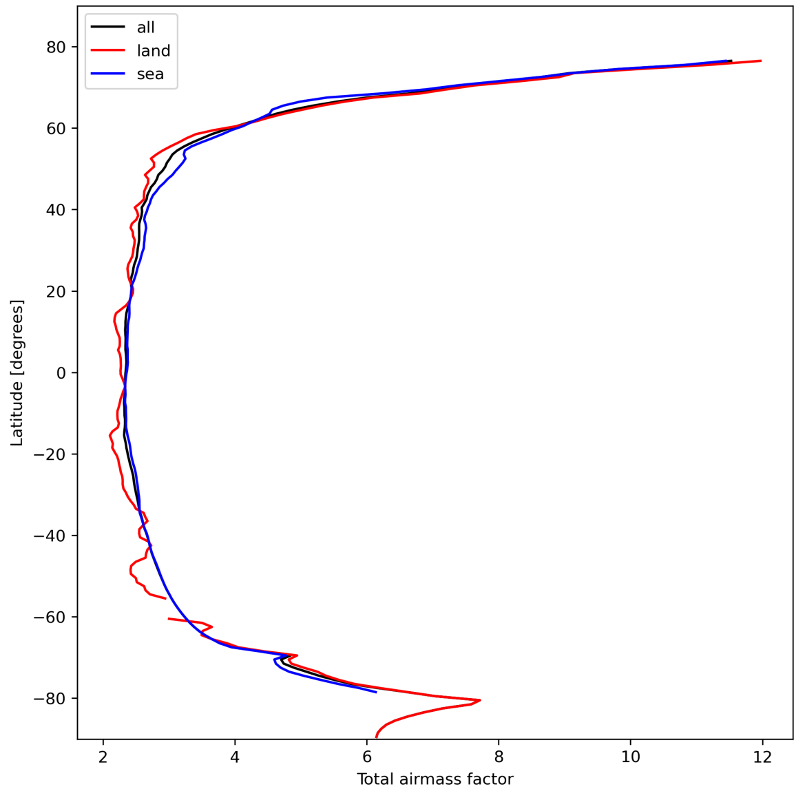
Figure 15: Zonal average of “Total airmass factor” for 2023-10-22 to 2023-10-24.
