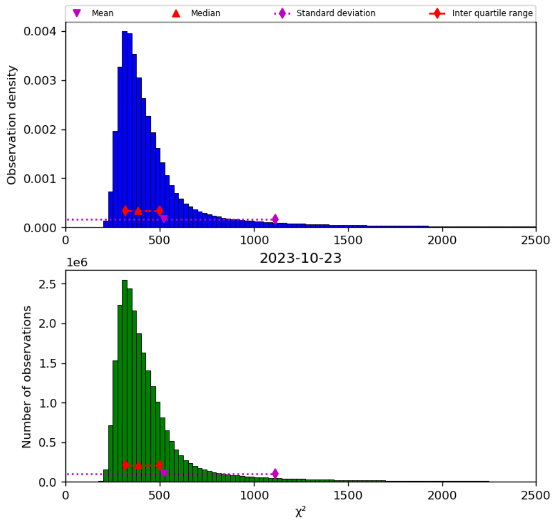
Figure 42: Histogram of “ \chi^2 ” for 2023-10-22 to 2023-10-24
