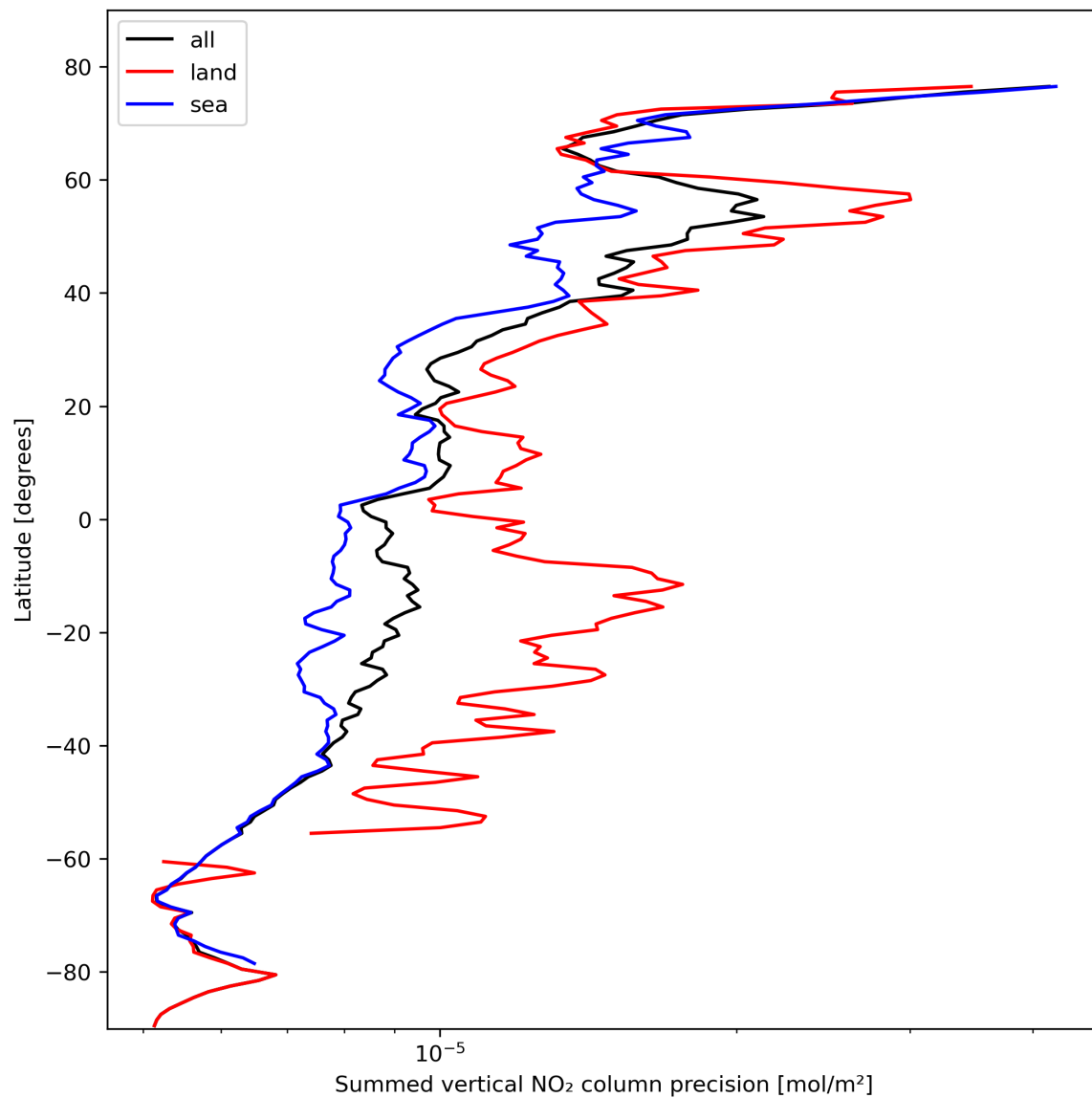
Figure 24: Zonal average of “Summed vertical NO 2 column precision” for 2023-10-22 to 2023-10-24.
