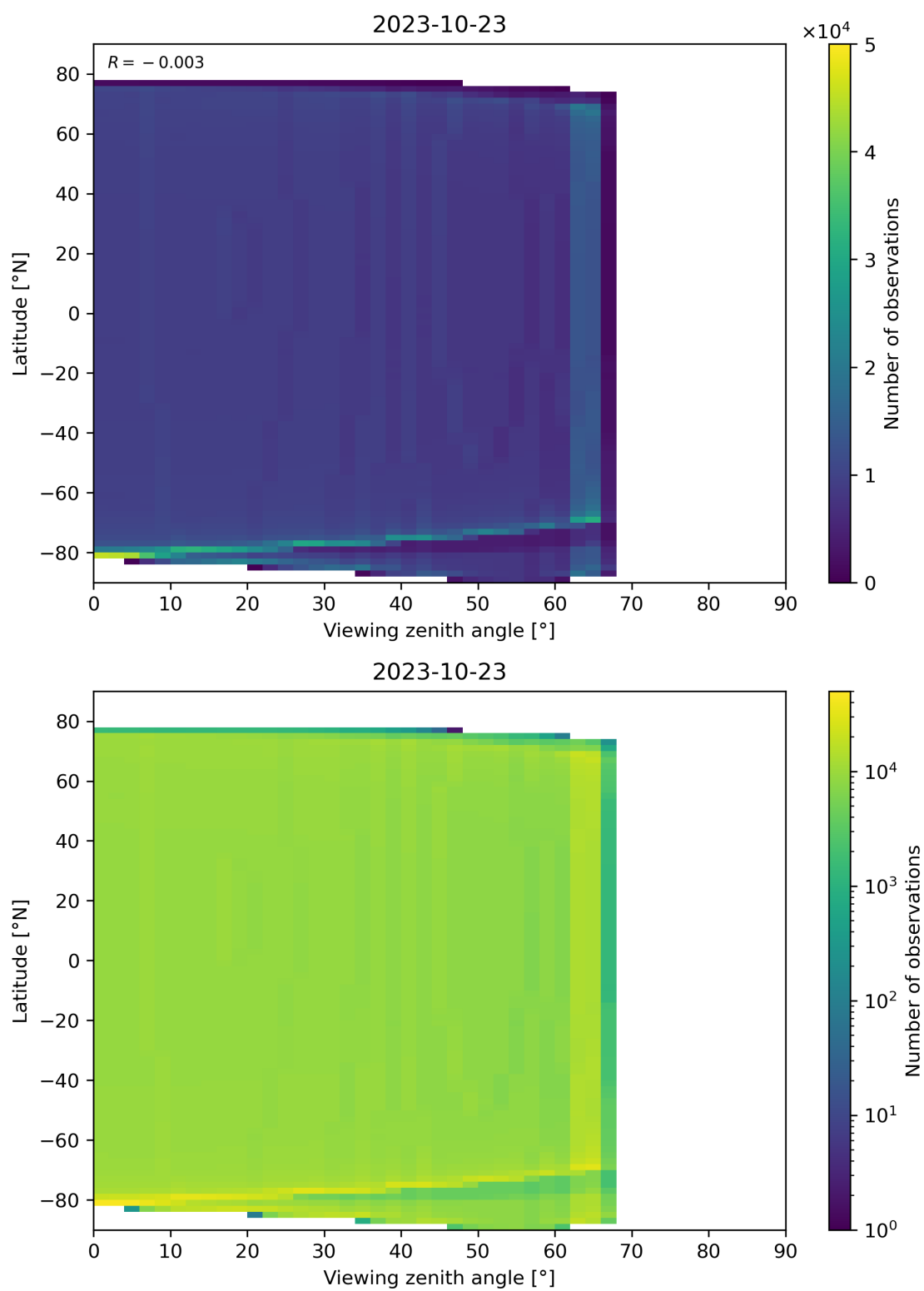
Figure 163: Scatter density plot of “Viewing zenith angle” against “Latitude” for 2023-10-22 to 2023-10-24.
