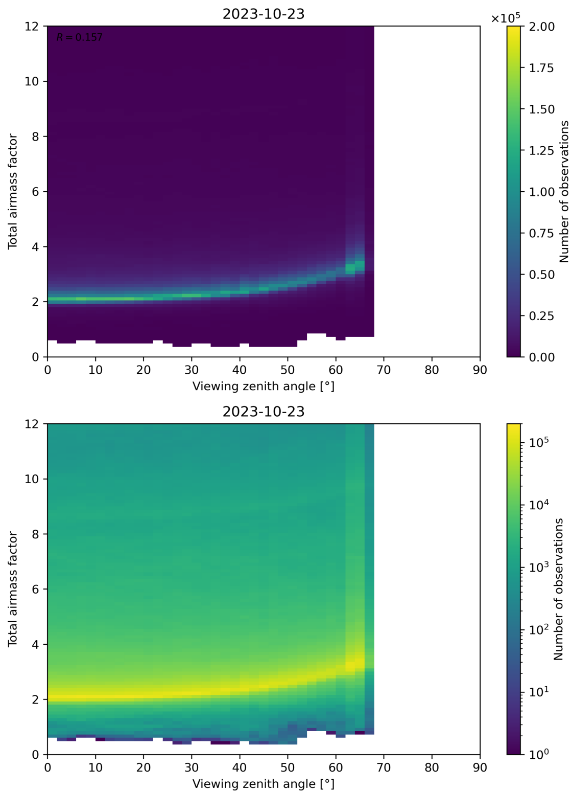
Figure 160: Scatter density plot of “Viewing zenith angle” against “Total airmass factor” for 2023-10-22 to 2023-10-24.
