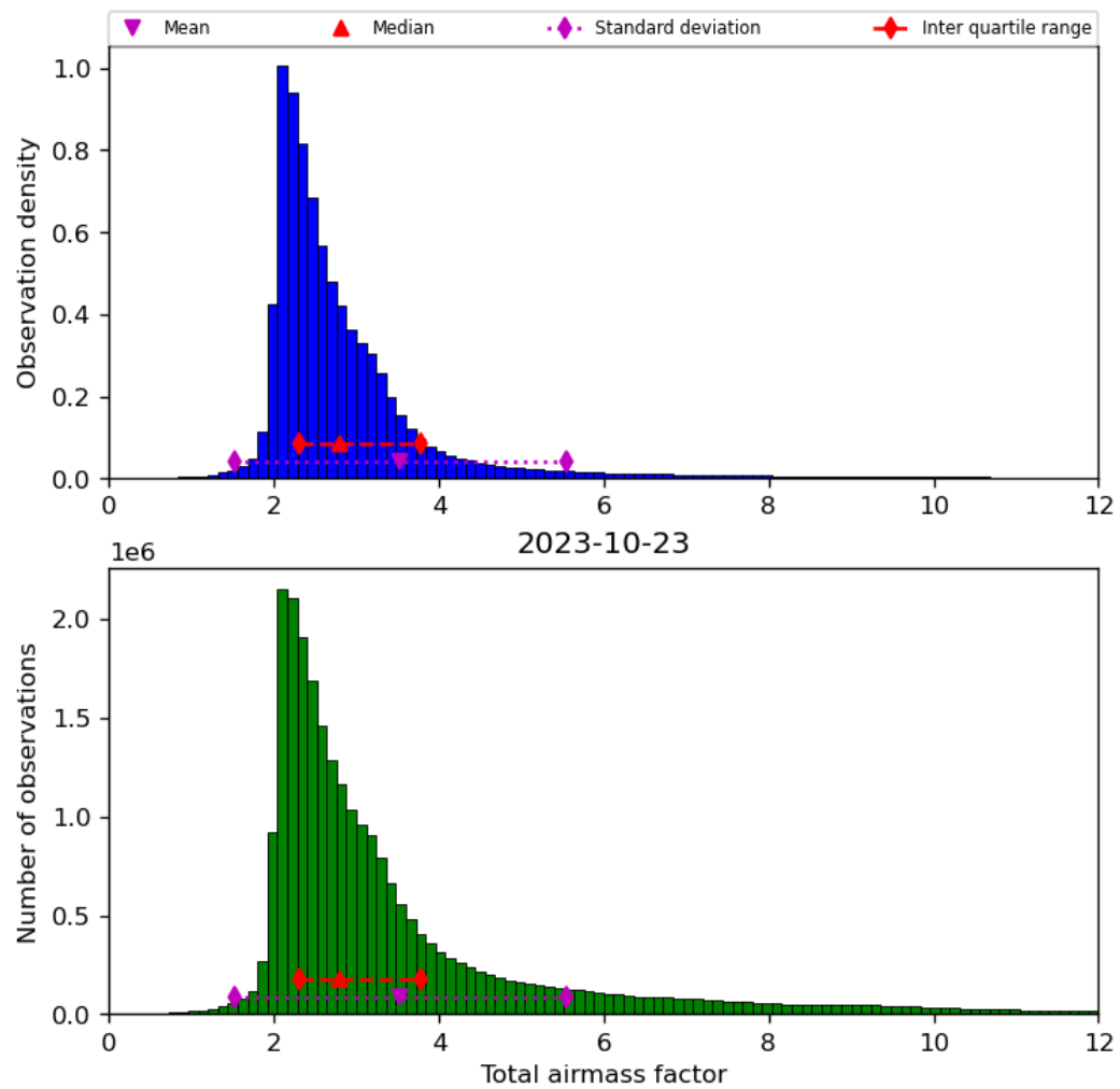
Figure 32: Histogram of “Total airmass factor” for 2023-10-22 to 2023-10-24
