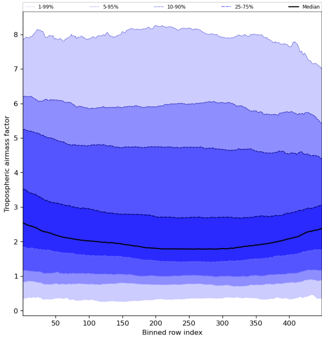
Figure 48: Along track statistics of “Tropospheric airmass factor” for 2023-10-22 to 2023-10-24
