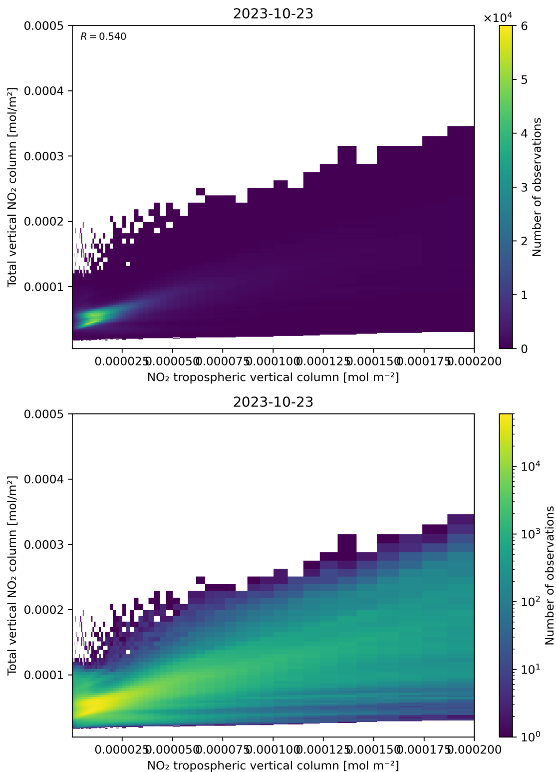
Figure 128: Scatter density plot of “NO 2 tropospheric vertical column” against “Total vertical NO 2 column” for 2023-10-22 to 2023-10-24.
