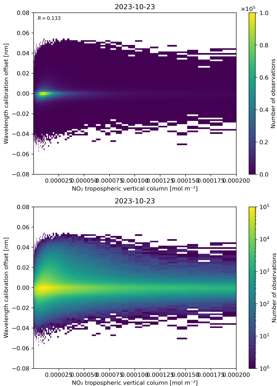
Figure 143: Scatter density plot of “NO 2 tropospheric vertical column” against “Wavelength calibration offset” for 2023-10-22 to 2023-10-24.
