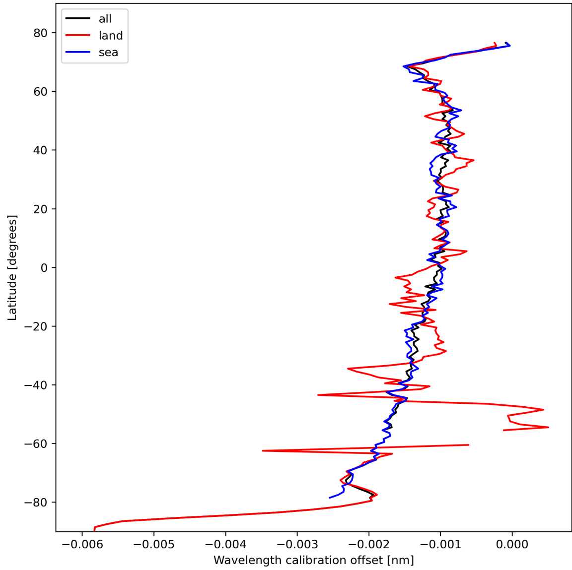
Figure 18: Zonal average of “Wavelength calibration offset” for 2023-10-22 to 2023-10-24.
