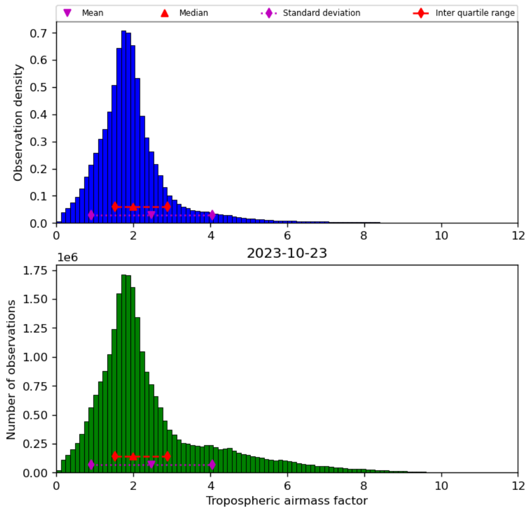
Figure 31: Histogram of “Tropospheric airmass factor” for 2023-10-22 to 2023-10-24
