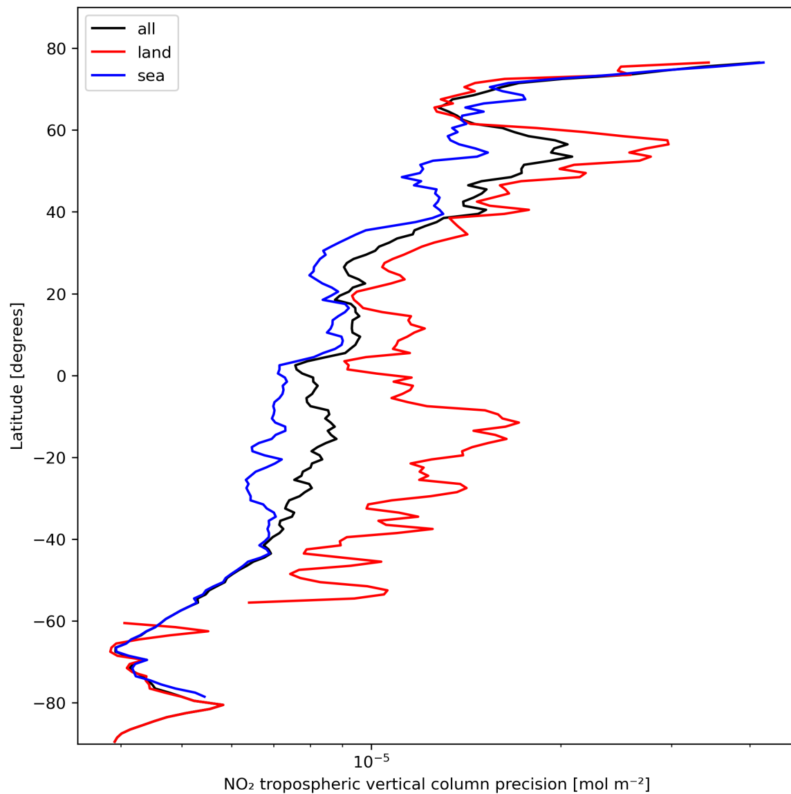
Figure 13: Zonal average of “NO 2 tropospheric vertical column precision” for 2023-10-22 to 2023-10-24.
