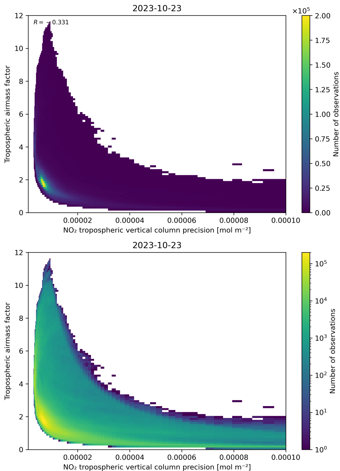
Figure 133: Scatter density plot of “NO 2 tropospheric vertical column precision” against “Tropospheric airmass factor” for 2023-10-22 to 2023-10-24.
