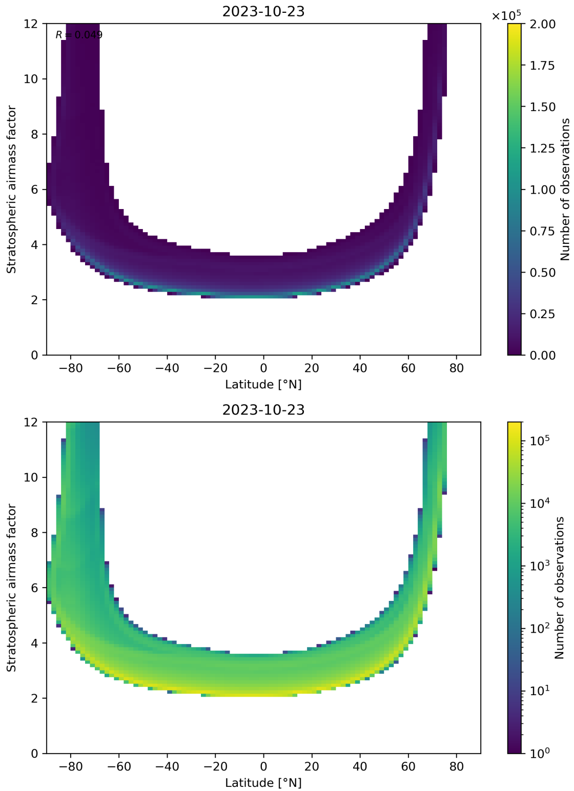
Figure 83: Scatter density plot of “Latitude” against “Stratospheric air mass factor” for 2023-10-22 to 2023-10-24.
