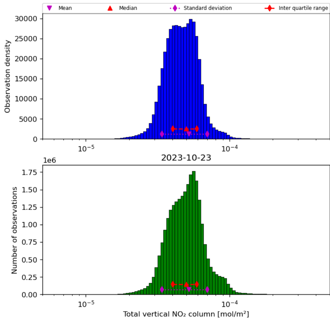
Figure 38: Histogram of “Total vertical NO 2 column” for 2023-10-22 to 2023-10-24
