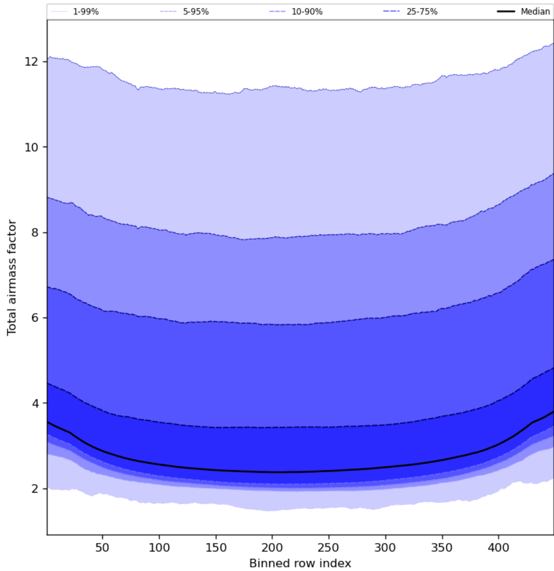
Figure 49: Along track statistics of “Total airmass factor” for 2023-10-22 to 2023-10-24
