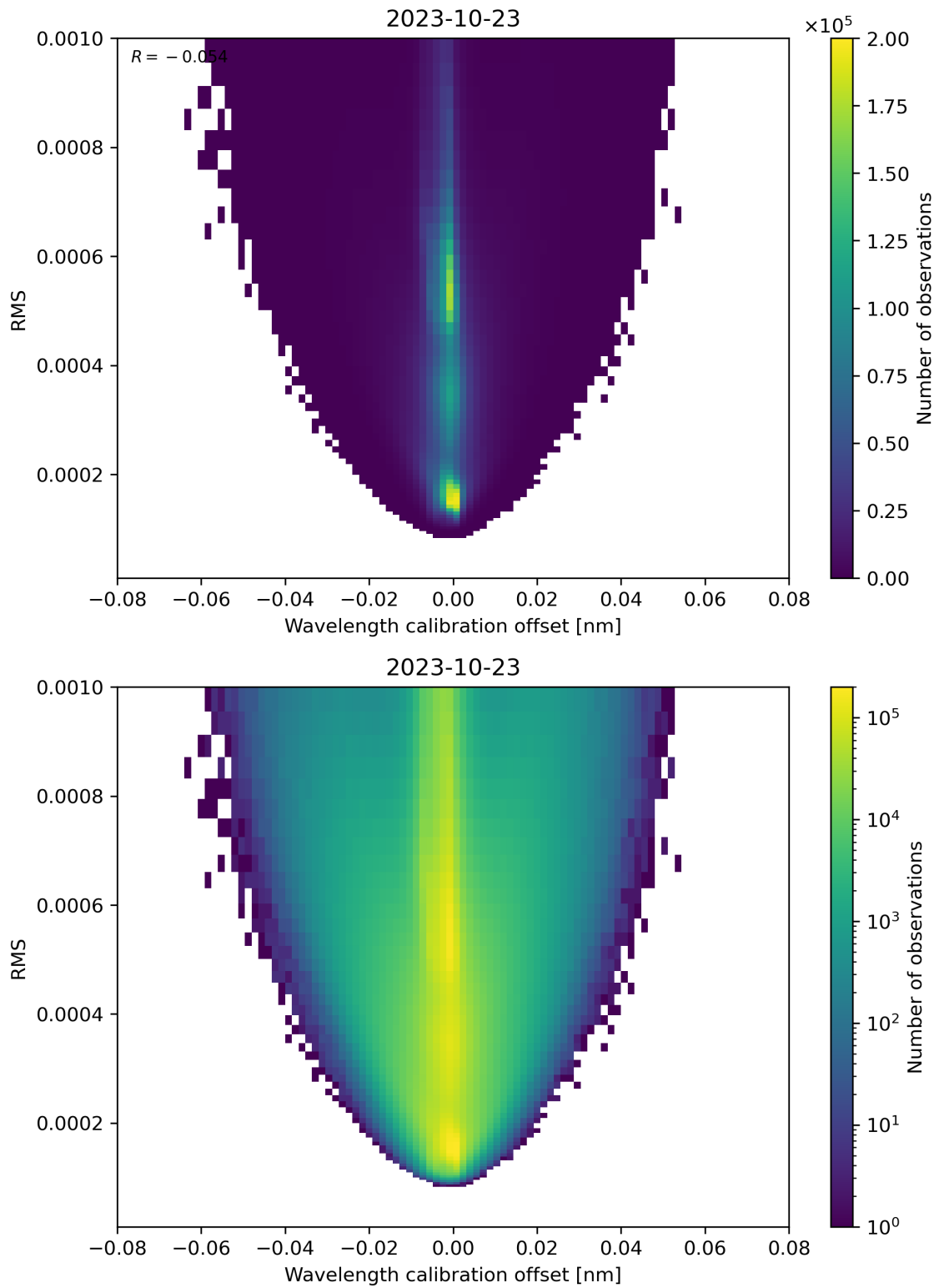
Figure 181: Scatter density plot of “Wavelength calibration offset” against “RMS” for 2023-10-22 to 2023-10-24.
