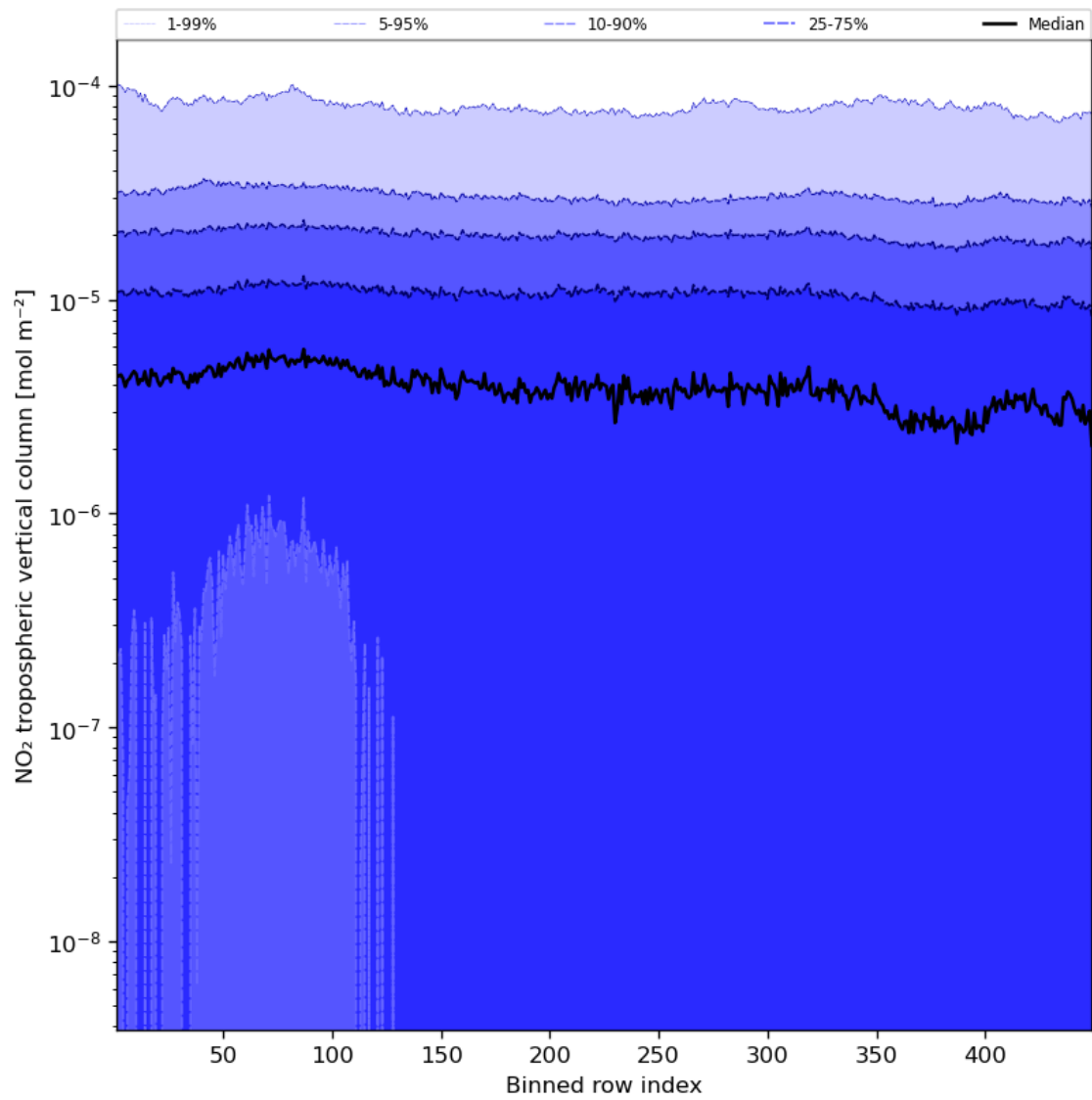
Figure 46: Along track statistics of “NO 2 tropospheric vertical column” for 2023-10-22 to 2023-10-24
