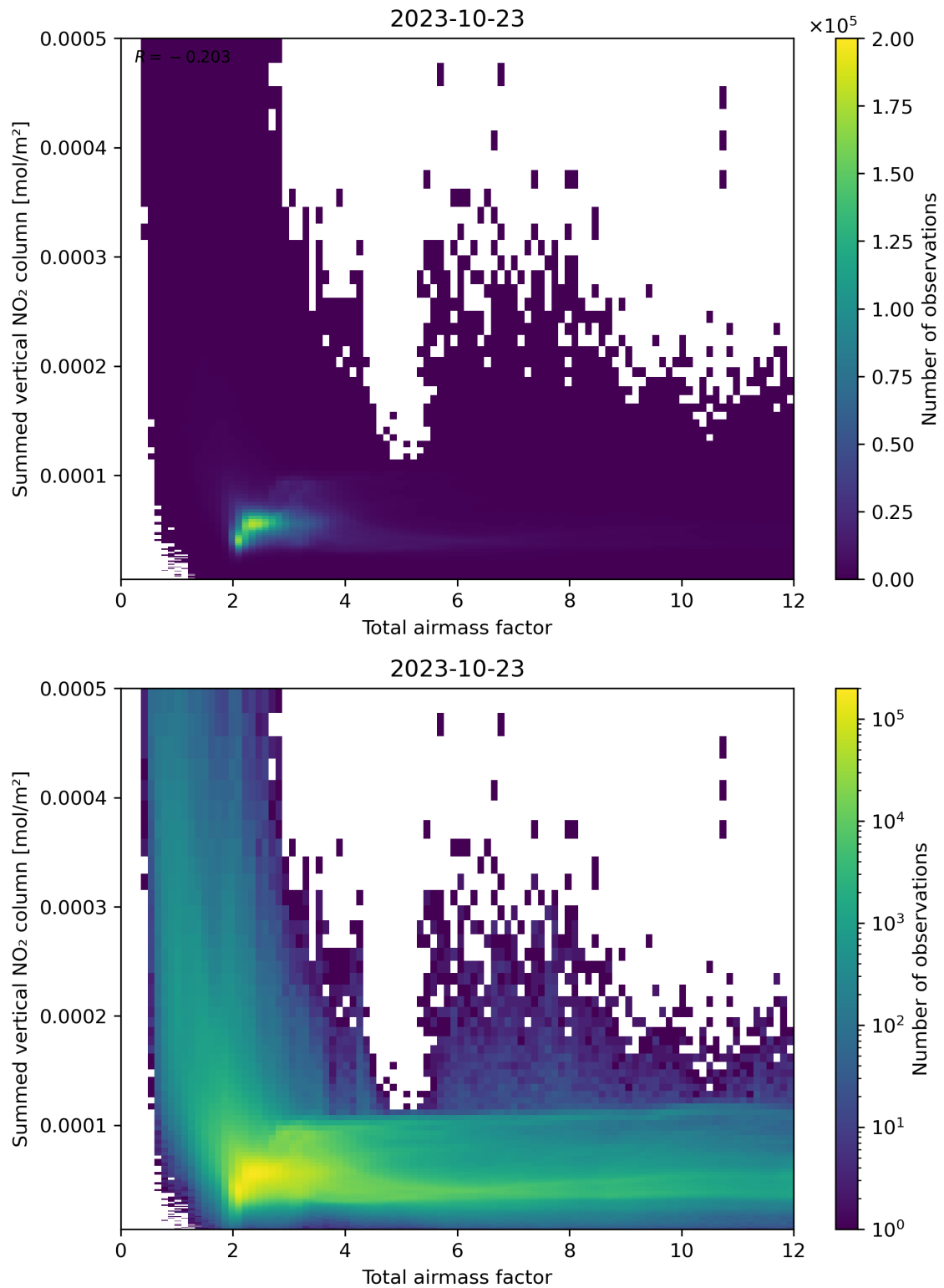
Figure 65: Scatter density plot of “Total airmass factor” against “Summed vertical NO 2 column” for 2023-10-22 to 2023-10-24.
