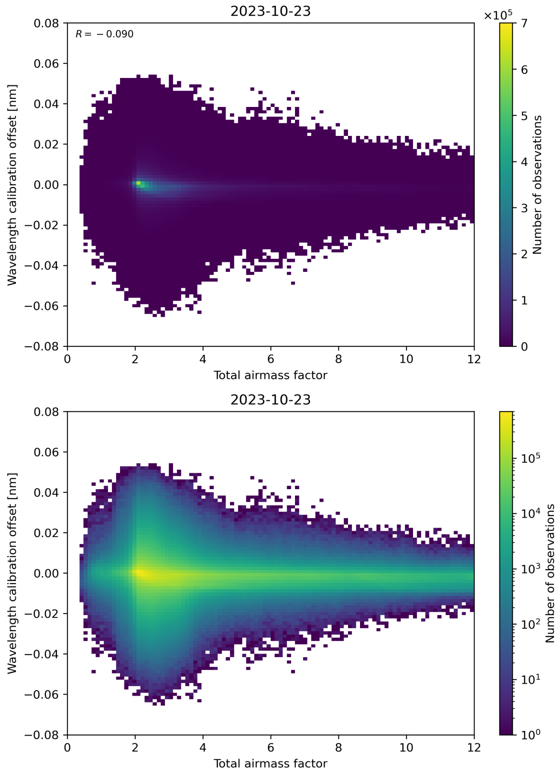
Figure 70: Scatter density plot of “Total airmass factor” against “Wavelength calibration offset” for 2023-10-22 to 2023-10-24.
