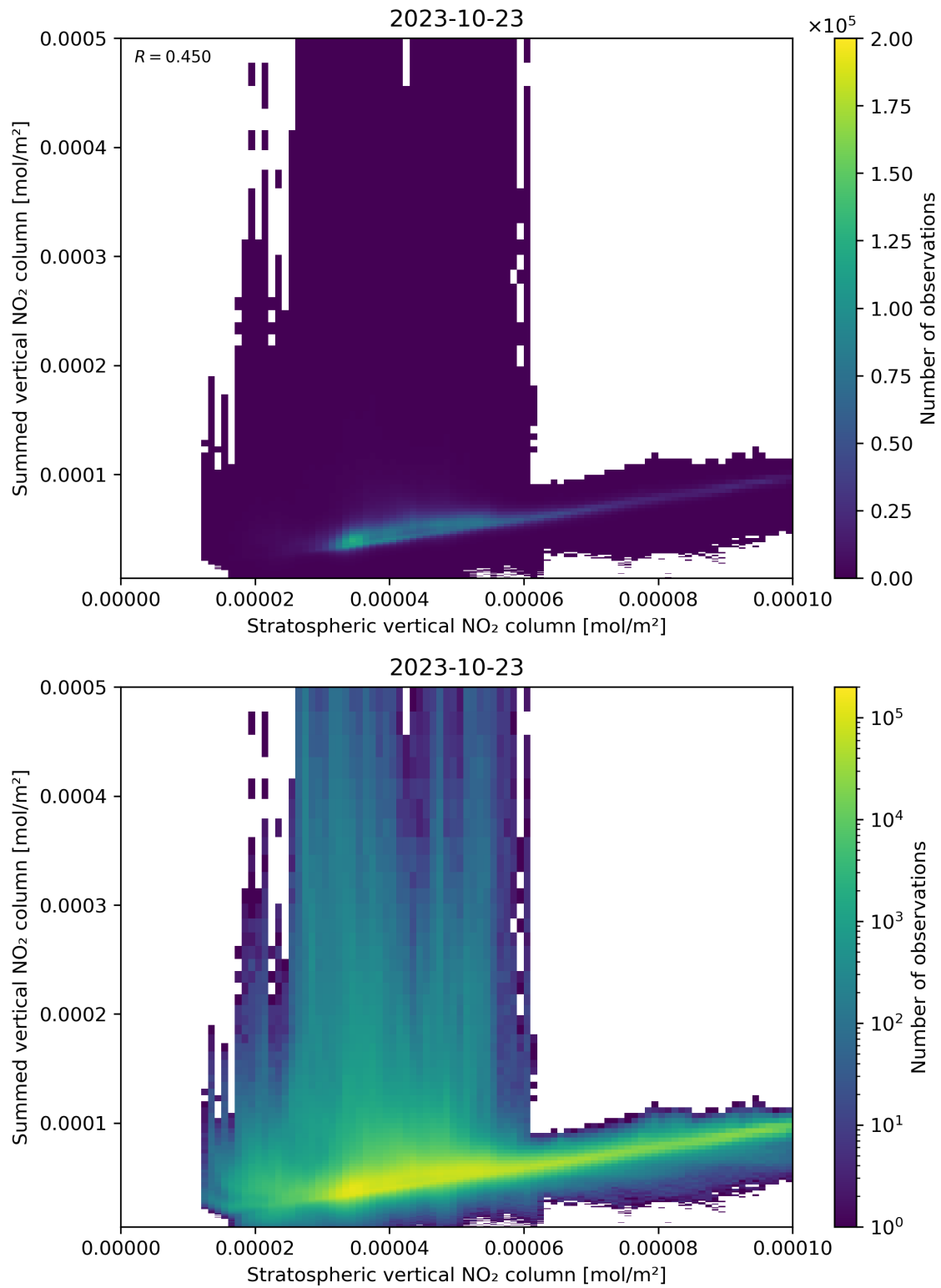
Figure 98: Scatter density plot of “Stratospheric vertical NO 2 column” against “Summed vertical NO 2 column” for 2023-10-22 to 2023-10-24.
