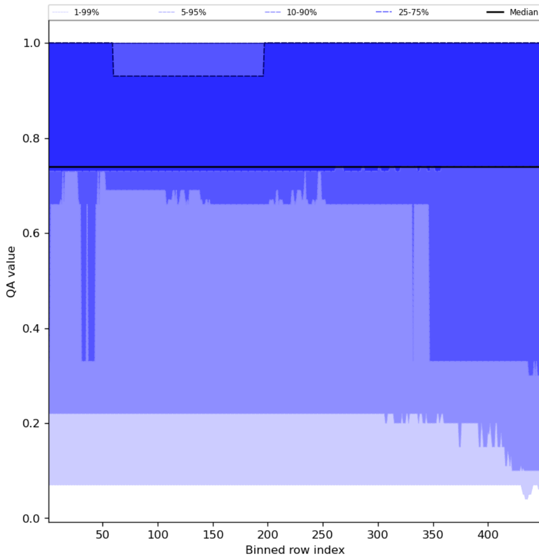
Figure 45: Along track statistics of “QA value” for 2023-10-22 to 2023-10-24
