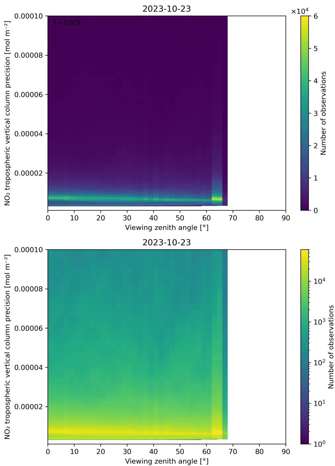
Figure 170: Scatter density plot of “Viewing zenith angle” against “NO 2 tropospheric vertical column precision” for 2023-10-22 to 2023-10-24.
