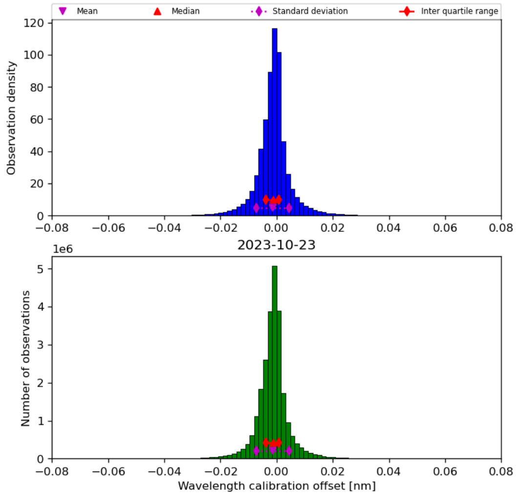
Figure 35: Histogram of “Wavelength calibration offset” for 2023-10-22 to 2023-10-24
