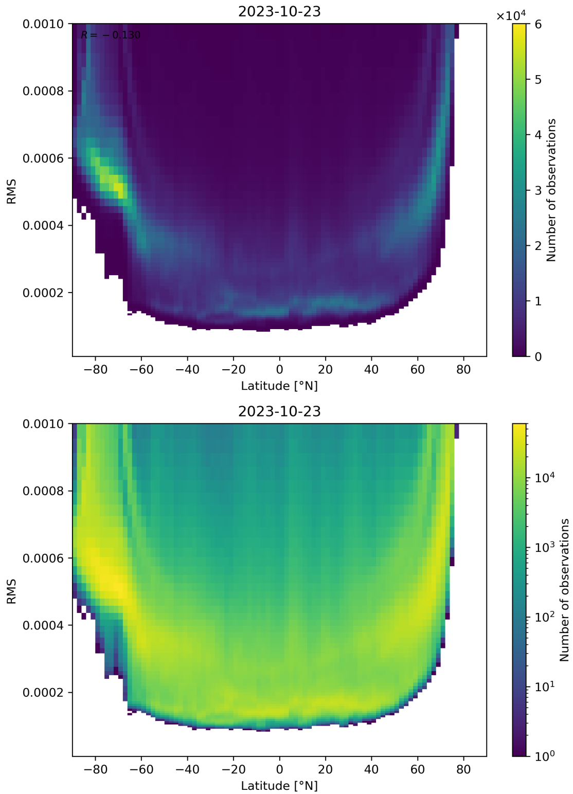
Figure 94: Scatter density plot of “Latitude” against “RMS” for 2023-10-22 to 2023-10-24.
