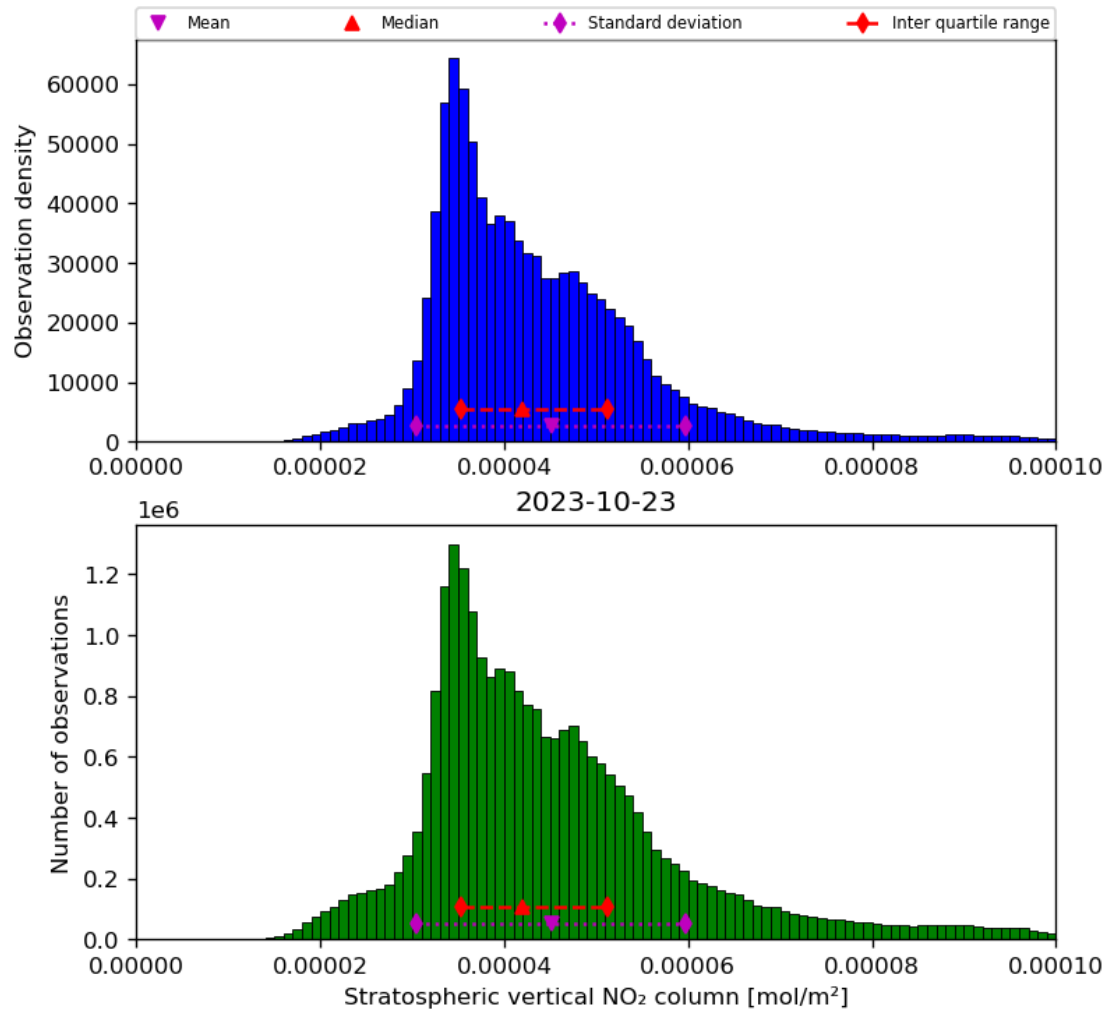
Figure 36: Histogram of “Stratospheric vertical NO 2 column” for 2023-10-22 to 2023-10-24
