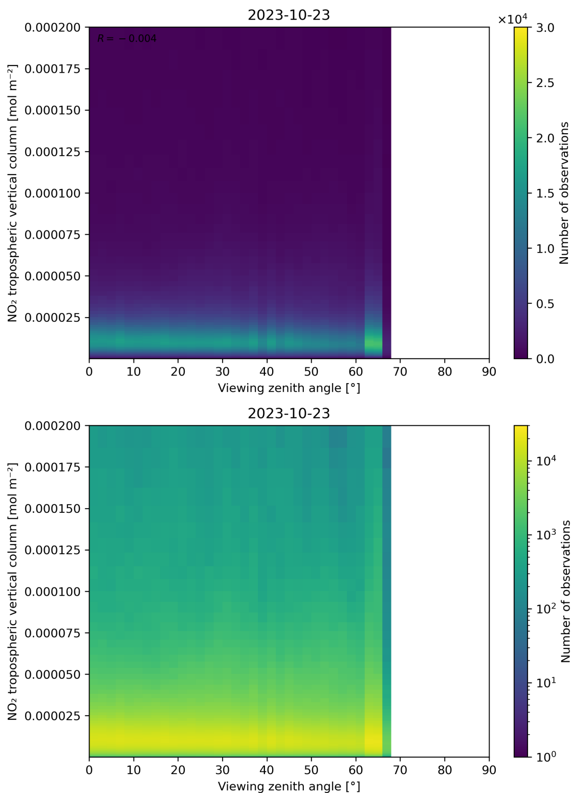
Figure 169: Scatter density plot of “Viewing zenith angle” against “NO 2 tropospheric vertical column” for 2023-10-22 to 2023-10-24.
