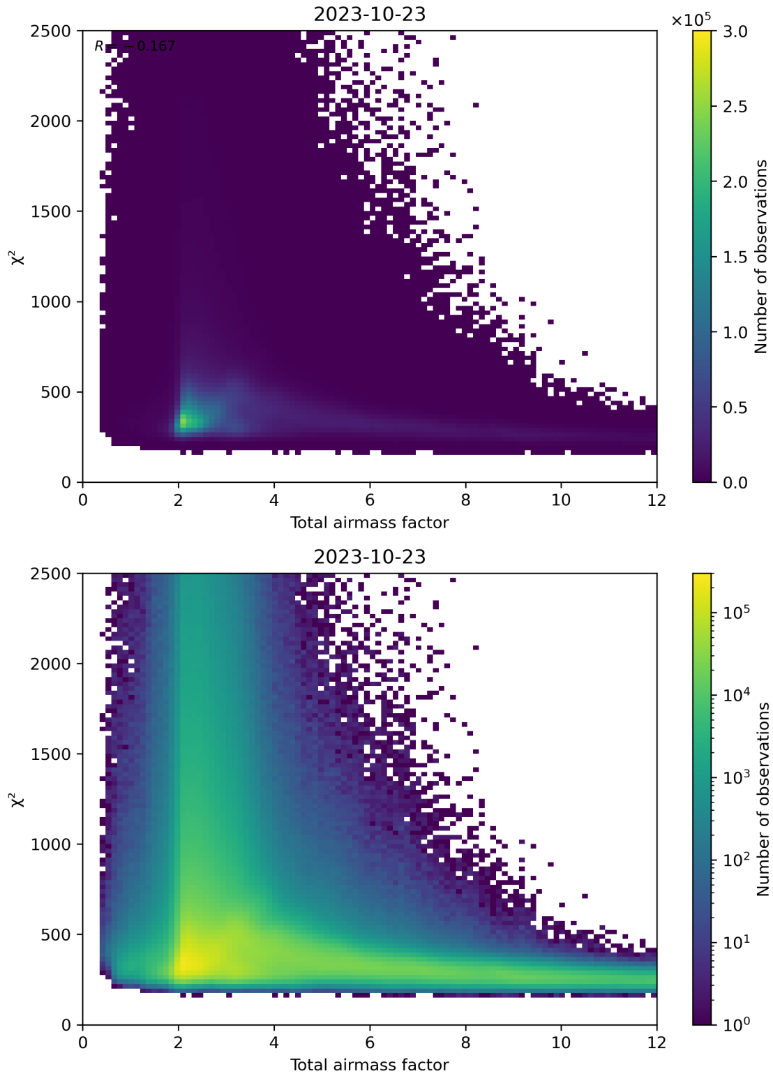
Figure 63: Scatter density plot of “Total airmass factor” against “ \chi^2 ” for 2023-10-22 to 2023-10-24.
