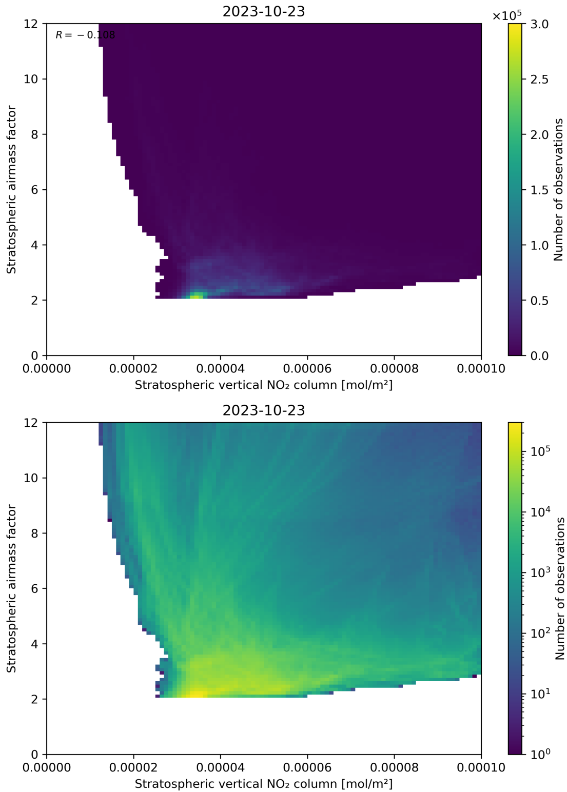
Figure 96: Scatter density plot of “Stratospheric vertical NO 2 column” against “Stratospheric airmass factor” for 2023-10-22 to 2023-10-24.
