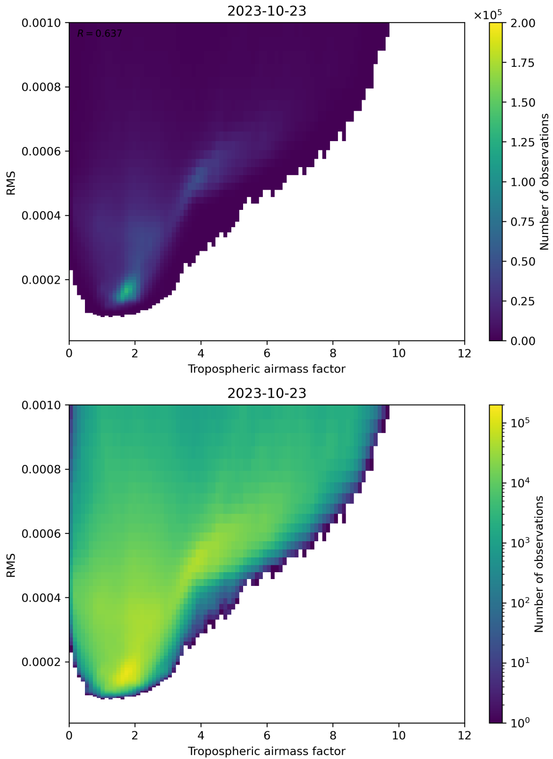
Figure 79: Scatter density plot of “Tropospheric airmass factor” against “RMS” for 2023-10-22 to 2023-10-24.
