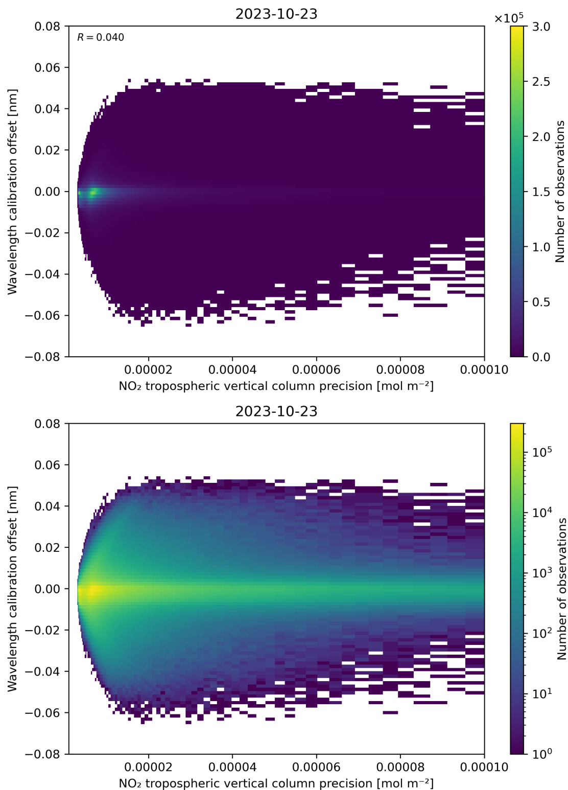
Figure 141: Scatter density plot of “NO 2 tropospheric vertical column precision” against “Wavelength calibration offset” for 2023-10-22 to 2023-10-24.
