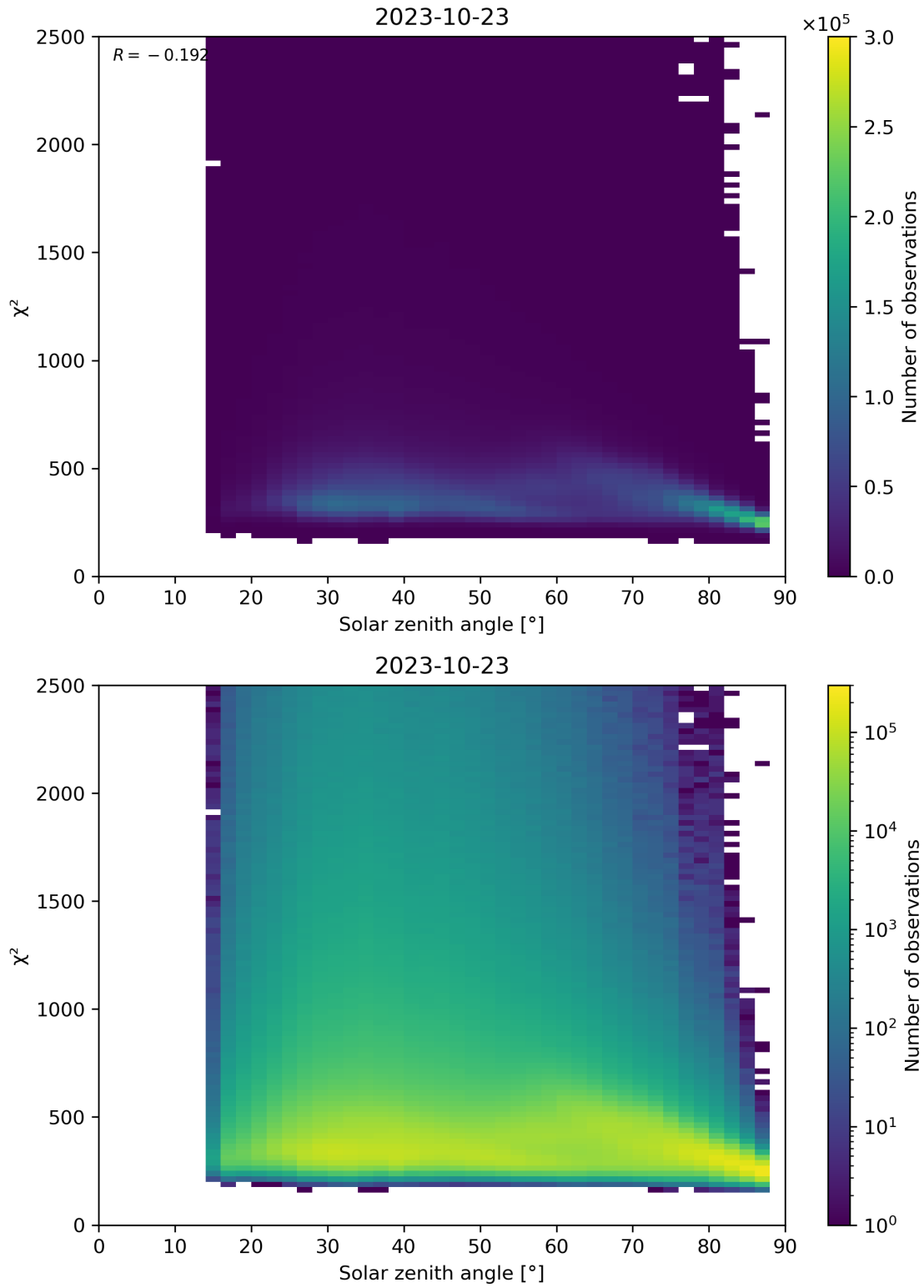
Figure 148: Scatter density plot of “Solar zenith angle” against “ \chi^2 ” for 2023-10-22 to 2023-10-24.
