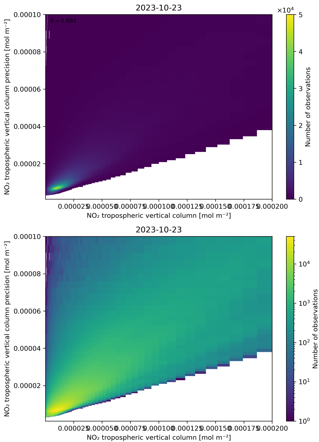
Figure 130: Scatter density plot of “NO 2 tropospheric vertical column” against “NO 2 tropospheric vertical column precision” for 2023-10-22 to 2023-10-24.
