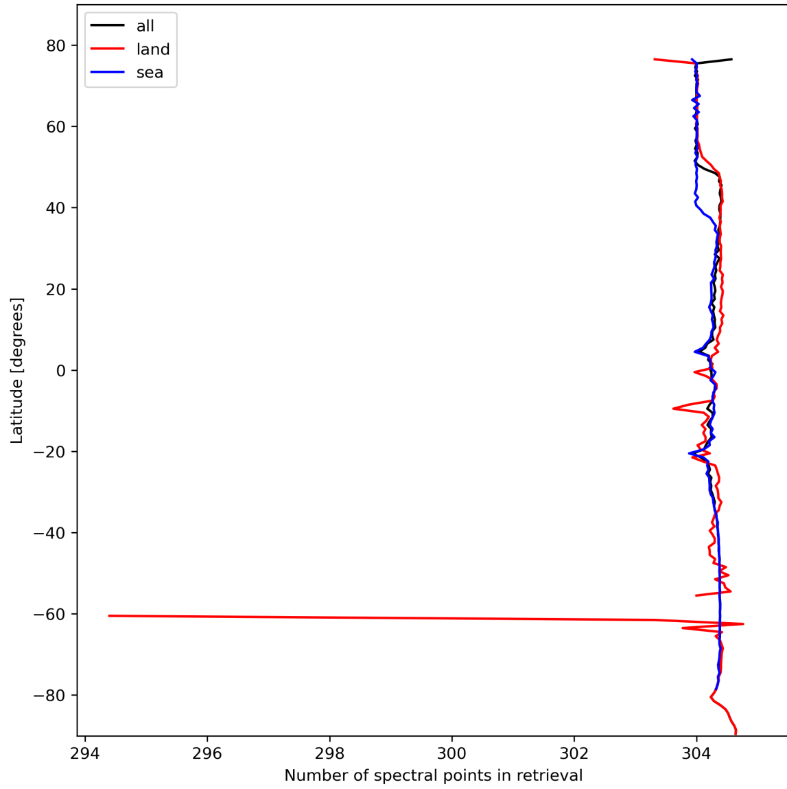
Figure 16: Zonal average of “Number of spectral points in retrieval” for 2023-10-23 to 2023-10-25.
