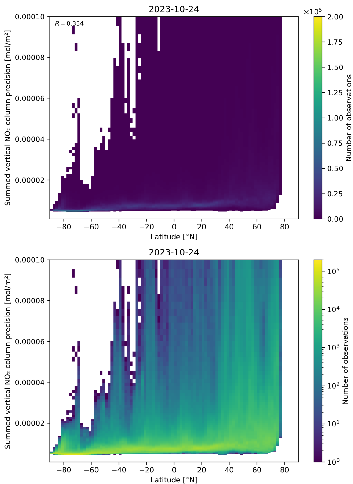
Figure 89: Scatter density plot of “Latitude” against “Summed vertical NO 2 column precision” for 2023-10-23 to 2023-10-25.
