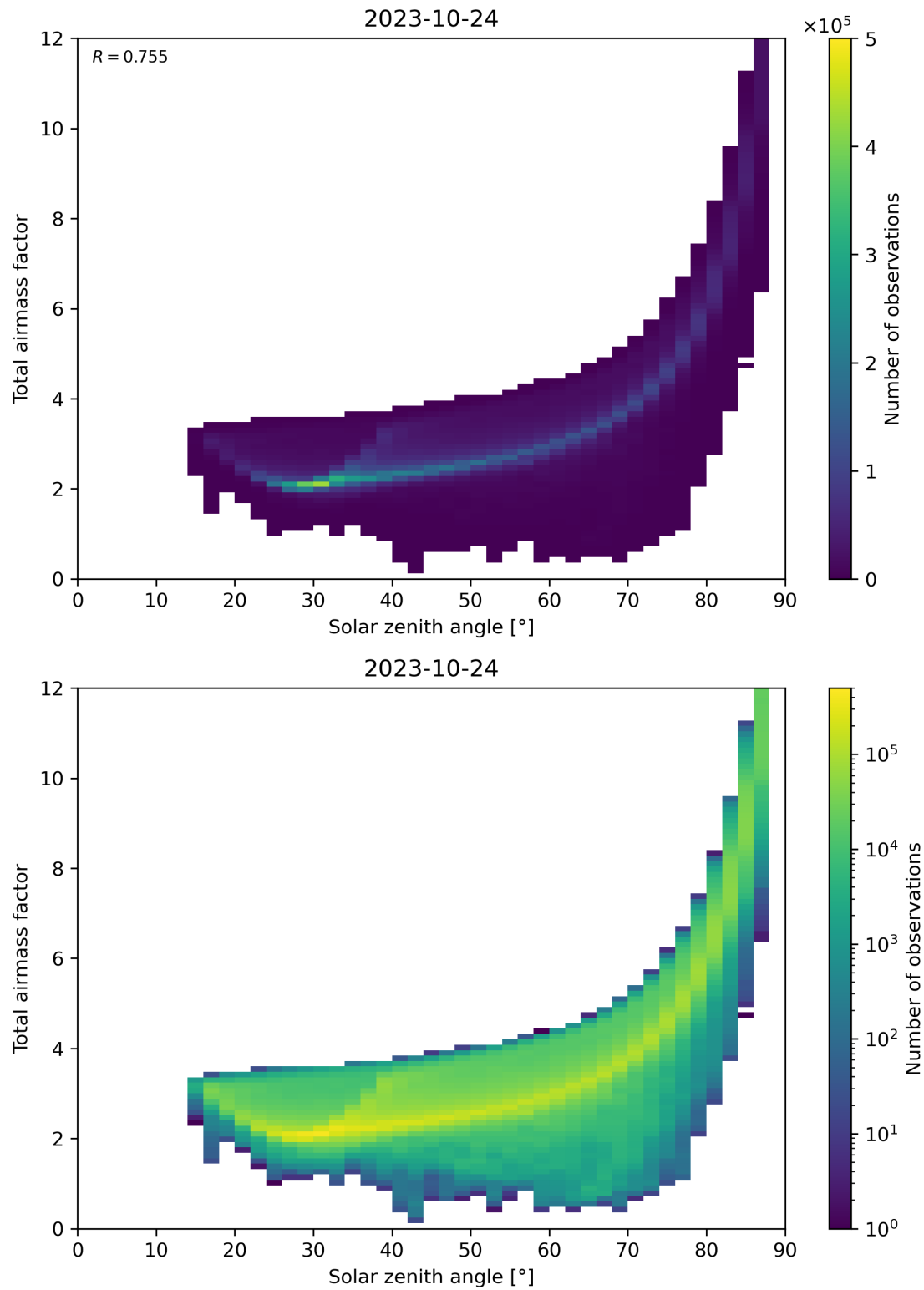
Figure 146: Scatter density plot of “Solar zenith angle” against “Total air mass factor” for 2023-10-23 to 2023-10-25.
