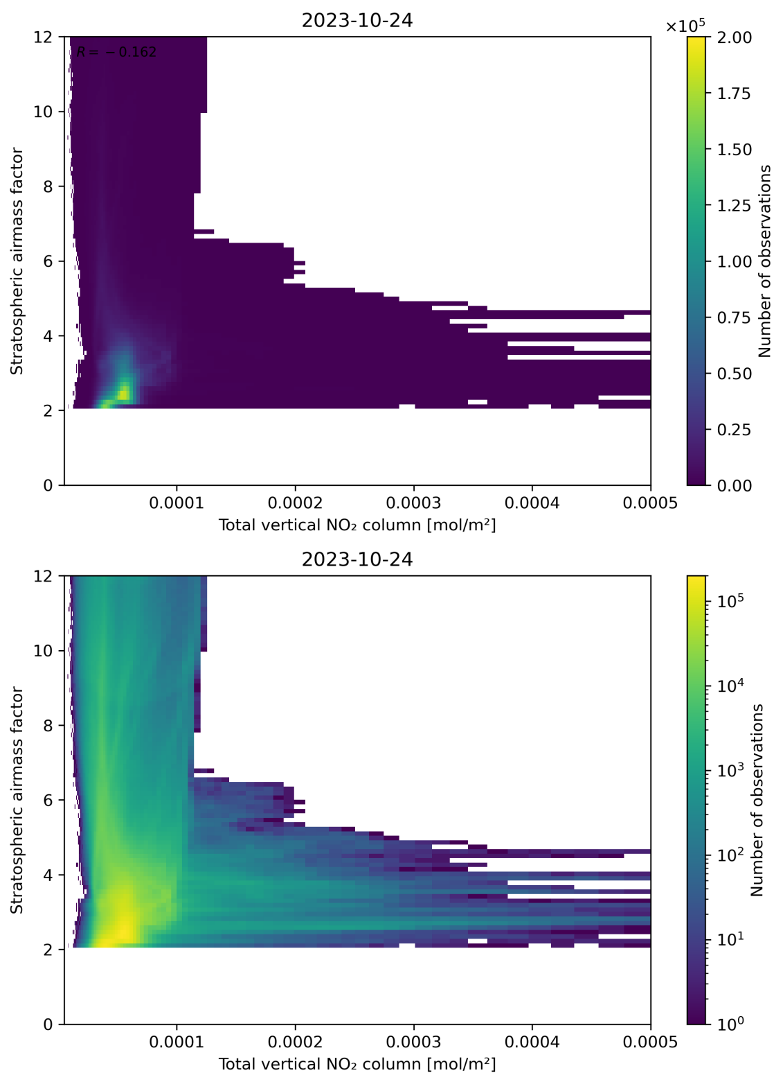
Figure 110: Scatter density plot of “Total vertical NO 2 column” against “Stratospheric airmass factor” for 2023-10-23 to 2023-10-25.
