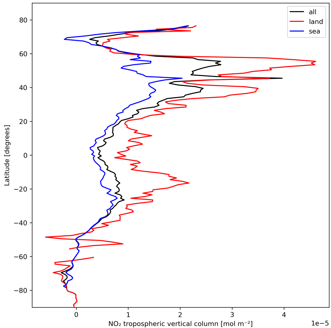
Figure 12: Zonal average of “NO 2 tropospheric vertical column” for 2023-10-23 to 2023-10-25.
