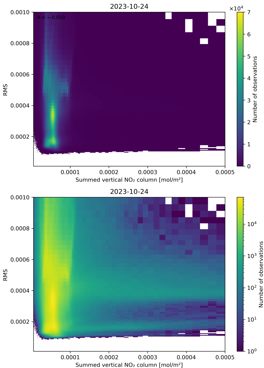
Figure 109: Scatter density plot of “Summed vertical NO 2 column” against “RMS” for 2023-10-23 to 2023-10-25.
