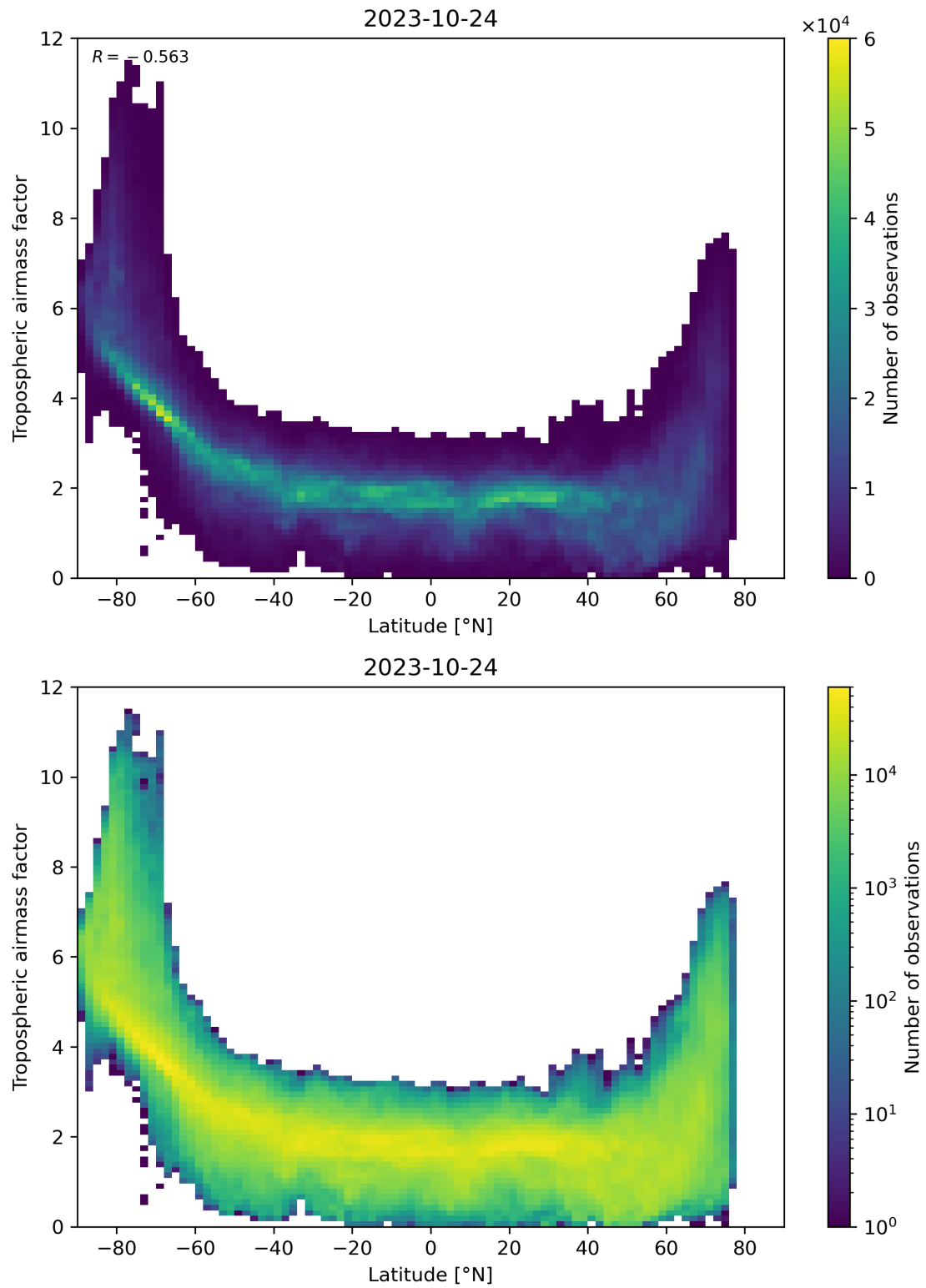
Figure 85: Scatter density plot of “Latitude” against “Tropospheric airmass factor” for 2023-10-23 to 2023-10-25.
