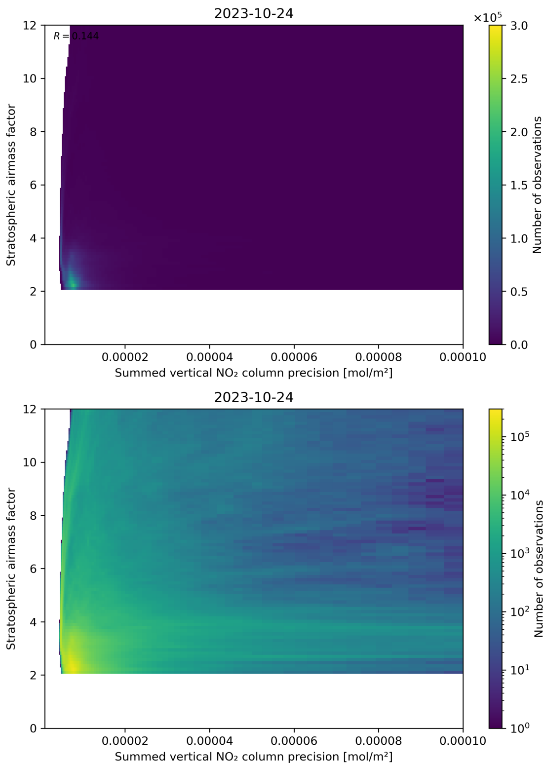
Figure 106: Scatter density plot of “Summed vertical NO 2 column precision” against “Stratospheric airmass factor” for 2023-10-23 to 2023-10-25.
