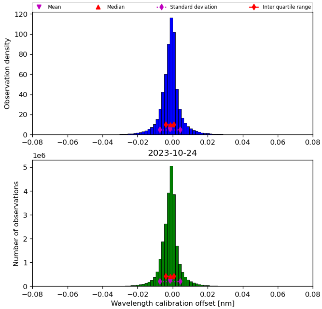
Figure 35: Histogram of “Wavelength calibration offset” for 2023-10-23 to 2023-10-25
