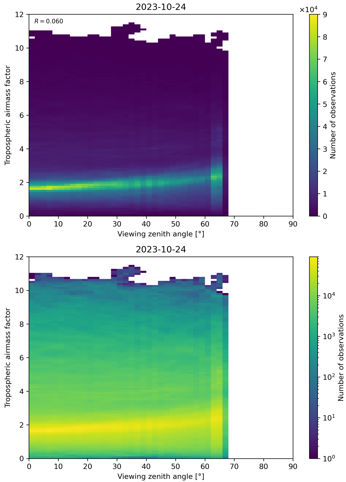
Figure 161: Scatter density plot of “Viewing zenith angle” against “Tropospheric airmass factor” for 2023-10-23 to 2023-10-25.
