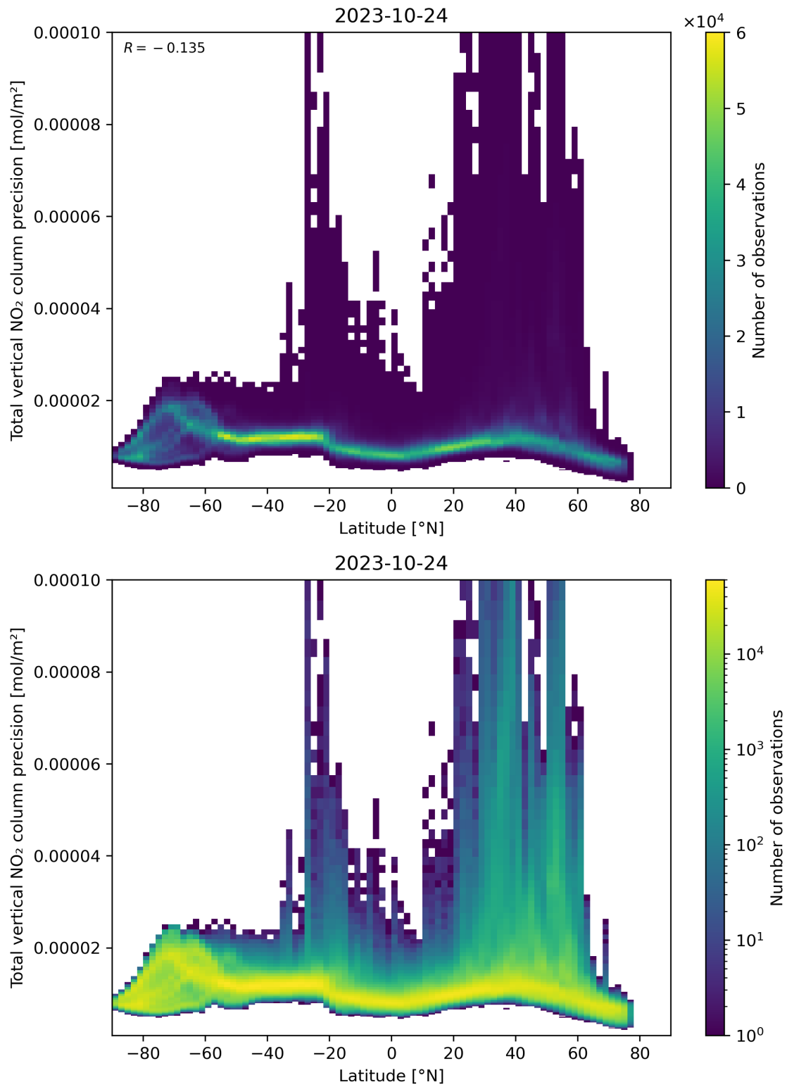
Figure 91: Scatter density plot of “Latitude” against “Total vertical NO 2 column precision” for 2023-10-23 to 2023-10-25.
