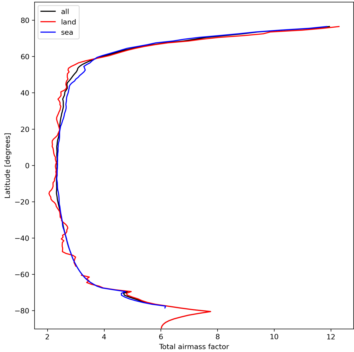
Figure 15: Zonal average of “Total airmass factor” for 2023-10-23 to 2023-10-25.
