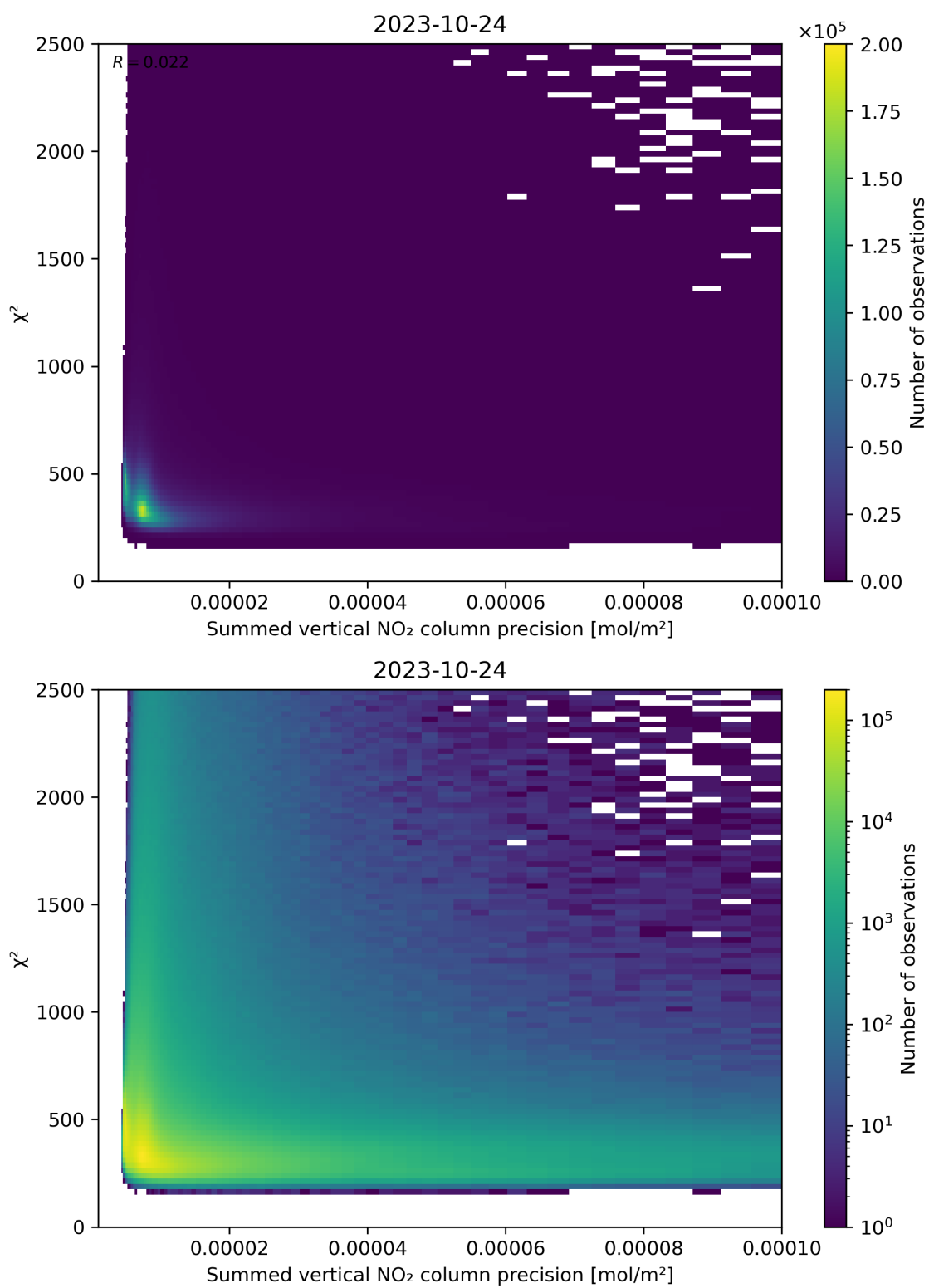
Figure 107: Scatter density plot of “Summed vertical NO 2 column precision” against “ \chi^2 ” for 2023-10-23 to 2023-10-25.
