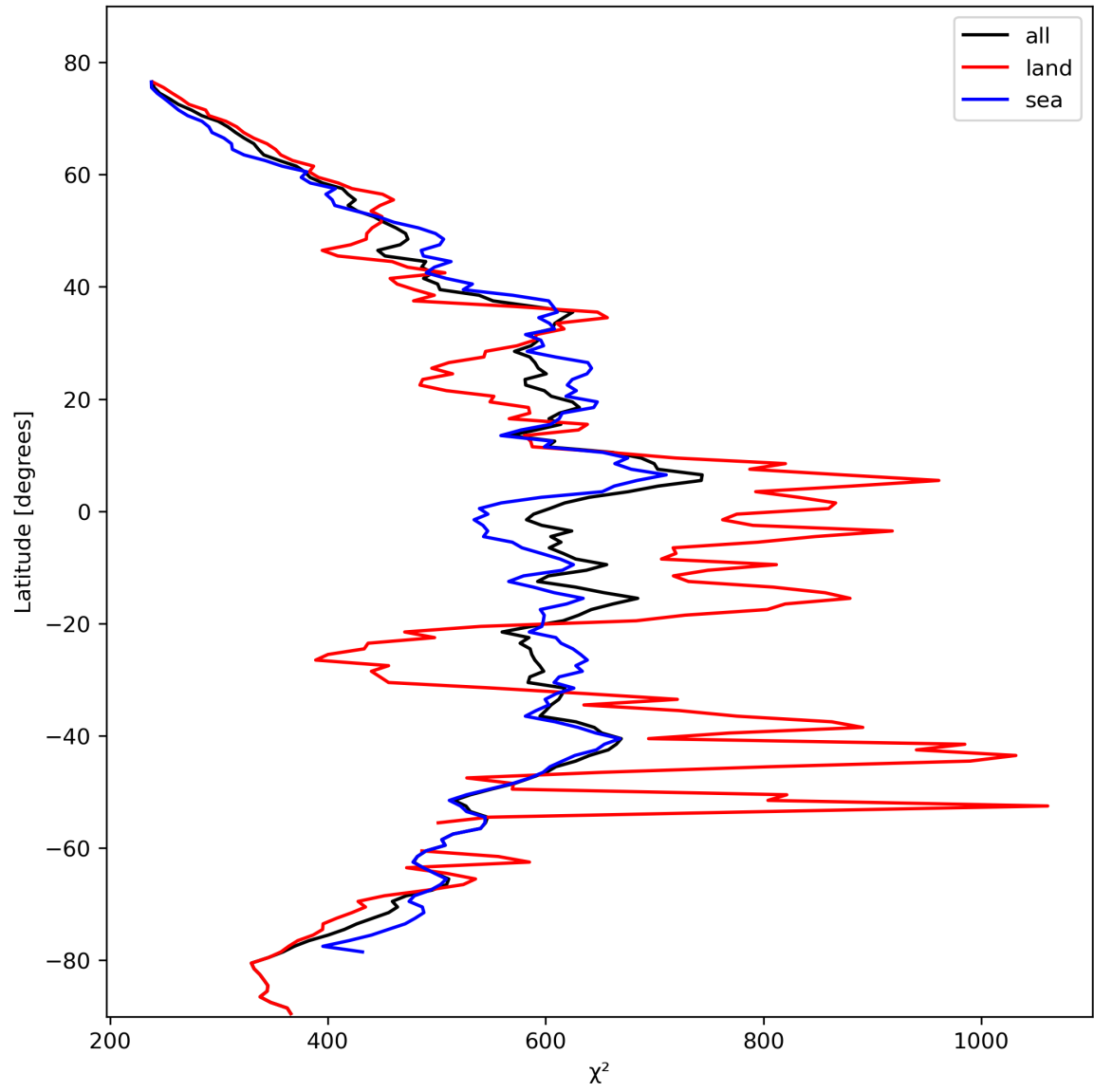
Figure 25: Zonal average of “ \chi^2 ” for 2023-10-23 to 2023-10-25.
