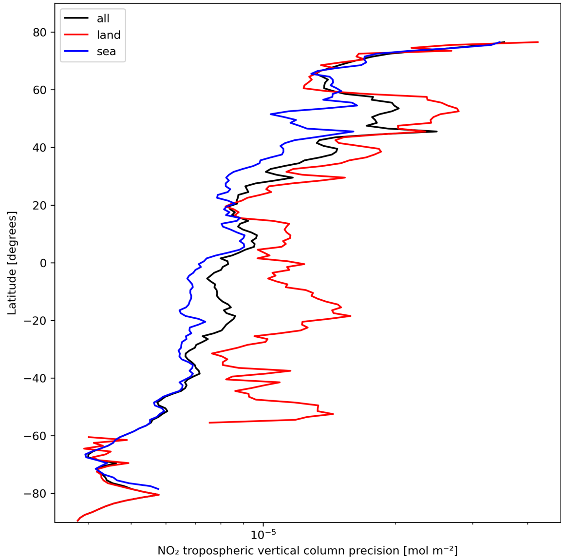
Figure 13: Zonal average of “NO 2 tropospheric vertical column precision” for 2023-10-23 to 2023-10-25.
