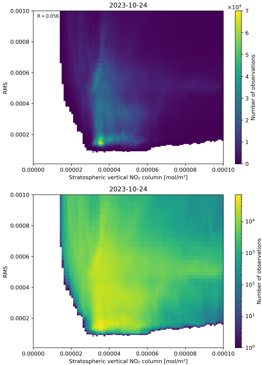
Figure 102: Scatter density plot of “Stratospheric vertical NO 2 column” against “RMS” for 2023-10-23 to 2023-10-25.
