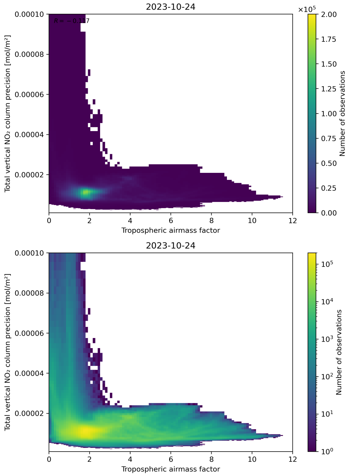
Figure 78: Scatter density plot of “Tropospheric air mass factor” against “Total vertical NO 2 column precision” for 2023-10-23 to 2023-10-25.
