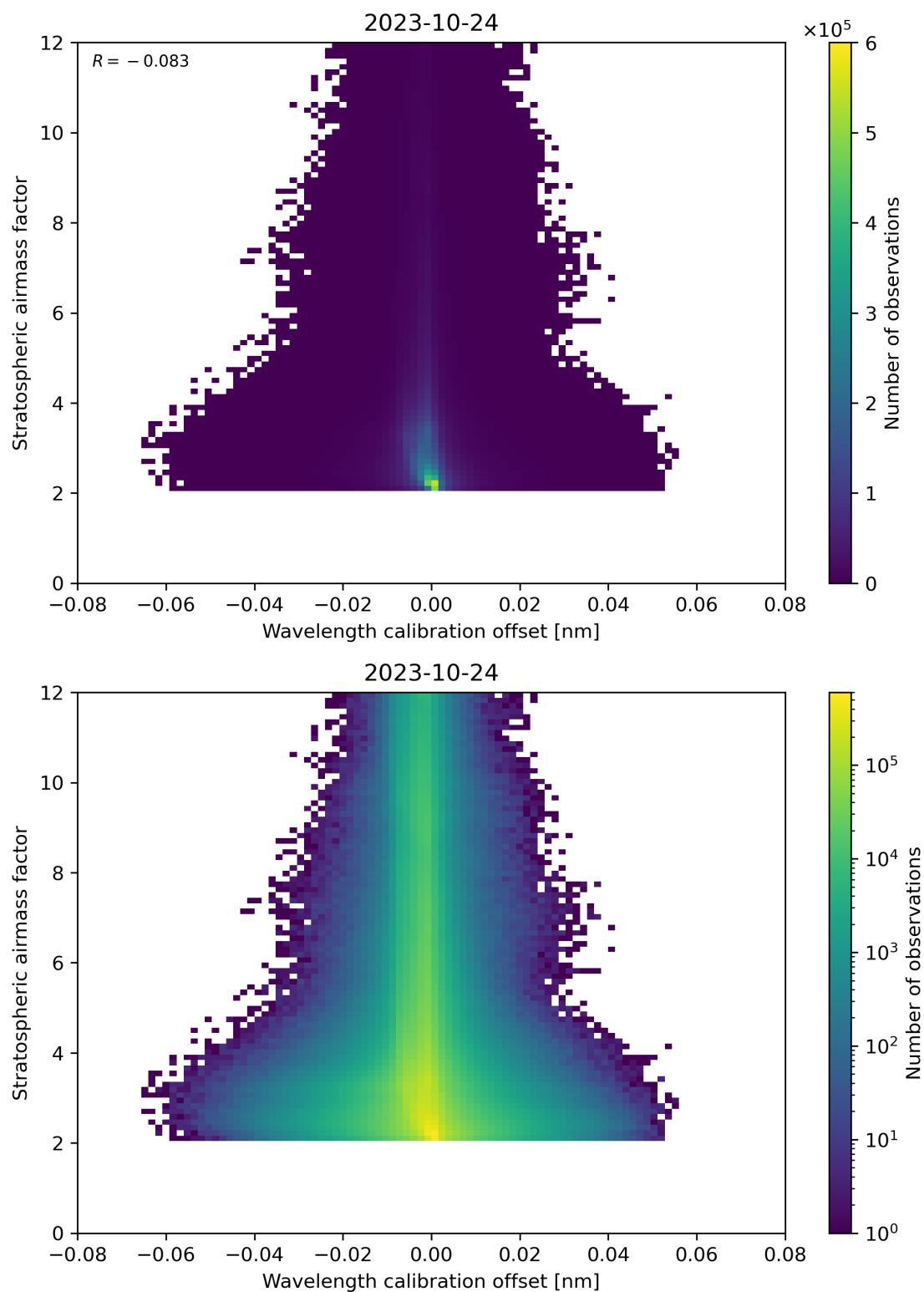
Figure 174: Scatter density plot of “Wavelength calibration offset” against “Stratospheric airmass factor” for 2023-10-23 to 2023-10-25.
