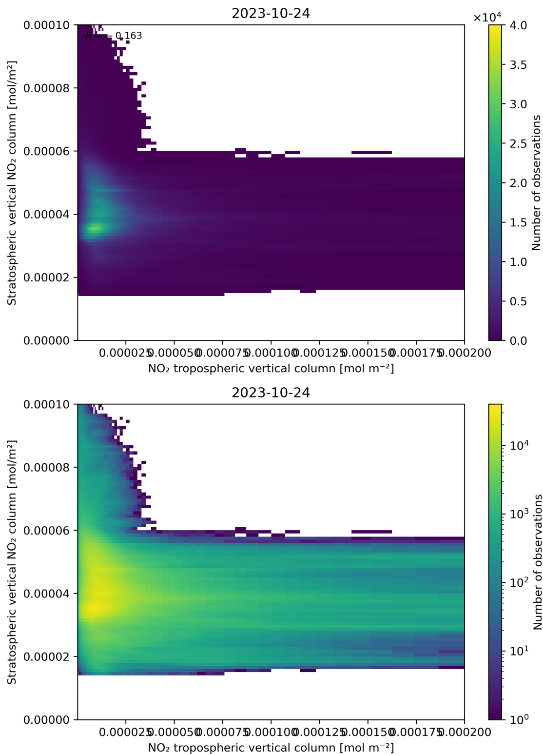
Figure 125: Scatter density plot of “NO 2 tropospheric vertical column” against “Stratospheric vertical NO 2 column” for 2023-10-23 to 2023-10-25.
