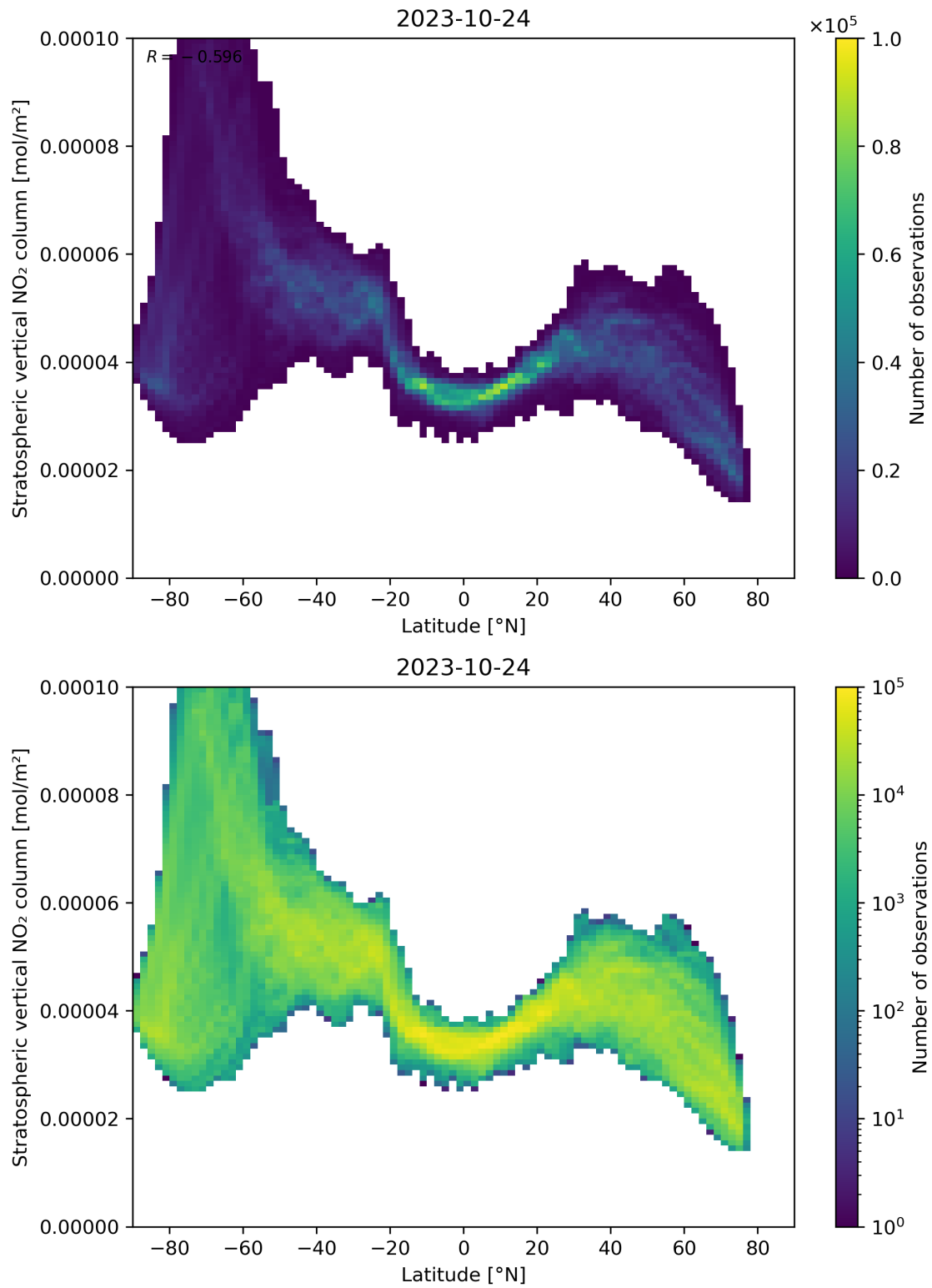
Figure 87: Scatter density plot of “Latitude” against “Stratospheric vertical NO 2 column” for 2023-10-23 to 2023-10-25.
