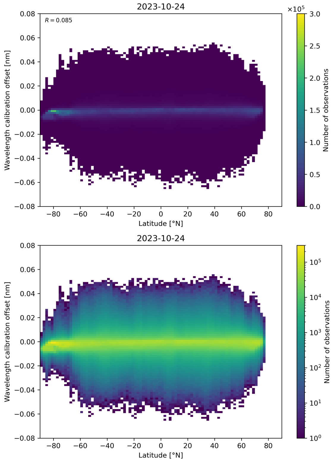
Figure 95: Scatter density plot of “Latitude” against “Wavelength calibration offset” for 2023-10-23 to 2023-10-25.
