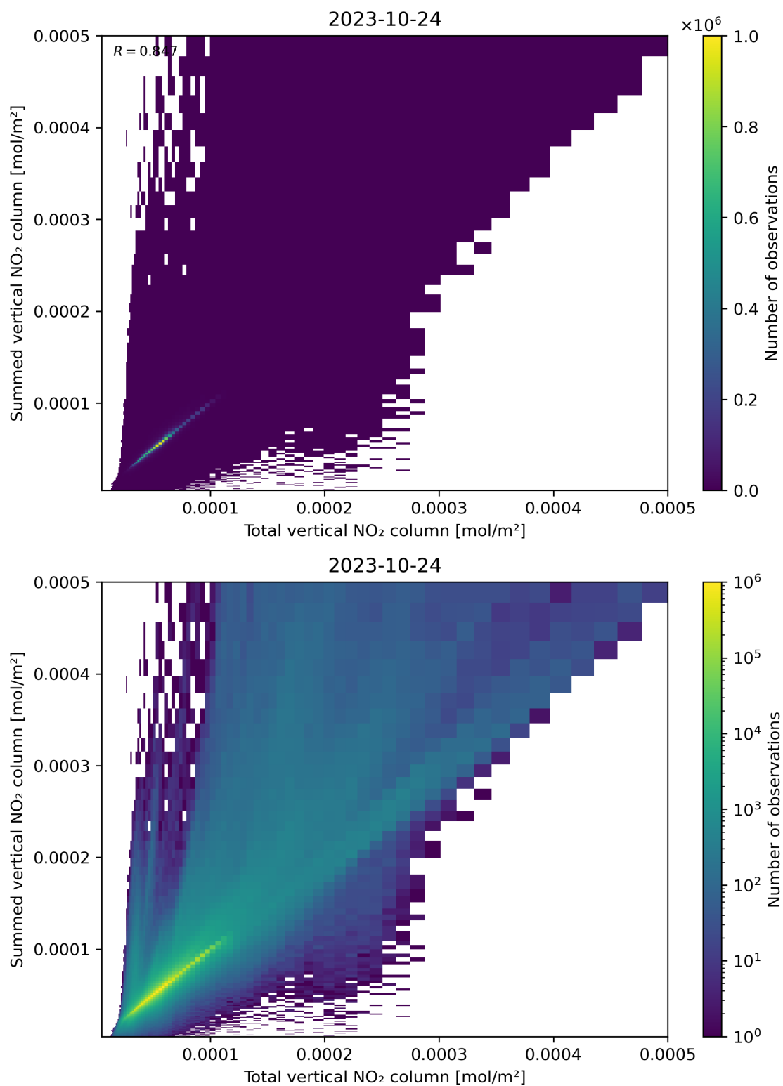
Figure 112: Scatter density plot of “Total vertical NO 2 column” against “Summed vertical NO 2 column” for 2023-10-23 to 2023-10-25.
