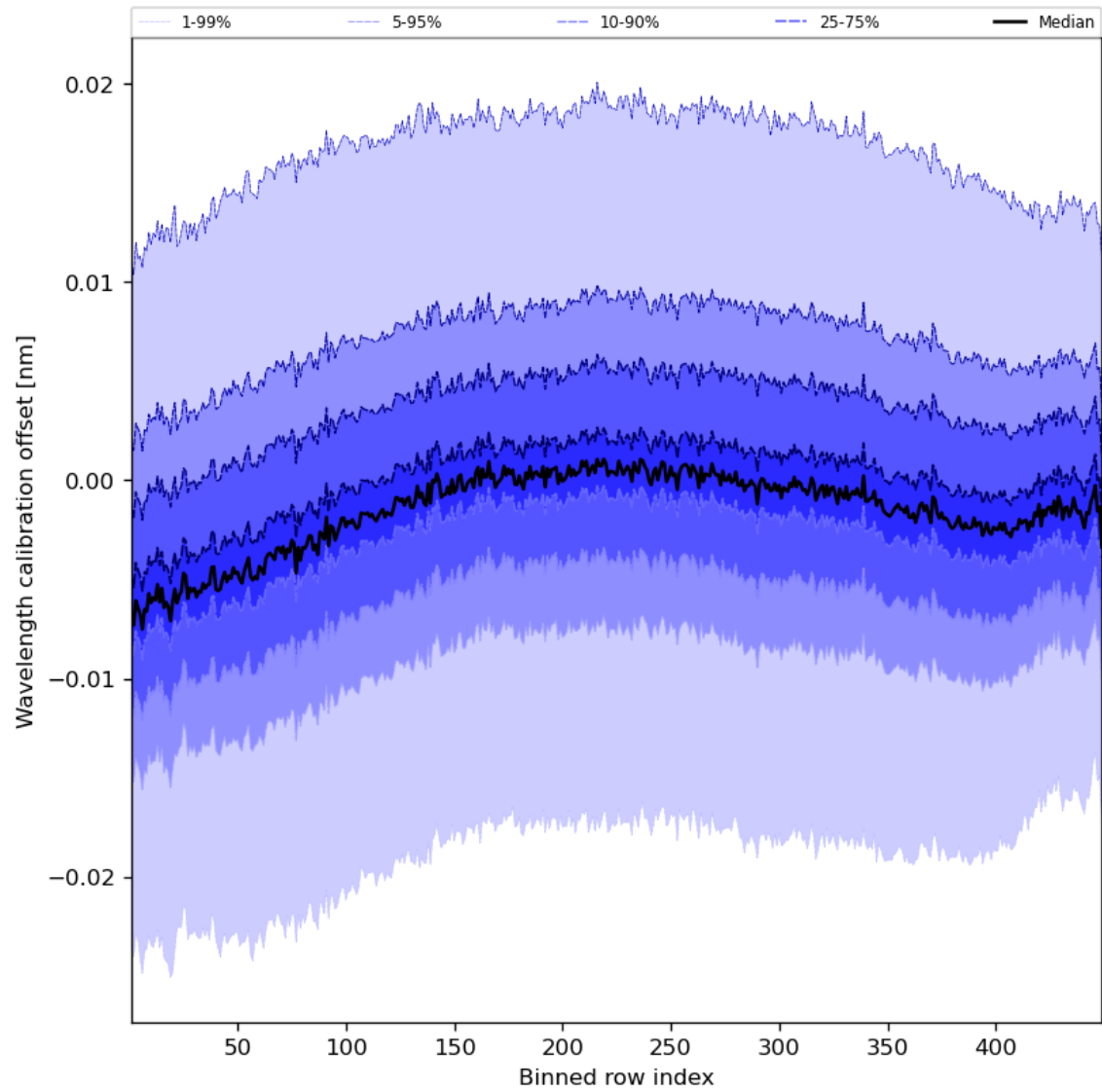
Figure 52: Along track statistics of “Wavelength calibration offset” for 2023-10-23 to 2023-10-25
