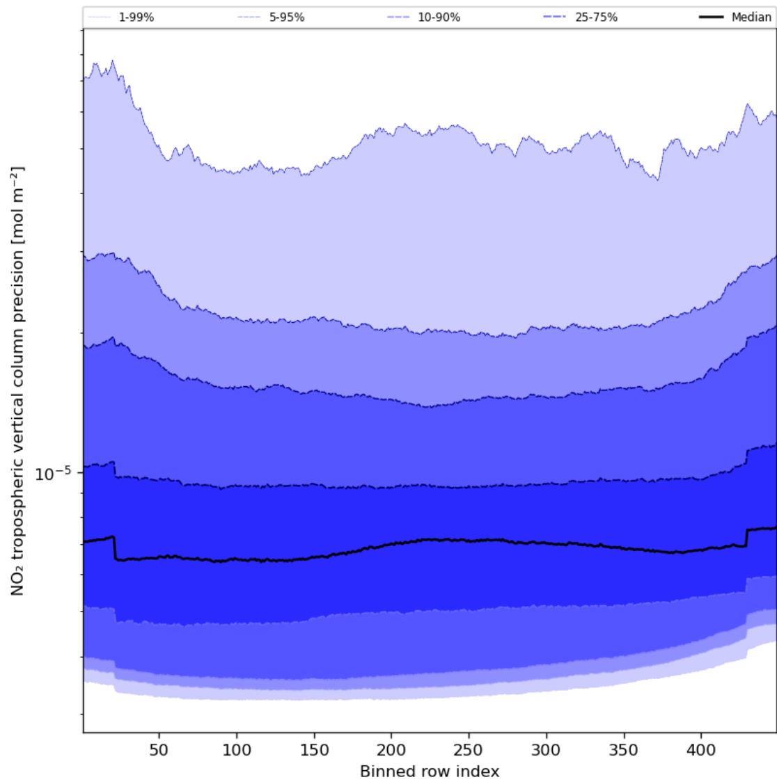
Figure 47: Along track statistics of “NO 2 tropospheric vertical column precision” for 2023-10-23 to 2023-10-25
