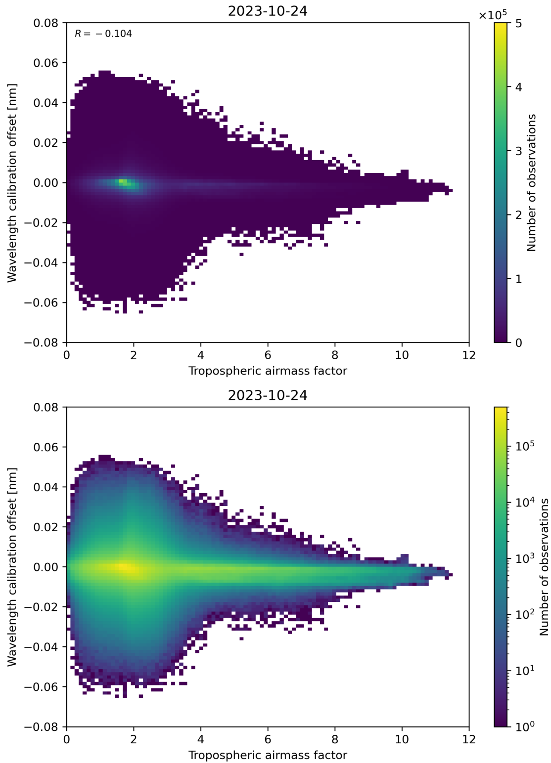
Figure 80: Scatter density plot of “Tropospheric airmass factor” against “Wavelength calibration offset” for 2023-10-23 to 2023-10-25.
