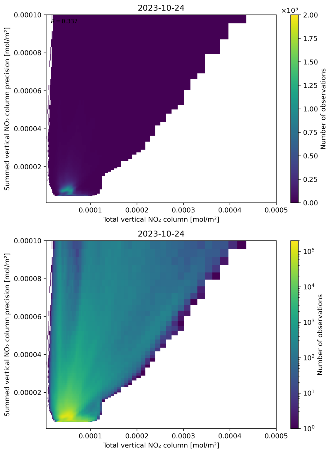
Figure 113: Scatter density plot of “Total vertical NO 2 column” against “Summed vertical NO 2 column precision” for 2023-10-23 to 2023-10-25.
