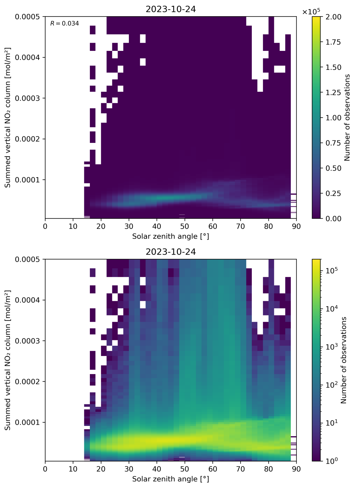
Figure 151: Scatter density plot of “Solar zenith angle” against “Summed vertical NO 2 column” for 2023-10-23 to 2023-10-25.
