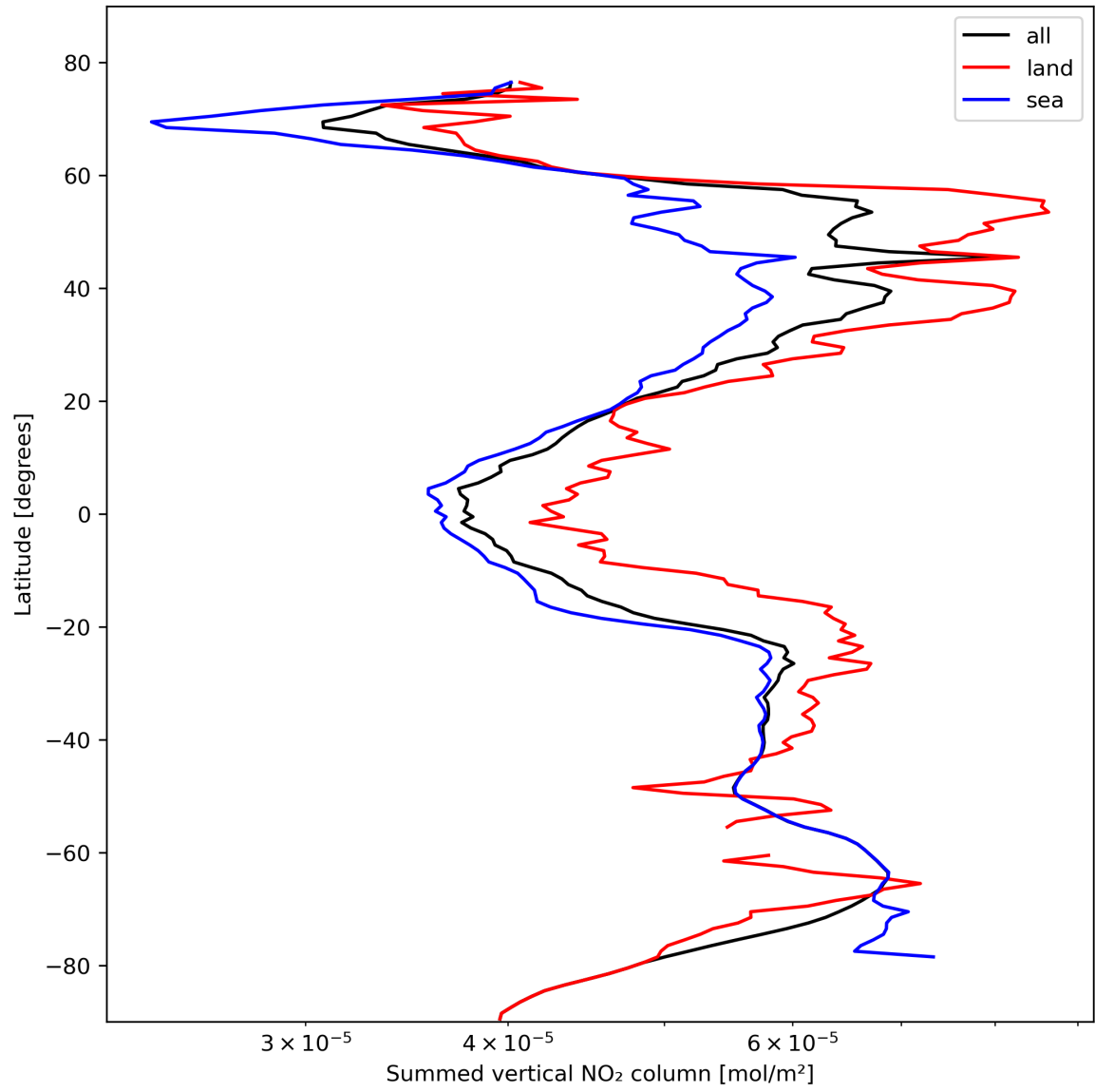
Figure 23: Zonal average of “Summed vertical NO 2 column” for 2023-10-23 to 2023-10-25.
