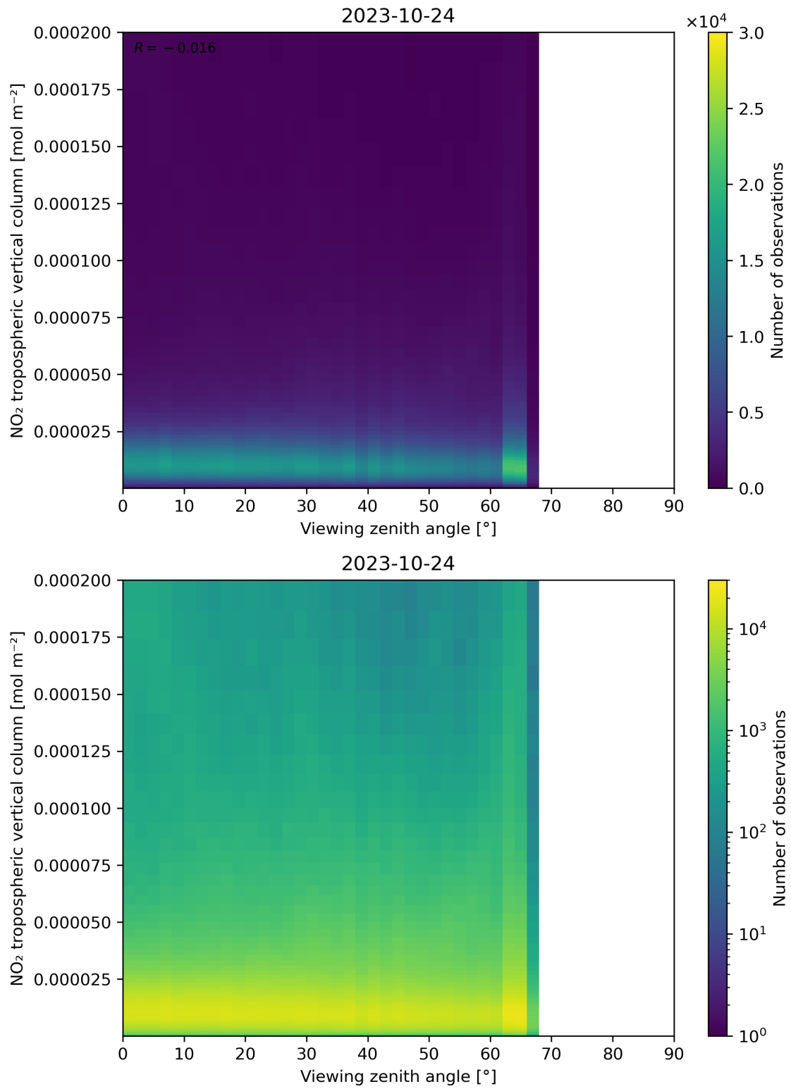
Figure 169: Scatter density plot of “Viewing zenith angle” against “NO 2 tropospheric vertical column” for 2023-10-23 to 2023-10-25.
