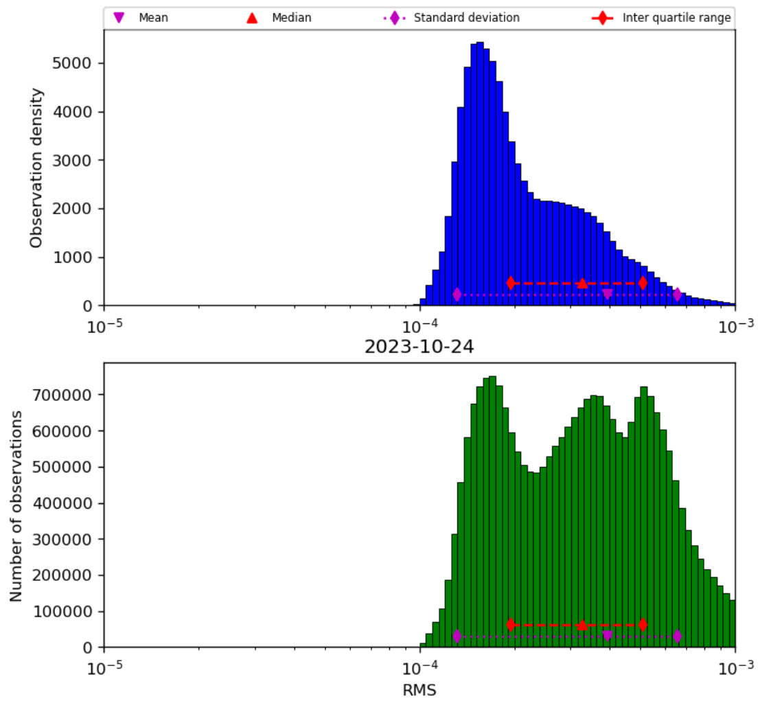
Figure 43: Histogram of “RMS” for 2023-10-23 to 2023-10-25
