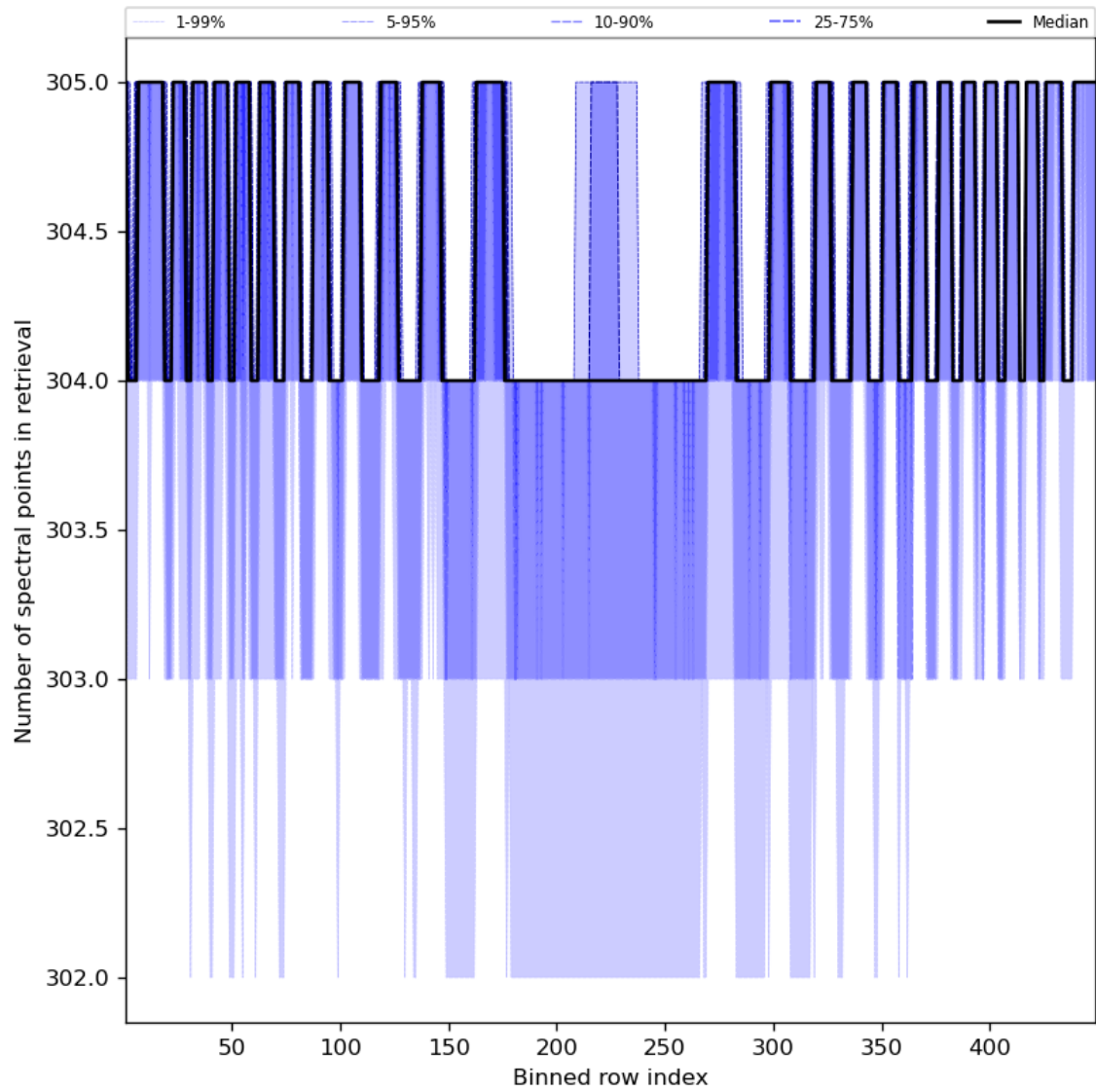
Figure 50: Along track statistics of “Number of spectral points in retrieval” for 2023-10-23 to 2023-10-25
