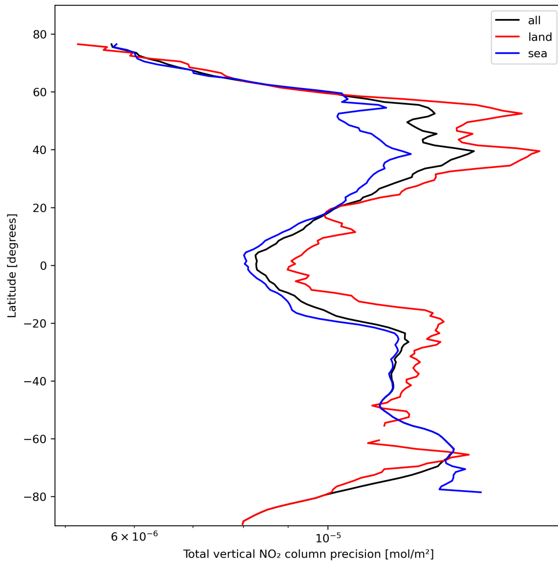
Figure 22: Zonal average of “Total vertical NO 2 column precision” for 2023-10-23 to 2023-10-25.
