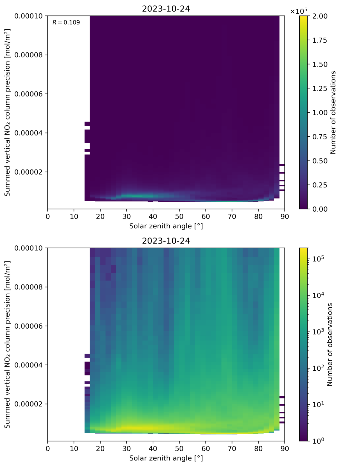
Figure 152: Scatter density plot of “Solar zenith angle” against “Summed vertical NO 2 column precision” for 2023-10-23 to 2023-10-25.
