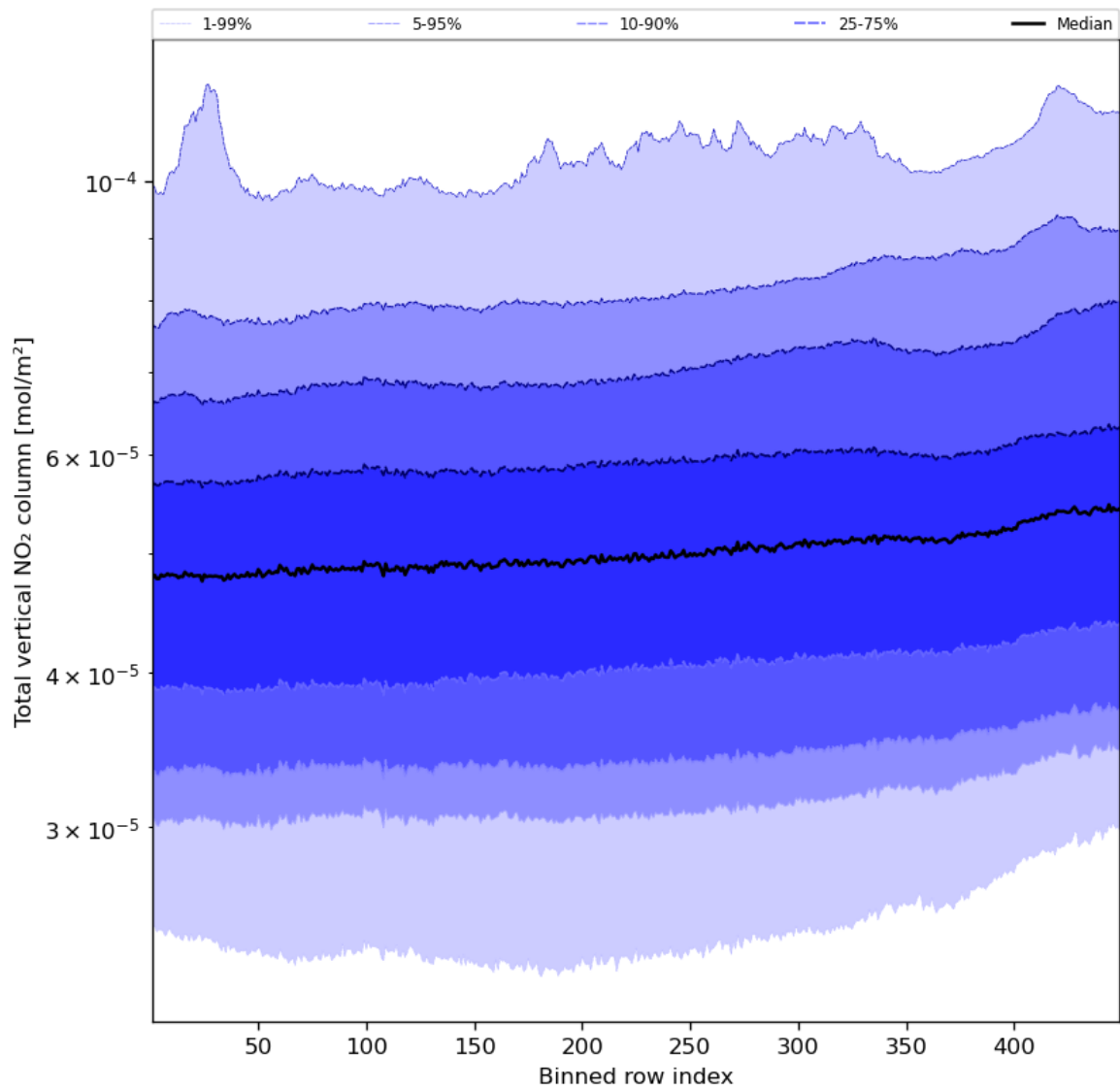
Figure 55: Along track statistics of “Total vertical NO 2 column” for 2023-10-23 to 2023-10-25
