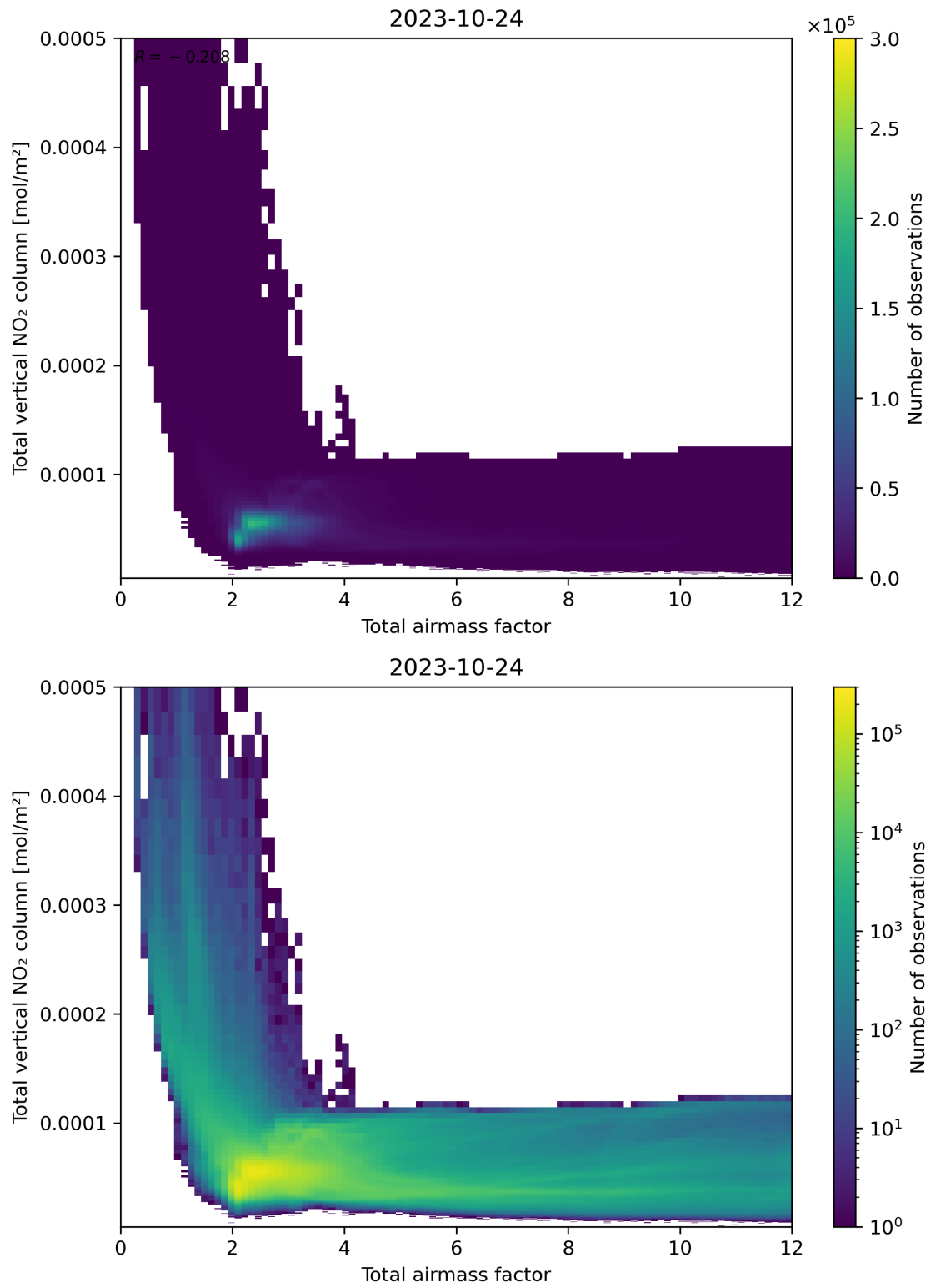
Figure 67: Scatter density plot of “Total airmass factor” against “Total vertical NO 2 column” for 2023-10-23 to 2023-10-25.
