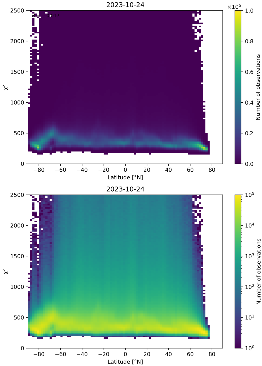
Figure 86: Scatter density plot of “Latitude” against “ \chi^2 ” for 2023-10-23 to 2023-10-25.
