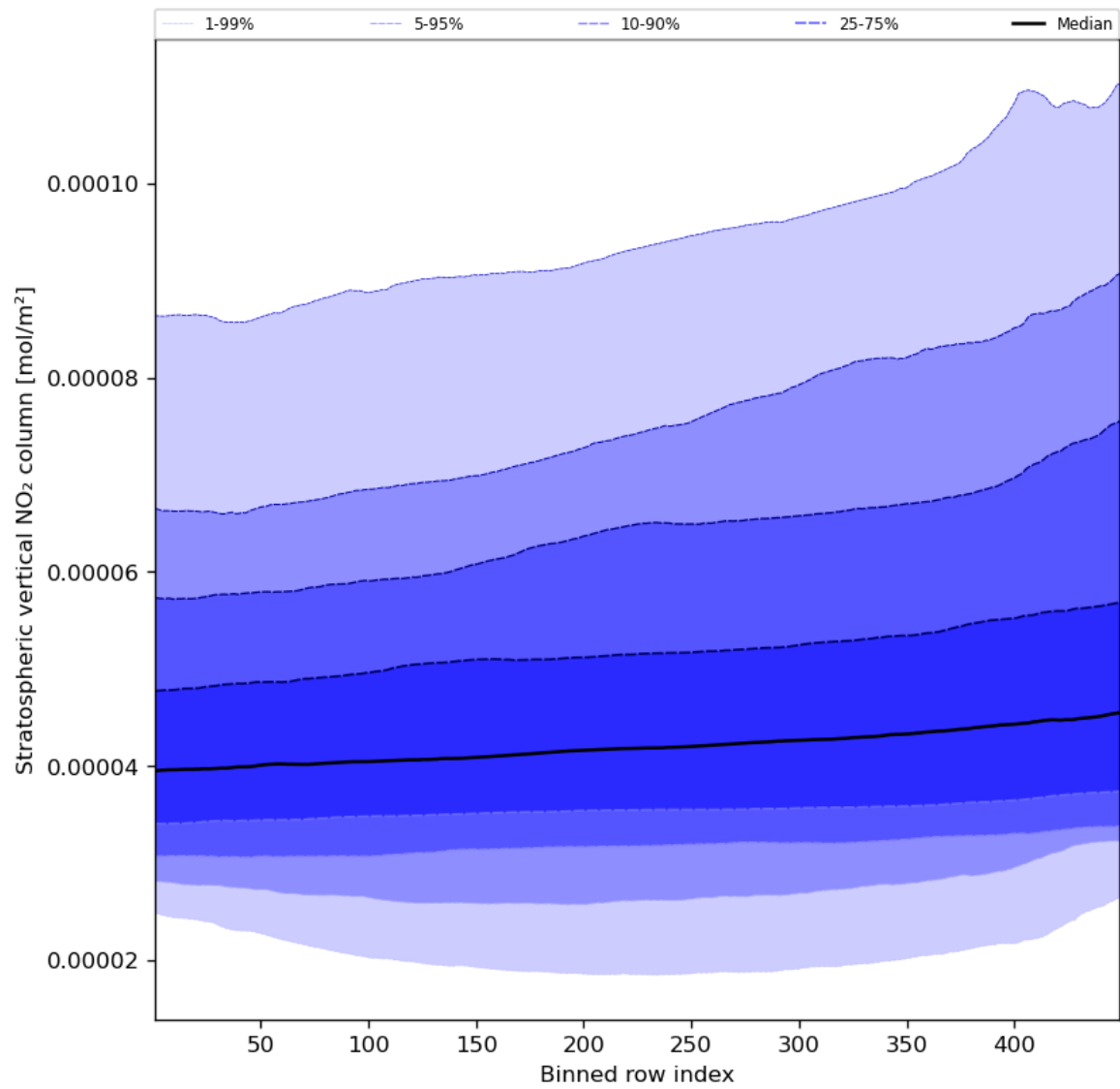
Figure 53: Along track statistics of “Stratospheric vertical NO 2 column” for 2023-10-23 to 2023-10-25
