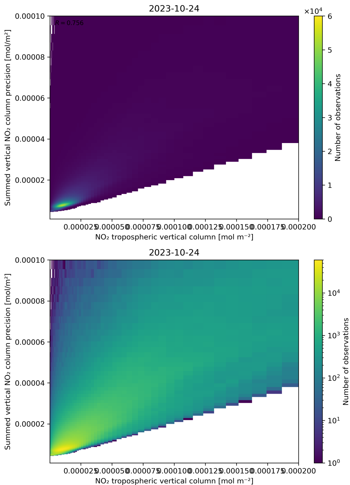
Figure 127: Scatter density plot of “NO 2 tropospheric vertical column” against “Summed vertical NO 2 column precision” for 2023-10-23 to 2023-10-25.
