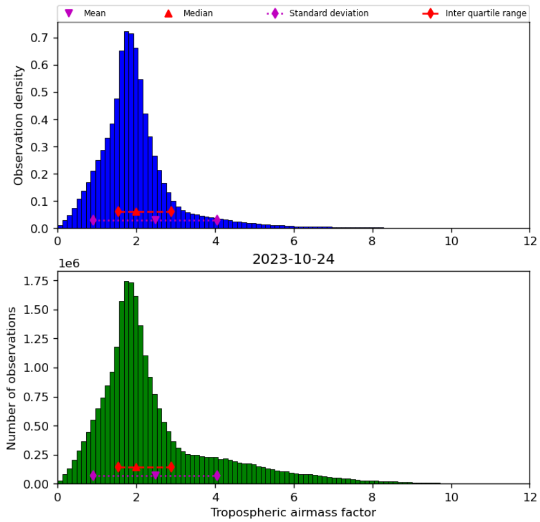
Figure 31: Histogram of “Tropospheric airmass factor” for 2023-10-23 to 2023-10-25
