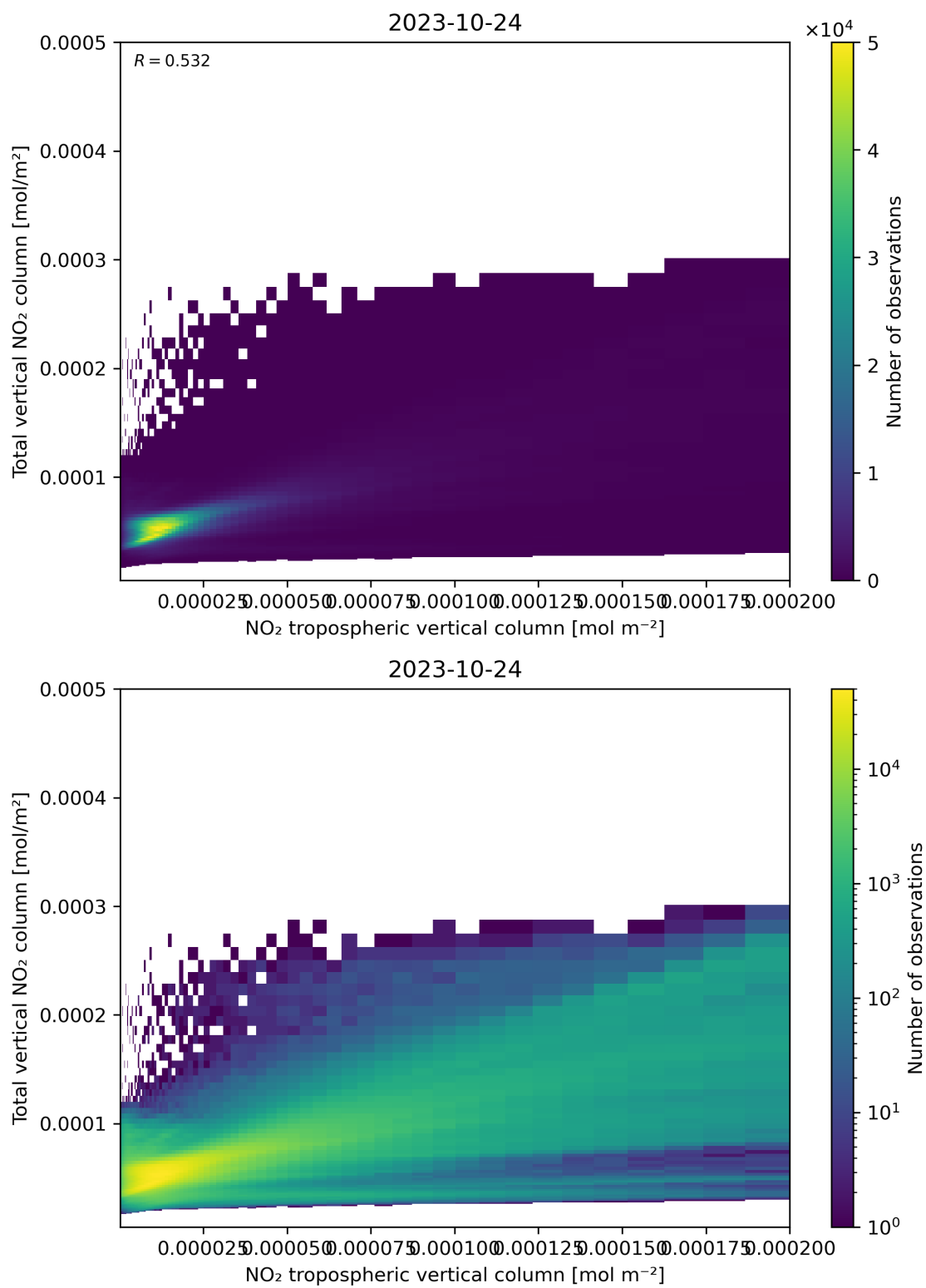
Figure 128: Scatter density plot of “NO 2 tropospheric vertical column” against “Total vertical NO 2 column” for 2023-10-23 to 2023-10-25.
