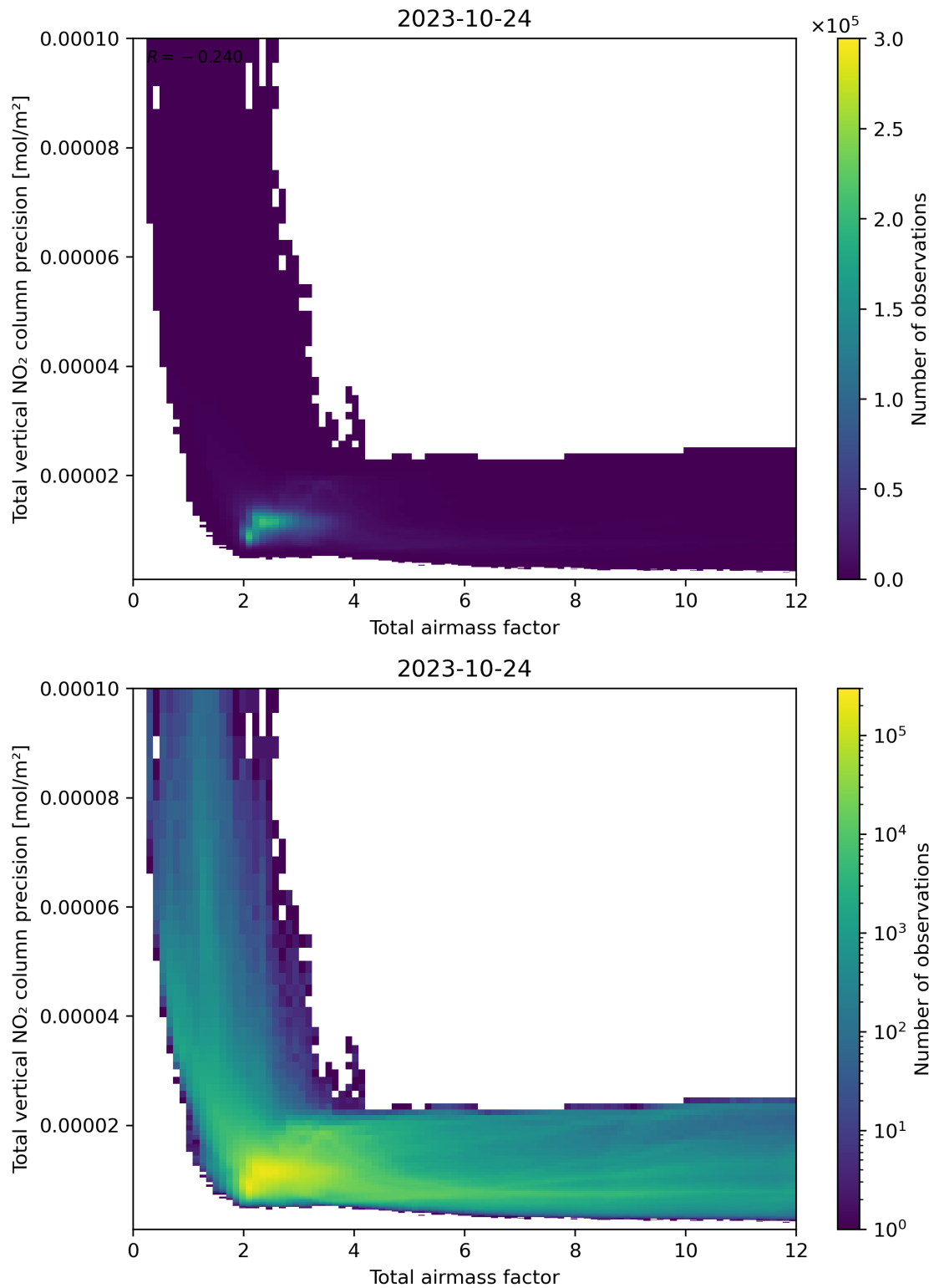
Figure 68: Scatter density plot of “Total airmass factor” against “Total vertical NO 2 column precision” for 2023-10-23 to 2023-10-25.
