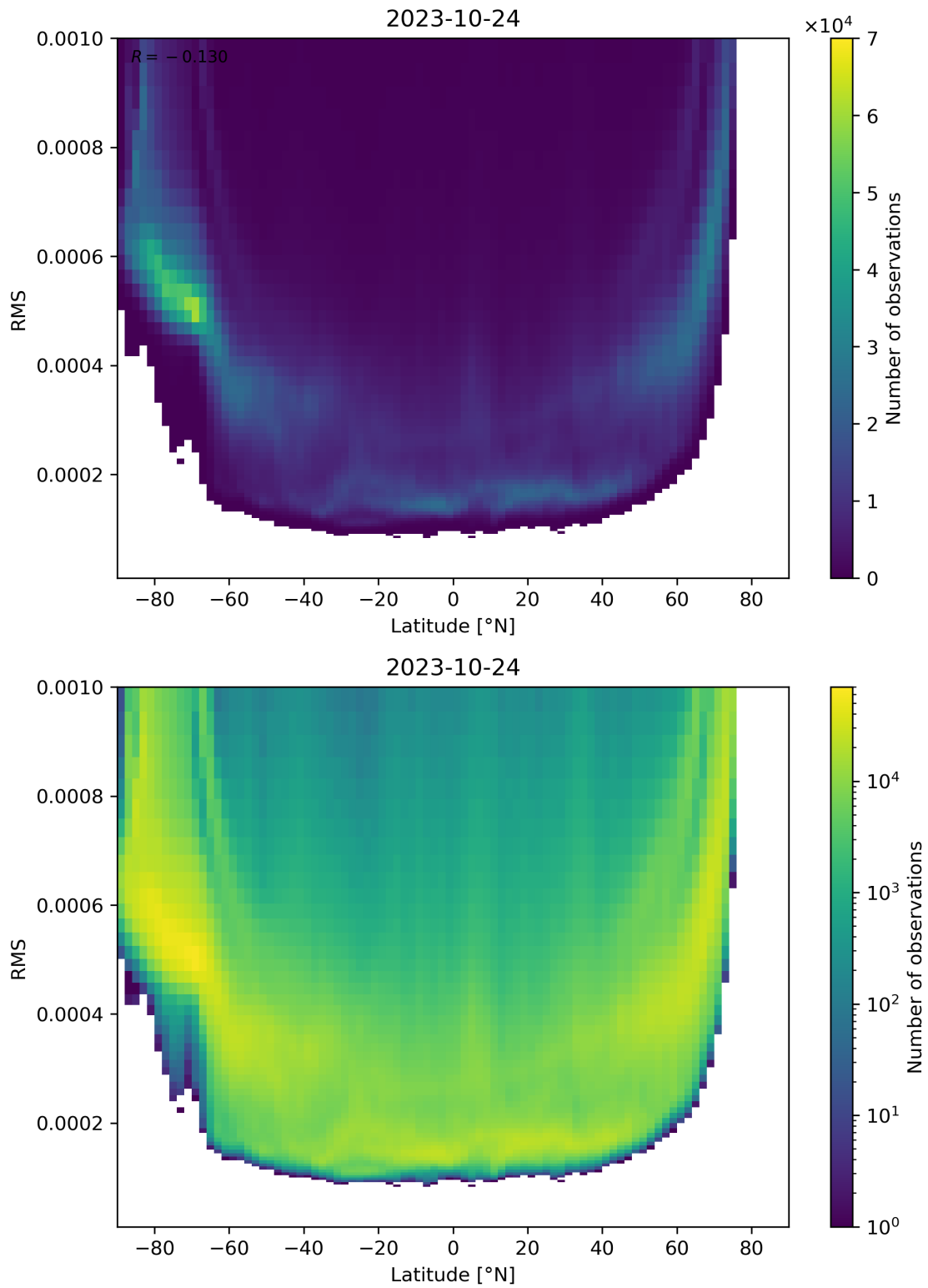
Figure 94: Scatter density plot of “Latitude” against “RMS” for 2023-10-23 to 2023-10-25.
