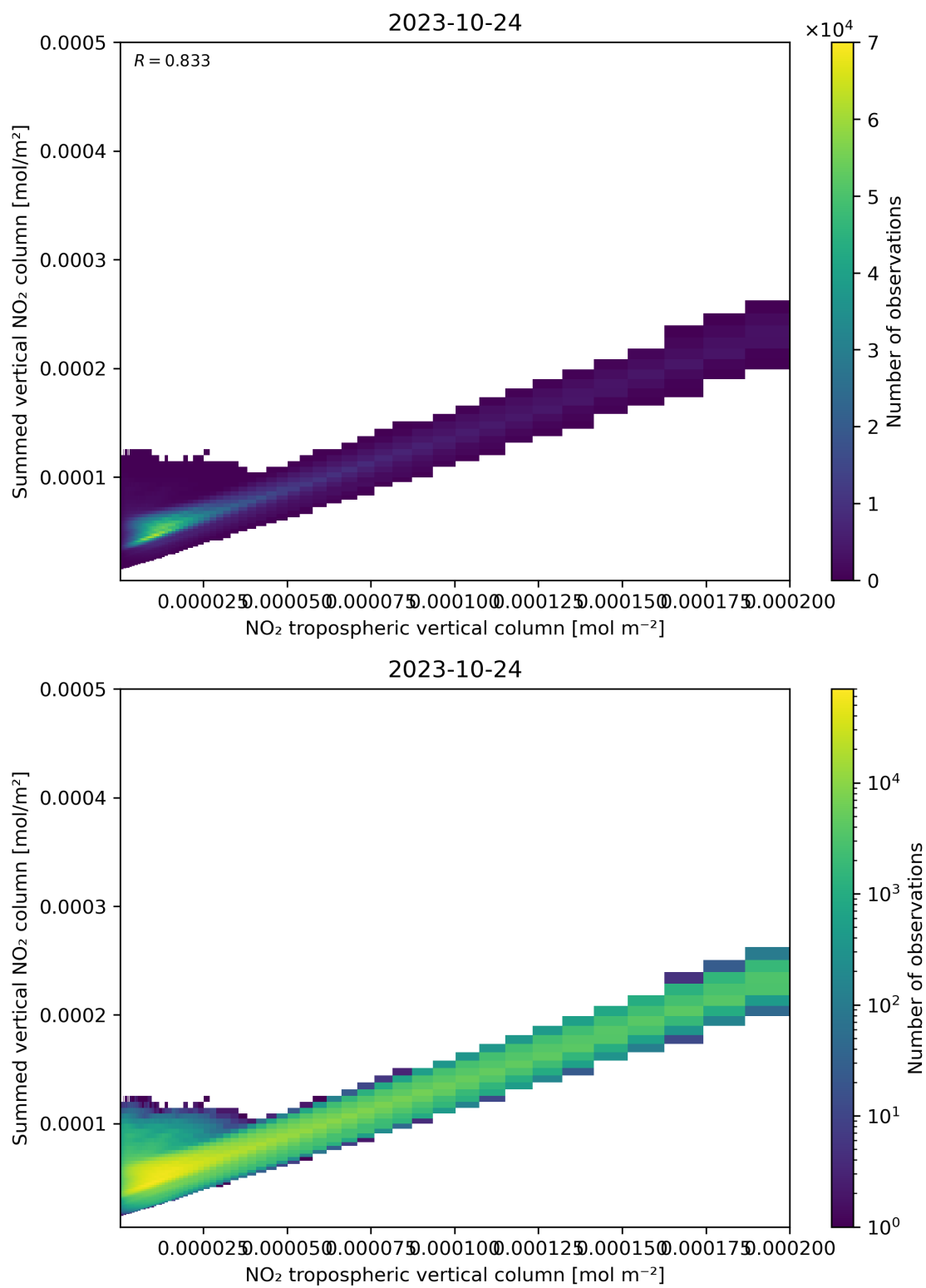
Figure 126: Scatter density plot of “NO 2 tropospheric vertical column” against “Summed vertical NO 2 column” for 2023-10-23 to 2023-10-25.
