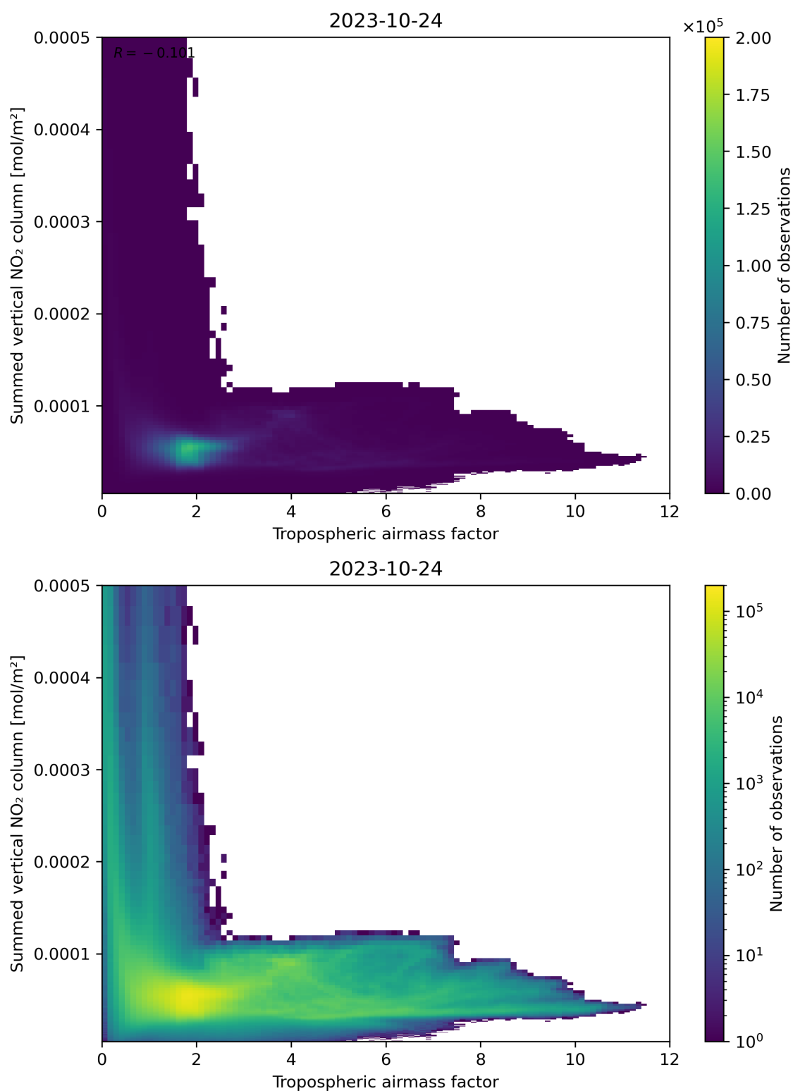
Figure 75: Scatter density plot of “Tropospheric airmass factor” against “Summed vertical NO 2 column” for 2023-10-23 to 2023-10-25.
