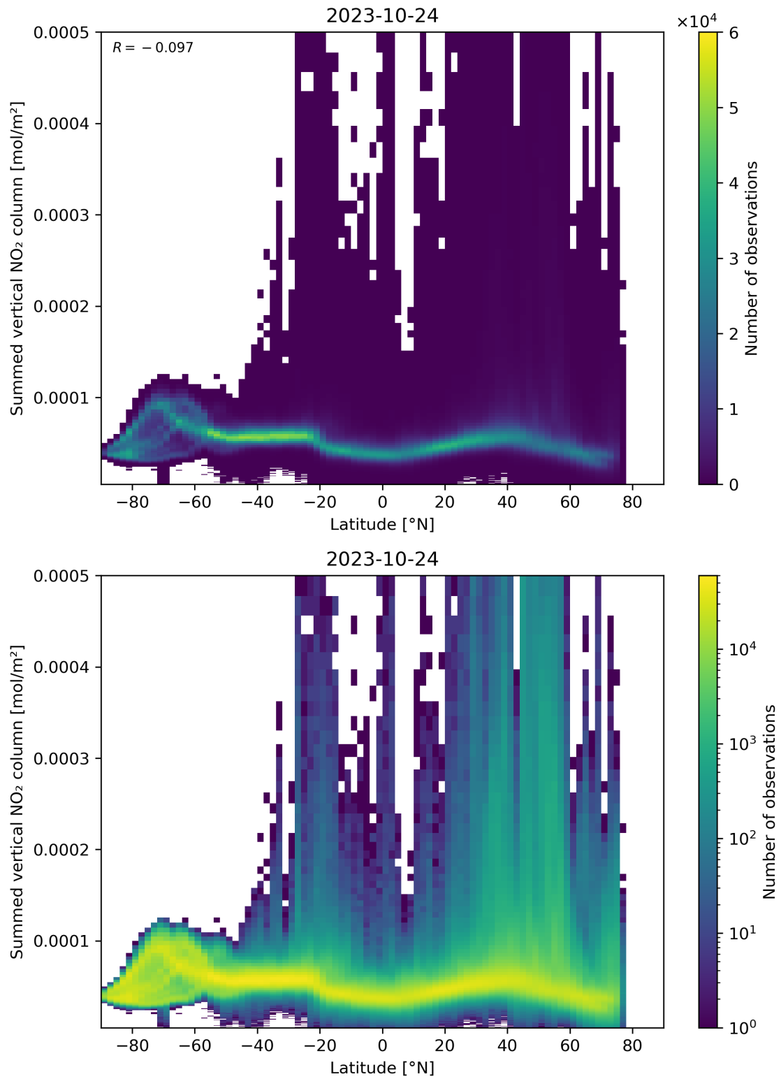
Figure 88: Scatter density plot of “Latitude” against “Summed vertical NO 2 column” for 2023-10-23 to 2023-10-25.
