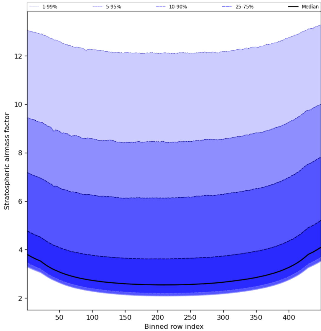
Figure 61: Along track statistics of “Stratospheric airmass factor” for 2023-10-23 to 2023-10-25
