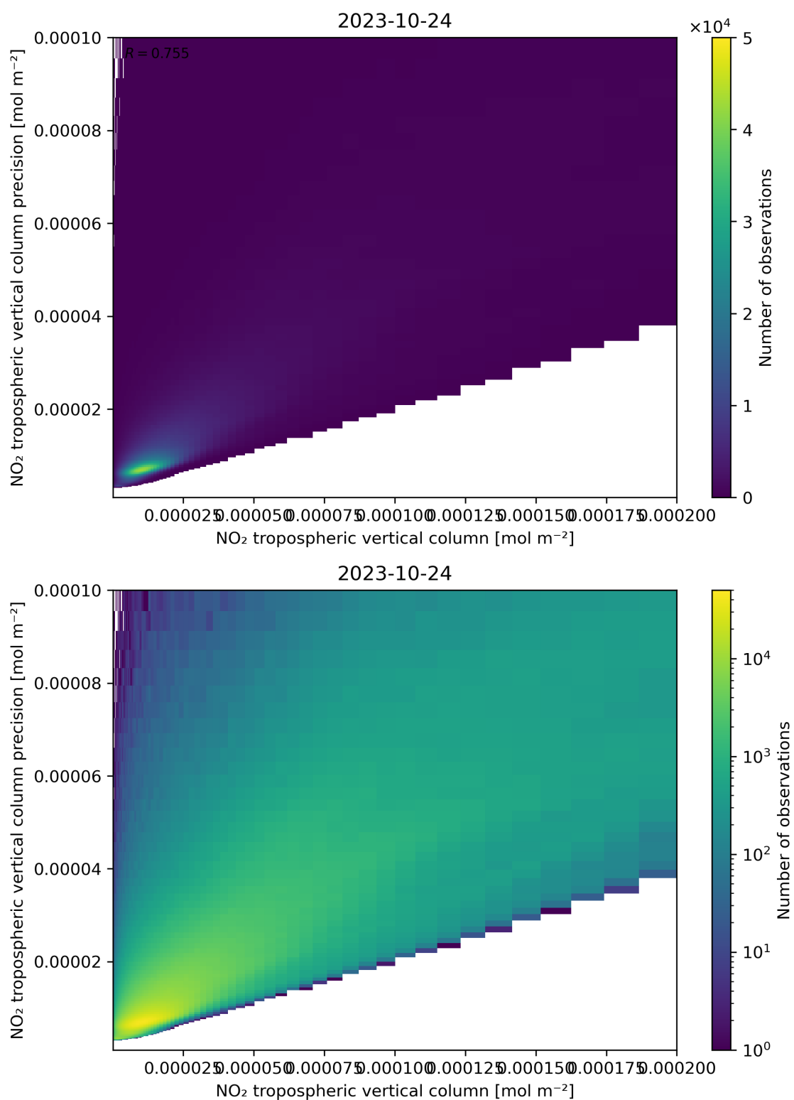
Figure 130: Scatter density plot of “NO 2 tropospheric vertical column” against “NO 2 tropospheric vertical column precision” for 2023-10-23 to 2023-10-25.
