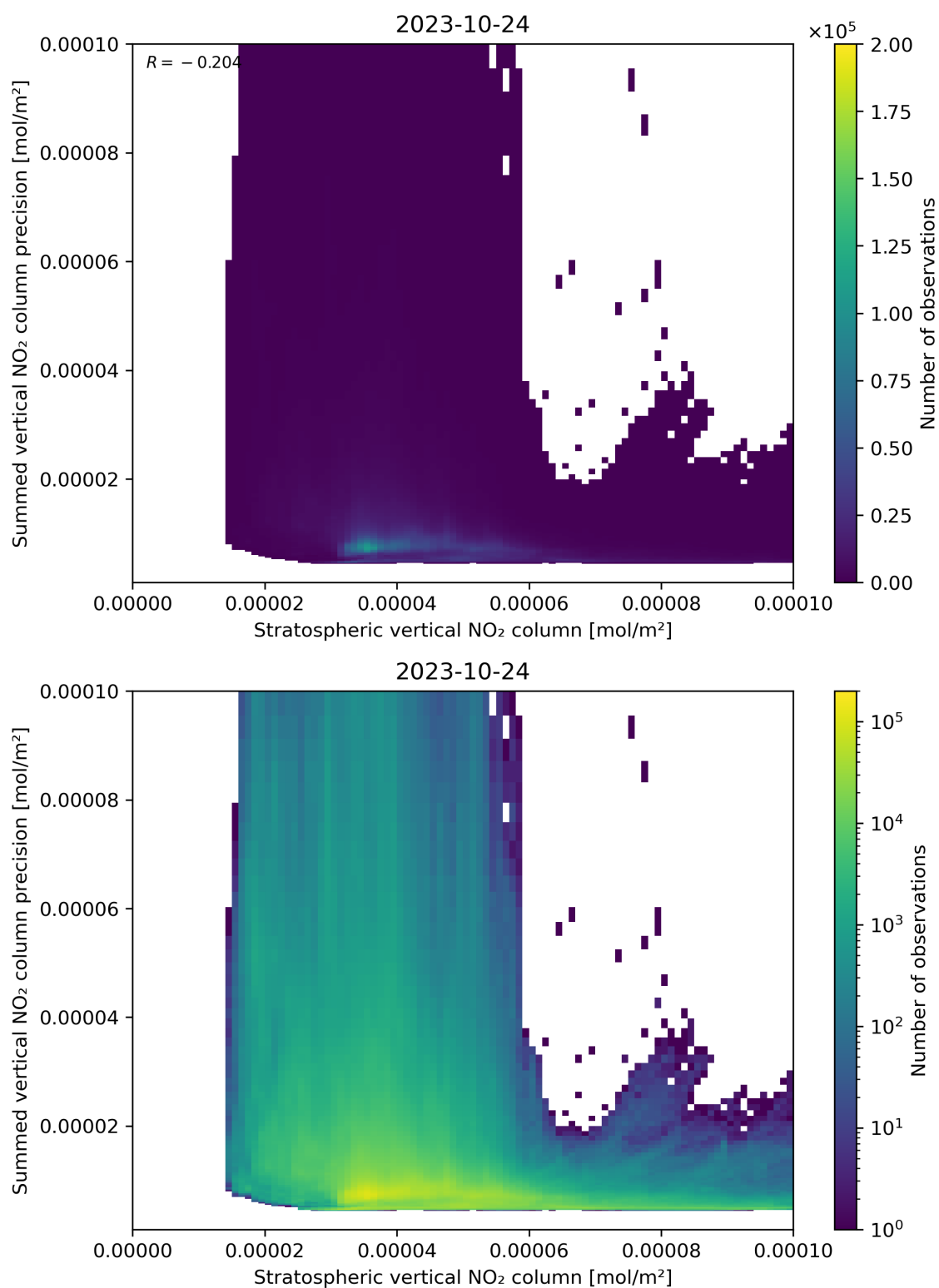
Figure 99: Scatter density plot of “Stratospheric vertical NO 2 column” against “Summed vertical NO 2 column precision” for 2023-10-23 to 2023-10-25.
