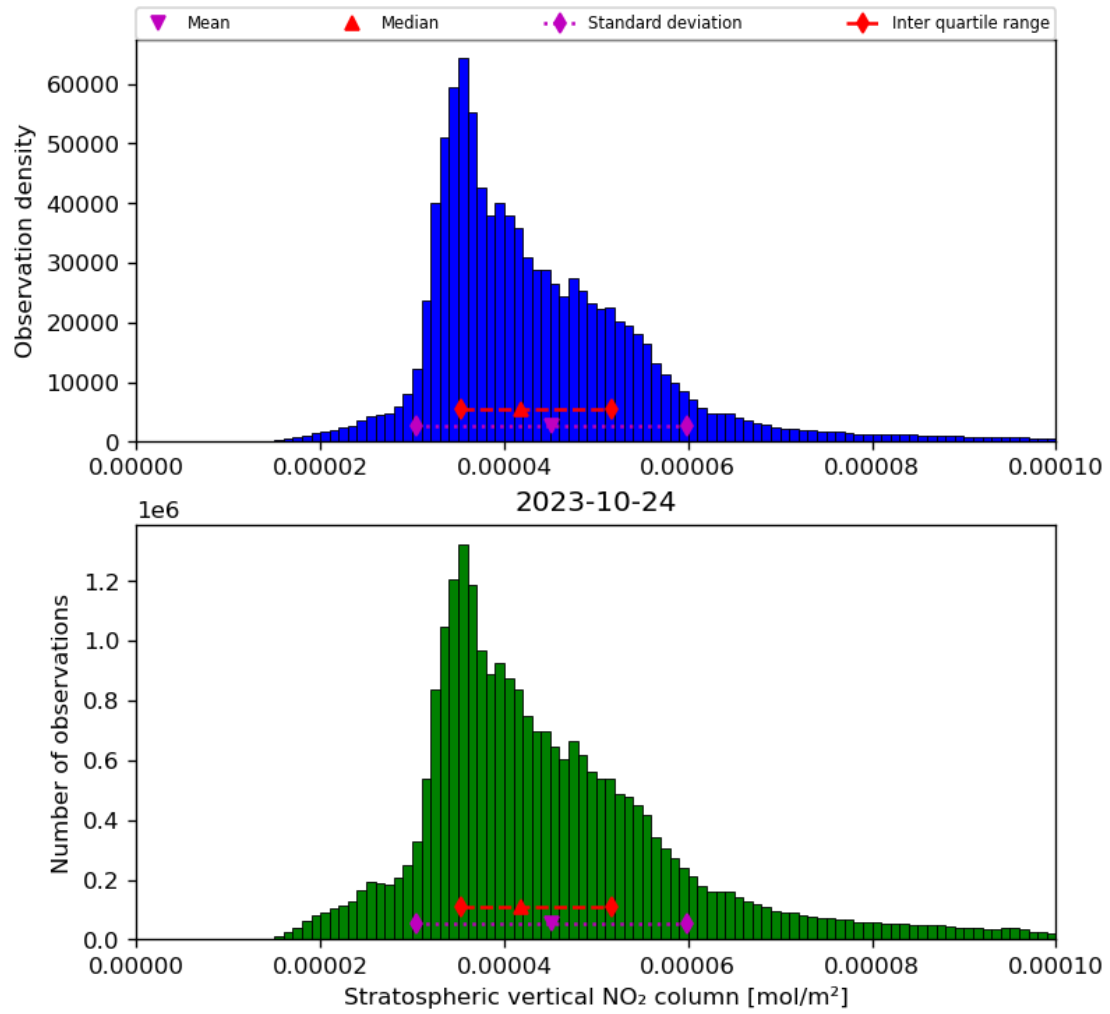
Figure 36: Histogram of “Stratospheric vertical NO 2 column” for 2023-10-23 to 2023-10-25
