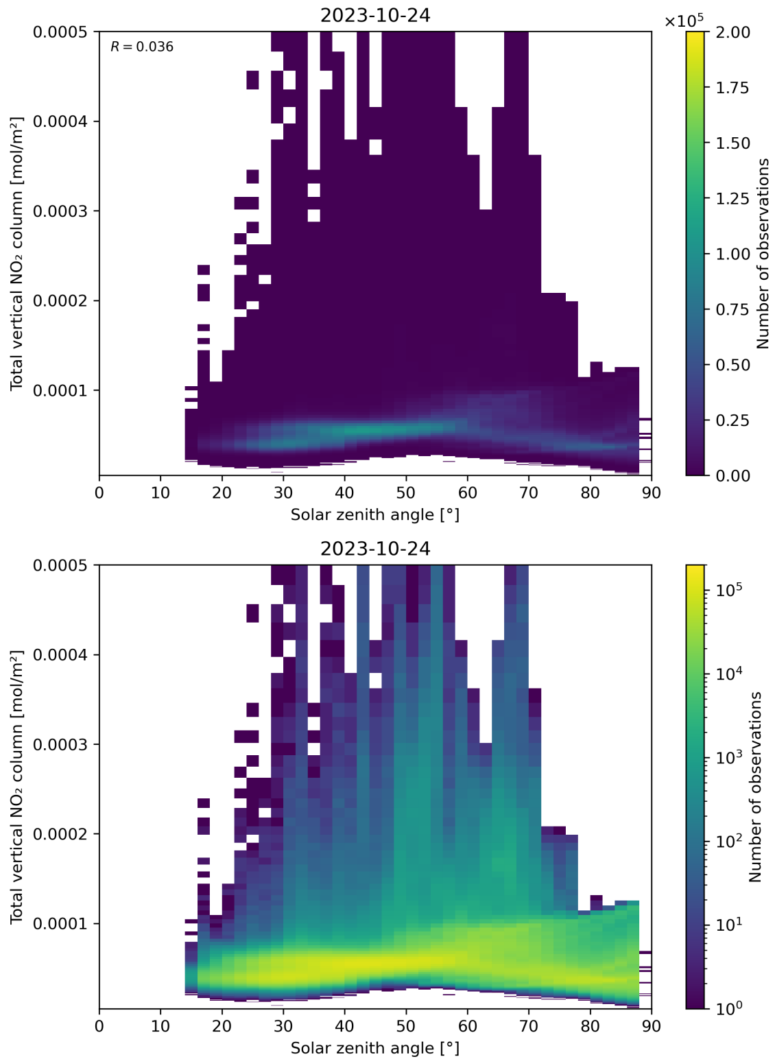
Figure 153: Scatter density plot of “Solar zenith angle” against “Total vertical NO 2 column” for 2023-10-23 to 2023-10-25.
