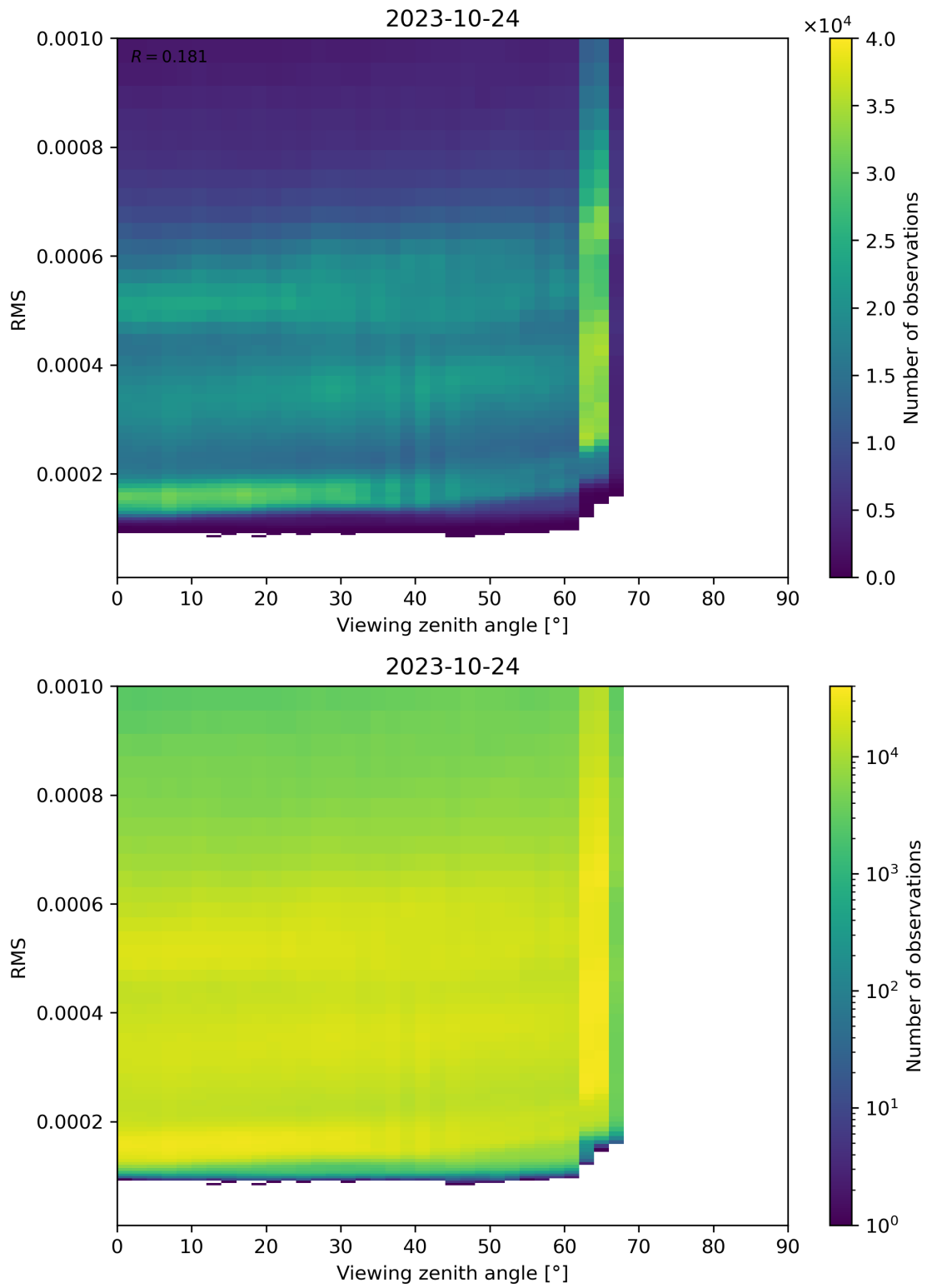
Figure 171: Scatter density plot of “Viewing zenith angle” against “RMS” for 2023-10-23 to 2023-10-25.
