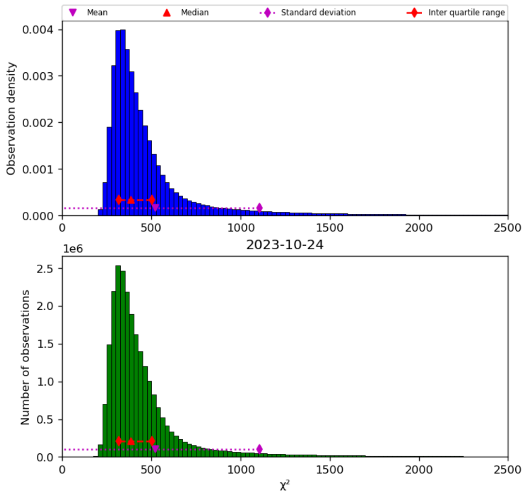
Figure 42: Histogram of “ \chi^2 ” for 2023-10-23 to 2023-10-25
