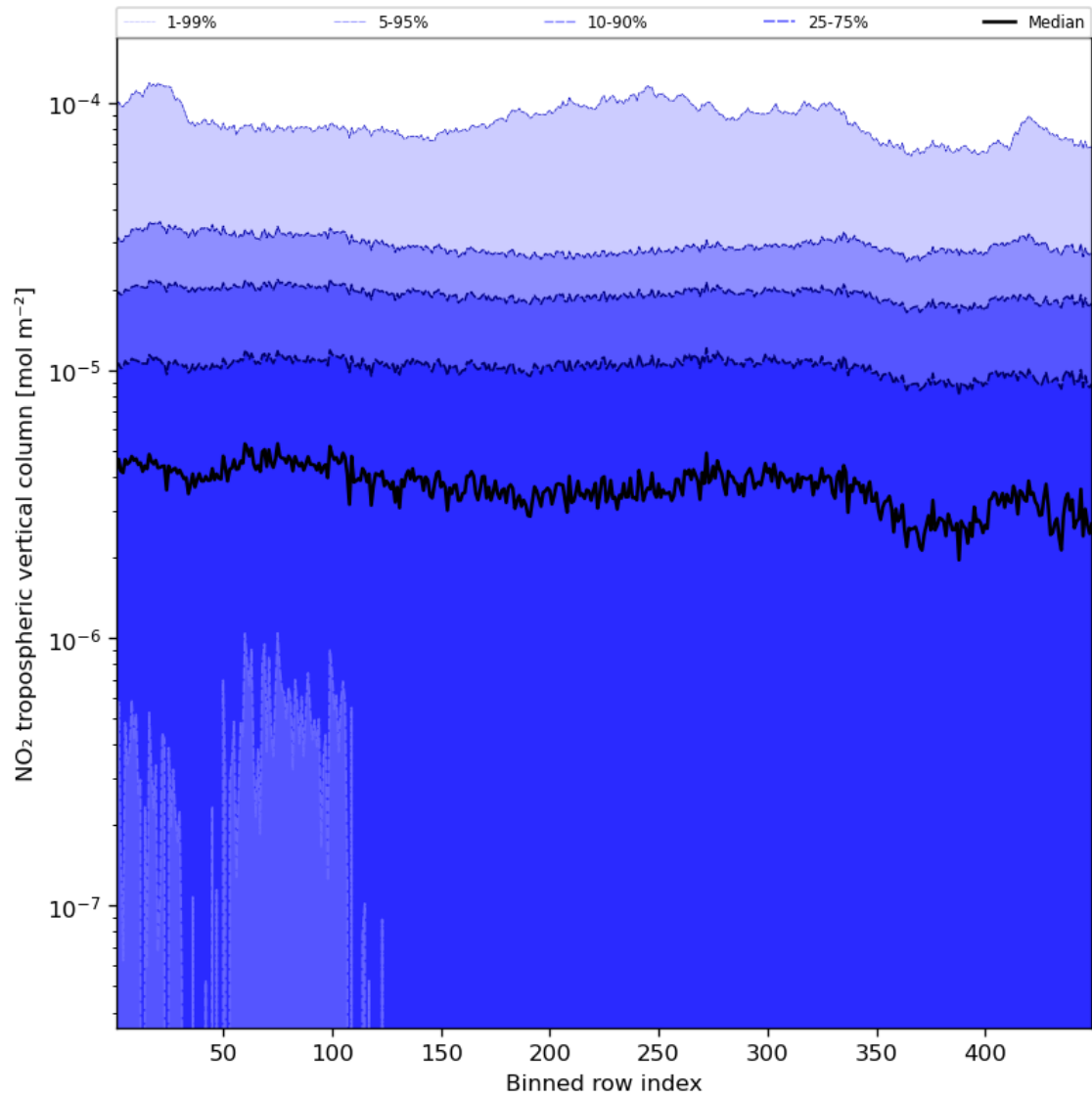
Figure 46: Along track statistics of “NO 2 tropospheric vertical column” for 2023-10-23 to 2023-10-25
