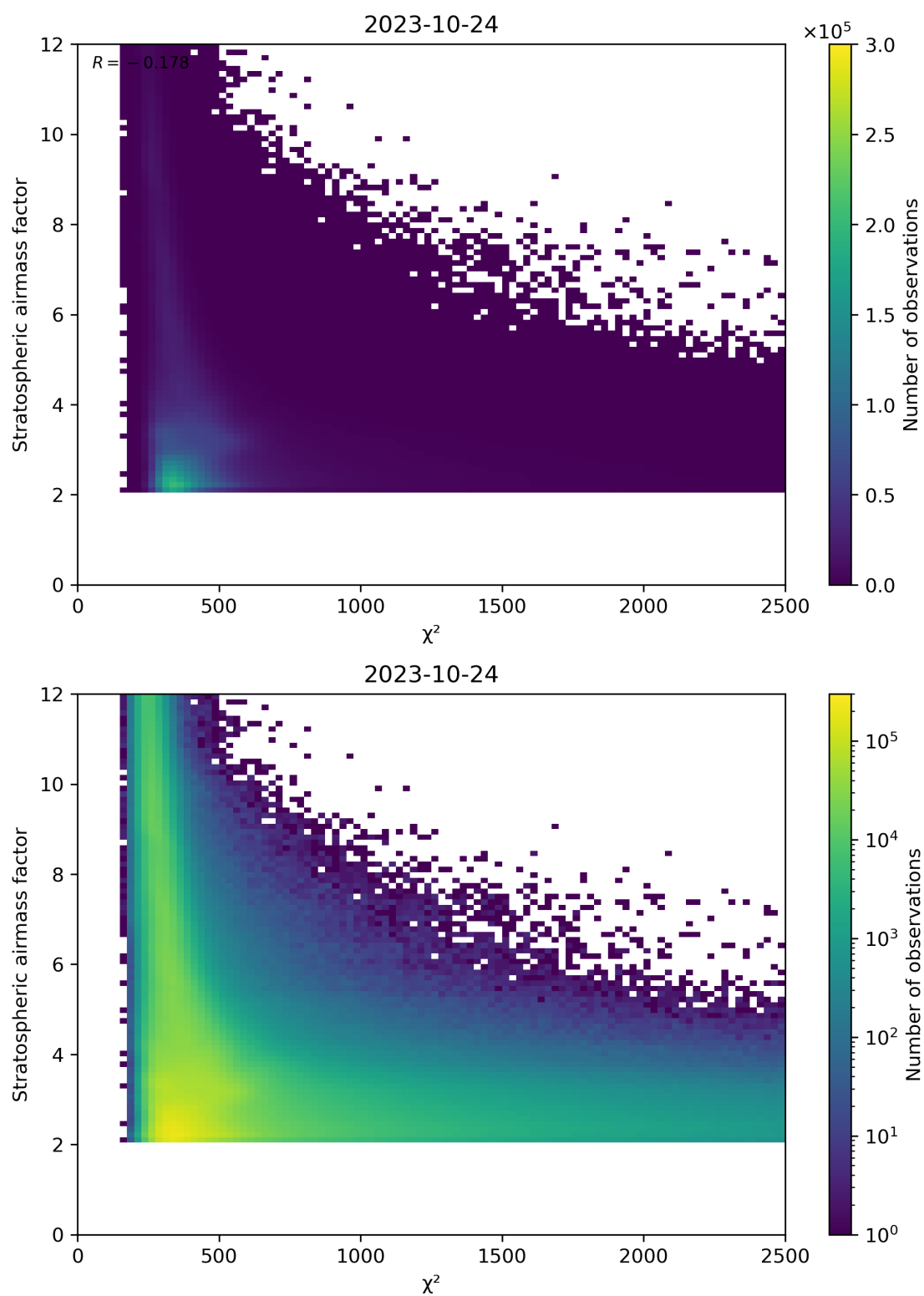
Figure 81: Scatter density plot of “ \chi^2 ” against “Stratospheric airmass factor” for 2023-10-23 to 2023-10-25.
