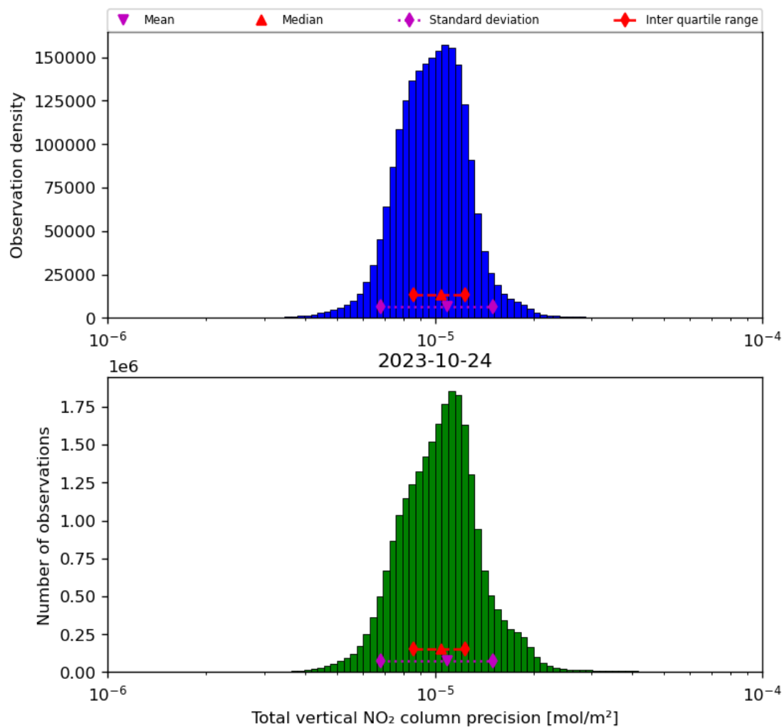
Figure 39: Histogram of “Total vertical NO 2 column precision” for 2023-10-23 to 2023-10-25
