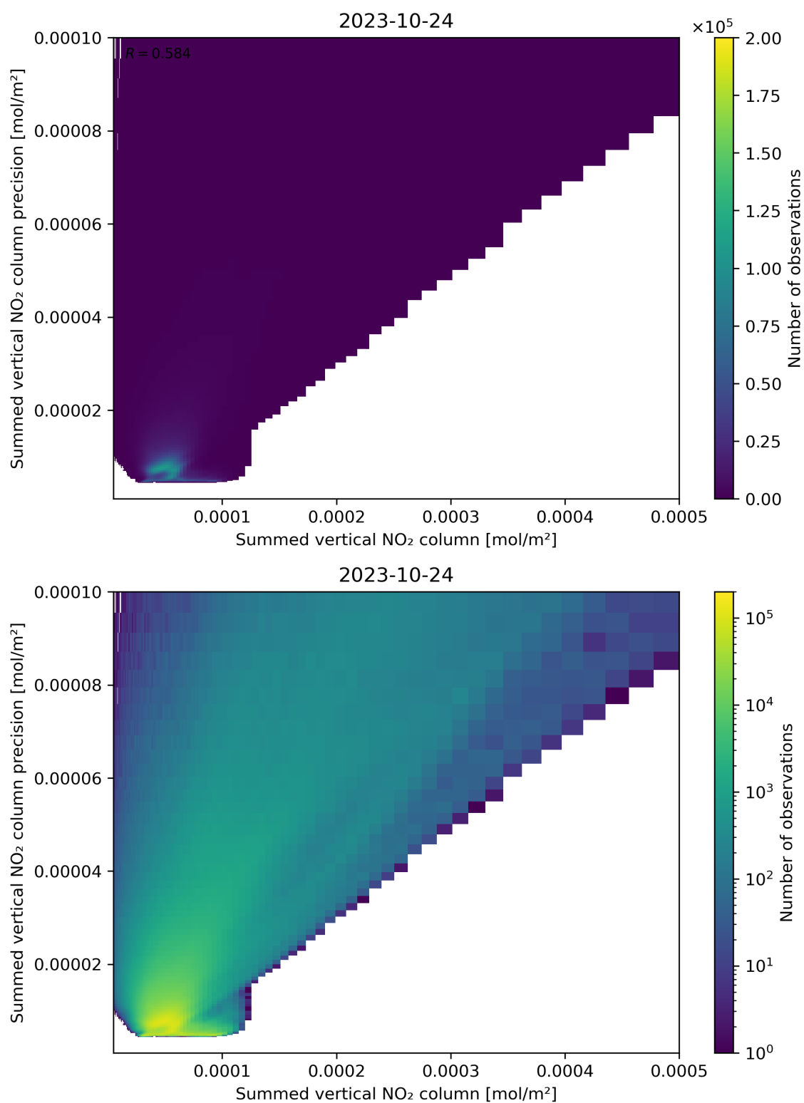
Figure 105: Scatter density plot of “Summed vertical NO 2 column” against “Summed vertical NO 2 column precision” for 2023-10-23 to 2023-10-25.
