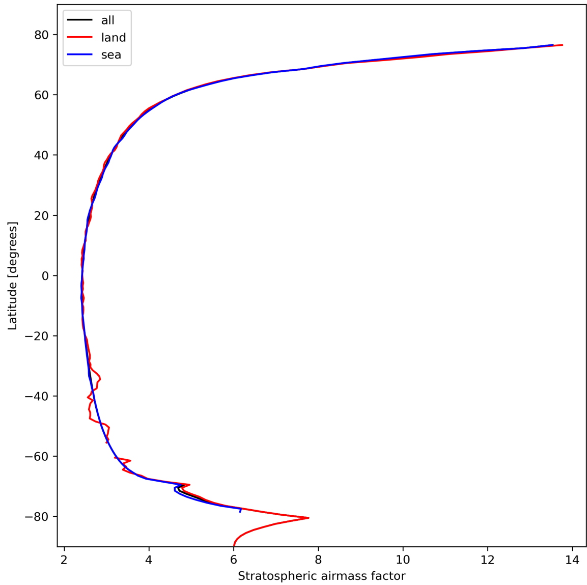
Figure 27: Zonal average of “Stratospheric air mass factor” for 2023-10-23 to 2023-10-25.
