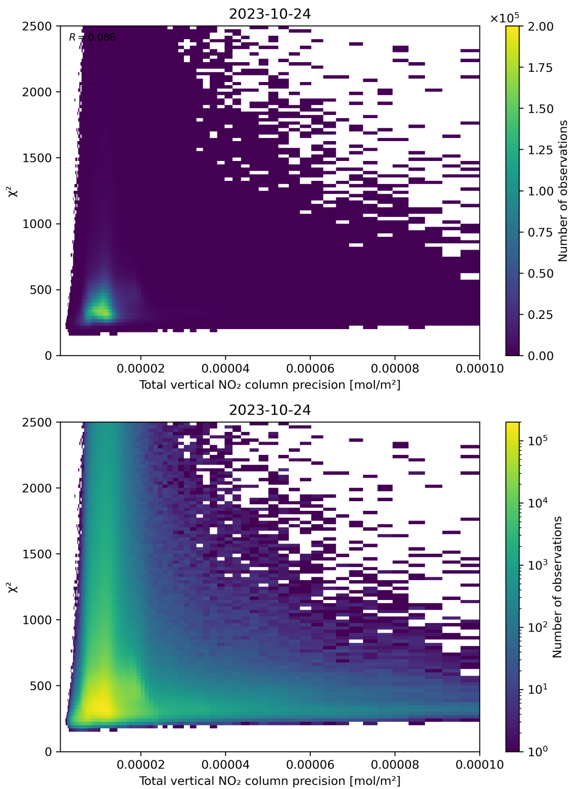
Figure 116: Scatter density plot of “Total vertical NO 2 column precision” against “ \chi^2 ” for 2023-10-23 to 2023-10-25.
