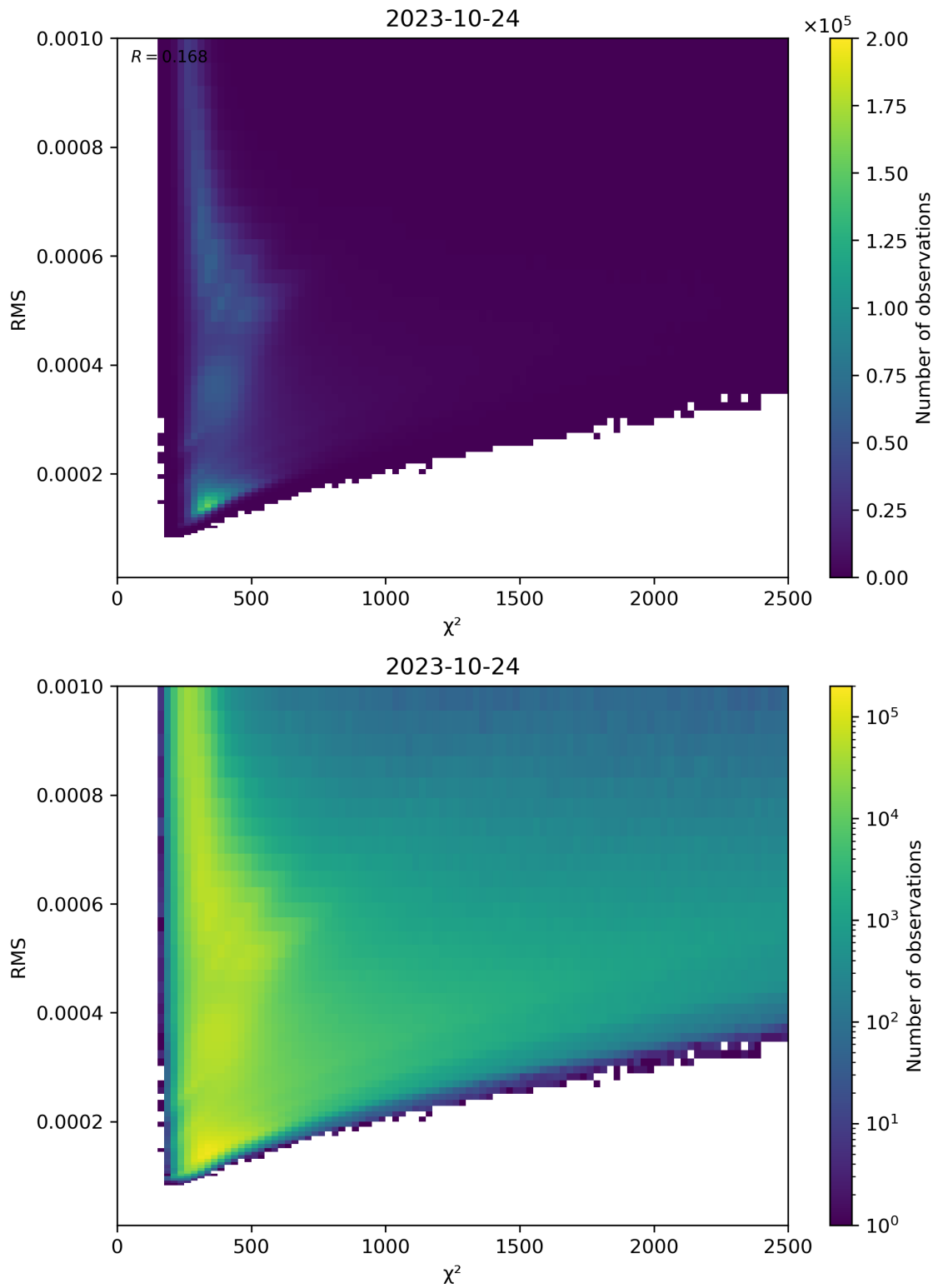
Figure 82: Scatter density plot of “ \chi^2 ” against “RMS” for 2023-10-23 to 2023-10-25.
