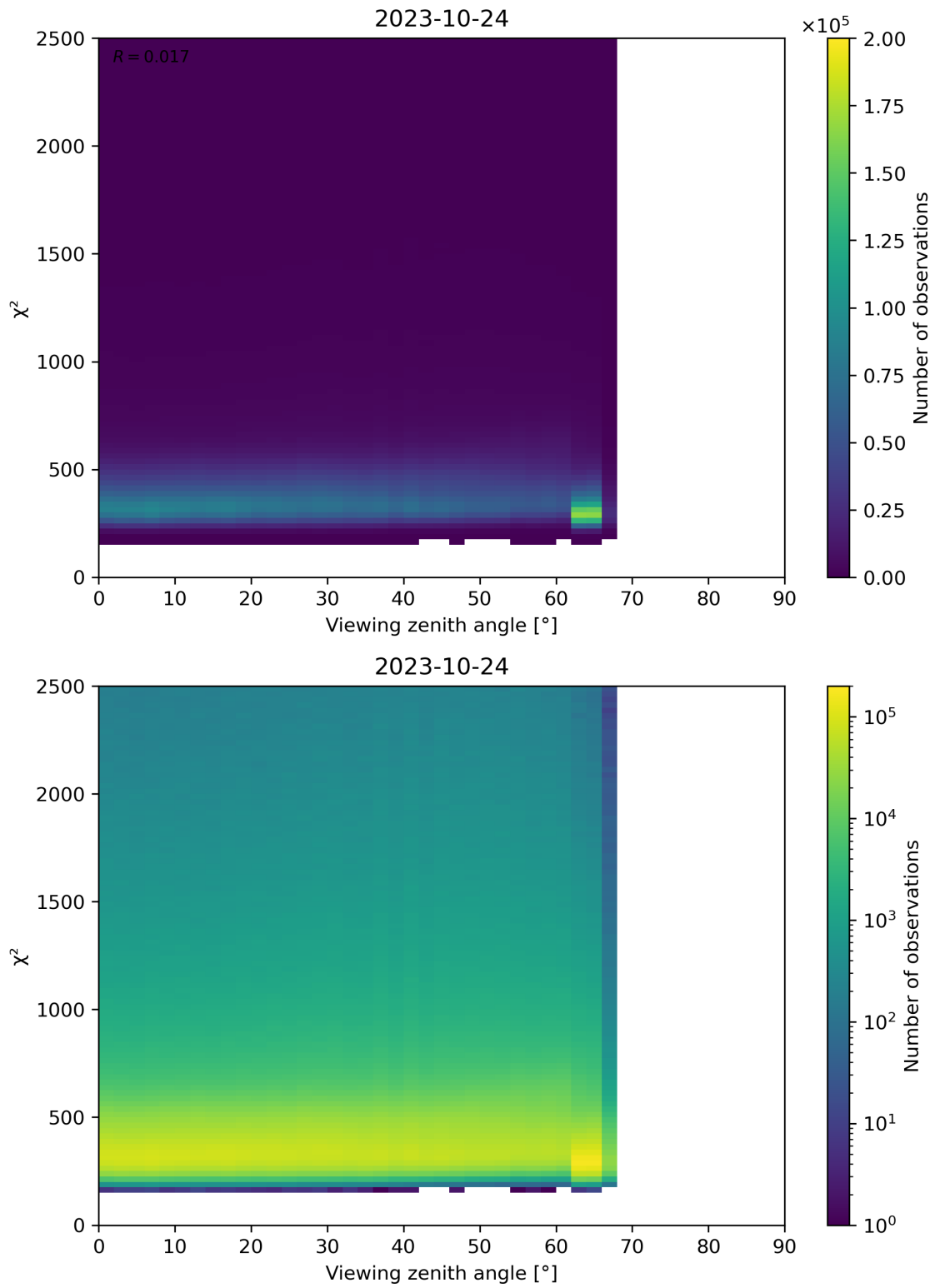
Figure 162: Scatter density plot of “Viewing zenith angle” against “ \chi^2 ” for 2023-10-23 to 2023-10-25.
