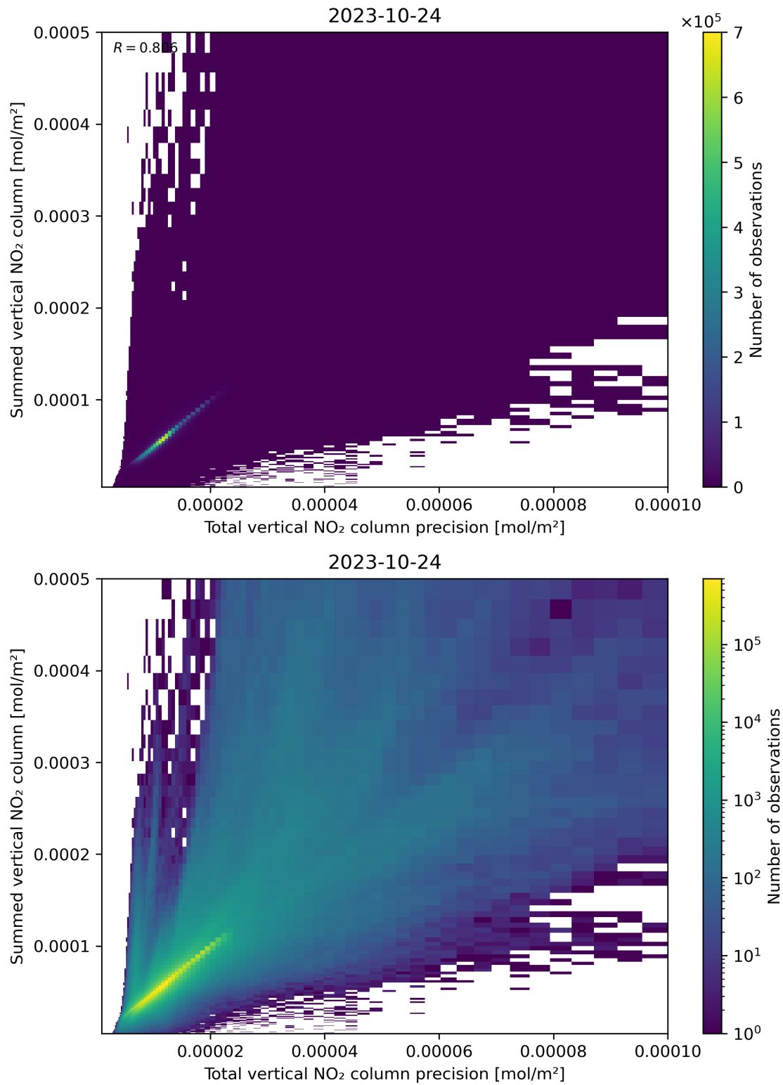
Figure 117: Scatter density plot of “Total vertical NO 2 column precision” against “Summed vertical NO 2 column” for 2023-10-23 to 2023-10-25.
