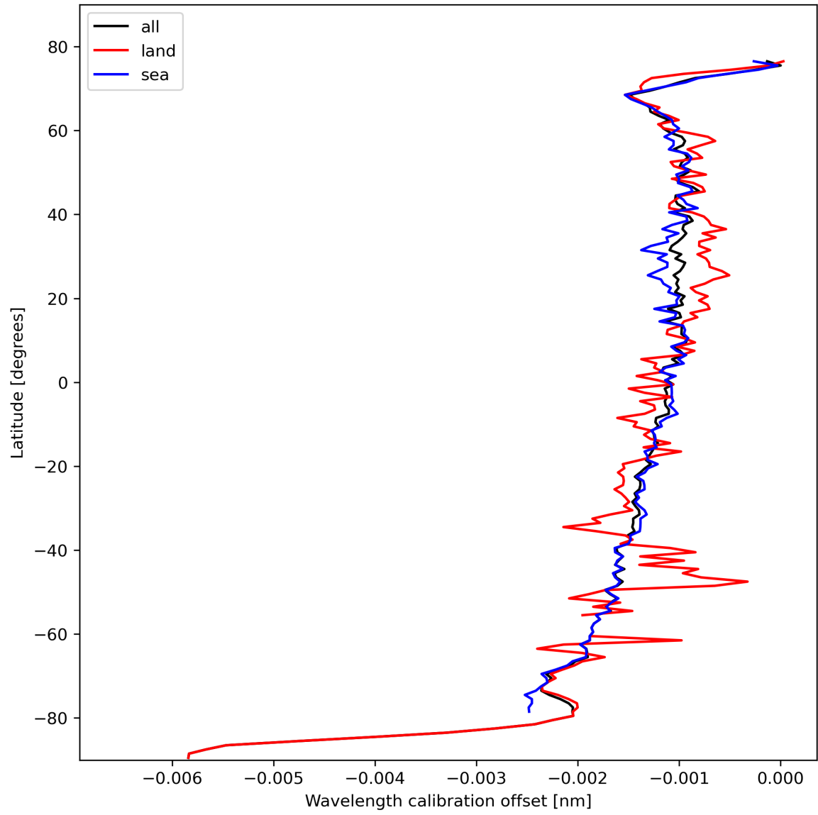
Figure 18: Zonal average of “Wavelength calibration offset” for 2023-10-23 to 2023-10-25.
