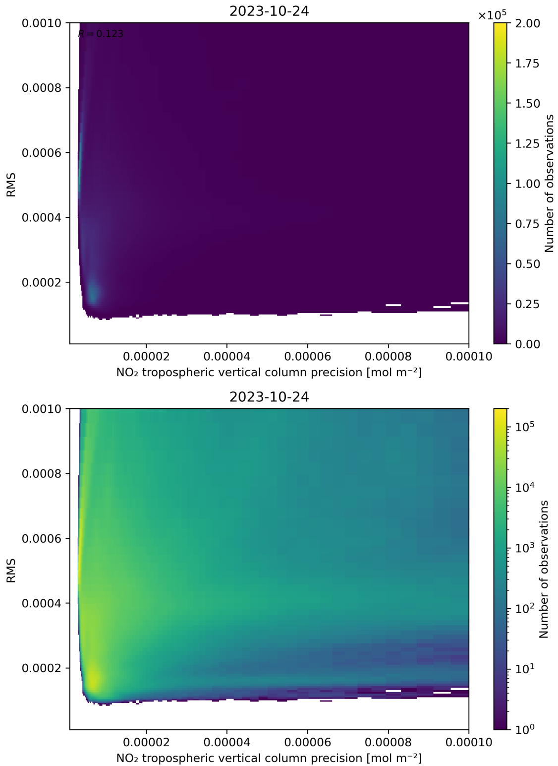
Figure 140: Scatter density plot of “NO 2 tropospheric vertical column precision” against “RMS” for 2023-10-23 to 2023-10-25.
