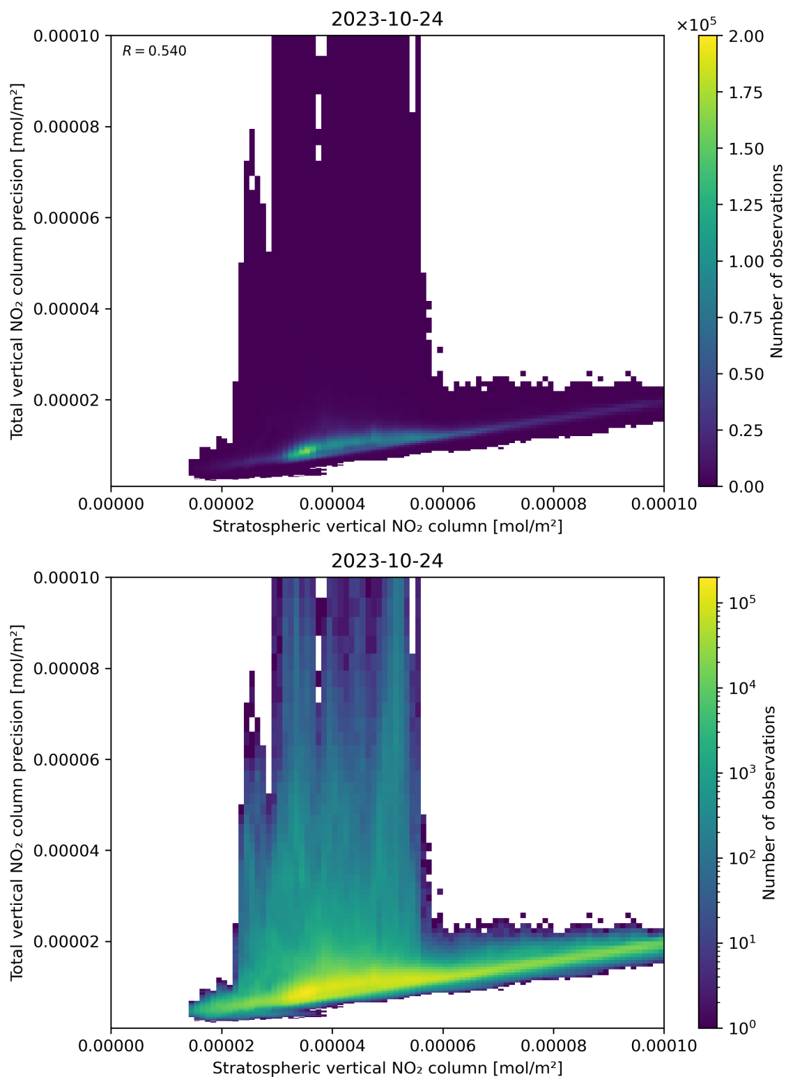
Figure 101: Scatter density plot of “Stratospheric vertical NO 2 column” against “Total vertical NO 2 column precision” for 2023-10-23 to 2023-10-25.
