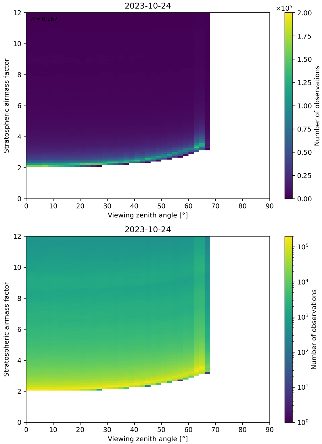
Figure 159: Scatter density plot of “Viewing zenith angle” against “Stratospheric airmass factor” for 2023-10-23 to 2023-10-25.
