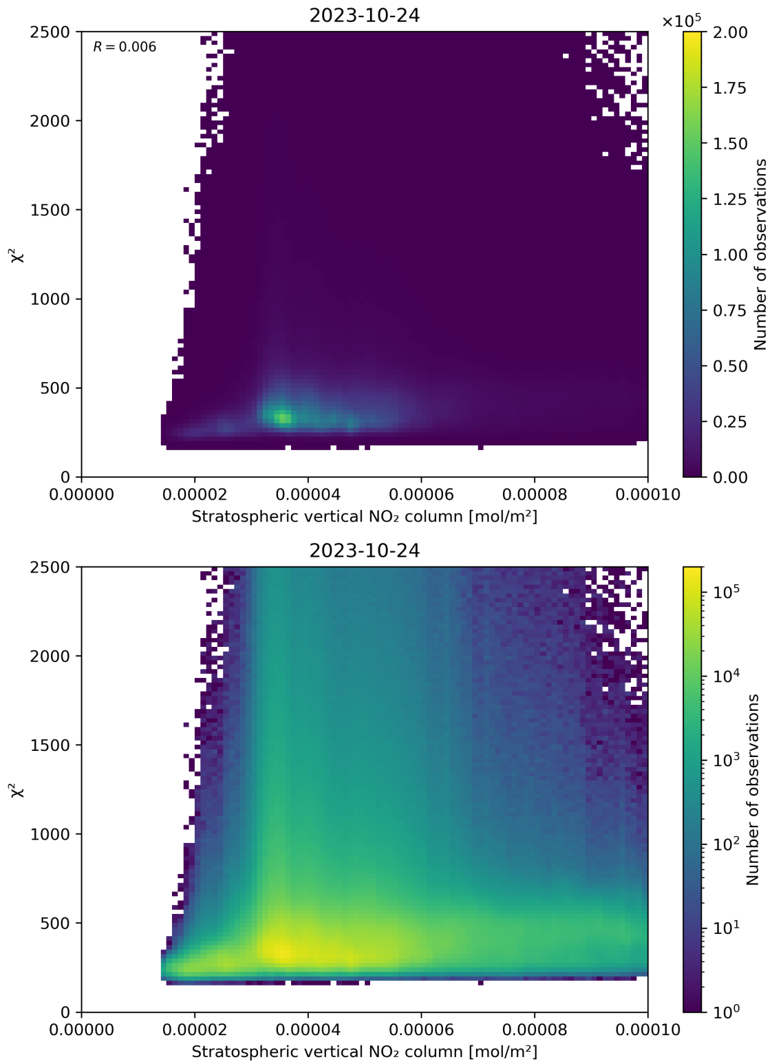
Figure 97: Scatter density plot of “Stratospheric vertical NO 2 column” against “ \chi^2 ” for 2023-10-23 to 2023-10-25.
