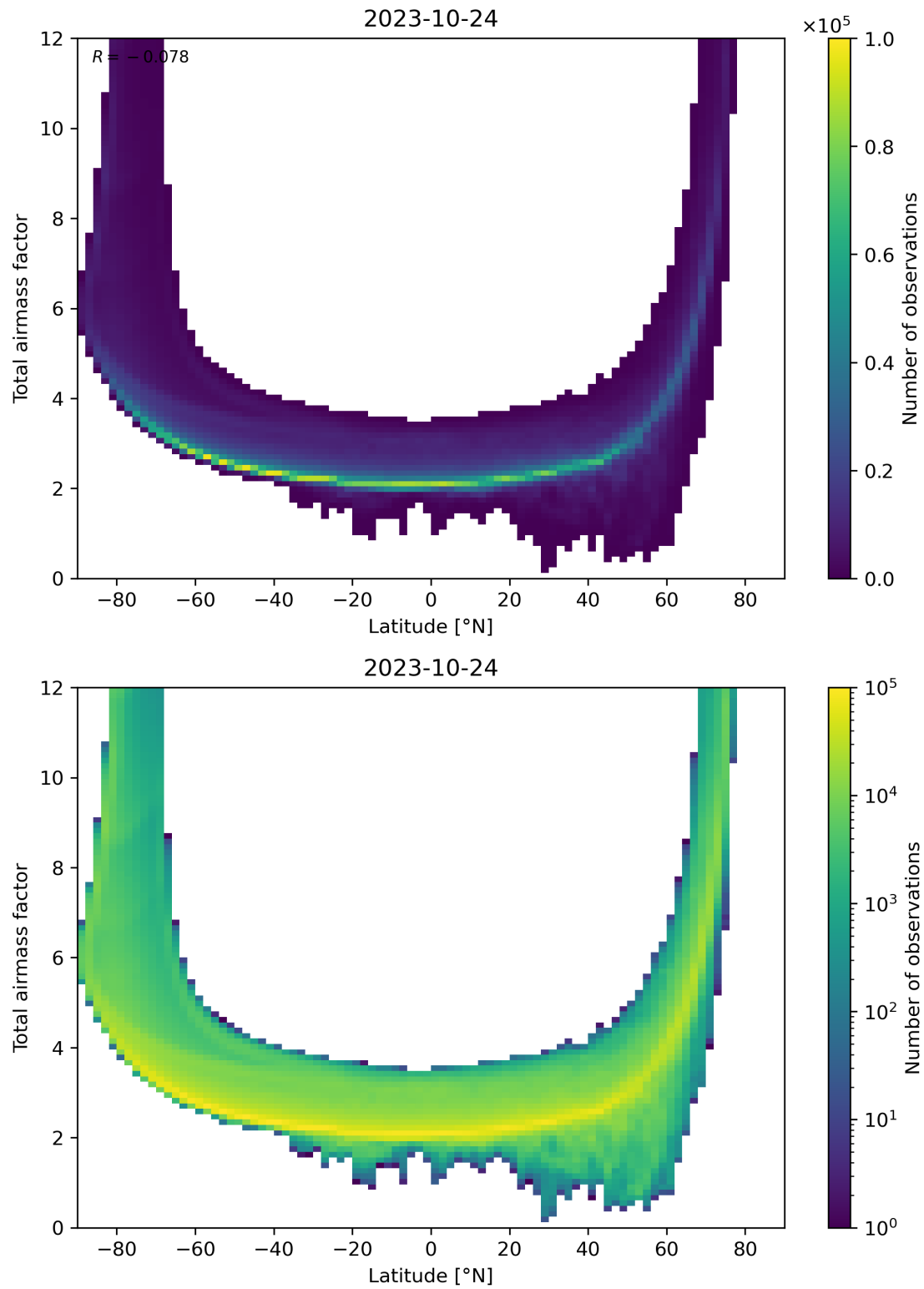
Figure 84: Scatter density plot of “Latitude” against “Total airmass factor” for 2023-10-23 to 2023-10-25.
