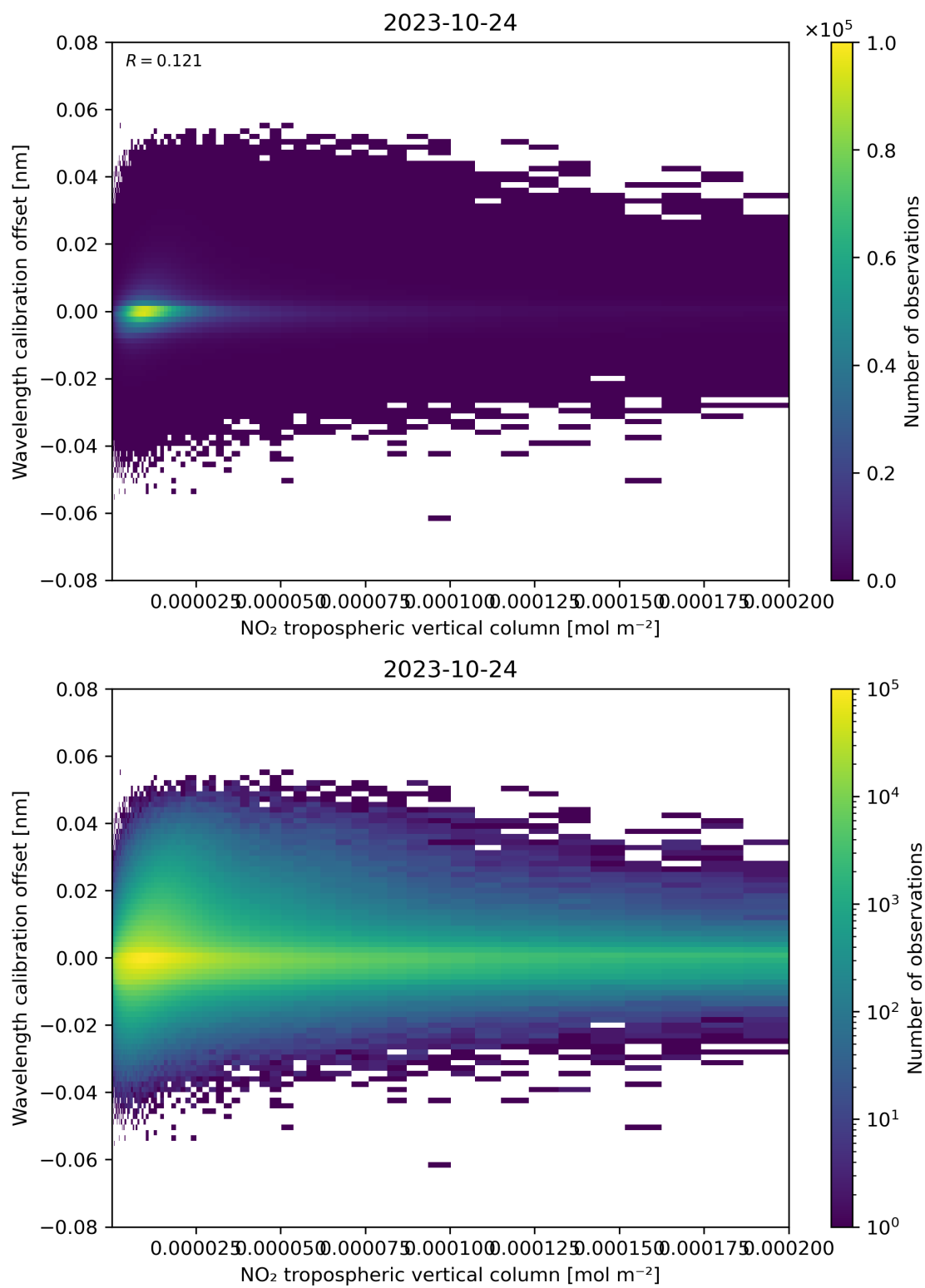
Figure 143: Scatter density plot of “NO 2 tropospheric vertical column” against “Wavelength calibration offset” for 2023-10-23 to 2023-10-25.
