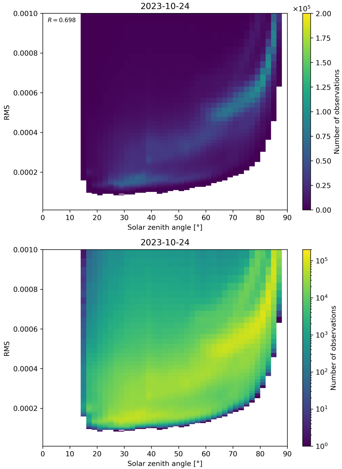
Figure 157: Scatter density plot of “Solar zenith angle” against “RMS” for 2023-10-23 to 2023-10-25.
