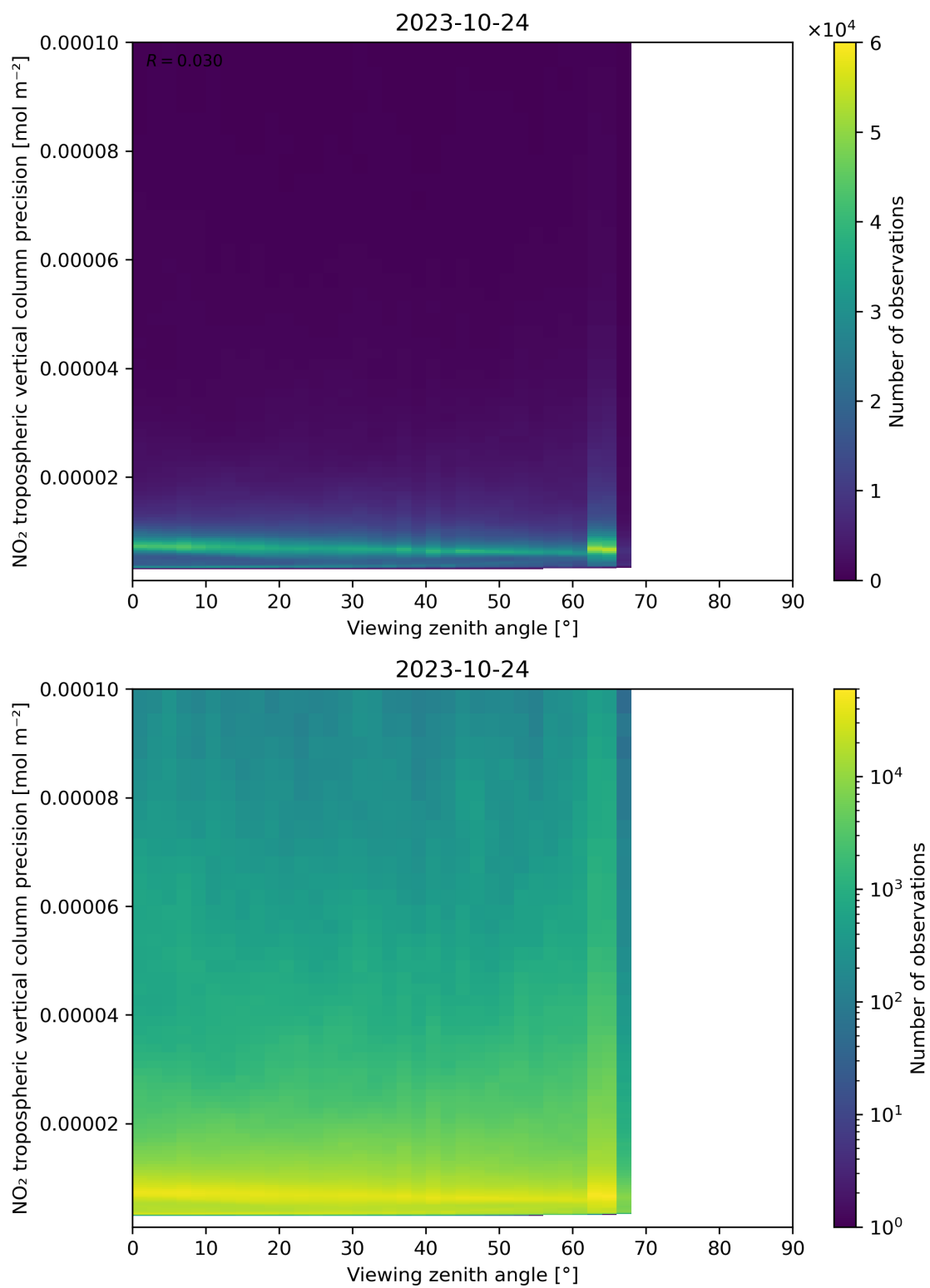
Figure 170: Scatter density plot of “Viewing zenith angle” against “NO 2 tropospheric vertical column precision” for 2023-10-23 to 2023-10-25.
