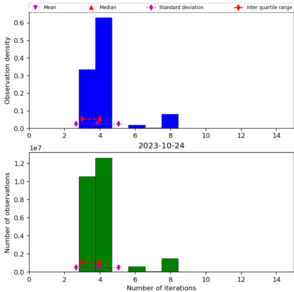
Figure 34: Histogram of “Number of iterations” for 2023-10-23 to 2023-10-25
