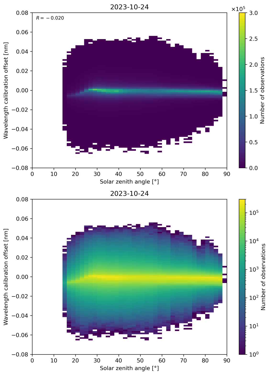
Figure 158: Scatter density plot of “Solar zenith angle” against “Wavelength calibration offset” for 2023-10-23 to 2023-10-25.
