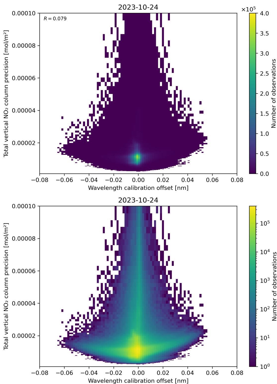
Figure 180: Scatter density plot of “Wavelength calibration offset” against “Total vertical NO 2 column precision” for 2023-10-23 to 2023-10-25.
