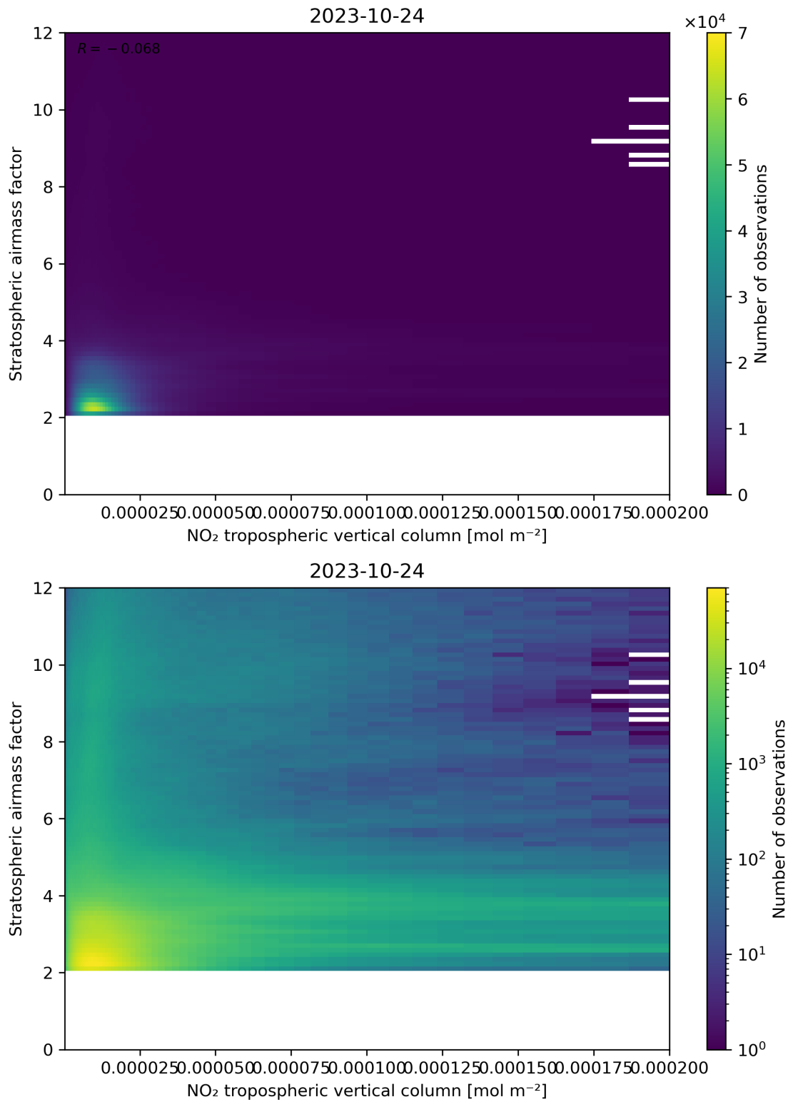
Figure 121: Scatter density plot of “NO 2 tropospheric vertical column” against “Stratospheric airmass factor” for 2023-10-23 to 2023-10-25.
