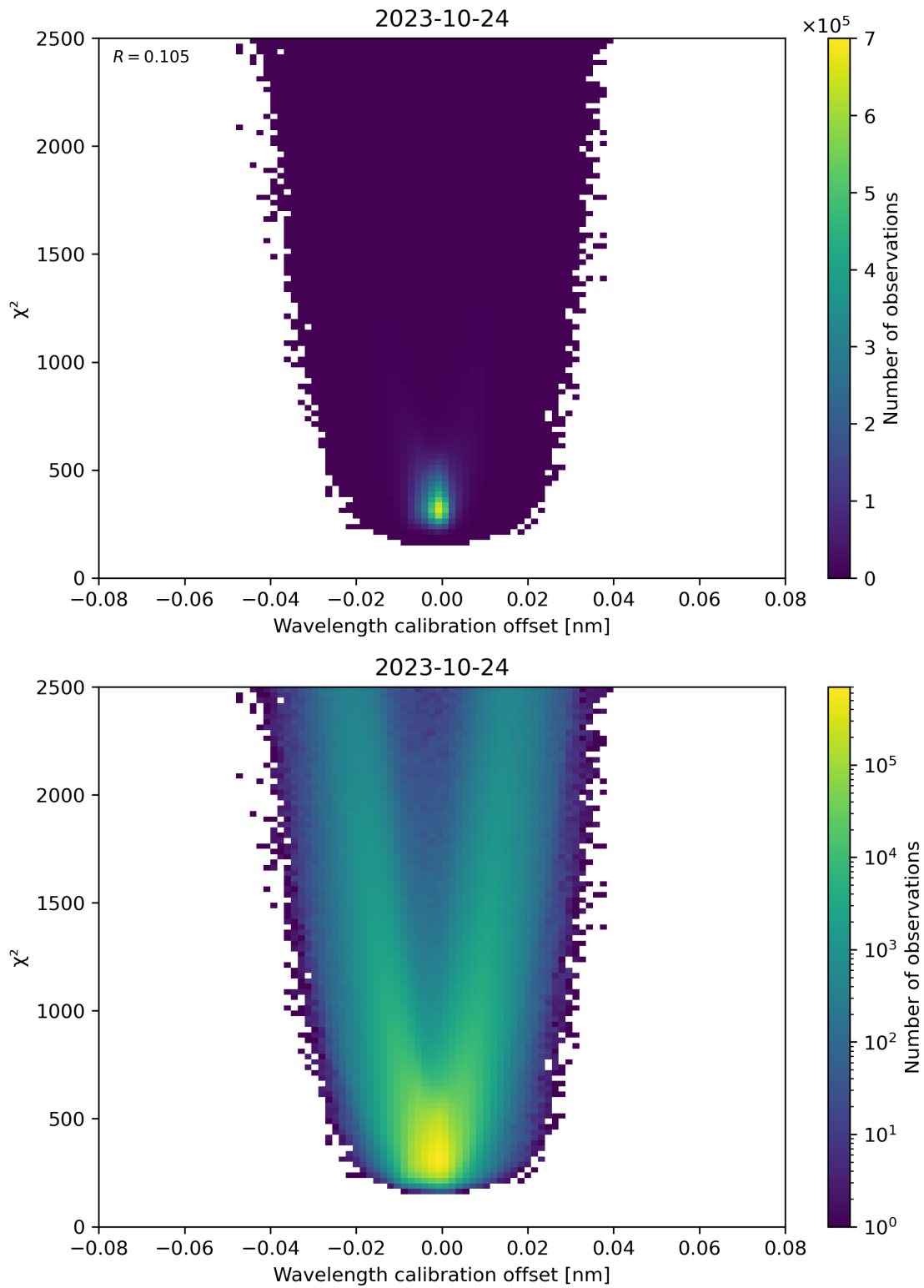
Figure 175: Scatter density plot of “Wavelength calibration offset” against “ \chi^2 ” for 2023-10-23 to 2023-10-25.
