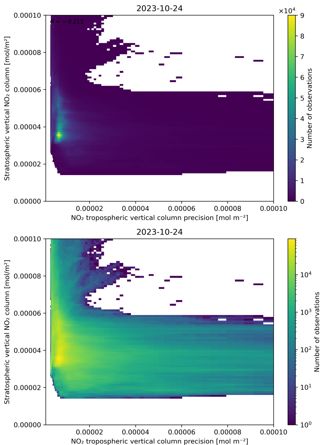
Figure 135: Scatter density plot of “NO 2 tropospheric vertical column precision” against “Stratospheric vertical NO 2 column” for 2023-10-23 to 2023-10-25.
