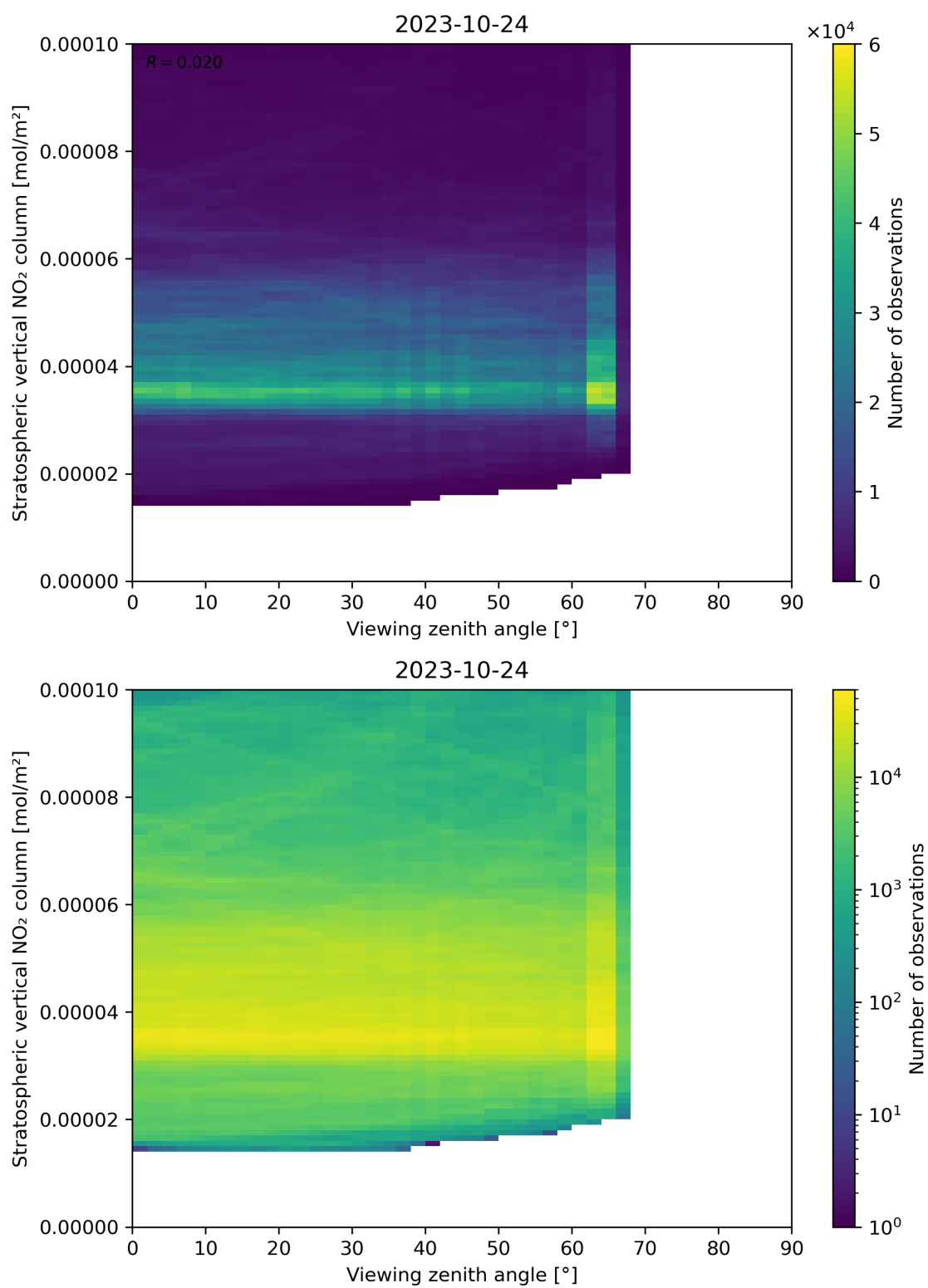
Figure 164: Scatter density plot of “Viewing zenith angle” against “Stratospheric vertical NO 2 column” for 2023-10-23 to 2023-10-25.
