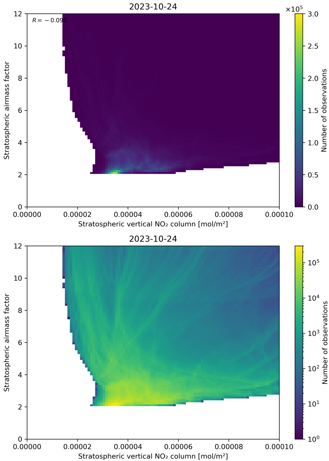
Figure 96: Scatter density plot of “Stratospheric vertical NO 2 column” against “Stratospheric airmass factor” for 2023-10-23 to 2023-10-25.
