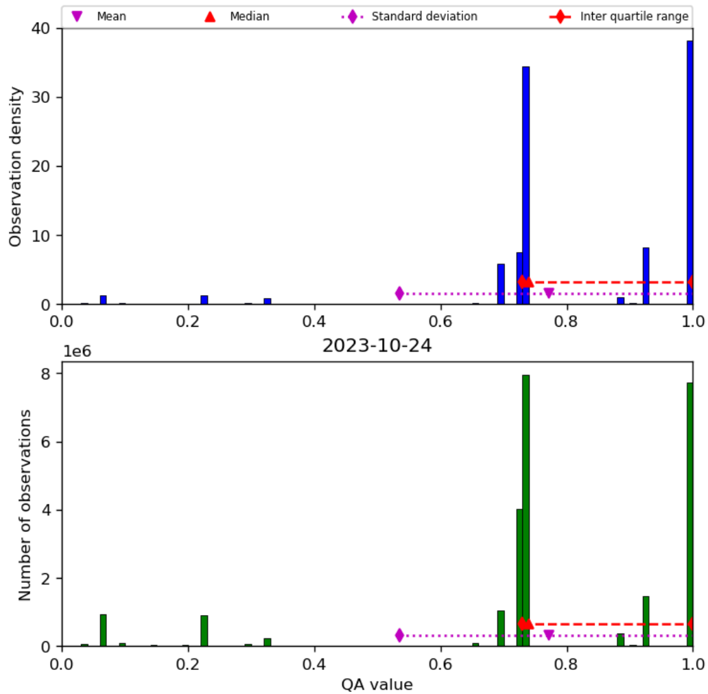
Figure 28: Histogram of “QA value” for 2023-10-23 to 2023-10-25
