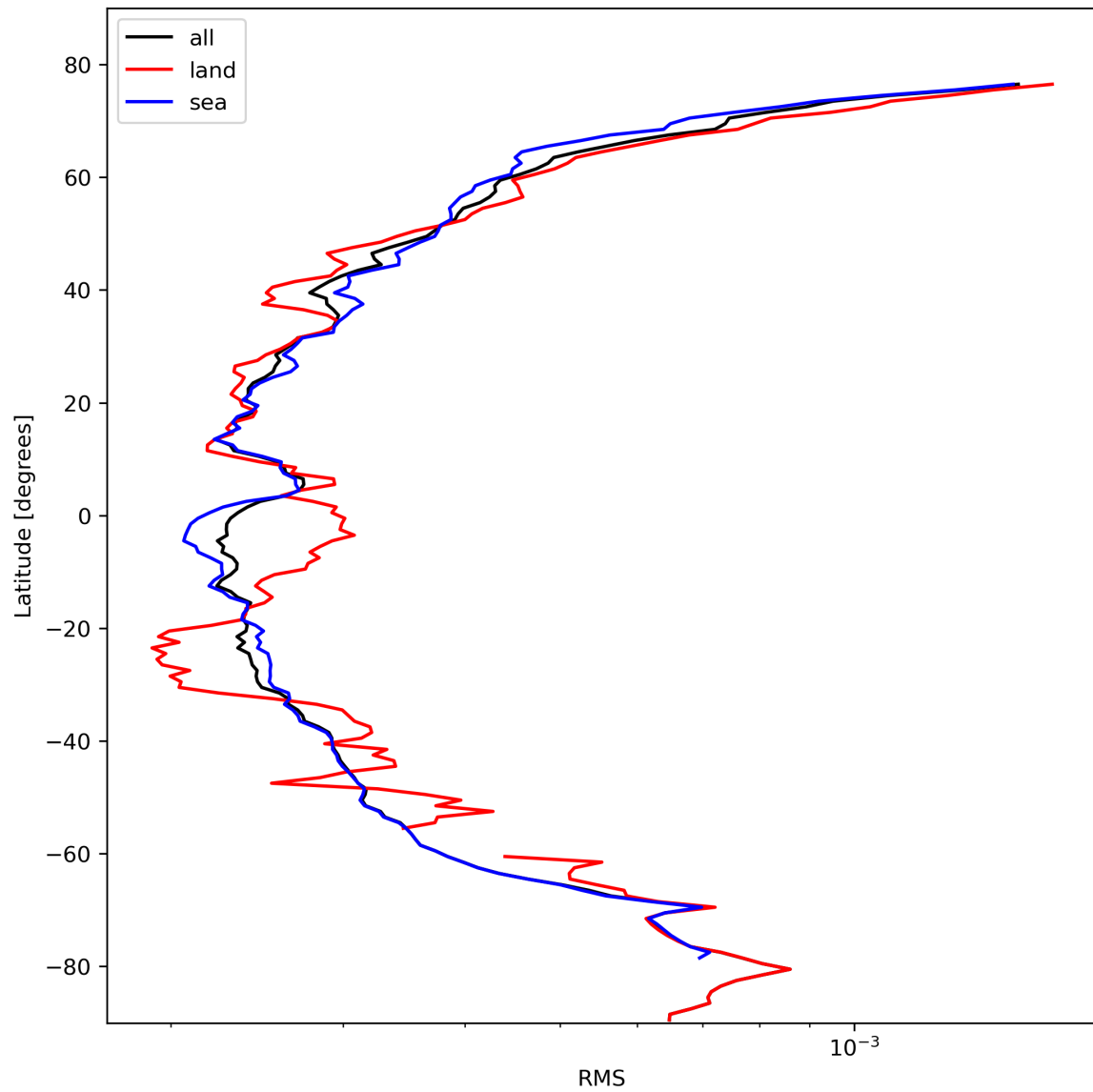
Figure 26: Zonal average of “RMS” for 2023-10-23 to 2023-10-25.
