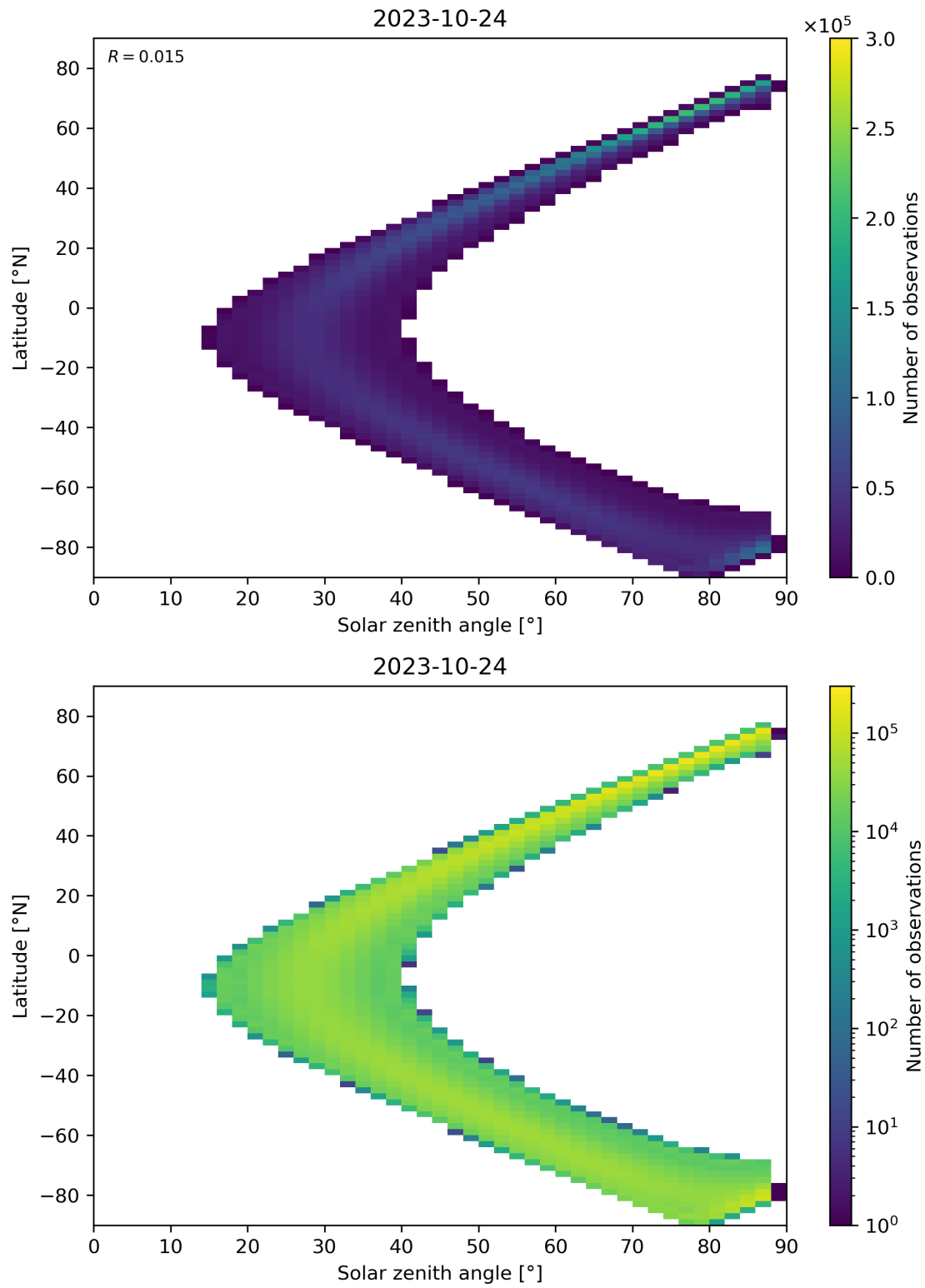
Figure 149: Scatter density plot of “Solar zenith angle” against “Latitude” for 2023-10-23 to 2023-10-25.
