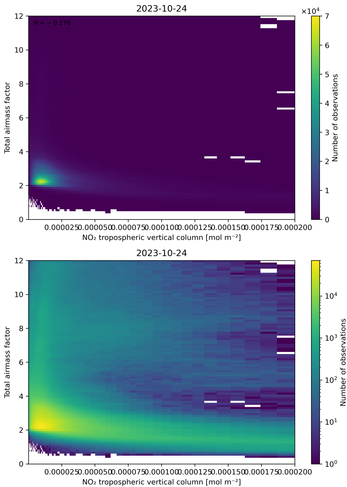
Figure 122: Scatter density plot of “NO 2 tropospheric vertical column” against “Total air mass factor” for 2023-10-23 to 2023-10-25.
