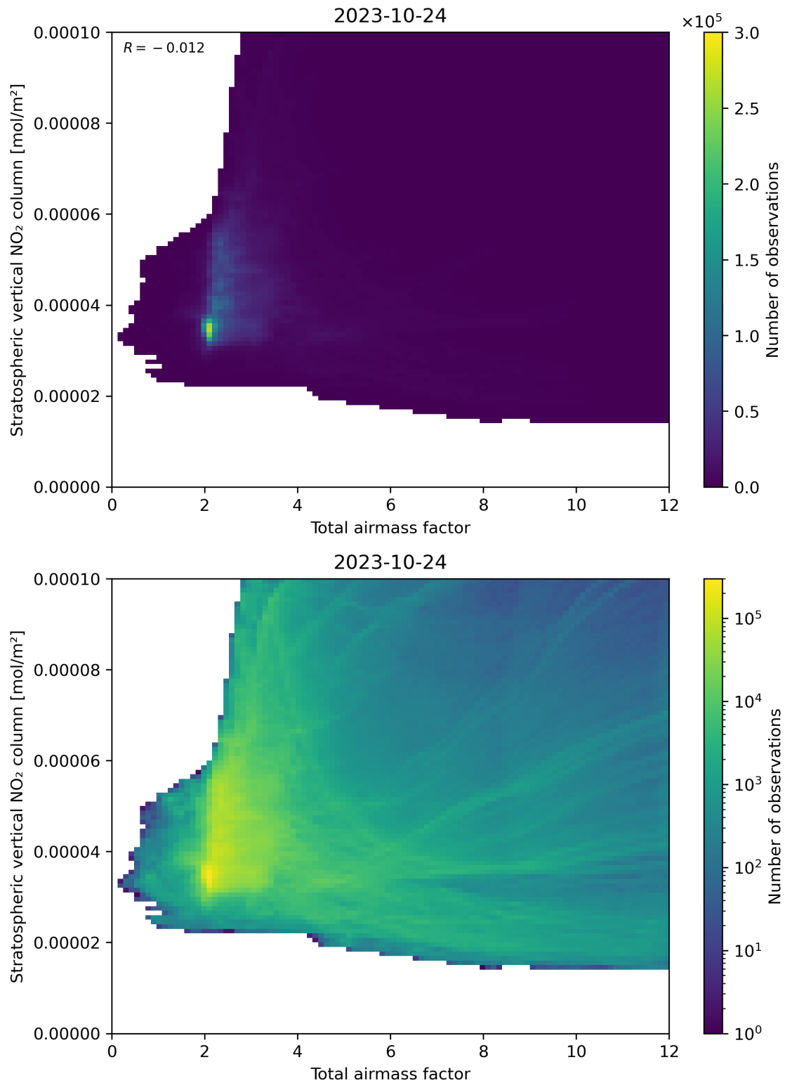
Figure 64: Scatter density plot of “Total airmass factor” against “Stratospheric vertical NO 2 column” for 2023-10-23 to 2023-10-25.
