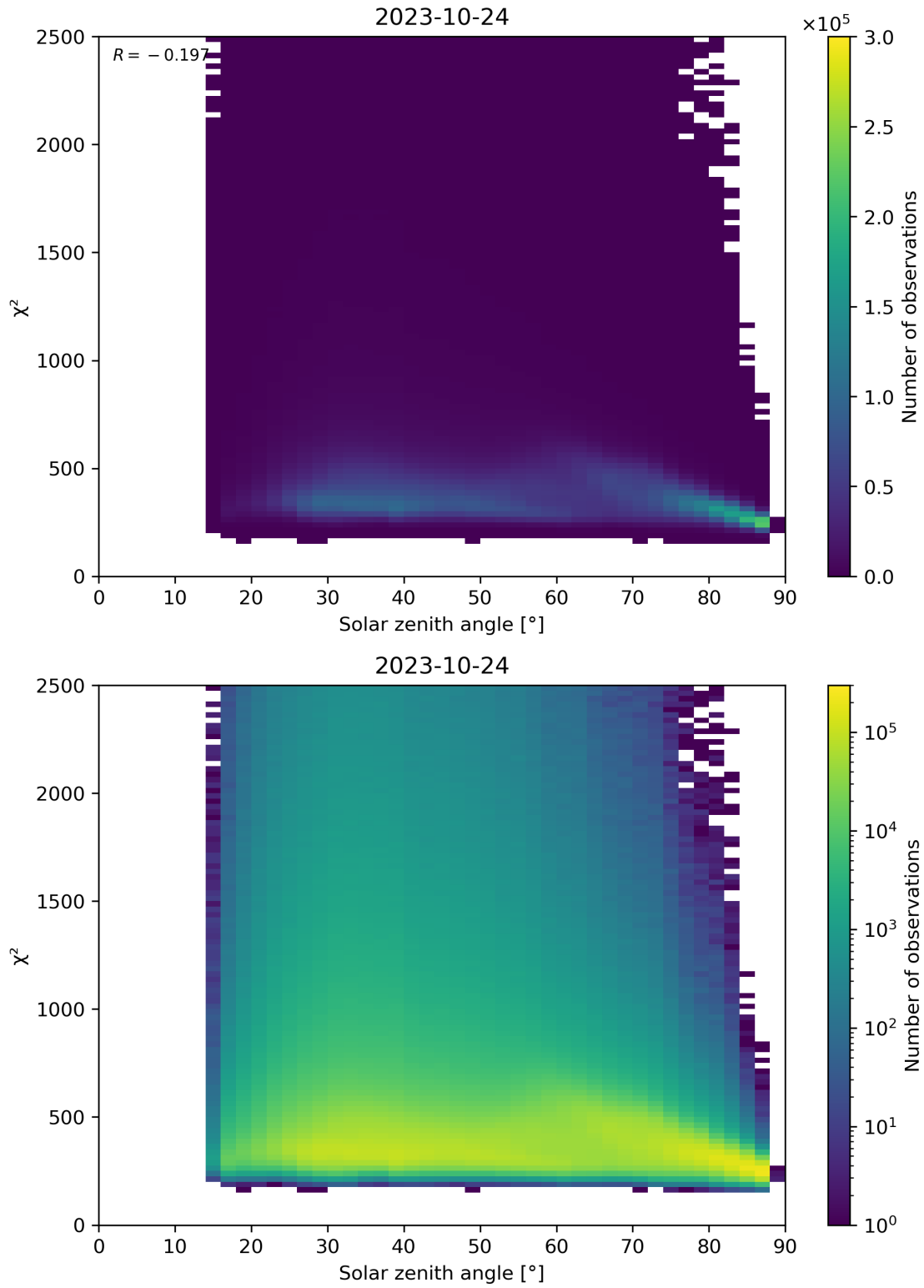
Figure 148: Scatter density plot of “Solar zenith angle” against “ \chi^2 ” for 2023-10-23 to 2023-10-25.
