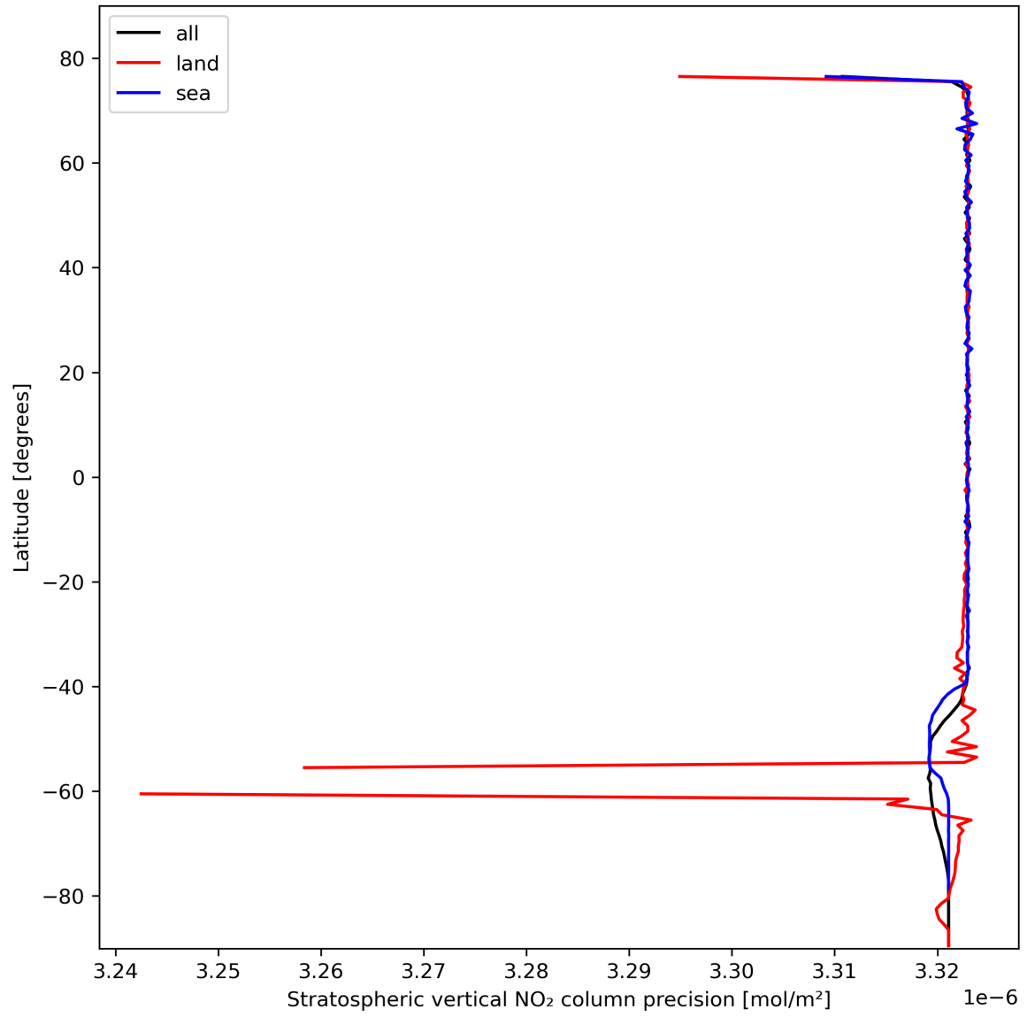
Figure 20: Zonal average of “Stratospheric vertical NO 2 column precision” for 2023-10-23 to 2023-10-25.
