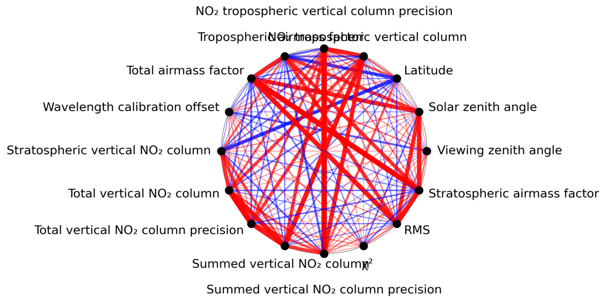
Figure 1: Map of correlation graph for 2023-10-23 to 2023-10-25.
