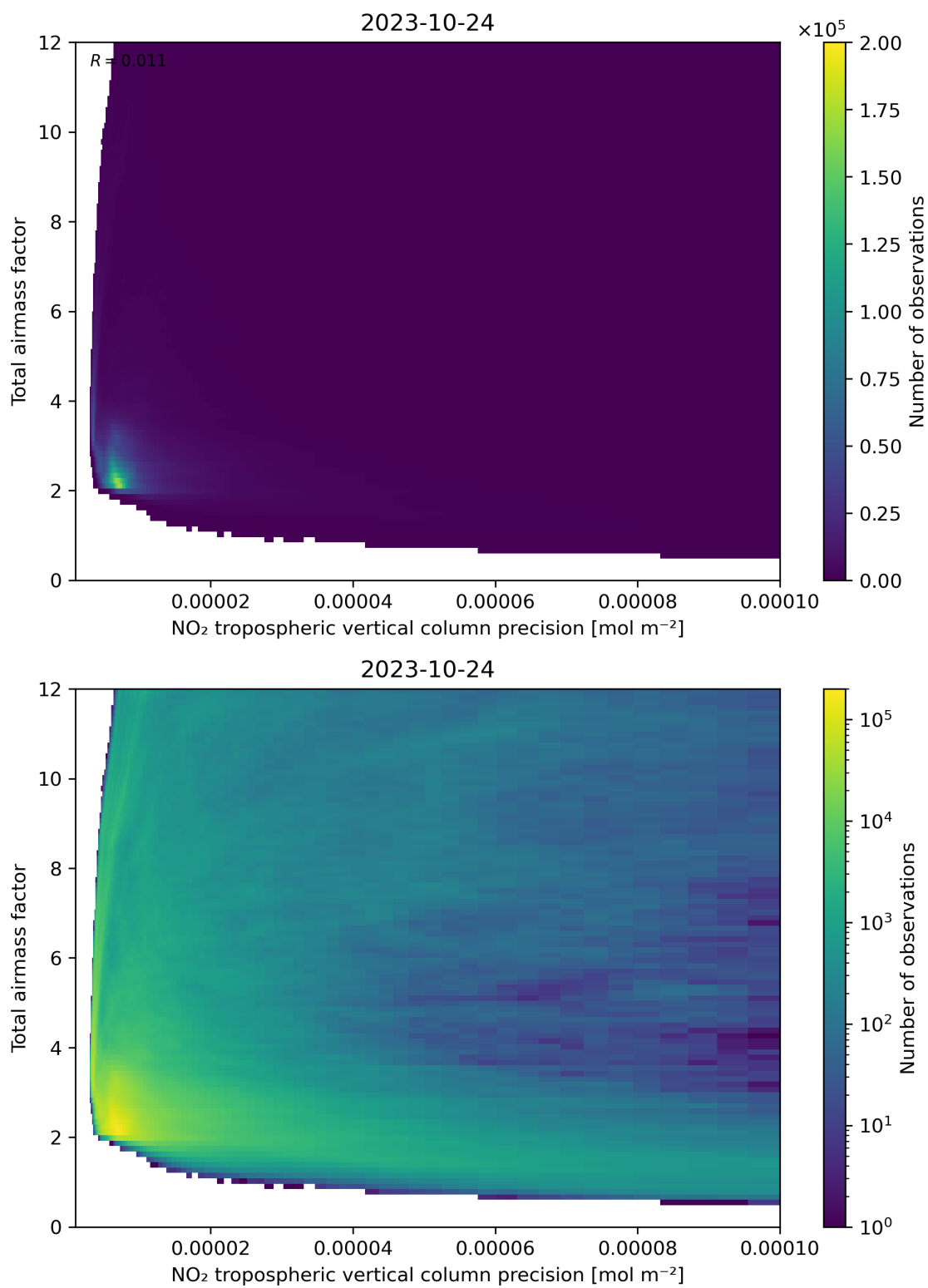
Figure 132: Scatter density plot of “NO 2 tropospheric vertical column precision” against “Total air mass factor” for 2023-10-23 to 2023-10-25.
