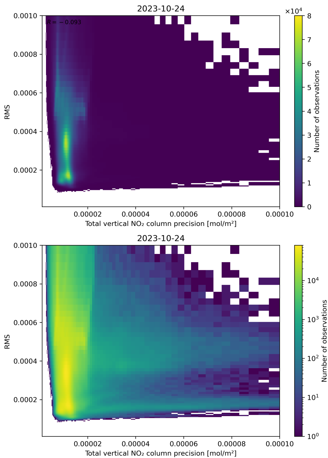
Figure 119: Scatter density plot of “Total vertical NO 2 column precision” against “RMS” for 2023-10-23 to 2023-10-25.
