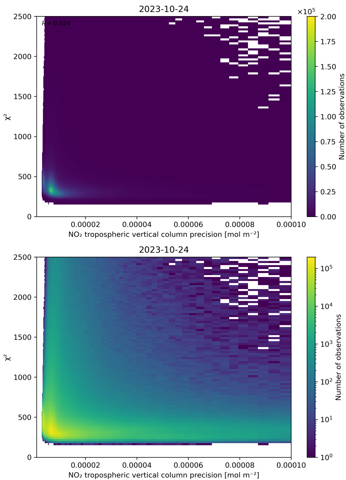
Figure 134: Scatter density plot of “NO 2 tropospheric vertical column precision” against “ \chi^2 ” for 2023-10-23 to 2023-10-25.
