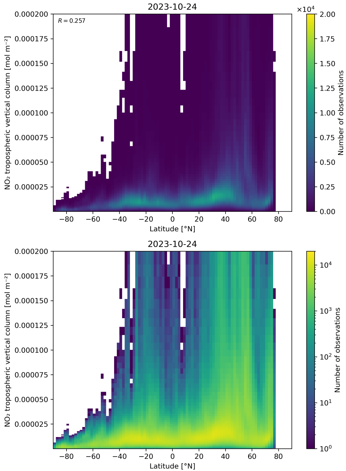
Figure 92: Scatter density plot of “Latitude” against “NO 2 tropospheric vertical column” for 2023-10-23 to 2023-10-25.
