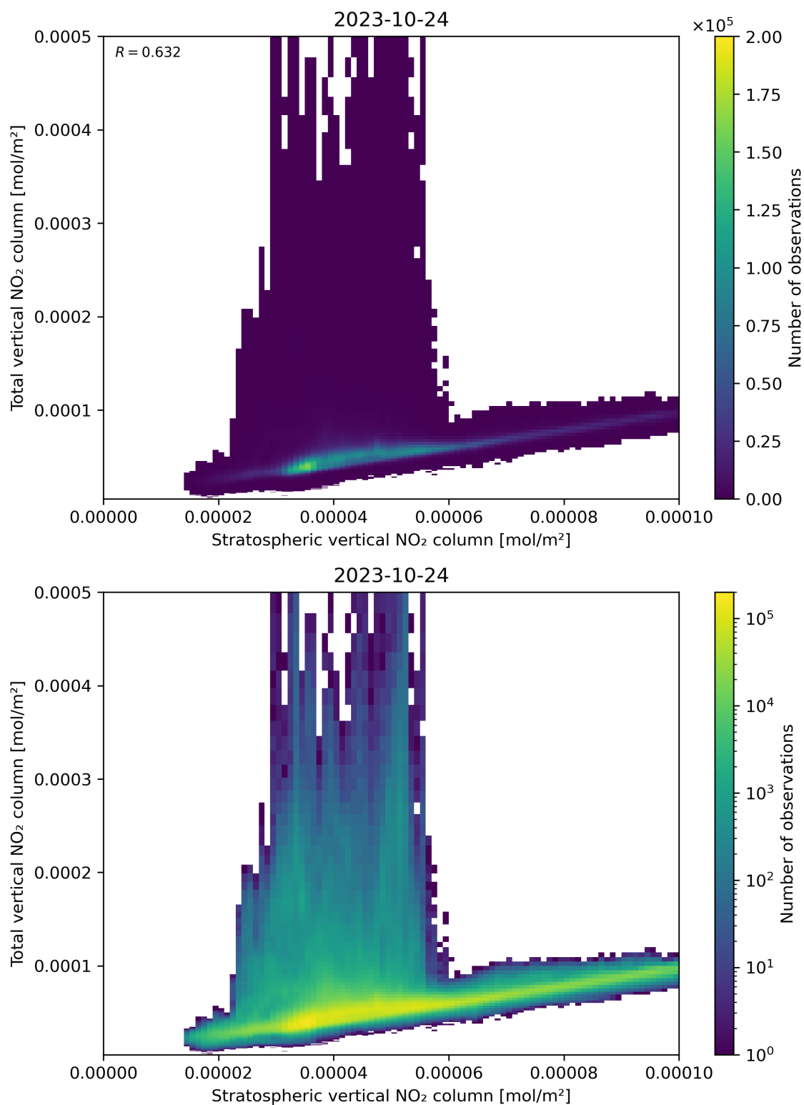
Figure 100: Scatter density plot of “Stratospheric vertical NO 2 column” against “Total vertical NO 2 column” for 2023-10-23 to 2023-10-25.
