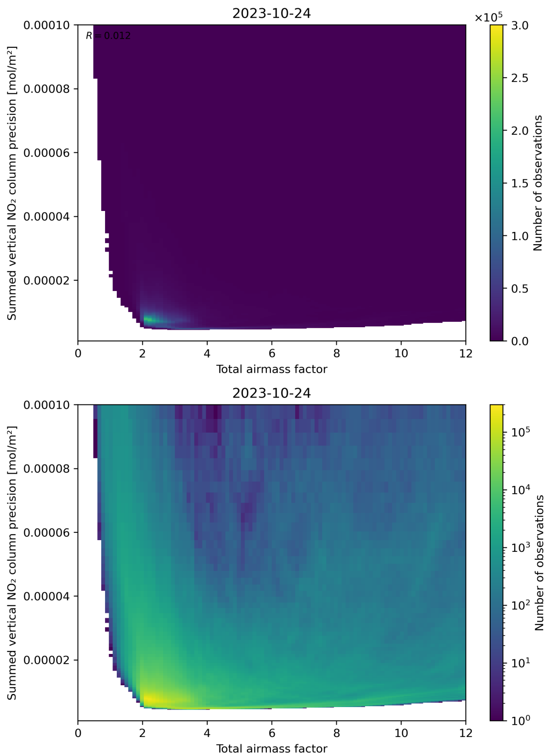
Figure 66: Scatter density plot of “Total airmass factor” against “Summed vertical NO 2 column precision” for 2023-10-23 to 2023-10-25.
