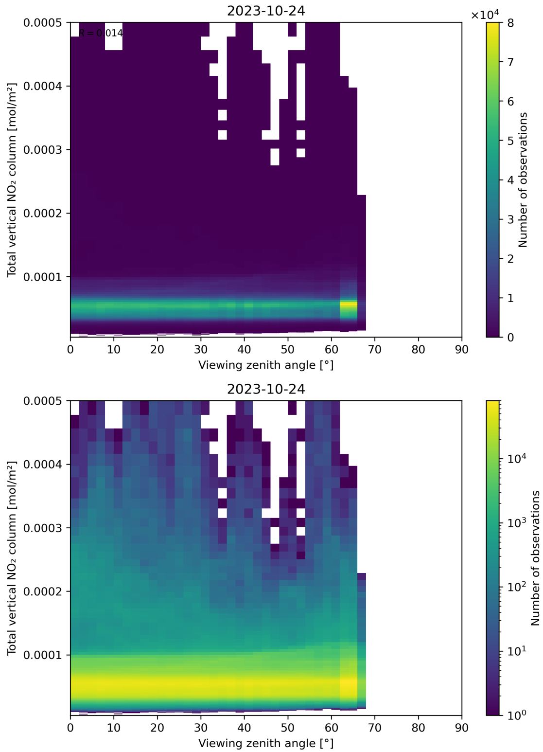
Figure 167: Scatter density plot of “Viewing zenith angle” against “Total vertical NO 2 column” for 2023-10-23 to 2023-10-25.
