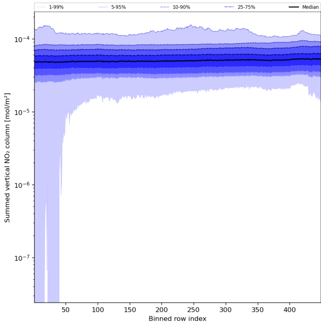
Figure 57: Along track statistics of “Summed vertical NO 2 column” for 2023-10-23 to 2023-10-25
