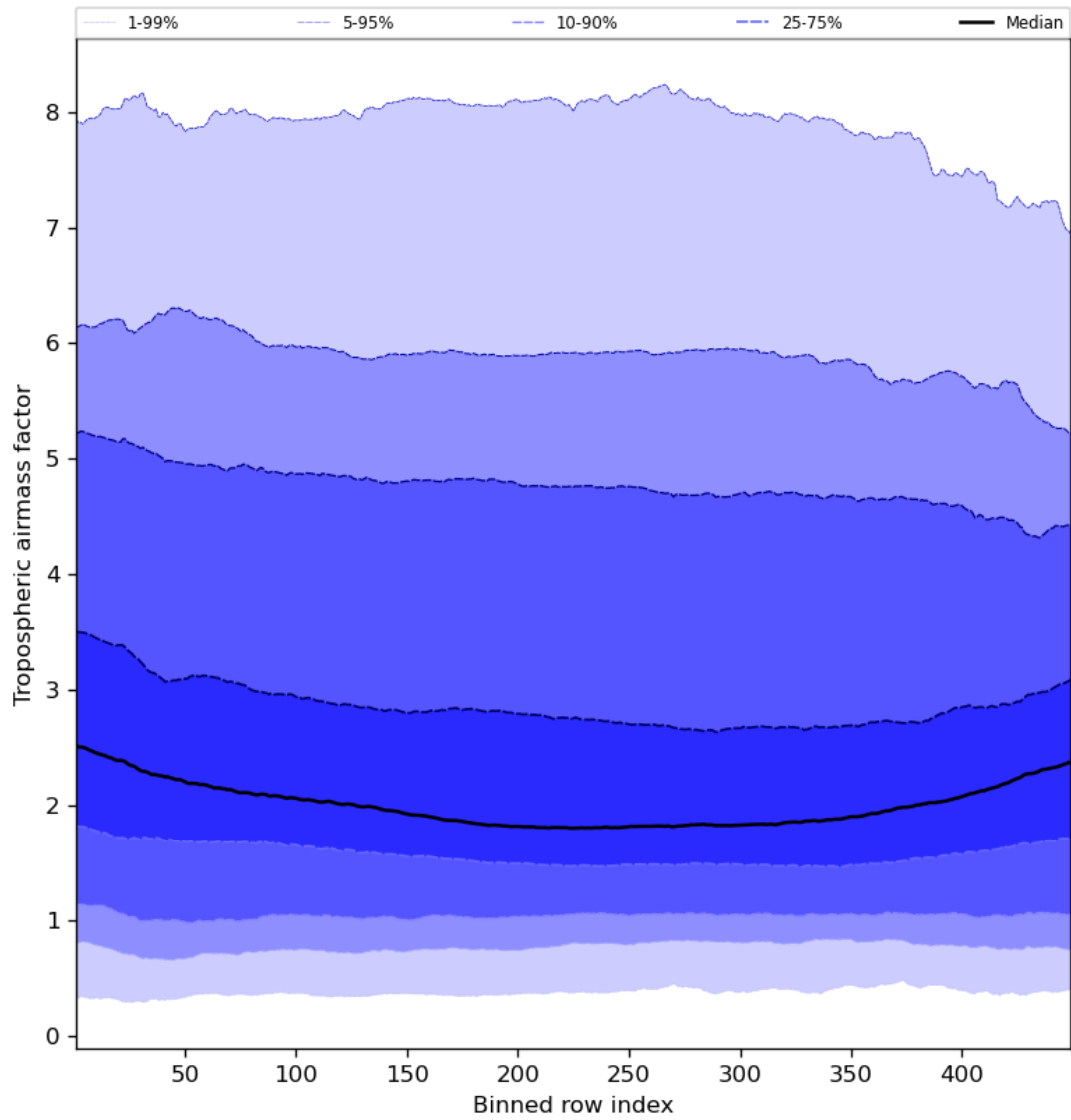
Figure 48: Along track statistics of “Tropospheric air mass factor” for 2023-10-23 to 2023-10-25
