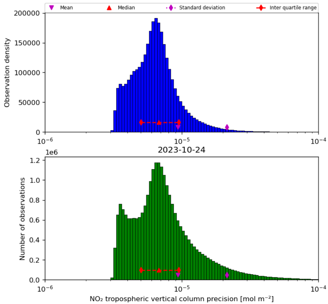
Figure 30: Histogram of “NO 2 tropospheric vertical column precision” for 2023-10-23 to 2023-10-25
