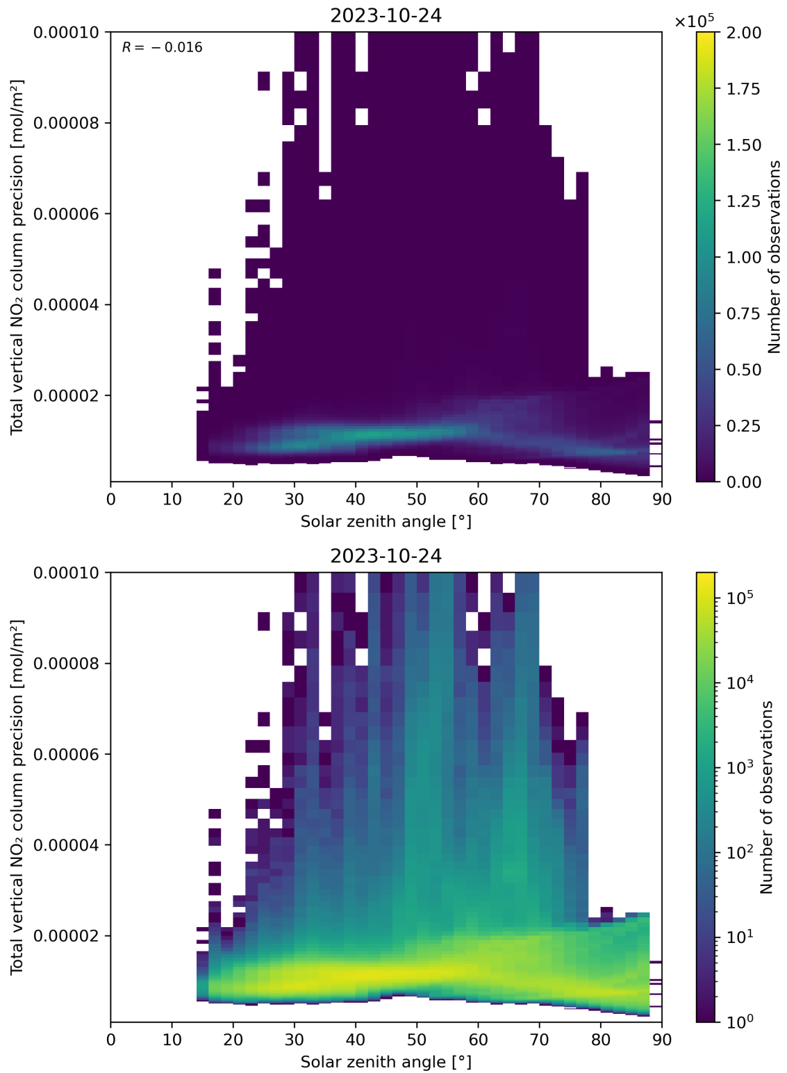
Figure 154: Scatter density plot of “Solar zenith angle” against “Total vertical NO 2 column precision” for 2023-10-23 to 2023-10-25.
