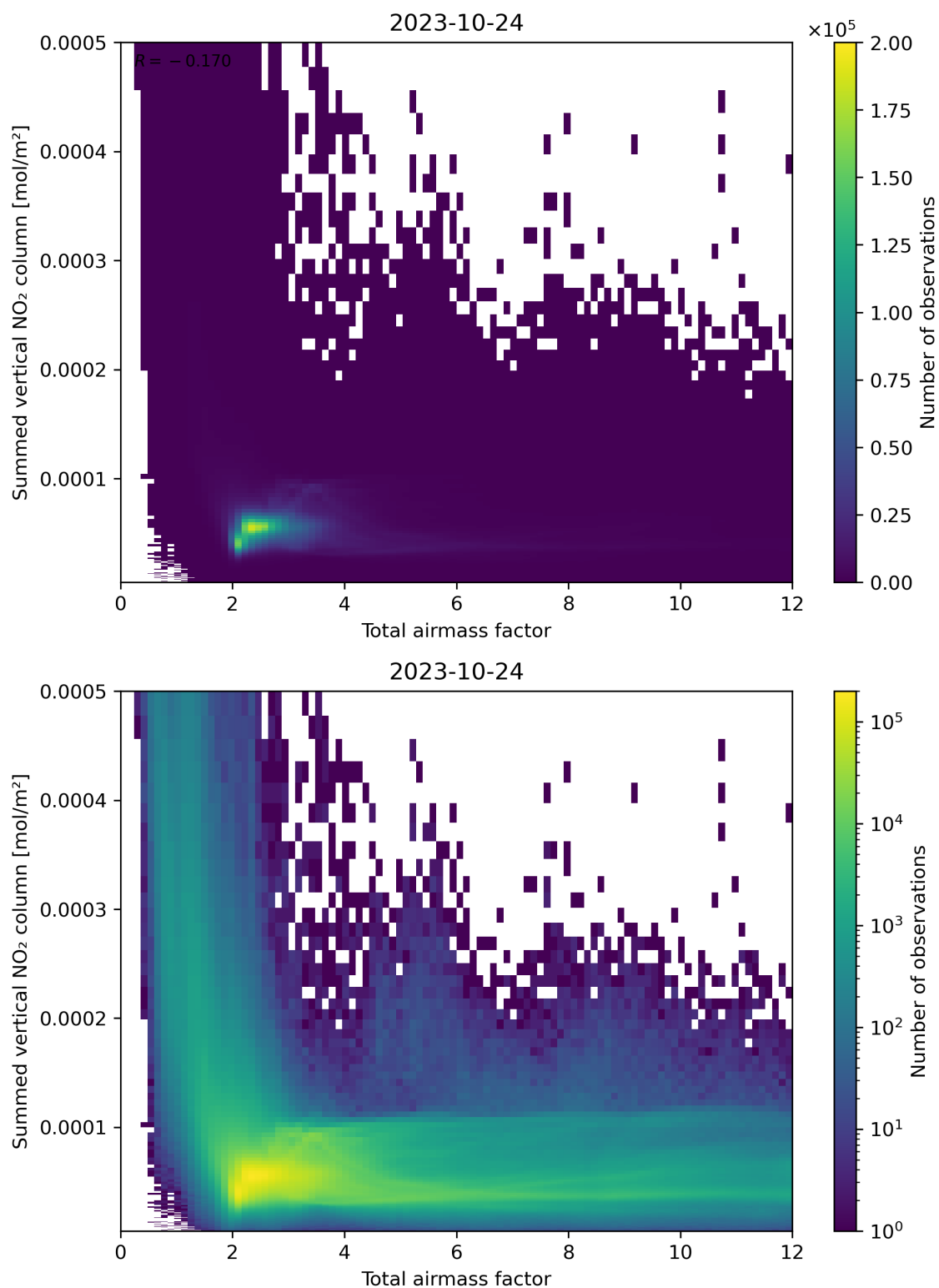
Figure 65: Scatter density plot of “Total airmass factor” against “Summed vertical NO 2 column” for 2023-10-23 to 2023-10-25.
