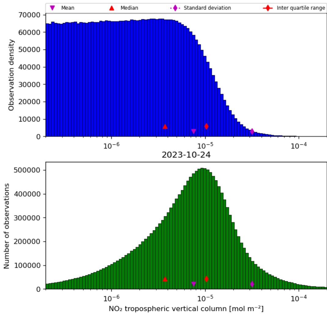
Figure 29: Histogram of “NO 2 tropospheric vertical column” for 2023-10-23 to 2023-10-25
