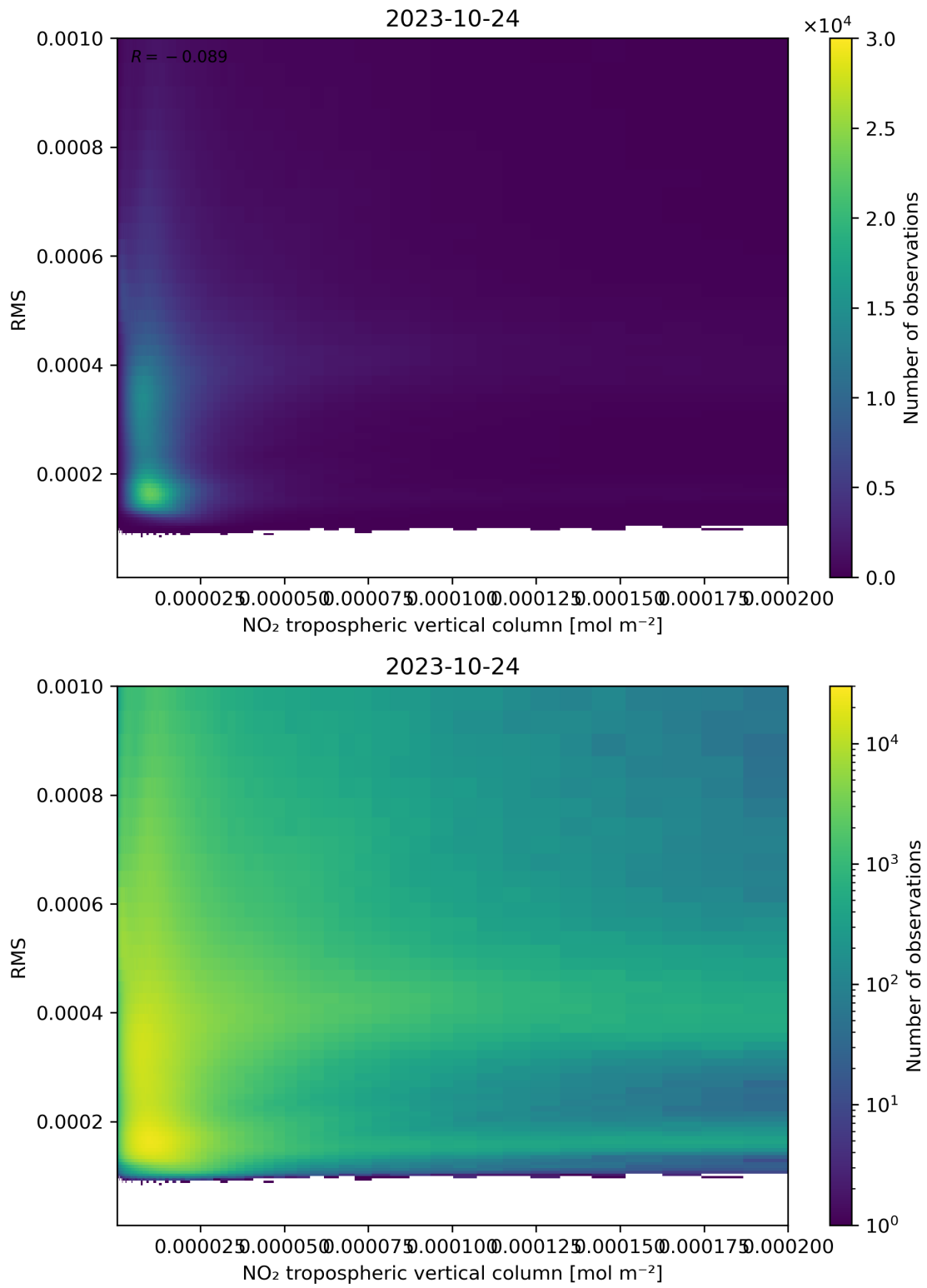
Figure 142: Scatter density plot of “NO 2 tropospheric vertical column” against “RMS” for 2023-10-23 to 2023-10-25.
