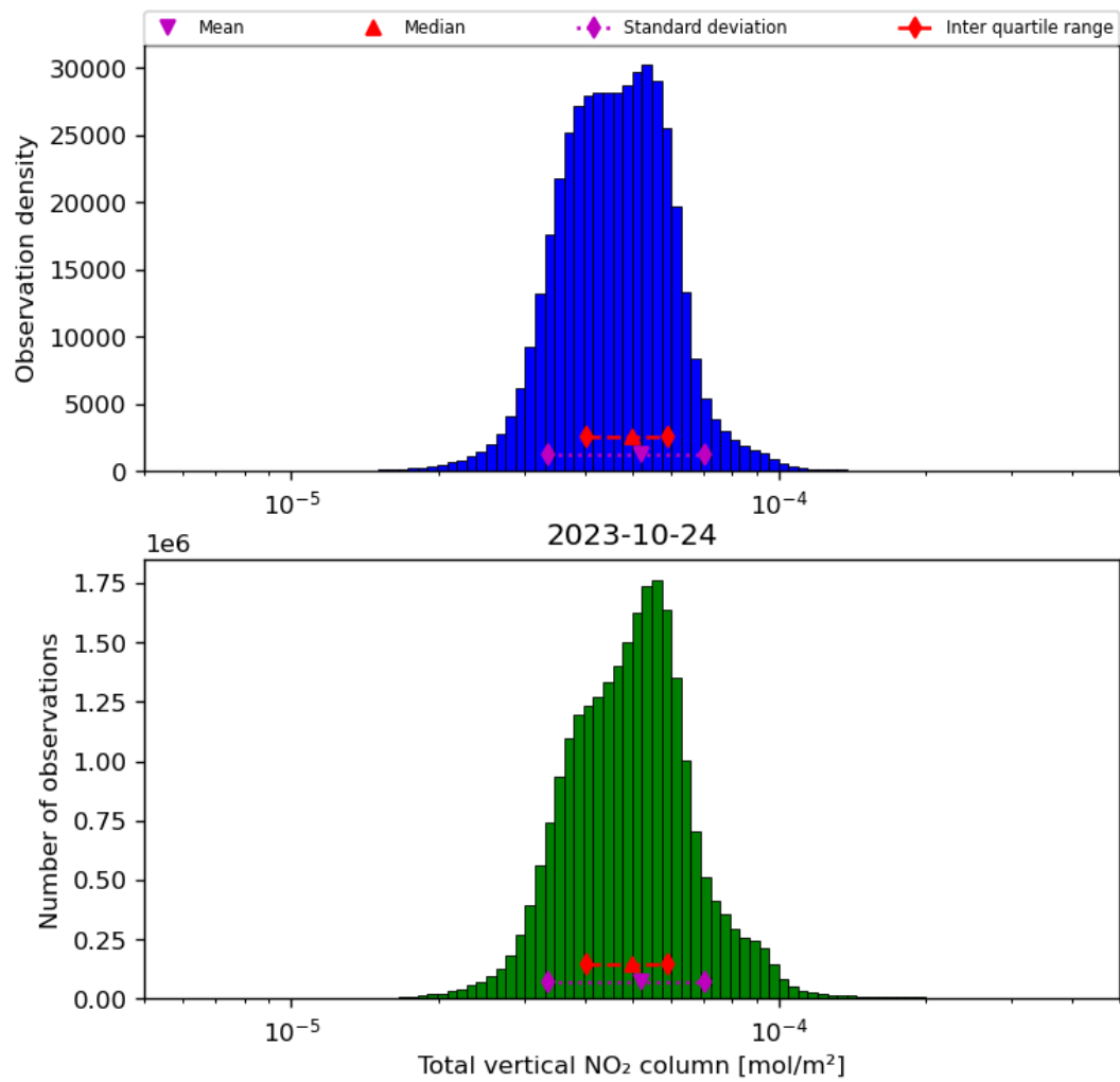
Figure 38: Histogram of “Total vertical NO 2 column” for 2023-10-23 to 2023-10-25
