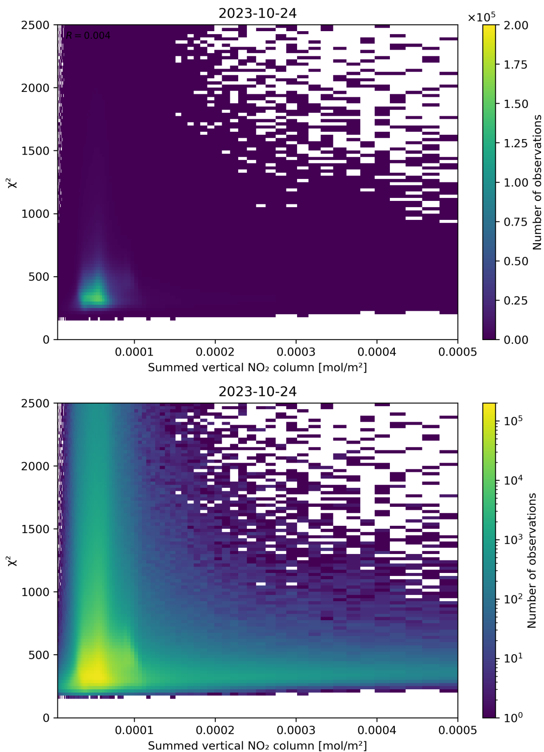
Figure 104: Scatter density plot of “Summed vertical NO 2 column” against “ \chi^2 ” for 2023-10-23 to 2023-10-25.
