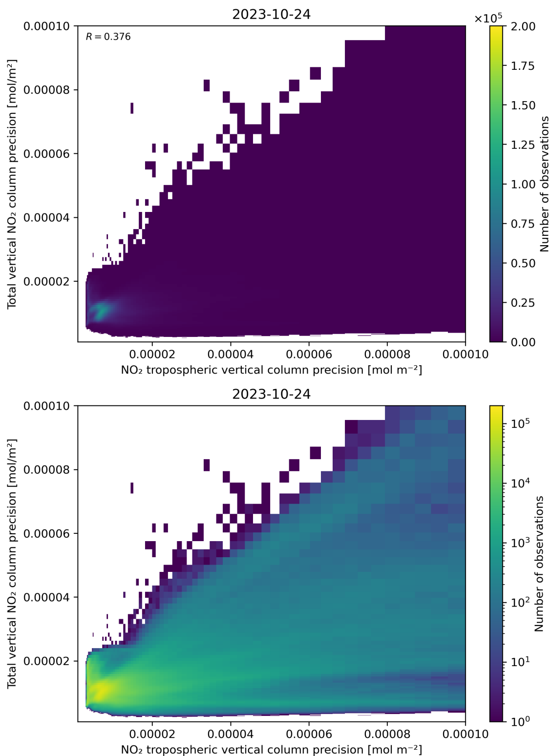
Figure 139: Scatter density plot of “NO 2 tropospheric vertical column precision” against “Total vertical NO 2 column precision” for 2023-10-23 to 2023-10-25.
