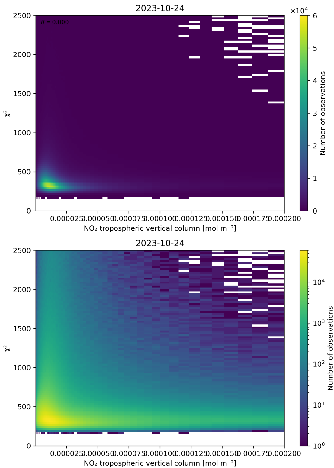
Figure 124: Scatter density plot of “NO 2 tropospheric vertical column” against “ \chi^2 ” for 2023-10-23 to 2023-10-25.
