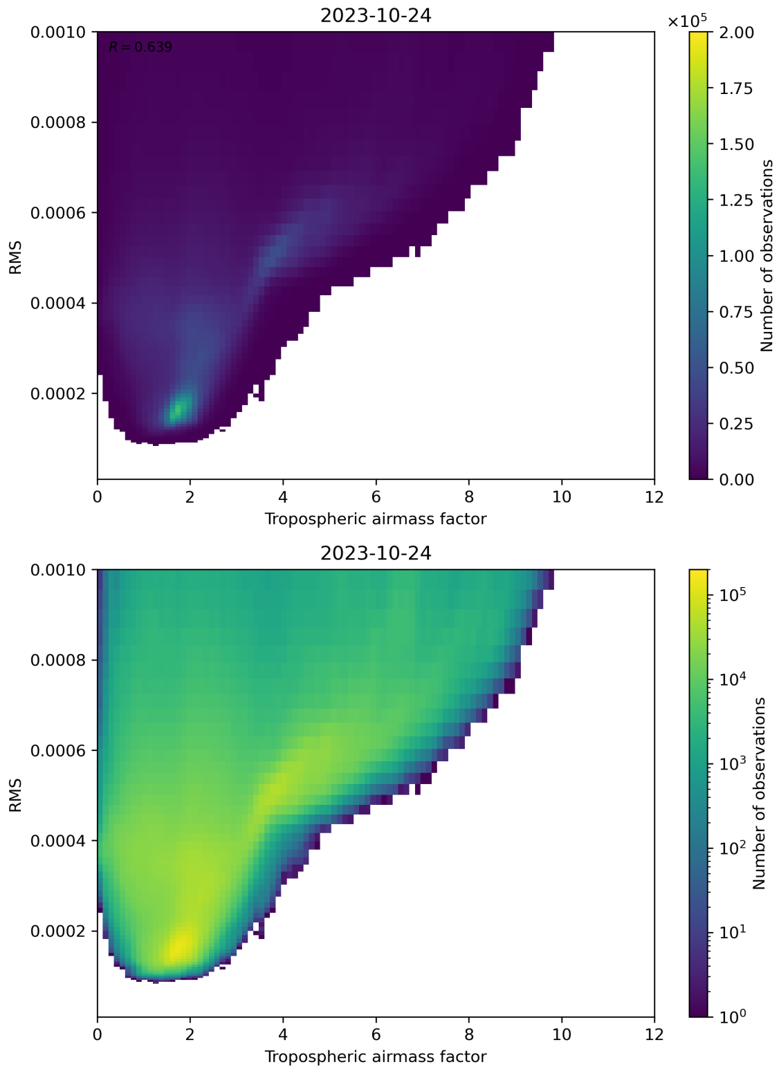
Figure 79: Scatter density plot of “Tropospheric airmass factor” against “RMS” for 2023-10-23 to 2023-10-25.
