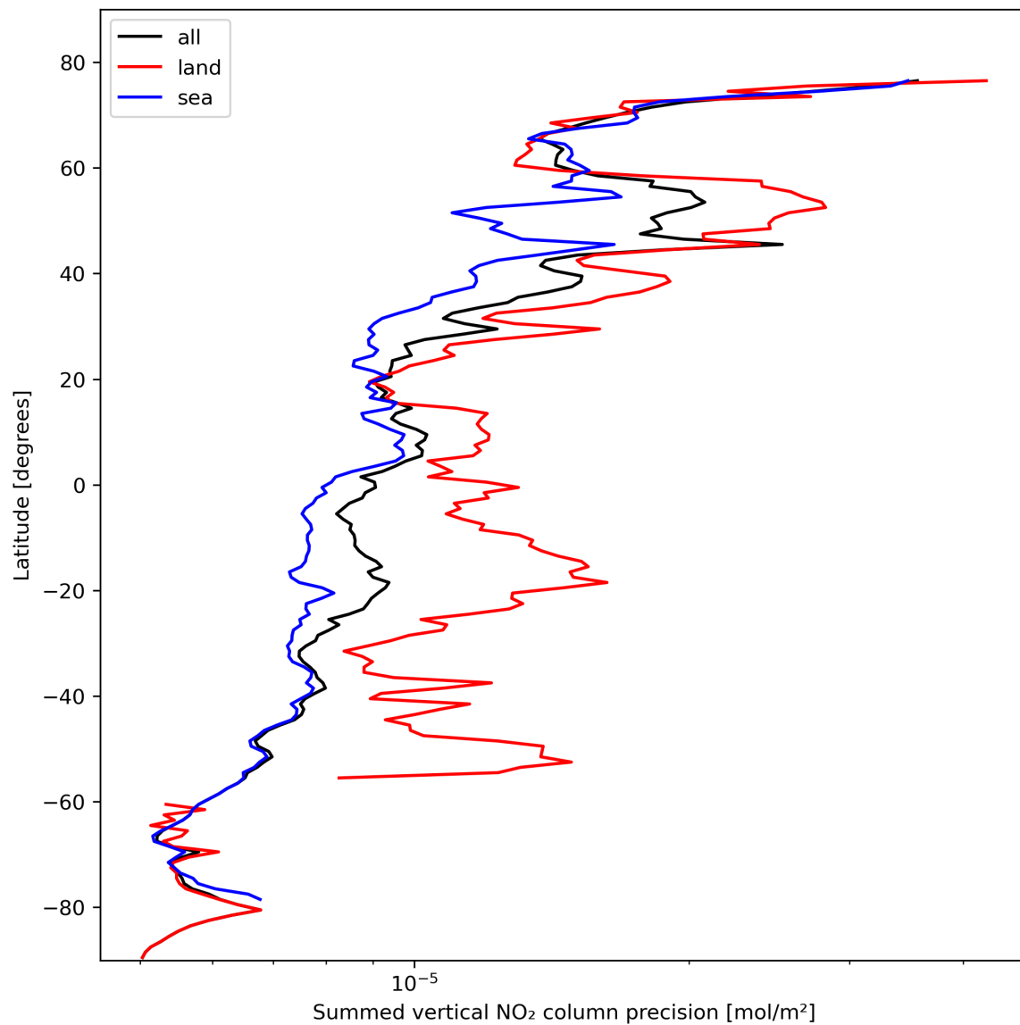
Figure 24: Zonal average of “Summed vertical NO 2 column precision” for 2023-10-23 to 2023-10-25.
