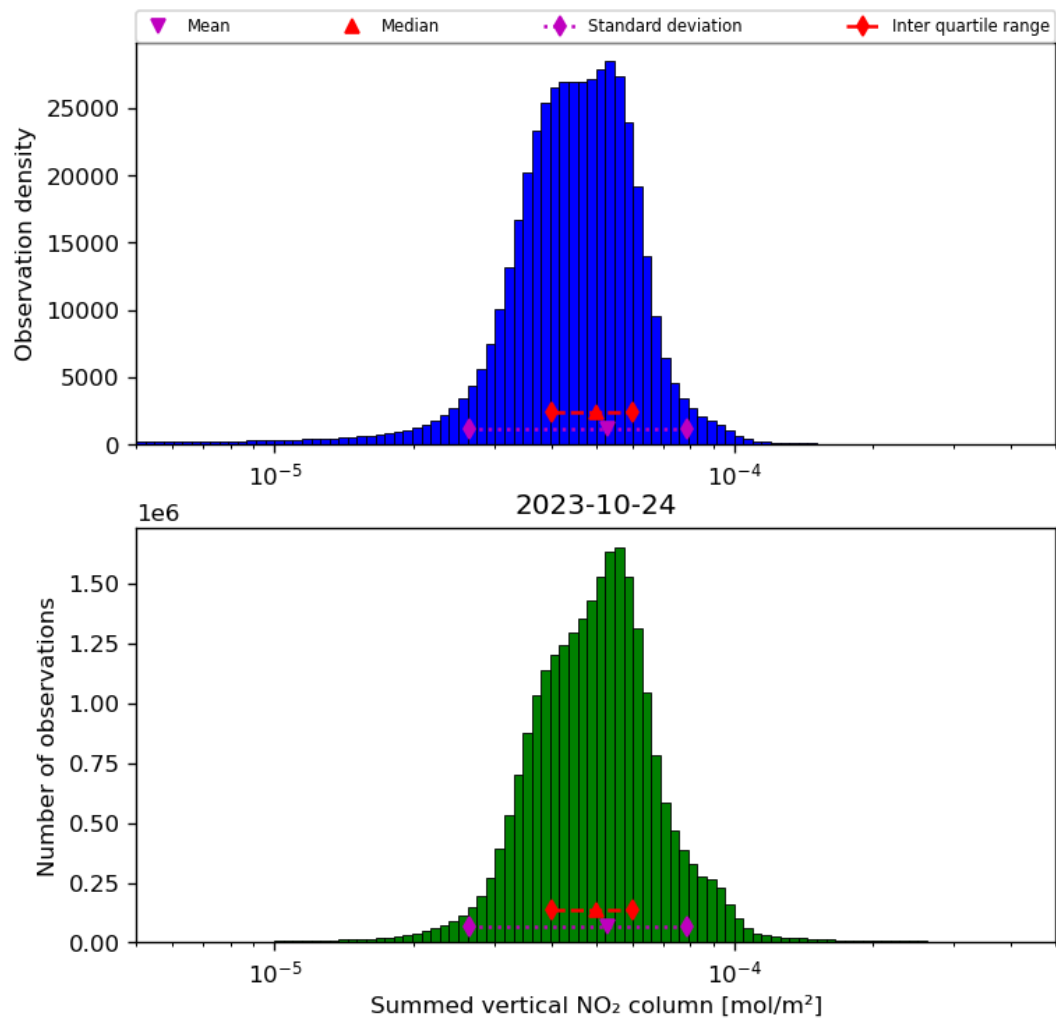
Figure 40: Histogram of “Summed vertical NO 2 column” for 2023-10-23 to 2023-10-25
