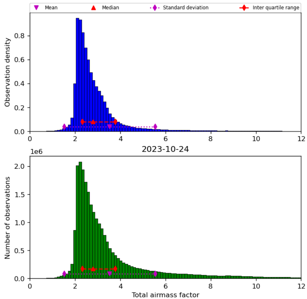
Figure 32: Histogram of “Total airmass factor” for 2023-10-23 to 2023-10-25
