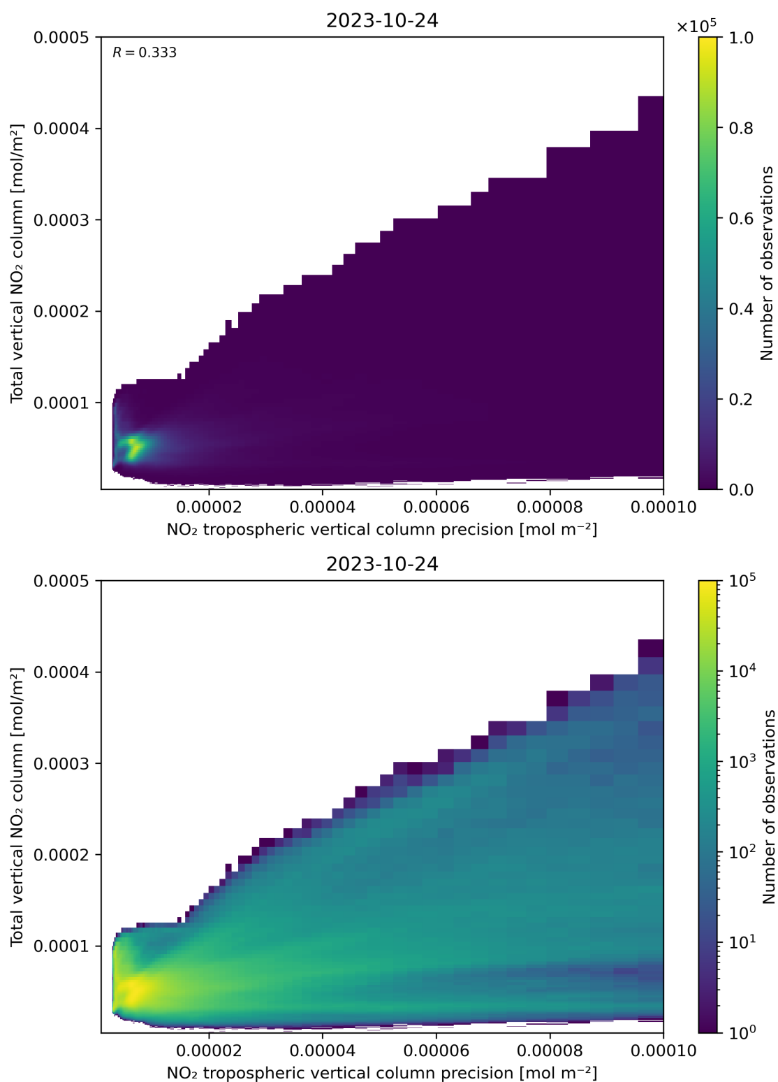
Figure 138: Scatter density plot of “NO 2 tropospheric vertical column precision” against “Total vertical NO 2 column” for 2023-10-23 to 2023-10-25.
