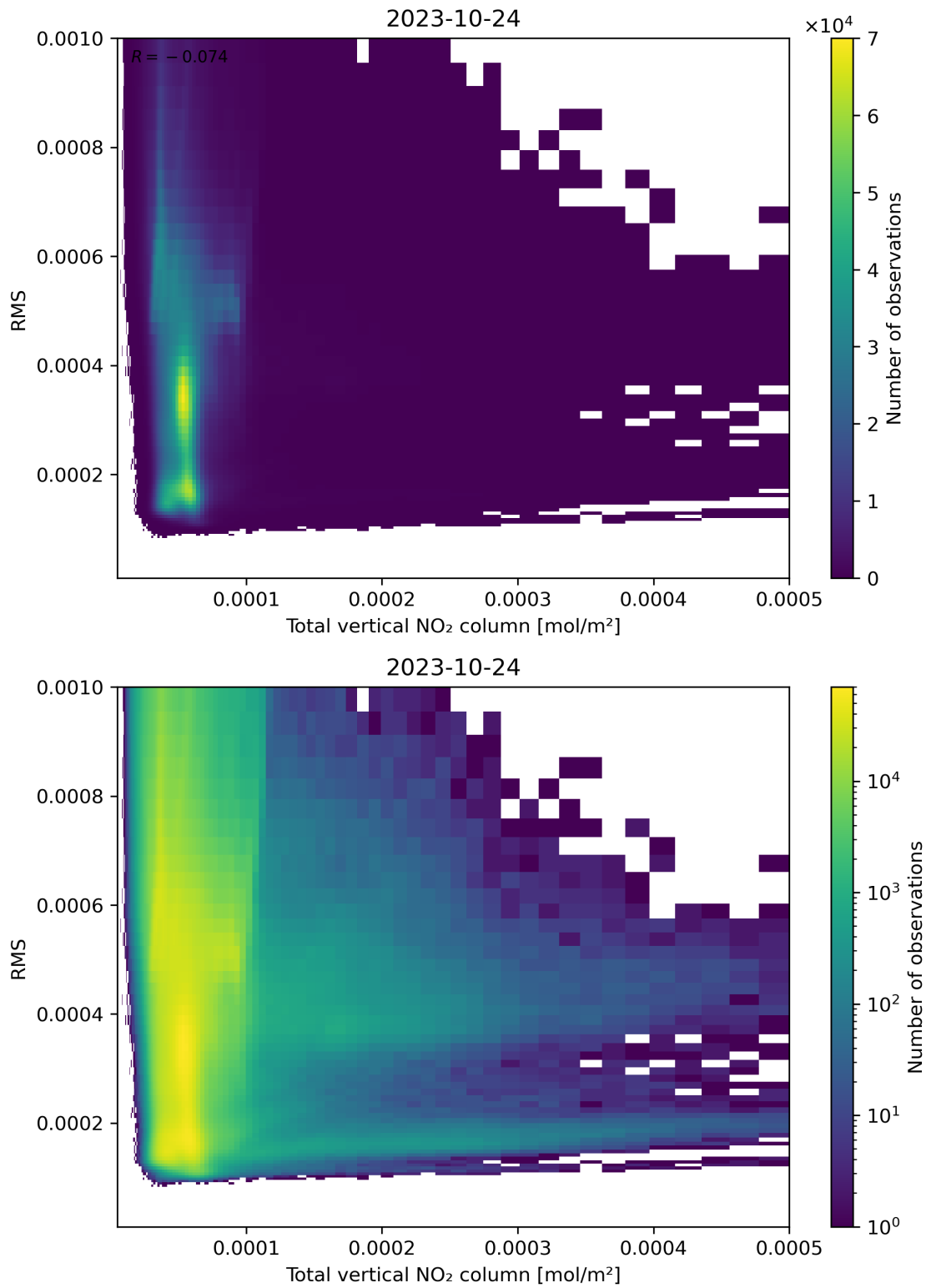
Figure 120: Scatter density plot of “Total vertical NO 2 column” against “RMS” for 2023-10-23 to 2023-10-25.
