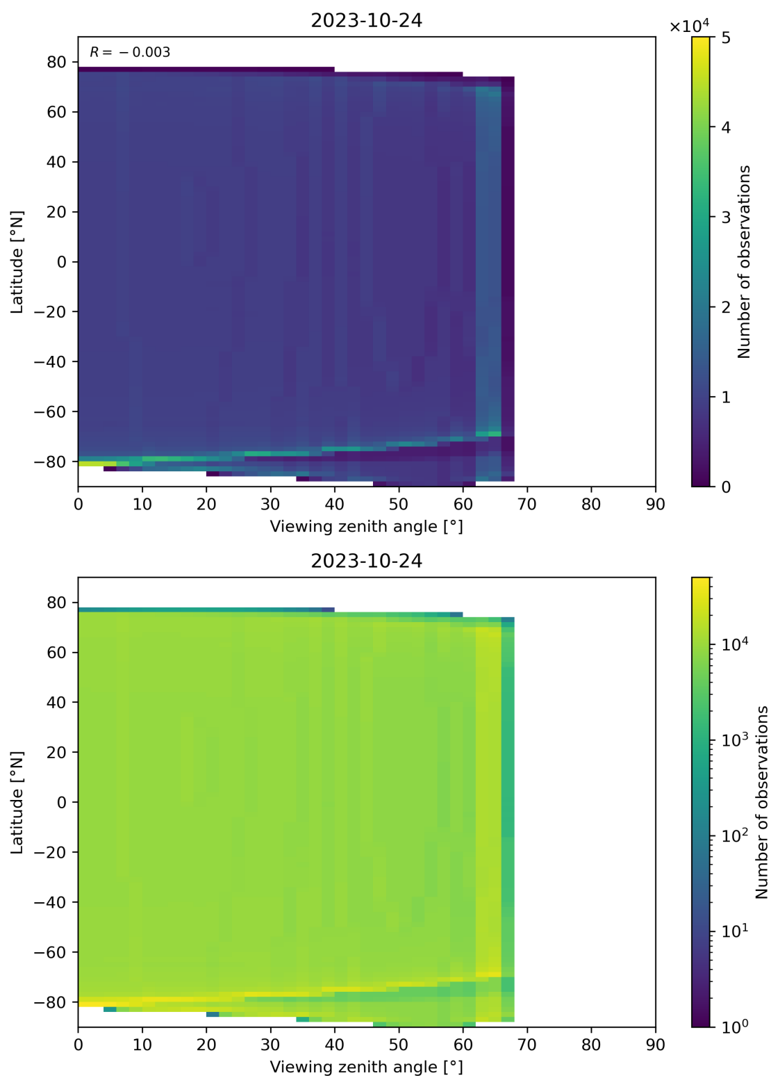
Figure 163: Scatter density plot of “Viewing zenith angle” against “Latitude” for 2023-10-23 to 2023-10-25.
