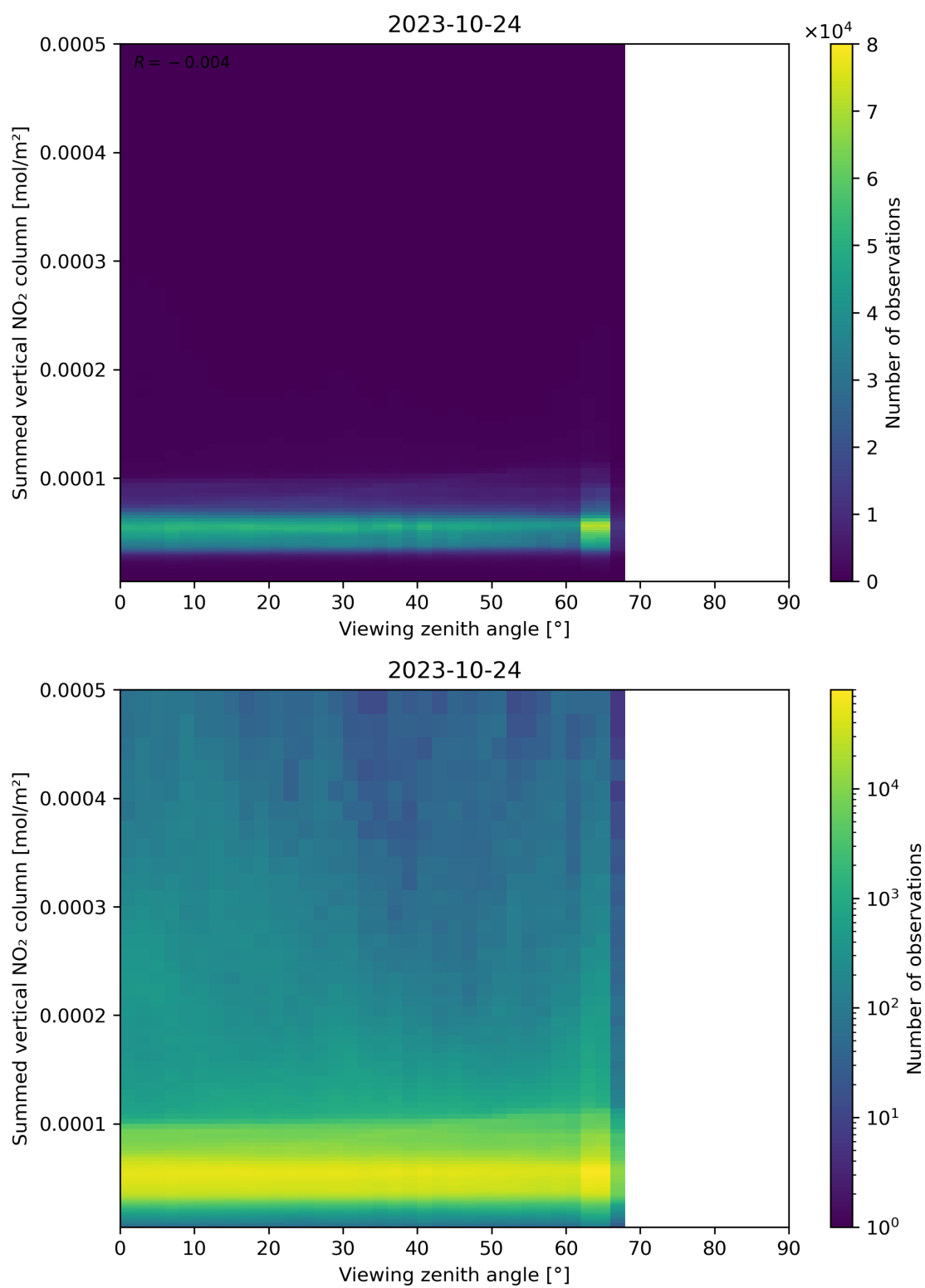
Figure 165: Scatter density plot of “Viewing zenith angle” against “Summed vertical NO 2 column” for 2023-10-23 to 2023-10-25.
