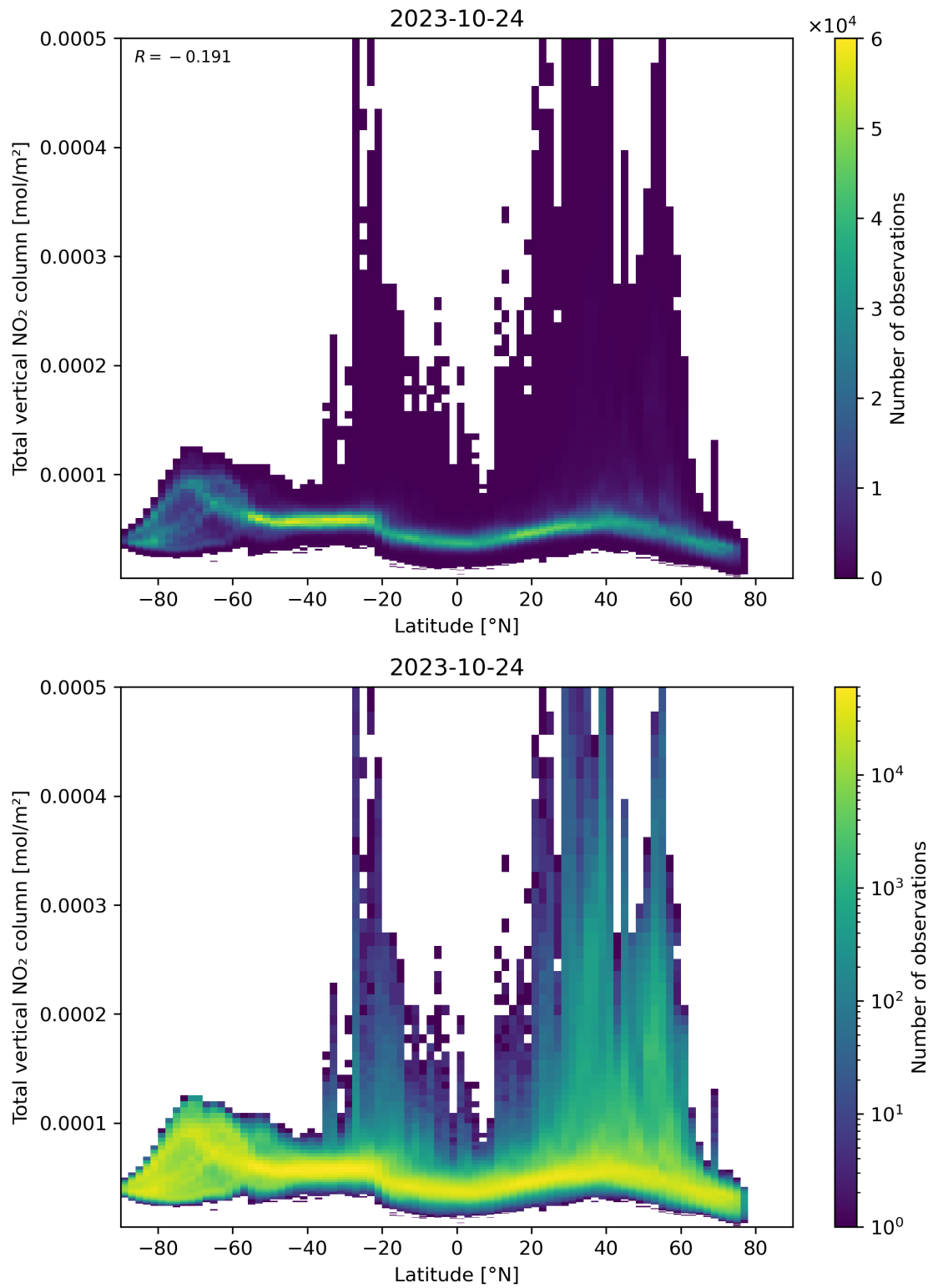
Figure 90: Scatter density plot of “Latitude” against “Total vertical NO 2 column” for 2023-10-23 to 2023-10-25.
