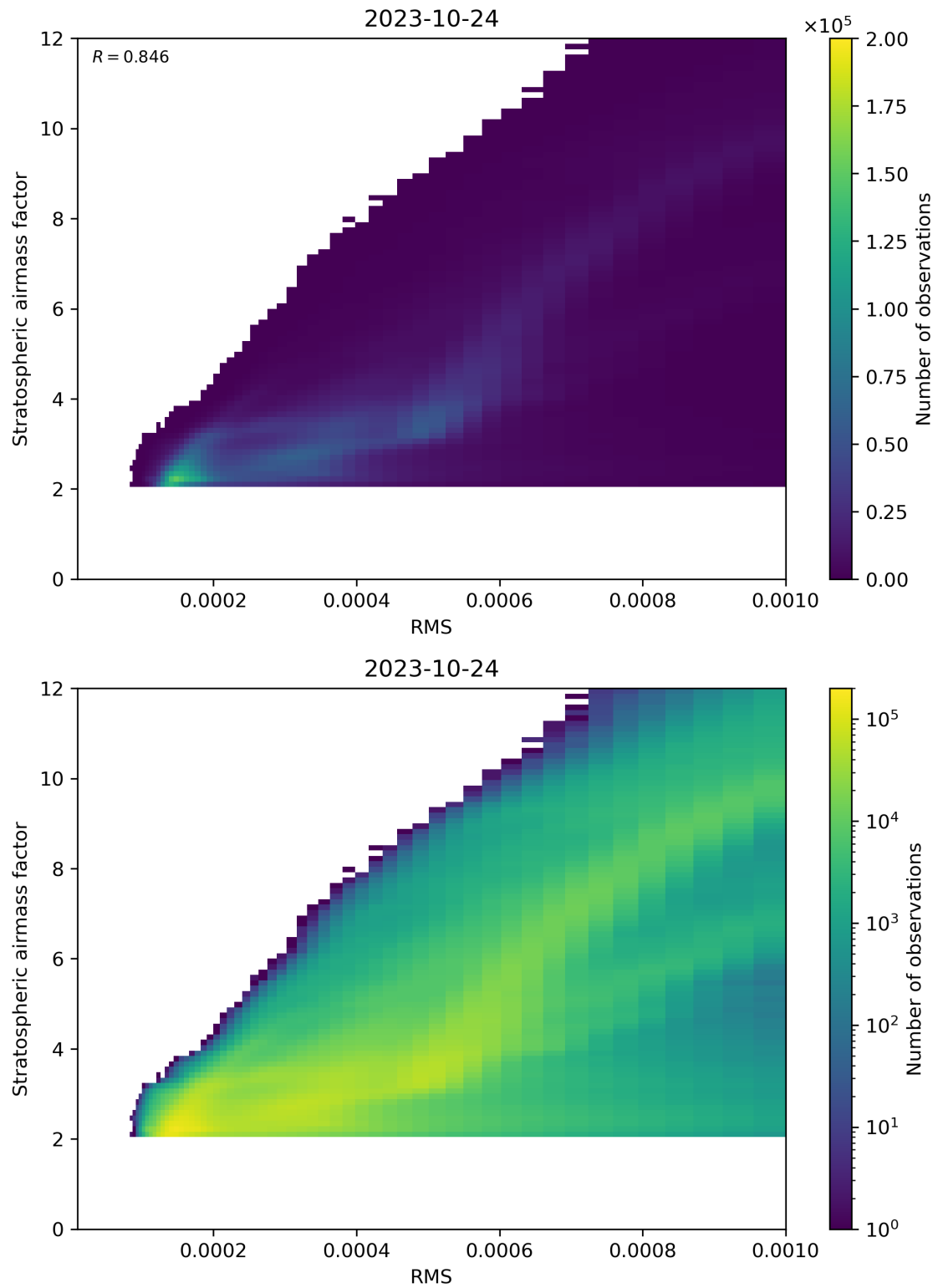
Figure 144: Scatter density plot of “RMS” against “Stratospheric airmass factor” for 2023-10-23 to 2023-10-25.
