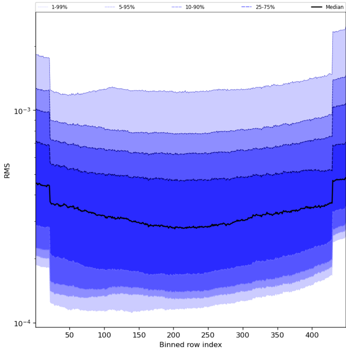
Figure 60: Along track statistics of “RMS” for 2023-10-23 to 2023-10-25
