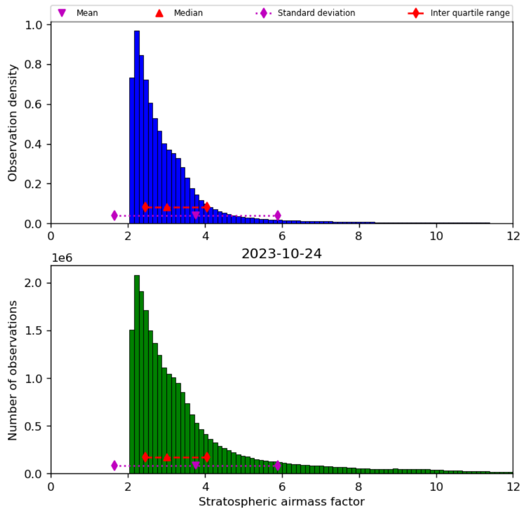
Figure 44: Histogram of “Stratospheric airmass factor” for 2023-10-23 to 2023-10-25
