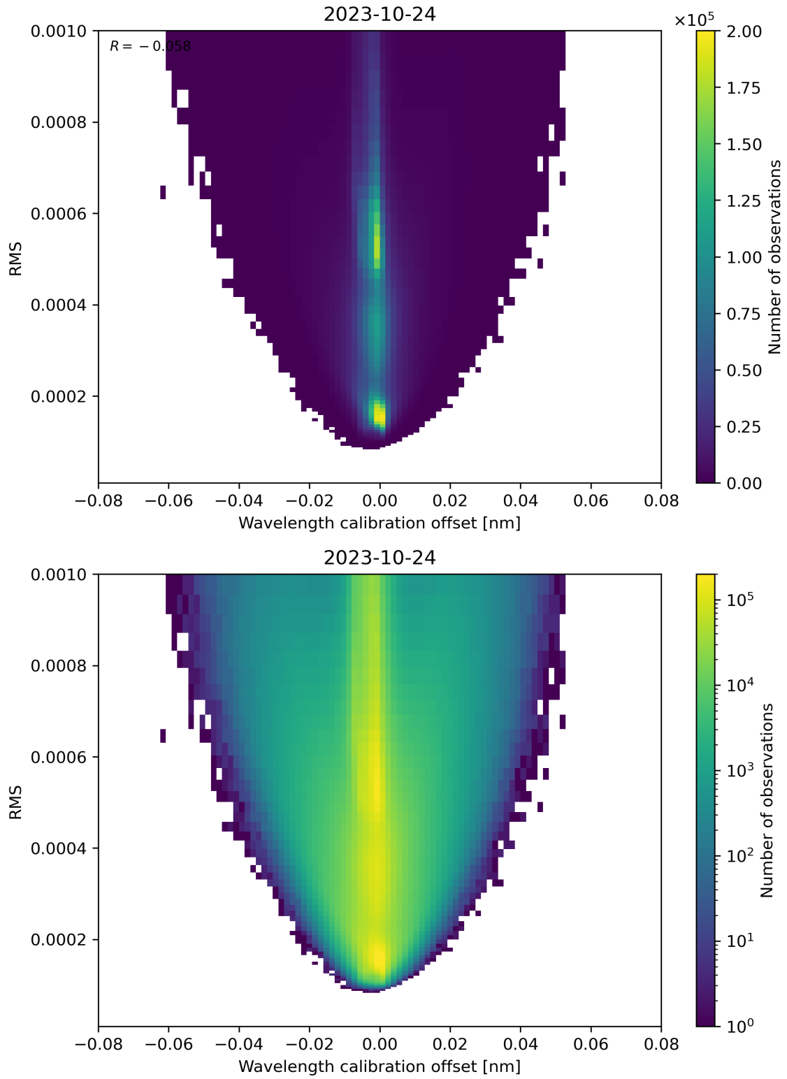
Figure 181: Scatter density plot of “Wavelength calibration offset” against “RMS” for 2023-10-23 to 2023-10-25.
