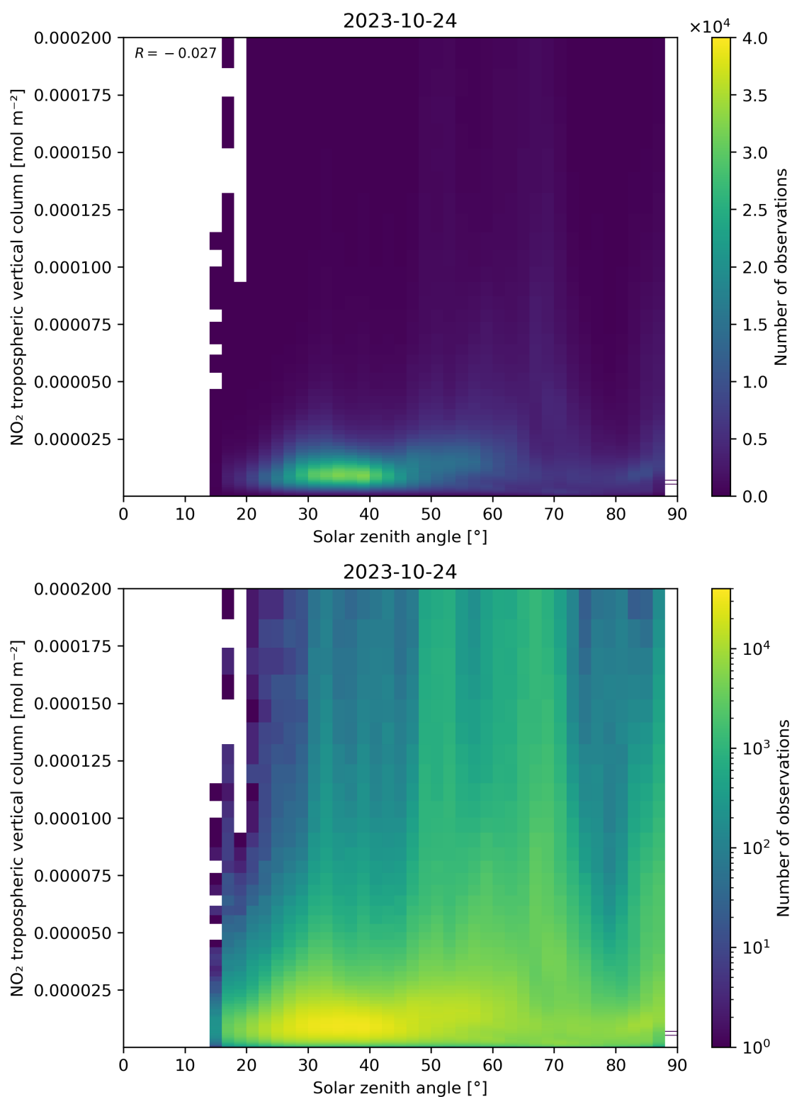
Figure 155: Scatter density plot of “Solar zenith angle” against “NO 2 tropospheric vertical column” for 2023-10-23 to 2023-10-25.
