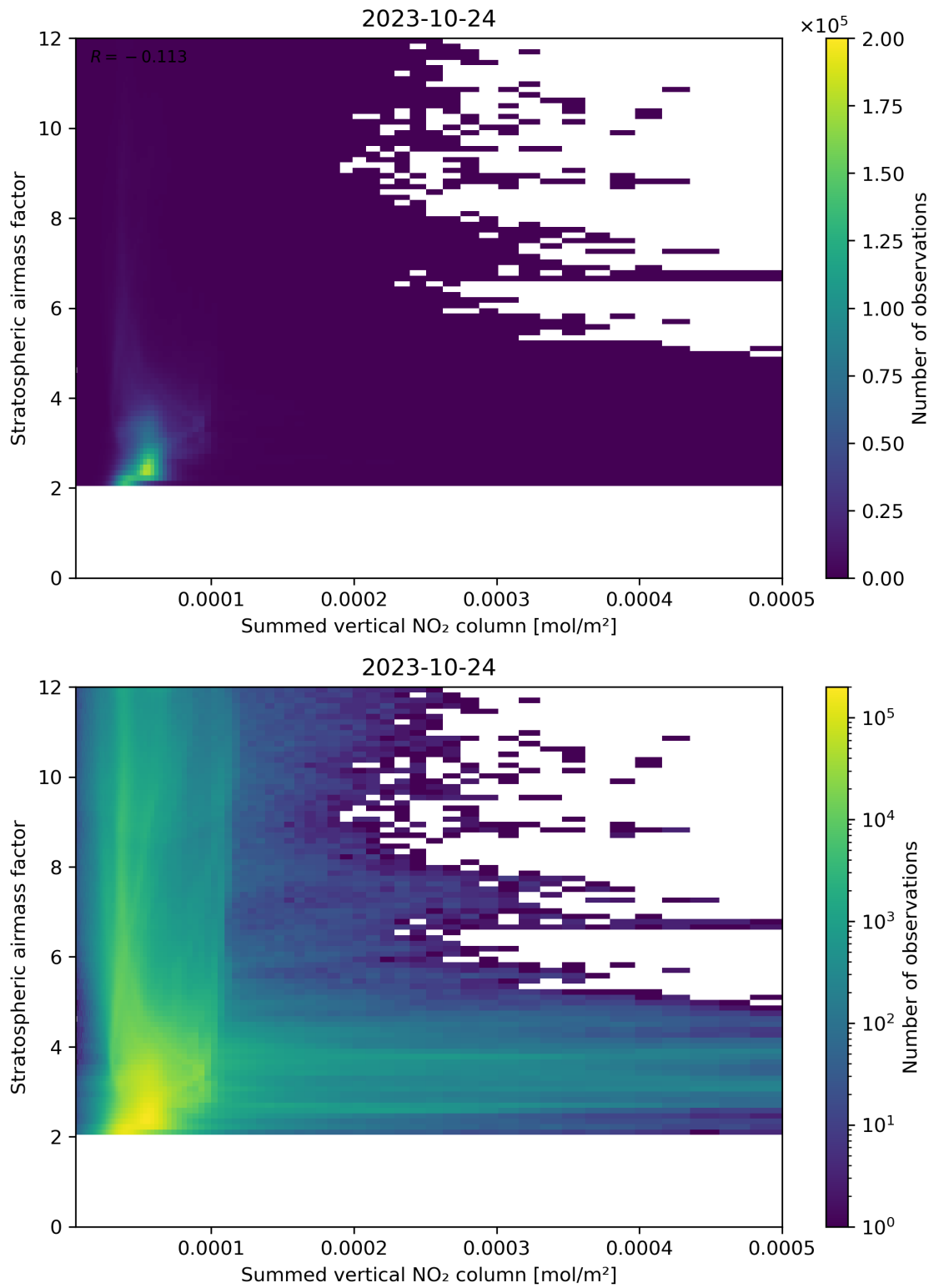
Figure 103: Scatter density plot of “Summed vertical NO 2 column” against “Stratospheric air mass factor” for 2023-10-23 to 2023-10-25.
