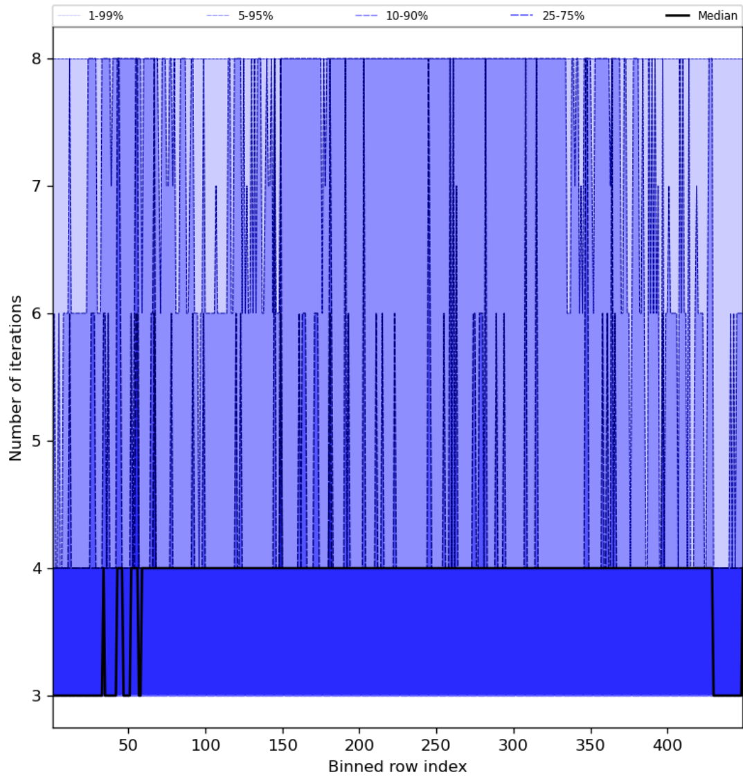
Figure 51: Along track statistics of “Number of iterations” for 2023-10-23 to 2023-10-25
