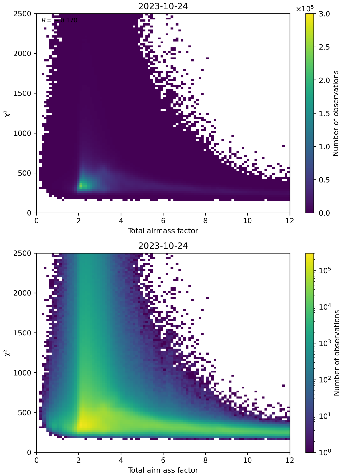
Figure 63: Scatter density plot of “Total airmass factor” against “ \chi^2 ” for 2023-10-23 to 2023-10-25.
