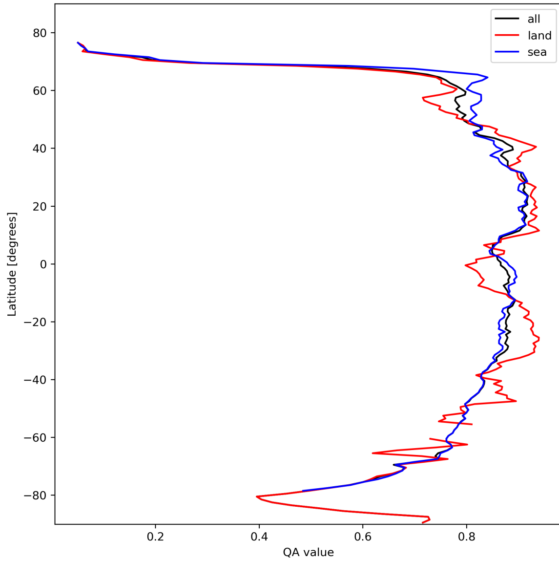
Figure 11: Zonal average of “QA value” for 2023-10-23 to 2023-10-25.
