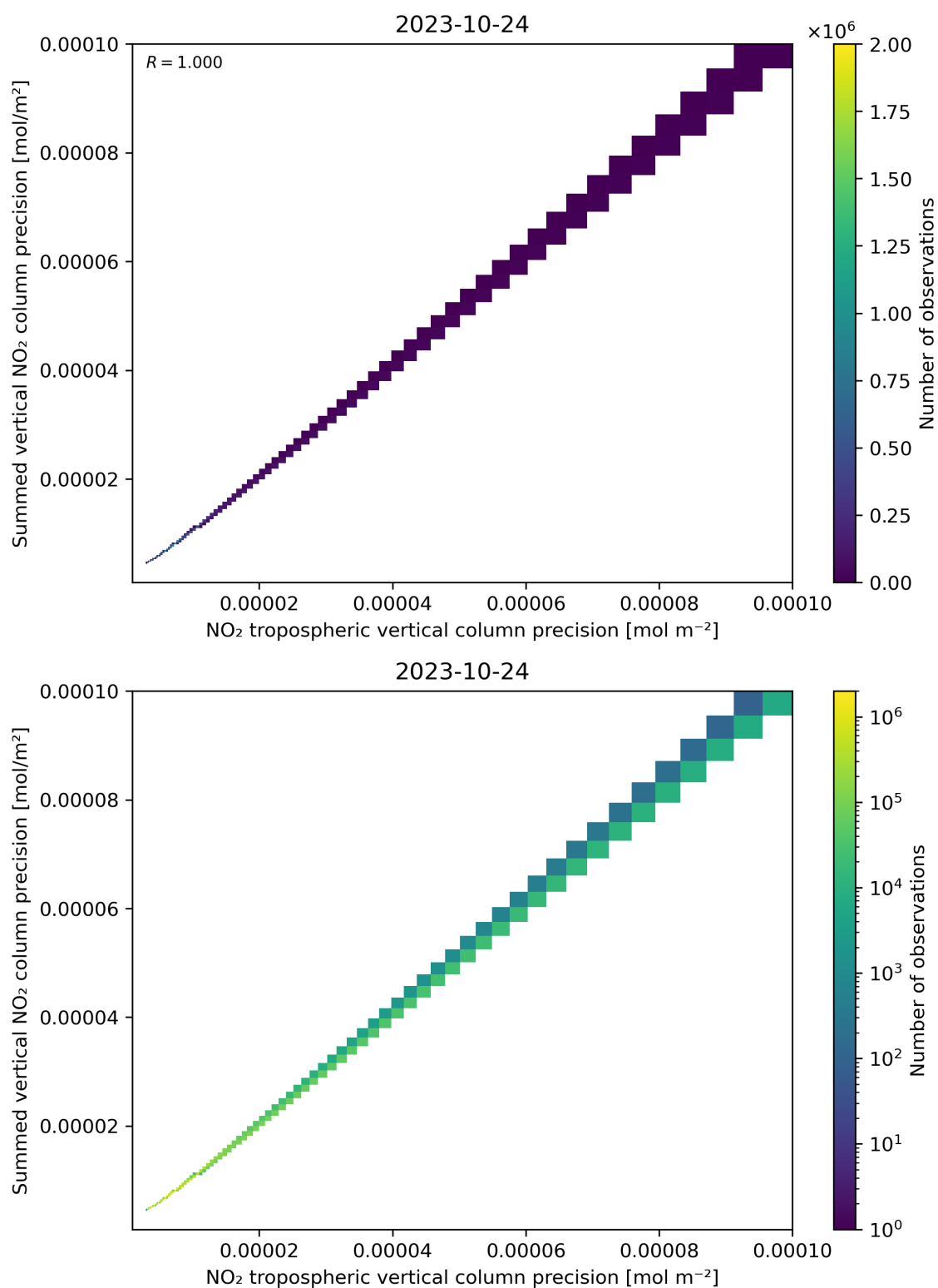
Figure 137: Scatter density plot of “NO 2 tropospheric vertical column precision” against “Summed vertical NO 2 column precision” for 2023-10-23 to 2023-10-25.
