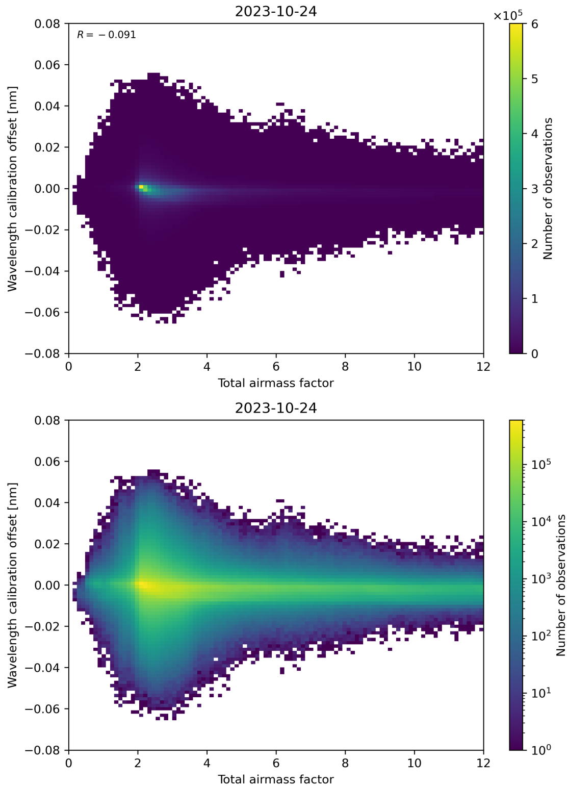
Figure 70: Scatter density plot of “Total airmass factor” against “Wavelength calibration offset” for 2023-10-23 to 2023-10-25.
