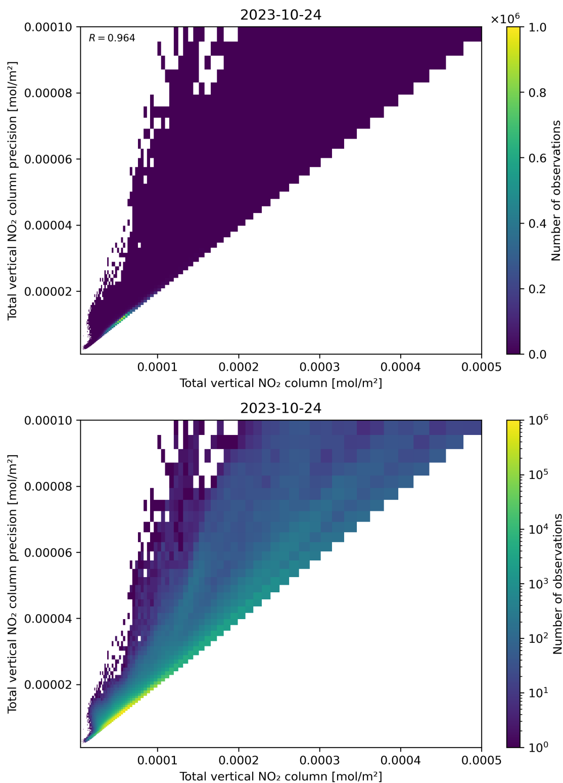
Figure 114: Scatter density plot of “Total vertical NO 2 column” against “Total vertical NO 2 column precision” for 2023-10-23 to 2023-10-25.
