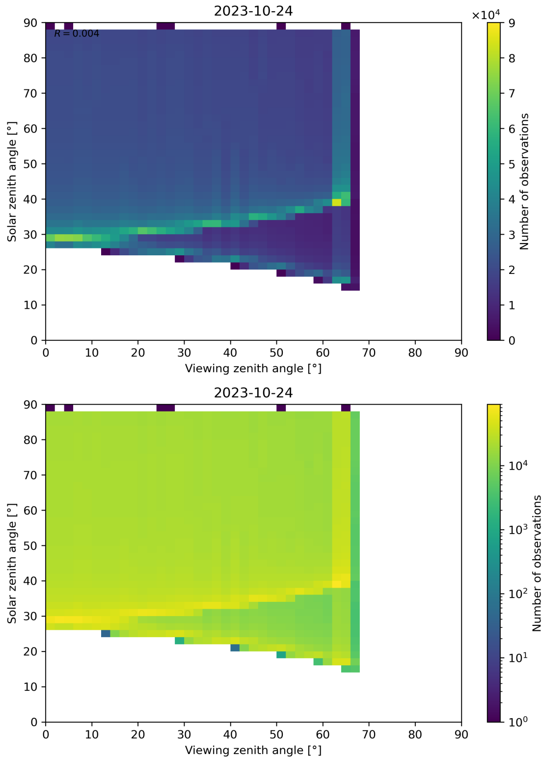
Figure 172: Scatter density plot of “Viewing zenith angle” against “Solar zenith angle” for 2023-10-23 to 2023-10-25.
