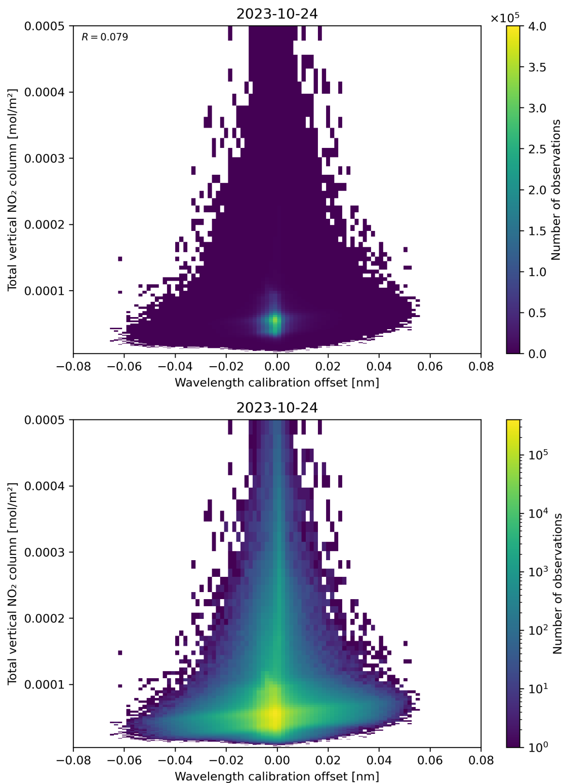
Figure 179: Scatter density plot of “Wavelength calibration offset” against “Total vertical NO 2 column” for 2023-10-23 to 2023-10-25.
