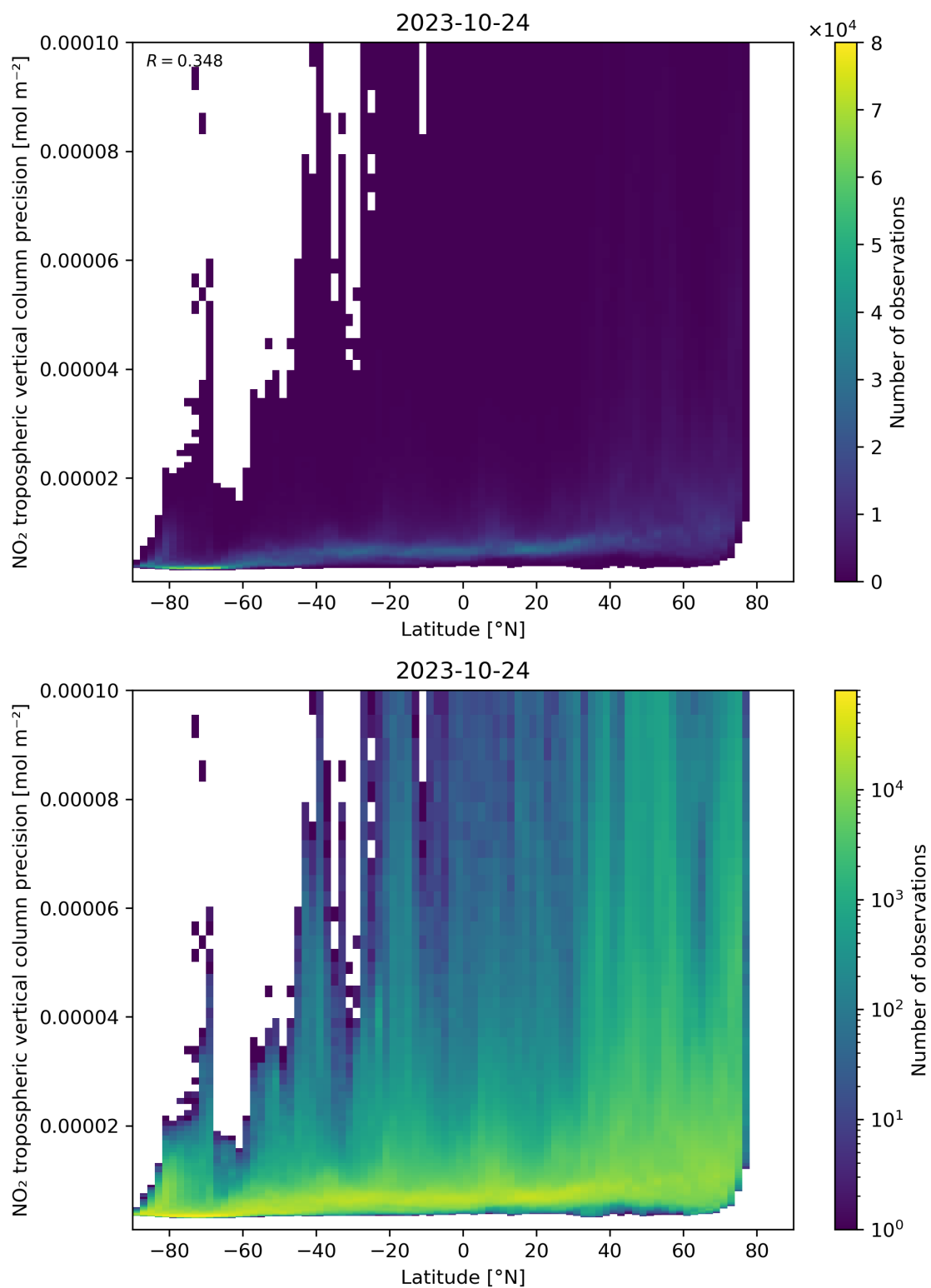
Figure 93: Scatter density plot of “Latitude” against “NO 2 tropospheric vertical column precision” for 2023-10-23 to 2023-10-25.
