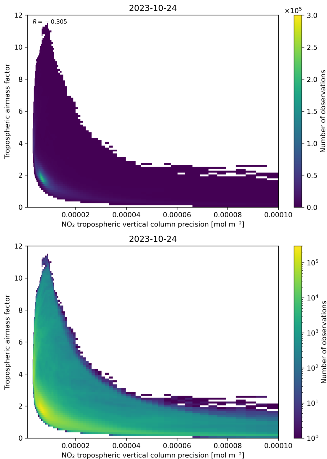
Figure 133: Scatter density plot of “NO 2 tropospheric vertical column precision” against “Tropospheric airmass factor” for 2023-10-23 to 2023-10-25.
