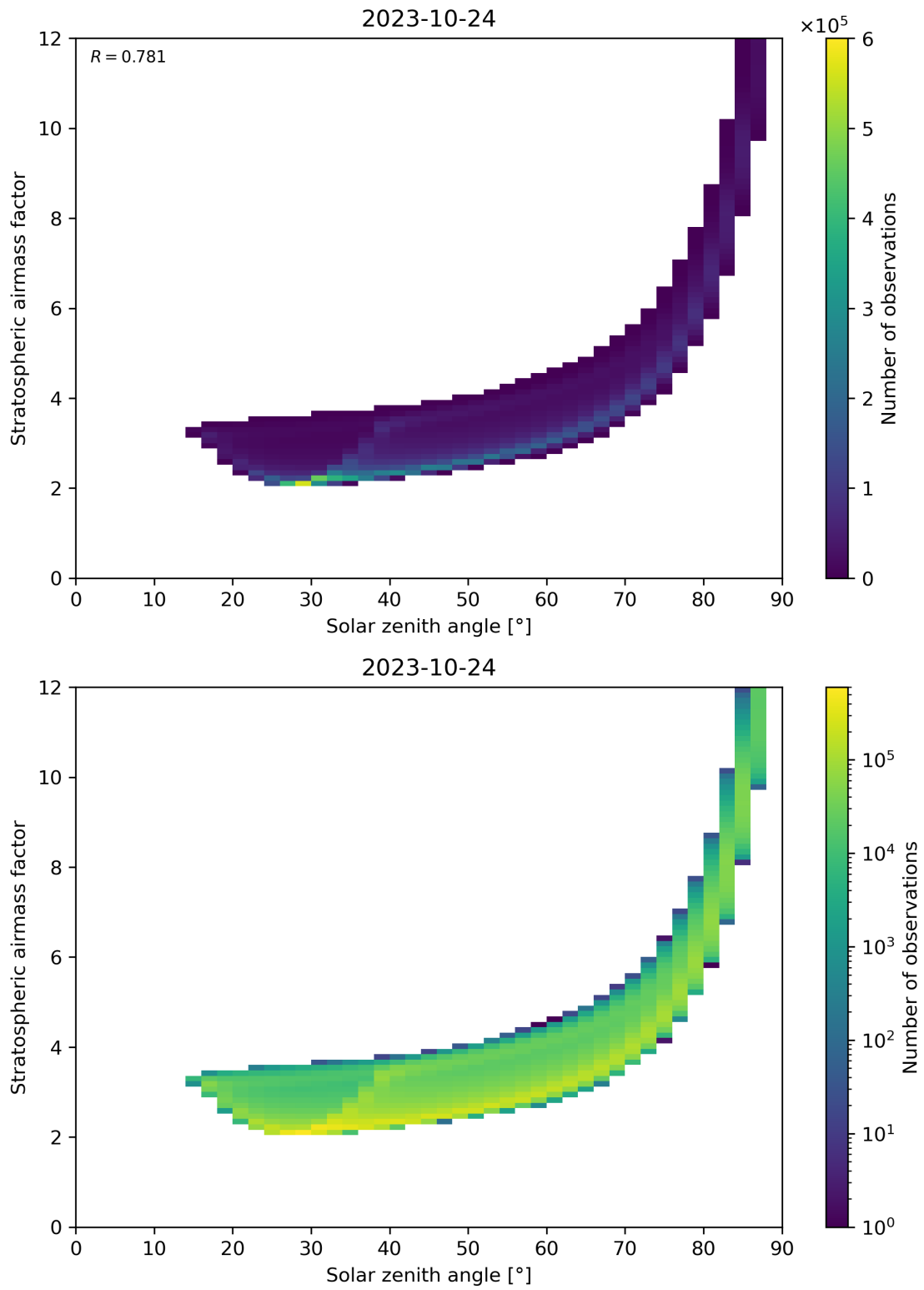
Figure 145: Scatter density plot of “Solar zenith angle” against “Stratospheric airmass factor” for 2023-10-23 to 2023-10-25.
