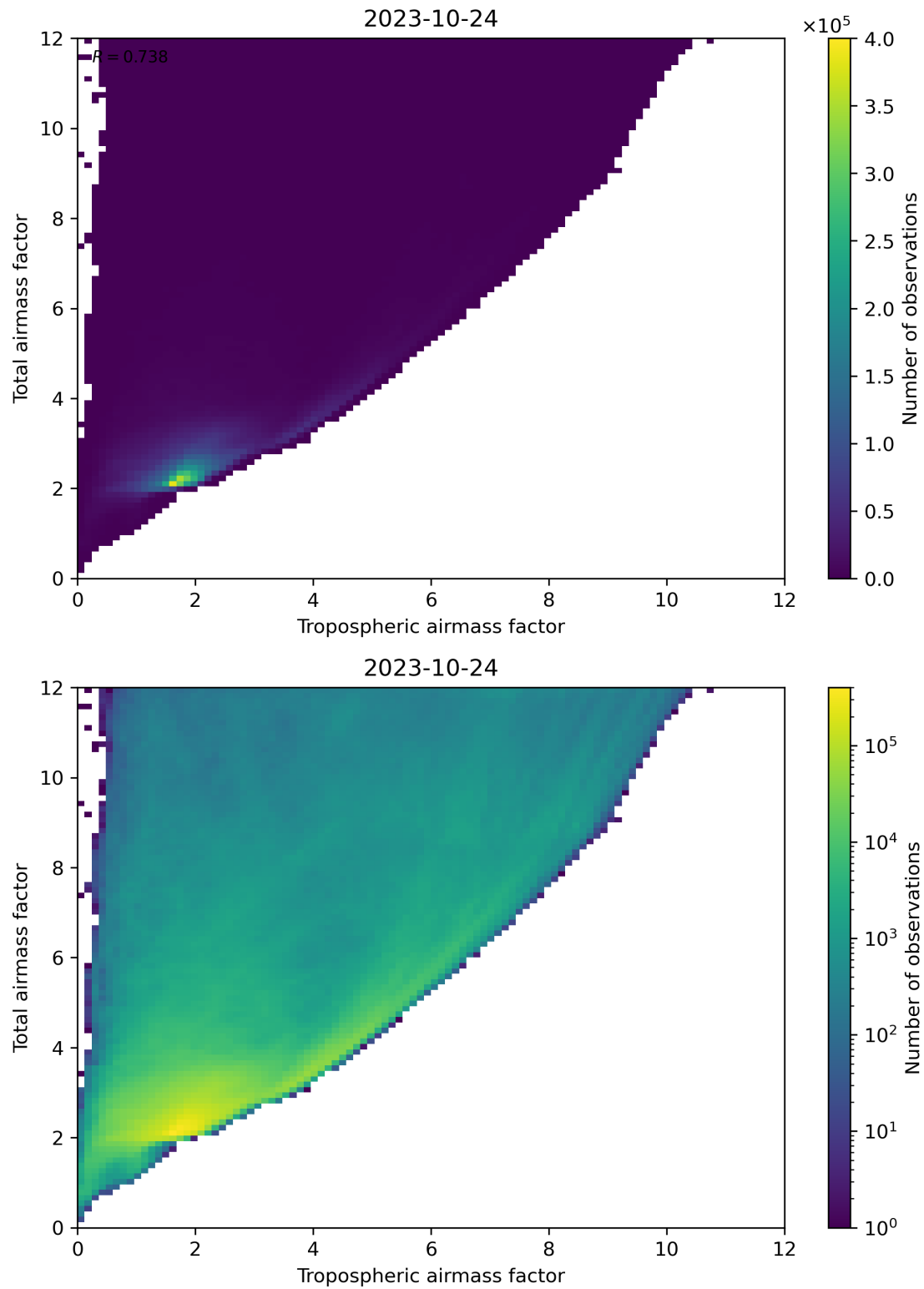
Figure 72: Scatter density plot of “Tropospheric airmass factor” against “Total airmass factor” for 2023-10-23 to 2023-10-25.
