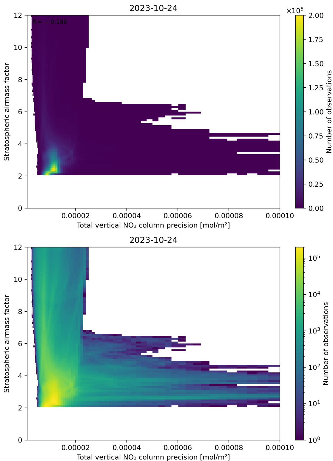
Figure 115: Scatter density plot of “Total vertical NO 2 column precision” against “Stratospheric airmass factor” for 2023-10-23 to 2023-10-25.
