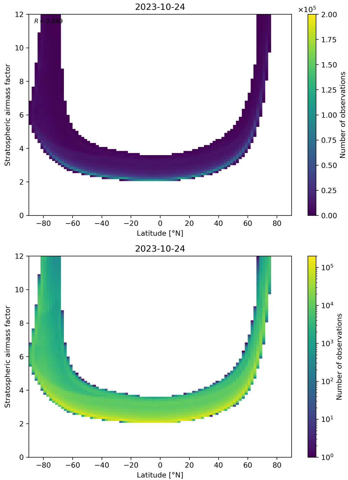
Figure 83: Scatter density plot of “Latitude” against “Stratospheric airmass factor” for 2023-10-23 to 2023-10-25.
