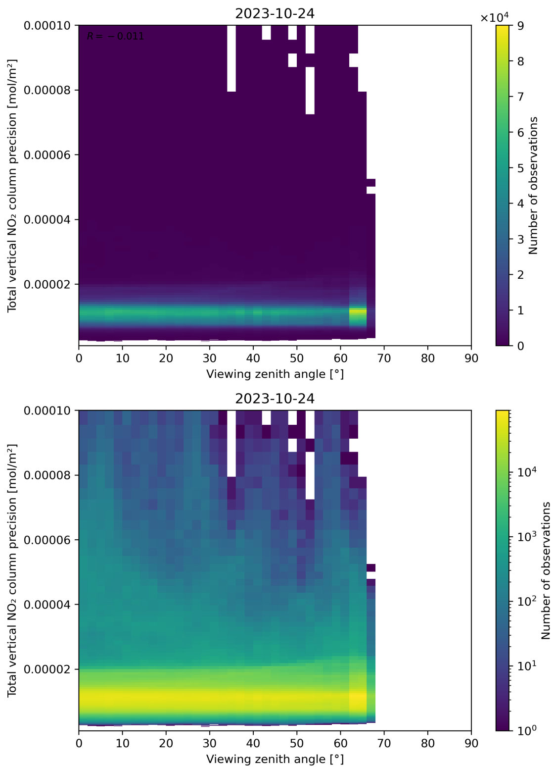
Figure 168: Scatter density plot of “Viewing zenith angle” against “Total vertical NO 2 column precision” for 2023-10-23 to 2023-10-25.
