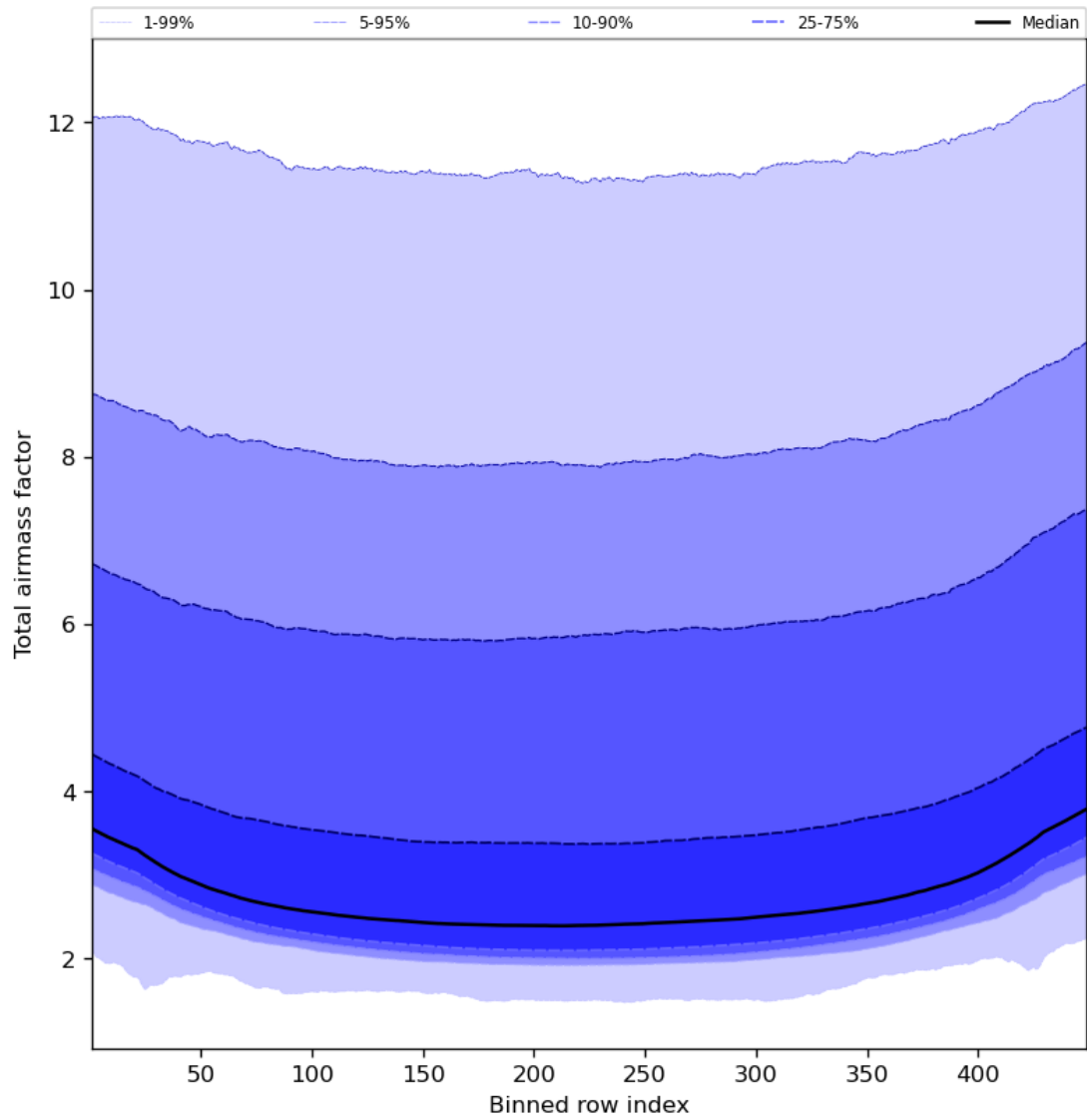
Figure 49: Along track statistics of “Total airmass factor” for 2023-10-23 to 2023-10-25
