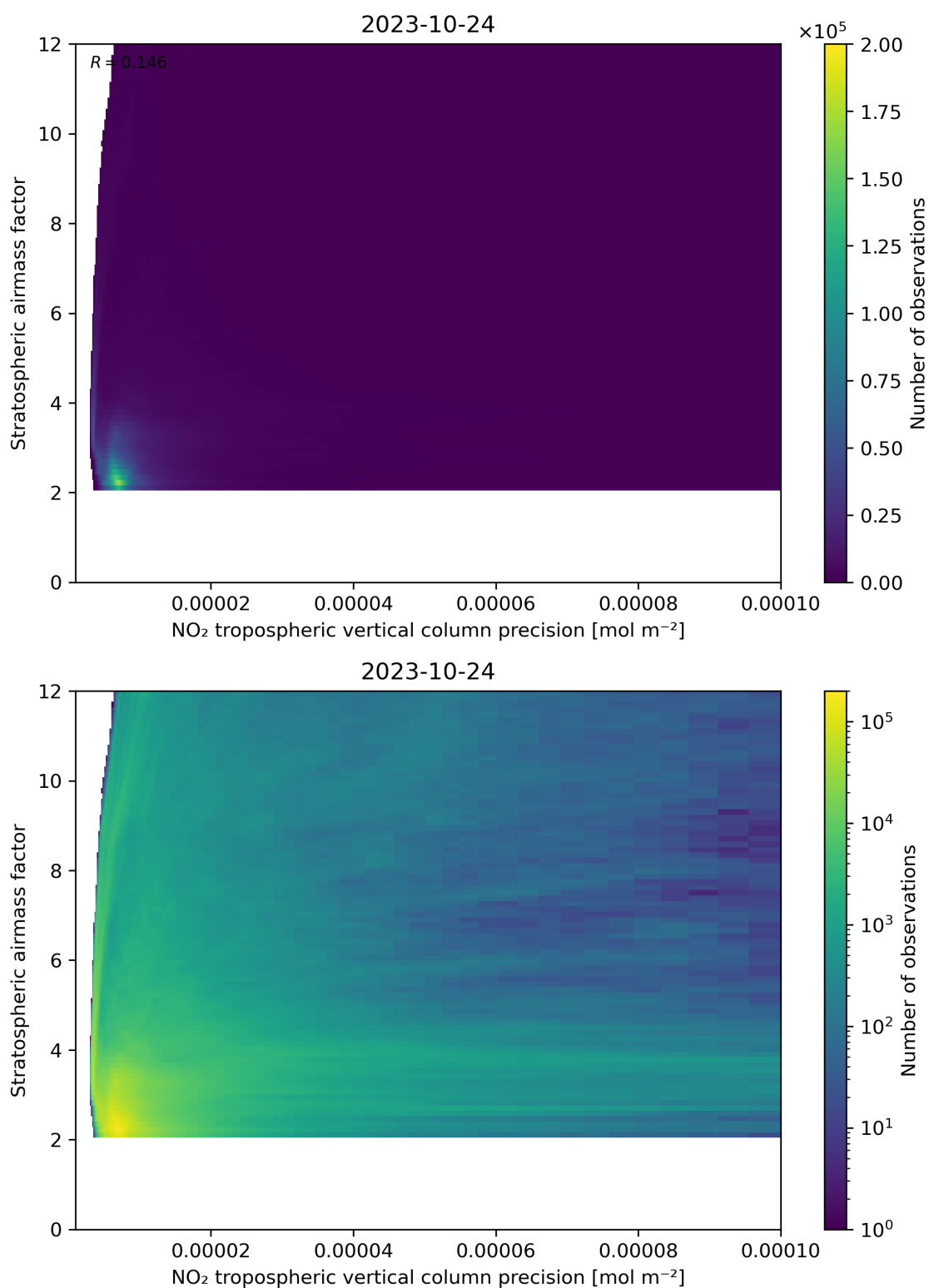
Figure 131: Scatter density plot of “NO 2 tropospheric vertical column precision” against “Stratospheric airmass factor” for 2023-10-23 to 2023-10-25.
