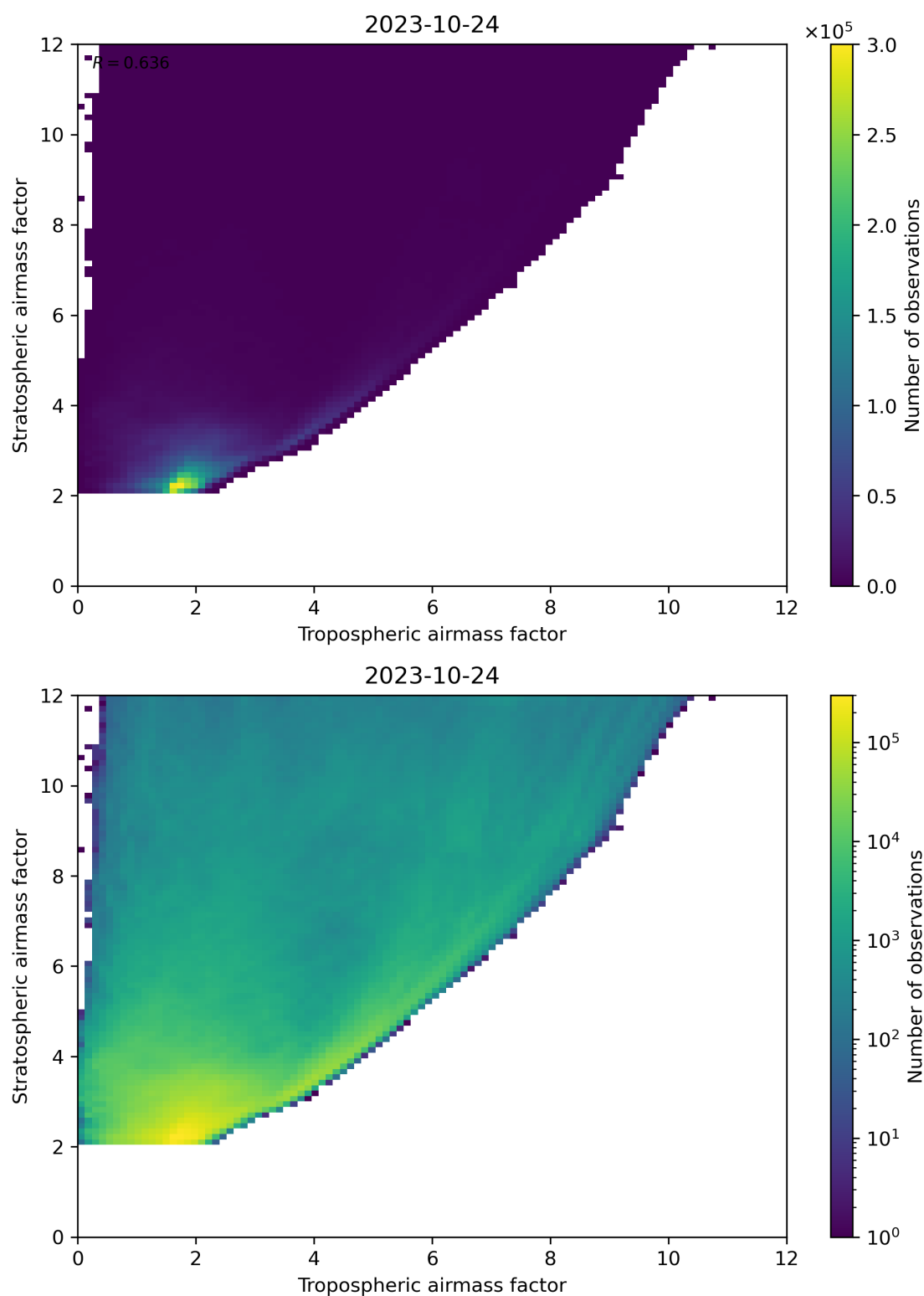
Figure 71: Scatter density plot of “Tropospheric airmass factor” against “Stratospheric airmass factor” for 2023-10-23 to 2023-10-25.
