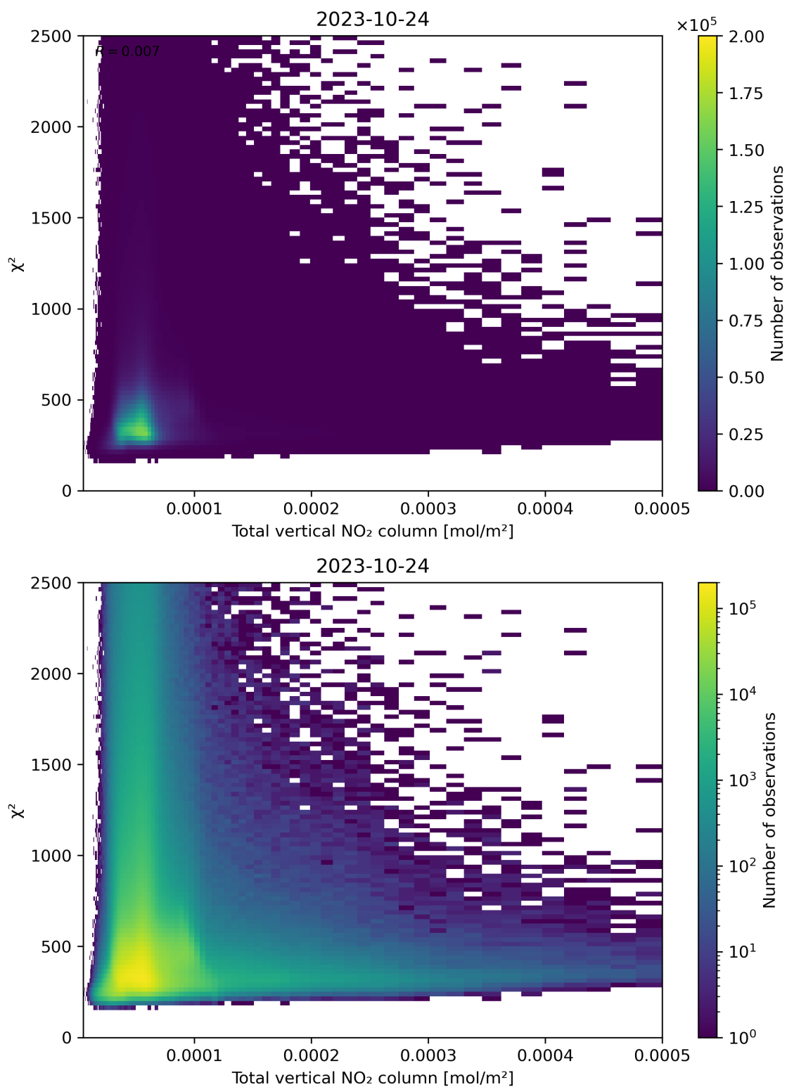
Figure 111: Scatter density plot of “Total vertical NO 2 column” against “ \chi^2 ” for 2023-10-23 to 2023-10-25.
