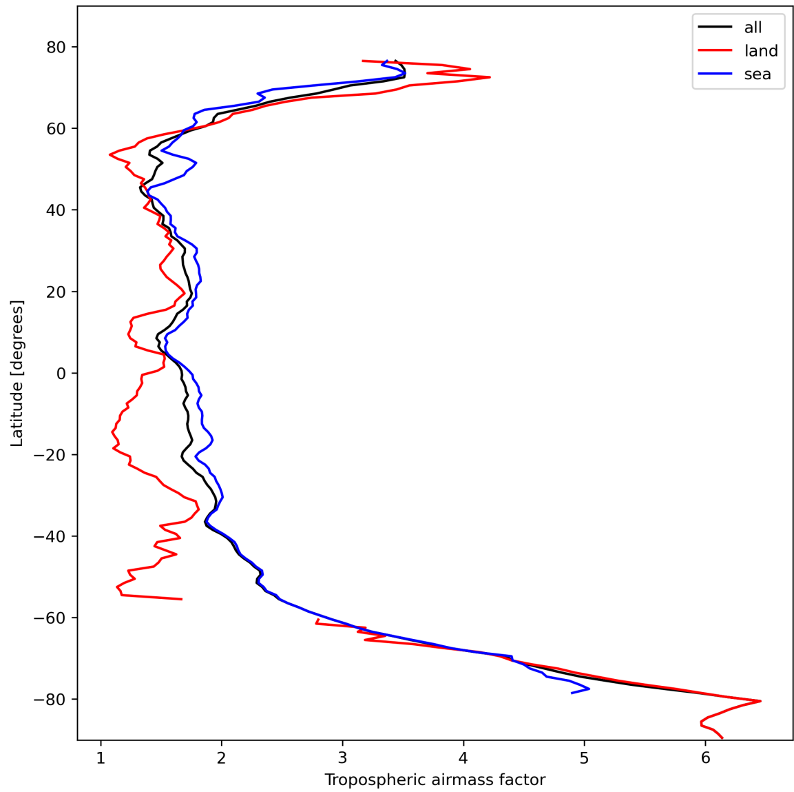
Figure 14: Zonal average of “Tropospheric airmass factor” for 2023-10-23 to 2023-10-25.
