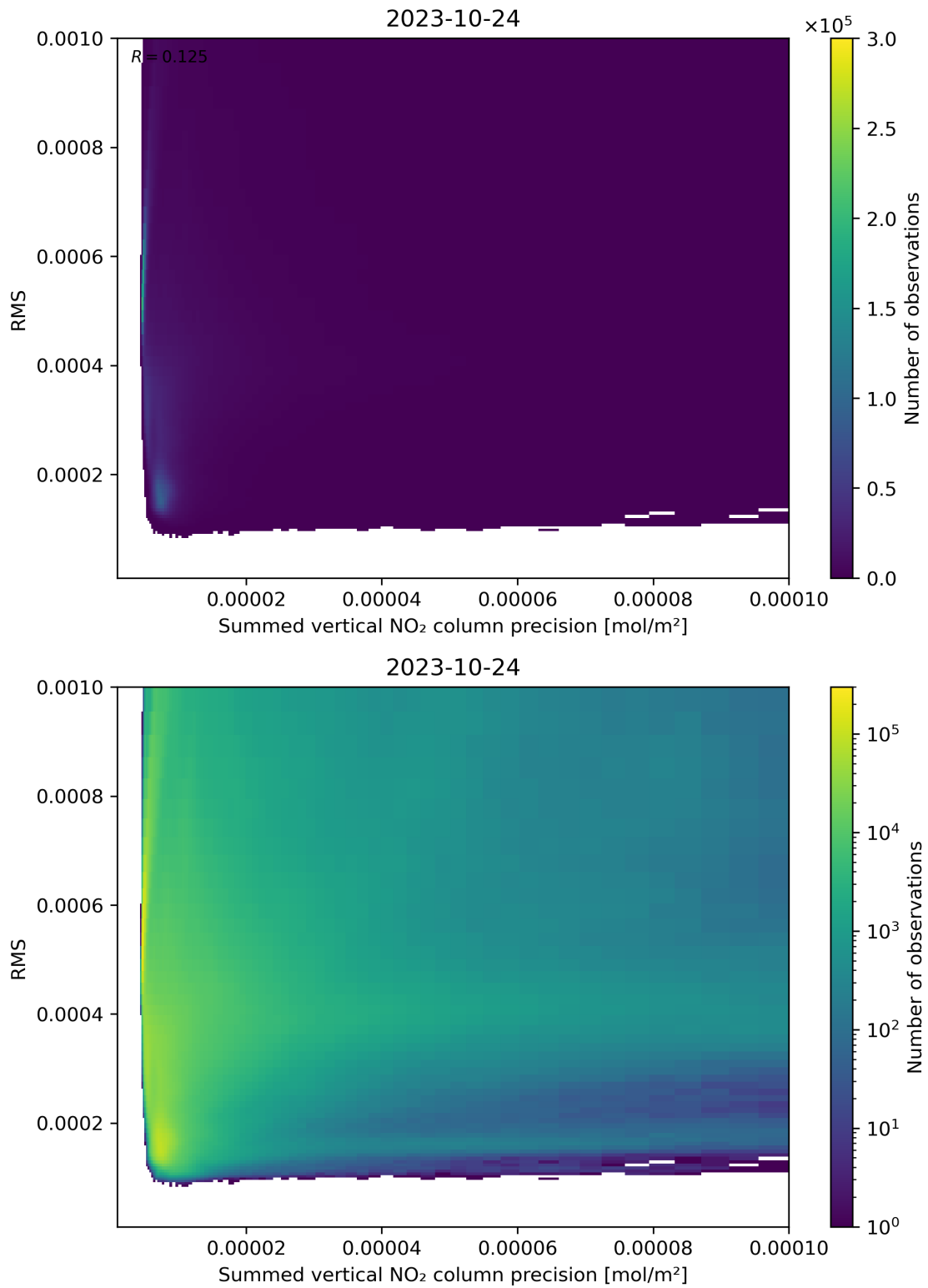
Figure 108: Scatter density plot of “Summed vertical NO 2 column precision” against “RMS” for 2023-10-23 to 2023-10-25.
