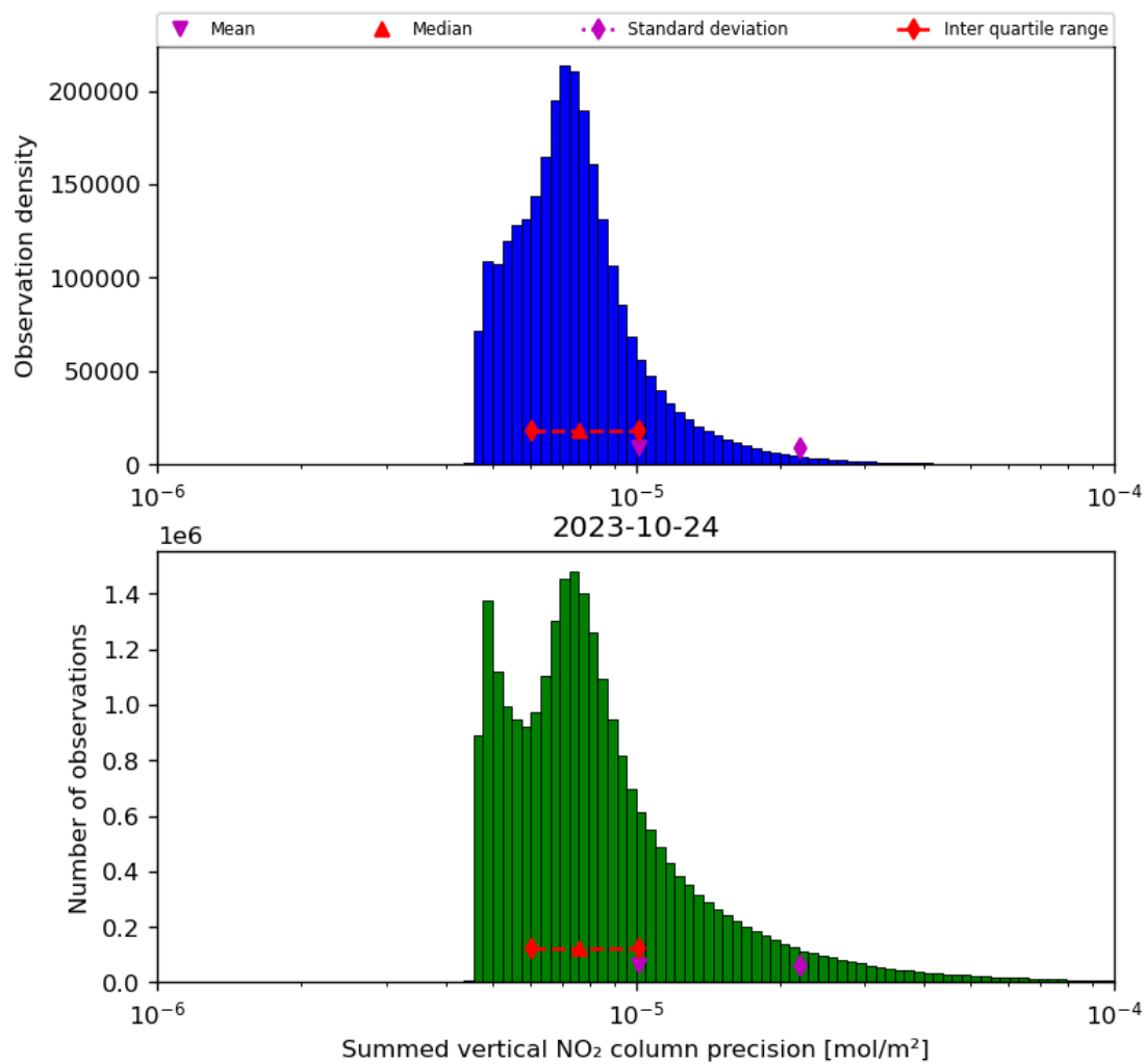
Figure 41: Histogram of "Summed vertical NO 2 column precision" for 2023-10-23 to 2023-10-25
