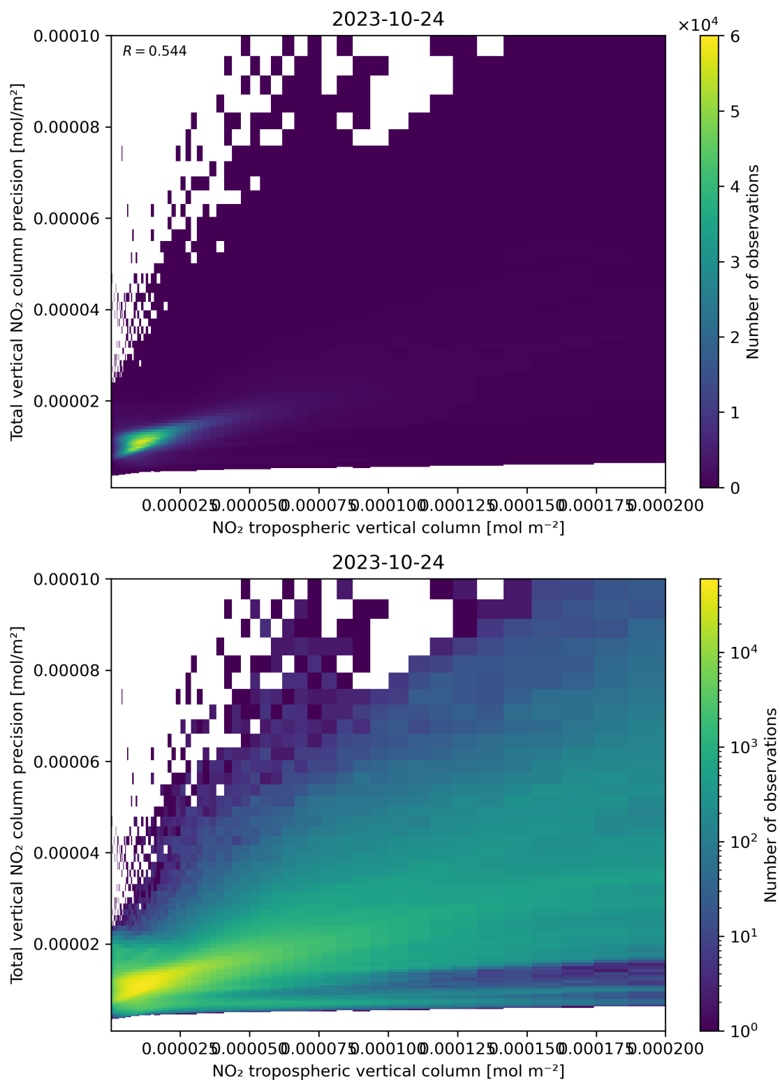
Figure 129: Scatter density plot of “NO 2 tropospheric vertical column” against “Total vertical NO 2 column precision” for 2023-10-23 to 2023-10-25.
