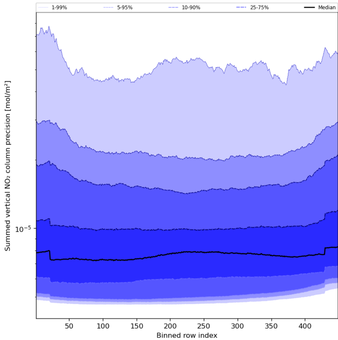
Figure 58: Along track statistics of “Summed vertical NO 2 column precision” for 2023-10-23 to 2023-10-25
