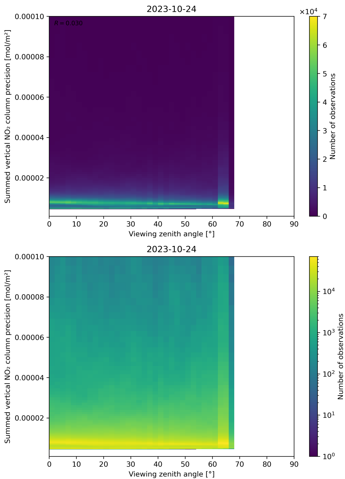
Figure 166: Scatter density plot of “Viewing zenith angle” against “Summed vertical NO 2 column precision” for 2023-10-23 to 2023-10-25.
