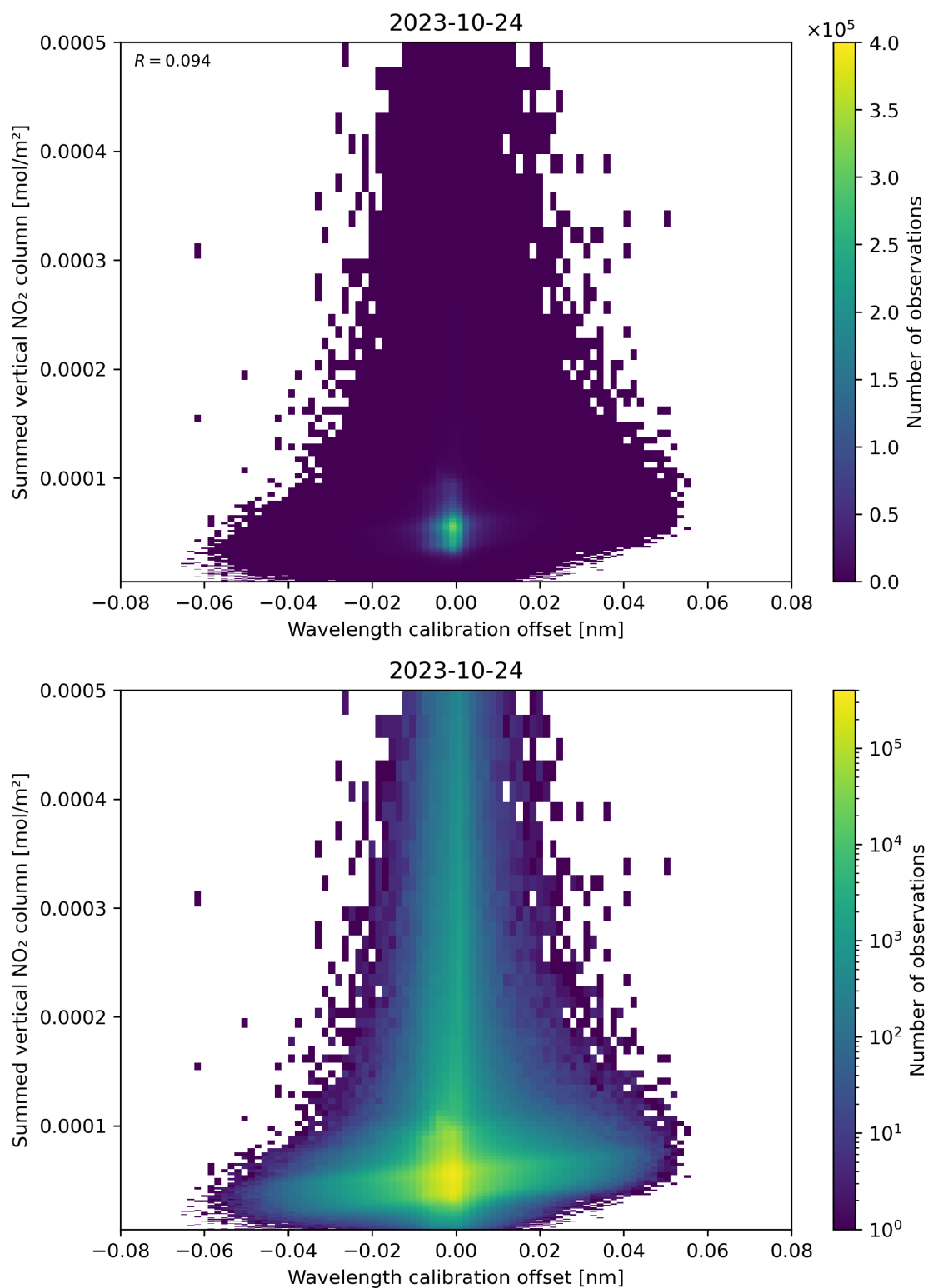
Figure 177: Scatter density plot of “Wavelength calibration offset” against “Summed vertical NO 2 column” for 2023-10-23 to 2023-10-25.
