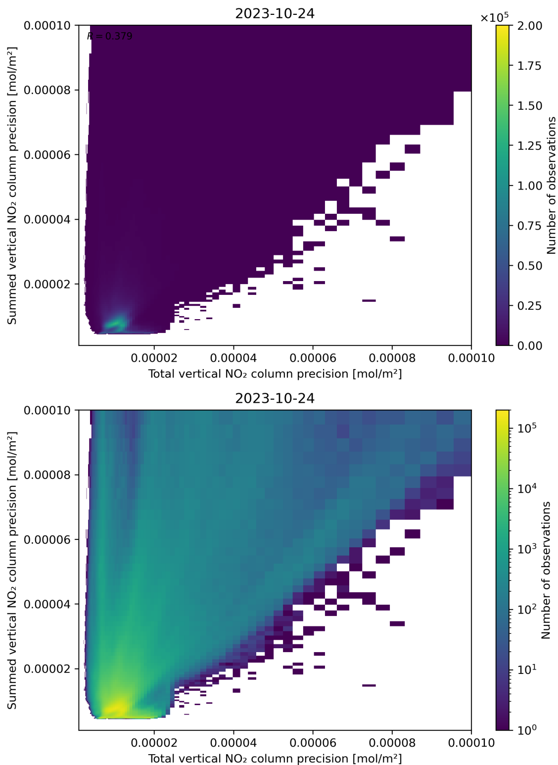
Figure 118: Scatter density plot of “Total vertical NO 2 column precision” against “Summed vertical NO 2 column precision” for 2023-10-23 to 2023-10-25.
