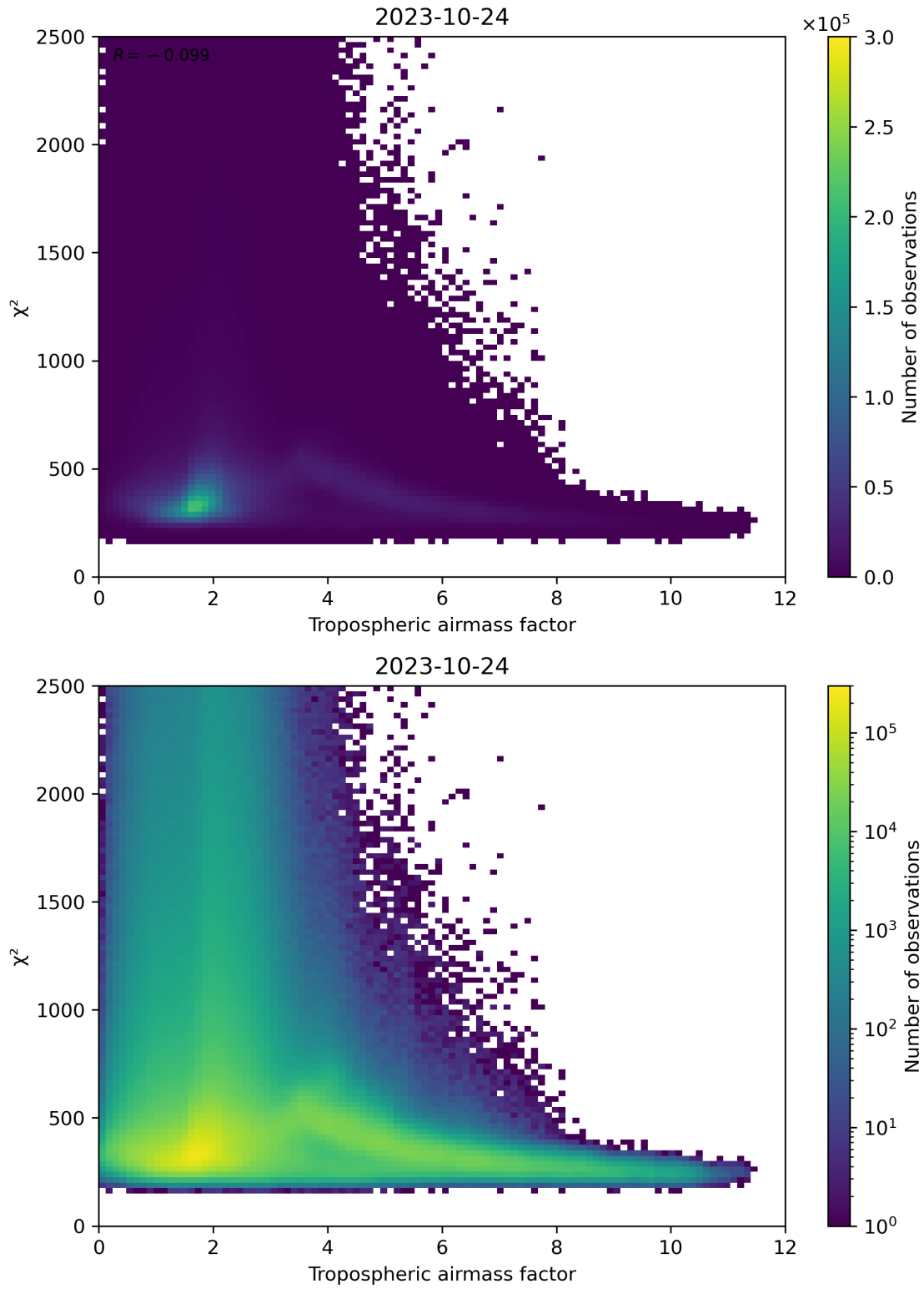
Figure 73: Scatter density plot of “Tropospheric airmass factor” against “ \chi^2 ” for 2023-10-23 to 2023-10-25.
