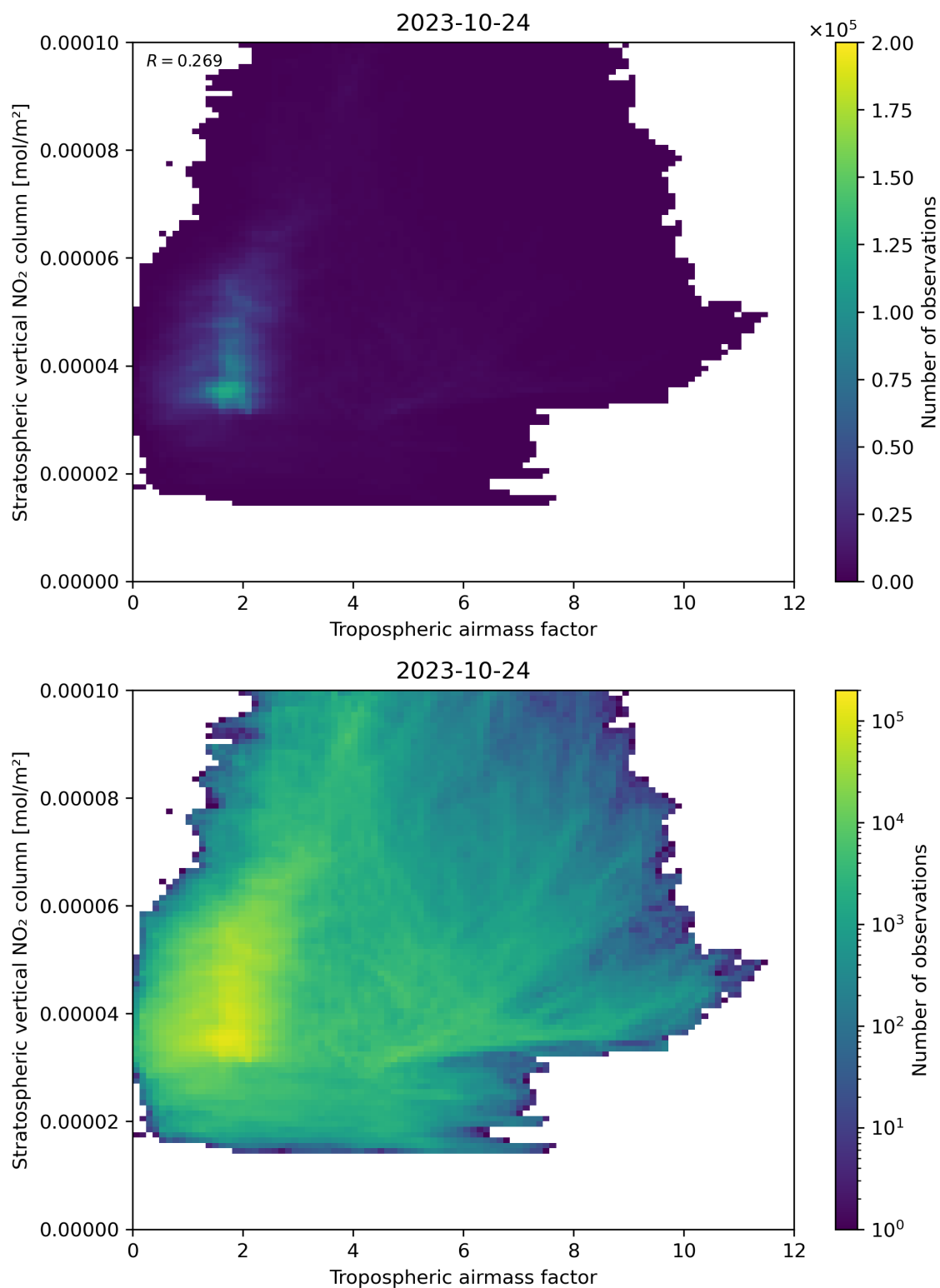
Figure 74: Scatter density plot of “Tropospheric airmass factor” against “Stratospheric vertical NO 2 column” for 2023-10-23 to 2023-10-25.
