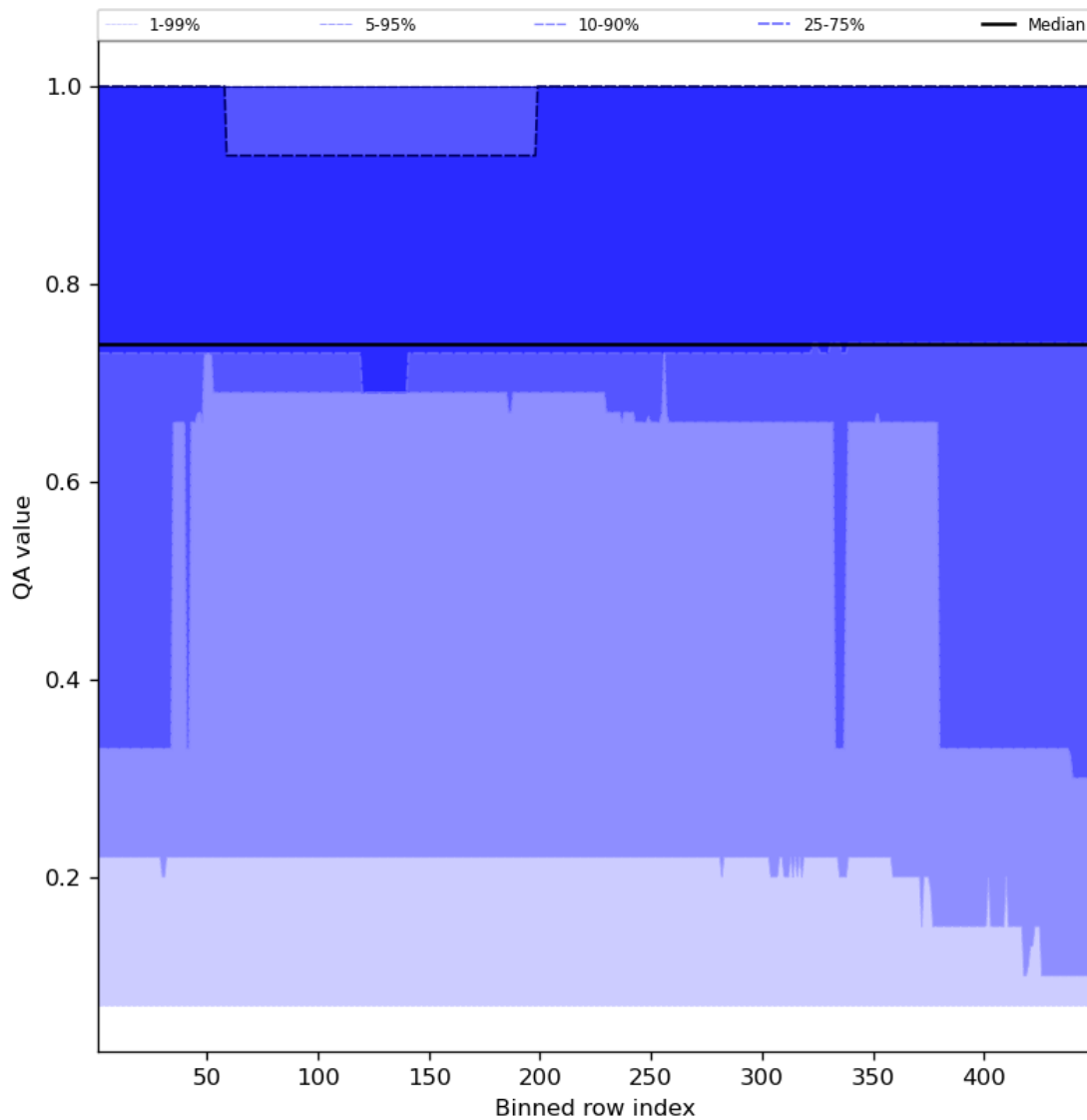
Figure 45: Along track statistics of “QA value” for 2023-10-23 to 2023-10-25
