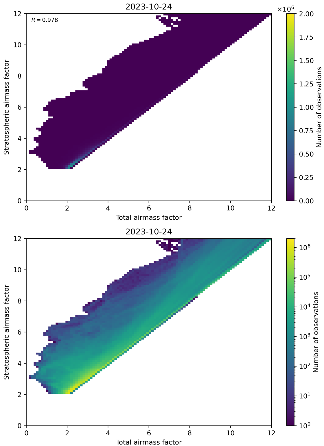
Figure 62: Scatter density plot of “Total air mass factor” against “Stratospheric air mass factor” for 2023-10-23 to 2023-10-25.
