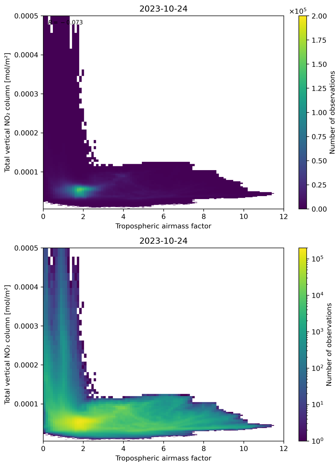
Figure 77: Scatter density plot of “Tropospheric airmass factor” against “Total vertical NO 2 column” for 2023-10-23 to 2023-10-25.
