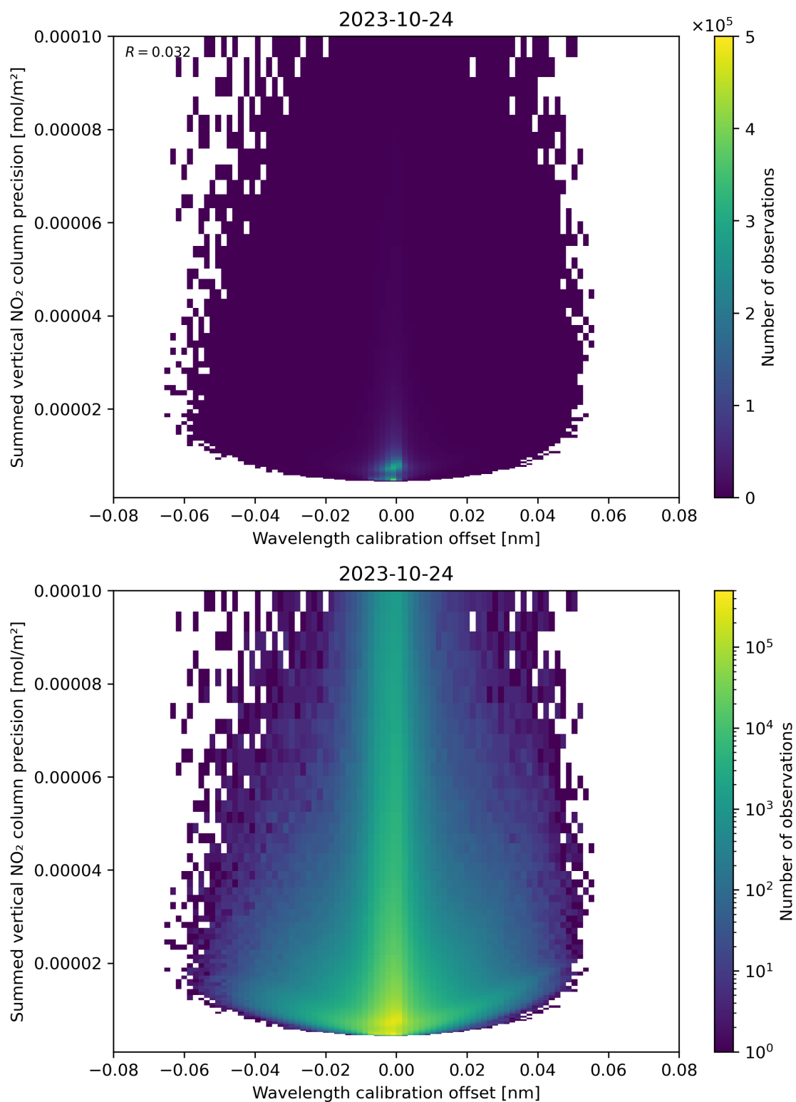
Figure 178: Scatter density plot of “Wavelength calibration offset” against “Summed vertical NO 2 column precision” for 2023-10-23 to 2023-10-25.
