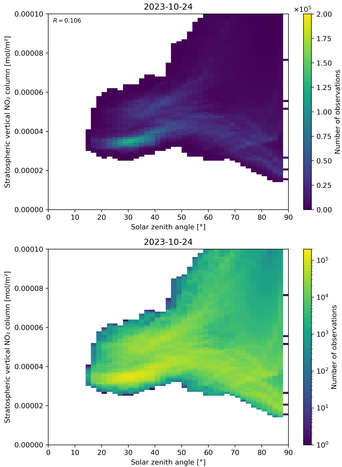
Figure 150: Scatter density plot of “Solar zenith angle” against “Stratospheric vertical NO 2 column” for 2023-10-23 to 2023-10-25.
