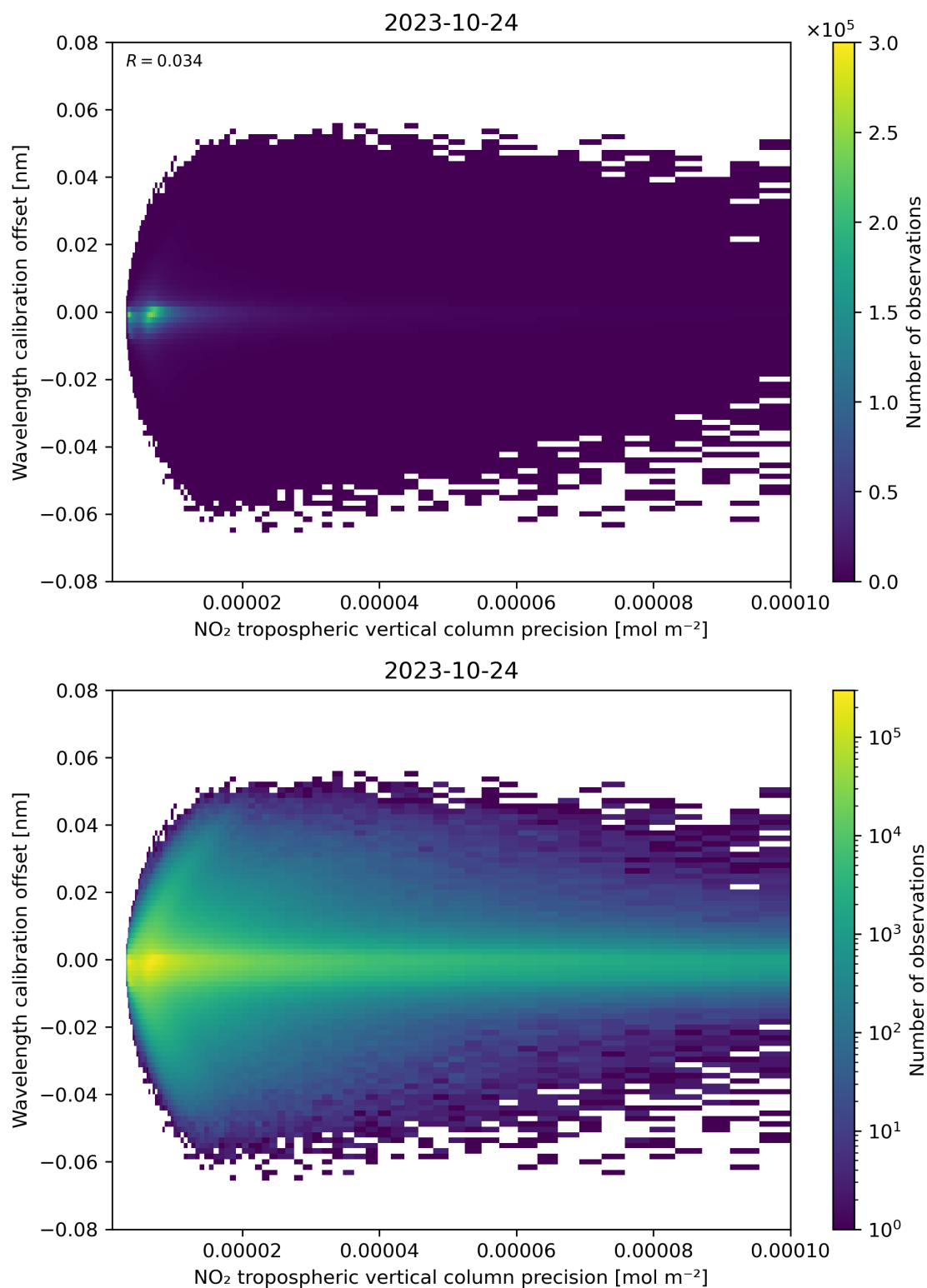
Figure 141: Scatter density plot of “NO 2 tropospheric vertical column precision” against “Wavelength calibration offset” for 2023-10-23 to 2023-10-25.
