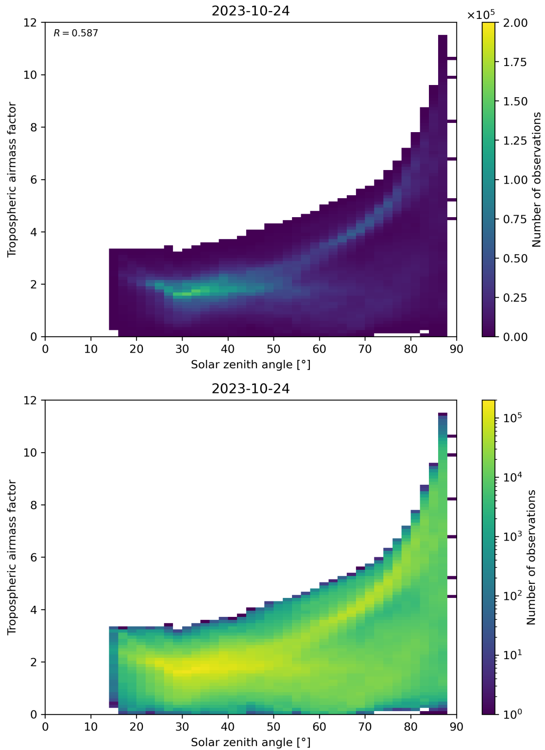
Figure 147: Scatter density plot of “Solar zenith angle” against “Tropospheric airmass factor” for 2023-10-23 to 2023-10-25.
