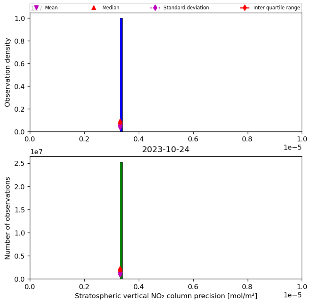
Figure 37: Histogram of “Stratospheric vertical NO 2 column precision” for 2023-10-23 to 2023-10-25
