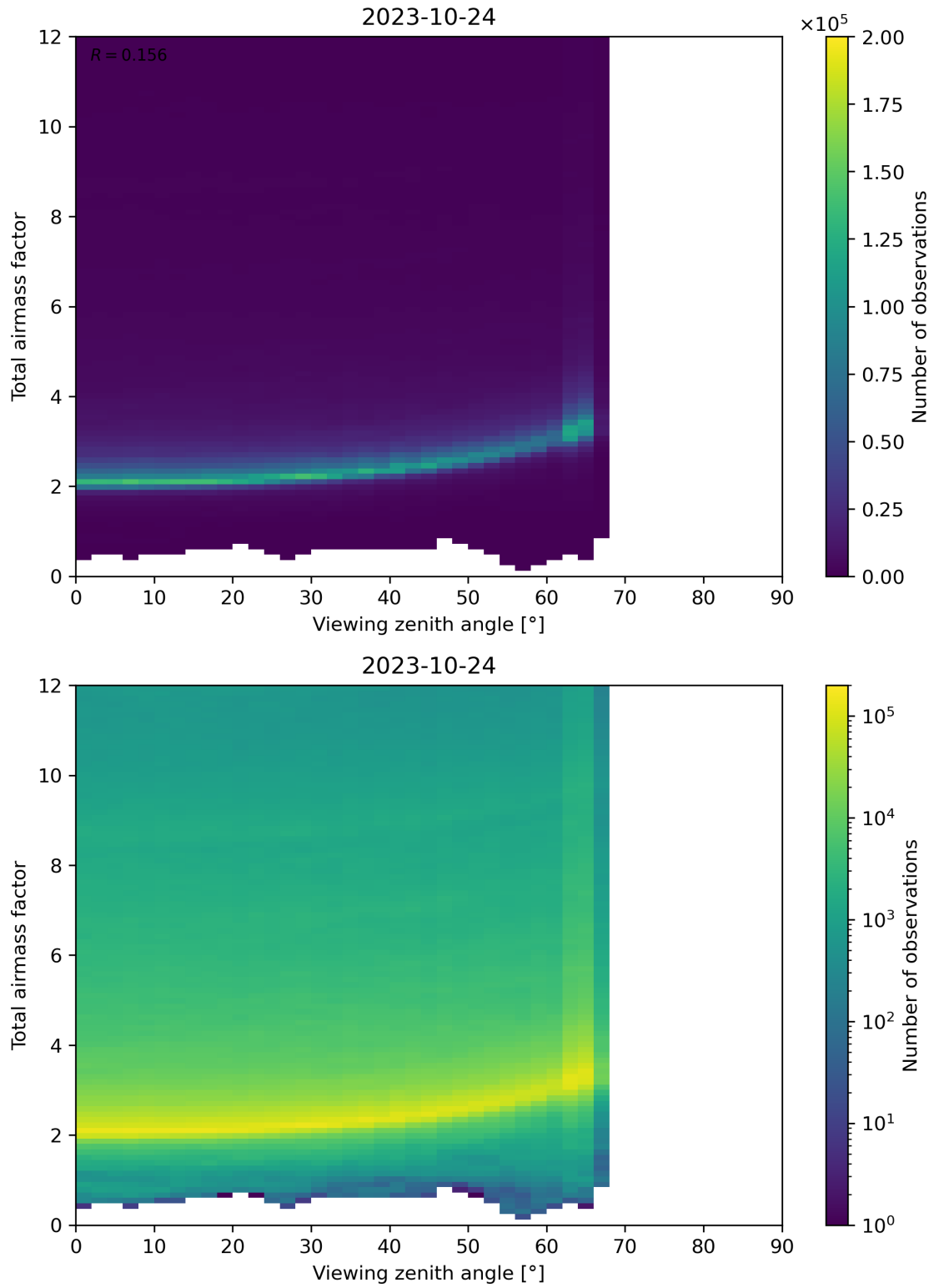
Figure 160: Scatter density plot of “Viewing zenith angle” against “Total airmass factor” for 2023-10-23 to 2023-10-25.
