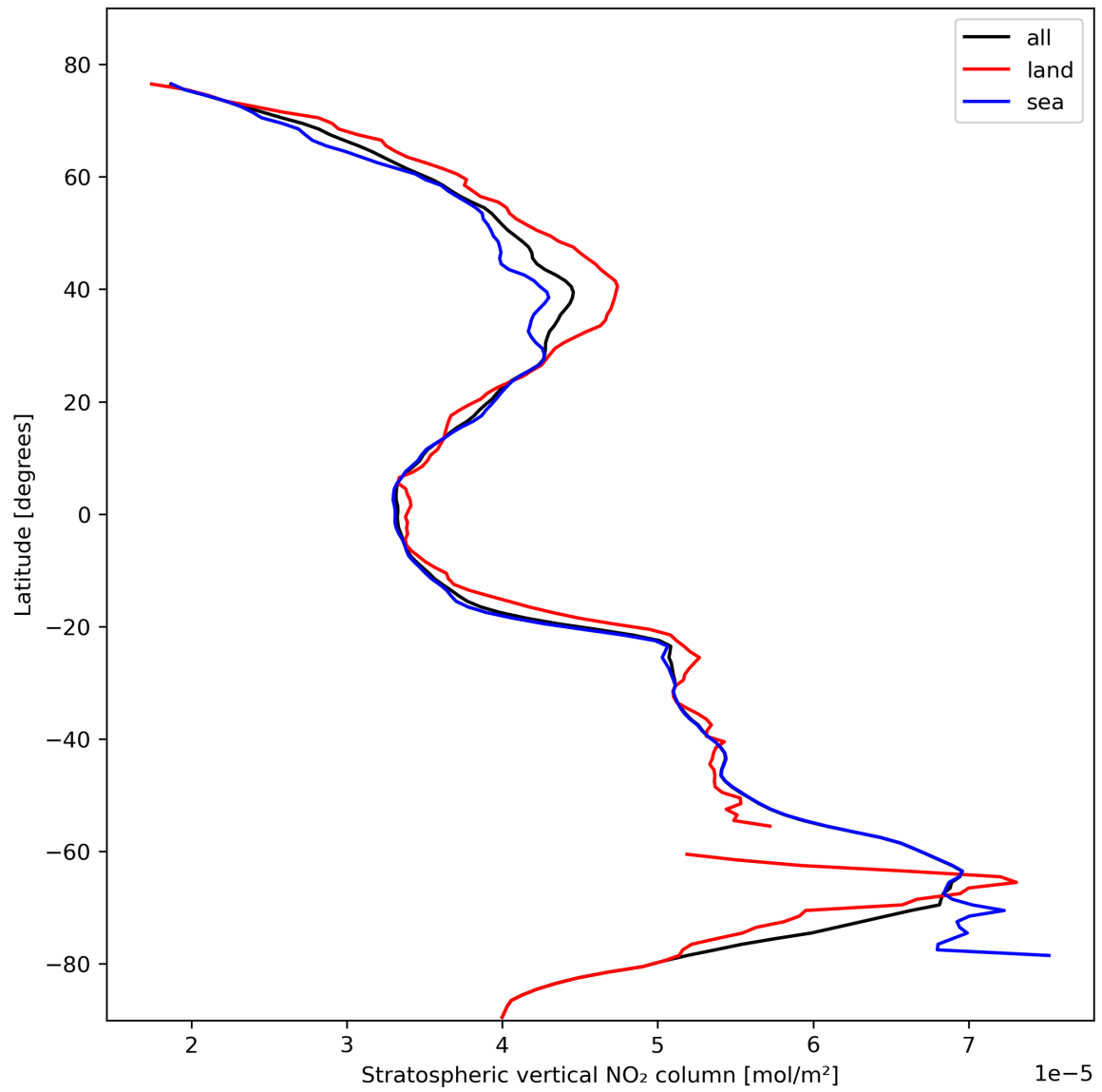
Figure 19: Zonal average of “Stratospheric vertical NO 2 column” for 2023-10-23 to 2023-10-25.
