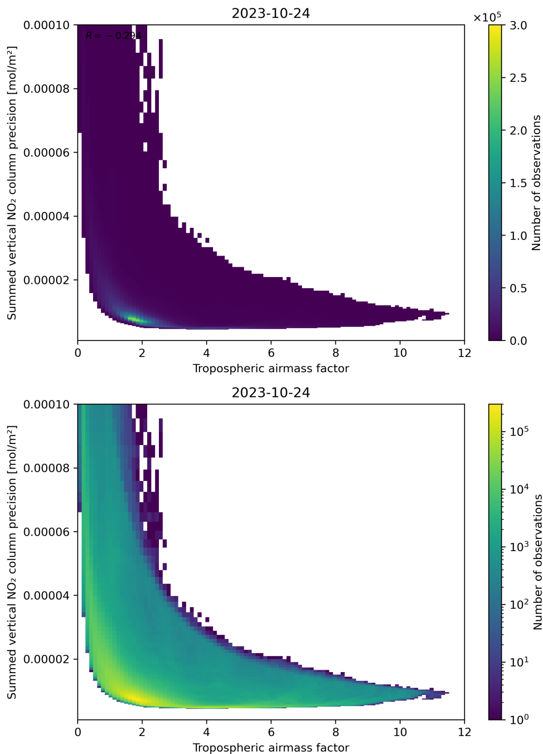
Figure 76: Scatter density plot of “Tropospheric air mass factor” against “Summed vertical NO 2 column precision” for 2023-10-23 to 2023-10-25.
