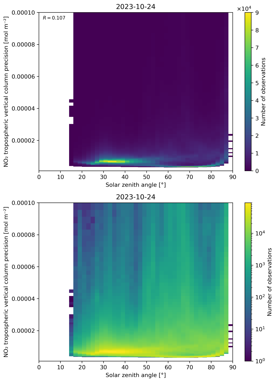
Figure 156: Scatter density plot of “Solar zenith angle” against “NO 2 tropospheric vertical column precision” for 2023-10-23 to 2023-10-25.
