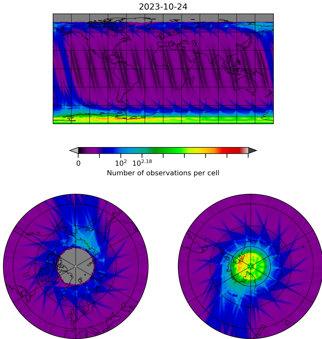
Figure 10: Map of the number of observations for 2023-10-23 to 2023-10-25
