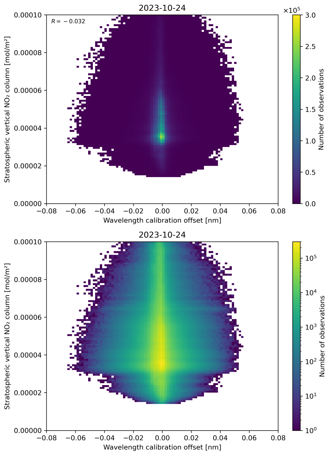
Figure 176: Scatter density plot of “Wavelength calibration offset” against “Stratospheric vertical NO 2 column” for 2023-10-23 to 2023-10-25.
