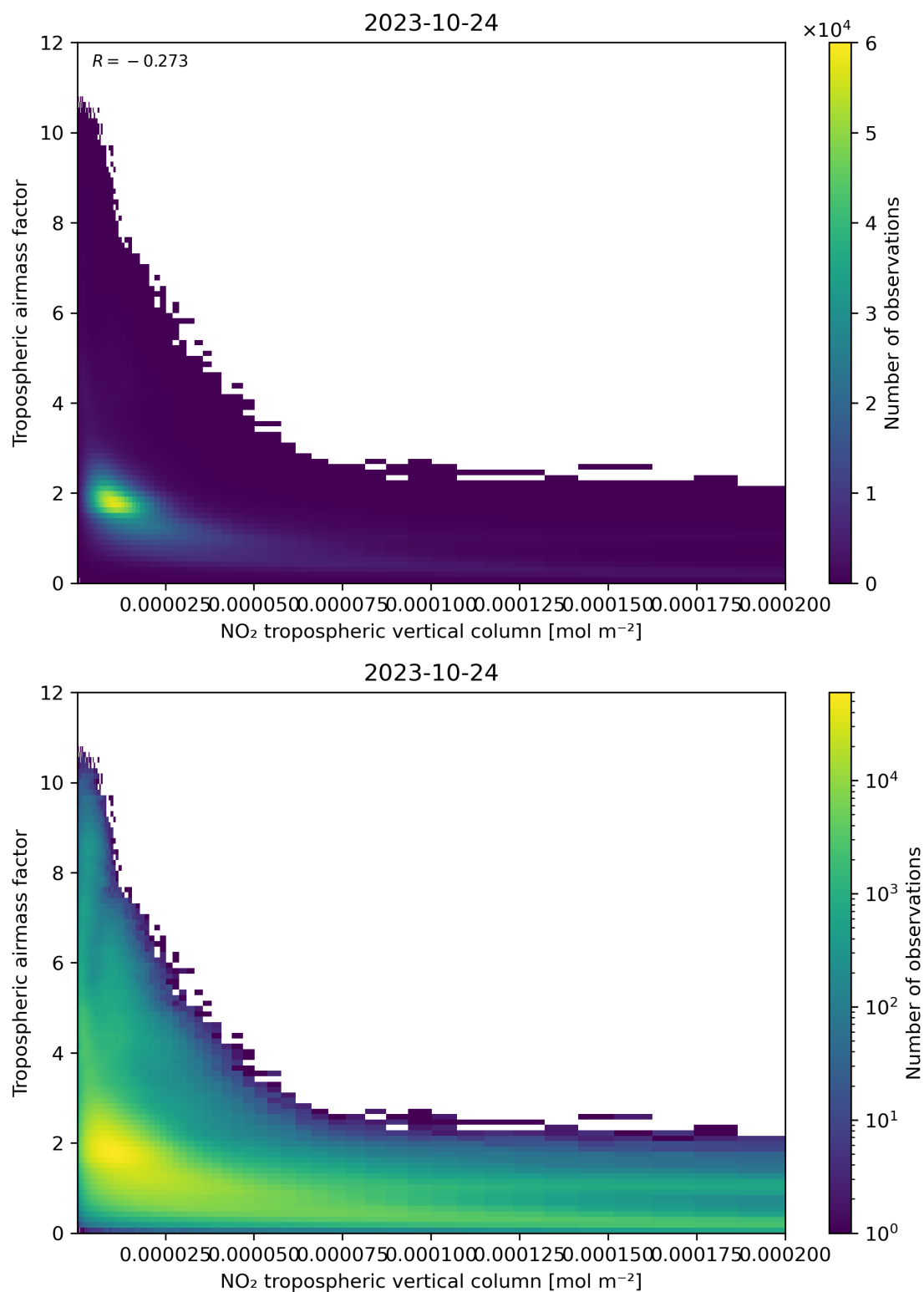
Figure 123: Scatter density plot of “NO 2 tropospheric vertical column” against “Tropospheric air mass factor” for 2023-10-23 to 2023-10-25.
