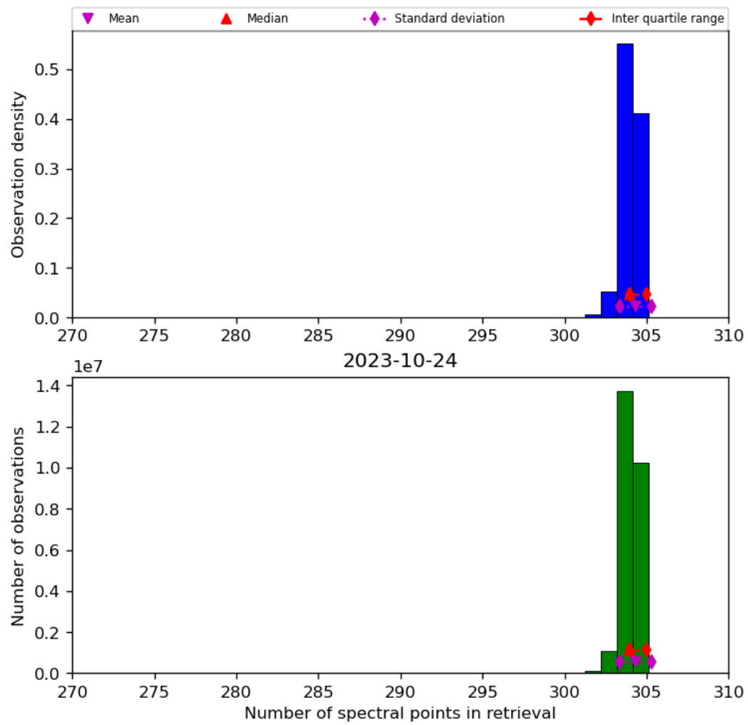
Figure 33: Histogram of “Number of spectral points in retrieval” for 2023-10-23 to 2023-10-25
