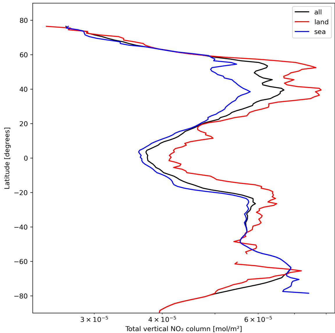
Figure 21: Zonal average of “Total vertical NO 2 column” for 2023-10-23 to 2023-10-25.
