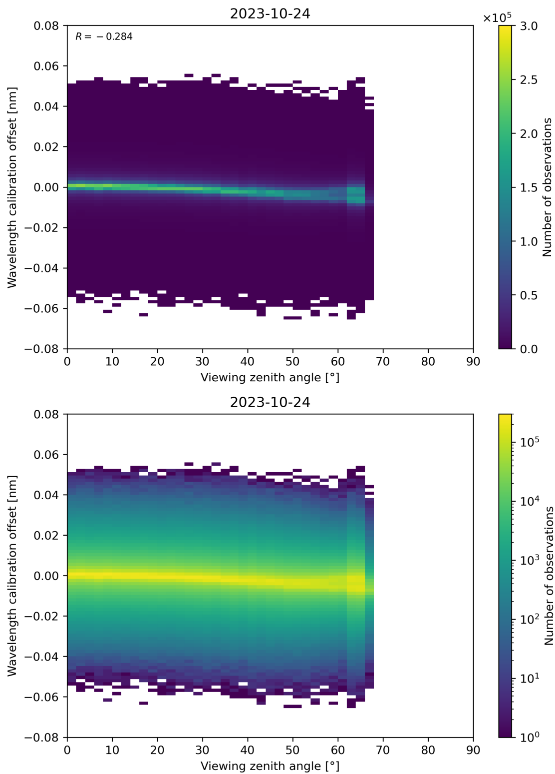
Figure 173: Scatter density plot of “Viewing zenith angle” against “Wavelength calibration offset” for 2023-10-23 to 2023-10-25.
