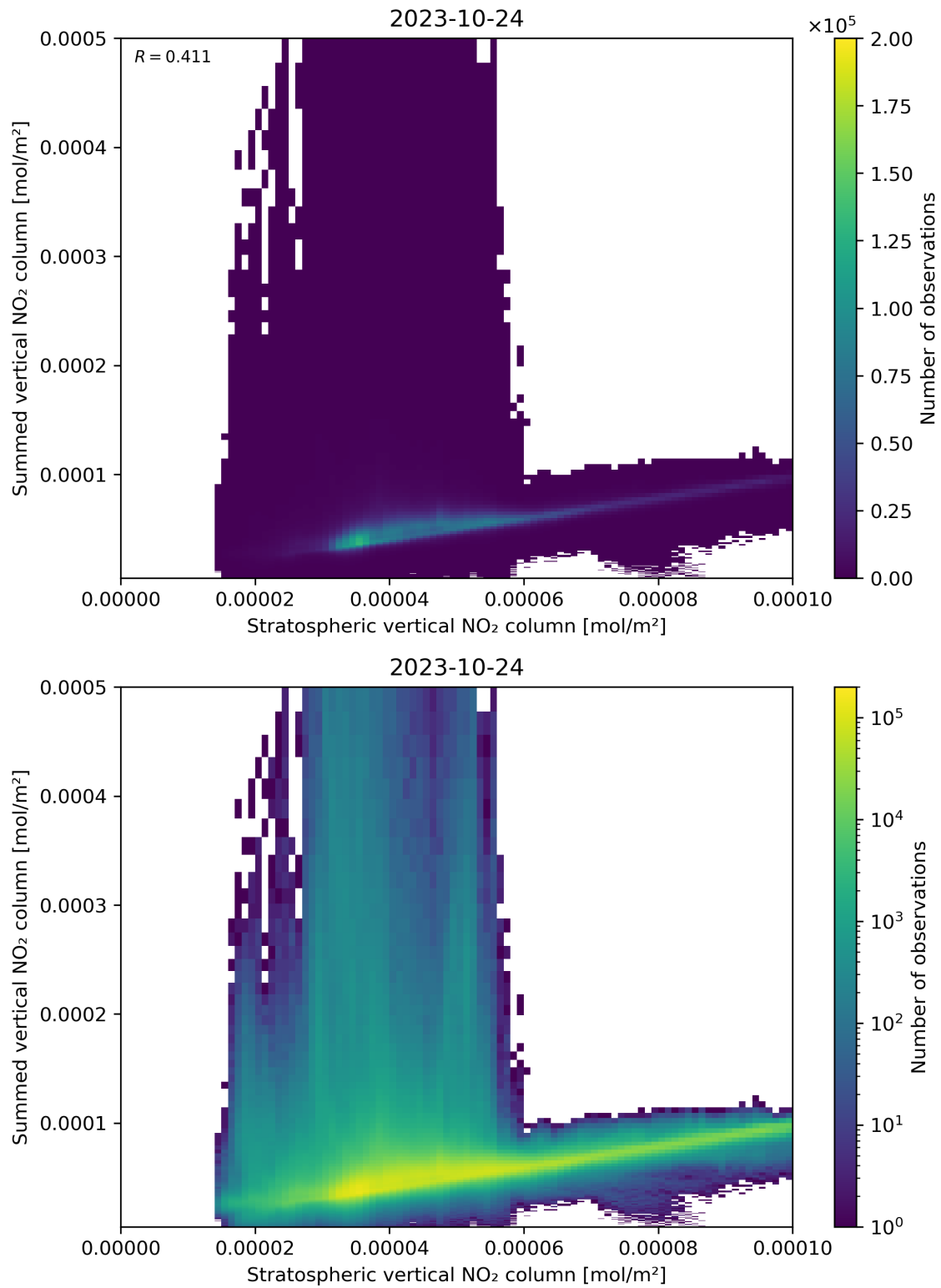
Figure 98: Scatter density plot of “Stratospheric vertical NO 2 column” against “Summed vertical NO 2 column” for 2023-10-23 to 2023-10-25.
