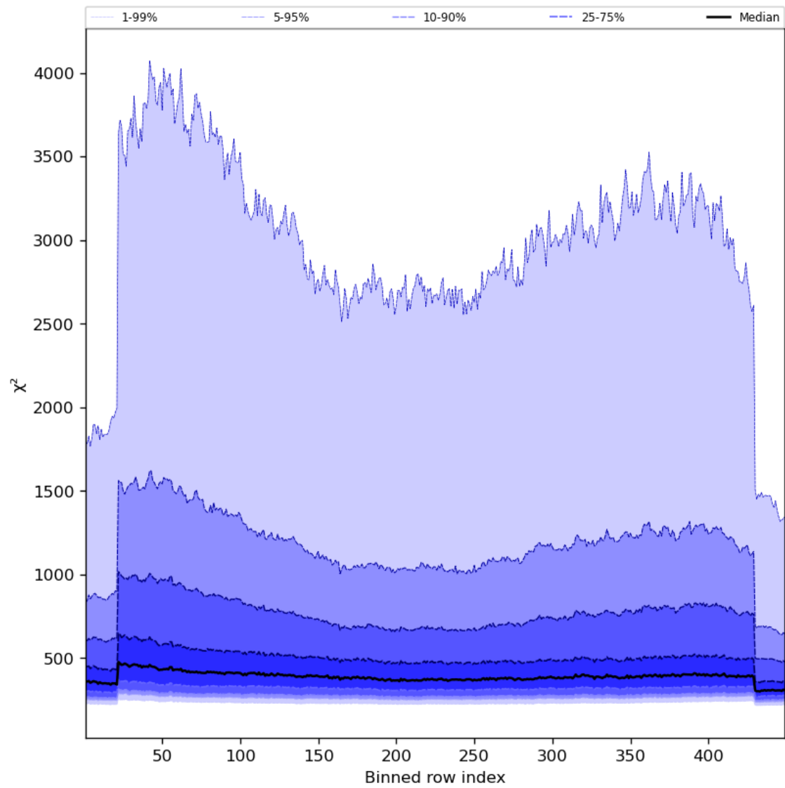
Figure 59: Along track statistics of “ \chi^2 ” for 2023-10-23 to 2023-10-25
