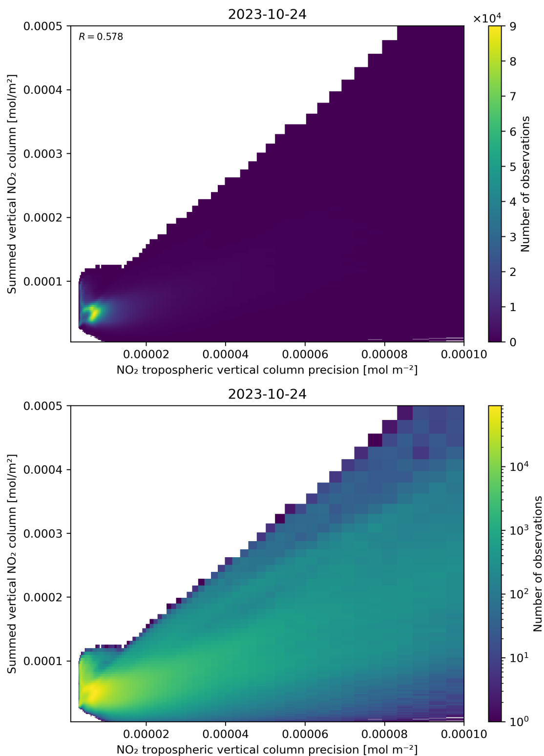
Figure 136: Scatter density plot of “NO 2 tropospheric vertical column precision” against “Summed vertical NO 2 column” for 2023-10-23 to 2023-10-25.
