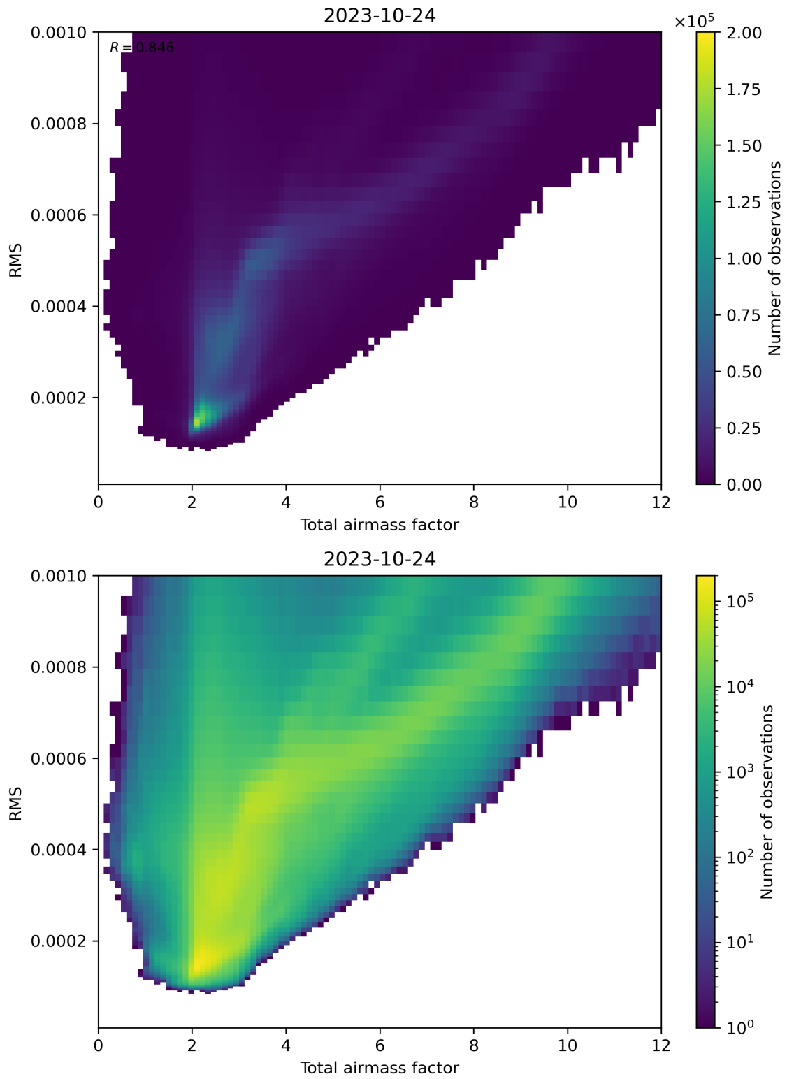
Figure 69: Scatter density plot of “Total airmass factor” against “RMS” for 2023-10-23 to 2023-10-25.
