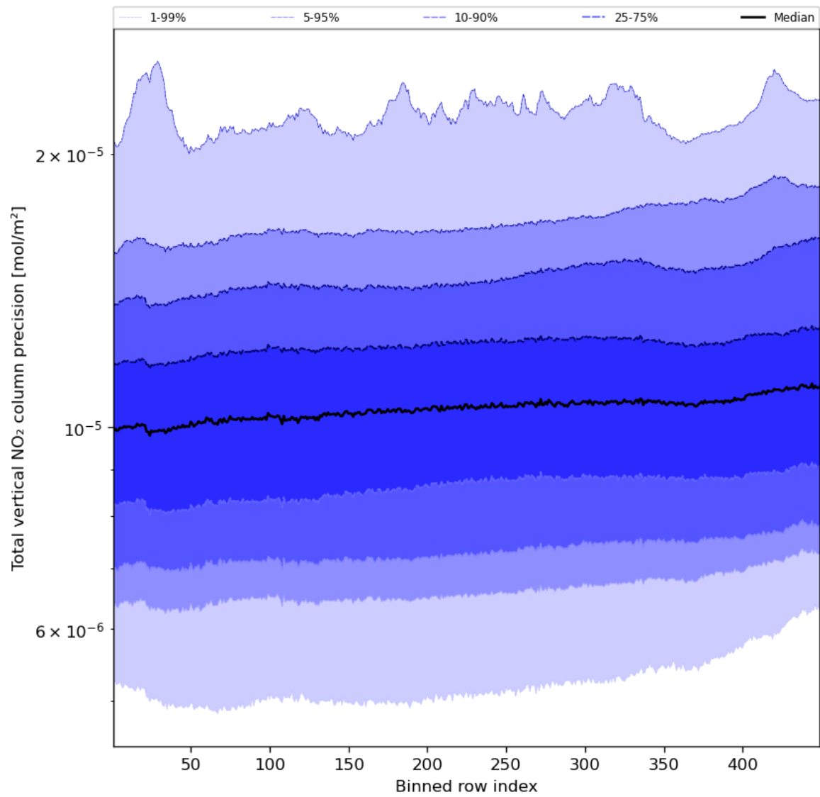
Figure 56: Along track statistics of “Total vertical NO 2 column precision” for 2023-10-23 to 2023-10-25
