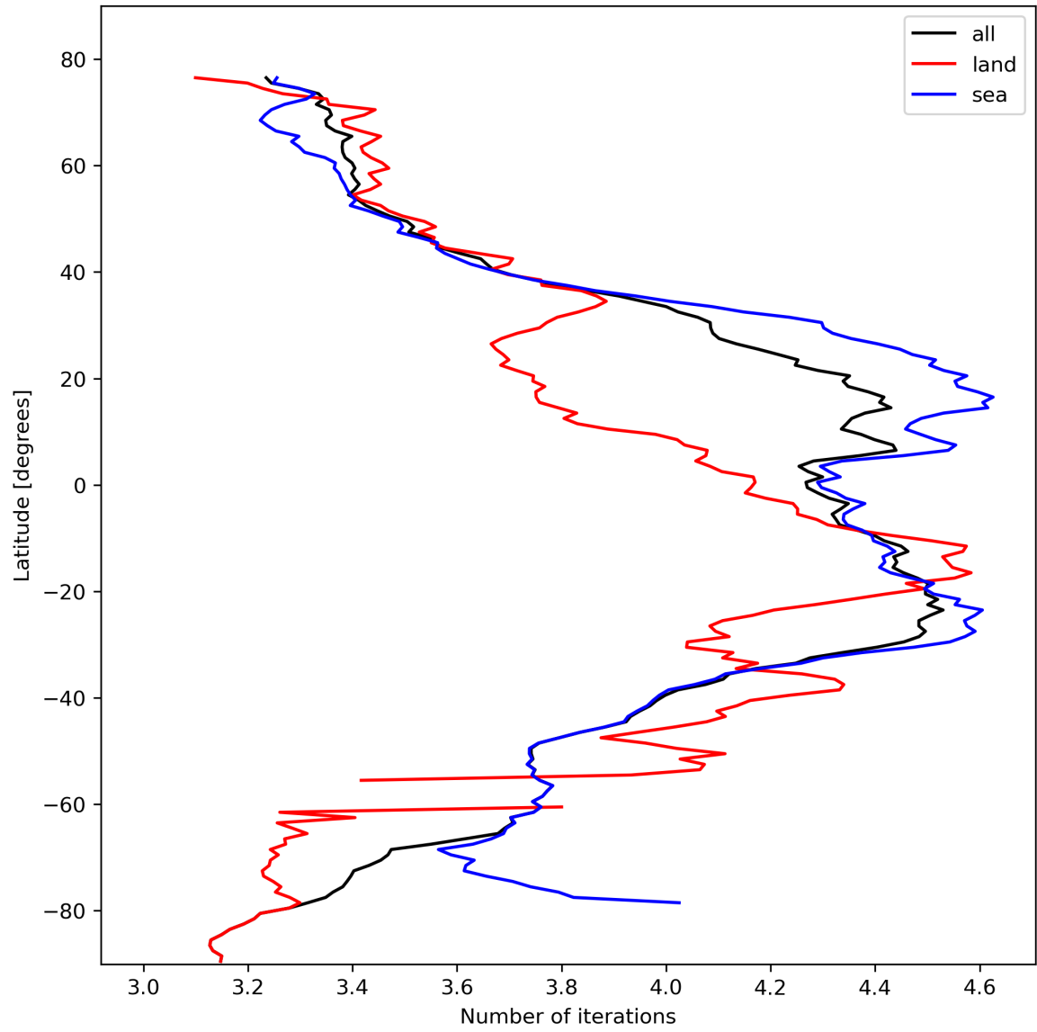
Figure 17: Zonal average of “Number of iterations” for 2023-10-23 to 2023-10-25.
