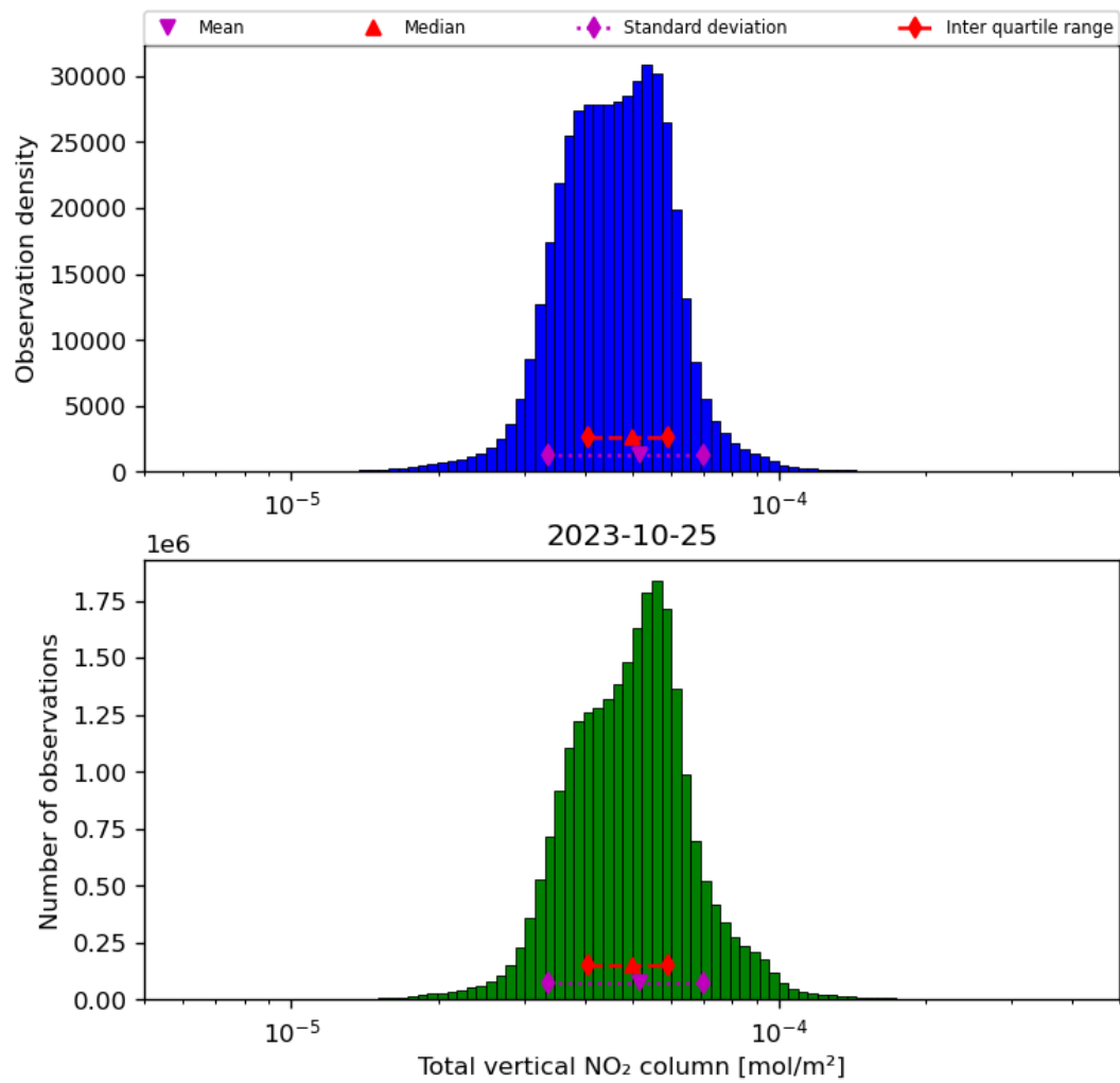
Figure 38: Histogram of "Total vertical NO 2 column" for 2023-10-24 to 2023-10-26
