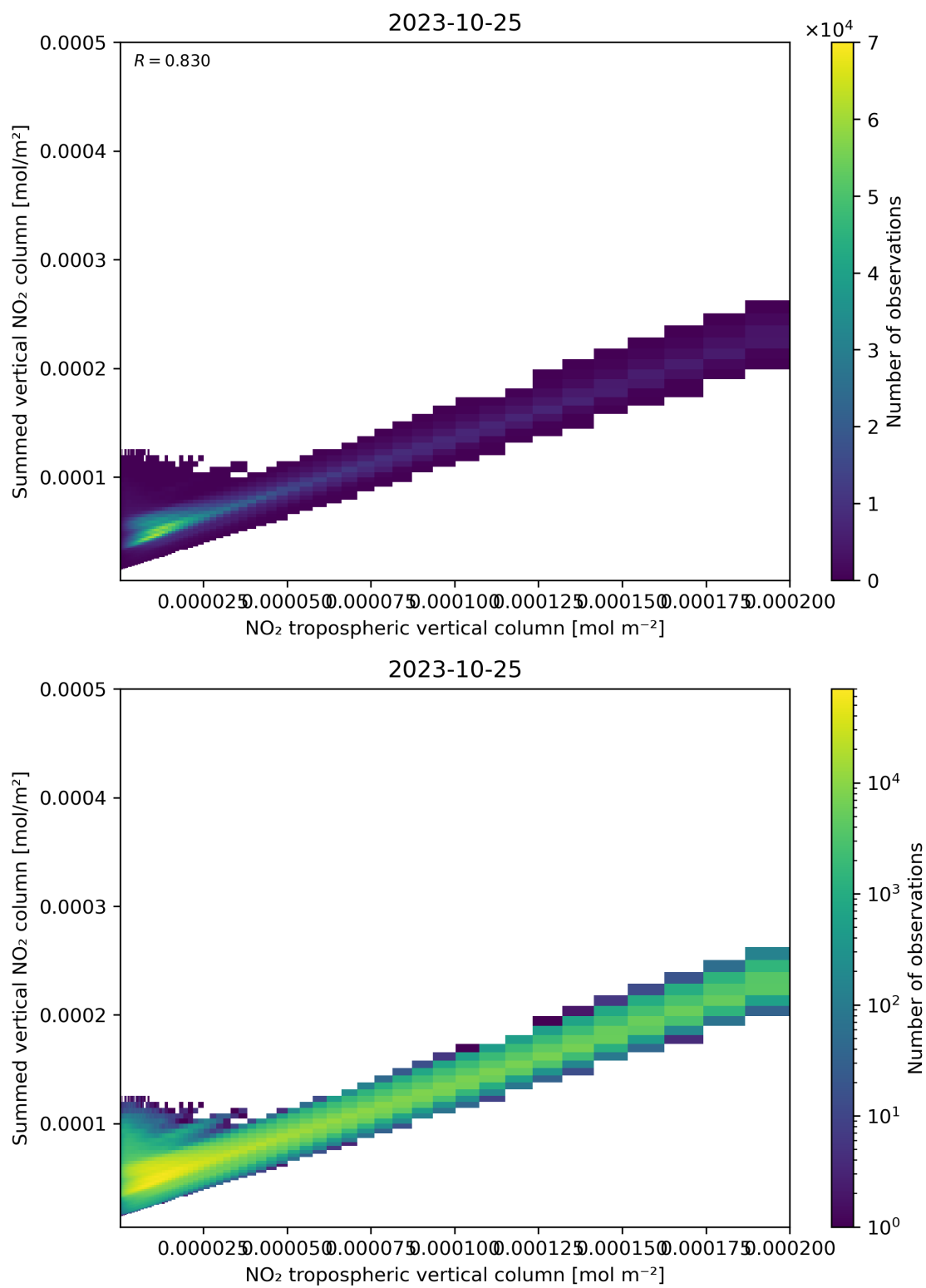
Figure 126: Scatter density plot of “NO 2 tropospheric vertical column” against “Summed vertical NO 2 column” for 2023-10-24 to 2023-10-26.
