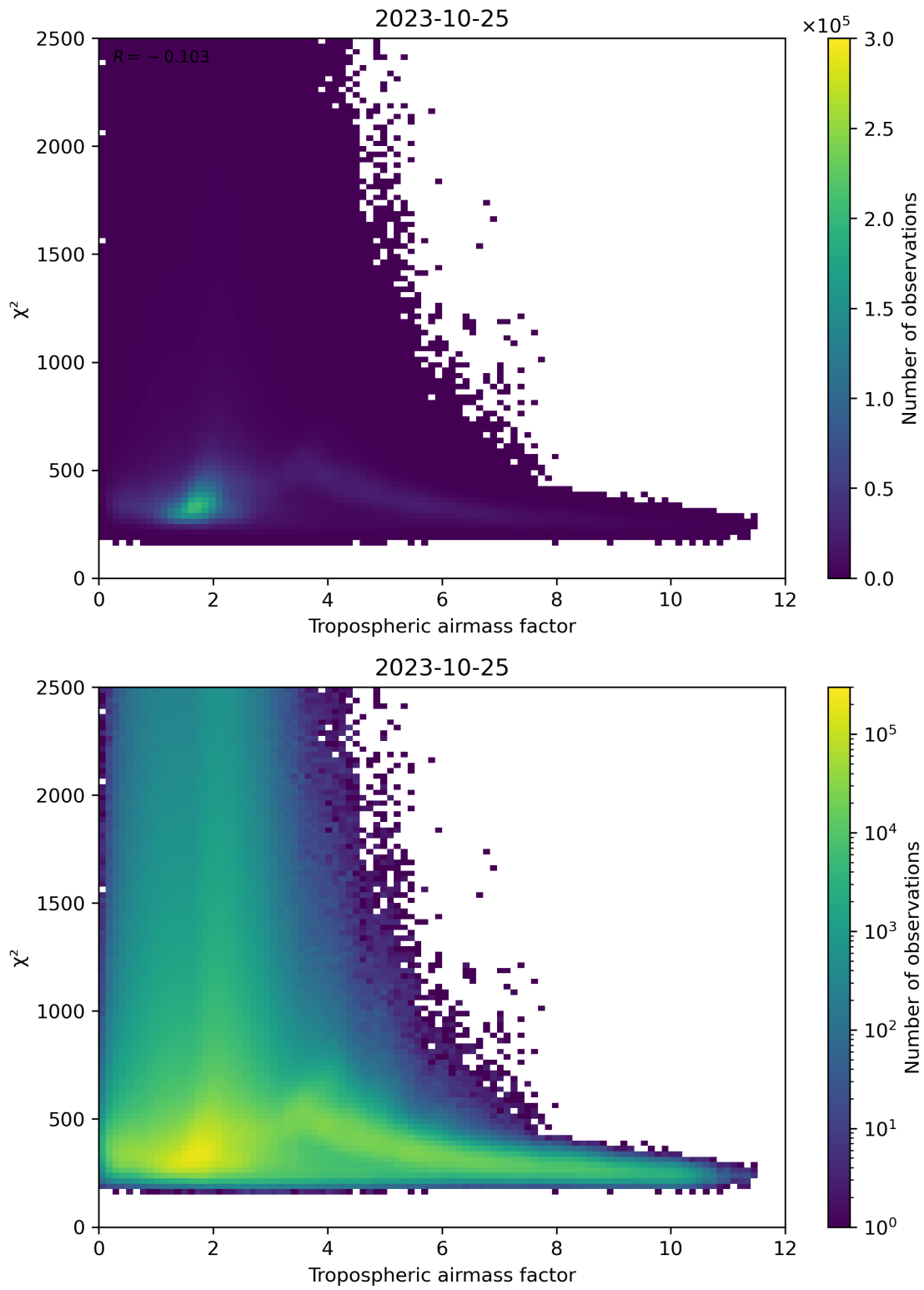
Figure 73: Scatter density plot of “Tropospheric airmass factor” against “ \chi^2 ” for 2023-10-24 to 2023-10-26.
