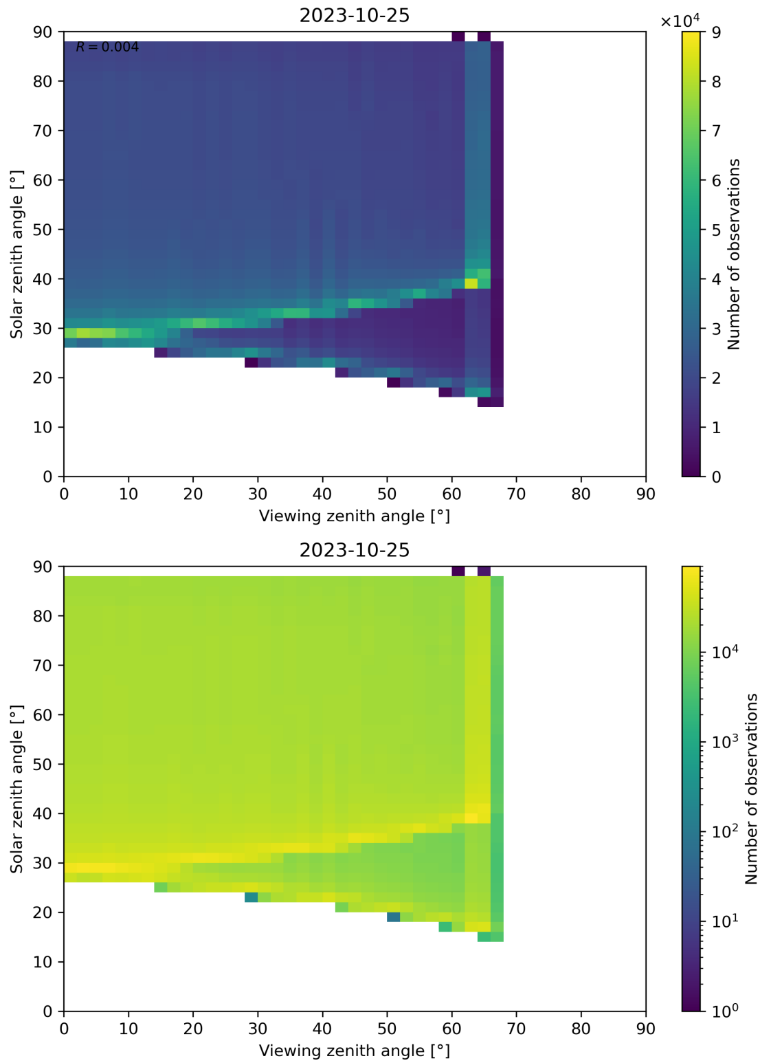
Figure 172: Scatter density plot of “Viewing zenith angle” against “Solar zenith angle” for 2023-10-24 to 2023-10-26.
