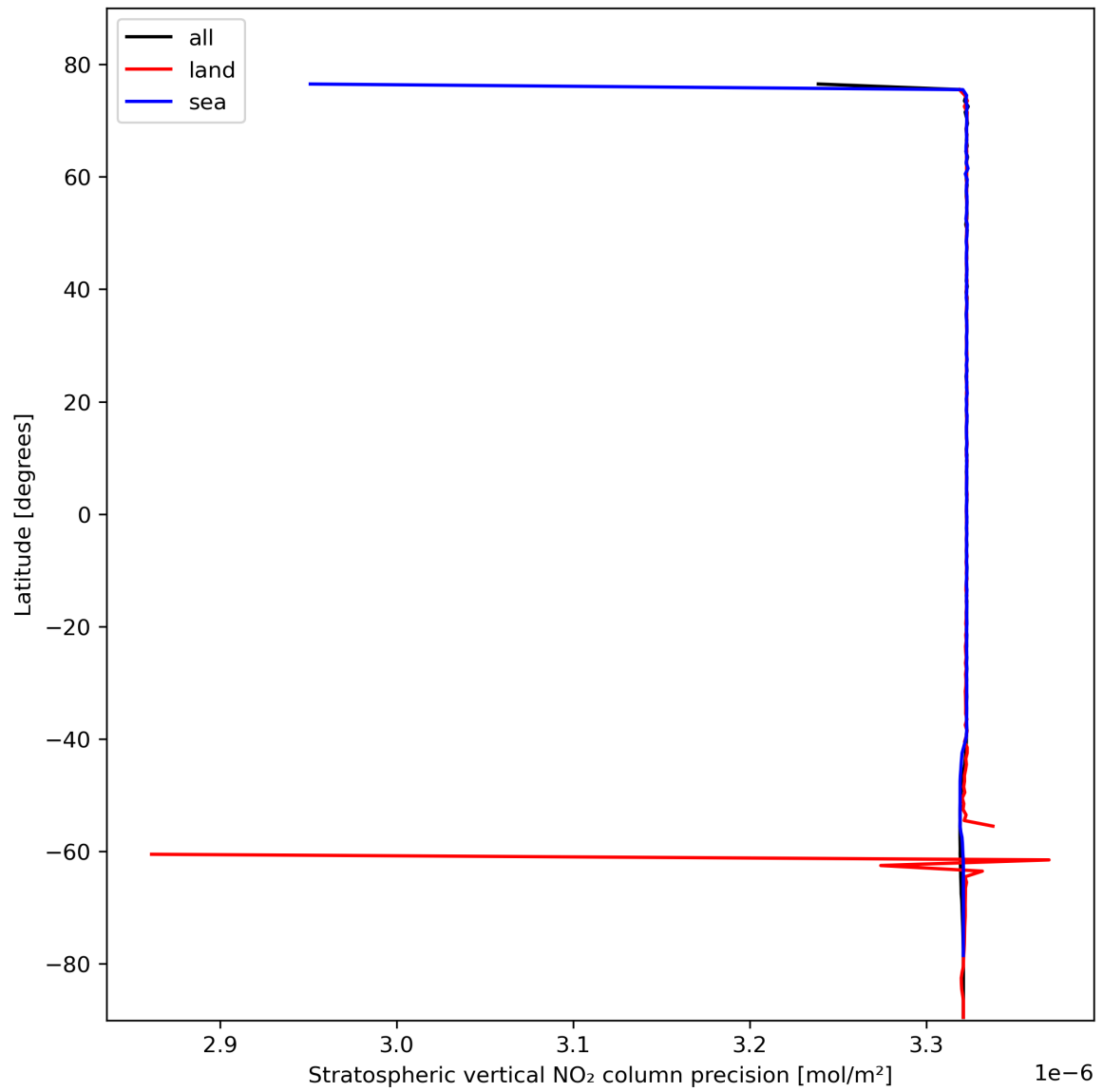
Figure 20: Zonal average of “Stratospheric vertical NO 2 column precision” for 2023-10-24 to 2023-10-26.
