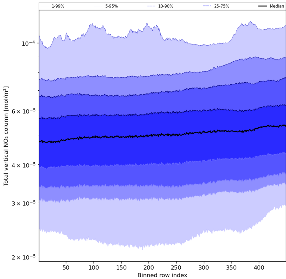
Figure 55: Along track statistics of “Total vertical NO 2 column” for 2023-10-24 to 2023-10-26
