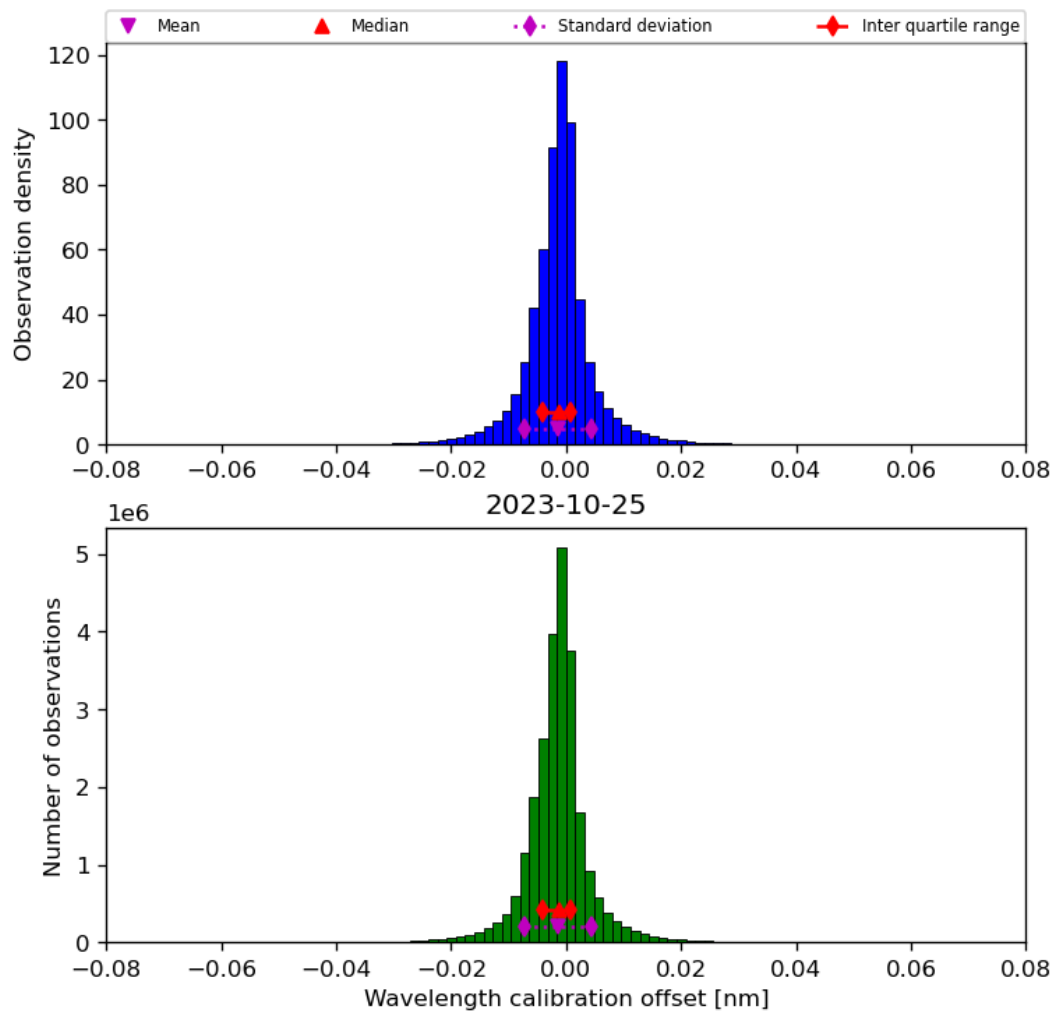
Figure 35: Histogram of “Wavelength calibration offset” for 2023-10-24 to 2023-10-26
