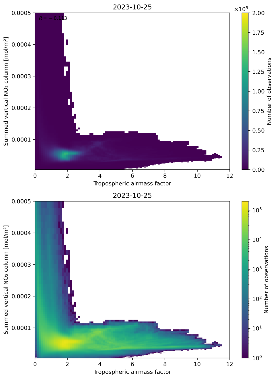
Figure 75: Scatter density plot of “Tropospheric airmass factor” against “Summed vertical NO 2 column” for 2023-10-24 to 2023-10-26.
