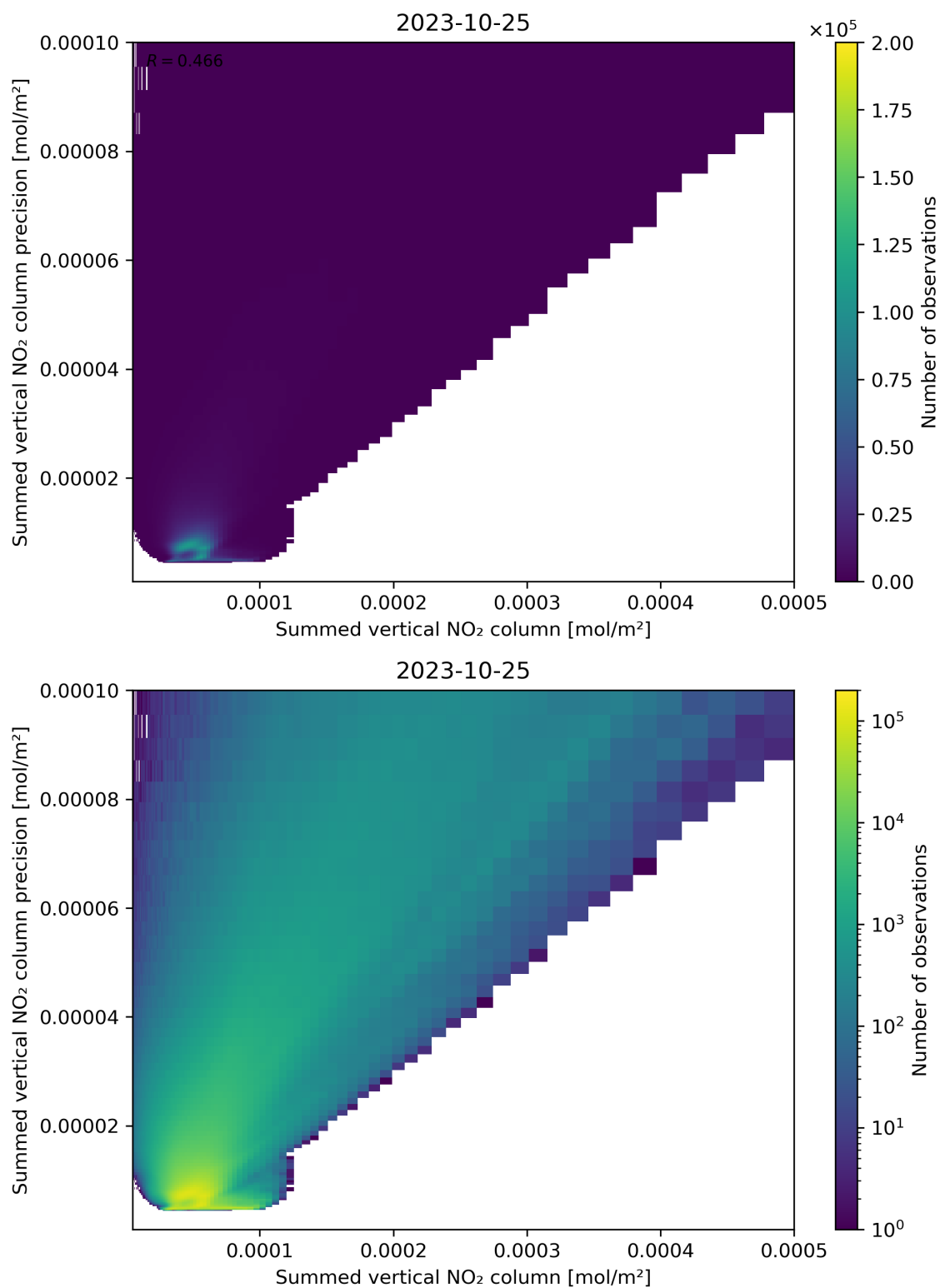
Figure 105: Scatter density plot of “Summed vertical NO 2 column” against “Summed vertical NO 2 column precision” for 2023-10-24 to 2023-10-26.
