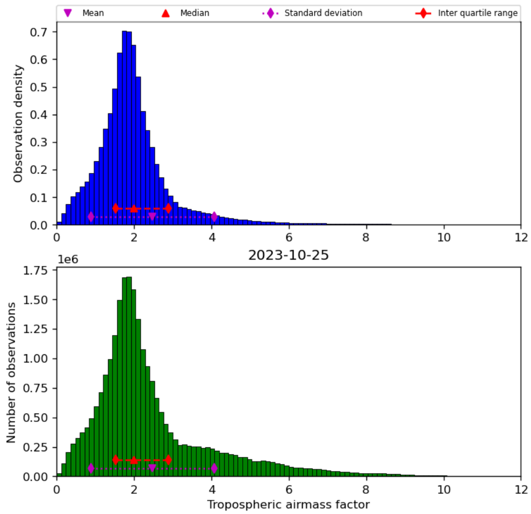
Figure 31: Histogram of “Tropospheric airmass factor” for 2023-10-24 to 2023-10-26
