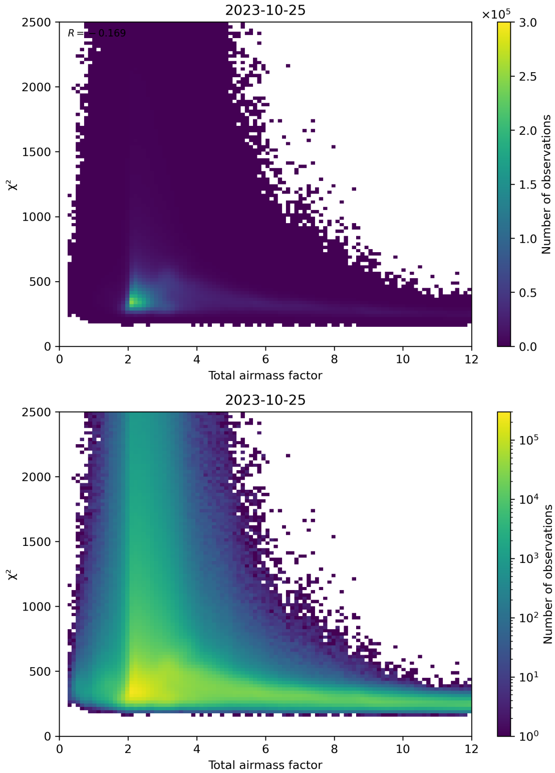
Figure 63: Scatter density plot of “Total airmass factor” against “ \chi^2 ” for 2023-10-24 to 2023-10-26.
