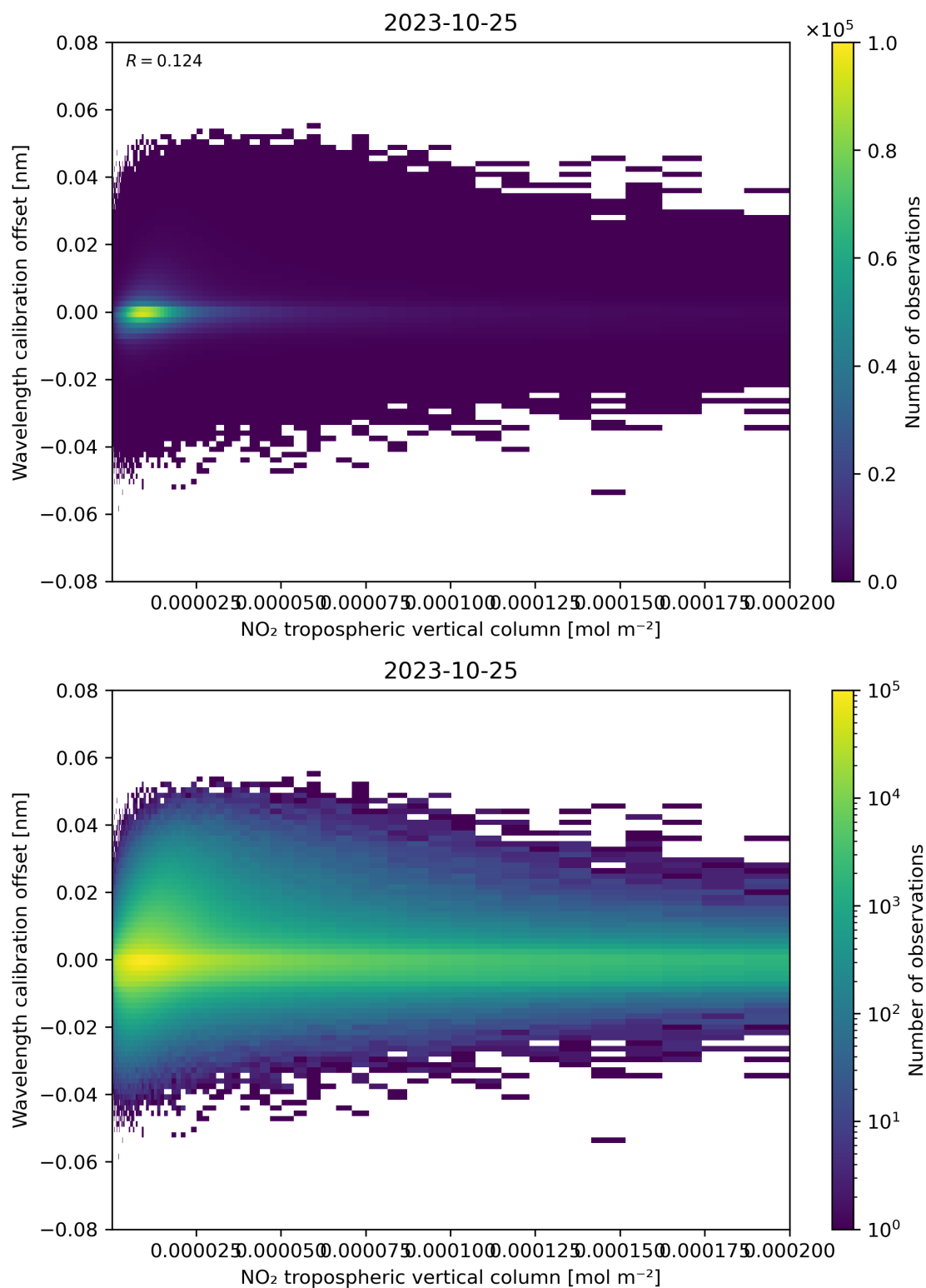
Figure 143: Scatter density plot of “NO 2 tropospheric vertical column” against “Wavelength calibration offset” for 2023-10-24 to 2023-10-26.
