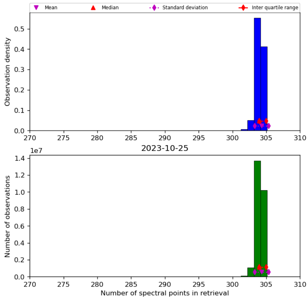
Figure 33: Histogram of “Number of spectral points in retrieval” for 2023-10-24 to 2023-10-26
