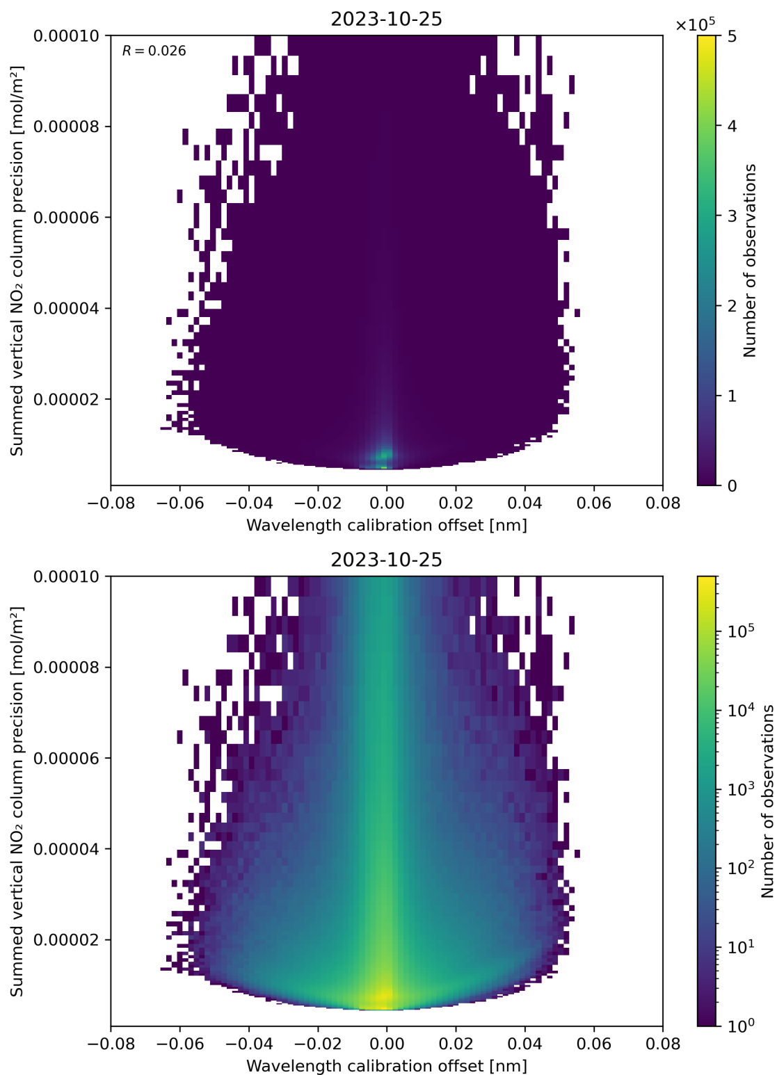
Figure 178: Scatter density plot of “Wavelength calibration offset” against “Summed vertical NO 2 column precision” for 2023-10-24 to 2023-10-26.
