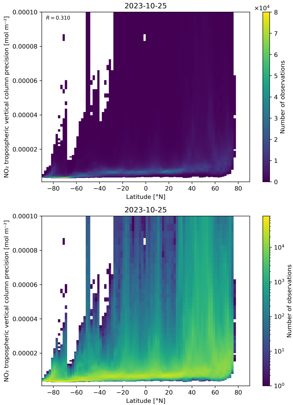
Figure 93: Scatter density plot of “Latitude” against “NO 2 tropospheric vertical column precision” for 2023-10-24 to 2023-10-26.
