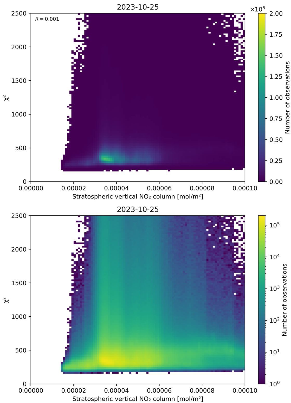
Figure 97: Scatter density plot of “Stratospheric vertical NO 2 column” against “ \chi^2 ” for 2023-10-24 to 2023-10-26.
