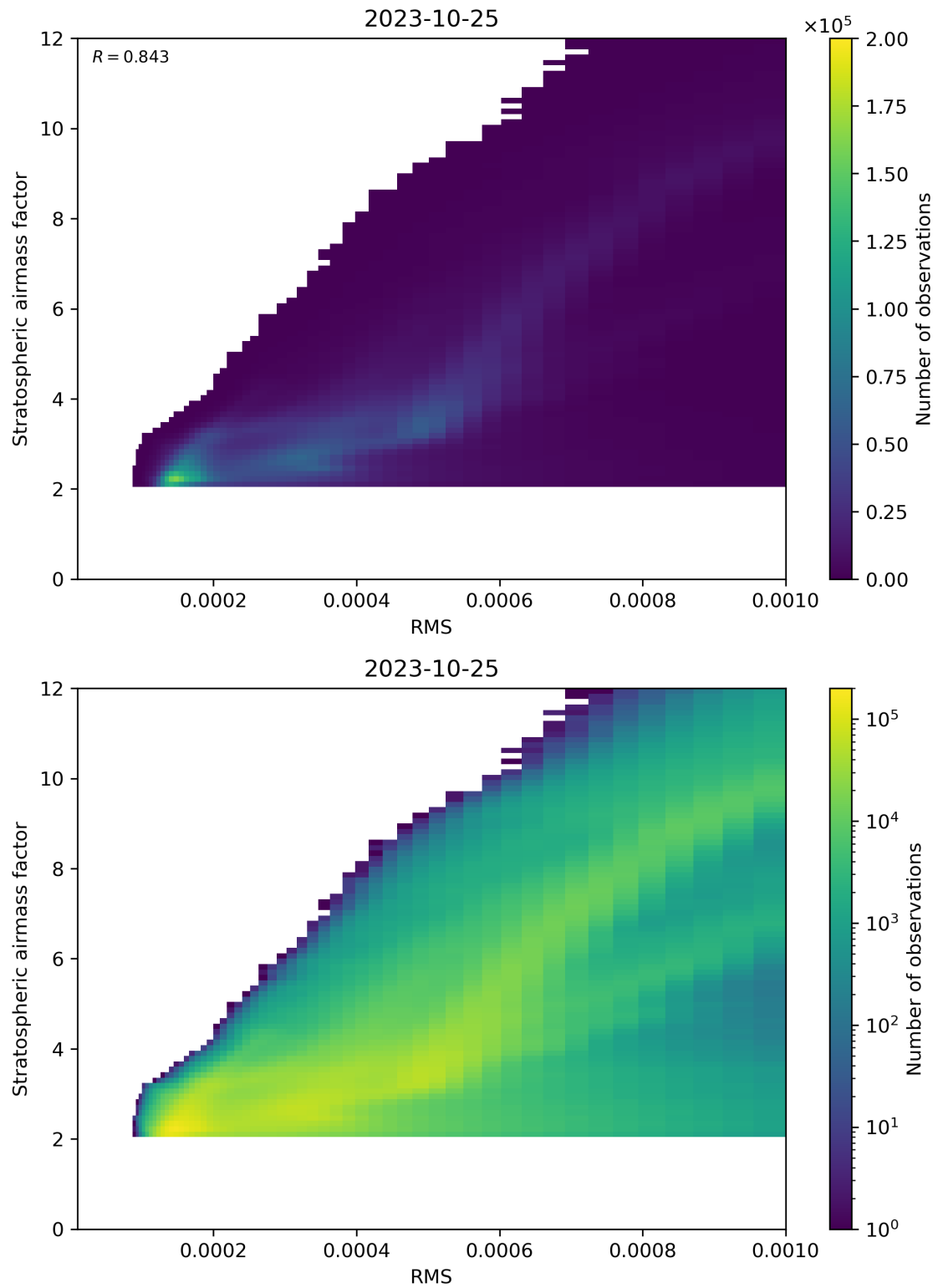
Figure 144: Scatter density plot of “RMS” against “Stratospheric airmass factor” for 2023-10-24 to 2023-10-26.
