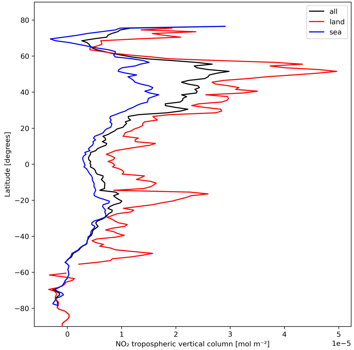
Figure 12: Zonal average of “NO 2 tropospheric vertical column” for 2023-10-24 to 2023-10-26.
