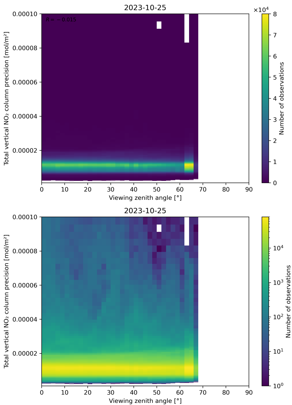
Figure 168: Scatter density plot of “Viewing zenith angle” against “Total vertical NO 2 column precision” for 2023-10-24 to 2023-10-26.
