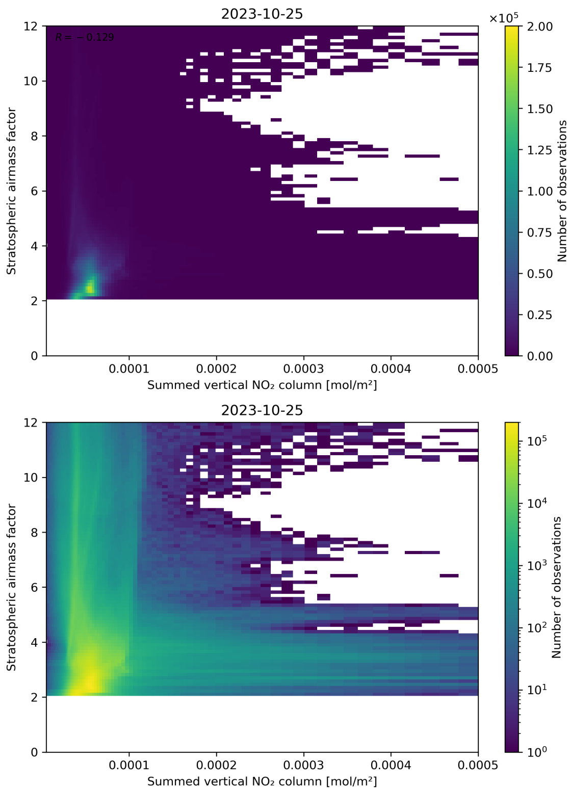
Figure 103: Scatter density plot of “Summed vertical NO 2 column” against “Stratospheric air mass factor” for 2023-10-24 to 2023-10-26.
