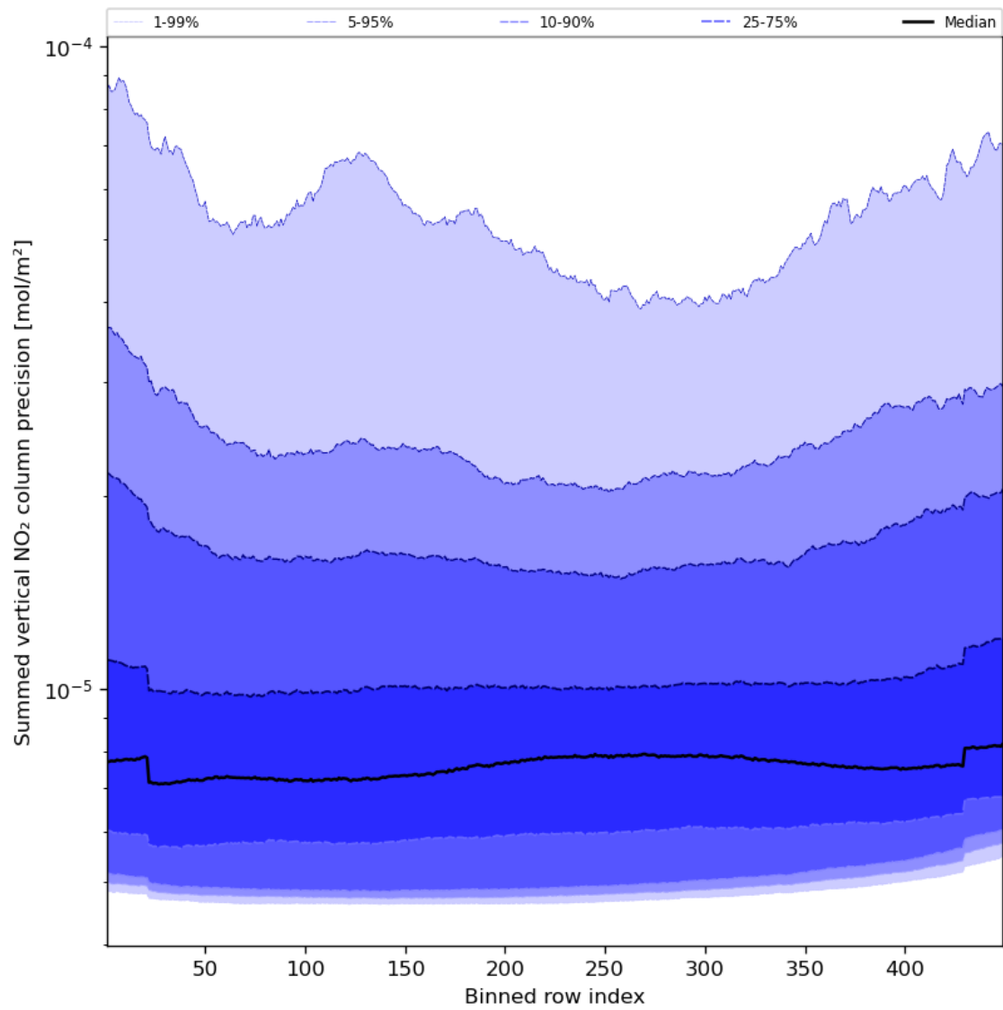
Figure 58: Along track statistics of “Summed vertical NO 2 column precision” for 2023-10-24 to 2023-10-26
