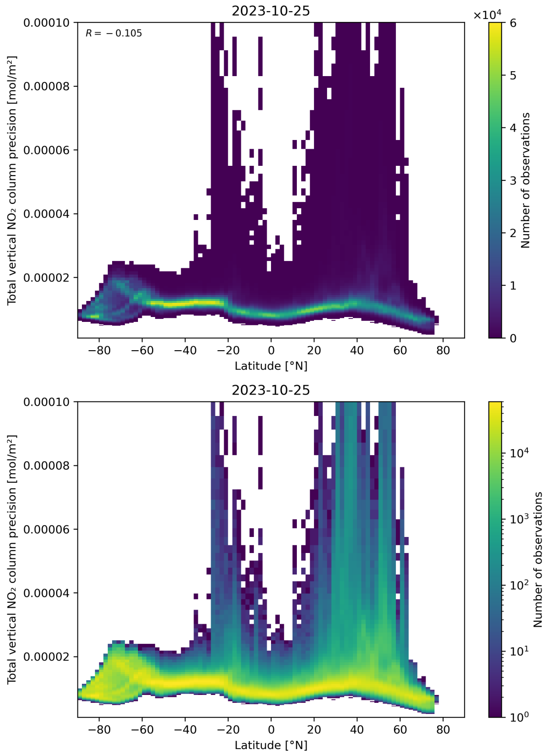
Figure 91: Scatter density plot of “Latitude” against “Total vertical NO 2 column precision” for 2023-10-24 to 2023-10-26.
