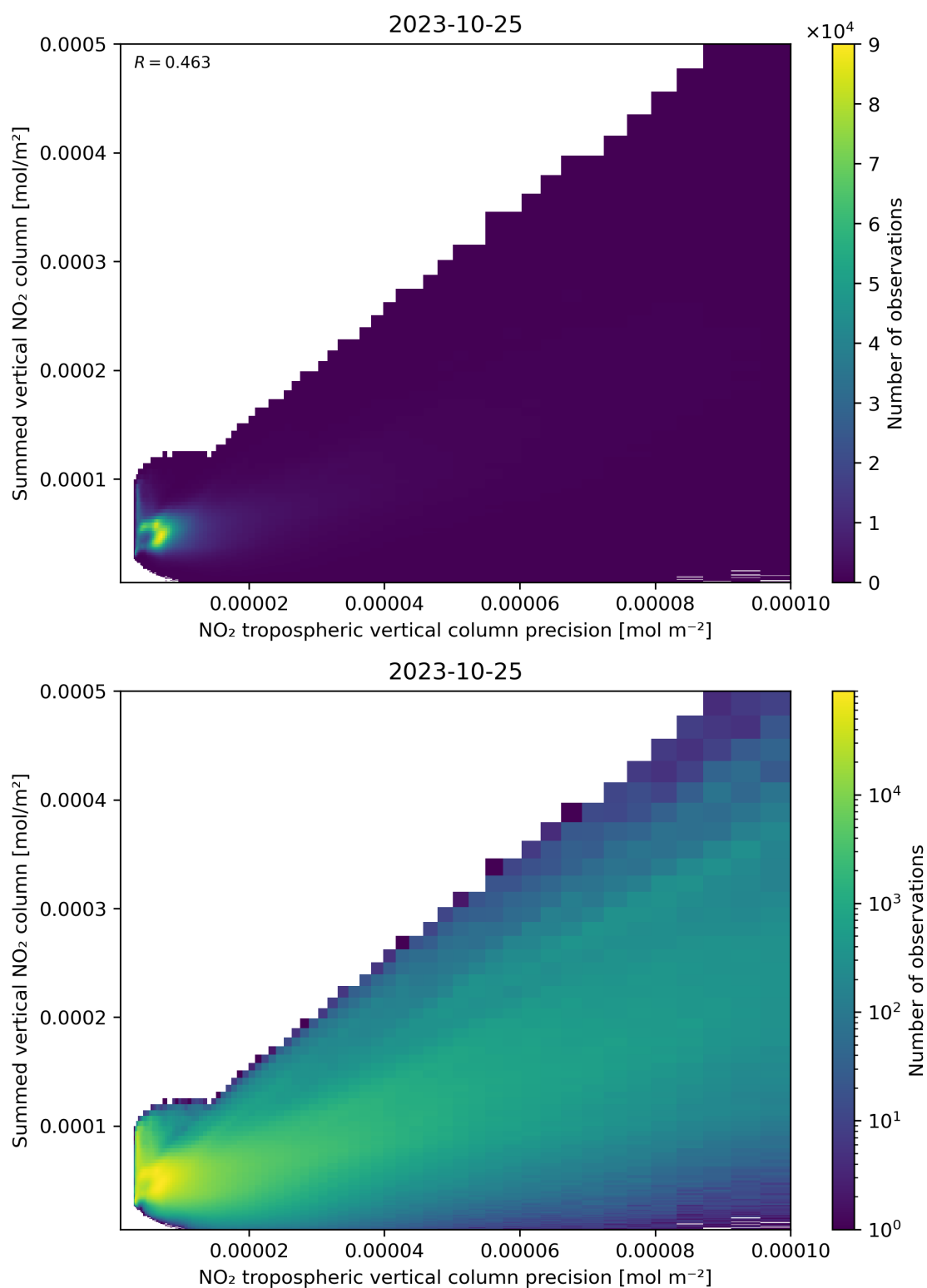
Figure 136: Scatter density plot of “NO 2 tropospheric vertical column precision” against “Summed vertical NO 2 column” for 2023-10-24 to 2023-10-26.
