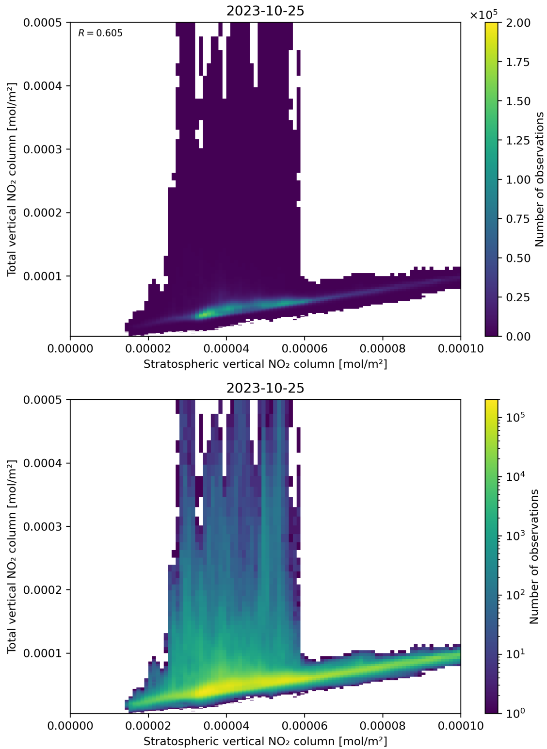
Figure 100: Scatter density plot of “Stratospheric vertical NO 2 column” against “Total vertical NO 2 column” for 2023-10-24 to 2023-10-26.
