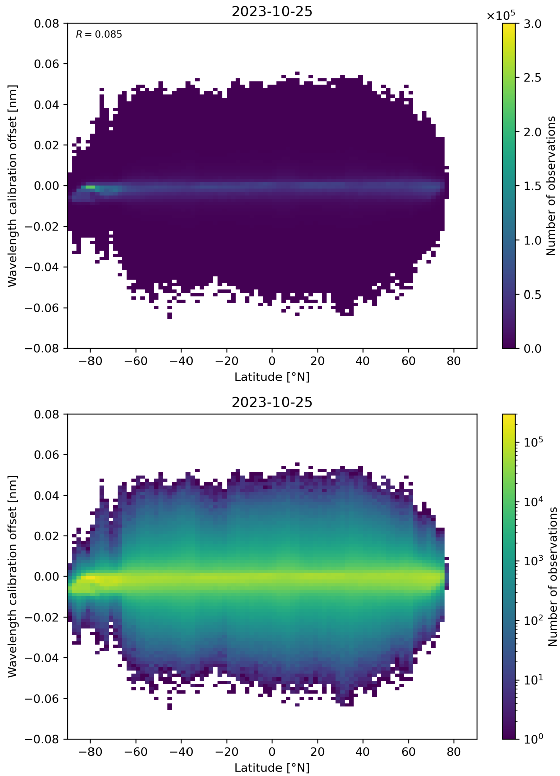
Figure 95: Scatter density plot of “Latitude” against “Wavelength calibration offset” for 2023-10-24 to 2023-10-26.
