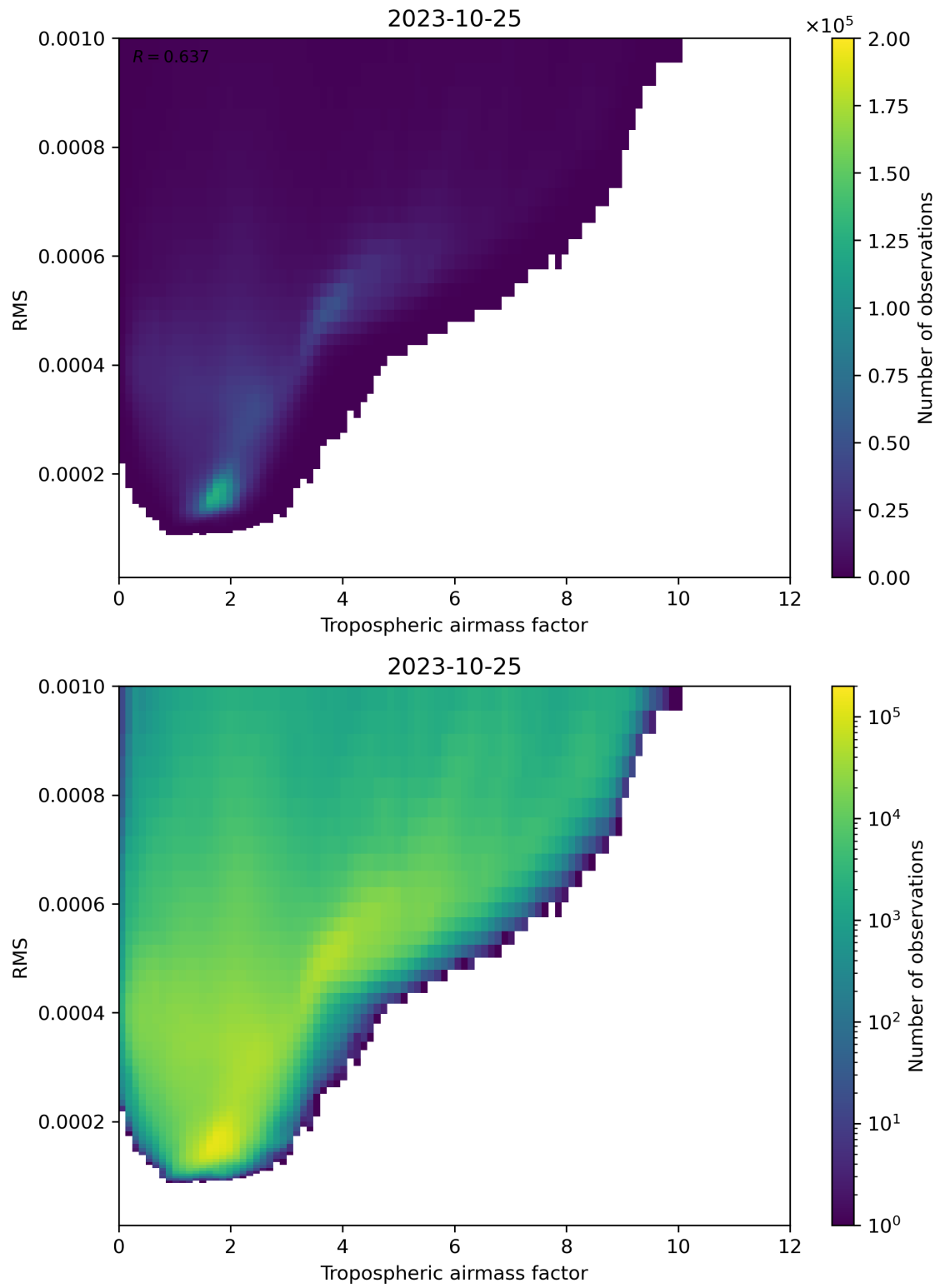
Figure 79: Scatter density plot of “Tropospheric airmass factor” against “RMS” for 2023-10-24 to 2023-10-26.
