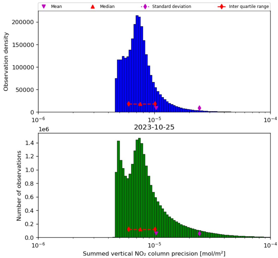
Figure 41: Histogram of "Summed vertical NO 2 column precision" for 2023-10-24 to 2023-10-26
