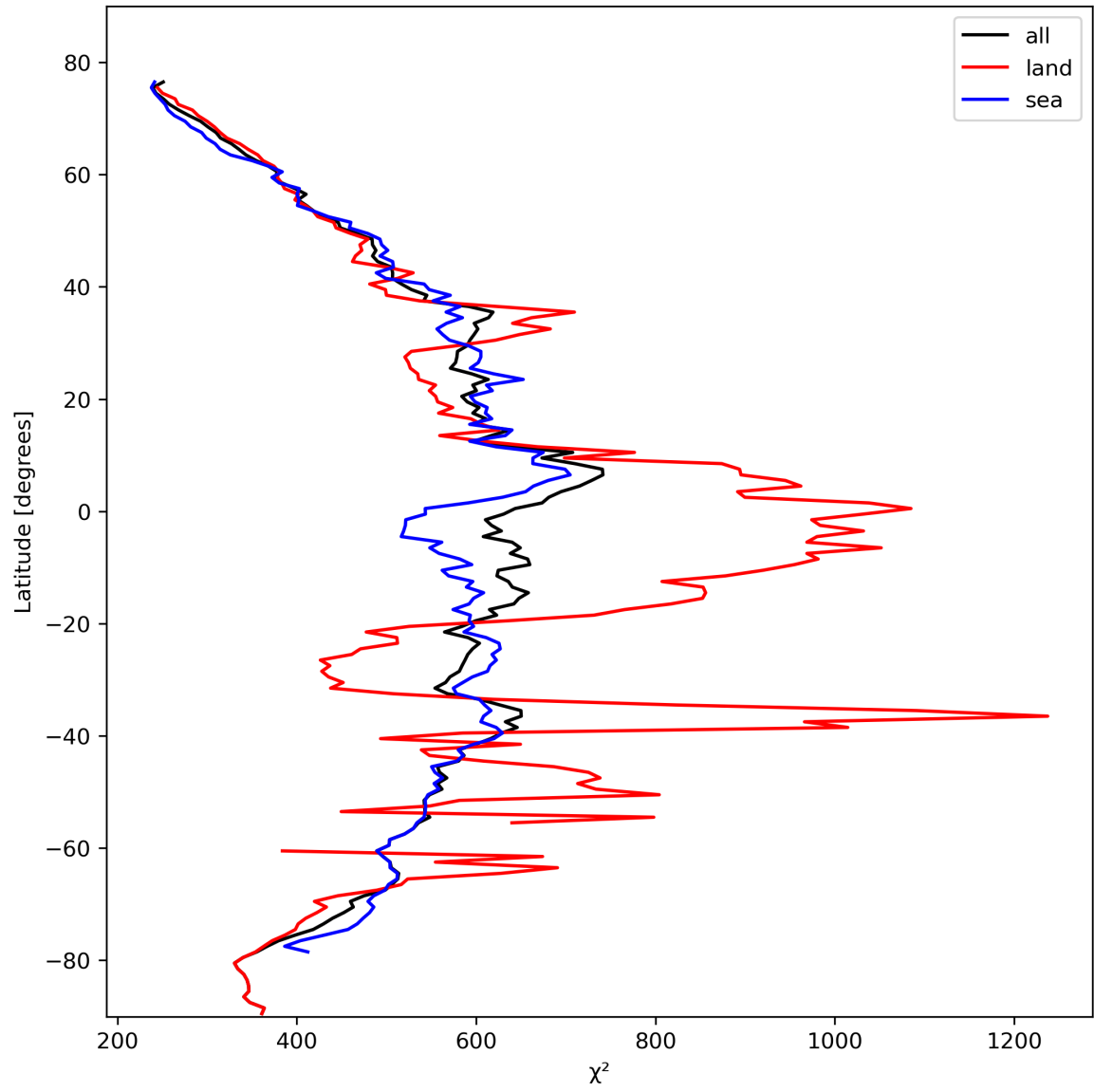
Figure 25: Zonal average of “ \chi^2 ” for 2023-10-24 to 2023-10-26.
