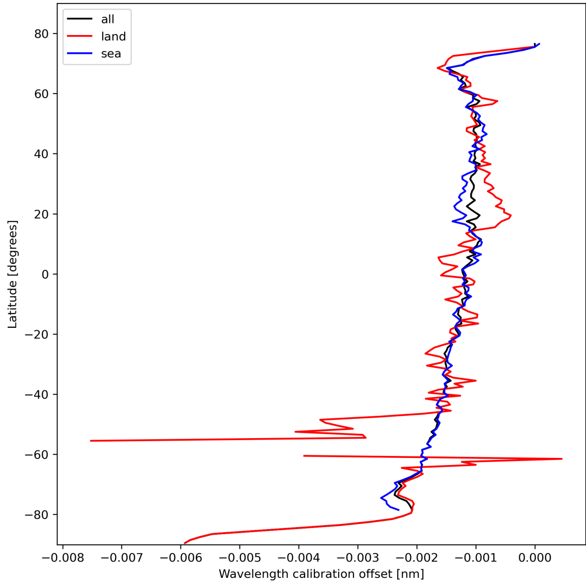
Figure 18: Zonal average of “Wavelength calibration offset” for 2023-10-24 to 2023-10-26.
