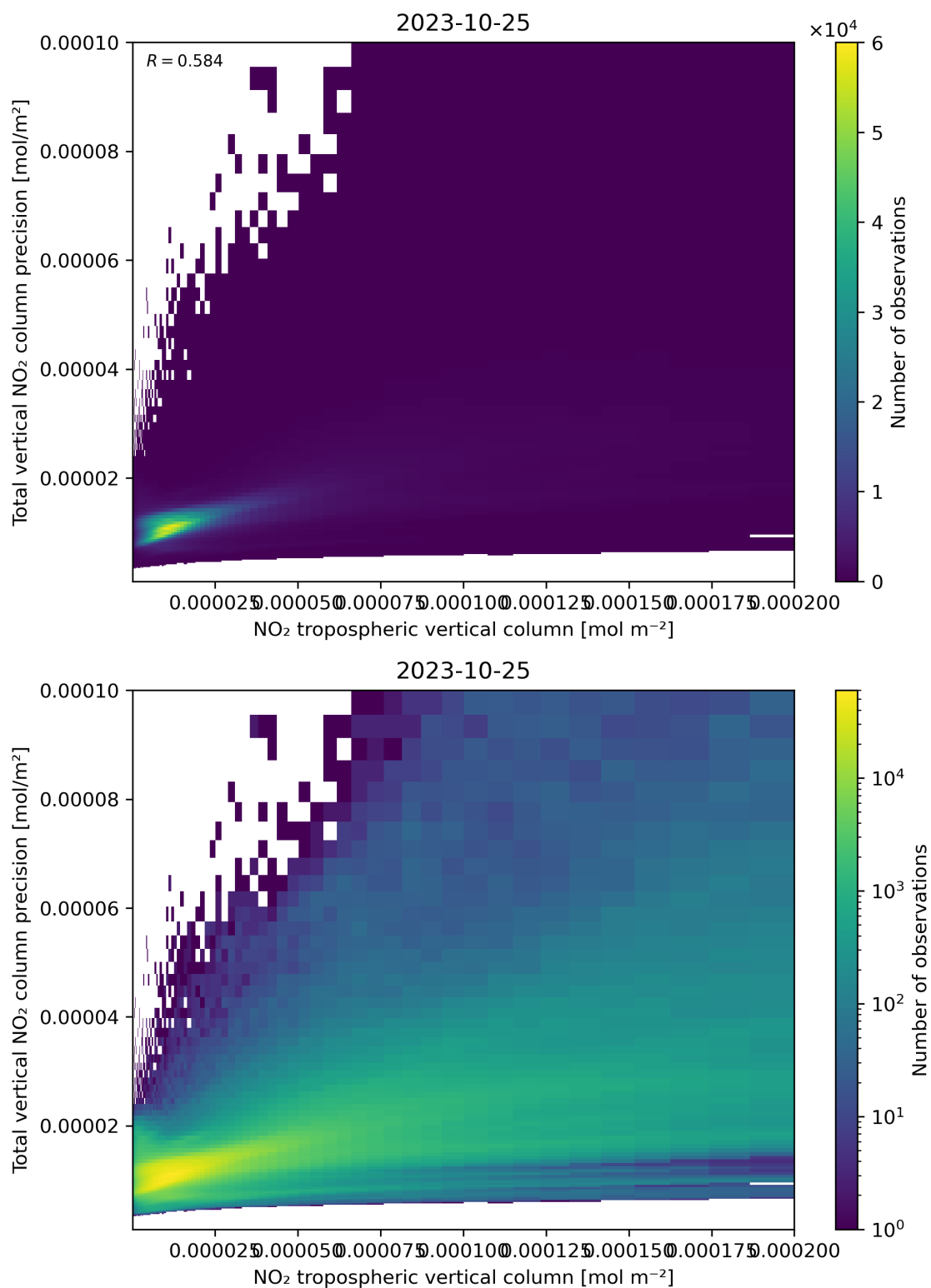
Figure 129: Scatter density plot of “NO 2 tropospheric vertical column” against “Total vertical NO 2 column precision” for 2023-10-24 to 2023-10-26.
