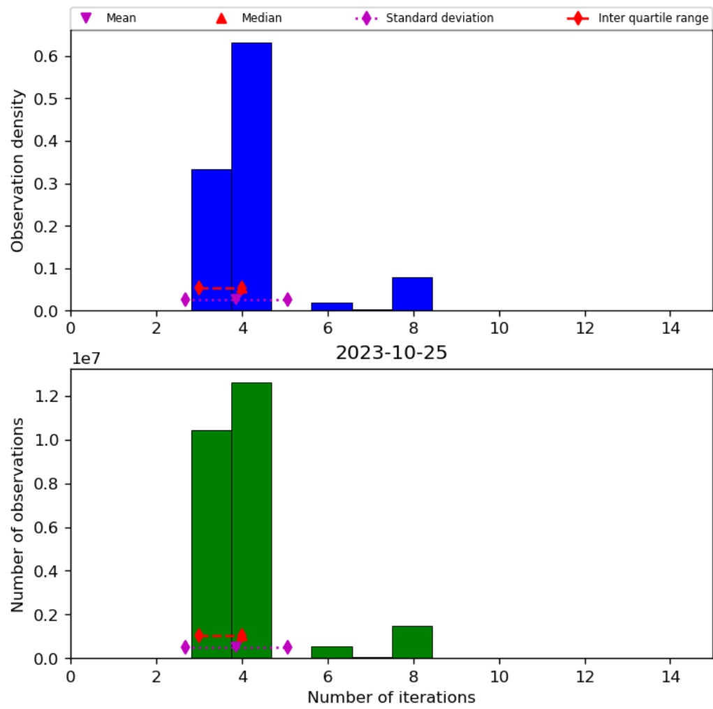
Figure 34: Histogram of “Number of iterations” for 2023-10-24 to 2023-10-26
