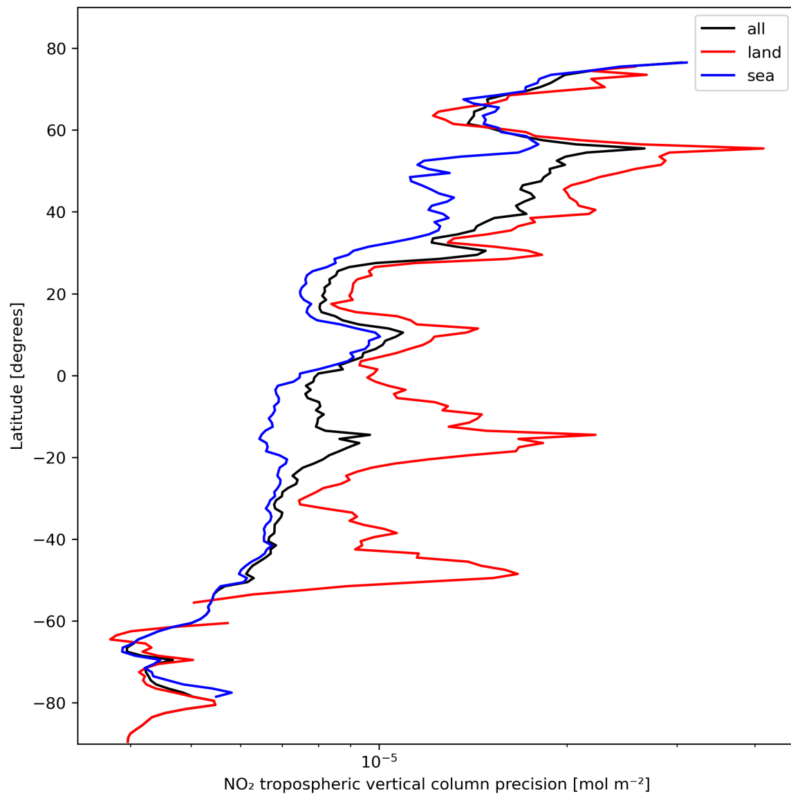
Figure 13: Zonal average of “NO 2 tropospheric vertical column precision” for 2023-10-24 to 2023-10-26.
