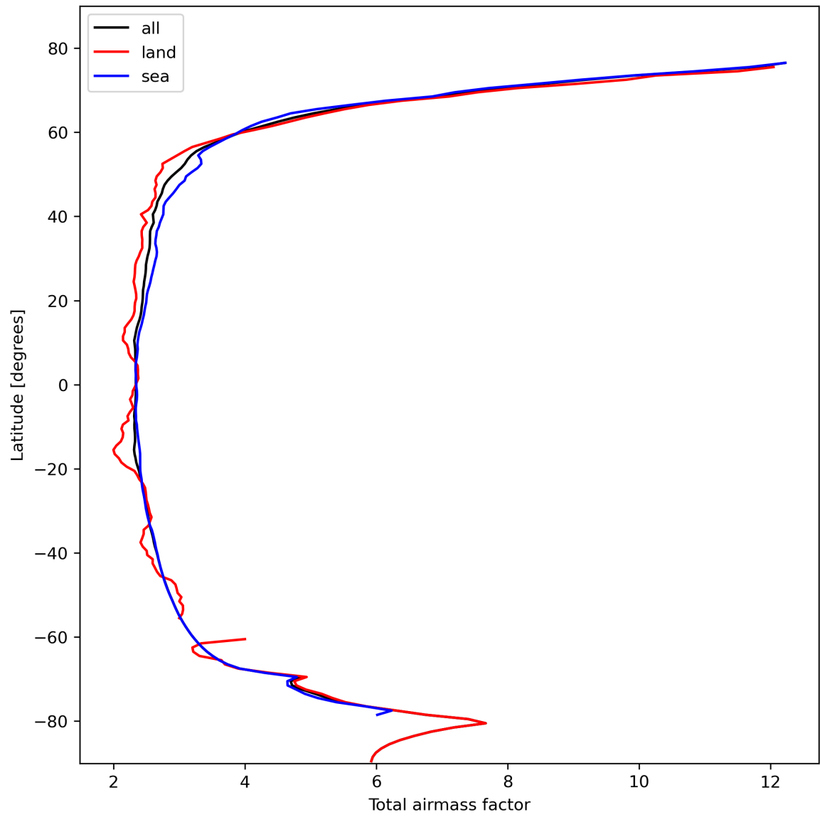
Figure 15: Zonal average of “Total airmass factor” for 2023-10-24 to 2023-10-26.
