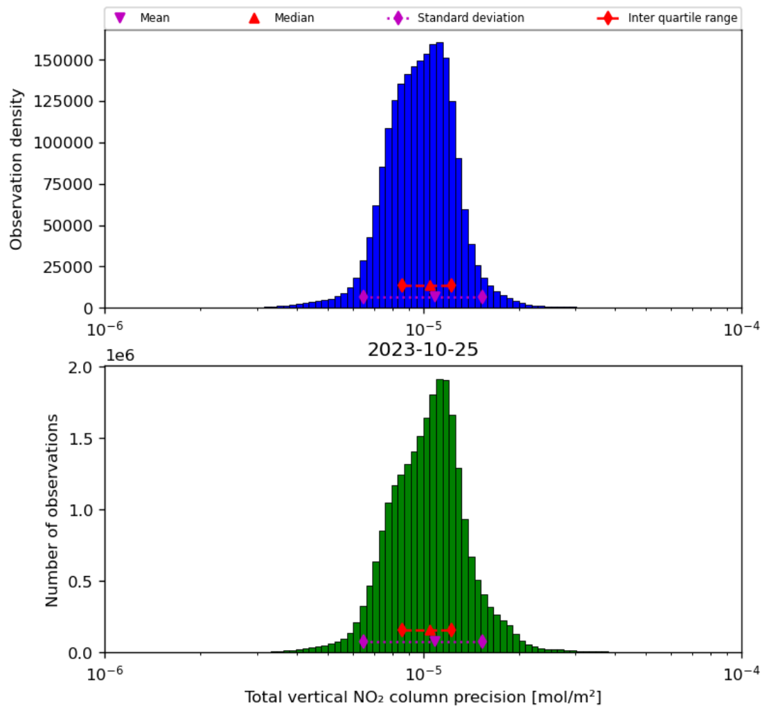
Figure 39: Histogram of "Total vertical NO 2 column precision" for 2023-10-24 to 2023-10-26
