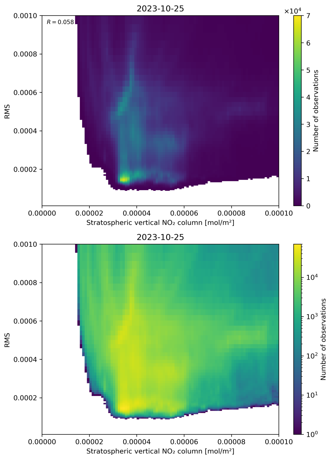
Figure 102: Scatter density plot of “Stratospheric vertical NO 2 column” against “RMS” for 2023-10-24 to 2023-10-26.
