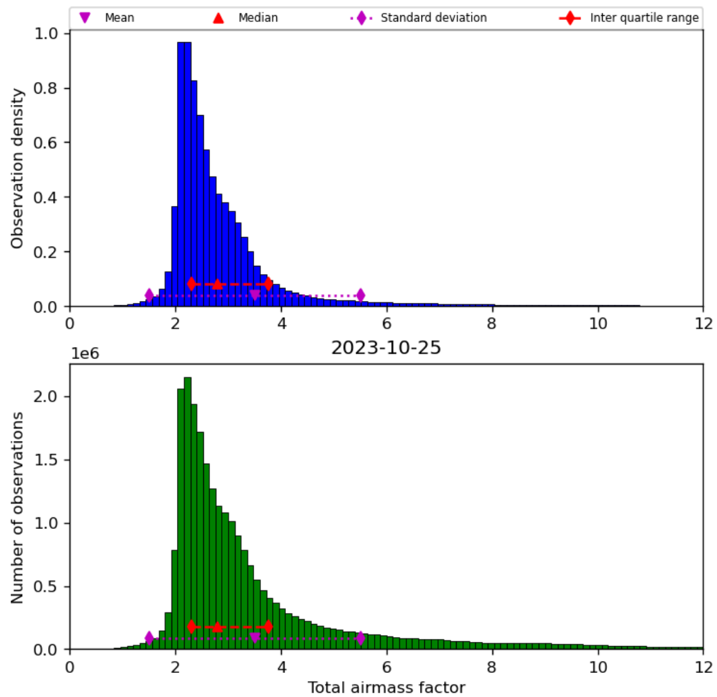
Figure 32: Histogram of “Total airmass factor” for 2023-10-24 to 2023-10-26
