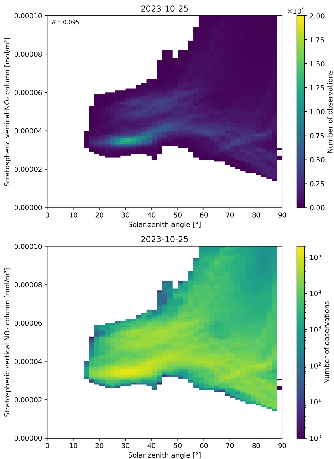
Figure 150: Scatter density plot of “Solar zenith angle” against “Stratospheric vertical NO 2 column” for 2023-10-24 to 2023-10-26.
