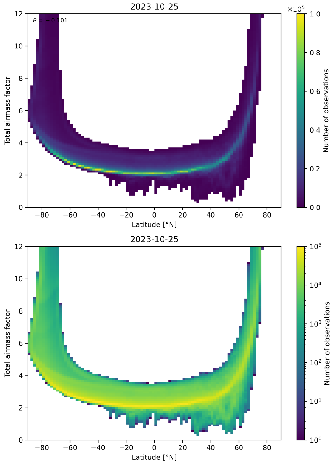
Figure 84: Scatter density plot of “Latitude” against “Total airmass factor” for 2023-10-24 to 2023-10-26.
