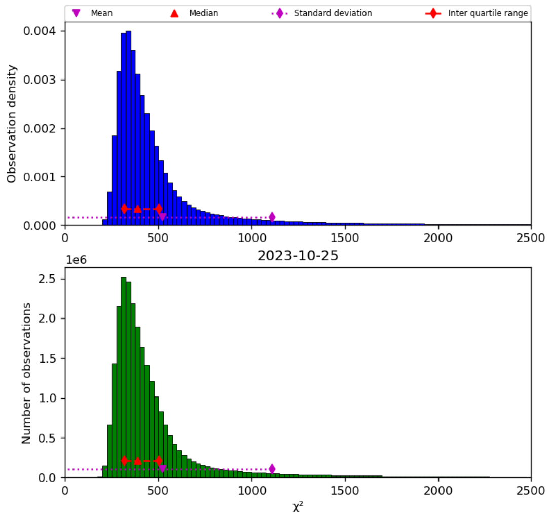
Figure 42: Histogram of “ \chi^2 ” for 2023-10-24 to 2023-10-26
