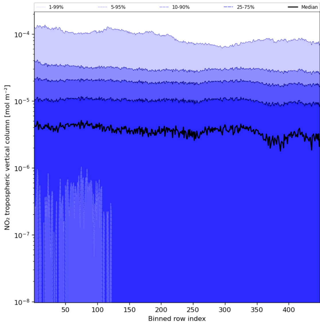
Figure 46: Along track statistics of “NO 2 tropospheric vertical column” for 2023-10-24 to 2023-10-26
