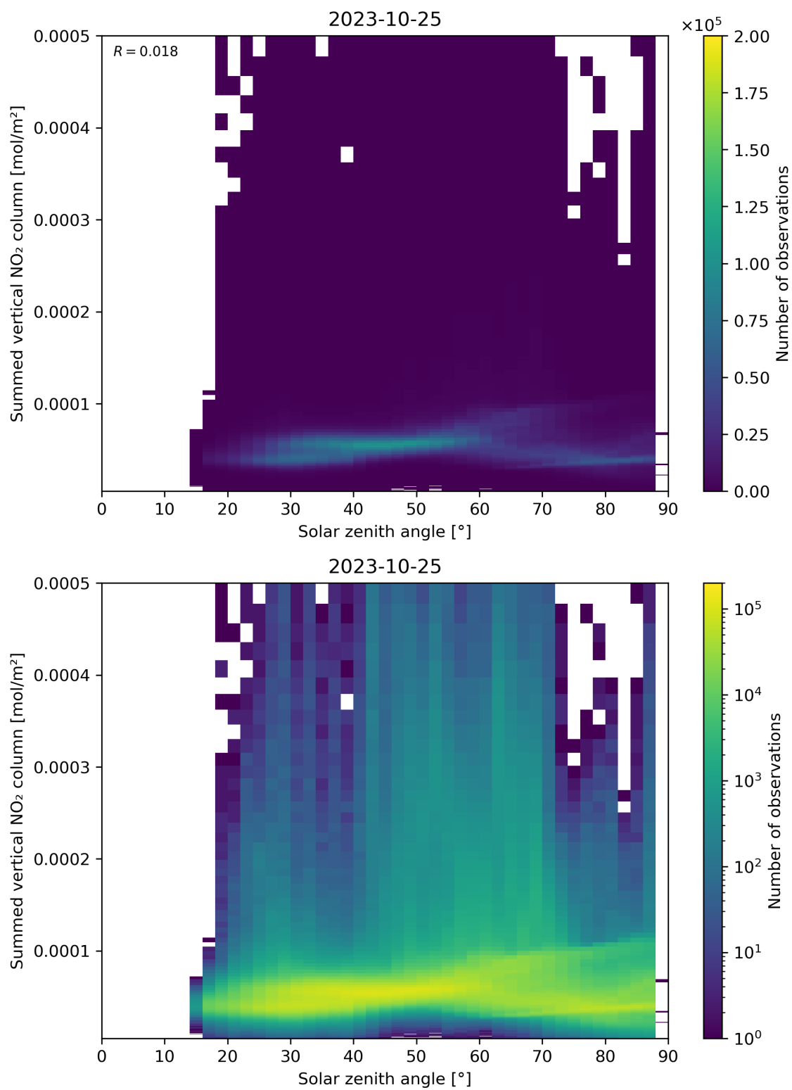
Figure 151: Scatter density plot of “Solar zenith angle” against “Summed vertical NO 2 column” for 2023-10-24 to 2023-10-26.
