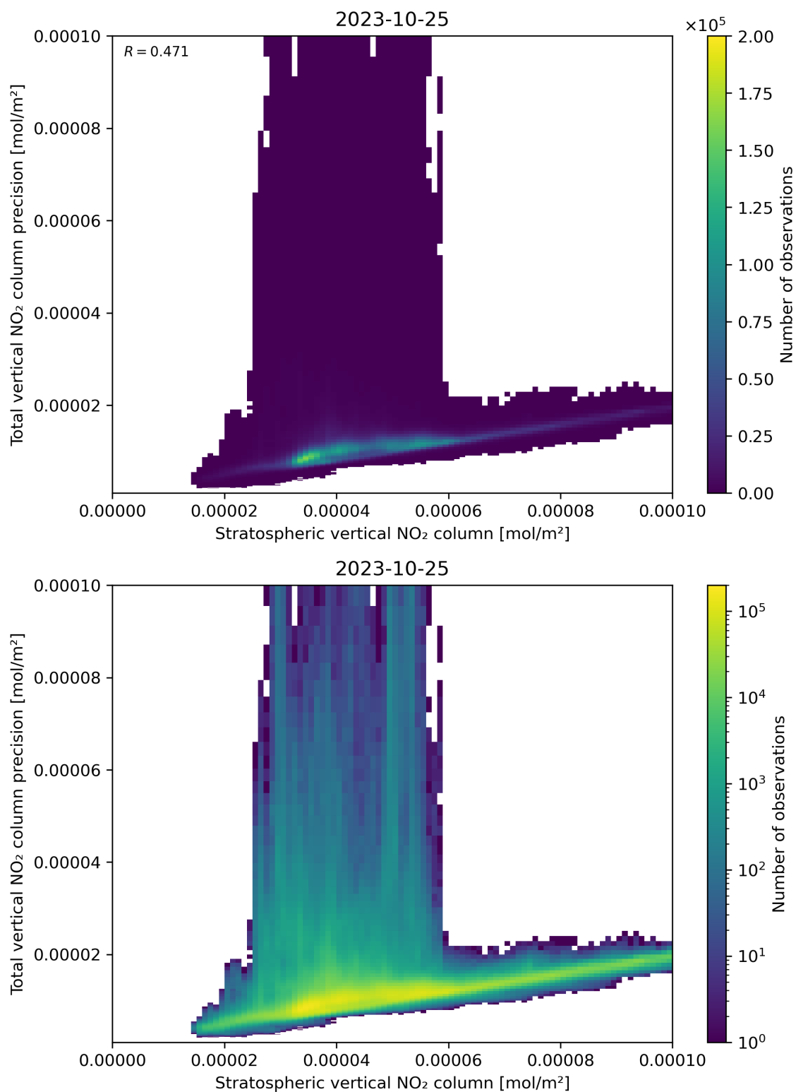
Figure 101: Scatter density plot of “Stratospheric vertical NO 2 column” against “Total vertical NO 2 column precision” for 2023-10-24 to 2023-10-26.
