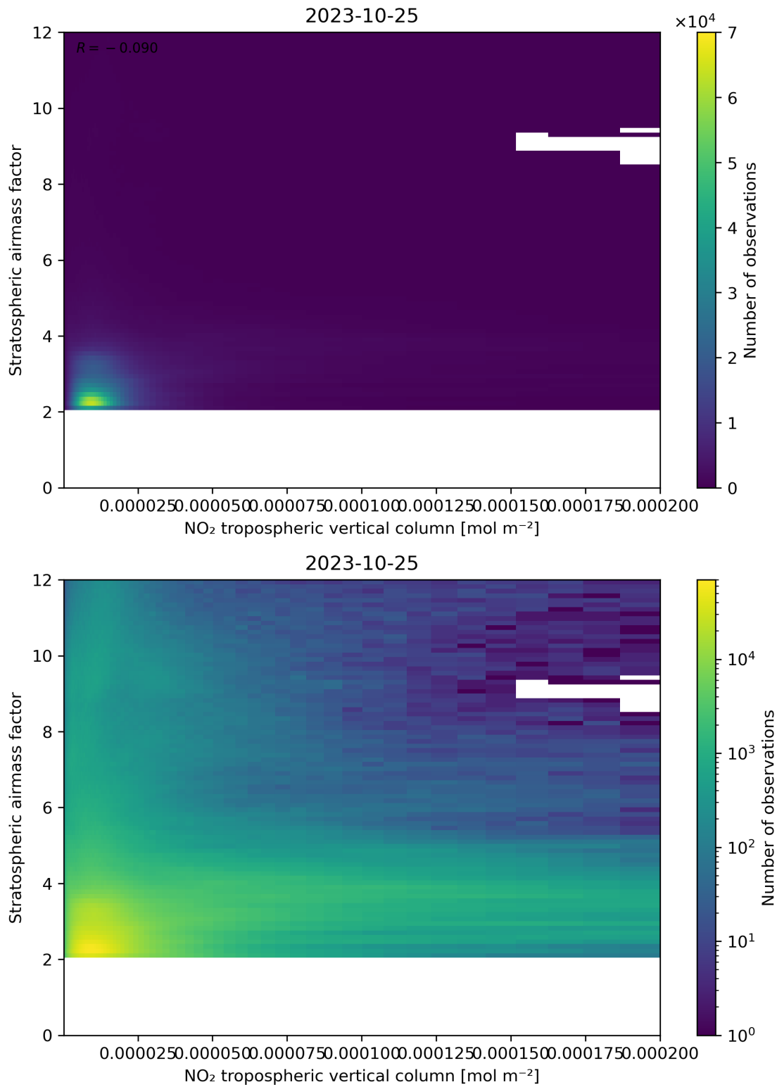
Figure 121: Scatter density plot of “NO 2 tropospheric vertical column” against “Stratospheric airmass factor” for 2023-10-24 to 2023-10-26.
