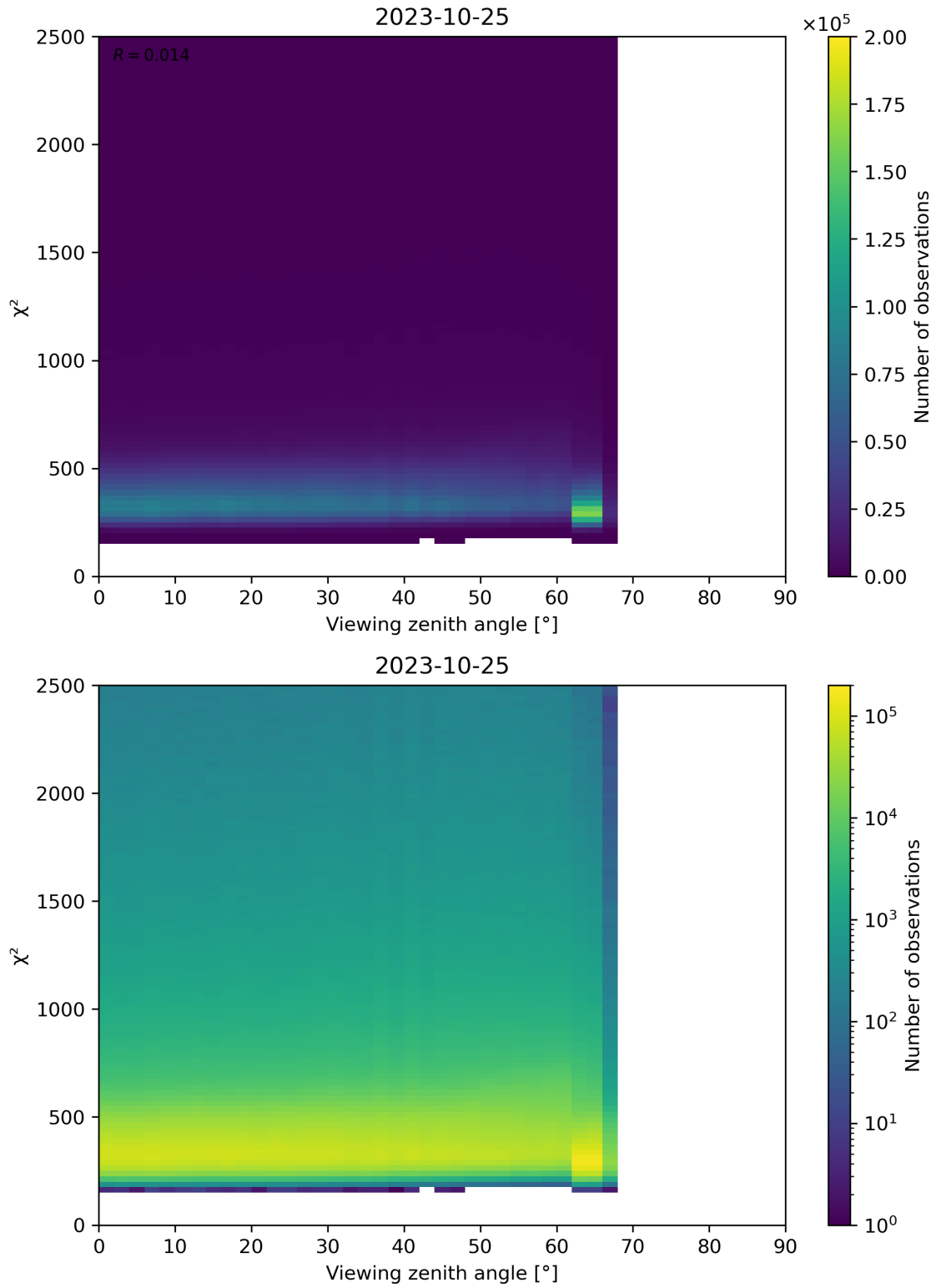
Figure 162: Scatter density plot of “Viewing zenith angle” against “ \chi^2 ” for 2023-10-24 to 2023-10-26.
