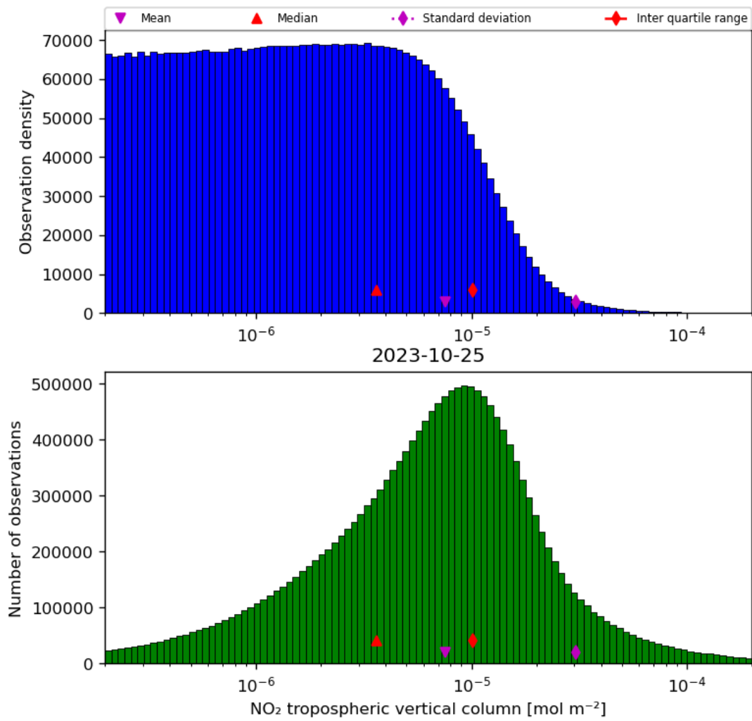
Figure 29: Histogram of “NO 2 tropospheric vertical column” for 2023-10-24 to 2023-10-26
