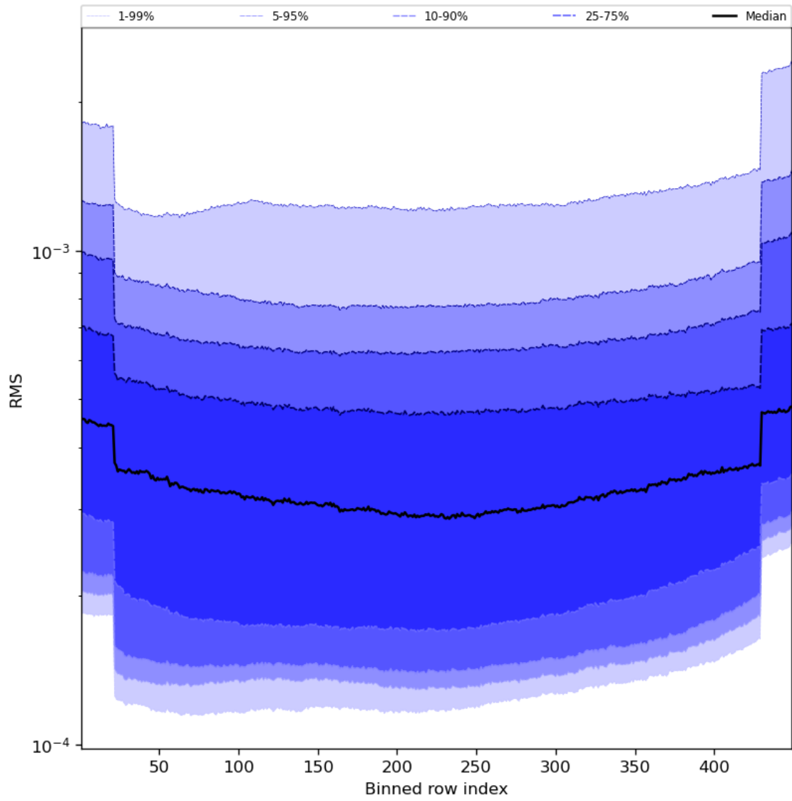
Figure 60: Along track statistics of “RMS” for 2023-10-24 to 2023-10-26
