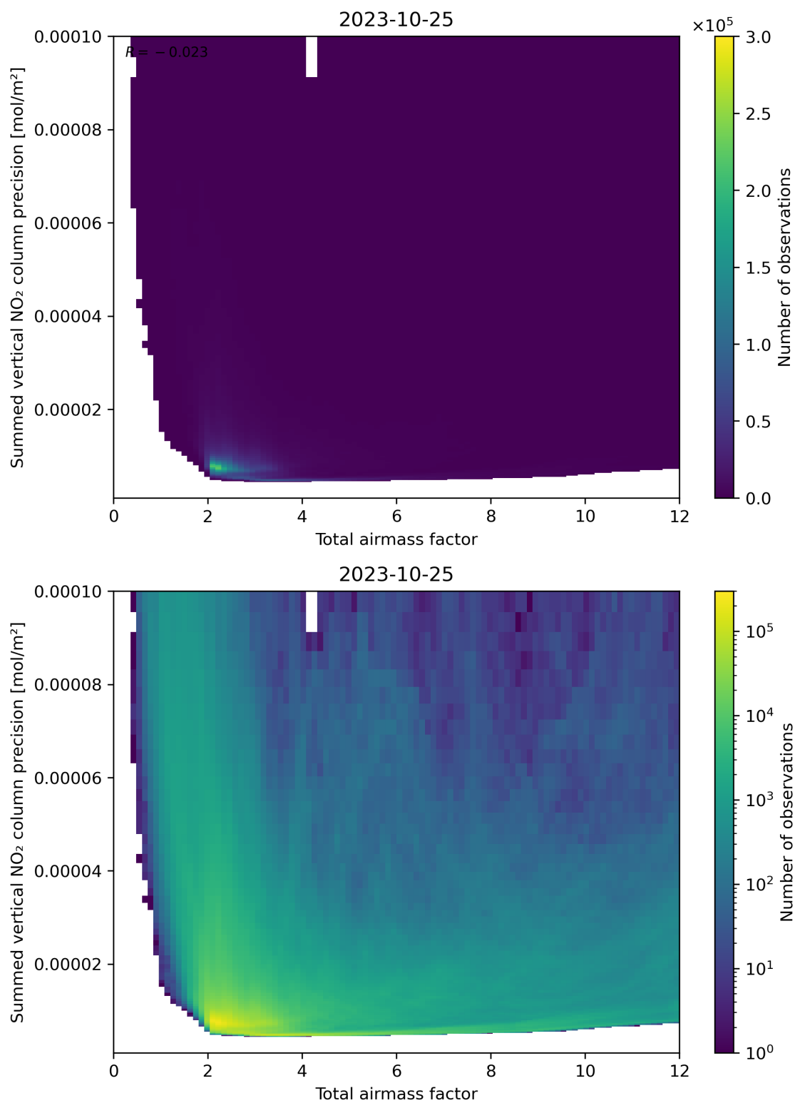
Figure 66: Scatter density plot of “Total airmass factor” against “Summed vertical NO 2 column precision” for 2023-10-24 to 2023-10-26.
