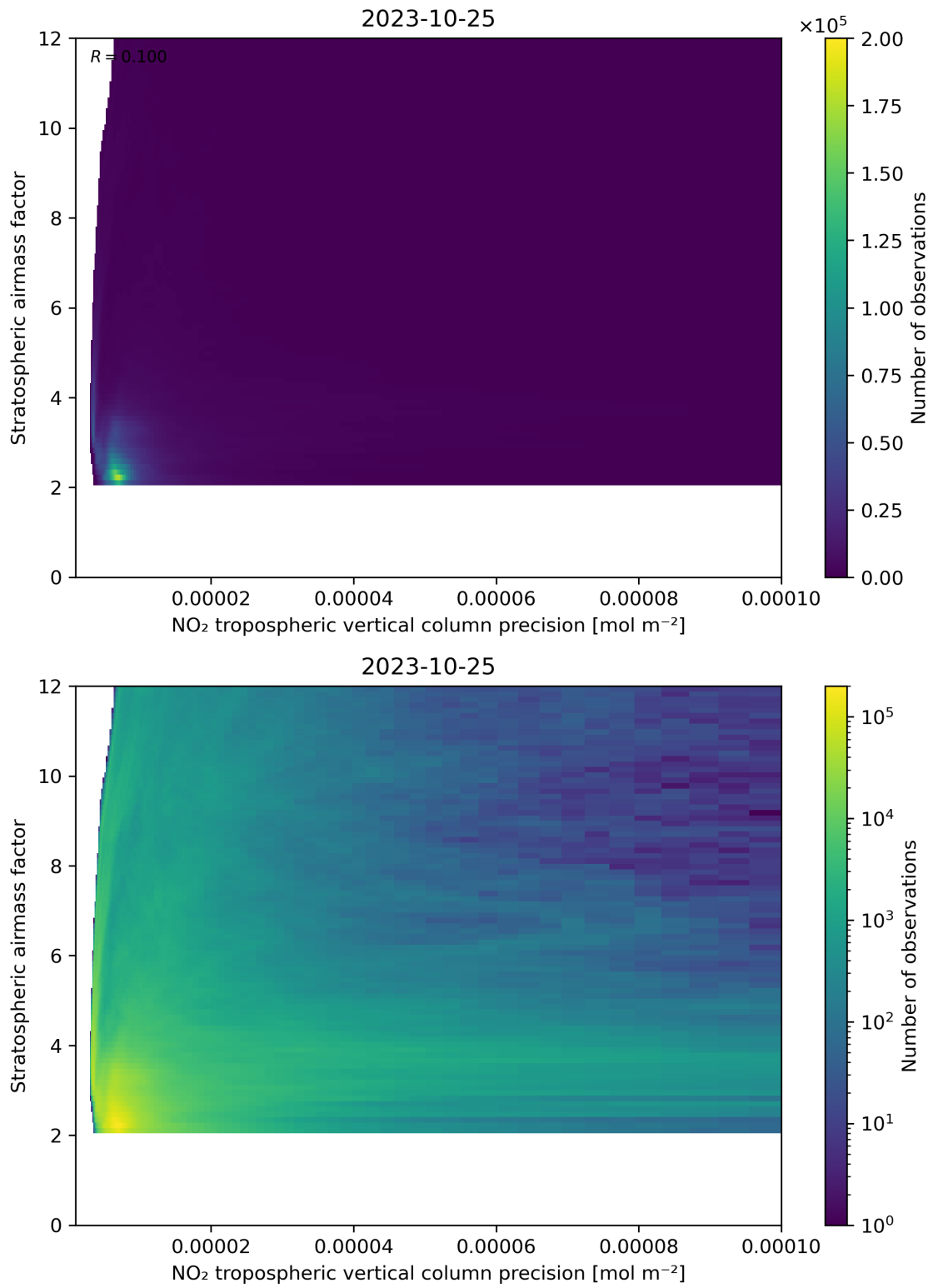
Figure 131: Scatter density plot of “NO 2 tropospheric vertical column precision” against “Stratospheric airmass factor” for 2023-10-24 to 2023-10-26.
