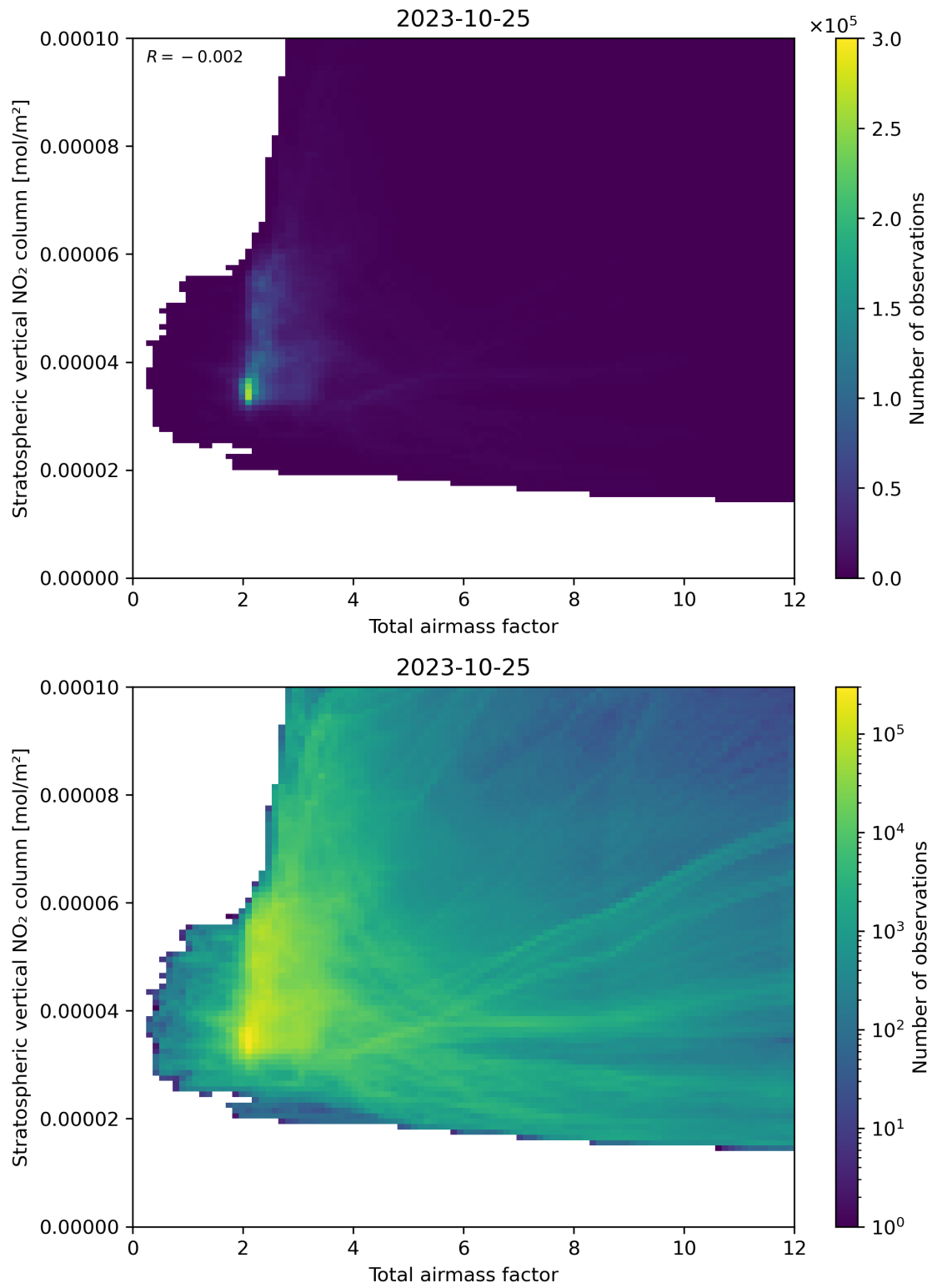
Figure 64: Scatter density plot of “Total airmass factor” against “Stratospheric vertical NO 2 column” for 2023-10-24 to 2023-10-26.
