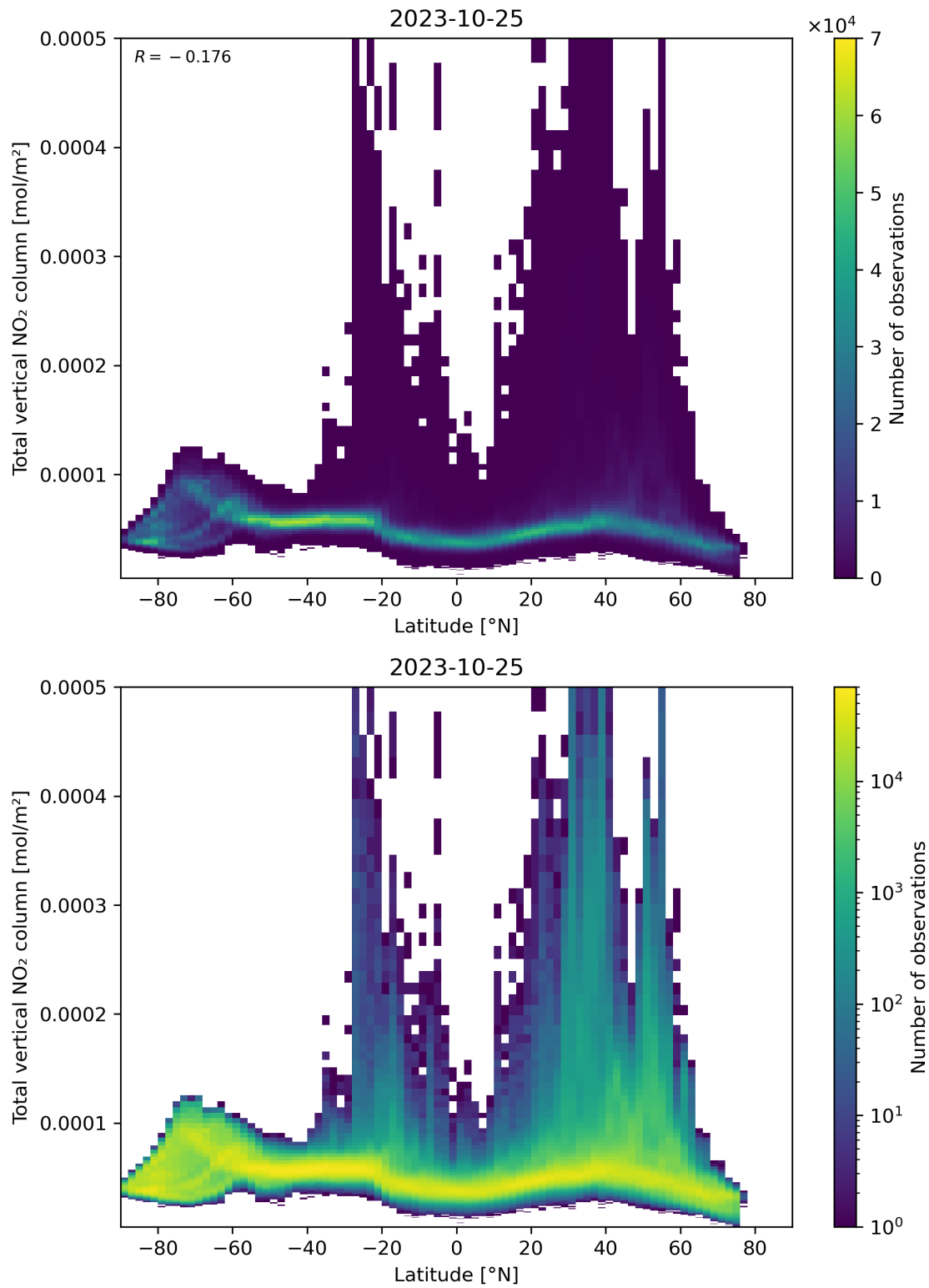
Figure 90: Scatter density plot of “Latitude” against “Total vertical NO 2 column” for 2023-10-24 to 2023-10-26.
