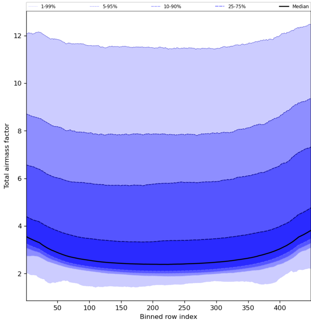
Figure 49: Along track statistics of “Total airmass factor” for 2023-10-24 to 2023-10-26
