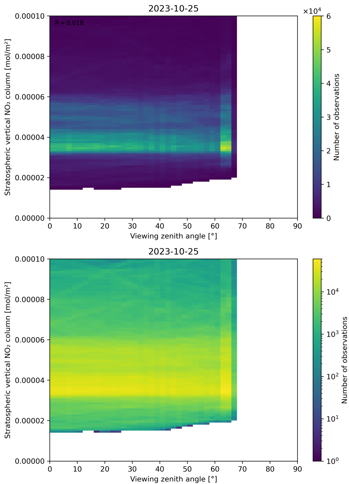
Figure 164: Scatter density plot of “Viewing zenith angle” against “Stratospheric vertical NO 2 column” for 2023-10-24 to 2023-10-26.
