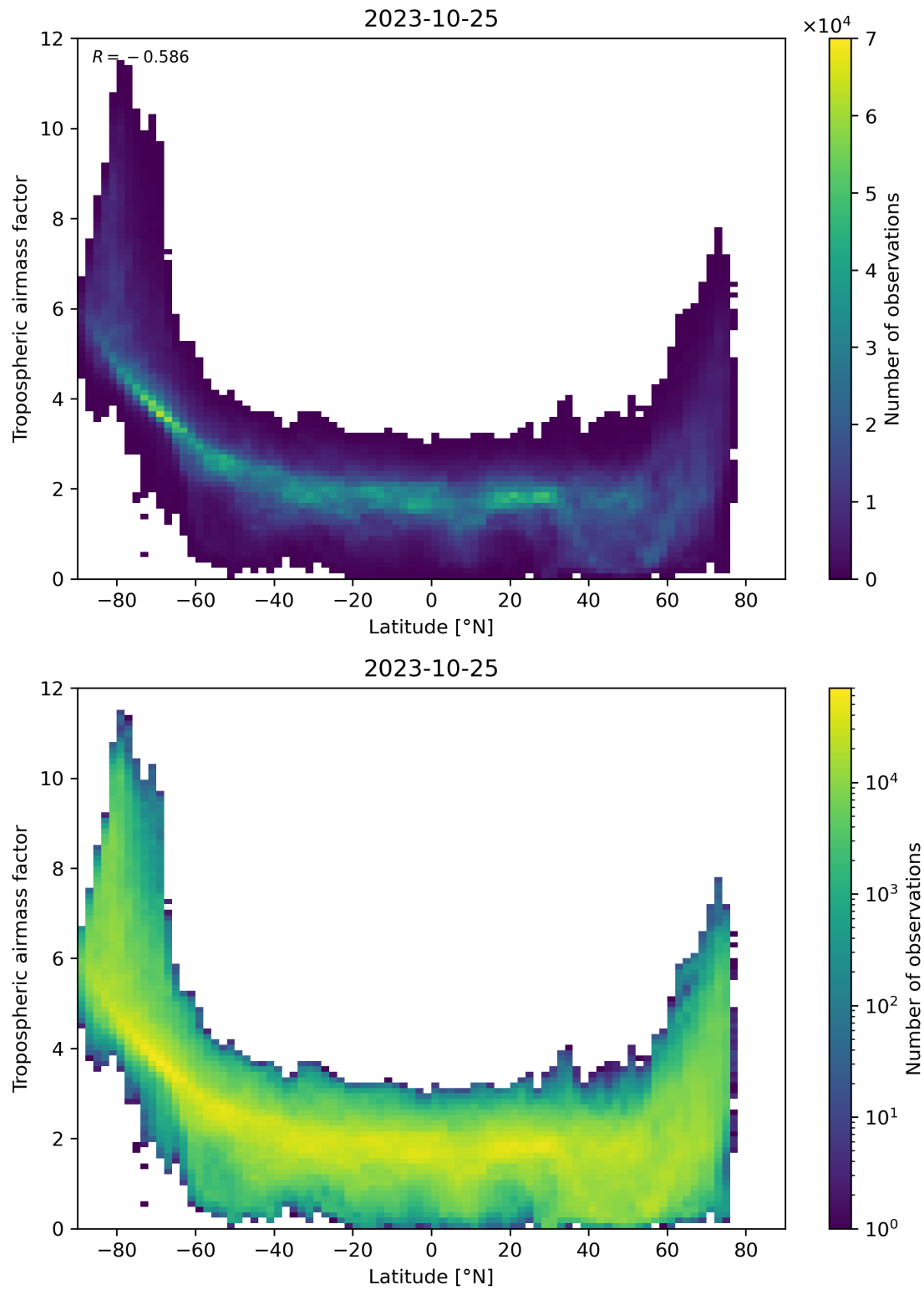
Figure 85: Scatter density plot of “Latitude” against “Tropospheric airmass factor” for 2023-10-24 to 2023-10-26.
