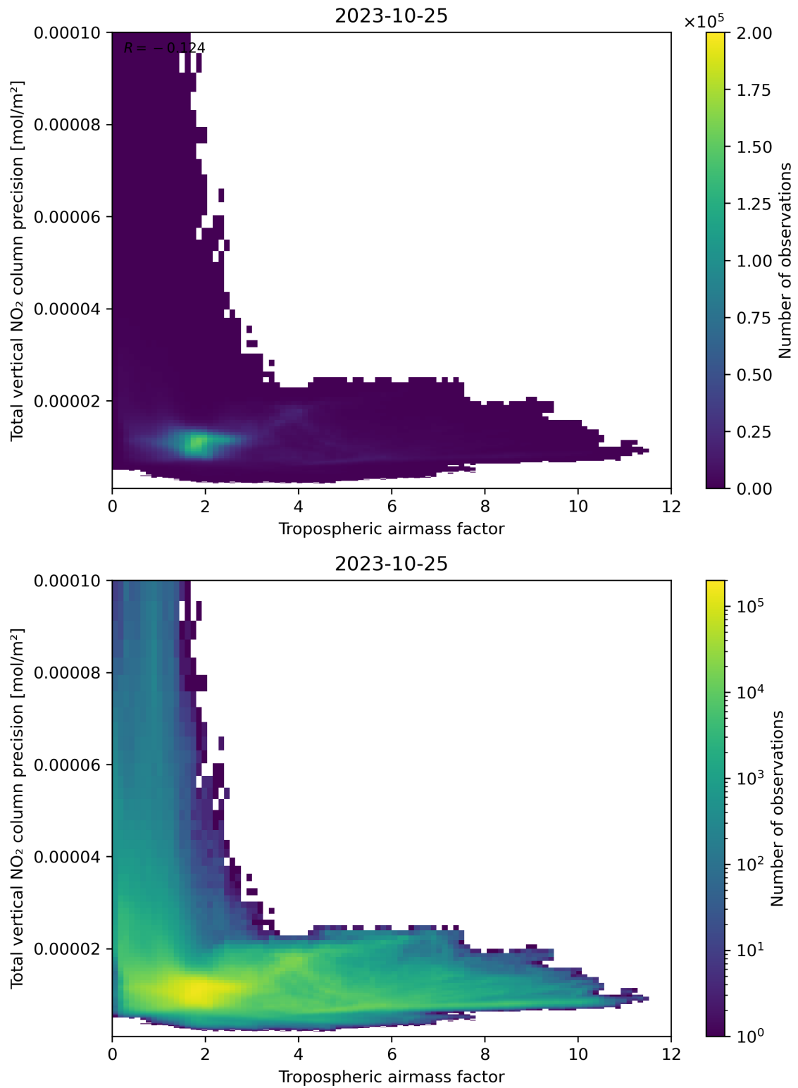
Figure 78: Scatter density plot of “Tropospheric air mass factor” against “Total vertical NO 2 column precision” for 2023-10-24 to 2023-10-26.
