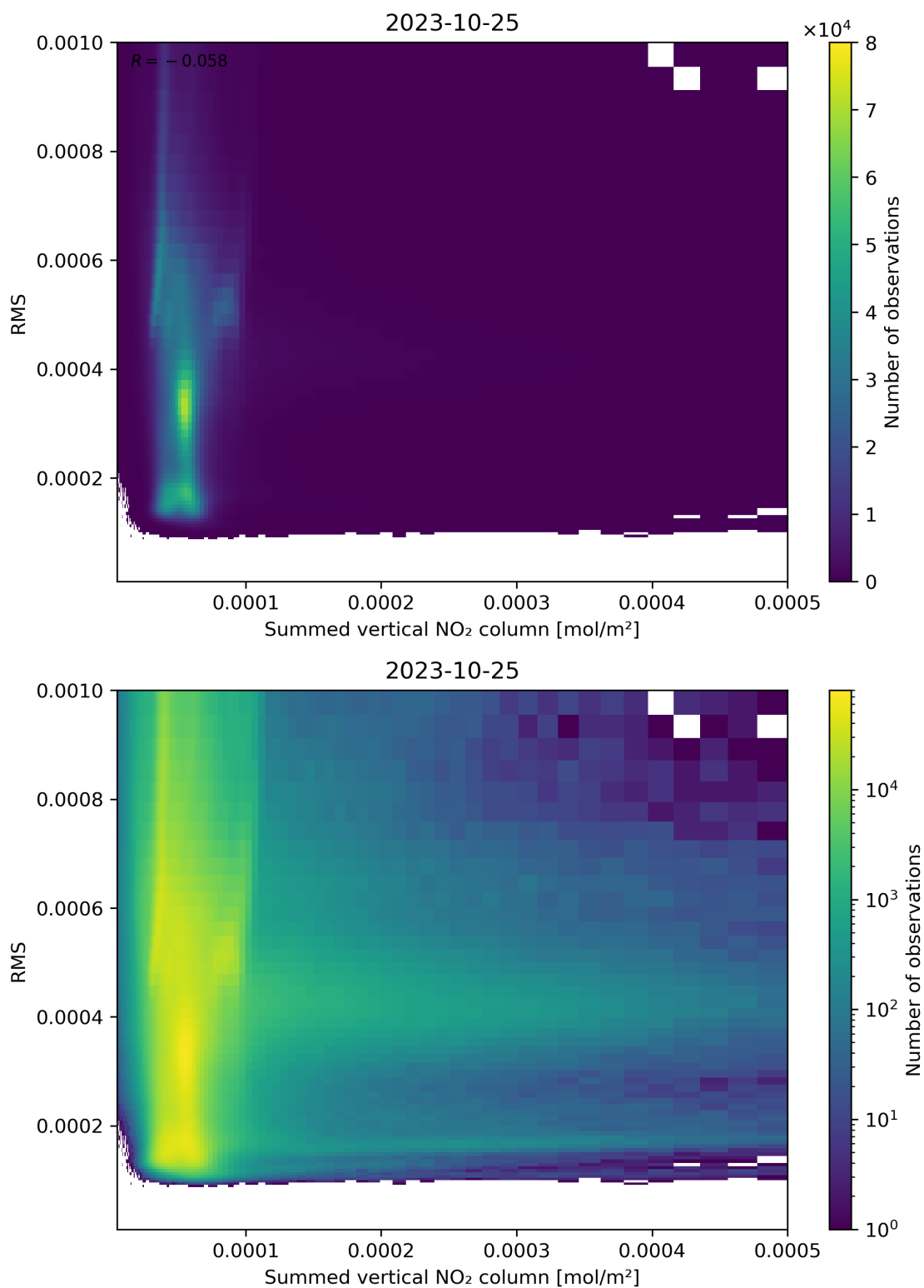
Figure 109: Scatter density plot of “Summed vertical NO 2 column” against “RMS” for 2023-10-24 to 2023-10-26.
