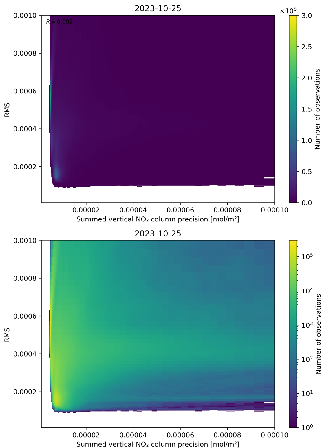
Figure 108: Scatter density plot of “Summed vertical NO 2 column precision” against “RMS” for 2023-10-24 to 2023-10-26.
