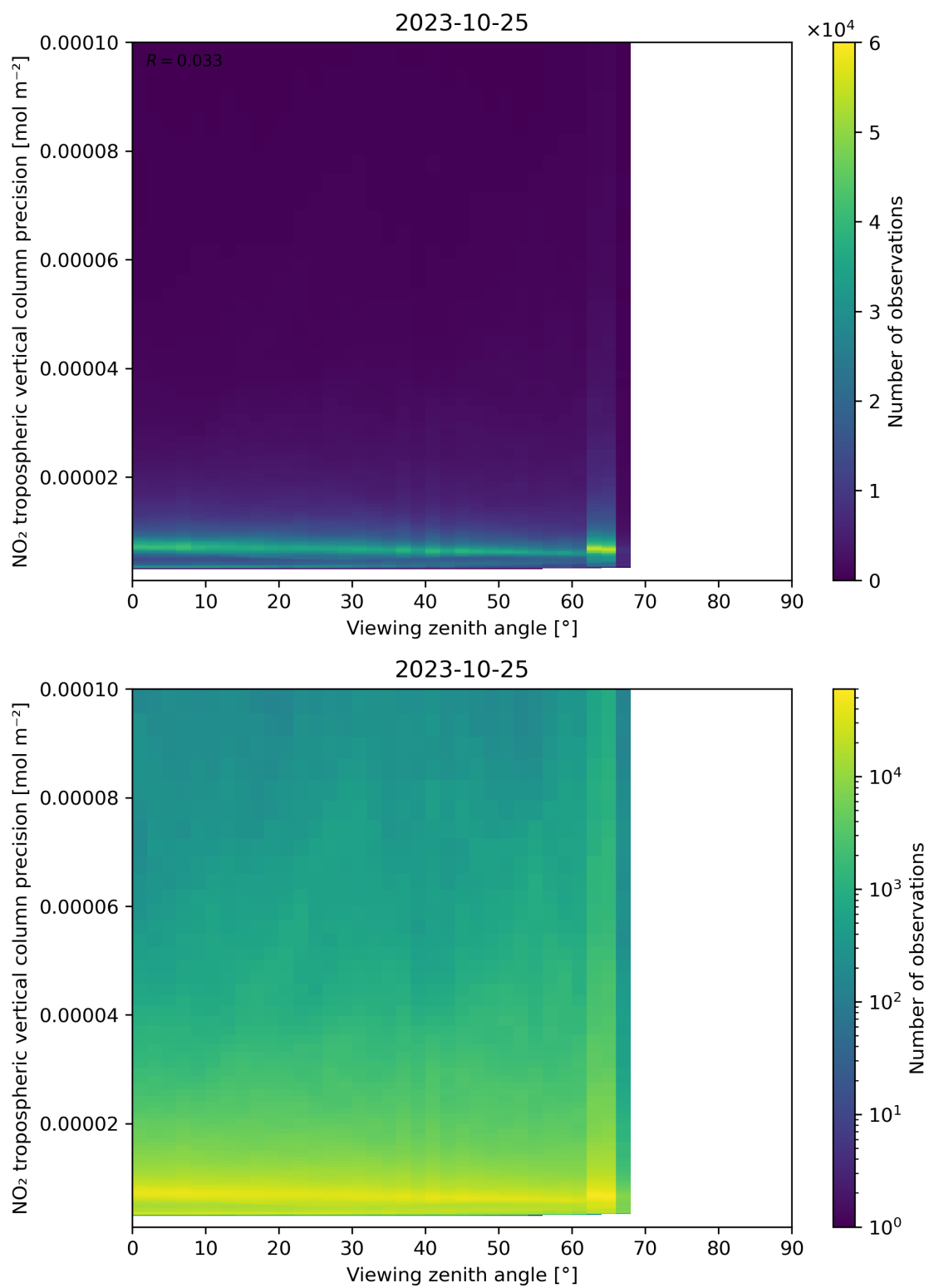
Figure 170: Scatter density plot of “Viewing zenith angle” against “NO 2 tropospheric vertical column precision” for 2023-10-24 to 2023-10-26.
