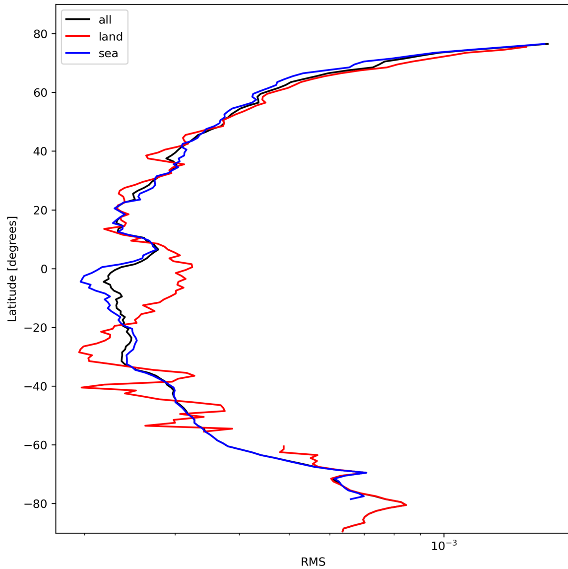
Figure 26: Zonal average of “RMS” for 2023-10-24 to 2023-10-26.
