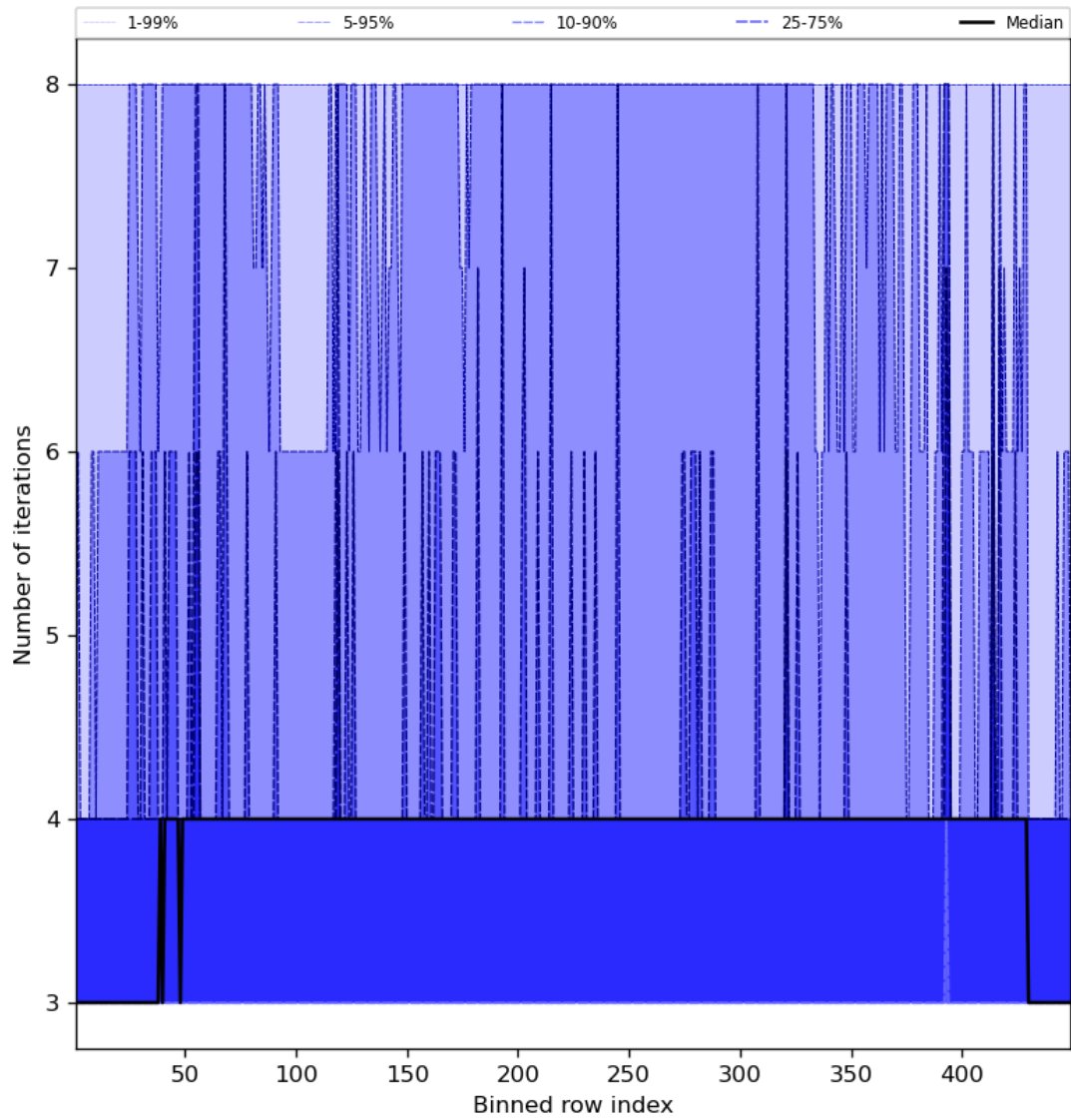
Figure 51: Along track statistics of “Number of iterations” for 2023-10-24 to 2023-10-26
