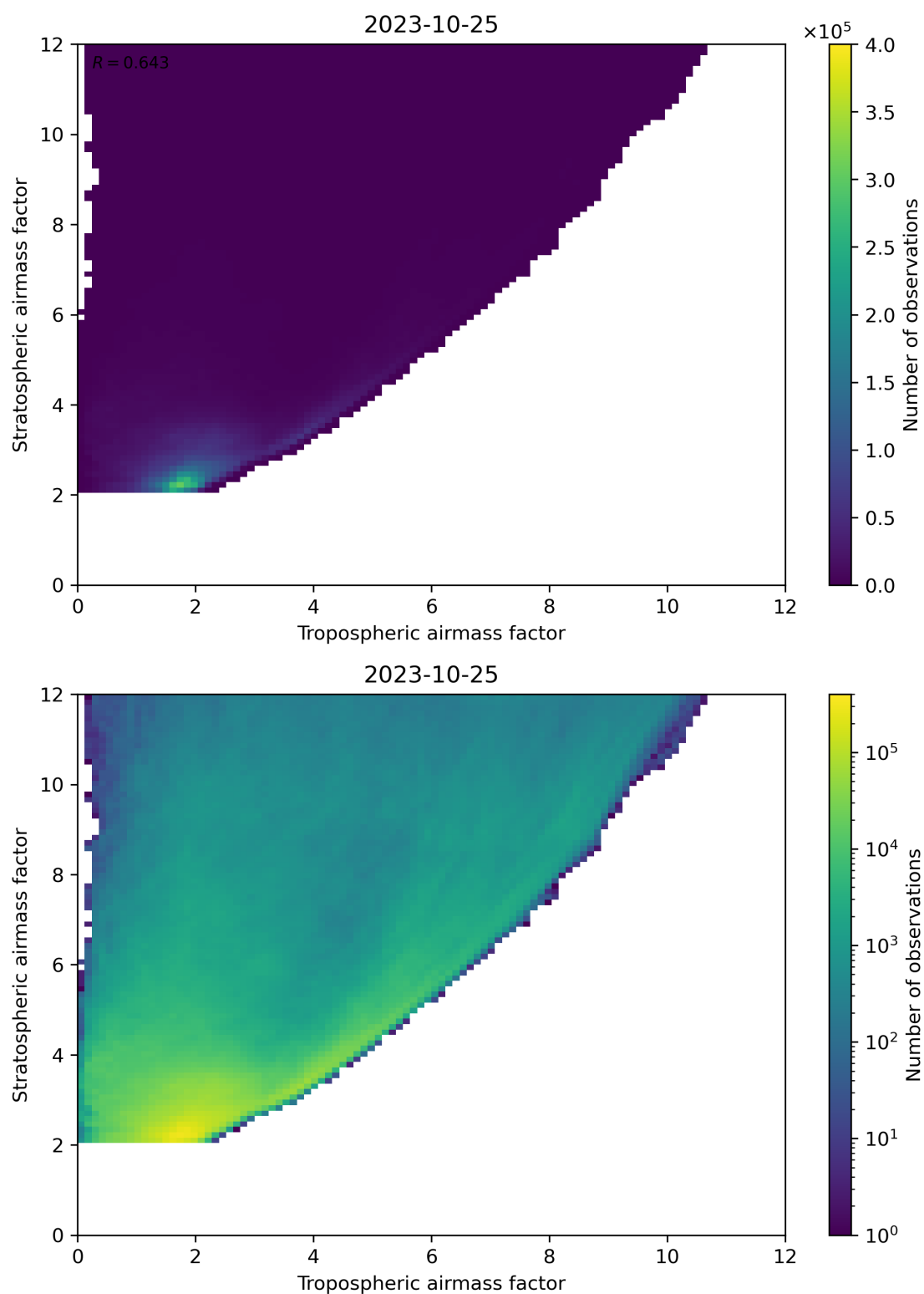
Figure 71: Scatter density plot of “Tropospheric airmass factor” against “Stratospheric airmass factor” for 2023-10-24 to 2023-10-26.
