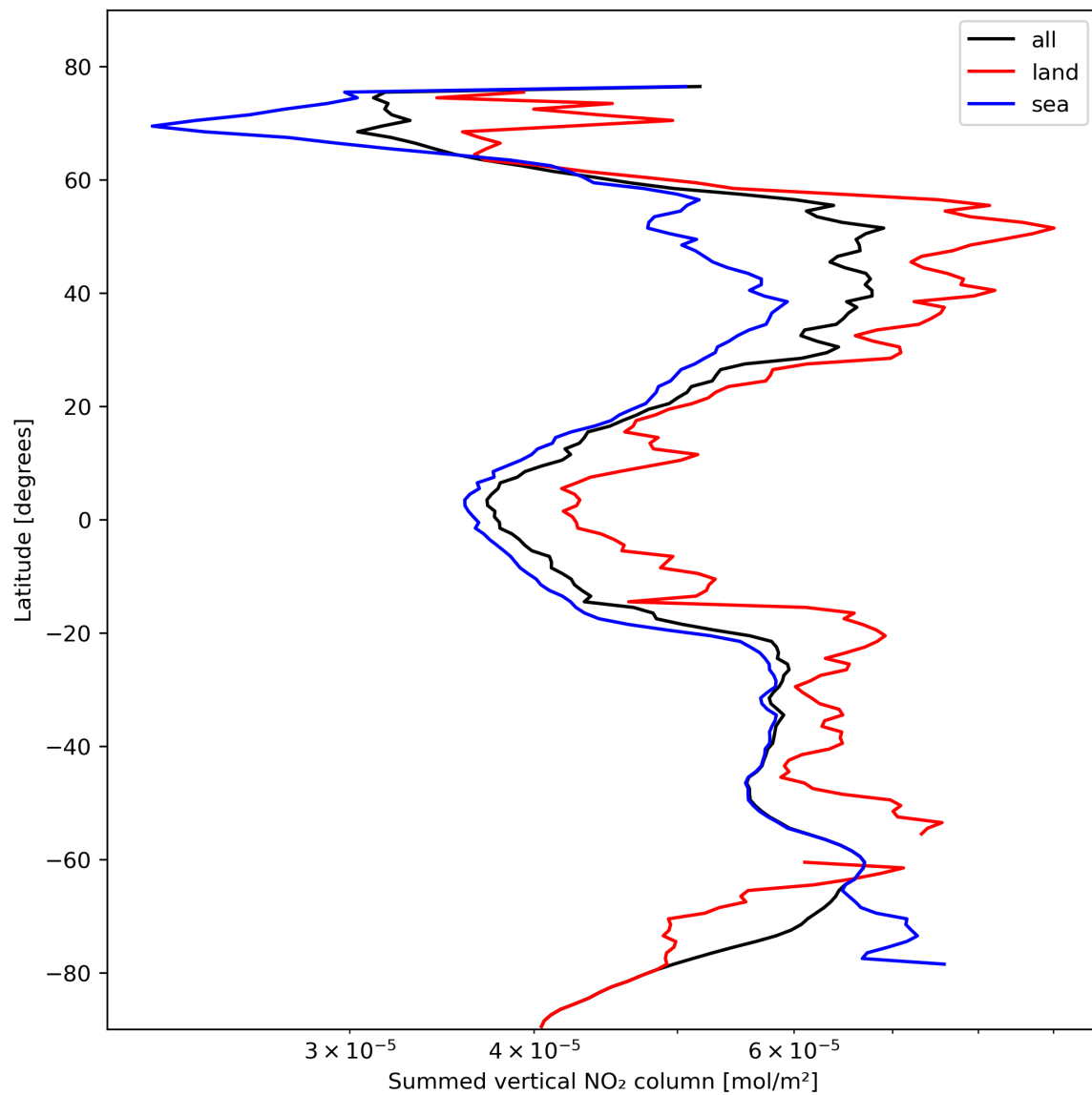
Figure 23: Zonal average of “Summed vertical NO 2 column” for 2023-10-24 to 2023-10-26.
