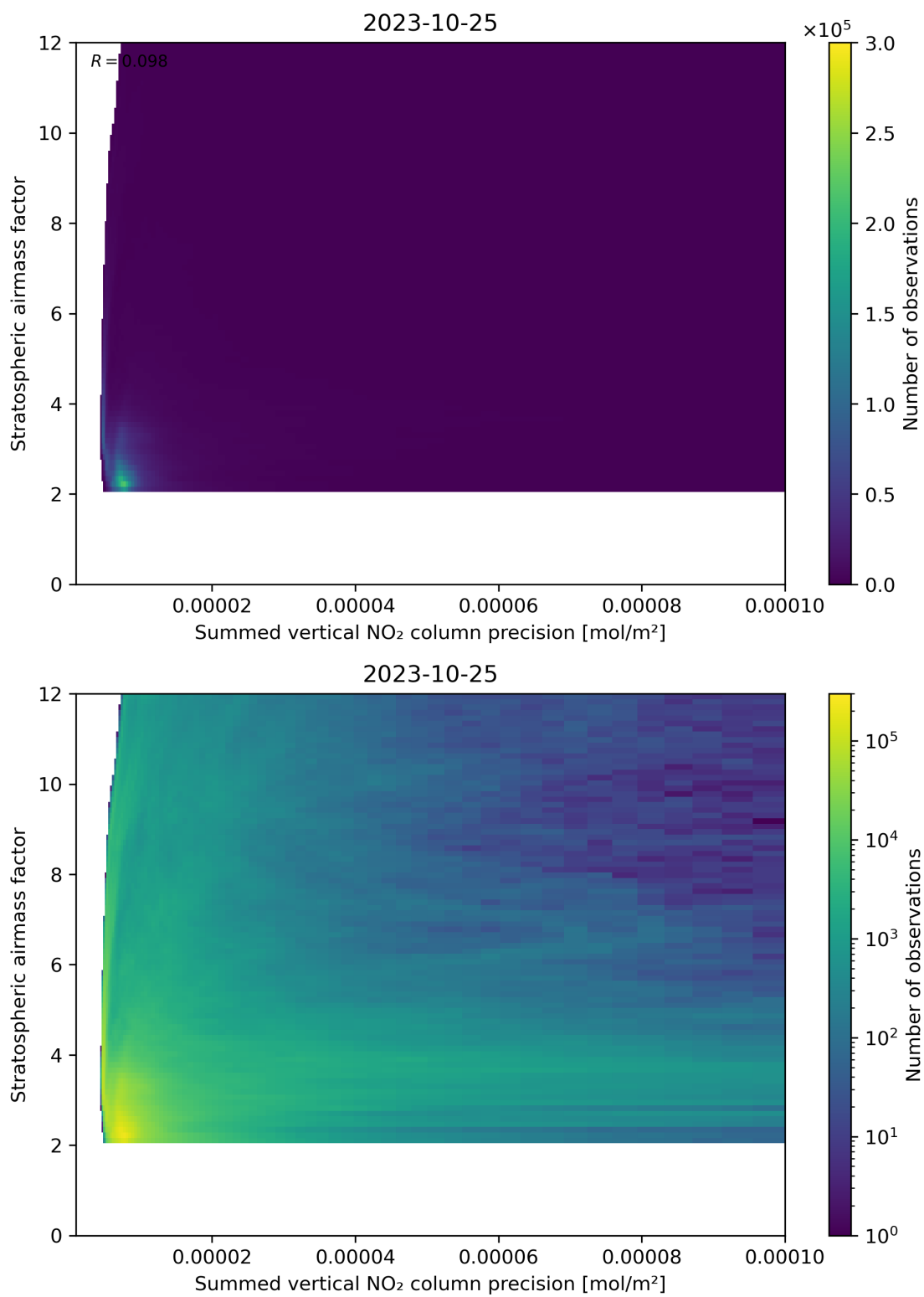
Figure 106: Scatter density plot of “Summed vertical NO 2 column precision” against “Stratospheric airmass factor” for 2023-10-24 to 2023-10-26.
