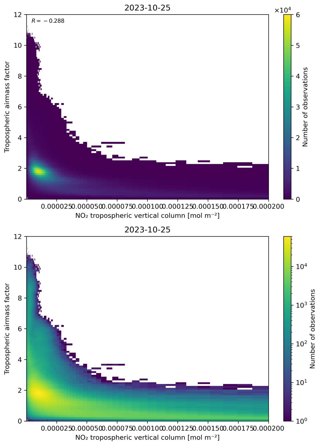
Figure 123: Scatter density plot of “NO 2 tropospheric vertical column” against “Tropospheric airmass factor” for 2023-10-24 to 2023-10-26.
