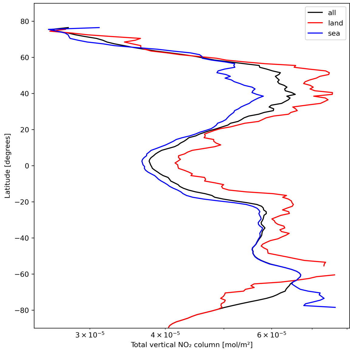
Figure 21: Zonal average of “Total vertical NO 2 column” for 2023-10-24 to 2023-10-26.
