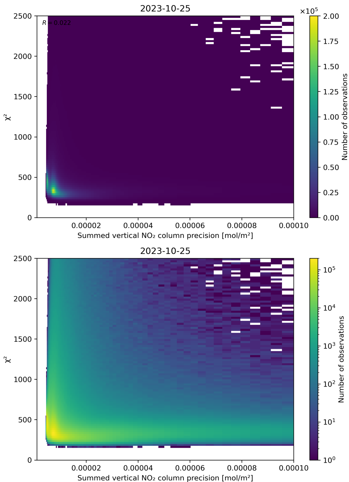
Figure 107: Scatter density plot of “Summed vertical NO 2 column precision” against “ \chi^2 ” for 2023-10-24 to 2023-10-26.
