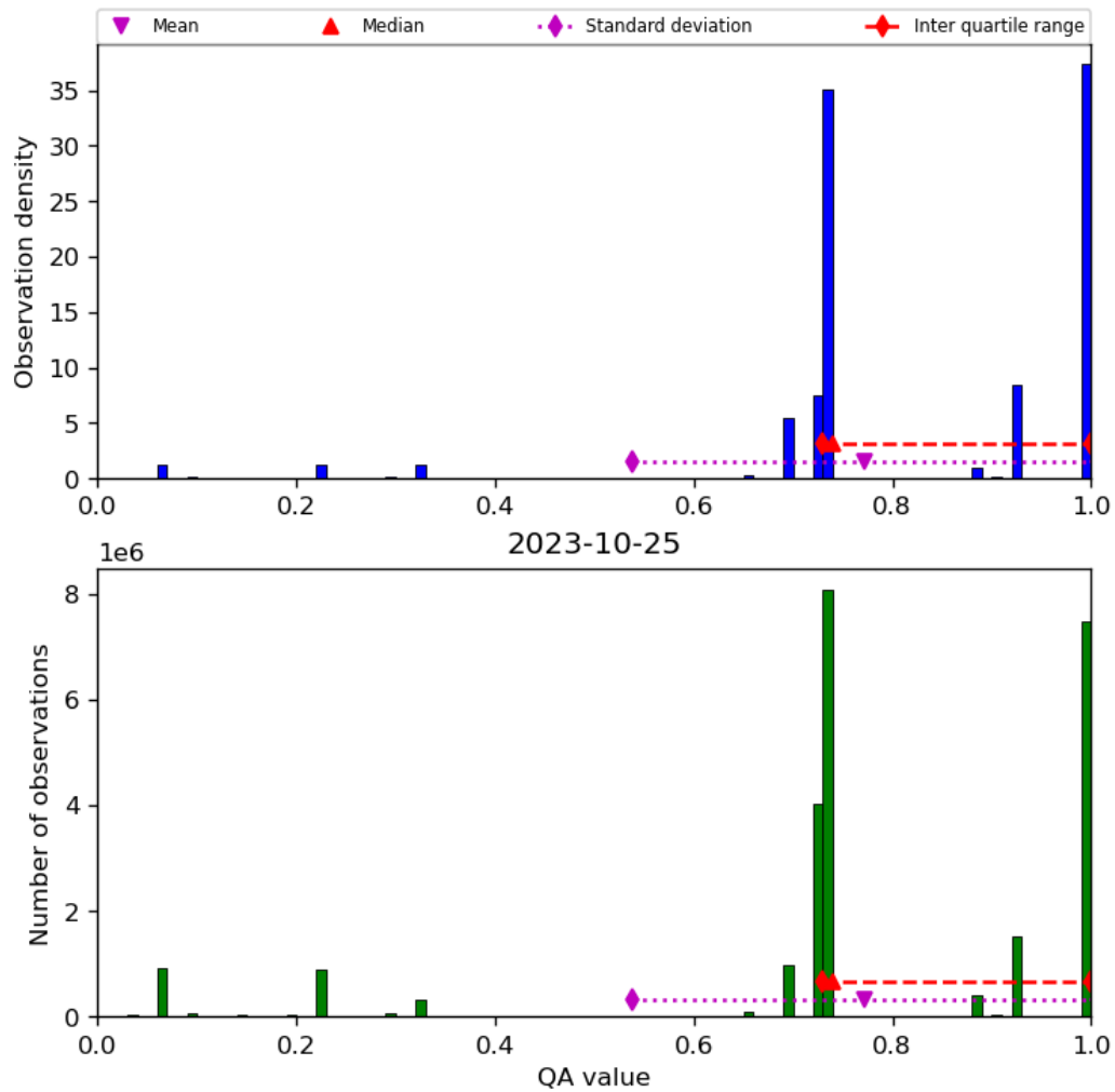
Figure 28: Histogram of “QA value” for 2023-10-24 to 2023-10-26
