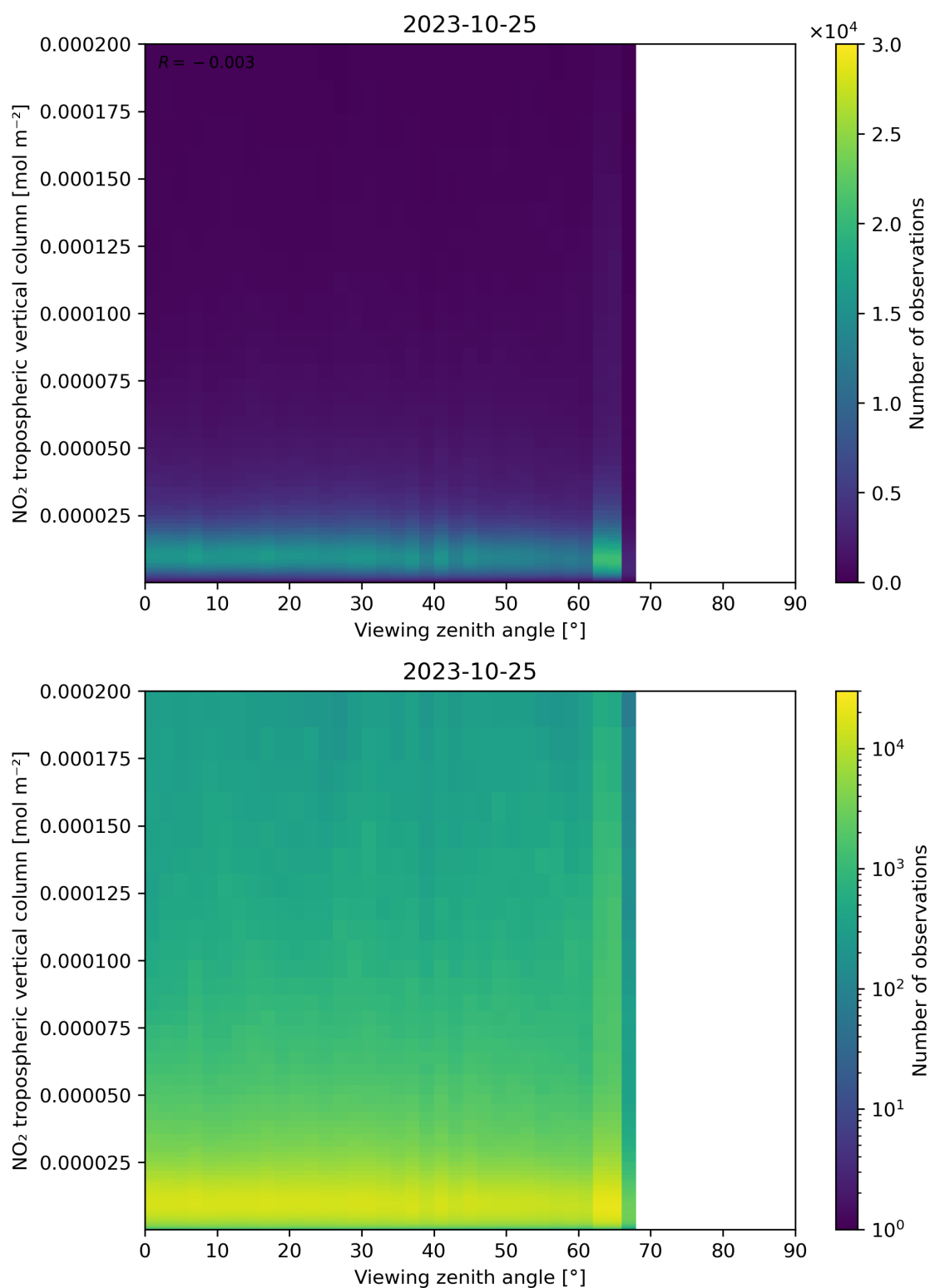
Figure 169: Scatter density plot of “Viewing zenith angle” against “NO 2 tropospheric vertical column” for 2023-10-24 to 2023-10-26.
