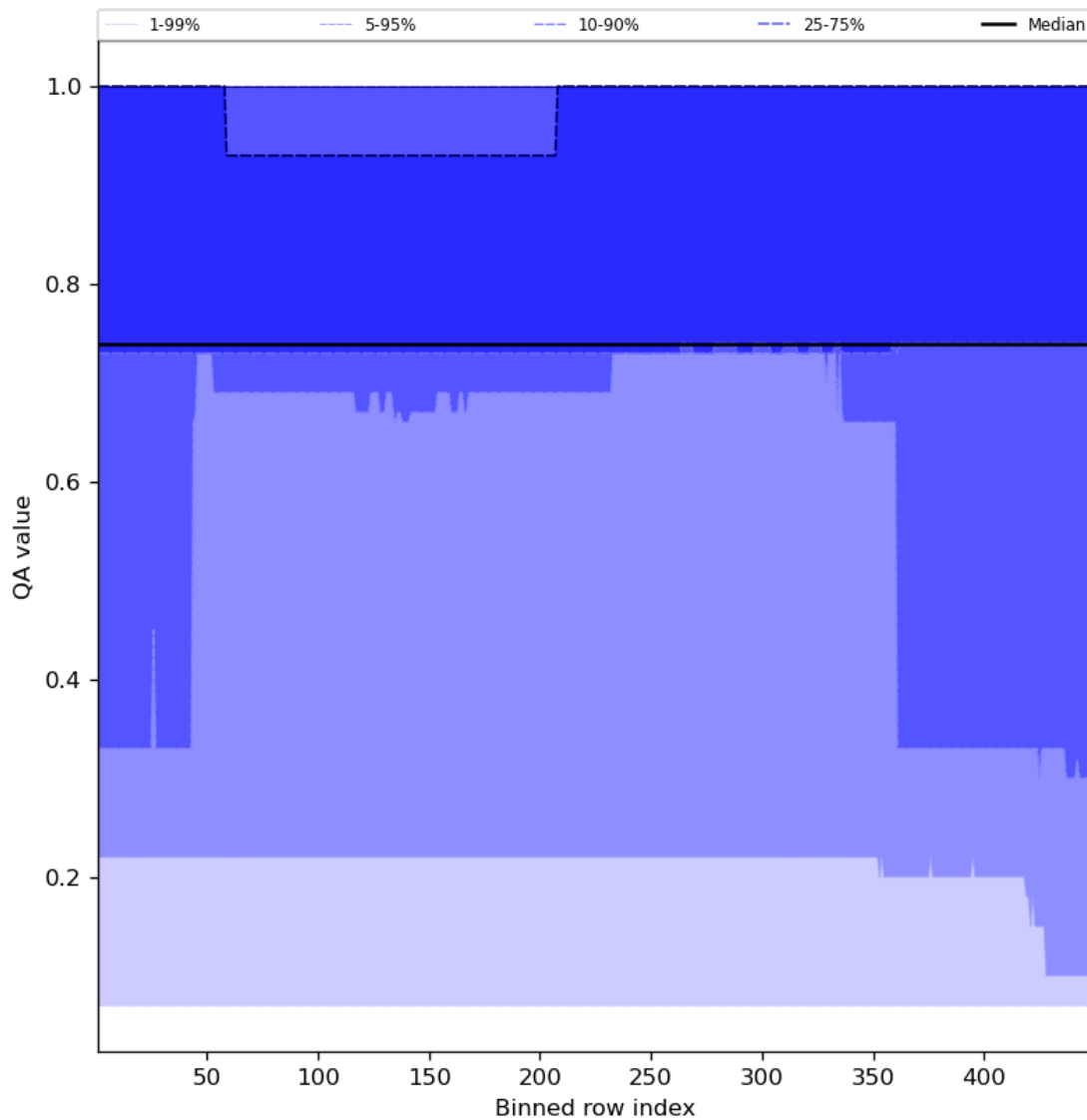
Figure 45: Along track statistics of “QA value” for 2023-10-24 to 2023-10-26
