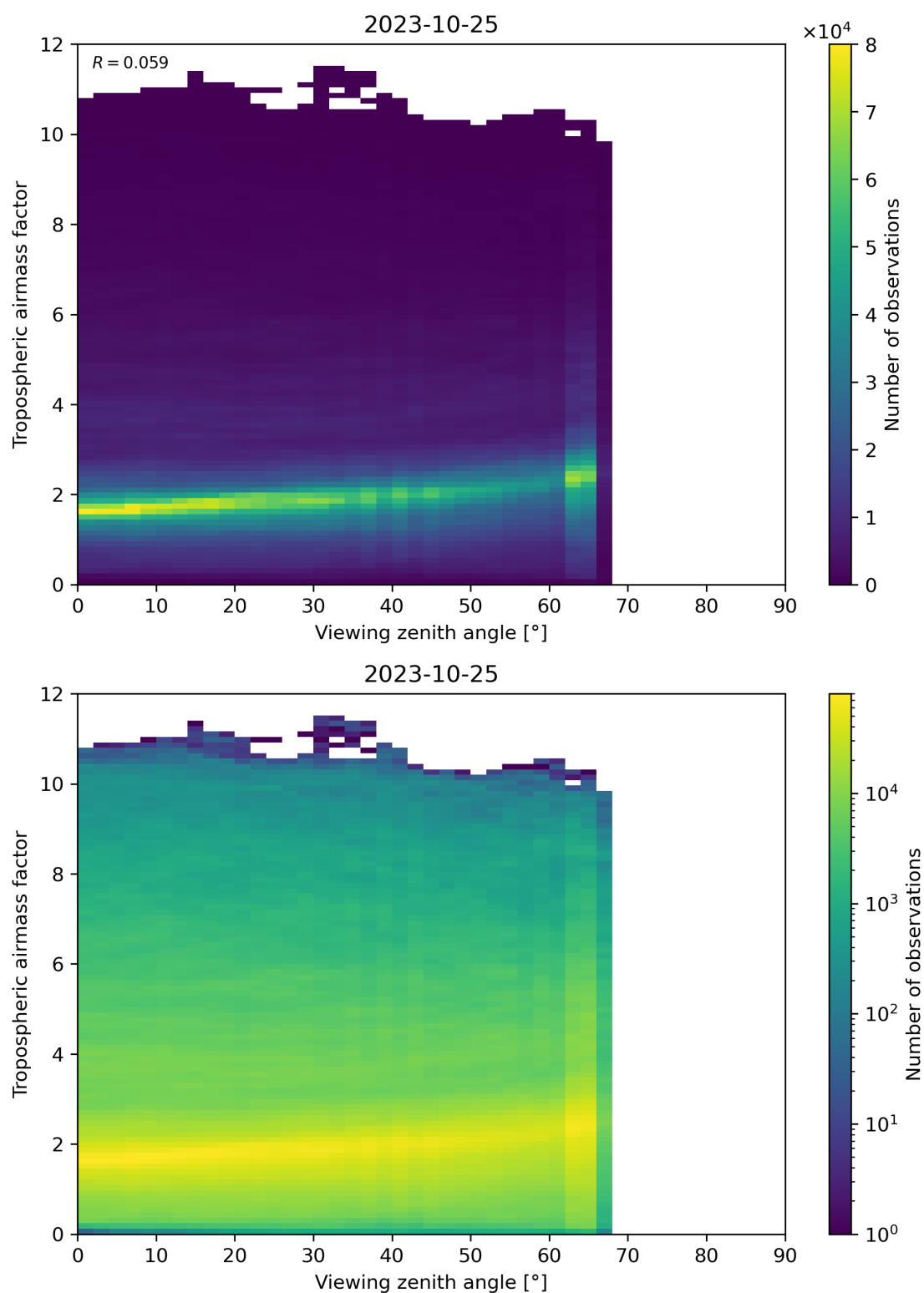
Figure 161: Scatter density plot of “Viewing zenith angle” against “Tropospheric airmass factor” for 2023-10-24 to 2023-10-26.
