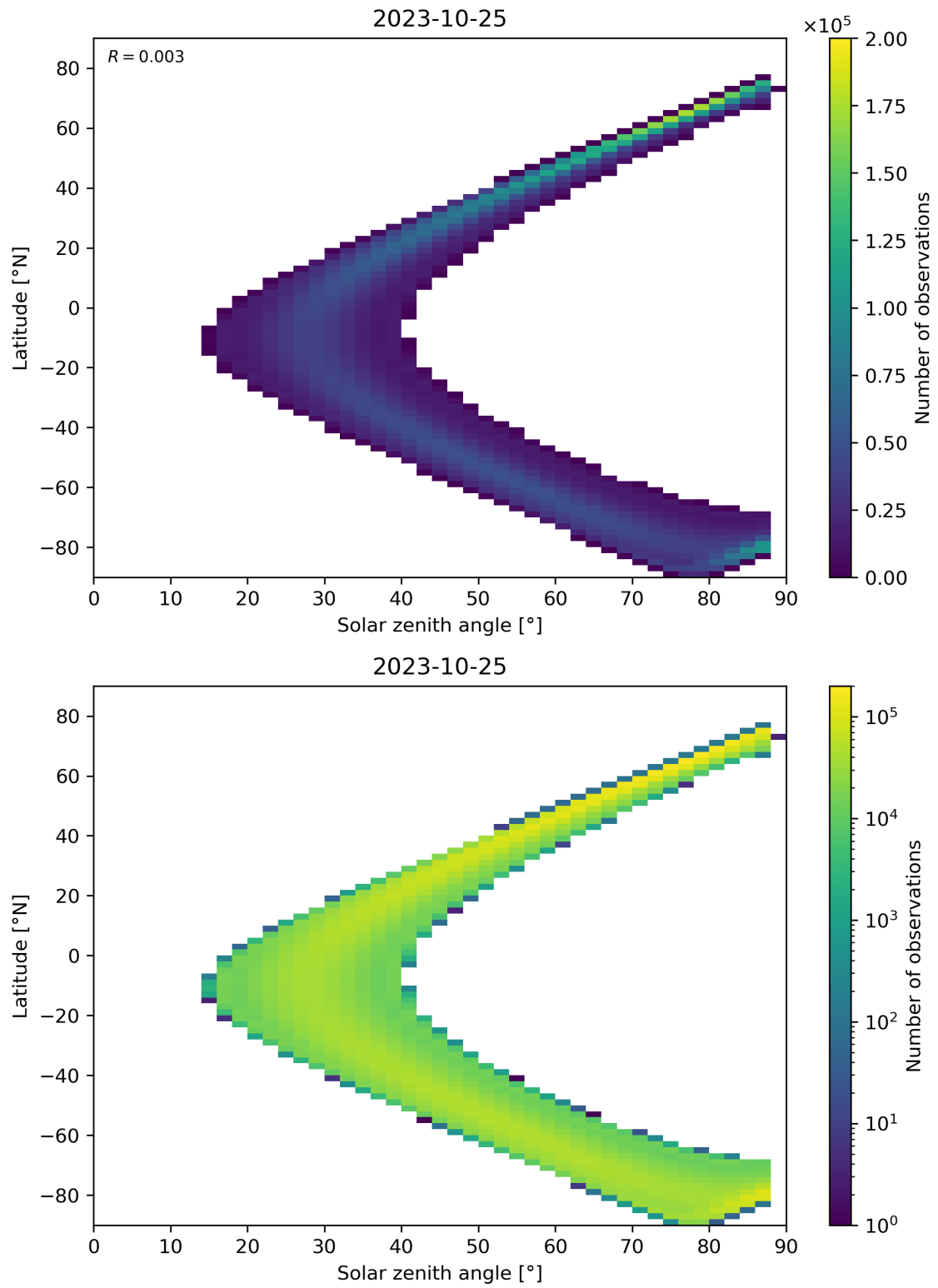
Figure 149: Scatter density plot of “Solar zenith angle” against “Latitude” for 2023-10-24 to 2023-10-26.
