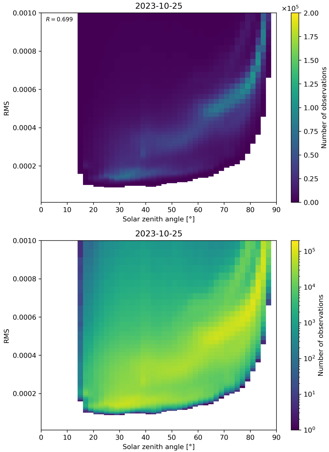
Figure 157: Scatter density plot of “Solar zenith angle” against “RMS” for 2023-10-24 to 2023-10-26.
