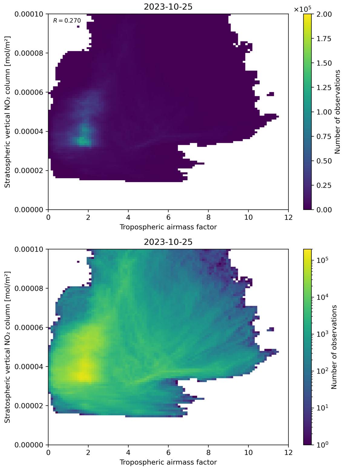
Figure 74: Scatter density plot of “Tropospheric air mass factor” against “Stratospheric vertical NO 2 column” for 2023-10-24 to 2023-10-26.
