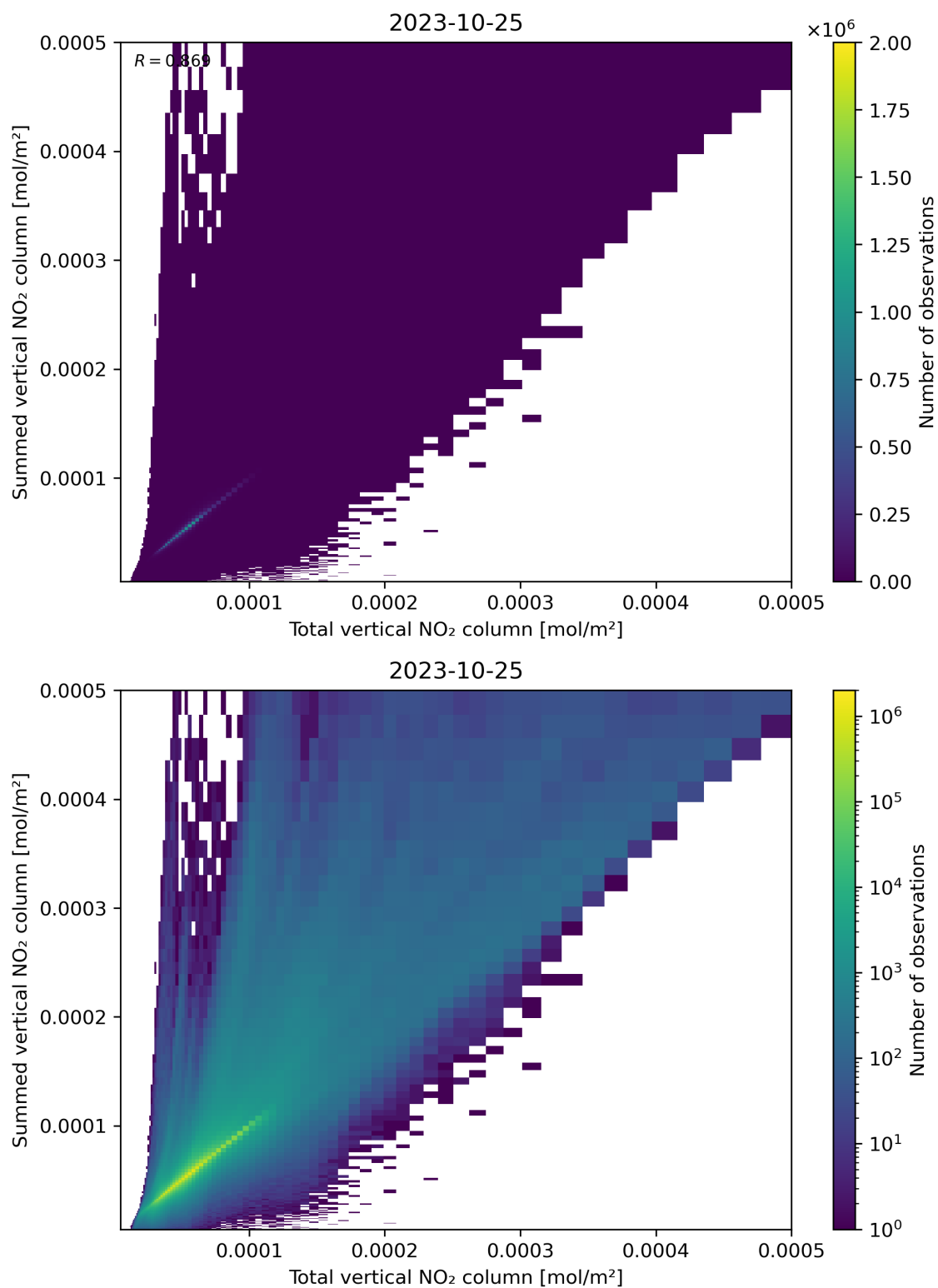
Figure 112: Scatter density plot of “Total vertical NO 2 column” against “Summed vertical NO 2 column” for 2023-10-24 to 2023-10-26.
