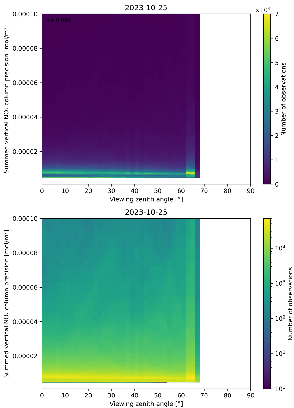
Figure 166: Scatter density plot of “Viewing zenith angle” against “Summed vertical NO 2 column precision” for 2023-10-24 to 2023-10-26.
