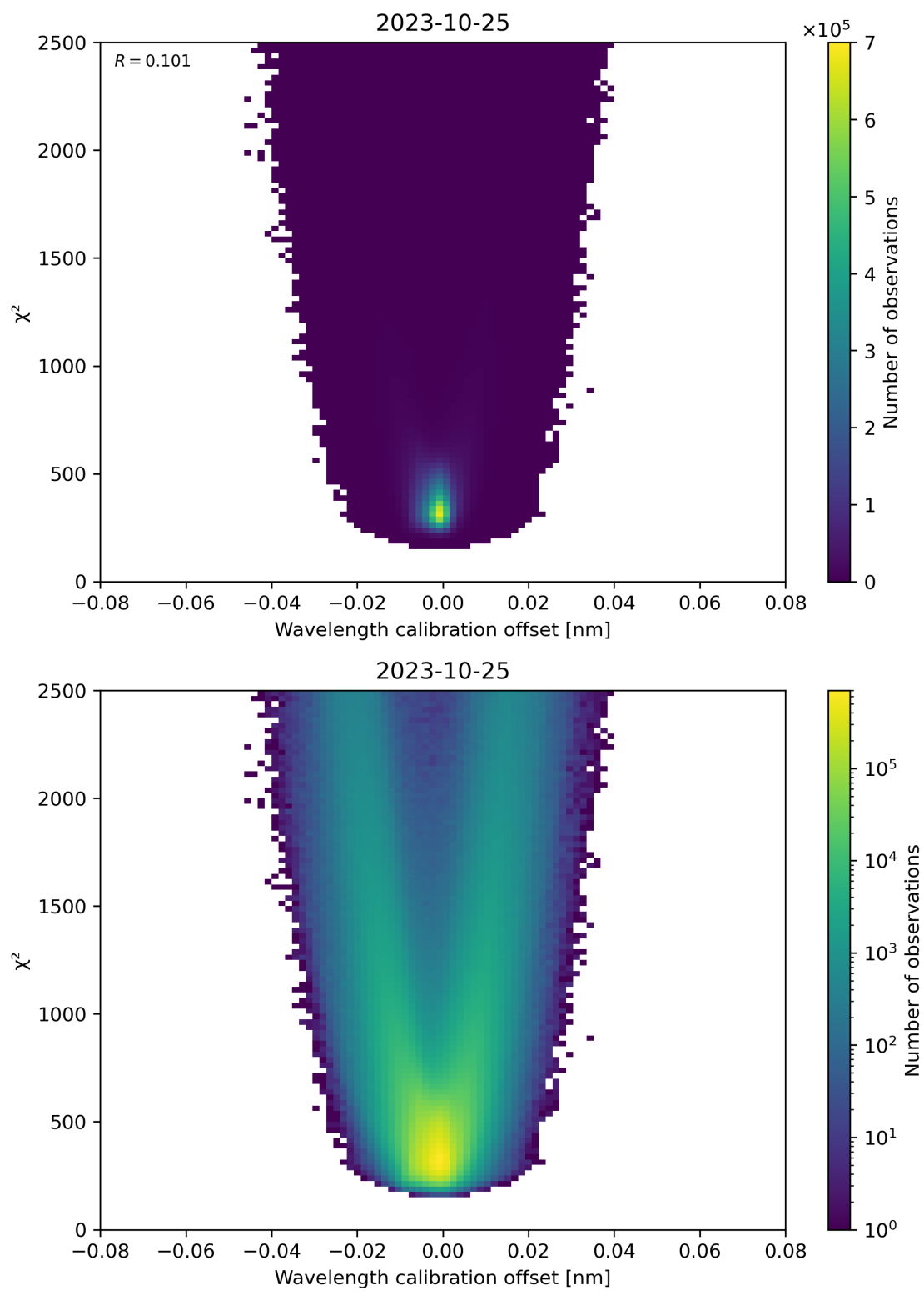
Figure 175: Scatter density plot of “Wavelength calibration offset” against “ \chi^2 ” for 2023-10-24 to 2023-10-26.
