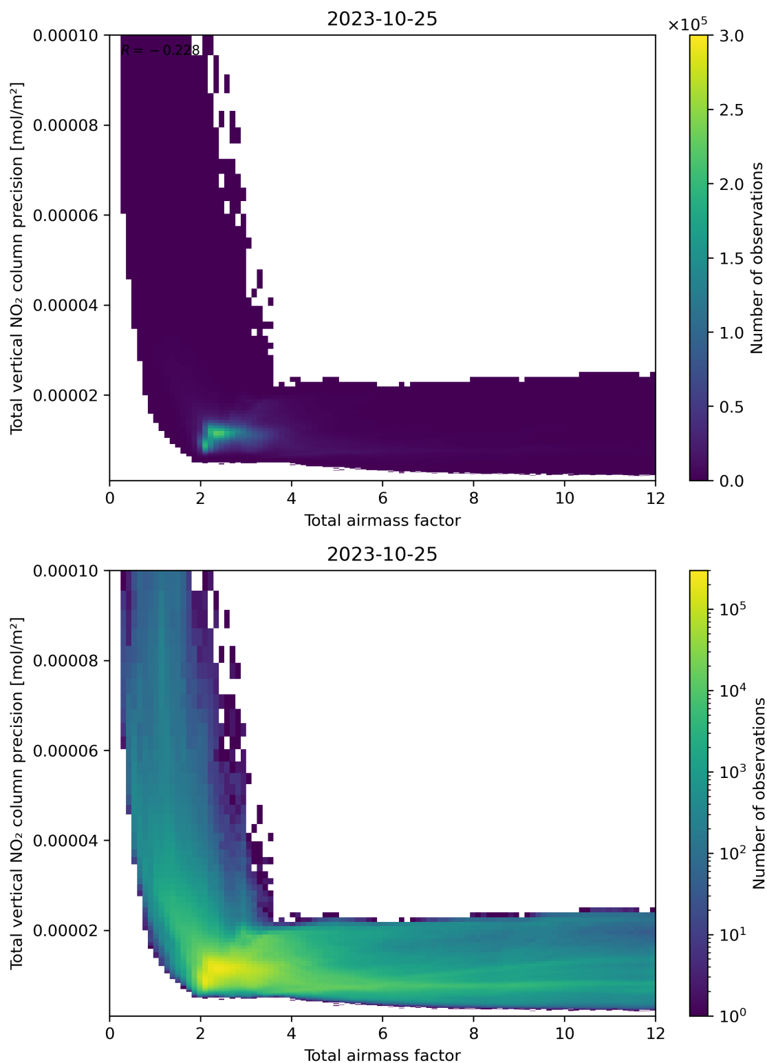
Figure 68: Scatter density plot of “Total airmass factor” against “Total vertical NO 2 column precision” for 2023-10-24 to 2023-10-26.
