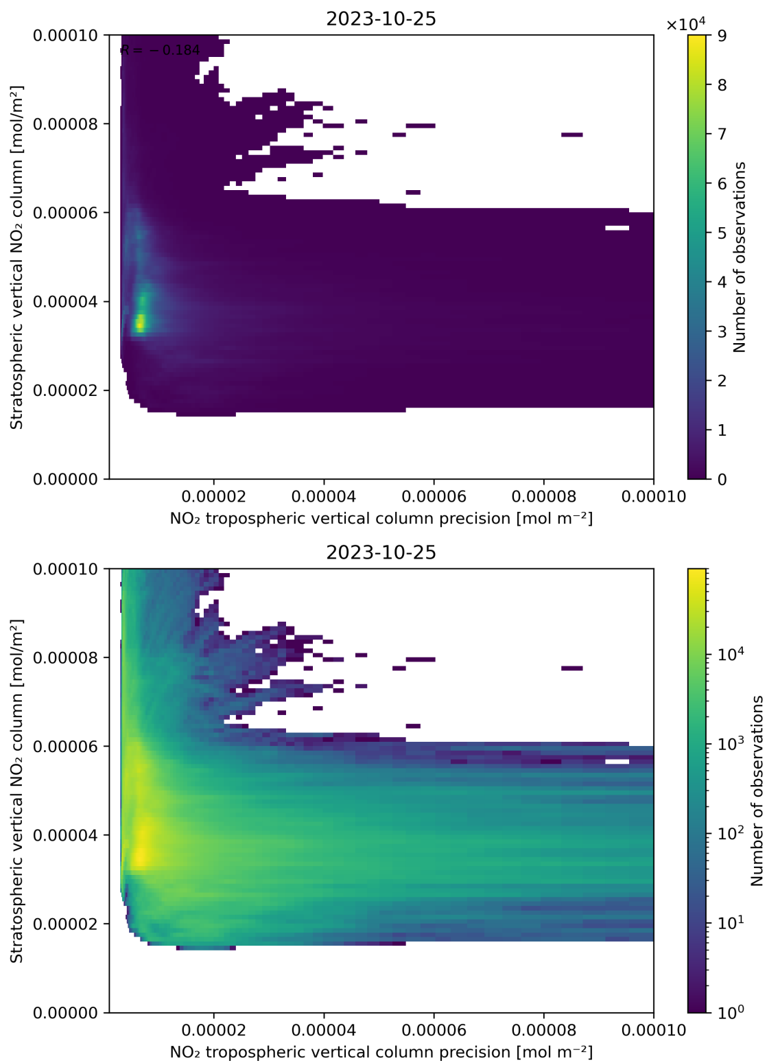
Figure 135: Scatter density plot of “NO 2 tropospheric vertical column precision” against “Stratospheric vertical NO 2 column” for 2023-10-24 to 2023-10-26.
