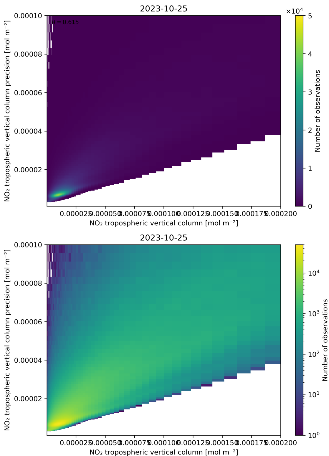
Figure 130: Scatter density plot of “NO 2 tropospheric vertical column” against “NO 2 tropospheric vertical column precision” for 2023-10-24 to 2023-10-26.
