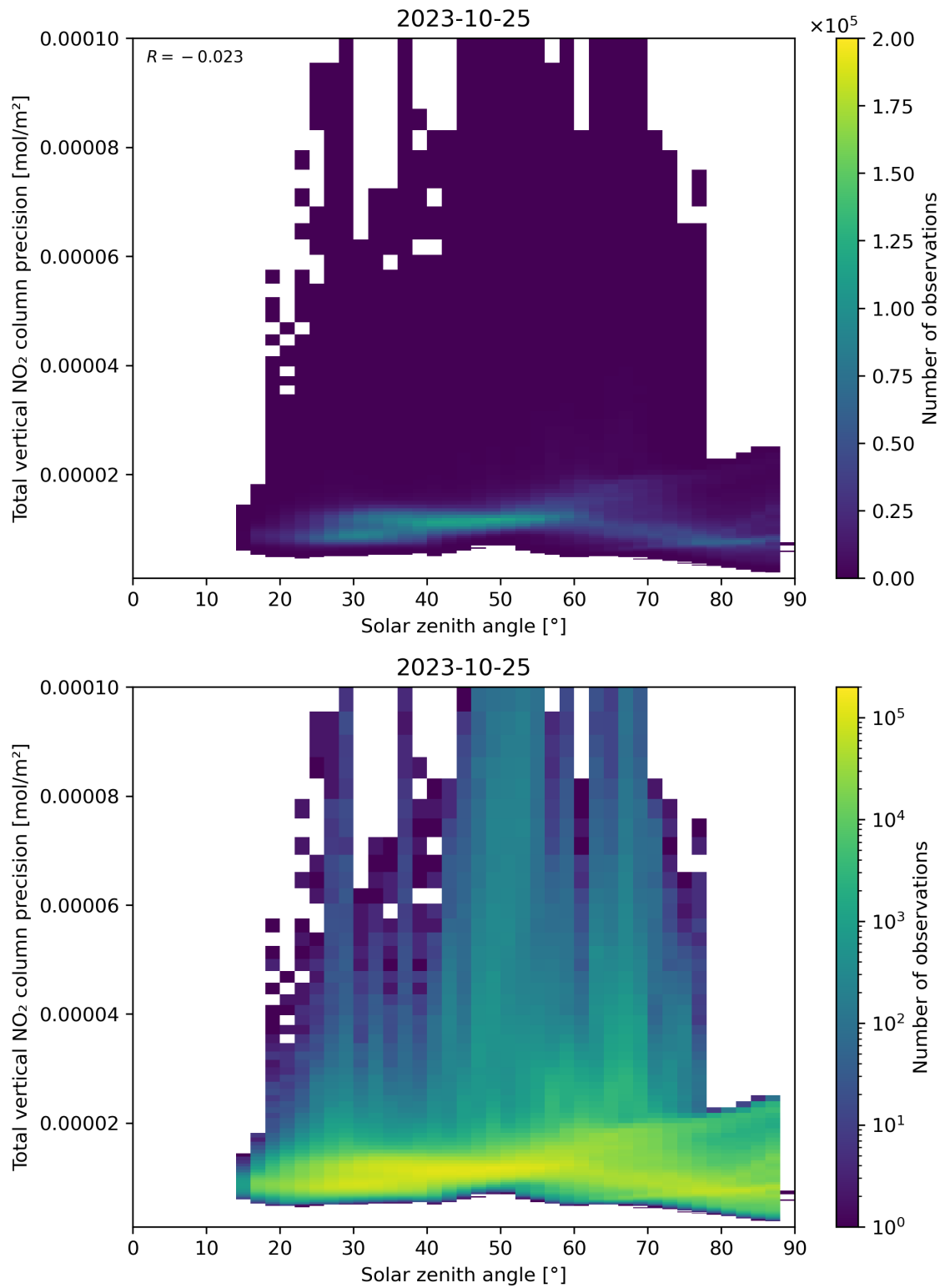
Figure 154: Scatter density plot of “Solar zenith angle” against “Total vertical NO 2 column precision” for 2023-10-24 to 2023-10-26.
