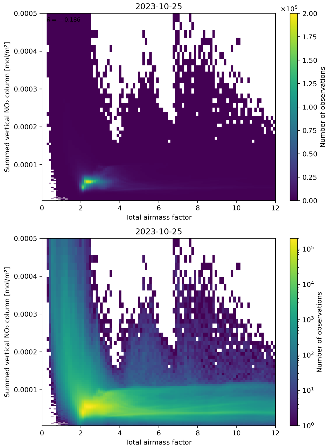
Figure 65: Scatter density plot of “Total airmass factor” against “Summed vertical NO 2 column” for 2023-10-24 to 2023-10-26.
