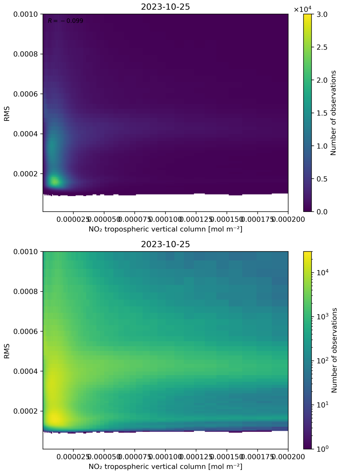
Figure 142: Scatter density plot of “NO 2 tropospheric vertical column” against “RMS” for 2023-10-24 to 2023-10-26.
