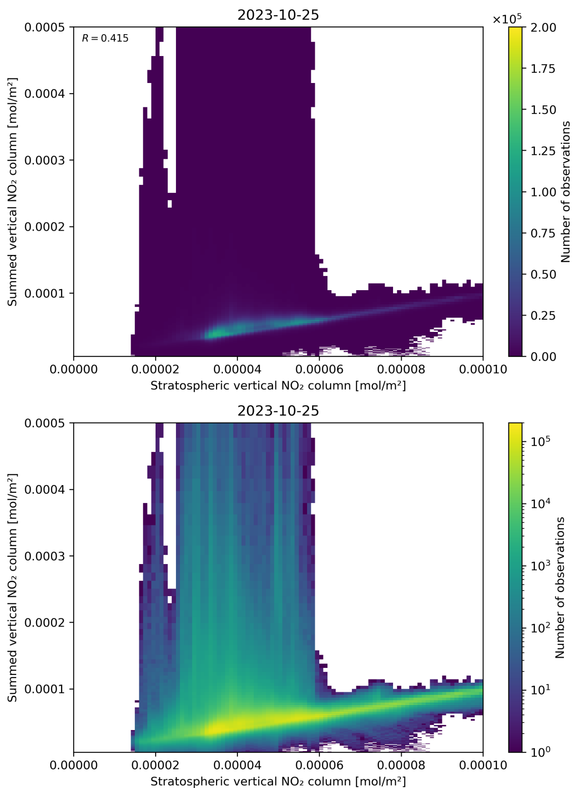
Figure 98: Scatter density plot of “Stratospheric vertical NO 2 column” against “Summed vertical NO 2 column” for 2023-10-24 to 2023-10-26.
