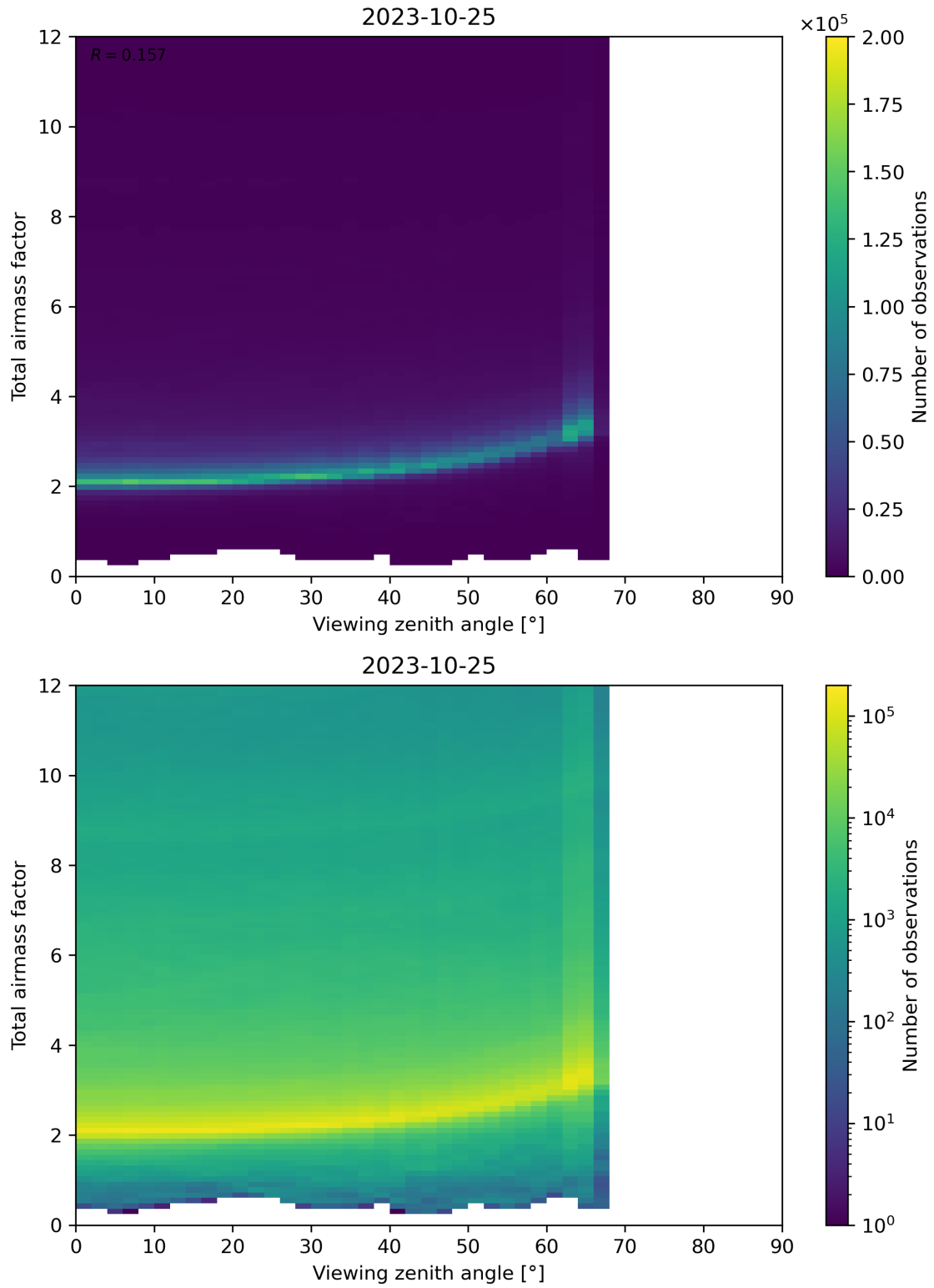
Figure 160: Scatter density plot of “Viewing zenith angle” against “Total airmass factor” for 2023-10-24 to 2023-10-26.
