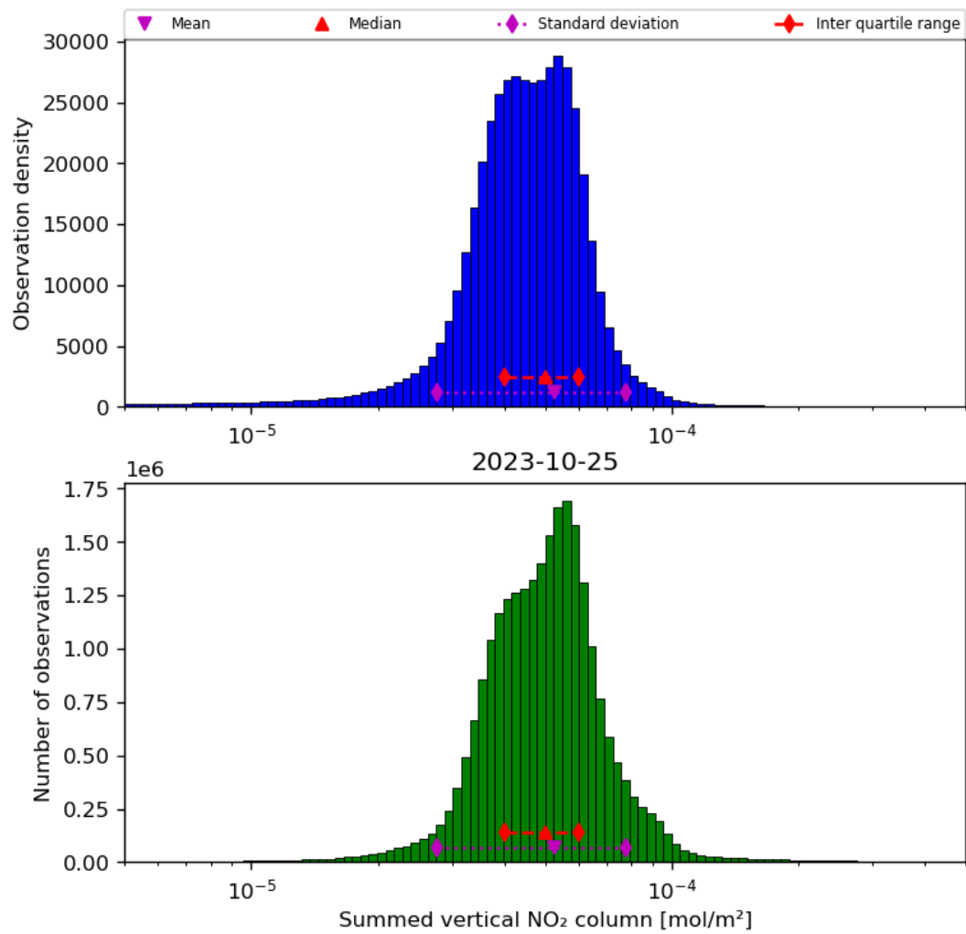
Figure 40: Histogram of "Summed vertical NO 2 column" for 2023-10-24 to 2023-10-26
