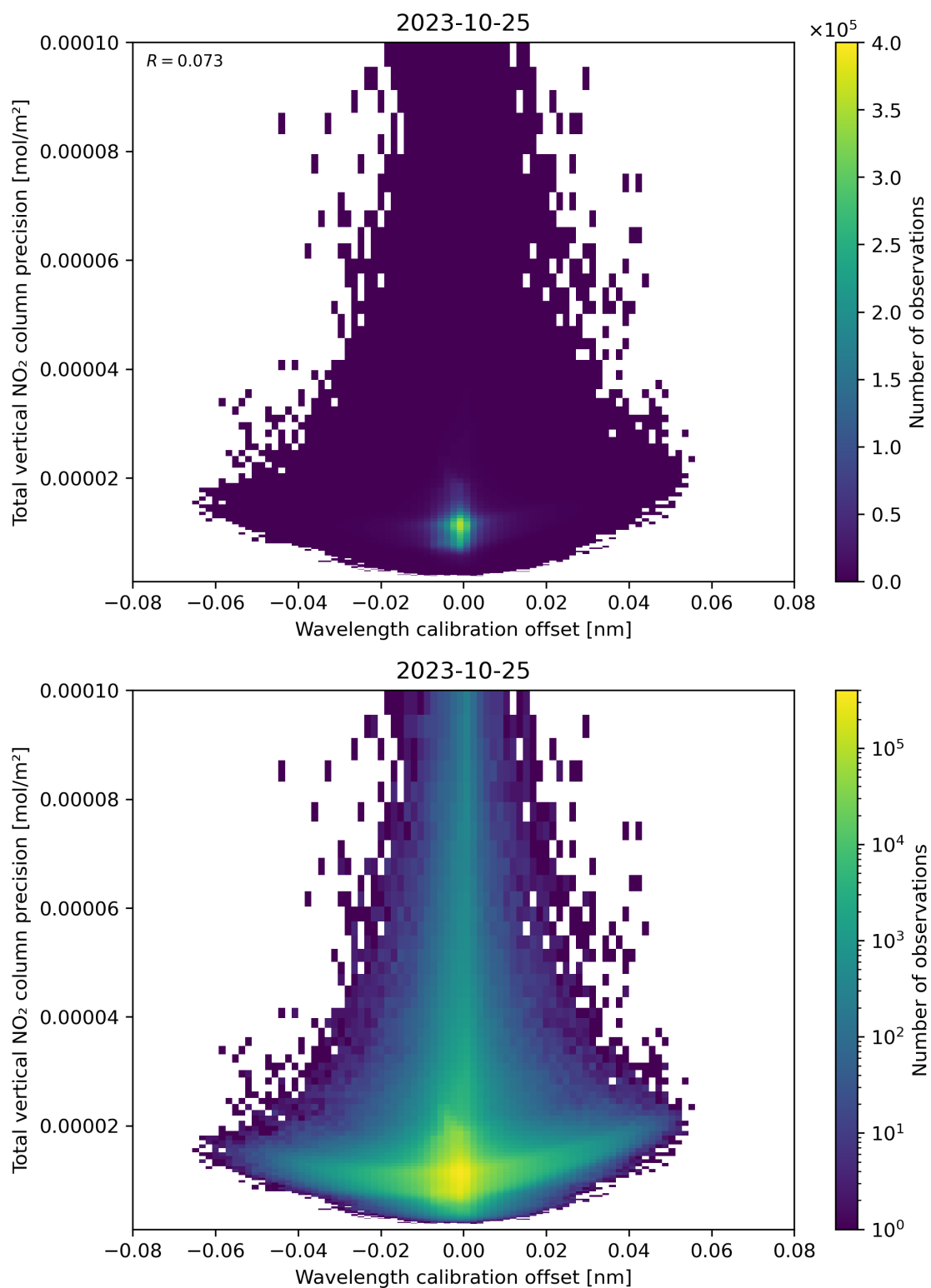
Figure 180: Scatter density plot of “Wavelength calibration offset” against “Total vertical NO 2 column precision” for 2023-10-24 to 2023-10-26.
