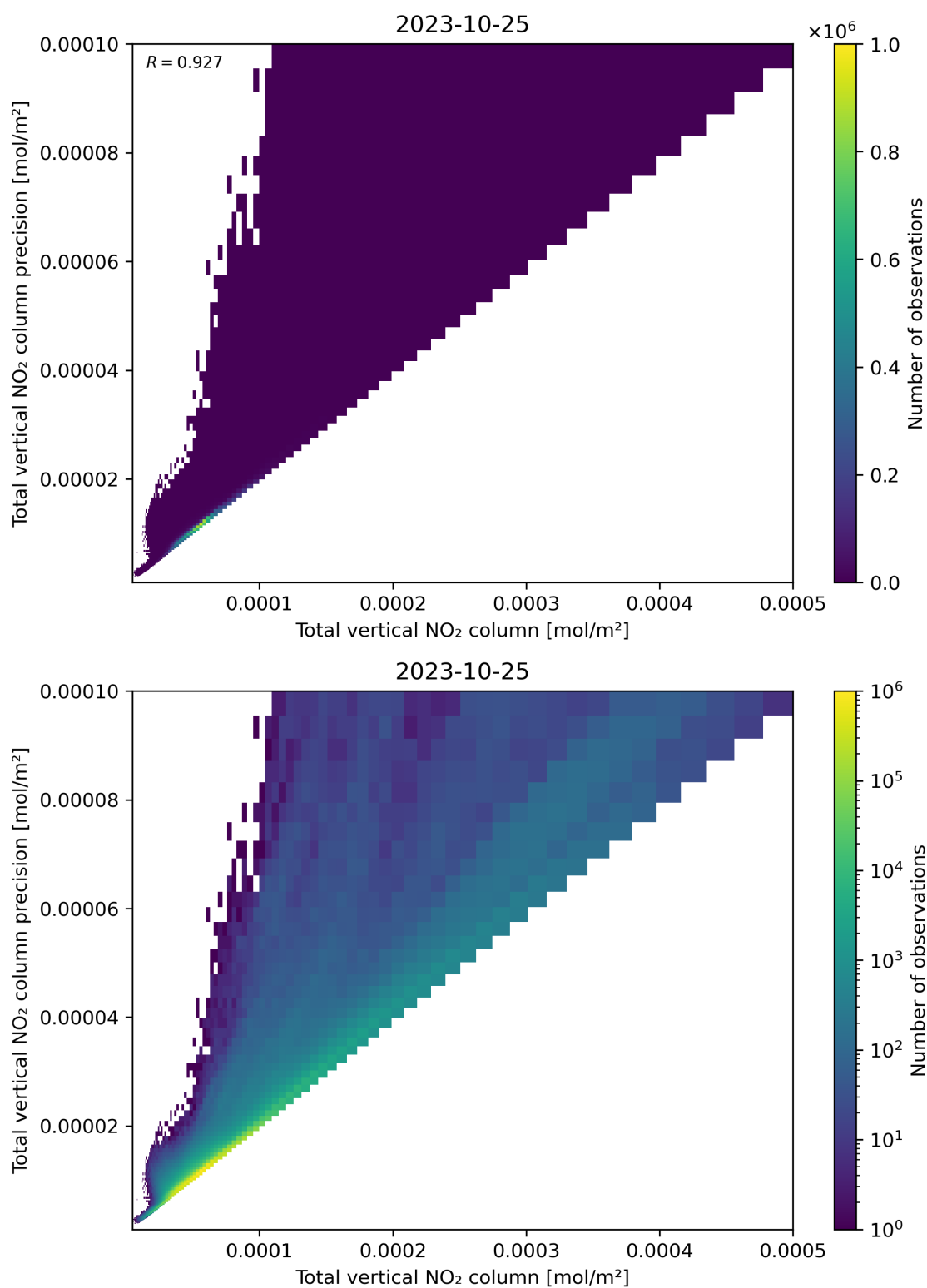
Figure 114: Scatter density plot of “Total vertical NO 2 column” against “Total vertical NO 2 column precision” for 2023-10-24 to 2023-10-26.
