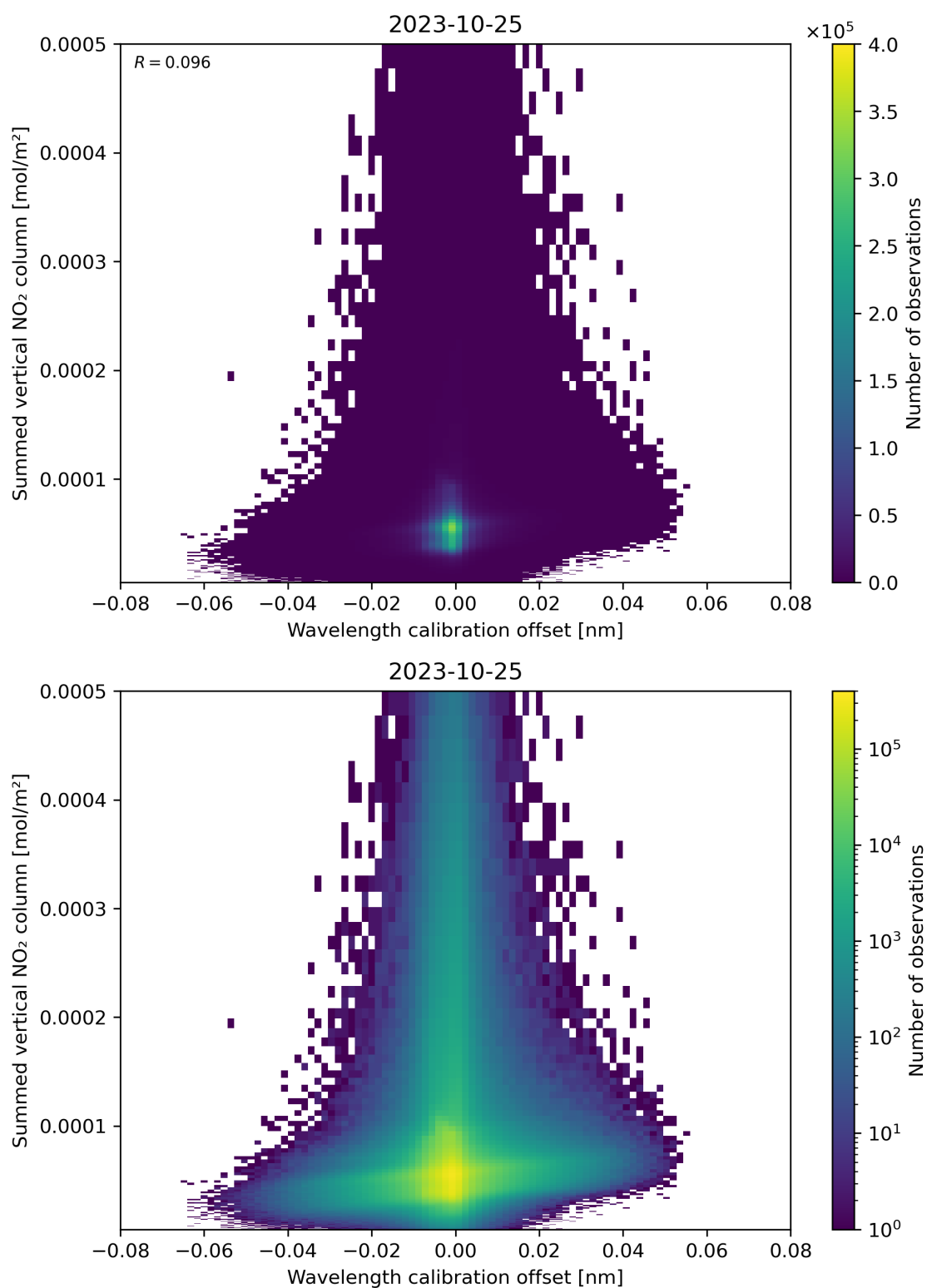
Figure 177: Scatter density plot of “Wavelength calibration offset” against “Summed vertical NO 2 column” for 2023-10-24 to 2023-10-26.
