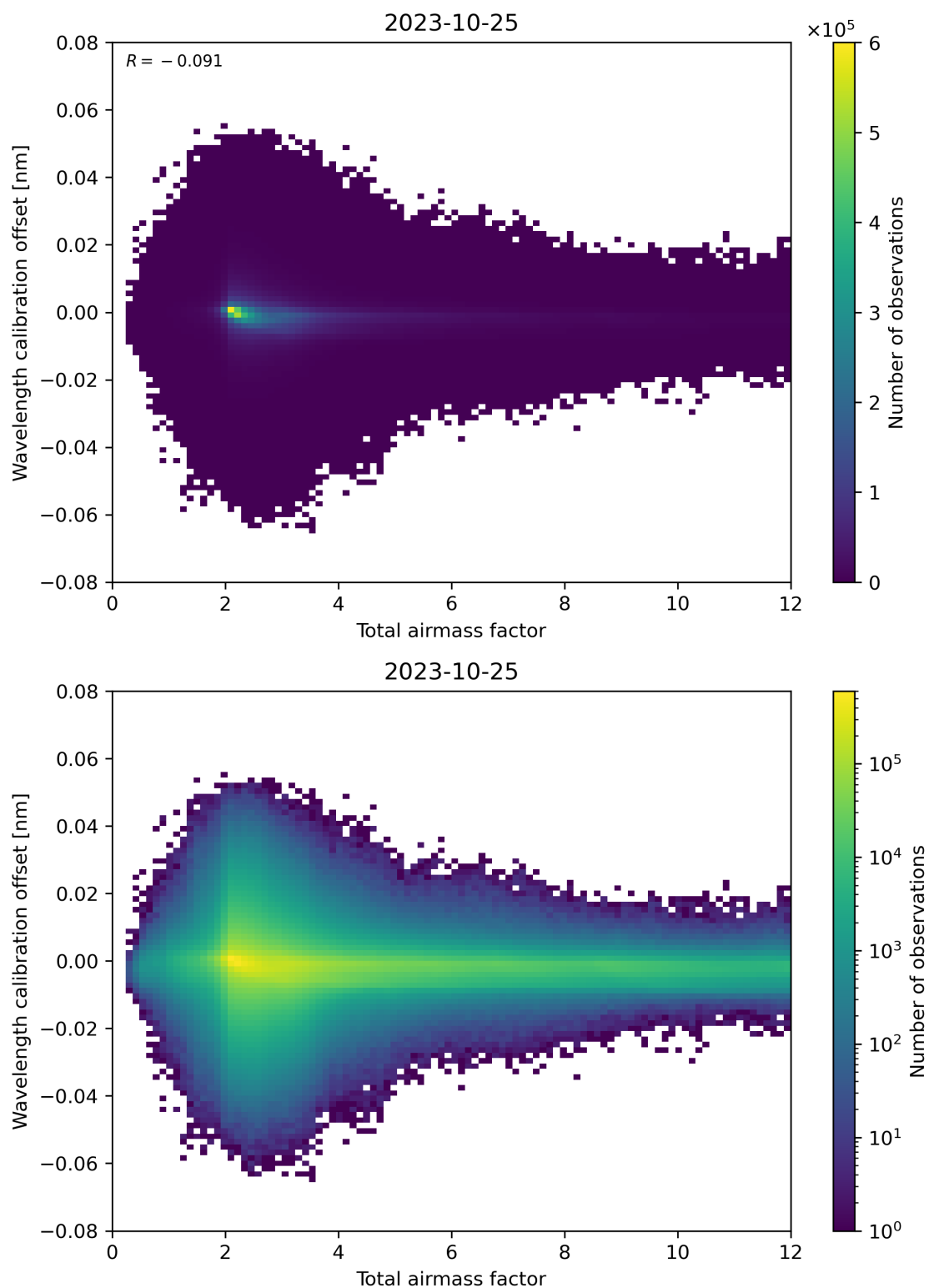
Figure 70: Scatter density plot of “Total airmass factor” against “Wavelength calibration offset” for 2023-10-24 to 2023-10-26.
