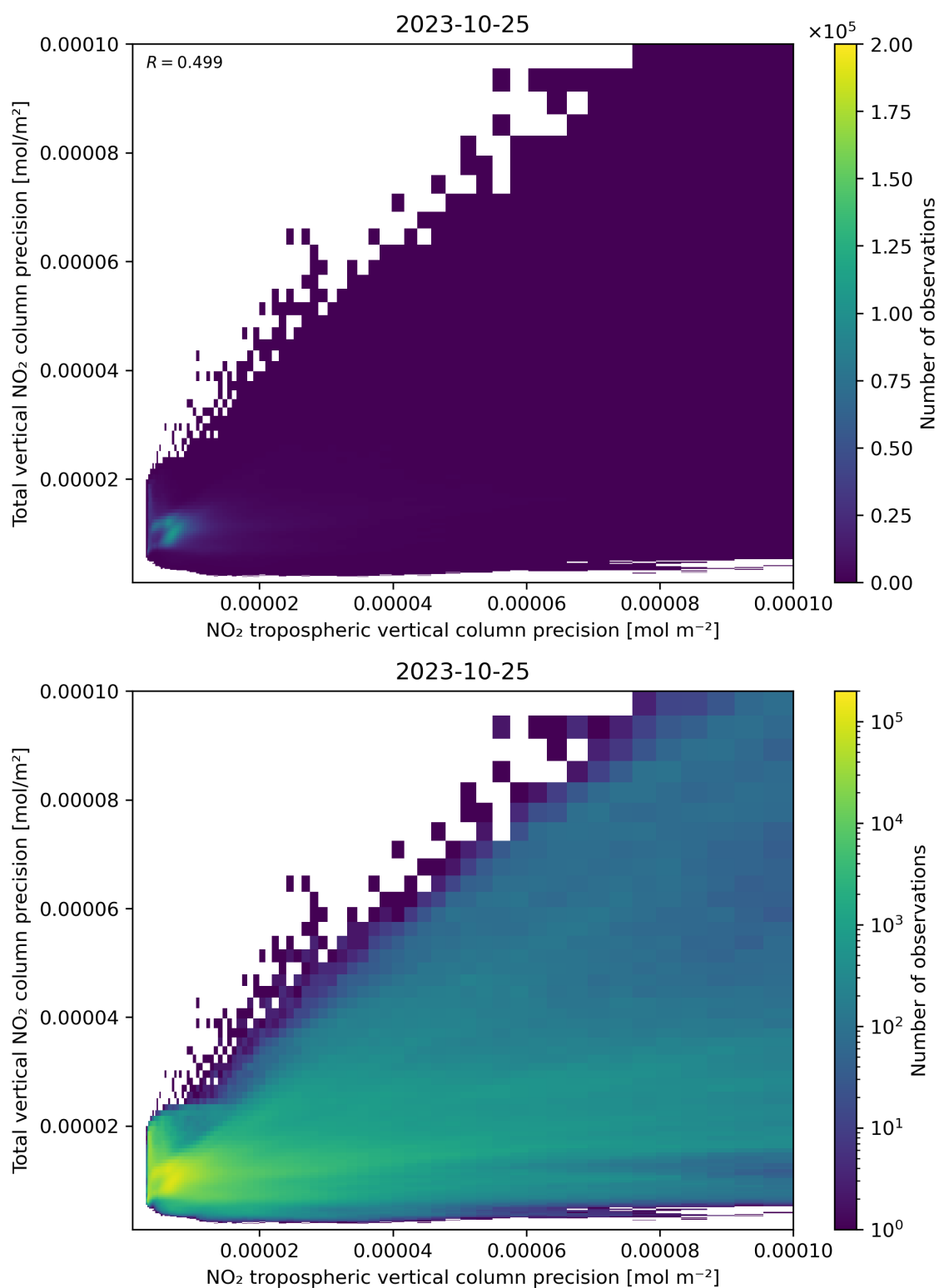
Figure 139: Scatter density plot of “NO 2 tropospheric vertical column precision” against “Total vertical NO 2 column precision” for 2023-10-24 to 2023-10-26.
