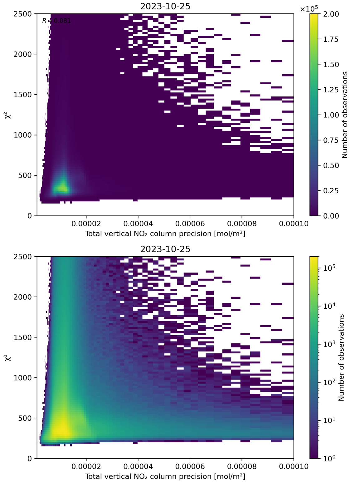
Figure 116: Scatter density plot of “Total vertical NO 2 column precision” against “ \chi^2 ” for 2023-10-24 to 2023-10-26.
