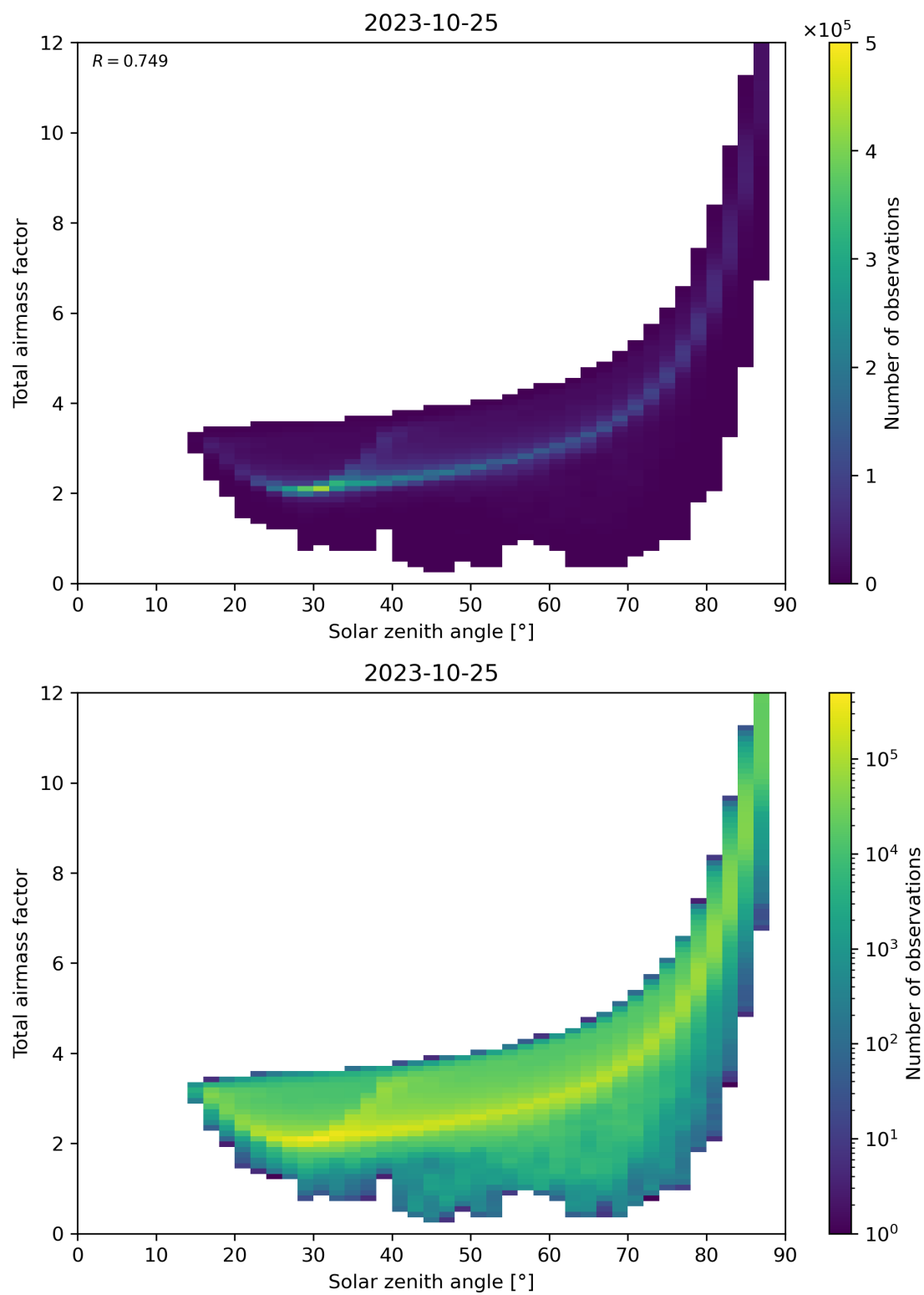
Figure 146: Scatter density plot of “Solar zenith angle” against “Total air mass factor” for 2023-10-24 to 2023-10-26.
