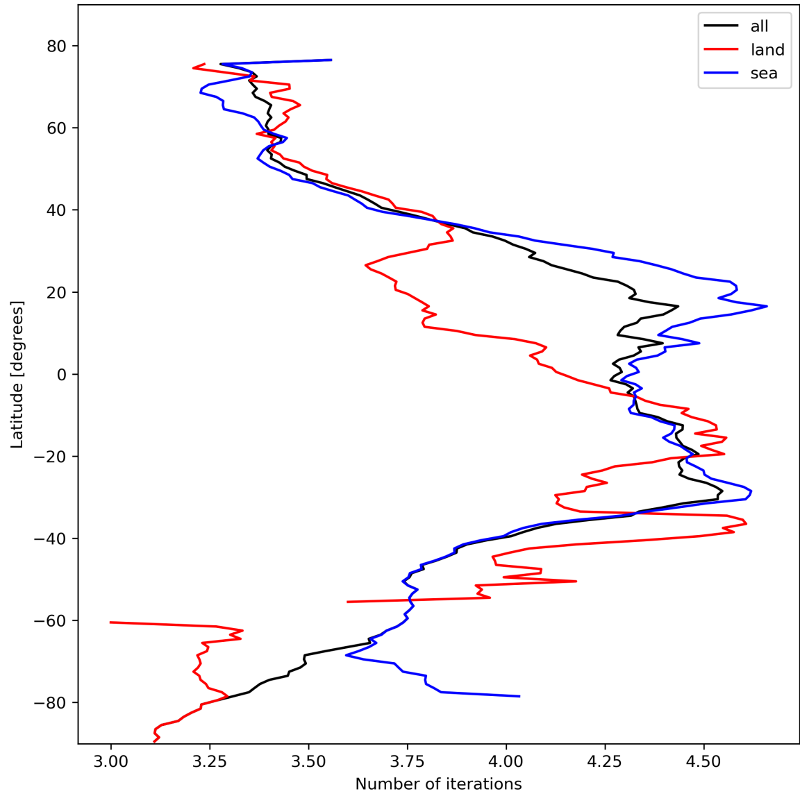
Figure 17: Zonal average of “Number of iterations” for 2023-10-24 to 2023-10-26.
