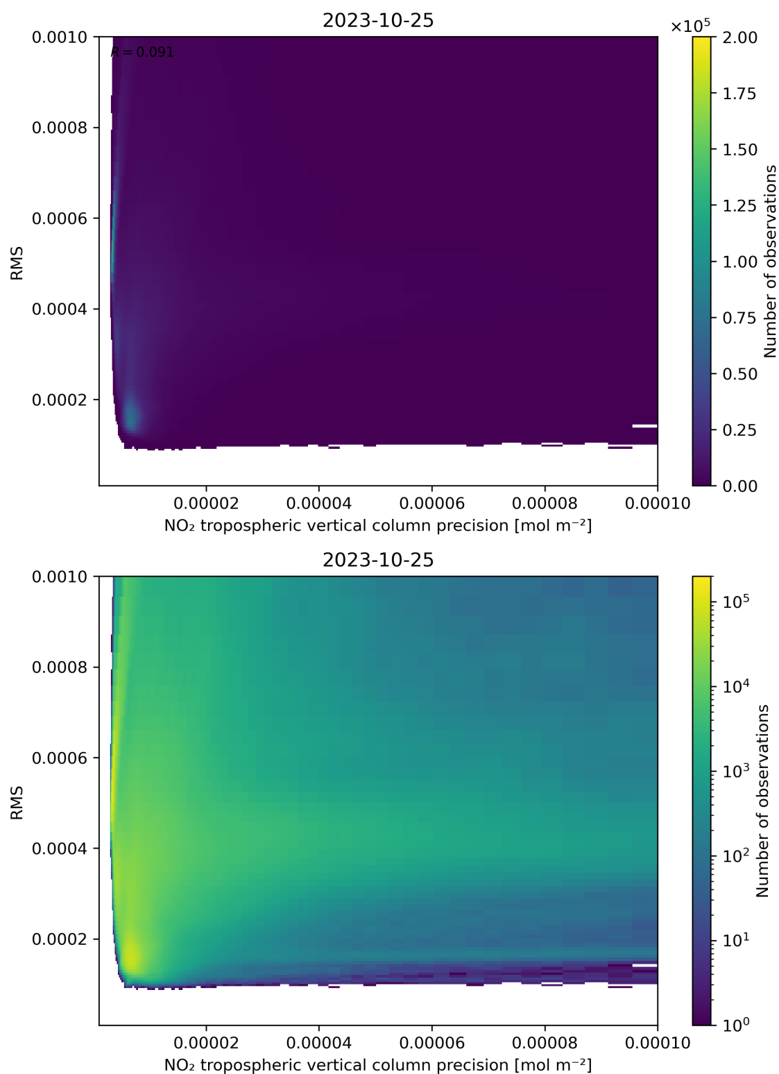
Figure 140: Scatter density plot of “NO 2 tropospheric vertical column precision” against “RMS” for 2023-10-24 to 2023-10-26.
