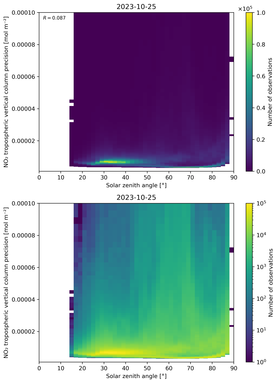
Figure 156: Scatter density plot of “Solar zenith angle” against “NO 2 tropospheric vertical column precision” for 2023-10-24 to 2023-10-26.
