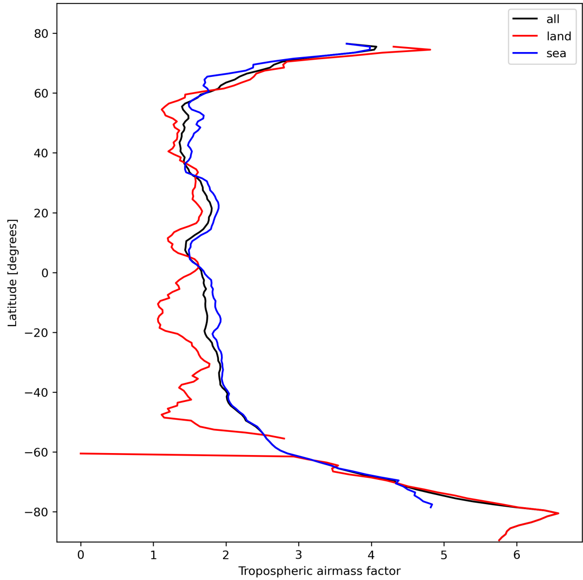
Figure 14: Zonal average of “Tropospheric airmass factor” for 2023-10-24 to 2023-10-26.
