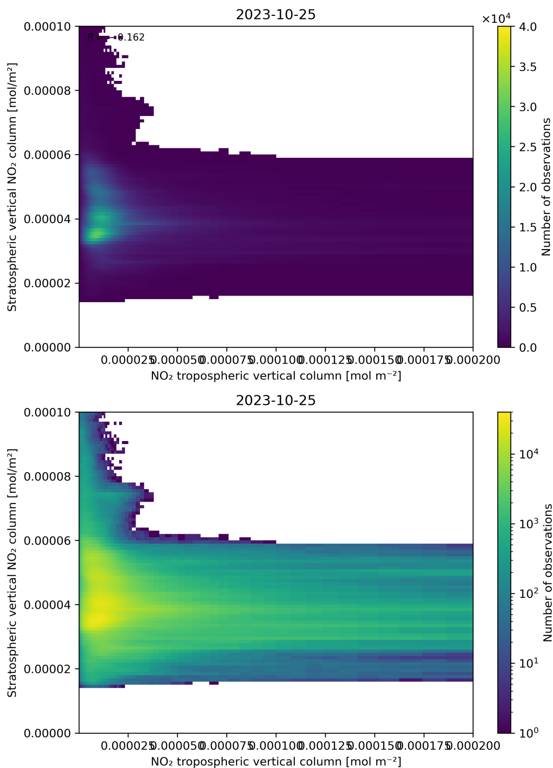
Figure 125: Scatter density plot of “NO 2 tropospheric vertical column” against “Stratospheric vertical NO 2 column” for 2023-10-24 to 2023-10-26.
