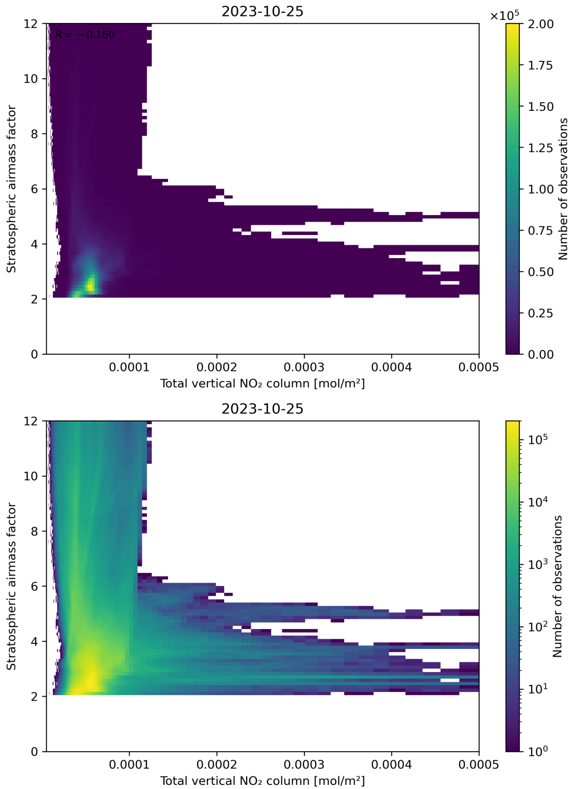
Figure 110: Scatter density plot of “Total vertical NO 2 column” against “Stratospheric airmass factor” for 2023-10-24 to 2023-10-26.
