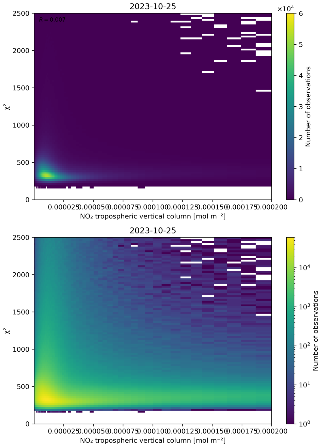
Figure 124: Scatter density plot of “NO 2 tropospheric vertical column” against “ \chi^2 ” for 2023-10-24 to 2023-10-26.
