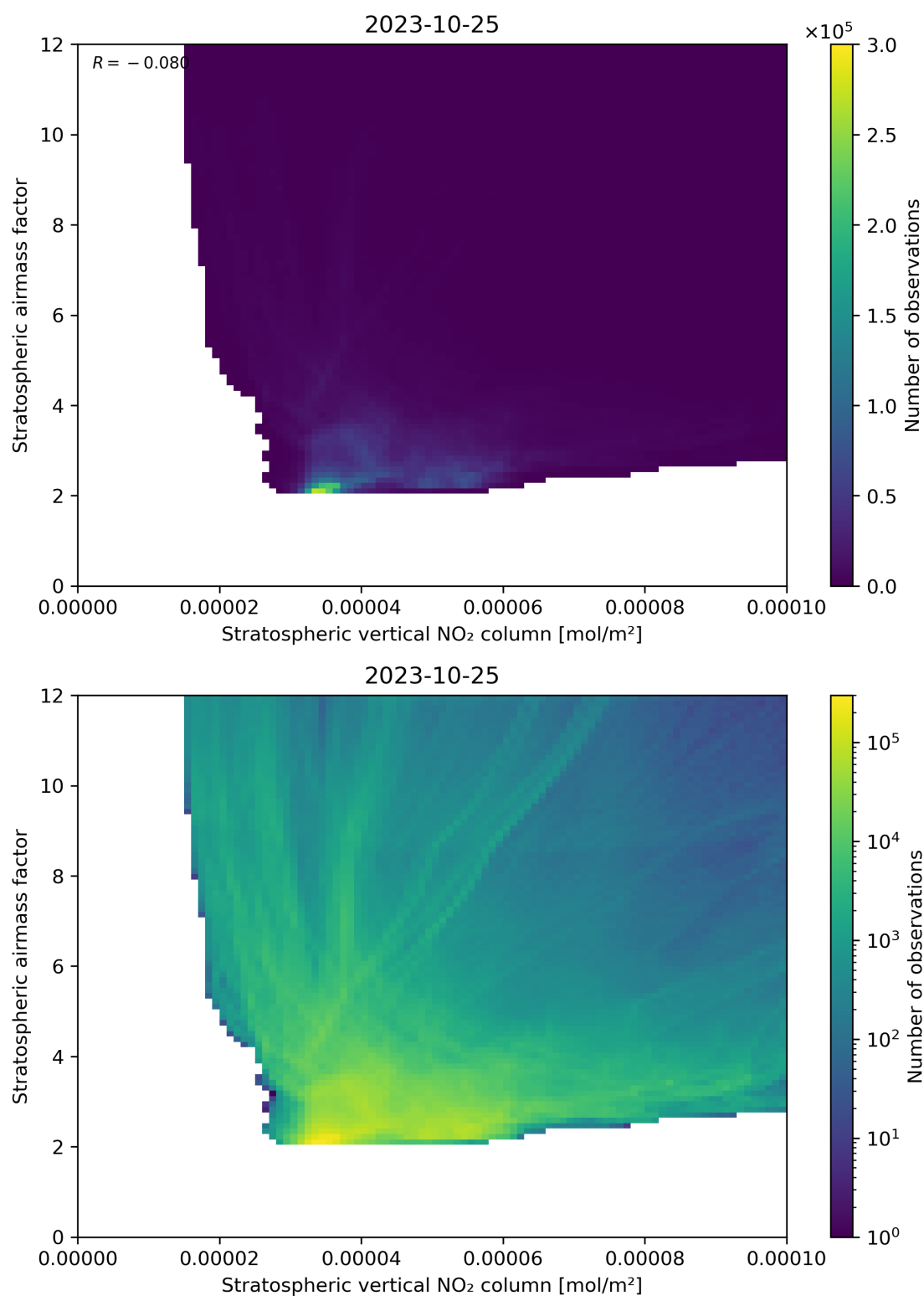
Figure 96: Scatter density plot of “Stratospheric vertical NO 2 column” against “Stratospheric airmass factor” for 2023-10-24 to 2023-10-26.
