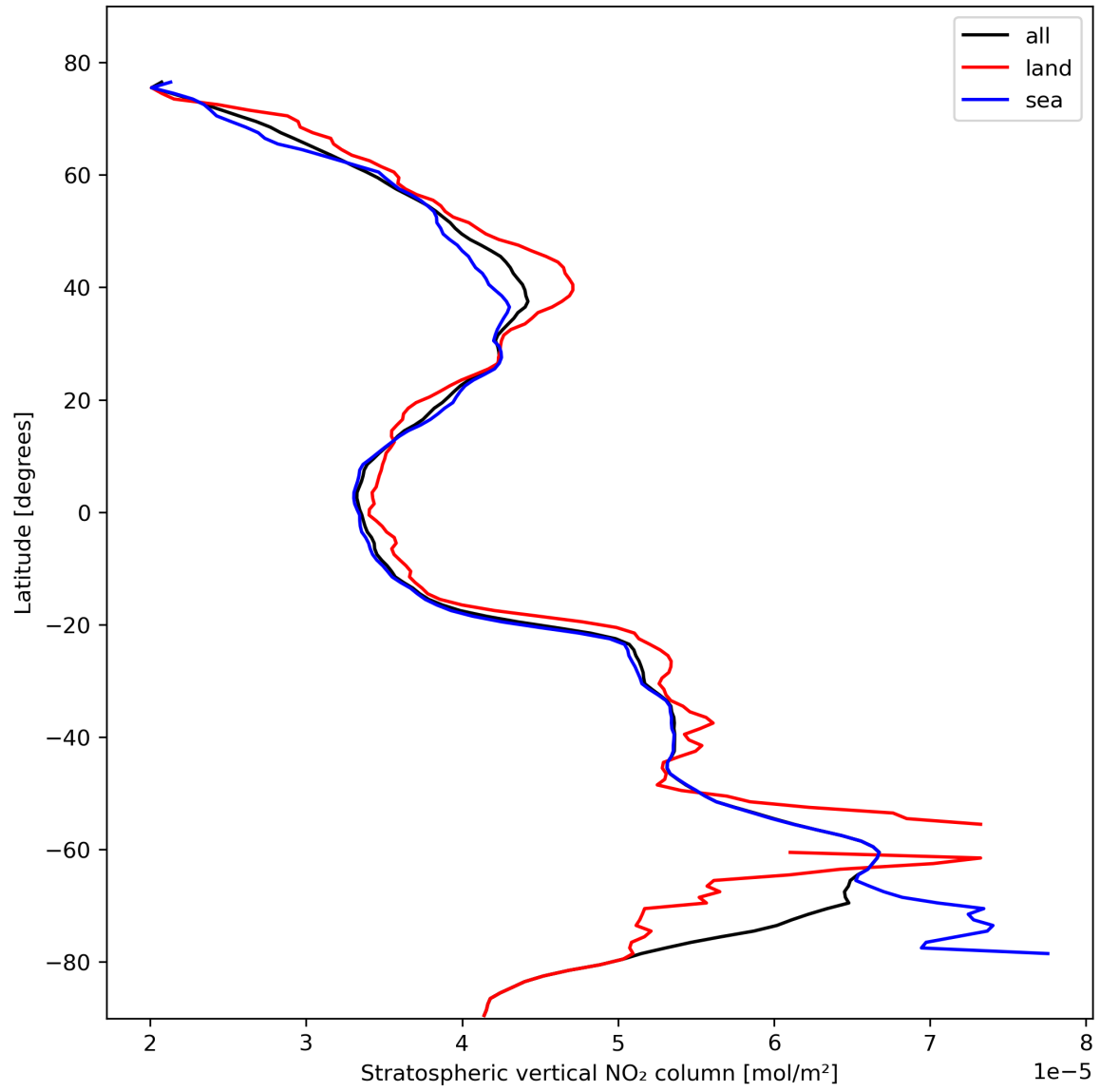
Figure 19: Zonal average of “Stratospheric vertical NO 2 column” for 2023-10-24 to 2023-10-26.
