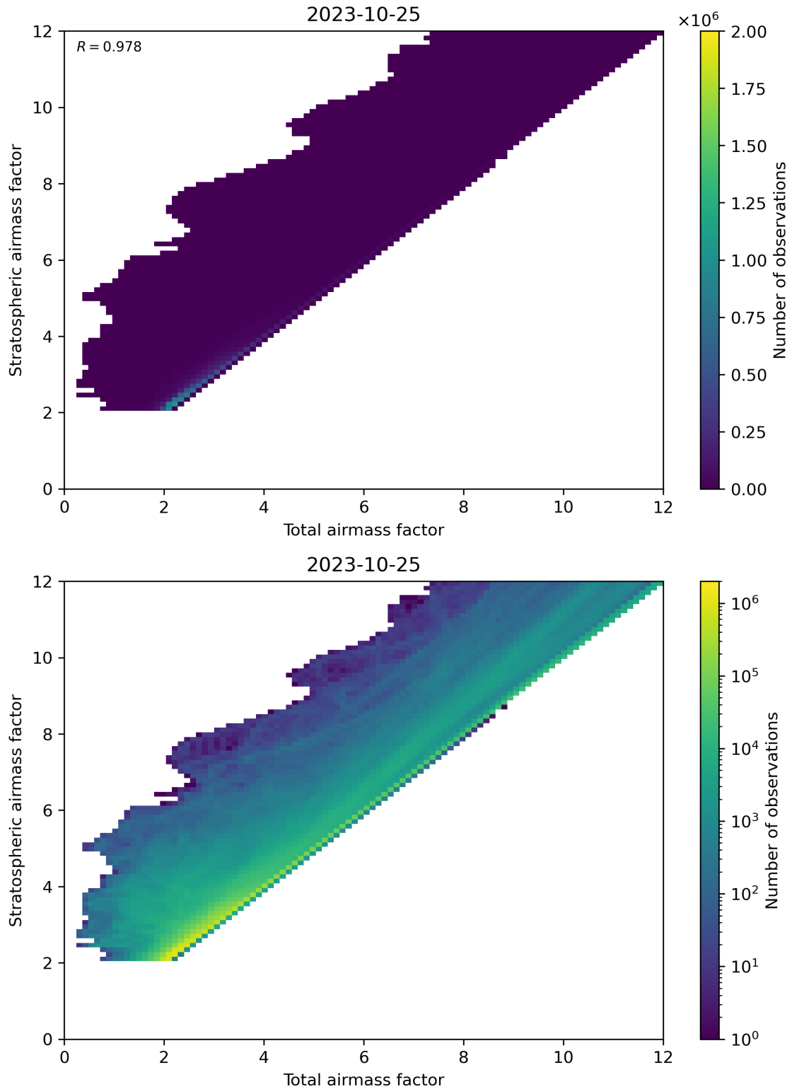
Figure 62: Scatter density plot of “Total airmass factor” against “Stratospheric airmass factor” for 2023-10-24 to 2023-10-26.
