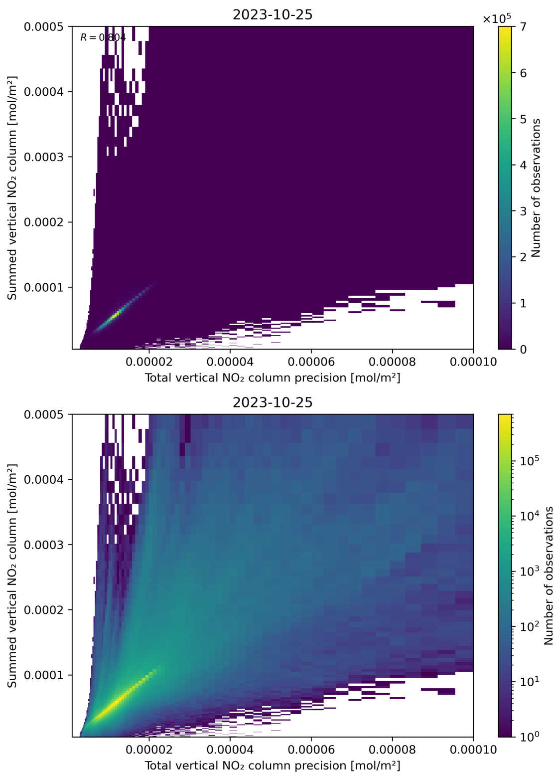
Figure 117: Scatter density plot of “Total vertical NO 2 column precision” against “Summed vertical NO 2 column” for 2023-10-24 to 2023-10-26.
