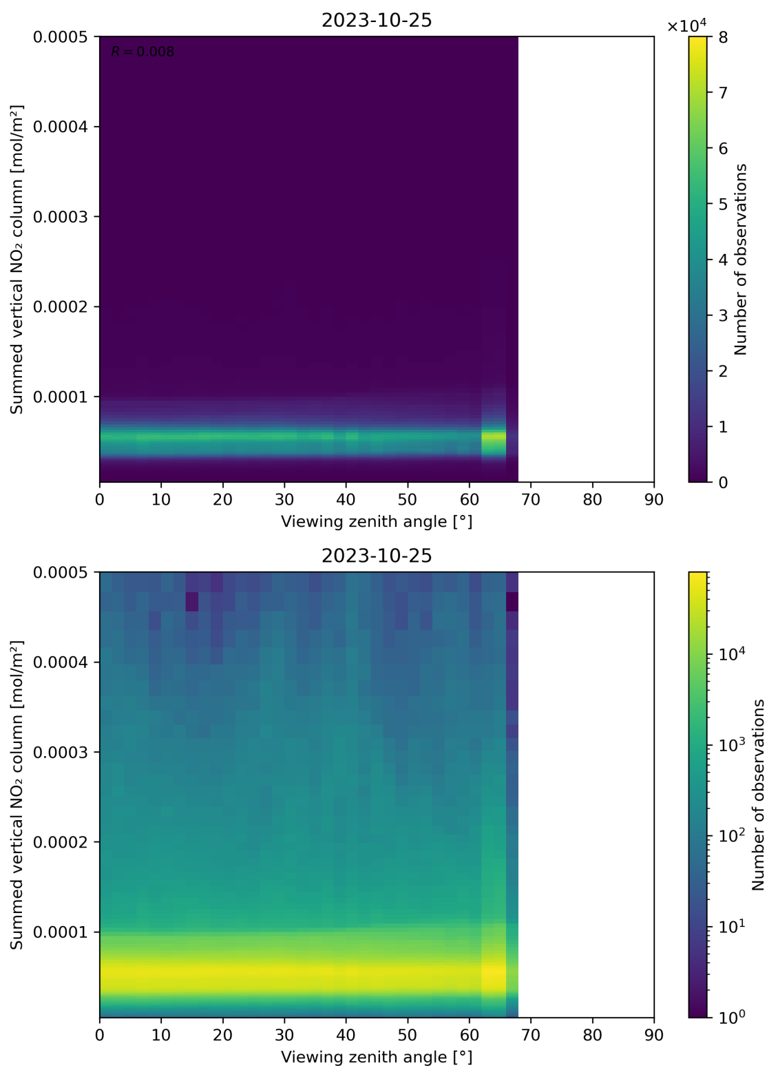
Figure 165: Scatter density plot of “Viewing zenith angle” against “Summed vertical NO 2 column” for 2023-10-24 to 2023-10-26.
