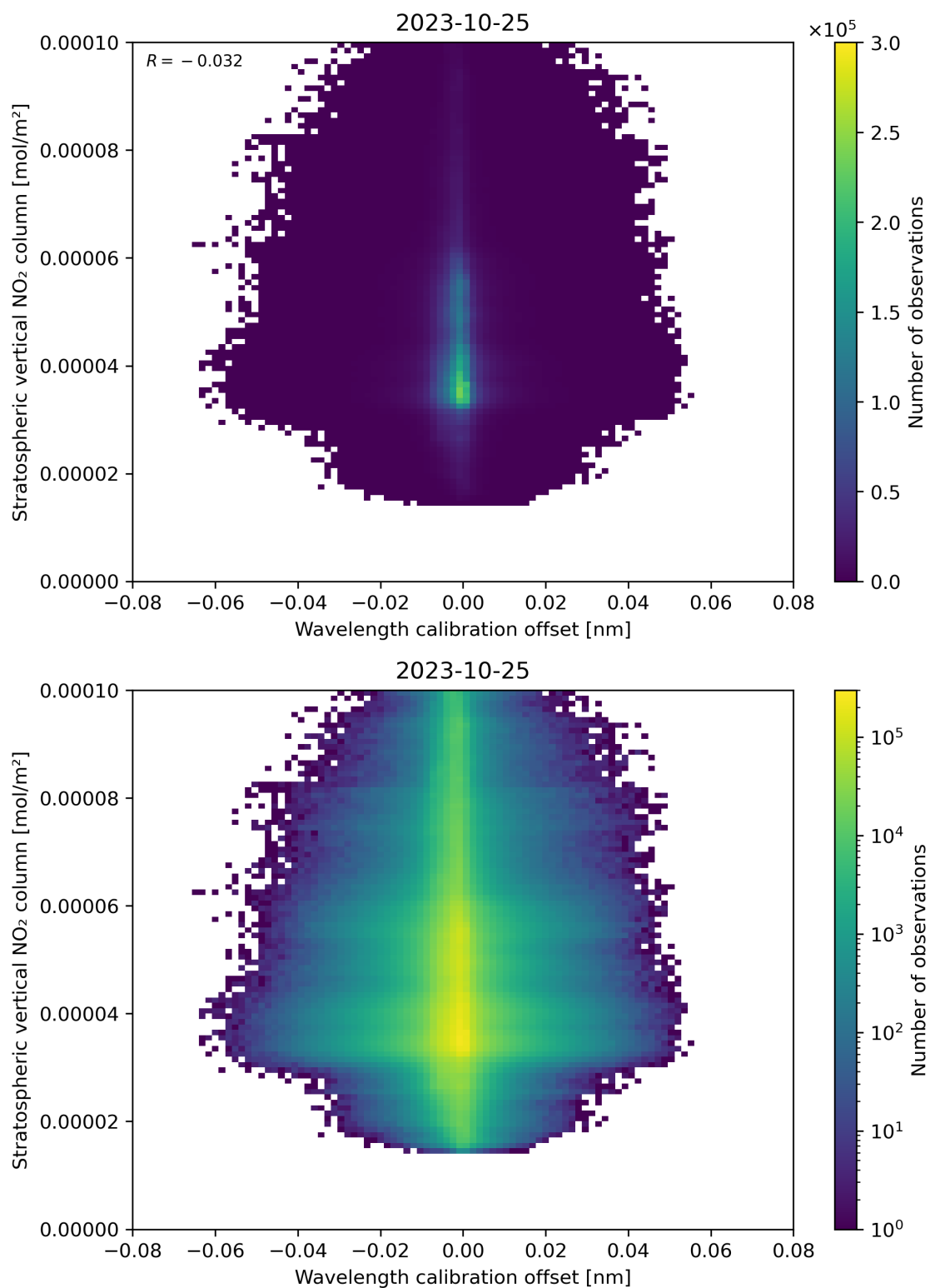
Figure 176: Scatter density plot of “Wavelength calibration offset” against “Stratospheric vertical NO 2 column” for 2023-10-24 to 2023-10-26.
