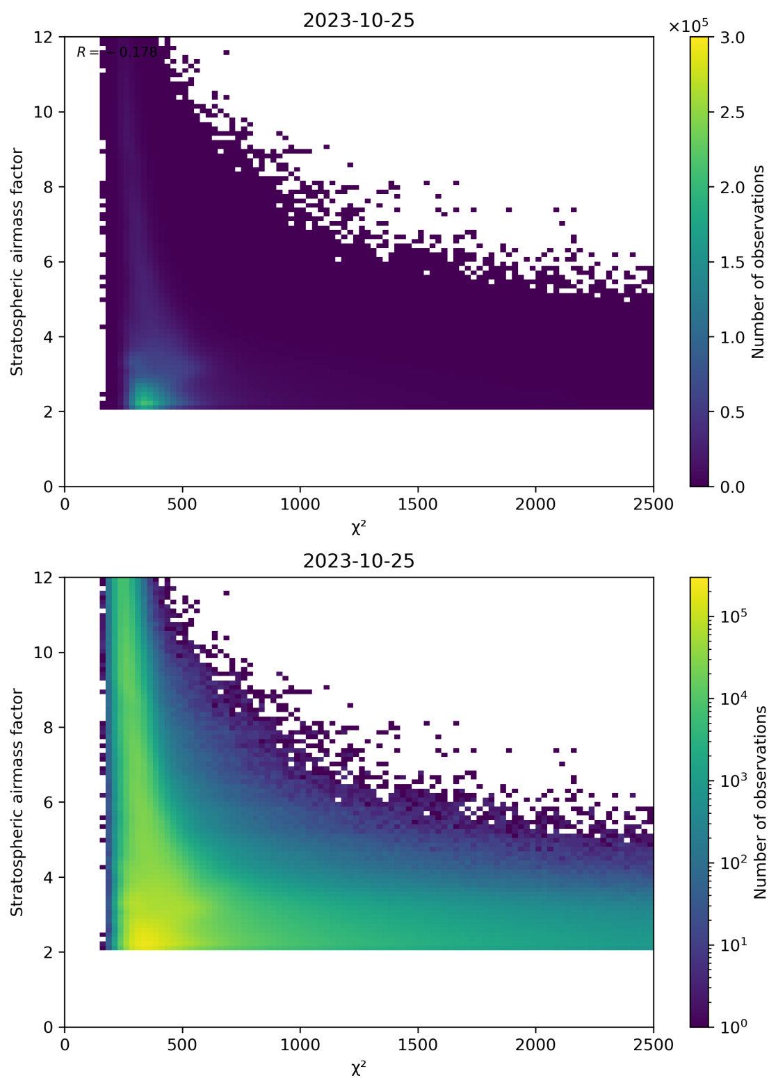
Figure 81: Scatter density plot of “ \chi^2 ” against “Stratospheric airmass factor” for 2023-10-24 to 2023-10-26.
