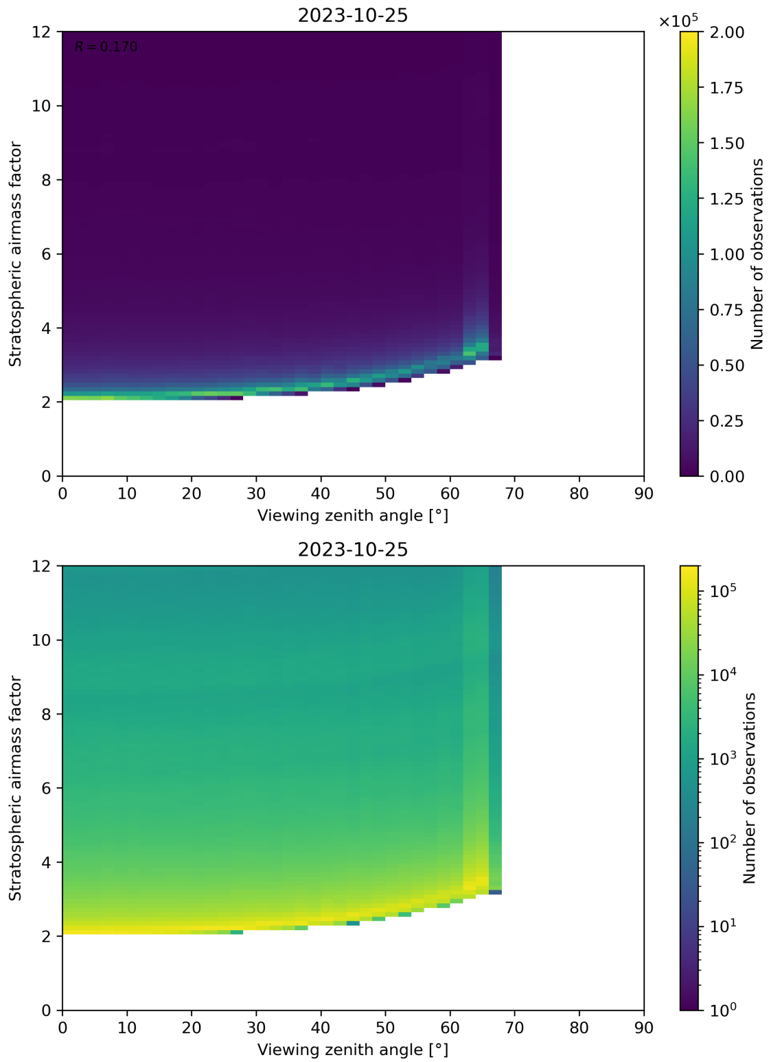
Figure 159: Scatter density plot of “Viewing zenith angle” against “Stratospheric airmass factor” for 2023-10-24 to 2023-10-26.
