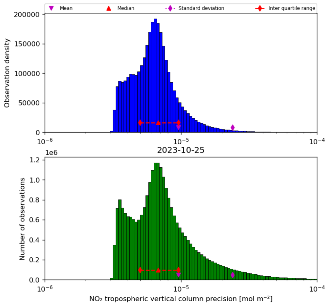
Figure 30: Histogram of “NO 2 tropospheric vertical column precision” for 2023-10-24 to 2023-10-26
