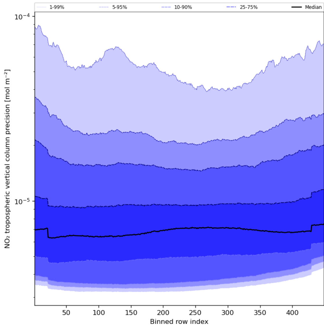
Figure 47: Along track statistics of “NO 2 tropospheric vertical column precision” for 2023-10-24 to 2023-10-26
