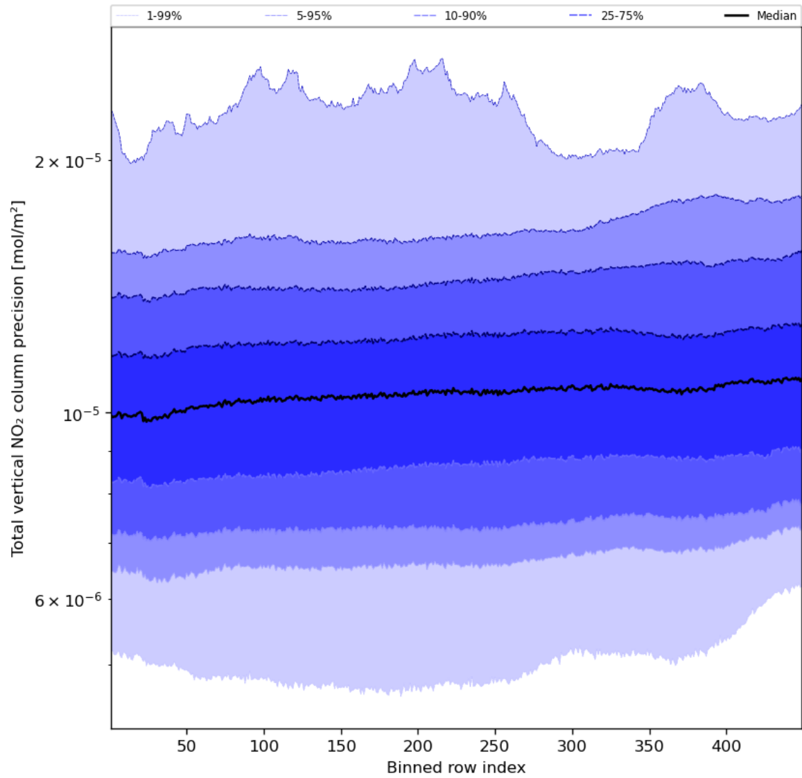
Figure 56: Along track statistics of “Total vertical NO 2 column precision” for 2023-10-24 to 2023-10-26
