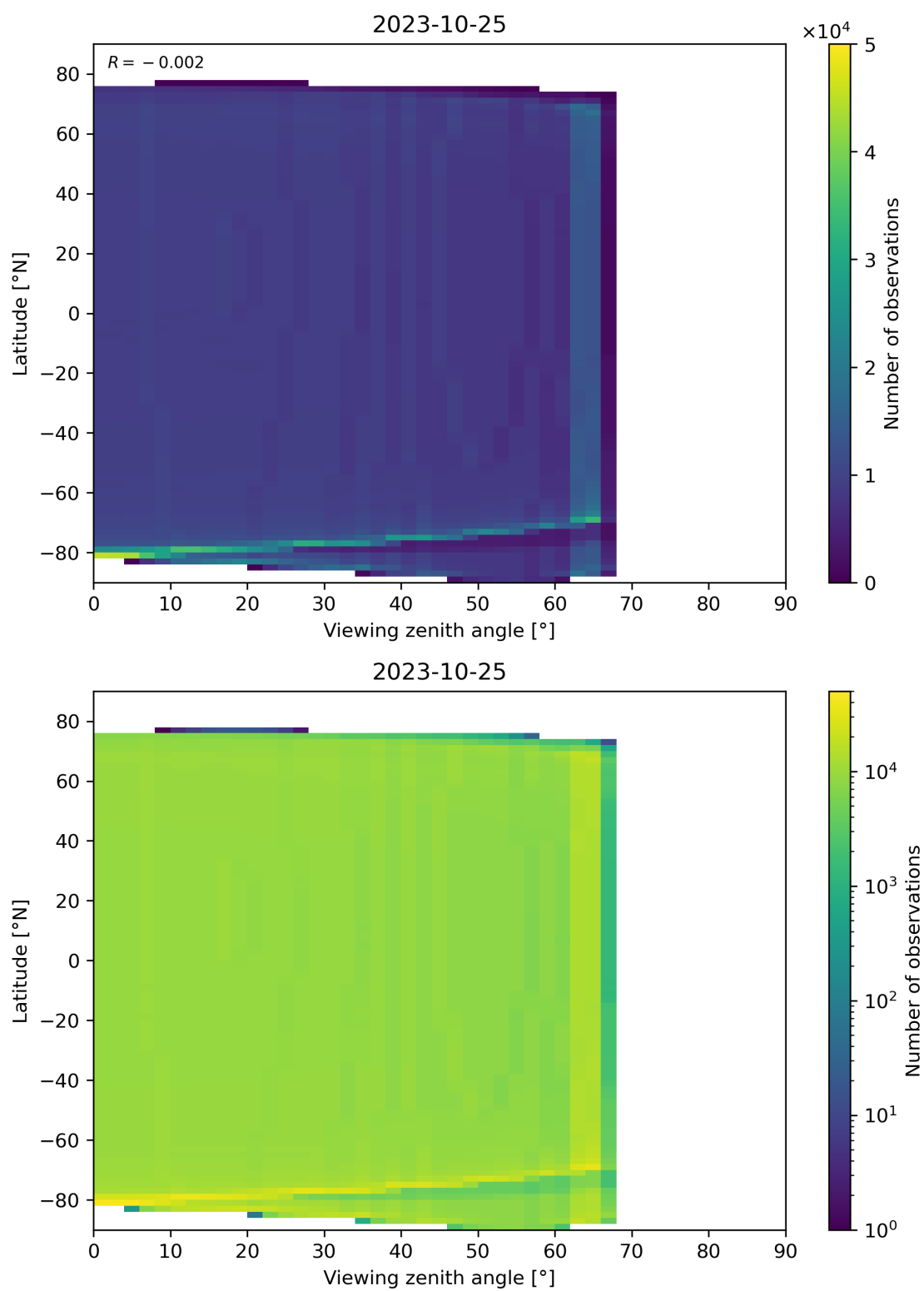
Figure 163: Scatter density plot of “Viewing zenith angle” against “Latitude” for 2023-10-24 to 2023-10-26.
