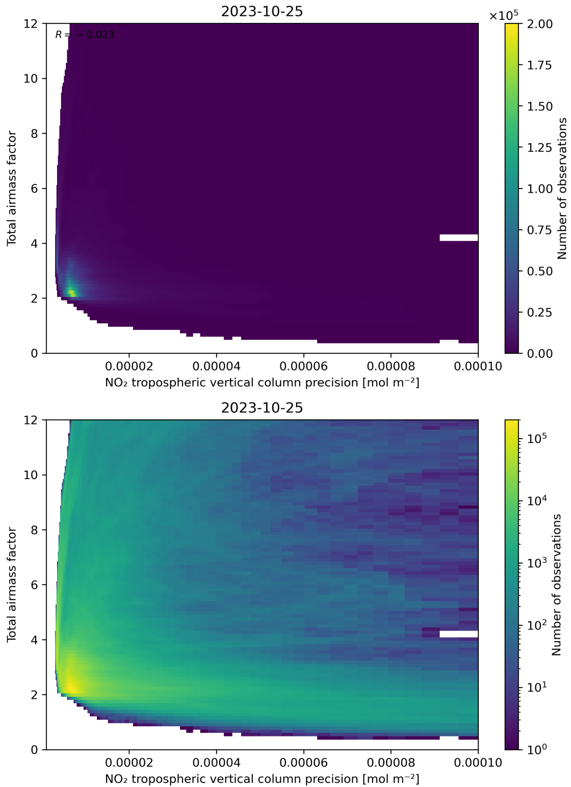
Figure 132: Scatter density plot of “NO 2 tropospheric vertical column precision” against “Total air mass factor” for 2023-10-24 to 2023-10-26.
