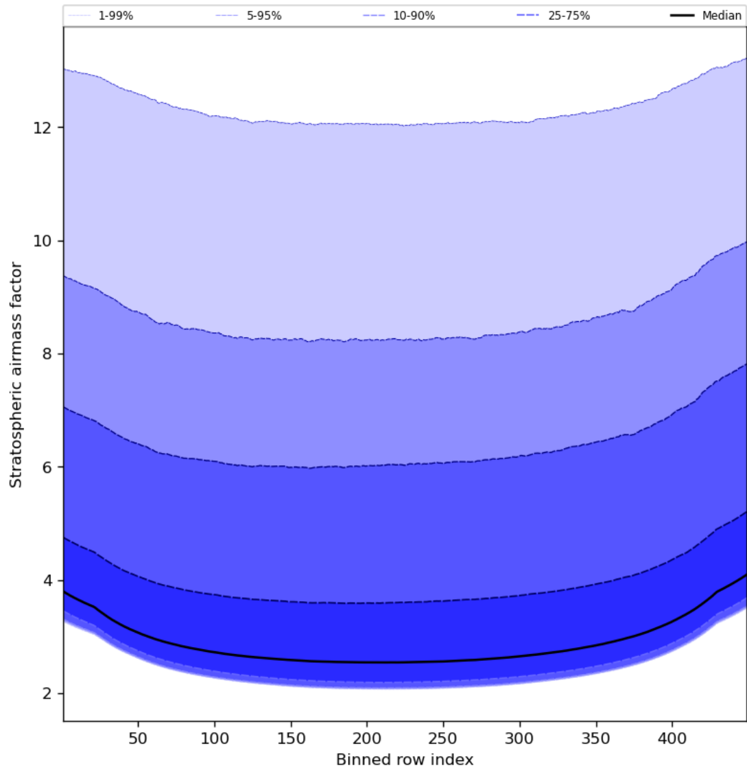
Figure 61: Along track statistics of “Stratospheric airmass factor” for 2023-10-24 to 2023-10-26
