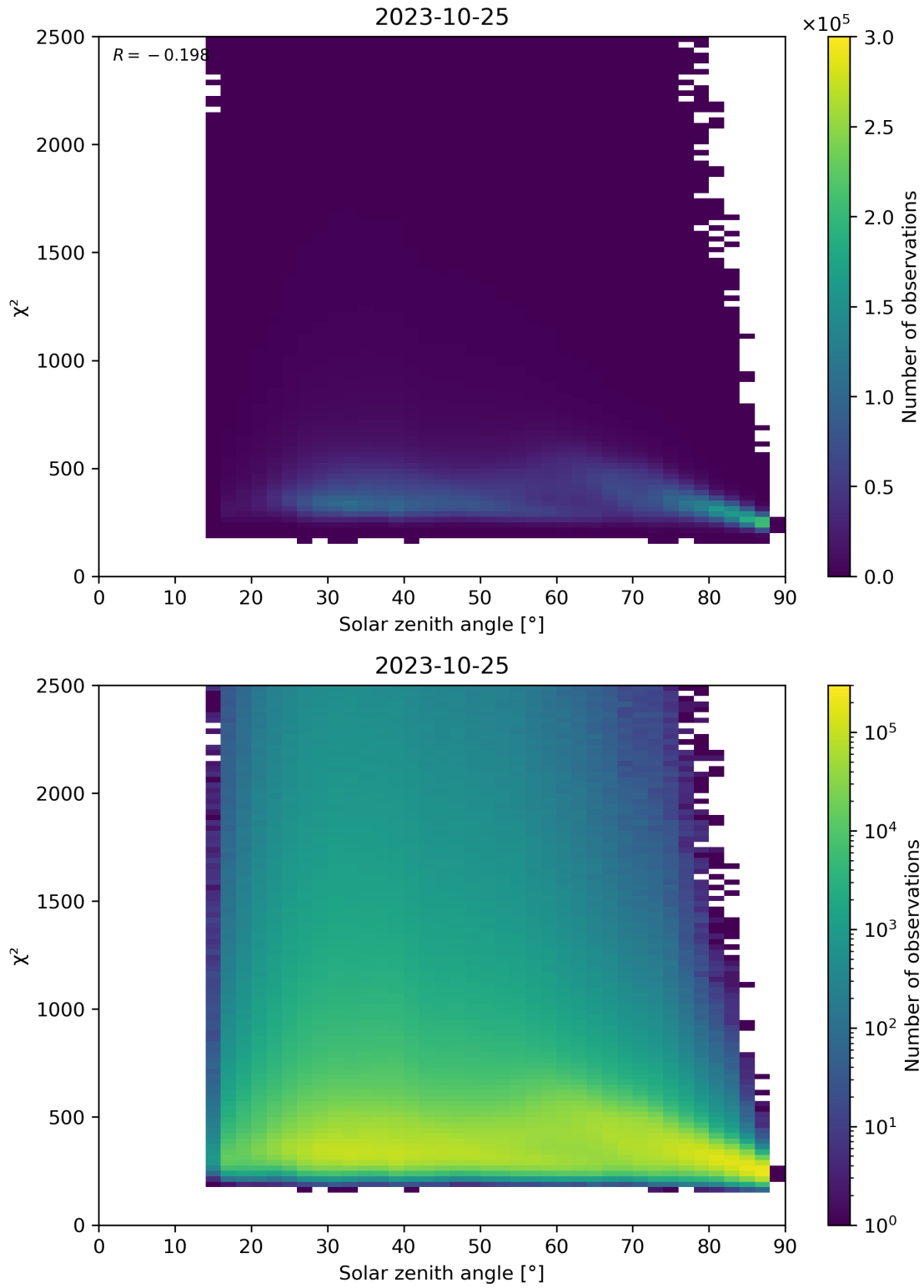
Figure 148: Scatter density plot of “Solar zenith angle” against “ \chi^2 ” for 2023-10-24 to 2023-10-26.
