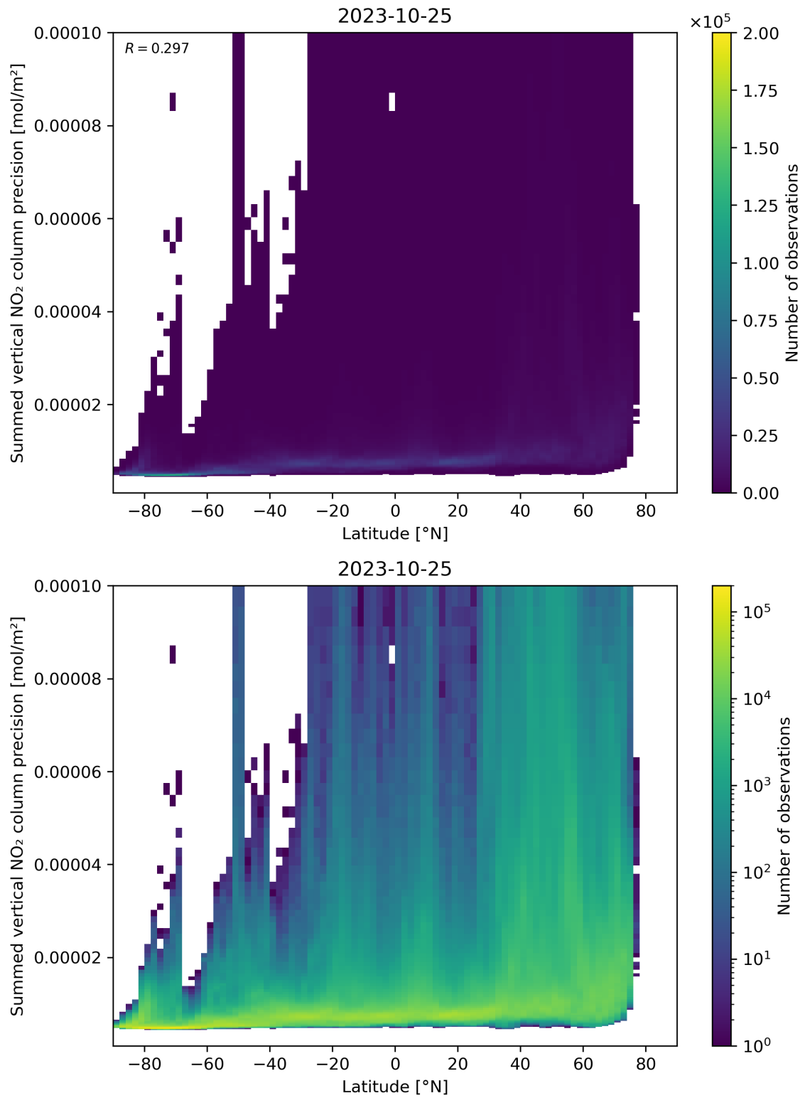
Figure 89: Scatter density plot of “Latitude” against “Summed vertical NO 2 column precision” for 2023-10-24 to 2023-10-26.
