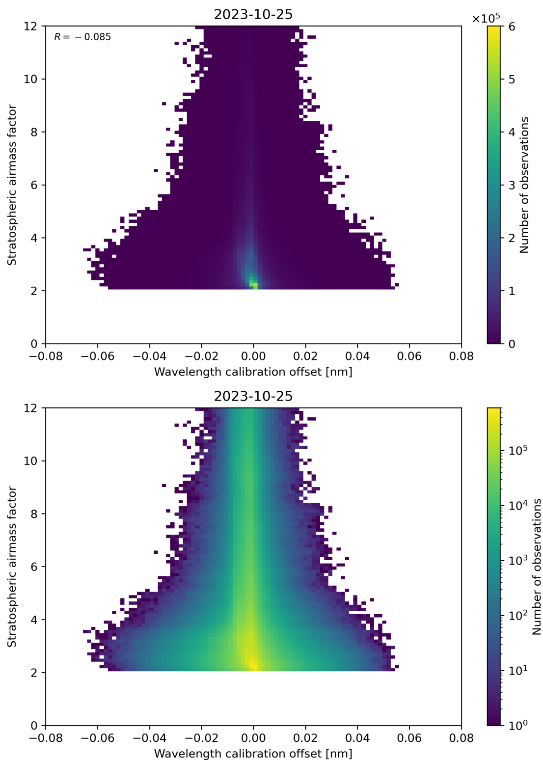
Figure 174: Scatter density plot of “Wavelength calibration offset” against “Stratospheric air mass factor” for 2023-10-24 to 2023-10-26.
