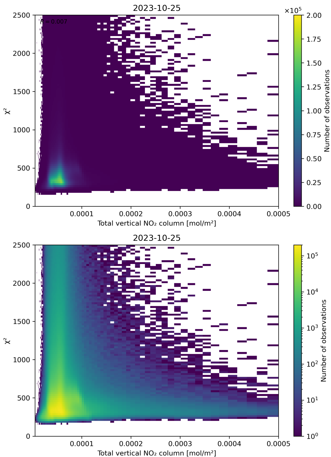
Figure 111: Scatter density plot of “Total vertical NO 2 column” against “ \chi^2 ” for 2023-10-24 to 2023-10-26.
