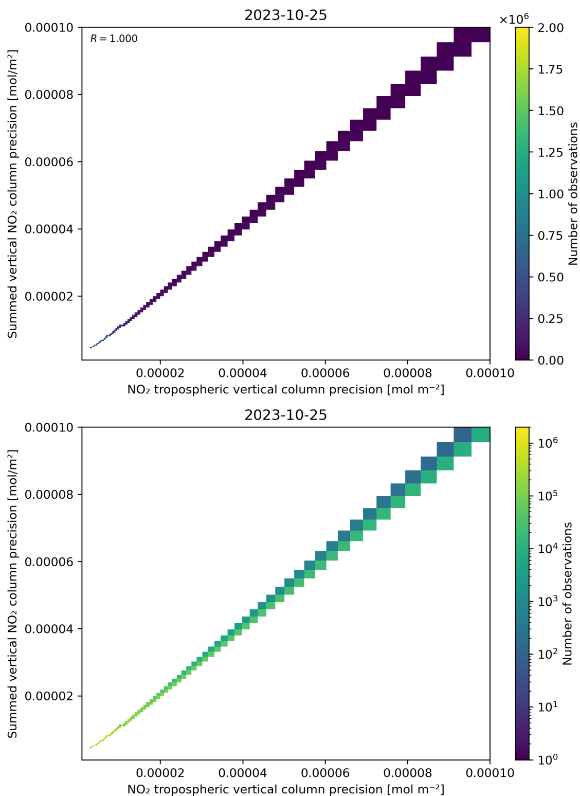
Figure 137: Scatter density plot of “NO 2 tropospheric vertical column precision” against “Summed vertical NO 2 column precision” for 2023-10-24 to 2023-10-26.
