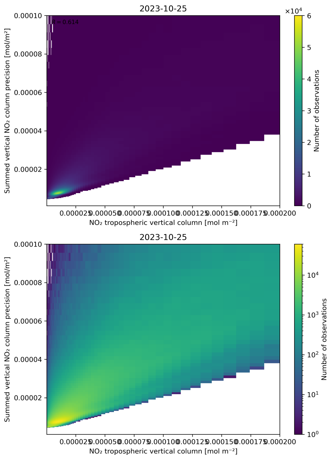
Figure 127: Scatter density plot of “NO 2 tropospheric vertical column” against “Summed vertical NO 2 column precision” for 2023-10-24 to 2023-10-26.
