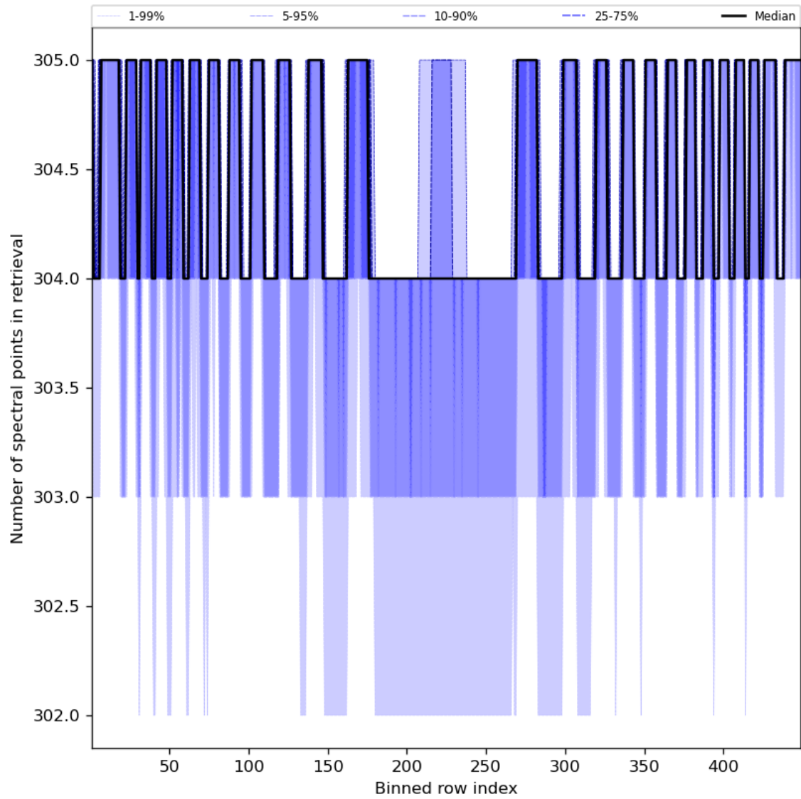
Figure 50: Along track statistics of “Number of spectral points in retrieval” for 2023-10-24 to 2023-10-26
