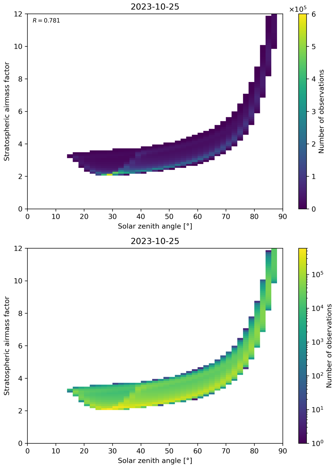
Figure 145: Scatter density plot of “Solar zenith angle” against “Stratospheric airmass factor” for 2023-10-24 to 2023-10-26.
