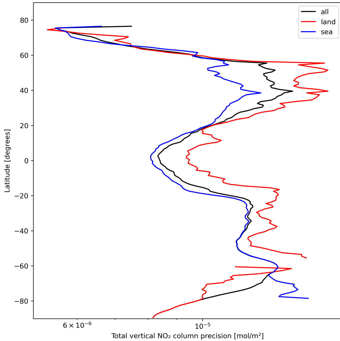
Figure 22: Zonal average of “Total vertical NO 2 column precision” for 2023-10-24 to 2023-10-26.
