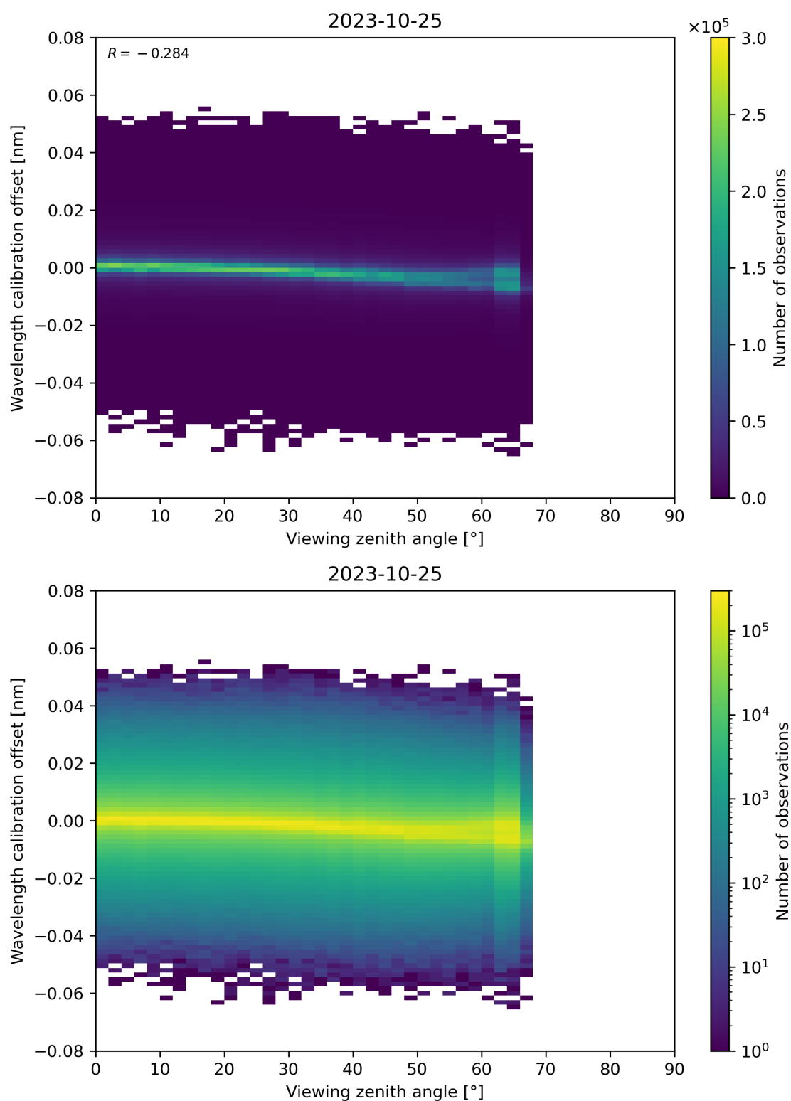
Figure 173: Scatter density plot of “Viewing zenith angle” against “Wavelength calibration offset” for 2023-10-24 to 2023-10-26.
