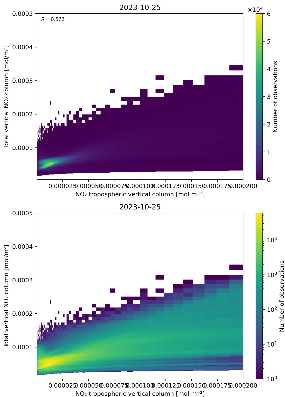
Figure 128: Scatter density plot of “NO 2 tropospheric vertical column” against “Total vertical NO 2 column” for 2023-10-24 to 2023-10-26.
