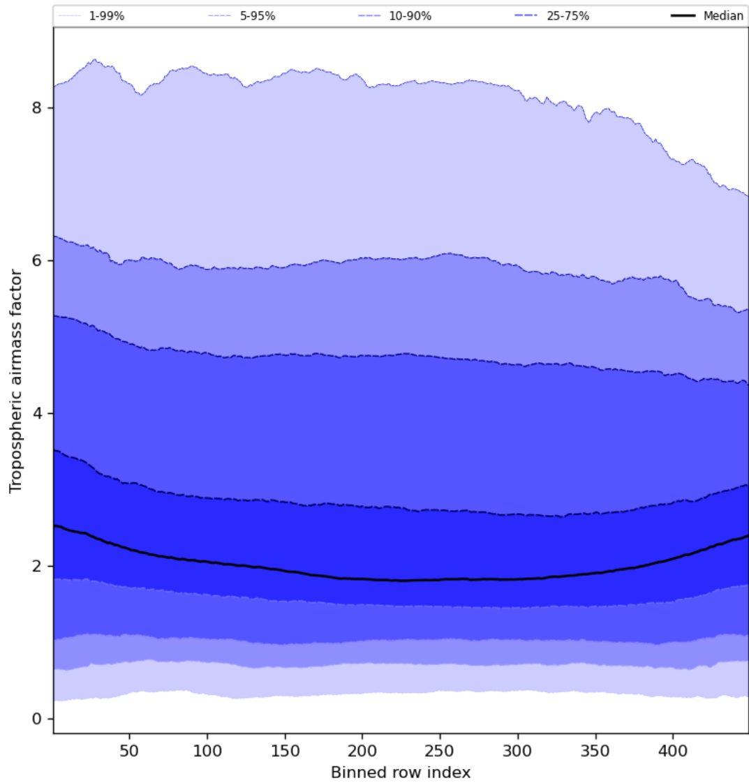
Figure 48: Along track statistics of “Tropospheric air mass factor” for 2023-10-24 to 2023-10-26
