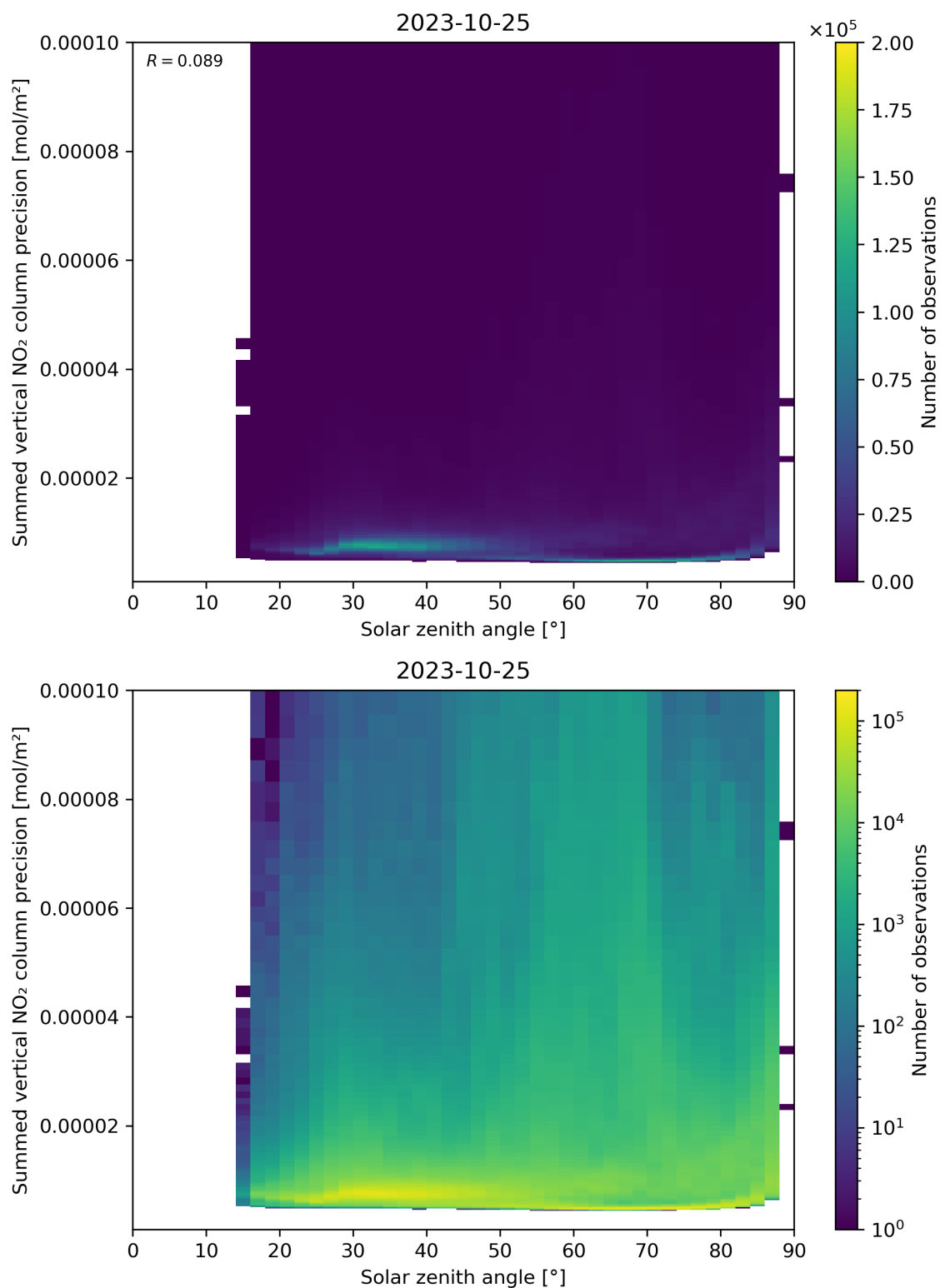
Figure 152: Scatter density plot of “Solar zenith angle” against “Summed vertical NO 2 column precision” for 2023-10-24 to 2023-10-26.
