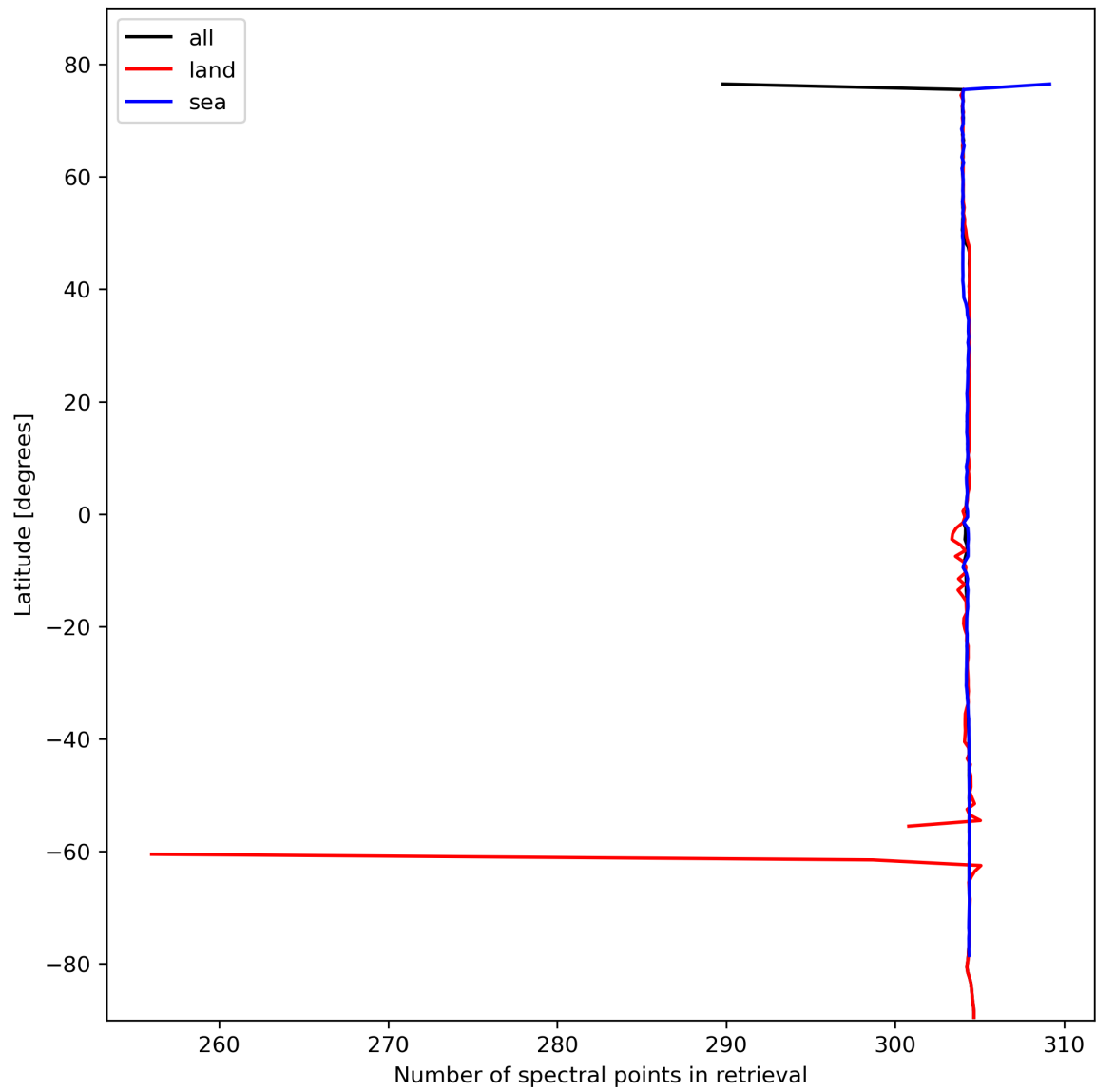
Figure 16: Zonal average of “Number of spectral points in retrieval” for 2023-10-24 to 2023-10-26.
