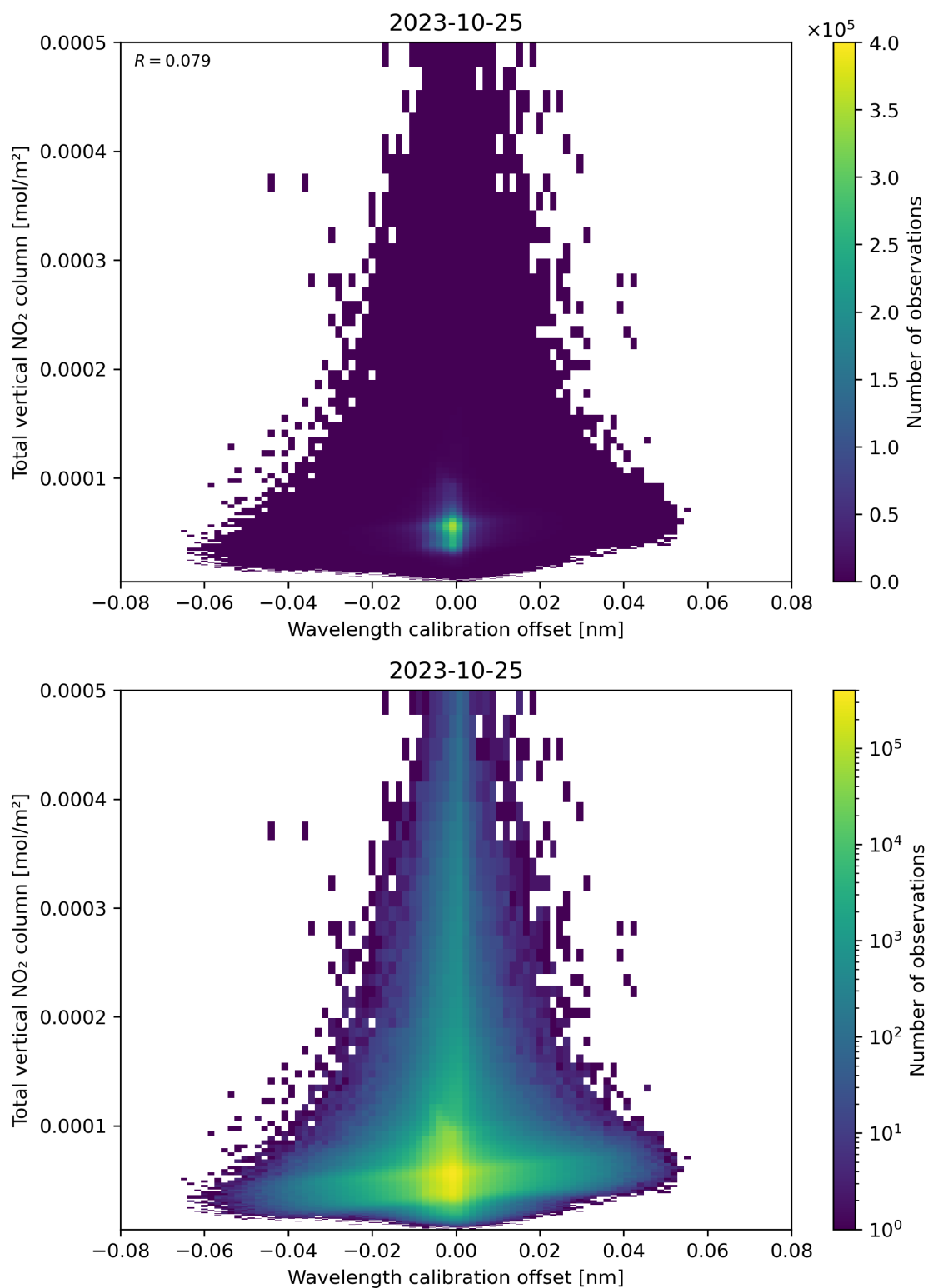
Figure 179: Scatter density plot of “Wavelength calibration offset” against “Total vertical NO 2 column” for 2023-10-24 to 2023-10-26.
