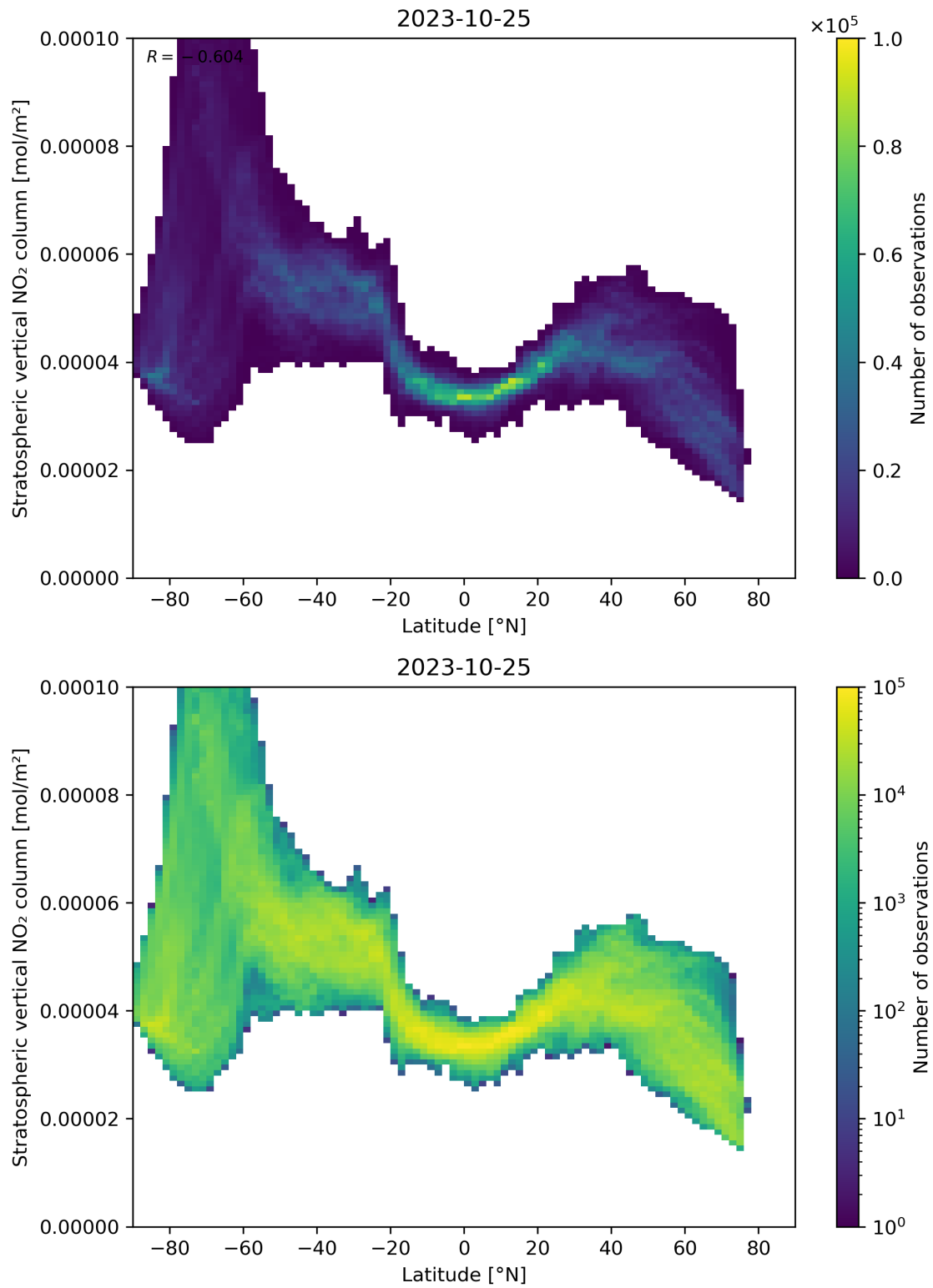
Figure 87: Scatter density plot of “Latitude” against “Stratospheric vertical NO 2 column” for 2023-10-24 to 2023-10-26.
