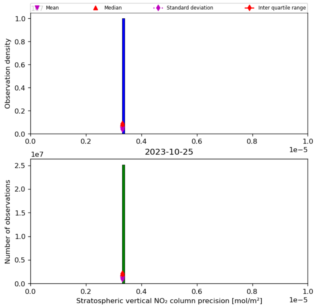
Figure 37: Histogram of “Stratospheric vertical NO 2 column precision” for 2023-10-24 to 2023-10-26
