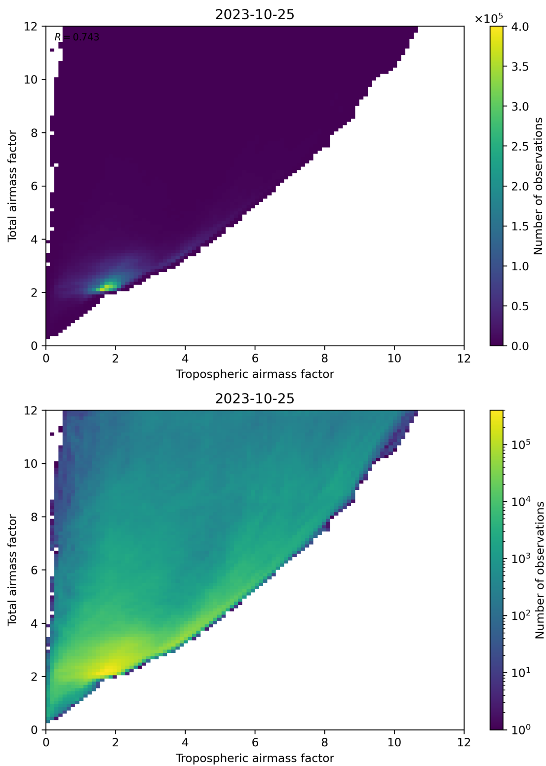
Figure 72: Scatter density plot of “Tropospheric airmass factor” against “Total airmass factor” for 2023-10-24 to 2023-10-26.
