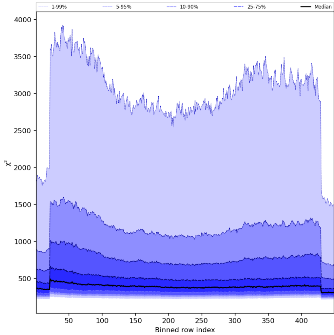
Figure 59: Along track statistics of “ \chi^2 ” for 2023-10-24 to 2023-10-26
