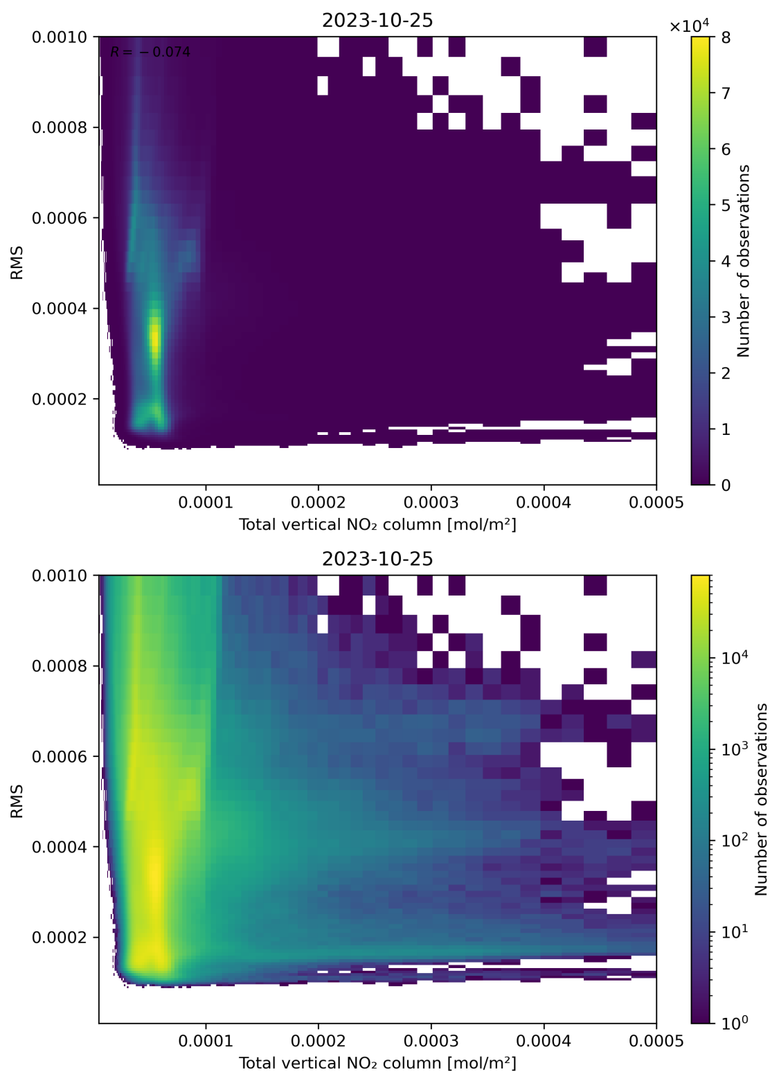
Figure 120: Scatter density plot of “Total vertical NO 2 column” against “RMS” for 2023-10-24 to 2023-10-26.
