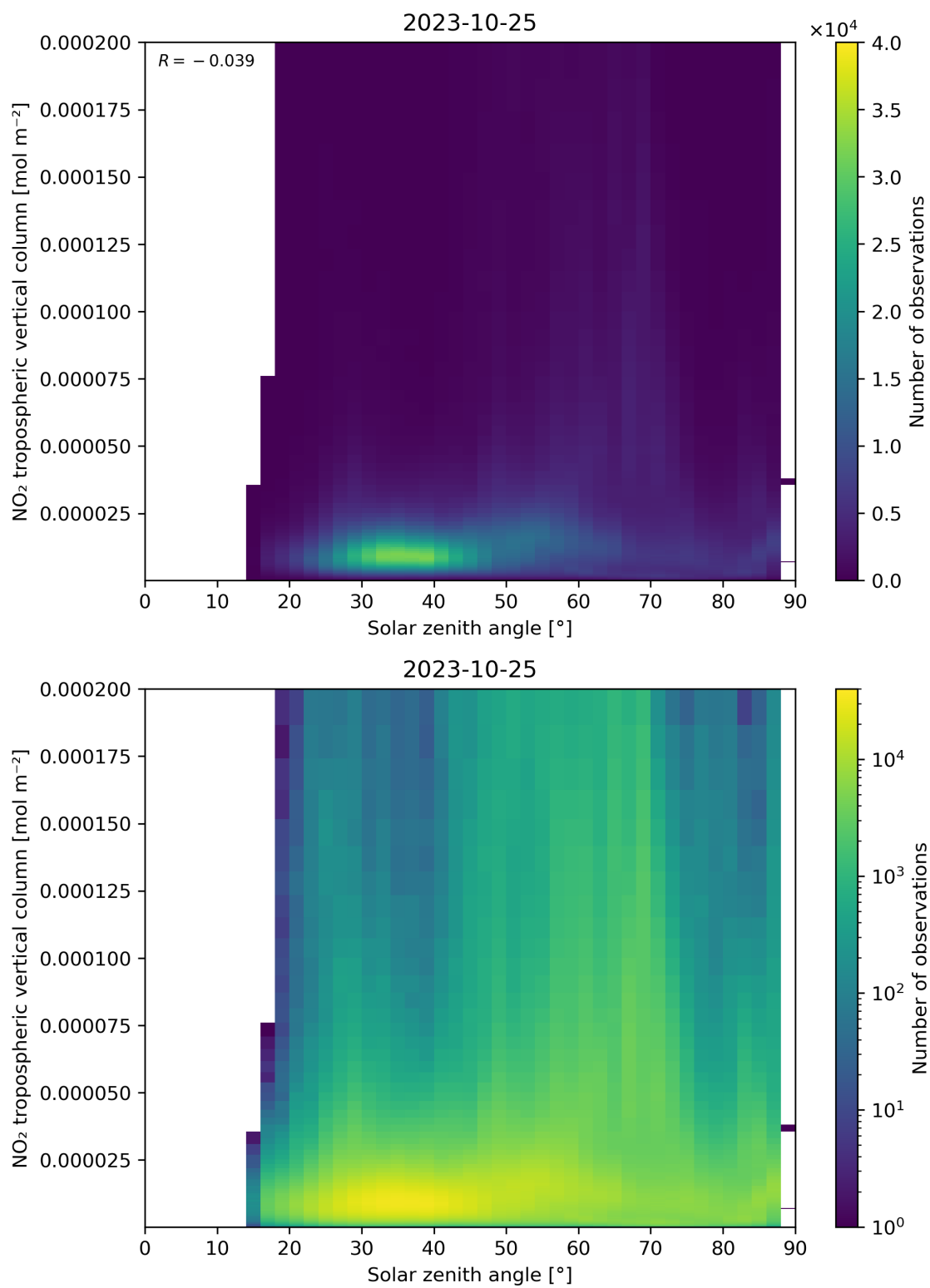
Figure 155: Scatter density plot of “Solar zenith angle” against “NO 2 tropospheric vertical column” for 2023-10-24 to 2023-10-26.
