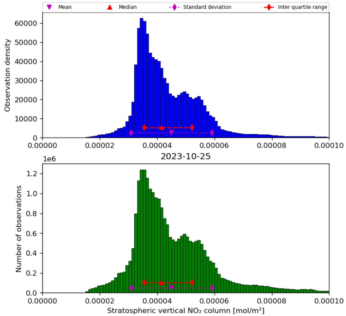
Figure 36: Histogram of “Stratospheric vertical NO 2 column” for 2023-10-24 to 2023-10-26
