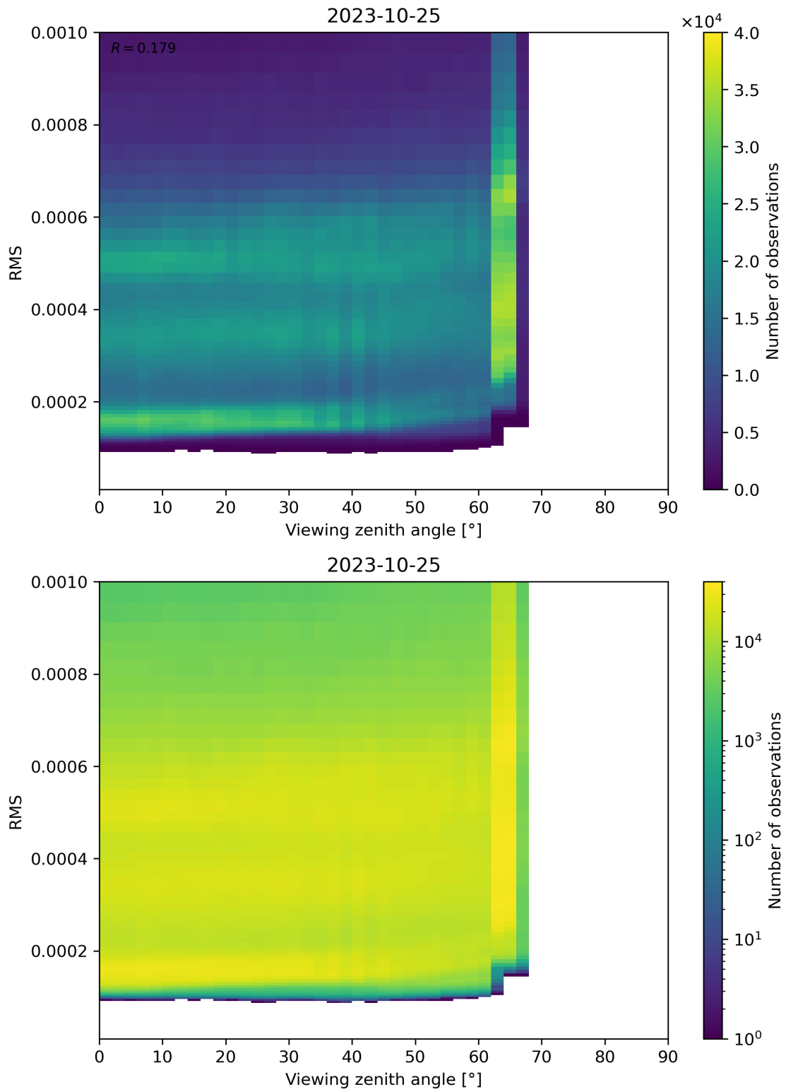
Figure 171: Scatter density plot of “Viewing zenith angle” against “RMS” for 2023-10-24 to 2023-10-26.
