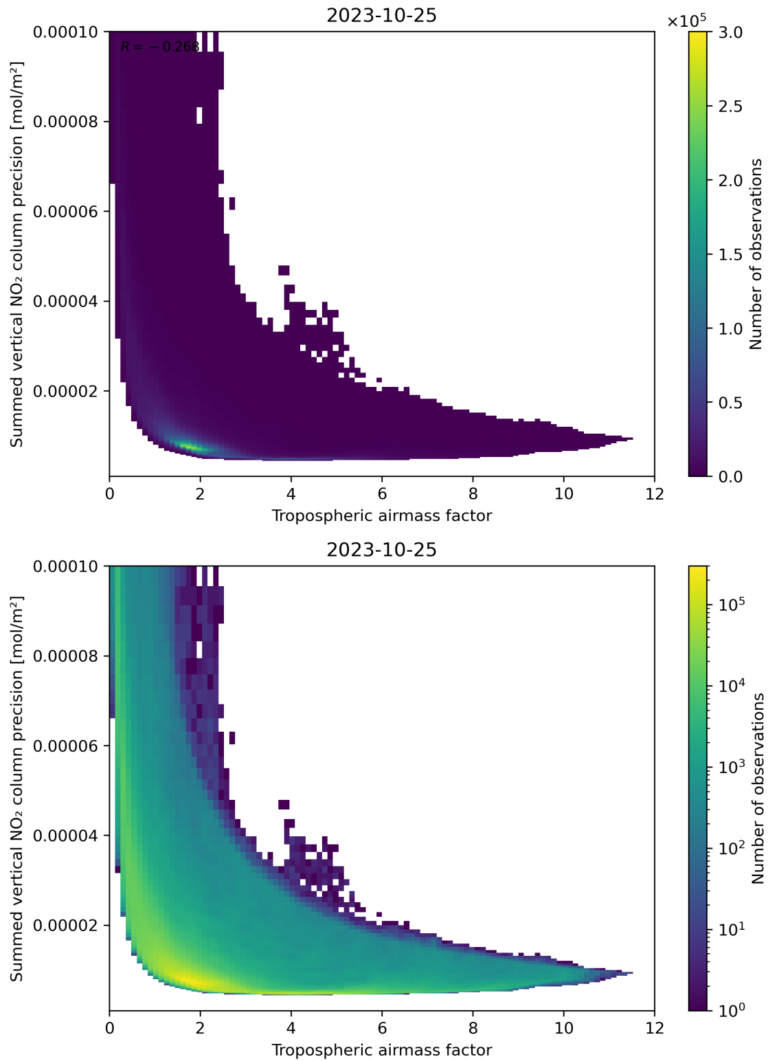
Figure 76: Scatter density plot of “Tropospheric air mass factor” against “Summed vertical NO 2 column precision” for 2023-10-24 to 2023-10-26.
