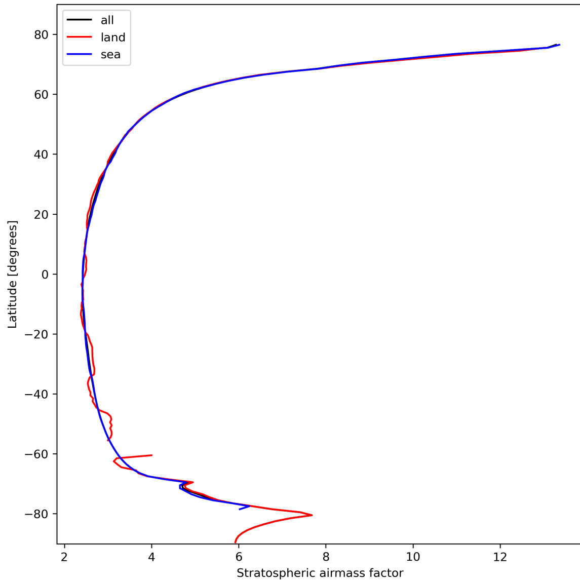
Figure 27: Zonal average of “Stratospheric airmass factor” for 2023-10-24 to 2023-10-26.
