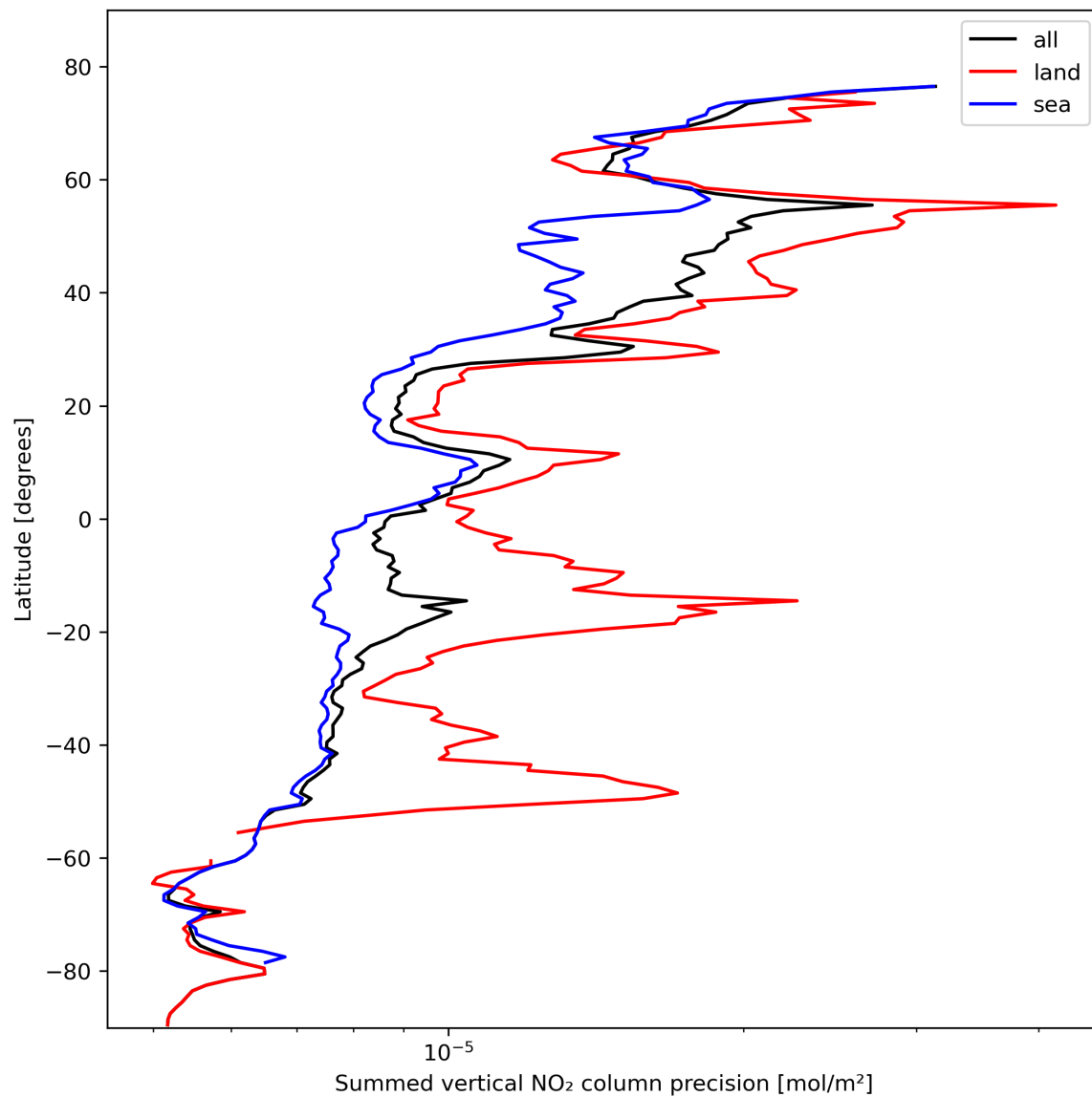
Figure 24: Zonal average of “Summed vertical NO 2 column precision” for 2023-10-24 to 2023-10-26.
