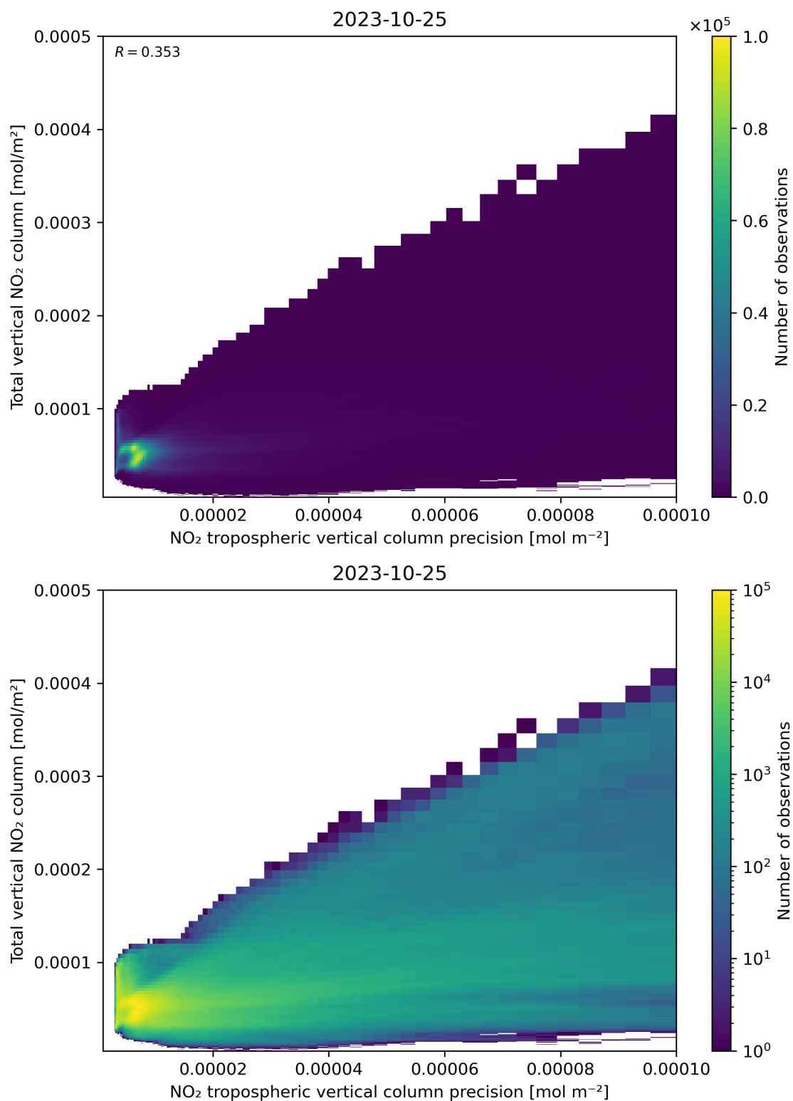
Figure 138: Scatter density plot of “NO 2 tropospheric vertical column precision” against “Total vertical NO 2 column” for 2023-10-24 to 2023-10-26.
