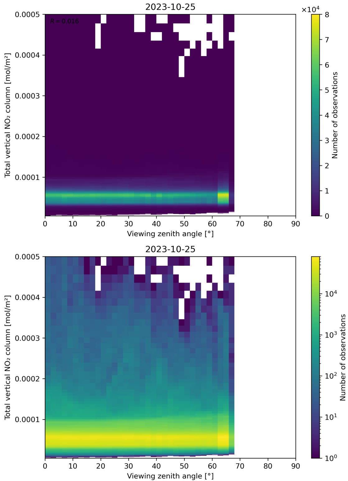
Figure 167: Scatter density plot of “Viewing zenith angle” against “Total vertical NO 2 column” for 2023-10-24 to 2023-10-26.
