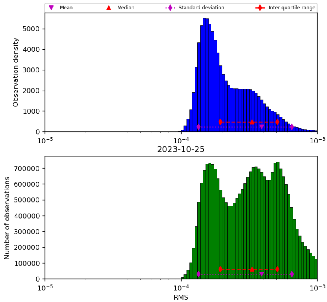
Figure 43: Histogram of “RMS” for 2023-10-24 to 2023-10-26
