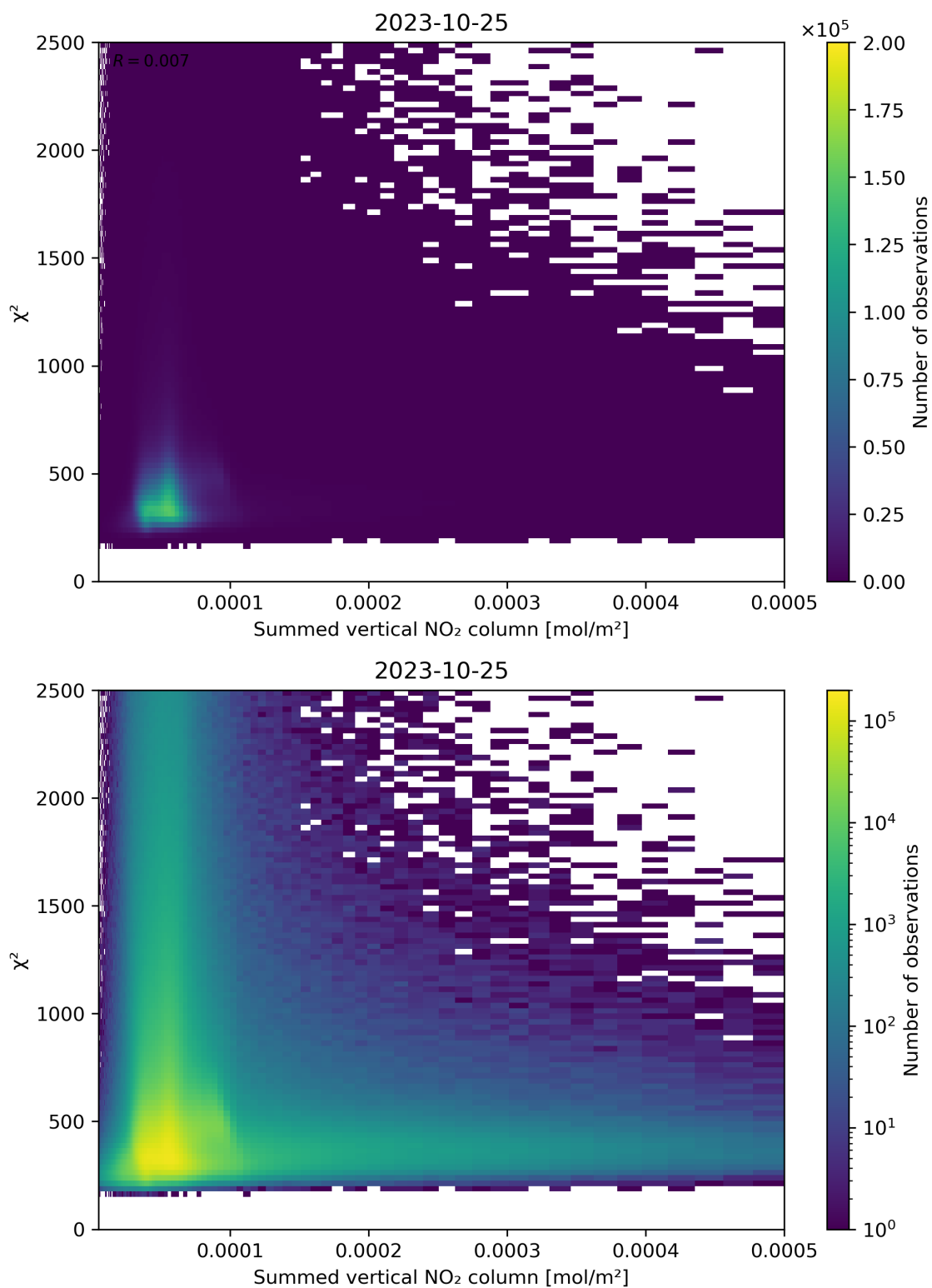
Figure 104: Scatter density plot of “Summed vertical NO 2 column” against “ \chi^2 ” for 2023-10-24 to 2023-10-26.
