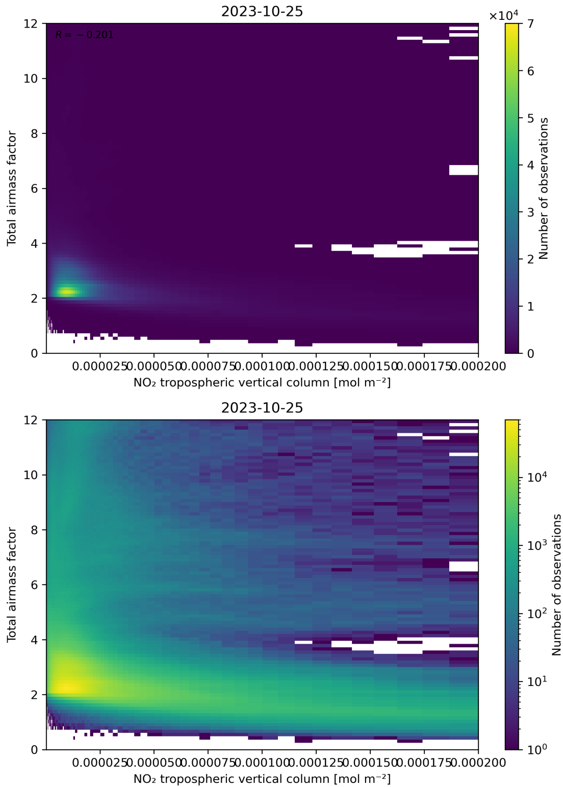
Figure 122: Scatter density plot of “NO 2 tropospheric vertical column” against “Total air mass factor” for 2023-10-24 to 2023-10-26.
