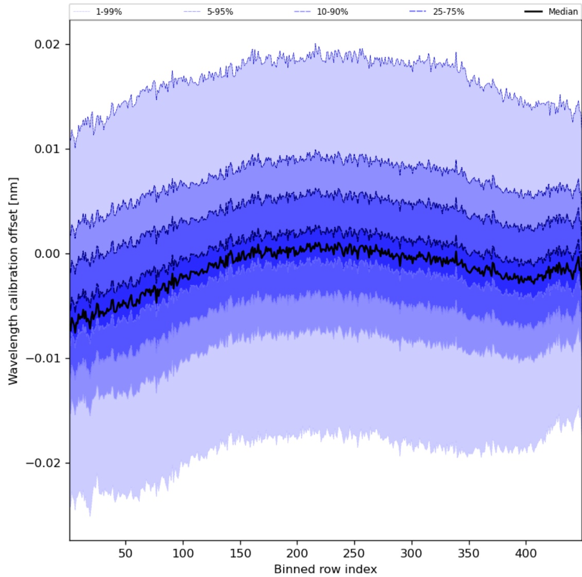
Figure 52: Along track statistics of “Wavelength calibration offset” for 2023-10-24 to 2023-10-26
