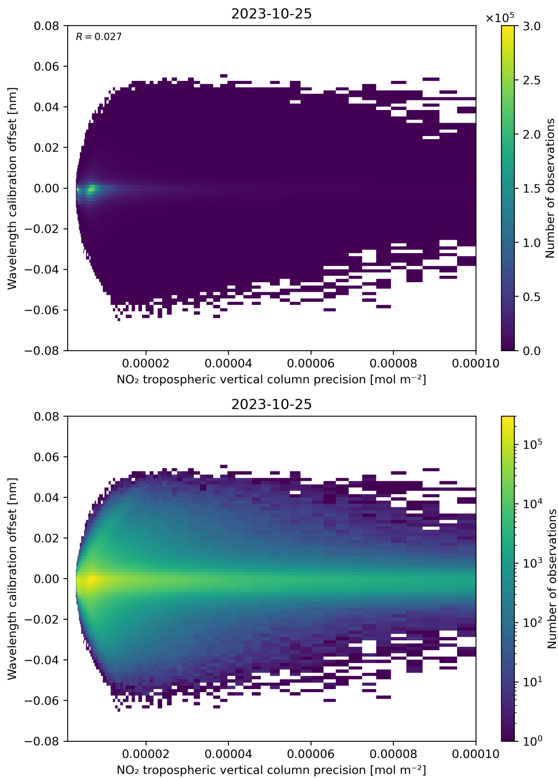
Figure 141: Scatter density plot of “NO 2 tropospheric vertical column precision” against “Wavelength calibration offset” for 2023-10-24 to 2023-10-26.
