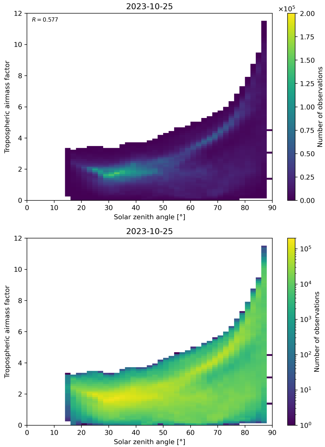
Figure 147: Scatter density plot of “Solar zenith angle” against “Tropospheric airmass factor” for 2023-10-24 to 2023-10-26.
