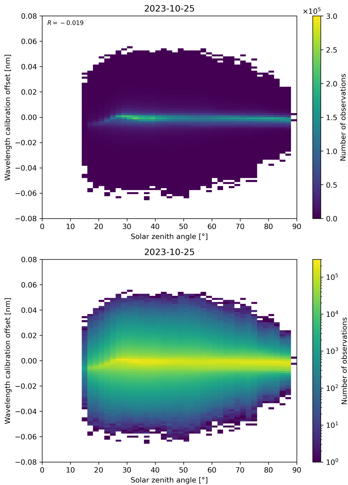
Figure 158: Scatter density plot of “Solar zenith angle” against “Wavelength calibration offset” for 2023-10-24 to 2023-10-26.
