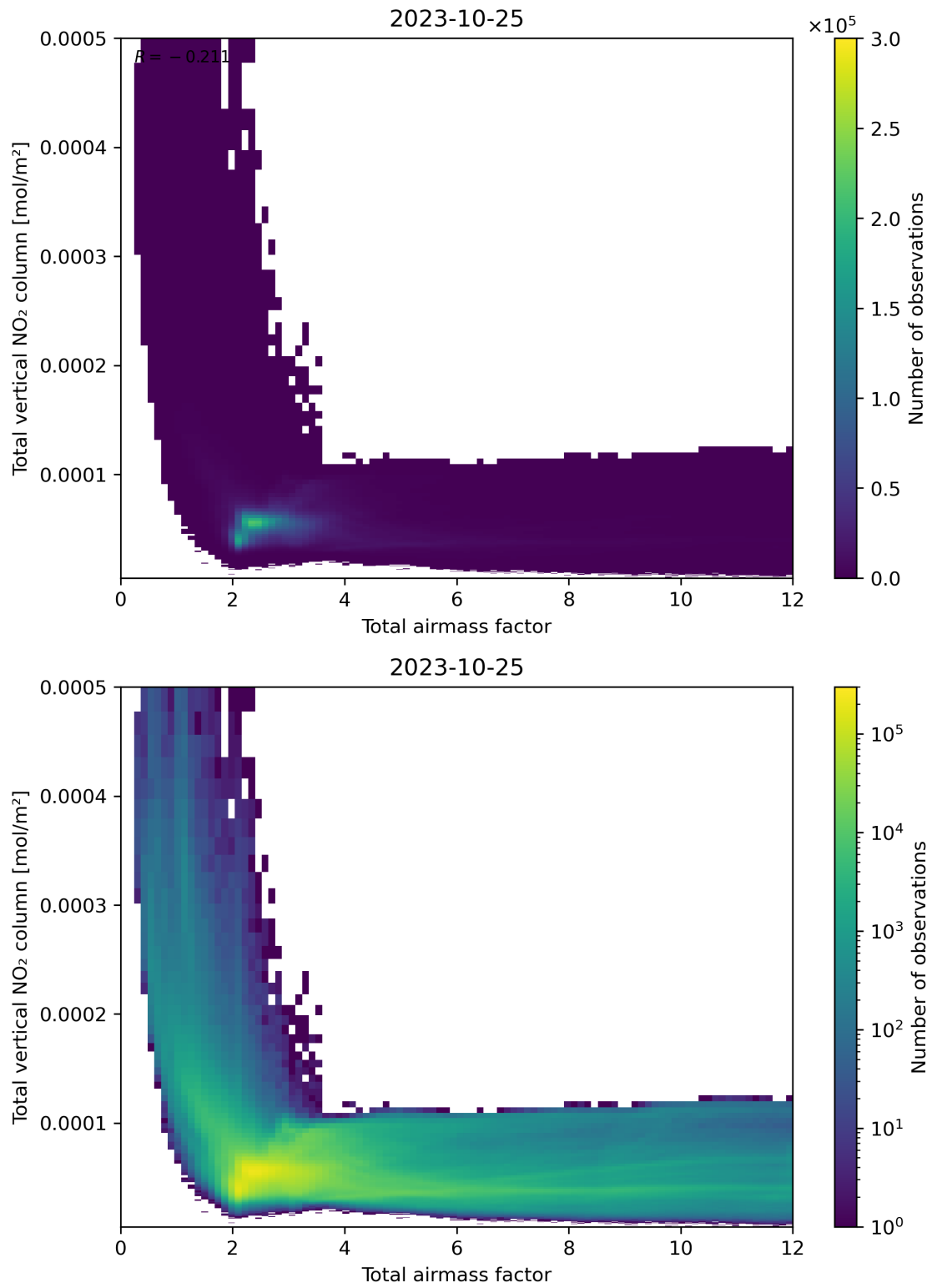
Figure 67: Scatter density plot of “Total airmass factor” against “Total vertical NO 2 column” for 2023-10-24 to 2023-10-26.
