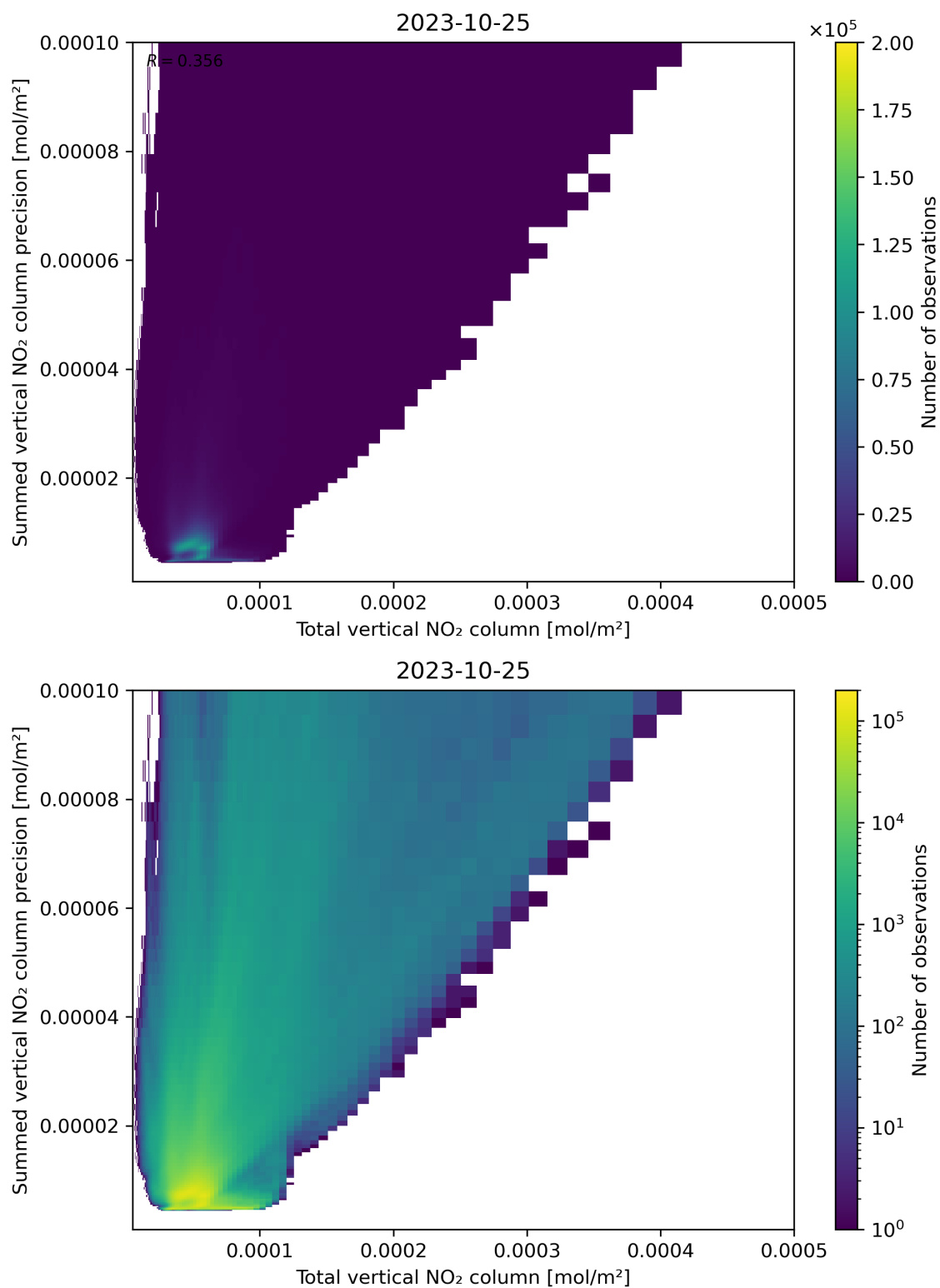
Figure 113: Scatter density plot of “Total vertical NO 2 column” against “Summed vertical NO 2 column precision” for 2023-10-24 to 2023-10-26.
