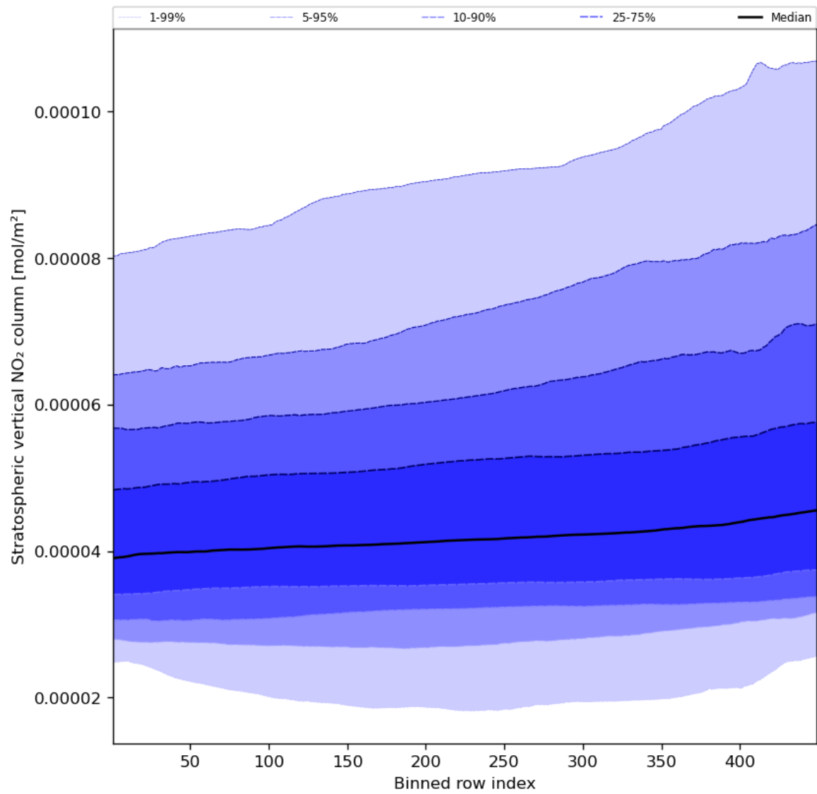
Figure 53: Along track statistics of “Stratospheric vertical NO 2 column” for 2023-10-24 to 2023-10-26
