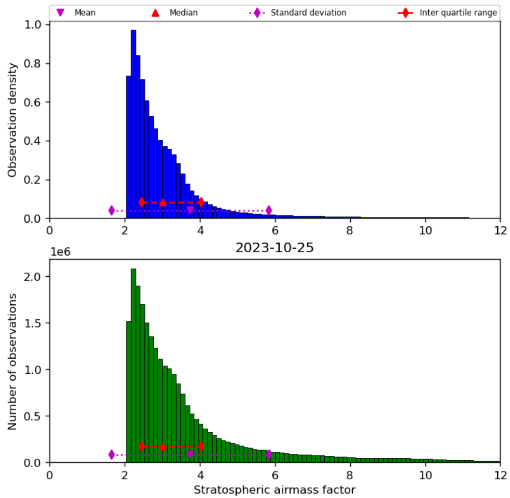
Figure 44: Histogram of “Stratospheric airmass factor” for 2023-10-24 to 2023-10-26
