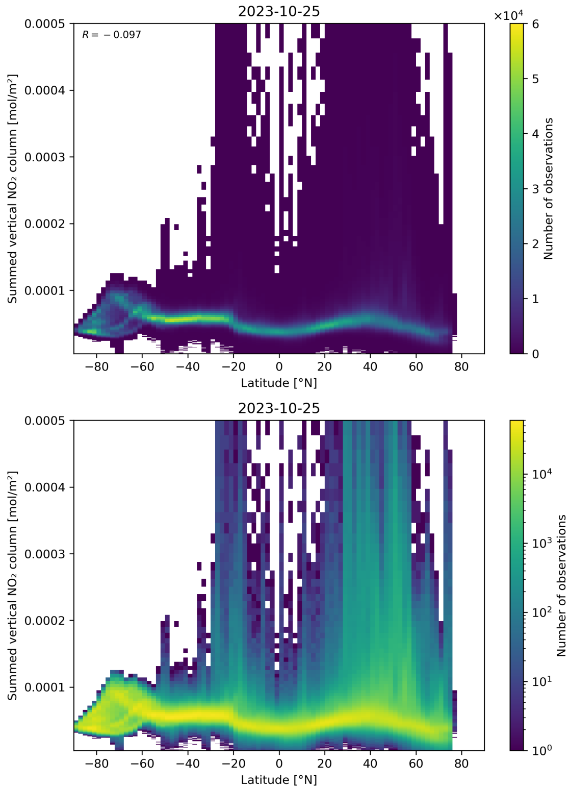
Figure 88: Scatter density plot of “Latitude” against “Summed vertical NO 2 column” for 2023-10-24 to 2023-10-26.
