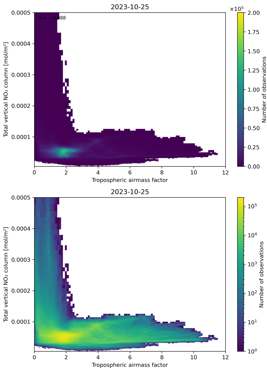
Figure 77: Scatter density plot of “Tropospheric airmass factor” against “Total vertical NO 2 column” for 2023-10-24 to 2023-10-26.
