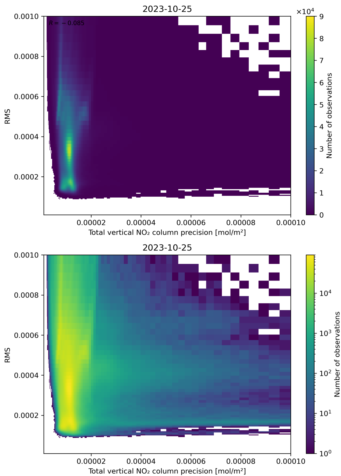
Figure 119: Scatter density plot of “Total vertical NO 2 column precision” against “RMS” for 2023-10-24 to 2023-10-26.
