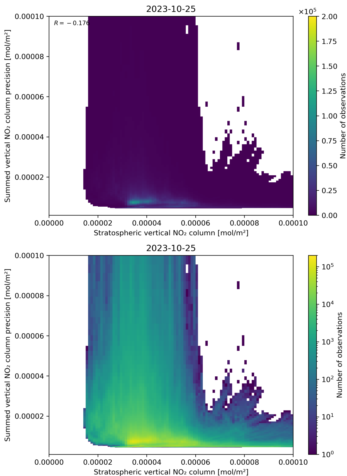
Figure 99: Scatter density plot of “Stratospheric vertical NO 2 column” against “Summed vertical NO 2 column precision” for 2023-10-24 to 2023-10-26.
