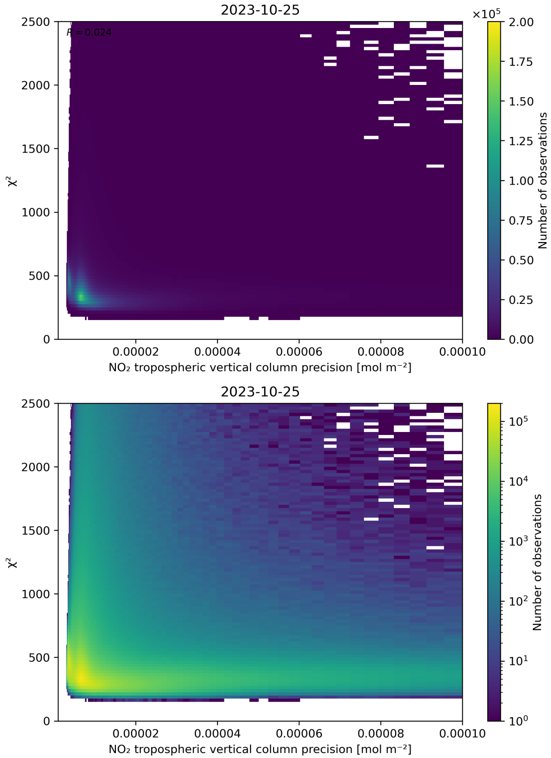
Figure 134: Scatter density plot of “NO 2 tropospheric vertical column precision” against “ \chi^2 ” for 2023-10-24 to 2023-10-26.
