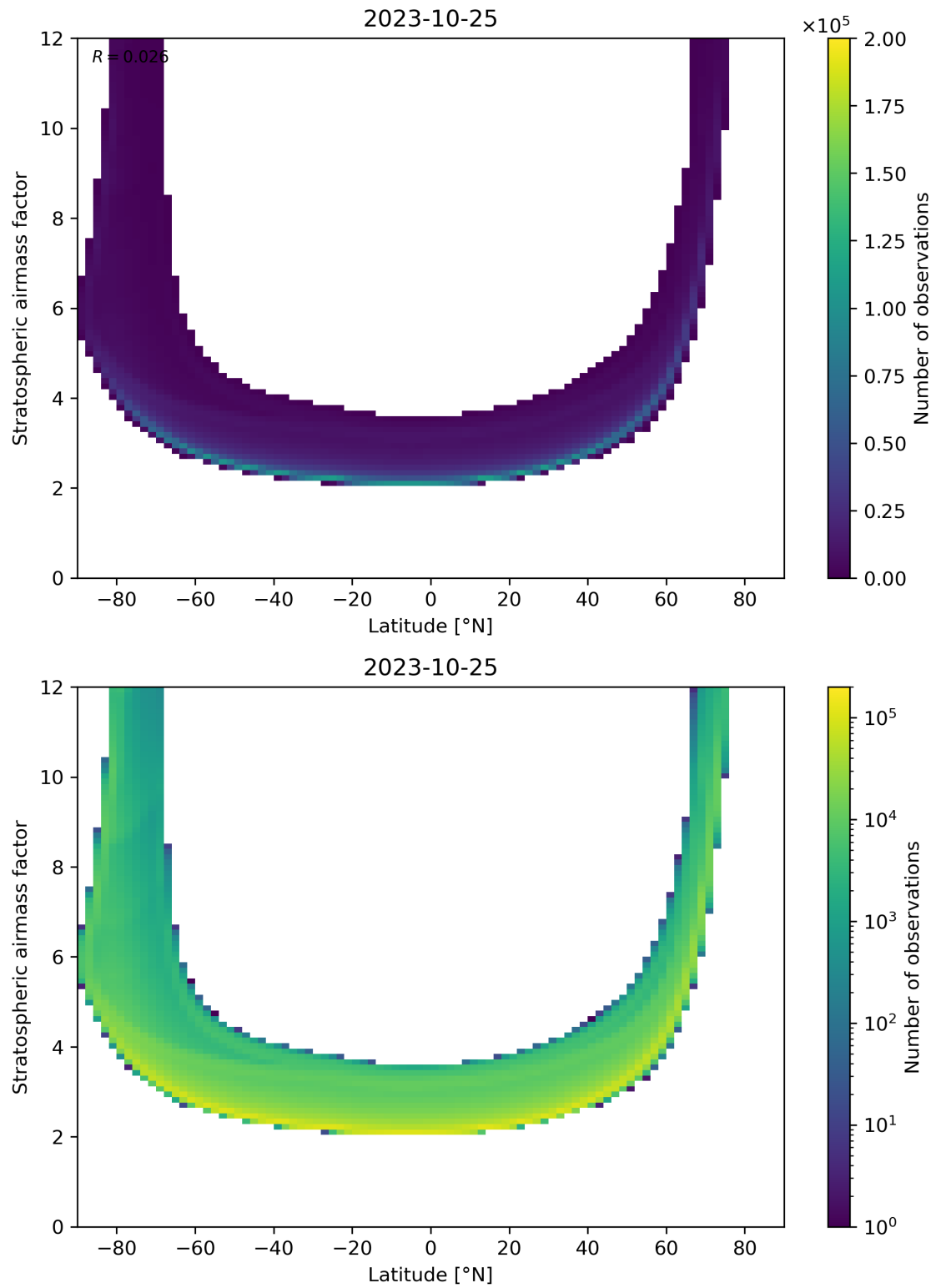
Figure 83: Scatter density plot of “Latitude” against “Stratospheric air mass factor” for 2023-10-24 to 2023-10-26.
