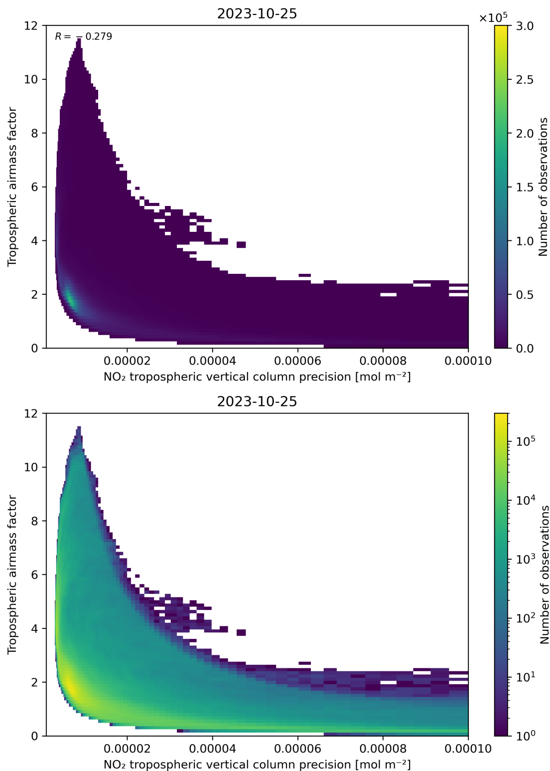
Figure 133: Scatter density plot of “NO 2 tropospheric vertical column precision” against “Tropospheric airmass factor” for 2023-10-24 to 2023-10-26.
