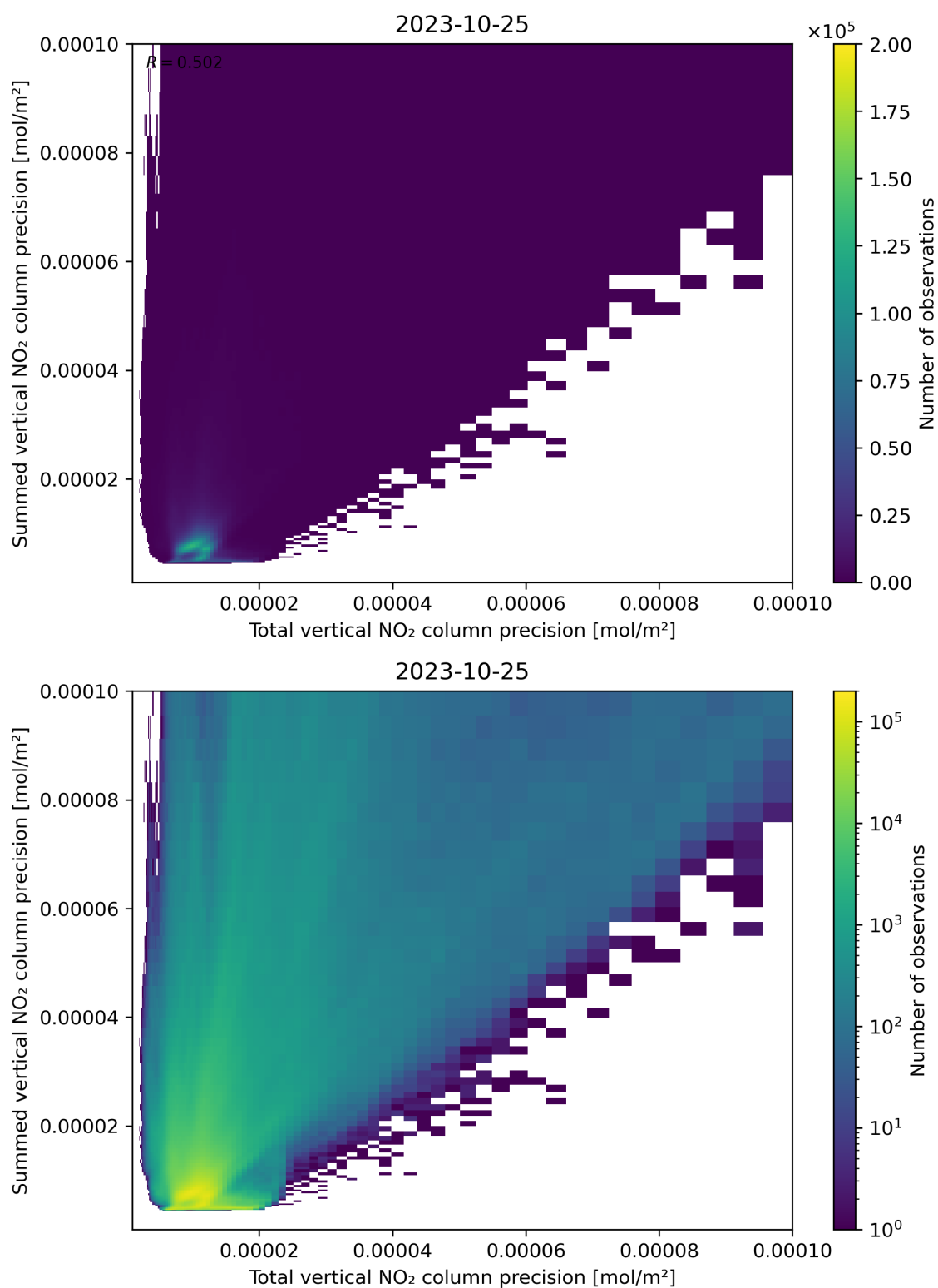
Figure 118: Scatter density plot of “Total vertical NO 2 column precision” against “Summed vertical NO 2 column precision” for 2023-10-24 to 2023-10-26.
