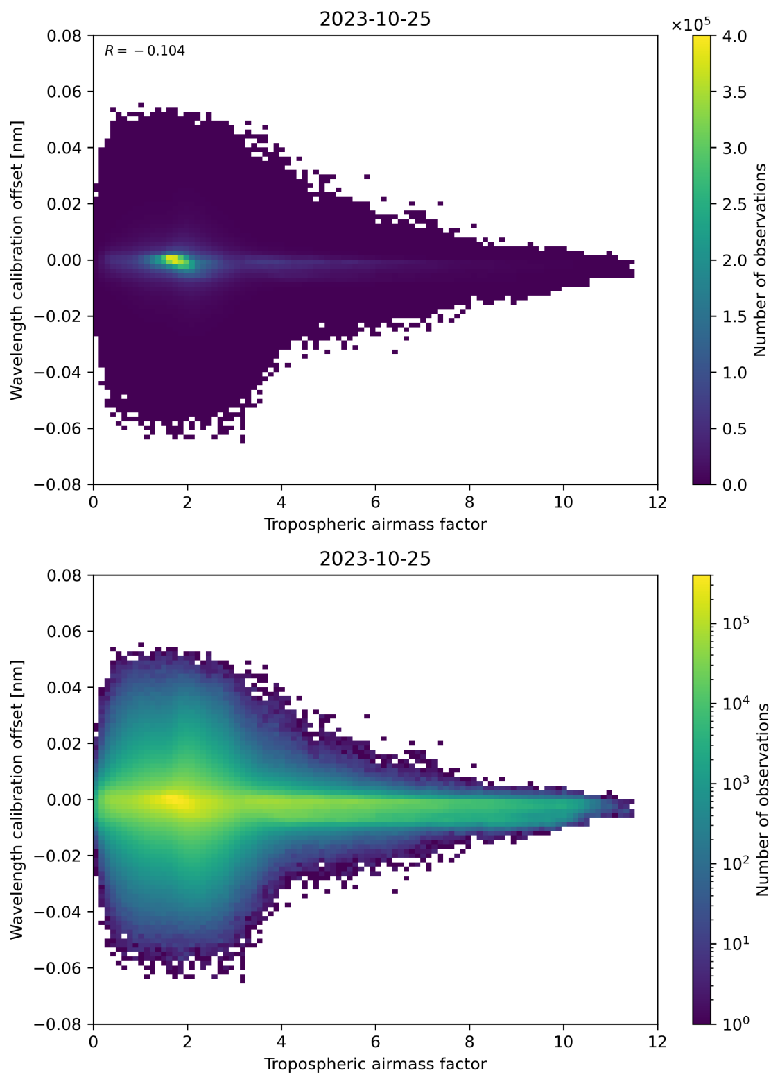
Figure 80: Scatter density plot of “Tropospheric airmass factor” against “Wavelength calibration offset” for 2023-10-24 to 2023-10-26.
