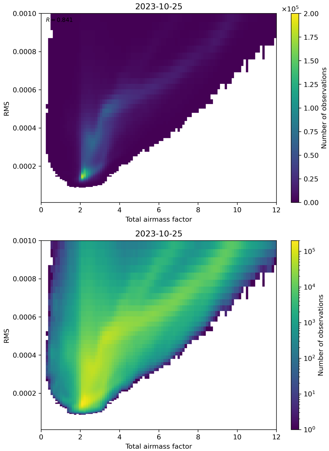
Figure 69: Scatter density plot of “Total airmass factor” against “RMS” for 2023-10-24 to 2023-10-26.
