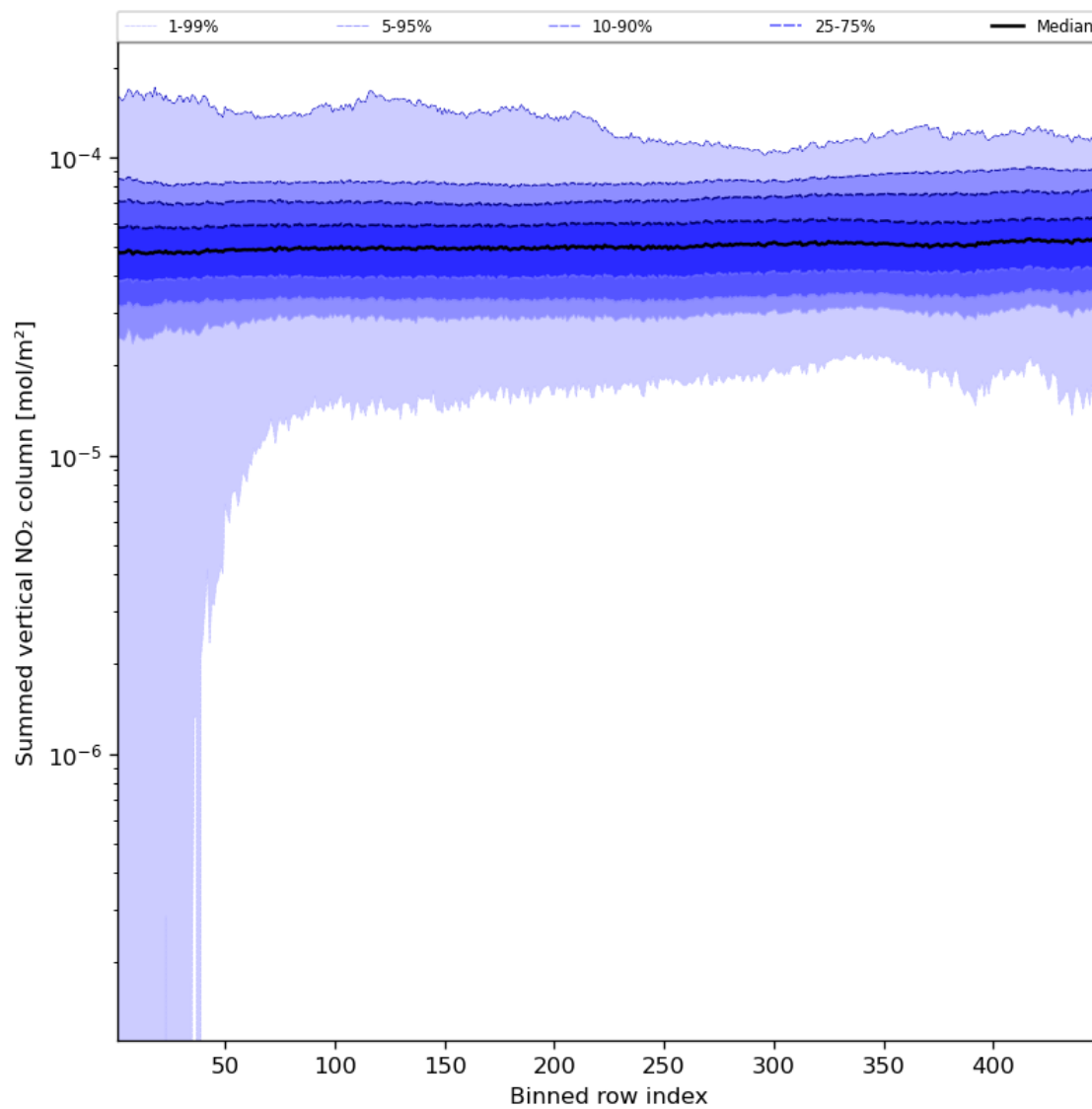
Figure 57: Along track statistics of “Summed vertical NO 2 column” for 2023-10-24 to 2023-10-26
