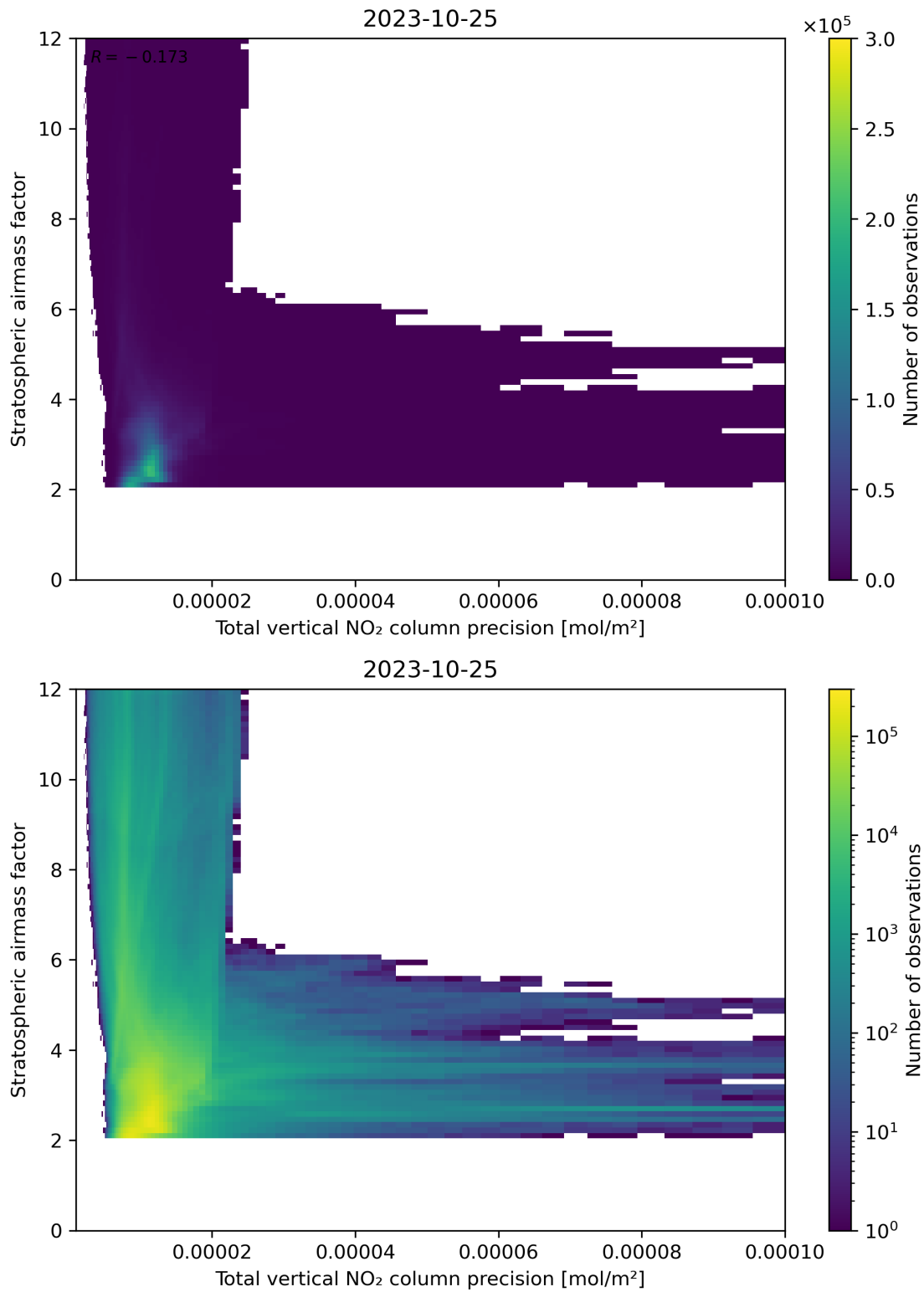
Figure 115: Scatter density plot of “Total vertical NO 2 column precision” against “Stratospheric airmass factor” for 2023-10-24 to 2023-10-26.
