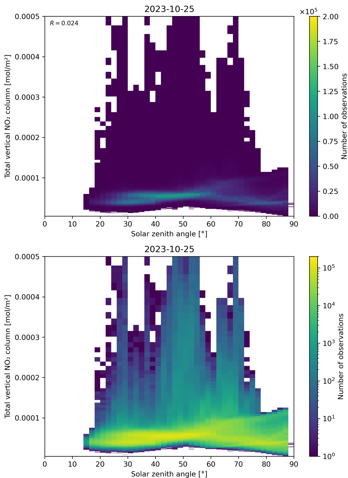
Figure 153: Scatter density plot of “Solar zenith angle” against “Total vertical NO 2 column” for 2023-10-24 to 2023-10-26.
