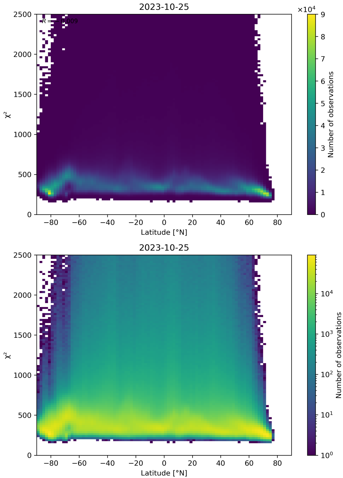
Figure 86: Scatter density plot of “Latitude” against “ \chi^2 ” for 2023-10-24 to 2023-10-26.
