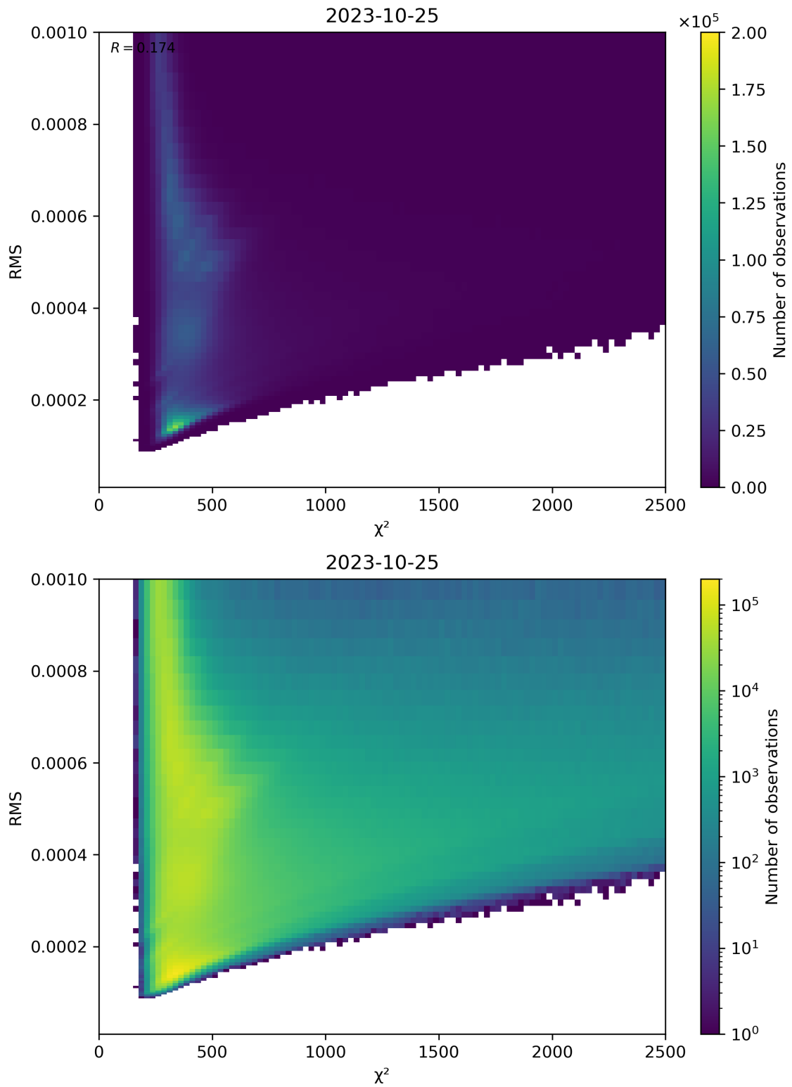
Figure 82: Scatter density plot of “ \chi^2 ” against “RMS” for 2023-10-24 to 2023-10-26.
