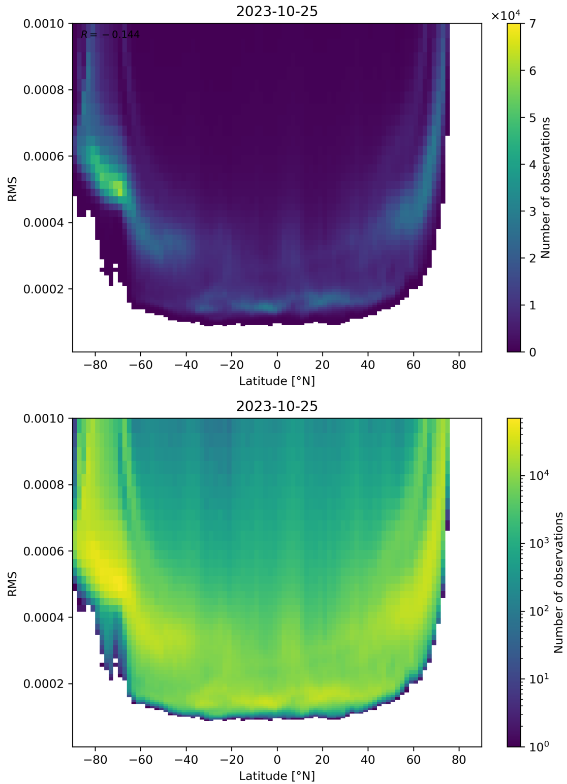
Figure 94: Scatter density plot of “Latitude” against “RMS” for 2023-10-24 to 2023-10-26.
