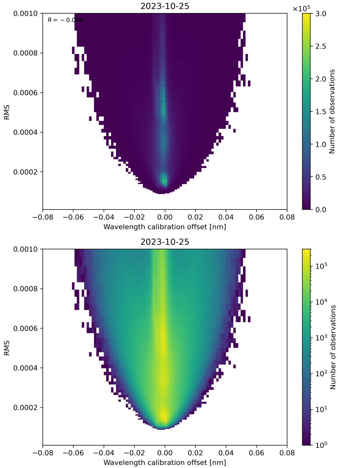
Figure 181: Scatter density plot of “Wavelength calibration offset” against “RMS” for 2023-10-24 to 2023-10-26.
