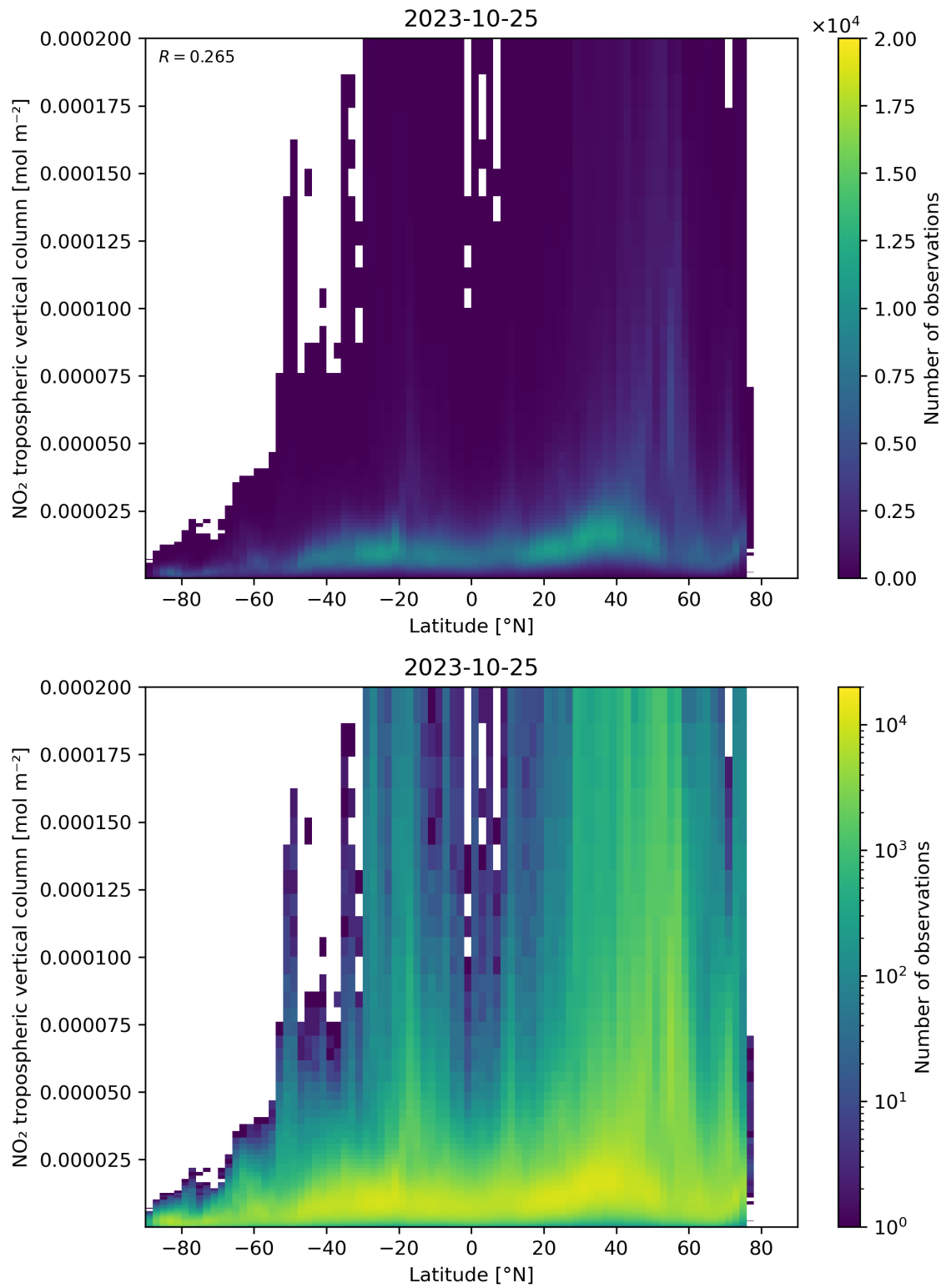
Figure 92: Scatter density plot of “Latitude” against “NO 2 tropospheric vertical column” for 2023-10-24 to 2023-10-26.
