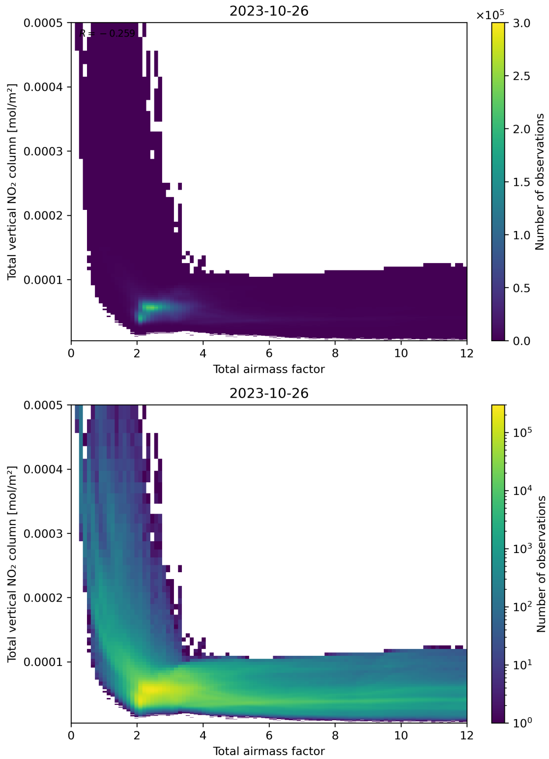
Figure 67: Scatter density plot of “Total airmass factor” against “Total vertical NO 2 column” for 2023-10-25 to 2023-10-27.
