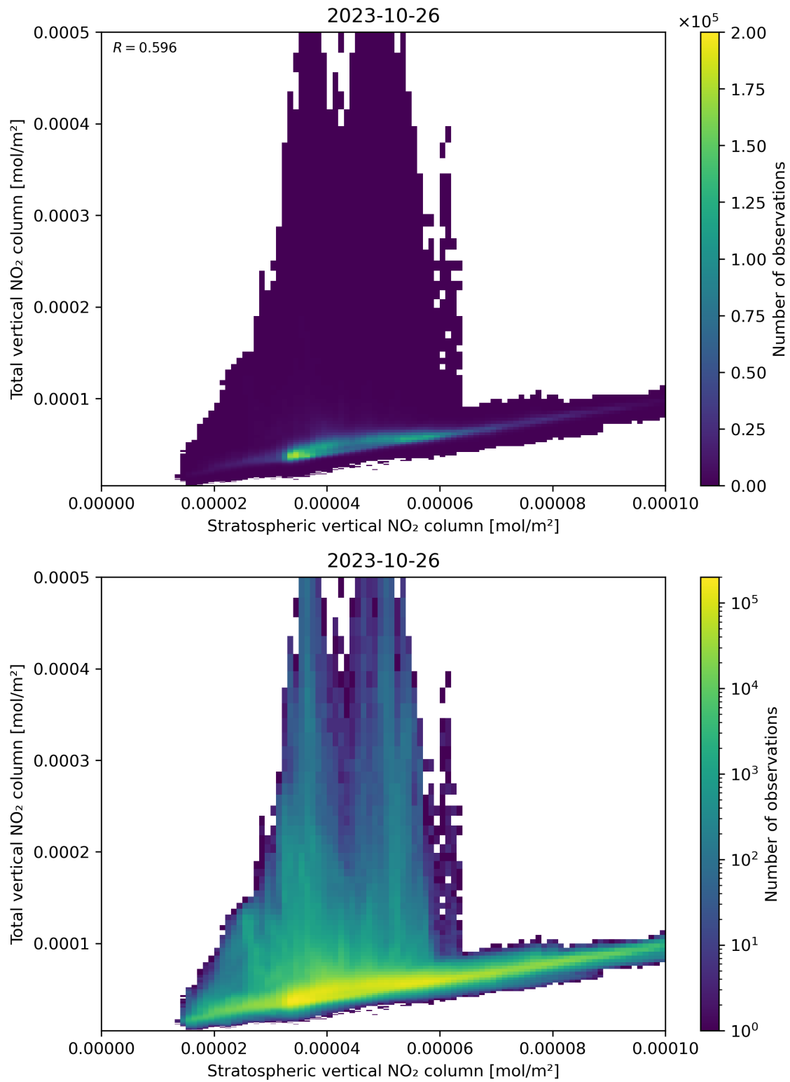
Figure 100: Scatter density plot of “Stratospheric vertical NO 2 column” against “Total vertical NO 2 column” for 2023-10-25 to 2023-10-27.
