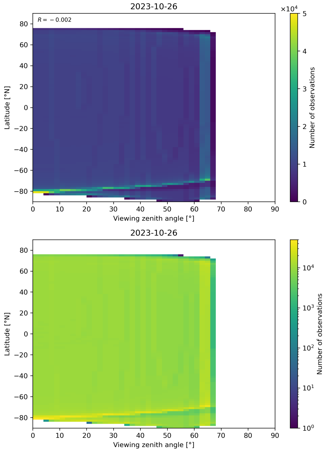
Figure 163: Scatter density plot of “Viewing zenith angle” against “Latitude” for 2023-10-25 to 2023-10-27.
