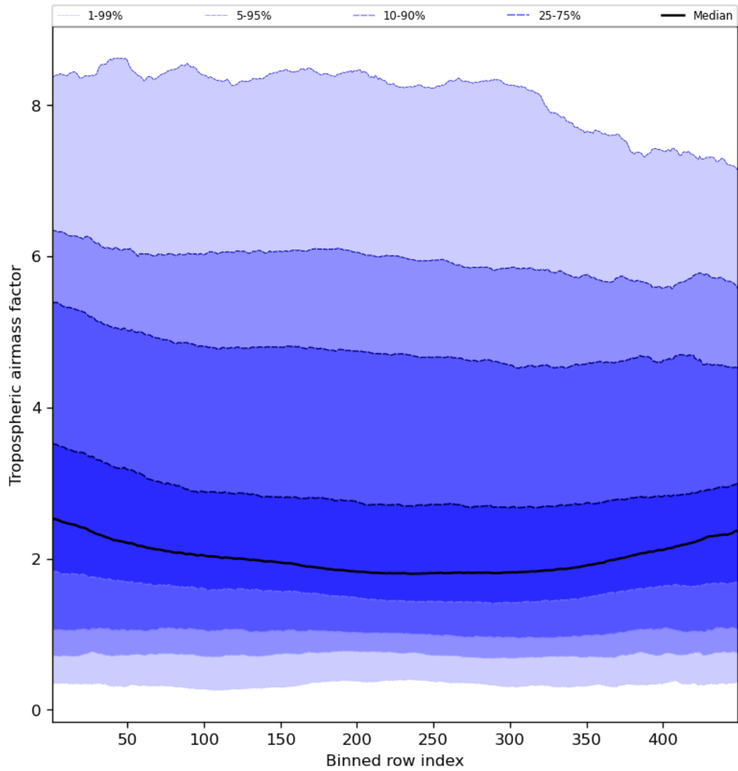
Figure 48: Along track statistics of “Tropospheric air mass factor” for 2023-10-25 to 2023-10-27
