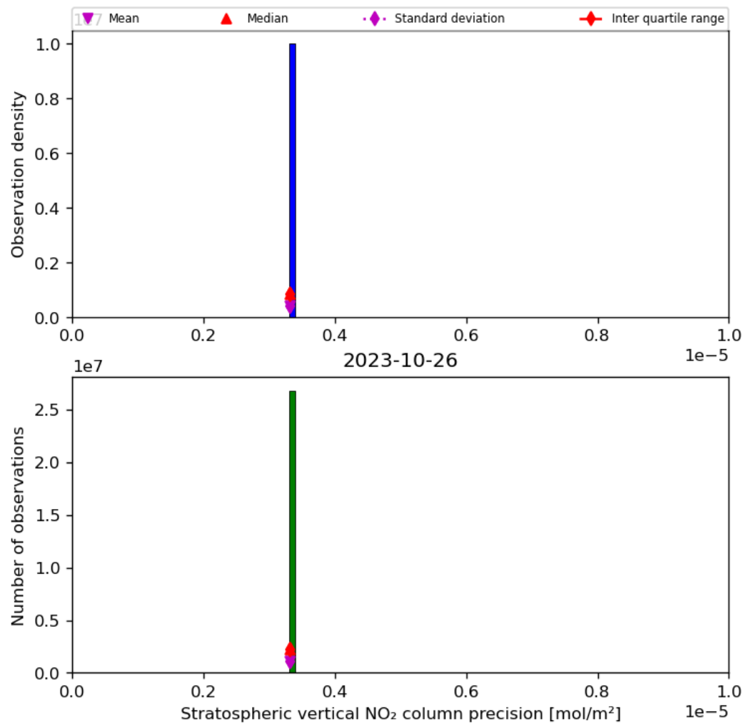
Figure 37: Histogram of “Stratospheric vertical NO 2 column precision” for 2023-10-25 to 2023-10-27
