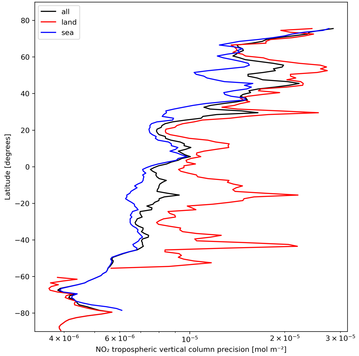
Figure 13: Zonal average of “NO 2 tropospheric vertical column precision” for 2023-10-25 to 2023-10-27.
