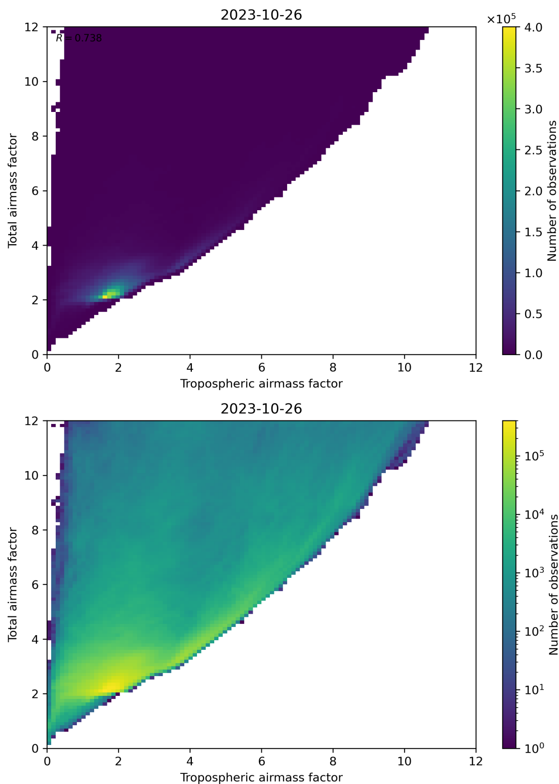
Figure 72: Scatter density plot of “Tropospheric airmass factor” against “Total airmass factor” for 2023-10-25 to 2023-10-27.
