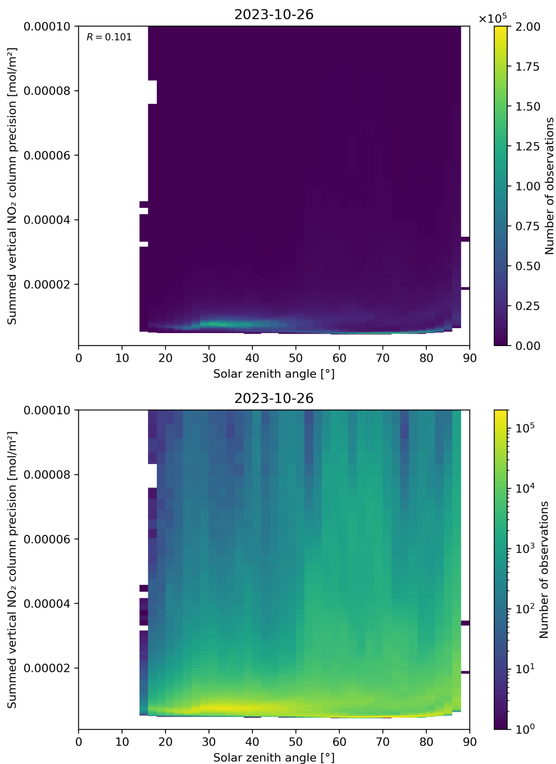
Figure 152: Scatter density plot of “Solar zenith angle” against “Summed vertical NO 2 column precision” for 2023-10-25 to 2023-10-27.
