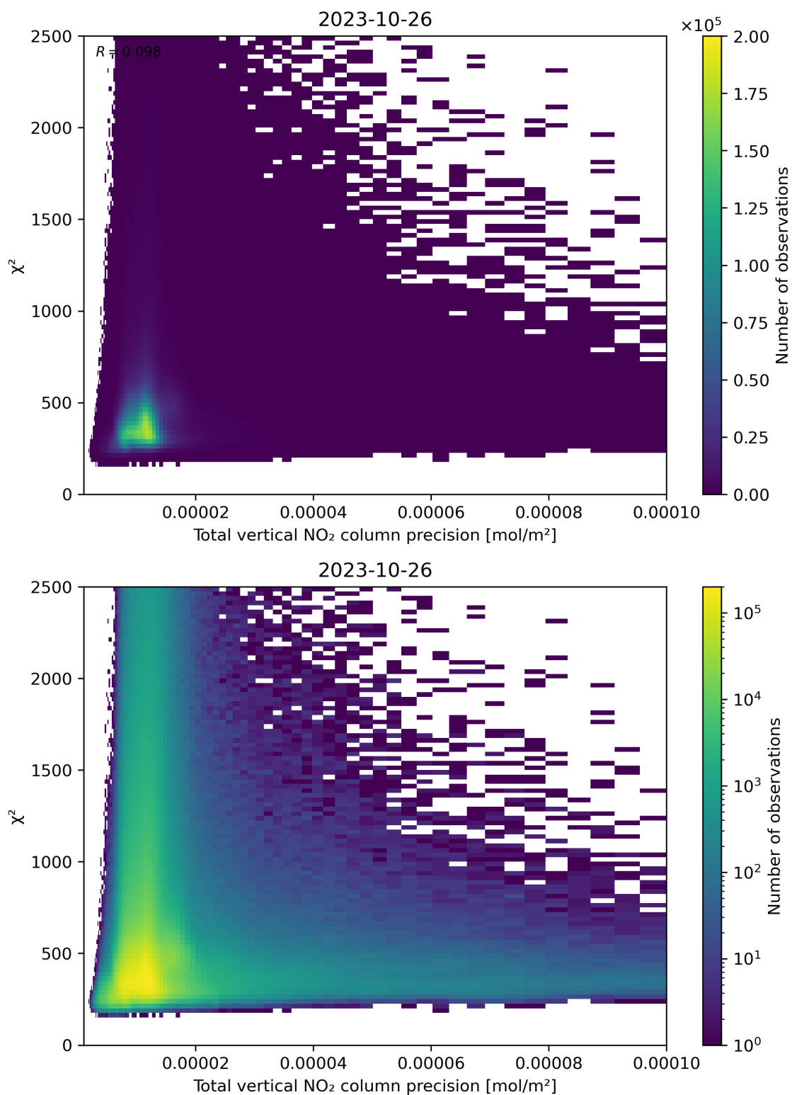
Figure 116: Scatter density plot of “Total vertical NO 2 column precision” against “ \chi^2 ” for 2023-10-25 to 2023-10-27.
