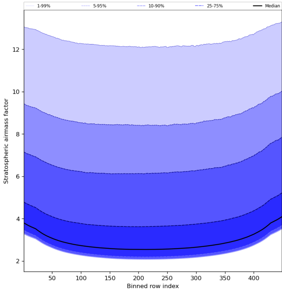
Figure 61: Along track statistics of “Stratospheric air mass factor” for 2023-10-25 to 2023-10-27
