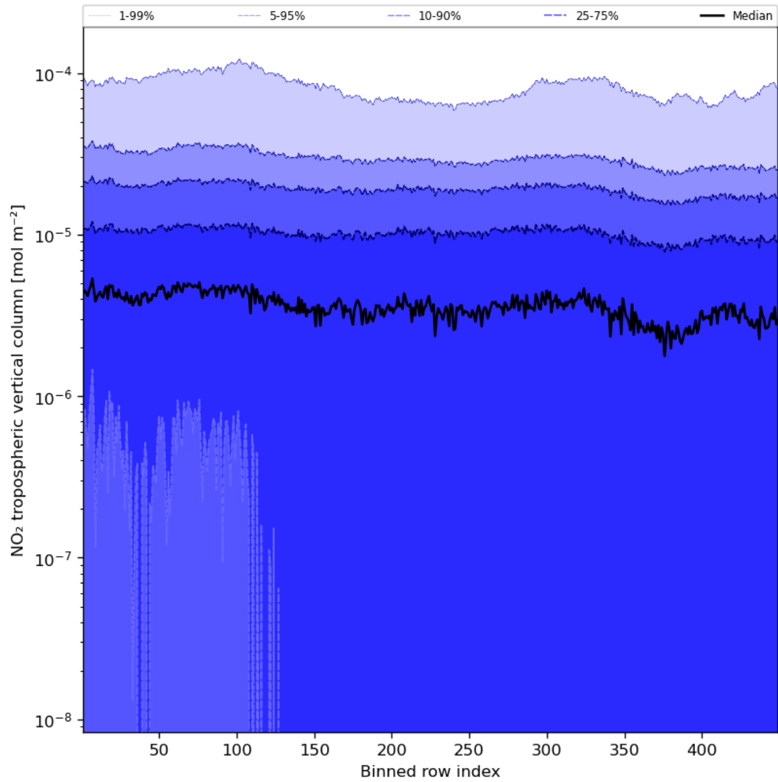
Figure 46: Along track statistics of “NO 2 tropospheric vertical column” for 2023-10-25 to 2023-10-27
