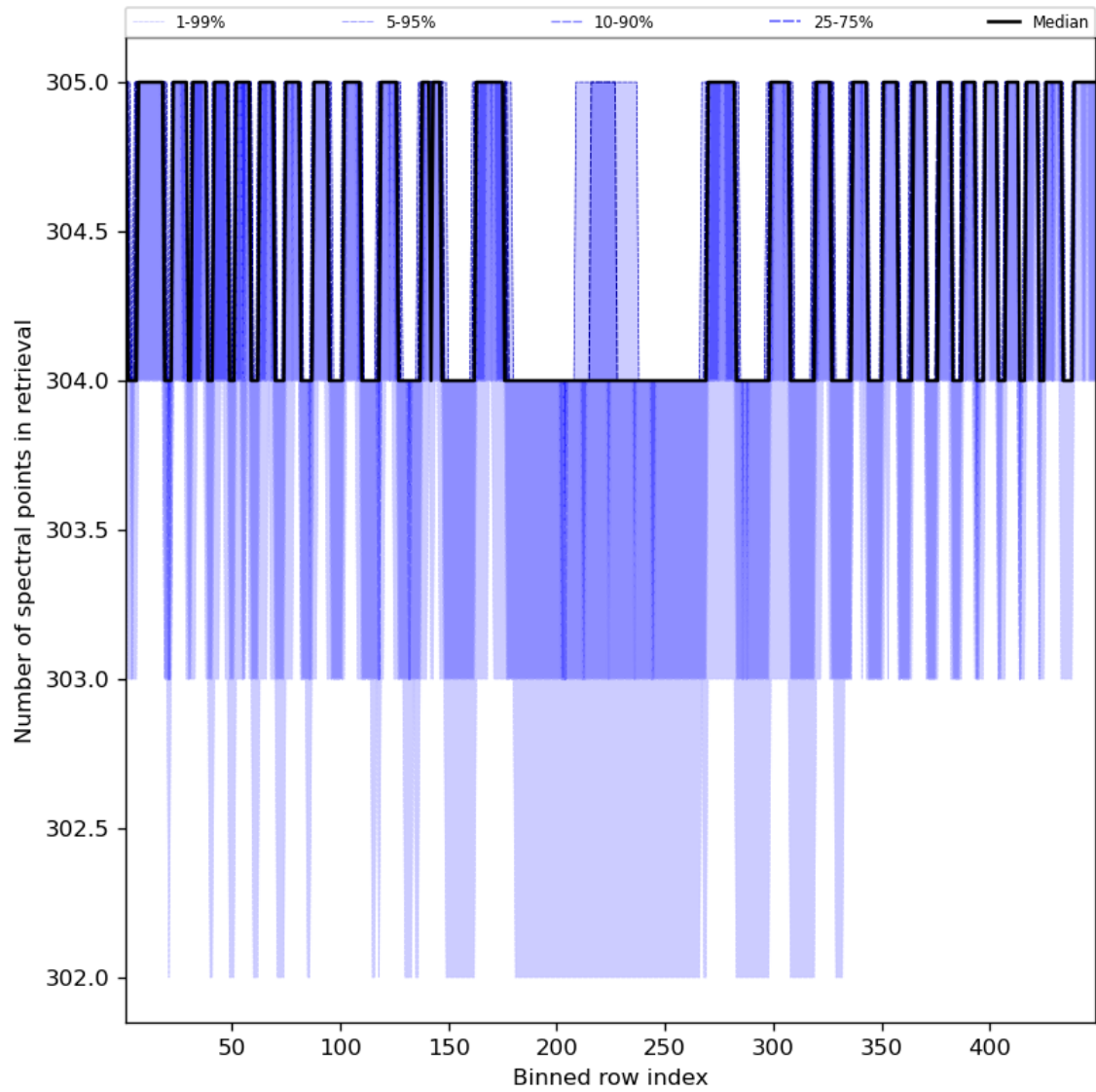
Figure 50: Along track statistics of “Number of spectral points in retrieval” for 2023-10-25 to 2023-10-27
