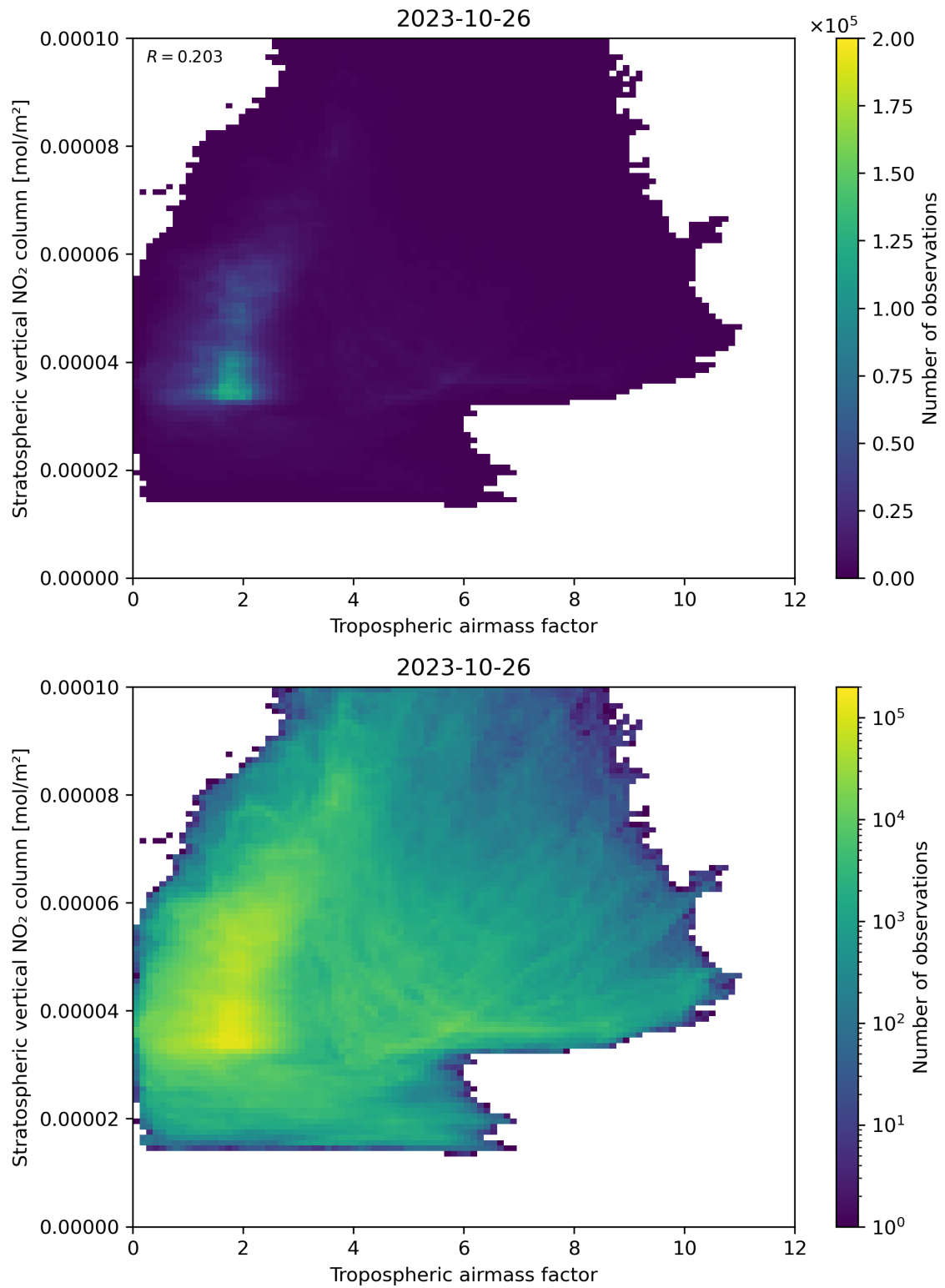
Figure 74: Scatter density plot of “Tropospheric air mass factor” against “Stratospheric vertical NO 2 column” for 2023-10-25 to 2023-10-27.
