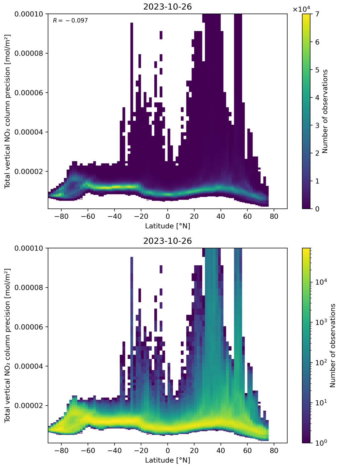
Figure 91: Scatter density plot of “Latitude” against “Total vertical NO 2 column precision” for 2023-10-25 to 2023-10-27.
