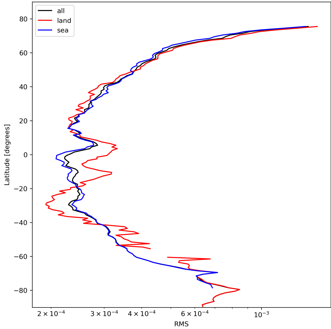
Figure 26: Zonal average of “RMS” for 2023-10-25 to 2023-10-27.
