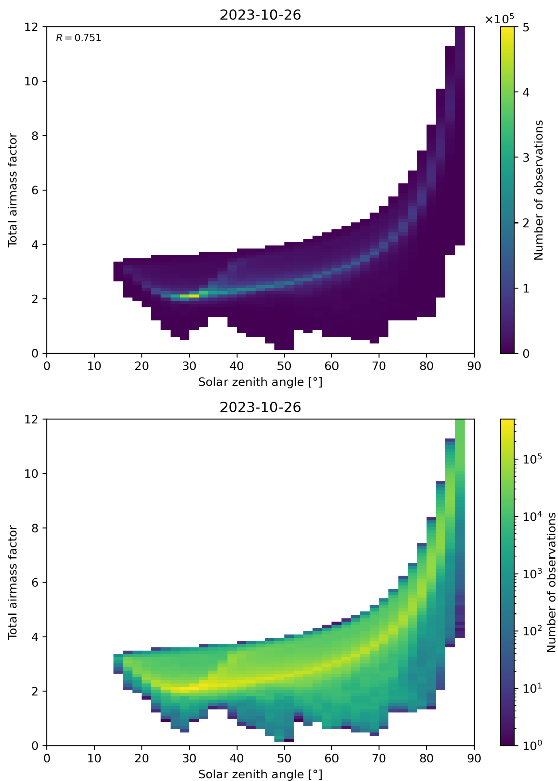
Figure 146: Scatter density plot of “Solar zenith angle” against “Total air mass factor” for 2023-10-25 to 2023-10-27.
