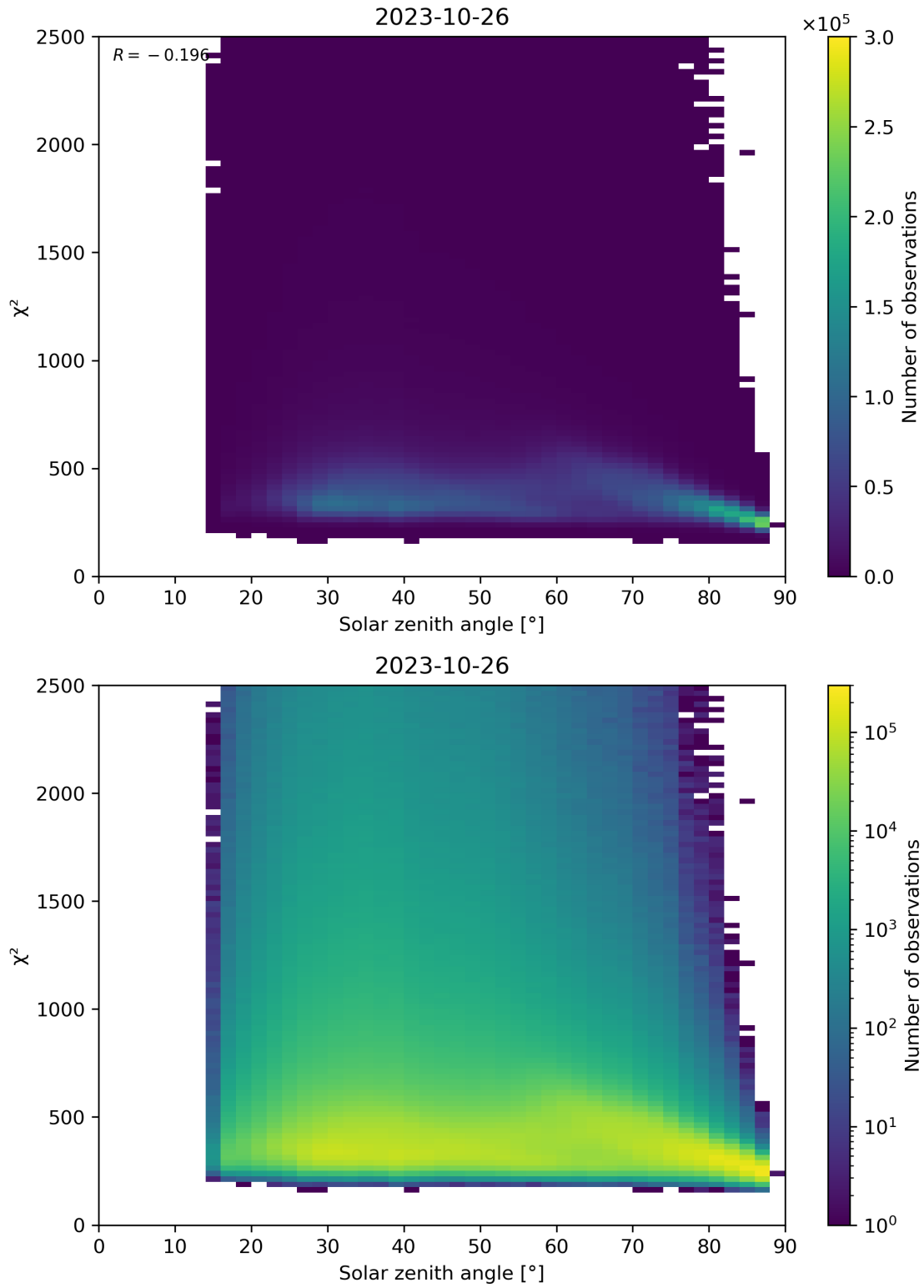
Figure 148: Scatter density plot of “Solar zenith angle” against “ \chi^2 ” for 2023-10-25 to 2023-10-27.
