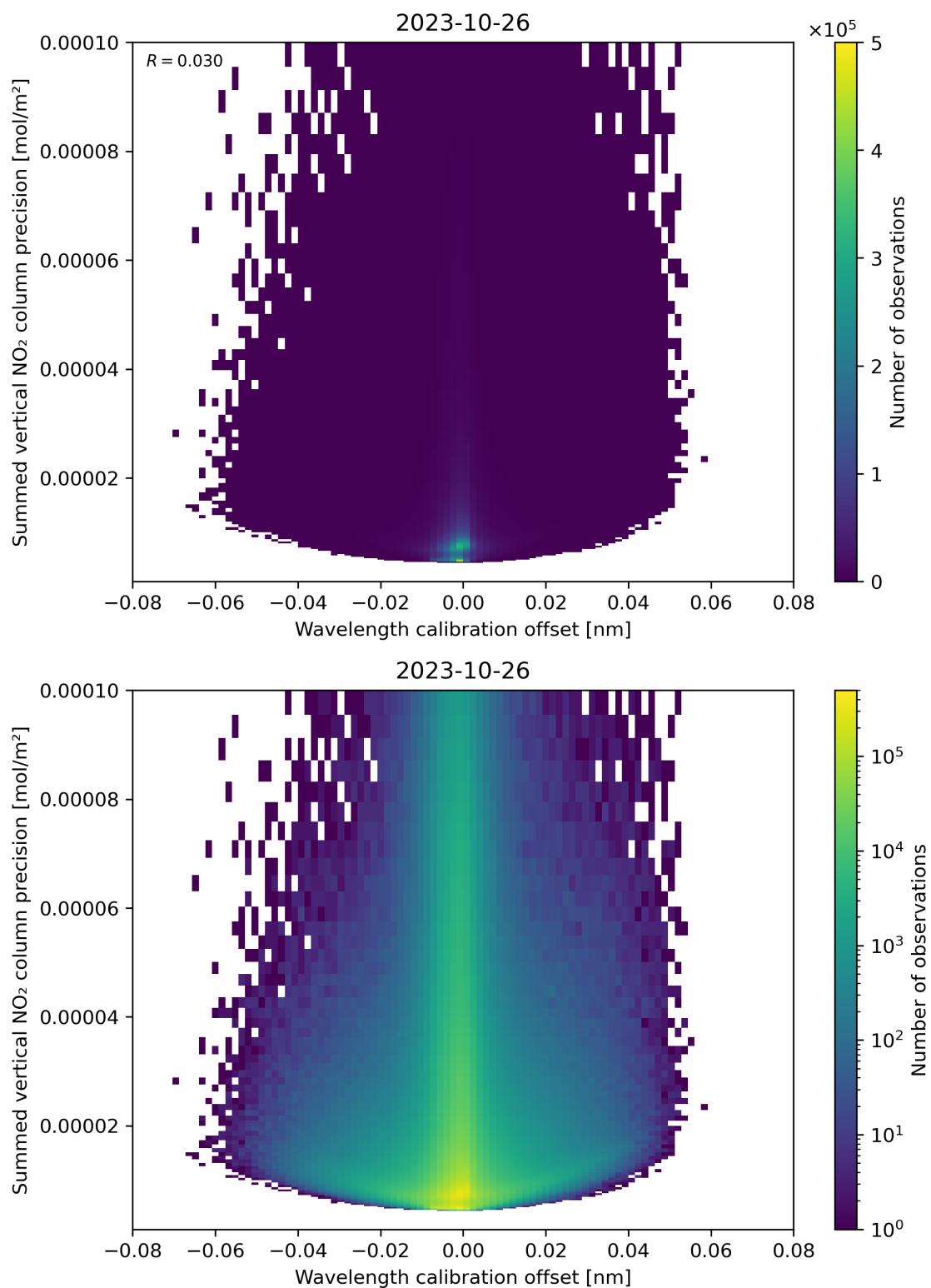
Figure 178: Scatter density plot of “Wavelength calibration offset” against “Summed vertical NO 2 column precision” for 2023-10-25 to 2023-10-27.
