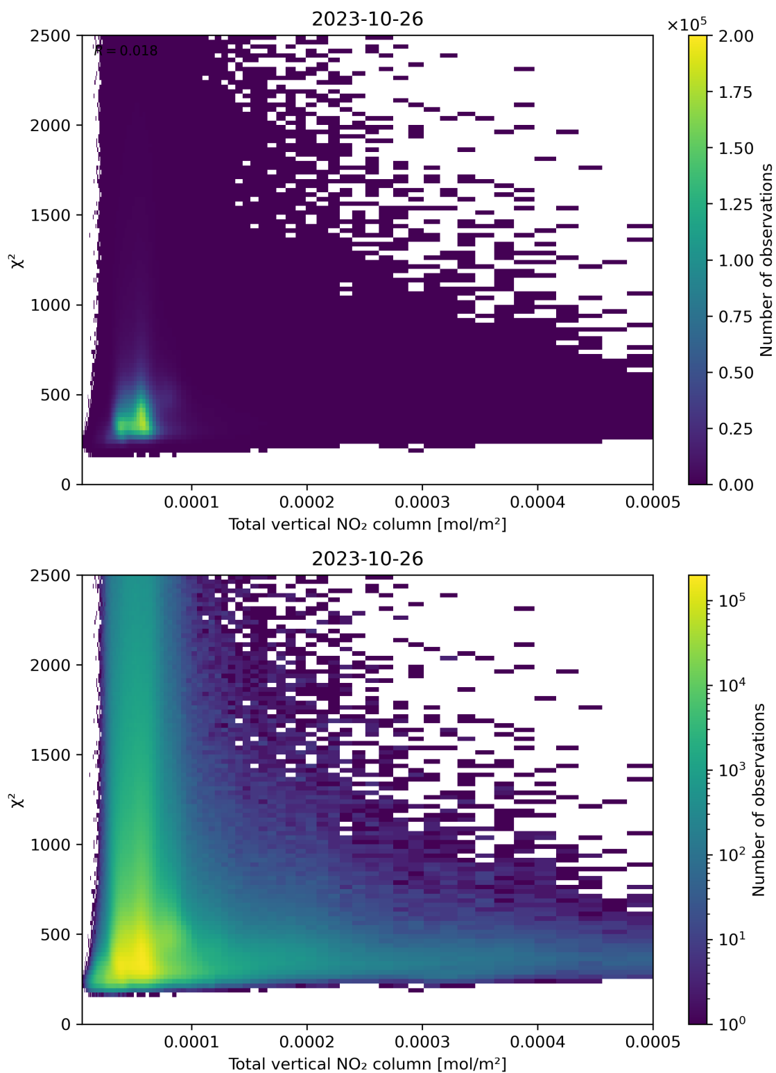
Figure 111: Scatter density plot of “Total vertical NO 2 column” against “ \chi^2 ” for 2023-10-25 to 2023-10-27.
