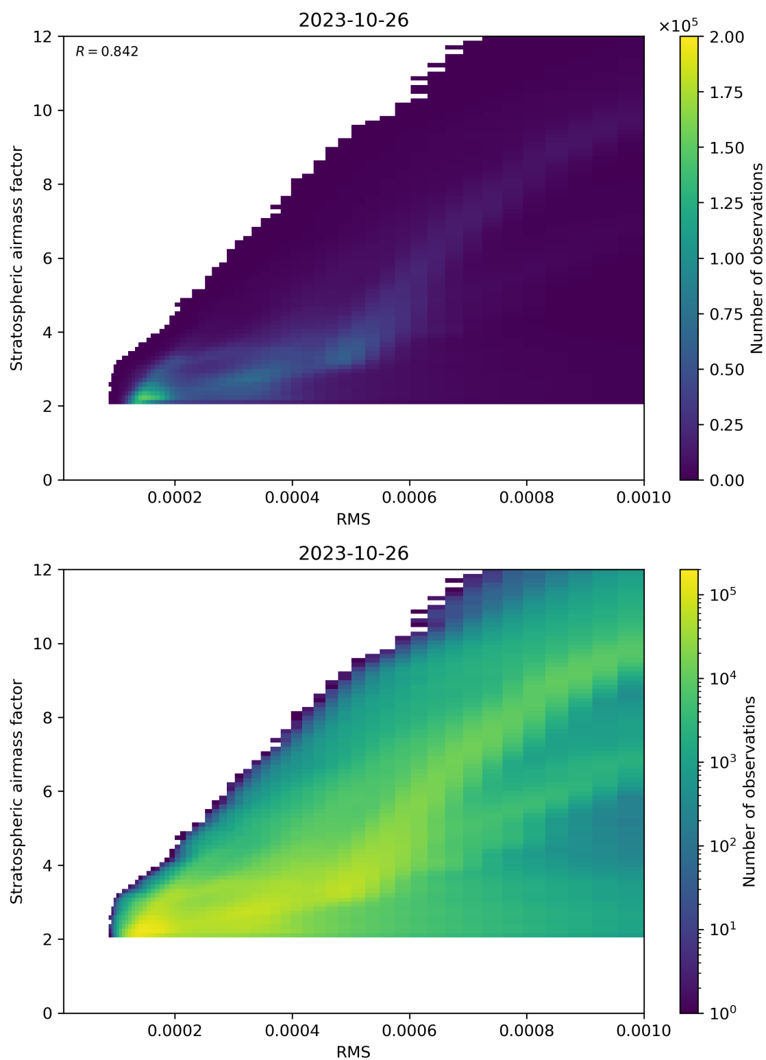
Figure 144: Scatter density plot of “RMS” against “Stratospheric airmass factor” for 2023-10-25 to 2023-10-27.
