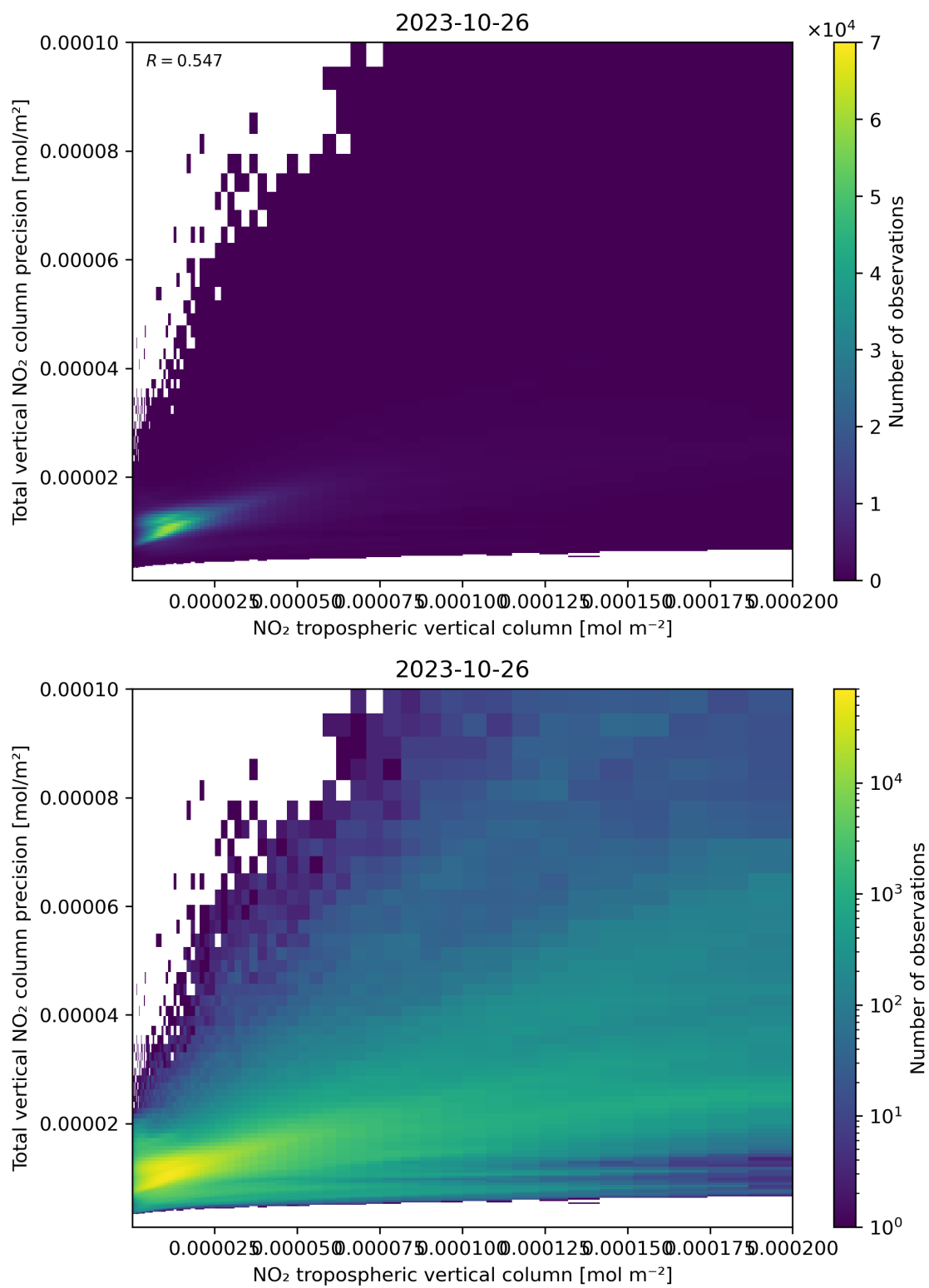
Figure 129: Scatter density plot of “NO 2 tropospheric vertical column” against “Total vertical NO 2 column precision” for 2023-10-25 to 2023-10-27.
