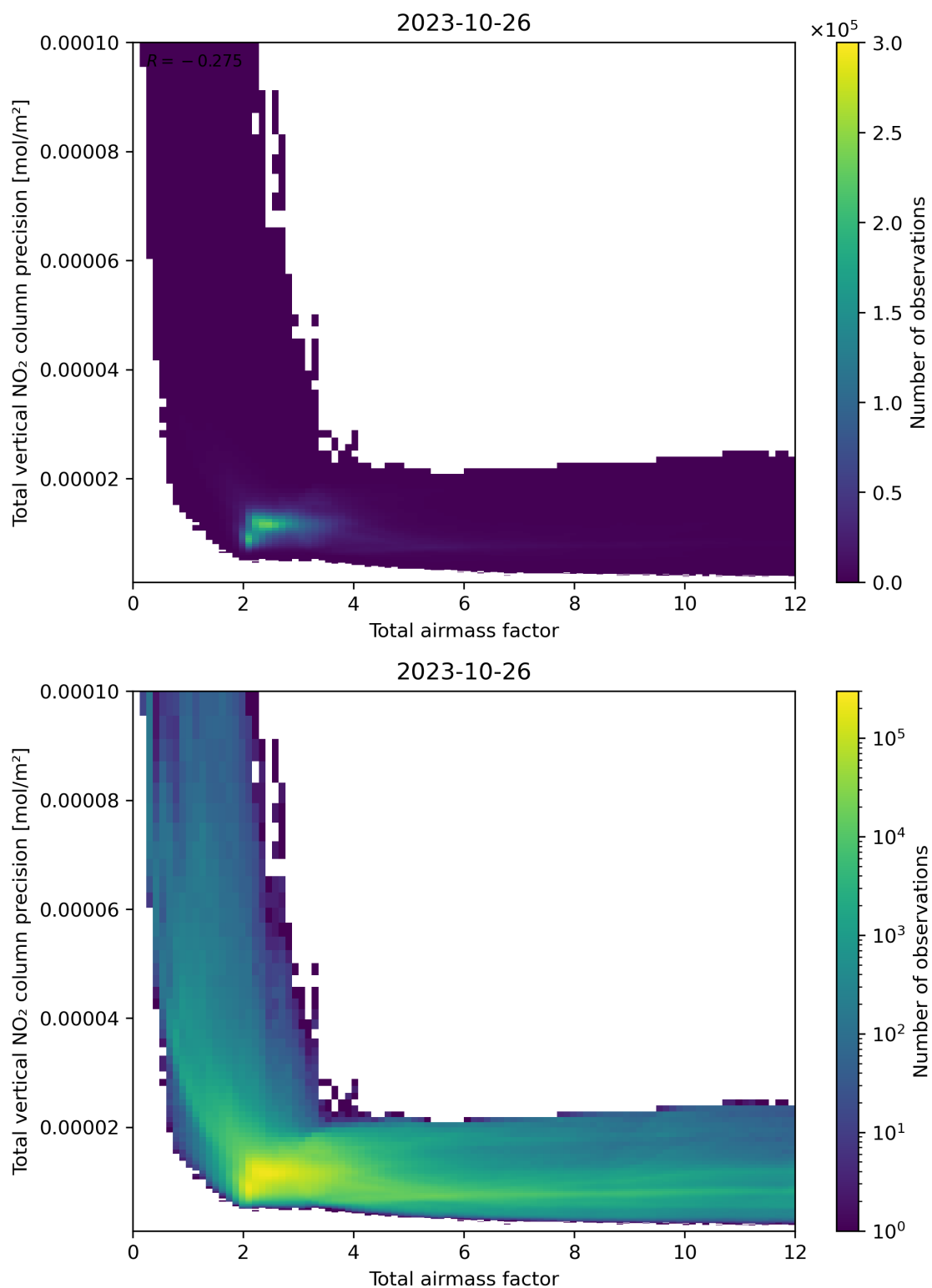
Figure 68: Scatter density plot of “Total airmass factor” against “Total vertical NO 2 column precision” for 2023-10-25 to 2023-10-27.
