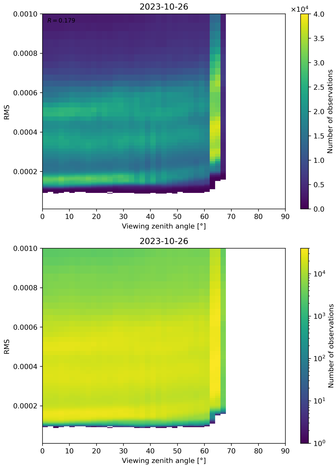
Figure 171: Scatter density plot of “Viewing zenith angle” against “RMS” for 2023-10-25 to 2023-10-27.
