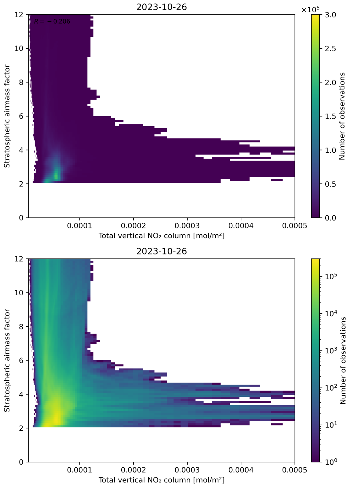
Figure 110: Scatter density plot of “Total vertical NO 2 column” against “Stratospheric airmass factor” for 2023-10-25 to 2023-10-27.
