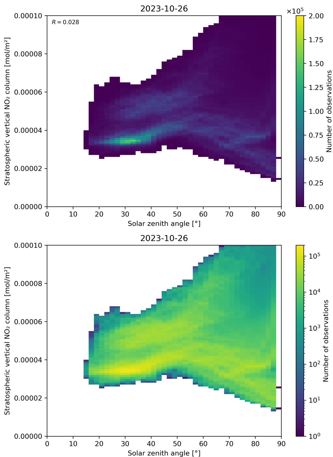
Figure 150: Scatter density plot of “Solar zenith angle” against “Stratospheric vertical NO 2 column” for 2023-10-25 to 2023-10-27.
