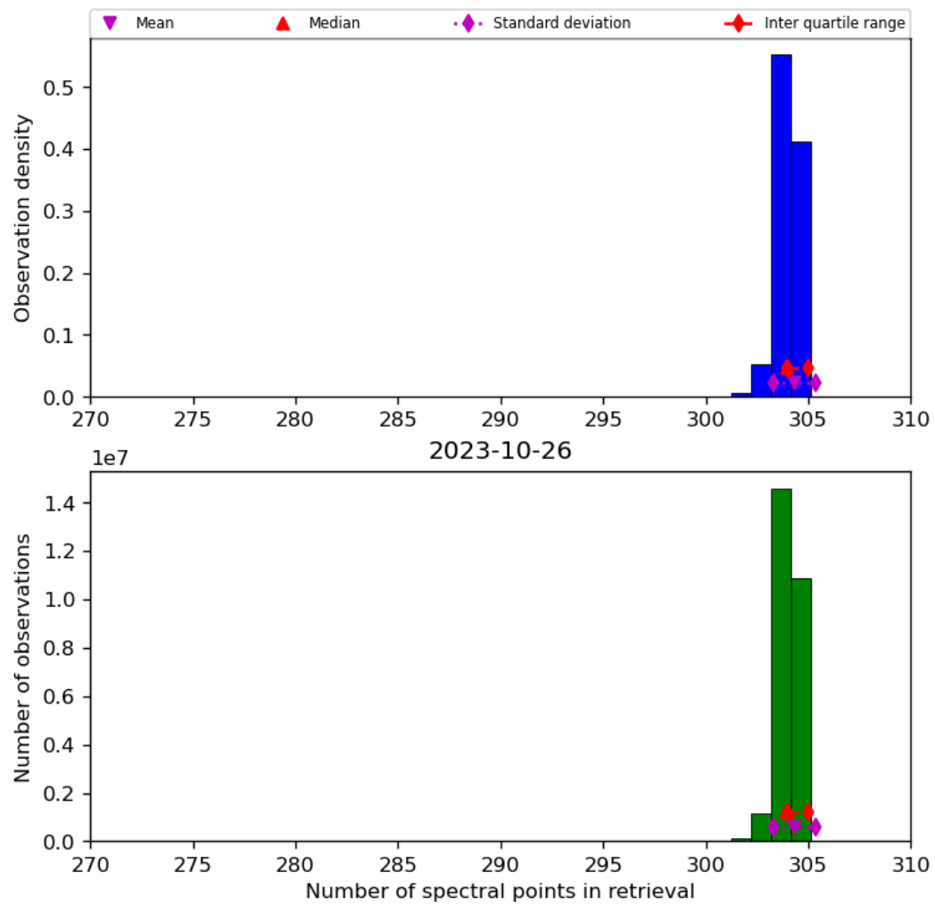
Figure 33: Histogram of “Number of spectral points in retrieval” for 2023-10-25 to 2023-10-27
