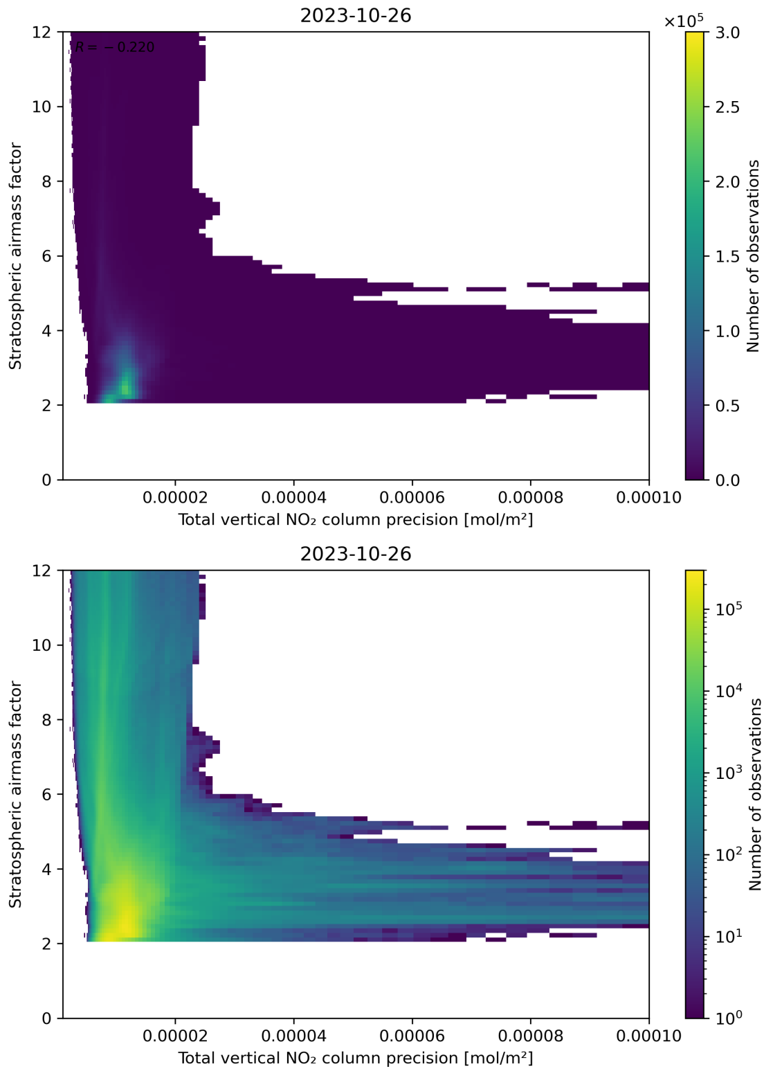
Figure 115: Scatter density plot of “Total vertical NO 2 column precision” against “Stratospheric air mass factor” for 2023-10-25 to 2023-10-27.
