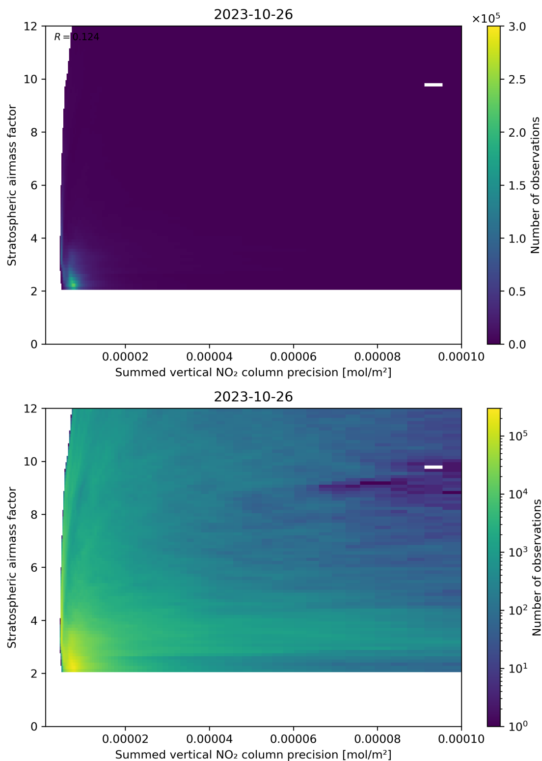
Figure 106: Scatter density plot of “Summed vertical NO 2 column precision” against “Stratospheric airmass factor” for 2023-10-25 to 2023-10-27.
