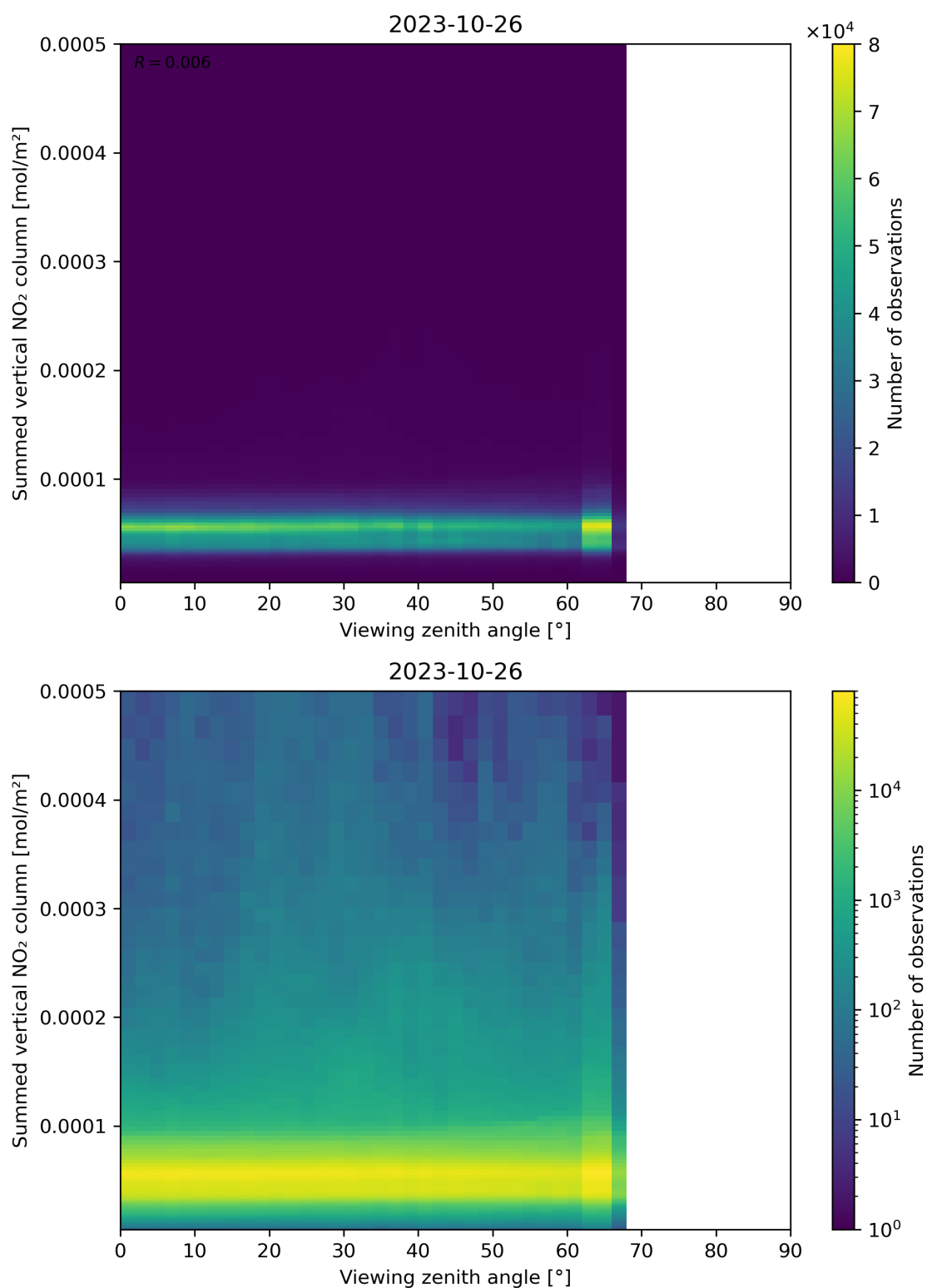
Figure 165: Scatter density plot of “Viewing zenith angle” against “Summed vertical NO 2 column” for 2023-10-25 to 2023-10-27.
