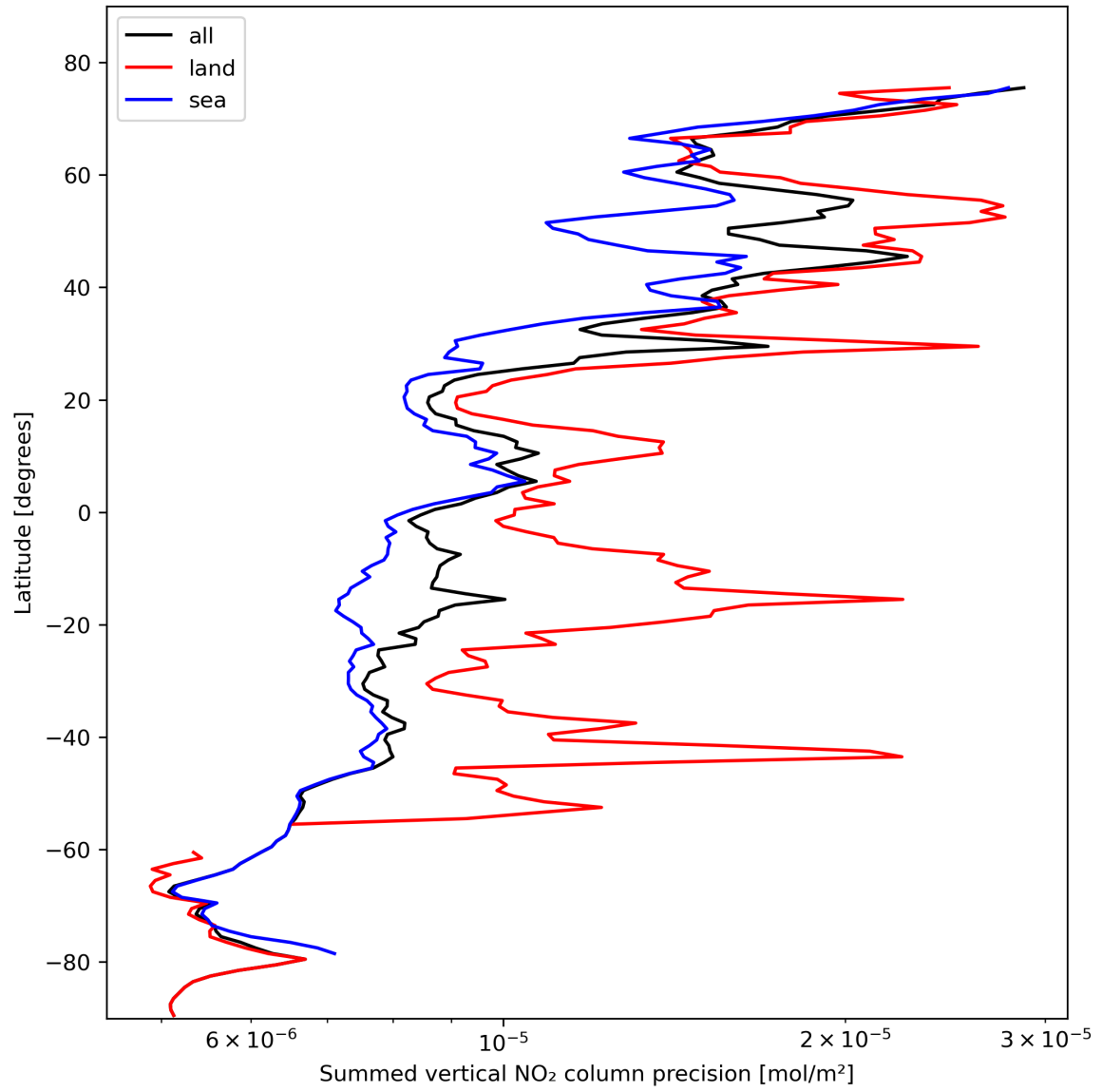
Figure 24: Zonal average of “Summed vertical NO 2 column precision” for 2023-10-25 to 2023-10-27.
