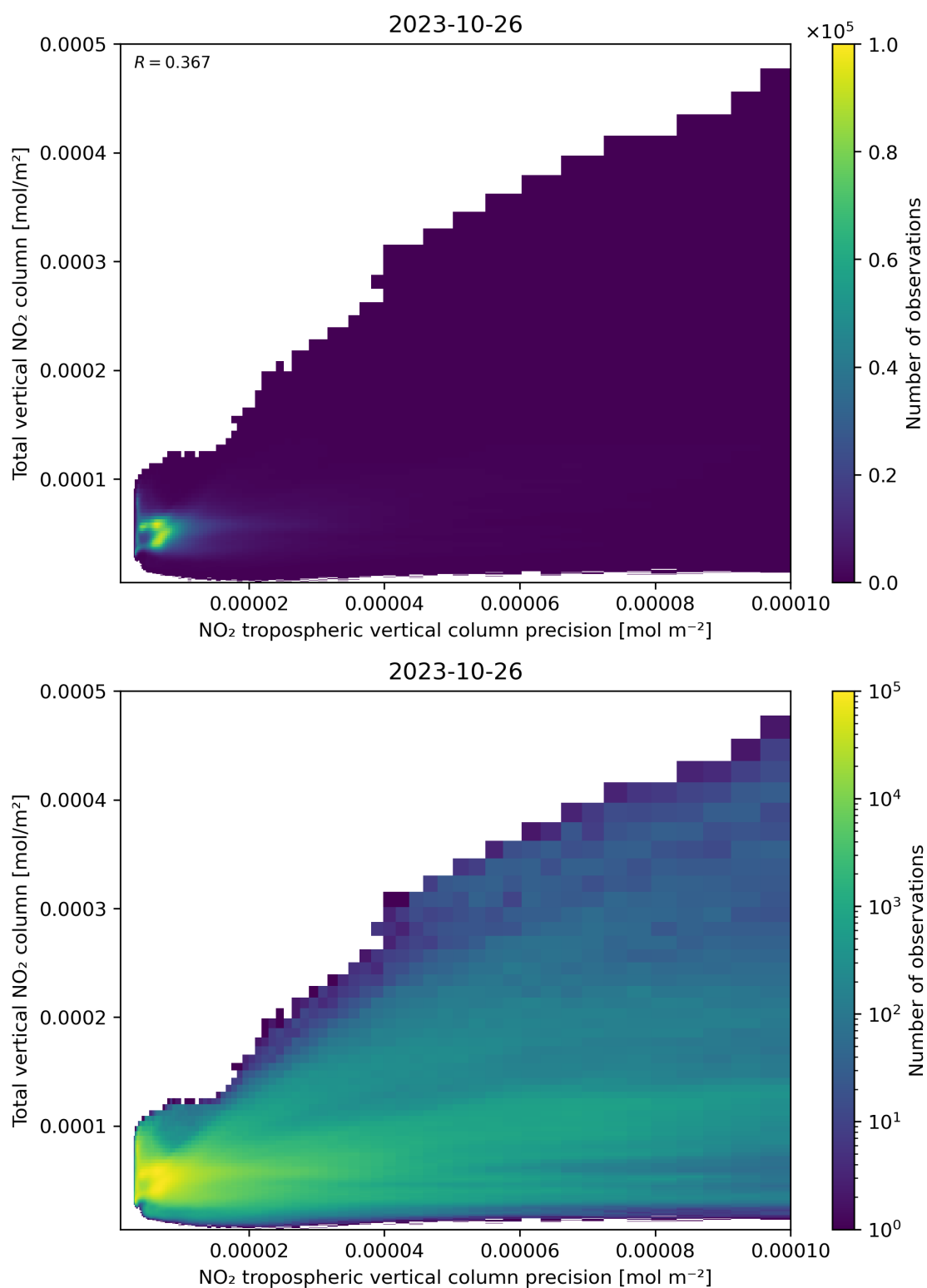
Figure 138: Scatter density plot of “NO 2 tropospheric vertical column precision” against “Total vertical NO 2 column” for 2023-10-25 to 2023-10-27.
