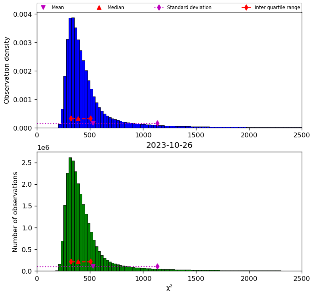
Figure 42: Histogram of “ \chi^2 ” for 2023-10-25 to 2023-10-27
