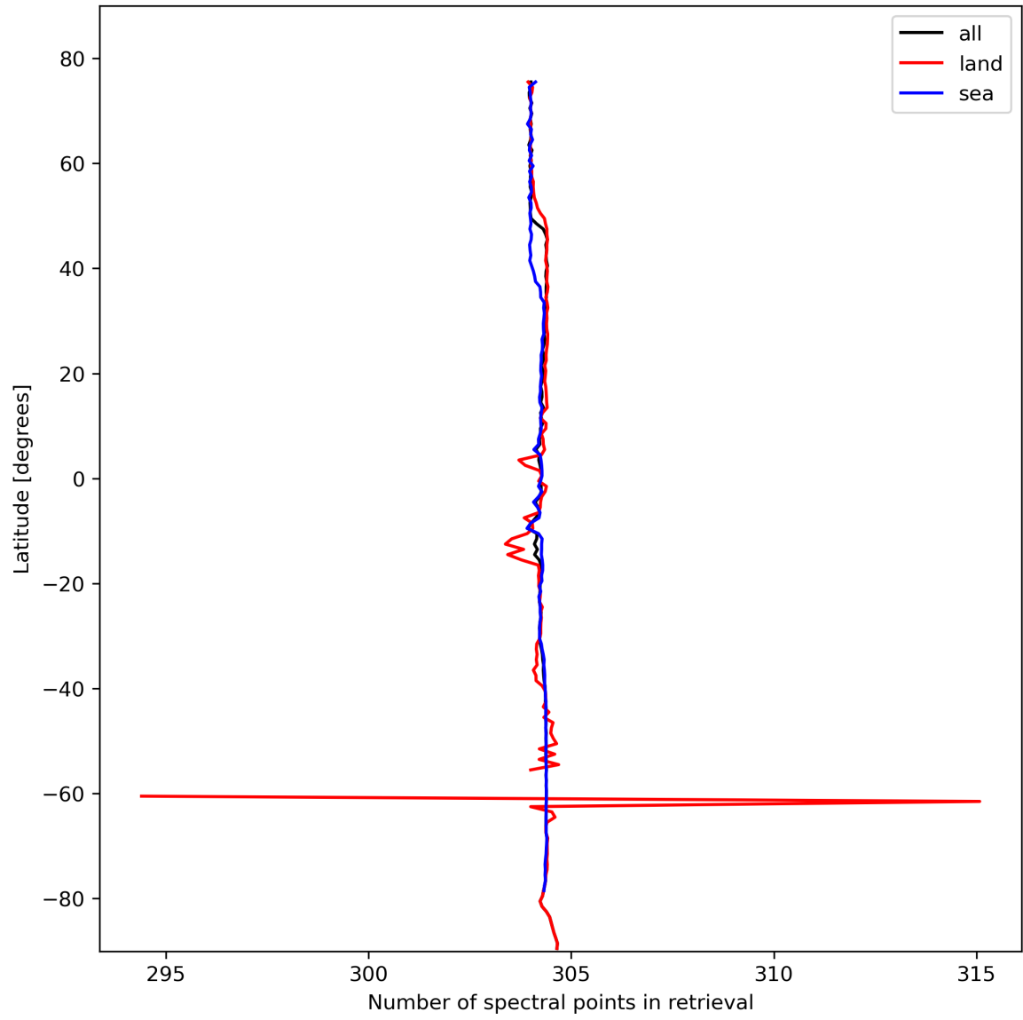
Figure 16: Zonal average of “Number of spectral points in retrieval” for 2023-10-25 to 2023-10-27.
