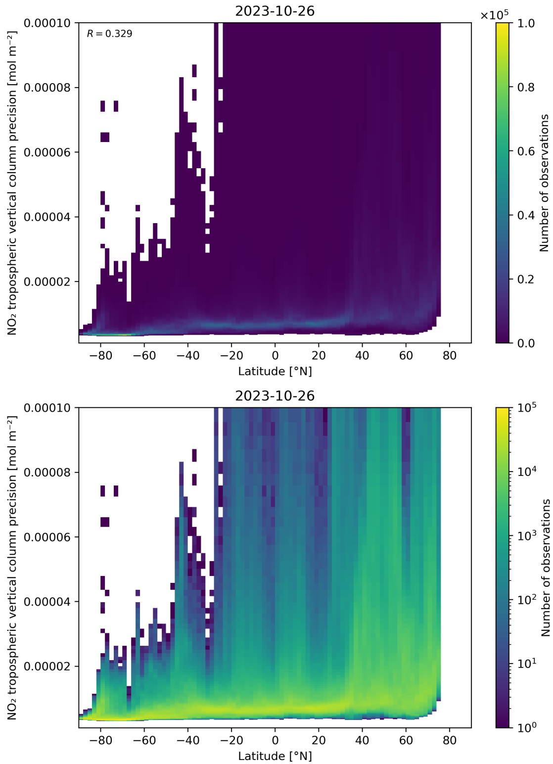
Figure 93: Scatter density plot of “Latitude” against “NO 2 tropospheric vertical column precision” for 2023-10-25 to 2023-10-27.
