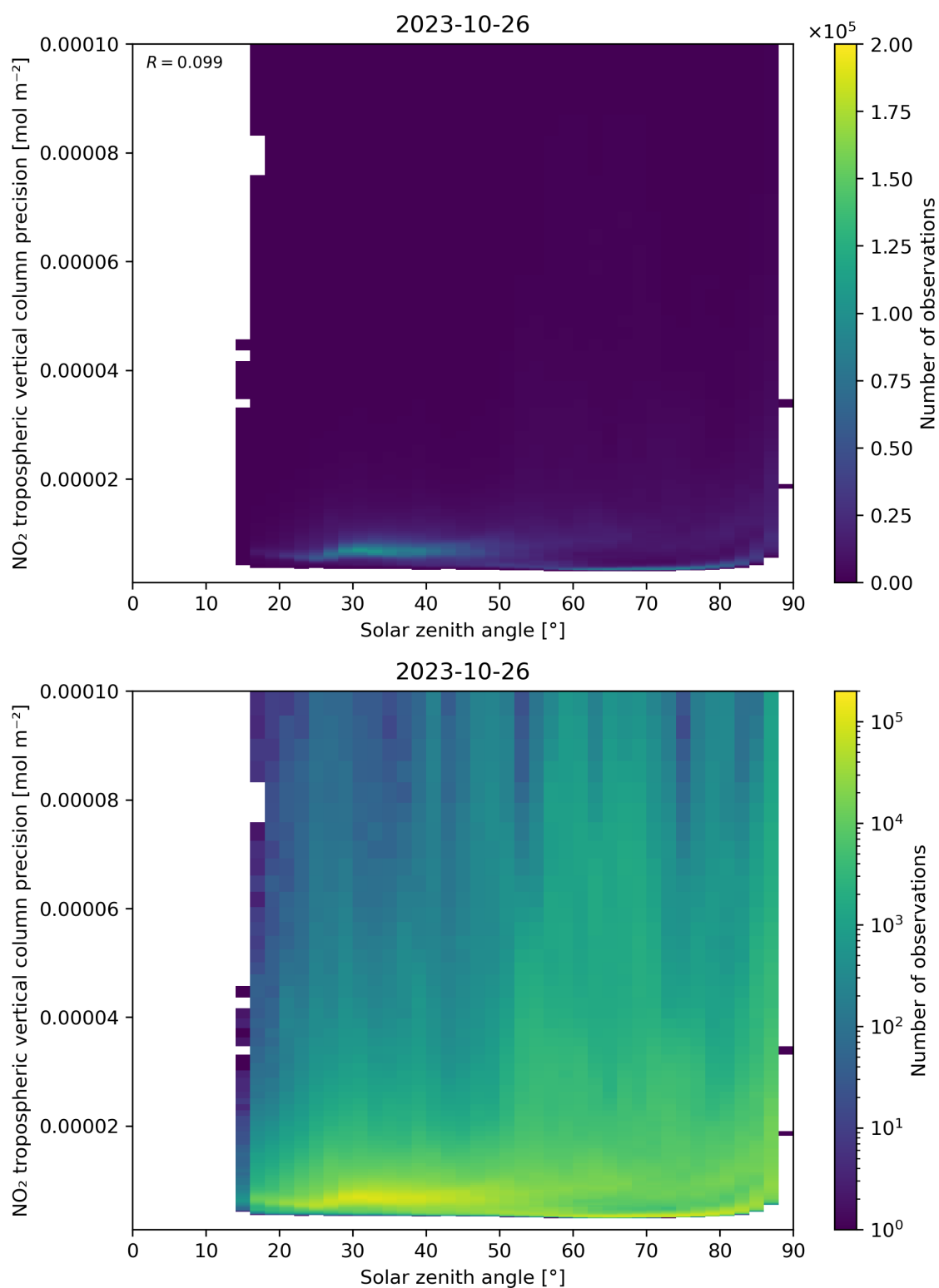
Figure 156: Scatter density plot of “Solar zenith angle” against “NO 2 tropospheric vertical column precision” for 2023-10-25 to 2023-10-27.
