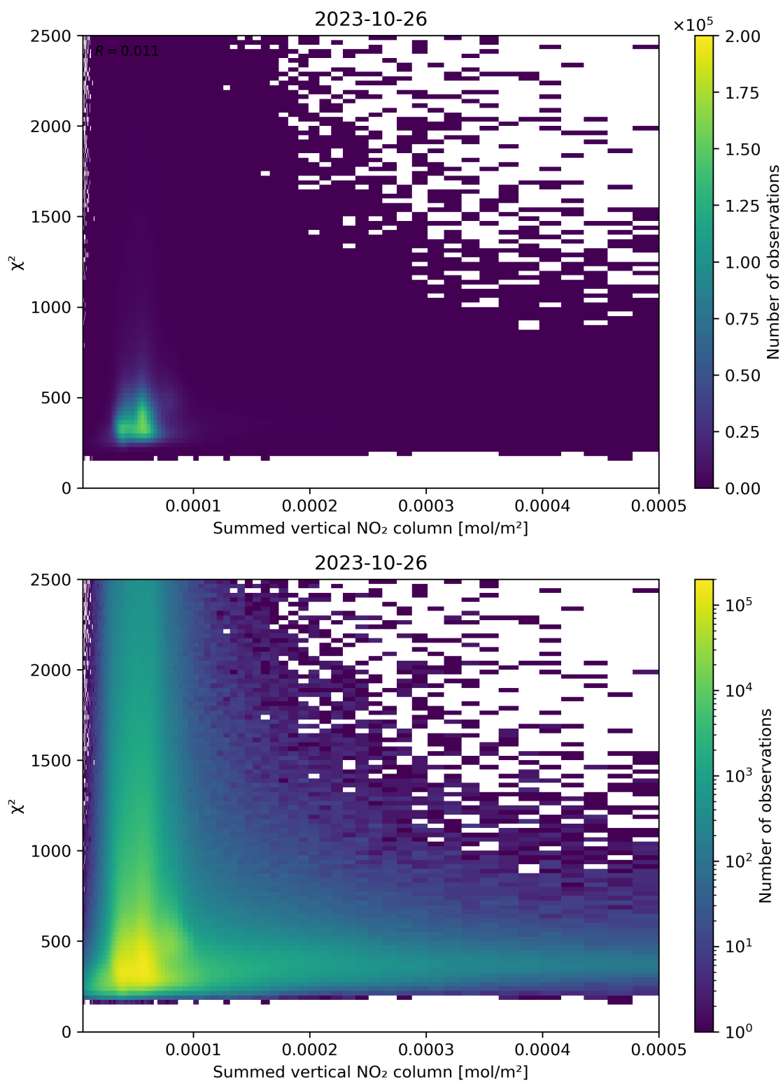
Figure 104: Scatter density plot of “Summed vertical NO 2 column” against “ \chi^2 ” for 2023-10-25 to 2023-10-27.
