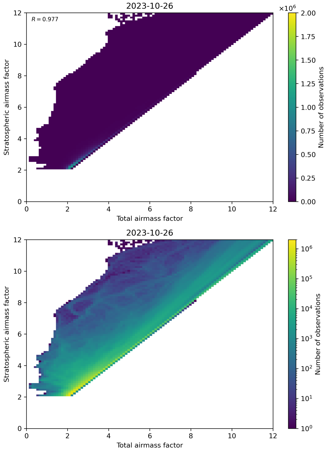
Figure 62: Scatter density plot of “Total airmass factor” against “Stratospheric airmass factor” for 2023-10-25 to 2023-10-27.
