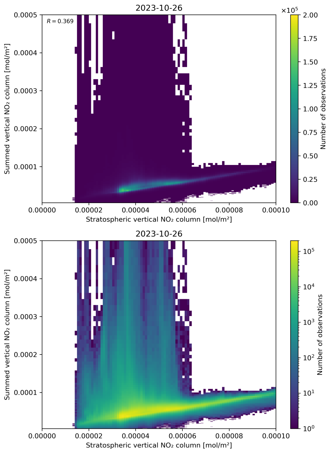
Figure 98: Scatter density plot of “Stratospheric vertical NO 2 column” against “Summed vertical NO 2 column” for 2023-10-25 to 2023-10-27.
