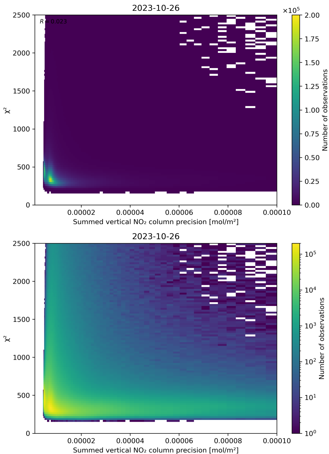
Figure 107: Scatter density plot of “Summed vertical NO 2 column precision” against “ \chi^2 ” for 2023-10-25 to 2023-10-27.
