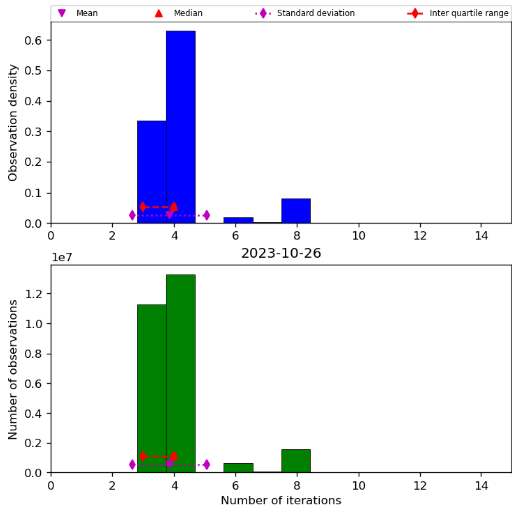
Figure 34: Histogram of “Number of iterations” for 2023-10-25 to 2023-10-27
