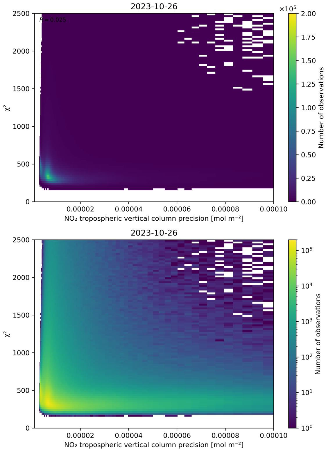
Figure 134: Scatter density plot of “NO 2 tropospheric vertical column precision” against “ \chi^2 ” for 2023-10-25 to 2023-10-27.
