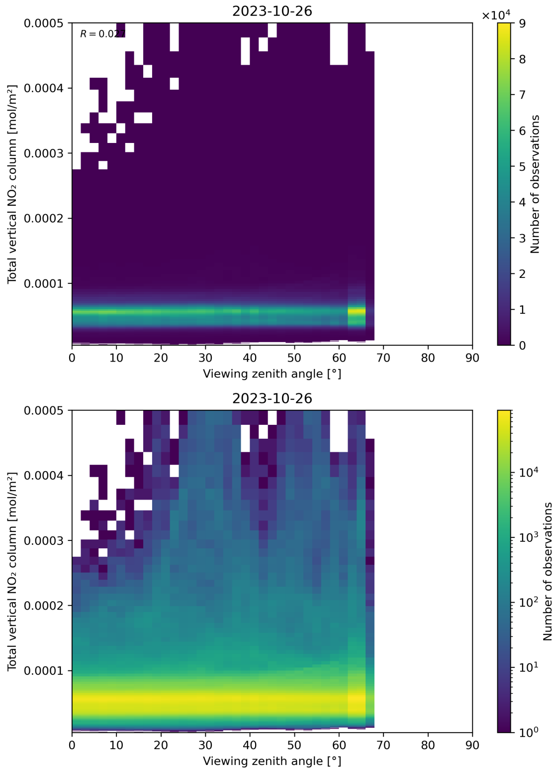
Figure 167: Scatter density plot of “Viewing zenith angle” against “Total vertical NO 2 column” for 2023-10-25 to 2023-10-27.
