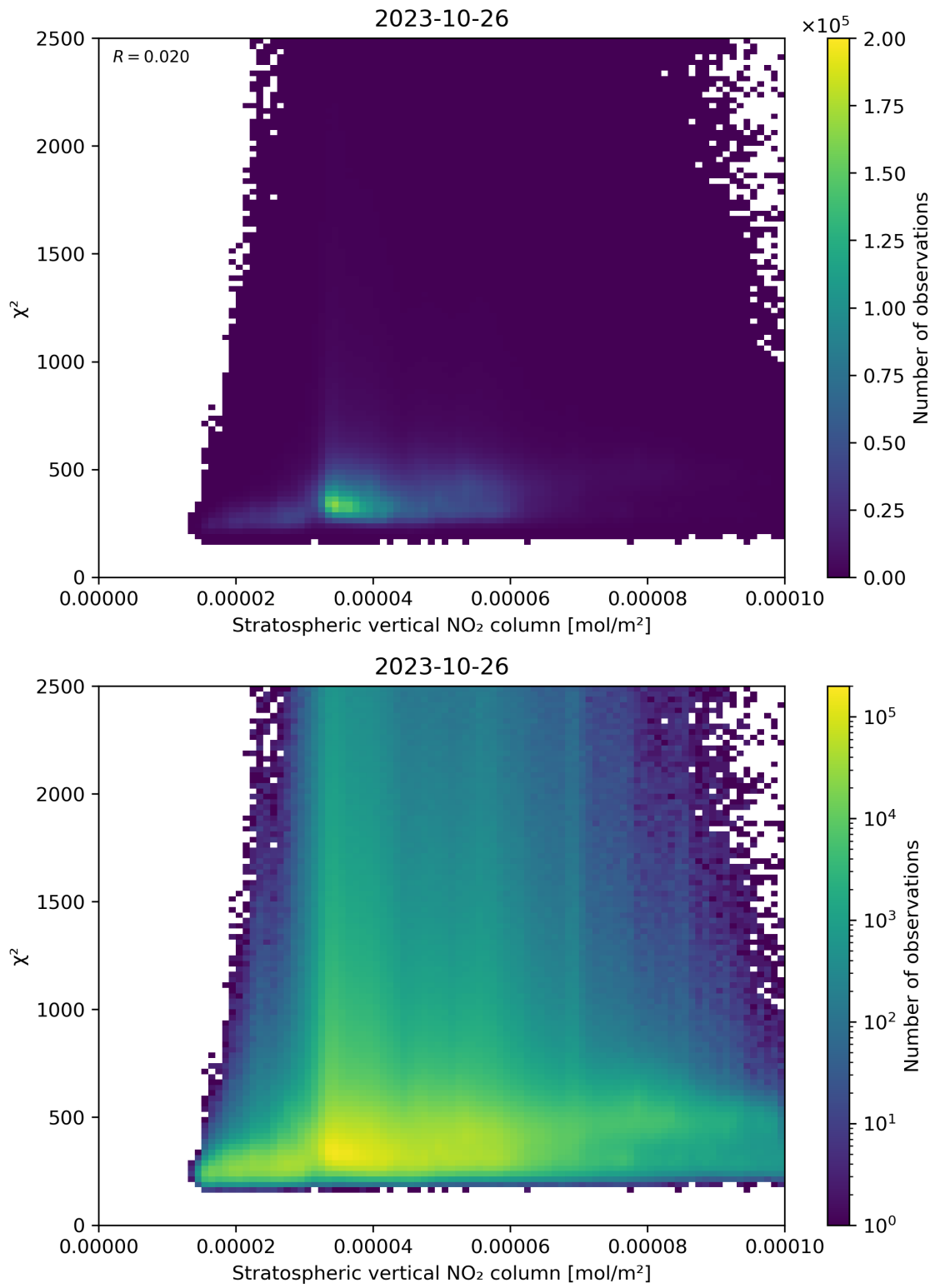
Figure 97: Scatter density plot of “Stratospheric vertical NO 2 column” against “ \chi^2 ” for 2023-10-25 to 2023-10-27.
