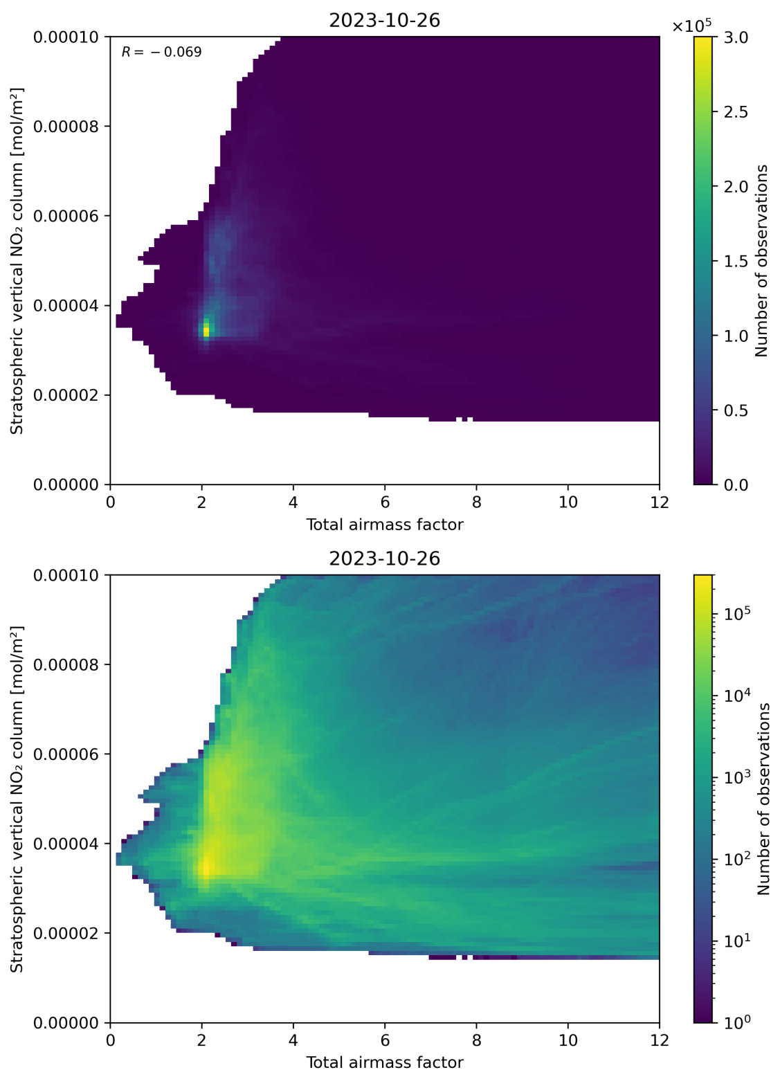
Figure 64: Scatter density plot of “Total airmass factor” against “Stratospheric vertical NO 2 column” for 2023-10-25 to 2023-10-27.
