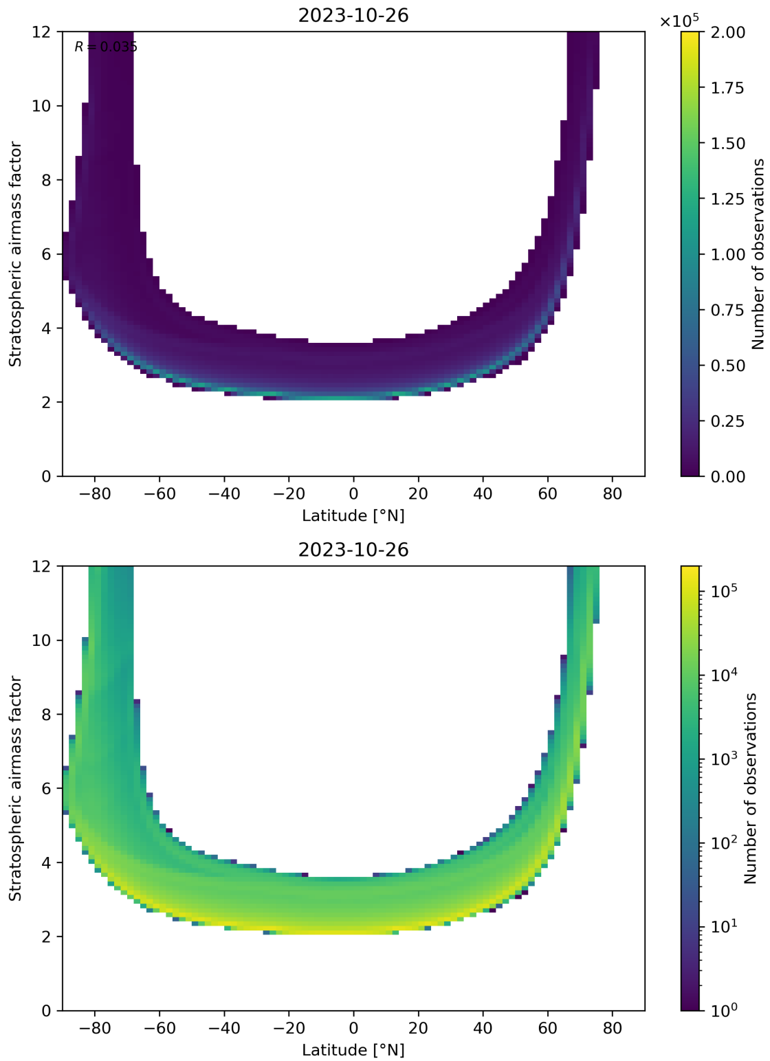
Figure 83: Scatter density plot of “Latitude” against “Stratospheric airmass factor” for 2023-10-25 to 2023-10-27.
