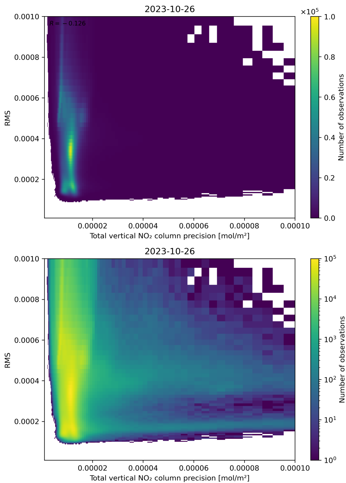
Figure 119: Scatter density plot of “Total vertical NO 2 column precision” against “RMS” for 2023-10-25 to 2023-10-27.
