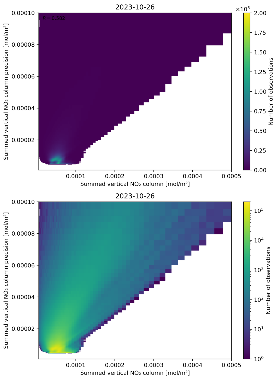
Figure 105: Scatter density plot of “Summed vertical NO 2 column” against “Summed vertical NO 2 column precision” for 2023-10-25 to 2023-10-27.
