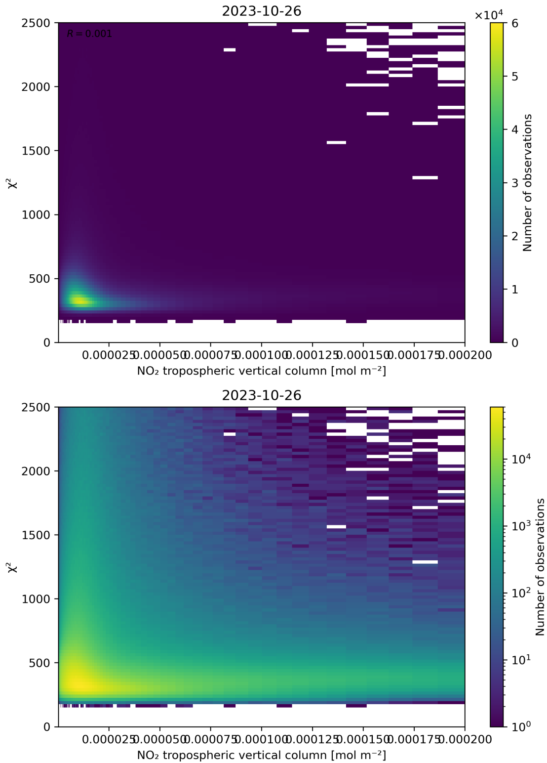
Figure 124: Scatter density plot of “NO 2 tropospheric vertical column” against “ \chi^2 ” for 2023-10-25 to 2023-10-27.
