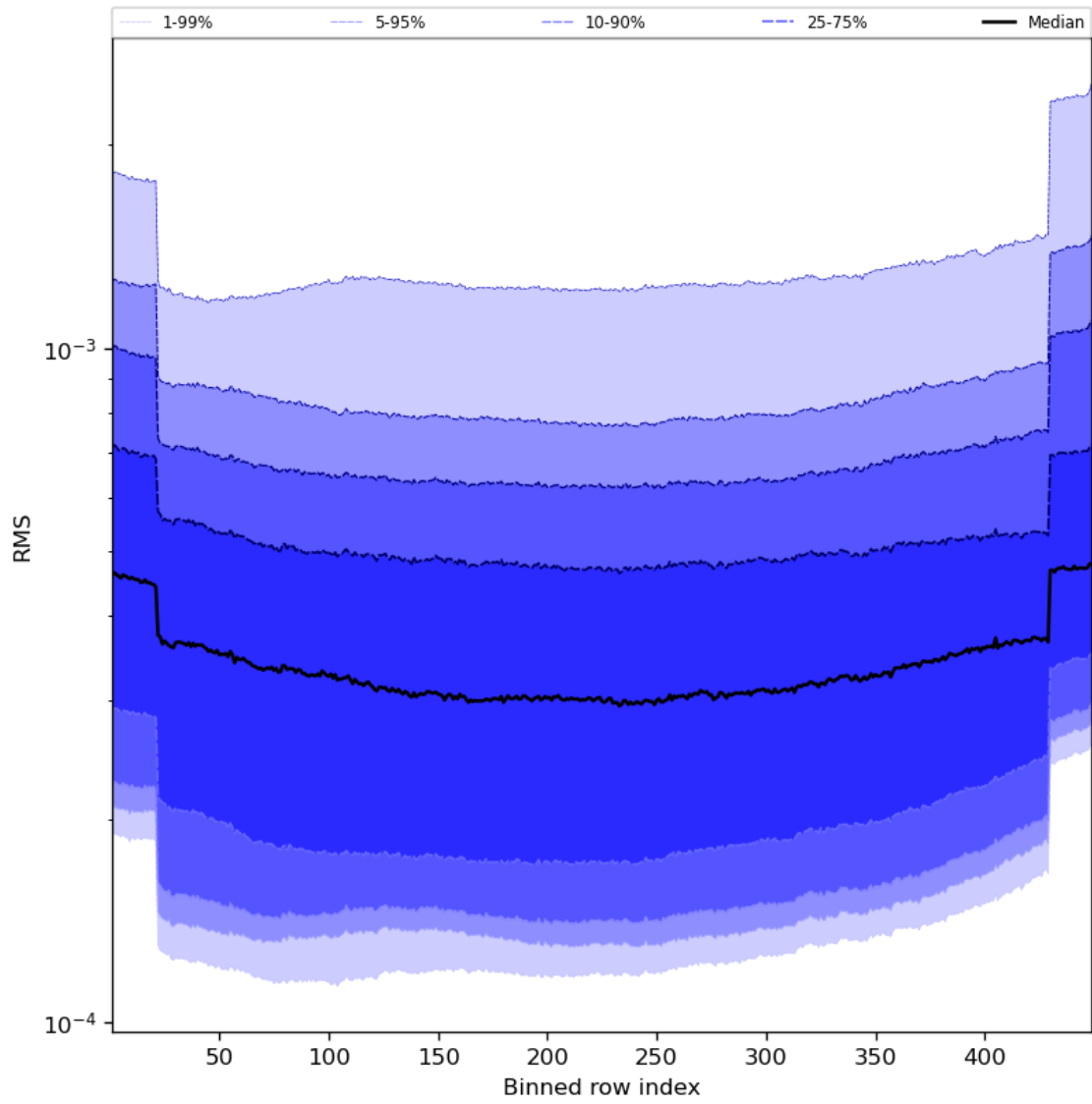
Figure 60: Along track statistics of “RMS” for 2023-10-25 to 2023-10-27
