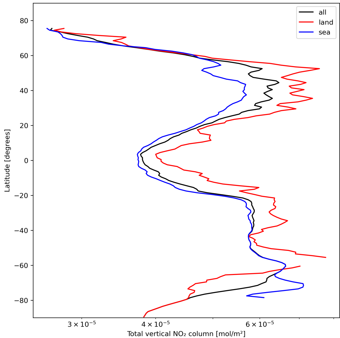
Figure 21: Zonal average of “Total vertical NO 2 column” for 2023-10-25 to 2023-10-27.
