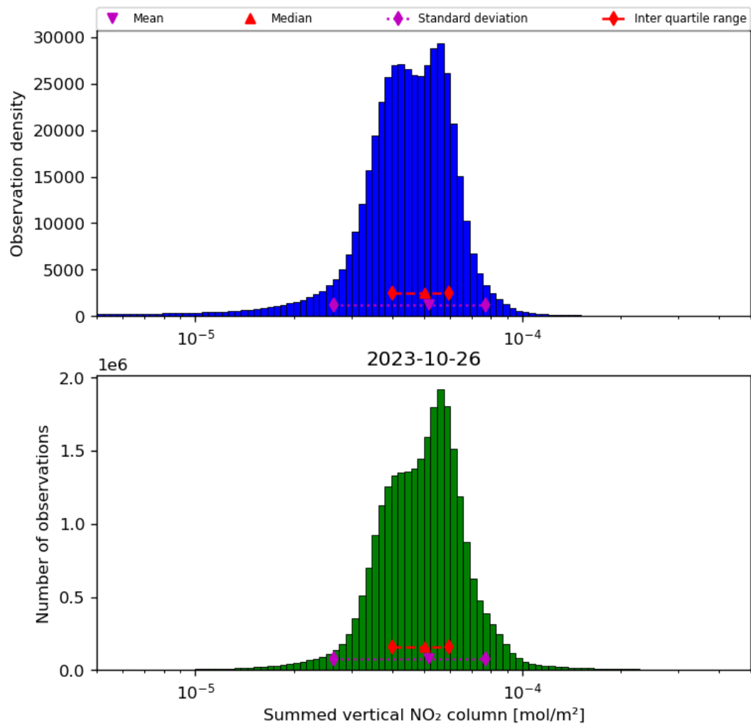
Figure 40: Histogram of “Summed vertical NO 2 column” for 2023-10-25 to 2023-10-27
