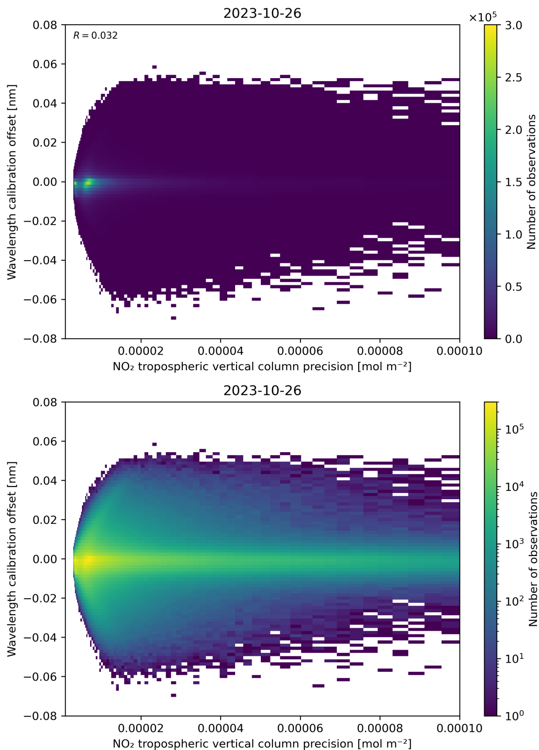
Figure 141: Scatter density plot of “NO 2 tropospheric vertical column precision” against “Wavelength calibration offset” for 2023-10-25 to 2023-10-27.
