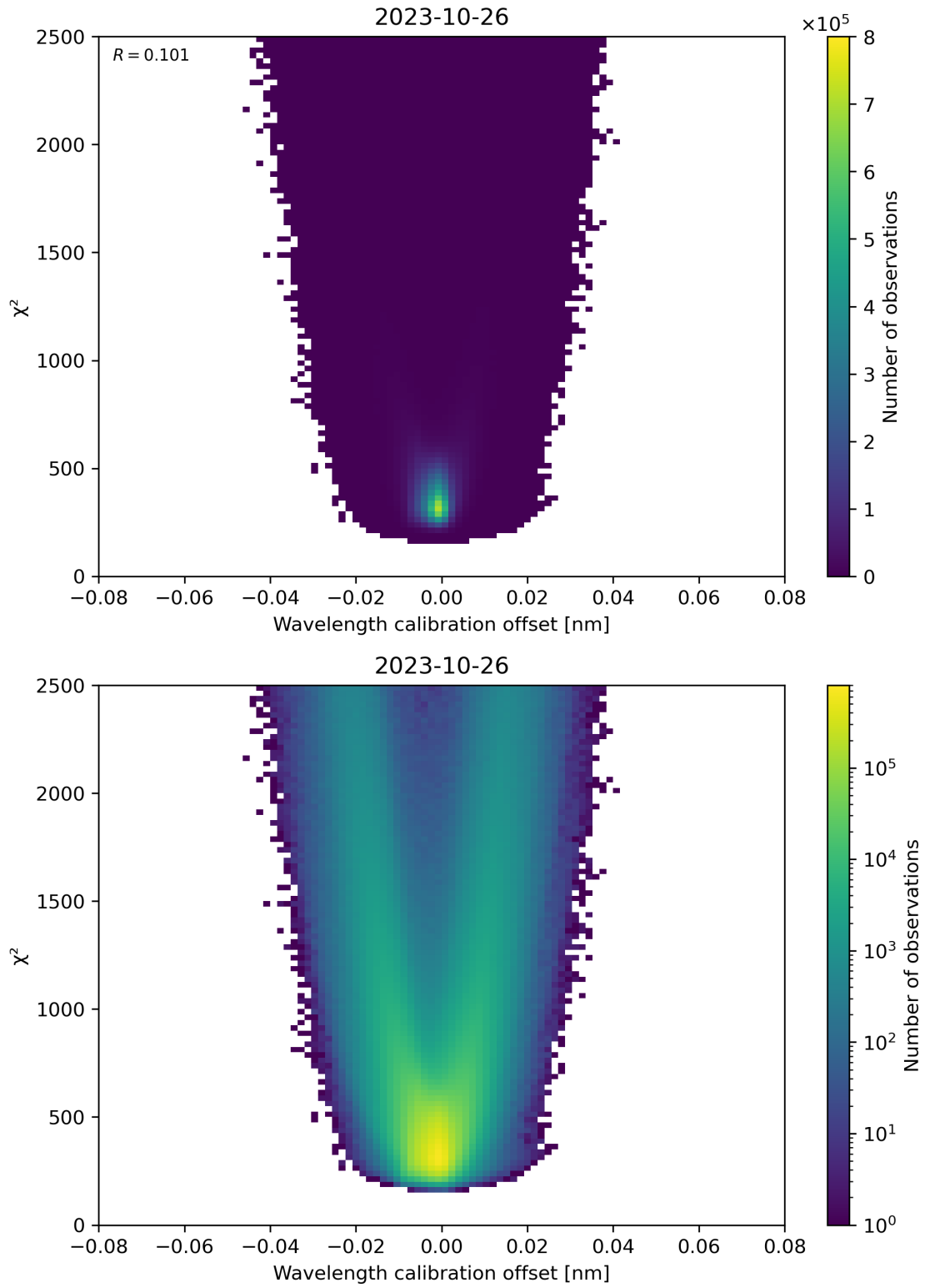
Figure 175: Scatter density plot of “Wavelength calibration offset” against “ \chi^2 ” for 2023-10-25 to 2023-10-27.
