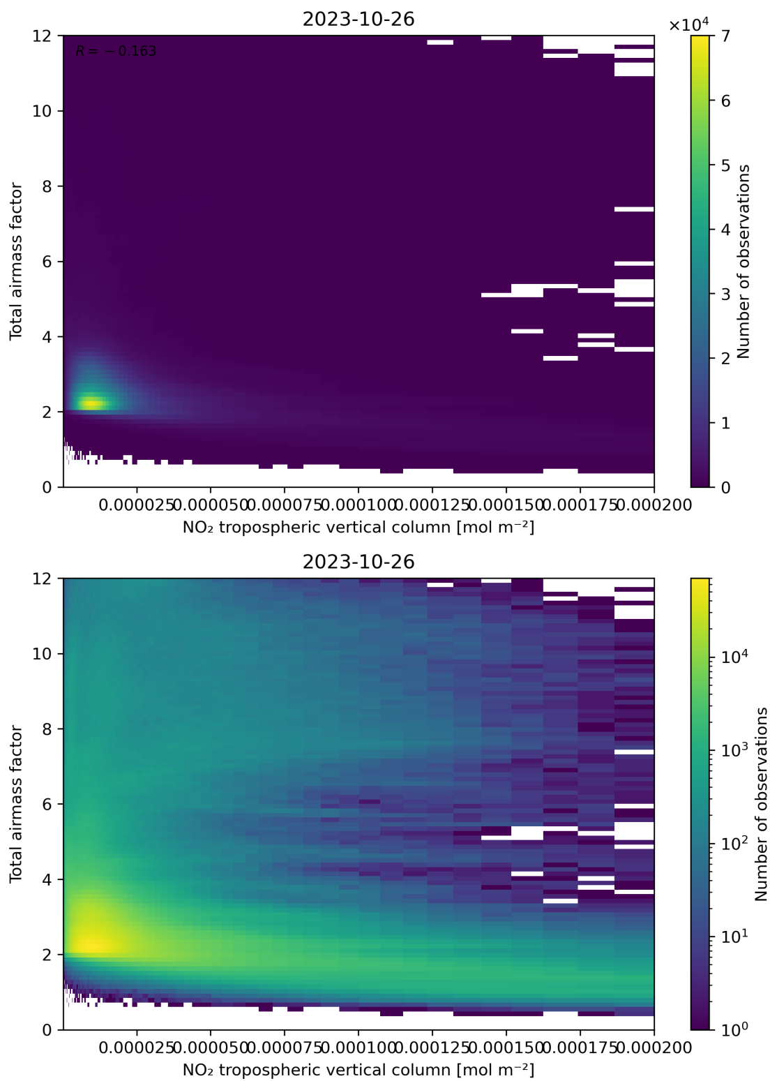
Figure 122: Scatter density plot of “NO 2 tropospheric vertical column” against “Total air mass factor” for 2023-10-25 to 2023-10-27.
