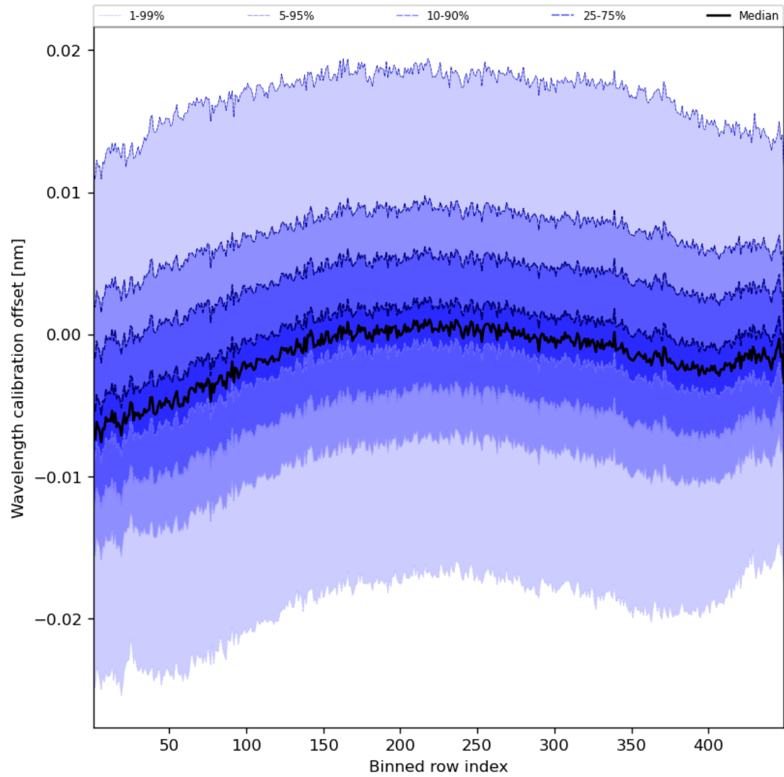
Figure 52: Along track statistics of “Wavelength calibration offset” for 2023-10-25 to 2023-10-27
