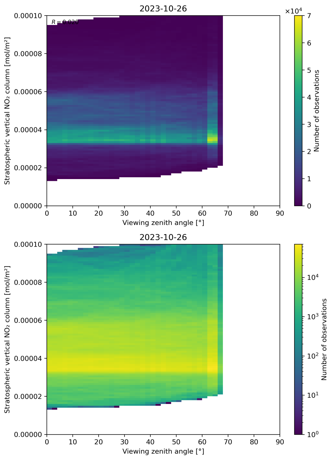
Figure 164: Scatter density plot of “Viewing zenith angle” against “Stratospheric vertical NO 2 column” for 2023-10-25 to 2023-10-27.
