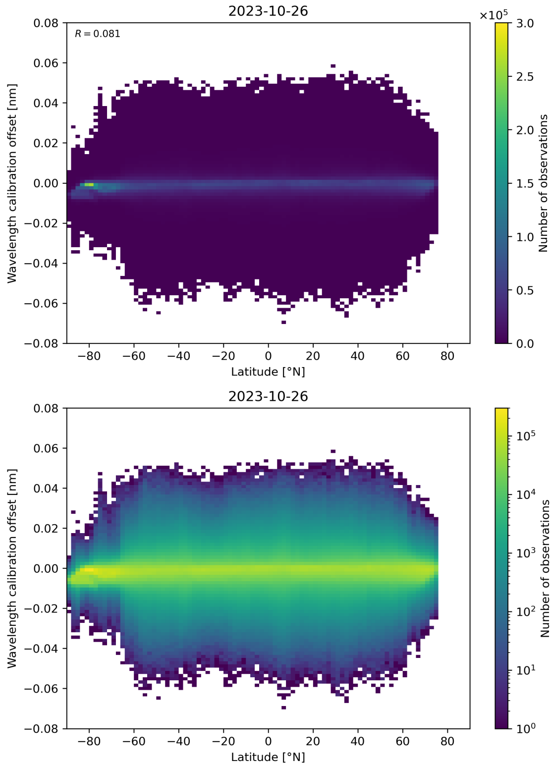
Figure 95: Scatter density plot of “Latitude” against “Wavelength calibration offset” for 2023-10-25 to 2023-10-27.
