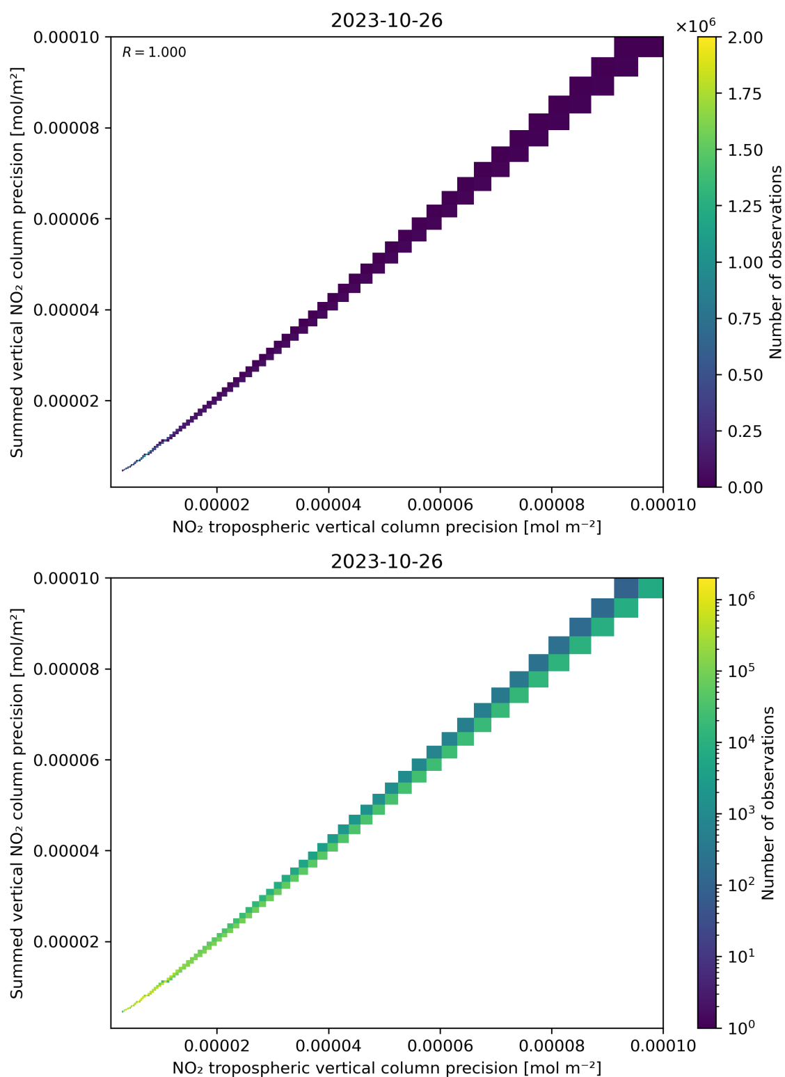
Figure 137: Scatter density plot of “NO 2 tropospheric vertical column precision” against “Summed vertical NO 2 column precision” for 2023-10-25 to 2023-10-27.
