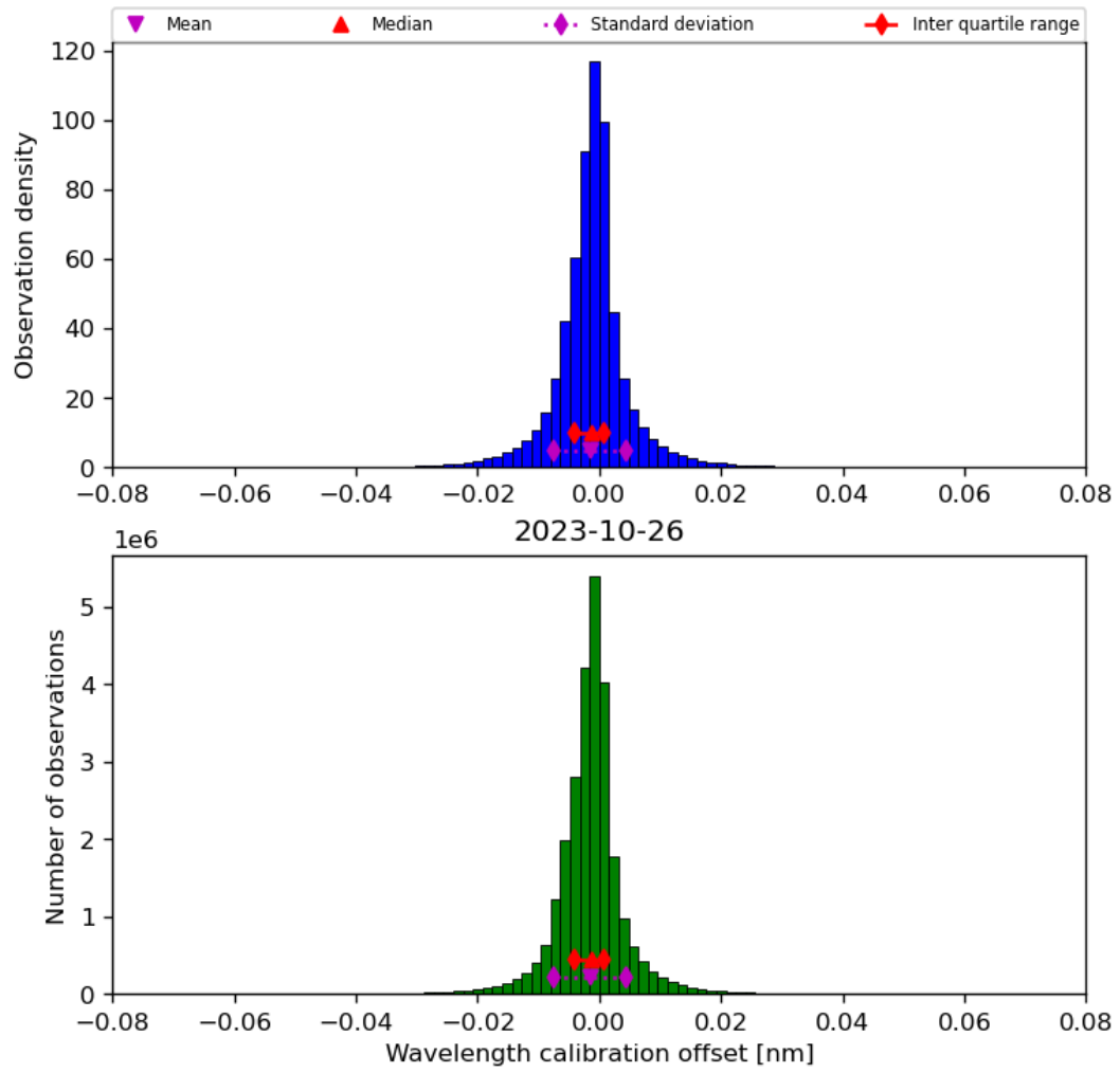
Figure 35: Histogram of “Wavelength calibration offset” for 2023-10-25 to 2023-10-27
