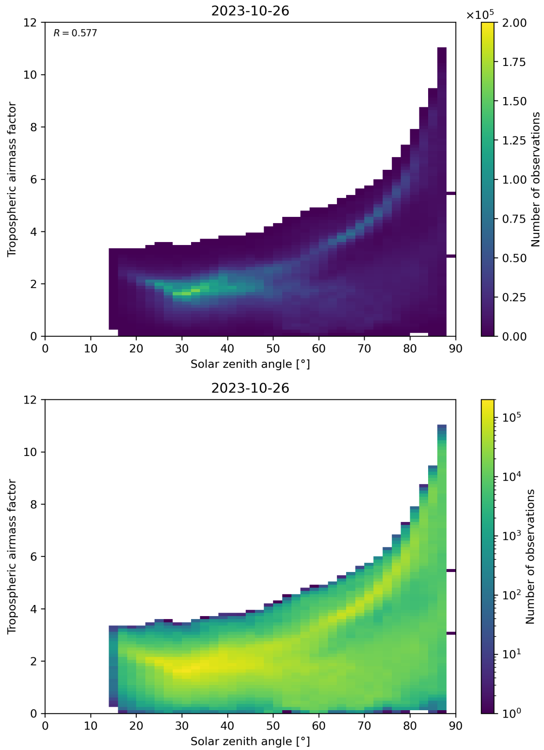
Figure 147: Scatter density plot of “Solar zenith angle” against “Tropospheric airmass factor” for 2023-10-25 to 2023-10-27.
