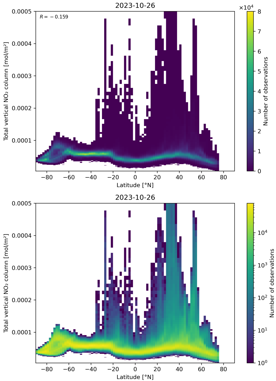
Figure 90: Scatter density plot of “Latitude” against “Total vertical NO 2 column” for 2023-10-25 to 2023-10-27.
