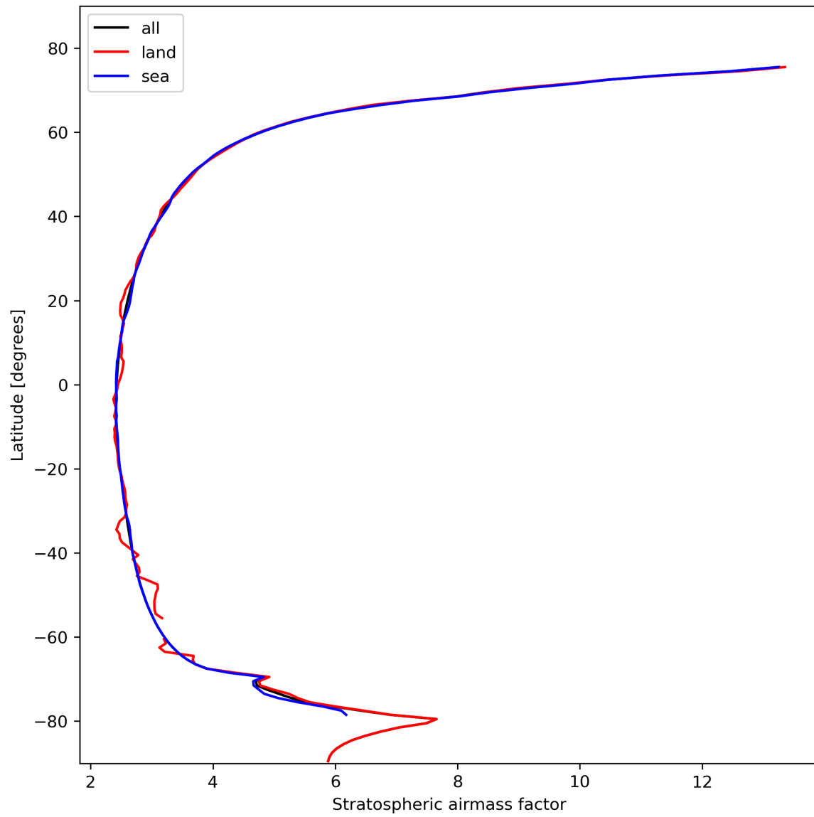
Figure 27: Zonal average of “Stratospheric airmass factor” for 2023-10-25 to 2023-10-27.
