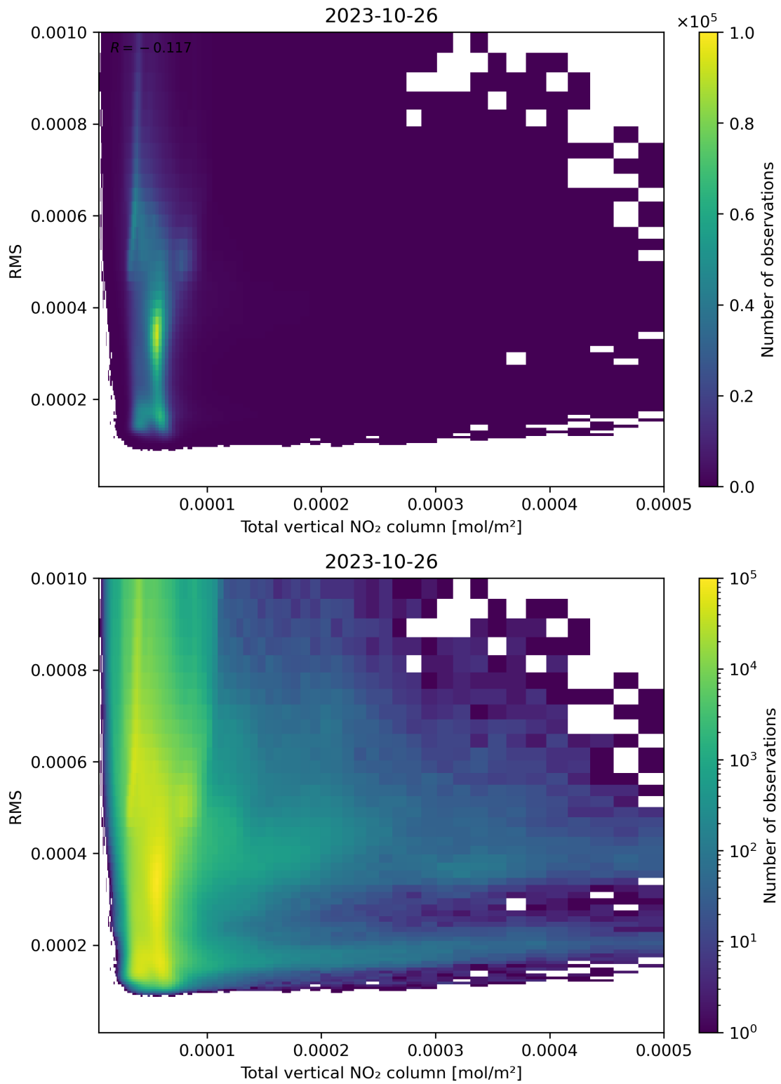
Figure 120: Scatter density plot of “Total vertical NO 2 column” against “RMS” for 2023-10-25 to 2023-10-27.
