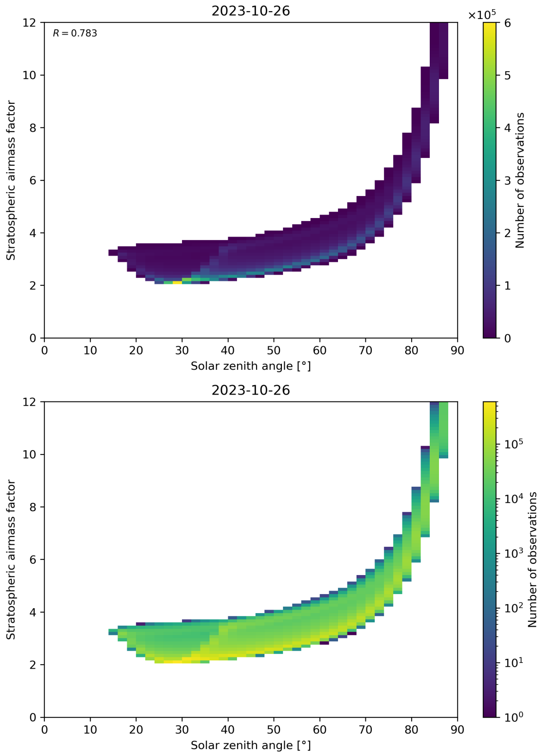
Figure 145: Scatter density plot of “Solar zenith angle” against “Stratospheric airmass factor” for 2023-10-25 to 2023-10-27.
