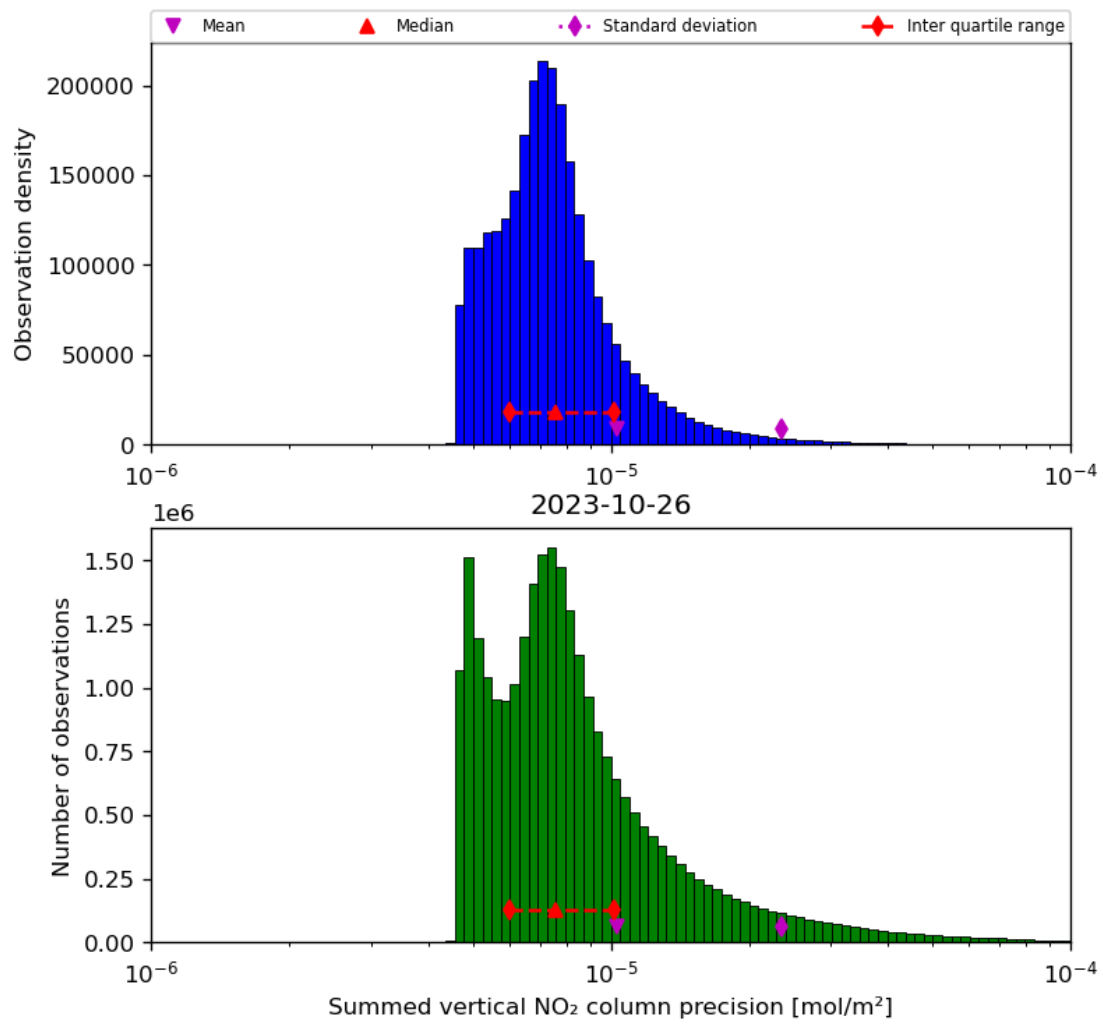
Figure 41: Histogram of "Summed vertical NO 2 column precision" for 2023-10-25 to 2023-10-27
