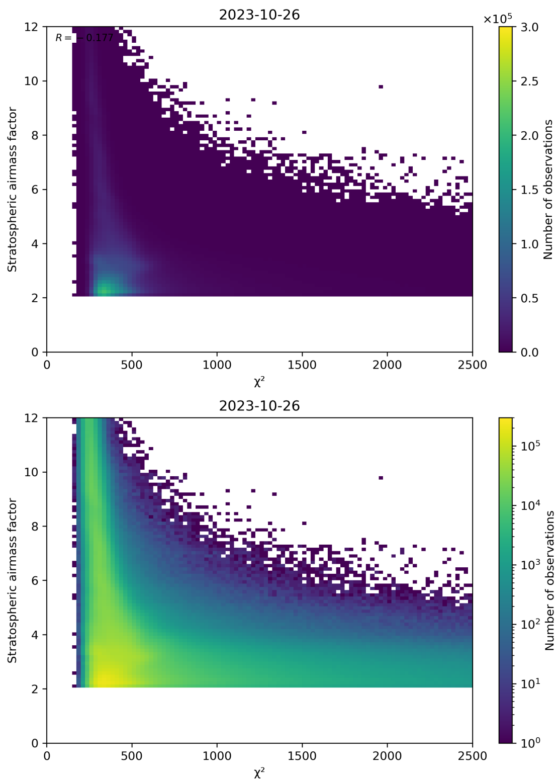
Figure 81: Scatter density plot of “ \chi^2 ” against “Stratospheric airmass factor” for 2023-10-25 to 2023-10-27.
