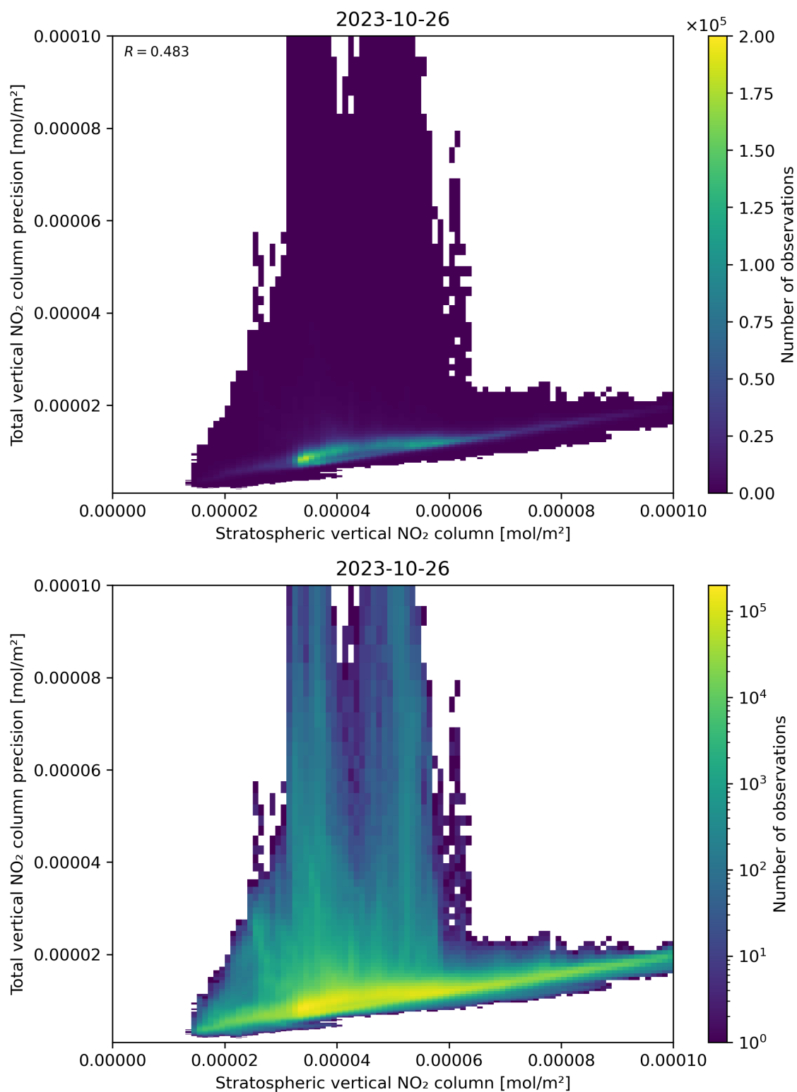
Figure 101: Scatter density plot of “Stratospheric vertical NO 2 column” against “Total vertical NO 2 column precision” for 2023-10-25 to 2023-10-27.
