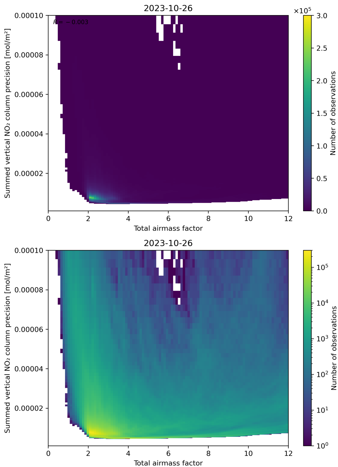
Figure 66: Scatter density plot of “Total airmass factor” against “Summed vertical NO 2 column precision” for 2023-10-25 to 2023-10-27.
