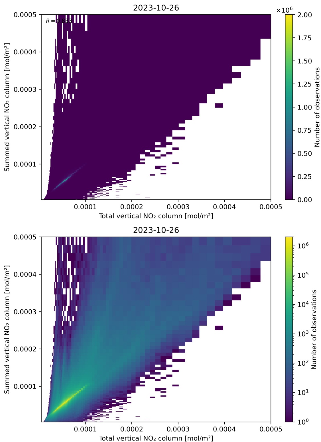
Figure 112: Scatter density plot of “Total vertical NO 2 column” against “Summed vertical NO 2 column” for 2023-10-25 to 2023-10-27.
