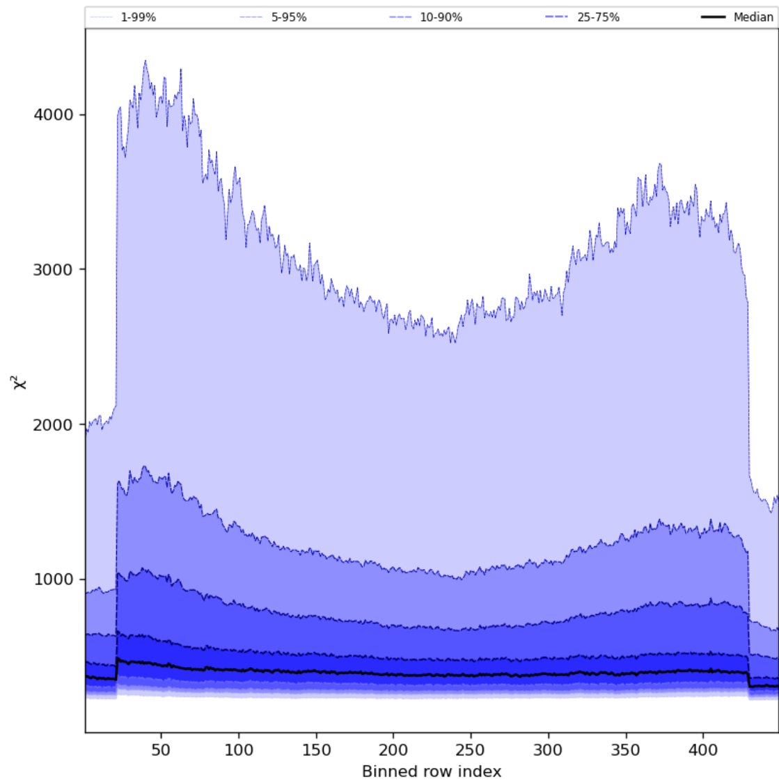
Figure 59: Along track statistics of “ \chi^2 ” for 2023-10-25 to 2023-10-27
