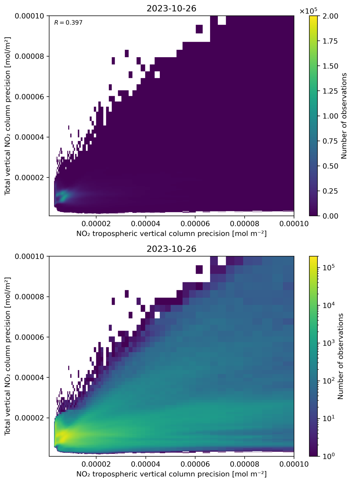
Figure 139: Scatter density plot of “NO 2 tropospheric vertical column precision” against “Total vertical NO 2 column precision” for 2023-10-25 to 2023-10-27.
