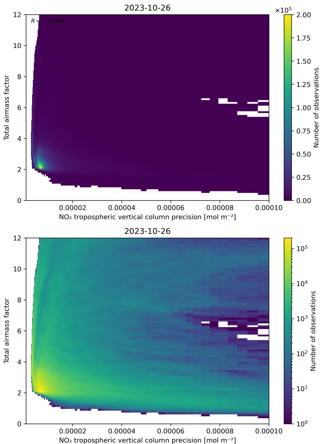
Figure 132: Scatter density plot of “NO 2 tropospheric vertical column precision” against “Total air mass factor” for 2023-10-25 to 2023-10-27.
