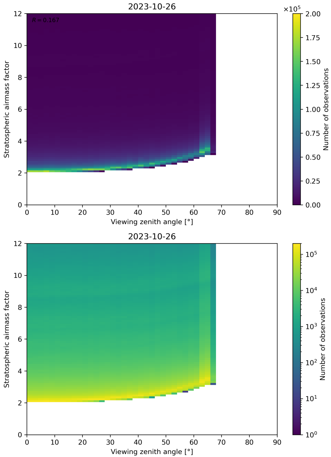
Figure 159: Scatter density plot of “Viewing zenith angle” against “Stratospheric airmass factor” for 2023-10-25 to 2023-10-27.
