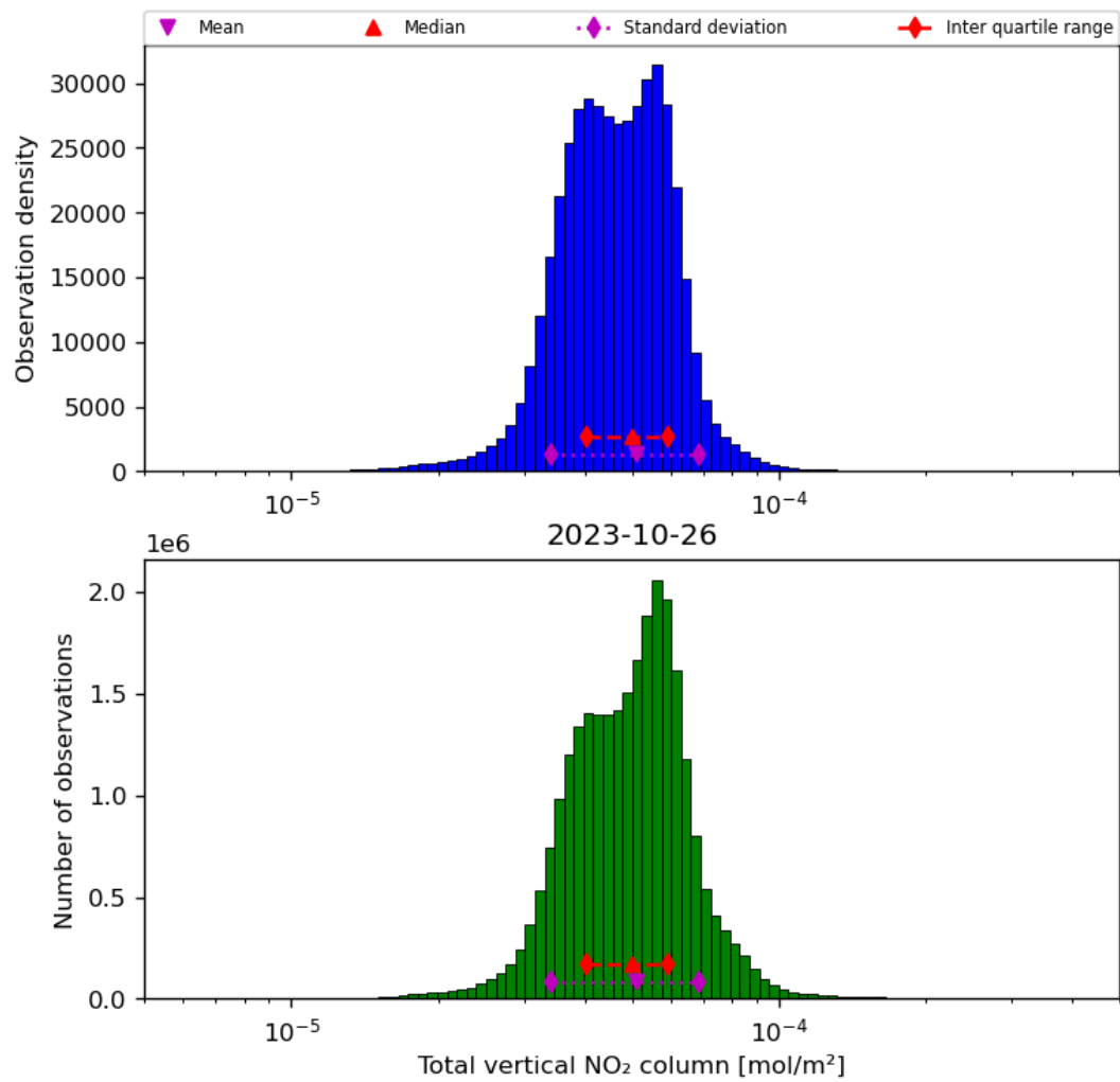
Figure 38: Histogram of “Total vertical NO 2 column” for 2023-10-25 to 2023-10-27
