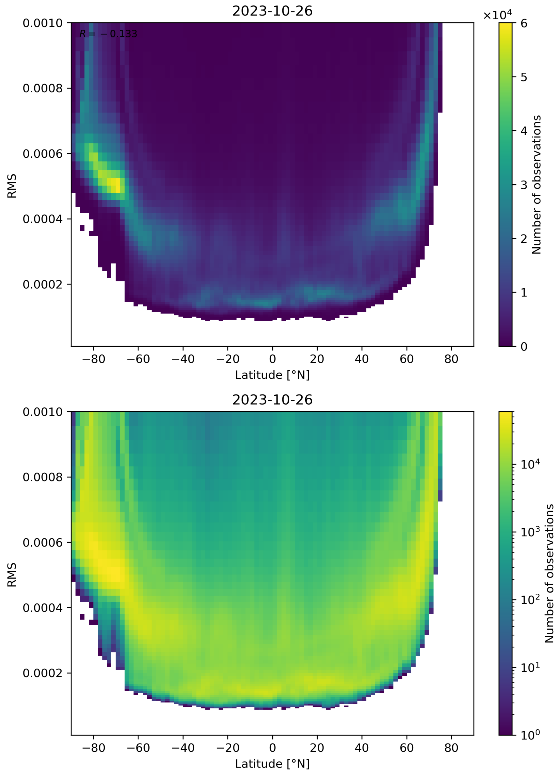
Figure 94: Scatter density plot of “Latitude” against “RMS” for 2023-10-25 to 2023-10-27.
