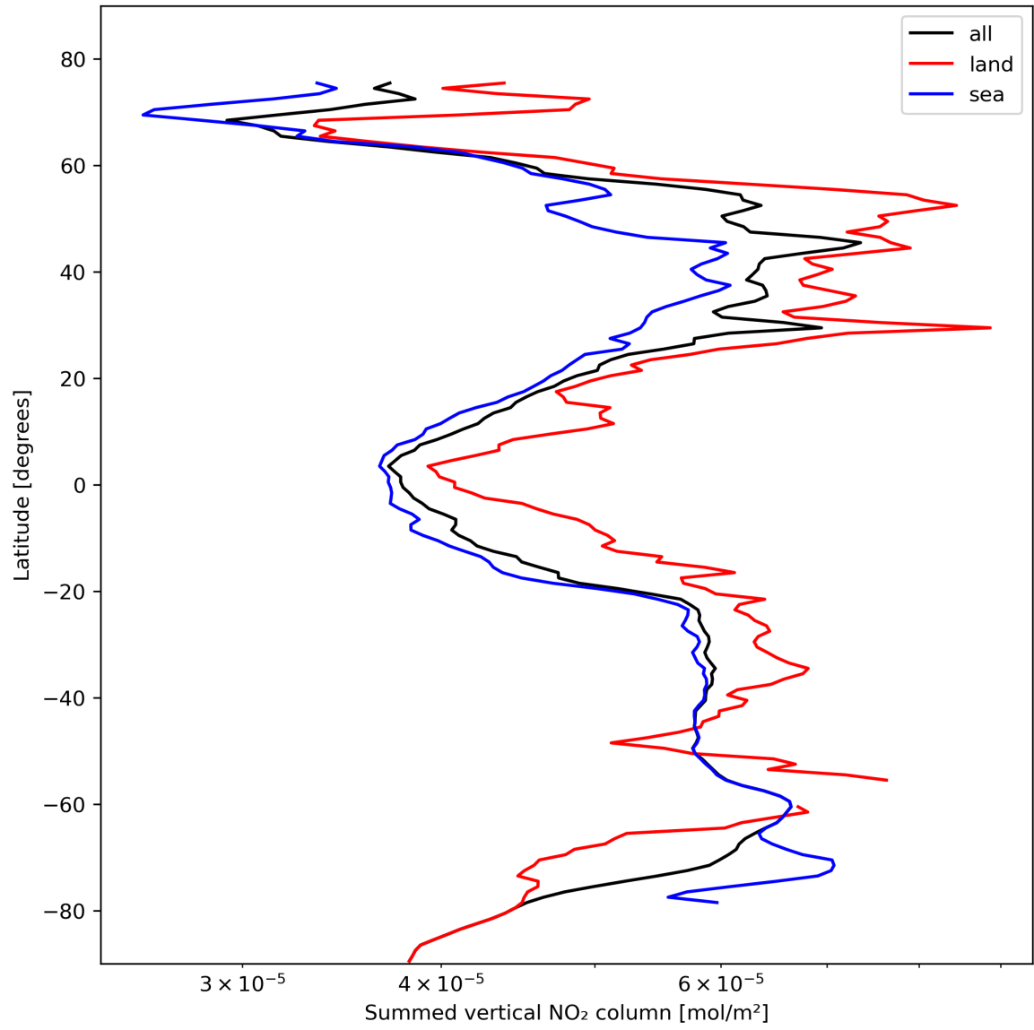
Figure 23: Zonal average of “Summed vertical NO 2 column” for 2023-10-25 to 2023-10-27.
