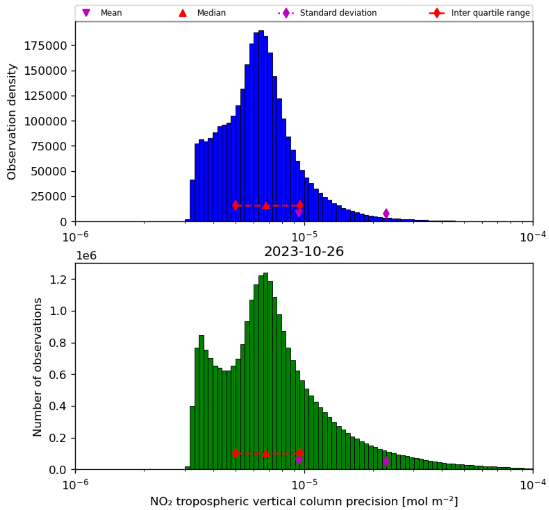
Figure 30: Histogram of “NO 2 tropospheric vertical column precision” for 2023-10-25 to 2023-10-27
