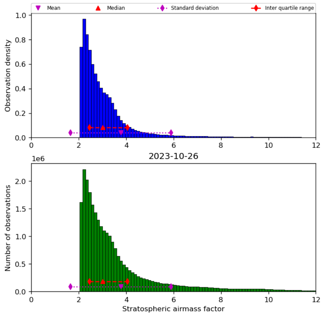
Figure 44: Histogram of “Stratospheric airmass factor” for 2023-10-25 to 2023-10-27
