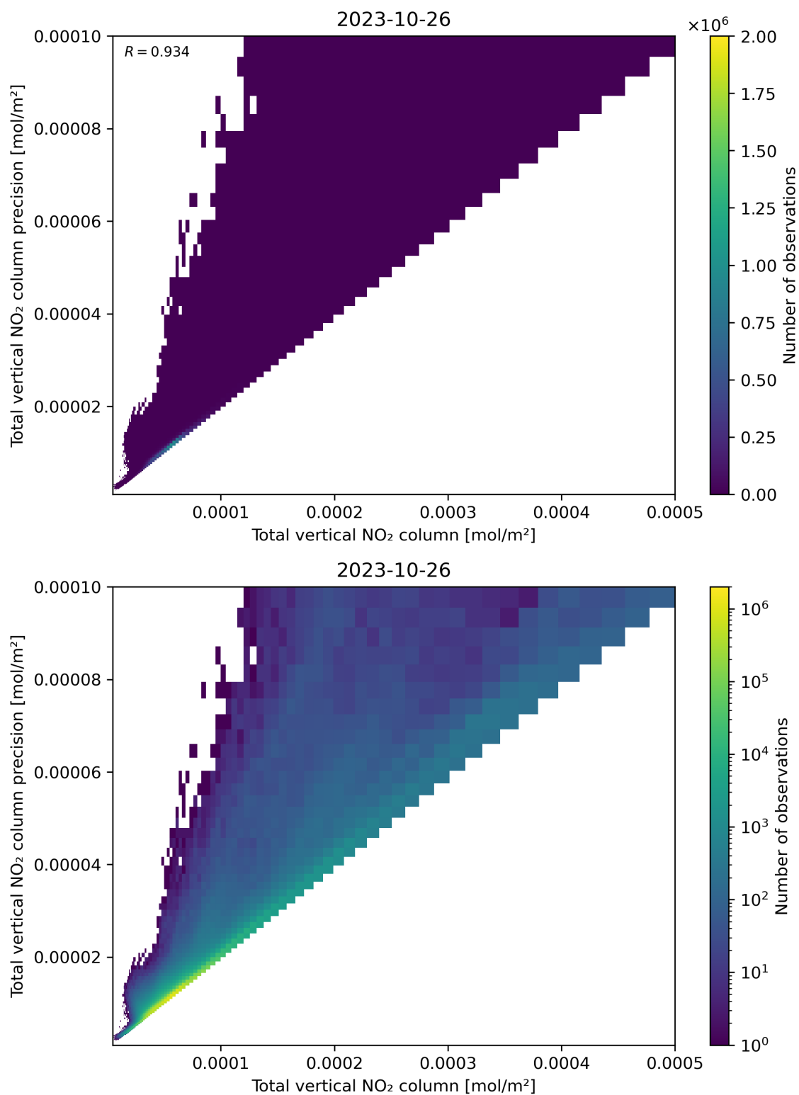
Figure 114: Scatter density plot of “Total vertical NO 2 column” against “Total vertical NO 2 column precision” for 2023-10-25 to 2023-10-27.
