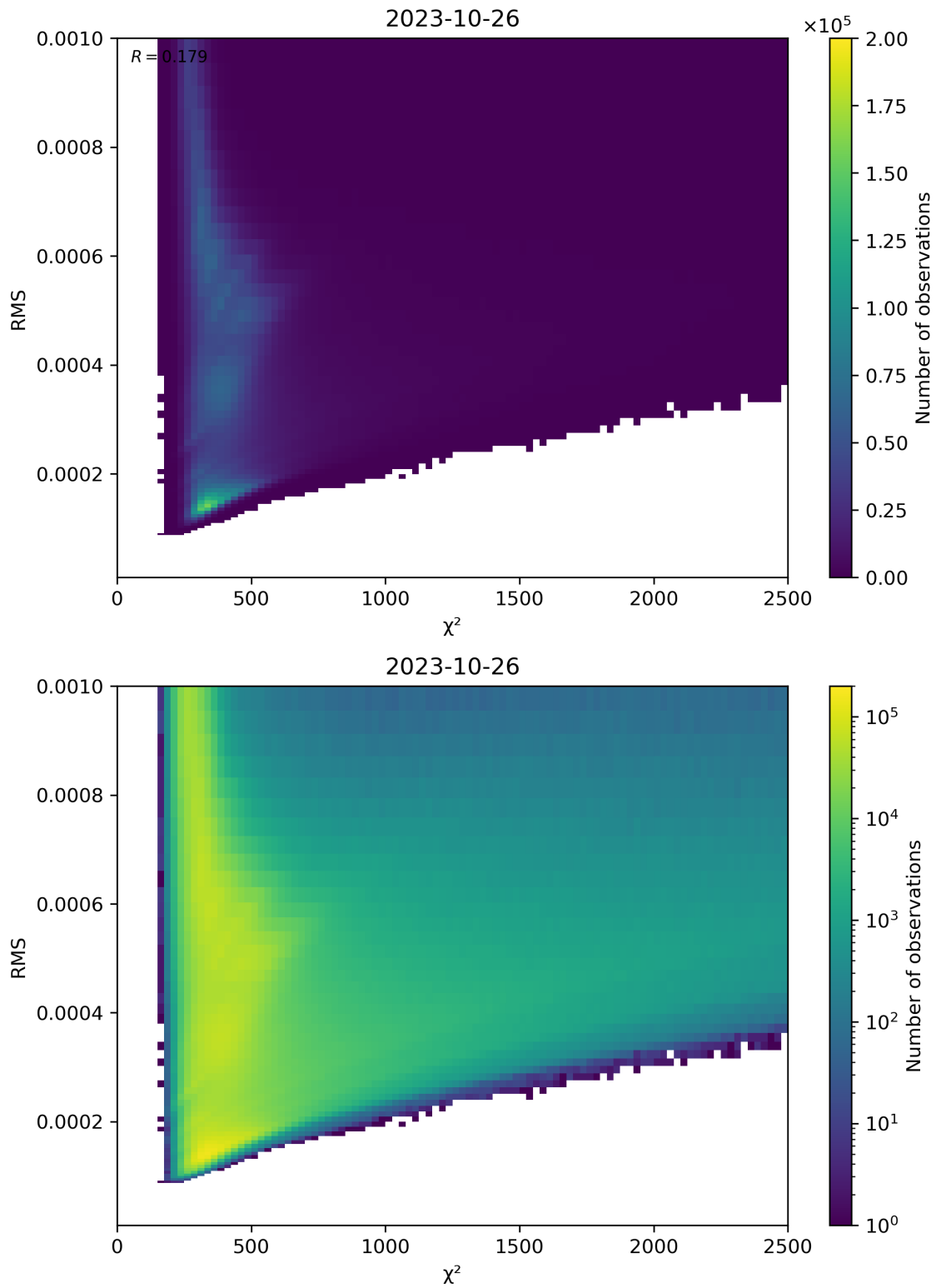
Figure 82: Scatter density plot of “ \chi^2 ” against “RMS” for 2023-10-25 to 2023-10-27.
