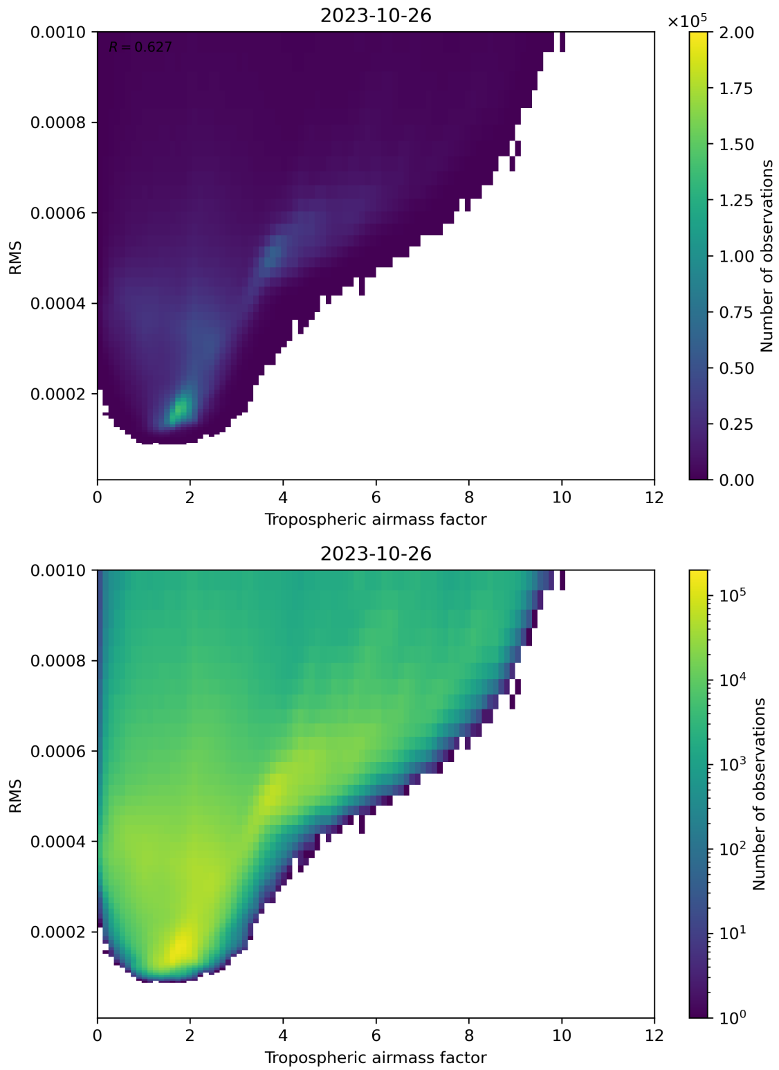
Figure 79: Scatter density plot of “Tropospheric airmass factor” against “RMS” for 2023-10-25 to 2023-10-27.
