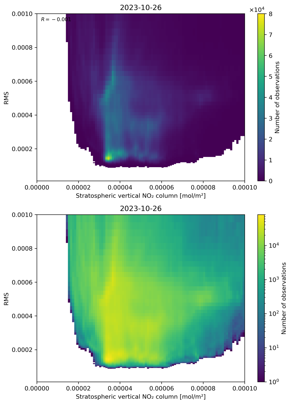
Figure 102: Scatter density plot of “Stratospheric vertical NO 2 column” against “RMS” for 2023-10-25 to 2023-10-27.
