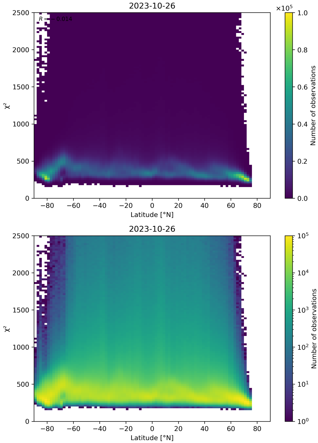
Figure 86: Scatter density plot of “Latitude” against “ \chi^2 ” for 2023-10-25 to 2023-10-27.
