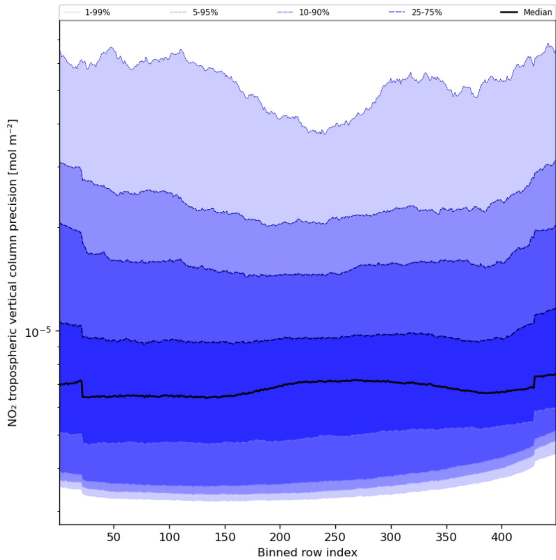
Figure 47: Along track statistics of “NO 2 tropospheric vertical column precision” for 2023-10-25 to 2023-10-27
