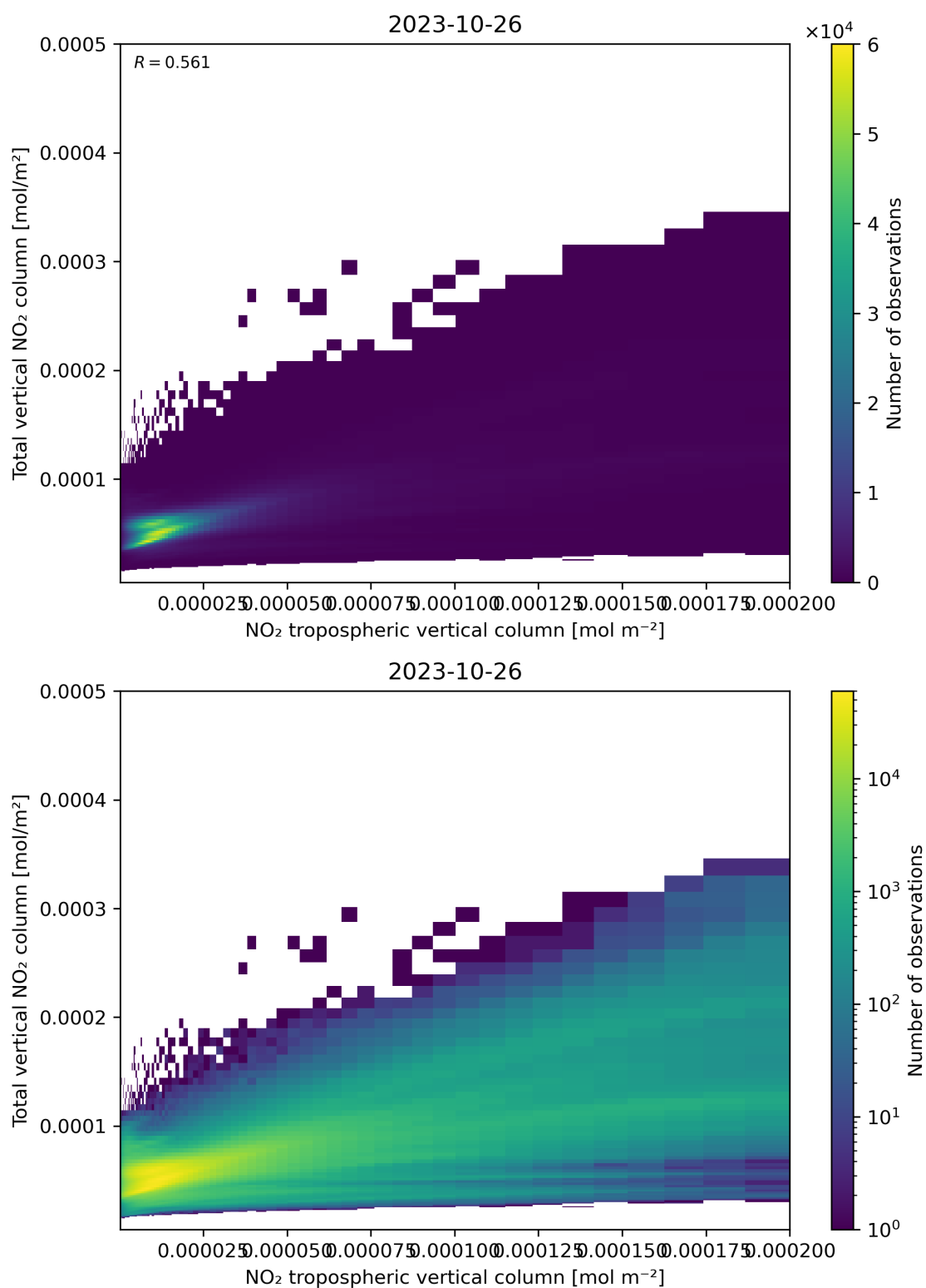
Figure 128: Scatter density plot of “NO 2 tropospheric vertical column” against “Total vertical NO 2 column” for 2023-10-25 to 2023-10-27.
