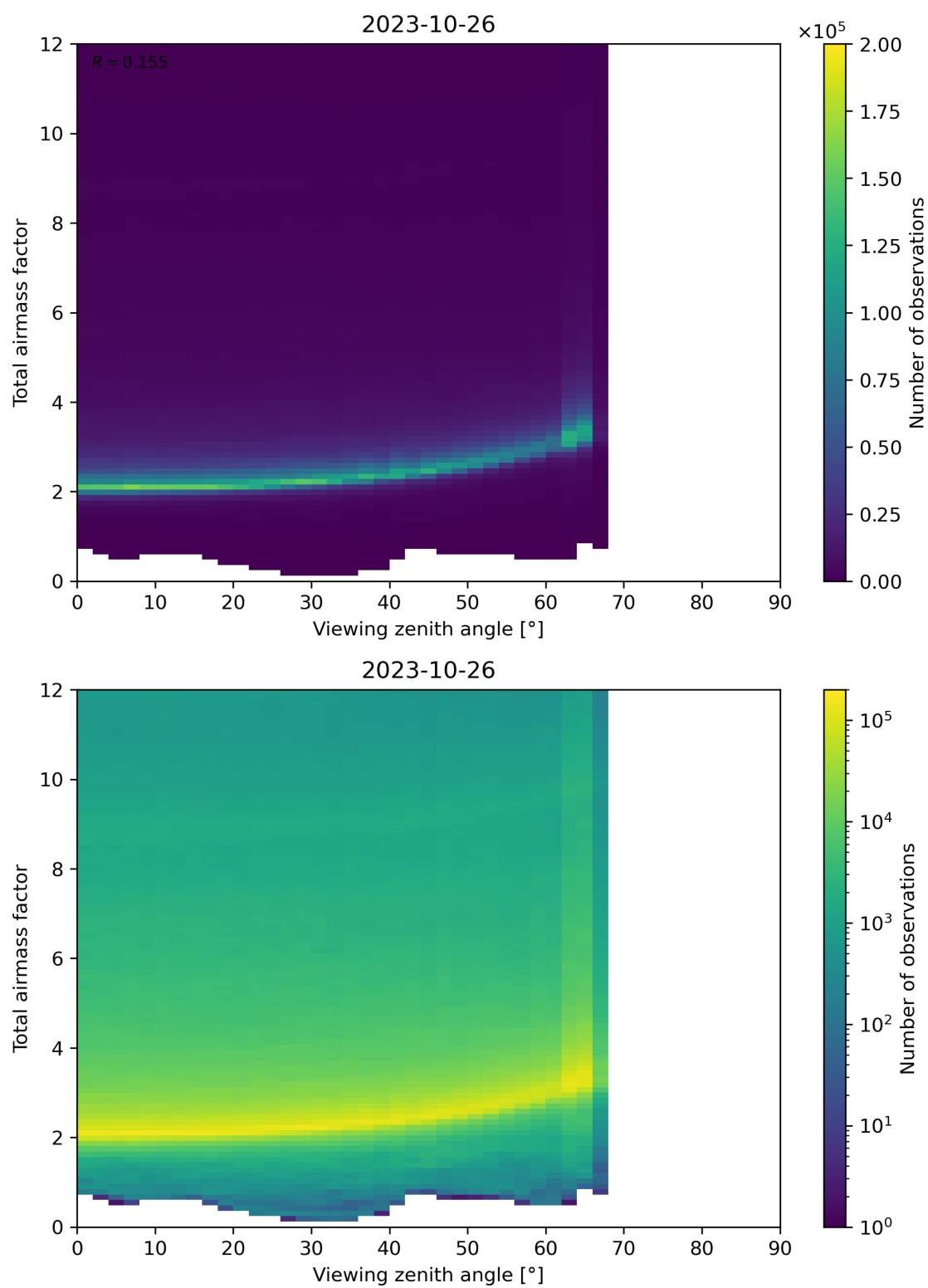
Figure 160: Scatter density plot of “Viewing zenith angle” against “Total airmass factor” for 2023-10-25 to 2023-10-27.
