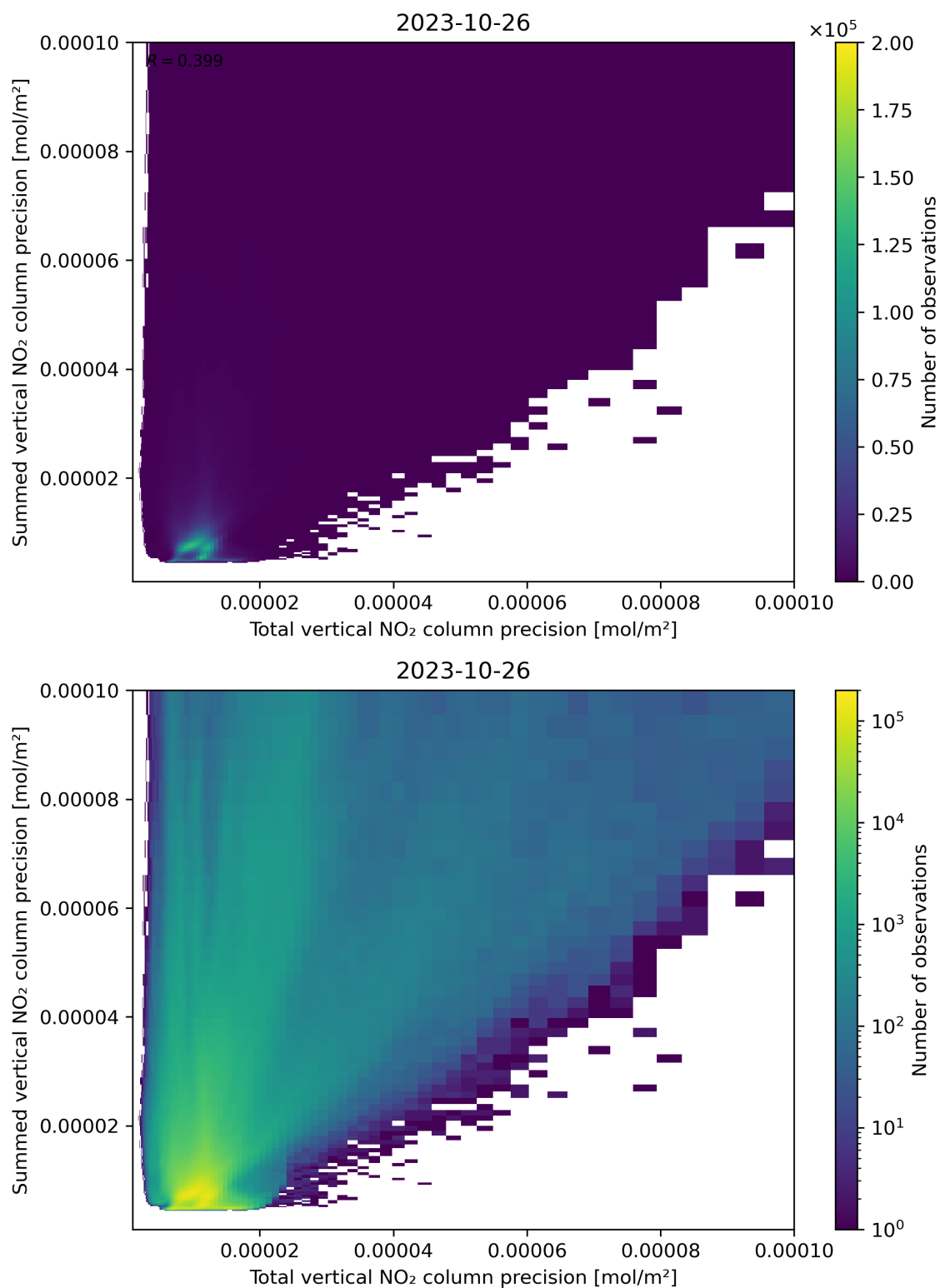
Figure 118: Scatter density plot of “Total vertical NO 2 column precision” against “Summed vertical NO 2 column precision” for 2023-10-25 to 2023-10-27.
