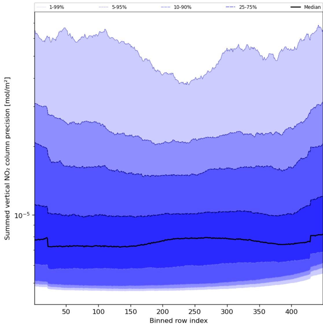
Figure 58: Along track statistics of “Summed vertical NO 2 column precision” for 2023-10-25 to 2023-10-27
