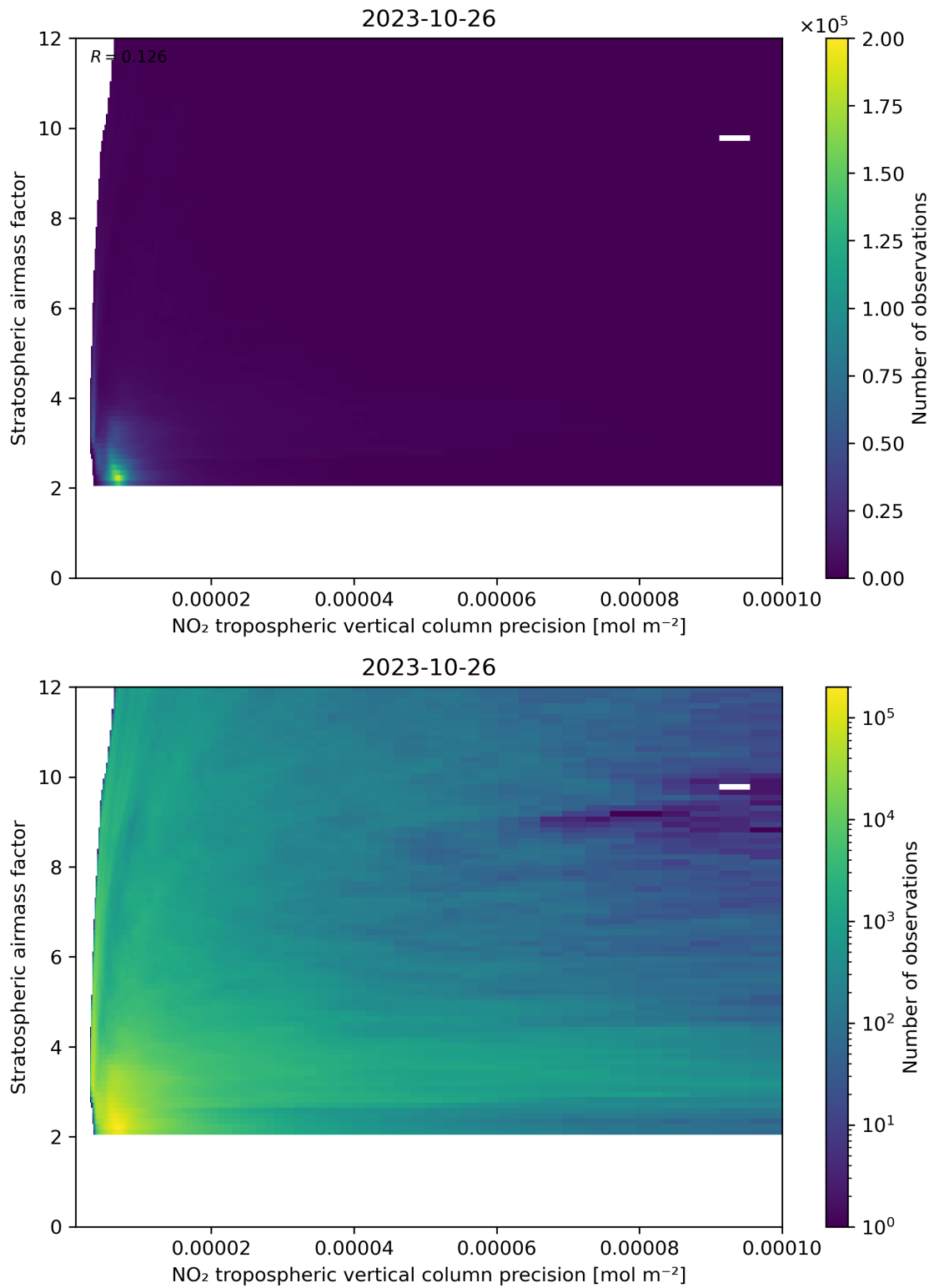
Figure 131: Scatter density plot of “NO 2 tropospheric vertical column precision” against “Stratospheric airmass factor” for 2023-10-25 to 2023-10-27.
