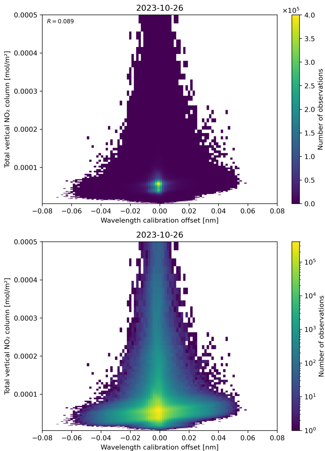
Figure 179: Scatter density plot of “Wavelength calibration offset” against “Total vertical NO 2 column” for 2023-10-25 to 2023-10-27.
