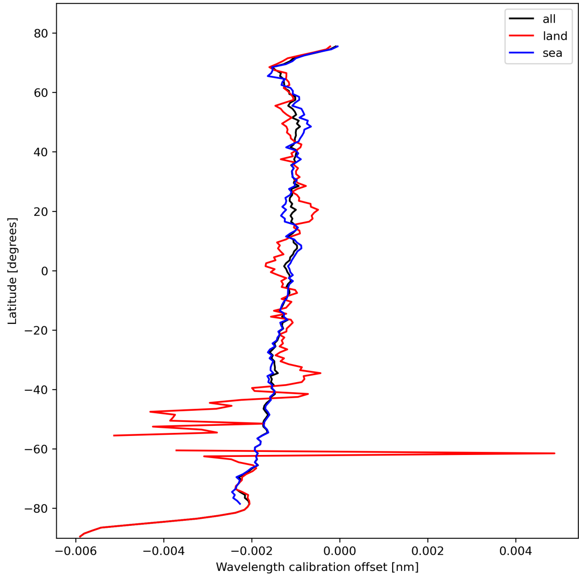
Figure 18: Zonal average of “Wavelength calibration offset” for 2023-10-25 to 2023-10-27.
