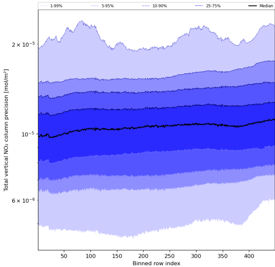
Figure 56: Along track statistics of “Total vertical NO 2 column precision” for 2023-10-25 to 2023-10-27
