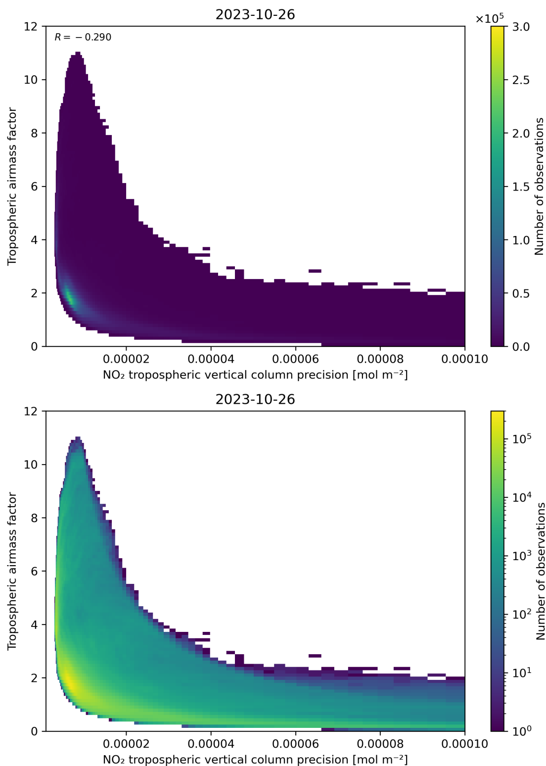
Figure 133: Scatter density plot of “NO 2 tropospheric vertical column precision” against “Tropospheric airmass factor” for 2023-10-25 to 2023-10-27.
