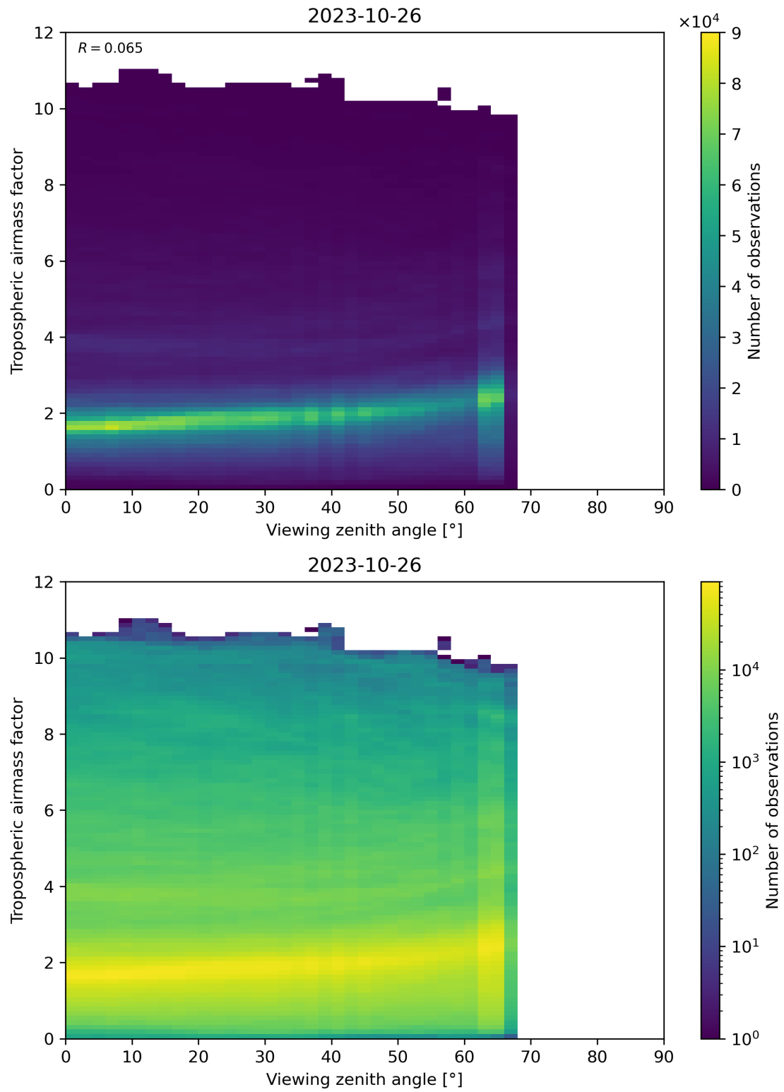
Figure 161: Scatter density plot of “Viewing zenith angle” against “Tropospheric airmass factor” for 2023-10-25 to 2023-10-27.
