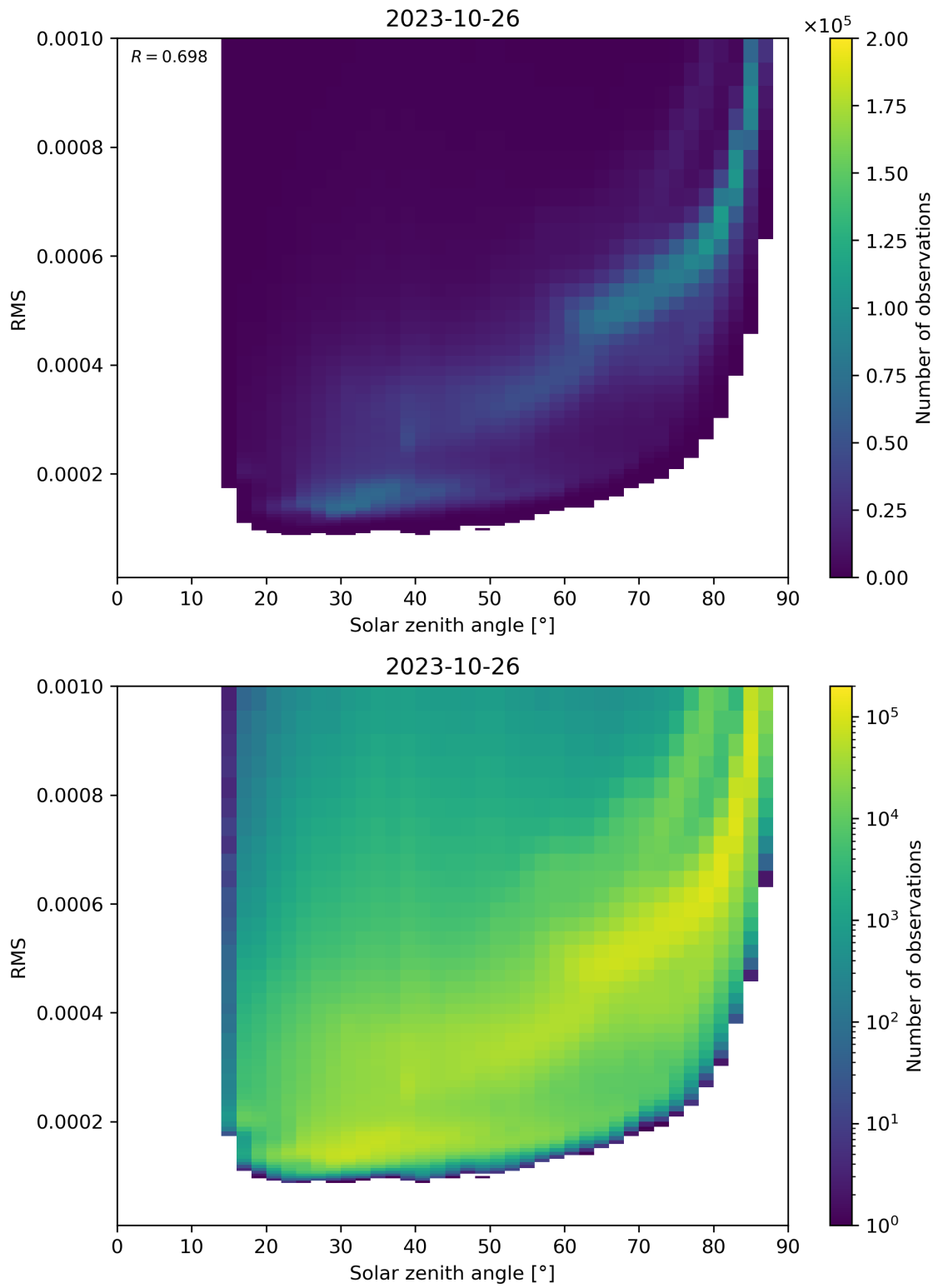
Figure 157: Scatter density plot of “Solar zenith angle” against “RMS” for 2023-10-25 to 2023-10-27.
