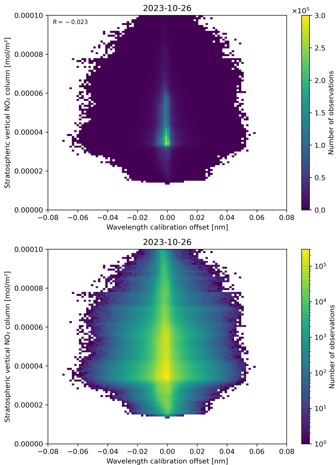
Figure 176: Scatter density plot of “Wavelength calibration offset” against “Stratospheric vertical NO 2 column” for 2023-10-25 to 2023-10-27.
