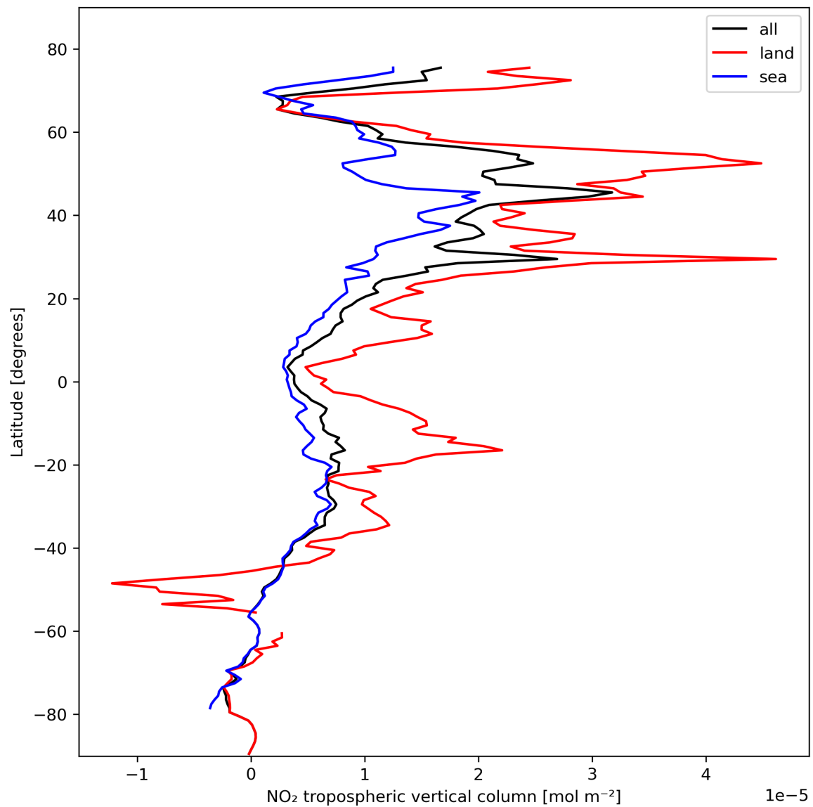
Figure 12: Zonal average of “NO 2 tropospheric vertical column” for 2023-10-25 to 2023-10-27.
