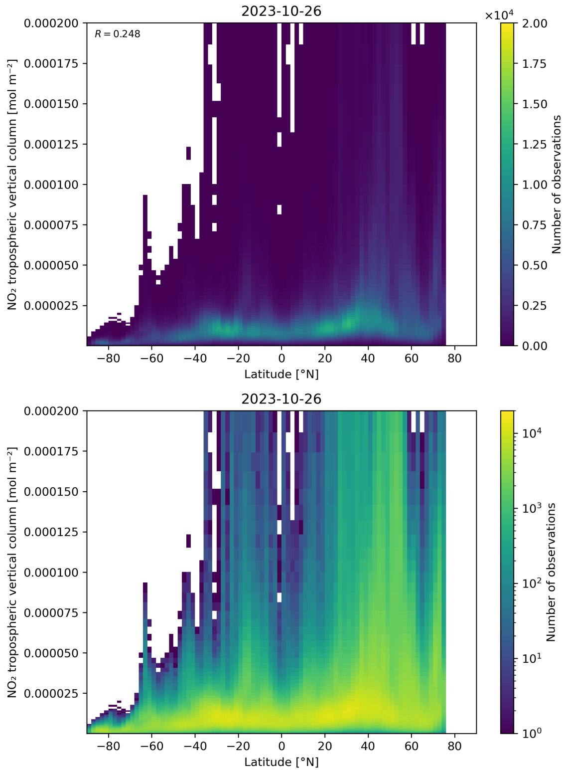
Figure 92: Scatter density plot of “Latitude” against “NO 2 tropospheric vertical column” for 2023-10-25 to 2023-10-27.
