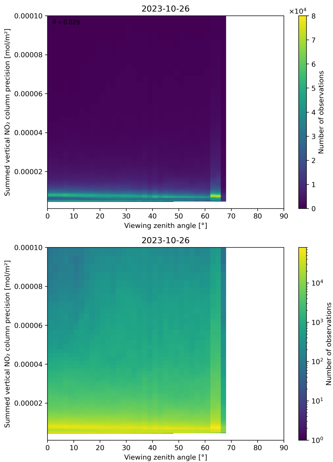
Figure 166: Scatter density plot of “Viewing zenith angle” against “Summed vertical NO 2 column precision” for 2023-10-25 to 2023-10-27.
