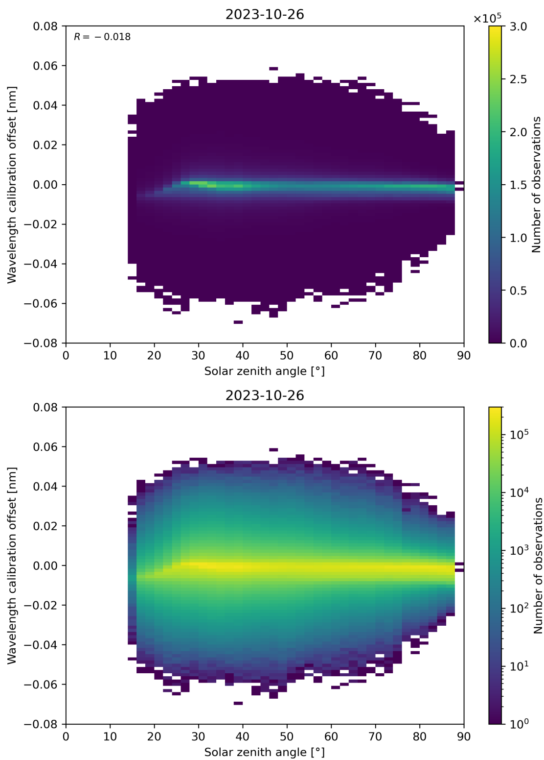
Figure 158: Scatter density plot of “Solar zenith angle” against “Wavelength calibration offset” for 2023-10-25 to 2023-10-27.
