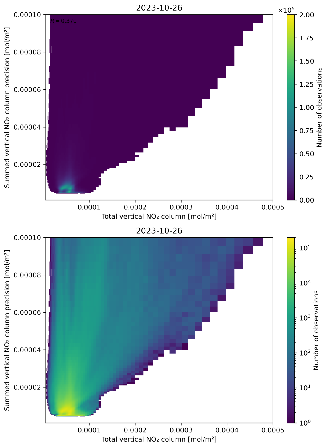
Figure 113: Scatter density plot of “Total vertical NO 2 column” against “Summed vertical NO 2 column precision” for 2023-10-25 to 2023-10-27.
