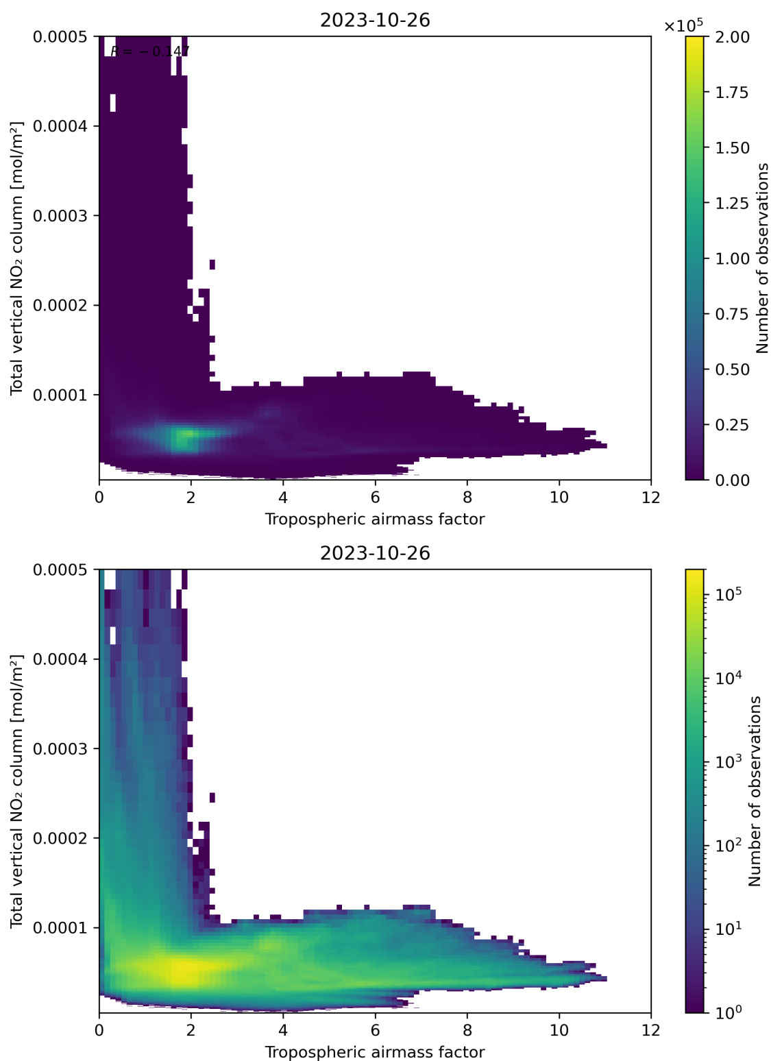
Figure 77: Scatter density plot of “Tropospheric airmass factor” against “Total vertical NO 2 column” for 2023-10-25 to 2023-10-27.
