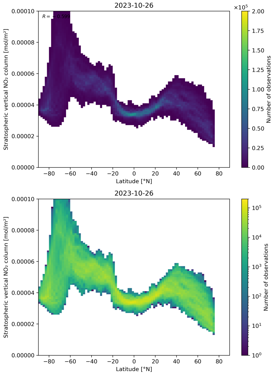
Figure 87: Scatter density plot of “Latitude” against “Stratospheric vertical NO 2 column” for 2023-10-25 to 2023-10-27.
