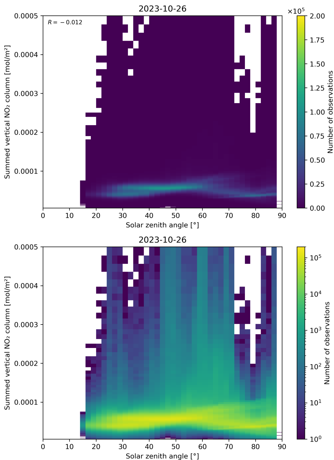
Figure 151: Scatter density plot of “Solar zenith angle” against “Summed vertical NO 2 column” for 2023-10-25 to 2023-10-27.
