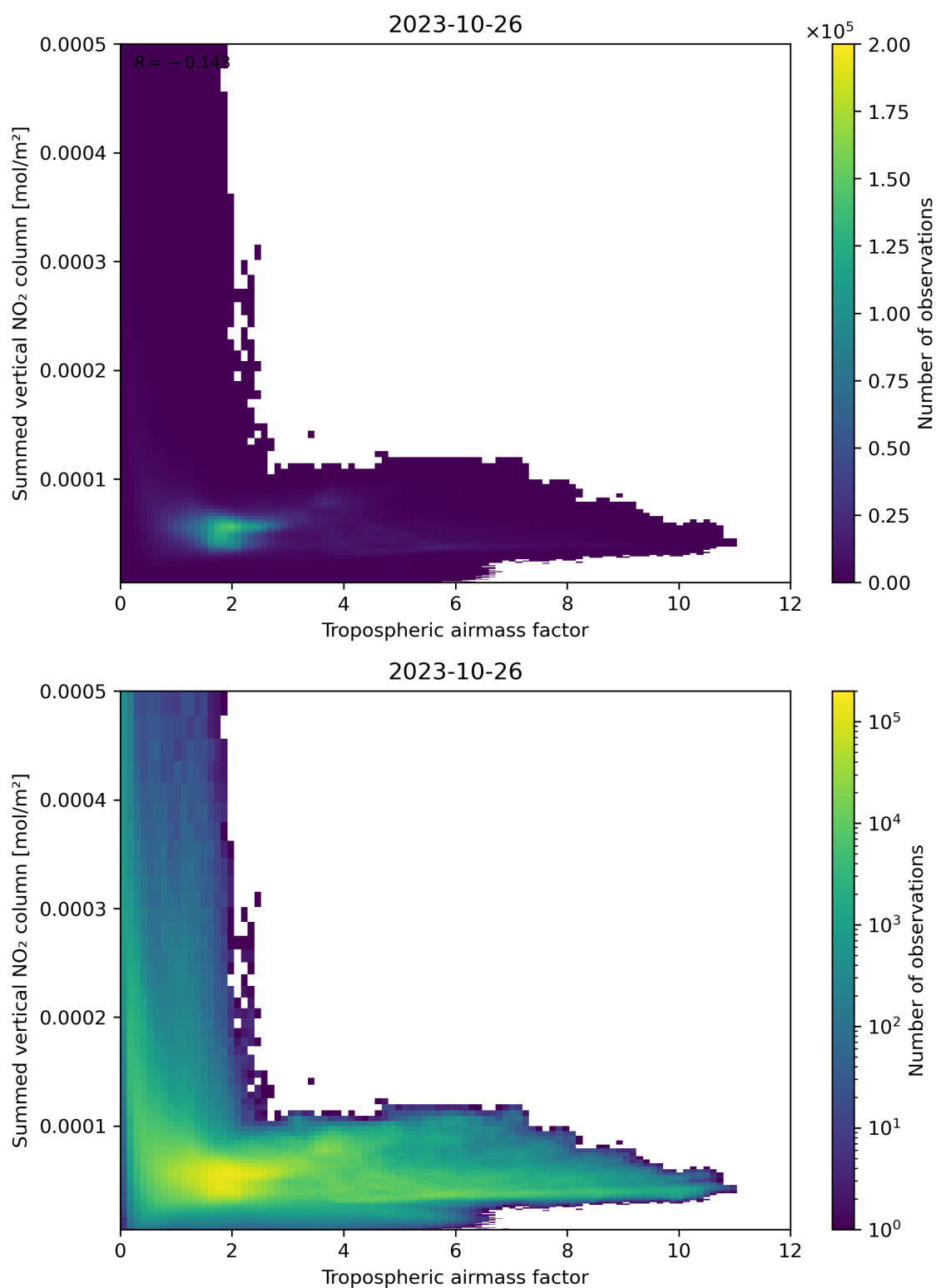
Figure 75: Scatter density plot of “Tropospheric airmass factor” against “Summed vertical NO 2 column” for 2023-10-25 to 2023-10-27.
