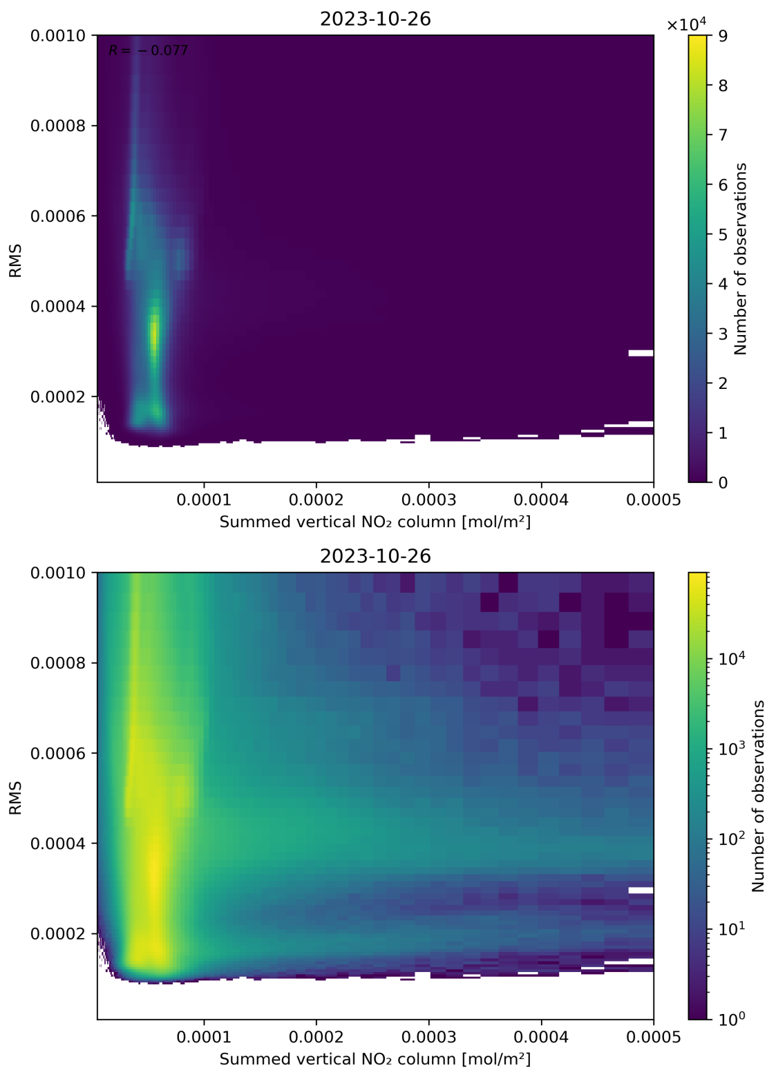
Figure 109: Scatter density plot of “Summed vertical NO 2 column” against “RMS” for 2023-10-25 to 2023-10-27.
