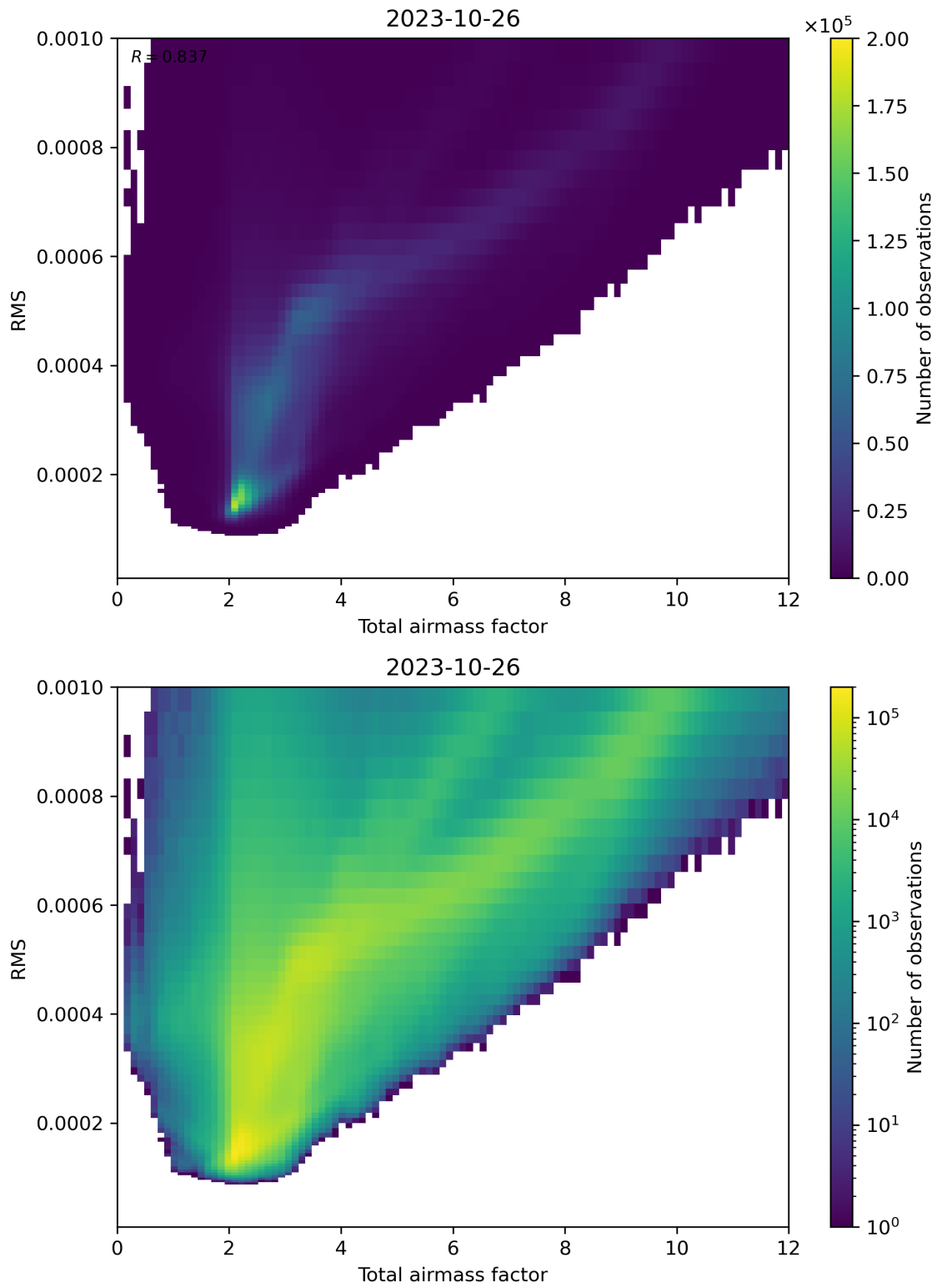
Figure 69: Scatter density plot of “Total airmass factor” against “RMS” for 2023-10-25 to 2023-10-27.
