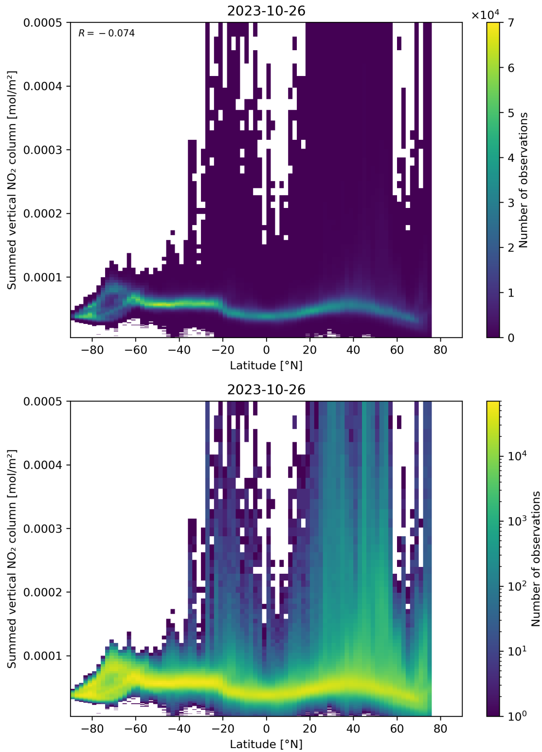
Figure 88: Scatter density plot of “Latitude” against “Summed vertical NO 2 column” for 2023-10-25 to 2023-10-27.
