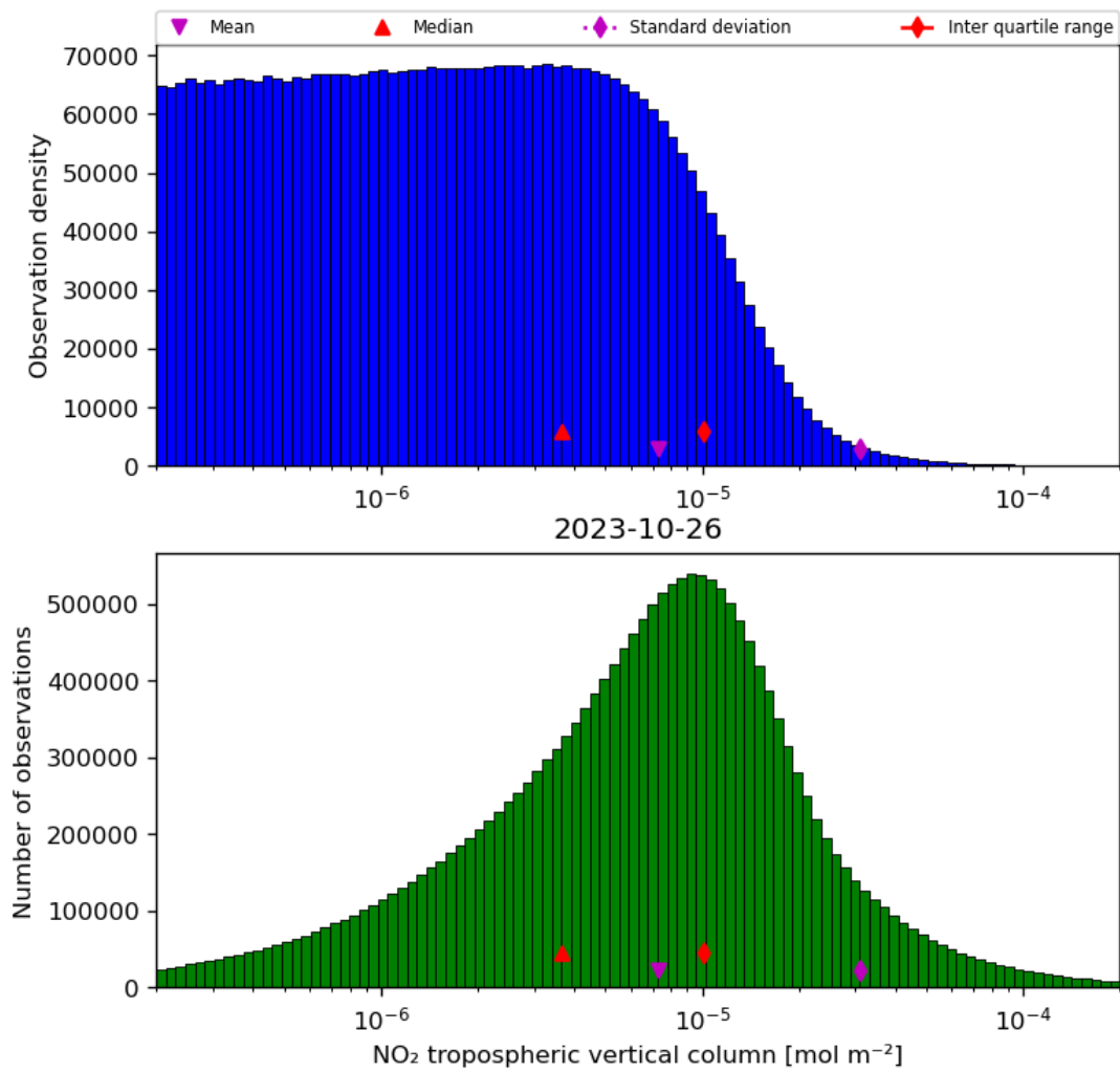
Figure 29: Histogram of “NO 2 tropospheric vertical column” for 2023-10-25 to 2023-10-27
