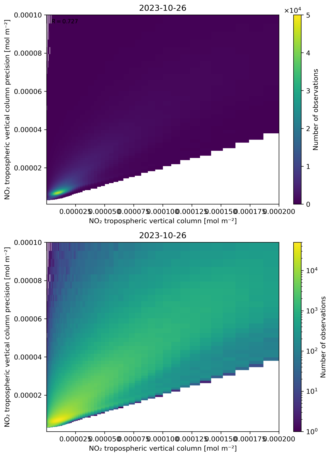
Figure 130: Scatter density plot of “NO 2 tropospheric vertical column” against “NO 2 tropospheric vertical column precision” for 2023-10-25 to 2023-10-27.
