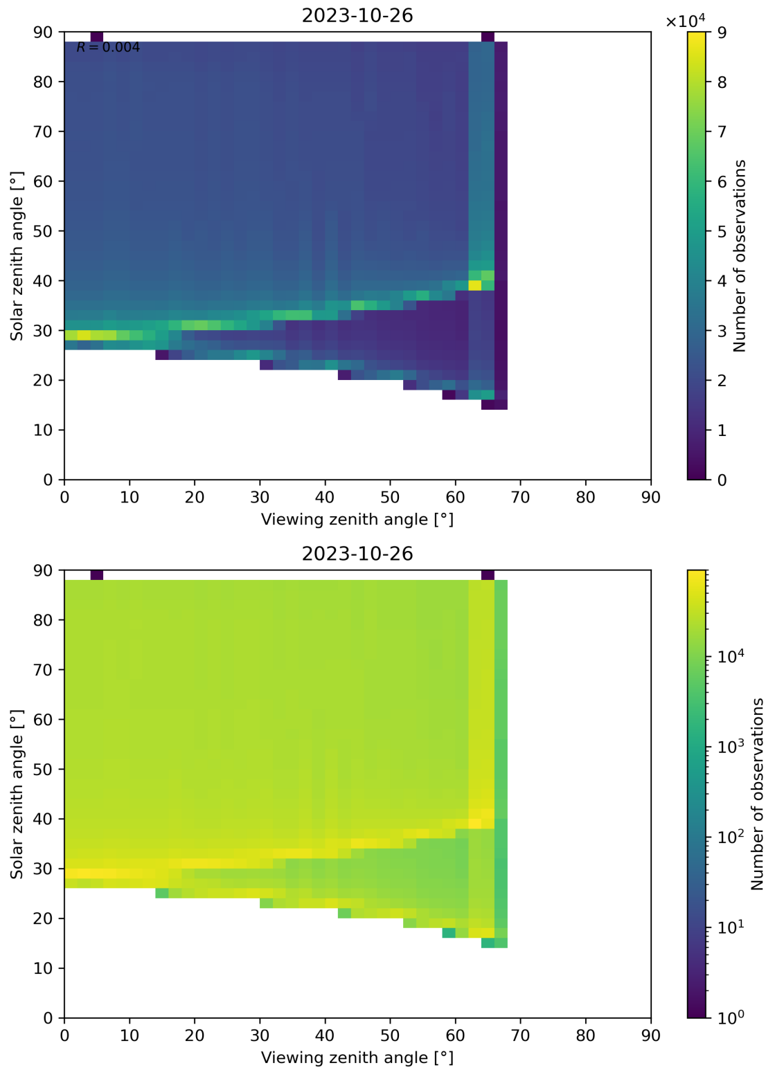
Figure 172: Scatter density plot of “Viewing zenith angle” against “Solar zenith angle” for 2023-10-25 to 2023-10-27.
