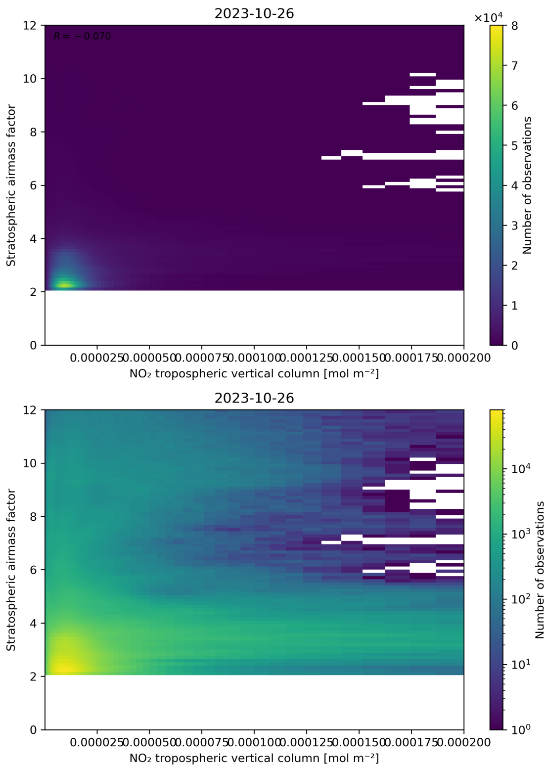
Figure 121: Scatter density plot of “NO 2 tropospheric vertical column” against “Stratospheric air mass factor” for 2023-10-25 to 2023-10-27.
