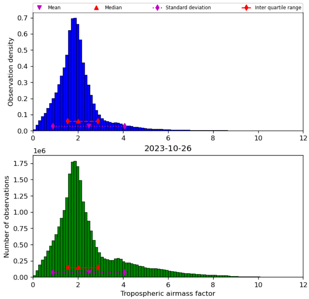
Figure 31: Histogram of “Tropospheric airmass factor” for 2023-10-25 to 2023-10-27
