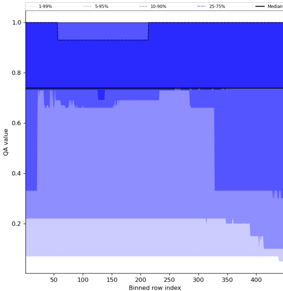
Figure 45: Along track statistics of “QA value” for 2023-10-25 to 2023-10-27
