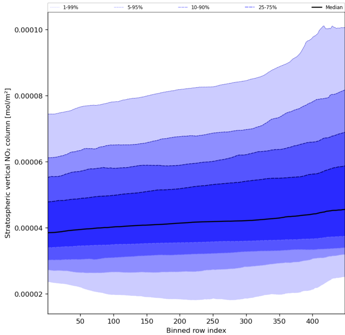
Figure 53: Along track statistics of “Stratospheric vertical NO 2 column” for 2023-10-25 to 2023-10-27
