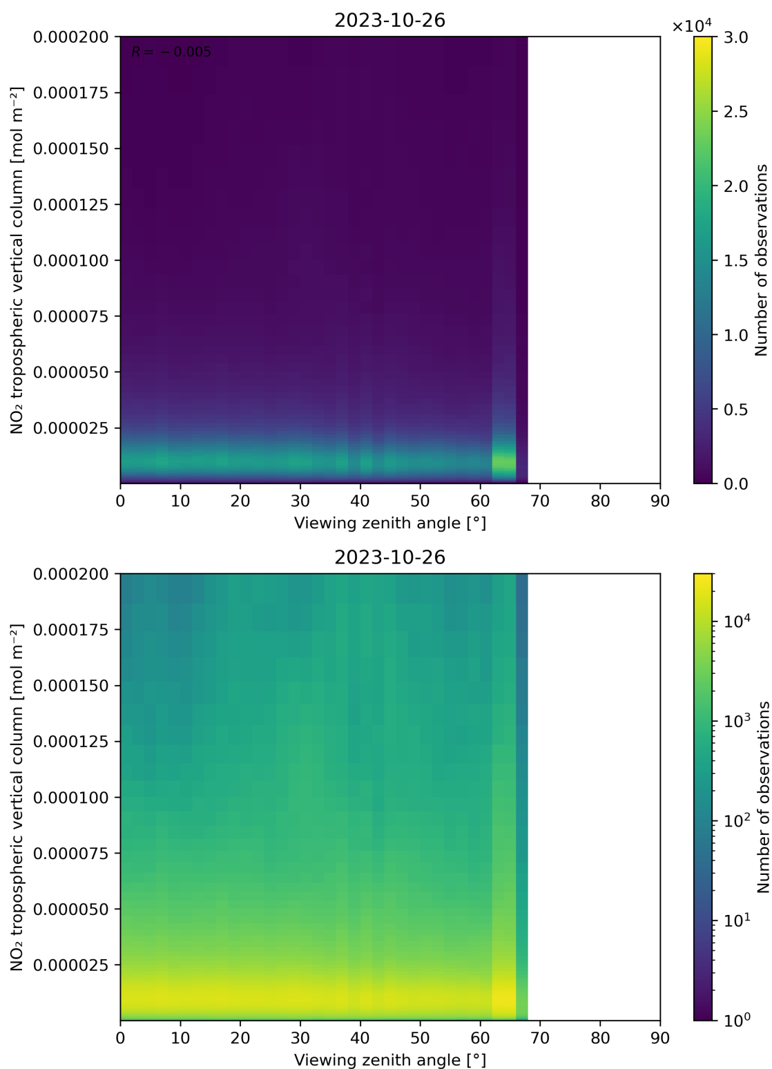
Figure 169: Scatter density plot of “Viewing zenith angle” against “NO 2 tropospheric vertical column” for 2023-10-25 to 2023-10-27.
