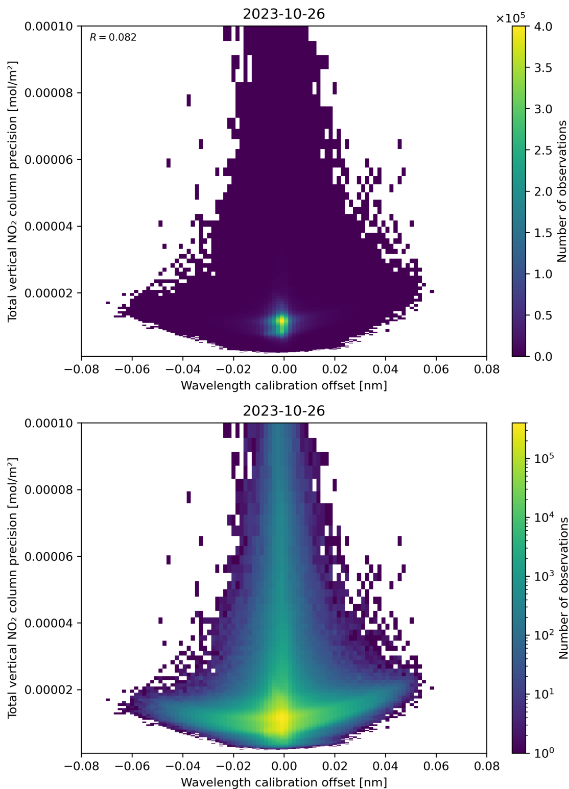
Figure 180: Scatter density plot of “Wavelength calibration offset” against “Total vertical NO 2 column precision” for 2023-10-25 to 2023-10-27.
