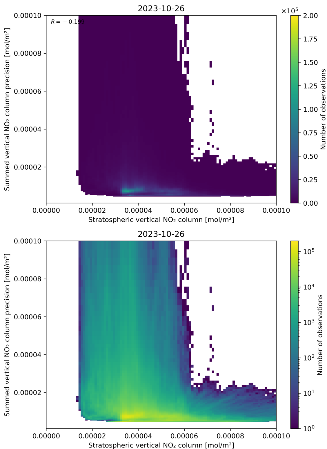
Figure 99: Scatter density plot of “Stratospheric vertical NO 2 column” against “Summed vertical NO 2 column precision” for 2023-10-25 to 2023-10-27.
