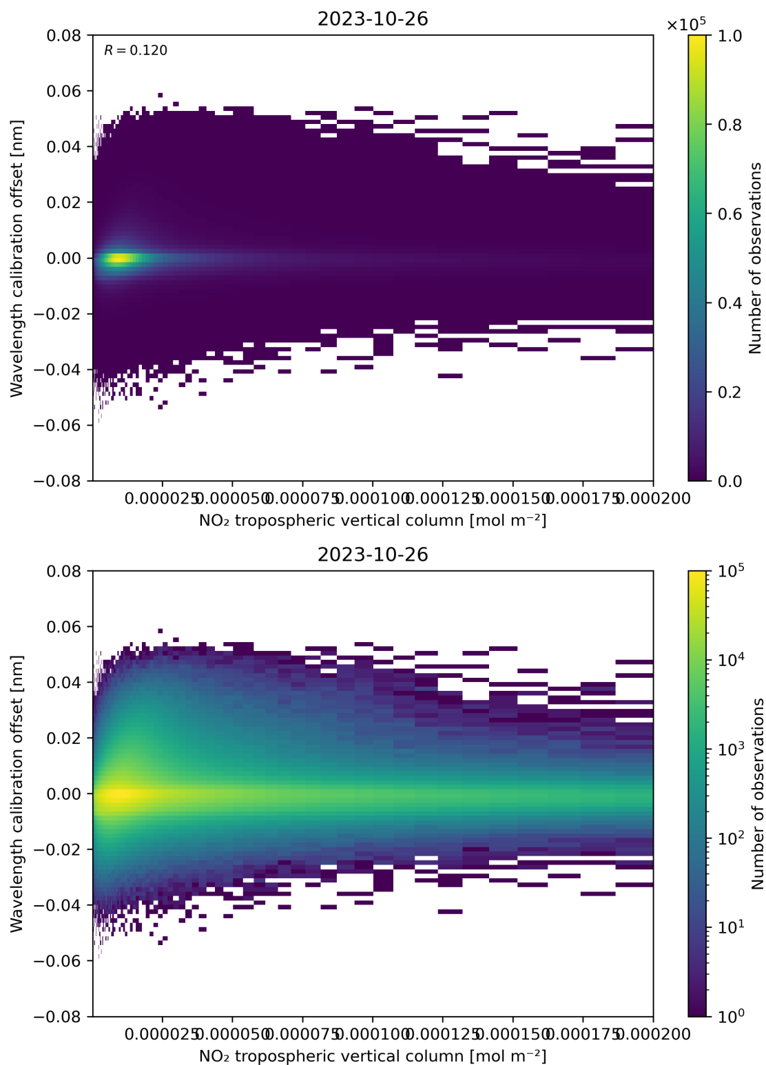
Figure 143: Scatter density plot of “NO 2 tropospheric vertical column” against “Wavelength calibration offset” for 2023-10-25 to 2023-10-27.
