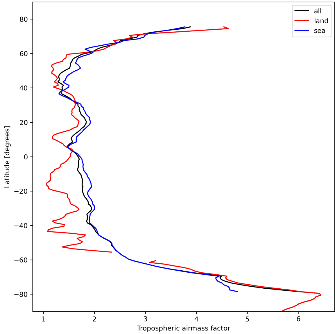
Figure 14: Zonal average of “Tropospheric airmass factor” for 2023-10-25 to 2023-10-27.
