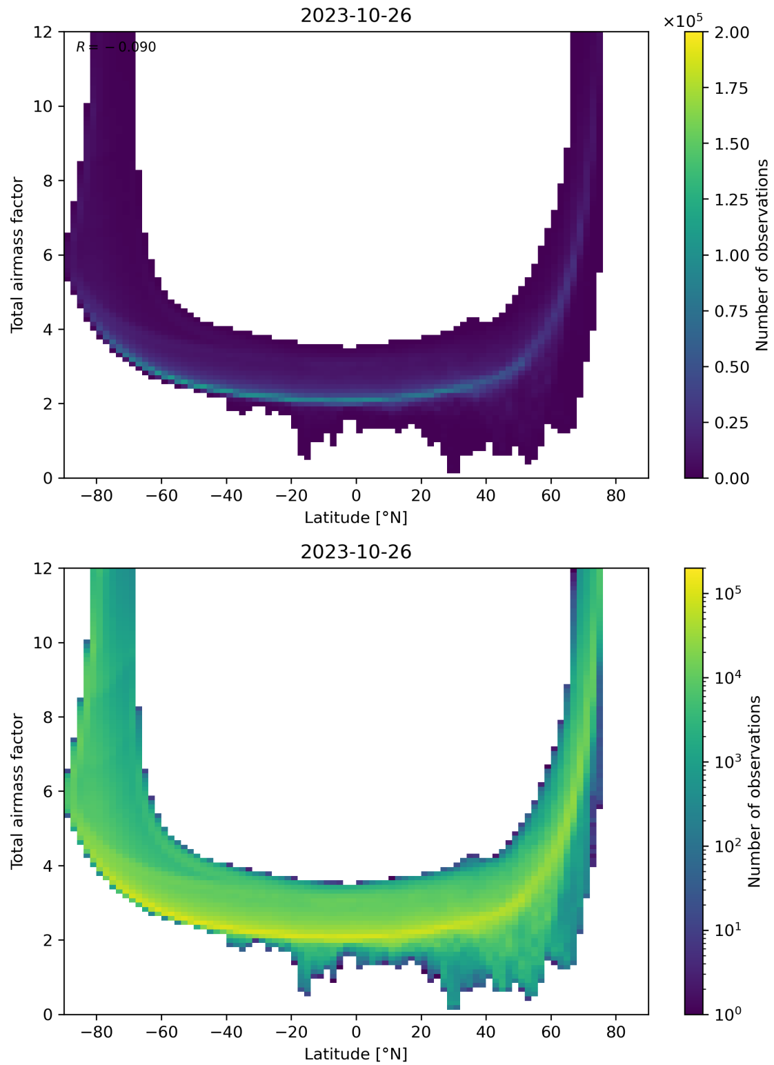
Figure 84: Scatter density plot of “Latitude” against “Total airmass factor” for 2023-10-25 to 2023-10-27.
