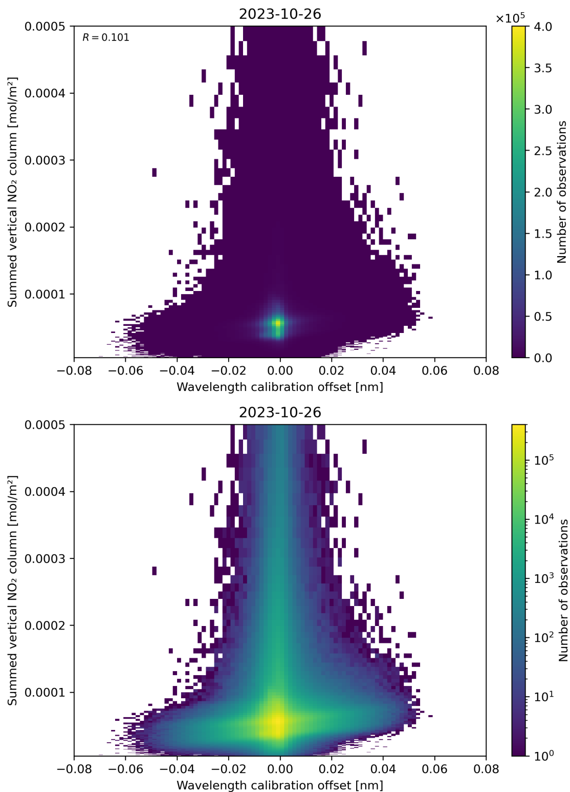
Figure 177: Scatter density plot of “Wavelength calibration offset” against “Summed vertical NO 2 column” for 2023-10-25 to 2023-10-27.
