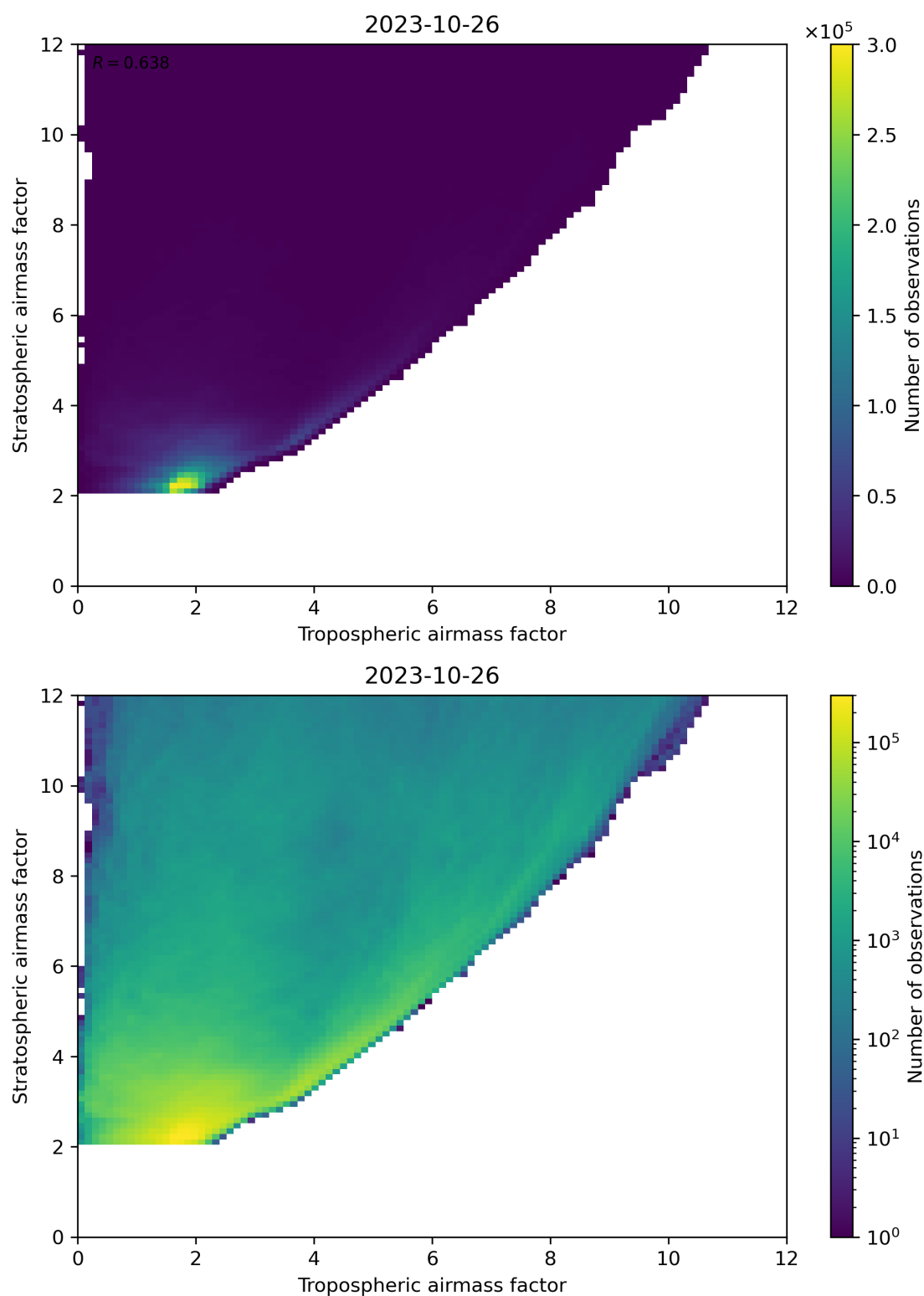
Figure 71: Scatter density plot of “Tropospheric airmass factor” against “Stratospheric airmass factor” for 2023-10-25 to 2023-10-27.
