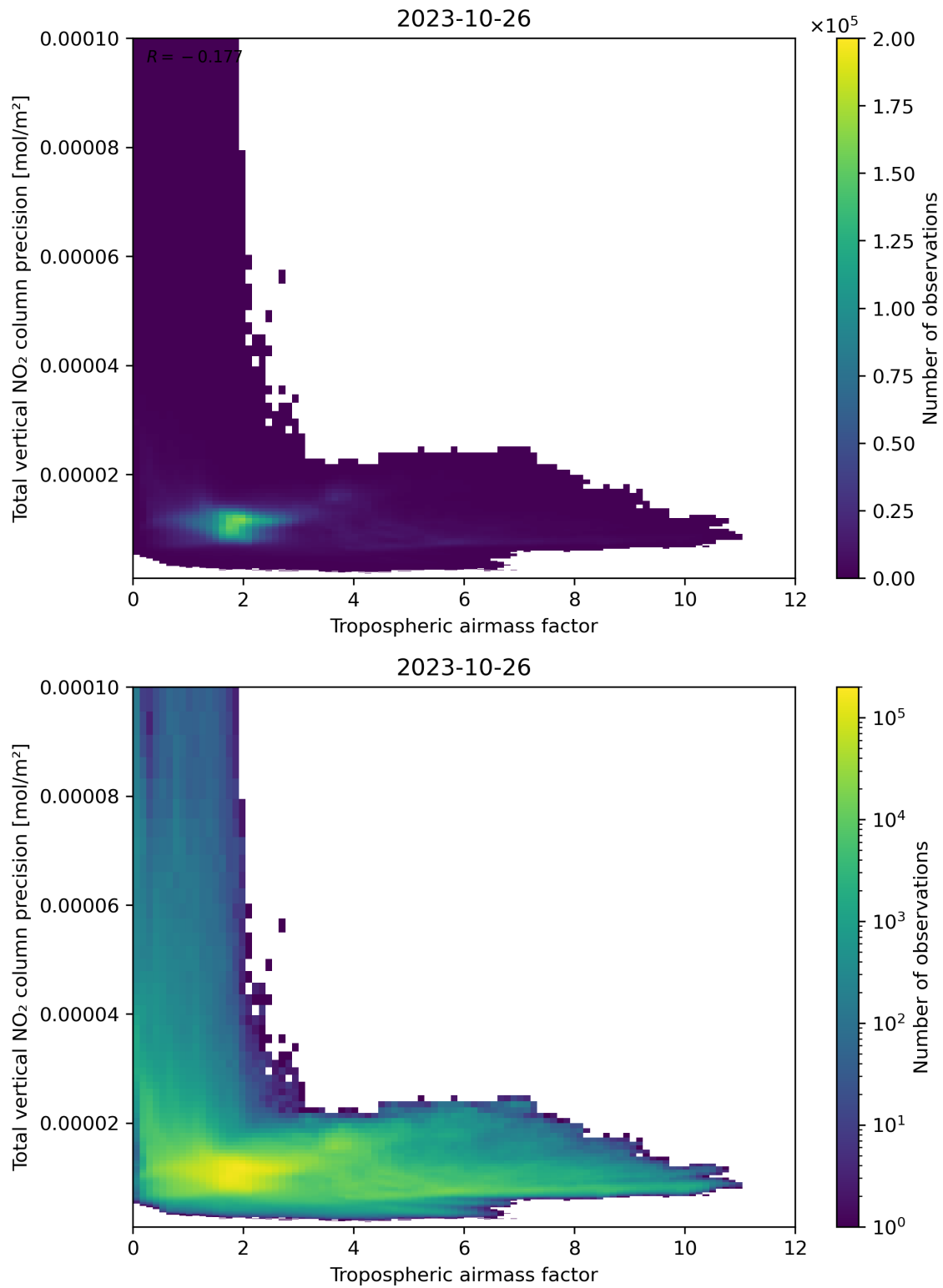
Figure 78: Scatter density plot of “Tropospheric air mass factor” against “Total vertical NO 2 column precision” for 2023-10-25 to 2023-10-27.
