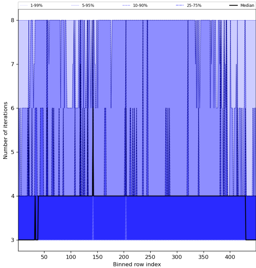
Figure 51: Along track statistics of “Number of iterations” for 2023-10-25 to 2023-10-27
