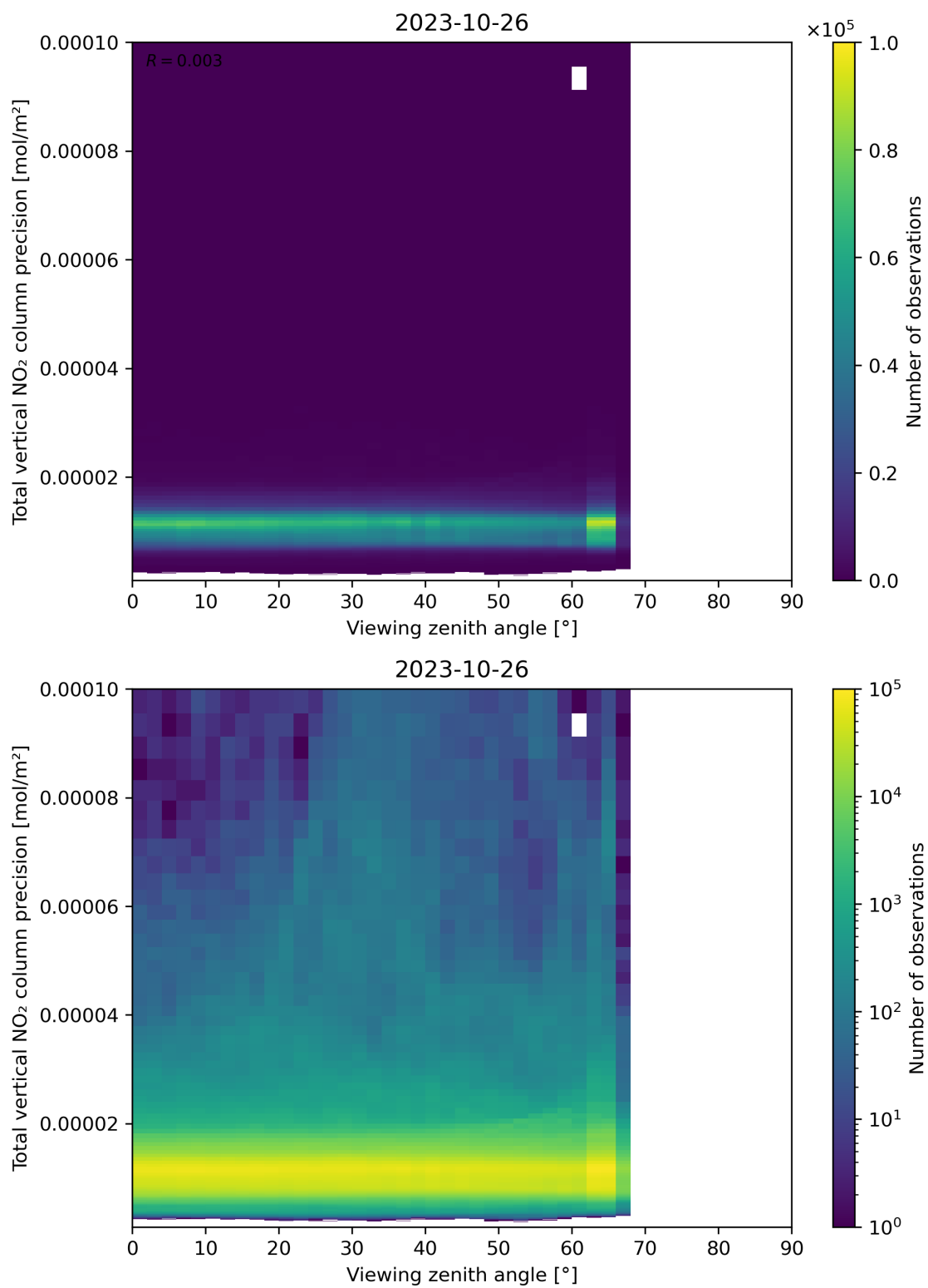
Figure 168: Scatter density plot of “Viewing zenith angle” against “Total vertical NO 2 column precision” for 2023-10-25 to 2023-10-27.
