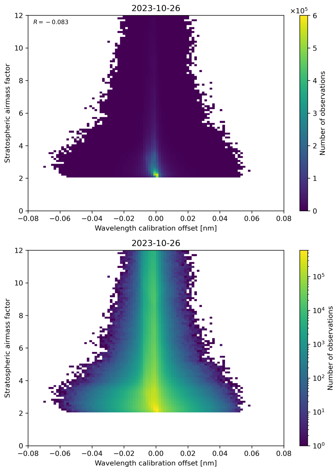
Figure 174: Scatter density plot of “Wavelength calibration offset” against “Stratospheric airmass factor” for 2023-10-25 to 2023-10-27.
