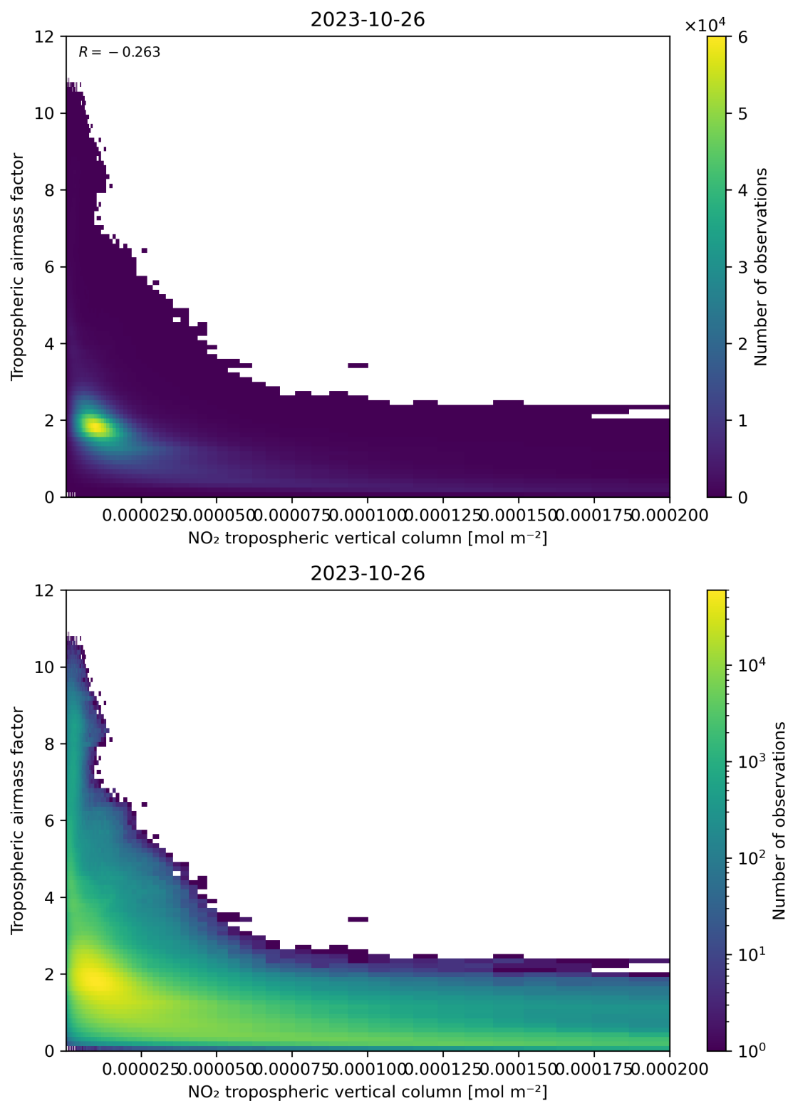
Figure 123: Scatter density plot of “NO 2 tropospheric vertical column” against “Tropospheric air mass factor” for 2023-10-25 to 2023-10-27.
