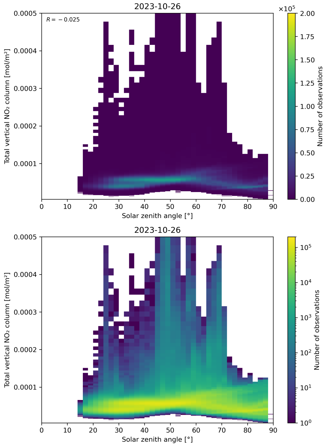
Figure 153: Scatter density plot of “Solar zenith angle” against “Total vertical NO 2 column” for 2023-10-25 to 2023-10-27.
