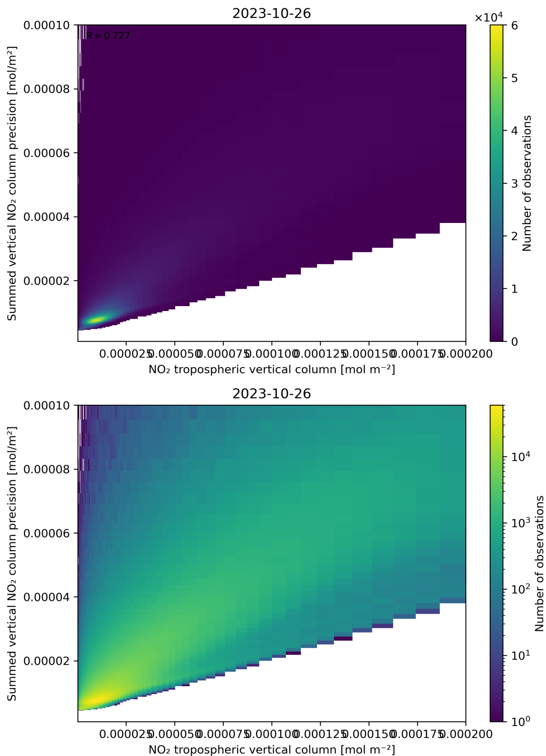
Figure 127: Scatter density plot of “NO 2 tropospheric vertical column” against “Summed vertical NO 2 column precision” for 2023-10-25 to 2023-10-27.
