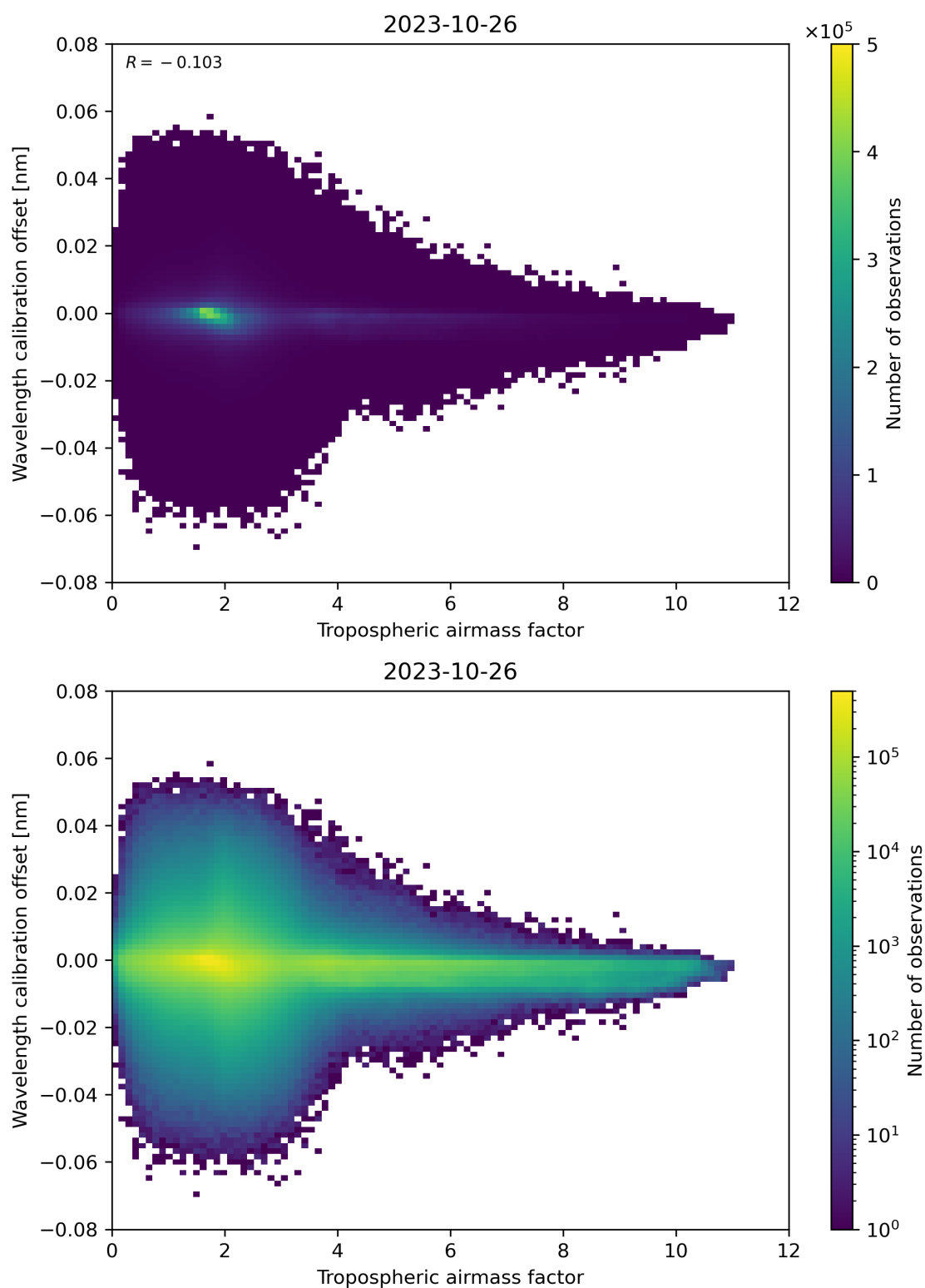
Figure 80: Scatter density plot of “Tropospheric airmass factor” against “Wavelength calibration offset” for 2023-10-25 to 2023-10-27.
