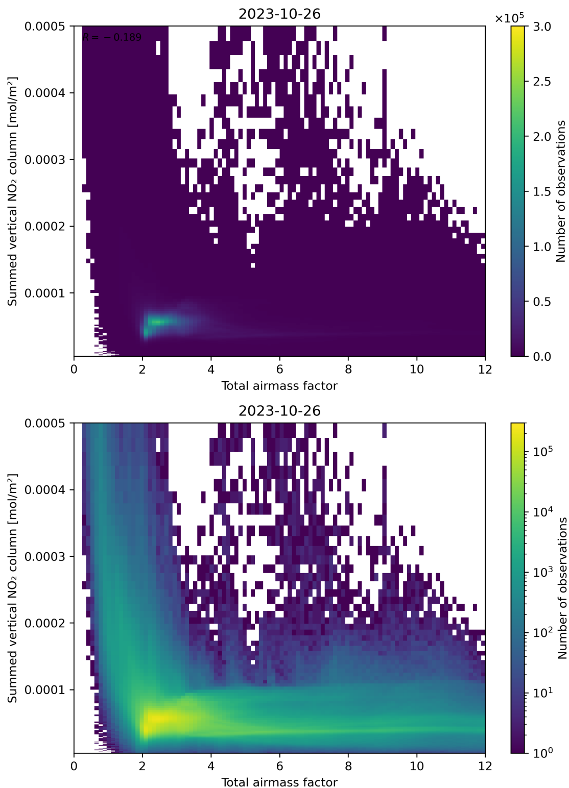
Figure 65: Scatter density plot of “Total airmass factor” against “Summed vertical NO 2 column” for 2023-10-25 to 2023-10-27.
