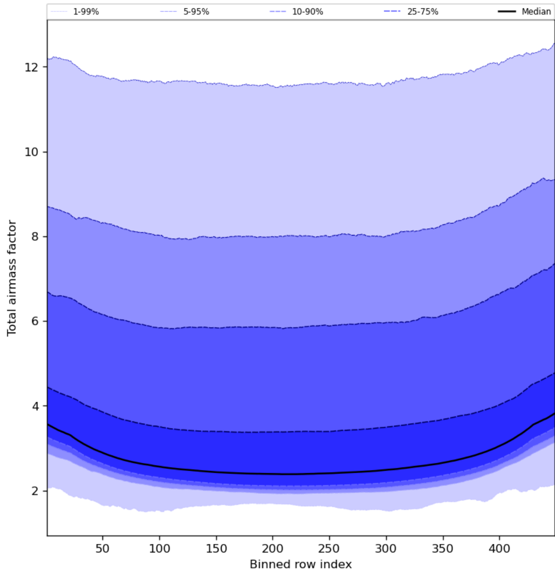
Figure 49: Along track statistics of “Total airmass factor” for 2023-10-25 to 2023-10-27
