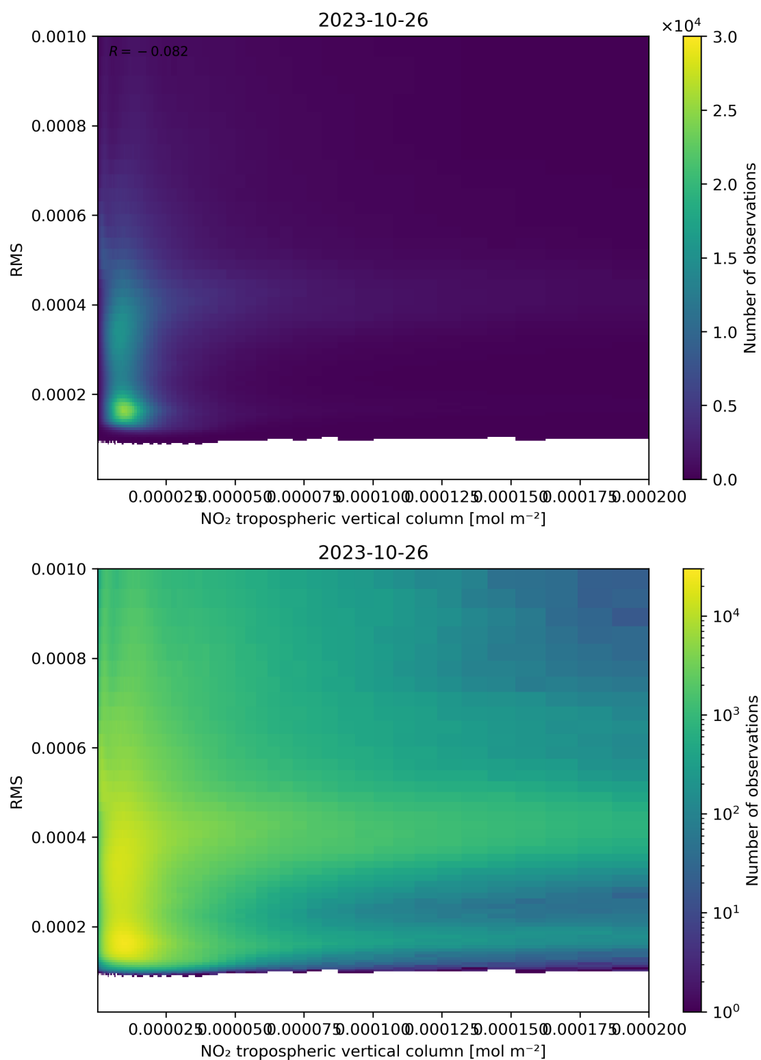
Figure 142: Scatter density plot of “NO 2 tropospheric vertical column” against “RMS” for 2023-10-25 to 2023-10-27.
