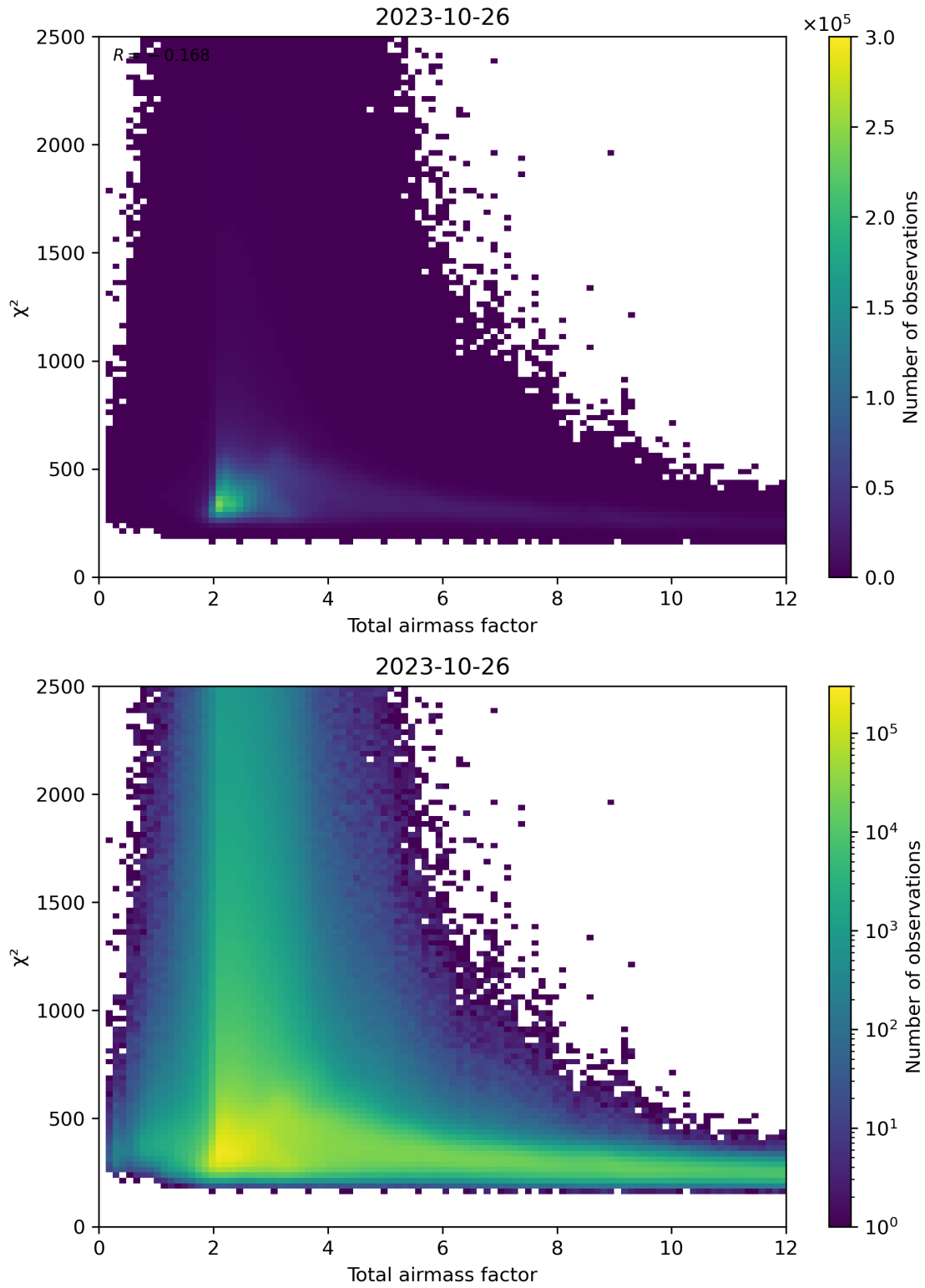
Figure 63: Scatter density plot of “Total airmass factor” against “ \chi^2 ” for 2023-10-25 to 2023-10-27.
