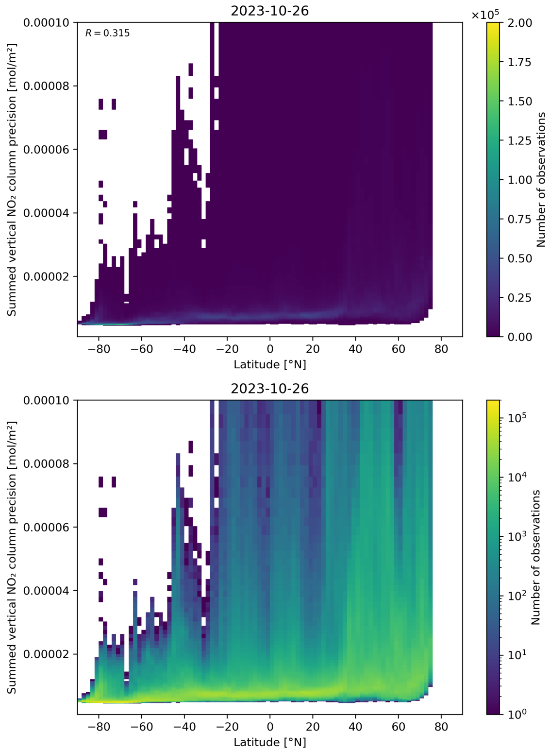
Figure 89: Scatter density plot of “Latitude” against “Summed vertical NO 2 column precision” for 2023-10-25 to 2023-10-27.
