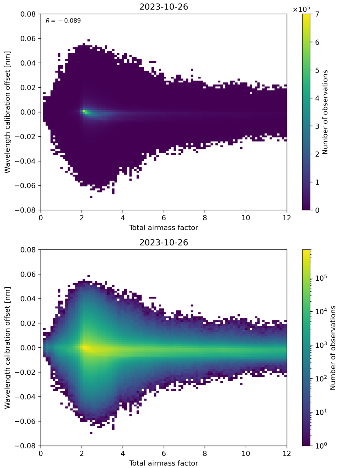
Figure 70: Scatter density plot of “Total airmass factor” against “Wavelength calibration offset” for 2023-10-25 to 2023-10-27.
