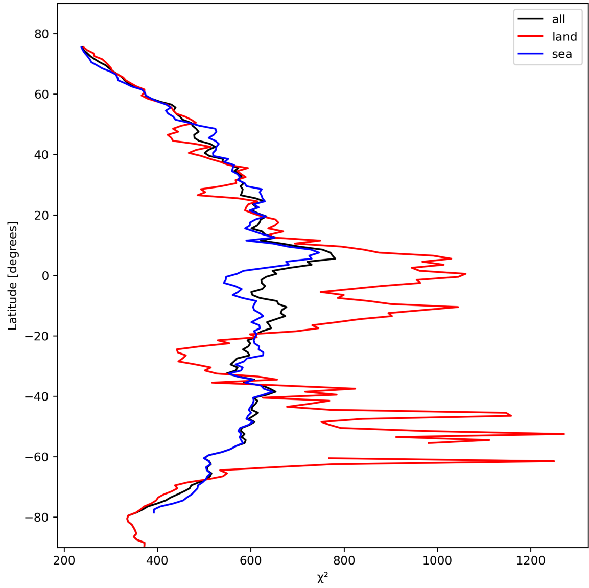
Figure 25: Zonal average of “ \chi^2 ” for 2023-10-25 to 2023-10-27.
