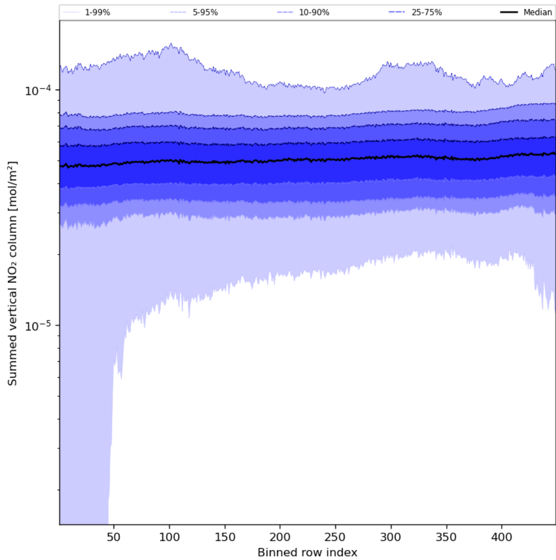
Figure 57: Along track statistics of “Summed vertical NO 2 column” for 2023-10-25 to 2023-10-27
