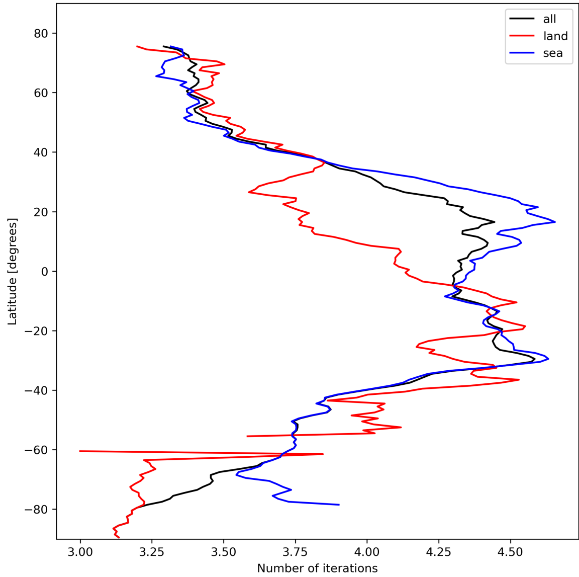
Figure 17: Zonal average of “Number of iterations” for 2023-10-25 to 2023-10-27.
