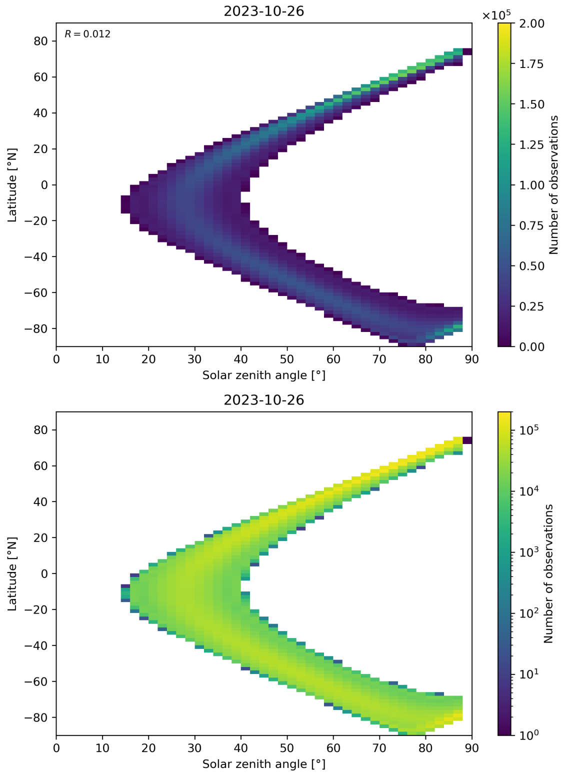
Figure 149: Scatter density plot of “Solar zenith angle” against “Latitude” for 2023-10-25 to 2023-10-27.
