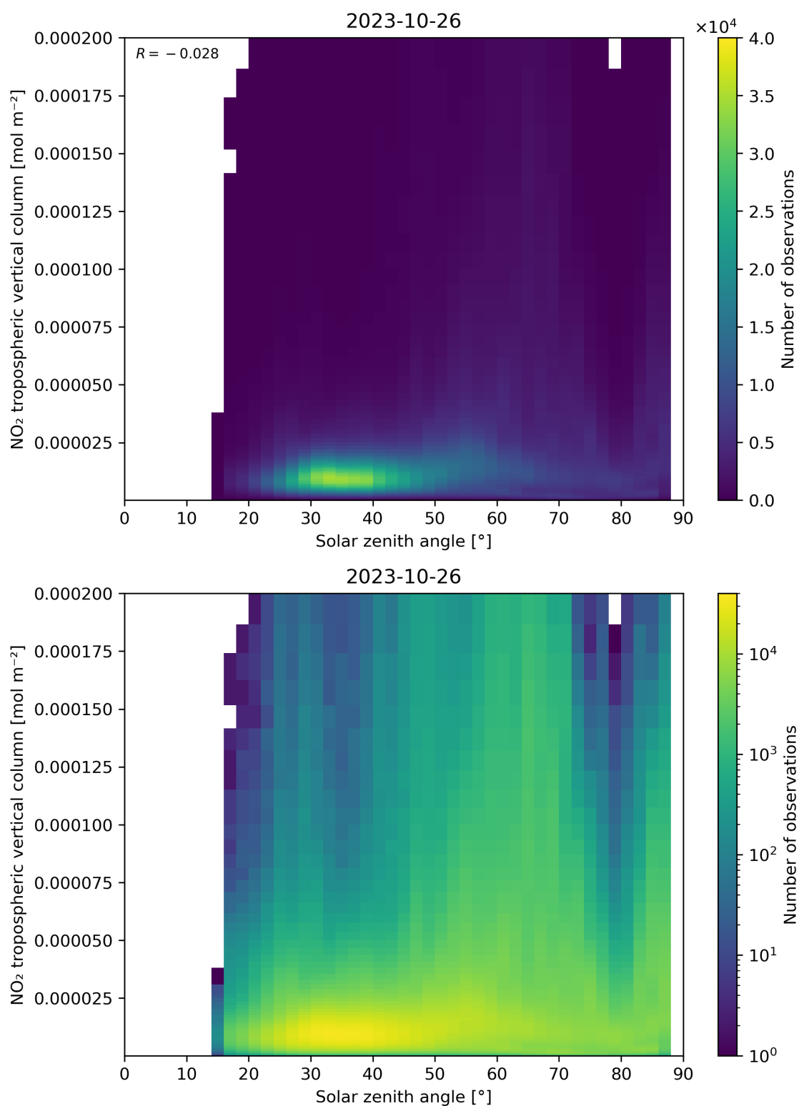
Figure 155: Scatter density plot of “Solar zenith angle” against “NO 2 tropospheric vertical column” for 2023-10-25 to 2023-10-27.
