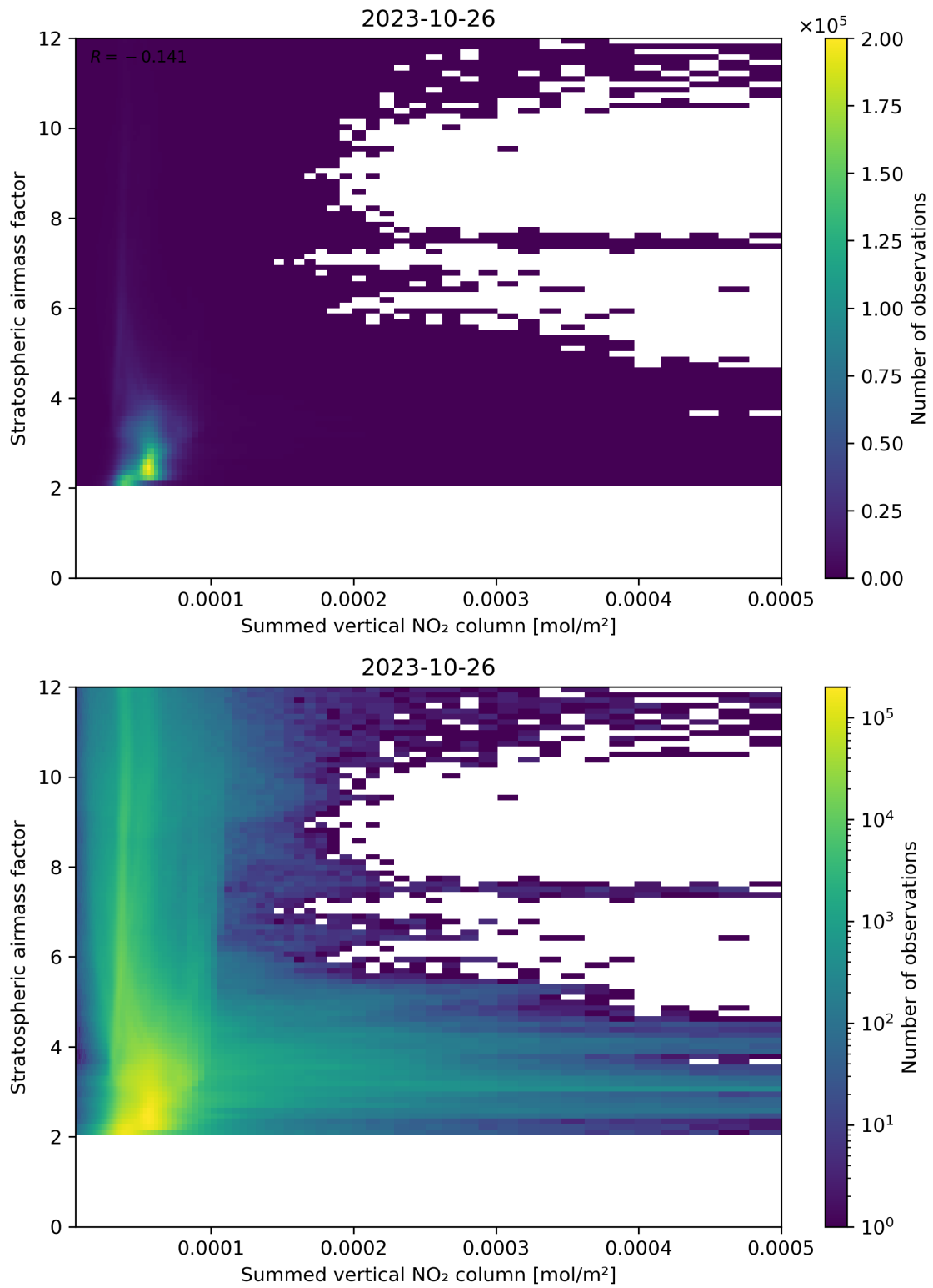
Figure 103: Scatter density plot of “Summed vertical NO 2 column” against “Stratospheric air mass factor” for 2023-10-25 to 2023-10-27.
