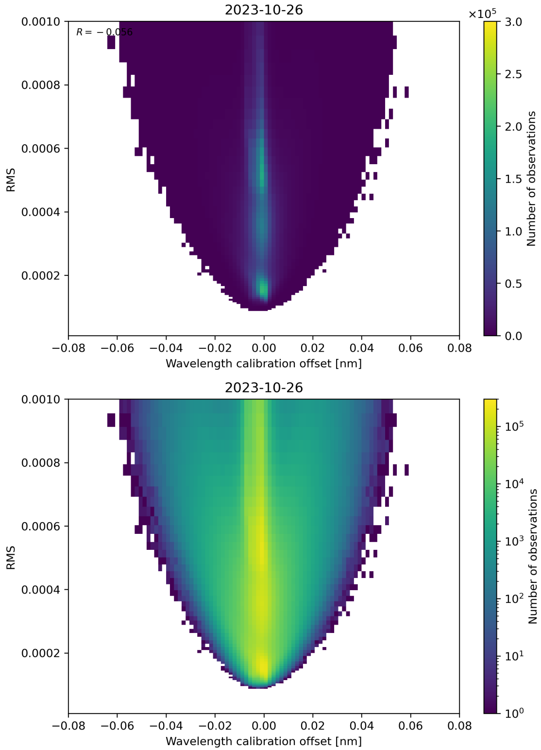
Figure 181: Scatter density plot of “Wavelength calibration offset” against “RMS” for 2023-10-25 to 2023-10-27.
