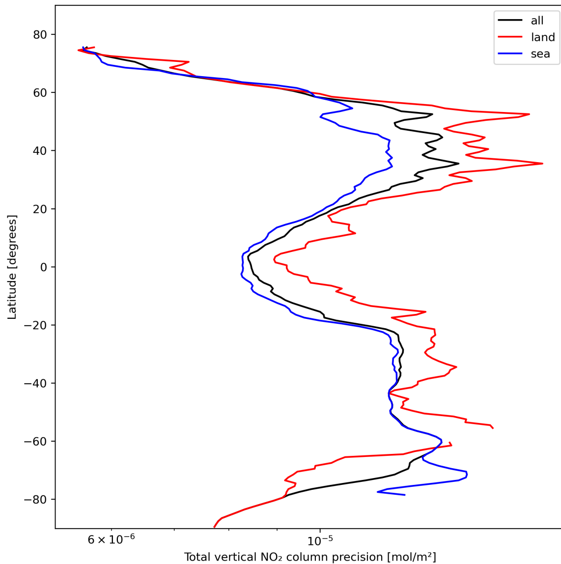
Figure 22: Zonal average of “Total vertical NO 2 column precision” for 2023-10-25 to 2023-10-27.
