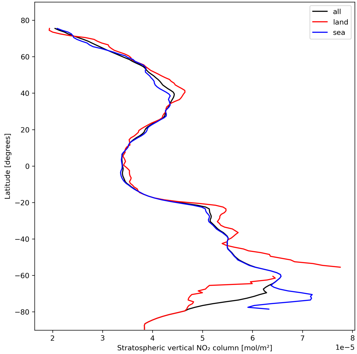
Figure 19: Zonal average of “Stratospheric vertical NO 2 column” for 2023-10-25 to 2023-10-27.
