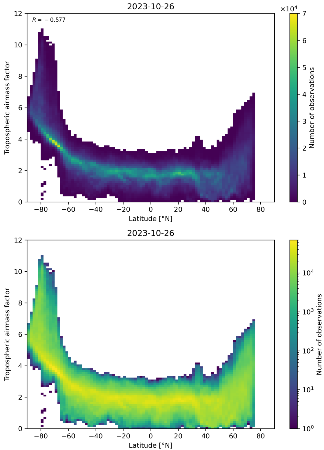
Figure 85: Scatter density plot of “Latitude” against “Tropospheric airmass factor” for 2023-10-25 to 2023-10-27.
