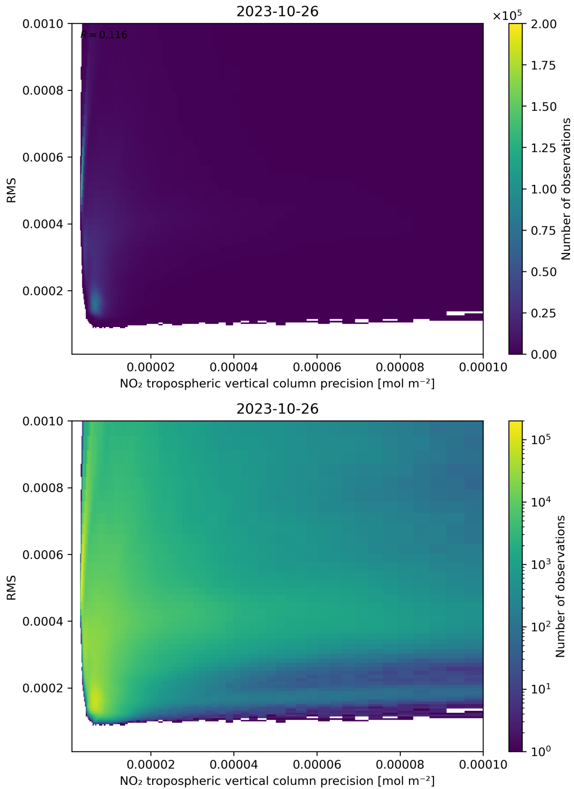
Figure 140: Scatter density plot of “NO 2 tropospheric vertical column precision” against “RMS” for 2023-10-25 to 2023-10-27.
