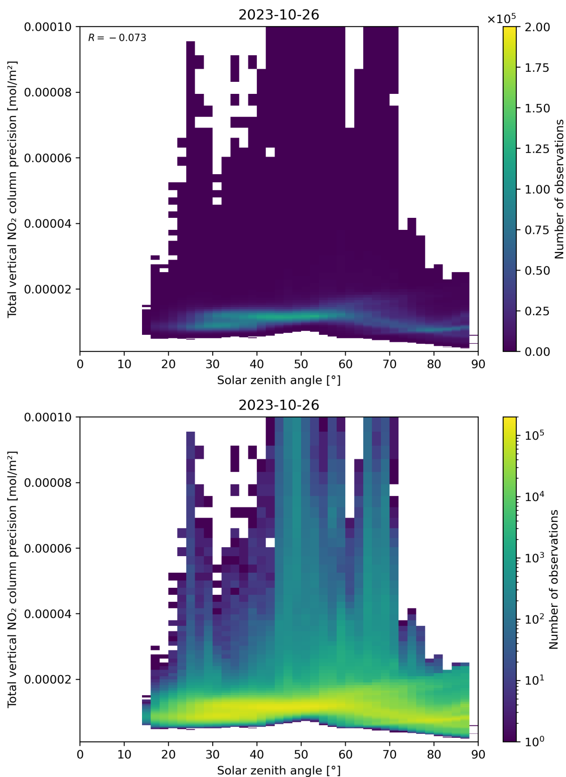
Figure 154: Scatter density plot of “Solar zenith angle” against “Total vertical NO 2 column precision” for 2023-10-25 to 2023-10-27.
