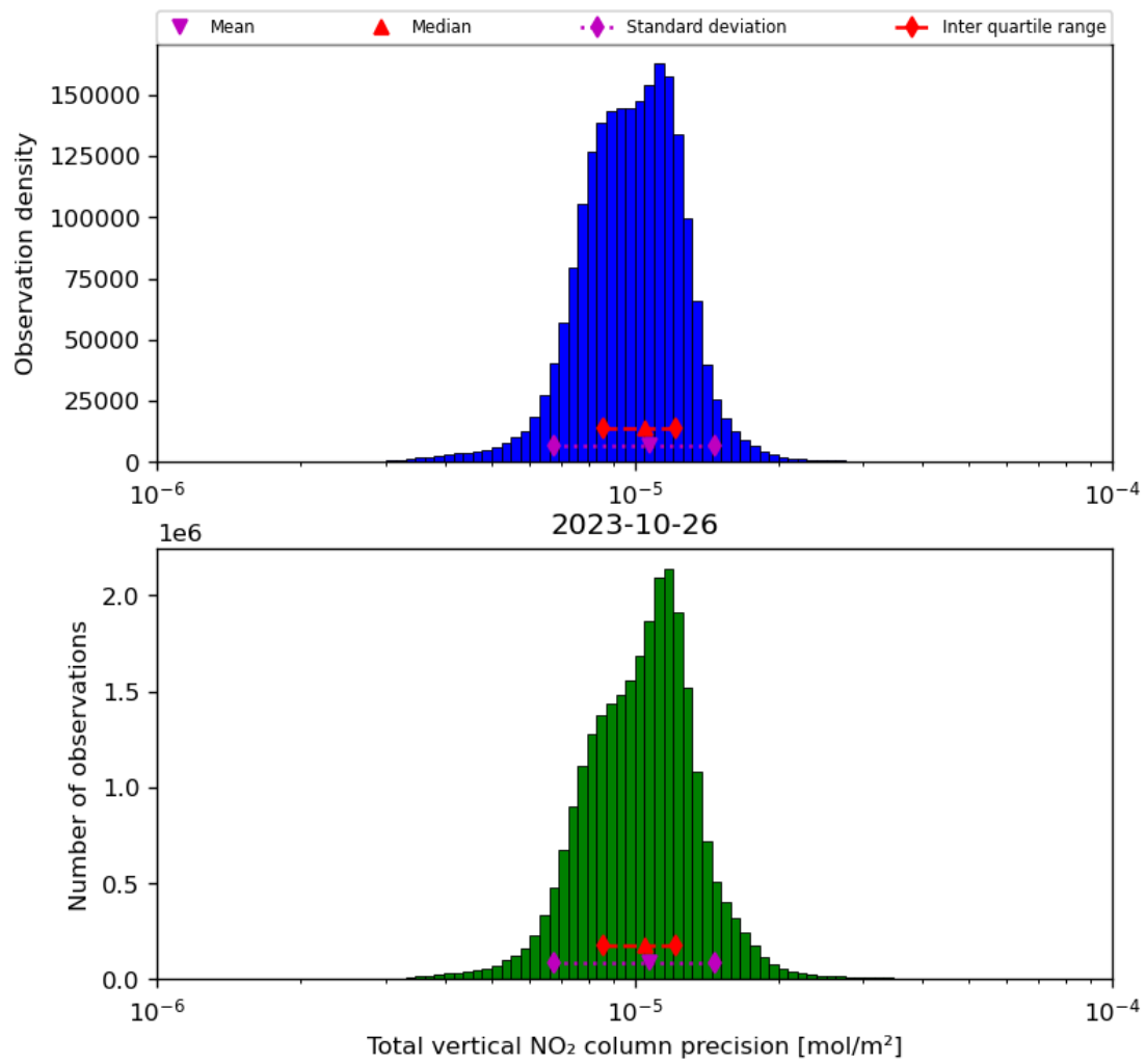
Figure 39: Histogram of "Total vertical NO 2 column precision" for 2023-10-25 to 2023-10-27
