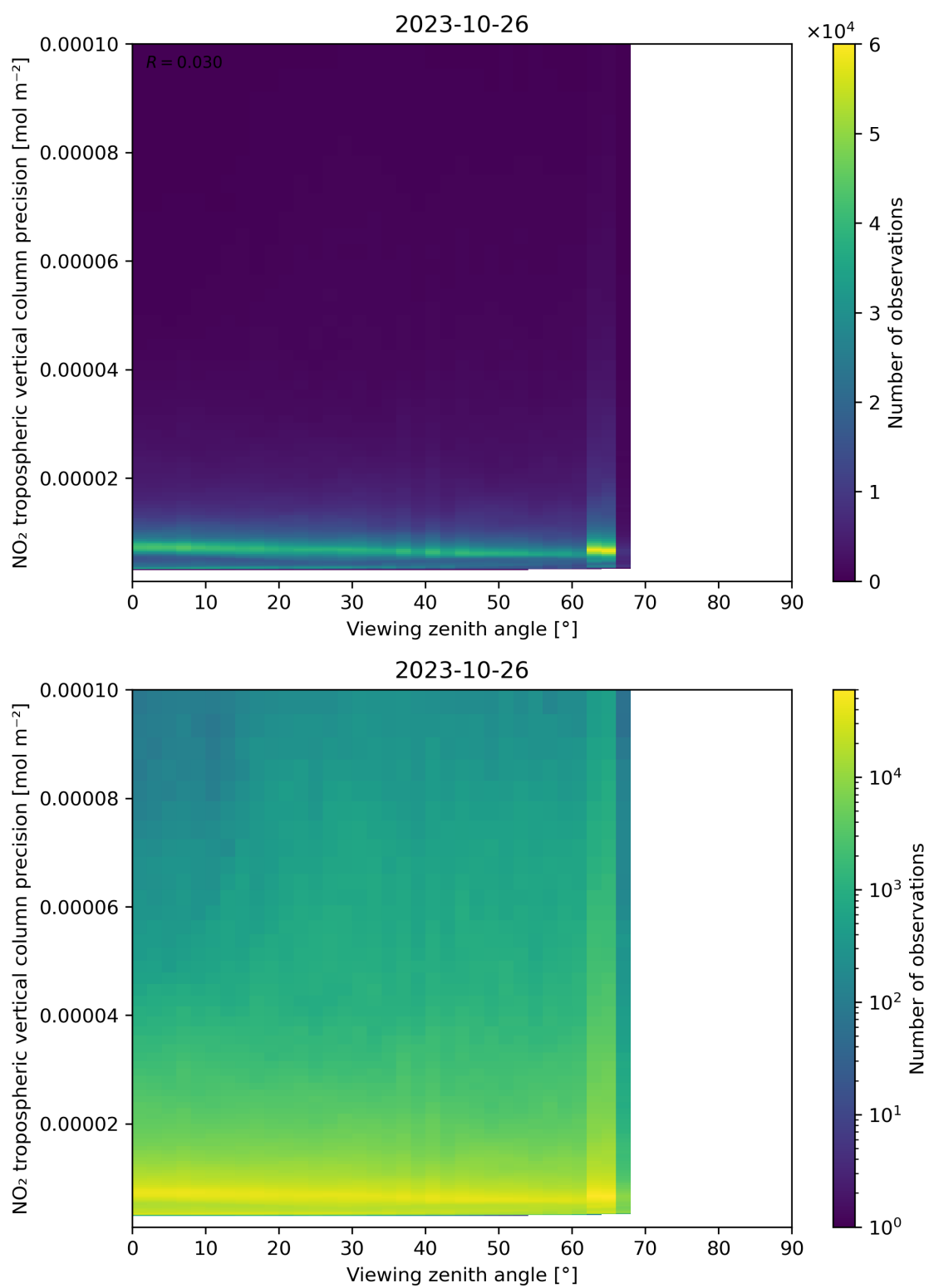
Figure 170: Scatter density plot of “Viewing zenith angle” against “NO 2 tropospheric vertical column precision” for 2023-10-25 to 2023-10-27.
