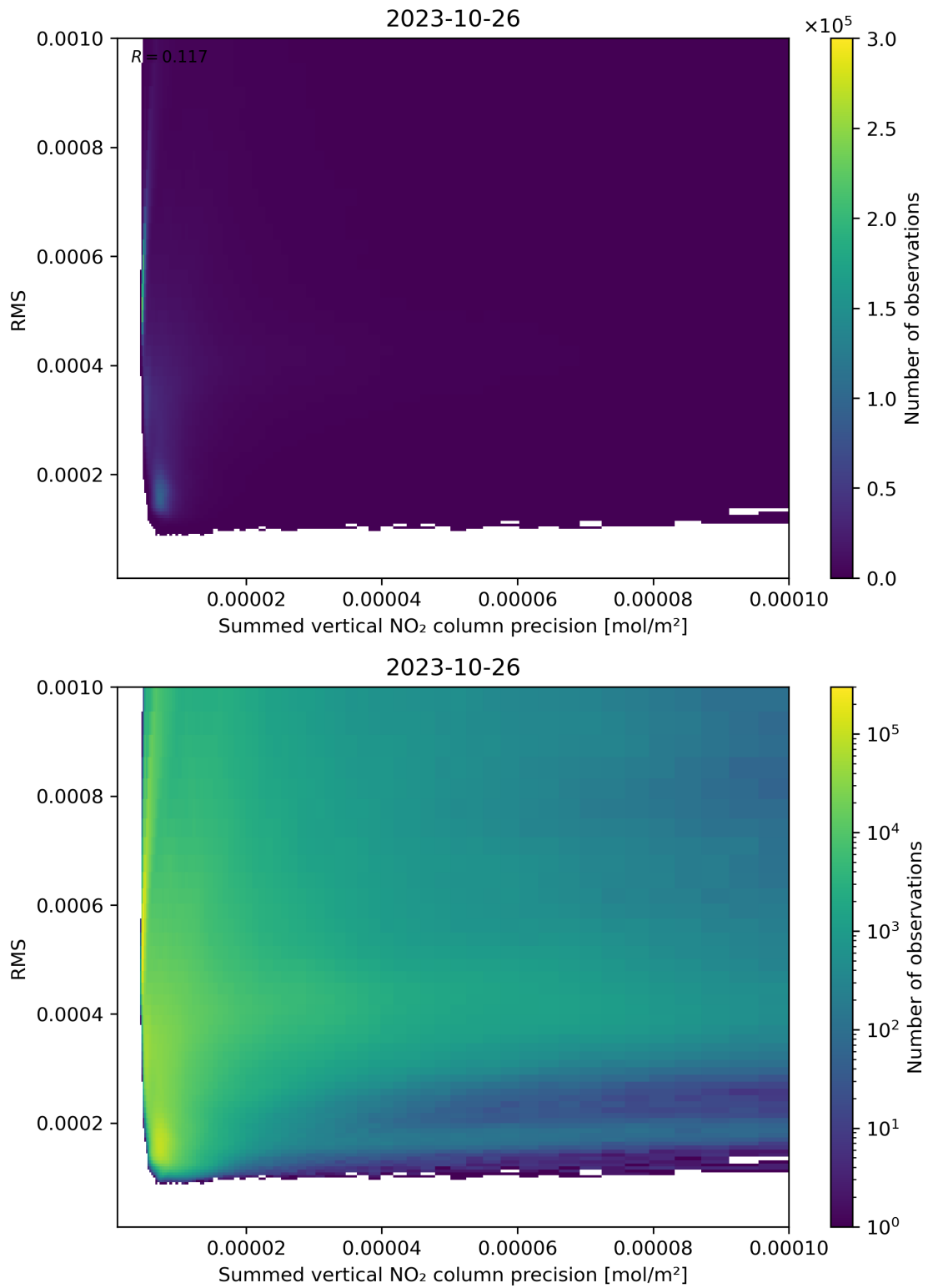
Figure 108: Scatter density plot of “Summed vertical NO 2 column precision” against “RMS” for 2023-10-25 to 2023-10-27.
