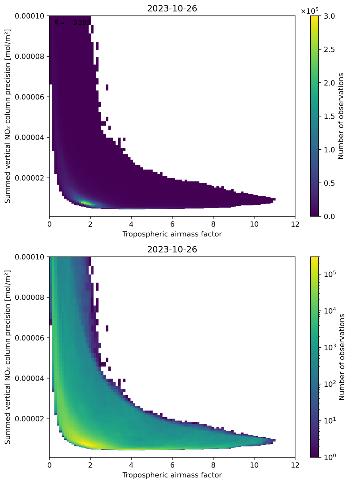
Figure 76: Scatter density plot of “Tropospheric air mass factor” against “Summed vertical NO 2 column precision” for 2023-10-25 to 2023-10-27.
