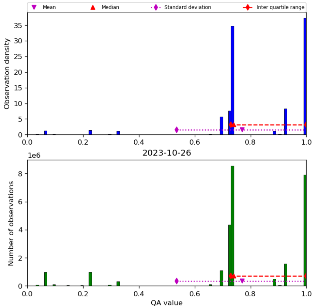
Figure 28: Histogram of “QA value” for 2023-10-25 to 2023-10-27
