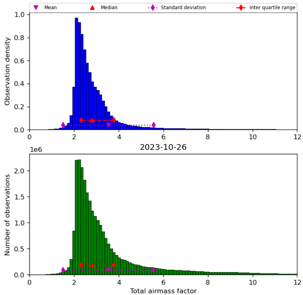
Figure 32: Histogram of “Total airmass factor” for 2023-10-25 to 2023-10-27
