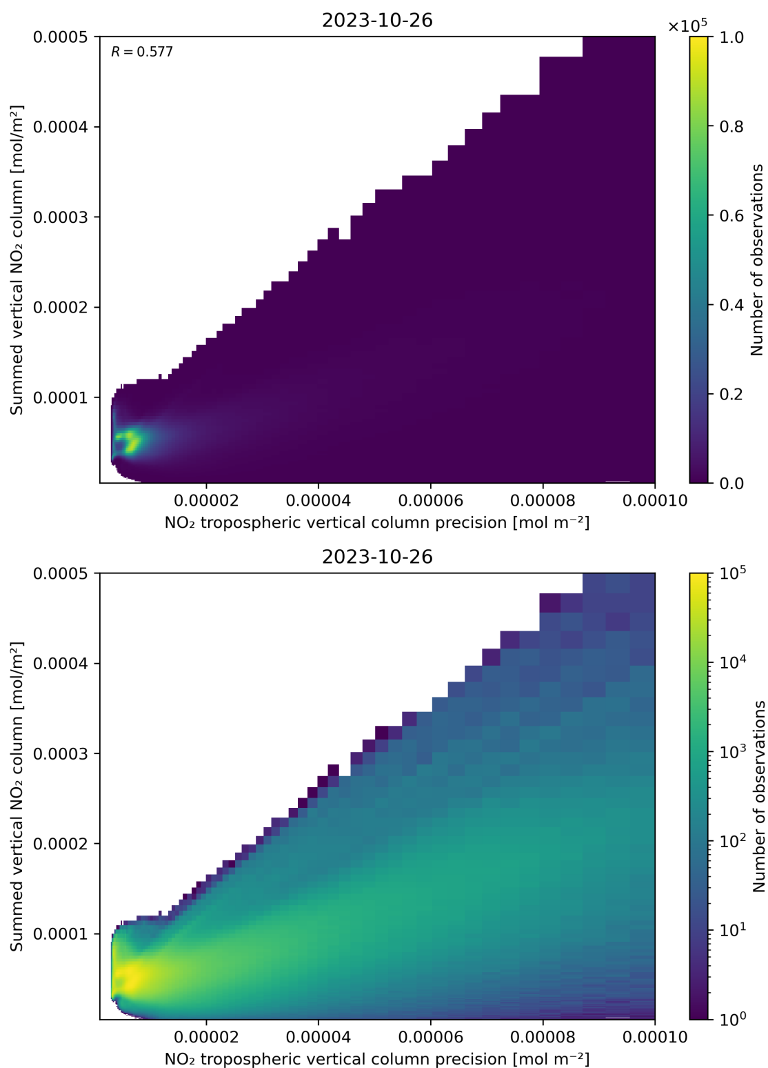
Figure 136: Scatter density plot of “NO 2 tropospheric vertical column precision” against “Summed vertical NO 2 column” for 2023-10-25 to 2023-10-27.
