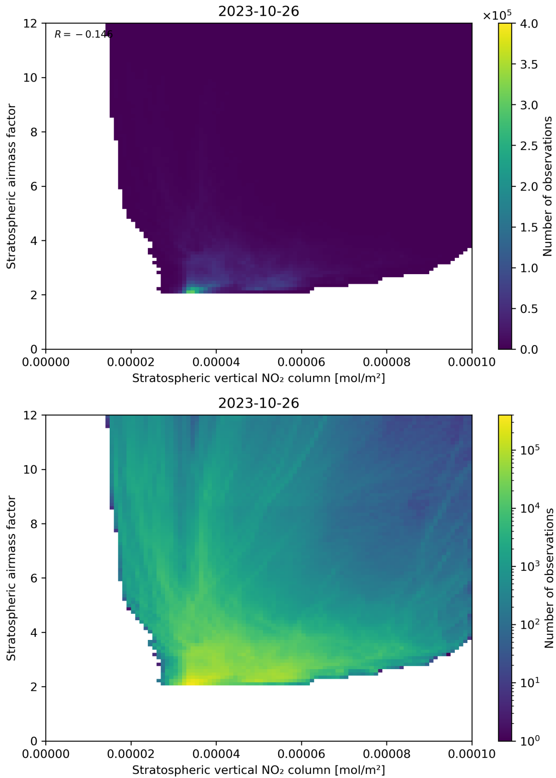
Figure 96: Scatter density plot of “Stratospheric vertical NO 2 column” against “Stratospheric airmass factor” for 2023-10-25 to 2023-10-27.
