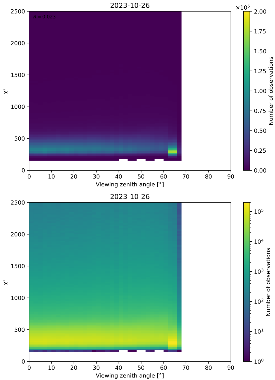
Figure 162: Scatter density plot of “Viewing zenith angle” against “ \chi^2 ” for 2023-10-25 to 2023-10-27.
