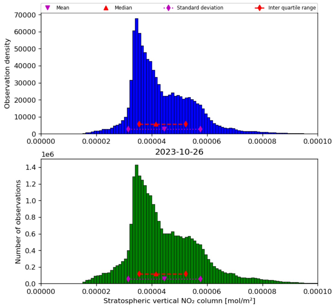
Figure 36: Histogram of “Stratospheric vertical NO 2 column” for 2023-10-25 to 2023-10-27
