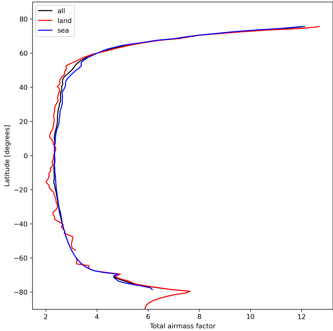
Figure 15: Zonal average of “Total airmass factor” for 2023-10-25 to 2023-10-27.
