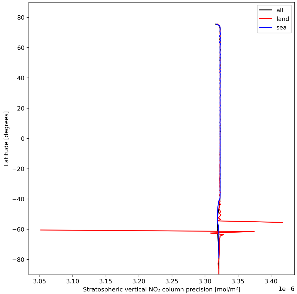
Figure 20: Zonal average of “Stratospheric vertical NO 2 column precision” for 2023-10-25 to 2023-10-27.
