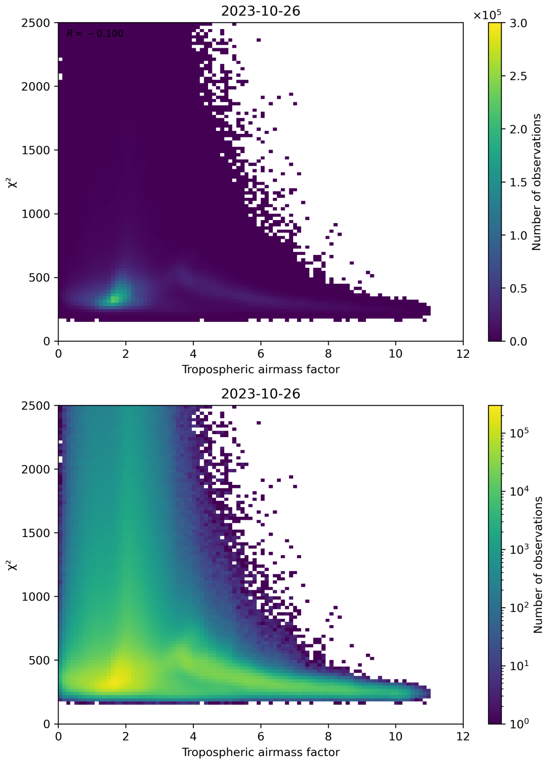
Figure 73: Scatter density plot of “Tropospheric airmass factor” against “ \chi^2 ” for 2023-10-25 to 2023-10-27.
