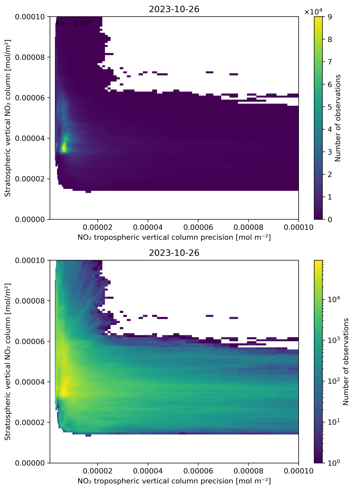
Figure 135: Scatter density plot of “NO 2 tropospheric vertical column precision” against “Stratospheric vertical NO 2 column” for 2023-10-25 to 2023-10-27.
