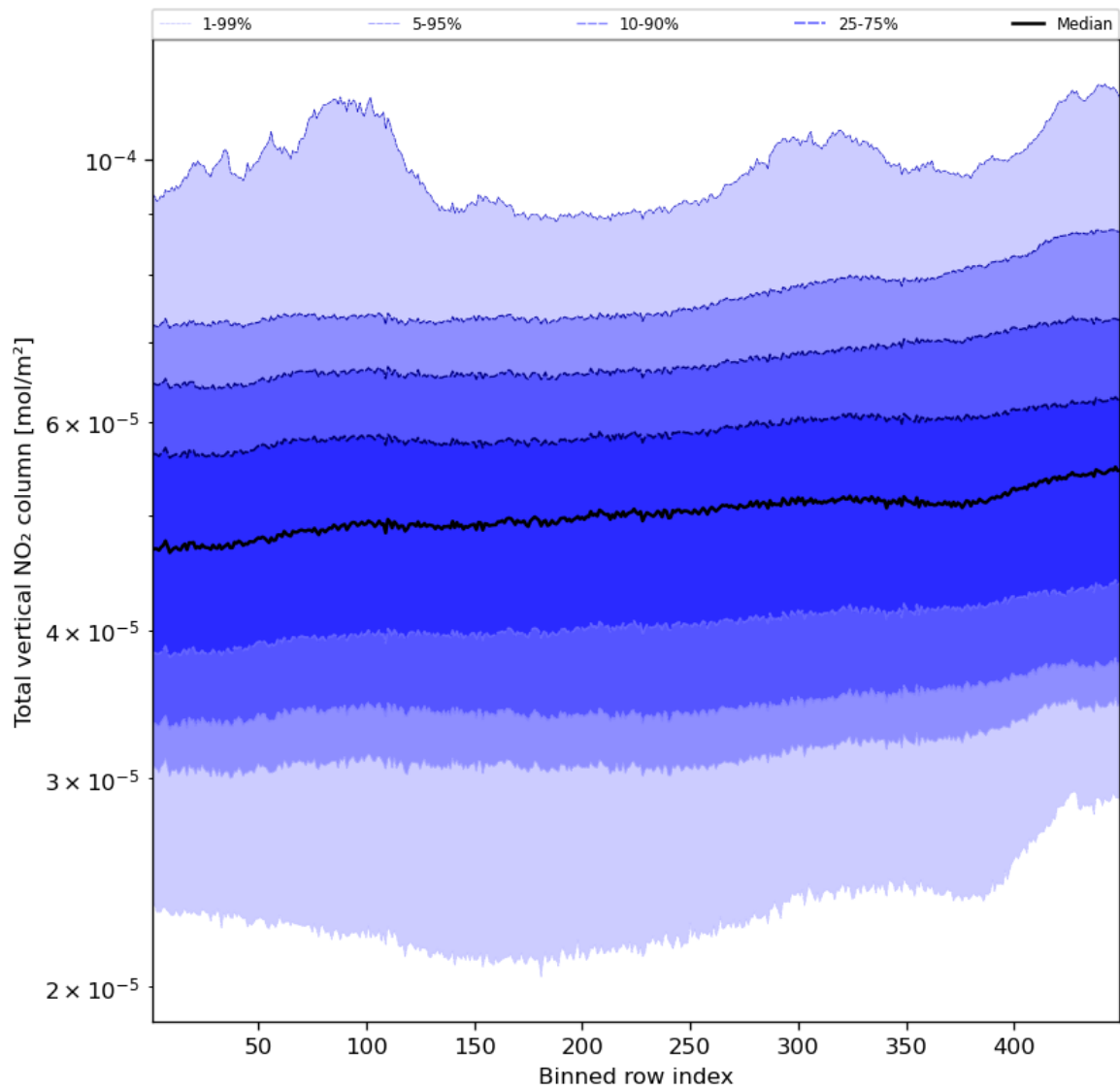
Figure 55: Along track statistics of “Total vertical NO 2 column” for 2023-10-25 to 2023-10-27
