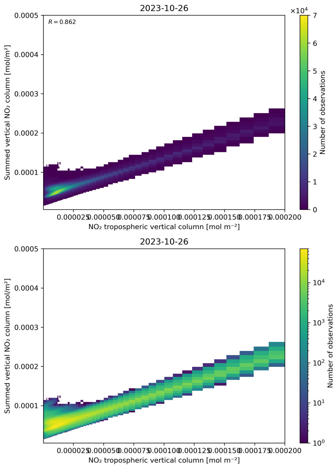
Figure 126: Scatter density plot of “NO 2 tropospheric vertical column” against “Summed vertical NO 2 column” for 2023-10-25 to 2023-10-27.
