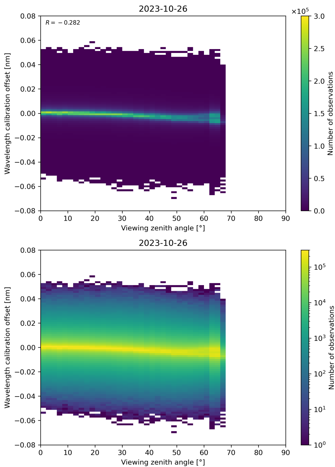
Figure 173: Scatter density plot of “Viewing zenith angle” against “Wavelength calibration offset” for 2023-10-25 to 2023-10-27.
