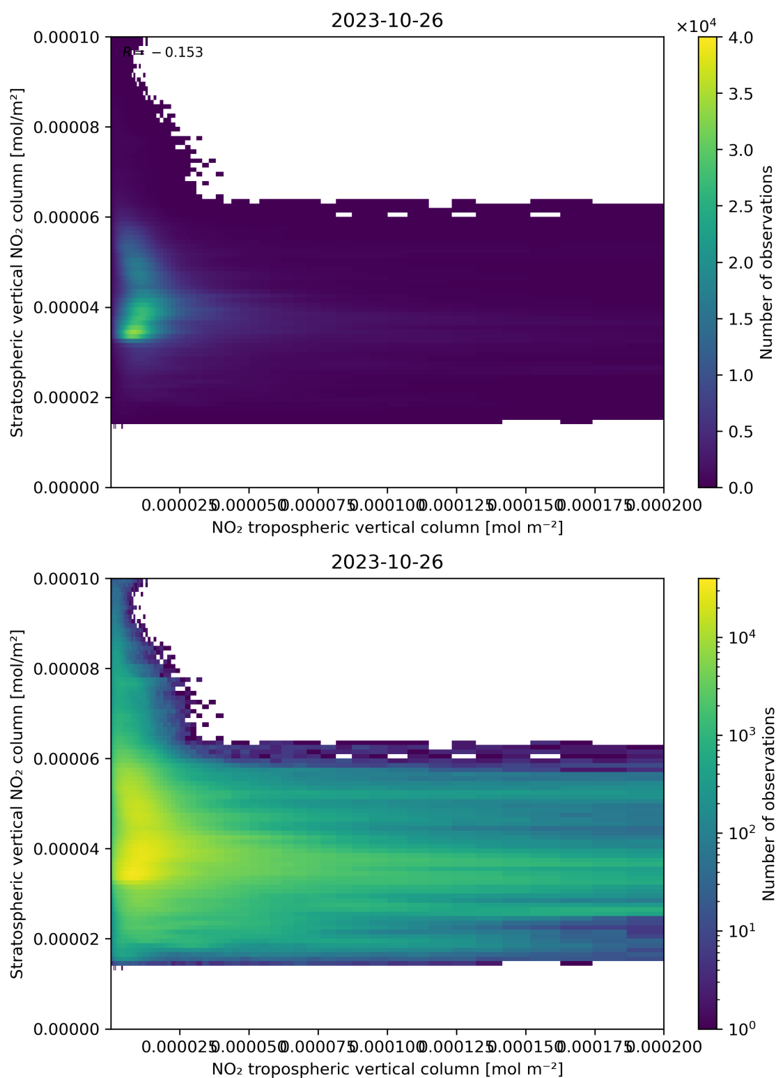
Figure 125: Scatter density plot of “NO 2 tropospheric vertical column” against “Stratospheric vertical NO 2 column” for 2023-10-25 to 2023-10-27.
