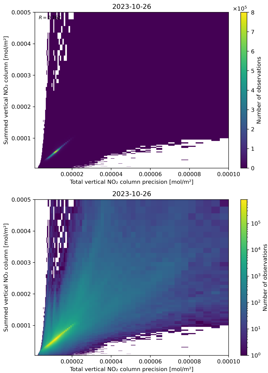
Figure 117: Scatter density plot of “Total vertical NO 2 column precision” against “Summed vertical NO 2 column” for 2023-10-25 to 2023-10-27.
