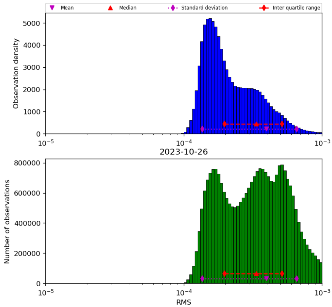
Figure 43: Histogram of “RMS” for 2023-10-25 to 2023-10-27
