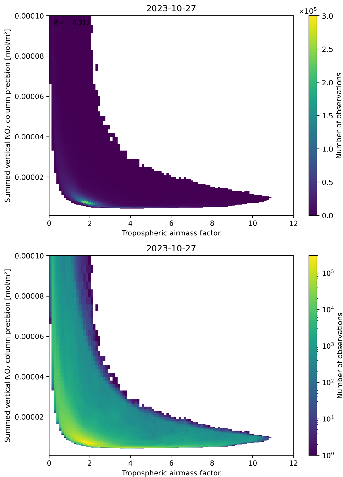
Figure 76: Scatter density plot of “Tropospheric air mass factor” against “Summed vertical NO 2 column precision” for 2023-10-27 to 2023-10-28.
