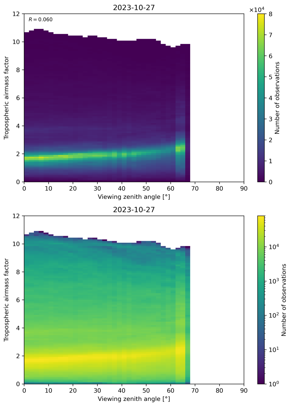
Figure 161: Scatter density plot of “Viewing zenith angle” against “Tropospheric airmass factor” for 2023-10-27 to 2023-10-28.
