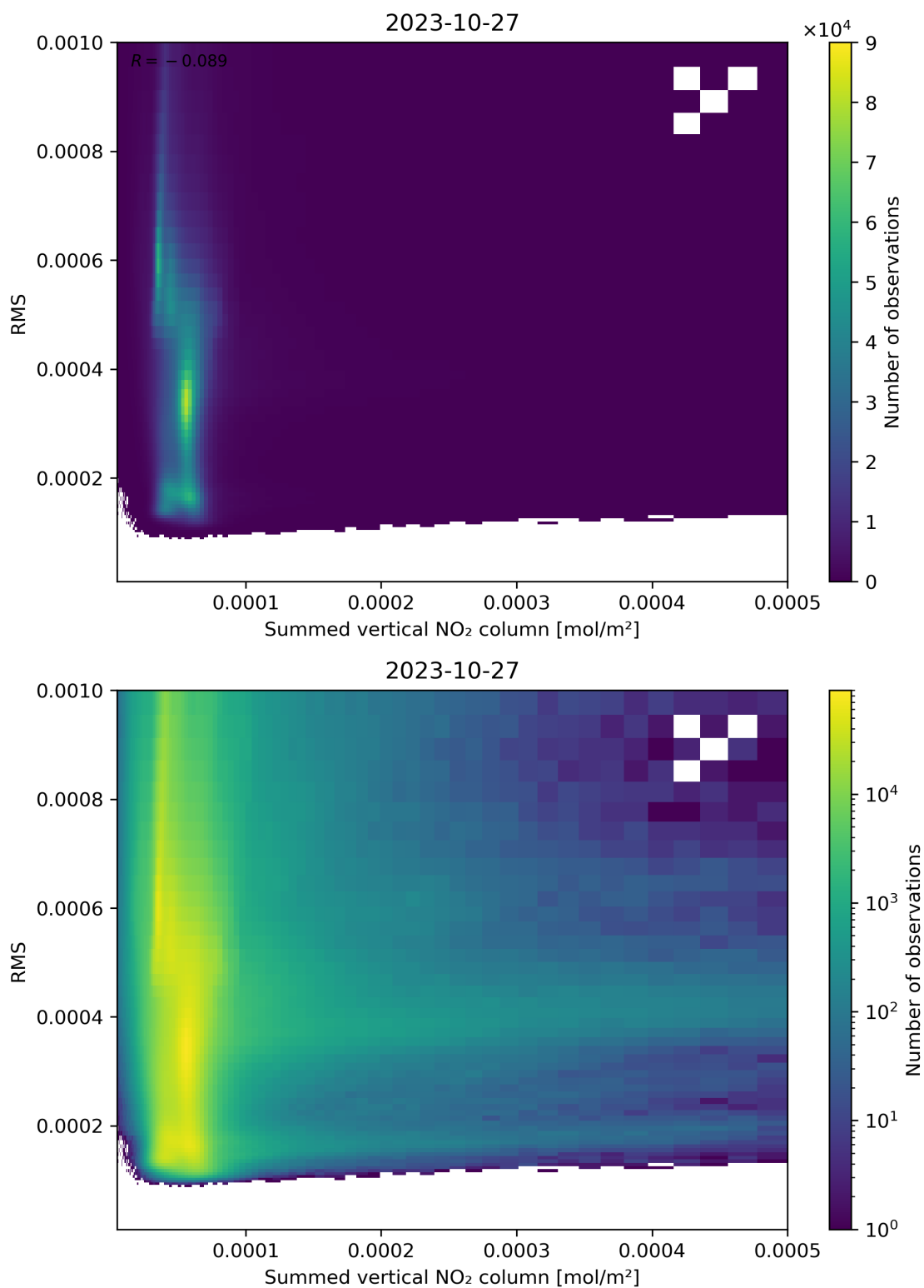
Figure 109: Scatter density plot of “Summed vertical NO 2 column” against “RMS” for 2023-10-27 to 2023-10-28.
