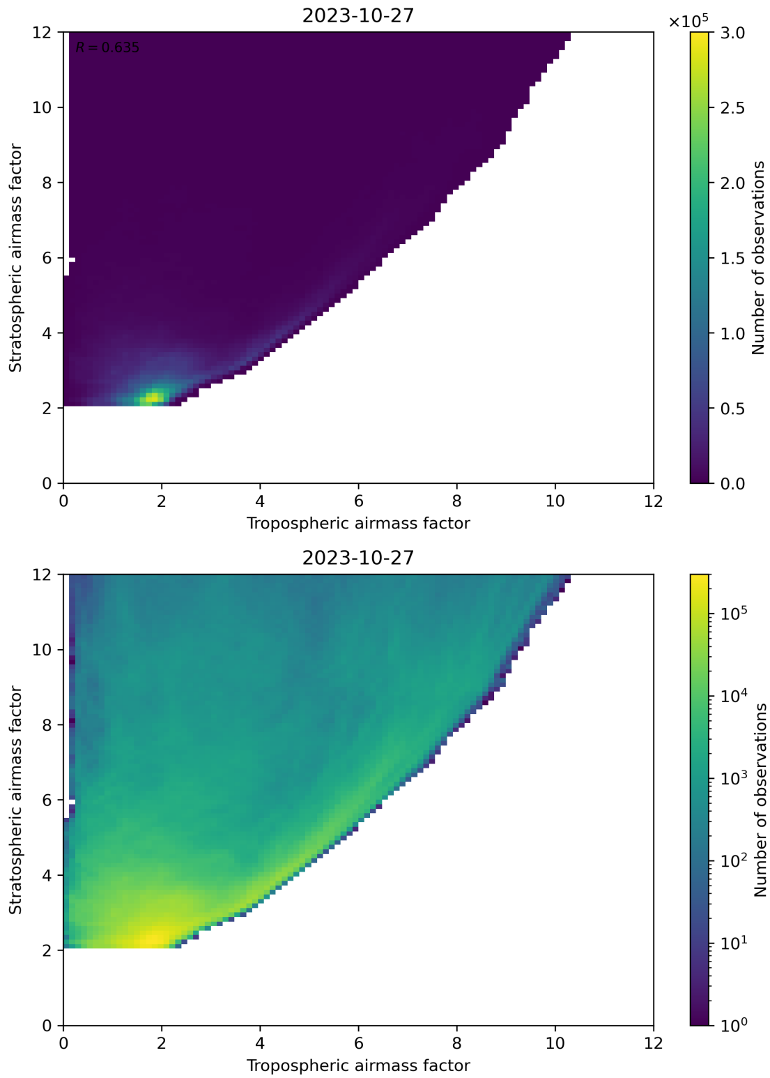
Figure 71: Scatter density plot of “Tropospheric airmass factor” against “Stratospheric airmass factor” for 2023-10-27 to 2023-10-28.
