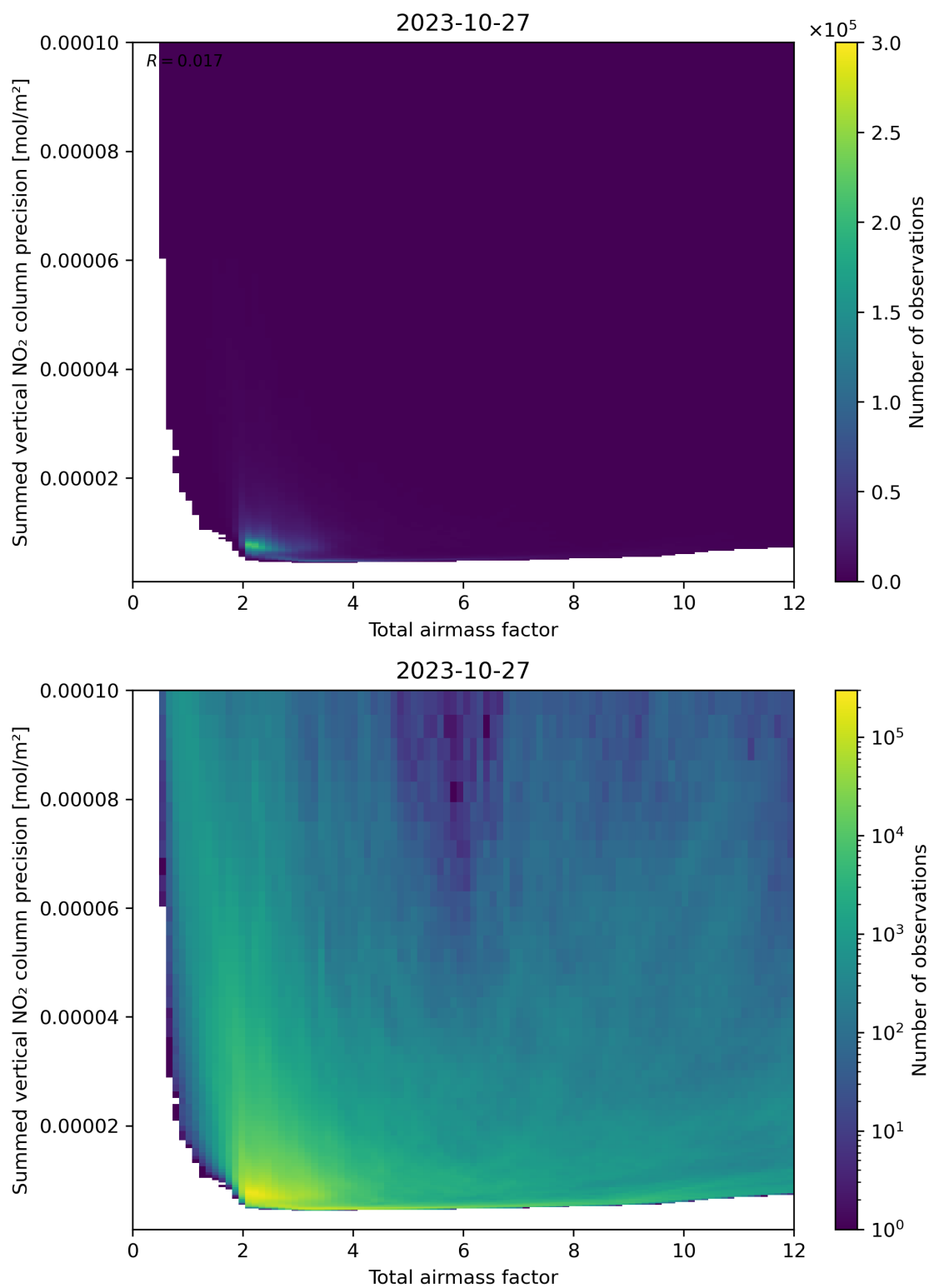
Figure 66: Scatter density plot of “Total airmass factor” against “Summed vertical NO 2 column precision” for 2023-10-27 to 2023-10-28.
