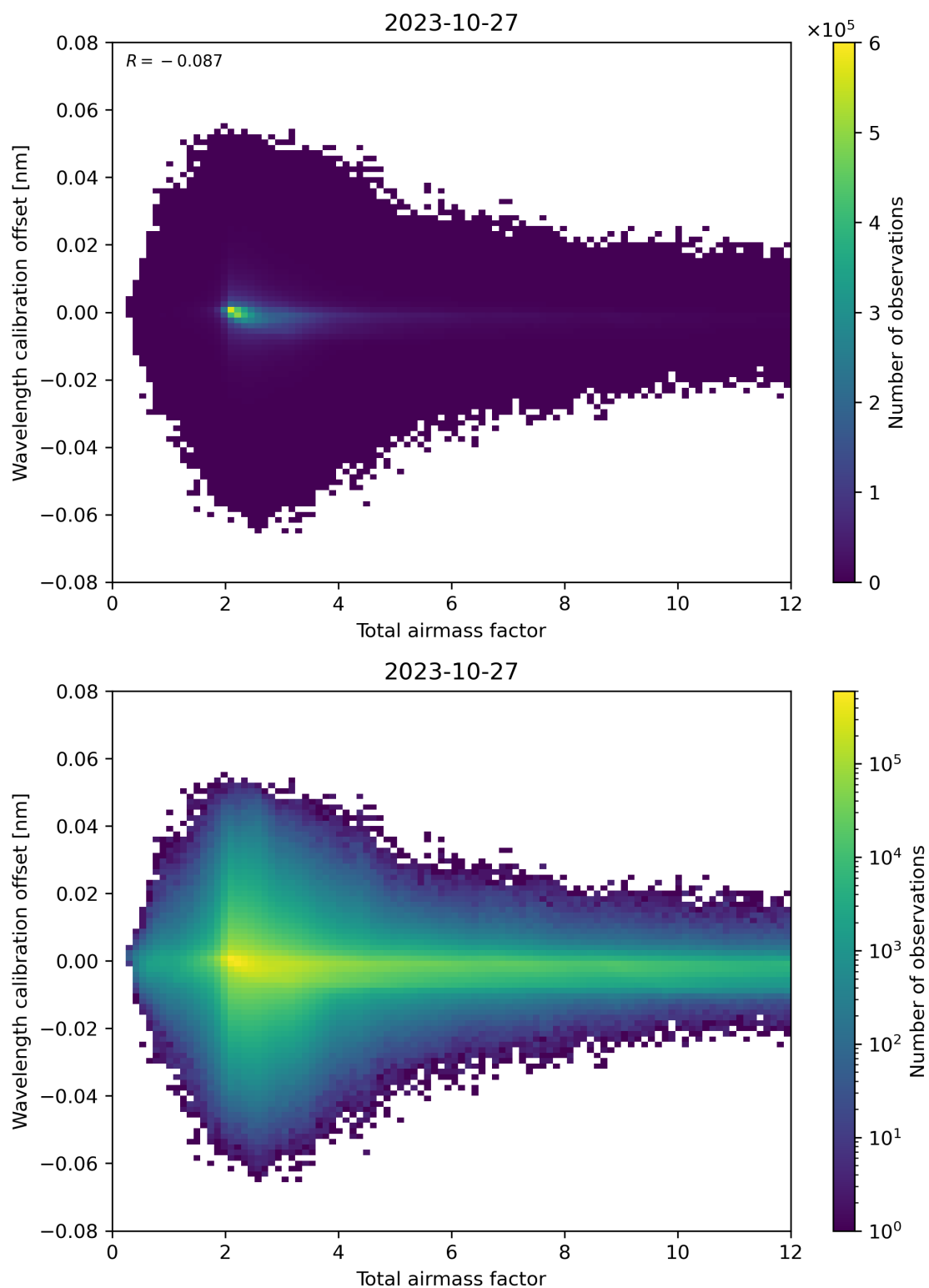
Figure 70: Scatter density plot of “Total airmass factor” against “Wavelength calibration offset” for 2023-10-27 to 2023-10-28.
