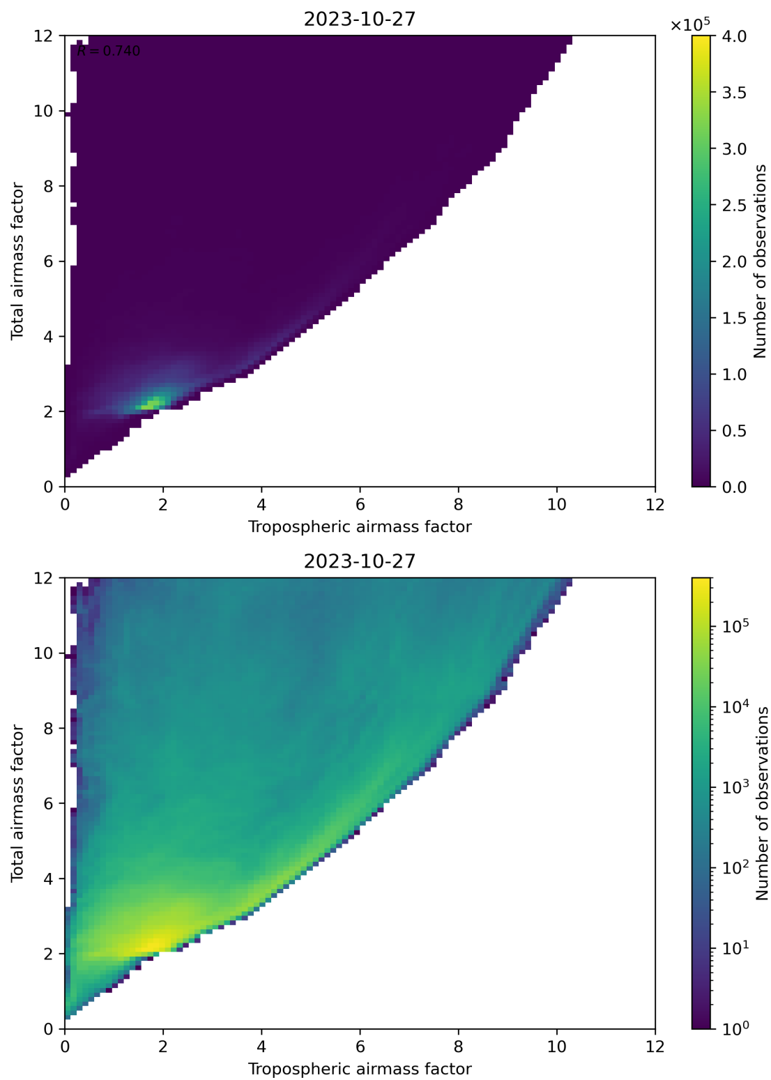
Figure 72: Scatter density plot of “Tropospheric airmass factor” against “Total airmass factor” for 2023-10-27 to 2023-10-28.
