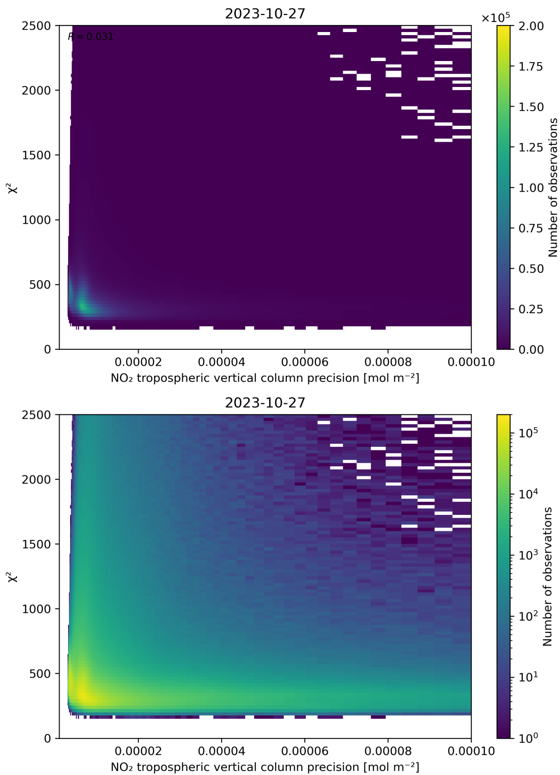
Figure 134: Scatter density plot of “NO 2 tropospheric vertical column precision” against “ \chi^2 ” for 2023-10-27 to 2023-10-28.
