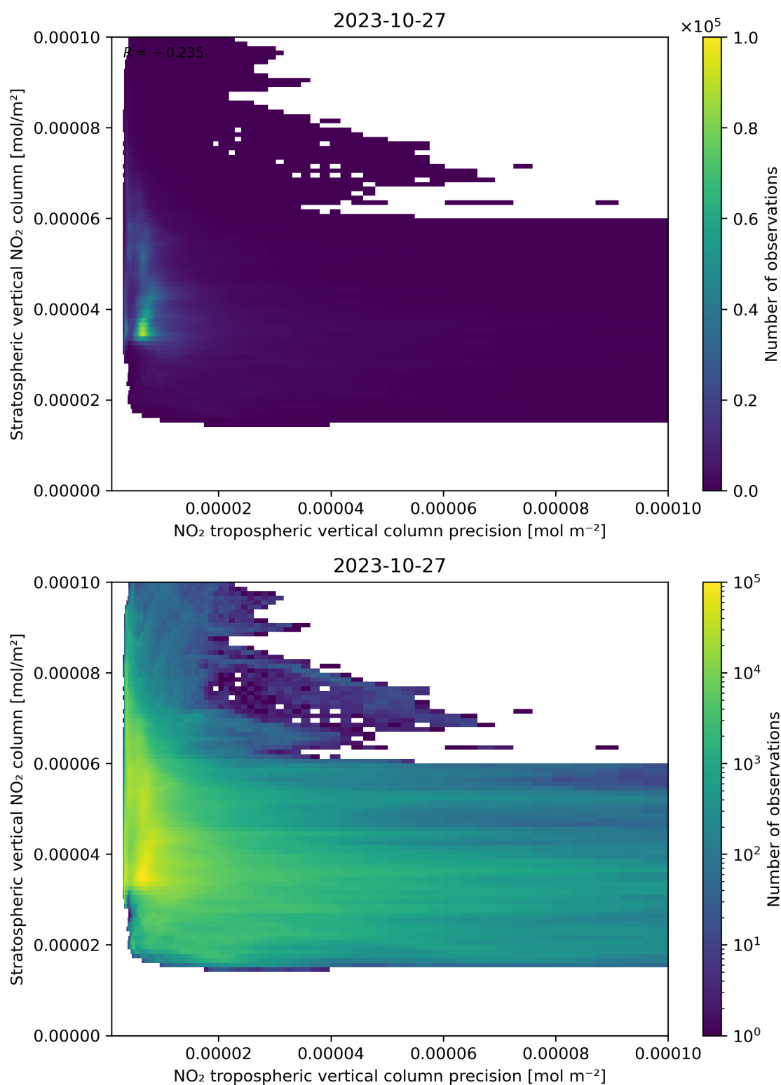
Figure 135: Scatter density plot of “NO 2 tropospheric vertical column precision” against “Stratospheric vertical NO 2 column” for 2023-10-27 to 2023-10-28.
