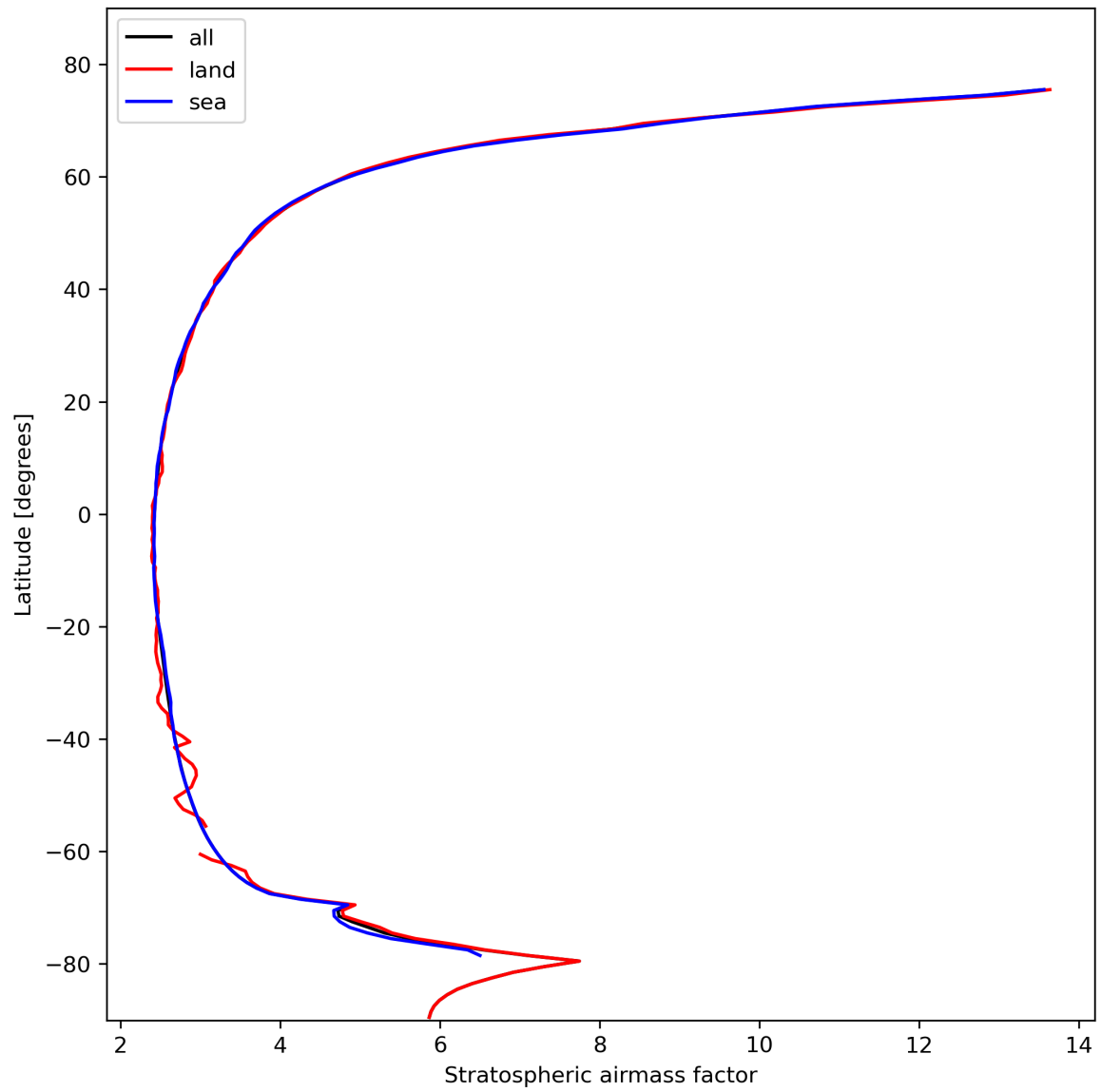
Figure 27: Zonal average of “Stratospheric airmass factor” for 2023-10-27 to 2023-10-28.
