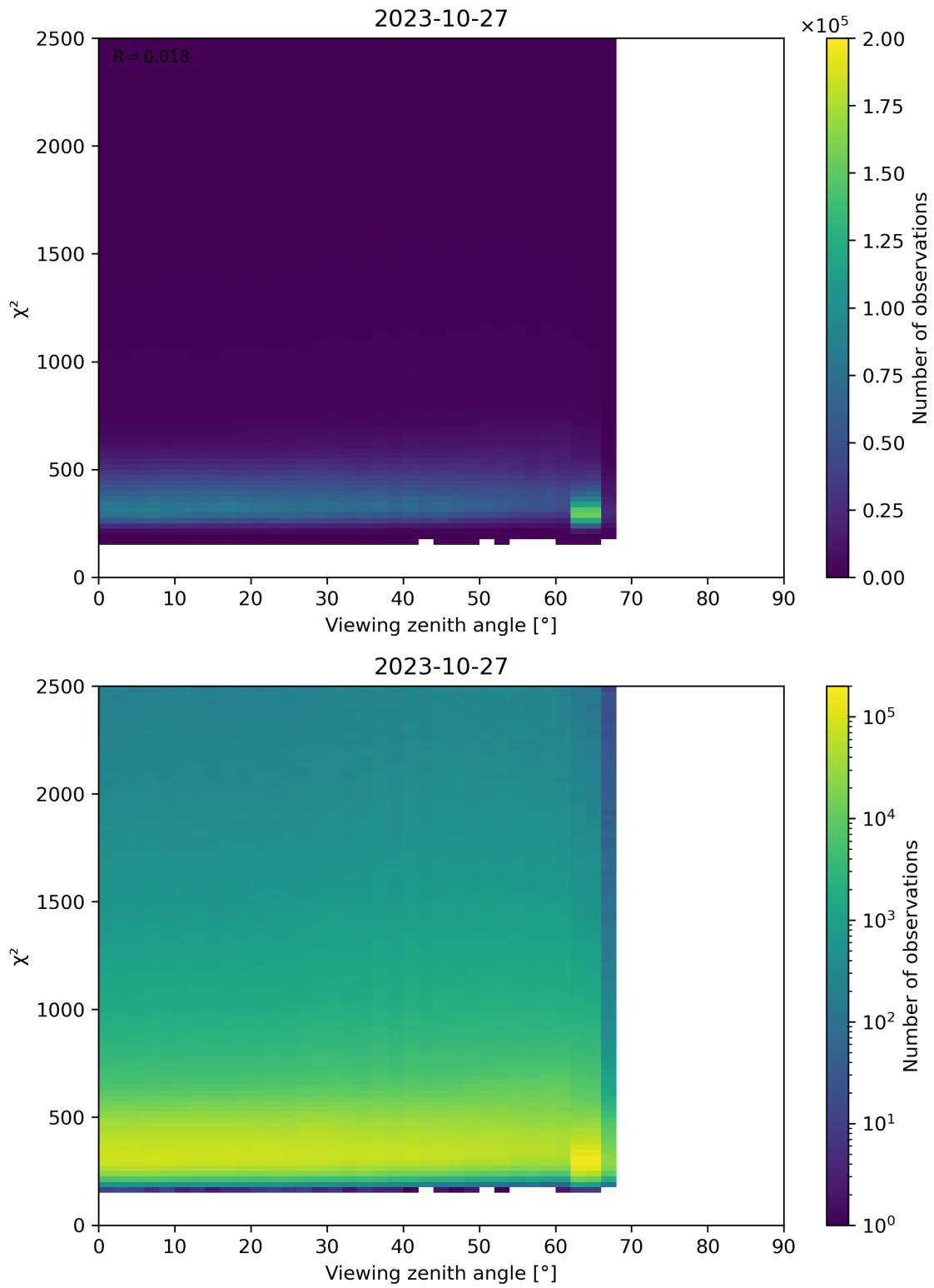
Figure 162: Scatter density plot of “Viewing zenith angle” against “ \chi^2 ” for 2023-10-27 to 2023-10-28.
