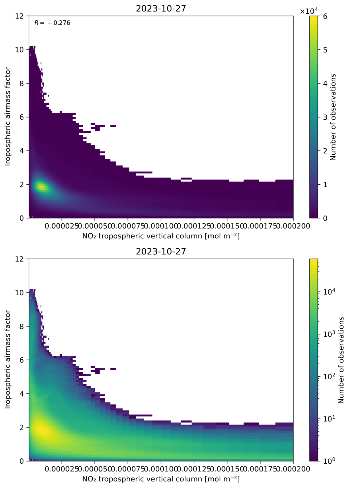
Figure 123: Scatter density plot of “NO 2 tropospheric vertical column” against “Tropospheric air mass factor” for 2023-10-27 to 2023-10-28.
