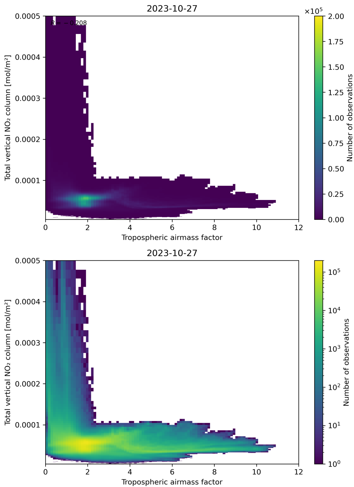
Figure 77: Scatter density plot of “Tropospheric airmass factor” against “Total vertical NO 2 column” for 2023-10-27 to 2023-10-28.
