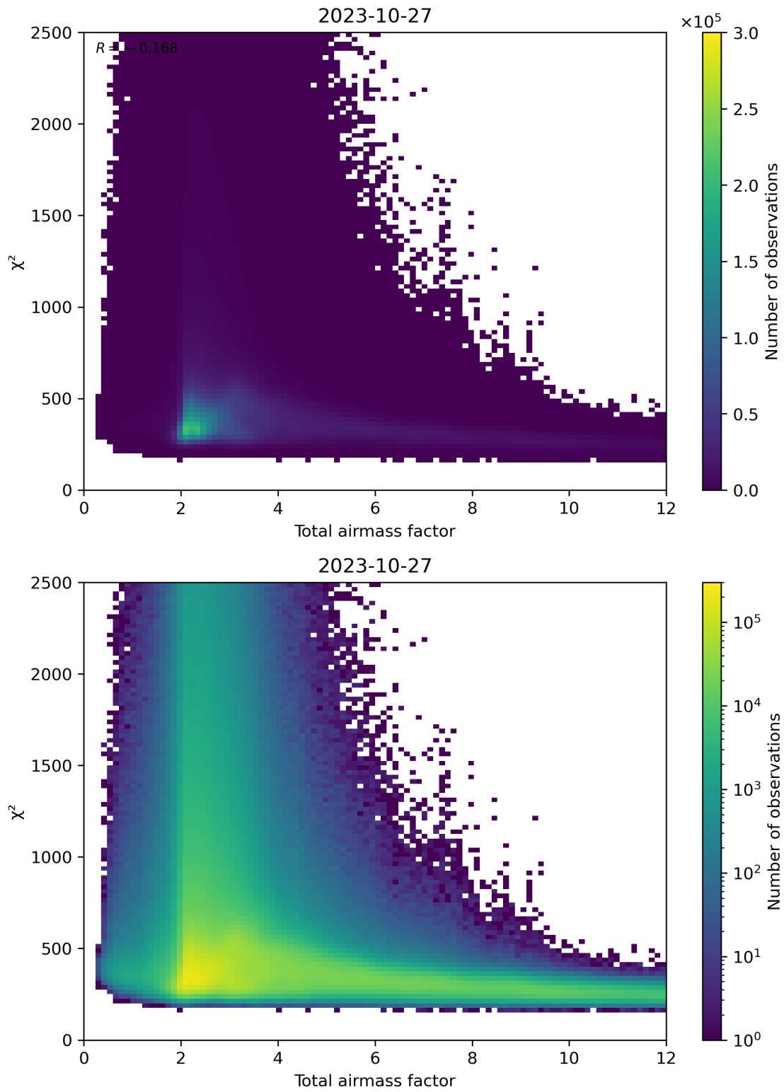
Figure 63: Scatter density plot of “Total airmass factor” against “ \chi^2 ” for 2023-10-27 to 2023-10-28.
