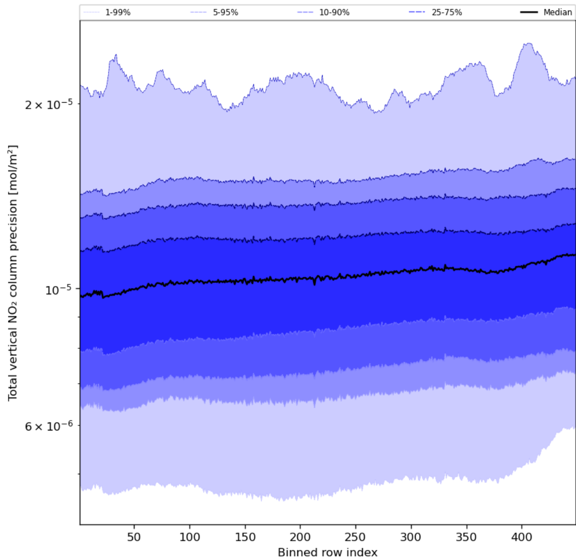
Figure 56: Along track statistics of “Total vertical NO 2 column precision” for 2023-10-27 to 2023-10-28
