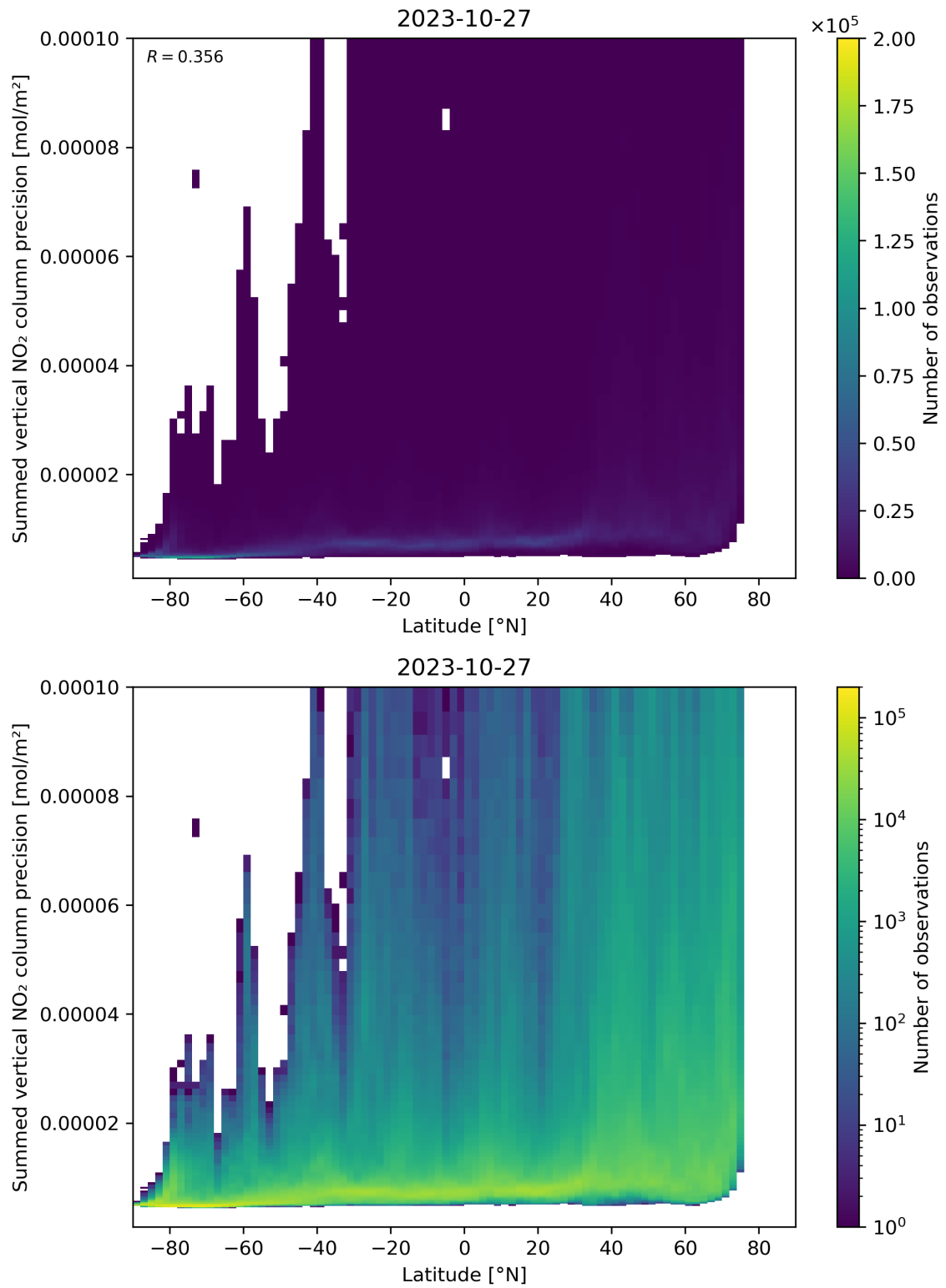
Figure 89: Scatter density plot of “Latitude” against “Summed vertical NO 2 column precision” for 2023-10-27 to 2023-10-28.
