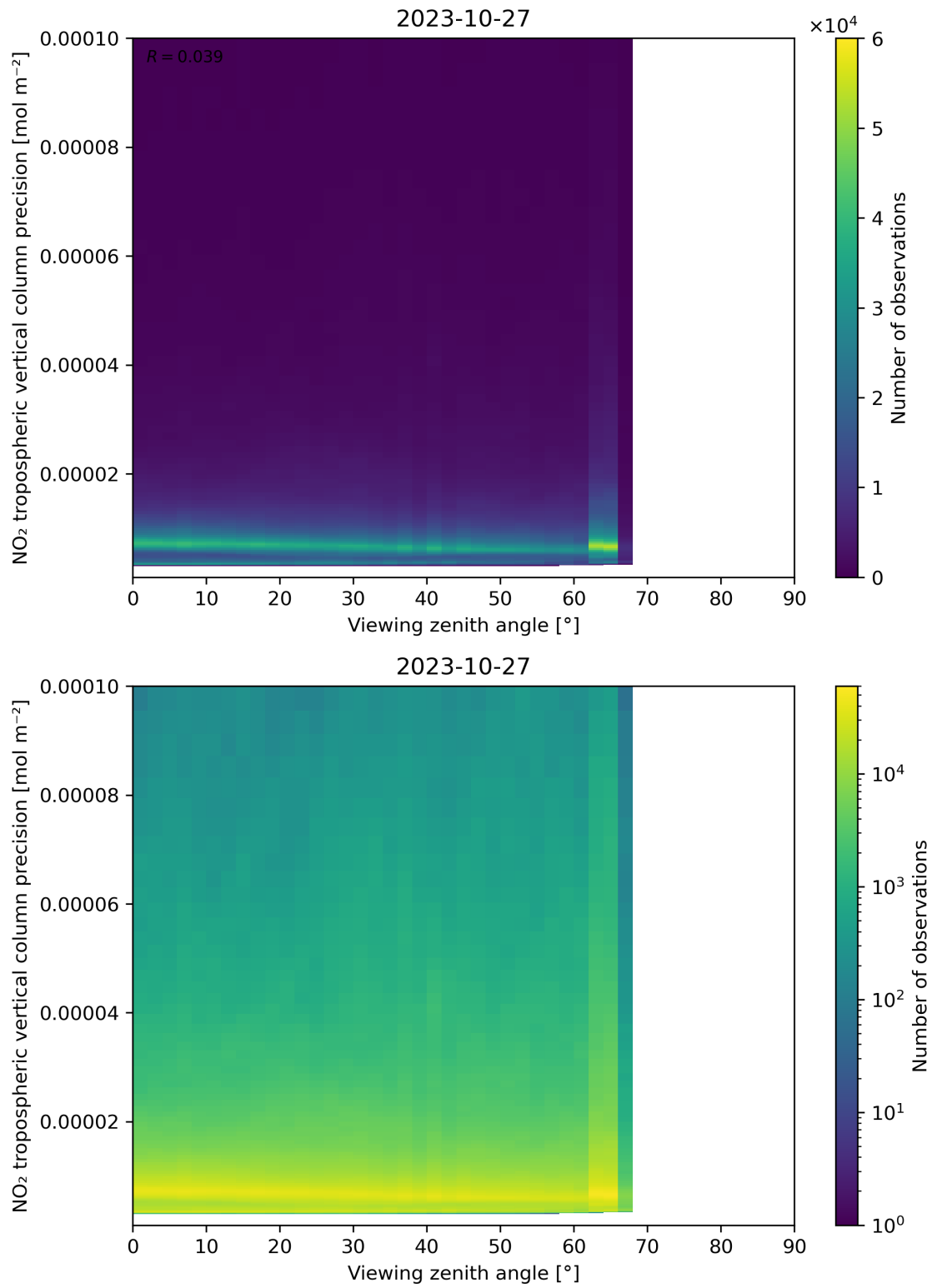
Figure 170: Scatter density plot of “Viewing zenith angle” against “NO 2 tropospheric vertical column precision” for 2023-10-27 to 2023-10-28.
