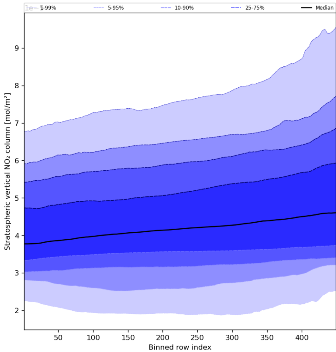
Figure 53: Along track statistics of “Stratospheric vertical NO 2 column” for 2023-10-27 to 2023-10-28
