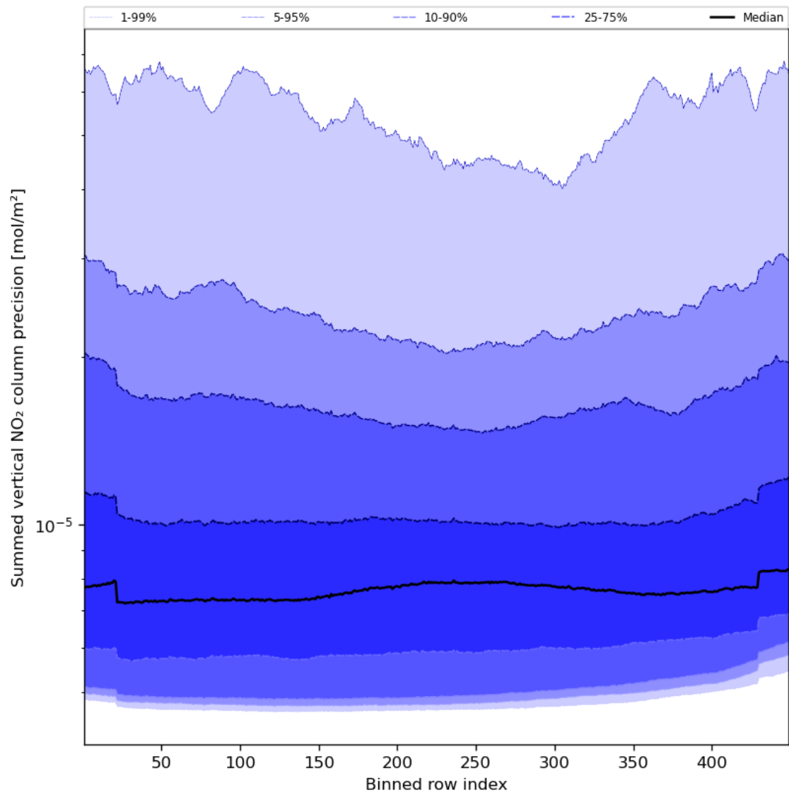
Figure 58: Along track statistics of “Summed vertical NO 2 column precision” for 2023-10-27 to 2023-10-28
