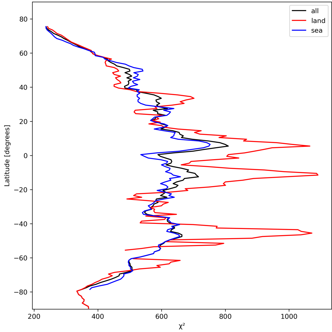
Figure 25: Zonal average of “ \chi^2 ” for 2023-10-27 to 2023-10-28.
