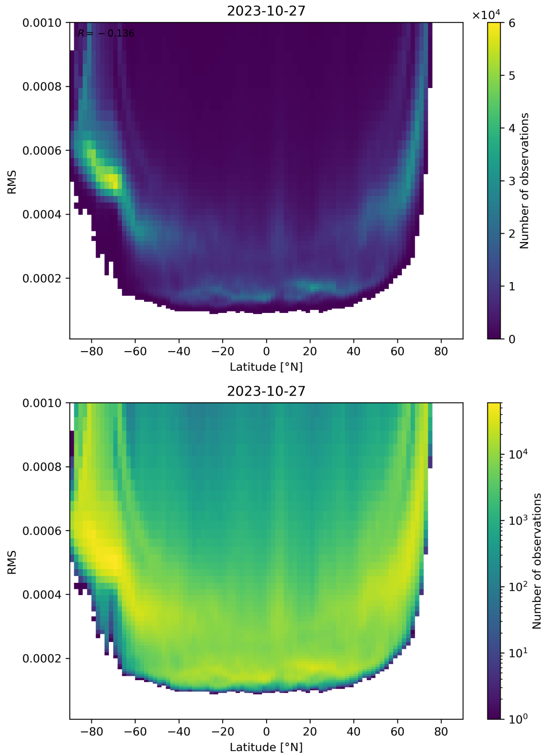
Figure 94: Scatter density plot of “Latitude” against “RMS” for 2023-10-27 to 2023-10-28.
