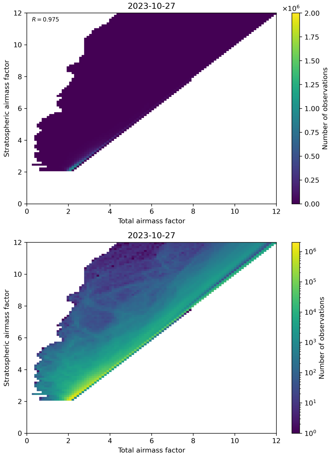
Figure 62: Scatter density plot of “Total airmass factor” against “Stratospheric airmass factor” for 2023-10-27 to 2023-10-28.
