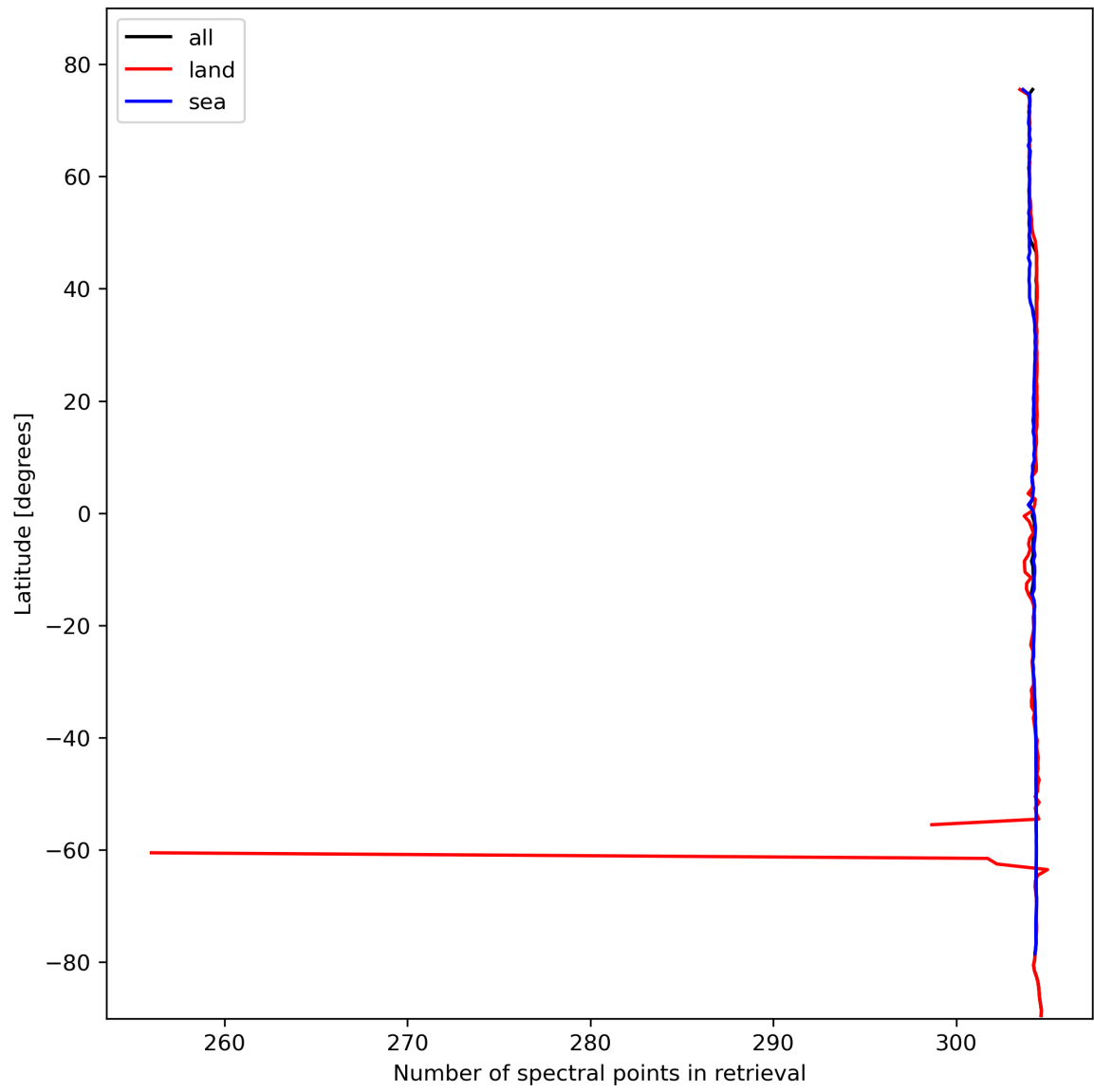
Figure 16: Zonal average of “Number of spectral points in retrieval” for 2023-10-27 to 2023-10-28.
