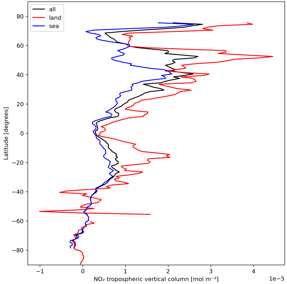
Figure 12: Zonal average of “NO 2 tropospheric vertical column” for 2023-10-27 to 2023-10-28.
