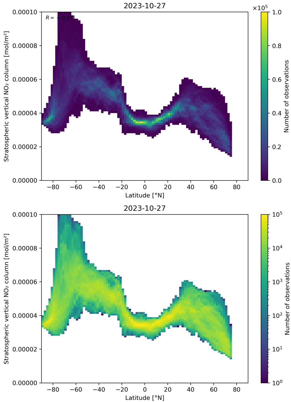
Figure 87: Scatter density plot of “Latitude” against “Stratospheric vertical NO 2 column” for 2023-10-27 to 2023-10-28.
