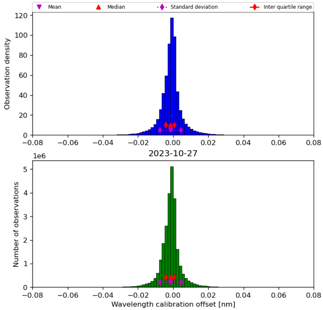
Figure 35: Histogram of “Wavelength calibration offset” for 2023-10-27 to 2023-10-28
