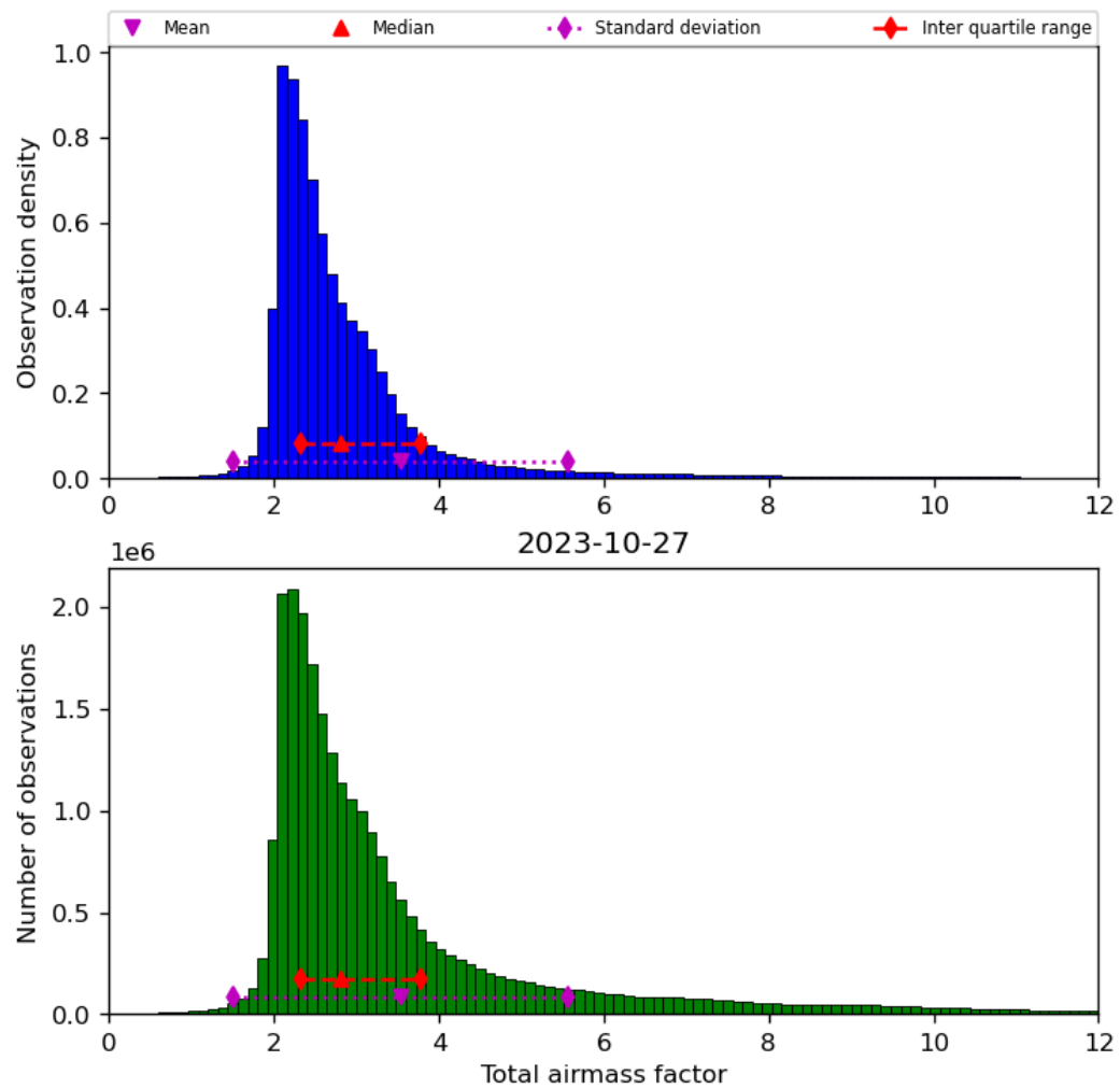
Figure 32: Histogram of “Total airmass factor” for 2023-10-27 to 2023-10-28
