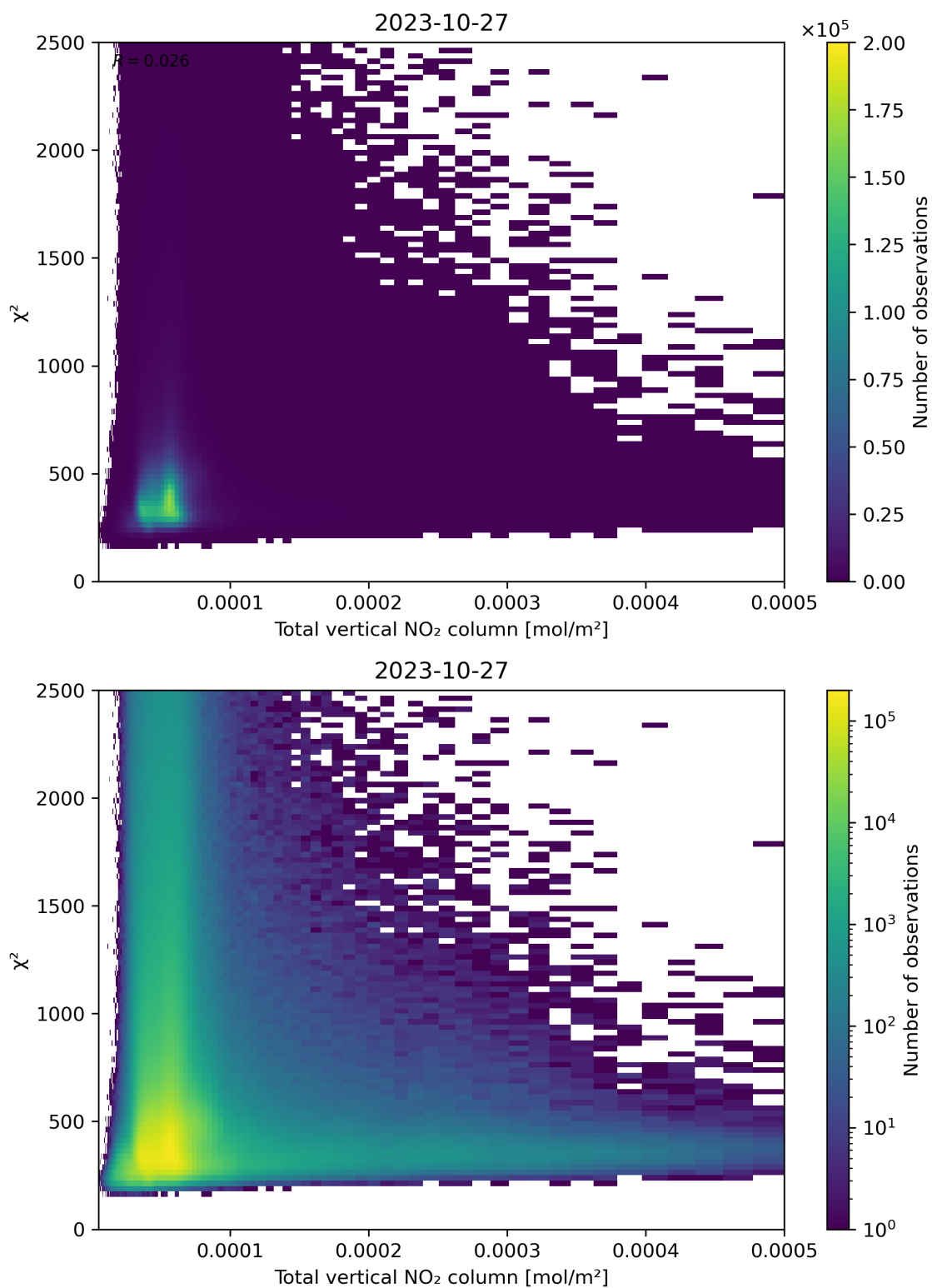
Figure 111: Scatter density plot of “Total vertical NO 2 column” against “ \chi^2 ” for 2023-10-27 to 2023-10-28.
