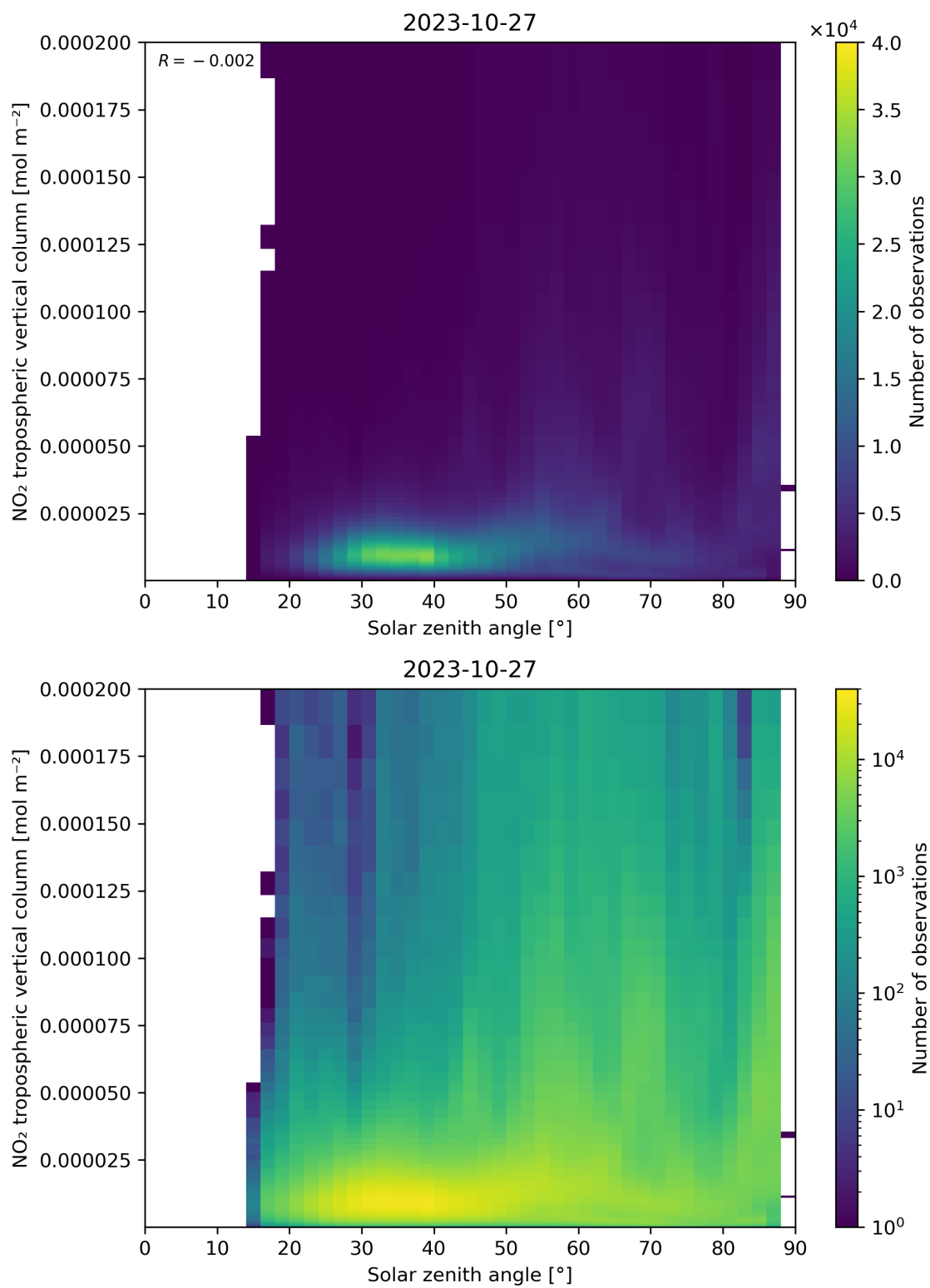
Figure 155: Scatter density plot of “Solar zenith angle” against “NO 2 tropospheric vertical column” for 2023-10-27 to 2023-10-28.
