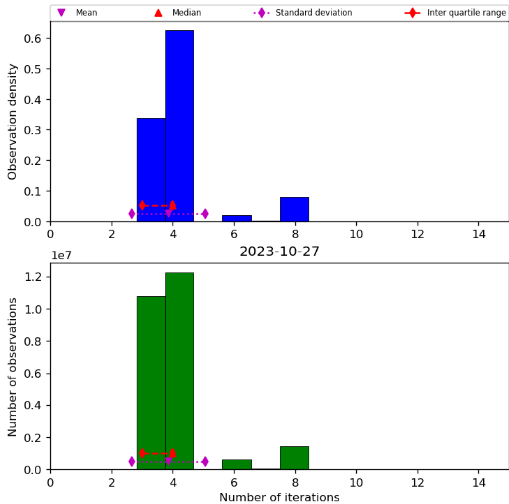
Figure 34: Histogram of “Number of iterations” for 2023-10-27 to 2023-10-28
