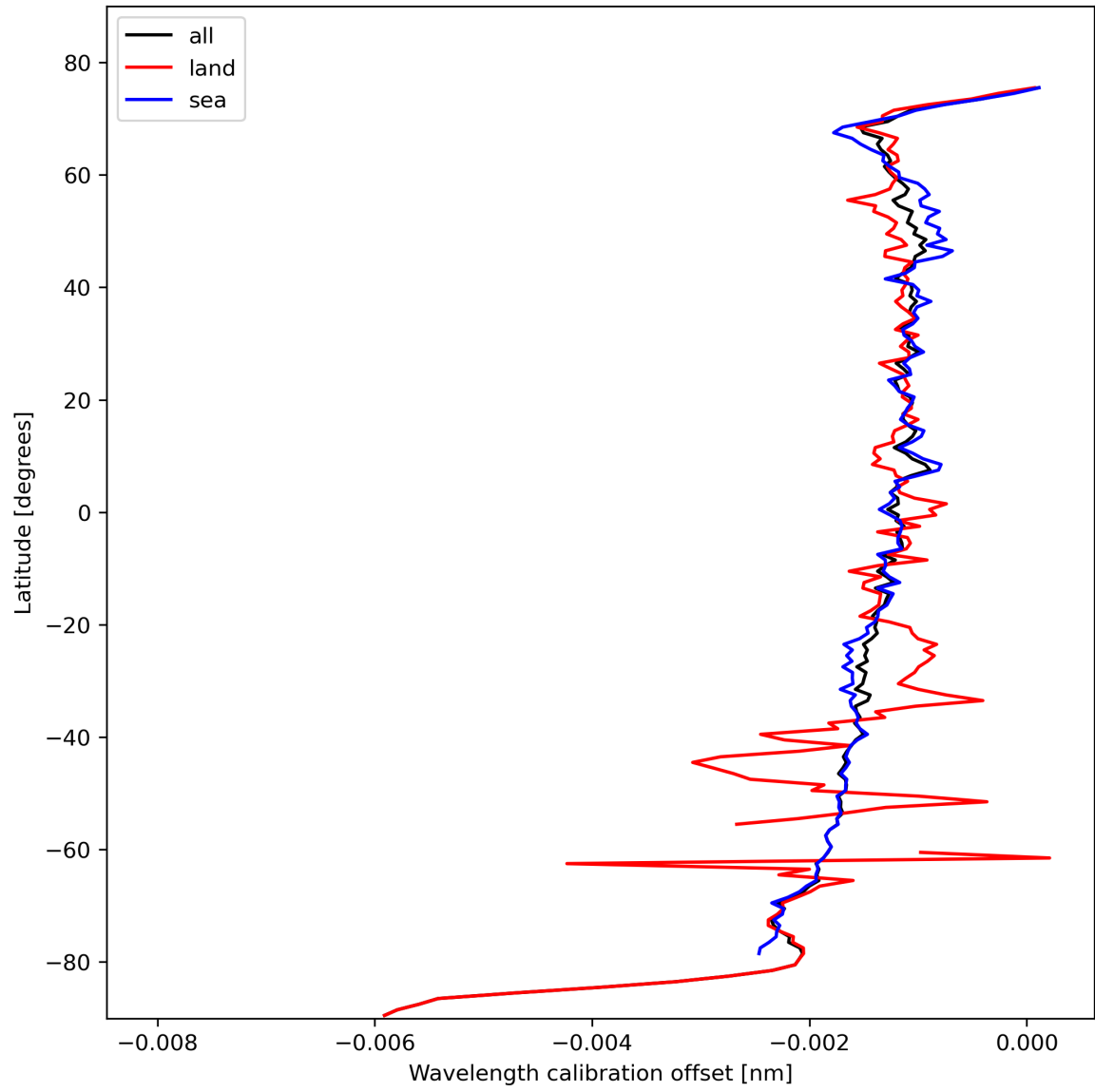
Figure 18: Zonal average of “Wavelength calibration offset” for 2023-10-27 to 2023-10-28.
