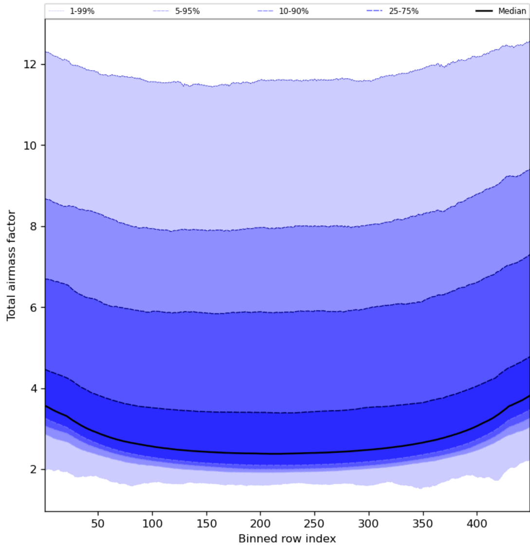
Figure 49: Along track statistics of “Total airmass factor” for 2023-10-27 to 2023-10-28
