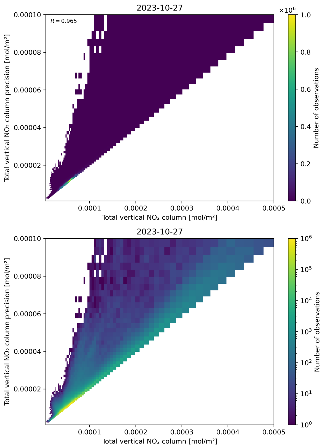
Figure 114: Scatter density plot of “Total vertical NO 2 column” against “Total vertical NO 2 column precision” for 2023-10-27 to 2023-10-28.
