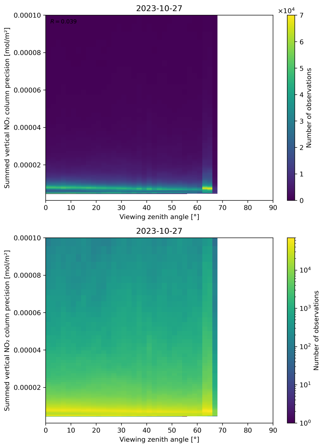
Figure 166: Scatter density plot of “Viewing zenith angle” against “Summed vertical NO 2 column precision” for 2023-10-27 to 2023-10-28.
