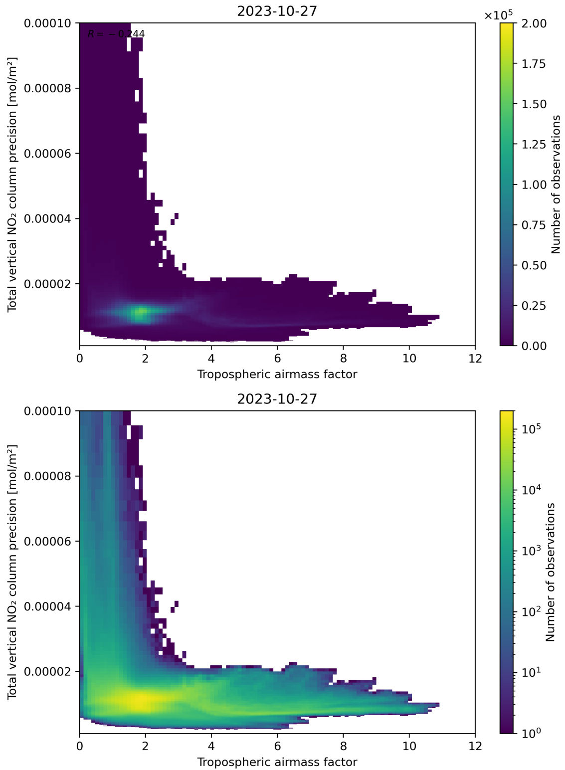
Figure 78: Scatter density plot of “Tropospheric air mass factor” against “Total vertical NO 2 column precision” for 2023-10-27 to 2023-10-28.
