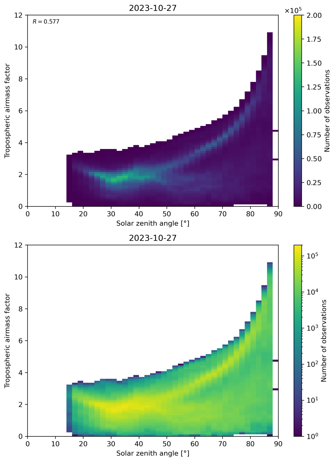
Figure 147: Scatter density plot of “Solar zenith angle” against “Tropospheric airmass factor” for 2023-10-27 to 2023-10-28.
