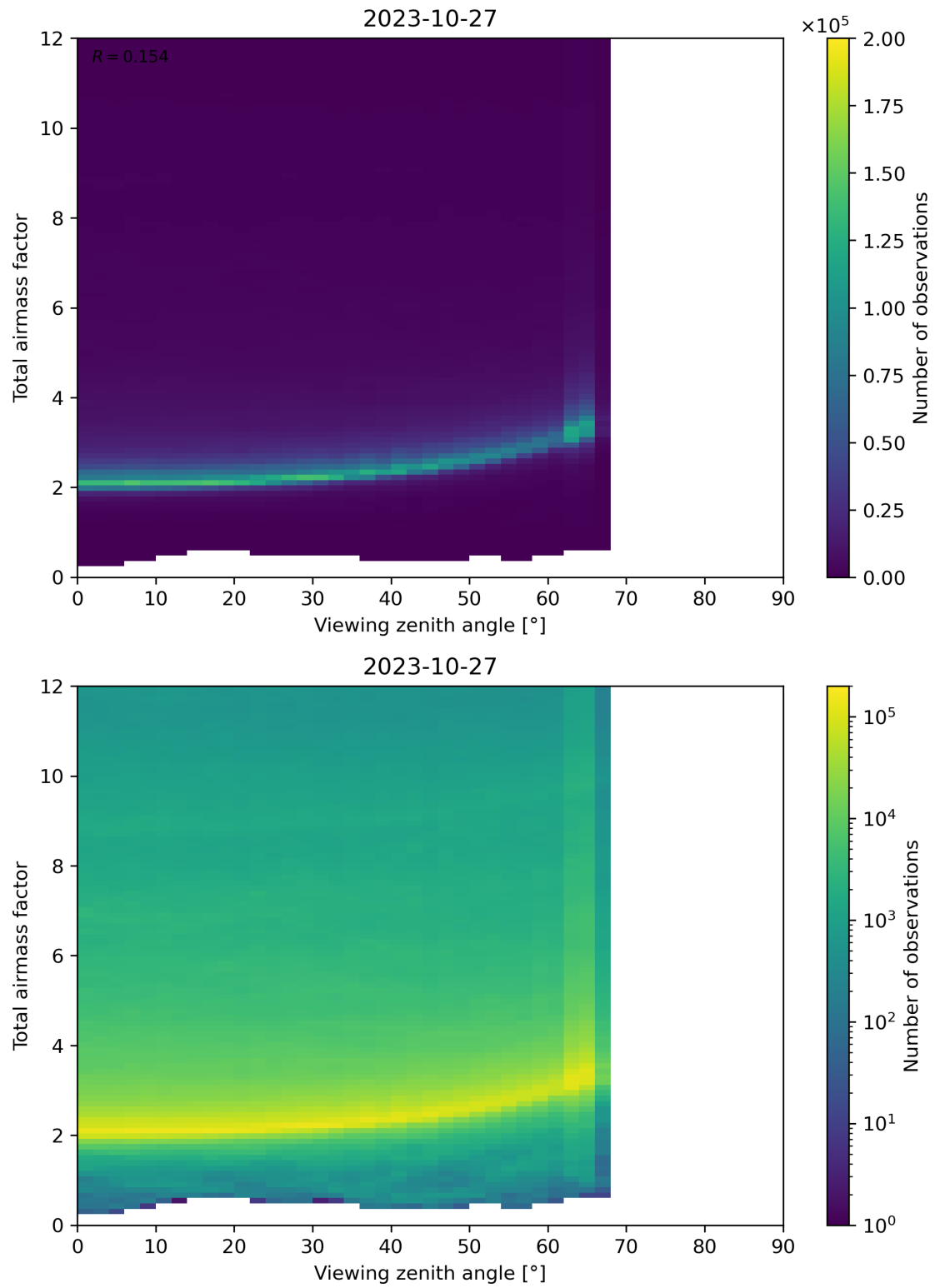
Figure 160: Scatter density plot of “Viewing zenith angle” against “Total airmass factor” for 2023-10-27 to 2023-10-28.
