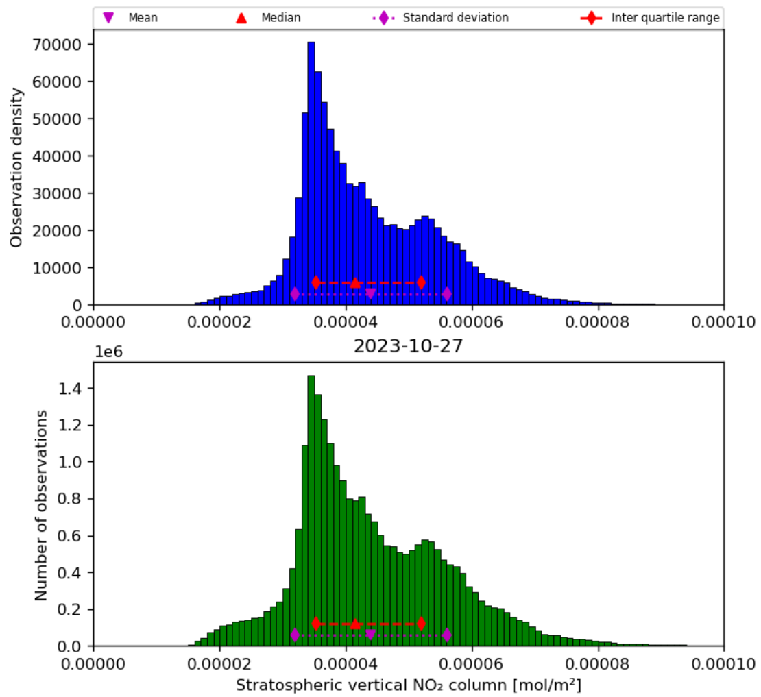
Figure 36: Histogram of “Stratospheric vertical NO 2 column” for 2023-10-27 to 2023-10-28
