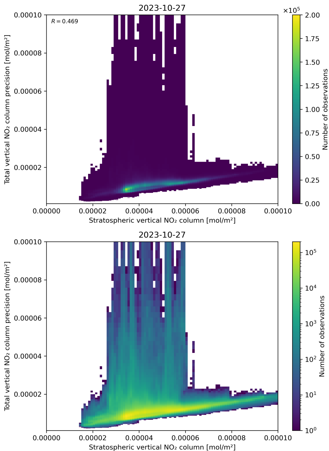
Figure 101: Scatter density plot of “Stratospheric vertical NO 2 column” against “Total vertical NO 2 column precision” for 2023-10-27 to 2023-10-28.
