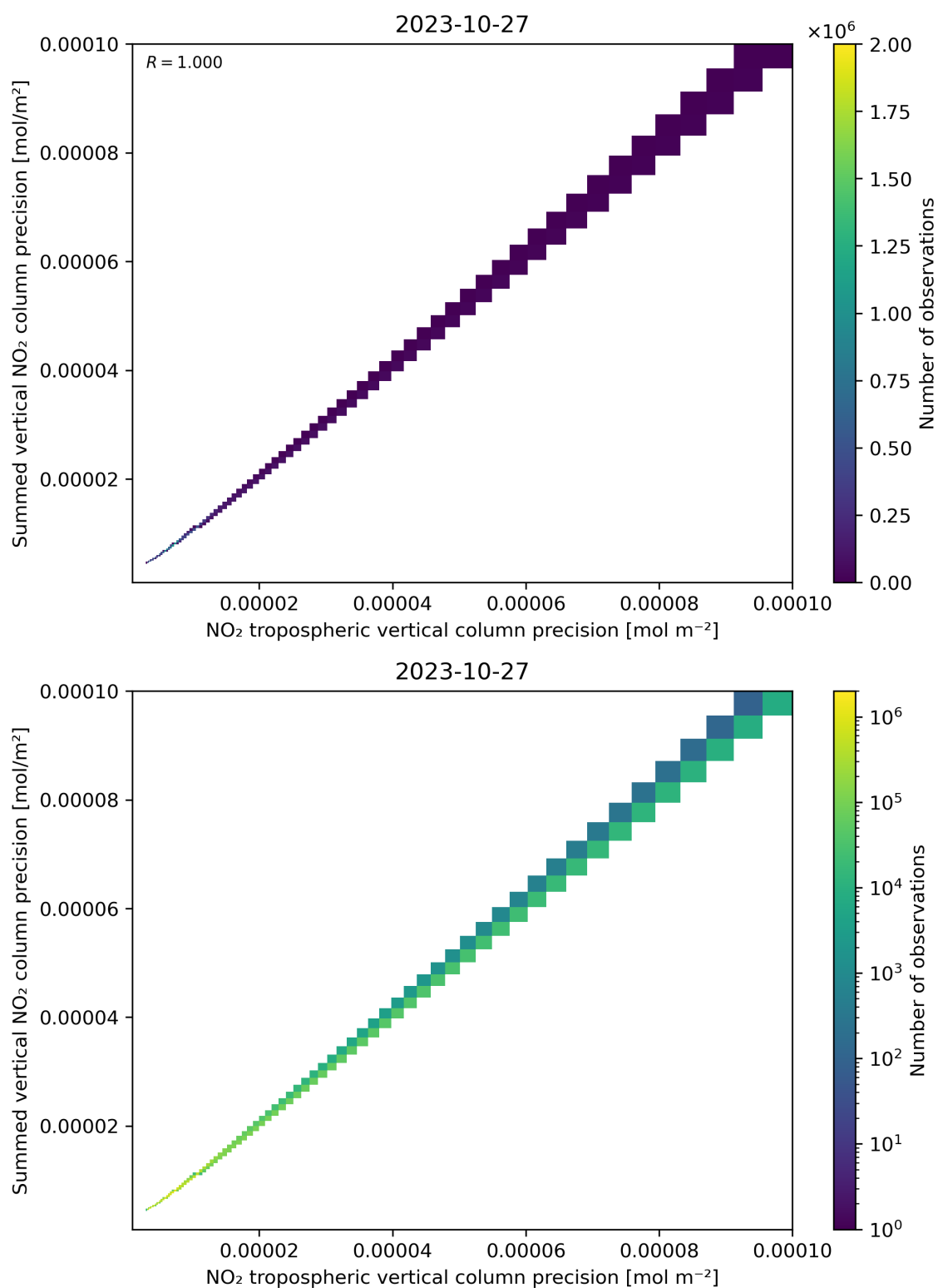
Figure 137: Scatter density plot of “NO 2 tropospheric vertical column precision” against “Summed vertical NO 2 column precision” for 2023-10-27 to 2023-10-28.
