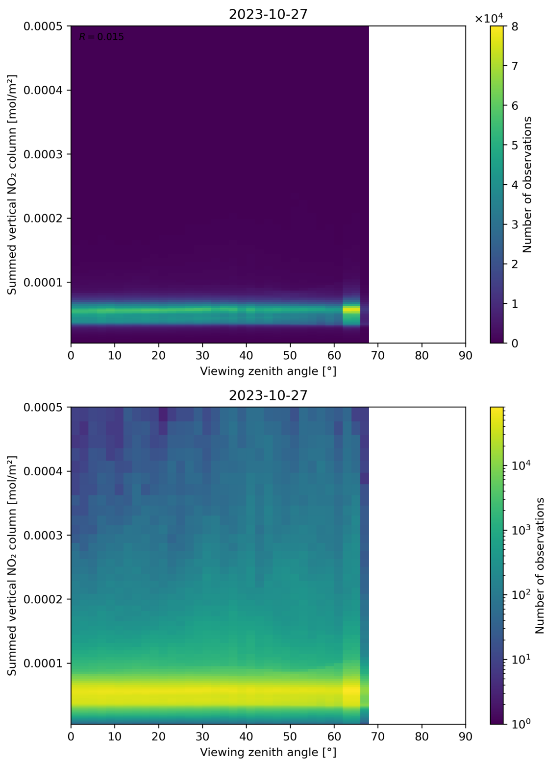
Figure 165: Scatter density plot of “Viewing zenith angle” against “Summed vertical NO 2 column” for 2023-10-27 to 2023-10-28.
