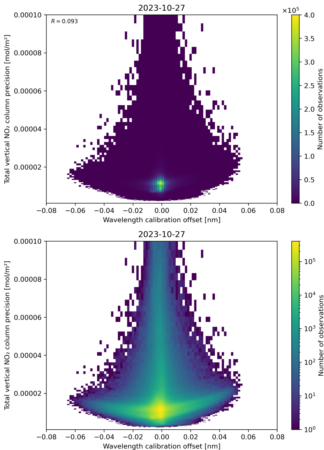
Figure 180: Scatter density plot of “Wavelength calibration offset” against “Total vertical NO 2 column precision” for 2023-10-27 to 2023-10-28.
