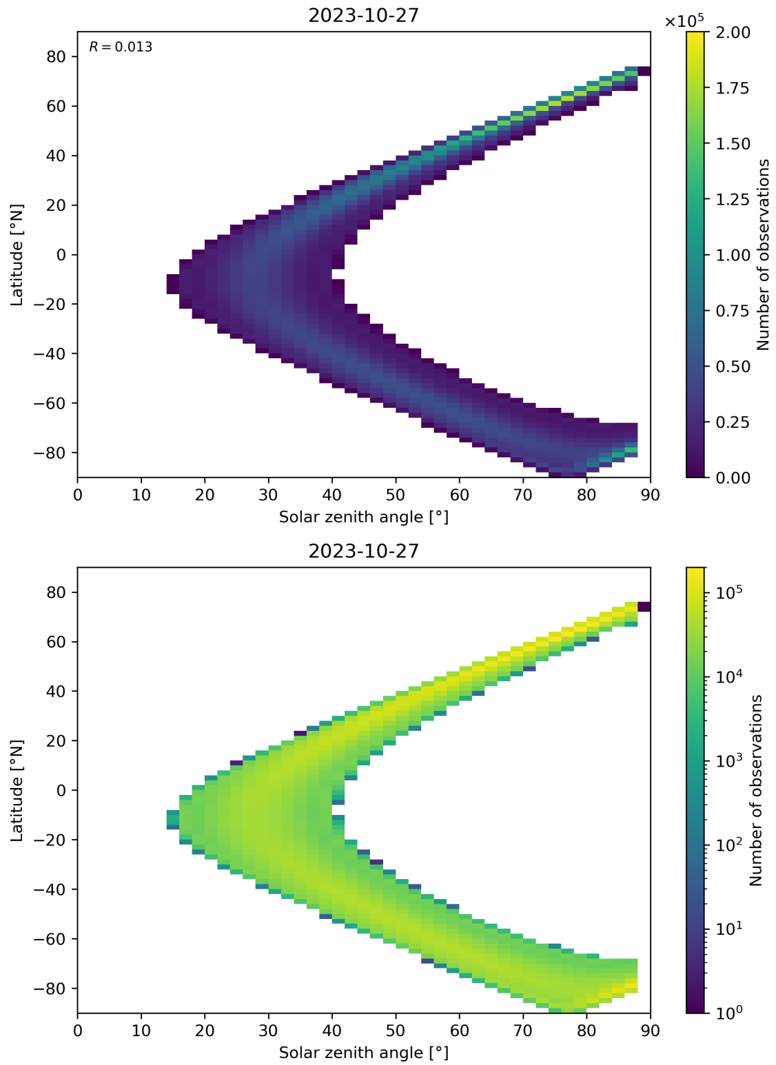
Figure 149: Scatter density plot of “Solar zenith angle” against “Latitude” for 2023-10-27 to 2023-10-28.
