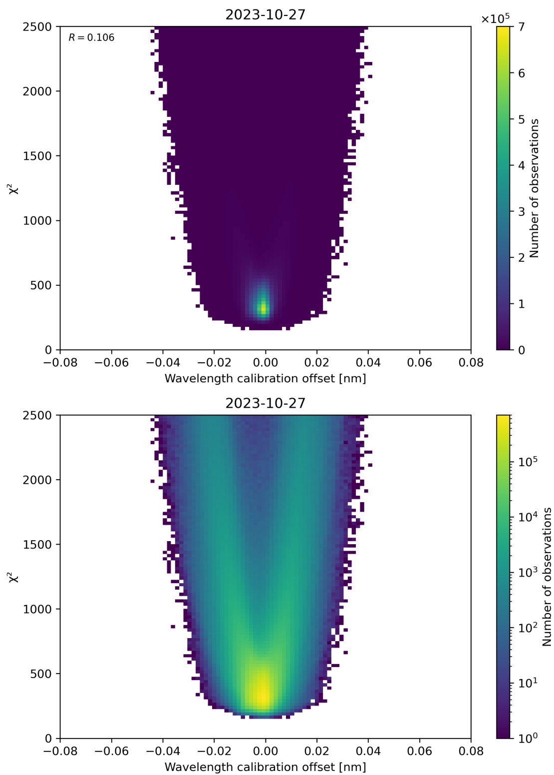
Figure 175: Scatter density plot of “Wavelength calibration offset” against “ \chi^2 ” for 2023-10-27 to 2023-10-28.
