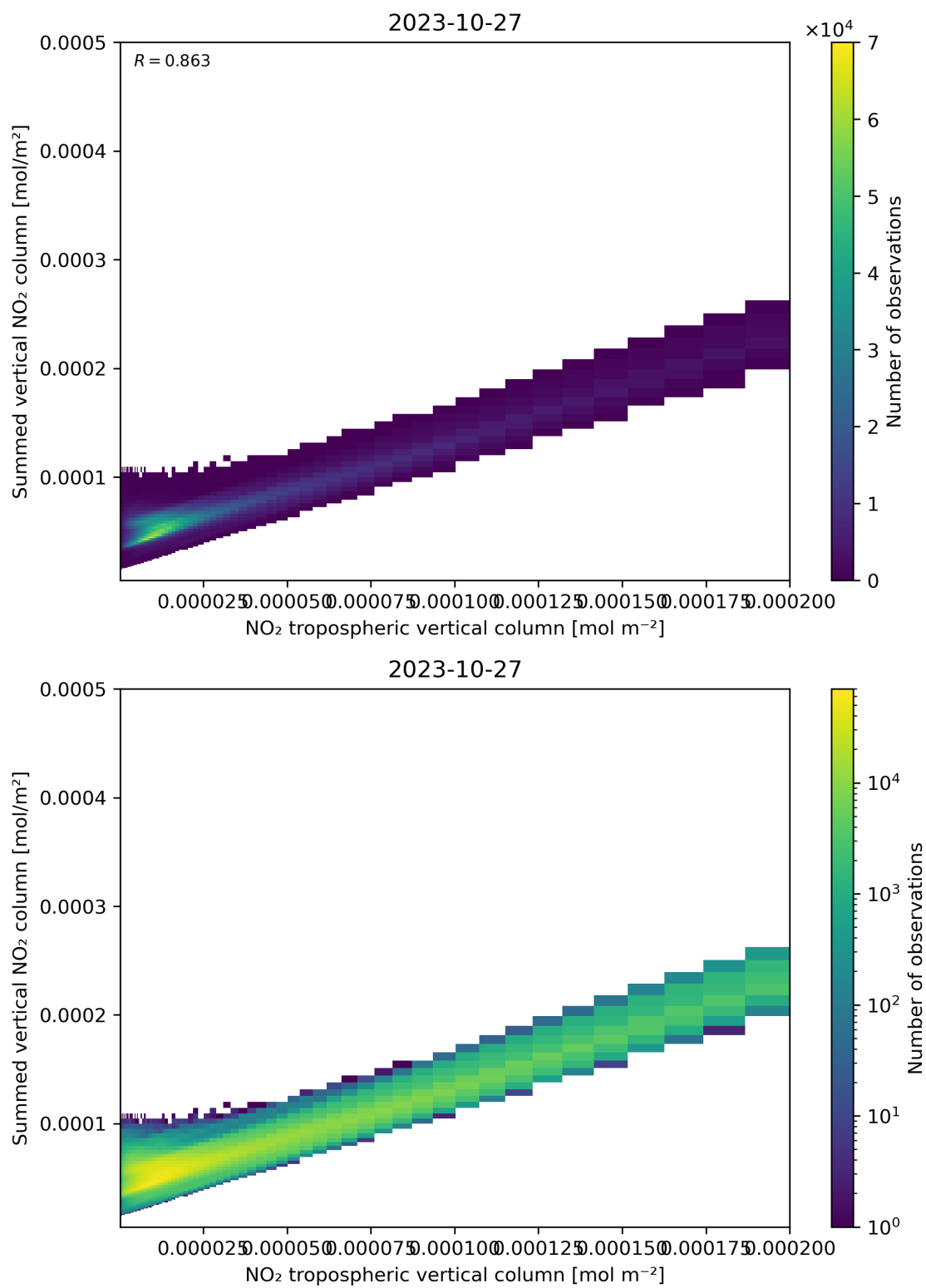
Figure 126: Scatter density plot of “NO 2 tropospheric vertical column” against “Summed vertical NO 2 column” for 2023-10-27 to 2023-10-28.
