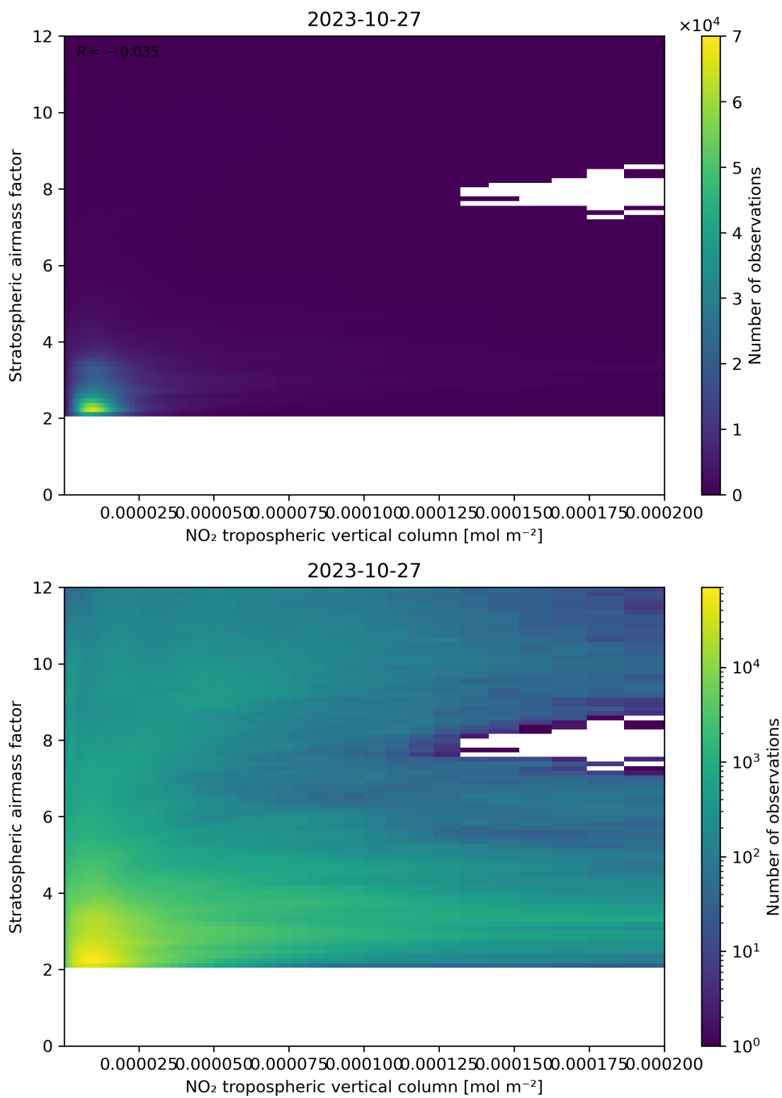
Figure 121: Scatter density plot of “NO 2 tropospheric vertical column” against “Stratospheric air mass factor” for 2023-10-27 to 2023-10-28.
