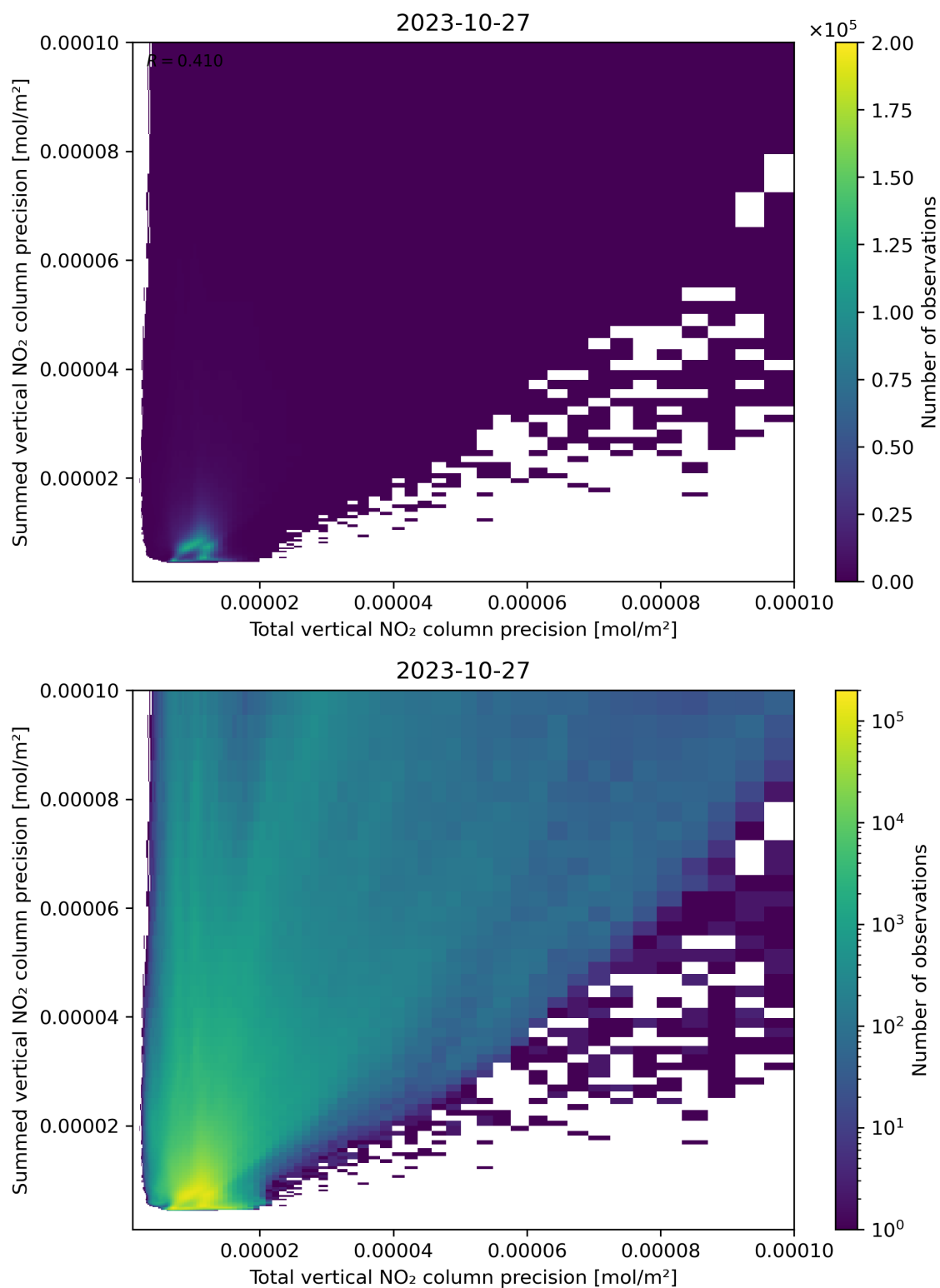
Figure 118: Scatter density plot of “Total vertical NO 2 column precision” against “Summed vertical NO 2 column precision” for 2023-10-27 to 2023-10-28.
