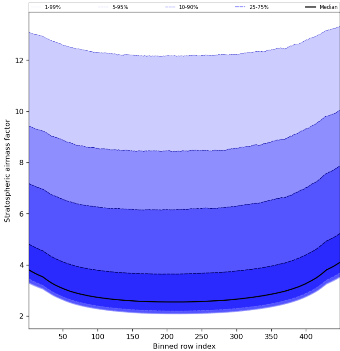
Figure 61: Along track statistics of “Stratospheric airmass factor” for 2023-10-27 to 2023-10-28
