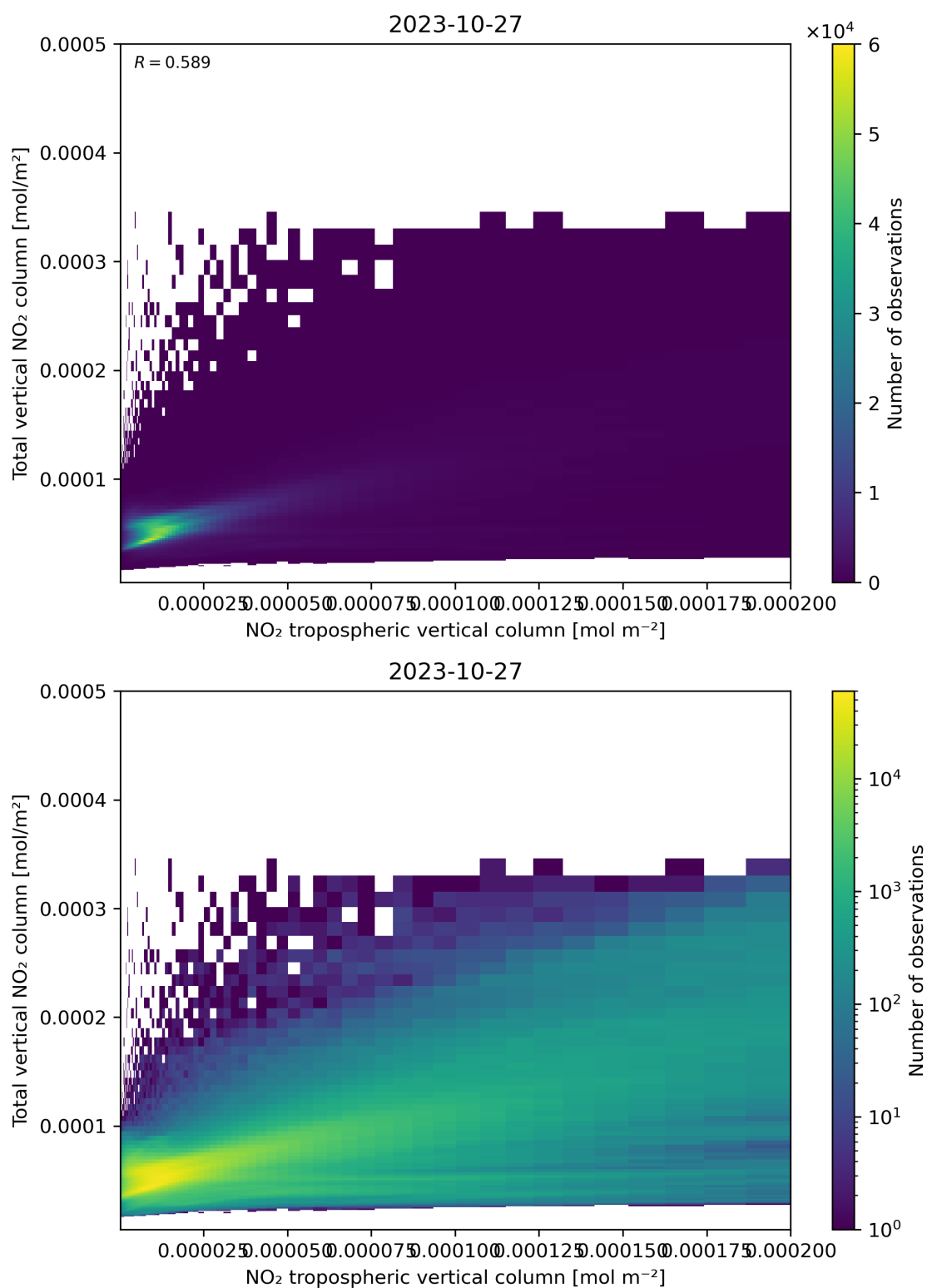
Figure 128: Scatter density plot of “NO 2 tropospheric vertical column” against “Total vertical NO 2 column” for 2023-10-27 to 2023-10-28.
