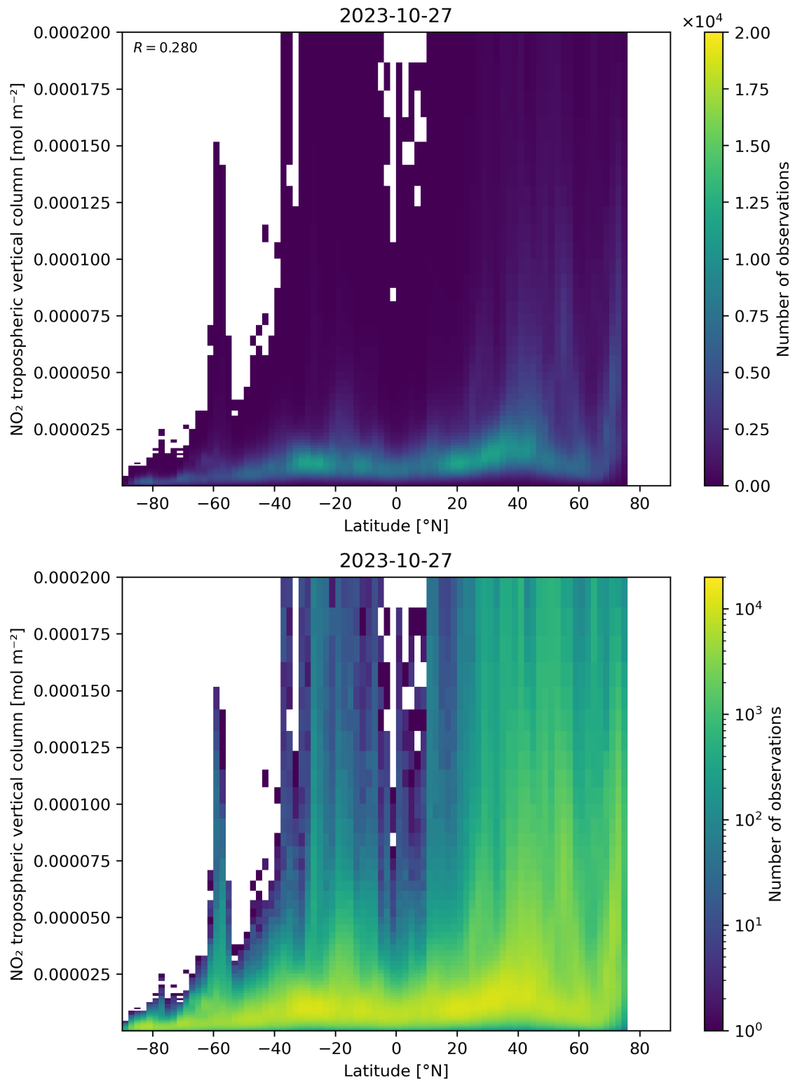
Figure 92: Scatter density plot of “Latitude” against “NO 2 tropospheric vertical column” for 2023-10-27 to 2023-10-28.
