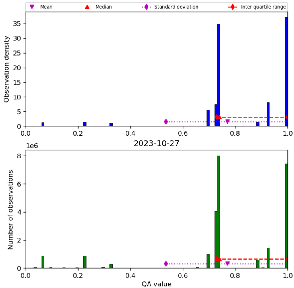
Figure 28: Histogram of “QA value” for 2023-10-27 to 2023-10-28
