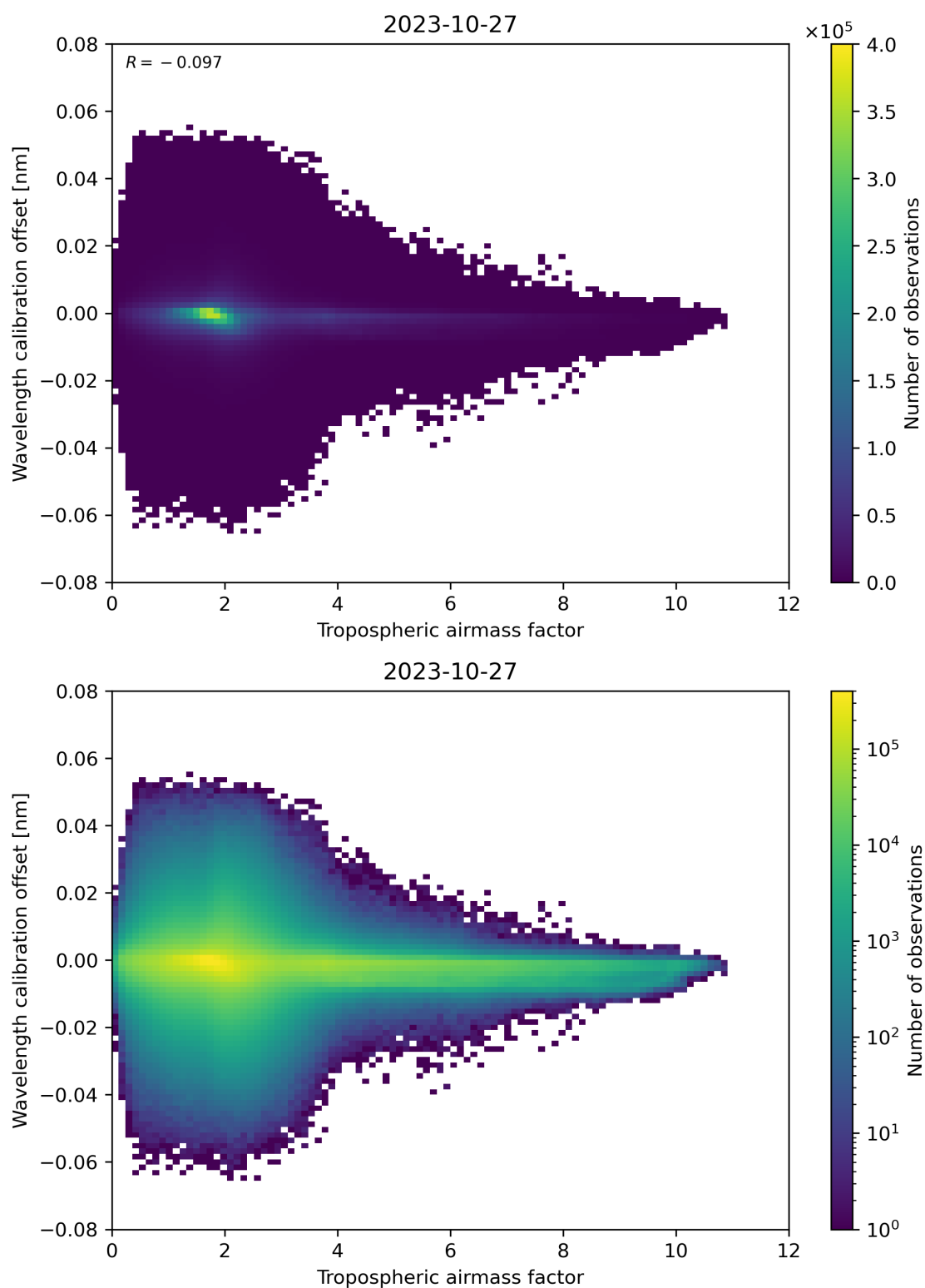
Figure 80: Scatter density plot of “Tropospheric airmass factor” against “Wavelength calibration offset” for 2023-10-27 to 2023-10-28.
