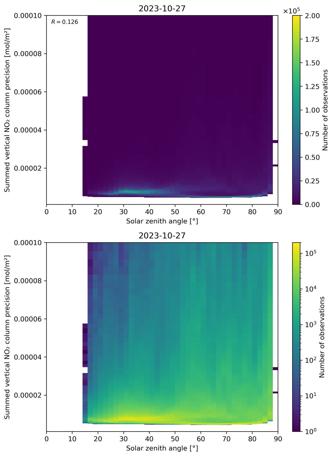
Figure 152: Scatter density plot of “Solar zenith angle” against “Summed vertical NO 2 column precision” for 2023-10-27 to 2023-10-28.
