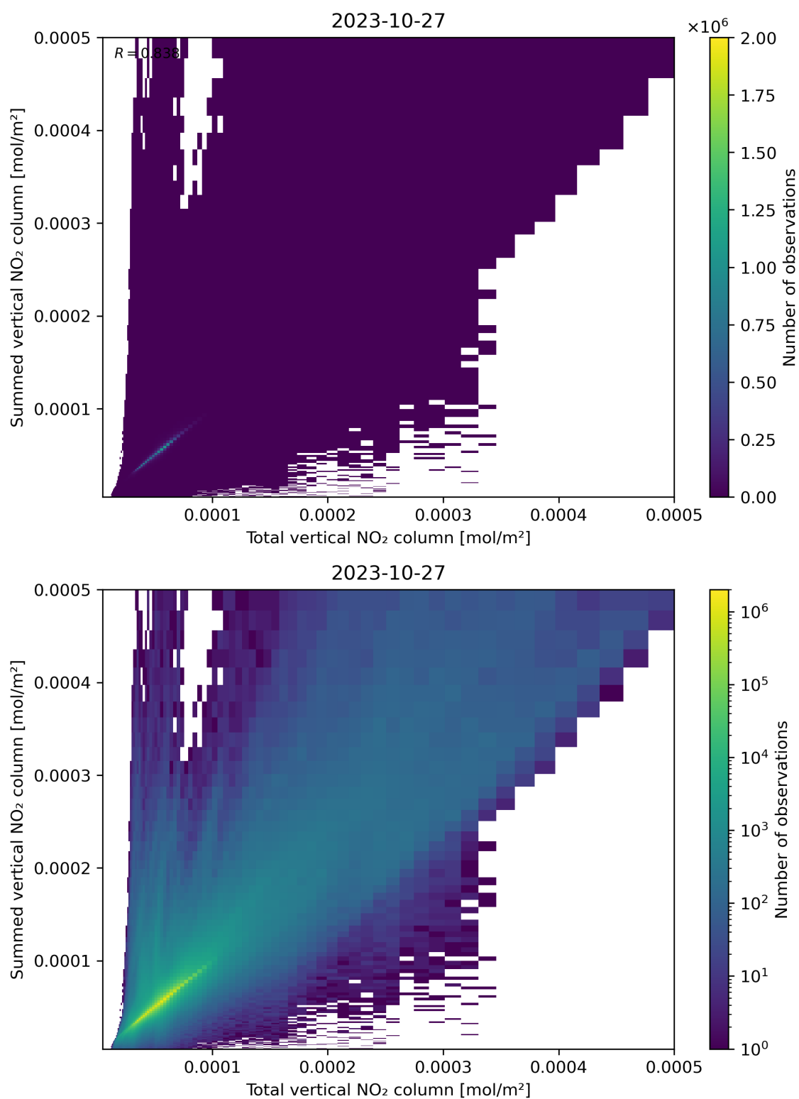
Figure 112: Scatter density plot of “Total vertical NO 2 column” against “Summed vertical NO 2 column” for 2023-10-27 to 2023-10-28.
