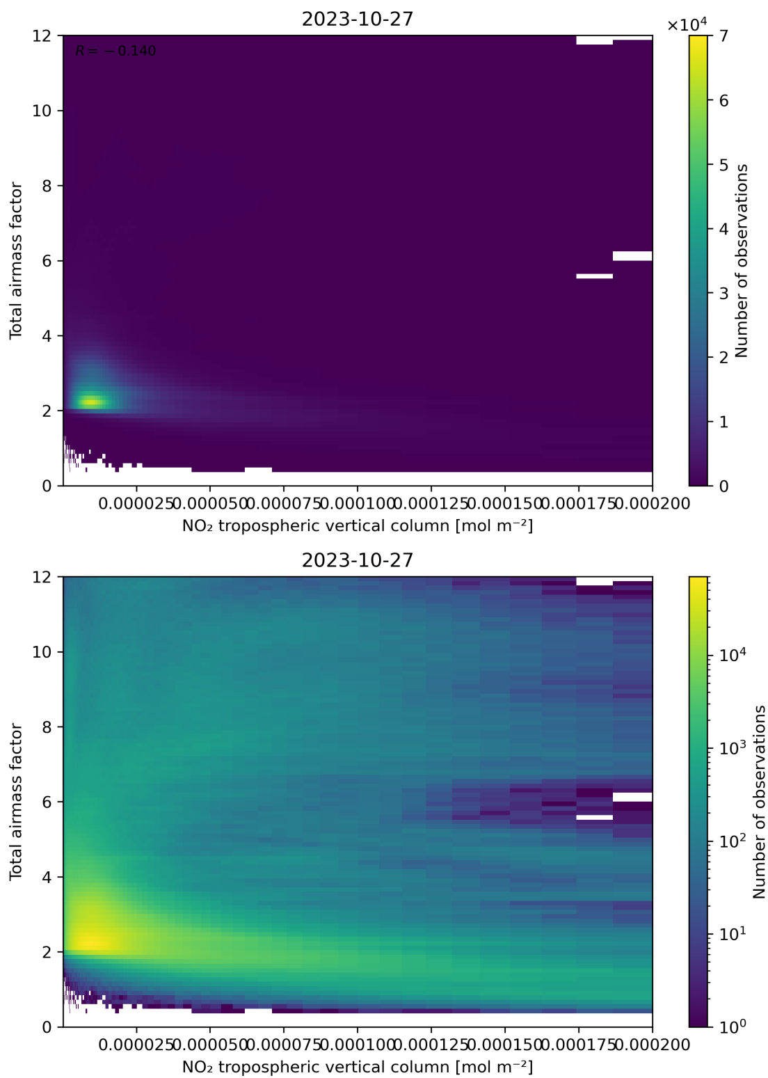
Figure 122: Scatter density plot of “NO 2 tropospheric vertical column” against “Total air mass factor” for 2023-10-27 to 2023-10-28.
