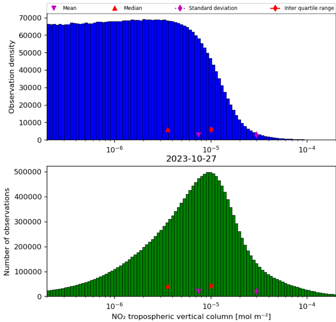
Figure 29: Histogram of “NO 2 tropospheric vertical column” for 2023-10-27 to 2023-10-28
