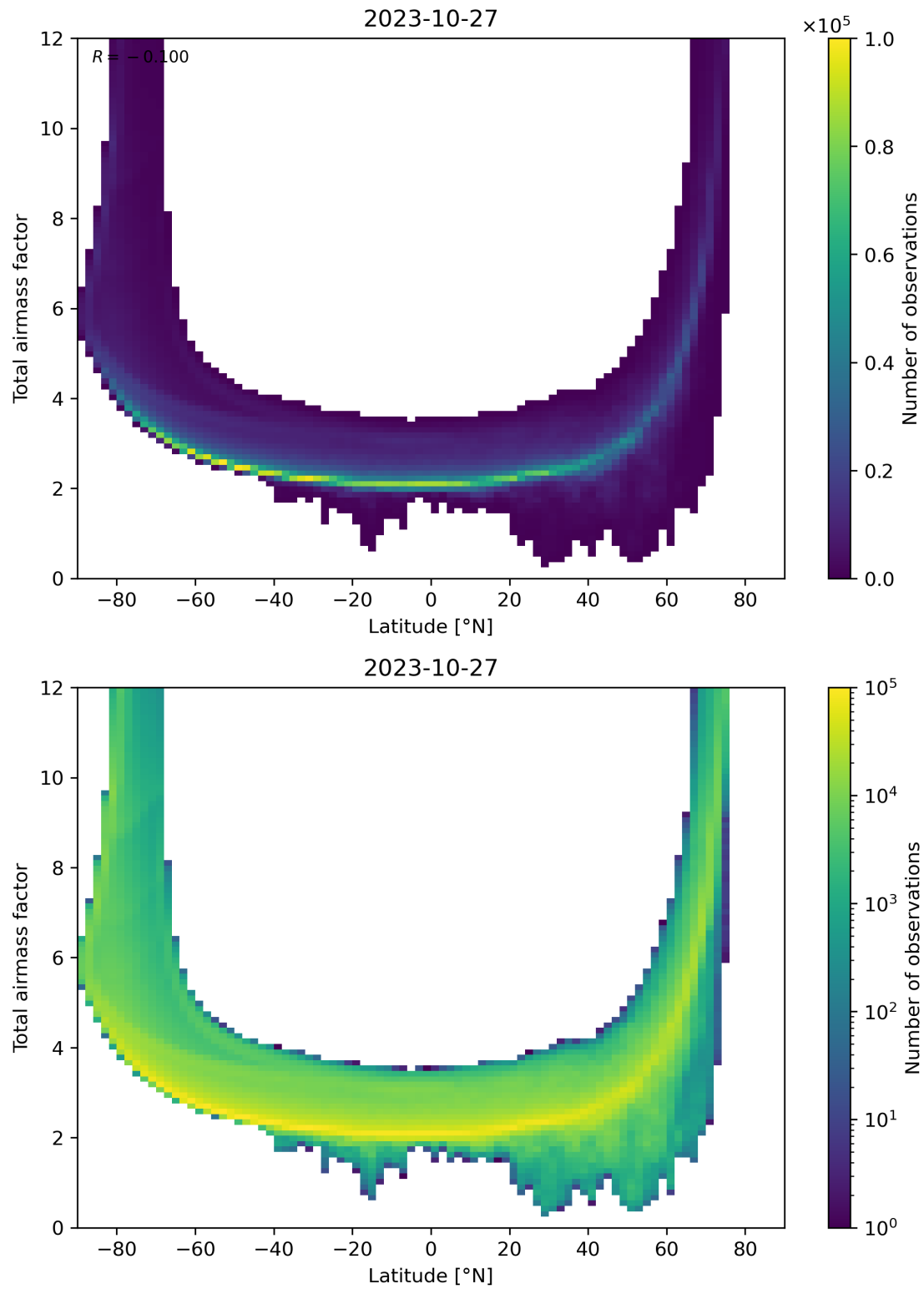
Figure 84: Scatter density plot of “Latitude” against “Total airmass factor” for 2023-10-27 to 2023-10-28.
