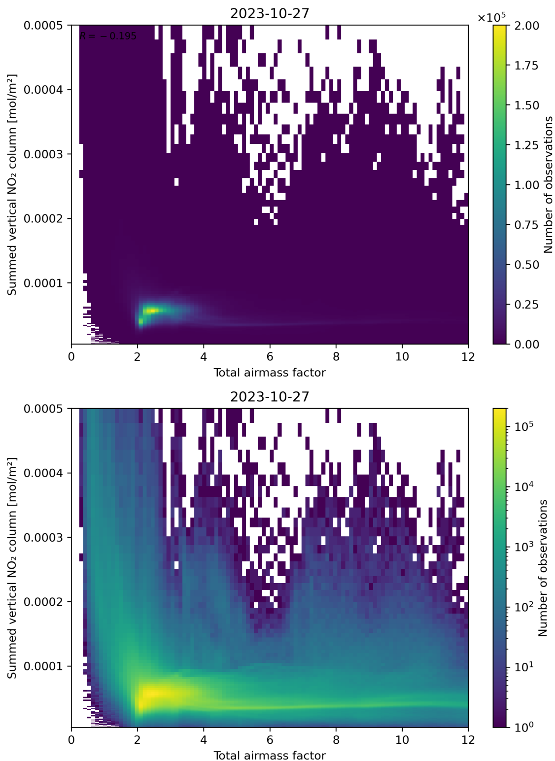
Figure 65: Scatter density plot of “Total airmass factor” against “Summed vertical NO 2 column” for 2023-10-27 to 2023-10-28.
