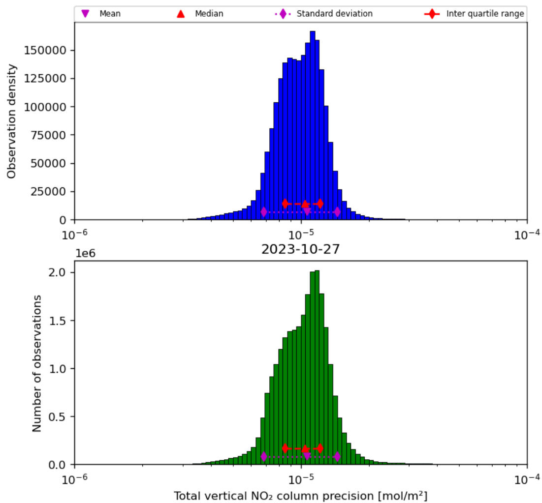
Figure 39: Histogram of “Total vertical NO 2 column precision” for 2023-10-27 to 2023-10-28
