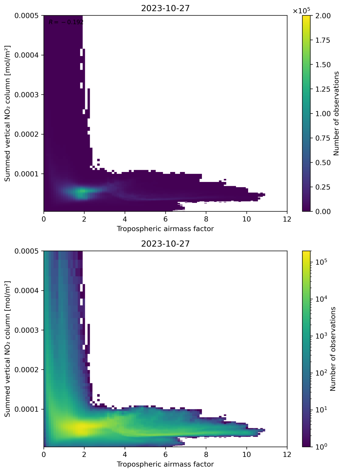
Figure 75: Scatter density plot of “Tropospheric airmass factor” against “Summed vertical NO 2 column” for 2023-10-27 to 2023-10-28.
