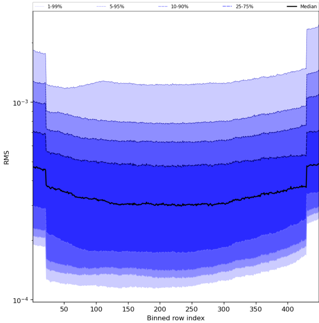
Figure 60: Along track statistics of “RMS” for 2023-10-27 to 2023-10-28
