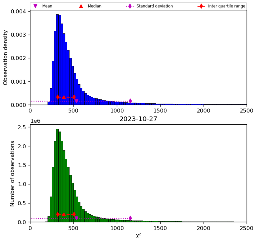
Figure 42: Histogram of " \chi^2 " for 2023-10-27 to 2023-10-28
