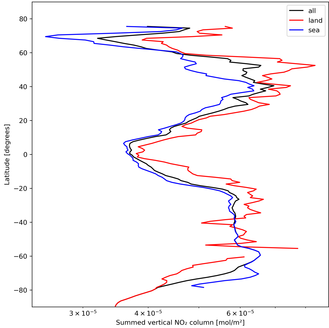
Figure 23: Zonal average of “Summed vertical NO 2 column” for 2023-10-27 to 2023-10-28.
