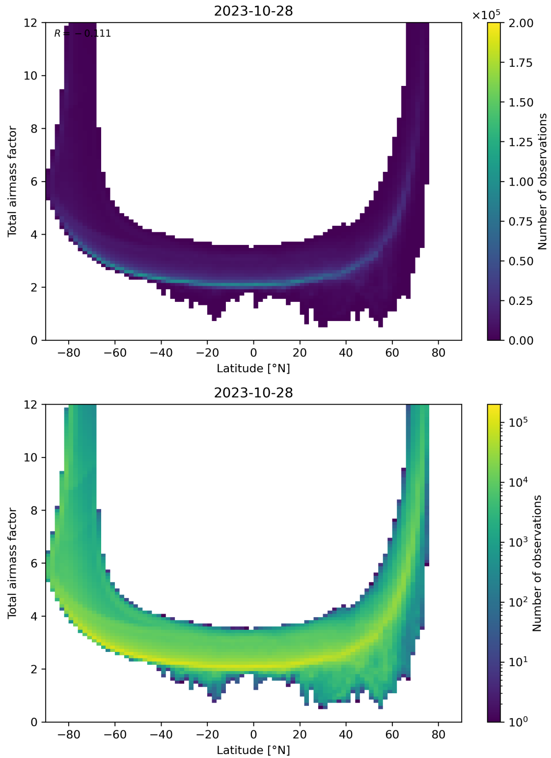
Figure 84: Scatter density plot of “Latitude” against “Total airmass factor” for 2023-10-28 to 2023-10-29.
