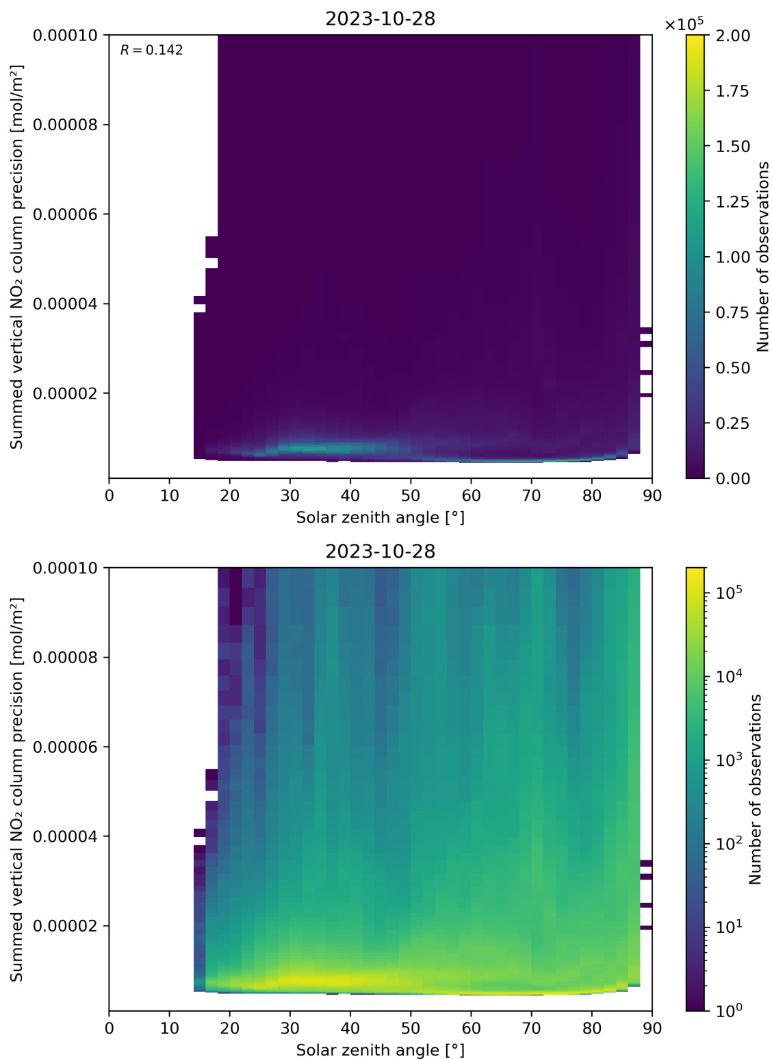
Figure 152: Scatter density plot of “Solar zenith angle” against “Summed vertical NO 2 column precision” for 2023-10-28 to 2023-10-29.
