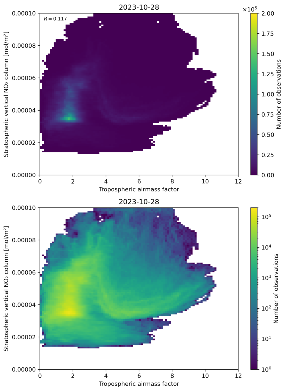
Figure 74: Scatter density plot of “Tropospheric air mass factor” against “Stratospheric vertical NO 2 column” for 2023-10-28 to 2023-10-29.
