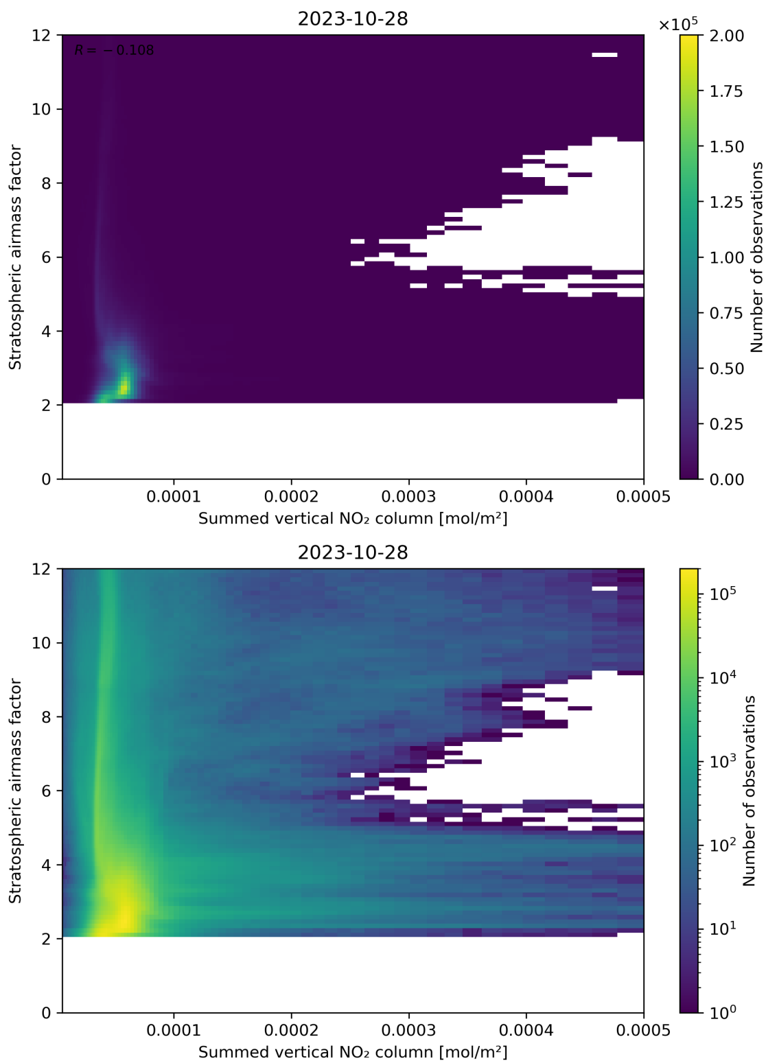
Figure 103: Scatter density plot of “Summed vertical NO 2 column” against “Stratospheric air mass factor” for 2023-10-28 to 2023-10-29.
