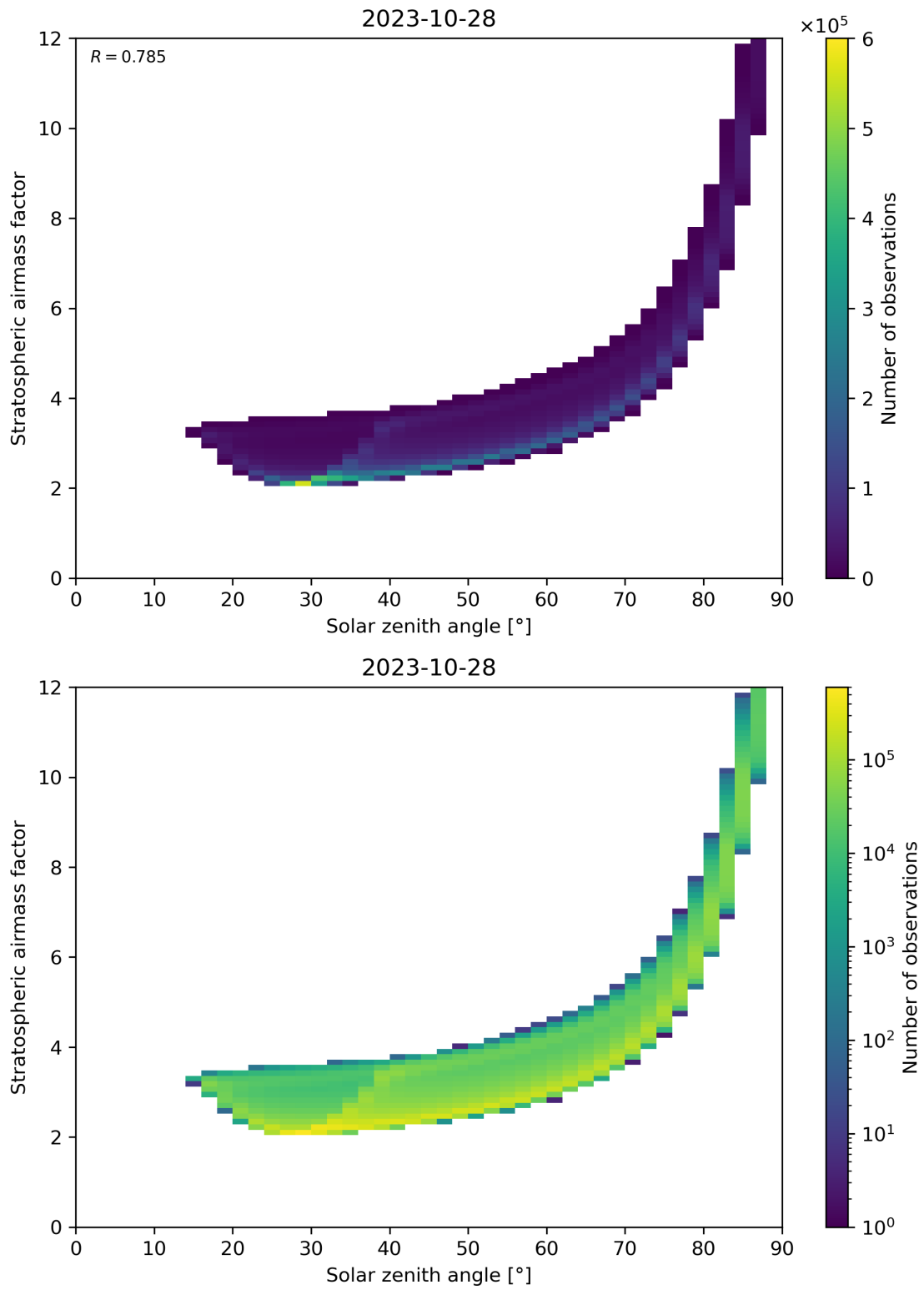
Figure 145: Scatter density plot of “Solar zenith angle” against “Stratospheric airmass factor” for 2023-10-28 to 2023-10-29.
