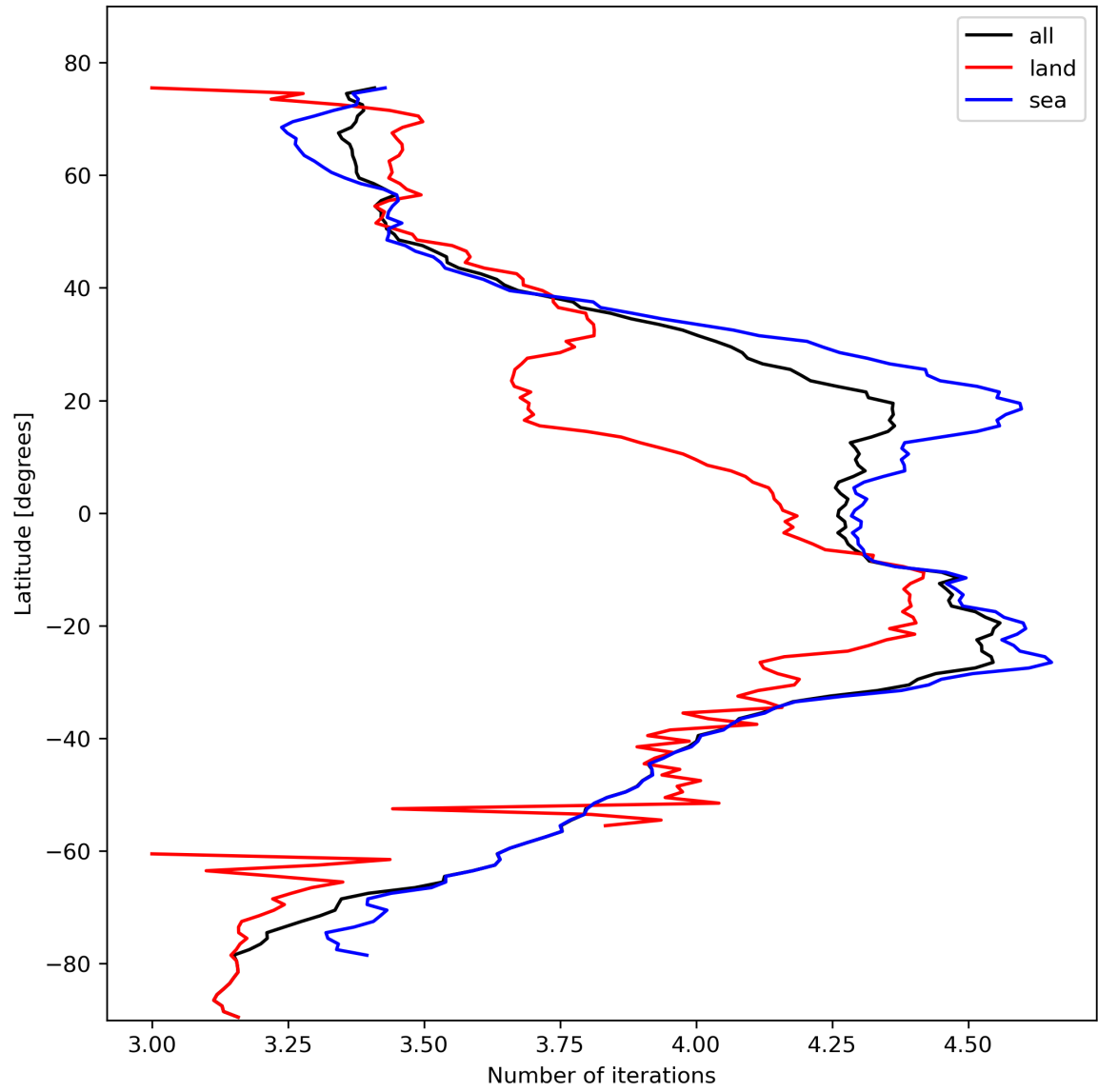
Figure 17: Zonal average of “Number of iterations” for 2023-10-28 to 2023-10-29.
