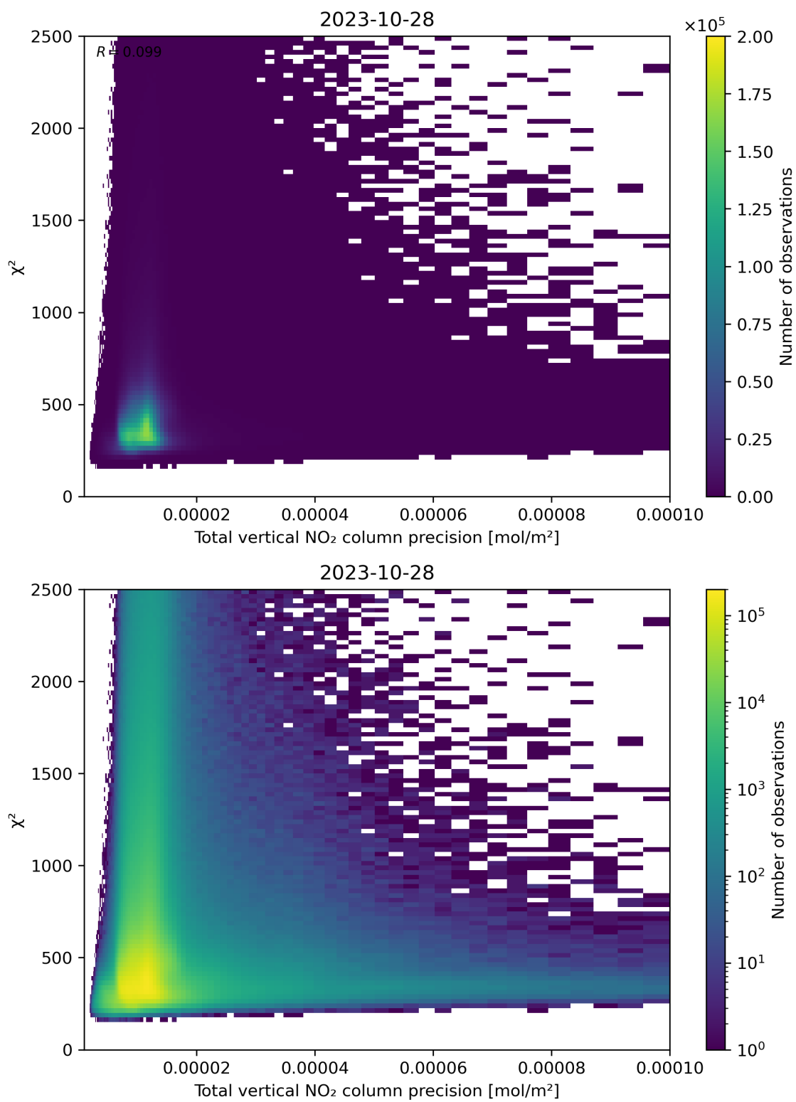
Figure 116: Scatter density plot of “Total vertical NO 2 column precision” against “ \chi^2 ” for 2023-10-28 to 2023-10-29.
