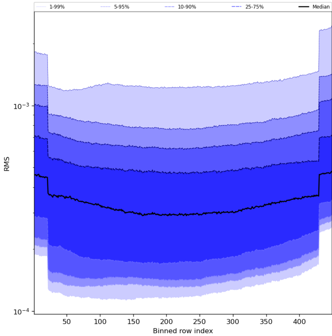
Figure 60: Along track statistics of “RMS” for 2023-10-28 to 2023-10-29
