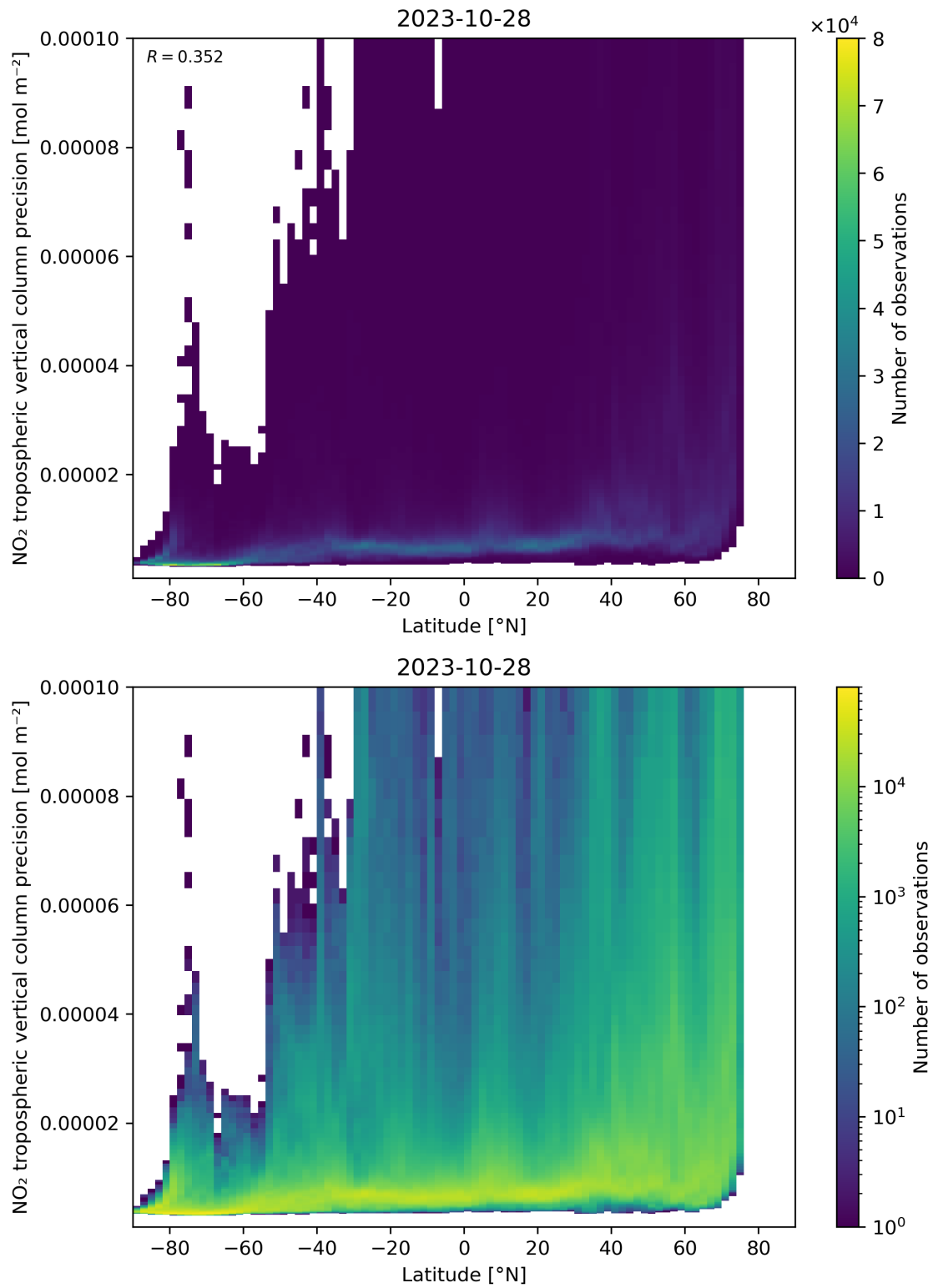
Figure 93: Scatter density plot of “Latitude” against “NO 2 tropospheric vertical column precision” for 2023-10-28 to 2023-10-29.
