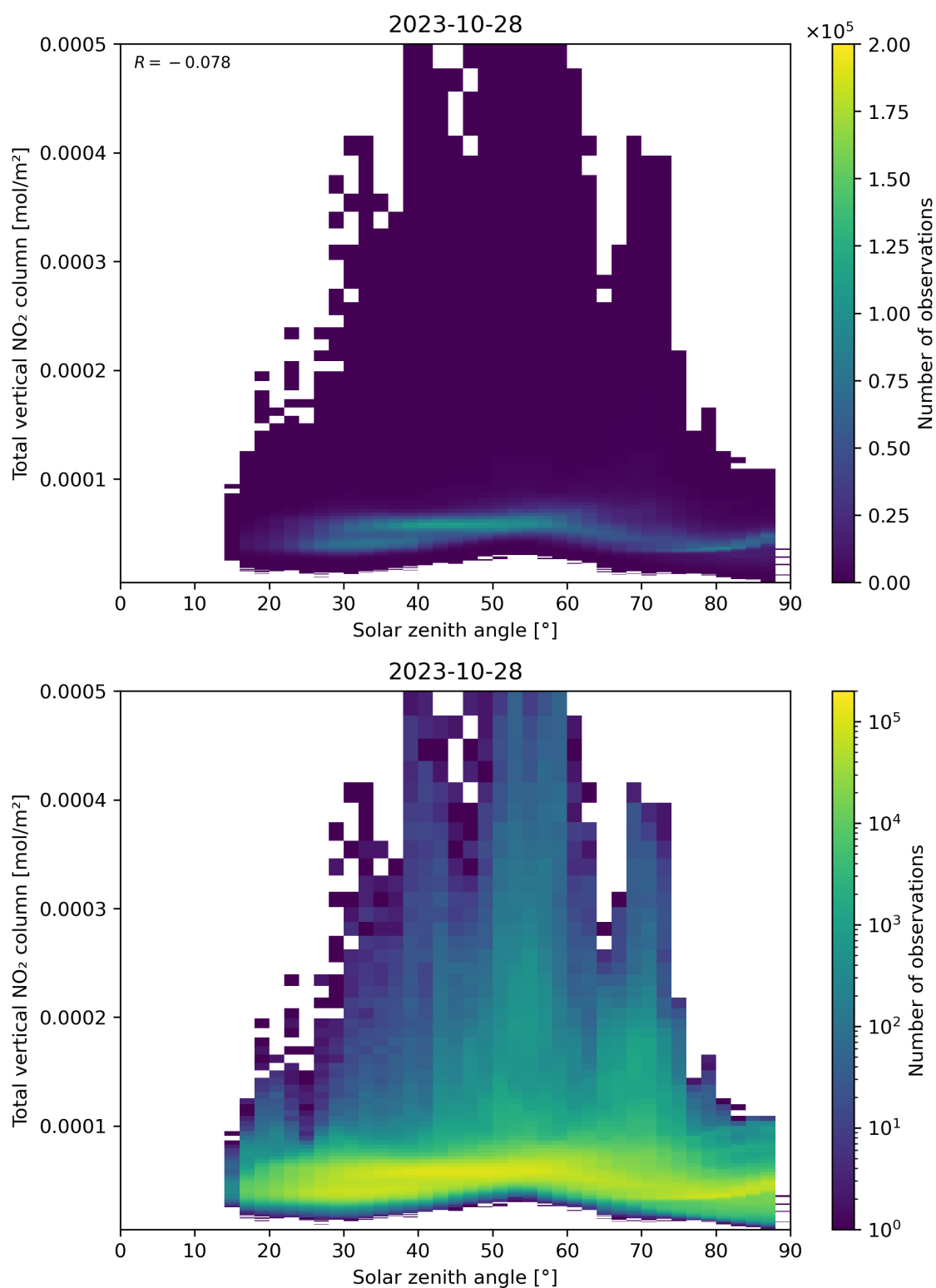
Figure 153: Scatter density plot of “Solar zenith angle” against “Total vertical NO 2 column” for 2023-10-28 to 2023-10-29.
