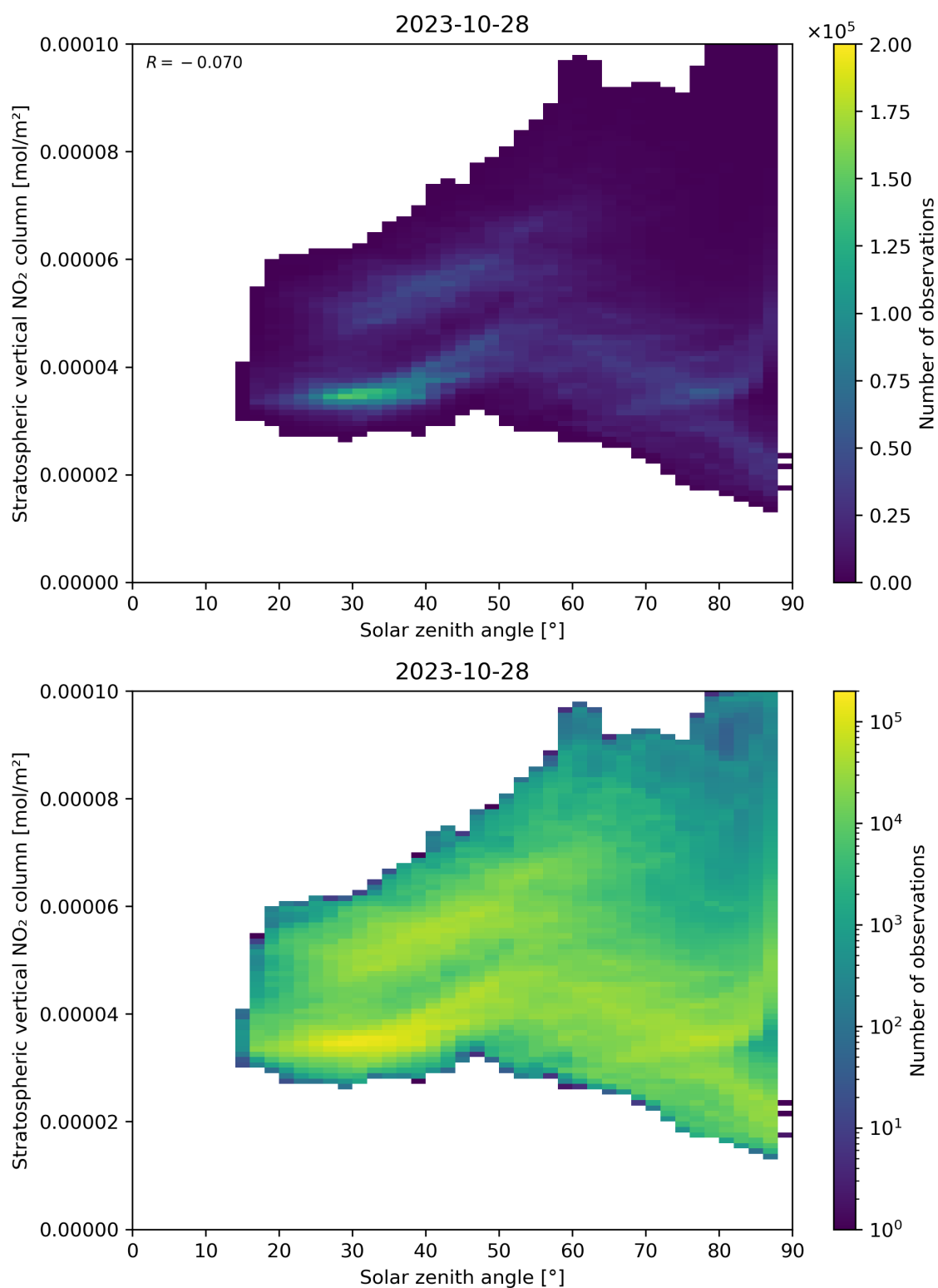
Figure 150: Scatter density plot of “Solar zenith angle” against “Stratospheric vertical NO 2 column” for 2023-10-28 to 2023-10-29.
