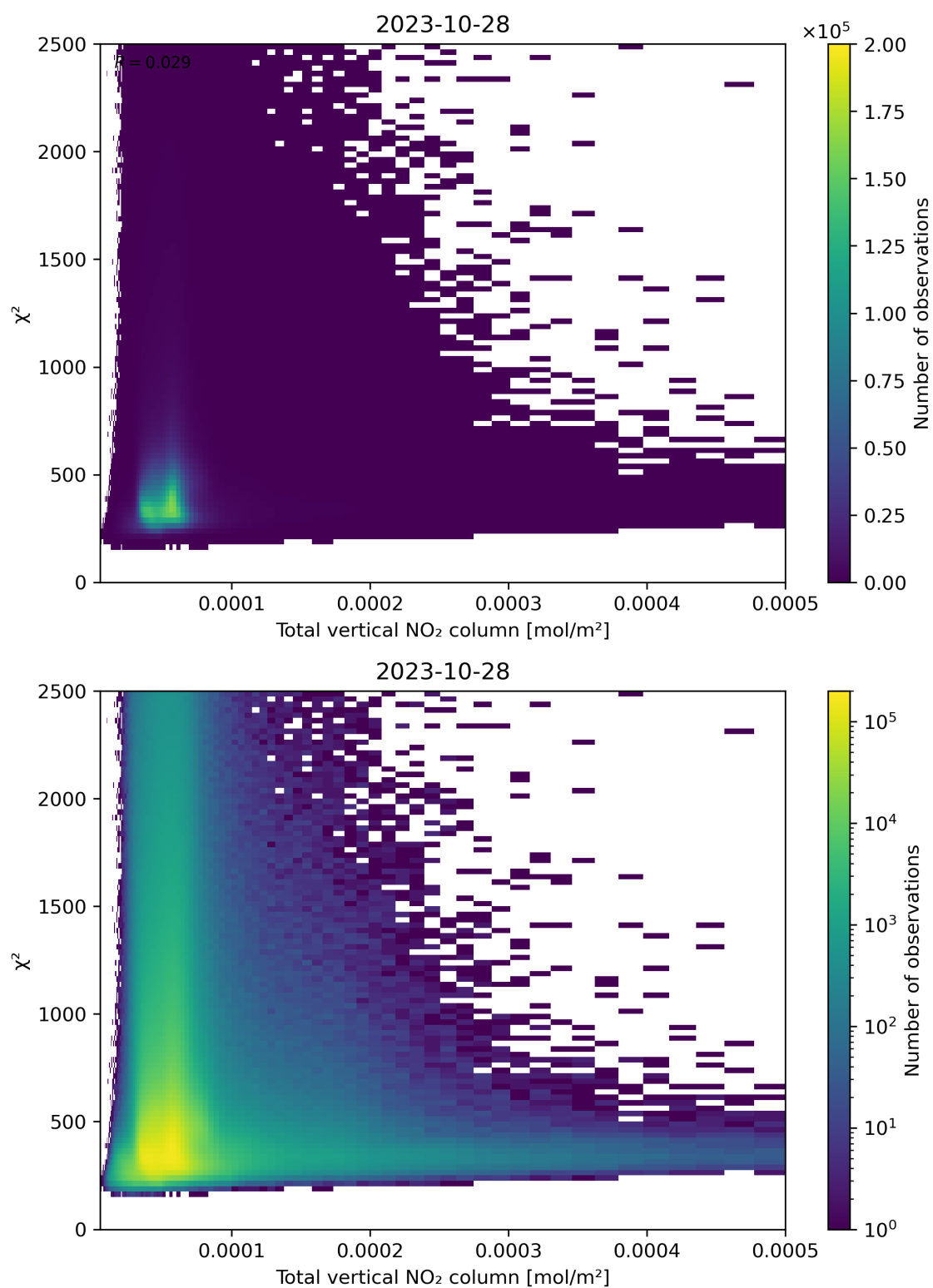
Figure 111: Scatter density plot of “Total vertical NO 2 column” against “ \chi^2 ” for 2023-10-28 to 2023-10-29.
