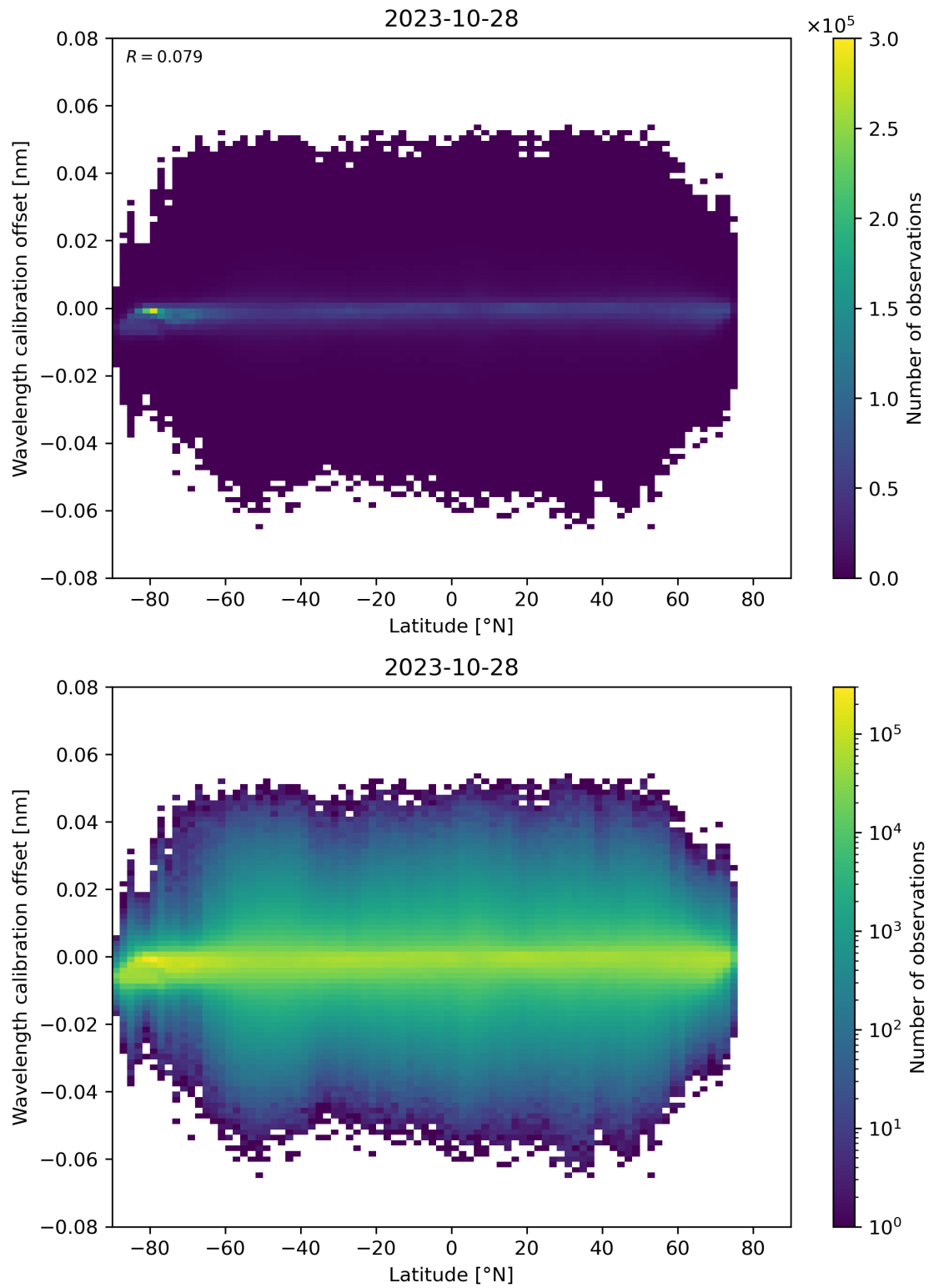
Figure 95: Scatter density plot of “Latitude” against “Wavelength calibration offset” for 2023-10-28 to 2023-10-29.
