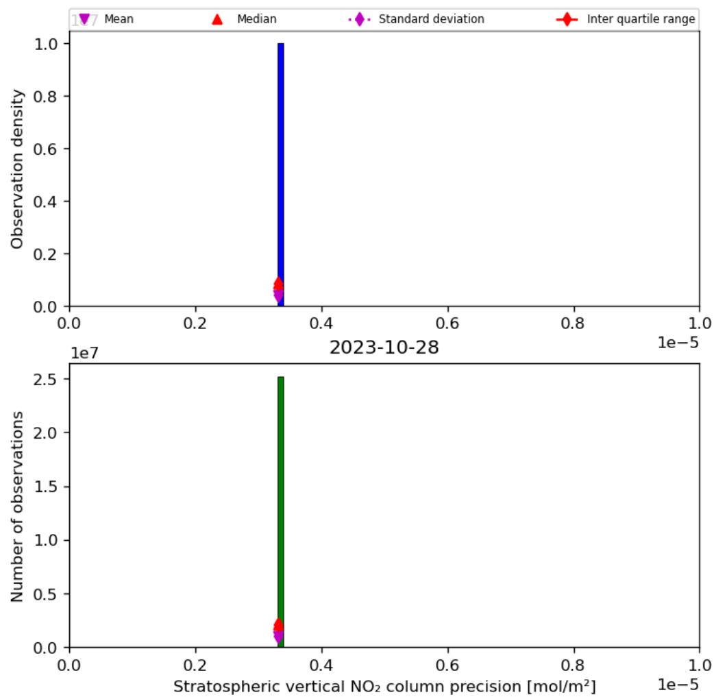
Figure 37: Histogram of “Stratospheric vertical NO 2 column precision” for 2023-10-28 to 2023-10-29
