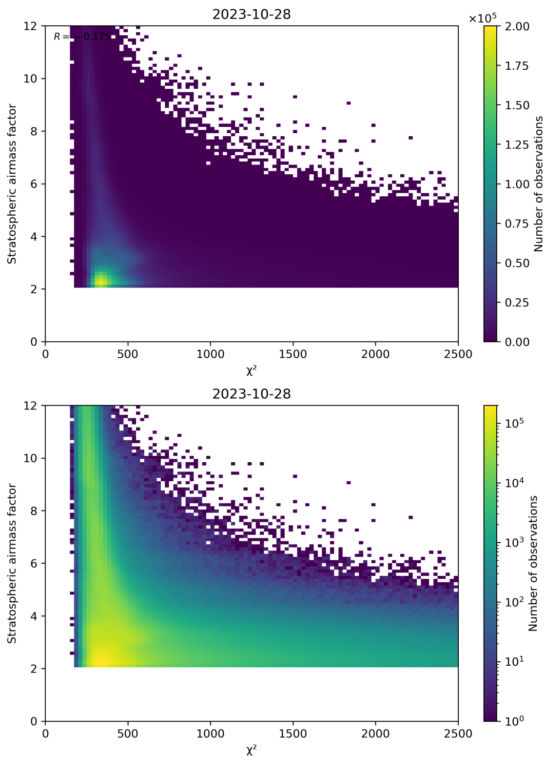
Figure 81: Scatter density plot of “ \chi^2 ” against “Stratospheric airmass factor” for 2023-10-28 to 2023-10-29.
