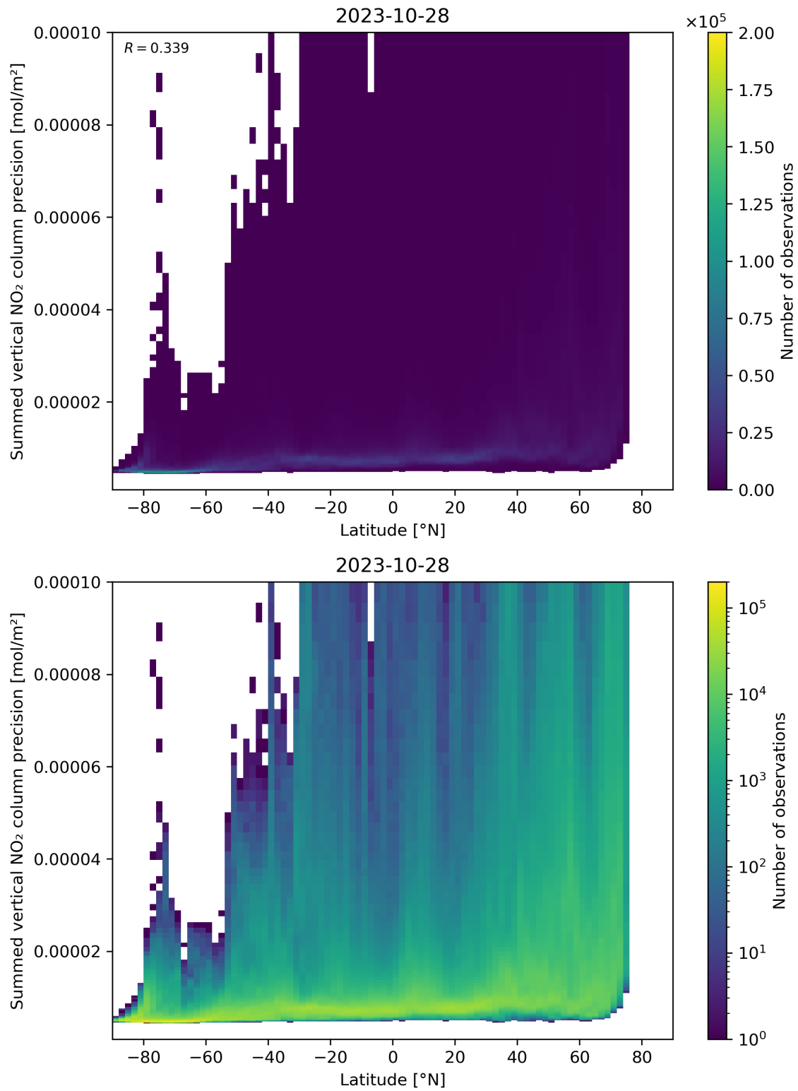
Figure 89: Scatter density plot of “Latitude” against “Summed vertical NO 2 column precision” for 2023-10-28 to 2023-10-29.
