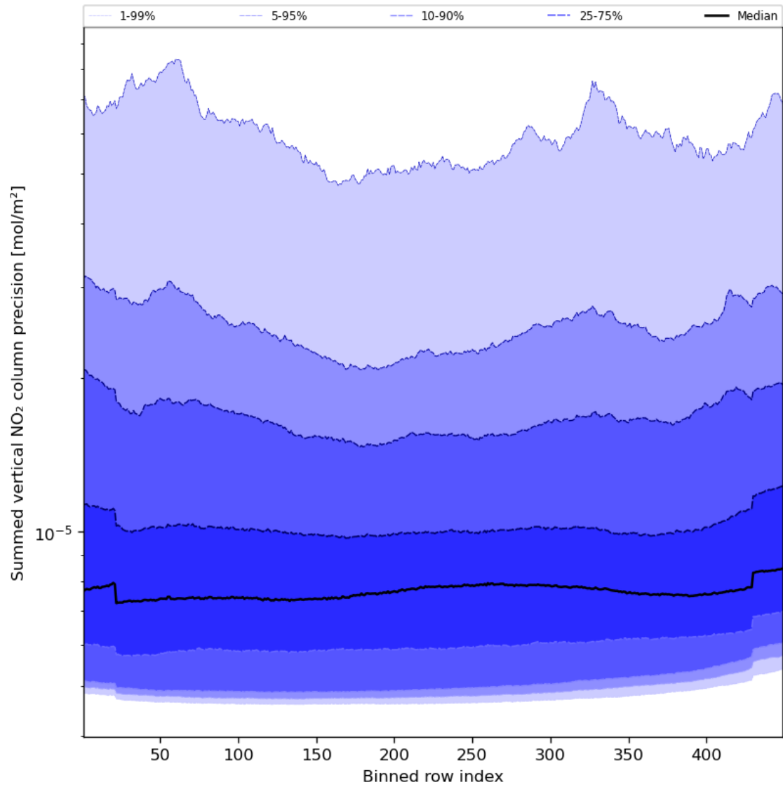
Figure 58: Along track statistics of “Summed vertical NO 2 column precision” for 2023-10-28 to 2023-10-29
