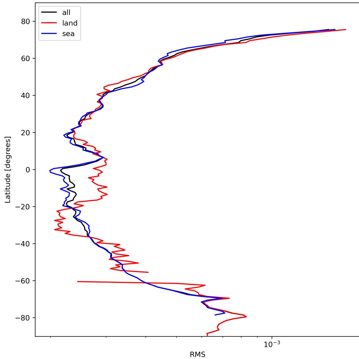
Figure 26: Zonal average of “RMS” for 2023-10-28 to 2023-10-29.
