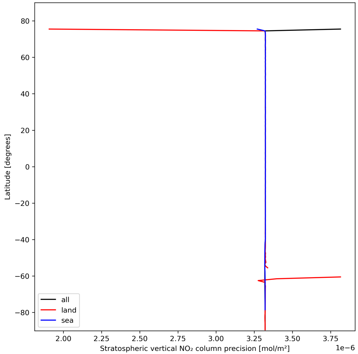
Figure 20: Zonal average of “Stratospheric vertical NO 2 column precision” for 2023-10-28 to 2023-10-29.
