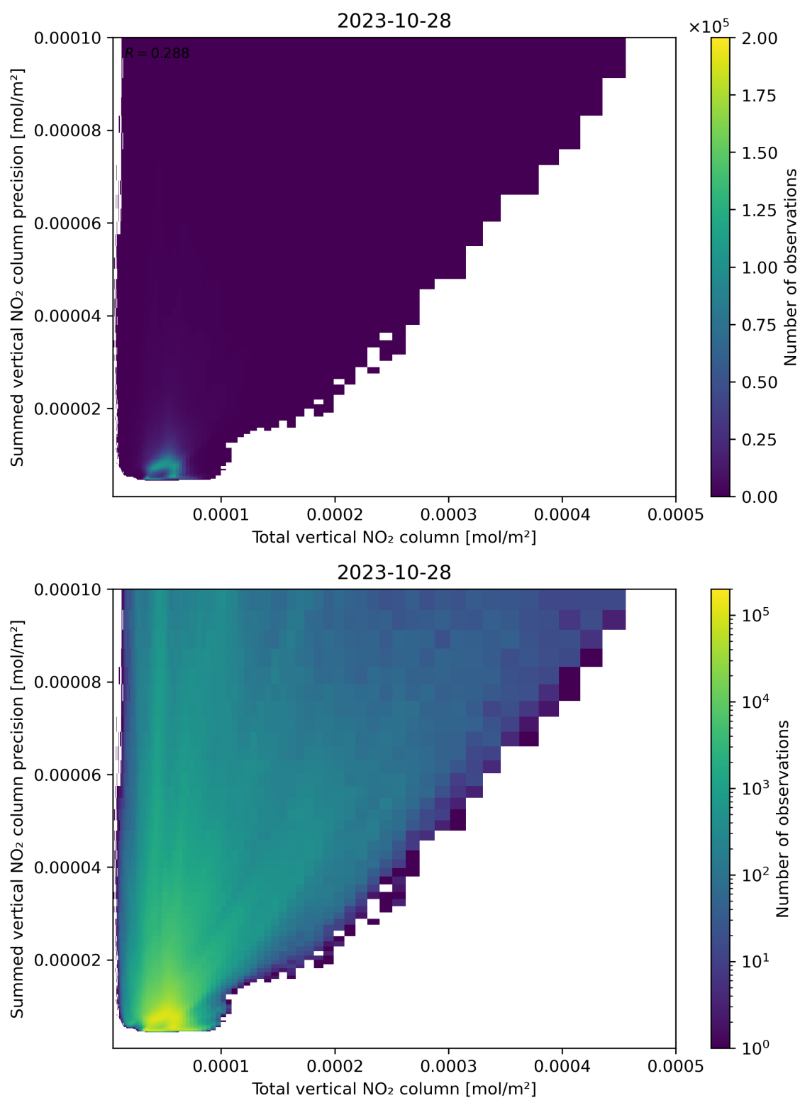
Figure 113: Scatter density plot of “Total vertical NO 2 column” against “Summed vertical NO 2 column precision” for 2023-10-28 to 2023-10-29.
