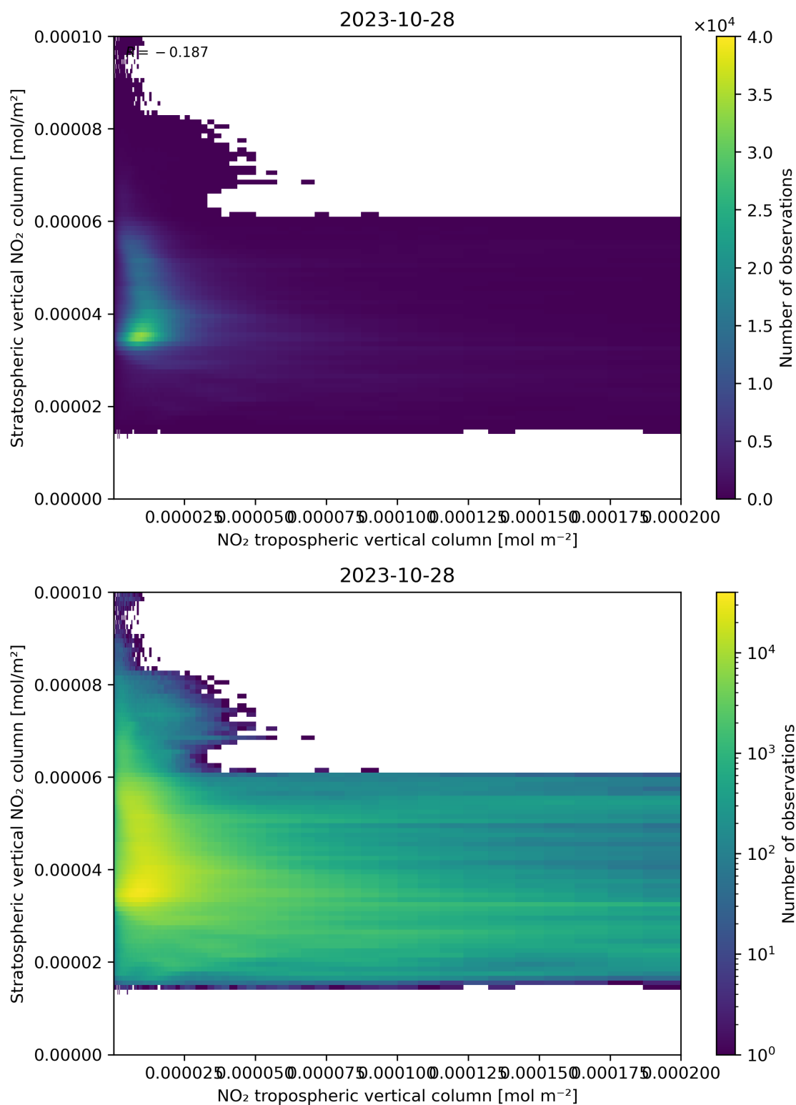
Figure 125: Scatter density plot of “NO 2 tropospheric vertical column” against “Stratospheric vertical NO 2 column” for 2023-10-28 to 2023-10-29.
