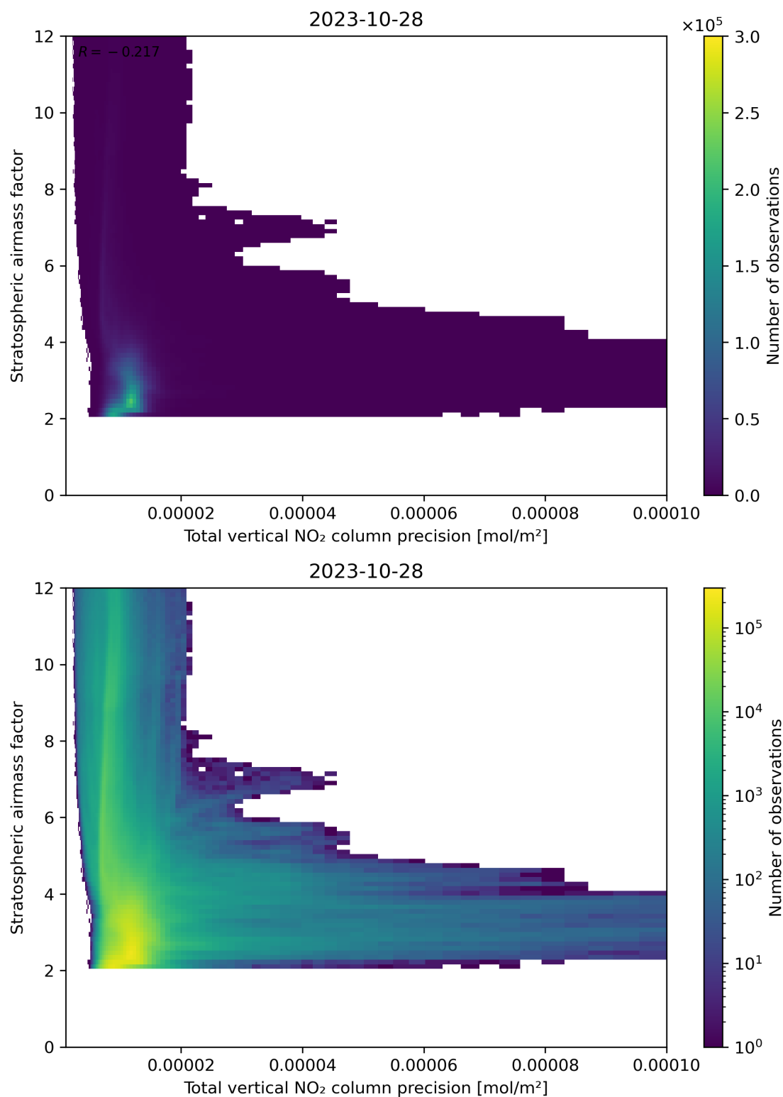
Figure 115: Scatter density plot of “Total vertical NO 2 column precision” against “Stratospheric airmass factor” for 2023-10-28 to 2023-10-29.
