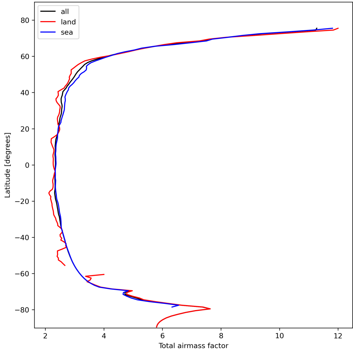
Figure 15: Zonal average of “Total airmass factor” for 2023-10-28 to 2023-10-29.
