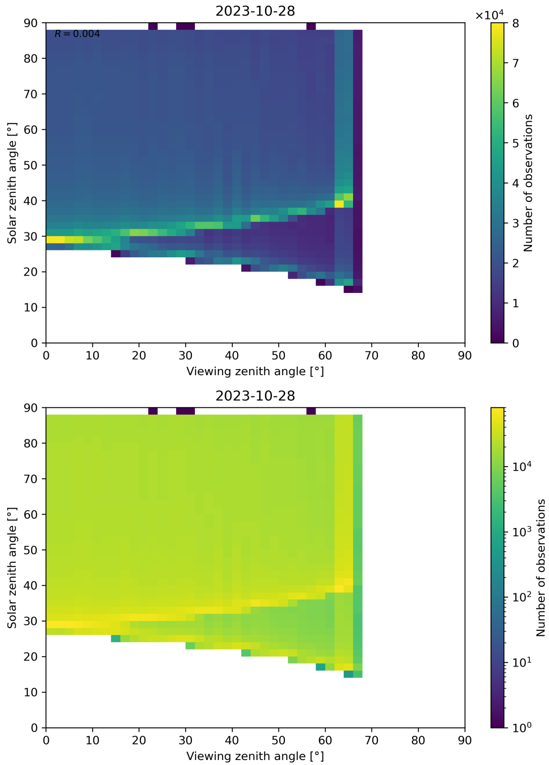
Figure 172: Scatter density plot of “Viewing zenith angle” against “Solar zenith angle” for 2023-10-28 to 2023-10-29.
