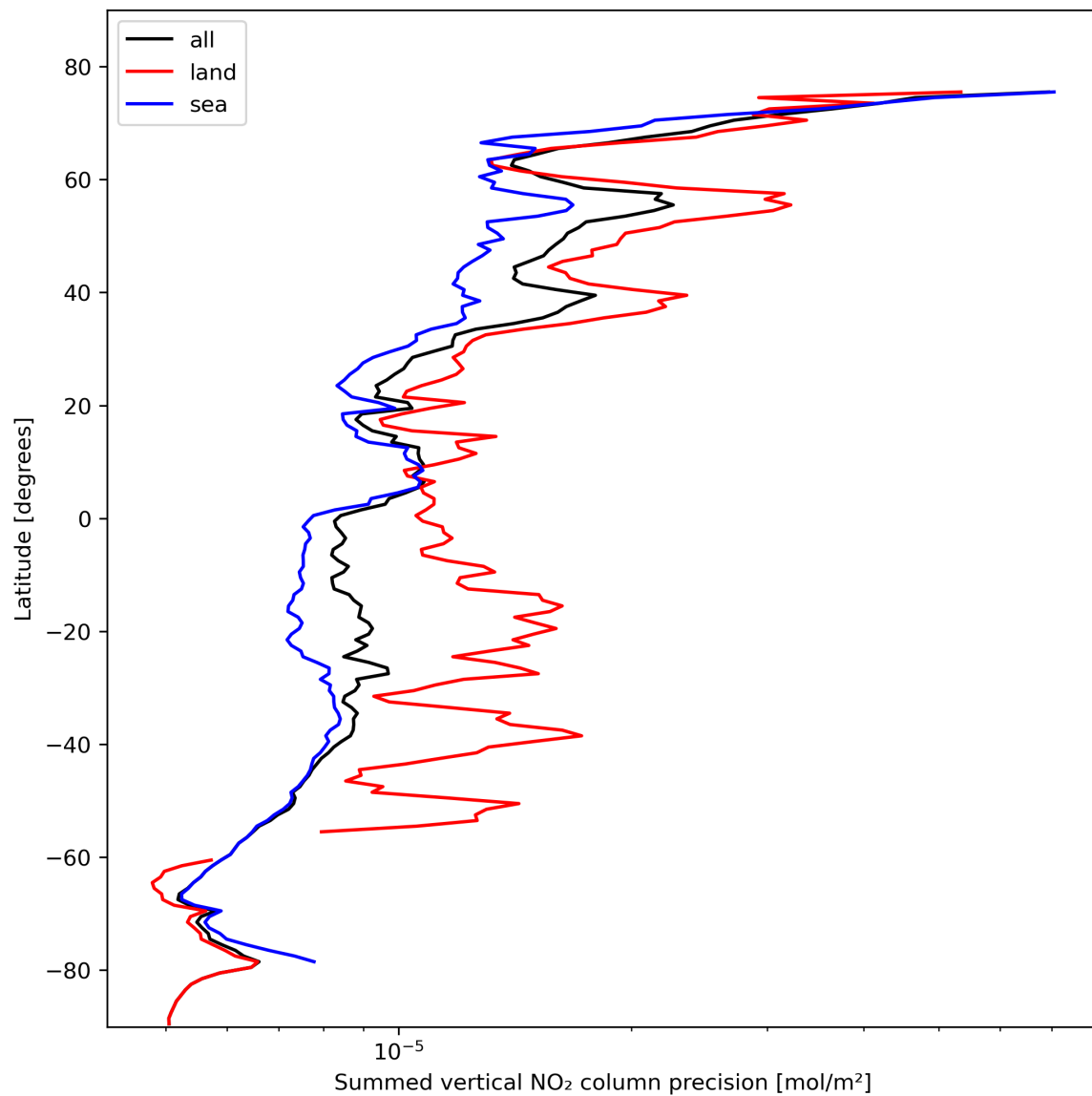
Figure 24: Zonal average of “Summed vertical NO 2 column precision” for 2023-10-28 to 2023-10-29.
