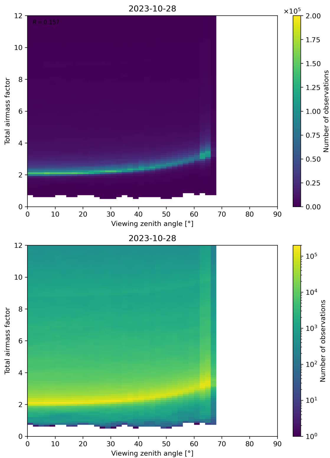
Figure 160: Scatter density plot of “Viewing zenith angle” against “Total airmass factor” for 2023-10-28 to 2023-10-29.
