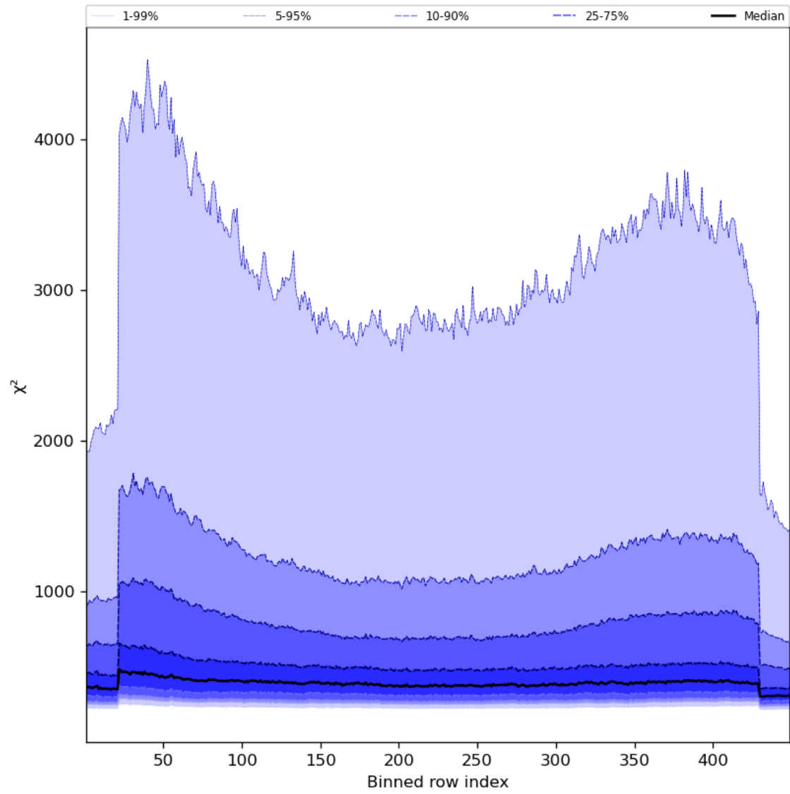
Figure 59: Along track statistics of “ \chi^2 ” for 2023-10-28 to 2023-10-29
