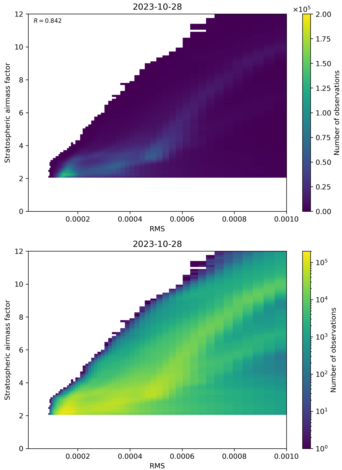
Figure 144: Scatter density plot of “RMS” against “Stratospheric airmass factor” for 2023-10-28 to 2023-10-29.
