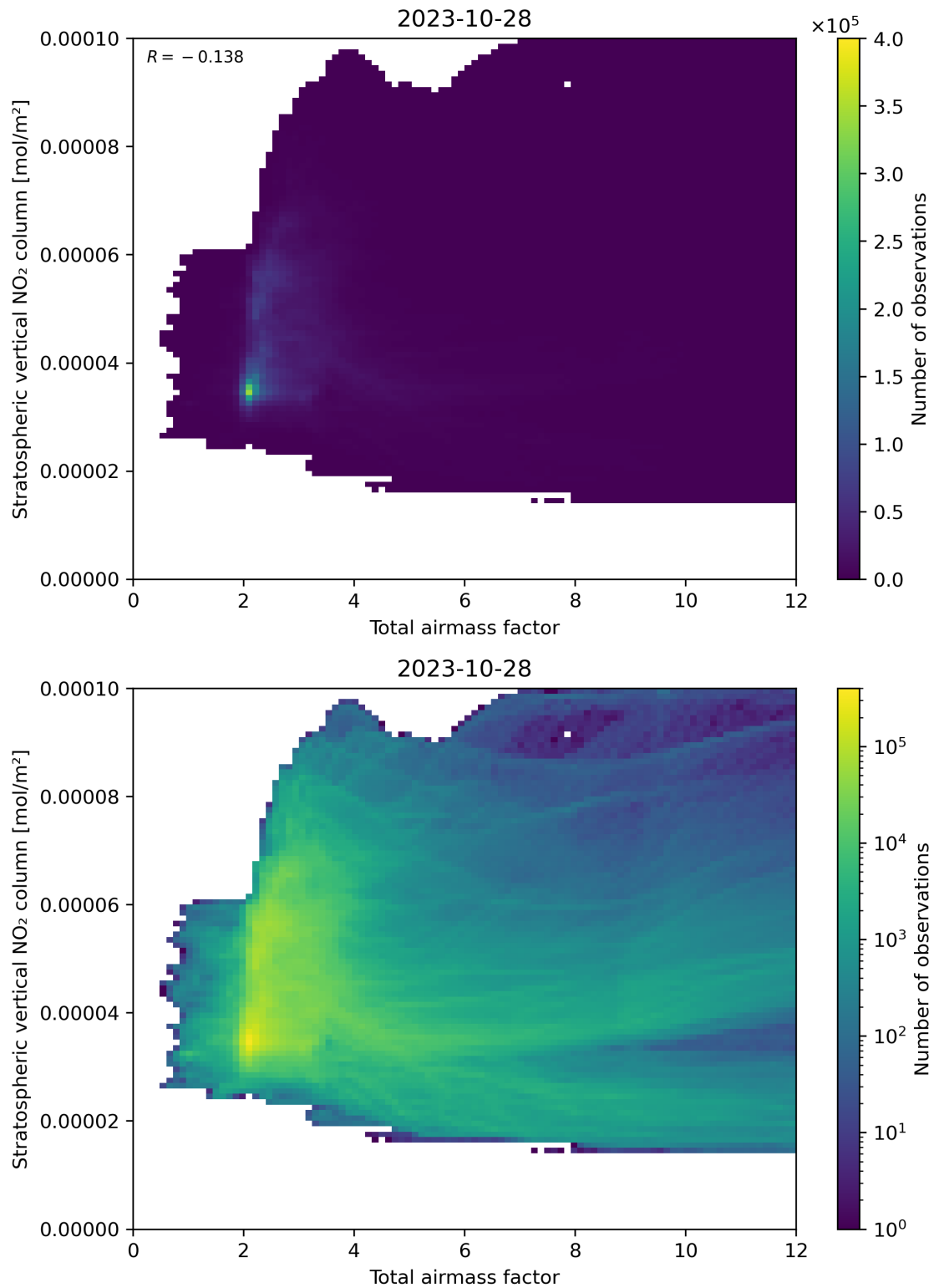
Figure 64: Scatter density plot of “Total airmass factor” against “Stratospheric vertical NO 2 column” for 2023-10-28 to 2023-10-29.
