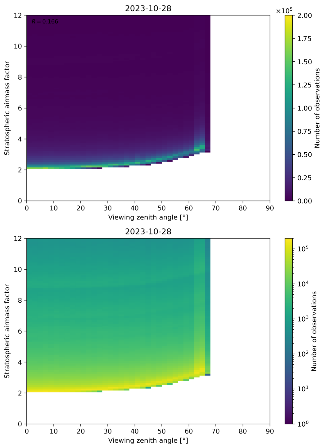
Figure 159: Scatter density plot of “Viewing zenith angle” against “Stratospheric airmass factor” for 2023-10-28 to 2023-10-29.
