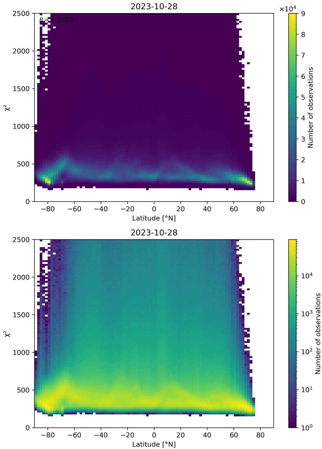
Figure 86: Scatter density plot of “Latitude” against “ \chi^2 ” for 2023-10-28 to 2023-10-29.
