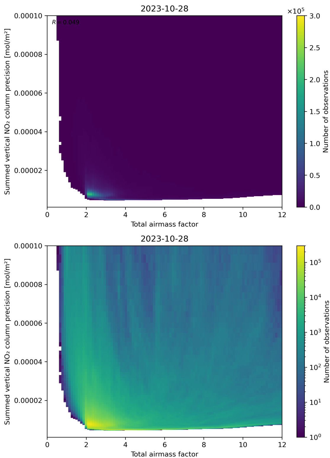
Figure 66: Scatter density plot of “Total airmass factor” against “Summed vertical NO 2 column precision” for 2023-10-28 to 2023-10-29.
