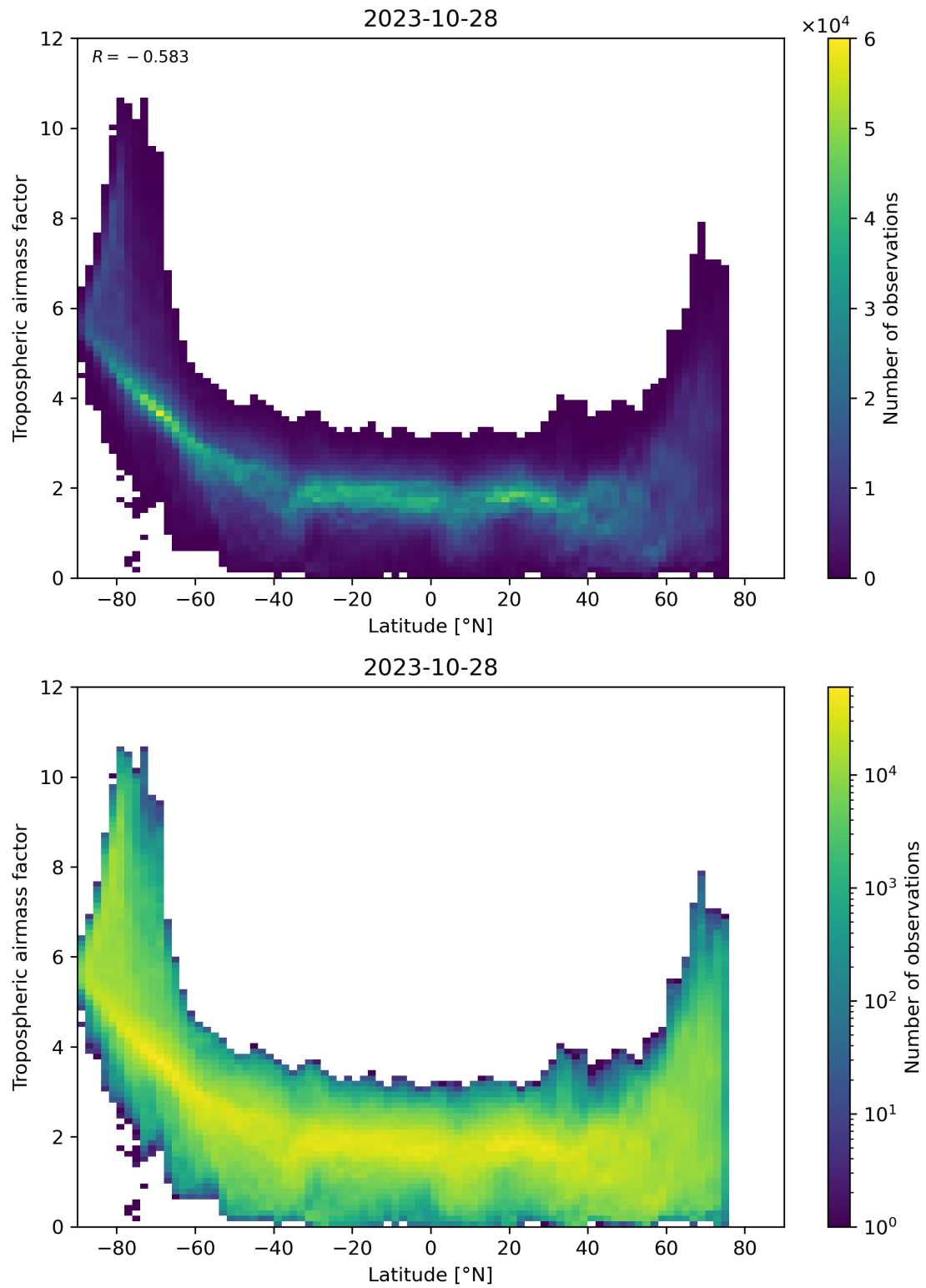
Figure 85: Scatter density plot of “Latitude” against “Tropospheric airmass factor” for 2023-10-28 to 2023-10-29.
