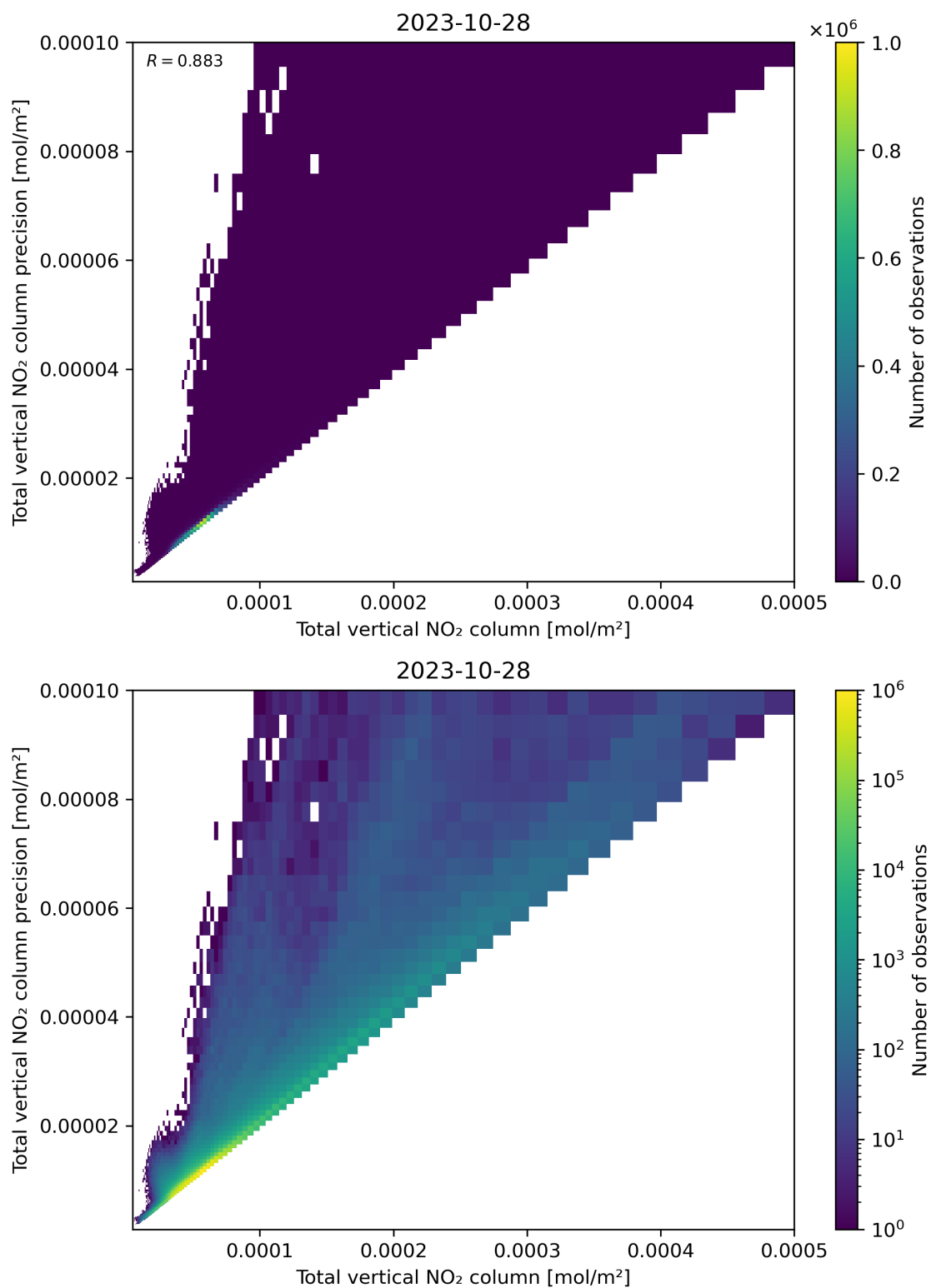
Figure 114: Scatter density plot of “Total vertical NO 2 column” against “Total vertical NO 2 column precision” for 2023-10-28 to 2023-10-29.
