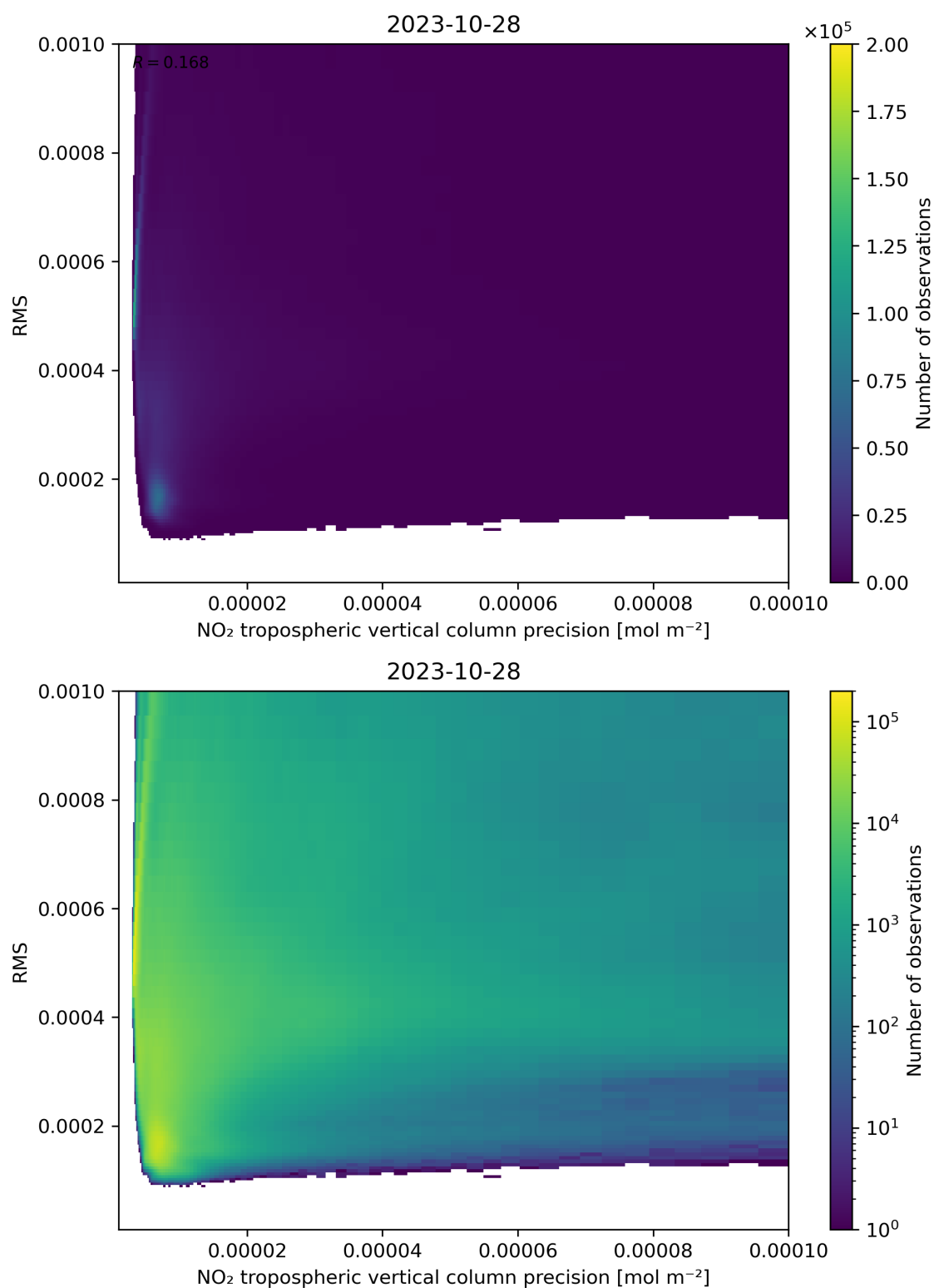
Figure 140: Scatter density plot of “NO 2 tropospheric vertical column precision” against “RMS” for 2023-10-28 to 2023-10-29.
