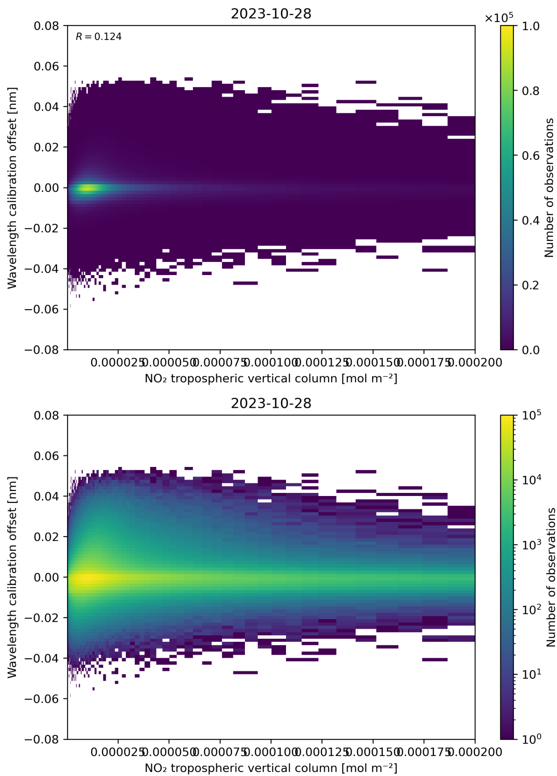
Figure 143: Scatter density plot of “NO 2 tropospheric vertical column” against “Wavelength calibration offset” for 2023-10-28 to 2023-10-29.
