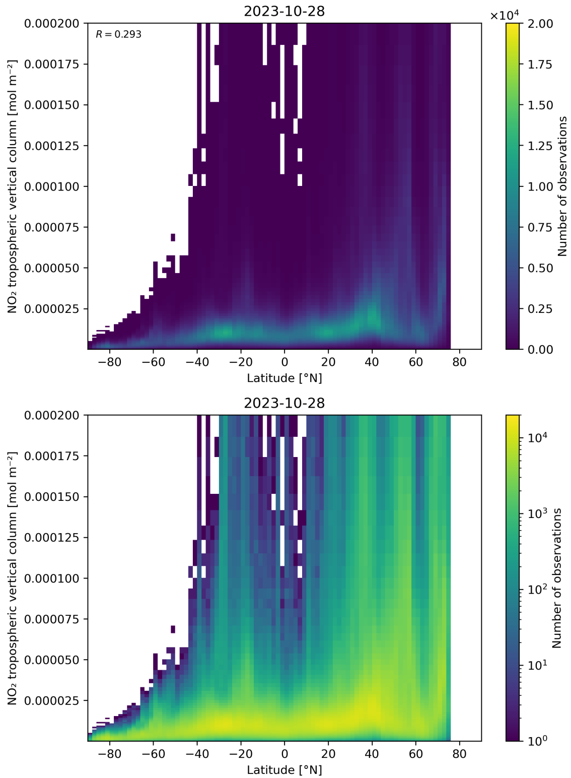
Figure 92: Scatter density plot of “Latitude” against “NO 2 tropospheric vertical column” for 2023-10-28 to 2023-10-29.
