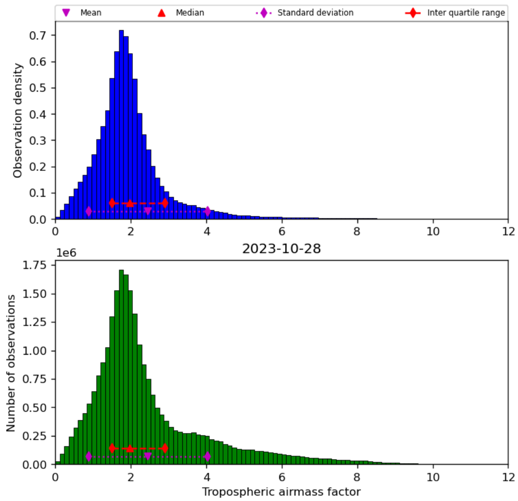
Figure 31: Histogram of “Tropospheric airmass factor” for 2023-10-28 to 2023-10-29
