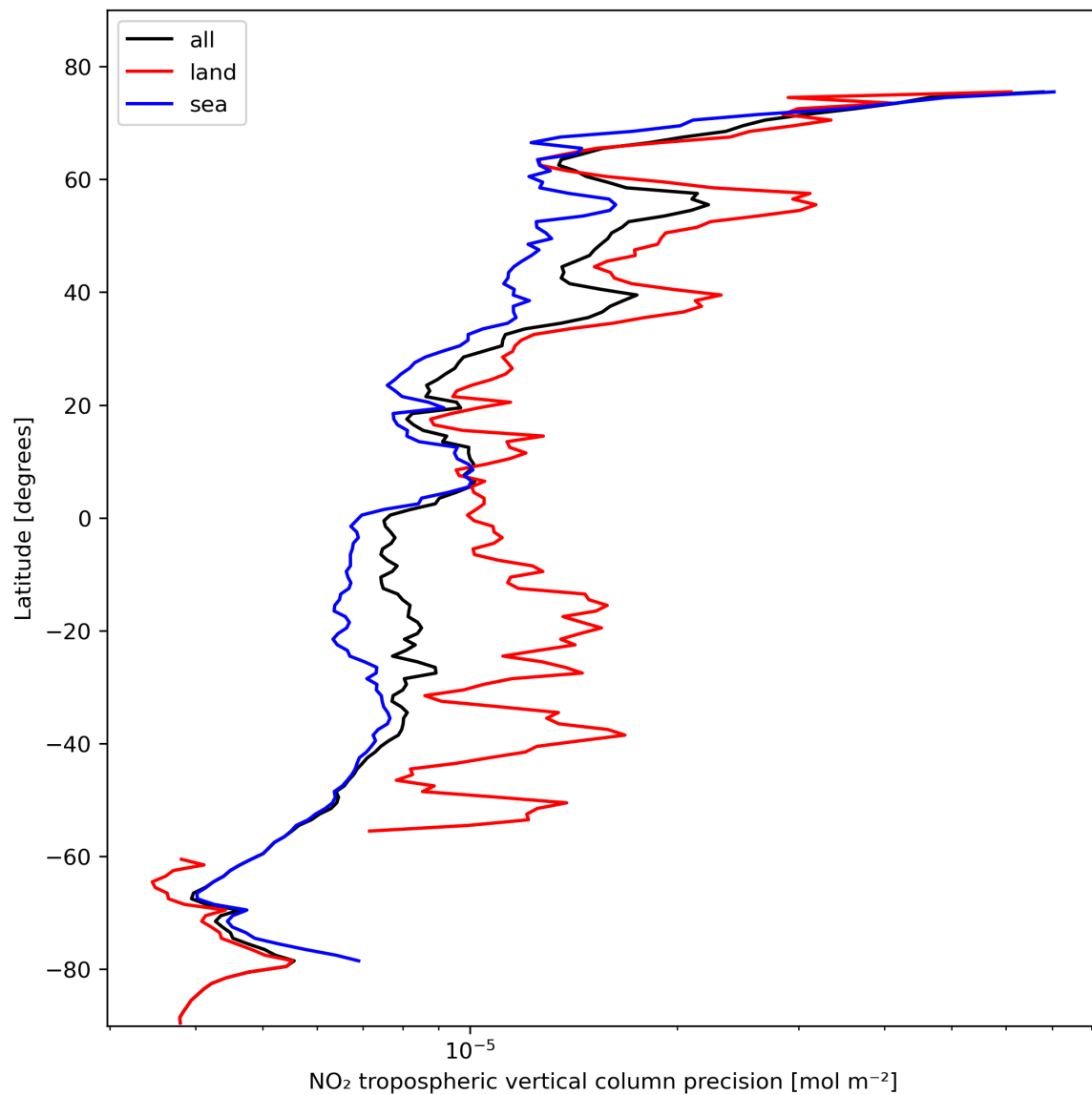
Figure 13: Zonal average of “NO 2 tropospheric vertical column precision” for 2023-10-28 to 2023-10-29.
