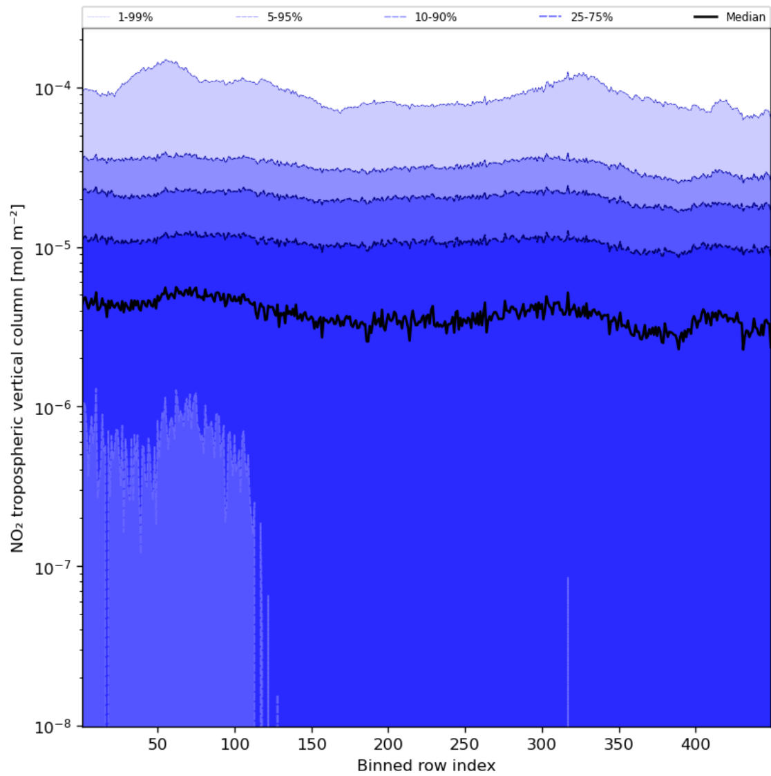
Figure 46: Along track statistics of “NO 2 tropospheric vertical column” for 2023-10-28 to 2023-10-29
