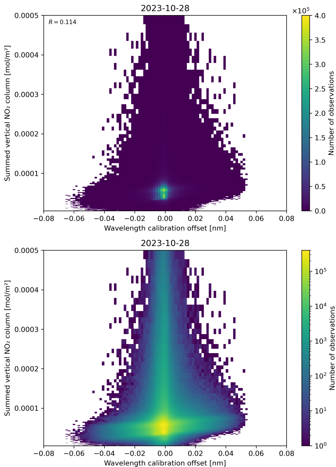
Figure 177: Scatter density plot of “Wavelength calibration offset” against “Summed vertical NO 2 column” for 2023-10-28 to 2023-10-29.
