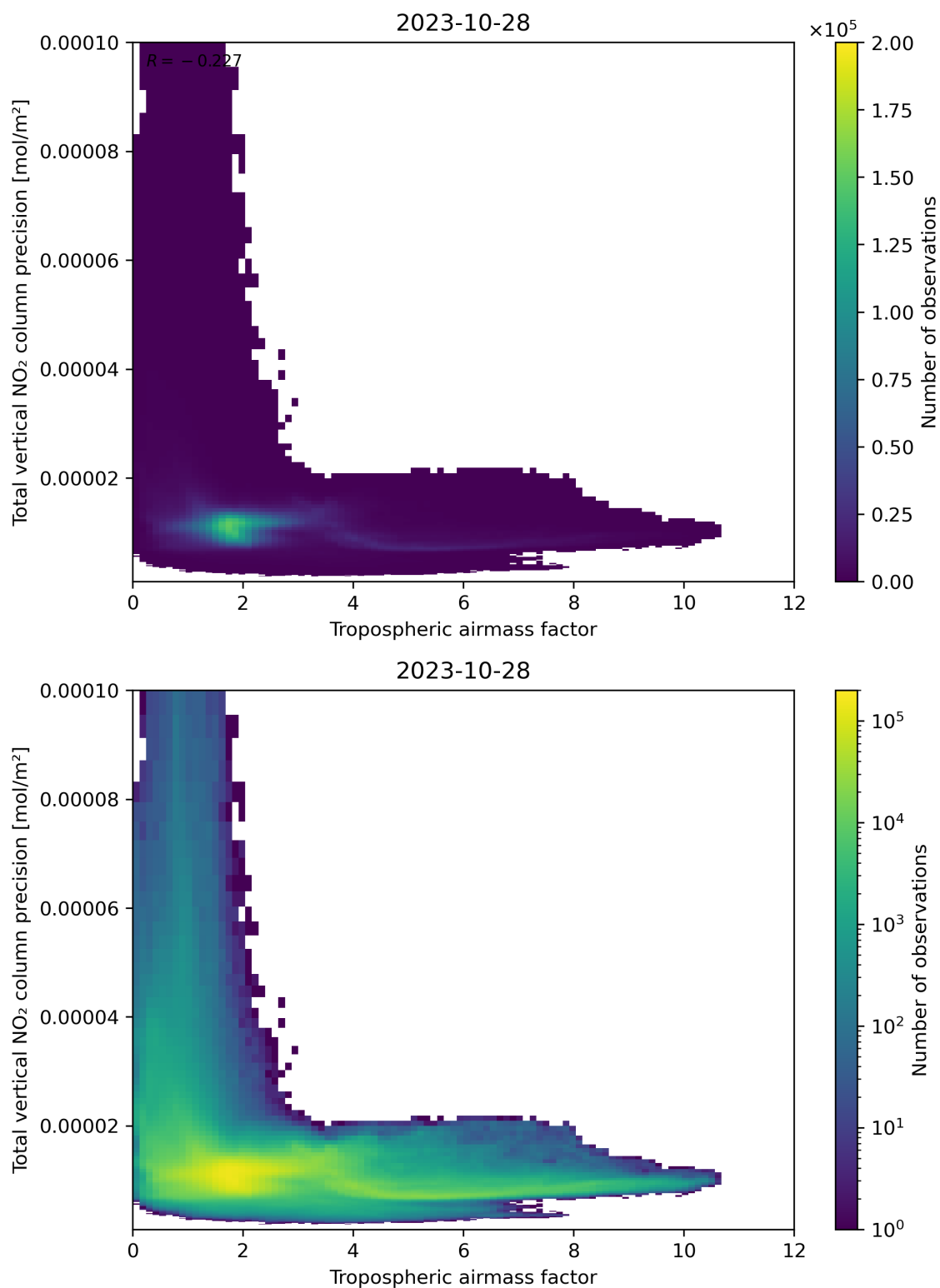
Figure 78: Scatter density plot of “Tropospheric air mass factor” against “Total vertical NO 2 column precision” for 2023-10-28 to 2023-10-29.
