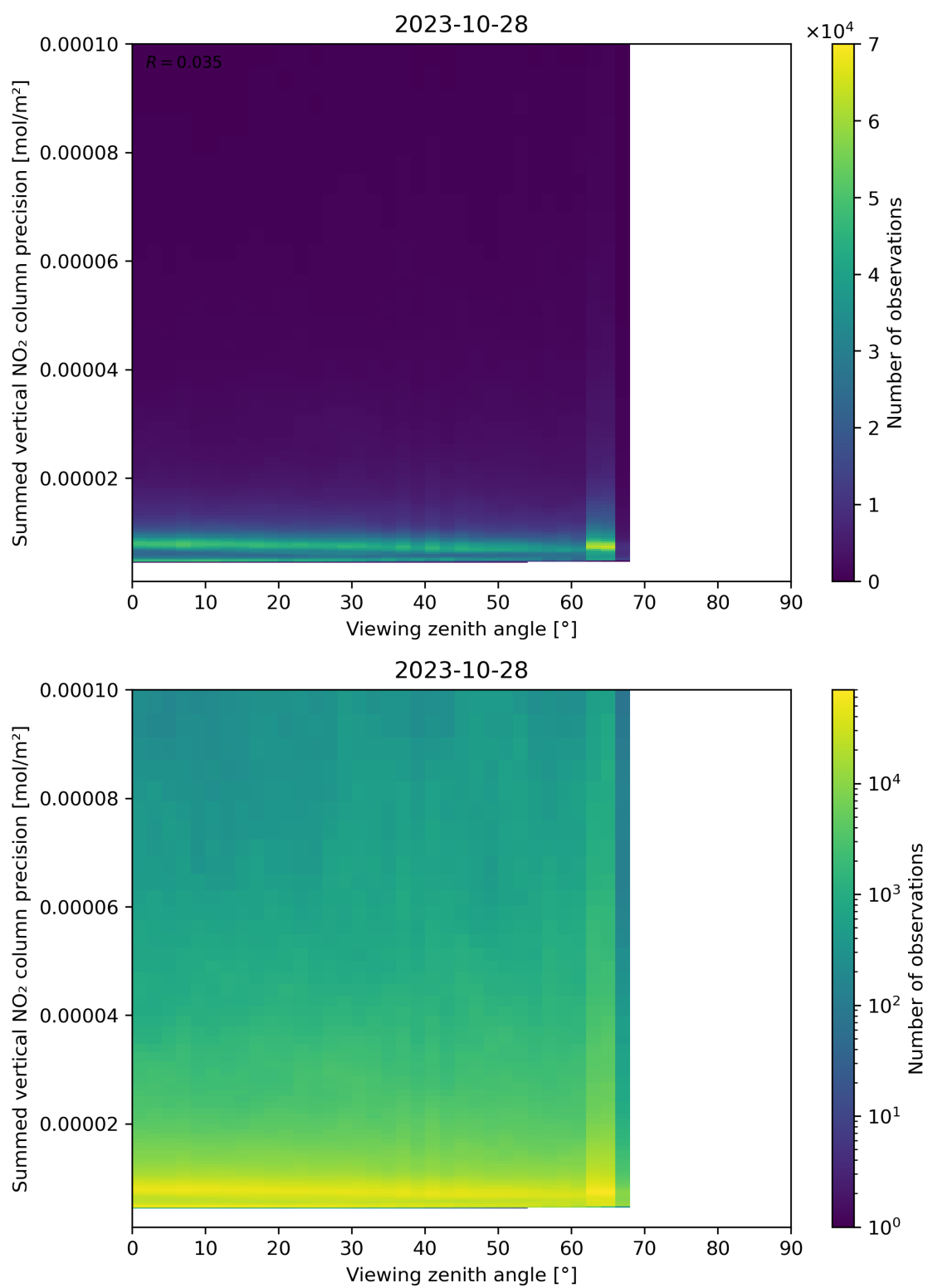
Figure 166: Scatter density plot of “Viewing zenith angle” against “Summed vertical NO 2 column precision” for 2023-10-28 to 2023-10-29.
