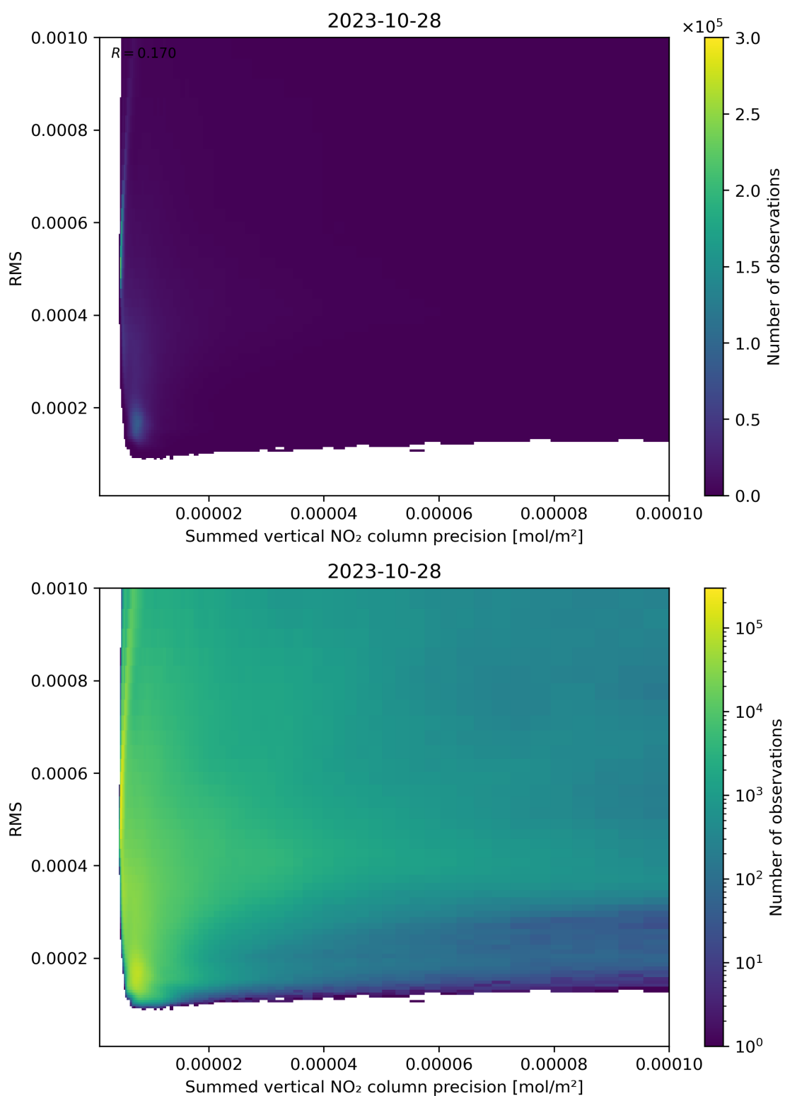
Figure 108: Scatter density plot of “Summed vertical NO 2 column precision” against “RMS” for 2023-10-28 to 2023-10-29.
