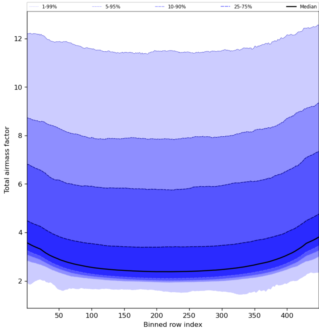
Figure 49: Along track statistics of “Total airmass factor” for 2023-10-28 to 2023-10-29
