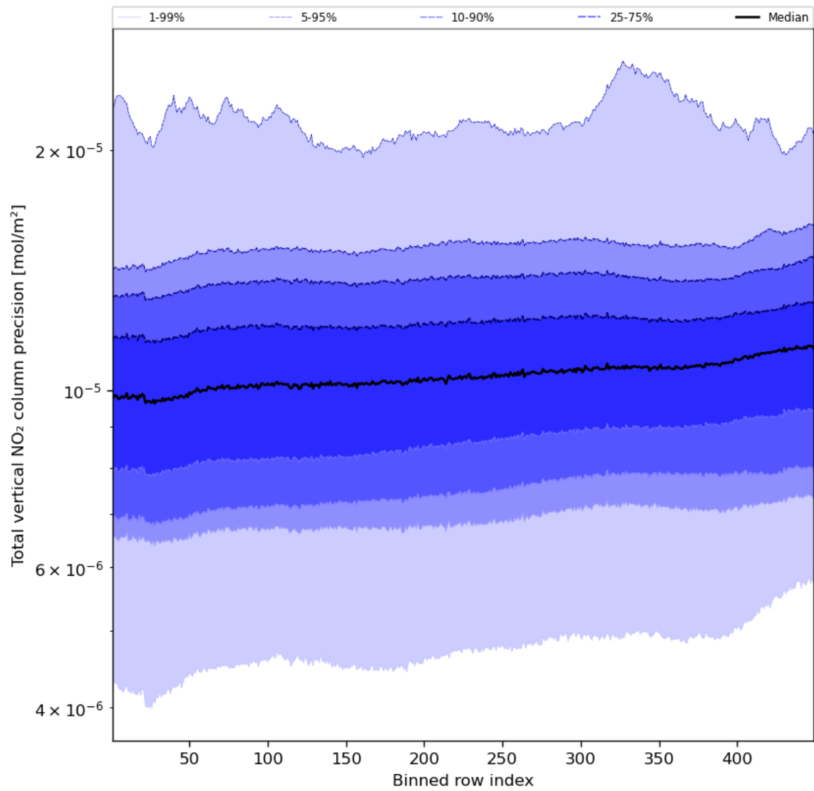
Figure 56: Along track statistics of “Total vertical NO 2 column precision” for 2023-10-28 to 2023-10-29
