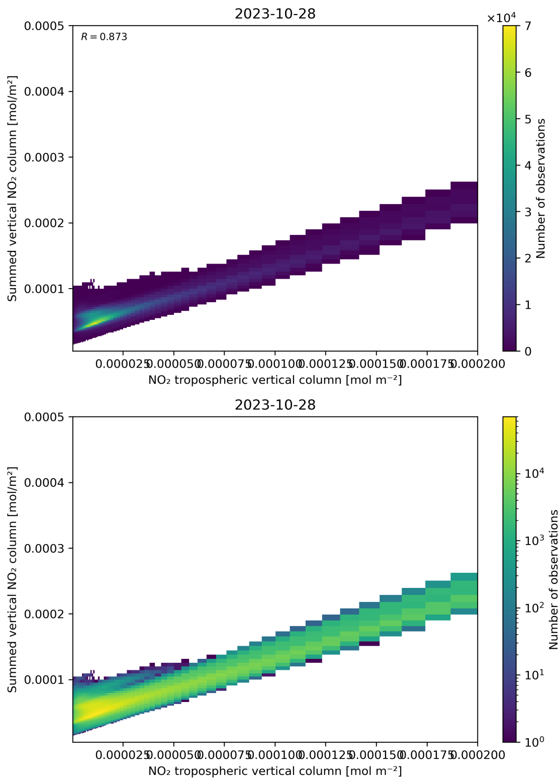
Figure 126: Scatter density plot of “NO 2 tropospheric vertical column” against “Summed vertical NO 2 column” for 2023-10-28 to 2023-10-29.
