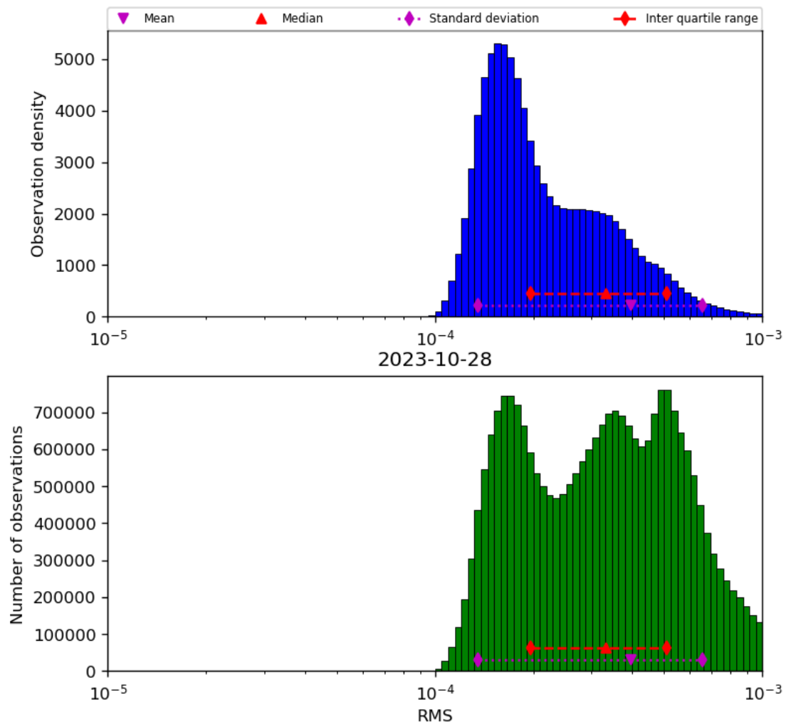
Figure 43: Histogram of “RMS” for 2023-10-28 to 2023-10-29
