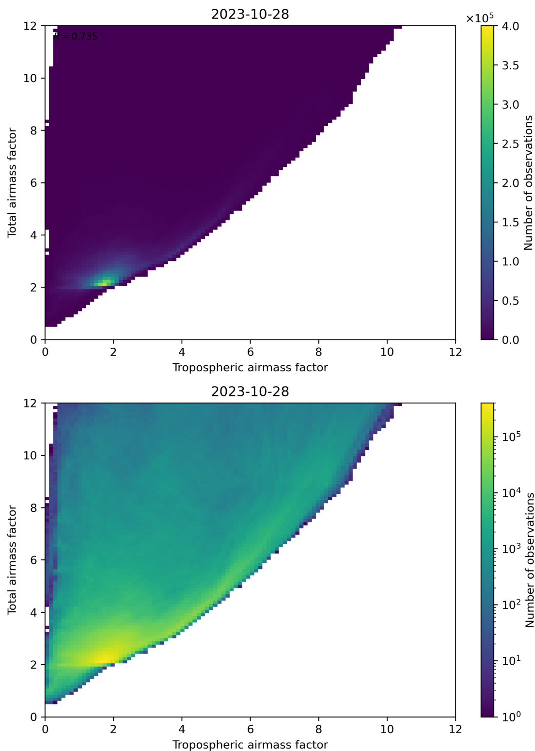
Figure 72: Scatter density plot of “Tropospheric airmass factor” against “Total airmass factor” for 2023-10-28 to 2023-10-29.
