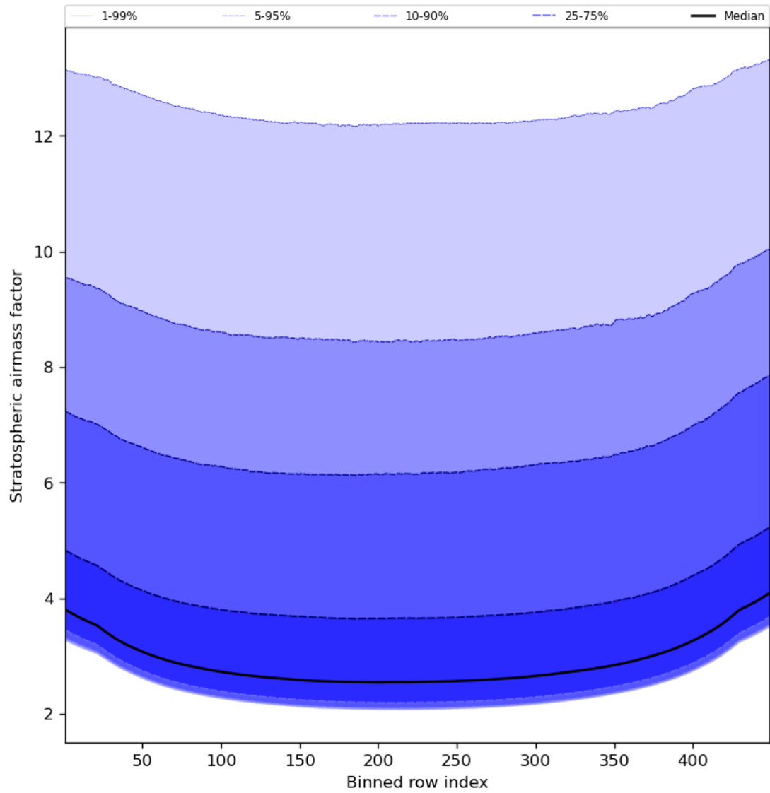
Figure 61: Along track statistics of “Stratospheric airmass factor” for 2023-10-28 to 2023-10-29
