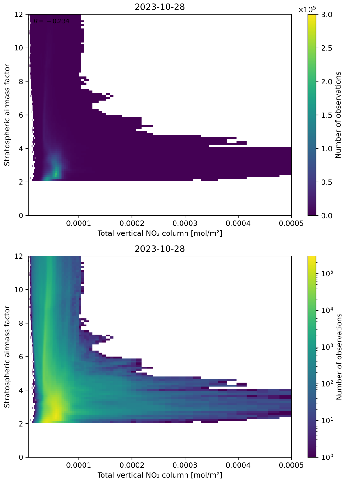
Figure 110: Scatter density plot of “Total vertical NO 2 column” against “Stratospheric airmass factor” for 2023-10-28 to 2023-10-29.
