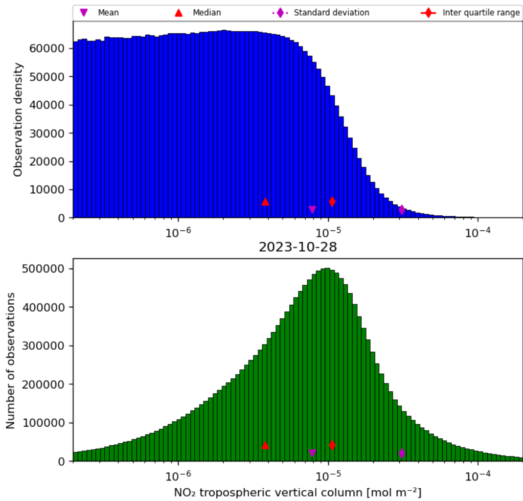
Figure 29: Histogram of “NO 2 tropospheric vertical column” for 2023-10-28 to 2023-10-29
