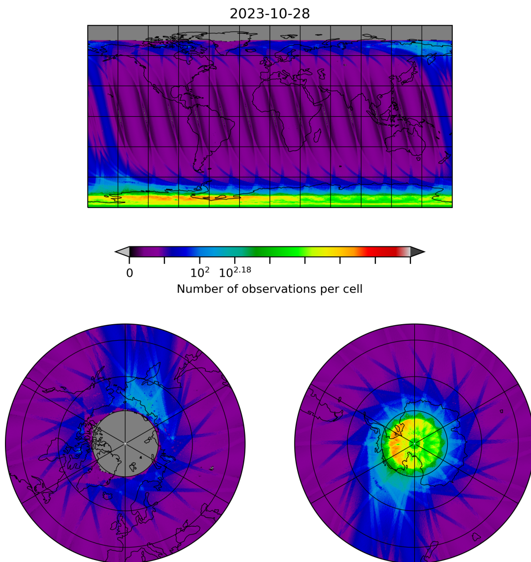
Figure 10: Map of the number of observations for 2023-10-28 to 2023-10-29
