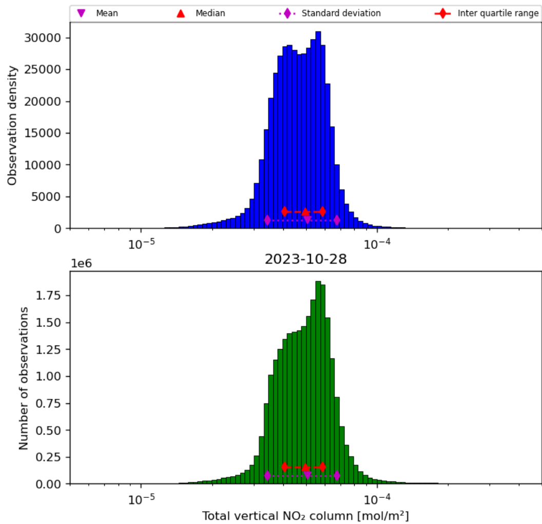
Figure 38: Histogram of “Total vertical NO 2 column” for 2023-10-28 to 2023-10-29
