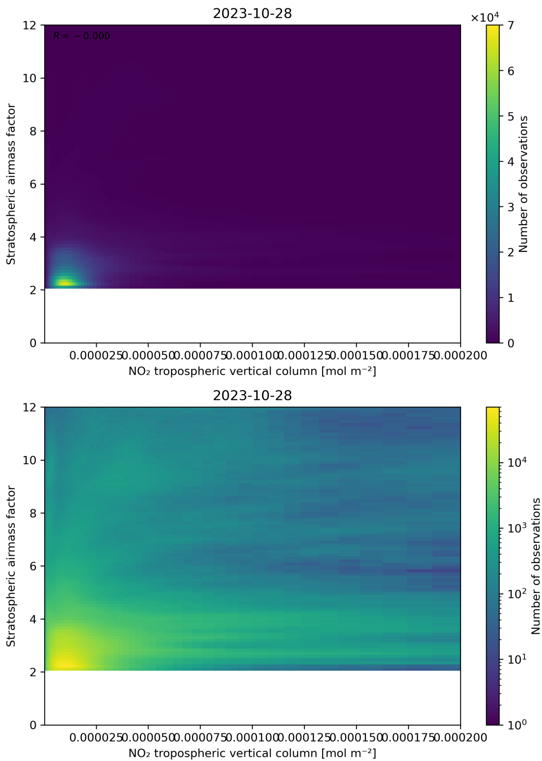
Figure 121: Scatter density plot of “NO 2 tropospheric vertical column” against “Stratospheric airmass factor” for 2023-10-28 to 2023-10-29.
