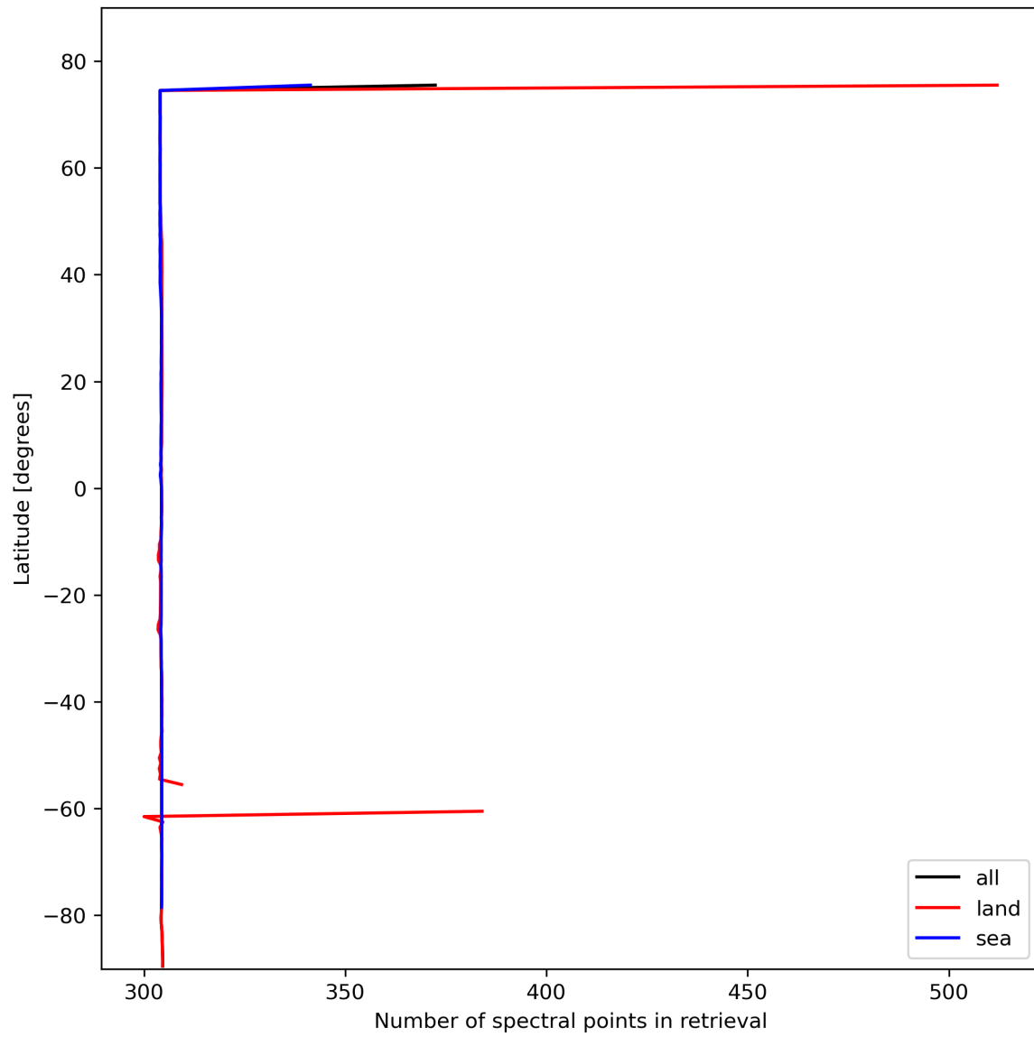
Figure 16: Zonal average of “Number of spectral points in retrieval” for 2023-10-28 to 2023-10-29.
