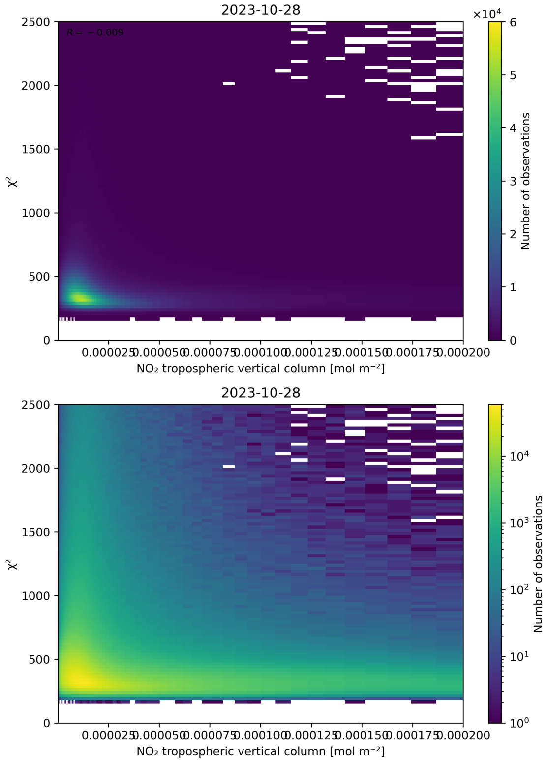
Figure 124: Scatter density plot of “NO 2 tropospheric vertical column” against “ \chi^2 ” for 2023-10-28 to 2023-10-29.
