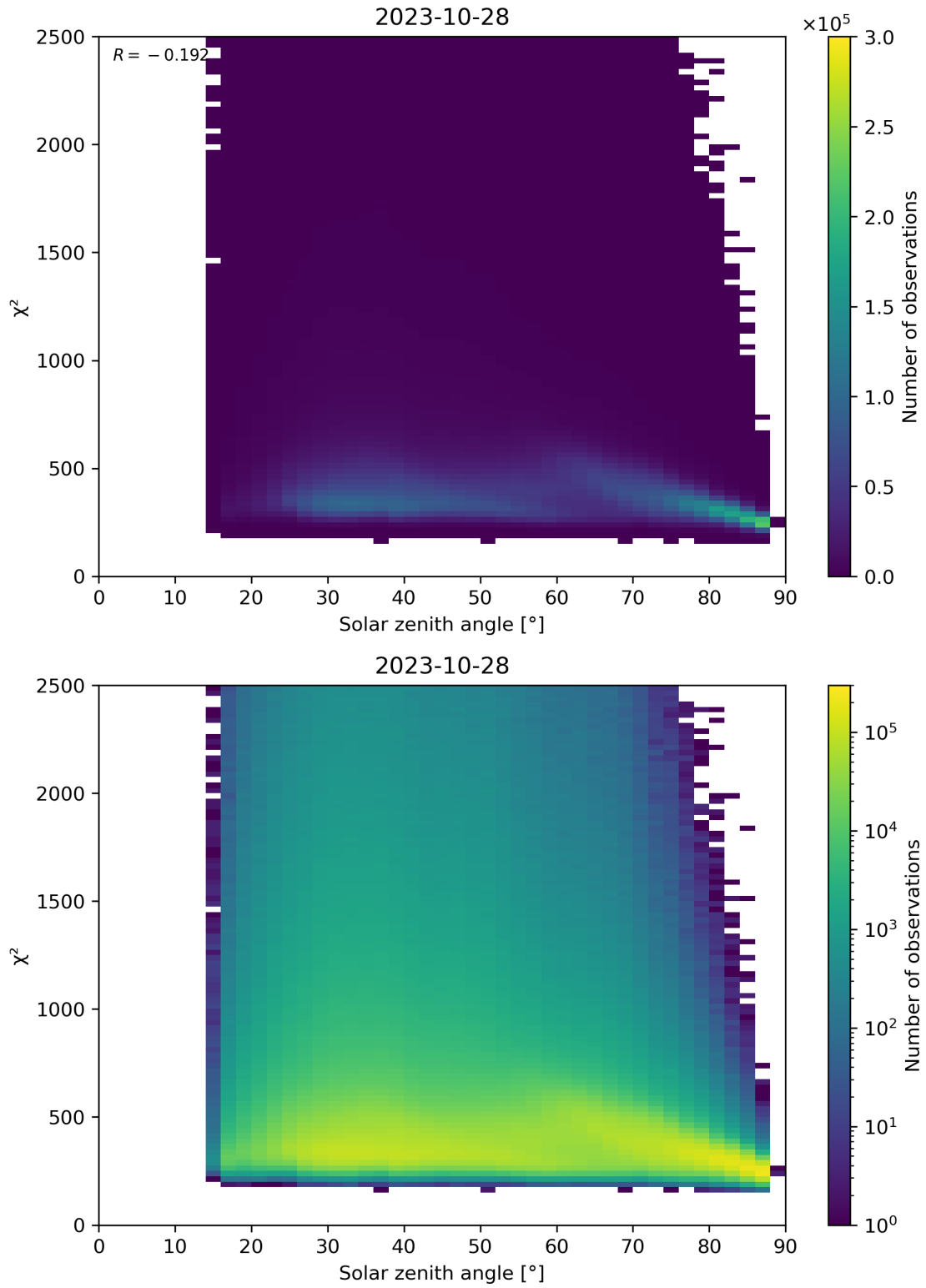
Figure 148: Scatter density plot of “Solar zenith angle” against “ \chi^2 ” for 2023-10-28 to 2023-10-29.
