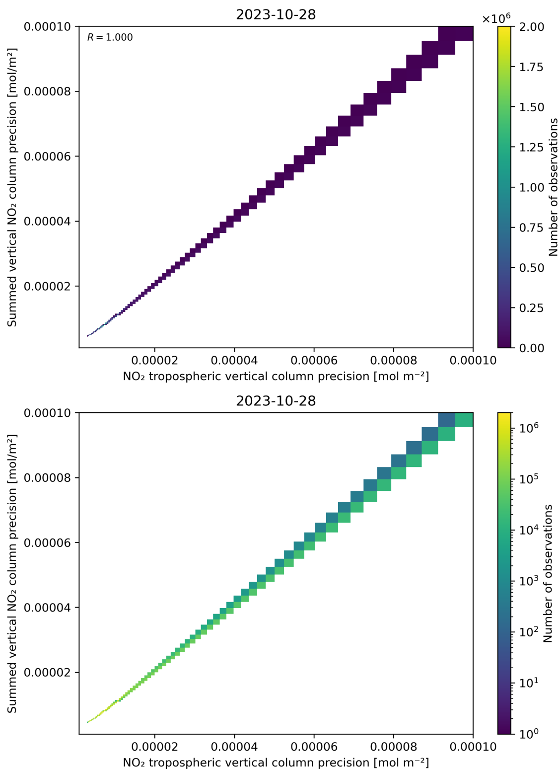
Figure 137: Scatter density plot of “NO 2 tropospheric vertical column precision” against “Summed vertical NO 2 column precision” for 2023-10-28 to 2023-10-29.
