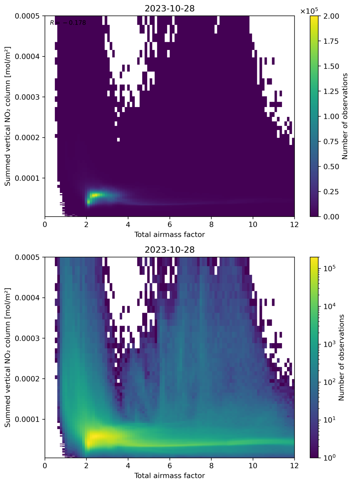
Figure 65: Scatter density plot of “Total airmass factor” against “Summed vertical NO 2 column” for 2023-10-28 to 2023-10-29.
