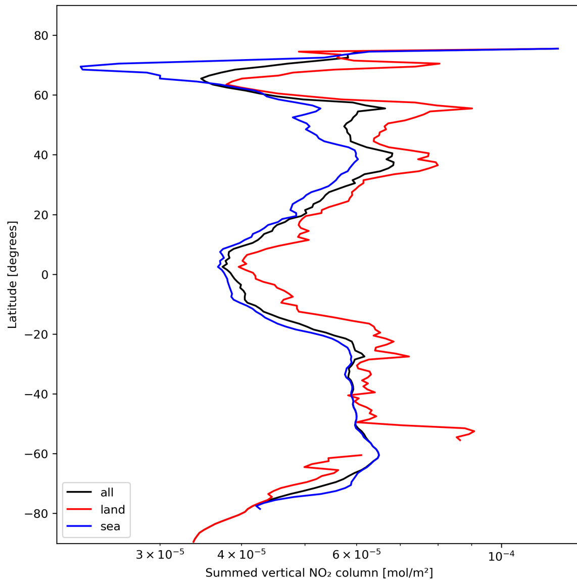
Figure 23: Zonal average of “Summed vertical NO 2 column” for 2023-10-28 to 2023-10-29.
