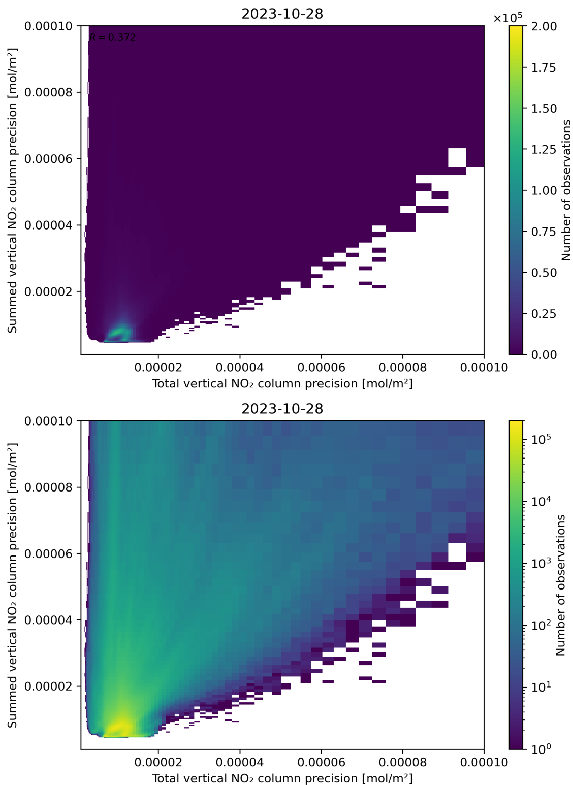
Figure 118: Scatter density plot of “Total vertical NO 2 column precision” against “Summed vertical NO 2 column precision” for 2023-10-28 to 2023-10-29.
