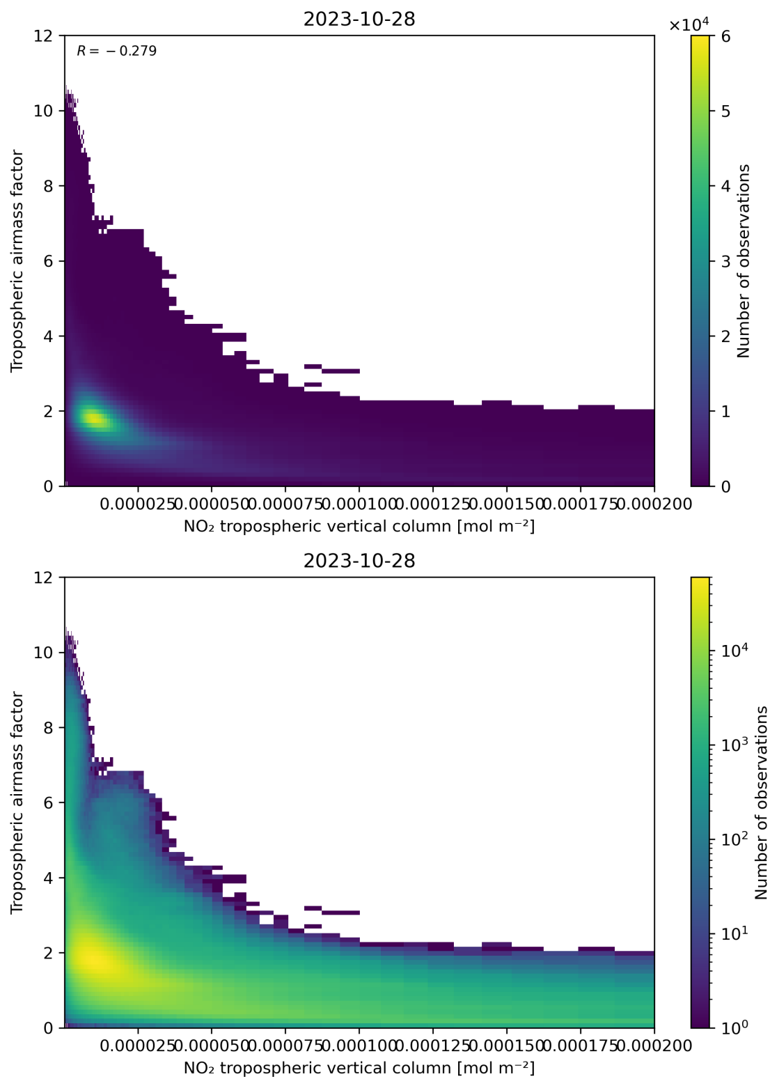
Figure 123: Scatter density plot of “NO 2 tropospheric vertical column” against “Tropospheric air mass factor” for 2023-10-28 to 2023-10-29.
