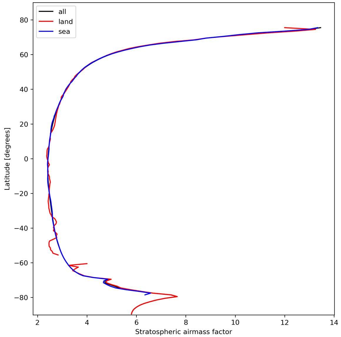
Figure 27: Zonal average of “Stratospheric airmass factor” for 2023-10-28 to 2023-10-29.
