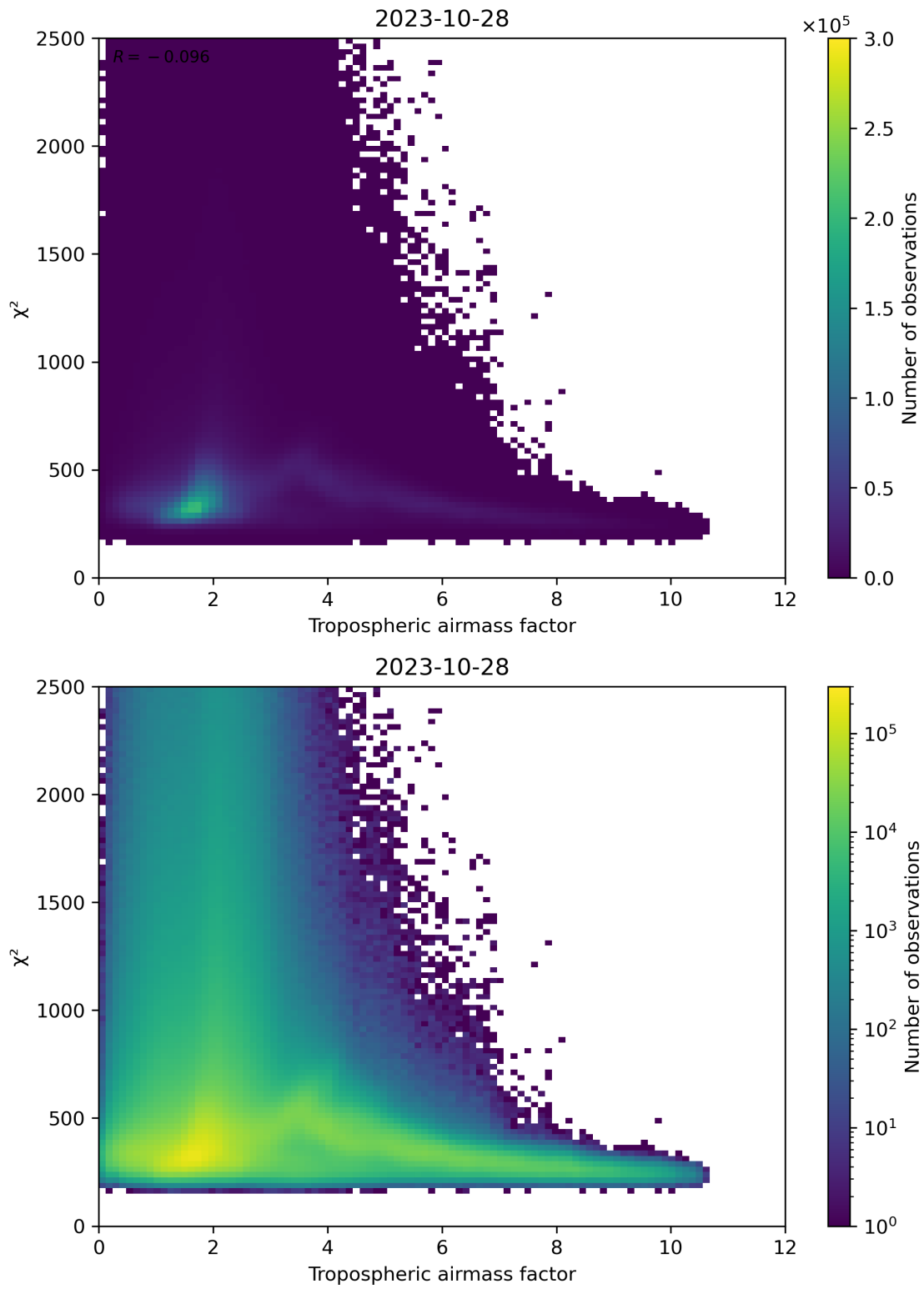
Figure 73: Scatter density plot of “Tropospheric airmass factor” against “ \chi^2 ” for 2023-10-28 to 2023-10-29.
