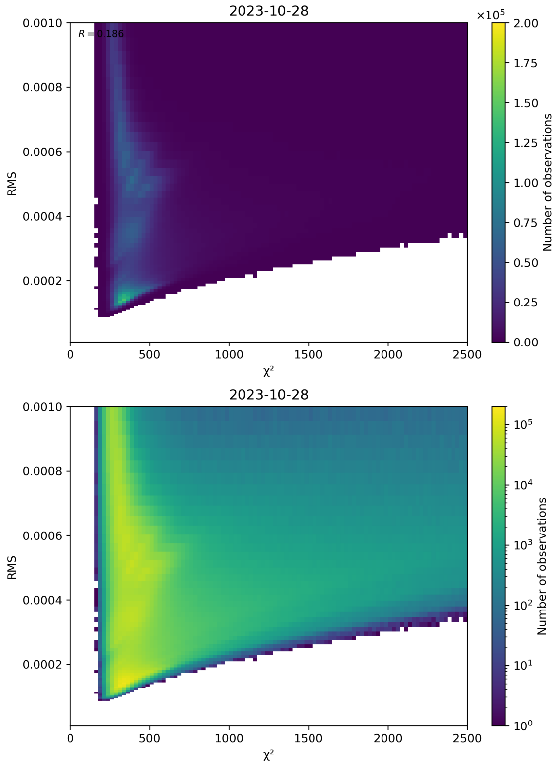
Figure 82: Scatter density plot of “ \chi^2 ” against “RMS” for 2023-10-28 to 2023-10-29.
