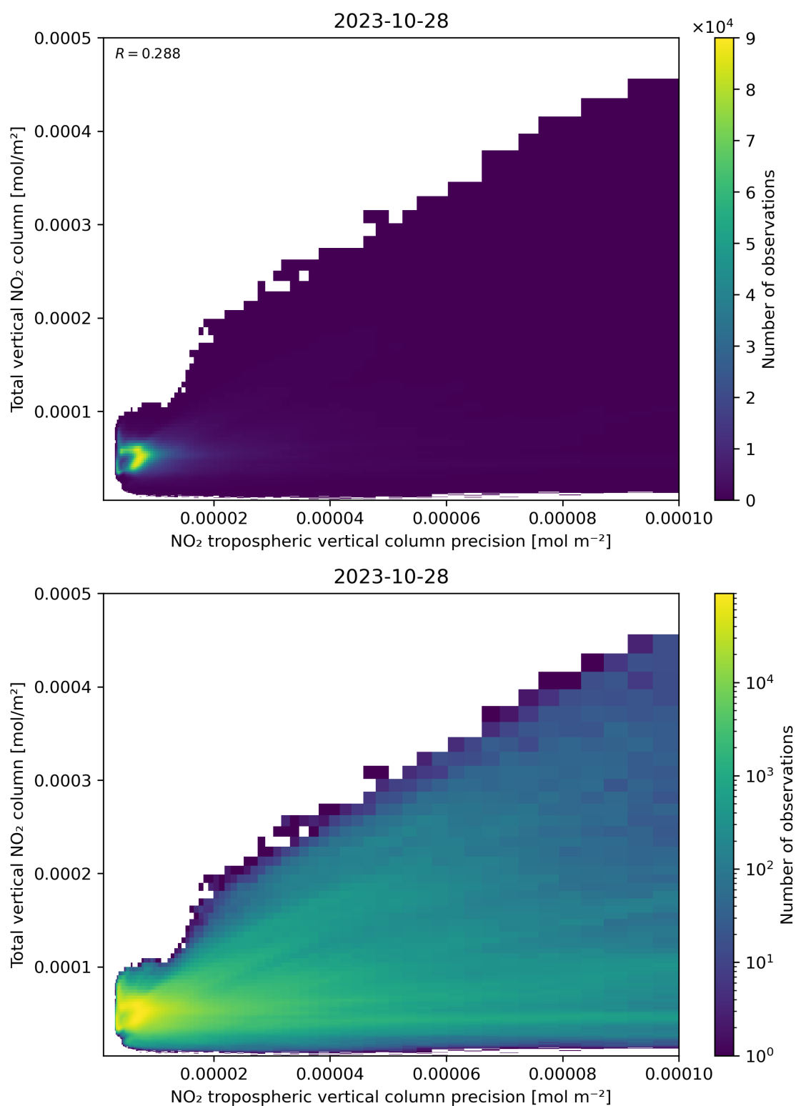
Figure 138: Scatter density plot of “NO 2 tropospheric vertical column precision” against “Total vertical NO 2 column” for 2023-10-28 to 2023-10-29.
