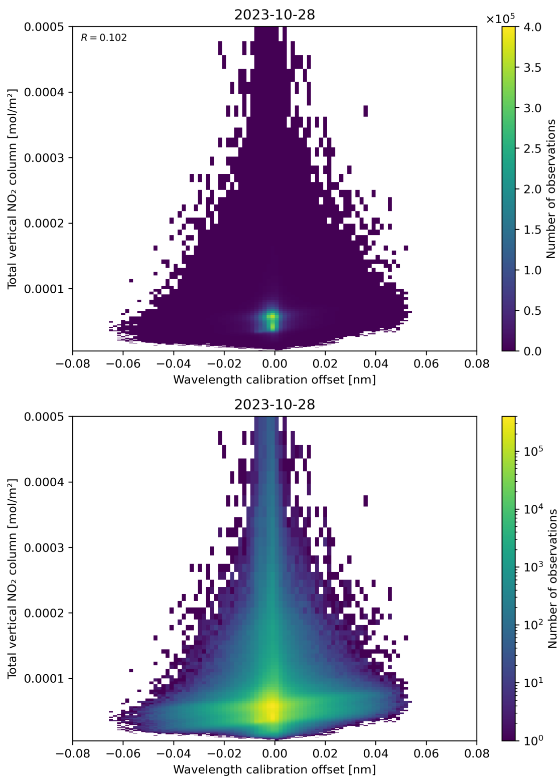
Figure 179: Scatter density plot of “Wavelength calibration offset” against “Total vertical NO 2 column” for 2023-10-28 to 2023-10-29.
