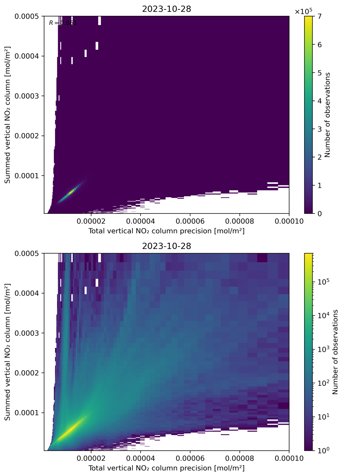
Figure 117: Scatter density plot of “Total vertical NO 2 column precision” against “Summed vertical NO 2 column” for 2023-10-28 to 2023-10-29.
