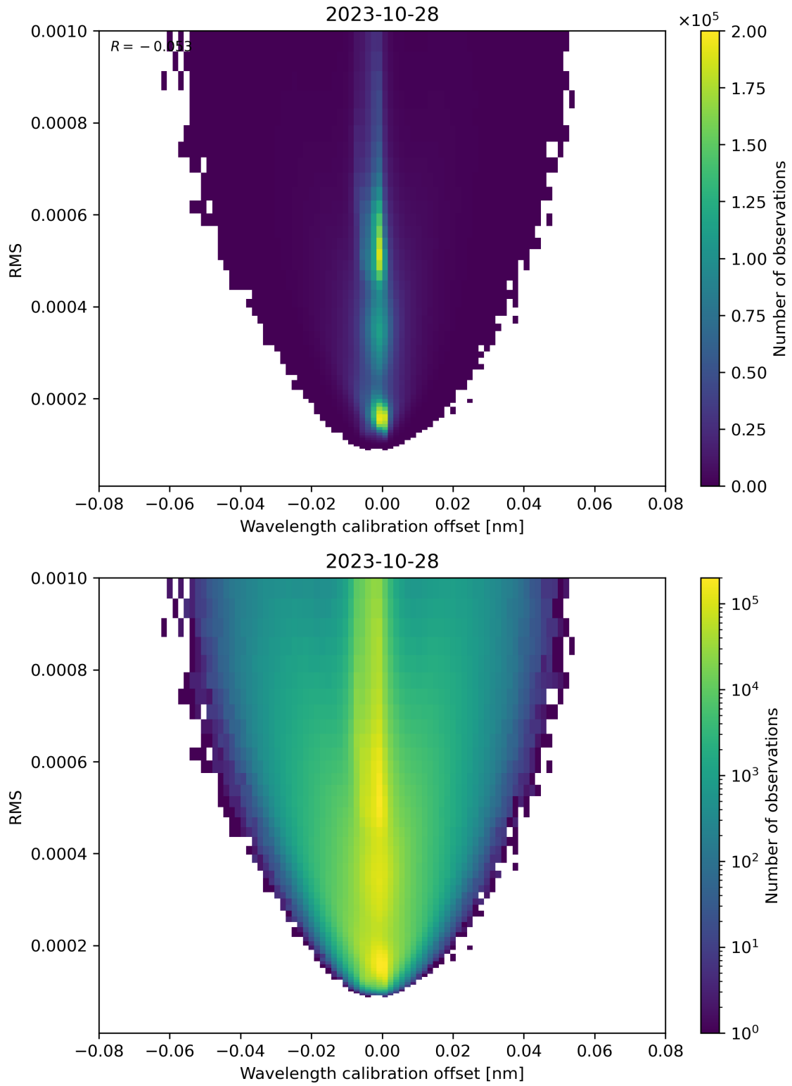
Figure 181: Scatter density plot of “Wavelength calibration offset” against “RMS” for 2023-10-28 to 2023-10-29.
