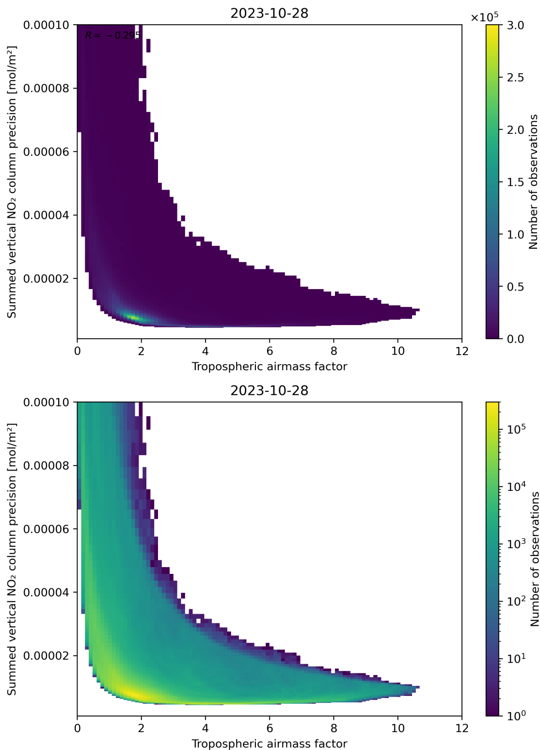
Figure 76: Scatter density plot of “Tropospheric air mass factor” against “Summed vertical NO 2 column precision” for 2023-10-28 to 2023-10-29.
