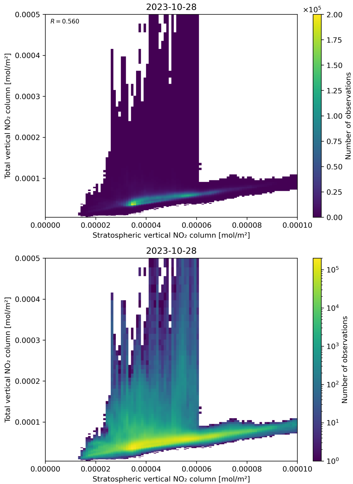
Figure 100: Scatter density plot of “Stratospheric vertical NO 2 column” against “Total vertical NO 2 column” for 2023-10-28 to 2023-10-29.
