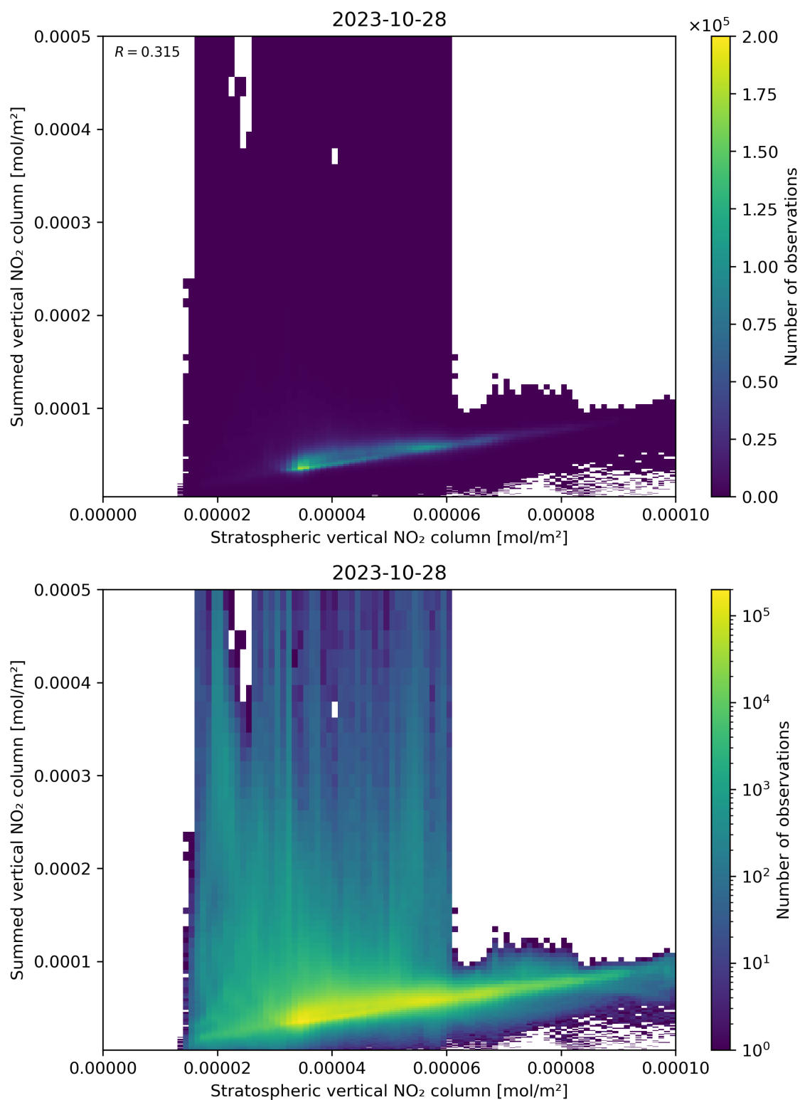
Figure 98: Scatter density plot of “Stratospheric vertical NO 2 column” against “Summed vertical NO 2 column” for 2023-10-28 to 2023-10-29.
