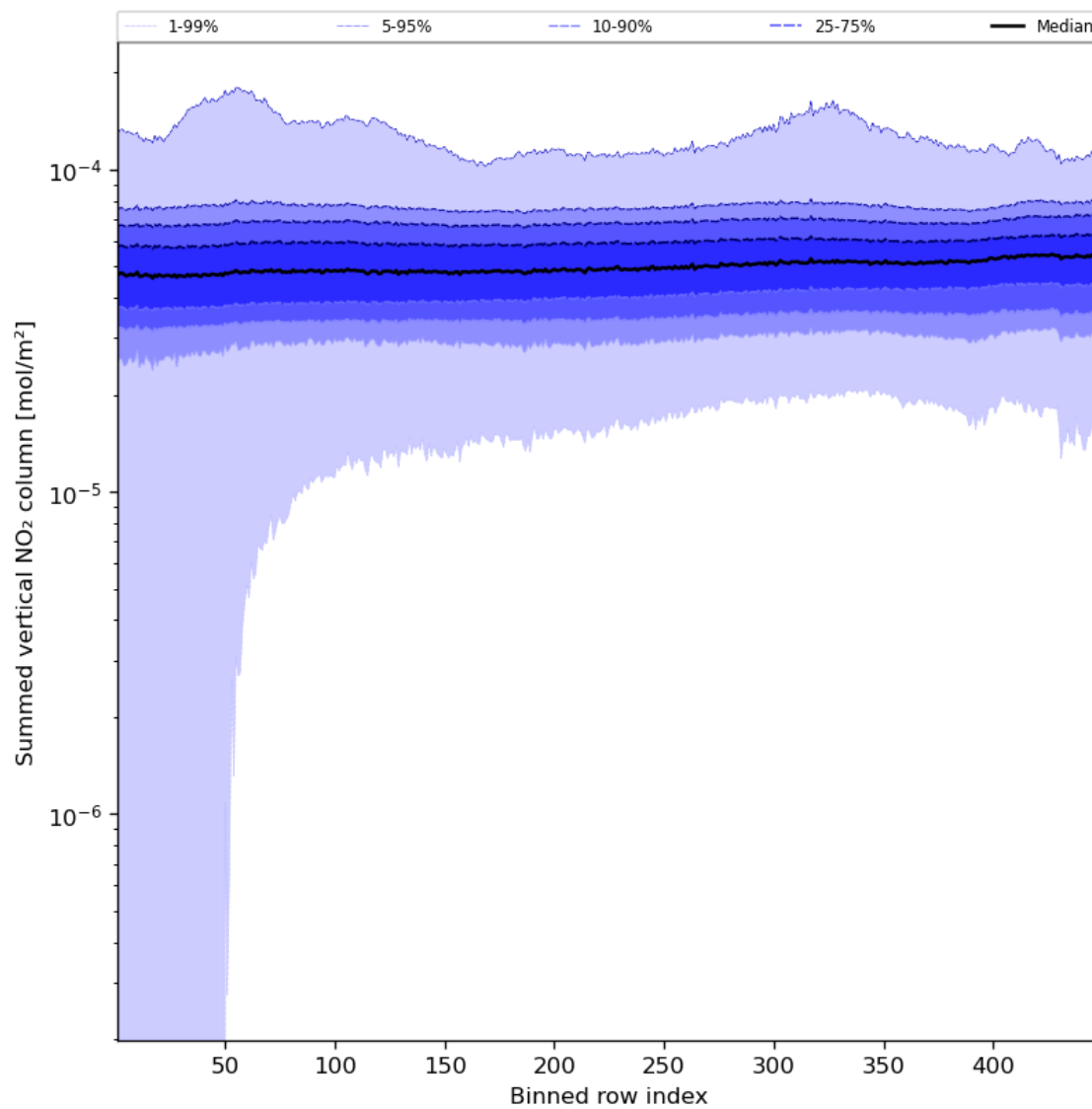
Figure 57: Along track statistics of “Summed vertical NO 2 column” for 2023-10-28 to 2023-10-29
