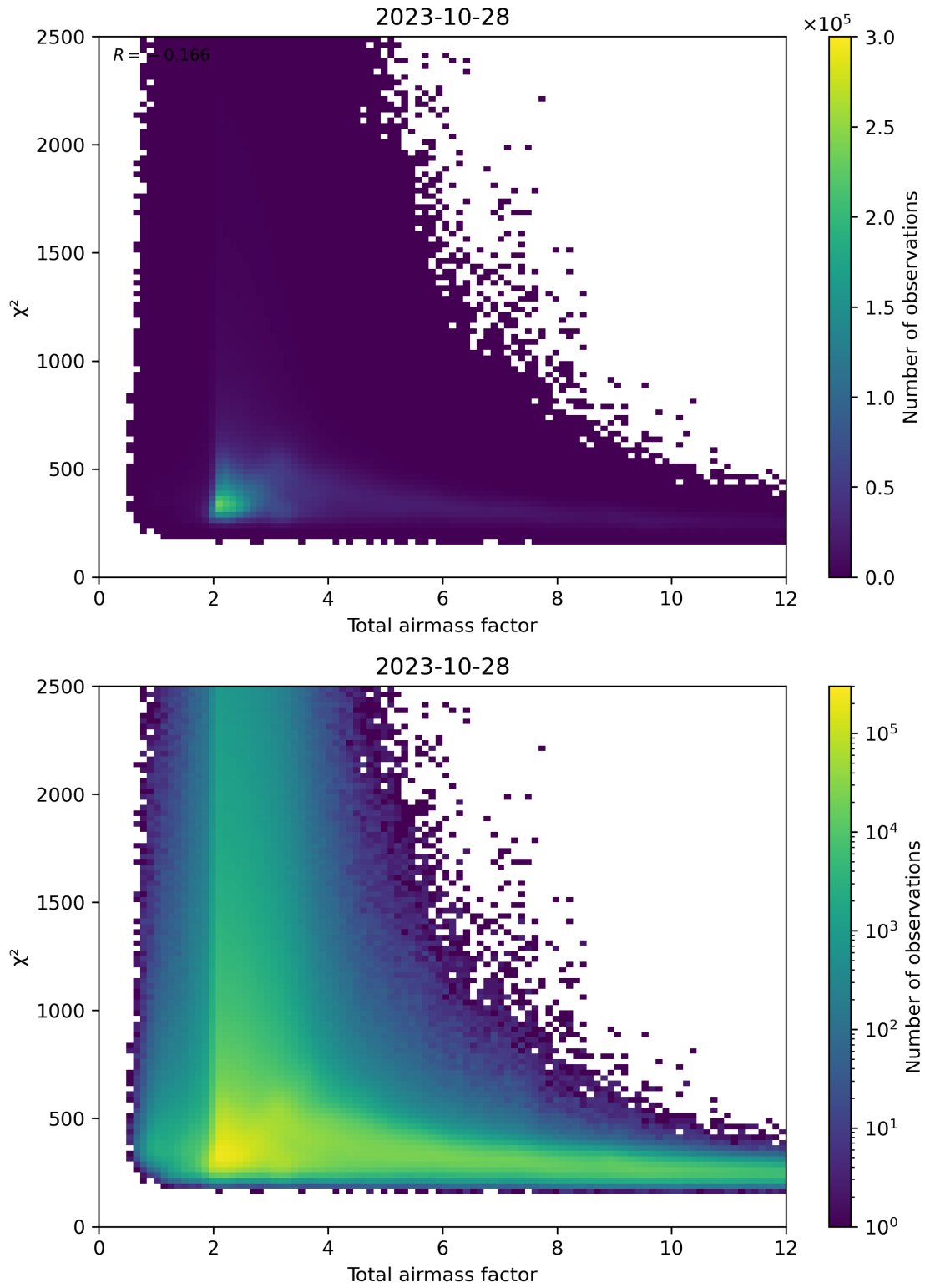
Figure 63: Scatter density plot of “Total airmass factor” against “ \chi^2 ” for 2023-10-28 to 2023-10-29.
