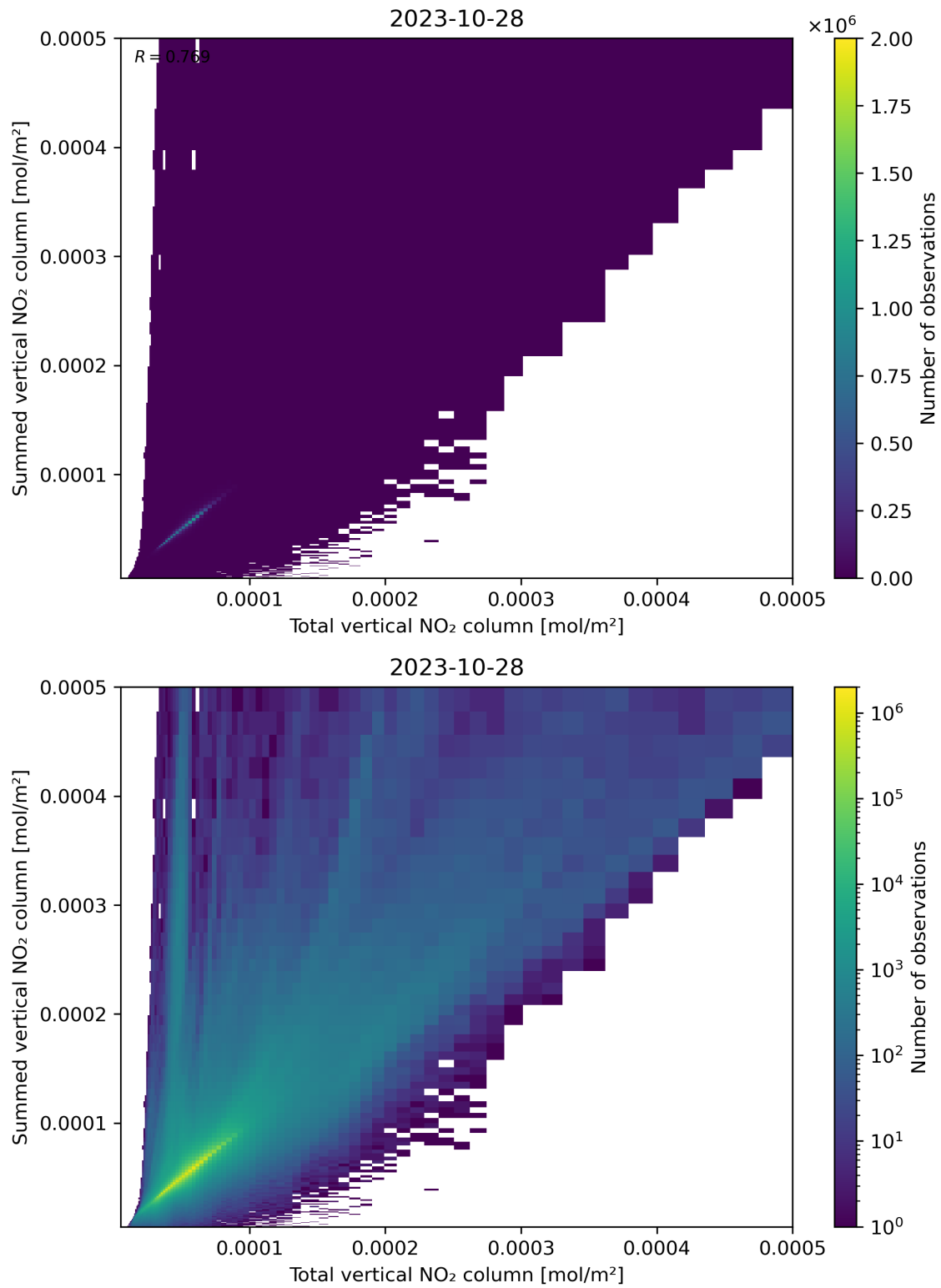
Figure 112: Scatter density plot of “Total vertical NO 2 column” against “Summed vertical NO 2 column” for 2023-10-28 to 2023-10-29.
