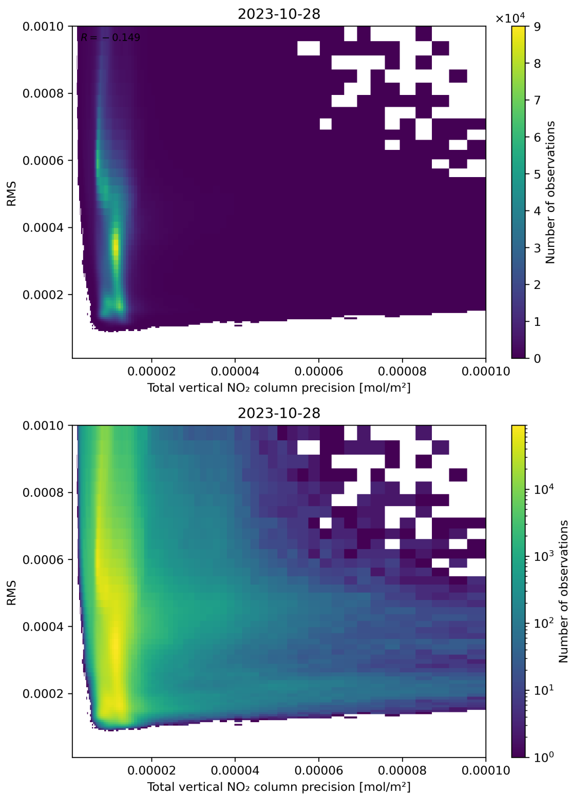
Figure 119: Scatter density plot of “Total vertical NO 2 column precision” against “RMS” for 2023-10-28 to 2023-10-29.
