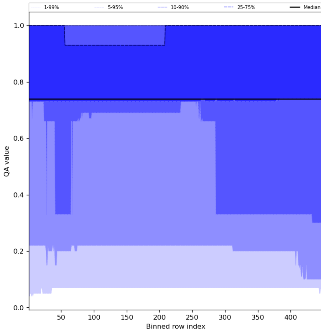
Figure 45: Along track statistics of "QA value" for 2023-10-28 to 2023-10-29
