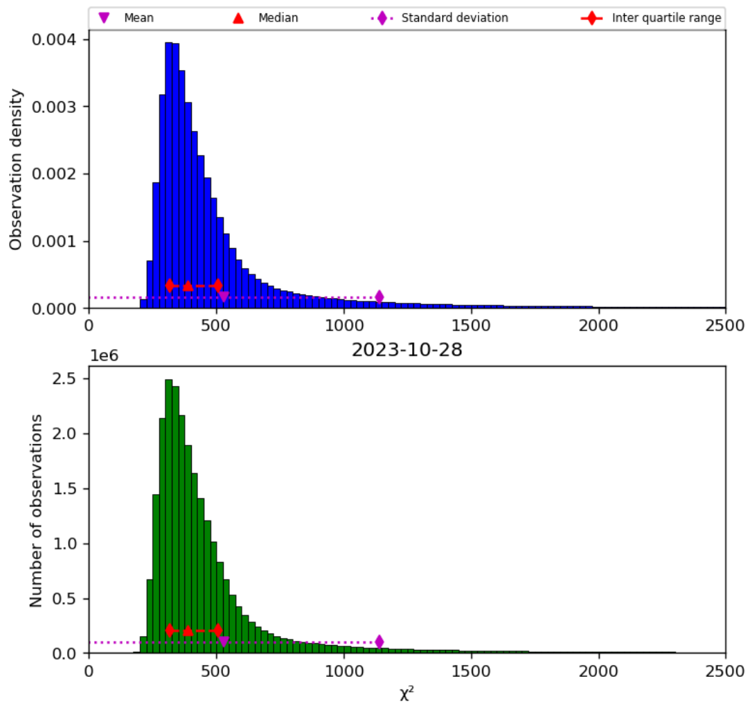
Figure 42: Histogram of “ \chi^2 ” for 2023-10-28 to 2023-10-29
