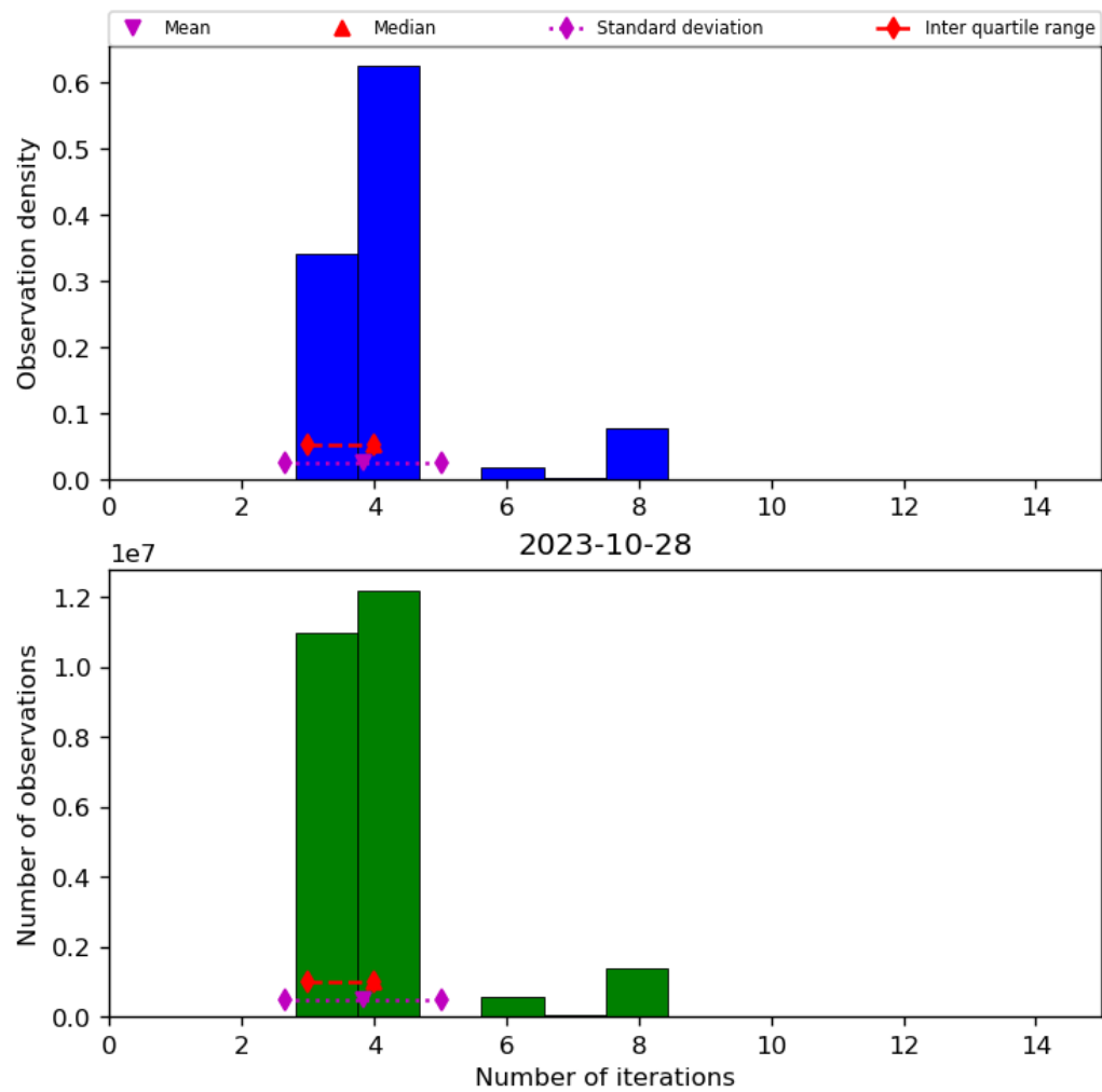
Figure 34: Histogram of “Number of iterations” for 2023-10-28 to 2023-10-29
