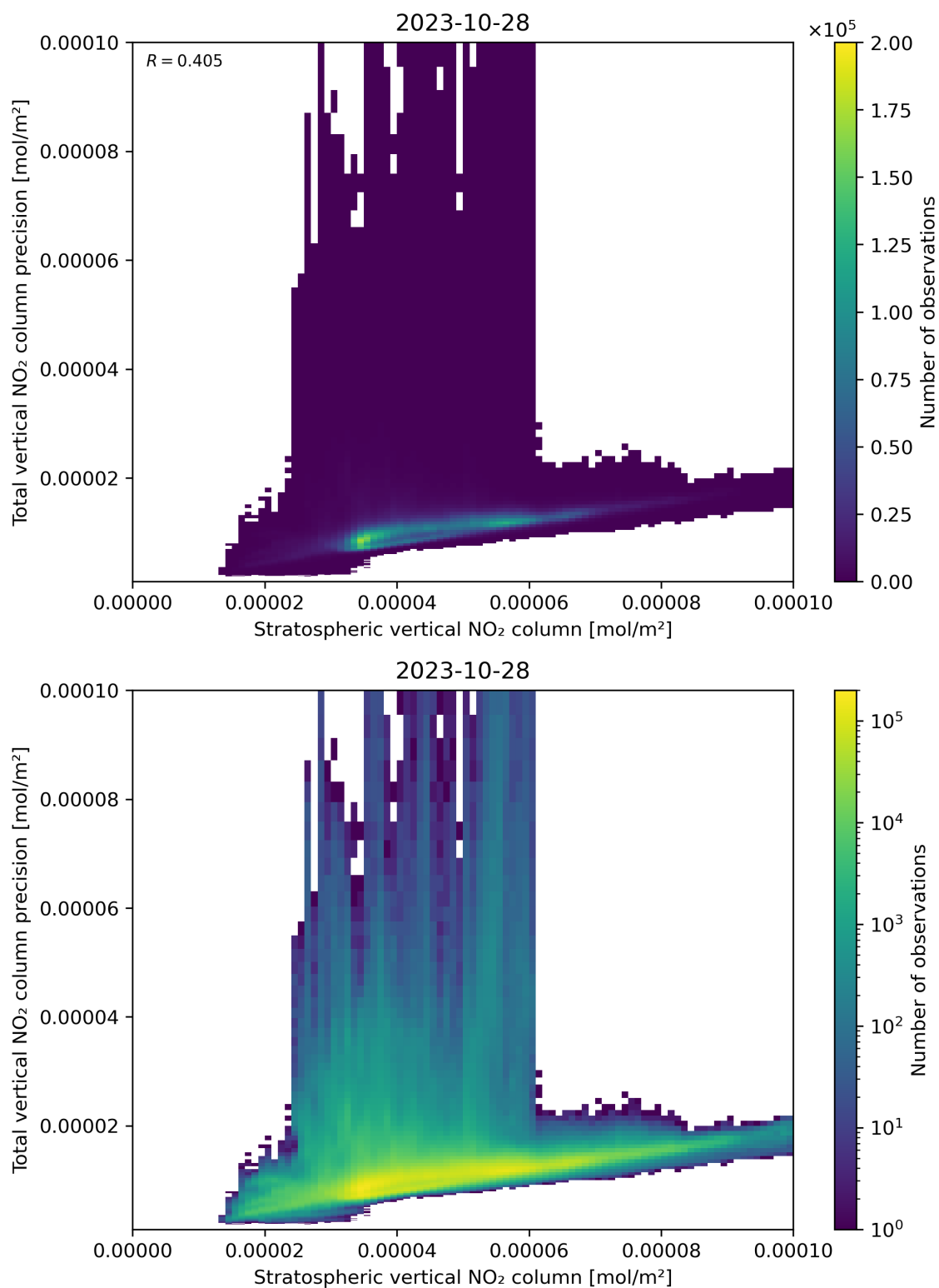
Figure 101: Scatter density plot of “Stratospheric vertical NO 2 column” against “Total vertical NO 2 column precision” for 2023-10-28 to 2023-10-29.
