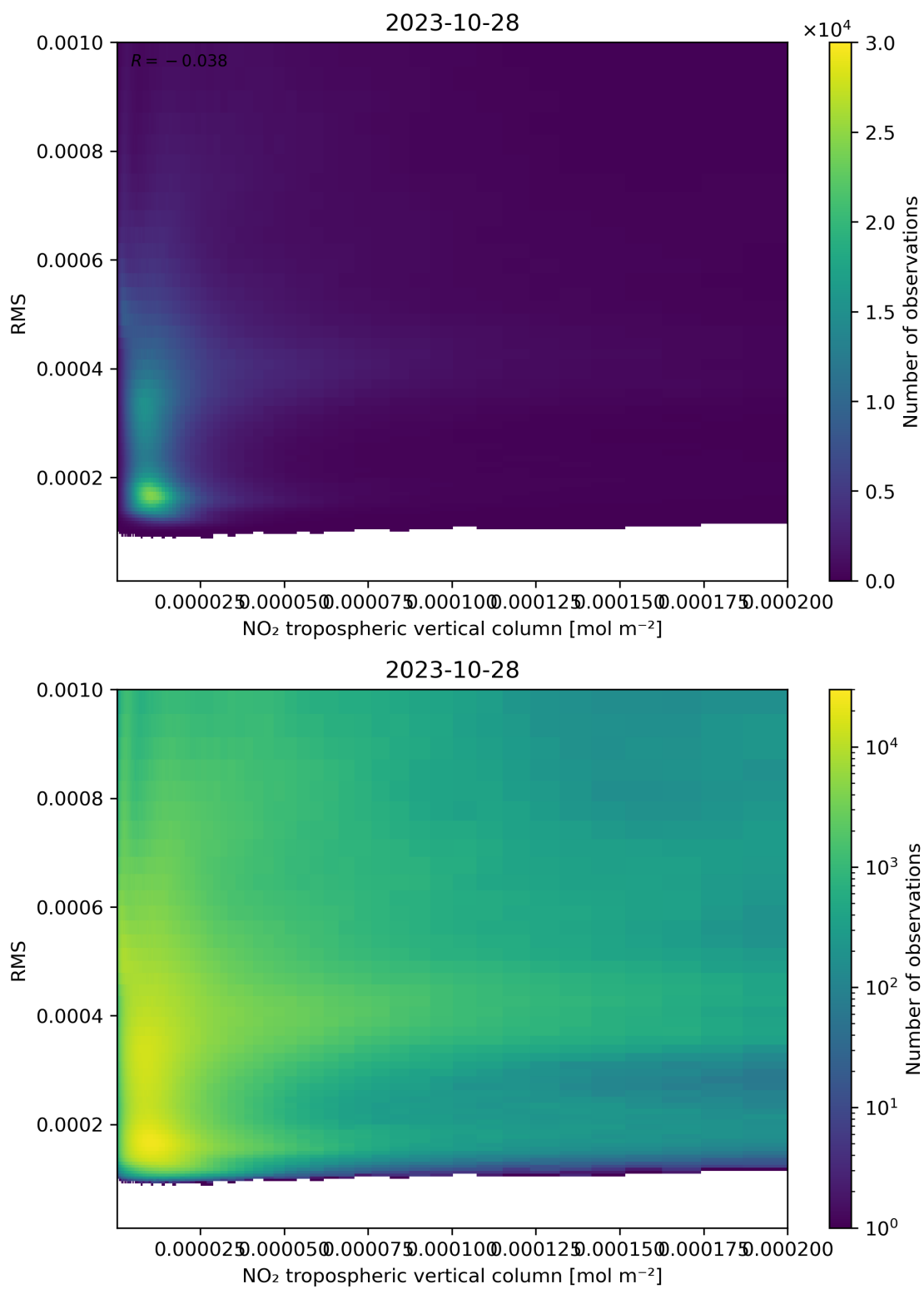
Figure 142: Scatter density plot of “NO 2 tropospheric vertical column” against “RMS” for 2023-10-28 to 2023-10-29.
