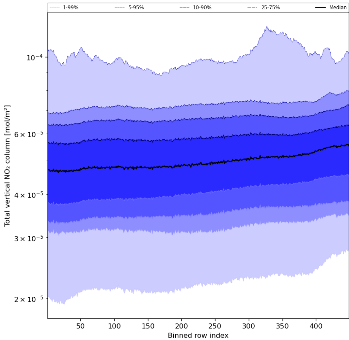
Figure 55: Along track statistics of “Total vertical NO 2 column” for 2023-10-28 to 2023-10-29
