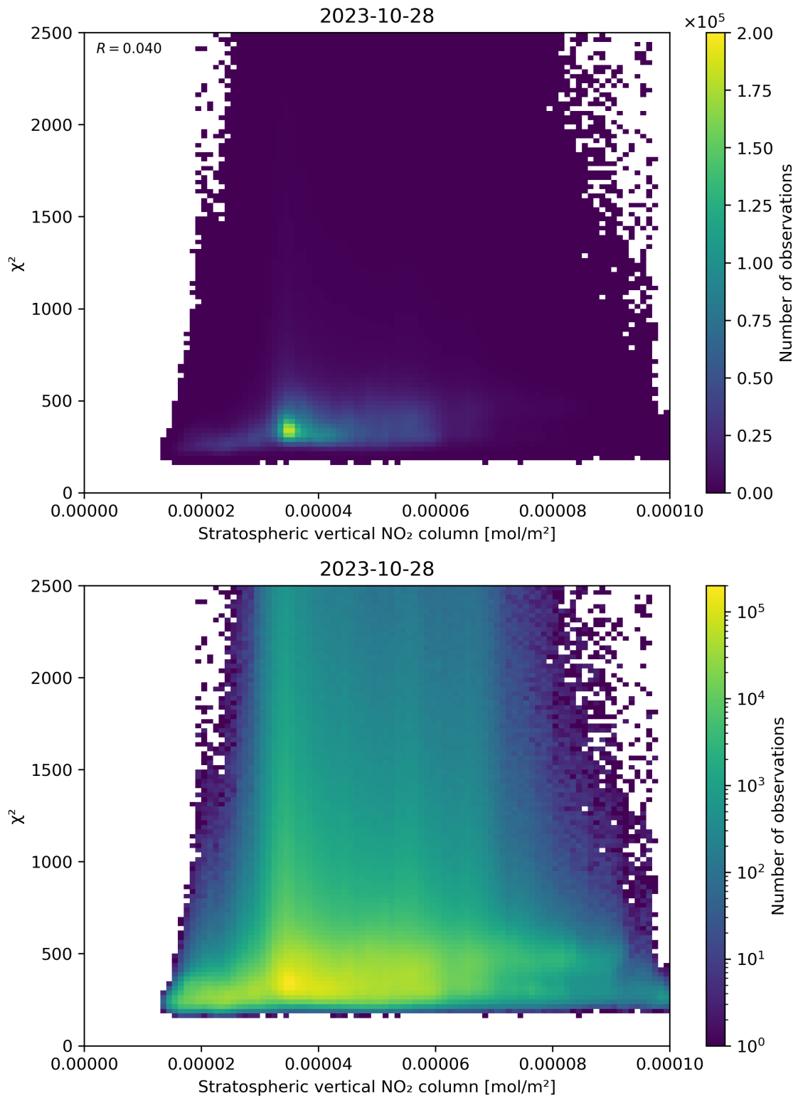
Figure 97: Scatter density plot of “Stratospheric vertical NO 2 column” against “ \chi^2 ” for 2023-10-28 to 2023-10-29.
