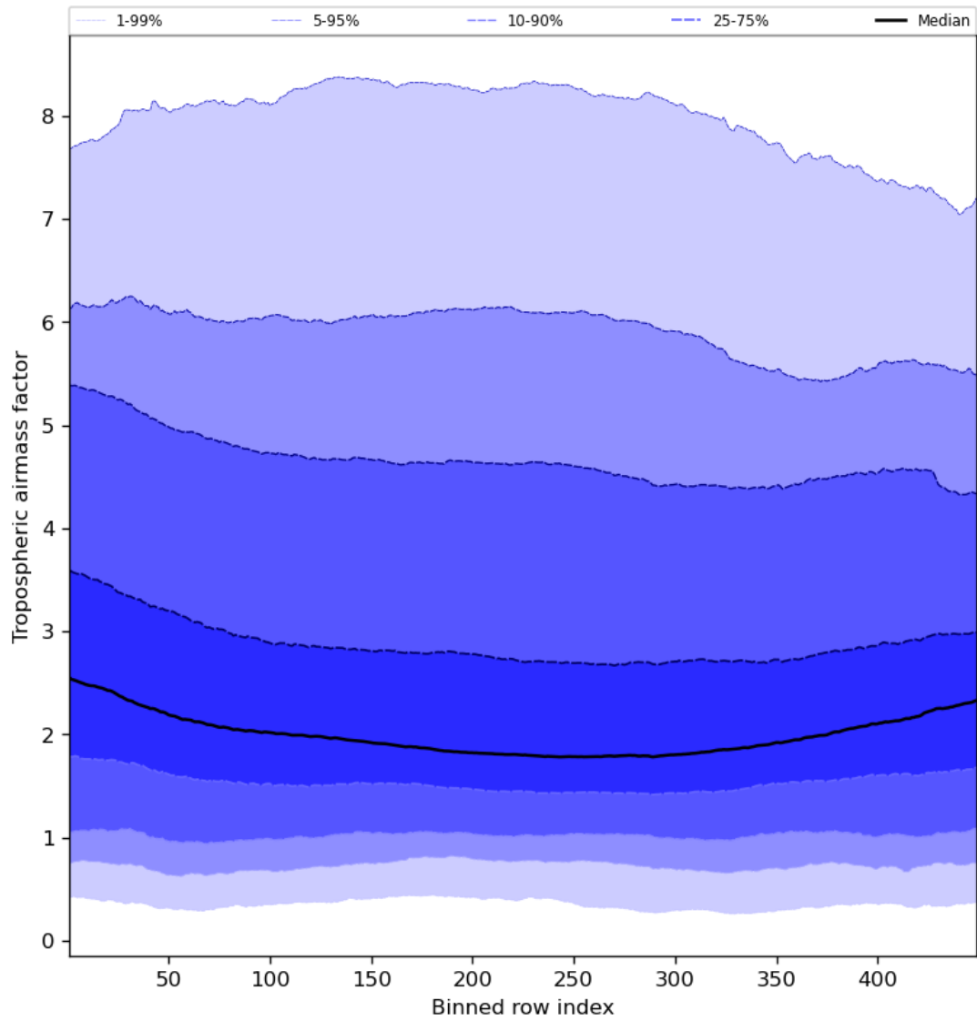
Figure 48: Along track statistics of “Tropospheric airmass factor” for 2023-10-28 to 2023-10-29
