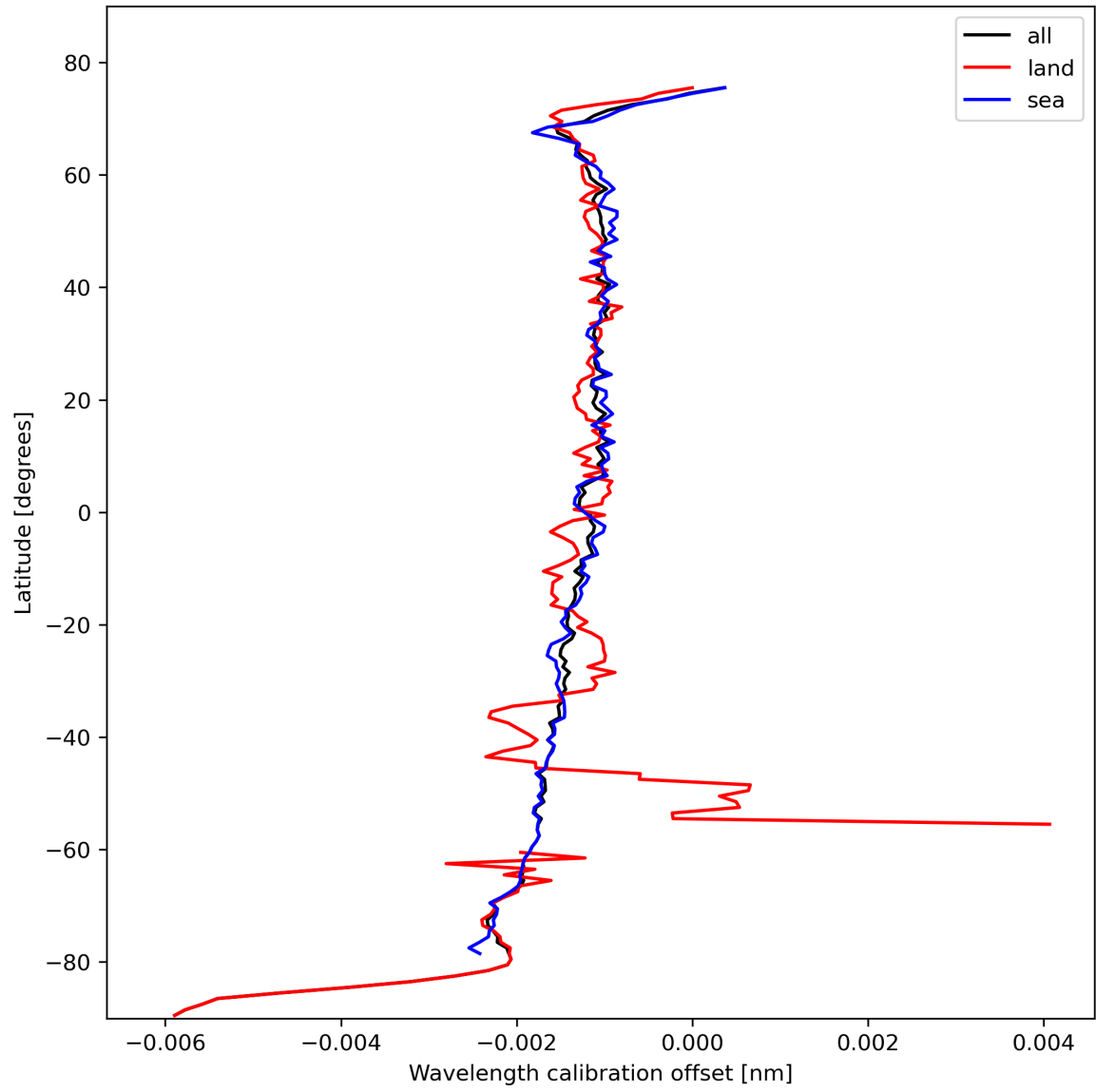
Figure 18: Zonal average of “Wavelength calibration offset” for 2023-10-28 to 2023-10-29.
