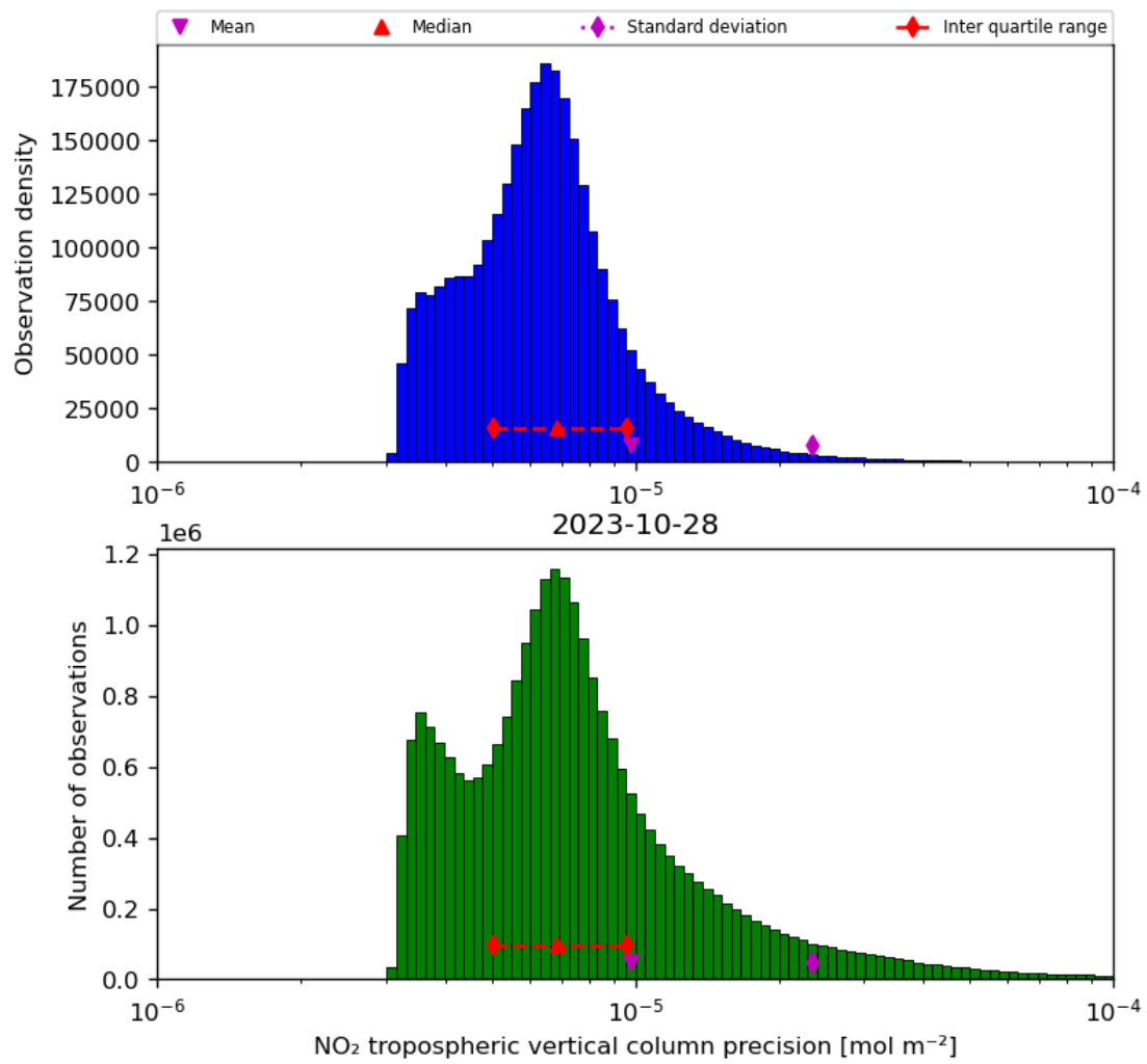
Figure 30: Histogram of “NO 2 tropospheric vertical column precision” for 2023-10-28 to 2023-10-29
