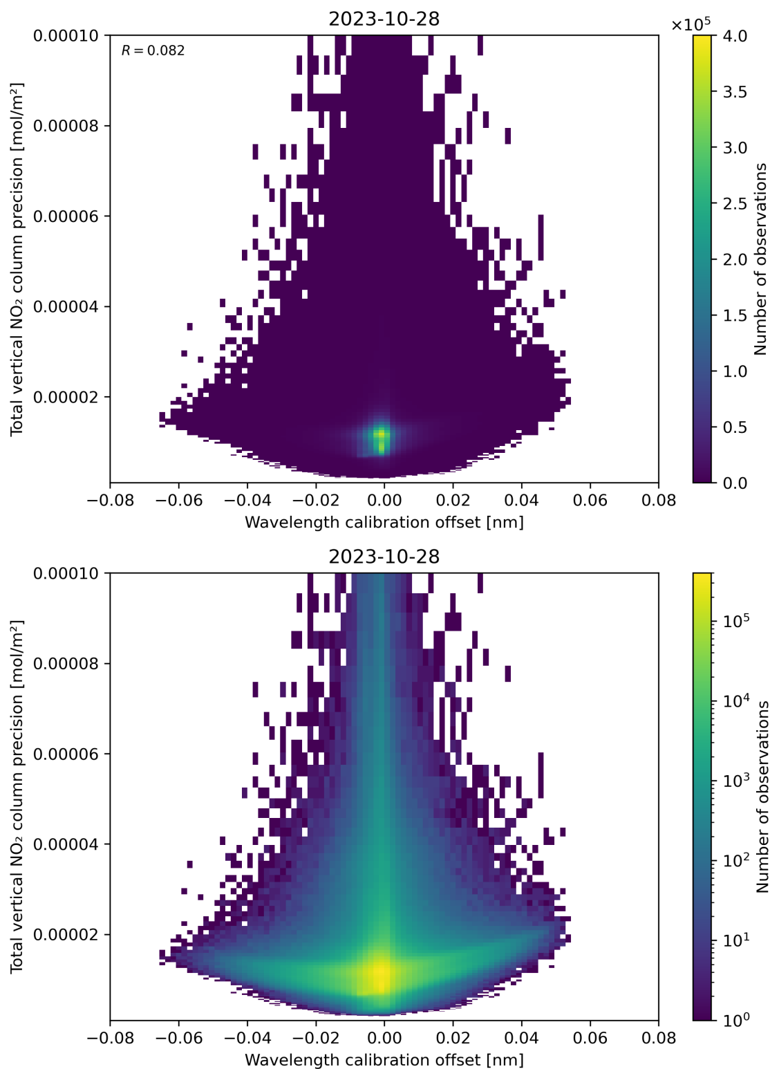
Figure 180: Scatter density plot of “Wavelength calibration offset” against “Total vertical NO 2 column precision” for 2023-10-28 to 2023-10-29.
