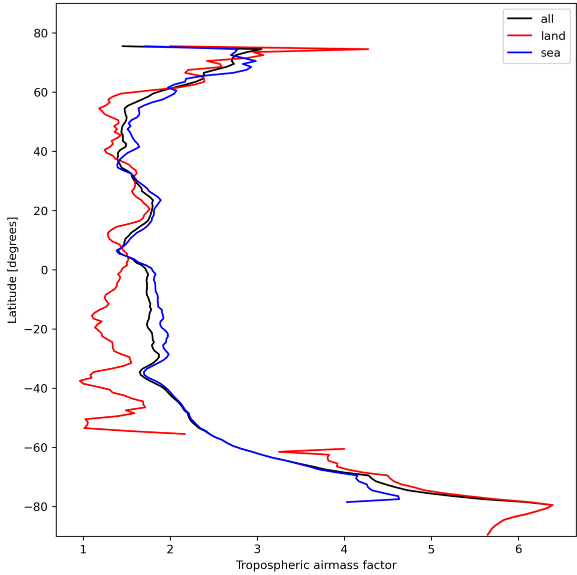
Figure 14: Zonal average of “Tropospheric airmass factor” for 2023-10-28 to 2023-10-29.
