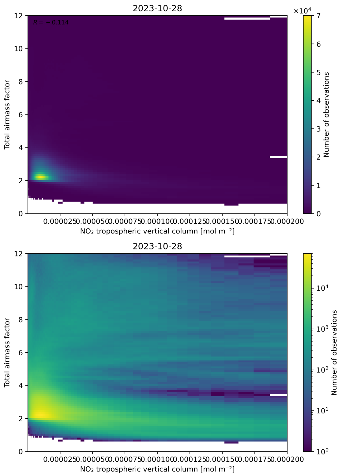
Figure 122: Scatter density plot of “NO 2 tropospheric vertical column” against “Total air mass factor” for 2023-10-28 to 2023-10-29.
