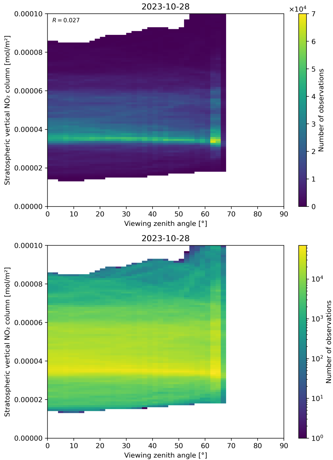
Figure 164: Scatter density plot of “Viewing zenith angle” against “Stratospheric vertical NO 2 column” for 2023-10-28 to 2023-10-29.
