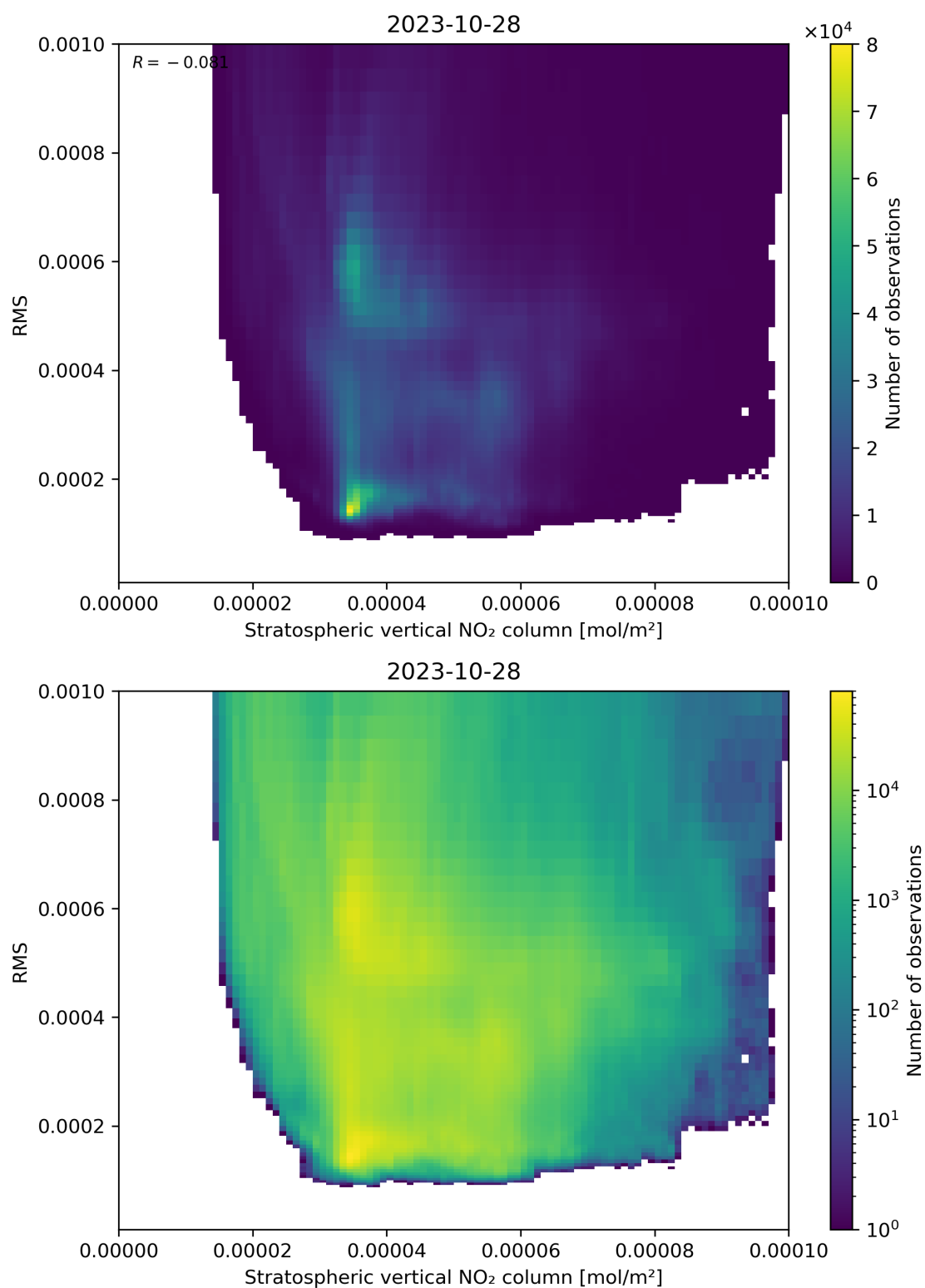
Figure 102: Scatter density plot of “Stratospheric vertical NO 2 column” against “RMS” for 2023-10-28 to 2023-10-29.
