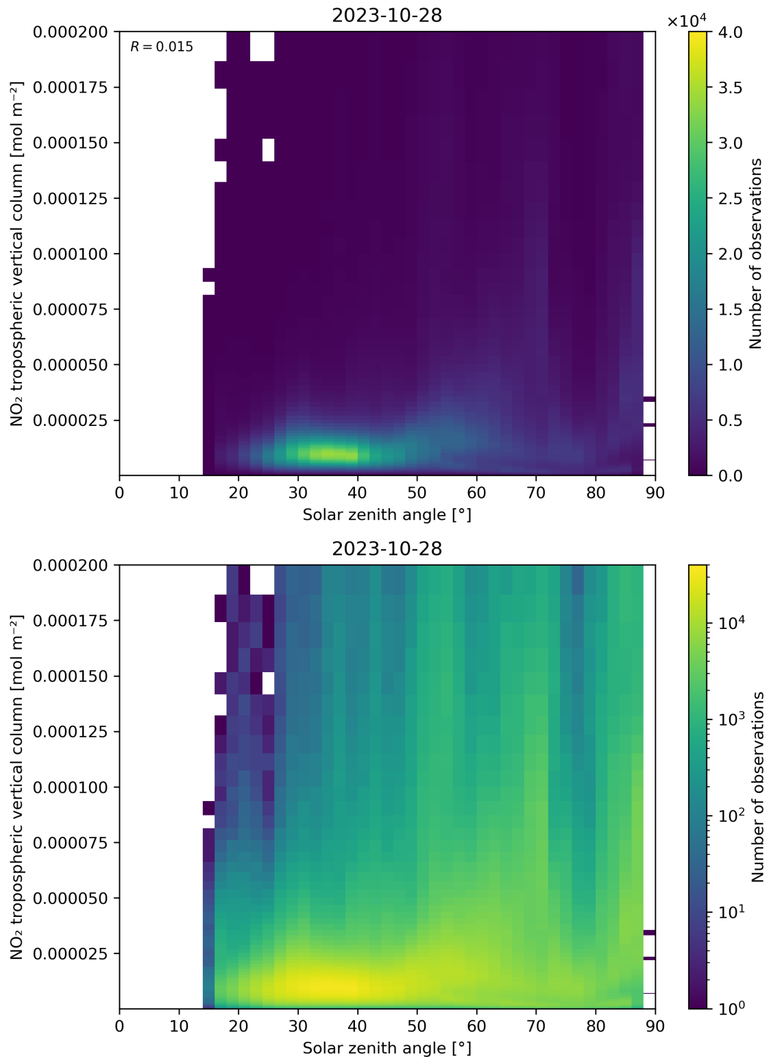
Figure 155: Scatter density plot of “Solar zenith angle” against “NO 2 tropospheric vertical column” for 2023-10-28 to 2023-10-29.
