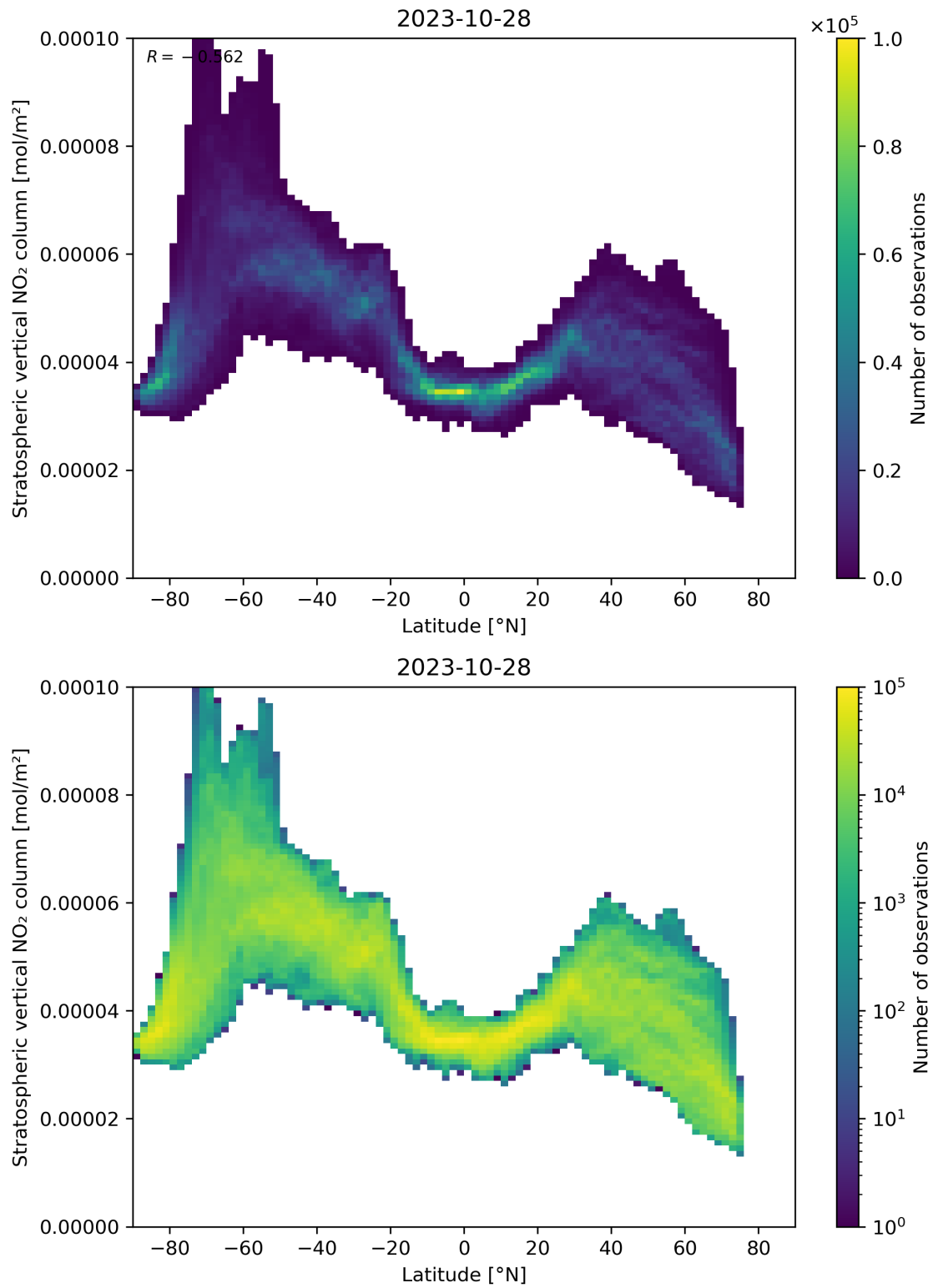
Figure 87: Scatter density plot of “Latitude” against “Stratospheric vertical NO 2 column” for 2023-10-28 to 2023-10-29.
