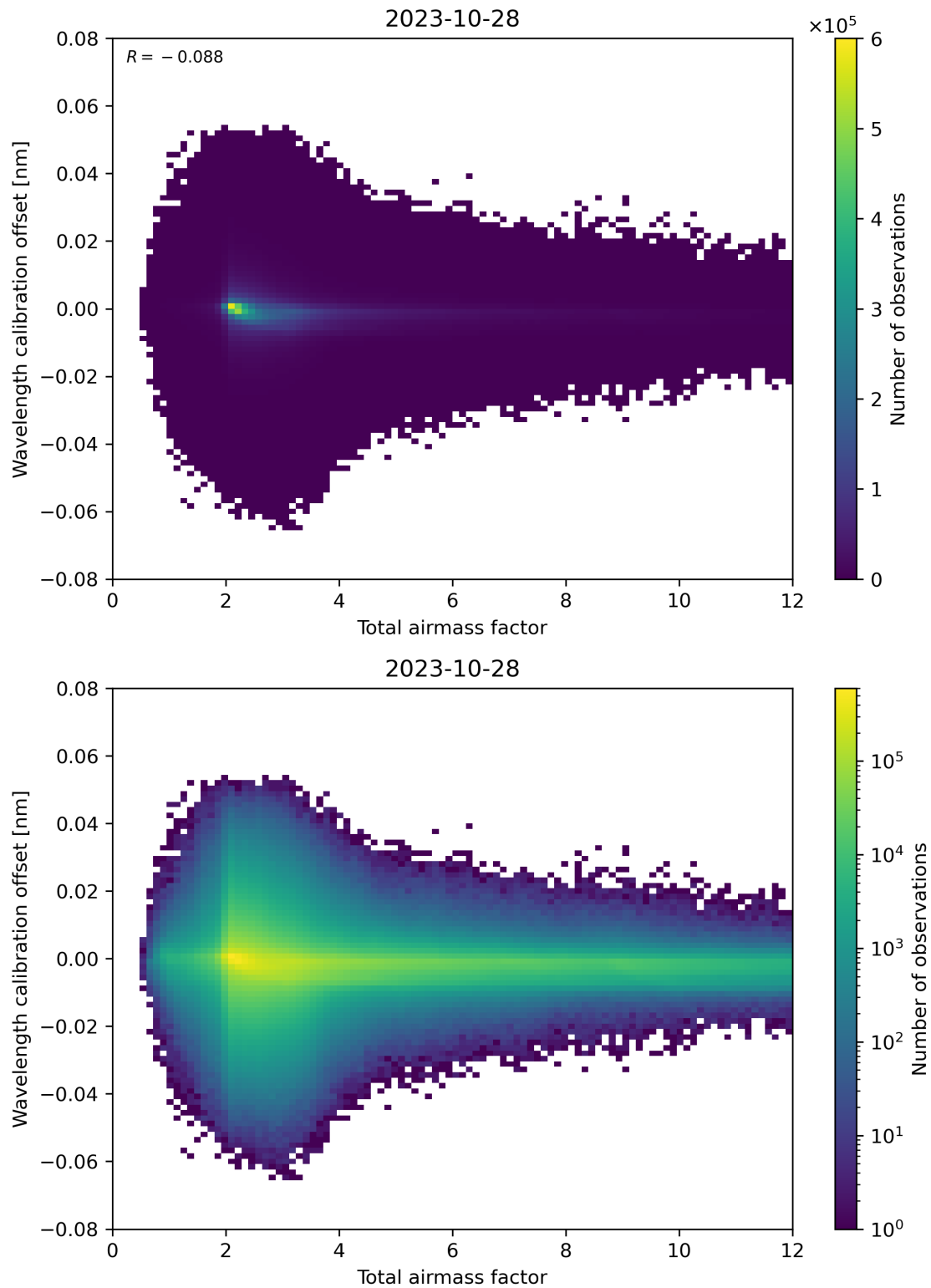
Figure 70: Scatter density plot of “Total airmass factor” against “Wavelength calibration offset” for 2023-10-28 to 2023-10-29.
