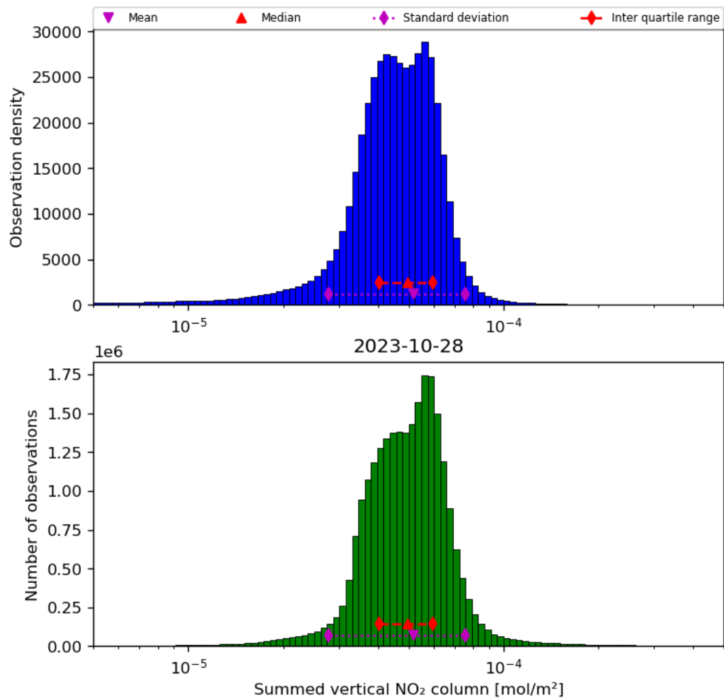
Figure 40: Histogram of “Summed vertical NO 2 column” for 2023-10-28 to 2023-10-29
