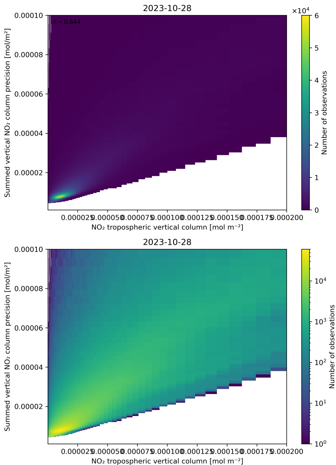
Figure 127: Scatter density plot of “NO 2 tropospheric vertical column” against “Summed vertical NO 2 column precision” for 2023-10-28 to 2023-10-29.
