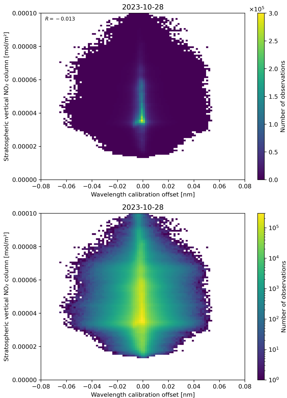
Figure 176: Scatter density plot of “Wavelength calibration offset” against “Stratospheric vertical NO 2 column” for 2023-10-28 to 2023-10-29.
