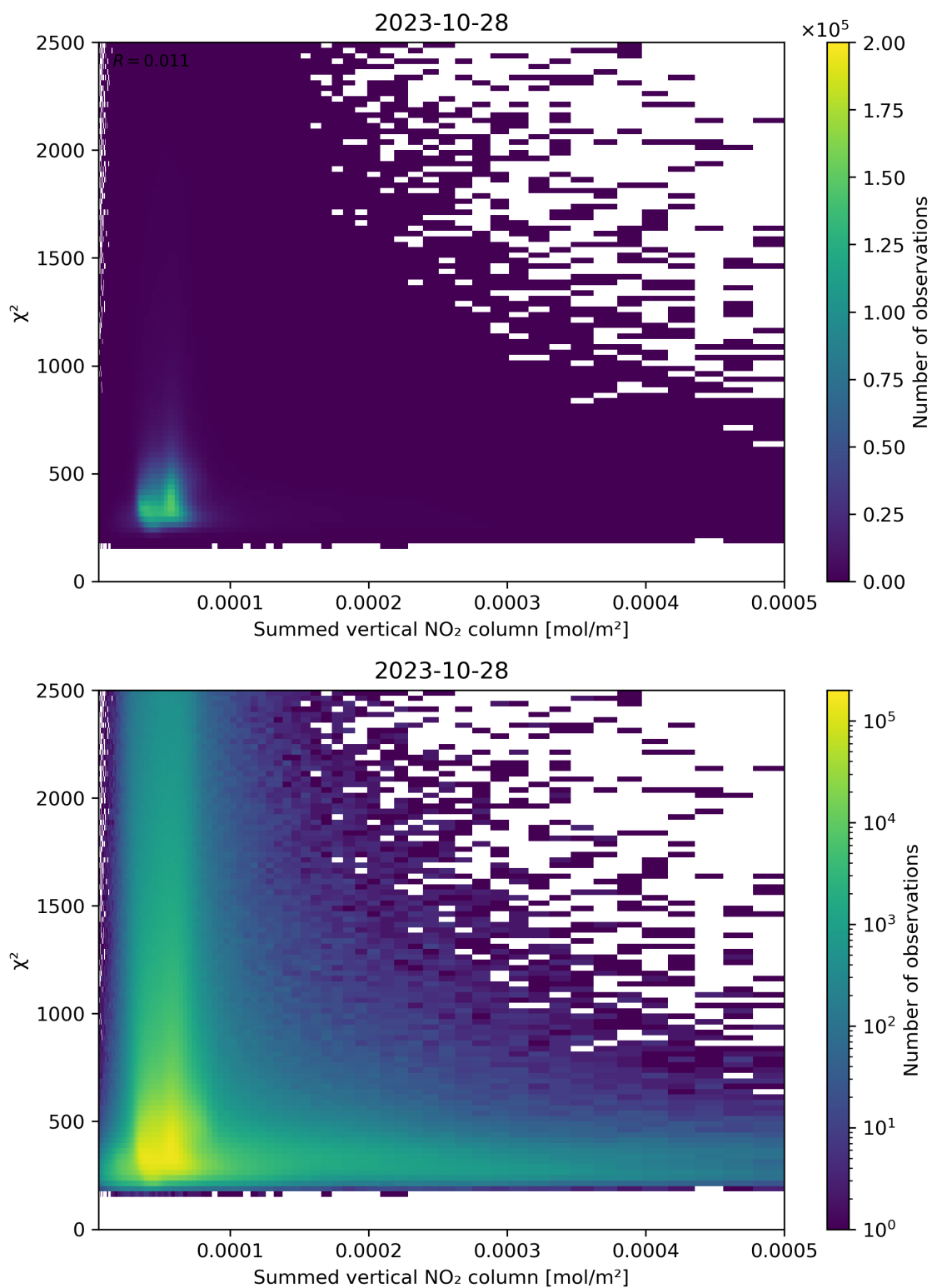
Figure 104: Scatter density plot of “Summed vertical NO 2 column” against “ \chi^2 ” for 2023-10-28 to 2023-10-29.
