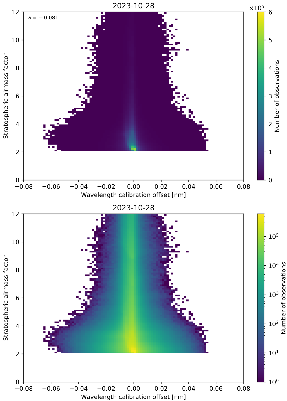
Figure 174: Scatter density plot of “Wavelength calibration offset” against “Stratospheric airmass factor” for 2023-10-28 to 2023-10-29.
