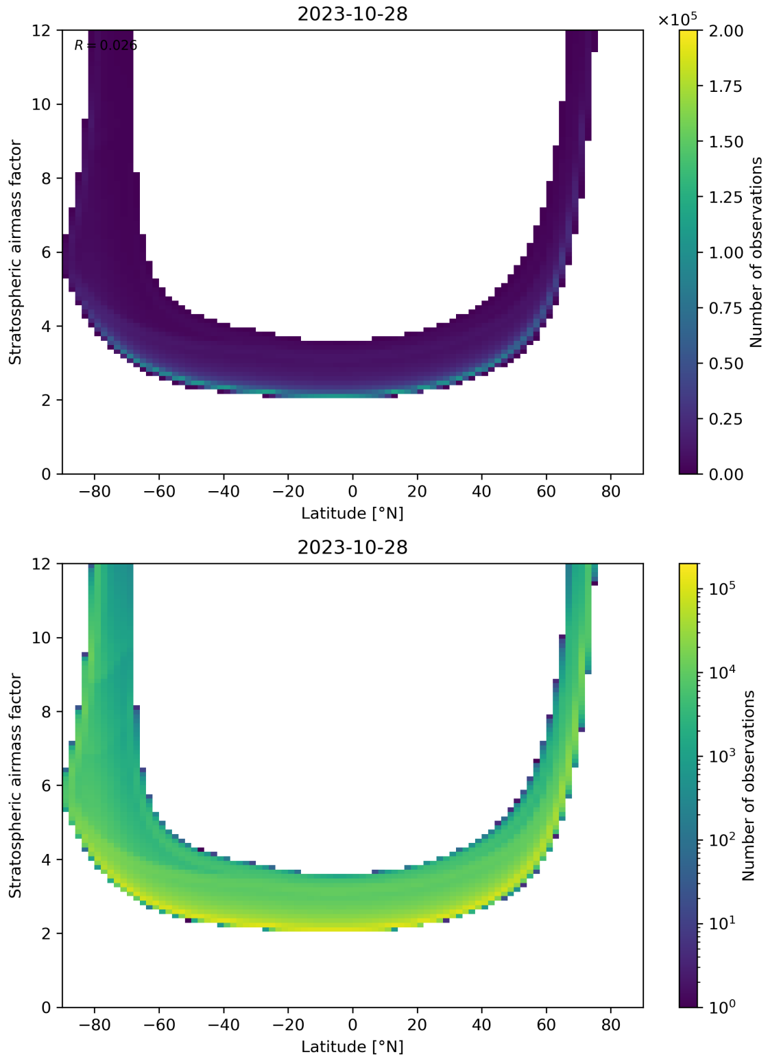
Figure 83: Scatter density plot of “Latitude” against “Stratospheric airmass factor” for 2023-10-28 to 2023-10-29.
