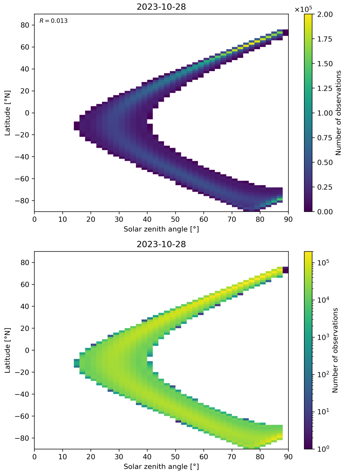
Figure 149: Scatter density plot of “Solar zenith angle” against “Latitude” for 2023-10-28 to 2023-10-29.
