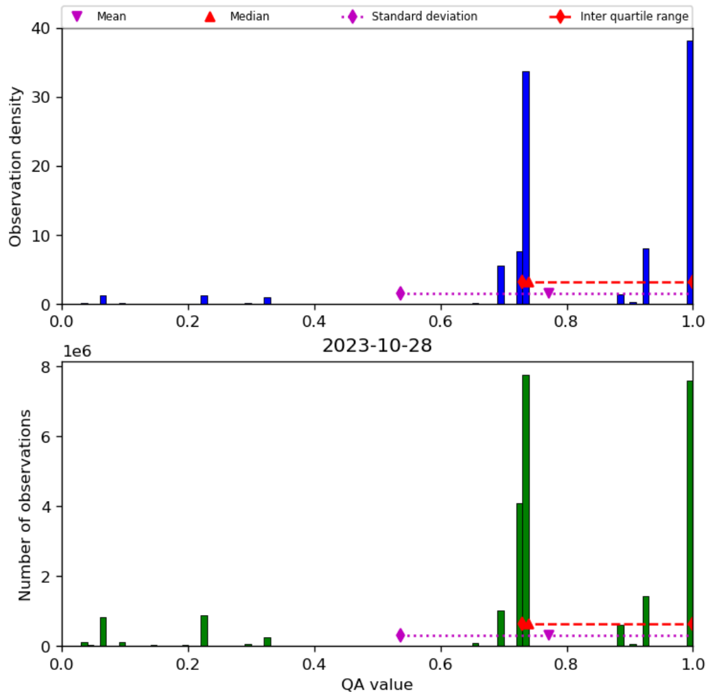
Figure 28: Histogram of “QA value” for 2023-10-28 to 2023-10-29
