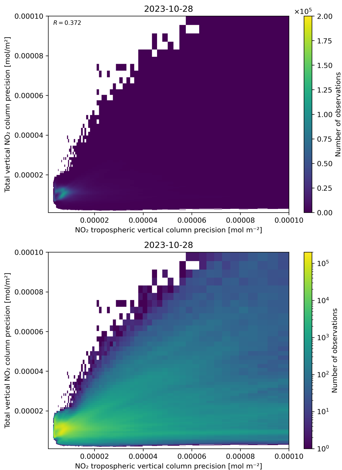
Figure 139: Scatter density plot of “NO 2 tropospheric vertical column precision” against “Total vertical NO 2 column precision” for 2023-10-28 to 2023-10-29.
