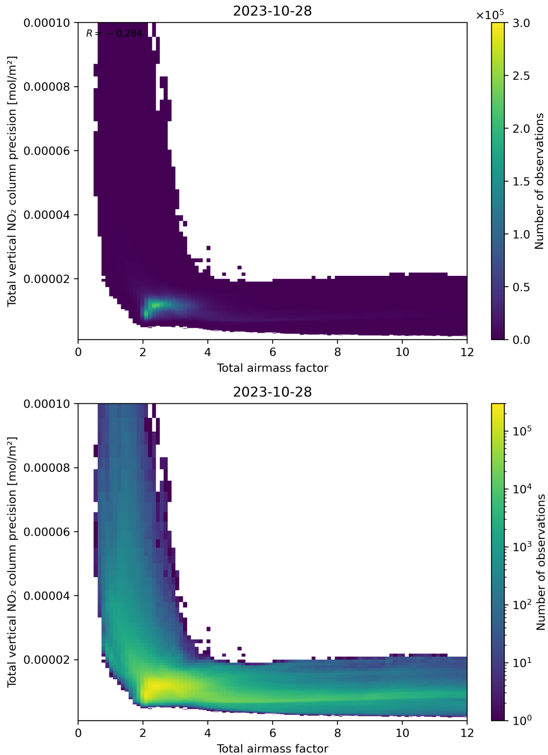
Figure 68: Scatter density plot of “Total airmass factor” against “Total vertical NO 2 column precision” for 2023-10-28 to 2023-10-29.
