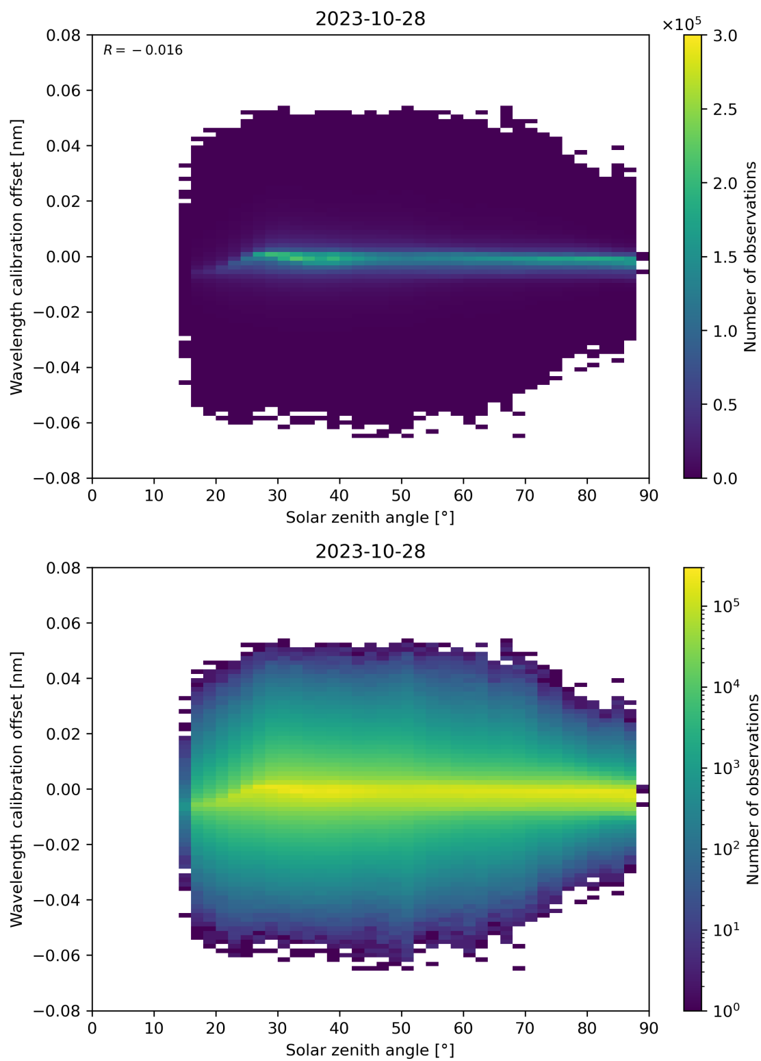
Figure 158: Scatter density plot of “Solar zenith angle” against “Wavelength calibration offset” for 2023-10-28 to 2023-10-29.
