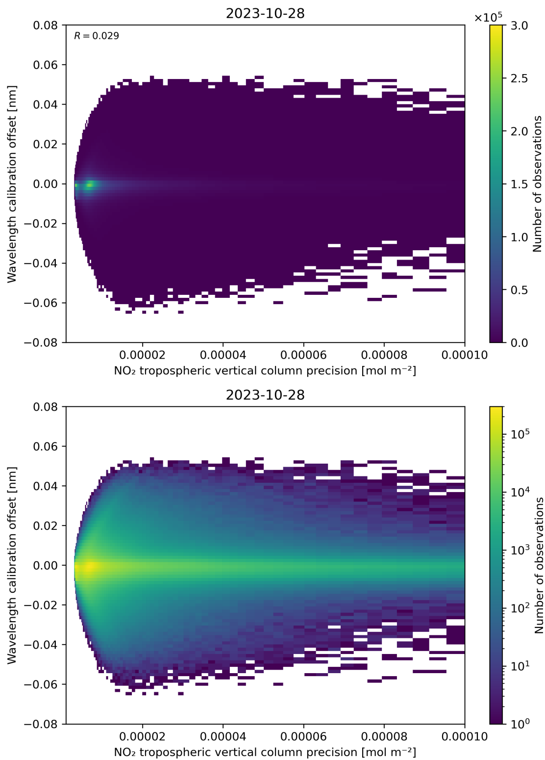
Figure 141: Scatter density plot of “NO 2 tropospheric vertical column precision” against “Wavelength calibration offset” for 2023-10-28 to 2023-10-29.
