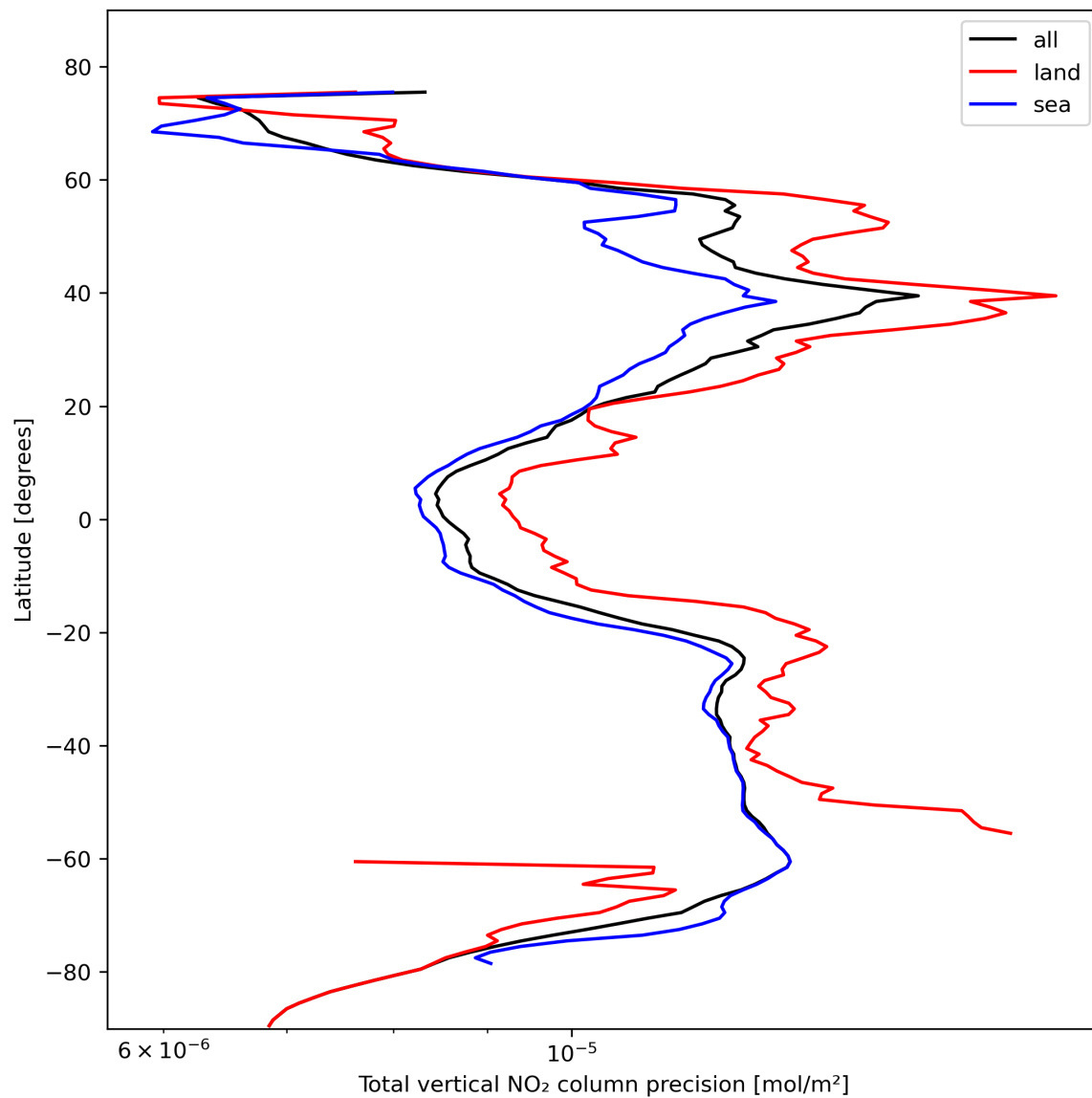
Figure 22: Zonal average of “Total vertical NO 2 column precision” for 2023-10-28 to 2023-10-29.
