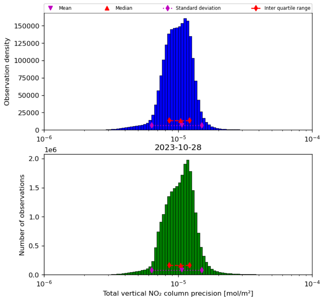
Figure 39: Histogram of “Total vertical NO 2 column precision” for 2023-10-28 to 2023-10-29
