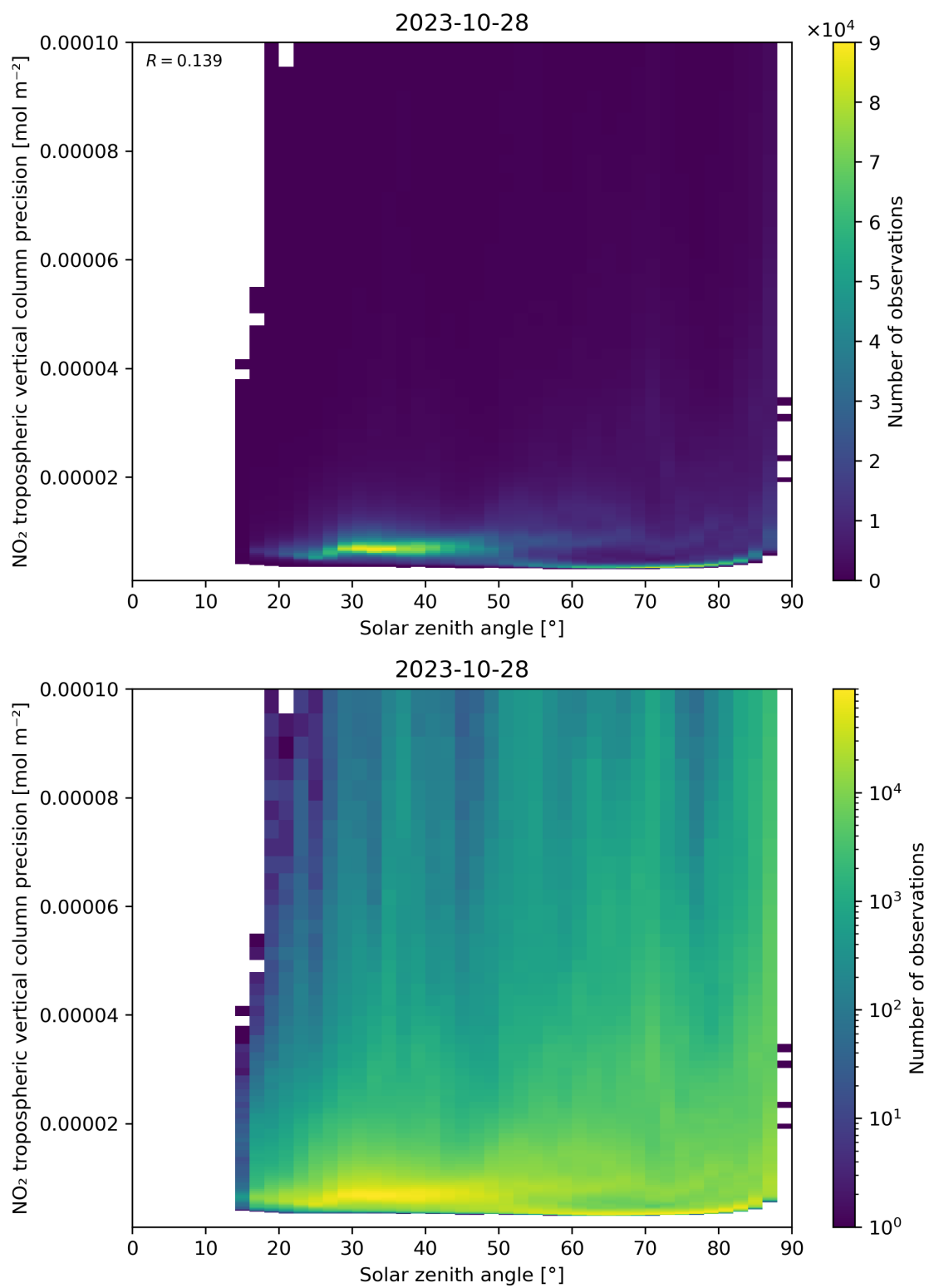
Figure 156: Scatter density plot of “Solar zenith angle” against “NO 2 tropospheric vertical column precision” for 2023-10-28 to 2023-10-29.
