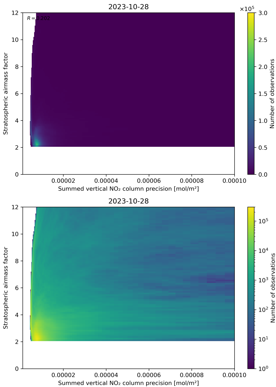
Figure 106: Scatter density plot of “Summed vertical NO 2 column precision” against “Stratospheric airmass factor” for 2023-10-28 to 2023-10-29.
