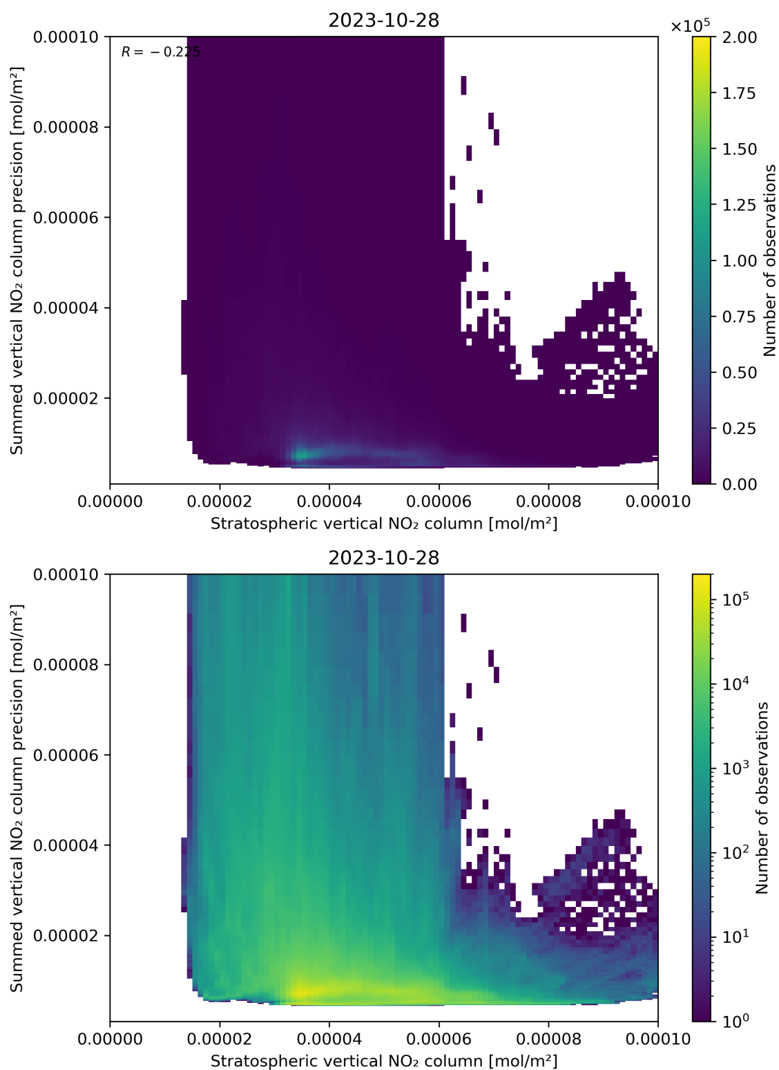
Figure 99: Scatter density plot of “Stratospheric vertical NO 2 column” against “Summed vertical NO 2 column precision” for 2023-10-28 to 2023-10-29.
