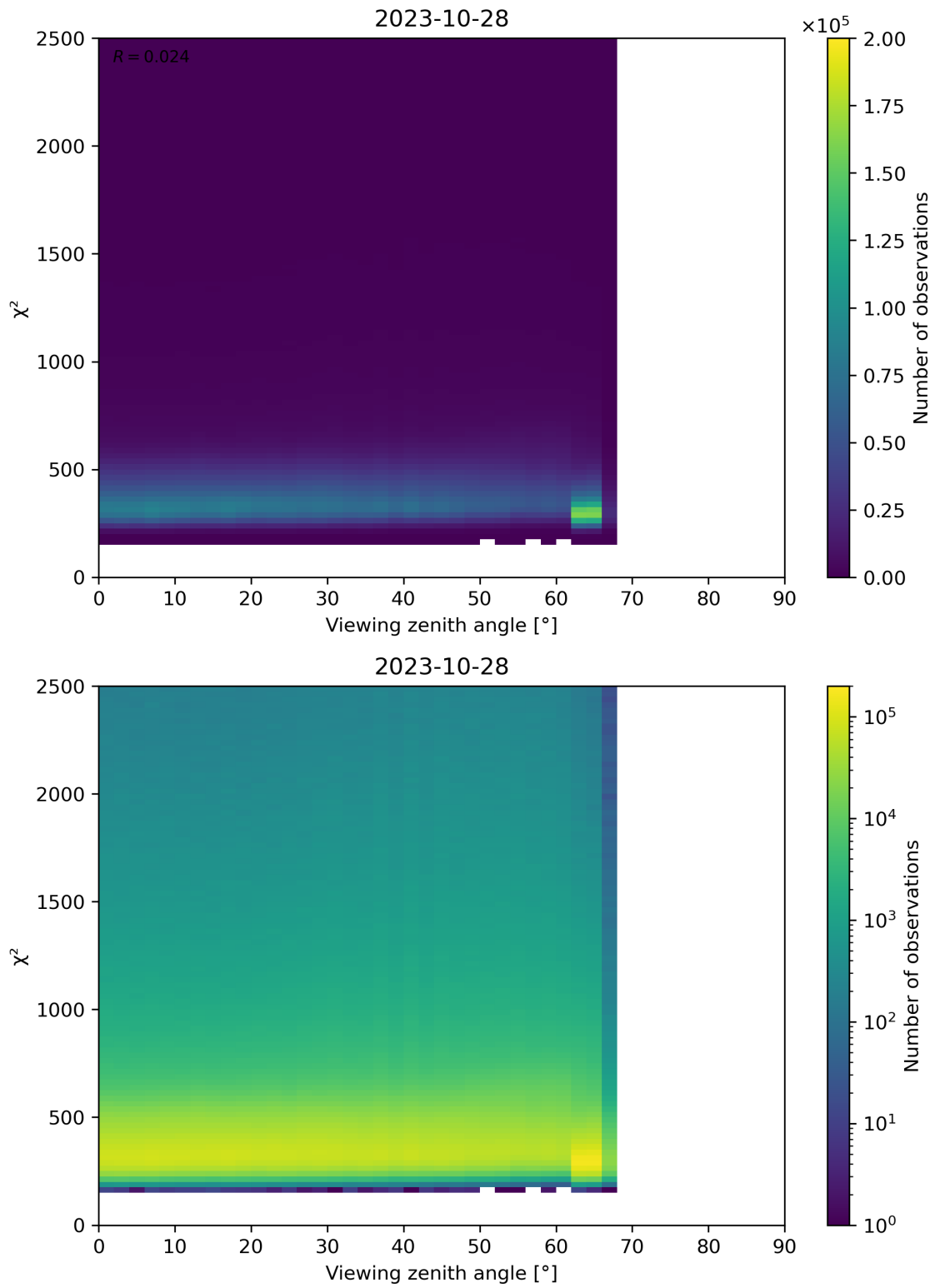
Figure 162: Scatter density plot of “Viewing zenith angle” against “ \chi^2 ” for 2023-10-28 to 2023-10-29.
