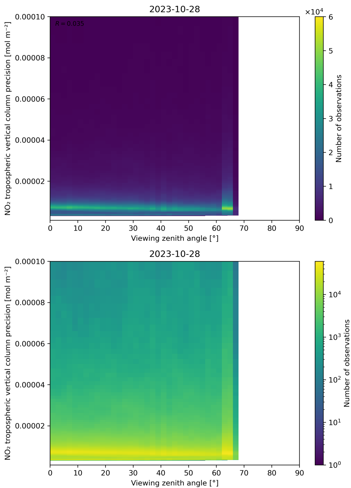
Figure 170: Scatter density plot of “Viewing zenith angle” against “NO 2 tropospheric vertical column precision” for 2023-10-28 to 2023-10-29.
