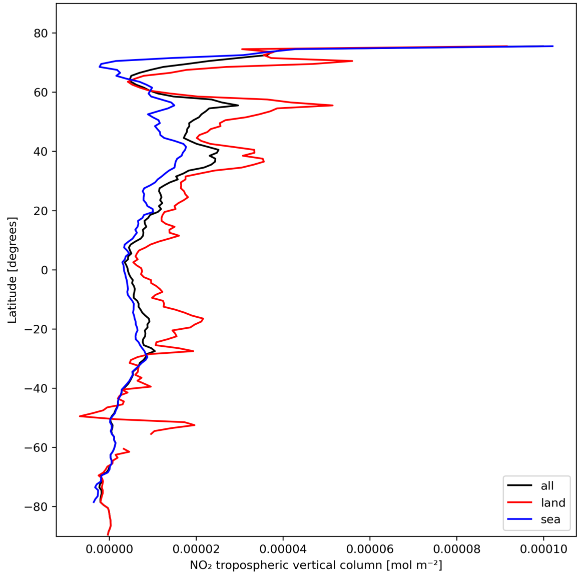
Figure 12: Zonal average of “NO 2 tropospheric vertical column” for 2023-10-28 to 2023-10-29.
