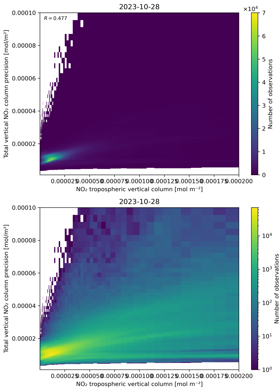
Figure 129: Scatter density plot of “NO 2 tropospheric vertical column” against “Total vertical NO 2 column precision” for 2023-10-28 to 2023-10-29.
