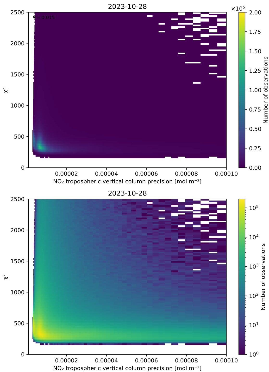
Figure 134: Scatter density plot of “NO 2 tropospheric vertical column precision” against “ \chi^2 ” for 2023-10-28 to 2023-10-29.
