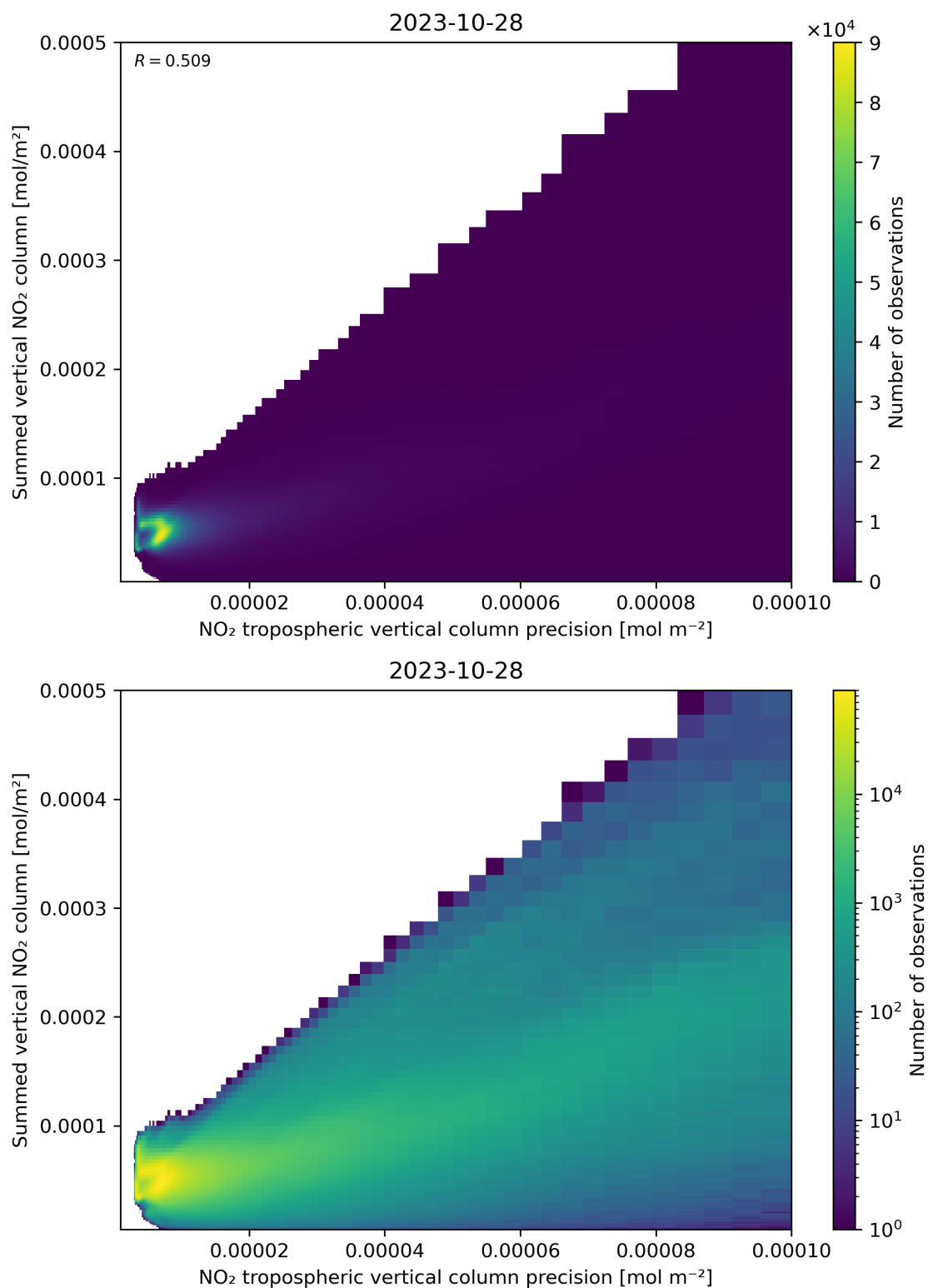
Figure 136: Scatter density plot of “NO 2 tropospheric vertical column precision” against “Summed vertical NO 2 column” for 2023-10-28 to 2023-10-29.
