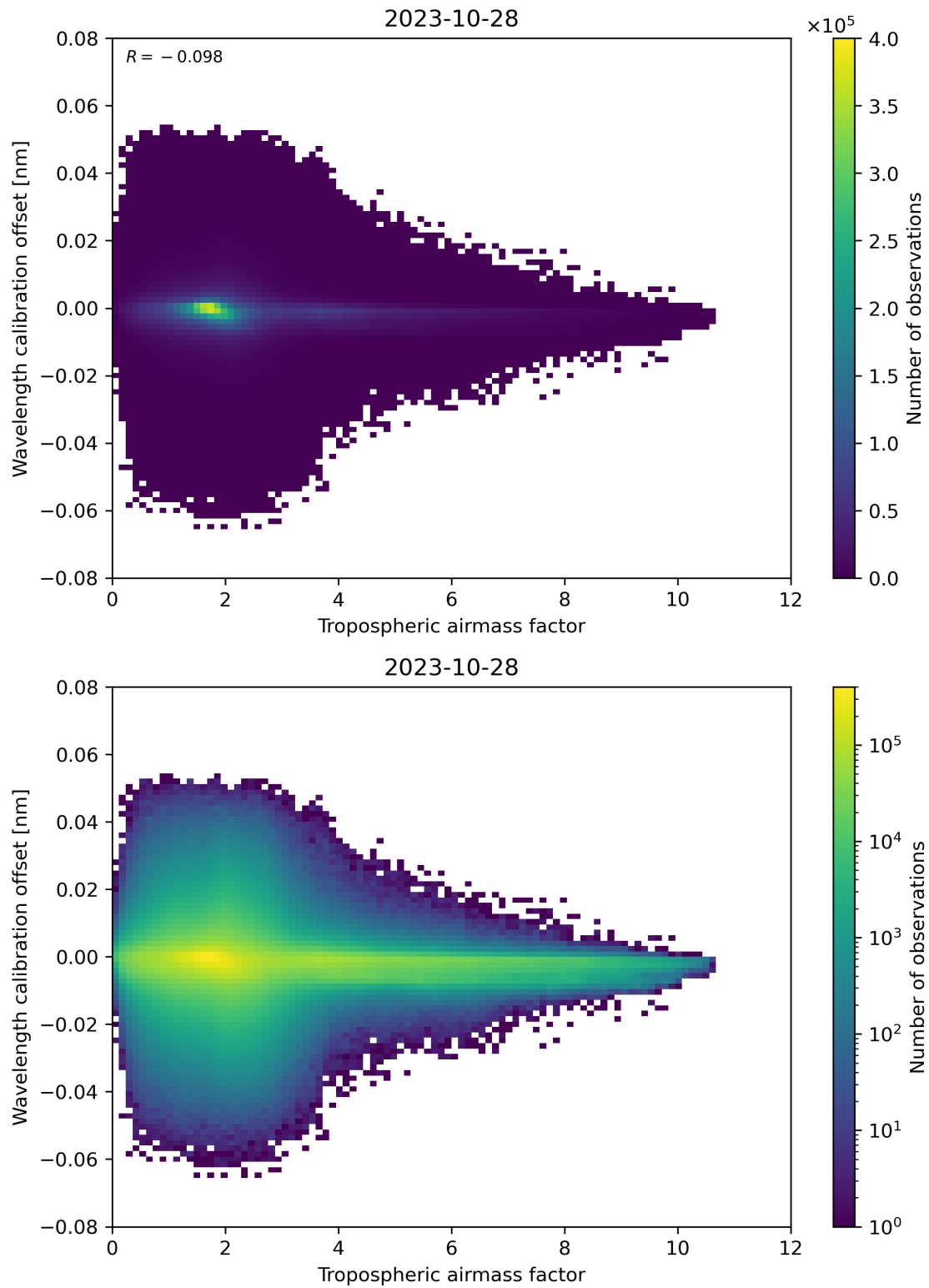
Figure 80: Scatter density plot of “Tropospheric air mass factor” against “Wavelength calibration offset” for 2023-10-28 to 2023-10-29.
