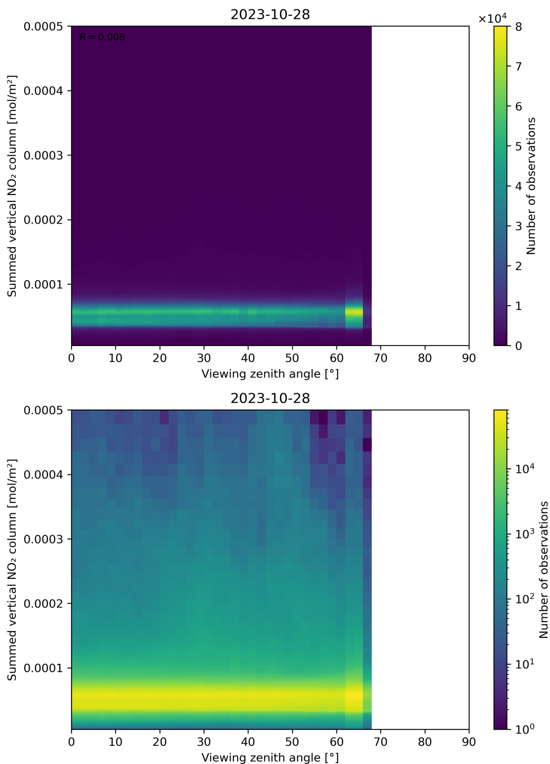
Figure 165: Scatter density plot of “Viewing zenith angle” against “Summed vertical NO 2 column” for 2023-10-28 to 2023-10-29.
