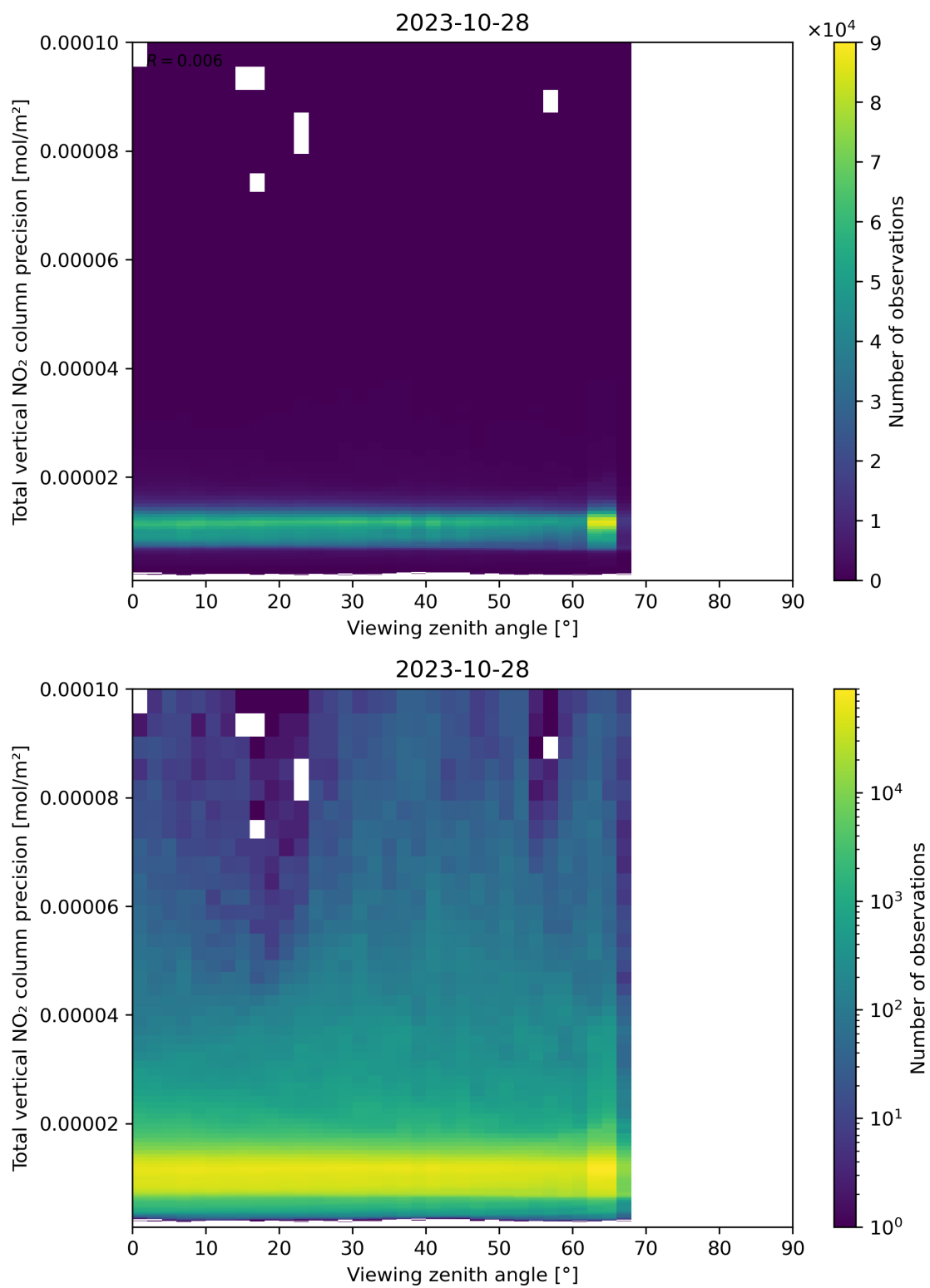
Figure 168: Scatter density plot of “Viewing zenith angle” against “Total vertical NO 2 column precision” for 2023-10-28 to 2023-10-29.
