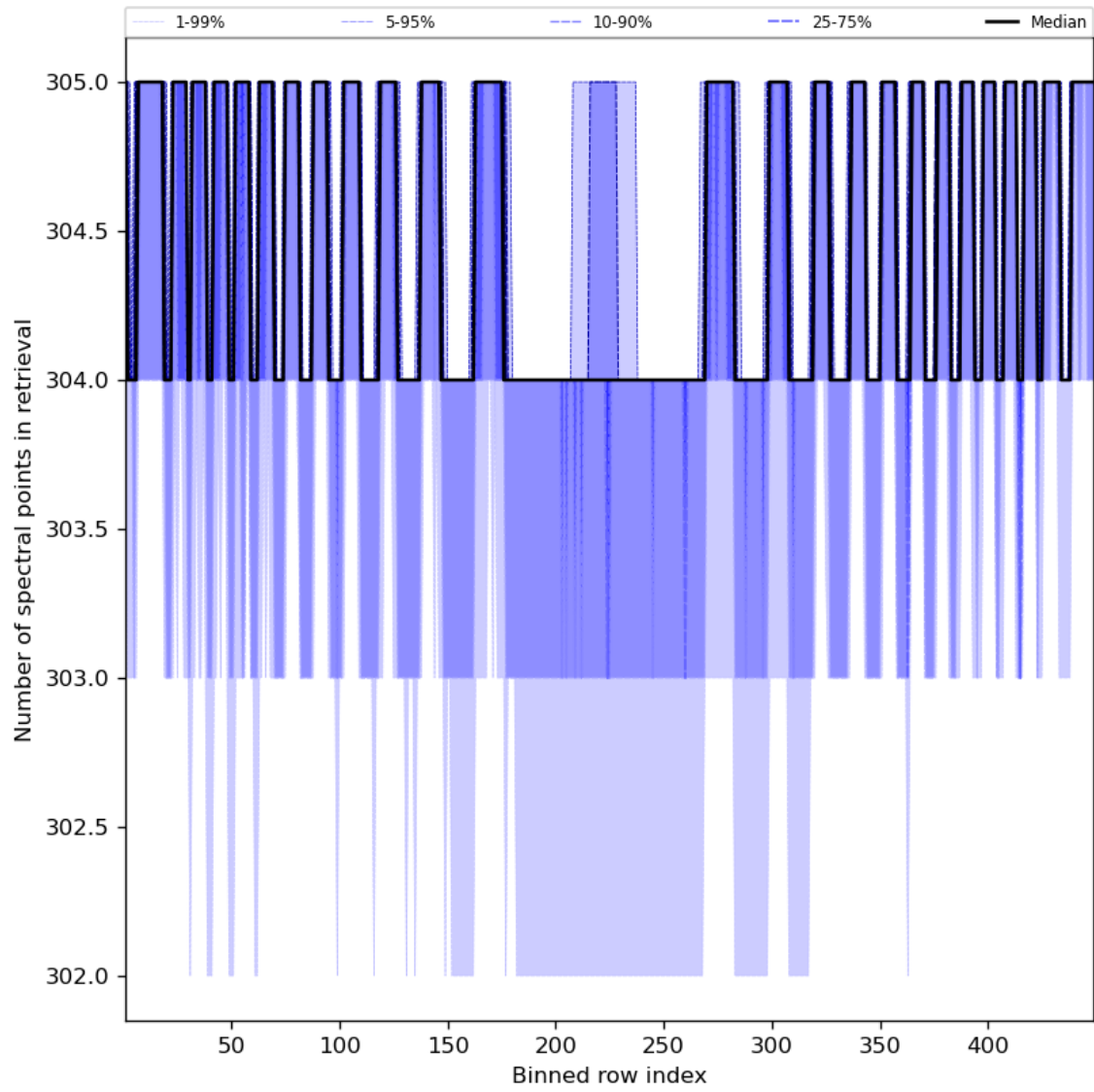
Figure 50: Along track statistics of “Number of spectral points in retrieval” for 2023-10-28 to 2023-10-29
