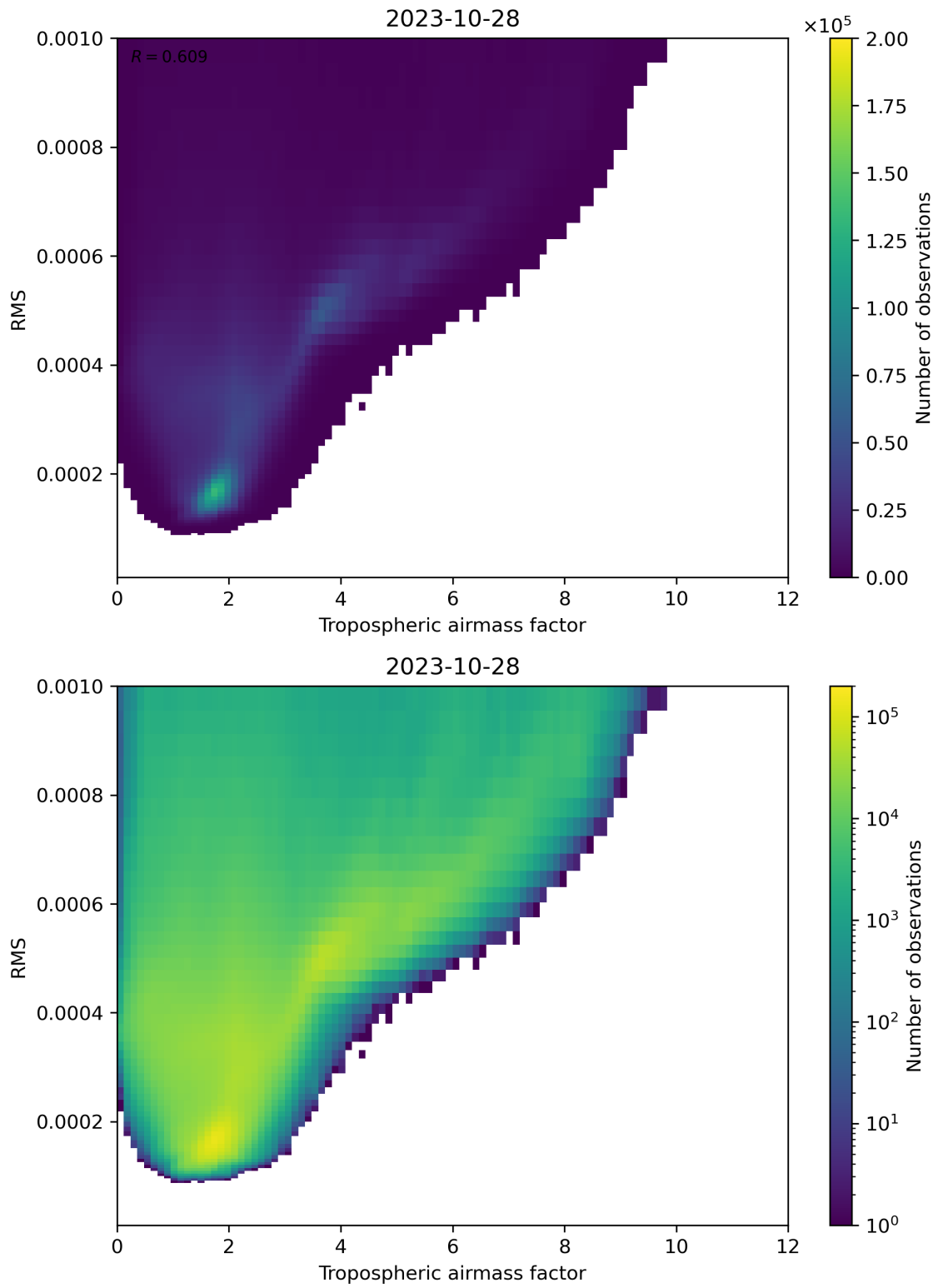
Figure 79: Scatter density plot of “Tropospheric airmass factor” against “RMS” for 2023-10-28 to 2023-10-29.
