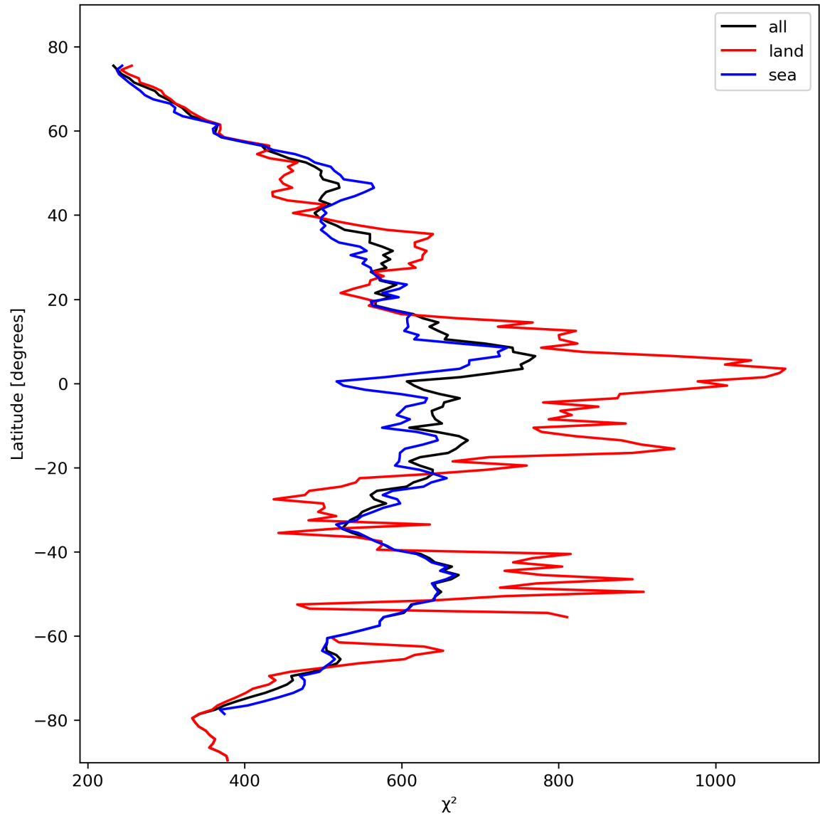
Figure 25: Zonal average of “ \chi^2 ” for 2023-10-28 to 2023-10-29.
