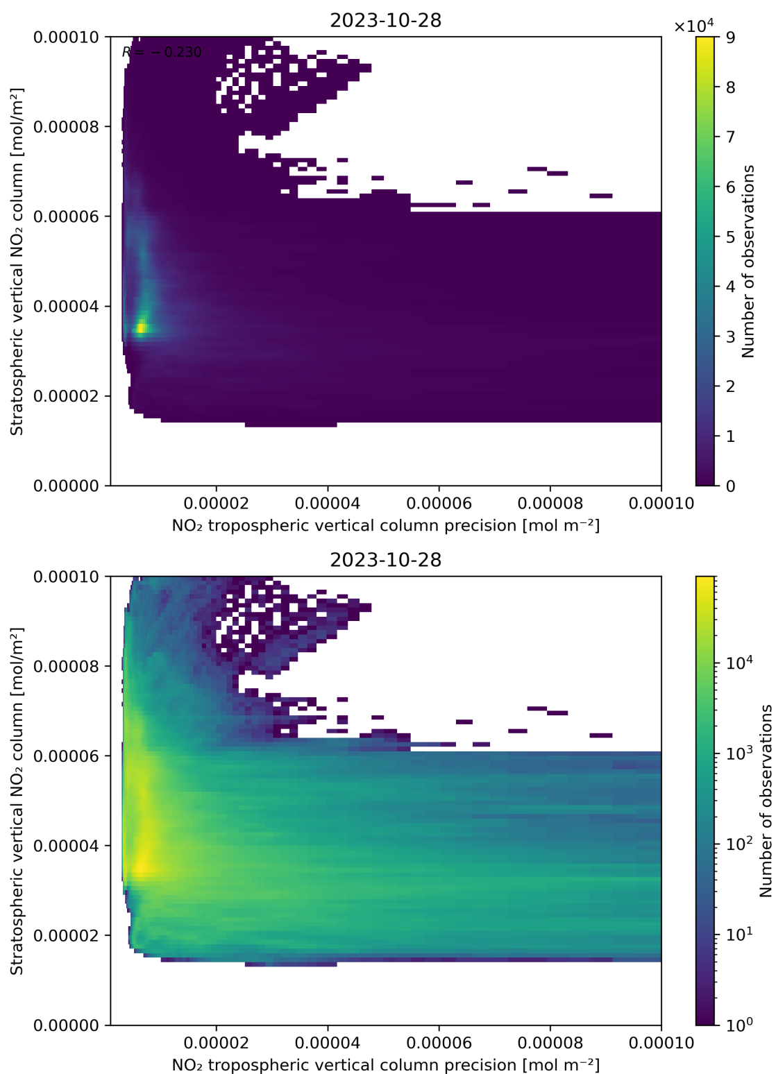
Figure 135: Scatter density plot of “NO 2 tropospheric vertical column precision” against “Stratospheric vertical NO 2 column” for 2023-10-28 to 2023-10-29.
