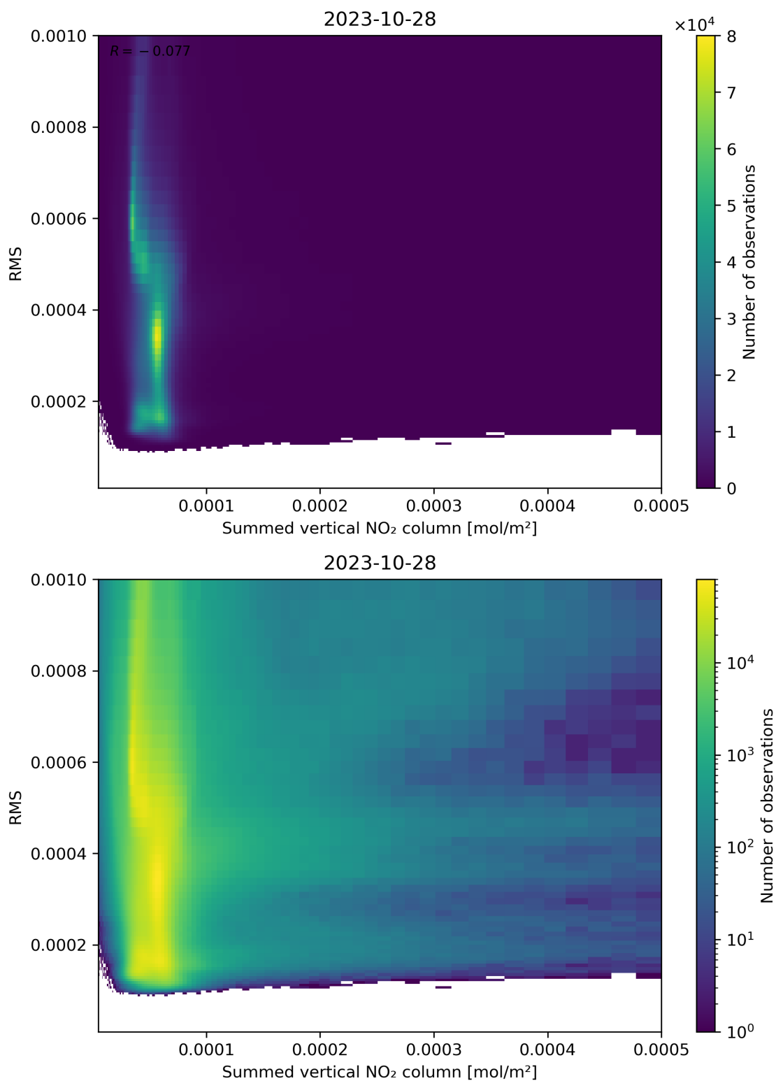
Figure 109: Scatter density plot of “Summed vertical NO 2 column” against “RMS” for 2023-10-28 to 2023-10-29.
