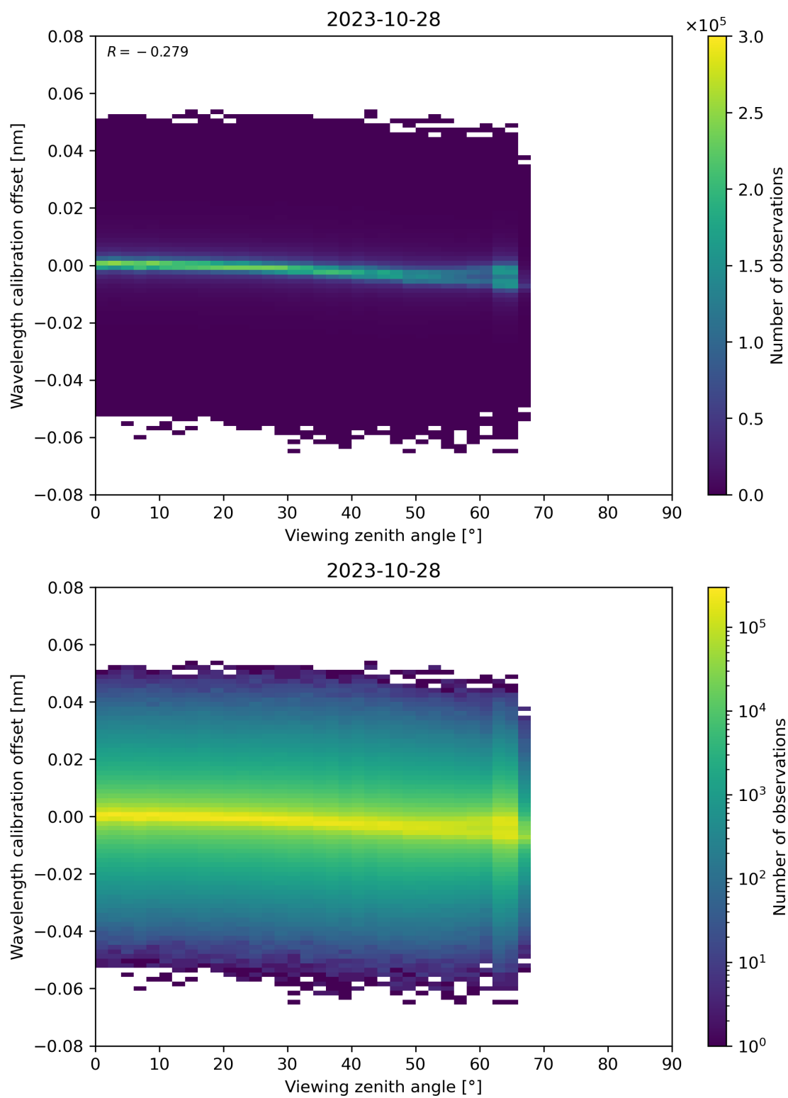
Figure 173: Scatter density plot of “Viewing zenith angle” against “Wavelength calibration offset” for 2023-10-28 to 2023-10-29.
