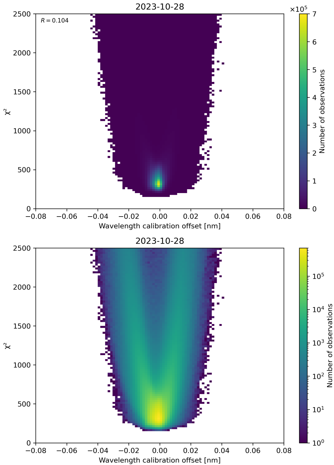
Figure 175: Scatter density plot of “Wavelength calibration offset” against “ \chi^2 ” for 2023-10-28 to 2023-10-29.
