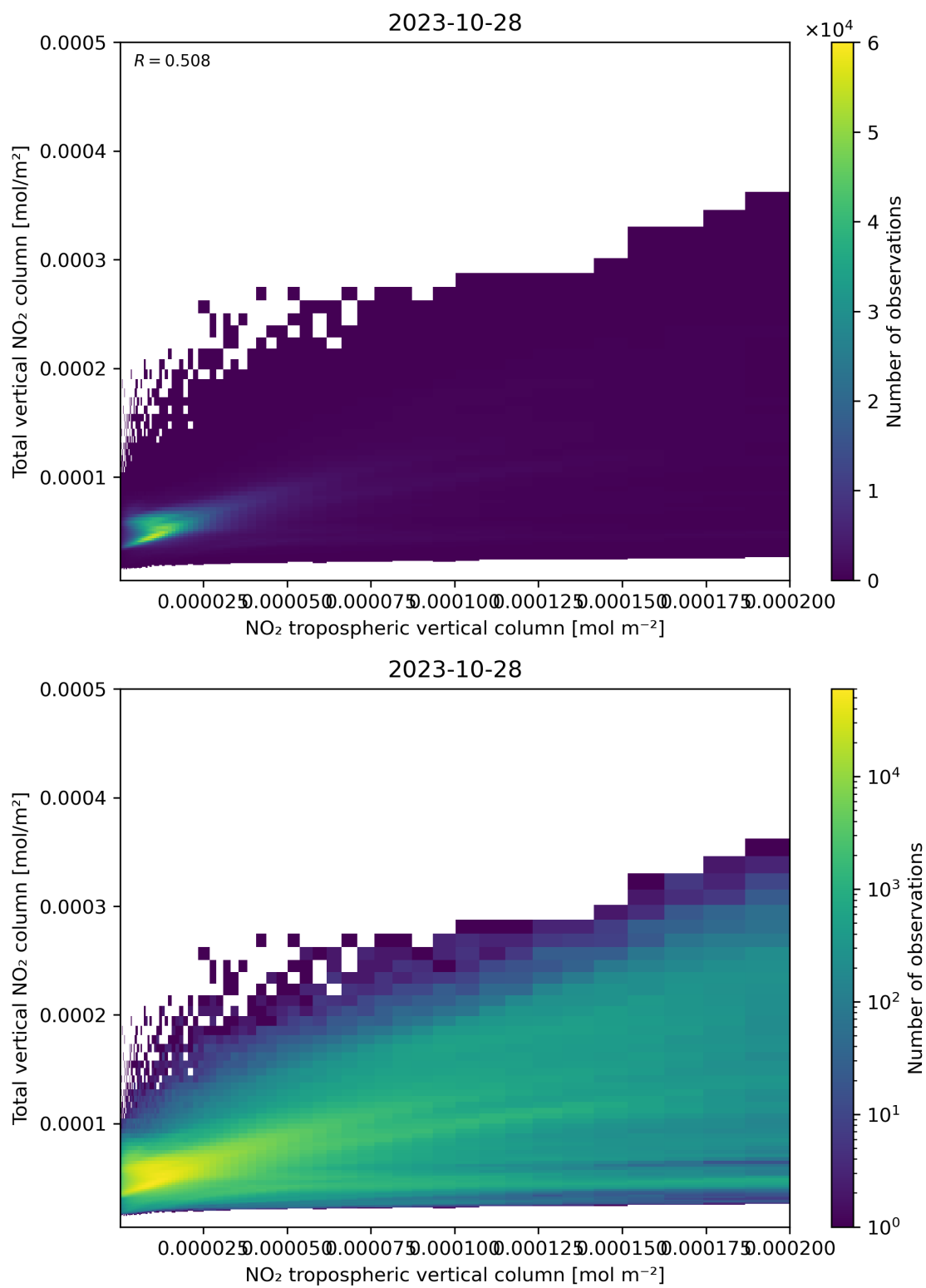
Figure 128: Scatter density plot of “NO 2 tropospheric vertical column” against “Total vertical NO 2 column” for 2023-10-28 to 2023-10-29.
