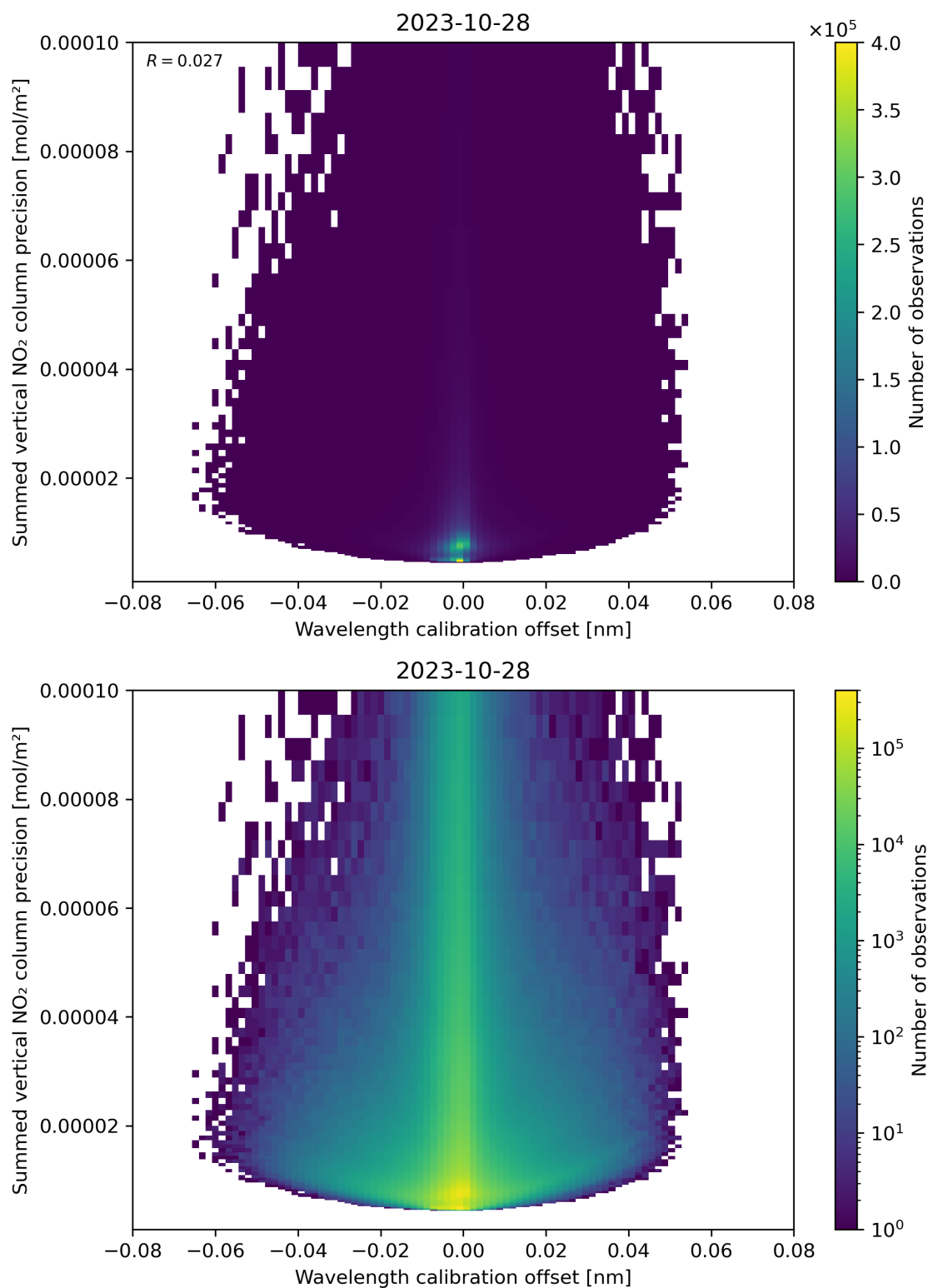
Figure 178: Scatter density plot of “Wavelength calibration offset” against “Summed vertical NO 2 column precision” for 2023-10-28 to 2023-10-29.
