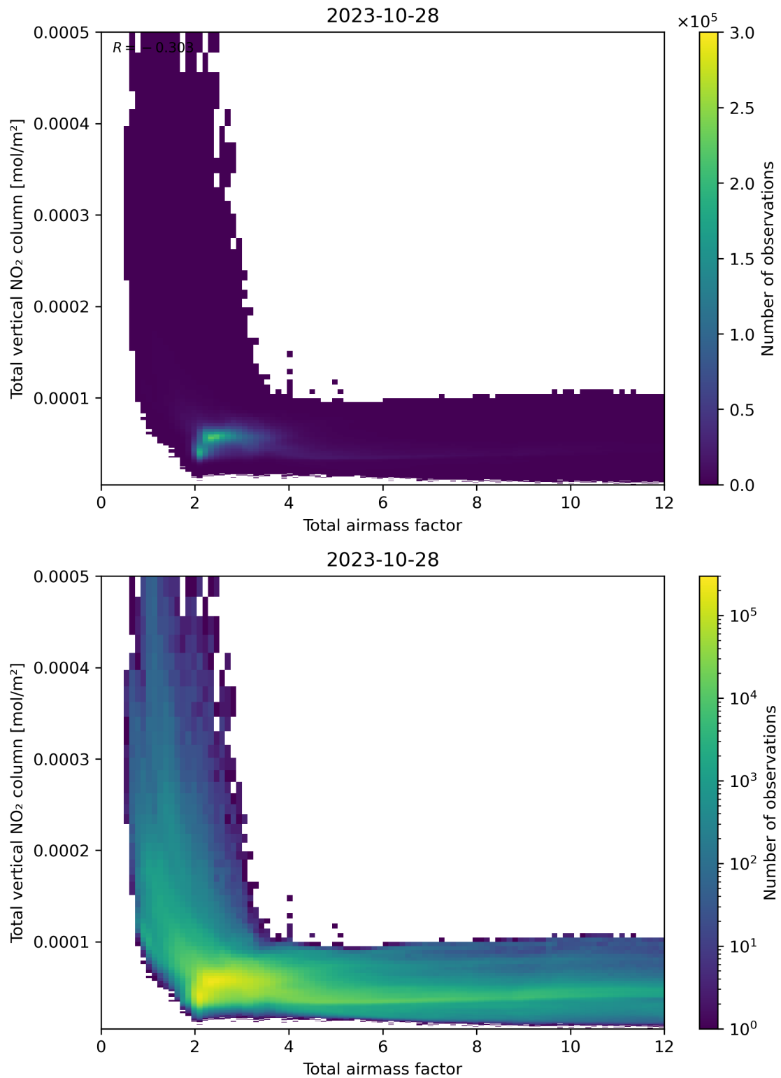
Figure 67: Scatter density plot of “Total airmass factor” against “Total vertical NO 2 column” for 2023-10-28 to 2023-10-29.
