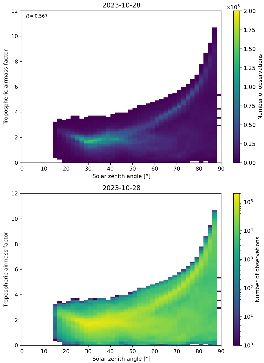
Figure 147: Scatter density plot of “Solar zenith angle” against “Tropospheric airmass factor” for 2023-10-28 to 2023-10-29.
