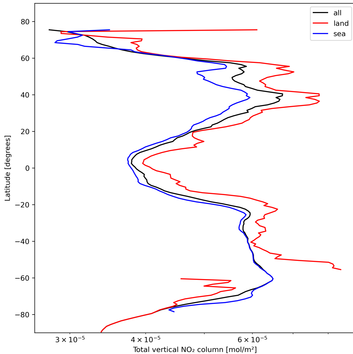
Figure 21: Zonal average of “Total vertical NO 2 column” for 2023-10-28 to 2023-10-29.
