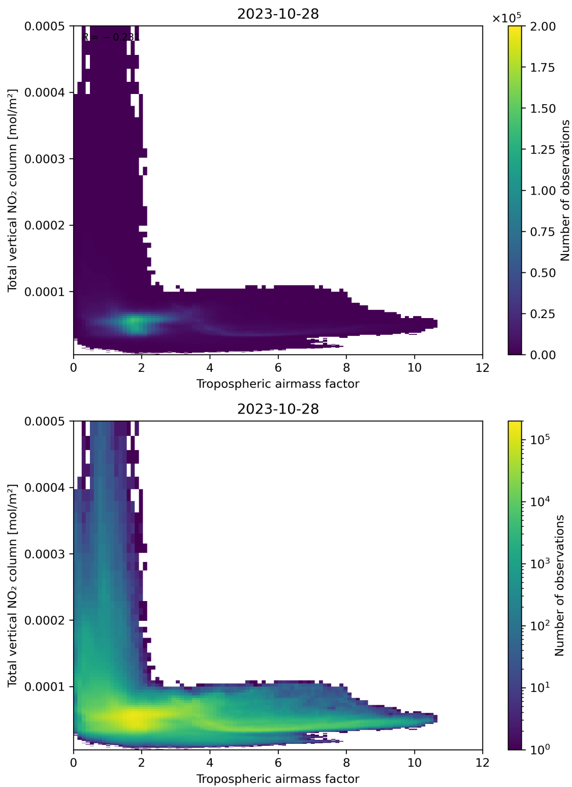
Figure 77: Scatter density plot of “Tropospheric airmass factor” against “Total vertical NO 2 column” for 2023-10-28 to 2023-10-29.
