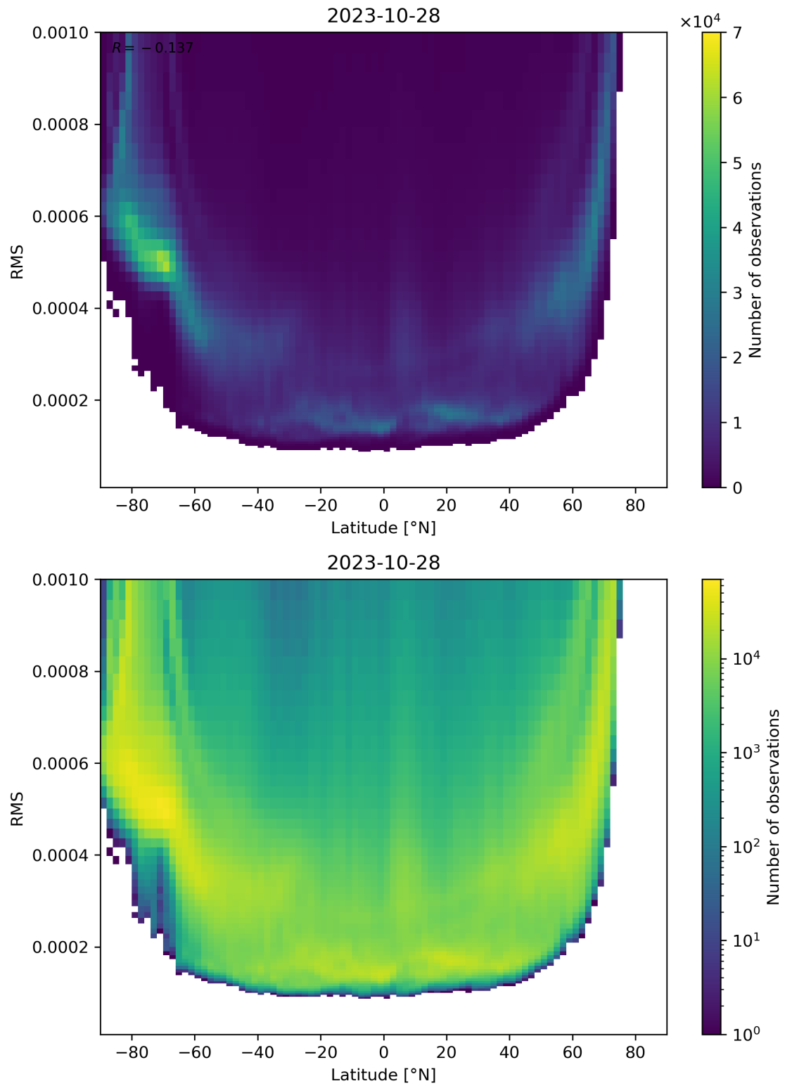
Figure 94: Scatter density plot of “Latitude” against “RMS” for 2023-10-28 to 2023-10-29.
