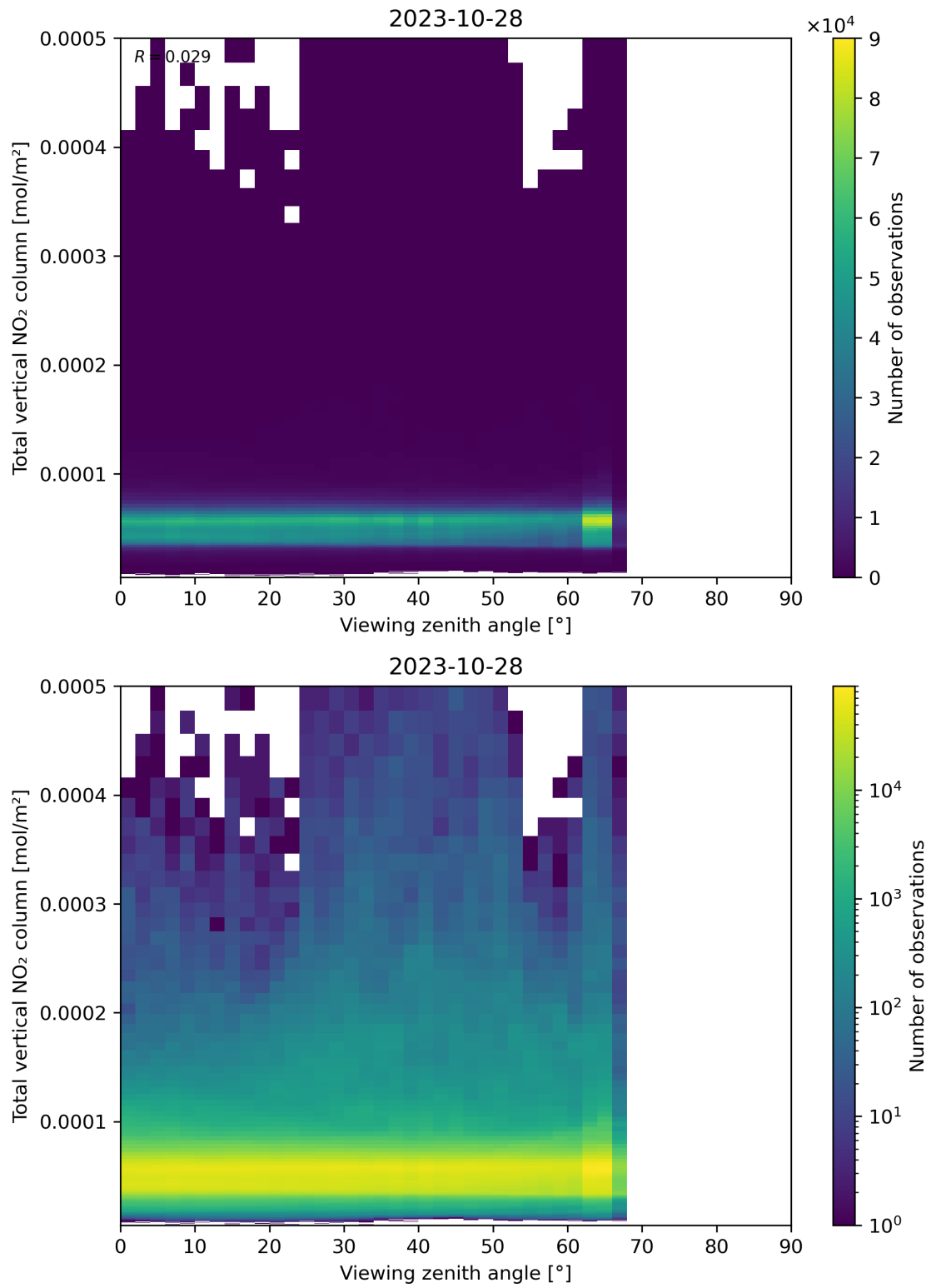
Figure 167: Scatter density plot of “Viewing zenith angle” against “Total vertical NO 2 column” for 2023-10-28 to 2023-10-29.
