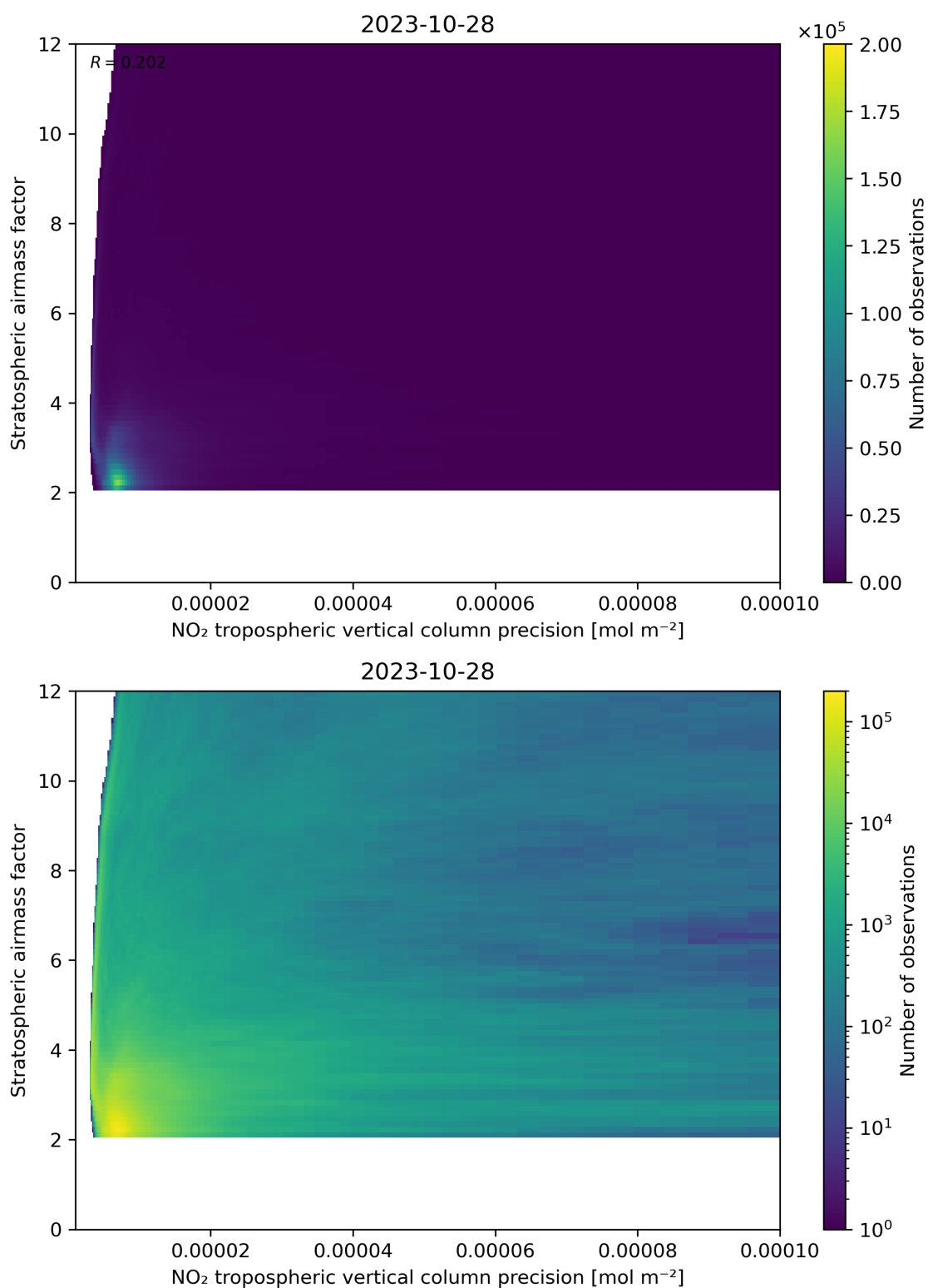
Figure 131: Scatter density plot of “NO 2 tropospheric vertical column precision” against “Stratospheric airmass factor” for 2023-10-28 to 2023-10-29.
