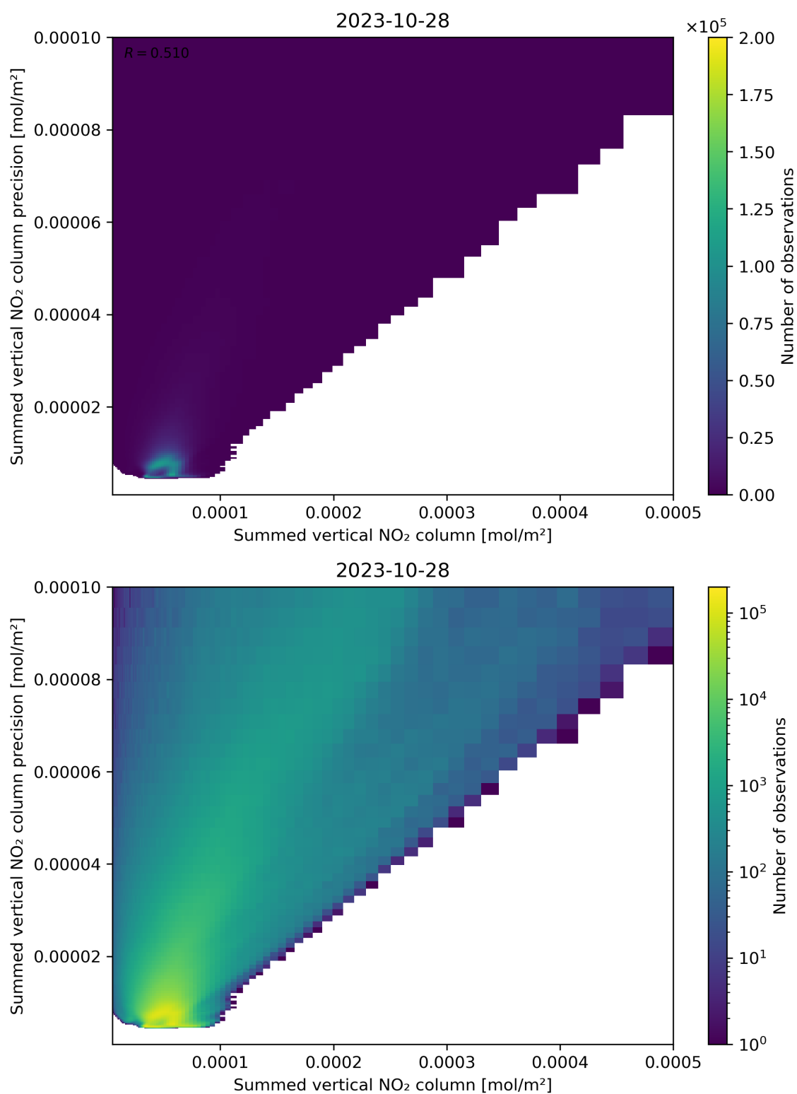
Figure 105: Scatter density plot of “Summed vertical NO 2 column” against “Summed vertical NO 2 column precision” for 2023-10-28 to 2023-10-29.
