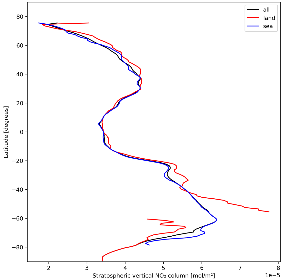
Figure 19: Zonal average of “Stratospheric vertical NO 2 column” for 2023-10-28 to 2023-10-29.
