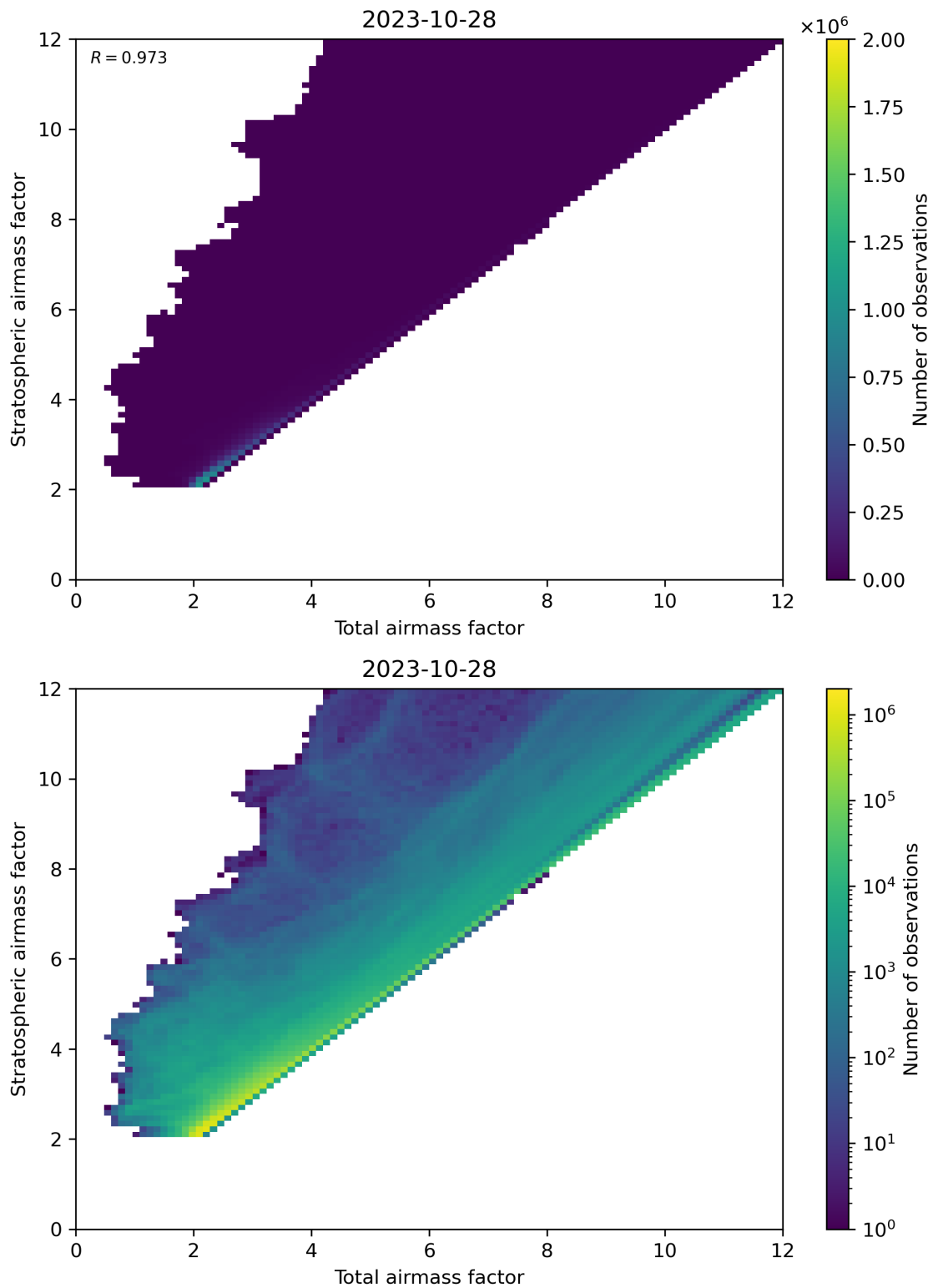
Figure 62: Scatter density plot of “Total airmass factor” against “Stratospheric airmass factor” for 2023-10-28 to 2023-10-29.
