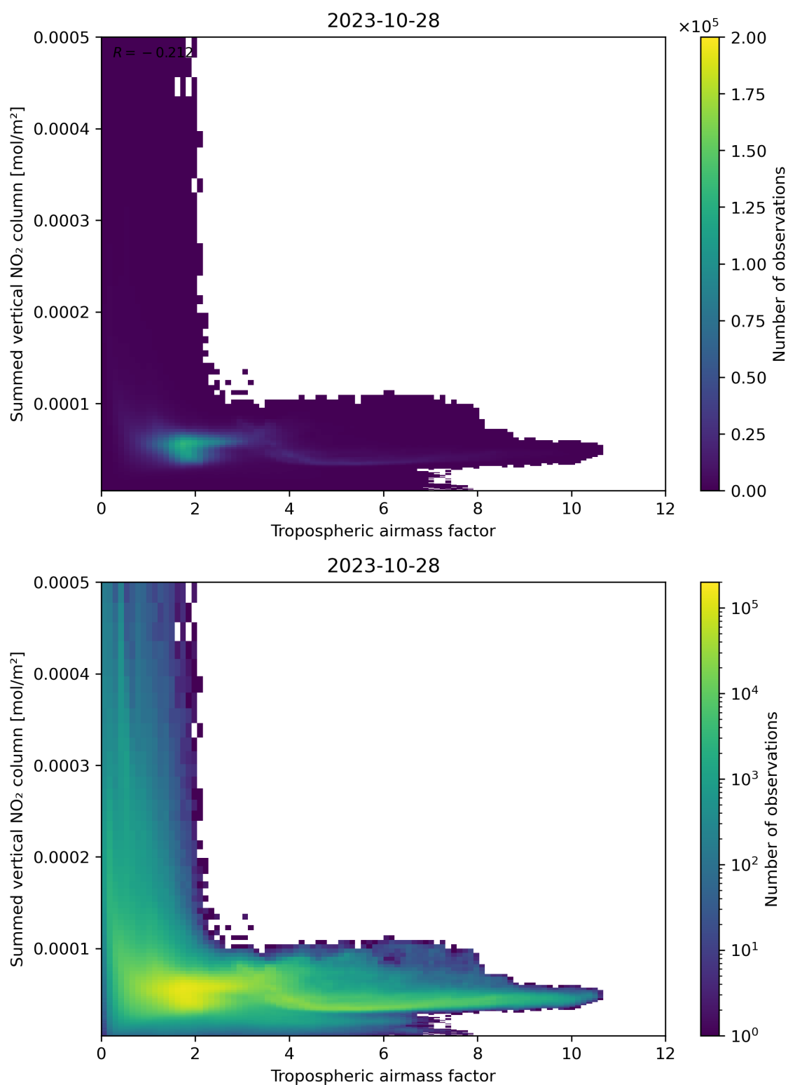
Figure 75: Scatter density plot of “Tropospheric air mass factor” against “Summed vertical NO 2 column” for 2023-10-28 to 2023-10-29.
