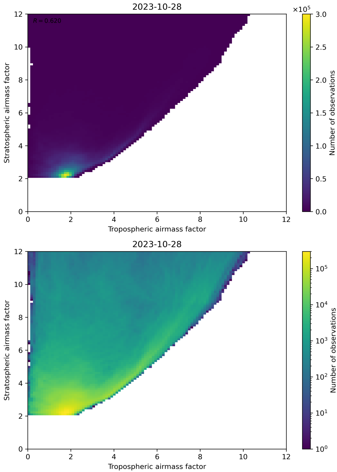
Figure 71: Scatter density plot of “Tropospheric airmass factor” against “Stratospheric airmass factor” for 2023-10-28 to 2023-10-29.
