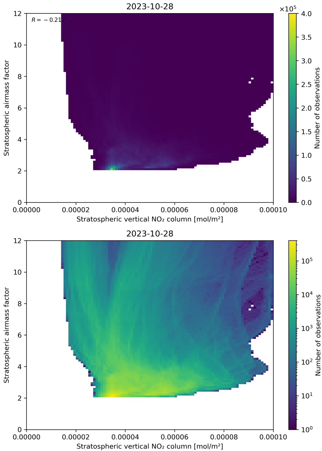
Figure 96: Scatter density plot of “Stratospheric vertical NO 2 column” against “Stratospheric airmass factor” for 2023-10-28 to 2023-10-29.
