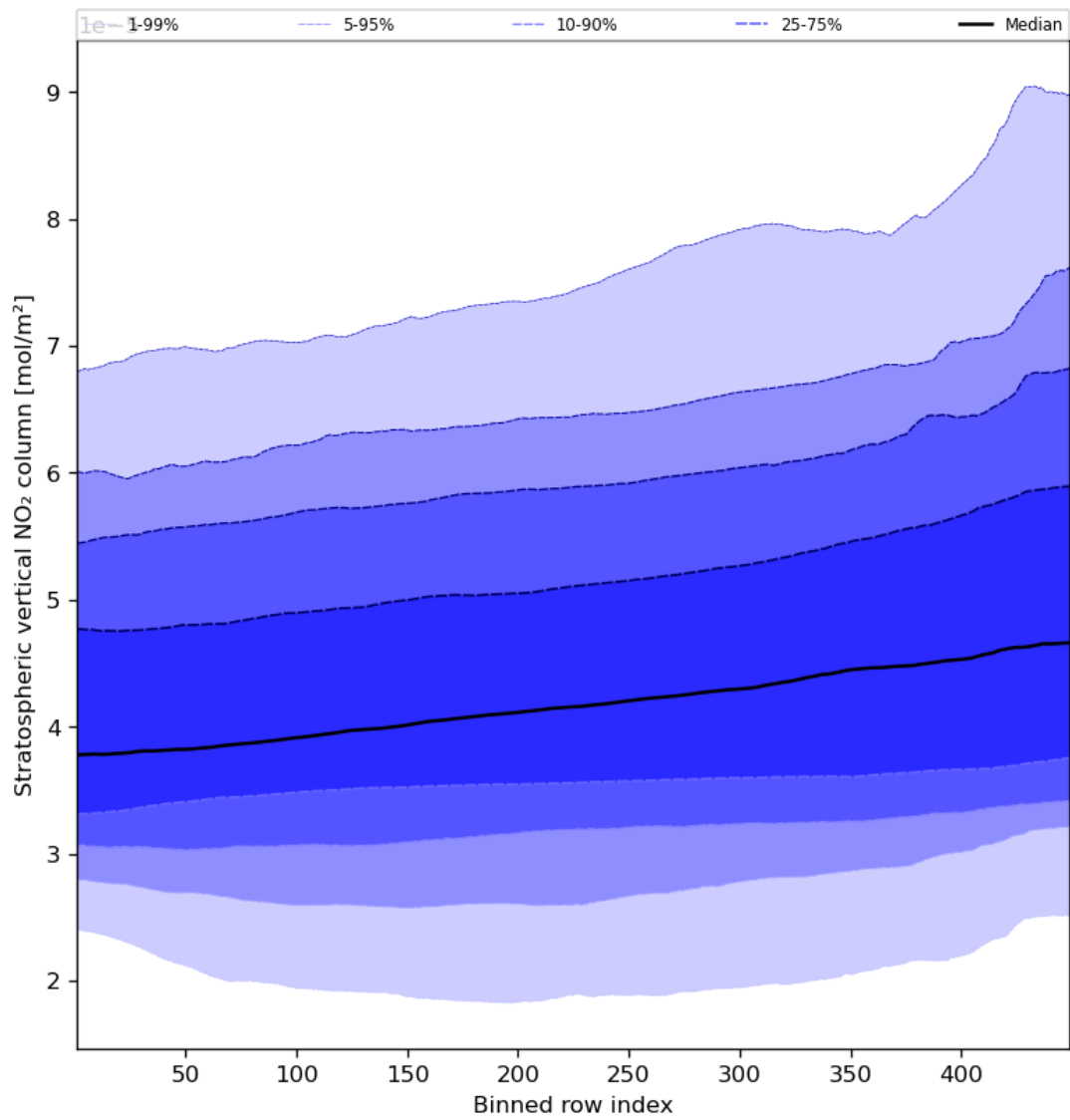
Figure 53: Along track statistics of “Stratospheric vertical NO 2 column” for 2023-10-28 to 2023-10-29
