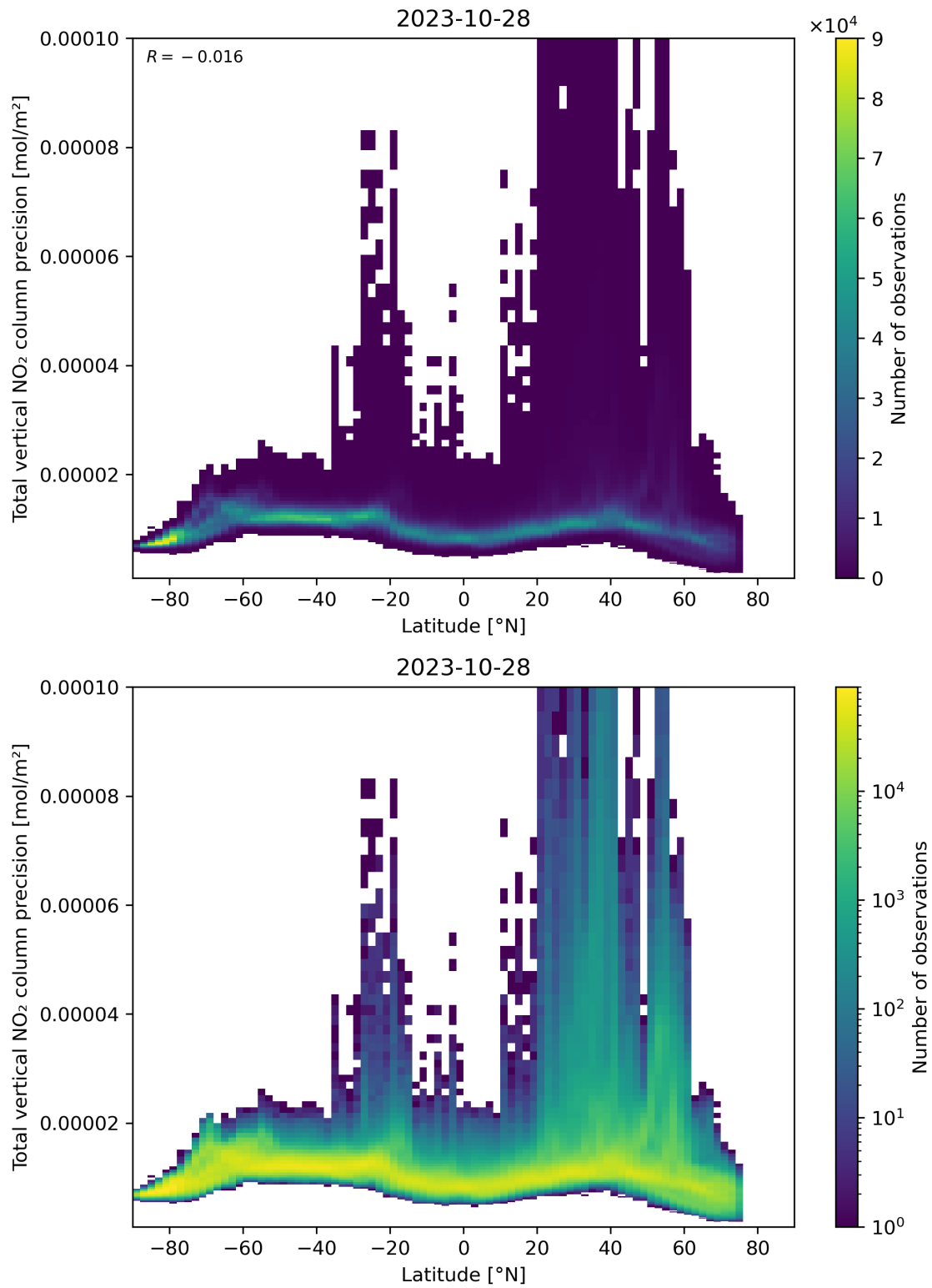
Figure 91: Scatter density plot of “Latitude” against “Total vertical NO 2 column precision” for 2023-10-28 to 2023-10-29.
