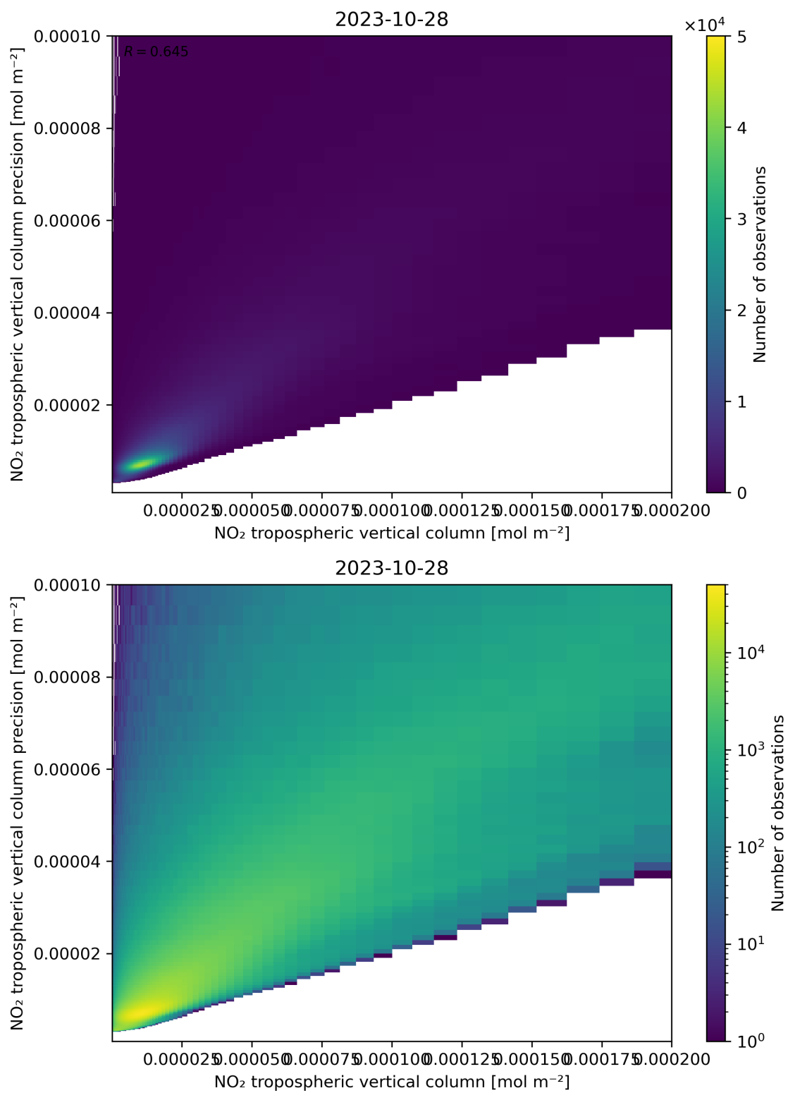
Figure 130: Scatter density plot of “NO 2 tropospheric vertical column” against “NO 2 tropospheric vertical column precision” for 2023-10-28 to 2023-10-29.
