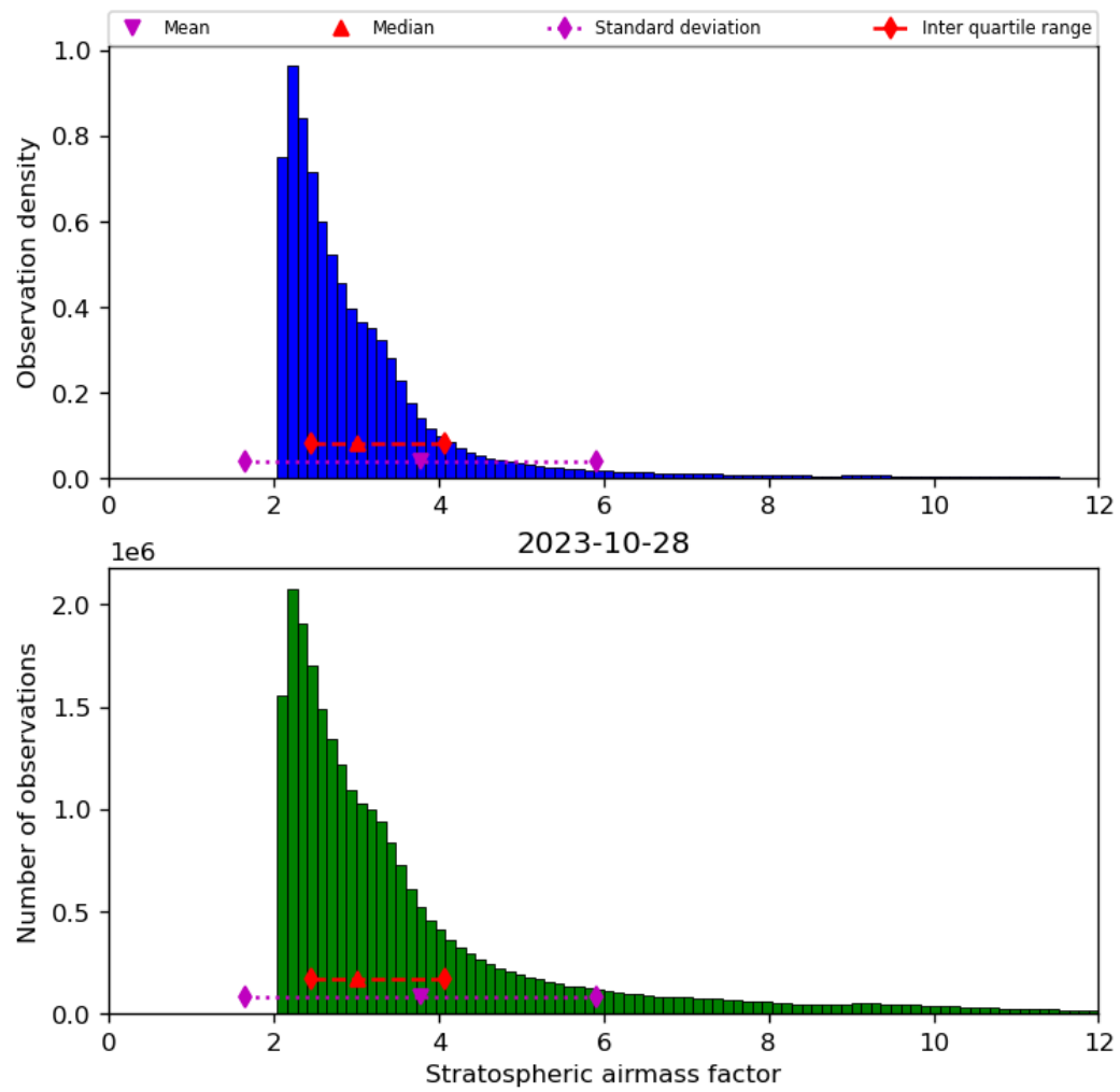
Figure 44: Histogram of “Stratospheric airmass factor” for 2023-10-28 to 2023-10-29
