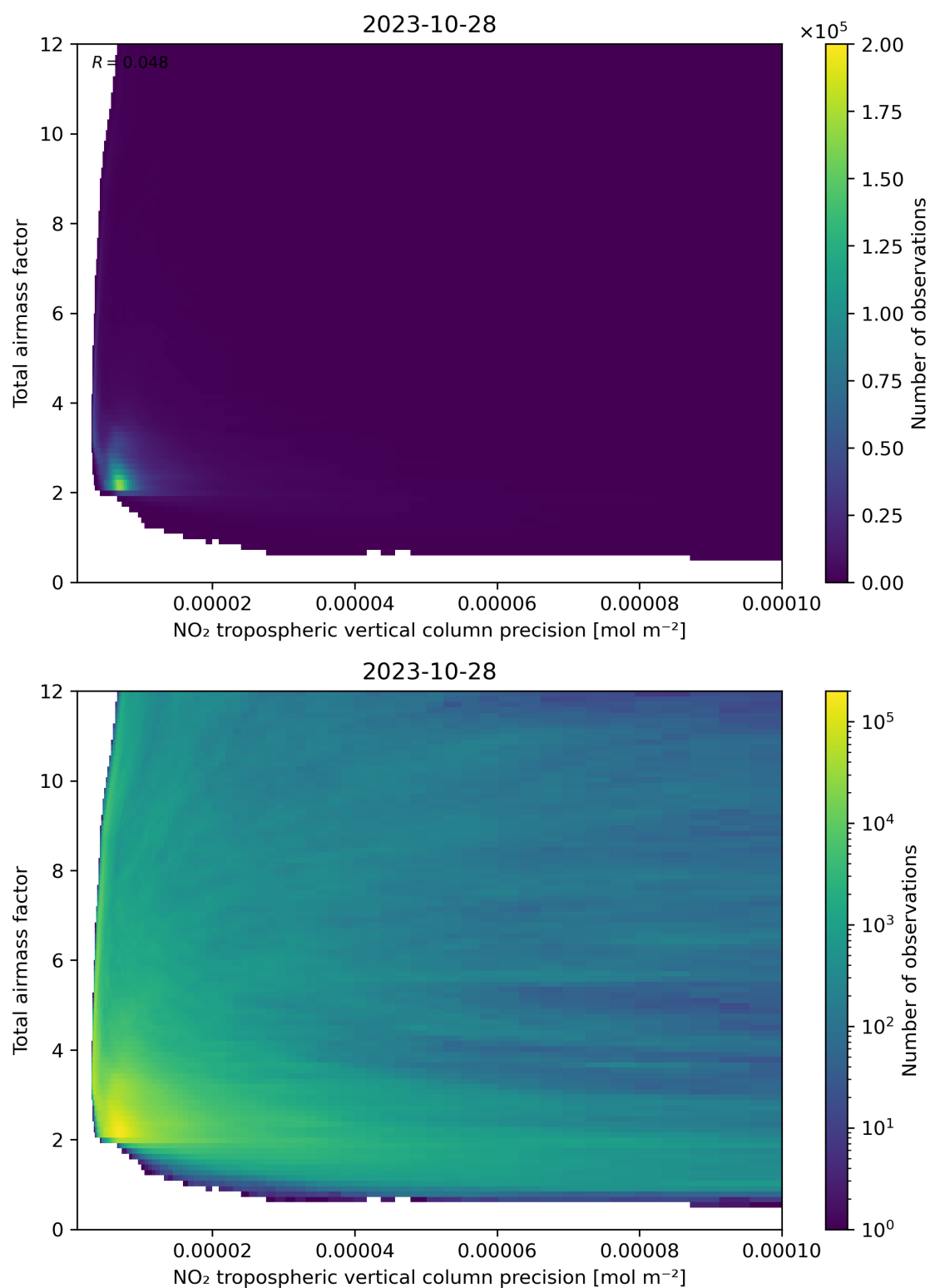
Figure 132: Scatter density plot of “NO 2 tropospheric vertical column precision” against “Total air mass factor” for 2023-10-28 to 2023-10-29.
