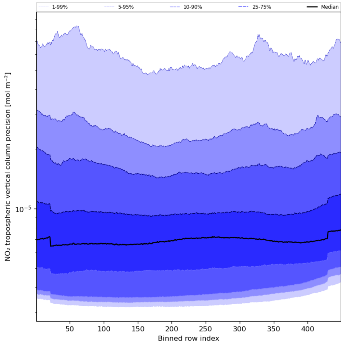
Figure 47: Along track statistics of “NO 2 tropospheric vertical column precision” for 2023-10-28 to 2023-10-29
