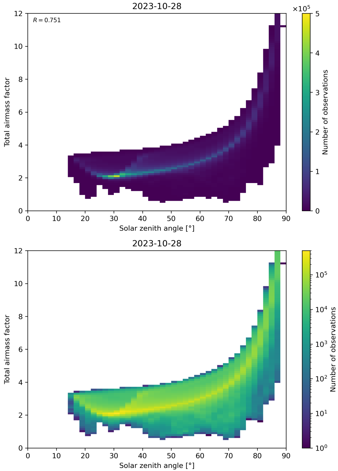
Figure 146: Scatter density plot of “Solar zenith angle” against “Total air mass factor” for 2023-10-28 to 2023-10-29.
