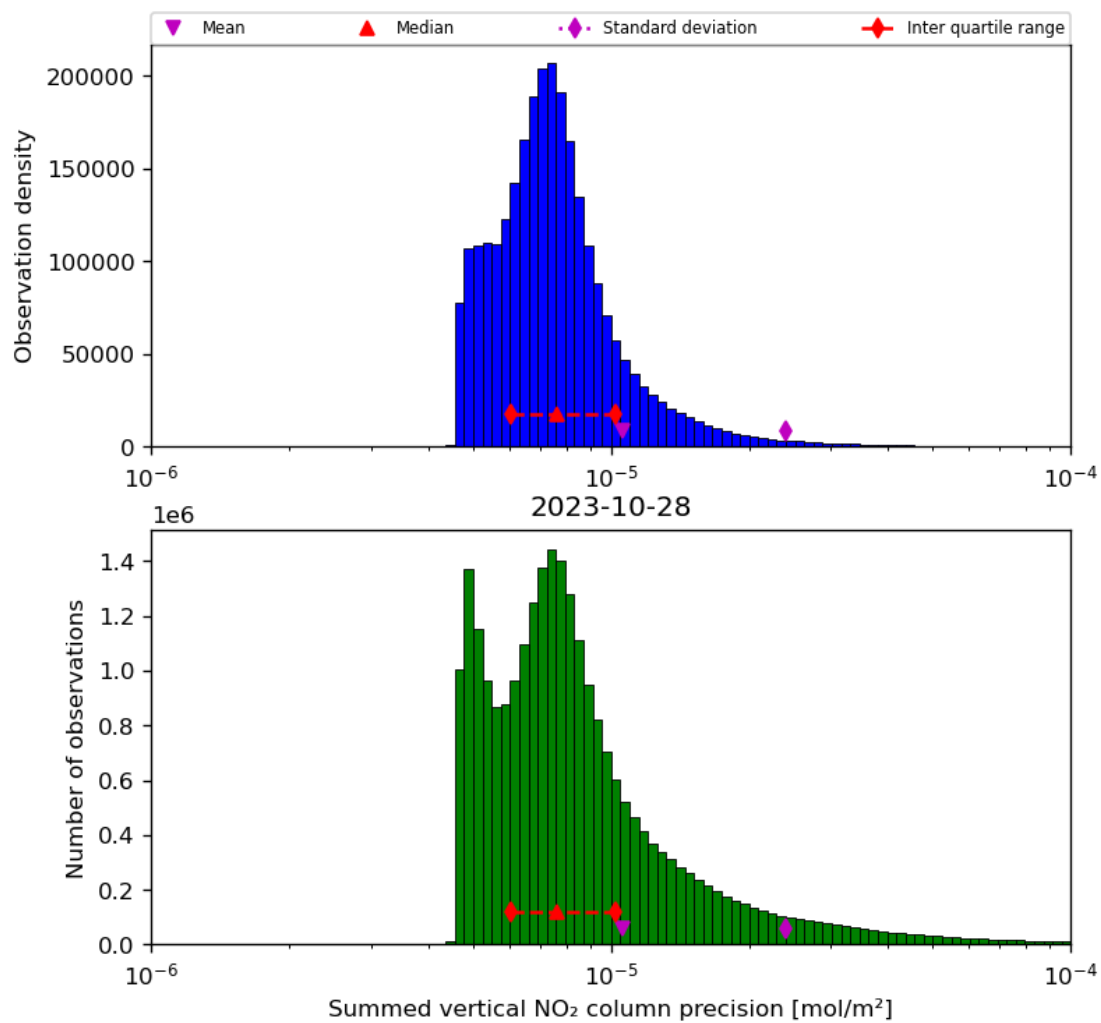
Figure 41: Histogram of “Summed vertical NO 2 column precision” for 2023-10-28 to 2023-10-29
