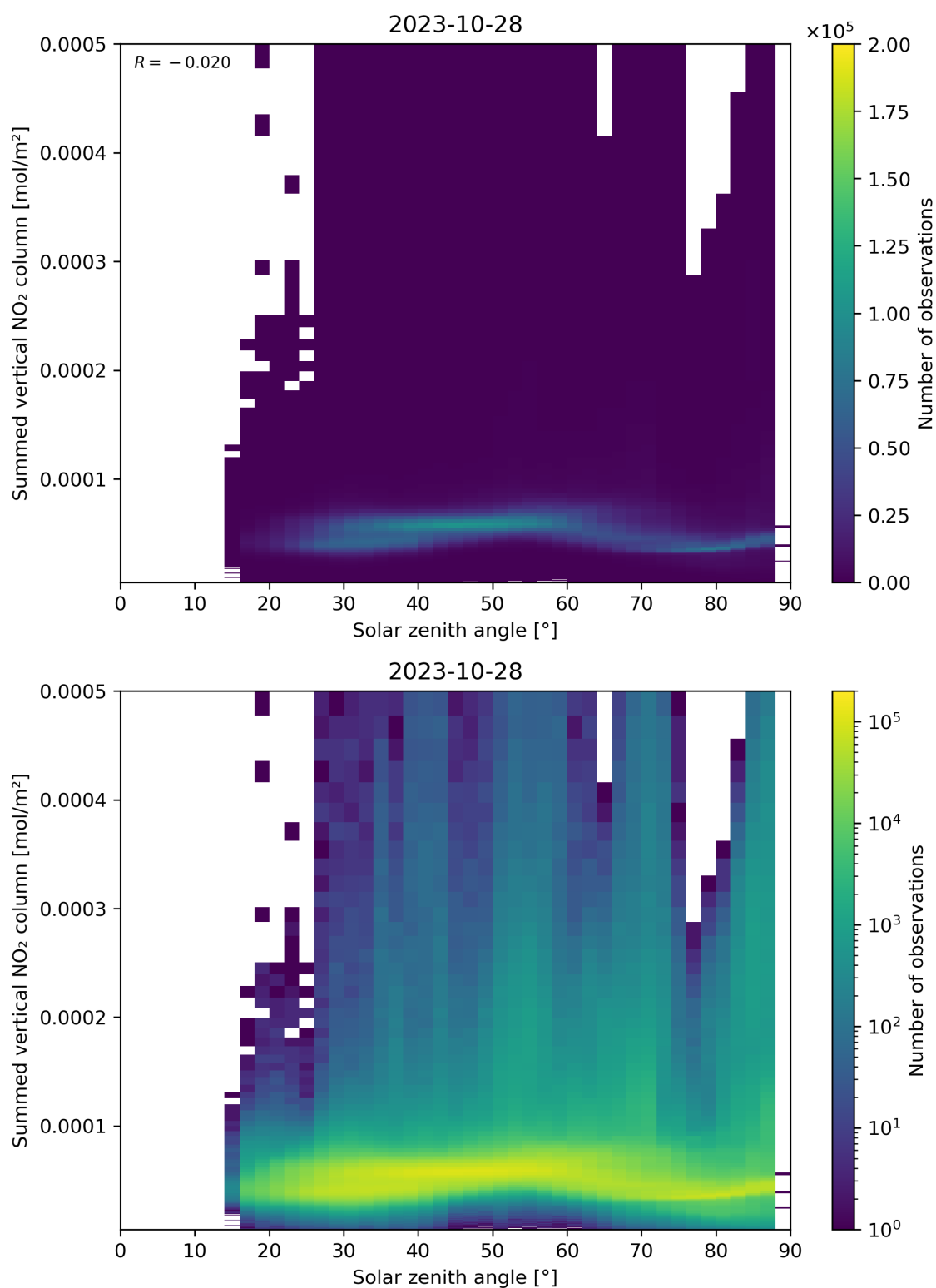
Figure 151: Scatter density plot of “Solar zenith angle” against “Summed vertical NO 2 column” for 2023-10-28 to 2023-10-29.
