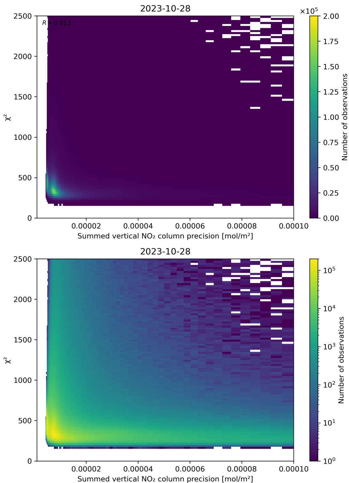
Figure 107: Scatter density plot of “Summed vertical NO 2 column precision” against “ \chi^2 ” for 2023-10-28 to 2023-10-29.
