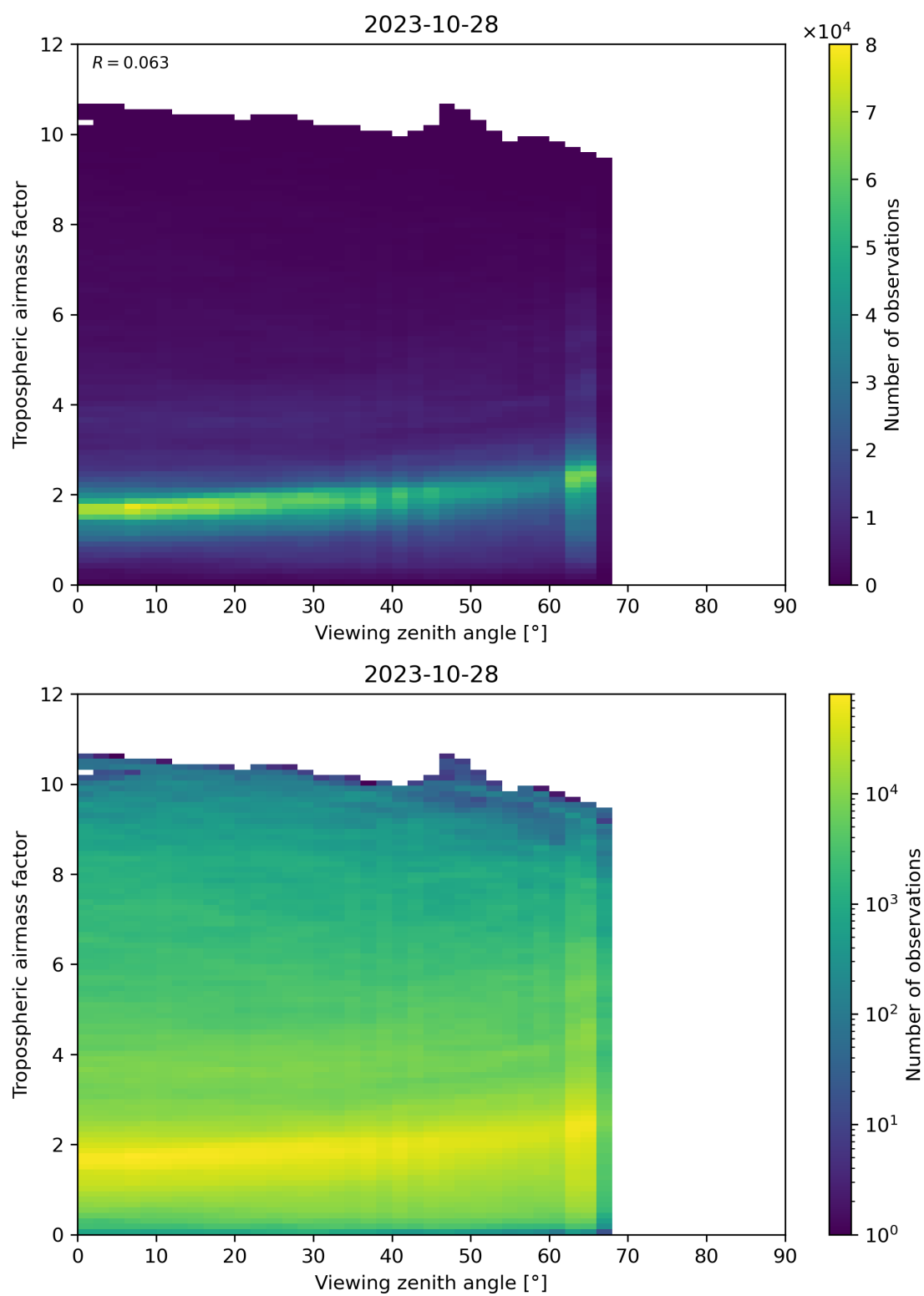
Figure 161: Scatter density plot of “Viewing zenith angle” against “Tropospheric airmass factor” for 2023-10-28 to 2023-10-29.
