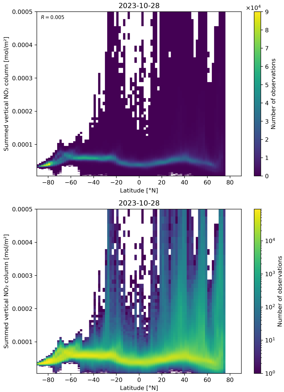
Figure 88: Scatter density plot of “Latitude” against “Summed vertical NO 2 column” for 2023-10-28 to 2023-10-29.
