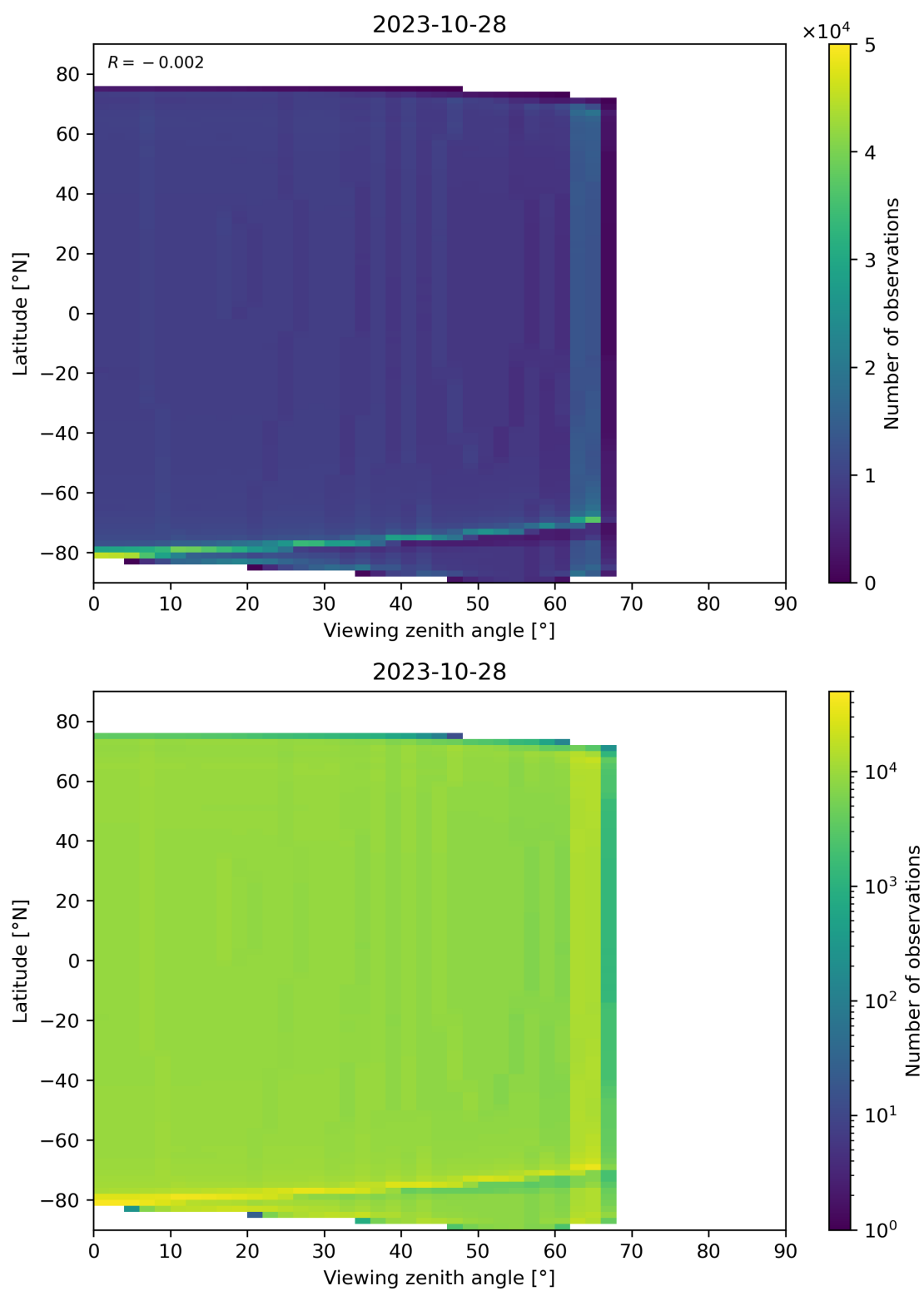
Figure 163: Scatter density plot of “Viewing zenith angle” against “Latitude” for 2023-10-28 to 2023-10-29.
