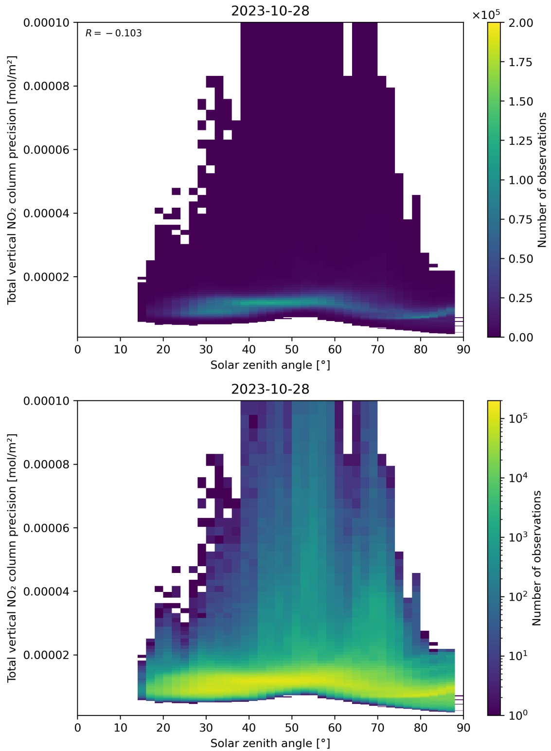
Figure 154: Scatter density plot of “Solar zenith angle” against “Total vertical NO 2 column precision” for 2023-10-28 to 2023-10-29.
