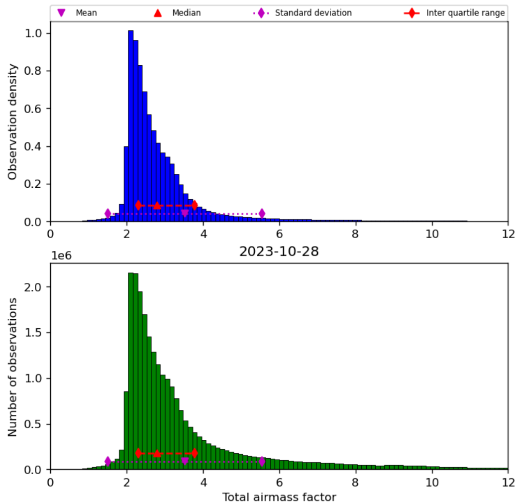
Figure 32: Histogram of “Total airmass factor” for 2023-10-28 to 2023-10-29
