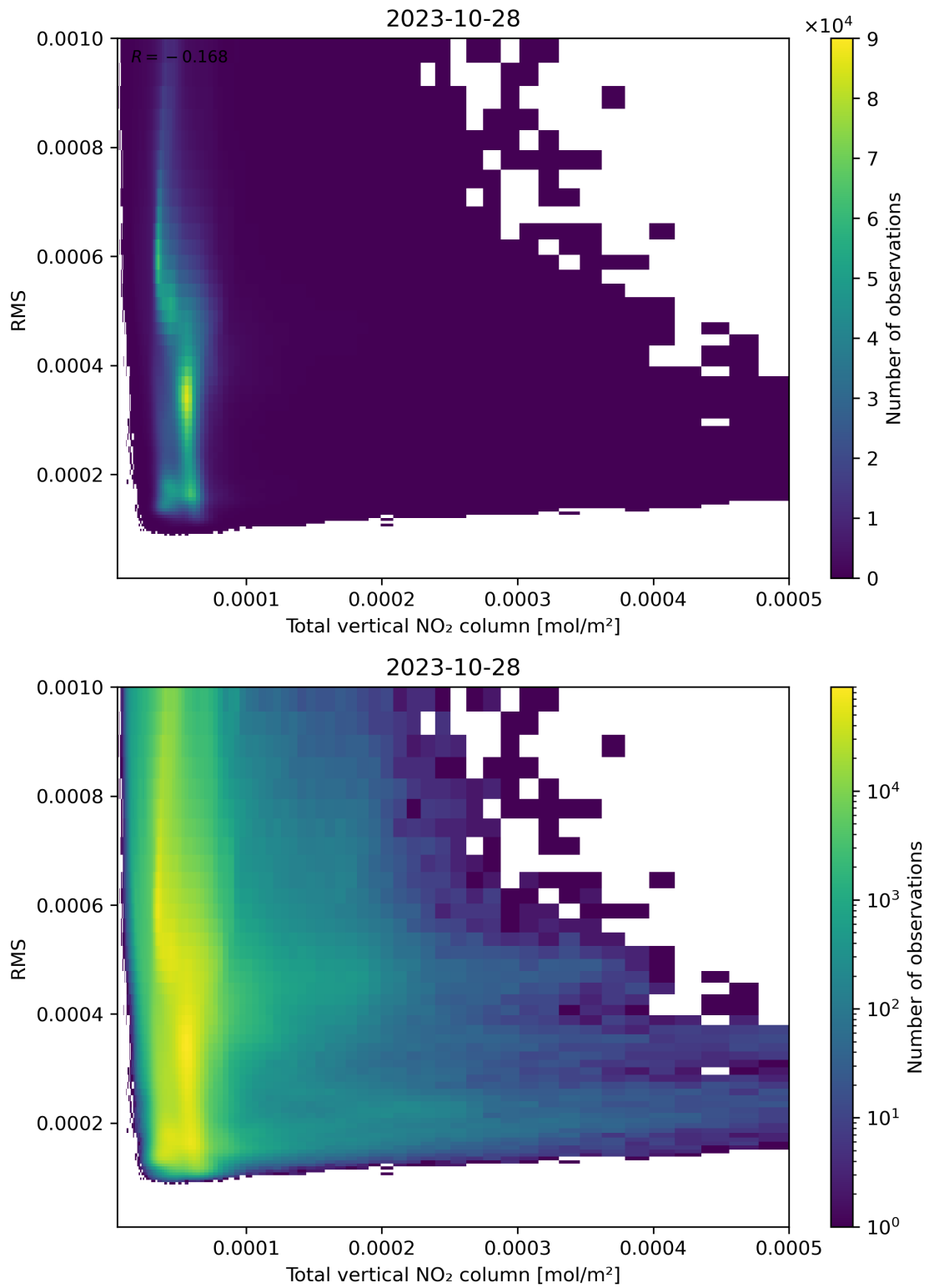
Figure 120: Scatter density plot of “Total vertical NO 2 column” against “RMS” for 2023-10-28 to 2023-10-29.
