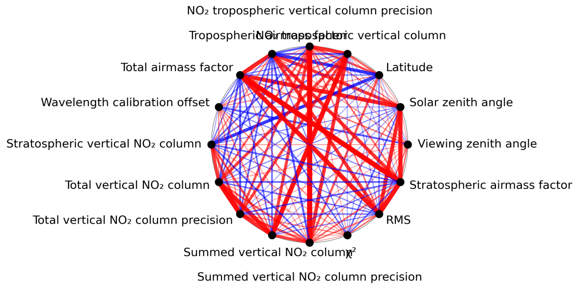
Figure 1: Map of correlation graph for 2023-10-28 to 2023-10-29.
