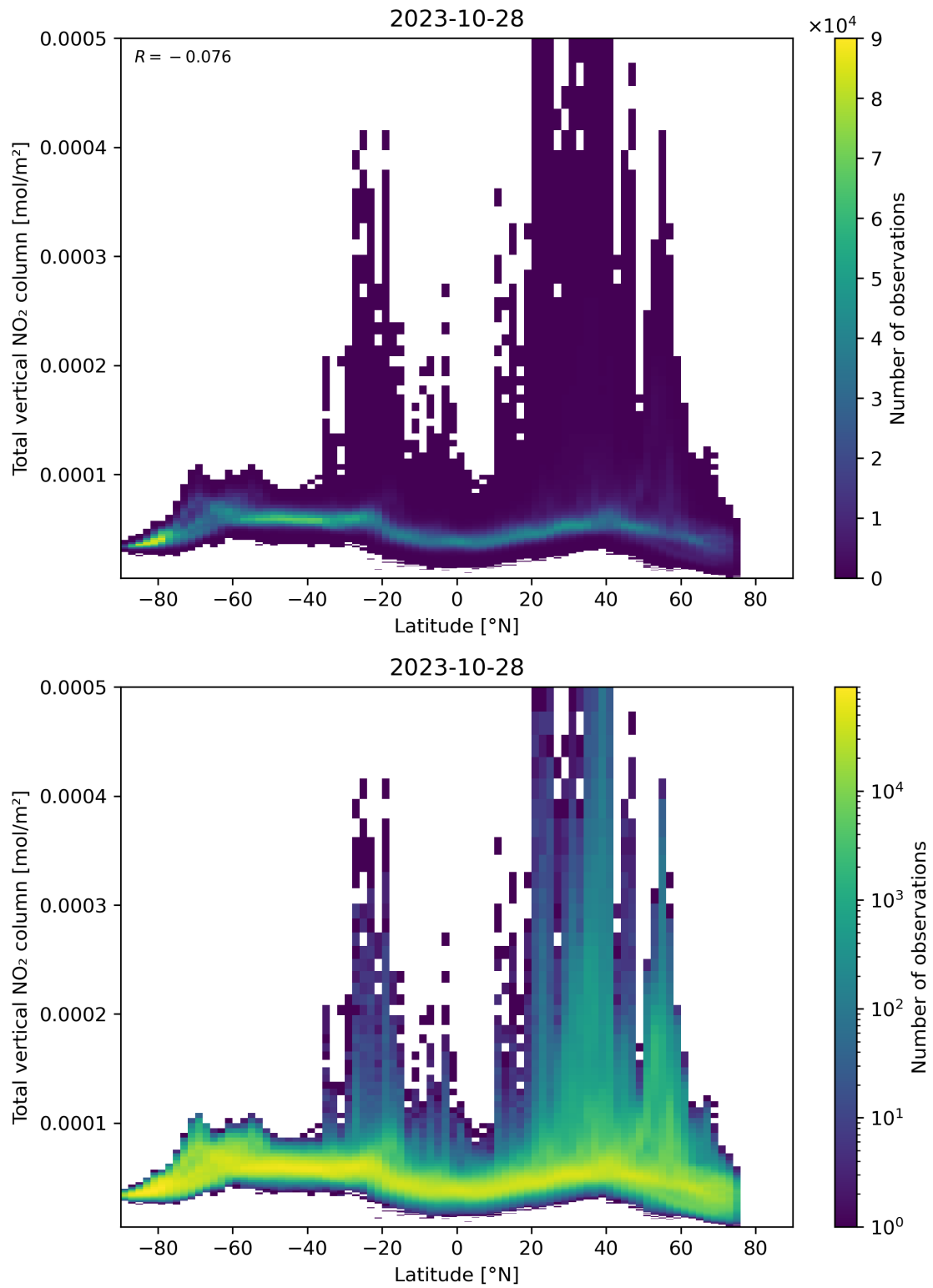
Figure 90: Scatter density plot of “Latitude” against “Total vertical NO 2 column” for 2023-10-28 to 2023-10-29.
