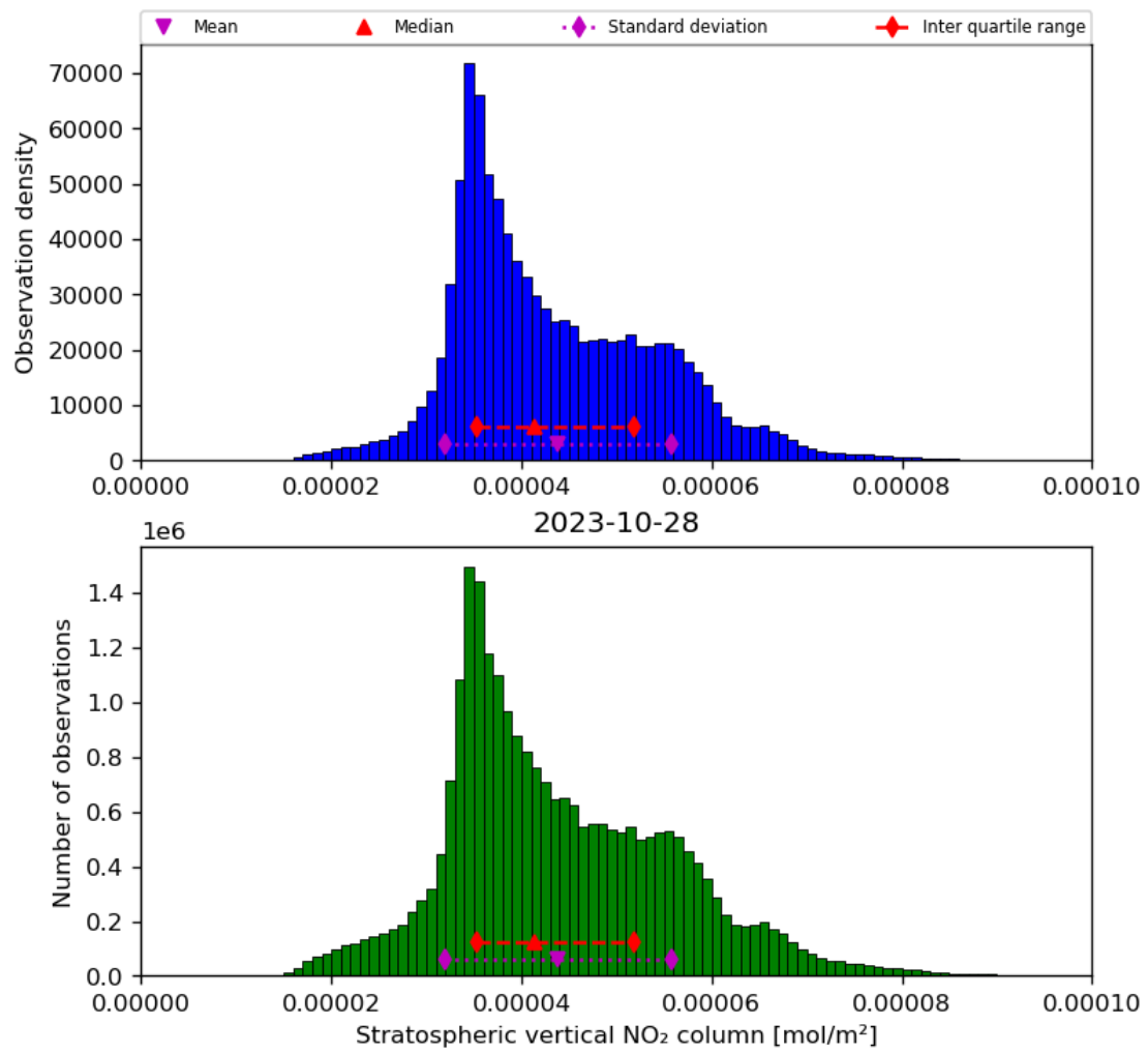
Figure 36: Histogram of “Stratospheric vertical NO 2 column” for 2023-10-28 to 2023-10-29
