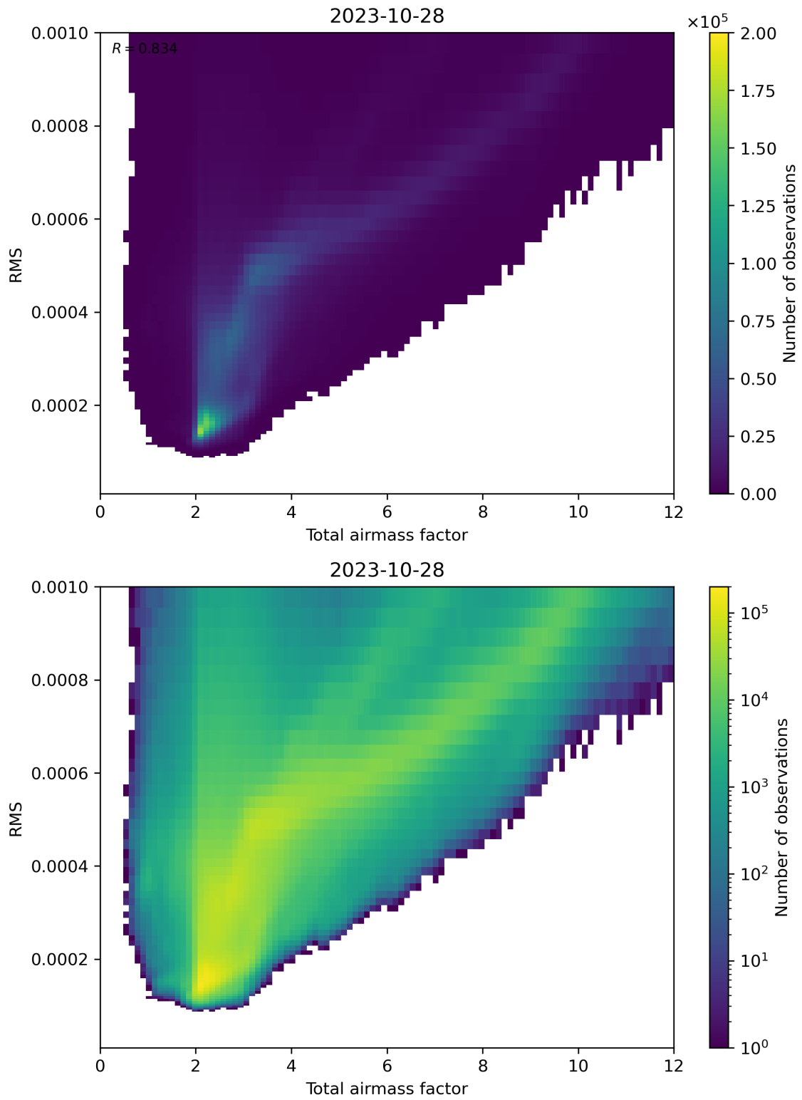
Figure 69: Scatter density plot of “Total airmass factor” against “RMS” for 2023-10-28 to 2023-10-29.
