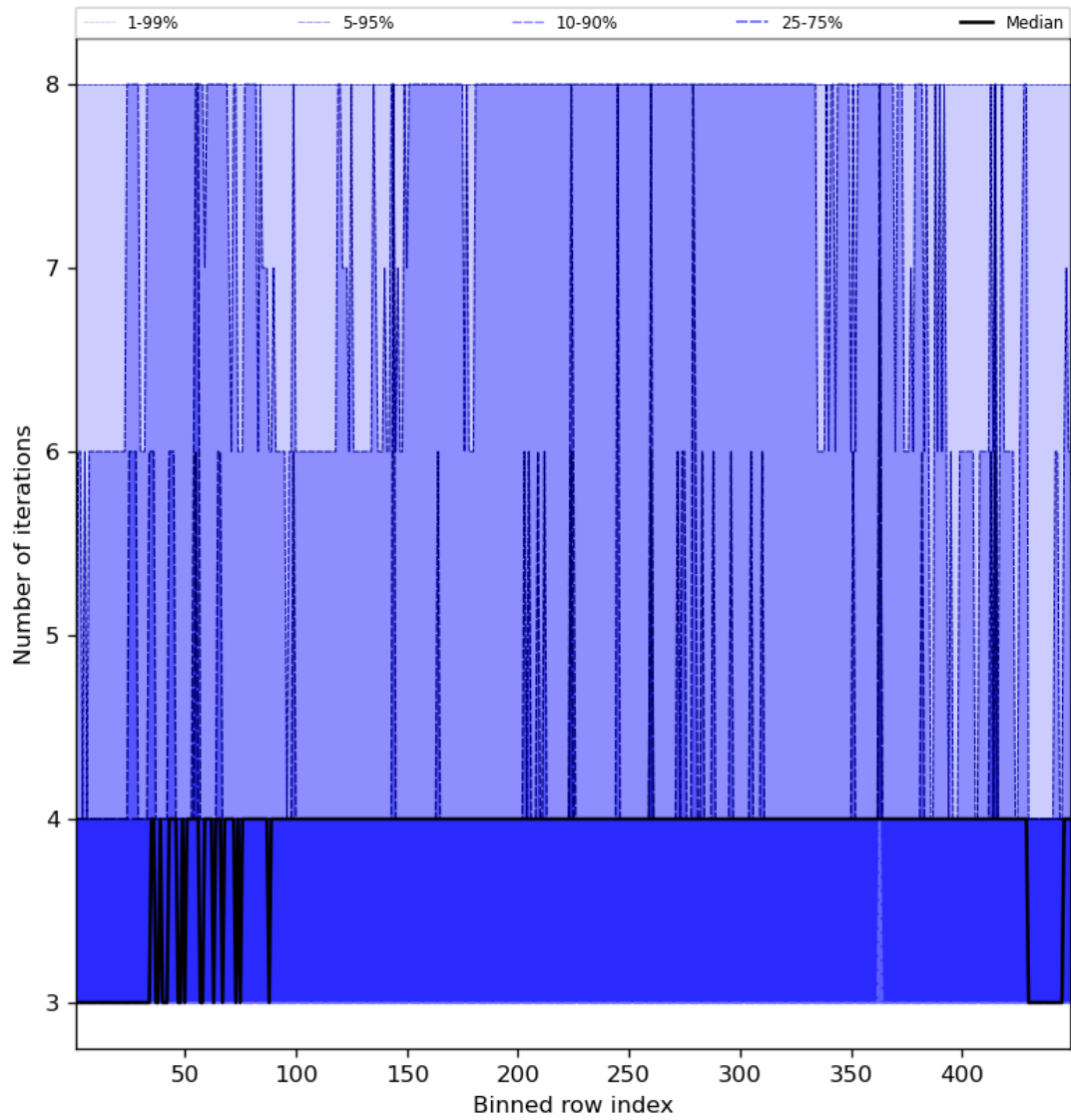
Figure 51: Along track statistics of “Number of iterations” for 2023-10-28 to 2023-10-29
