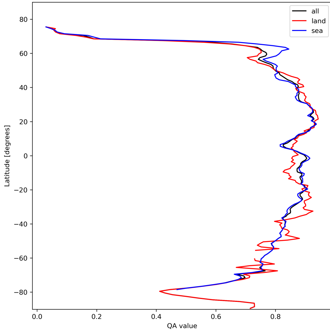
Figure 11: Zonal average of “QA value” for 2023-10-28 to 2023-10-29.
