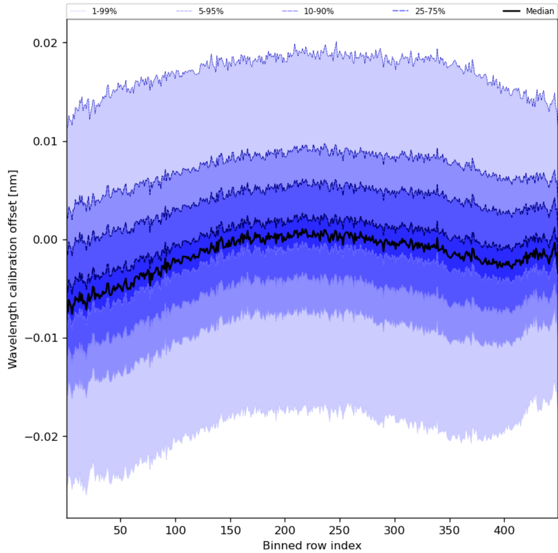
Figure 52: Along track statistics of “Wavelength calibration offset” for 2023-10-28 to 2023-10-29
