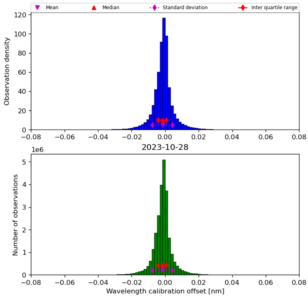
Figure 35: Histogram of “Wavelength calibration offset” for 2023-10-28 to 2023-10-29
