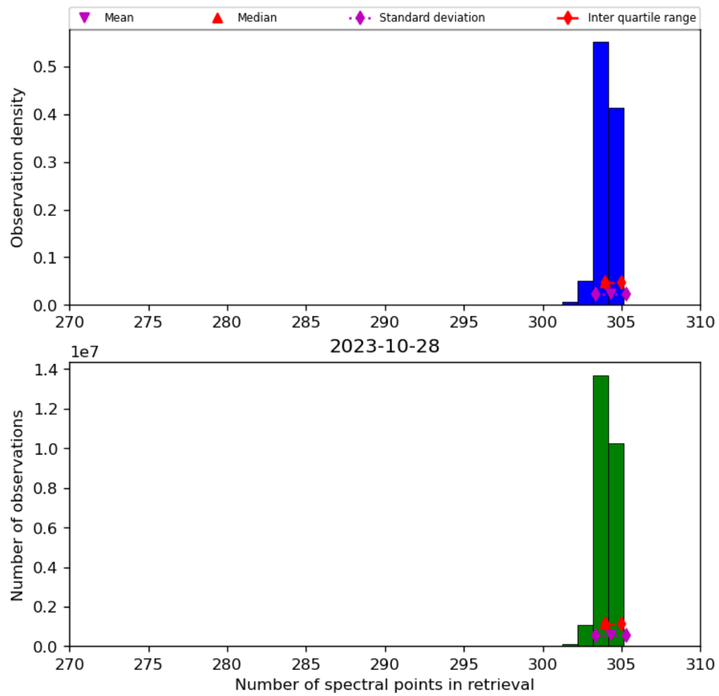
Figure 33: Histogram of “Number of spectral points in retrieval” for 2023-10-28 to 2023-10-29
