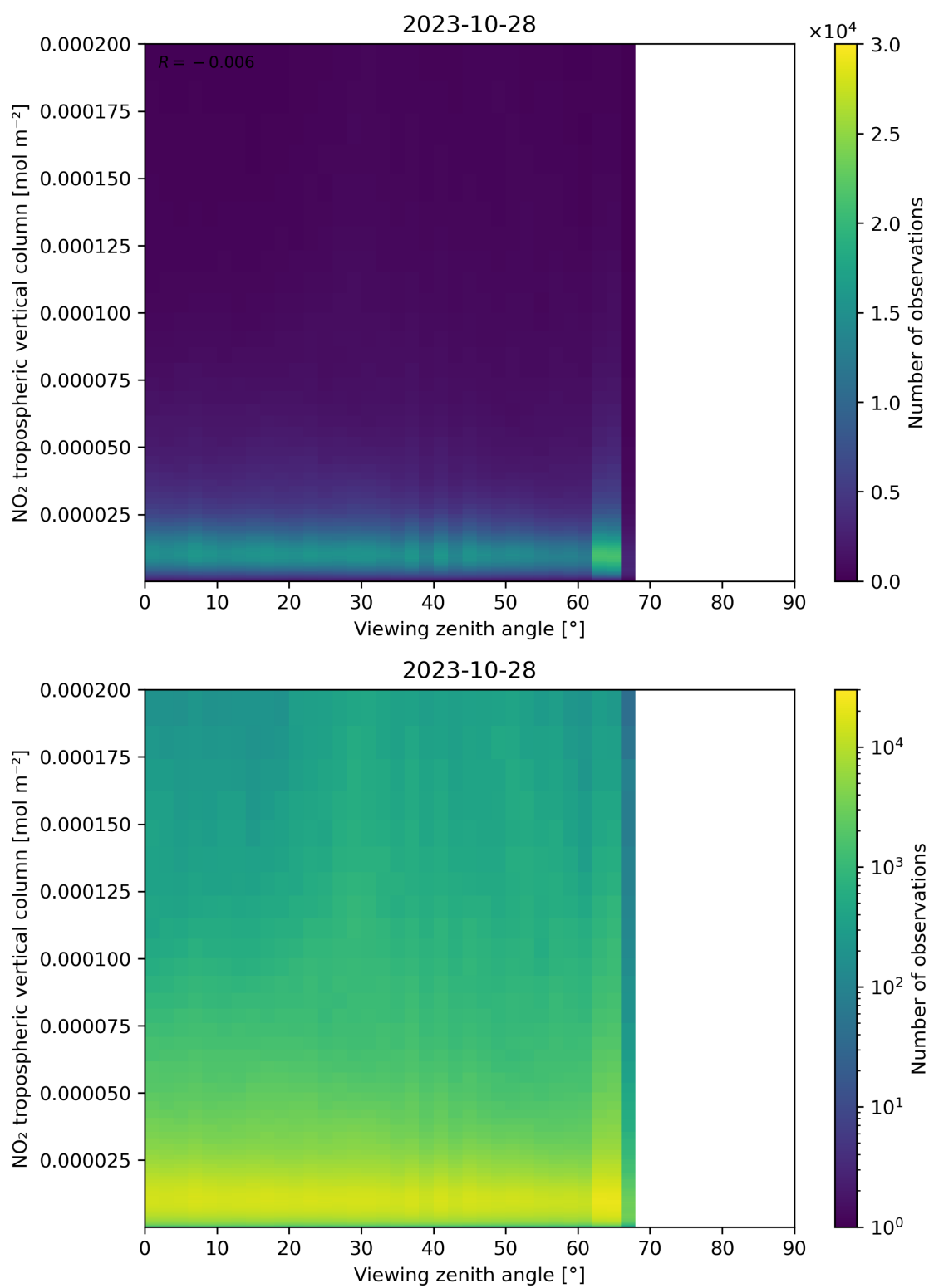
Figure 169: Scatter density plot of “Viewing zenith angle” against “NO 2 tropospheric vertical column” for 2023-10-28 to 2023-10-29.
