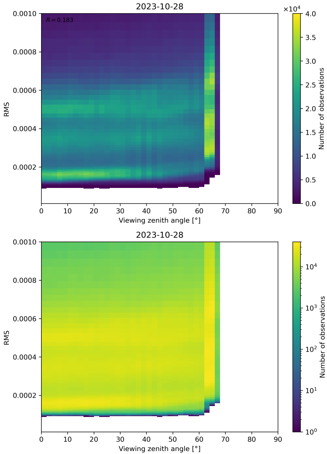
Figure 171: Scatter density plot of “Viewing zenith angle” against “RMS” for 2023-10-28 to 2023-10-29.
