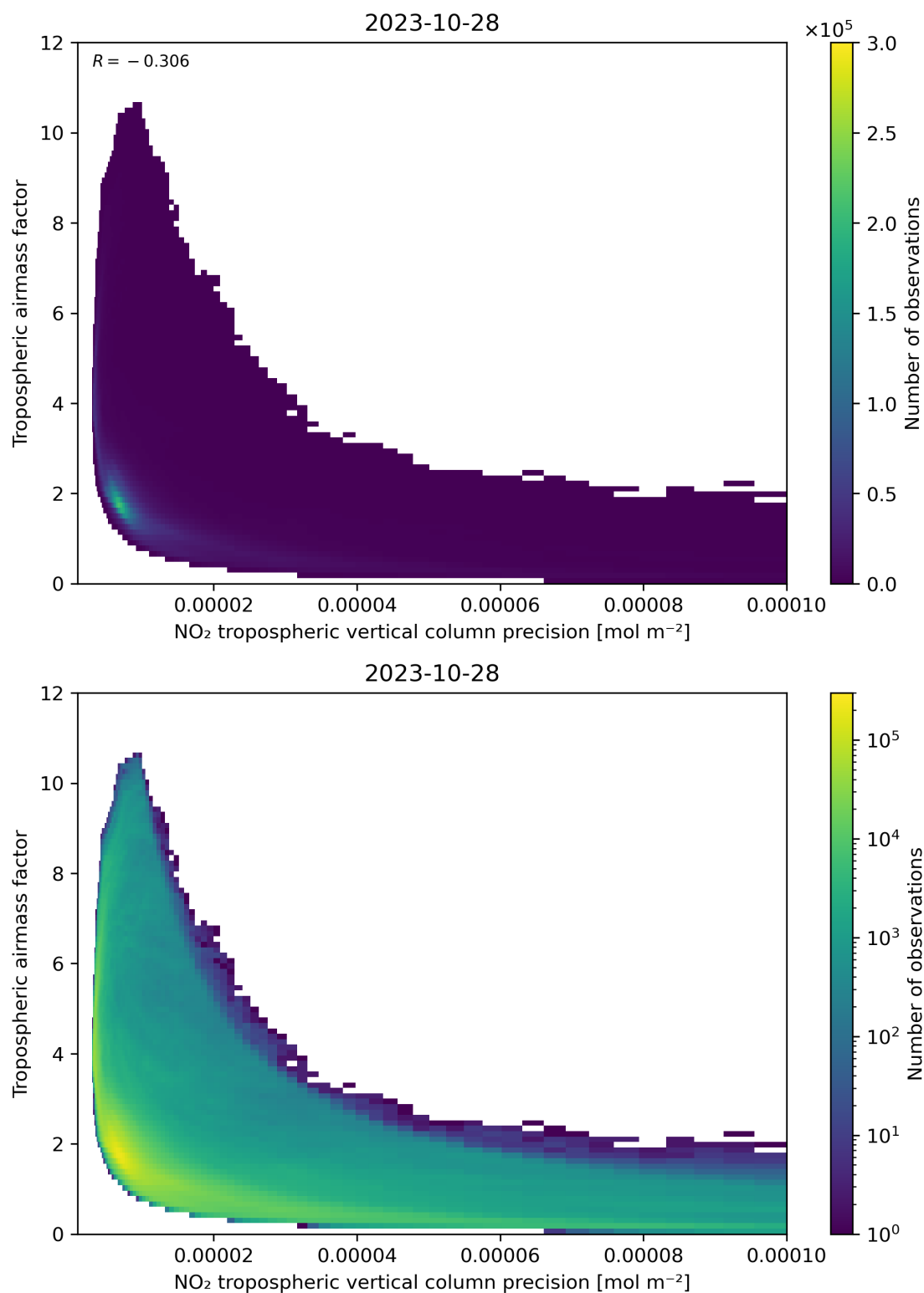
Figure 133: Scatter density plot of “NO 2 tropospheric vertical column precision” against “Tropospheric airmass factor” for 2023-10-28 to 2023-10-29.
