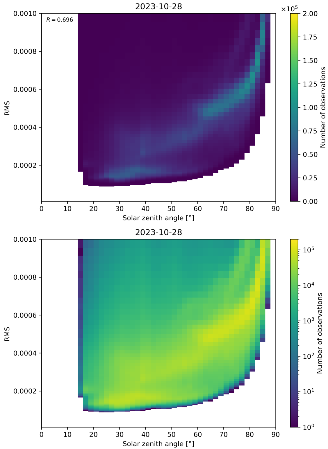
Figure 157: Scatter density plot of “Solar zenith angle” against “RMS” for 2023-10-28 to 2023-10-29.
