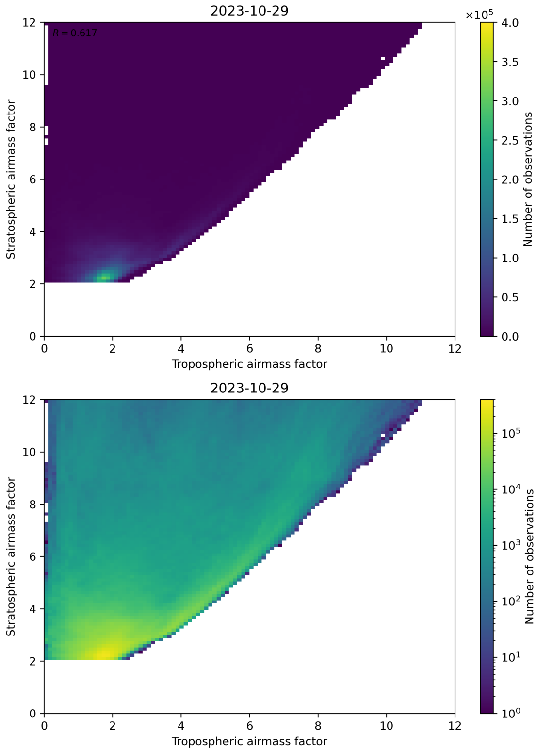
Figure 71: Scatter density plot of “Tropospheric airmass factor” against “Stratospheric airmass factor” for 2023-10-28 to 2023-10-30.
