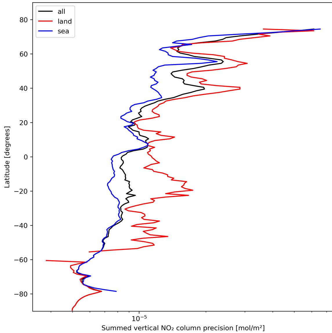
Figure 24: Zonal average of “Summed vertical NO 2 column precision” for 2023-10-28 to 2023-10-30.
