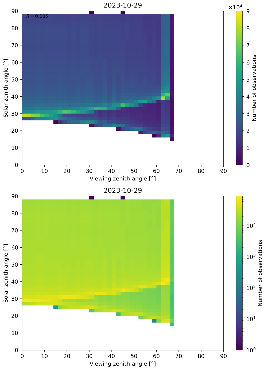
Figure 172: Scatter density plot of “Viewing zenith angle” against “Solar zenith angle” for 2023-10-28 to 2023-10-30.
