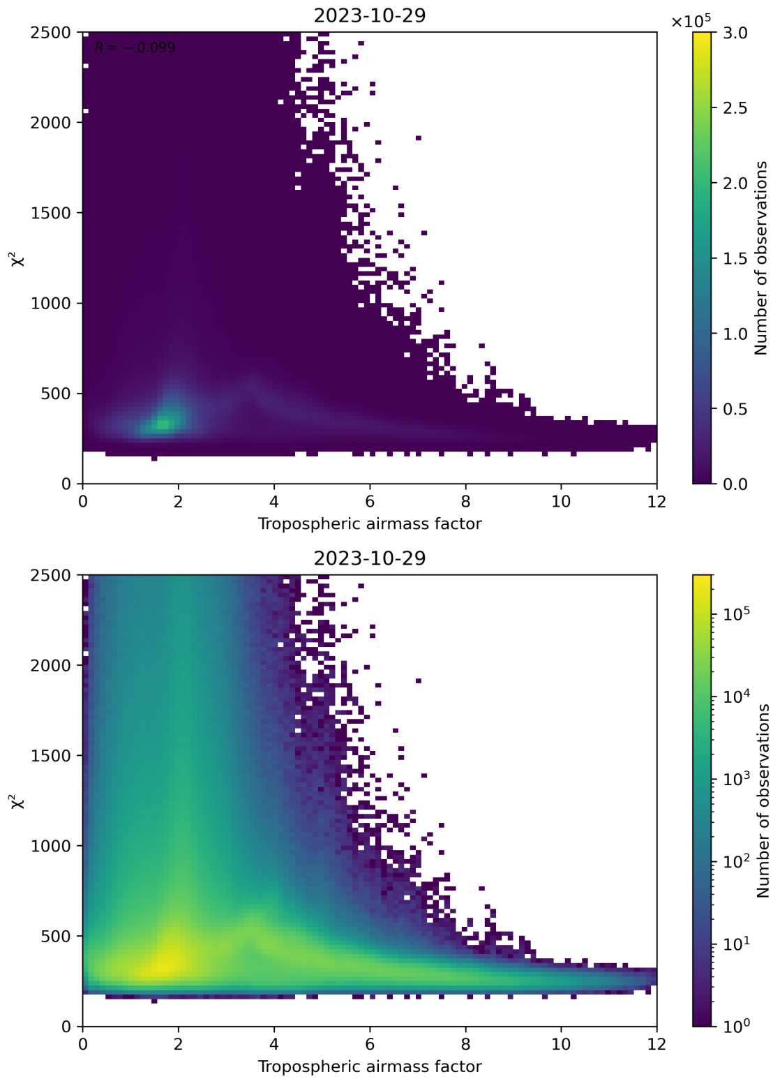
Figure 73: Scatter density plot of “Tropospheric airmass factor” against “ \chi^2 ” for 2023-10-28 to 2023-10-30.
