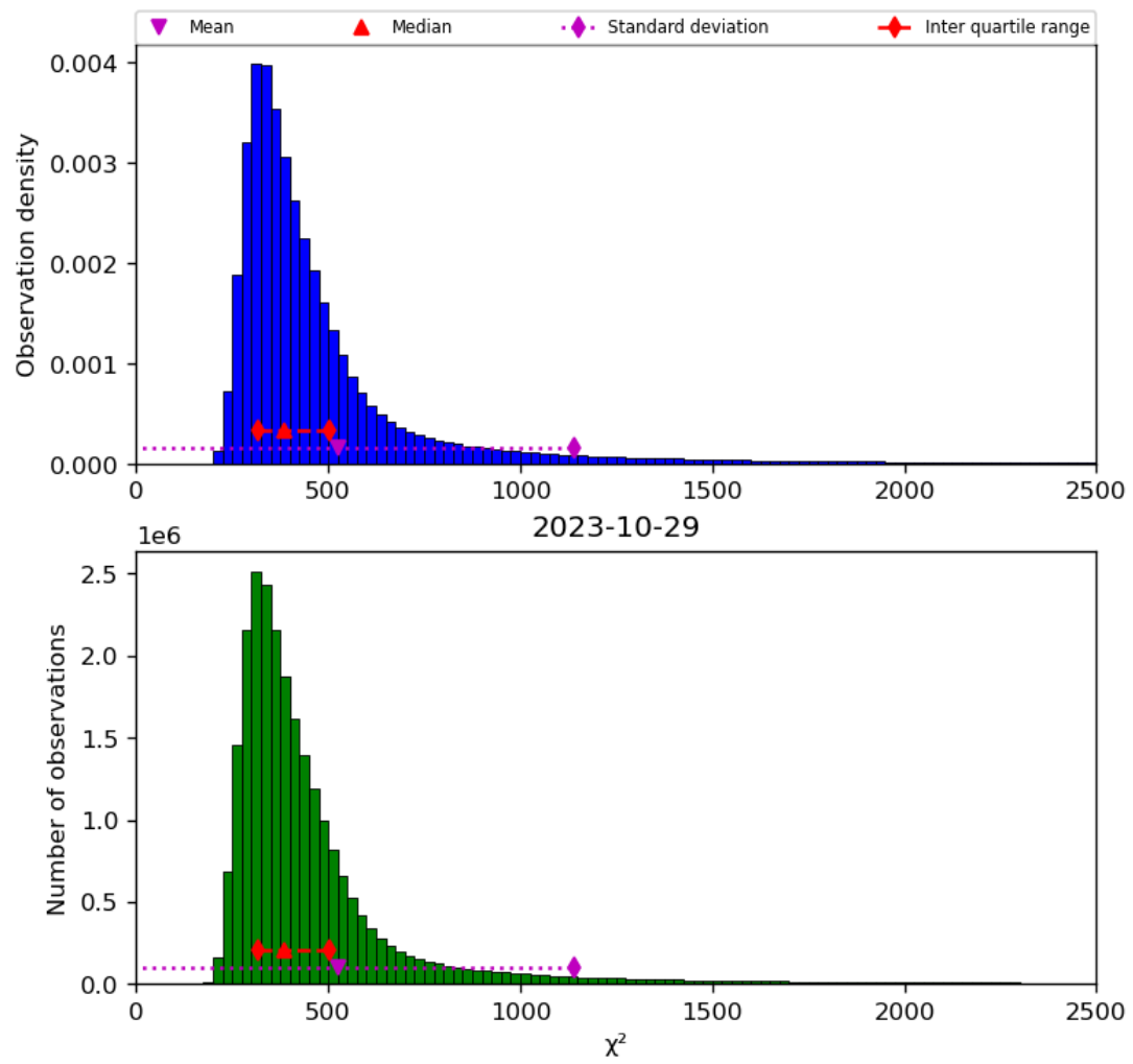
Figure 42: Histogram of “ \chi^2 ” for 2023-10-28 to 2023-10-30
