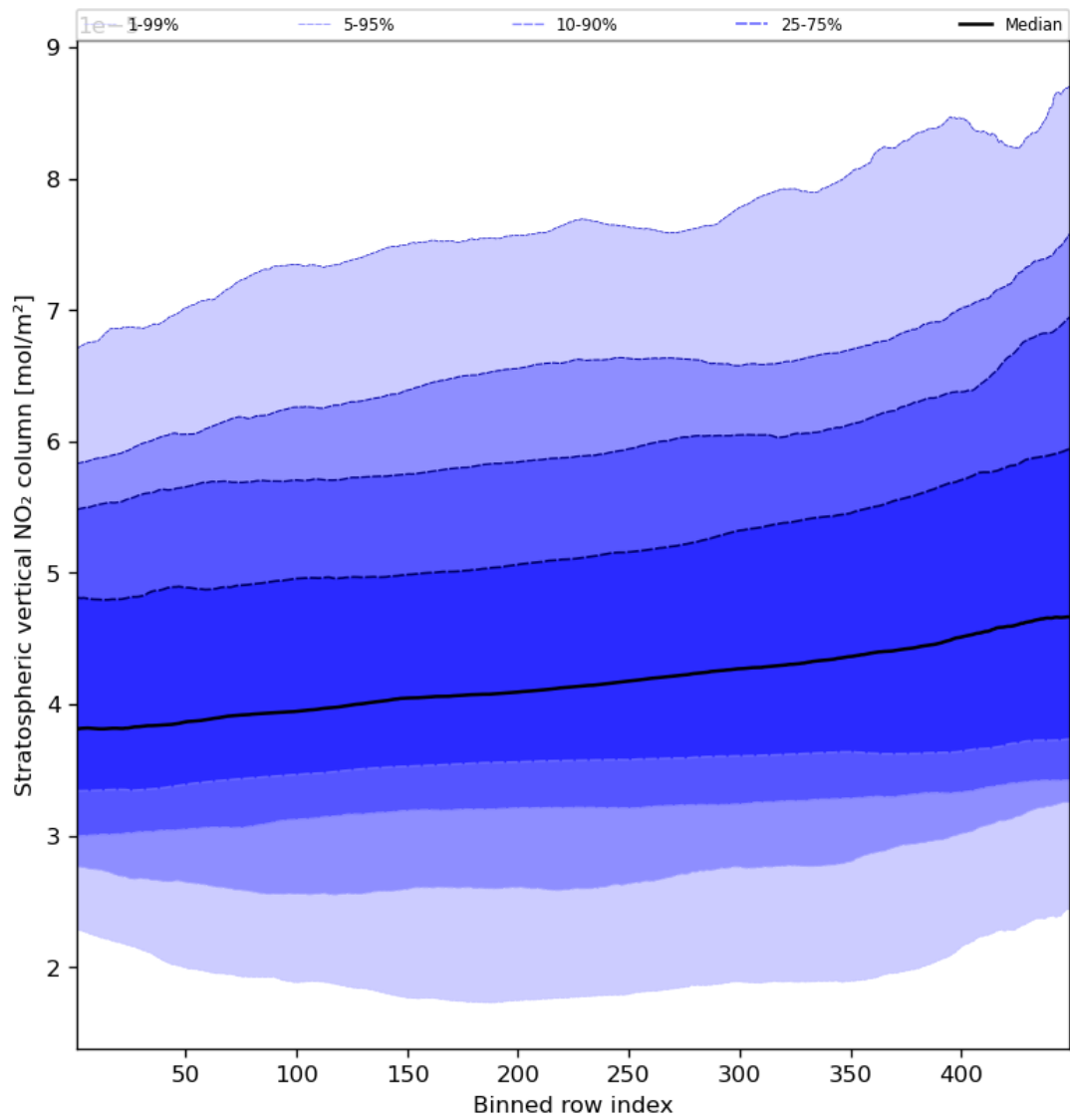
Figure 53: Along track statistics of “Stratospheric vertical NO 2 column” for 2023-10-28 to 2023-10-30
