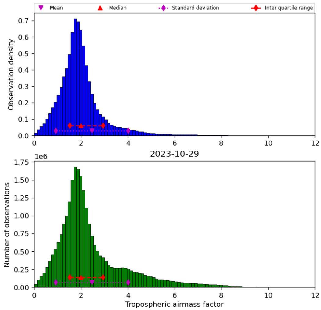
Figure 31: Histogram of “Tropospheric airmass factor” for 2023-10-28 to 2023-10-30
