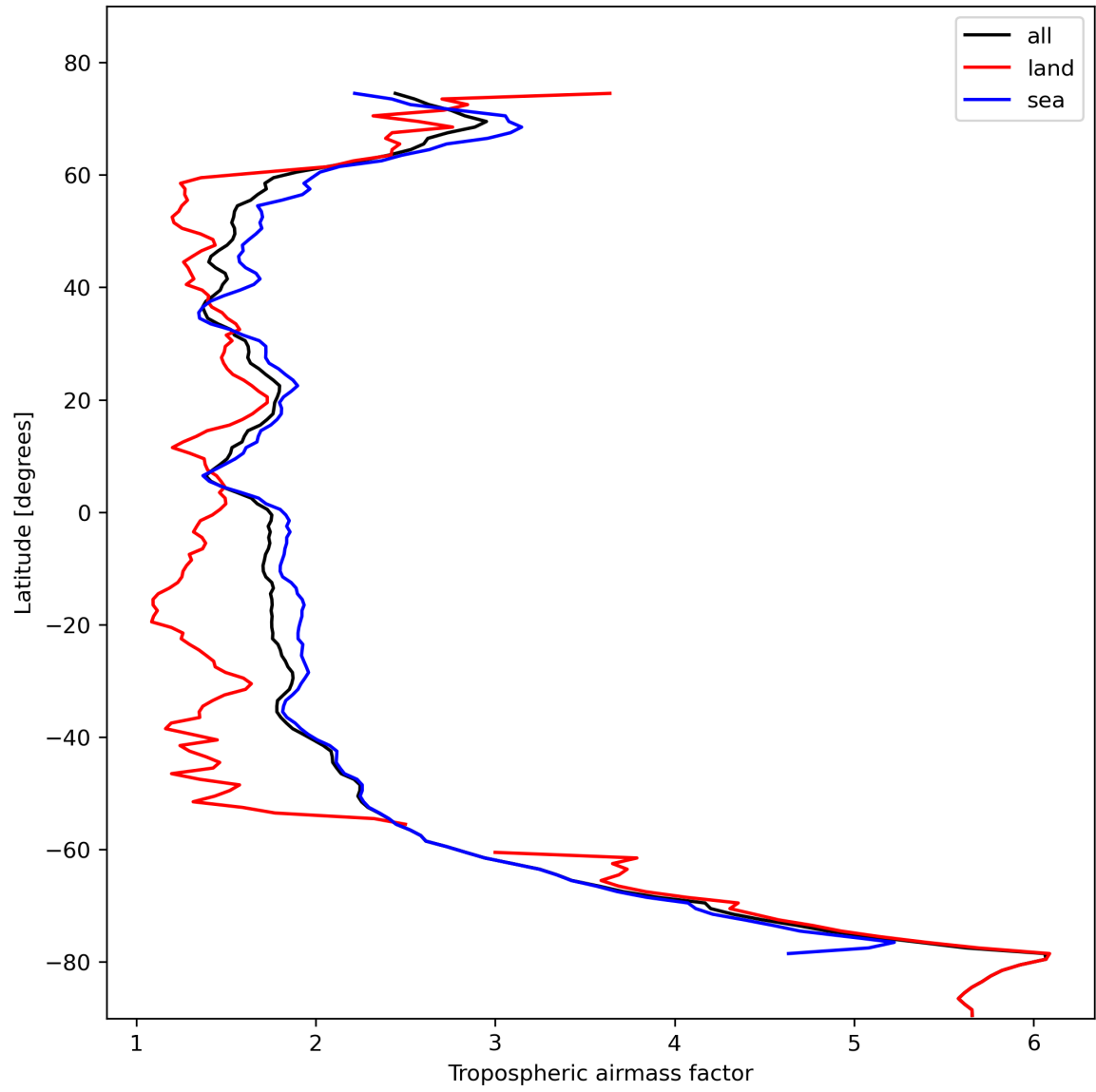
Figure 14: Zonal average of “Tropospheric airmass factor” for 2023-10-28 to 2023-10-30.
