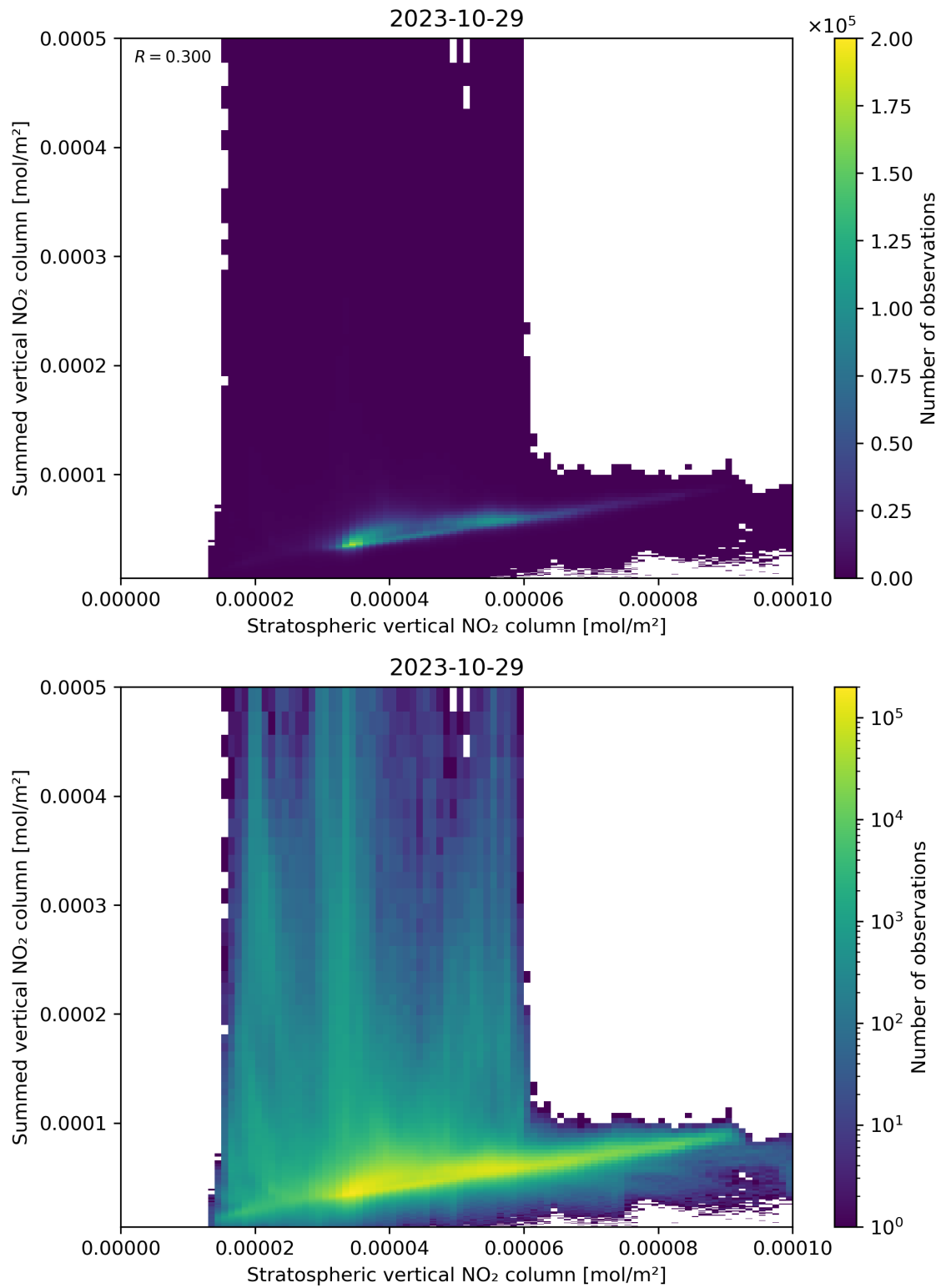
Figure 98: Scatter density plot of “Stratospheric vertical NO 2 column” against “Summed vertical NO 2 column” for 2023-10-28 to 2023-10-30.
