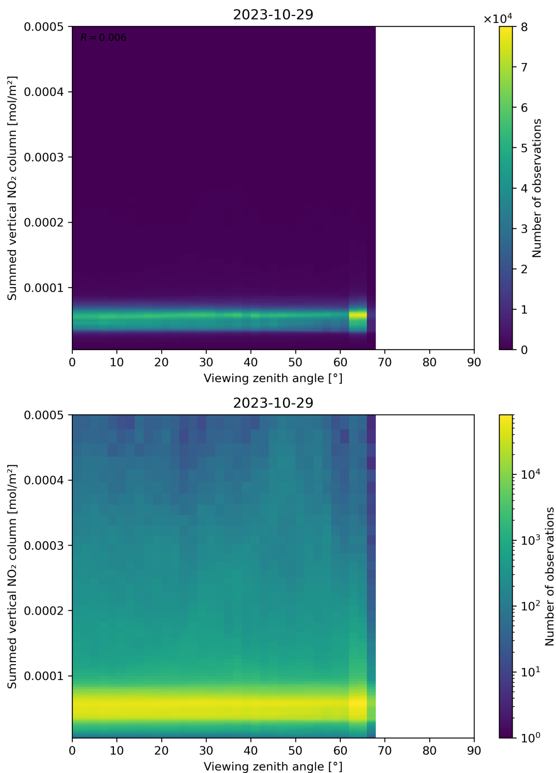
Figure 165: Scatter density plot of “Viewing zenith angle” against “Summed vertical NO 2 column” for 2023-10-28 to 2023-10-30.
