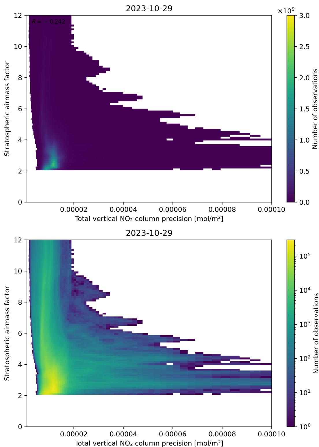
Figure 115: Scatter density plot of “Total vertical NO 2 column precision” against “Stratospheric air mass factor” for 2023-10-28 to 2023-10-30.
