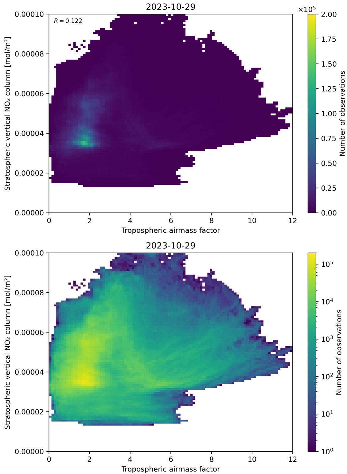
Figure 74: Scatter density plot of “Tropospheric air mass factor” against “Stratospheric vertical NO 2 column” for 2023-10-28 to 2023-10-30.
