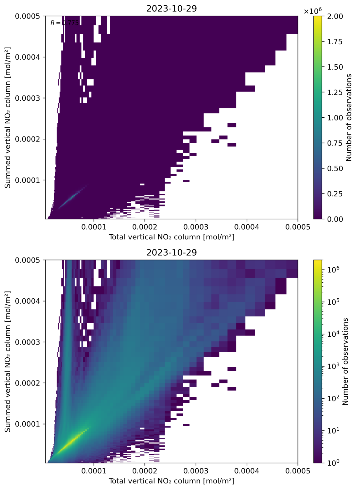
Figure 112: Scatter density plot of “Total vertical NO 2 column” against “Summed vertical NO 2 column” for 2023-10-28 to 2023-10-30.
