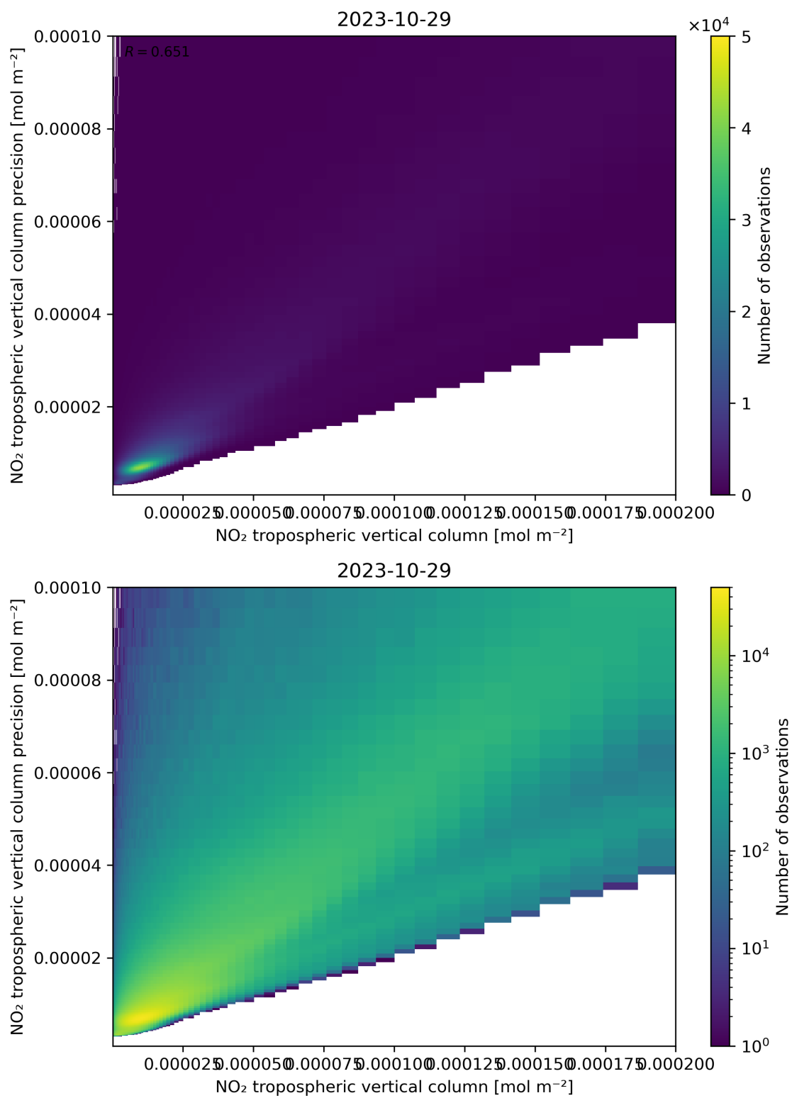
Figure 130: Scatter density plot of “NO 2 tropospheric vertical column” against “NO 2 tropospheric vertical column precision” for 2023-10-28 to 2023-10-30.
