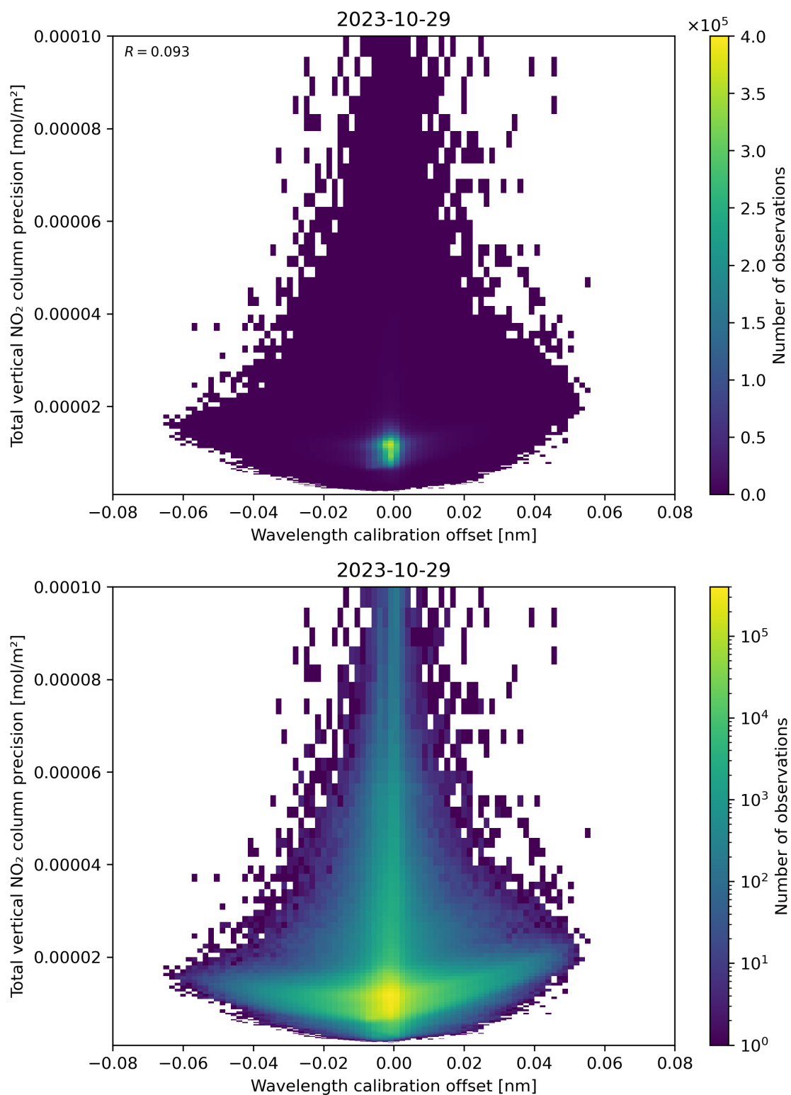
Figure 180: Scatter density plot of “Wavelength calibration offset” against “Total vertical NO 2 column precision” for 2023-10-28 to 2023-10-30.
