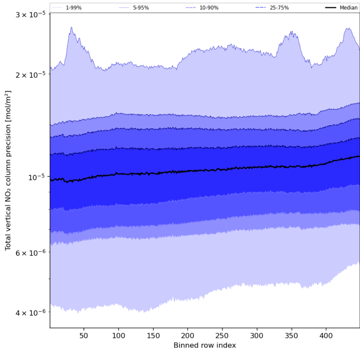
Figure 56: Along track statistics of “Total vertical NO 2 column precision” for 2023-10-28 to 2023-10-30
