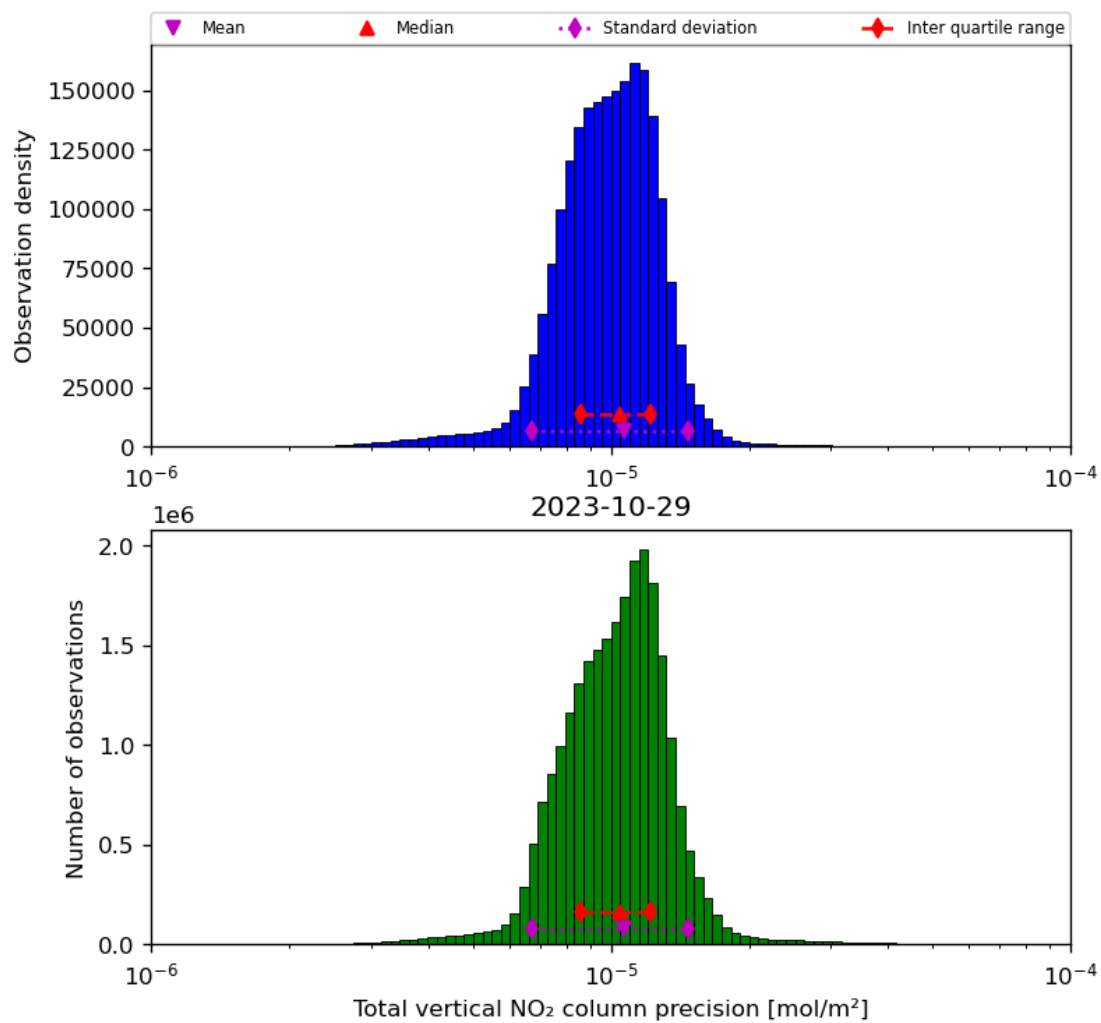
Figure 39: Histogram of "Total vertical NO 2 column precision" for 2023-10-28 to 2023-10-30
