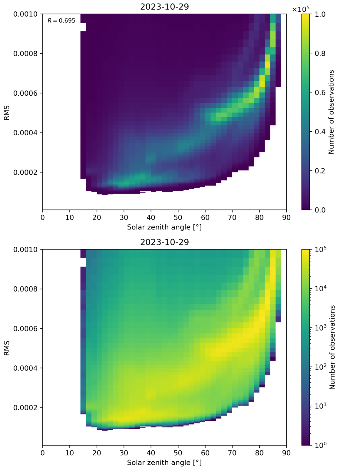
Figure 157: Scatter density plot of “Solar zenith angle” against “RMS” for 2023-10-28 to 2023-10-30.
