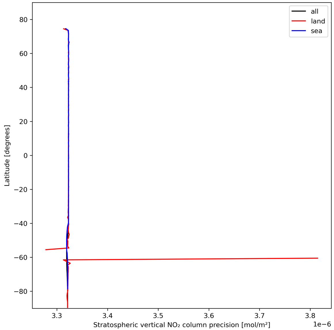
Figure 20: Zonal average of “Stratospheric vertical NO 2 column precision” for 2023-10-28 to 2023-10-30.
