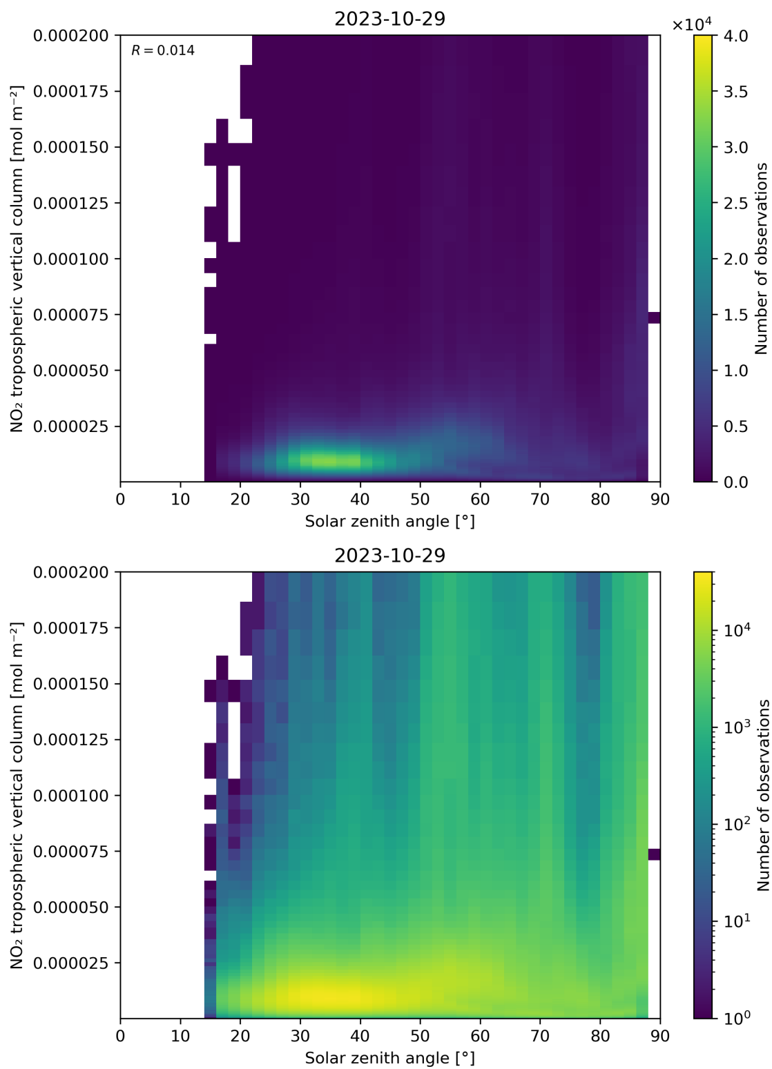
Figure 155: Scatter density plot of “Solar zenith angle” against “NO 2 tropospheric vertical column” for 2023-10-28 to 2023-10-30.
