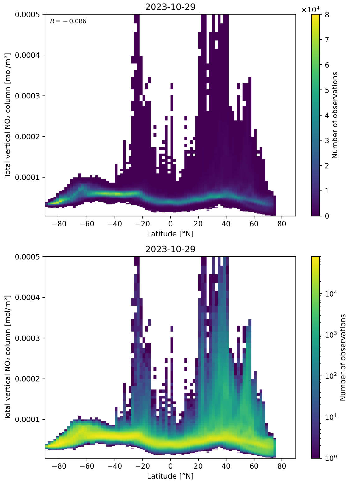
Figure 90: Scatter density plot of “Latitude” against “Total vertical NO 2 column” for 2023-10-28 to 2023-10-30.
