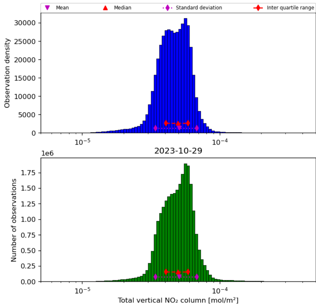
Figure 38: Histogram of “Total vertical NO 2 column” for 2023-10-28 to 2023-10-30
