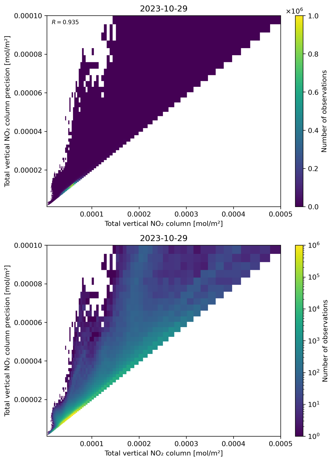
Figure 114: Scatter density plot of “Total vertical NO 2 column” against “Total vertical NO 2 column precision” for 2023-10-28 to 2023-10-30.
