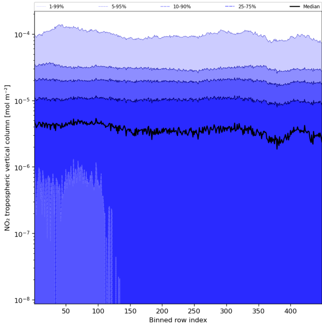
Figure 46: Along track statistics of “ \text{NO}_2 tropospheric vertical column” for 2023-10-28 to 2023-10-30
