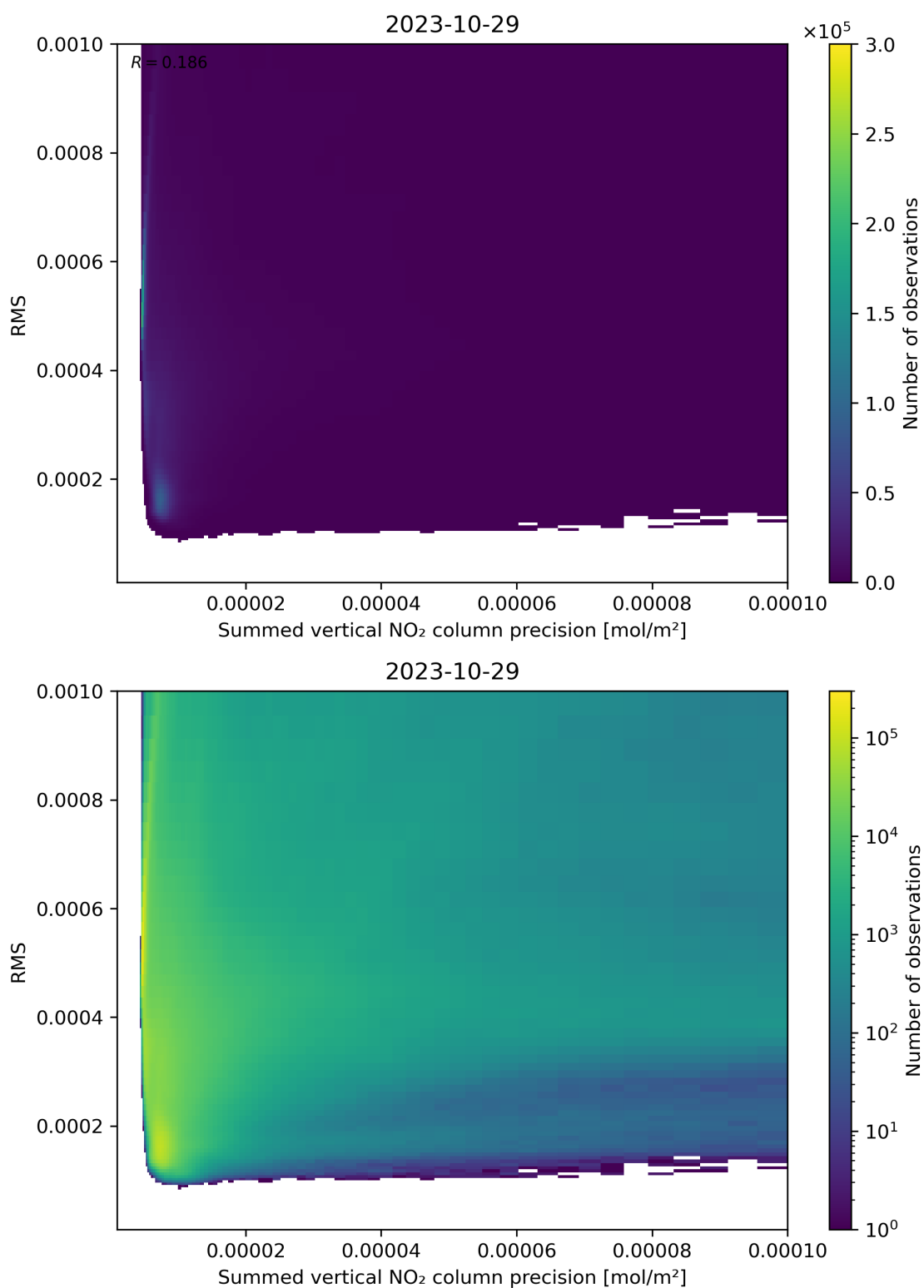
Figure 108: Scatter density plot of “Summed vertical NO 2 column precision” against “RMS” for 2023-10-28 to 2023-10-30.
