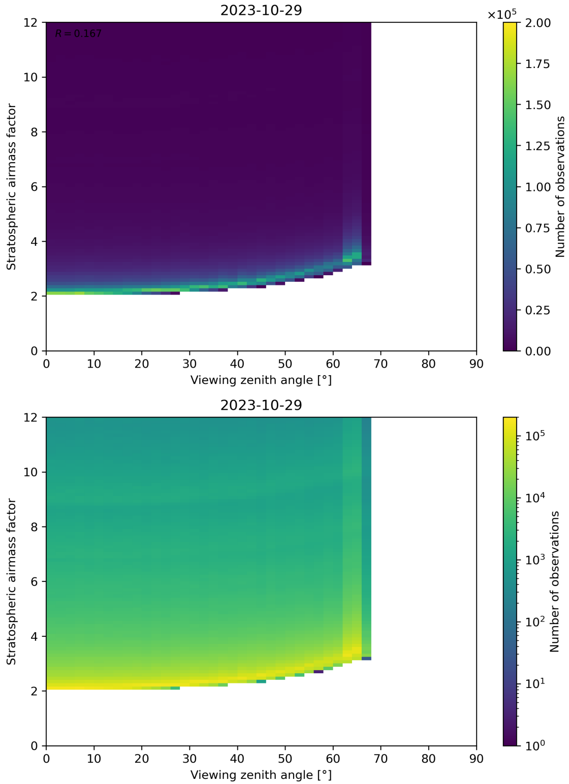
Figure 159: Scatter density plot of “Viewing zenith angle” against “Stratospheric airmass factor” for 2023-10-28 to 2023-10-30.
