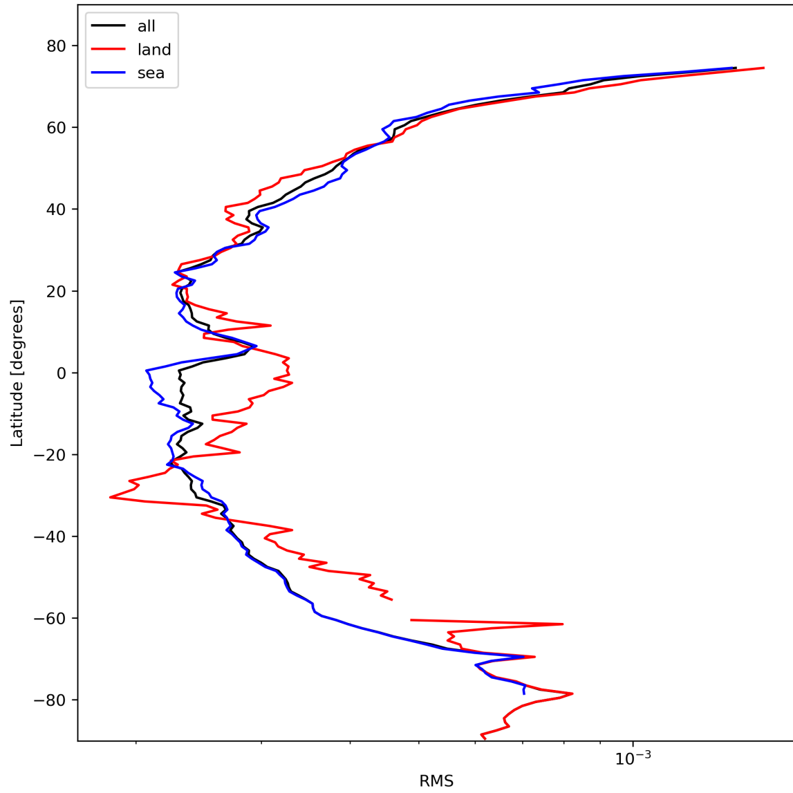
Figure 26: Zonal average of “RMS” for 2023-10-28 to 2023-10-30.
