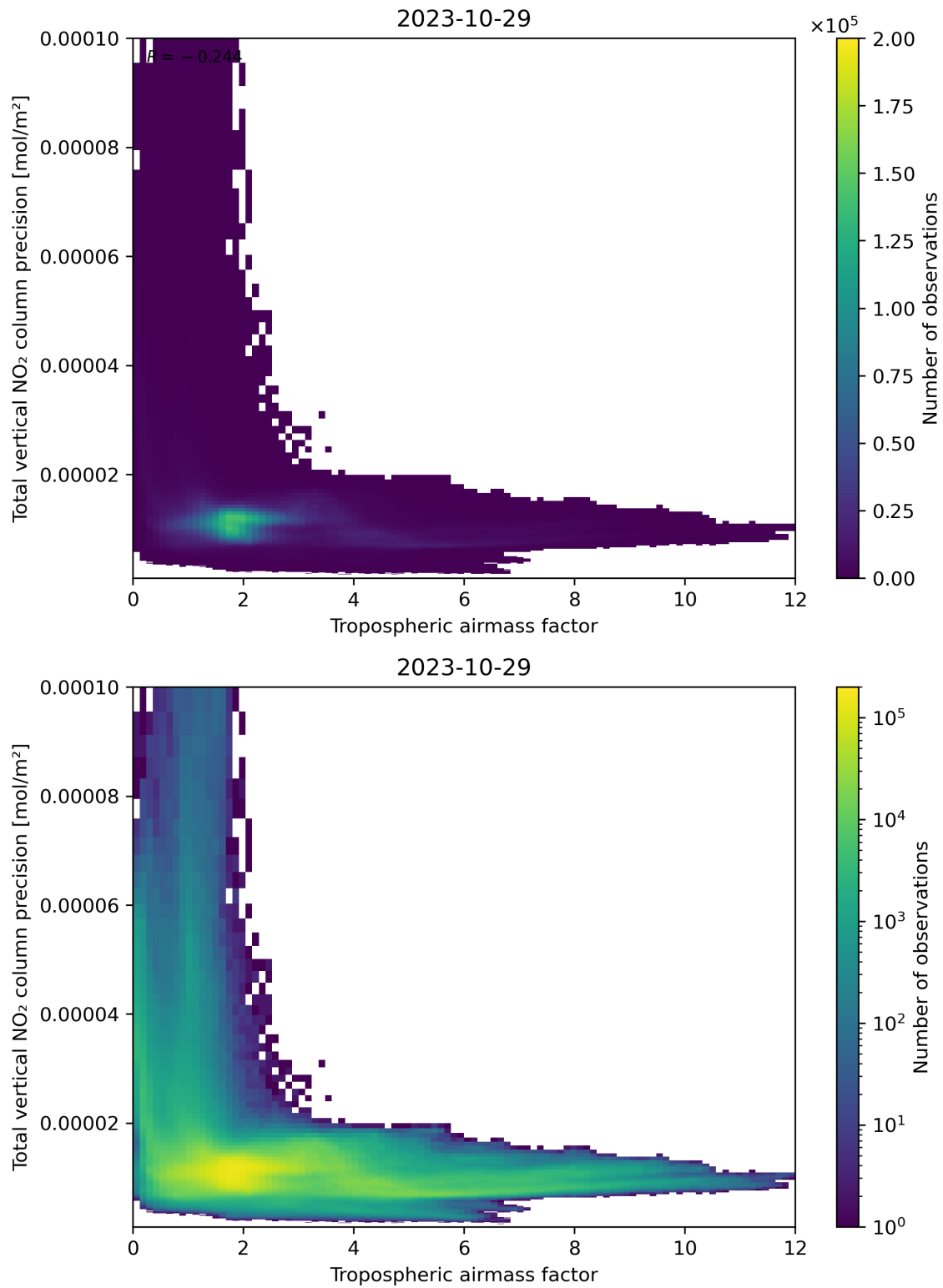
Figure 78: Scatter density plot of “Tropospheric air mass factor” against “Total vertical NO 2 column precision” for 2023-10-28 to 2023-10-30.
