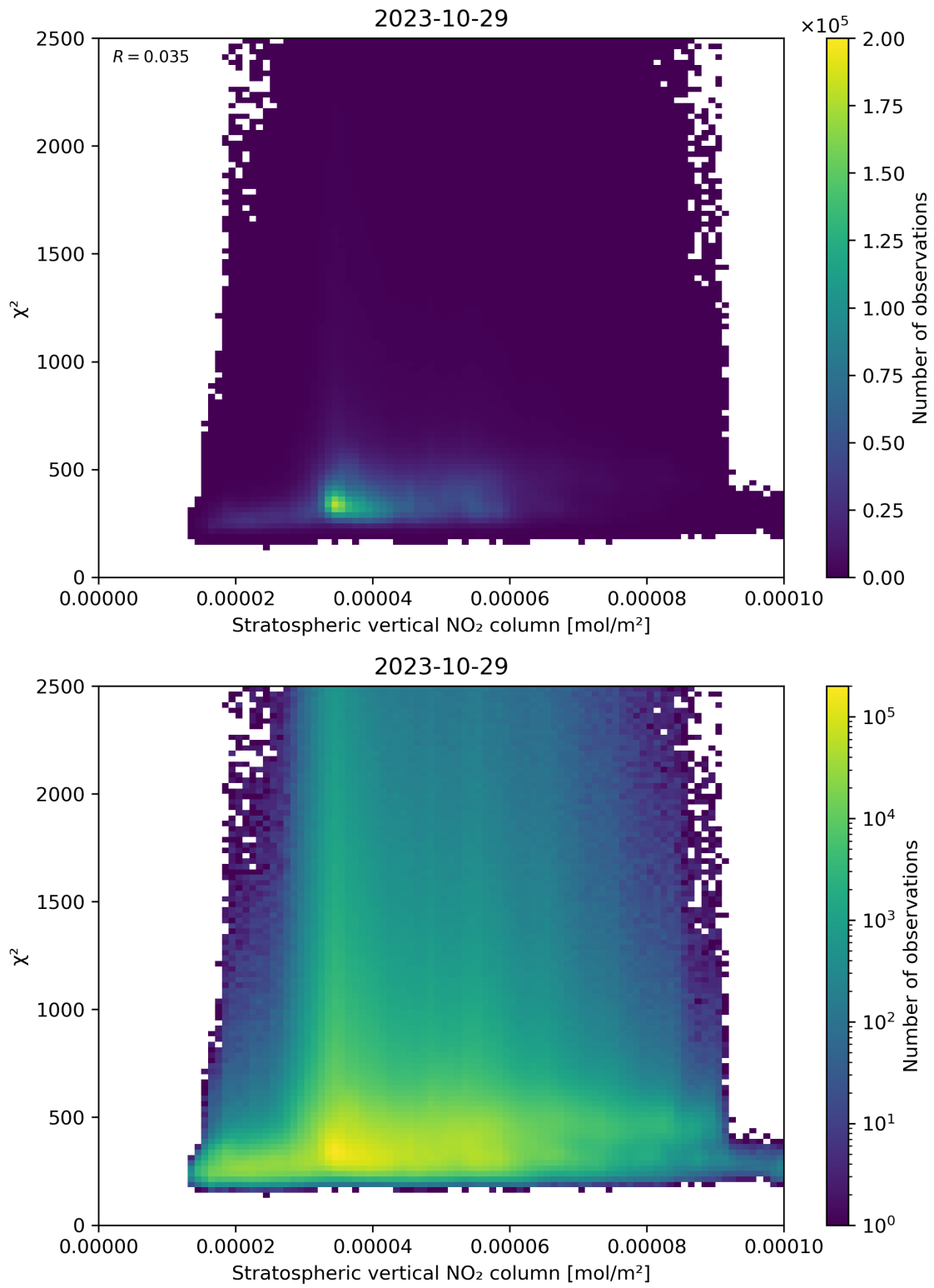
Figure 97: Scatter density plot of “Stratospheric vertical NO 2 column” against “ \chi^2 ” for 2023-10-28 to 2023-10-30.
