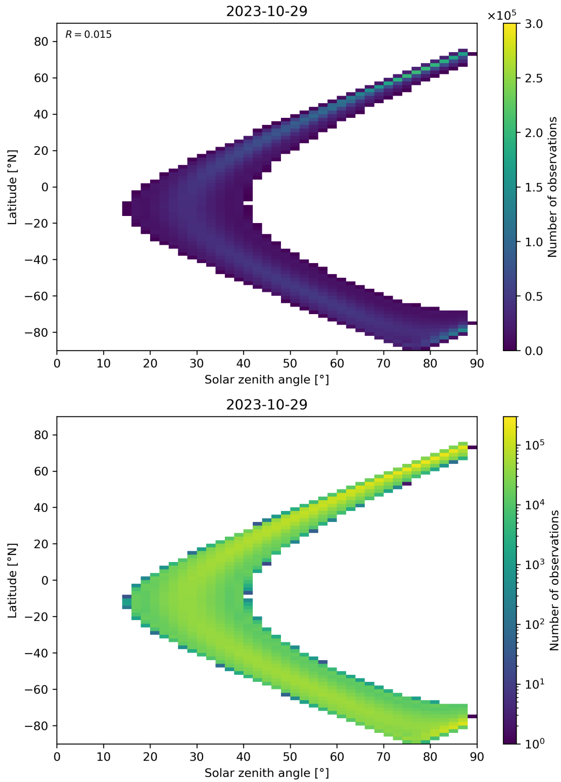
Figure 149: Scatter density plot of “Solar zenith angle” against “Latitude” for 2023-10-28 to 2023-10-30.
