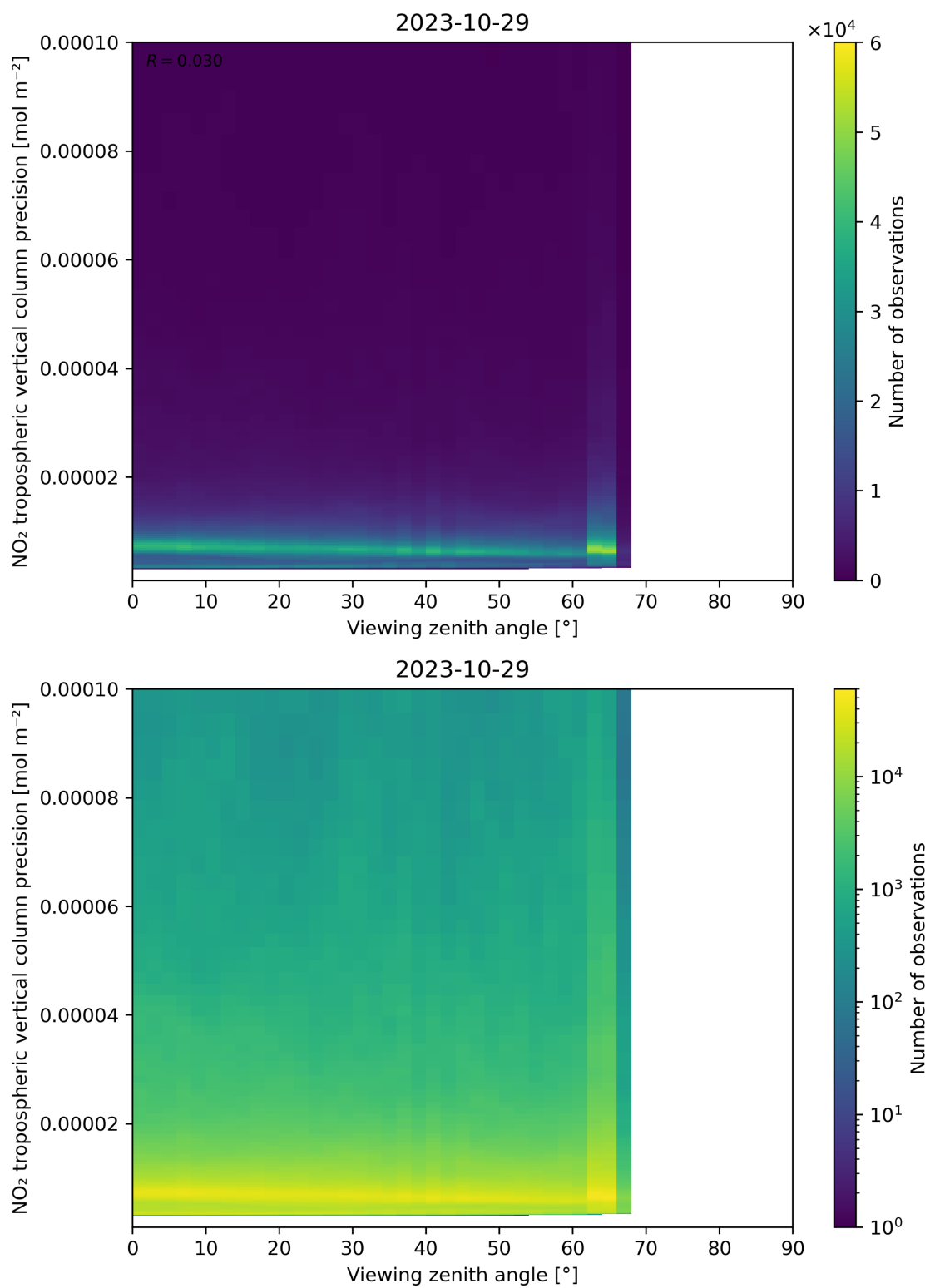
Figure 170: Scatter density plot of “Viewing zenith angle” against “NO 2 tropospheric vertical column precision” for 2023-10-28 to 2023-10-30.
