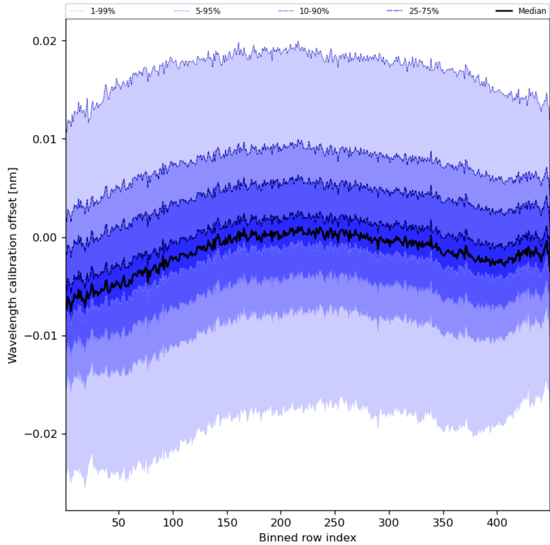
Figure 52: Along track statistics of “Wavelength calibration offset” for 2023-10-28 to 2023-10-30
