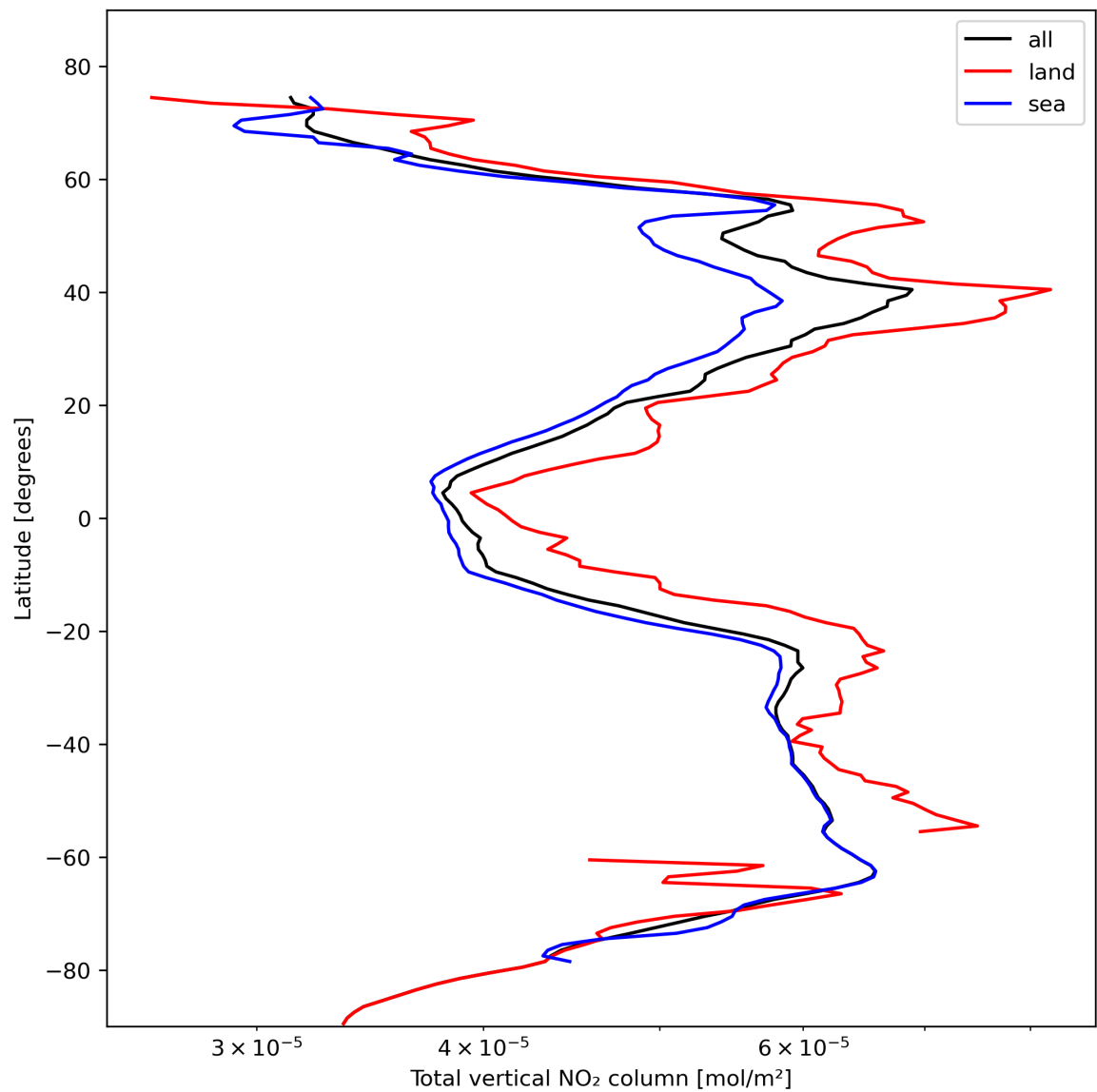
Figure 21: Zonal average of “Total vertical NO 2 column” for 2023-10-28 to 2023-10-30.
