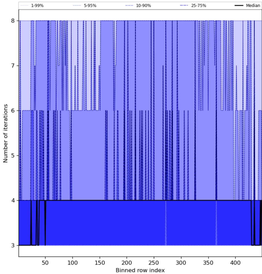
Figure 51: Along track statistics of “Number of iterations” for 2023-10-28 to 2023-10-30
