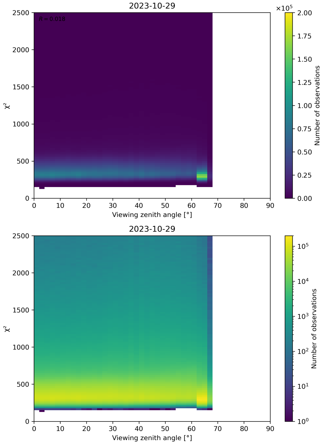
Figure 162: Scatter density plot of “Viewing zenith angle” against “ \chi^2 ” for 2023-10-28 to 2023-10-30.
