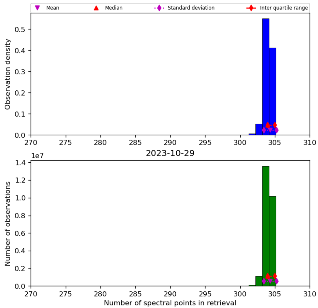
Figure 33: Histogram of “Number of spectral points in retrieval” for 2023-10-28 to 2023-10-30
