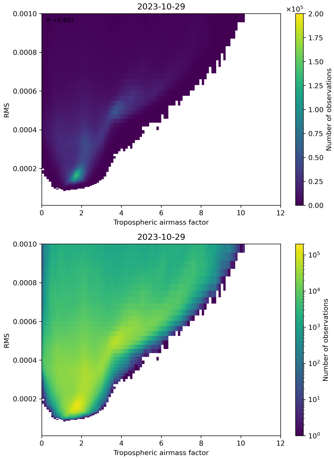
Figure 79: Scatter density plot of “Tropospheric airmass factor” against “RMS” for 2023-10-28 to 2023-10-30.
