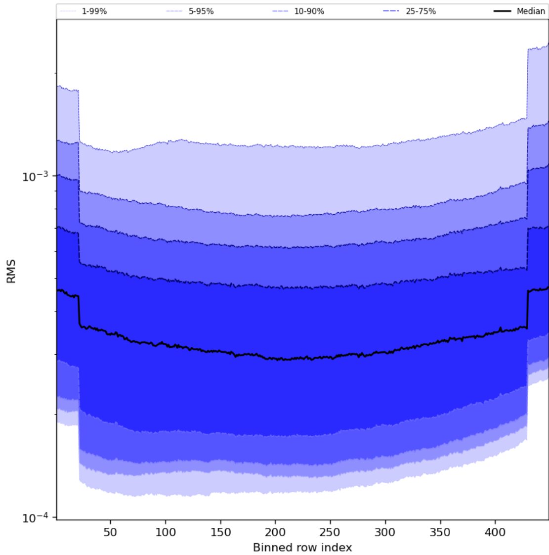
Figure 60: Along track statistics of “RMS” for 2023-10-28 to 2023-10-30
