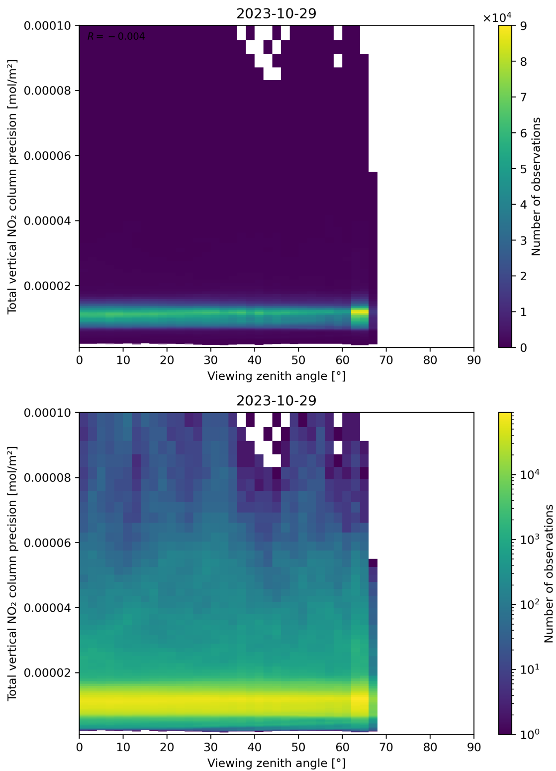
Figure 168: Scatter density plot of “Viewing zenith angle” against “Total vertical NO 2 column precision” for 2023-10-28 to 2023-10-30.
