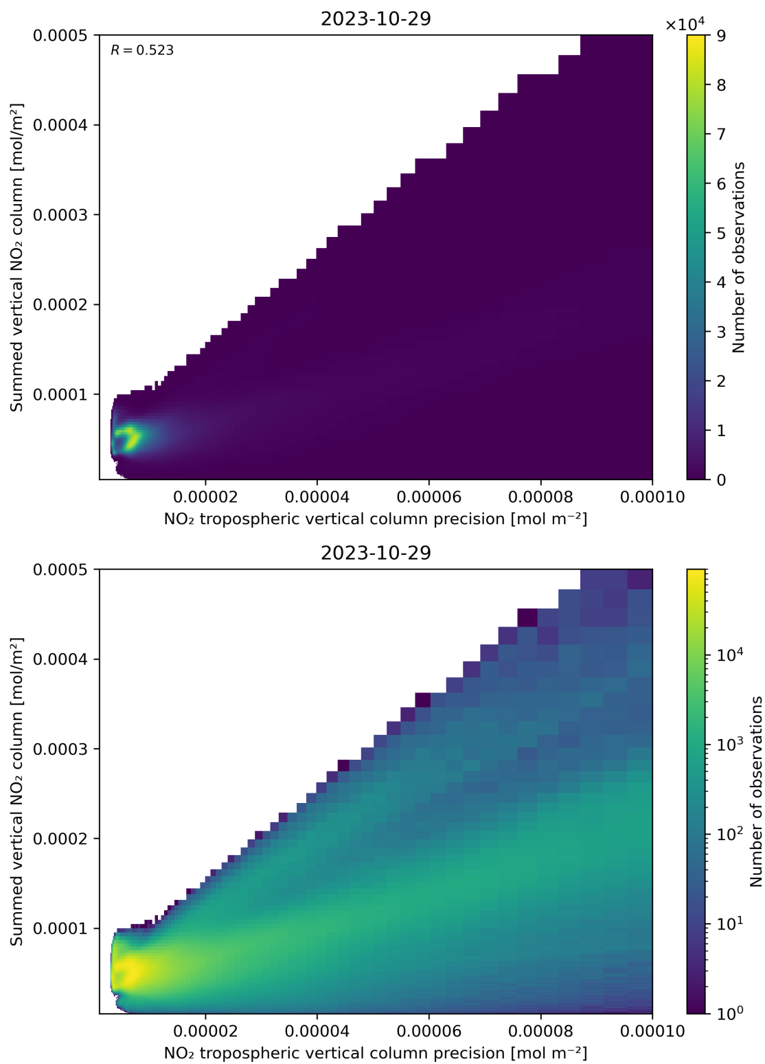
Figure 136: Scatter density plot of “NO 2 tropospheric vertical column precision” against “Summed vertical NO 2 column” for 2023-10-28 to 2023-10-30.
