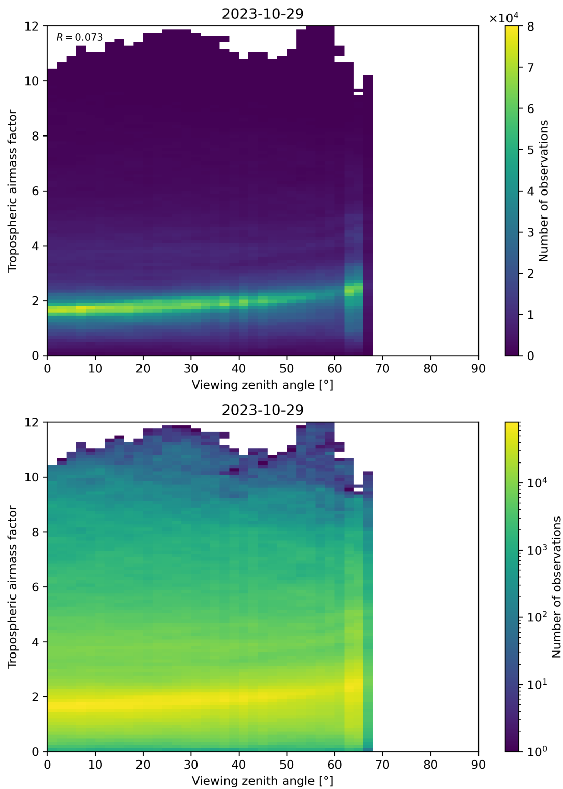
Figure 161: Scatter density plot of “Viewing zenith angle” against “Tropospheric airmass factor” for 2023-10-28 to 2023-10-30.
