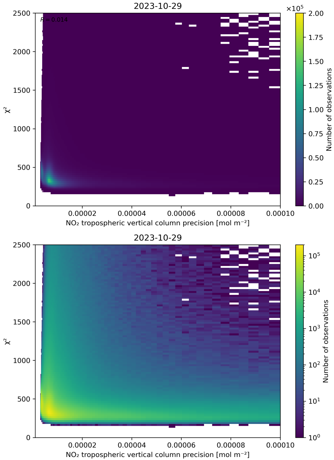
Figure 134: Scatter density plot of “NO 2 tropospheric vertical column precision” against “ \chi^2 ” for 2023-10-28 to 2023-10-30.
