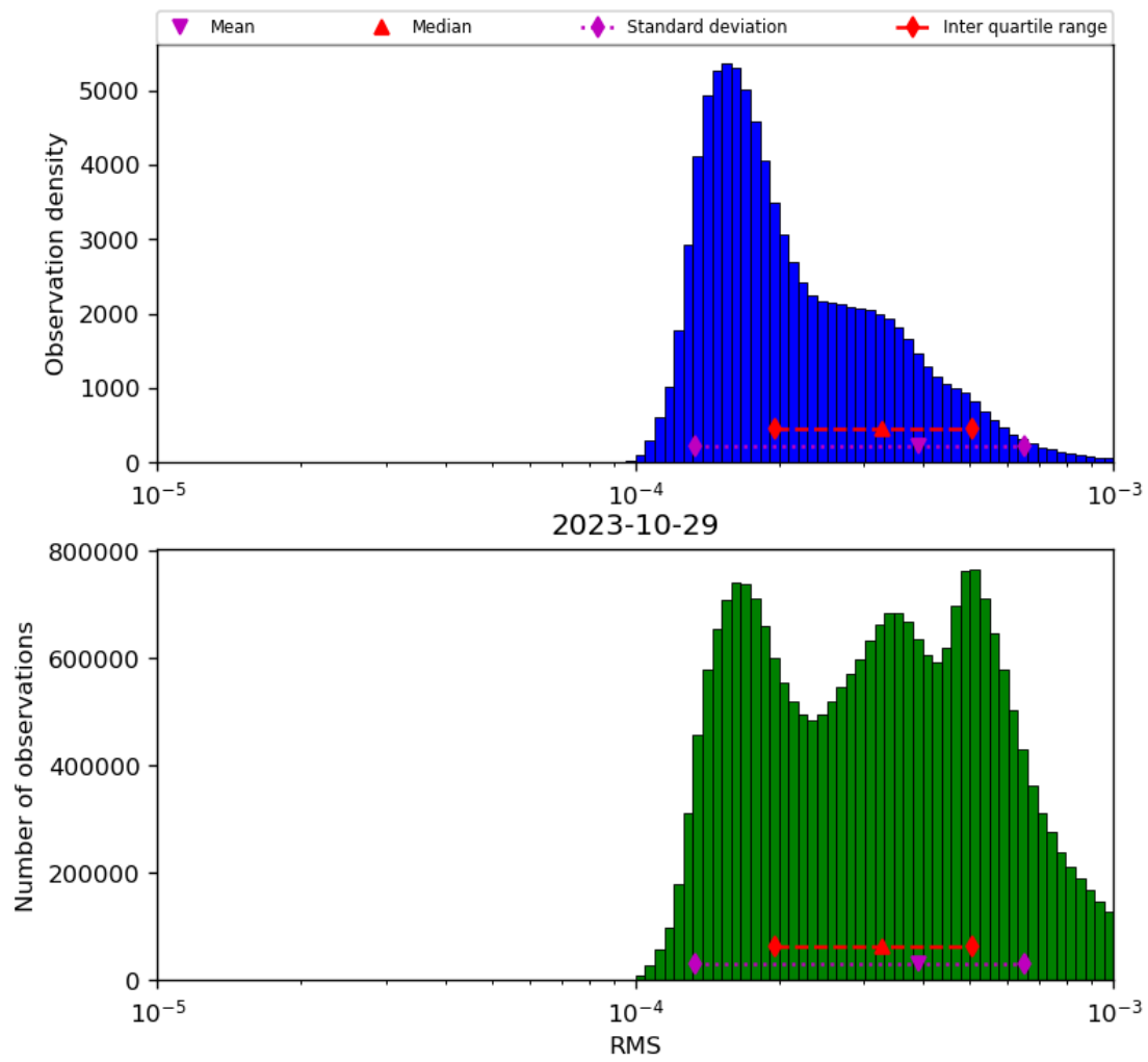
Figure 43: Histogram of “RMS” for 2023-10-28 to 2023-10-30
