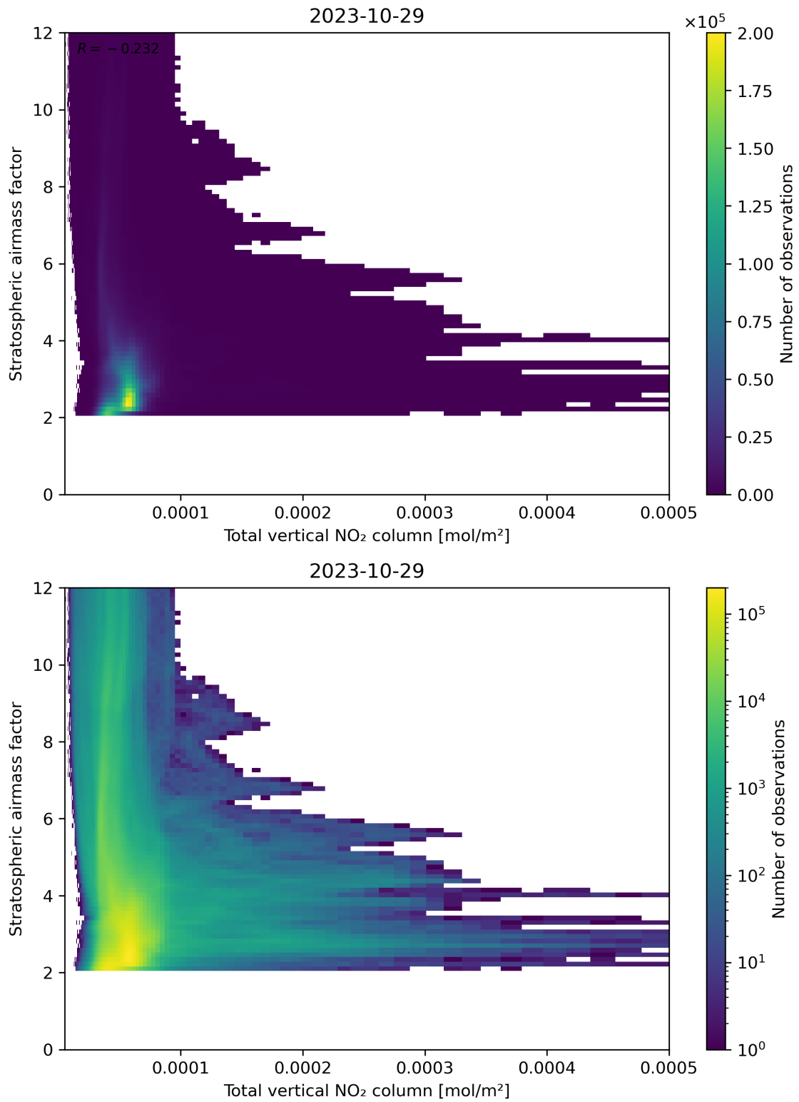
Figure 110: Scatter density plot of “Total vertical NO 2 column” against “Stratospheric airmass factor” for 2023-10-28 to 2023-10-30.
