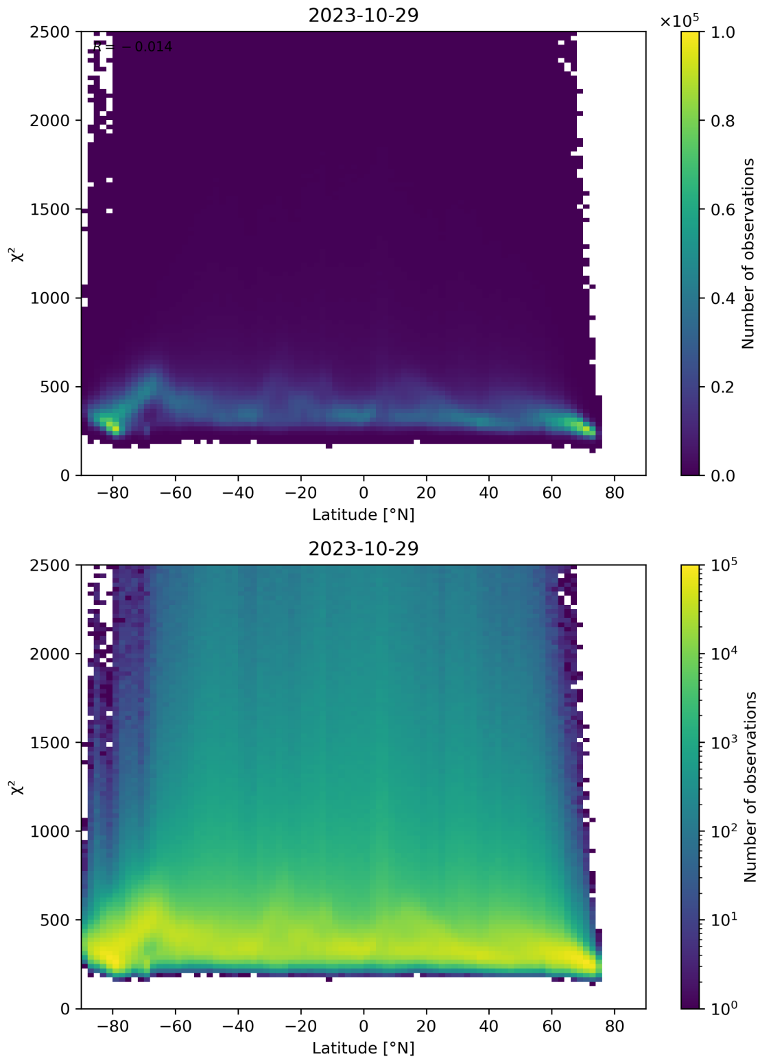
Figure 86: Scatter density plot of “Latitude” against “ \chi^2 ” for 2023-10-28 to 2023-10-30.
