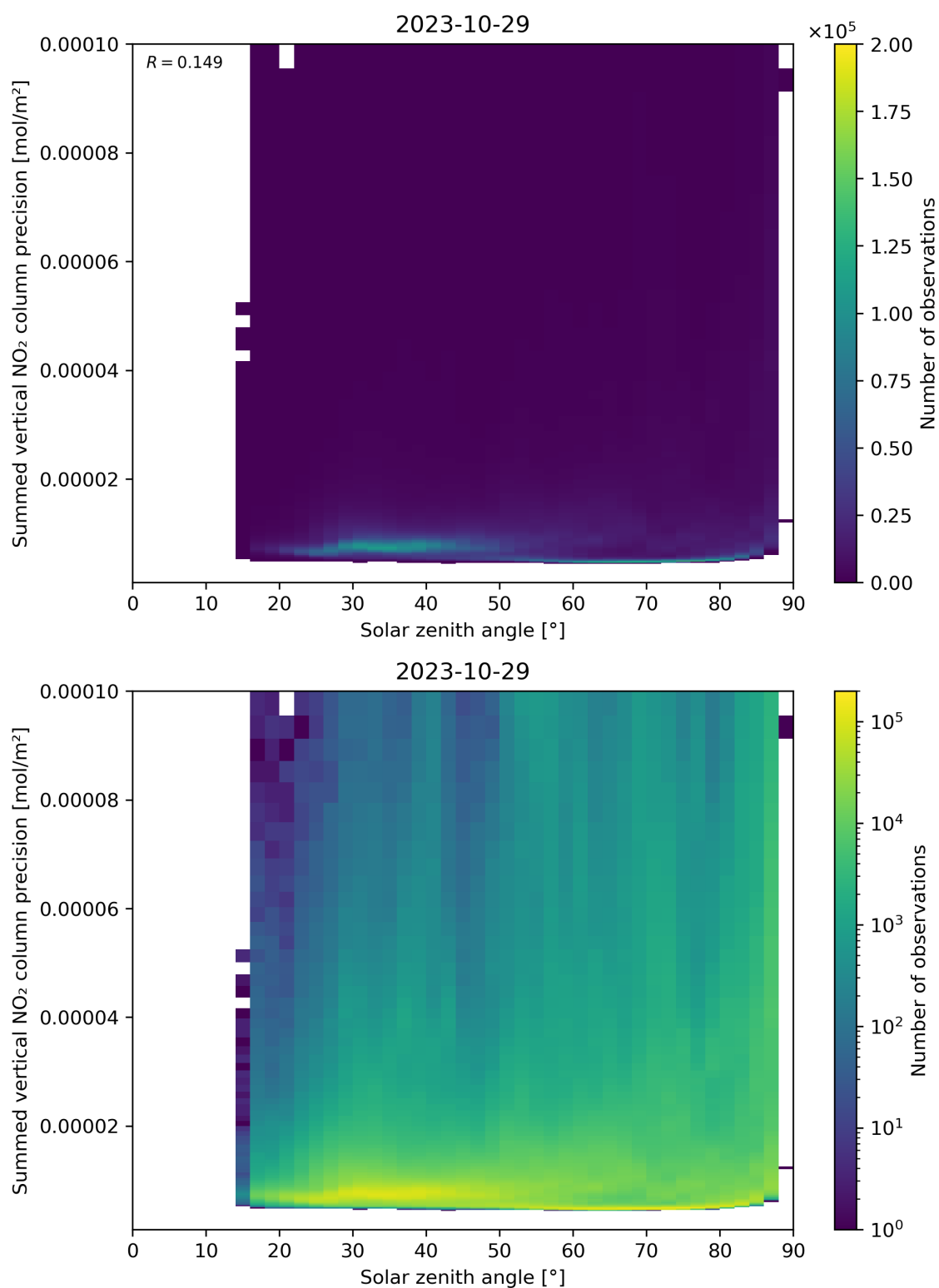
Figure 152: Scatter density plot of “Solar zenith angle” against “Summed vertical NO 2 column precision” for 2023-10-28 to 2023-10-30.
