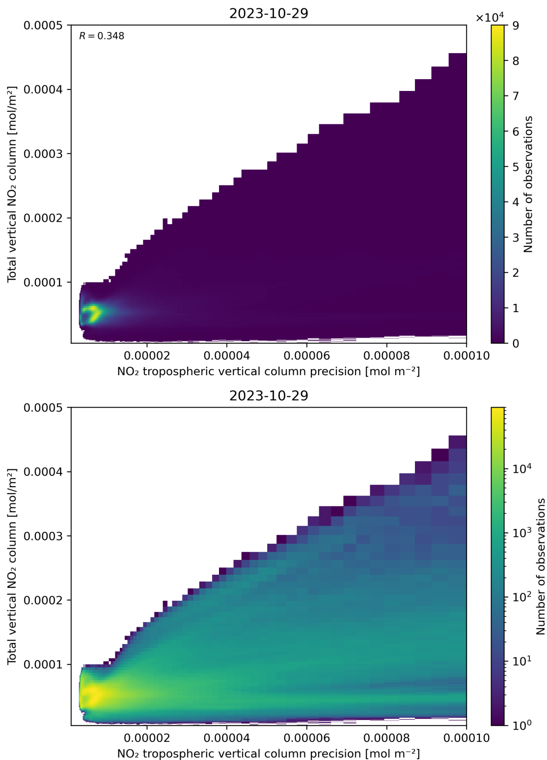
Figure 138: Scatter density plot of “NO 2 tropospheric vertical column precision” against “Total vertical NO 2 column” for 2023-10-28 to 2023-10-30.
