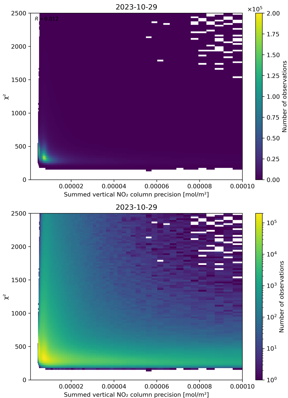
Figure 107: Scatter density plot of “Summed vertical NO 2 column precision” against “ \chi^2 ” for 2023-10-28 to 2023-10-30.
