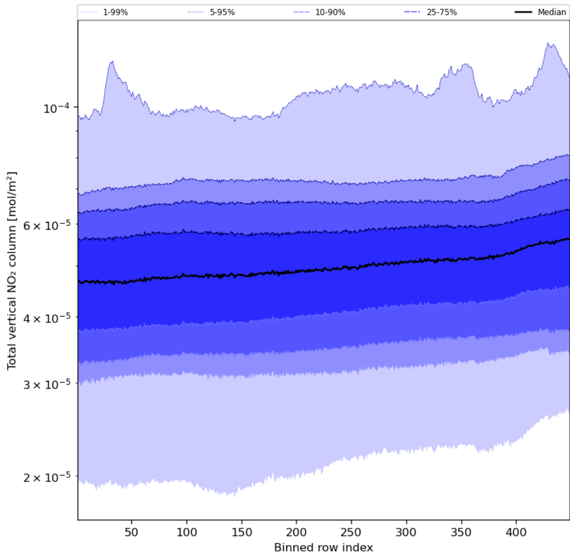
Figure 55: Along track statistics of “Total vertical NO 2 column” for 2023-10-28 to 2023-10-30
