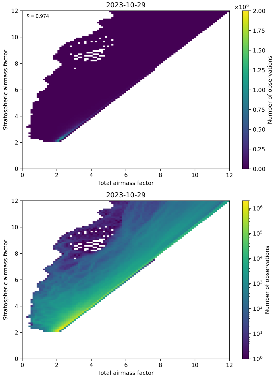
Figure 62: Scatter density plot of “Total airmass factor” against “Stratospheric airmass factor” for 2023-10-28 to 2023-10-30.
