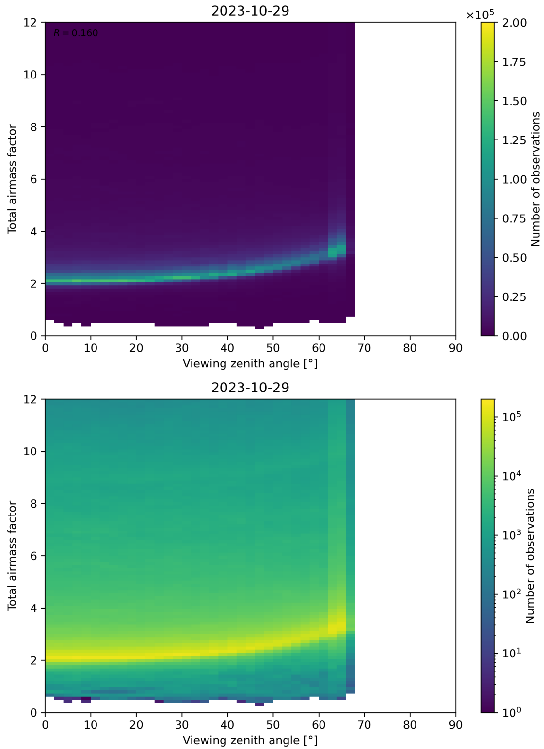
Figure 160: Scatter density plot of “Viewing zenith angle” against “Total airmass factor” for 2023-10-28 to 2023-10-30.
