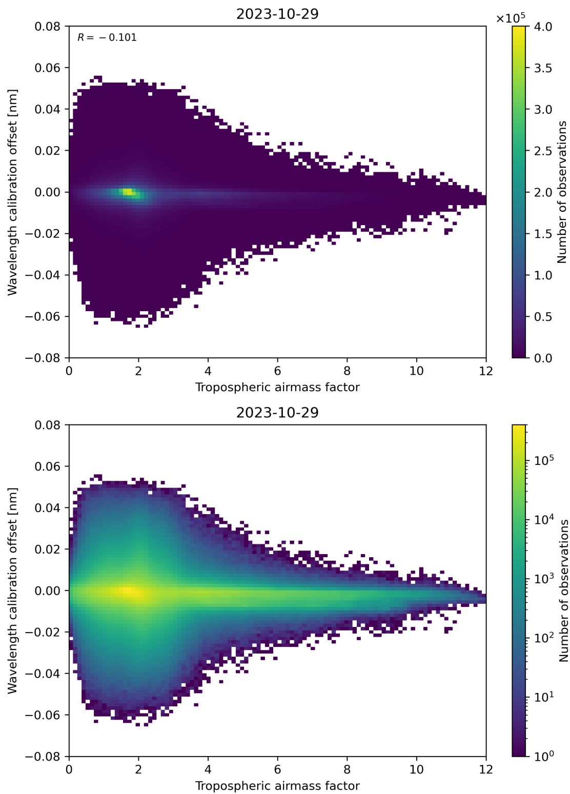
Figure 80: Scatter density plot of “Tropospheric airmass factor” against “Wavelength calibration offset” for 2023-10-28 to 2023-10-30.
