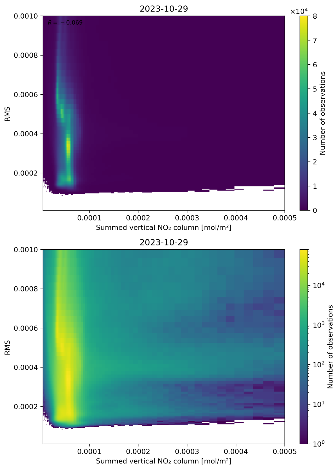
Figure 109: Scatter density plot of “Summed vertical NO 2 column” against “RMS” for 2023-10-28 to 2023-10-30.
