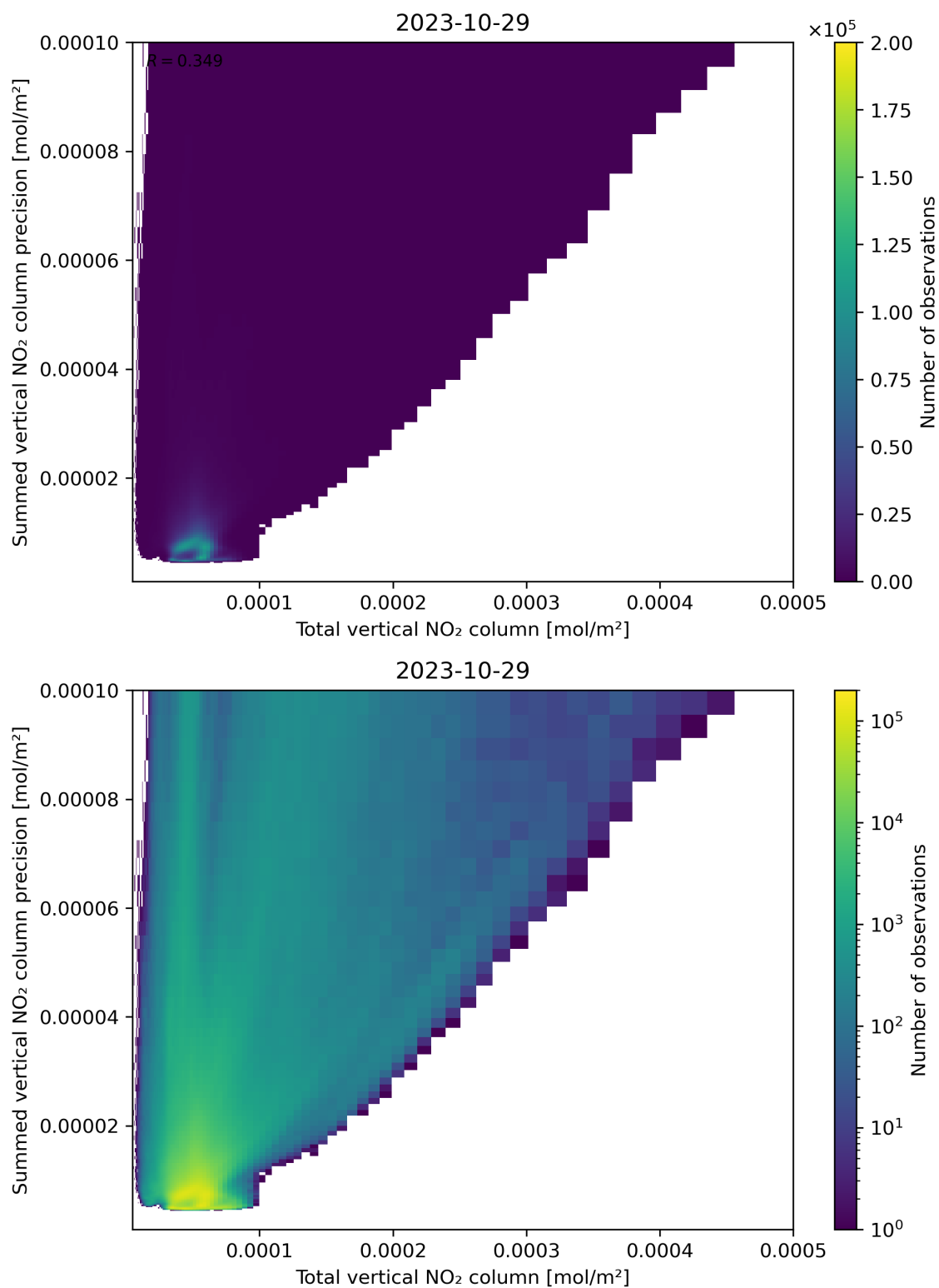
Figure 113: Scatter density plot of “Total vertical NO 2 column” against “Summed vertical NO 2 column precision” for 2023-10-28 to 2023-10-30.
