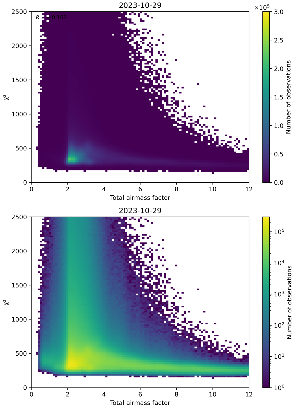
Figure 63: Scatter density plot of “Total airmass factor” against “ \chi^2 ” for 2023-10-28 to 2023-10-30.
