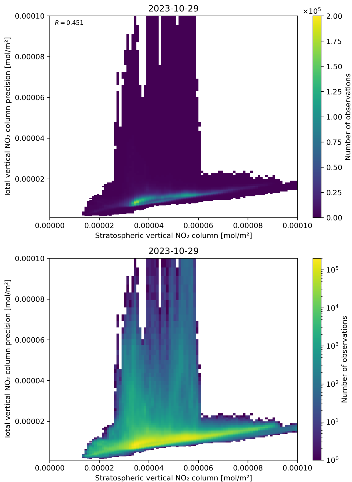
Figure 101: Scatter density plot of “Stratospheric vertical NO 2 column” against “Total vertical NO 2 column precision” for 2023-10-28 to 2023-10-30.
