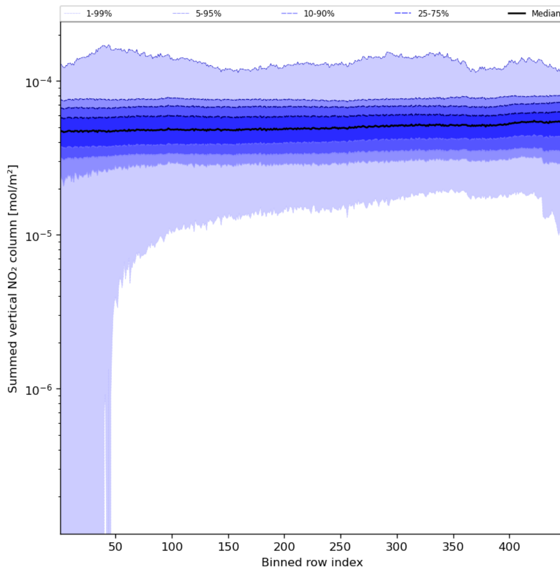
Figure 57: Along track statistics of “Summed vertical NO 2 column” for 2023-10-28 to 2023-10-30
