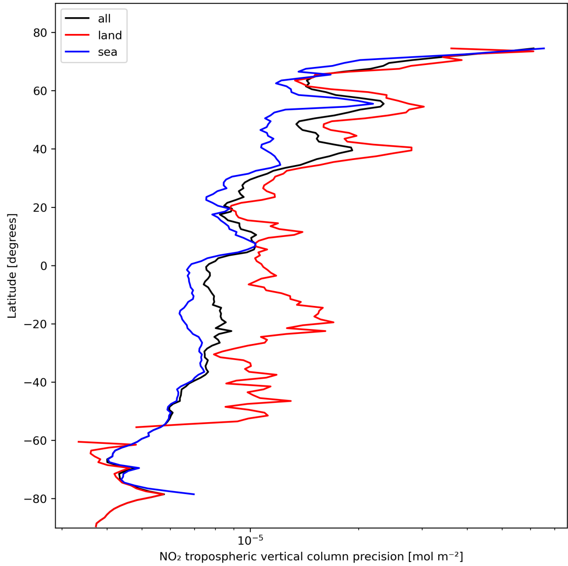
Figure 13: Zonal average of “NO 2 tropospheric vertical column precision” for 2023-10-28 to 2023-10-30.
