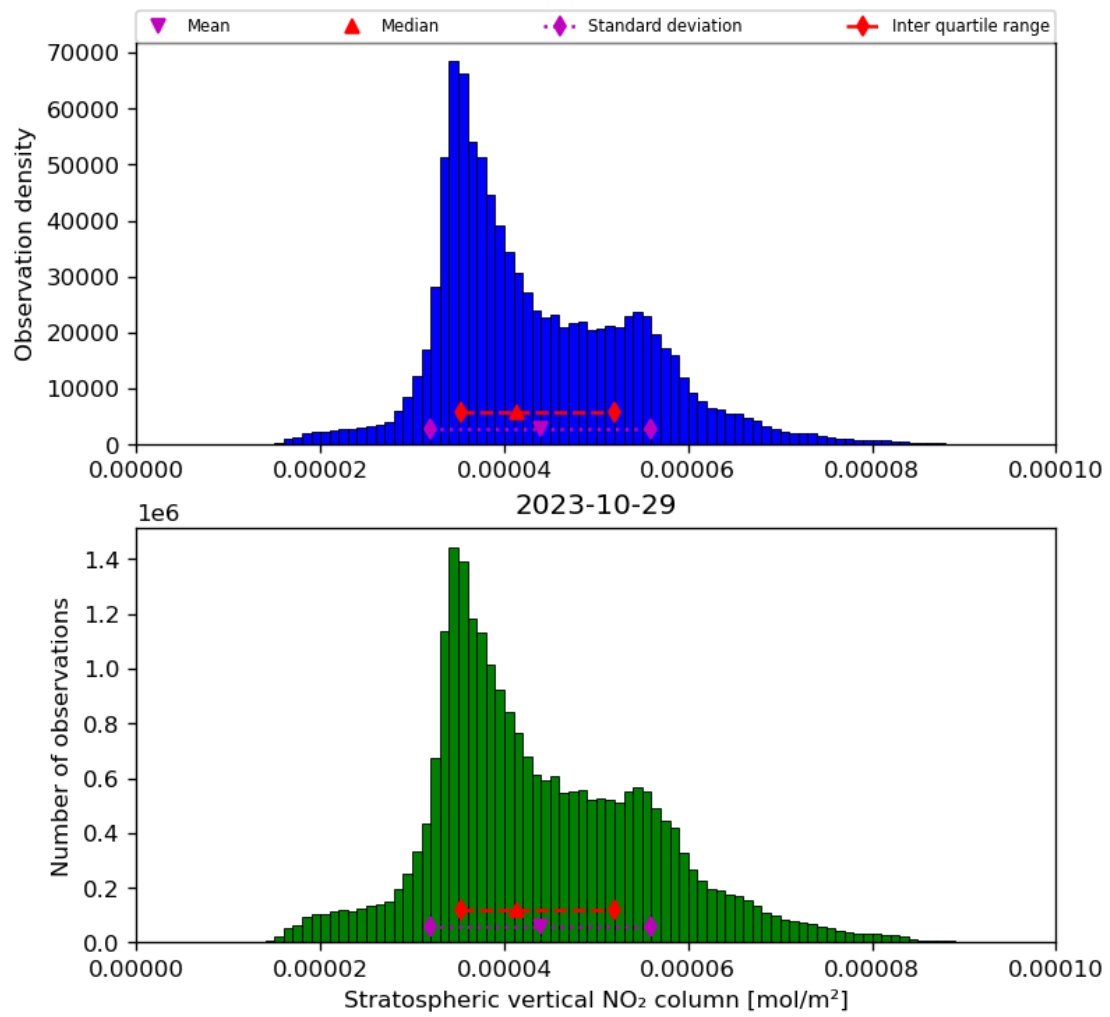
Figure 36: Histogram of “Stratospheric vertical NO 2 column” for 2023-10-28 to 2023-10-30
