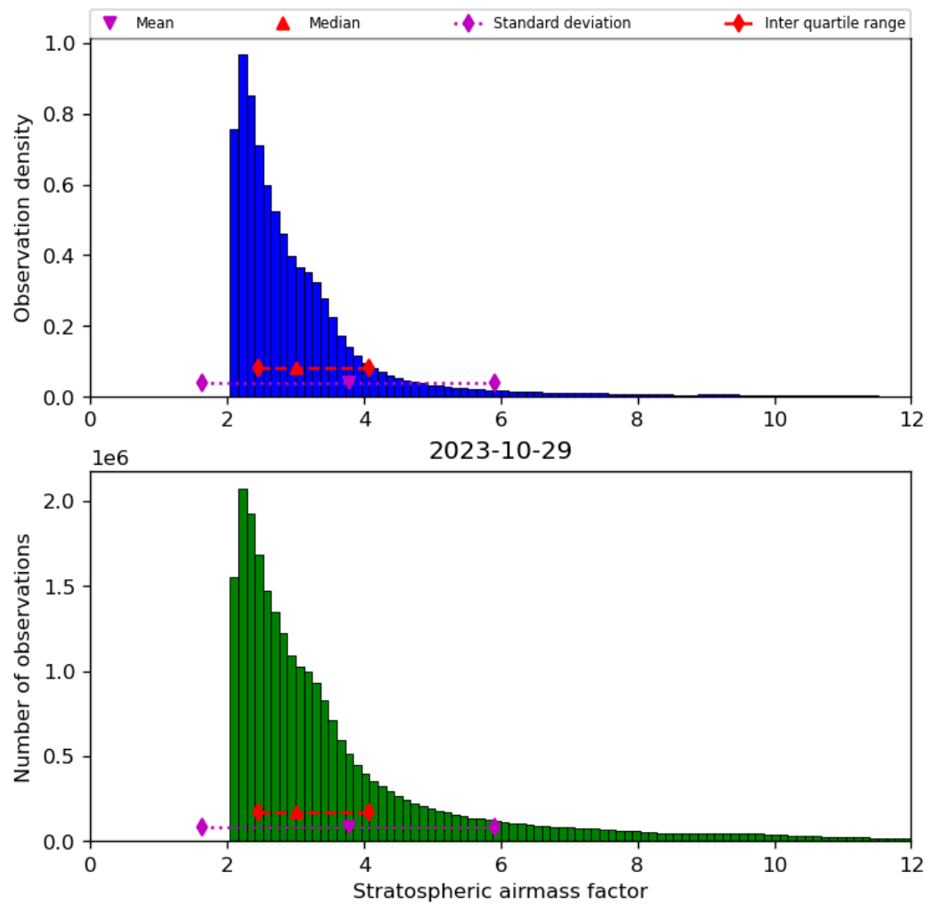
Figure 44: Histogram of “Stratospheric airmass factor” for 2023-10-28 to 2023-10-30
