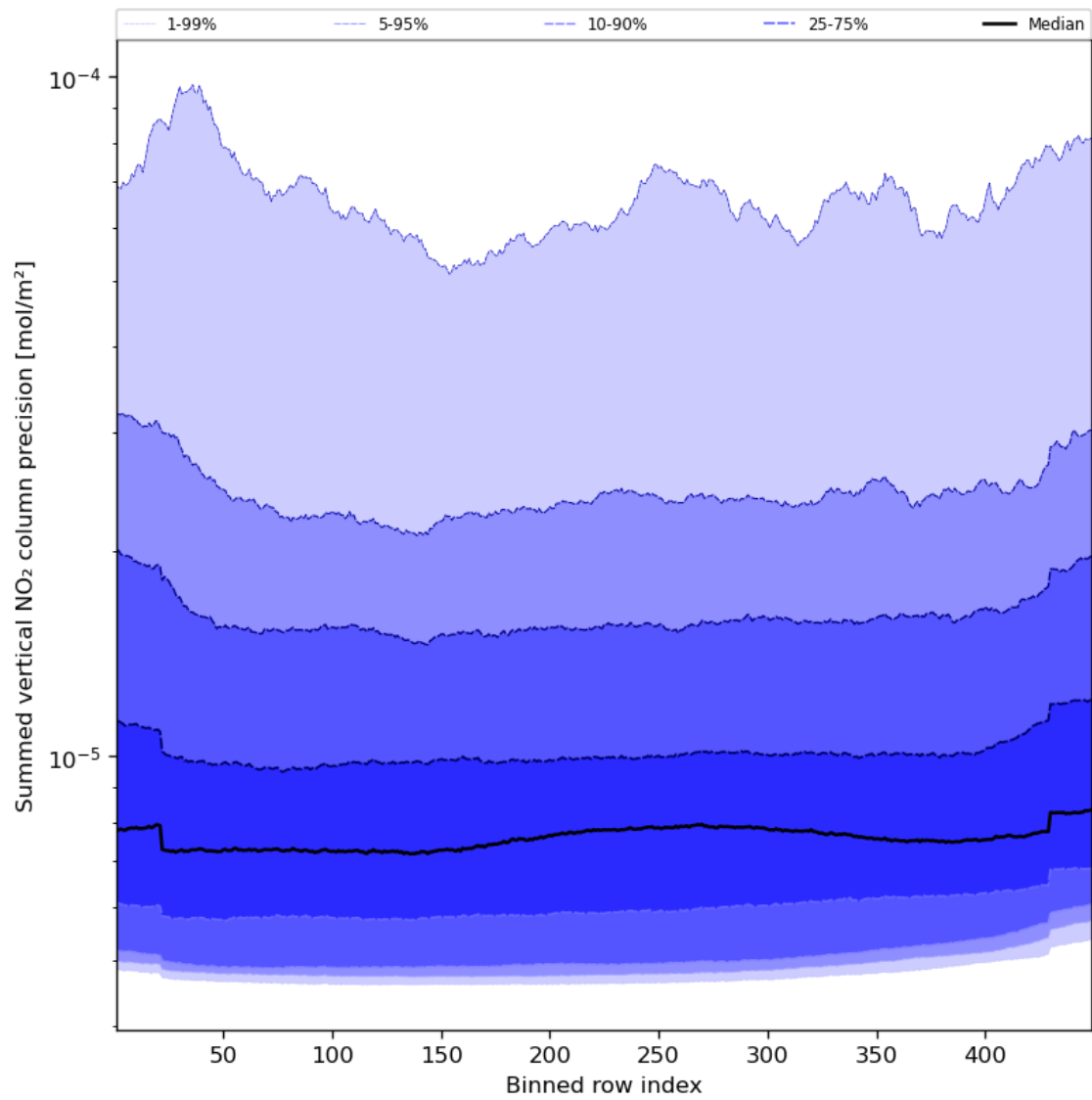
Figure 58: Along track statistics of “Summed vertical NO 2 column precision” for 2023-10-28 to 2023-10-30
