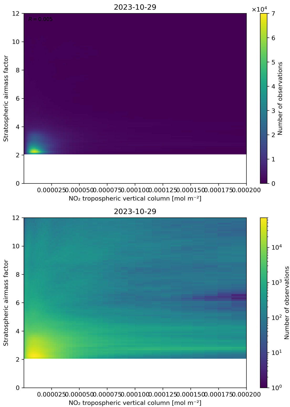
Figure 121: Scatter density plot of “NO 2 tropospheric vertical column” against “Stratospheric airmass factor” for 2023-10-28 to 2023-10-30.
