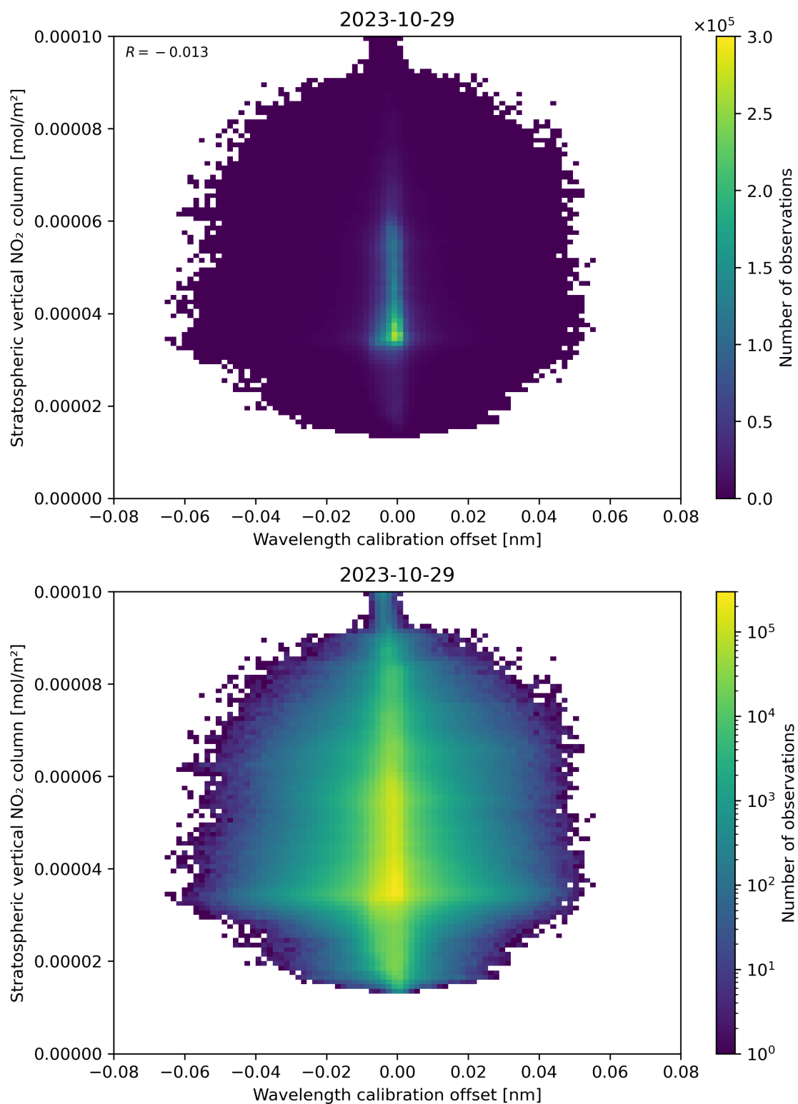
Figure 176: Scatter density plot of “Wavelength calibration offset” against “Stratospheric vertical NO 2 column” for 2023-10-28 to 2023-10-30.
