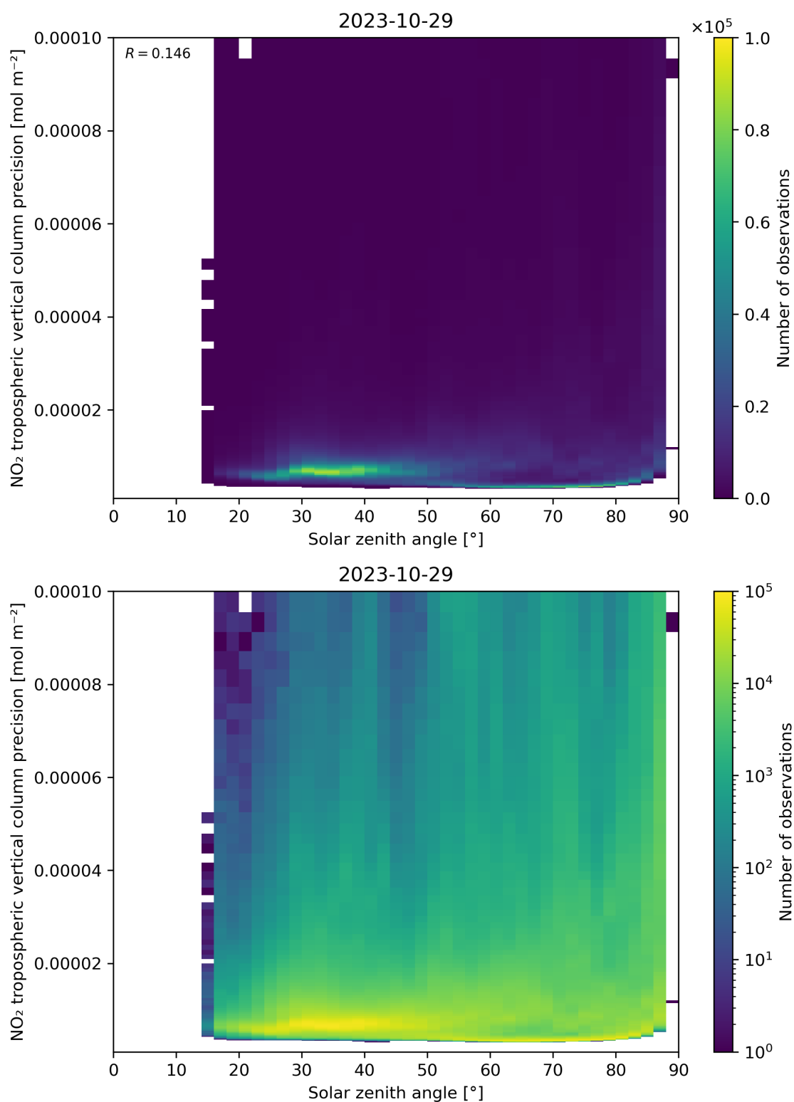
Figure 156: Scatter density plot of “Solar zenith angle” against “NO 2 tropospheric vertical column precision” for 2023-10-28 to 2023-10-30.
