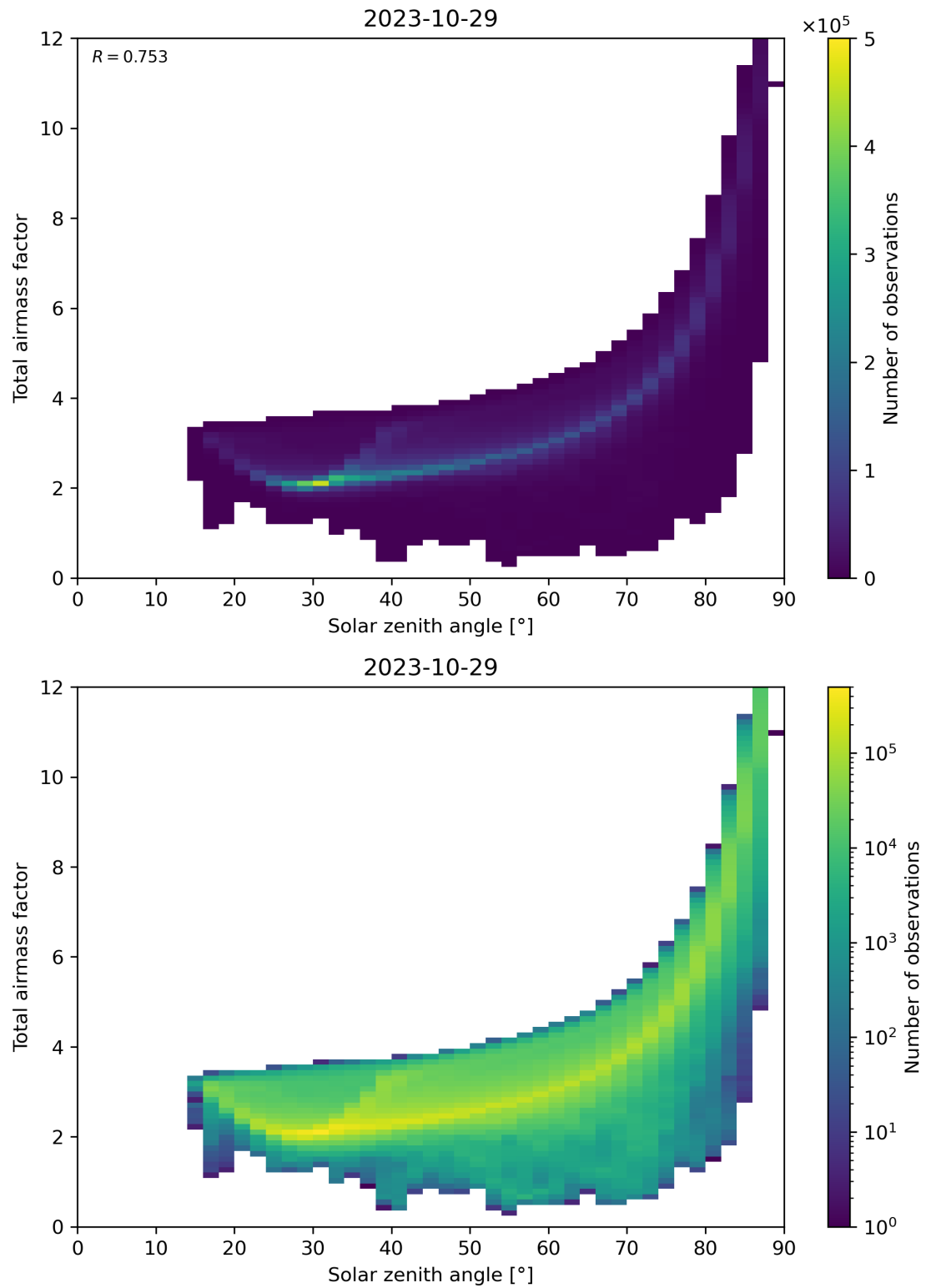
Figure 146: Scatter density plot of “Solar zenith angle” against “Total air mass factor” for 2023-10-28 to 2023-10-30.
