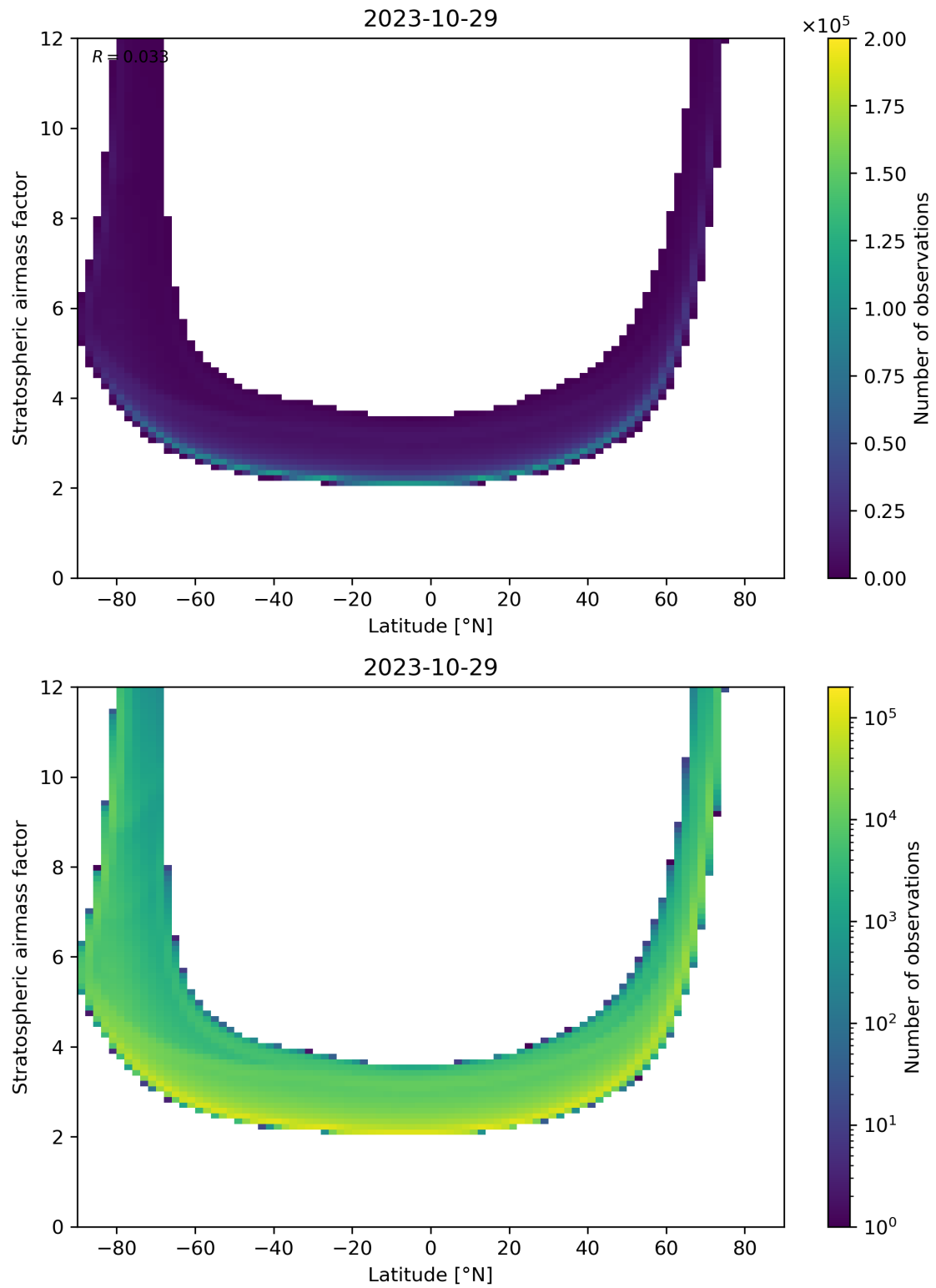
Figure 83: Scatter density plot of “Latitude” against “Stratospheric air mass factor” for 2023-10-28 to 2023-10-30.
