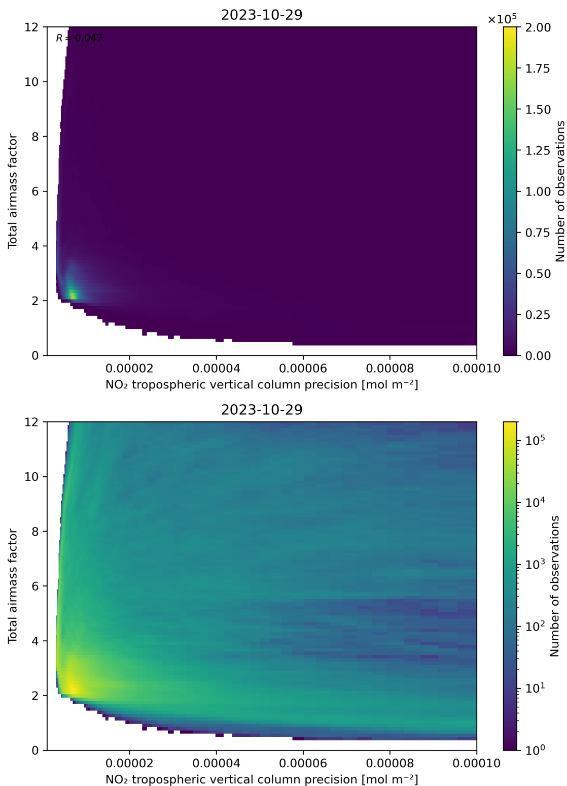
Figure 132: Scatter density plot of “NO 2 tropospheric vertical column precision” against “Total air mass factor” for 2023-10-28 to 2023-10-30.
