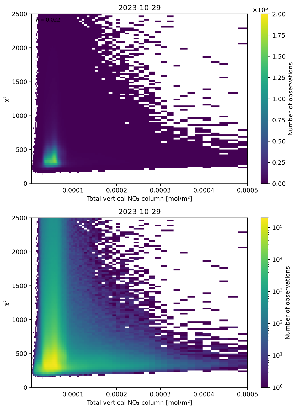
Figure 111: Scatter density plot of “Total vertical NO 2 column” against “ \chi^2 ” for 2023-10-28 to 2023-10-30.
