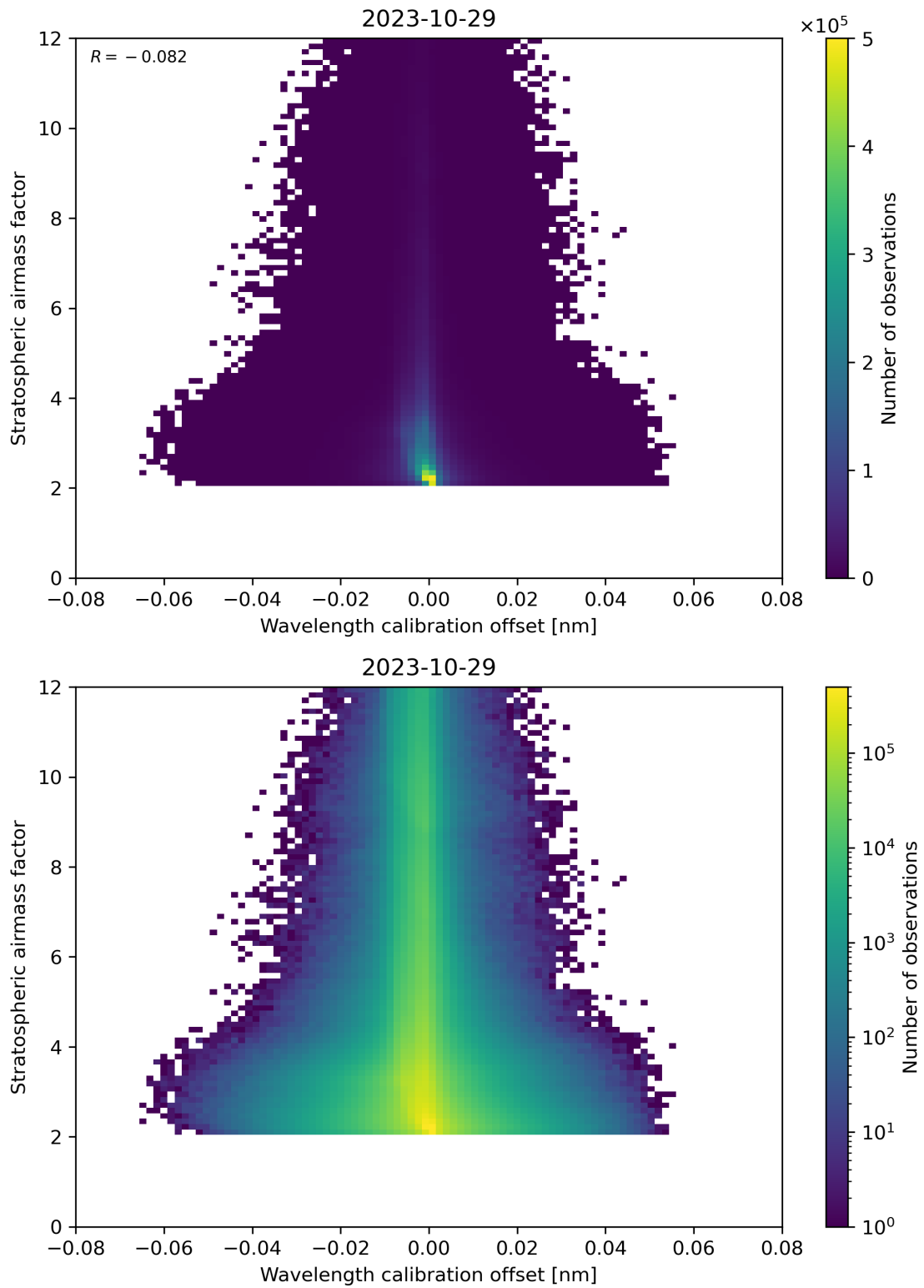
Figure 174: Scatter density plot of “Wavelength calibration offset” against “Stratospheric airmass factor” for 2023-10-28 to 2023-10-30.
