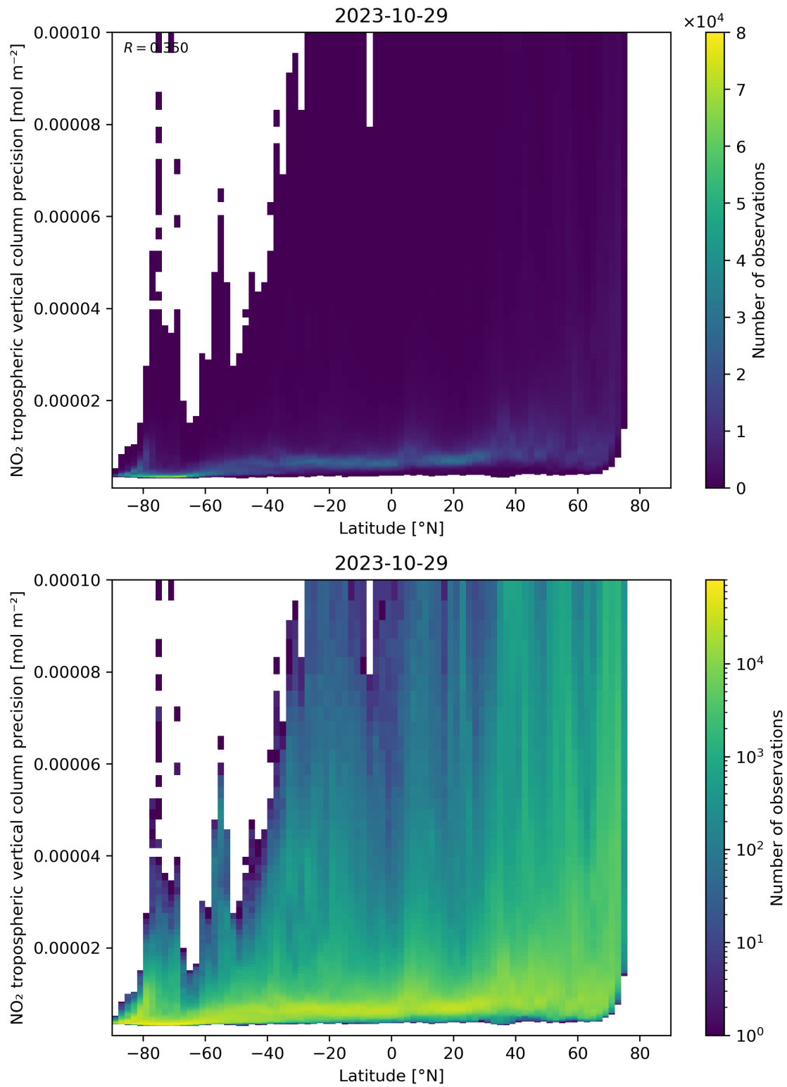
Figure 93: Scatter density plot of “Latitude” against “NO 2 tropospheric vertical column precision” for 2023-10-28 to 2023-10-30.
