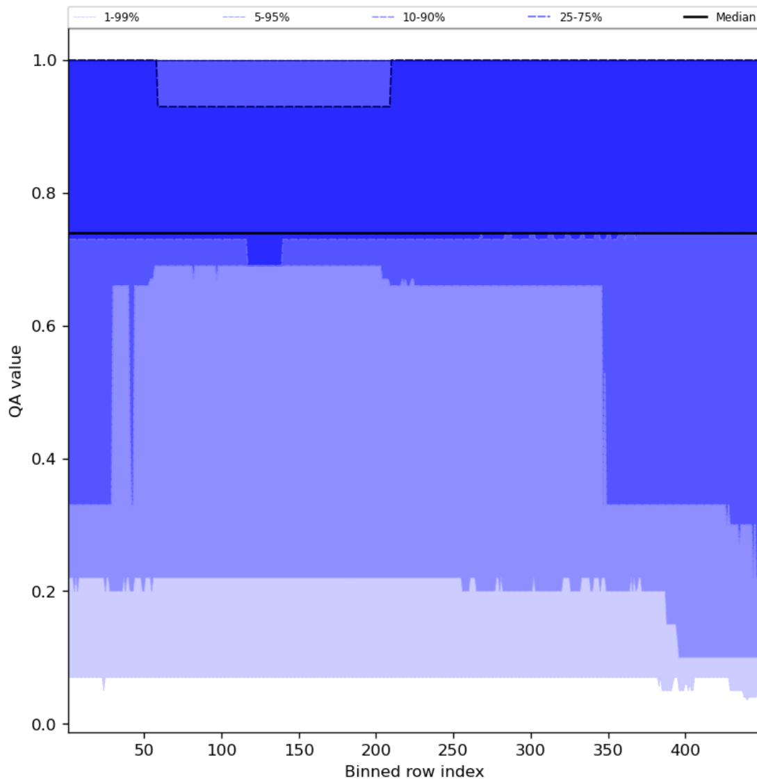
Figure 45: Along track statistics of “QA value” for 2023-10-28 to 2023-10-30
