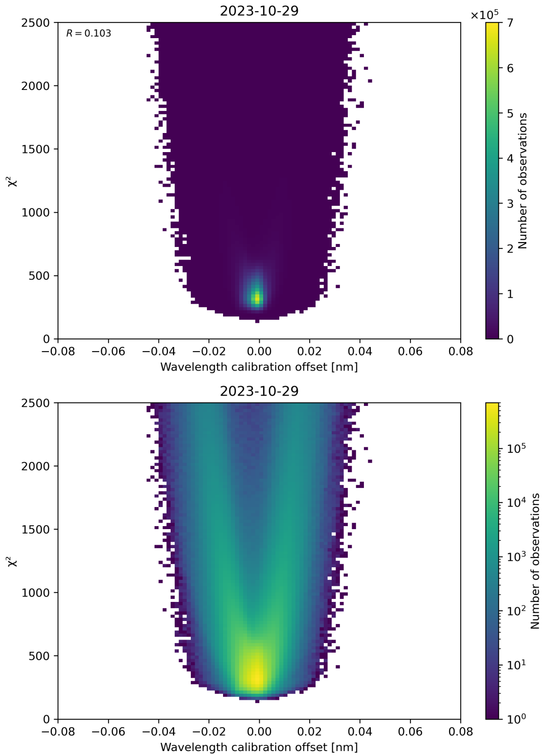
Figure 175: Scatter density plot of “Wavelength calibration offset” against “ \chi^2 ” for 2023-10-28 to 2023-10-30.
