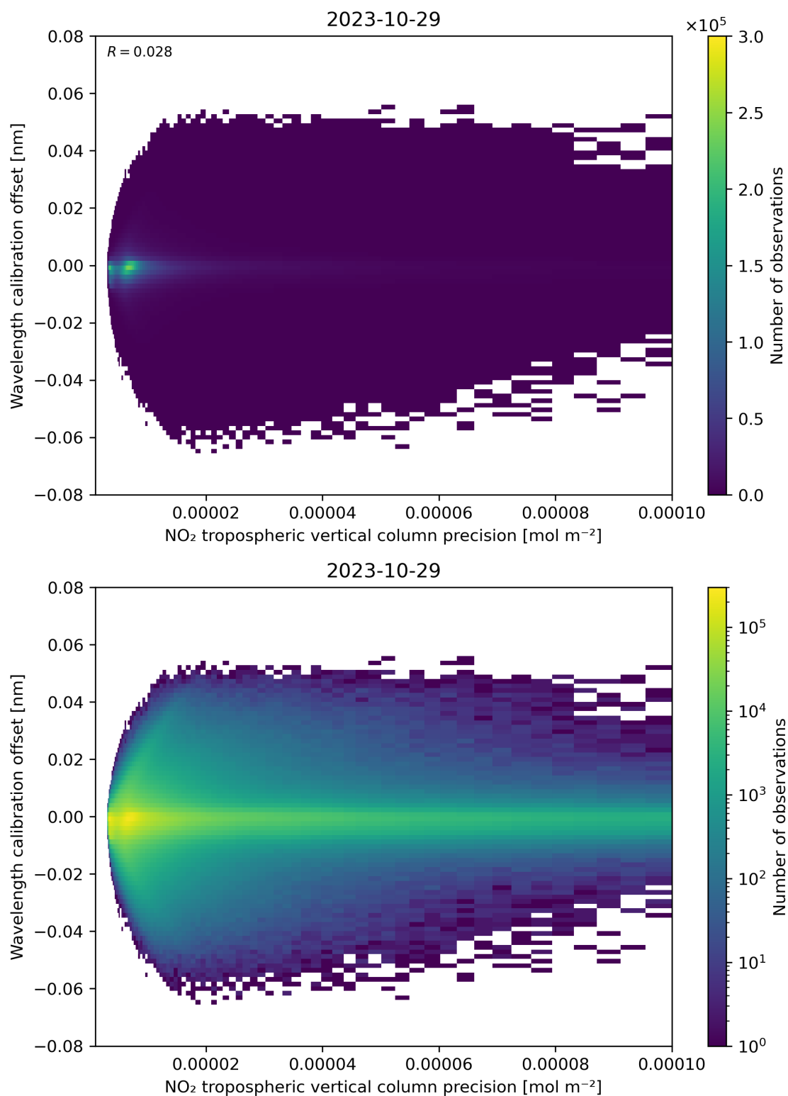
Figure 141: Scatter density plot of “NO 2 tropospheric vertical column precision” against “Wavelength calibration offset” for 2023-10-28 to 2023-10-30.
