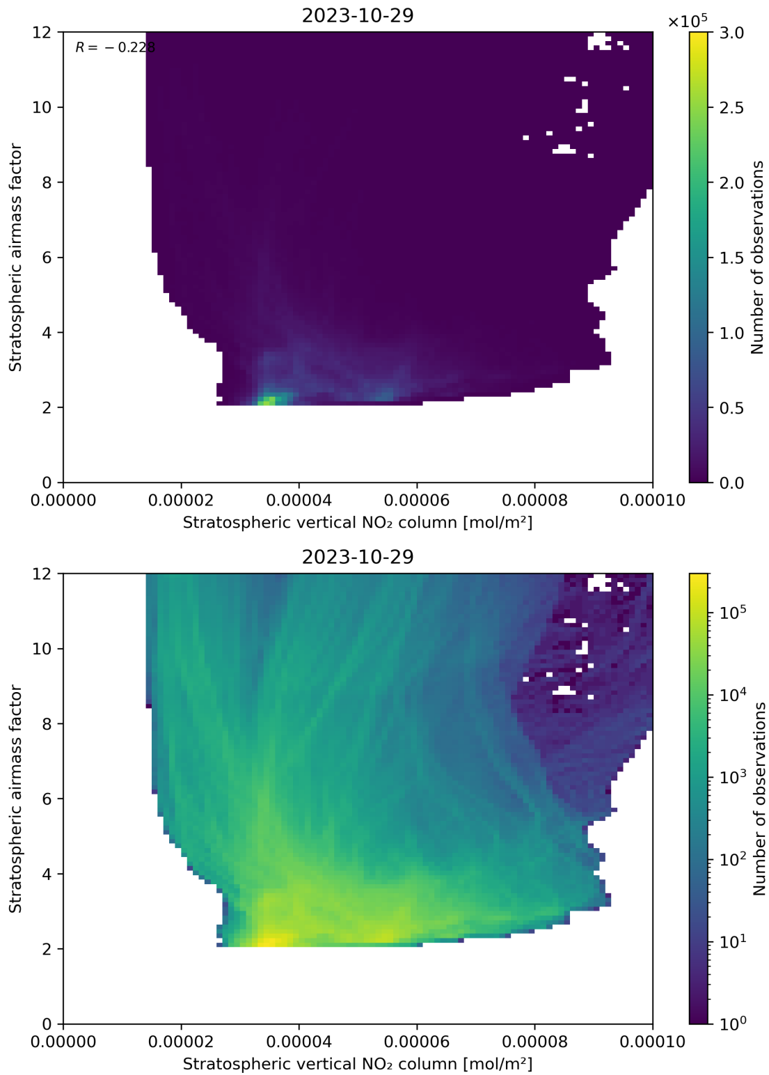
Figure 96: Scatter density plot of “Stratospheric vertical NO 2 column” against “Stratospheric airmass factor” for 2023-10-28 to 2023-10-30.
