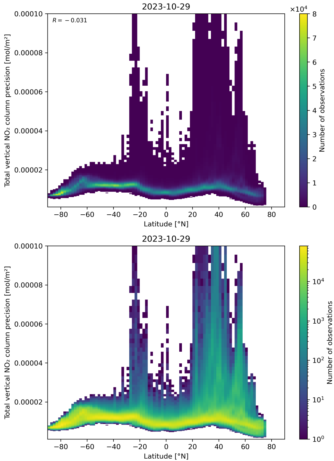
Figure 91: Scatter density plot of “Latitude” against “Total vertical NO 2 column precision” for 2023-10-28 to 2023-10-30.
