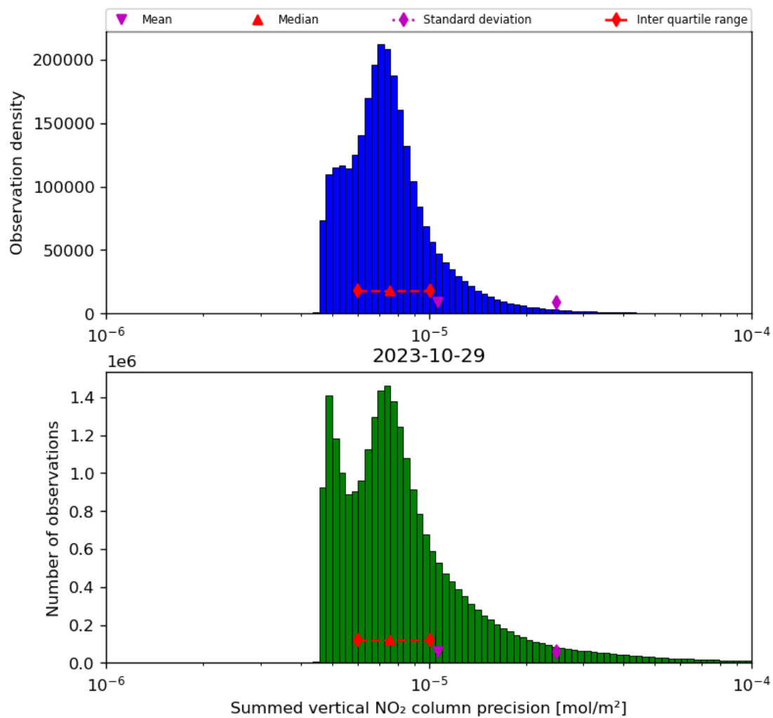
Figure 41: Histogram of "Summed vertical NO 2 column precision" for 2023-10-28 to 2023-10-30
