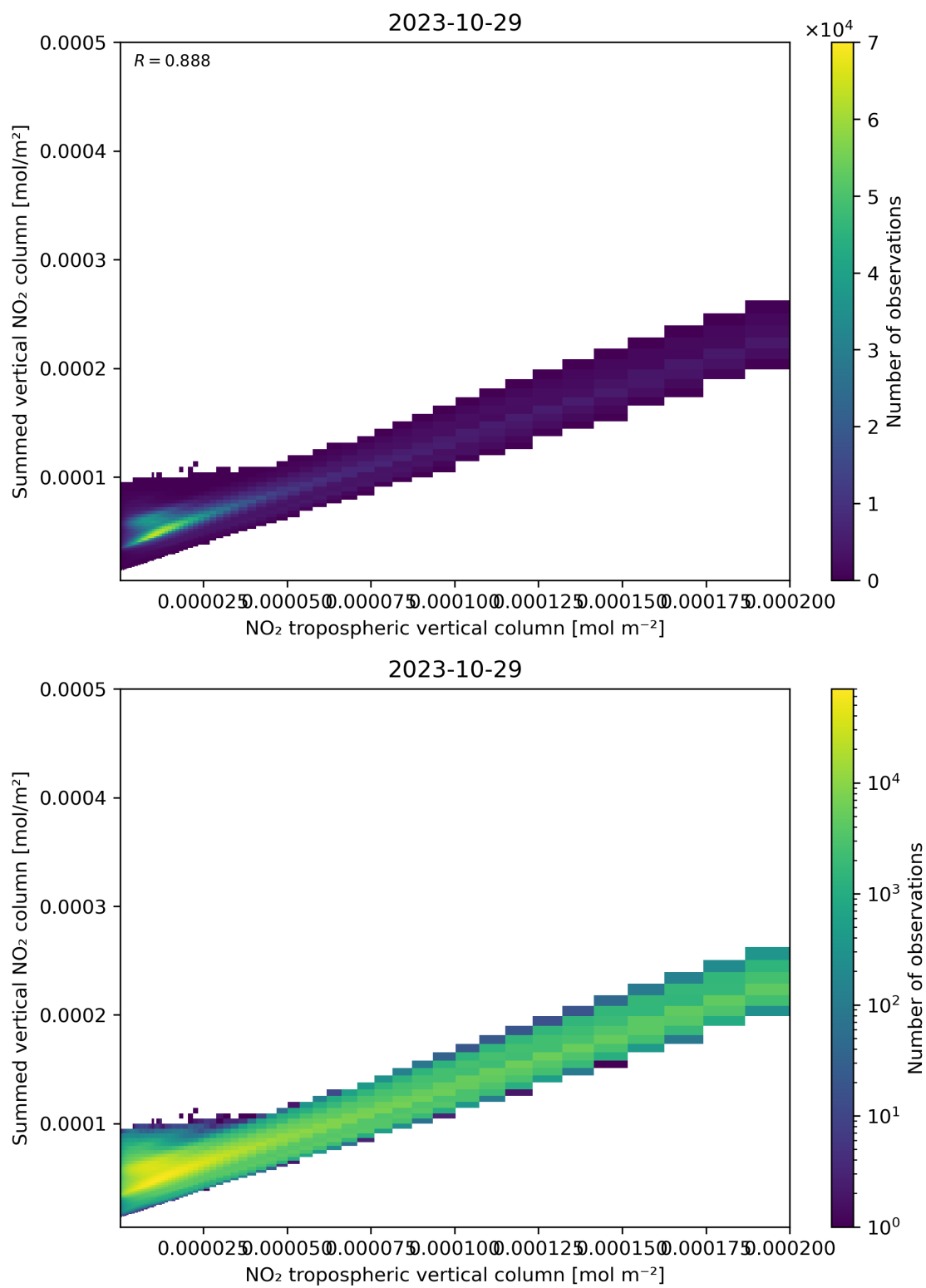
Figure 126: Scatter density plot of “NO 2 tropospheric vertical column” against “Summed vertical NO 2 column” for 2023-10-28 to 2023-10-30.
