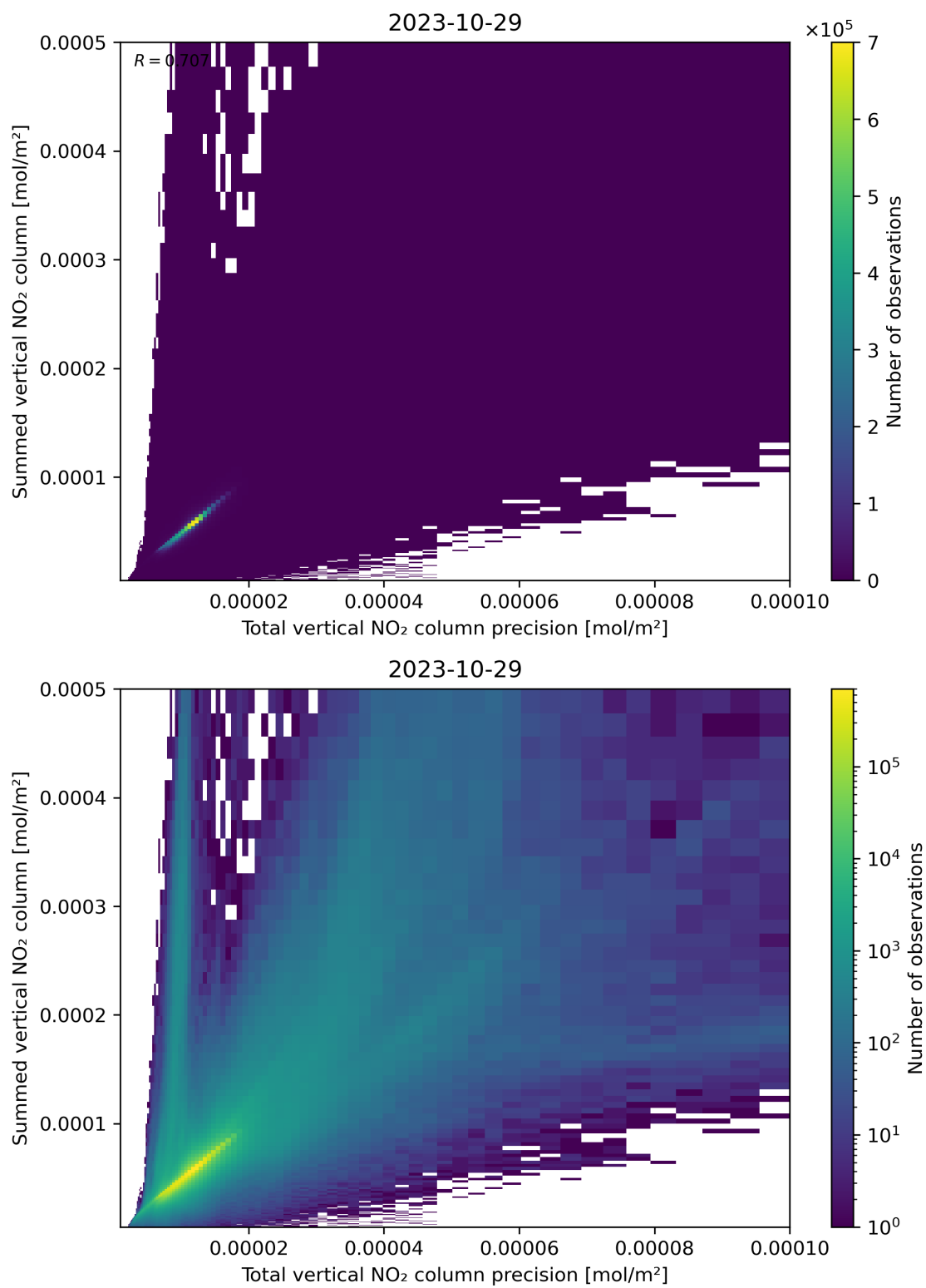
Figure 117: Scatter density plot of “Total vertical NO 2 column precision” against “Summed vertical NO 2 column” for 2023-10-28 to 2023-10-30.
