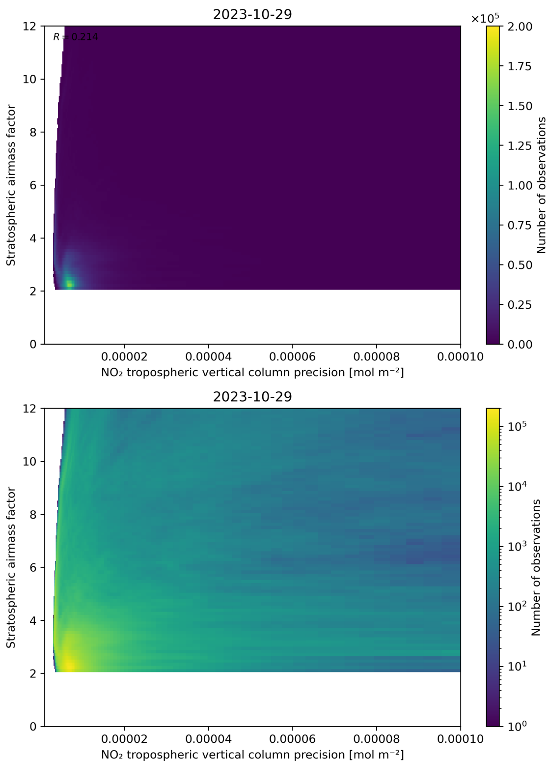
Figure 131: Scatter density plot of “NO 2 tropospheric vertical column precision” against “Stratospheric airmass factor” for 2023-10-28 to 2023-10-30.
