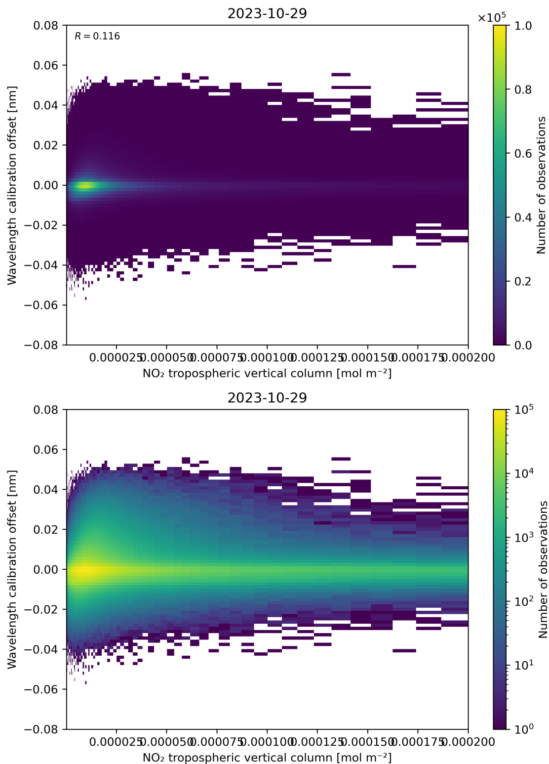
Figure 143: Scatter density plot of “NO 2 tropospheric vertical column” against “Wavelength calibration offset” for 2023-10-28 to 2023-10-30.
