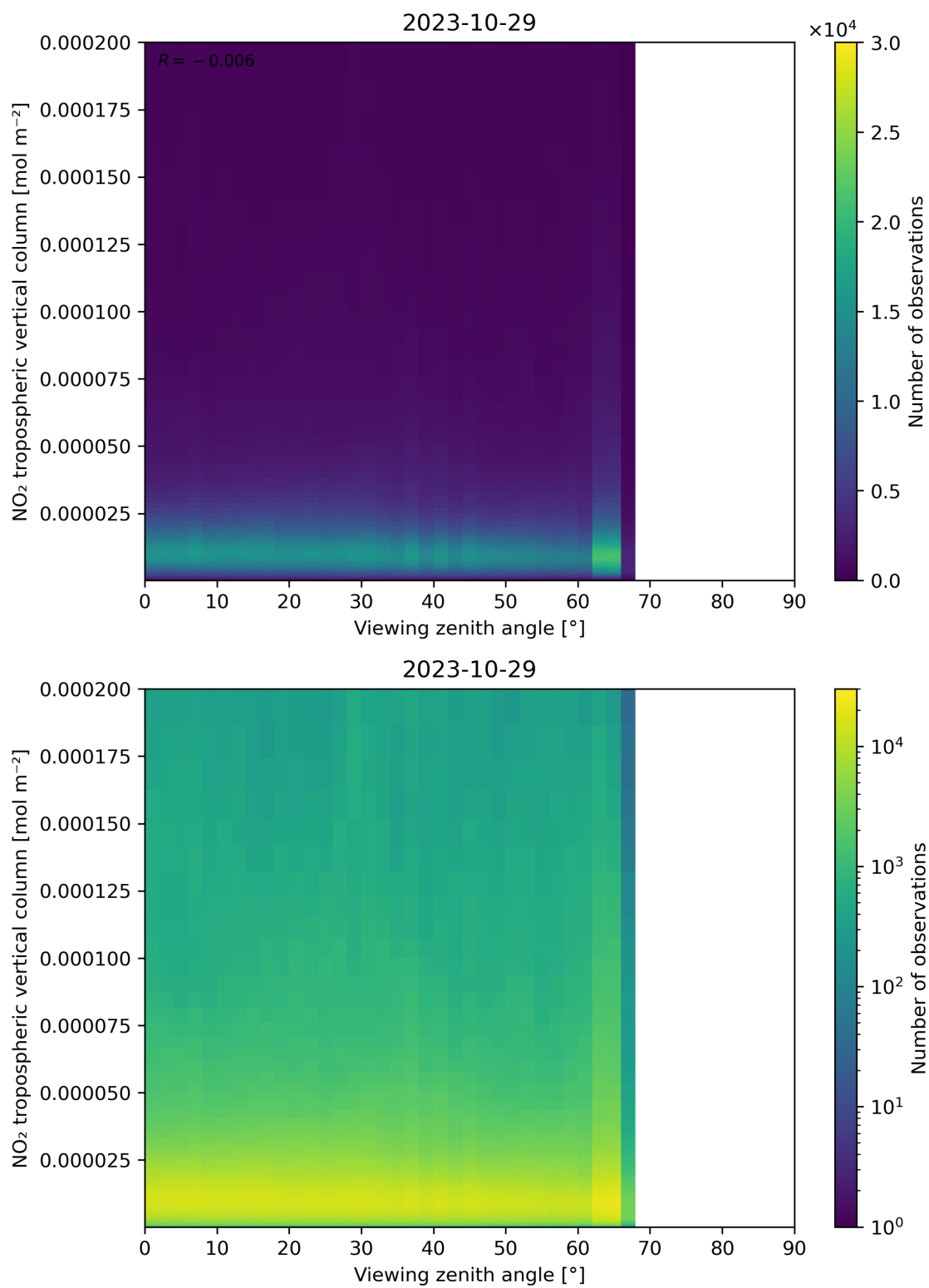
Figure 169: Scatter density plot of “Viewing zenith angle” against “NO 2 tropospheric vertical column” for 2023-10-28 to 2023-10-30.
