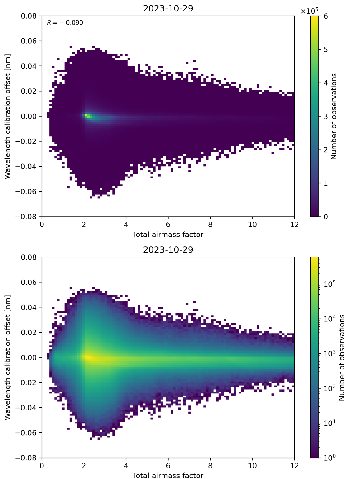
Figure 70: Scatter density plot of “Total airmass factor” against “Wavelength calibration offset” for 2023-10-28 to 2023-10-30.
