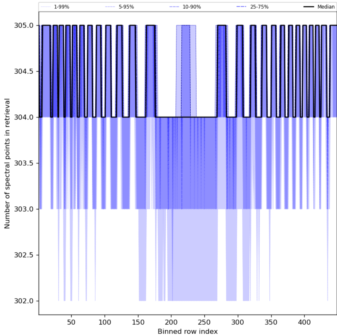
Figure 50: Along track statistics of “Number of spectral points in retrieval” for 2023-10-28 to 2023-10-30
