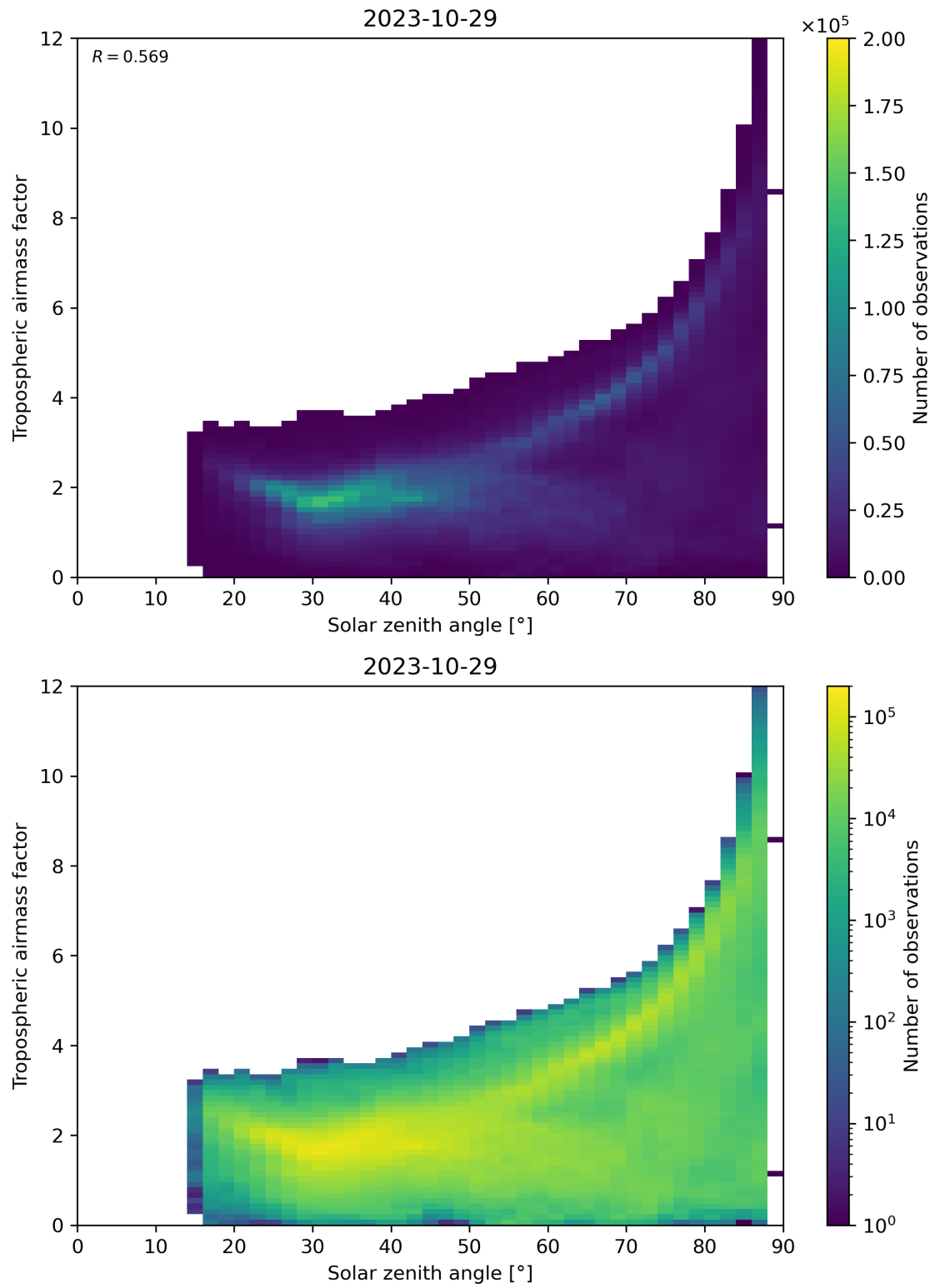
Figure 147: Scatter density plot of “Solar zenith angle” against “Tropospheric airmass factor” for 2023-10-28 to 2023-10-30.
