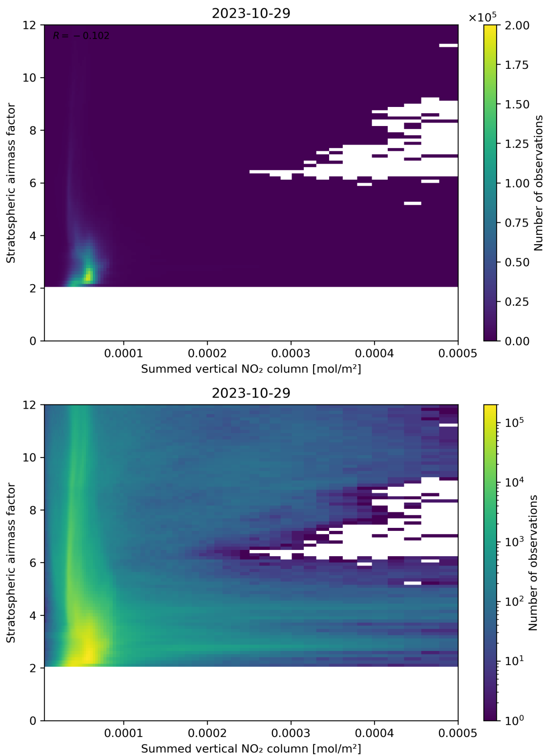
Figure 103: Scatter density plot of “Summed vertical NO 2 column” against “Stratospheric air mass factor” for 2023-10-28 to 2023-10-30.
