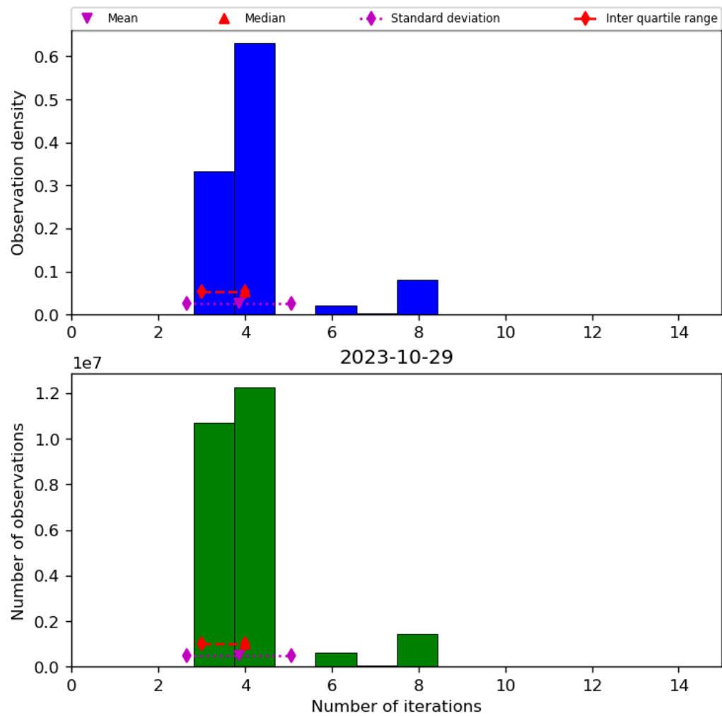
Figure 34: Histogram of “Number of iterations” for 2023-10-28 to 2023-10-30
