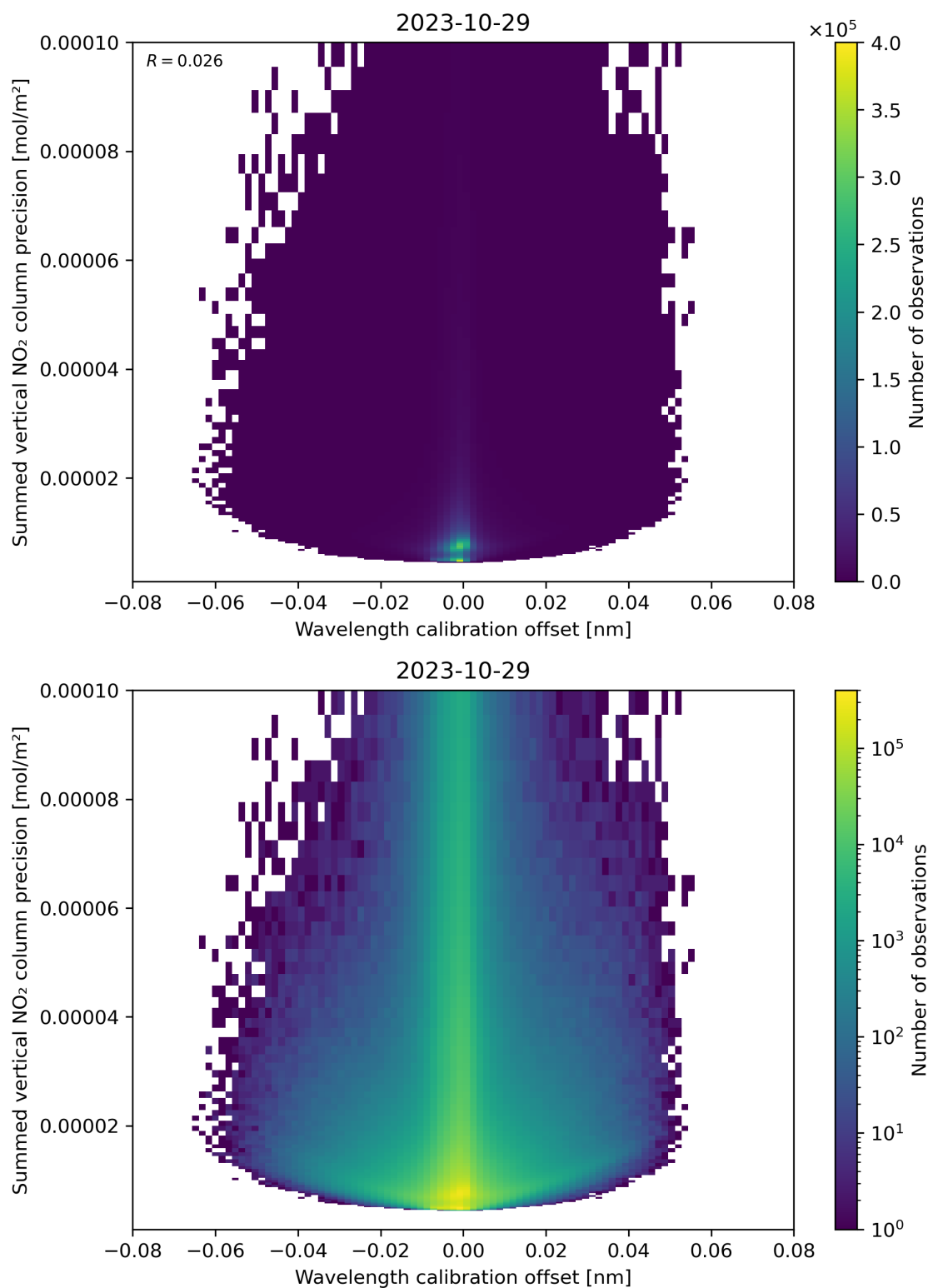
Figure 178: Scatter density plot of “Wavelength calibration offset” against “Summed vertical NO 2 column precision” for 2023-10-28 to 2023-10-30.
