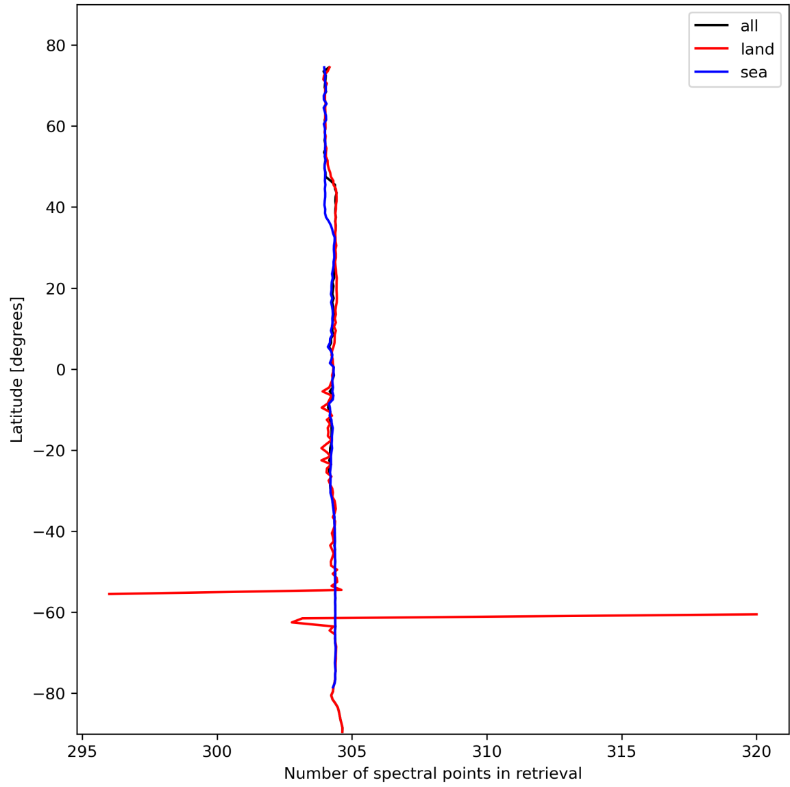
Figure 16: Zonal average of “Number of spectral points in retrieval” for 2023-10-28 to 2023-10-30.
