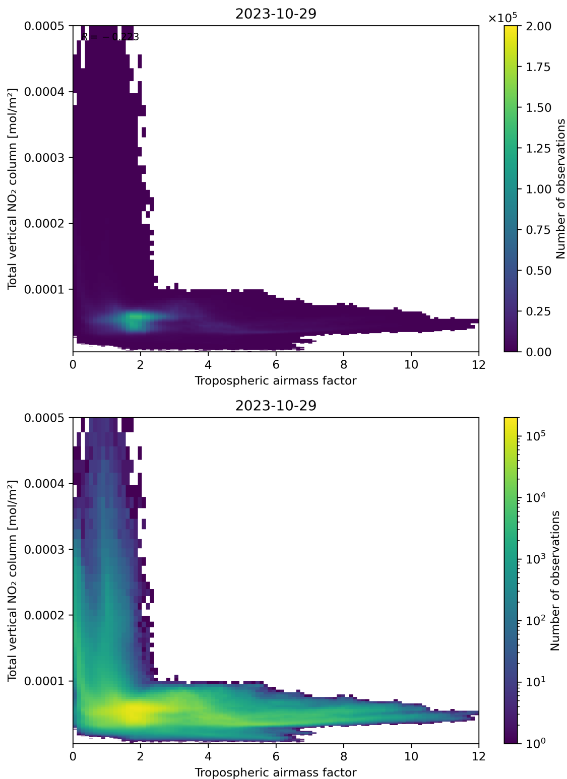
Figure 77: Scatter density plot of “Tropospheric airmass factor” against “Total vertical \text{NO}_2 column” for 2023-10-28 to 2023-10-30.
