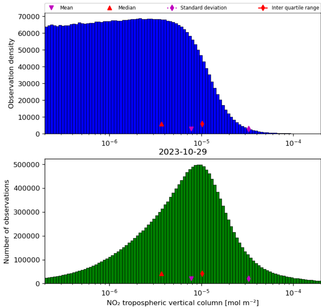
Figure 29: Histogram of “NO 2 tropospheric vertical column” for 2023-10-28 to 2023-10-30
