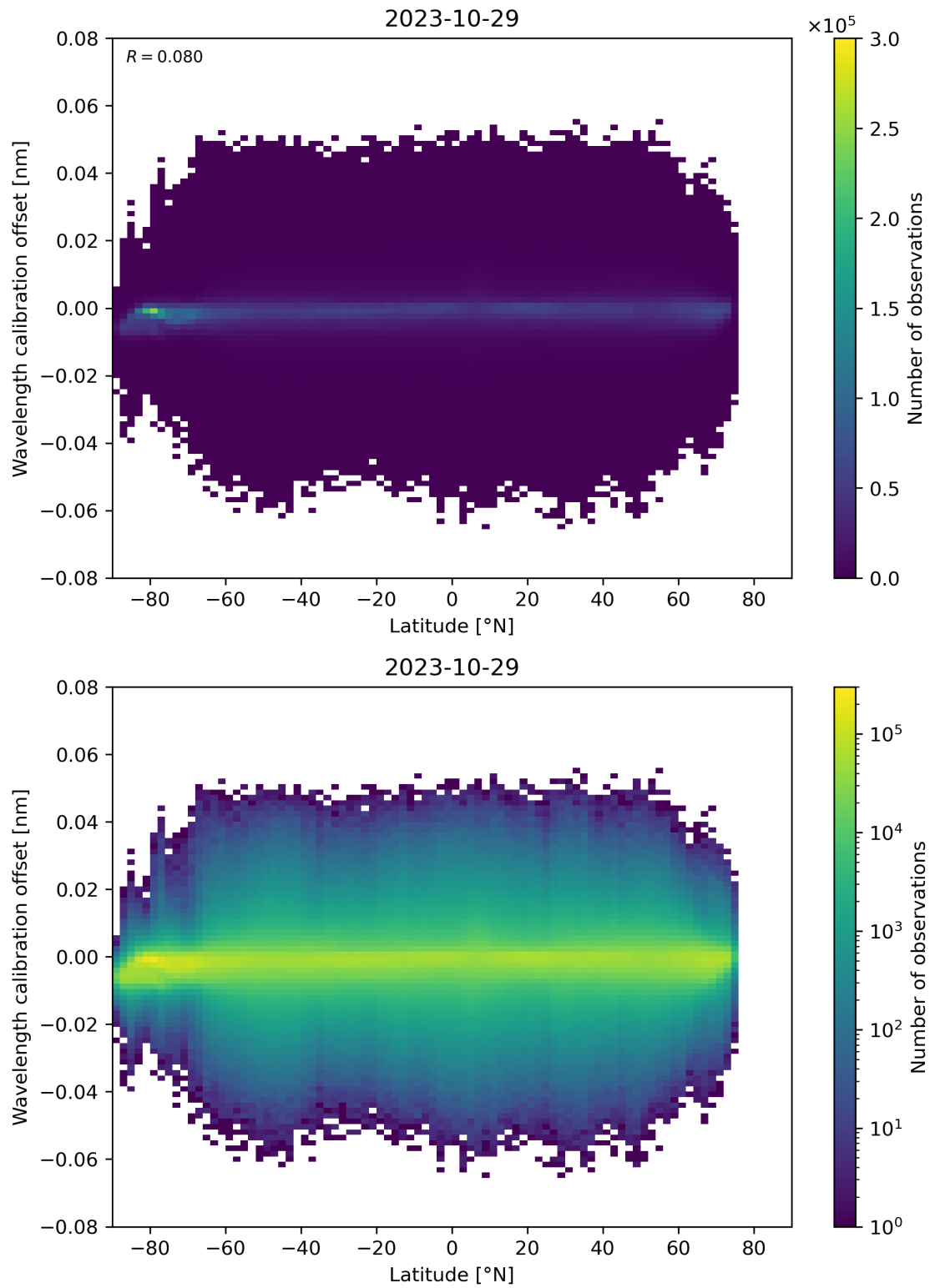
Figure 95: Scatter density plot of “Latitude” against “Wavelength calibration offset” for 2023-10-28 to 2023-10-30.
