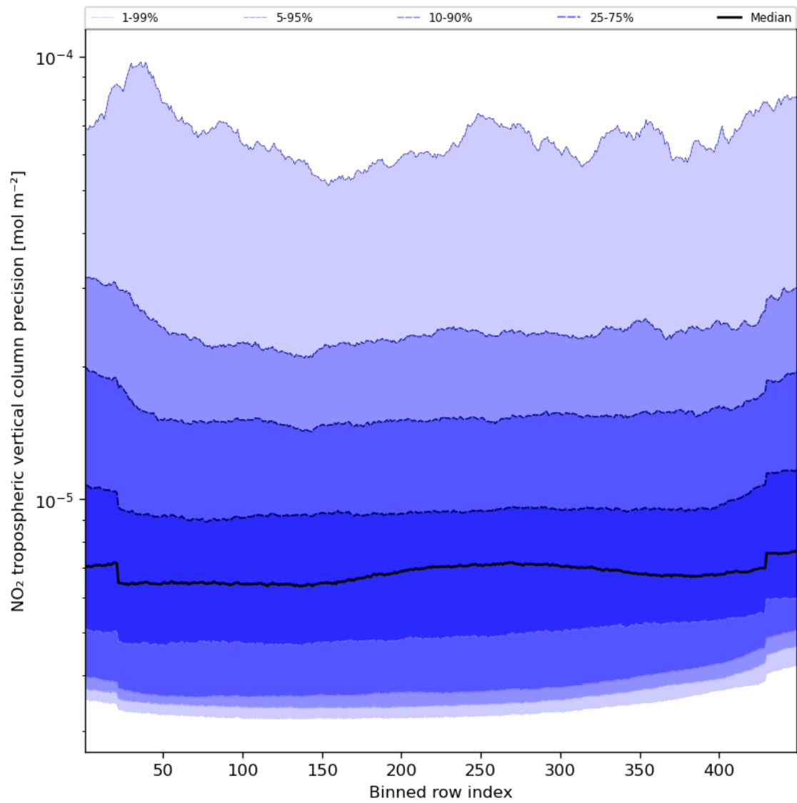
Figure 47: Along track statistics of “NO 2 tropospheric vertical column precision” for 2023-10-28 to 2023-10-30
