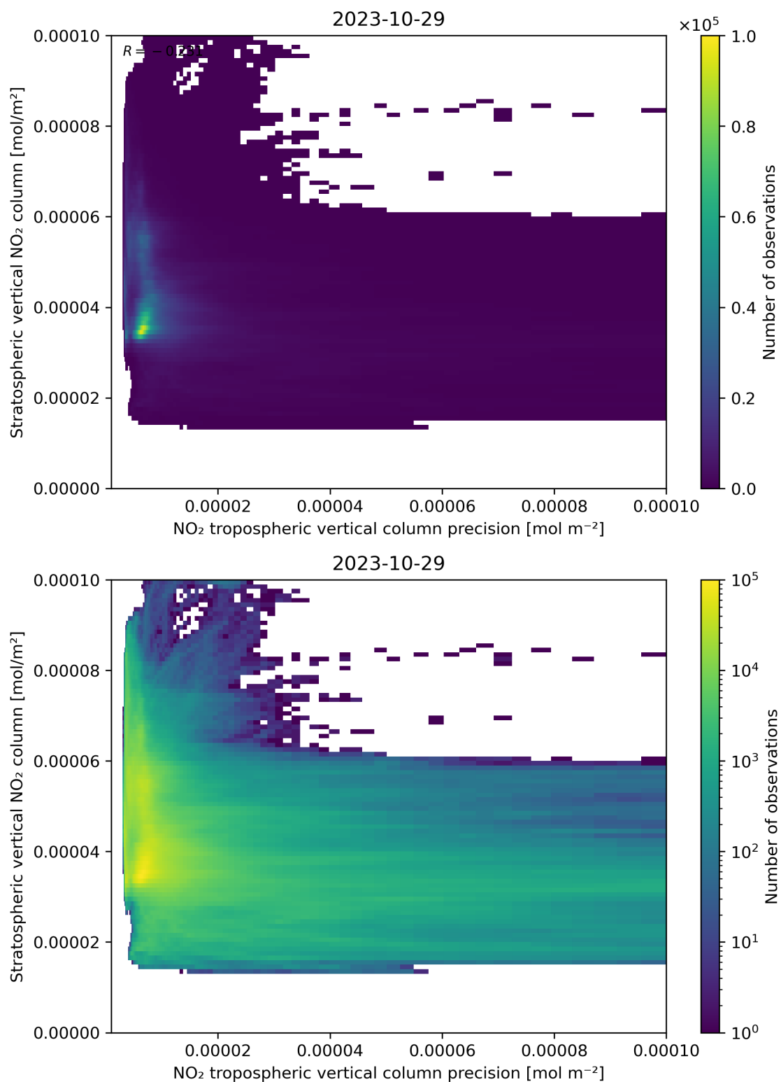
Figure 135: Scatter density plot of “NO 2 tropospheric vertical column precision” against “Stratospheric vertical NO 2 column” for 2023-10-28 to 2023-10-30.
