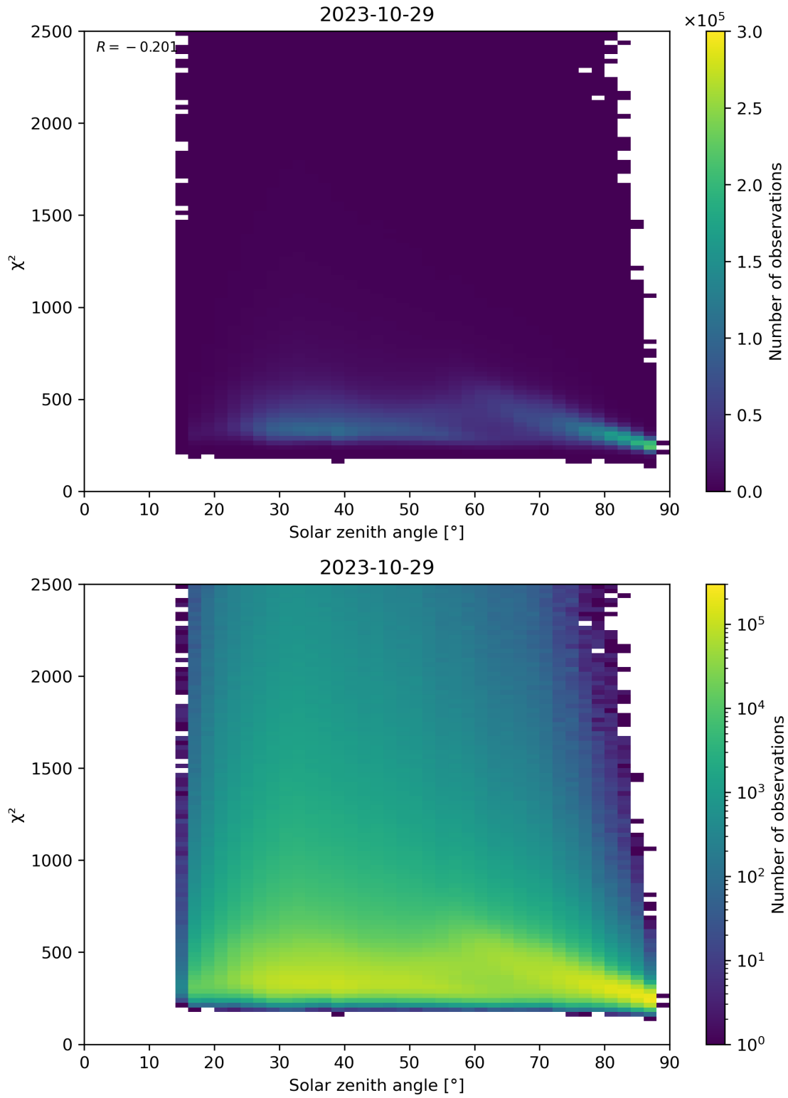
Figure 148: Scatter density plot of “Solar zenith angle” against “ \chi^2 ” for 2023-10-28 to 2023-10-30.
