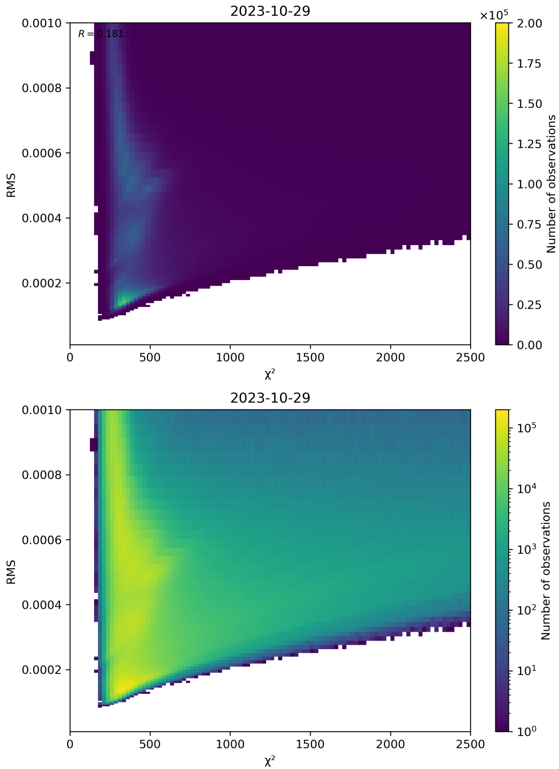
Figure 82: Scatter density plot of “ \chi^2 ” against “RMS” for 2023-10-28 to 2023-10-30.
