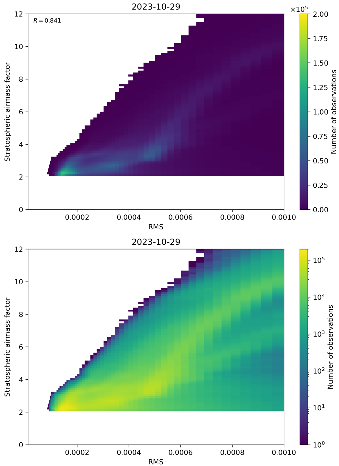
Figure 144: Scatter density plot of “RMS” against “Stratospheric airmass factor” for 2023-10-28 to 2023-10-30.
