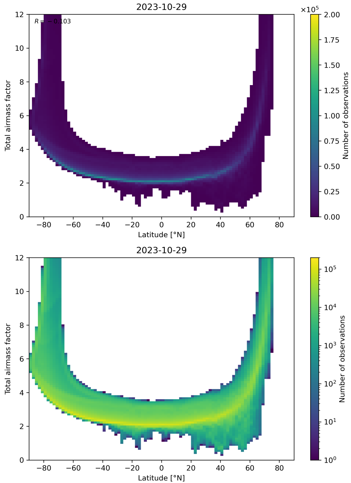
Figure 84: Scatter density plot of “Latitude” against “Total airmass factor” for 2023-10-28 to 2023-10-30.
