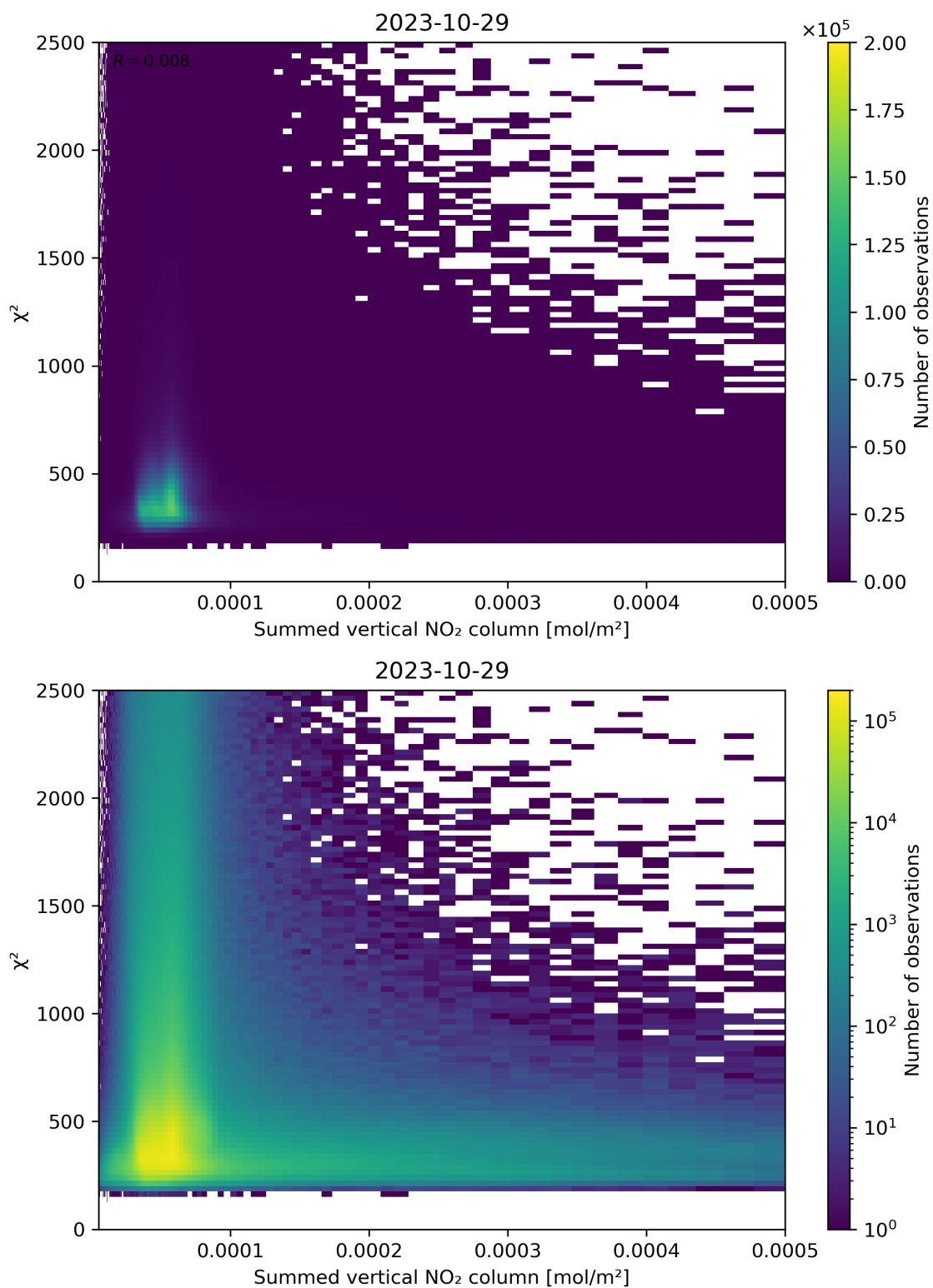
Figure 104: Scatter density plot of “Summed vertical NO 2 column” against “ \chi^2 ” for 2023-10-28 to 2023-10-30.
