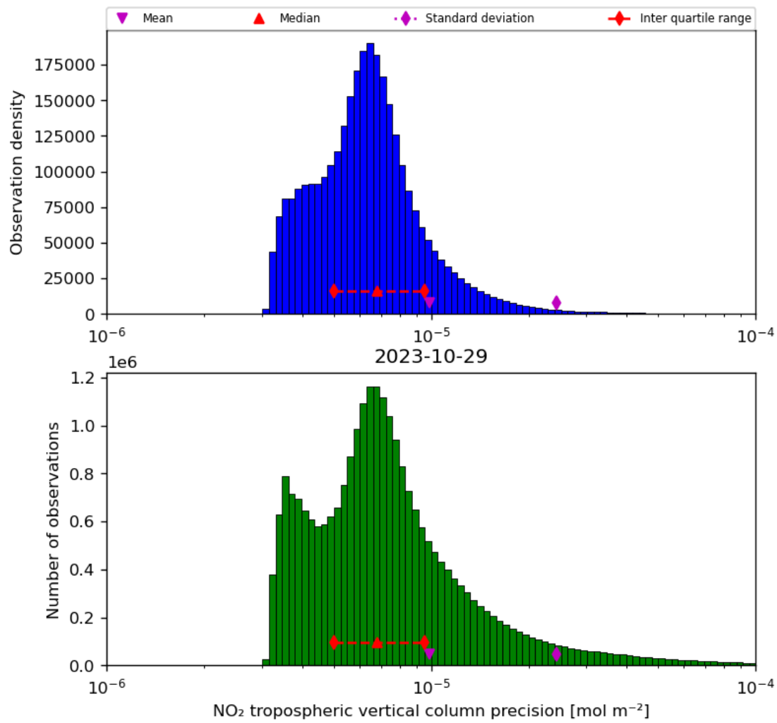
Figure 30: Histogram of “NO 2 tropospheric vertical column precision” for 2023-10-28 to 2023-10-30
