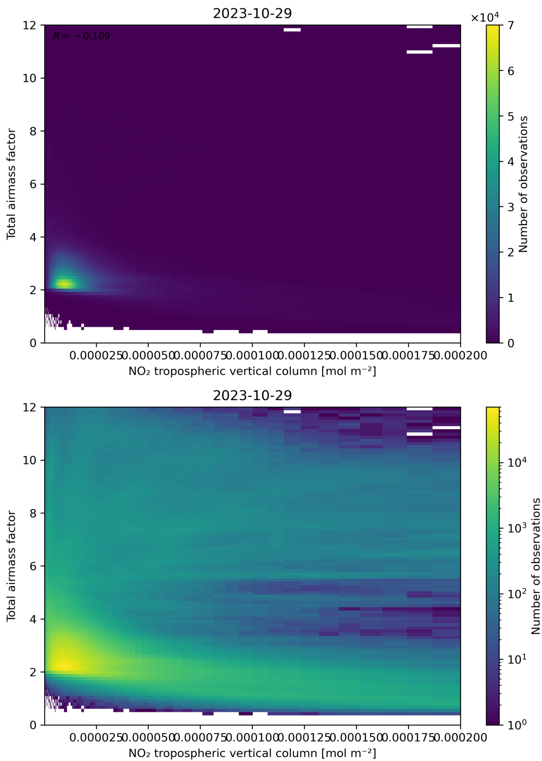
Figure 122: Scatter density plot of “NO 2 tropospheric vertical column” against “Total air mass factor” for 2023-10-28 to 2023-10-30.
