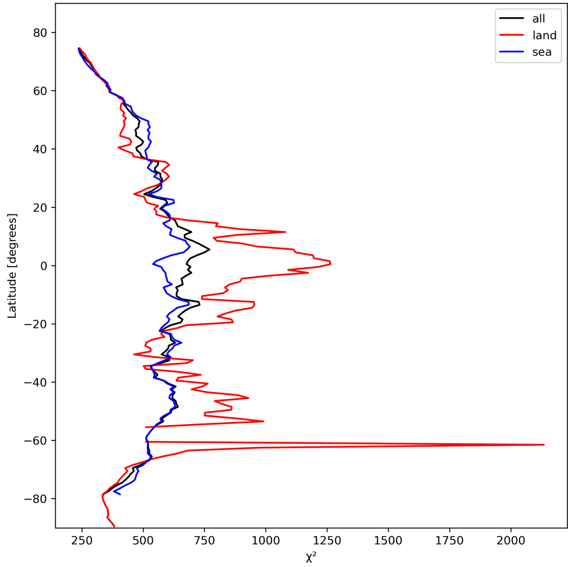
Figure 25: Zonal average of “ \chi^2 ” for 2023-10-28 to 2023-10-30.
