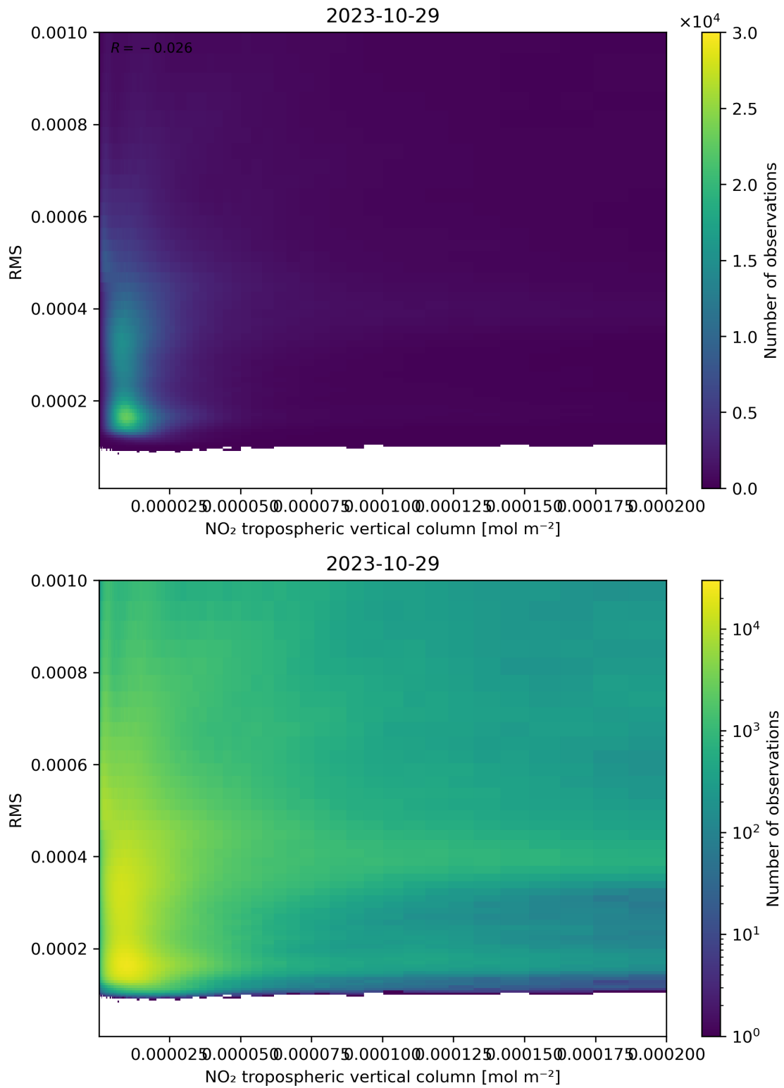
Figure 142: Scatter density plot of “NO 2 tropospheric vertical column” against “RMS” for 2023-10-28 to 2023-10-30.
