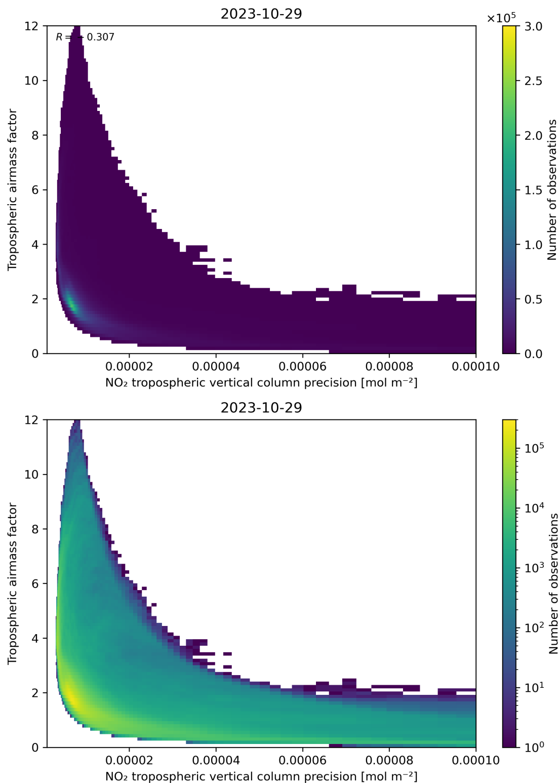
Figure 133: Scatter density plot of “NO 2 tropospheric vertical column precision” against “Tropospheric airmass factor” for 2023-10-28 to 2023-10-30.
