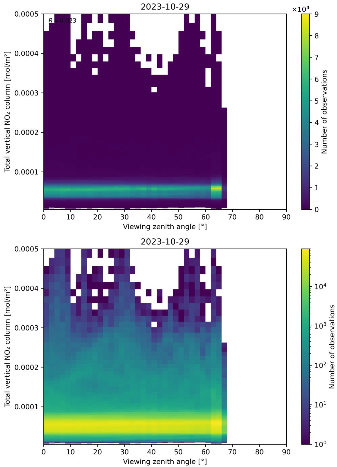
Figure 167: Scatter density plot of “Viewing zenith angle” against “Total vertical NO 2 column” for 2023-10-28 to 2023-10-30.
