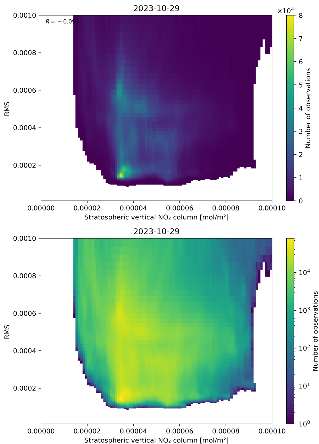
Figure 102: Scatter density plot of “Stratospheric vertical NO 2 column” against “RMS” for 2023-10-28 to 2023-10-30.
