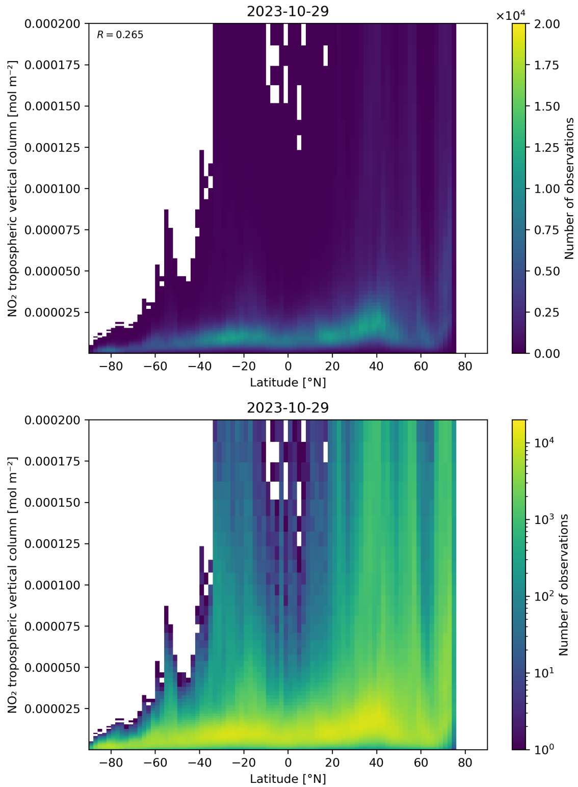
Figure 92: Scatter density plot of “Latitude” against “NO 2 tropospheric vertical column” for 2023-10-28 to 2023-10-30.
