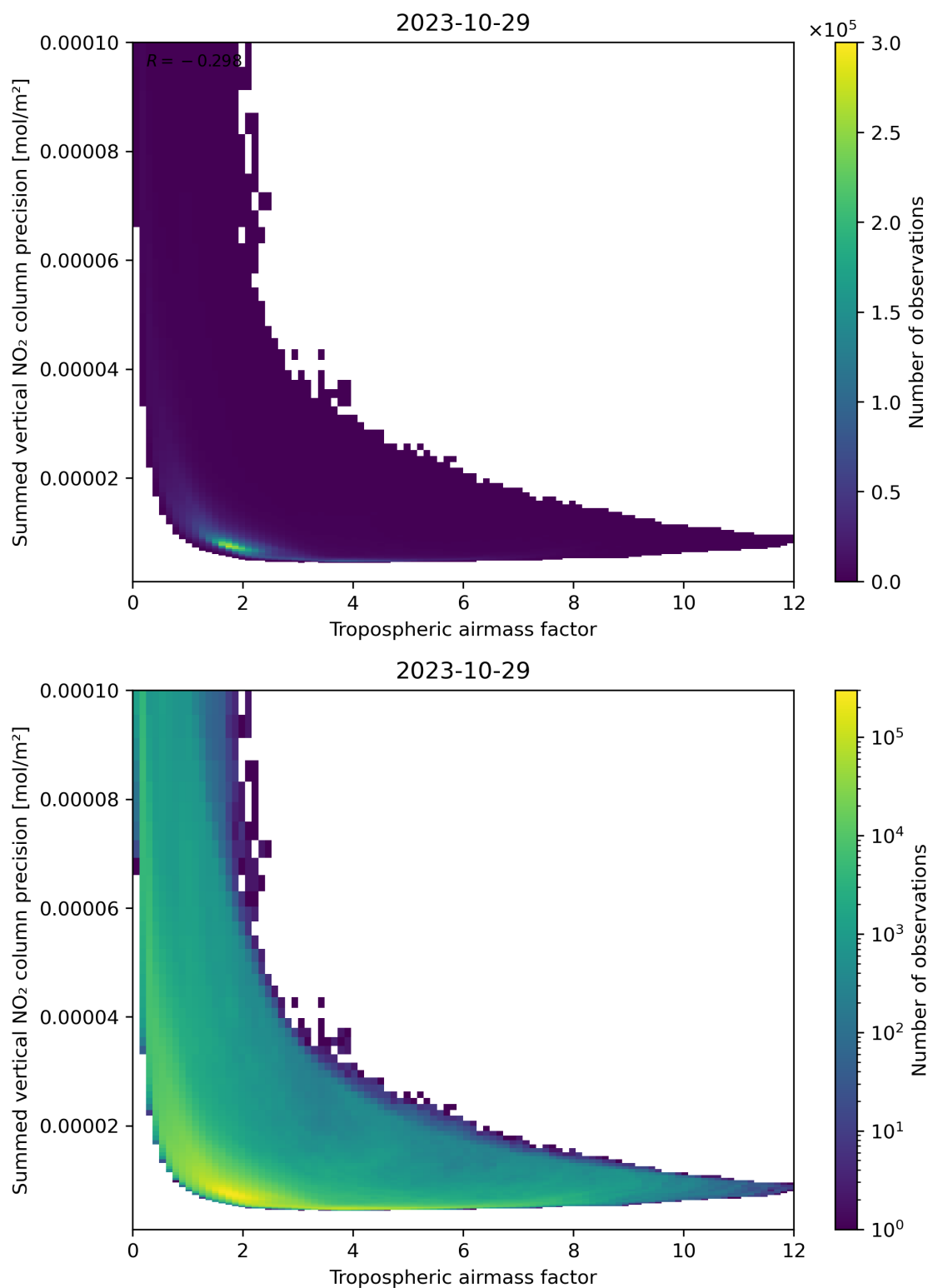
Figure 76: Scatter density plot of “Tropospheric air mass factor” against “Summed vertical NO 2 column precision” for 2023-10-28 to 2023-10-30.
