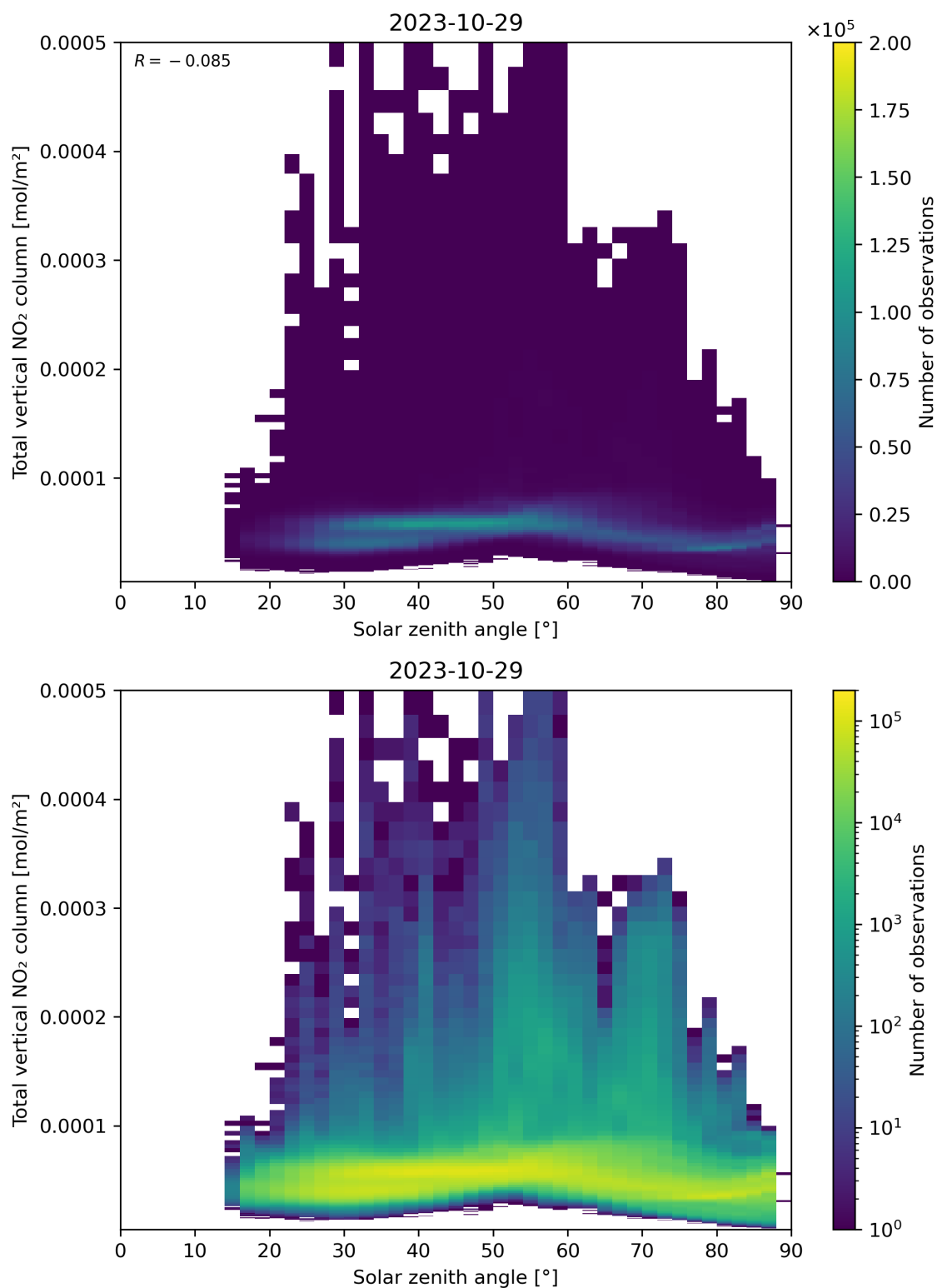
Figure 153: Scatter density plot of “Solar zenith angle” against “Total vertical NO 2 column” for 2023-10-28 to 2023-10-30.
