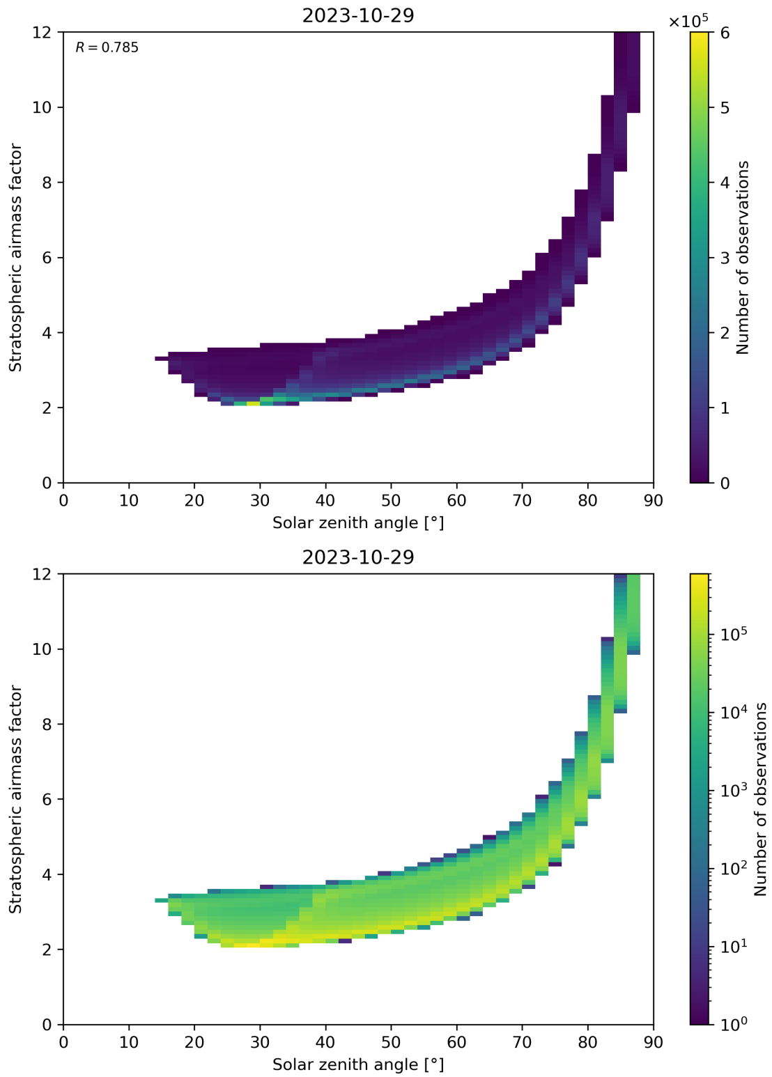
Figure 145: Scatter density plot of “Solar zenith angle” against “Stratospheric airmass factor” for 2023-10-28 to 2023-10-30.
