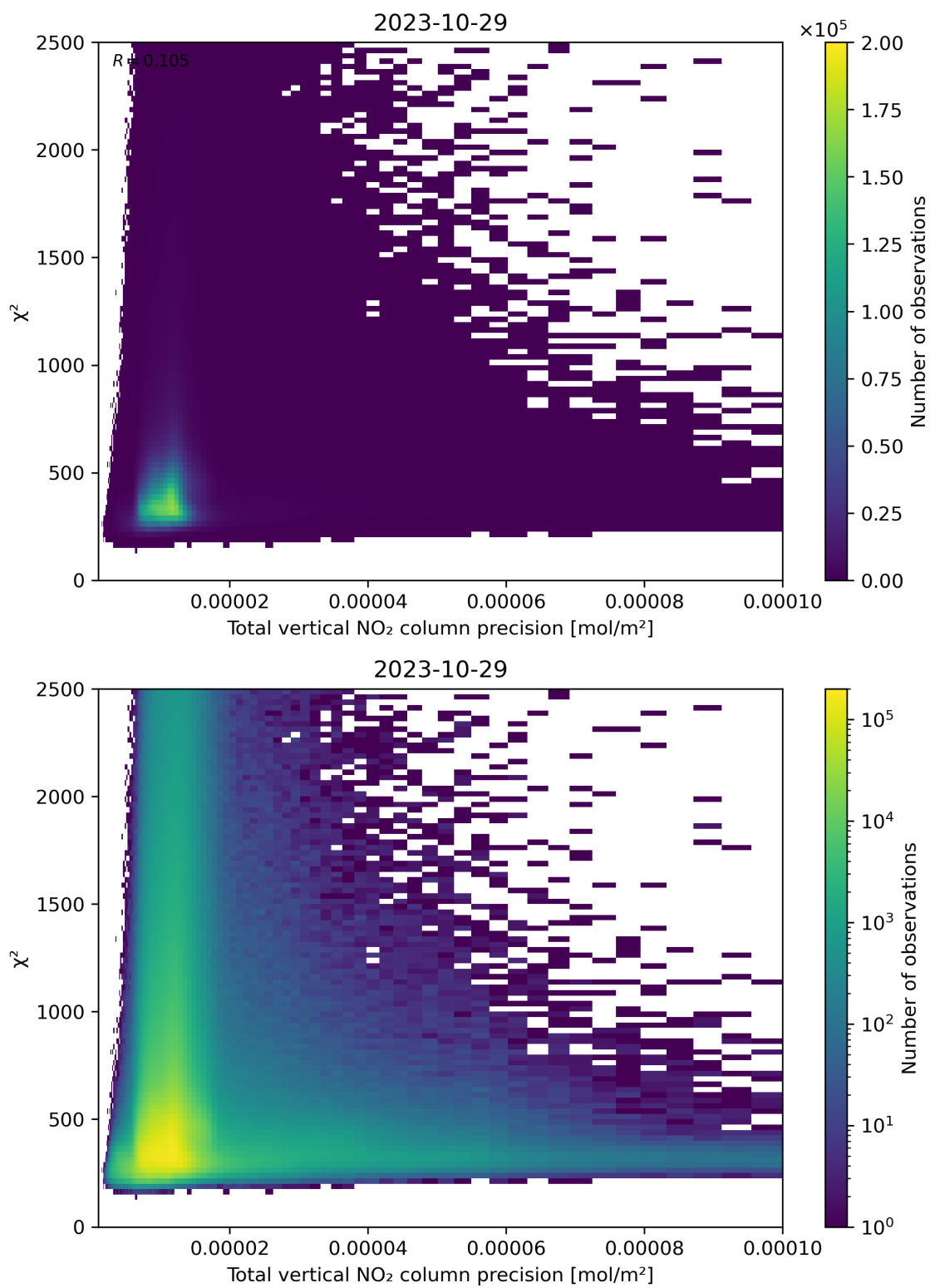
Figure 116: Scatter density plot of “Total vertical NO 2 column precision” against “ \chi^2 ” for 2023-10-28 to 2023-10-30.
