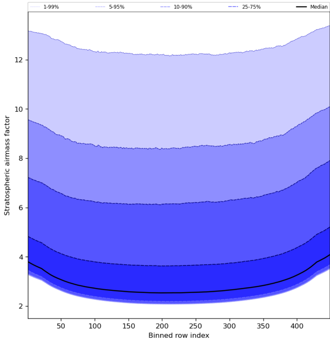
Figure 61: Along track statistics of “Stratospheric airmass factor” for 2023-10-28 to 2023-10-30
