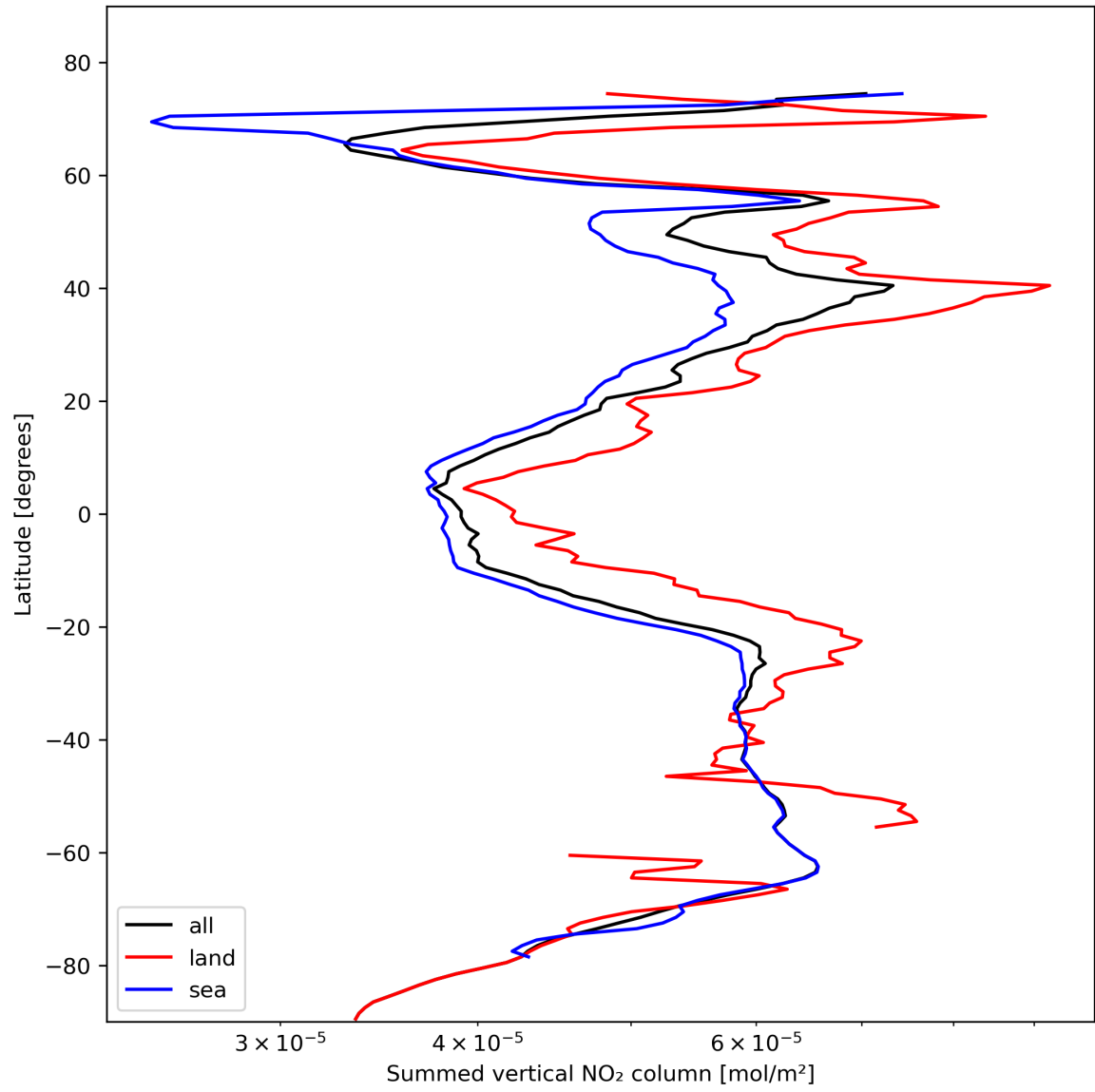
Figure 23: Zonal average of “Summed vertical NO 2 column” for 2023-10-28 to 2023-10-30.
