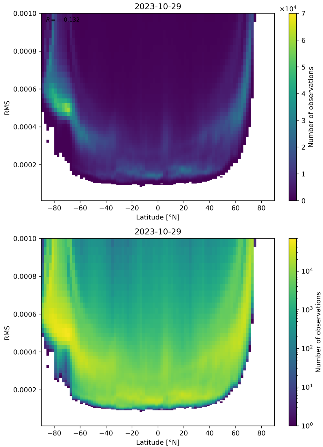
Figure 94: Scatter density plot of “Latitude” against “RMS” for 2023-10-28 to 2023-10-30.
