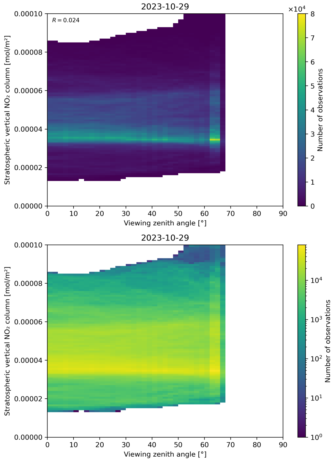
Figure 164: Scatter density plot of “Viewing zenith angle” against “Stratospheric vertical NO 2 column” for 2023-10-28 to 2023-10-30.
