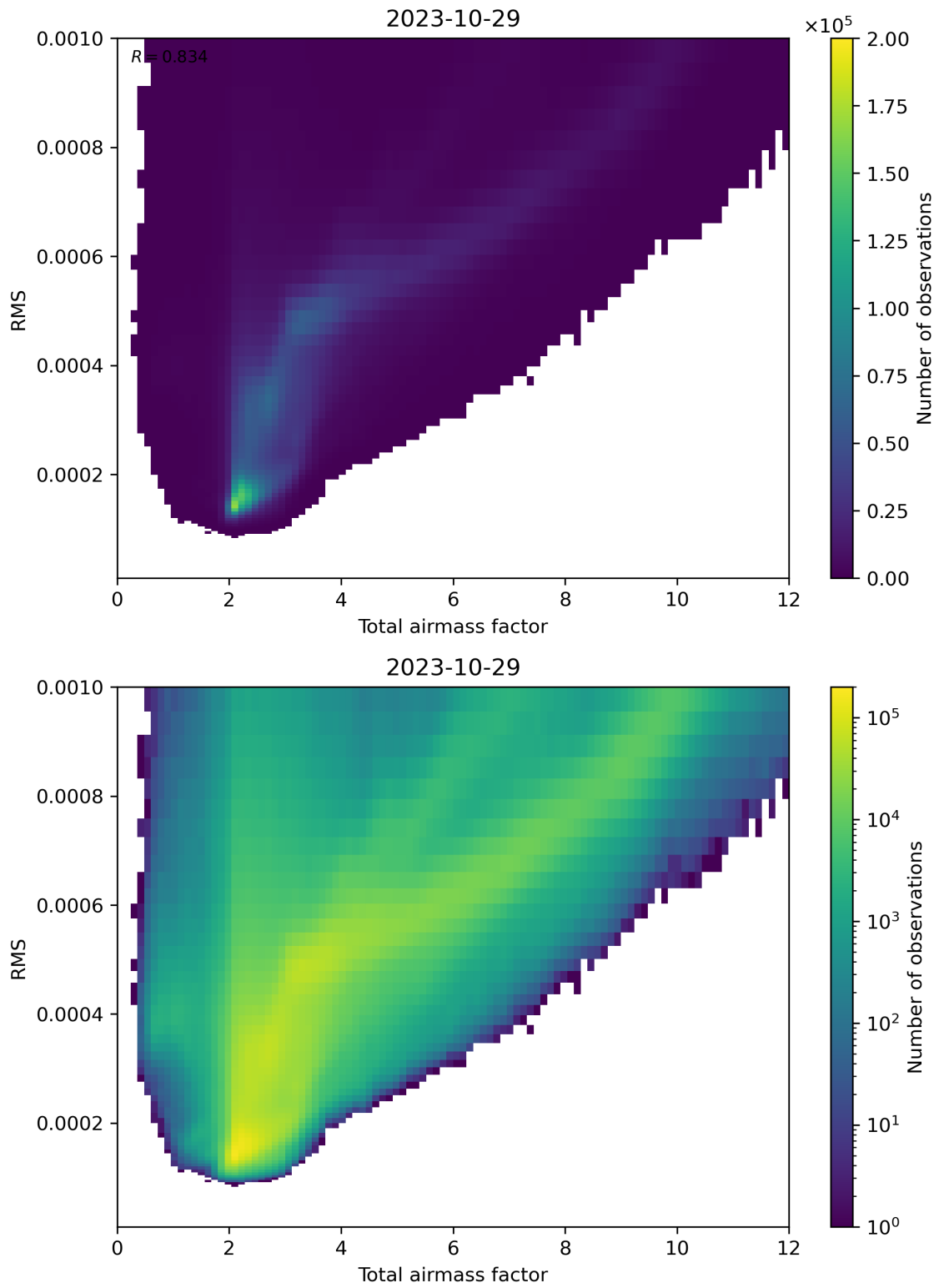
Figure 69: Scatter density plot of “Total airmass factor” against “RMS” for 2023-10-28 to 2023-10-30.
