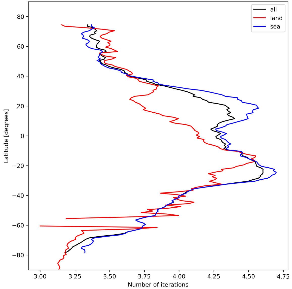
Figure 17: Zonal average of “Number of iterations” for 2023-10-28 to 2023-10-30.
