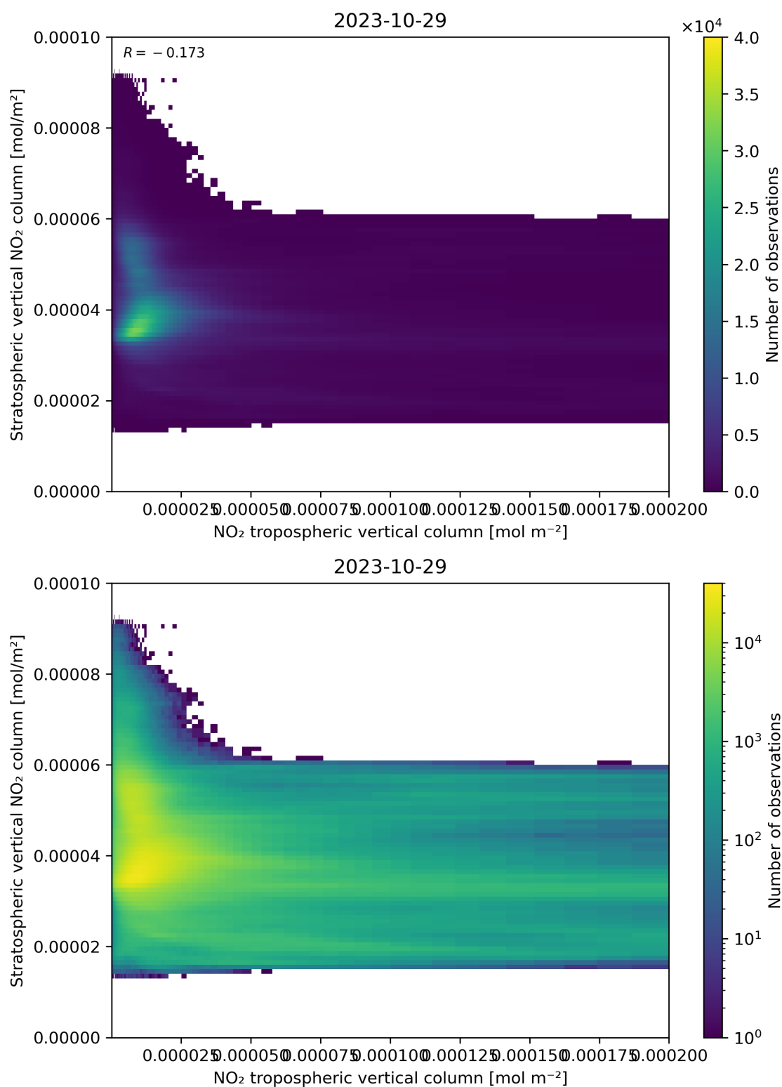
Figure 125: Scatter density plot of “NO 2 tropospheric vertical column” against “Stratospheric vertical NO 2 column” for 2023-10-28 to 2023-10-30.
