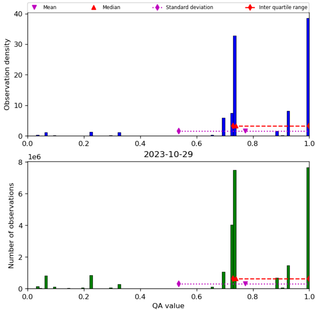
Figure 28: Histogram of “QA value” for 2023-10-28 to 2023-10-30
