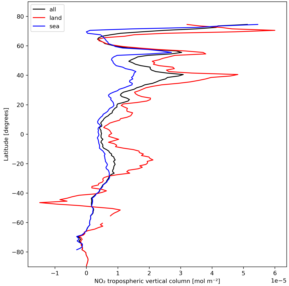
Figure 12: Zonal average of “NO 2 tropospheric vertical column” for 2023-10-28 to 2023-10-30.
