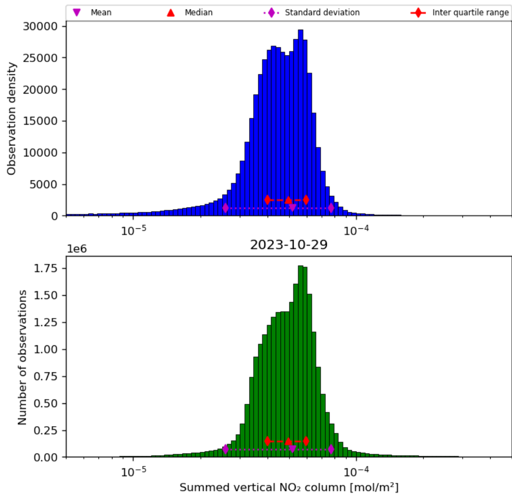
Figure 40: Histogram of “Summed vertical NO 2 column” for 2023-10-28 to 2023-10-30
