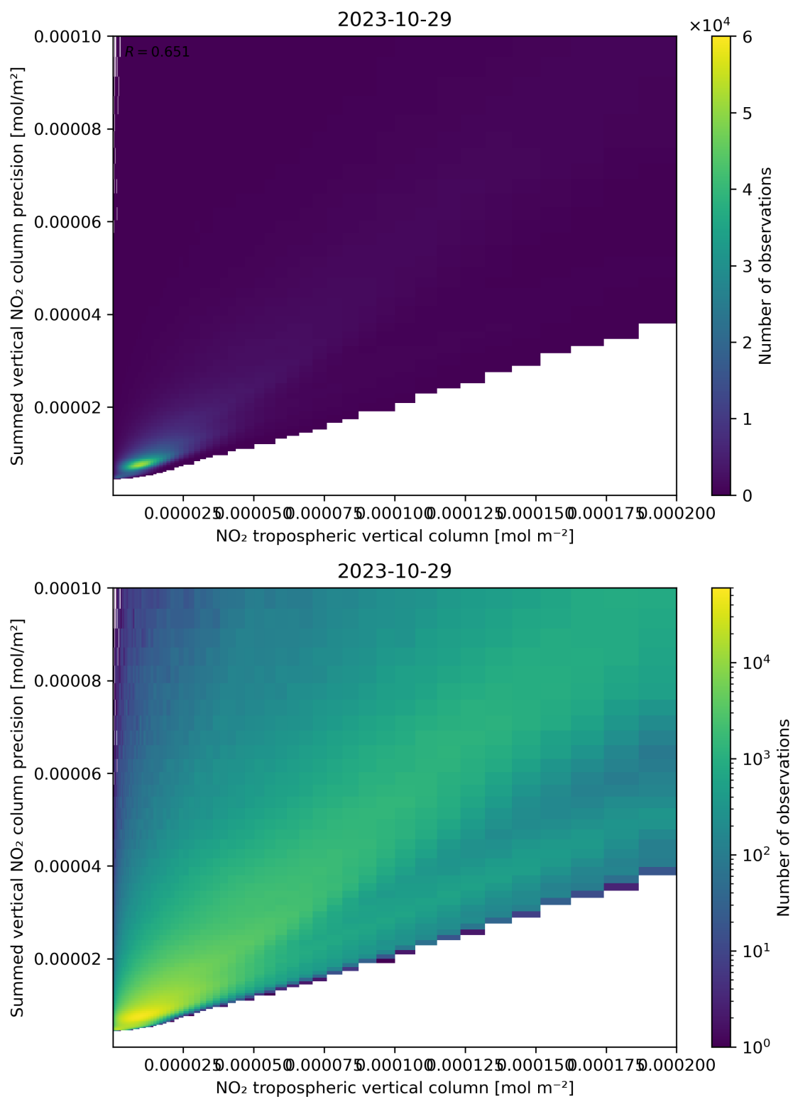
Figure 127: Scatter density plot of “NO 2 tropospheric vertical column” against “Summed vertical NO 2 column precision” for 2023-10-28 to 2023-10-30.
