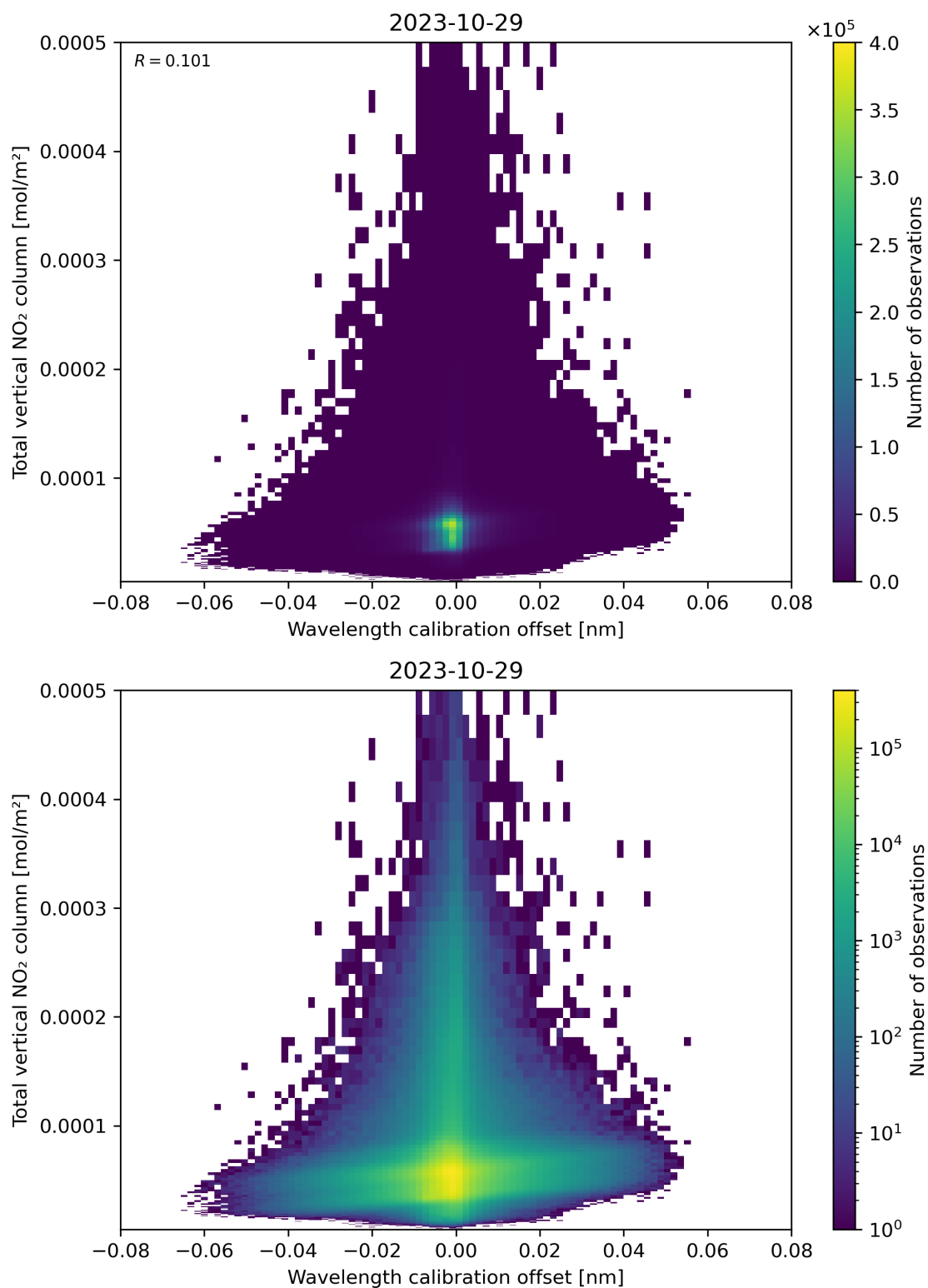
Figure 179: Scatter density plot of “Wavelength calibration offset” against “Total vertical NO 2 column” for 2023-10-28 to 2023-10-30.
