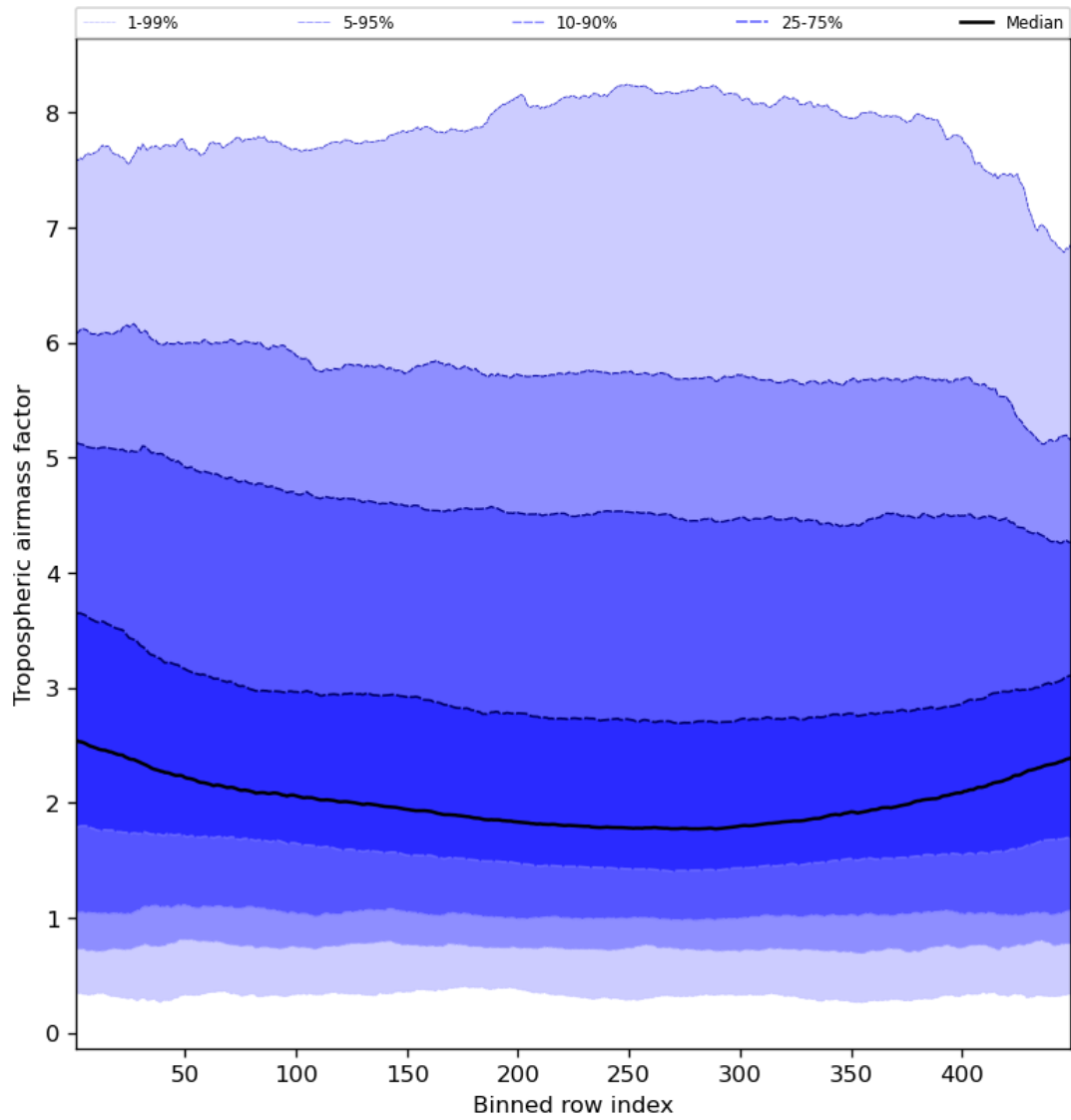
Figure 48: Along track statistics of “Tropospheric air mass factor” for 2023-10-28 to 2023-10-30
