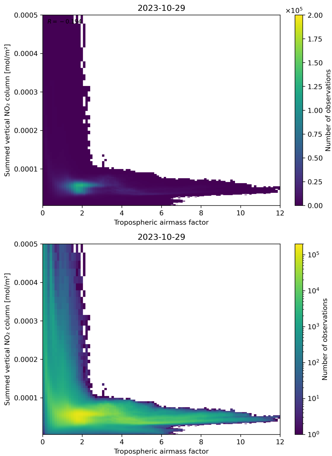
Figure 75: Scatter density plot of “Tropospheric airmass factor” against “Summed vertical NO 2 column” for 2023-10-28 to 2023-10-30.
