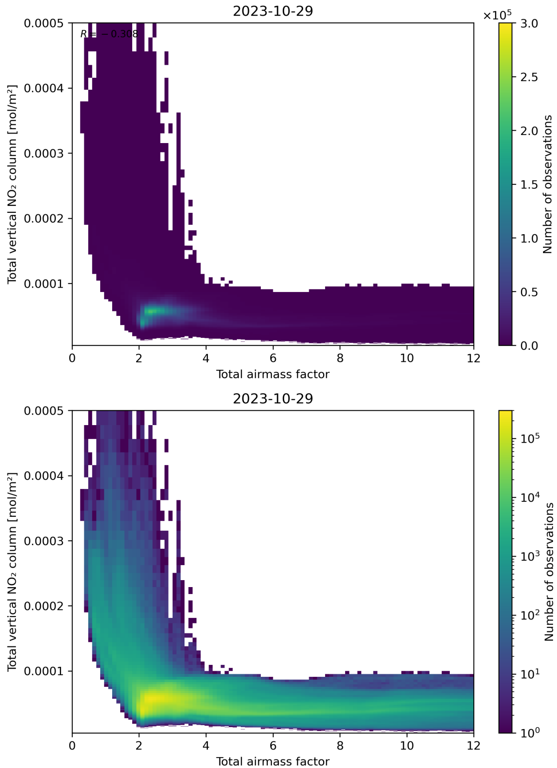
Figure 67: Scatter density plot of “Total airmass factor” against “Total vertical NO 2 column” for 2023-10-28 to 2023-10-30.
