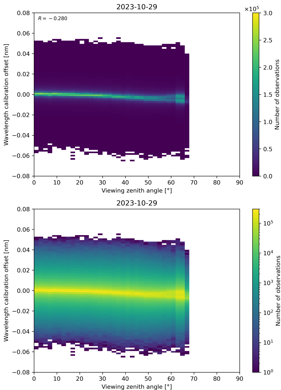
Figure 173: Scatter density plot of “Viewing zenith angle” against “Wavelength calibration offset” for 2023-10-28 to 2023-10-30.
