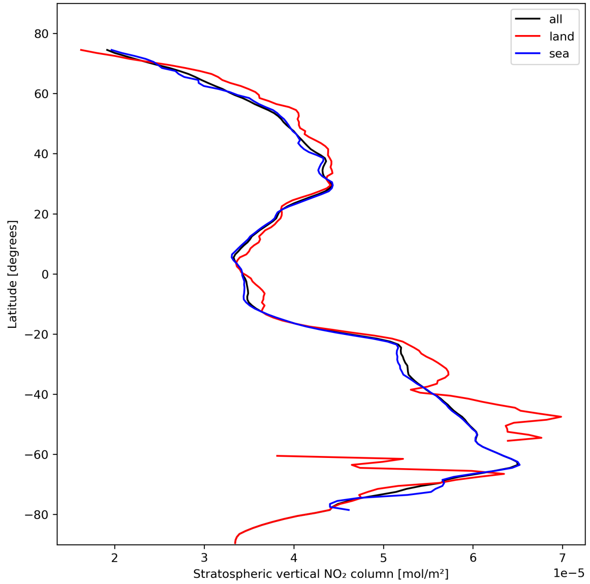
Figure 19: Zonal average of “Stratospheric vertical NO 2 column” for 2023-10-28 to 2023-10-30.
