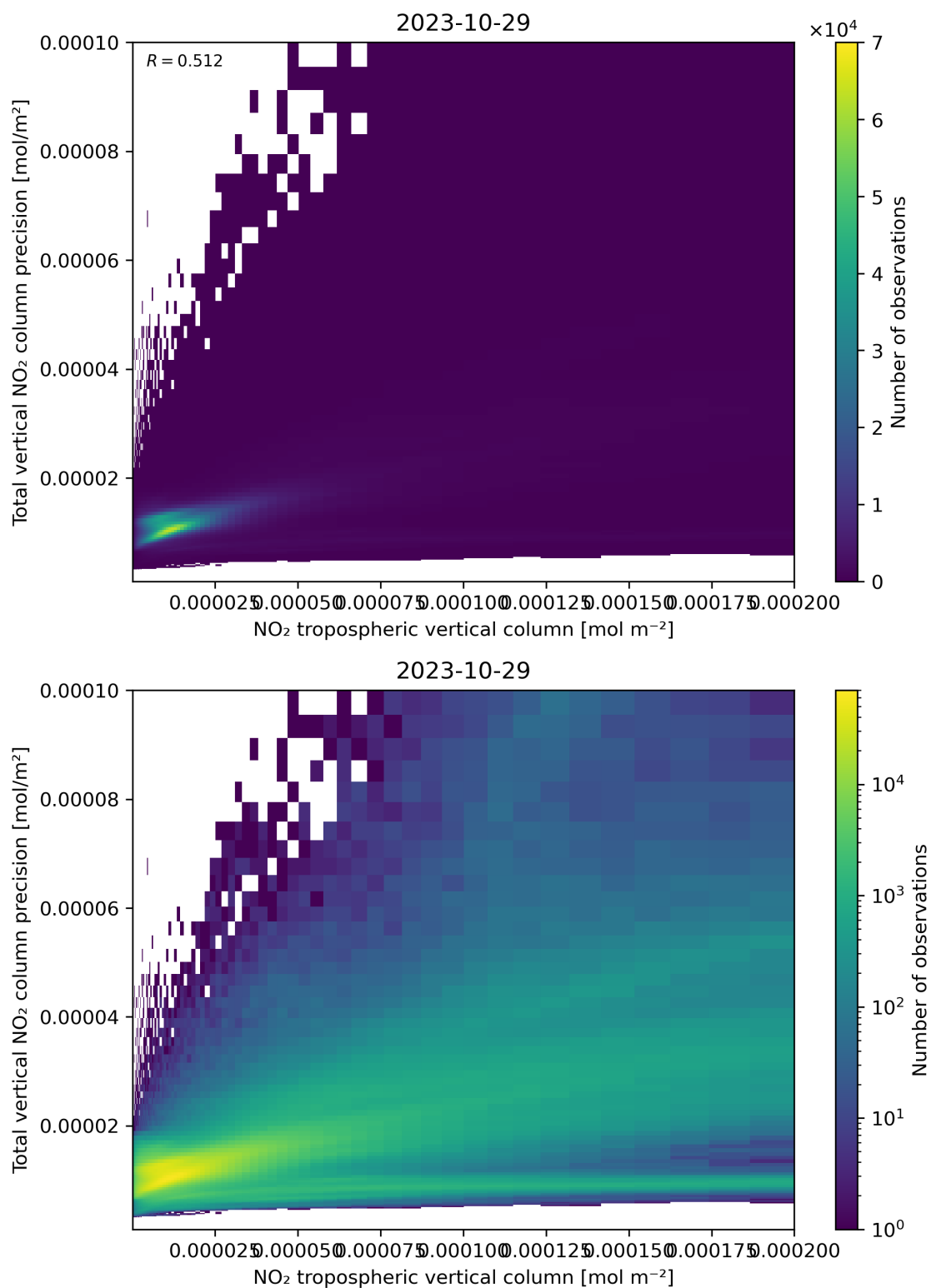
Figure 129: Scatter density plot of “NO 2 tropospheric vertical column” against “Total vertical NO 2 column precision” for 2023-10-28 to 2023-10-30.
