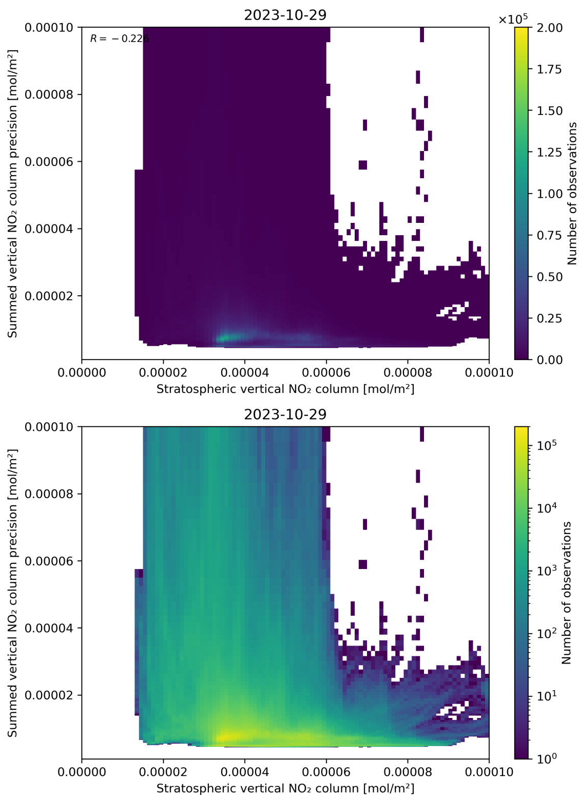
Figure 99: Scatter density plot of “Stratospheric vertical NO 2 column” against “Summed vertical NO 2 column precision” for 2023-10-28 to 2023-10-30.
