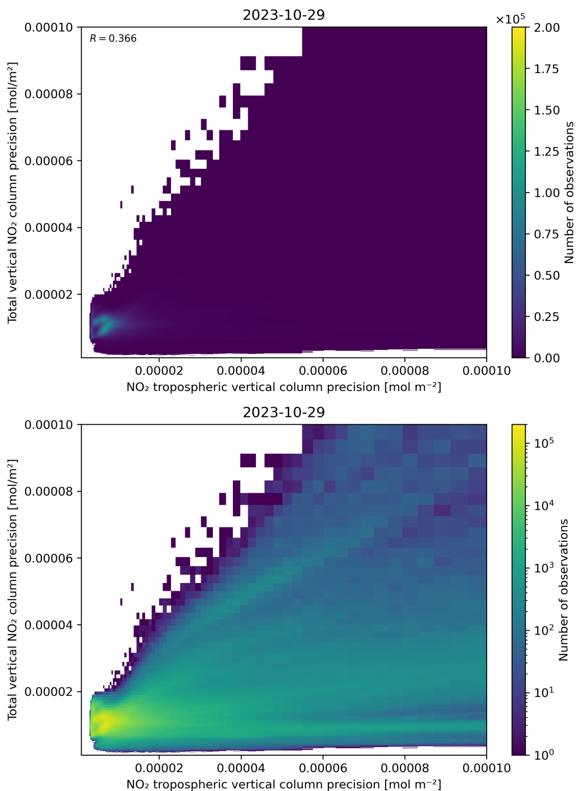
Figure 139: Scatter density plot of “NO 2 tropospheric vertical column precision” against “Total vertical NO 2 column precision” for 2023-10-28 to 2023-10-30.
