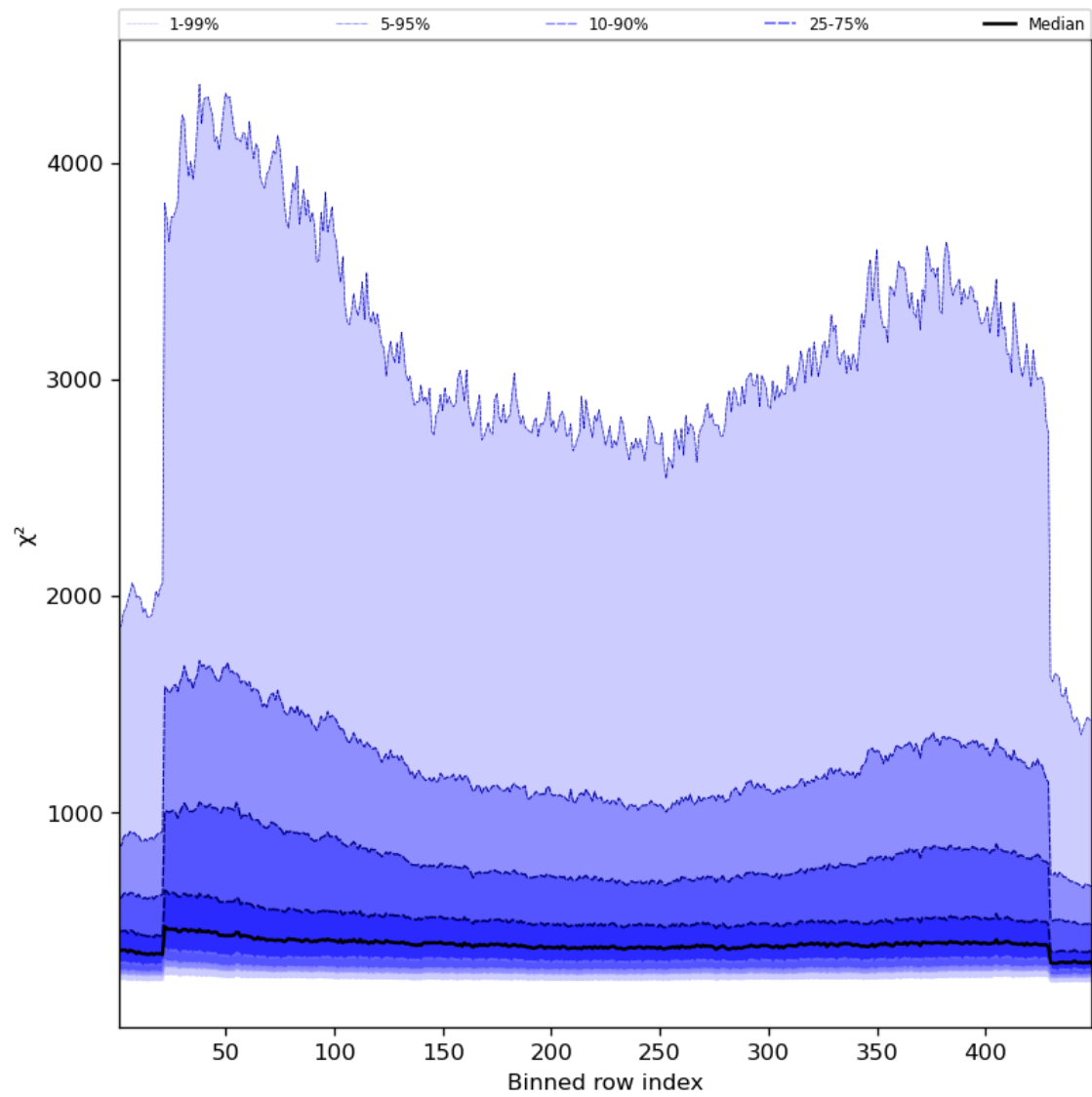
Figure 59: Along track statistics of “ \chi^2 ” for 2023-10-28 to 2023-10-30
