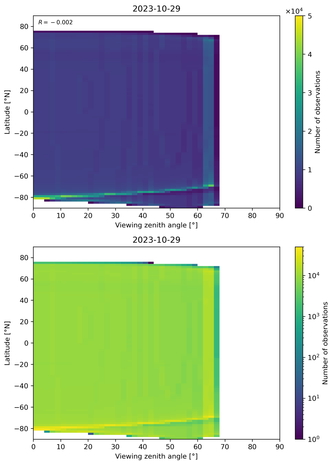
Figure 163: Scatter density plot of “Viewing zenith angle” against “Latitude” for 2023-10-28 to 2023-10-30.
