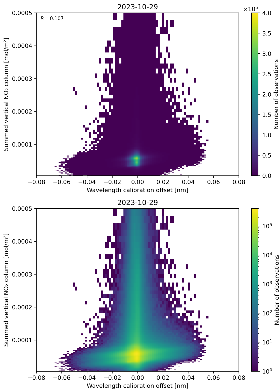
Figure 177: Scatter density plot of “Wavelength calibration offset” against “Summed vertical NO 2 column” for 2023-10-28 to 2023-10-30.
