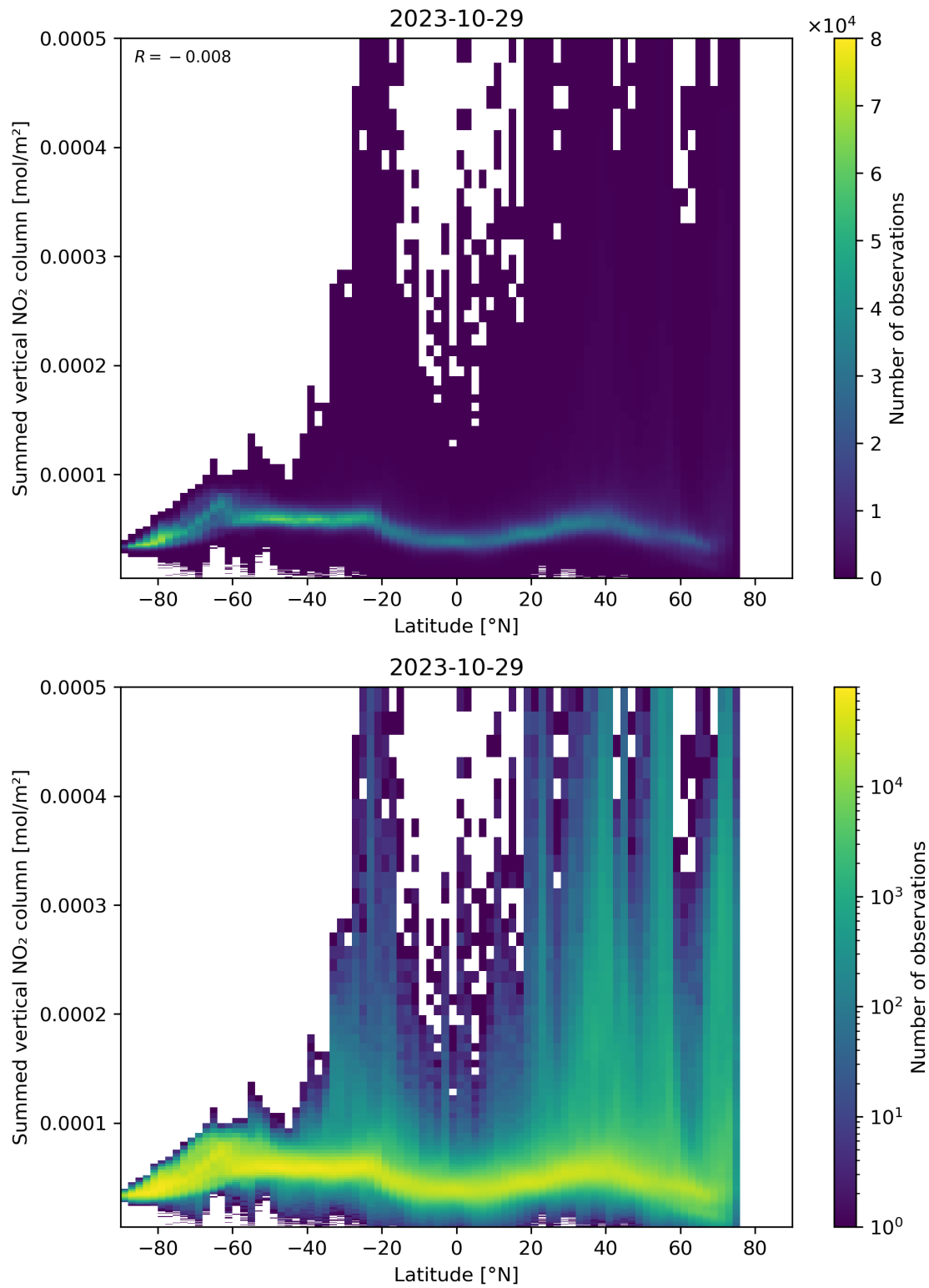
Figure 88: Scatter density plot of “Latitude” against “Summed vertical NO 2 column” for 2023-10-28 to 2023-10-30.
