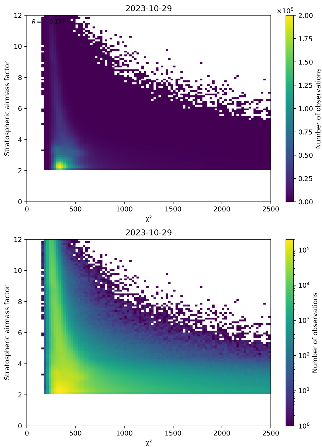
Figure 81: Scatter density plot of “ \chi^2 ” against “Stratospheric airmass factor” for 2023-10-28 to 2023-10-30.
