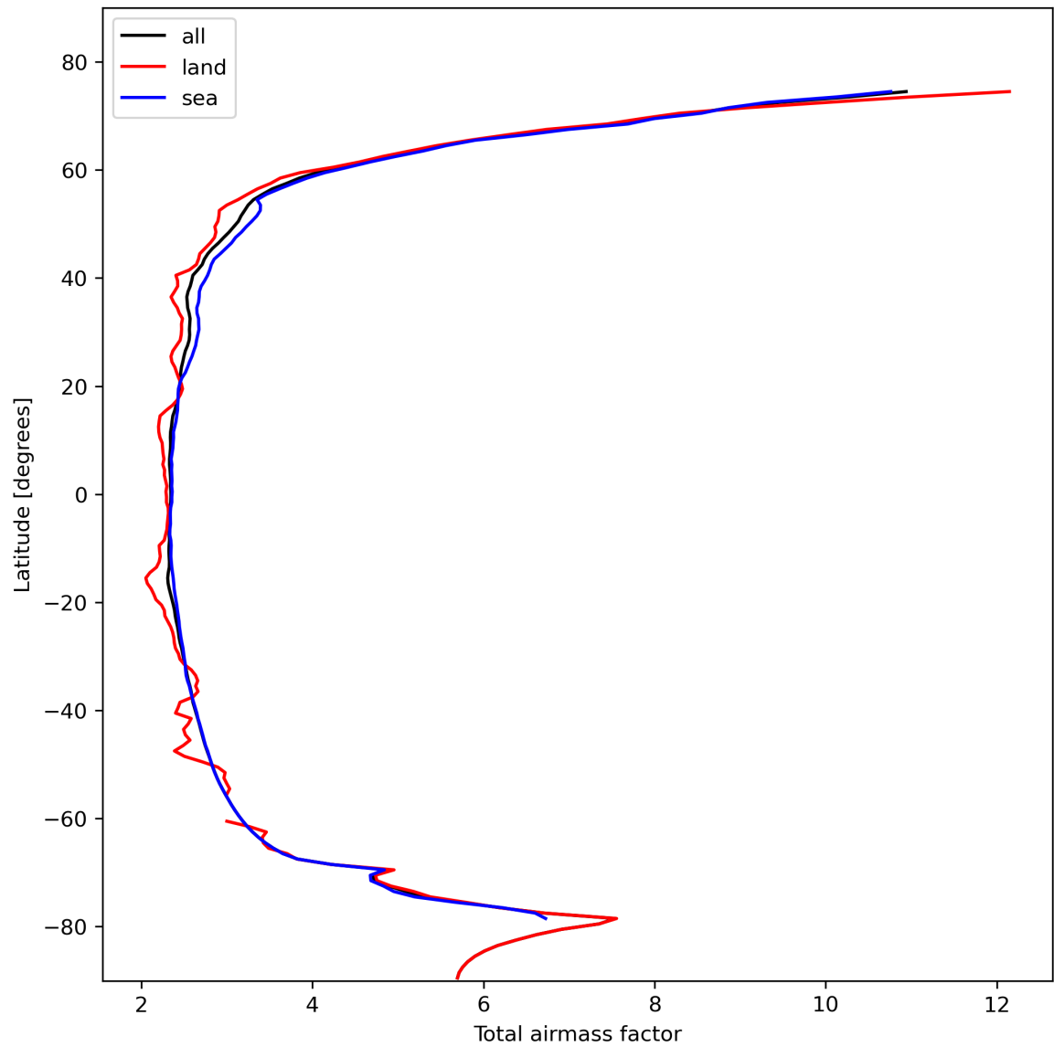
Figure 15: Zonal average of “Total airmass factor” for 2023-10-28 to 2023-10-30.
