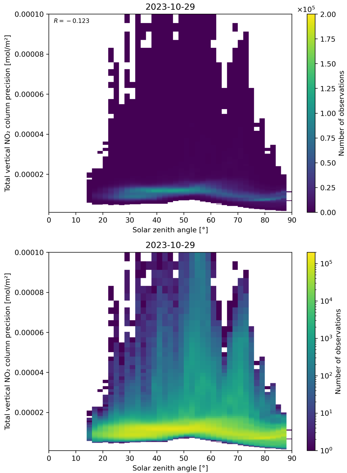
Figure 154: Scatter density plot of “Solar zenith angle” against “Total vertical NO 2 column precision” for 2023-10-28 to 2023-10-30.
