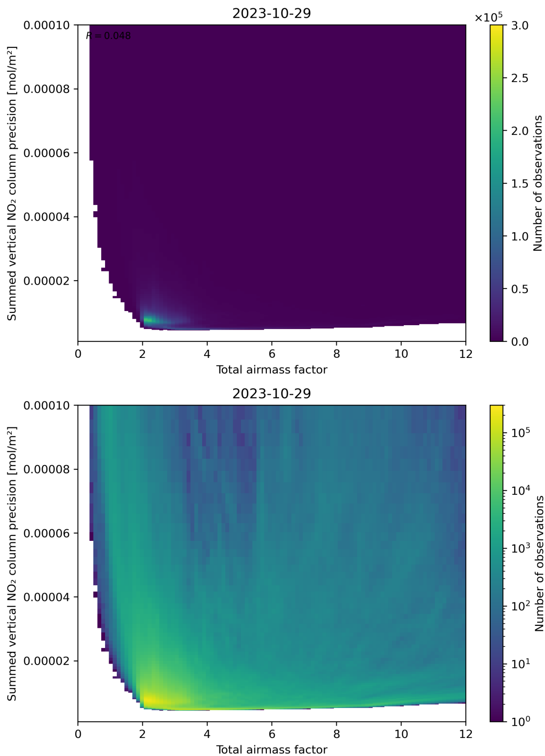
Figure 66: Scatter density plot of “Total airmass factor” against “Summed vertical NO 2 column precision” for 2023-10-28 to 2023-10-30.
