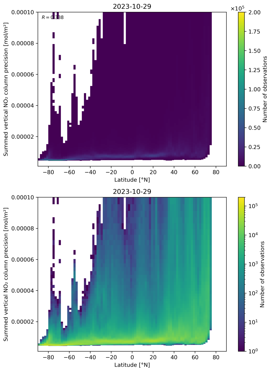
Figure 89: Scatter density plot of “Latitude” against “Summed vertical NO 2 column precision” for 2023-10-28 to 2023-10-30.
