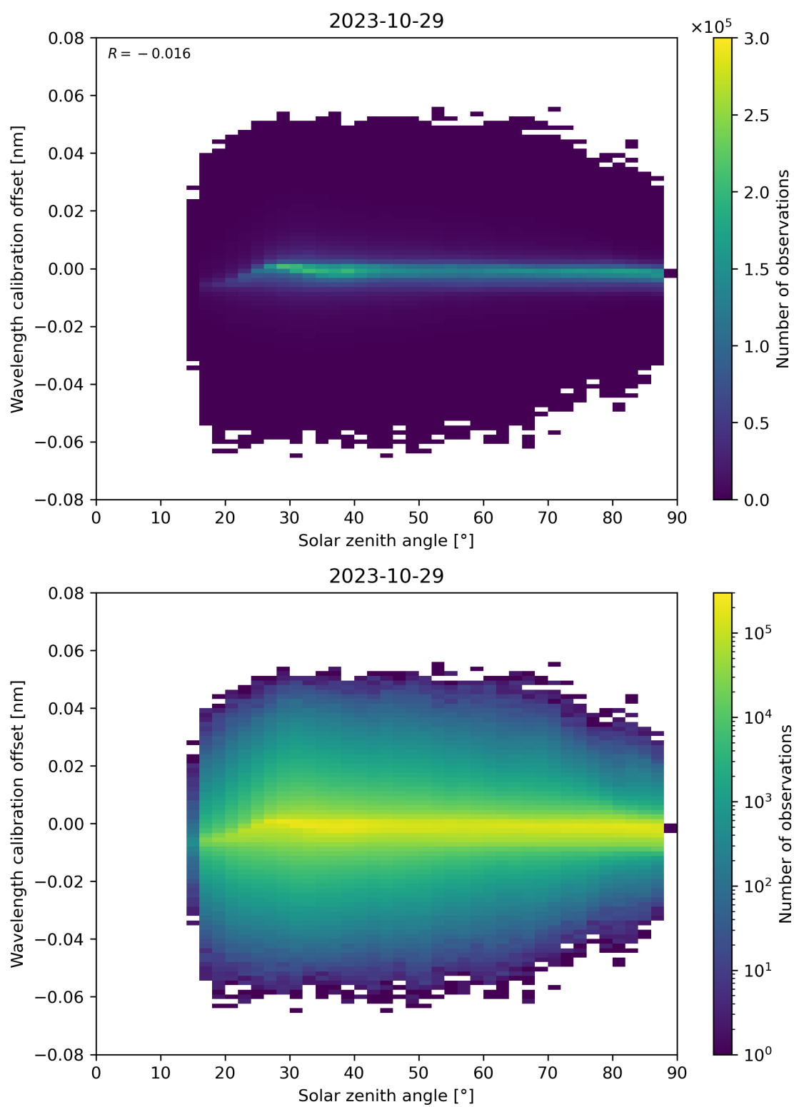
Figure 158: Scatter density plot of “Solar zenith angle” against “Wavelength calibration offset” for 2023-10-28 to 2023-10-30.
