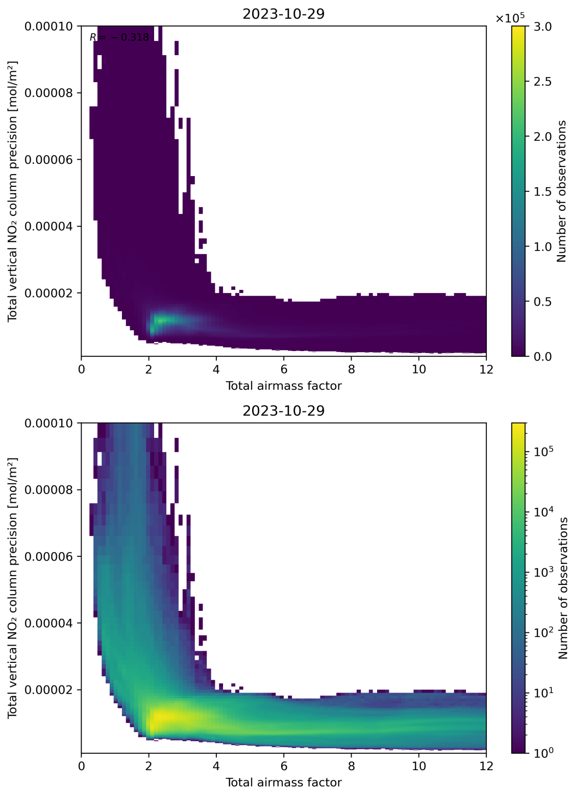
Figure 68: Scatter density plot of “Total airmass factor” against “Total vertical NO 2 column precision” for 2023-10-28 to 2023-10-30.
