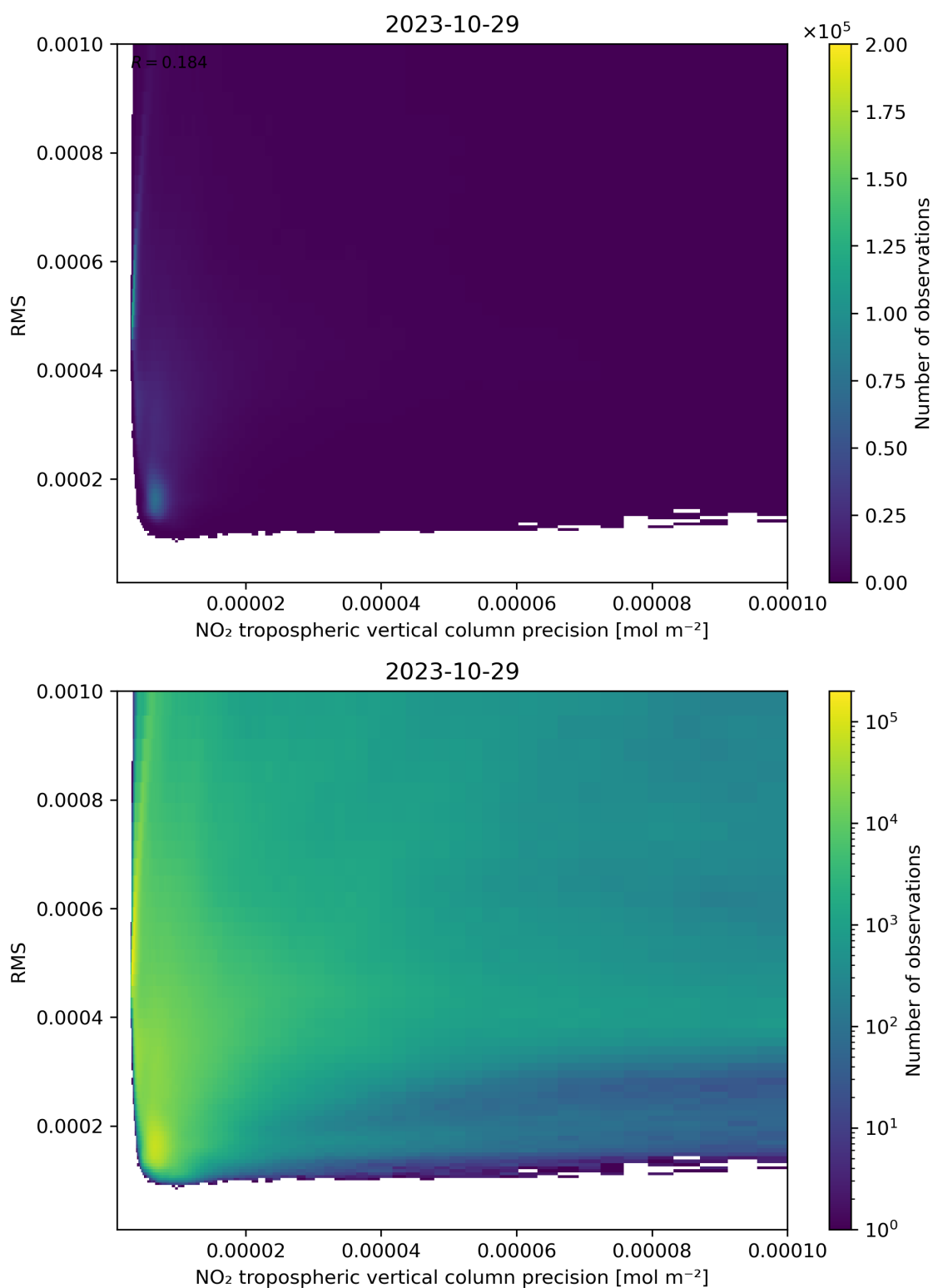
Figure 140: Scatter density plot of “NO 2 tropospheric vertical column precision” against “RMS” for 2023-10-28 to 2023-10-30.
