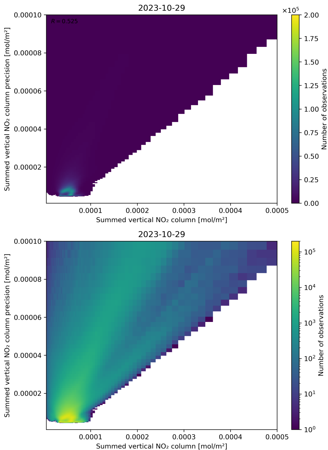
Figure 105: Scatter density plot of “Summed vertical NO 2 column” against “Summed vertical NO 2 column precision” for 2023-10-28 to 2023-10-30.
