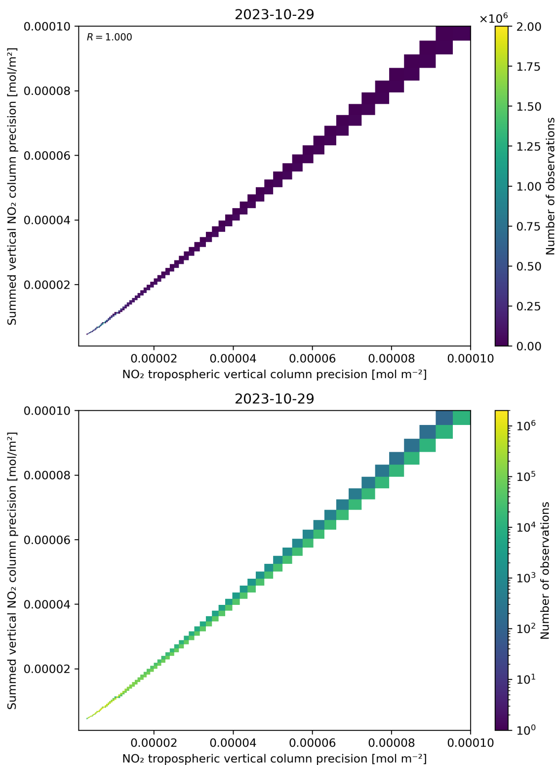
Figure 137: Scatter density plot of “NO 2 tropospheric vertical column precision” against “Summed vertical NO 2 column precision” for 2023-10-28 to 2023-10-30.
