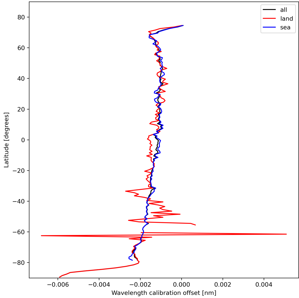
Figure 18: Zonal average of “Wavelength calibration offset” for 2023-10-28 to 2023-10-30.
