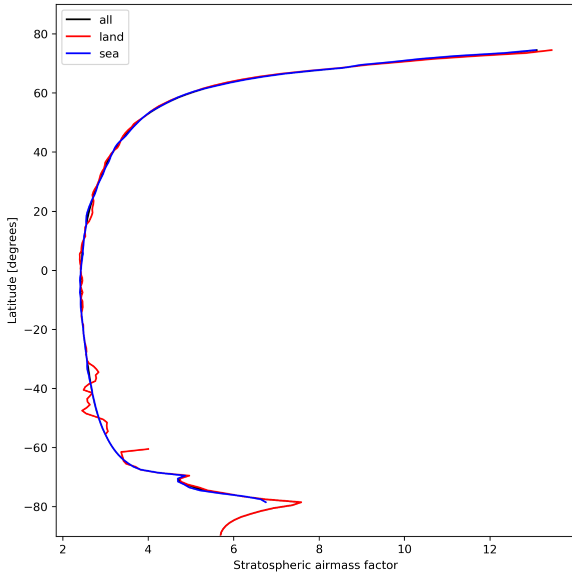
Figure 27: Zonal average of “Stratospheric air mass factor” for 2023-10-28 to 2023-10-30.
