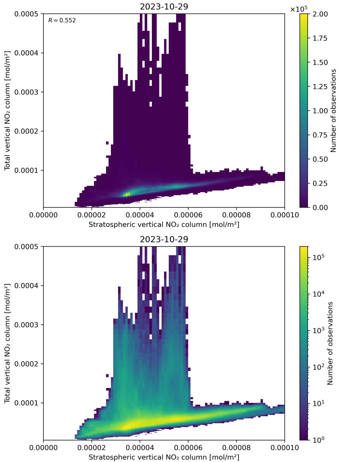
Figure 100: Scatter density plot of “Stratospheric vertical NO 2 column” against “Total vertical NO 2 column” for 2023-10-28 to 2023-10-30.
