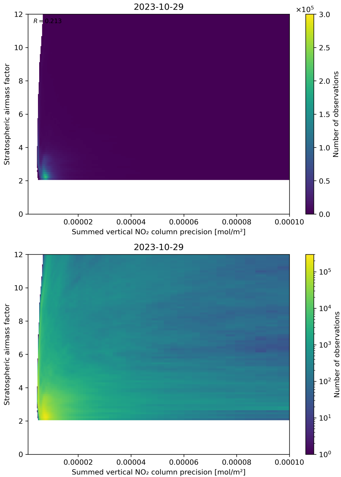
Figure 106: Scatter density plot of “Summed vertical NO 2 column precision” against “Stratospheric airmass factor” for 2023-10-28 to 2023-10-30.
