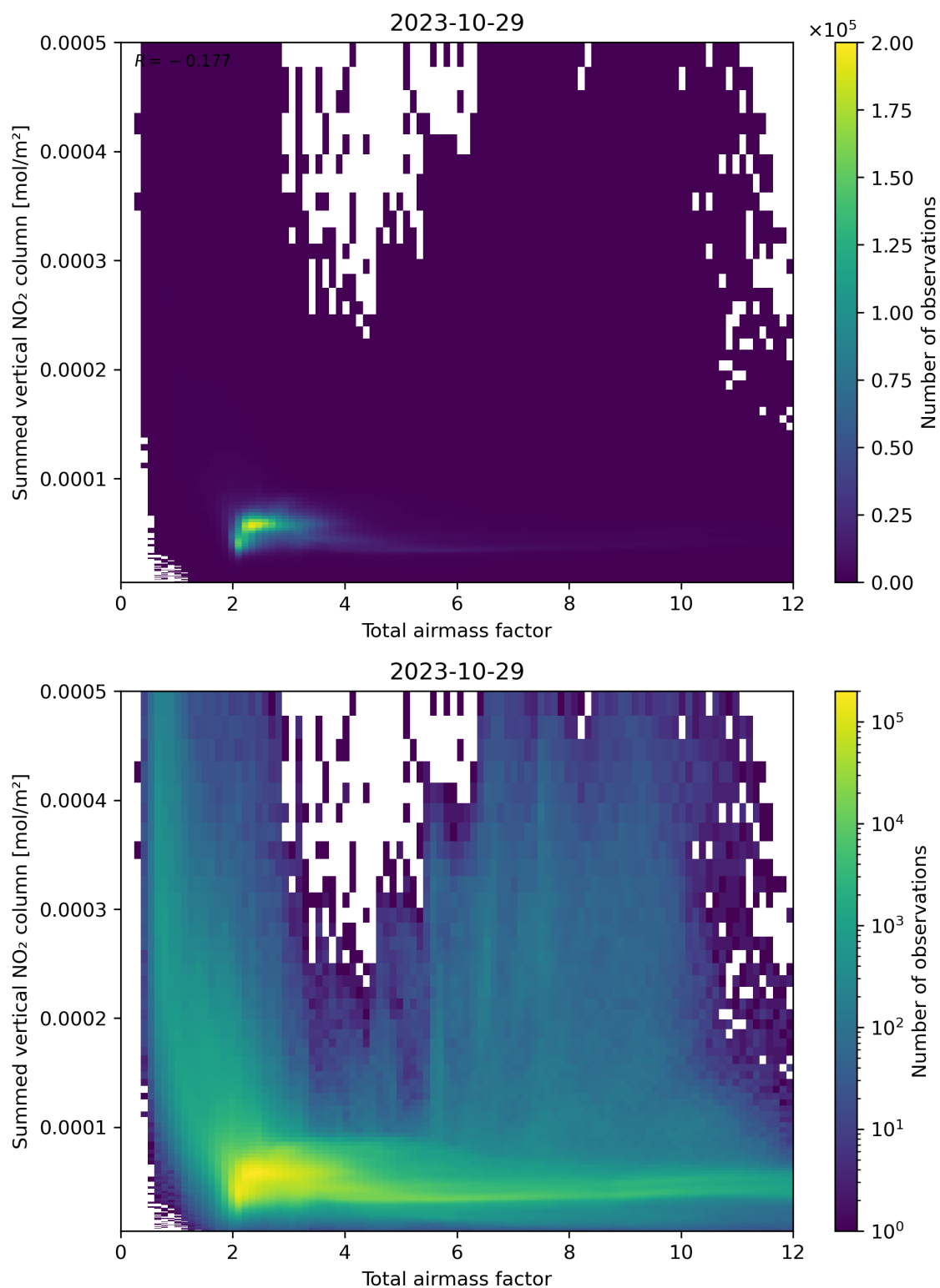
Figure 65: Scatter density plot of “Total airmass factor” against “Summed vertical NO 2 column” for 2023-10-28 to 2023-10-30.
