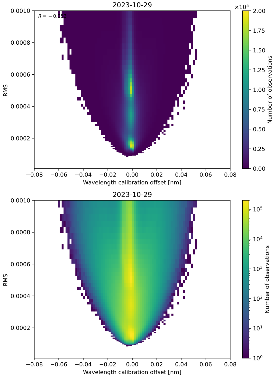
Figure 181: Scatter density plot of “Wavelength calibration offset” against “RMS” for 2023-10-28 to 2023-10-30.
