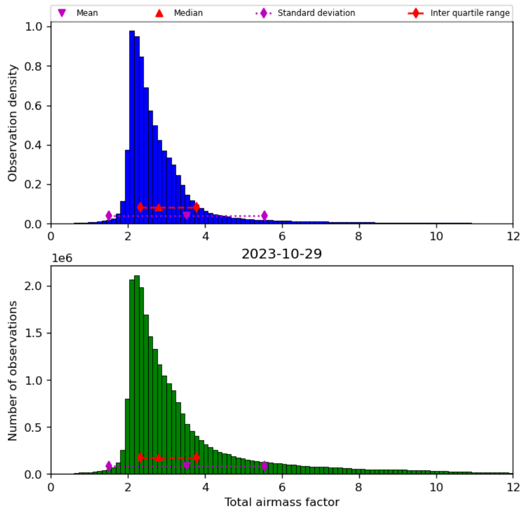
Figure 32: Histogram of “Total airmass factor” for 2023-10-28 to 2023-10-30
