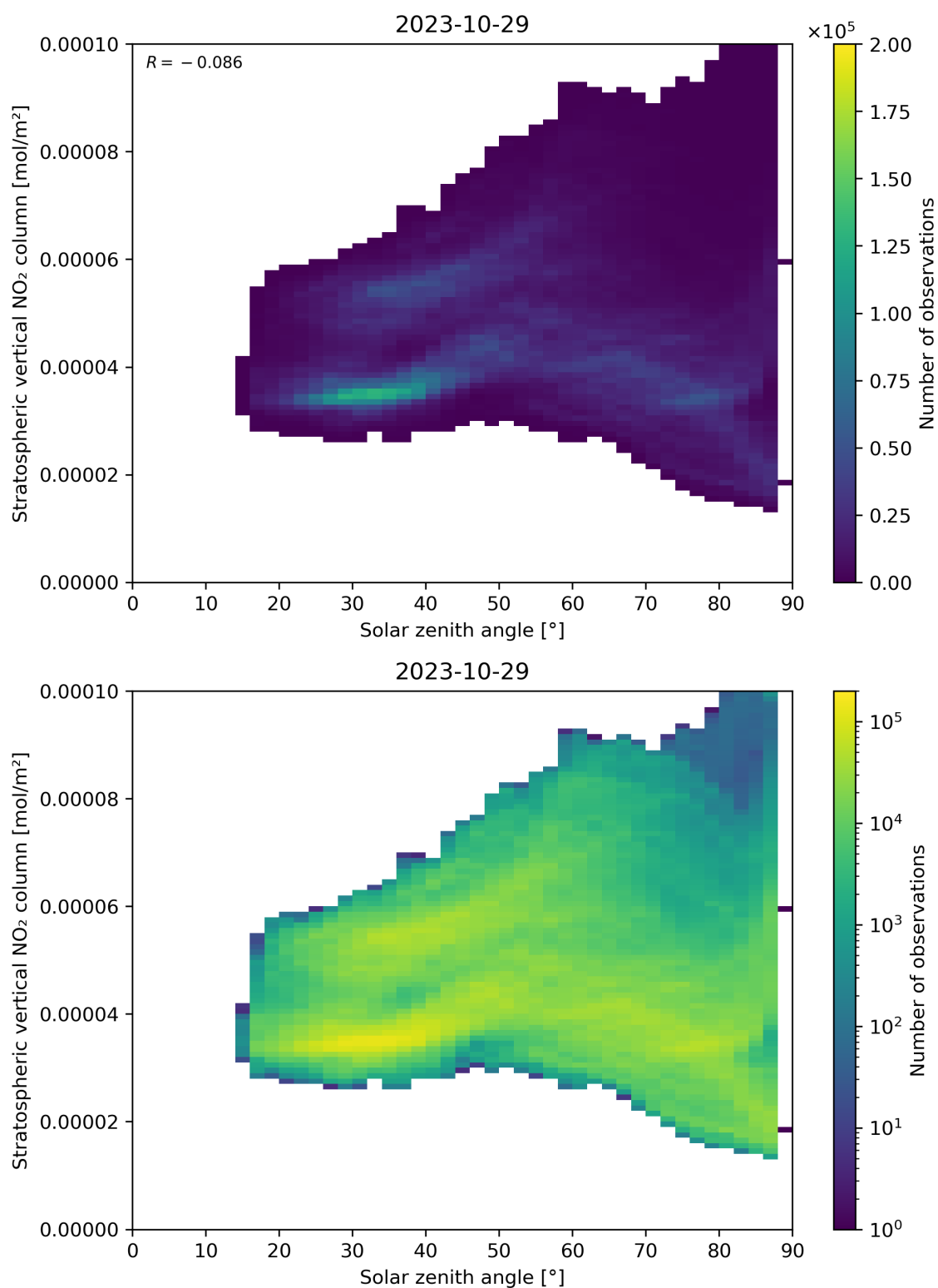
Figure 150: Scatter density plot of “Solar zenith angle” against “Stratospheric vertical NO 2 column” for 2023-10-28 to 2023-10-30.
