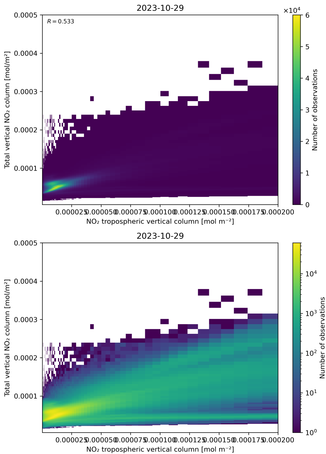
Figure 128: Scatter density plot of “NO 2 tropospheric vertical column” against “Total vertical NO 2 column” for 2023-10-28 to 2023-10-30.
