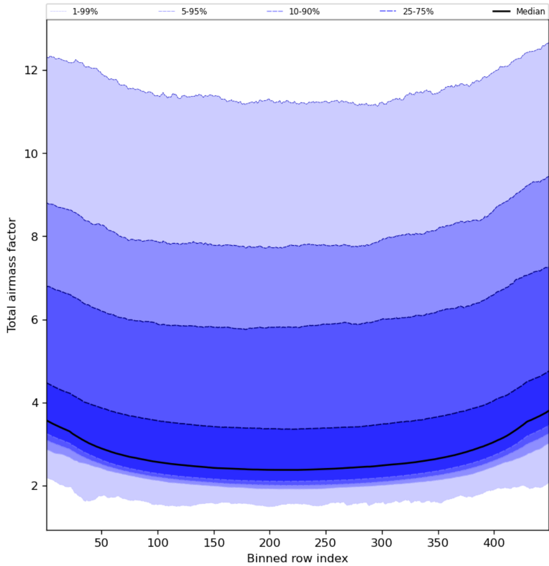
Figure 49: Along track statistics of “Total airmass factor” for 2023-10-28 to 2023-10-30
