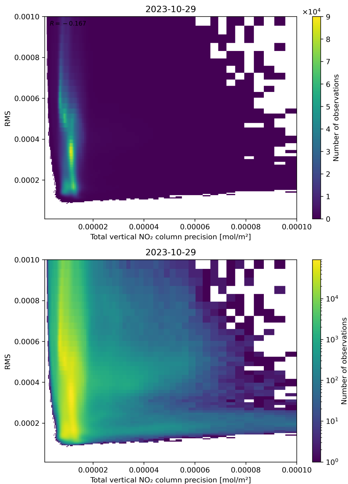
Figure 119: Scatter density plot of “Total vertical NO 2 column precision” against “RMS” for 2023-10-28 to 2023-10-30.
