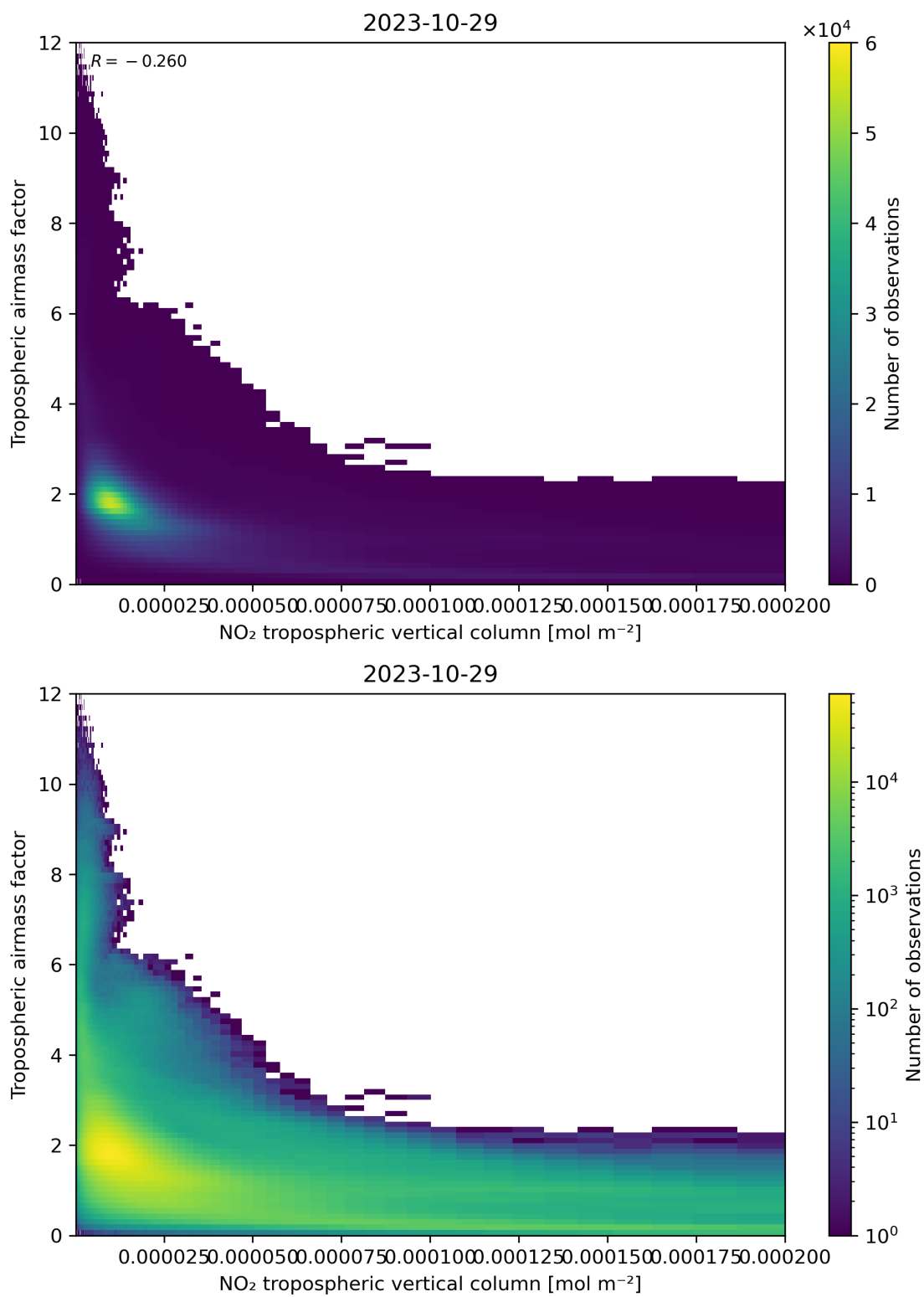
Figure 123: Scatter density plot of “NO 2 tropospheric vertical column” against “Tropospheric air mass factor” for 2023-10-28 to 2023-10-30.
