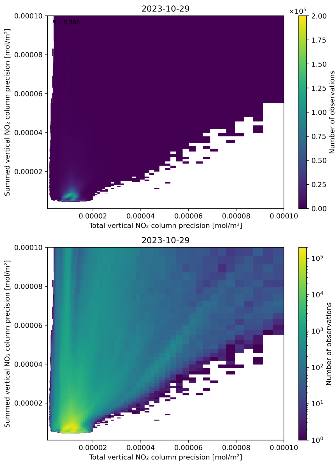
Figure 118: Scatter density plot of “Total vertical NO 2 column precision” against “Summed vertical NO 2 column precision” for 2023-10-28 to 2023-10-30.
