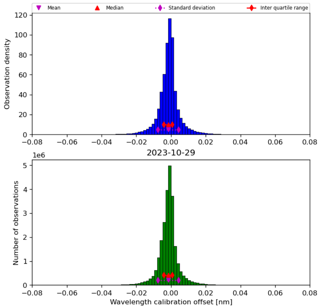
Figure 35: Histogram of “Wavelength calibration offset” for 2023-10-28 to 2023-10-30
