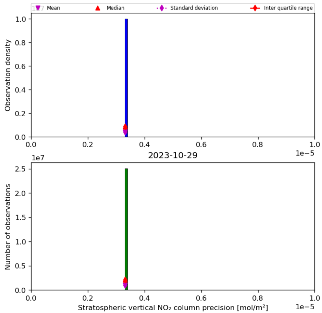
Figure 37: Histogram of “Stratospheric vertical NO 2 column precision” for 2023-10-28 to 2023-10-30
