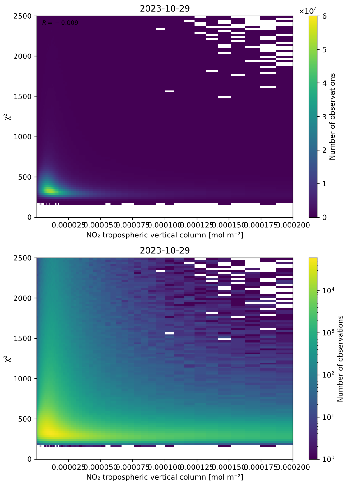
Figure 124: Scatter density plot of “NO 2 tropospheric vertical column” against “ \chi^2 ” for 2023-10-28 to 2023-10-30.
