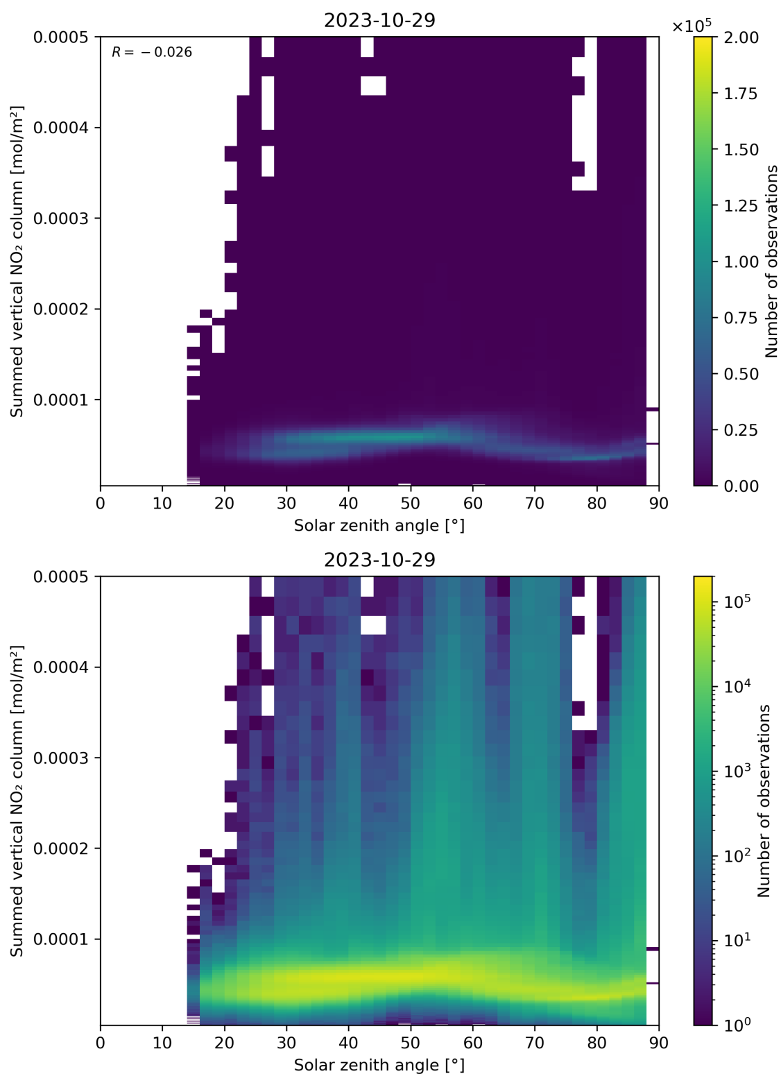
Figure 151: Scatter density plot of “Solar zenith angle” against “Summed vertical NO 2 column” for 2023-10-28 to 2023-10-30.
