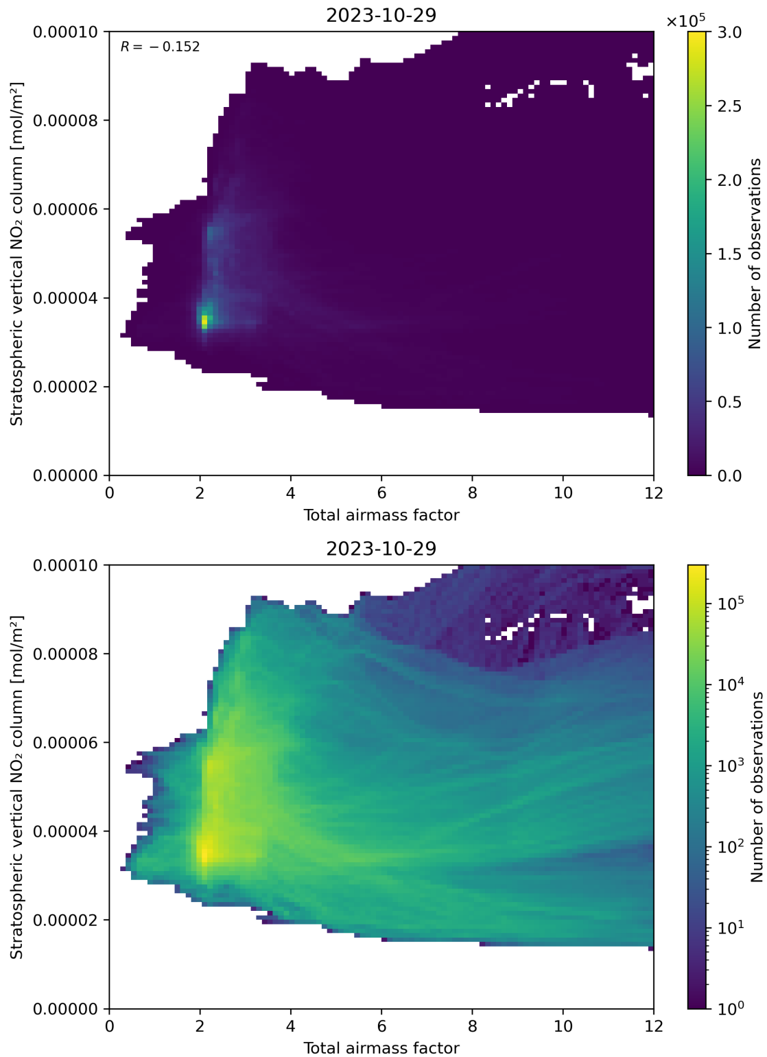
Figure 64: Scatter density plot of “Total airmass factor” against “Stratospheric vertical \text{NO}_2 column” for 2023-10-28 to 2023-10-30.
