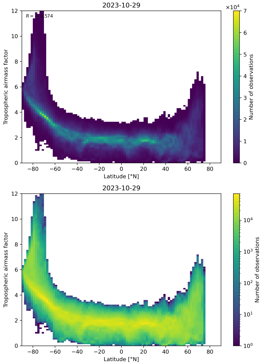
Figure 85: Scatter density plot of “Latitude” against “Tropospheric air mass factor” for 2023-10-28 to 2023-10-30.
