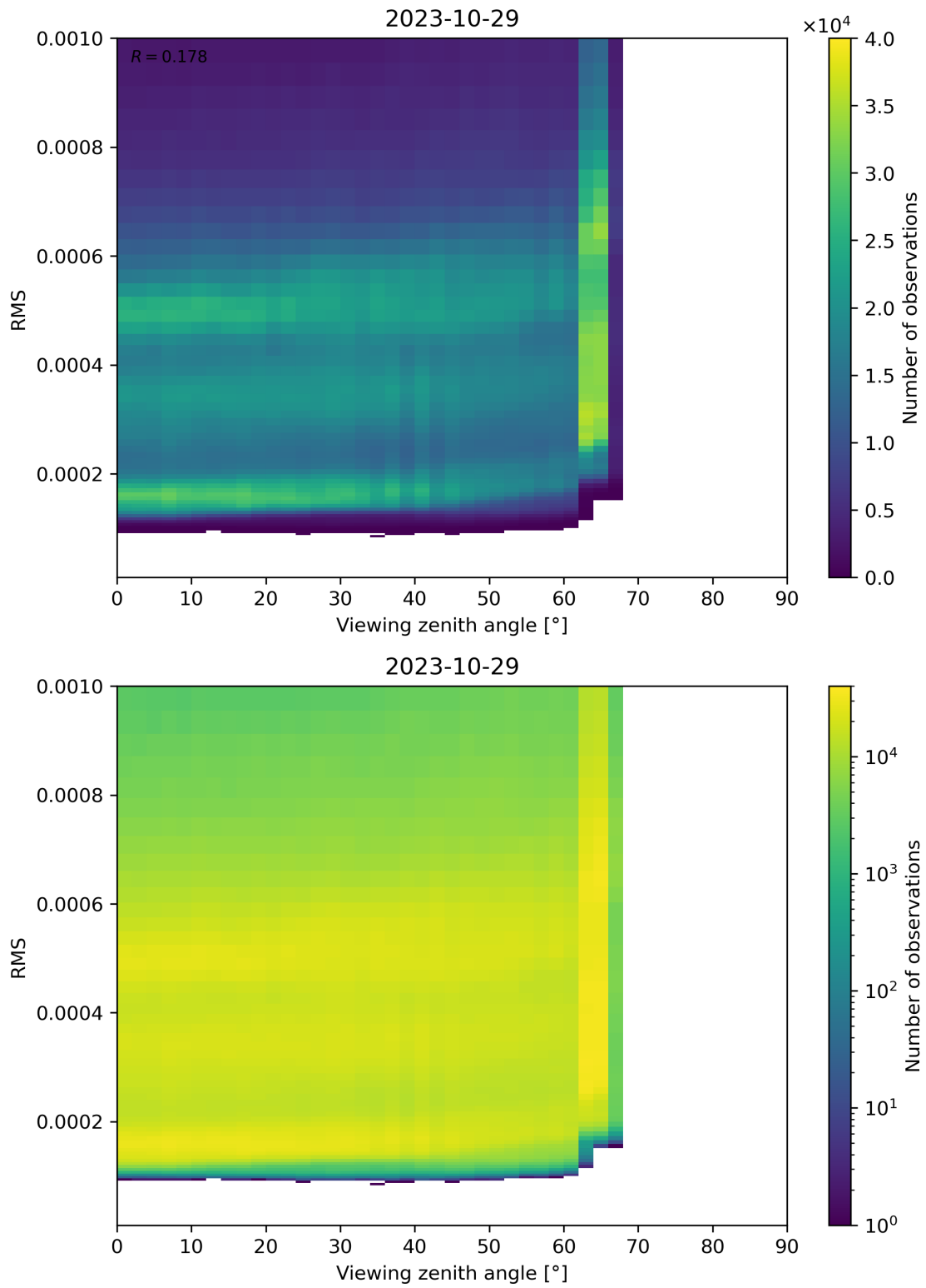
Figure 171: Scatter density plot of “Viewing zenith angle” against “RMS” for 2023-10-28 to 2023-10-30.
