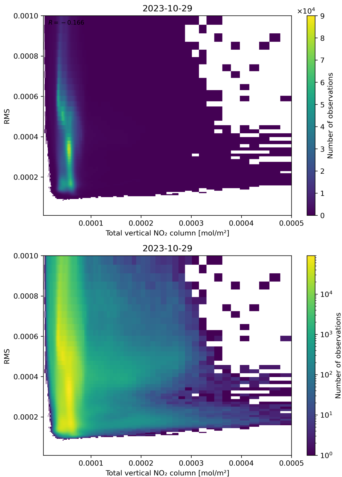
Figure 120: Scatter density plot of “Total vertical NO 2 column” against “RMS” for 2023-10-28 to 2023-10-30.
