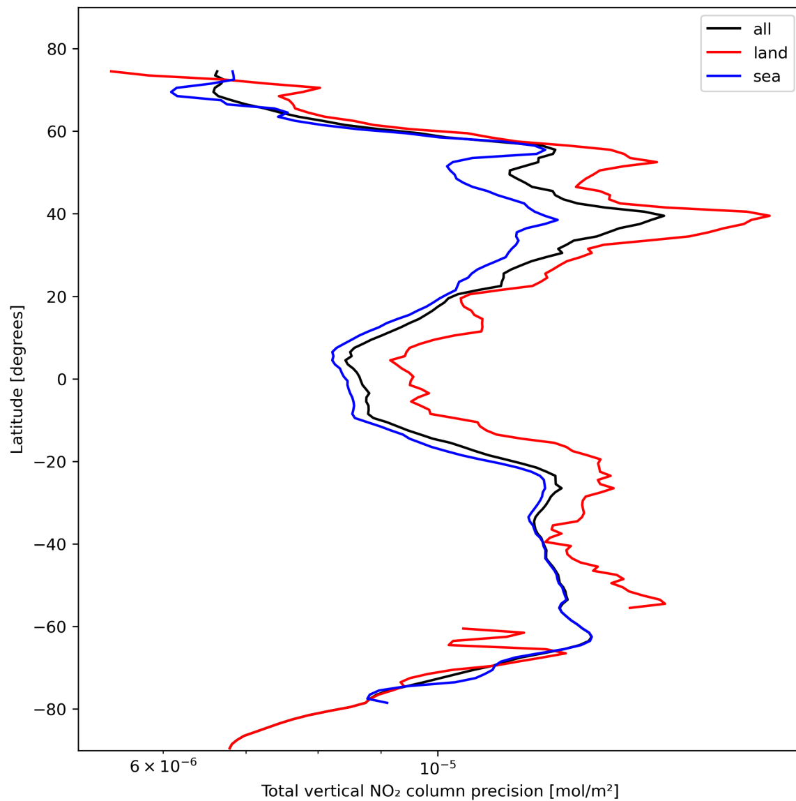
Figure 22: Zonal average of “Total vertical NO 2 column precision” for 2023-10-28 to 2023-10-30.
