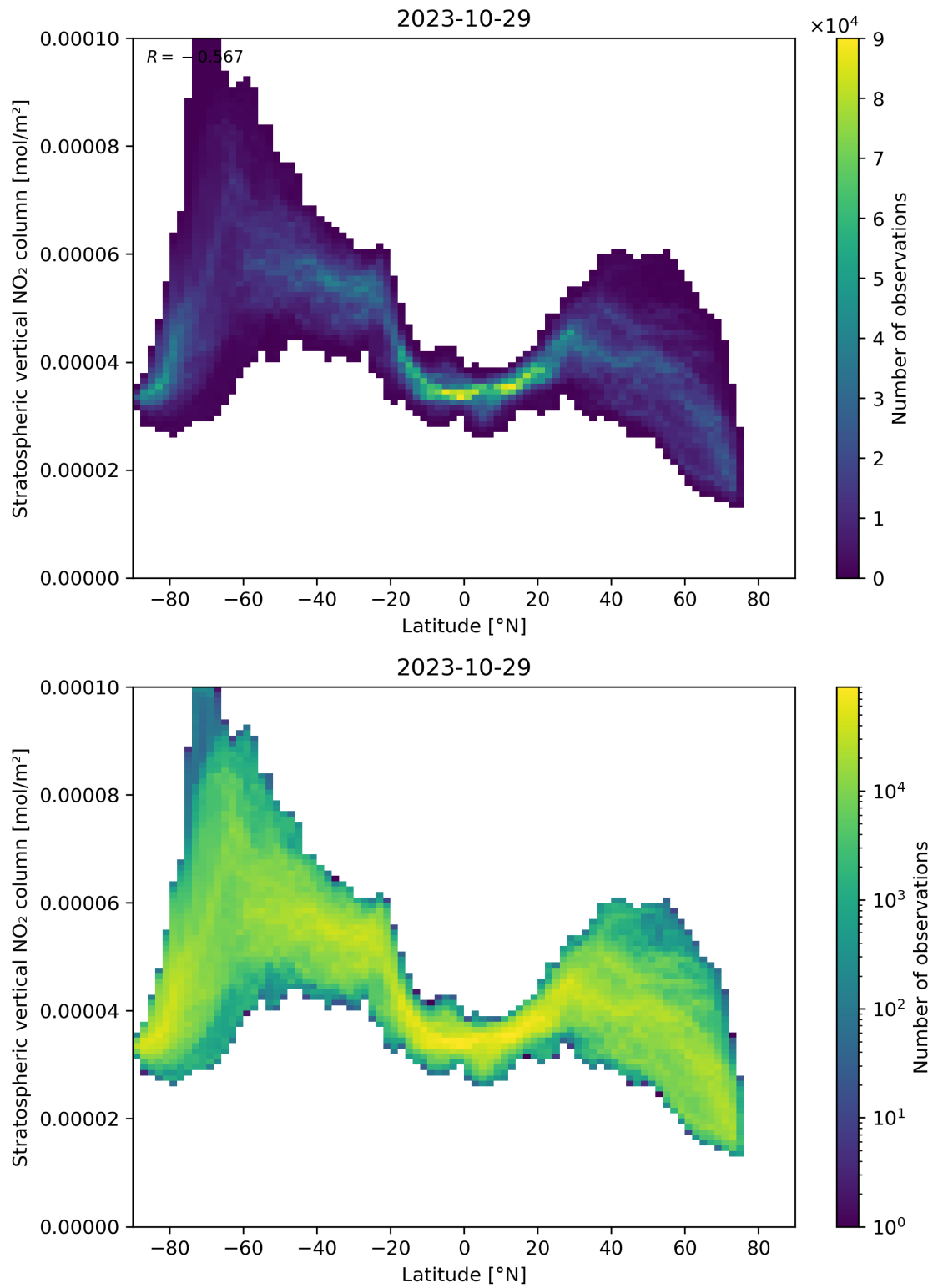
Figure 87: Scatter density plot of “Latitude” against “Stratospheric vertical NO 2 column” for 2023-10-28 to 2023-10-30.
