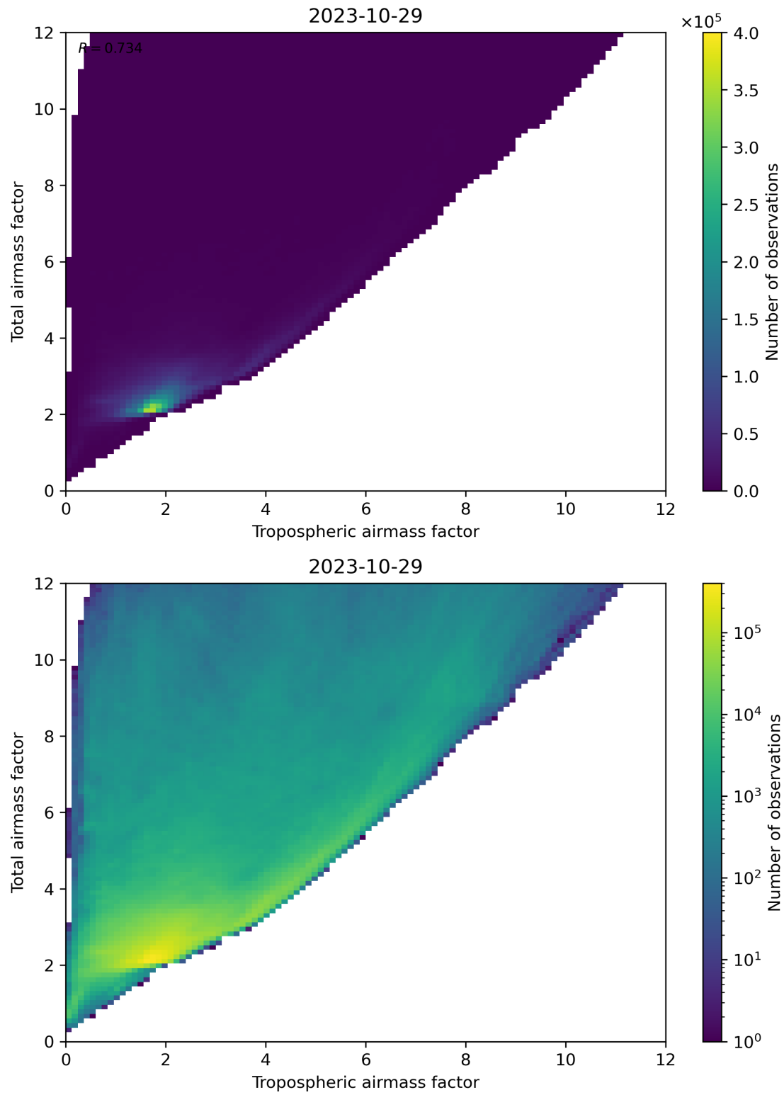
Figure 72: Scatter density plot of “Tropospheric airmass factor” against “Total airmass factor” for 2023-10-28 to 2023-10-30.
