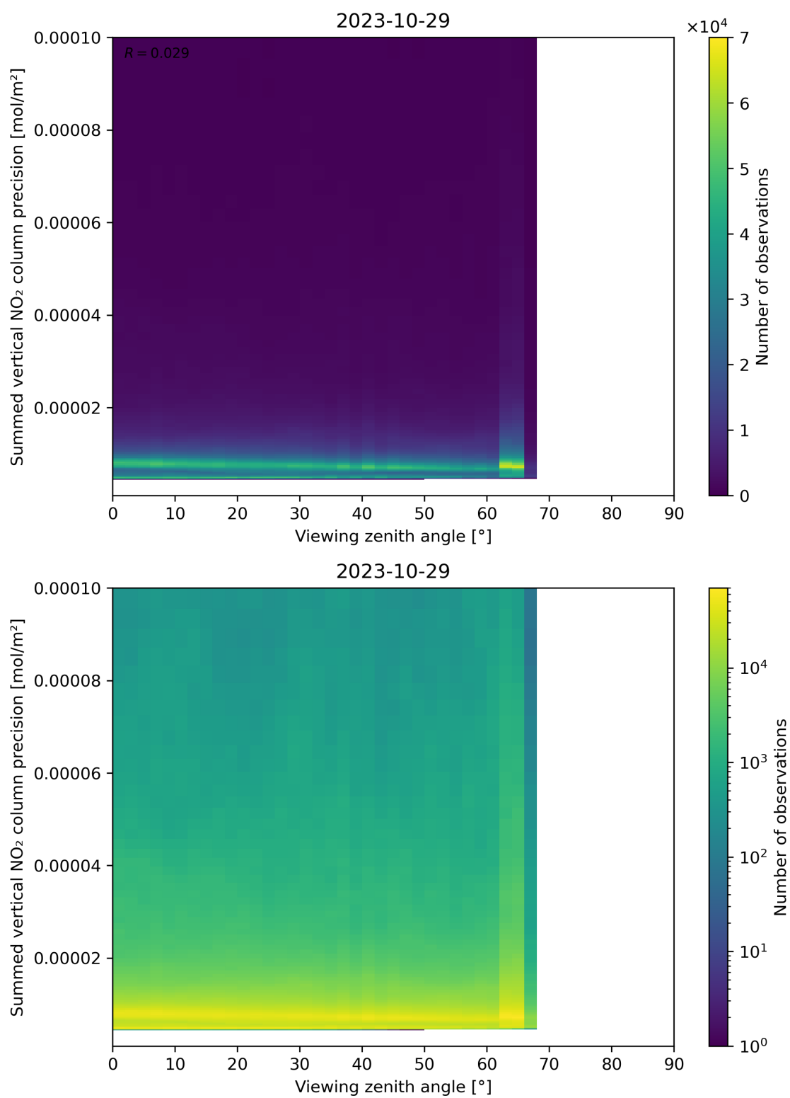
Figure 166: Scatter density plot of “Viewing zenith angle” against “Summed vertical NO 2 column precision” for 2023-10-28 to 2023-10-30.
