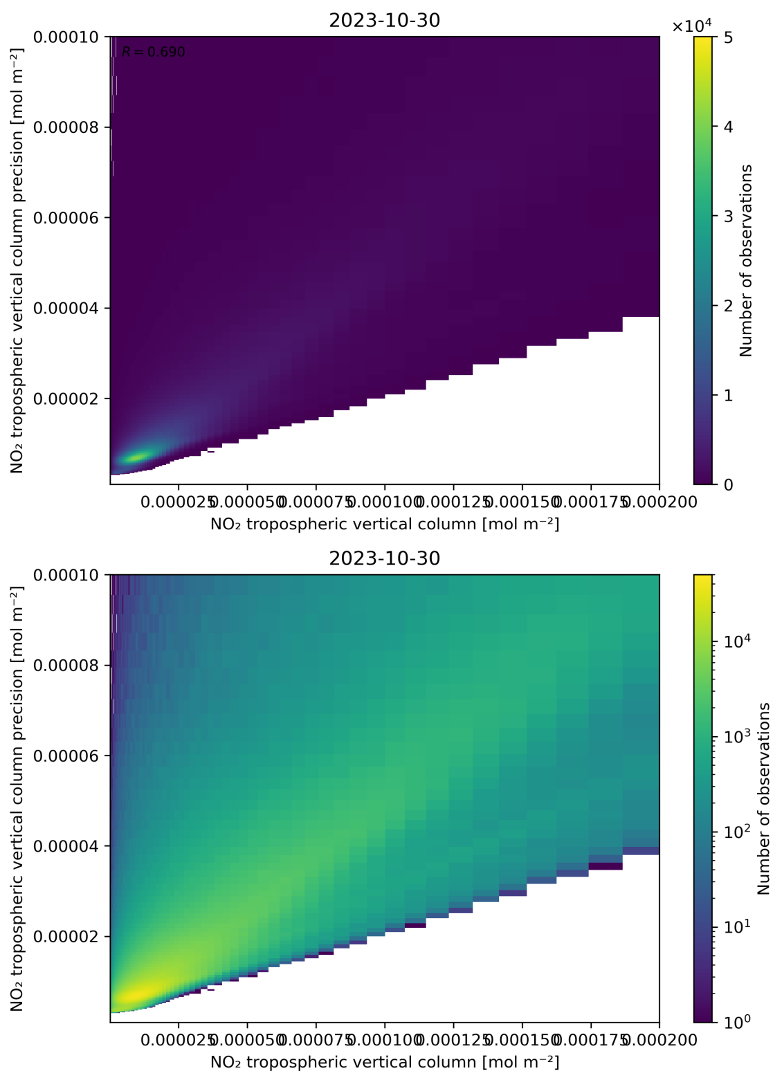
Figure 130: Scatter density plot of “NO 2 tropospheric vertical column” against “NO 2 tropospheric vertical column precision” for 2023-10-29 to 2023-10-31.
