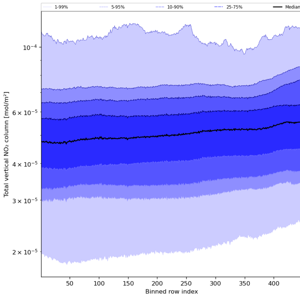
Figure 55: Along track statistics of “Total vertical NO 2 column” for 2023-10-29 to 2023-10-31
