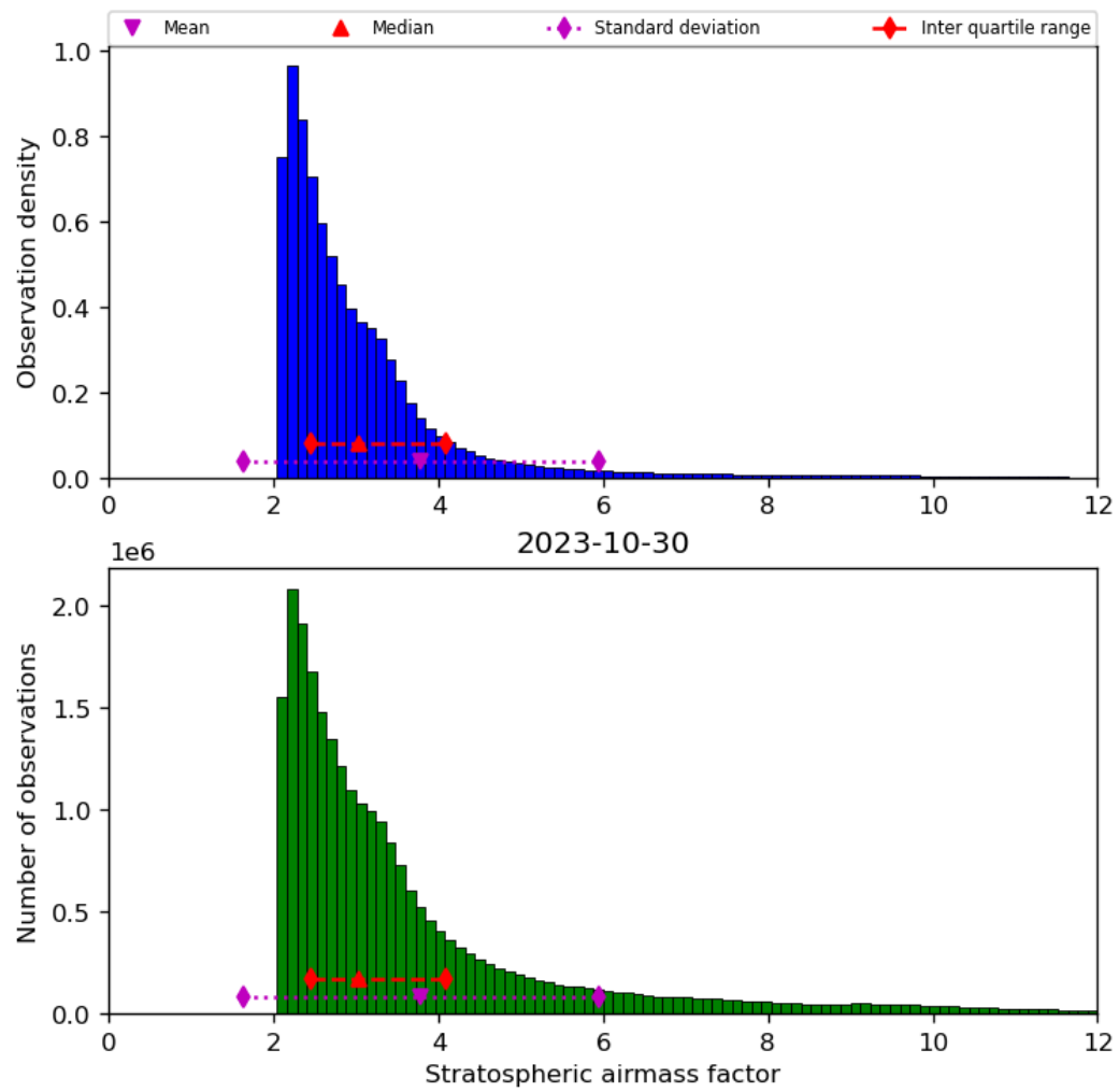
Figure 44: Histogram of “Stratospheric airmass factor” for 2023-10-29 to 2023-10-31
