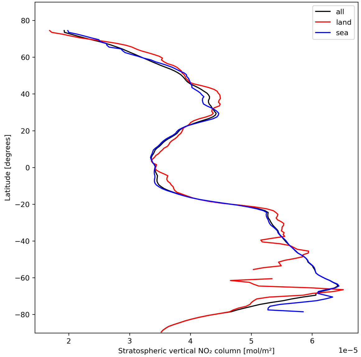
Figure 19: Zonal average of “Stratospheric vertical NO 2 column” for 2023-10-29 to 2023-10-31.
