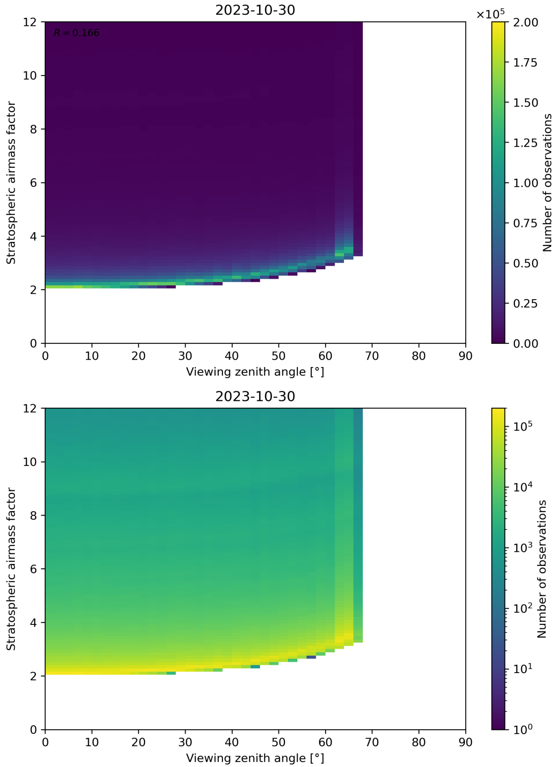
Figure 159: Scatter density plot of “Viewing zenith angle” against “Stratospheric airmass factor” for 2023-10-29 to 2023-10-31.
