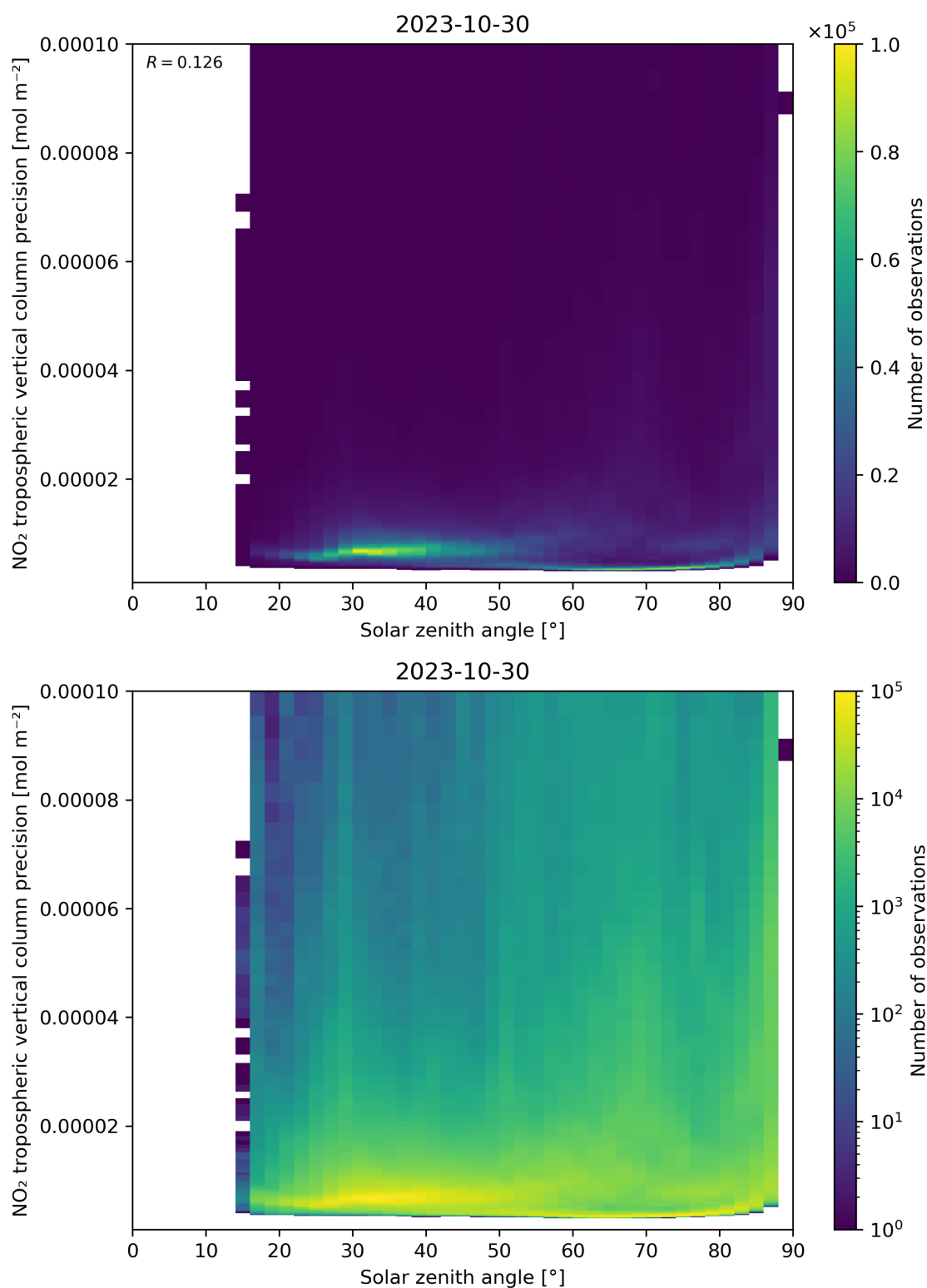
Figure 156: Scatter density plot of “Solar zenith angle” against “NO 2 tropospheric vertical column precision” for 2023-10-29 to 2023-10-31.
