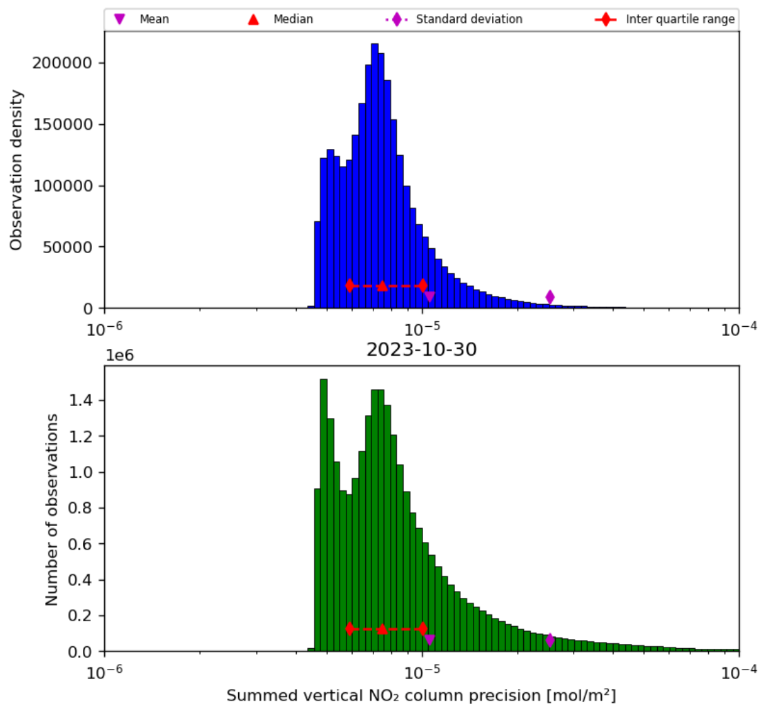
Figure 41: Histogram of “Summed vertical NO 2 column precision” for 2023-10-29 to 2023-10-31
