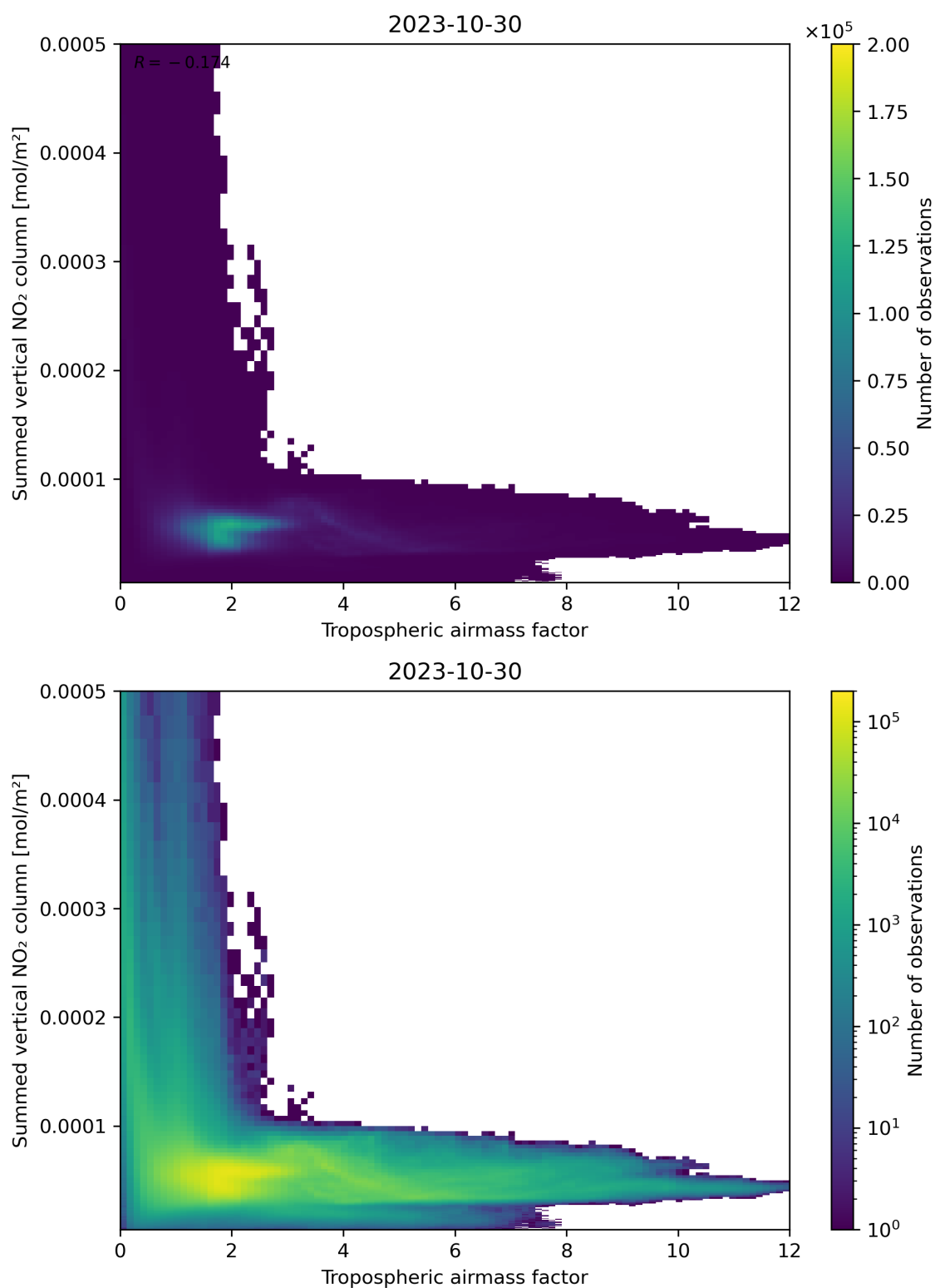
Figure 75: Scatter density plot of “Tropospheric air mass factor” against “Summed vertical NO 2 column” for 2023-10-29 to 2023-10-31.
