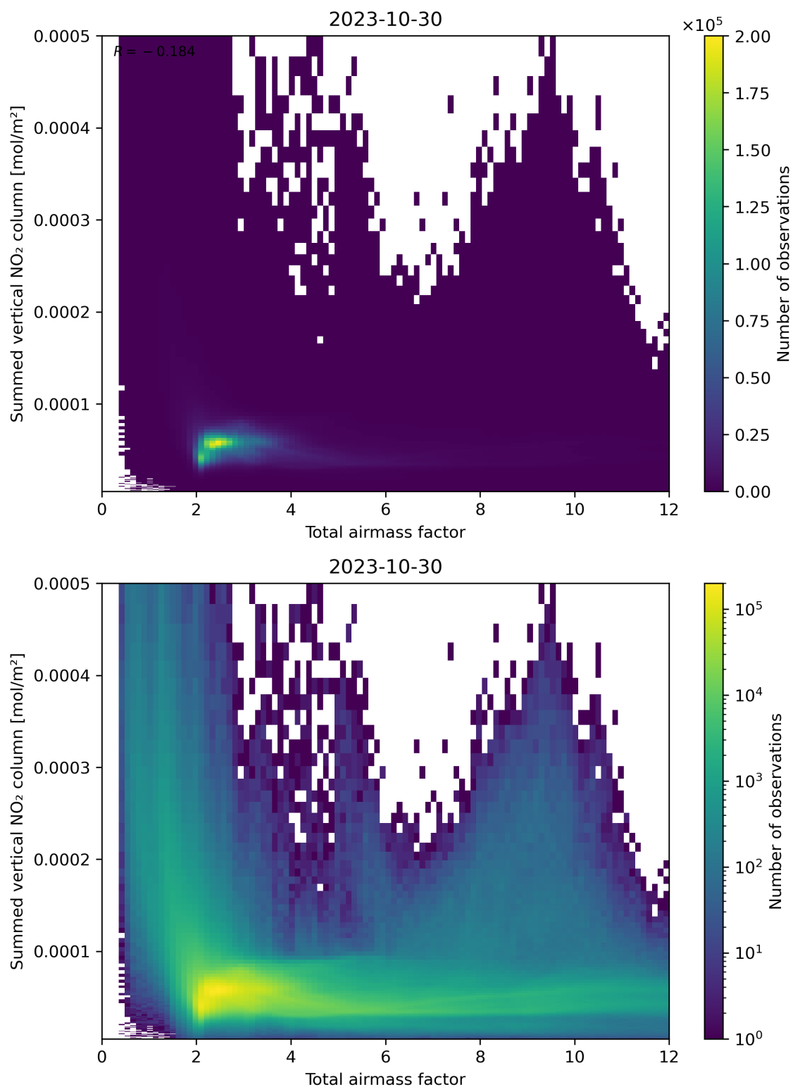
Figure 65: Scatter density plot of “Total airmass factor” against “Summed vertical NO 2 column” for 2023-10-29 to 2023-10-31.
