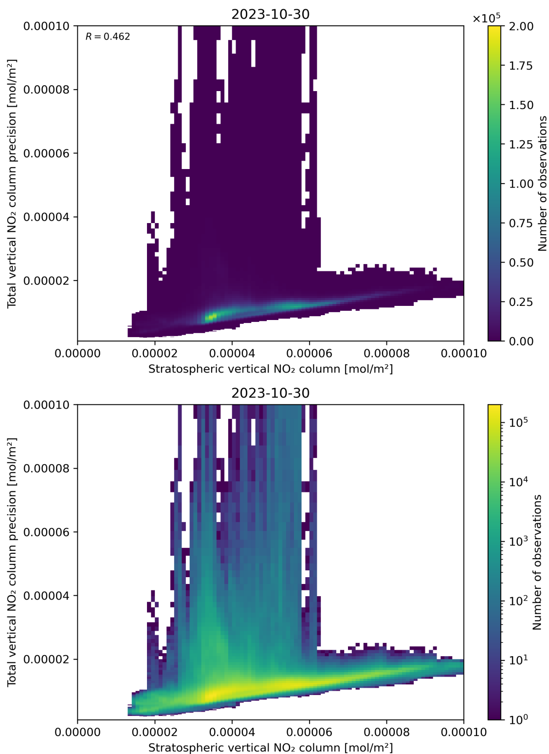
Figure 101: Scatter density plot of “Stratospheric vertical NO 2 column” against “Total vertical NO 2 column precision” for 2023-10-29 to 2023-10-31.
