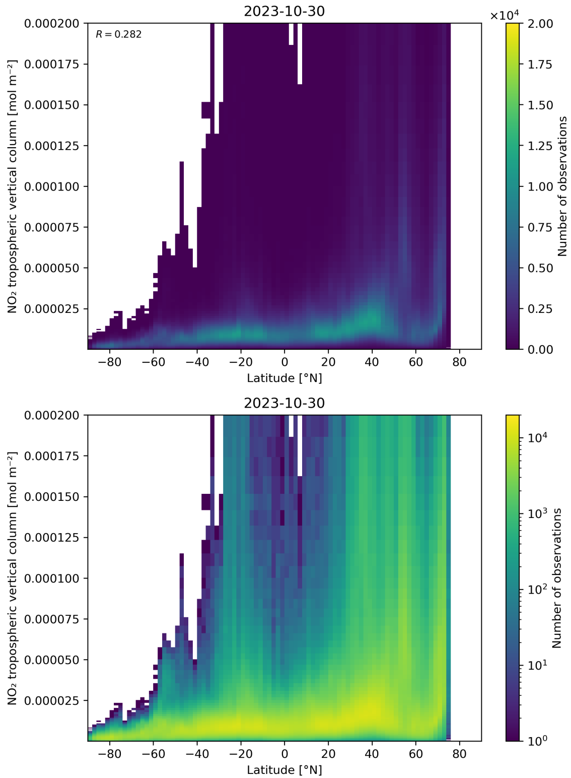
Figure 92: Scatter density plot of “Latitude” against “NO 2 tropospheric vertical column” for 2023-10-29 to 2023-10-31.
