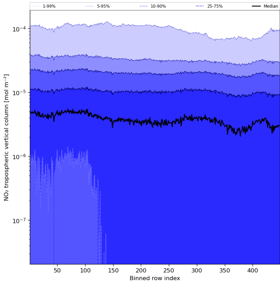
Figure 46: Along track statistics of “NO 2 tropospheric vertical column” for 2023-10-29 to 2023-10-31
