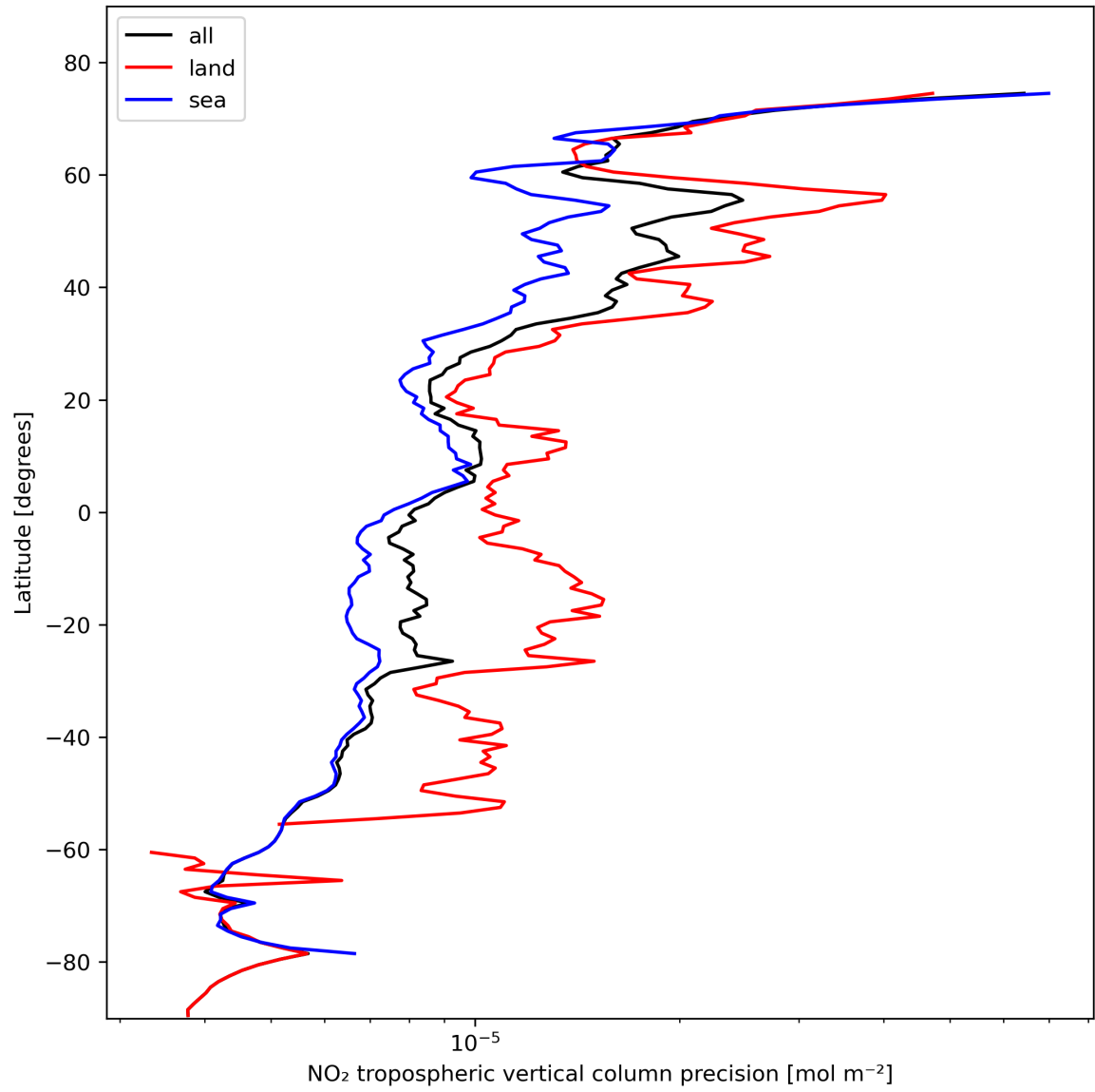
Figure 13: Zonal average of "NO 2 tropospheric vertical column precision" for 2023-10-29 to 2023-10-31.
