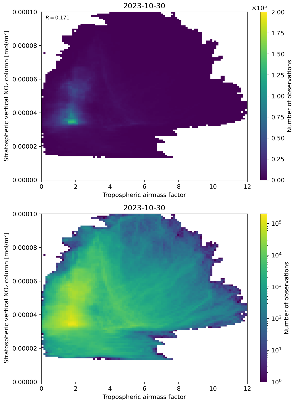
Figure 74: Scatter density plot of “Tropospheric air mass factor” against “Stratospheric vertical NO 2 column” for 2023-10-29 to 2023-10-31.
