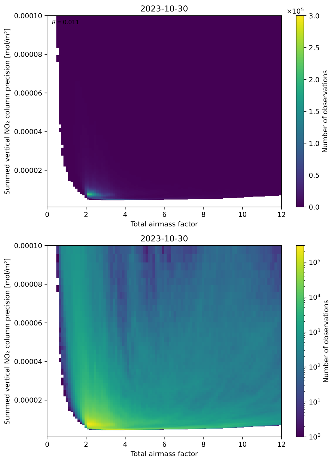
Figure 66: Scatter density plot of “Total airmass factor” against “Summed vertical NO 2 column precision” for 2023-10-29 to 2023-10-31.
