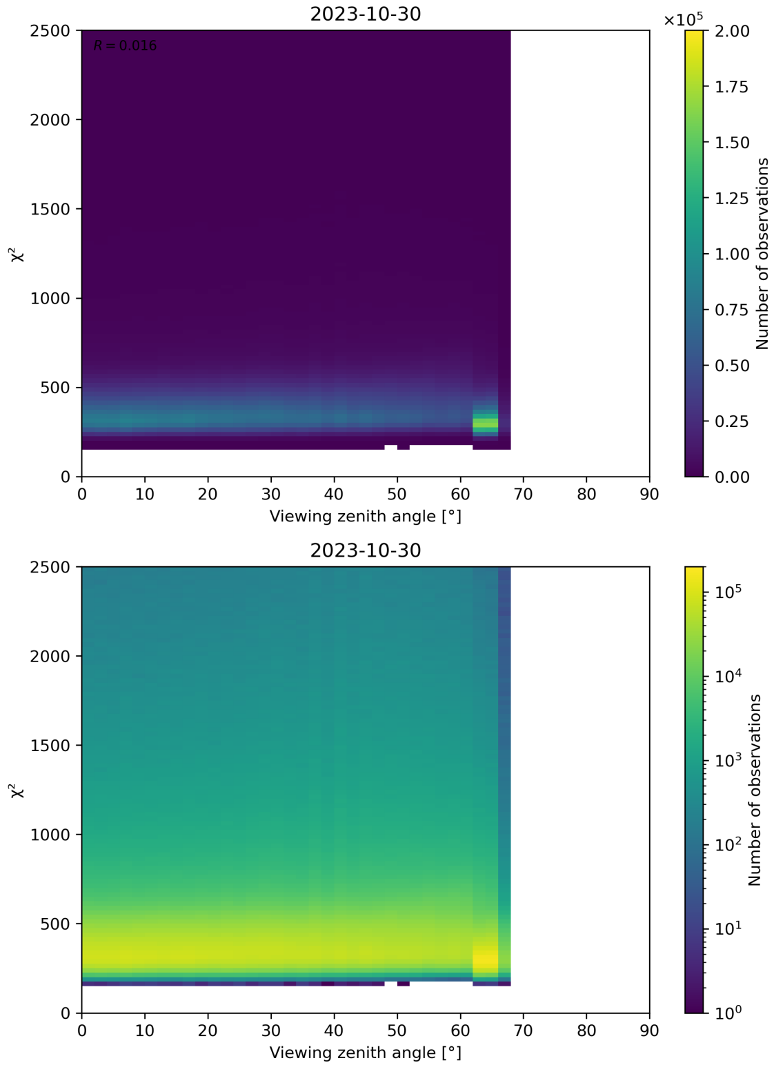
Figure 162: Scatter density plot of “Viewing zenith angle” against “ \chi^2 ” for 2023-10-29 to 2023-10-31.
