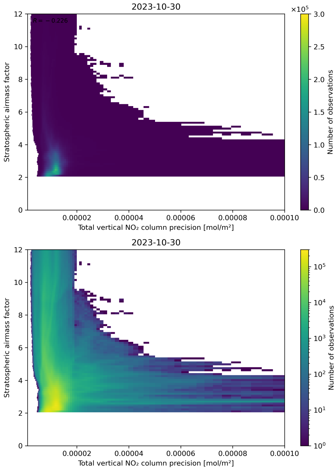
Figure 115: Scatter density plot of “Total vertical NO 2 column precision” against “Stratospheric air mass factor” for 2023-10-29 to 2023-10-31.
