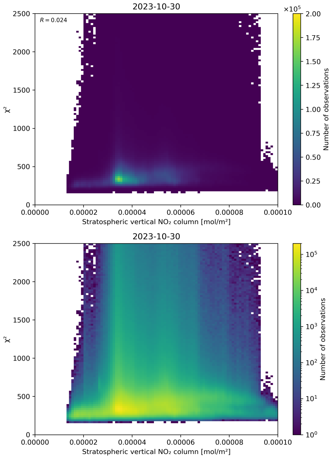
Figure 97: Scatter density plot of “Stratospheric vertical NO 2 column” against “ \chi^2 ” for 2023-10-29 to 2023-10-31.
