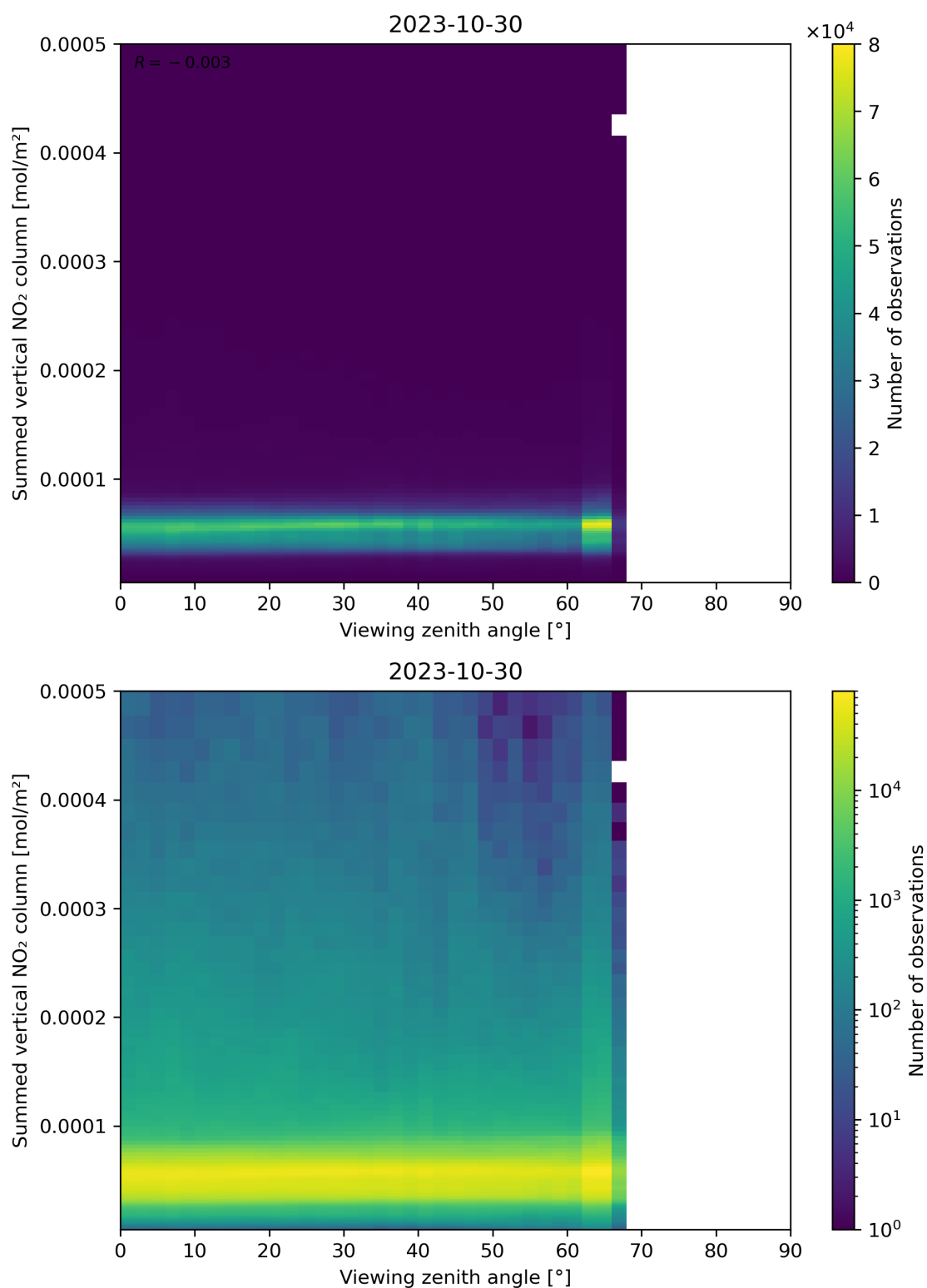
Figure 165: Scatter density plot of “Viewing zenith angle” against “Summed vertical NO 2 column” for 2023-10-29 to 2023-10-31.
