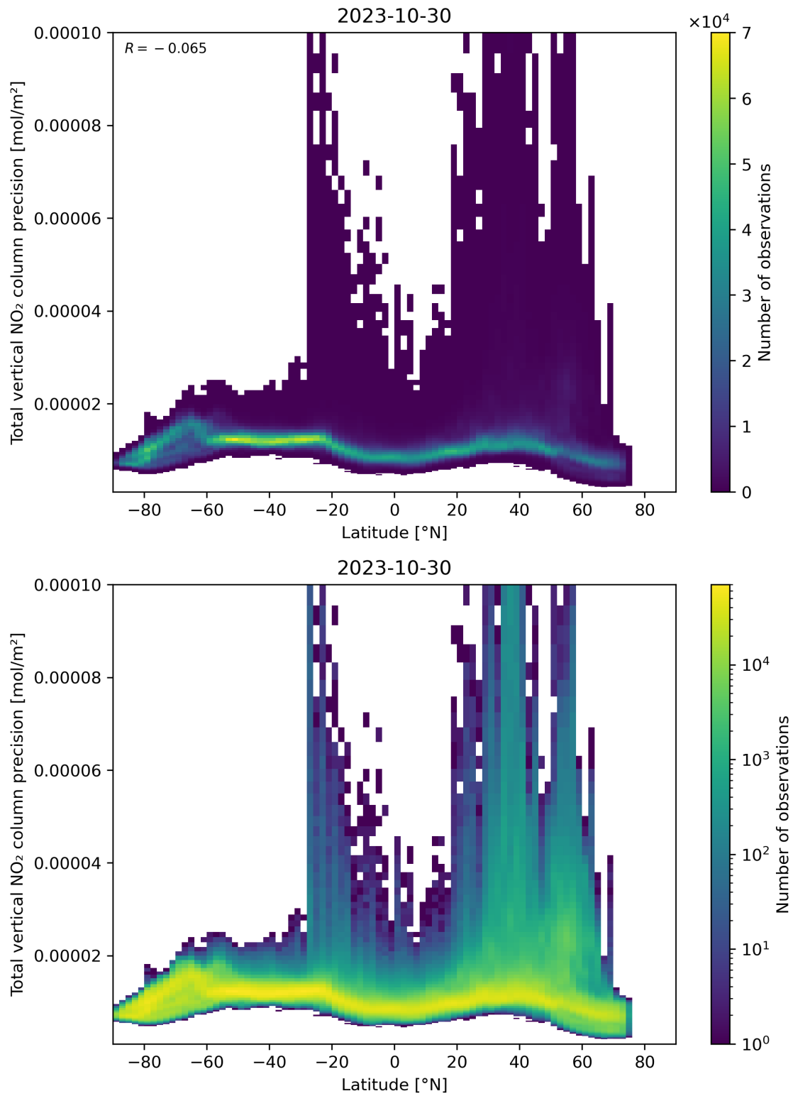
Figure 91: Scatter density plot of “Latitude” against “Total vertical NO 2 column precision” for 2023-10-29 to 2023-10-31.
