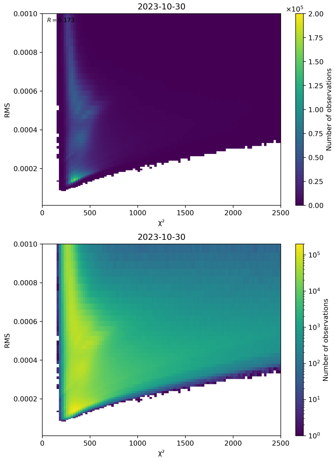
Figure 82: Scatter density plot of “ \chi^2 ” against “RMS” for 2023-10-29 to 2023-10-31.
