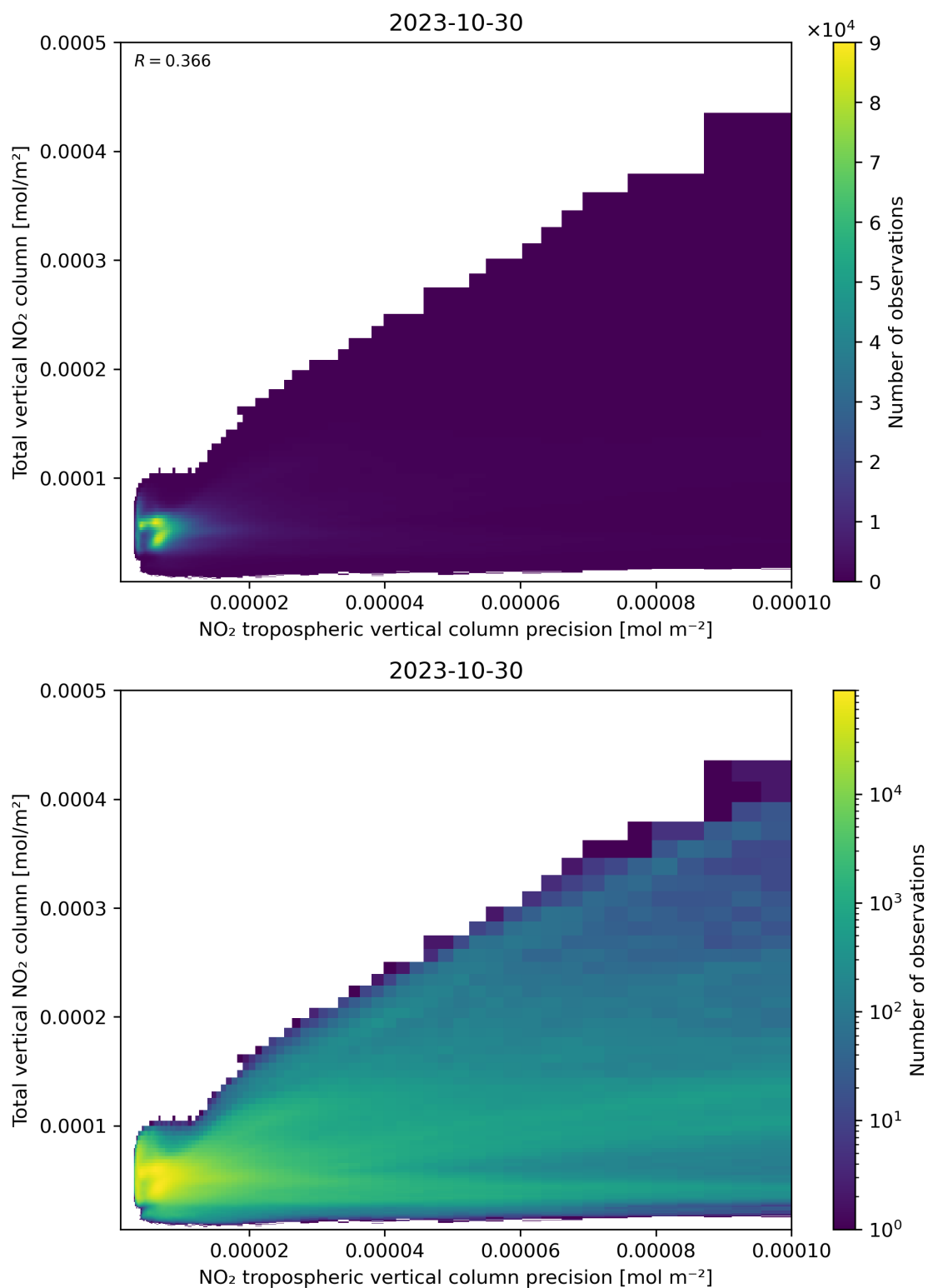
Figure 138: Scatter density plot of “NO 2 tropospheric vertical column precision” against “Total vertical NO 2 column” for 2023-10-29 to 2023-10-31.
