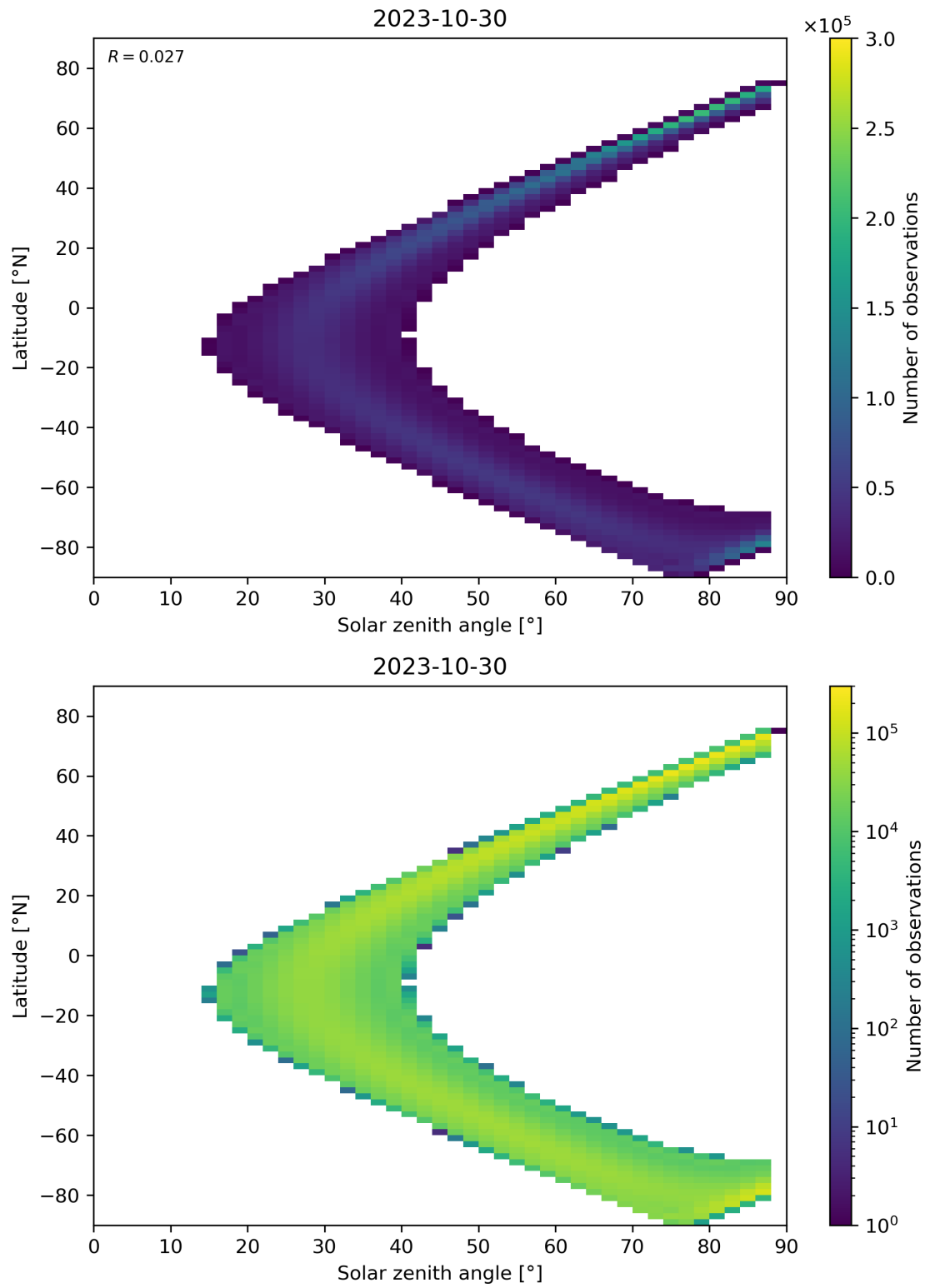
Figure 149: Scatter density plot of “Solar zenith angle” against “Latitude” for 2023-10-29 to 2023-10-31.
