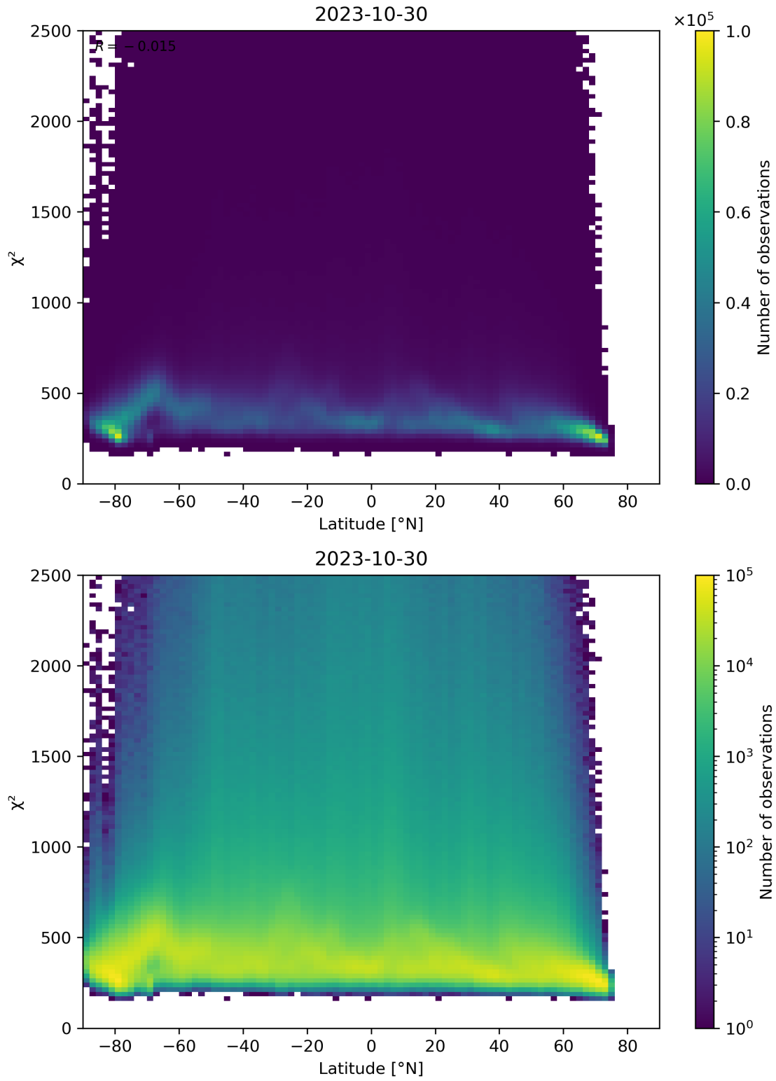
Figure 86: Scatter density plot of “Latitude” against “ \chi^2 ” for 2023-10-29 to 2023-10-31.
