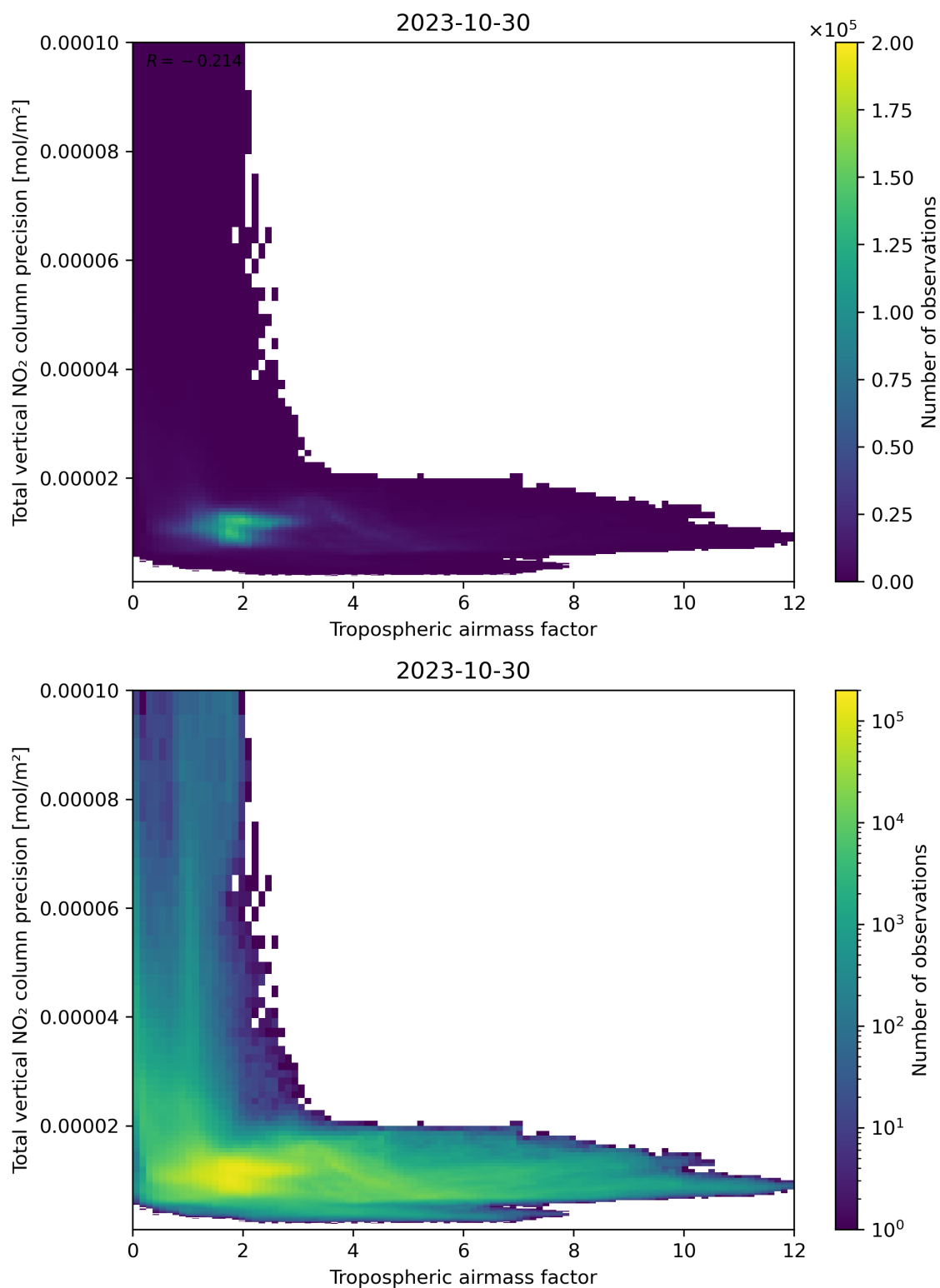
Figure 78: Scatter density plot of “Tropospheric air mass factor” against “Total vertical NO 2 column precision” for 2023-10-29 to 2023-10-31.
