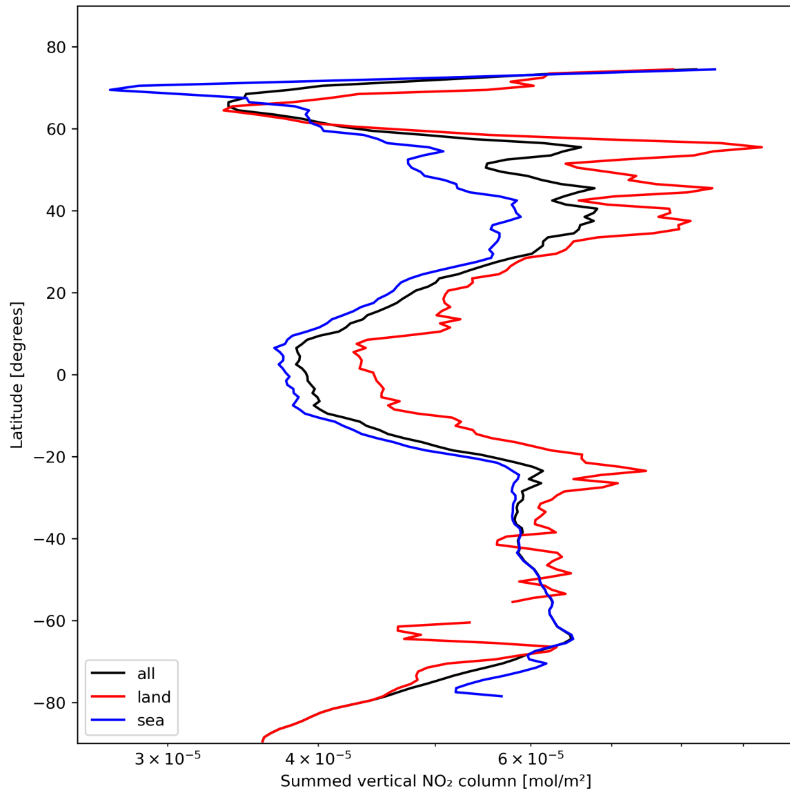
Figure 23: Zonal average of “Summed vertical NO 2 column” for 2023-10-29 to 2023-10-31.
