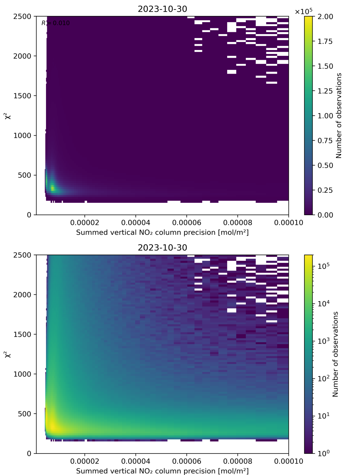
Figure 107: Scatter density plot of “Summed vertical NO 2 column precision” against “ \chi^2 ” for 2023-10-29 to 2023-10-31.
