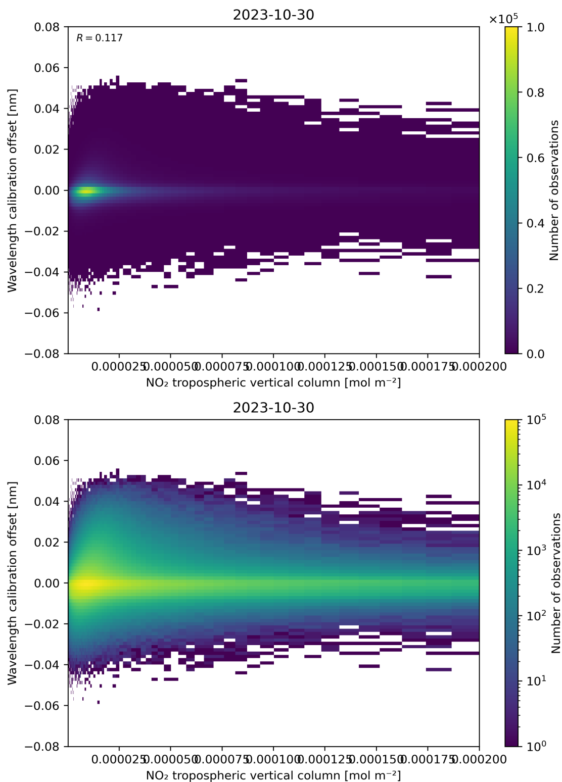
Figure 143: Scatter density plot of “NO 2 tropospheric vertical column” against “Wavelength calibration offset” for 2023-10-29 to 2023-10-31.
