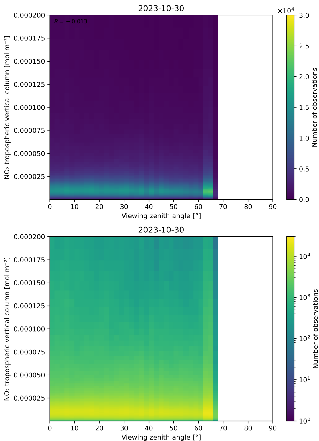
Figure 169: Scatter density plot of “Viewing zenith angle” against “NO 2 tropospheric vertical column” for 2023-10-29 to 2023-10-31.
