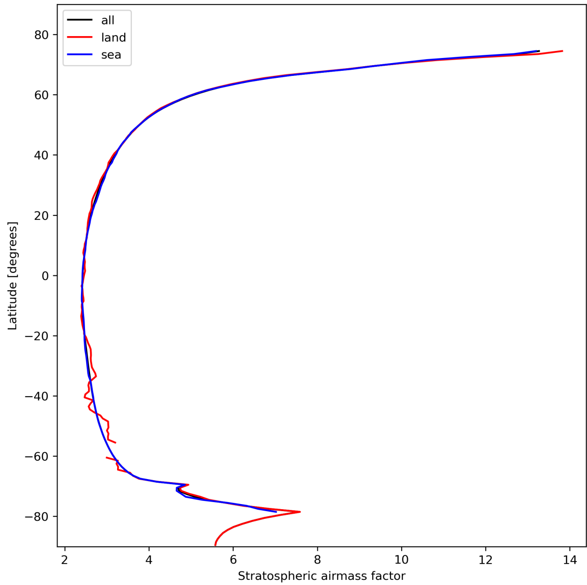
Figure 27: Zonal average of “Stratospheric airmass factor” for 2023-10-29 to 2023-10-31.
