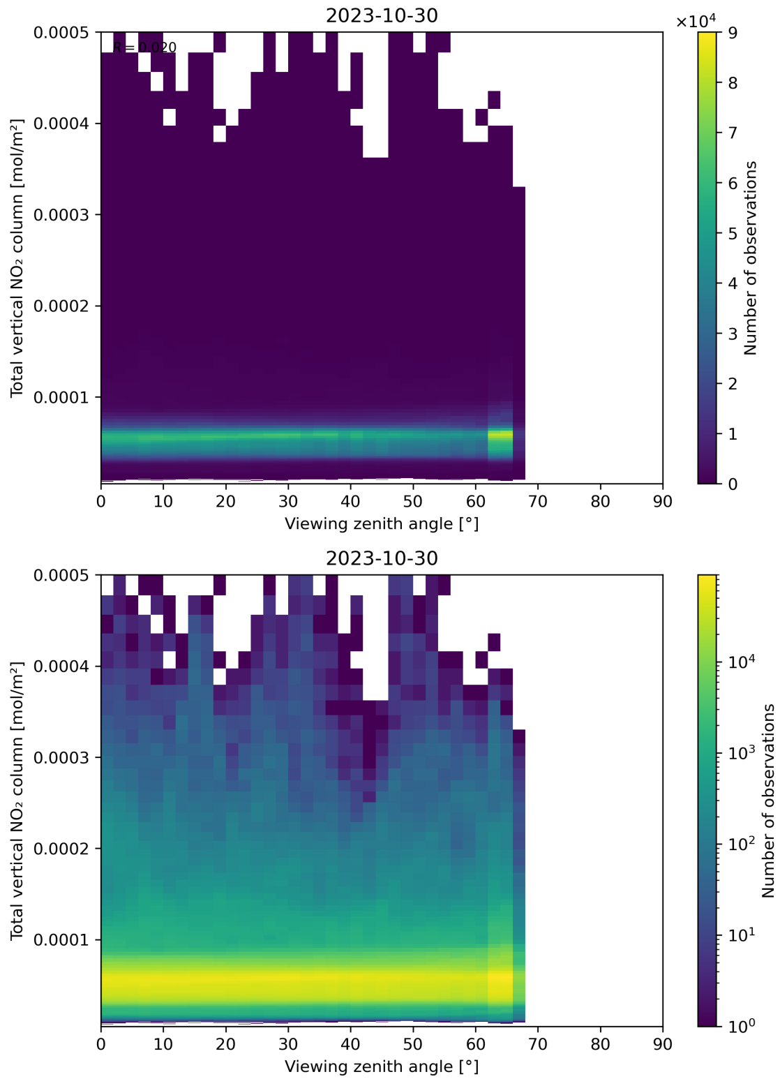
Figure 167: Scatter density plot of “Viewing zenith angle” against “Total vertical NO 2 column” for 2023-10-29 to 2023-10-31.
