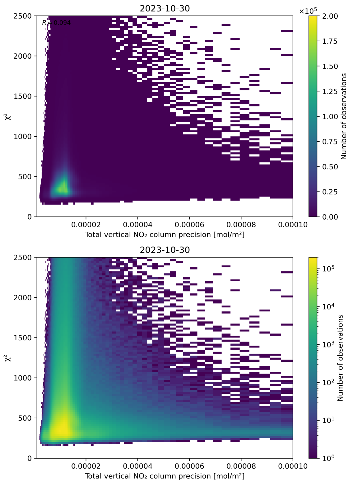
Figure 116: Scatter density plot of “Total vertical NO 2 column precision” against “ \chi^2 ” for 2023-10-29 to 2023-10-31.
