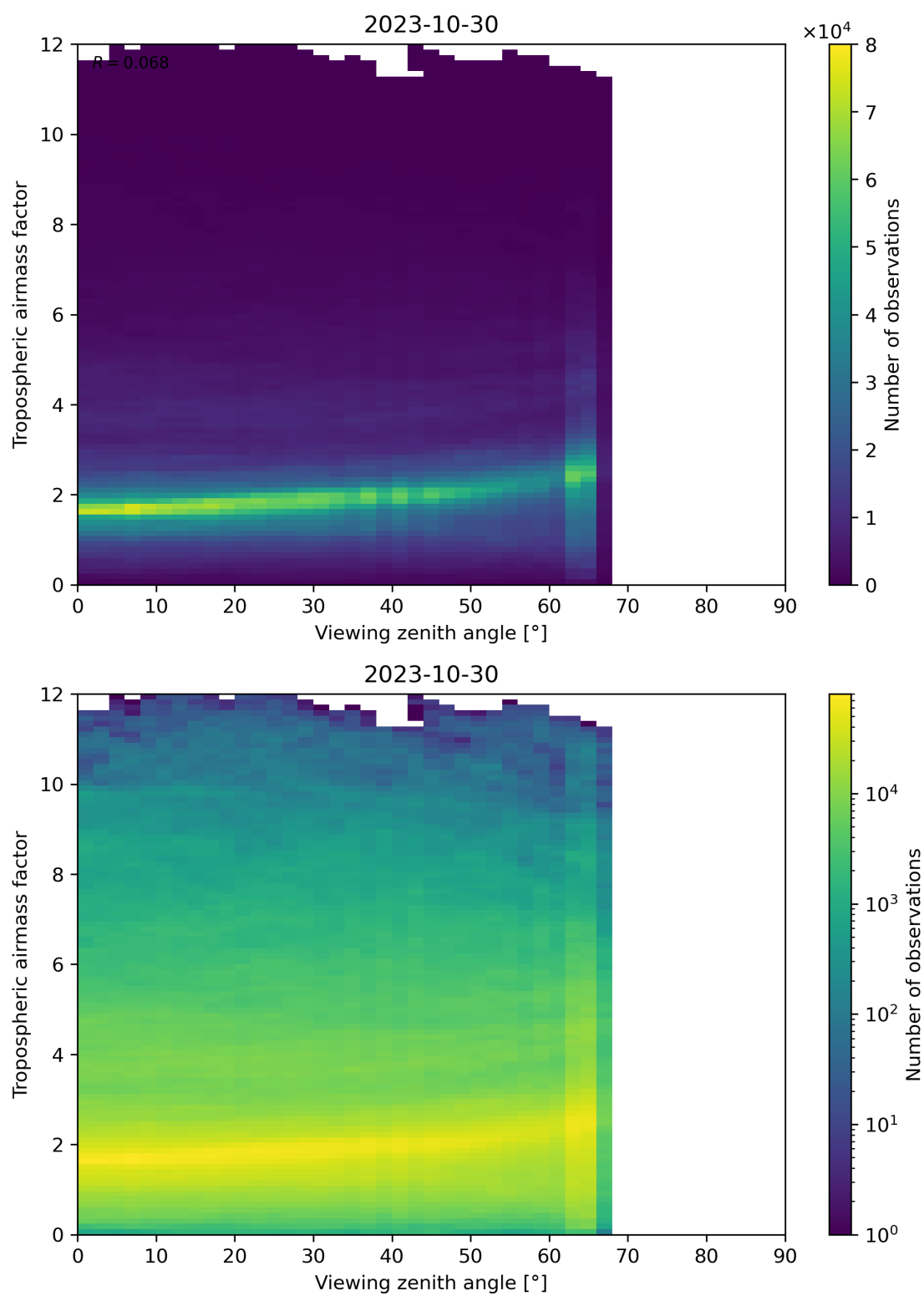
Figure 161: Scatter density plot of “Viewing zenith angle” against “Tropospheric airmass factor” for 2023-10-29 to 2023-10-31.
