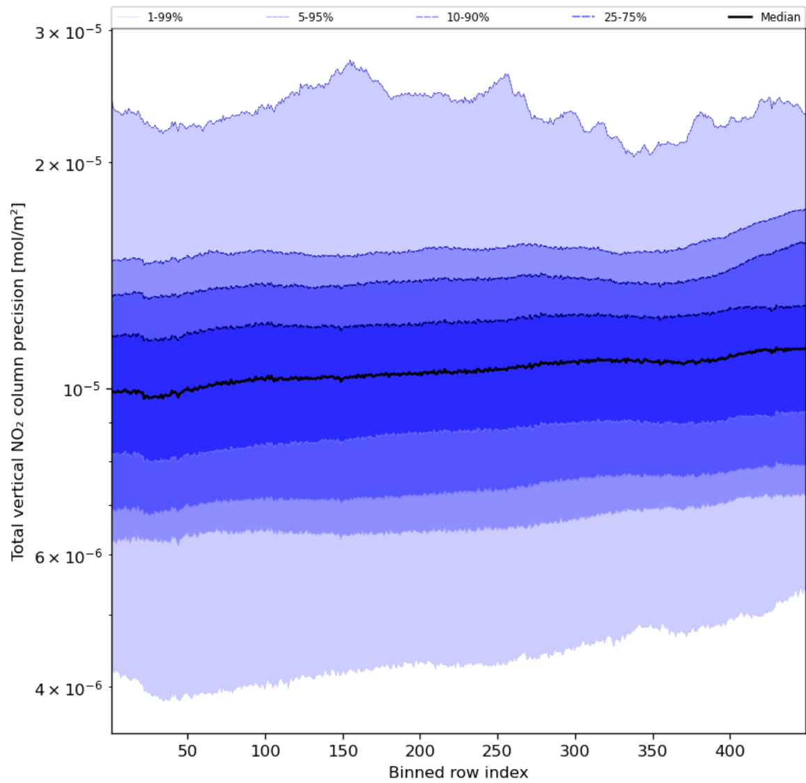
Figure 56: Along track statistics of “Total vertical NO 2 column precision” for 2023-10-29 to 2023-10-31
