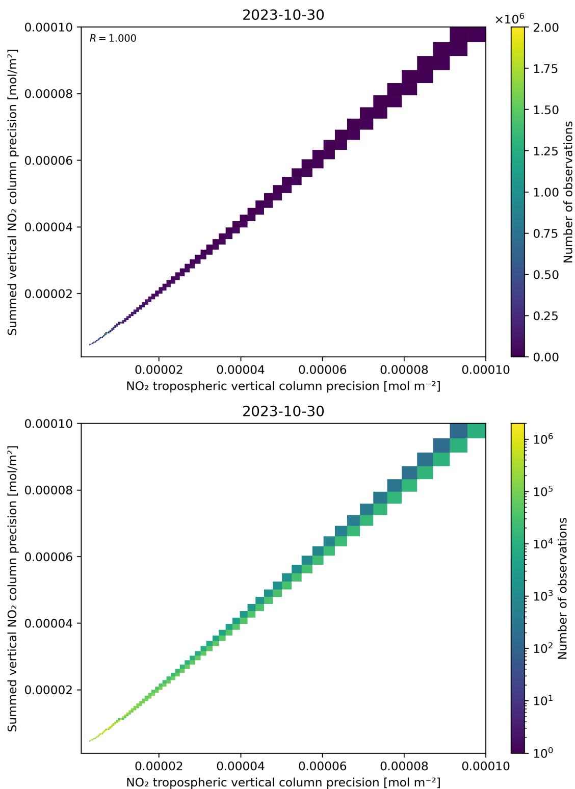
Figure 137: Scatter density plot of “NO 2 tropospheric vertical column precision” against “Summed vertical NO 2 column precision” for 2023-10-29 to 2023-10-31.
