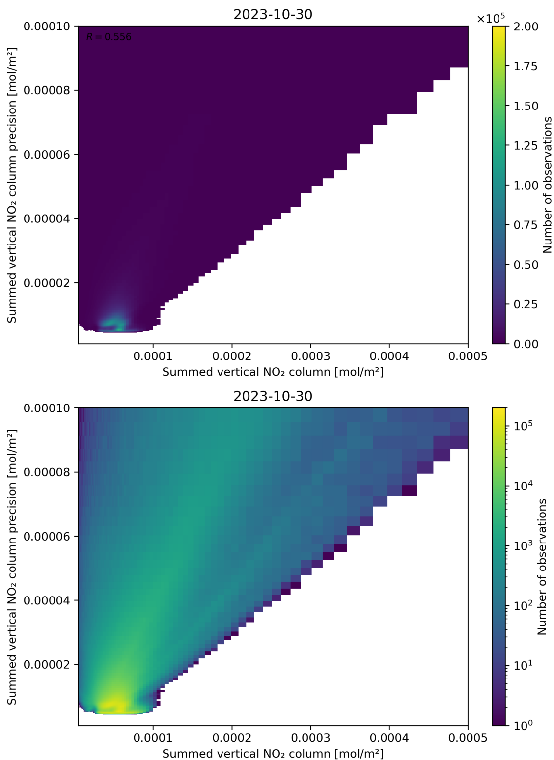
Figure 105: Scatter density plot of “Summed vertical NO 2 column” against “Summed vertical NO 2 column precision” for 2023-10-29 to 2023-10-31.
