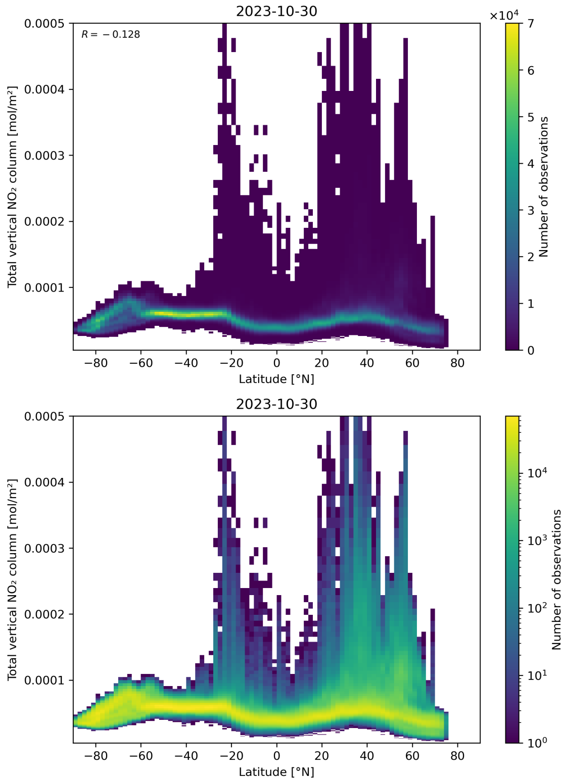
Figure 90: Scatter density plot of “Latitude” against “Total vertical NO 2 column” for 2023-10-29 to 2023-10-31.
