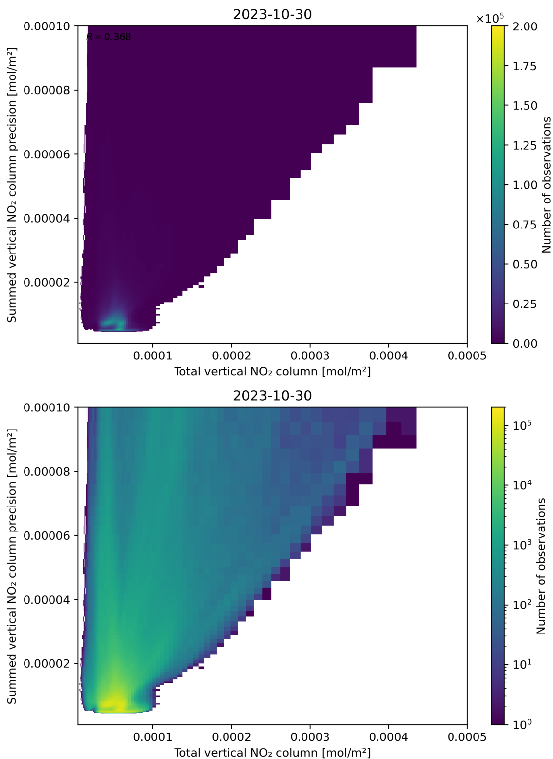
Figure 113: Scatter density plot of “Total vertical NO 2 column” against “Summed vertical NO 2 column precision” for 2023-10-29 to 2023-10-31.
