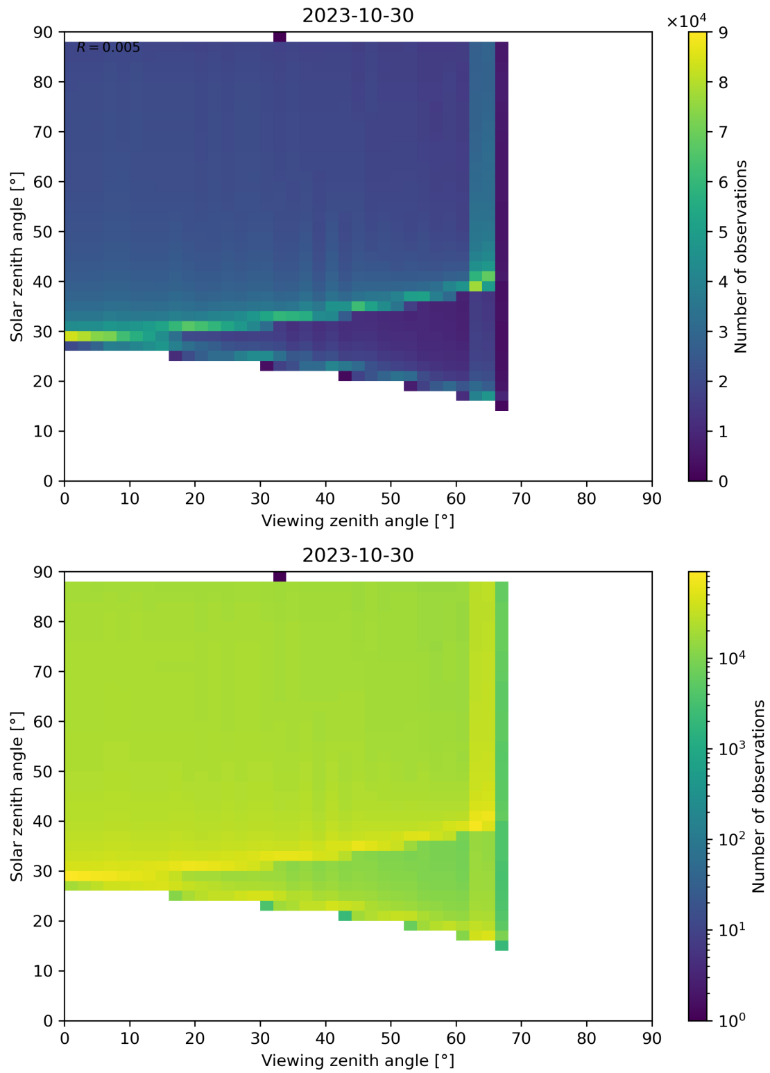
Figure 172: Scatter density plot of “Viewing zenith angle” against “Solar zenith angle” for 2023-10-29 to 2023-10-31.
