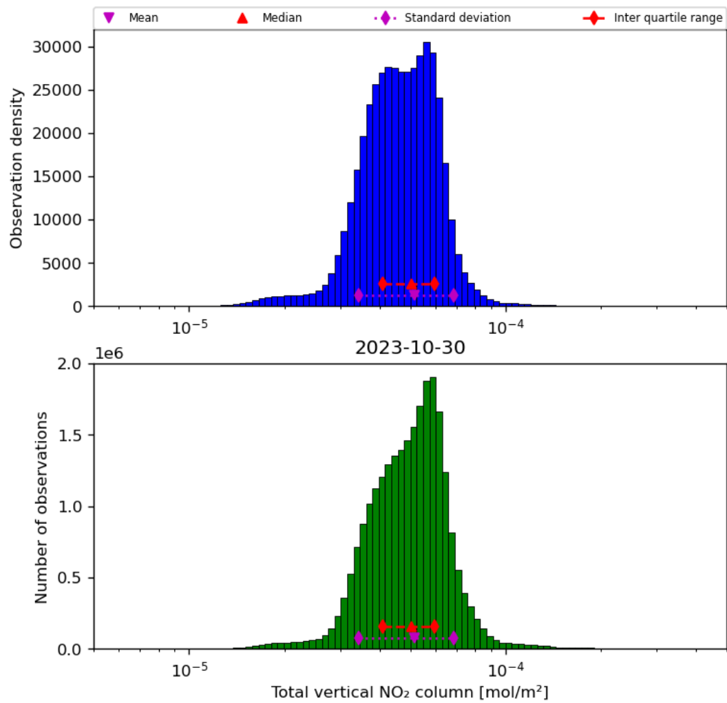
Figure 38: Histogram of "Total vertical NO 2 column" for 2023-10-29 to 2023-10-31
