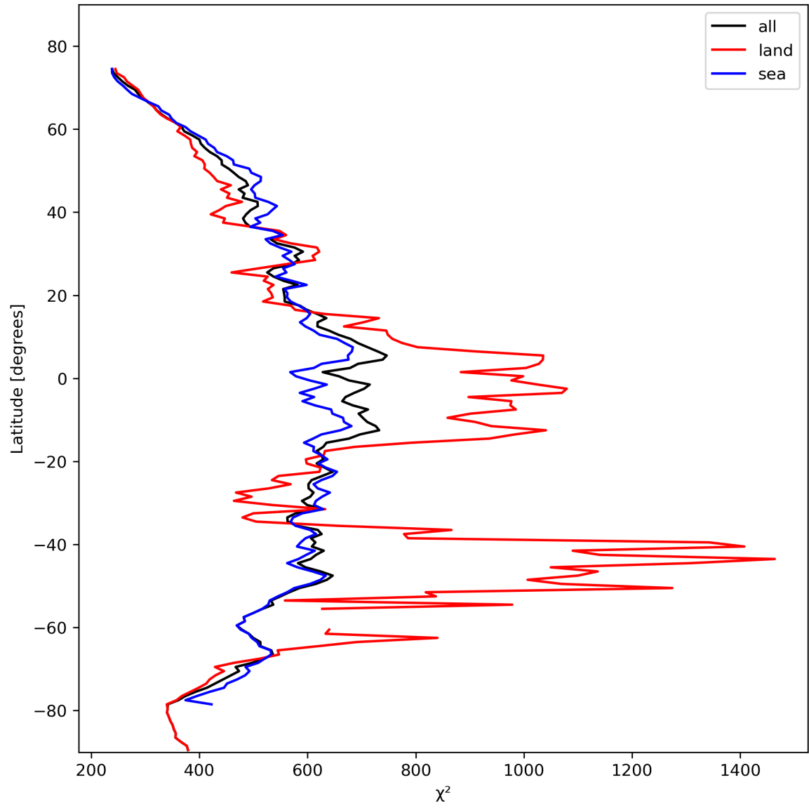
Figure 25: Zonal average of “ \chi^2 ” for 2023-10-29 to 2023-10-31.
