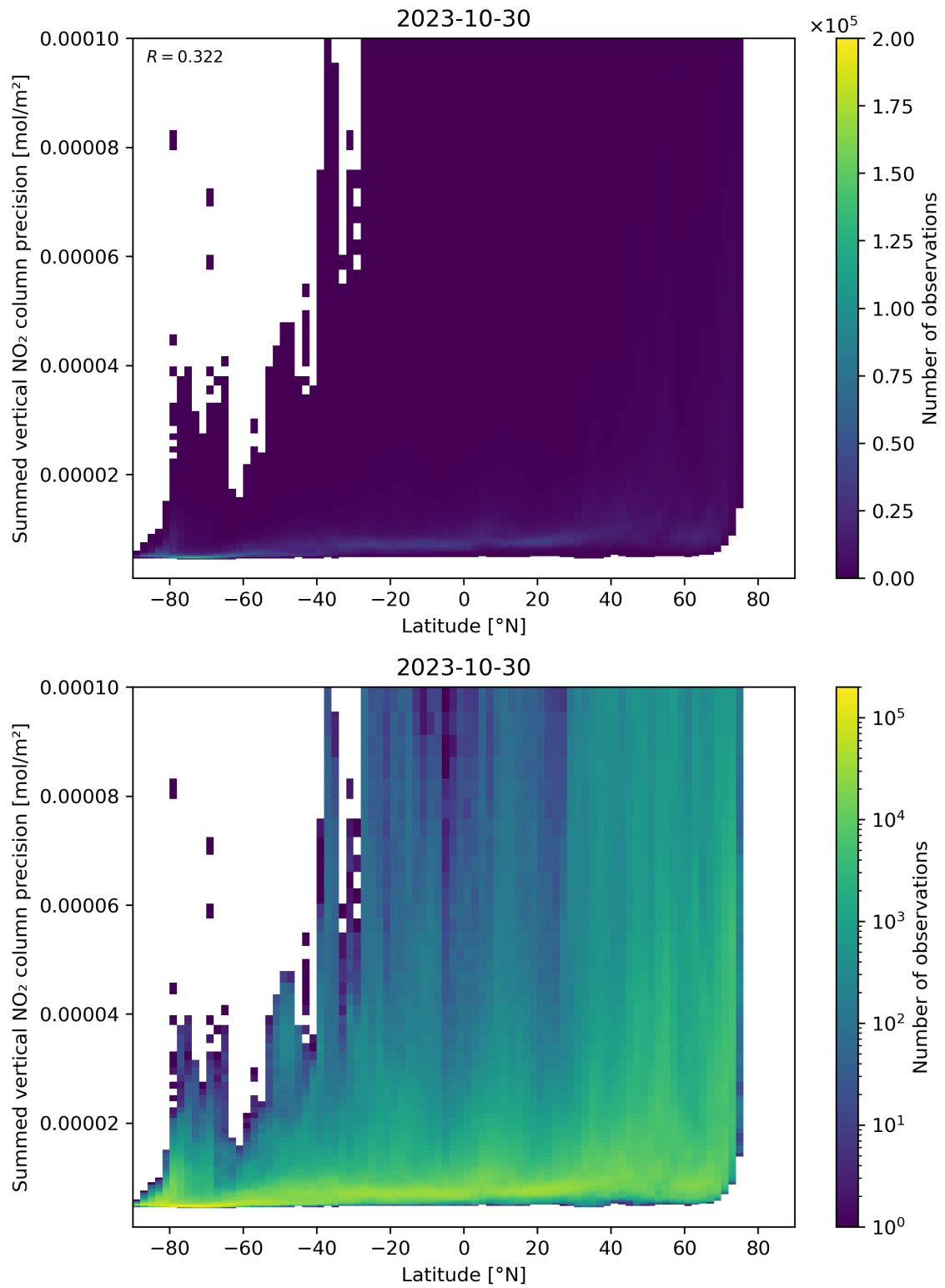
Figure 89: Scatter density plot of “Latitude” against “Summed vertical NO 2 column precision” for 2023-10-29 to 2023-10-31.
