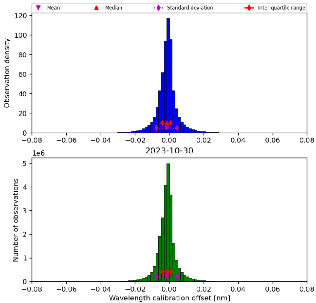
Figure 35: Histogram of “Wavelength calibration offset” for 2023-10-29 to 2023-10-31
