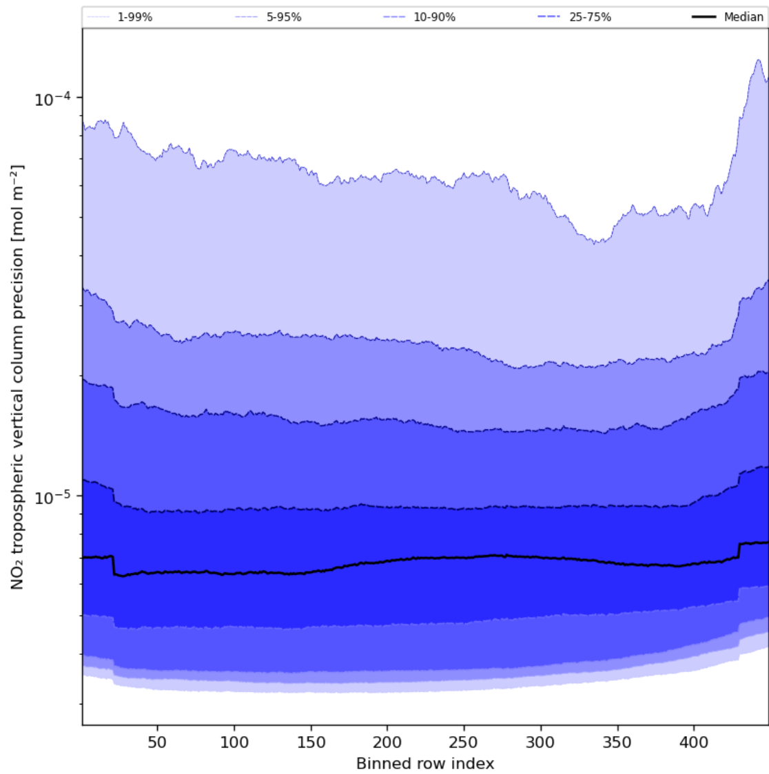
Figure 47: Along track statistics of “NO 2 tropospheric vertical column precision” for 2023-10-29 to 2023-10-31
