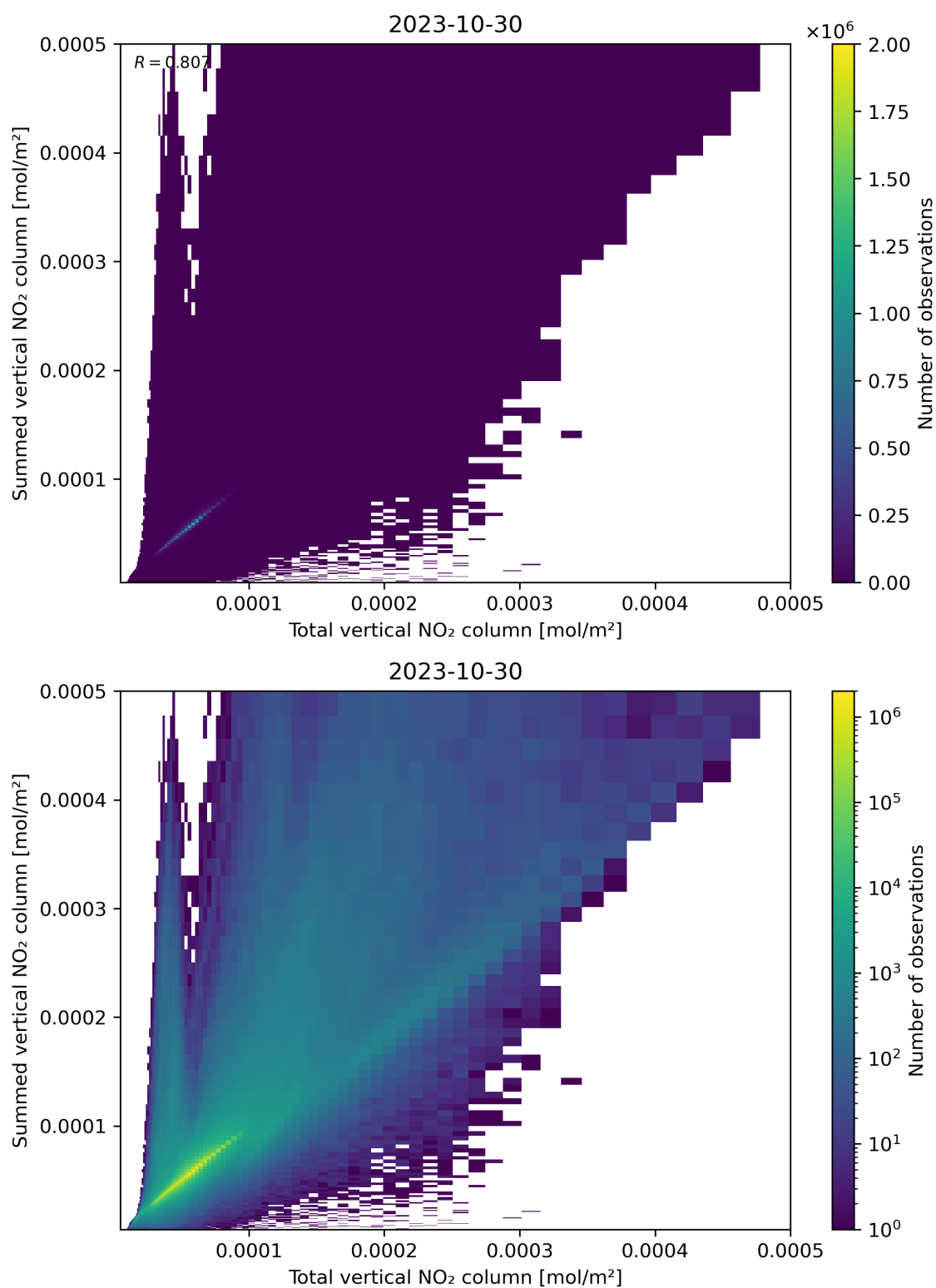
Figure 112: Scatter density plot of “Total vertical NO 2 column” against “Summed vertical NO 2 column” for 2023-10-29 to 2023-10-31.
