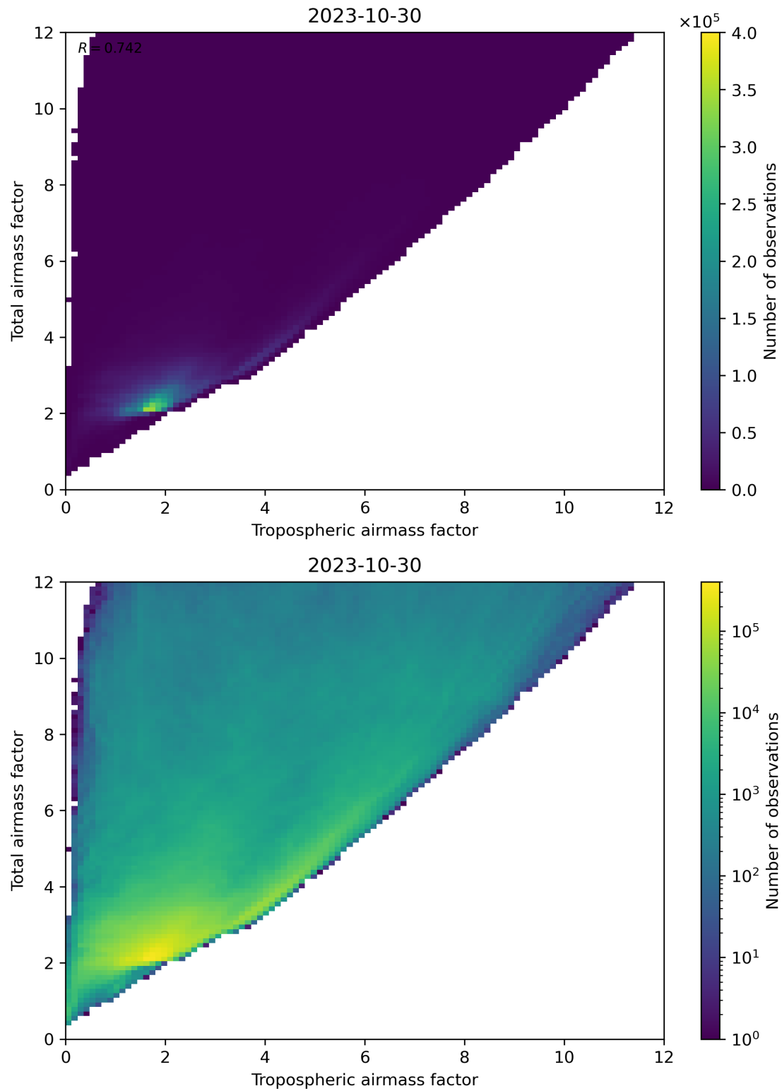
Figure 72: Scatter density plot of “Tropospheric airmass factor” against “Total airmass factor” for 2023-10-29 to 2023-10-31.
