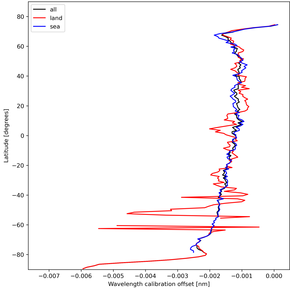
Figure 18: Zonal average of “Wavelength calibration offset” for 2023-10-29 to 2023-10-31.
