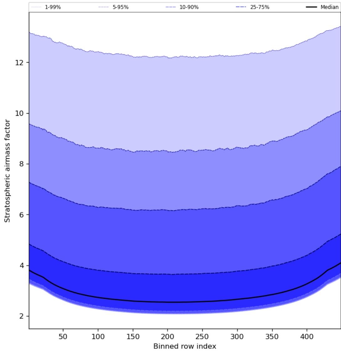
Figure 61: Along track statistics of “Stratospheric airmass factor” for 2023-10-29 to 2023-10-31
