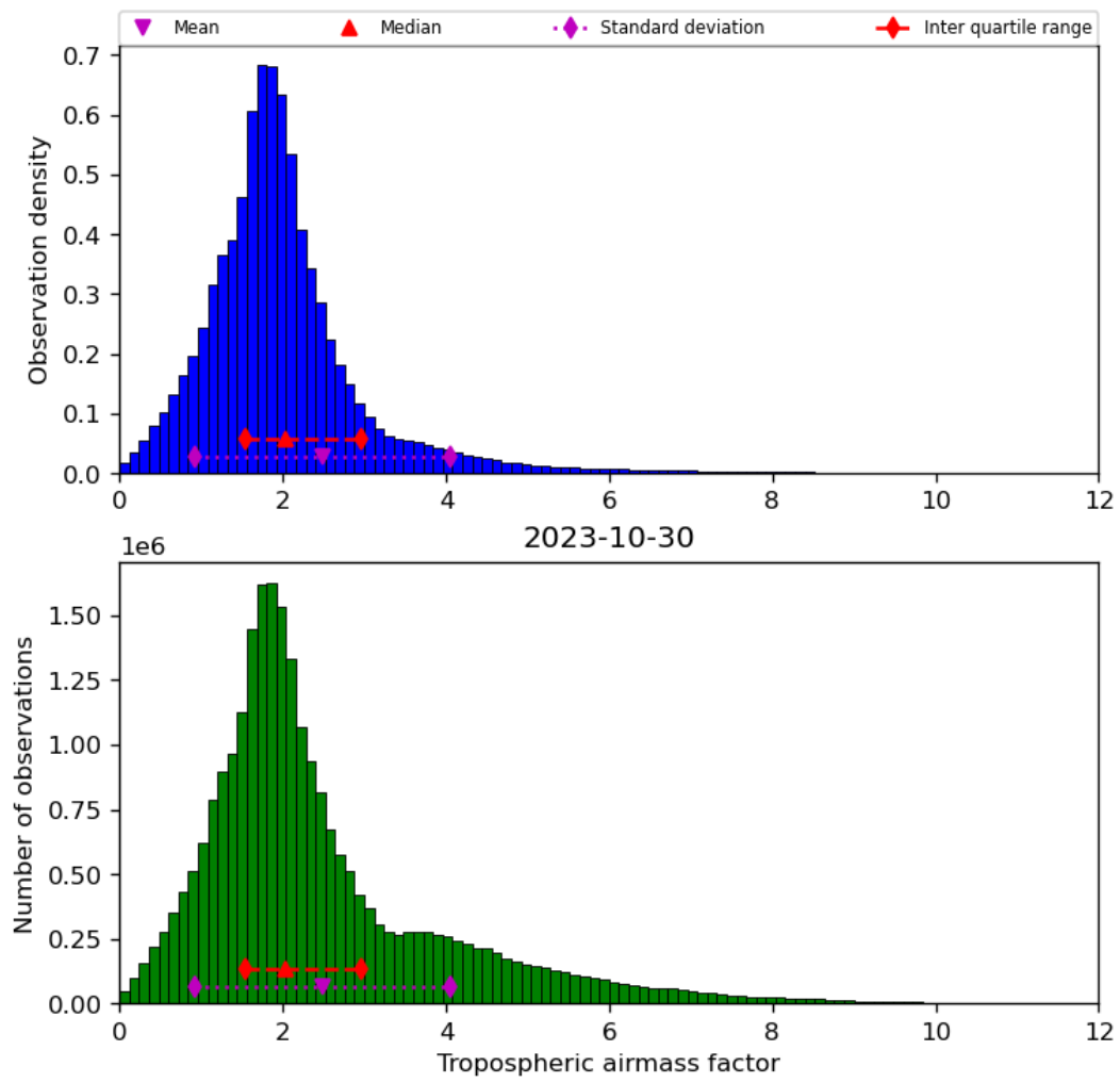
Figure 31: Histogram of “Tropospheric airmass factor” for 2023-10-29 to 2023-10-31
