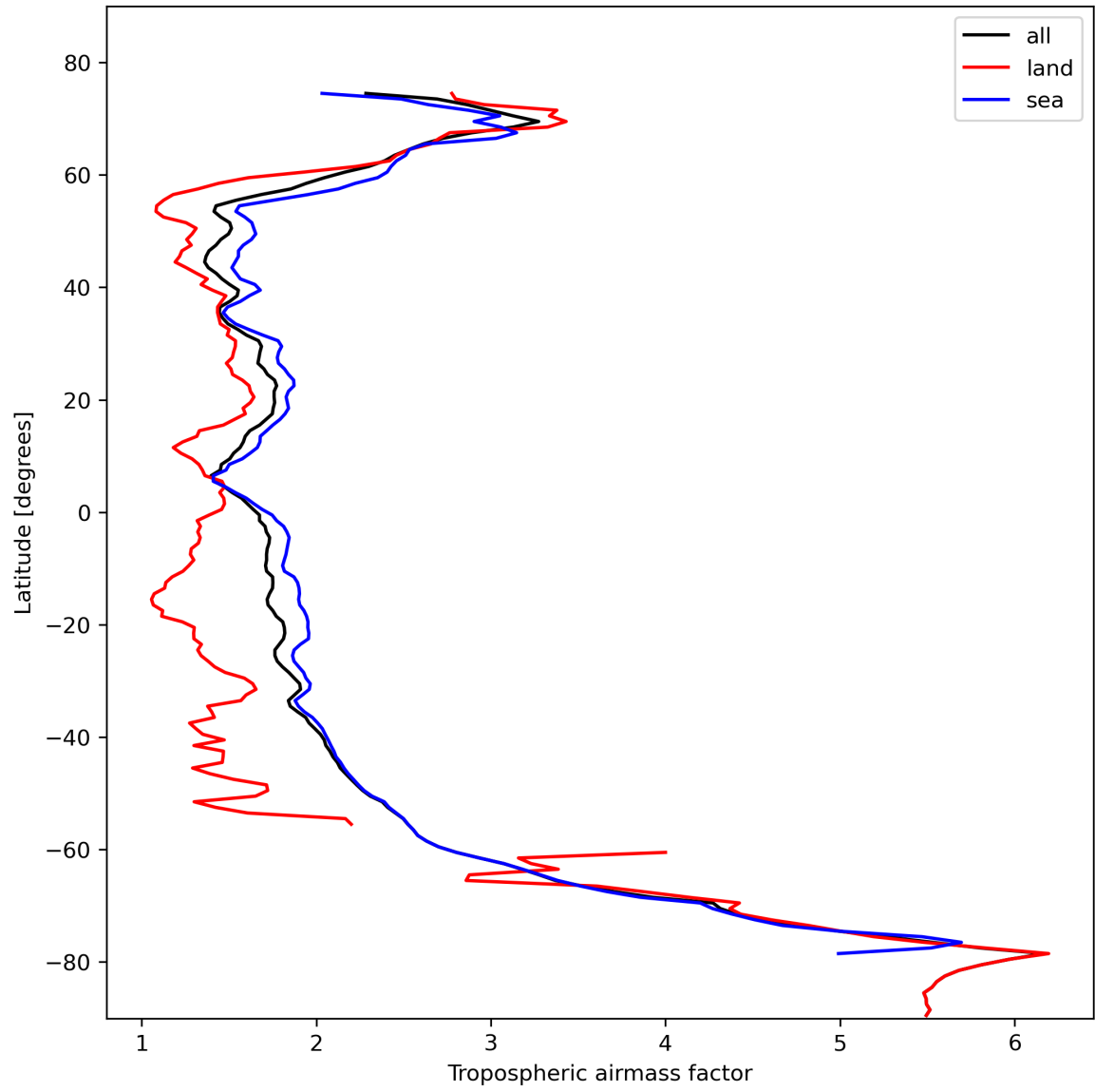
Figure 14: Zonal average of “Tropospheric airmass factor” for 2023-10-29 to 2023-10-31.
