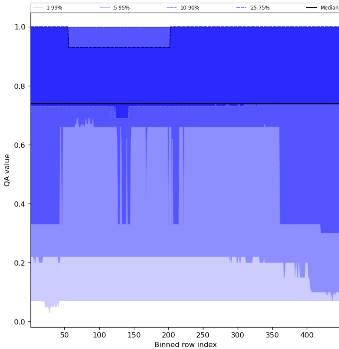
Figure 45: Along track statistics of “QA value” for 2023-10-29 to 2023-10-31
