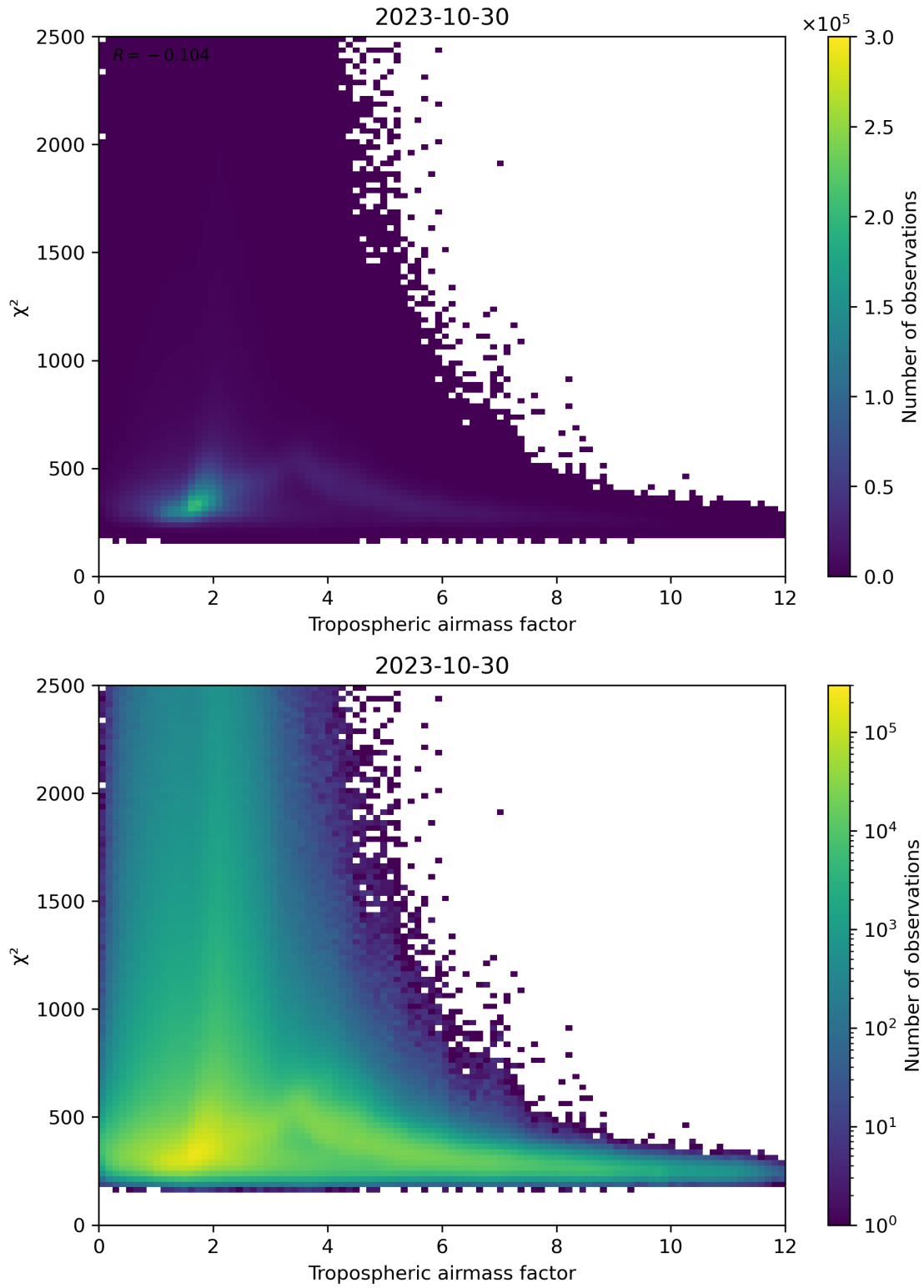
Figure 73: Scatter density plot of “Tropospheric airmass factor” against “ \chi^2 ” for 2023-10-29 to 2023-10-31.
