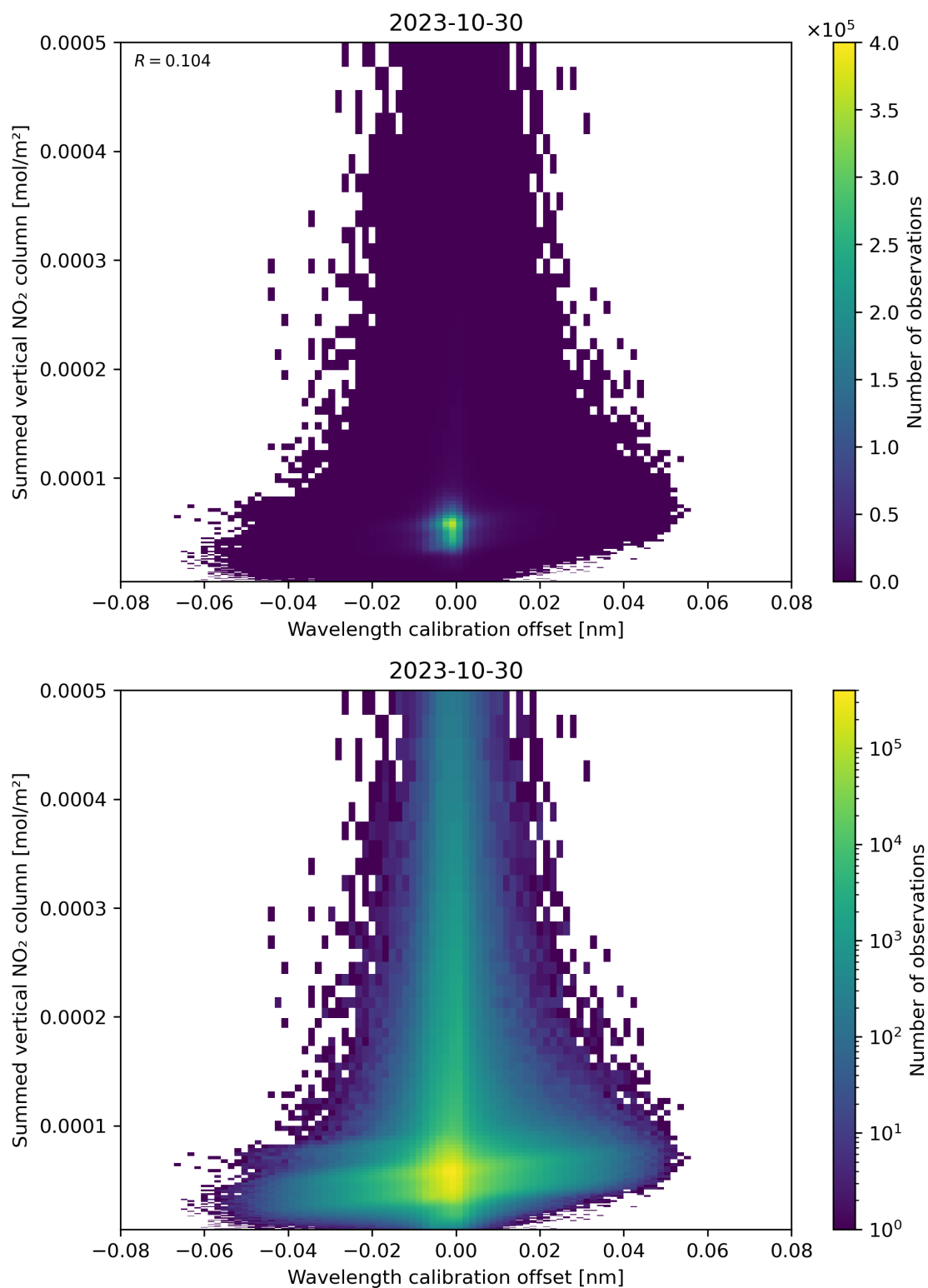
Figure 177: Scatter density plot of “Wavelength calibration offset” against “Summed vertical NO 2 column” for 2023-10-29 to 2023-10-31.
