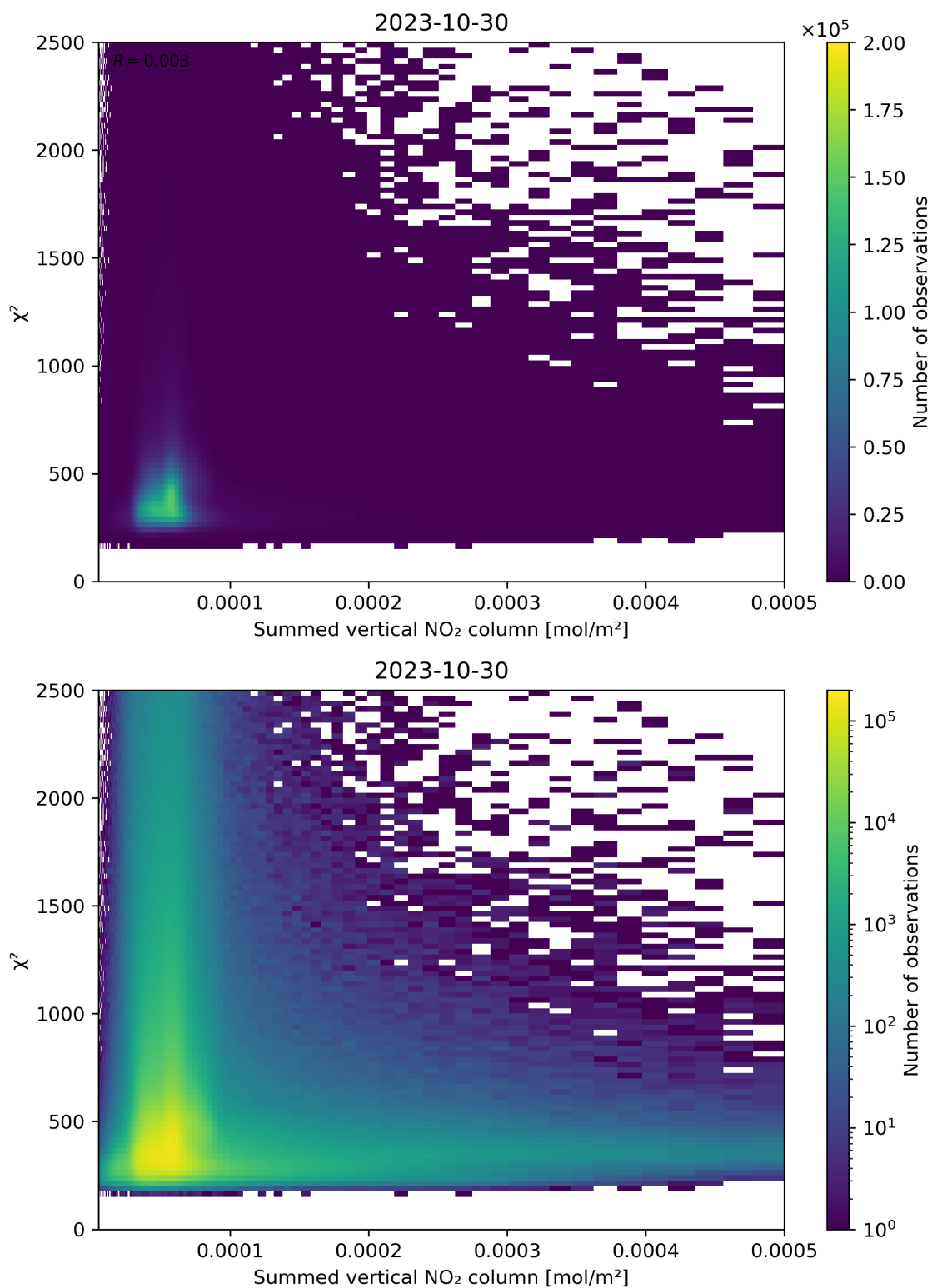
Figure 104: Scatter density plot of “Summed vertical NO 2 column” against “ \chi^2 ” for 2023-10-29 to 2023-10-31.
