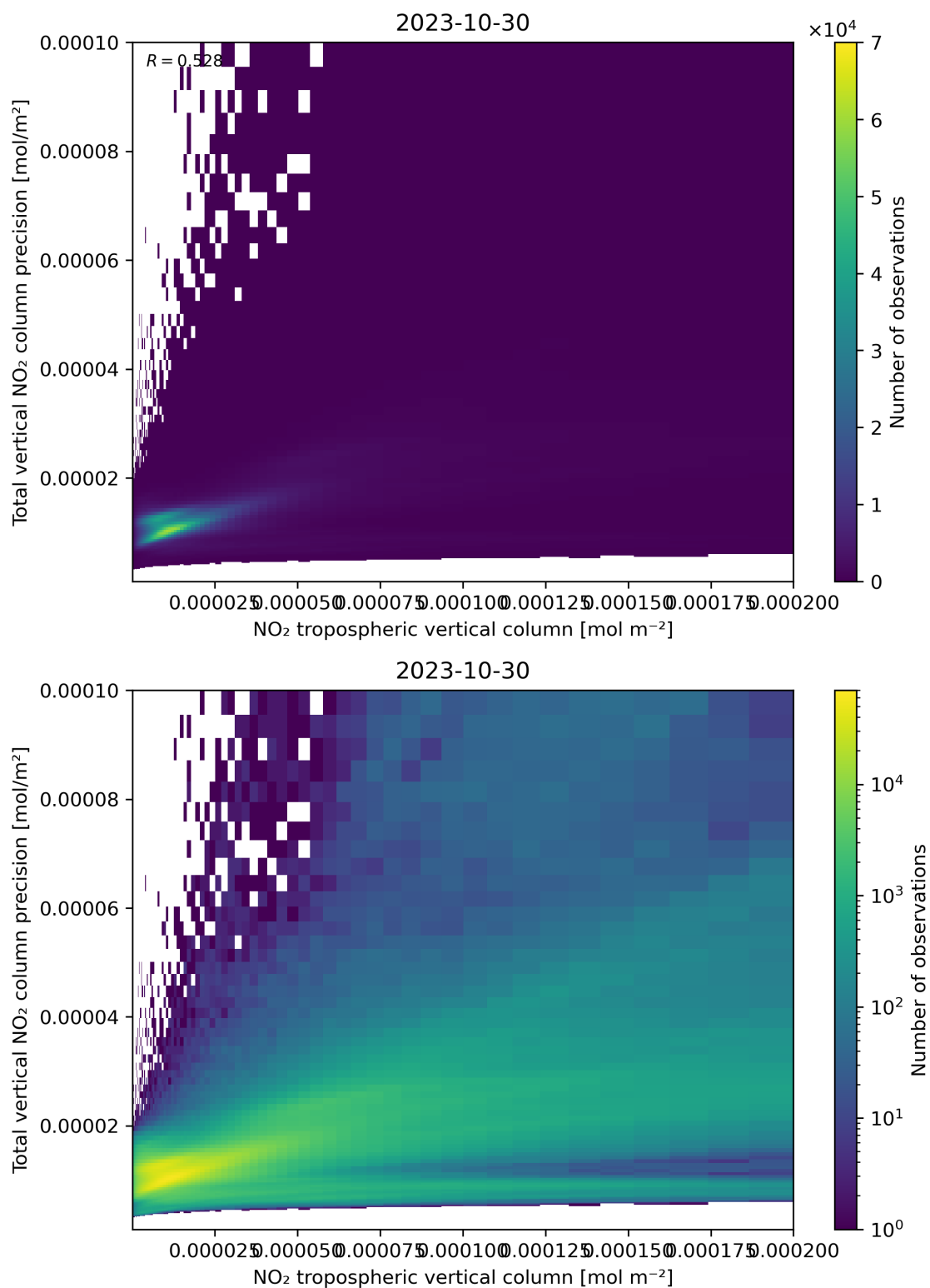
Figure 129: Scatter density plot of “NO 2 tropospheric vertical column” against “Total vertical NO 2 column precision” for 2023-10-29 to 2023-10-31.
