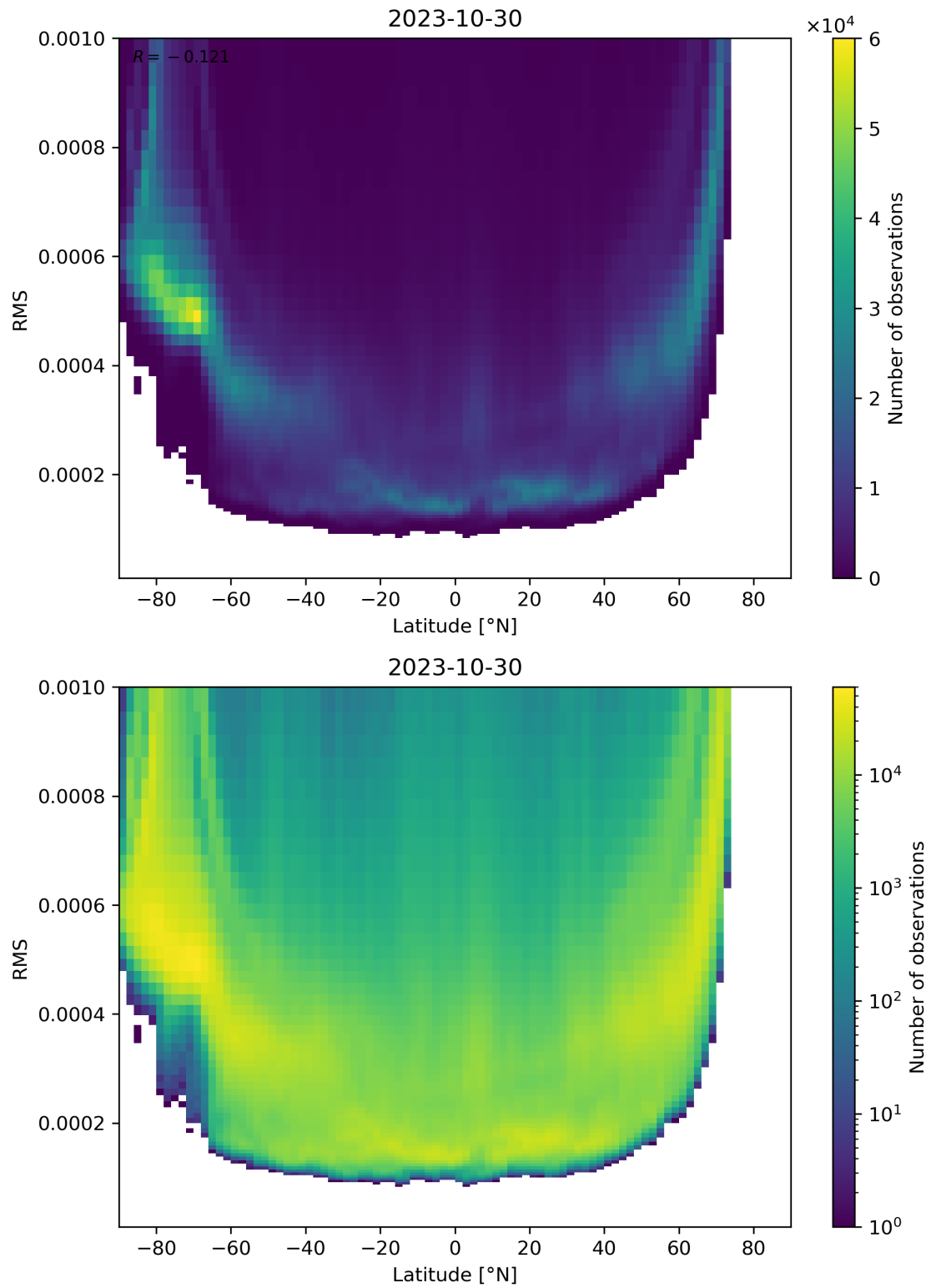
Figure 94: Scatter density plot of “Latitude” against “RMS” for 2023-10-29 to 2023-10-31.
