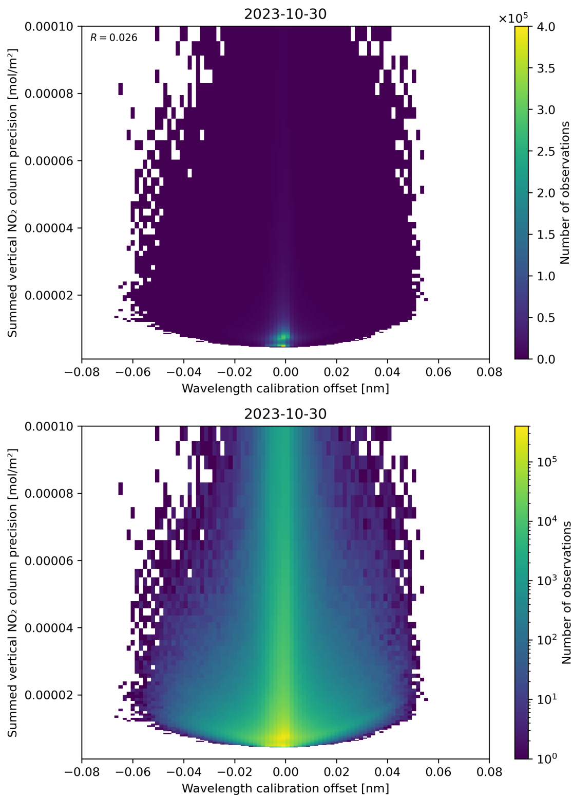
Figure 178: Scatter density plot of “Wavelength calibration offset” against “Summed vertical NO 2 column precision” for 2023-10-29 to 2023-10-31.
