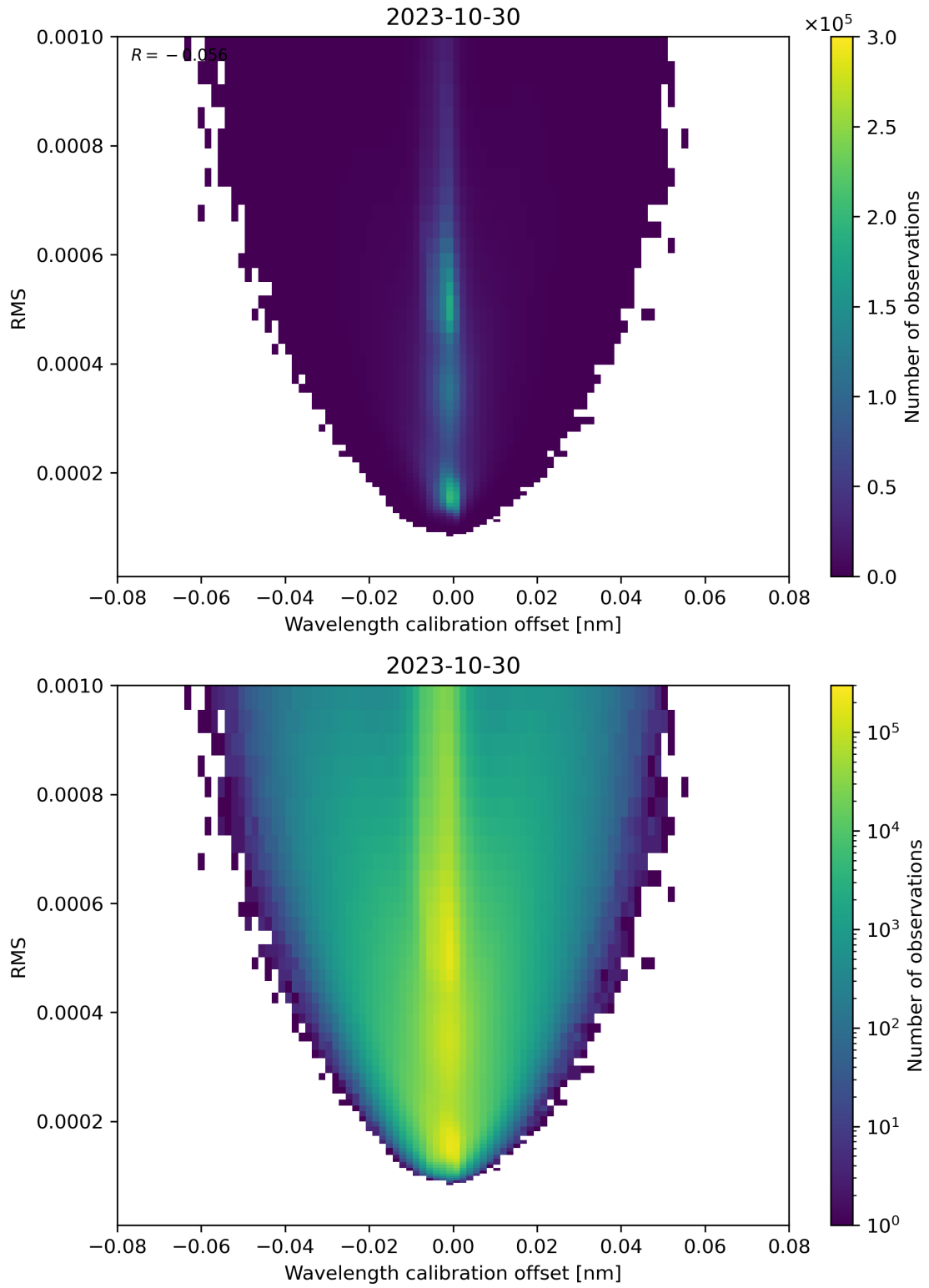
Figure 181: Scatter density plot of “Wavelength calibration offset” against “RMS” for 2023-10-29 to 2023-10-31.
