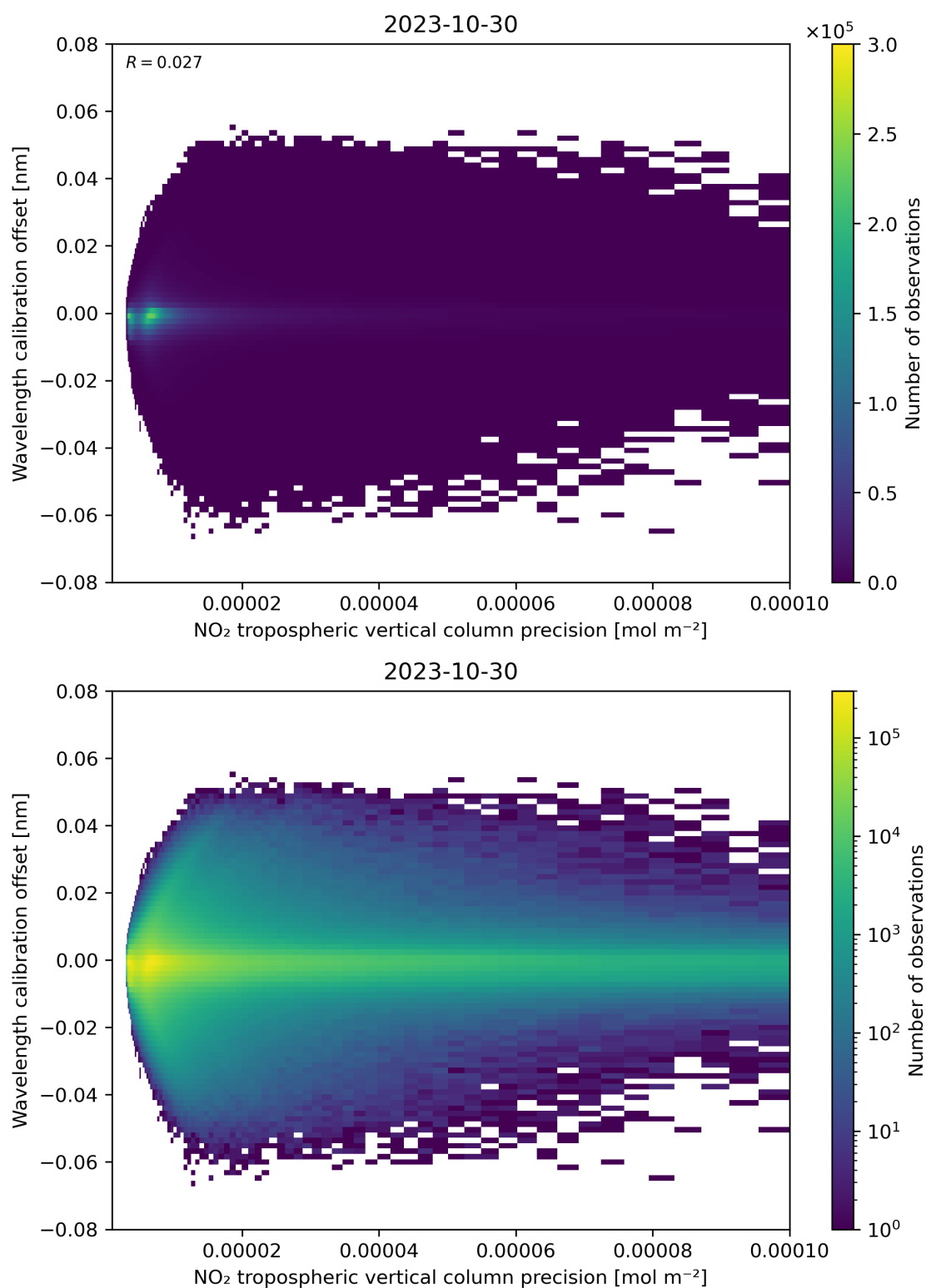
Figure 141: Scatter density plot of “NO 2 tropospheric vertical column precision” against “Wavelength calibration offset” for 2023-10-29 to 2023-10-31.
