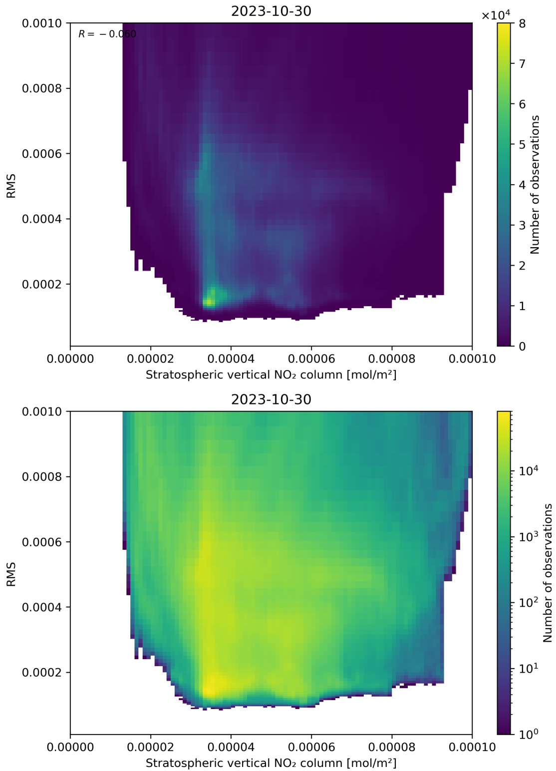
Figure 102: Scatter density plot of “Stratospheric vertical NO 2 column” against “RMS” for 2023-10-29 to 2023-10-31.
