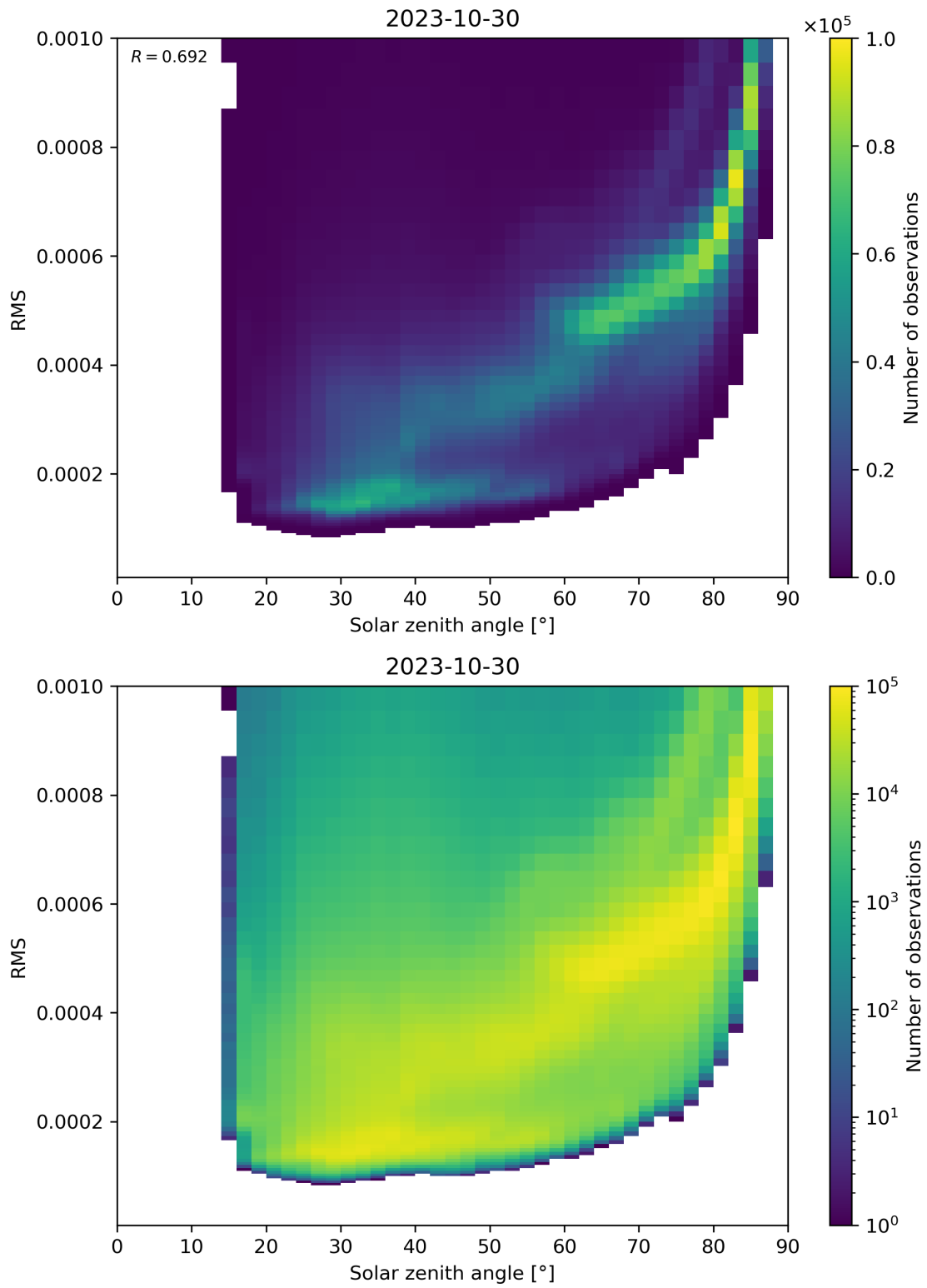
Figure 157: Scatter density plot of “Solar zenith angle” against “RMS” for 2023-10-29 to 2023-10-31.
