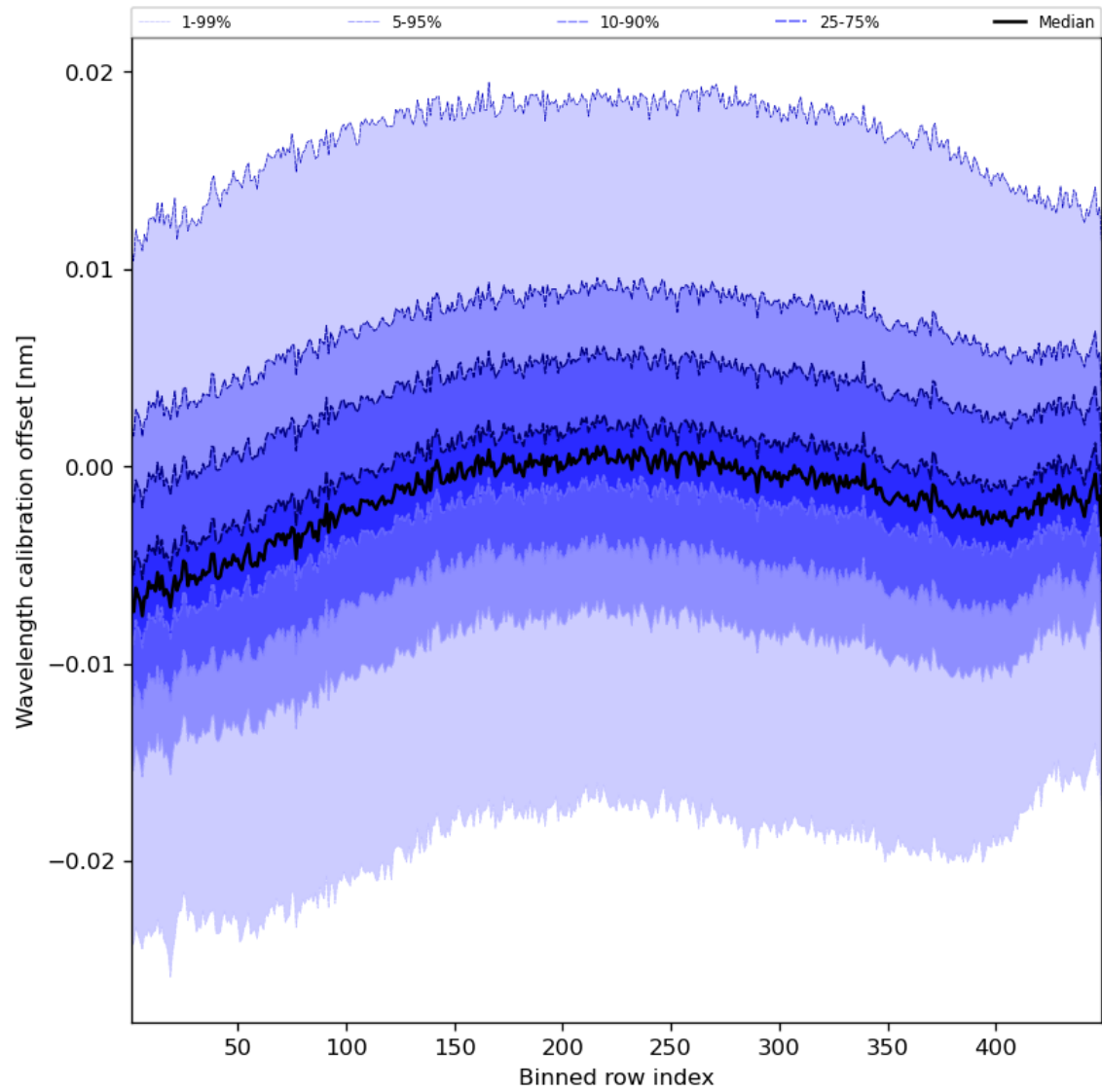
Figure 52: Along track statistics of “Wavelength calibration offset” for 2023-10-29 to 2023-10-31
