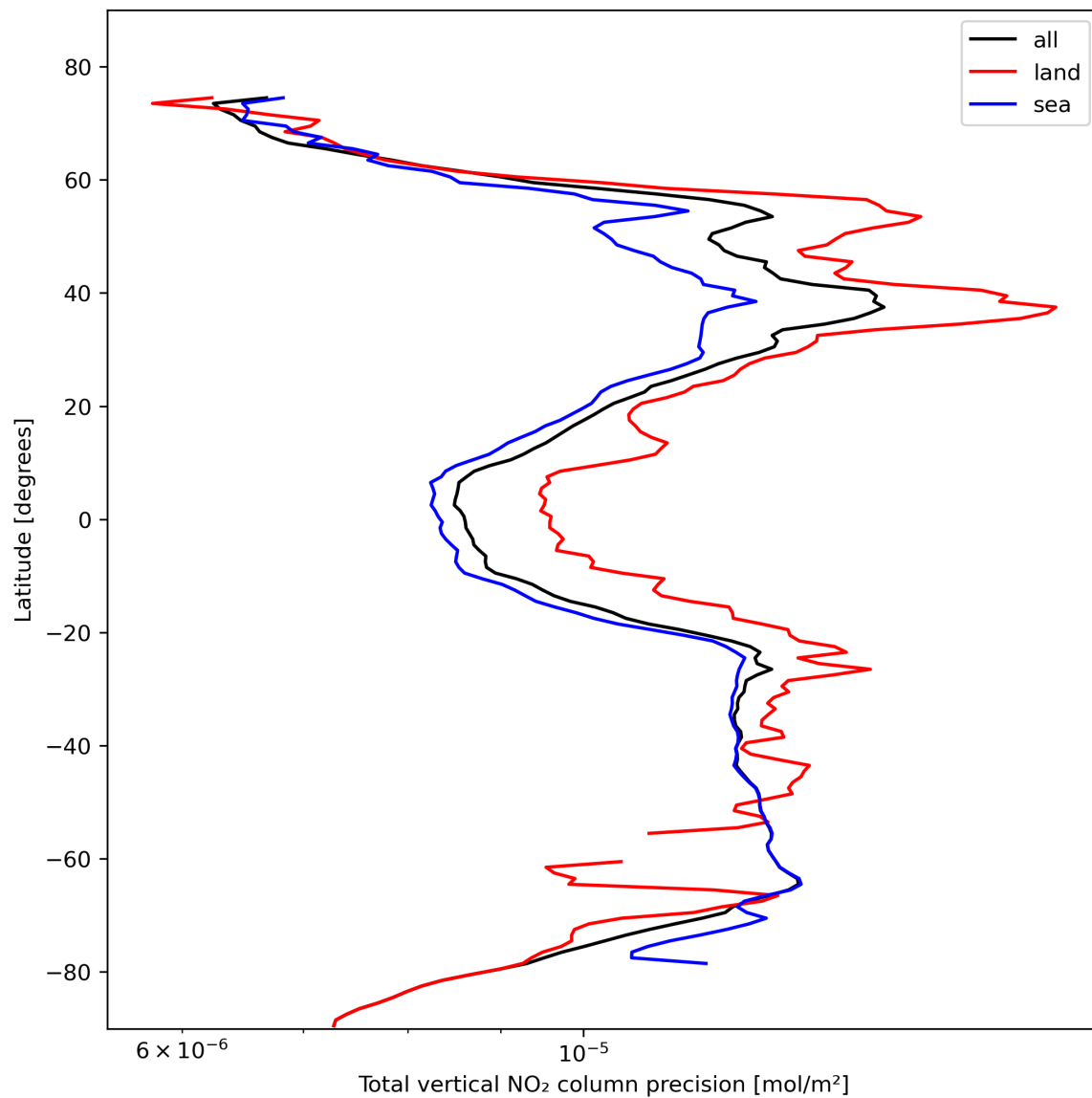
Figure 22: Zonal average of “Total vertical NO 2 column precision” for 2023-10-29 to 2023-10-31.
