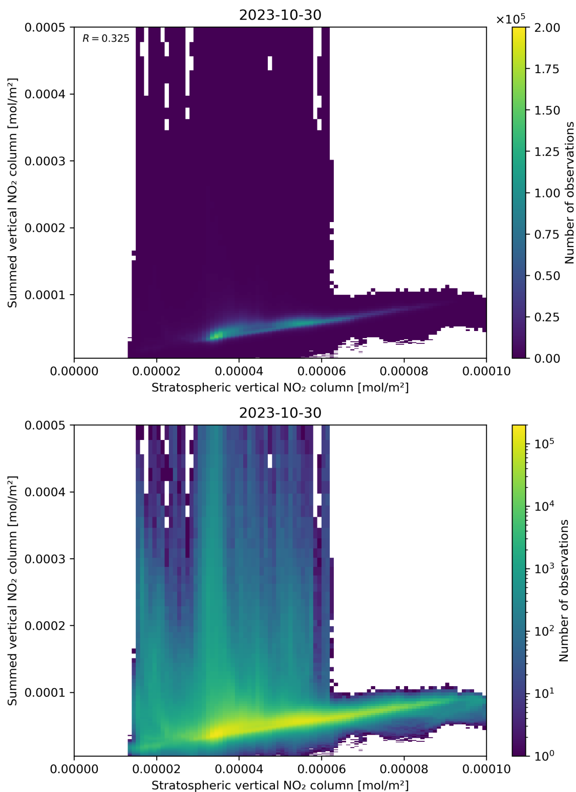
Figure 98: Scatter density plot of “Stratospheric vertical NO 2 column” against “Summed vertical NO 2 column” for 2023-10-29 to 2023-10-31.
