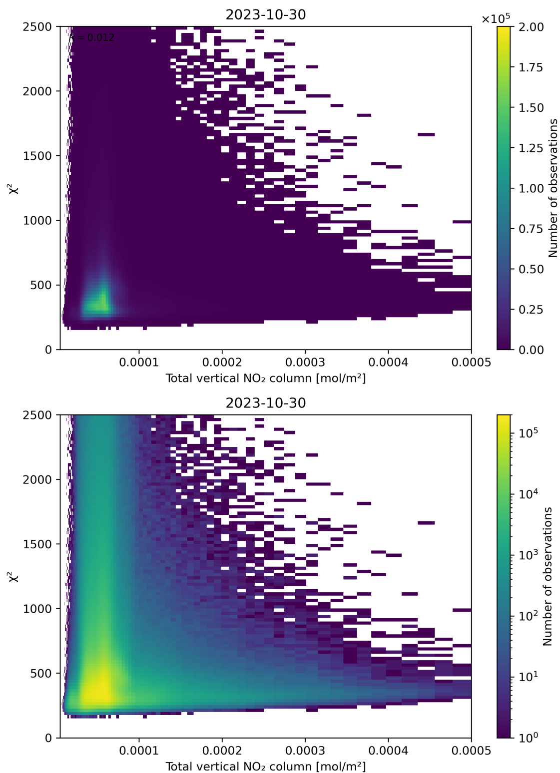
Figure 111: Scatter density plot of “Total vertical NO 2 column” against “ \chi^2 ” for 2023-10-29 to 2023-10-31.
