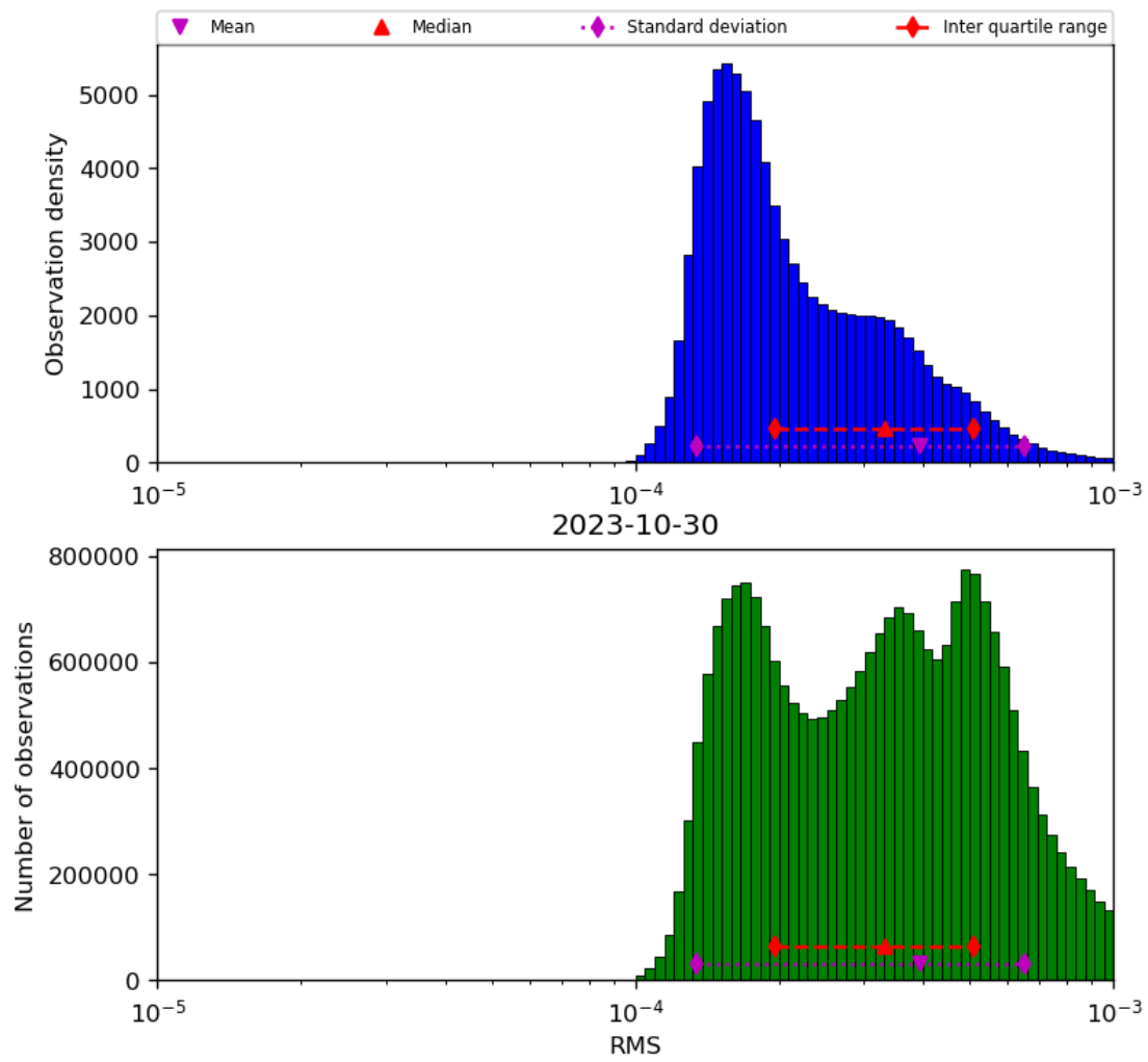
Figure 43: Histogram of “RMS” for 2023-10-29 to 2023-10-31
