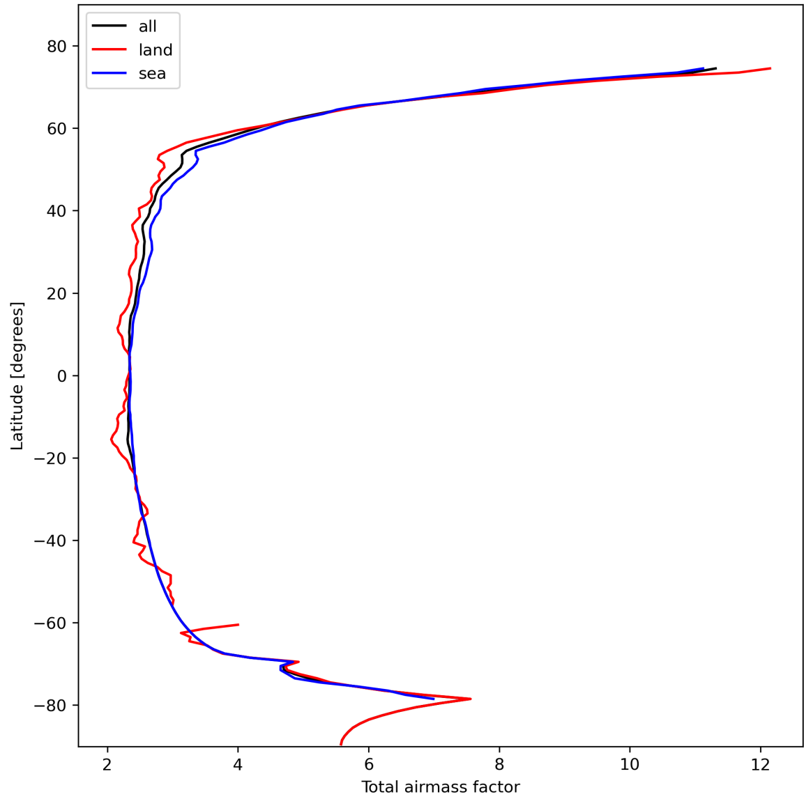
Figure 15: Zonal average of “Total airmass factor” for 2023-10-29 to 2023-10-31.
