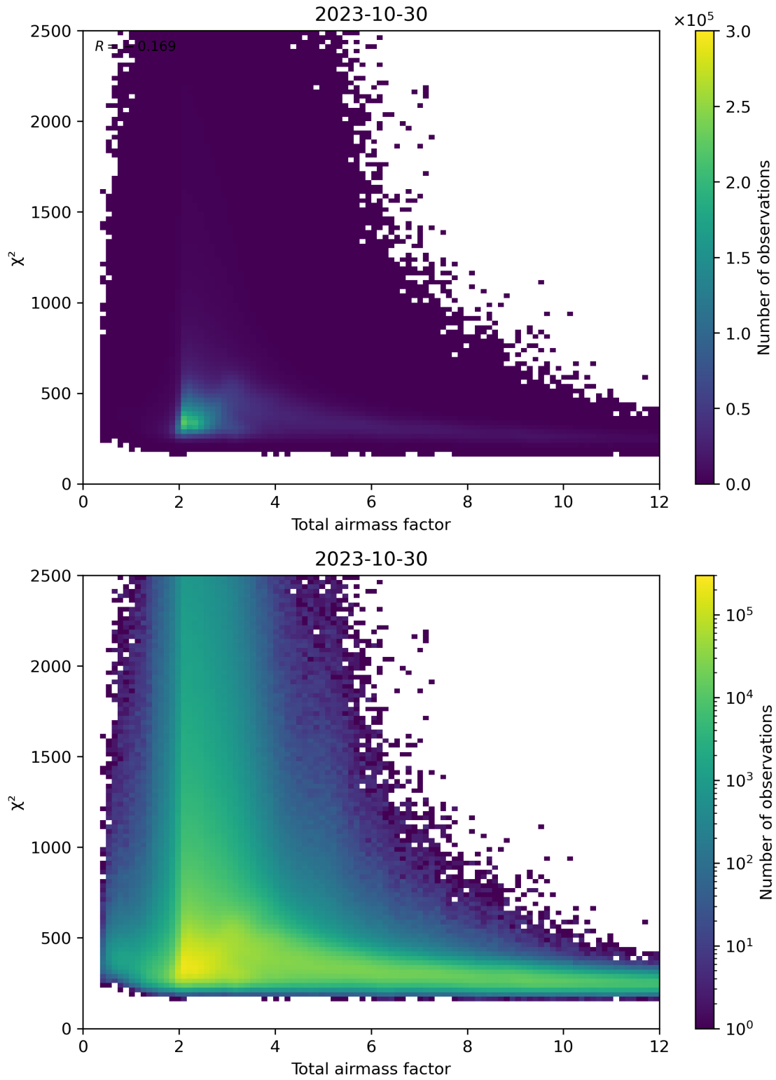
Figure 63: Scatter density plot of “Total airmass factor” against “ \chi^2 ” for 2023-10-29 to 2023-10-31.
