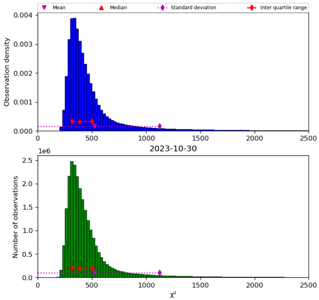
Figure 42: Histogram of “ \chi^2 ” for 2023-10-29 to 2023-10-31
