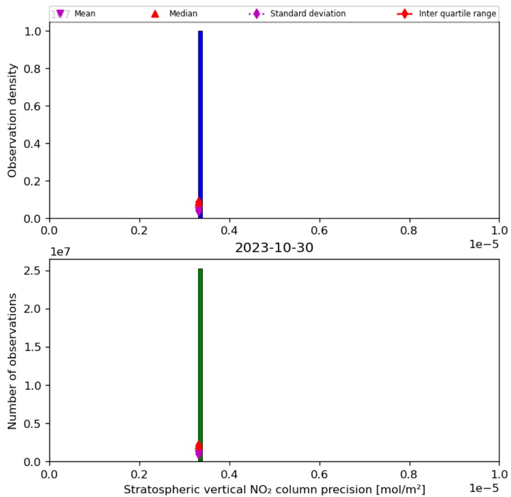
Figure 37: Histogram of “Stratospheric vertical NO 2 column precision” for 2023-10-29 to 2023-10-31
