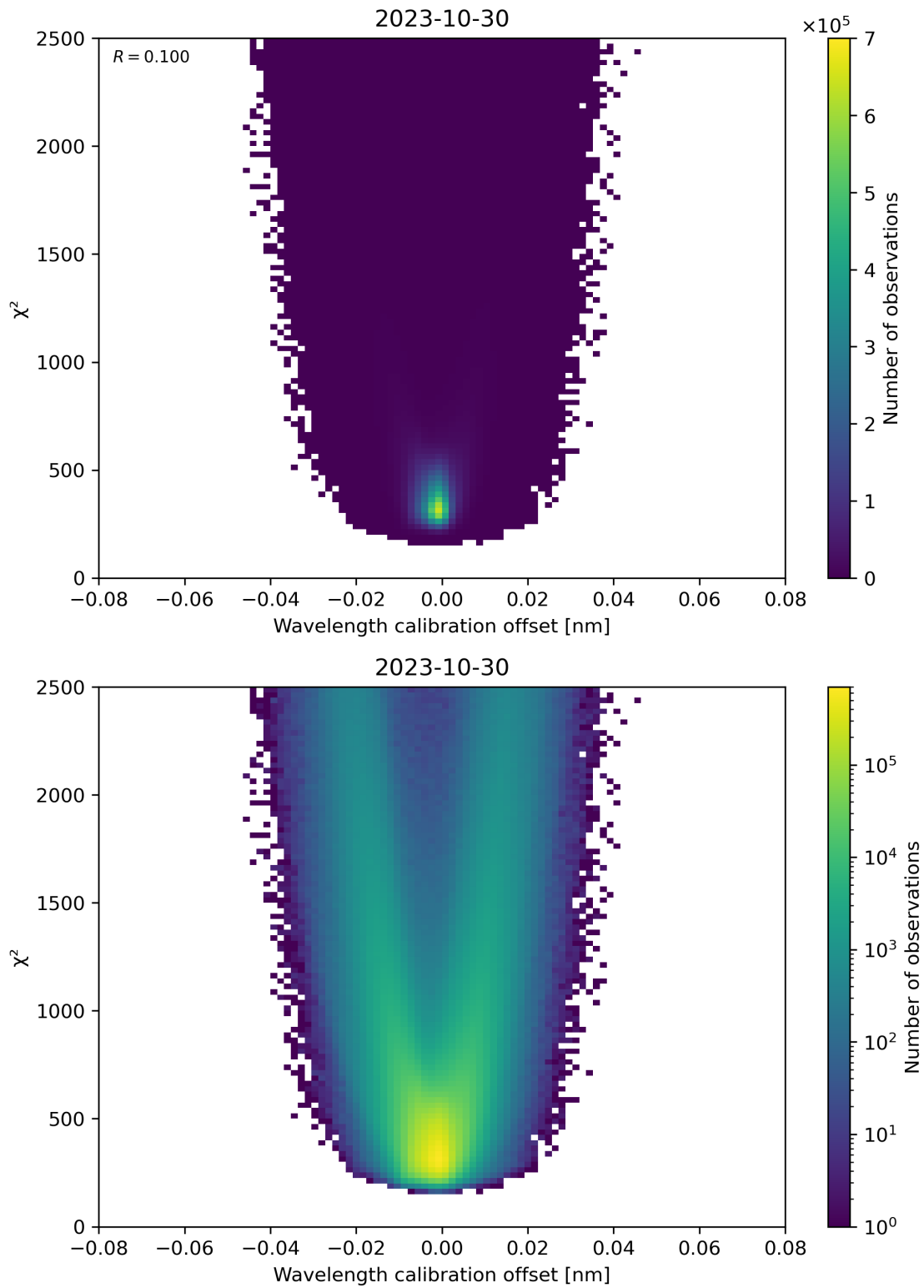
Figure 175: Scatter density plot of “Wavelength calibration offset” against “ \chi^2 ” for 2023-10-29 to 2023-10-31.
