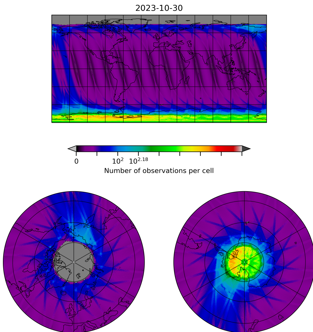
Figure 10: Map of the number of observations for 2023-10-29 to 2023-10-31
