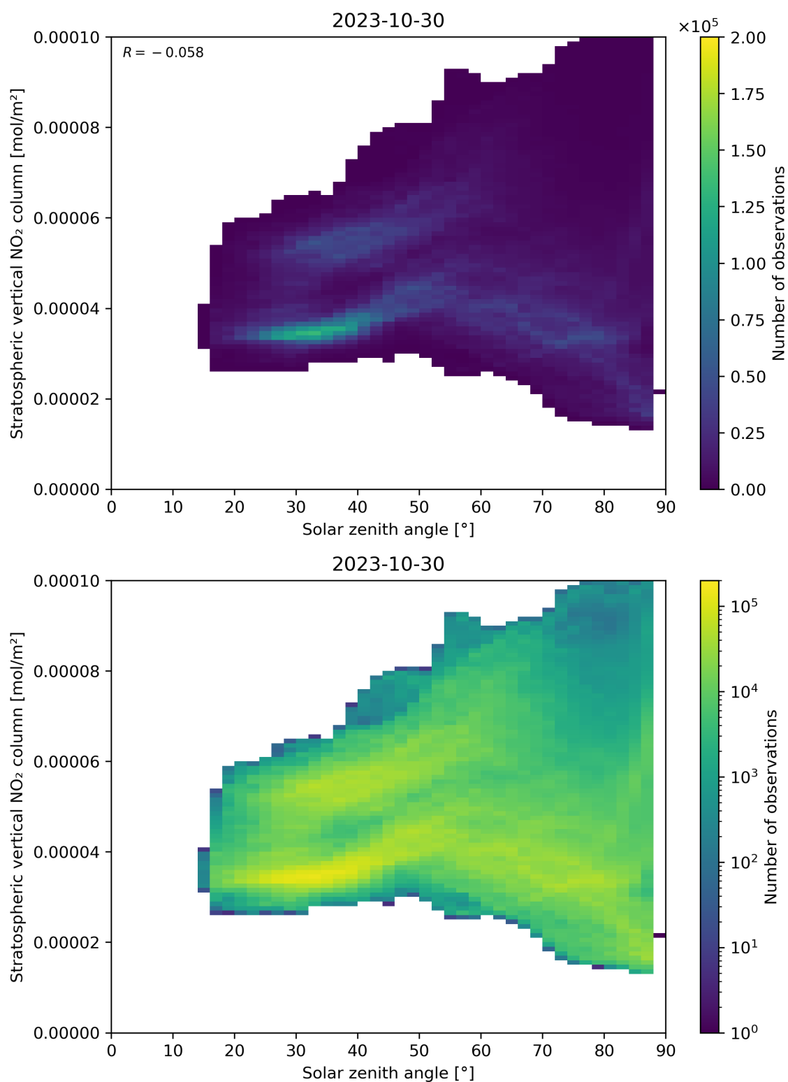
Figure 150: Scatter density plot of “Solar zenith angle” against “Stratospheric vertical NO 2 column” for 2023-10-29 to 2023-10-31.
