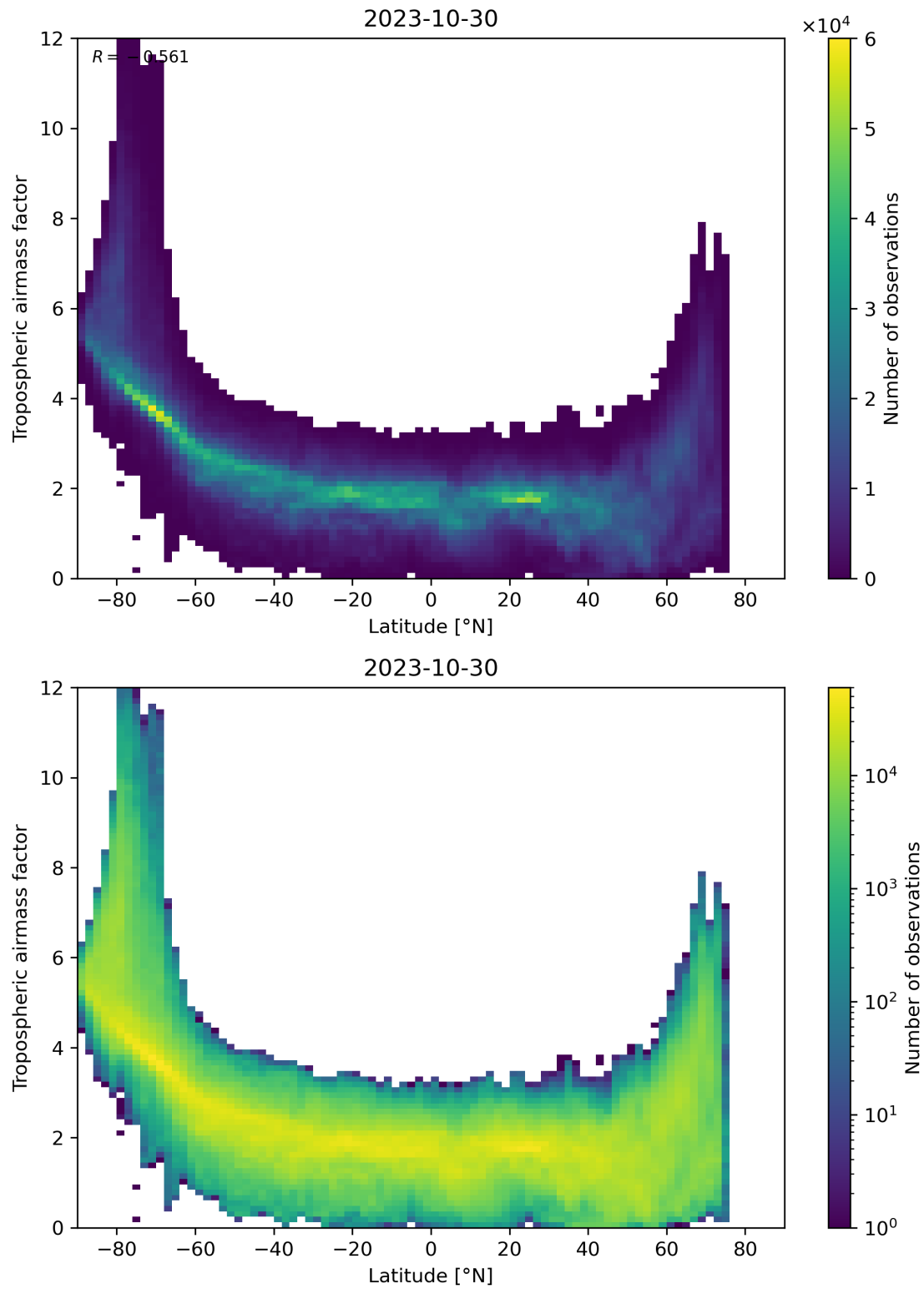
Figure 85: Scatter density plot of “Latitude” against “Tropospheric air mass factor” for 2023-10-29 to 2023-10-31.
