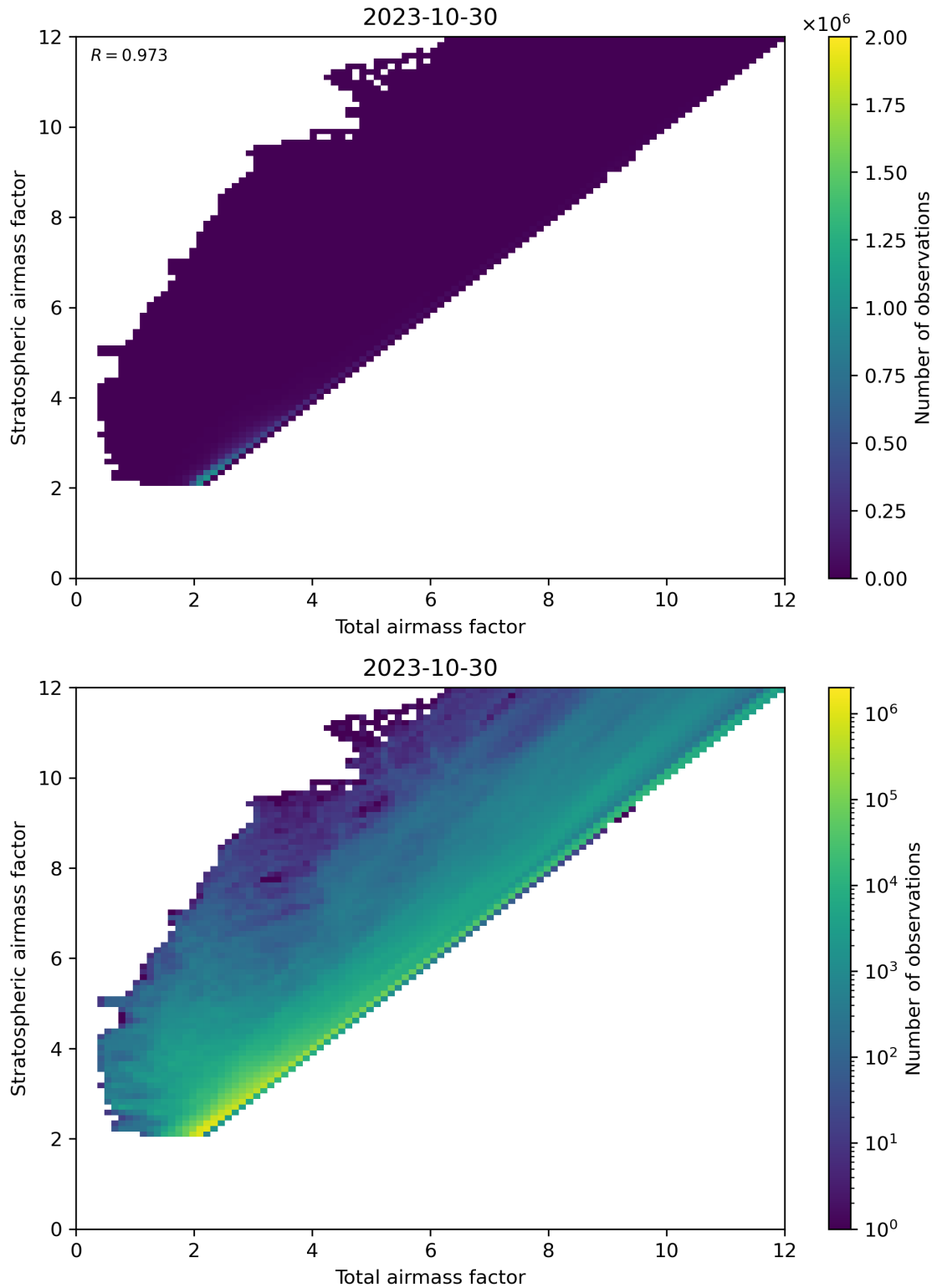
Figure 62: Scatter density plot of “Total airmass factor” against “Stratospheric airmass factor” for 2023-10-29 to 2023-10-31.
