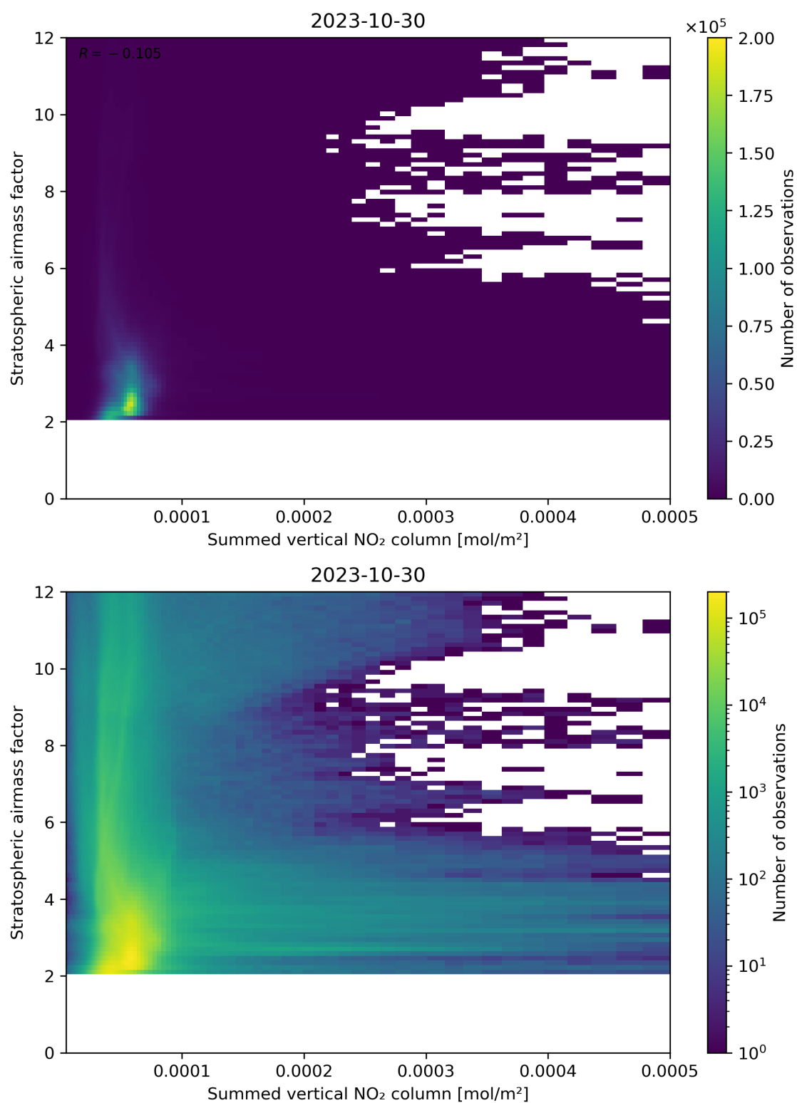
Figure 103: Scatter density plot of “Summed vertical NO 2 column” against “Stratospheric air mass factor” for 2023-10-29 to 2023-10-31.
