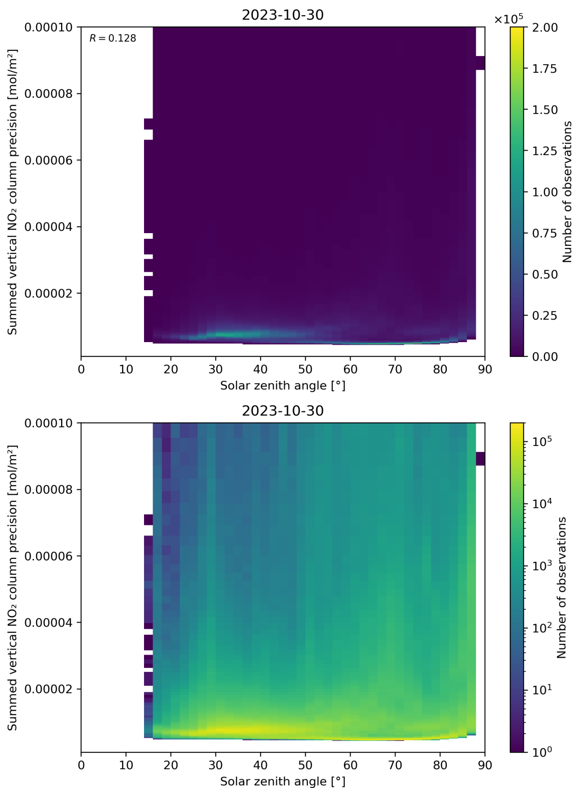
Figure 152: Scatter density plot of “Solar zenith angle” against “Summed vertical NO 2 column precision” for 2023-10-29 to 2023-10-31.
