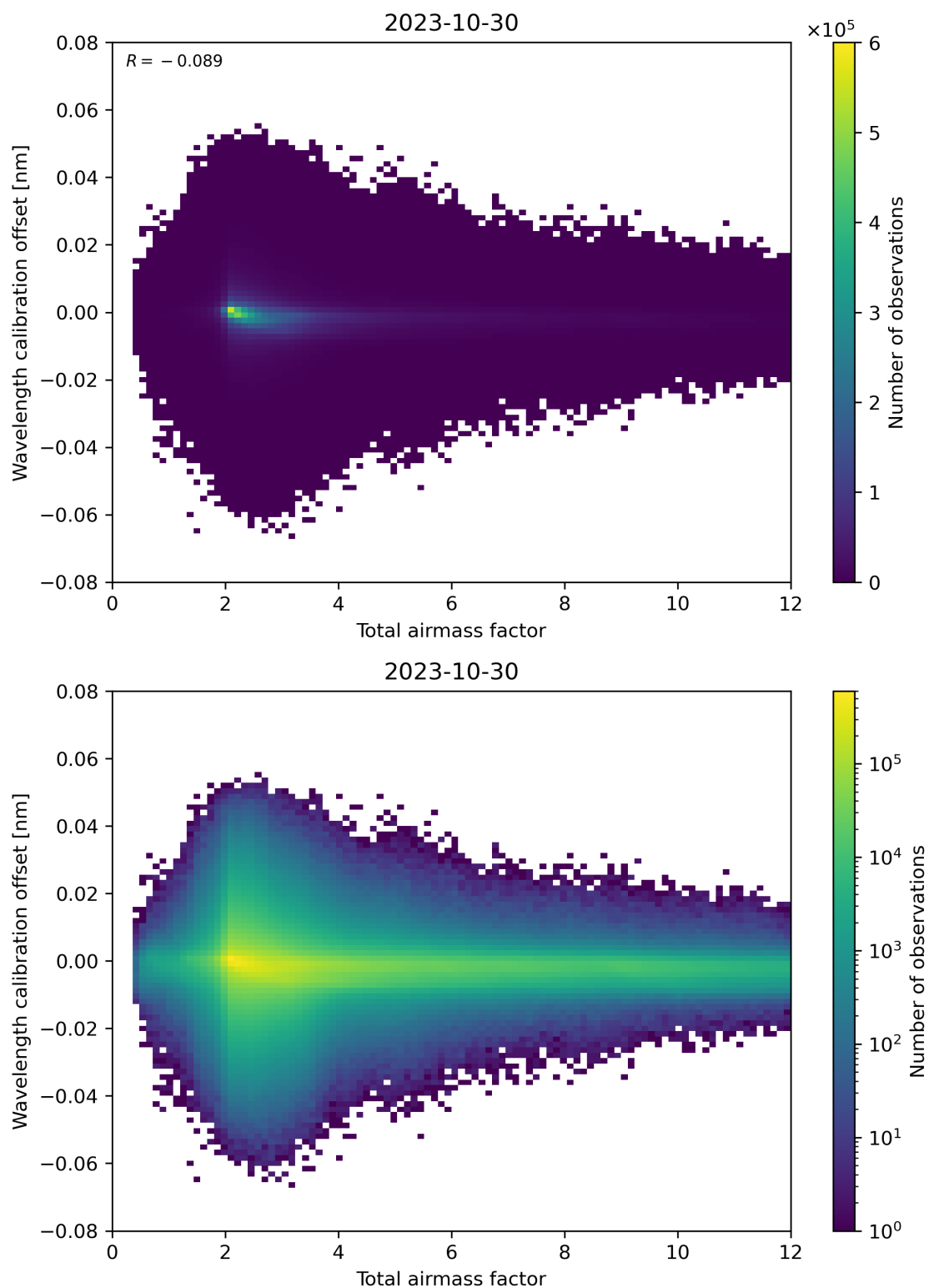
Figure 70: Scatter density plot of “Total airmass factor” against “Wavelength calibration offset” for 2023-10-29 to 2023-10-31.
