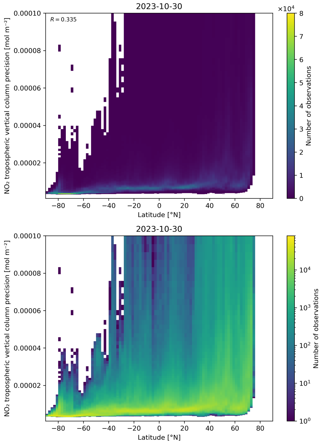
Figure 93: Scatter density plot of “Latitude” against “NO 2 tropospheric vertical column precision” for 2023-10-29 to 2023-10-31.
