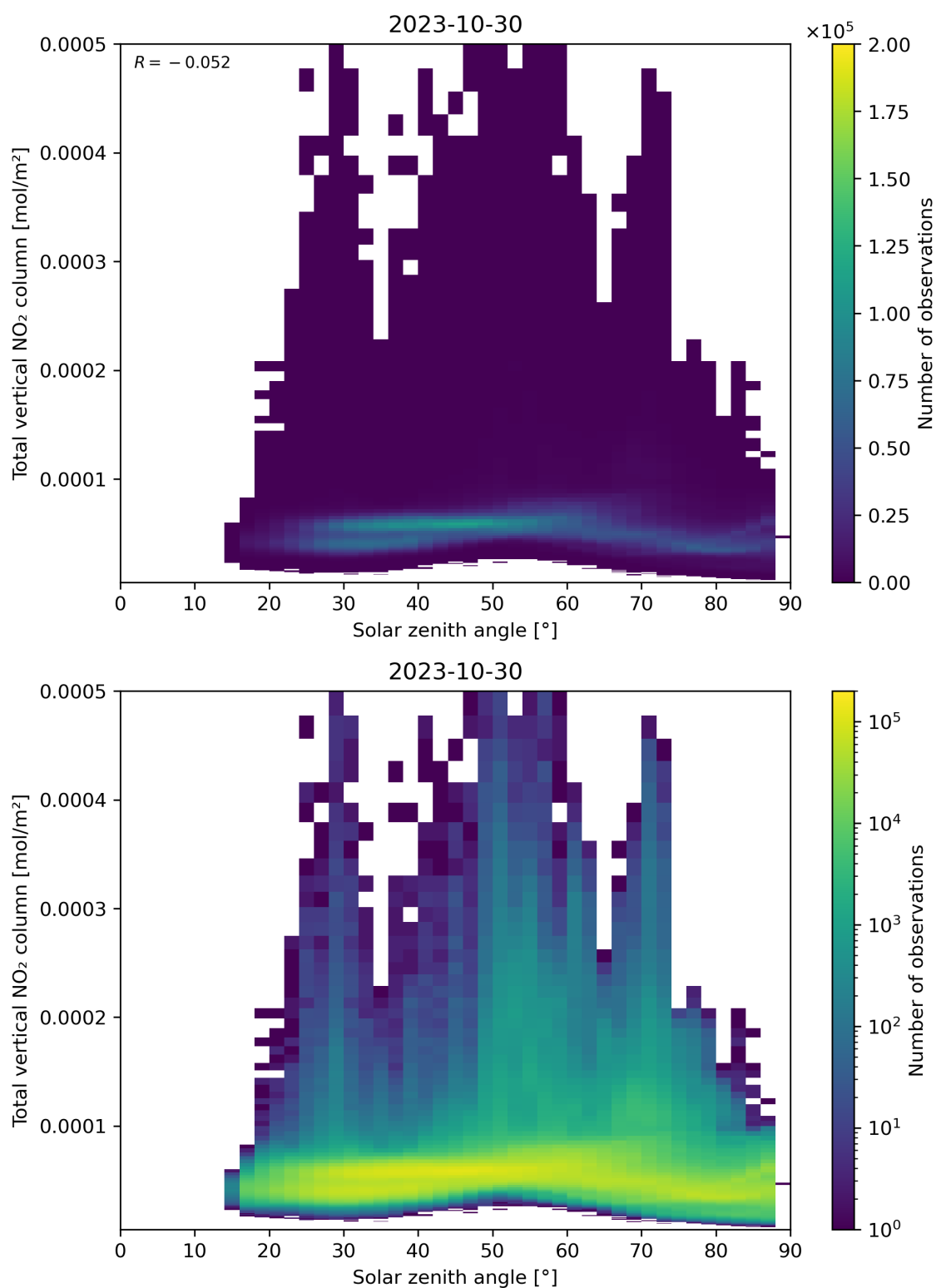
Figure 153: Scatter density plot of “Solar zenith angle” against “Total vertical NO 2 column” for 2023-10-29 to 2023-10-31.
