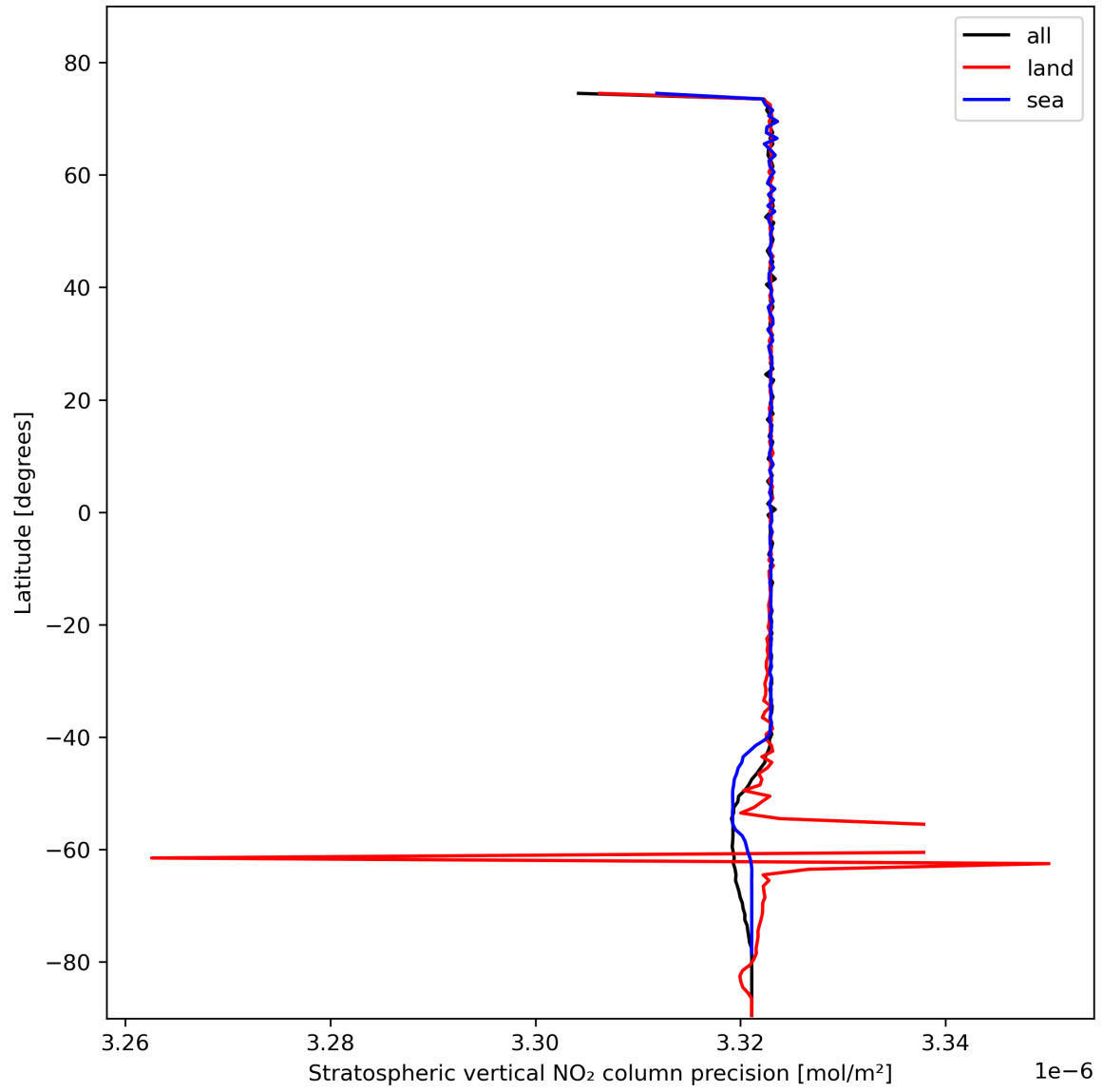
Figure 20: Zonal average of “Stratospheric vertical NO 2 column precision” for 2023-10-29 to 2023-10-31.
