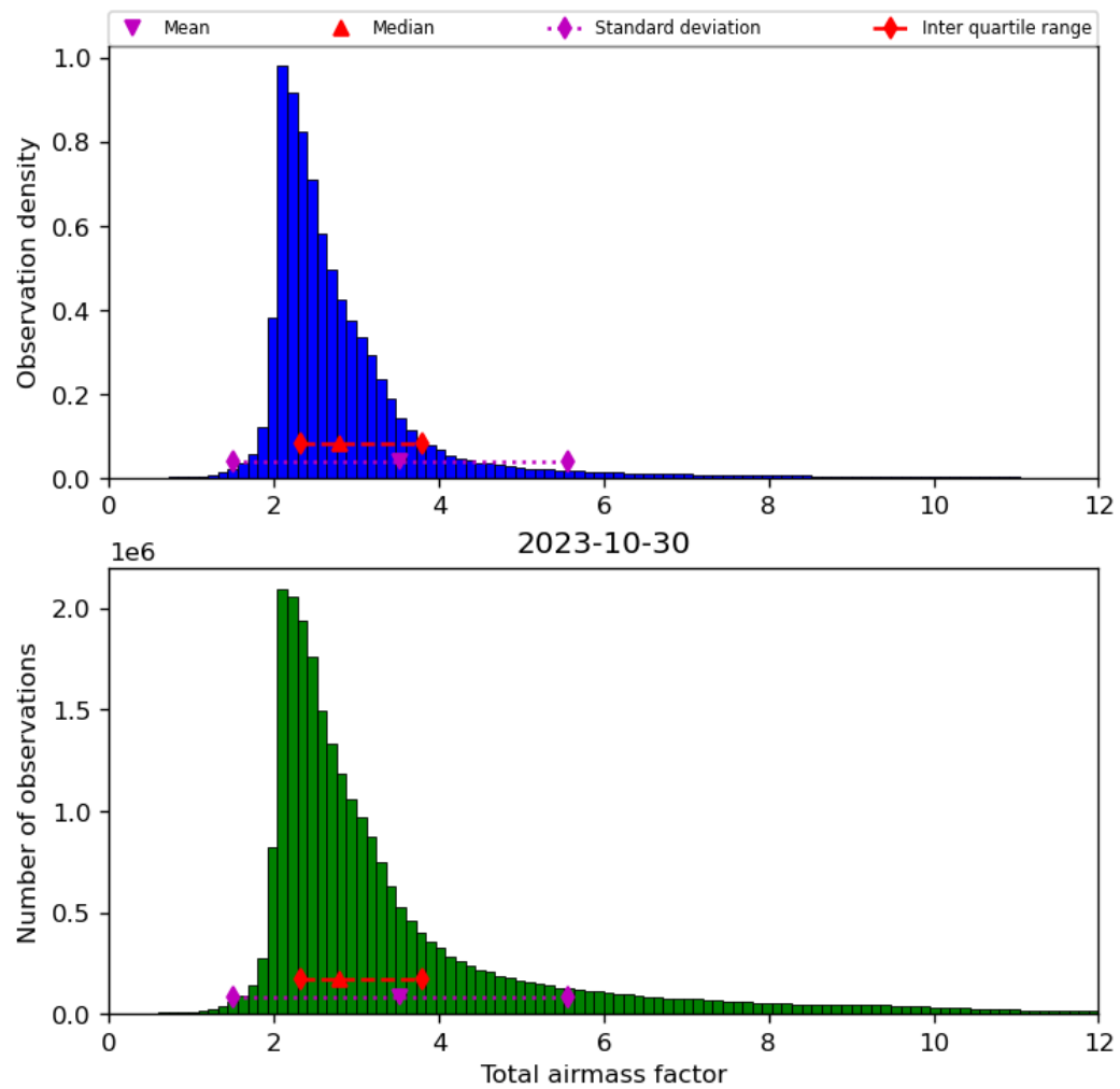
Figure 32: Histogram of “Total airmass factor” for 2023-10-29 to 2023-10-31
