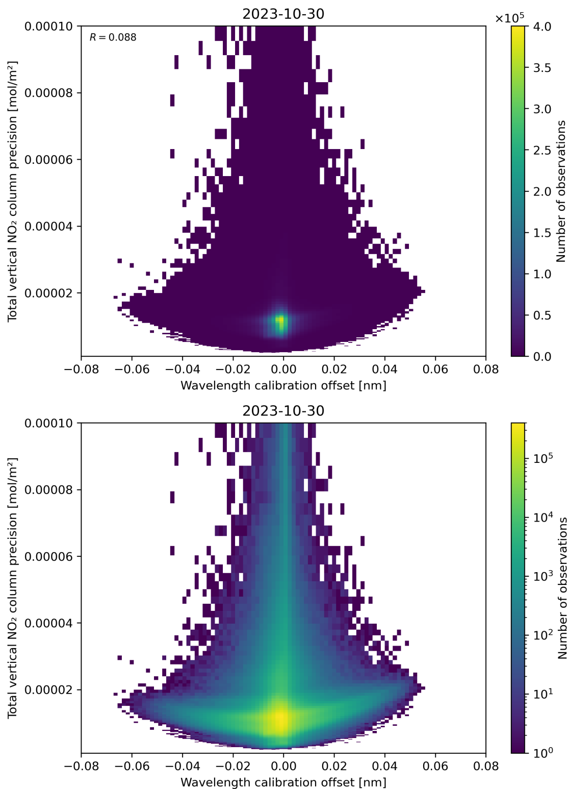
Figure 180: Scatter density plot of “Wavelength calibration offset” against “Total vertical NO 2 column precision” for 2023-10-29 to 2023-10-31.
