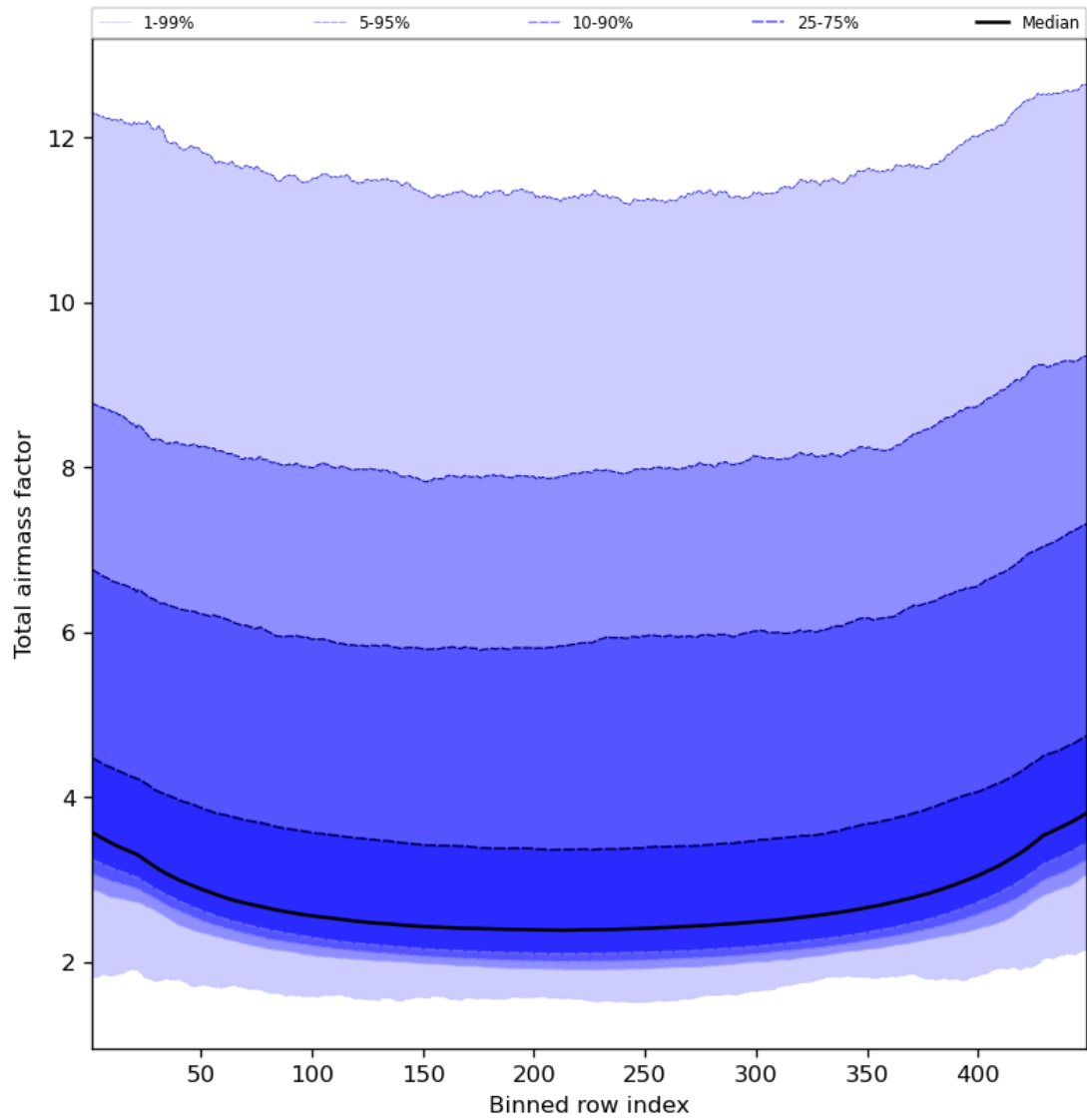
Figure 49: Along track statistics of “Total airmass factor” for 2023-10-29 to 2023-10-31
