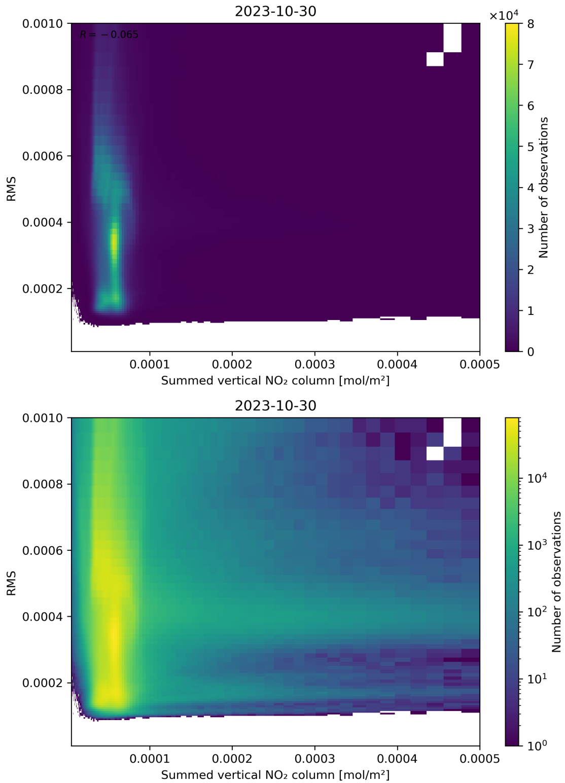
Figure 109: Scatter density plot of “Summed vertical NO 2 column” against “RMS” for 2023-10-29 to 2023-10-31.
