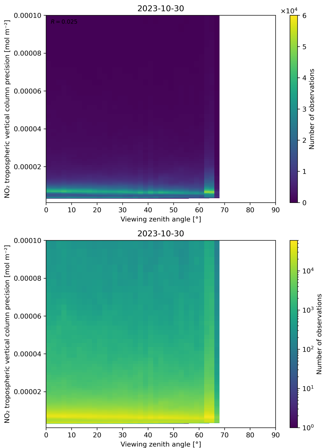
Figure 170: Scatter density plot of “Viewing zenith angle” against “NO 2 tropospheric vertical column precision” for 2023-10-29 to 2023-10-31.
