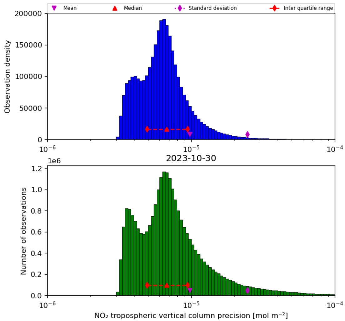
Figure 30: Histogram of “NO 2 tropospheric vertical column precision” for 2023-10-29 to 2023-10-31
