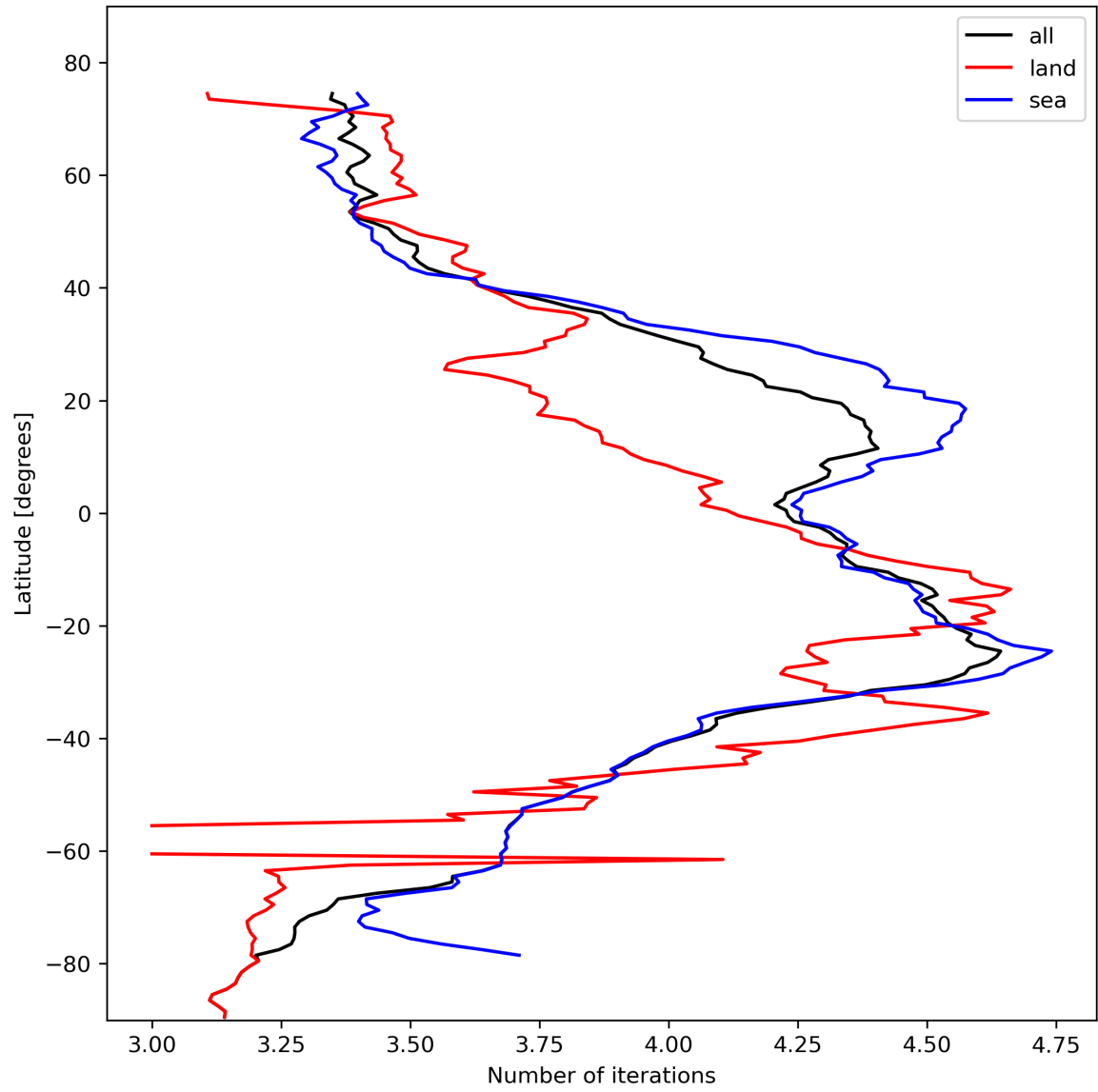
Figure 17: Zonal average of “Number of iterations” for 2023-10-29 to 2023-10-31.
