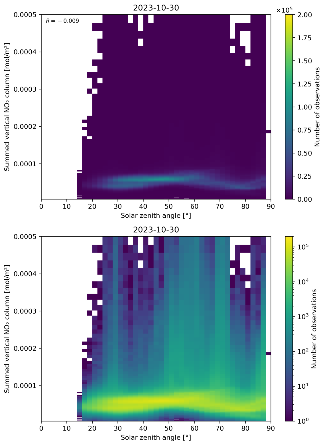
Figure 151: Scatter density plot of “Solar zenith angle” against “Summed vertical NO 2 column” for 2023-10-29 to 2023-10-31.
