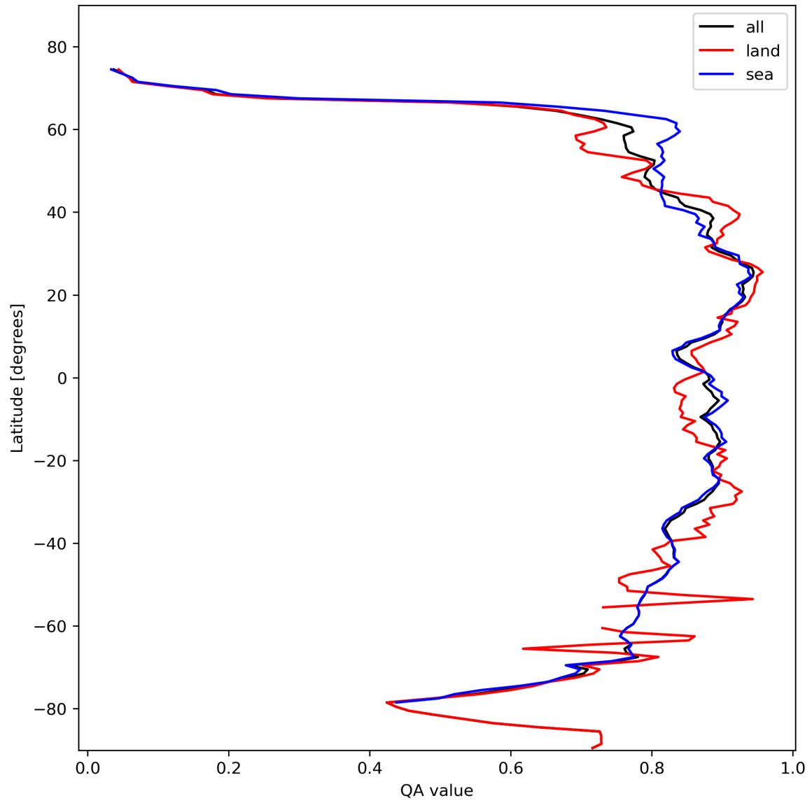
Figure 11: Zonal average of “QA value” for 2023-10-29 to 2023-10-31.
