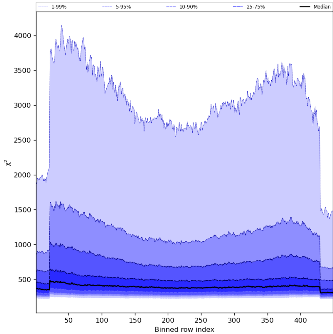
Figure 59: Along track statistics of “ \chi^2 ” for 2023-10-29 to 2023-10-31
