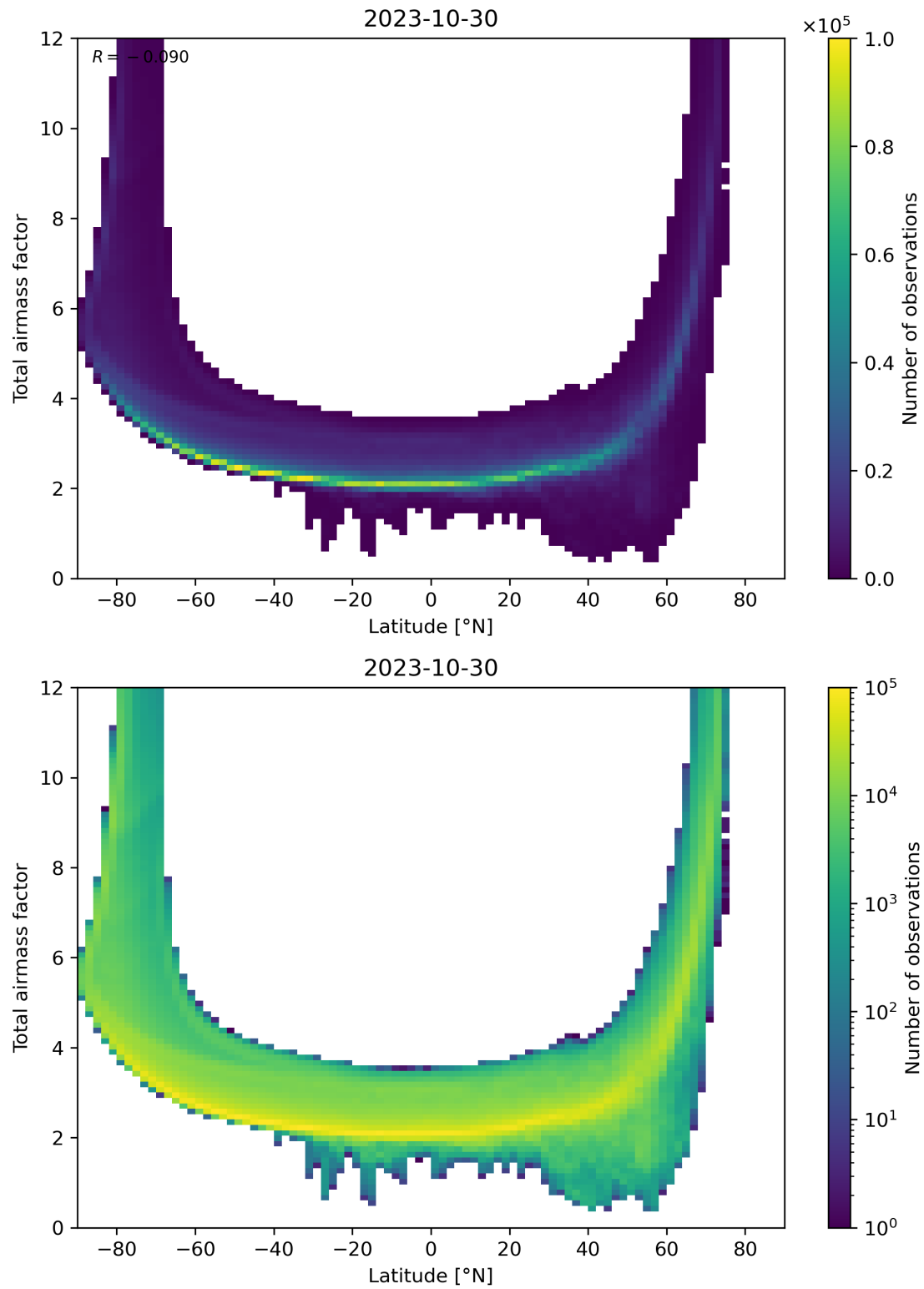
Figure 84: Scatter density plot of “Latitude” against “Total airmass factor” for 2023-10-29 to 2023-10-31.
