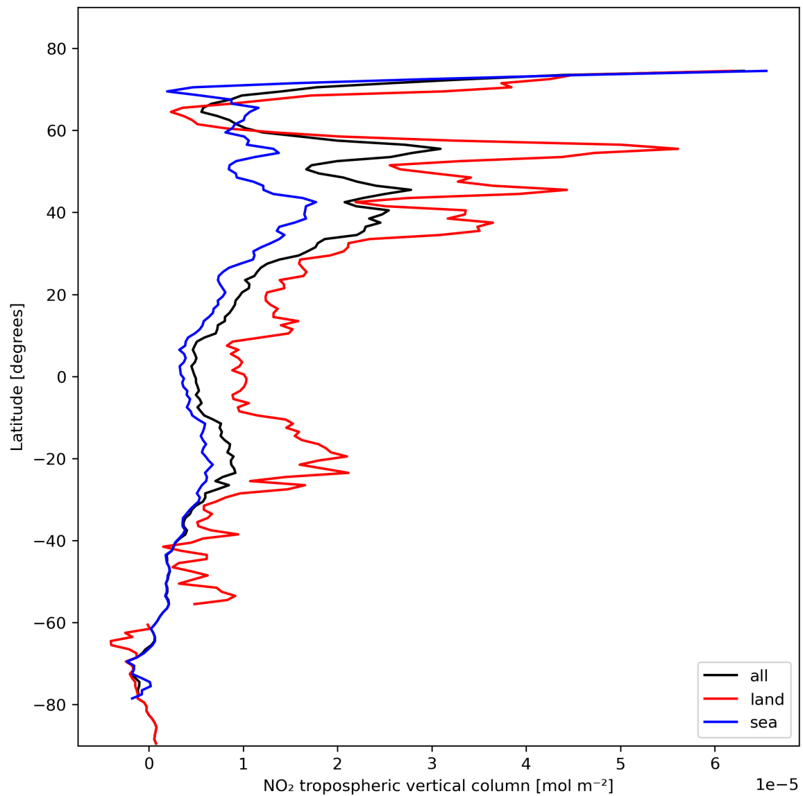
Figure 12: Zonal average of “NO 2 tropospheric vertical column” for 2023-10-29 to 2023-10-31.
