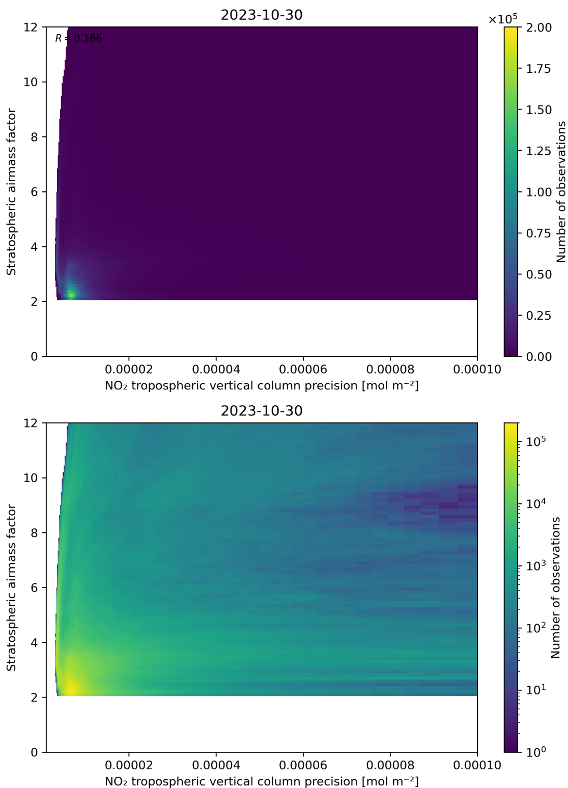
Figure 131: Scatter density plot of “NO 2 tropospheric vertical column precision” against “Stratospheric airmass factor” for 2023-10-29 to 2023-10-31.
