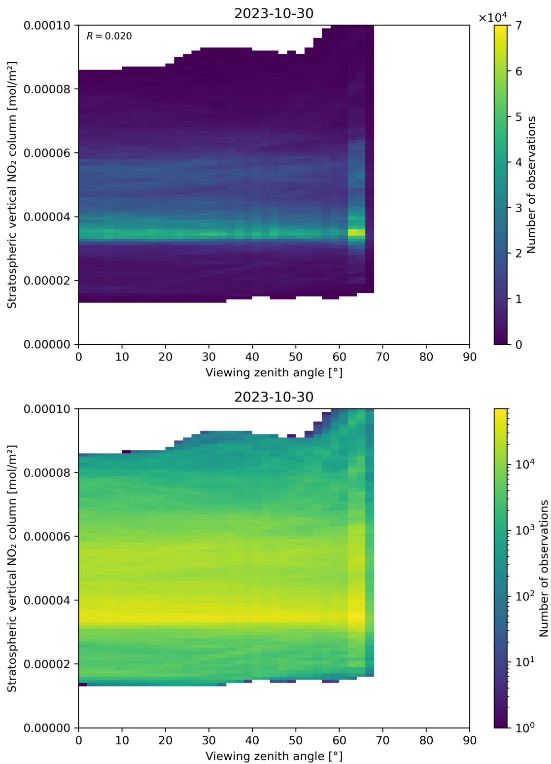
Figure 164: Scatter density plot of “Viewing zenith angle” against “Stratospheric vertical NO 2 column” for 2023-10-29 to 2023-10-31.
