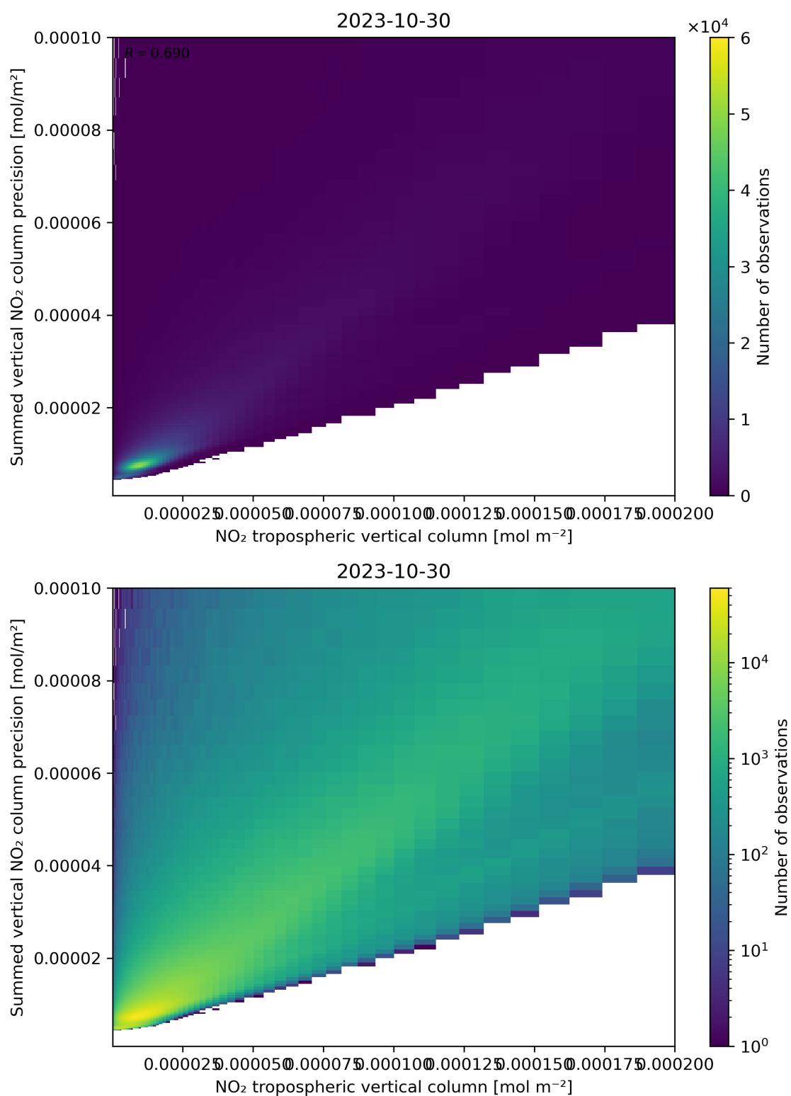
Figure 127: Scatter density plot of “NO 2 tropospheric vertical column” against “Summed vertical NO 2 column precision” for 2023-10-29 to 2023-10-31.
