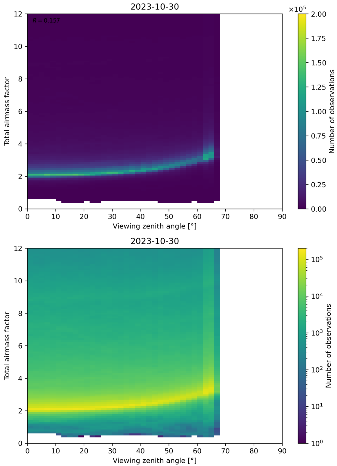
Figure 160: Scatter density plot of “Viewing zenith angle” against “Total airmass factor” for 2023-10-29 to 2023-10-31.
