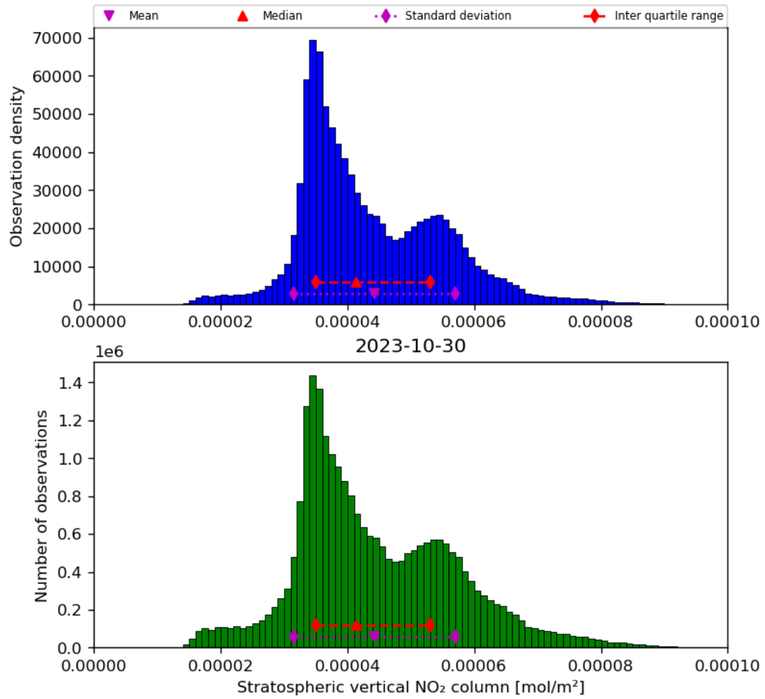
Figure 36: Histogram of “Stratospheric vertical NO 2 column” for 2023-10-29 to 2023-10-31
