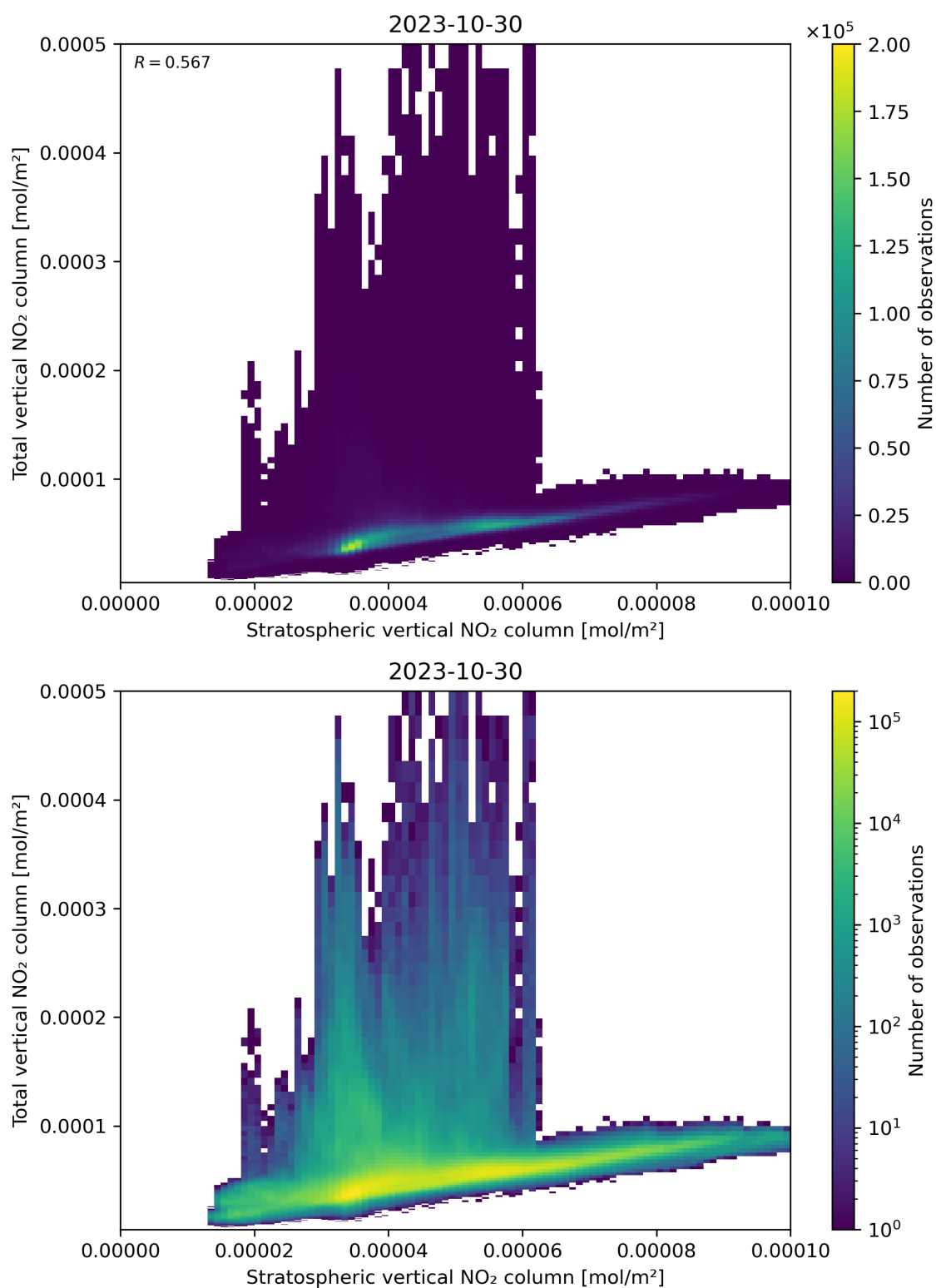
Figure 100: Scatter density plot of “Stratospheric vertical NO 2 column” against “Total vertical NO 2 column” for 2023-10-29 to 2023-10-31.
