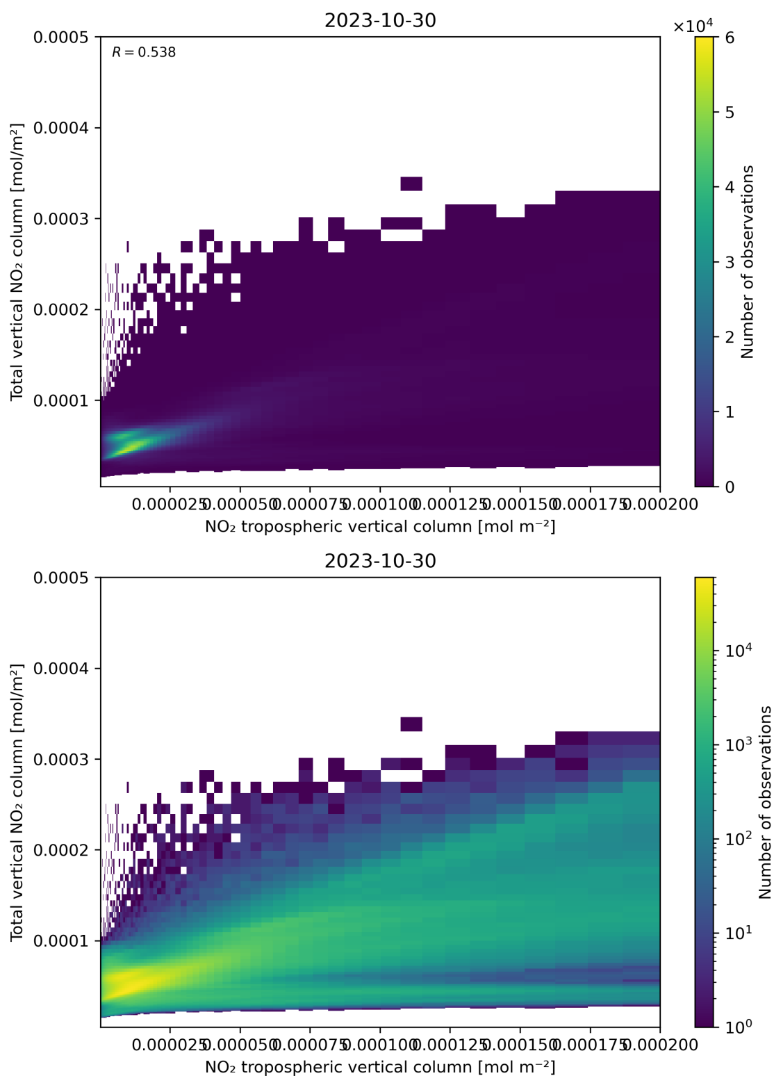
Figure 128: Scatter density plot of “NO 2 tropospheric vertical column” against “Total vertical NO 2 column” for 2023-10-29 to 2023-10-31.
