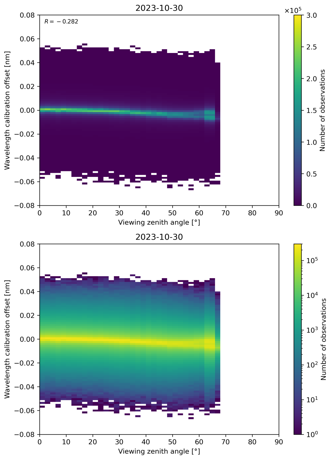
Figure 173: Scatter density plot of “Viewing zenith angle” against “Wavelength calibration offset” for 2023-10-29 to 2023-10-31.
