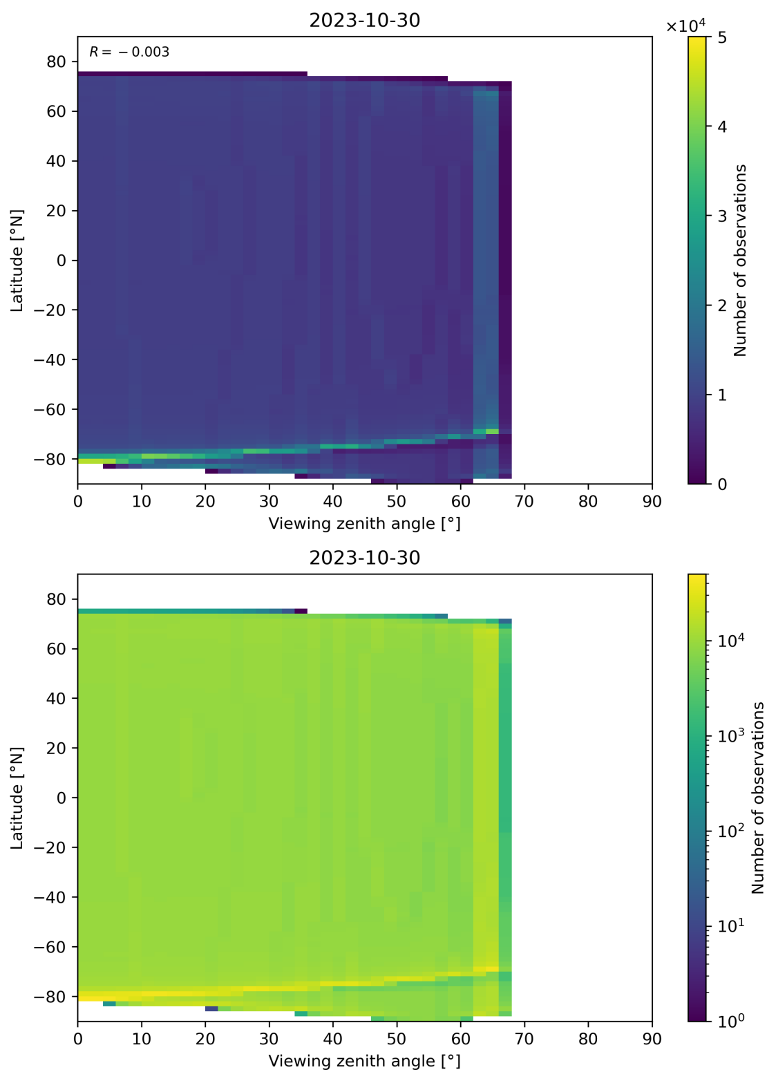
Figure 163: Scatter density plot of “Viewing zenith angle” against “Latitude” for 2023-10-29 to 2023-10-31.
