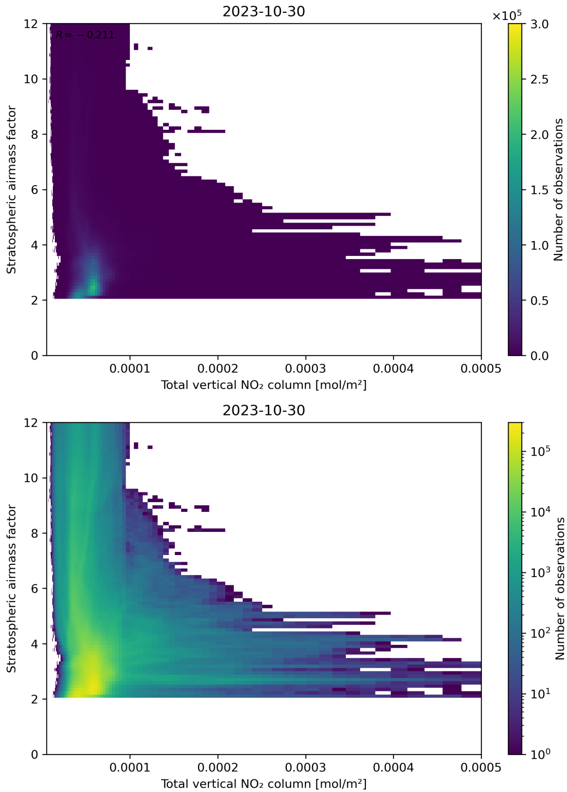
Figure 110: Scatter density plot of “Total vertical NO 2 column” against “Stratospheric air mass factor” for 2023-10-29 to 2023-10-31.
