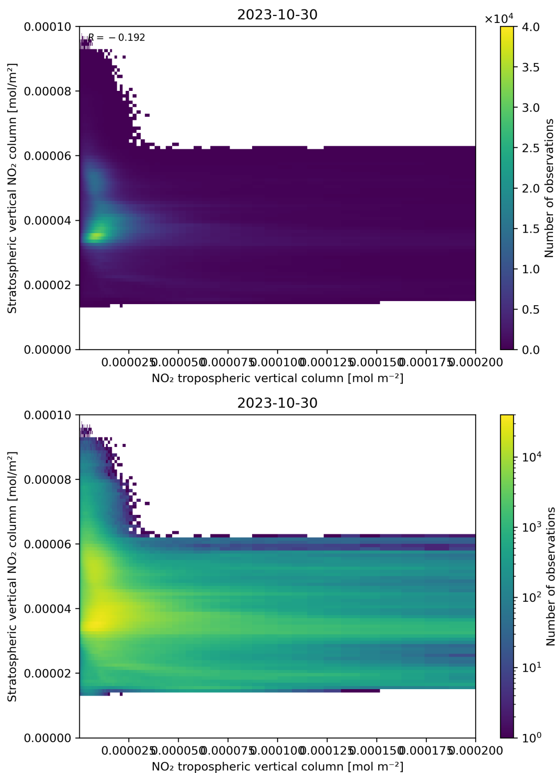
Figure 125: Scatter density plot of “NO 2 tropospheric vertical column” against “Stratospheric vertical NO 2 column” for 2023-10-29 to 2023-10-31.
