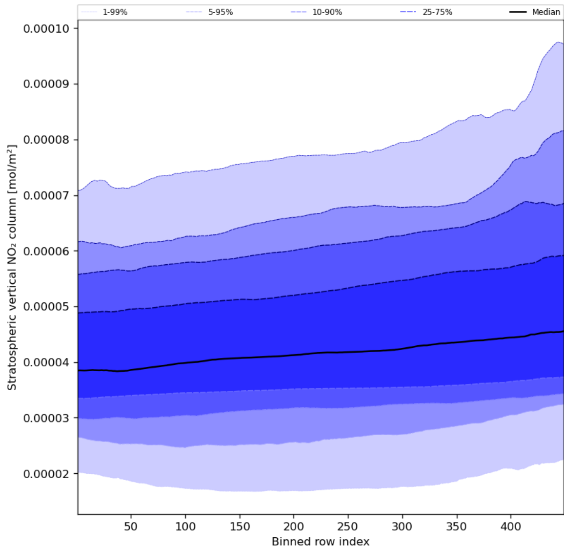
Figure 53: Along track statistics of “Stratospheric vertical NO 2 column” for 2023-10-29 to 2023-10-31
