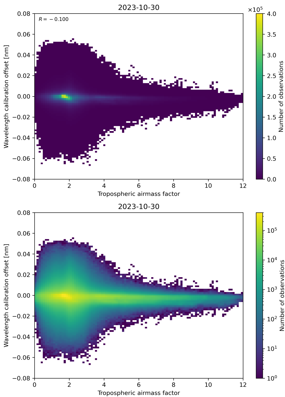
Figure 80: Scatter density plot of “Tropospheric airmass factor” against “Wavelength calibration offset” for 2023-10-29 to 2023-10-31.
