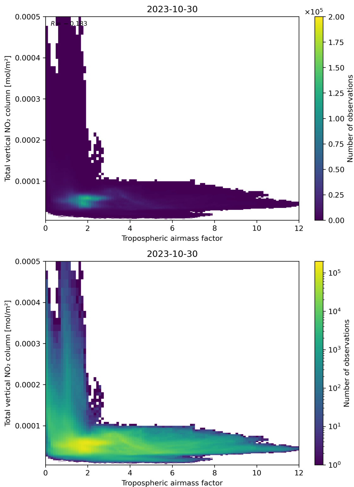
Figure 77: Scatter density plot of “Tropospheric airmass factor” against “Total vertical NO 2 column” for 2023-10-29 to 2023-10-31.
