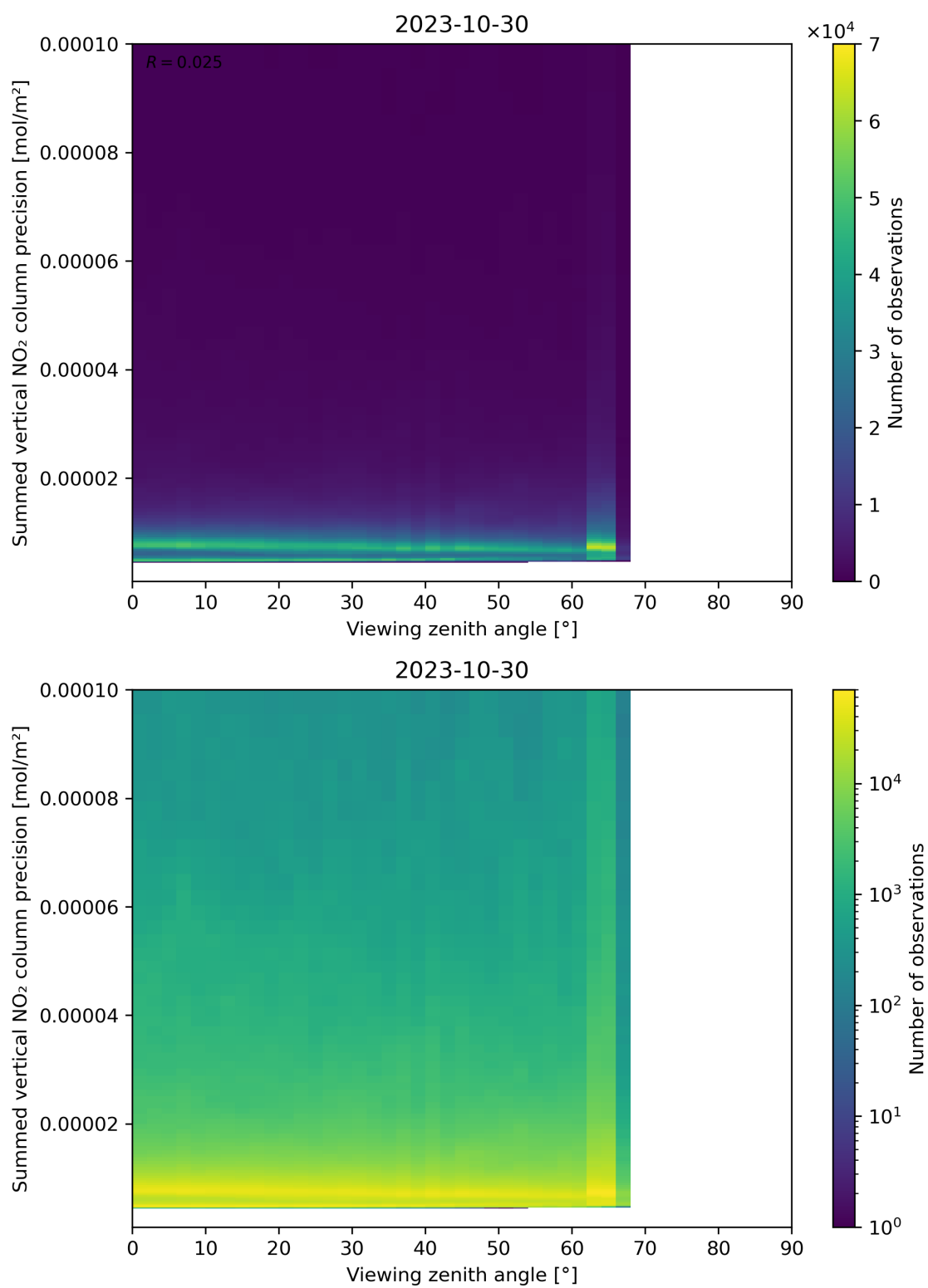
Figure 166: Scatter density plot of “Viewing zenith angle” against “Summed vertical NO 2 column precision” for 2023-10-29 to 2023-10-31.
