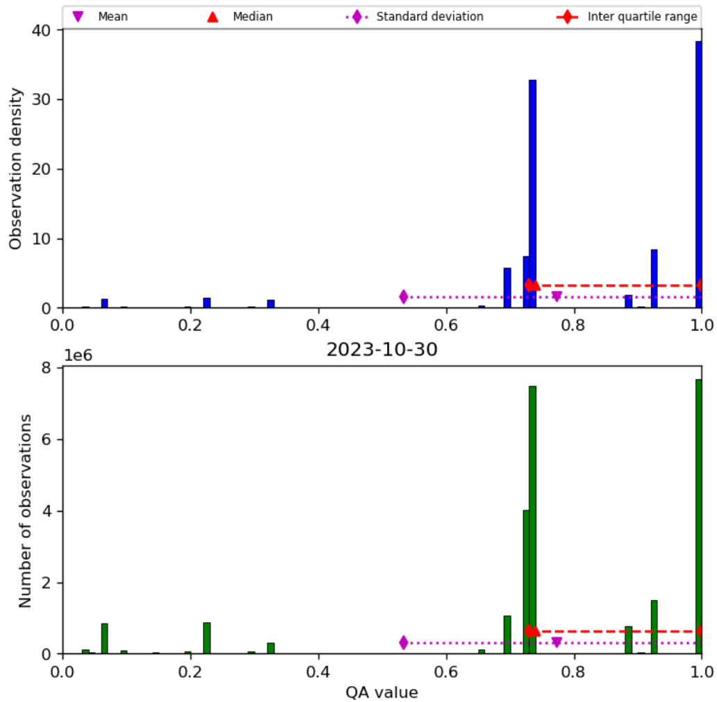
Figure 28: Histogram of “QA value” for 2023-10-29 to 2023-10-31
