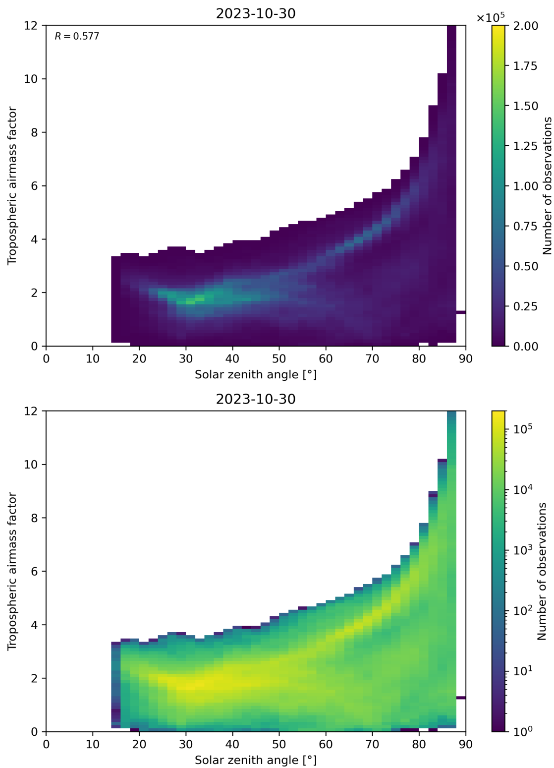
Figure 147: Scatter density plot of “Solar zenith angle” against “Tropospheric airmass factor” for 2023-10-29 to 2023-10-31.
