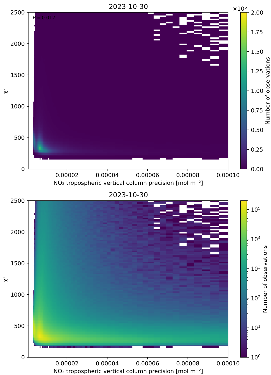
Figure 134: Scatter density plot of “NO 2 tropospheric vertical column precision” against “ \chi^2 ” for 2023-10-29 to 2023-10-31.
