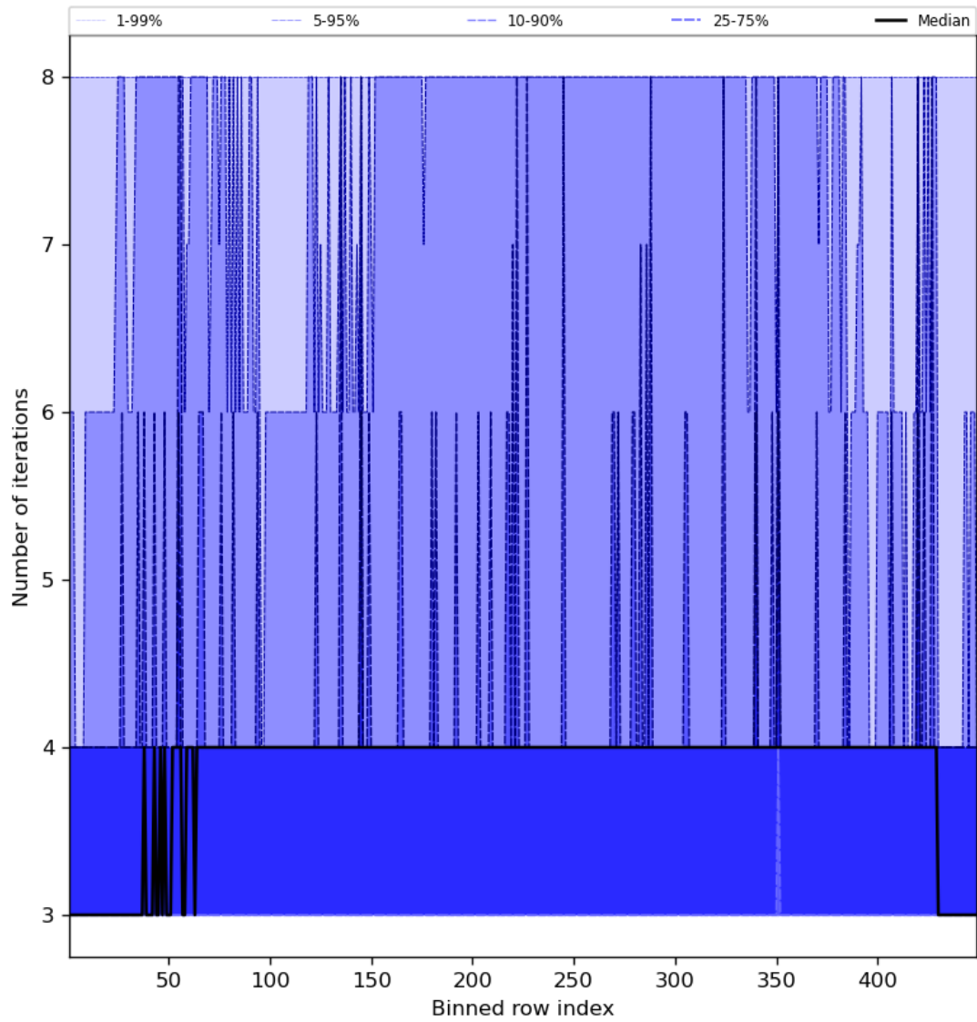
Figure 51: Along track statistics of “Number of iterations” for 2023-10-29 to 2023-10-31
