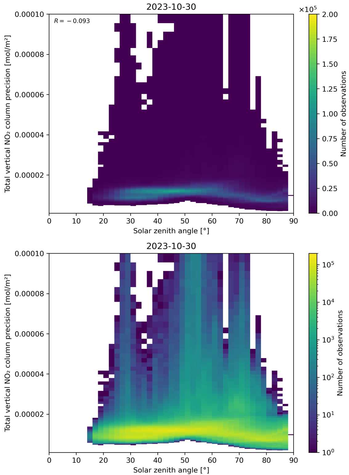
Figure 154: Scatter density plot of “Solar zenith angle” against “Total vertical NO 2 column precision” for 2023-10-29 to 2023-10-31.
