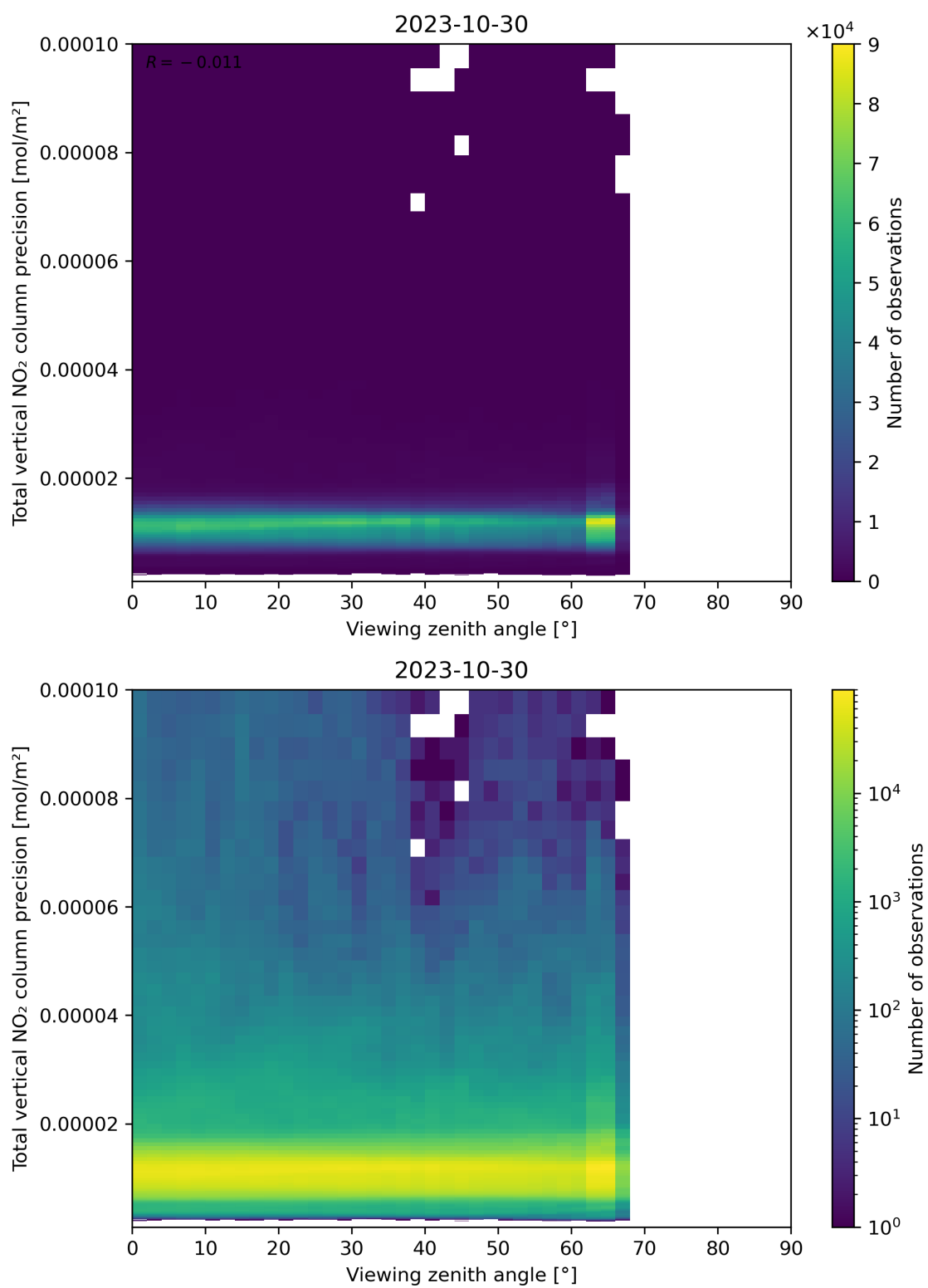
Figure 168: Scatter density plot of “Viewing zenith angle” against “Total vertical NO 2 column precision” for 2023-10-29 to 2023-10-31.
