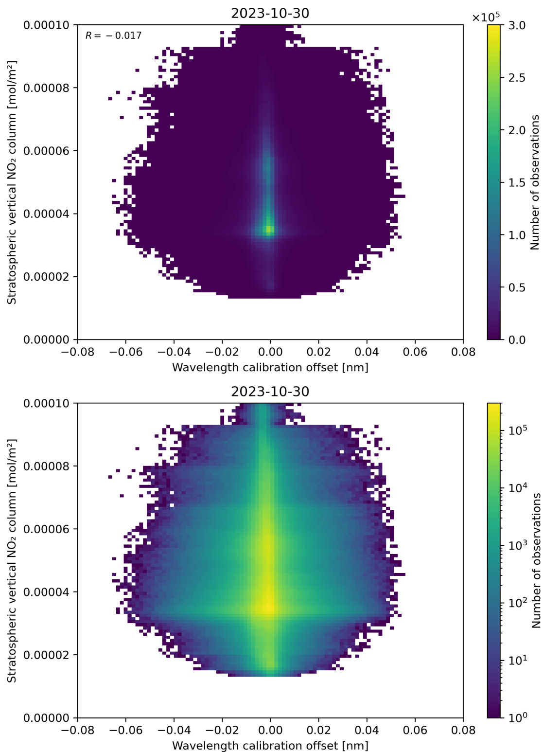
Figure 176: Scatter density plot of “Wavelength calibration offset” against “Stratospheric vertical NO 2 column” for 2023-10-29 to 2023-10-31.
