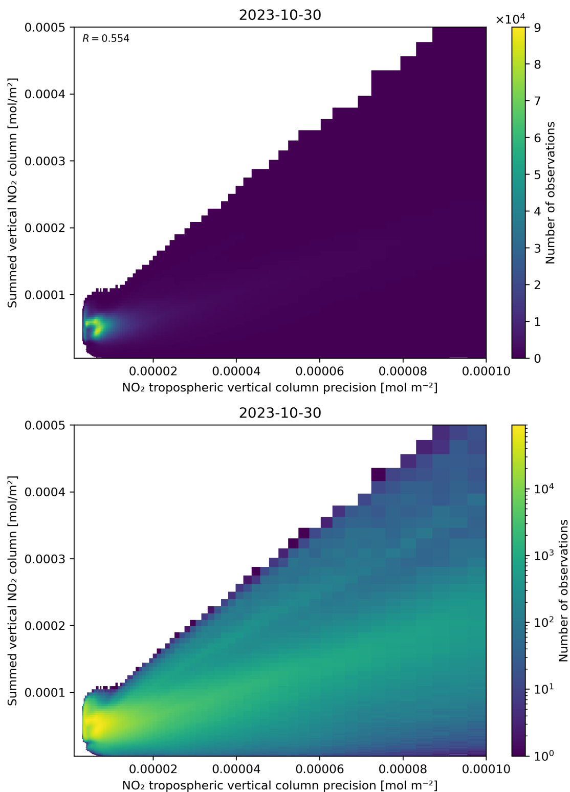
Figure 136: Scatter density plot of “NO 2 tropospheric vertical column precision” against “Summed vertical NO 2 column” for 2023-10-29 to 2023-10-31.
