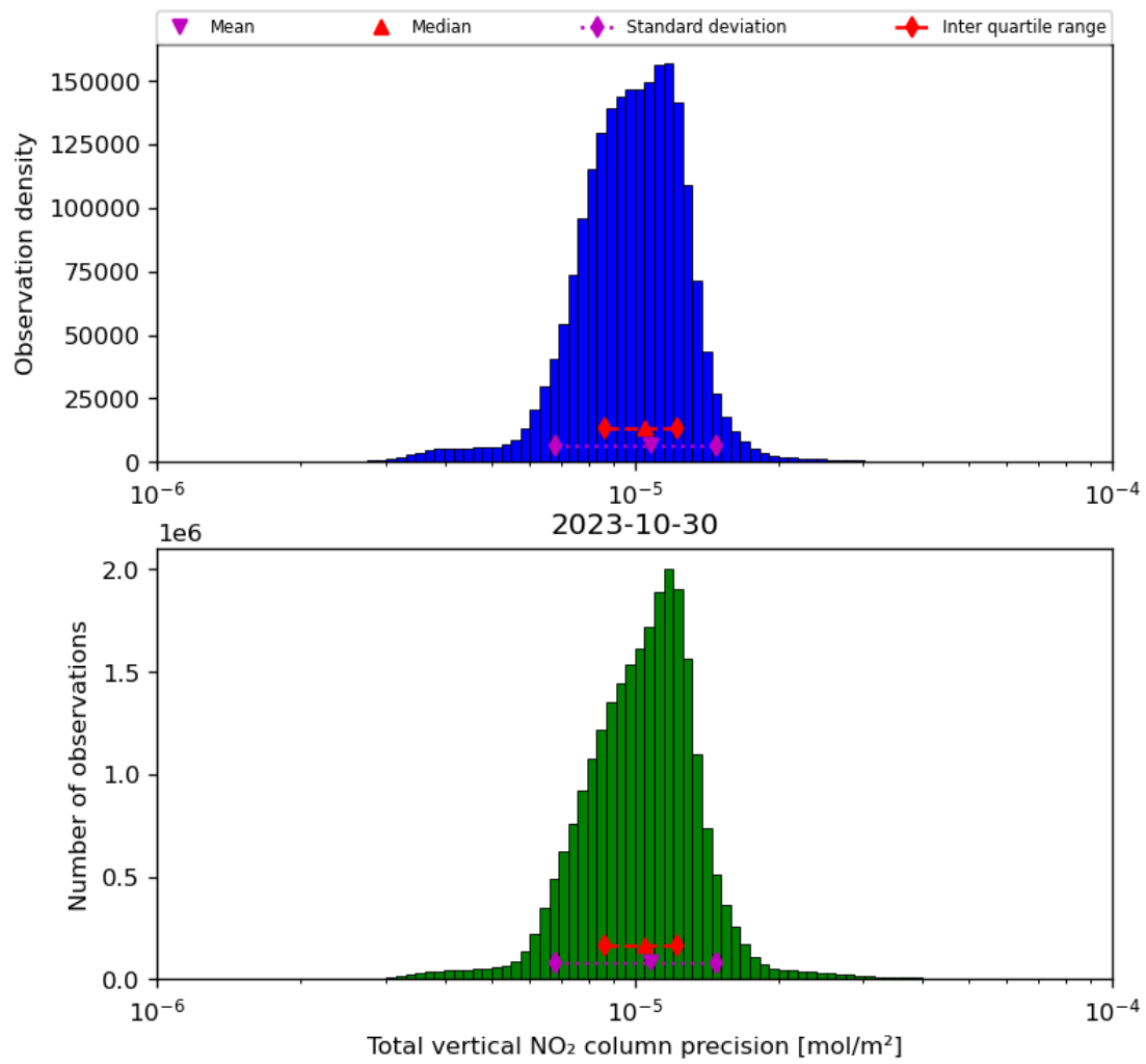
Figure 39: Histogram of “Total vertical NO 2 column precision” for 2023-10-29 to 2023-10-31
