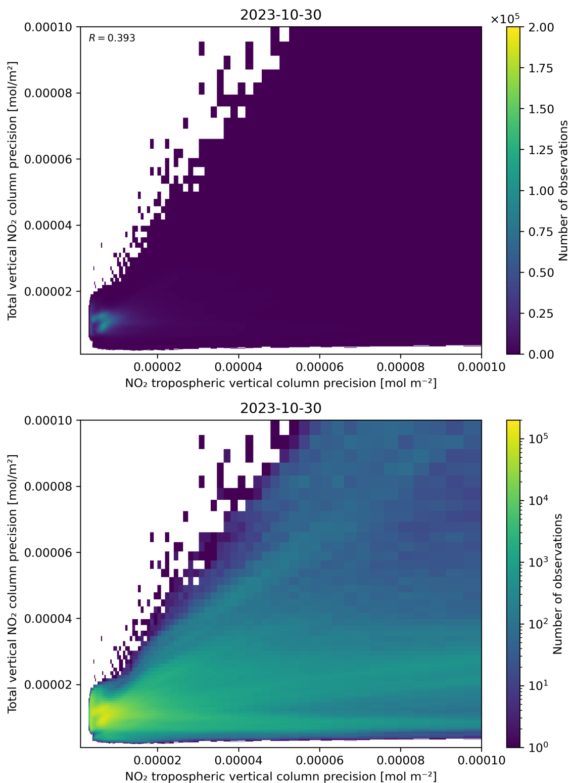
Figure 139: Scatter density plot of “NO 2 tropospheric vertical column precision” against “Total vertical NO 2 column precision” for 2023-10-29 to 2023-10-31.
