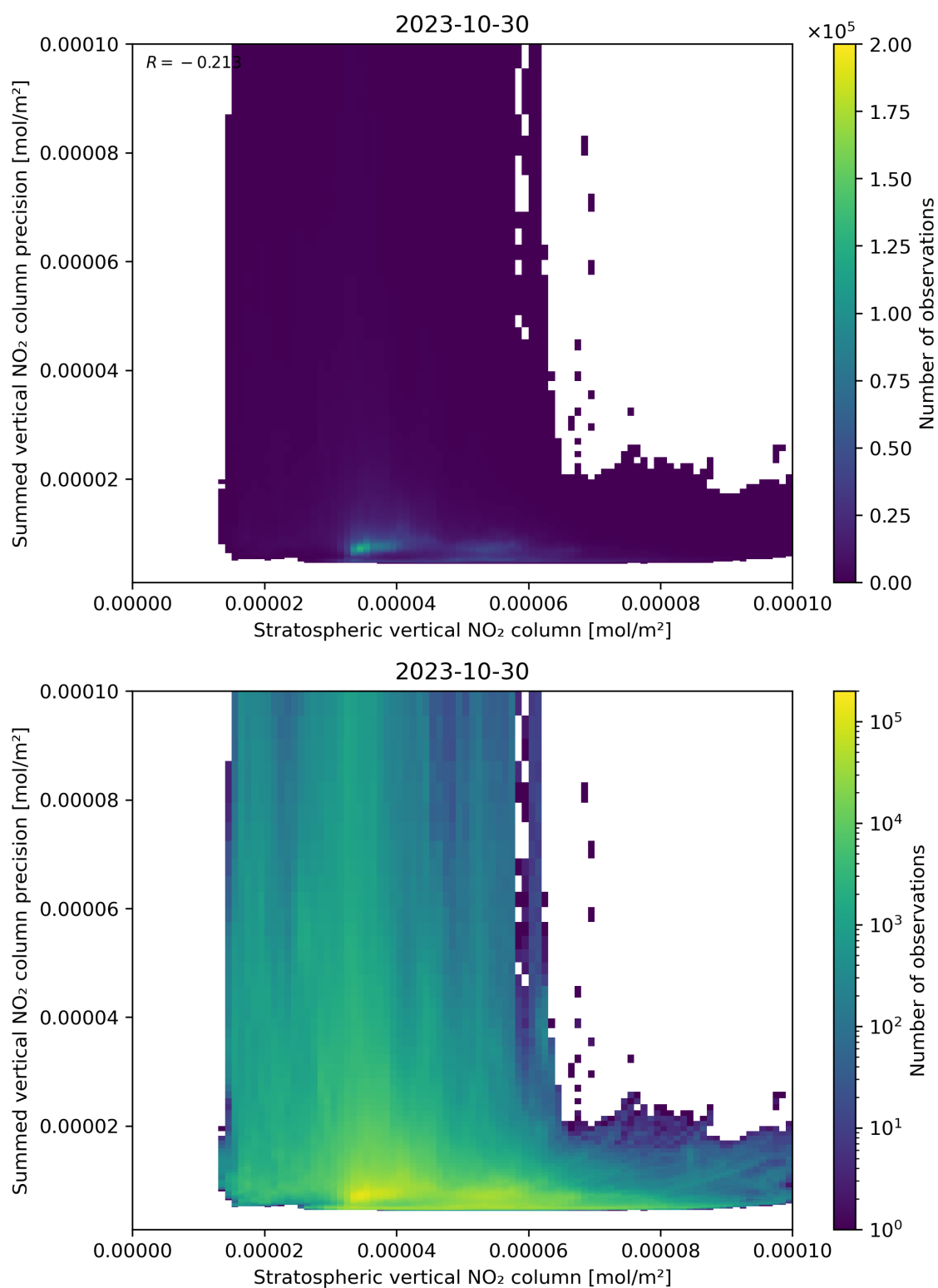
Figure 99: Scatter density plot of “Stratospheric vertical NO 2 column” against “Summed vertical NO 2 column precision” for 2023-10-29 to 2023-10-31.
