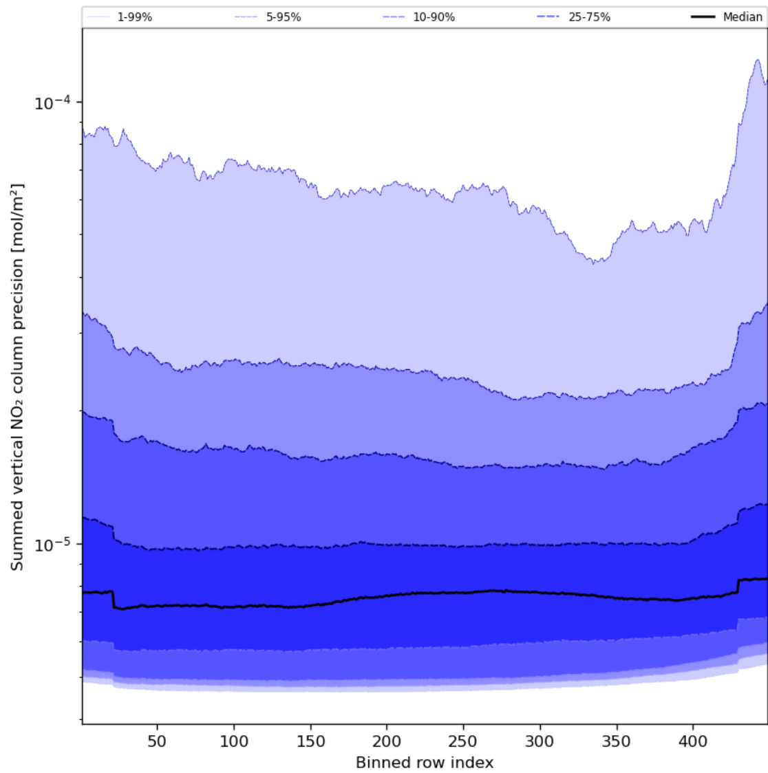
Figure 58: Along track statistics of “Summed vertical NO 2 column precision” for 2023-10-29 to 2023-10-31
