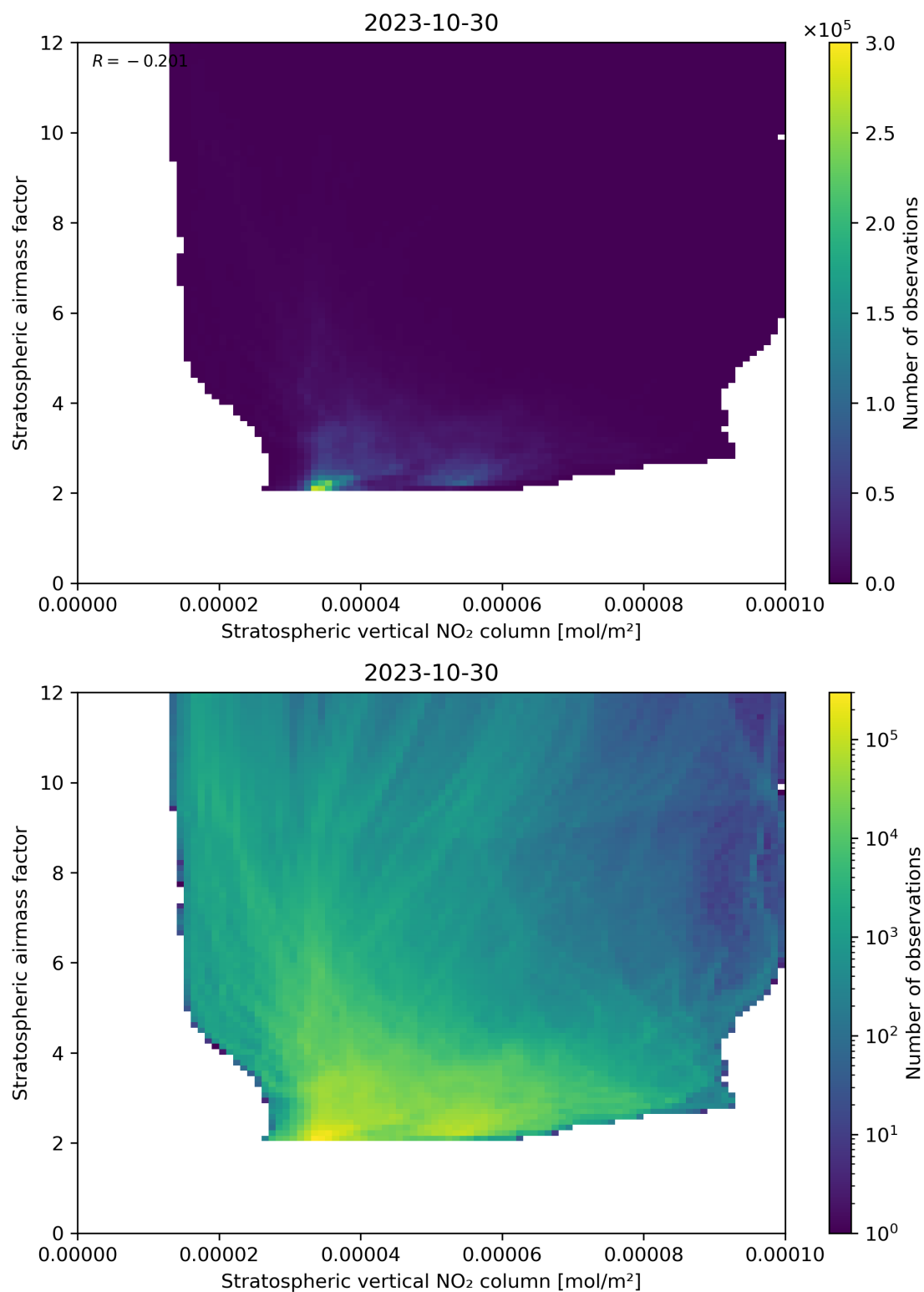
Figure 96: Scatter density plot of “Stratospheric vertical NO 2 column” against “Stratospheric airmass factor” for 2023-10-29 to 2023-10-31.
