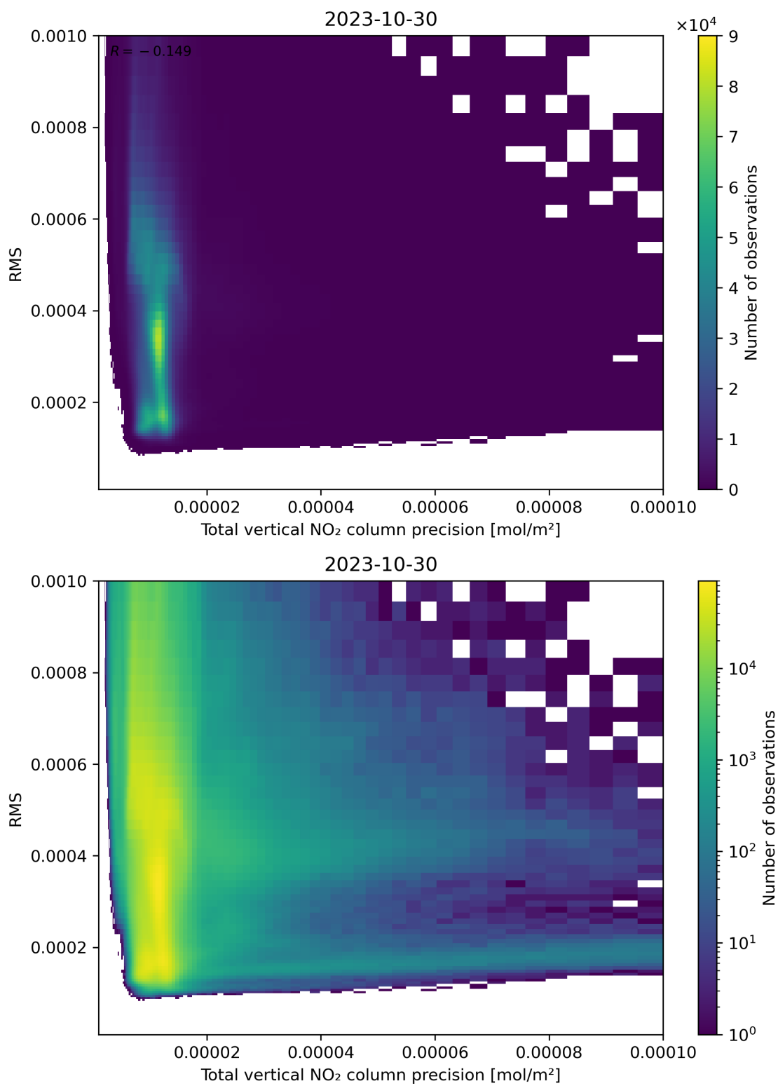
Figure 119: Scatter density plot of “Total vertical NO 2 column precision” against “RMS” for 2023-10-29 to 2023-10-31.
