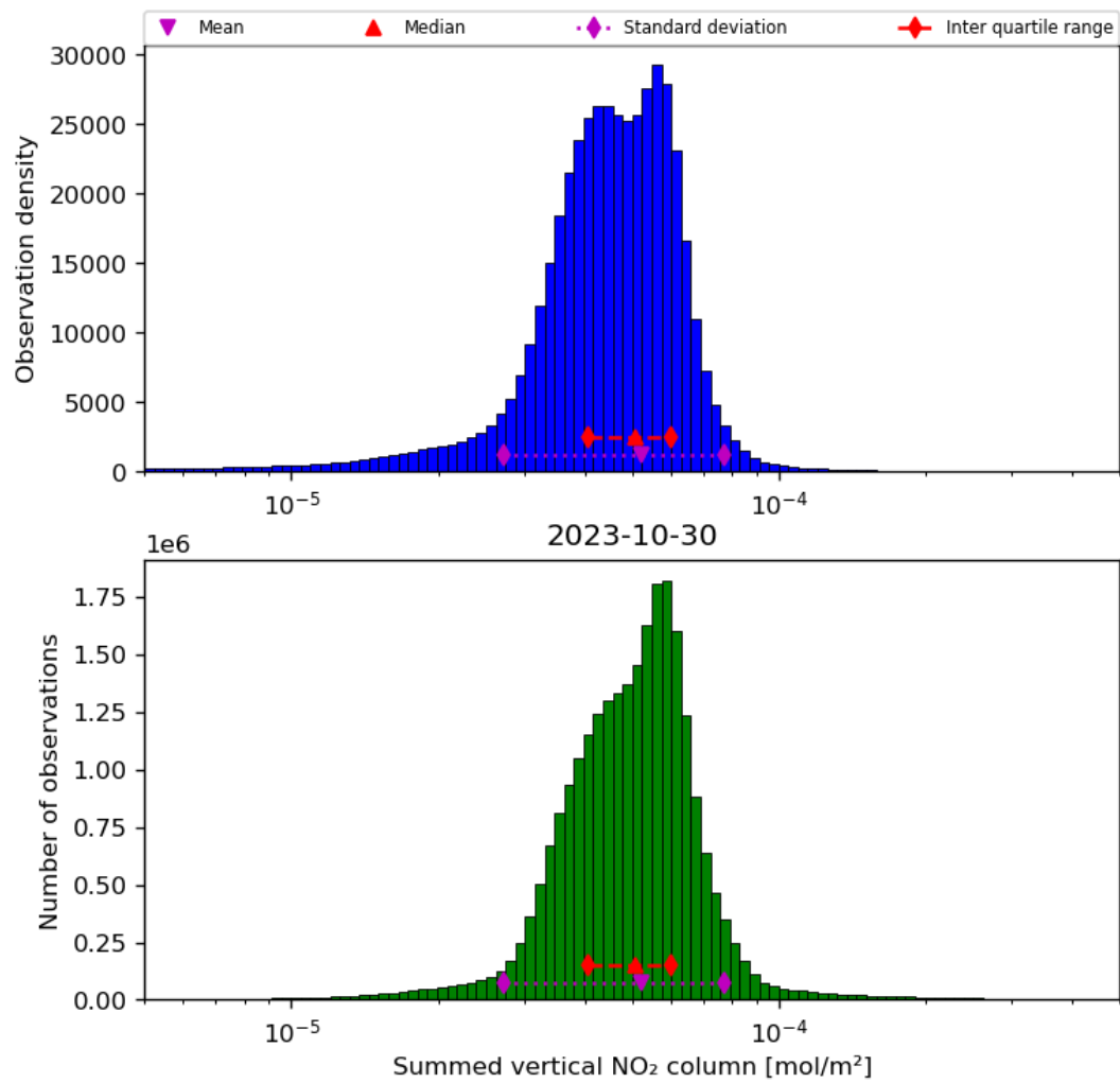
Figure 40: Histogram of “Summed vertical NO 2 column” for 2023-10-29 to 2023-10-31
