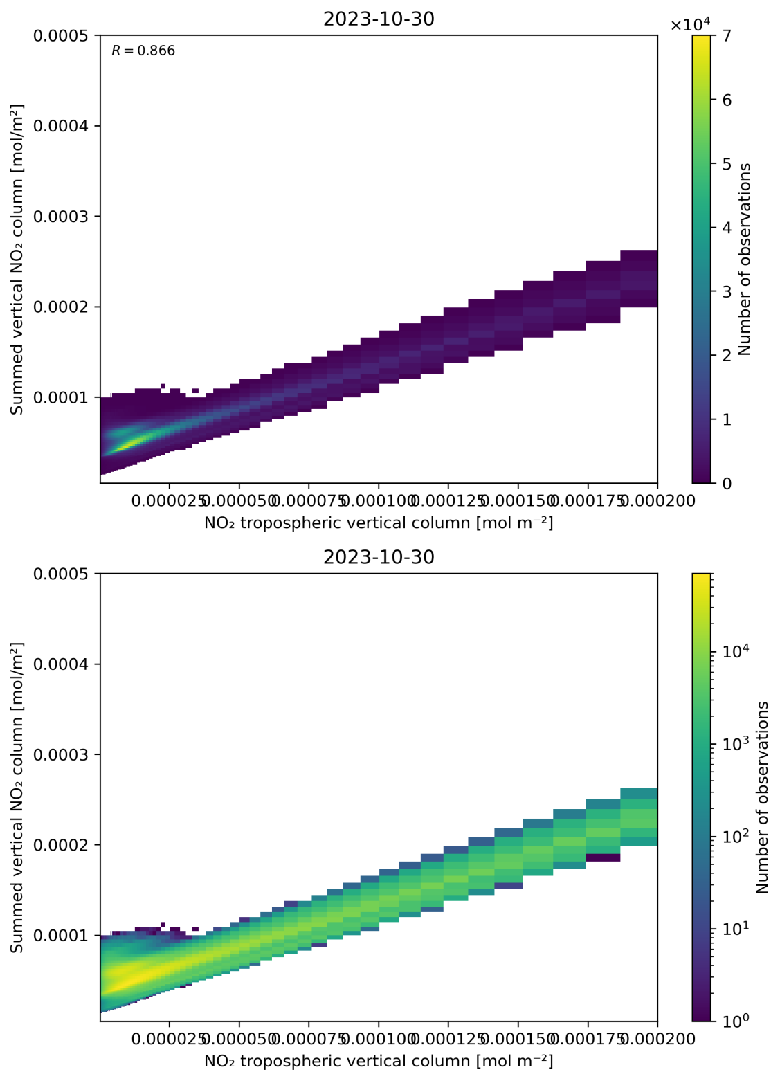
Figure 126: Scatter density plot of “NO 2 tropospheric vertical column” against “Summed vertical NO 2 column” for 2023-10-29 to 2023-10-31.
