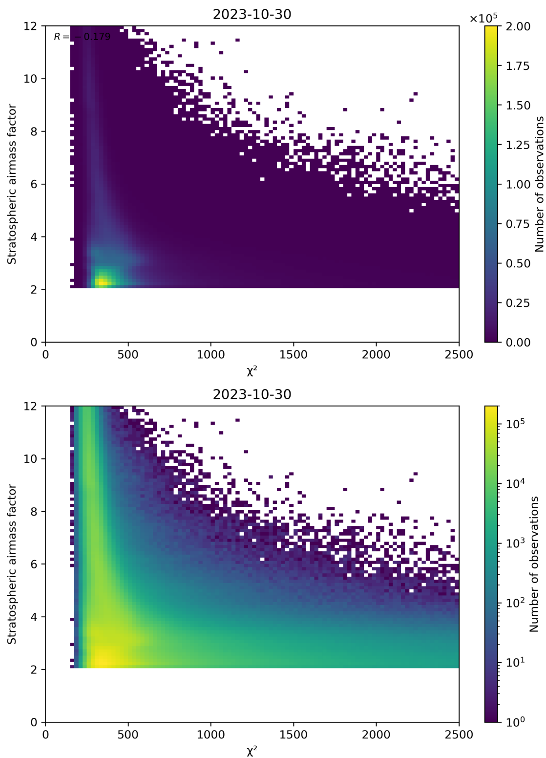
Figure 81: Scatter density plot of “ \chi^2 ” against “Stratospheric airmass factor” for 2023-10-29 to 2023-10-31.
