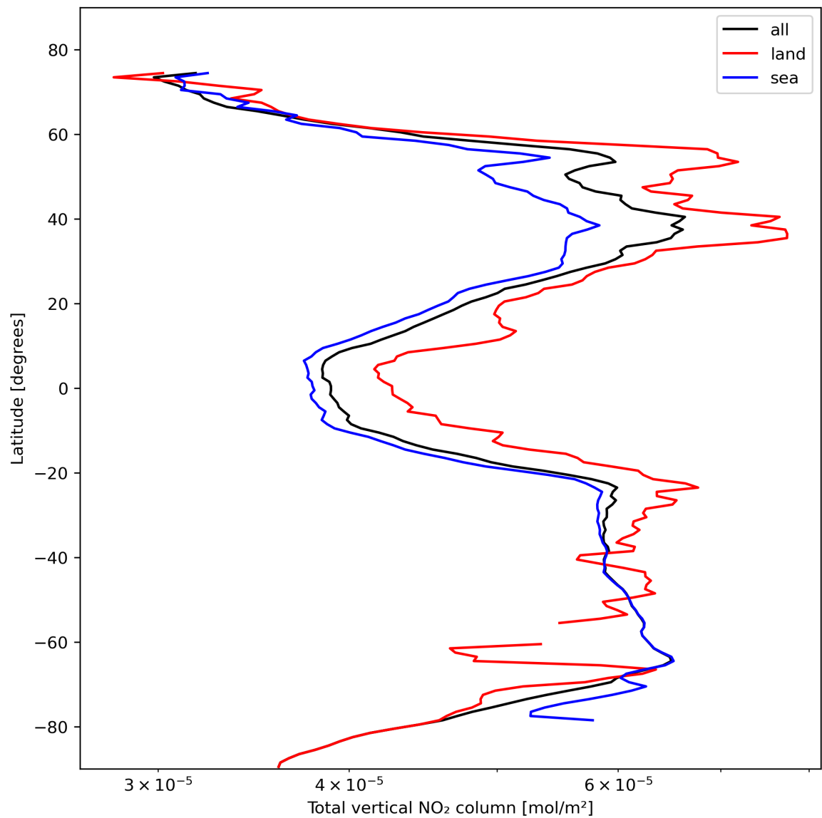
Figure 21: Zonal average of “Total vertical NO 2 column” for 2023-10-29 to 2023-10-31.
