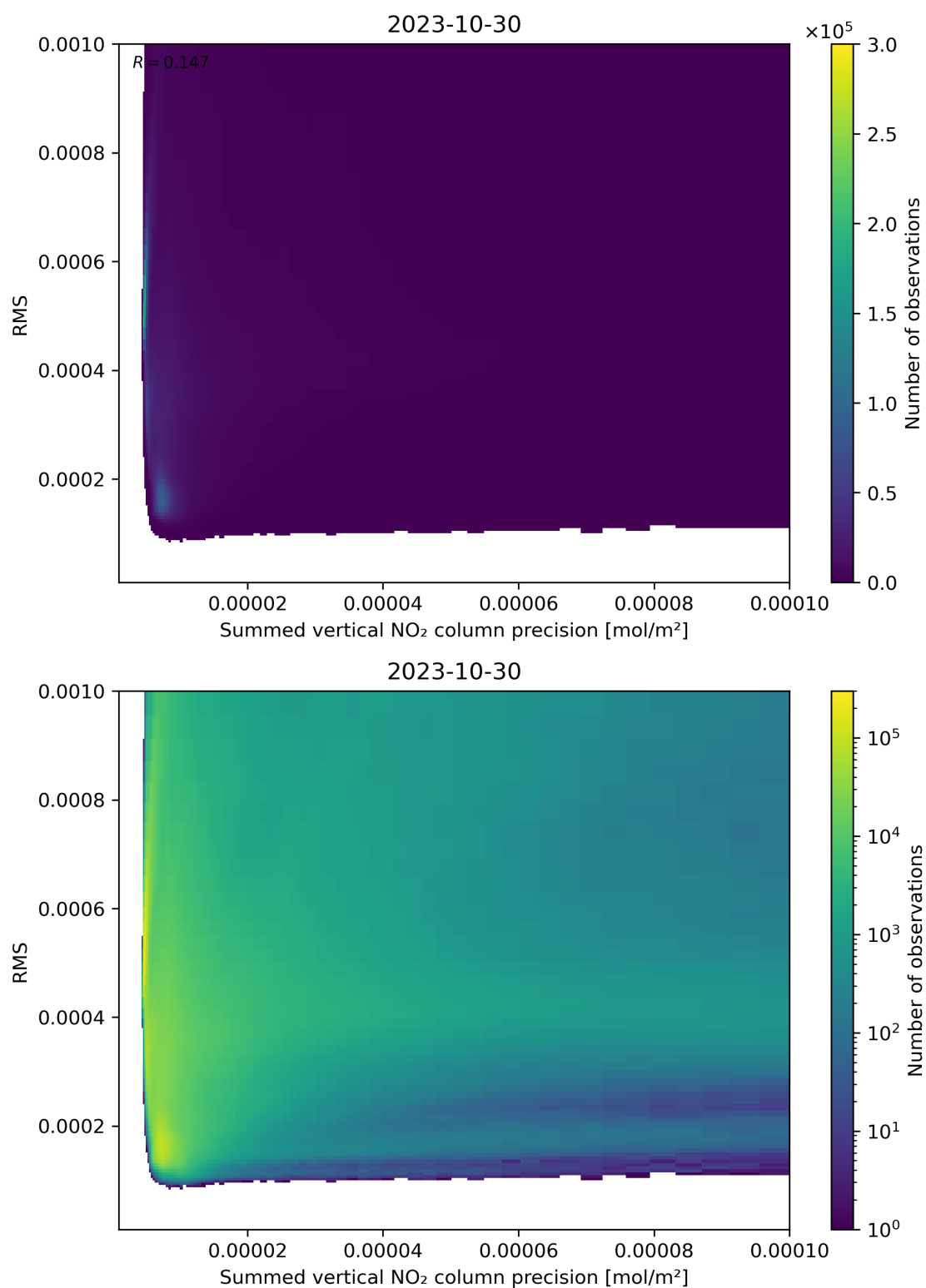
Figure 108: Scatter density plot of “Summed vertical NO 2 column precision” against “RMS” for 2023-10-29 to 2023-10-31.
