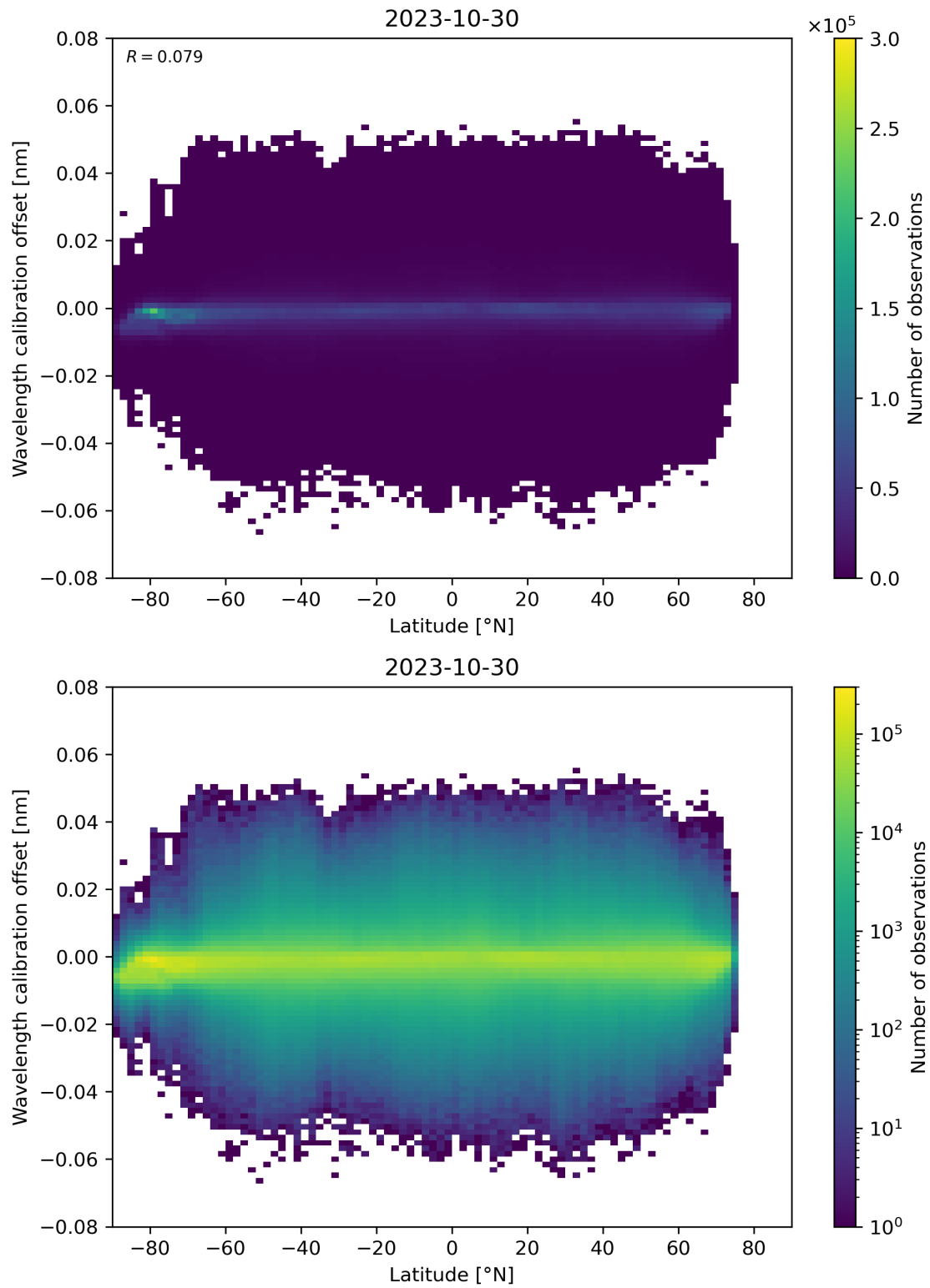
Figure 95: Scatter density plot of “Latitude” against “Wavelength calibration offset” for 2023-10-29 to 2023-10-31.
