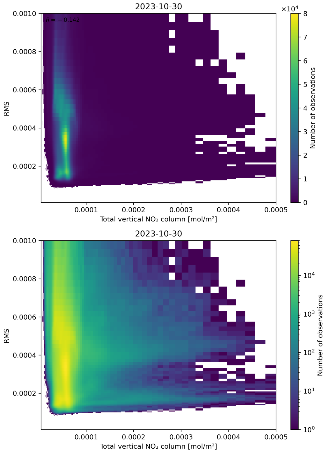
Figure 120: Scatter density plot of “Total vertical NO 2 column” against “RMS” for 2023-10-29 to 2023-10-31.
