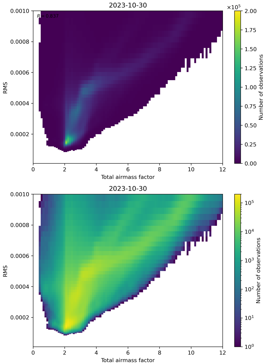
Figure 69: Scatter density plot of “Total airmass factor” against “RMS” for 2023-10-29 to 2023-10-31.
