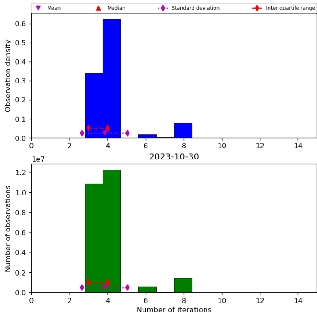
Figure 34: Histogram of “Number of iterations” for 2023-10-29 to 2023-10-31
