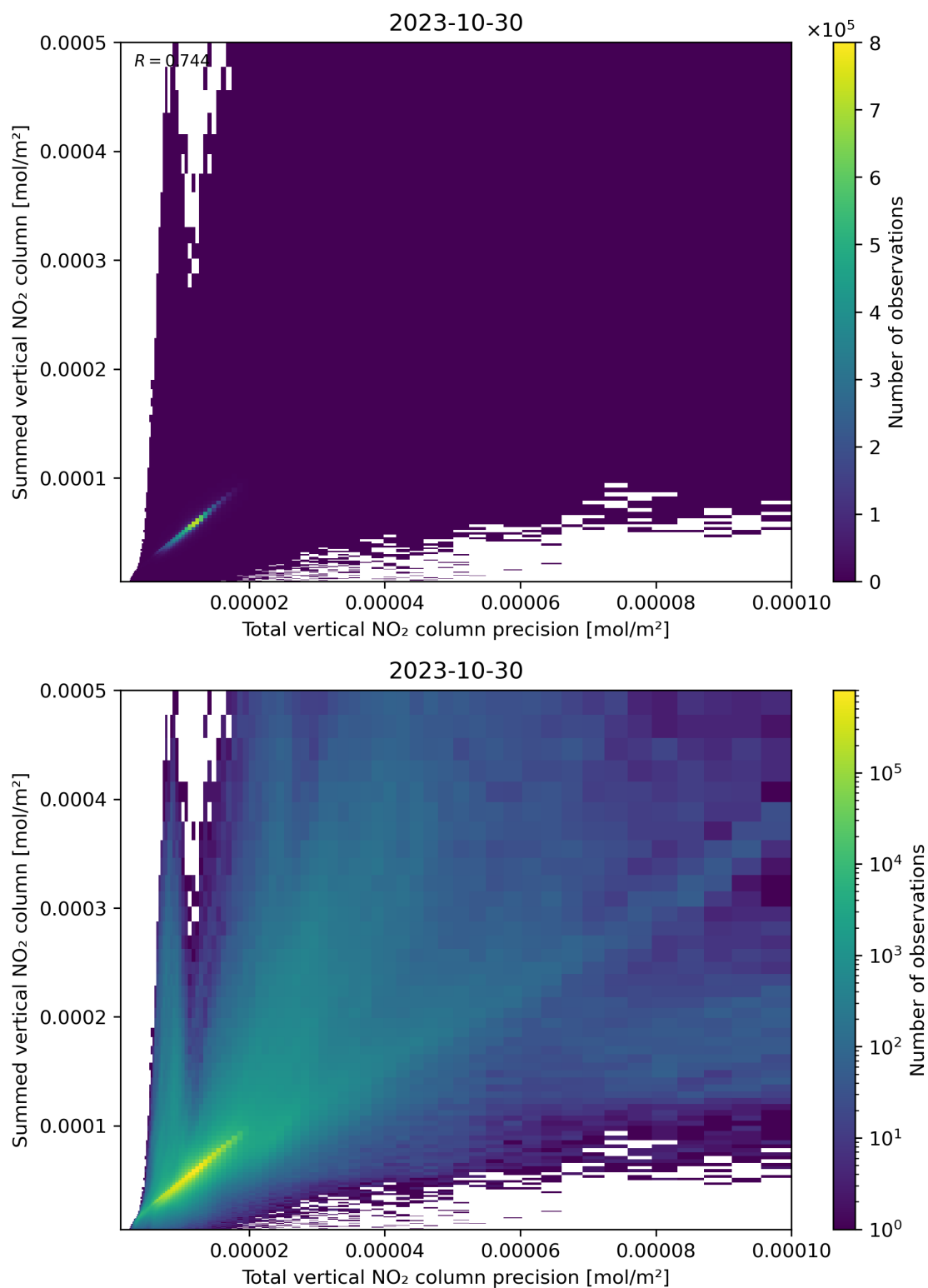
Figure 117: Scatter density plot of “Total vertical NO 2 column precision” against “Summed vertical NO 2 column” for 2023-10-29 to 2023-10-31.
