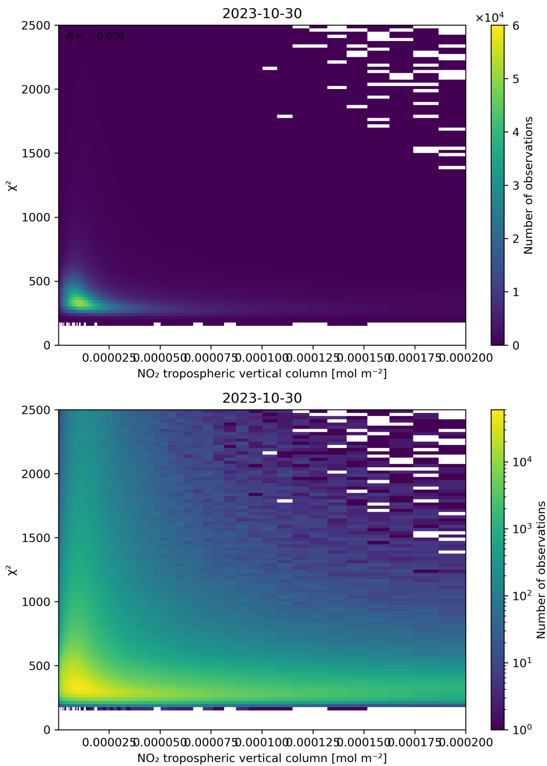
Figure 124: Scatter density plot of “NO 2 tropospheric vertical column” against “ \chi^2 ” for 2023-10-29 to 2023-10-31.
