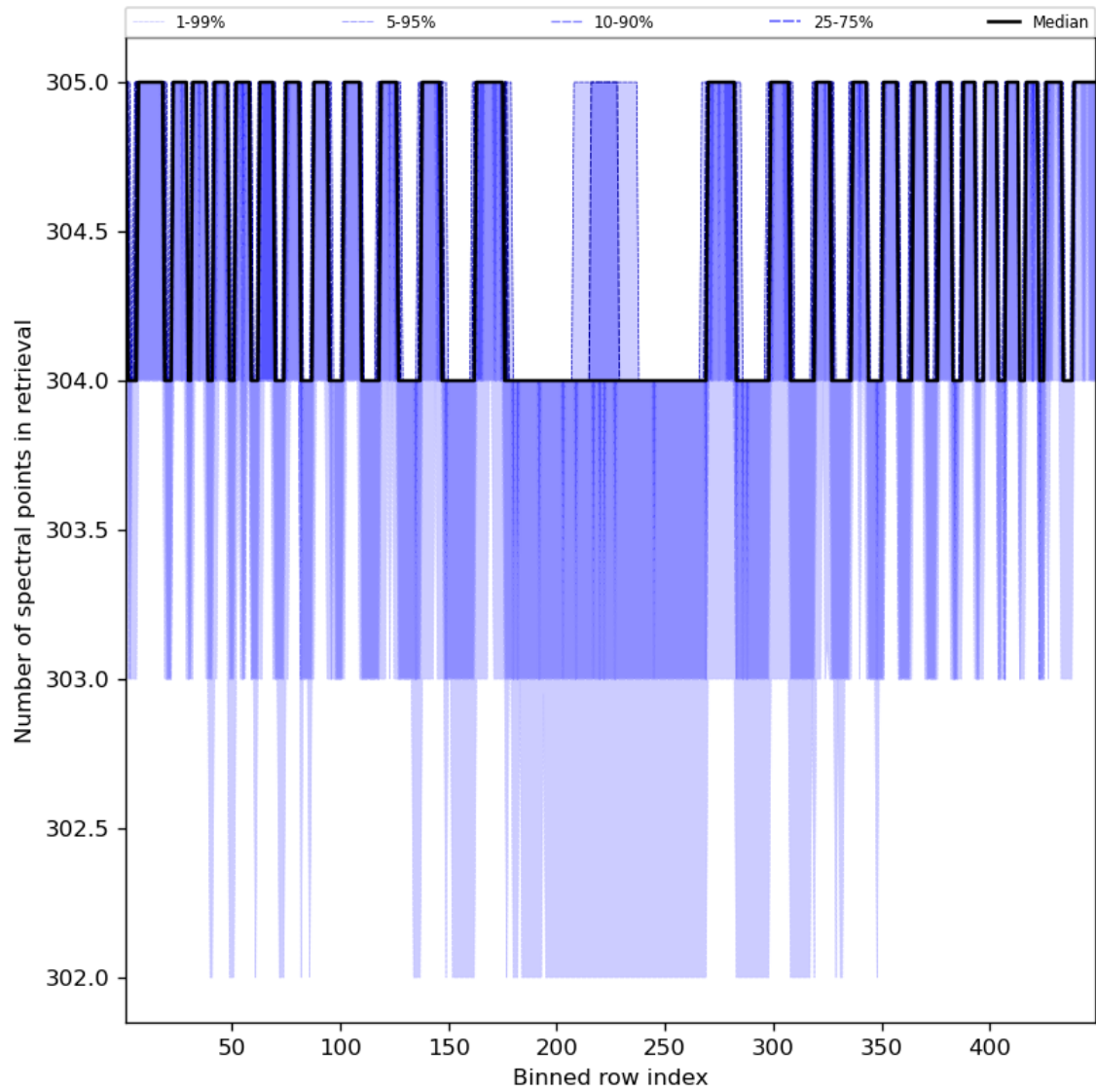
Figure 50: Along track statistics of “Number of spectral points in retrieval” for 2023-10-29 to 2023-10-31
