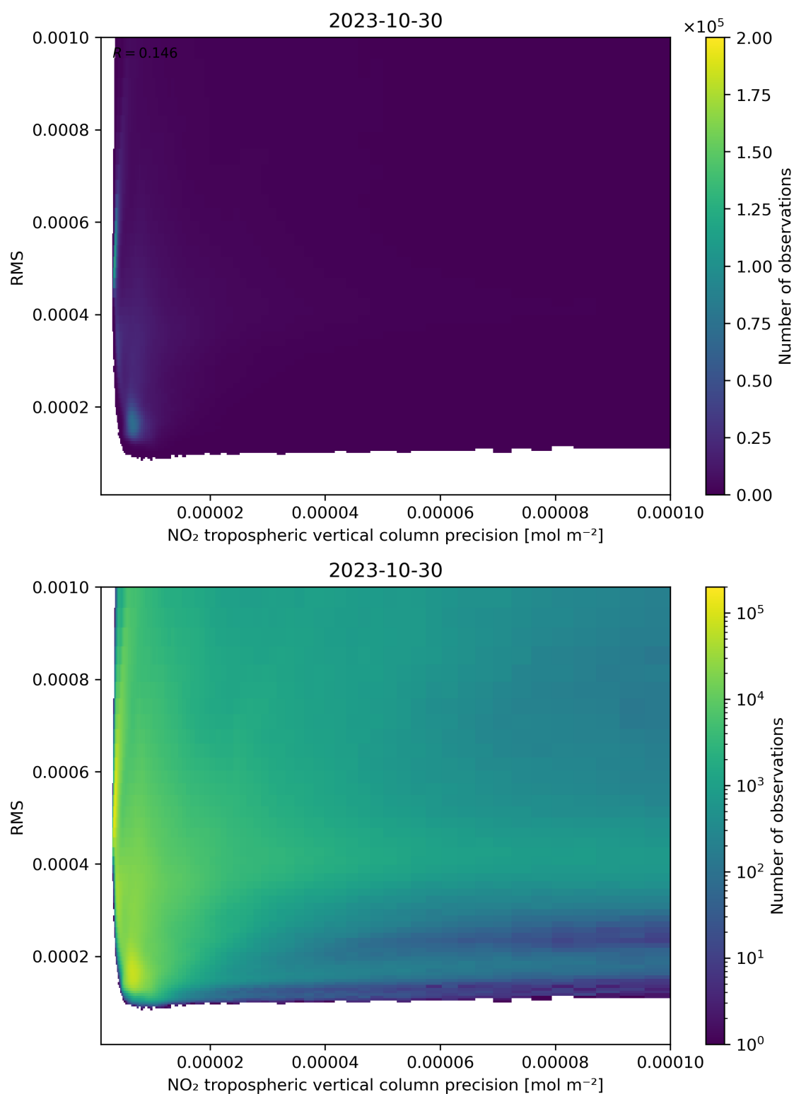
Figure 140: Scatter density plot of “NO 2 tropospheric vertical column precision” against “RMS” for 2023-10-29 to 2023-10-31.
