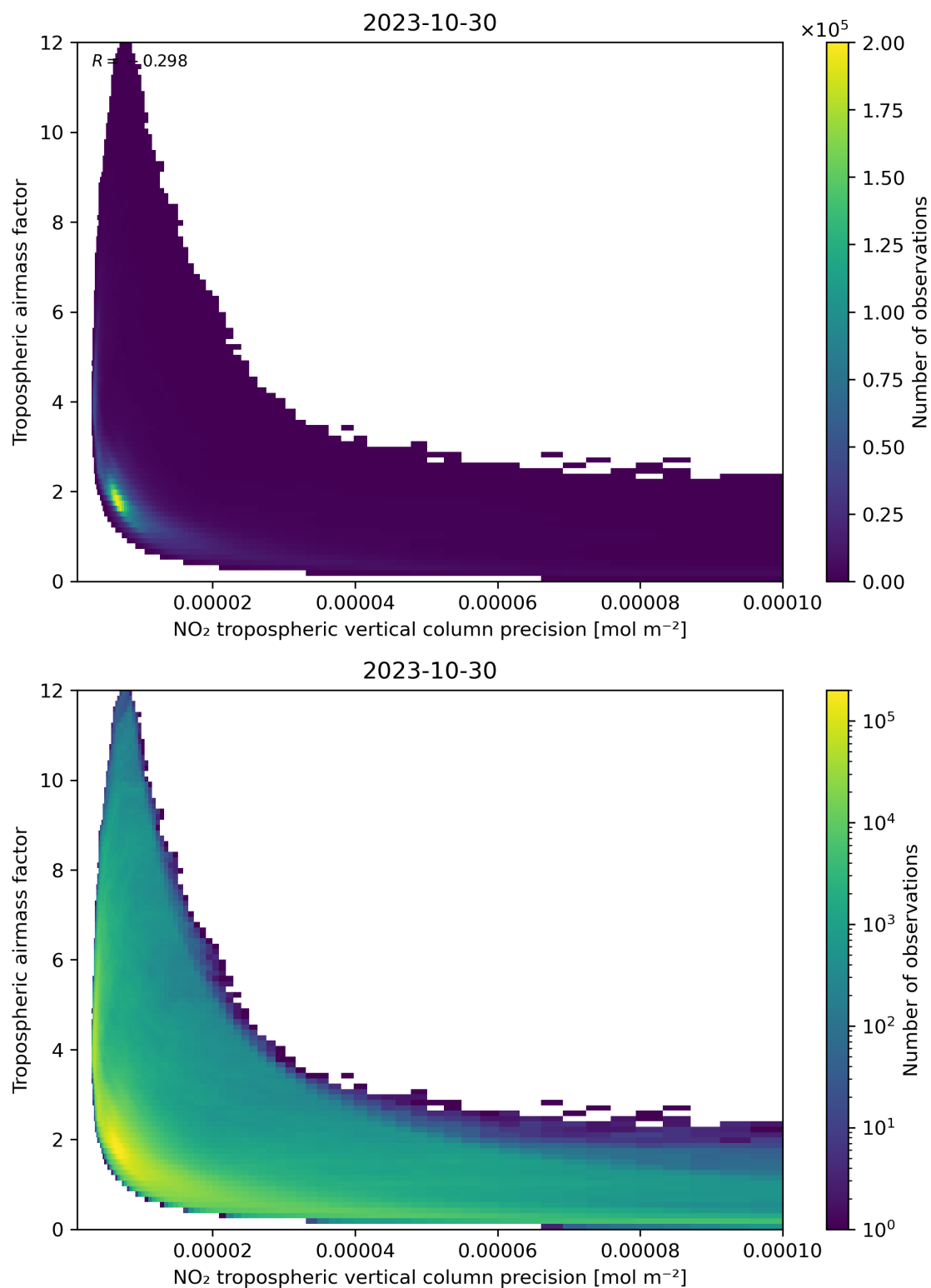
Figure 133: Scatter density plot of “NO 2 tropospheric vertical column precision” against “Tropospheric airmass factor” for 2023-10-29 to 2023-10-31.
