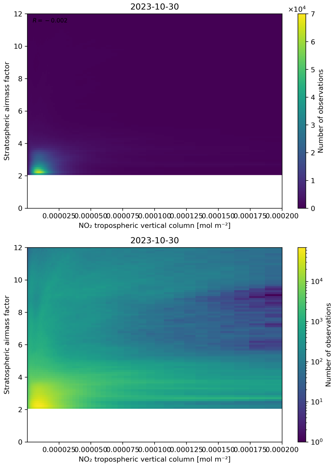
Figure 121: Scatter density plot of “NO 2 tropospheric vertical column” against “Stratospheric airmass factor” for 2023-10-29 to 2023-10-31.
