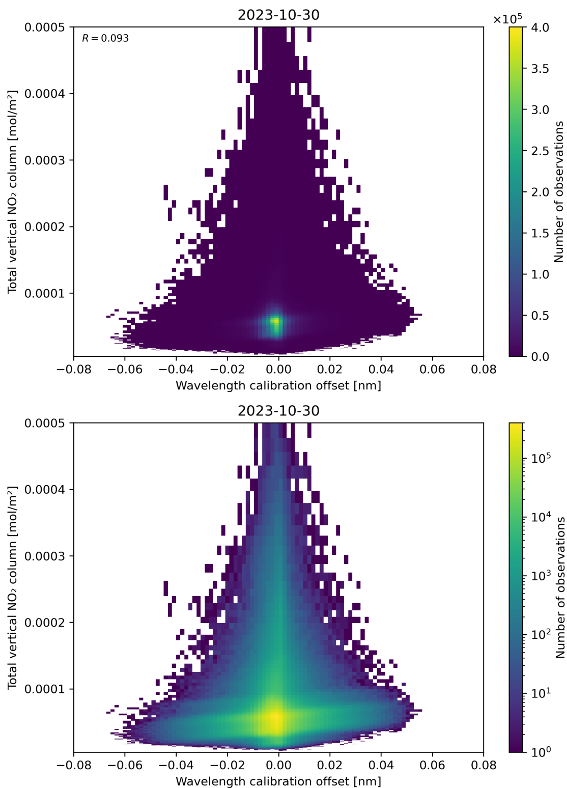
Figure 179: Scatter density plot of “Wavelength calibration offset” against “Total vertical NO 2 column” for 2023-10-29 to 2023-10-31.
