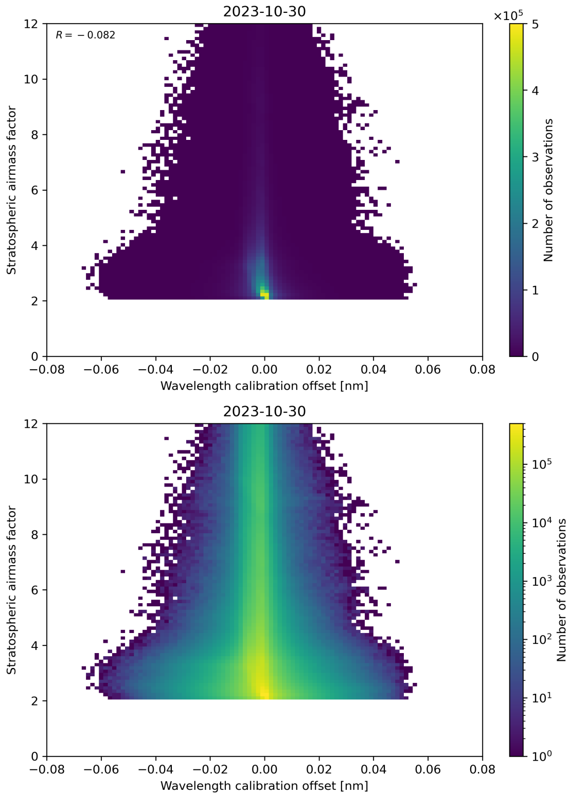
Figure 174: Scatter density plot of “Wavelength calibration offset” against “Stratospheric airmass factor” for 2023-10-29 to 2023-10-31.
