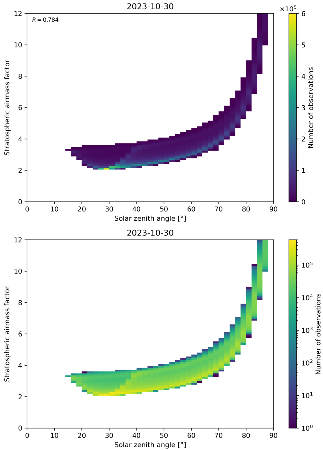
Figure 145: Scatter density plot of “Solar zenith angle” against “Stratospheric airmass factor” for 2023-10-29 to 2023-10-31.
