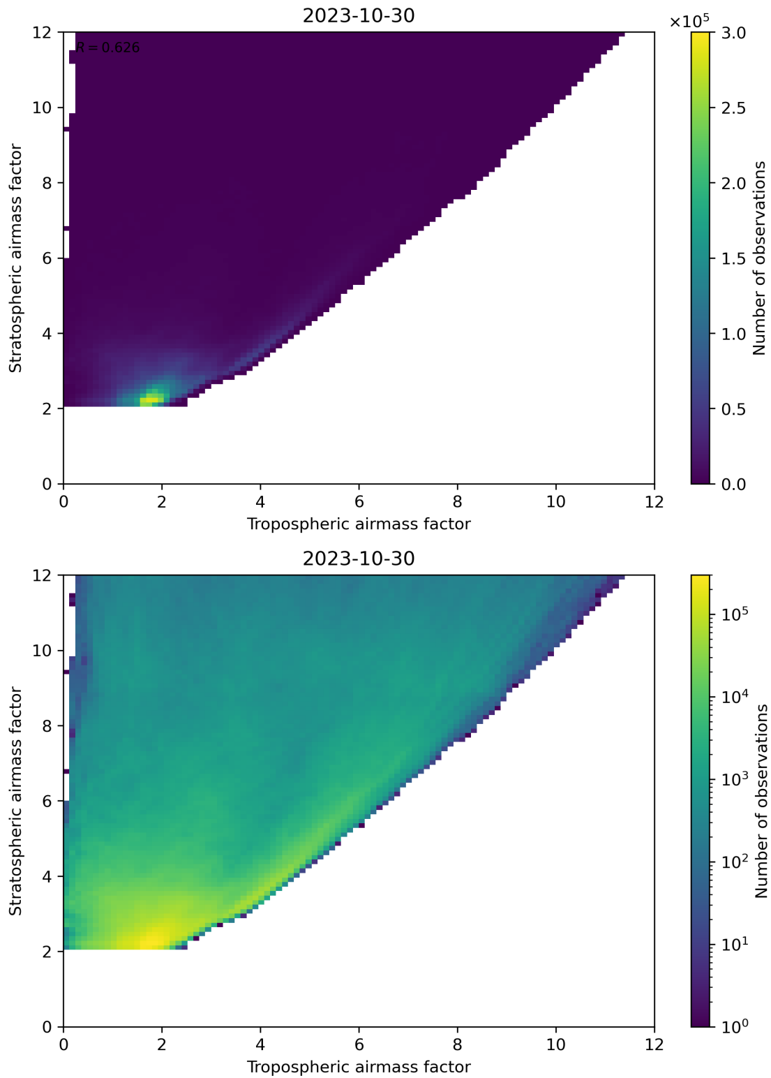
Figure 71: Scatter density plot of “Tropospheric airmass factor” against “Stratospheric airmass factor” for 2023-10-29 to 2023-10-31.
