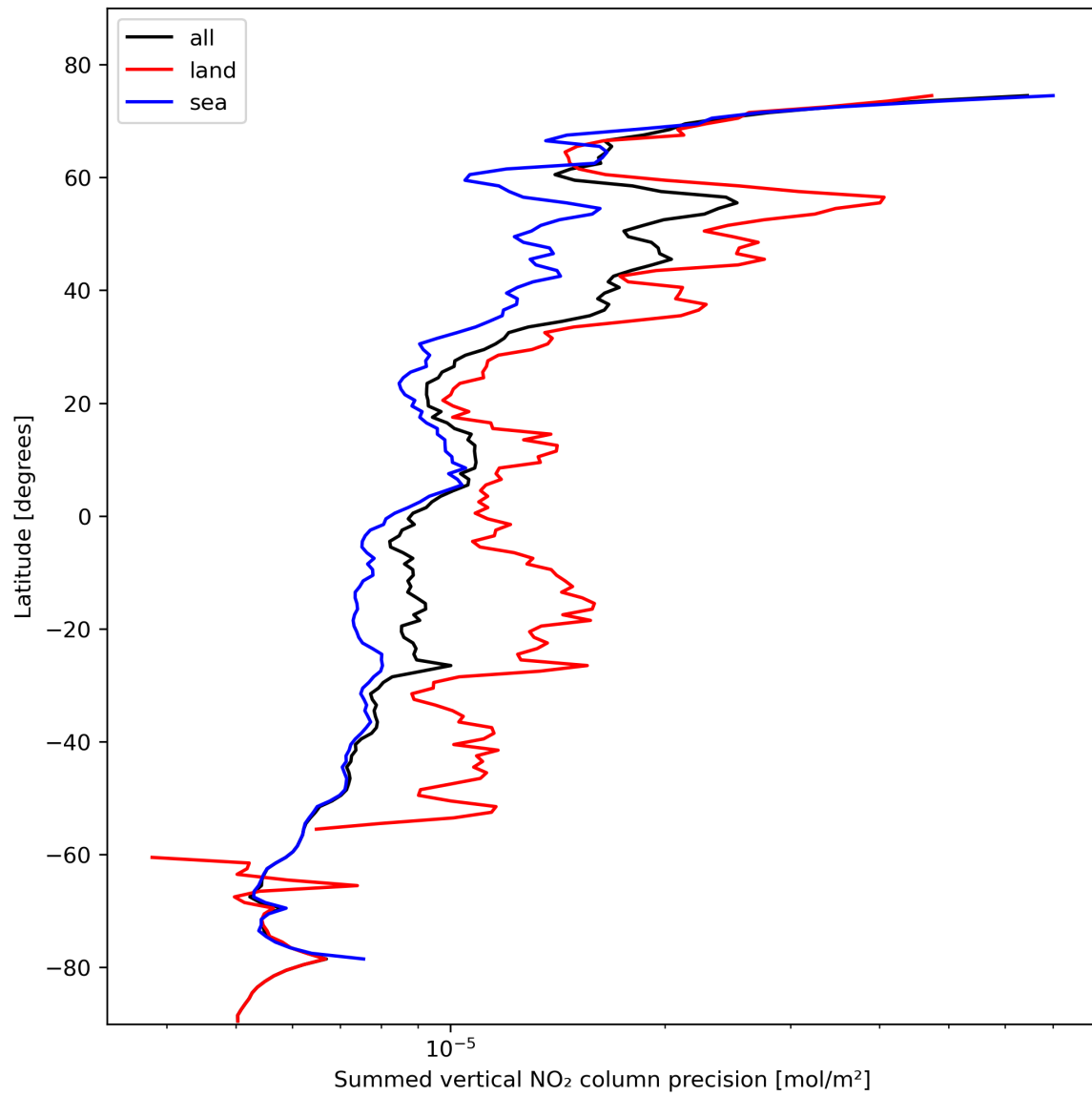
Figure 24: Zonal average of “Summed vertical NO 2 column precision” for 2023-10-29 to 2023-10-31.
