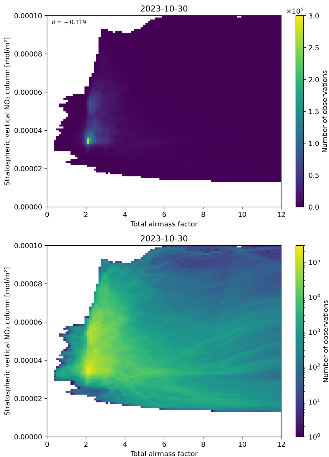
Figure 64: Scatter density plot of “Total airmass factor” against “Stratospheric vertical NO 2 column” for 2023-10-29 to 2023-10-31.
