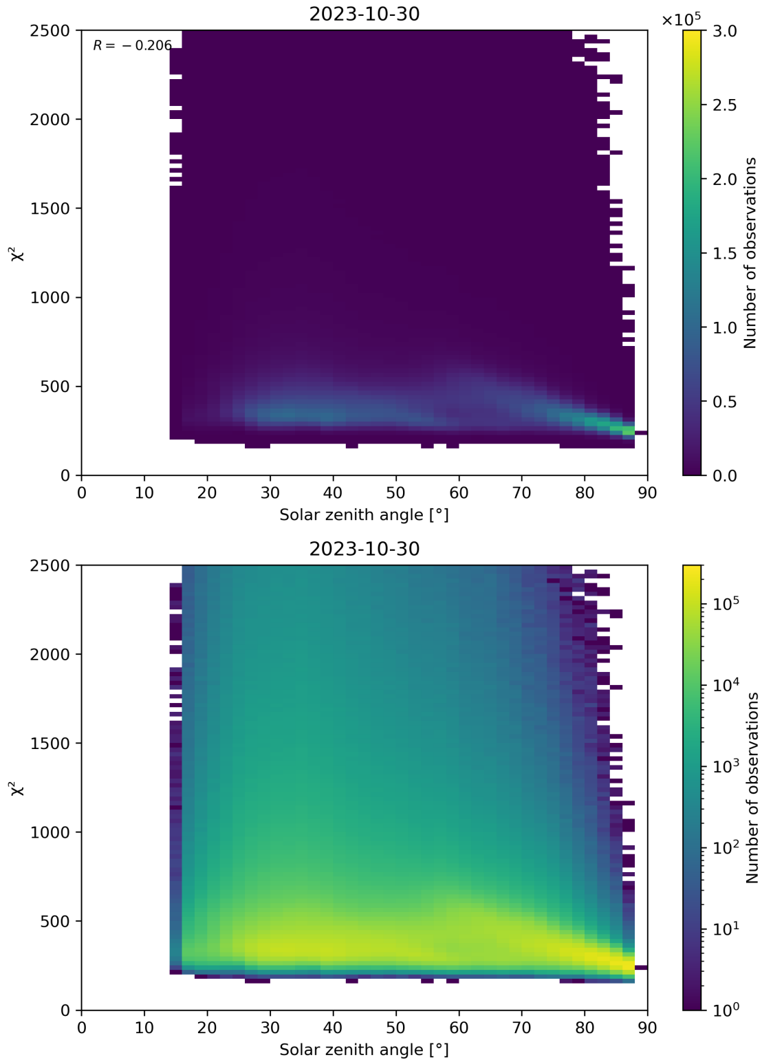
Figure 148: Scatter density plot of “Solar zenith angle” against “ \chi^2 ” for 2023-10-29 to 2023-10-31.
