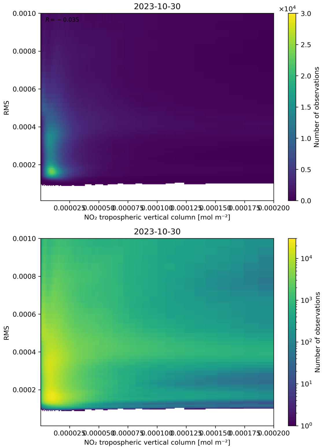
Figure 142: Scatter density plot of “NO 2 tropospheric vertical column” against “RMS” for 2023-10-29 to 2023-10-31.
