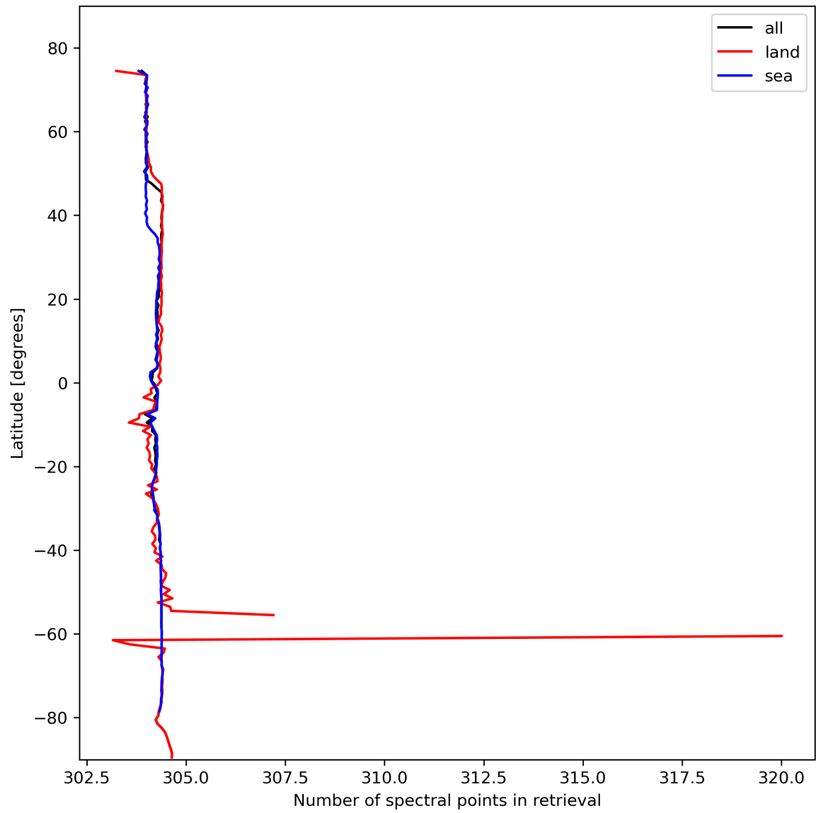
Figure 16: Zonal average of “Number of spectral points in retrieval” for 2023-10-29 to 2023-10-31.
