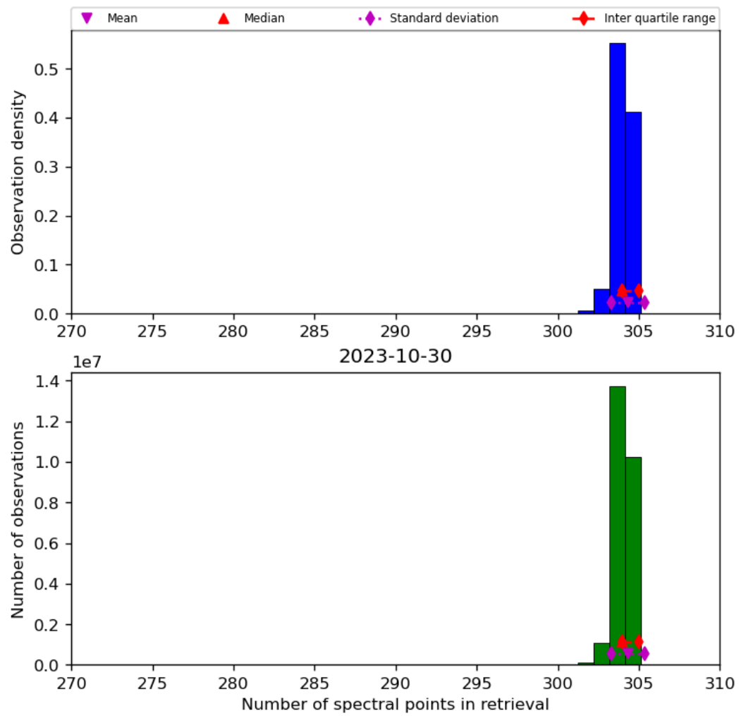
Figure 33: Histogram of “Number of spectral points in retrieval” for 2023-10-29 to 2023-10-31
