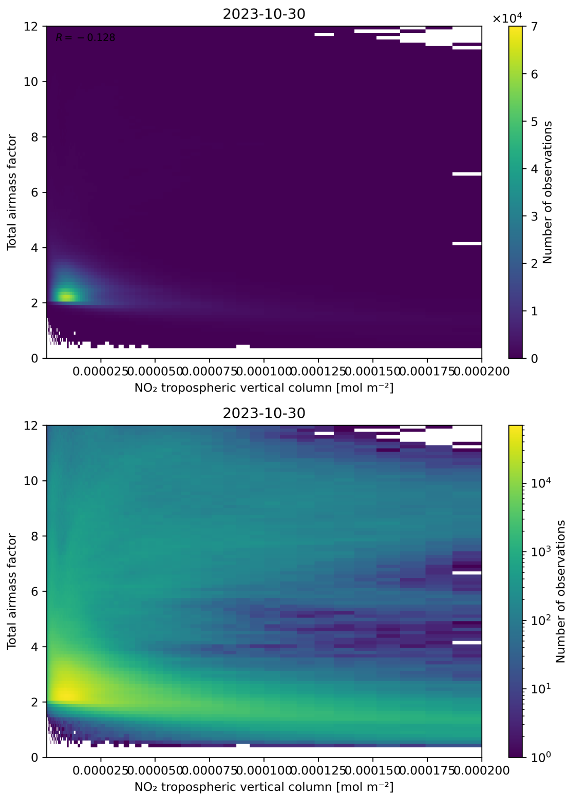
Figure 122: Scatter density plot of “NO 2 tropospheric vertical column” against “Total air mass factor” for 2023-10-29 to 2023-10-31.
