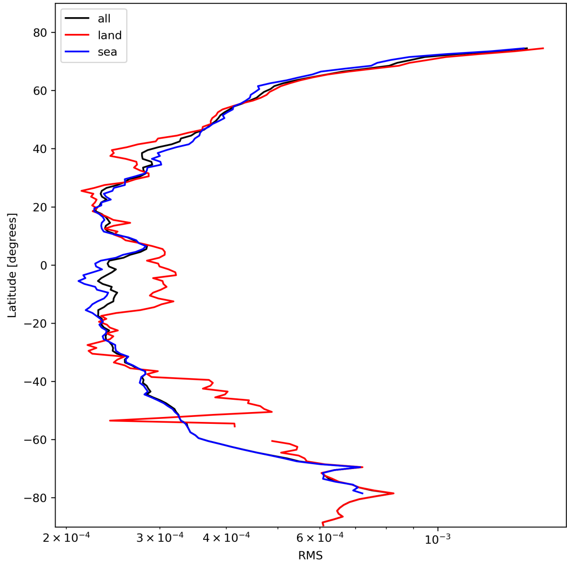
Figure 26: Zonal average of “RMS” for 2023-10-29 to 2023-10-31.
