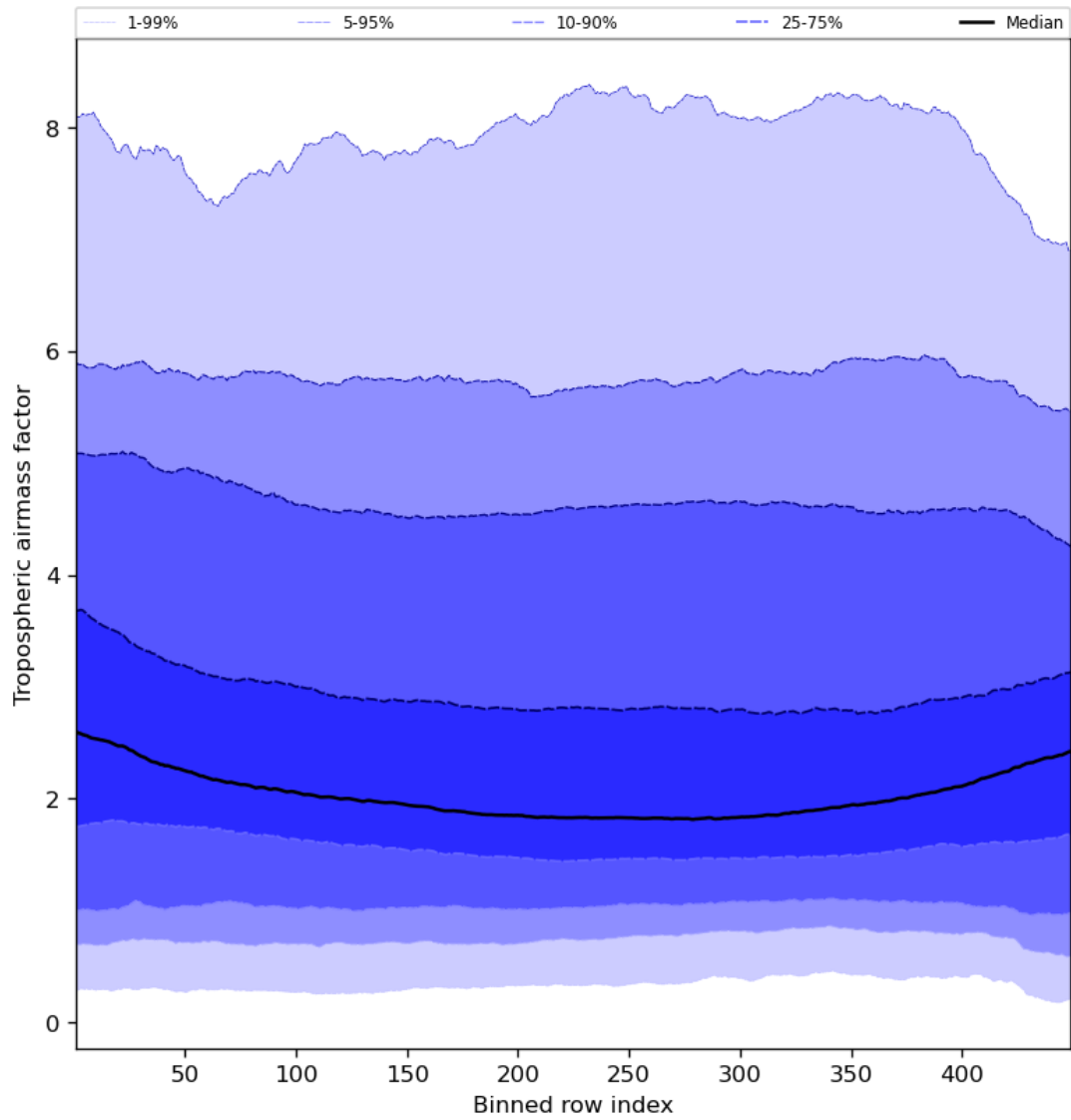
Figure 48: Along track statistics of “Tropospheric air mass factor” for 2023-10-29 to 2023-10-31
