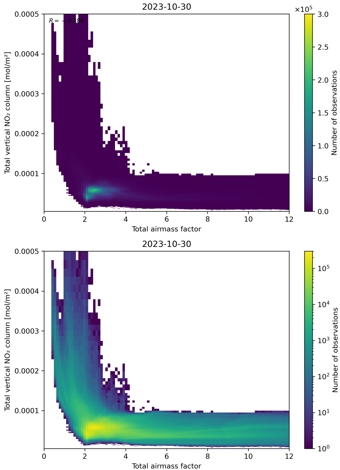
Figure 67: Scatter density plot of “Total airmass factor” against “Total vertical NO 2 column” for 2023-10-29 to 2023-10-31.
