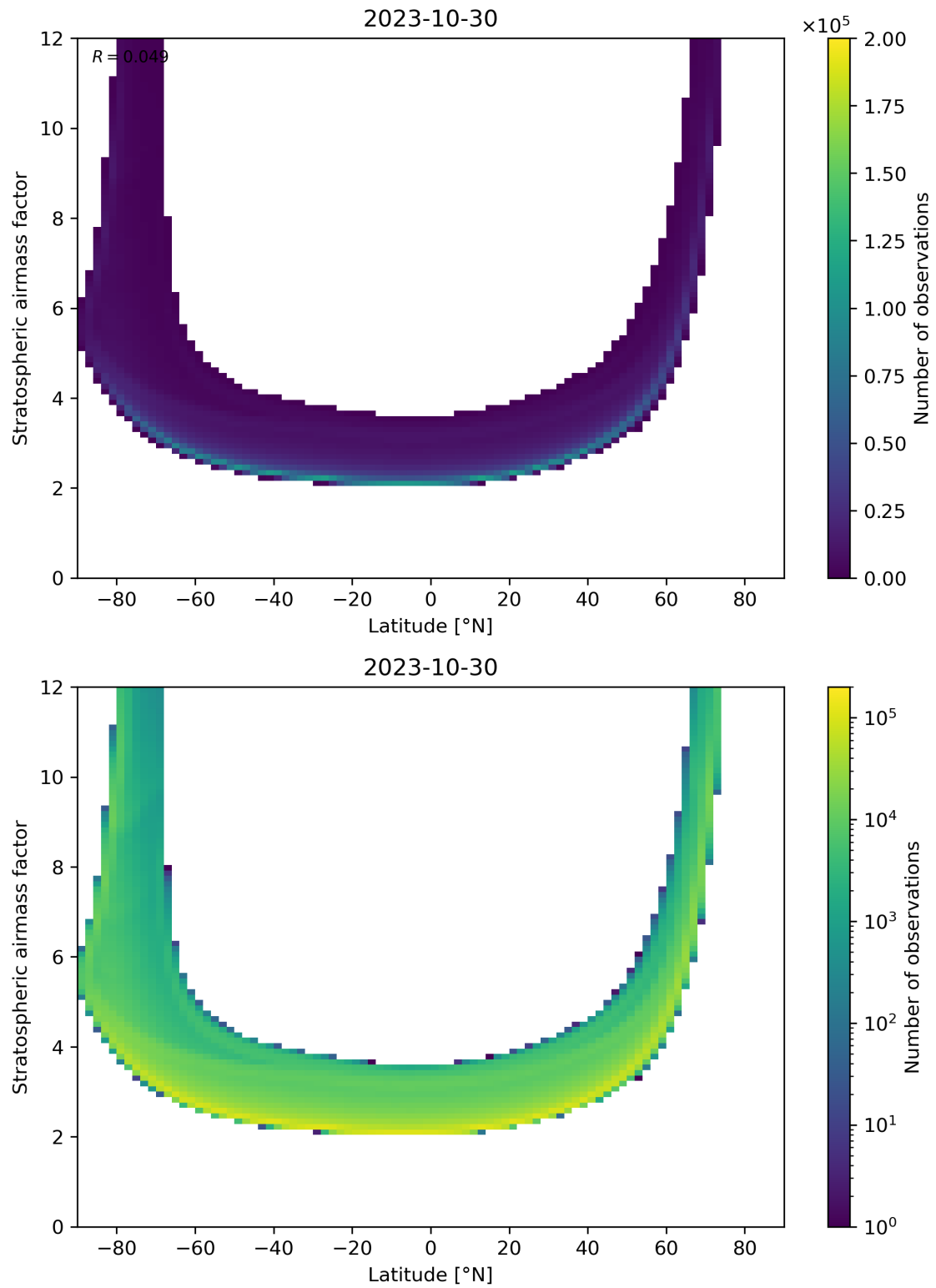
Figure 83: Scatter density plot of “Latitude” against “Stratospheric air mass factor” for 2023-10-29 to 2023-10-31.
