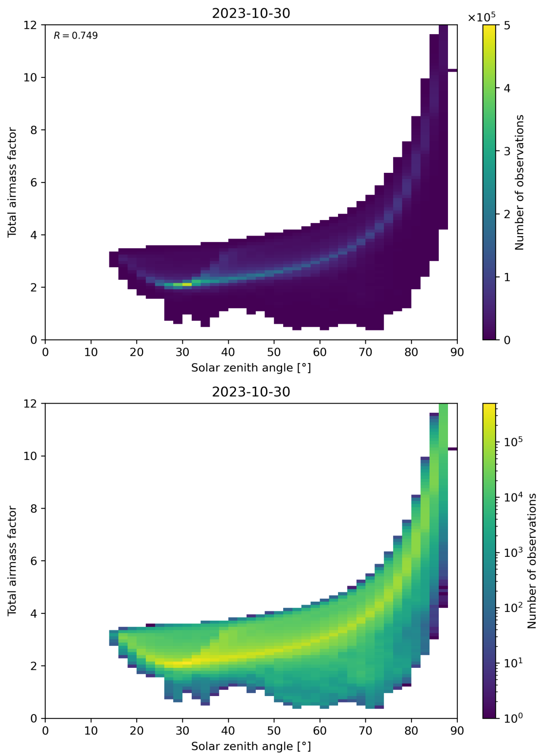
Figure 146: Scatter density plot of “Solar zenith angle” against “Total airmass factor” for 2023-10-29 to 2023-10-31.
