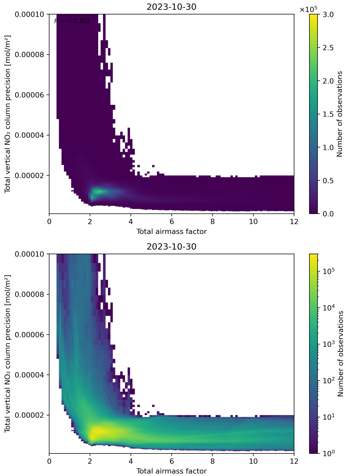
Figure 68: Scatter density plot of “Total airmass factor” against “Total vertical NO 2 column precision” for 2023-10-29 to 2023-10-31.
