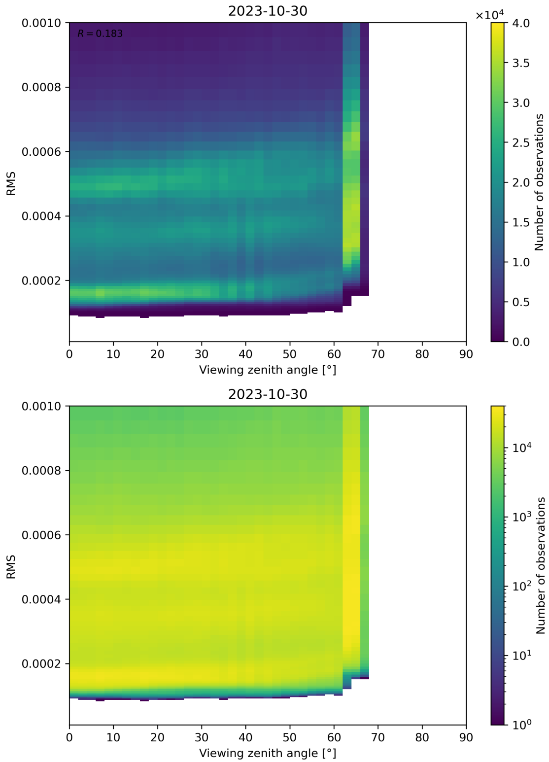
Figure 171: Scatter density plot of “Viewing zenith angle” against “RMS” for 2023-10-29 to 2023-10-31.
