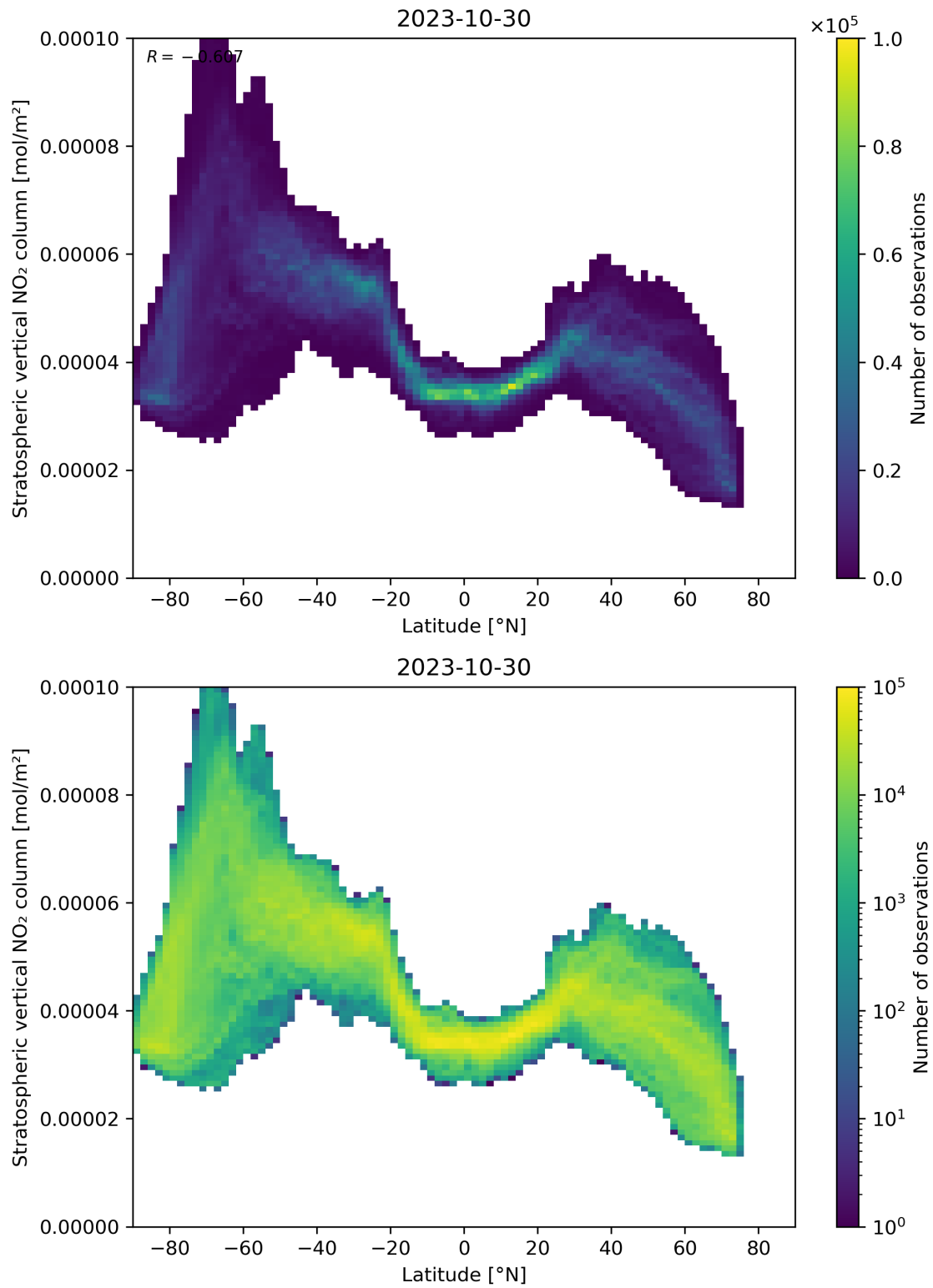
Figure 87: Scatter density plot of “Latitude” against “Stratospheric vertical NO 2 column” for 2023-10-29 to 2023-10-31.
