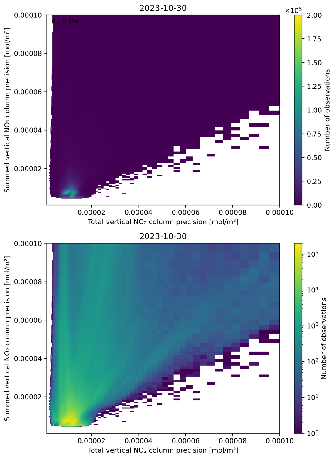
Figure 118: Scatter density plot of “Total vertical NO 2 column precision” against “Summed vertical NO 2 column precision” for 2023-10-29 to 2023-10-31.
