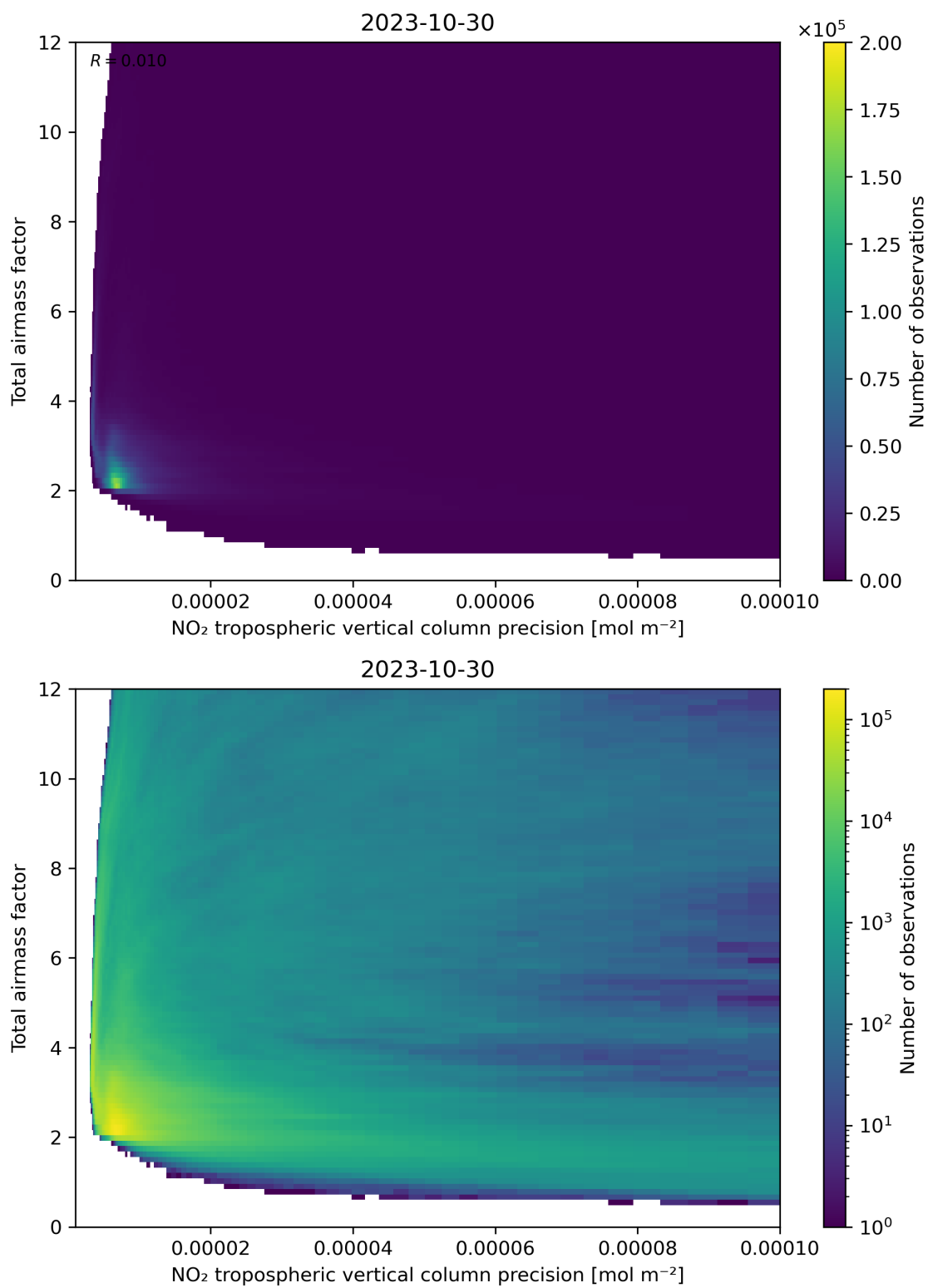
Figure 132: Scatter density plot of “NO 2 tropospheric vertical column precision” against “Total air mass factor” for 2023-10-29 to 2023-10-31.
