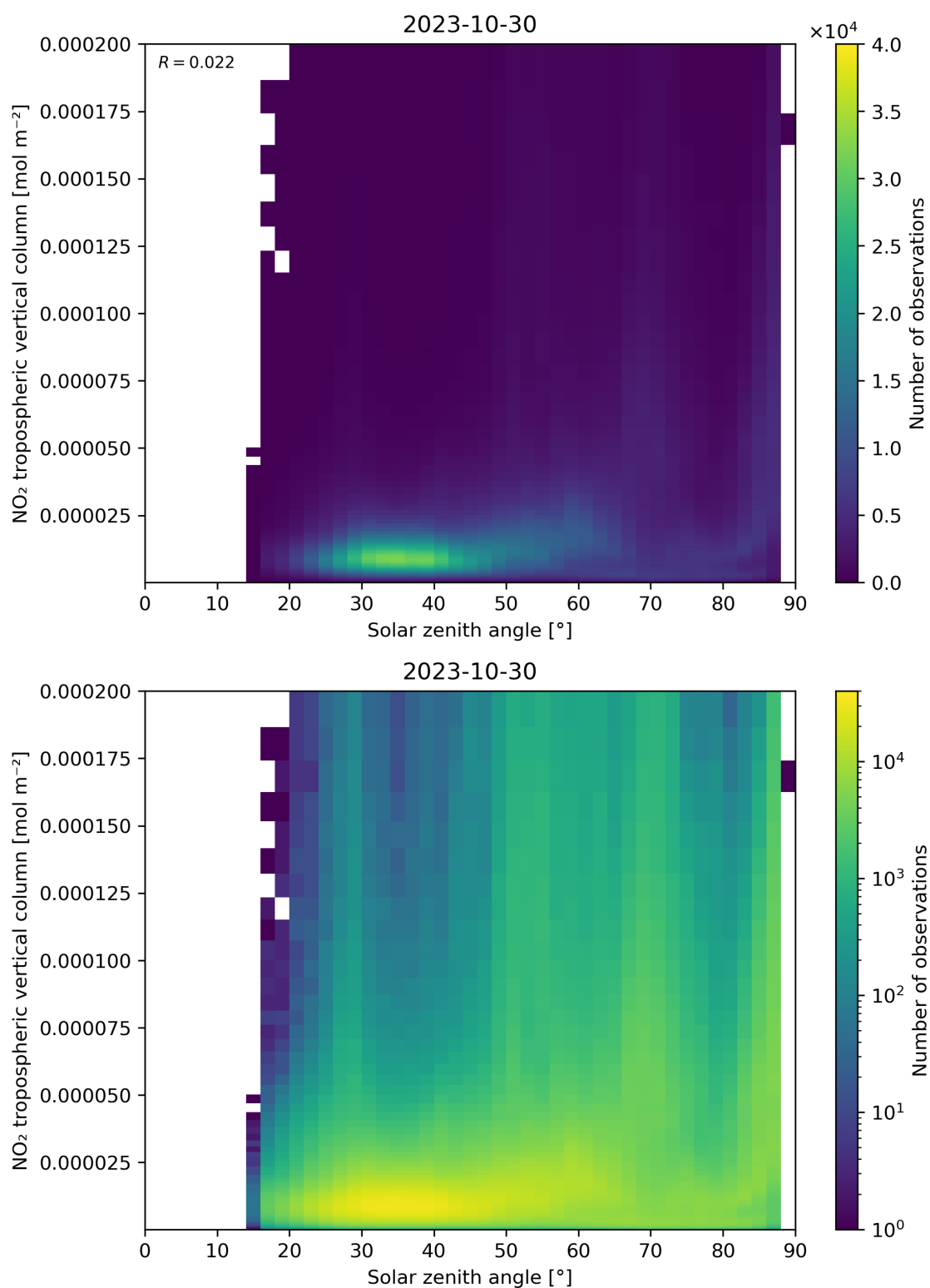
Figure 155: Scatter density plot of “Solar zenith angle” against “NO 2 tropospheric vertical column” for 2023-10-29 to 2023-10-31.
