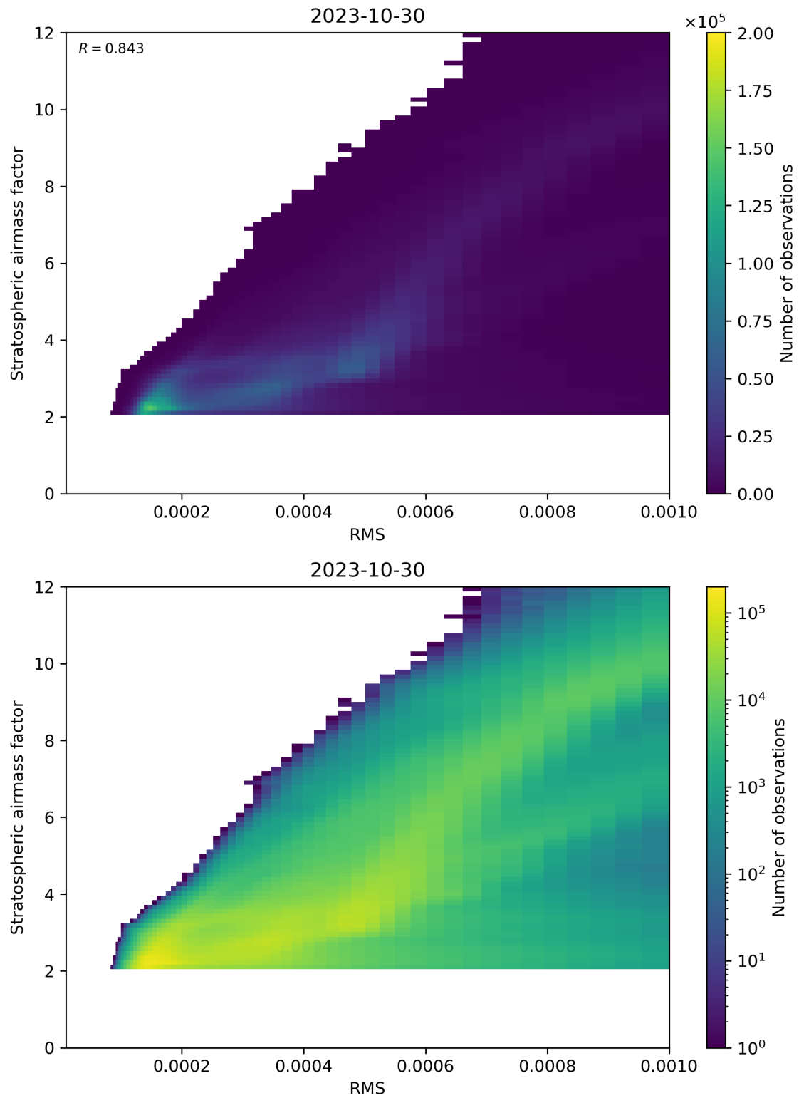
Figure 144: Scatter density plot of “RMS” against “Stratospheric airmass factor” for 2023-10-29 to 2023-10-31.
