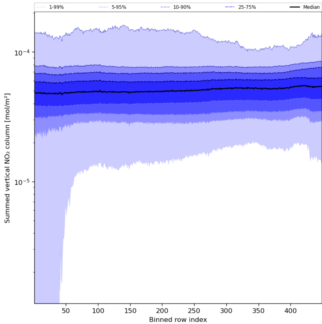
Figure 57: Along track statistics of “Summed vertical NO 2 column” for 2023-10-29 to 2023-10-31
