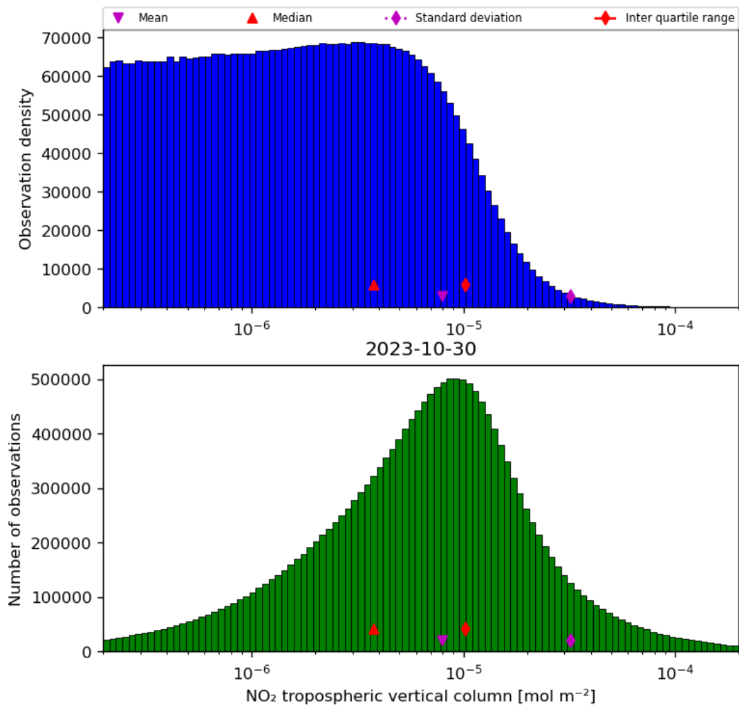
Figure 29: Histogram of “NO 2 tropospheric vertical column” for 2023-10-29 to 2023-10-31
