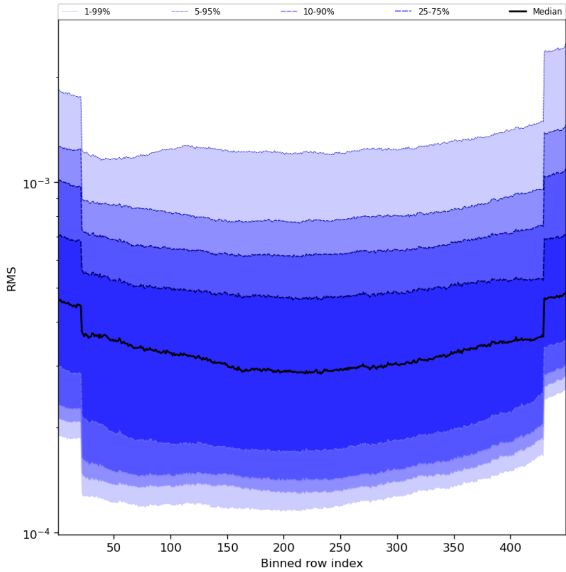
Figure 60: Along track statistics of “RMS” for 2023-10-29 to 2023-10-31
