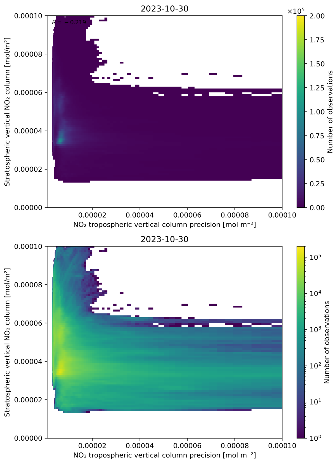
Figure 135: Scatter density plot of “NO 2 tropospheric vertical column precision” against “Stratospheric vertical NO 2 column” for 2023-10-29 to 2023-10-31.
