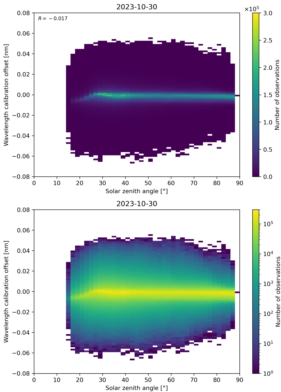
Figure 158: Scatter density plot of “Solar zenith angle” against “Wavelength calibration offset” for 2023-10-29 to 2023-10-31.
