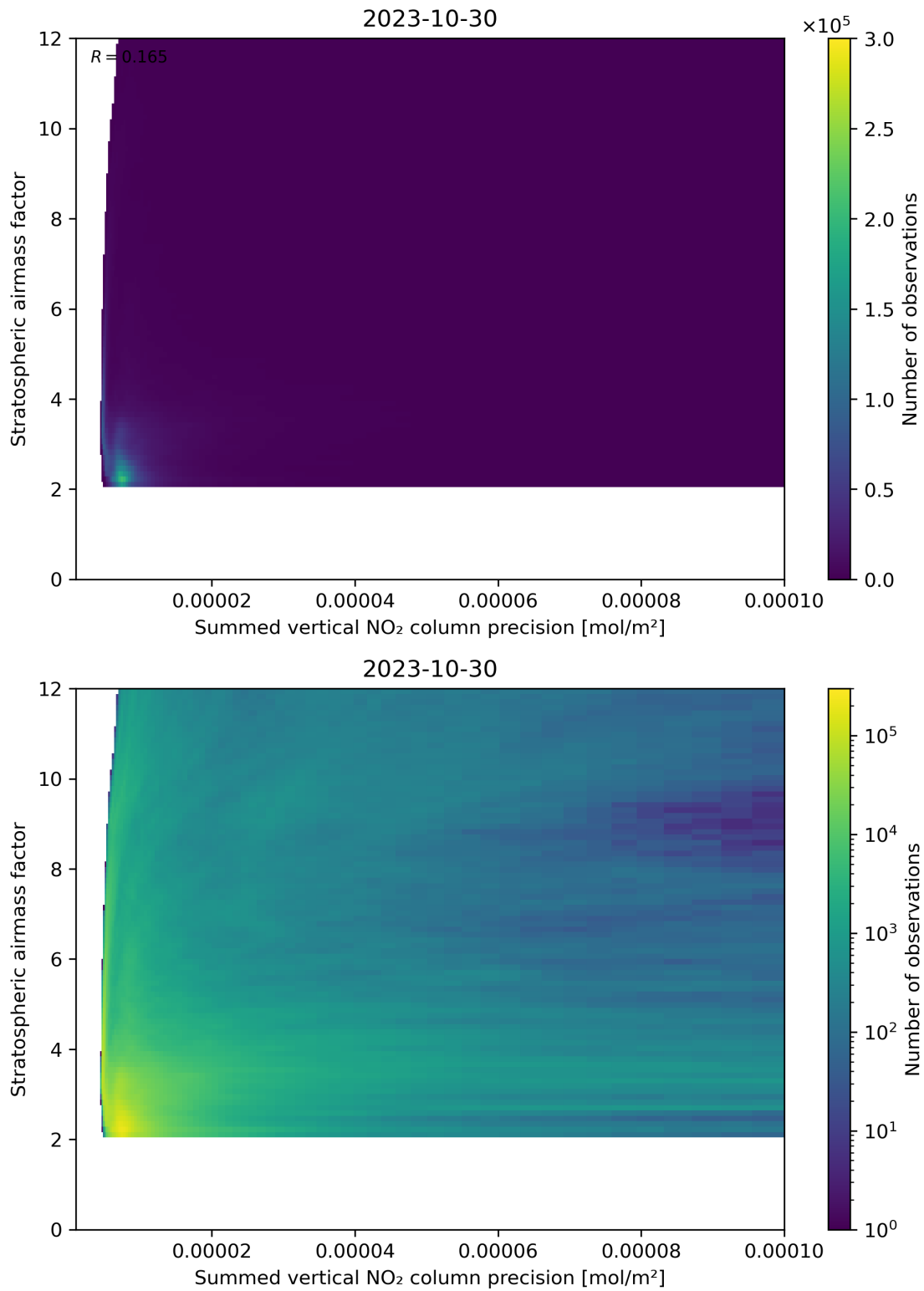
Figure 106: Scatter density plot of “Summed vertical NO 2 column precision” against “Stratospheric airmass factor” for 2023-10-29 to 2023-10-31.
