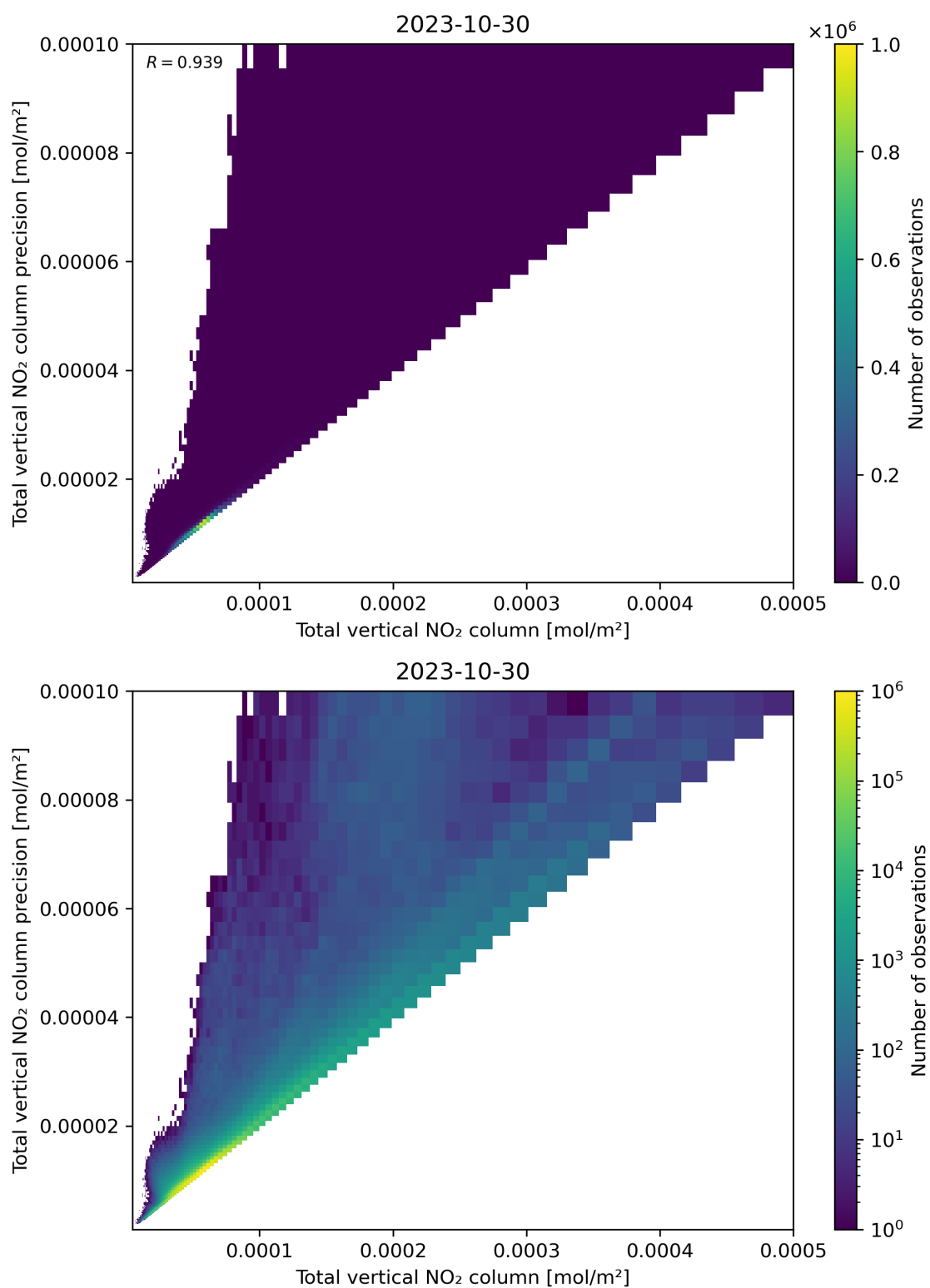
Figure 114: Scatter density plot of “Total vertical NO 2 column” against “Total vertical NO 2 column precision” for 2023-10-29 to 2023-10-31.
