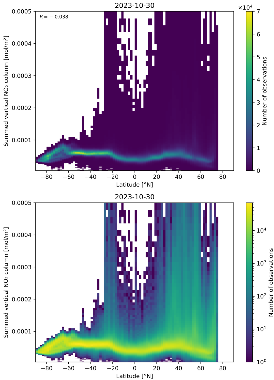
Figure 88: Scatter density plot of “Latitude” against “Summed vertical NO 2 column” for 2023-10-29 to 2023-10-31.
