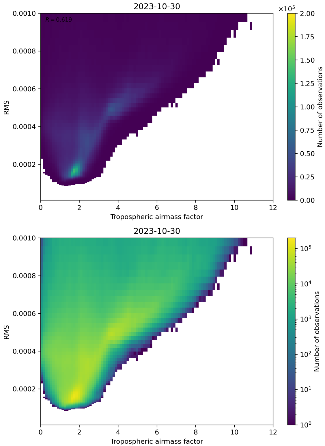
Figure 79: Scatter density plot of “Tropospheric airmass factor” against “RMS” for 2023-10-29 to 2023-10-31.
