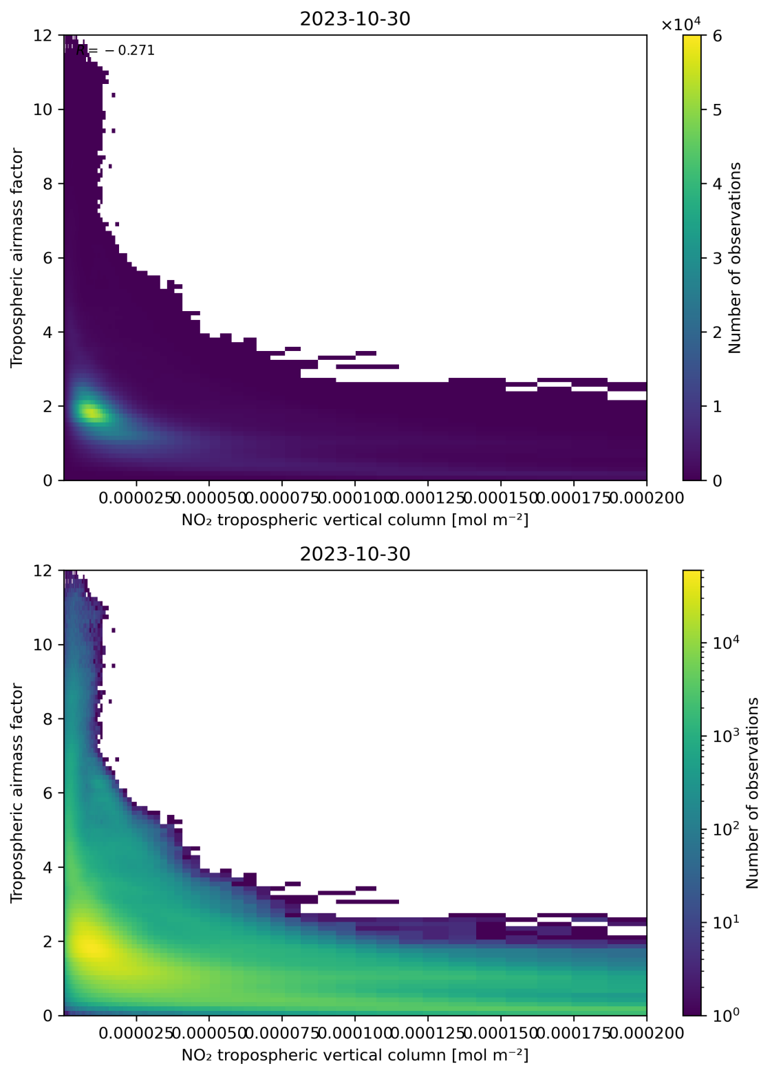
Figure 123: Scatter density plot of “NO 2 tropospheric vertical column” against “Tropospheric air mass factor” for 2023-10-29 to 2023-10-31.
