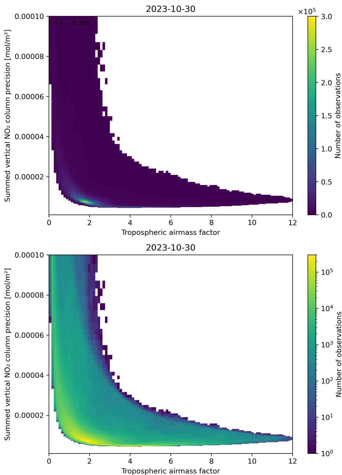
Figure 76: Scatter density plot of “Tropospheric air mass factor” against “Summed vertical NO 2 column precision” for 2023-10-29 to 2023-10-31.
