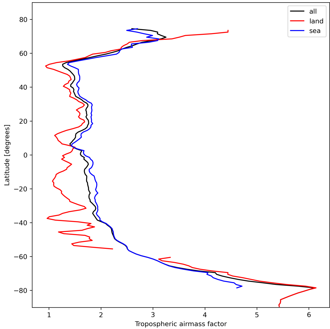
Figure 14: Zonal average of “Tropospheric airmass factor” for 2023-10-30 to 2023-11-01.
