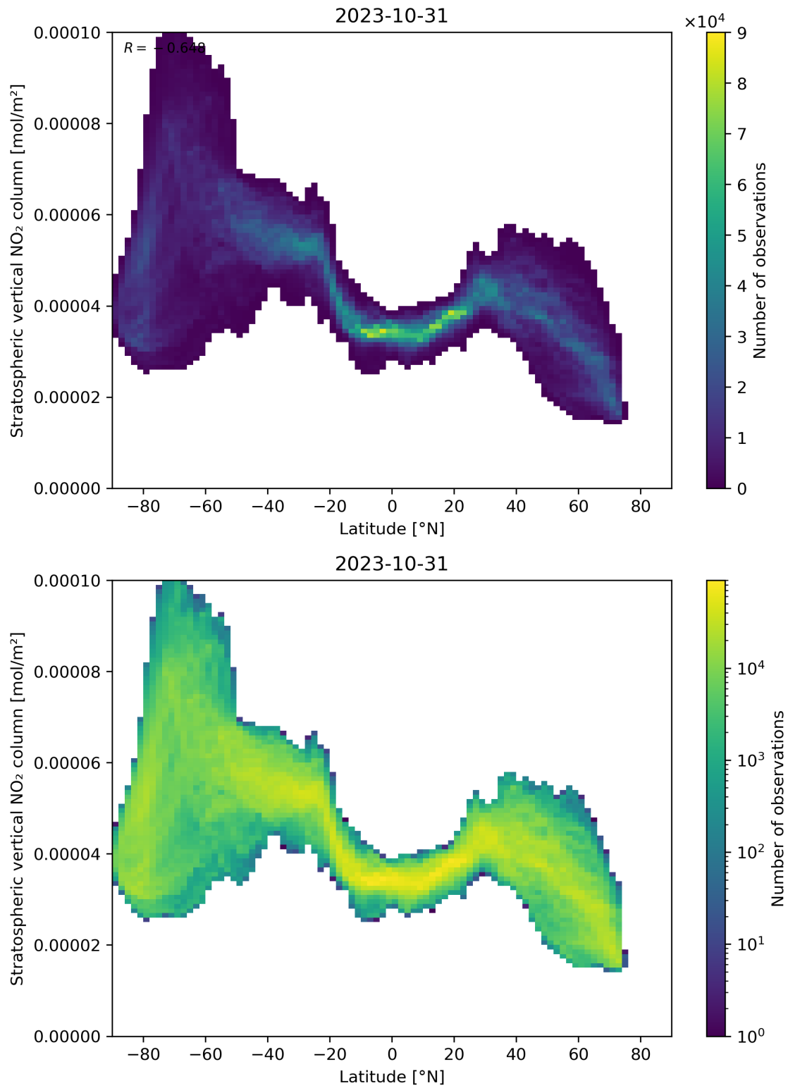
Figure 87: Scatter density plot of “Latitude” against “Stratospheric vertical NO 2 column” for 2023-10-30 to 2023-11-01.
