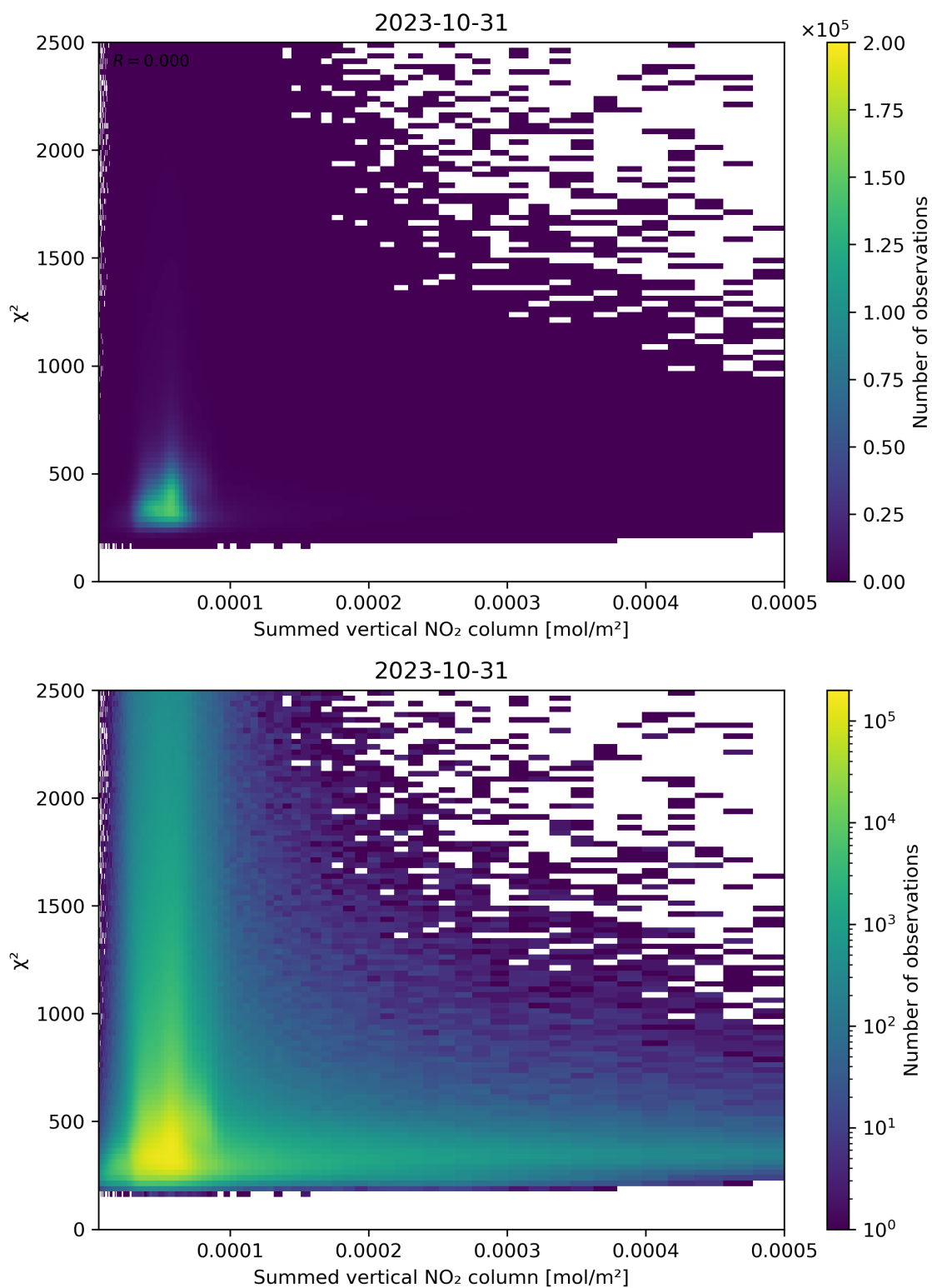
Figure 104: Scatter density plot of “Summed vertical NO 2 column” against “ \chi^2 ” for 2023-10-30 to 2023-11-01.
