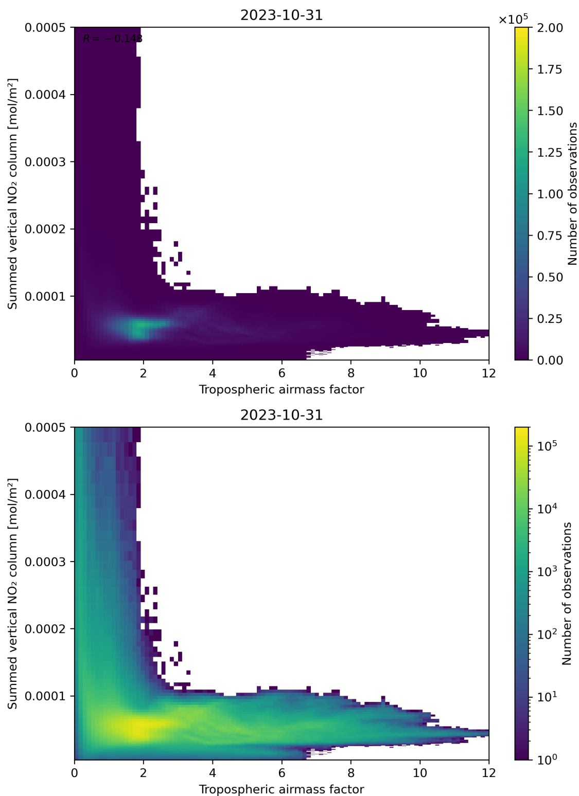
Figure 75: Scatter density plot of “Tropospheric airmass factor” against “Summed vertical NO 2 column” for 2023-10-30 to 2023-11-01.
