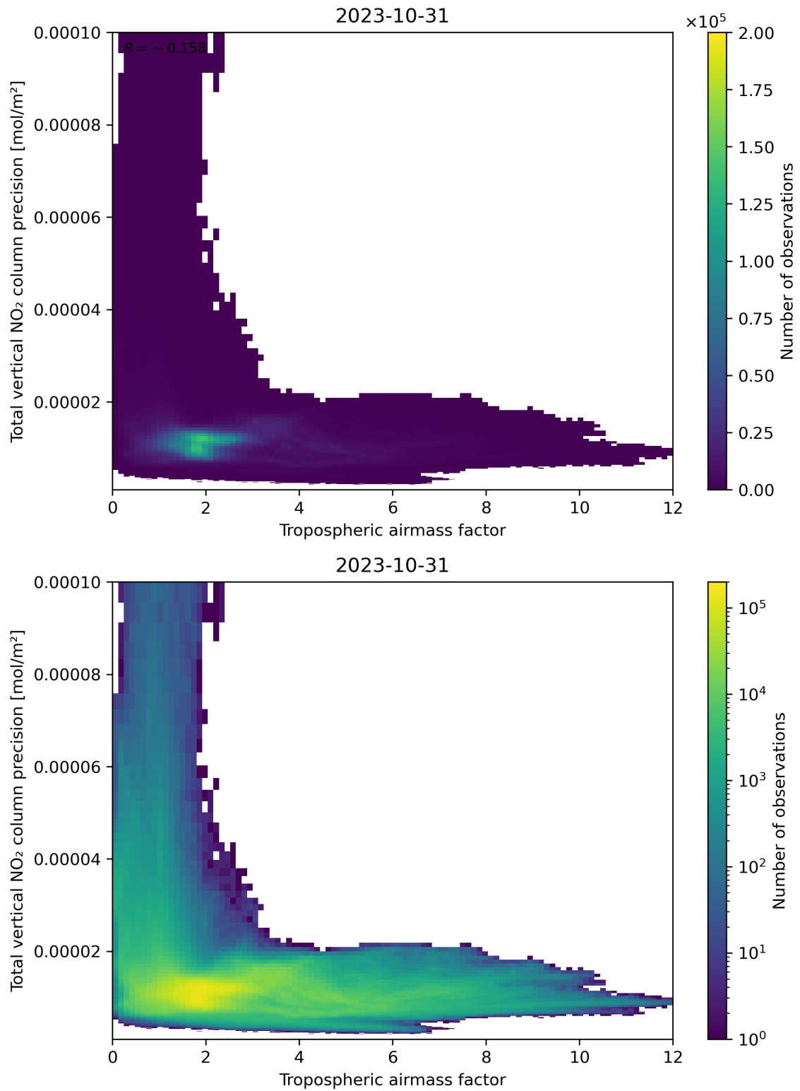
Figure 78: Scatter density plot of “Tropospheric air mass factor” against “Total vertical NO 2 column precision” for 2023-10-30 to 2023-11-01.
