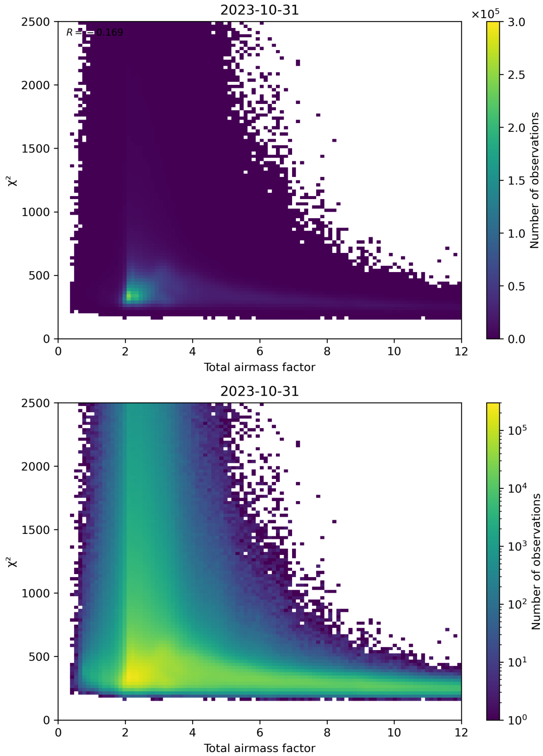
Figure 63: Scatter density plot of “Total airmass factor” against “ \chi^2 ” for 2023-10-30 to 2023-11-01.
