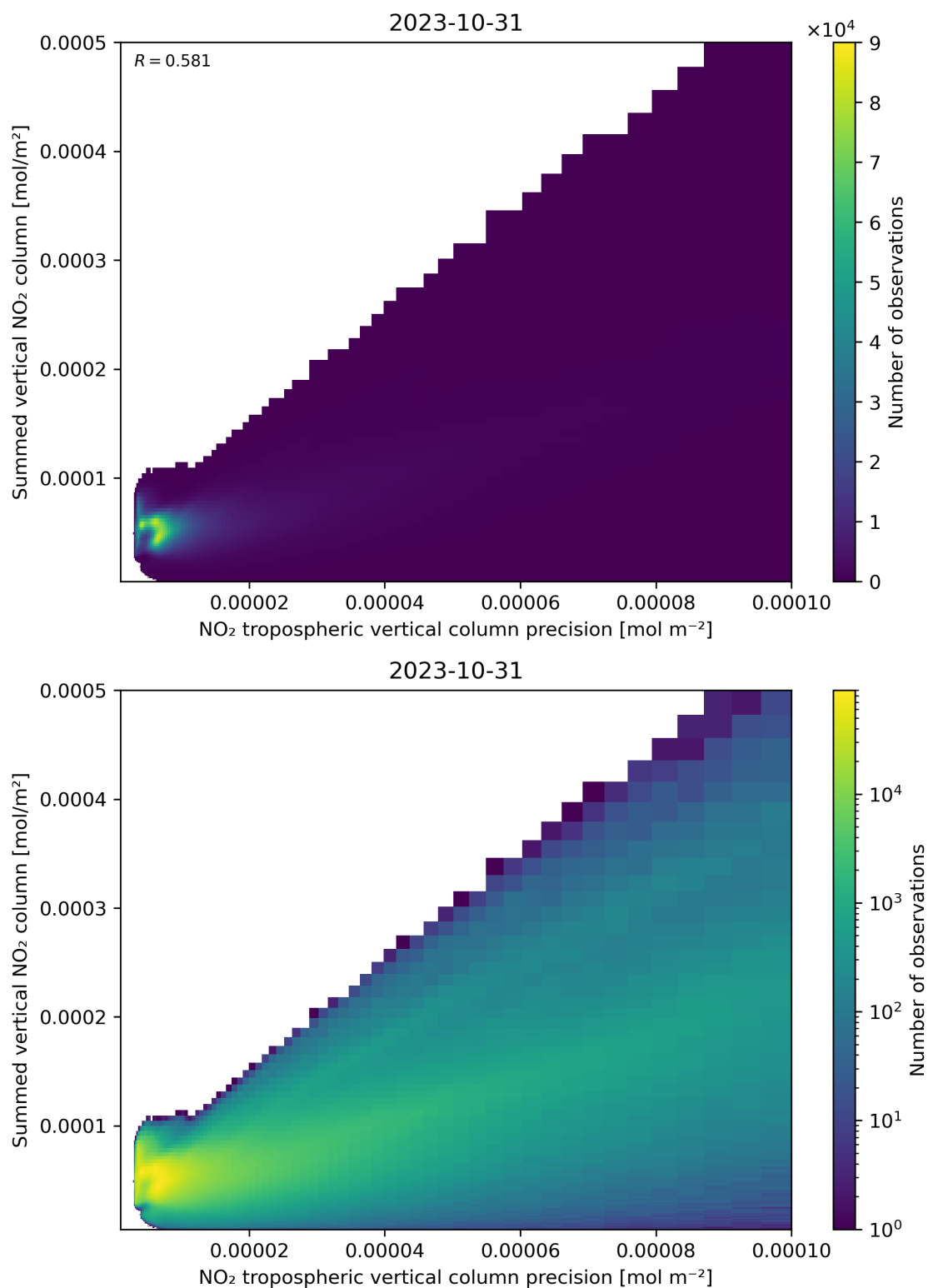
Figure 136: Scatter density plot of “NO 2 tropospheric vertical column precision” against “Summed vertical NO 2 column” for 2023-10-30 to 2023-11-01.
