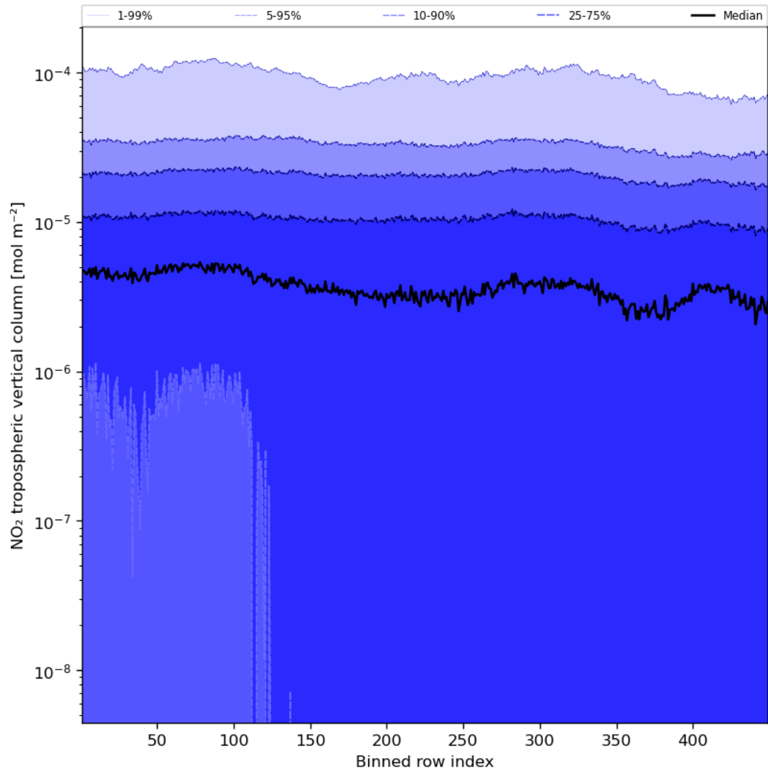
Figure 46: Along track statistics of “NO 2 tropospheric vertical column” for 2023-10-30 to 2023-11-01
