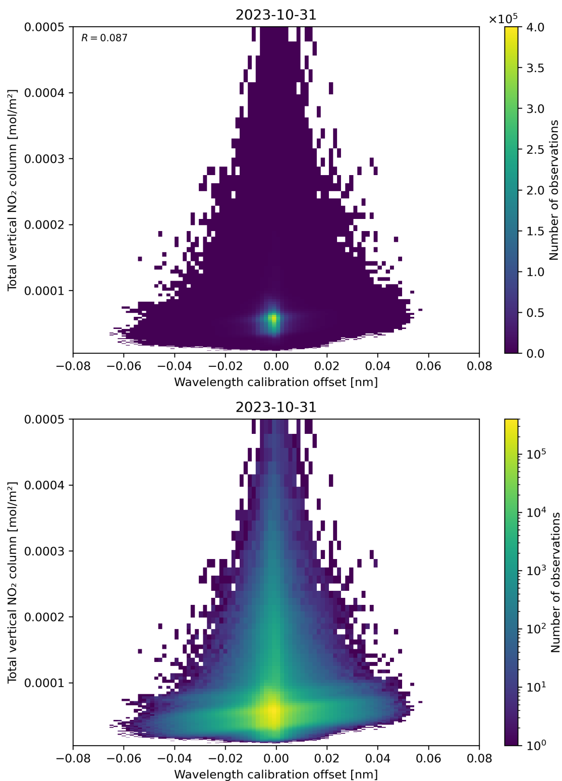
Figure 179: Scatter density plot of “Wavelength calibration offset” against “Total vertical NO 2 column” for 2023-10-30 to 2023-11-01.
