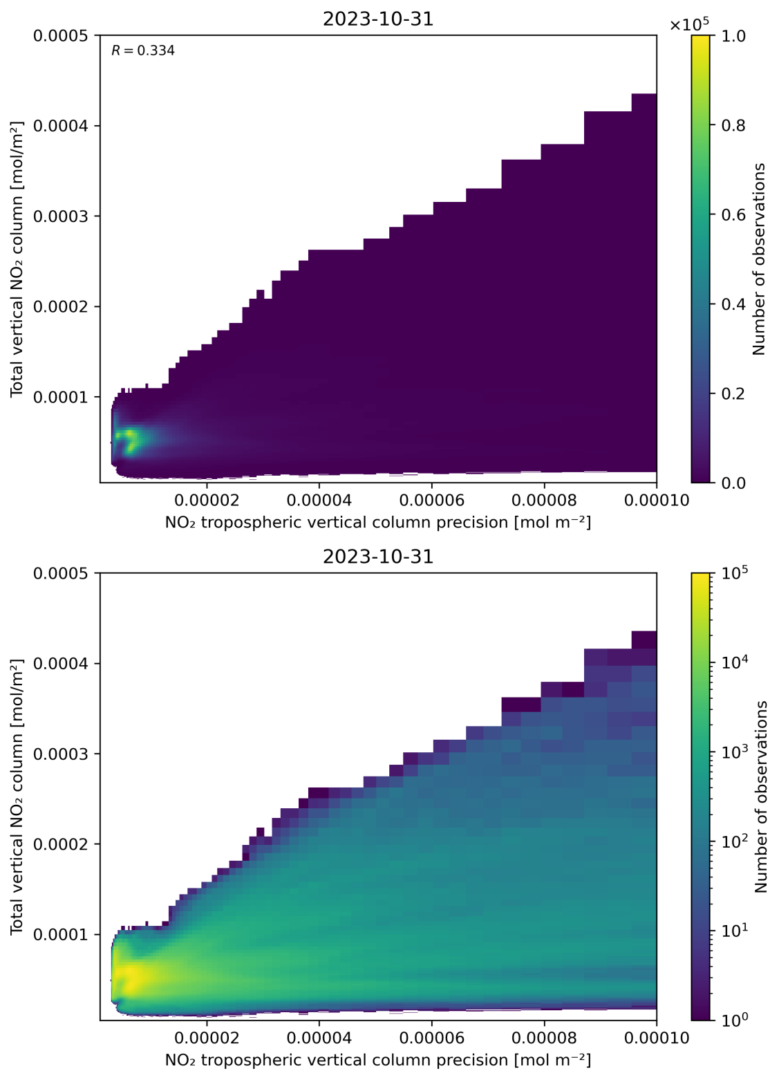
Figure 138: Scatter density plot of “NO 2 tropospheric vertical column precision” against “Total vertical NO 2 column” for 2023-10-30 to 2023-11-01.
