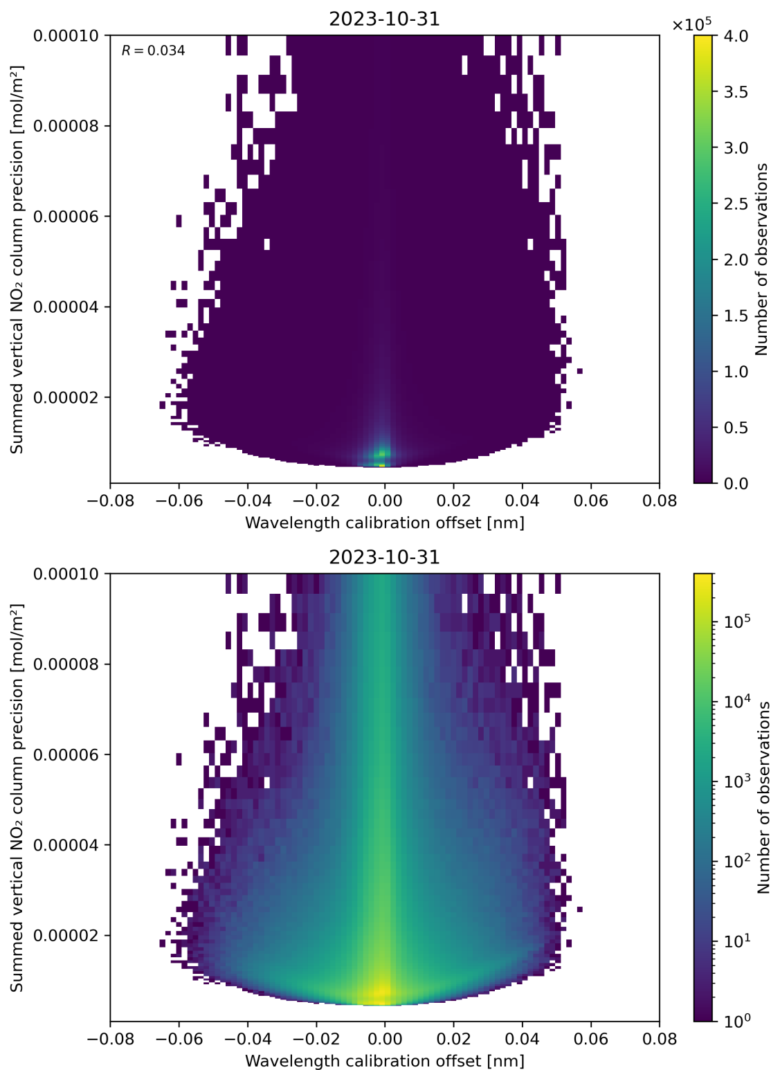
Figure 178: Scatter density plot of “Wavelength calibration offset” against “Summed vertical NO 2 column precision” for 2023-10-30 to 2023-11-01.
