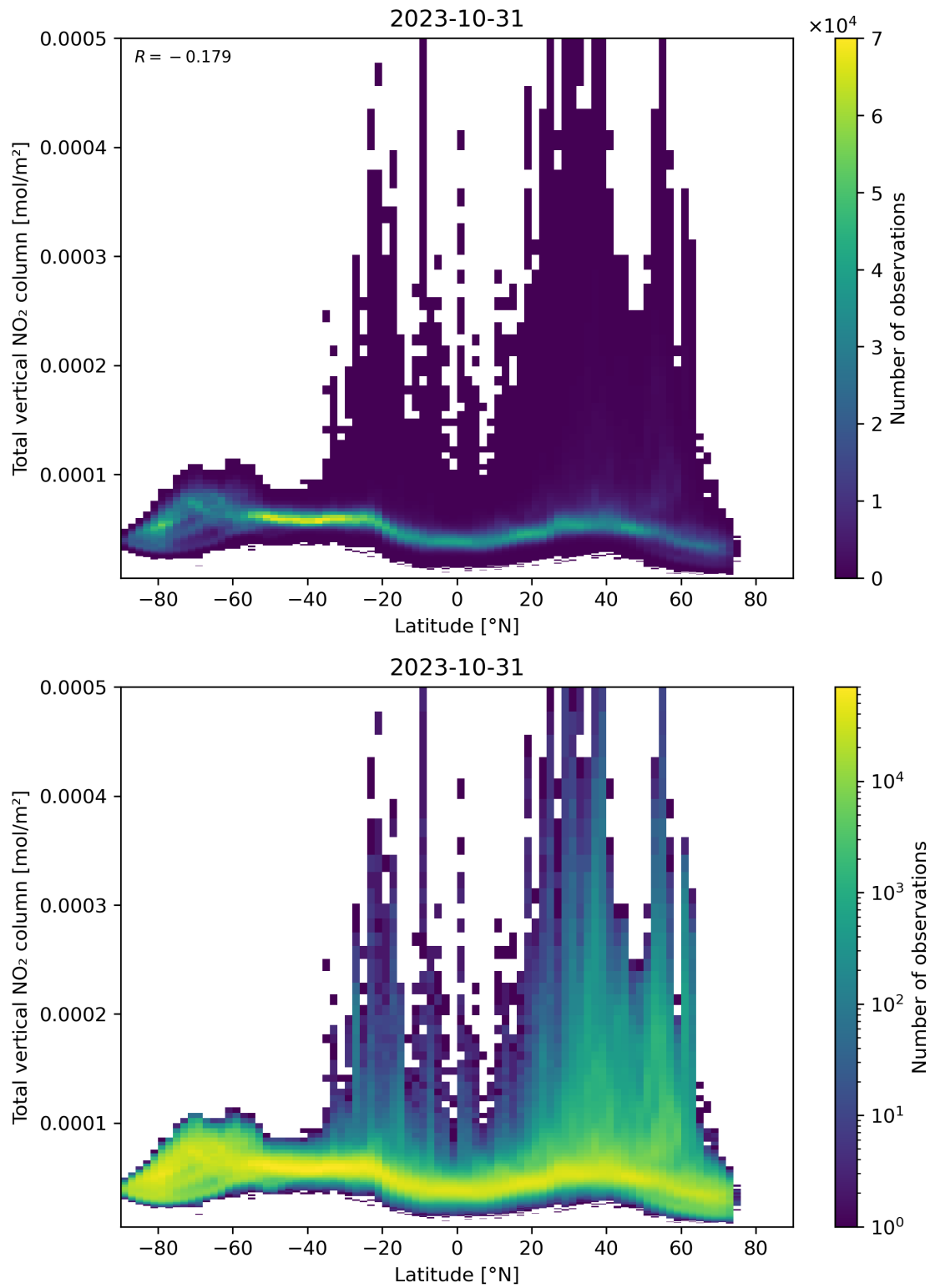
Figure 90: Scatter density plot of “Latitude” against “Total vertical NO 2 column” for 2023-10-30 to 2023-11-01.
