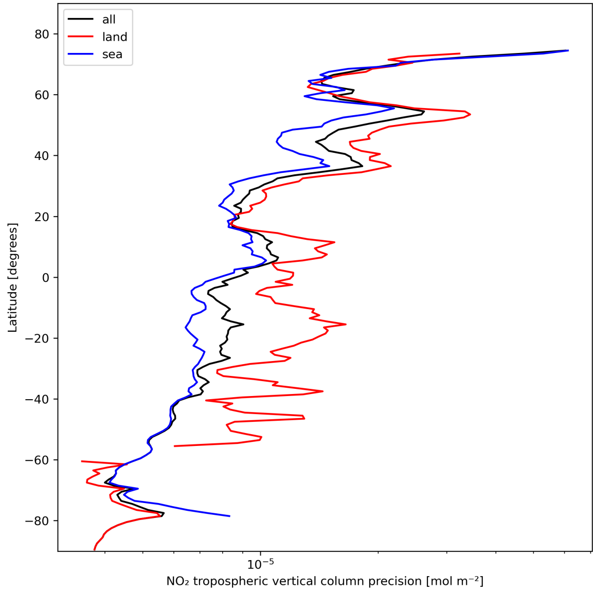
Figure 13: Zonal average of “NO 2 tropospheric vertical column precision” for 2023-10-30 to 2023-11-01.
