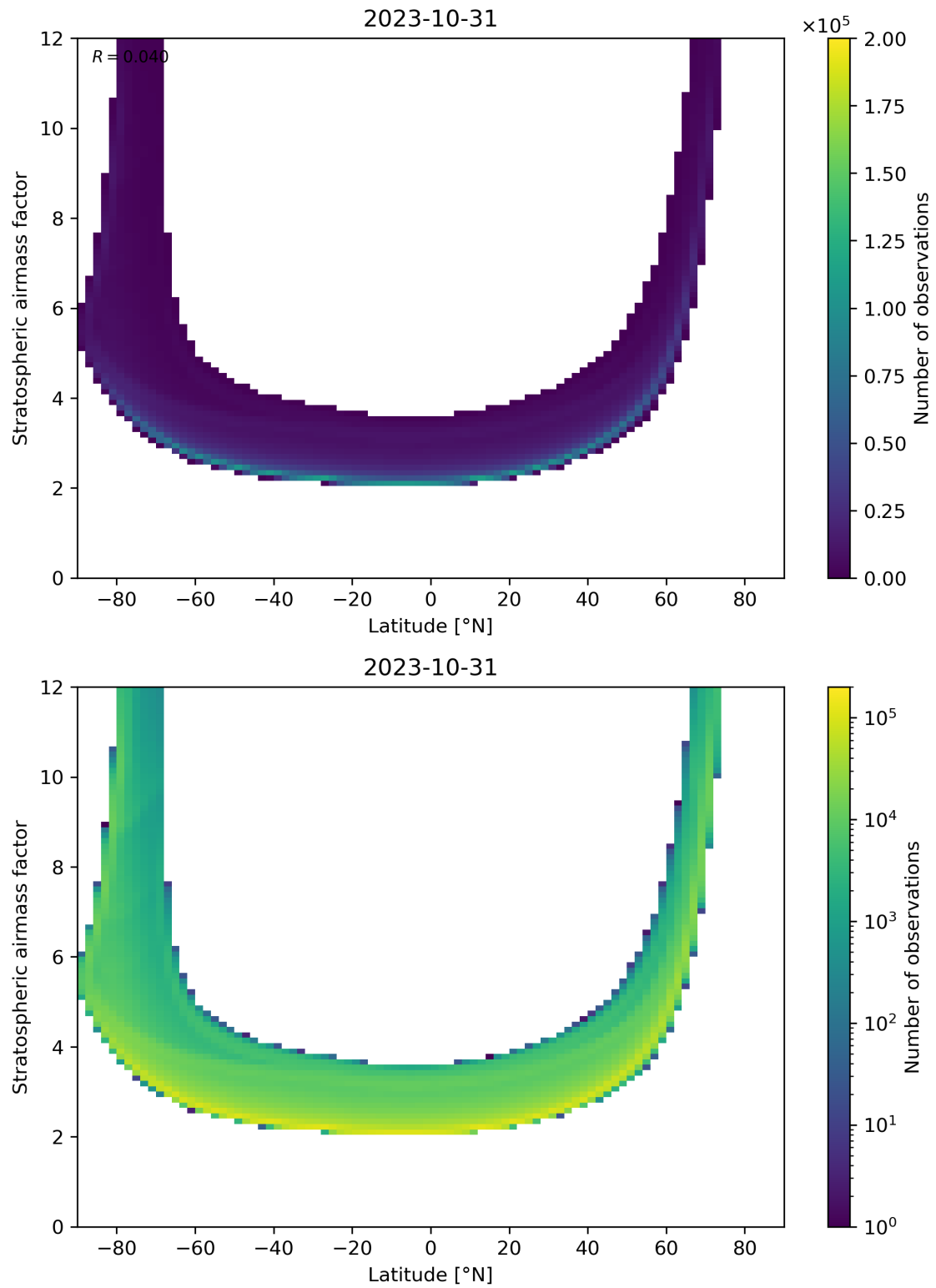
Figure 83: Scatter density plot of “Latitude” against “Stratospheric airmass factor” for 2023-10-30 to 2023-11-01.
