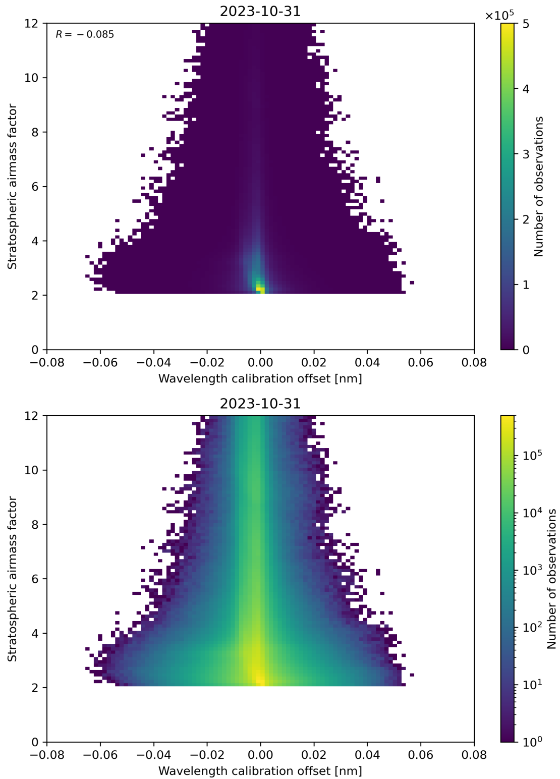
Figure 174: Scatter density plot of “Wavelength calibration offset” against “Stratospheric airmass factor” for 2023-10-30 to 2023-11-01.
