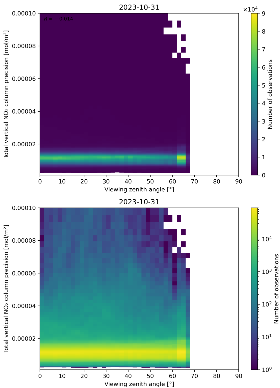
Figure 168: Scatter density plot of “Viewing zenith angle” against “Total vertical NO 2 column precision” for 2023-10-30 to 2023-11-01.
