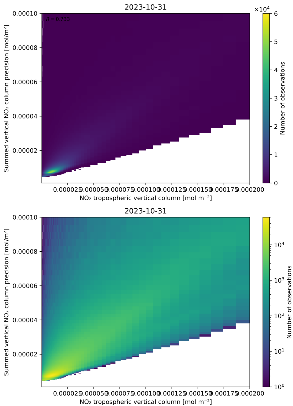
Figure 127: Scatter density plot of “NO 2 tropospheric vertical column” against “Summed vertical NO 2 column precision” for 2023-10-30 to 2023-11-01.
