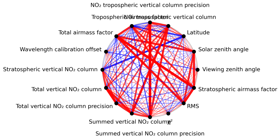
Figure 1: Map of correlation graph for 2023-10-30 to 2023-11-01.
