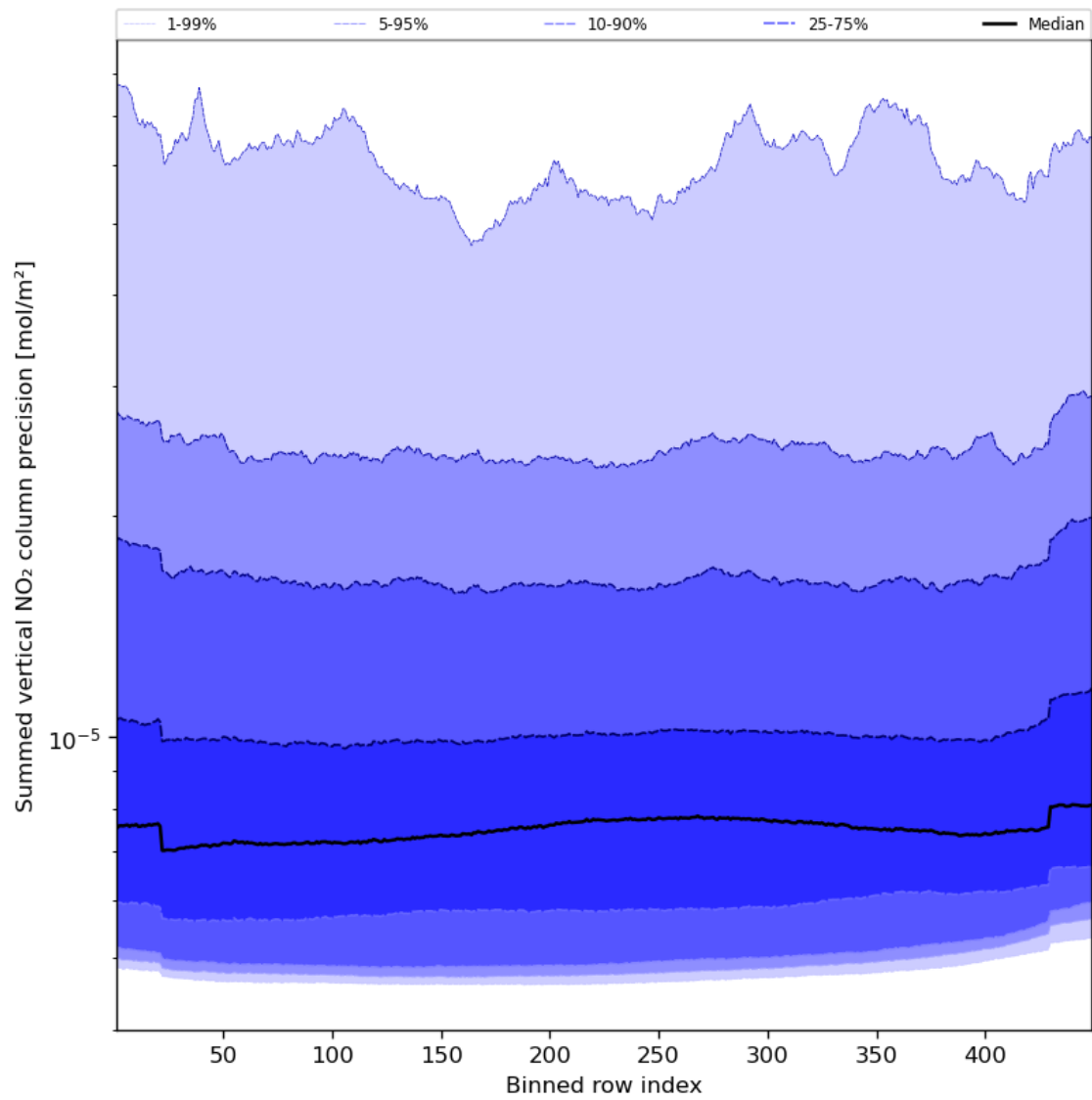
Figure 58: Along track statistics of “Summed vertical NO 2 column precision” for 2023-10-30 to 2023-11-01
