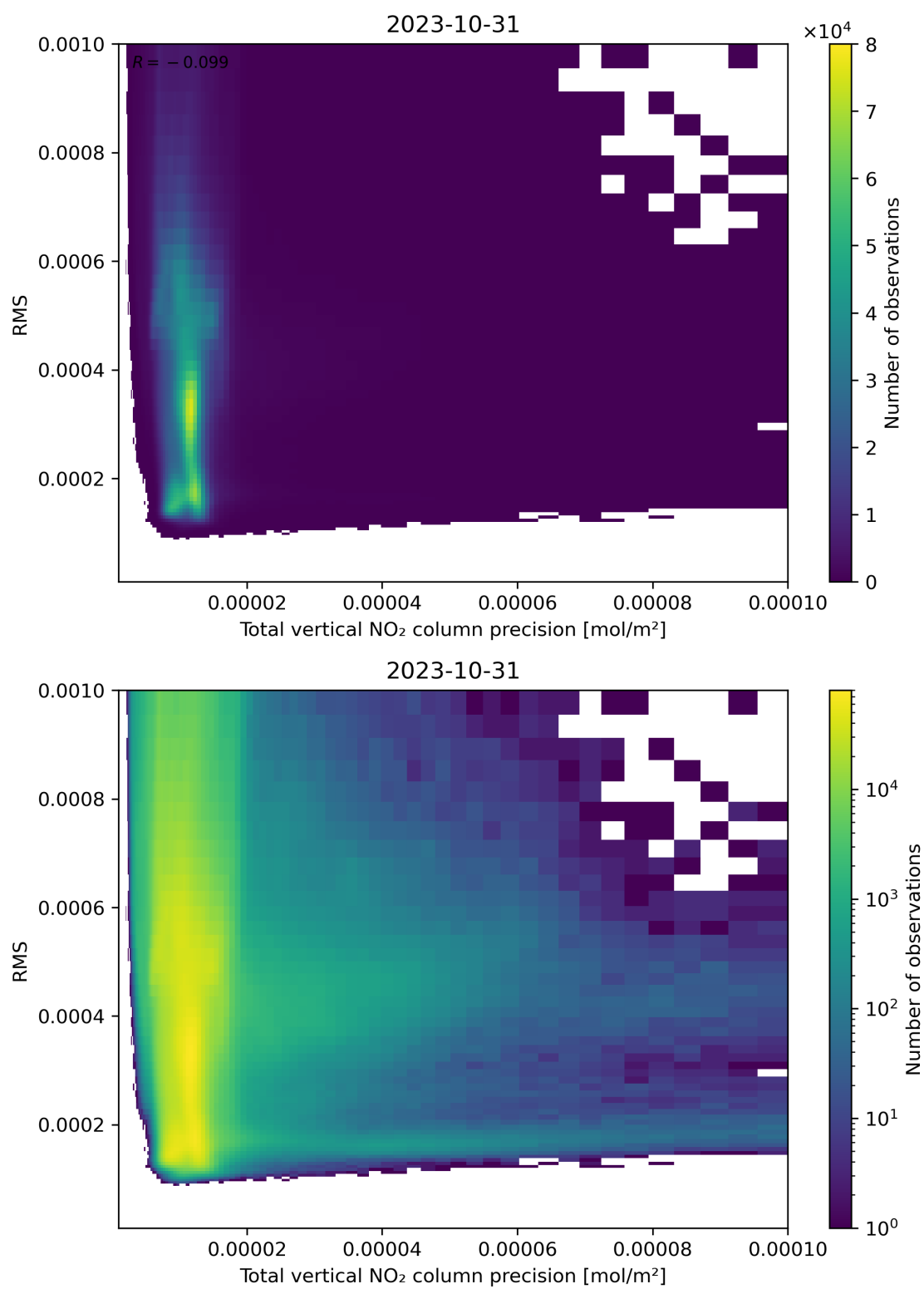
Figure 119: Scatter density plot of “Total vertical NO 2 column precision” against “RMS” for 2023-10-30 to 2023-11-01.
