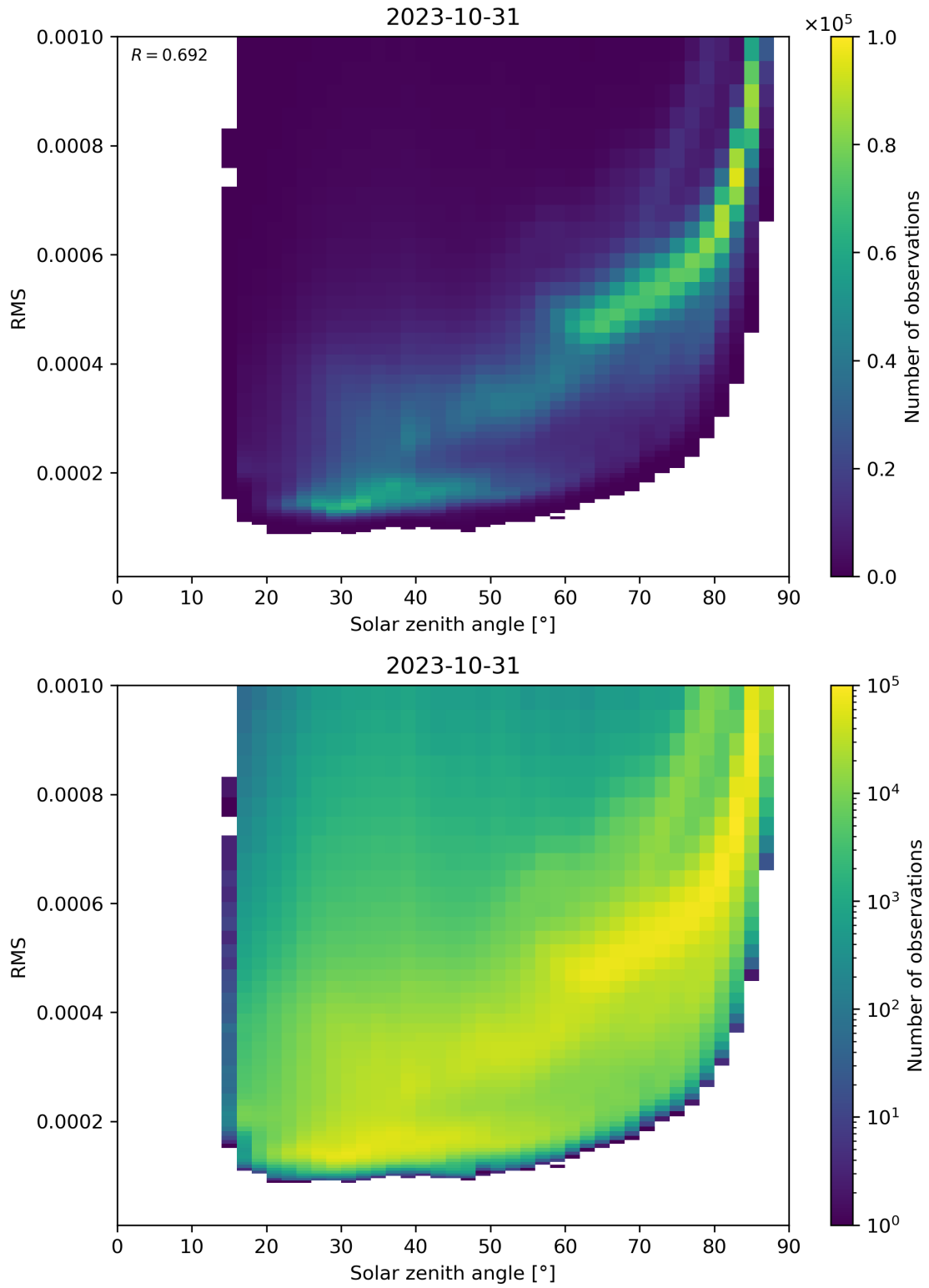
Figure 157: Scatter density plot of “Solar zenith angle” against “RMS” for 2023-10-30 to 2023-11-01.
