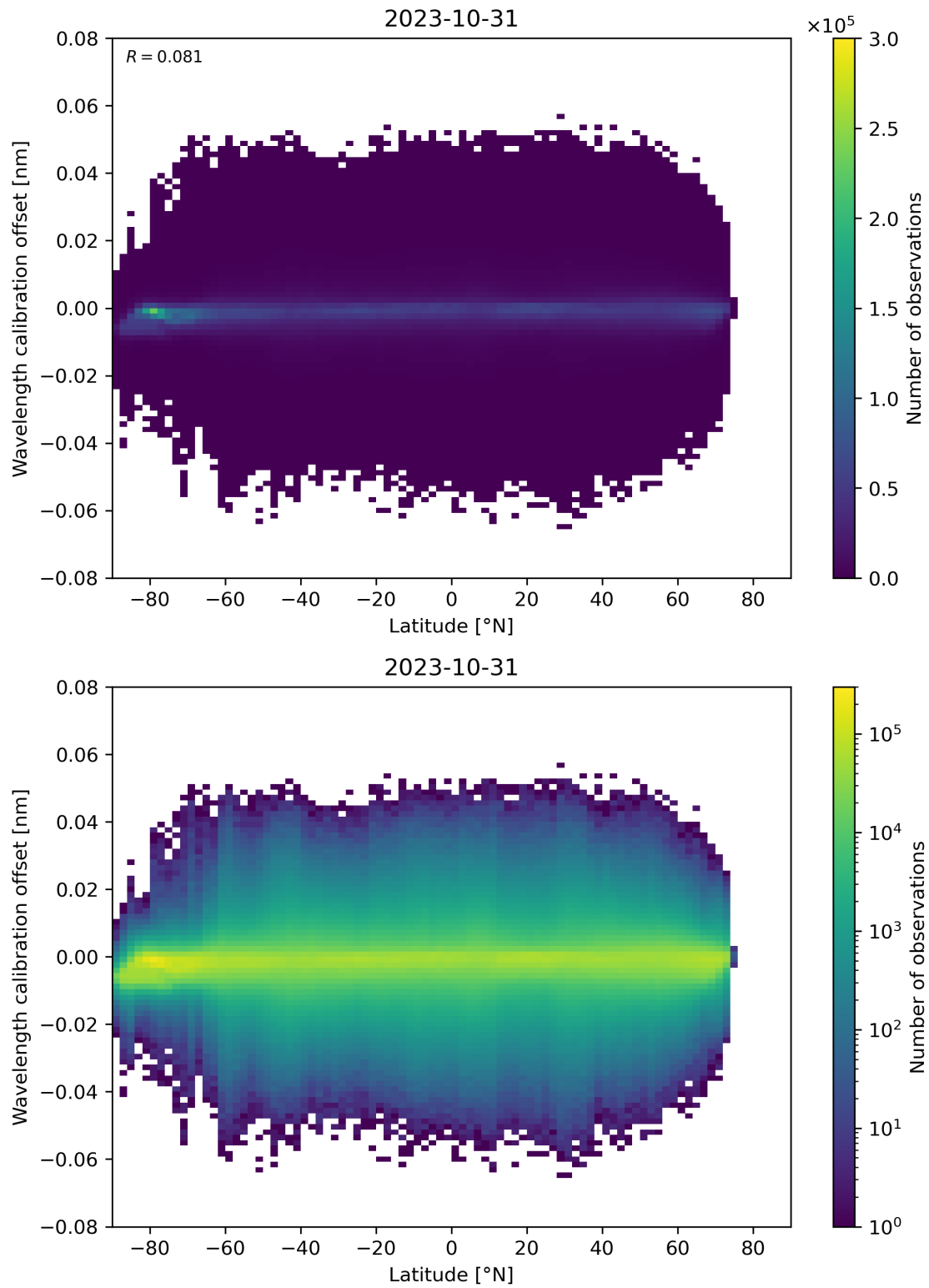
Figure 95: Scatter density plot of “Latitude” against “Wavelength calibration offset” for 2023-10-30 to 2023-11-01.
