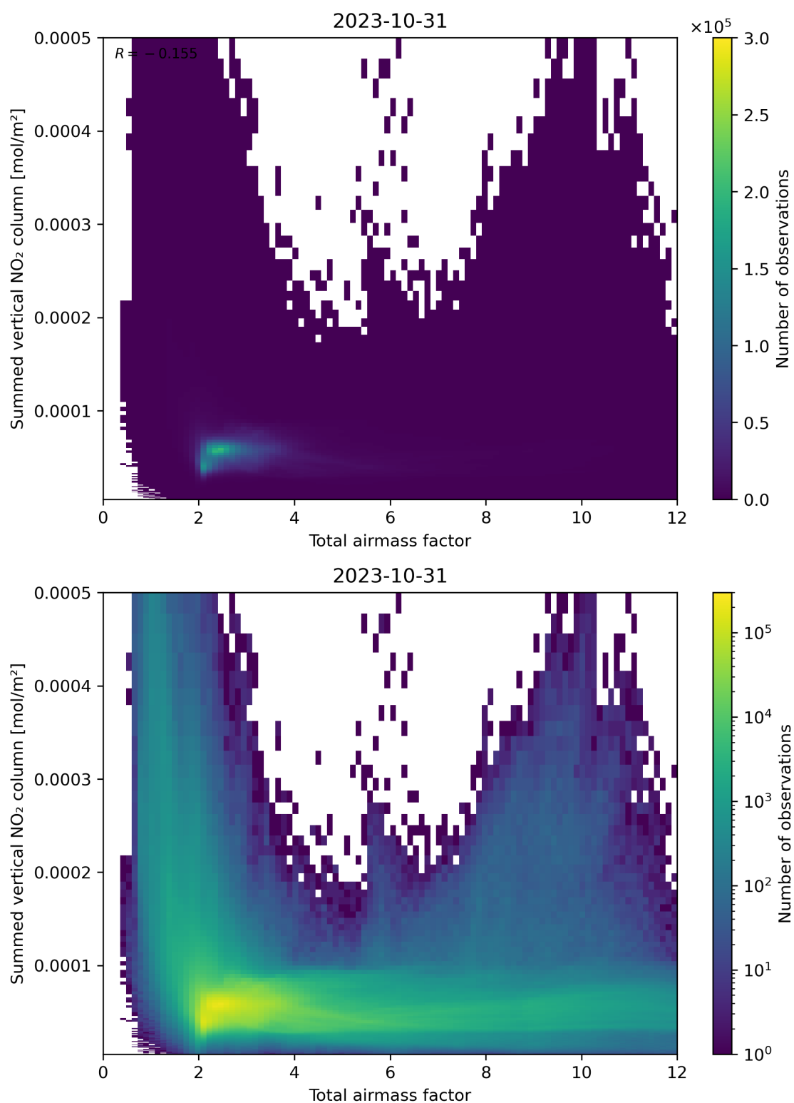
Figure 65: Scatter density plot of “Total airmass factor” against “Summed vertical NO 2 column” for 2023-10-30 to 2023-11-01.
