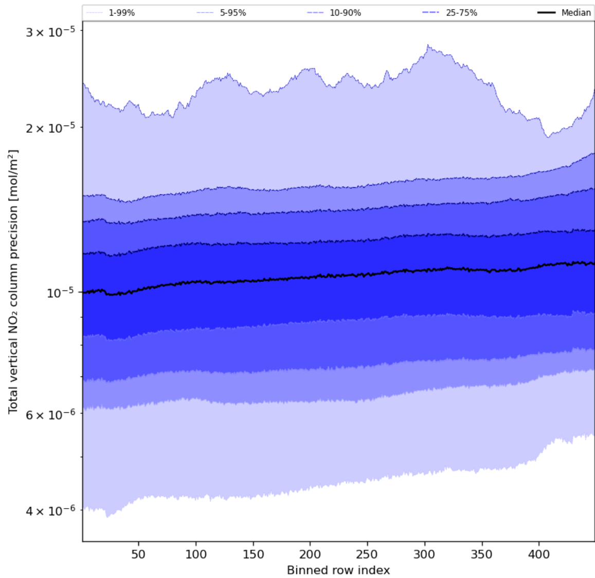
Figure 56: Along track statistics of “Total vertical NO 2 column precision” for 2023-10-30 to 2023-11-01
