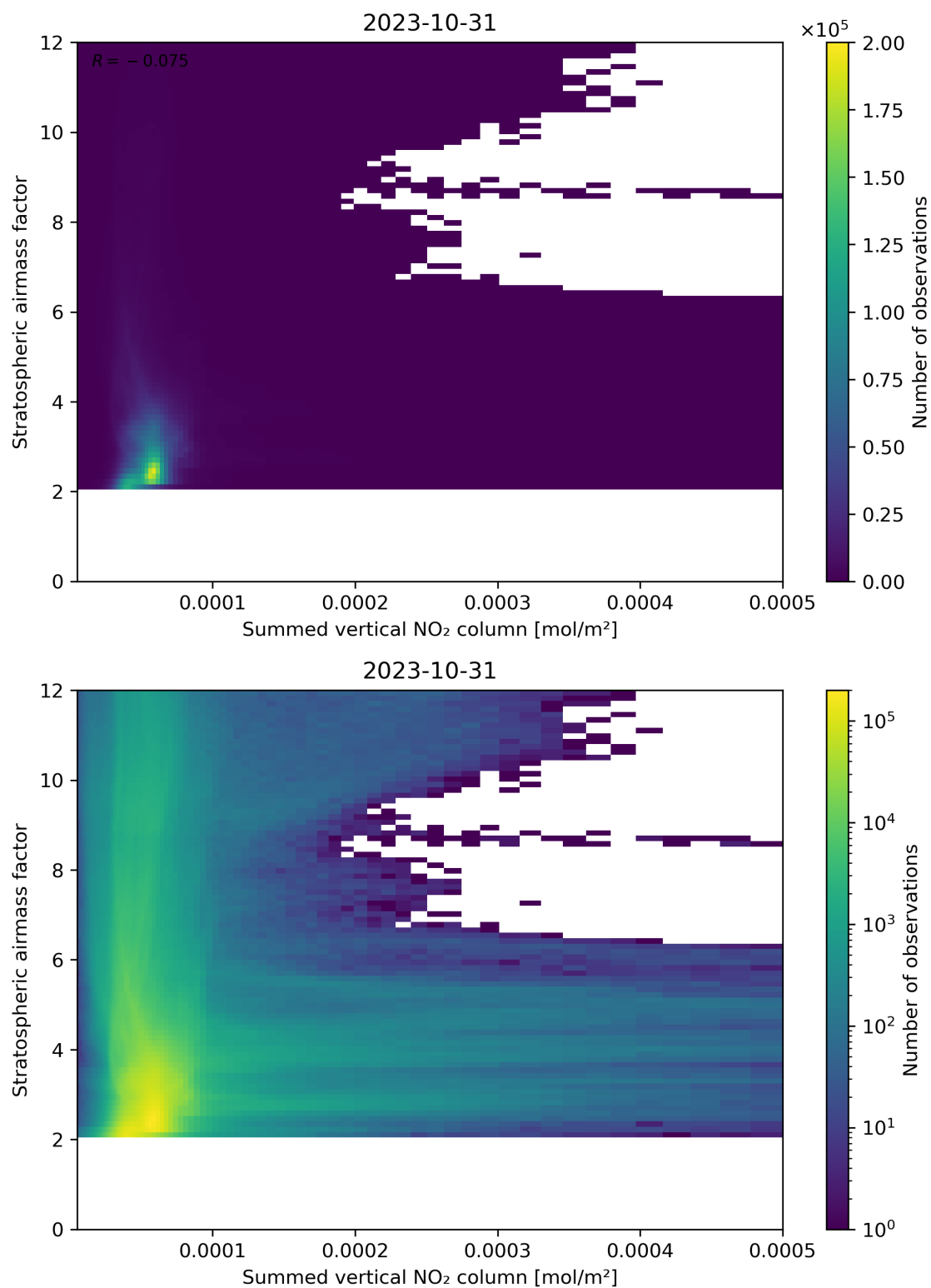
Figure 103: Scatter density plot of “Summed vertical NO 2 column” against “Stratospheric air mass factor” for 2023-10-30 to 2023-11-01.
