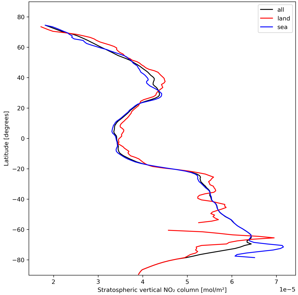
Figure 19: Zonal average of “Stratospheric vertical NO 2 column” for 2023-10-30 to 2023-11-01.
