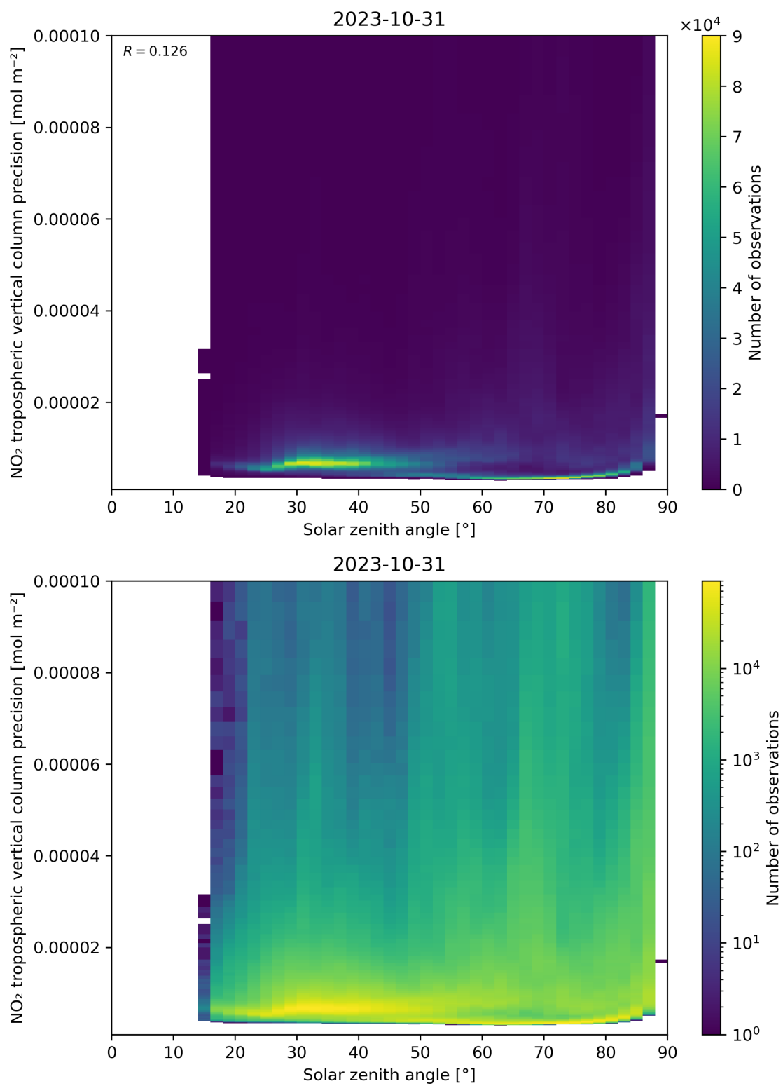
Figure 156: Scatter density plot of “Solar zenith angle” against “NO 2 tropospheric vertical column precision” for 2023-10-30 to 2023-11-01.
