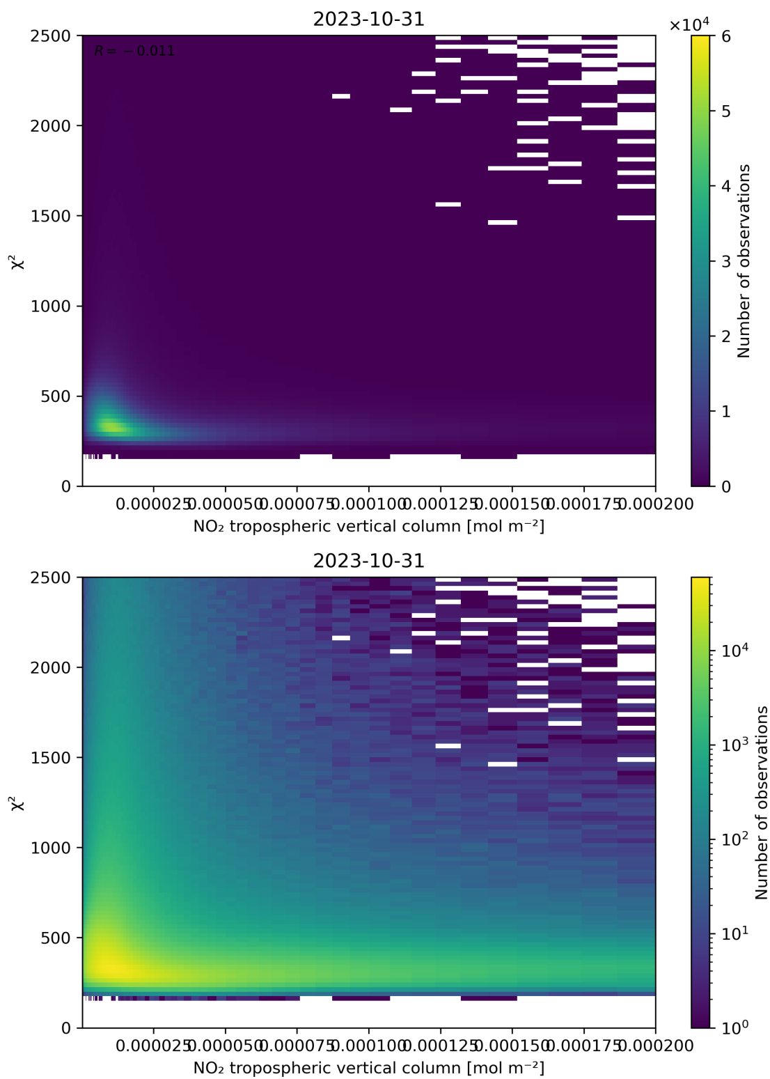
Figure 124: Scatter density plot of “NO 2 tropospheric vertical column” against “ \chi^2 ” for 2023-10-30 to 2023-11-01.
