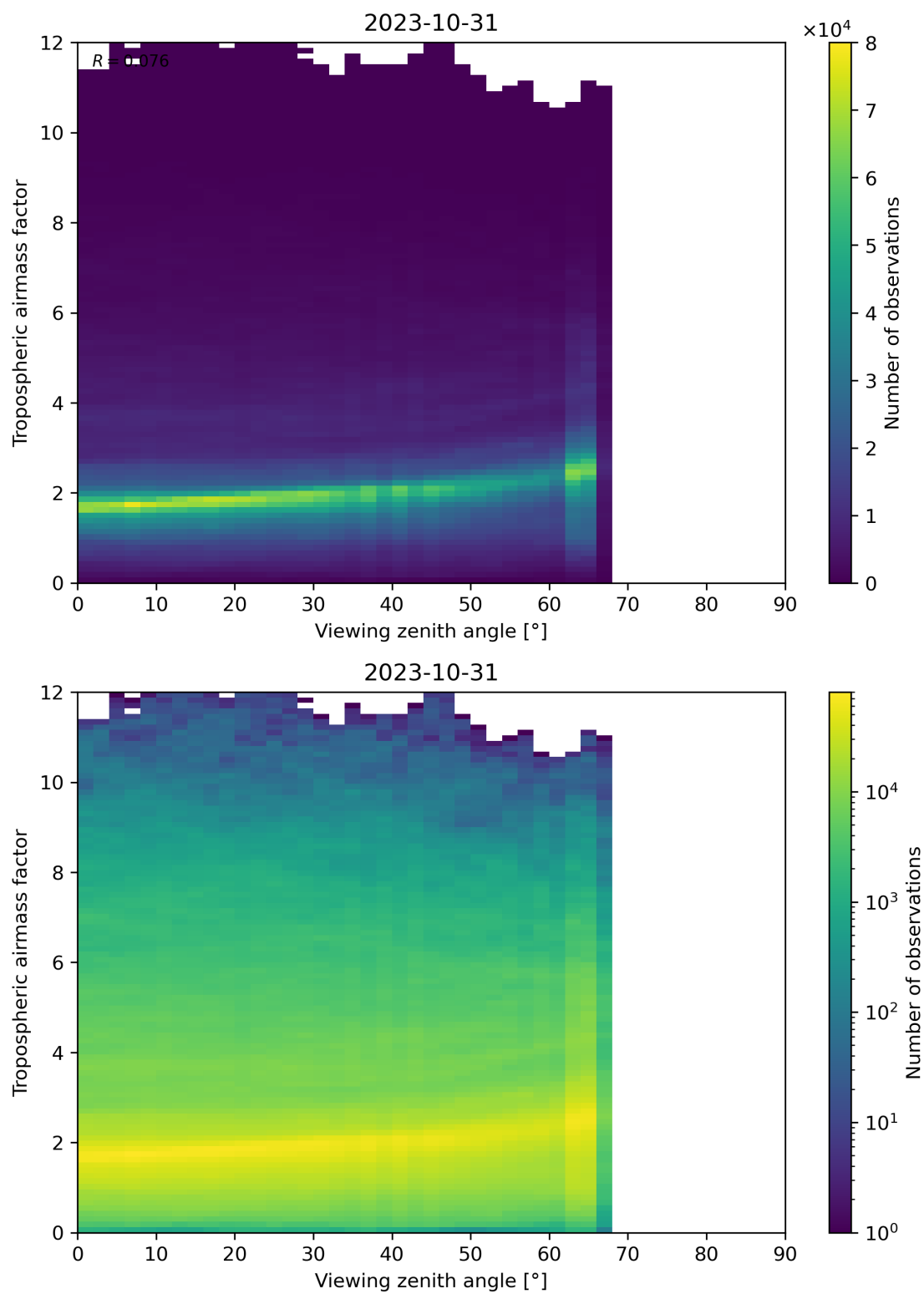
Figure 161: Scatter density plot of “Viewing zenith angle” against “Tropospheric airmass factor” for 2023-10-30 to 2023-11-01.
