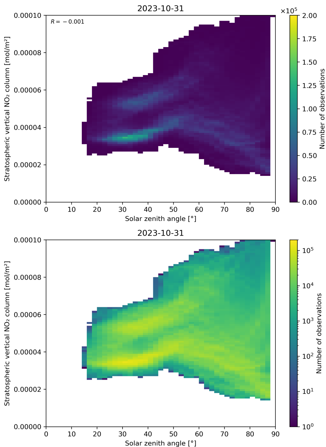
Figure 150: Scatter density plot of “Solar zenith angle” against “Stratospheric vertical NO 2 column” for 2023-10-30 to 2023-11-01.
