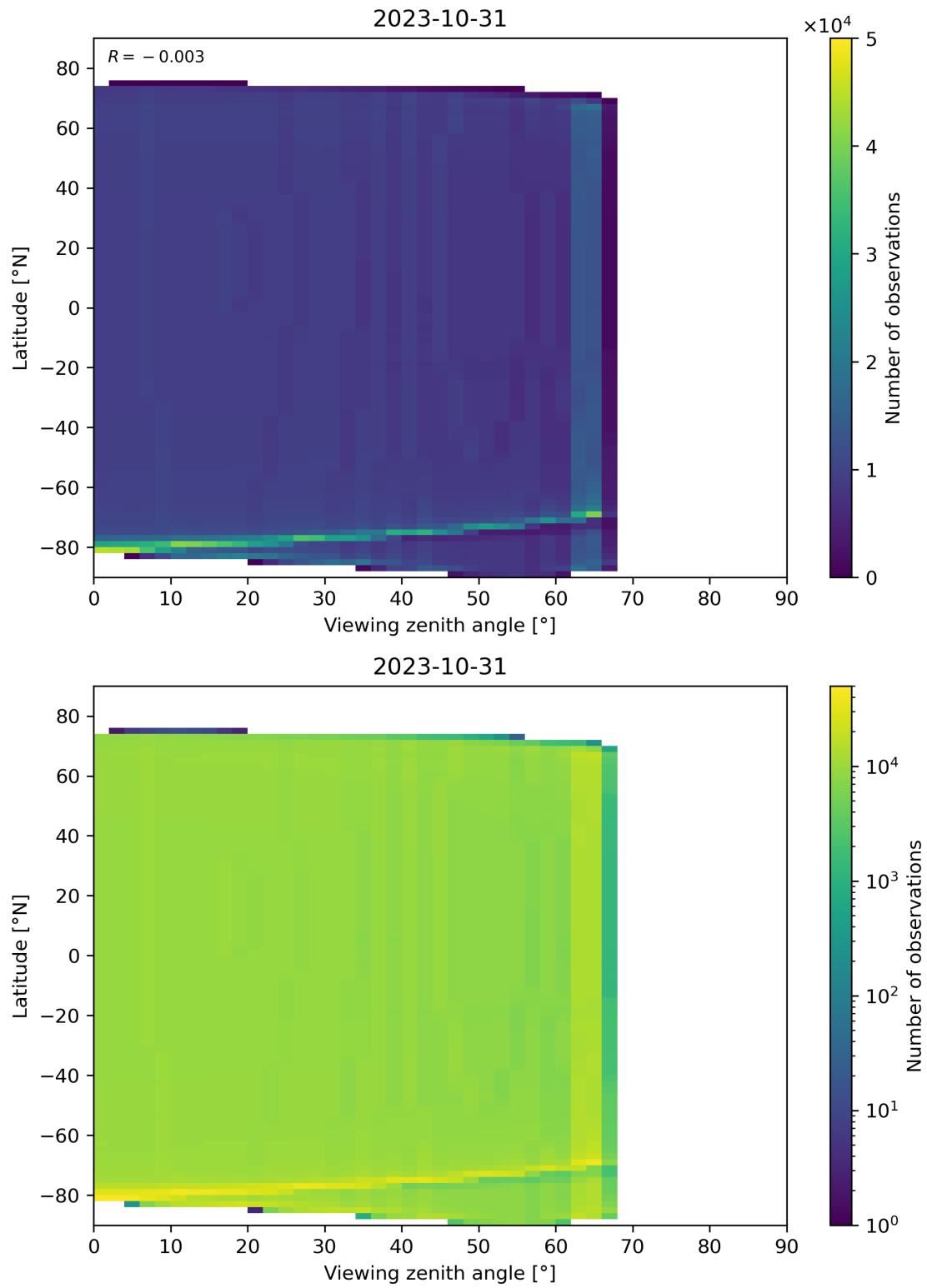
Figure 163: Scatter density plot of “Viewing zenith angle” against “Latitude” for 2023-10-30 to 2023-11-01.
