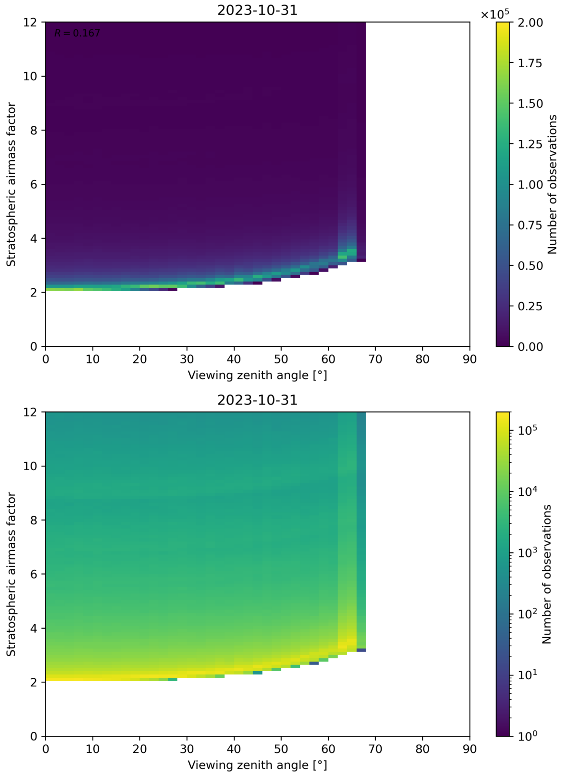
Figure 159: Scatter density plot of “Viewing zenith angle” against “Stratospheric airmass factor” for 2023-10-30 to 2023-11-01.
