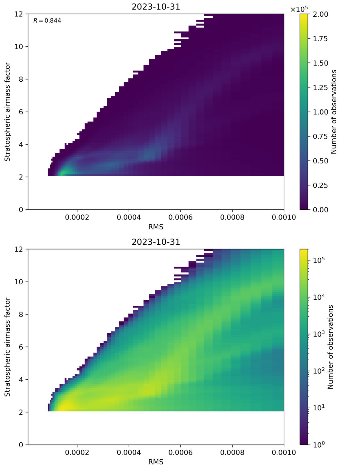
Figure 144: Scatter density plot of “RMS” against “Stratospheric airmass factor” for 2023-10-30 to 2023-11-01.
