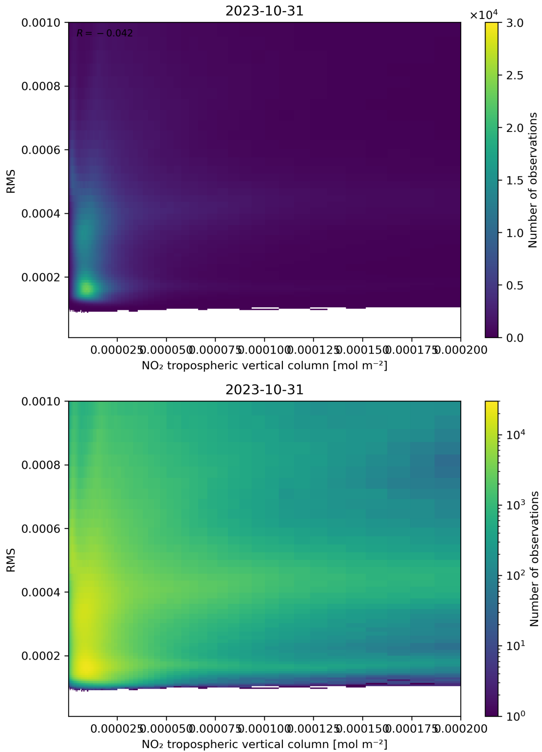
Figure 142: Scatter density plot of “NO 2 tropospheric vertical column” against “RMS” for 2023-10-30 to 2023-11-01.
