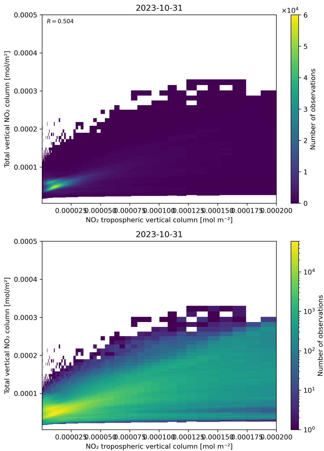
Figure 128: Scatter density plot of “NO 2 tropospheric vertical column” against “Total vertical NO 2 column” for 2023-10-30 to 2023-11-01.
