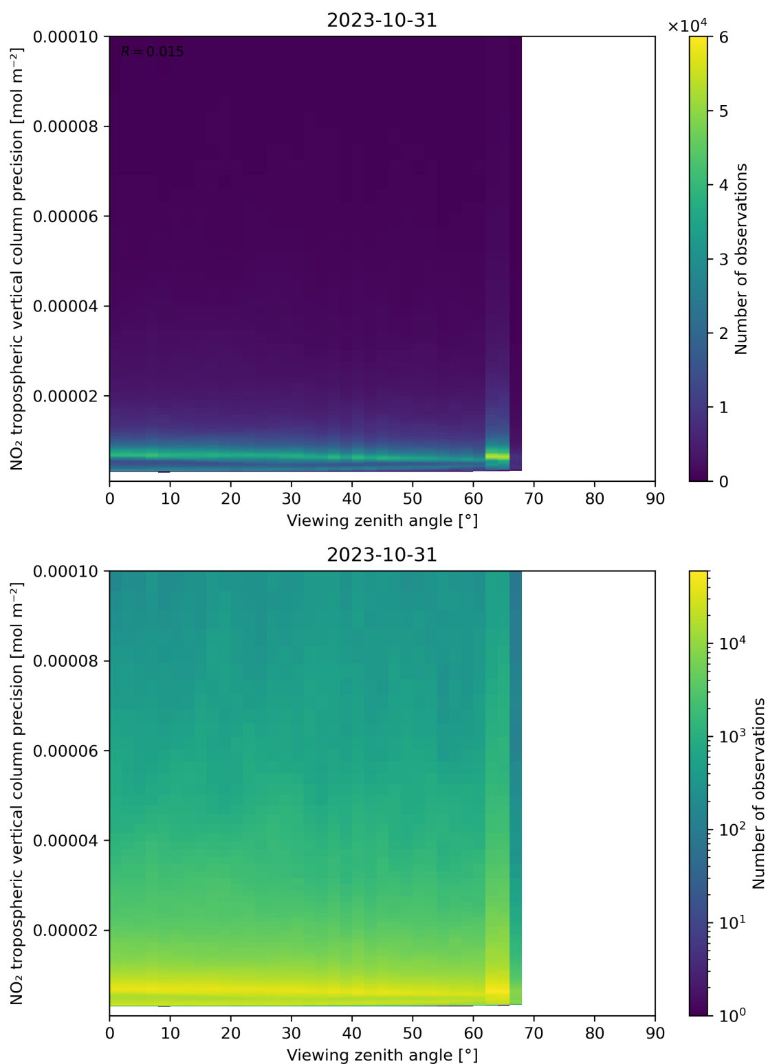
Figure 170: Scatter density plot of “Viewing zenith angle” against “NO 2 tropospheric vertical column precision” for 2023-10-30 to 2023-11-01.
