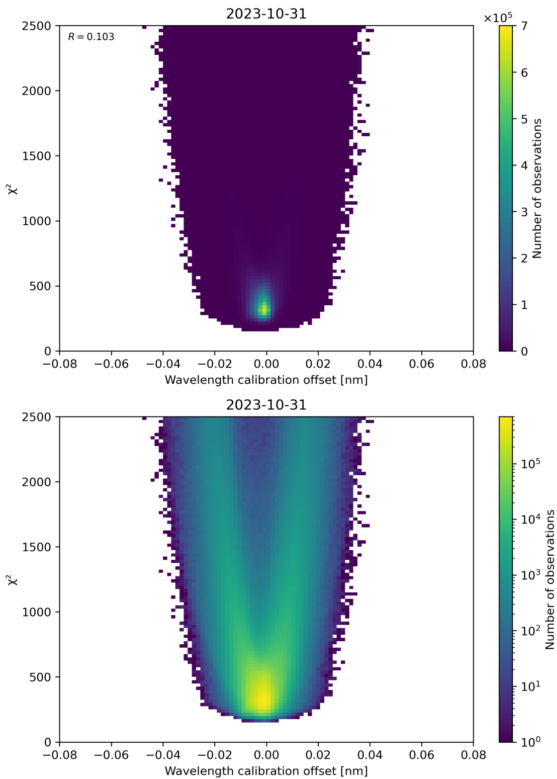
Figure 175: Scatter density plot of “Wavelength calibration offset” against “ \chi^2 ” for 2023-10-30 to 2023-11-01.
