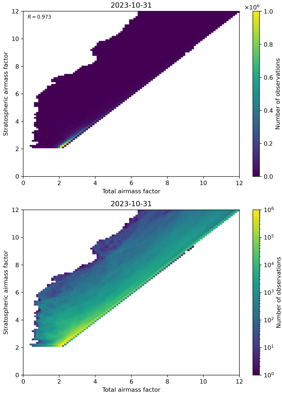
Figure 62: Scatter density plot of “Total air mass factor” against “Stratospheric air mass factor” for 2023-10-30 to 2023-11-01.
