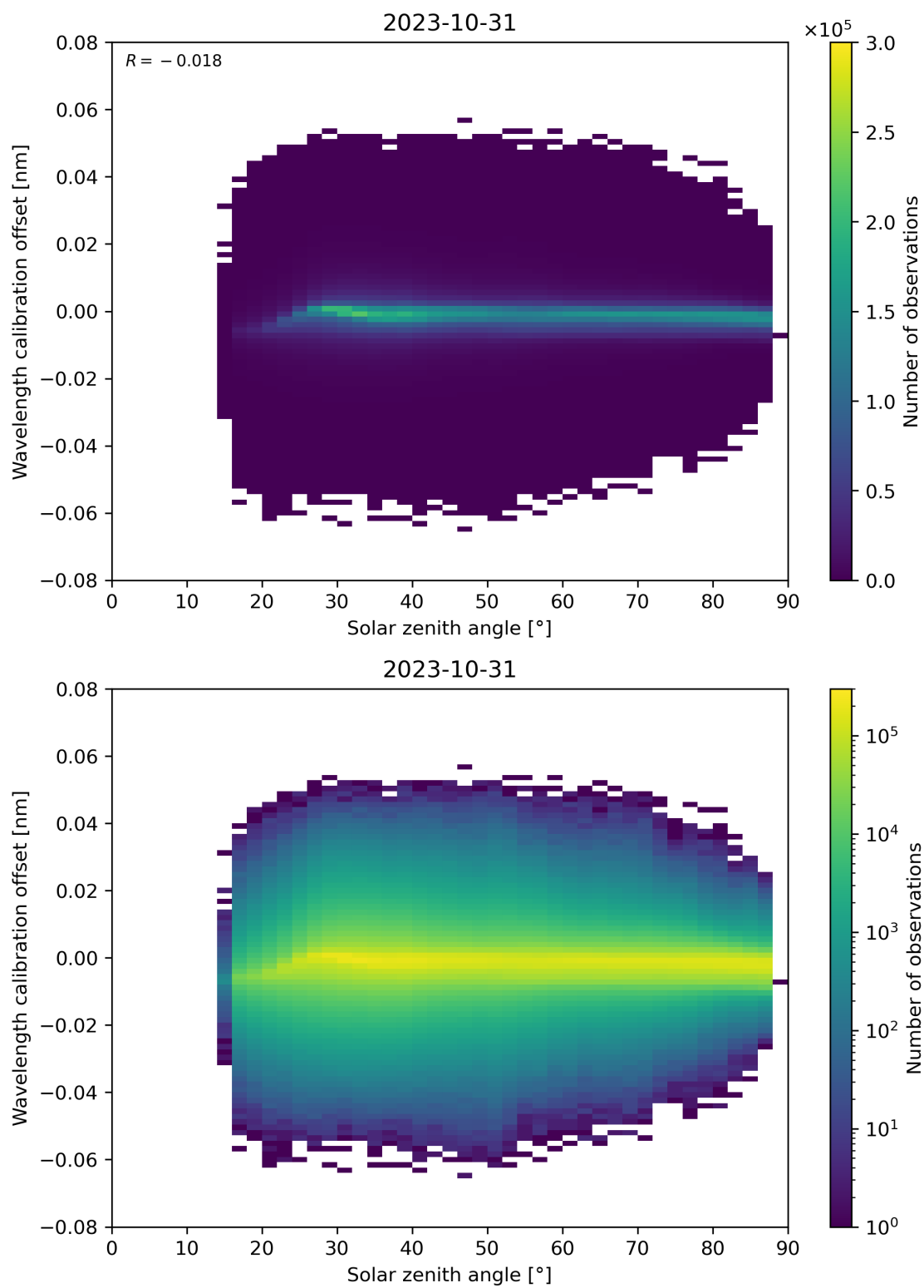
Figure 158: Scatter density plot of “Solar zenith angle” against “Wavelength calibration offset” for 2023-10-30 to 2023-11-01.
