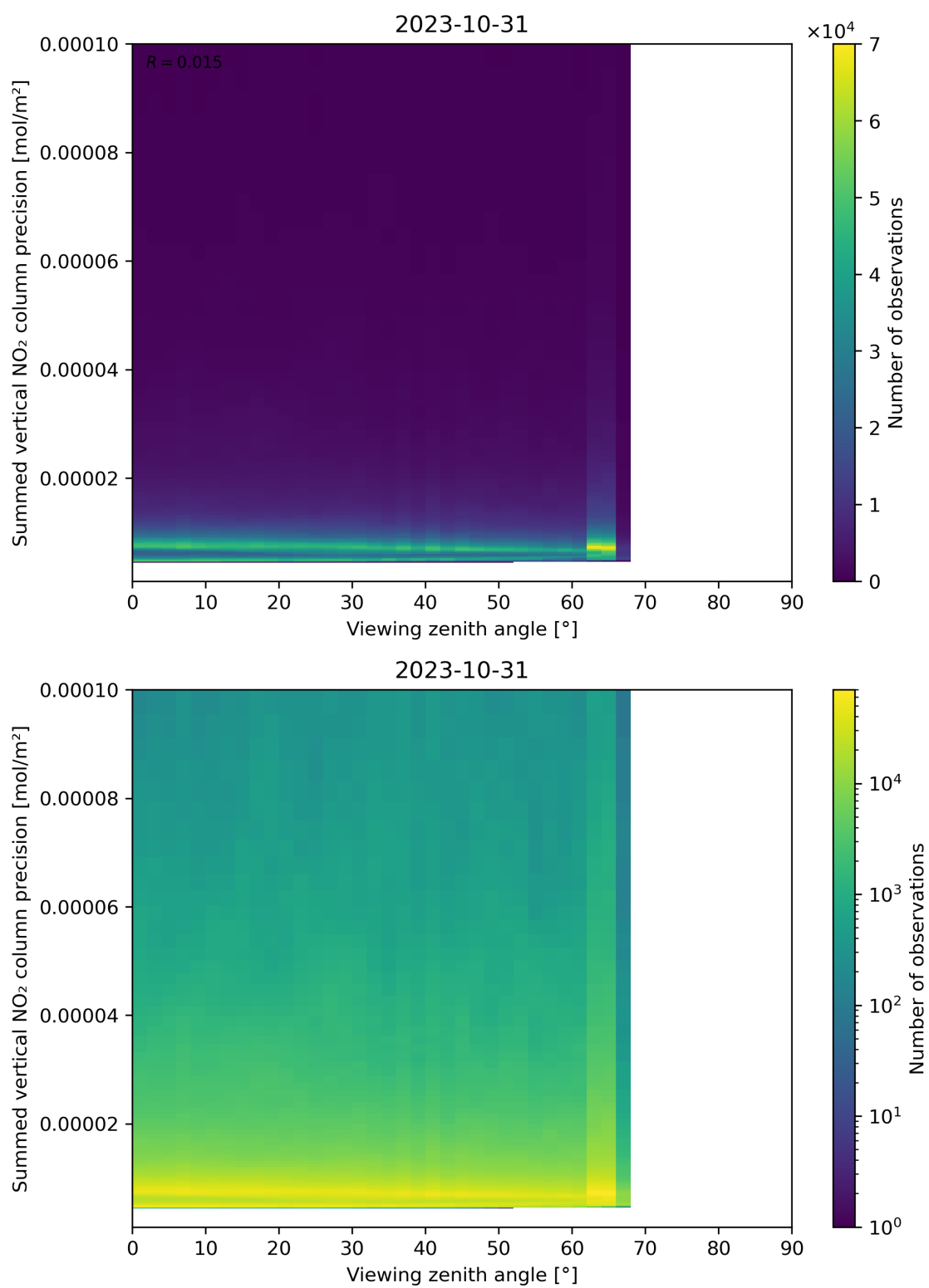
Figure 166: Scatter density plot of “Viewing zenith angle” against “Summed vertical NO 2 column precision” for 2023-10-30 to 2023-11-01.
