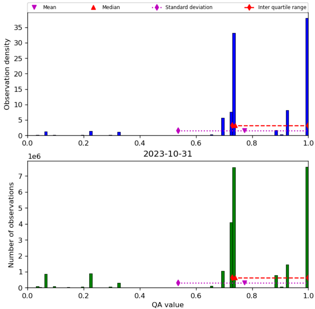
Figure 28: Histogram of “QA value” for 2023-10-30 to 2023-11-01
