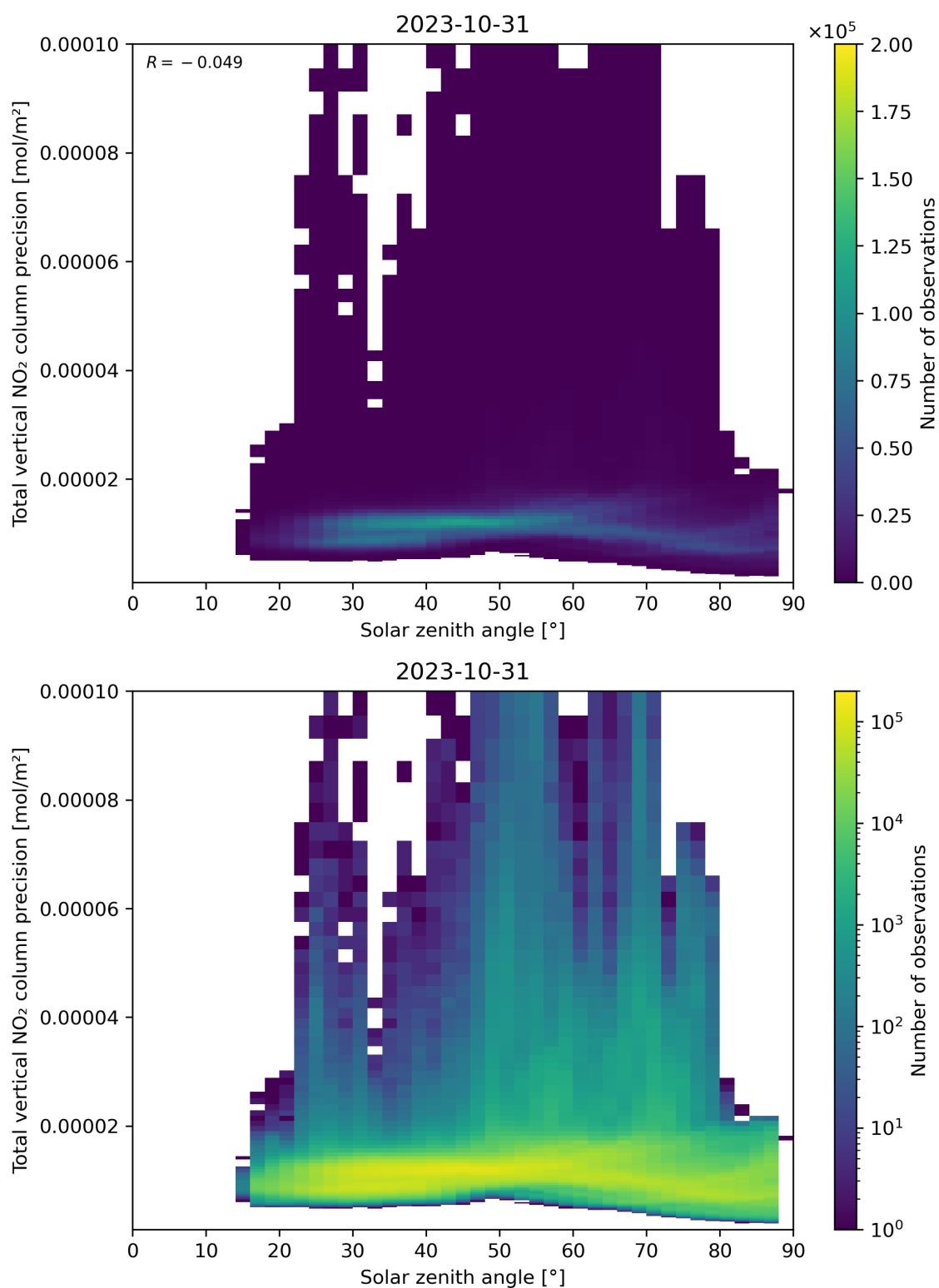
Figure 154: Scatter density plot of “Solar zenith angle” against “Total vertical NO 2 column precision” for 2023-10-30 to 2023-11-01.
