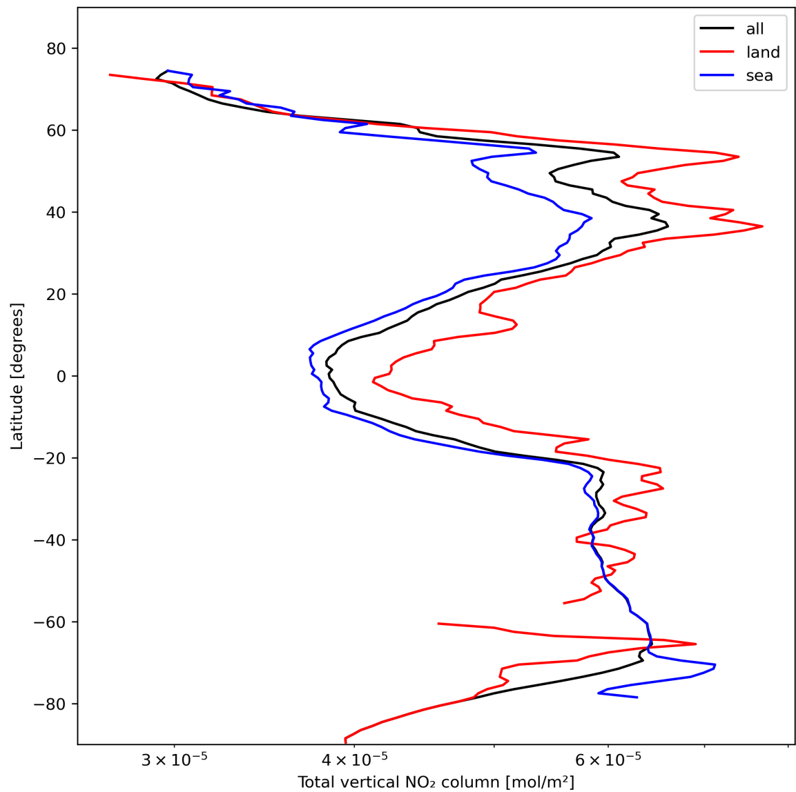
Figure 21: Zonal average of “Total vertical NO 2 column” for 2023-10-30 to 2023-11-01.
