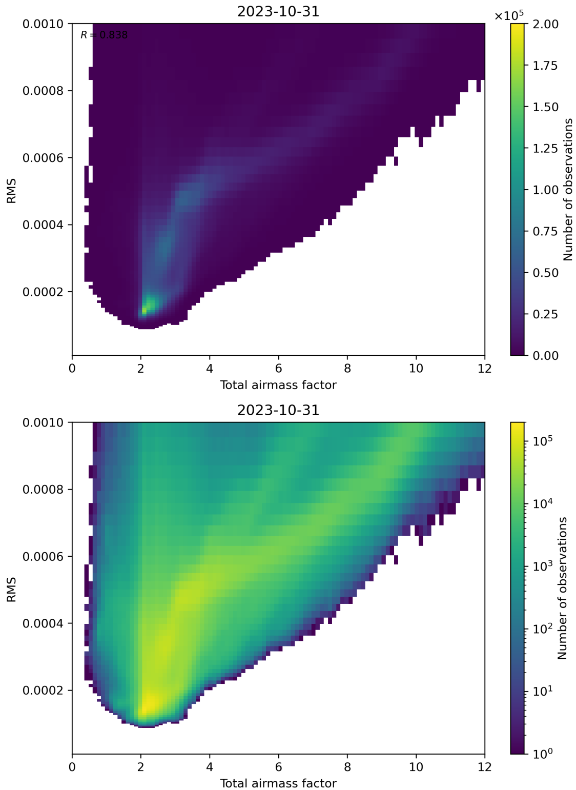
Figure 69: Scatter density plot of “Total airmass factor” against “RMS” for 2023-10-30 to 2023-11-01.
