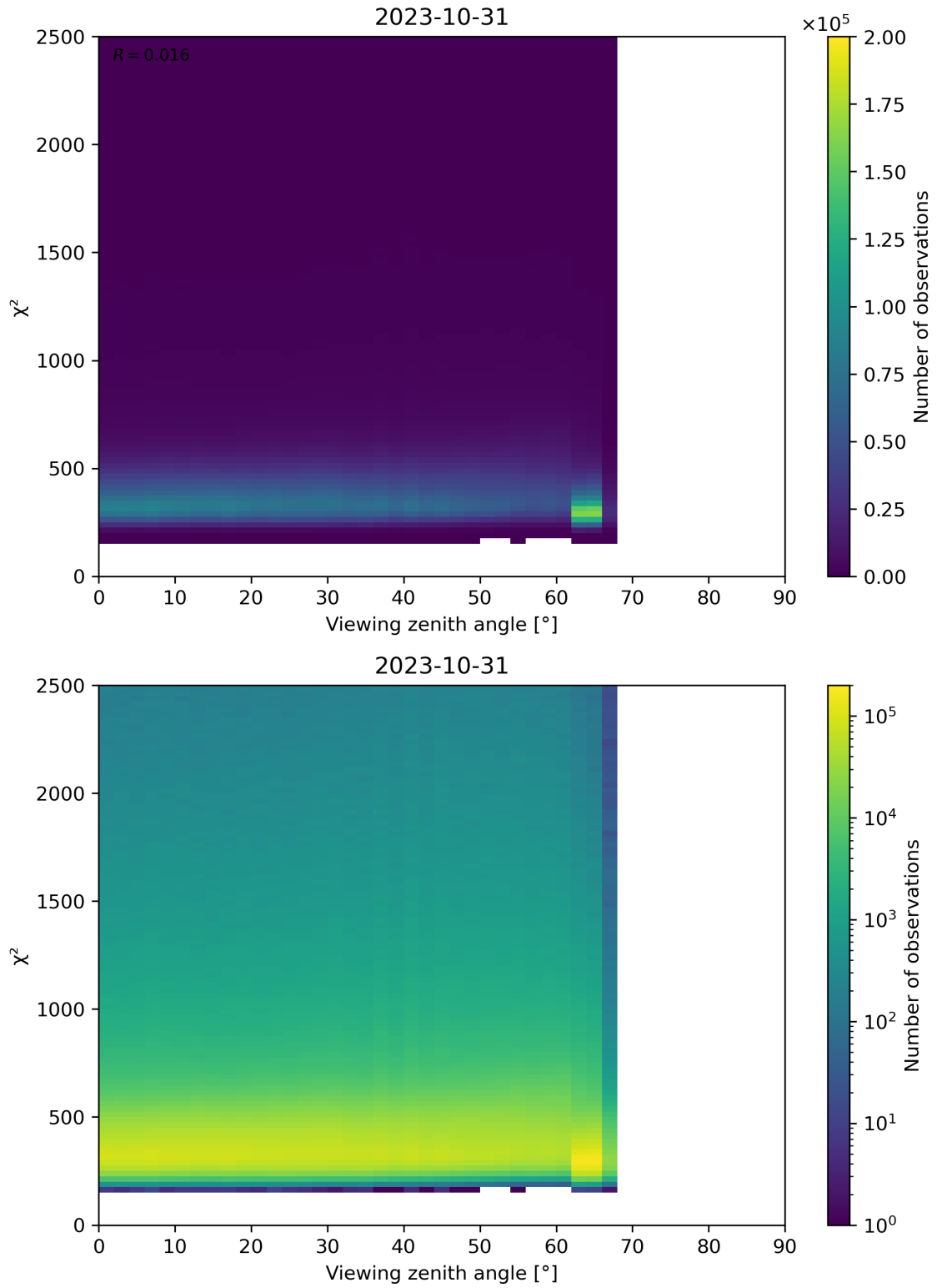
Figure 162: Scatter density plot of “Viewing zenith angle” against “ \chi^2 ” for 2023-10-30 to 2023-11-01.
