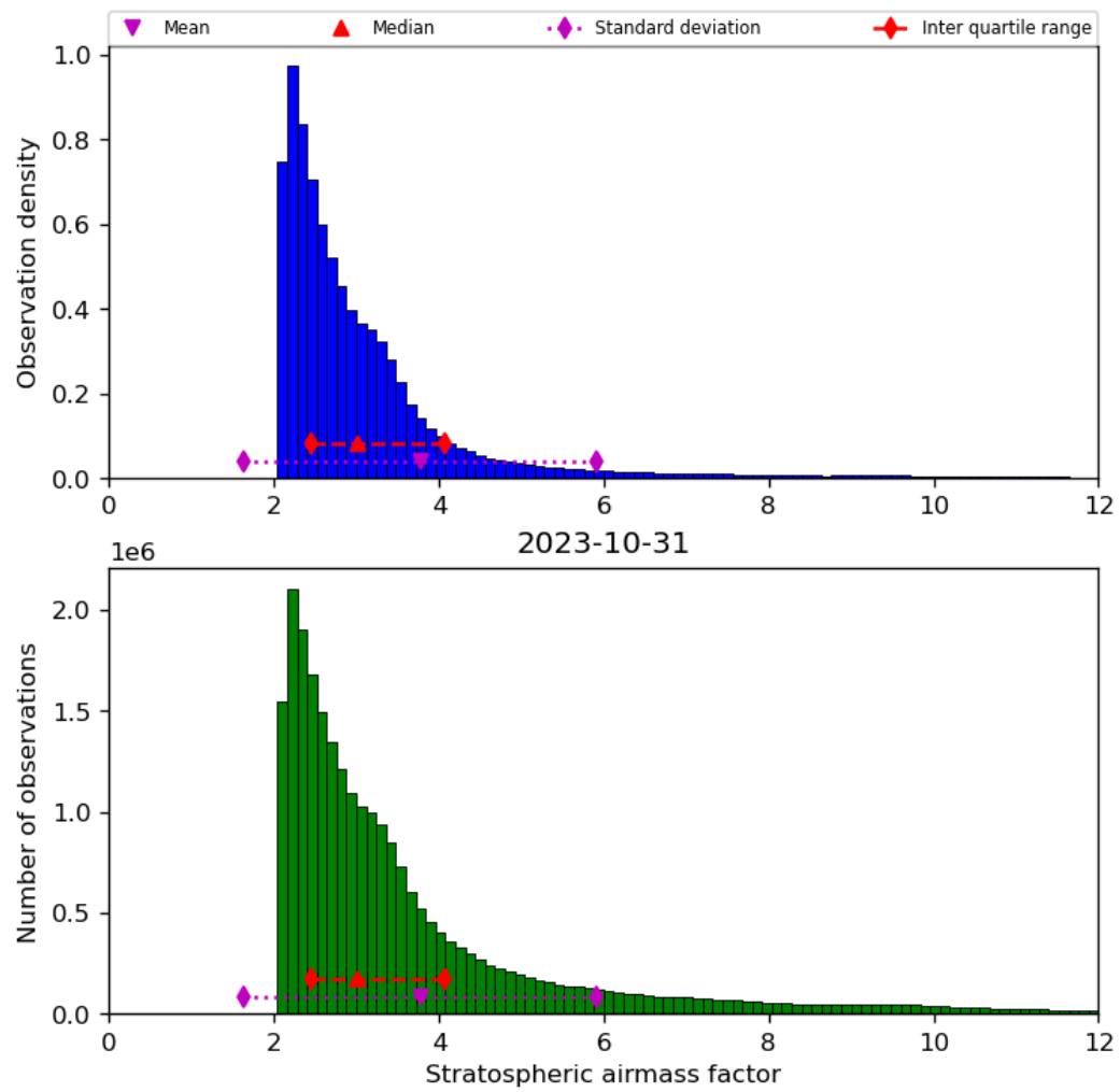
Figure 44: Histogram of “Stratospheric airmass factor” for 2023-10-30 to 2023-11-01
