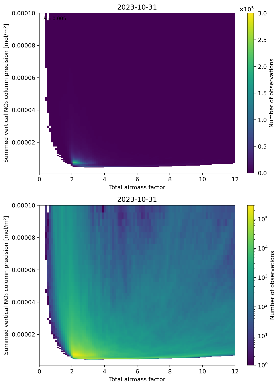
Figure 66: Scatter density plot of “Total airmass factor” against “Summed vertical NO 2 column precision” for 2023-10-30 to 2023-11-01.
