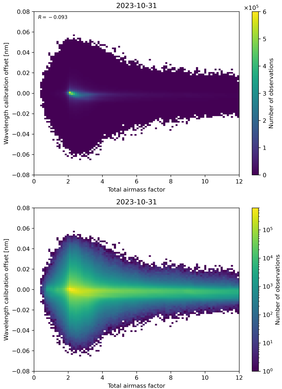
Figure 70: Scatter density plot of “Total airmass factor” against “Wavelength calibration offset” for 2023-10-30 to 2023-11-01.
