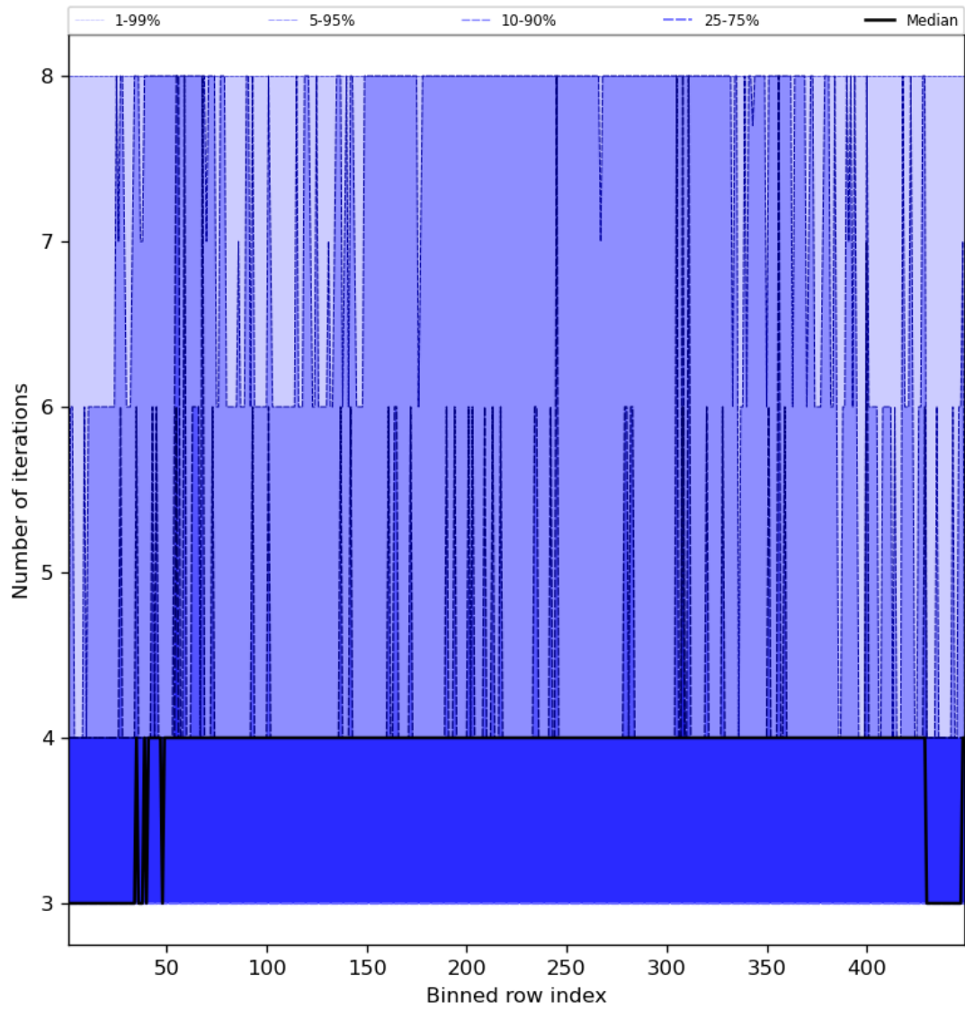
Figure 51: Along track statistics of “Number of iterations” for 2023-10-30 to 2023-11-01
