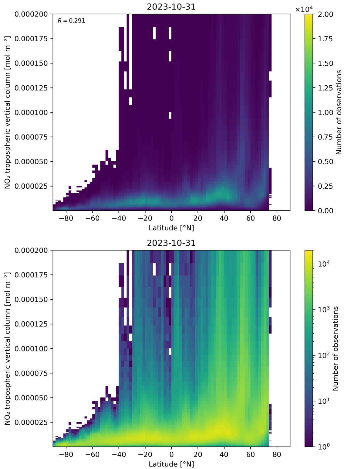
Figure 92: Scatter density plot of “Latitude” against “NO 2 tropospheric vertical column” for 2023-10-30 to 2023-11-01.
