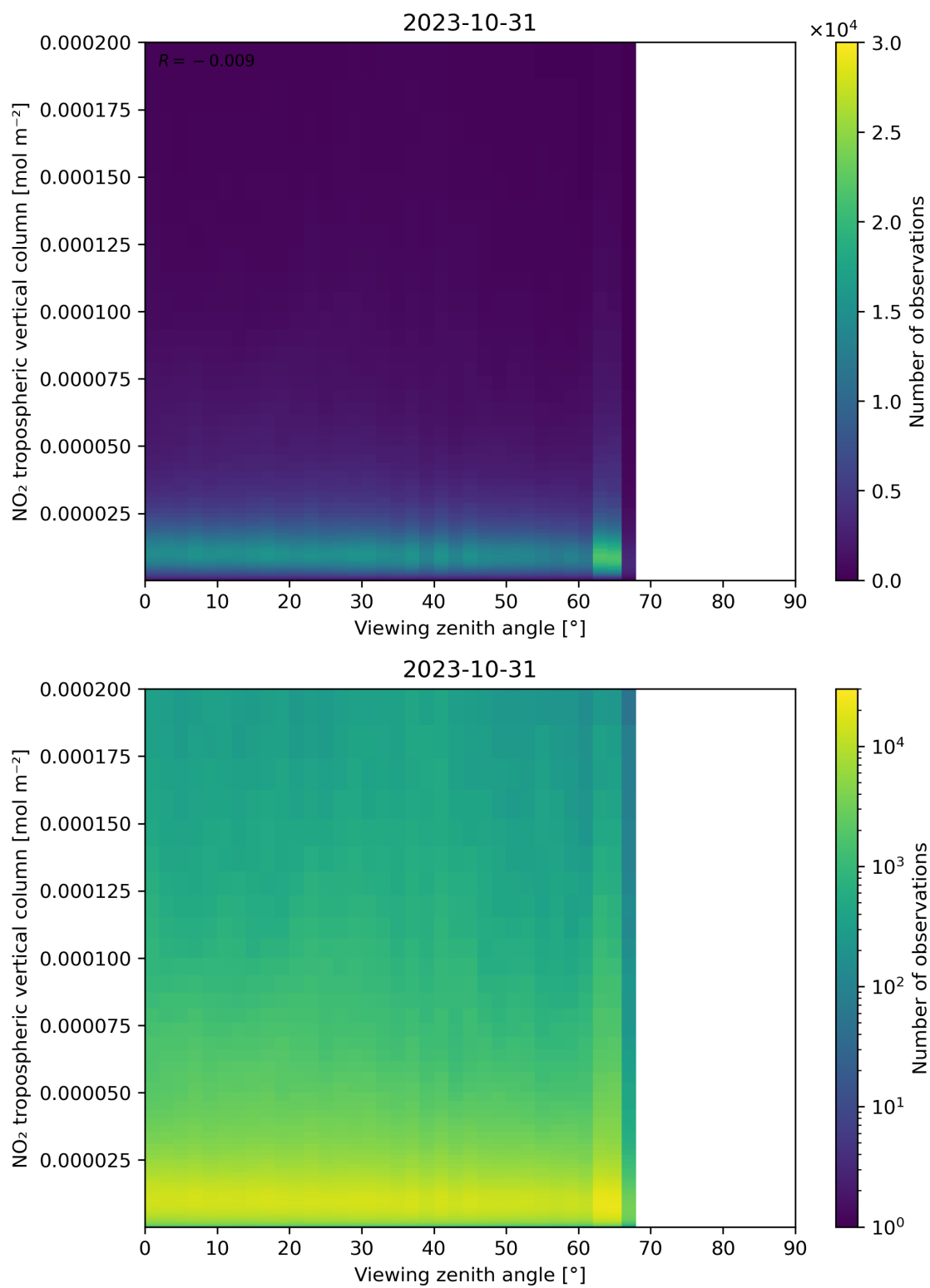
Figure 169: Scatter density plot of “Viewing zenith angle” against “NO 2 tropospheric vertical column” for 2023-10-30 to 2023-11-01.
