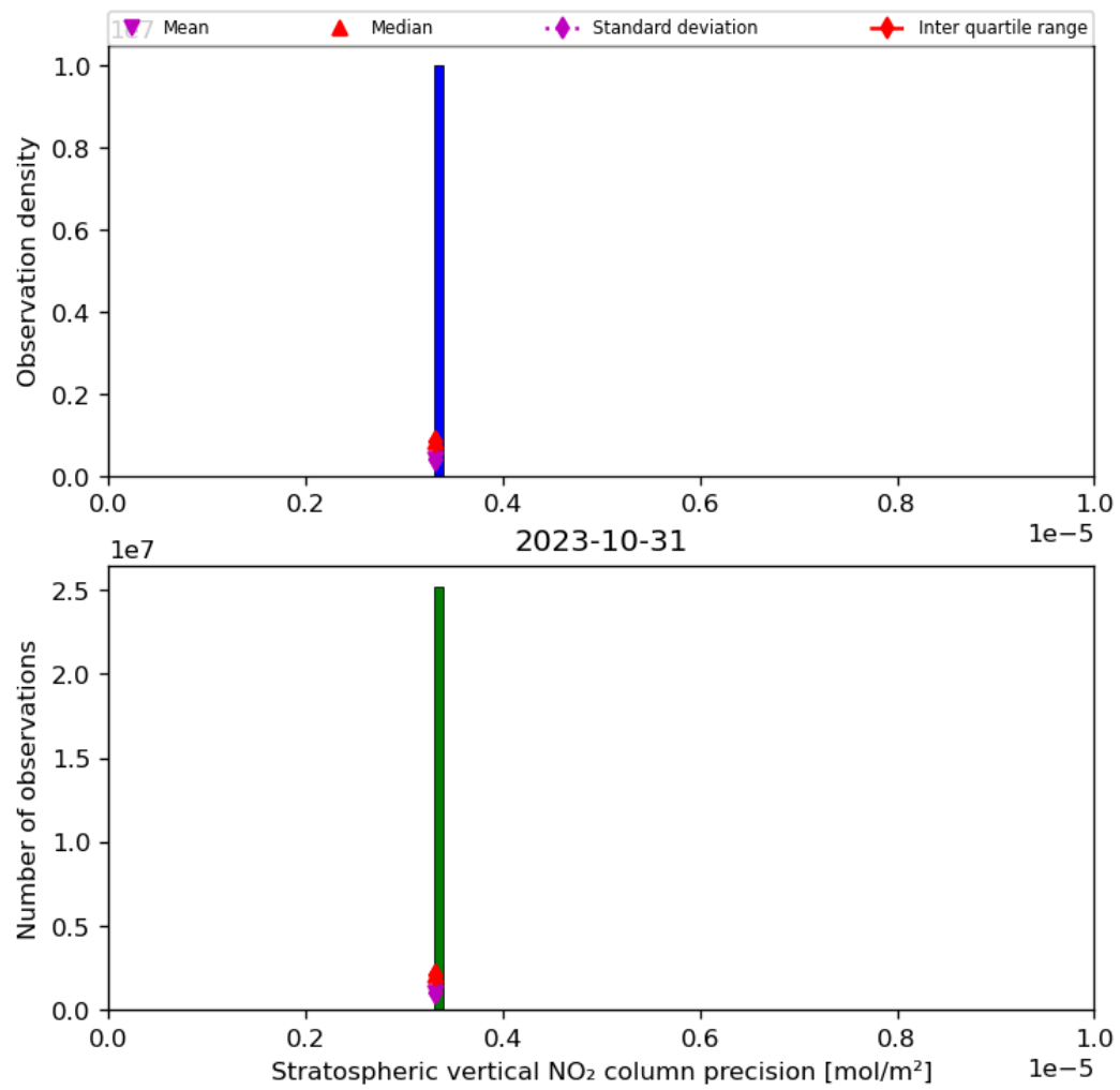
Figure 37: Histogram of “Stratospheric vertical NO 2 column precision” for 2023-10-30 to 2023-11-01
