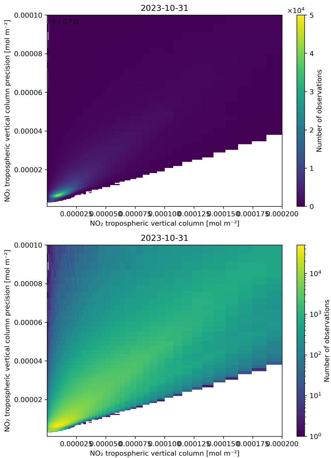
Figure 130: Scatter density plot of “NO 2 tropospheric vertical column” against “NO 2 tropospheric vertical column precision” for 2023-10-30 to 2023-11-01.
