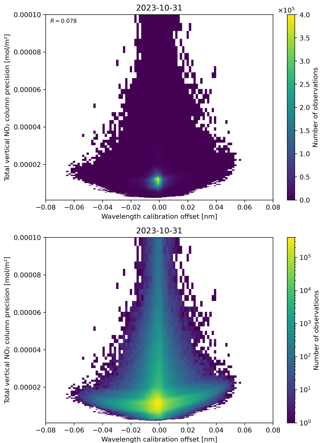
Figure 180: Scatter density plot of “Wavelength calibration offset” against “Total vertical NO 2 column precision” for 2023-10-30 to 2023-11-01.
