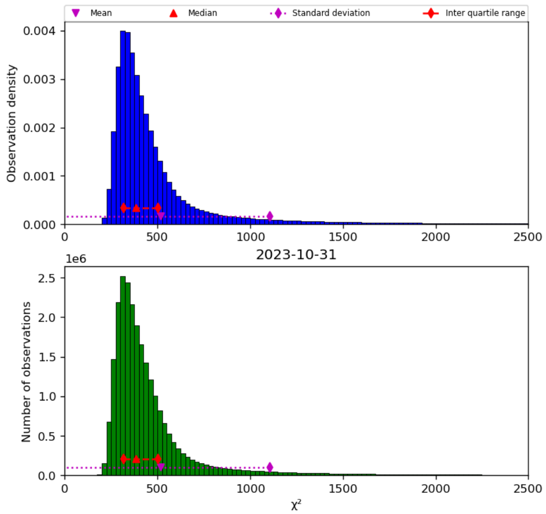
Figure 42: Histogram of " \chi^2 " for 2023-10-30 to 2023-11-01
