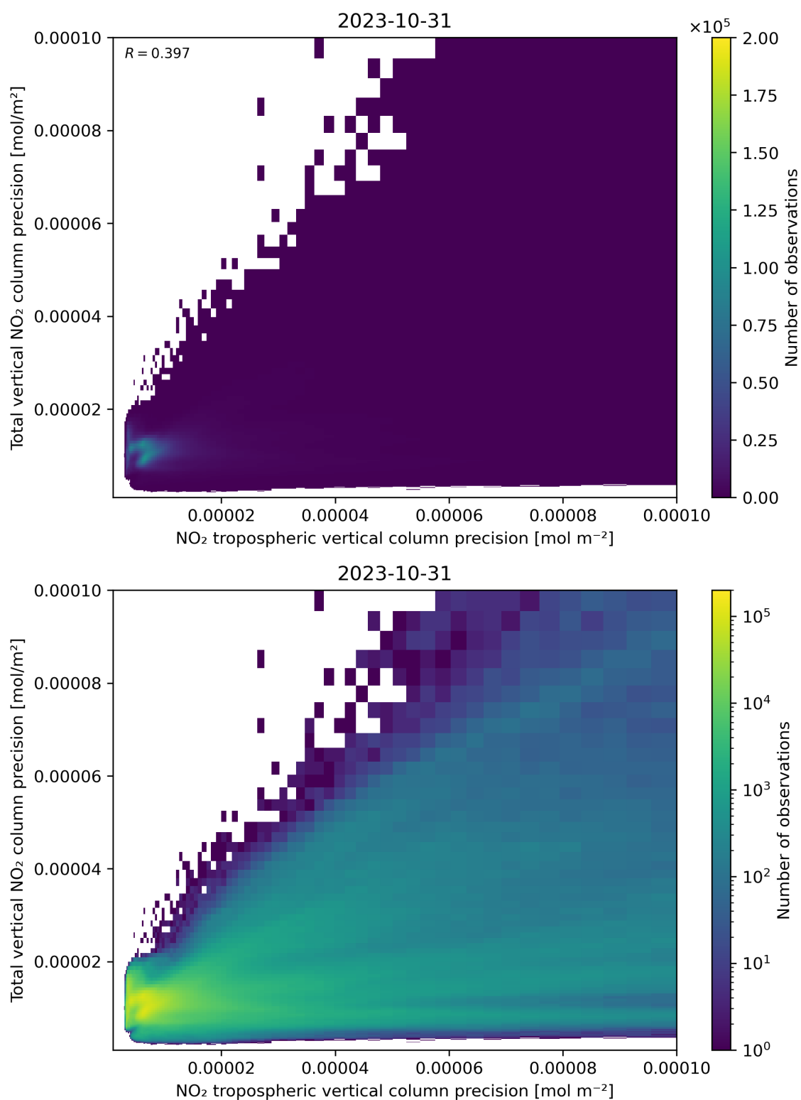
Figure 139: Scatter density plot of “NO 2 tropospheric vertical column precision” against “Total vertical NO 2 column precision” for 2023-10-30 to 2023-11-01.
