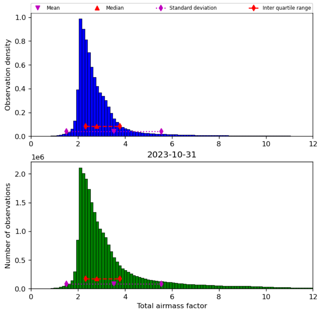
Figure 32: Histogram of “Total airmass factor” for 2023-10-30 to 2023-11-01
