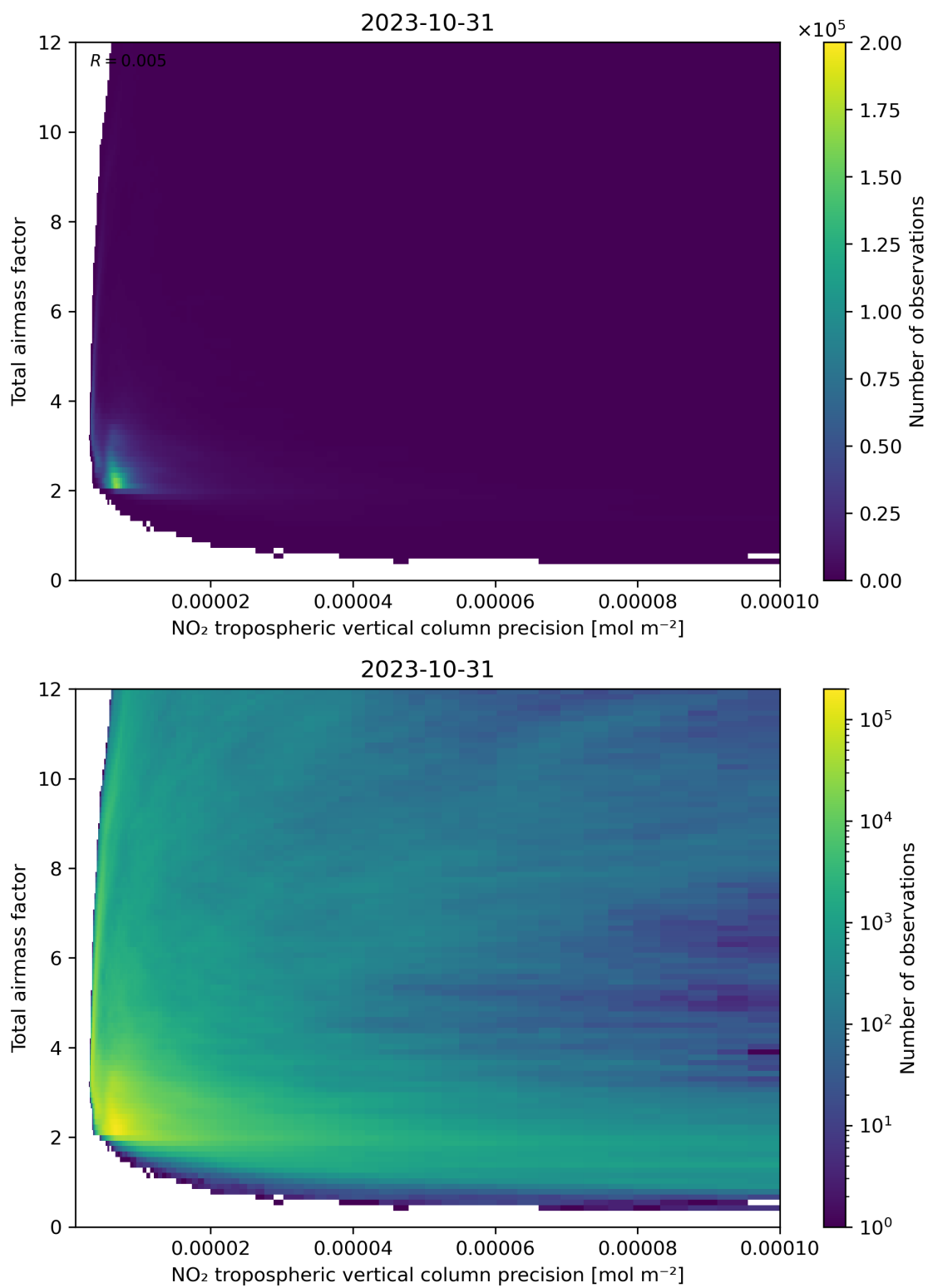
Figure 132: Scatter density plot of “NO 2 tropospheric vertical column precision” against “Total airmass factor” for 2023-10-30 to 2023-11-01.
