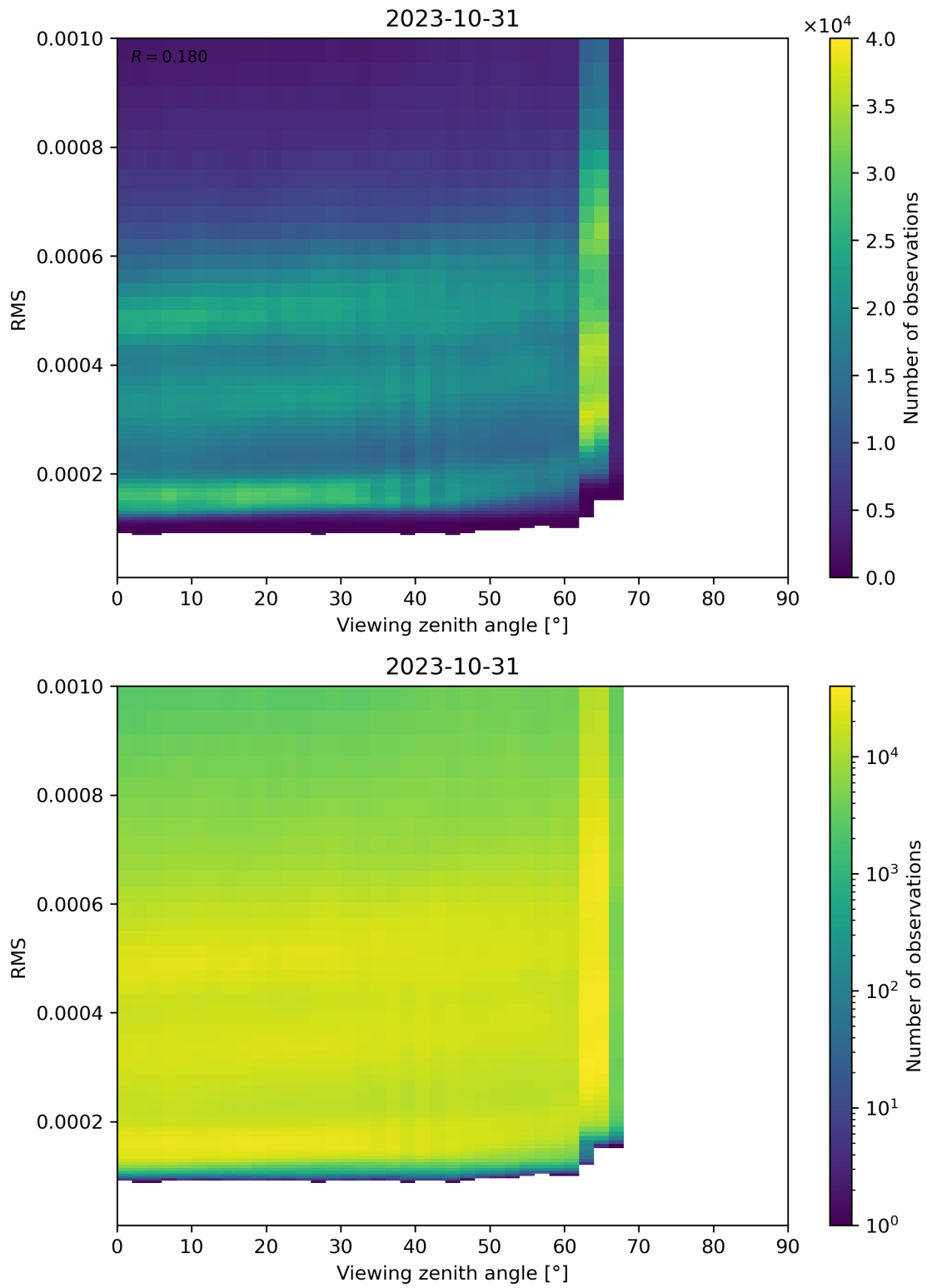
Figure 171: Scatter density plot of “Viewing zenith angle” against “RMS” for 2023-10-30 to 2023-11-01.
