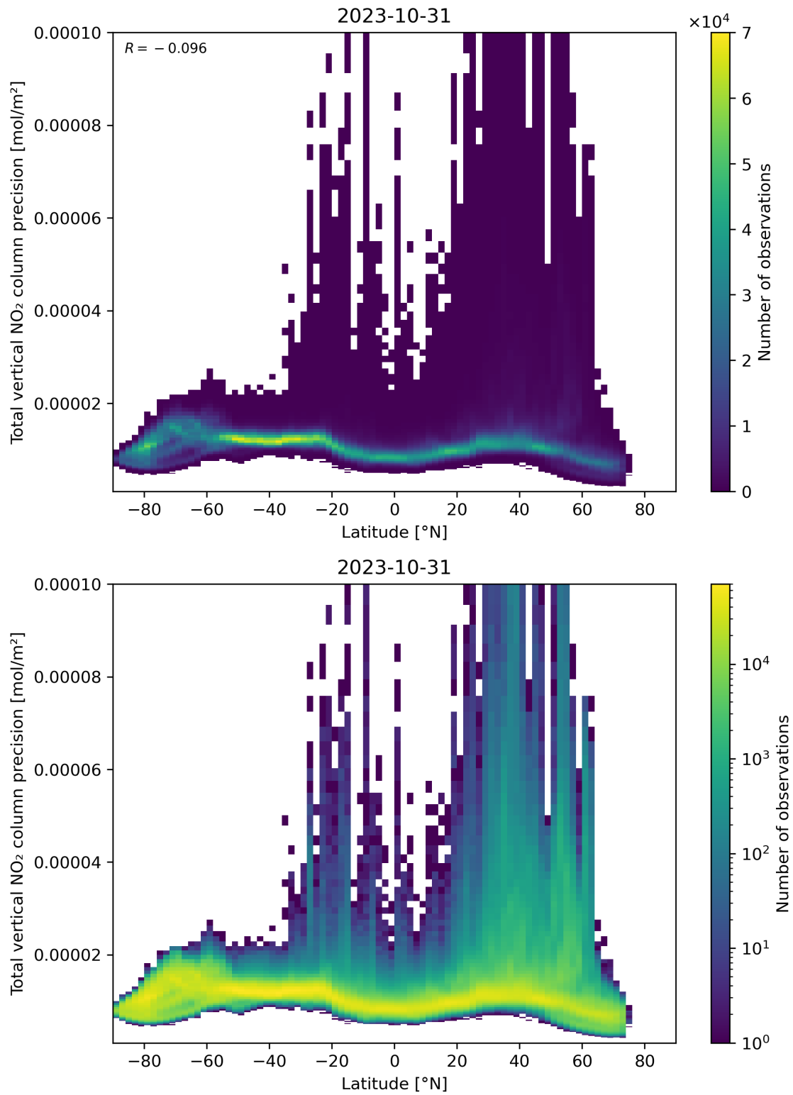
Figure 91: Scatter density plot of “Latitude” against “Total vertical NO 2 column precision” for 2023-10-30 to 2023-11-01.
