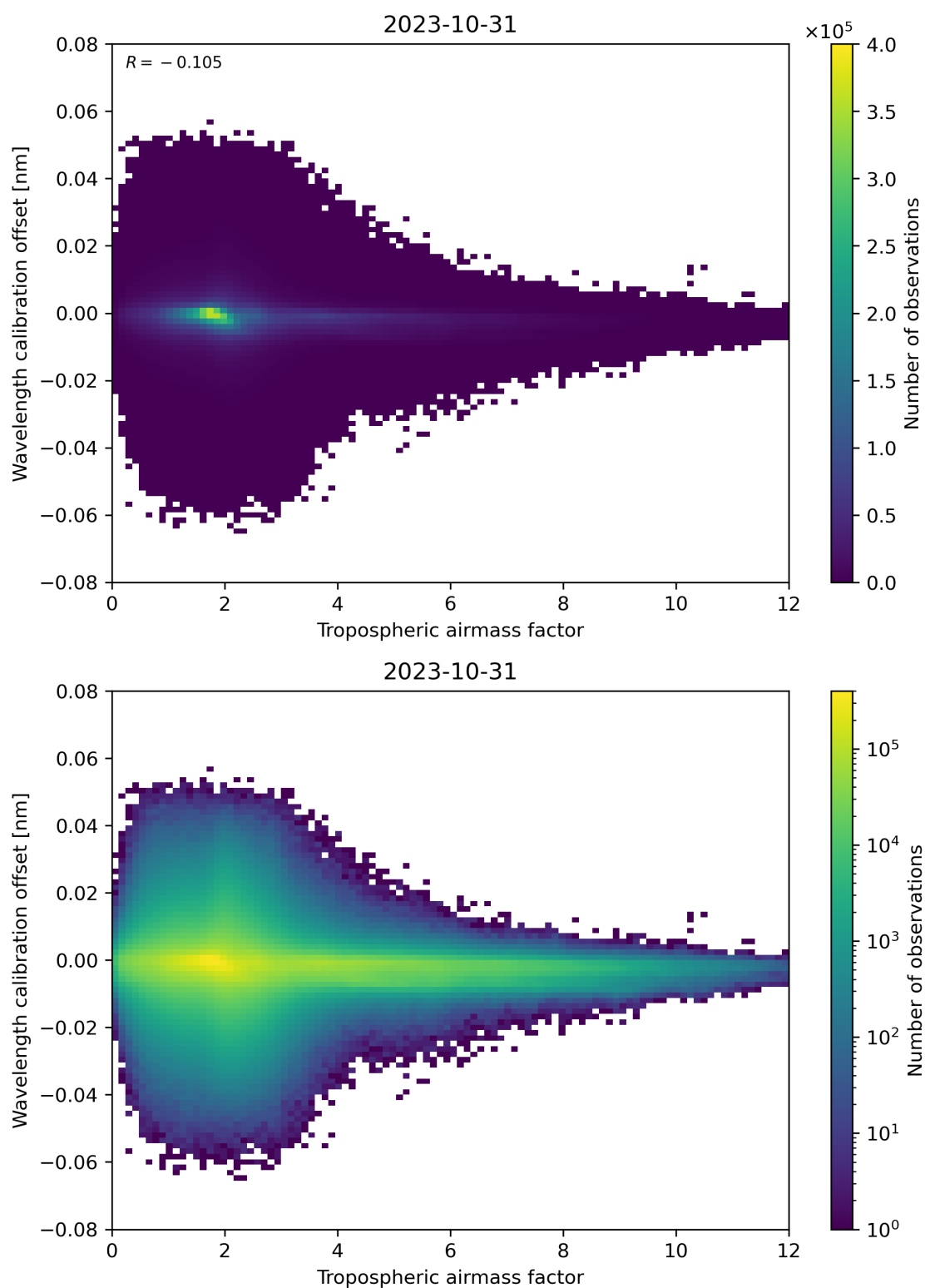
Figure 80: Scatter density plot of “Tropospheric airmass factor” against “Wavelength calibration offset” for 2023-10-30 to 2023-11-01.
