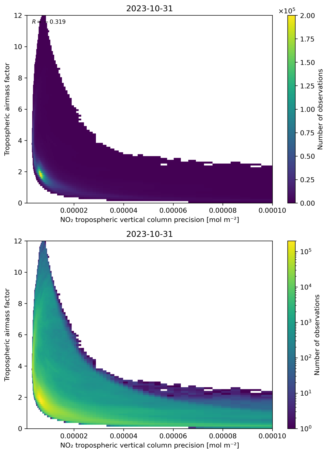
Figure 133: Scatter density plot of “NO 2 tropospheric vertical column precision” against “Tropospheric airmass factor” for 2023-10-30 to 2023-11-01.
