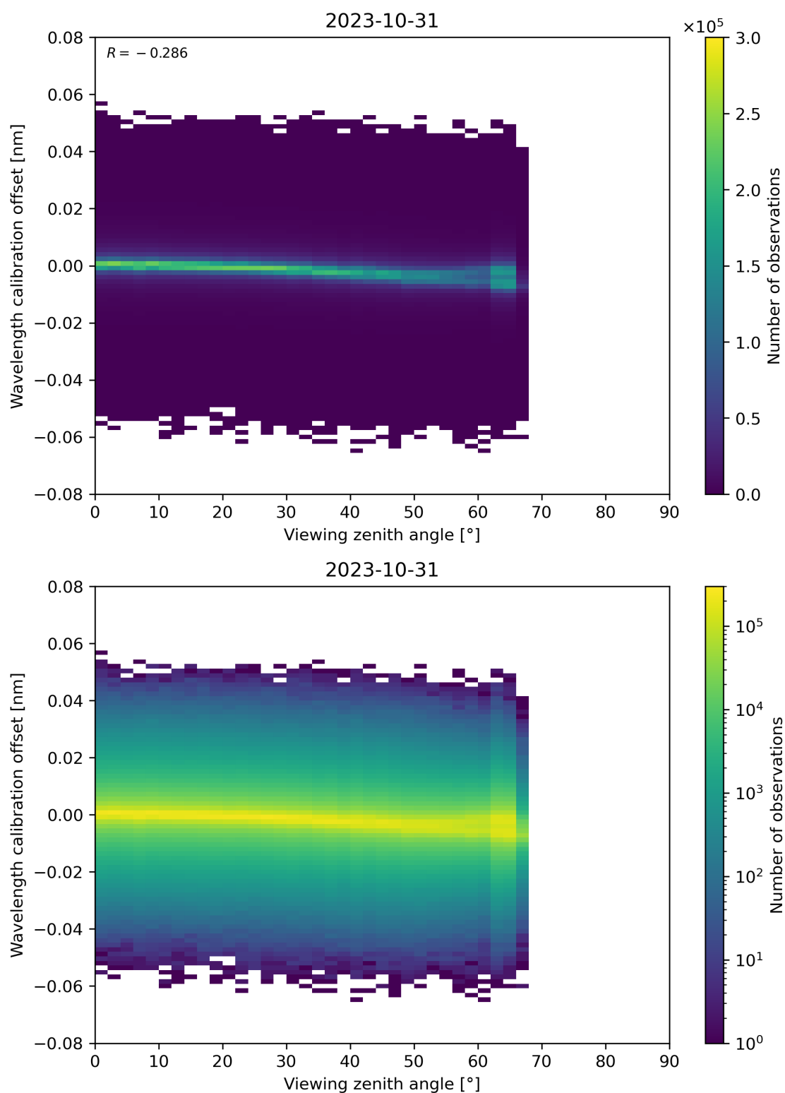
Figure 173: Scatter density plot of “Viewing zenith angle” against “Wavelength calibration offset” for 2023-10-30 to 2023-11-01.
