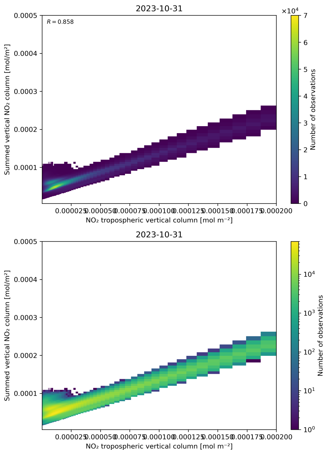
Figure 126: Scatter density plot of “NO 2 tropospheric vertical column” against “Summed vertical NO 2 column” for 2023-10-30 to 2023-11-01.
