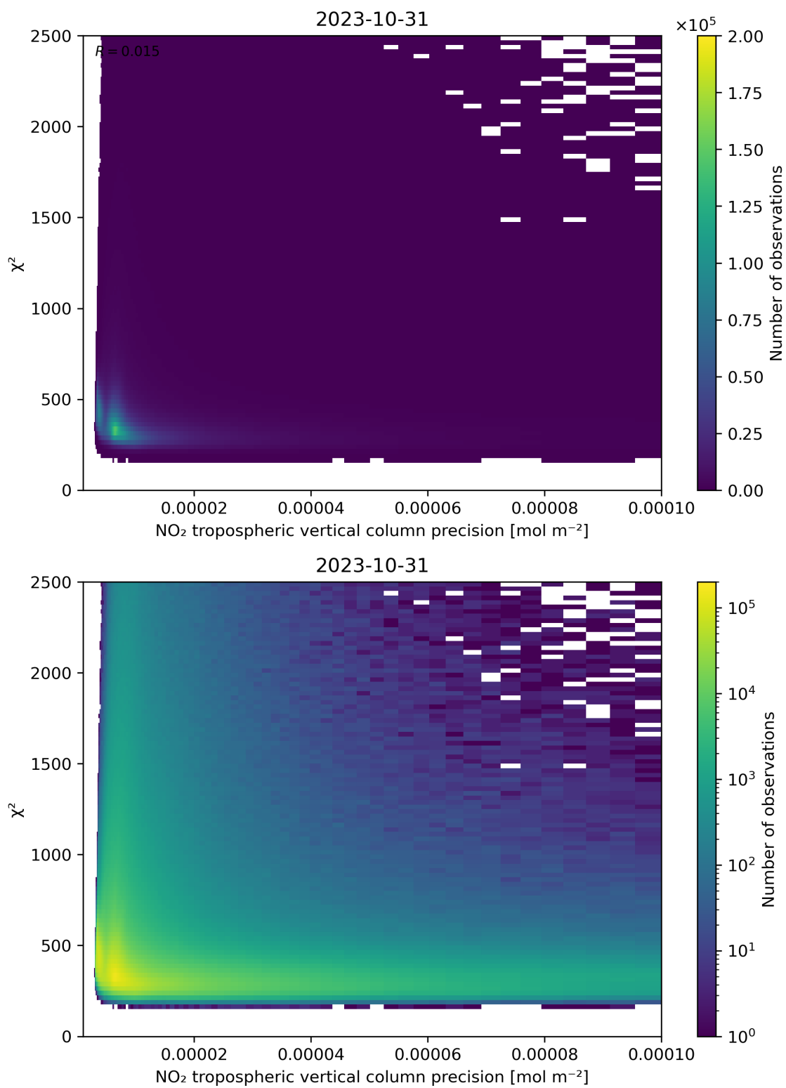
Figure 134: Scatter density plot of “NO 2 tropospheric vertical column precision” against “ \chi^2 ” for 2023-10-30 to 2023-11-01.
