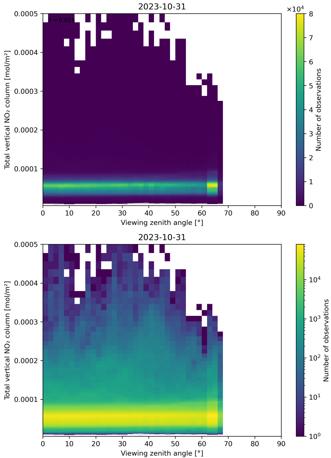
Figure 167: Scatter density plot of “Viewing zenith angle” against “Total vertical NO 2 column” for 2023-10-30 to 2023-11-01.
