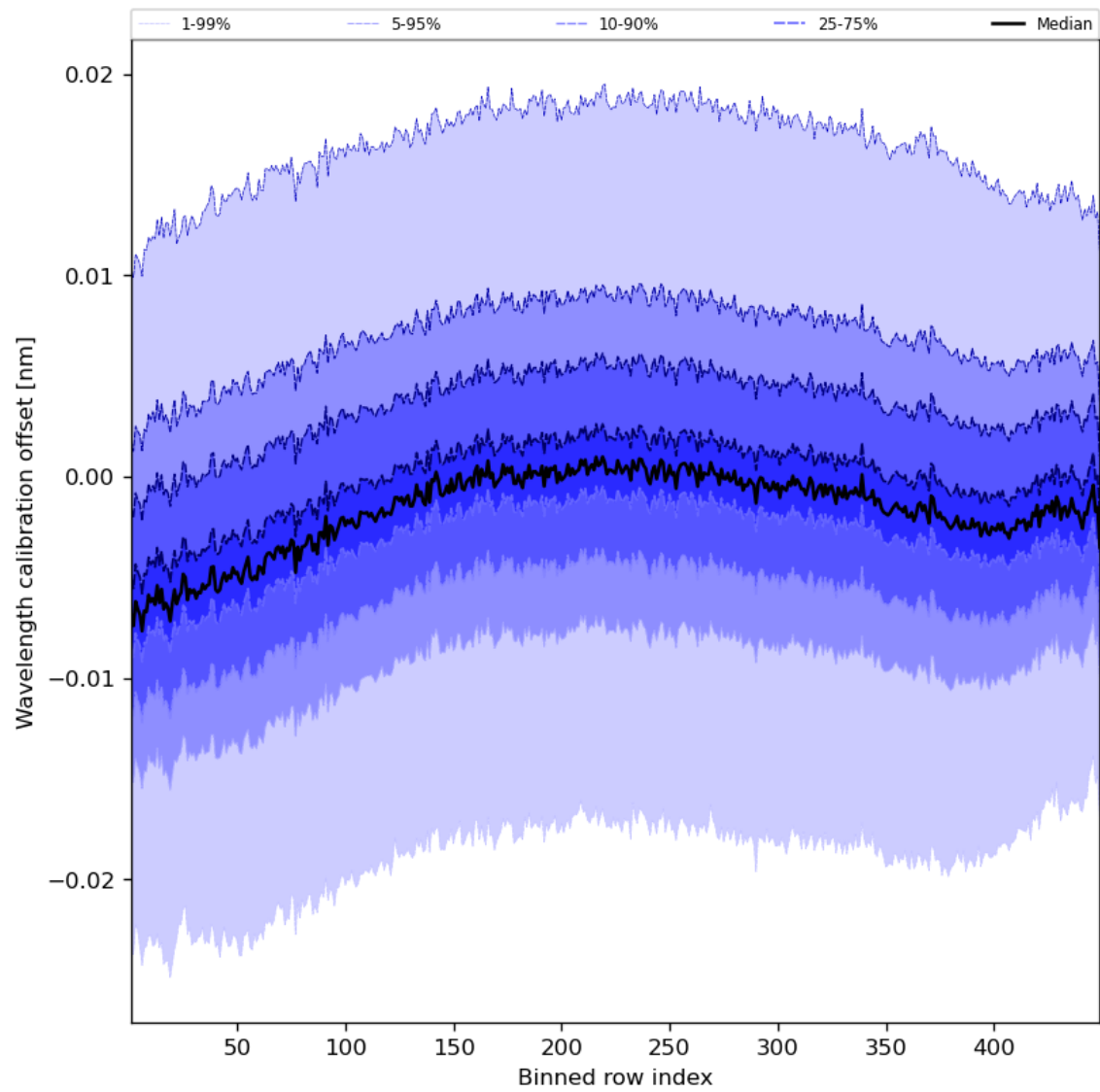
Figure 52: Along track statistics of “Wavelength calibration offset” for 2023-10-30 to 2023-11-01
