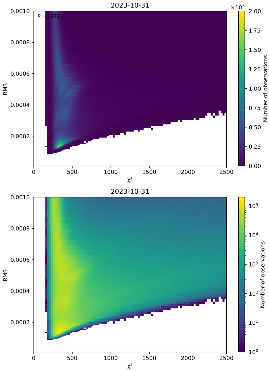
Figure 82: Scatter density plot of “ \chi^2 ” against “RMS” for 2023-10-30 to 2023-11-01.
