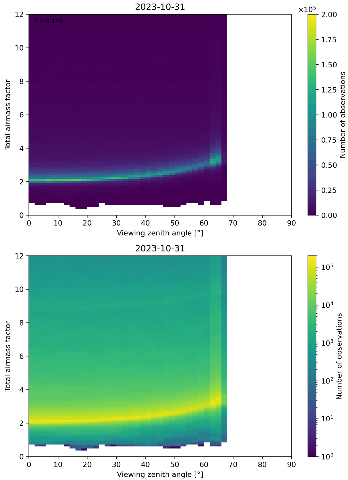
Figure 160: Scatter density plot of “Viewing zenith angle” against “Total airmass factor” for 2023-10-30 to 2023-11-01.
