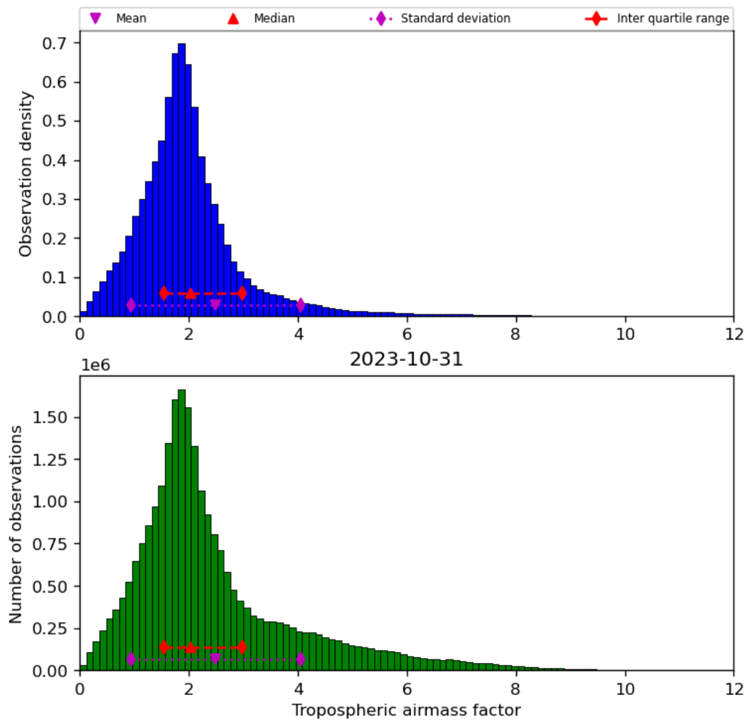
Figure 31: Histogram of “Tropospheric airmass factor” for 2023-10-30 to 2023-11-01
