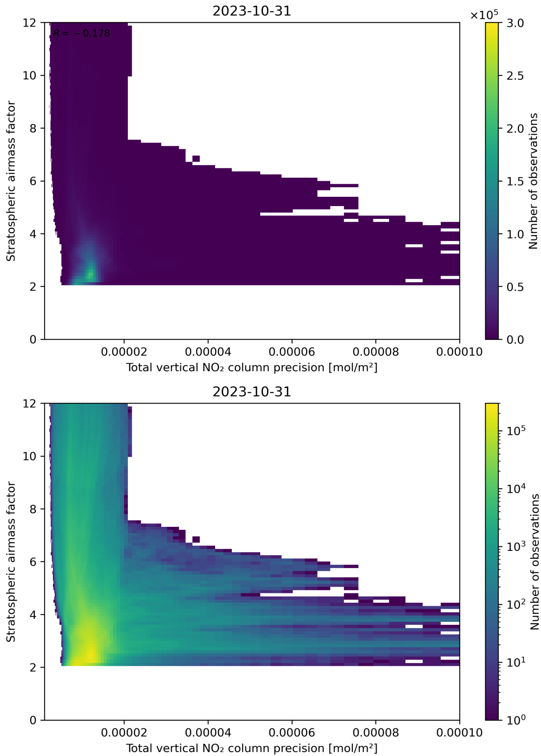
Figure 115: Scatter density plot of “Total vertical NO 2 column precision” against “Stratospheric air mass factor” for 2023-10-30 to 2023-11-01.
