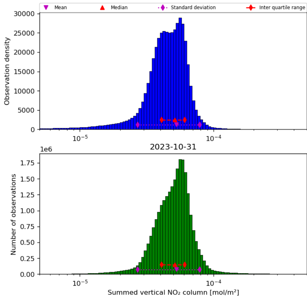
Figure 40: Histogram of “Summed vertical NO 2 column” for 2023-10-30 to 2023-11-01
