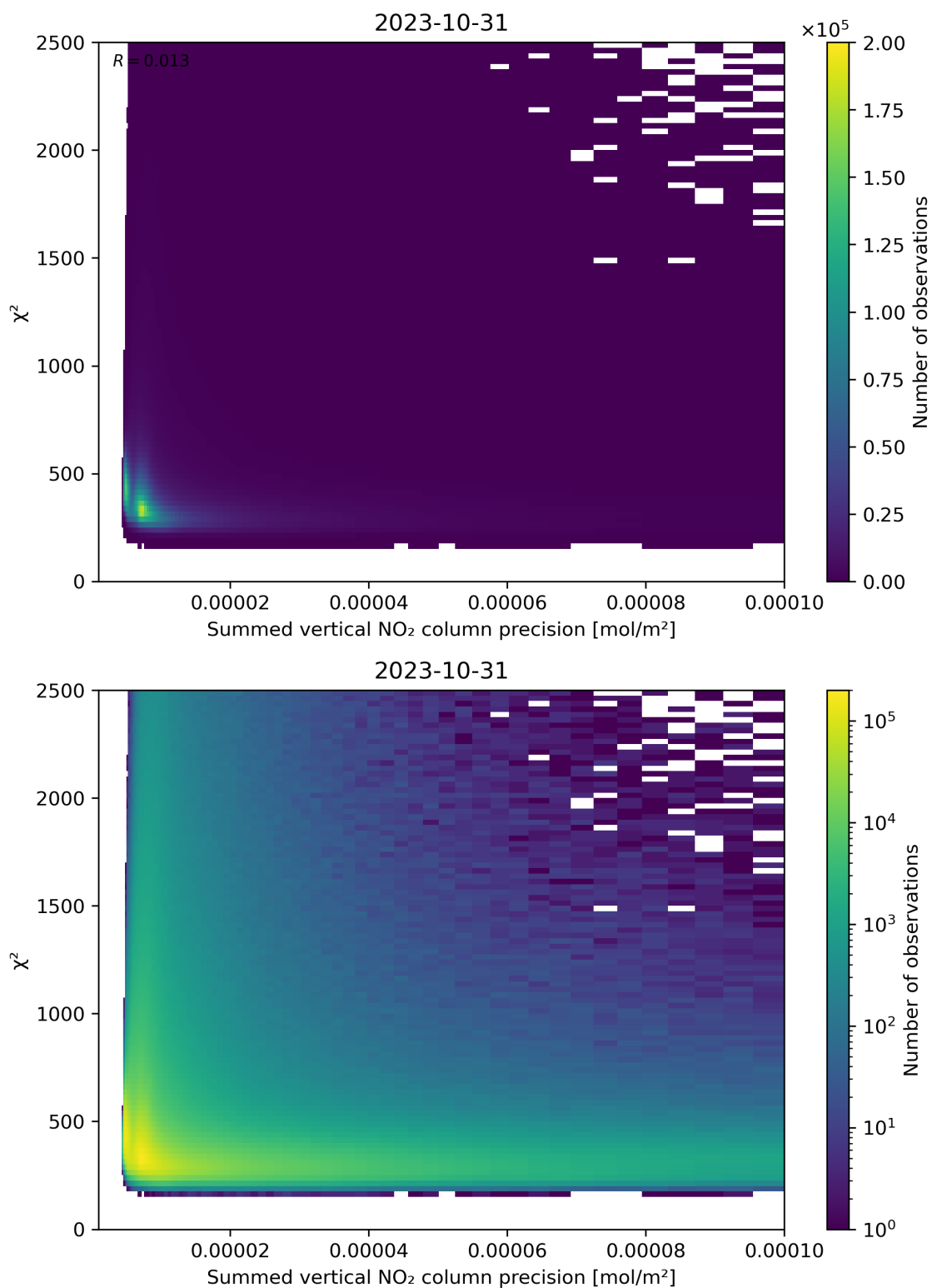
Figure 107: Scatter density plot of “Summed vertical NO 2 column precision” against “ \chi^2 ” for 2023-10-30 to 2023-11-01.
