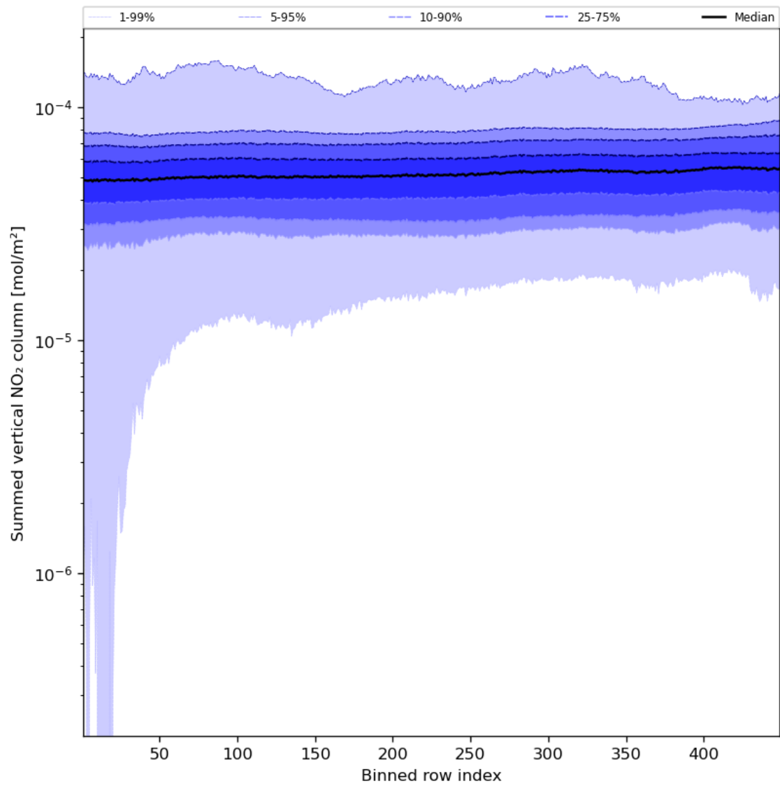
Figure 57: Along track statistics of “Summed vertical NO 2 column” for 2023-10-30 to 2023-11-01
