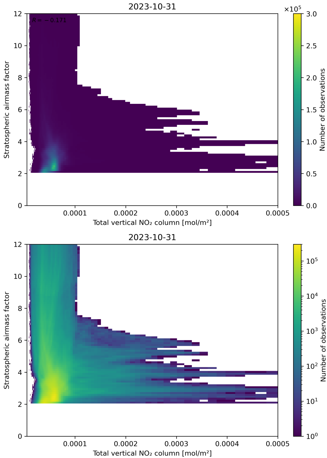
Figure 110: Scatter density plot of “Total vertical NO 2 column” against “Stratospheric air mass factor” for 2023-10-30 to 2023-11-01.
