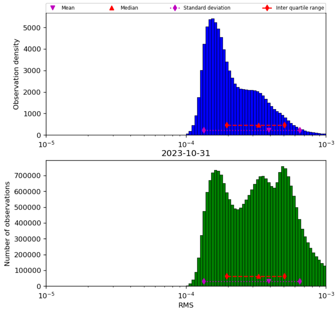
Figure 43: Histogram of “RMS” for 2023-10-30 to 2023-11-01
