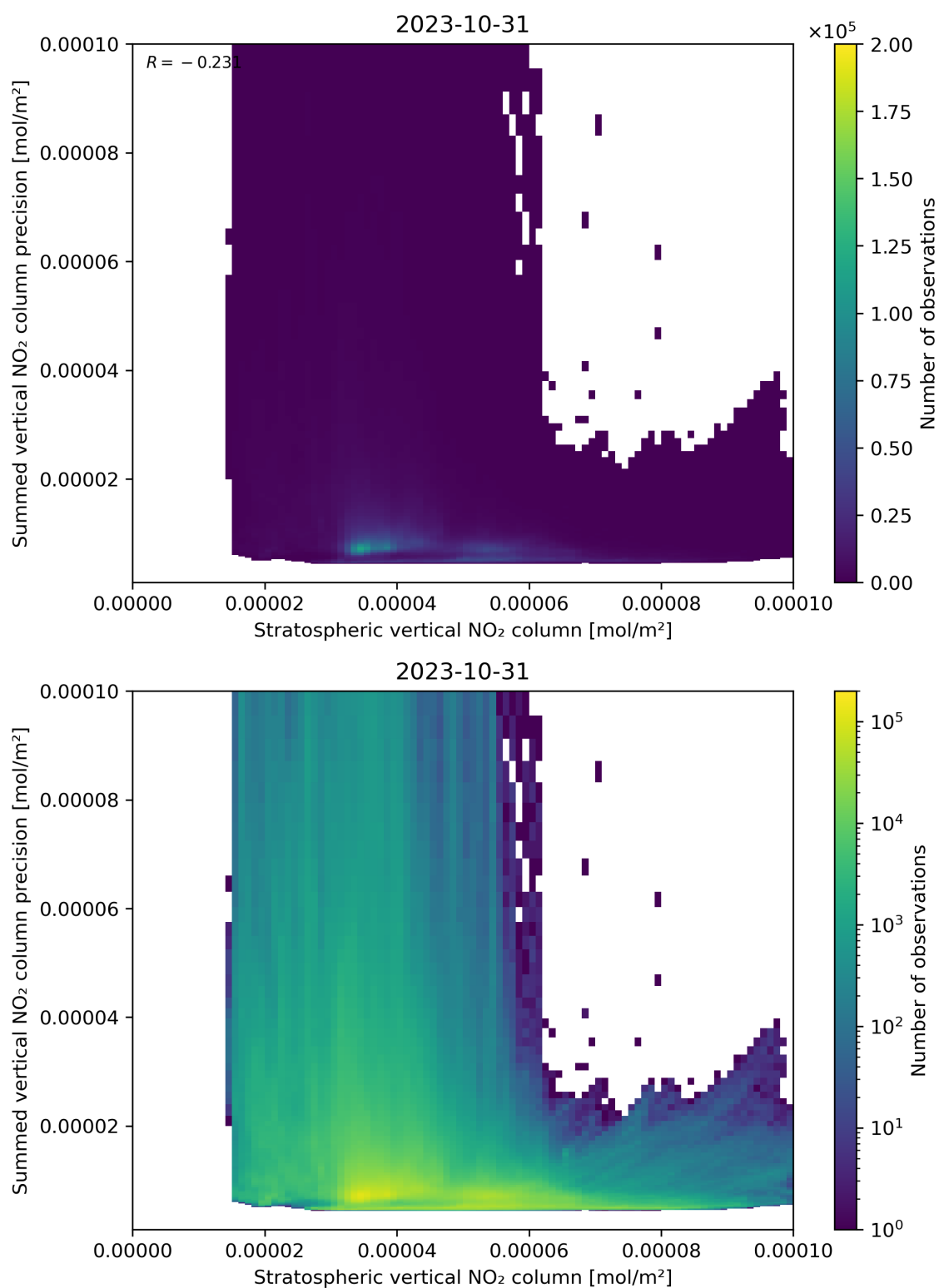
Figure 99: Scatter density plot of “Stratospheric vertical NO 2 column” against “Summed vertical NO 2 column precision” for 2023-10-30 to 2023-11-01.
