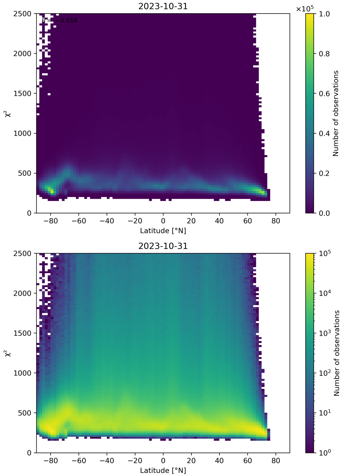
Figure 86: Scatter density plot of “Latitude” against “ \chi^2 ” for 2023-10-30 to 2023-11-01.
