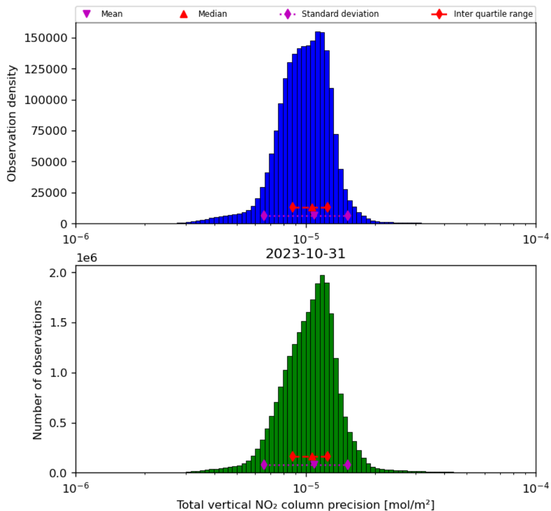
Figure 39: Histogram of “Total vertical NO 2 column precision” for 2023-10-30 to 2023-11-01
