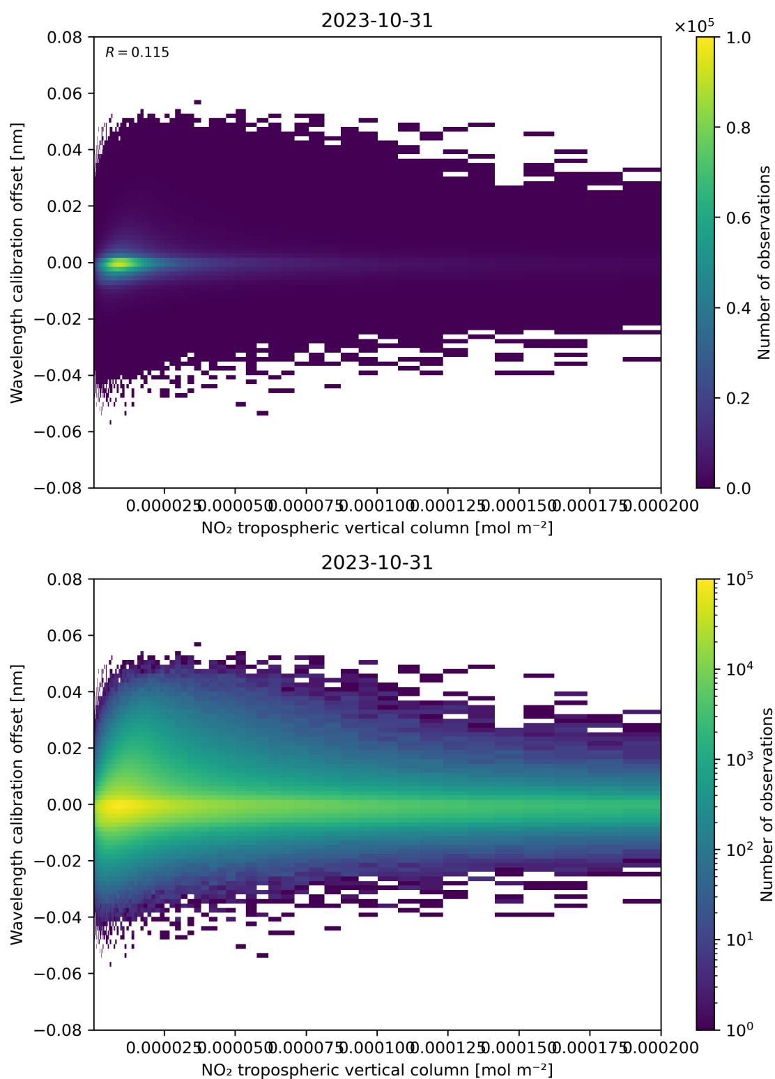
Figure 143: Scatter density plot of “NO 2 tropospheric vertical column” against “Wavelength calibration offset” for 2023-10-30 to 2023-11-01.
