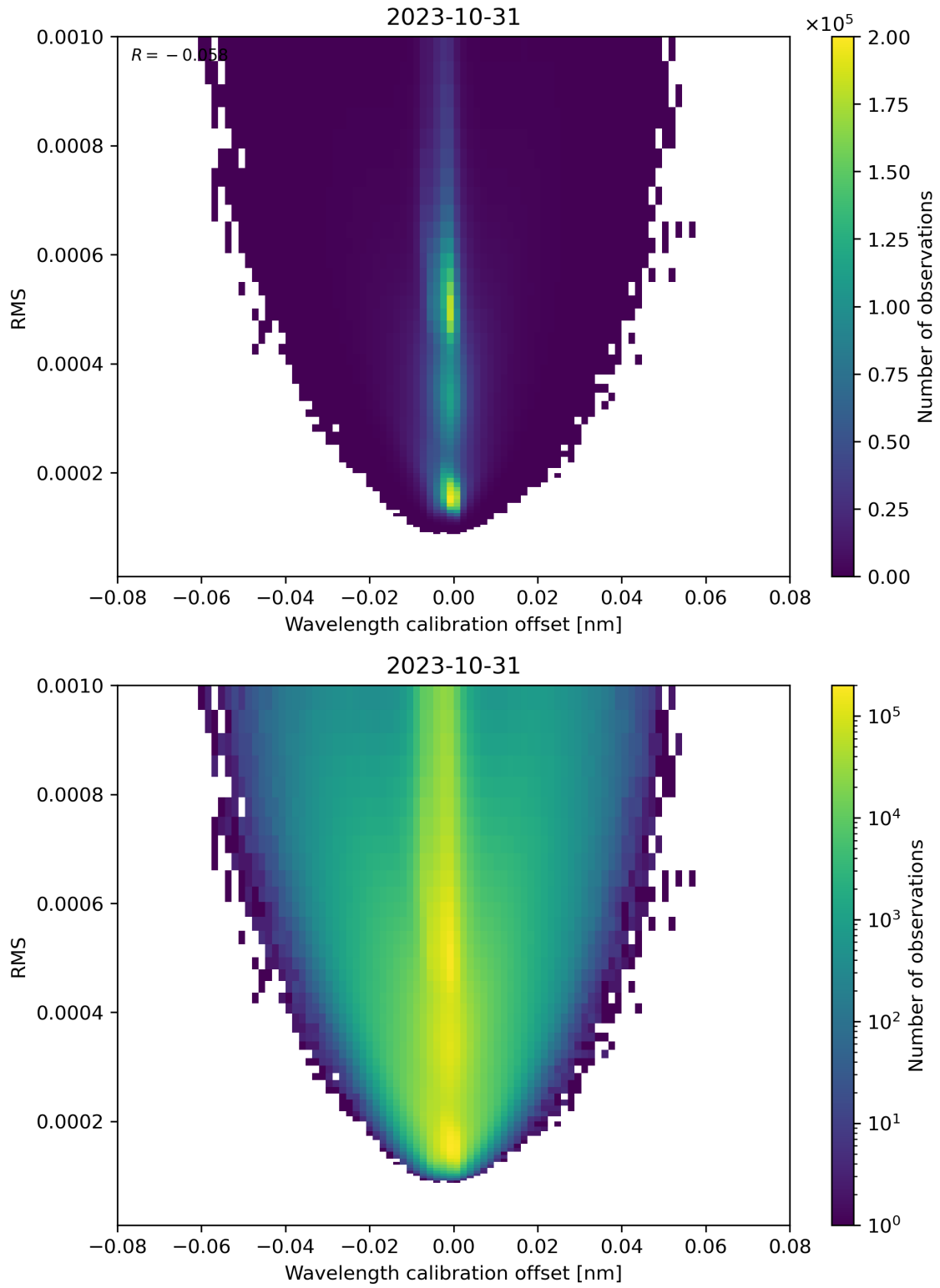
Figure 181: Scatter density plot of “Wavelength calibration offset” against “RMS” for 2023-10-30 to 2023-11-01.
