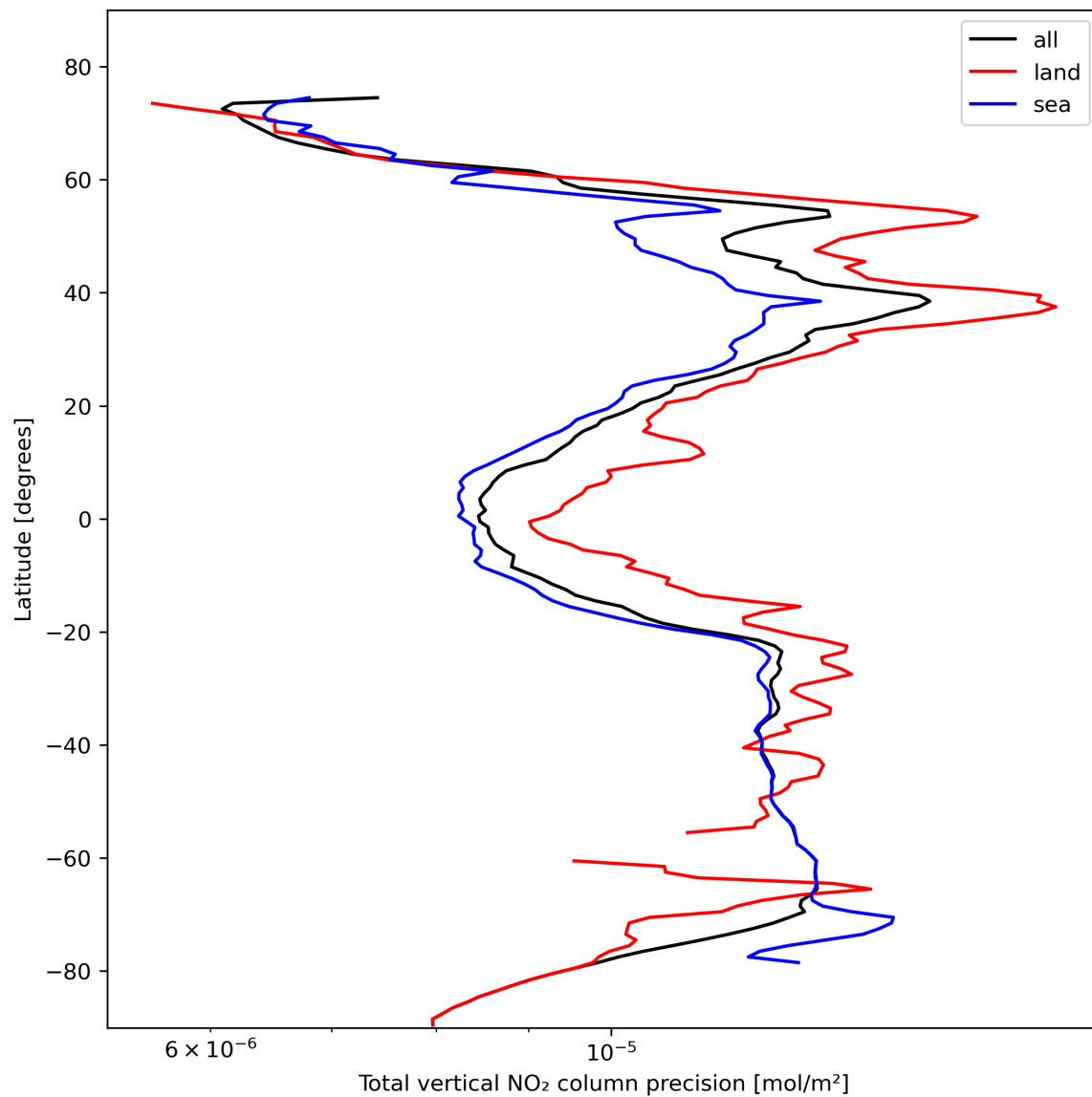
Figure 22: Zonal average of “Total vertical NO 2 column precision” for 2023-10-30 to 2023-11-01.
