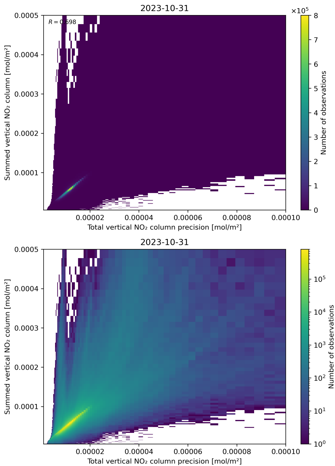
Figure 117: Scatter density plot of “Total vertical NO 2 column precision” against “Summed vertical NO 2 column” for 2023-10-30 to 2023-11-01.
