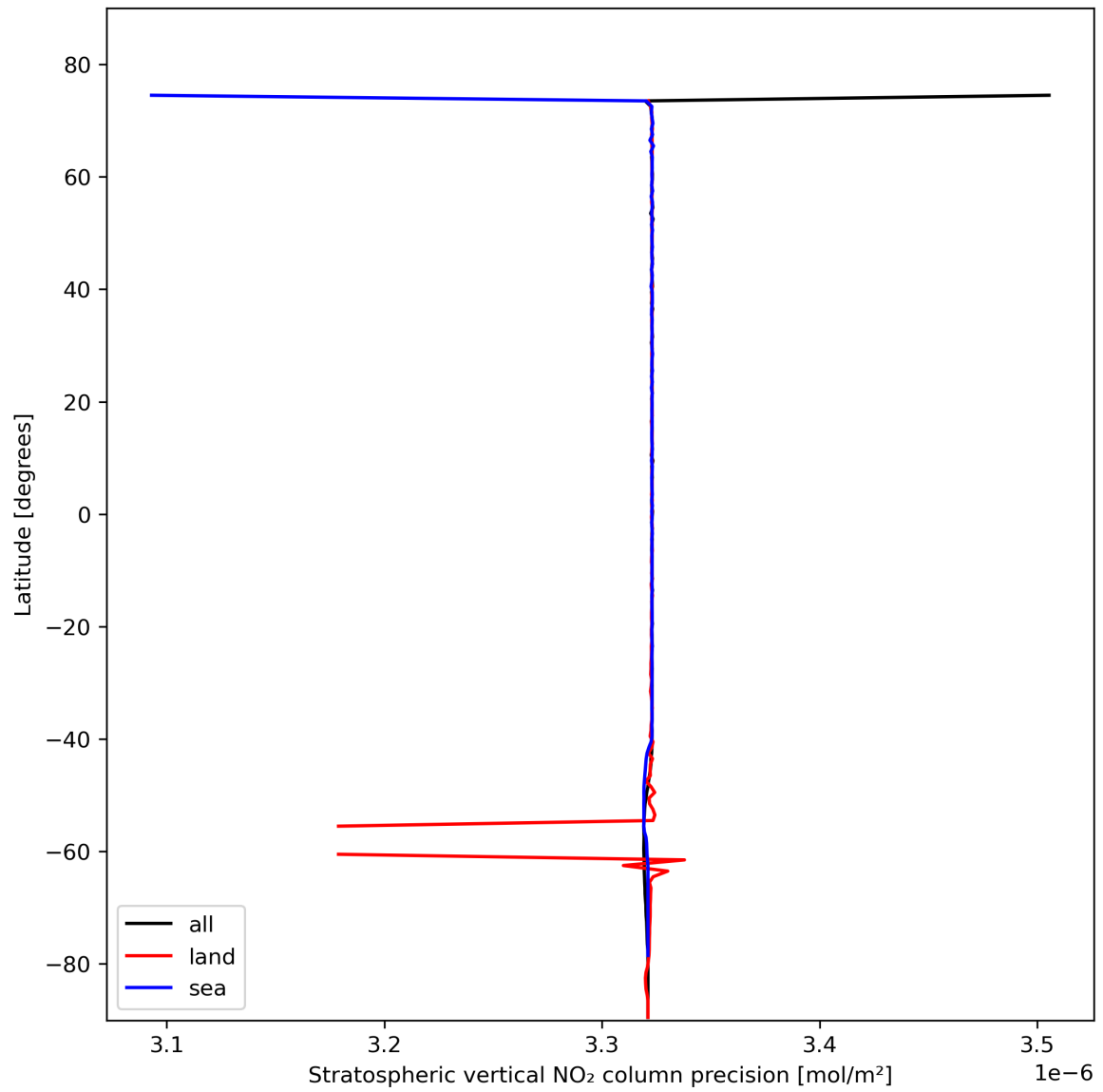
Figure 20: Zonal average of “Stratospheric vertical NO 2 column precision” for 2023-10-30 to 2023-11-01.
