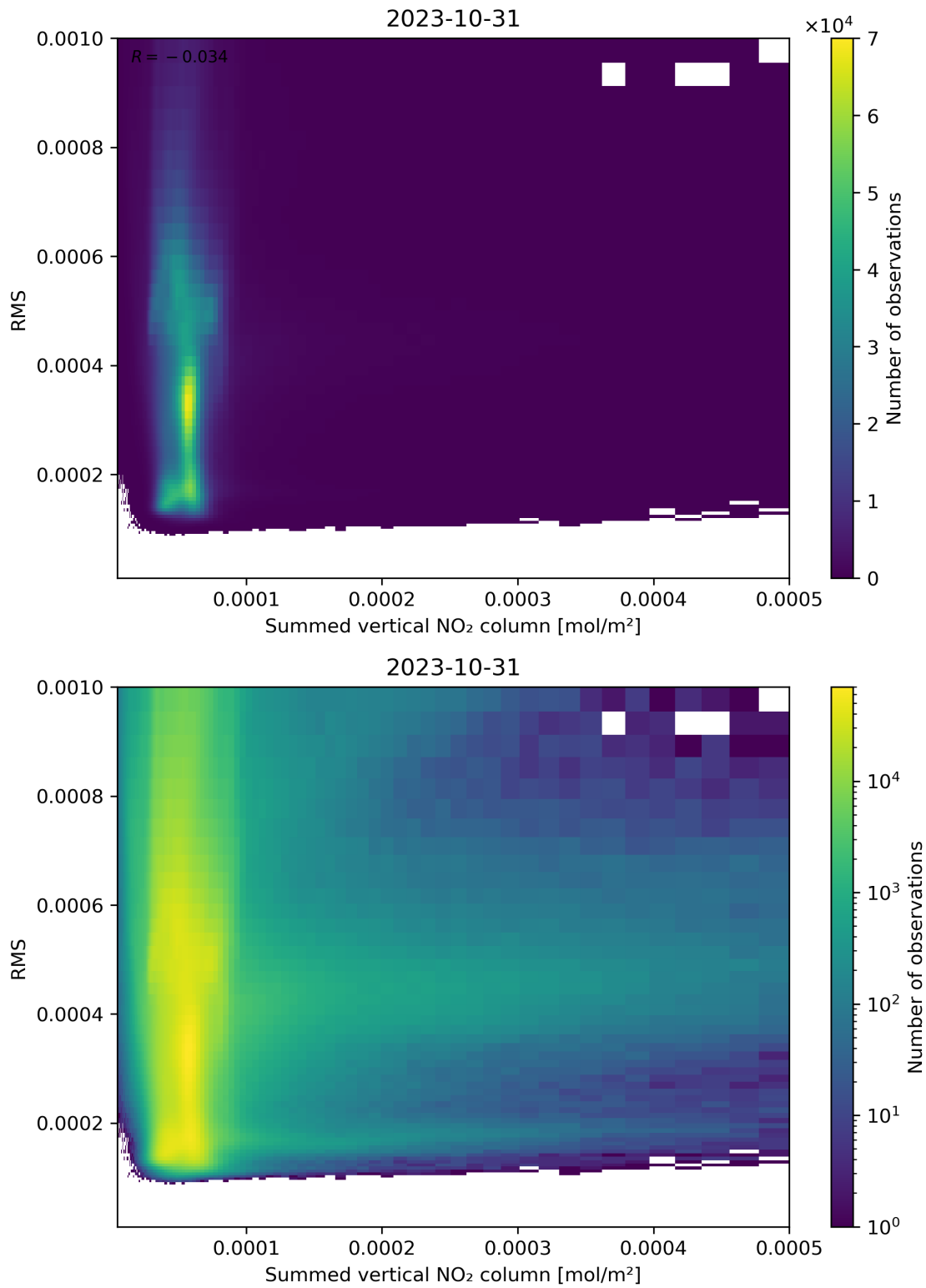
Figure 109: Scatter density plot of “Summed vertical NO 2 column” against “RMS” for 2023-10-30 to 2023-11-01.
