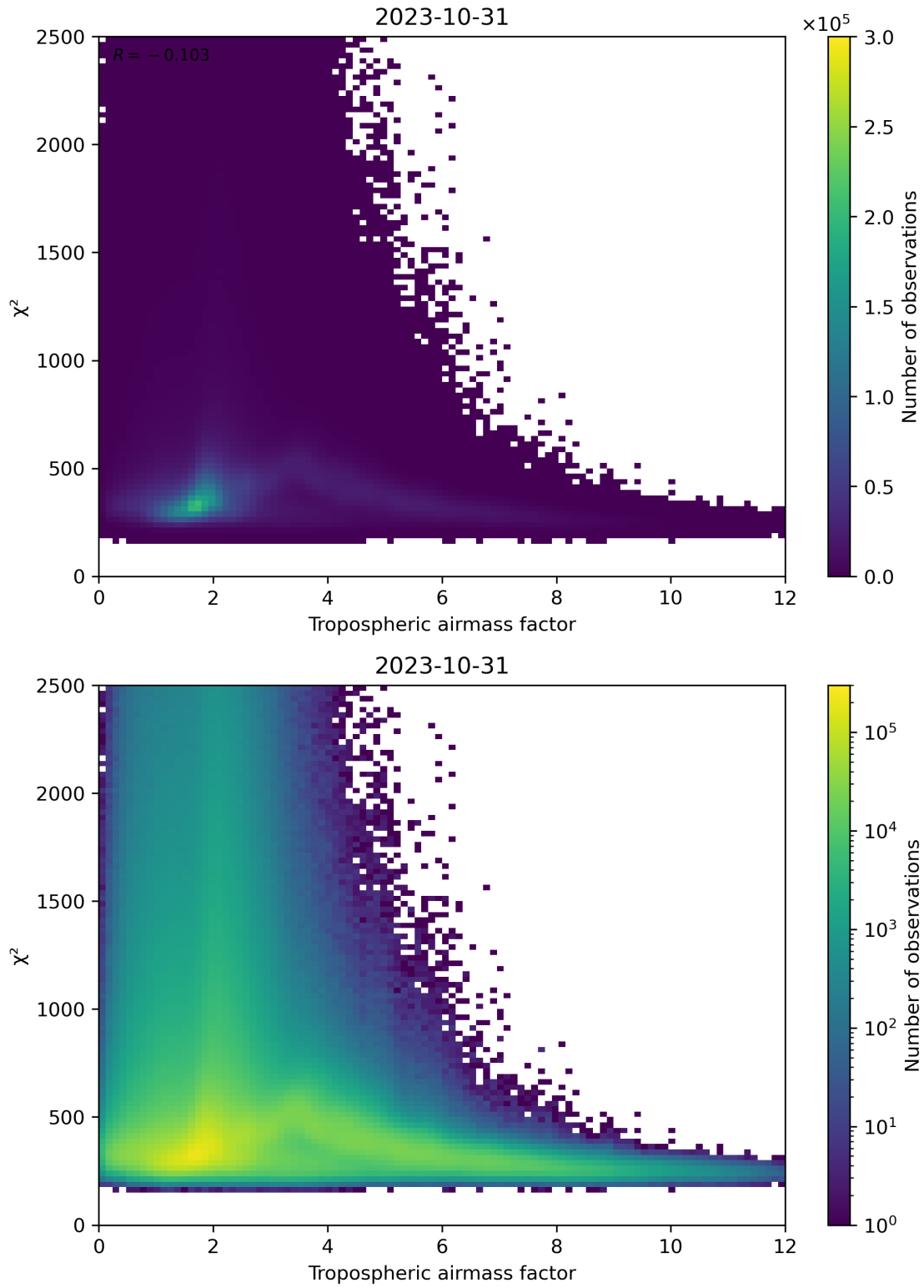
Figure 73: Scatter density plot of “Tropospheric airmass factor” against “ \chi^2 ” for 2023-10-30 to 2023-11-01.
