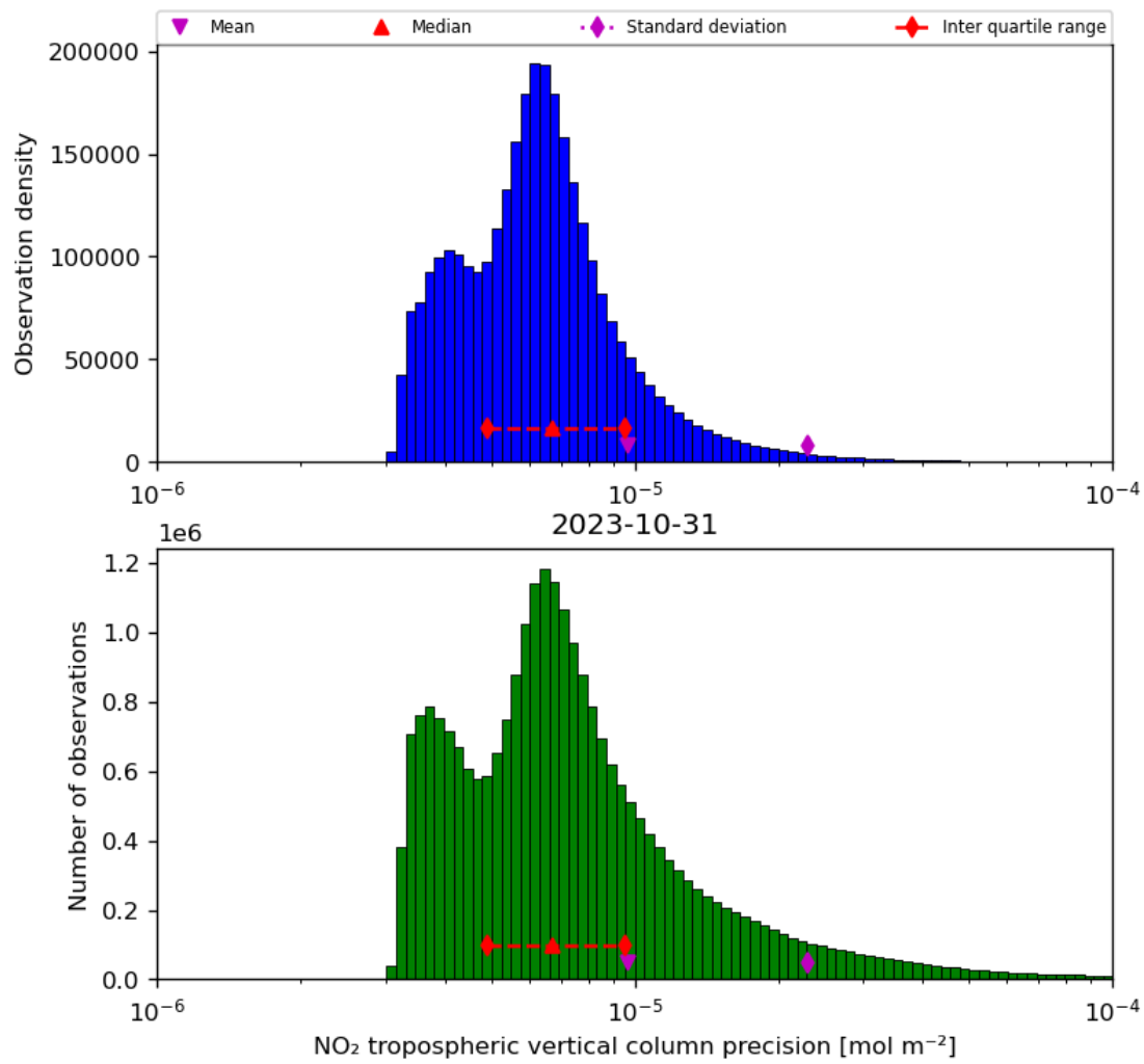
Figure 30: Histogram of “NO 2 tropospheric vertical column precision” for 2023-10-30 to 2023-11-01
