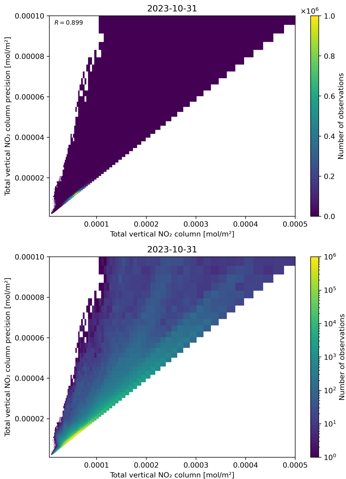
Figure 114: Scatter density plot of “Total vertical NO 2 column” against “Total vertical NO 2 column precision” for 2023-10-30 to 2023-11-01.
