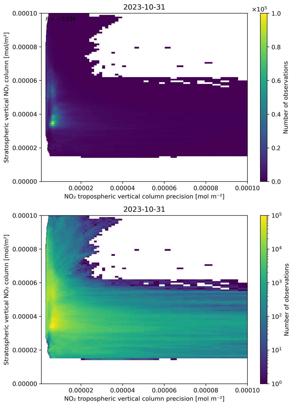
Figure 135: Scatter density plot of “NO 2 tropospheric vertical column precision” against “Stratospheric vertical NO 2 column” for 2023-10-30 to 2023-11-01.
