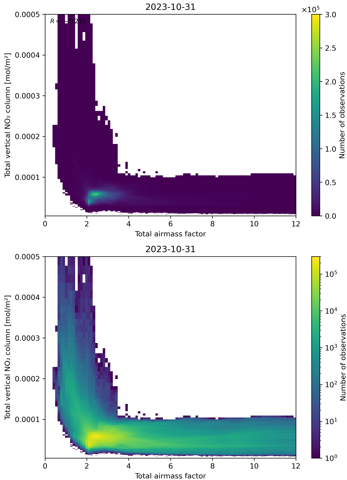
Figure 67: Scatter density plot of “Total airmass factor” against “Total vertical NO 2 column” for 2023-10-30 to 2023-11-01.
