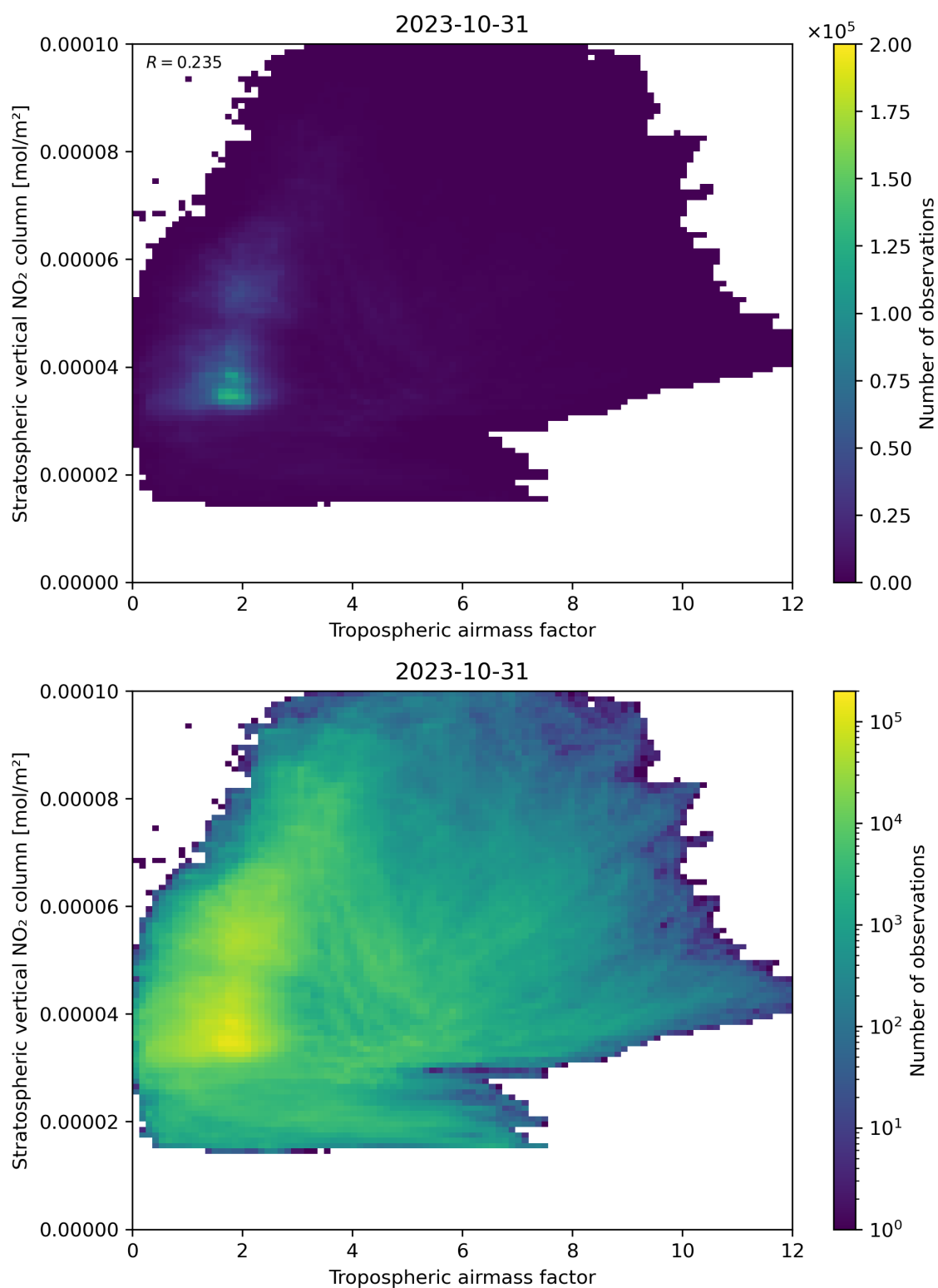
Figure 74: Scatter density plot of “Tropospheric air mass factor” against “Stratospheric vertical NO 2 column” for 2023-10-30 to 2023-11-01.
