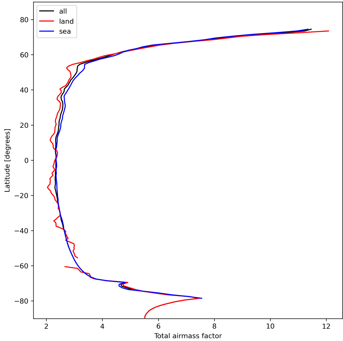
Figure 15: Zonal average of “Total airmass factor” for 2023-10-30 to 2023-11-01.
