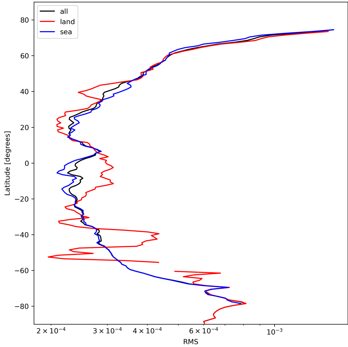
Figure 26: Zonal average of “RMS” for 2023-10-30 to 2023-11-01.
