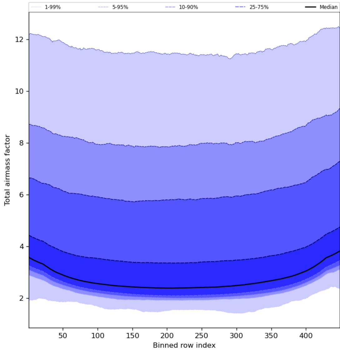
Figure 49: Along track statistics of “Total airmass factor” for 2023-10-30 to 2023-11-01
