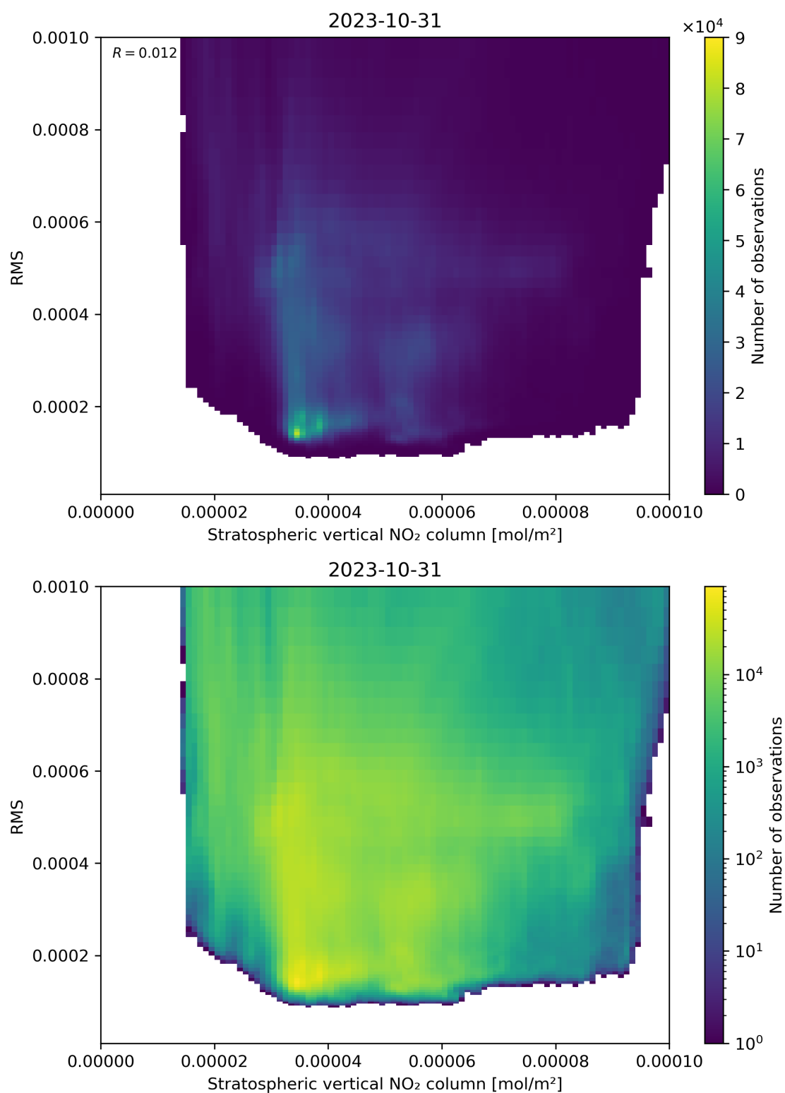
Figure 102: Scatter density plot of “Stratospheric vertical NO 2 column” against “RMS” for 2023-10-30 to 2023-11-01.
