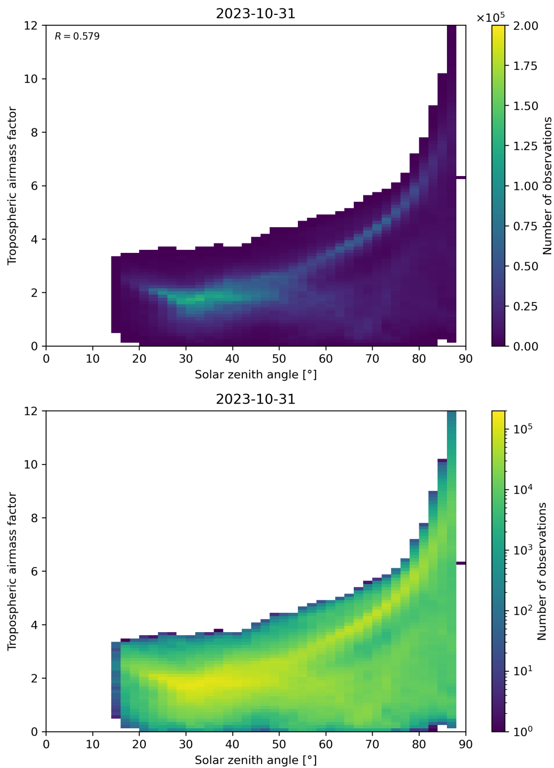
Figure 147: Scatter density plot of “Solar zenith angle” against “Tropospheric airmass factor” for 2023-10-30 to 2023-11-01.
