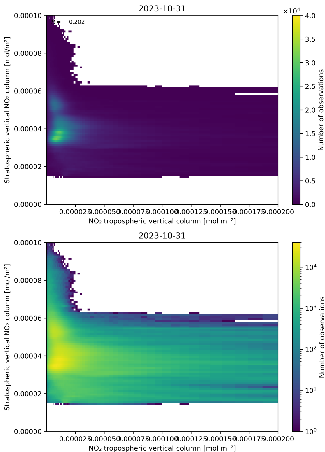
Figure 125: Scatter density plot of “NO 2 tropospheric vertical column” against “Stratospheric vertical NO 2 column” for 2023-10-30 to 2023-11-01.
