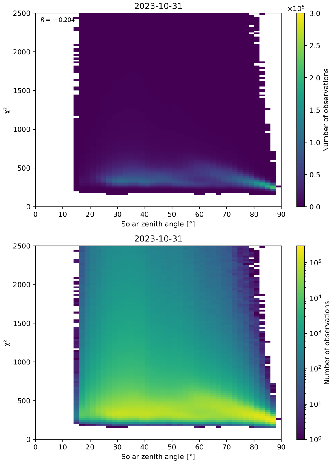
Figure 148: Scatter density plot of “Solar zenith angle” against “ \chi^2 ” for 2023-10-30 to 2023-11-01.
