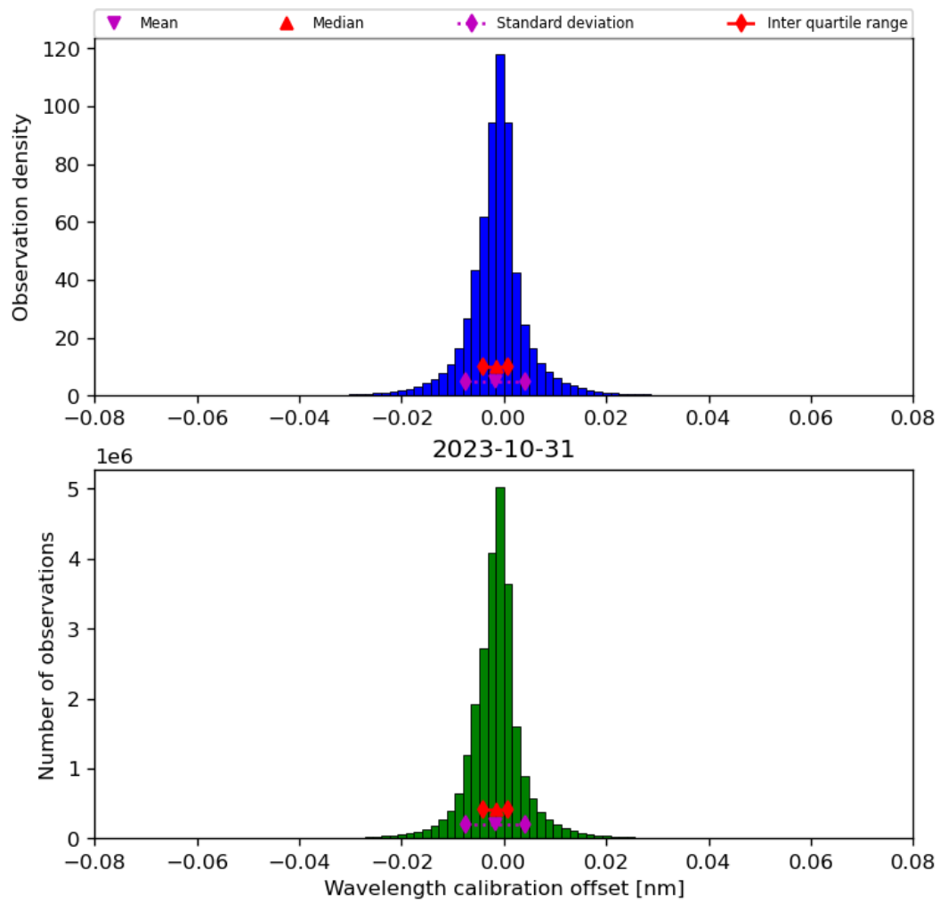
Figure 35: Histogram of “Wavelength calibration offset” for 2023-10-30 to 2023-11-01
