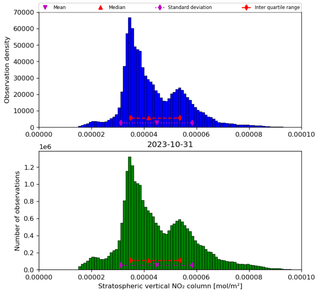
Figure 36: Histogram of “Stratospheric vertical NO 2 column” for 2023-10-30 to 2023-11-01
