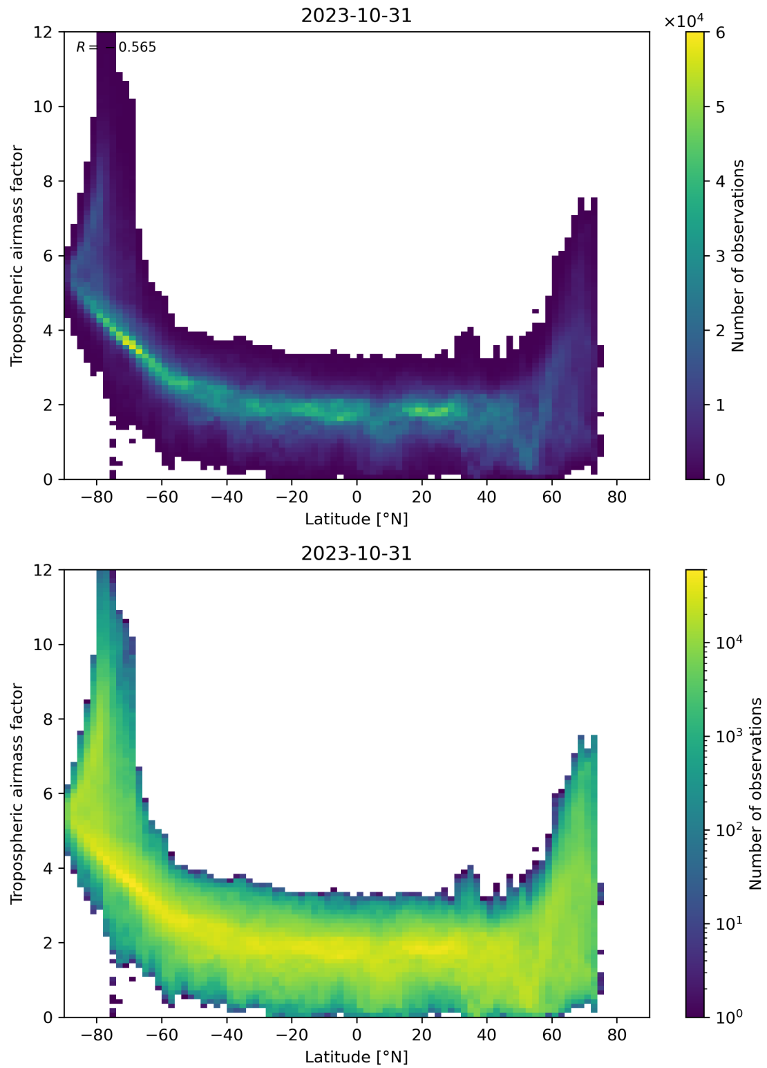
Figure 85: Scatter density plot of “Latitude” against “Tropospheric air mass factor” for 2023-10-30 to 2023-11-01.
