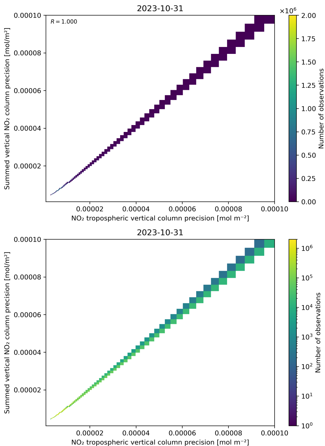
Figure 137: Scatter density plot of “NO 2 tropospheric vertical column precision” against “Summed vertical NO 2 column precision” for 2023-10-30 to 2023-11-01.
