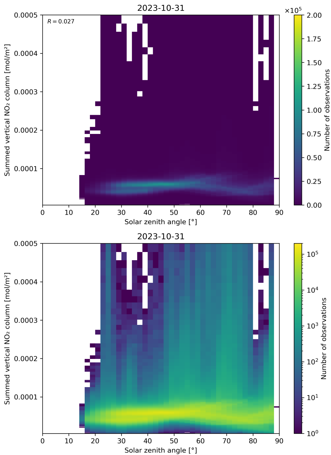
Figure 151: Scatter density plot of “Solar zenith angle” against “Summed vertical NO 2 column” for 2023-10-30 to 2023-11-01.
