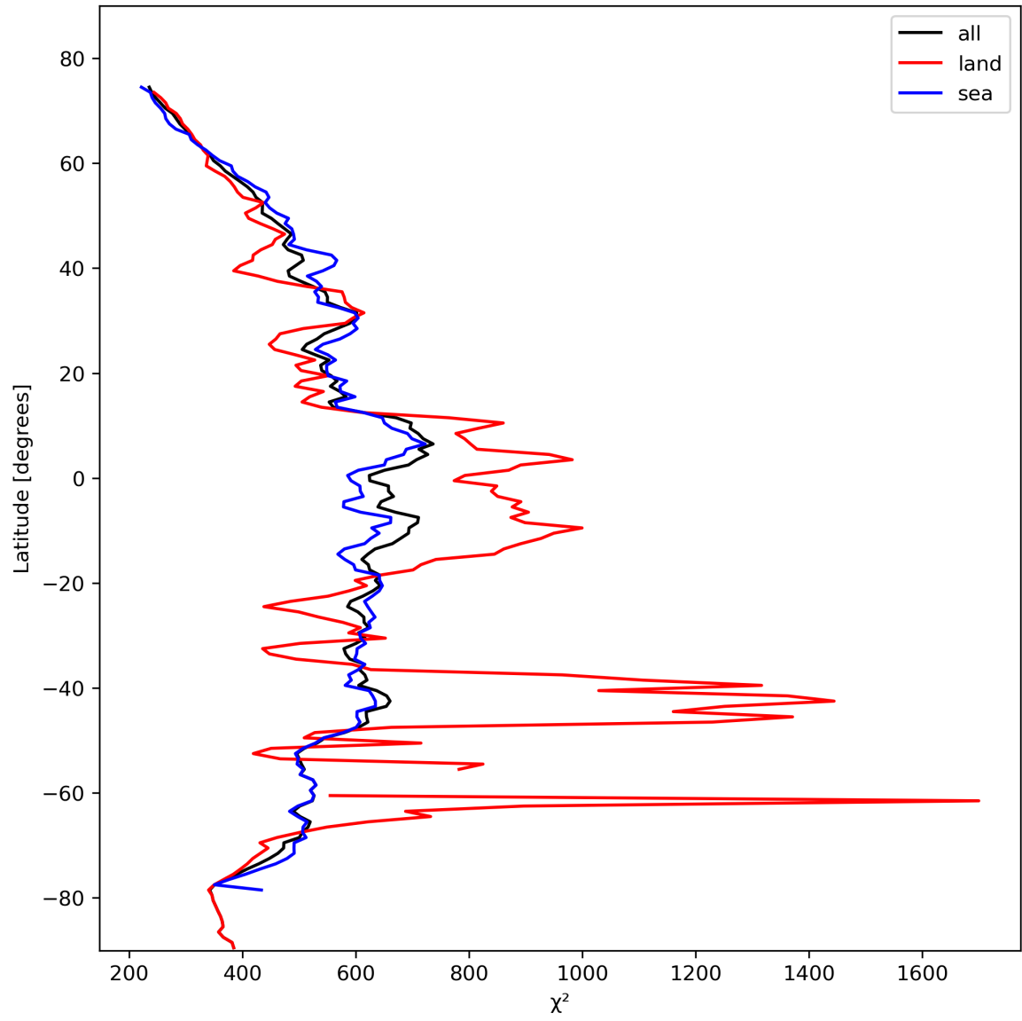
Figure 25: Zonal average of “ \chi^2 ” for 2023-10-30 to 2023-11-01.
