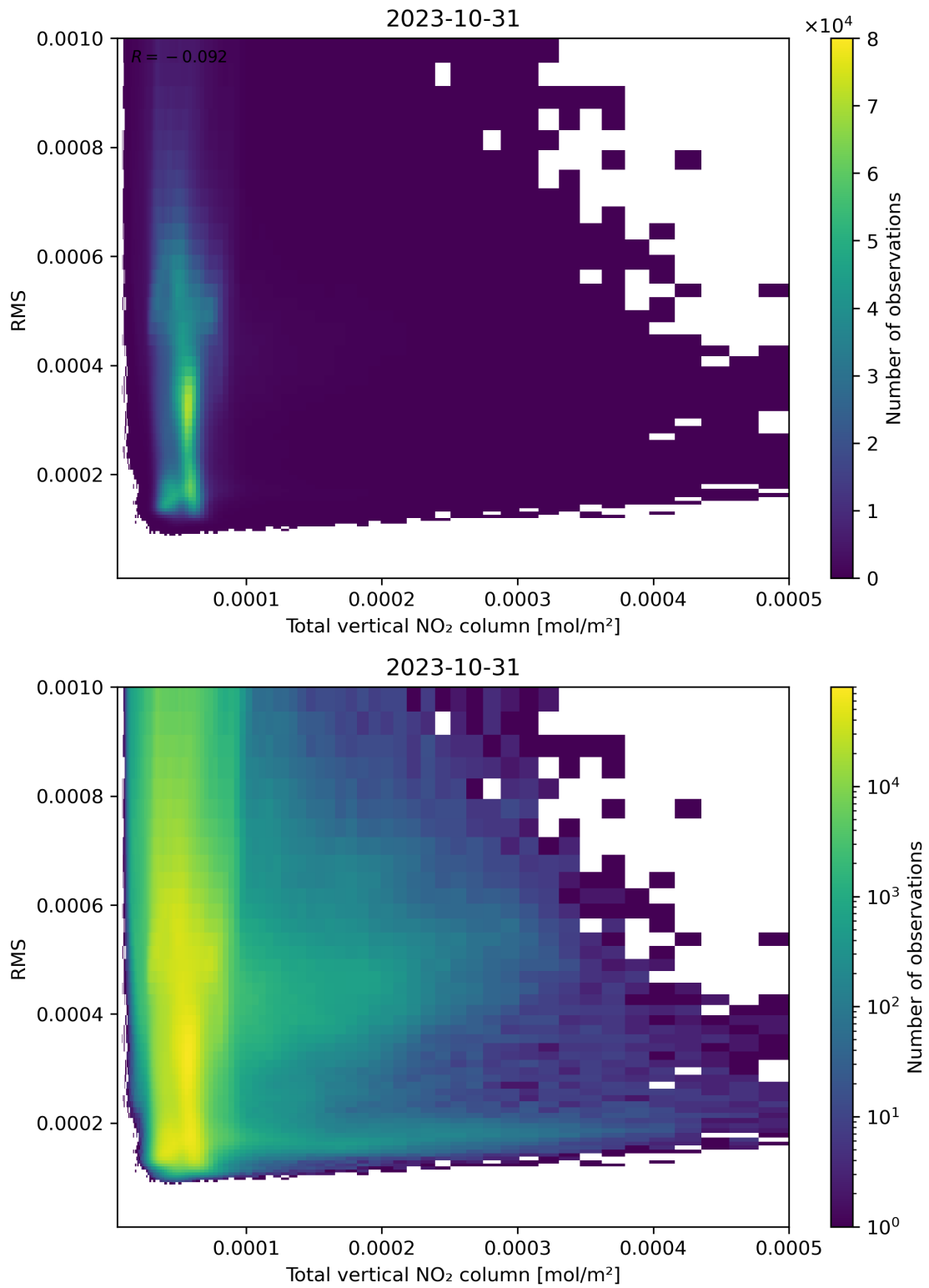
Figure 120: Scatter density plot of “Total vertical NO 2 column” against “RMS” for 2023-10-30 to 2023-11-01.
