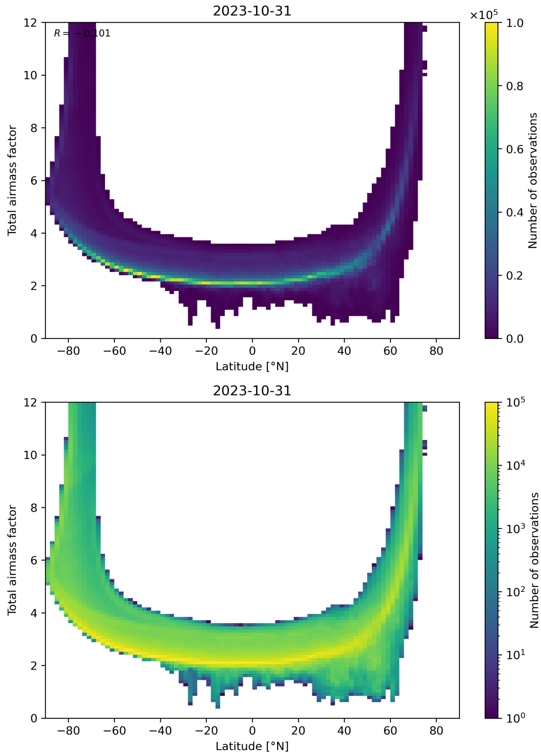
Figure 84: Scatter density plot of “Latitude” against “Total airmass factor” for 2023-10-30 to 2023-11-01.
