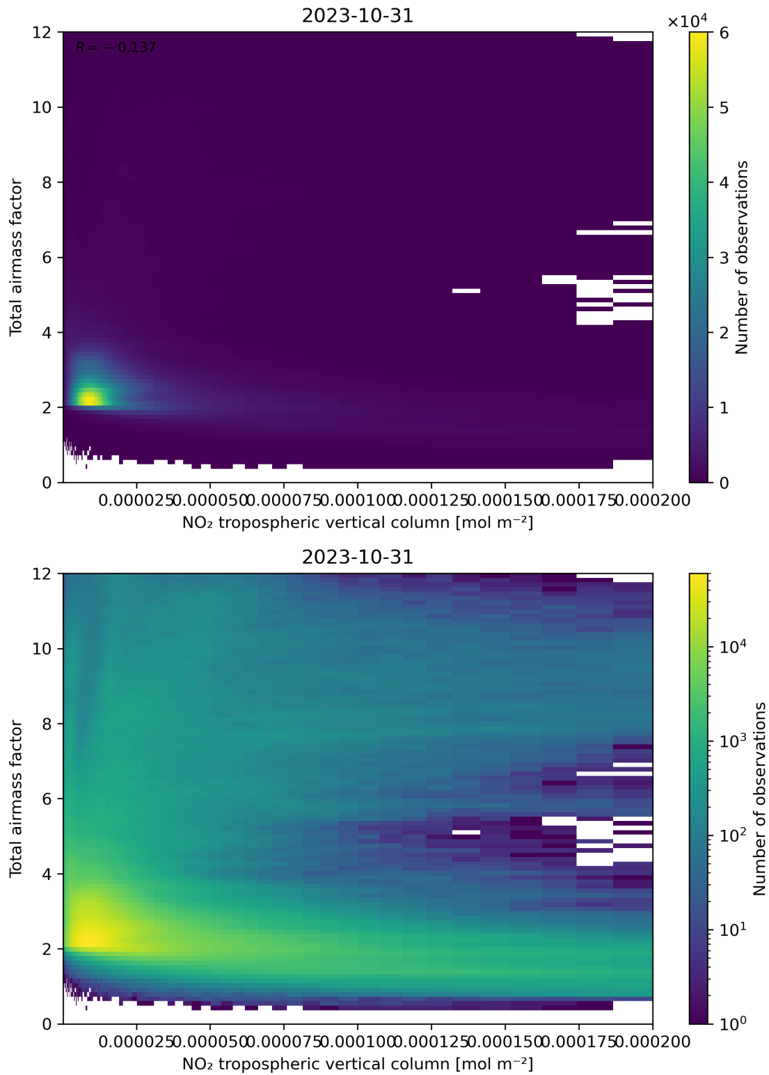
Figure 122: Scatter density plot of “NO 2 tropospheric vertical column” against “Total air mass factor” for 2023-10-30 to 2023-11-01.
