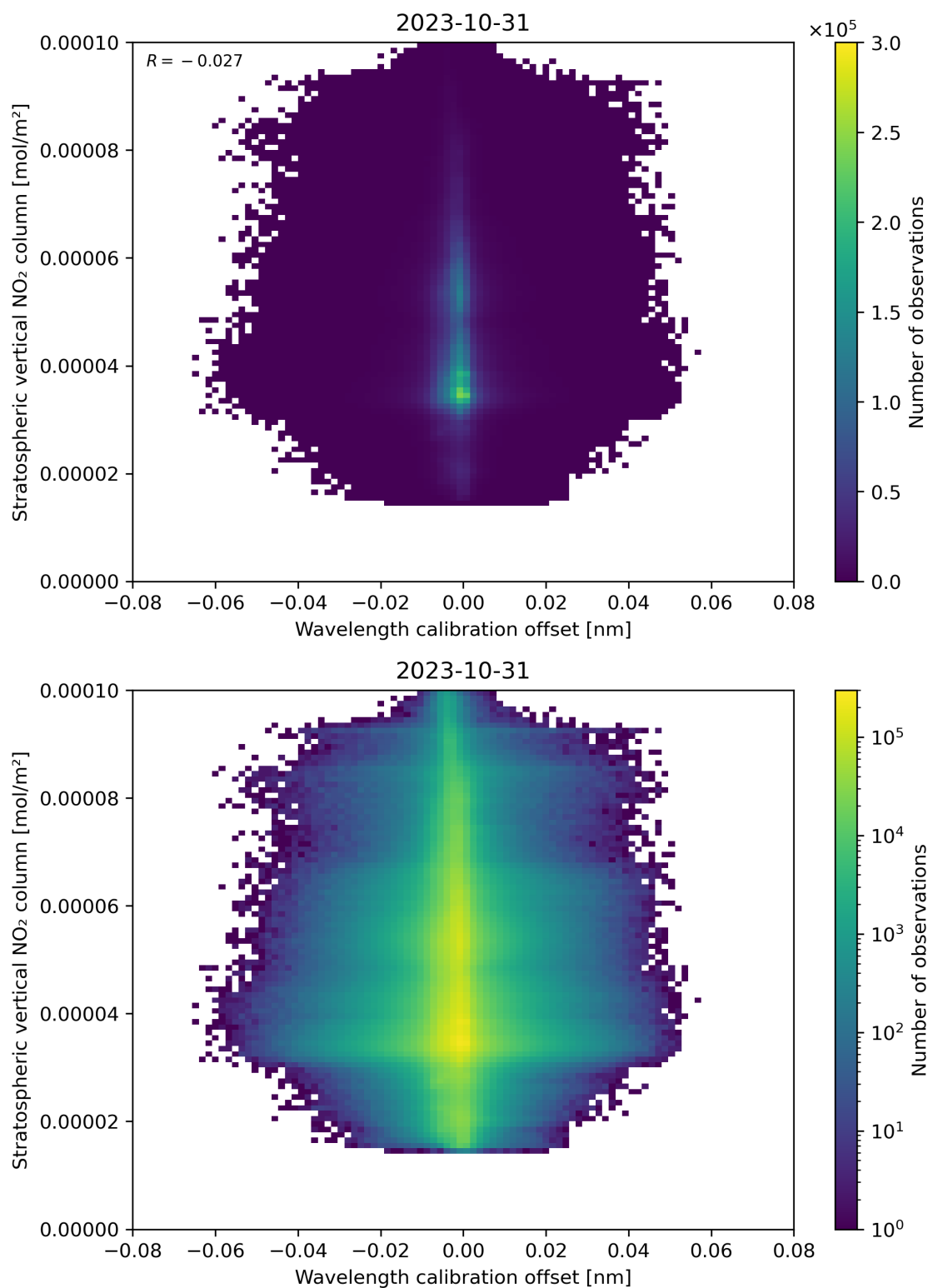
Figure 176: Scatter density plot of “Wavelength calibration offset” against “Stratospheric vertical NO 2 column” for 2023-10-30 to 2023-11-01.
