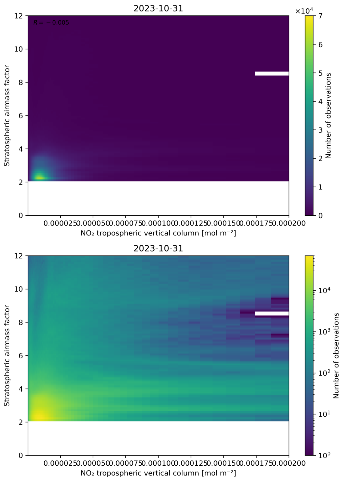
Figure 121: Scatter density plot of “NO 2 tropospheric vertical column” against “Stratospheric airmass factor” for 2023-10-30 to 2023-11-01.
