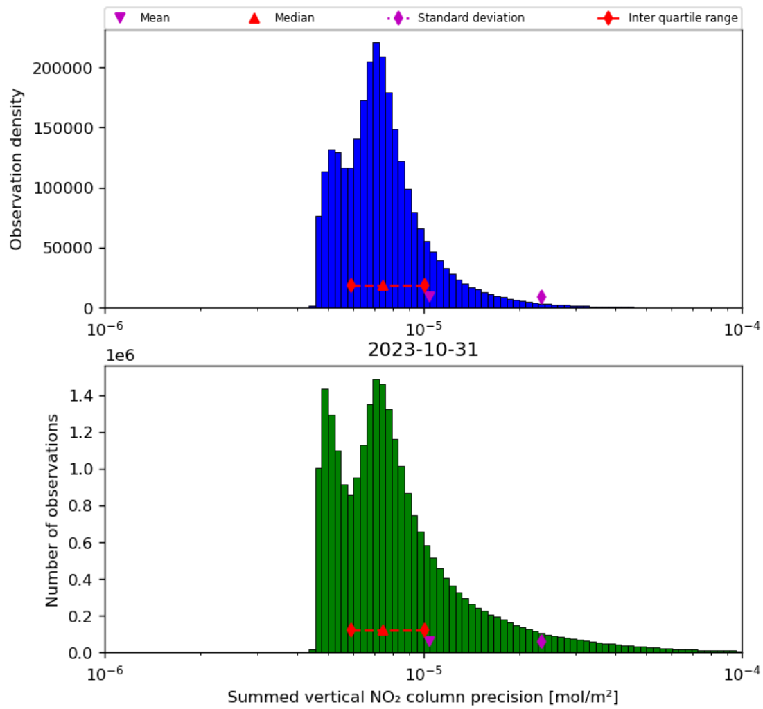
Figure 41: Histogram of "Summed vertical NO 2 column precision" for 2023-10-30 to 2023-11-01
