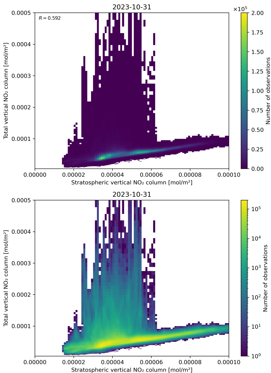
Figure 100: Scatter density plot of “Stratospheric vertical NO 2 column” against “Total vertical NO 2 column” for 2023-10-30 to 2023-11-01.
