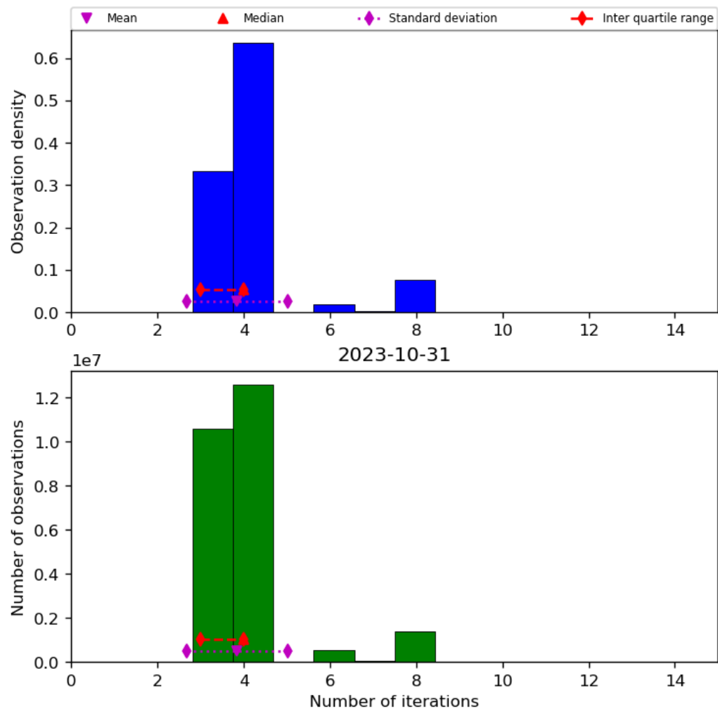
Figure 34: Histogram of "Number of iterations" for 2023-10-30 to 2023-11-01
