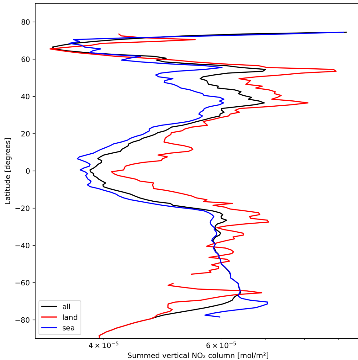
Figure 23: Zonal average of “Summed vertical NO 2 column” for 2023-10-30 to 2023-11-01.
