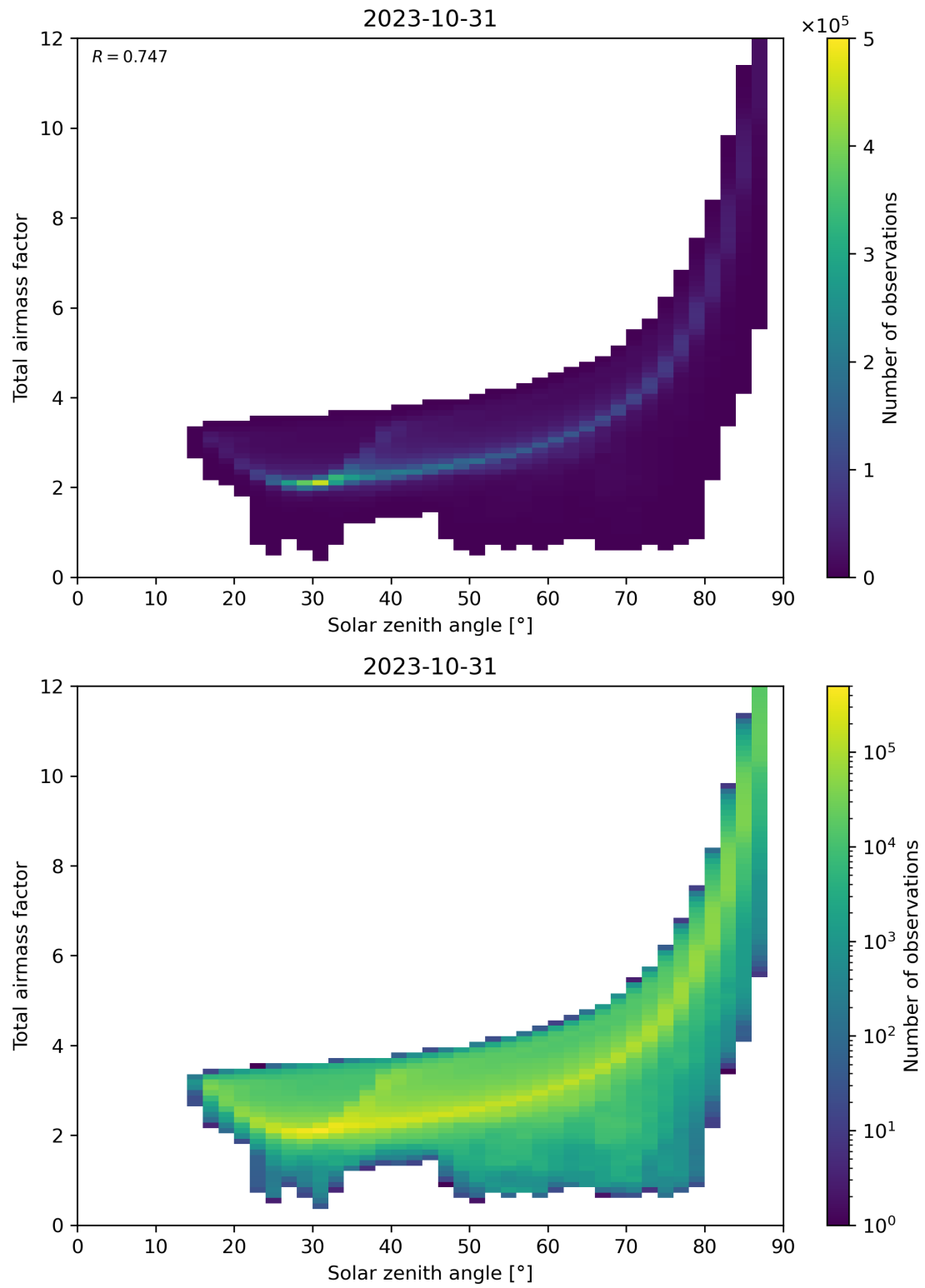
Figure 146: Scatter density plot of “Solar zenith angle” against “Total air mass factor” for 2023-10-30 to 2023-11-01.
