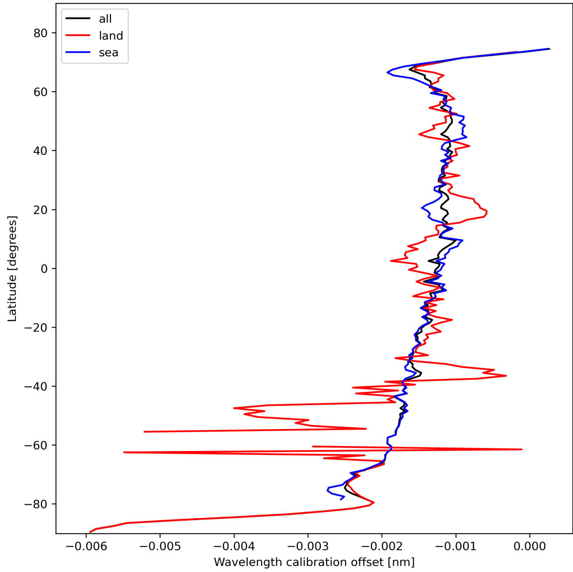
Figure 18: Zonal average of “Wavelength calibration offset” for 2023-10-30 to 2023-11-01.
