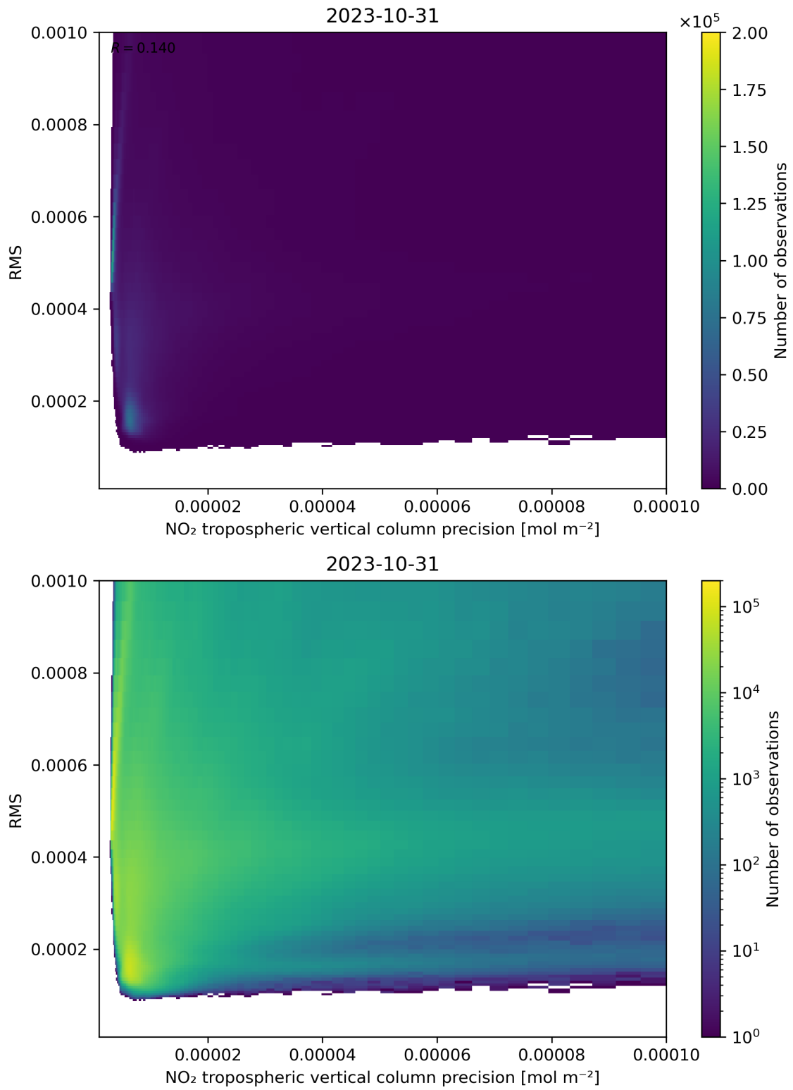
Figure 140: Scatter density plot of “NO 2 tropospheric vertical column precision” against “RMS” for 2023-10-30 to 2023-11-01.
