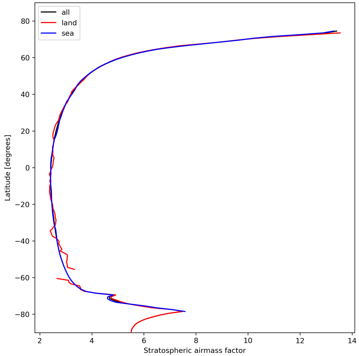
Figure 27: Zonal average of “Stratospheric air mass factor” for 2023-10-30 to 2023-11-01.
