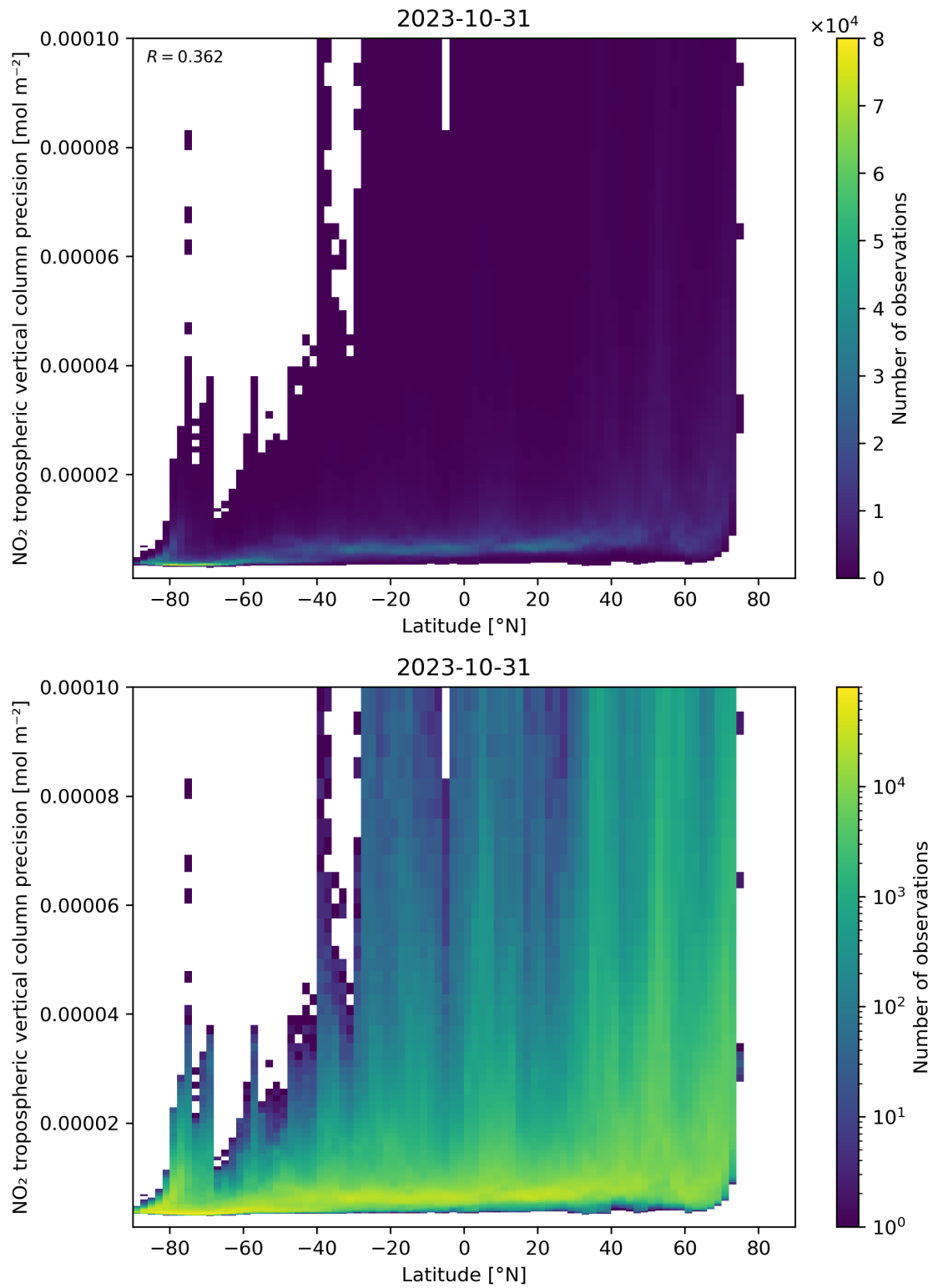
Figure 93: Scatter density plot of “Latitude” against “NO 2 tropospheric vertical column precision” for 2023-10-30 to 2023-11-01.
