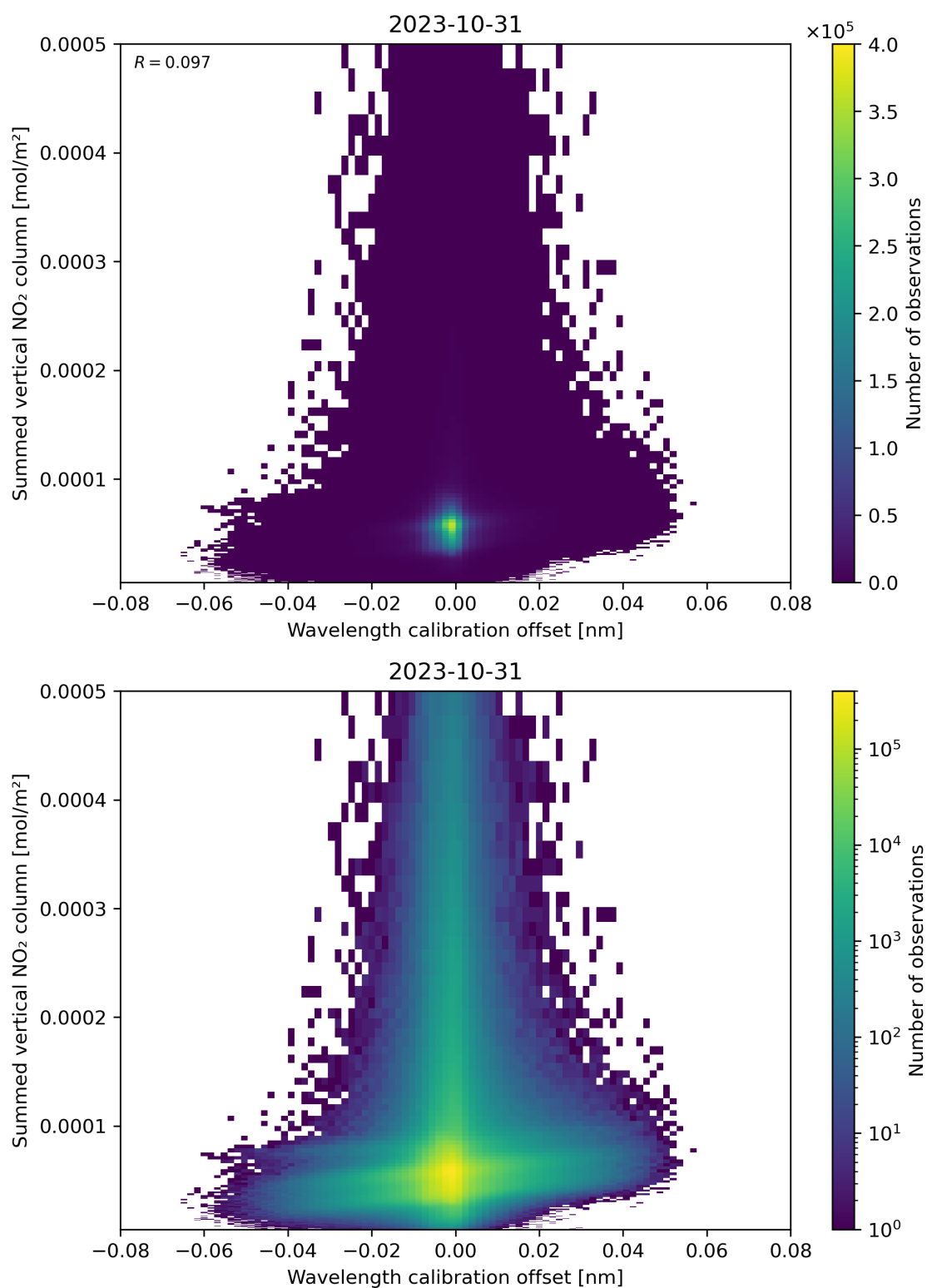
Figure 177: Scatter density plot of “Wavelength calibration offset” against “Summed vertical NO 2 column” for 2023-10-30 to 2023-11-01.
