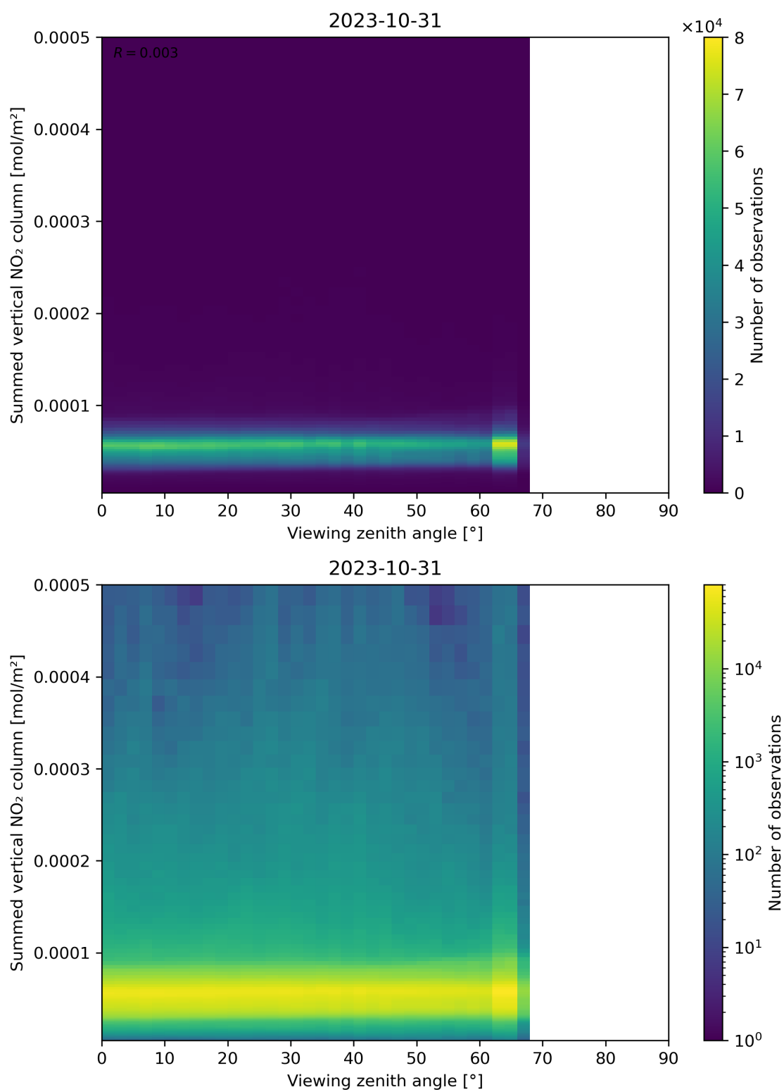
Figure 165: Scatter density plot of “Viewing zenith angle” against “Summed vertical NO 2 column” for 2023-10-30 to 2023-11-01.
