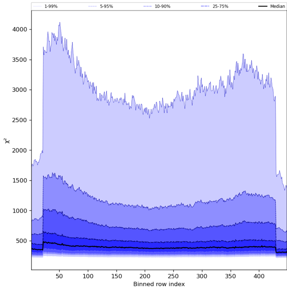
Figure 59: Along track statistics of “ \chi^2 ” for 2023-10-30 to 2023-11-01
