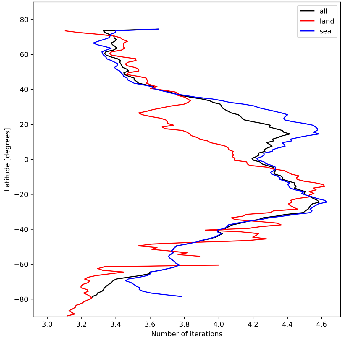
Figure 17: Zonal average of “Number of iterations” for 2023-10-30 to 2023-11-01.
