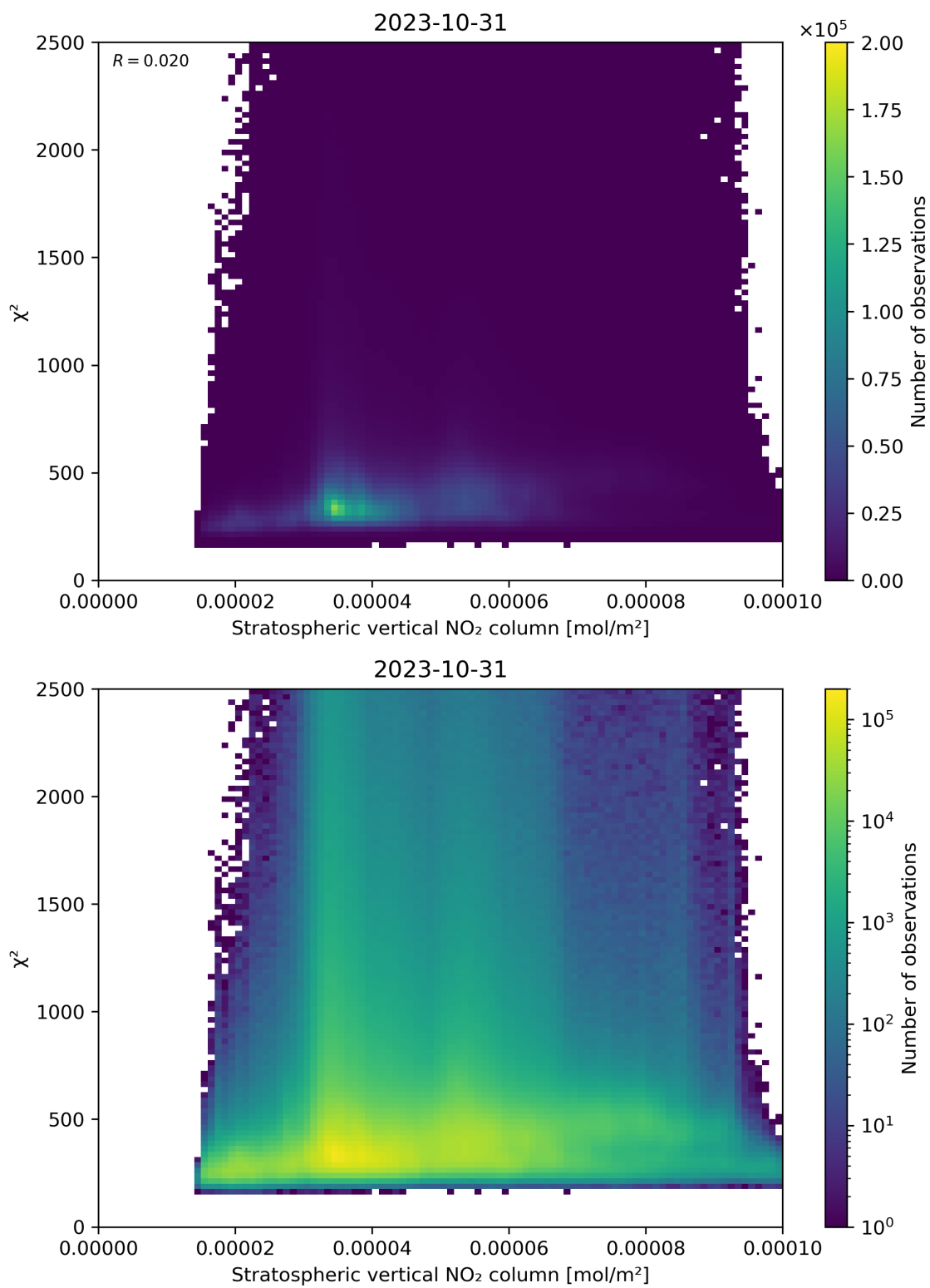
Figure 97: Scatter density plot of “Stratospheric vertical NO 2 column” against “ \chi^2 ” for 2023-10-30 to 2023-11-01.
