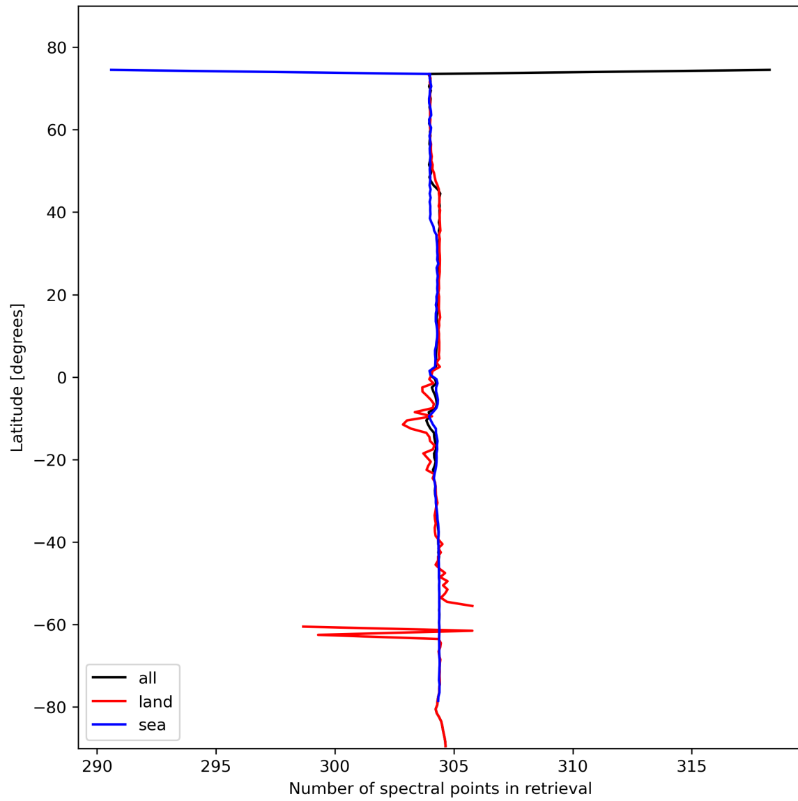
Figure 16: Zonal average of “Number of spectral points in retrieval” for 2023-10-30 to 2023-11-01.
