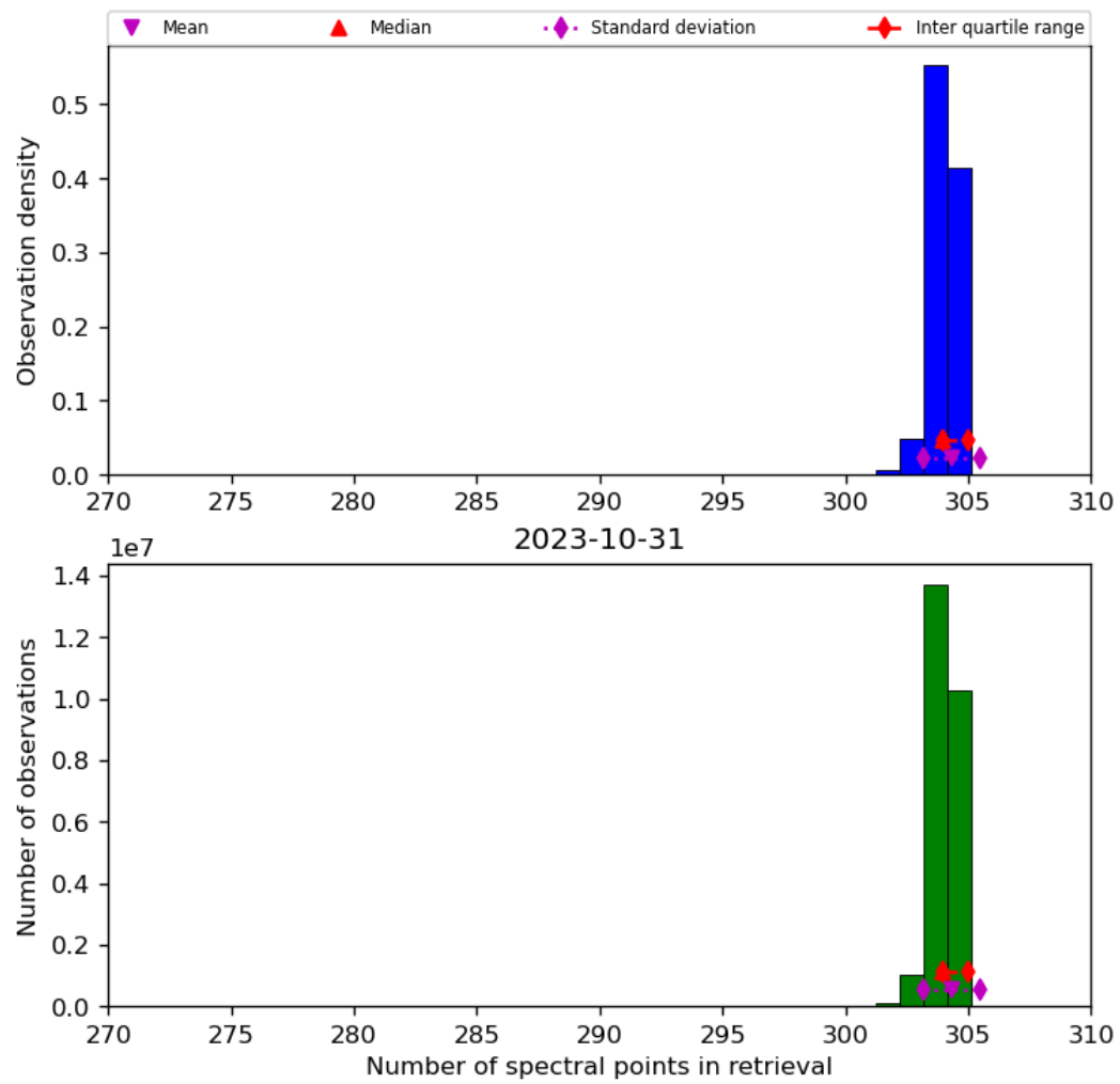
Figure 33: Histogram of “Number of spectral points in retrieval” for 2023-10-30 to 2023-11-01
