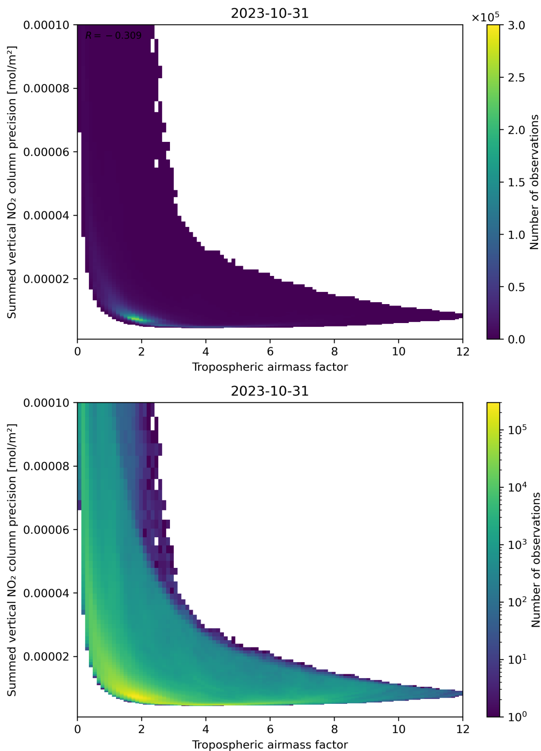
Figure 76: Scatter density plot of “Tropospheric air mass factor” against “Summed vertical NO 2 column precision” for 2023-10-30 to 2023-11-01.
