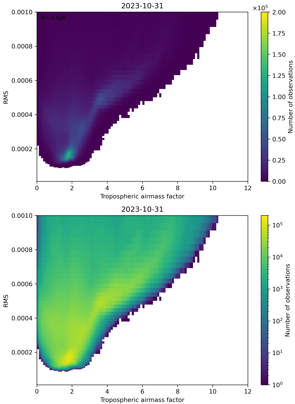
Figure 79: Scatter density plot of “Tropospheric airmass factor” against “RMS” for 2023-10-30 to 2023-11-01.
