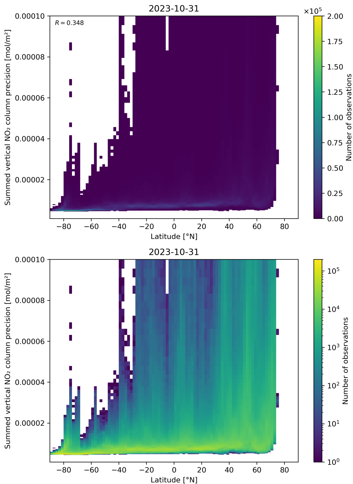
Figure 89: Scatter density plot of “Latitude” against “Summed vertical NO 2 column precision” for 2023-10-30 to 2023-11-01.
