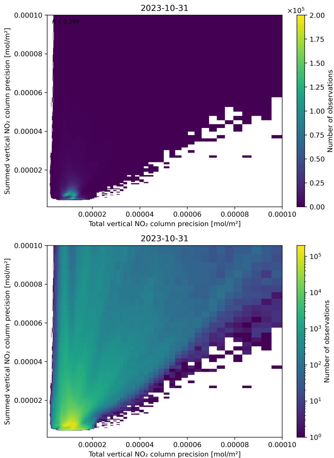
Figure 118: Scatter density plot of “Total vertical NO 2 column precision” against “Summed vertical NO 2 column precision” for 2023-10-30 to 2023-11-01.
