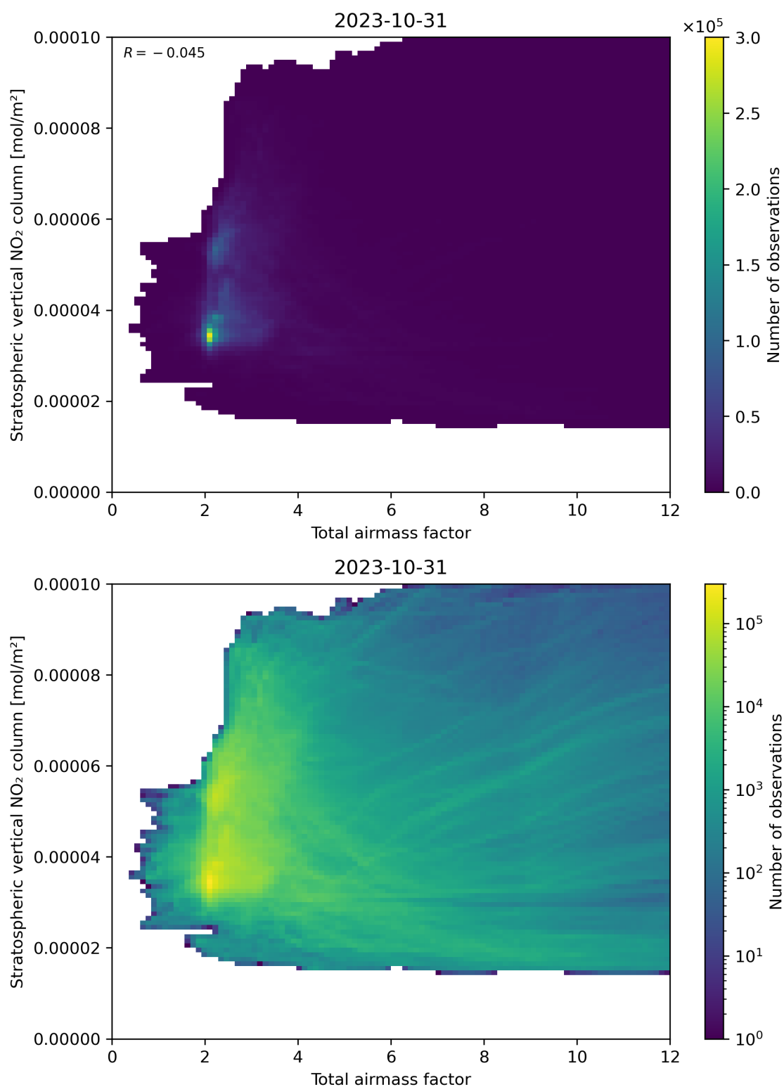
Figure 64: Scatter density plot of “Total airmass factor” against “Stratospheric vertical NO 2 column” for 2023-10-30 to 2023-11-01.
