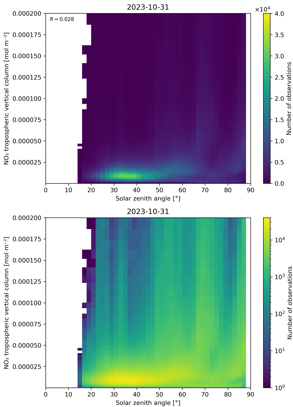
Figure 155: Scatter density plot of “Solar zenith angle” against “NO 2 tropospheric vertical column” for 2023-10-30 to 2023-11-01.
