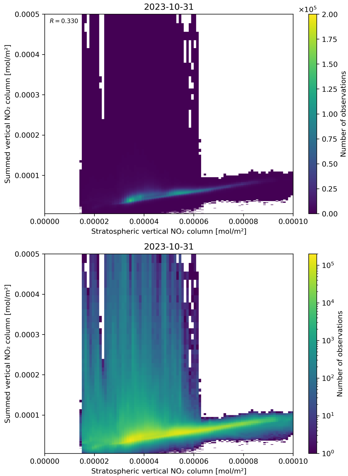
Figure 98: Scatter density plot of “Stratospheric vertical NO 2 column” against “Summed vertical NO 2 column” for 2023-10-30 to 2023-11-01.
