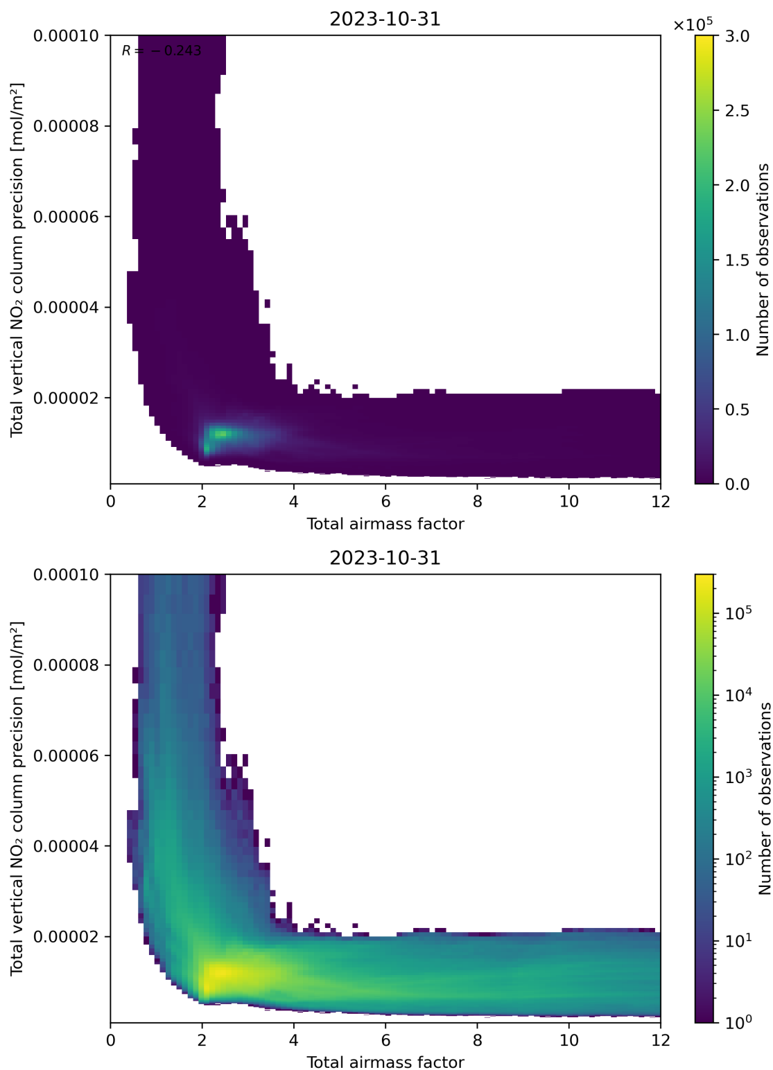
Figure 68: Scatter density plot of “Total airmass factor” against “Total vertical NO 2 column precision” for 2023-10-30 to 2023-11-01.
