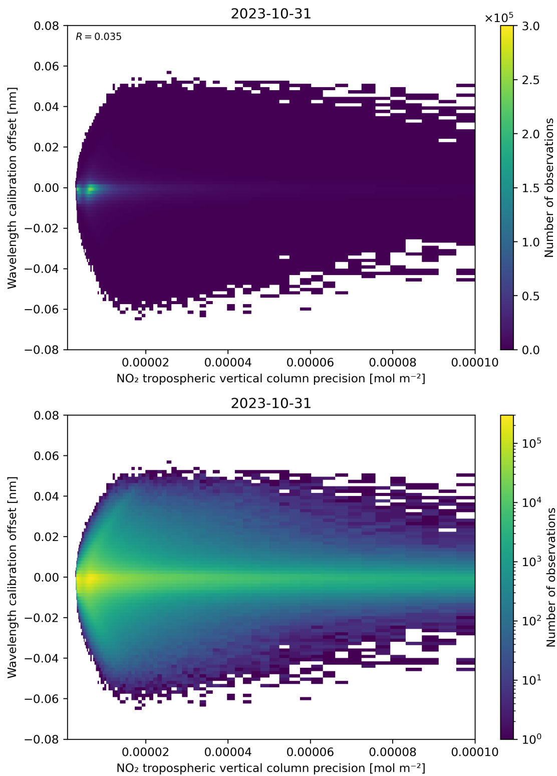
Figure 141: Scatter density plot of “NO 2 tropospheric vertical column precision” against “Wavelength calibration offset” for 2023-10-30 to 2023-11-01.
