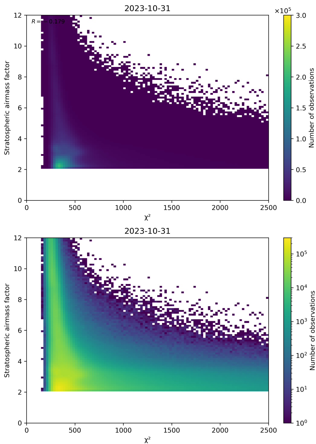
Figure 81: Scatter density plot of “ \chi^2 ” against “Stratospheric airmass factor” for 2023-10-30 to 2023-11-01.
