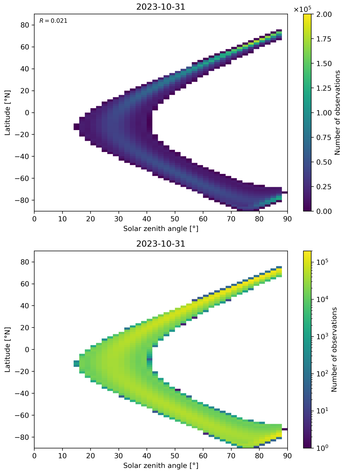
Figure 149: Scatter density plot of “Solar zenith angle” against “Latitude” for 2023-10-30 to 2023-11-01.
