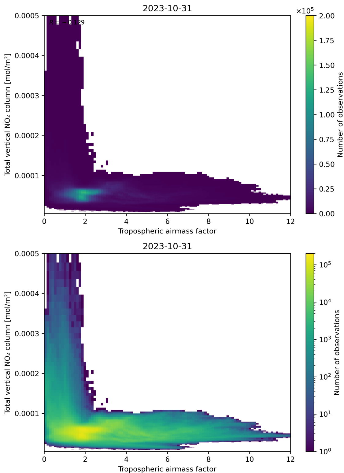
Figure 77: Scatter density plot of “Tropospheric airmass factor” against “Total vertical NO 2 column” for 2023-10-30 to 2023-11-01.
