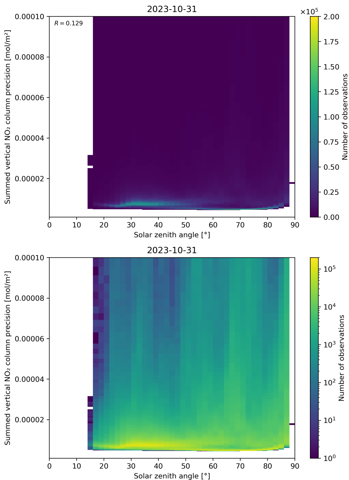
Figure 152: Scatter density plot of “Solar zenith angle” against “Summed vertical NO 2 column precision” for 2023-10-30 to 2023-11-01.
