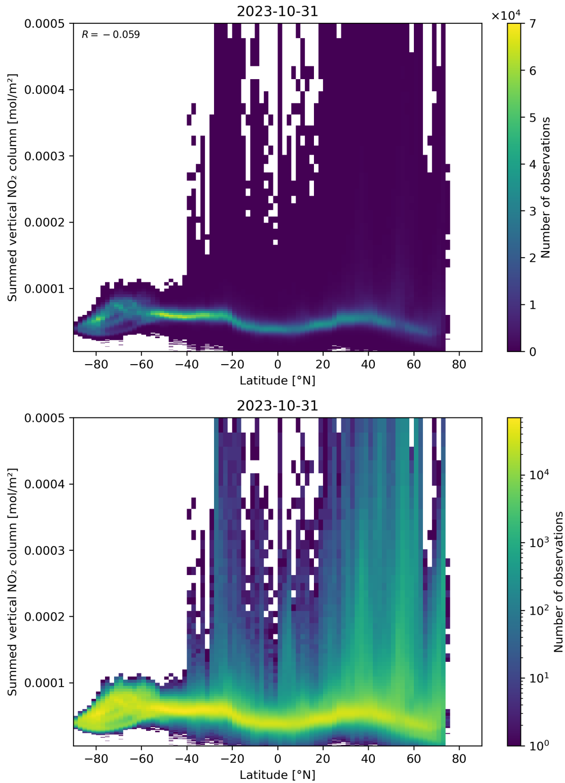
Figure 88: Scatter density plot of “Latitude” against “Summed vertical NO 2 column” for 2023-10-30 to 2023-11-01.
