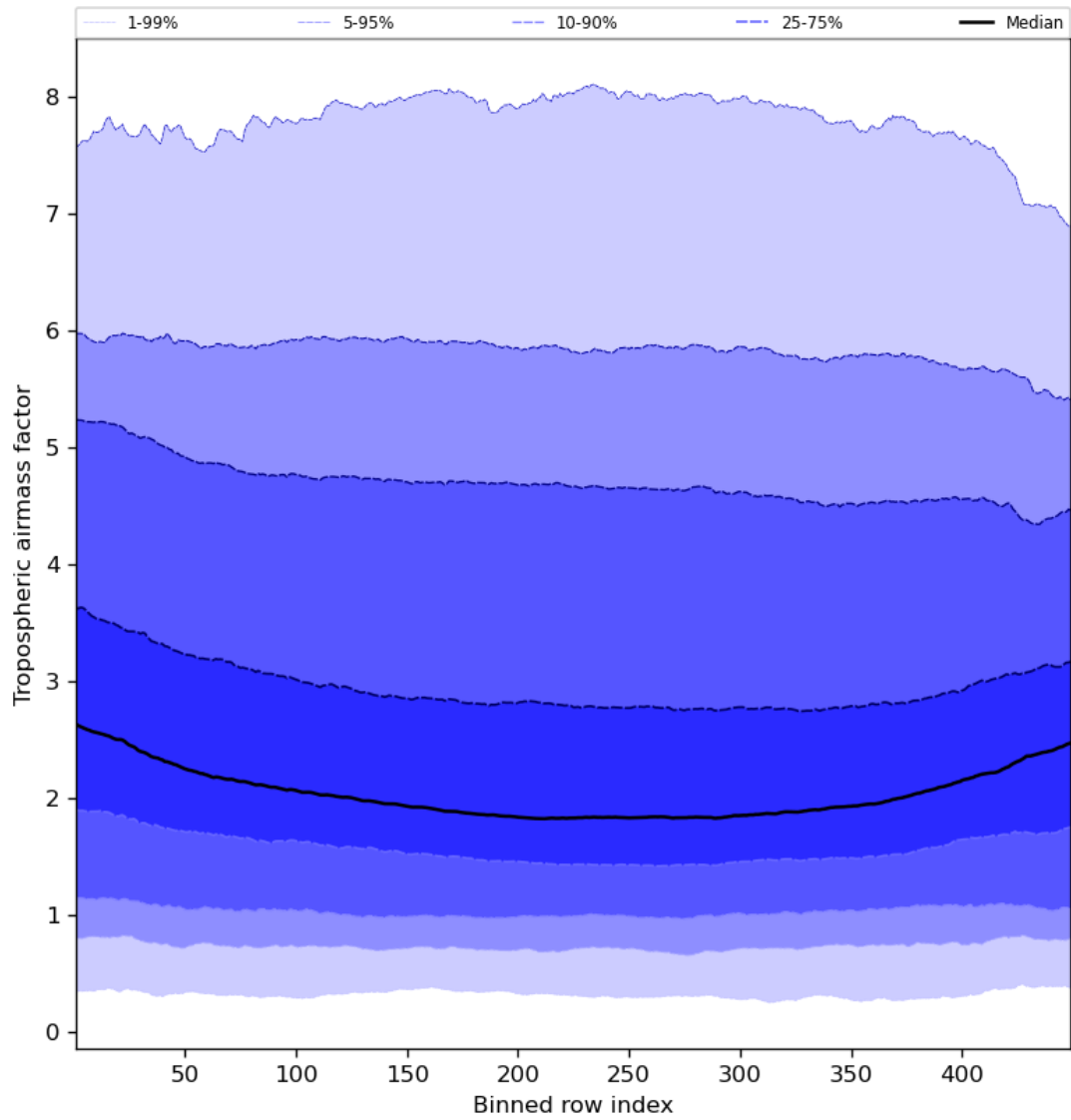
Figure 48: Along track statistics of “Tropospheric air mass factor” for 2023-10-30 to 2023-11-01
