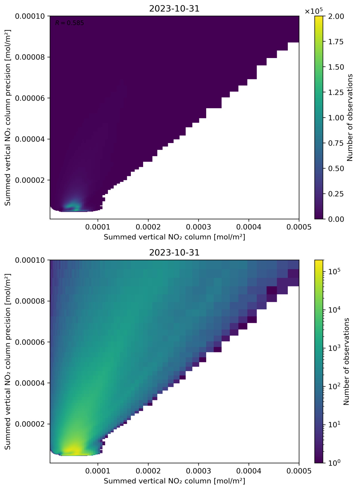
Figure 105: Scatter density plot of “Summed vertical NO 2 column” against “Summed vertical NO 2 column precision” for 2023-10-30 to 2023-11-01.
