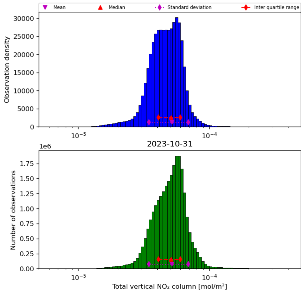
Figure 38: Histogram of “Total vertical NO 2 column” for 2023-10-30 to 2023-11-01
