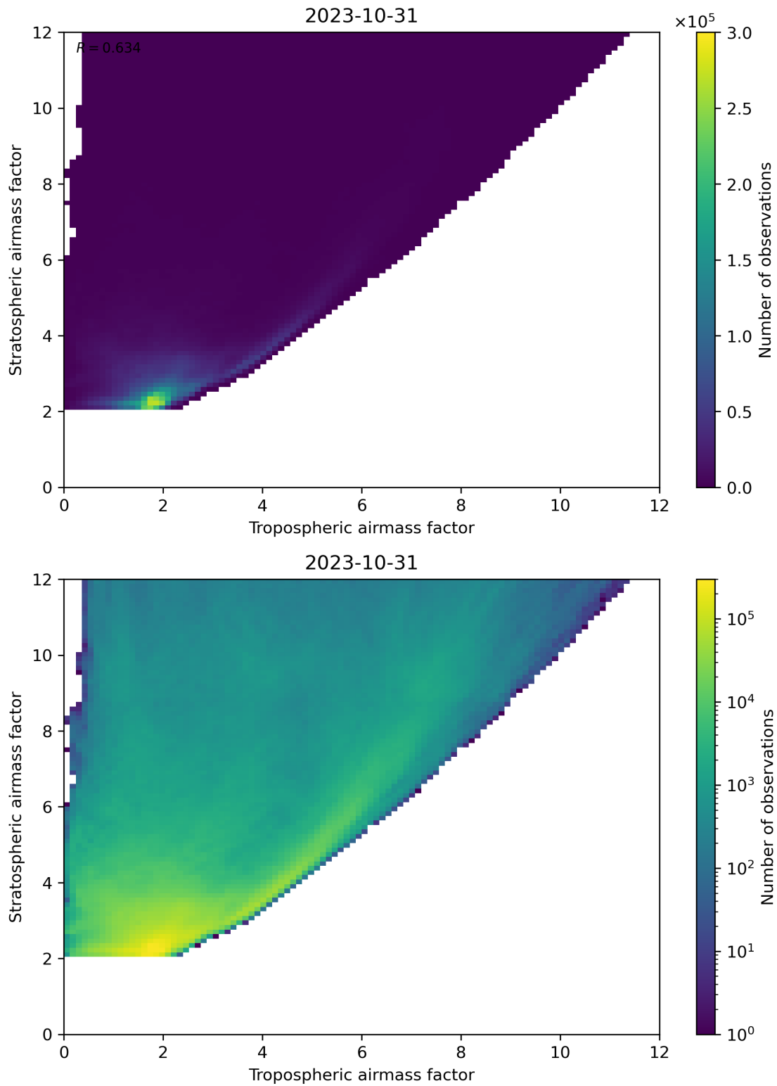
Figure 71: Scatter density plot of “Tropospheric airmass factor” against “Stratospheric airmass factor” for 2023-10-30 to 2023-11-01.
