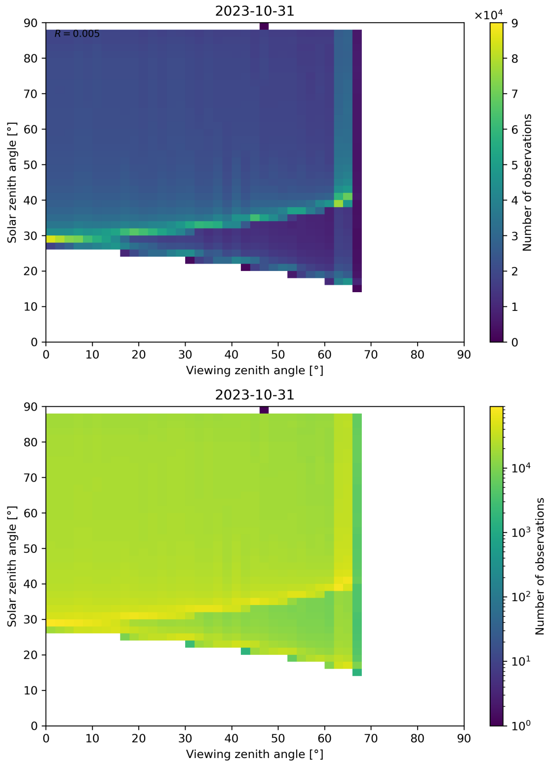
Figure 172: Scatter density plot of “Viewing zenith angle” against “Solar zenith angle” for 2023-10-30 to 2023-11-01.
