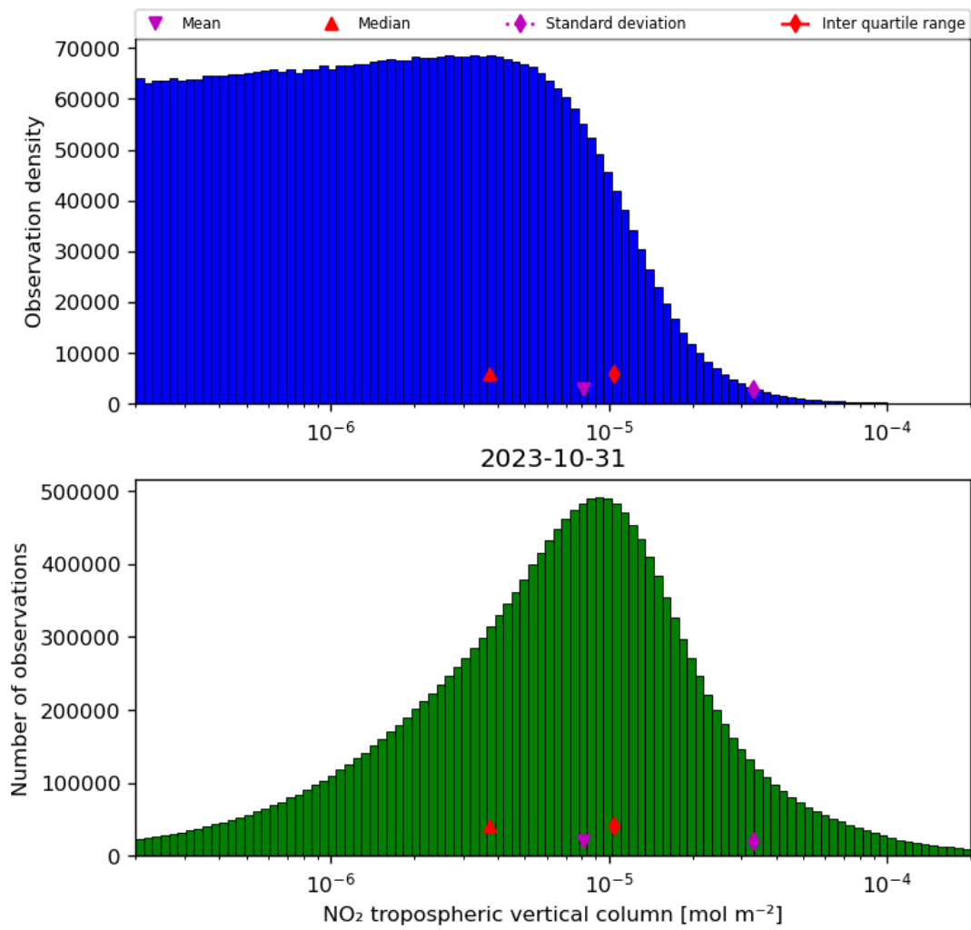
Figure 29: Histogram of “NO 2 tropospheric vertical column” for 2023-10-30 to 2023-11-01
