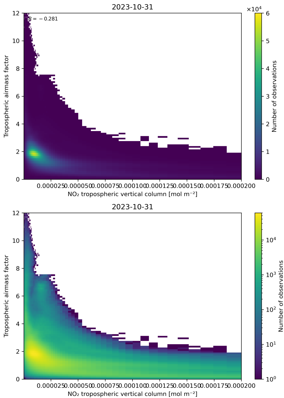
Figure 123: Scatter density plot of “NO 2 tropospheric vertical column” against “Tropospheric air mass factor” for 2023-10-30 to 2023-11-01.
