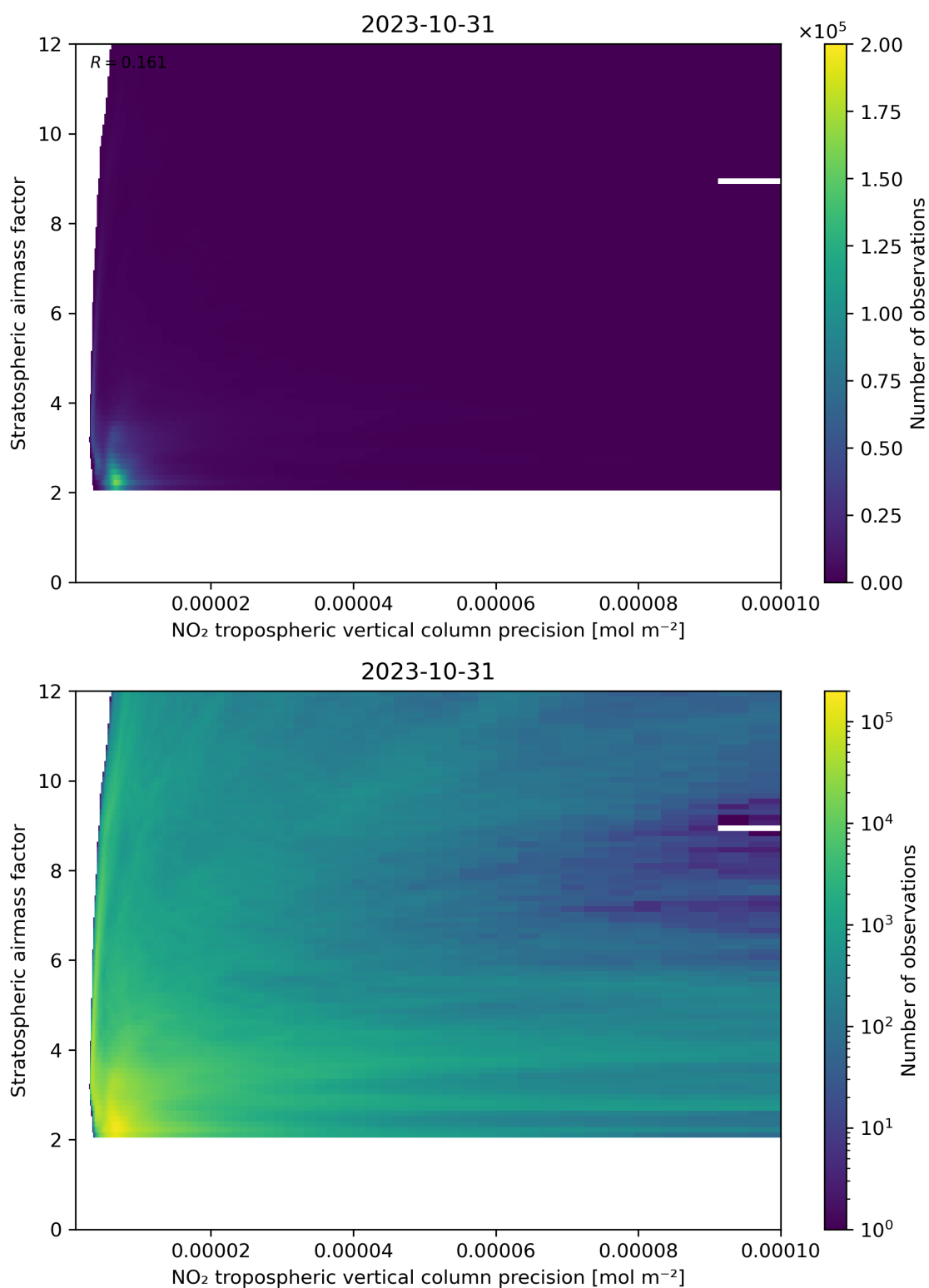
Figure 131: Scatter density plot of “NO 2 tropospheric vertical column precision” against “Stratospheric airmass factor” for 2023-10-30 to 2023-11-01.
