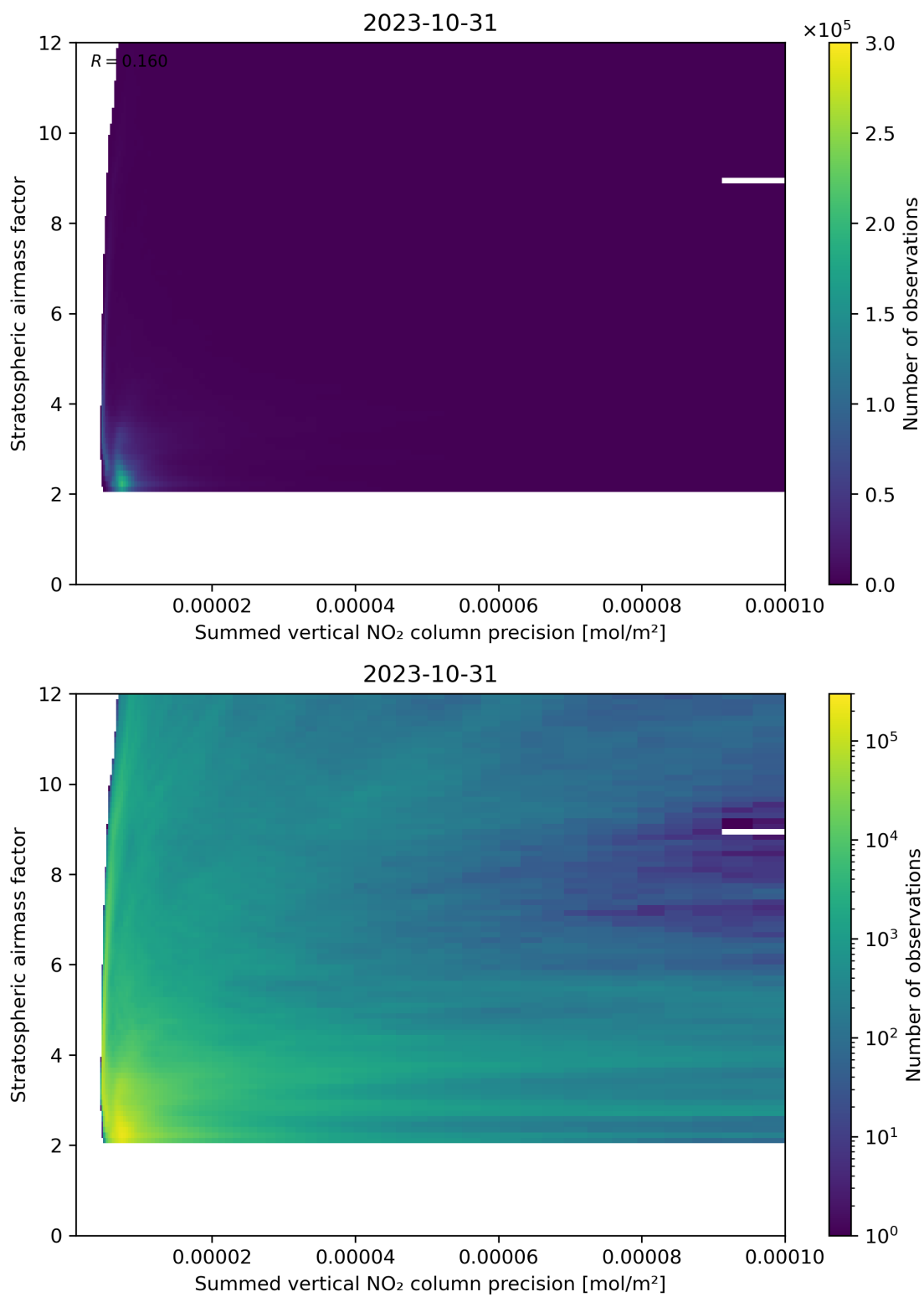
Figure 106: Scatter density plot of “Summed vertical NO 2 column precision” against “Stratospheric airmass factor” for 2023-10-30 to 2023-11-01.
