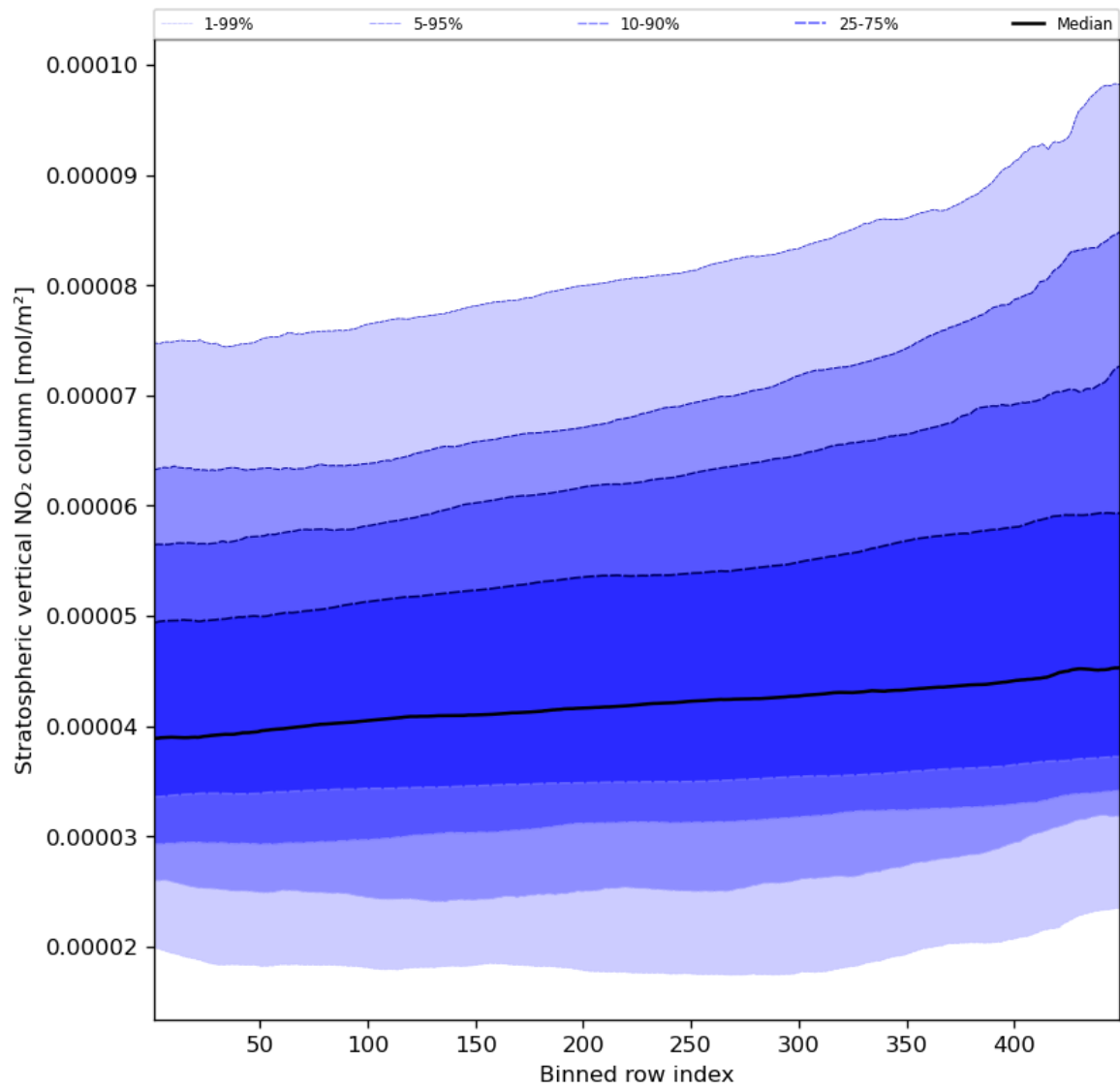
Figure 53: Along track statistics of “Stratospheric vertical NO 2 column” for 2023-10-30 to 2023-11-01
