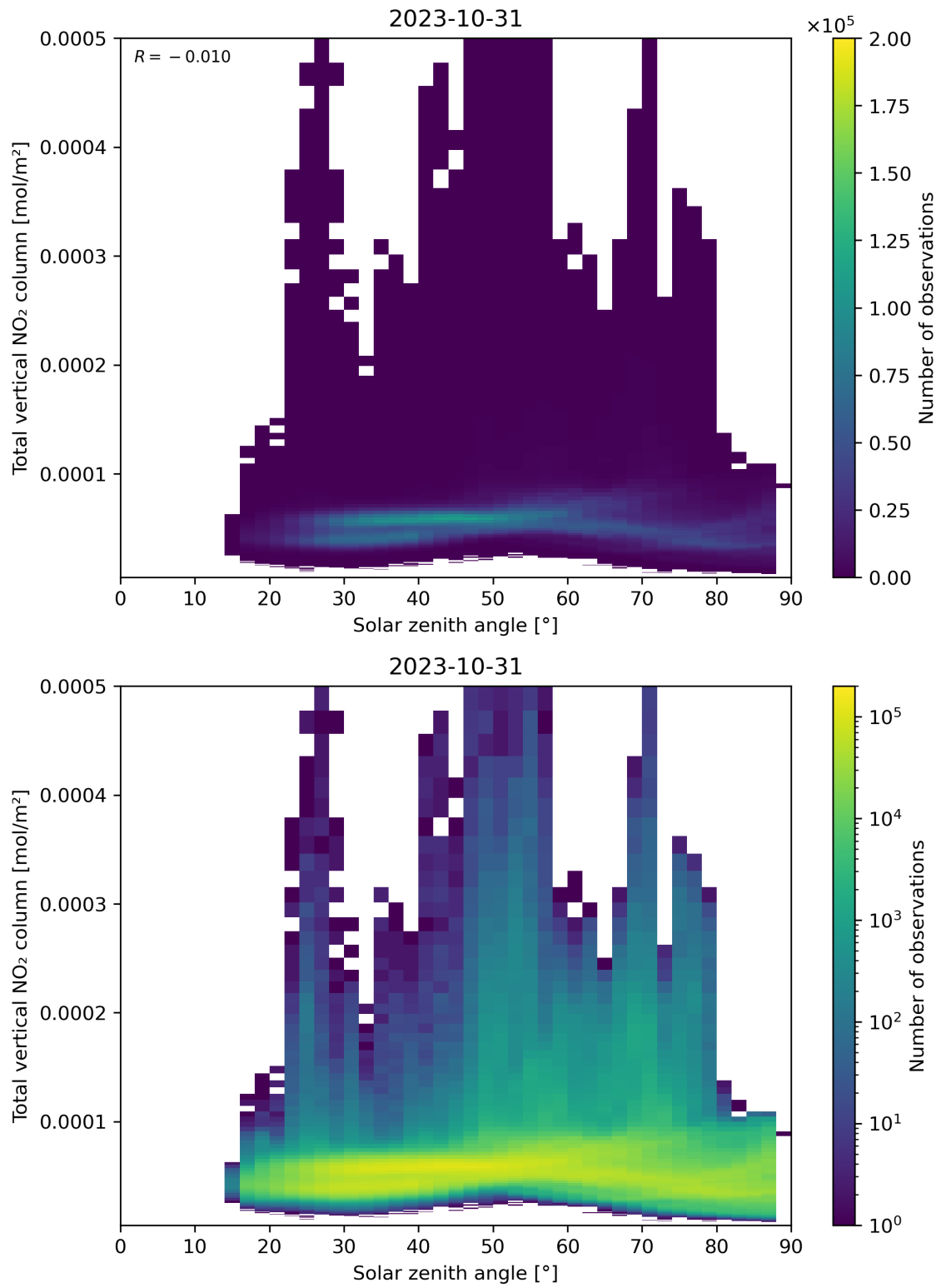
Figure 153: Scatter density plot of “Solar zenith angle” against “Total vertical NO 2 column” for 2023-10-30 to 2023-11-01.
