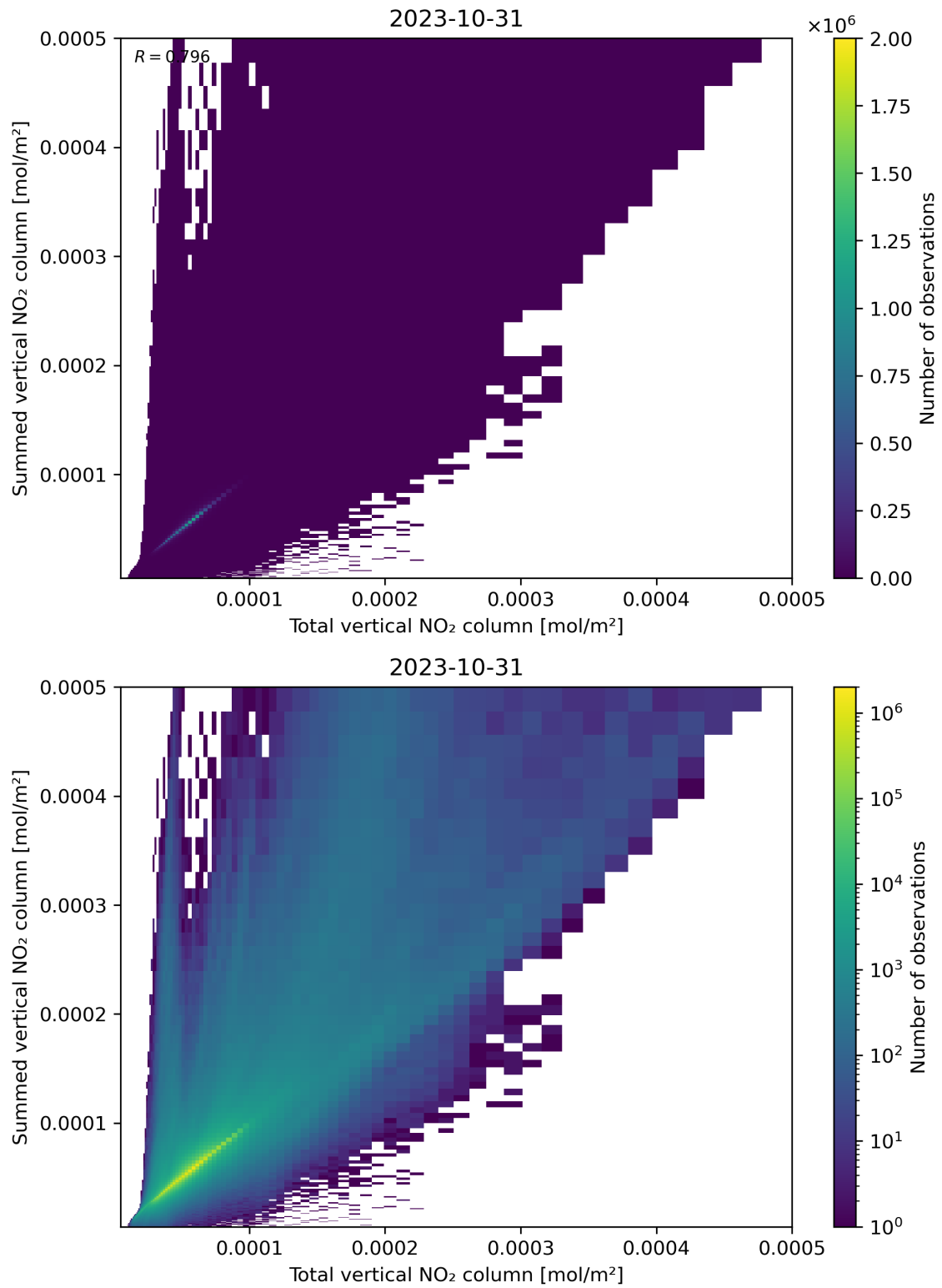
Figure 112: Scatter density plot of “Total vertical NO 2 column” against “Summed vertical NO 2 column” for 2023-10-30 to 2023-11-01.
