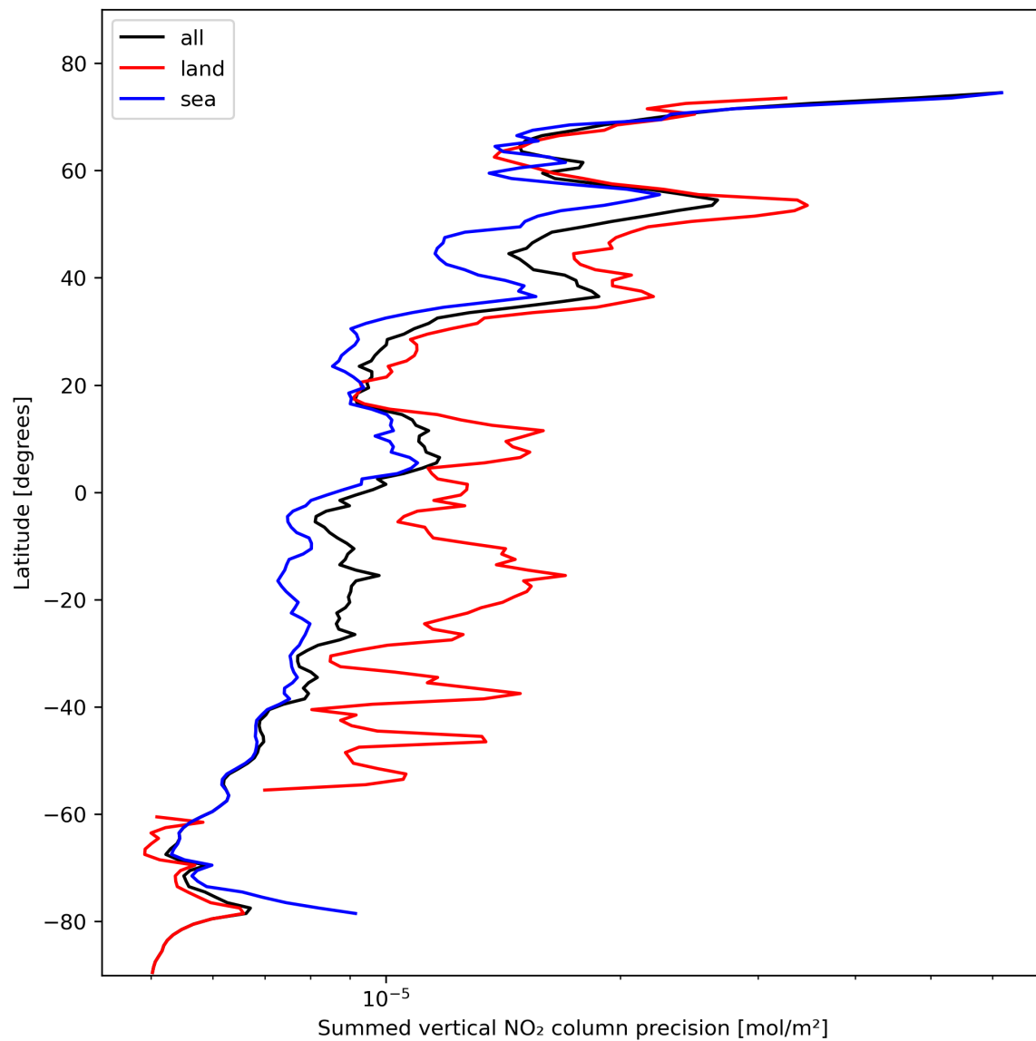
Figure 24: Zonal average of “Summed vertical NO 2 column precision” for 2023-10-30 to 2023-11-01.
