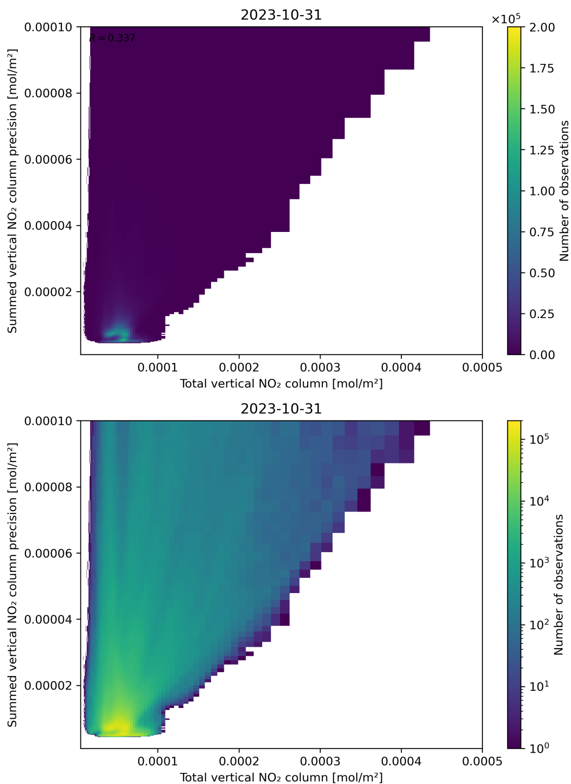
Figure 113: Scatter density plot of “Total vertical NO 2 column” against “Summed vertical NO 2 column precision” for 2023-10-30 to 2023-11-01.
