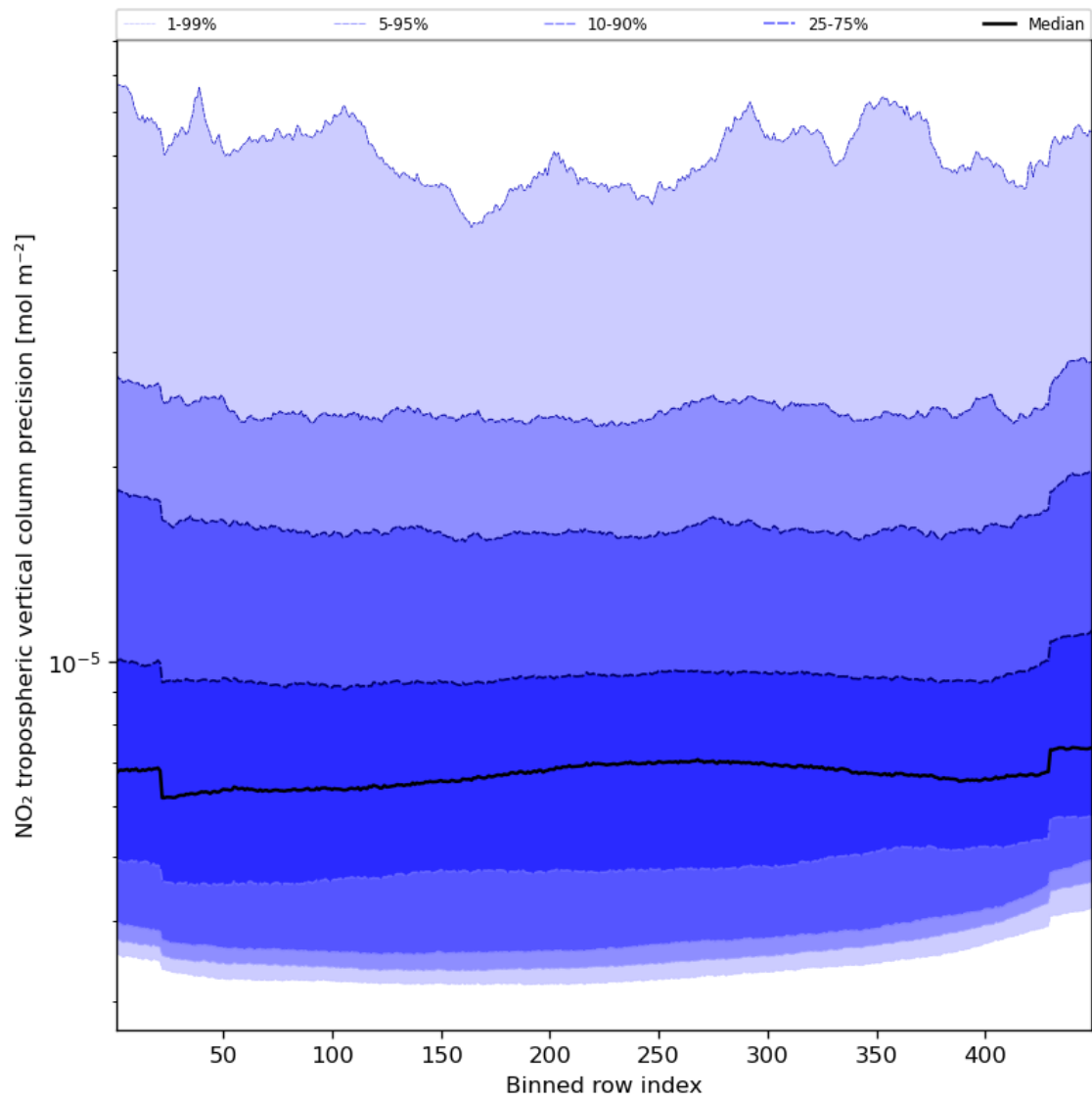
Figure 47: Along track statistics of “NO 2 tropospheric vertical column precision” for 2023-10-30 to 2023-11-01
