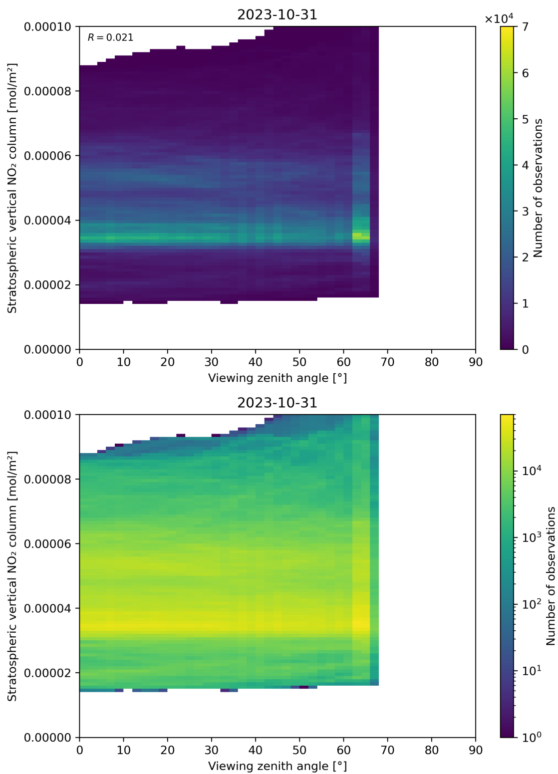
Figure 164: Scatter density plot of “Viewing zenith angle” against “Stratospheric vertical NO 2 column” for 2023-10-30 to 2023-11-01.
