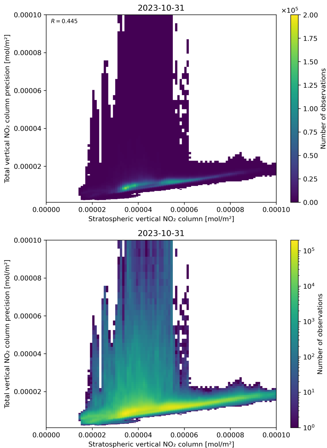
Figure 101: Scatter density plot of “Stratospheric vertical NO 2 column” against “Total vertical NO 2 column precision” for 2023-10-30 to 2023-11-01.
