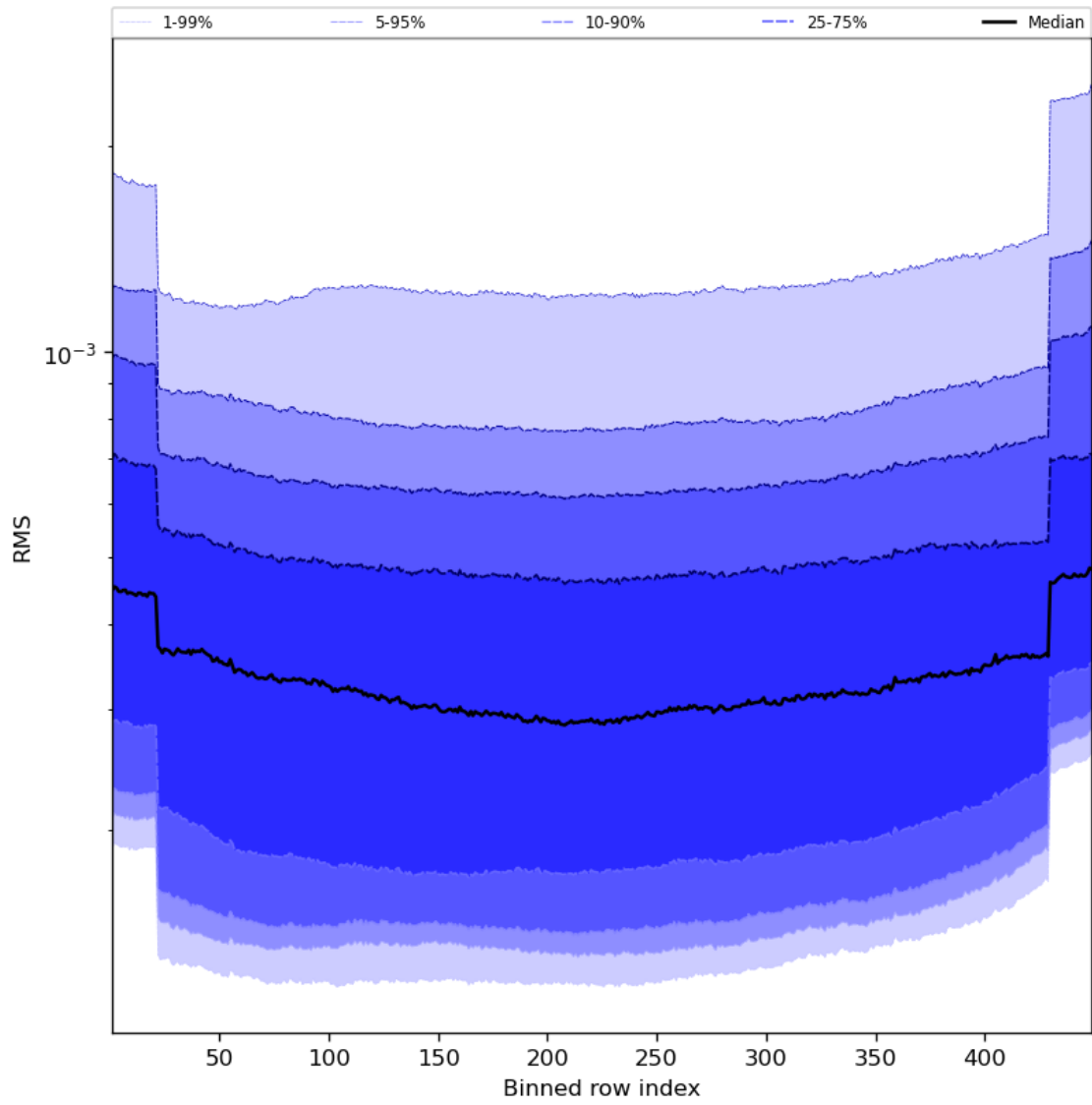
Figure 60: Along track statistics of “RMS” for 2023-10-30 to 2023-11-01
