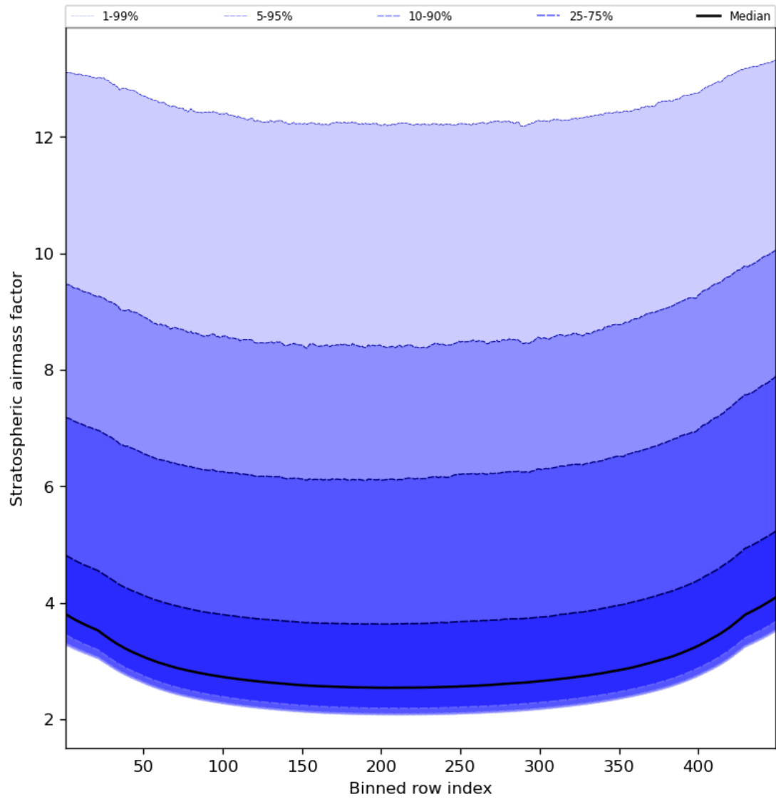
Figure 61: Along track statistics of “Stratospheric airmass factor” for 2023-10-30 to 2023-11-01
