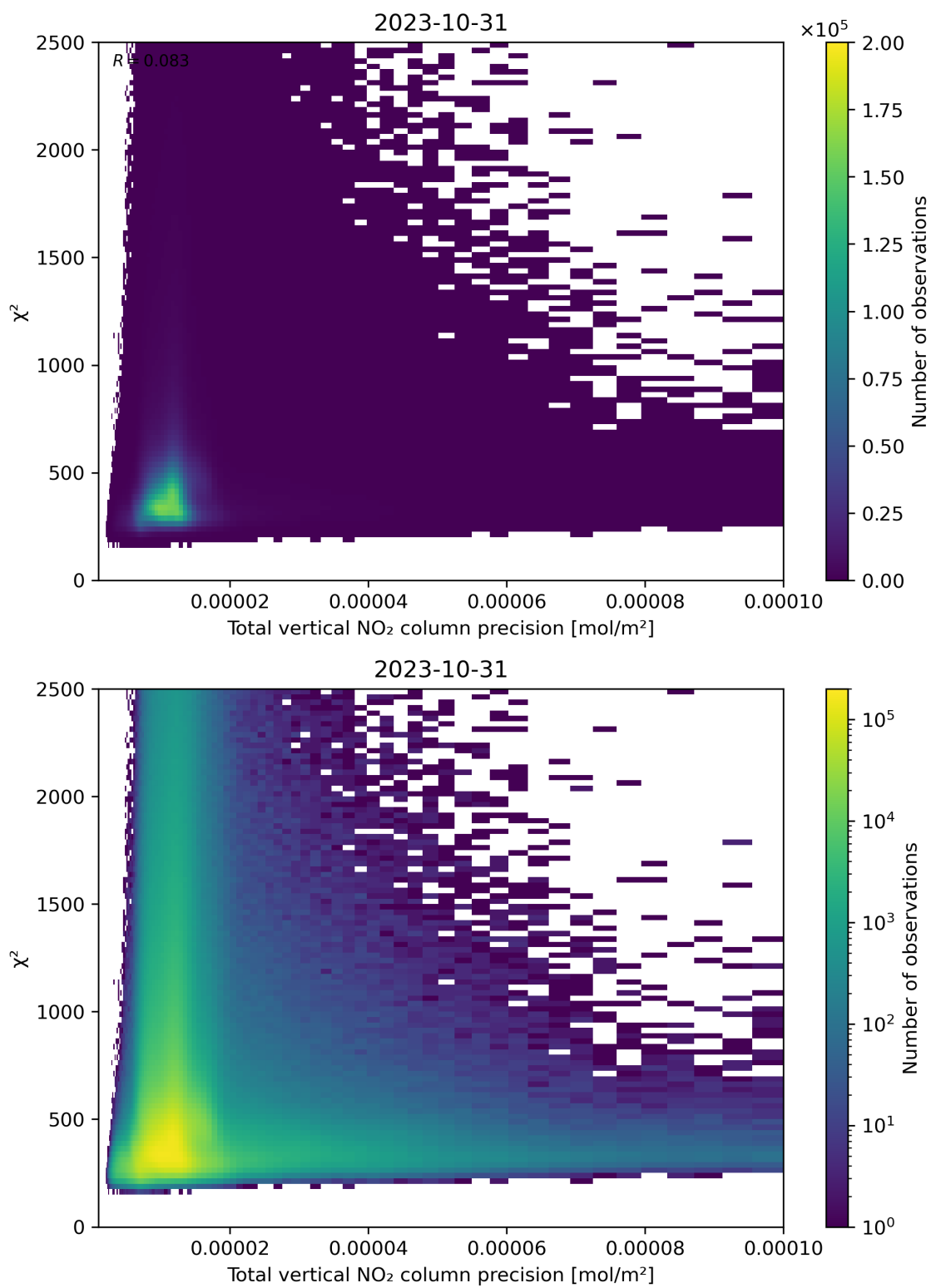
Figure 116: Scatter density plot of “Total vertical NO 2 column precision” against “ \chi^2 ” for 2023-10-30 to 2023-11-01.
