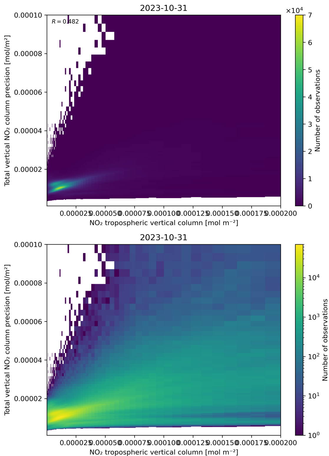
Figure 129: Scatter density plot of “NO 2 tropospheric vertical column” against “Total vertical NO 2 column precision” for 2023-10-30 to 2023-11-01.
