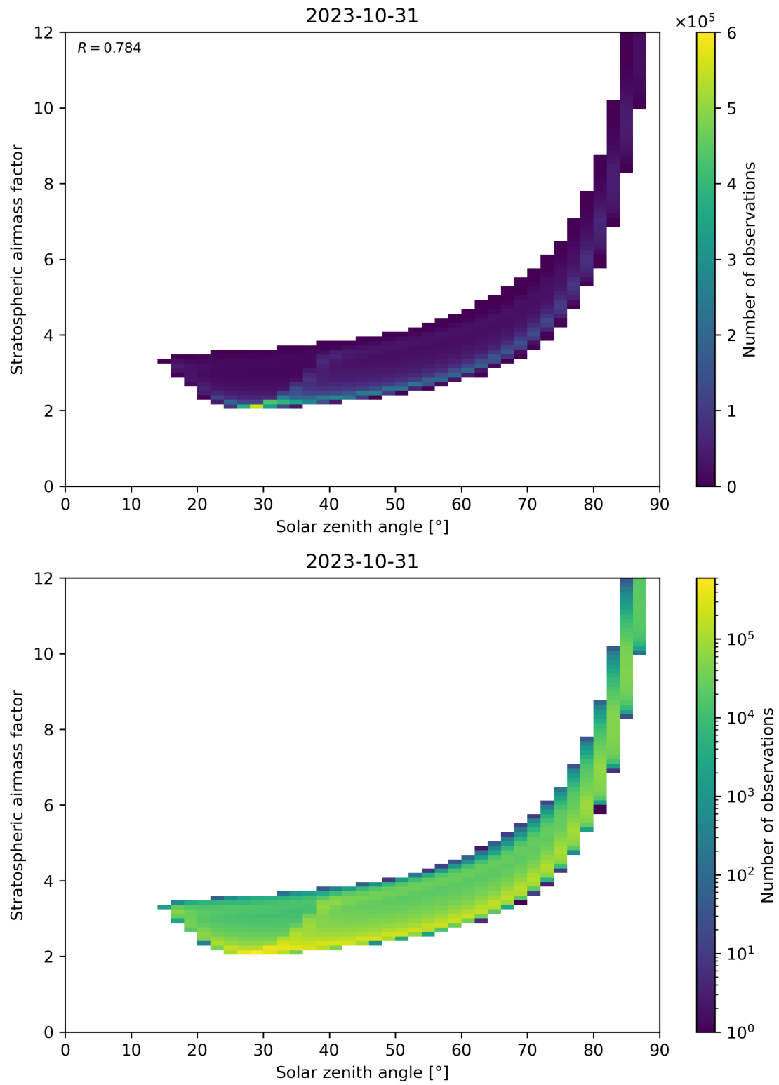
Figure 145: Scatter density plot of “Solar zenith angle” against “Stratospheric airmass factor” for 2023-10-30 to 2023-11-01.
