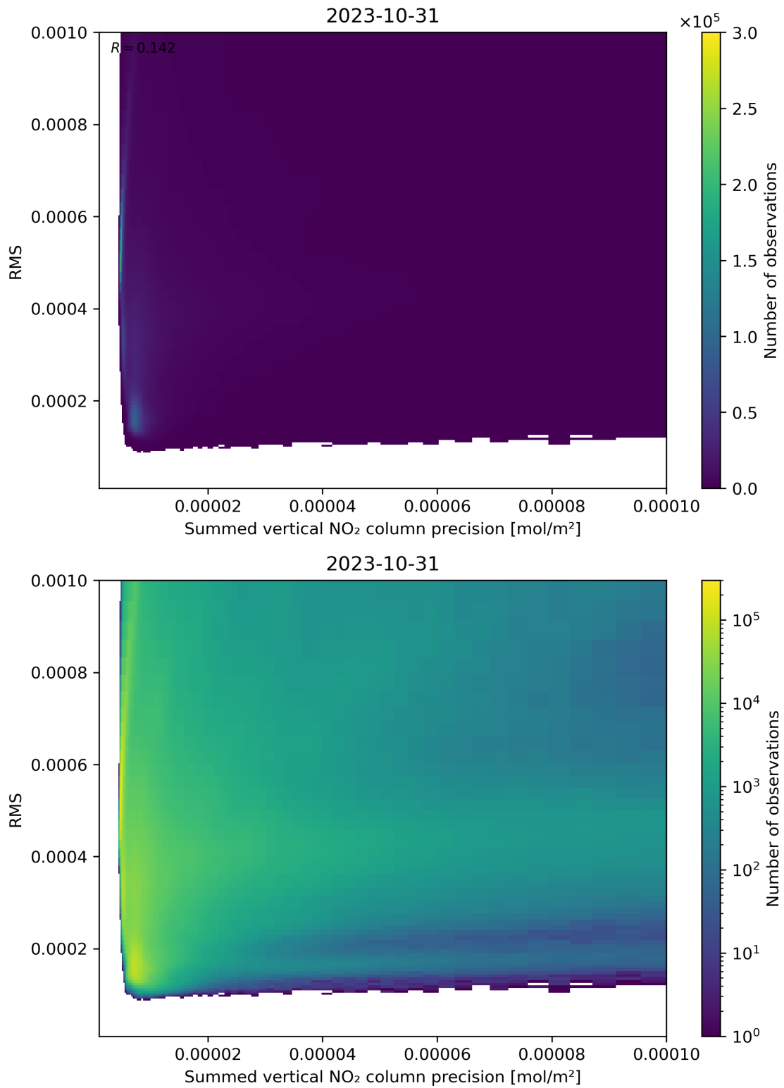
Figure 108: Scatter density plot of “Summed vertical NO 2 column precision” against “RMS” for 2023-10-30 to 2023-11-01.
