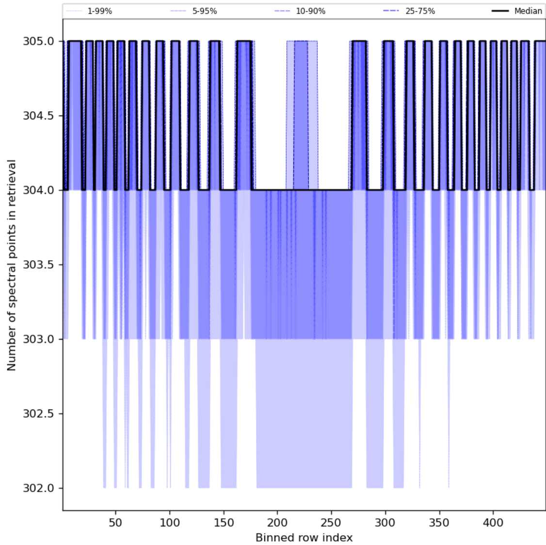
Figure 50: Along track statistics of “Number of spectral points in retrieval” for 2023-10-30 to 2023-11-01
