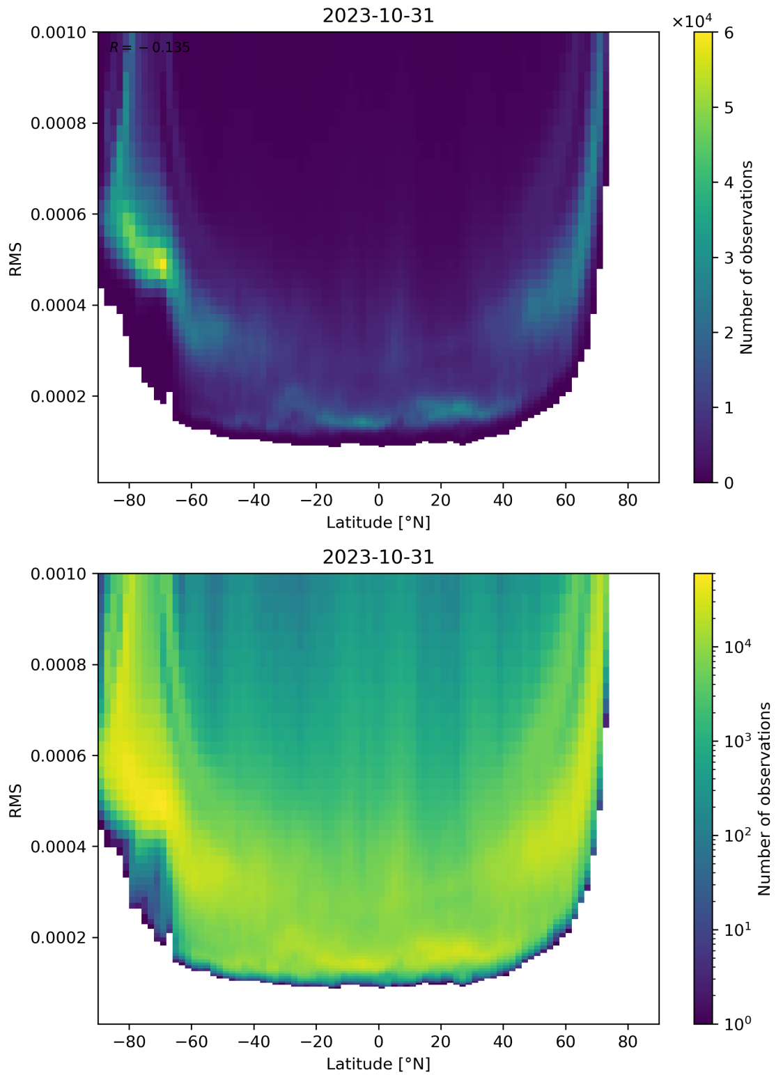
Figure 94: Scatter density plot of “Latitude” against “RMS” for 2023-10-30 to 2023-11-01.
