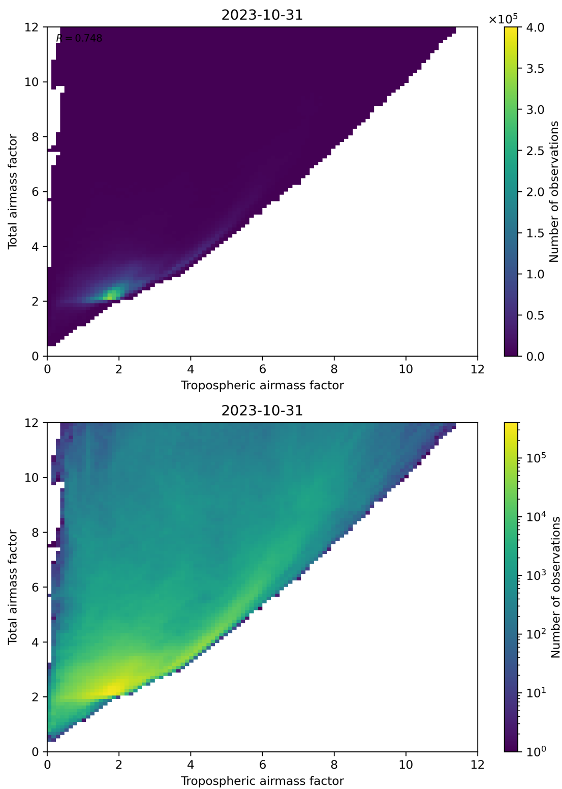
Figure 72: Scatter density plot of “Tropospheric airmass factor” against “Total airmass factor” for 2023-10-30 to 2023-11-01.
