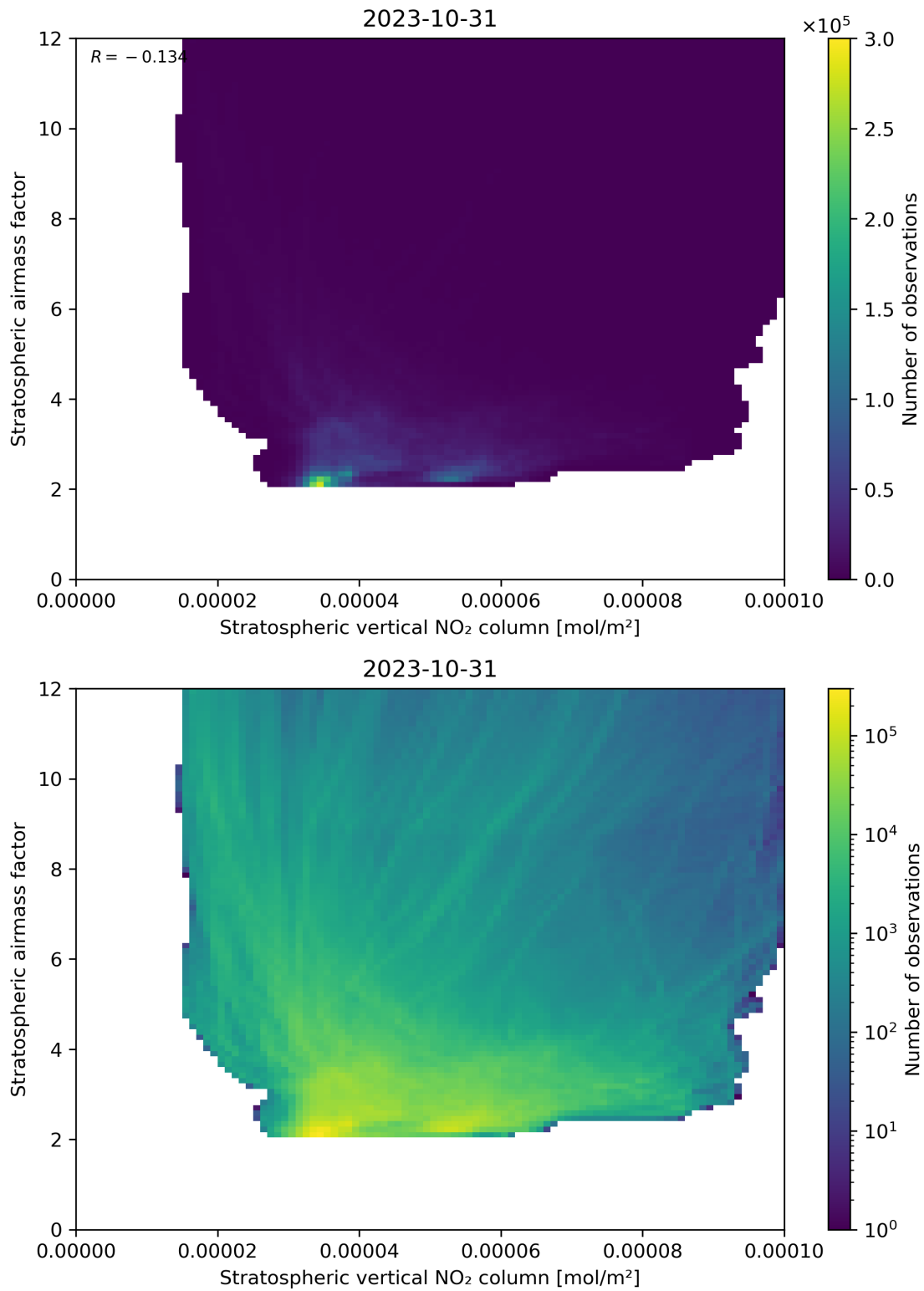
Figure 96: Scatter density plot of “Stratospheric vertical NO 2 column” against “Stratospheric airmass factor” for 2023-10-30 to 2023-11-01.
