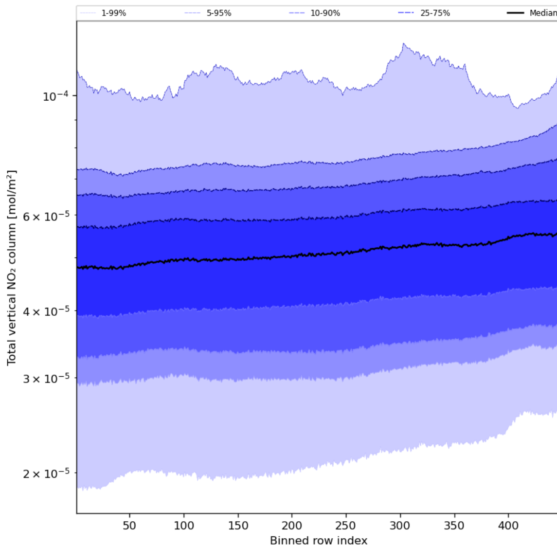
Figure 55: Along track statistics of “Total vertical NO 2 column” for 2023-10-30 to 2023-11-01
