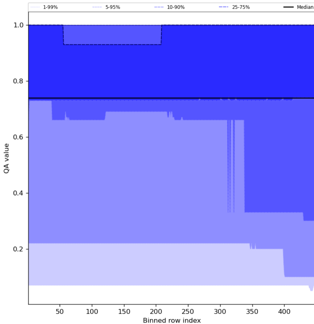
Figure 45: Along track statistics of “QA value” for 2023-10-30 to 2023-11-01
