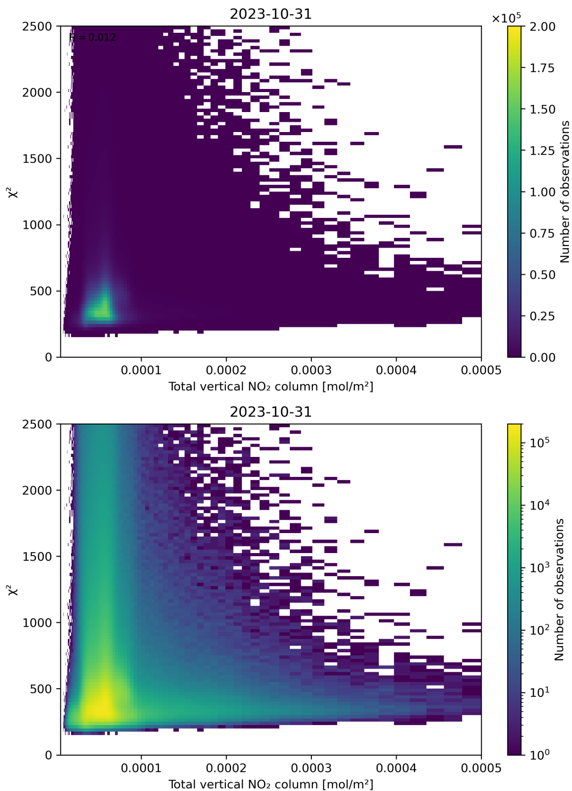
Figure 111: Scatter density plot of “Total vertical NO 2 column” against “ \chi^2 ” for 2023-10-30 to 2023-11-01.
