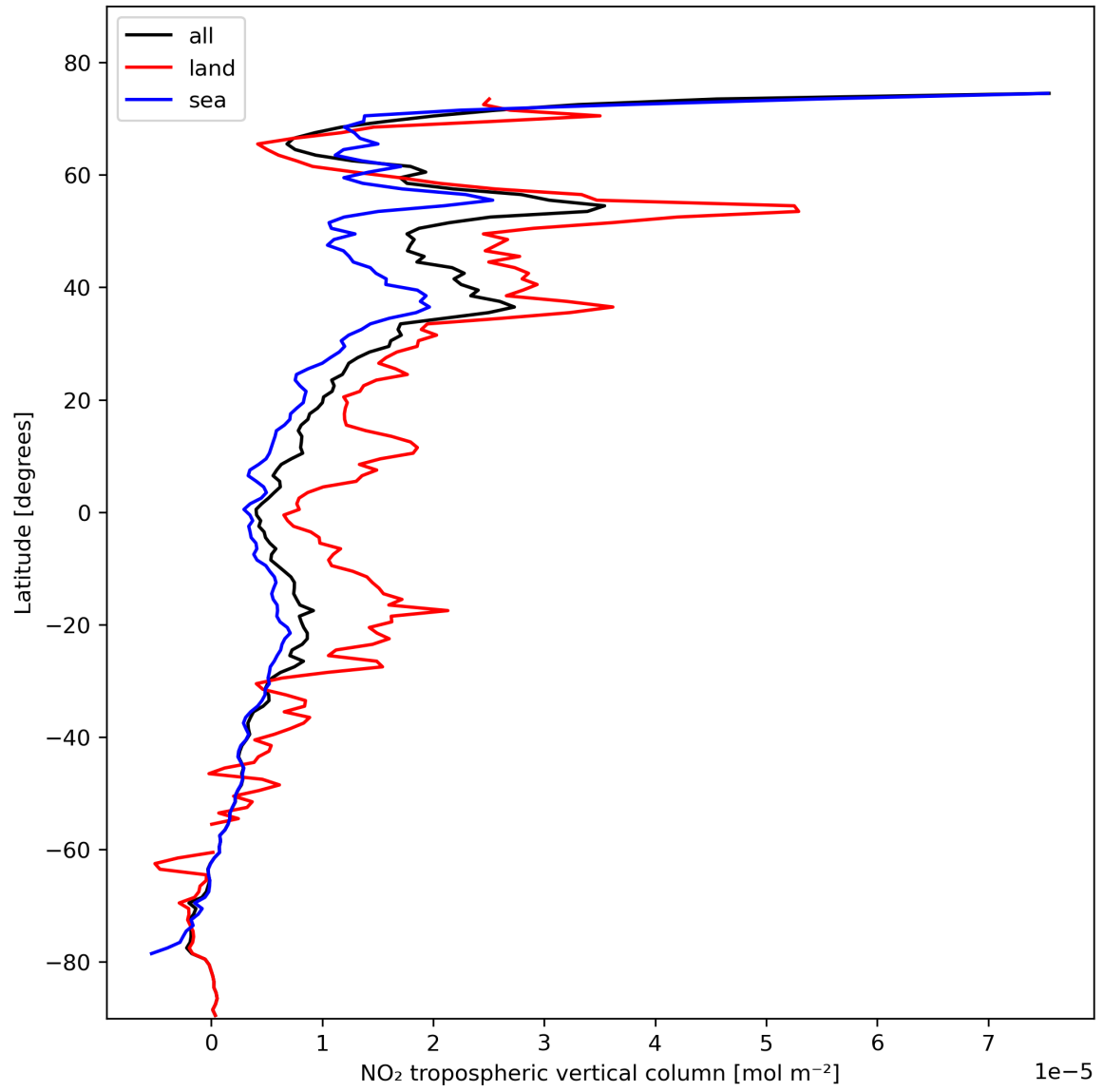
Figure 12: Zonal average of “NO 2 tropospheric vertical column” for 2023-10-30 to 2023-11-01.
