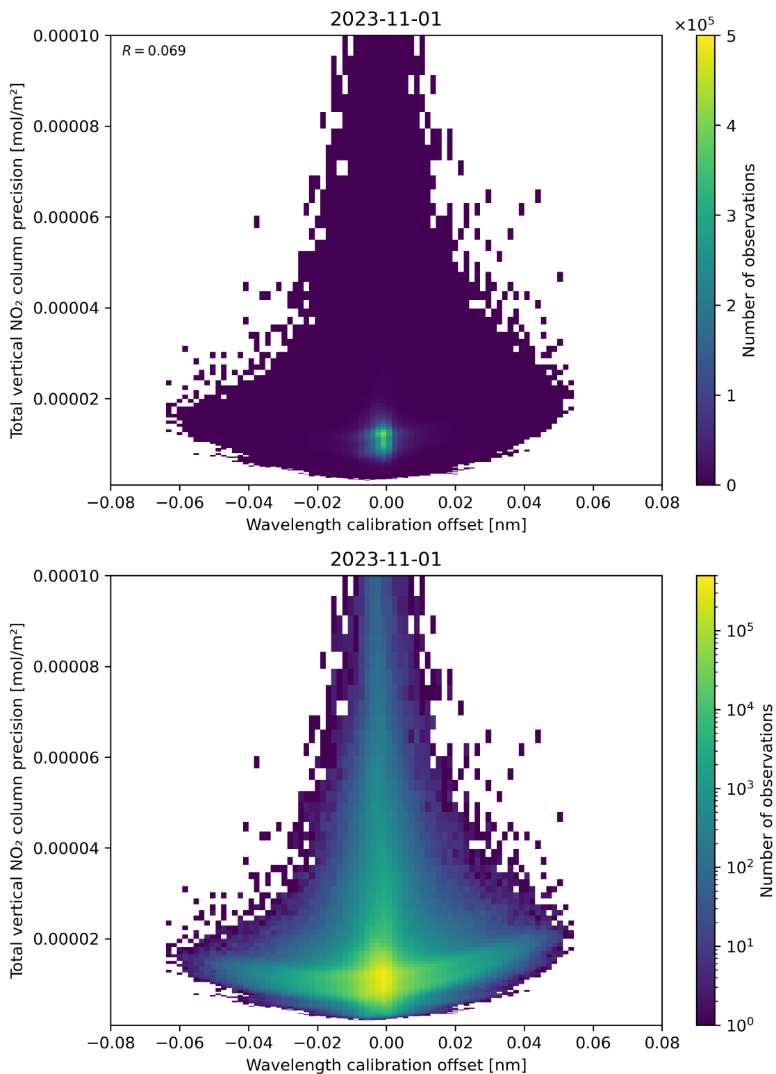
Figure 180: Scatter density plot of “Wavelength calibration offset” against “Total vertical NO 2 column precision” for 2023-10-31 to 2023-11-02.
