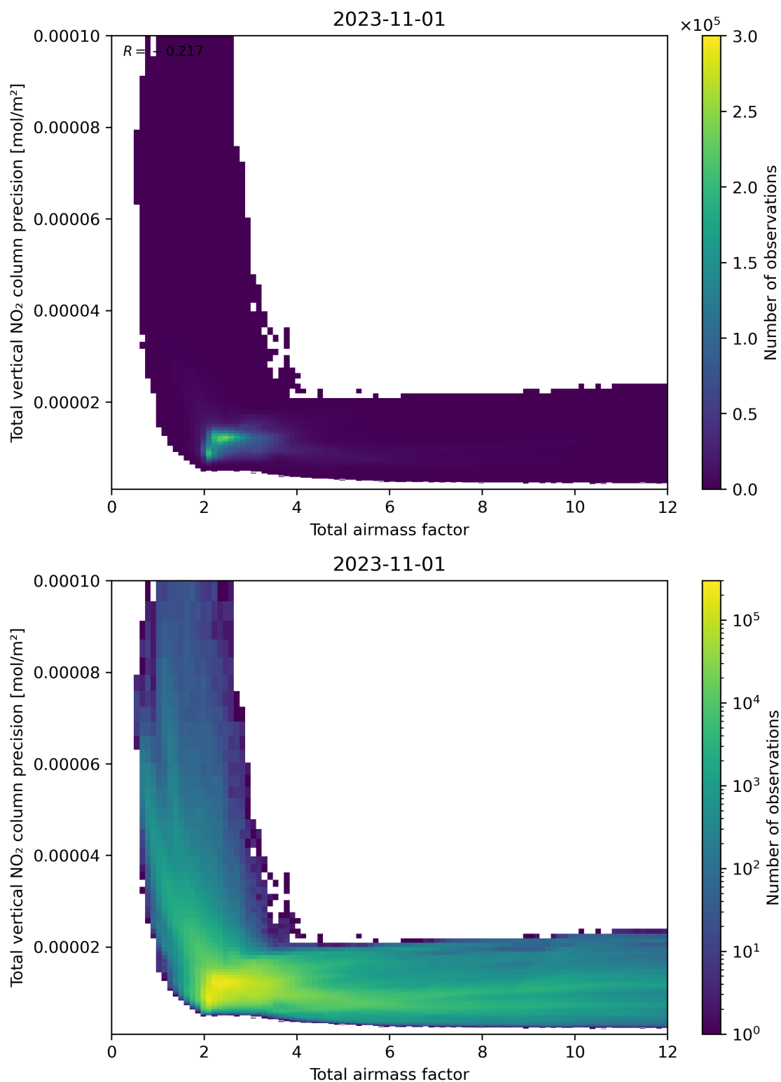
Figure 68: Scatter density plot of “Total airmass factor” against “Total vertical NO 2 column precision” for 2023-10-31 to 2023-11-02.
