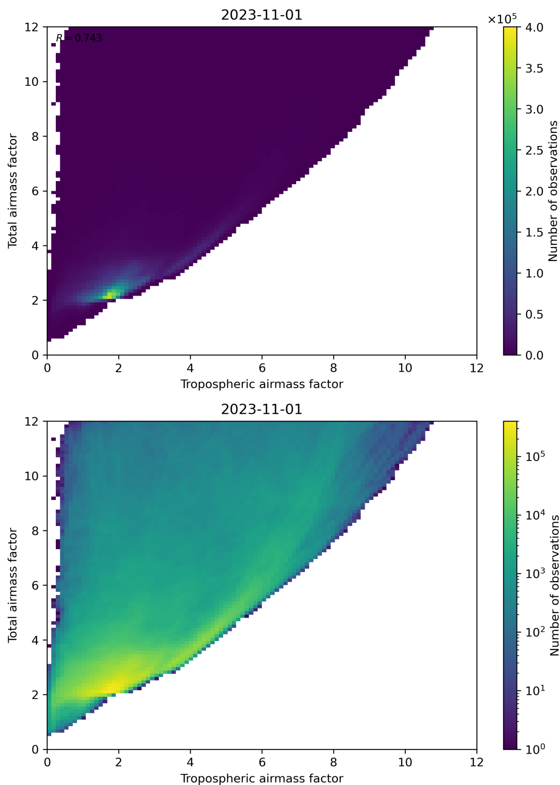
Figure 72: Scatter density plot of “Tropospheric airmass factor” against “Total airmass factor” for 2023-10-31 to 2023-11-02.
