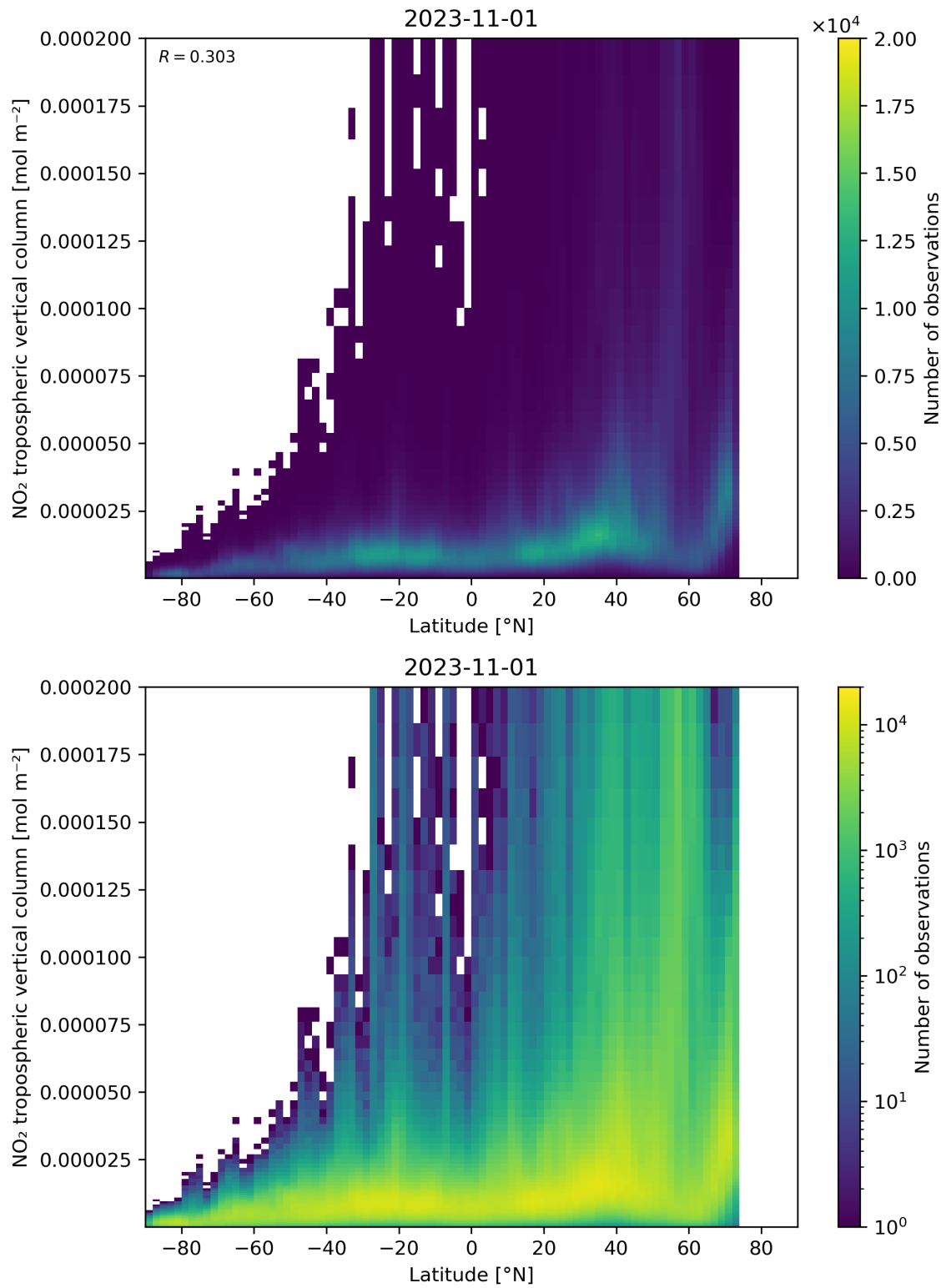
Figure 92: Scatter density plot of “Latitude” against “NO 2 tropospheric vertical column” for 2023-10-31 to 2023-11-02.
