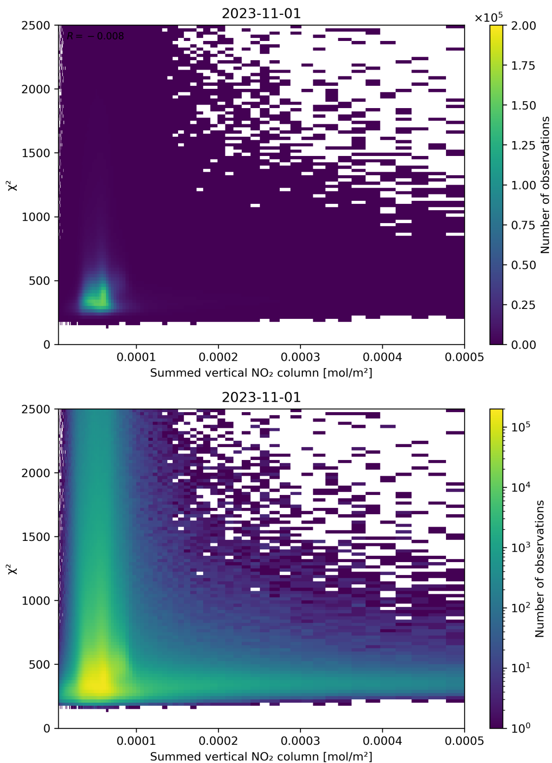
Figure 104: Scatter density plot of “Summed vertical NO 2 column” against “ \chi^2 ” for 2023-10-31 to 2023-11-02.
