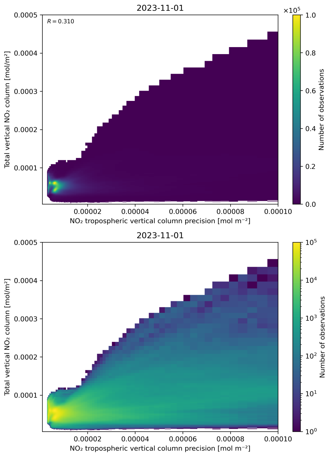
Figure 138: Scatter density plot of “NO 2 tropospheric vertical column precision” against “Total vertical NO 2 column” for 2023-10-31 to 2023-11-02.
