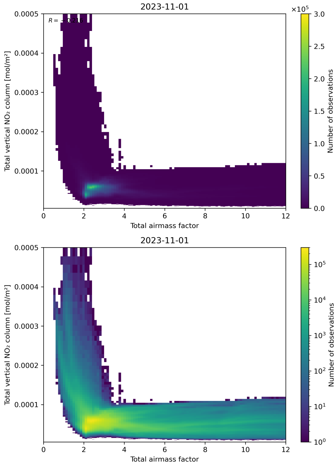
Figure 67: Scatter density plot of “Total airmass factor” against “Total vertical NO 2 column” for 2023-10-31 to 2023-11-02.
