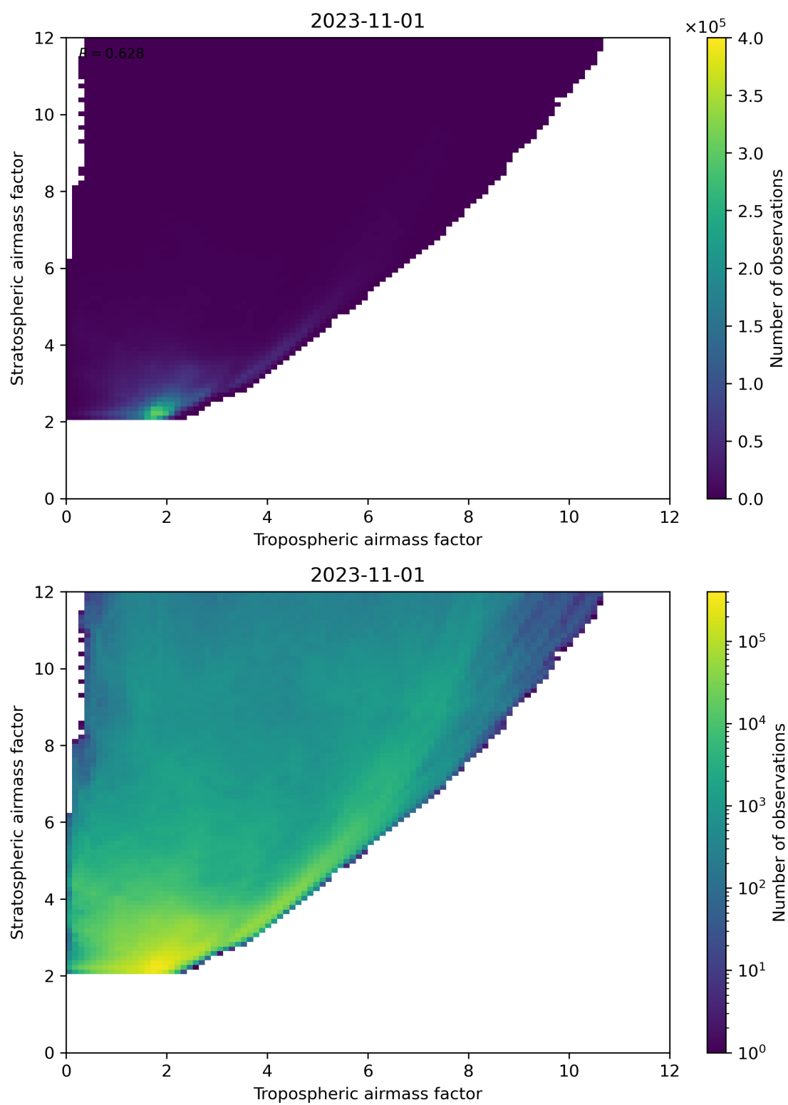
Figure 71: Scatter density plot of “Tropospheric airmass factor” against “Stratospheric airmass factor” for 2023-10-31 to 2023-11-02.
