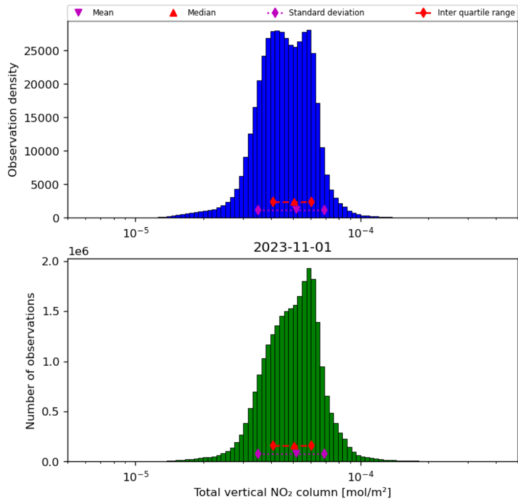
Figure 38: Histogram of "Total vertical NO 2 column" for 2023-10-31 to 2023-11-02
