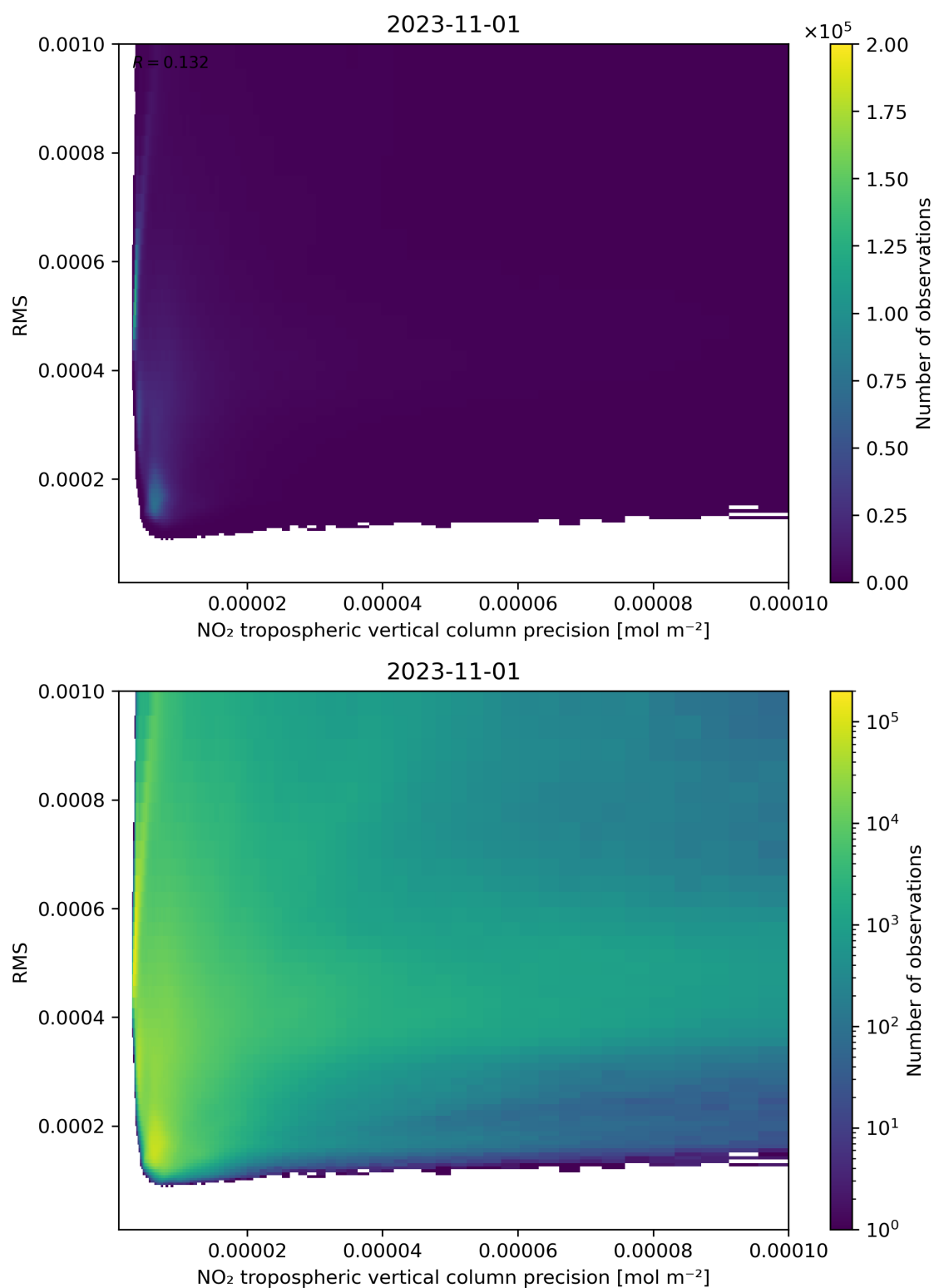
Figure 140: Scatter density plot of “NO 2 tropospheric vertical column precision” against “RMS” for 2023-10-31 to 2023-11-02.
