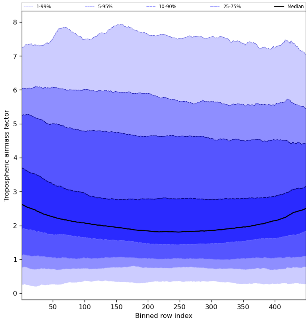
Figure 48: Along track statistics of “Tropospheric airmass factor” for 2023-10-31 to 2023-11-02
