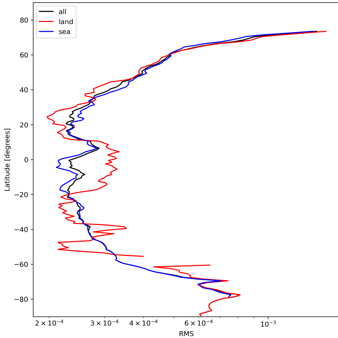
Figure 26: Zonal average of “RMS” for 2023-10-31 to 2023-11-02.
