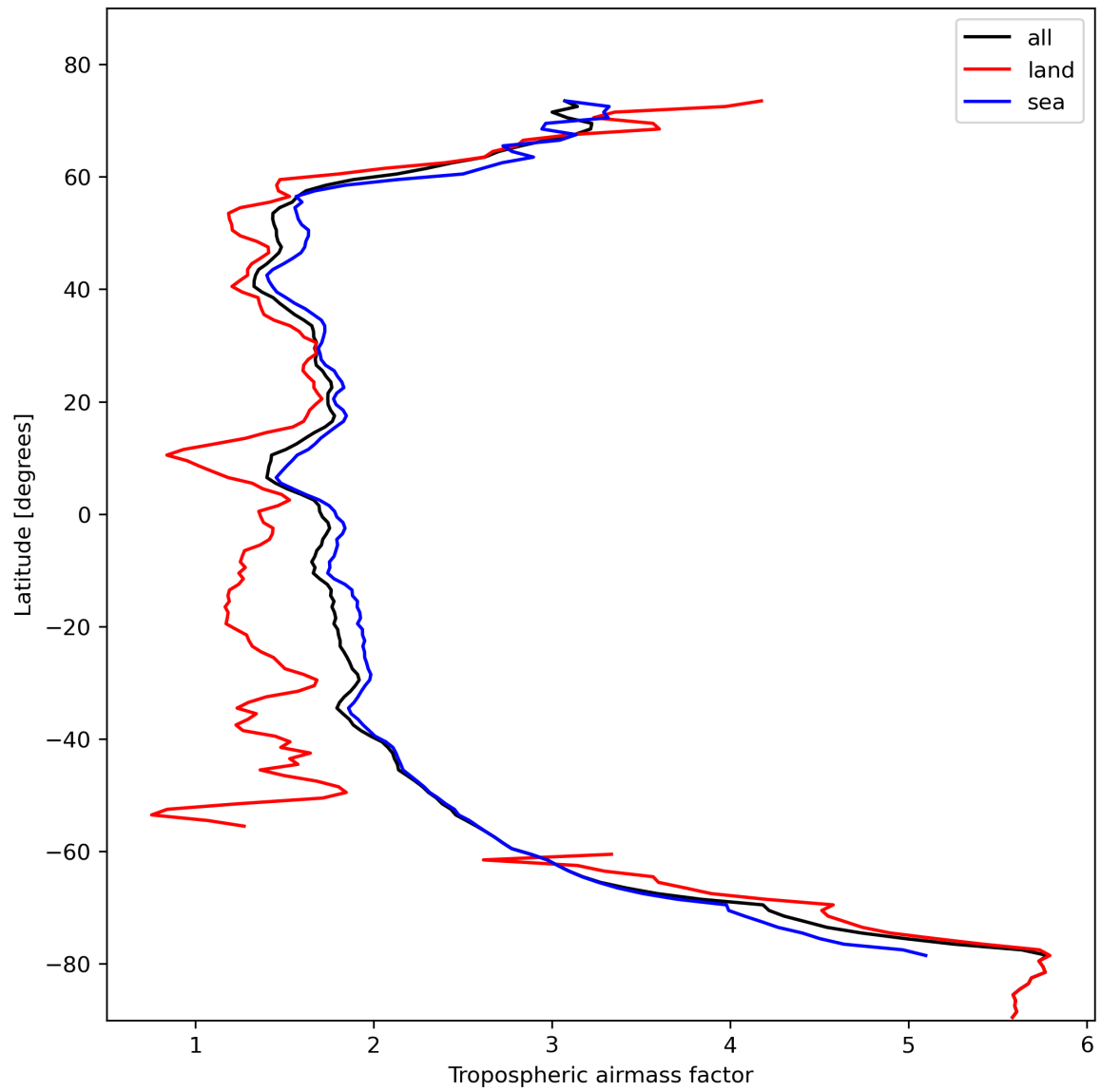
Figure 14: Zonal average of “Tropospheric airmass factor” for 2023-10-31 to 2023-11-02.
