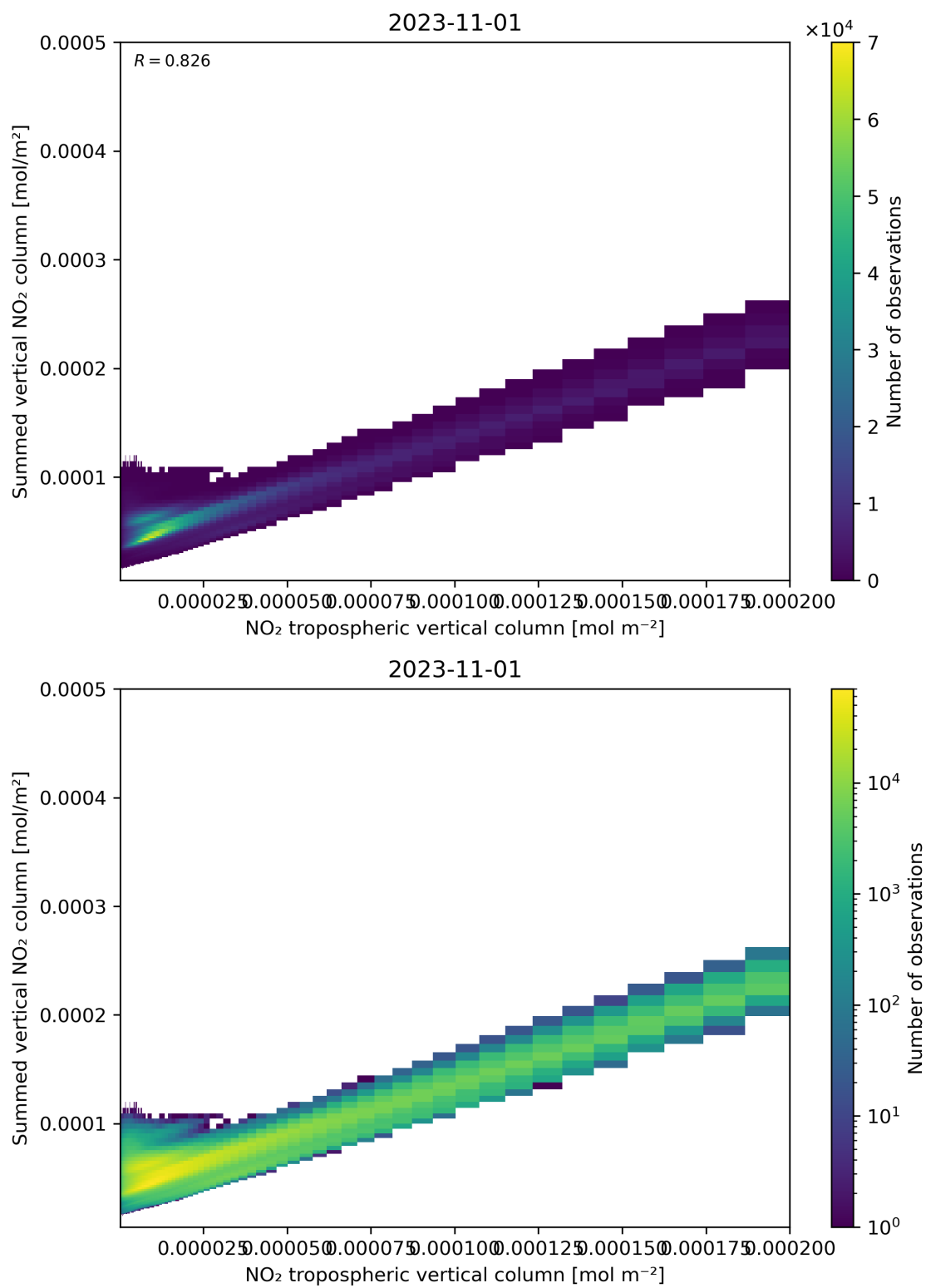
Figure 126: Scatter density plot of “NO 2 tropospheric vertical column” against “Summed vertical NO 2 column” for 2023-10-31 to 2023-11-02.
