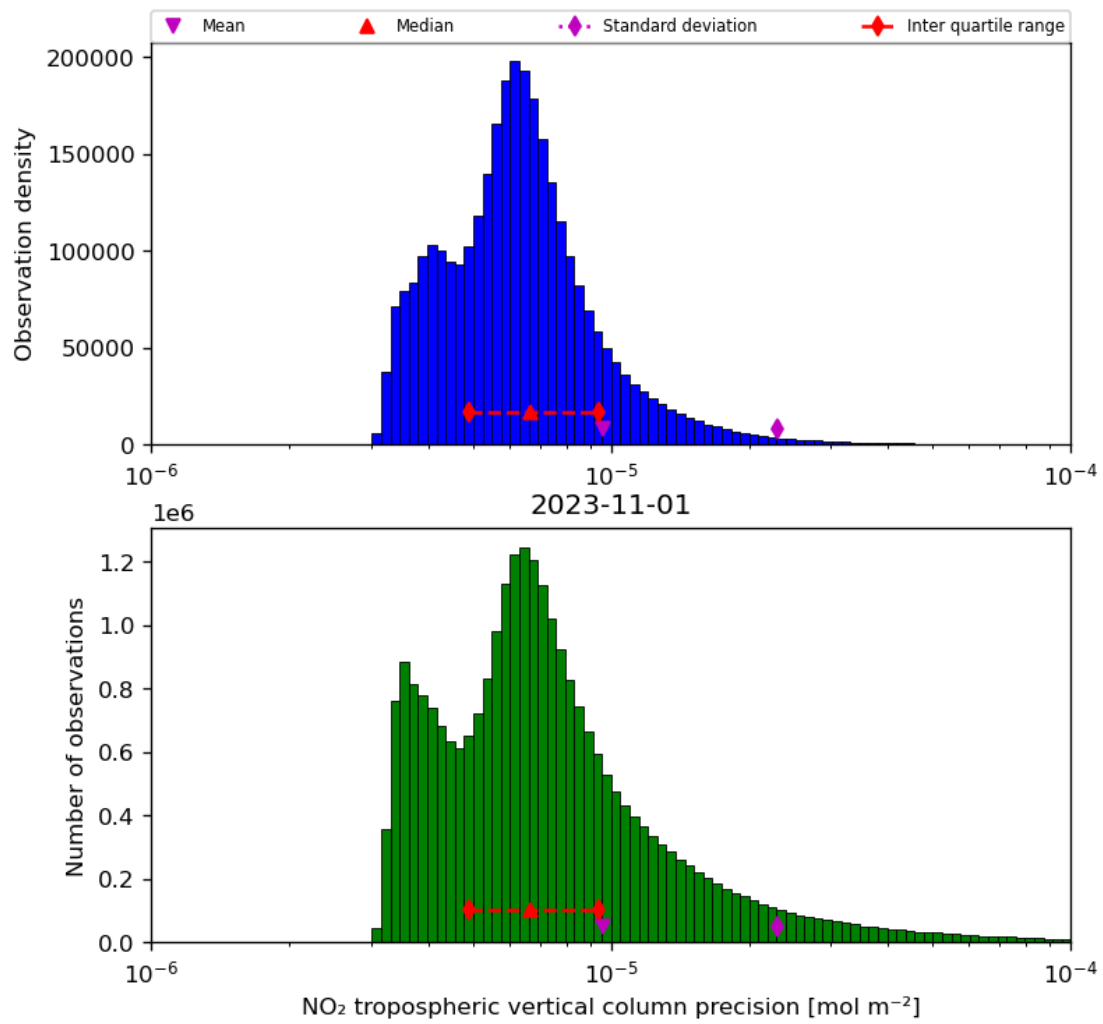
Figure 30: Histogram of “NO 2 tropospheric vertical column precision” for 2023-10-31 to 2023-11-02
