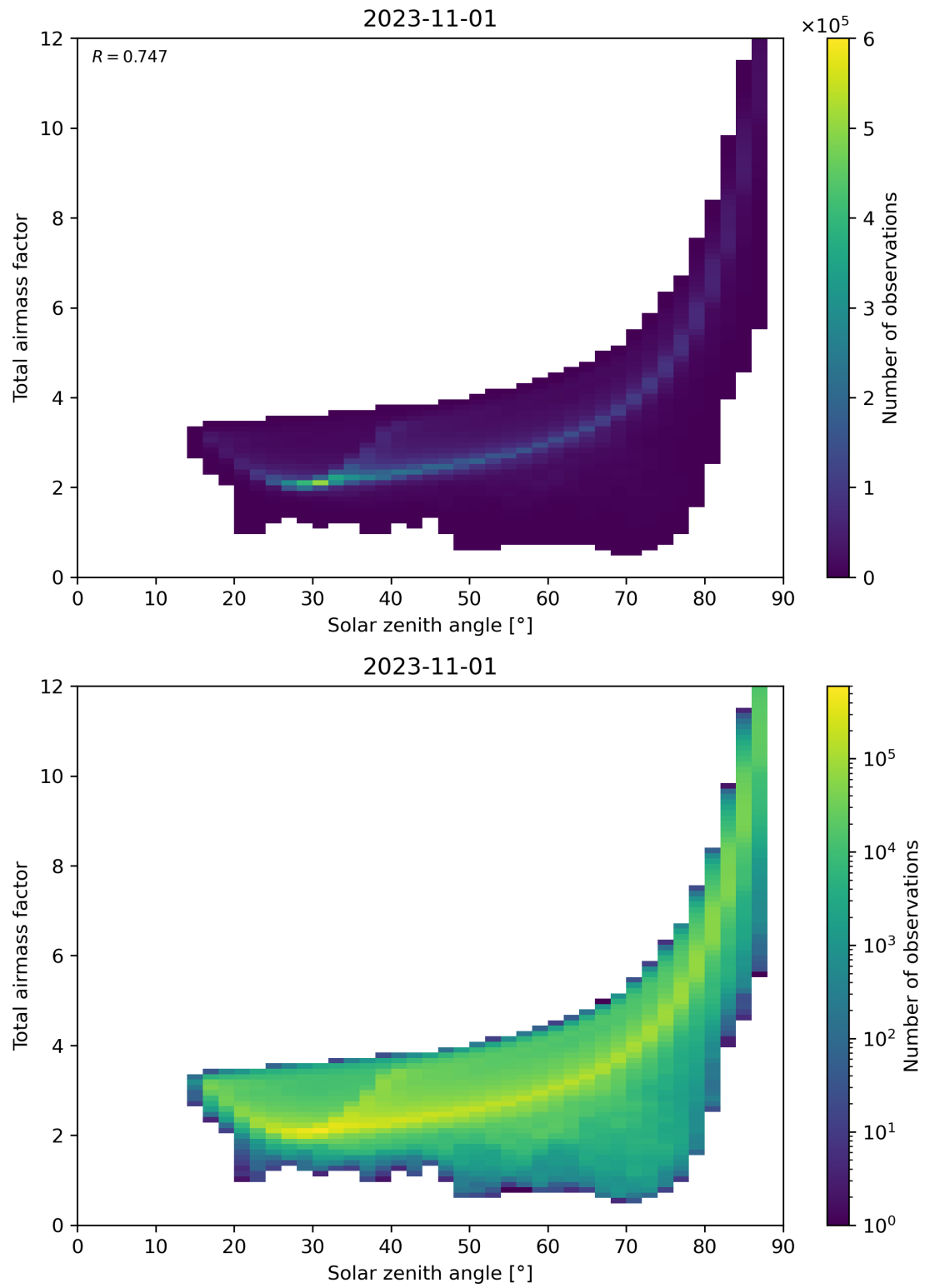
Figure 146: Scatter density plot of “Solar zenith angle” against “Total airmass factor” for 2023-10-31 to 2023-11-02.
