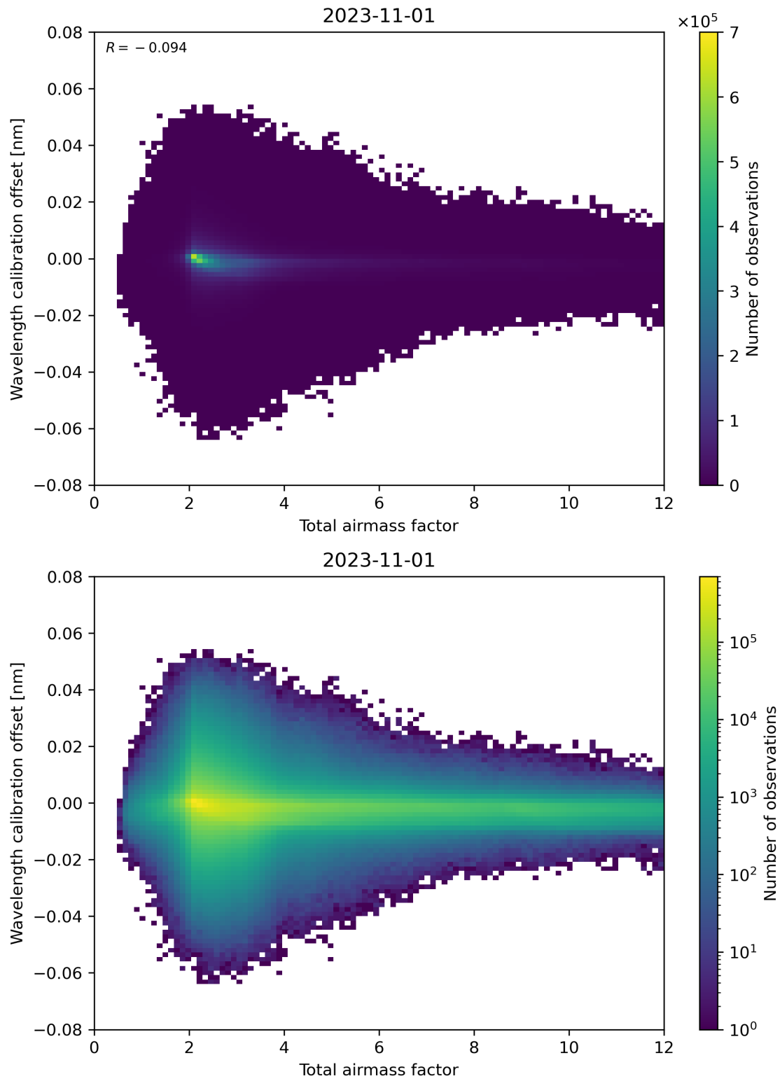
Figure 70: Scatter density plot of “Total airmass factor” against “Wavelength calibration offset” for 2023-10-31 to 2023-11-02.
