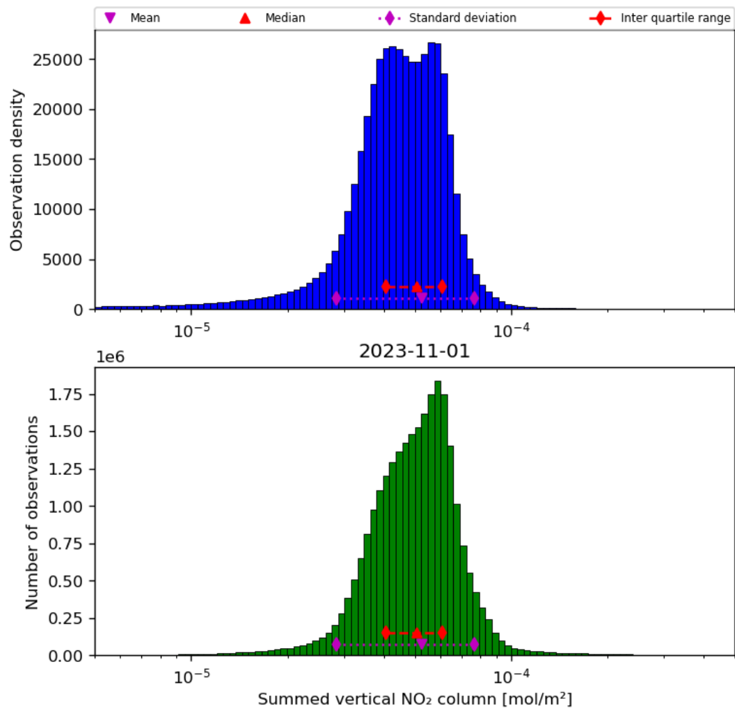
Figure 40: Histogram of “Summed vertical NO 2 column” for 2023-10-31 to 2023-11-02
