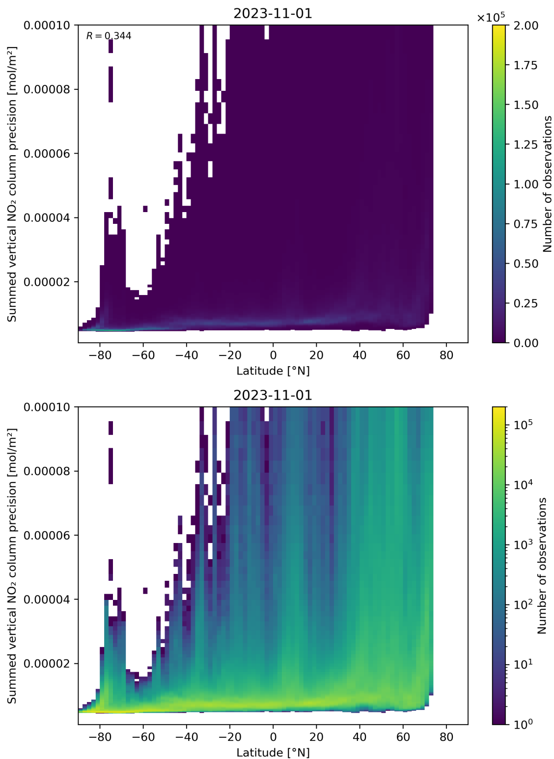
Figure 89: Scatter density plot of “Latitude” against “Summed vertical NO 2 column precision” for 2023-10-31 to 2023-11-02.
