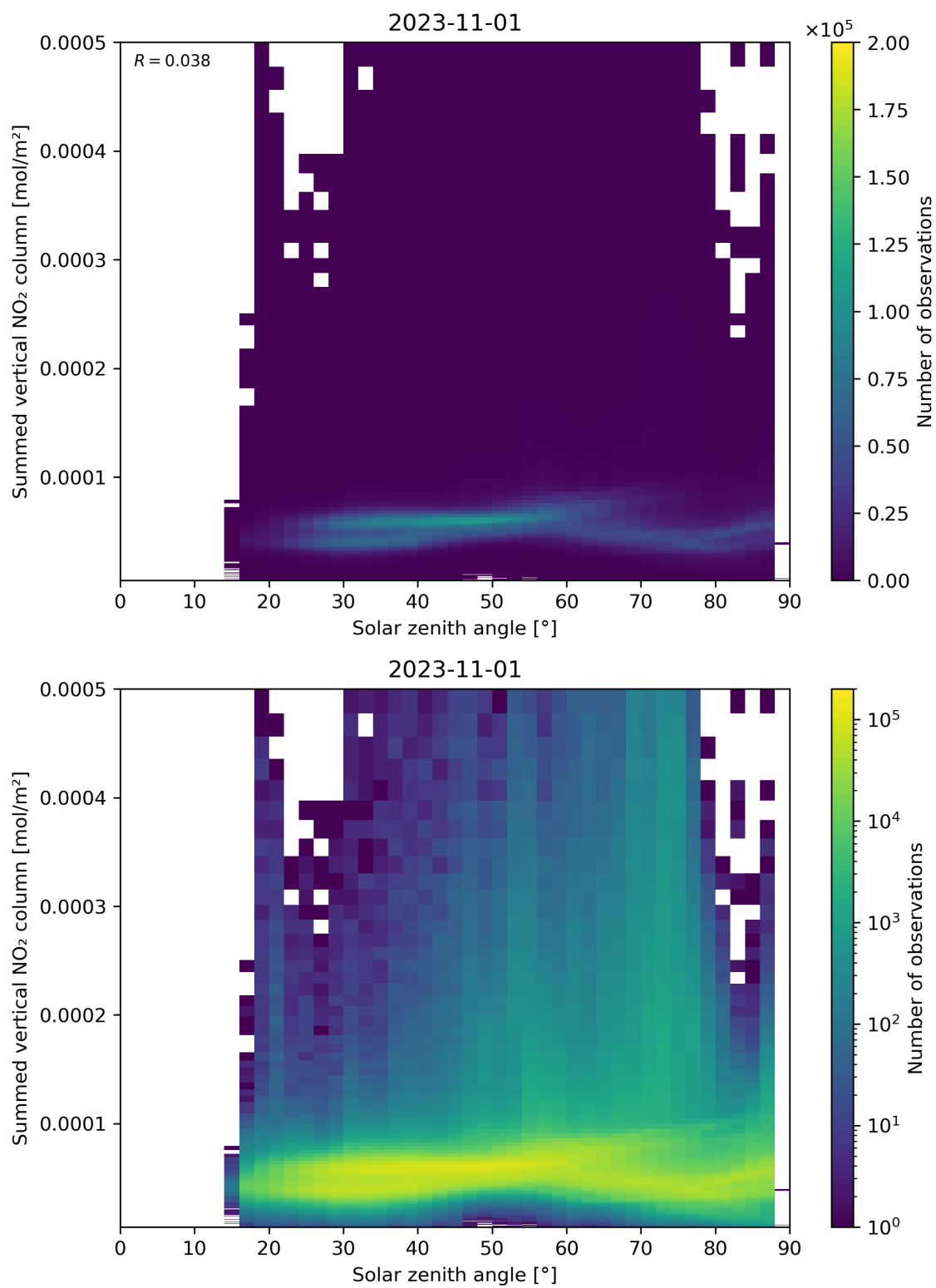
Figure 151: Scatter density plot of “Solar zenith angle” against “Summed vertical NO 2 column” for 2023-10-31 to 2023-11-02.
