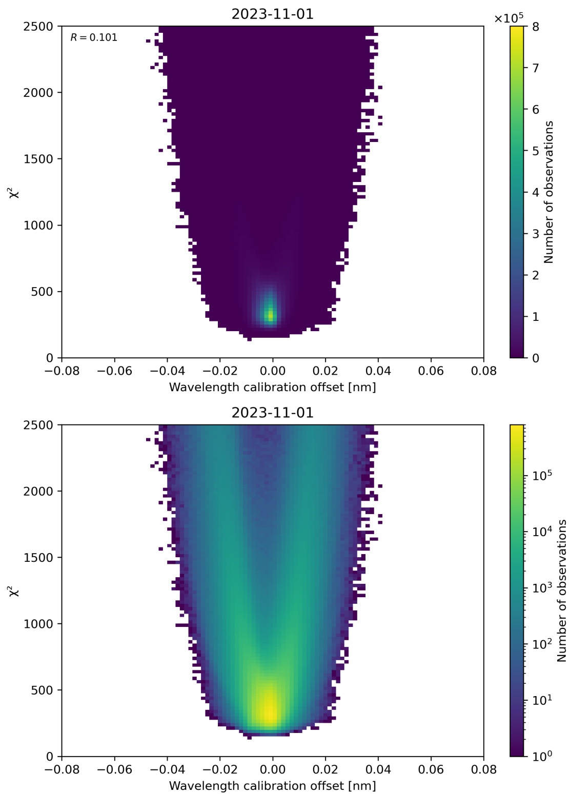
Figure 175: Scatter density plot of “Wavelength calibration offset” against “ \chi^2 ” for 2023-10-31 to 2023-11-02.
