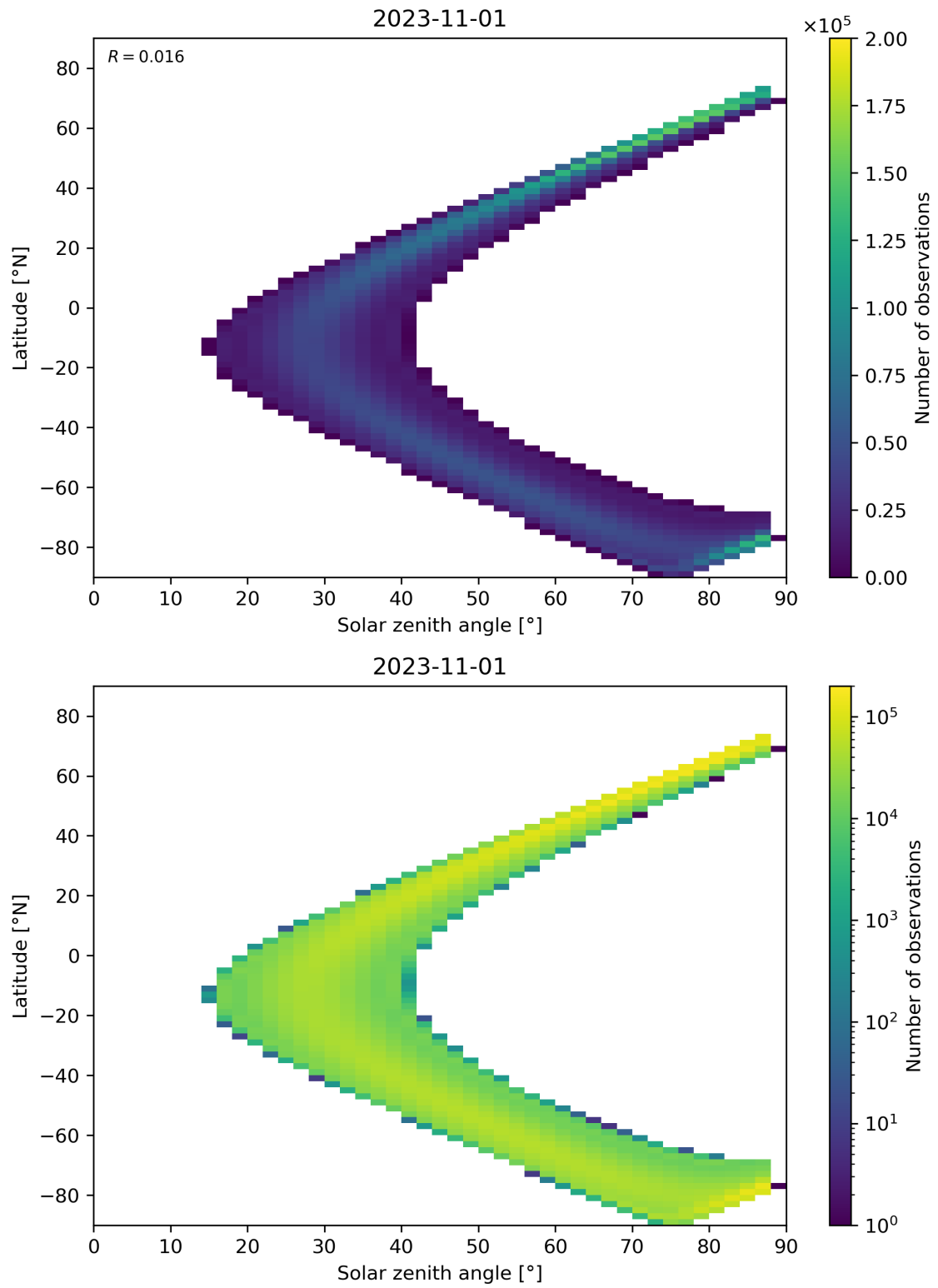
Figure 149: Scatter density plot of “Solar zenith angle” against “Latitude” for 2023-10-31 to 2023-11-02.
