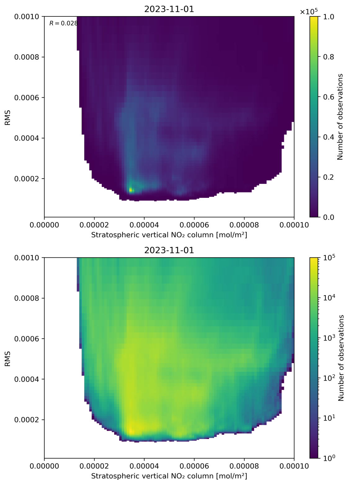
Figure 102: Scatter density plot of “Stratospheric vertical NO 2 column” against “RMS” for 2023-10-31 to 2023-11-02.
