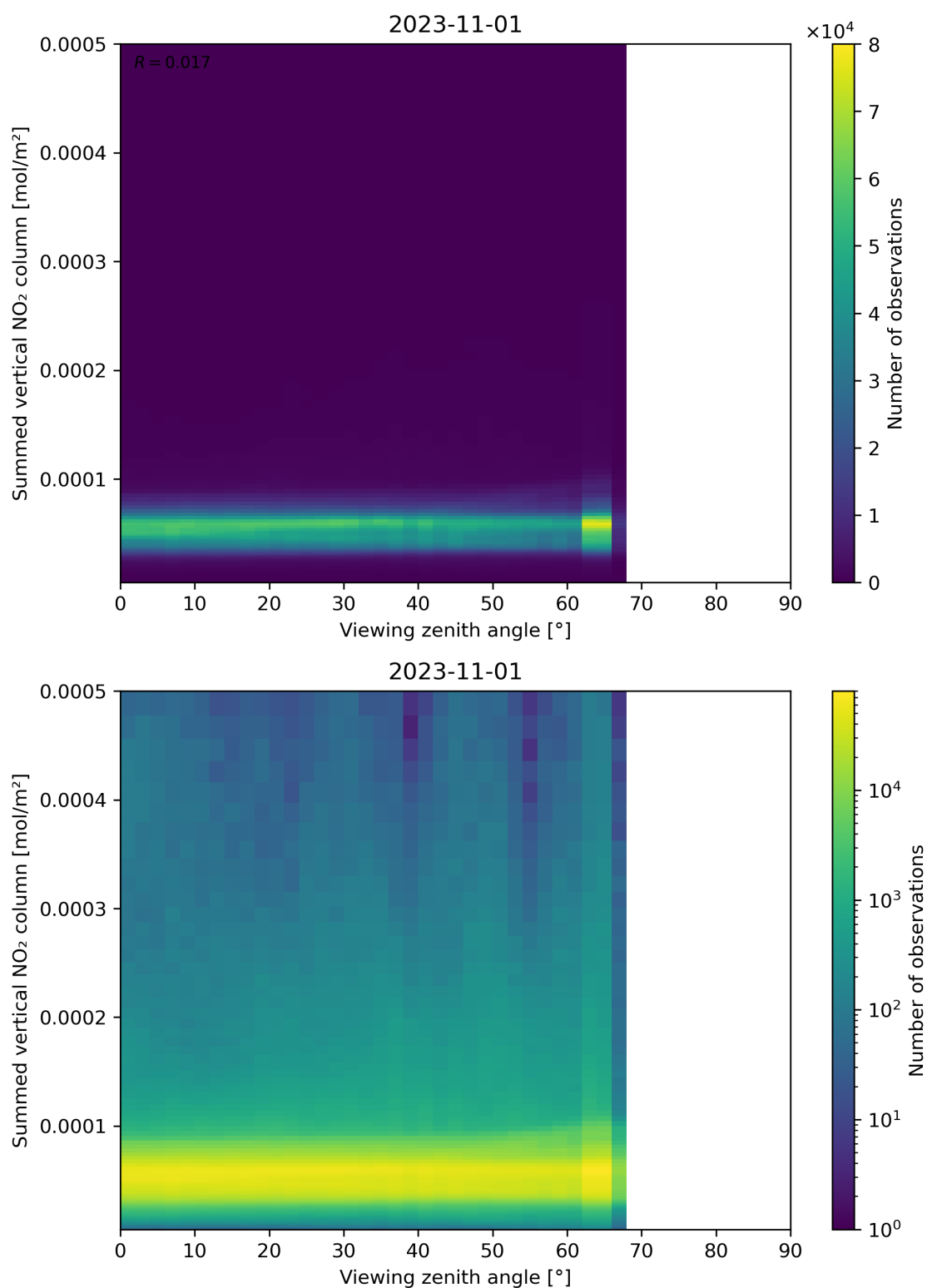
Figure 165: Scatter density plot of “Viewing zenith angle” against “Summed vertical NO 2 column” for 2023-10-31 to 2023-11-02.
