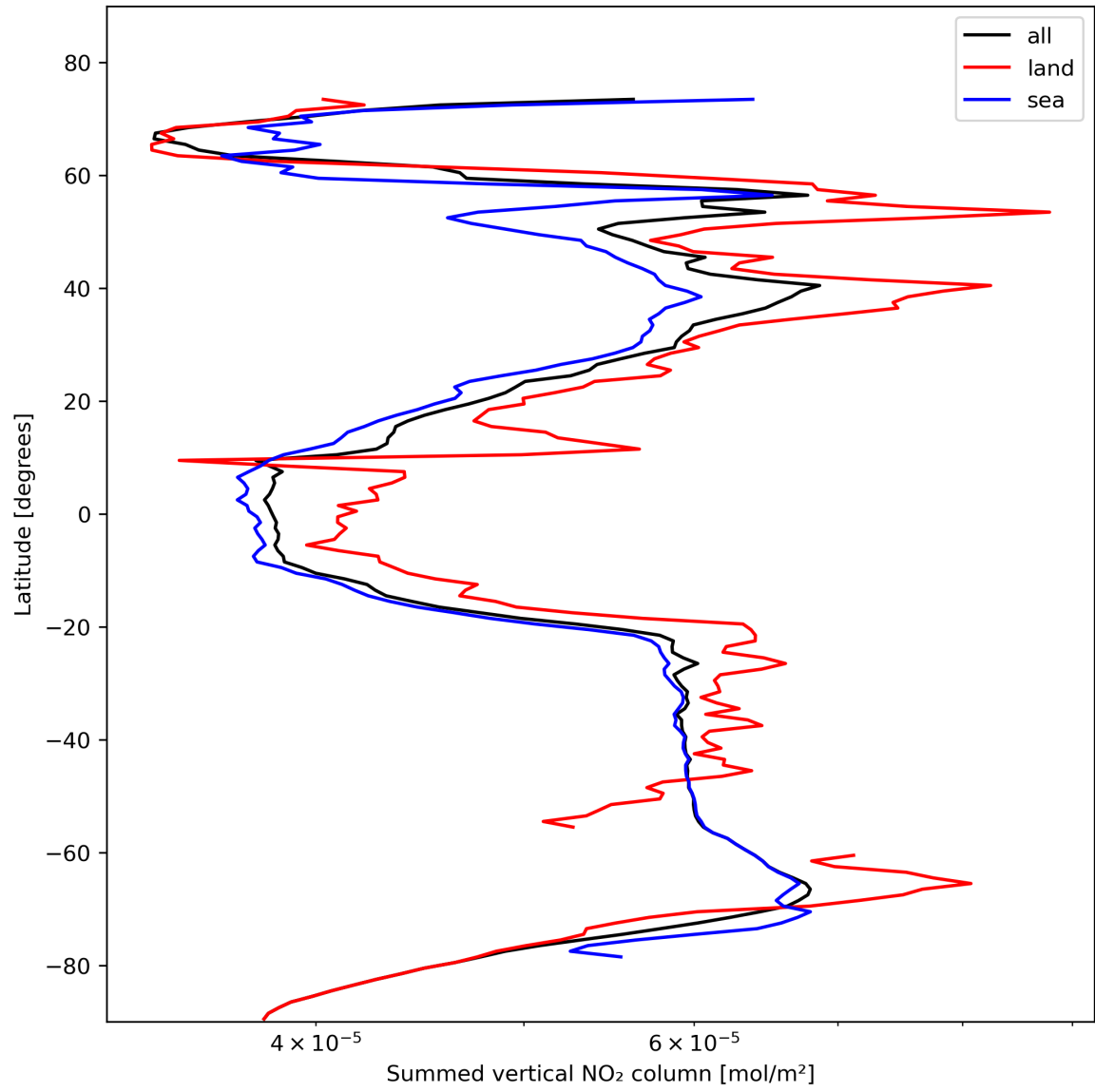
Figure 23: Zonal average of “Summed vertical NO 2 column” for 2023-10-31 to 2023-11-02.
