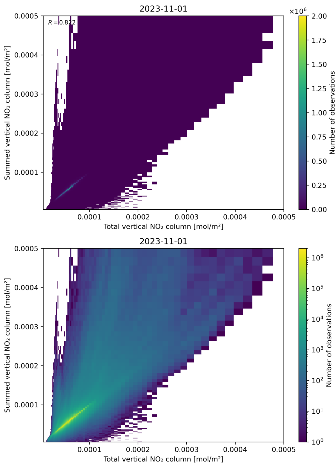
Figure 112: Scatter density plot of “Total vertical NO 2 column” against “Summed vertical NO 2 column” for 2023-10-31 to 2023-11-02.
