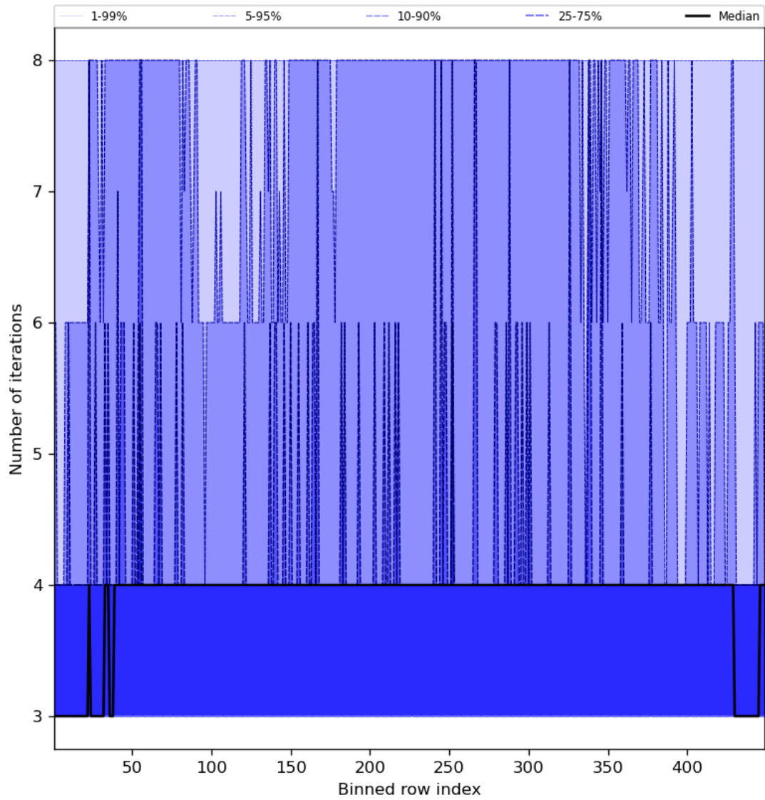
Figure 51: Along track statistics of “Number of iterations” for 2023-10-31 to 2023-11-02
