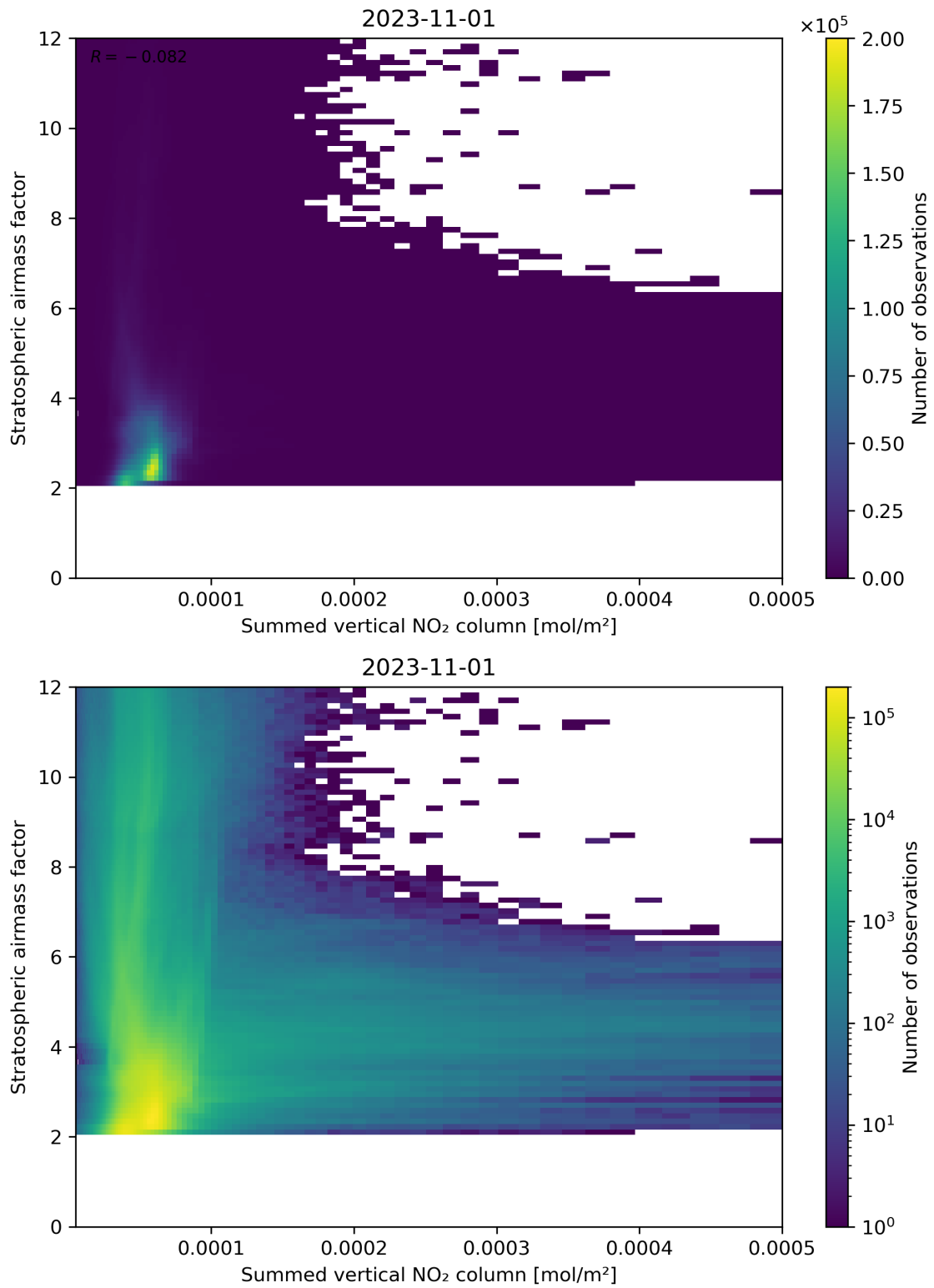
Figure 103: Scatter density plot of “Summed vertical NO 2 column” against “Stratospheric air mass factor” for 2023-10-31 to 2023-11-02.
