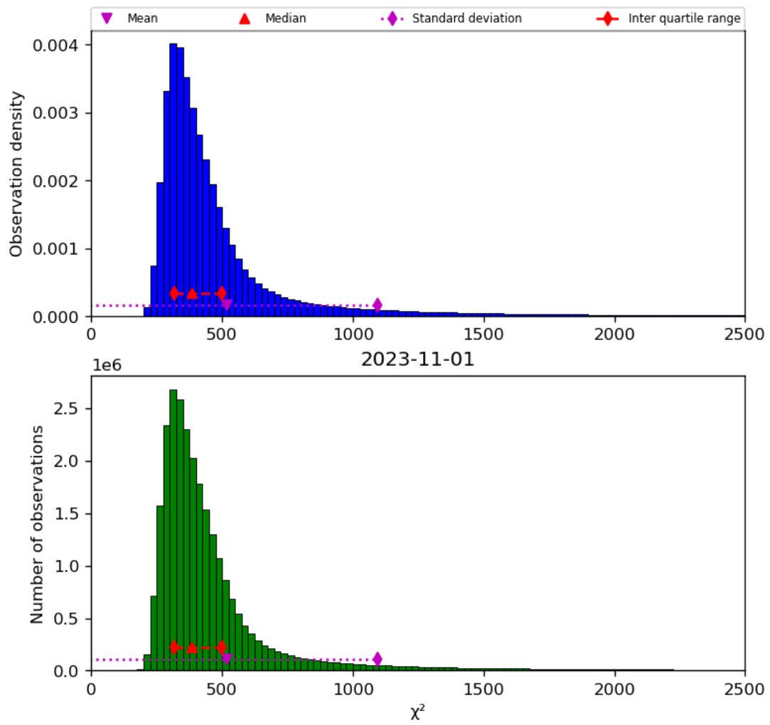
Figure 42: Histogram of “ \chi^2 ” for 2023-10-31 to 2023-11-02
