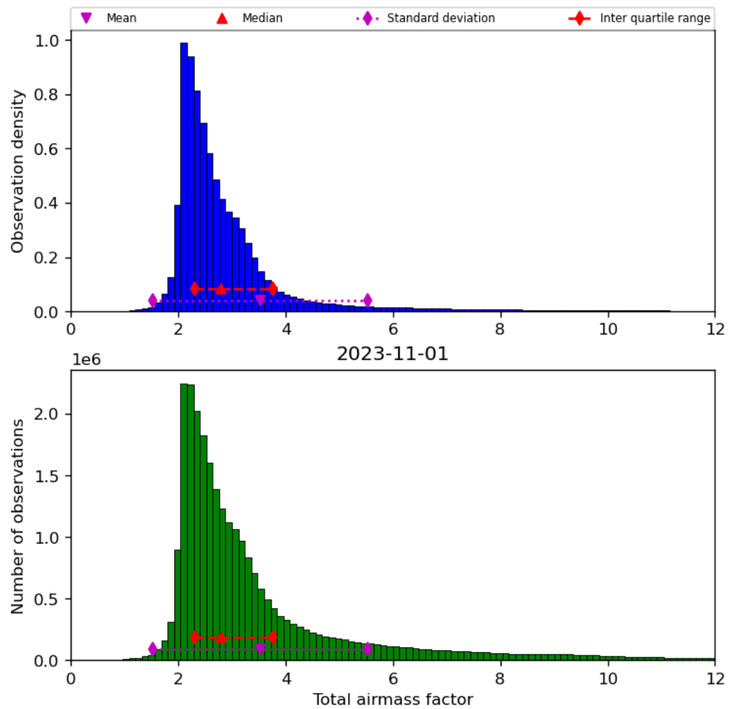
Figure 32: Histogram of “Total airmass factor” for 2023-10-31 to 2023-11-02
