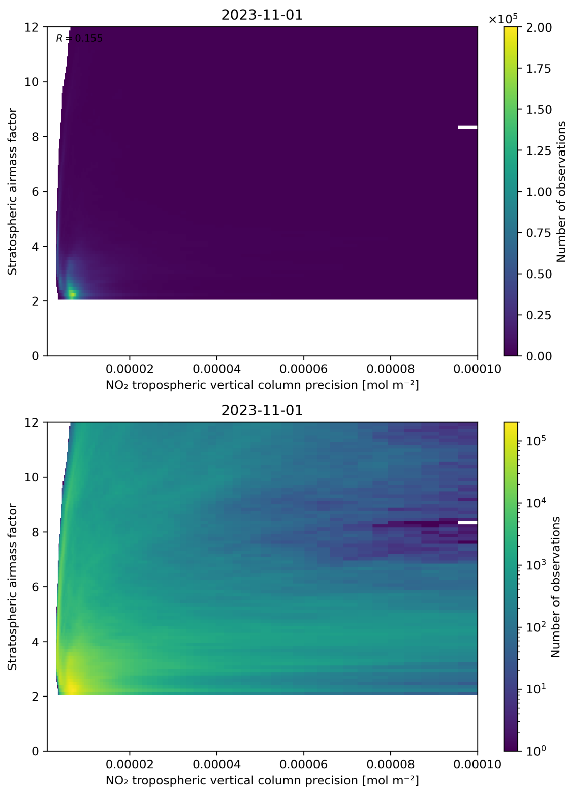
Figure 131: Scatter density plot of “NO 2 tropospheric vertical column precision” against “Stratospheric airmass factor” for 2023-10-31 to 2023-11-02.
