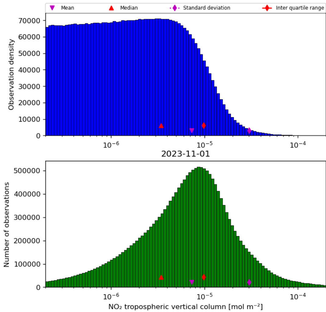
Figure 29: Histogram of “NO 2 tropospheric vertical column” for 2023-10-31 to 2023-11-02
