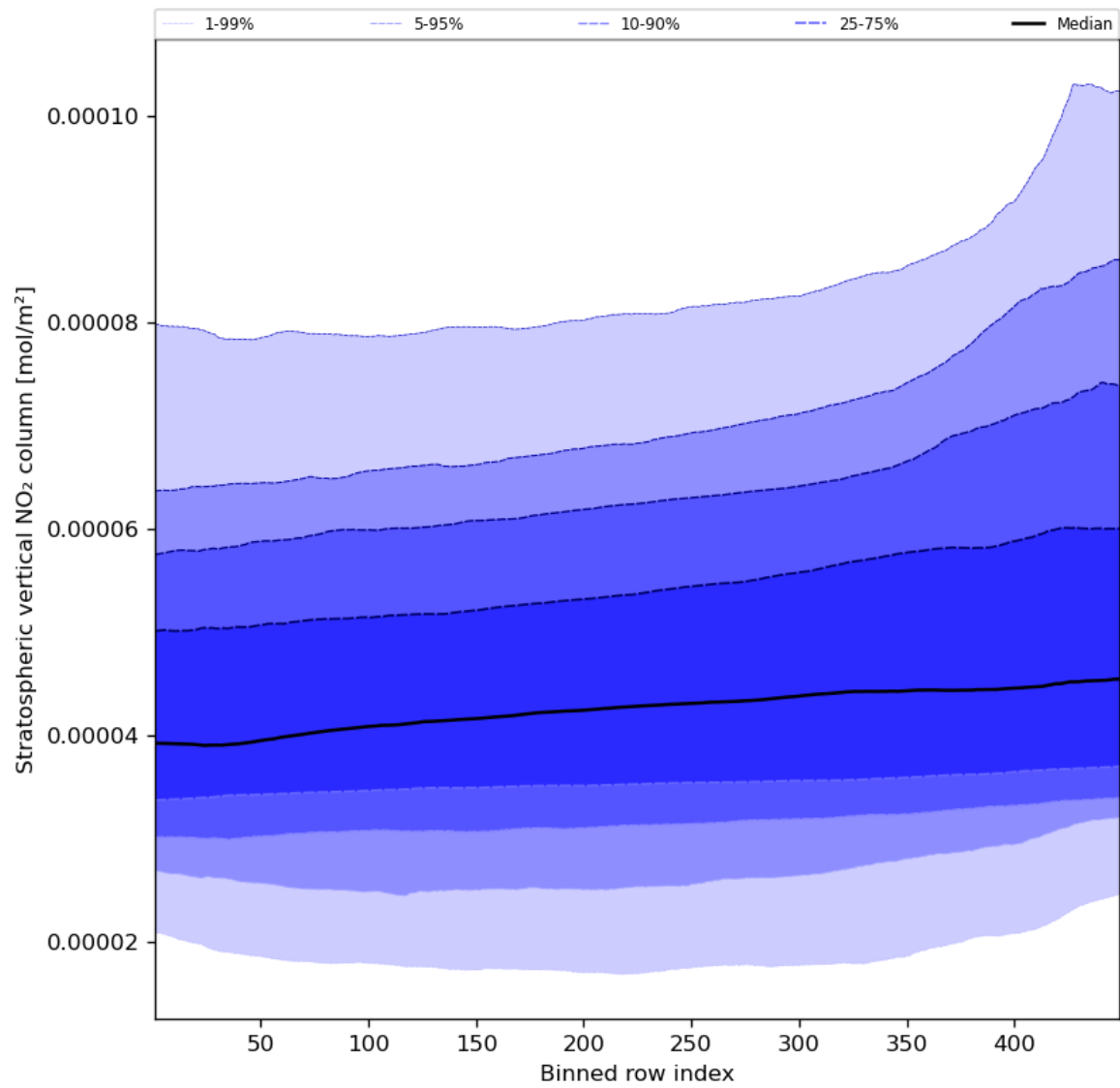
Figure 53: Along track statistics of “Stratospheric vertical NO 2 column” for 2023-10-31 to 2023-11-02
