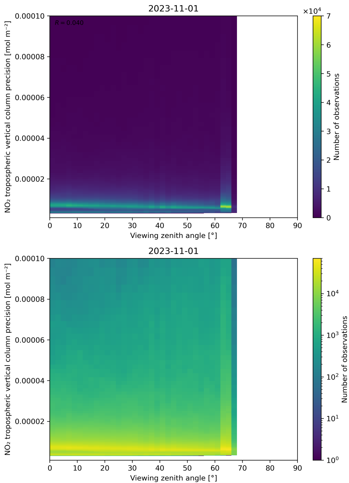
Figure 170: Scatter density plot of “Viewing zenith angle” against “NO 2 tropospheric vertical column precision” for 2023-10-31 to 2023-11-02.
