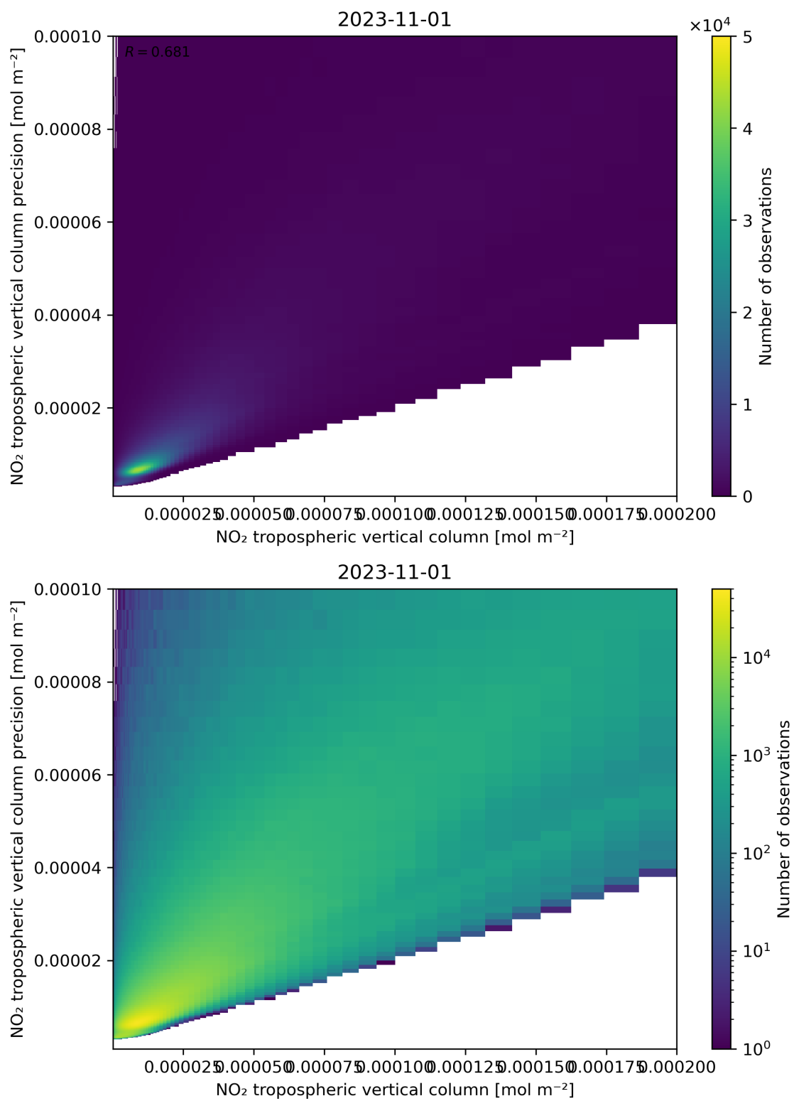
Figure 130: Scatter density plot of “NO 2 tropospheric vertical column” against “NO 2 tropospheric vertical column precision” for 2023-10-31 to 2023-11-02.
