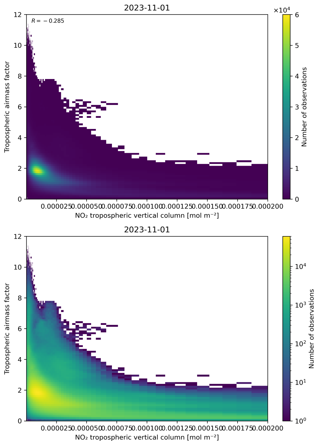
Figure 123: Scatter density plot of “NO 2 tropospheric vertical column” against “Tropospheric air mass factor” for 2023-10-31 to 2023-11-02.
