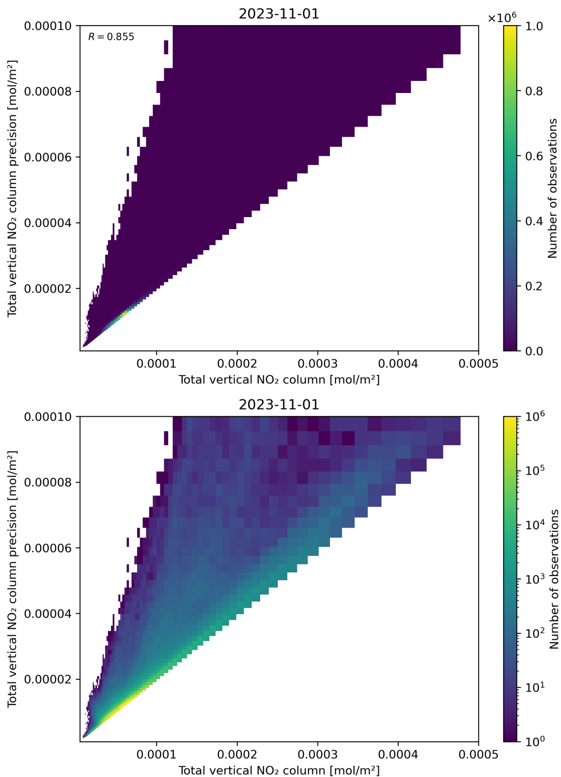
Figure 114: Scatter density plot of “Total vertical NO 2 column” against “Total vertical NO 2 column precision” for 2023-10-31 to 2023-11-02.
