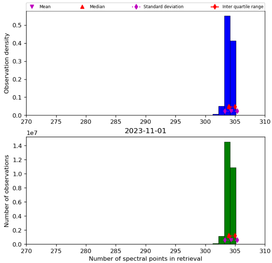
Figure 33: Histogram of “Number of spectral points in retrieval” for 2023-10-31 to 2023-11-02
