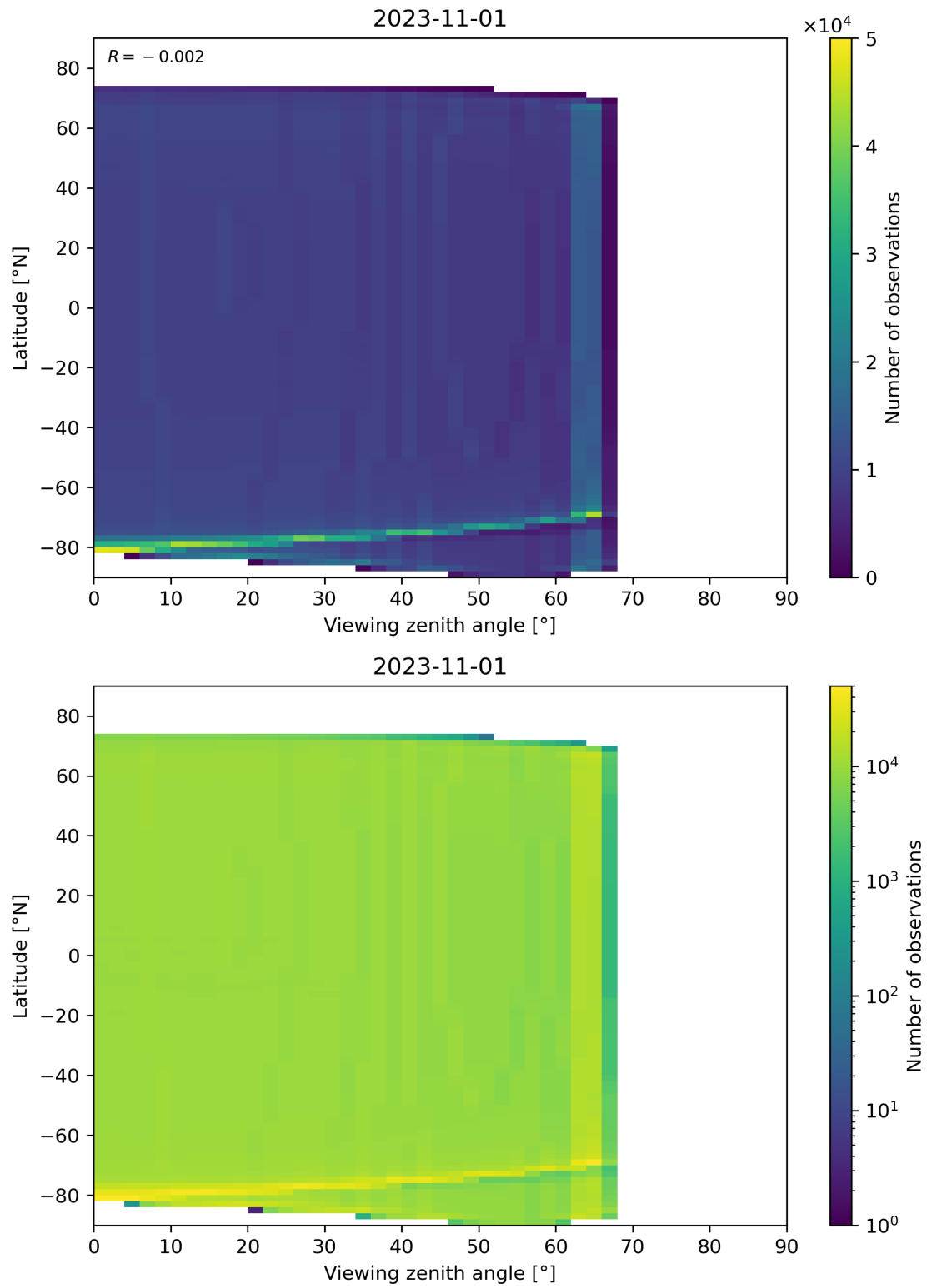
Figure 163: Scatter density plot of “Viewing zenith angle” against “Latitude” for 2023-10-31 to 2023-11-02.
