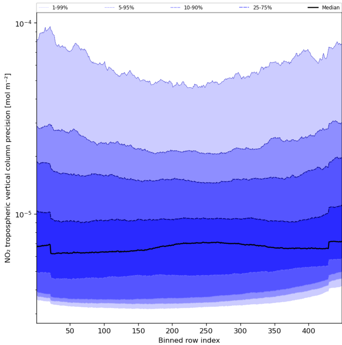
Figure 47: Along track statistics of “NO 2 tropospheric vertical column precision” for 2023-10-31 to 2023-11-02
