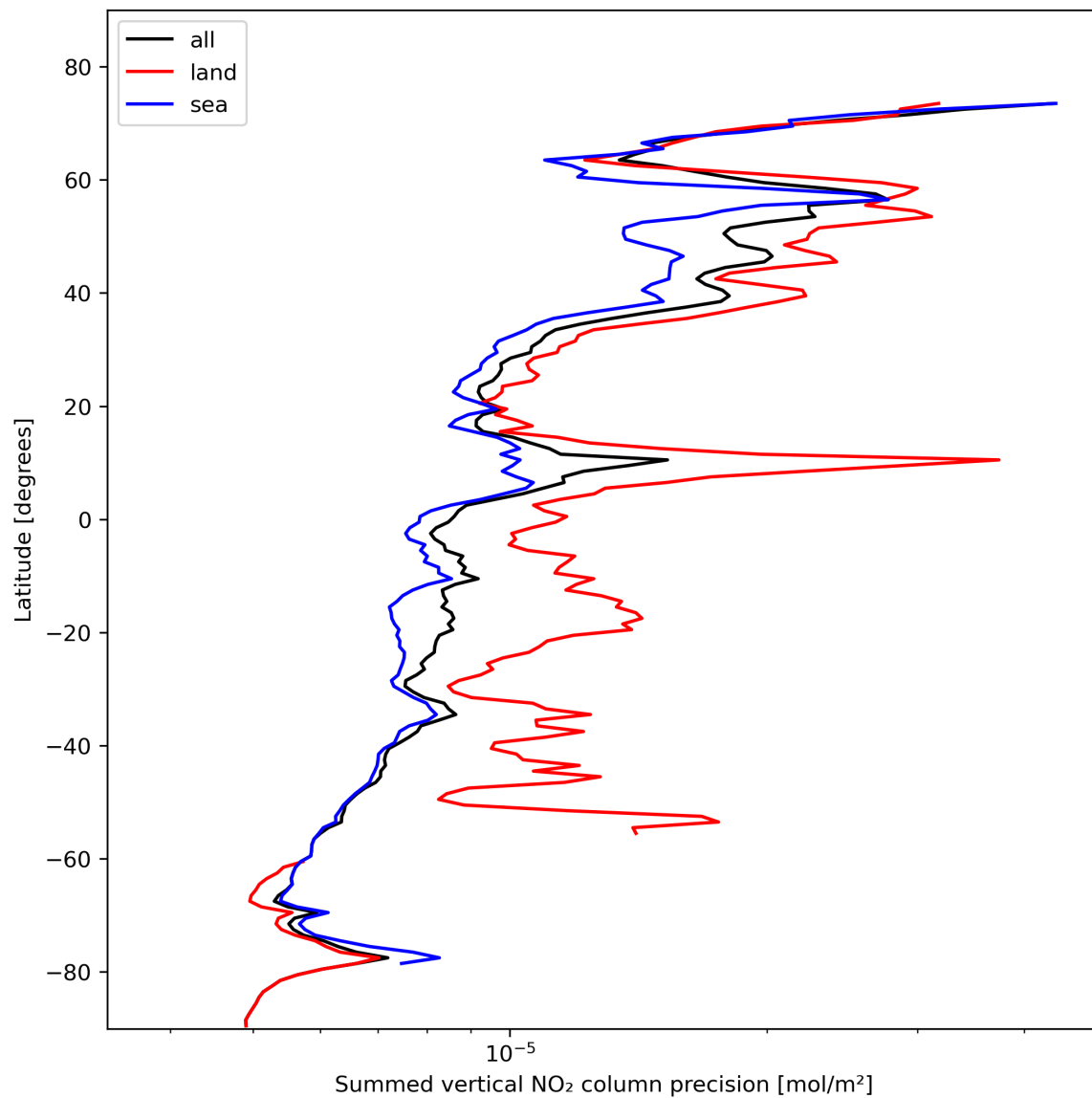
Figure 24: Zonal average of “Summed vertical NO 2 column precision” for 2023-10-31 to 2023-11-02.
