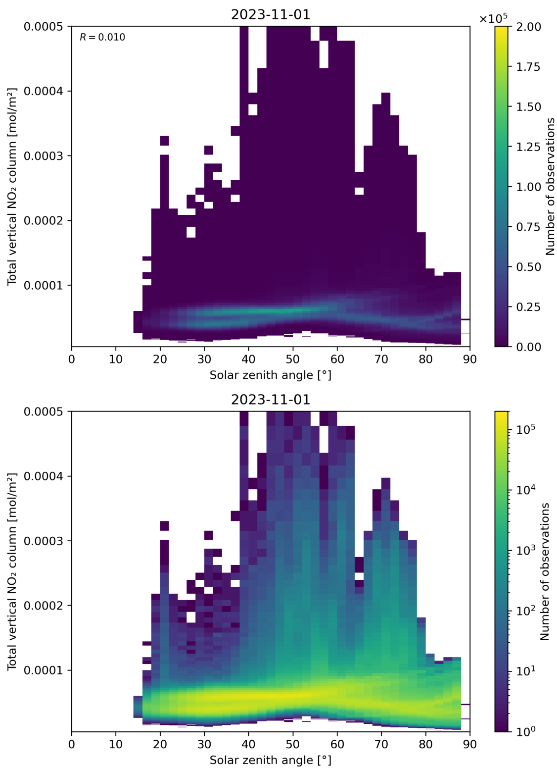
Figure 153: Scatter density plot of “Solar zenith angle” against “Total vertical NO 2 column” for 2023-10-31 to 2023-11-02.
