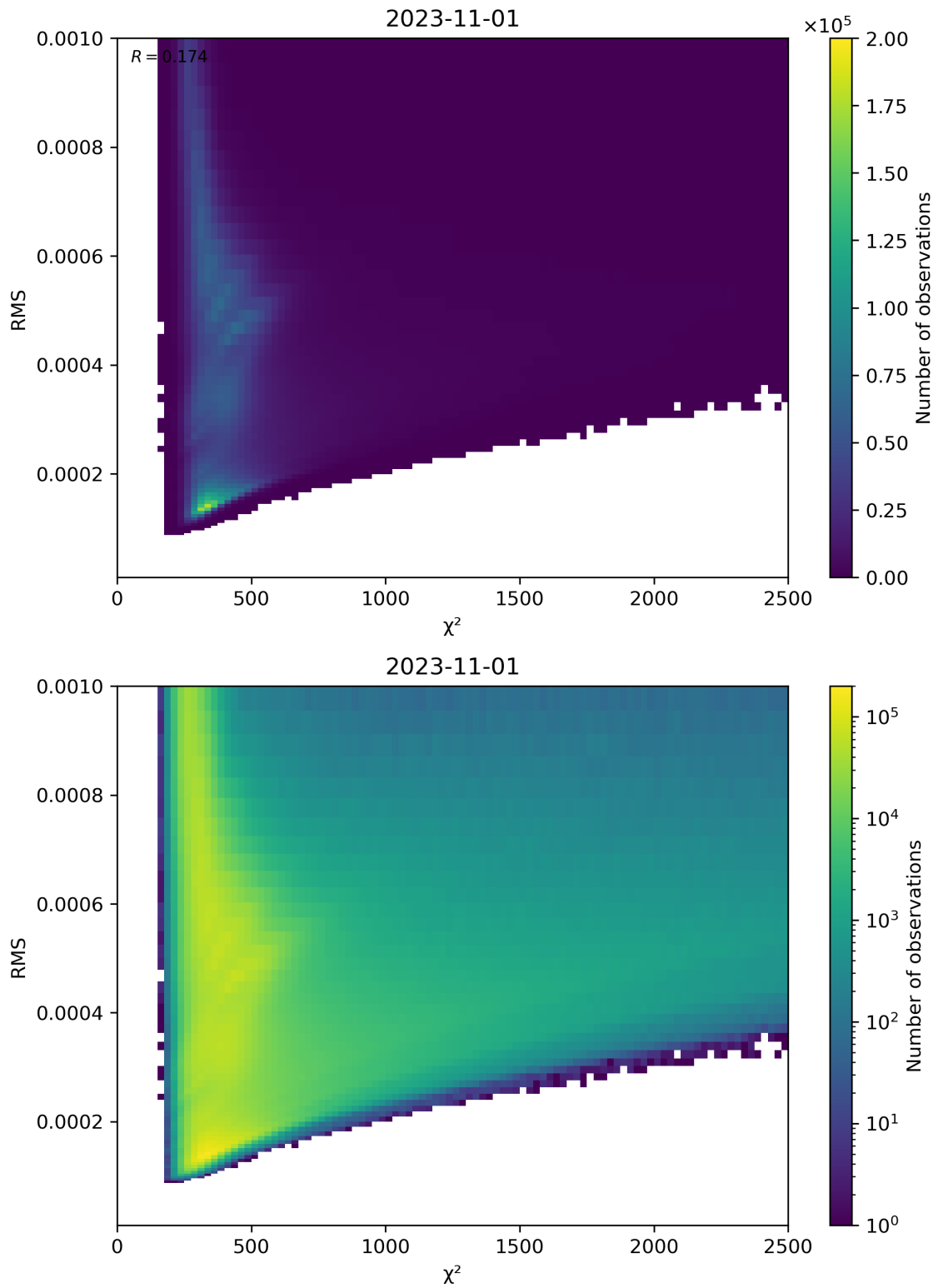
Figure 82: Scatter density plot of “ \chi^2 ” against “RMS” for 2023-10-31 to 2023-11-02.
