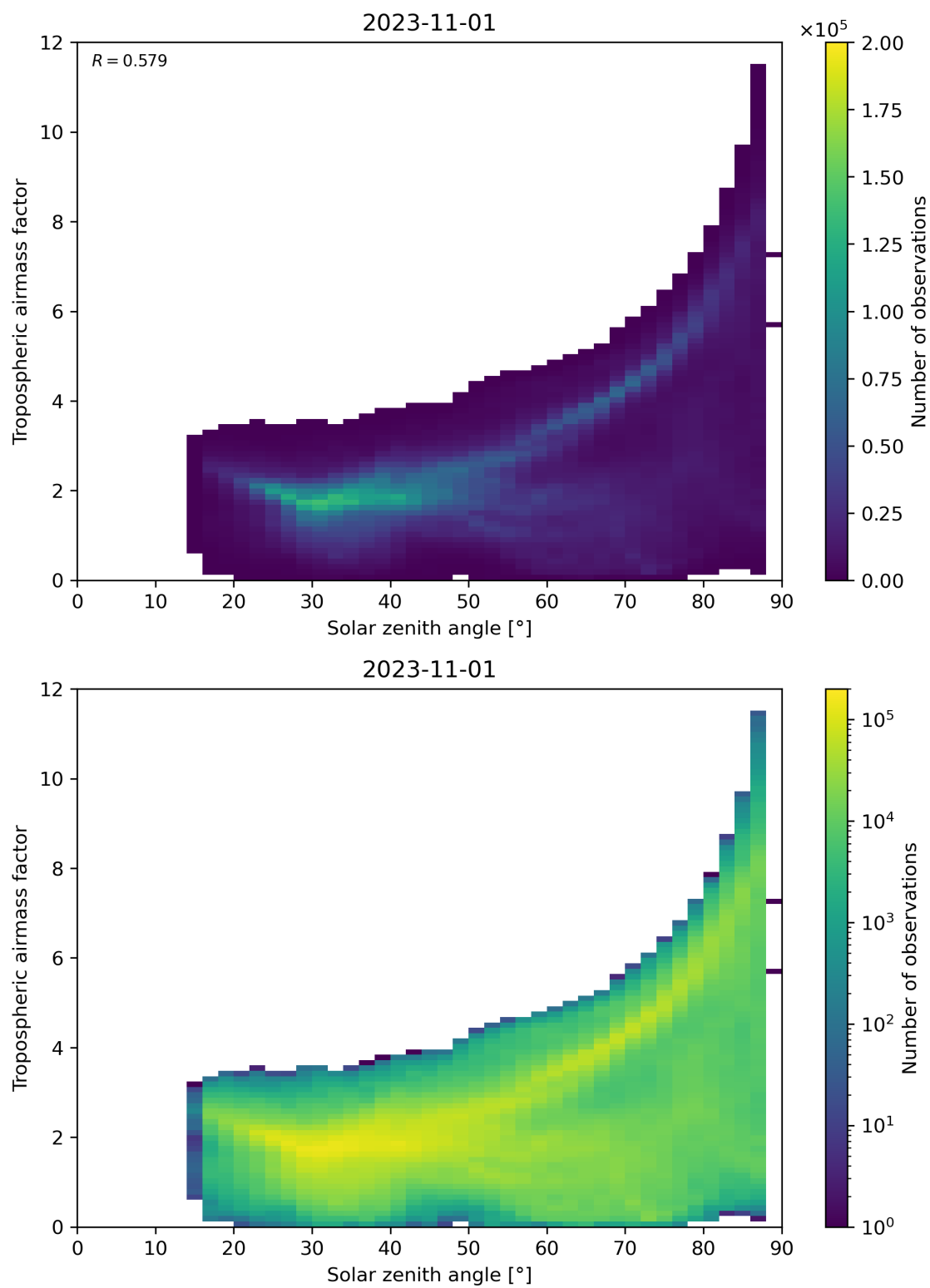
Figure 147: Scatter density plot of “Solar zenith angle” against “Tropospheric airmass factor” for 2023-10-31 to 2023-11-02.
