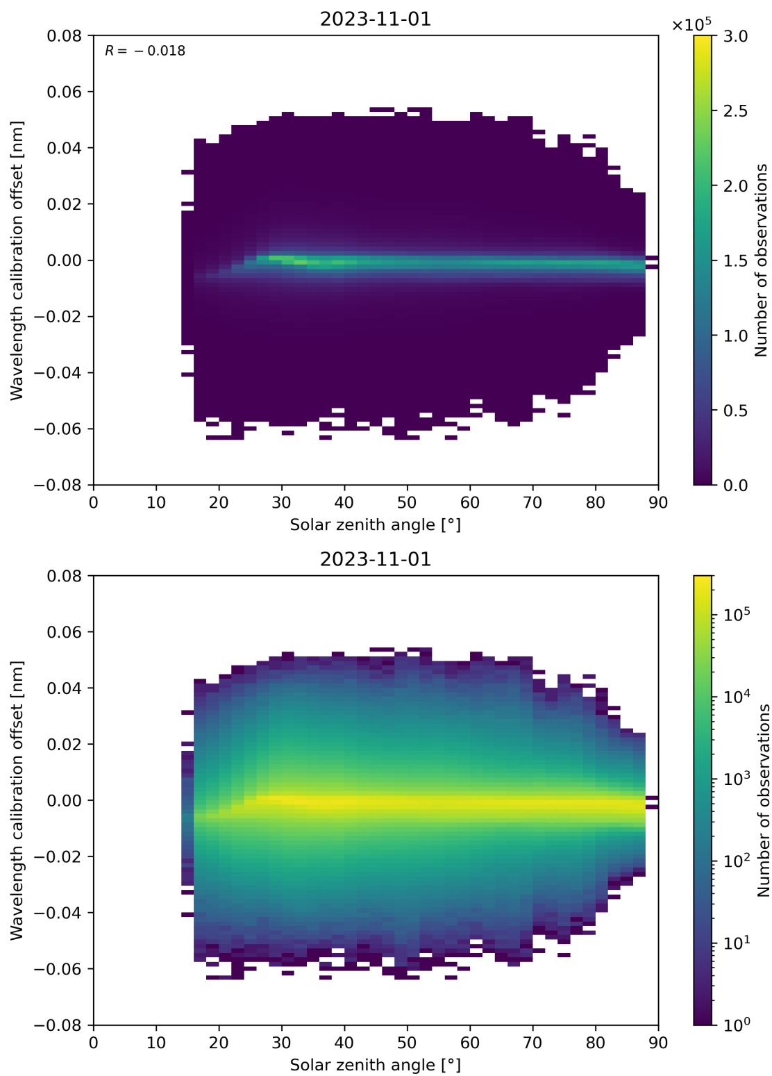
Figure 158: Scatter density plot of “Solar zenith angle” against “Wavelength calibration offset” for 2023-10-31 to 2023-11-02.
