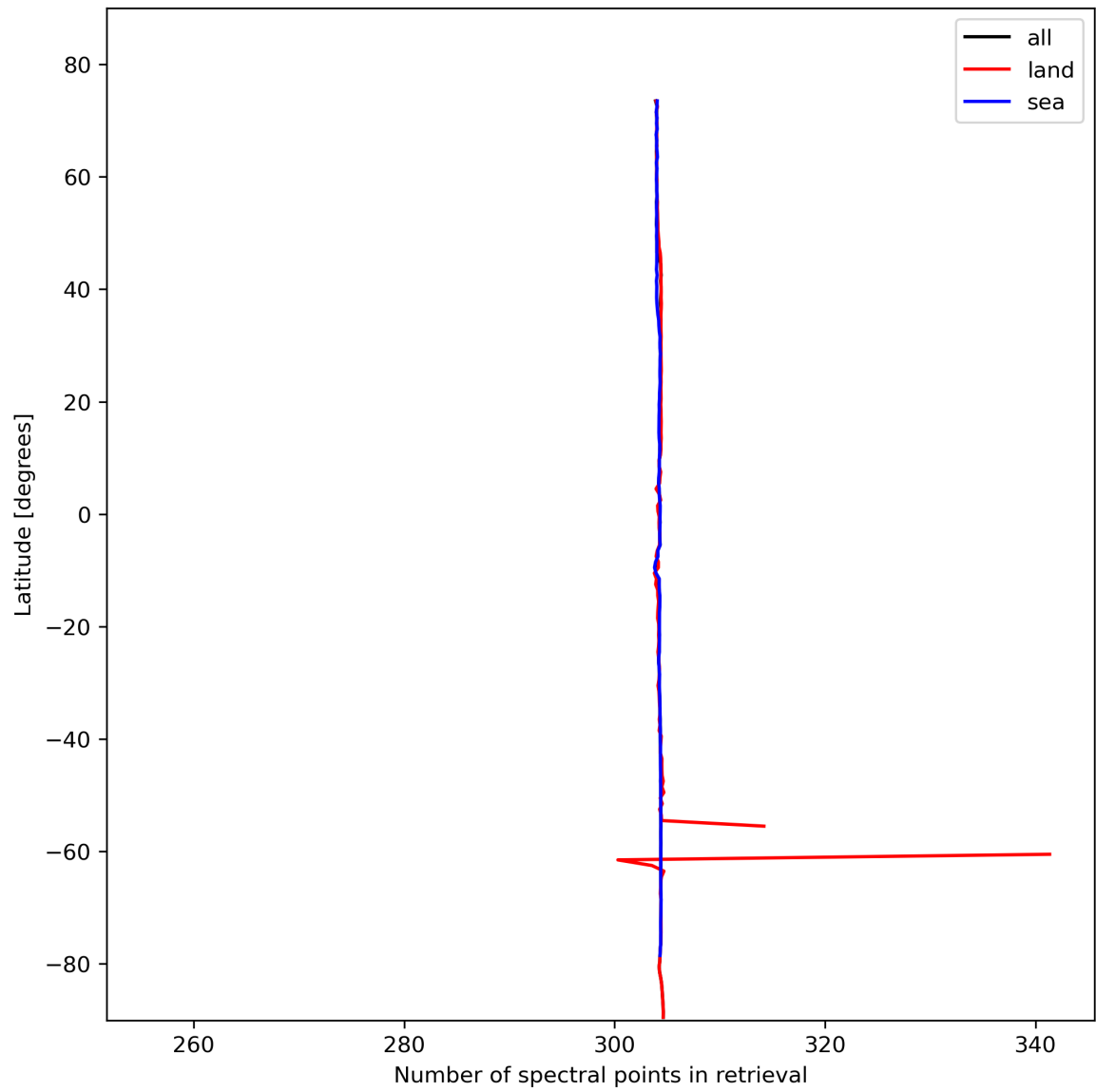
Figure 16: Zonal average of “Number of spectral points in retrieval” for 2023-10-31 to 2023-11-02.
