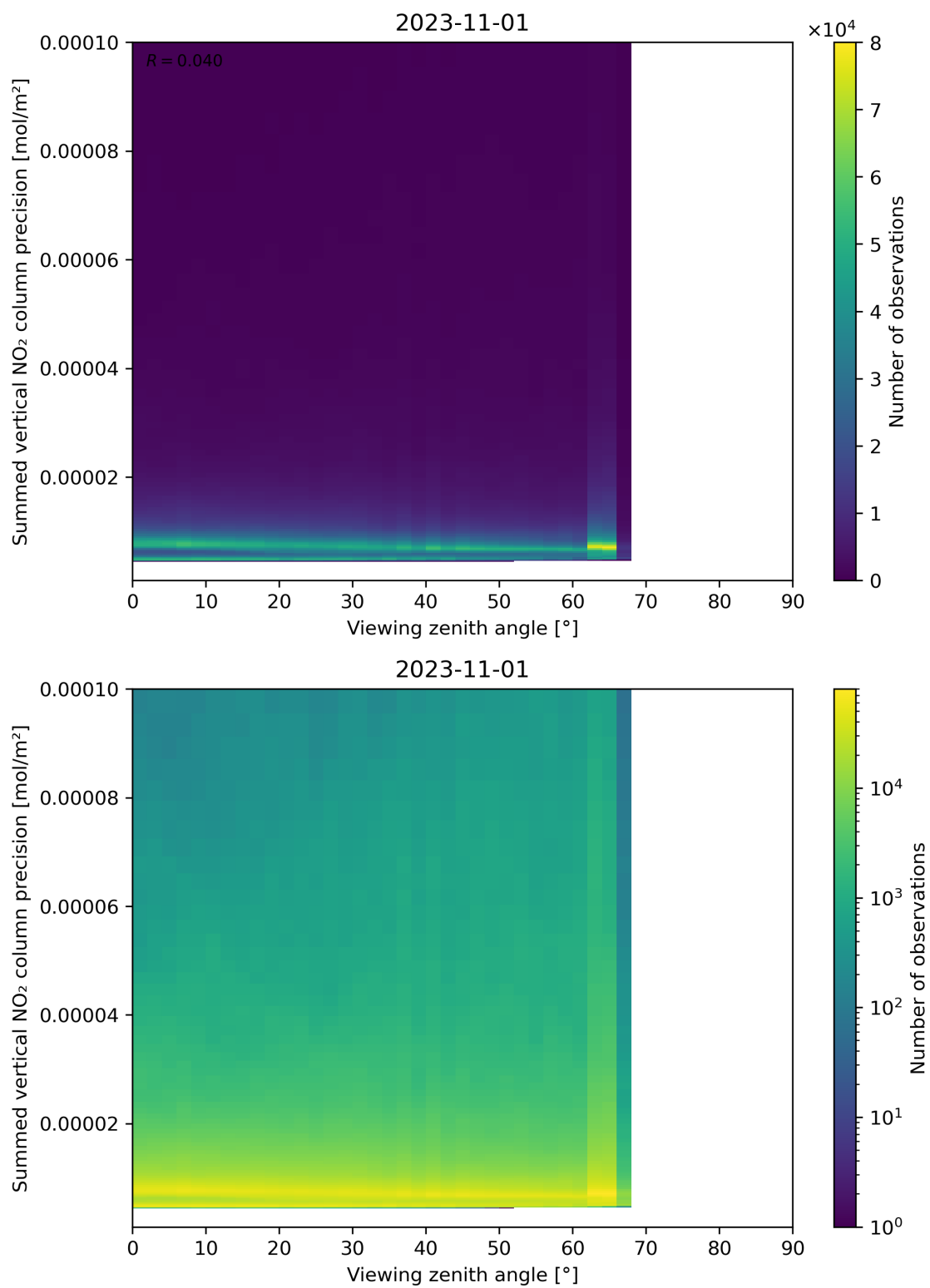
Figure 166: Scatter density plot of “Viewing zenith angle” against “Summed vertical NO 2 column precision” for 2023-10-31 to 2023-11-02.
