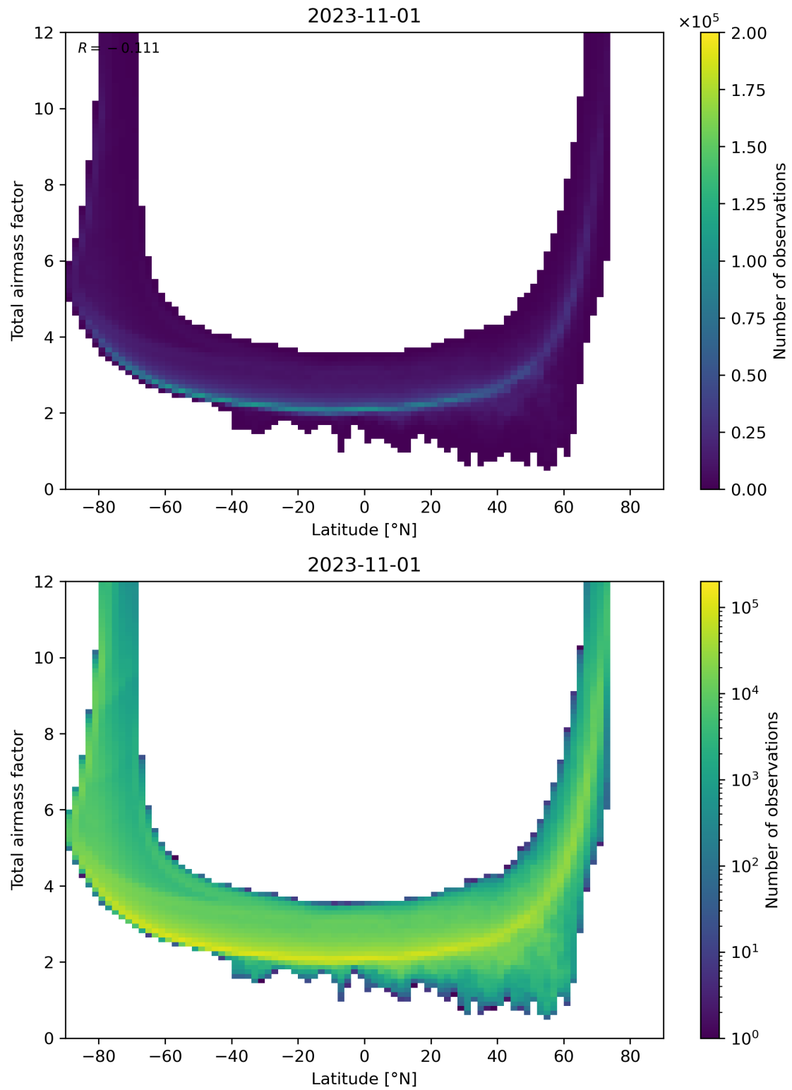
Figure 84: Scatter density plot of “Latitude” against “Total airmass factor” for 2023-10-31 to 2023-11-02.
