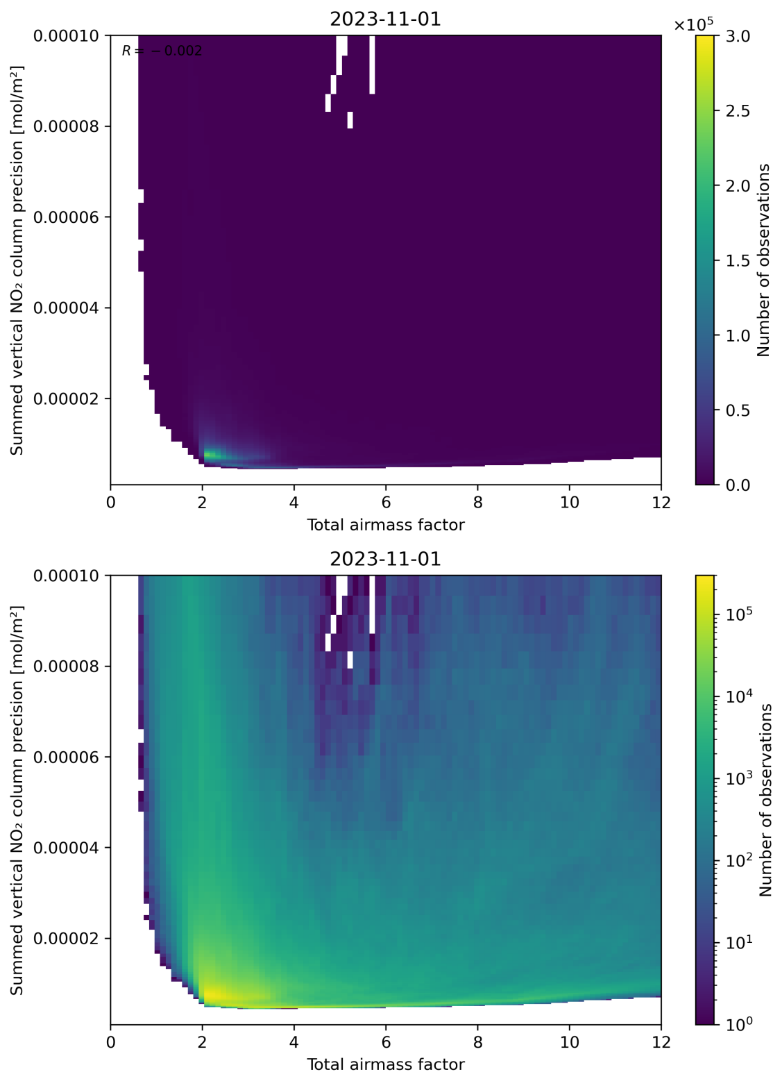
Figure 66: Scatter density plot of “Total airmass factor” against “Summed vertical NO 2 column precision” for 2023-10-31 to 2023-11-02.
