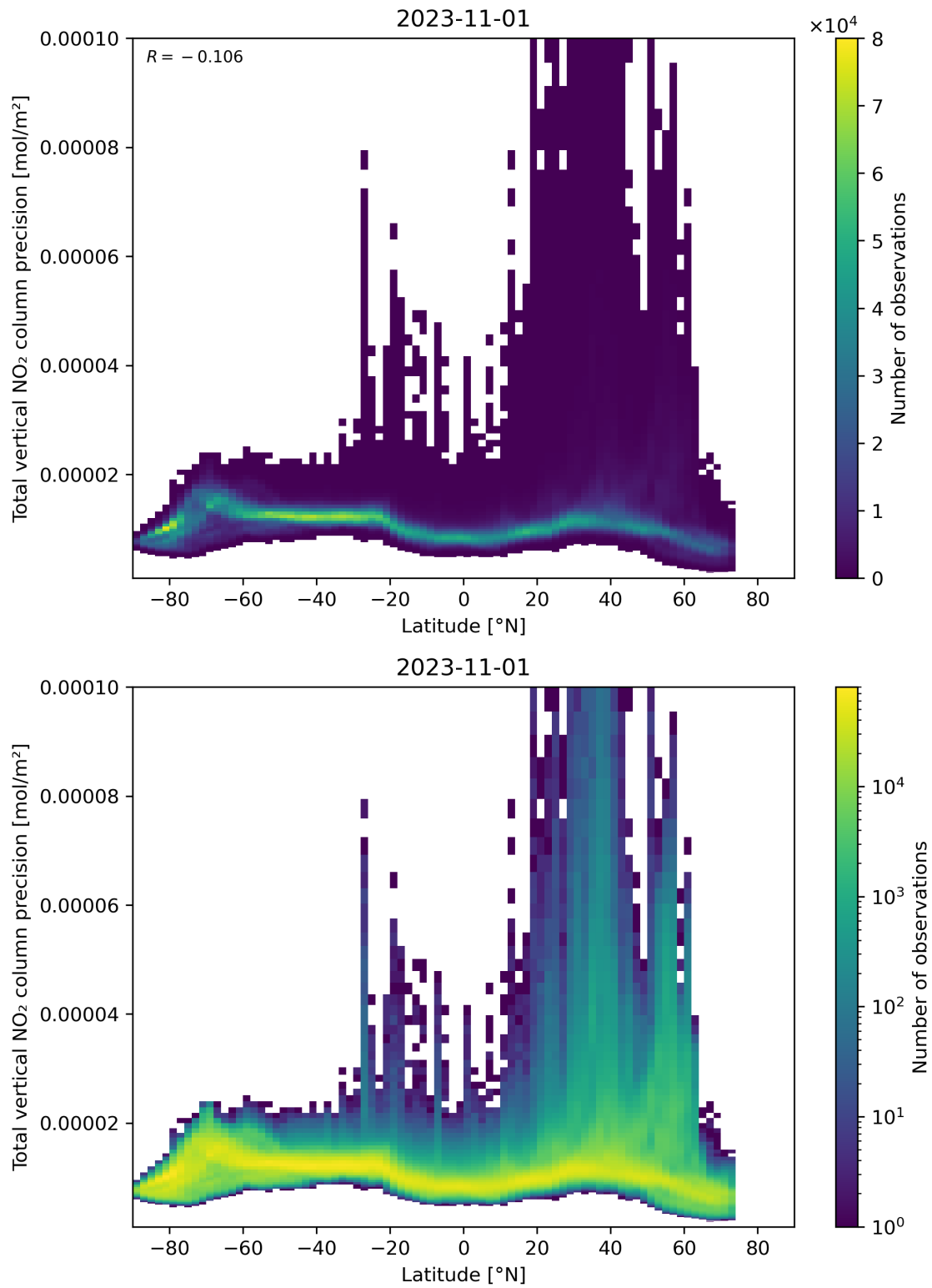
Figure 91: Scatter density plot of “Latitude” against “Total vertical NO 2 column precision” for 2023-10-31 to 2023-11-02.
