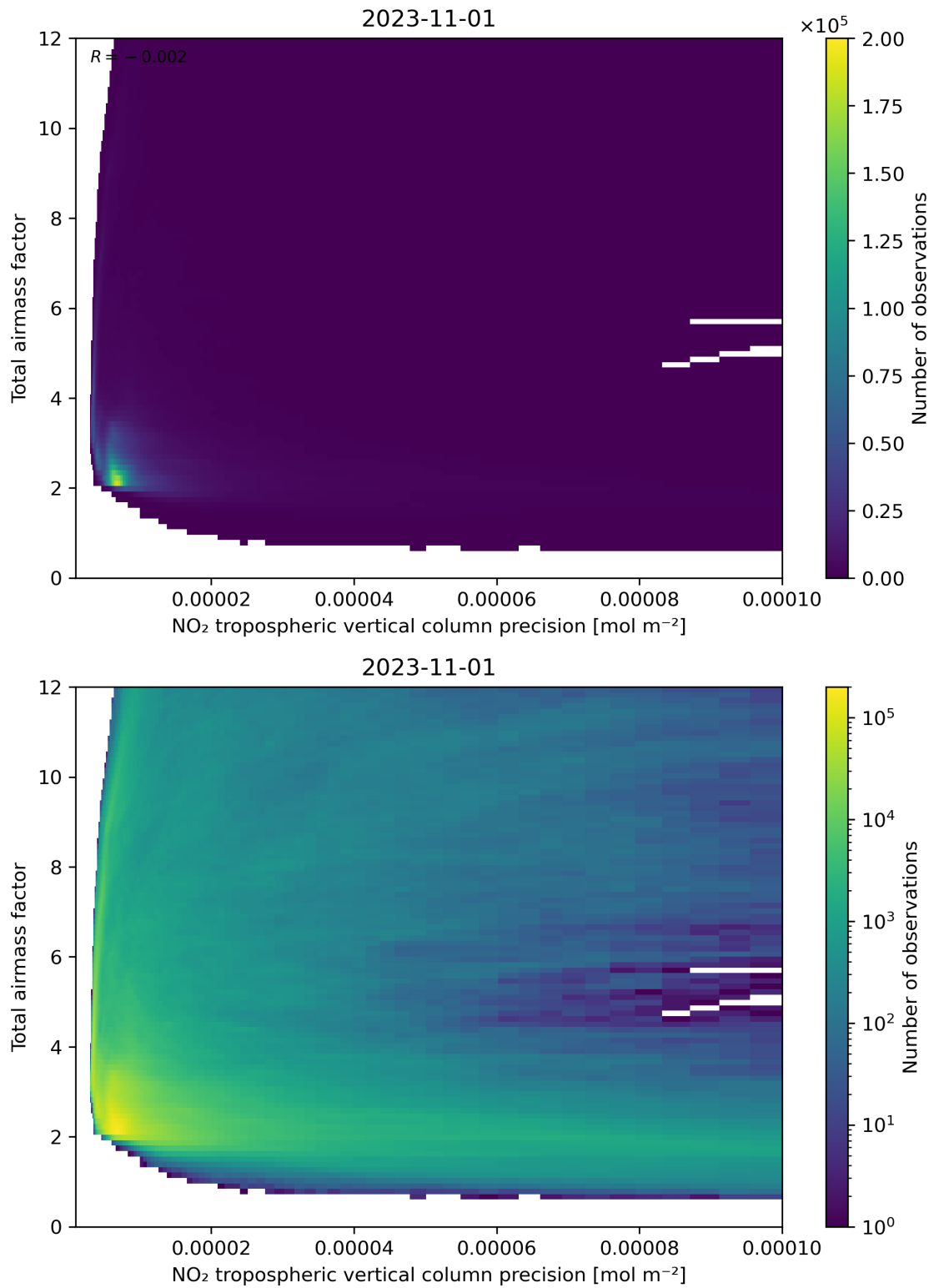
Figure 132: Scatter density plot of “NO 2 tropospheric vertical column precision” against “Total air mass factor” for 2023-10-31 to 2023-11-02.
