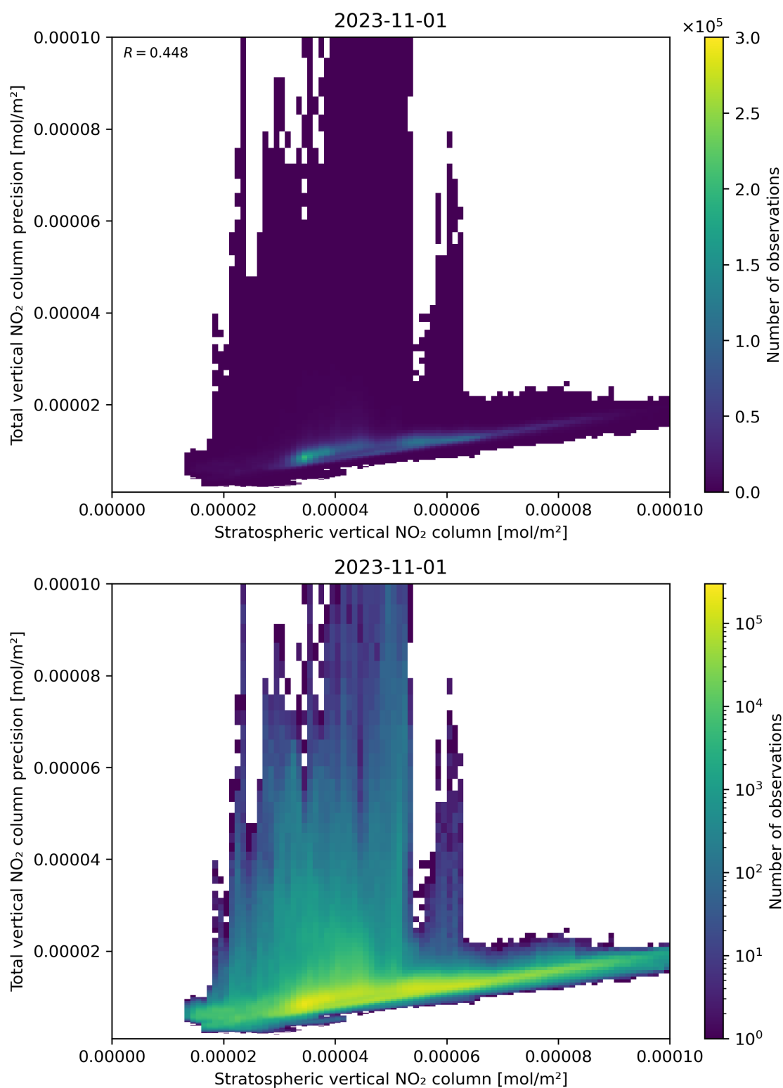
Figure 101: Scatter density plot of “Stratospheric vertical NO 2 column” against “Total vertical NO 2 column precision” for 2023-10-31 to 2023-11-02.
