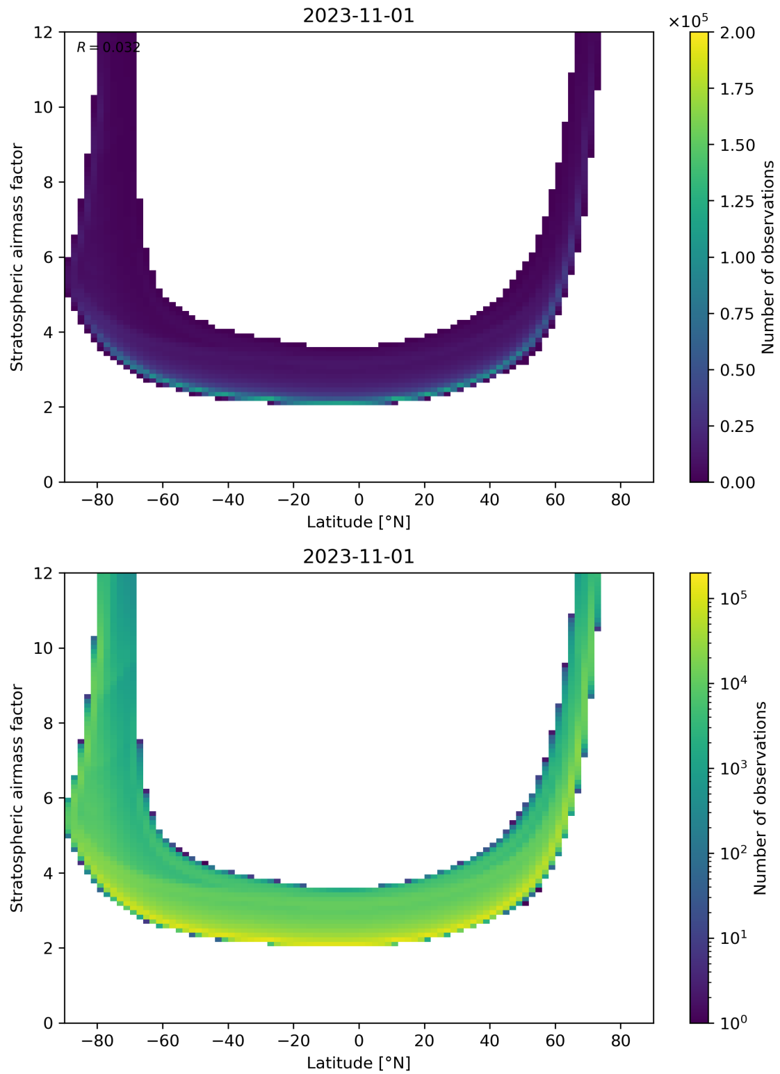
Figure 83: Scatter density plot of “Latitude” against “Stratospheric airmass factor” for 2023-10-31 to 2023-11-02.
