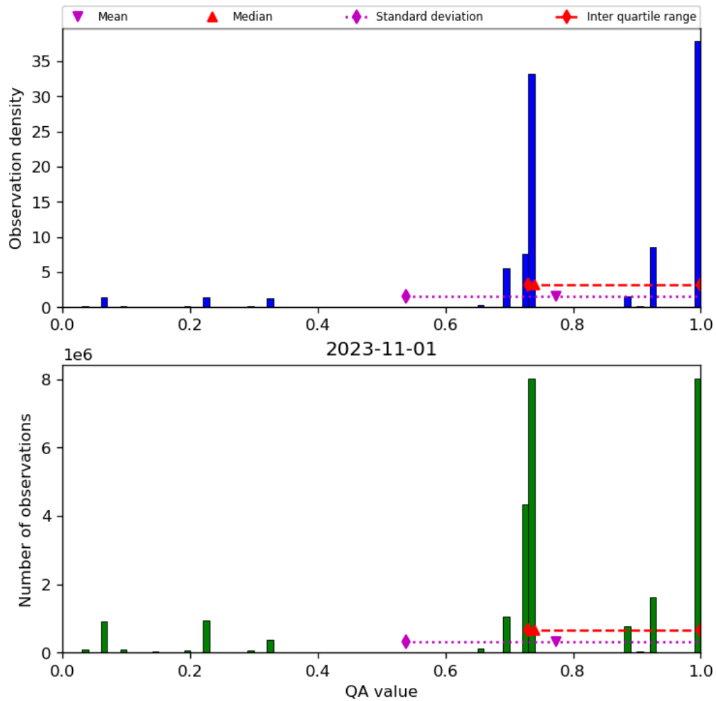
Figure 28: Histogram of “QA value” for 2023-10-31 to 2023-11-02
