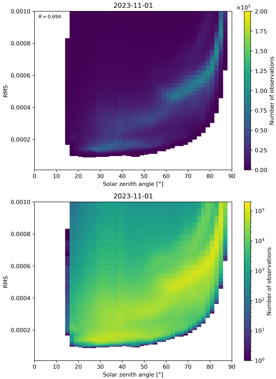
Figure 157: Scatter density plot of “Solar zenith angle” against “RMS” for 2023-10-31 to 2023-11-02.
