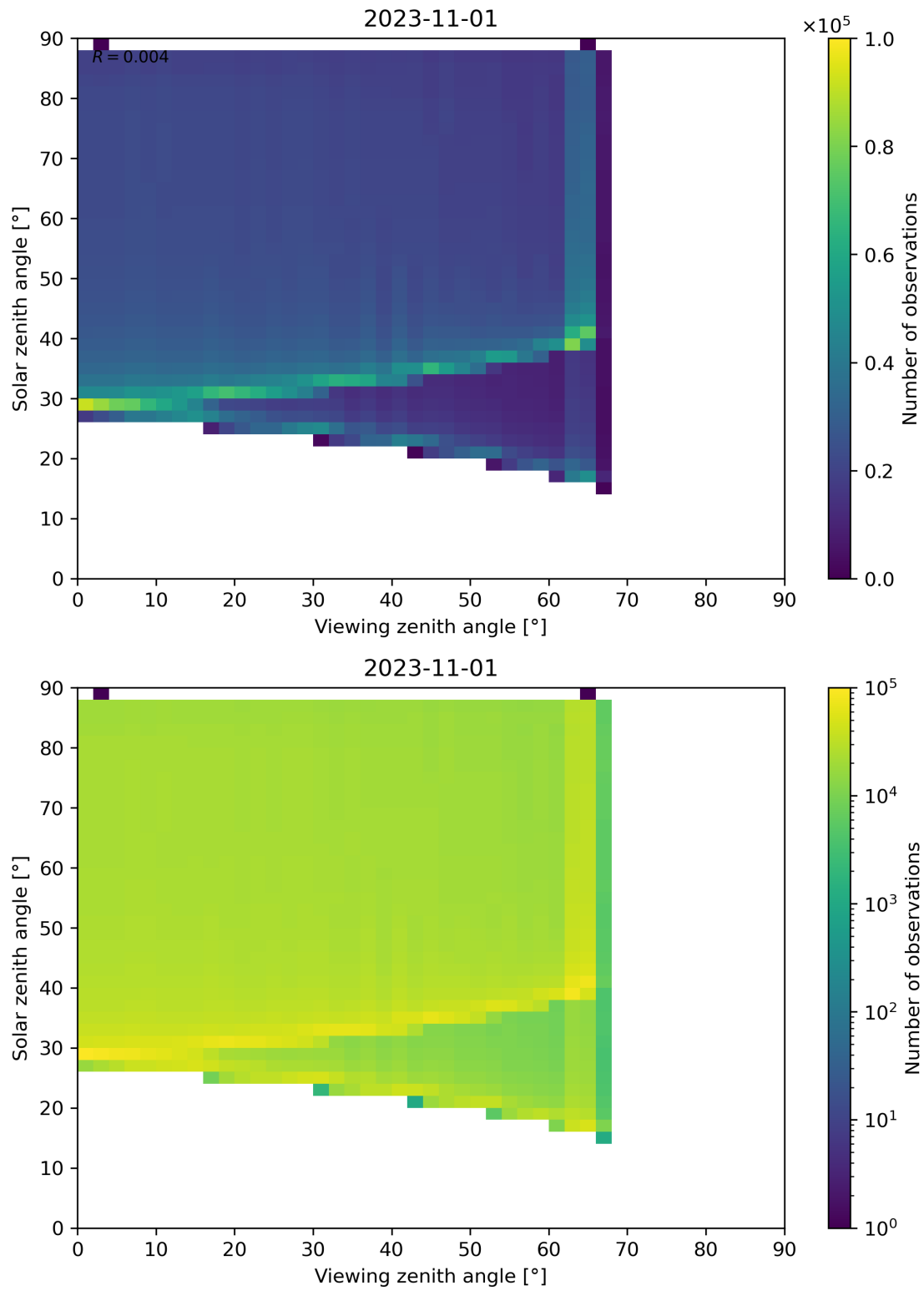
Figure 172: Scatter density plot of “Viewing zenith angle” against “Solar zenith angle” for 2023-10-31 to 2023-11-02.
