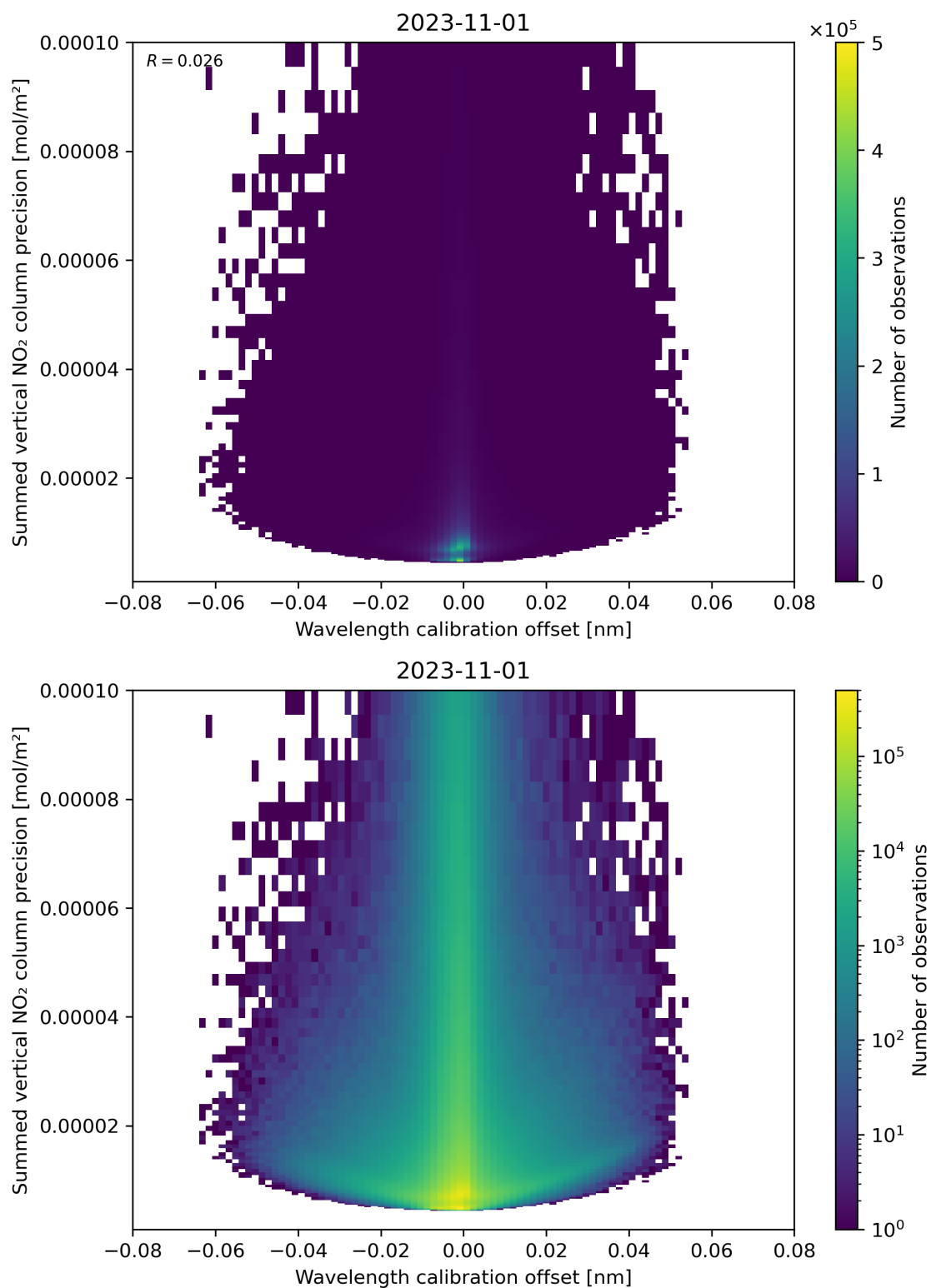
Figure 178: Scatter density plot of “Wavelength calibration offset” against “Summed vertical NO 2 column precision” for 2023-10-31 to 2023-11-02.
