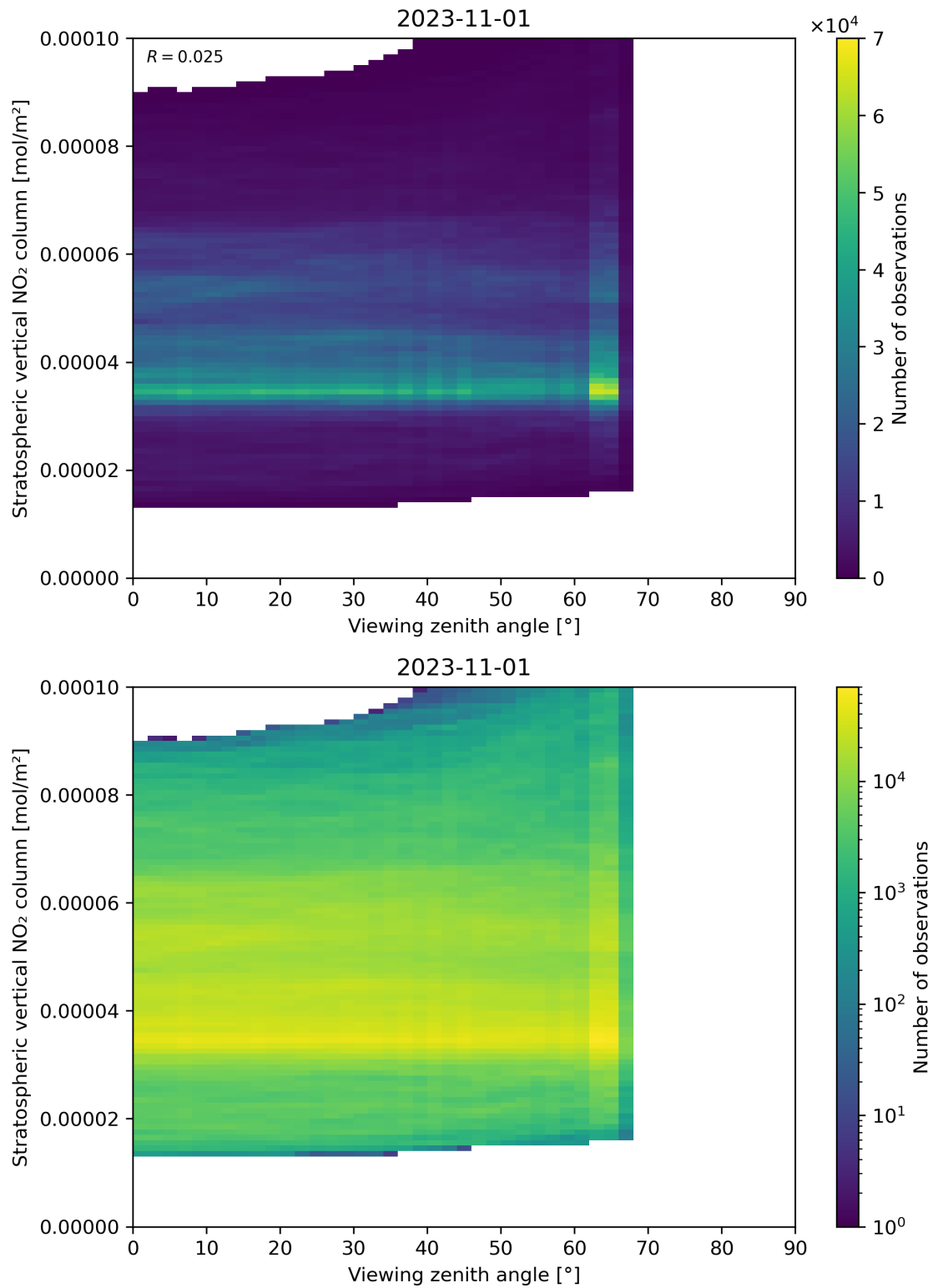
Figure 164: Scatter density plot of “Viewing zenith angle” against “Stratospheric vertical NO 2 column” for 2023-10-31 to 2023-11-02.
