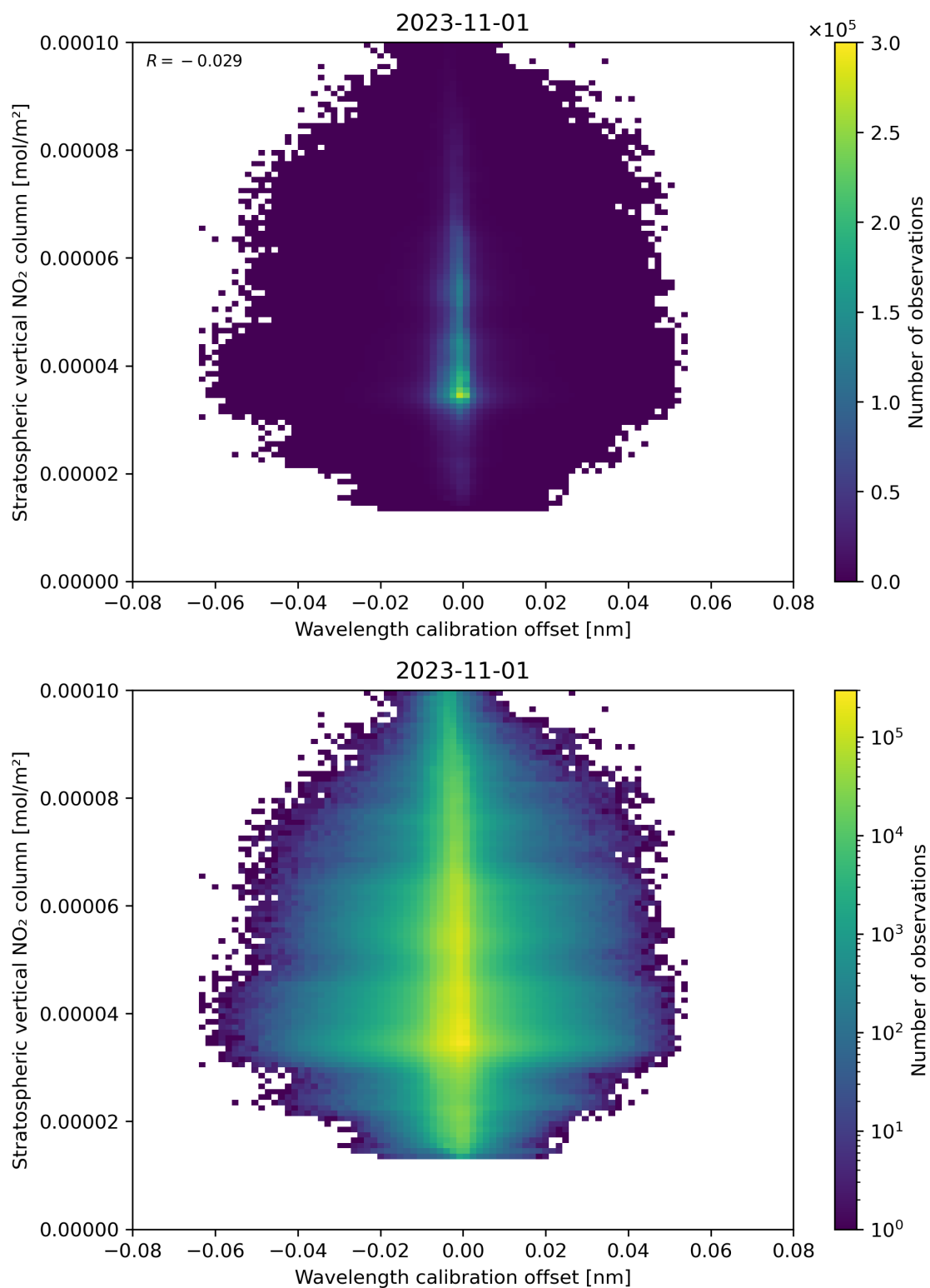
Figure 176: Scatter density plot of “Wavelength calibration offset” against “Stratospheric vertical NO 2 column” for 2023-10-31 to 2023-11-02.
