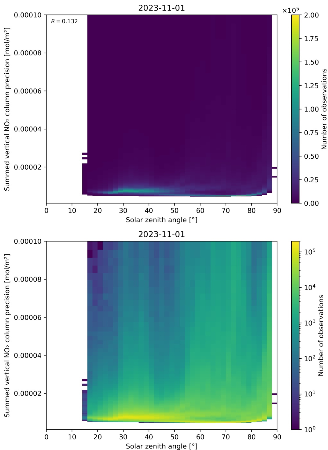
Figure 152: Scatter density plot of “Solar zenith angle” against “Summed vertical NO 2 column precision” for 2023-10-31 to 2023-11-02.
