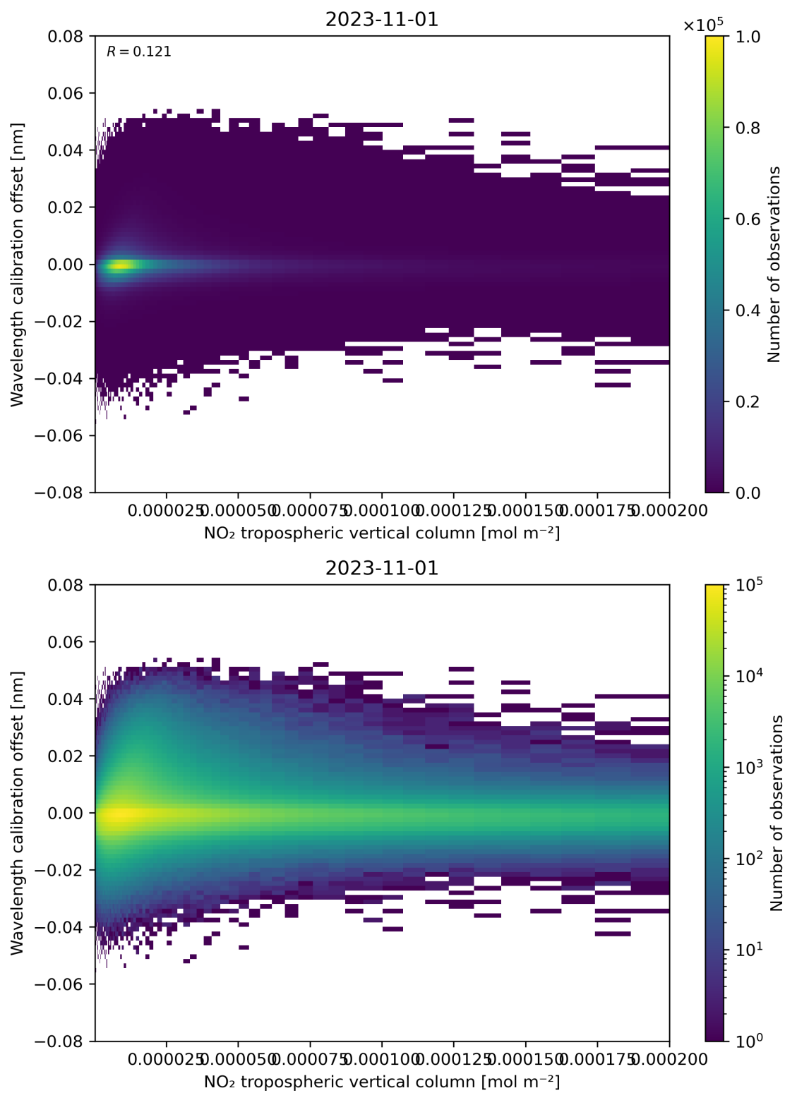
Figure 143: Scatter density plot of “NO 2 tropospheric vertical column” against “Wavelength calibration offset” for 2023-10-31 to 2023-11-02.
