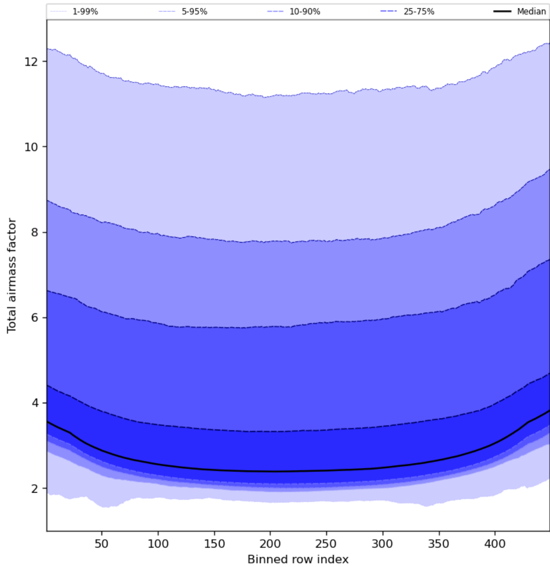
Figure 49: Along track statistics of “Total airmass factor” for 2023-10-31 to 2023-11-02
