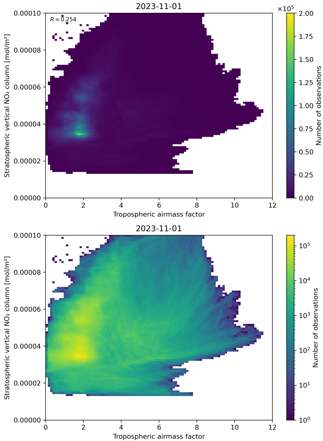
Figure 74: Scatter density plot of “Tropospheric air mass factor” against “Stratospheric vertical NO 2 column” for 2023-10-31 to 2023-11-02.
