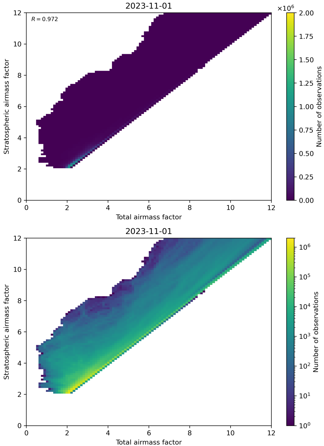
Figure 62: Scatter density plot of “Total airmass factor” against “Stratospheric airmass factor” for 2023-10-31 to 2023-11-02.
