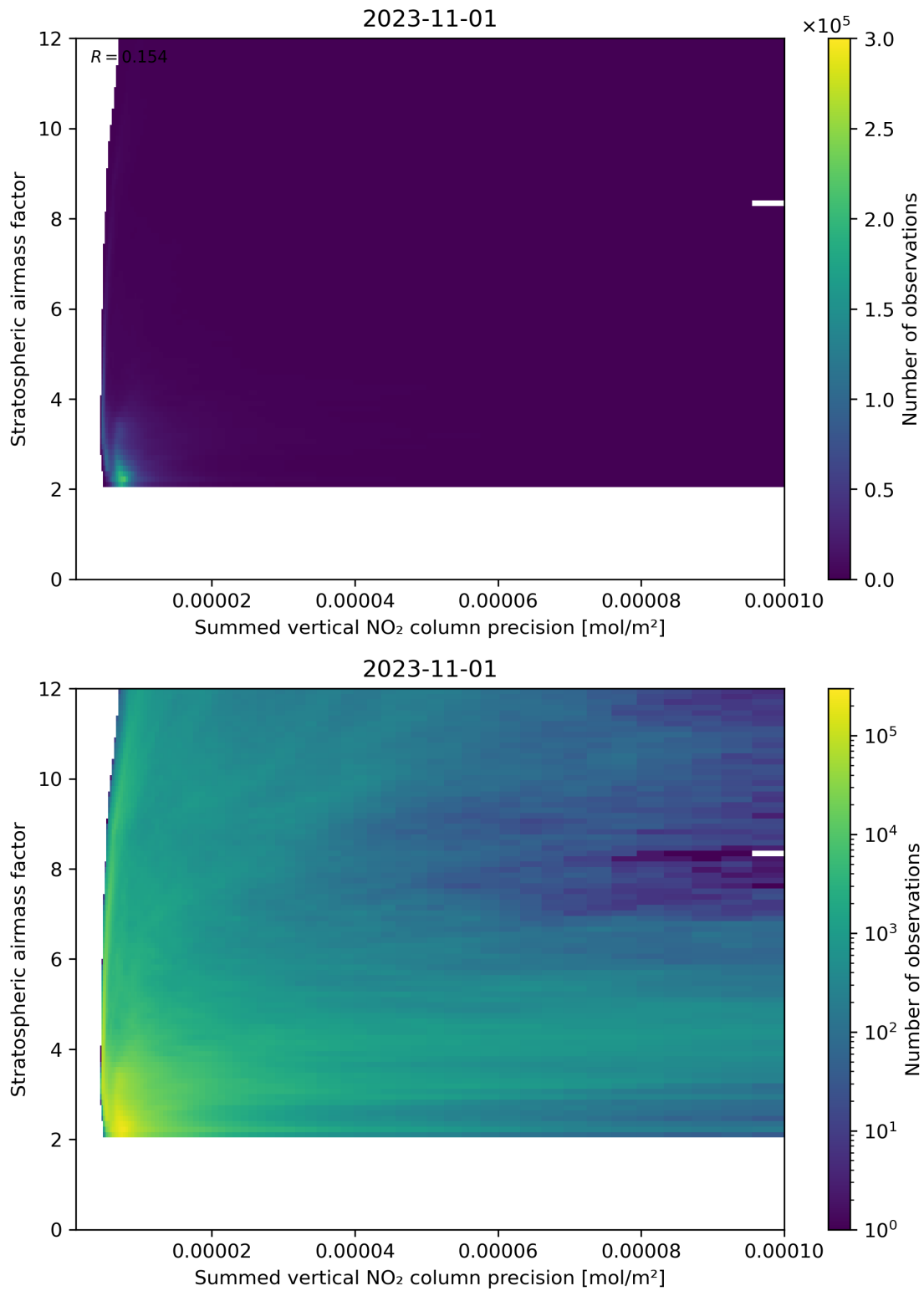
Figure 106: Scatter density plot of “Summed vertical NO 2 column precision” against “Stratospheric airmass factor” for 2023-10-31 to 2023-11-02.
