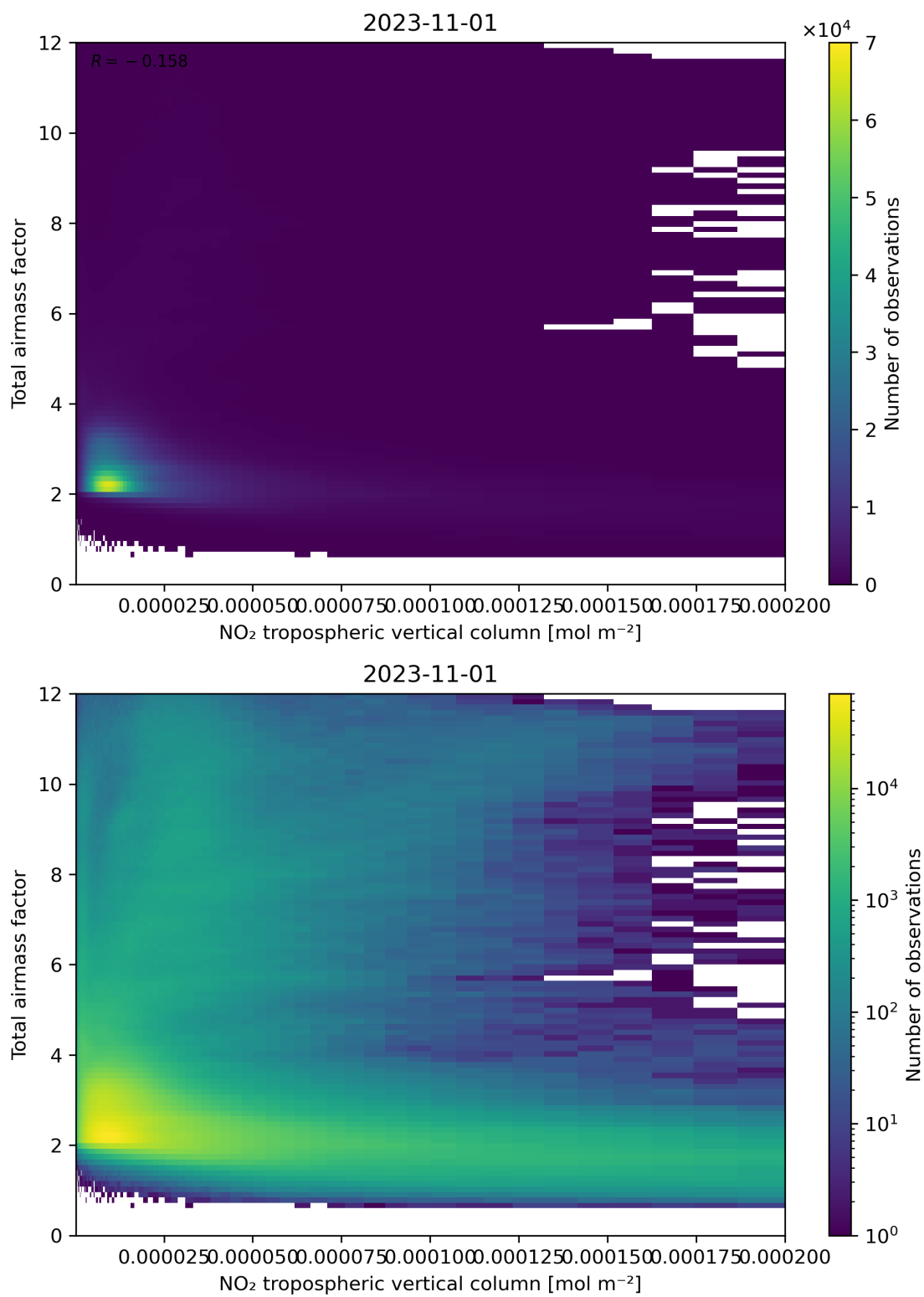
Figure 122: Scatter density plot of “NO 2 tropospheric vertical column” against “Total air mass factor” for 2023-10-31 to 2023-11-02.
