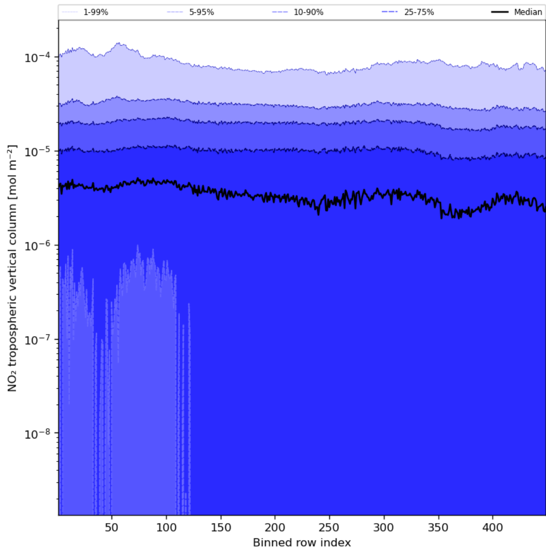
Figure 46: Along track statistics of “NO 2 tropospheric vertical column” for 2023-10-31 to 2023-11-02
