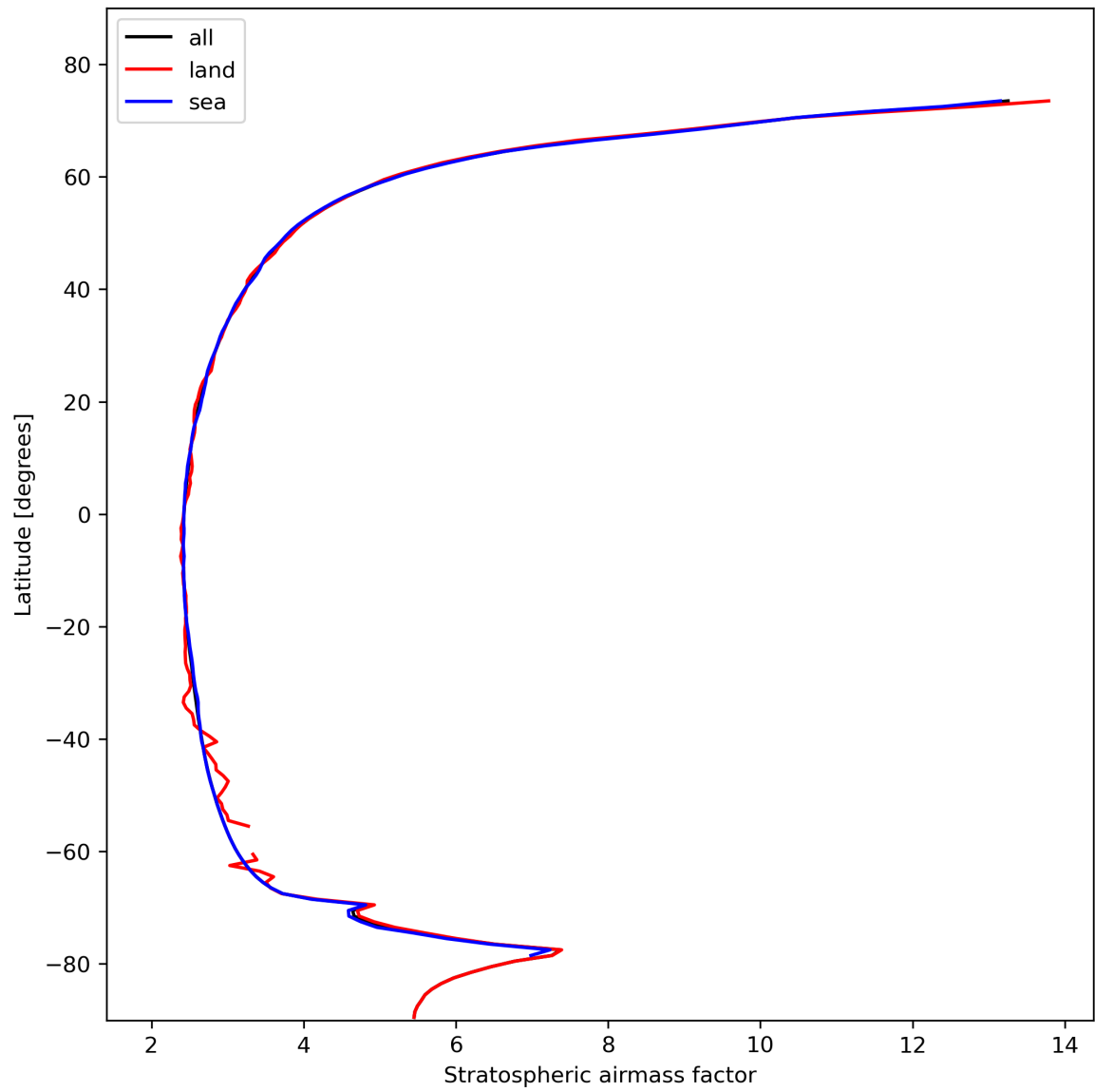
Figure 27: Zonal average of “Stratospheric air mass factor” for 2023-10-31 to 2023-11-02.
