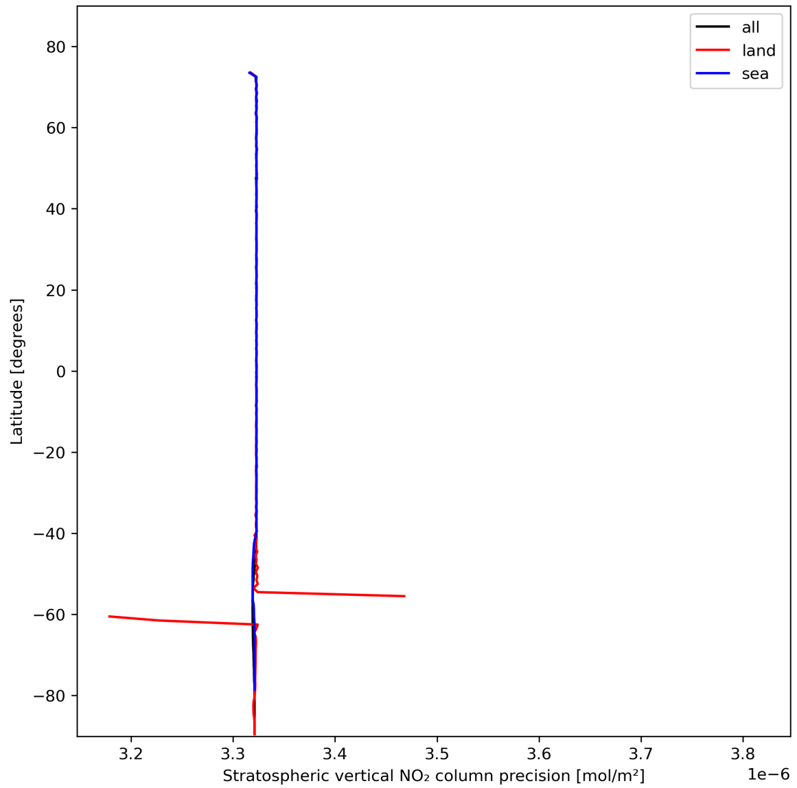
Figure 20: Zonal average of “Stratospheric vertical NO 2 column precision” for 2023-10-31 to 2023-11-02.
