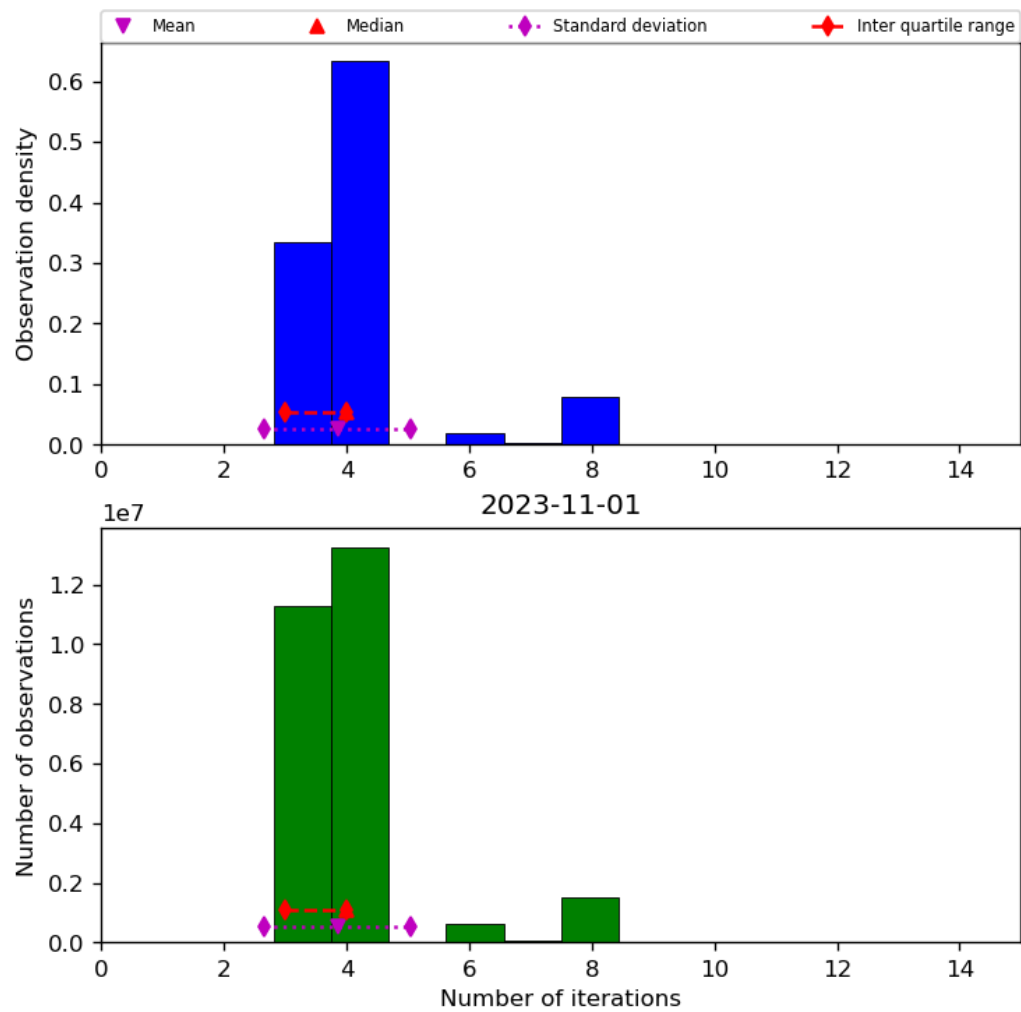
Figure 34: Histogram of “Number of iterations” for 2023-10-31 to 2023-11-02
