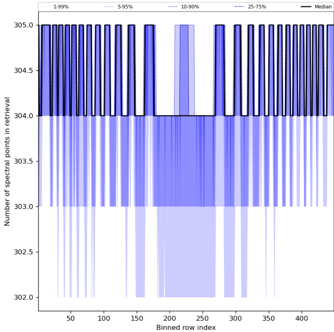
Figure 50: Along track statistics of “Number of spectral points in retrieval” for 2023-10-31 to 2023-11-02
