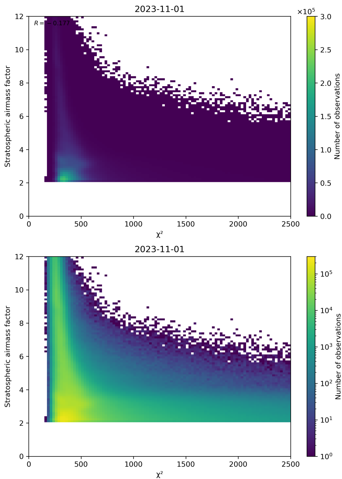
Figure 81: Scatter density plot of “ \chi^2 ” against “Stratospheric airmass factor” for 2023-10-31 to 2023-11-02.
