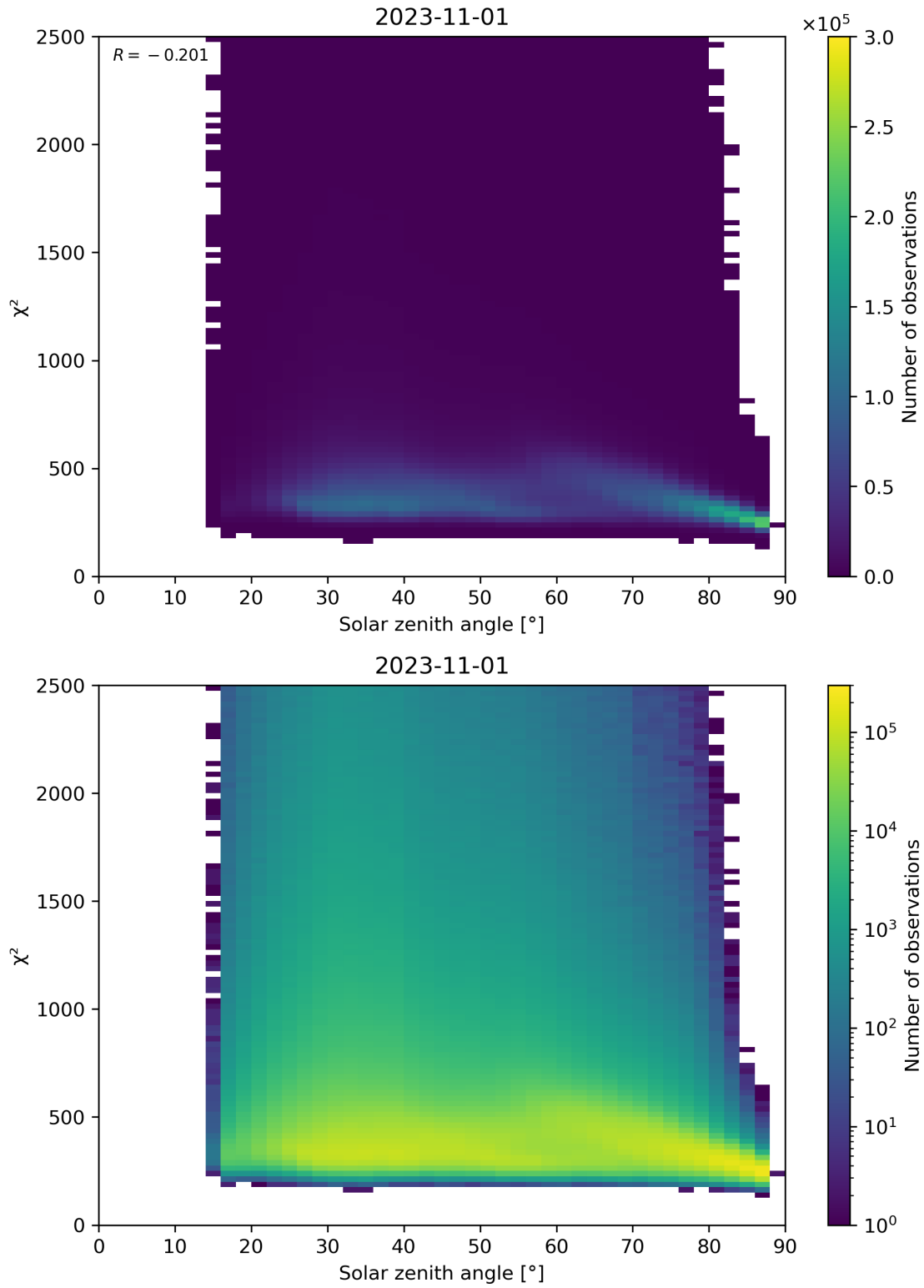
Figure 148: Scatter density plot of “Solar zenith angle” against “ \chi^2 ” for 2023-10-31 to 2023-11-02.
