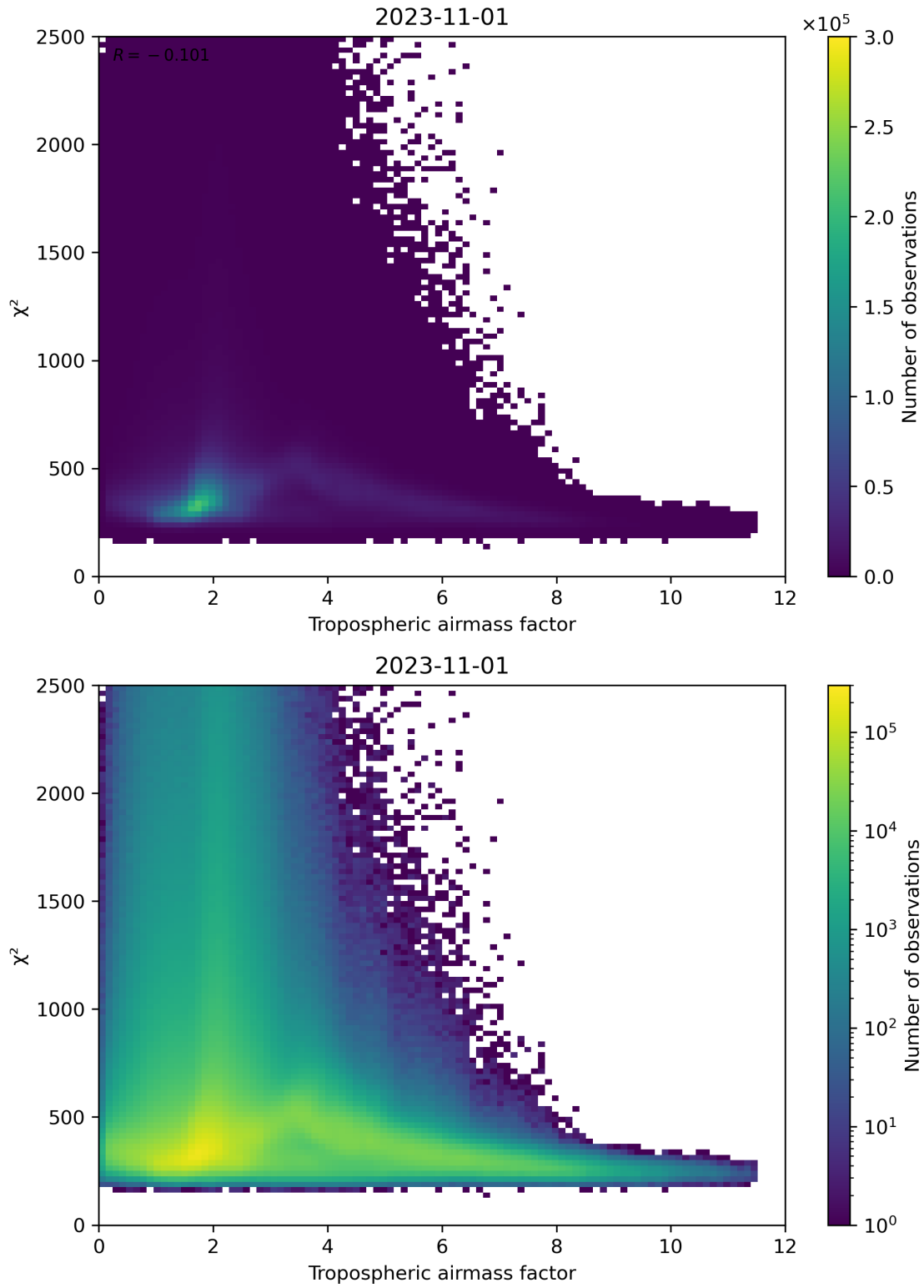
Figure 73: Scatter density plot of “Tropospheric airmass factor” against “ \chi^2 ” for 2023-10-31 to 2023-11-02.
