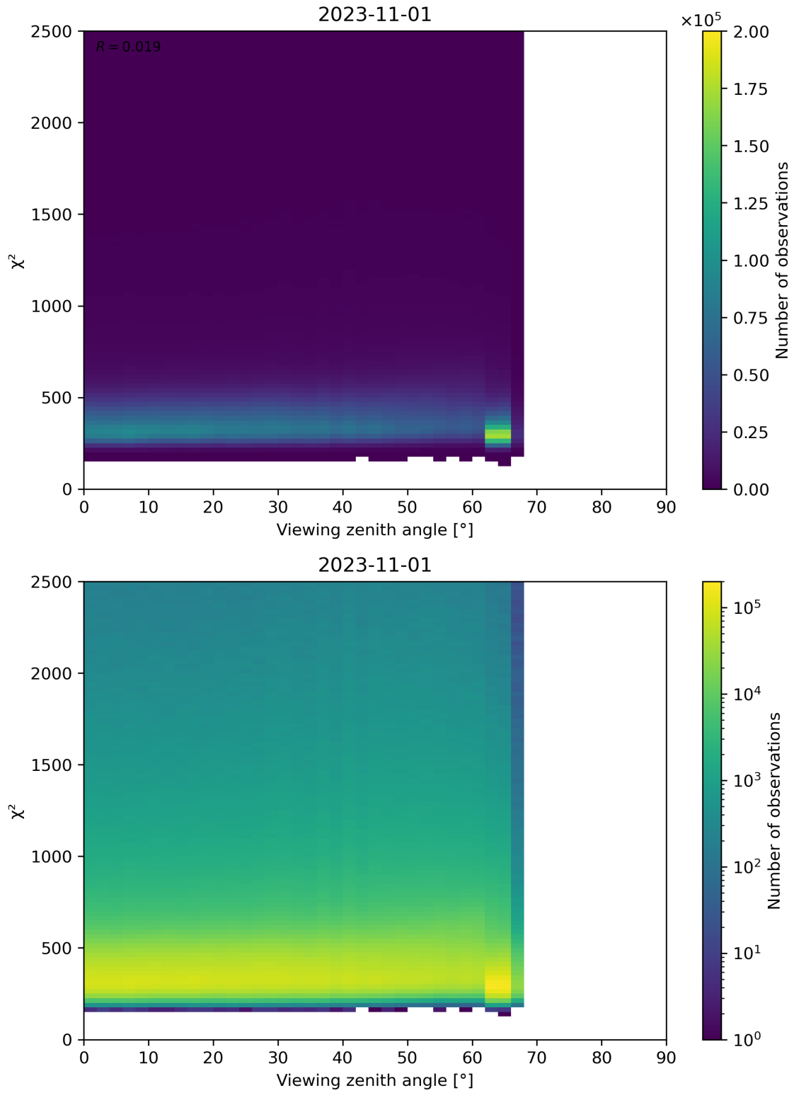
Figure 162: Scatter density plot of “Viewing zenith angle” against “ \chi^2 ” for 2023-10-31 to 2023-11-02.
