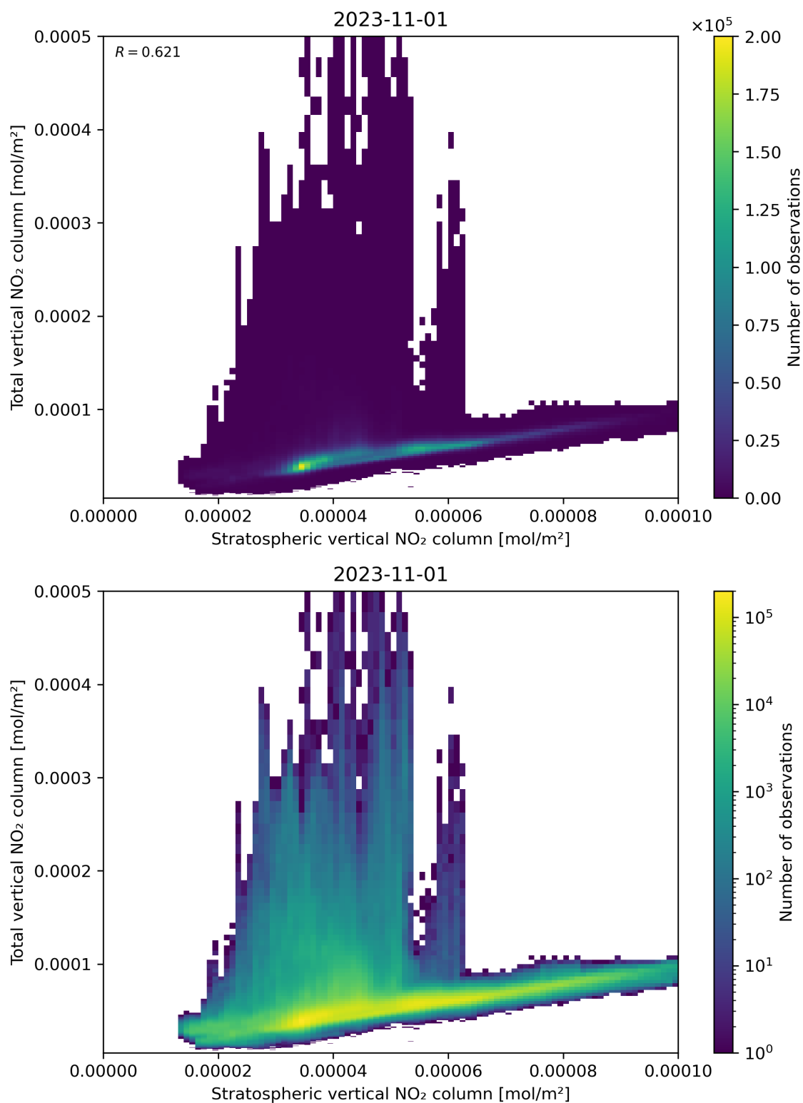
Figure 100: Scatter density plot of “Stratospheric vertical NO 2 column” against “Total vertical NO 2 column” for 2023-10-31 to 2023-11-02.
