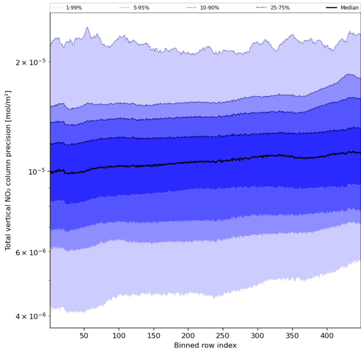
Figure 56: Along track statistics of “Total vertical NO 2 column precision” for 2023-10-31 to 2023-11-02
