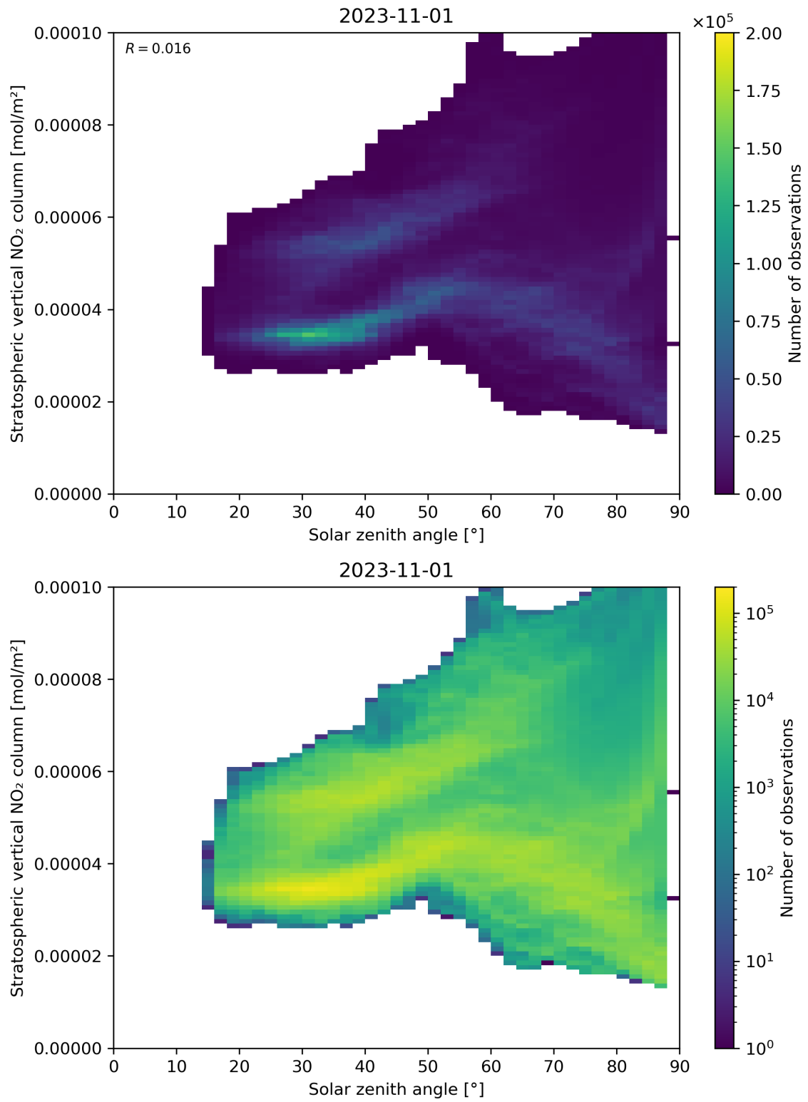
Figure 150: Scatter density plot of “Solar zenith angle” against “Stratospheric vertical NO 2 column” for 2023-10-31 to 2023-11-02.
