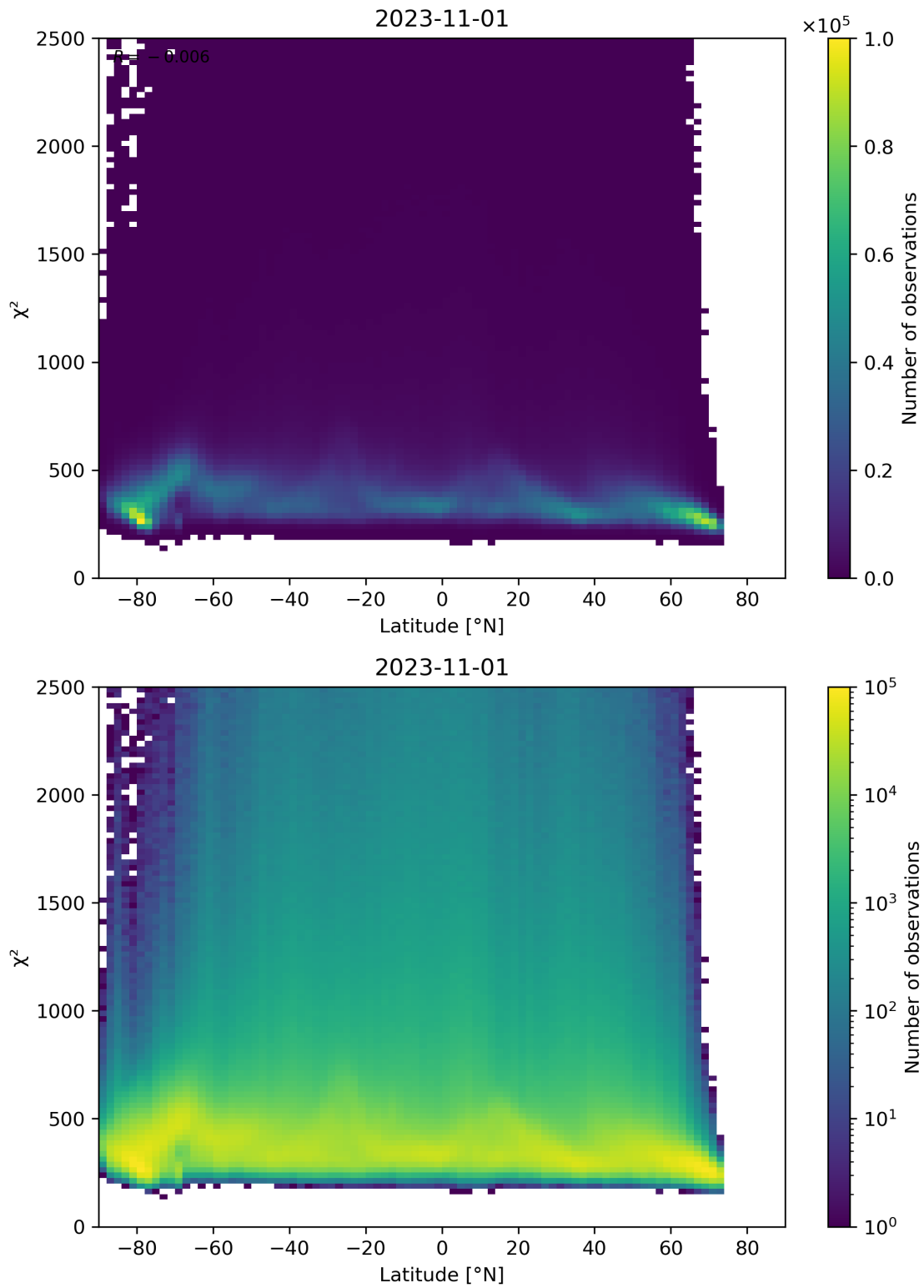
Figure 86: Scatter density plot of “Latitude” against “ \chi^2 ” for 2023-10-31 to 2023-11-02.
