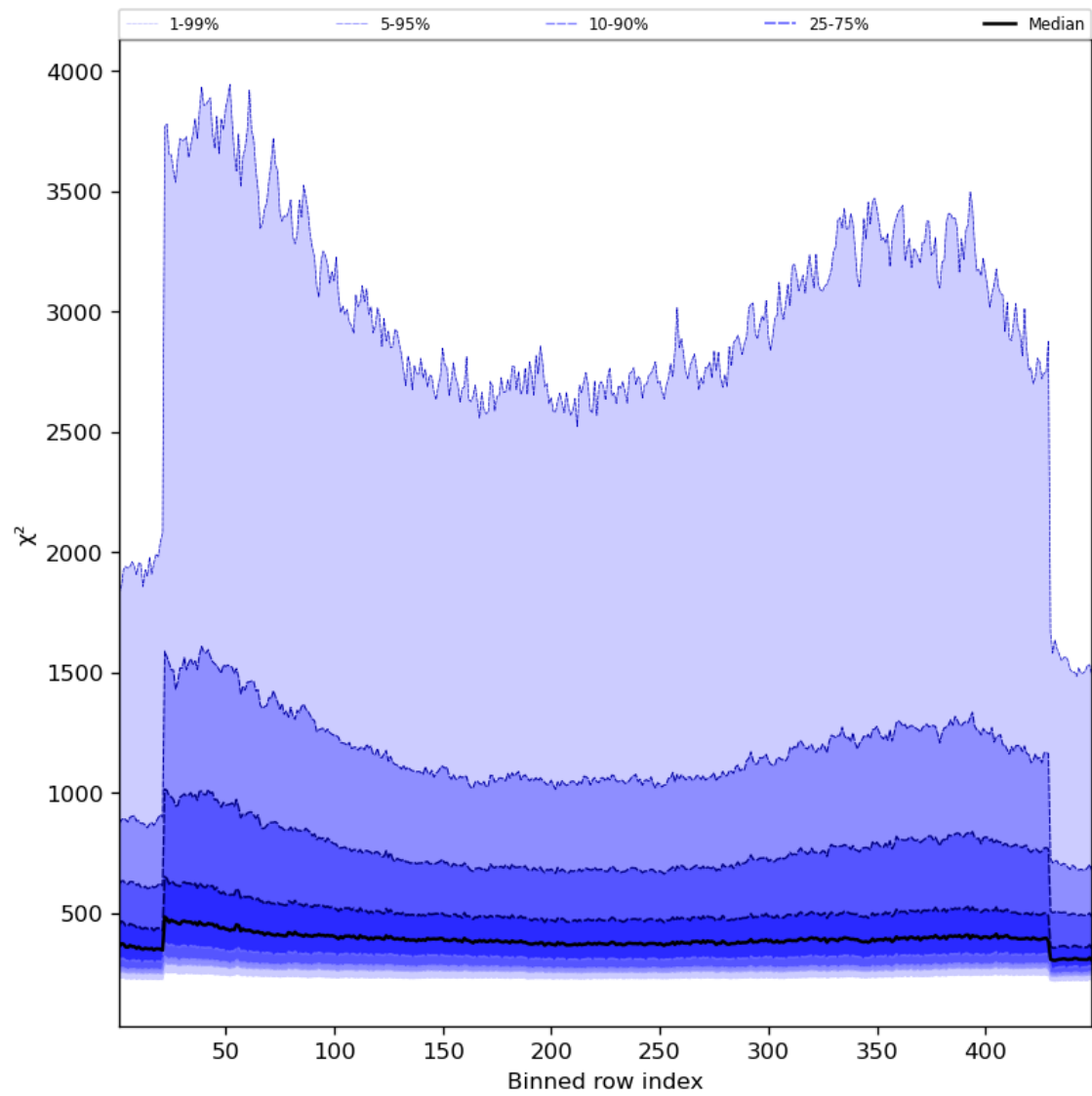
Figure 59: Along track statistics of “ \chi^2 ” for 2023-10-31 to 2023-11-02
