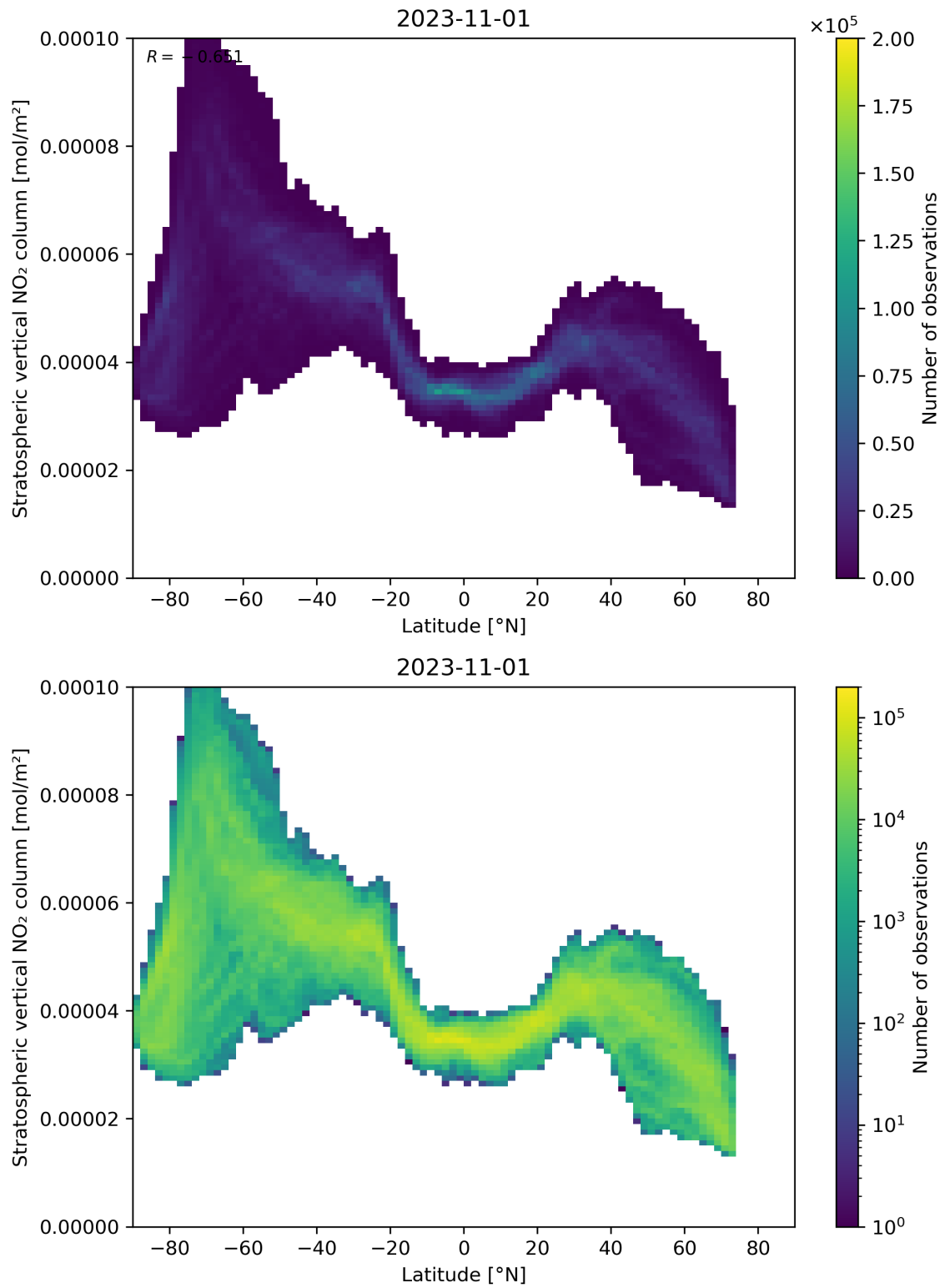
Figure 87: Scatter density plot of “Latitude” against “Stratospheric vertical NO 2 column” for 2023-10-31 to 2023-11-02.
