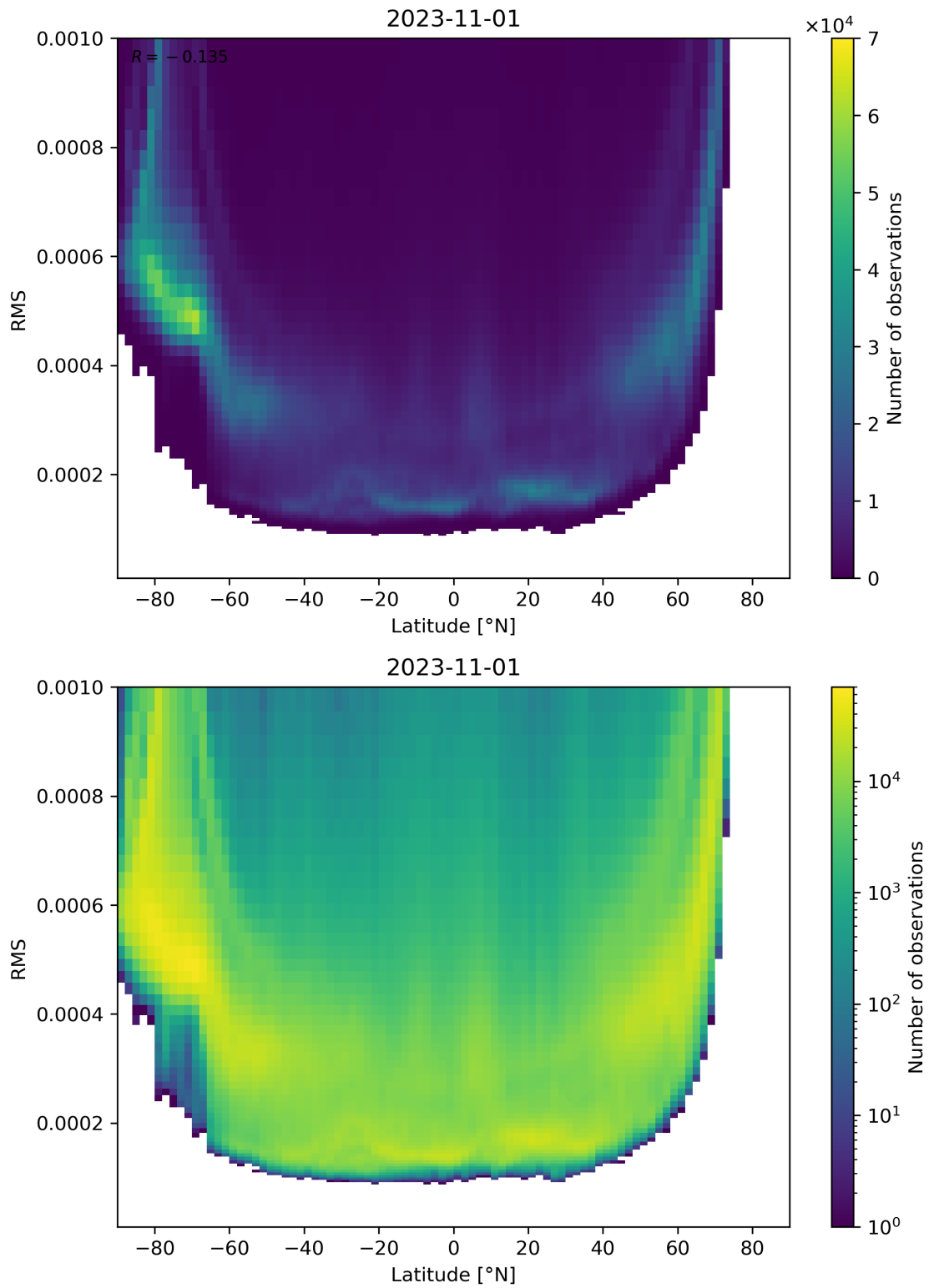
Figure 94: Scatter density plot of “Latitude” against “RMS” for 2023-10-31 to 2023-11-02.
