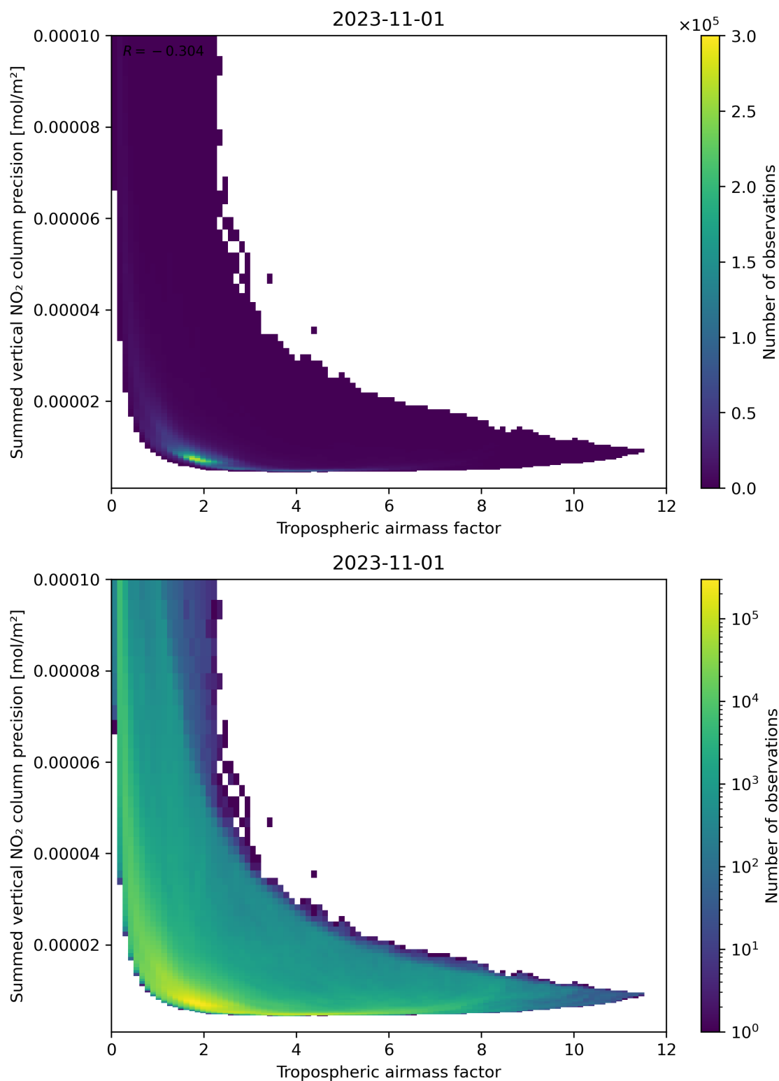
Figure 76: Scatter density plot of “Tropospheric air mass factor” against “Summed vertical NO 2 column precision” for 2023-10-31 to 2023-11-02.
