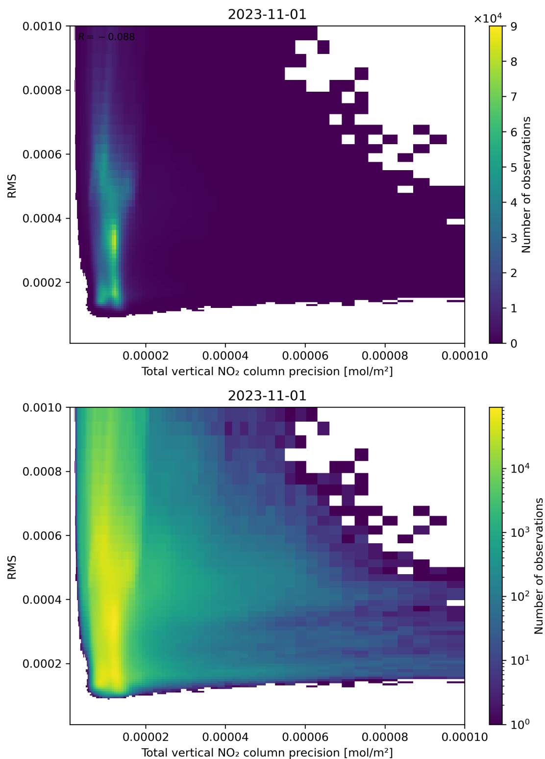
Figure 119: Scatter density plot of “Total vertical NO 2 column precision” against “RMS” for 2023-10-31 to 2023-11-02.
