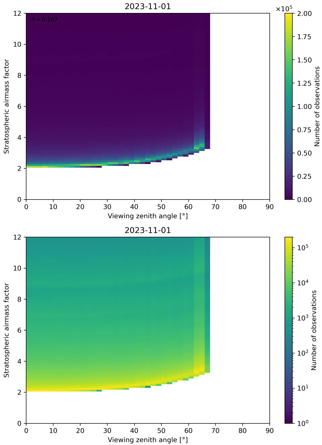
Figure 159: Scatter density plot of “Viewing zenith angle” against “Stratospheric airmass factor” for 2023-10-31 to 2023-11-02.
