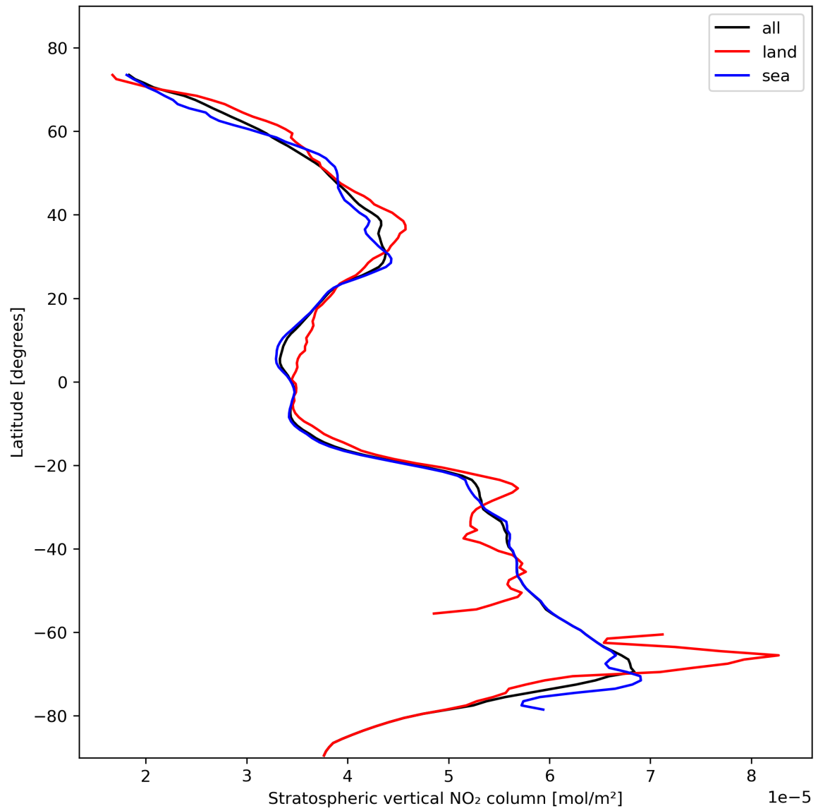
Figure 19: Zonal average of “Stratospheric vertical NO 2 column” for 2023-10-31 to 2023-11-02.
