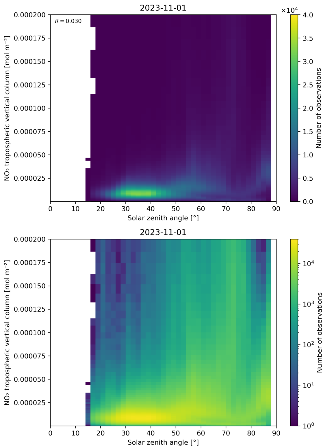
Figure 155: Scatter density plot of “Solar zenith angle” against “NO 2 tropospheric vertical column” for 2023-10-31 to 2023-11-02.
