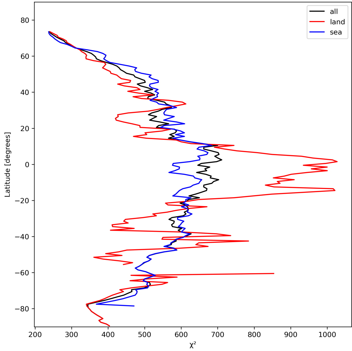
Figure 25: Zonal average of “ \chi^2 ” for 2023-10-31 to 2023-11-02.
