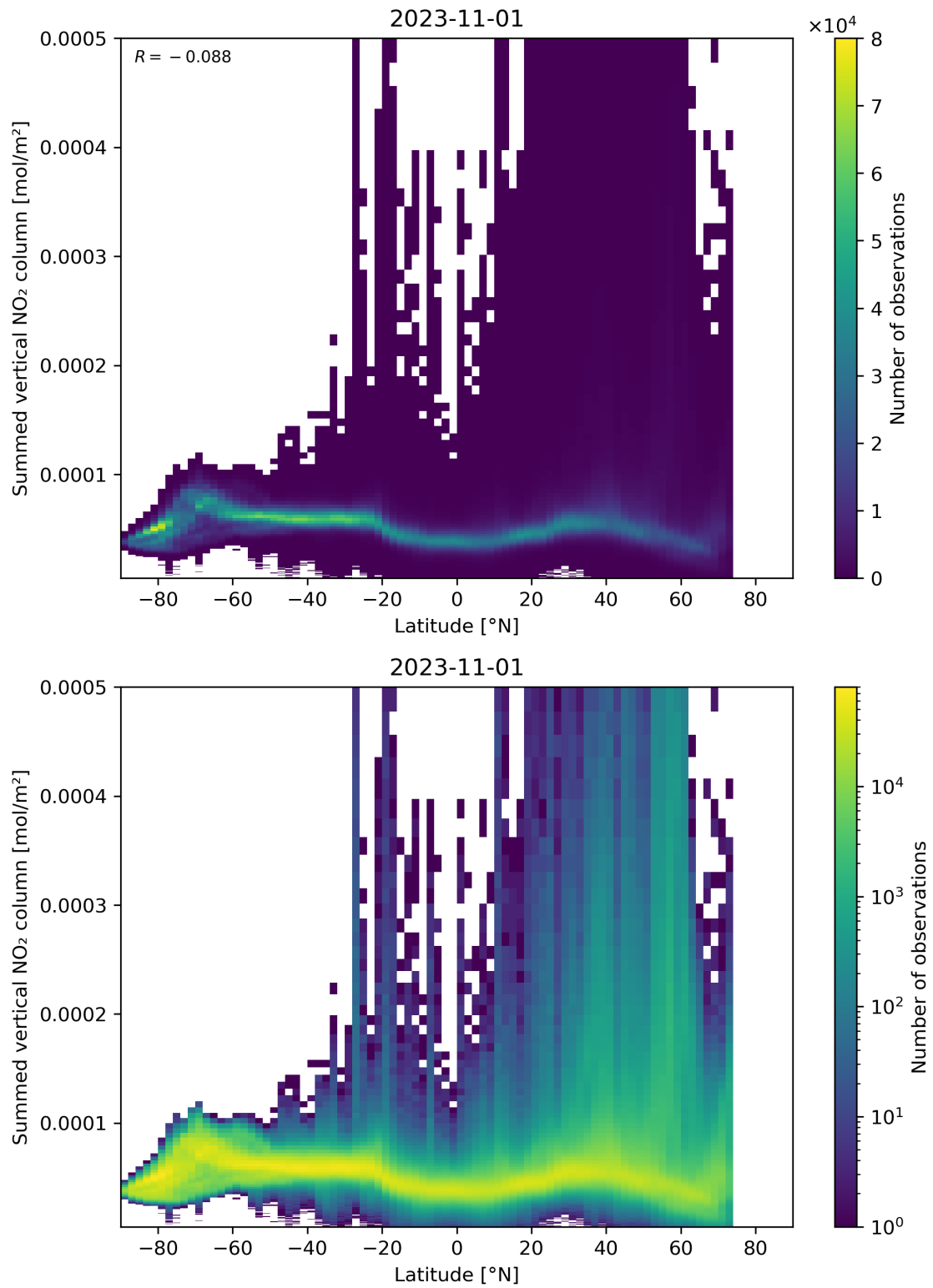
Figure 88: Scatter density plot of “Latitude” against “Summed vertical NO 2 column” for 2023-10-31 to 2023-11-02.
