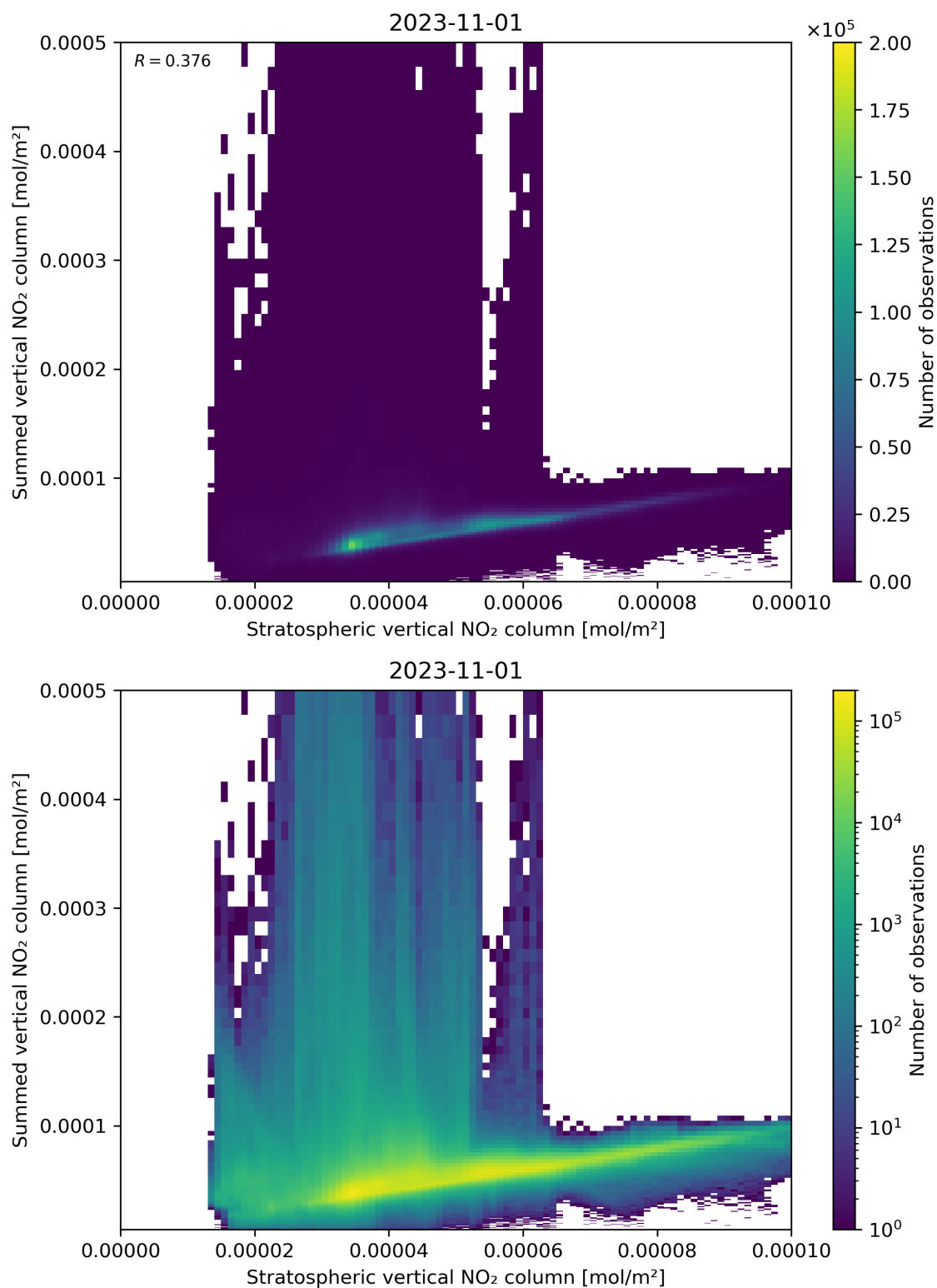
Figure 98: Scatter density plot of “Stratospheric vertical NO 2 column” against “Summed vertical NO 2 column” for 2023-10-31 to 2023-11-02.
