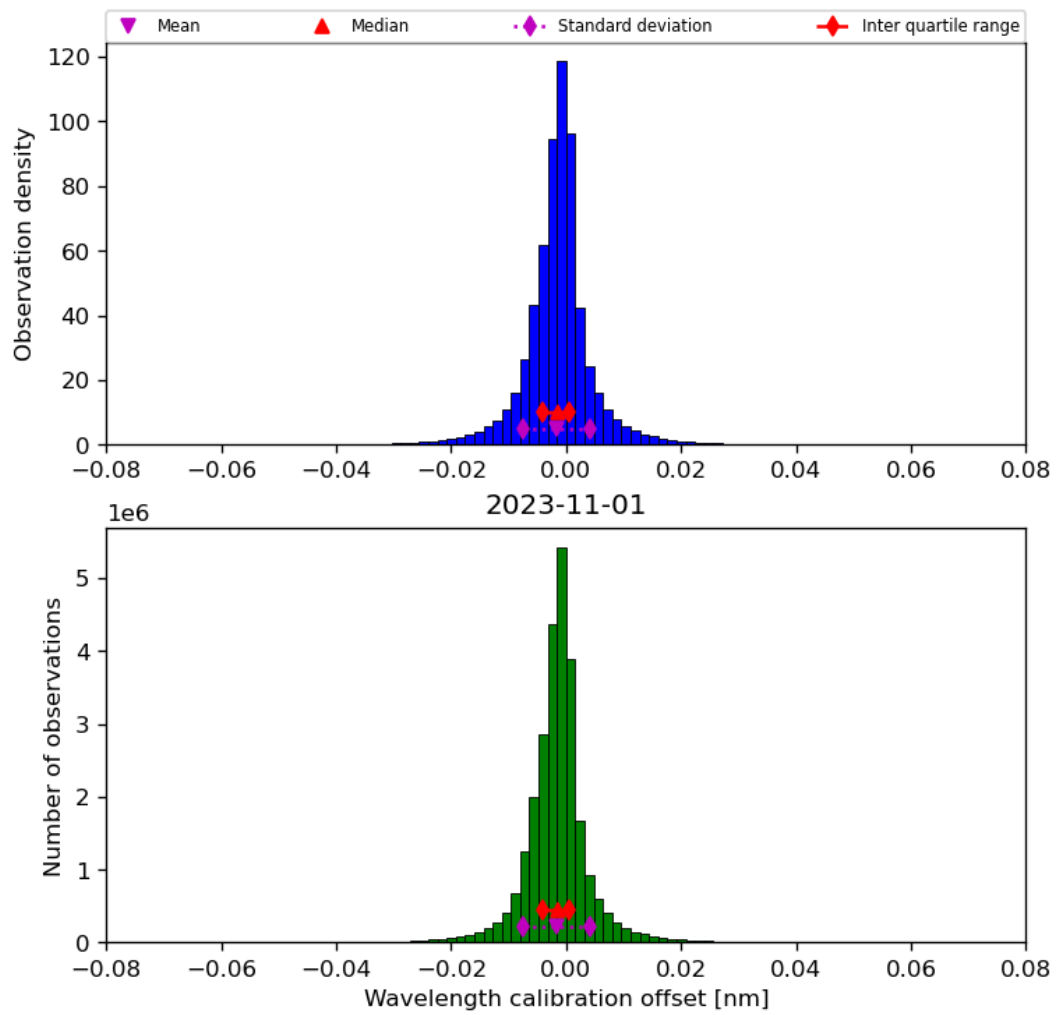
Figure 35: Histogram of “Wavelength calibration offset” for 2023-10-31 to 2023-11-02
