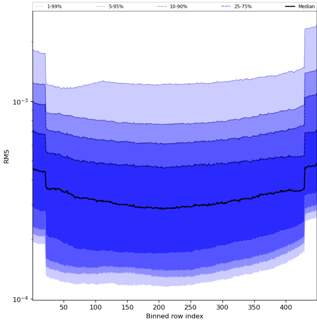
Figure 60: Along track statistics of “RMS” for 2023-10-31 to 2023-11-02
