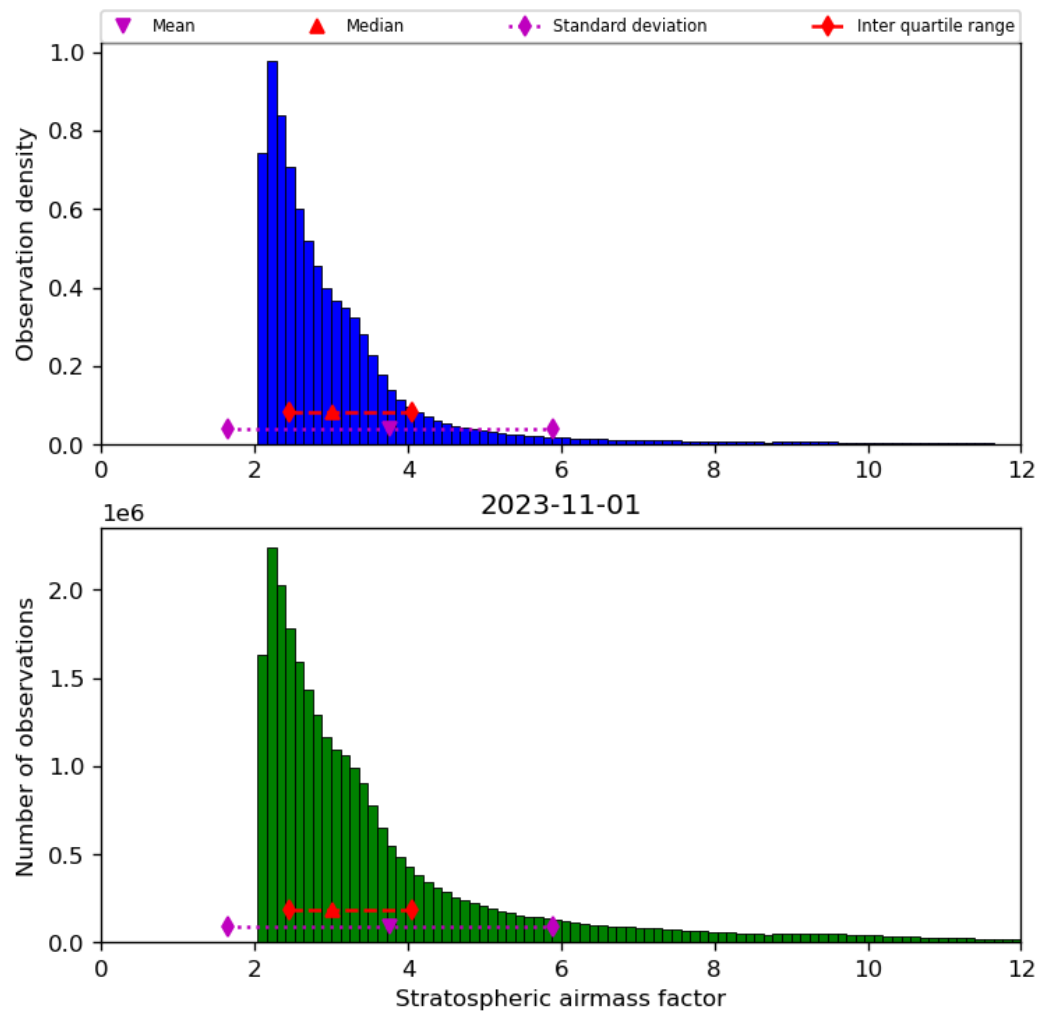
Figure 44: Histogram of “Stratospheric airmass factor” for 2023-10-31 to 2023-11-02
