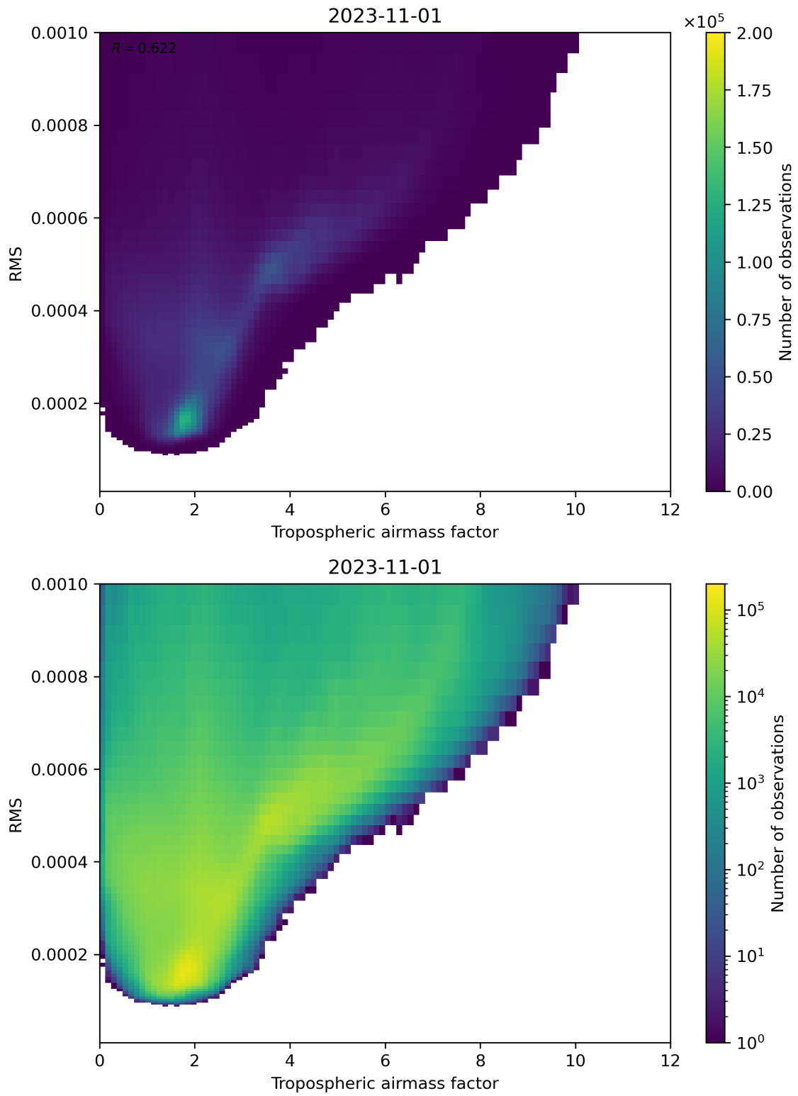
Figure 79: Scatter density plot of “Tropospheric airmass factor” against “RMS” for 2023-10-31 to 2023-11-02.
