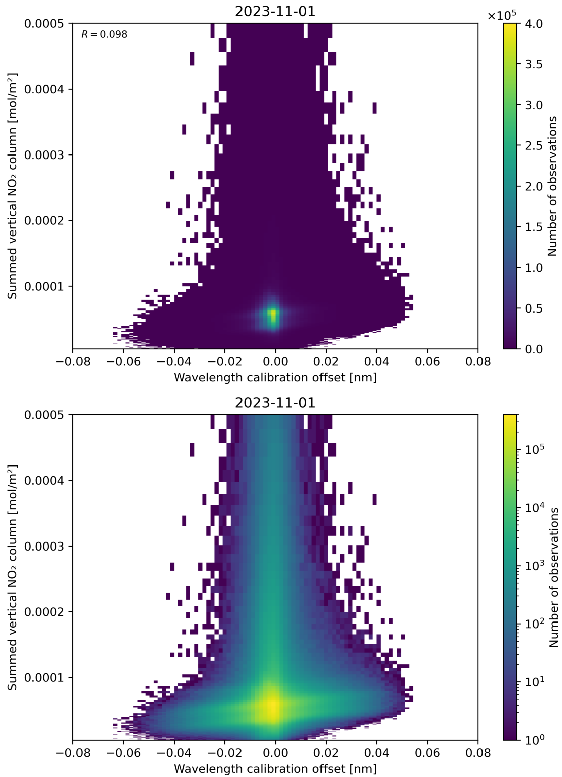
Figure 177: Scatter density plot of “Wavelength calibration offset” against “Summed vertical NO 2 column” for 2023-10-31 to 2023-11-02.
