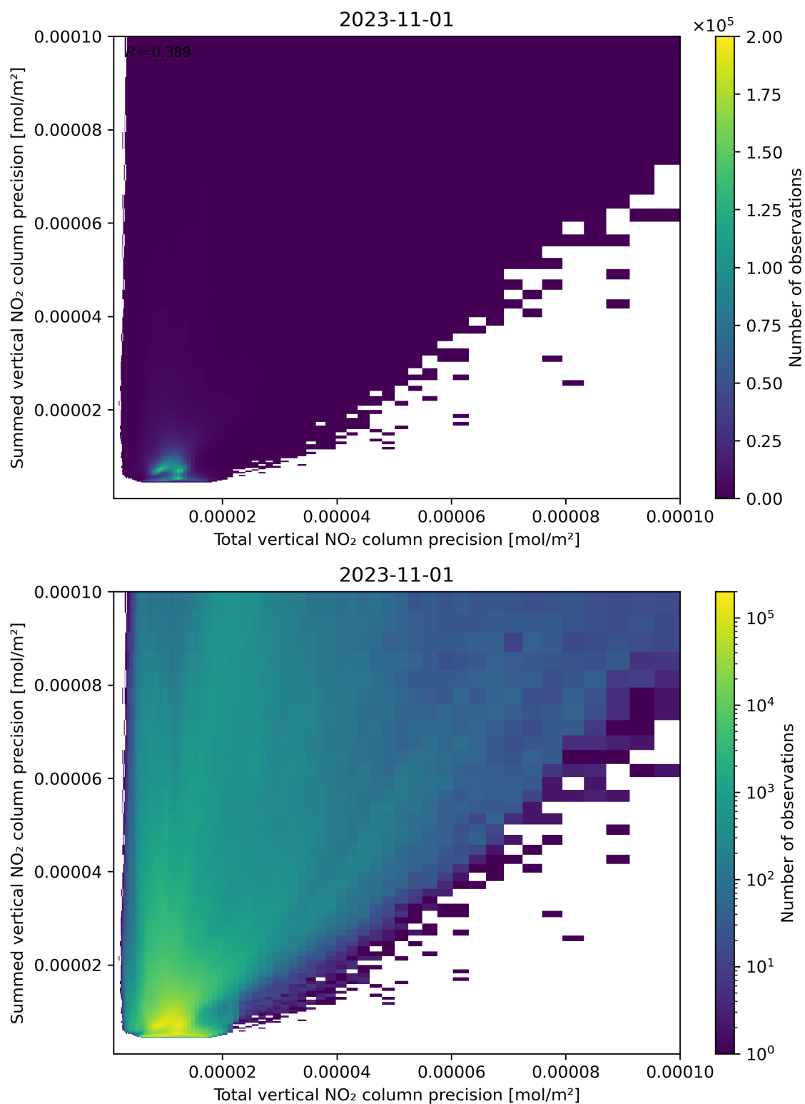
Figure 118: Scatter density plot of “Total vertical NO 2 column precision” against “Summed vertical NO 2 column precision” for 2023-10-31 to 2023-11-02.
