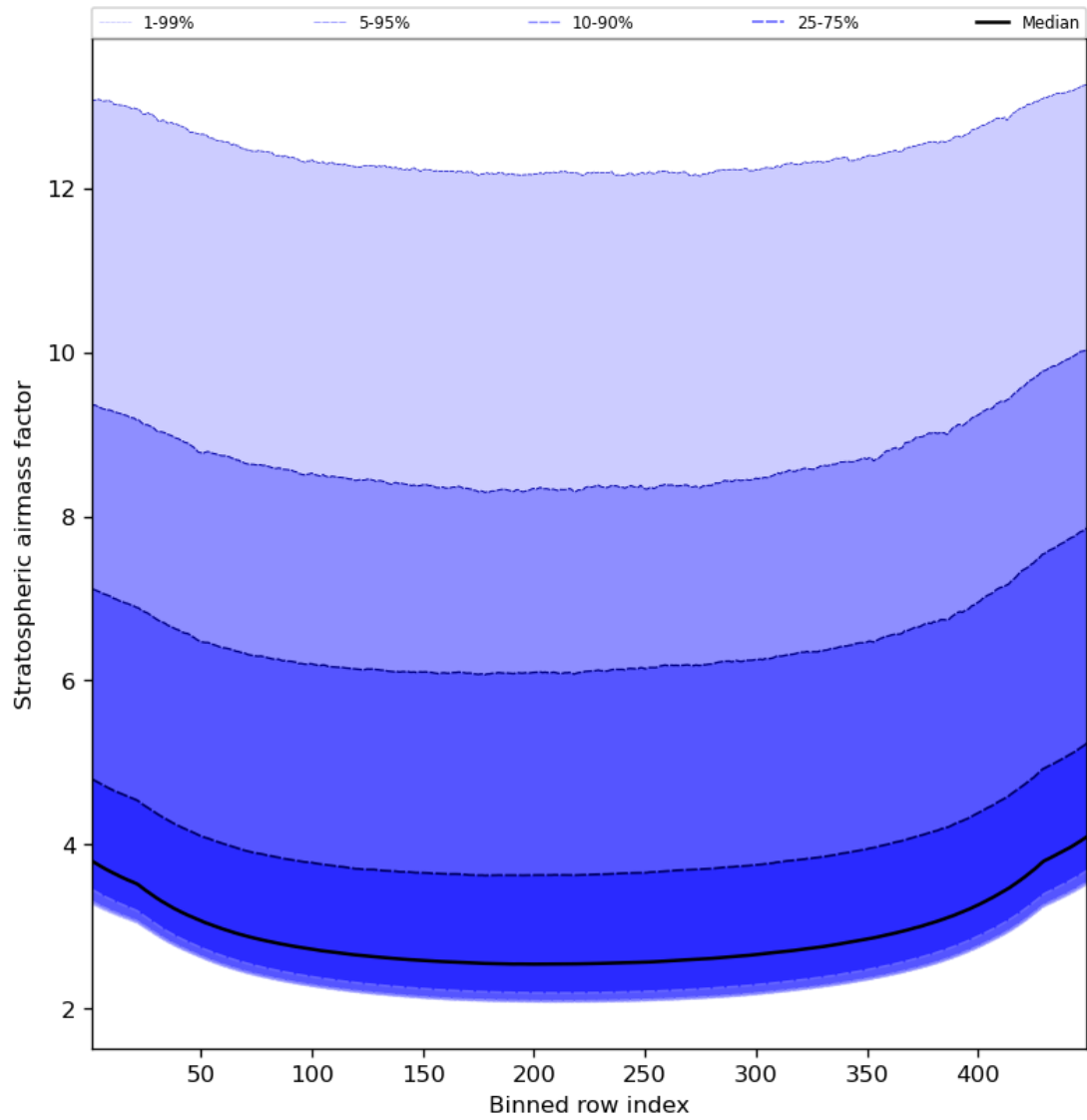
Figure 61: Along track statistics of “Stratospheric airmass factor” for 2023-10-31 to 2023-11-02
