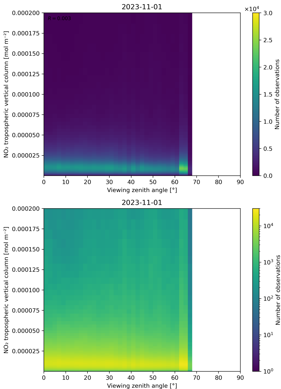
Figure 169: Scatter density plot of “Viewing zenith angle” against “NO 2 tropospheric vertical column” for 2023-10-31 to 2023-11-02.
