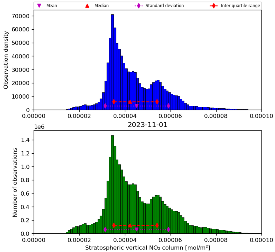
Figure 36: Histogram of “Stratospheric vertical NO 2 column” for 2023-10-31 to 2023-11-02
