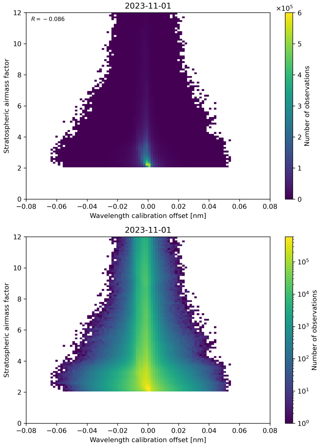
Figure 174: Scatter density plot of “Wavelength calibration offset” against “Stratospheric airmass factor” for 2023-10-31 to 2023-11-02.
