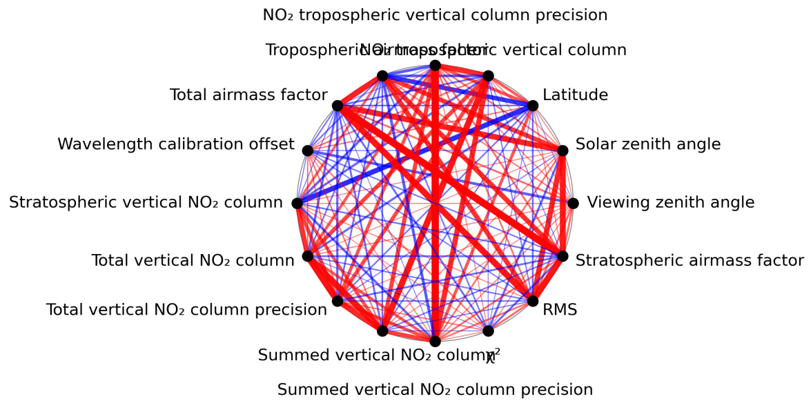
Figure 1: Map of correlation graph for 2023-10-31 to 2023-11-02.
