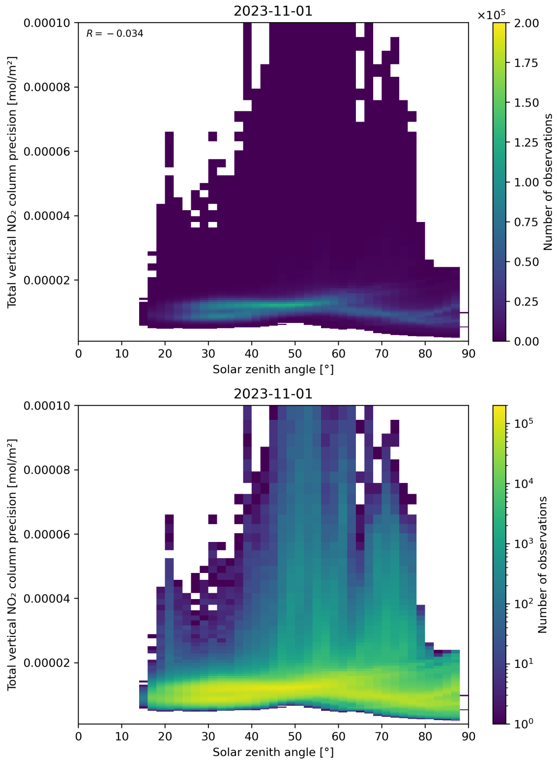
Figure 154: Scatter density plot of “Solar zenith angle” against “Total vertical NO 2 column precision” for 2023-10-31 to 2023-11-02.
