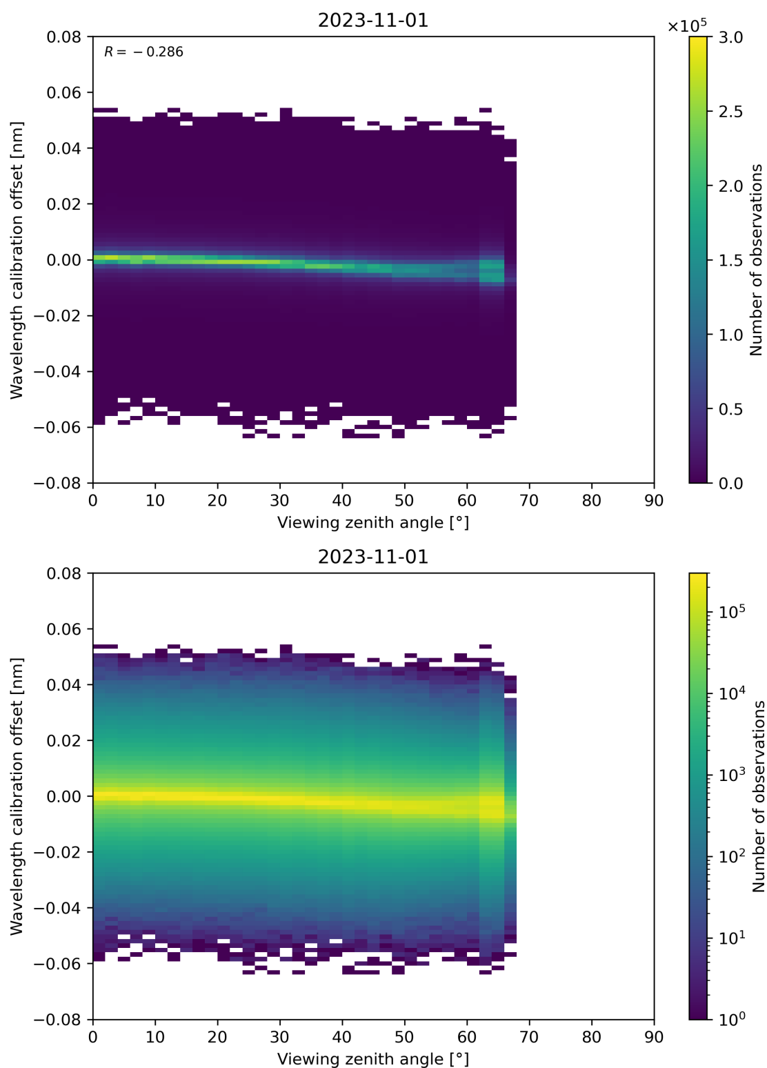
Figure 173: Scatter density plot of “Viewing zenith angle” against “Wavelength calibration offset” for 2023-10-31 to 2023-11-02.
