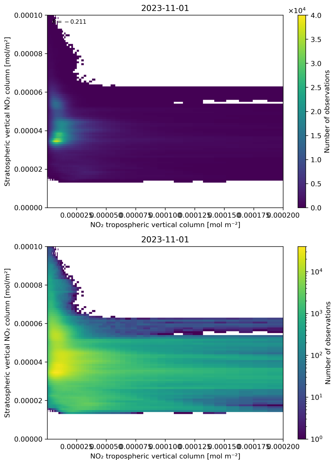
Figure 125: Scatter density plot of “NO 2 tropospheric vertical column” against “Stratospheric vertical NO 2 column” for 2023-10-31 to 2023-11-02.
