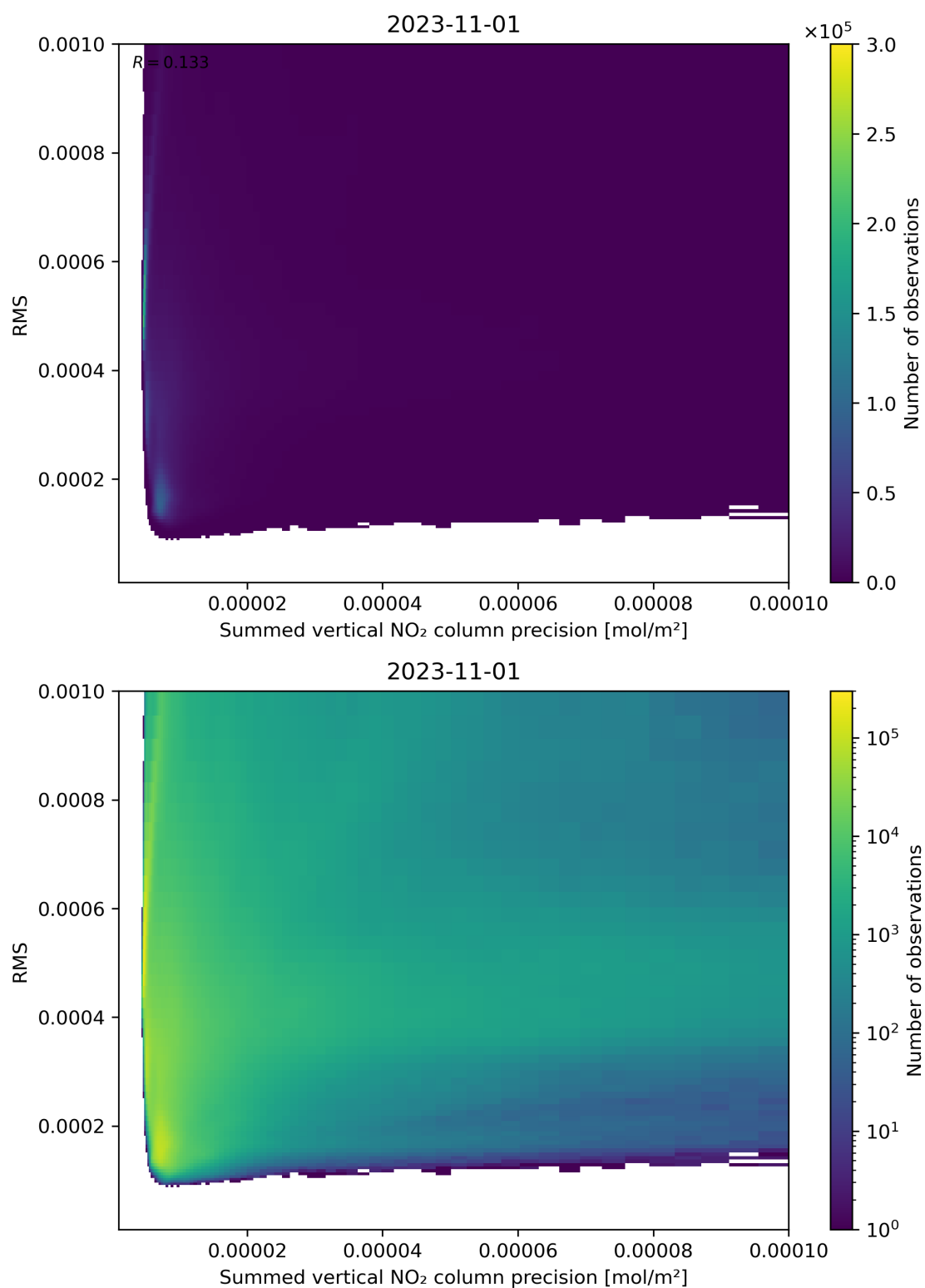
Figure 108: Scatter density plot of “Summed vertical NO 2 column precision” against “RMS” for 2023-10-31 to 2023-11-02.
