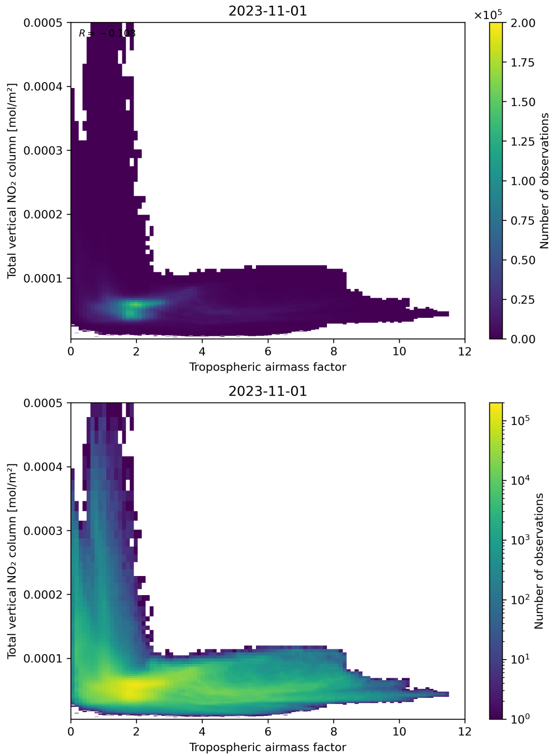
Figure 77: Scatter density plot of “Tropospheric airmass factor” against “Total vertical NO 2 column” for 2023-10-31 to 2023-11-02.
