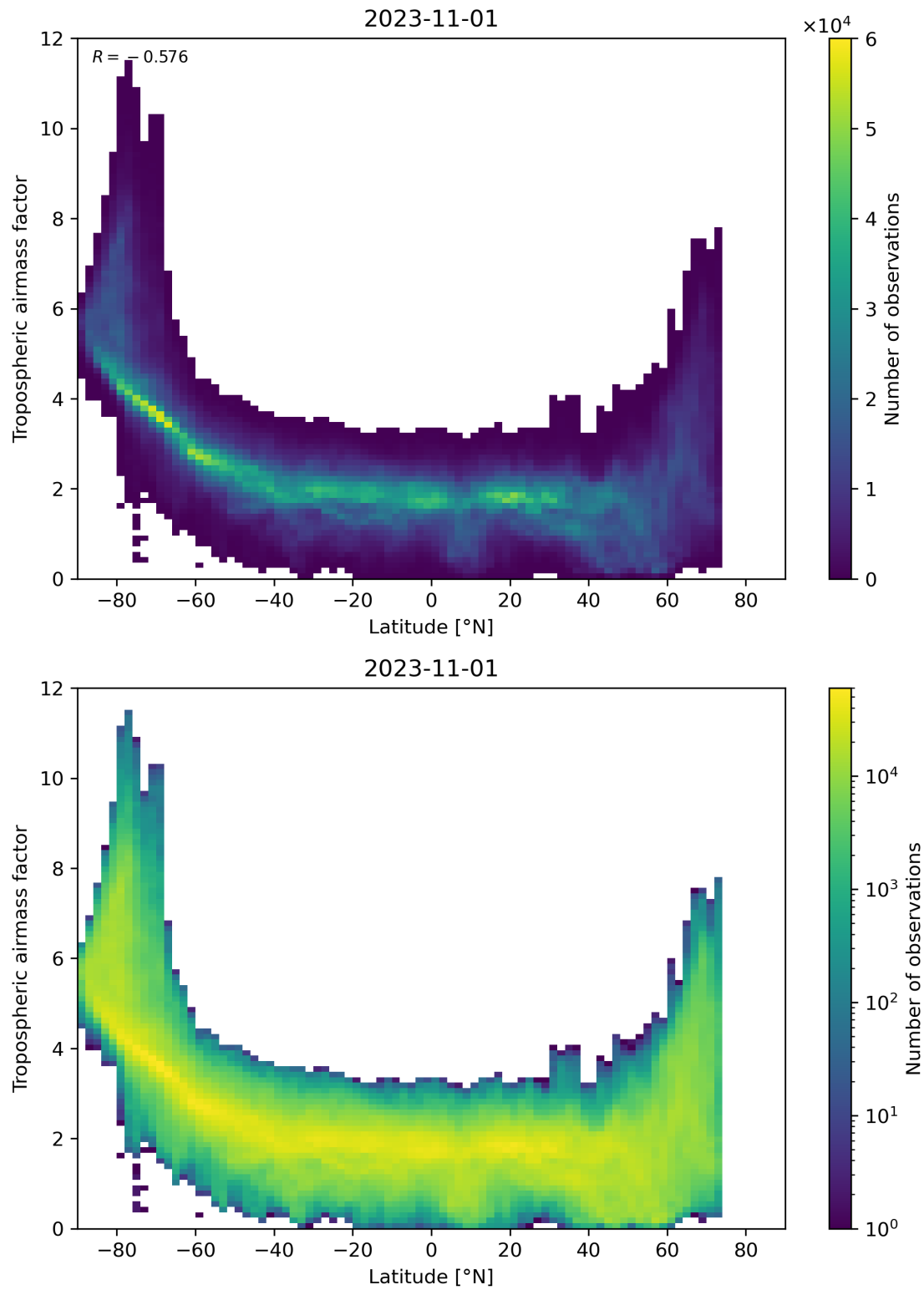
Figure 85: Scatter density plot of “Latitude” against “Tropospheric airmass factor” for 2023-10-31 to 2023-11-02.
