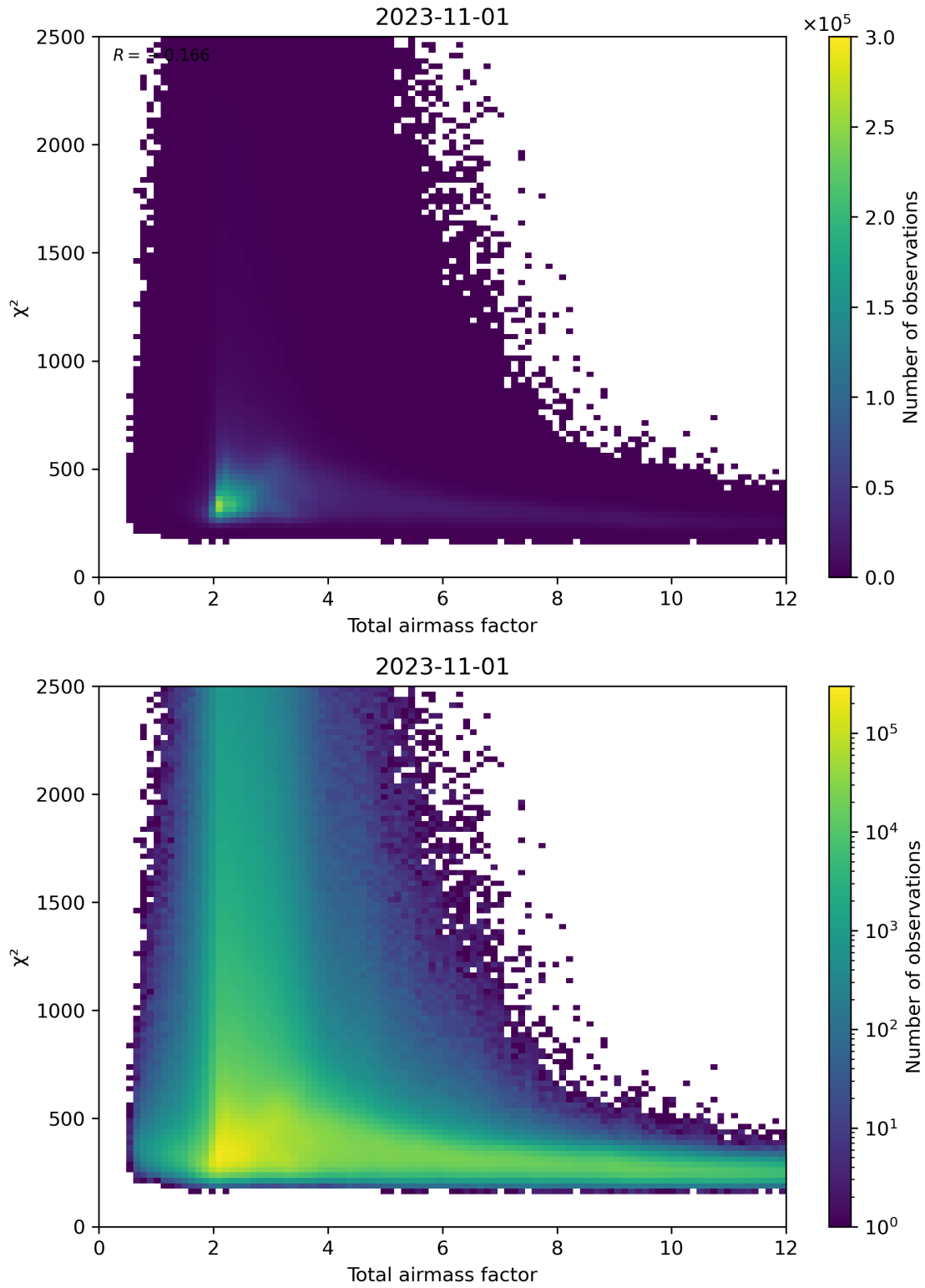
Figure 63: Scatter density plot of “Total airmass factor” against “ \chi^2 ” for 2023-10-31 to 2023-11-02.
