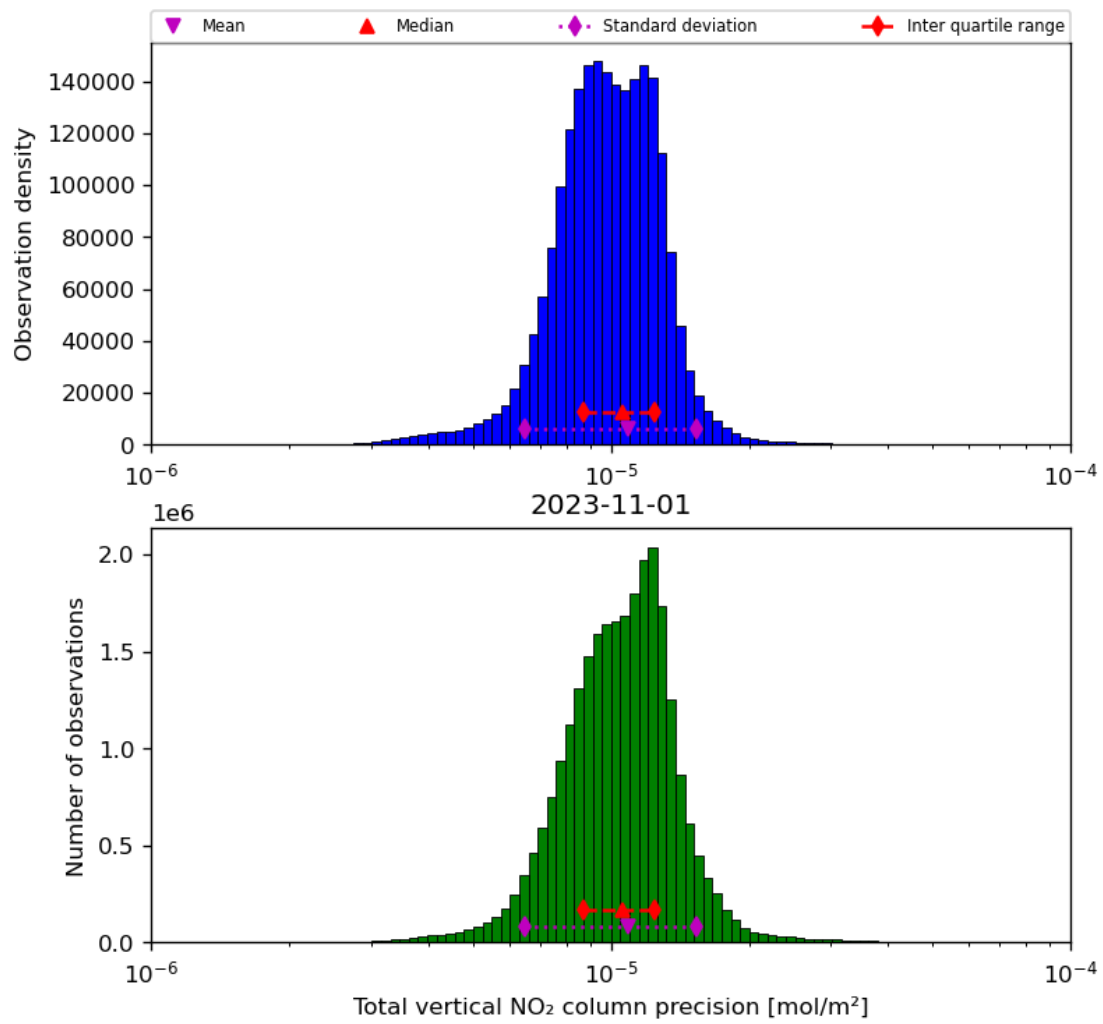
Figure 39: Histogram of "Total vertical NO 2 column precision" for 2023-10-31 to 2023-11-02
