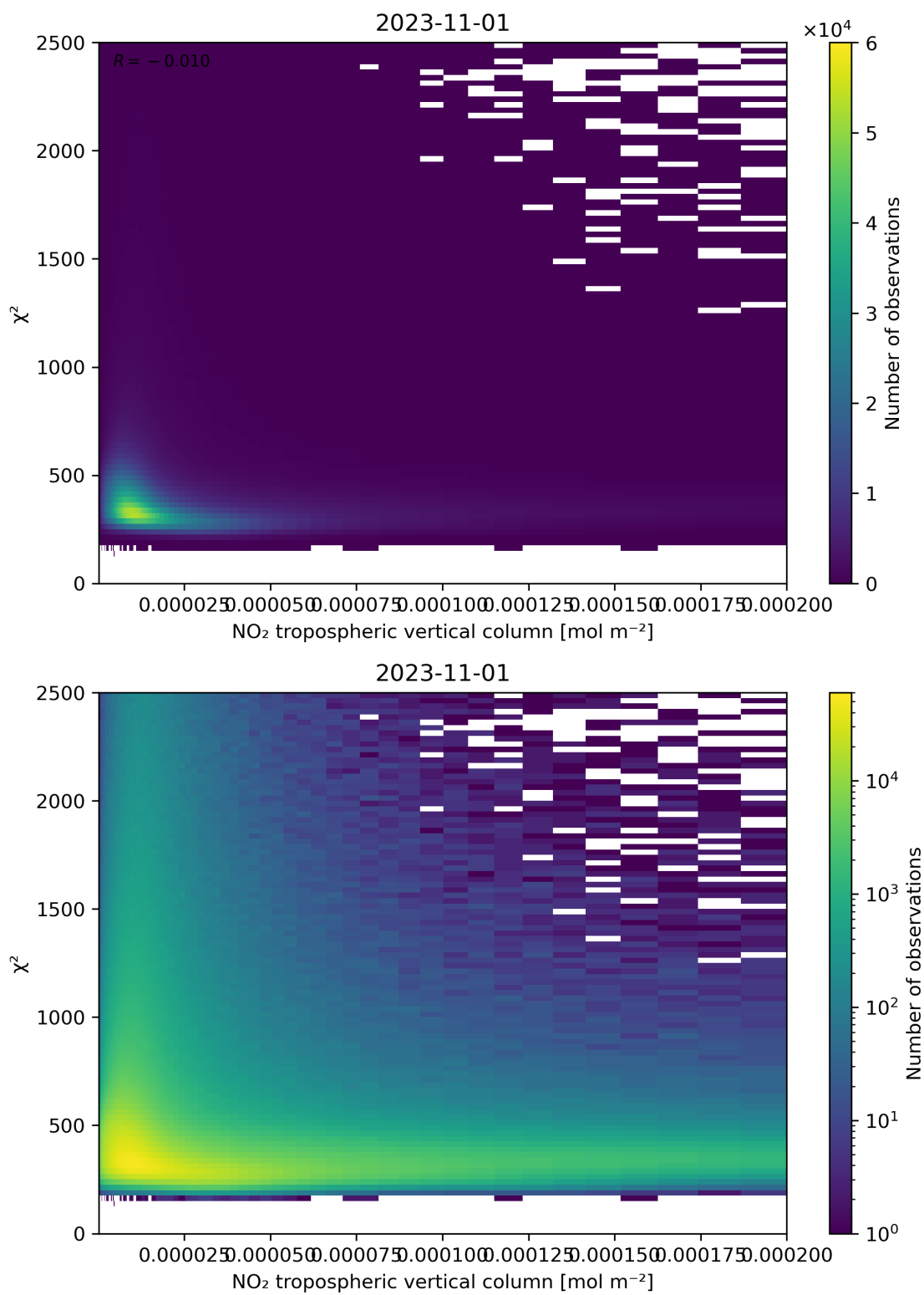
Figure 124: Scatter density plot of “NO 2 tropospheric vertical column” against “ \chi^2 ” for 2023-10-31 to 2023-11-02.
