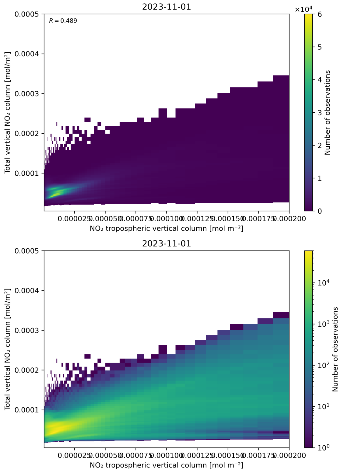
Figure 128: Scatter density plot of “NO 2 tropospheric vertical column” against “Total vertical NO 2 column” for 2023-10-31 to 2023-11-02.
