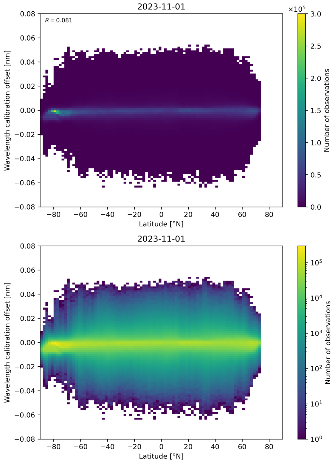
Figure 95: Scatter density plot of “Latitude” against “Wavelength calibration offset” for 2023-10-31 to 2023-11-02.
