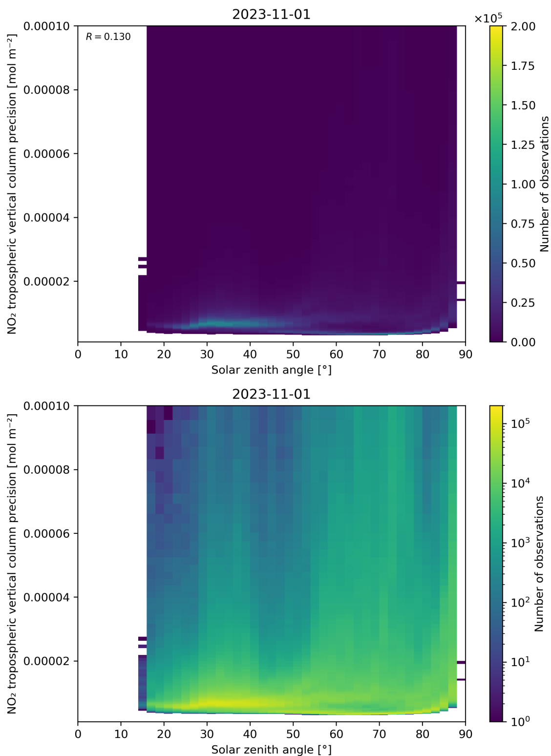
Figure 156: Scatter density plot of “Solar zenith angle” against “NO 2 tropospheric vertical column precision” for 2023-10-31 to 2023-11-02.
