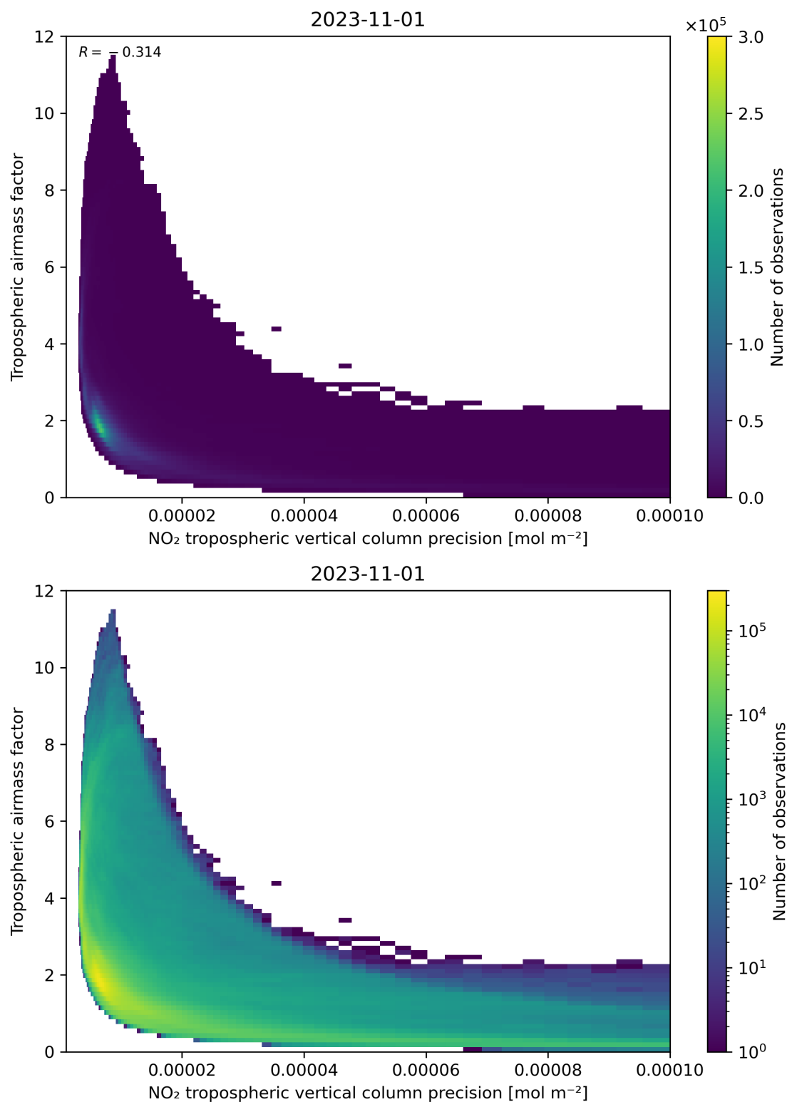
Figure 133: Scatter density plot of “NO 2 tropospheric vertical column precision” against “Tropospheric air mass factor” for 2023-10-31 to 2023-11-02.
