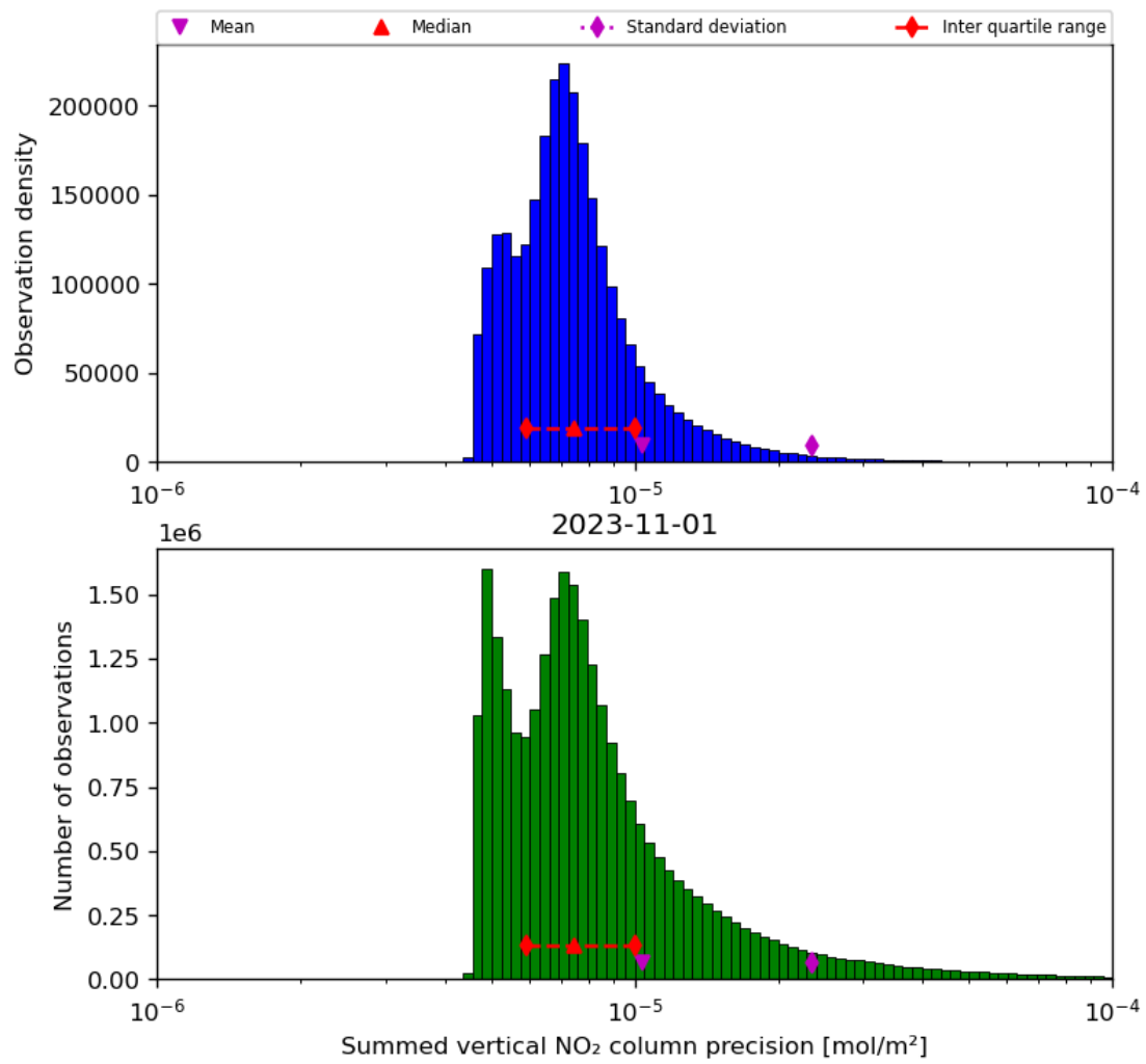
Figure 41: Histogram of “Summed vertical NO 2 column precision” for 2023-10-31 to 2023-11-02
