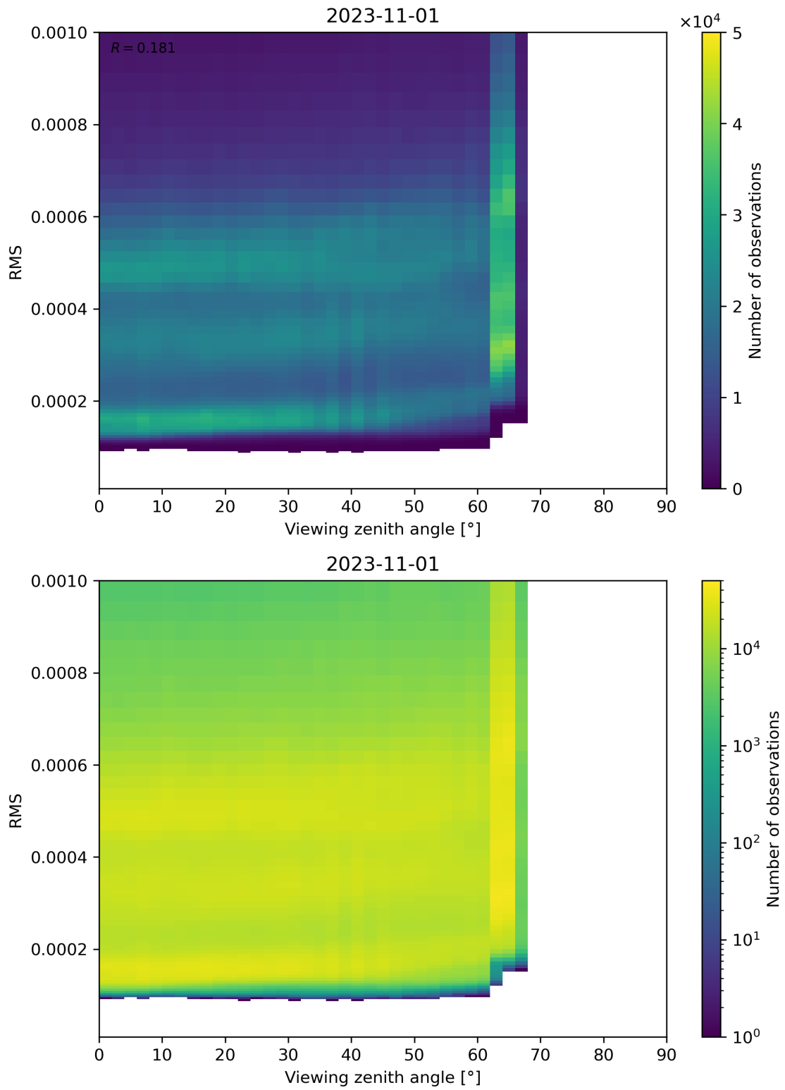
Figure 171: Scatter density plot of “Viewing zenith angle” against “RMS” for 2023-10-31 to 2023-11-02.
