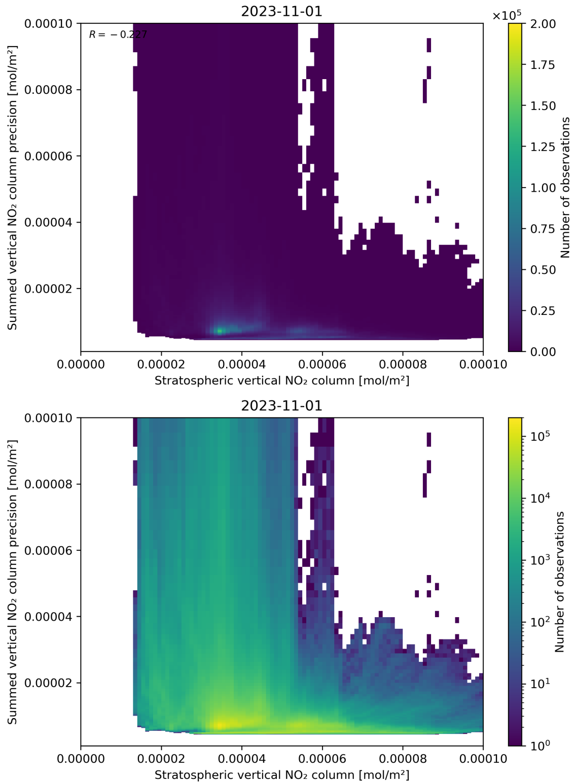
Figure 99: Scatter density plot of “Stratospheric vertical NO 2 column” against “Summed vertical NO 2 column precision” for 2023-10-31 to 2023-11-02.
