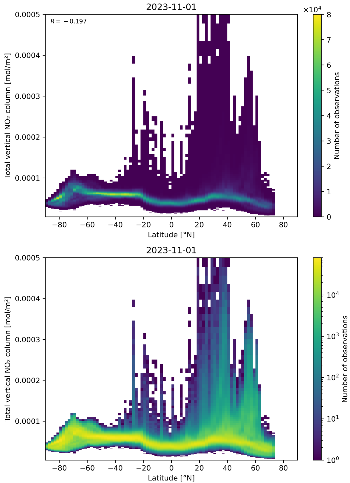
Figure 90: Scatter density plot of “Latitude” against “Total vertical NO 2 column” for 2023-10-31 to 2023-11-02.
