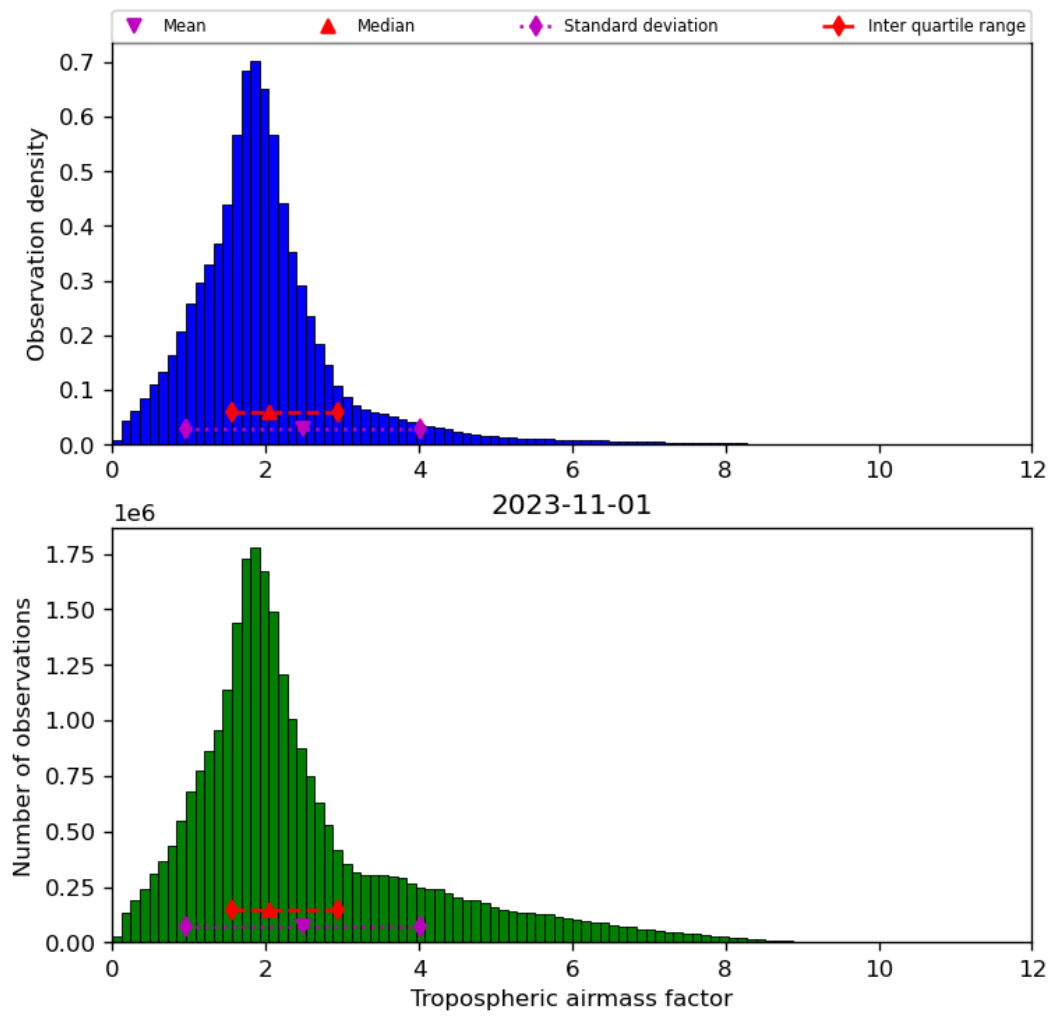
Figure 31: Histogram of “Tropospheric airmass factor” for 2023-10-31 to 2023-11-02
