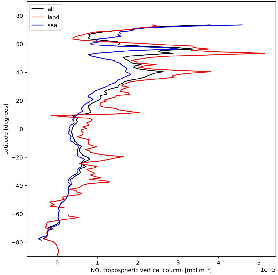
Figure 12: Zonal average of “NO 2 tropospheric vertical column” for 2023-10-31 to 2023-11-02.
