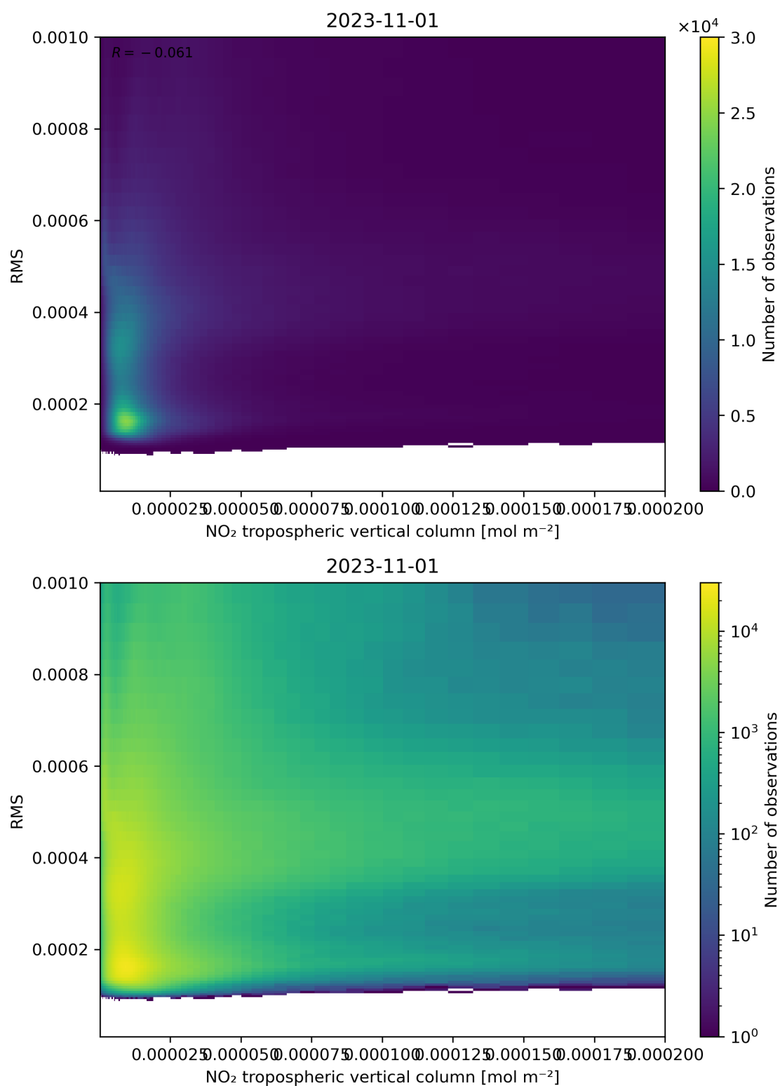
Figure 142: Scatter density plot of “NO 2 tropospheric vertical column” against “RMS” for 2023-10-31 to 2023-11-02.
