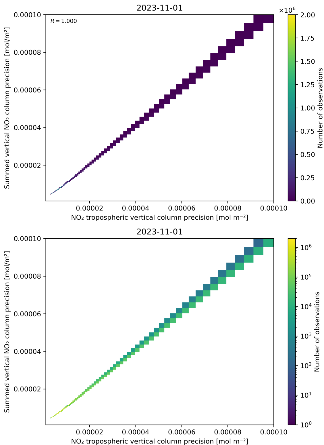
Figure 137: Scatter density plot of “NO 2 tropospheric vertical column precision” against “Summed vertical NO 2 column precision” for 2023-10-31 to 2023-11-02.
