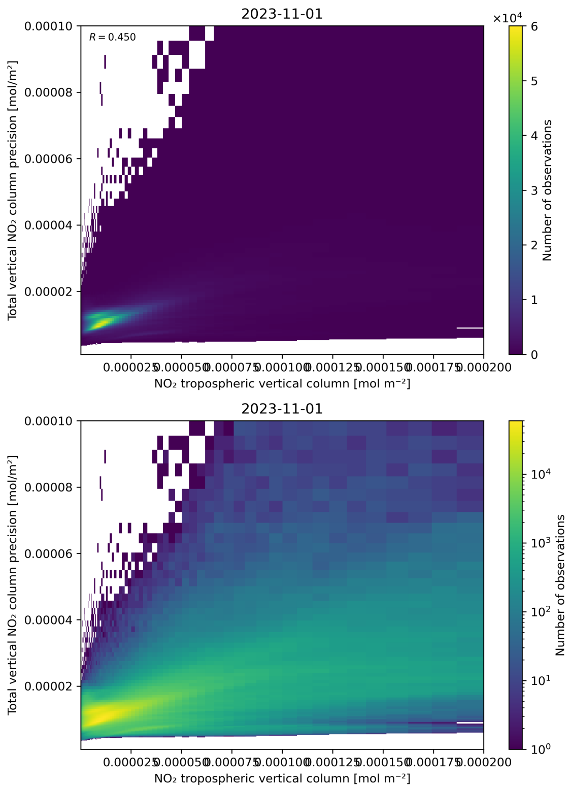
Figure 129: Scatter density plot of “NO 2 tropospheric vertical column” against “Total vertical NO 2 column precision” for 2023-10-31 to 2023-11-02.
