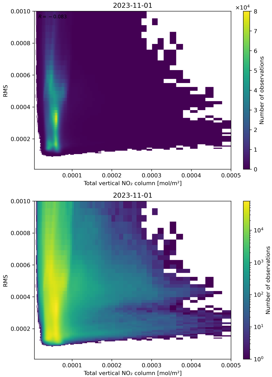
Figure 120: Scatter density plot of “Total vertical NO 2 column” against “RMS” for 2023-10-31 to 2023-11-02.
