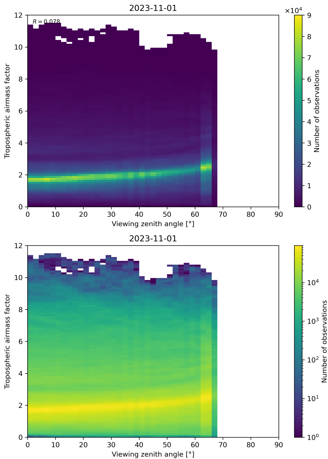
Figure 161: Scatter density plot of “Viewing zenith angle” against “Tropospheric airmass factor” for 2023-10-31 to 2023-11-02.
