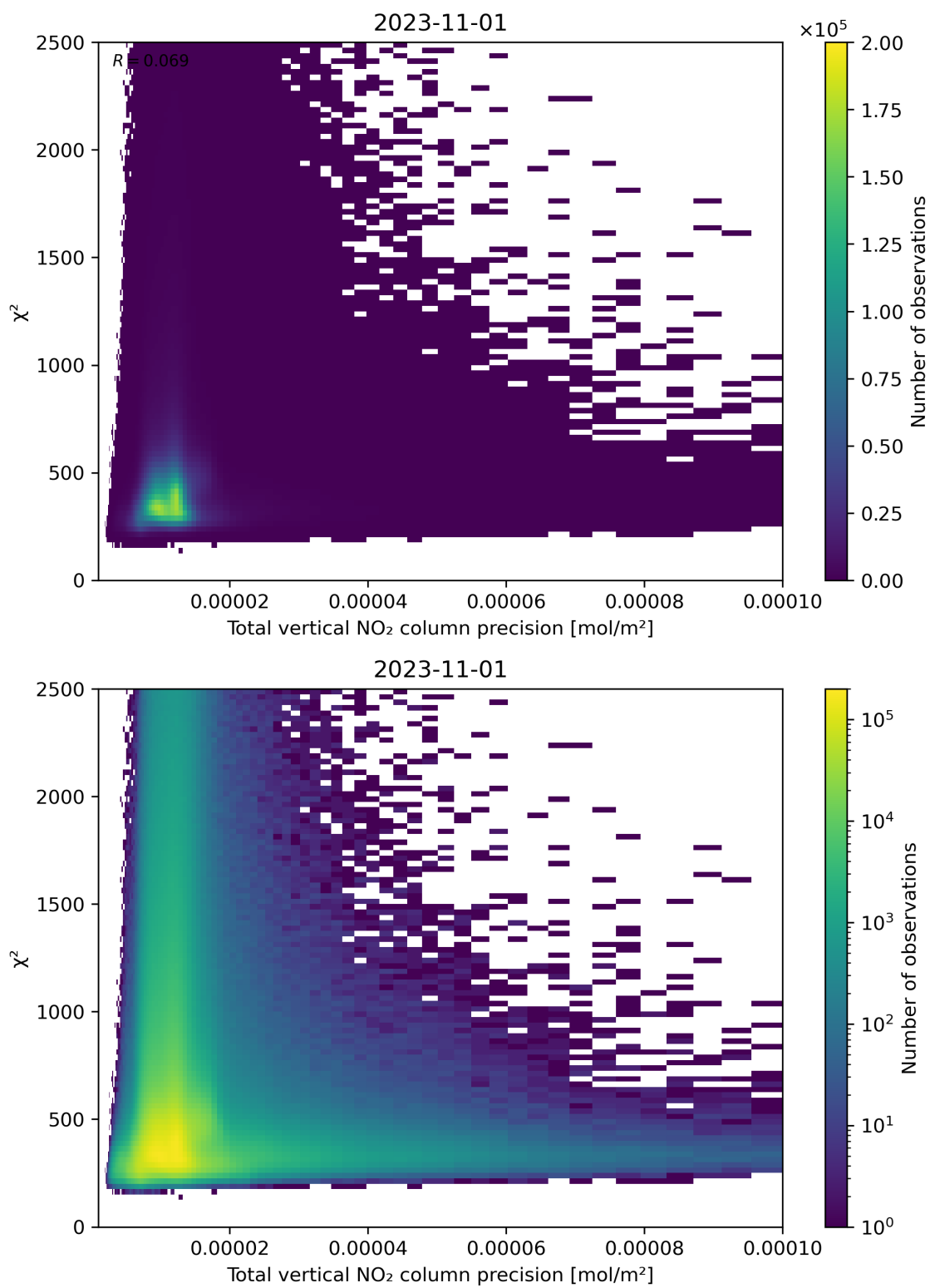
Figure 116: Scatter density plot of “Total vertical NO 2 column precision” against “ \chi^2 ” for 2023-10-31 to 2023-11-02.
