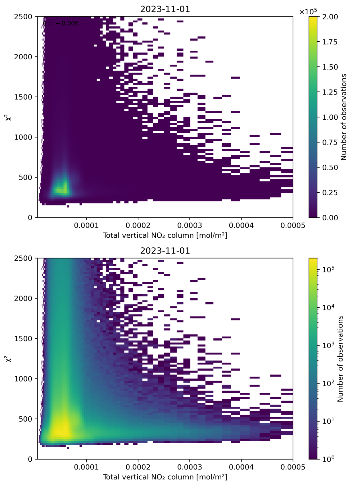
Figure 111: Scatter density plot of “Total vertical NO 2 column” against “ \chi^2 ” for 2023-10-31 to 2023-11-02.
