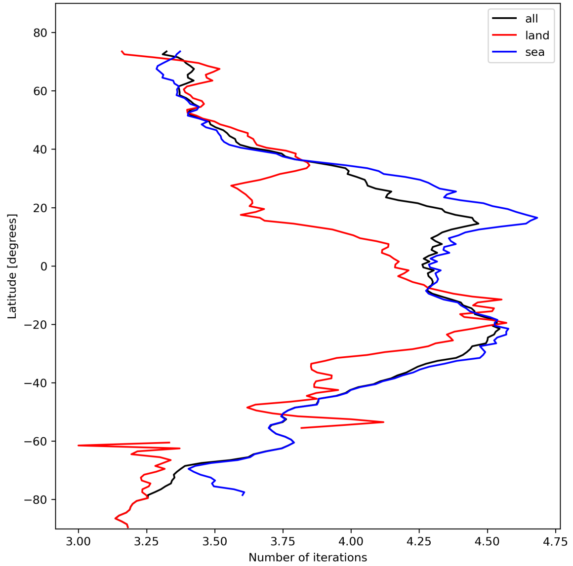
Figure 17: Zonal average of “Number of iterations” for 2023-10-31 to 2023-11-02.
