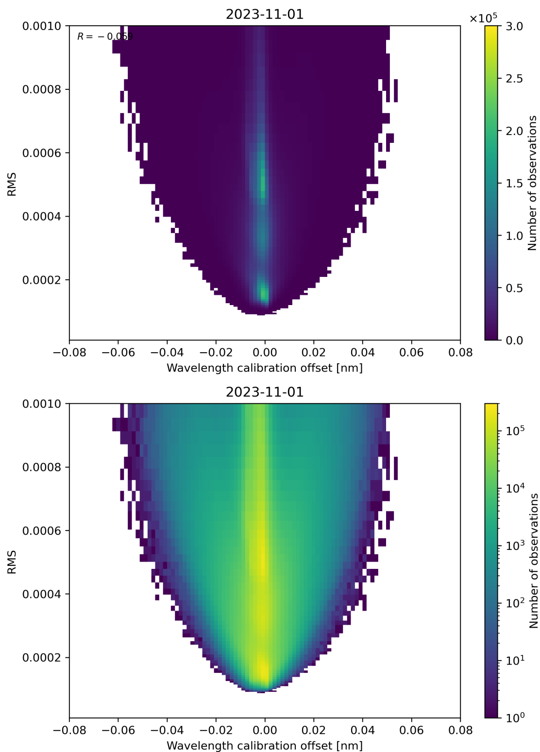
Figure 181: Scatter density plot of “Wavelength calibration offset” against “RMS” for 2023-10-31 to 2023-11-02.
