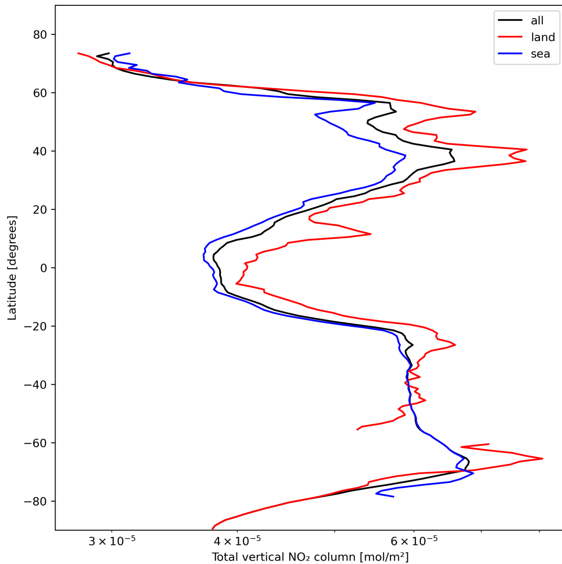
Figure 21: Zonal average of “Total vertical NO 2 column” for 2023-10-31 to 2023-11-02.
