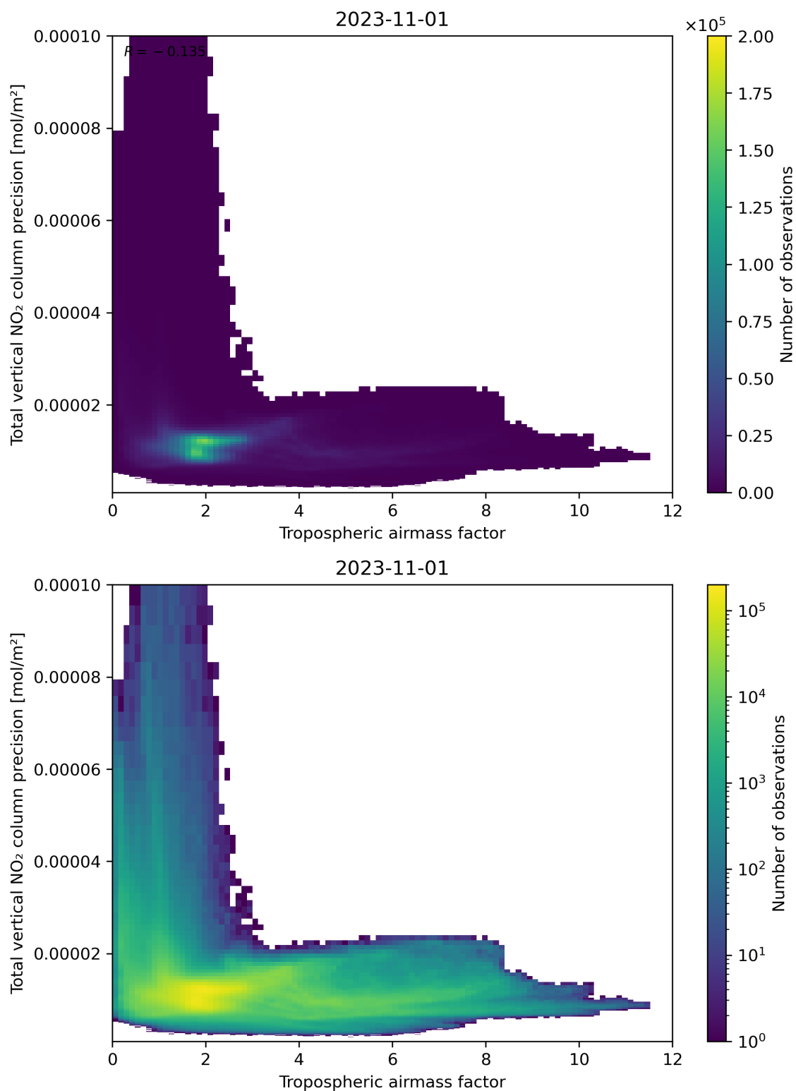
Figure 78: Scatter density plot of “Tropospheric air mass factor” against “Total vertical NO 2 column precision” for 2023-10-31 to 2023-11-02.
