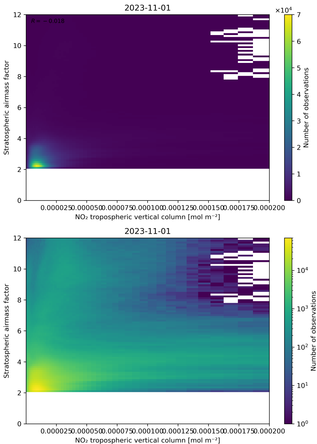
Figure 121: Scatter density plot of “NO 2 tropospheric vertical column” against “Stratospheric airmass factor” for 2023-10-31 to 2023-11-02.
