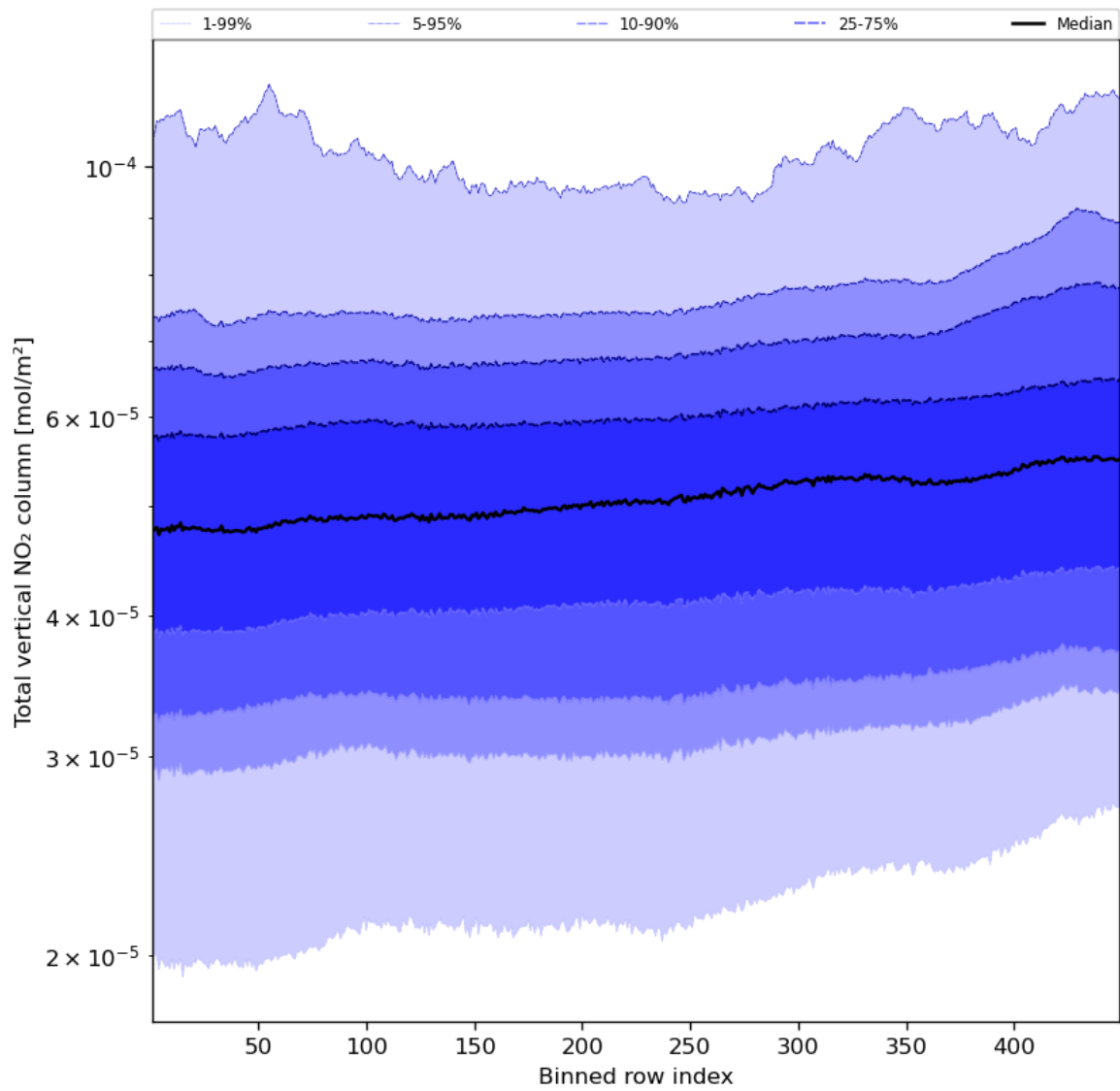
Figure 55: Along track statistics of “Total vertical NO 2 column” for 2023-10-31 to 2023-11-02
