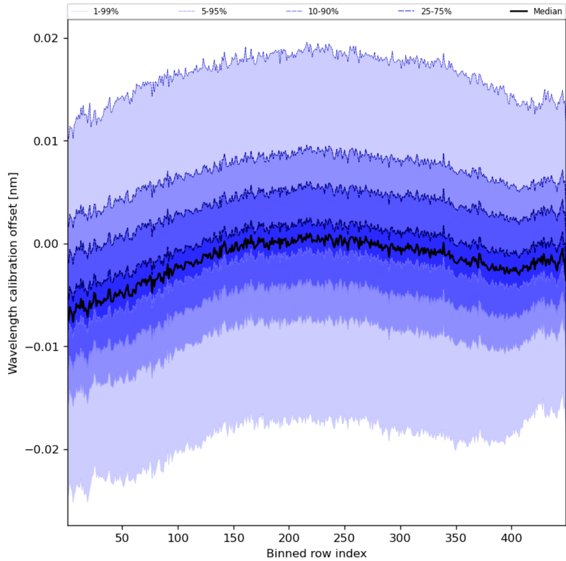
Figure 52: Along track statistics of “Wavelength calibration offset” for 2023-10-31 to 2023-11-02
