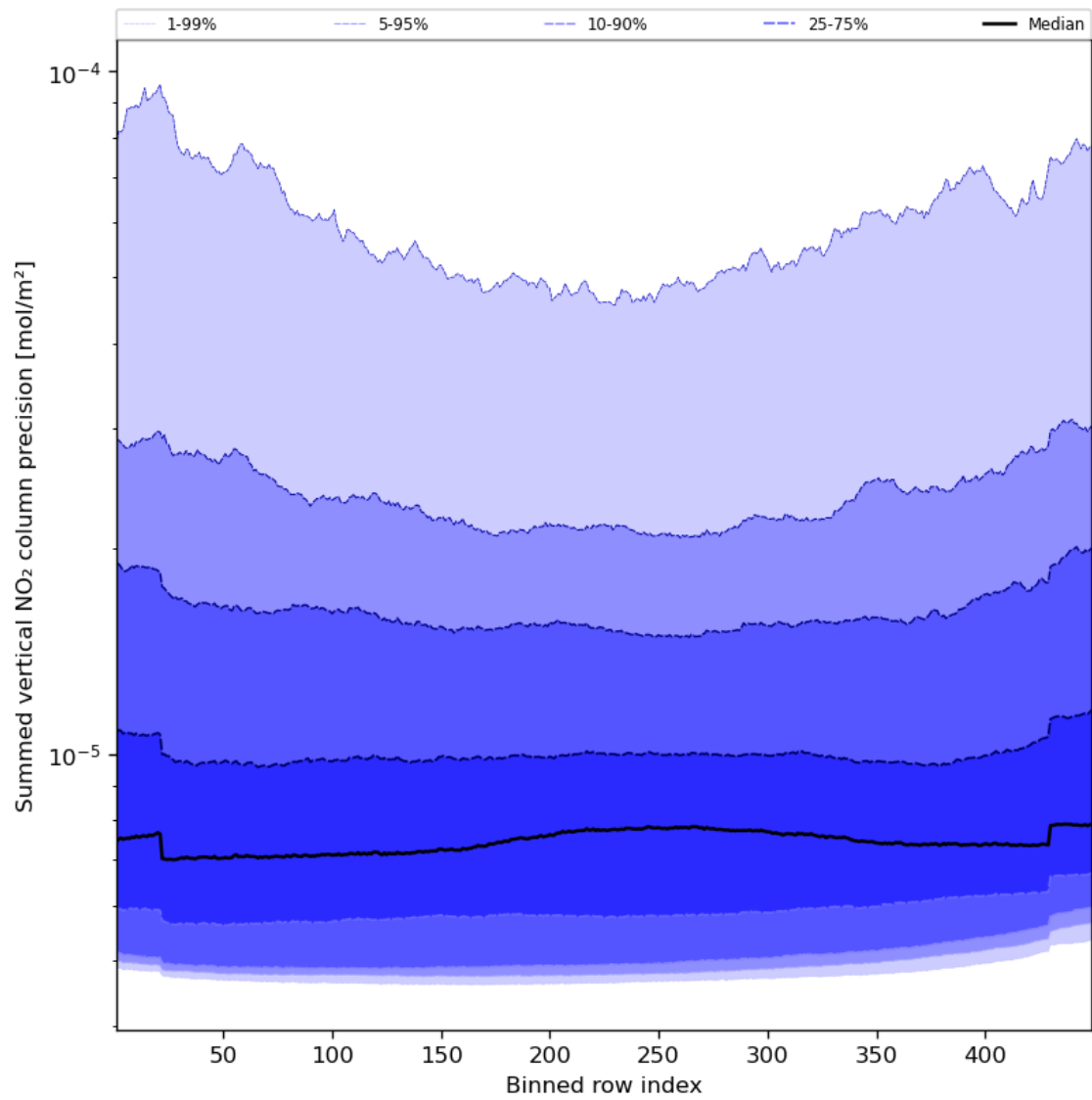
Figure 58: Along track statistics of “Summed vertical NO 2 column precision” for 2023-10-31 to 2023-11-02
