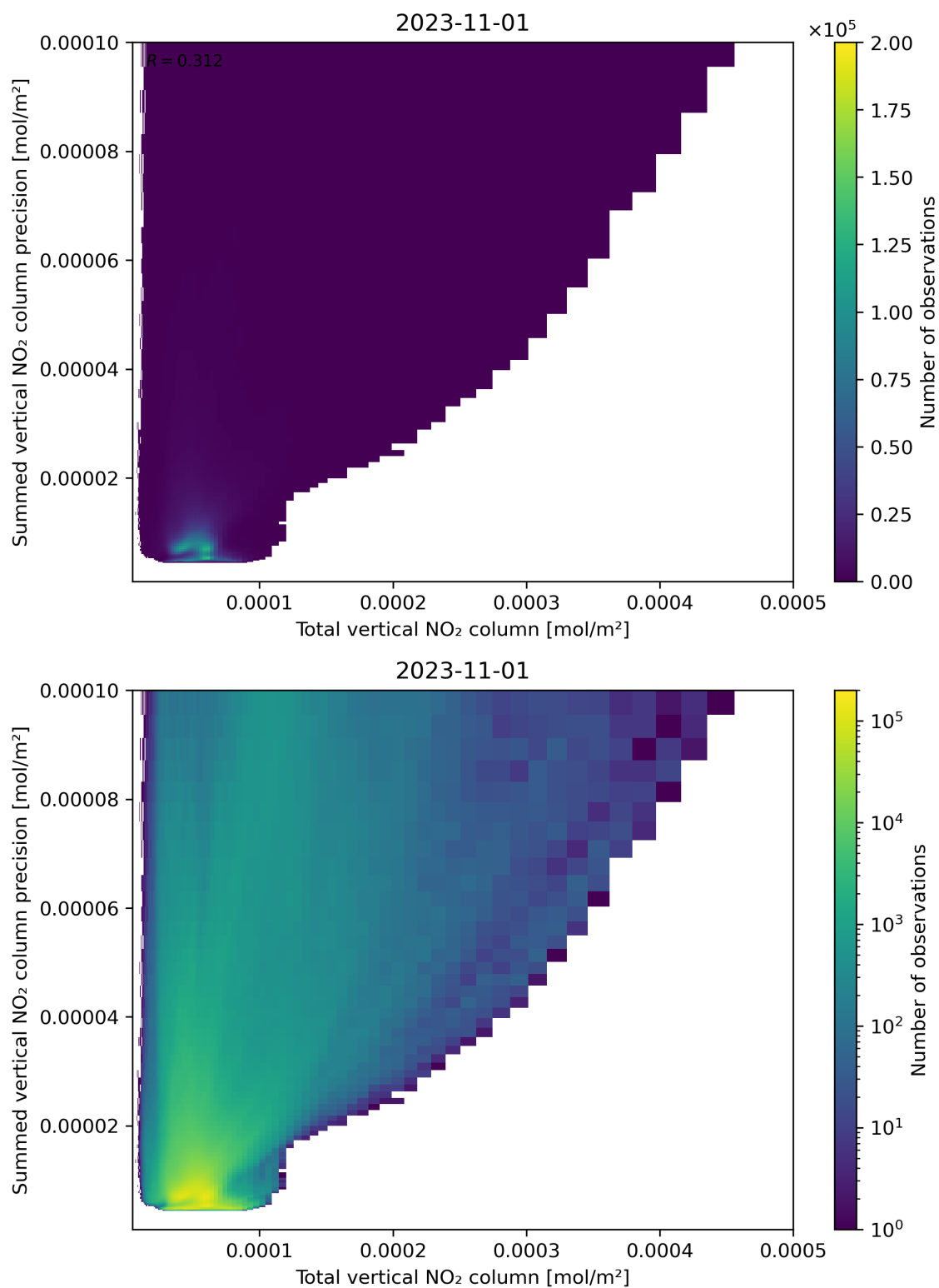
Figure 113: Scatter density plot of “Total vertical NO 2 column” against “Summed vertical NO 2 column precision” for 2023-10-31 to 2023-11-02.
