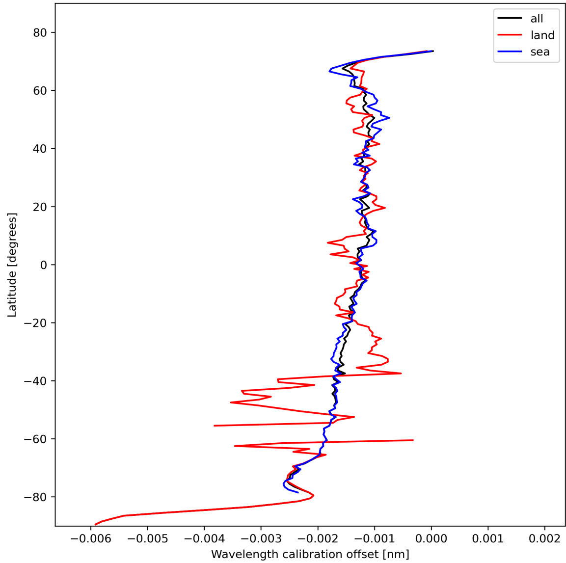
Figure 18: Zonal average of “Wavelength calibration offset” for 2023-10-31 to 2023-11-02.
