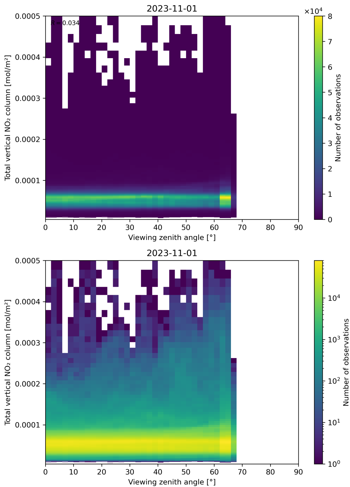
Figure 167: Scatter density plot of “Viewing zenith angle” against “Total vertical NO 2 column” for 2023-10-31 to 2023-11-02.
