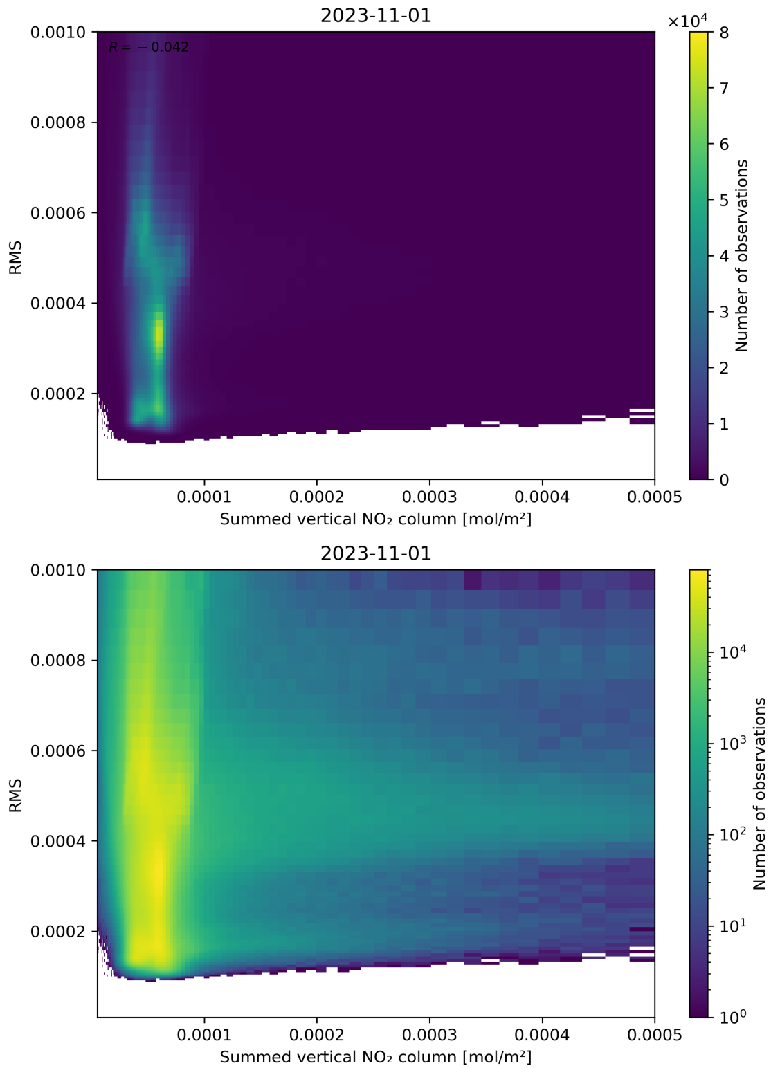
Figure 109: Scatter density plot of “Summed vertical NO 2 column” against “RMS” for 2023-10-31 to 2023-11-02.
