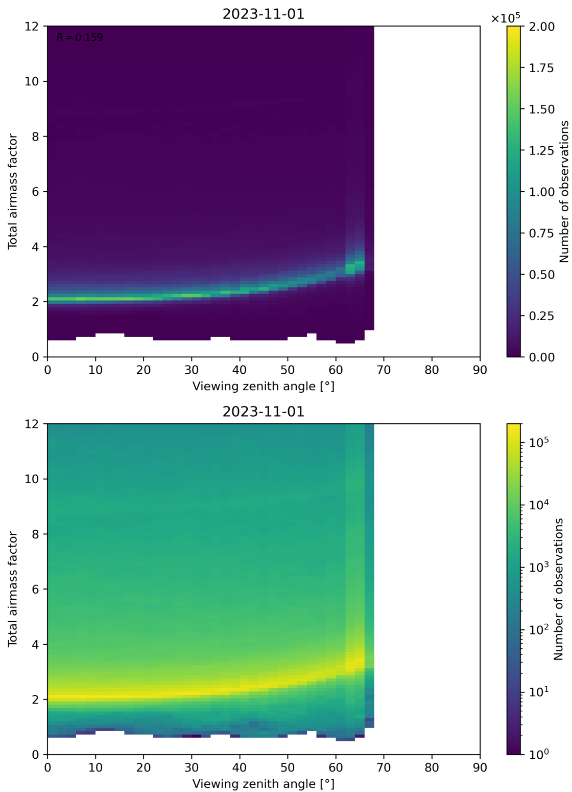
Figure 160: Scatter density plot of “Viewing zenith angle” against “Total airmass factor” for 2023-10-31 to 2023-11-02.
