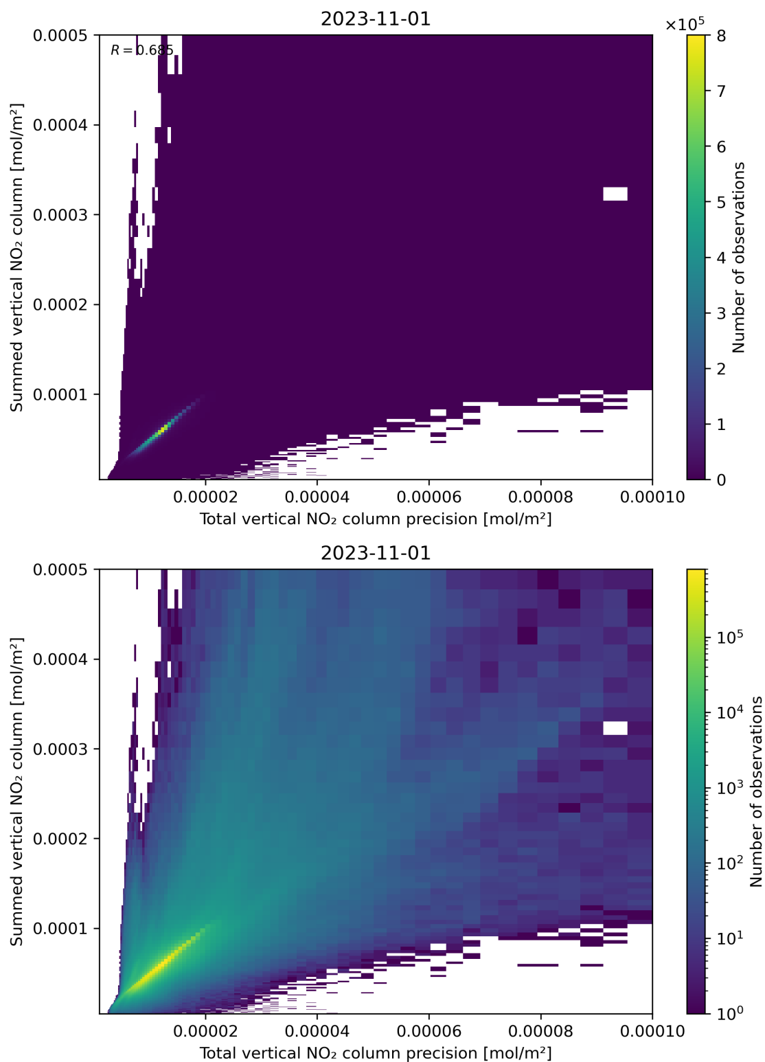
Figure 117: Scatter density plot of “Total vertical NO 2 column precision” against “Summed vertical NO 2 column” for 2023-10-31 to 2023-11-02.
