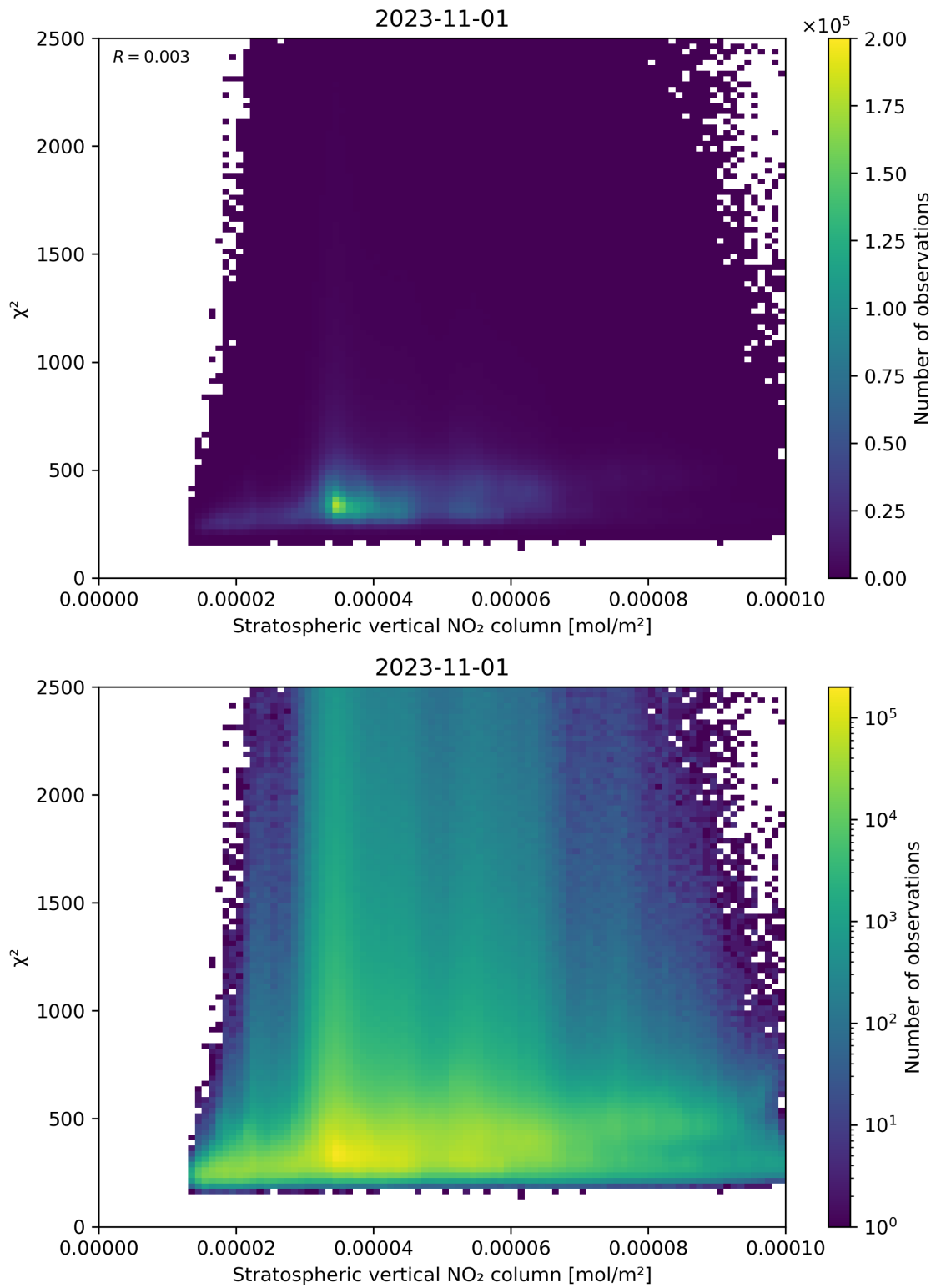
Figure 97: Scatter density plot of “Stratospheric vertical NO 2 column” against “ \chi^2 ” for 2023-10-31 to 2023-11-02.
