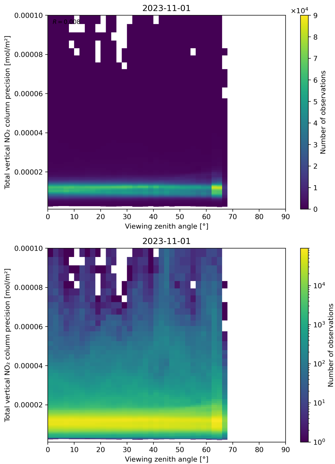
Figure 168: Scatter density plot of “Viewing zenith angle” against “Total vertical NO 2 column precision” for 2023-10-31 to 2023-11-02.
