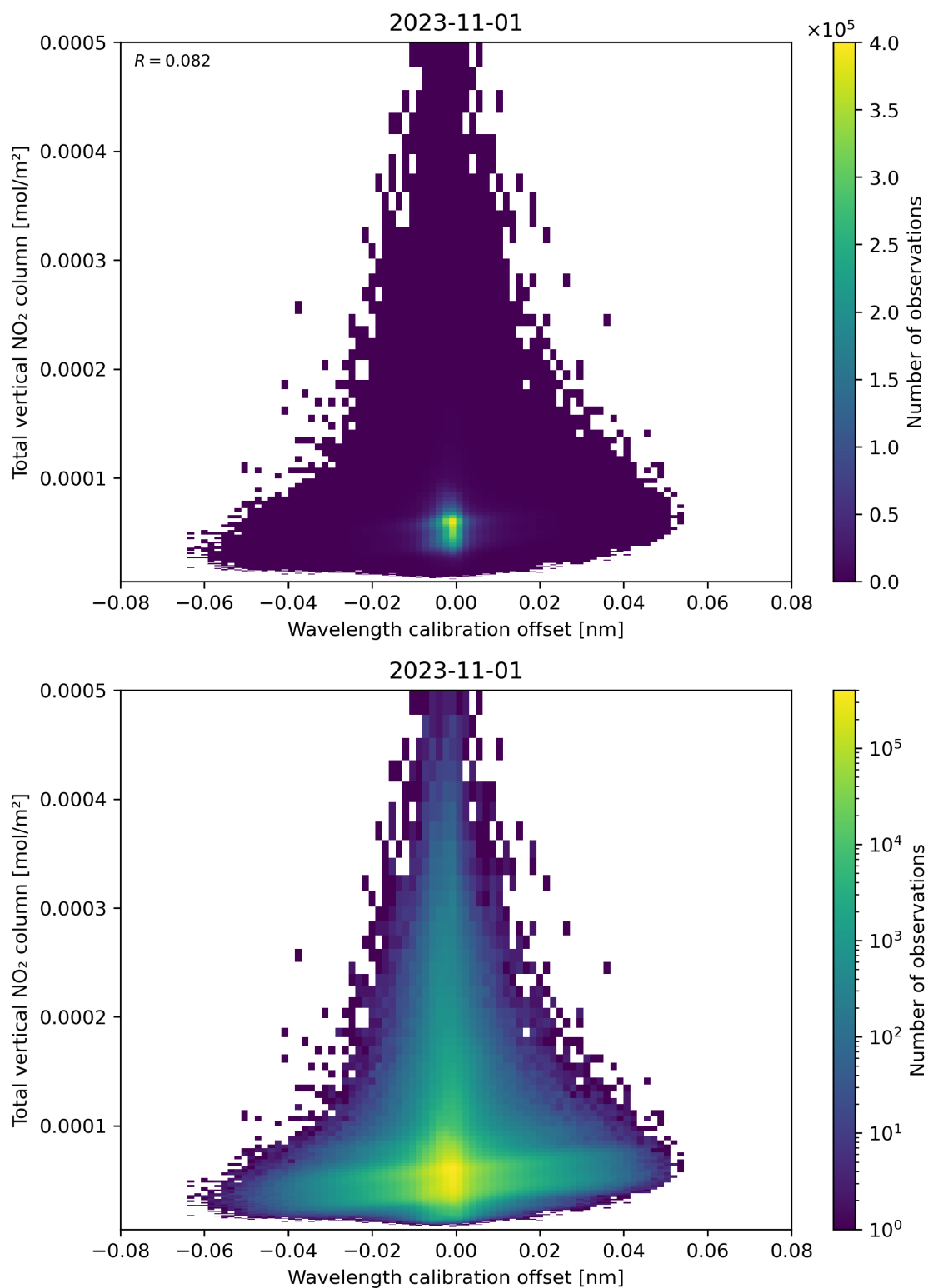
Figure 179: Scatter density plot of “Wavelength calibration offset” against “Total vertical NO 2 column” for 2023-10-31 to 2023-11-02.
