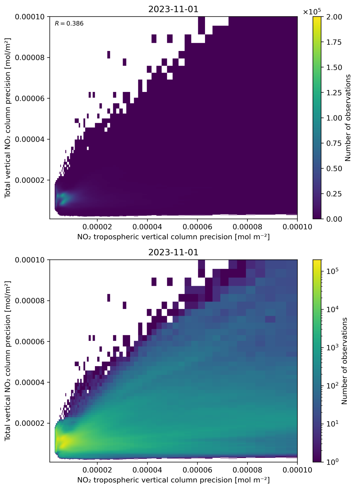
Figure 139: Scatter density plot of “NO 2 tropospheric vertical column precision” against “Total vertical NO 2 column precision” for 2023-10-31 to 2023-11-02.
