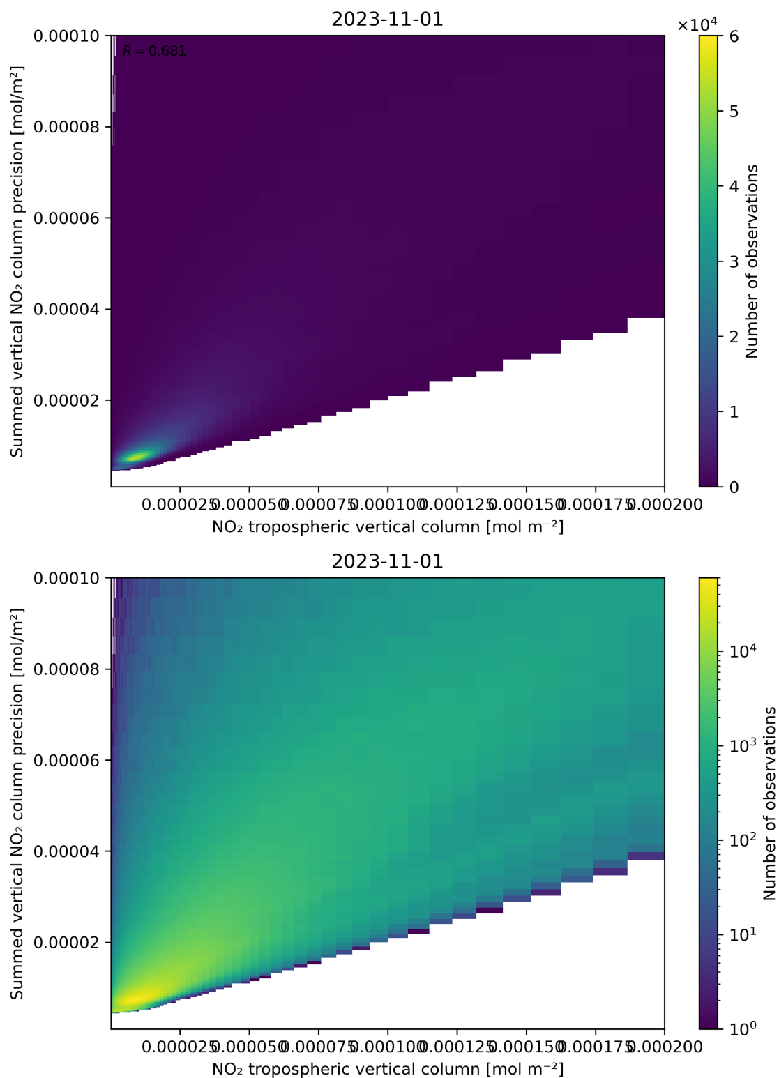
Figure 127: Scatter density plot of “NO 2 tropospheric vertical column” against “Summed vertical NO 2 column precision” for 2023-10-31 to 2023-11-02.
