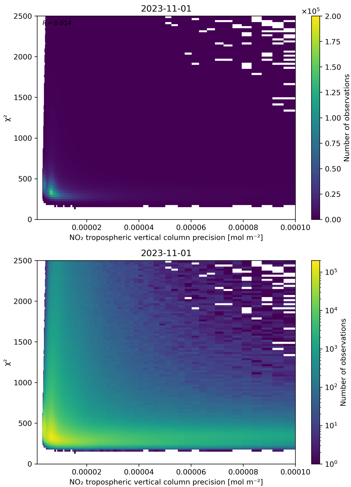
Figure 134: Scatter density plot of “NO 2 tropospheric vertical column precision” against “ \chi^2 ” for 2023-10-31 to 2023-11-02.
