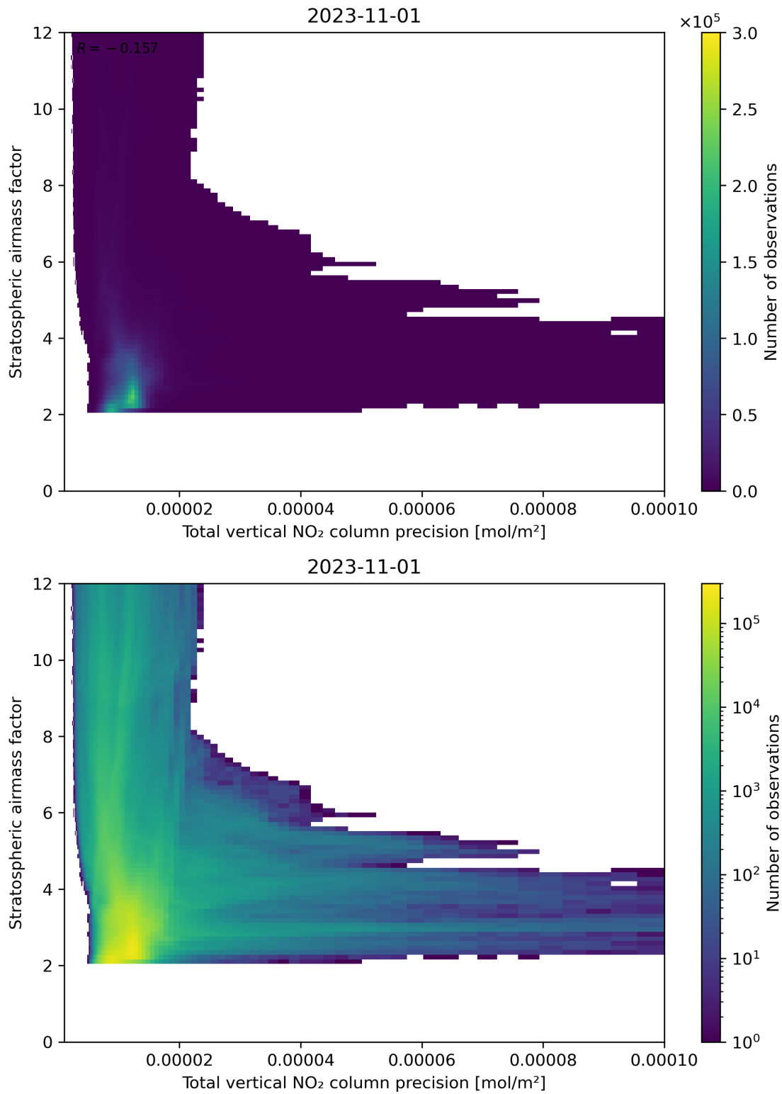
Figure 115: Scatter density plot of “Total vertical NO 2 column precision” against “Stratospheric air mass factor” for 2023-10-31 to 2023-11-02.
