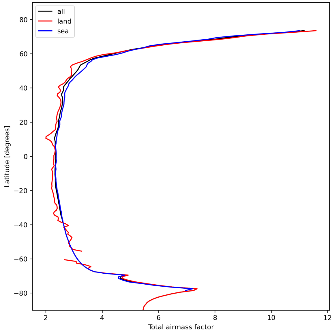
Figure 15: Zonal average of “Total airmass factor” for 2023-10-31 to 2023-11-02.
