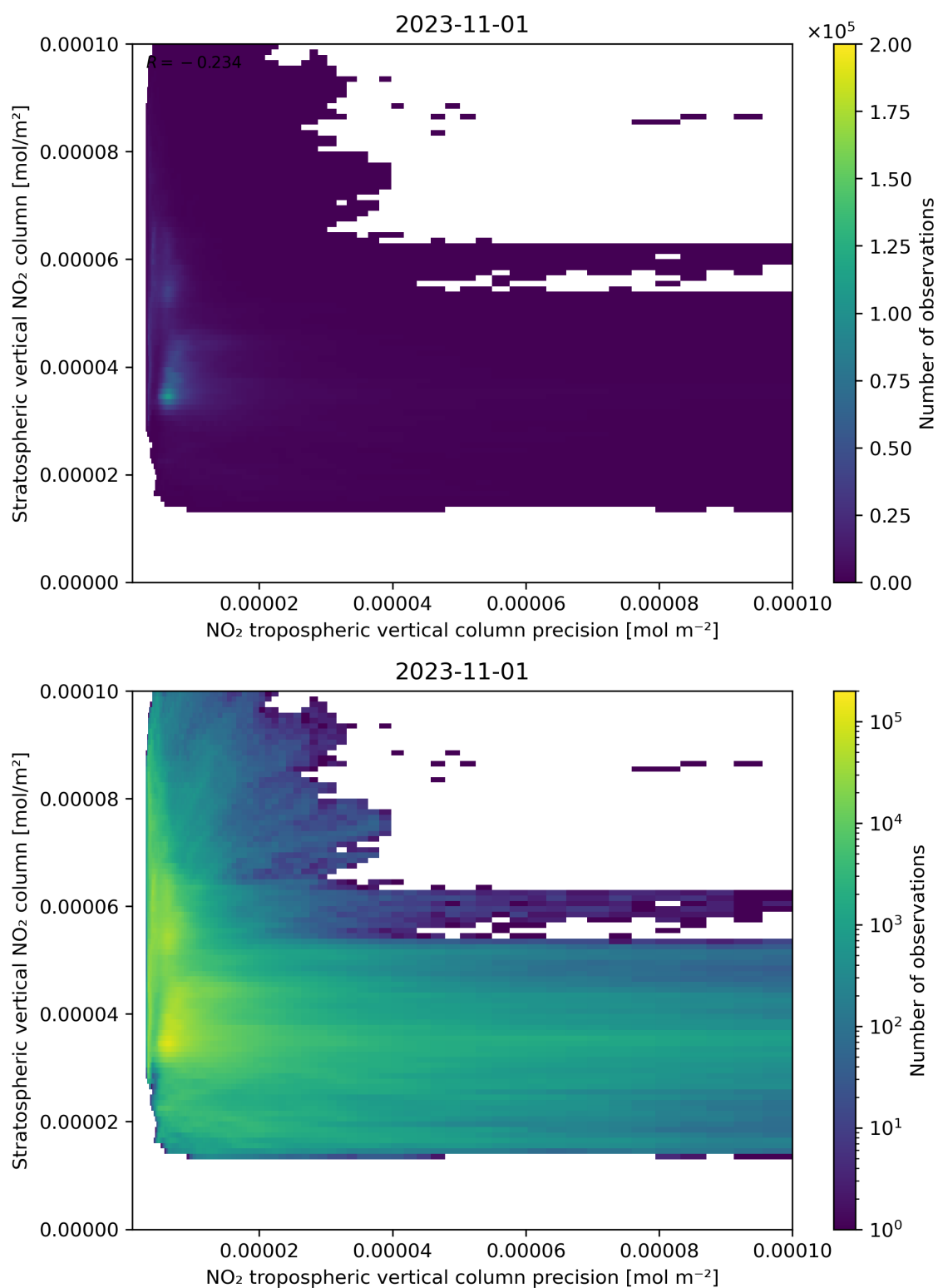
Figure 135: Scatter density plot of “NO 2 tropospheric vertical column precision” against “Stratospheric vertical NO 2 column” for 2023-10-31 to 2023-11-02.
