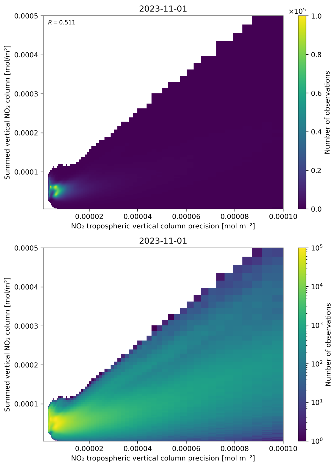
Figure 136: Scatter density plot of “NO 2 tropospheric vertical column precision” against “Summed vertical NO 2 column” for 2023-10-31 to 2023-11-02.
