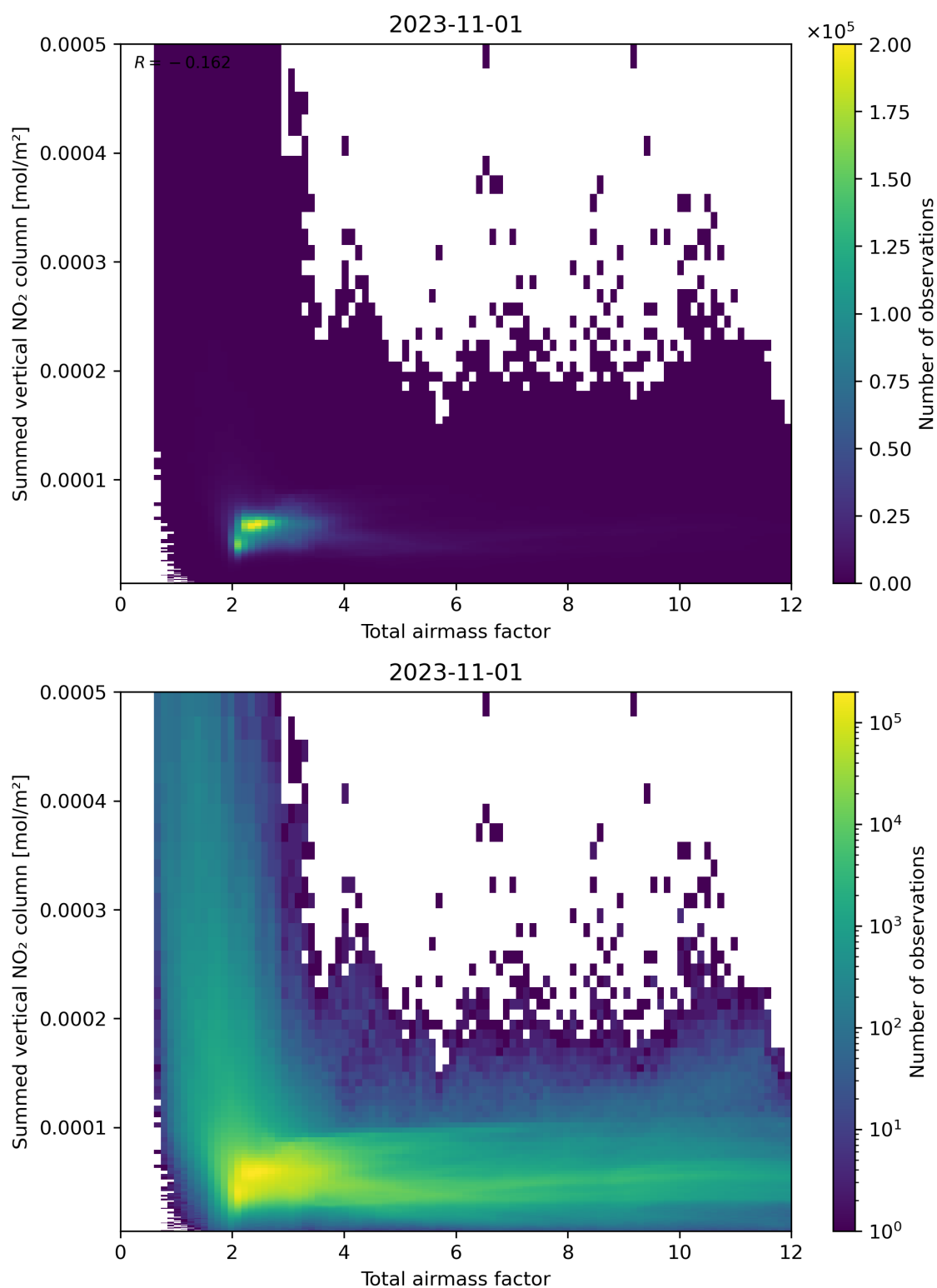
Figure 65: Scatter density plot of “Total airmass factor” against “Summed vertical NO 2 column” for 2023-10-31 to 2023-11-02.
