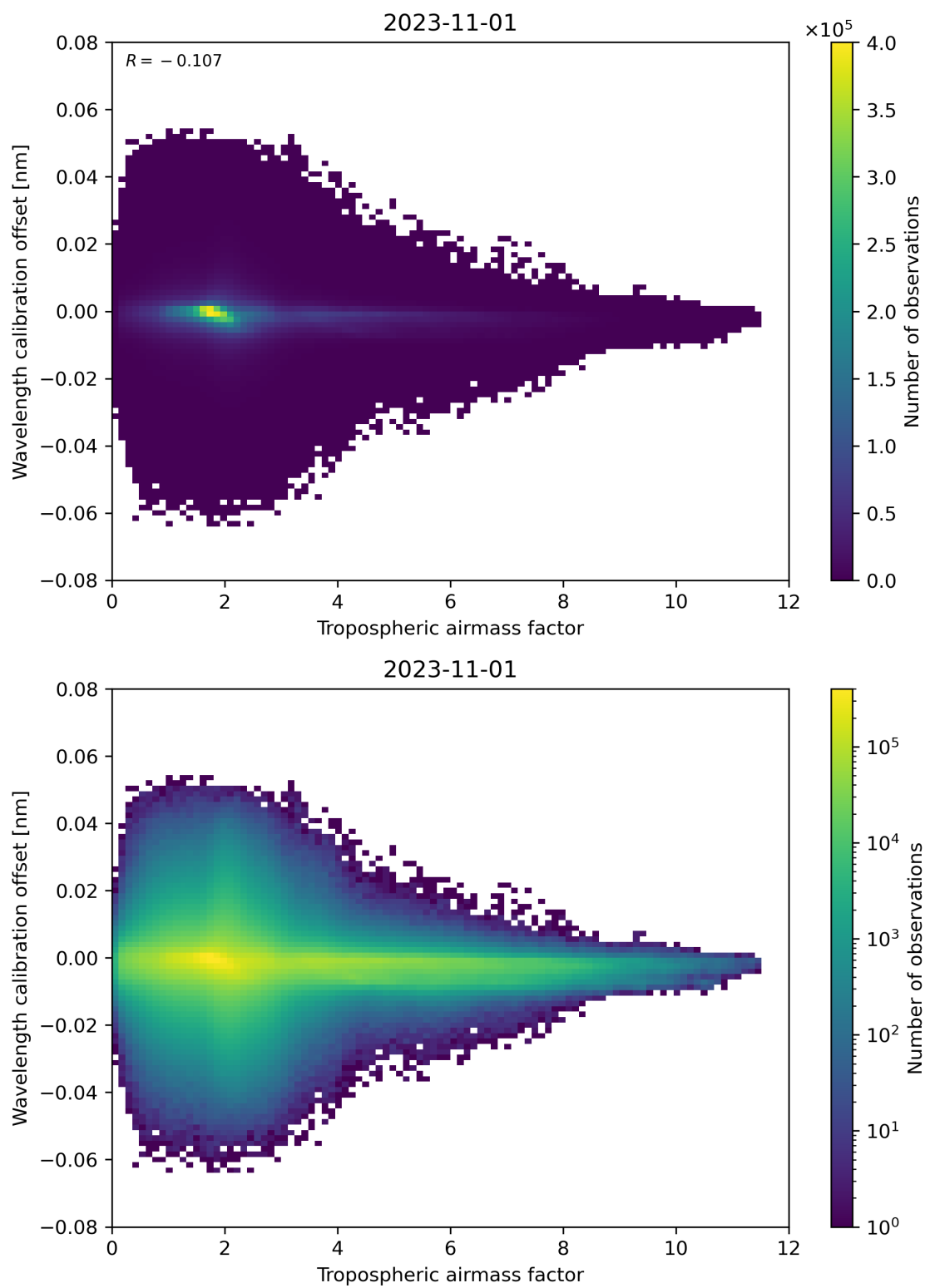
Figure 80: Scatter density plot of “Tropospheric airmass factor” against “Wavelength calibration offset” for 2023-10-31 to 2023-11-02.
