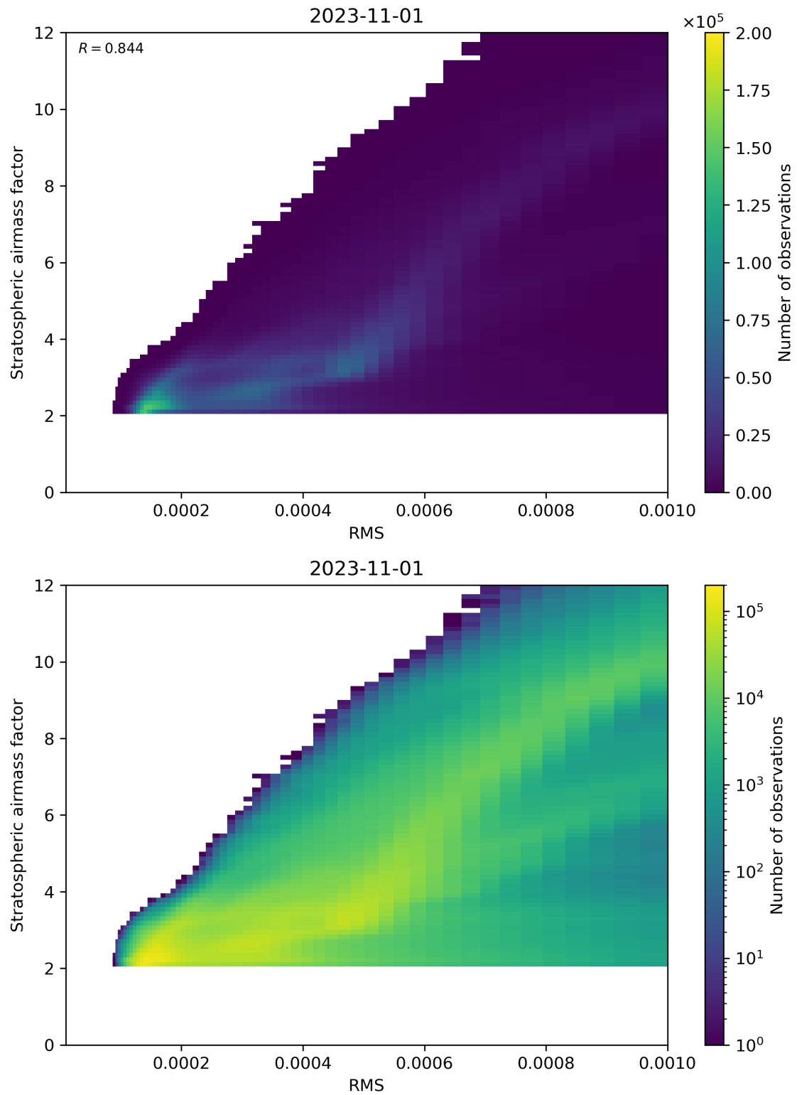
Figure 144: Scatter density plot of “RMS” against “Stratospheric airmass factor” for 2023-10-31 to 2023-11-02.
