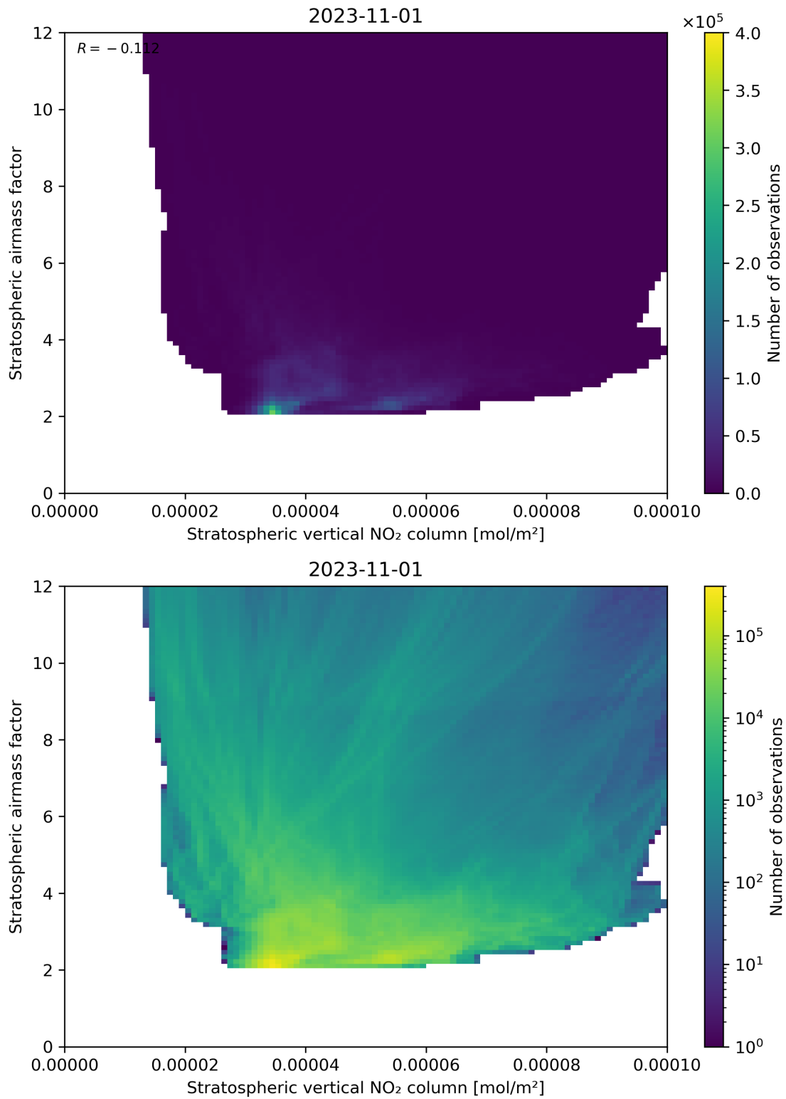
Figure 96: Scatter density plot of “Stratospheric vertical NO 2 column” against “Stratospheric airmass factor” for 2023-10-31 to 2023-11-02.
