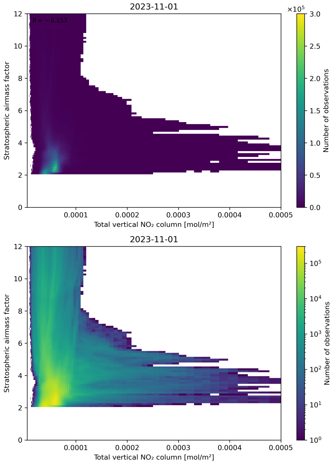
Figure 110: Scatter density plot of “Total vertical NO 2 column” against “Stratospheric airmass factor” for 2023-10-31 to 2023-11-02.
