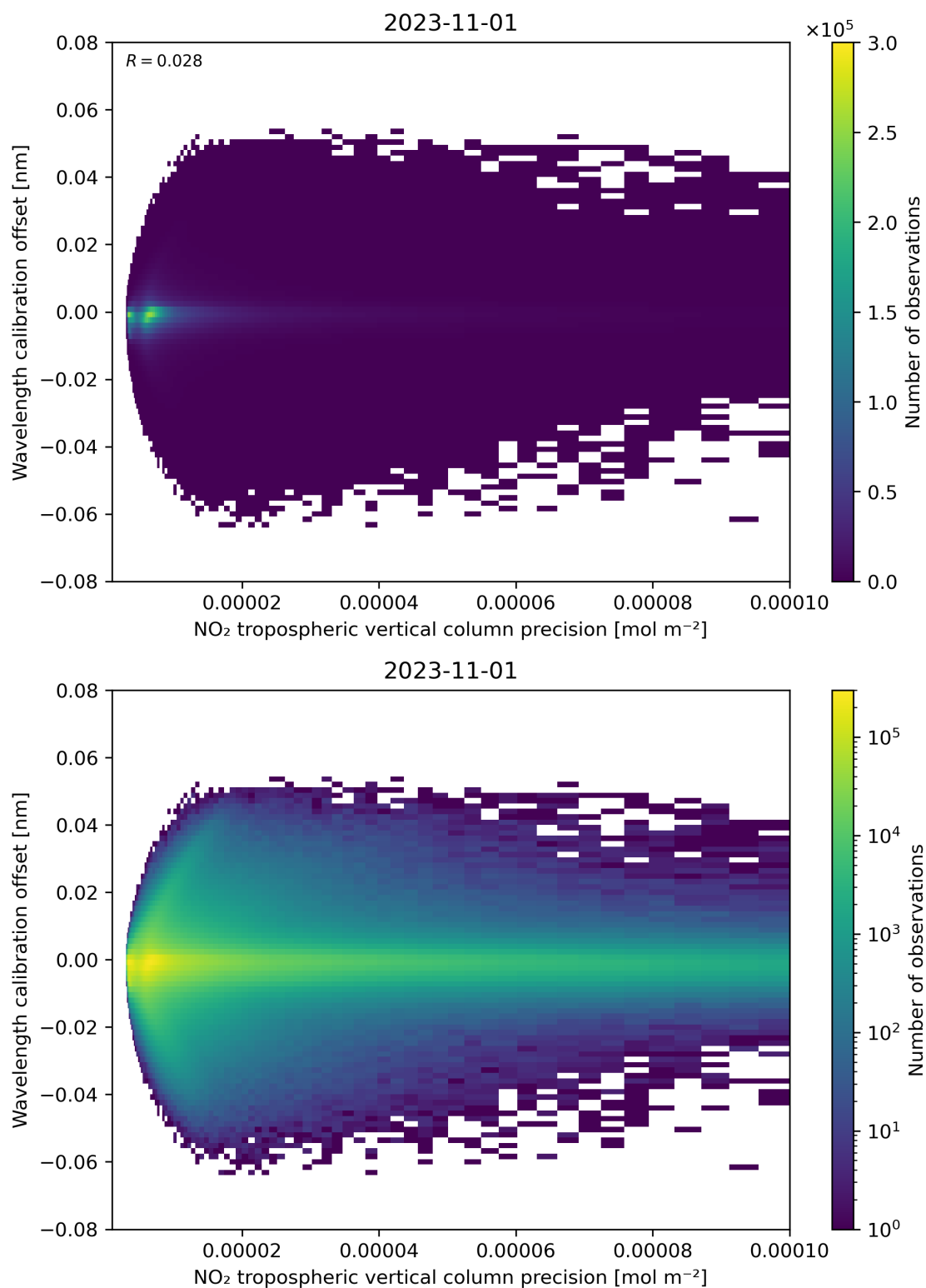
Figure 141: Scatter density plot of “NO 2 tropospheric vertical column precision” against “Wavelength calibration offset” for 2023-10-31 to 2023-11-02.
