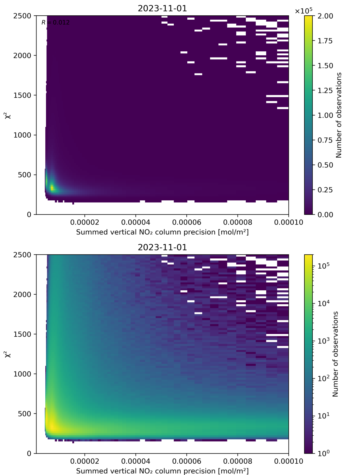
Figure 107: Scatter density plot of “Summed vertical NO 2 column precision” against “ \chi^2 ” for 2023-10-31 to 2023-11-02.
