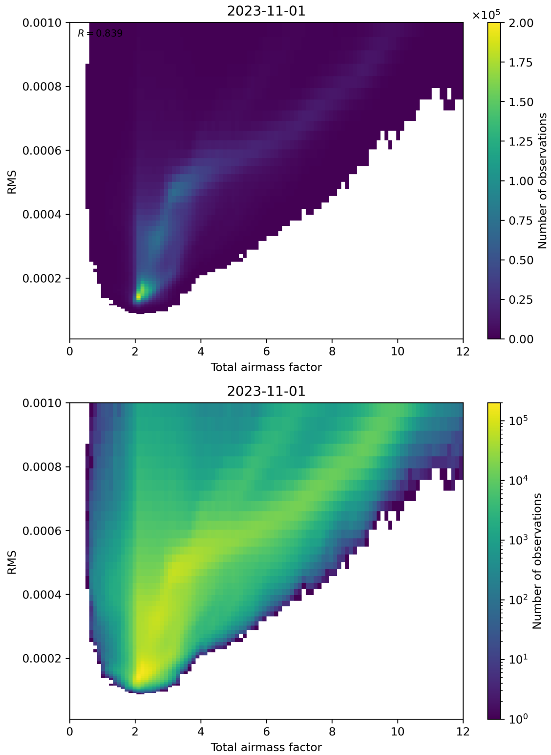
Figure 69: Scatter density plot of “Total airmass factor” against “RMS” for 2023-10-31 to 2023-11-02.
