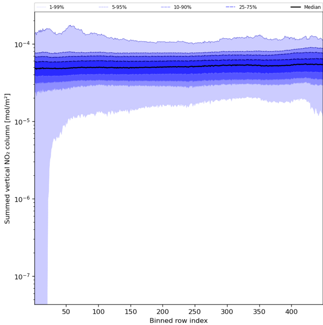
Figure 57: Along track statistics of “Summed vertical NO 2 column” for 2023-10-31 to 2023-11-02
