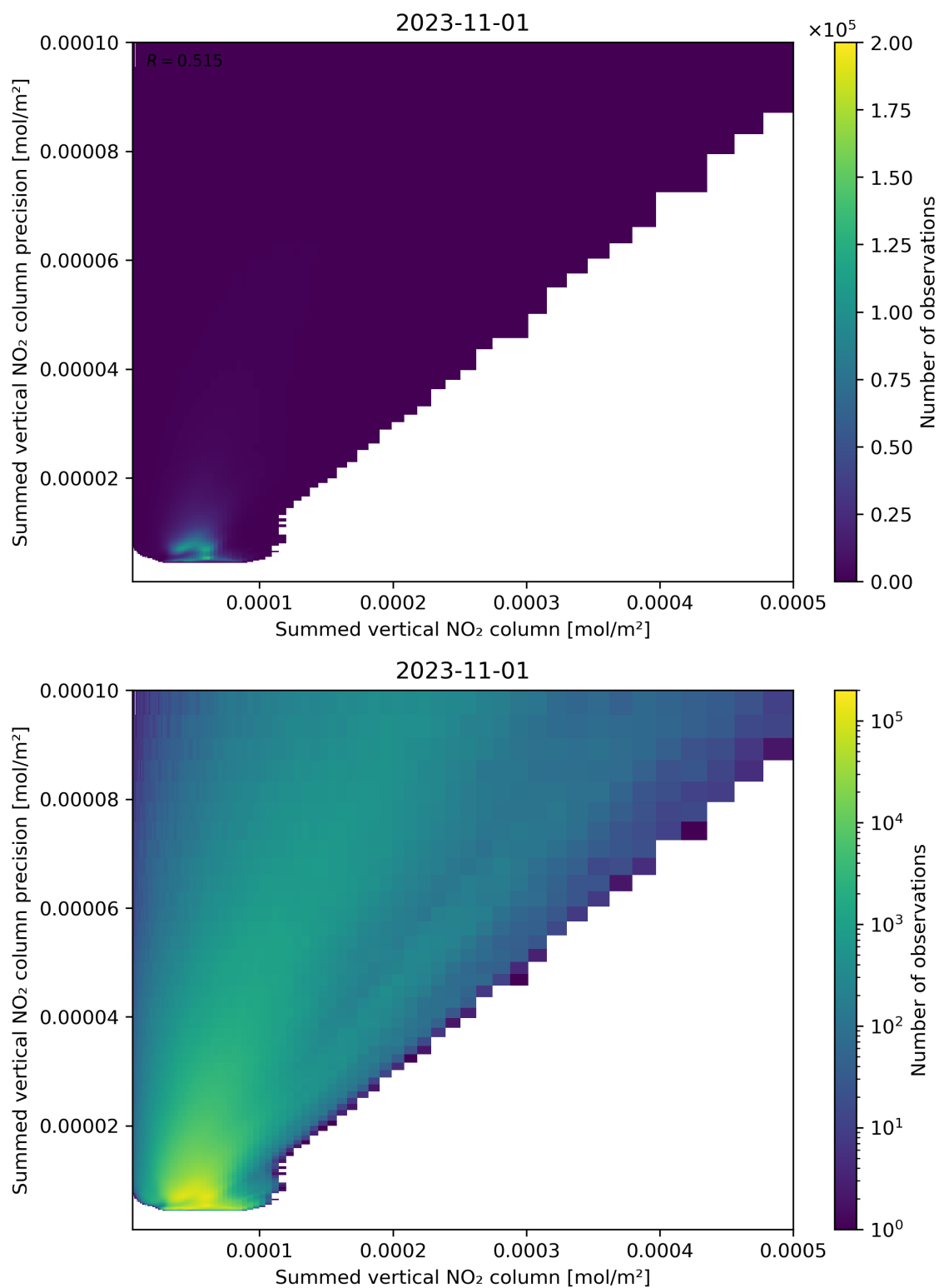
Figure 105: Scatter density plot of “Summed vertical NO 2 column” against “Summed vertical NO 2 column precision” for 2023-10-31 to 2023-11-02.
