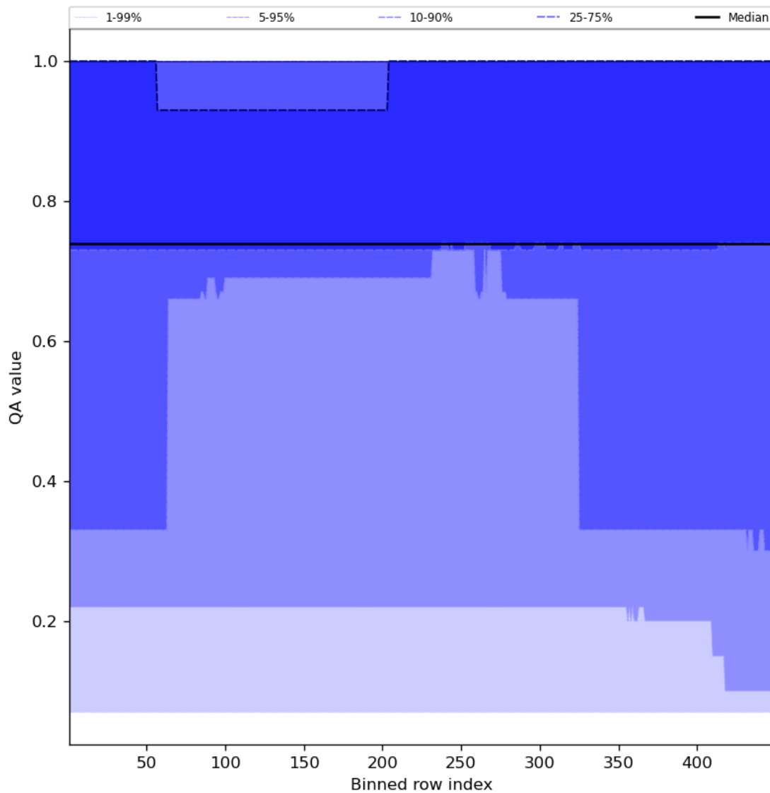
Figure 45: Along track statistics of “QA value” for 2023-10-31 to 2023-11-02
