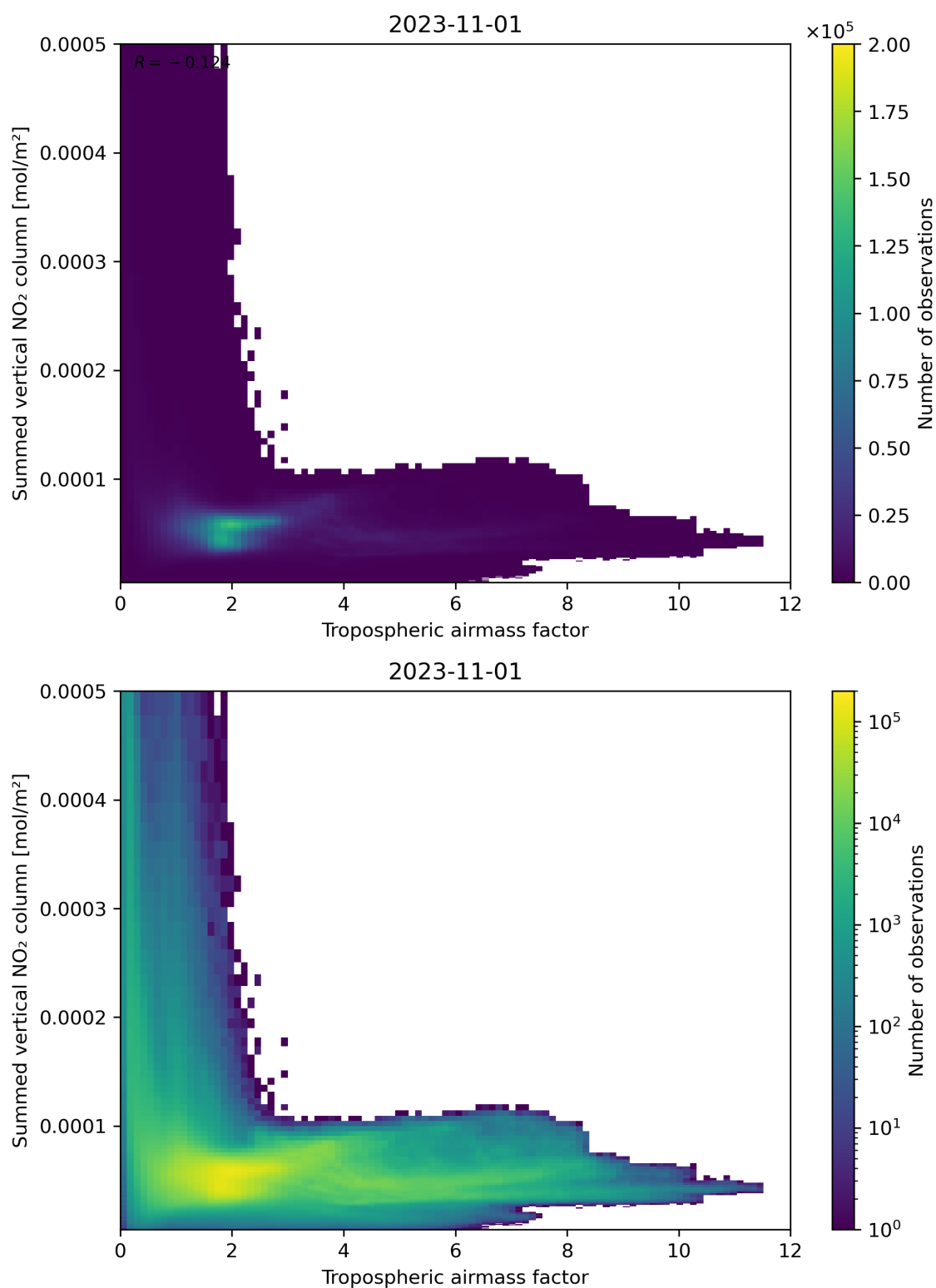
Figure 75: Scatter density plot of “Tropospheric airmass factor” against “Summed vertical NO 2 column” for 2023-10-31 to 2023-11-02.
