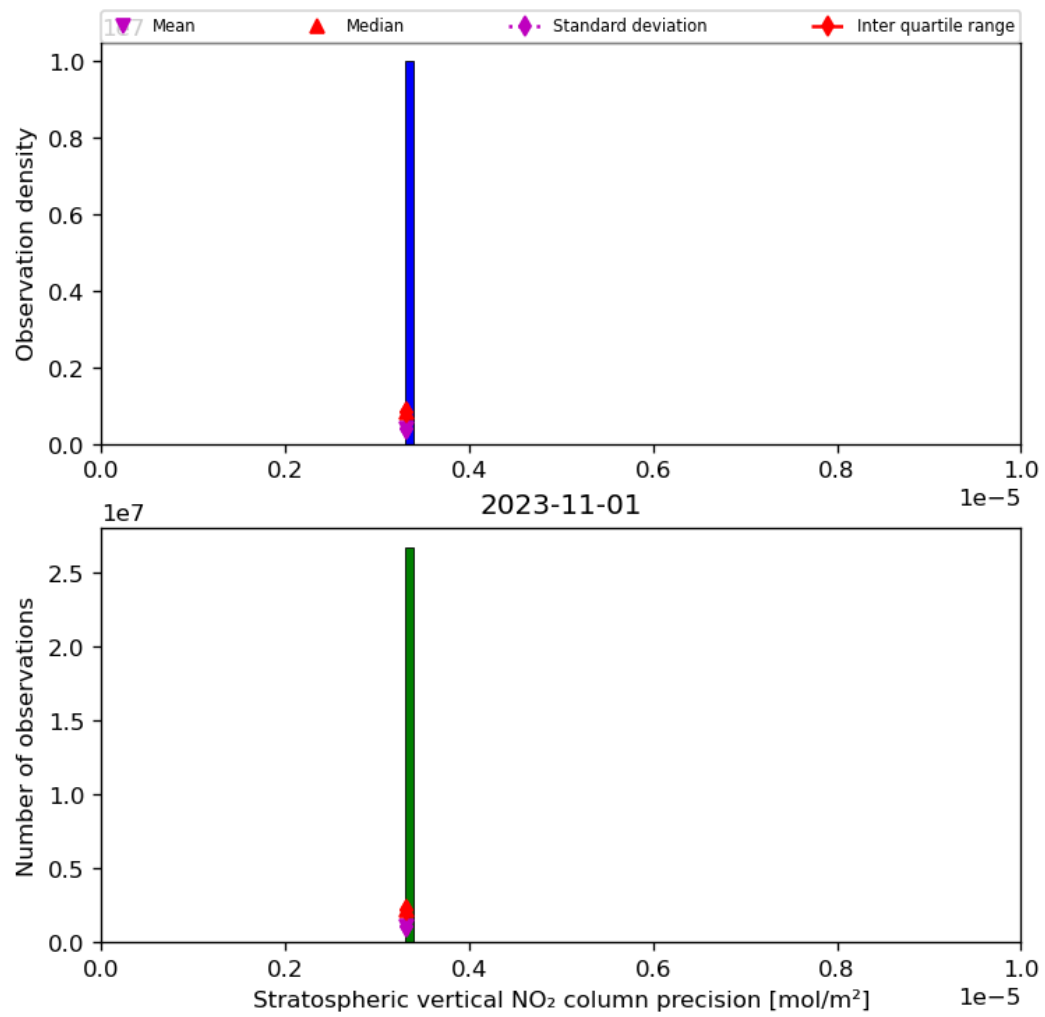
Figure 37: Histogram of “Stratospheric vertical NO 2 column precision” for 2023-10-31 to 2023-11-02
