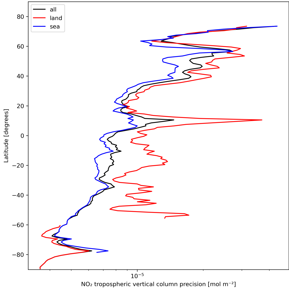
Figure 13: Zonal average of "NO 2 tropospheric vertical column precision" for 2023-10-31 to 2023-11-02.
