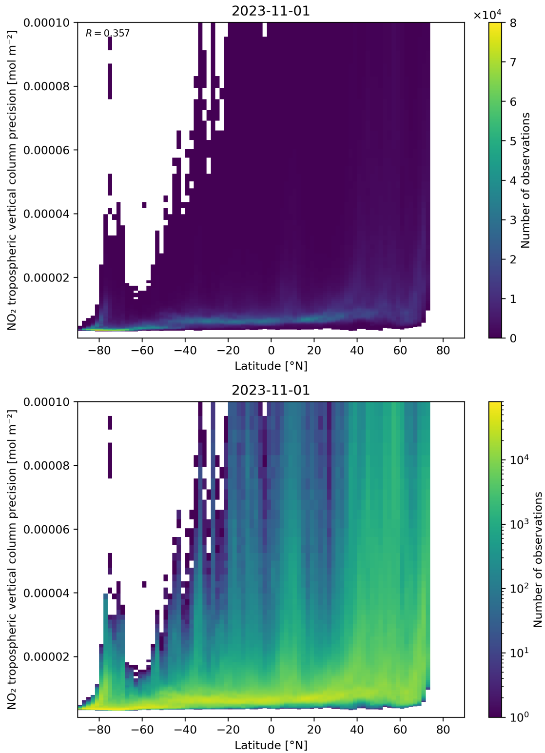
Figure 93: Scatter density plot of “Latitude” against “NO 2 tropospheric vertical column precision” for 2023-10-31 to 2023-11-02.
