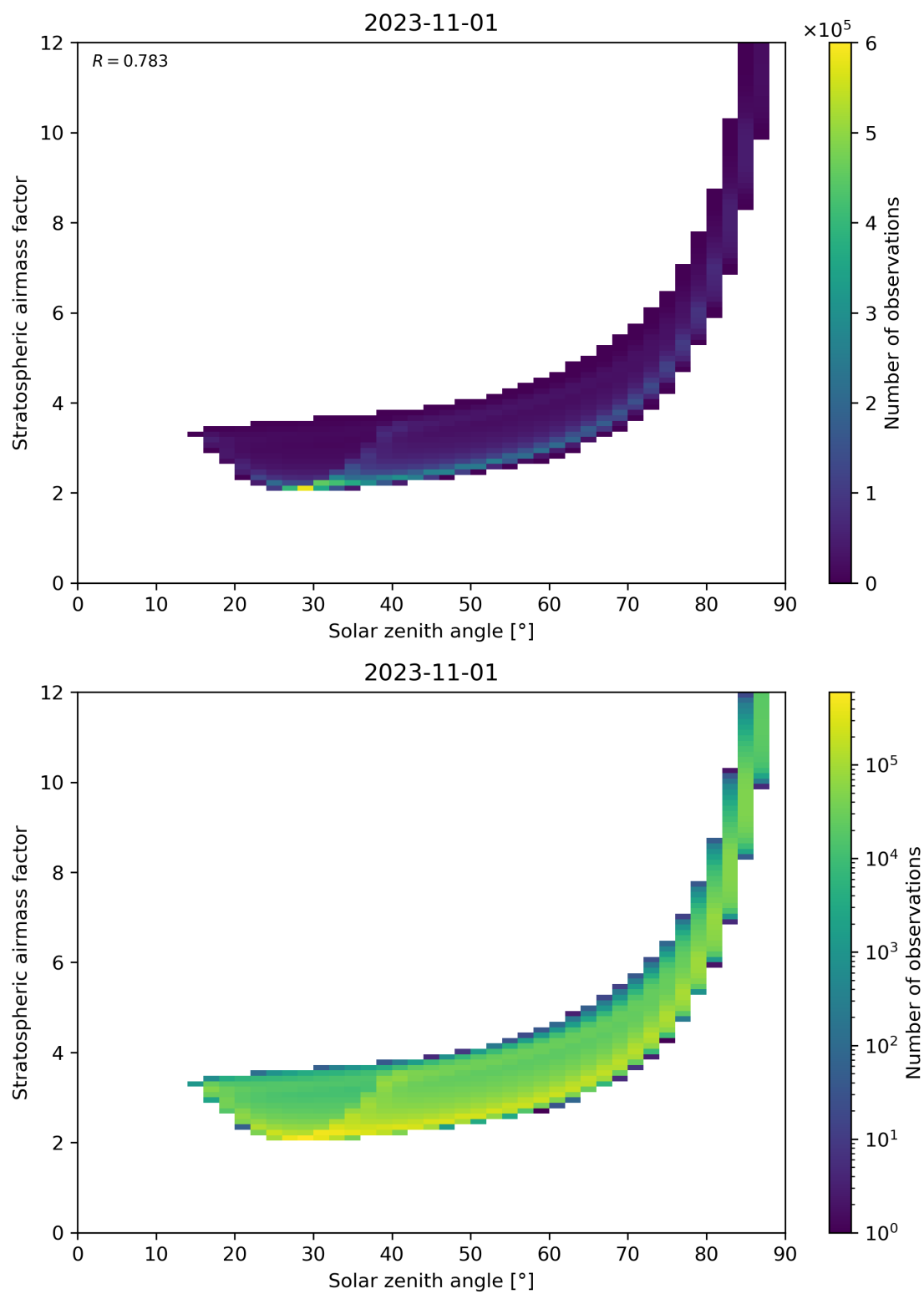
Figure 145: Scatter density plot of “Solar zenith angle” against “Stratospheric airmass factor” for 2023-10-31 to 2023-11-02.
