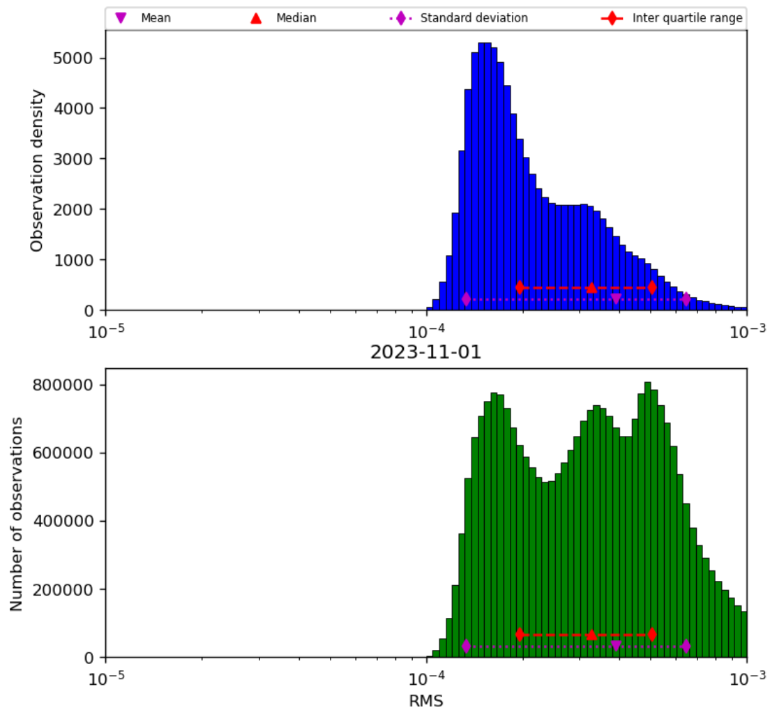
Figure 43: Histogram of “RMS” for 2023-10-31 to 2023-11-02
