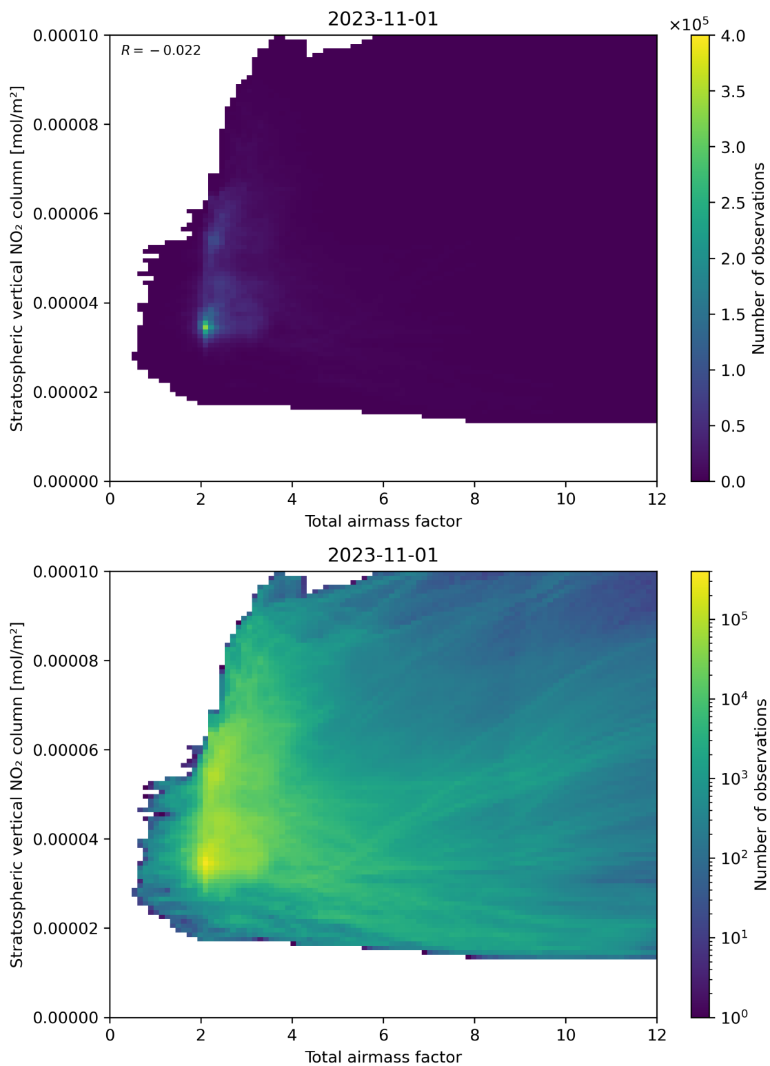
Figure 64: Scatter density plot of “Total airmass factor” against “Stratospheric vertical NO 2 column” for 2023-10-31 to 2023-11-02.
