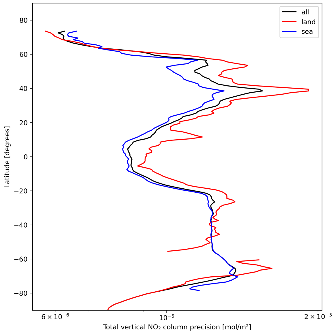
Figure 22: Zonal average of “Total vertical NO 2 column precision” for 2023-10-31 to 2023-11-02.
