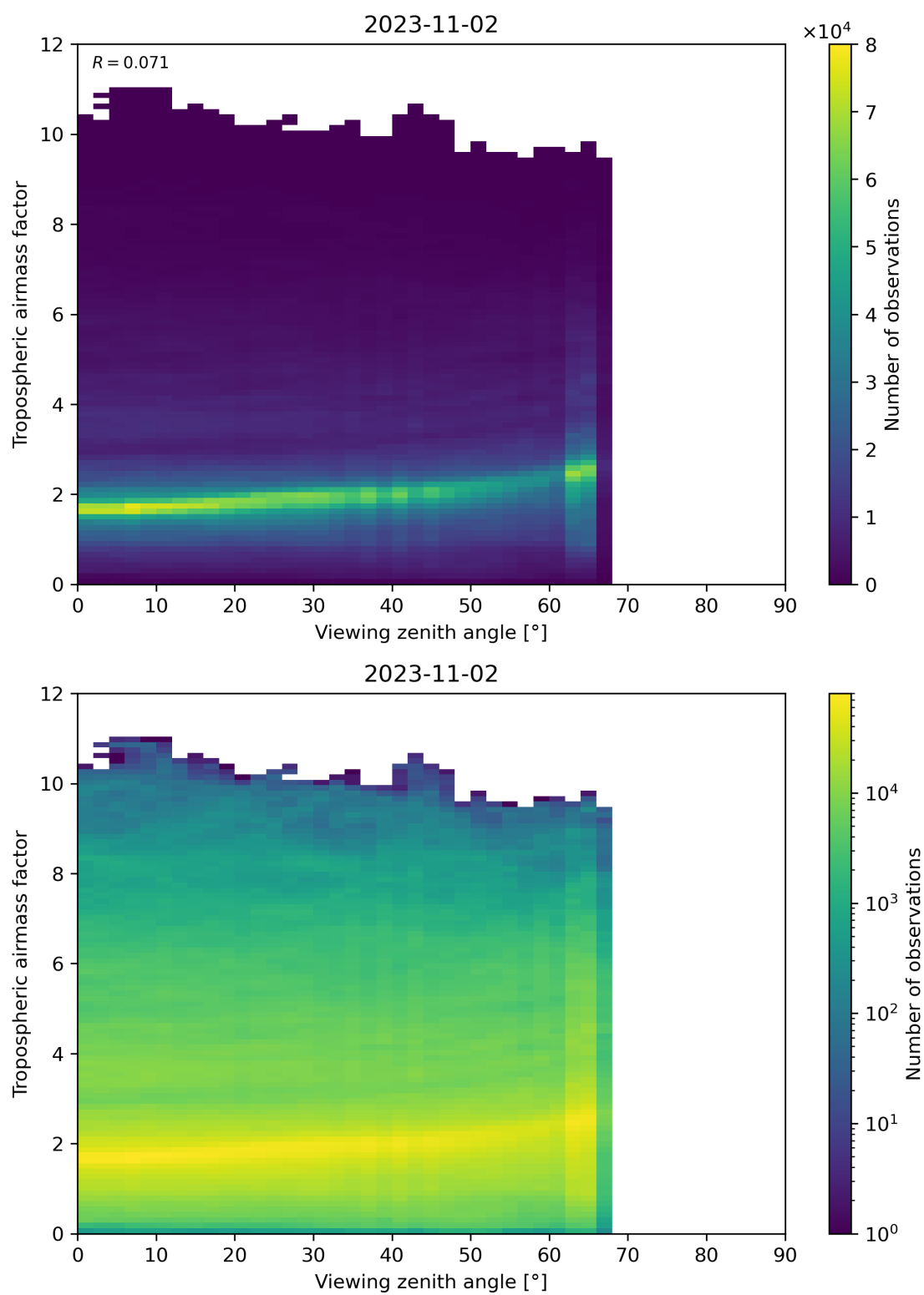
Figure 161: Scatter density plot of “Viewing zenith angle” against “Tropospheric airmass factor” for 2023-11-02 to 2023-11-03.
