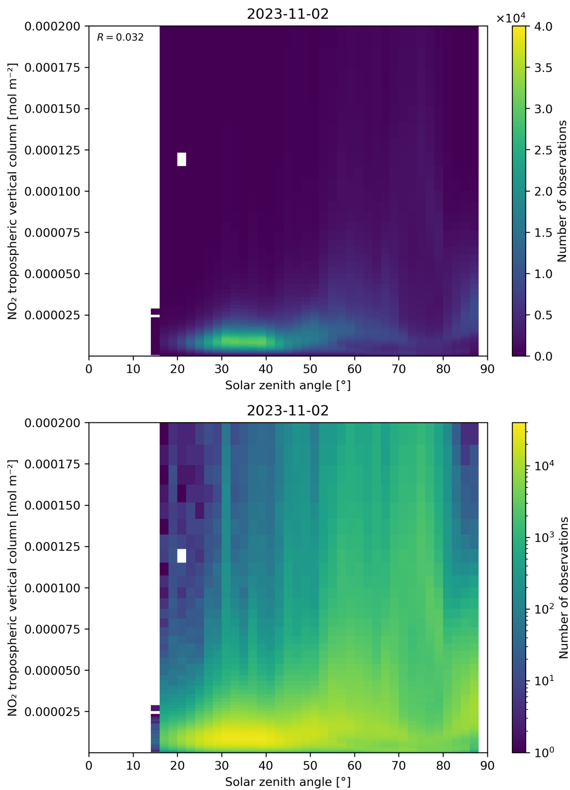
Figure 155: Scatter density plot of “Solar zenith angle” against “NO 2 tropospheric vertical column” for 2023-11-02 to 2023-11-03.
