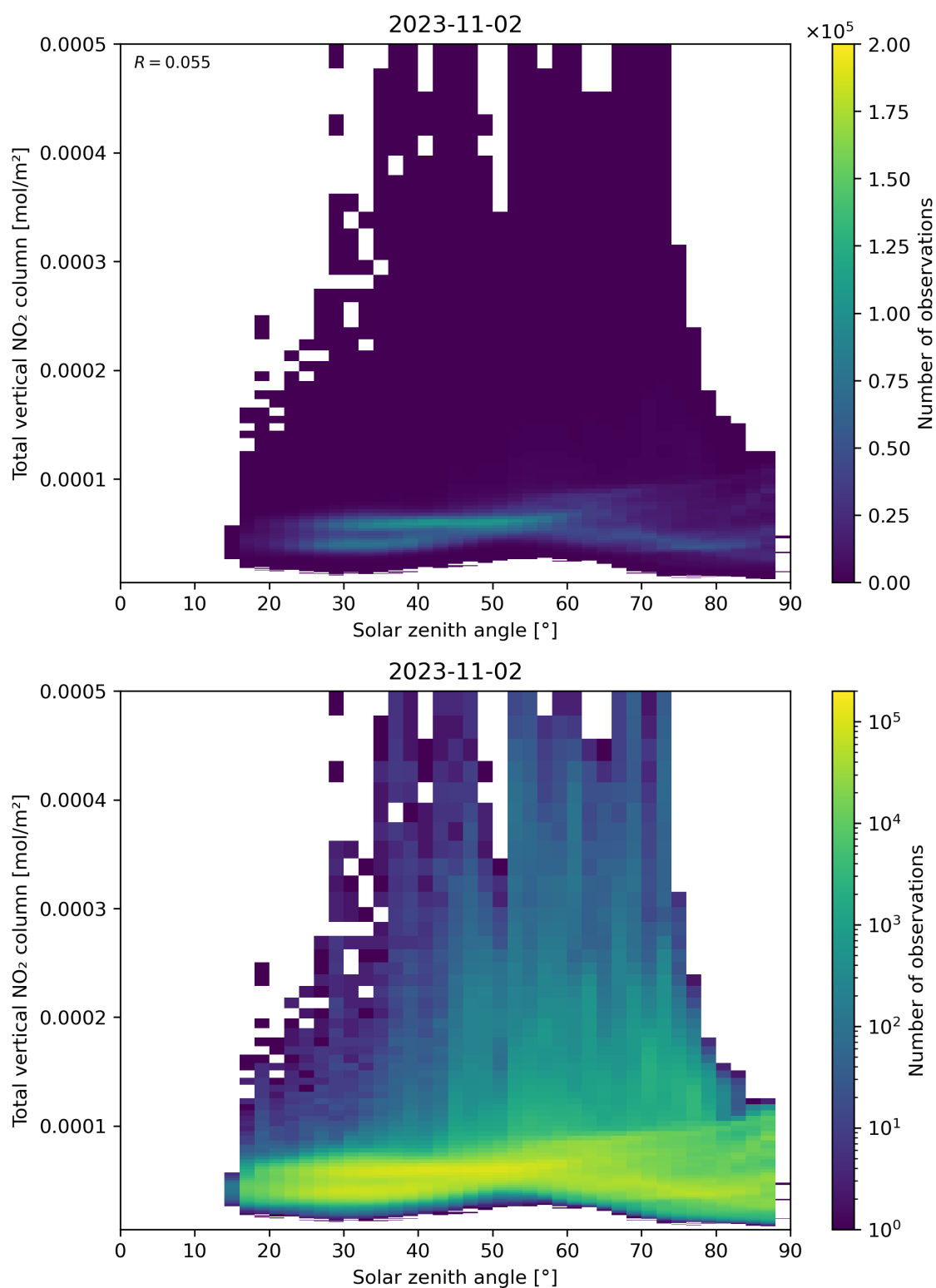
Figure 153: Scatter density plot of “Solar zenith angle” against “Total vertical NO 2 column” for 2023-11-02 to 2023-11-03.
