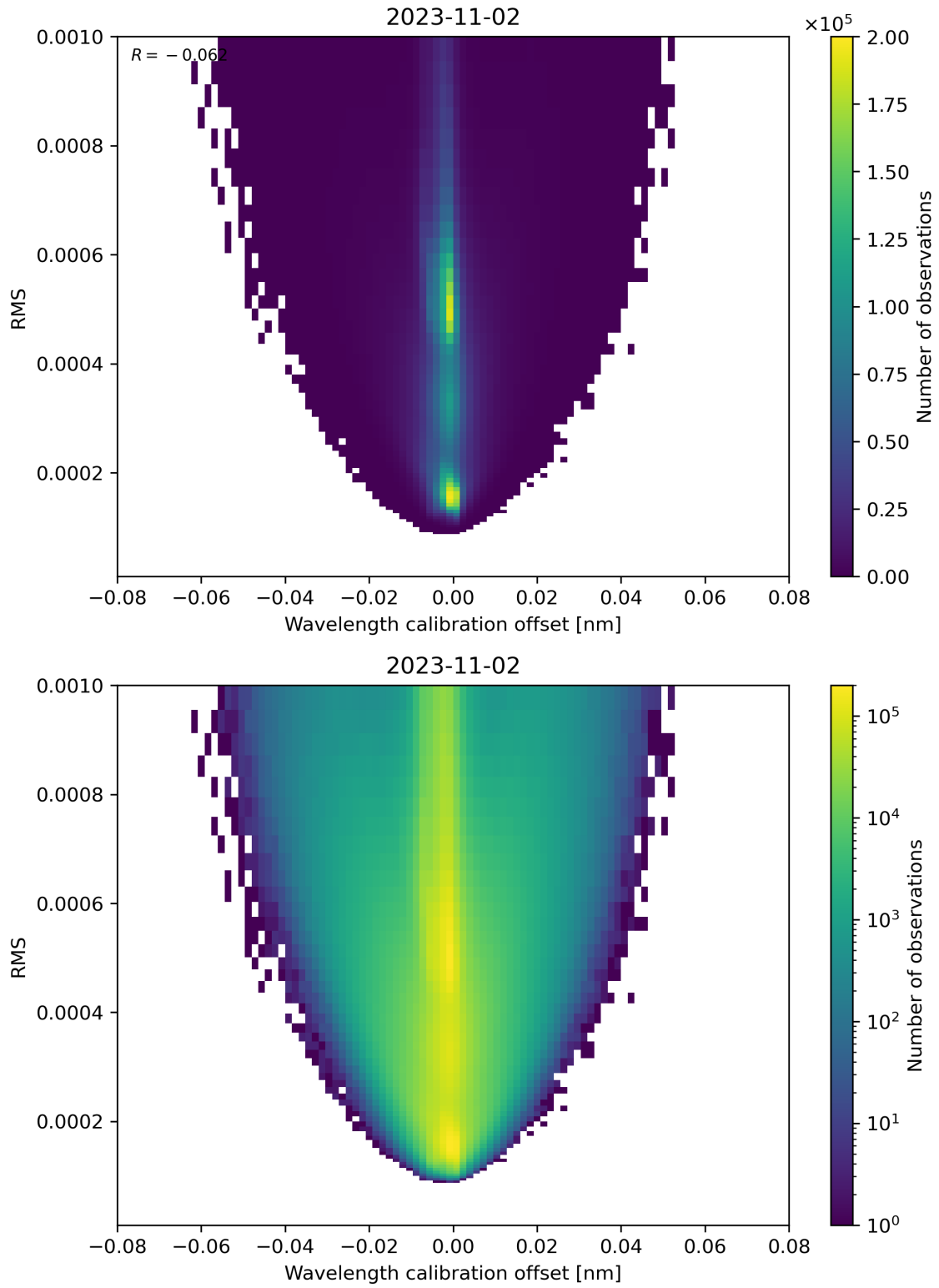
Figure 181: Scatter density plot of “Wavelength calibration offset” against “RMS” for 2023-11-02 to 2023-11-03.
