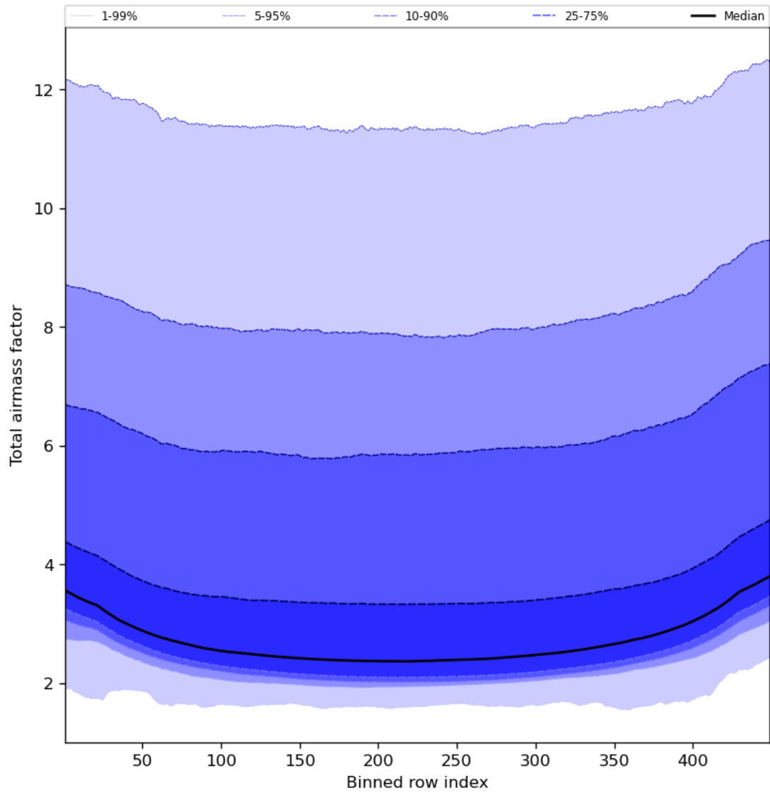
Figure 49: Along track statistics of “Total airmass factor” for 2023-11-02 to 2023-11-03
