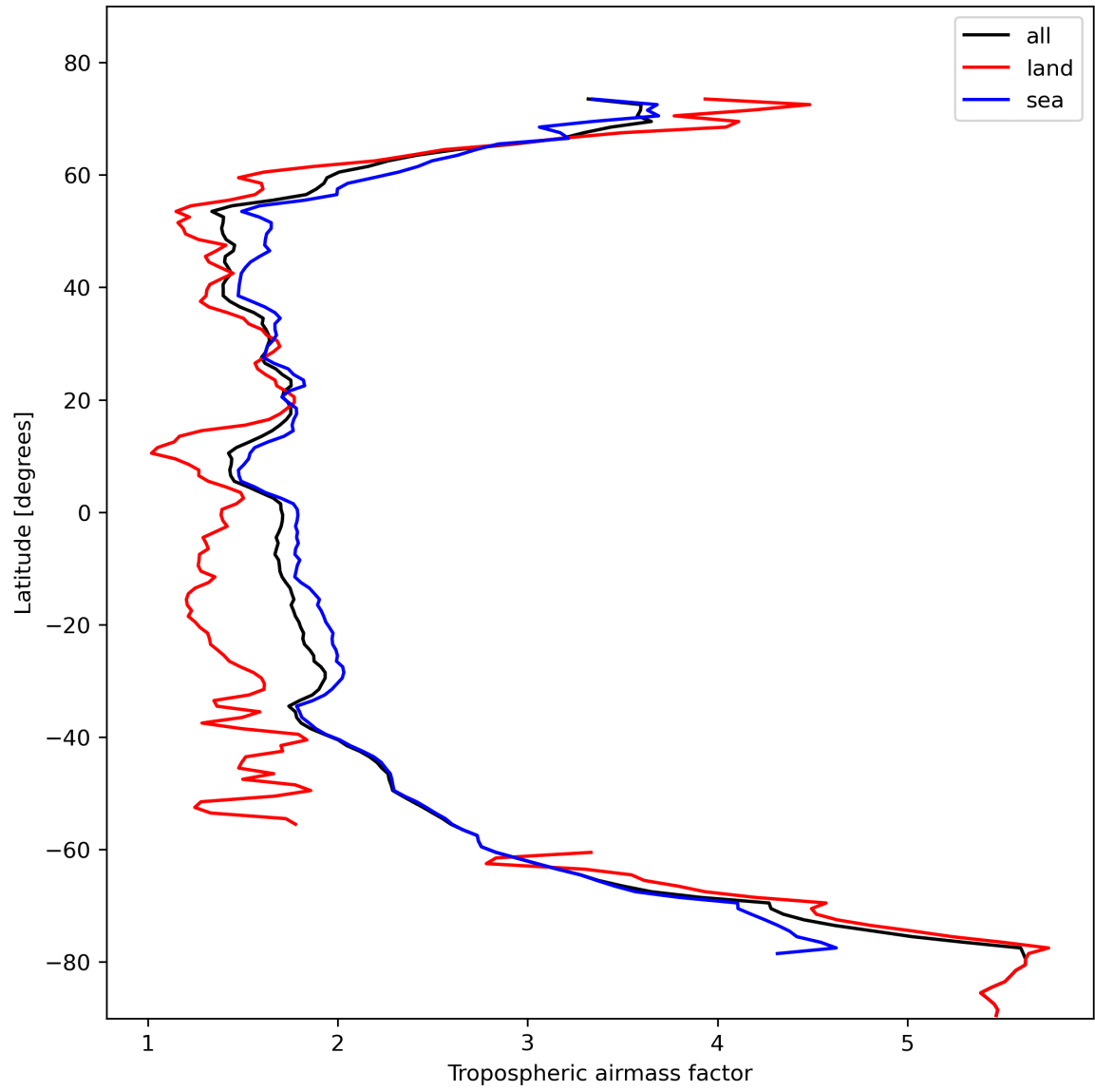
Figure 14: Zonal average of “Tropospheric airmass factor” for 2023-11-02 to 2023-11-03.
