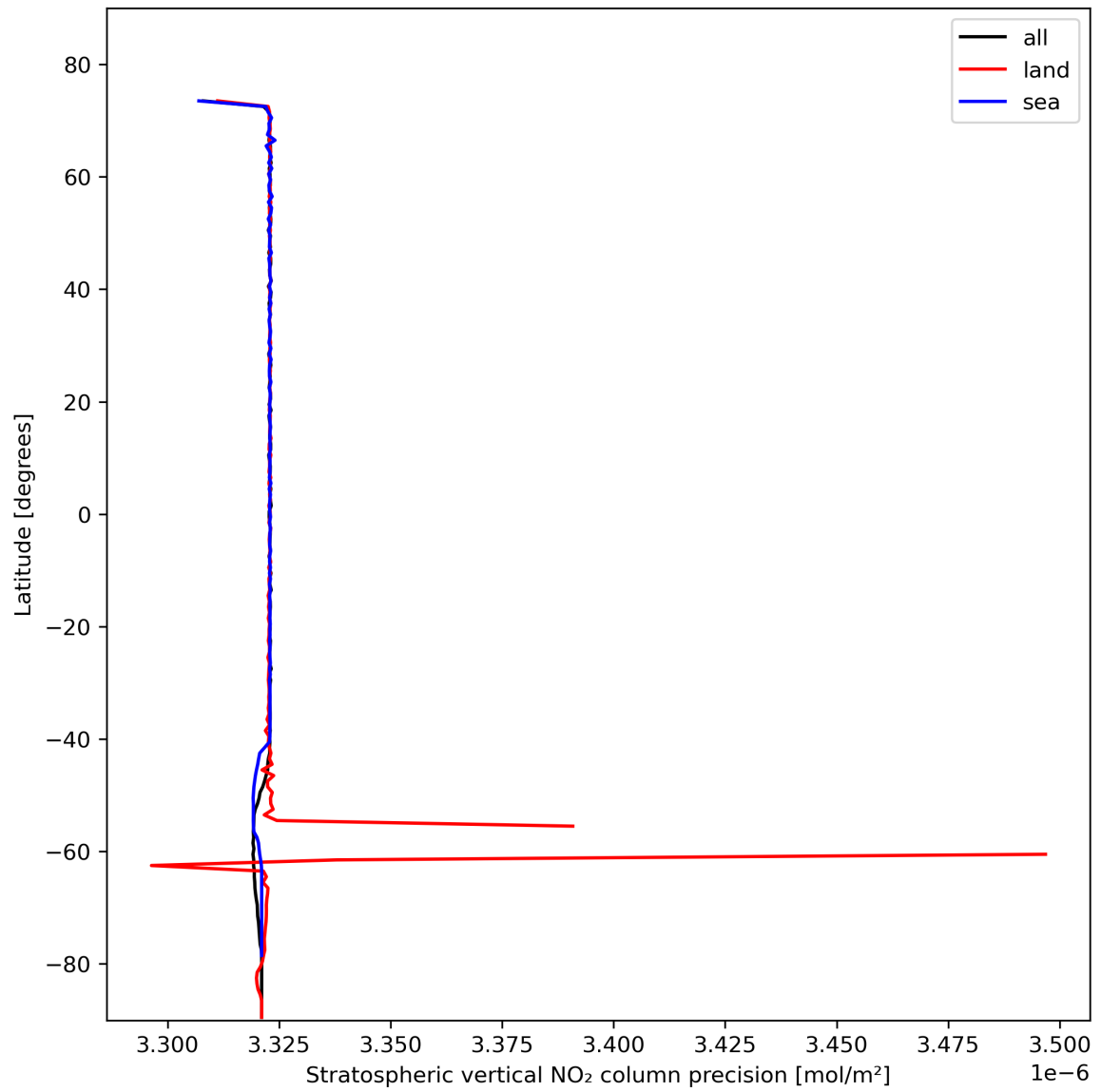
Figure 20: Zonal average of “Stratospheric vertical NO 2 column precision” for 2023-11-02 to 2023-11-03.
