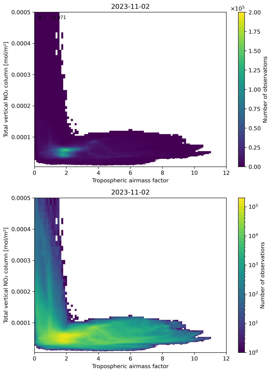
Figure 77: Scatter density plot of “Tropospheric airmass factor” against “Total vertical NO 2 column” for 2023-11-02 to 2023-11-03.
