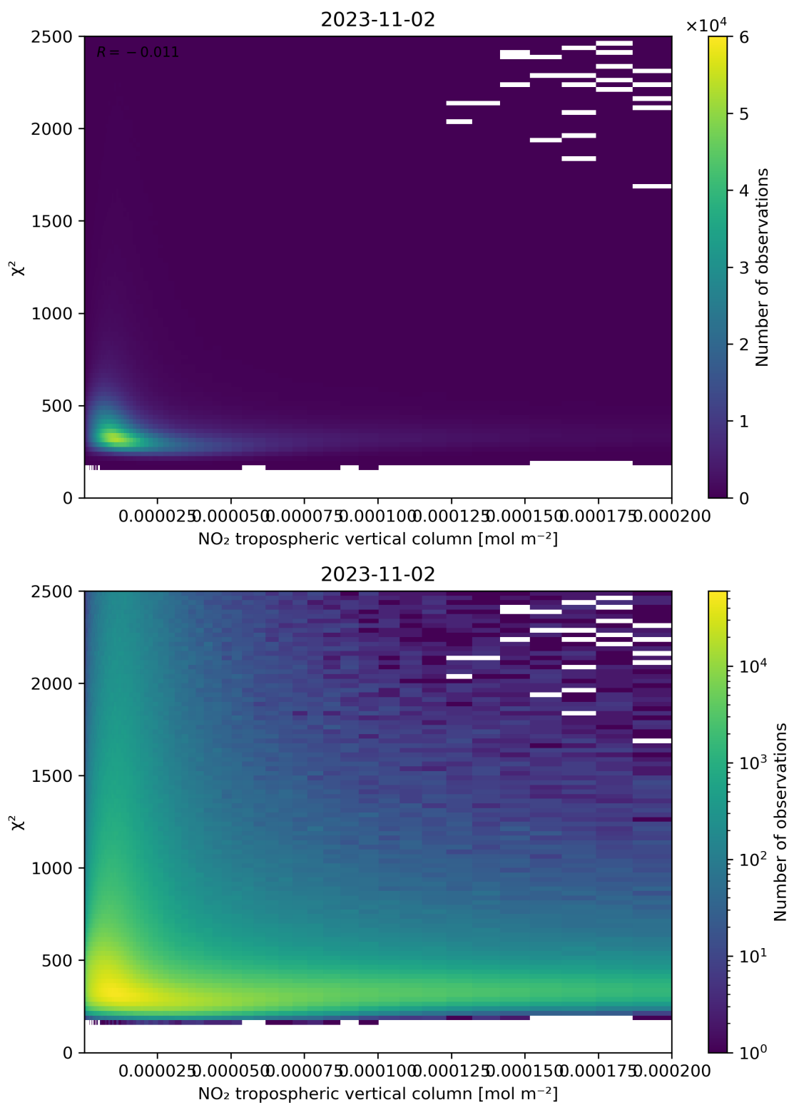
Figure 124: Scatter density plot of “NO 2 tropospheric vertical column” against “ \chi^2 ” for 2023-11-02 to 2023-11-03.
