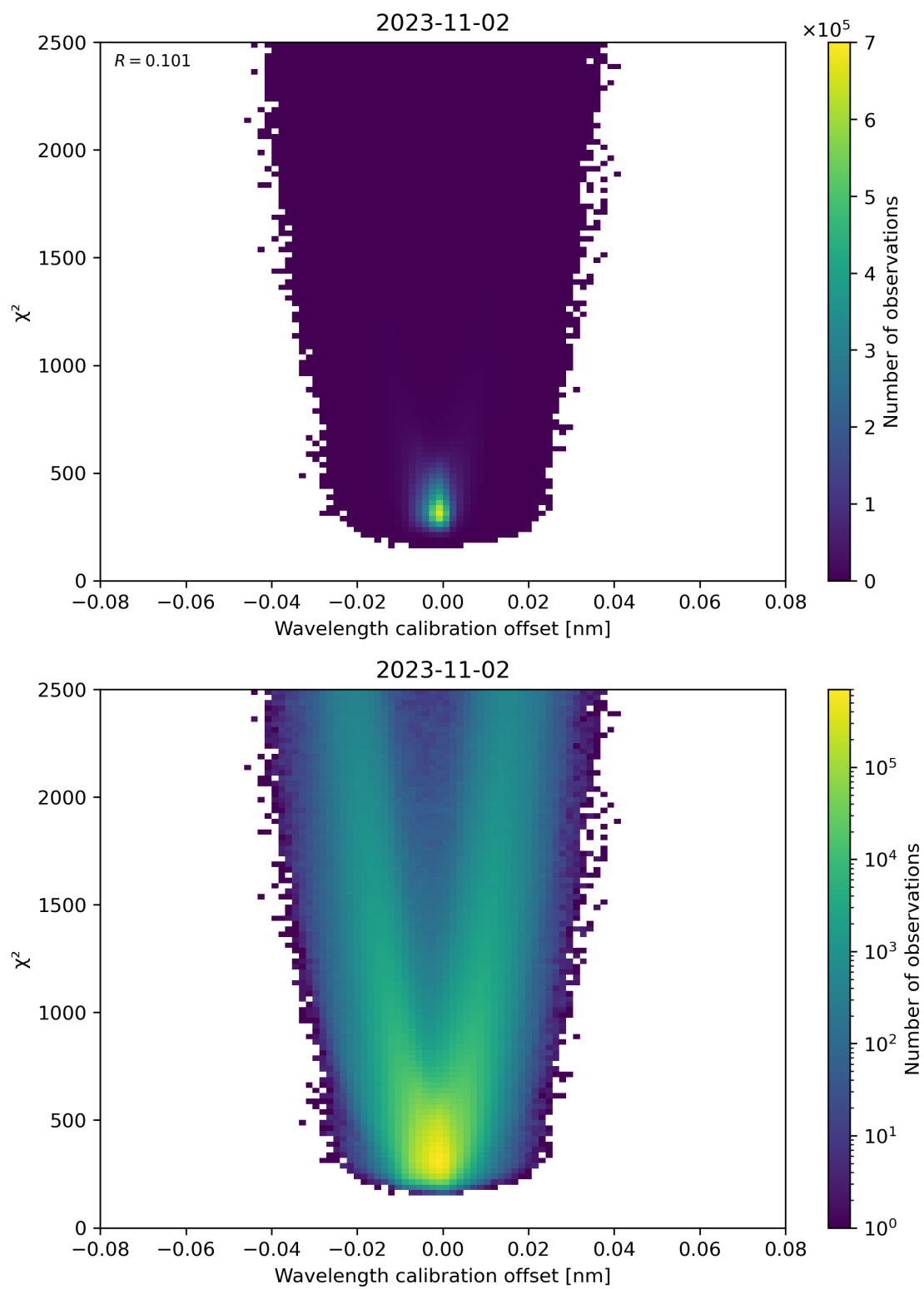
Figure 175: Scatter density plot of “Wavelength calibration offset” against “ \chi^2 ” for 2023-11-02 to 2023-11-03.
