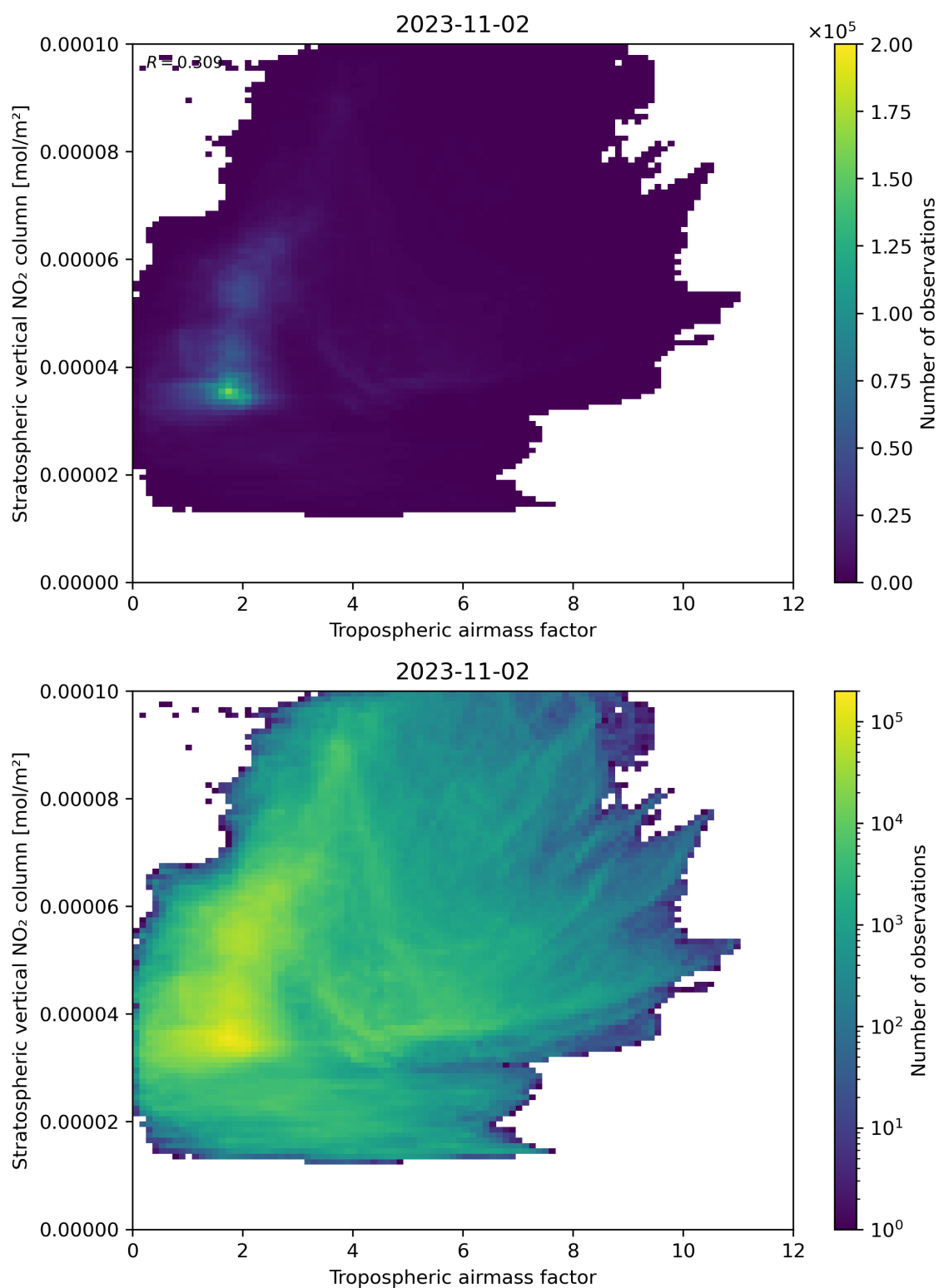
Figure 74: Scatter density plot of “Tropospheric air mass factor” against “Stratospheric vertical NO 2 column” for 2023-11-02 to 2023-11-03.
