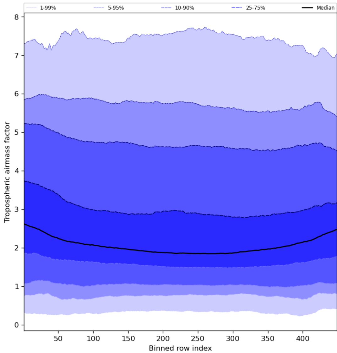
Figure 48: Along track statistics of “Tropospheric air mass factor” for 2023-11-02 to 2023-11-03
