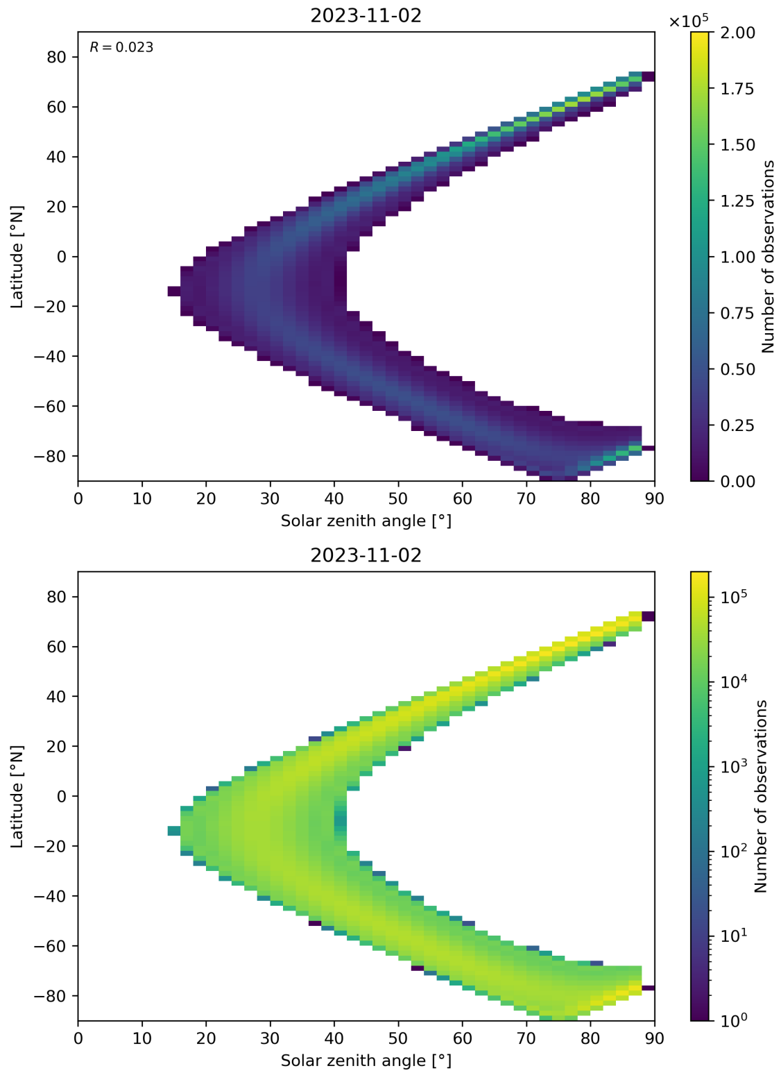
Figure 149: Scatter density plot of “Solar zenith angle” against “Latitude” for 2023-11-02 to 2023-11-03.
