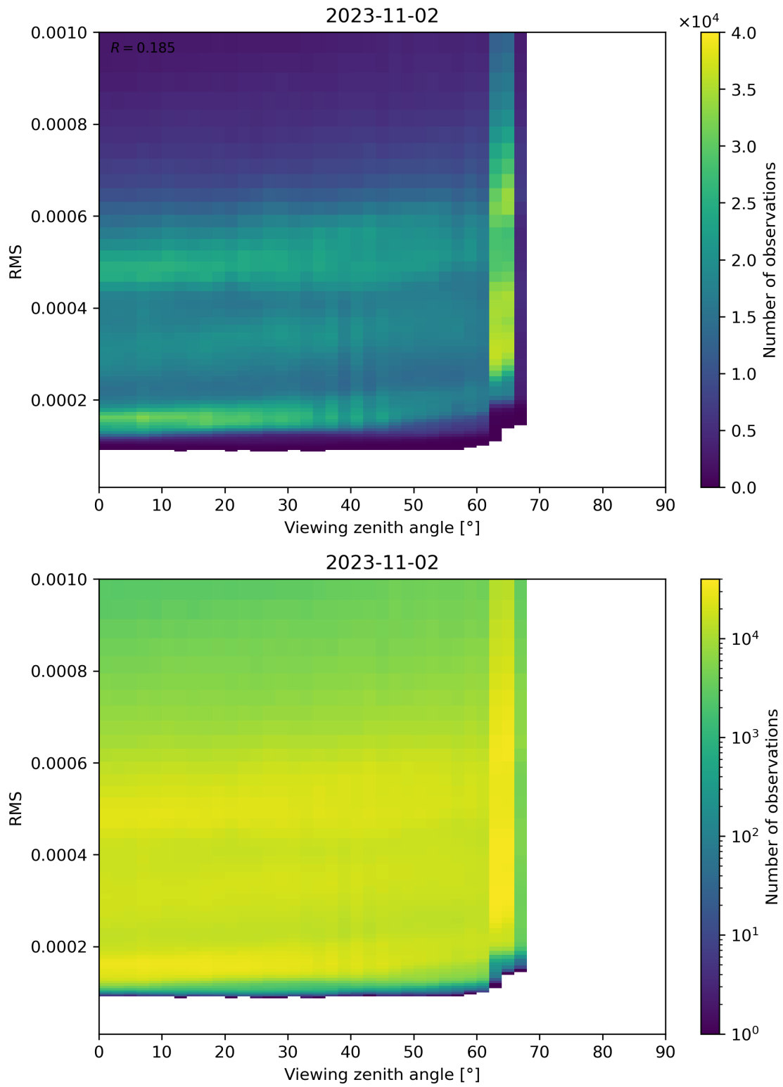
Figure 171: Scatter density plot of “Viewing zenith angle” against “RMS” for 2023-11-02 to 2023-11-03.
