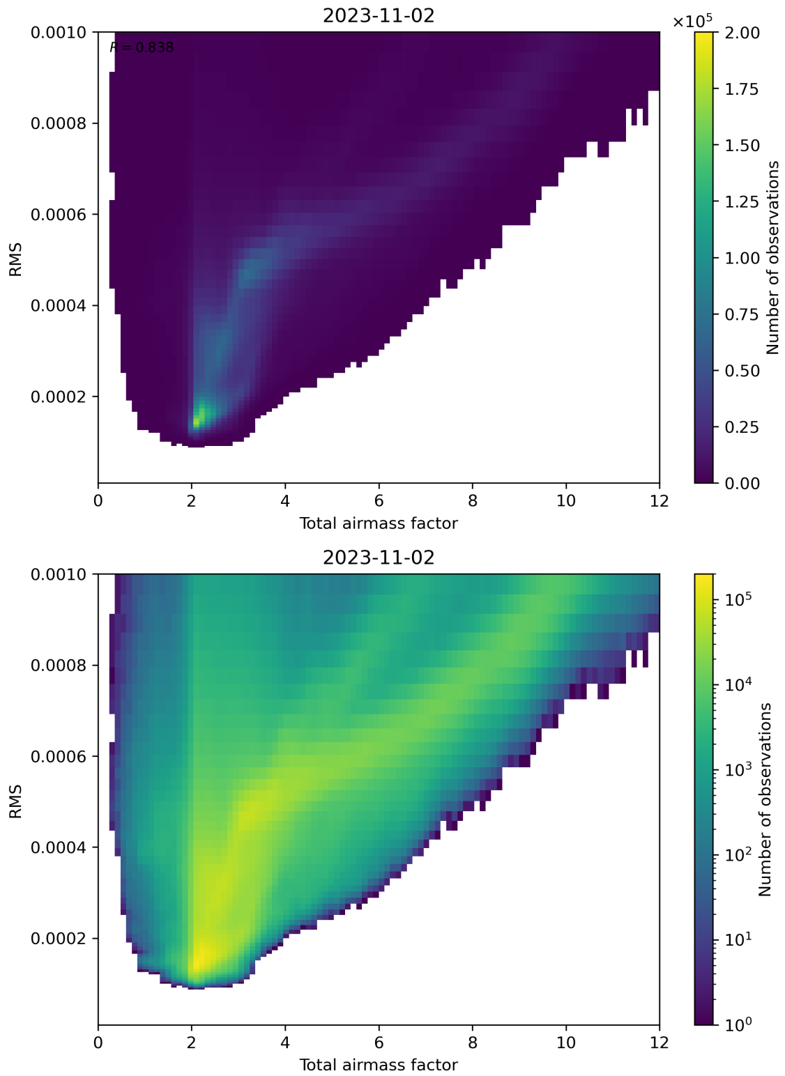
Figure 69: Scatter density plot of “Total airmass factor” against “RMS” for 2023-11-02 to 2023-11-03.
