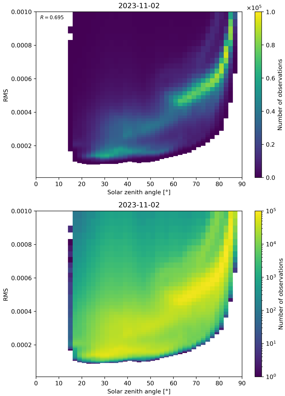
Figure 157: Scatter density plot of “Solar zenith angle” against “RMS” for 2023-11-02 to 2023-11-03.
