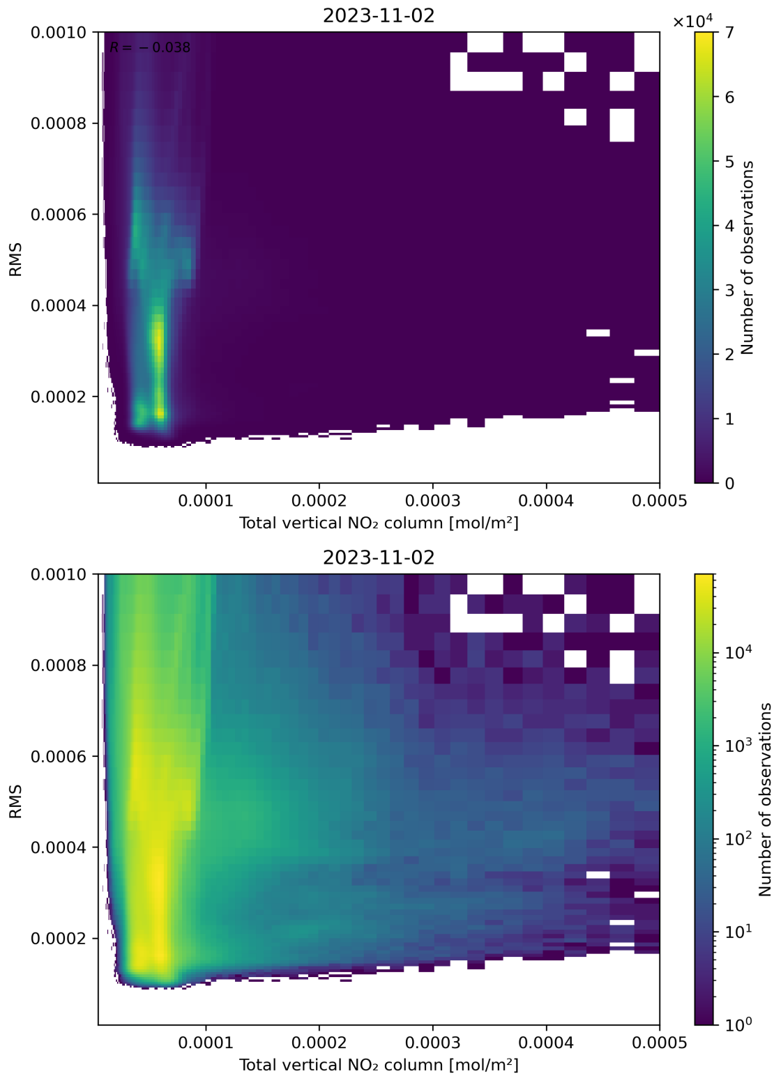
Figure 120: Scatter density plot of “Total vertical NO 2 column” against “RMS” for 2023-11-02 to 2023-11-03.
