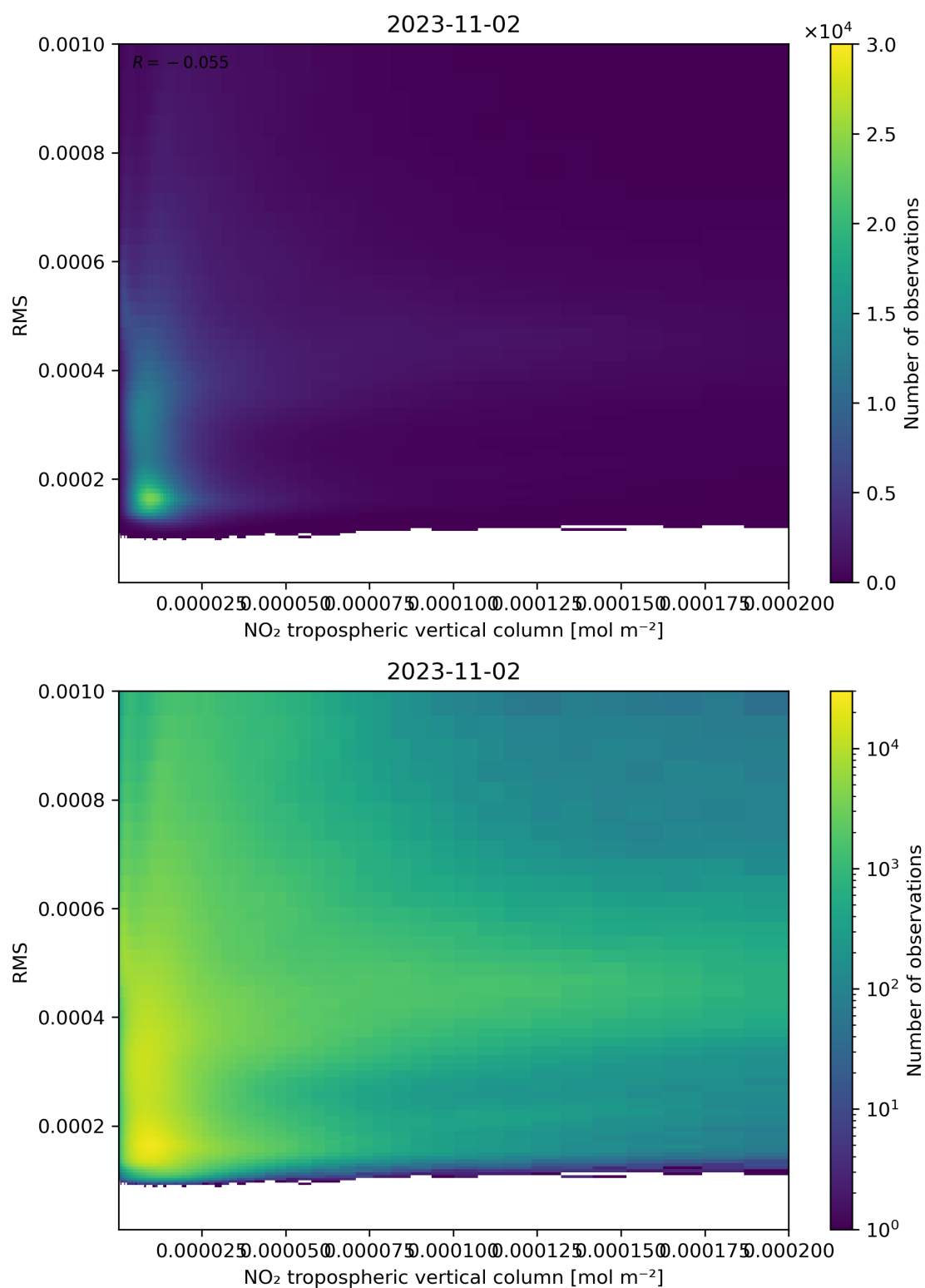
Figure 142: Scatter density plot of “NO 2 tropospheric vertical column” against “RMS” for 2023-11-02 to 2023-11-03.
