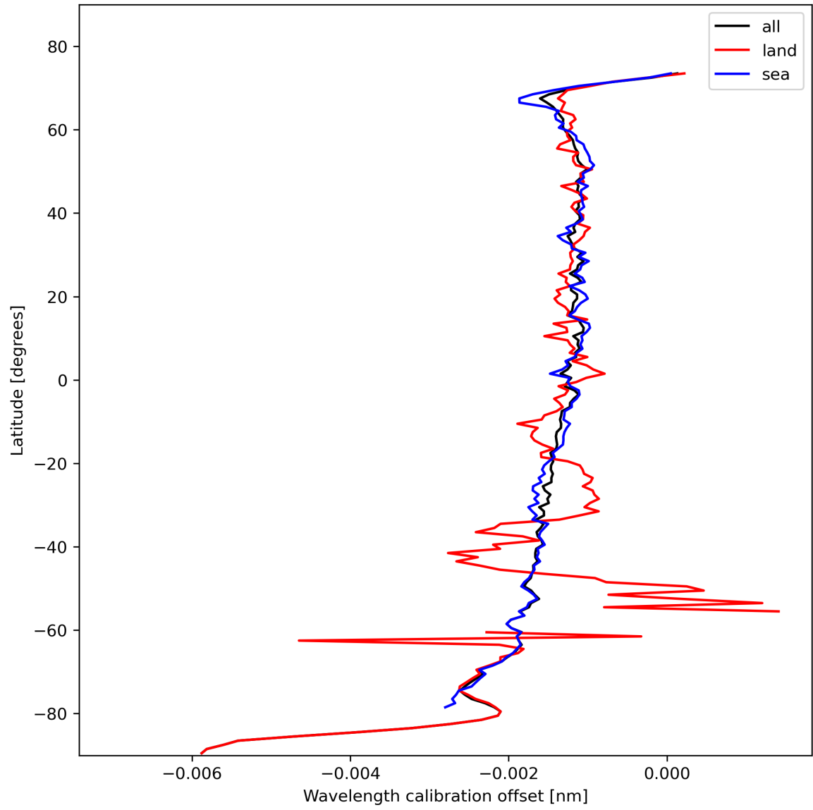
Figure 18: Zonal average of “Wavelength calibration offset” for 2023-11-02 to 2023-11-03.
