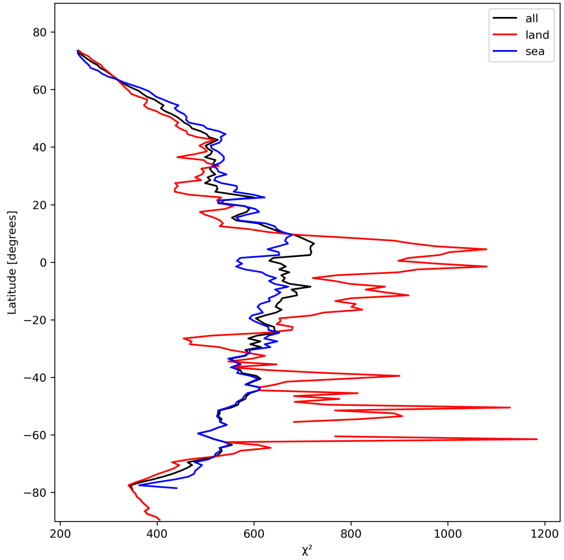
Figure 25: Zonal average of “ \chi^2 ” for 2023-11-02 to 2023-11-03.
