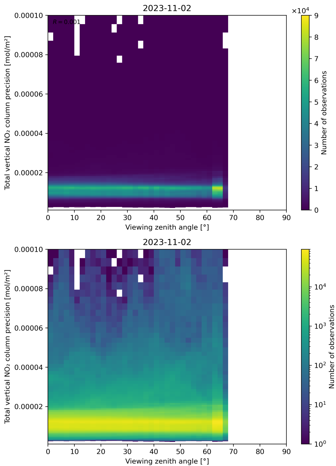
Figure 168: Scatter density plot of “Viewing zenith angle” against “Total vertical NO 2 column precision” for 2023-11-02 to 2023-11-03.
