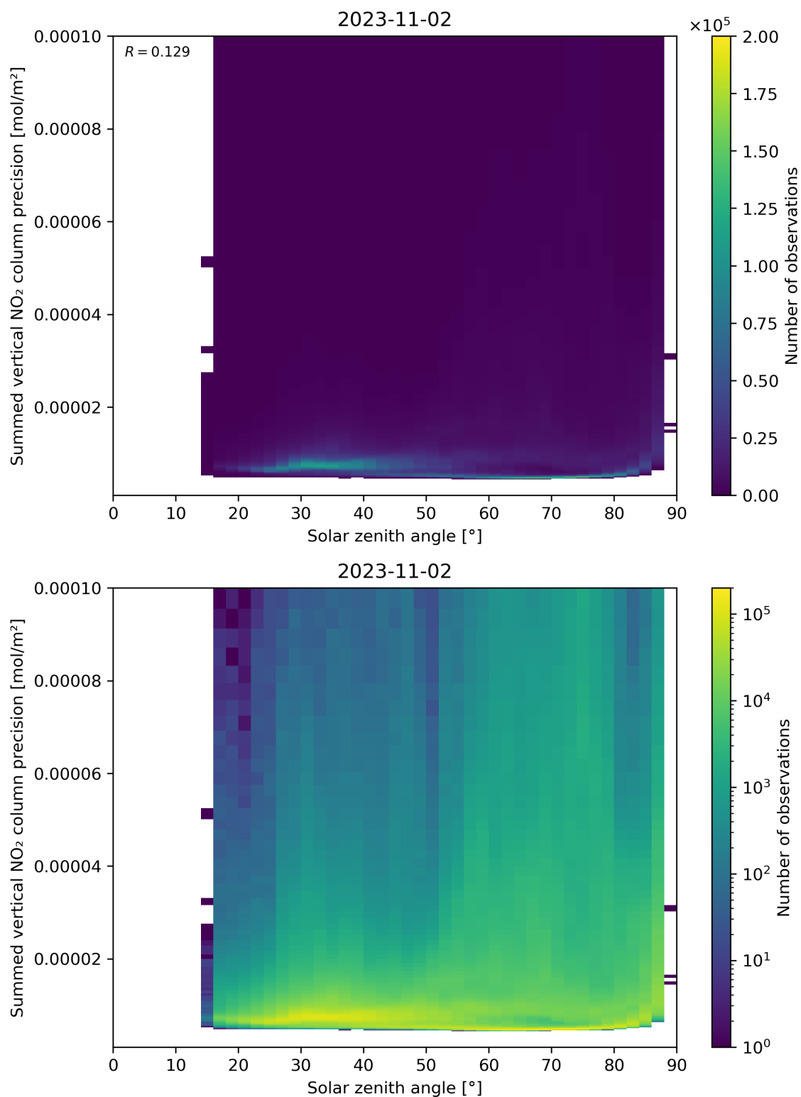
Figure 152: Scatter density plot of “Solar zenith angle” against “Summed vertical NO 2 column precision” for 2023-11-02 to 2023-11-03.
