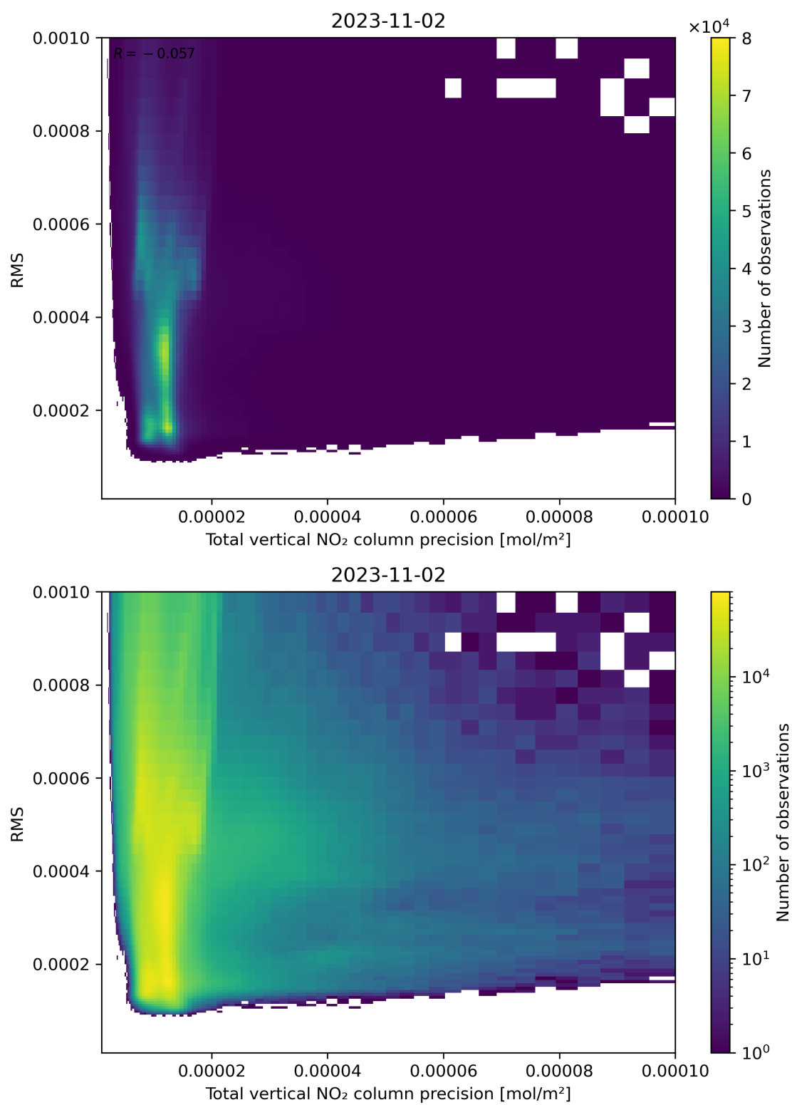
Figure 119: Scatter density plot of “Total vertical NO 2 column precision” against “RMS” for 2023-11-02 to 2023-11-03.
