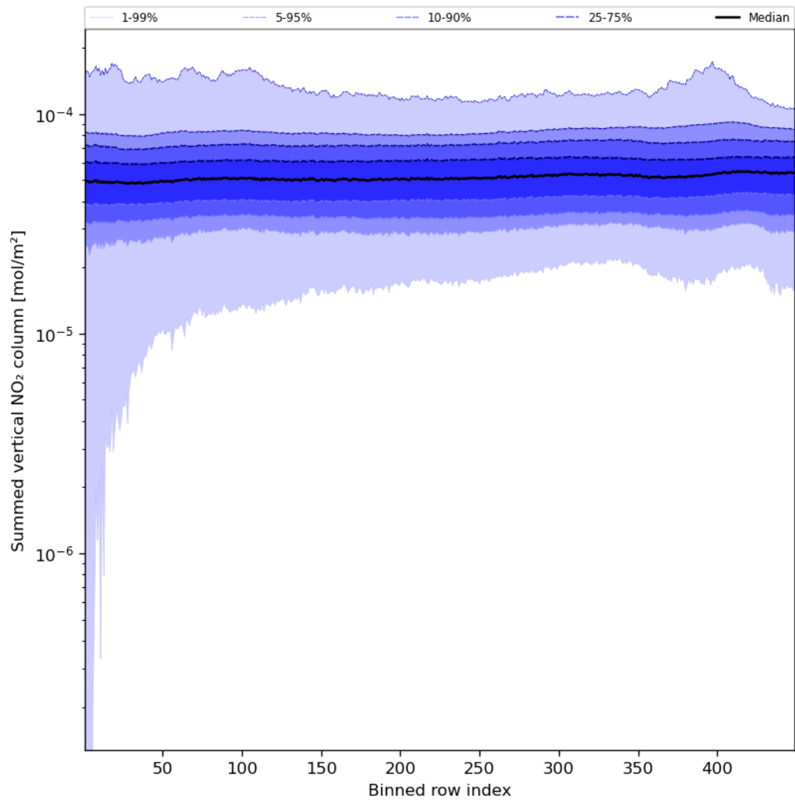
Figure 57: Along track statistics of “Summed vertical NO 2 column” for 2023-11-02 to 2023-11-03
