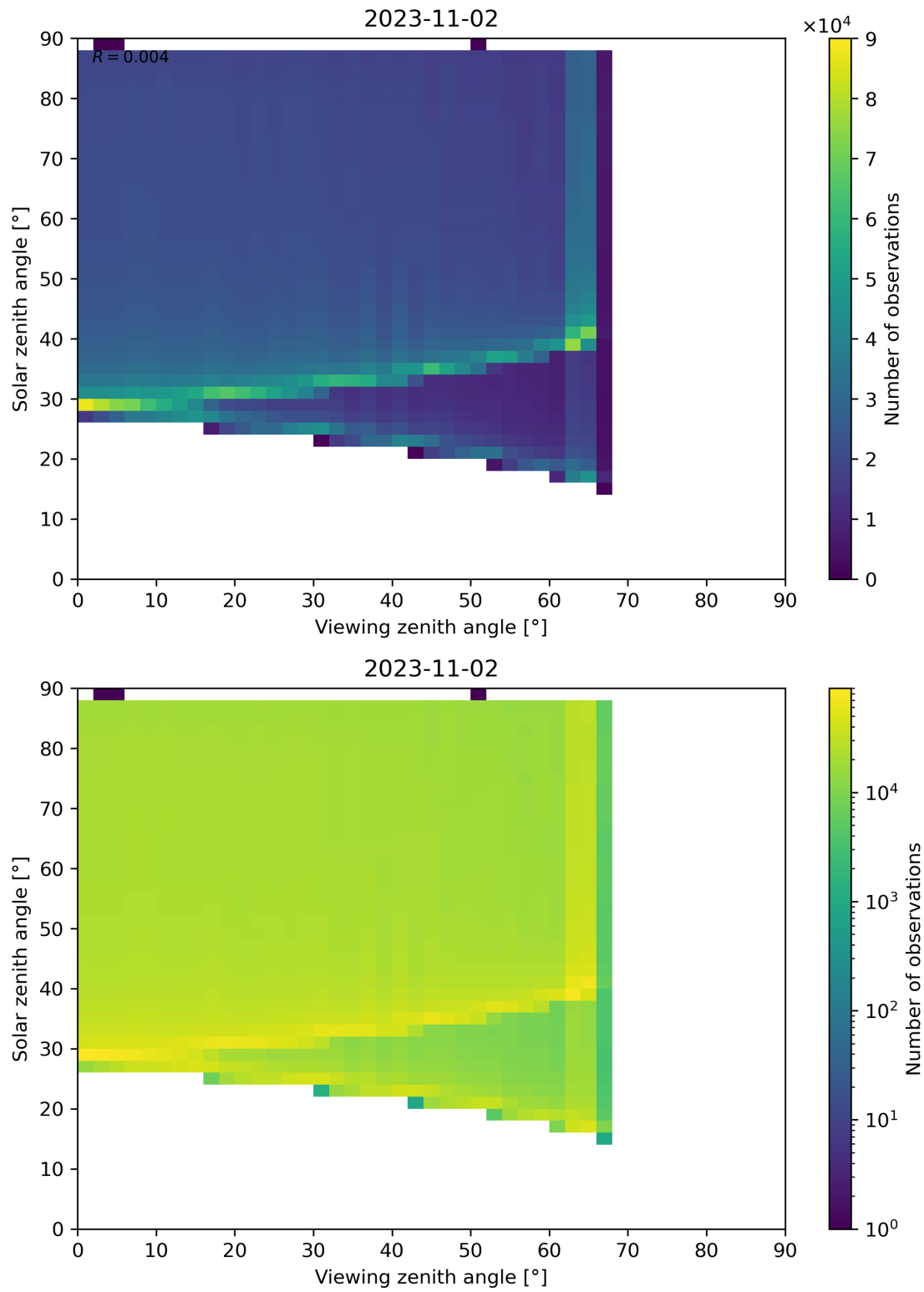
Figure 172: Scatter density plot of “Viewing zenith angle” against “Solar zenith angle” for 2023-11-02 to 2023-11-03.
