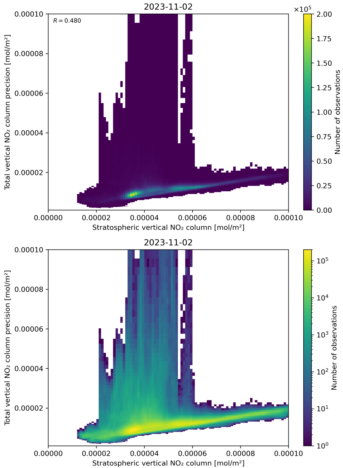
Figure 101: Scatter density plot of “Stratospheric vertical NO 2 column” against “Total vertical NO 2 column precision” for 2023-11-02 to 2023-11-03.
