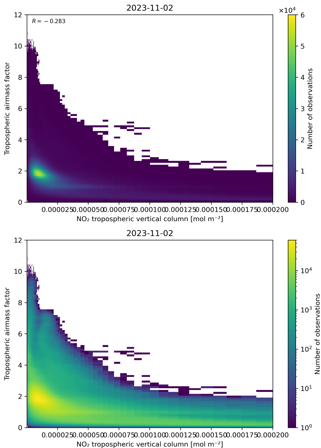
Figure 123: Scatter density plot of “NO 2 tropospheric vertical column” against “Tropospheric air mass factor” for 2023-11-02 to 2023-11-03.
