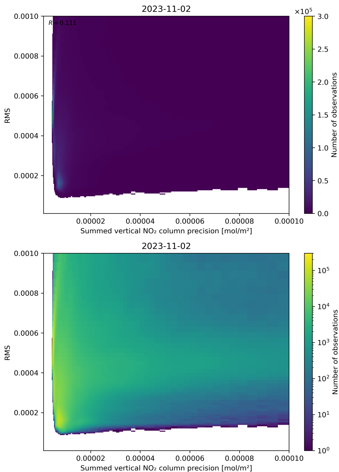
Figure 108: Scatter density plot of “Summed vertical NO 2 column precision” against “RMS” for 2023-11-02 to 2023-11-03.
