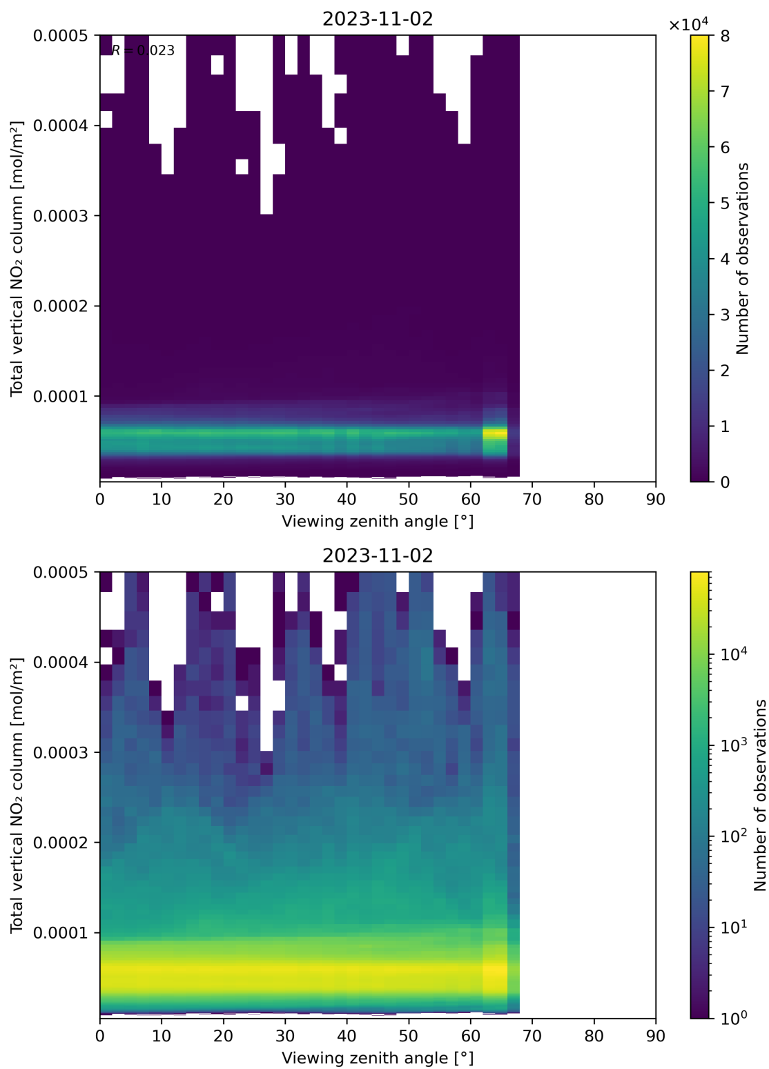
Figure 167: Scatter density plot of “Viewing zenith angle” against “Total vertical NO 2 column” for 2023-11-02 to 2023-11-03.
