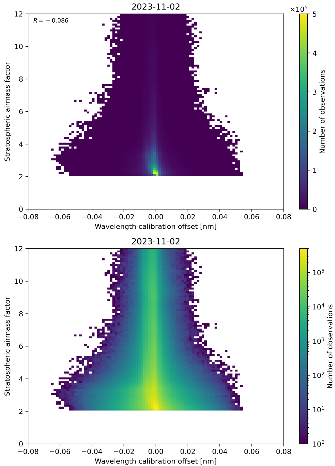
Figure 174: Scatter density plot of “Wavelength calibration offset” against “Stratospheric airmass factor” for 2023-11-02 to 2023-11-03.
