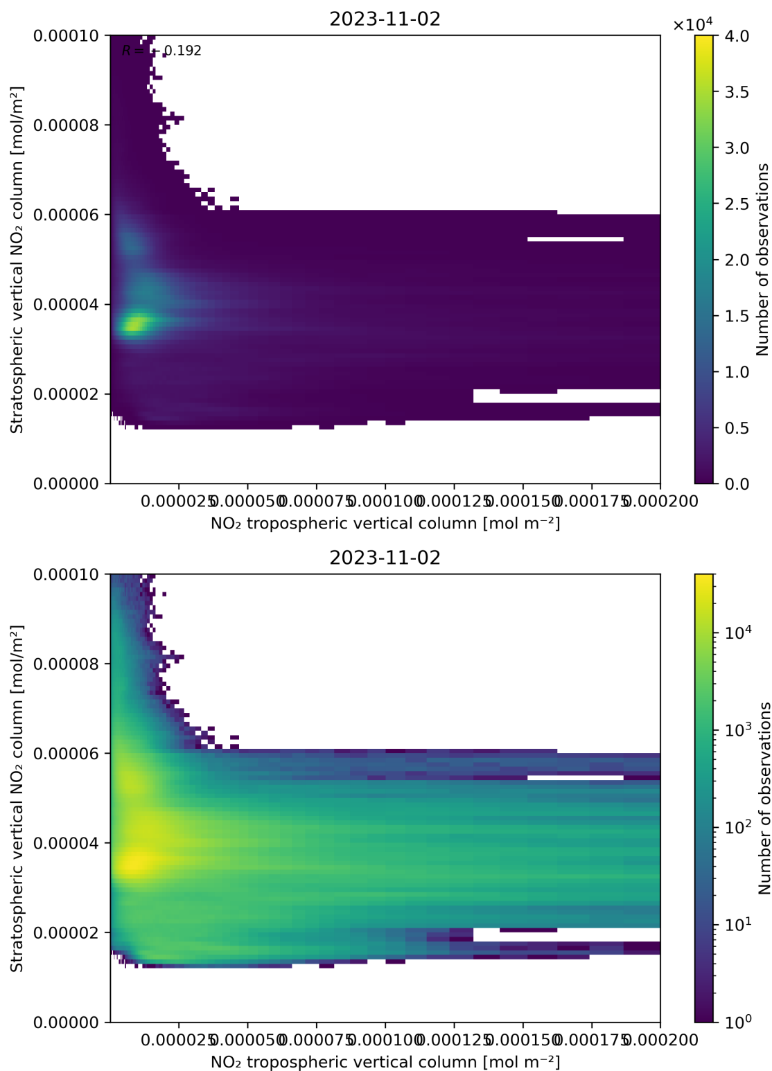
Figure 125: Scatter density plot of “NO 2 tropospheric vertical column” against “Stratospheric vertical NO 2 column” for 2023-11-02 to 2023-11-03.
