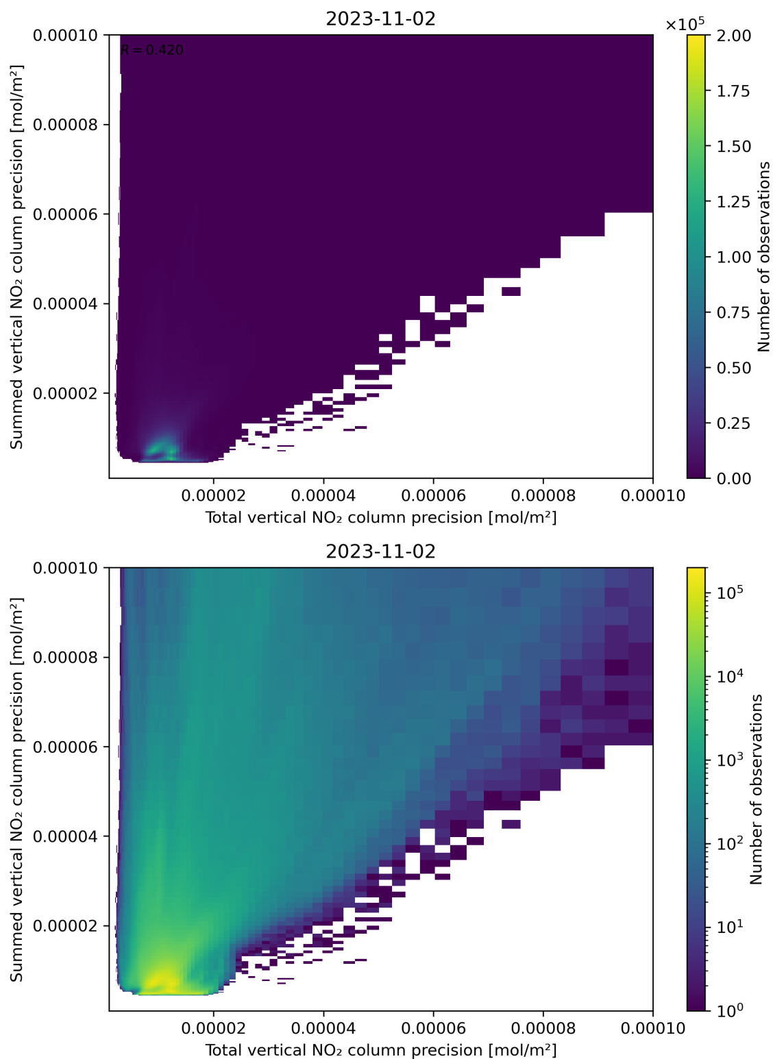
Figure 118: Scatter density plot of “Total vertical NO 2 column precision” against “Summed vertical NO 2 column precision” for 2023-11-02 to 2023-11-03.
