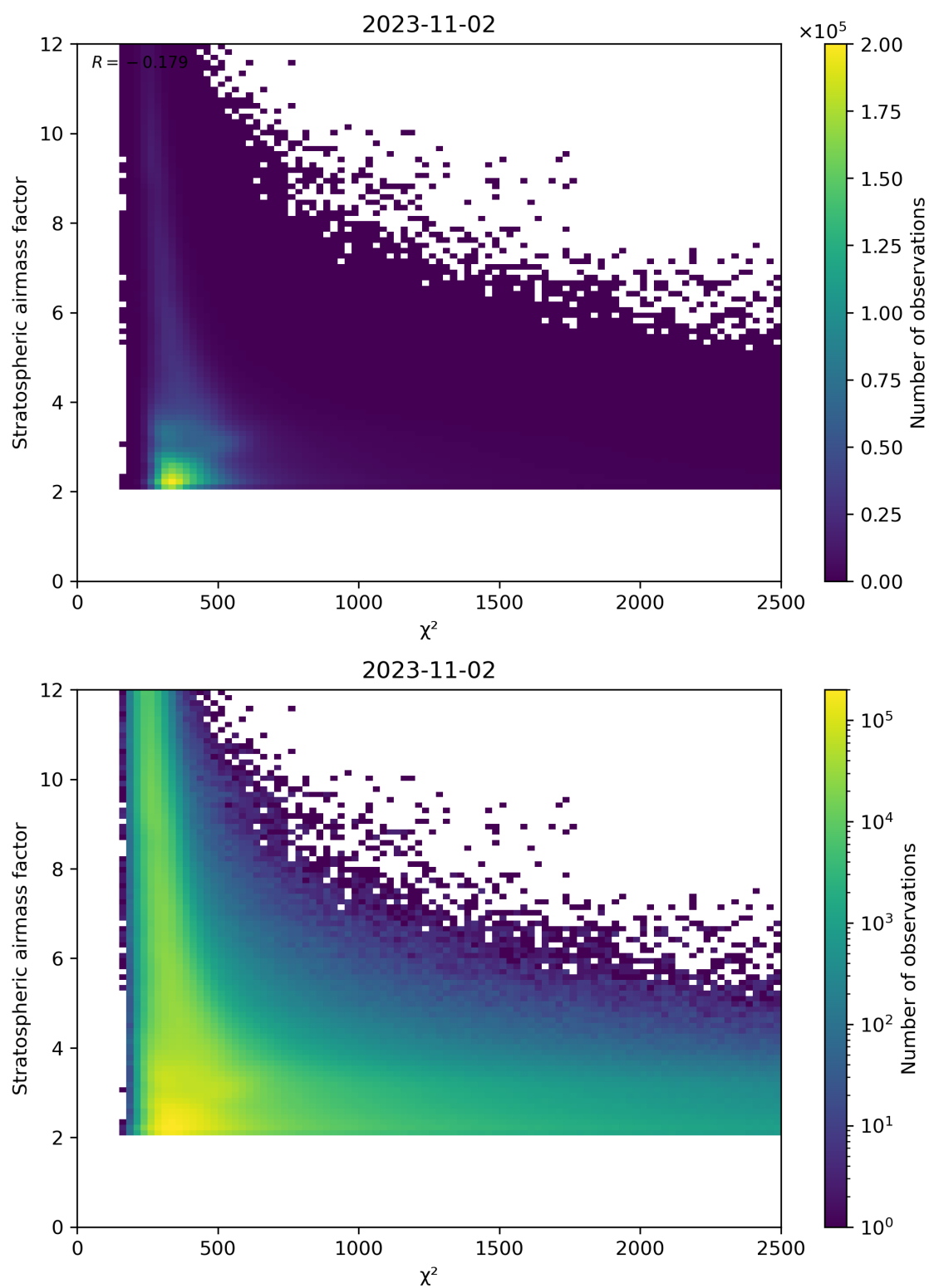
Figure 81: Scatter density plot of “ \chi^2 ” against “Stratospheric airmass factor” for 2023-11-02 to 2023-11-03.
