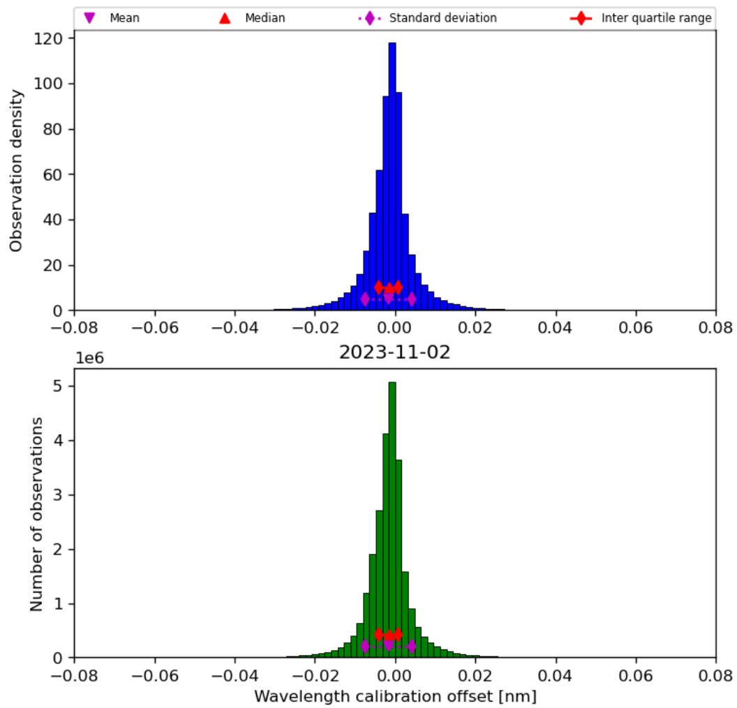
Figure 35: Histogram of “Wavelength calibration offset” for 2023-11-02 to 2023-11-03
