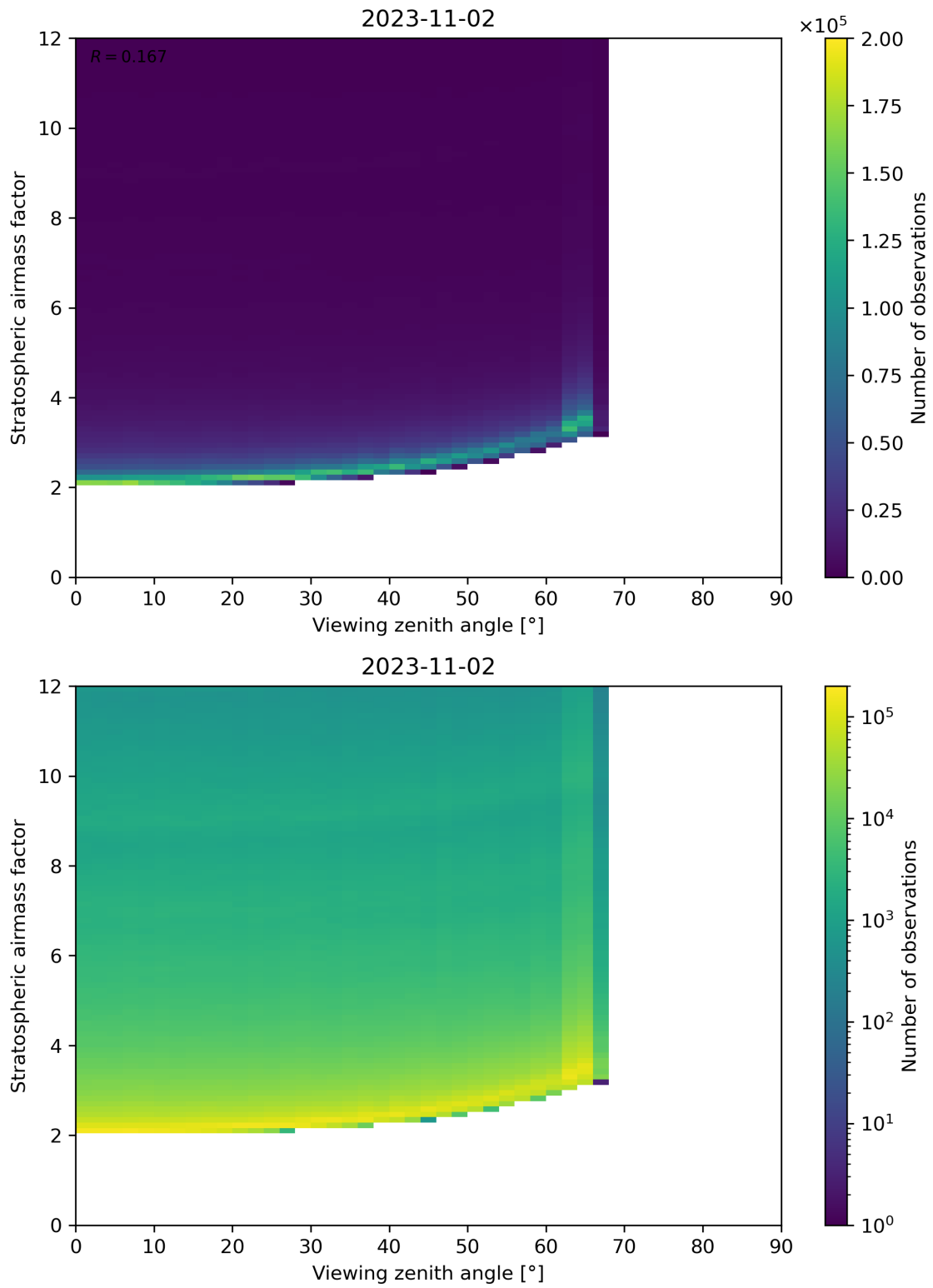
Figure 159: Scatter density plot of “Viewing zenith angle” against “Stratospheric airmass factor” for 2023-11-02 to 2023-11-03.
