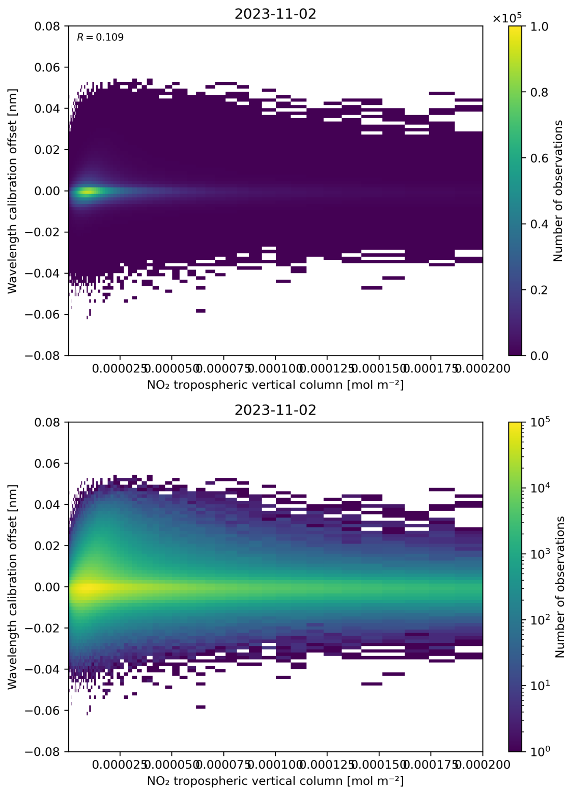
Figure 143: Scatter density plot of “NO 2 tropospheric vertical column” against “Wavelength calibration offset” for 2023-11-02 to 2023-11-03.
