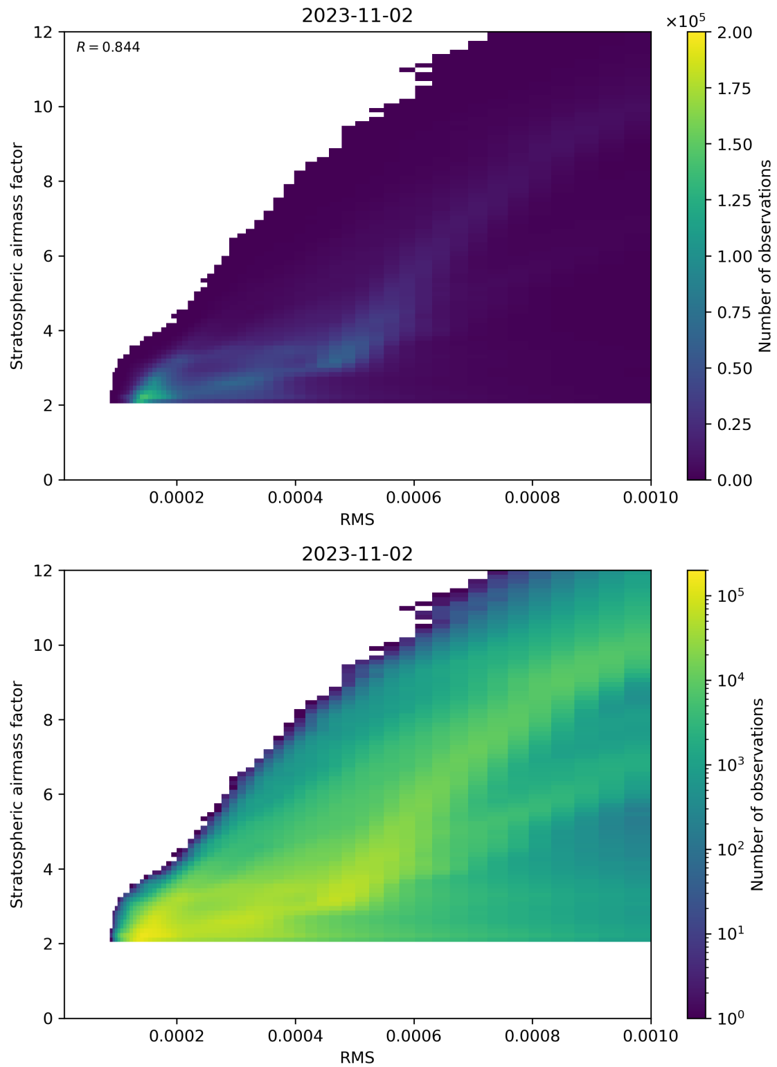
Figure 144: Scatter density plot of “RMS” against “Stratospheric airmass factor” for 2023-11-02 to 2023-11-03.
