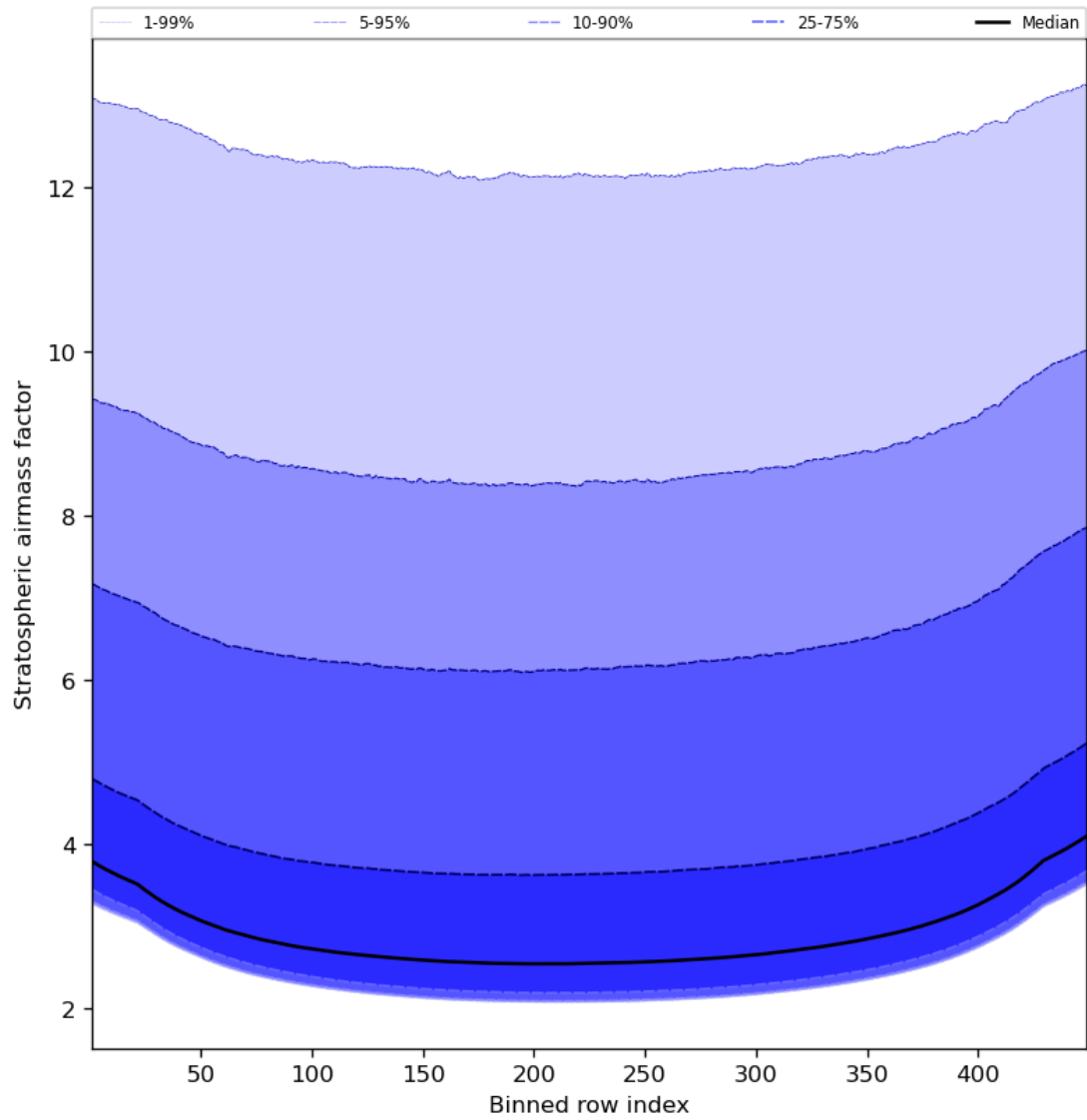
Figure 61: Along track statistics of “Stratospheric airmass factor” for 2023-11-02 to 2023-11-03
