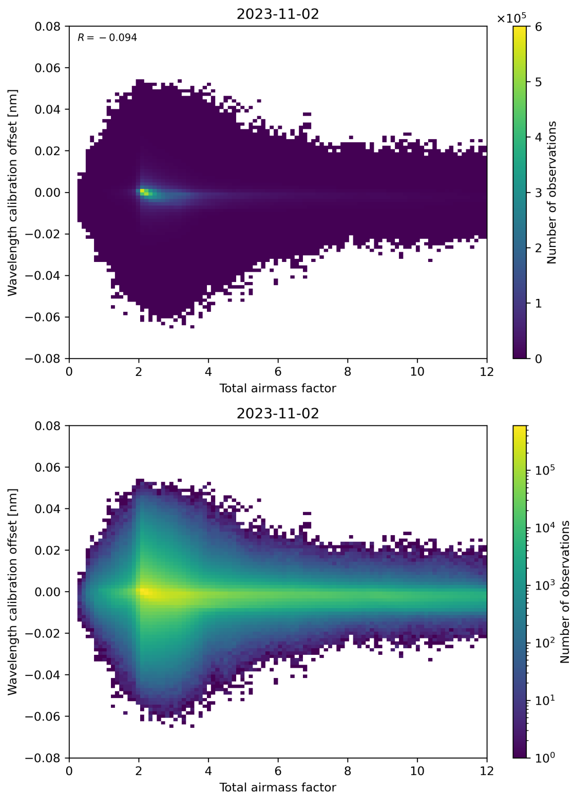
Figure 70: Scatter density plot of “Total airmass factor” against “Wavelength calibration offset” for 2023-11-02 to 2023-11-03.
