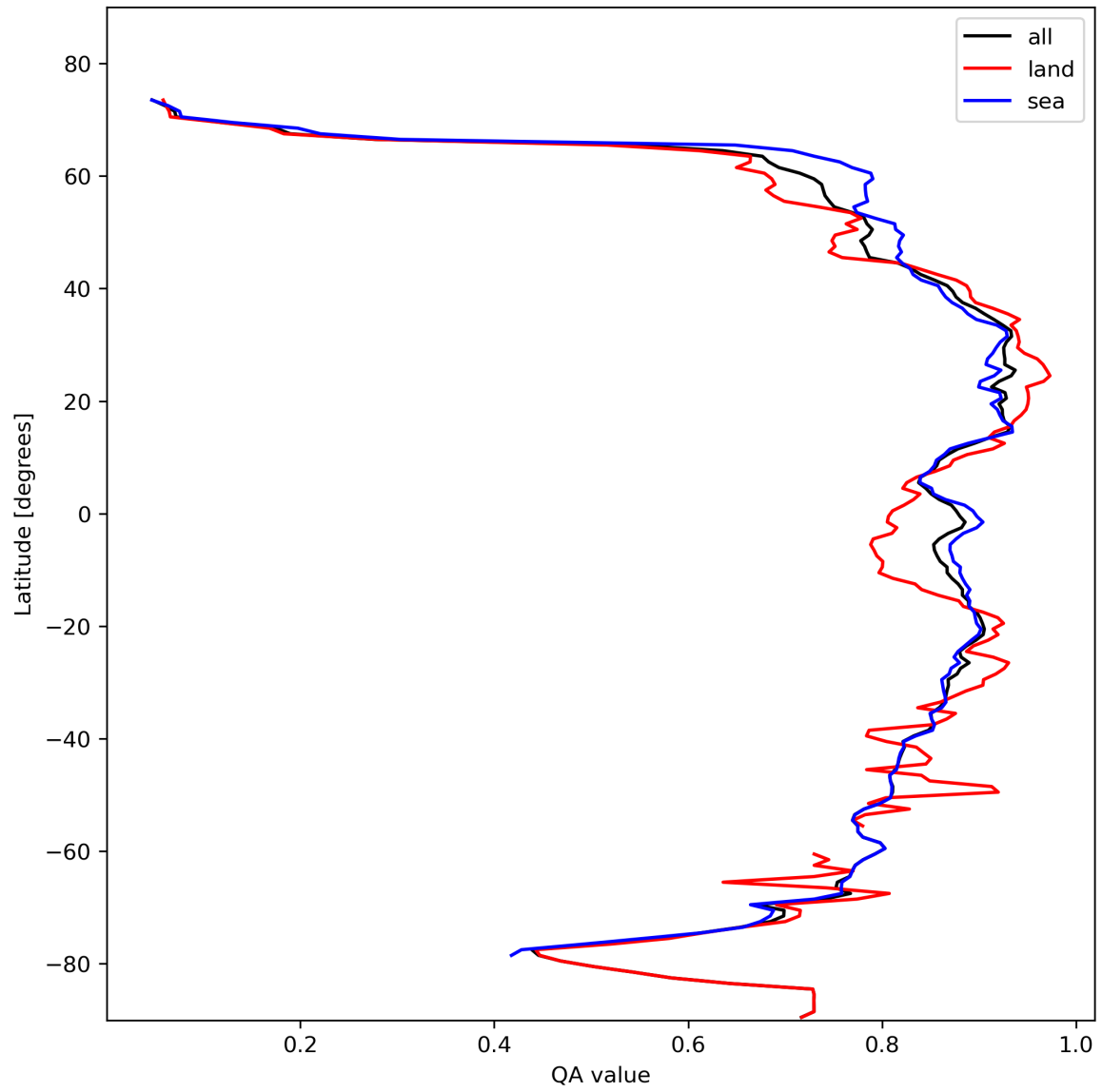
Figure 11: Zonal average of “QA value” for 2023-11-02 to 2023-11-03.
