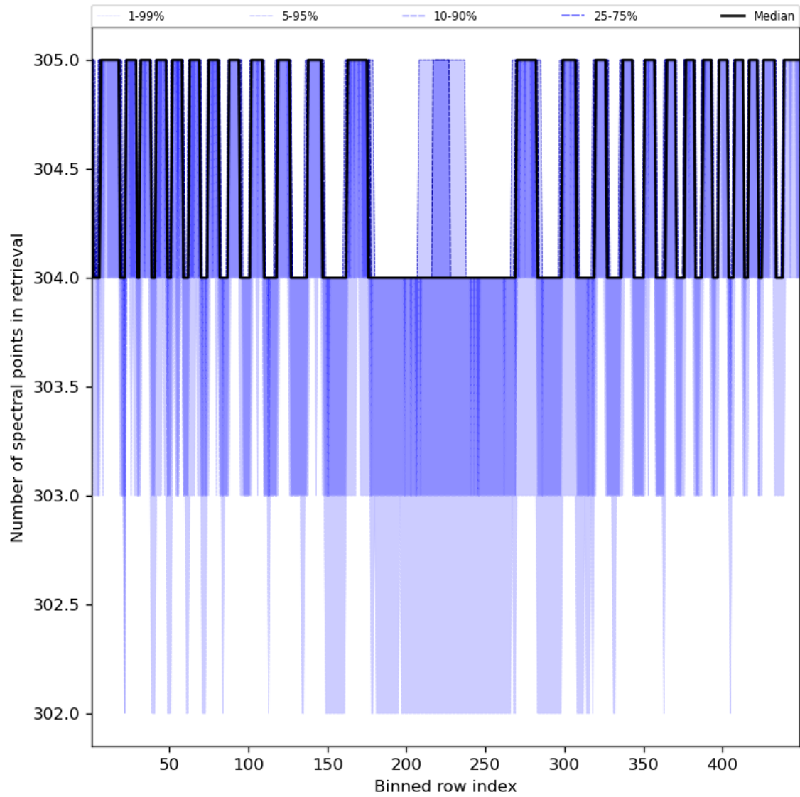
Figure 50: Along track statistics of “Number of spectral points in retrieval” for 2023-11-02 to 2023-11-03
