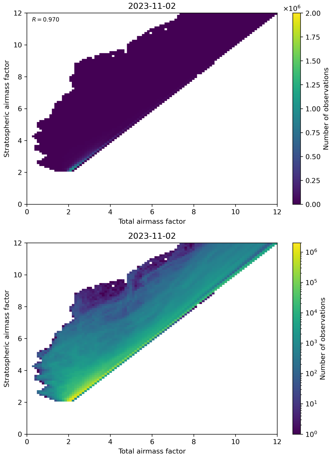
Figure 62: Scatter density plot of “Total airmass factor” against “Stratospheric airmass factor” for 2023-11-02 to 2023-11-03.
