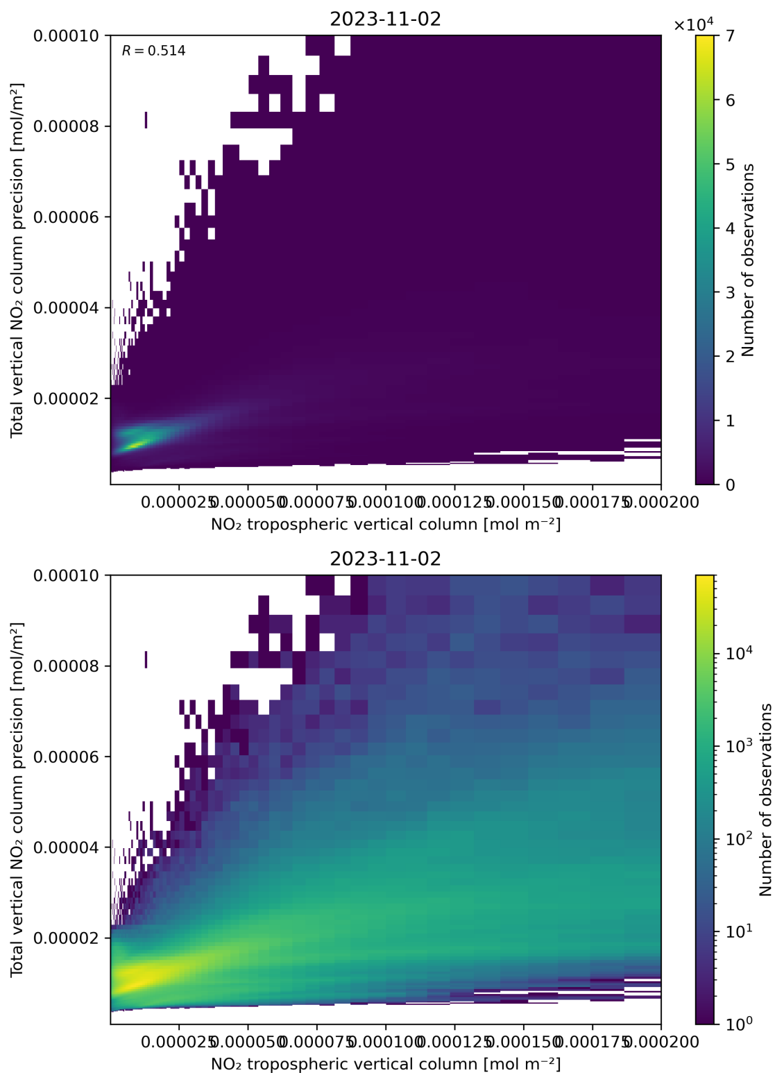
Figure 129: Scatter density plot of “NO 2 tropospheric vertical column” against “Total vertical NO 2 column precision” for 2023-11-02 to 2023-11-03.
