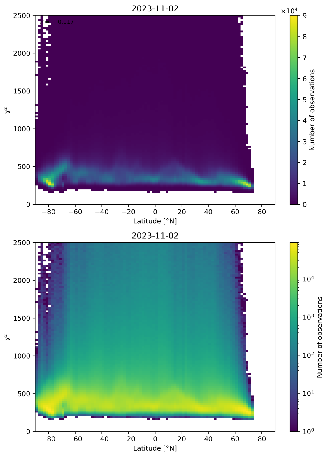
Figure 86: Scatter density plot of “Latitude” against “ \chi^2 ” for 2023-11-02 to 2023-11-03.
