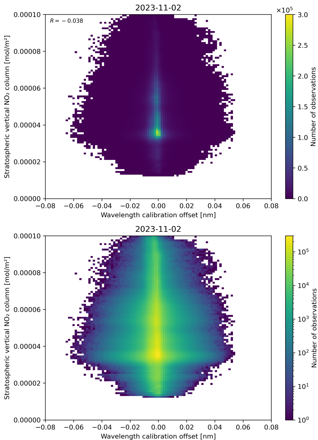
Figure 176: Scatter density plot of “Wavelength calibration offset” against “Stratospheric vertical NO 2 column” for 2023-11-02 to 2023-11-03.
