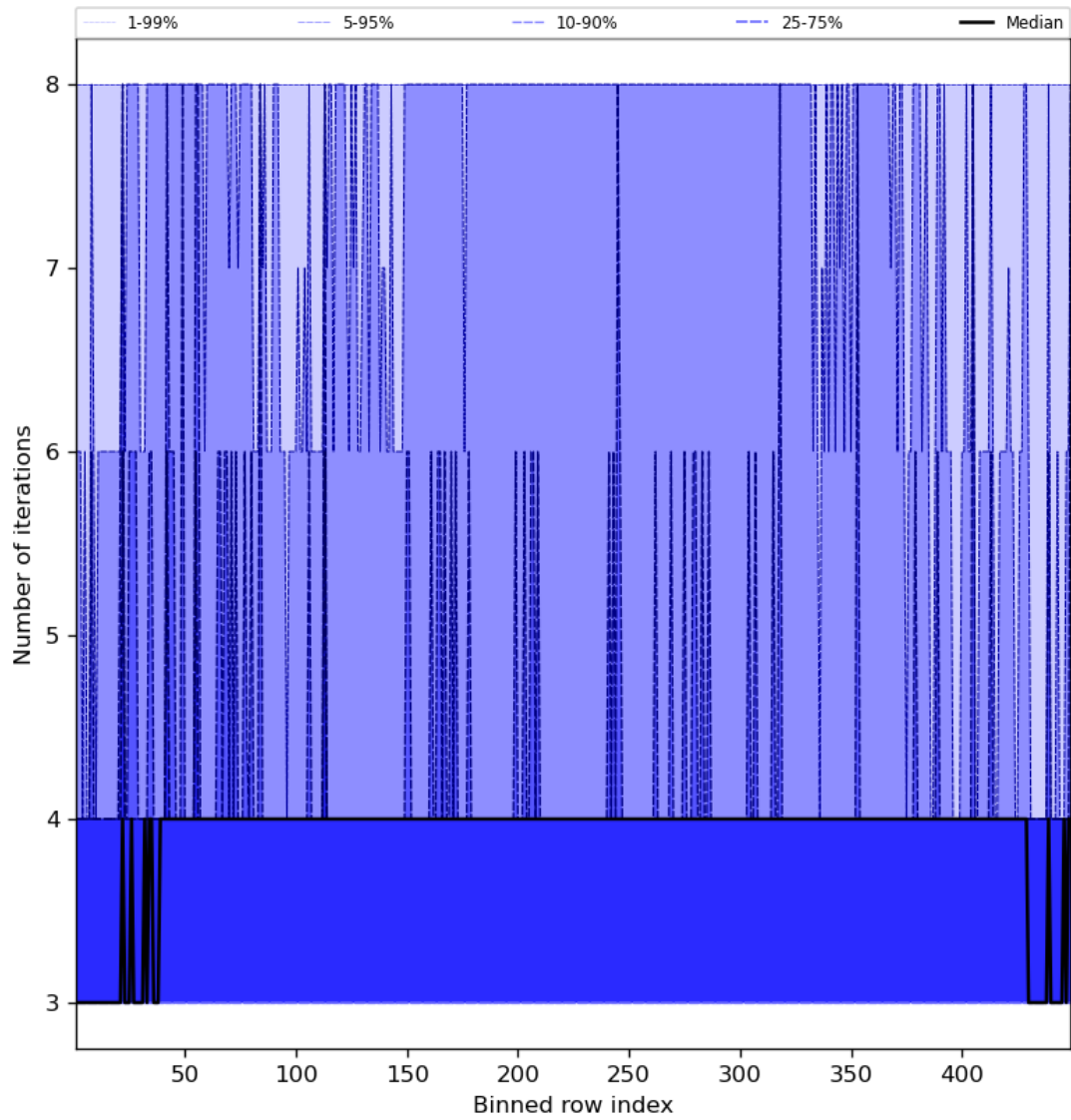
Figure 51: Along track statistics of “Number of iterations” for 2023-11-02 to 2023-11-03
