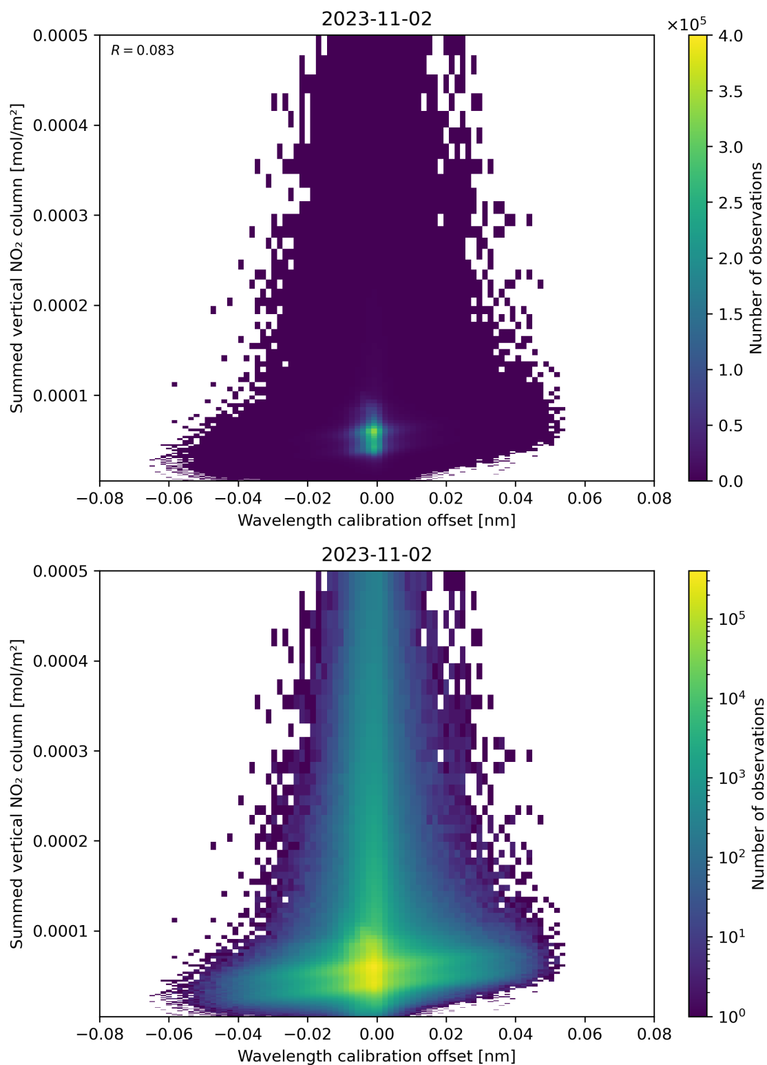
Figure 177: Scatter density plot of “Wavelength calibration offset” against “Summed vertical NO 2 column” for 2023-11-02 to 2023-11-03.
