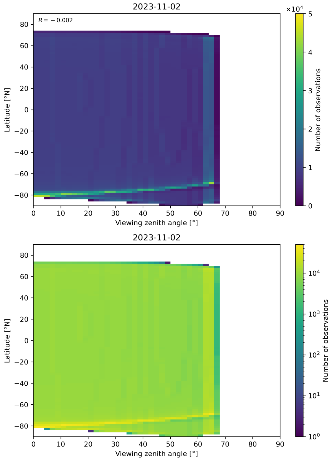
Figure 163: Scatter density plot of “Viewing zenith angle” against “Latitude” for 2023-11-02 to 2023-11-03.
