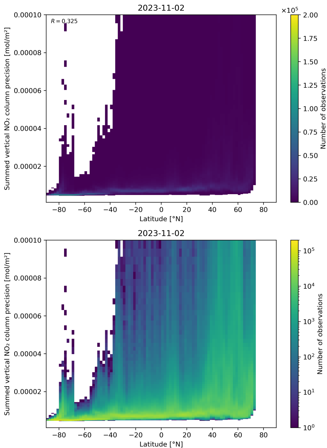
Figure 89: Scatter density plot of “Latitude” against “Summed vertical NO 2 column precision” for 2023-11-02 to 2023-11-03.
