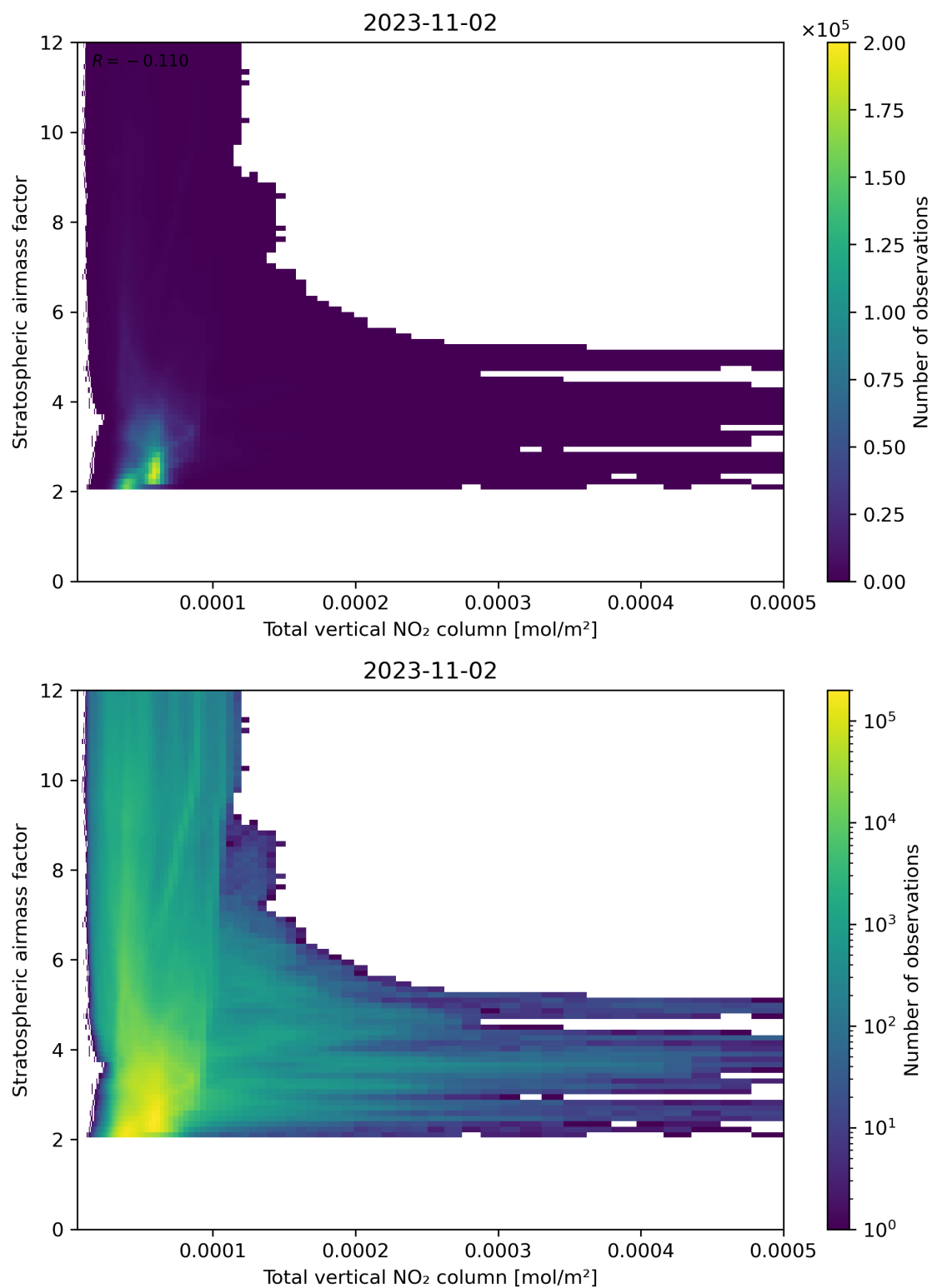
Figure 110: Scatter density plot of “Total vertical NO 2 column” against “Stratospheric airmass factor” for 2023-11-02 to 2023-11-03.
