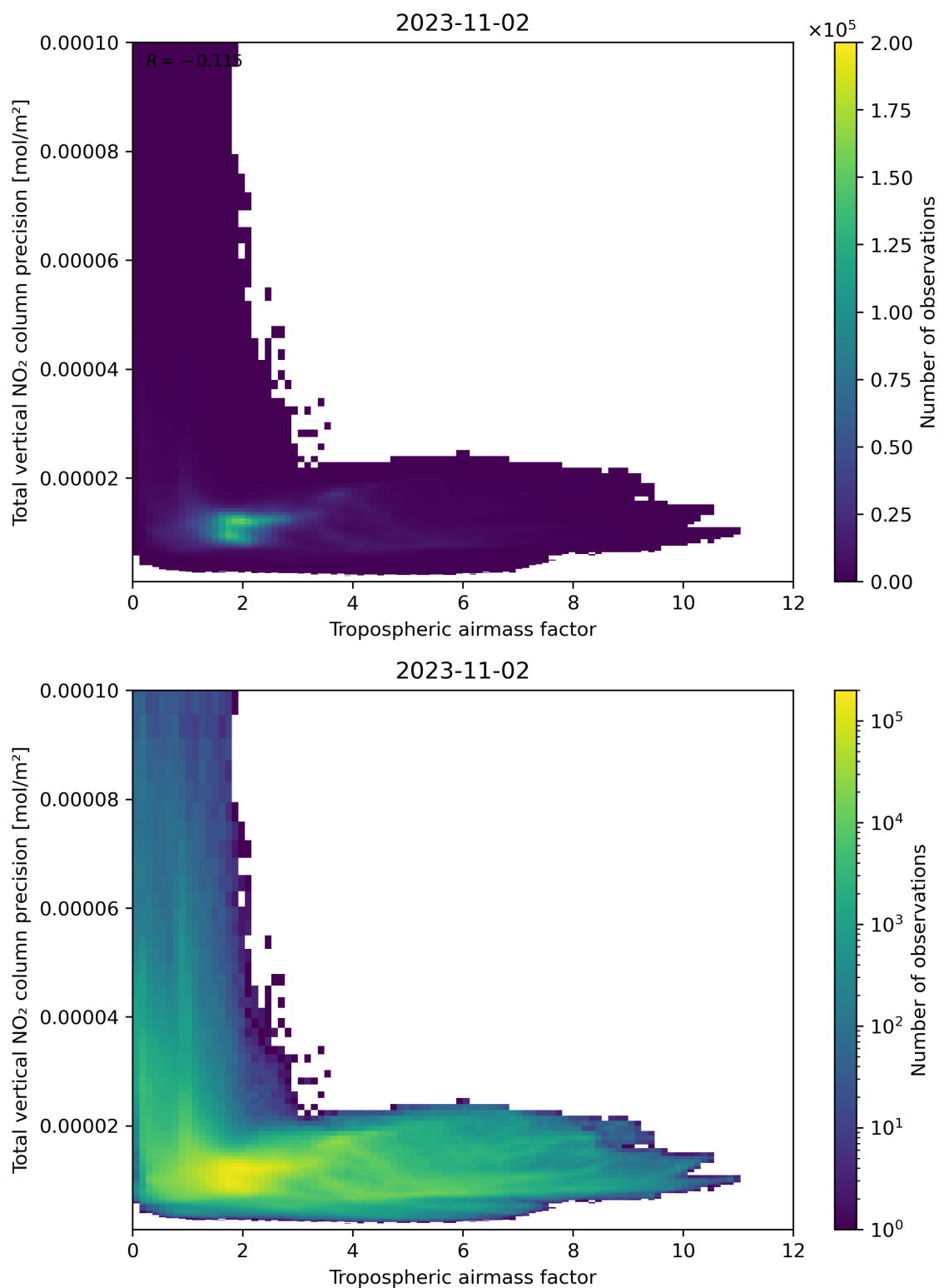
Figure 78: Scatter density plot of “Tropospheric air mass factor” against “Total vertical NO 2 column precision” for 2023-11-02 to 2023-11-03.
