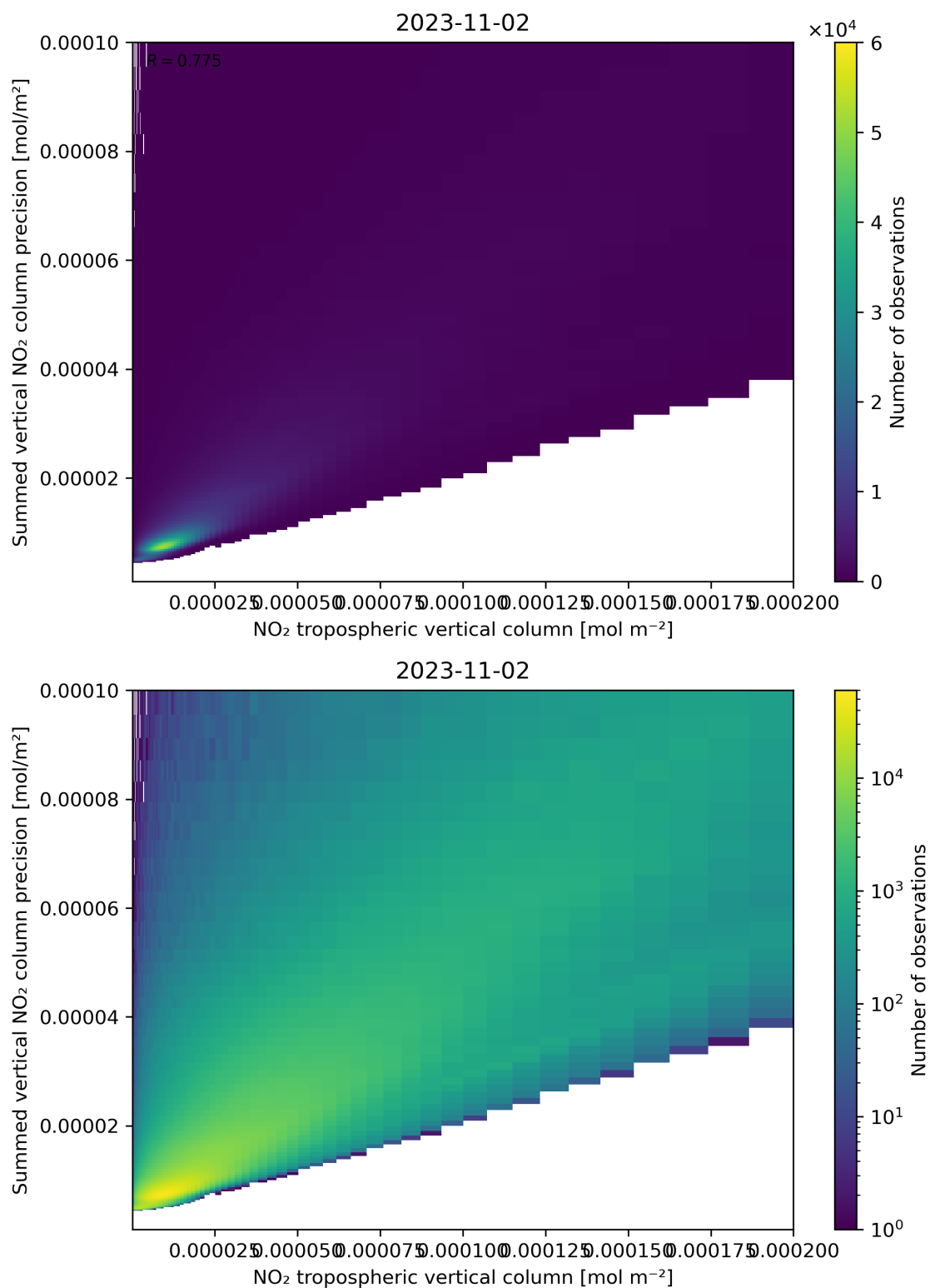
Figure 127: Scatter density plot of “NO 2 tropospheric vertical column” against “Summed vertical NO 2 column precision” for 2023-11-02 to 2023-11-03.
