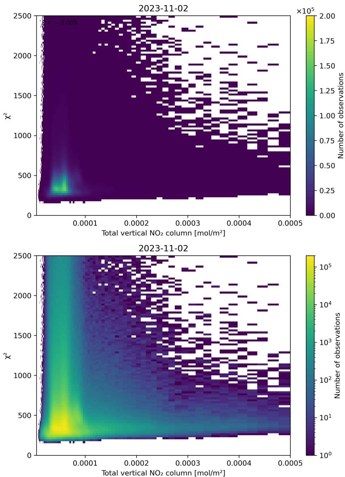
Figure 111: Scatter density plot of “Total vertical NO 2 column” against “ \chi^2 ” for 2023-11-02 to 2023-11-03.
