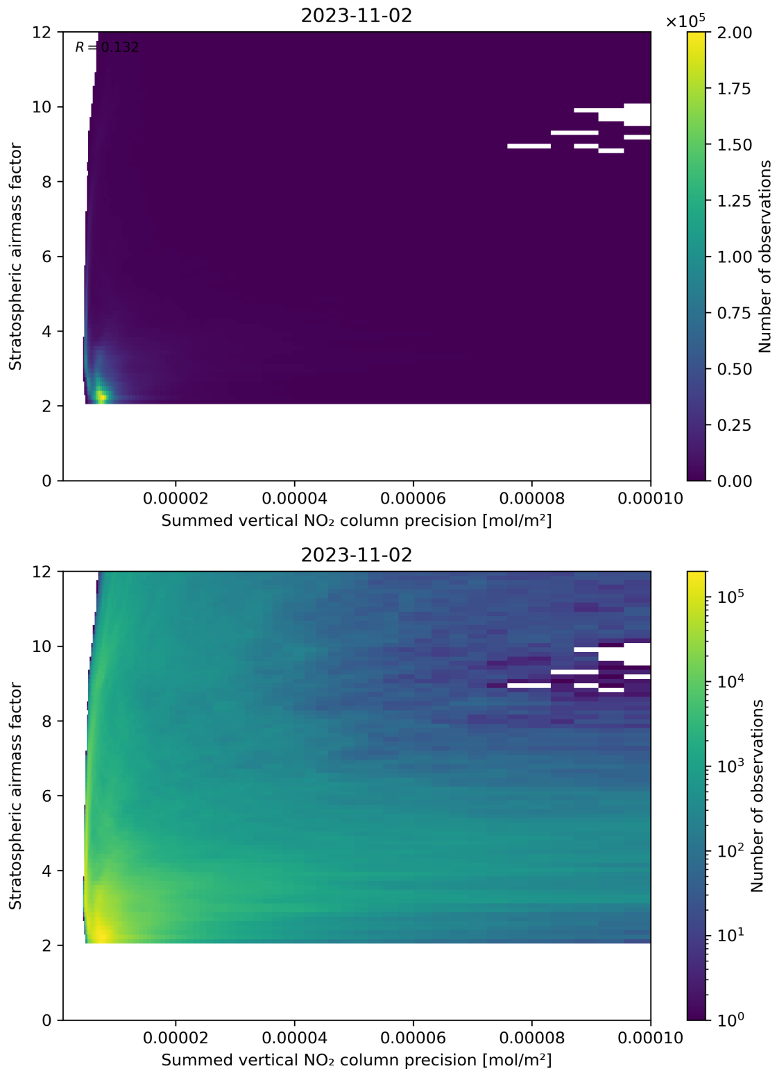
Figure 106: Scatter density plot of “Summed vertical NO 2 column precision” against “Stratospheric airmass factor” for 2023-11-02 to 2023-11-03.
