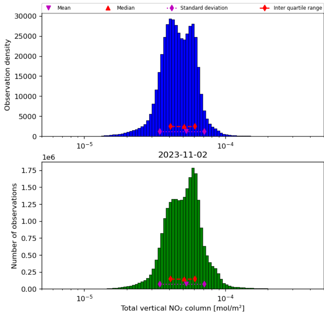
Figure 38: Histogram of “Total vertical NO 2 column” for 2023-11-02 to 2023-11-03
