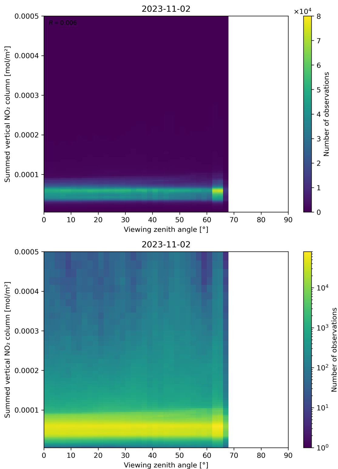
Figure 165: Scatter density plot of “Viewing zenith angle” against “Summed vertical NO 2 column” for 2023-11-02 to 2023-11-03.
