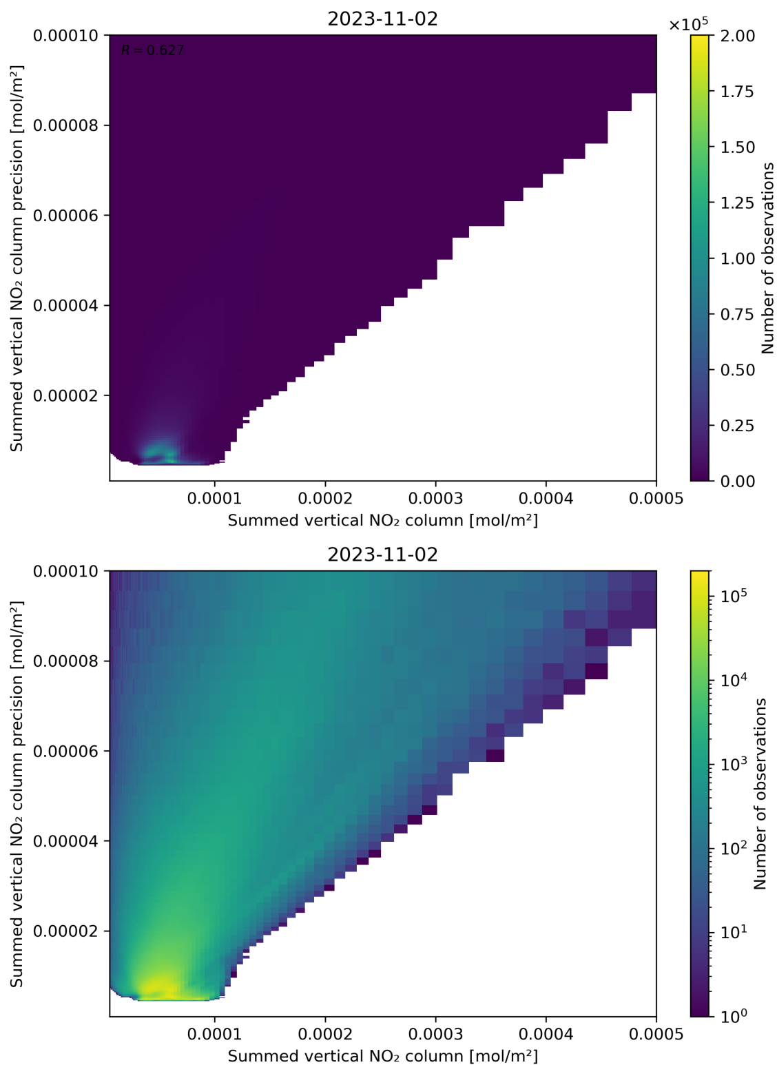
Figure 105: Scatter density plot of “Summed vertical NO 2 column” against “Summed vertical NO 2 column precision” for 2023-11-02 to 2023-11-03.
