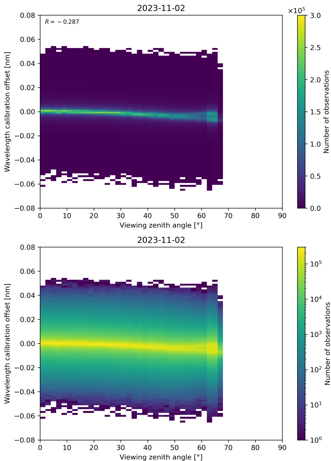
Figure 173: Scatter density plot of “Viewing zenith angle” against “Wavelength calibration offset” for 2023-11-02 to 2023-11-03.
