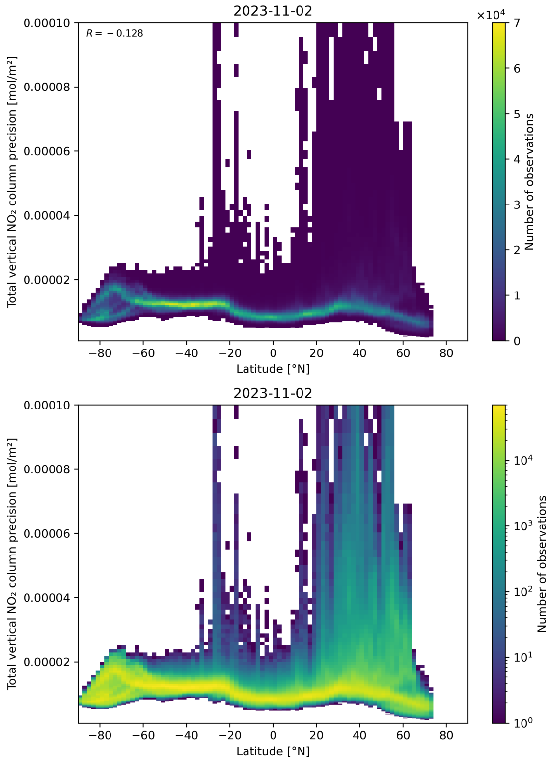
Figure 91: Scatter density plot of “Latitude” against “Total vertical NO 2 column precision” for 2023-11-02 to 2023-11-03.
