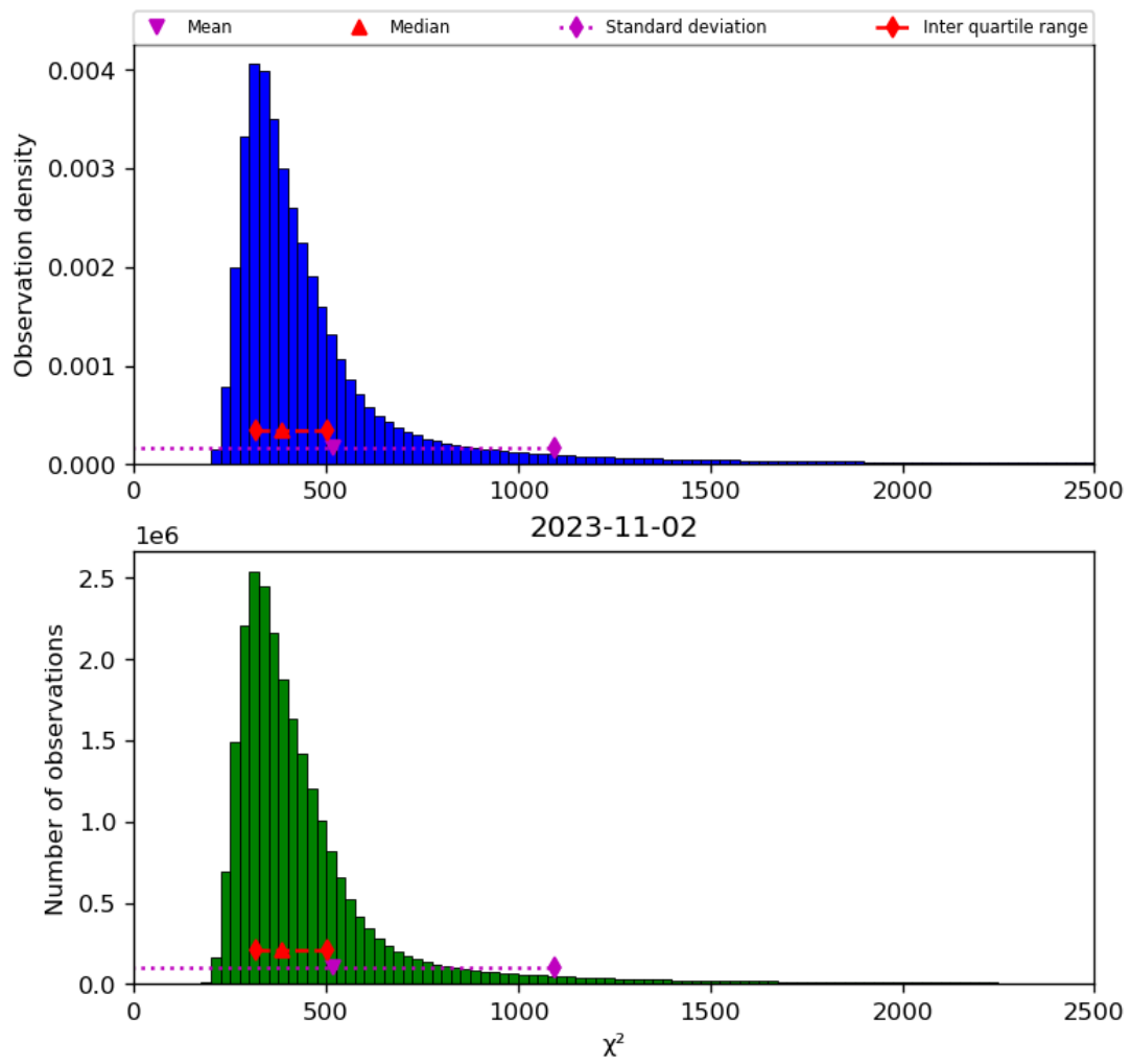
Figure 42: Histogram of “ \chi^2 ” for 2023-11-02 to 2023-11-03
