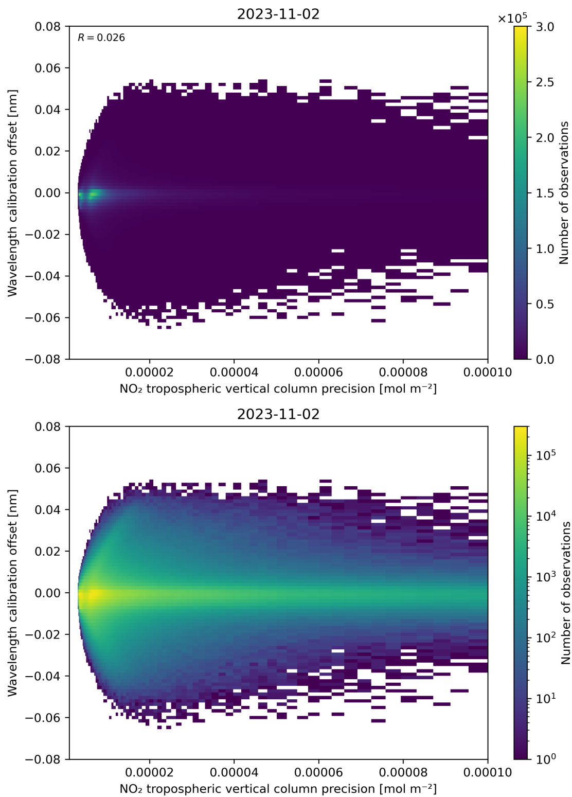
Figure 141: Scatter density plot of “NO 2 tropospheric vertical column precision” against “Wavelength calibration offset” for 2023-11-02 to 2023-11-03.
