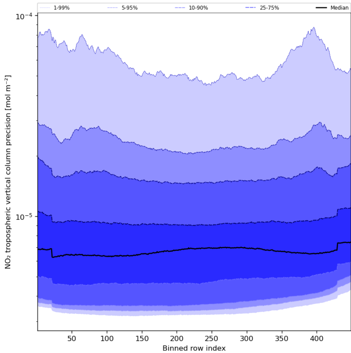
Figure 47: Along track statistics of “NO 2 tropospheric vertical column precision” for 2023-11-02 to 2023-11-03
