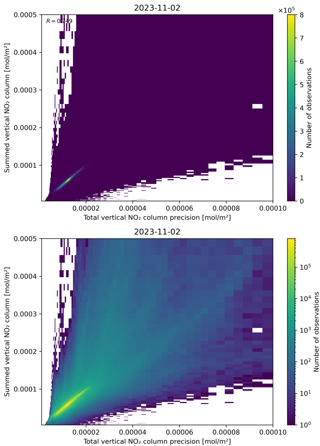
Figure 117: Scatter density plot of “Total vertical NO 2 column precision” against “Summed vertical NO 2 column” for 2023-11-02 to 2023-11-03.
