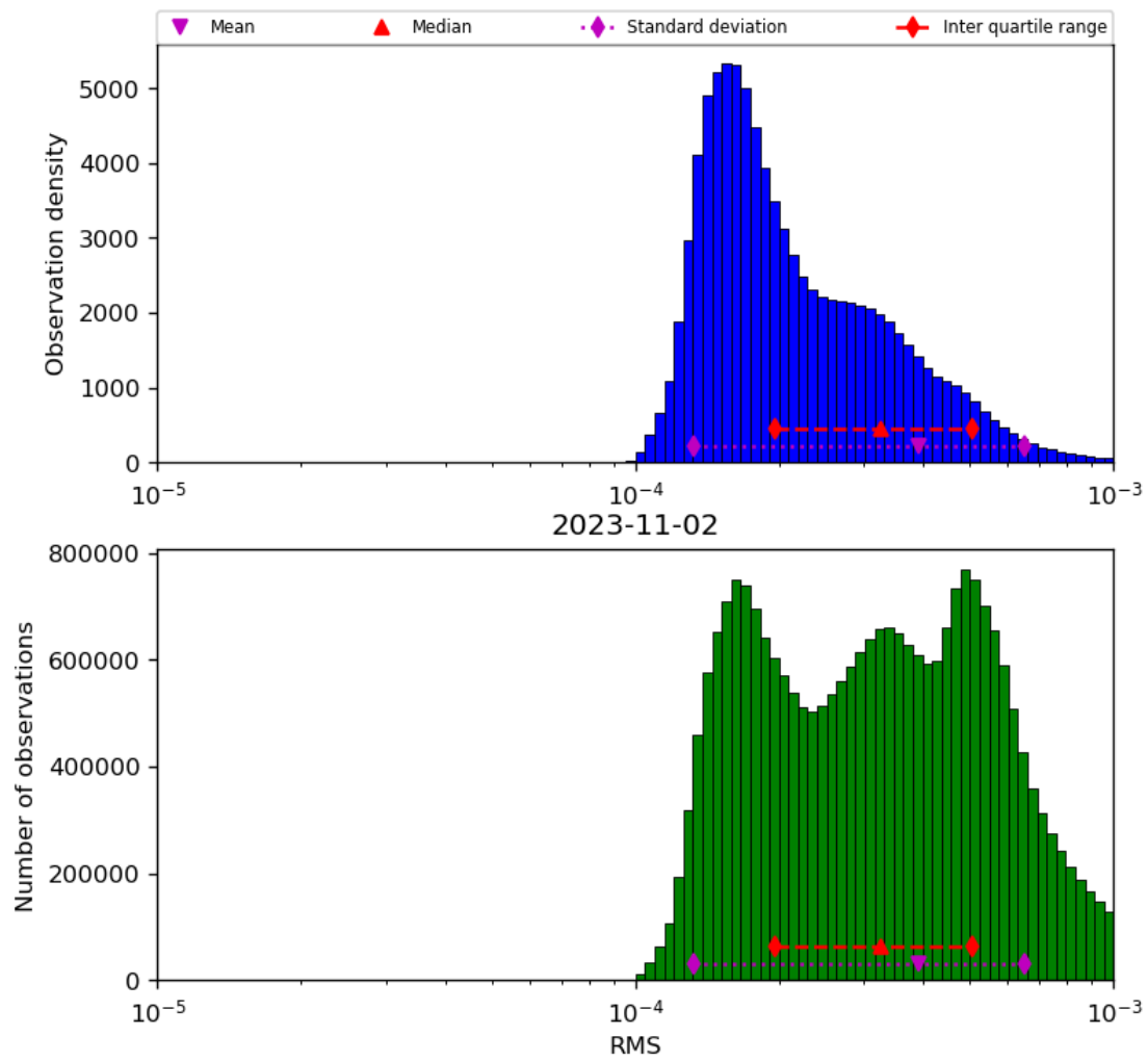
Figure 43: Histogram of “RMS” for 2023-11-02 to 2023-11-03
