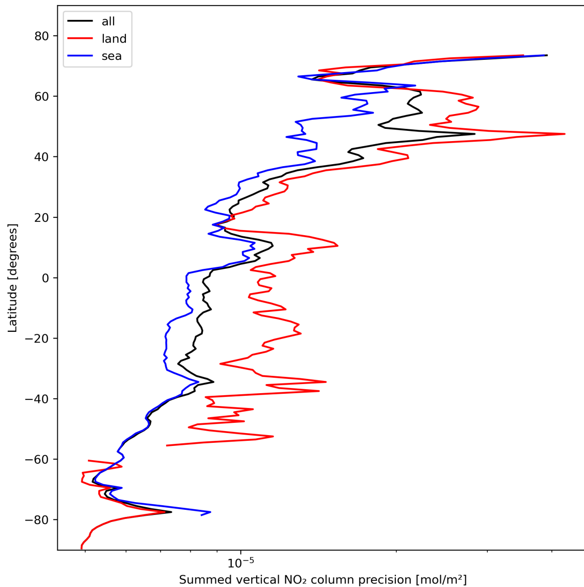
Figure 24: Zonal average of “Summed vertical NO 2 column precision” for 2023-11-02 to 2023-11-03.
