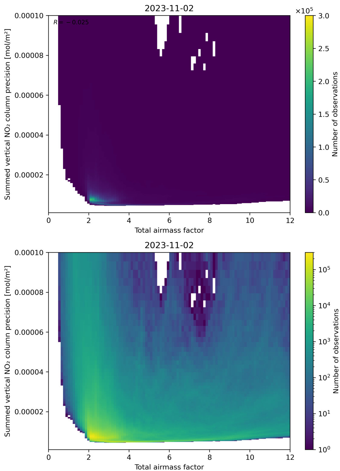
Figure 66: Scatter density plot of “Total airmass factor” against “Summed vertical NO 2 column precision” for 2023-11-02 to 2023-11-03.
