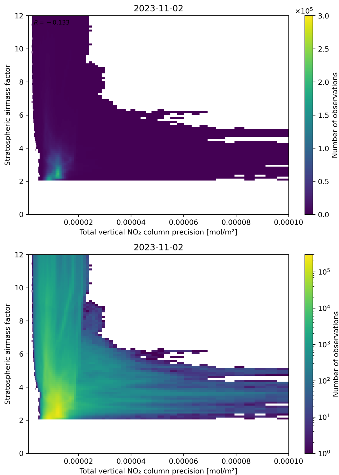
Figure 115: Scatter density plot of “Total vertical NO 2 column precision” against “Stratospheric air mass factor” for 2023-11-02 to 2023-11-03.
