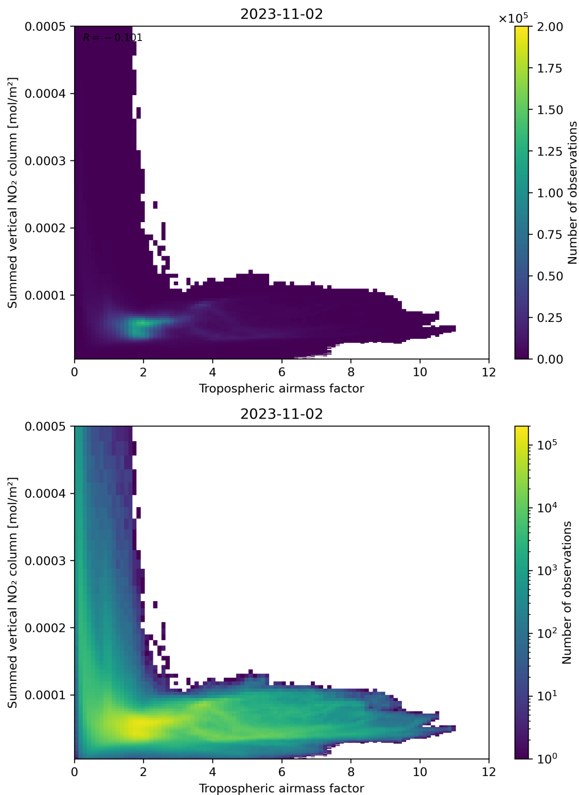
Figure 75: Scatter density plot of “Tropospheric airmass factor” against “Summed vertical NO 2 column” for 2023-11-02 to 2023-11-03.
