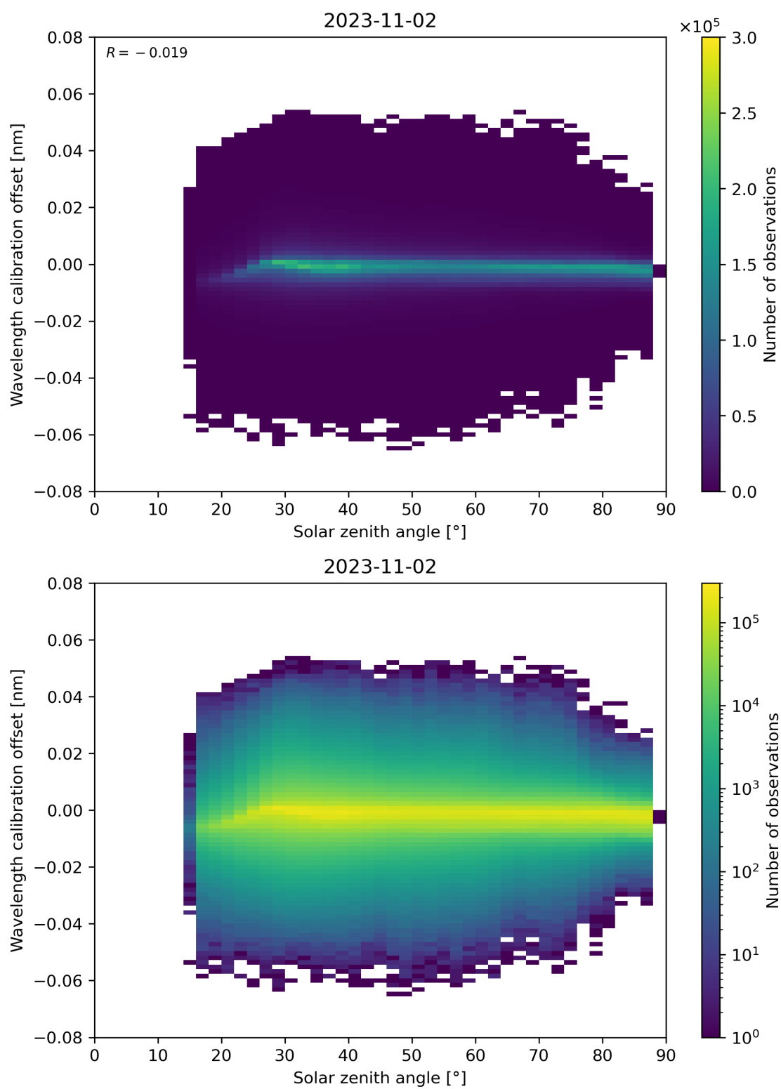
Figure 158: Scatter density plot of “Solar zenith angle” against “Wavelength calibration offset” for 2023-11-02 to 2023-11-03.
