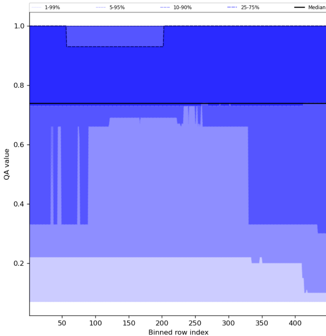
Figure 45: Along track statistics of “QA value” for 2023-11-02 to 2023-11-03
