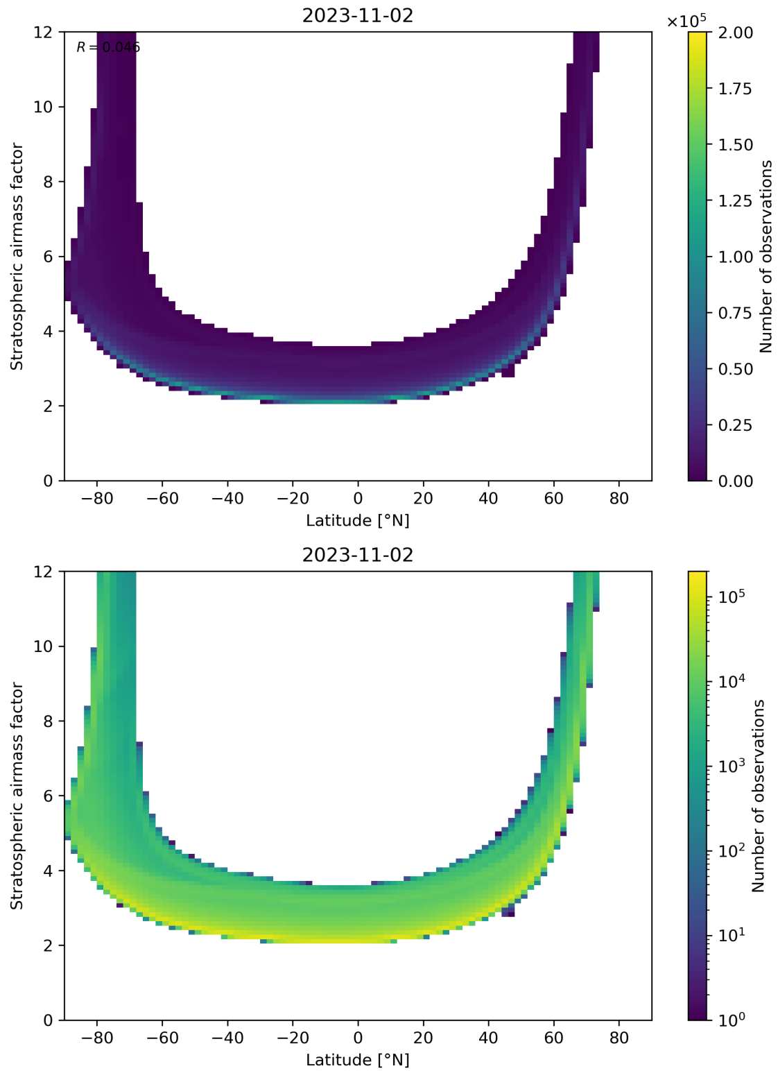
Figure 83: Scatter density plot of “Latitude” against “Stratospheric airmass factor” for 2023-11-02 to 2023-11-03.
