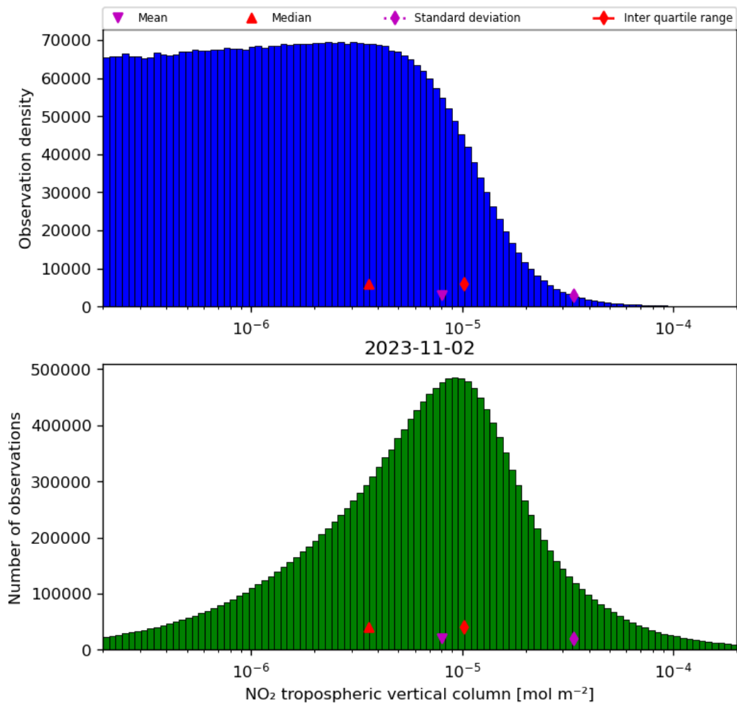
Figure 29: Histogram of “NO 2 tropospheric vertical column” for 2023-11-02 to 2023-11-03
