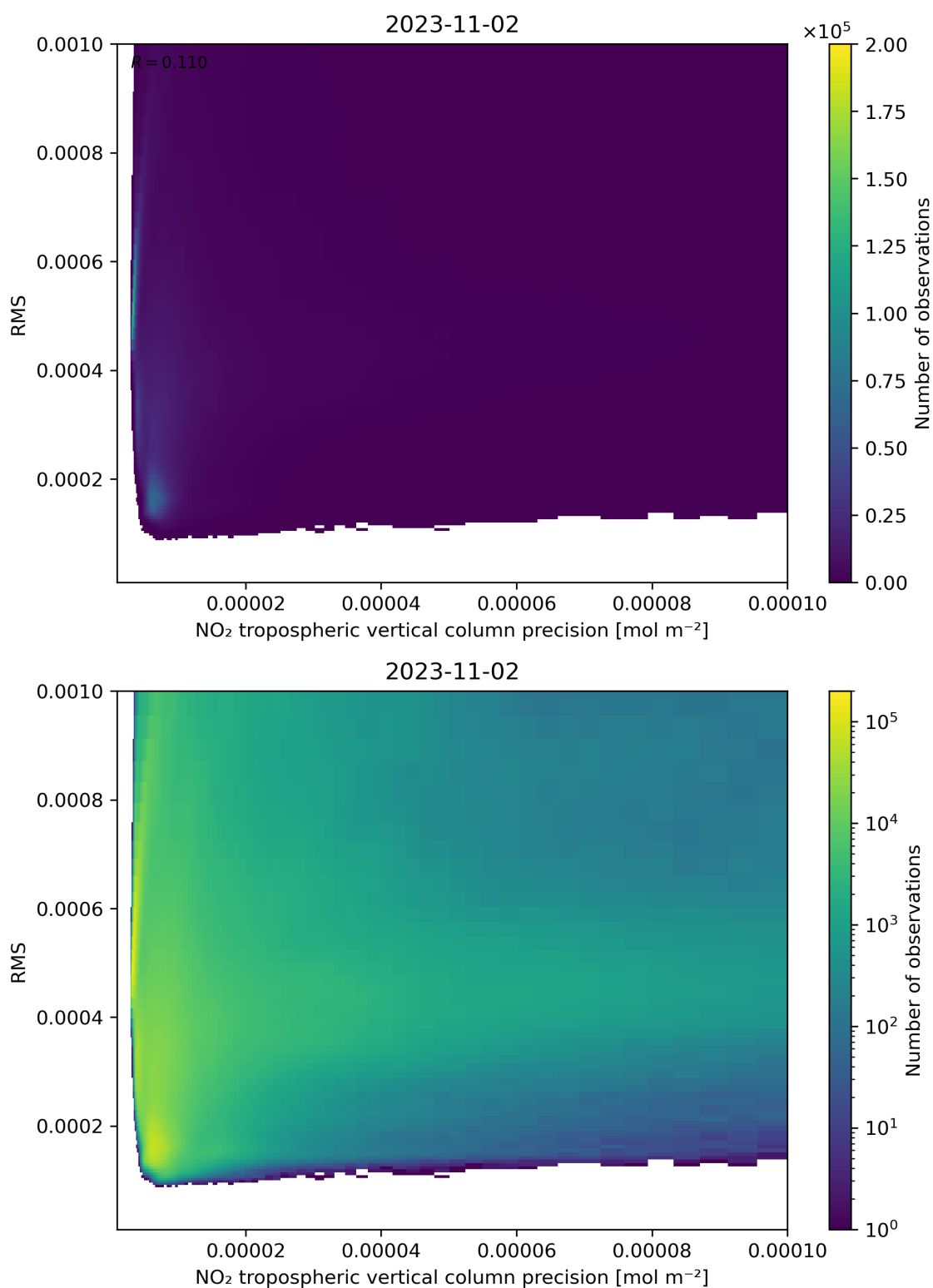
Figure 140: Scatter density plot of “NO 2 tropospheric vertical column precision” against “RMS” for 2023-11-02 to 2023-11-03.
