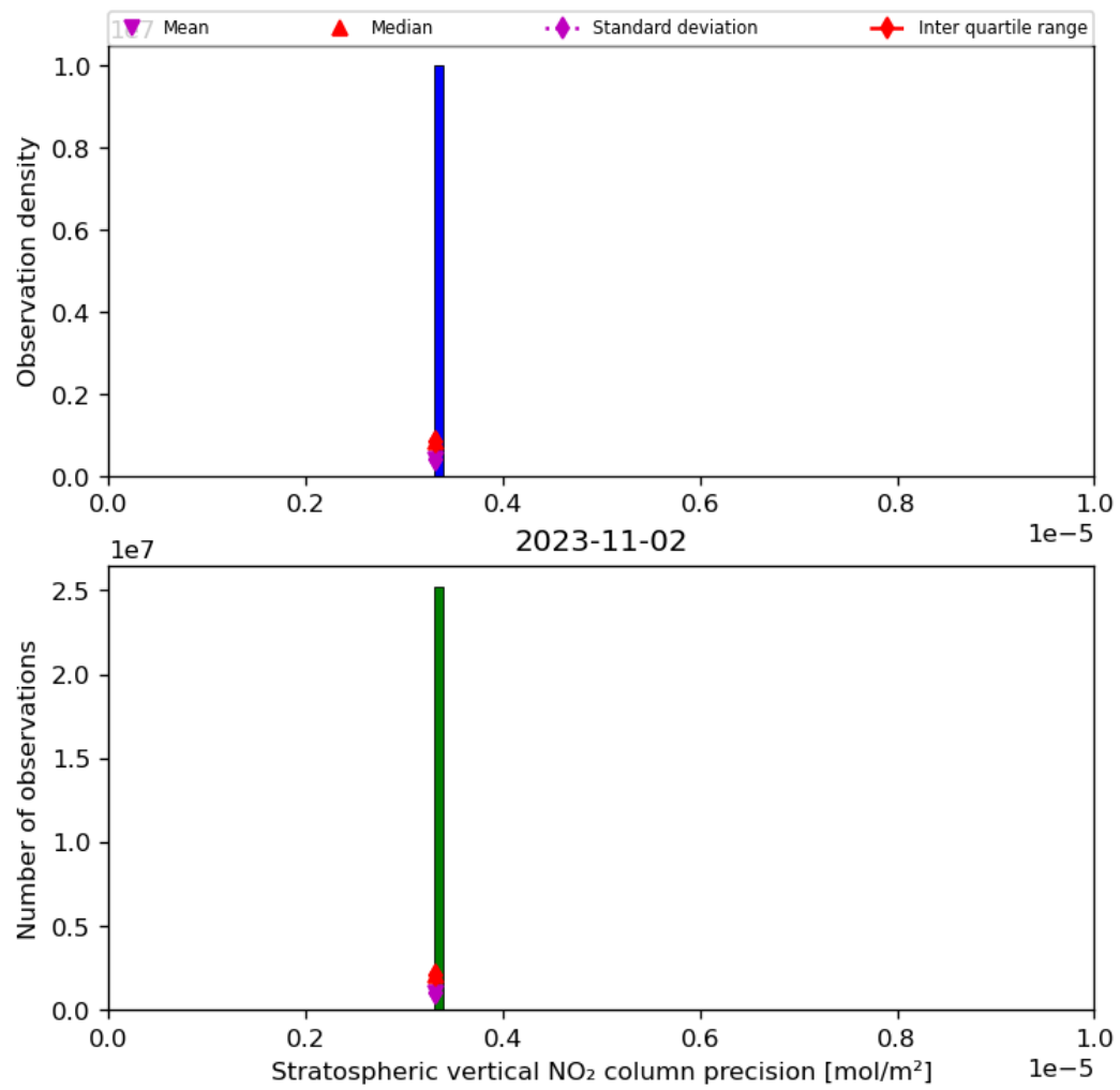
Figure 37: Histogram of “Stratospheric vertical NO 2 column precision” for 2023-11-02 to 2023-11-03
