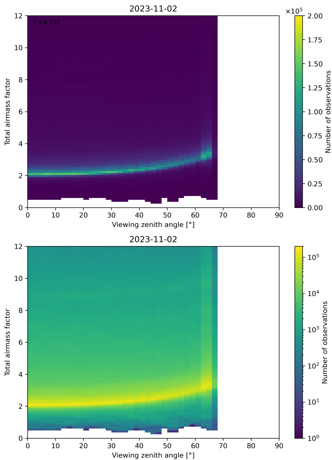
Figure 160: Scatter density plot of “Viewing zenith angle” against “Total airmass factor” for 2023-11-02 to 2023-11-03.
