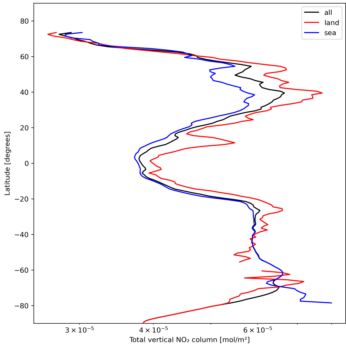
Figure 21: Zonal average of “Total vertical NO 2 column” for 2023-11-02 to 2023-11-03.
