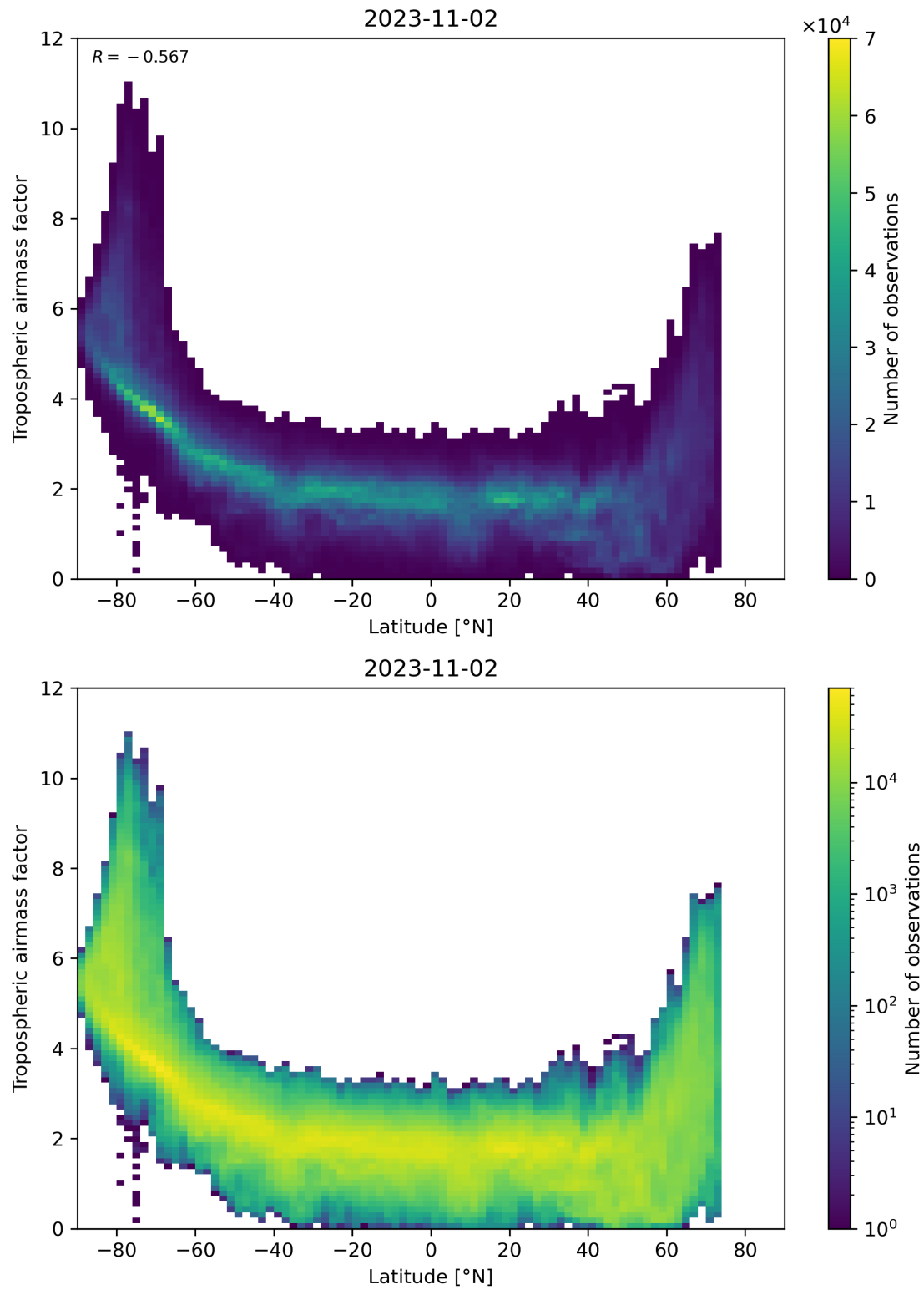
Figure 85: Scatter density plot of “Latitude” against “Tropospheric airmass factor” for 2023-11-02 to 2023-11-03.
