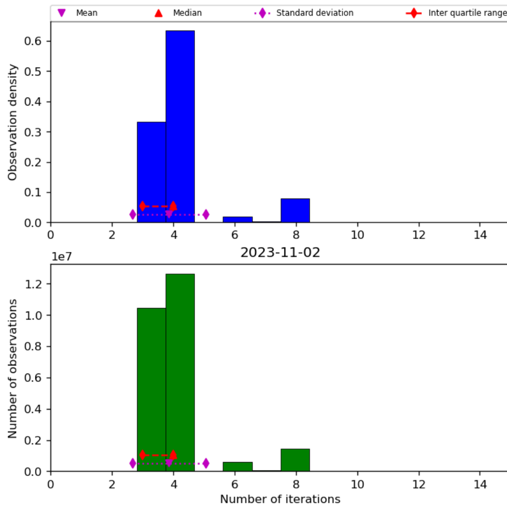
Figure 34: Histogram of “Number of iterations” for 2023-11-02 to 2023-11-03
