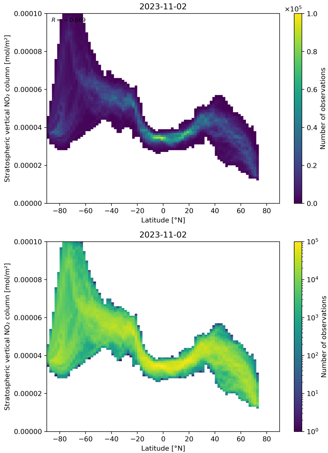
Figure 87: Scatter density plot of “Latitude” against “Stratospheric vertical NO 2 column” for 2023-11-02 to 2023-11-03.
