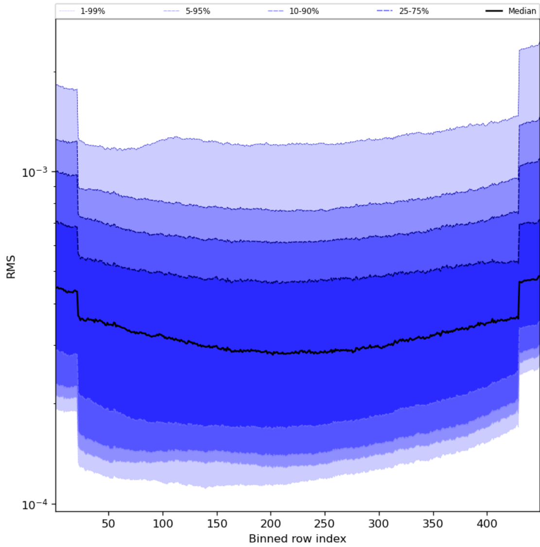
Figure 60: Along track statistics of “RMS” for 2023-11-02 to 2023-11-03
