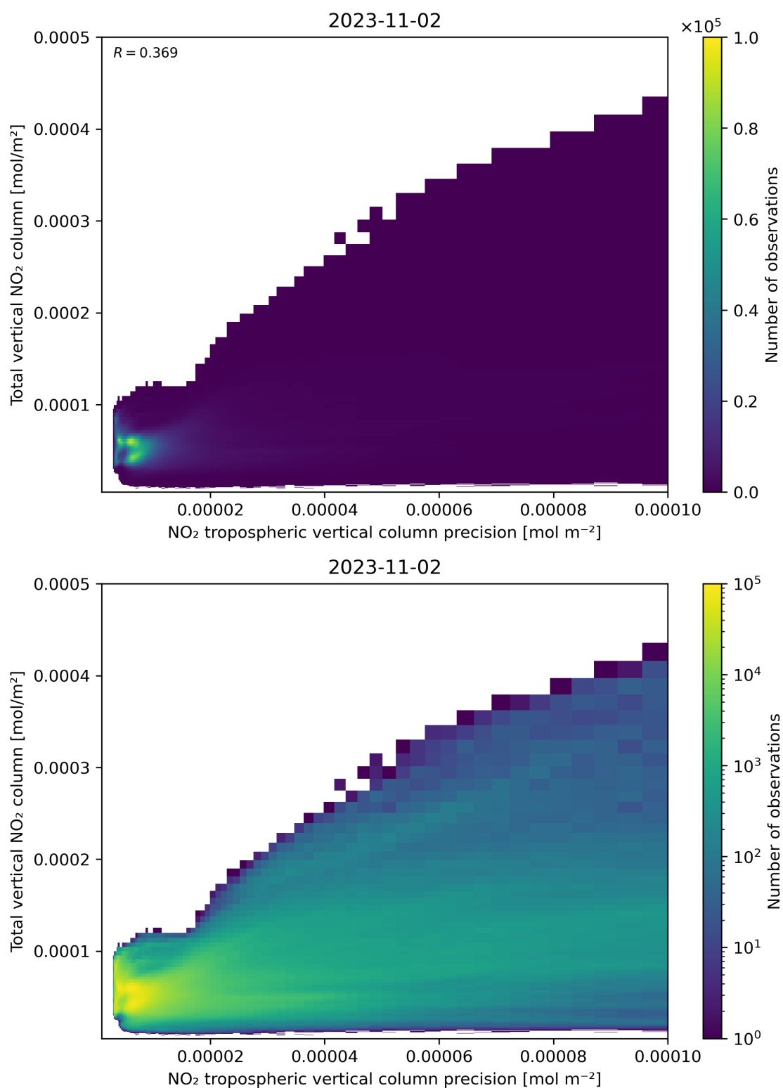
Figure 138: Scatter density plot of “NO 2 tropospheric vertical column precision” against “Total vertical NO 2 column” for 2023-11-02 to 2023-11-03.
