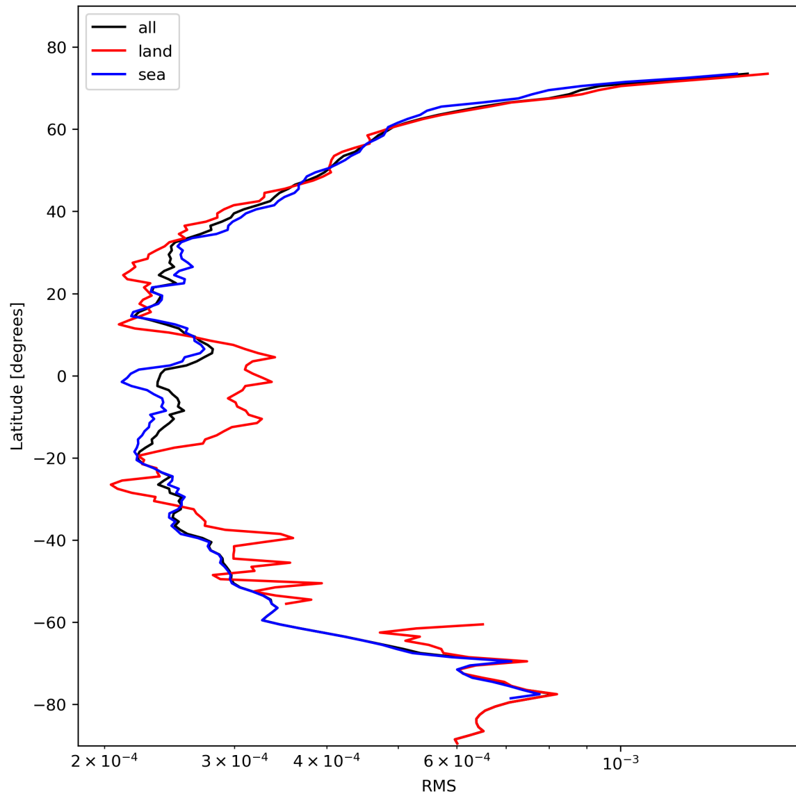
Figure 26: Zonal average of “RMS” for 2023-11-02 to 2023-11-03.
