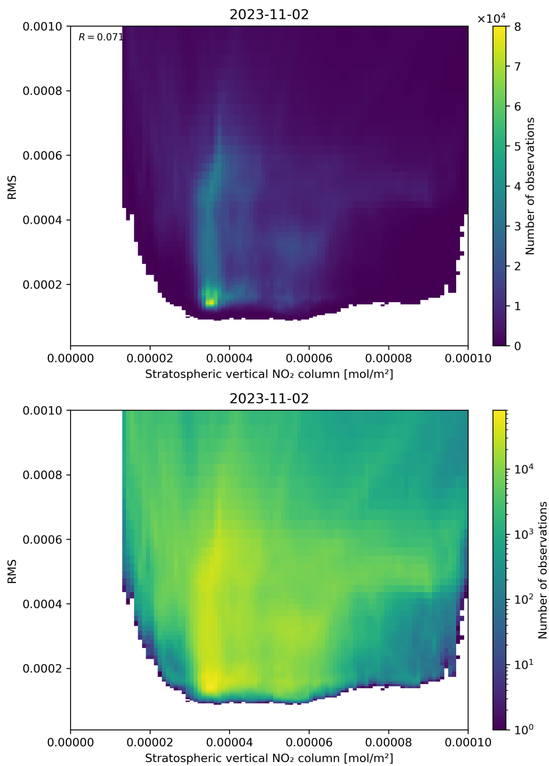
Figure 102: Scatter density plot of “Stratospheric vertical NO 2 column” against “RMS” for 2023-11-02 to 2023-11-03.
