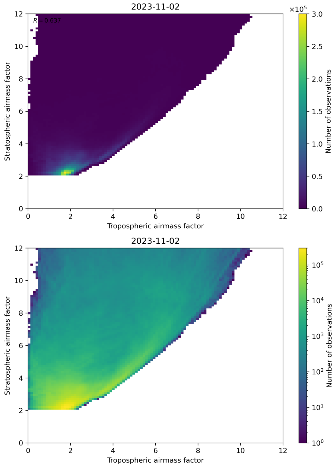
Figure 71: Scatter density plot of “Tropospheric airmass factor” against “Stratospheric airmass factor” for 2023-11-02 to 2023-11-03.
