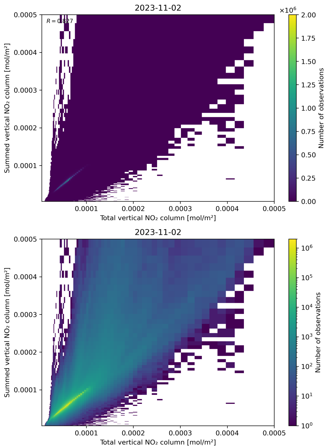
Figure 112: Scatter density plot of “Total vertical NO 2 column” against “Summed vertical NO 2 column” for 2023-11-02 to 2023-11-03.
