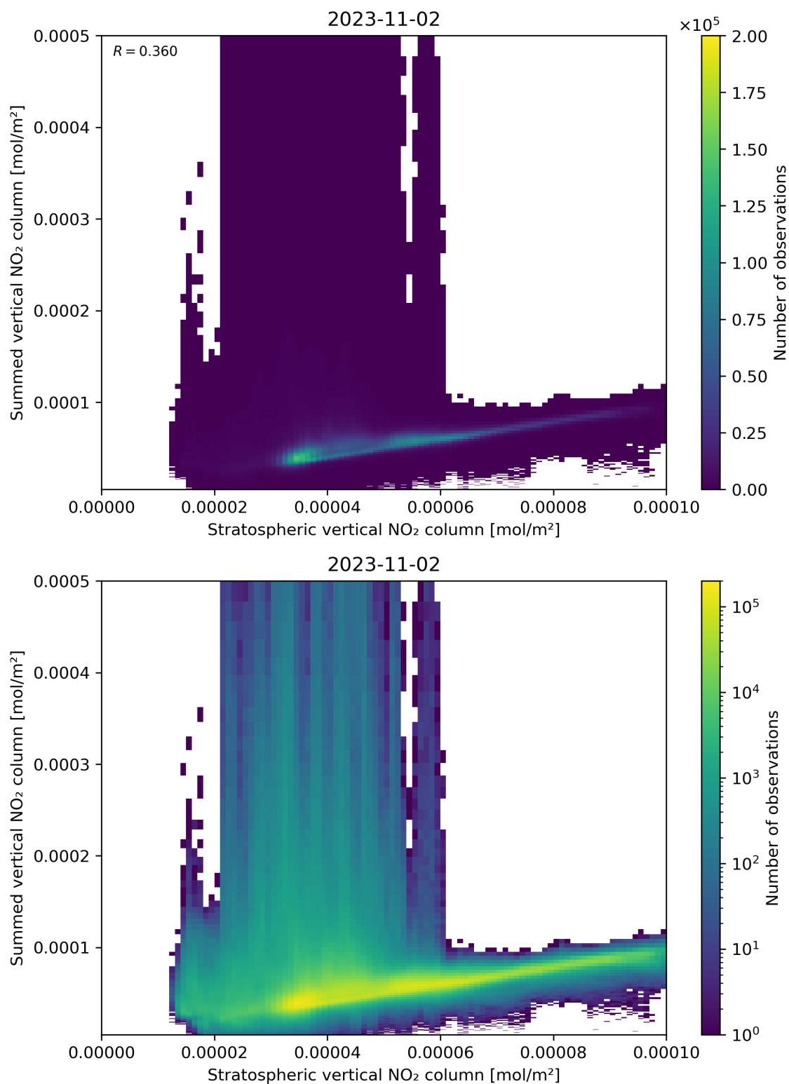
Figure 98: Scatter density plot of “Stratospheric vertical NO 2 column” against “Summed vertical NO 2 column” for 2023-11-02 to 2023-11-03.
