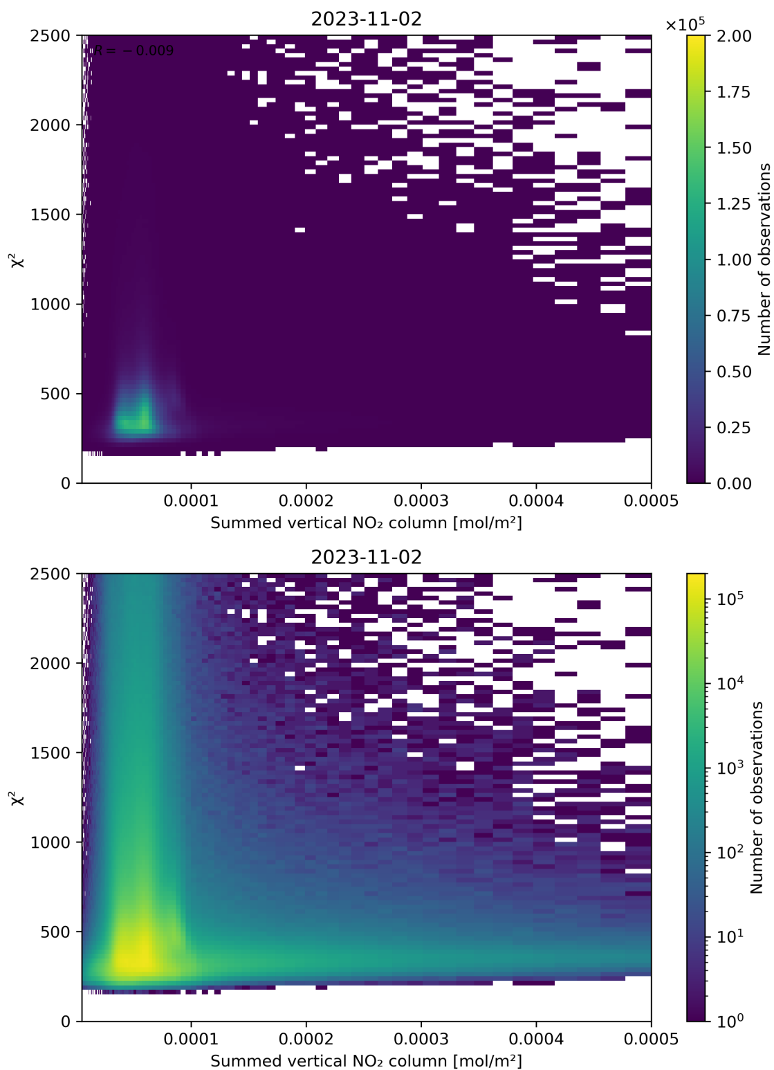
Figure 104: Scatter density plot of “Summed vertical NO 2 column” against “ \chi^2 ” for 2023-11-02 to 2023-11-03.
