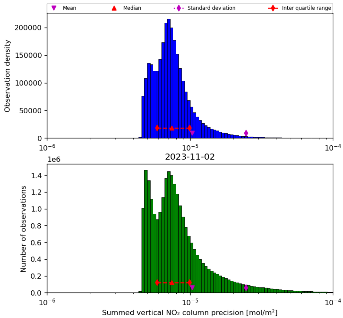
Figure 41: Histogram of “Summed vertical NO 2 column precision” for 2023-11-02 to 2023-11-03
