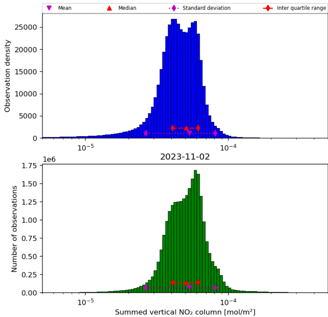
Figure 40: Histogram of “Summed vertical NO 2 column” for 2023-11-02 to 2023-11-03
