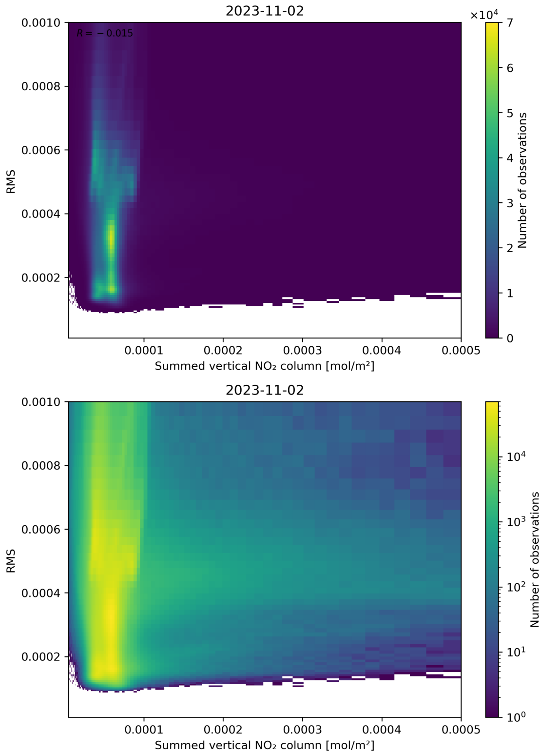
Figure 109: Scatter density plot of “Summed vertical NO 2 column” against “RMS” for 2023-11-02 to 2023-11-03.
