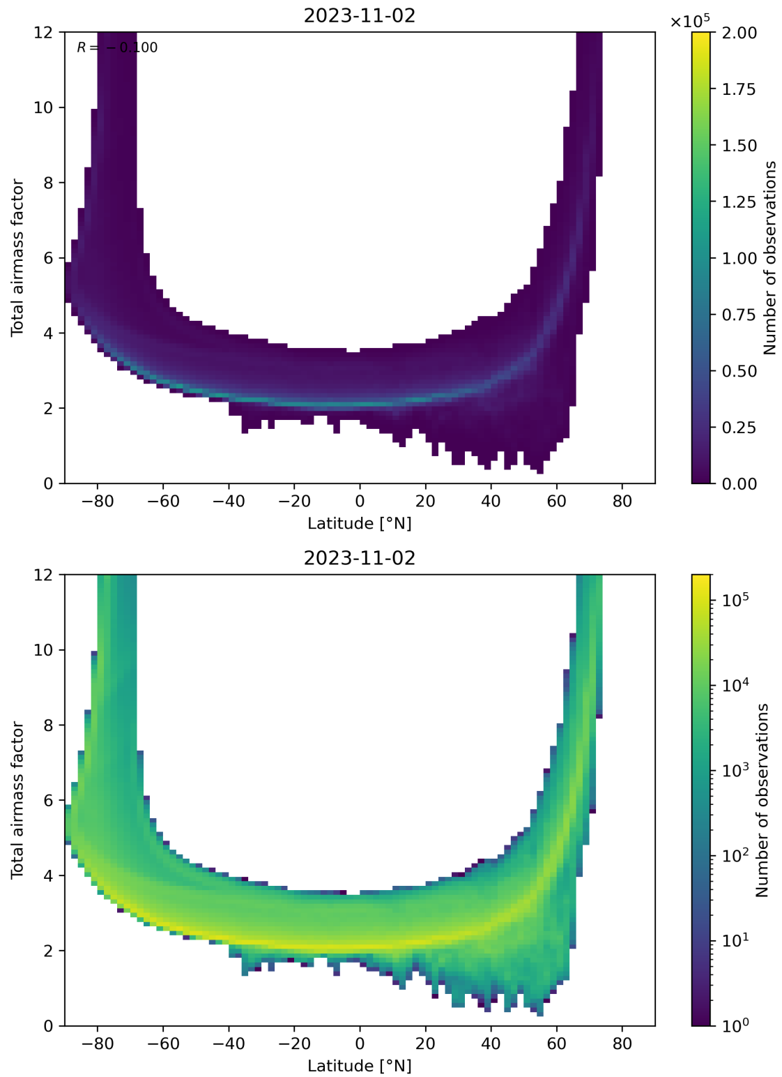
Figure 84: Scatter density plot of “Latitude” against “Total airmass factor” for 2023-11-02 to 2023-11-03.
