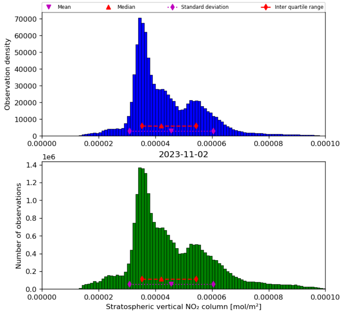
Figure 36: Histogram of “Stratospheric vertical NO 2 column” for 2023-11-02 to 2023-11-03
