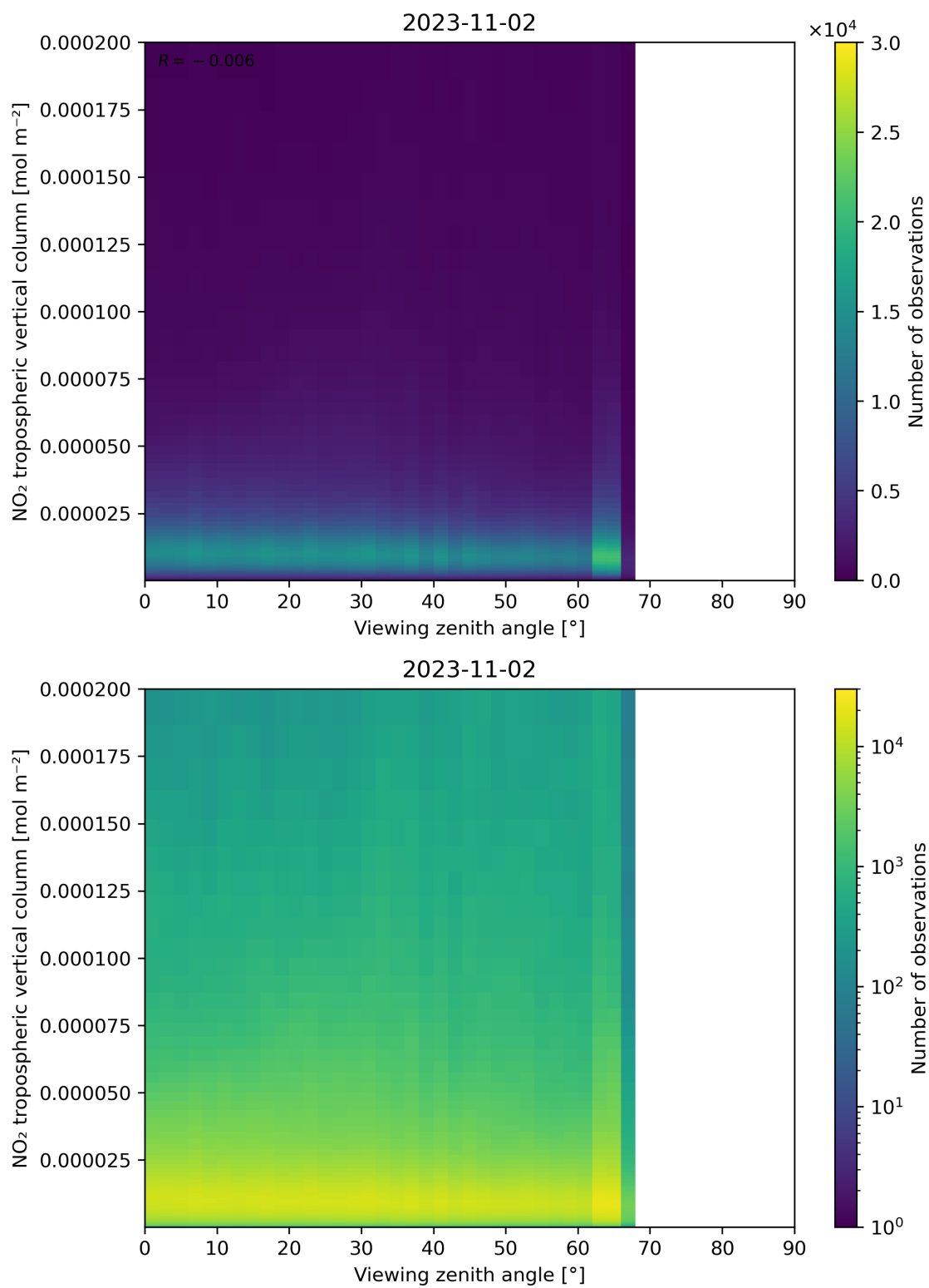
Figure 169: Scatter density plot of “Viewing zenith angle” against “NO 2 tropospheric vertical column” for 2023-11-02 to 2023-11-03.
