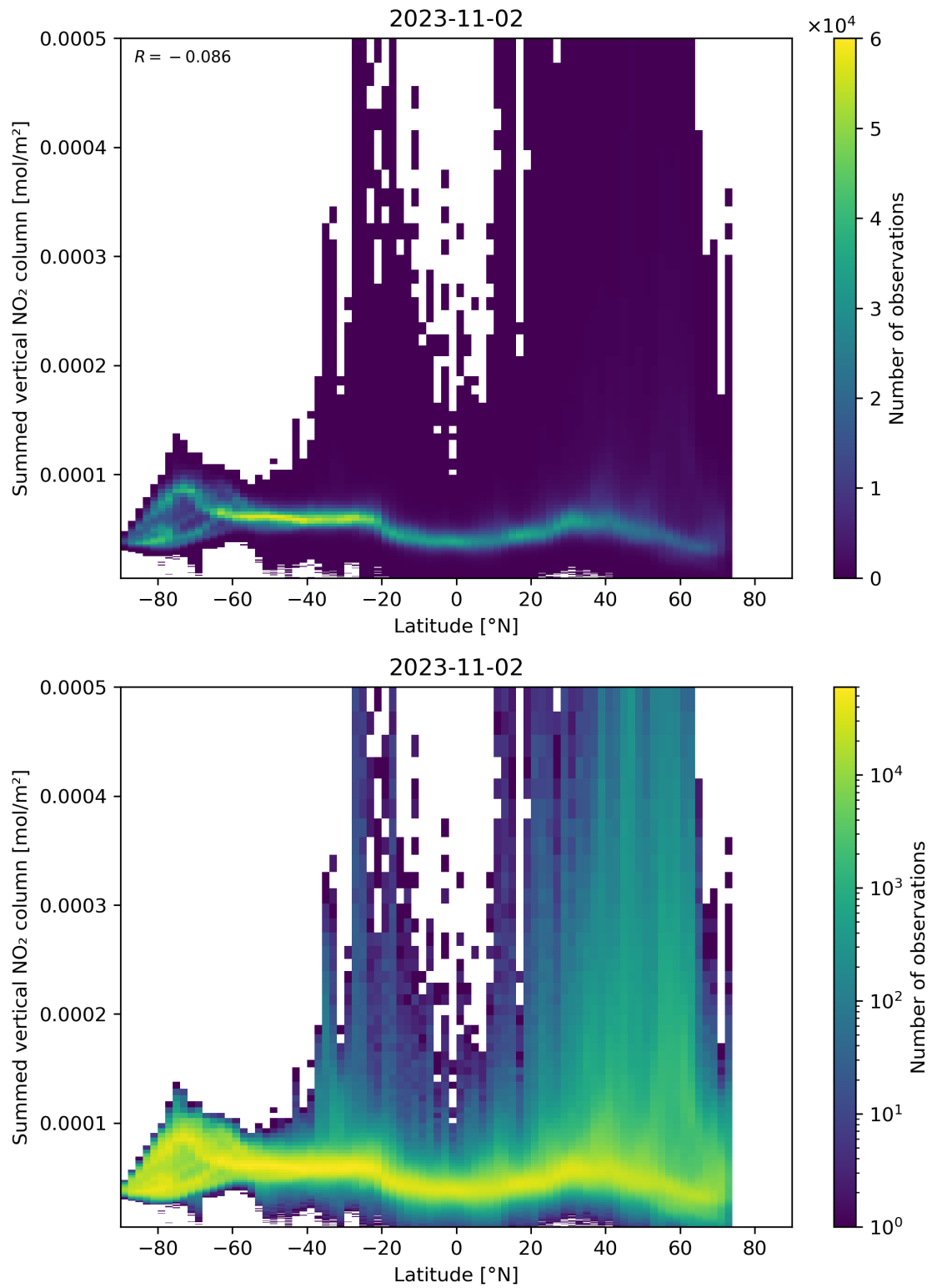
Figure 88: Scatter density plot of “Latitude” against “Summed vertical NO 2 column” for 2023-11-02 to 2023-11-03.
