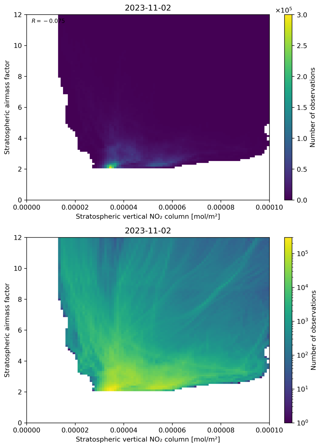
Figure 96: Scatter density plot of “Stratospheric vertical NO 2 column” against “Stratospheric airmass factor” for 2023-11-02 to 2023-11-03.
