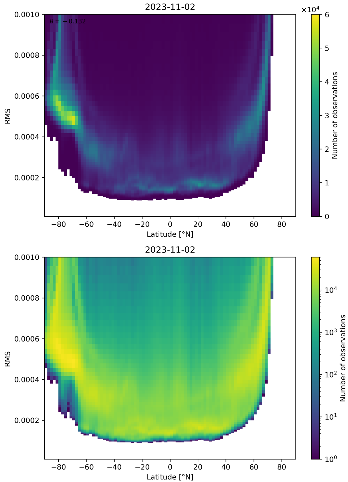
Figure 94: Scatter density plot of “Latitude” against “RMS” for 2023-11-02 to 2023-11-03.
