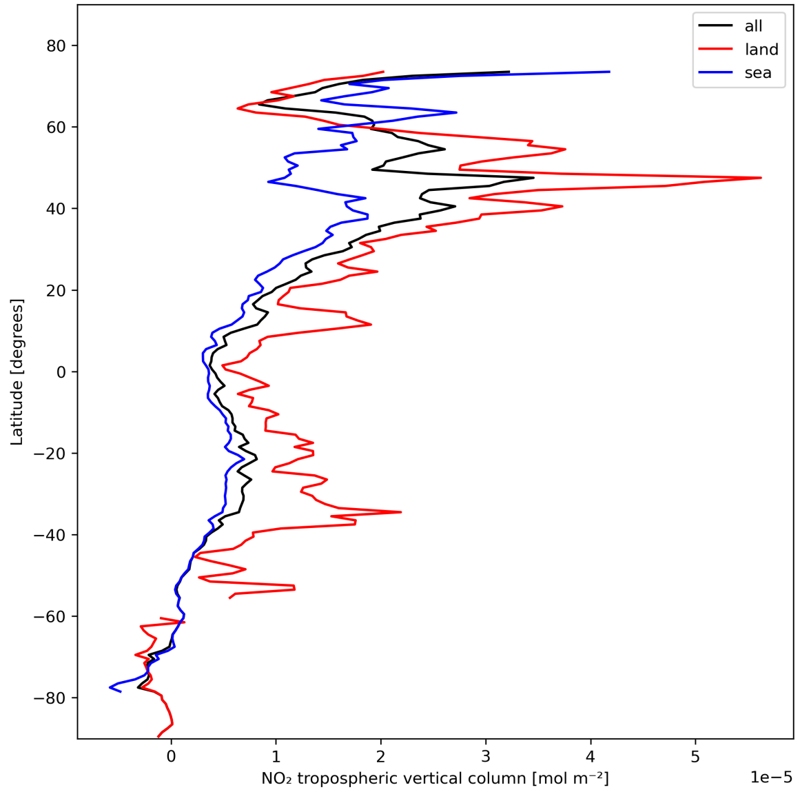
Figure 12: Zonal average of “NO 2 tropospheric vertical column” for 2023-11-02 to 2023-11-03.
