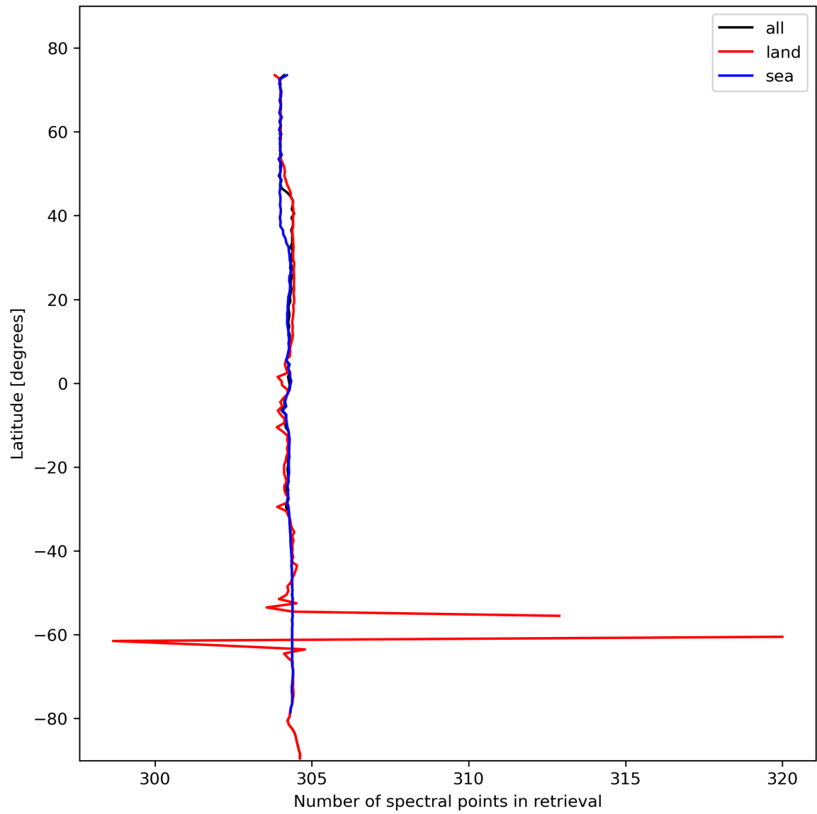
Figure 16: Zonal average of “Number of spectral points in retrieval” for 2023-11-02 to 2023-11-03.
