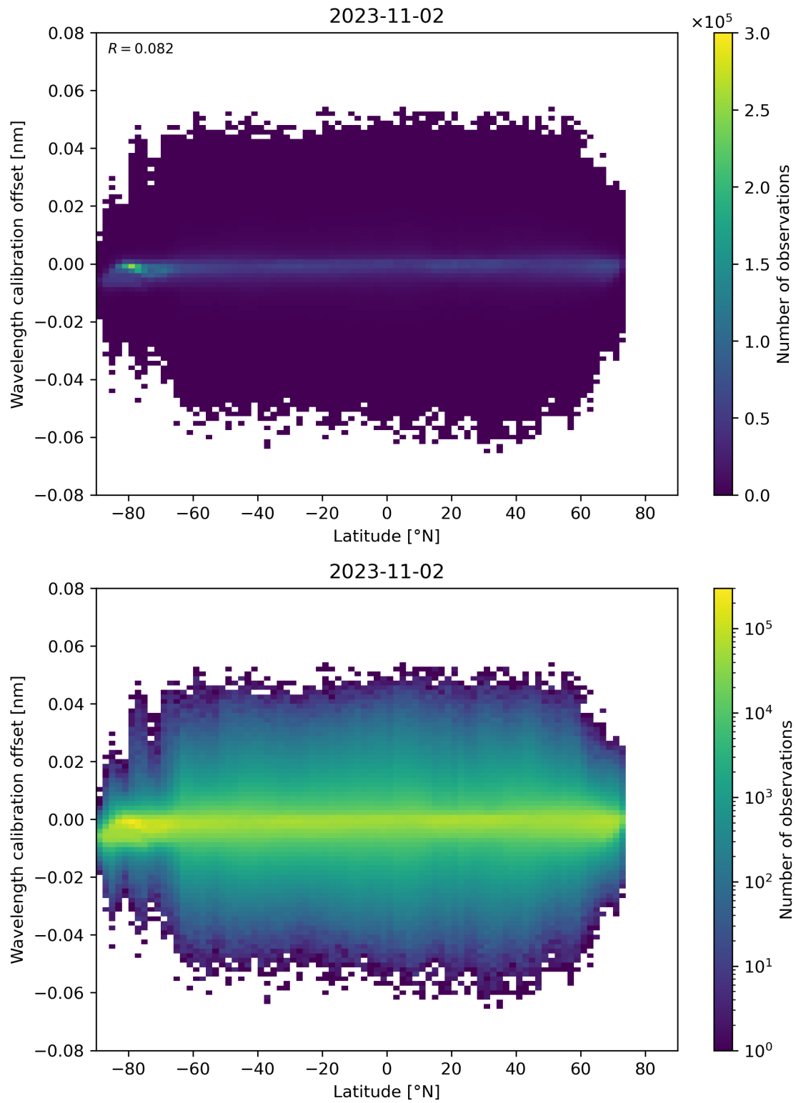
Figure 95: Scatter density plot of “Latitude” against “Wavelength calibration offset” for 2023-11-02 to 2023-11-03.
