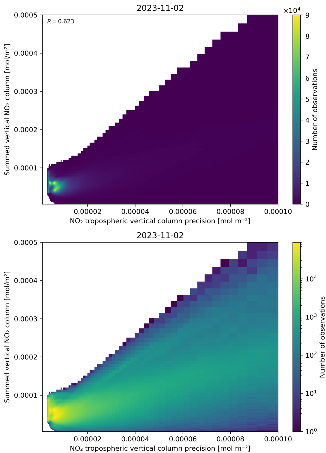
Figure 136: Scatter density plot of “NO 2 tropospheric vertical column precision” against “Summed vertical NO 2 column” for 2023-11-02 to 2023-11-03.
