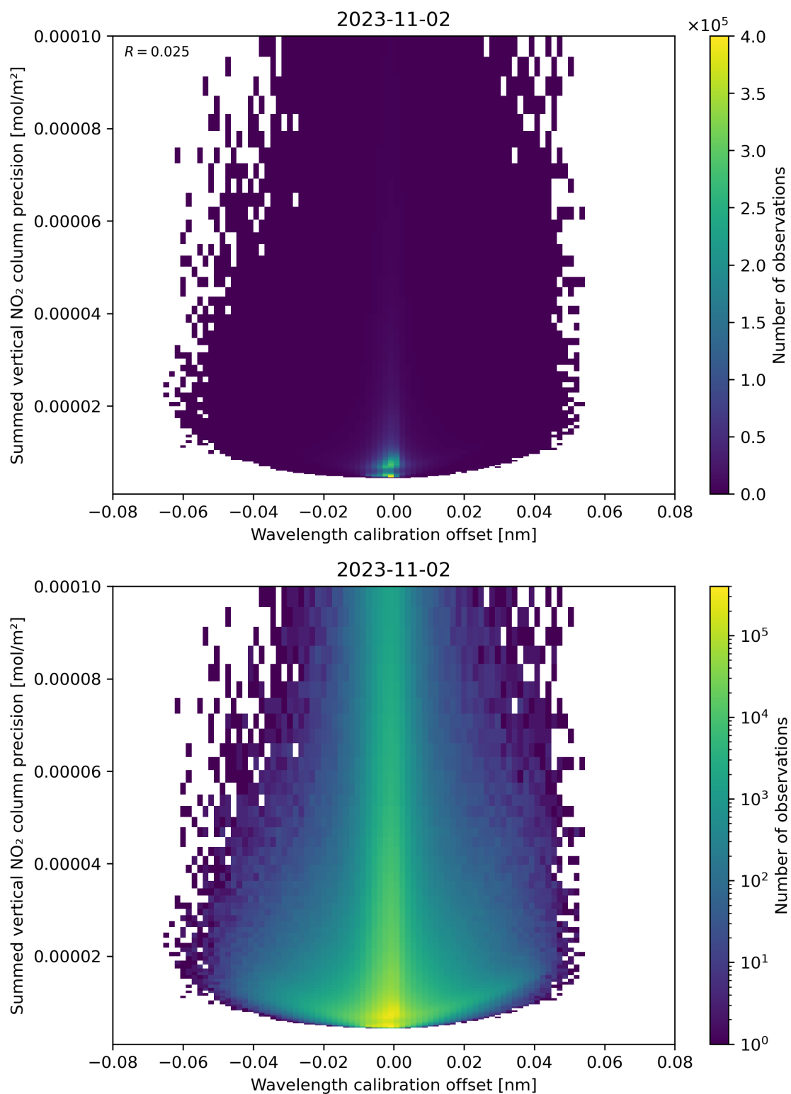
Figure 178: Scatter density plot of “Wavelength calibration offset” against “Summed vertical NO 2 column precision” for 2023-11-02 to 2023-11-03.
