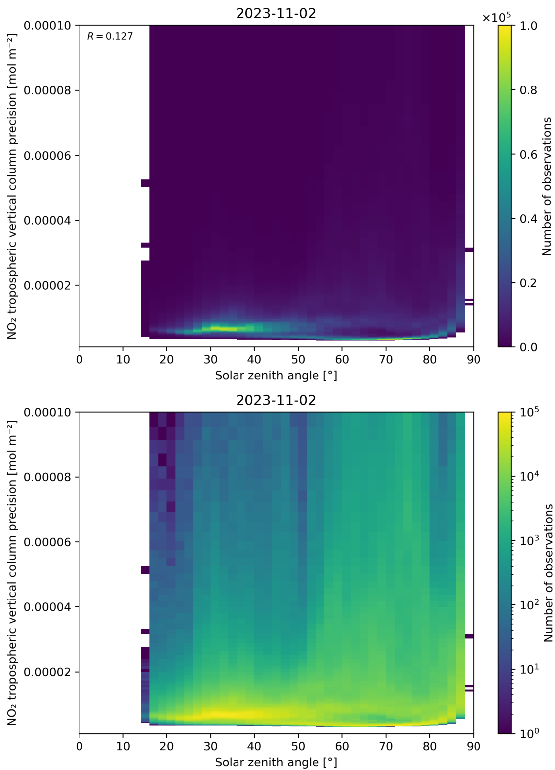
Figure 156: Scatter density plot of “Solar zenith angle” against “NO 2 tropospheric vertical column precision” for 2023-11-02 to 2023-11-03.
