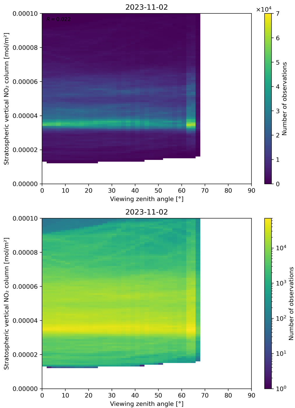
Figure 164: Scatter density plot of “Viewing zenith angle” against “Stratospheric vertical NO 2 column” for 2023-11-02 to 2023-11-03.
