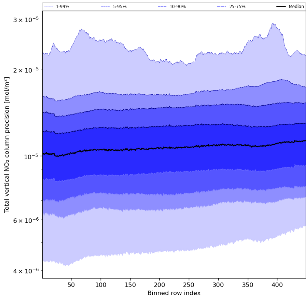
Figure 56: Along track statistics of "Total vertical NO 2 column precision" for 2023-11-02 to 2023-11-03
