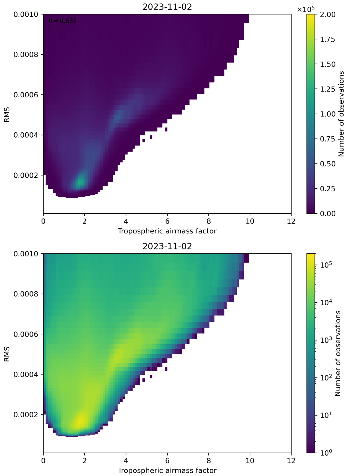
Figure 79: Scatter density plot of “Tropospheric airmass factor” against “RMS” for 2023-11-02 to 2023-11-03.
