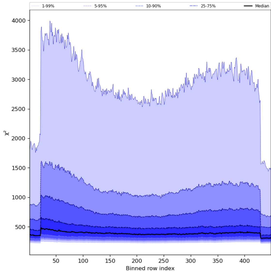
Figure 59: Along track statistics of “ \chi^2 ” for 2023-11-02 to 2023-11-03
