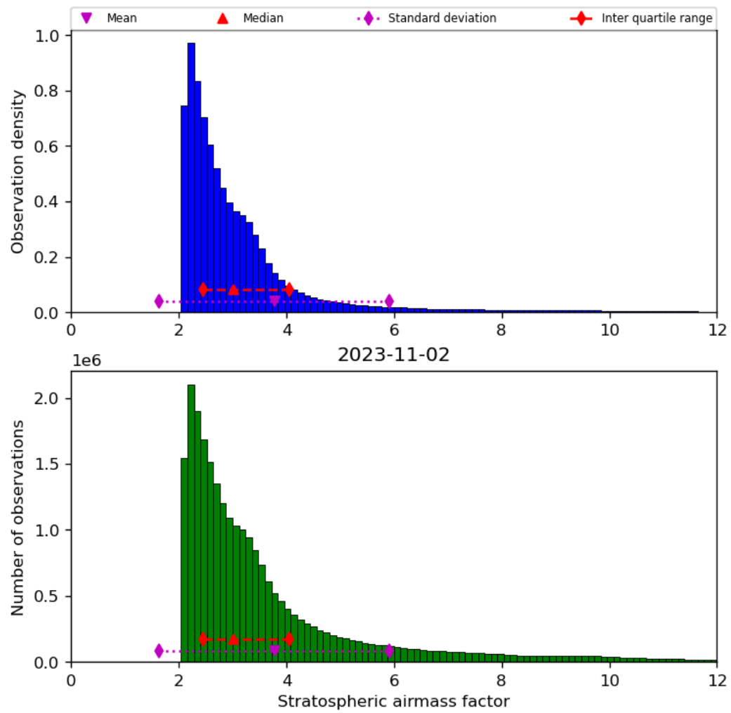
Figure 44: Histogram of “Stratospheric airmass factor” for 2023-11-02 to 2023-11-03
