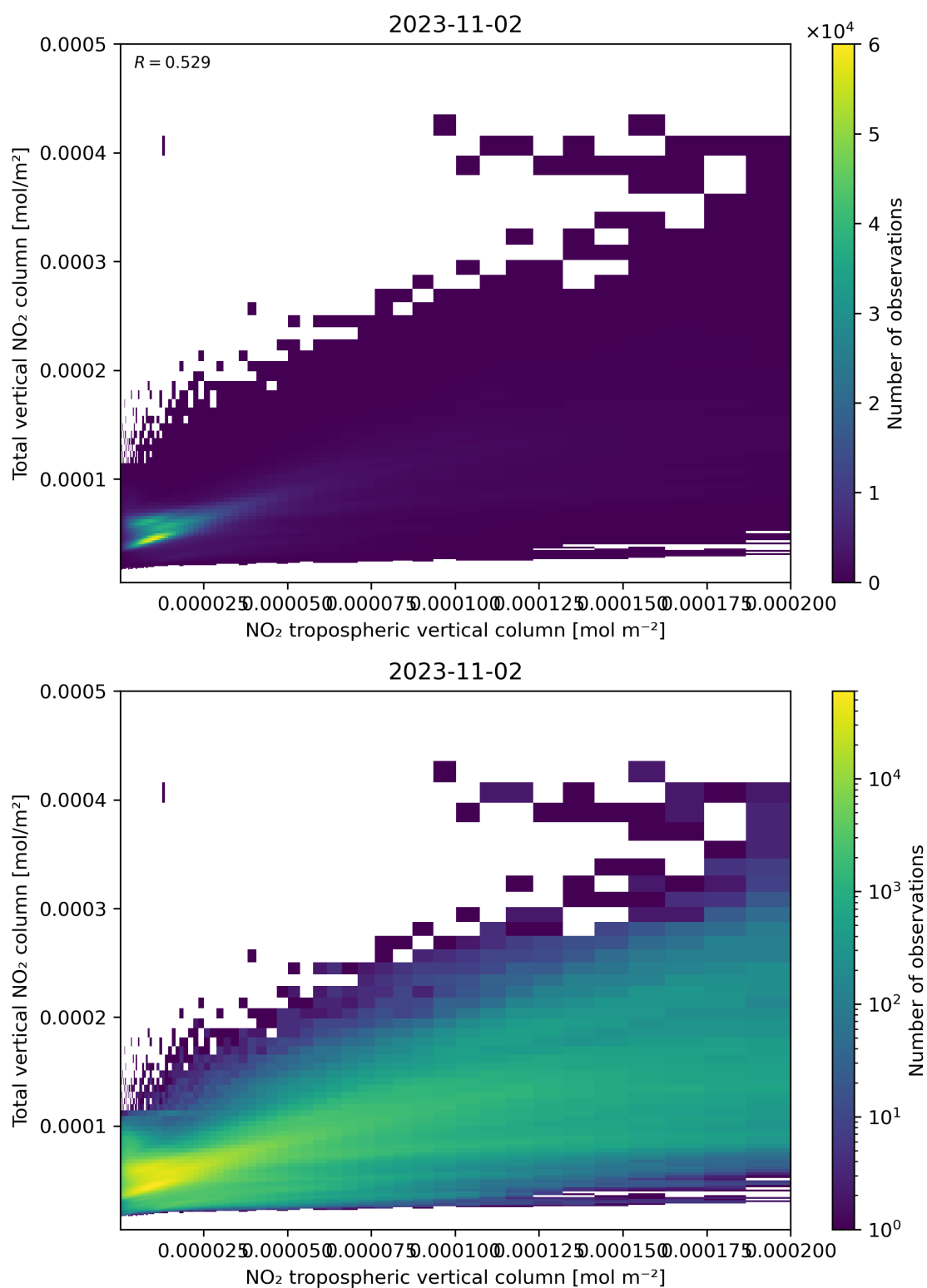
Figure 128: Scatter density plot of “NO 2 tropospheric vertical column” against “Total vertical NO 2 column” for 2023-11-02 to 2023-11-03.
