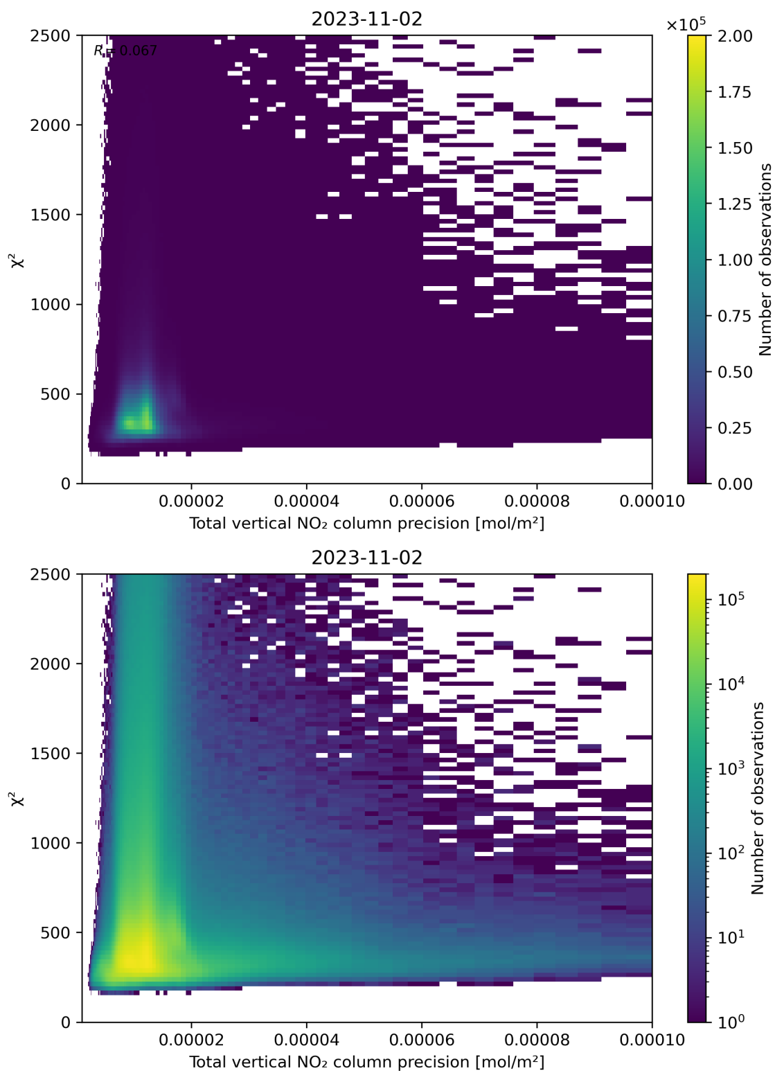
Figure 116: Scatter density plot of “Total vertical NO 2 column precision” against “ \chi^2 ” for 2023-11-02 to 2023-11-03.
