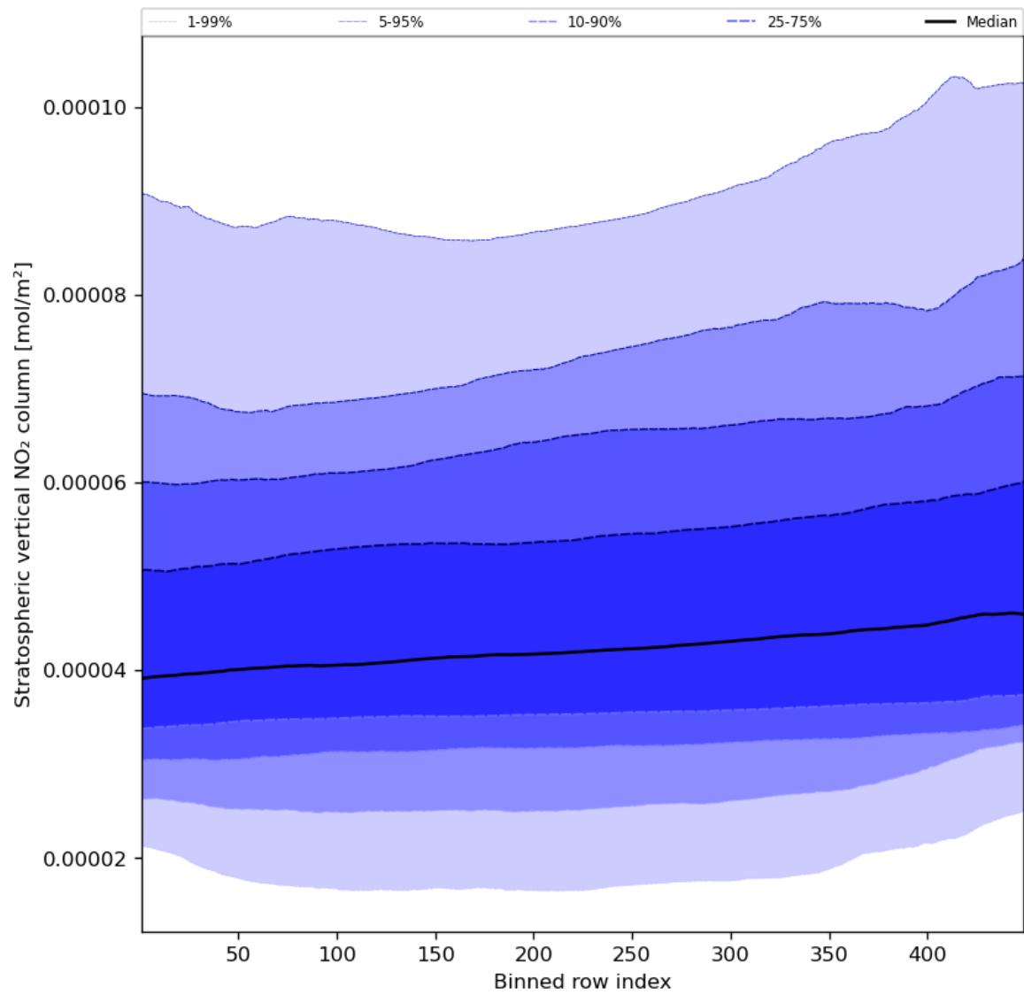
Figure 53: Along track statistics of “Stratospheric vertical NO 2 column” for 2023-11-02 to 2023-11-03
