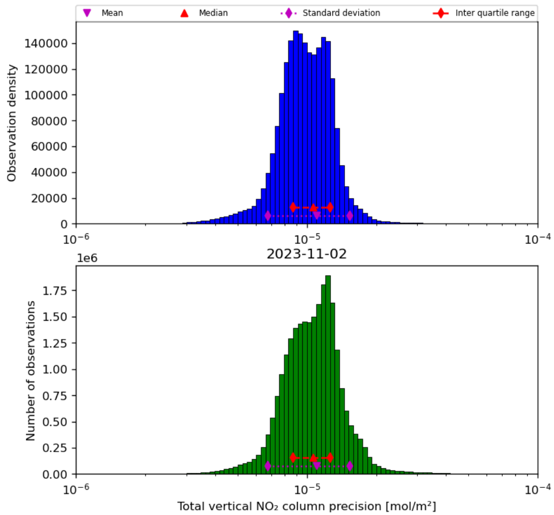
Figure 39: Histogram of “Total vertical NO 2 column precision” for 2023-11-02 to 2023-11-03
