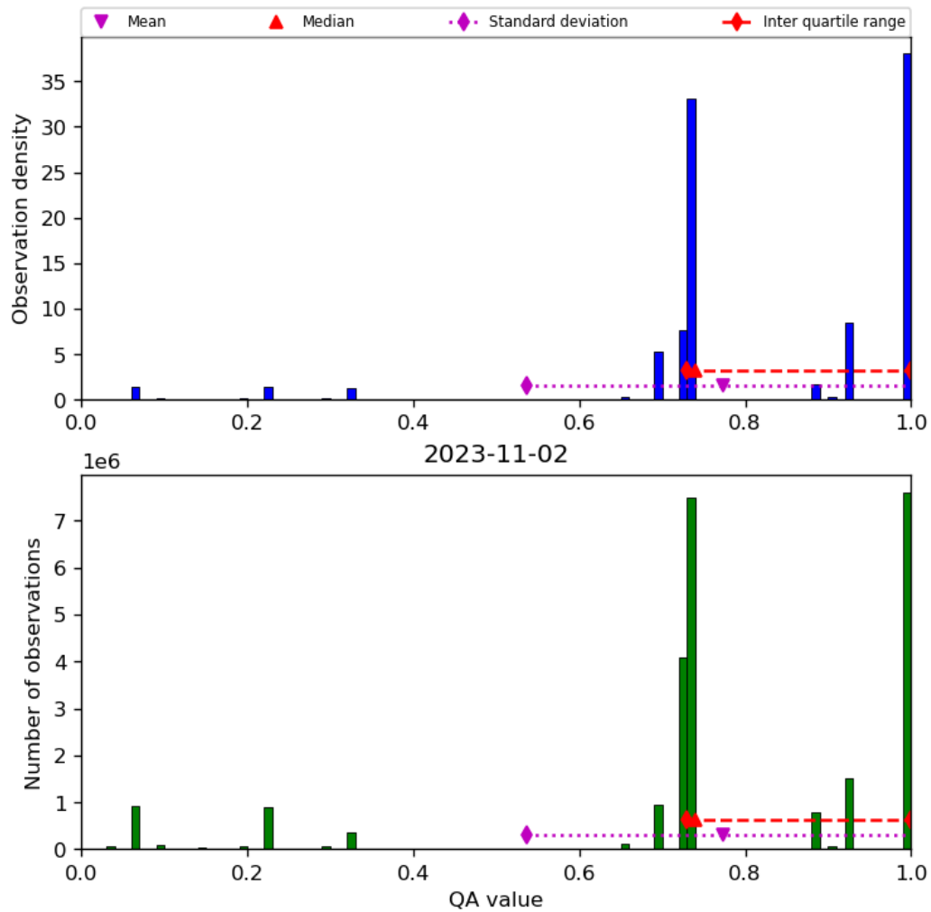
Figure 28: Histogram of “QA value” for 2023-11-02 to 2023-11-03
