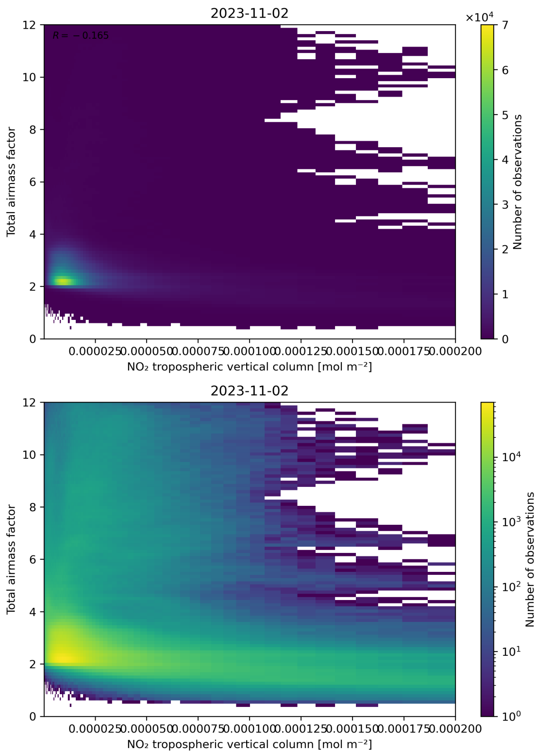
Figure 122: Scatter density plot of “NO 2 tropospheric vertical column” against “Total air mass factor” for 2023-11-02 to 2023-11-03.
