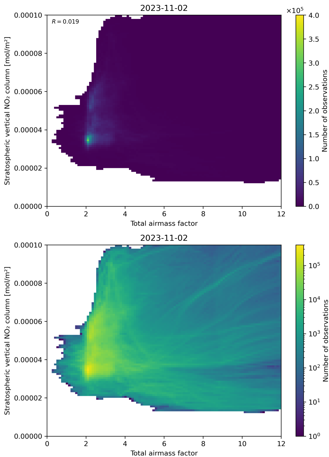
Figure 64: Scatter density plot of “Total airmass factor” against “Stratospheric vertical NO 2 column” for 2023-11-02 to 2023-11-03.
