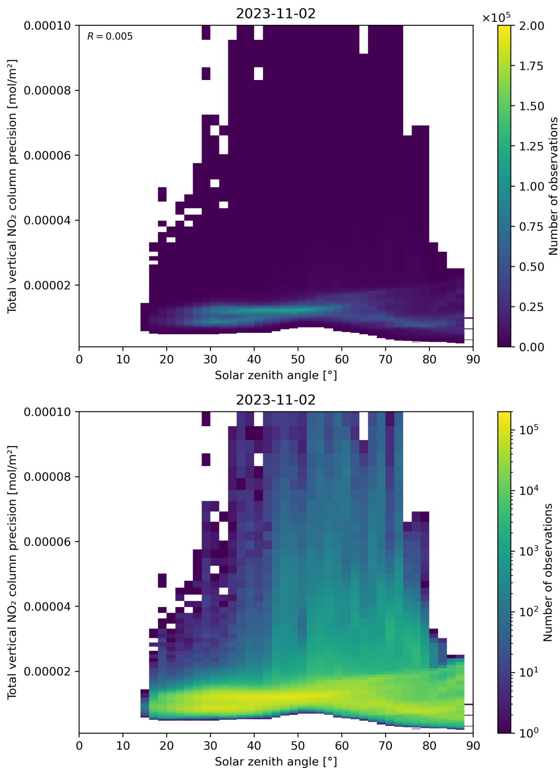
Figure 154: Scatter density plot of “Solar zenith angle” against “Total vertical NO 2 column precision” for 2023-11-02 to 2023-11-03.
