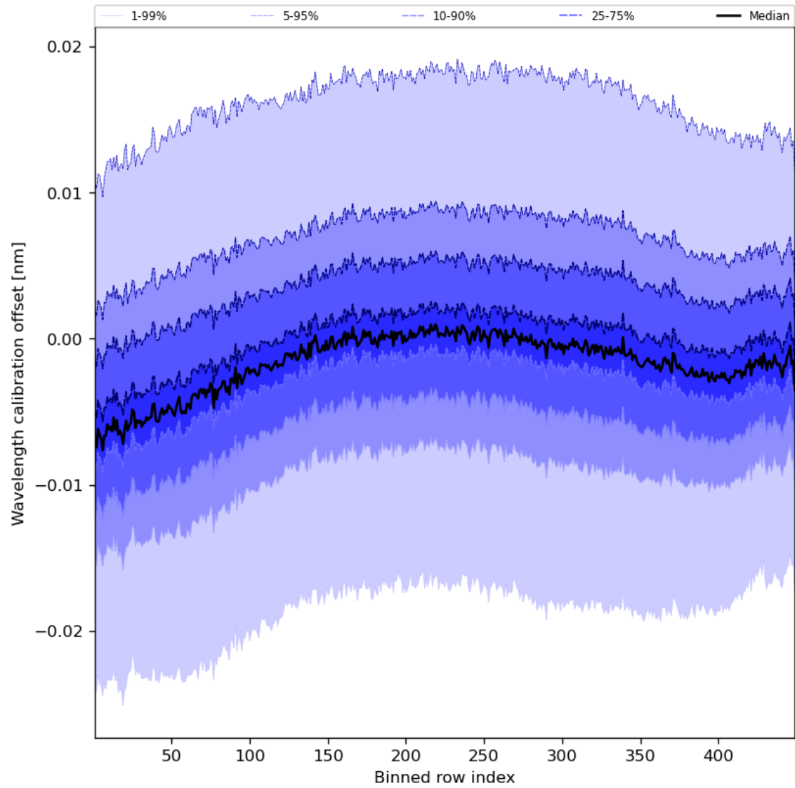
Figure 52: Along track statistics of “Wavelength calibration offset” for 2023-11-02 to 2023-11-03
