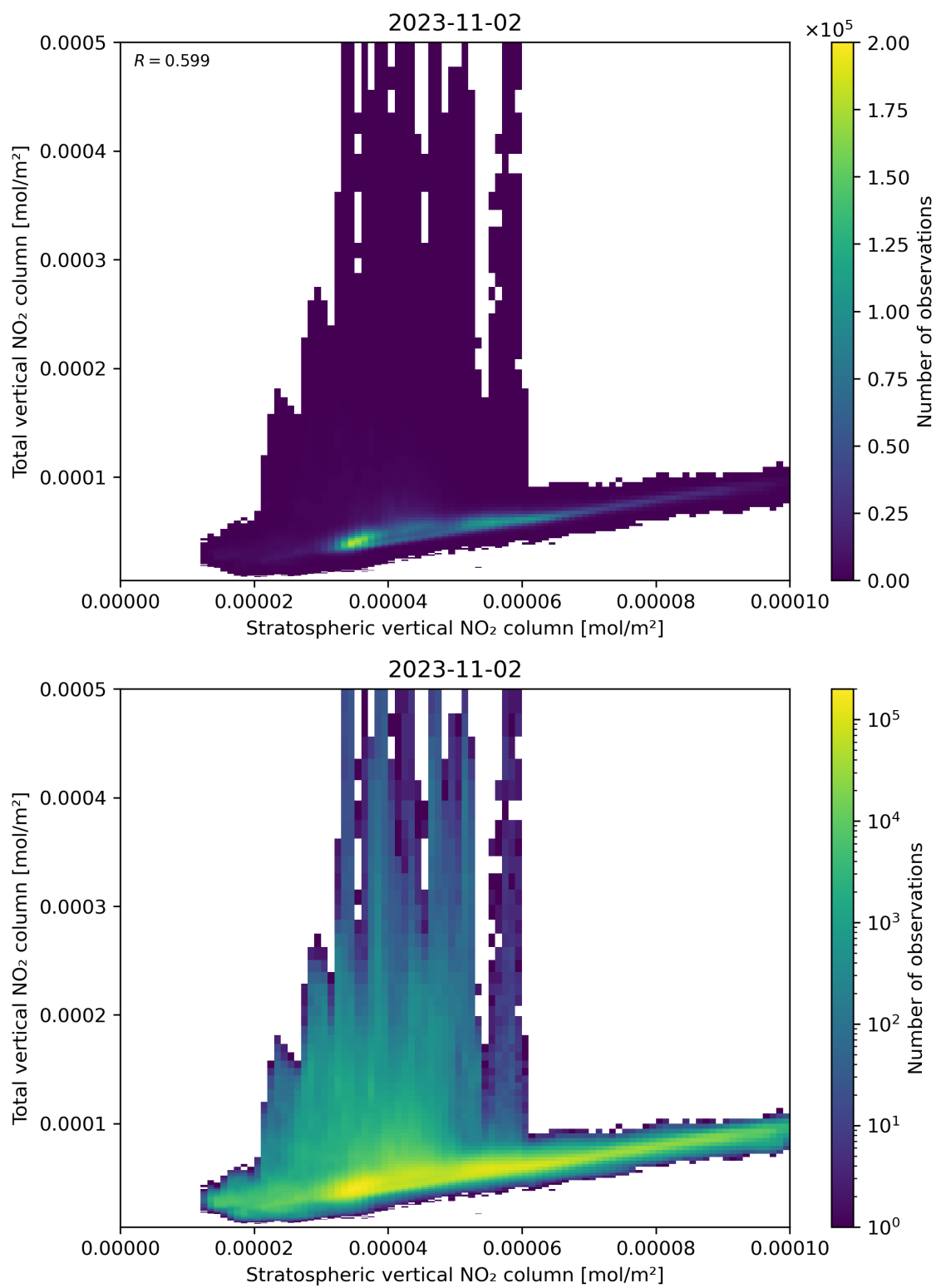
Figure 100: Scatter density plot of “Stratospheric vertical NO 2 column” against “Total vertical NO 2 column” for 2023-11-02 to 2023-11-03.
