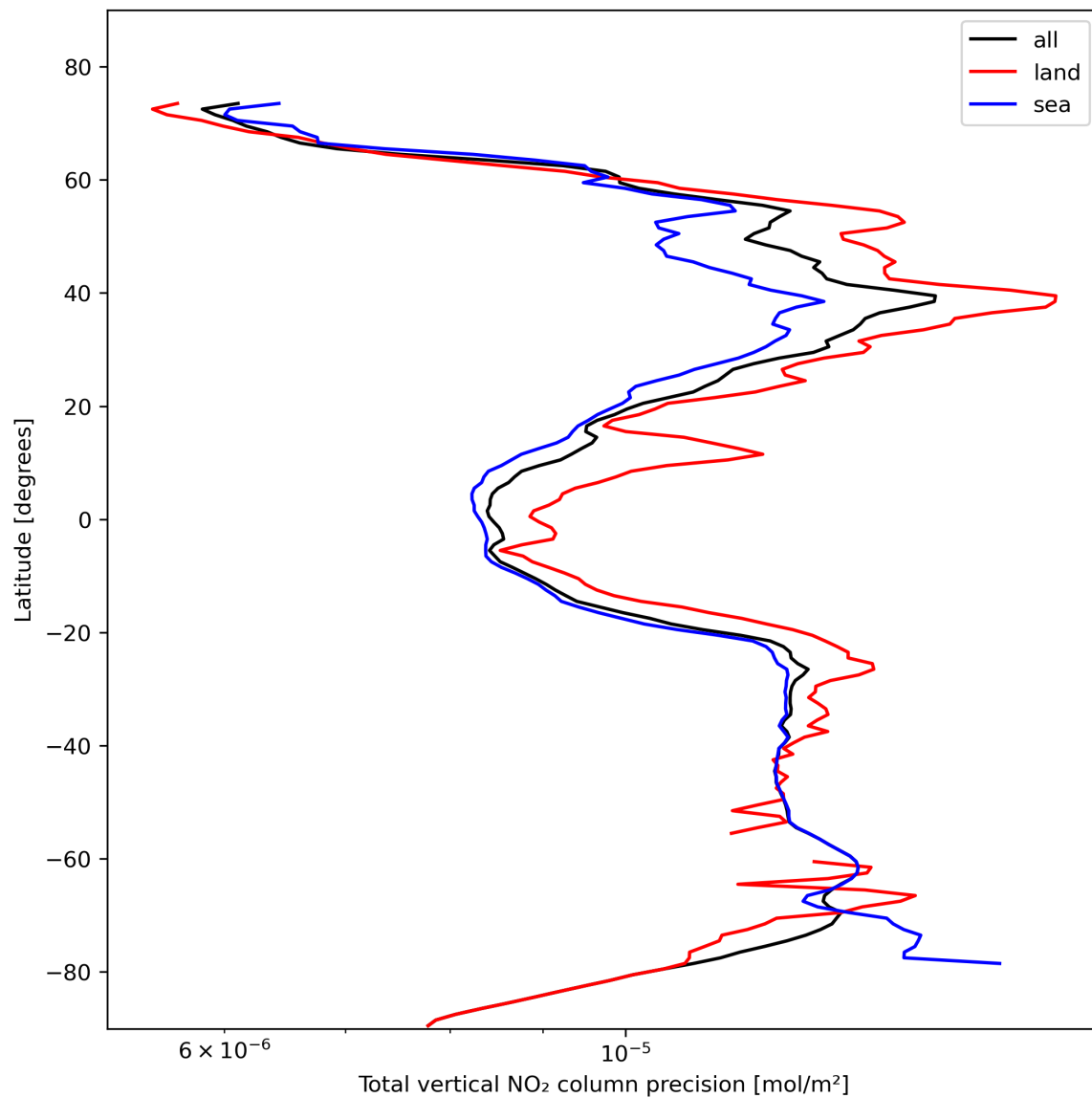
Figure 22: Zonal average of “Total vertical NO 2 column precision” for 2023-11-02 to 2023-11-03.
