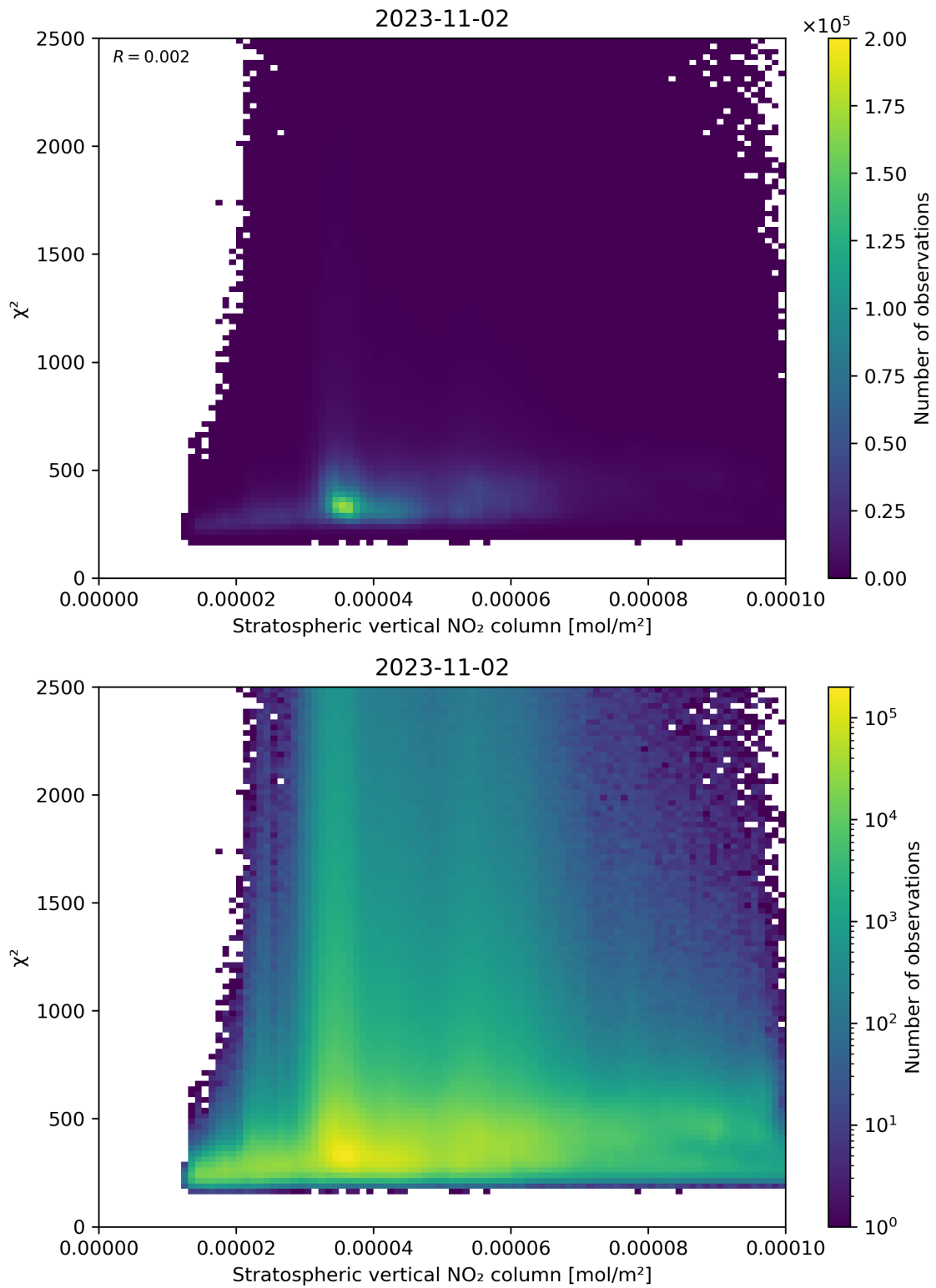
Figure 97: Scatter density plot of “Stratospheric vertical NO 2 column” against “ \chi^2 ” for 2023-11-02 to 2023-11-03.
