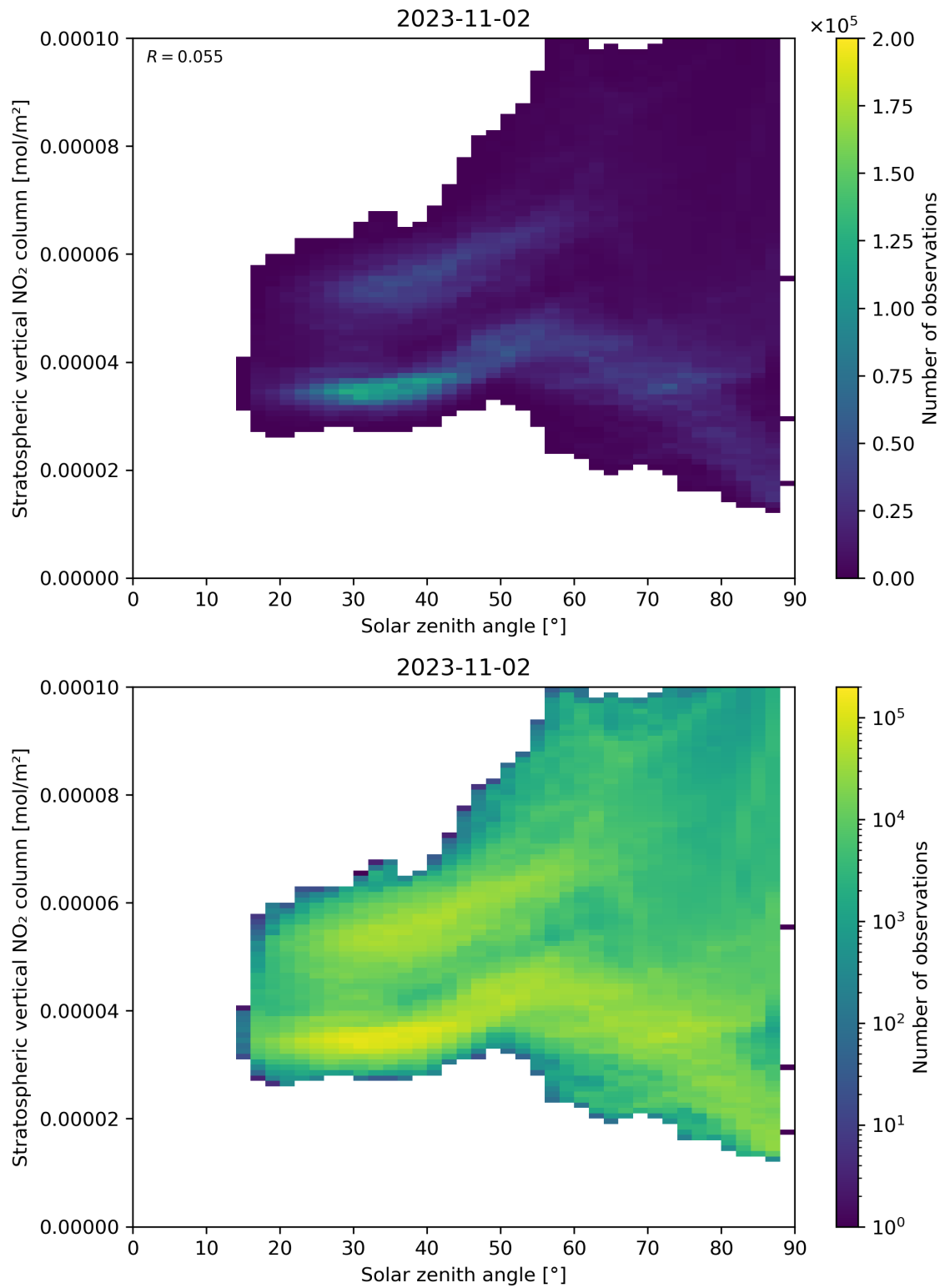
Figure 150: Scatter density plot of “Solar zenith angle” against “Stratospheric vertical NO 2 column” for 2023-11-02 to 2023-11-03.
