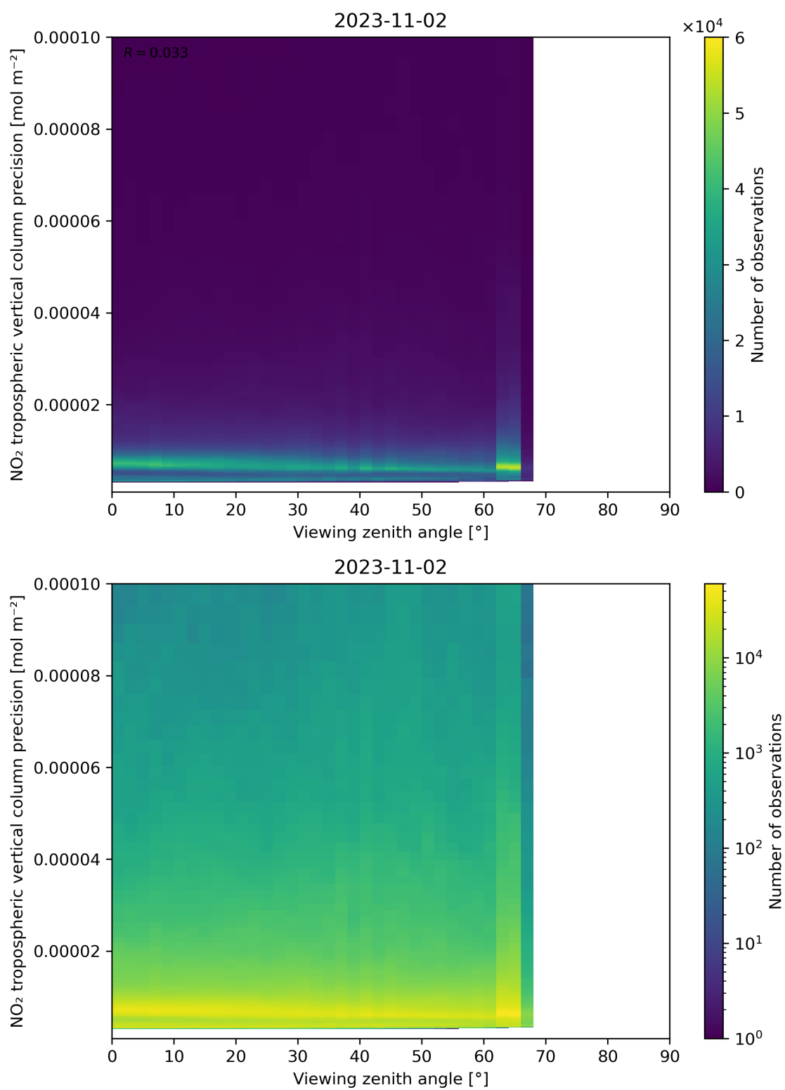
Figure 170: Scatter density plot of “Viewing zenith angle” against “NO 2 tropospheric vertical column precision” for 2023-11-02 to 2023-11-03.
