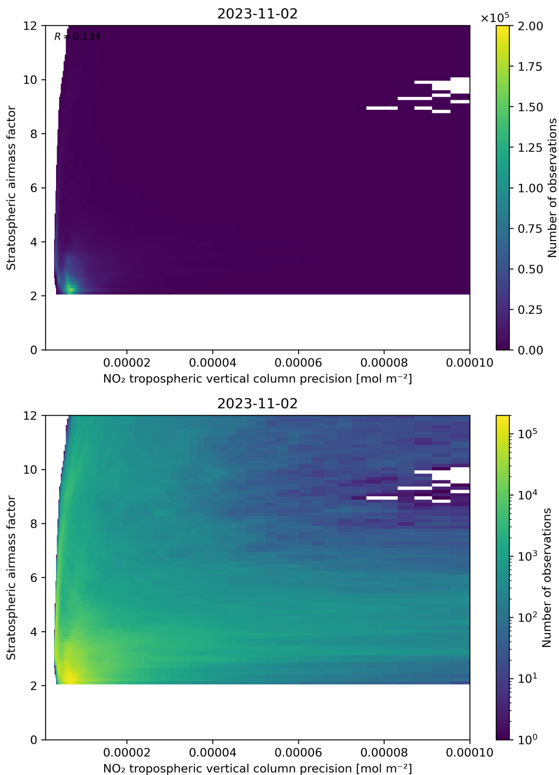
Figure 131: Scatter density plot of “NO 2 tropospheric vertical column precision” against “Stratospheric airmass factor” for 2023-11-02 to 2023-11-03.
