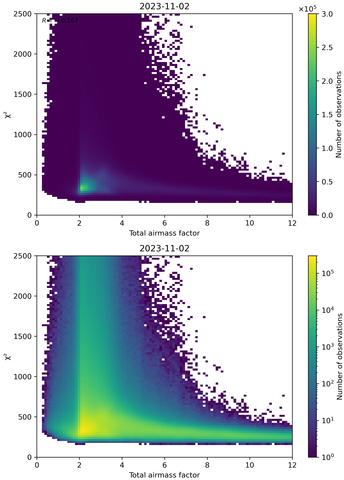
Figure 63: Scatter density plot of “Total airmass factor” against “ \chi^2 ” for 2023-11-02 to 2023-11-03.
