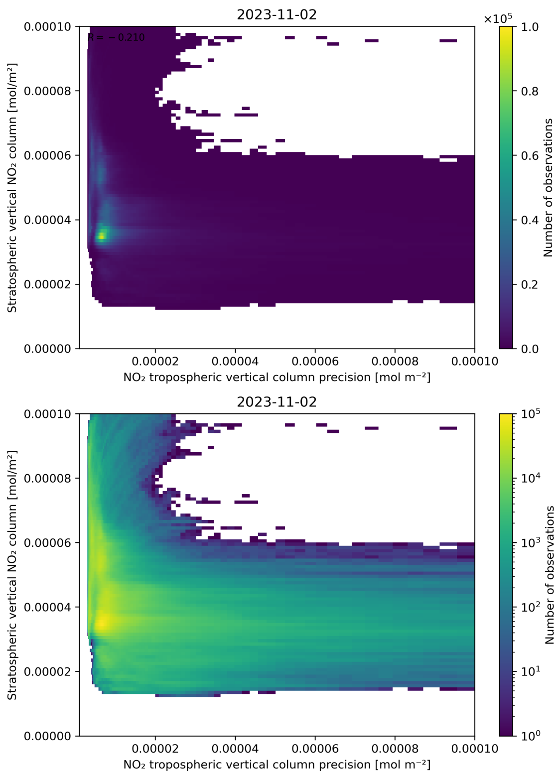
Figure 135: Scatter density plot of “NO 2 tropospheric vertical column precision” against “Stratospheric vertical NO 2 column” for 2023-11-02 to 2023-11-03.
