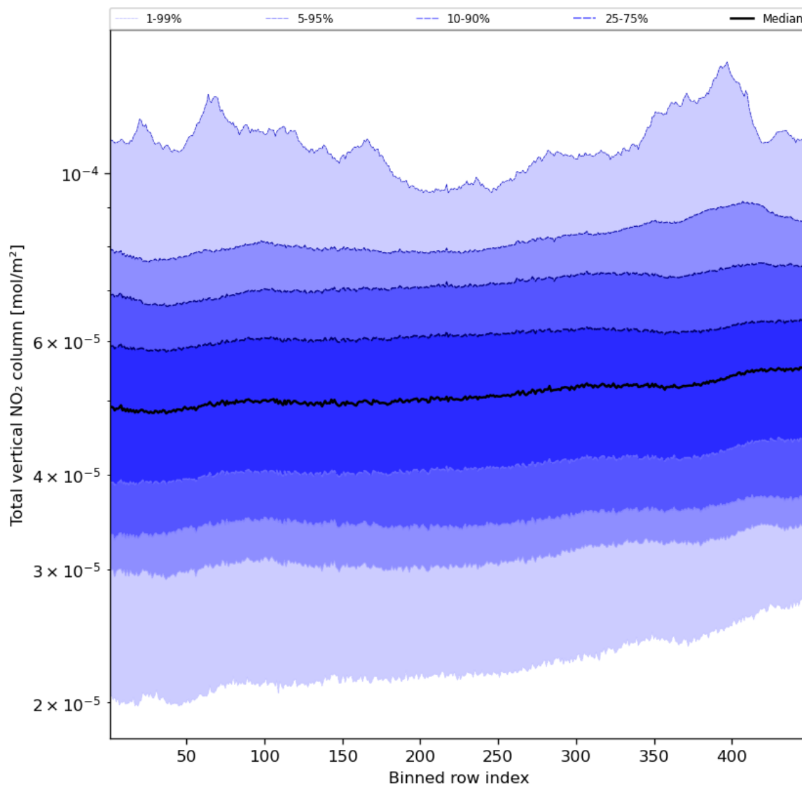
Figure 55: Along track statistics of “Total vertical NO 2 column” for 2023-11-02 to 2023-11-03
