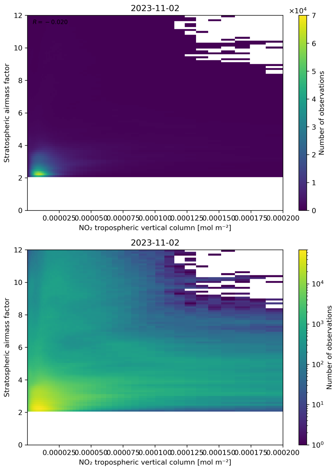
Figure 121: Scatter density plot of “NO 2 tropospheric vertical column” against “Stratospheric airmass factor” for 2023-11-02 to 2023-11-03.
