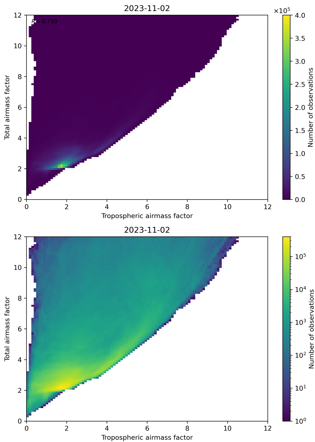
Figure 72: Scatter density plot of “Tropospheric airmass factor” against “Total airmass factor” for 2023-11-02 to 2023-11-03.
