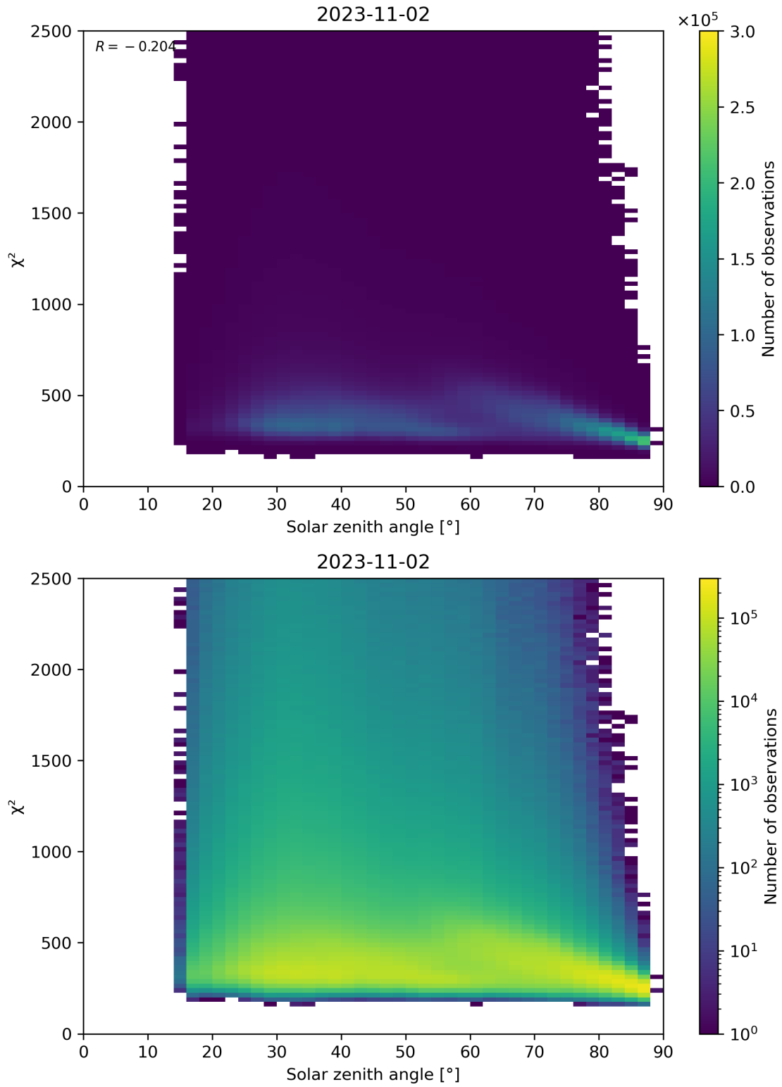
Figure 148: Scatter density plot of “Solar zenith angle” against “ \chi^2 ” for 2023-11-02 to 2023-11-03.
