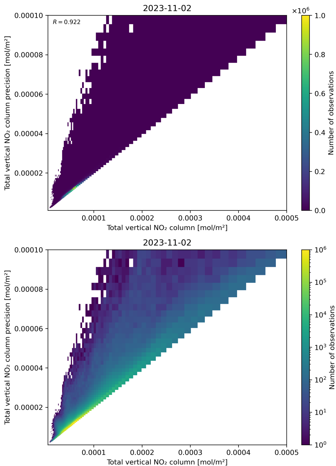
Figure 114: Scatter density plot of “Total vertical NO 2 column” against “Total vertical NO 2 column precision” for 2023-11-02 to 2023-11-03.
