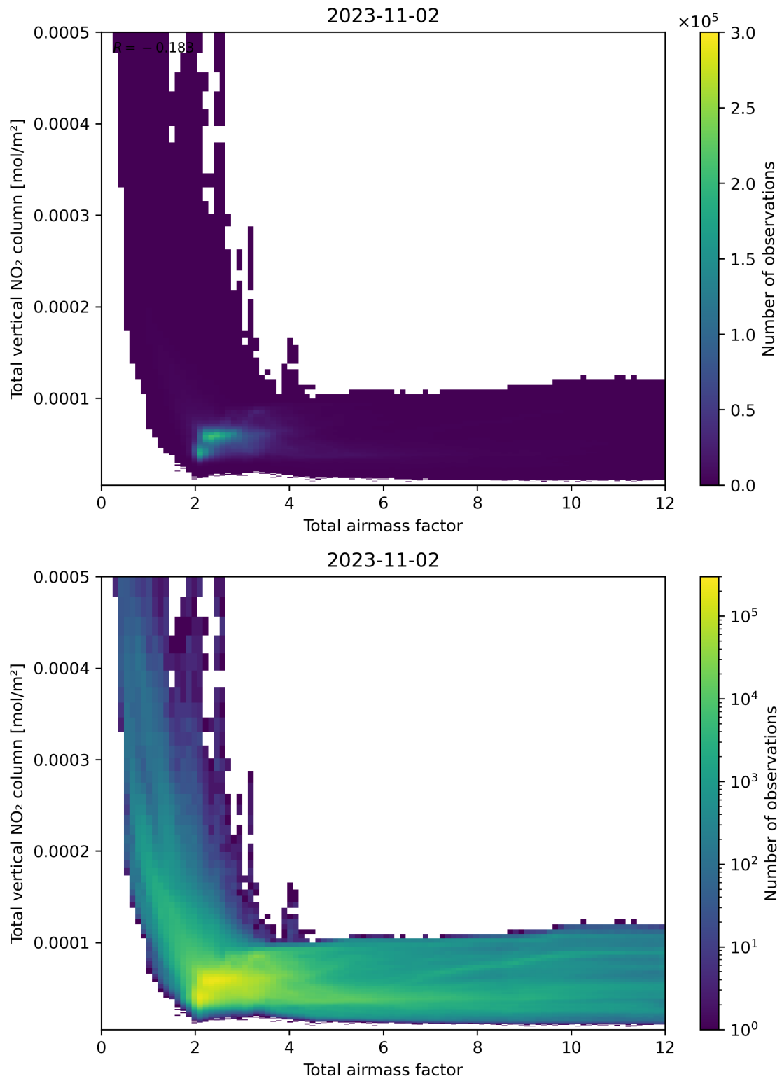
Figure 67: Scatter density plot of “Total airmass factor” against “Total vertical NO 2 column” for 2023-11-02 to 2023-11-03.
