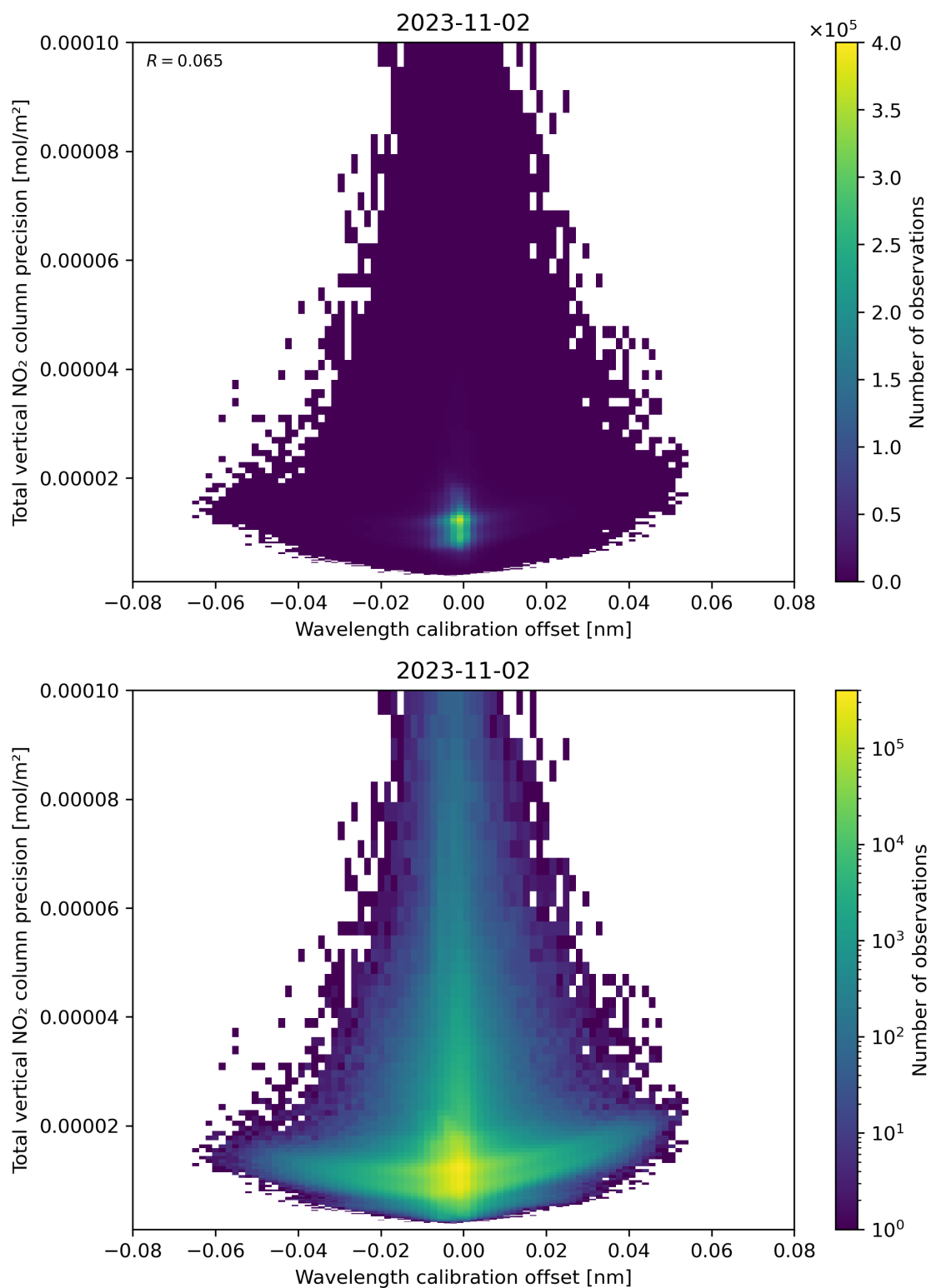
Figure 180: Scatter density plot of “Wavelength calibration offset” against “Total vertical NO 2 column precision” for 2023-11-02 to 2023-11-03.
