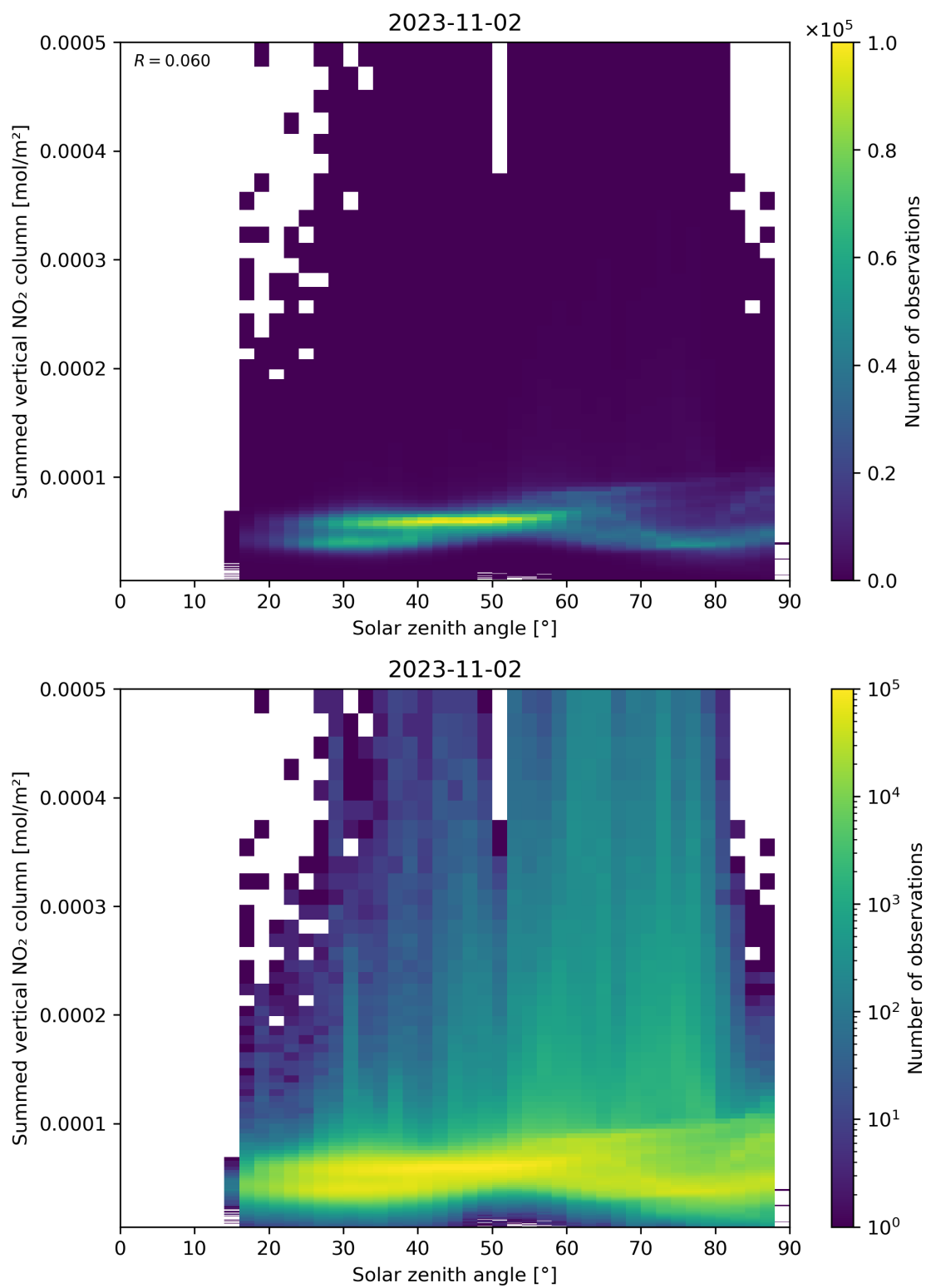
Figure 151: Scatter density plot of “Solar zenith angle” against “Summed vertical NO 2 column” for 2023-11-02 to 2023-11-03.
