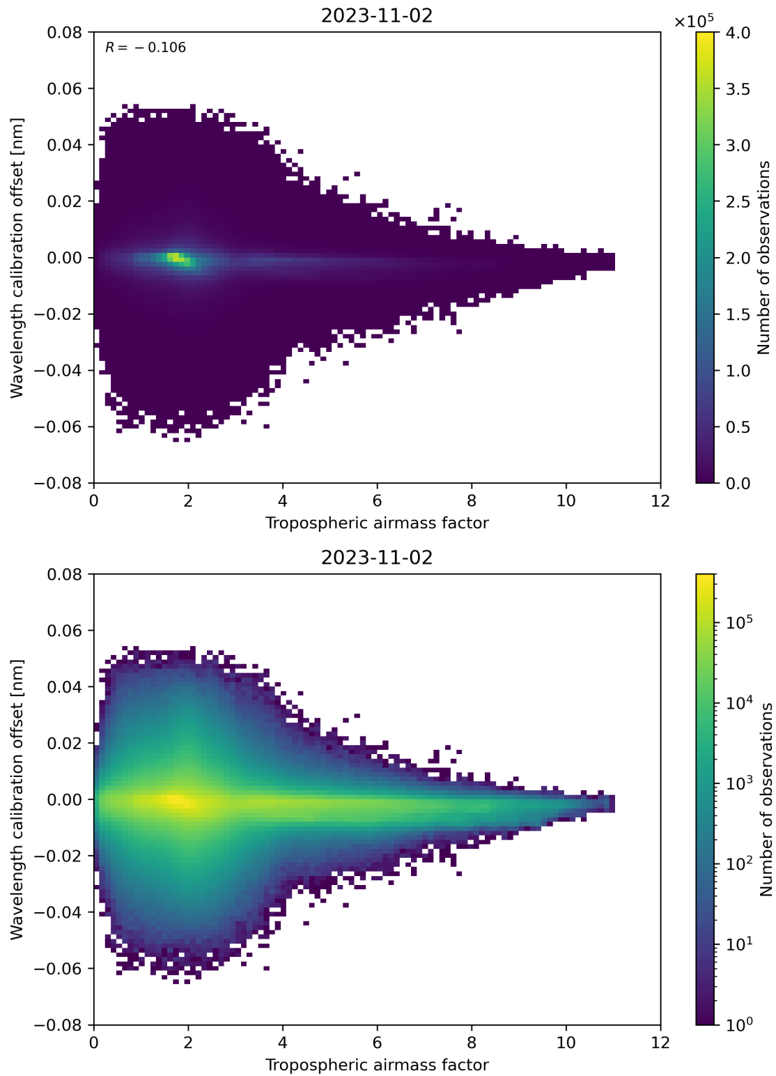
Figure 80: Scatter density plot of “Tropospheric air mass factor” against “Wavelength calibration offset” for 2023-11-02 to 2023-11-03.
