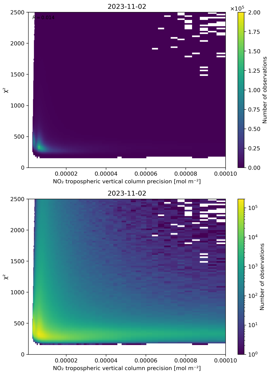
Figure 134: Scatter density plot of “NO 2 tropospheric vertical column precision” against “ \chi^2 ” for 2023-11-02 to 2023-11-03.
