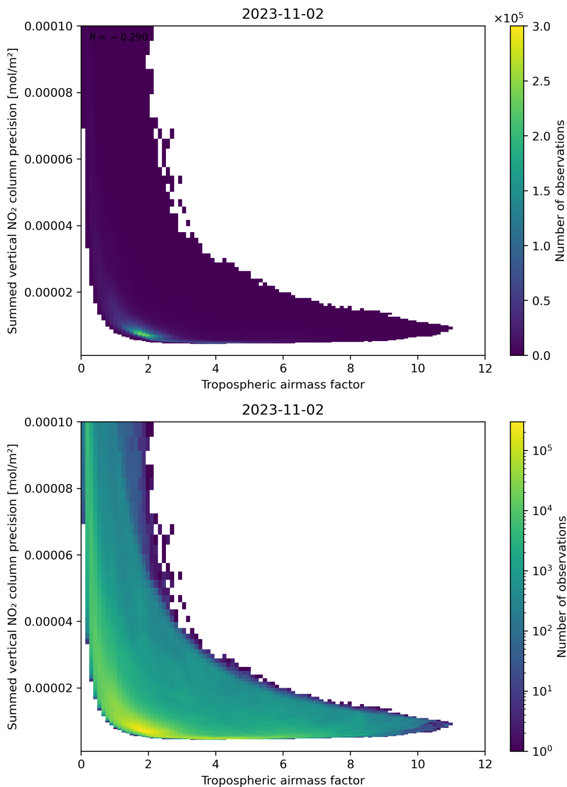
Figure 76: Scatter density plot of “Tropospheric air mass factor” against “Summed vertical NO 2 column precision” for 2023-11-02 to 2023-11-03.
