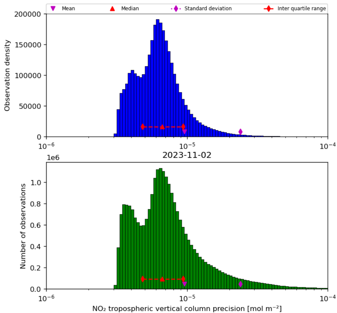
Figure 30: Histogram of “NO 2 tropospheric vertical column precision” for 2023-11-02 to 2023-11-03
