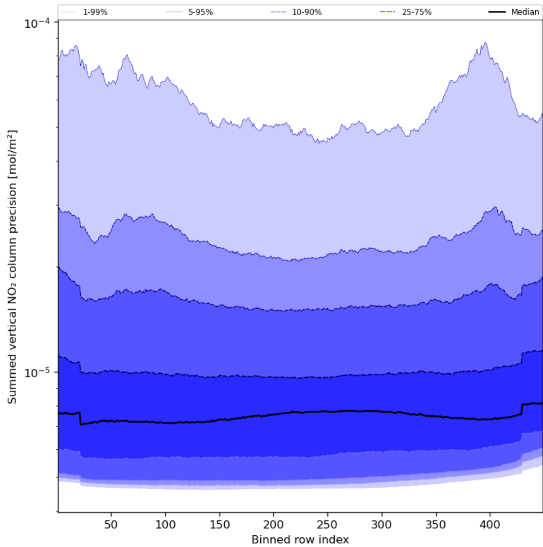
Figure 58: Along track statistics of “Summed vertical NO 2 column precision” for 2023-11-02 to 2023-11-03
