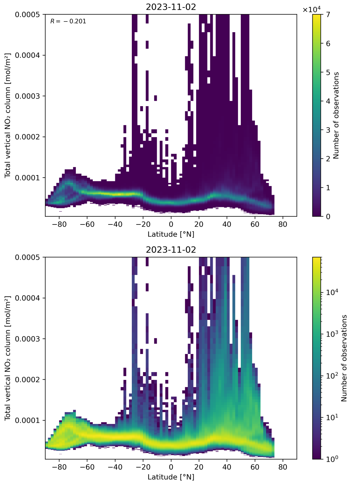
Figure 90: Scatter density plot of “Latitude” against “Total vertical NO 2 column” for 2023-11-02 to 2023-11-03.
