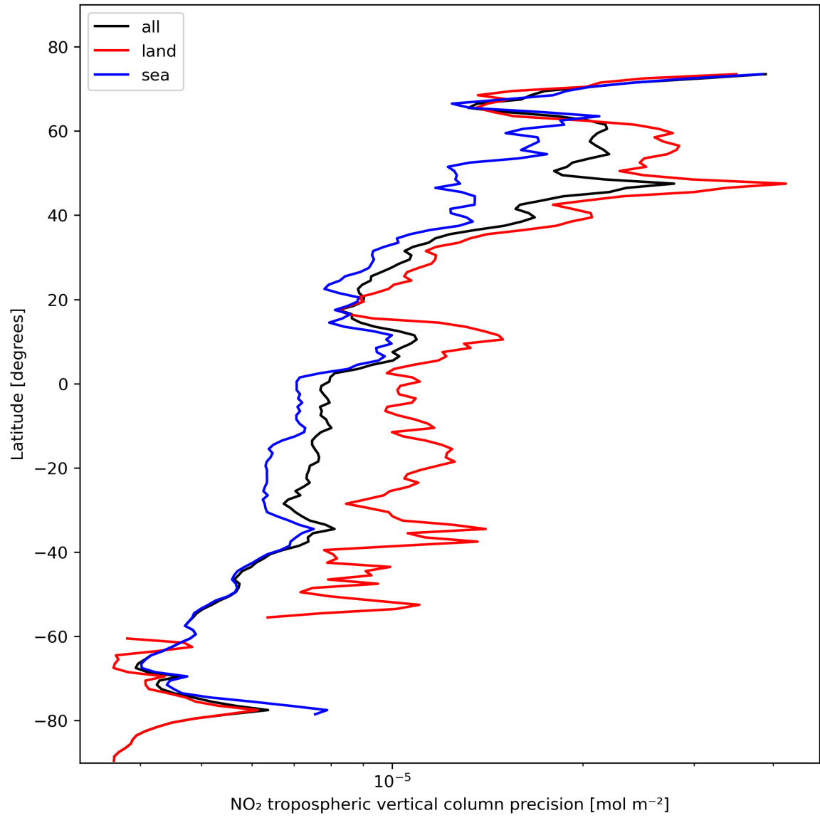
Figure 13: Zonal average of “NO 2 tropospheric vertical column precision” for 2023-11-02 to 2023-11-03.
