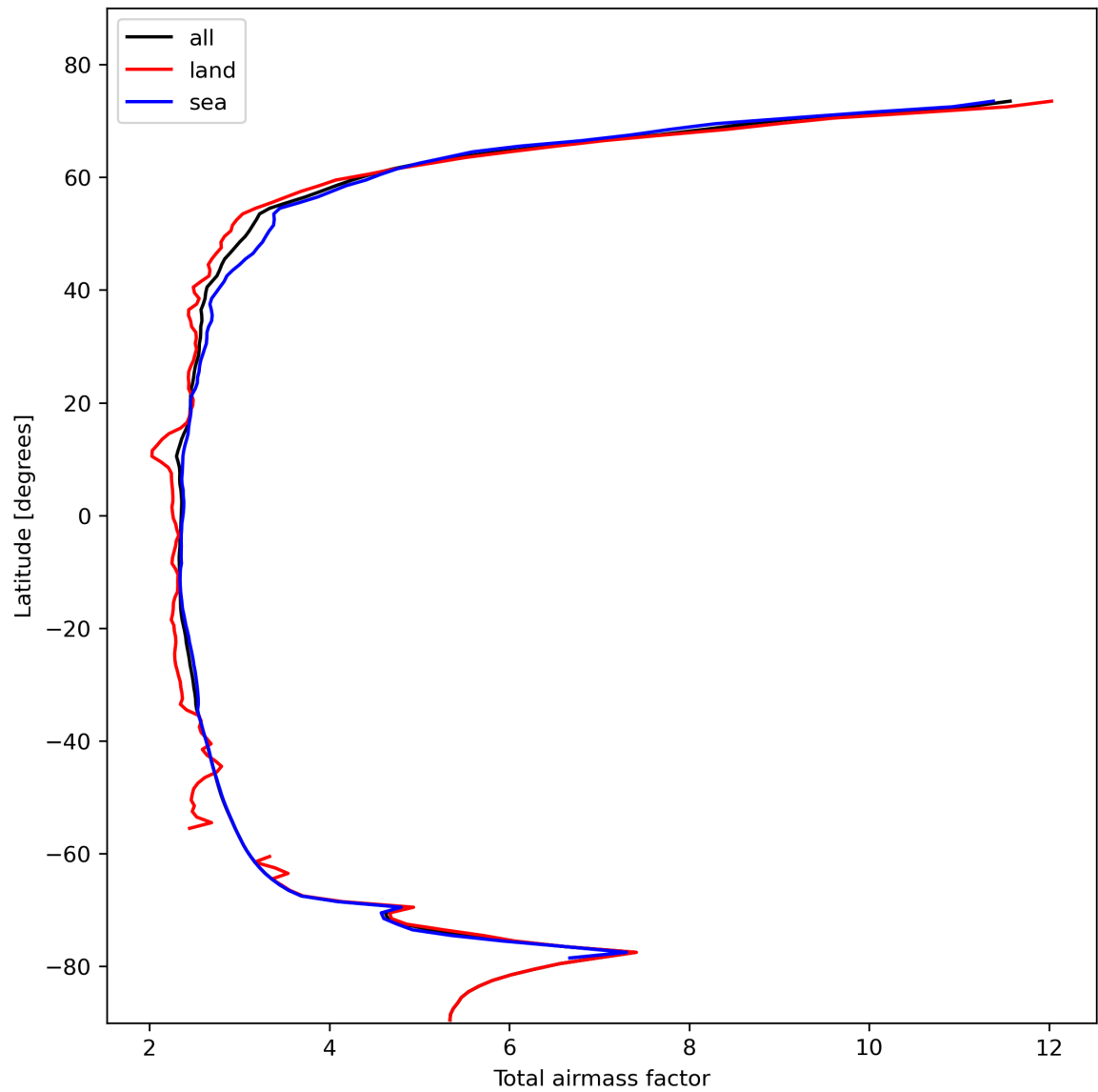
Figure 15: Zonal average of “Total airmass factor” for 2023-11-02 to 2023-11-03.
