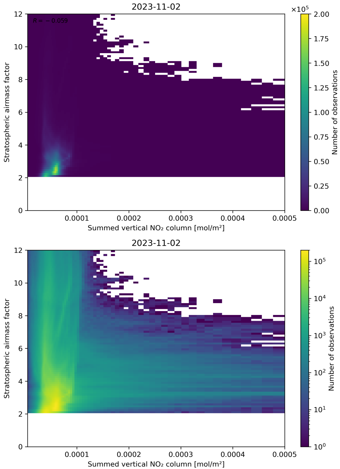
Figure 103: Scatter density plot of “Summed vertical NO 2 column” against “Stratospheric airmass factor” for 2023-11-02 to 2023-11-03.
