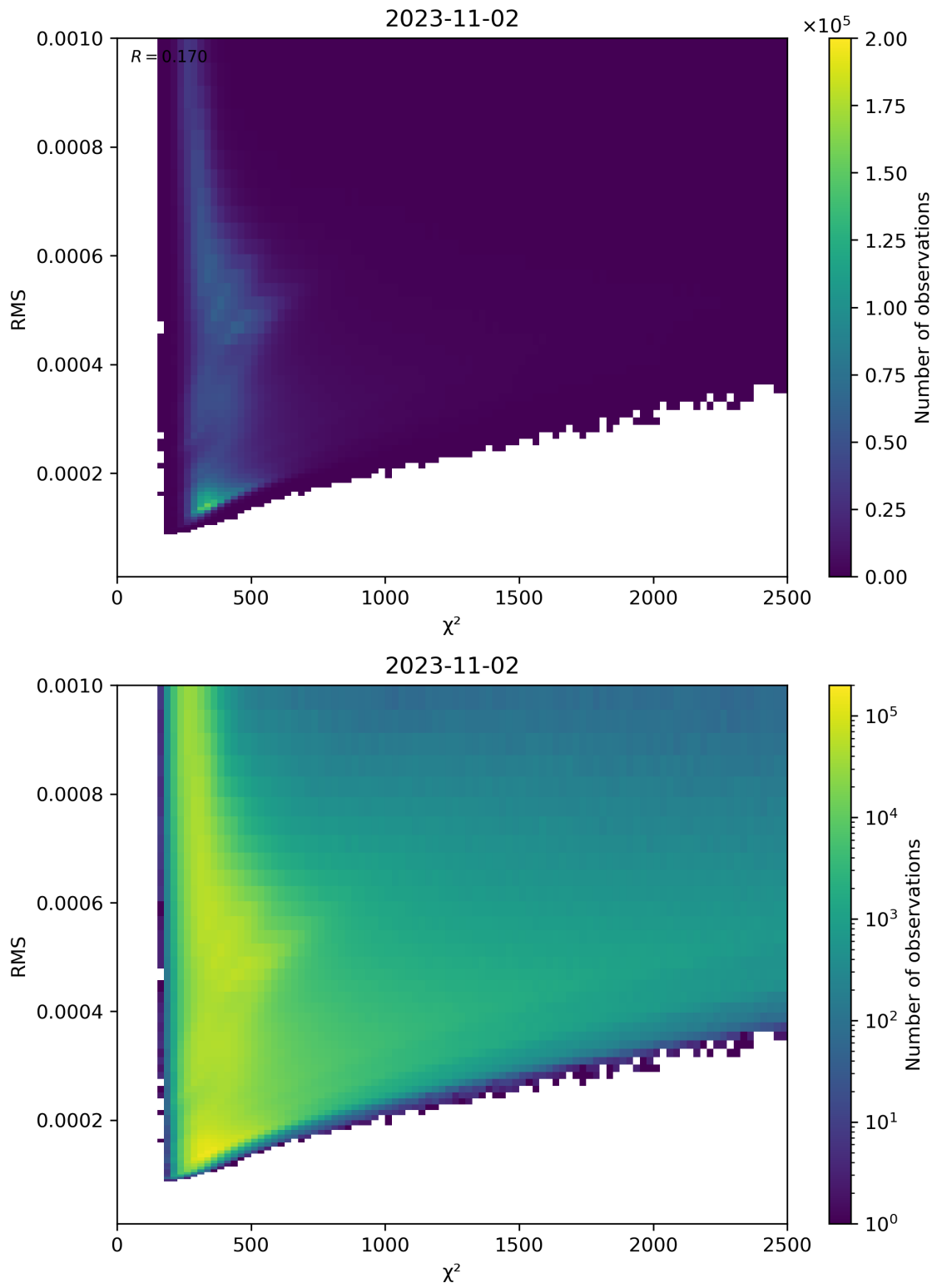
Figure 82: Scatter density plot of “ \chi^2 ” against “RMS” for 2023-11-02 to 2023-11-03.
