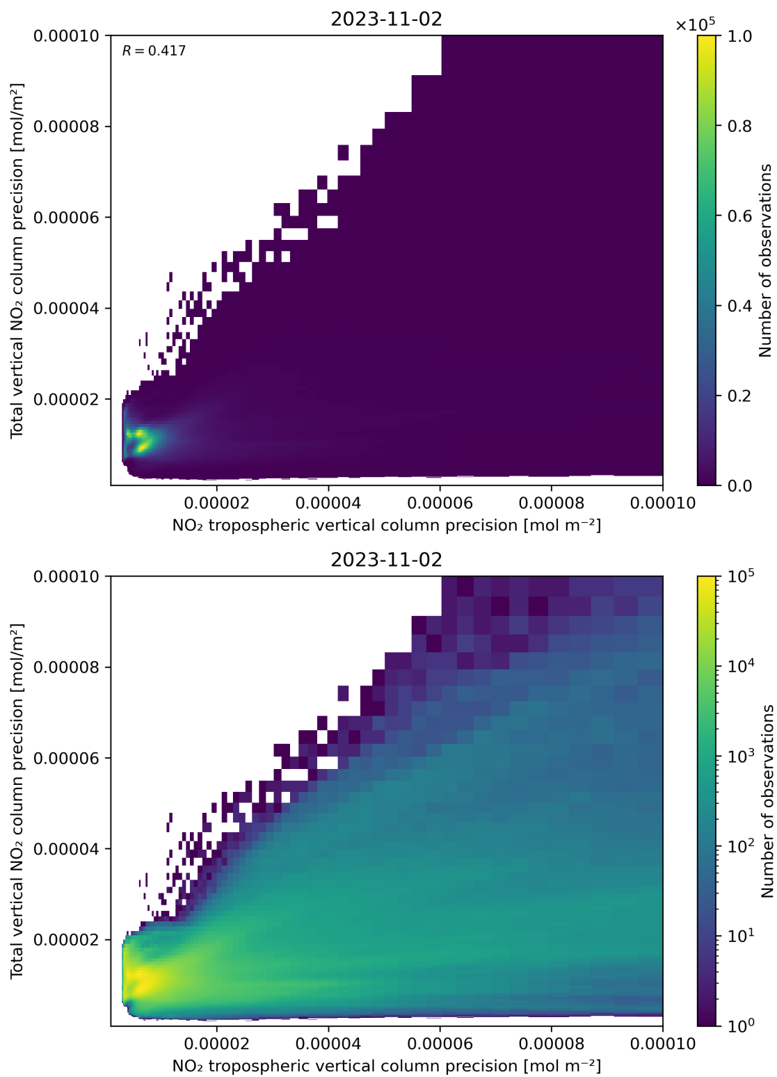
Figure 139: Scatter density plot of “NO 2 tropospheric vertical column precision” against “Total vertical NO 2 column precision” for 2023-11-02 to 2023-11-03.
