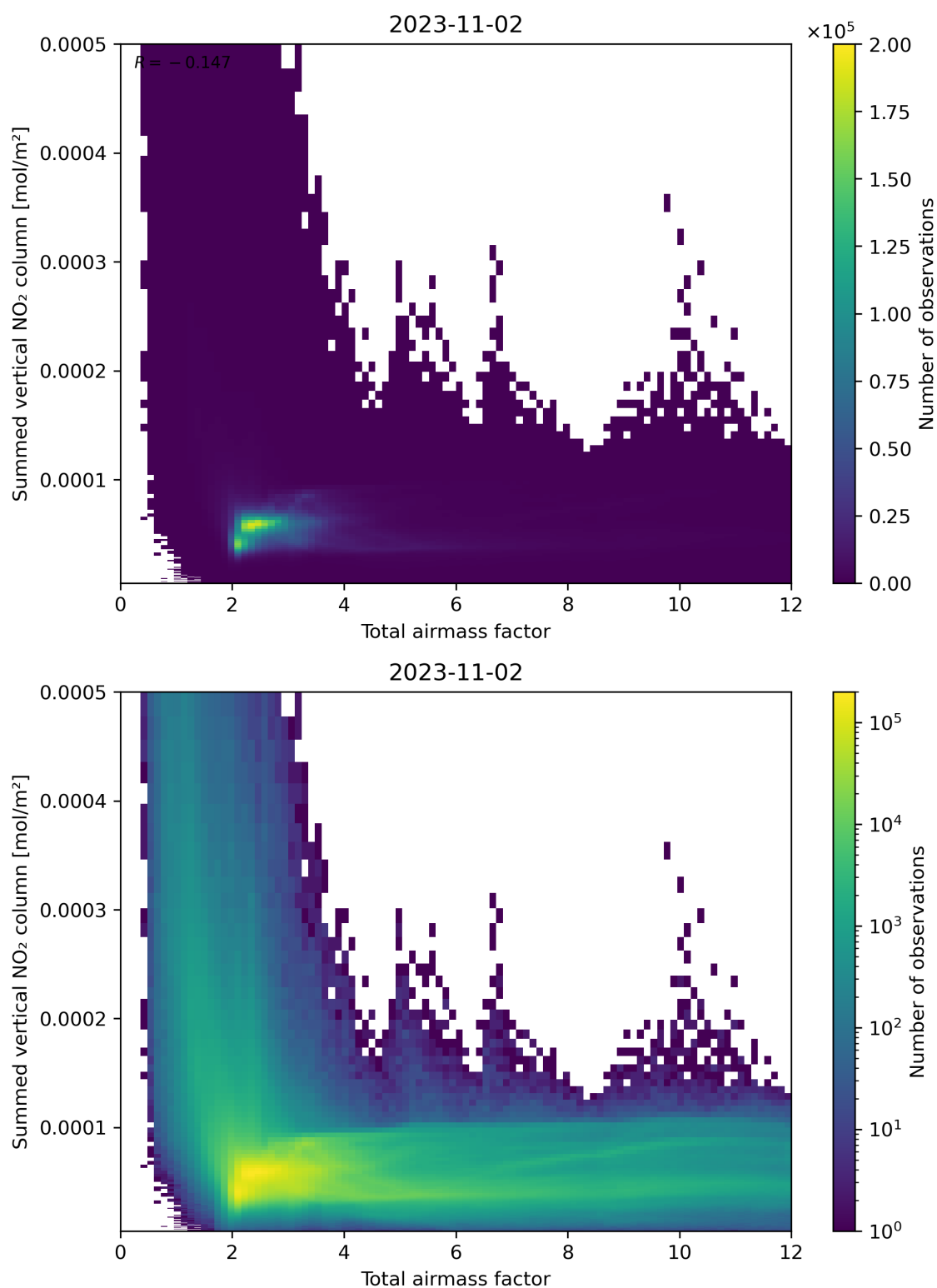
Figure 65: Scatter density plot of “Total airmass factor” against “Summed vertical NO 2 column” for 2023-11-02 to 2023-11-03.
