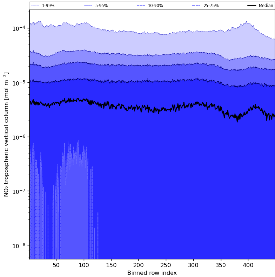
Figure 46: Along track statistics of “NO 2 tropospheric vertical column” for 2023-11-02 to 2023-11-03
