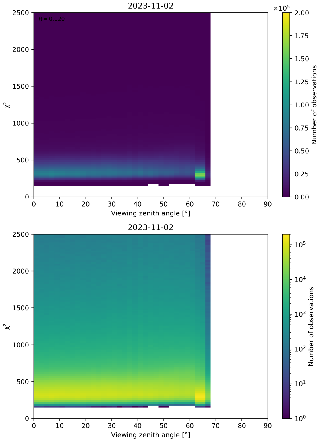
Figure 162: Scatter density plot of “Viewing zenith angle” against “ \chi^2 ” for 2023-11-02 to 2023-11-03.
