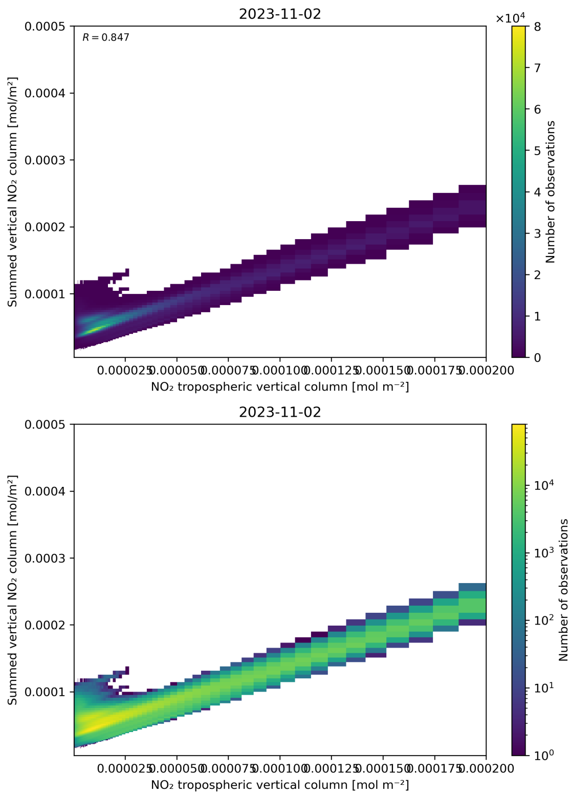
Figure 126: Scatter density plot of “NO 2 tropospheric vertical column” against “Summed vertical NO 2 column” for 2023-11-02 to 2023-11-03.
