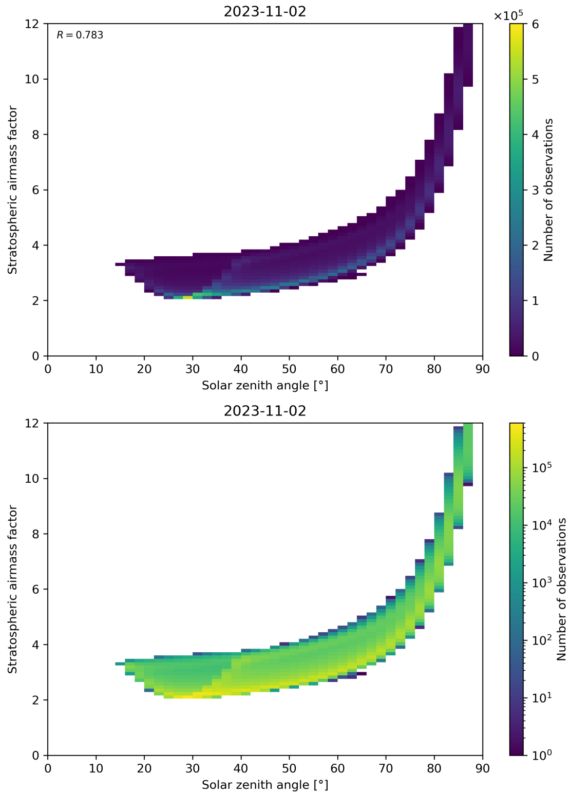
Figure 145: Scatter density plot of “Solar zenith angle” against “Stratospheric airmass factor” for 2023-11-02 to 2023-11-03.
