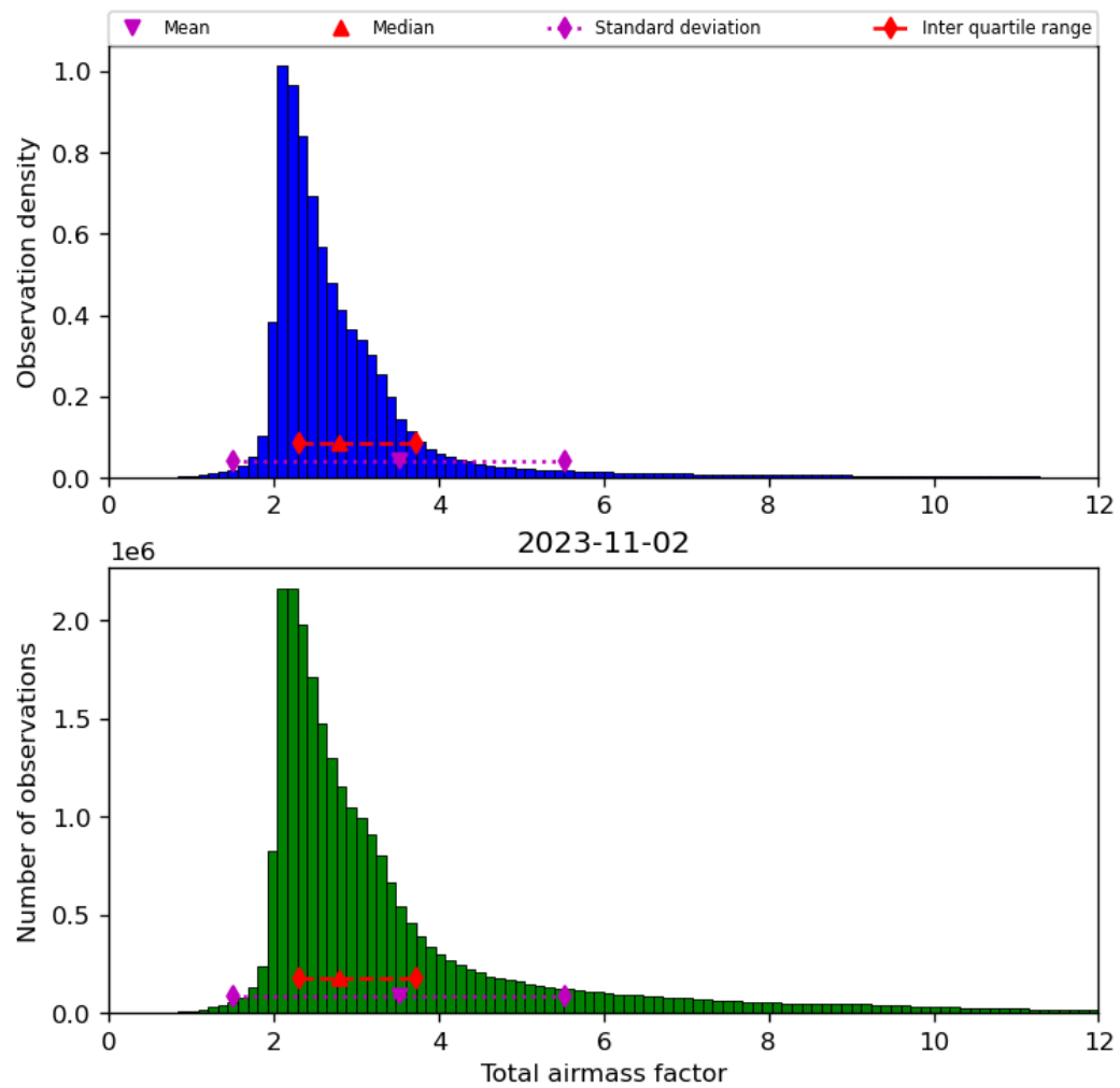
Figure 32: Histogram of “Total airmass factor” for 2023-11-02 to 2023-11-03
