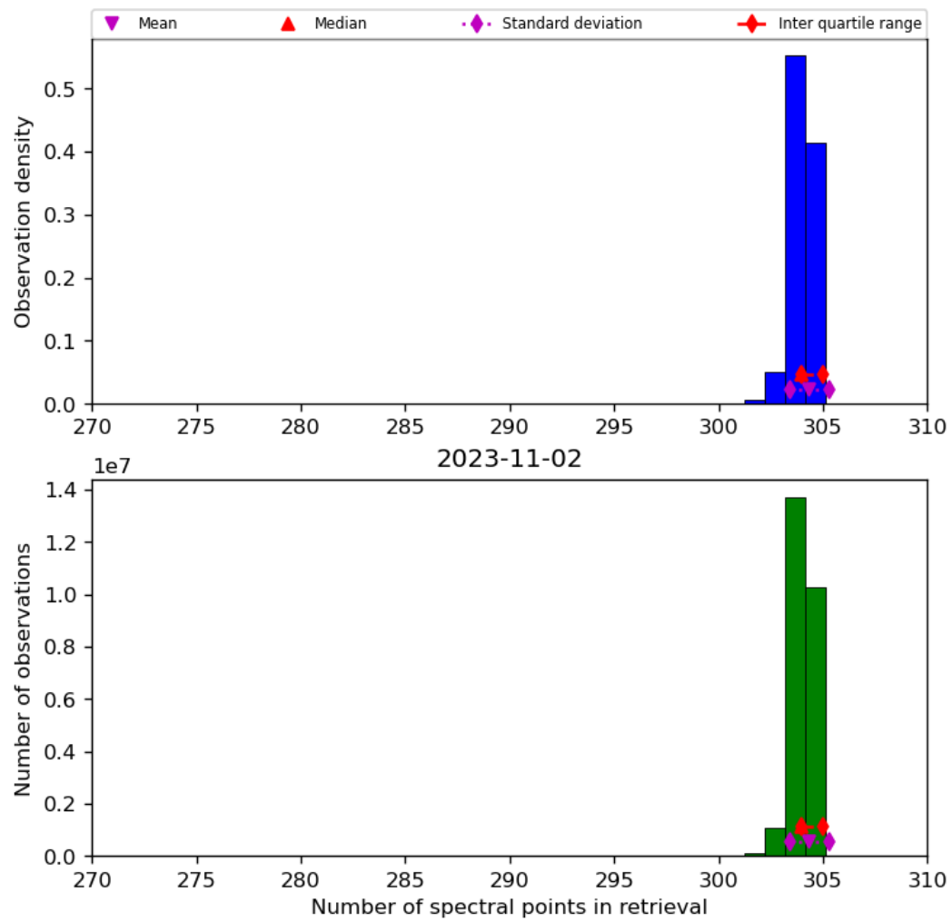
Figure 33: Histogram of “Number of spectral points in retrieval” for 2023-11-02 to 2023-11-03
