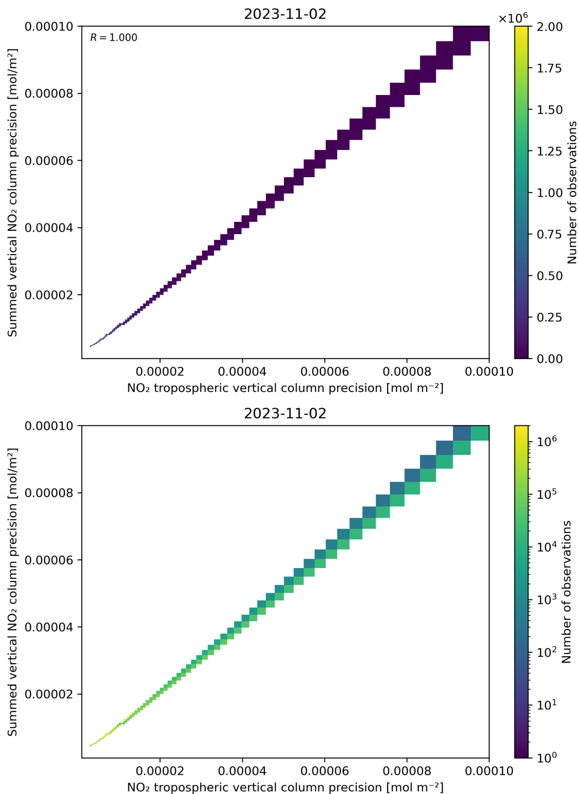
Figure 137: Scatter density plot of “NO 2 tropospheric vertical column precision” against “Summed vertical NO 2 column precision” for 2023-11-02 to 2023-11-03.
