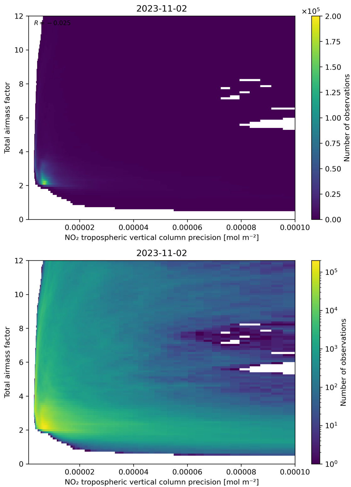
Figure 132: Scatter density plot of “NO 2 tropospheric vertical column precision” against “Total air mass factor” for 2023-11-02 to 2023-11-03.
