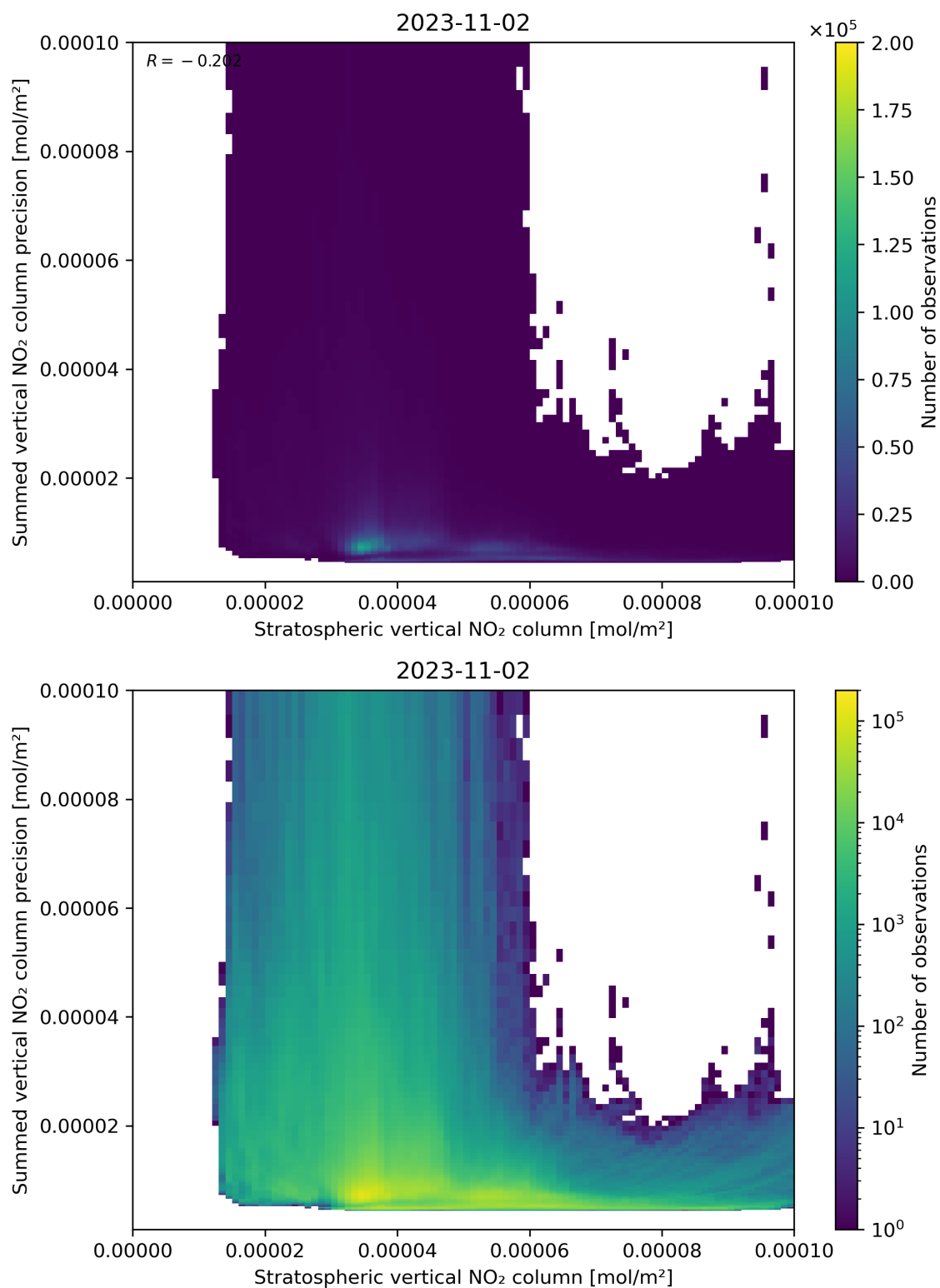
Figure 99: Scatter density plot of “Stratospheric vertical NO 2 column” against “Summed vertical NO 2 column precision” for 2023-11-02 to 2023-11-03.
