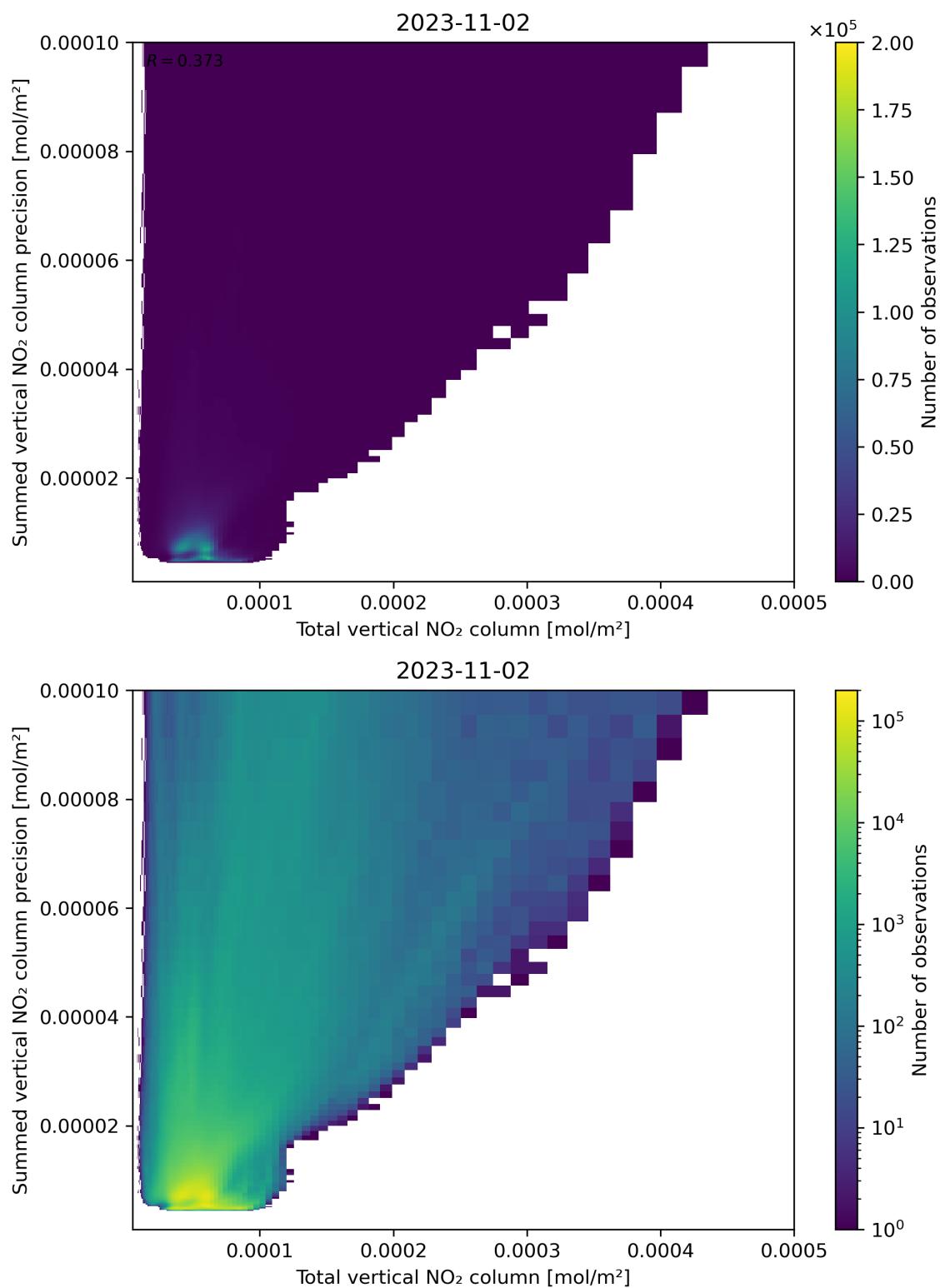
Figure 113: Scatter density plot of “Total vertical NO 2 column” against “Summed vertical NO 2 column precision” for 2023-11-02 to 2023-11-03.
