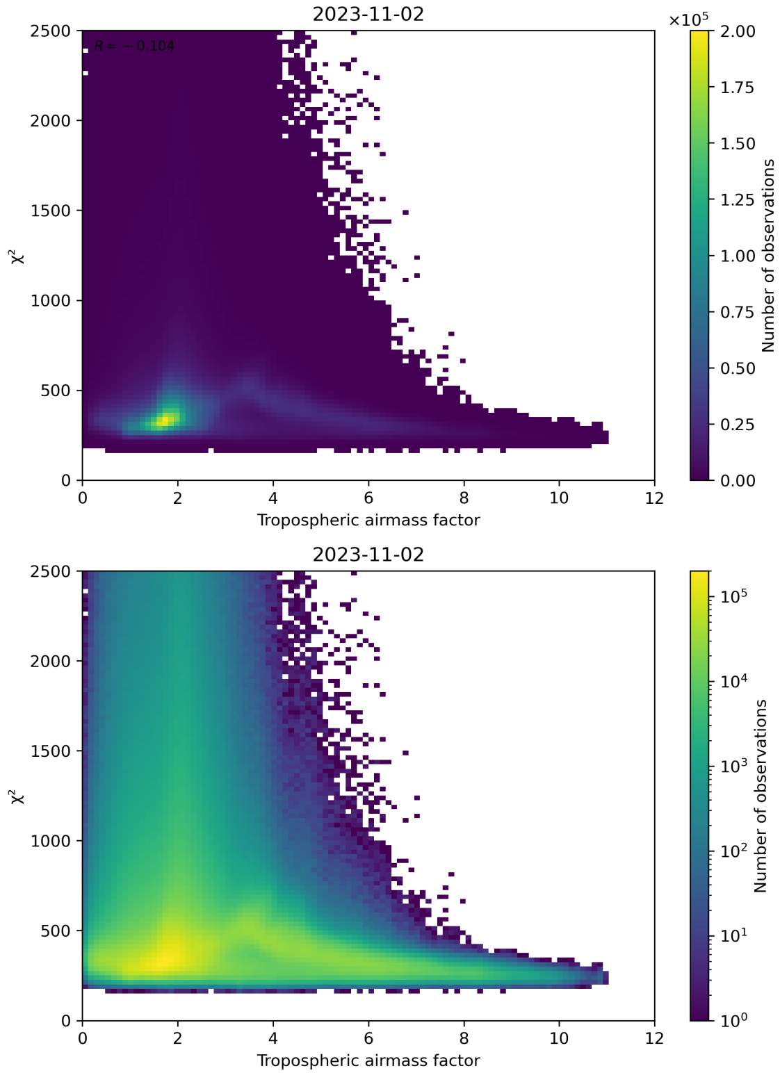
Figure 73: Scatter density plot of “Tropospheric airmass factor” against “ \chi^2 ” for 2023-11-02 to 2023-11-03.
