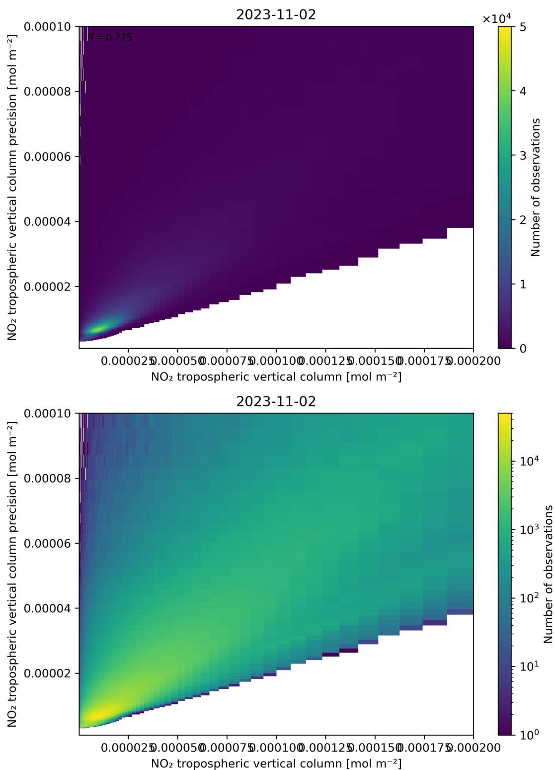
Figure 130: Scatter density plot of “NO 2 tropospheric vertical column” against “NO 2 tropospheric vertical column precision” for 2023-11-02 to 2023-11-03.
