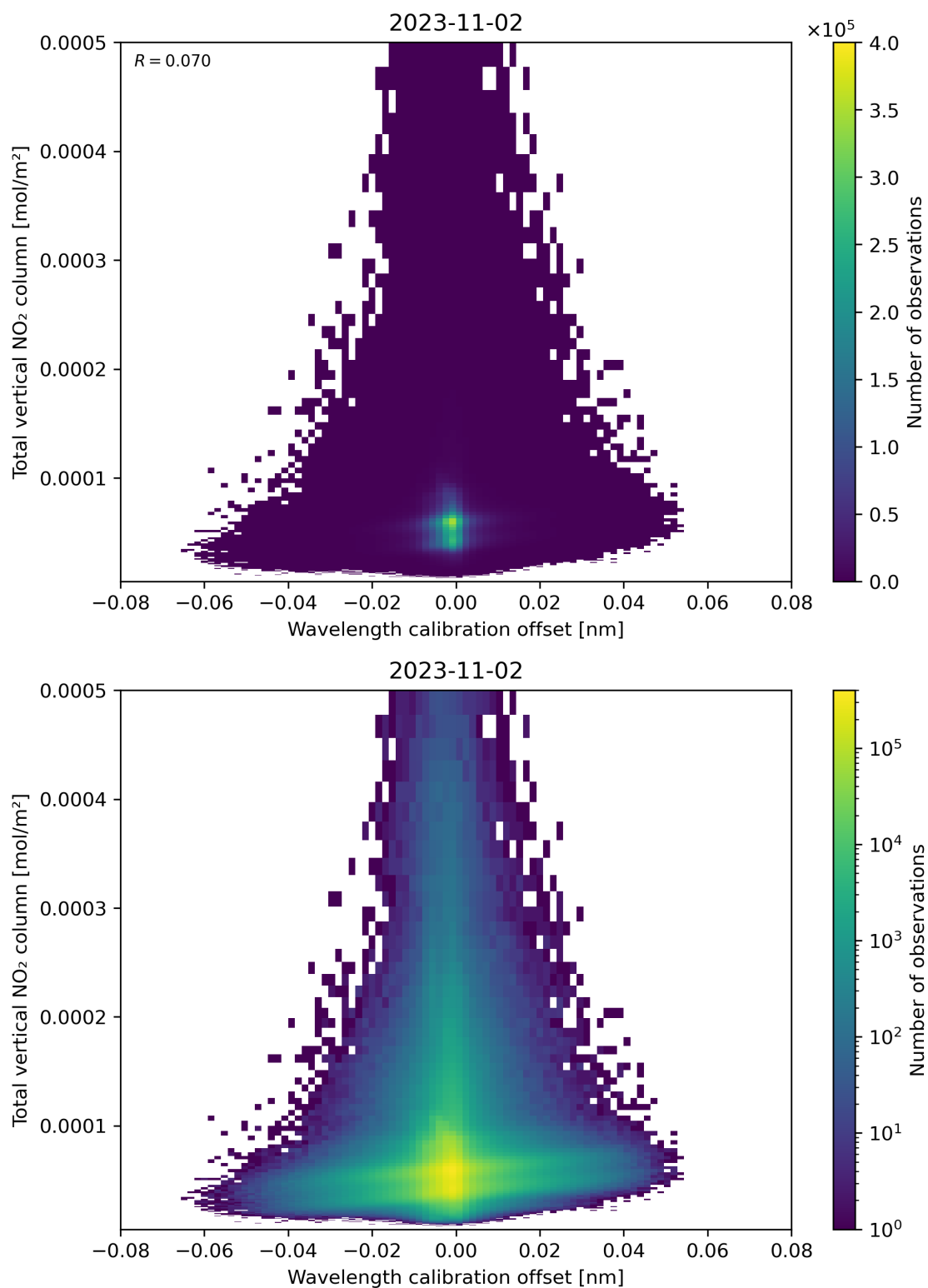
Figure 179: Scatter density plot of “Wavelength calibration offset” against “Total vertical NO 2 column” for 2023-11-02 to 2023-11-03.
