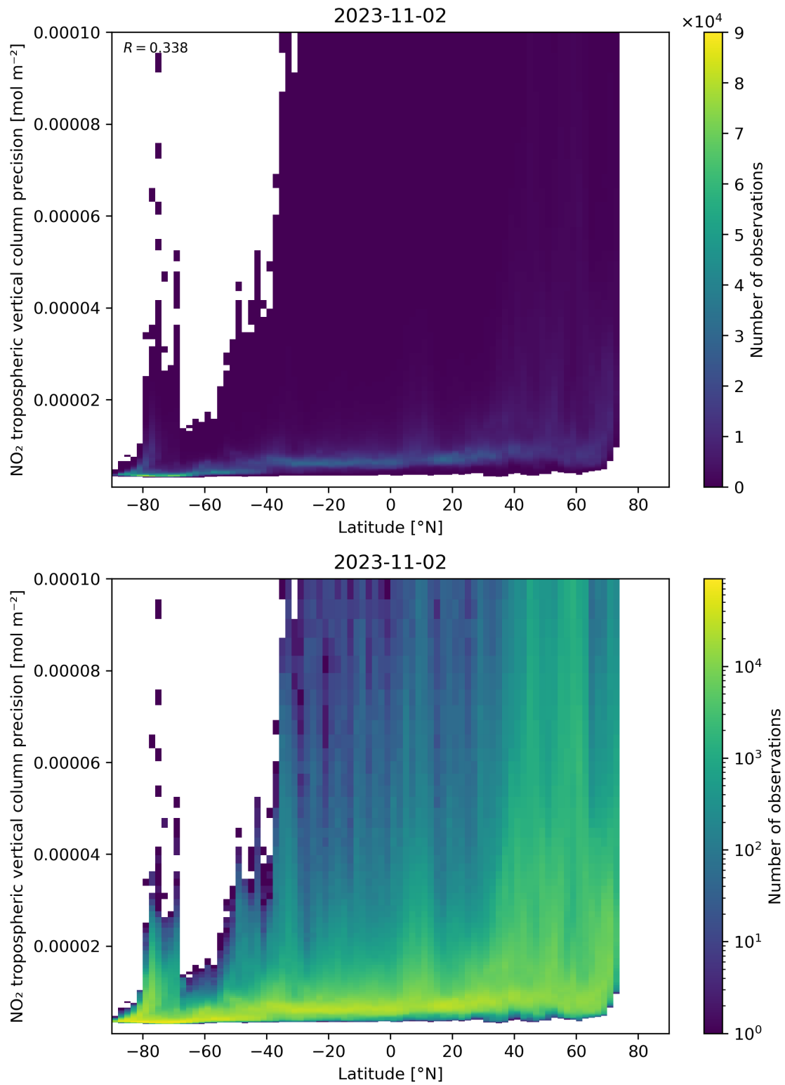
Figure 93: Scatter density plot of “Latitude” against “NO 2 tropospheric vertical column precision” for 2023-11-02 to 2023-11-03.
