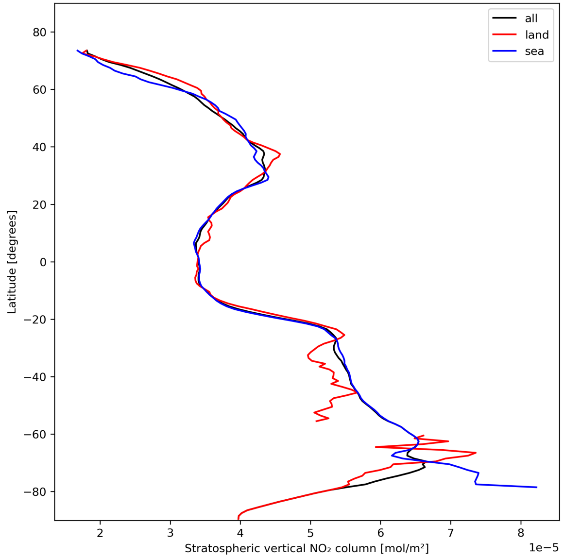
Figure 19: Zonal average of “Stratospheric vertical NO 2 column” for 2023-11-02 to 2023-11-03.
