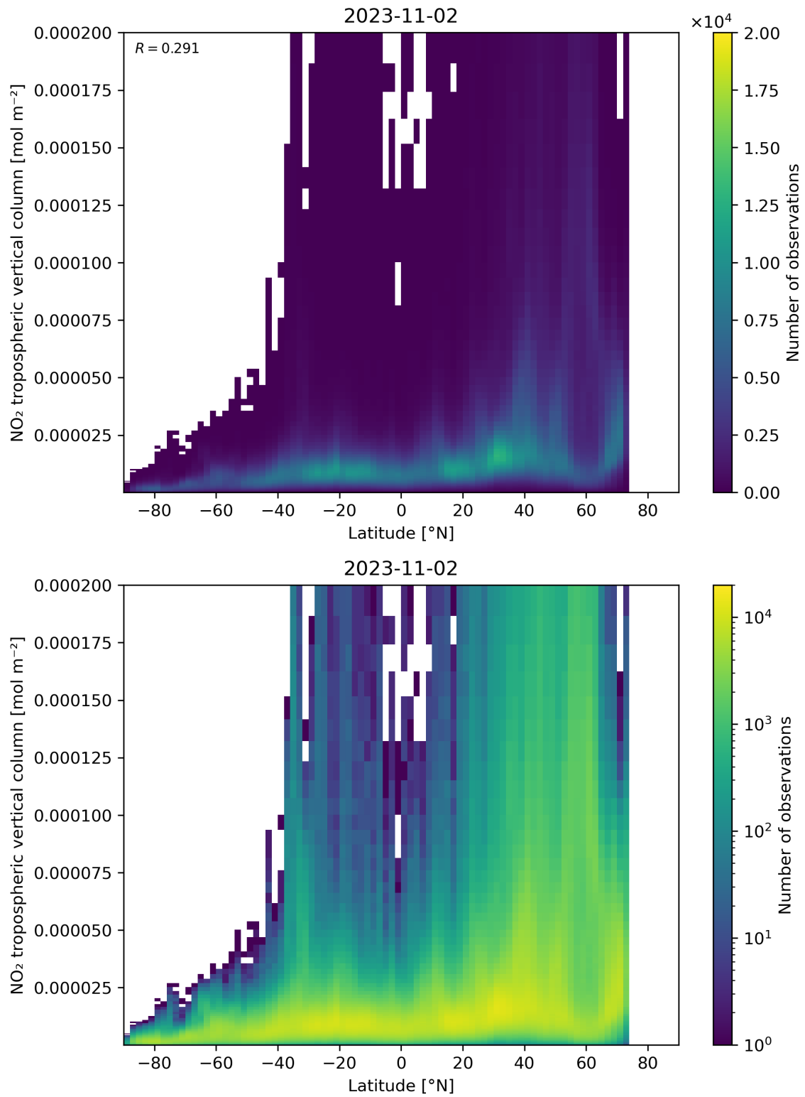
Figure 92: Scatter density plot of “Latitude” against “NO 2 tropospheric vertical column” for 2023-11-02 to 2023-11-03.
