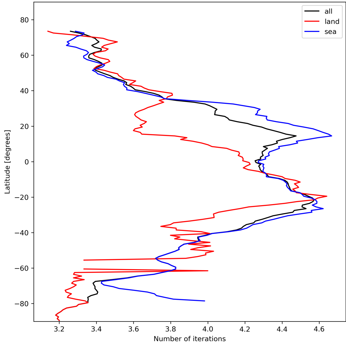
Figure 17: Zonal average of “Number of iterations” for 2023-11-02 to 2023-11-03.
