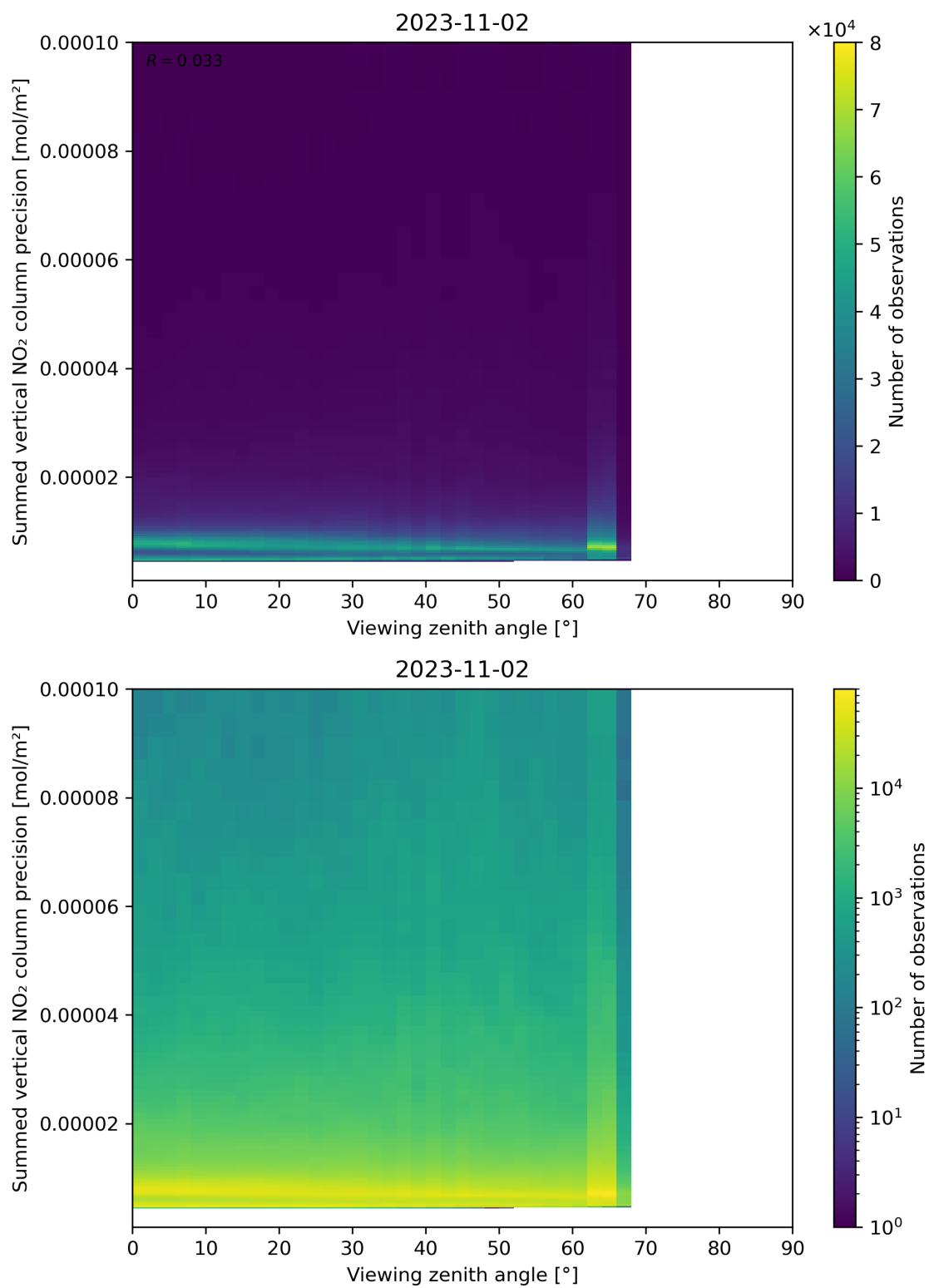
Figure 166: Scatter density plot of “Viewing zenith angle” against “Summed vertical NO 2 column precision” for 2023-11-02 to 2023-11-03.
