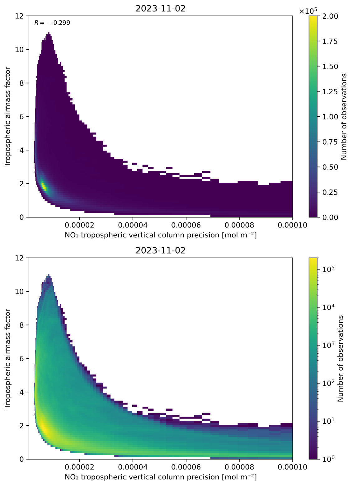
Figure 133: Scatter density plot of “NO 2 tropospheric vertical column precision” against “Tropospheric airmass factor” for 2023-11-02 to 2023-11-03.
