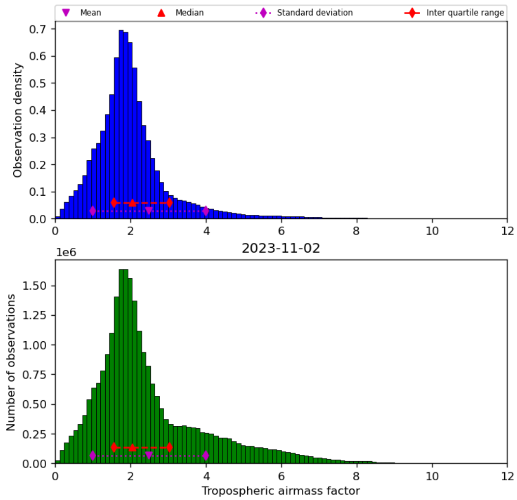
Figure 31: Histogram of “Tropospheric airmass factor” for 2023-11-02 to 2023-11-03
