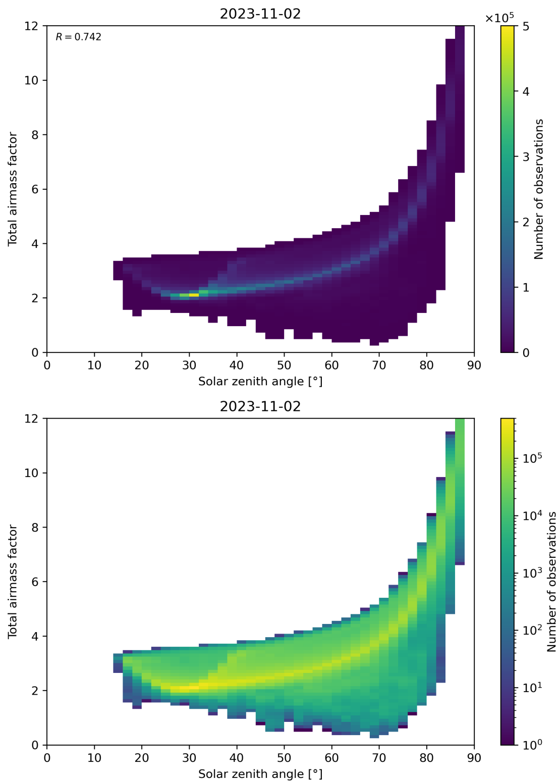
Figure 146: Scatter density plot of “Solar zenith angle” against “Total air mass factor” for 2023-11-02 to 2023-11-03.
