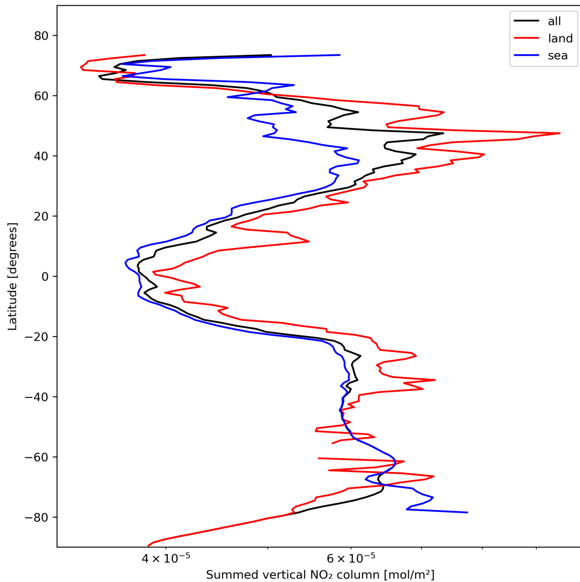
Figure 23: Zonal average of “Summed vertical NO 2 column” for 2023-11-02 to 2023-11-03.
