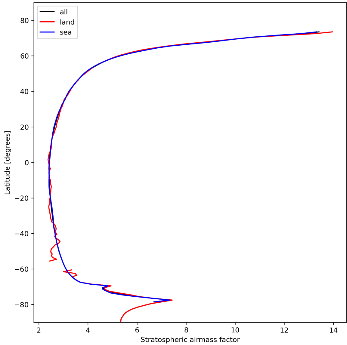
Figure 27: Zonal average of “Stratospheric air mass factor” for 2023-11-02 to 2023-11-03.
