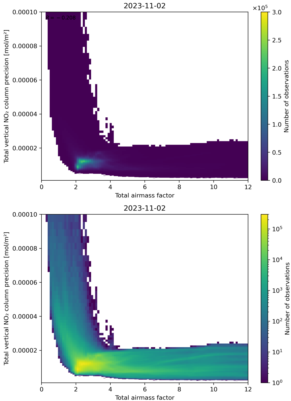
Figure 68: Scatter density plot of “Total airmass factor” against “Total vertical NO 2 column precision” for 2023-11-02 to 2023-11-03.
