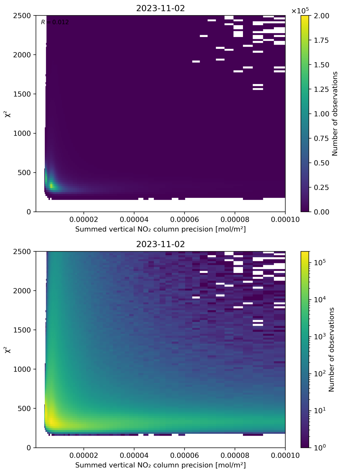
Figure 107: Scatter density plot of “Summed vertical NO 2 column precision” against “ \chi^2 ” for 2023-11-02 to 2023-11-03.
