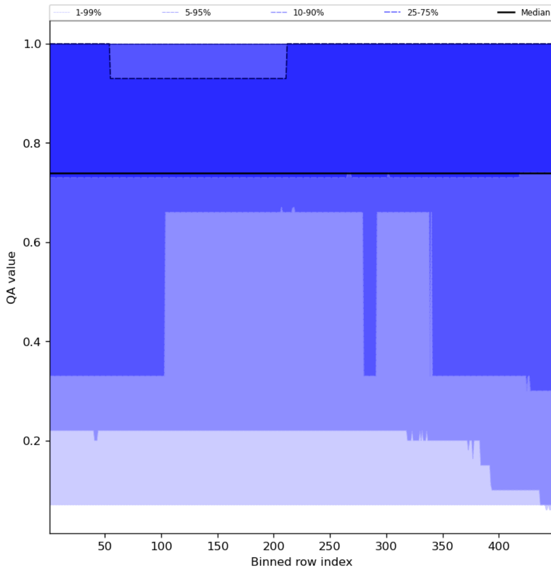
Figure 45: Along track statistics of “QA value” for 2023-11-02 to 2023-11-04
