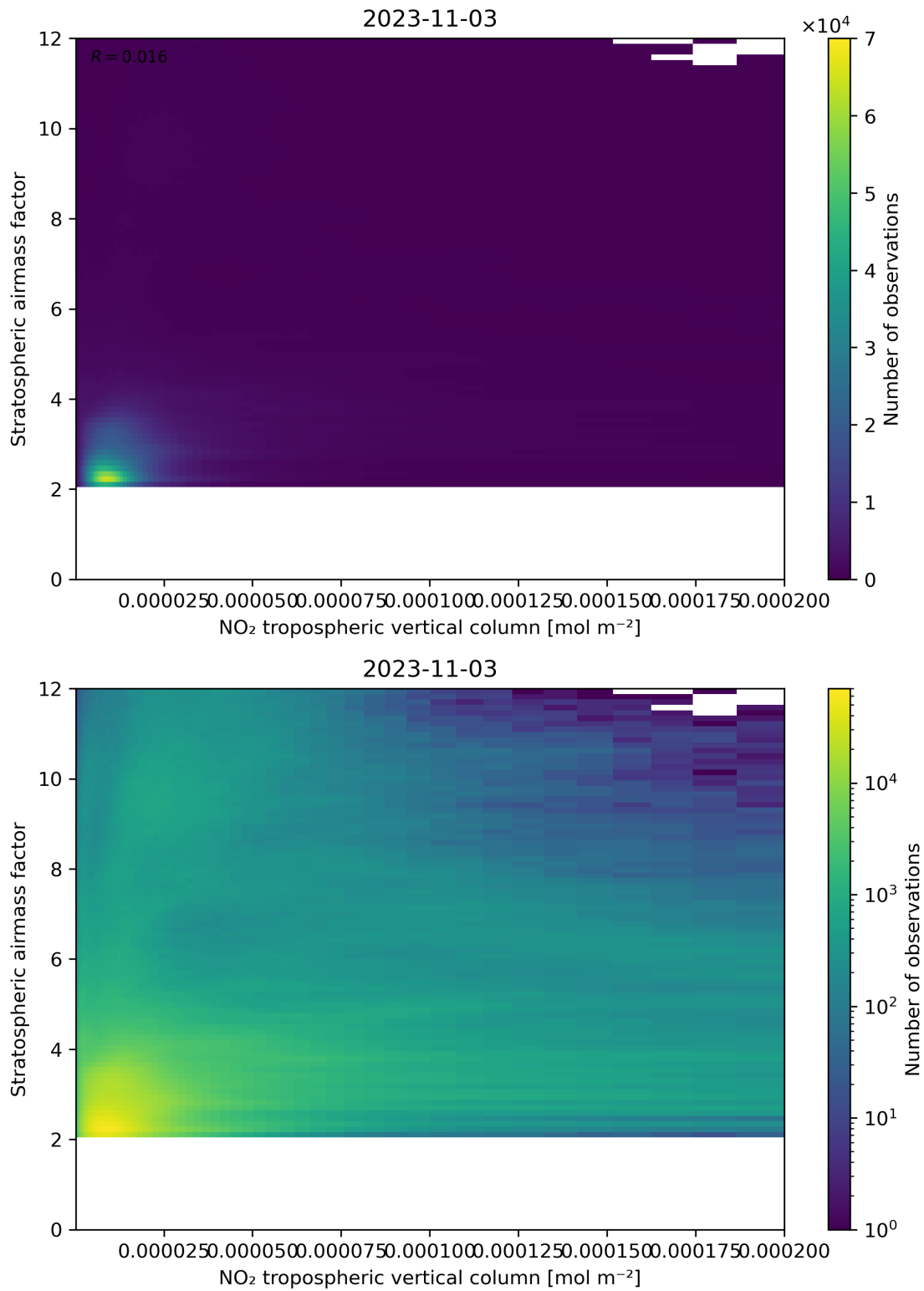
Figure 121: Scatter density plot of “NO 2 tropospheric vertical column” against “Stratospheric airmass factor” for 2023-11-02 to 2023-11-04.
