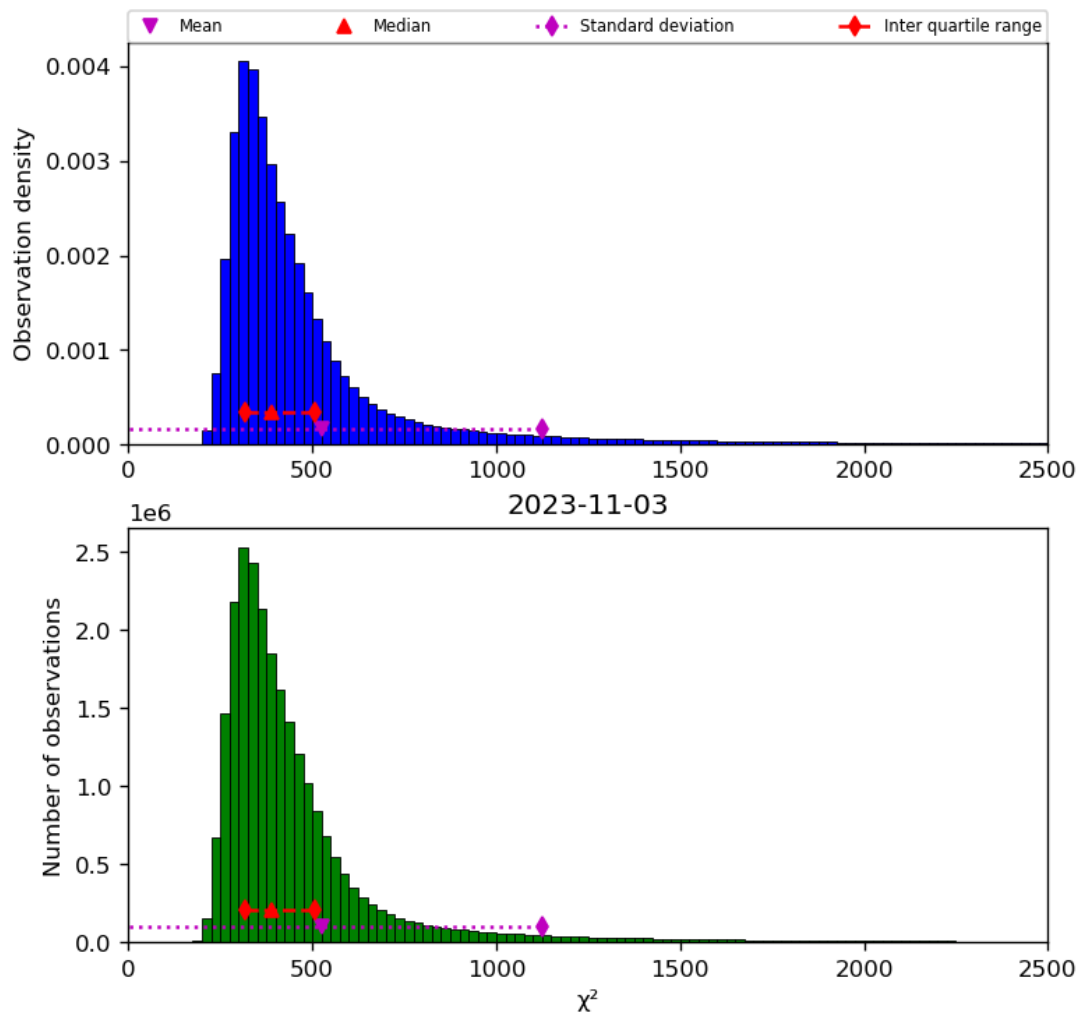
Figure 42: Histogram of “ \chi^2 ” for 2023-11-02 to 2023-11-04
