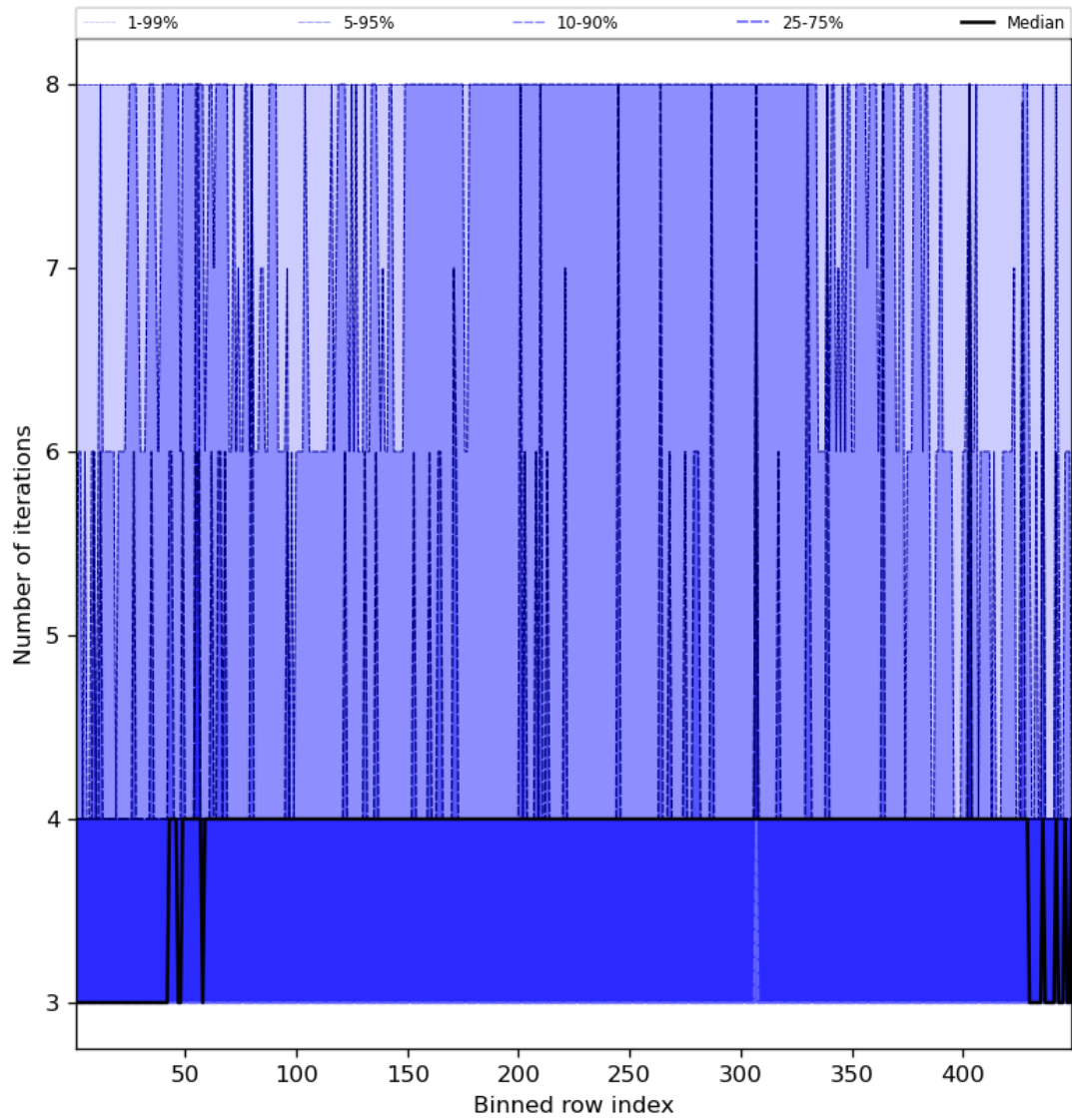
Figure 51: Along track statistics of “Number of iterations” for 2023-11-02 to 2023-11-04
