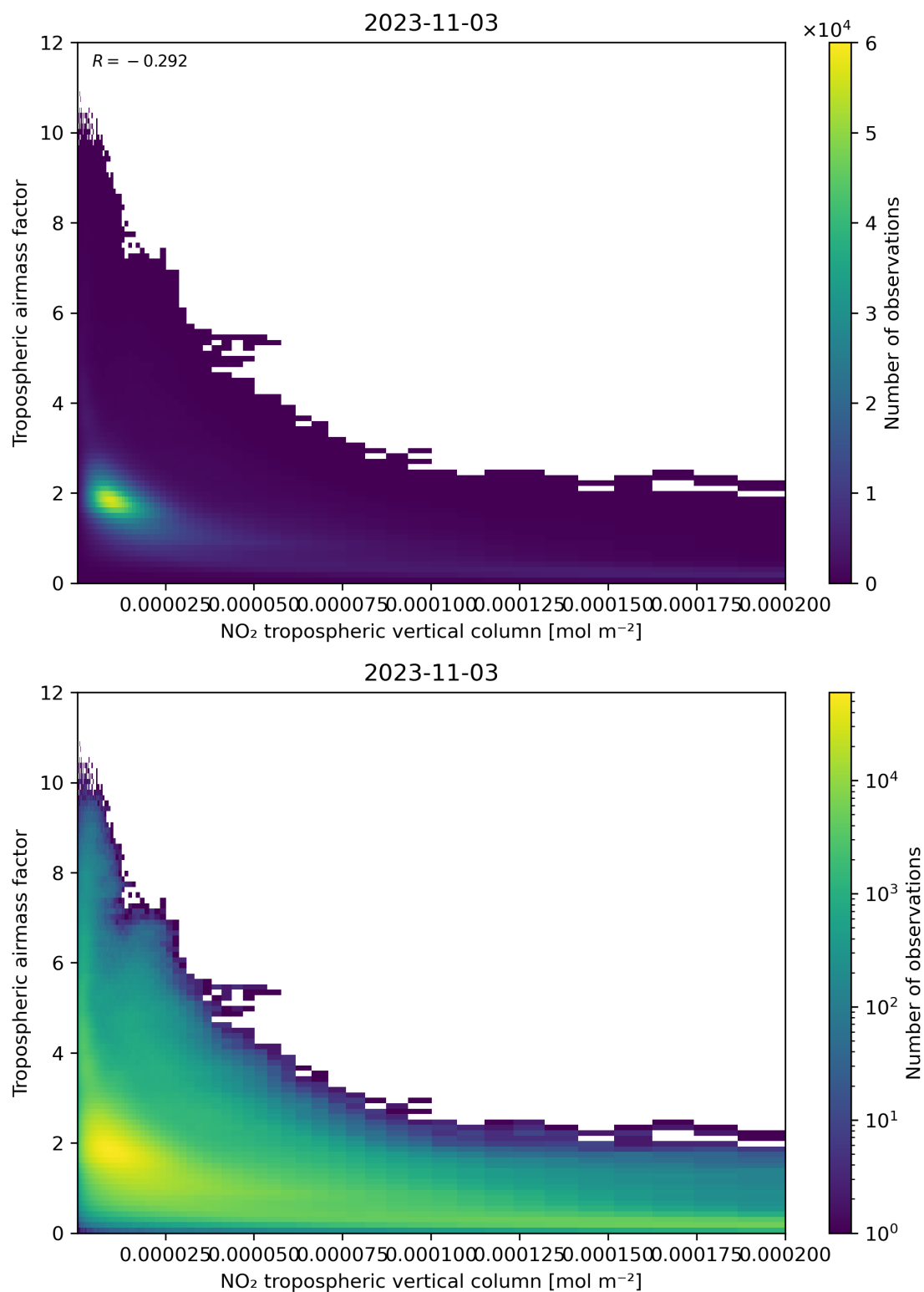
Figure 123: Scatter density plot of “NO 2 tropospheric vertical column” against “Tropospheric air mass factor” for 2023-11-02 to 2023-11-04.
