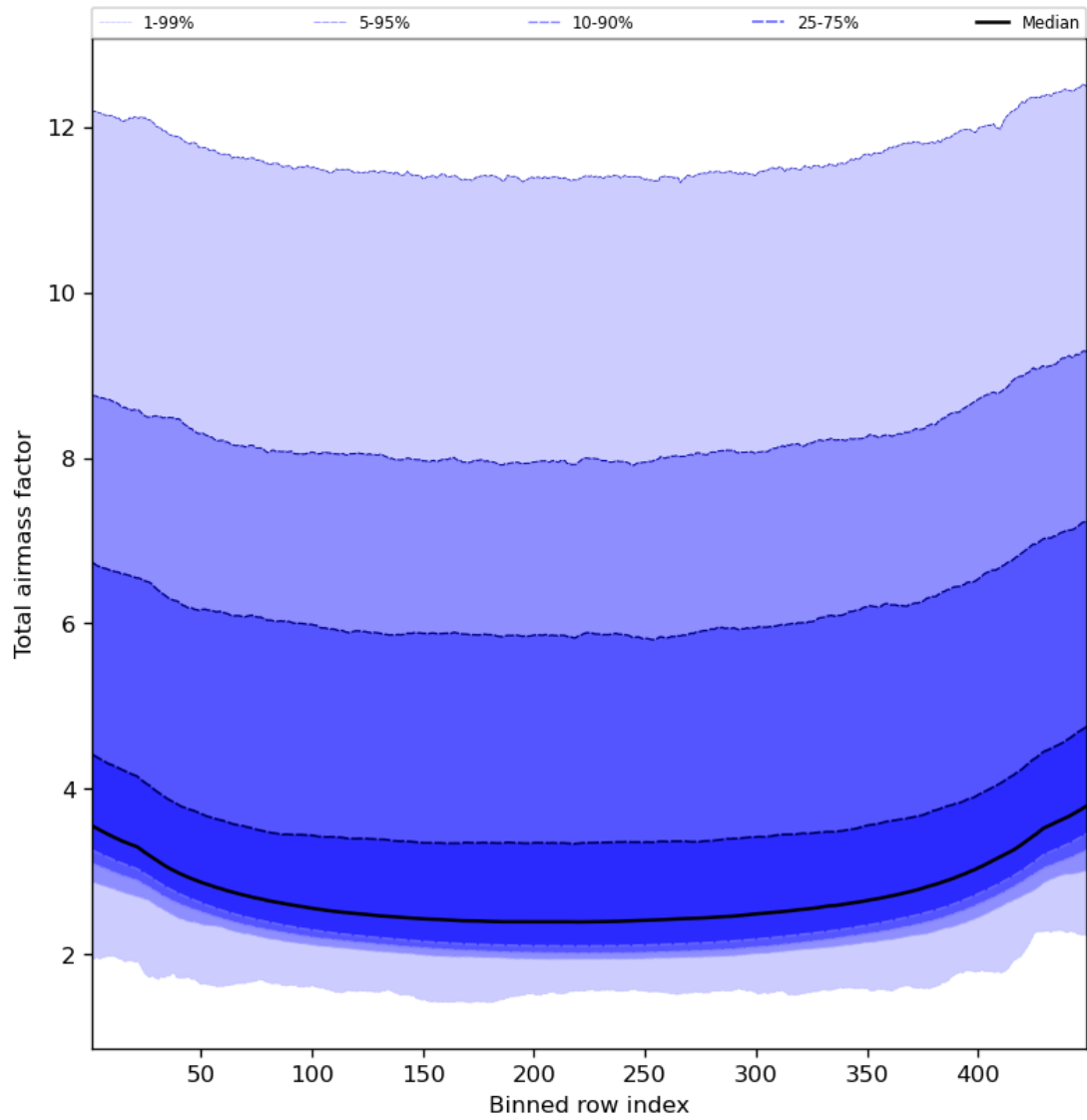
Figure 49: Along track statistics of “Total airmass factor” for 2023-11-02 to 2023-11-04
