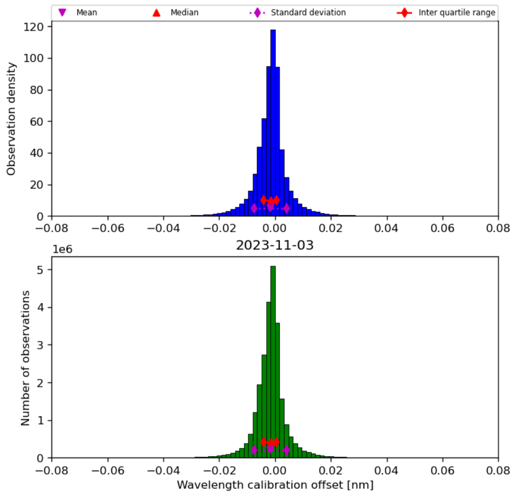
Figure 35: Histogram of “Wavelength calibration offset” for 2023-11-02 to 2023-11-04
