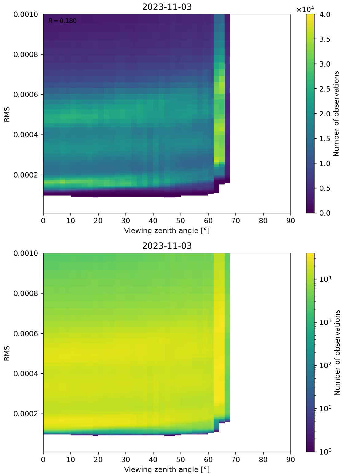
Figure 171: Scatter density plot of “Viewing zenith angle” against “RMS” for 2023-11-02 to 2023-11-04.
