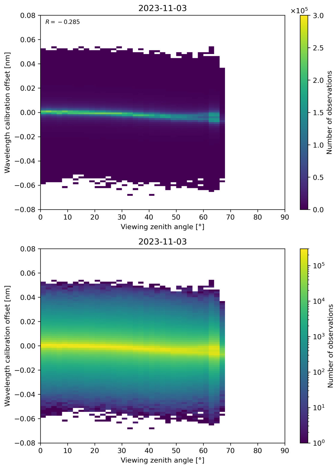
Figure 173: Scatter density plot of “Viewing zenith angle” against “Wavelength calibration offset” for 2023-11-02 to 2023-11-04.
