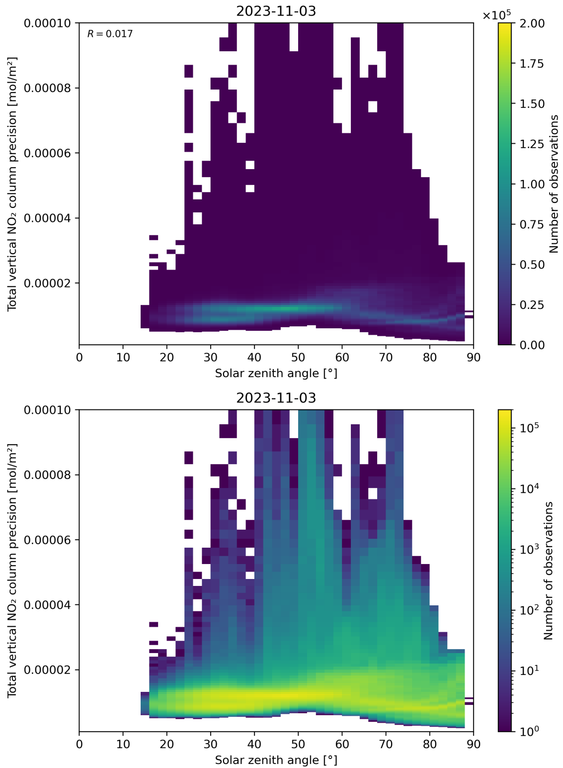
Figure 154: Scatter density plot of “Solar zenith angle” against “Total vertical NO 2 column precision” for 2023-11-02 to 2023-11-04.
