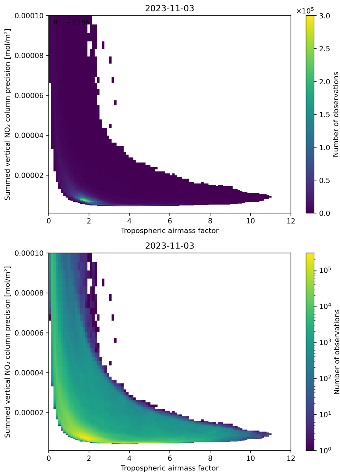
Figure 76: Scatter density plot of “Tropospheric air mass factor” against “Summed vertical NO 2 column precision” for 2023-11-02 to 2023-11-04.
