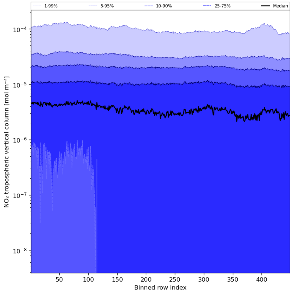
Figure 46: Along track statistics of “NO 2 tropospheric vertical column” for 2023-11-02 to 2023-11-04
