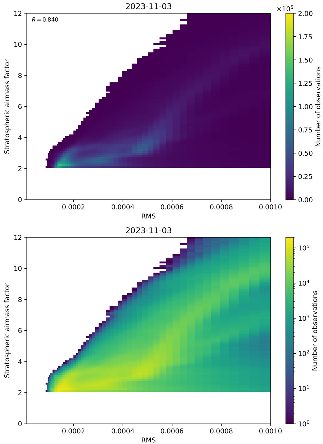
Figure 144: Scatter density plot of “RMS” against “Stratospheric airmass factor” for 2023-11-02 to 2023-11-04.
