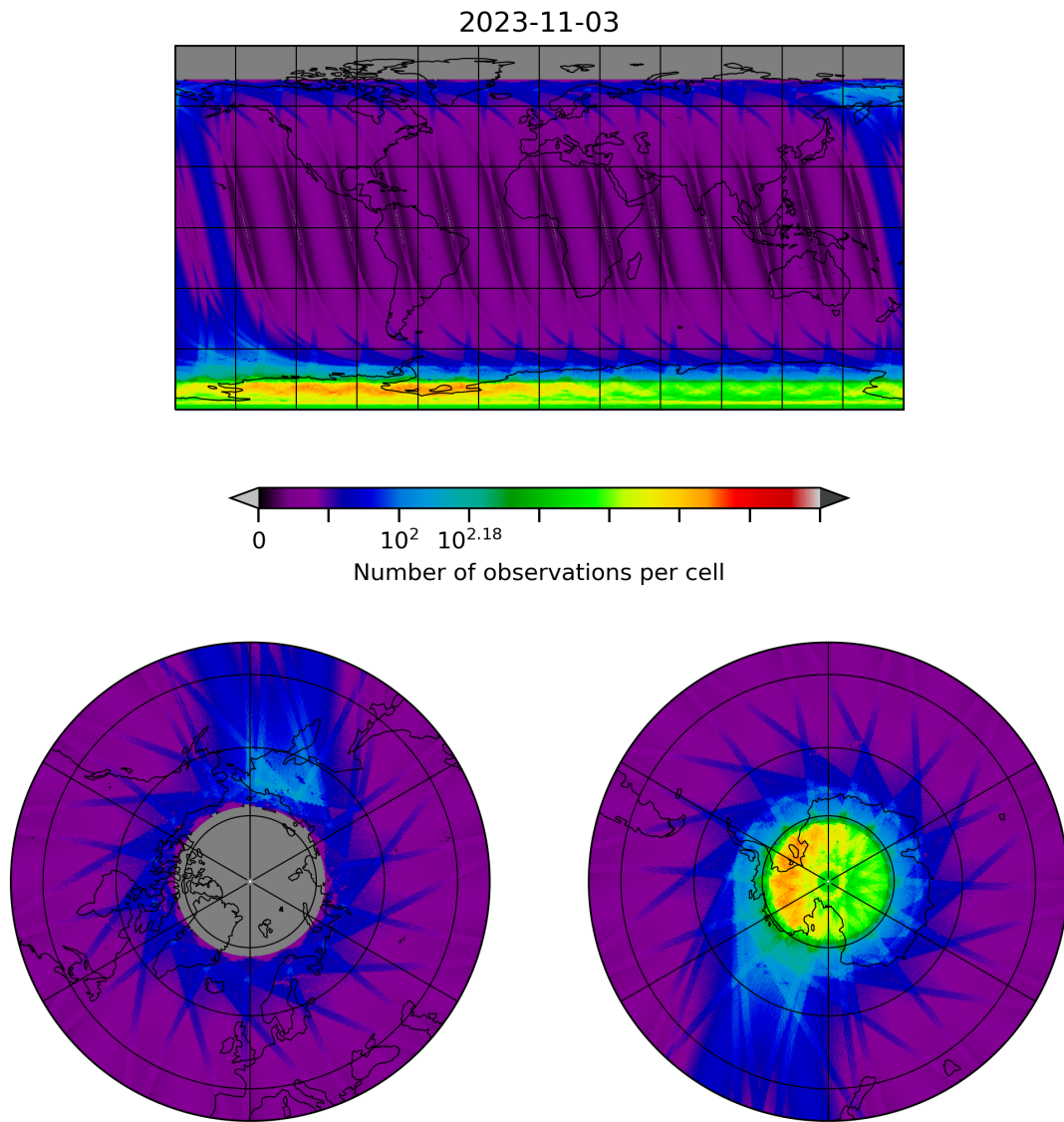
Figure 10: Map of the number of observations for 2023-11-02 to 2023-11-04
