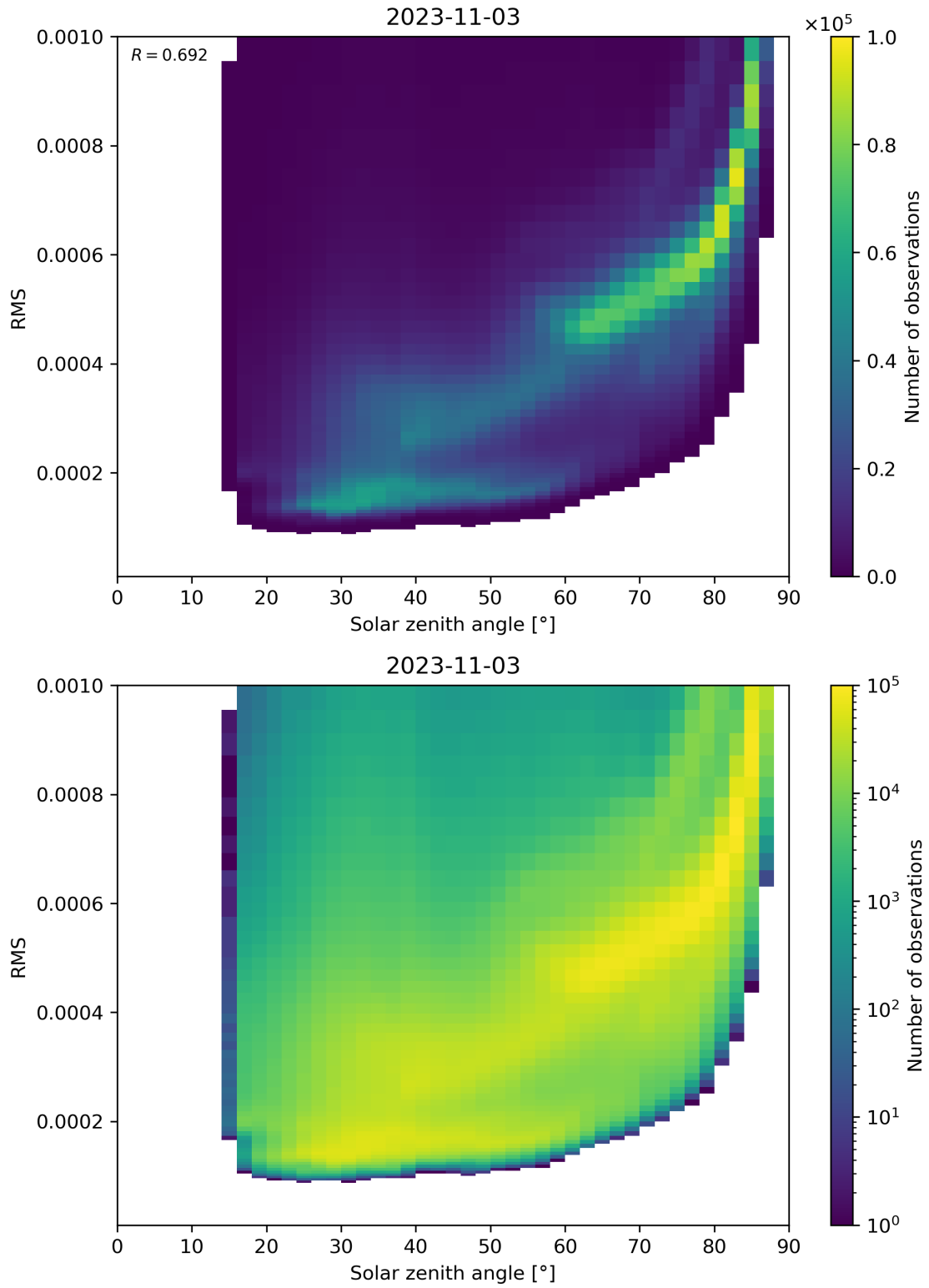
Figure 157: Scatter density plot of “Solar zenith angle” against “RMS” for 2023-11-02 to 2023-11-04.
