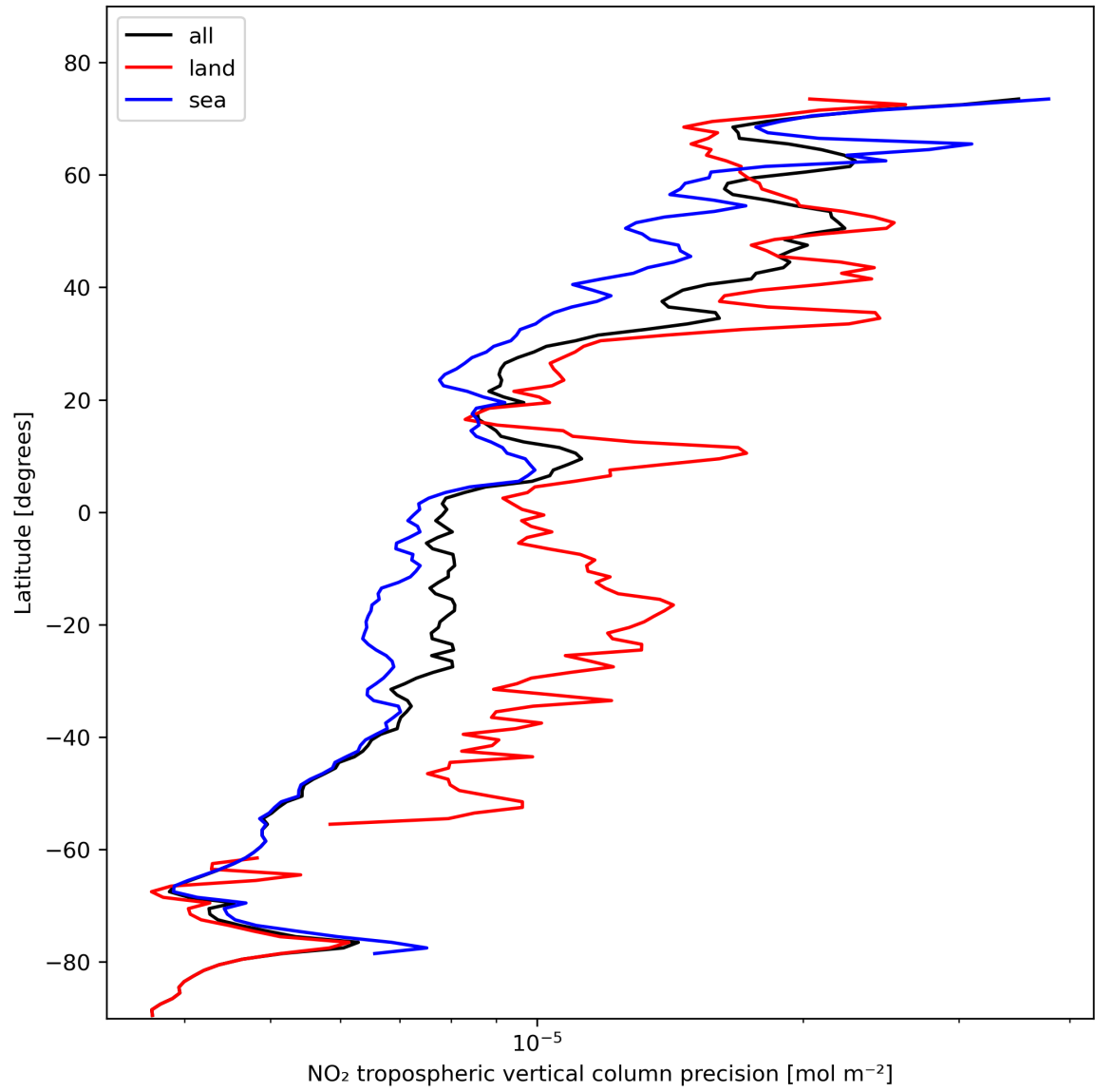
Figure 13: Zonal average of “NO 2 tropospheric vertical column precision” for 2023-11-02 to 2023-11-04.
