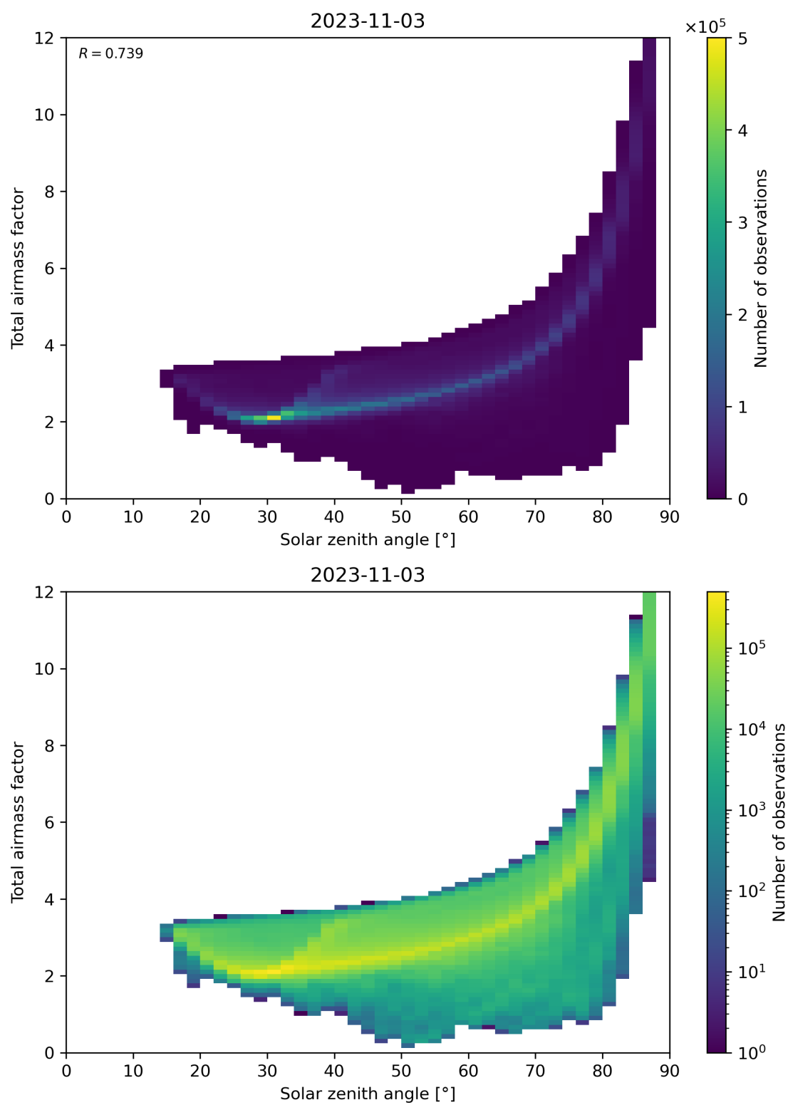
Figure 146: Scatter density plot of “Solar zenith angle” against “Total air mass factor” for 2023-11-02 to 2023-11-04.
