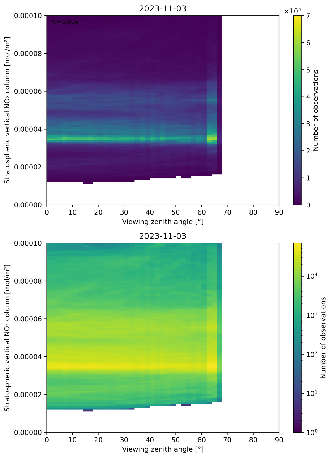
Figure 164: Scatter density plot of “Viewing zenith angle” against “Stratospheric vertical NO 2 column” for 2023-11-02 to 2023-11-04.
