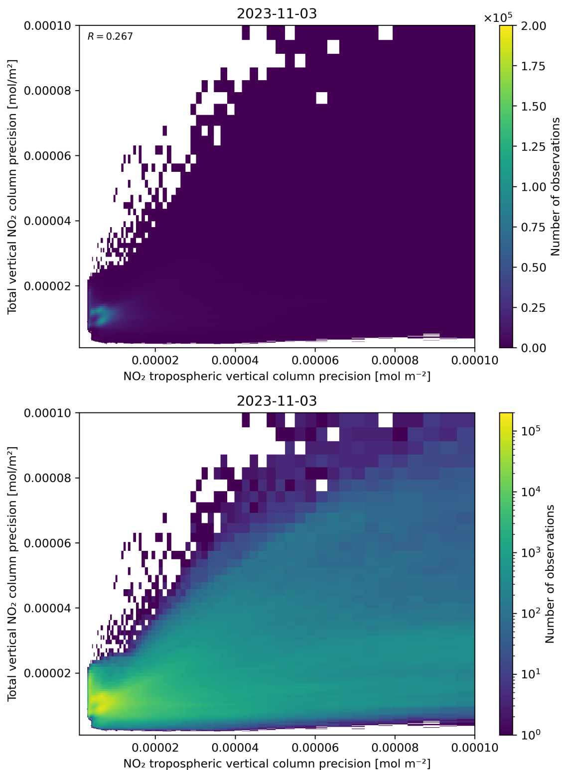
Figure 139: Scatter density plot of “NO 2 tropospheric vertical column precision” against “Total vertical NO 2 column precision” for 2023-11-02 to 2023-11-04.
