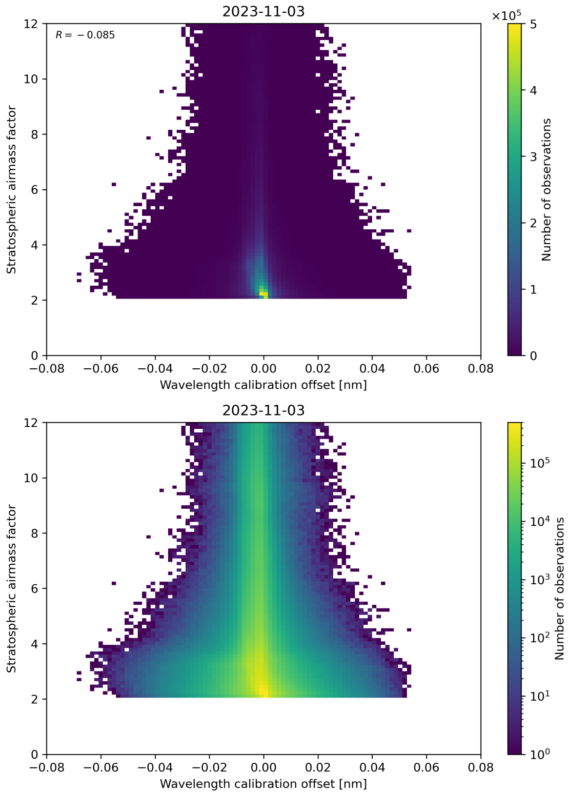
Figure 174: Scatter density plot of “Wavelength calibration offset” against “Stratospheric airmass factor” for 2023-11-02 to 2023-11-04.
