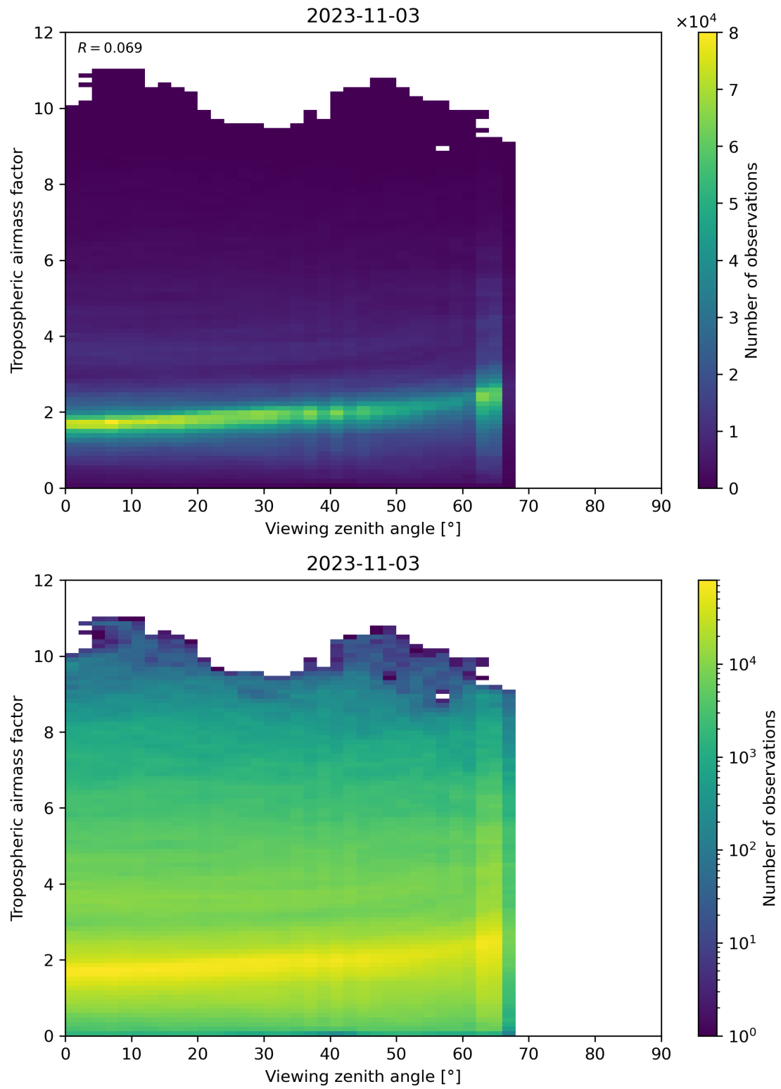
Figure 161: Scatter density plot of “Viewing zenith angle” against “Tropospheric airmass factor” for 2023-11-02 to 2023-11-04.
