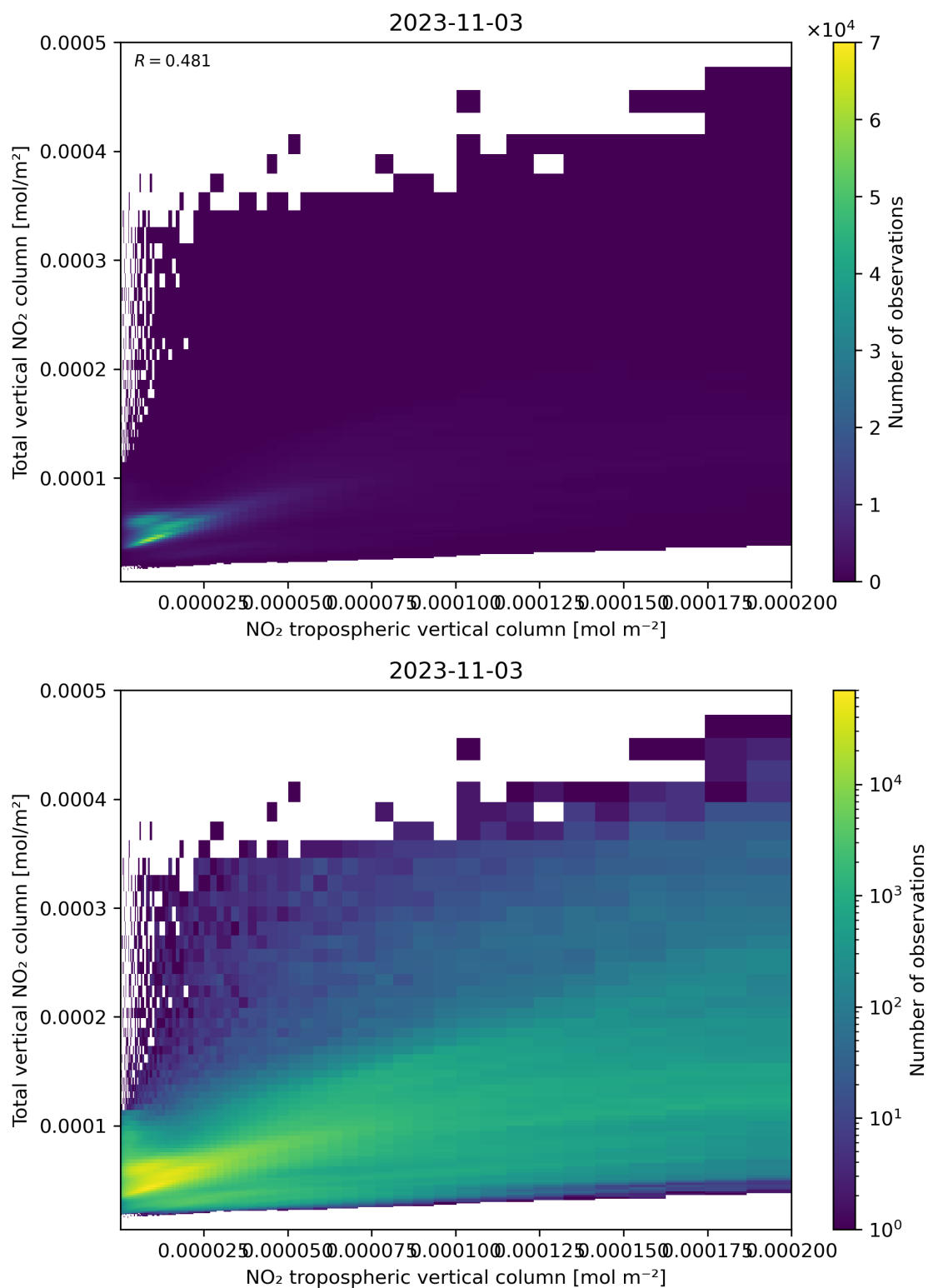
Figure 128: Scatter density plot of “NO 2 tropospheric vertical column” against “Total vertical NO 2 column” for 2023-11-02 to 2023-11-04.
