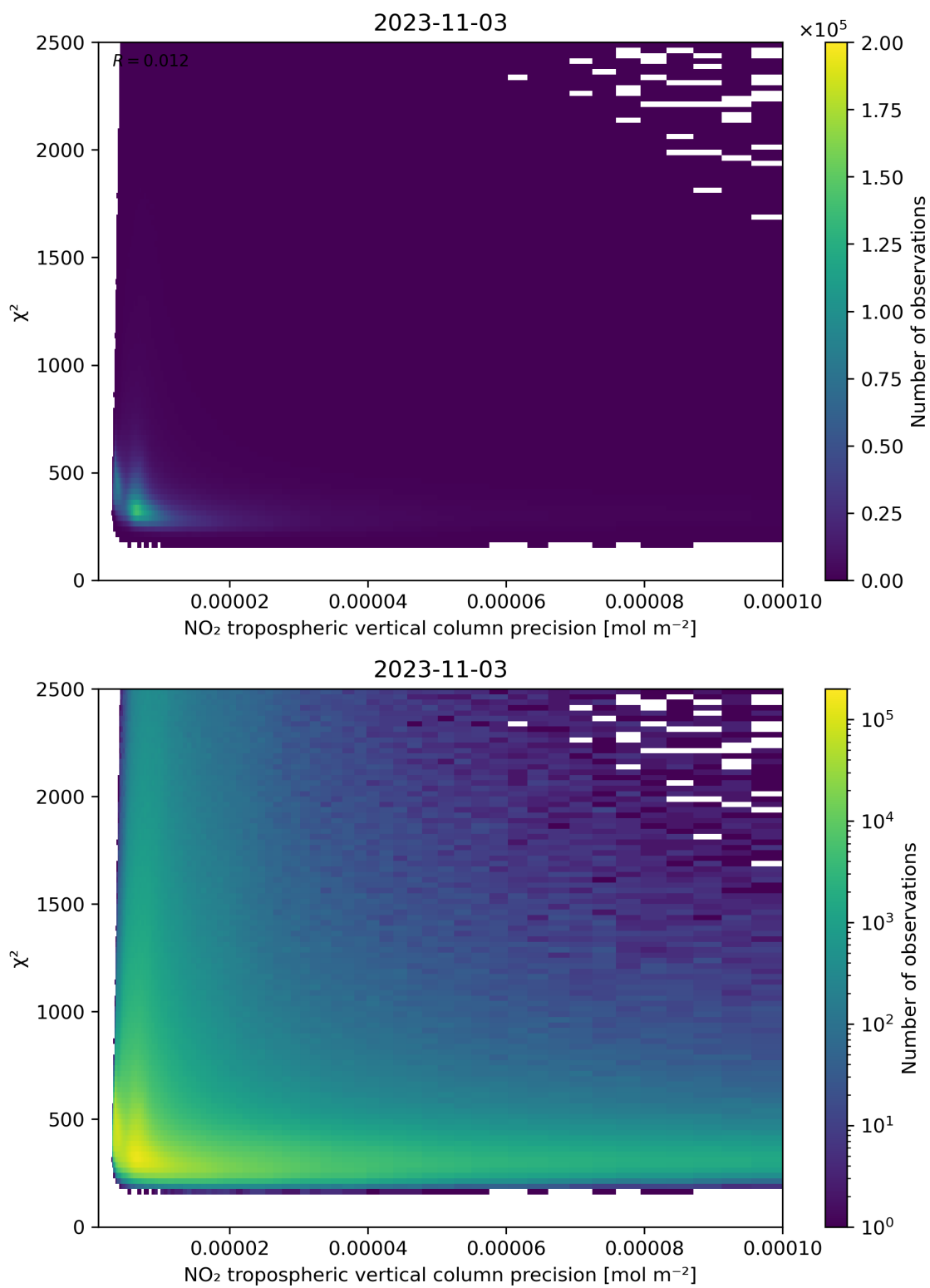
Figure 134: Scatter density plot of “NO 2 tropospheric vertical column precision” against “ \chi^2 ” for 2023-11-02 to 2023-11-04.
