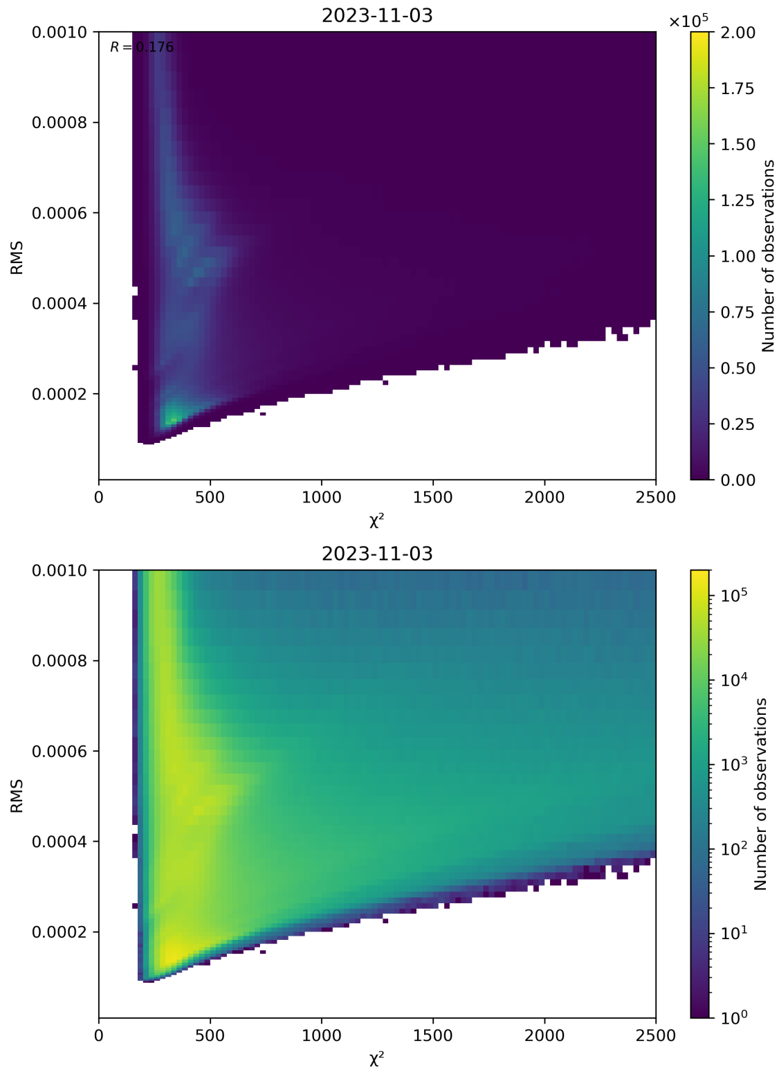
Figure 82: Scatter density plot of “ \chi^2 ” against “RMS” for 2023-11-02 to 2023-11-04.
