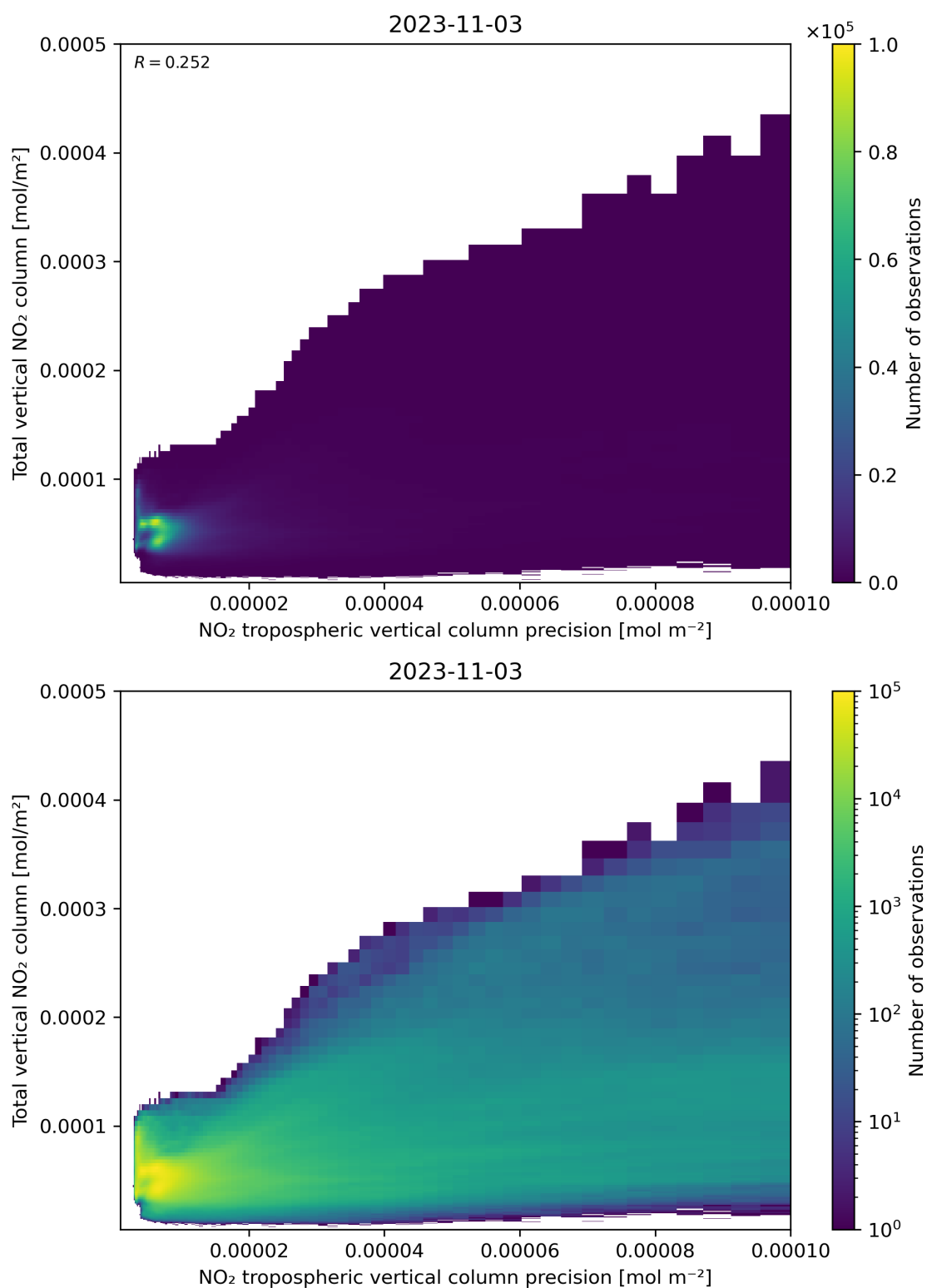
Figure 138: Scatter density plot of “NO 2 tropospheric vertical column precision” against “Total vertical NO 2 column” for 2023-11-02 to 2023-11-04.
