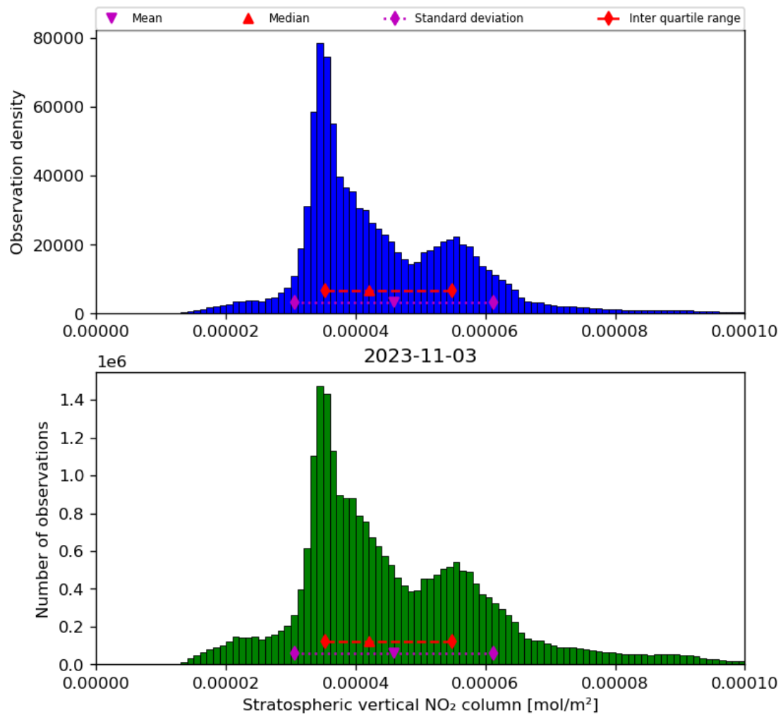
Figure 36: Histogram of “Stratospheric vertical NO 2 column” for 2023-11-02 to 2023-11-04
