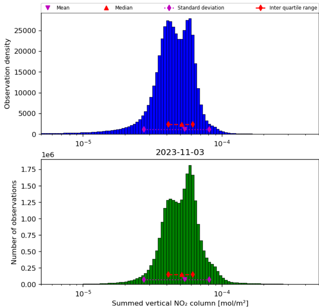
Figure 40: Histogram of “Summed vertical NO 2 column” for 2023-11-02 to 2023-11-04
