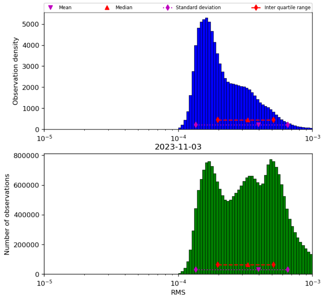
Figure 43: Histogram of “RMS” for 2023-11-02 to 2023-11-04
