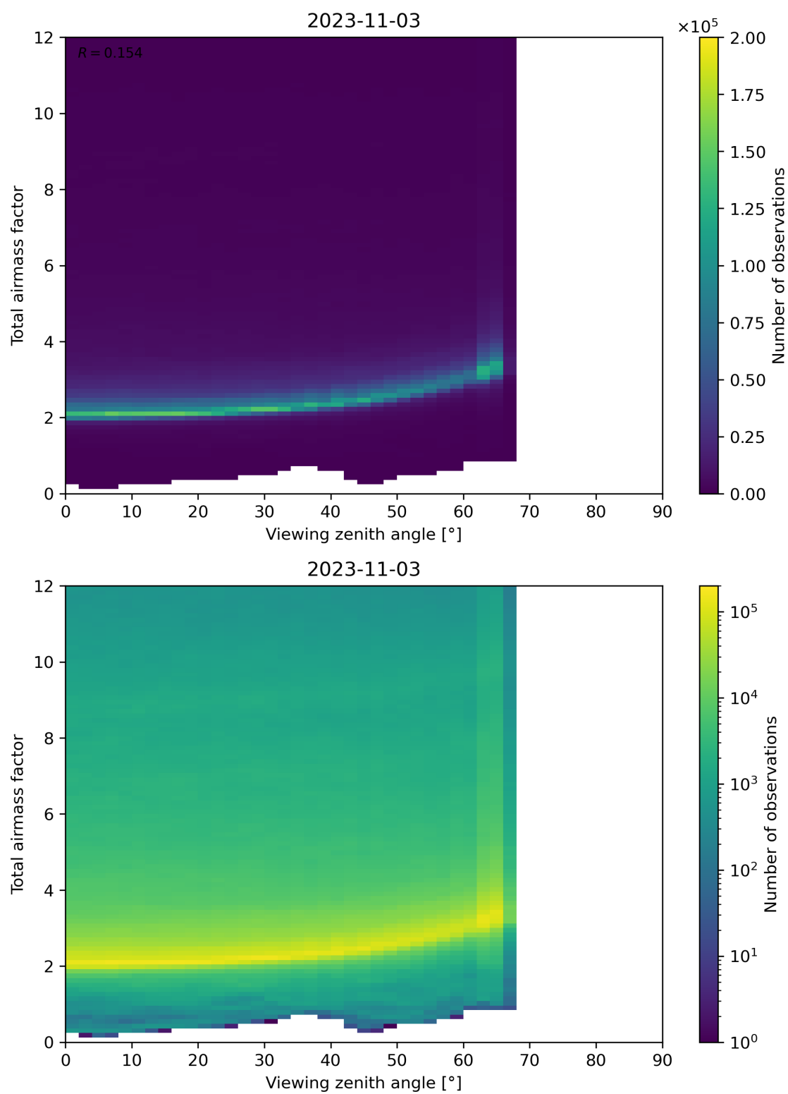
Figure 160: Scatter density plot of “Viewing zenith angle” against “Total airmass factor” for 2023-11-02 to 2023-11-04.
