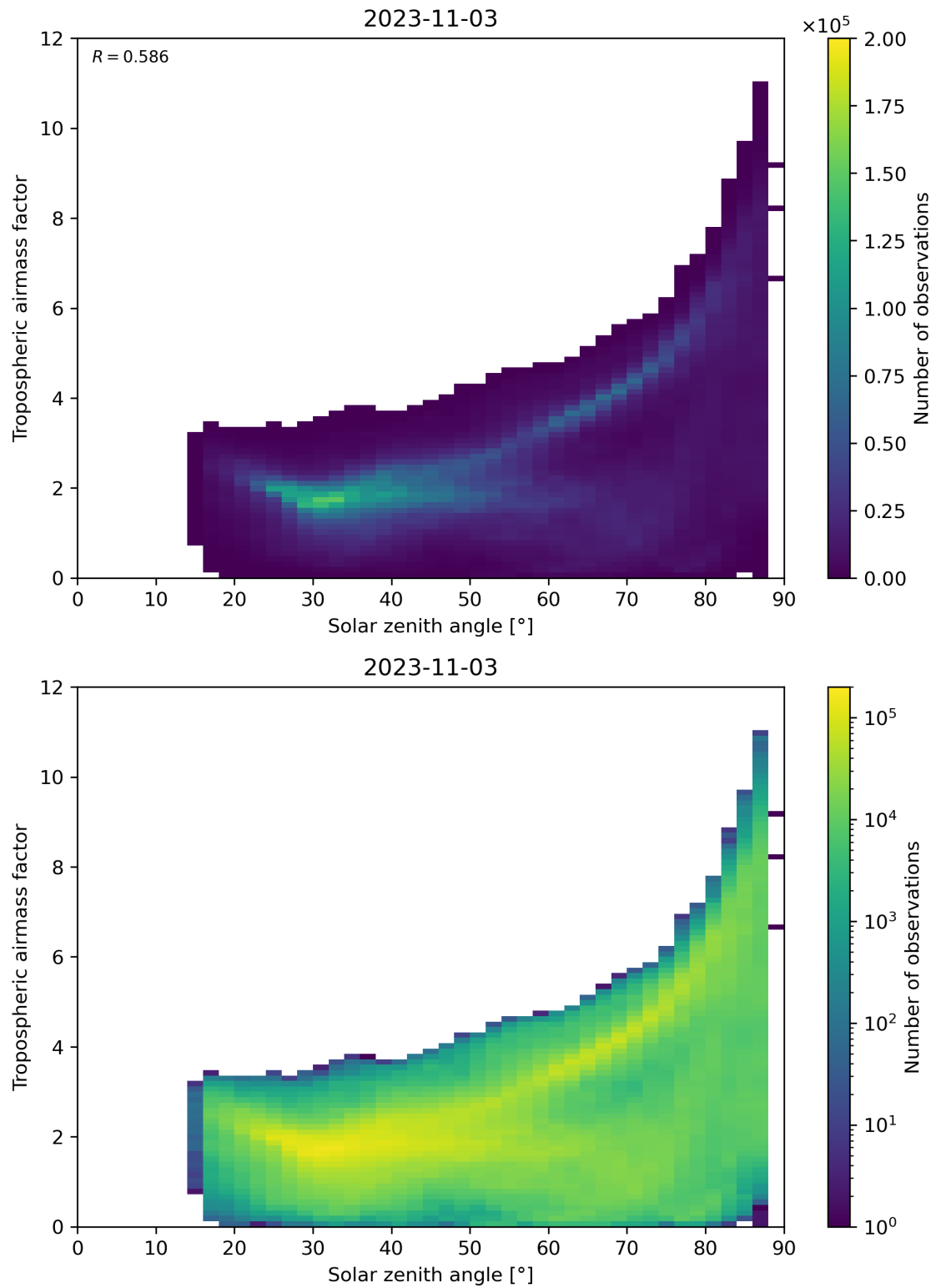
Figure 147: Scatter density plot of “Solar zenith angle” against “Tropospheric airmass factor” for 2023-11-02 to 2023-11-04.
