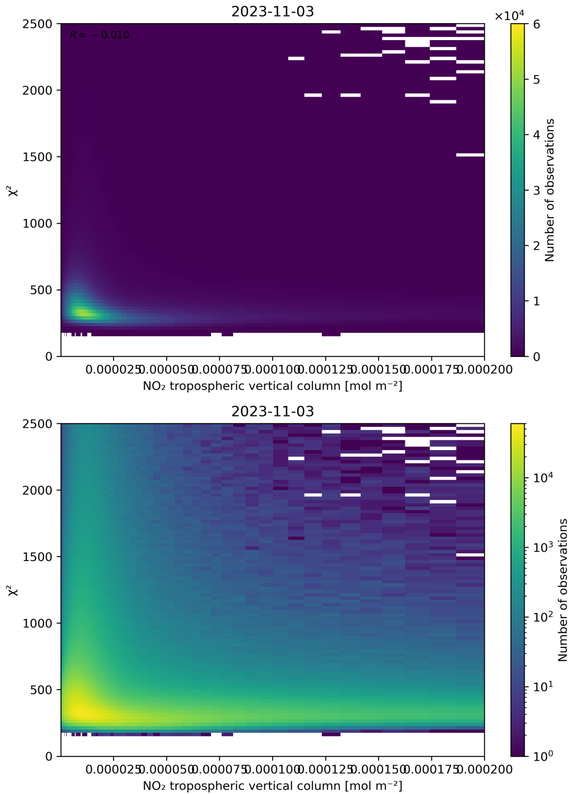
Figure 124: Scatter density plot of “NO 2 tropospheric vertical column” against “ \chi^2 ” for 2023-11-02 to 2023-11-04.
