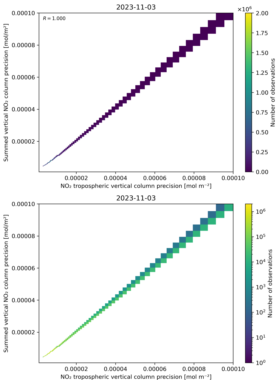
Figure 137: Scatter density plot of “NO 2 tropospheric vertical column precision” against “Summed vertical NO 2 column precision” for 2023-11-02 to 2023-11-04.
