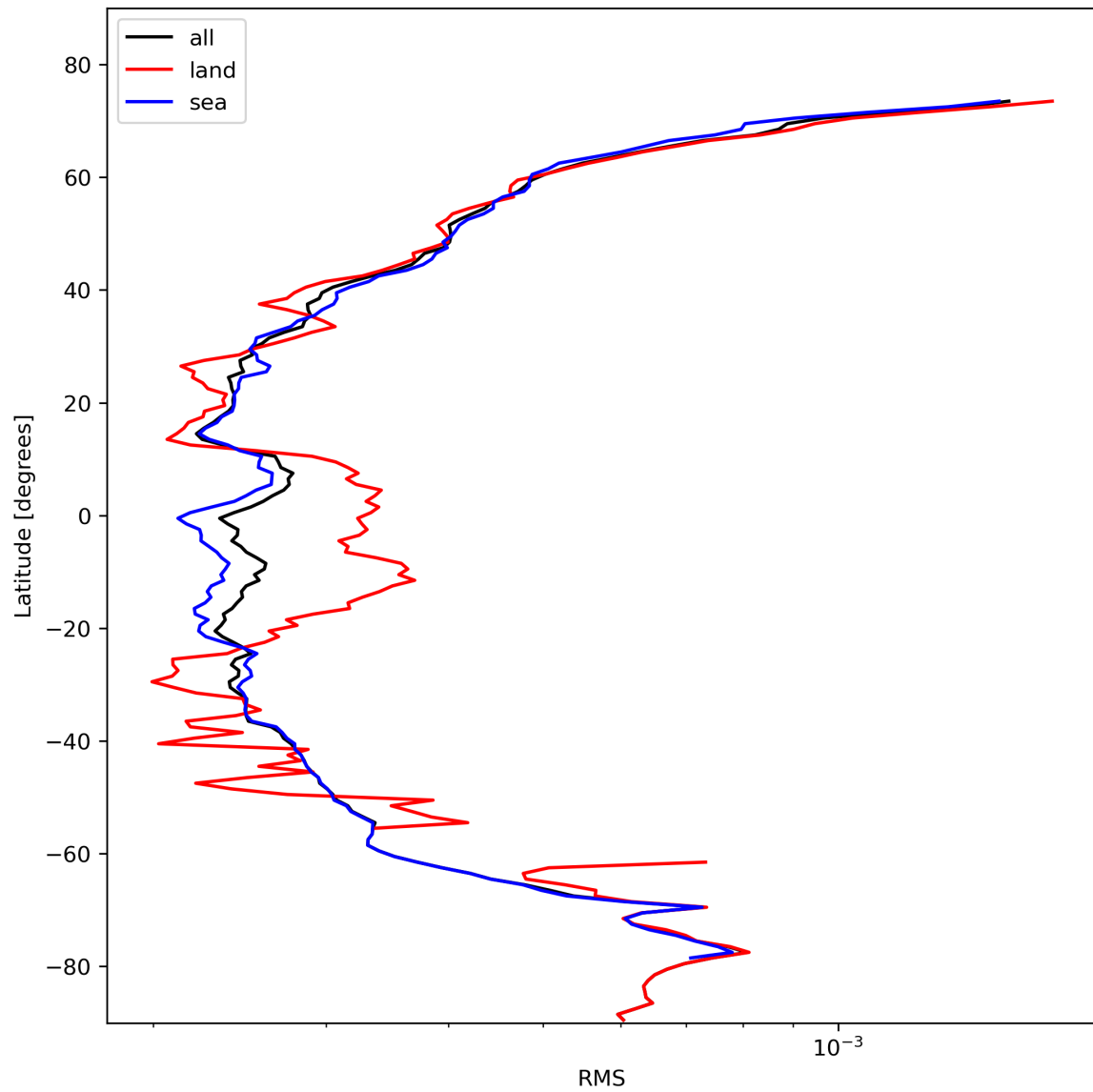
Figure 26: Zonal average of “RMS” for 2023-11-02 to 2023-11-04.
