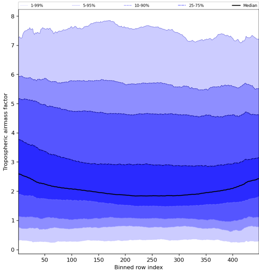
Figure 48: Along track statistics of “Tropospheric airmass factor” for 2023-11-02 to 2023-11-04
