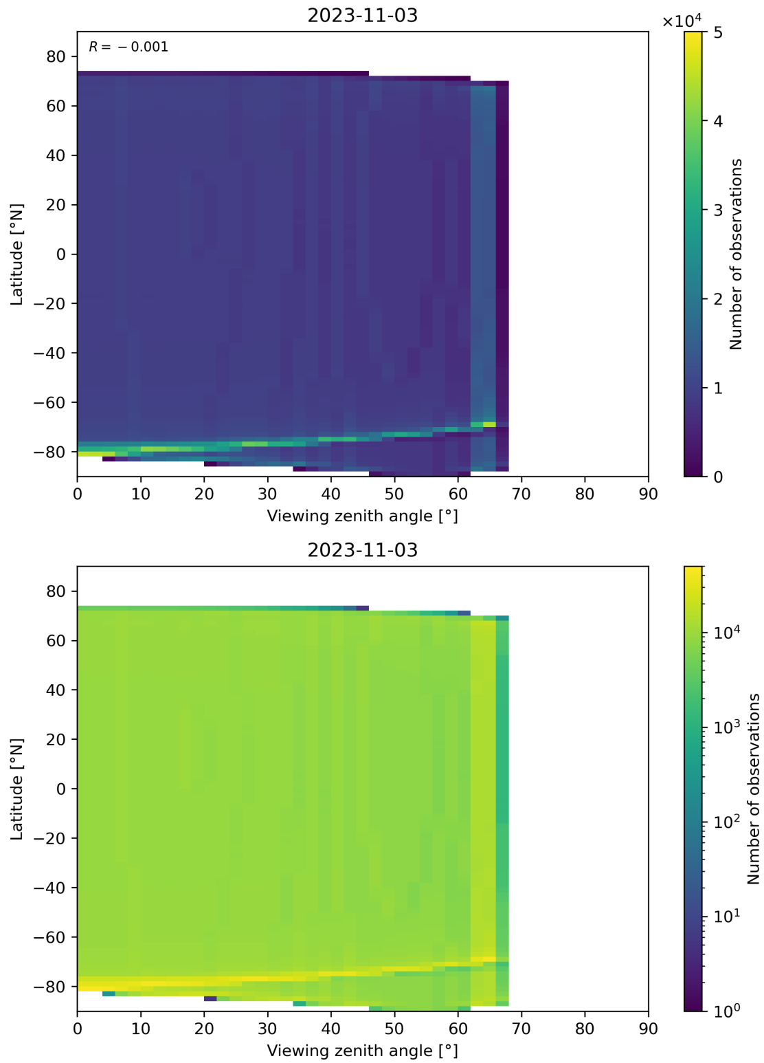
Figure 163: Scatter density plot of “Viewing zenith angle” against “Latitude” for 2023-11-02 to 2023-11-04.
