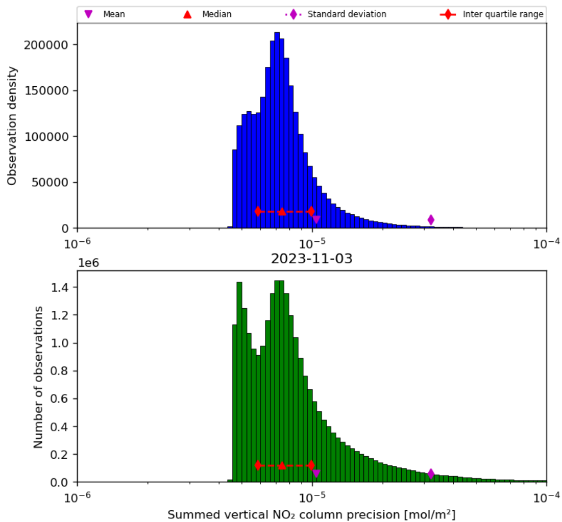
Figure 41: Histogram of "Summed vertical NO 2 column precision" for 2023-11-02 to 2023-11-04
