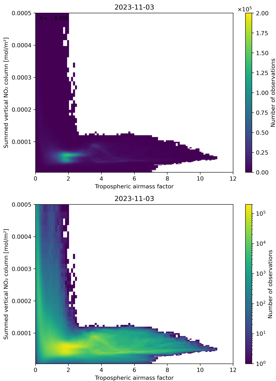
Figure 75: Scatter density plot of “Tropospheric airmass factor” against “Summed vertical NO 2 column” for 2023-11-02 to 2023-11-04.
