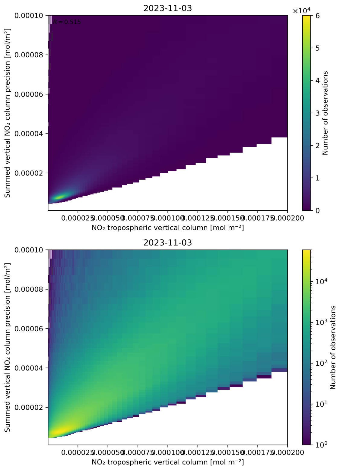
Figure 127: Scatter density plot of “NO 2 tropospheric vertical column” against “Summed vertical NO 2 column precision” for 2023-11-02 to 2023-11-04.
