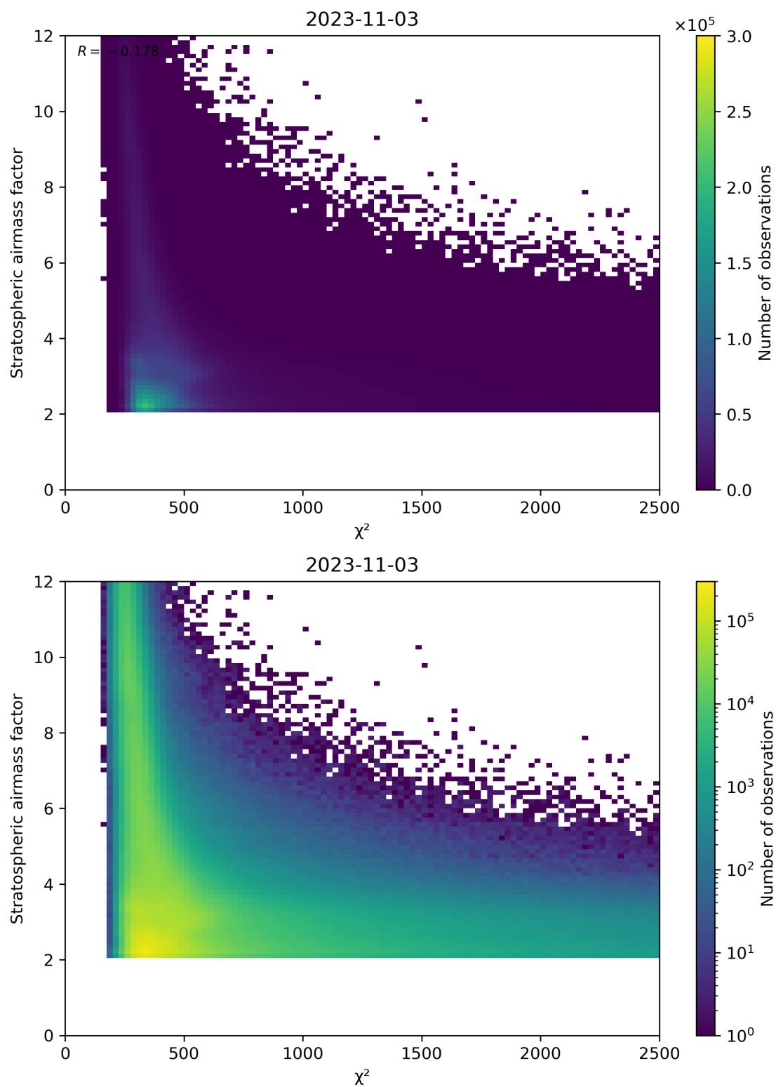
Figure 81: Scatter density plot of “ \chi^2 ” against “Stratospheric airmass factor” for 2023-11-02 to 2023-11-04.
