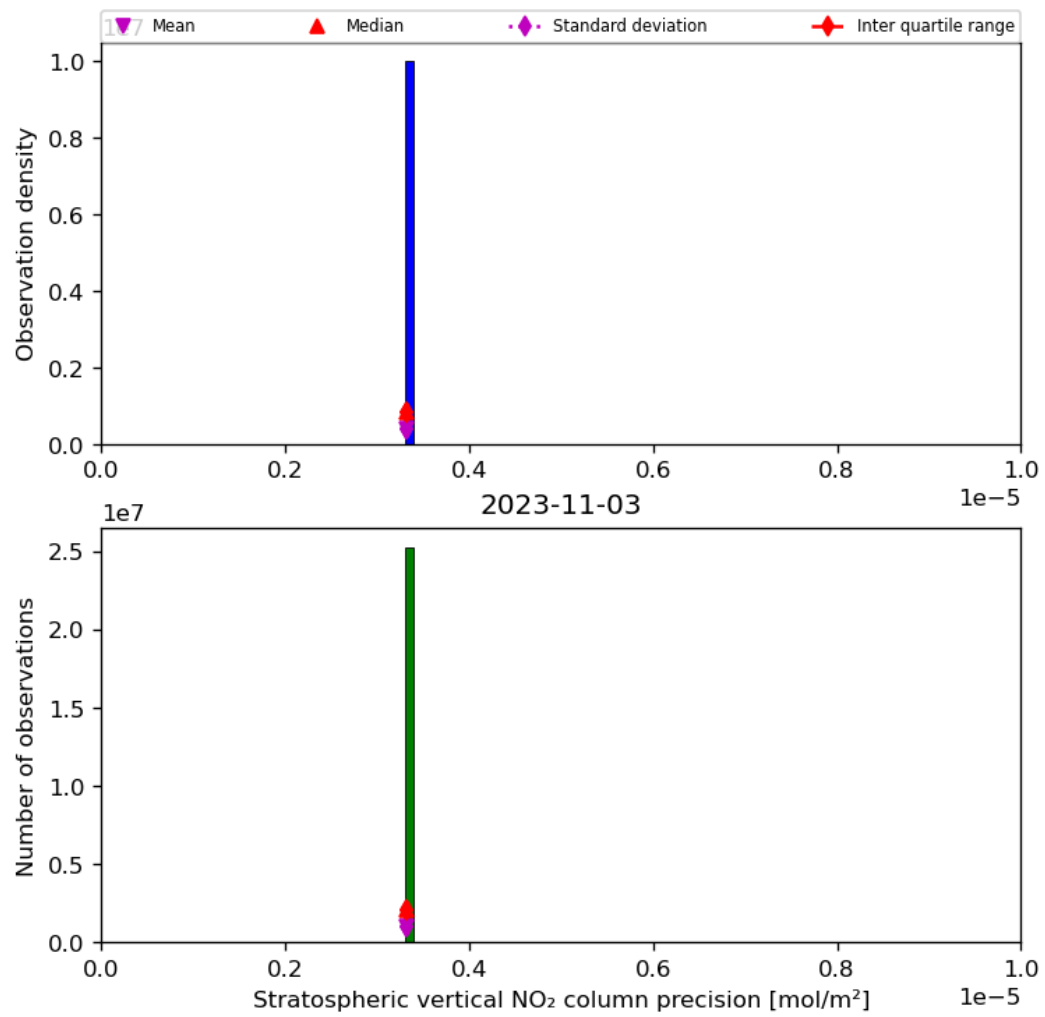
Figure 37: Histogram of “Stratospheric vertical NO 2 column precision” for 2023-11-02 to 2023-11-04
