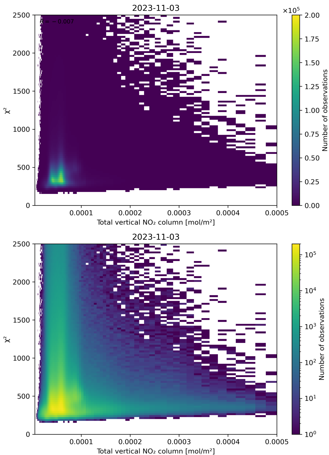
Figure 111: Scatter density plot of “Total vertical NO 2 column” against “ \chi^2 ” for 2023-11-02 to 2023-11-04.
