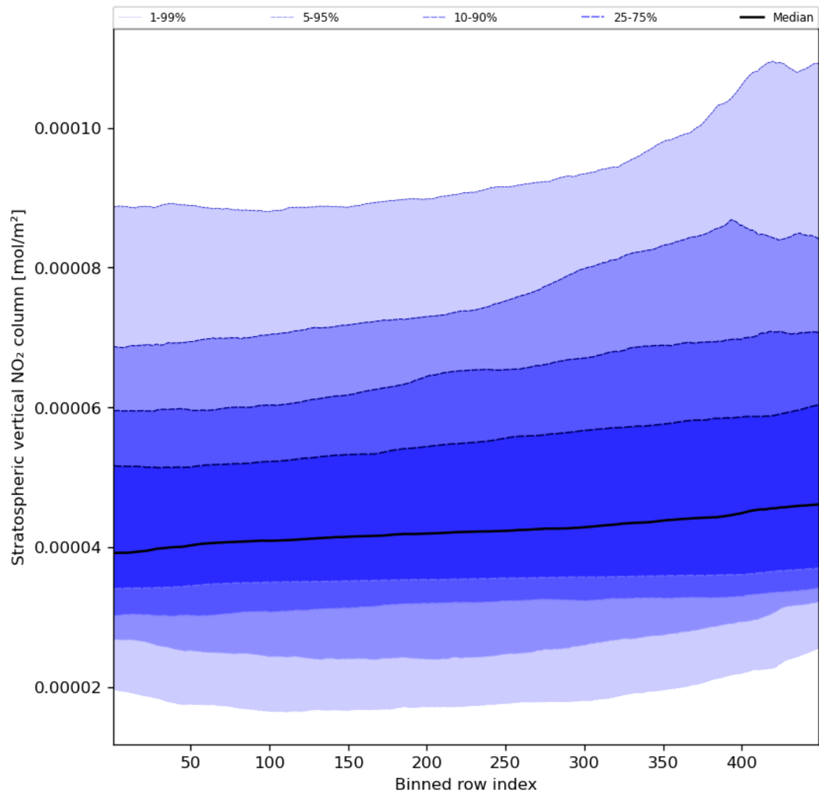
Figure 53: Along track statistics of “Stratospheric vertical NO 2 column” for 2023-11-02 to 2023-11-04
