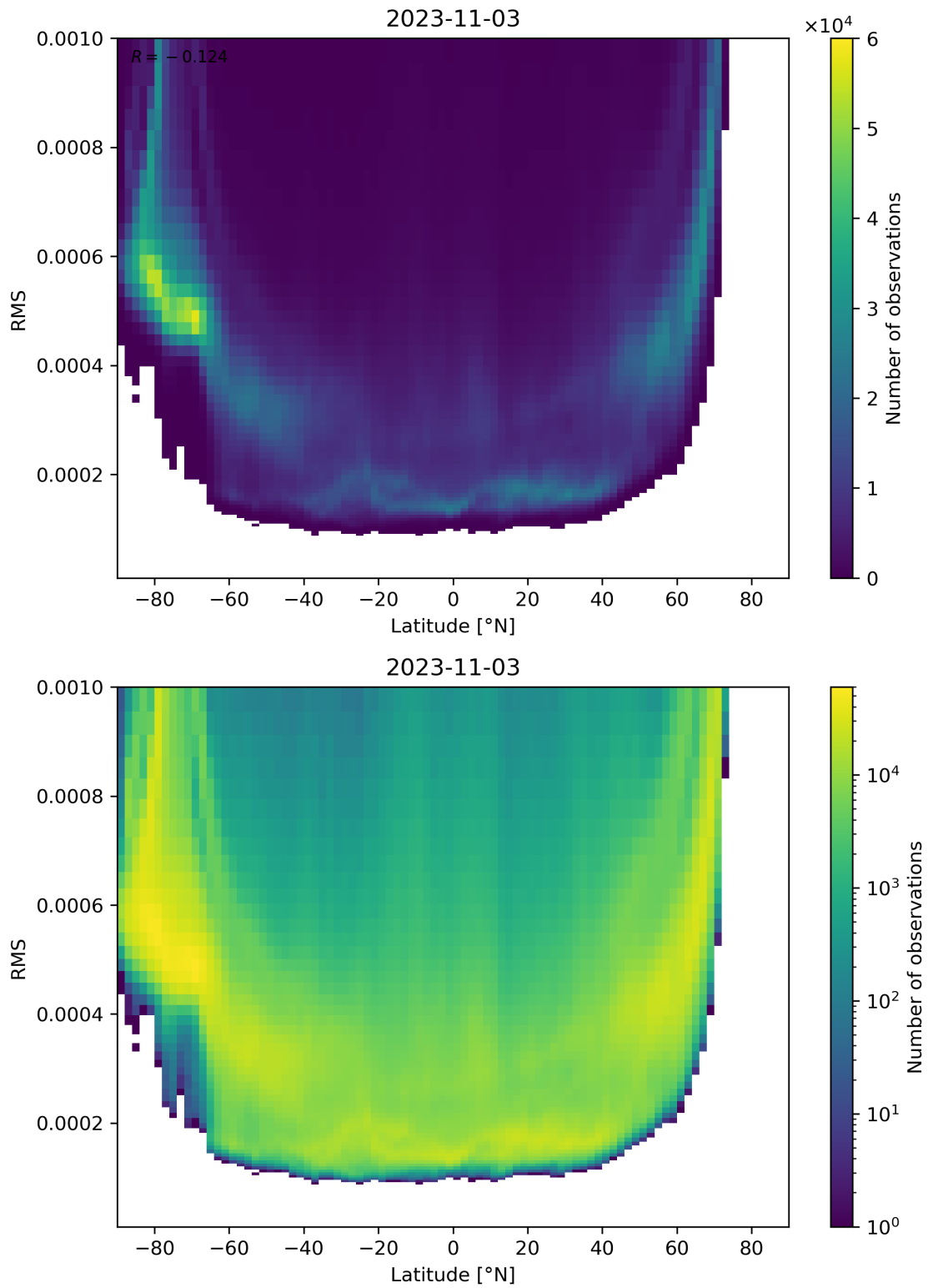
Figure 94: Scatter density plot of “Latitude” against “RMS” for 2023-11-02 to 2023-11-04.
