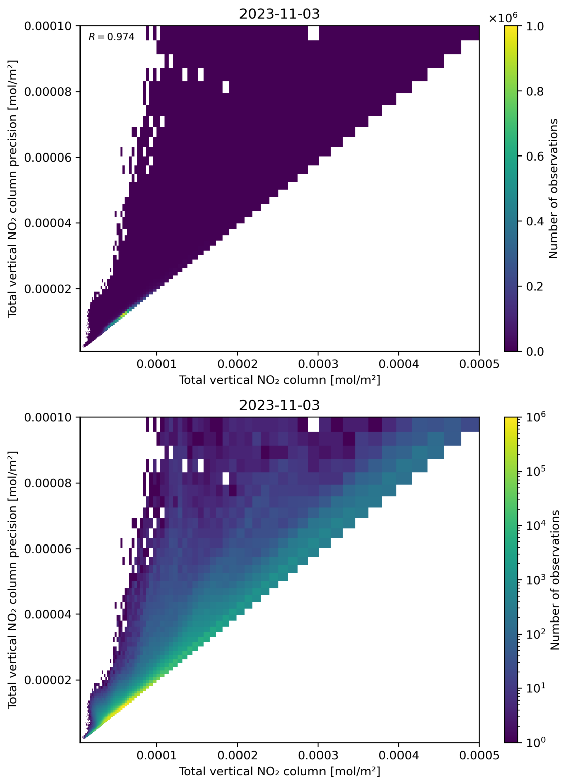
Figure 114: Scatter density plot of “Total vertical NO 2 column” against “Total vertical NO 2 column precision” for 2023-11-02 to 2023-11-04.
