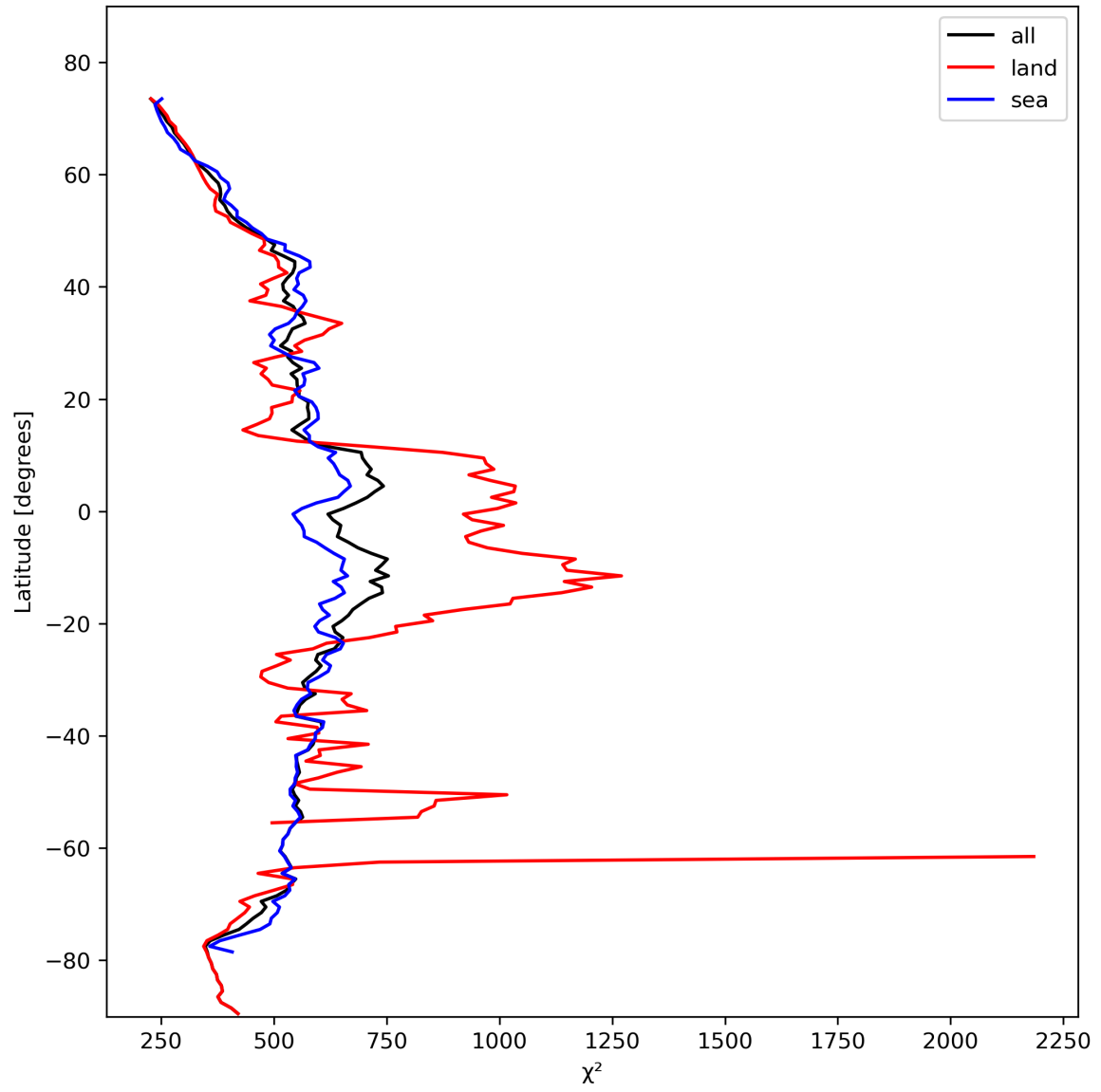
Figure 25: Zonal average of “ \chi^2 ” for 2023-11-02 to 2023-11-04.
