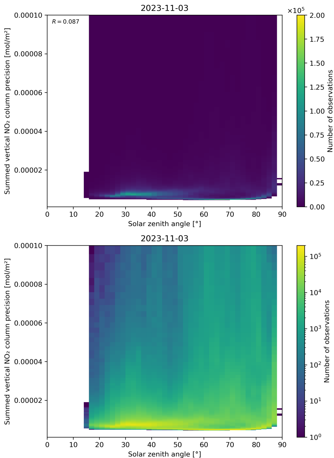
Figure 152: Scatter density plot of “Solar zenith angle” against “Summed vertical NO 2 column precision” for 2023-11-02 to 2023-11-04.
