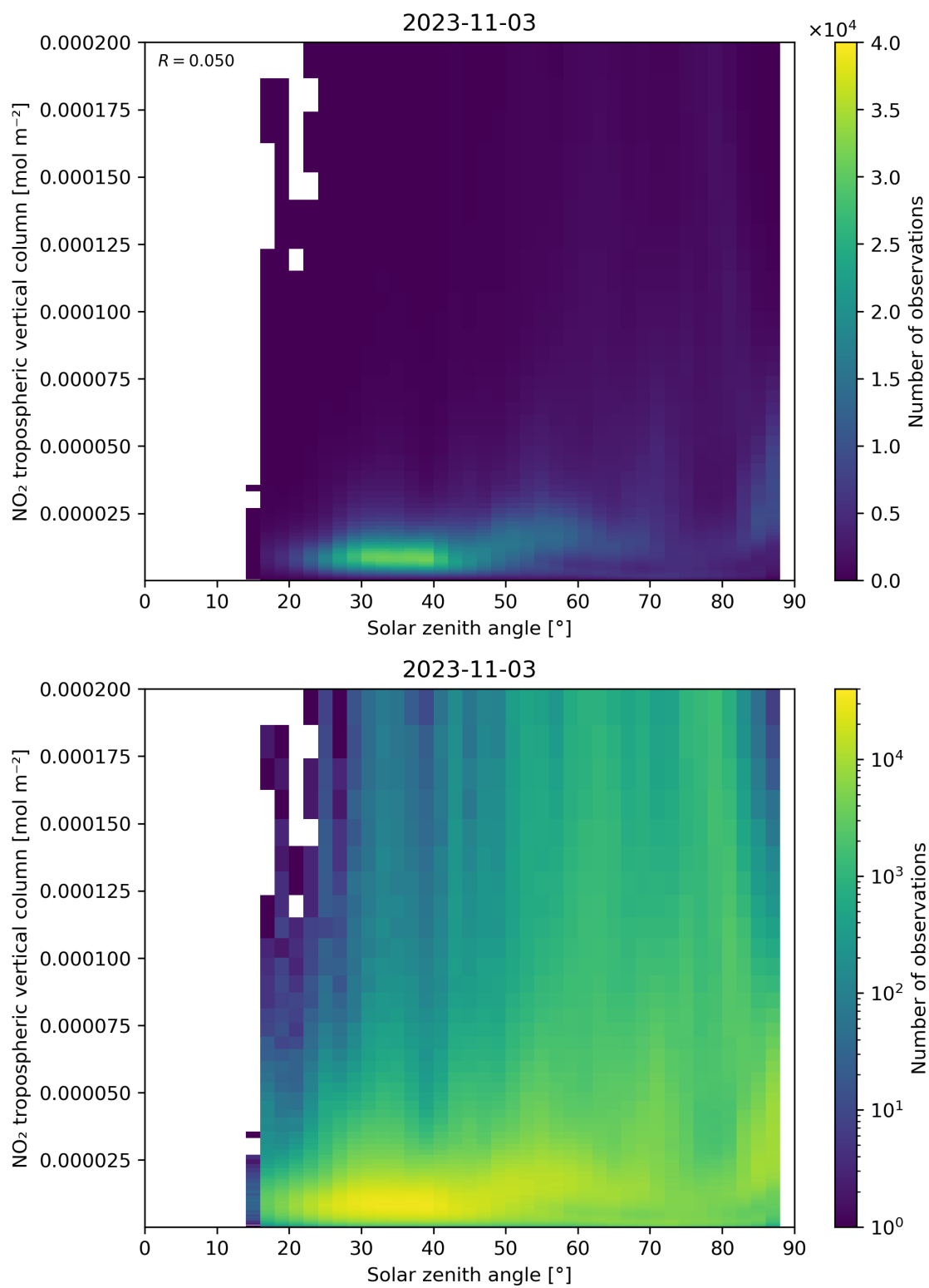
Figure 155: Scatter density plot of “Solar zenith angle” against “NO 2 tropospheric vertical column” for 2023-11-02 to 2023-11-04.
