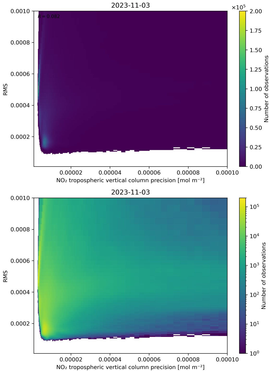
Figure 140: Scatter density plot of “NO 2 tropospheric vertical column precision” against “RMS” for 2023-11-02 to 2023-11-04.
