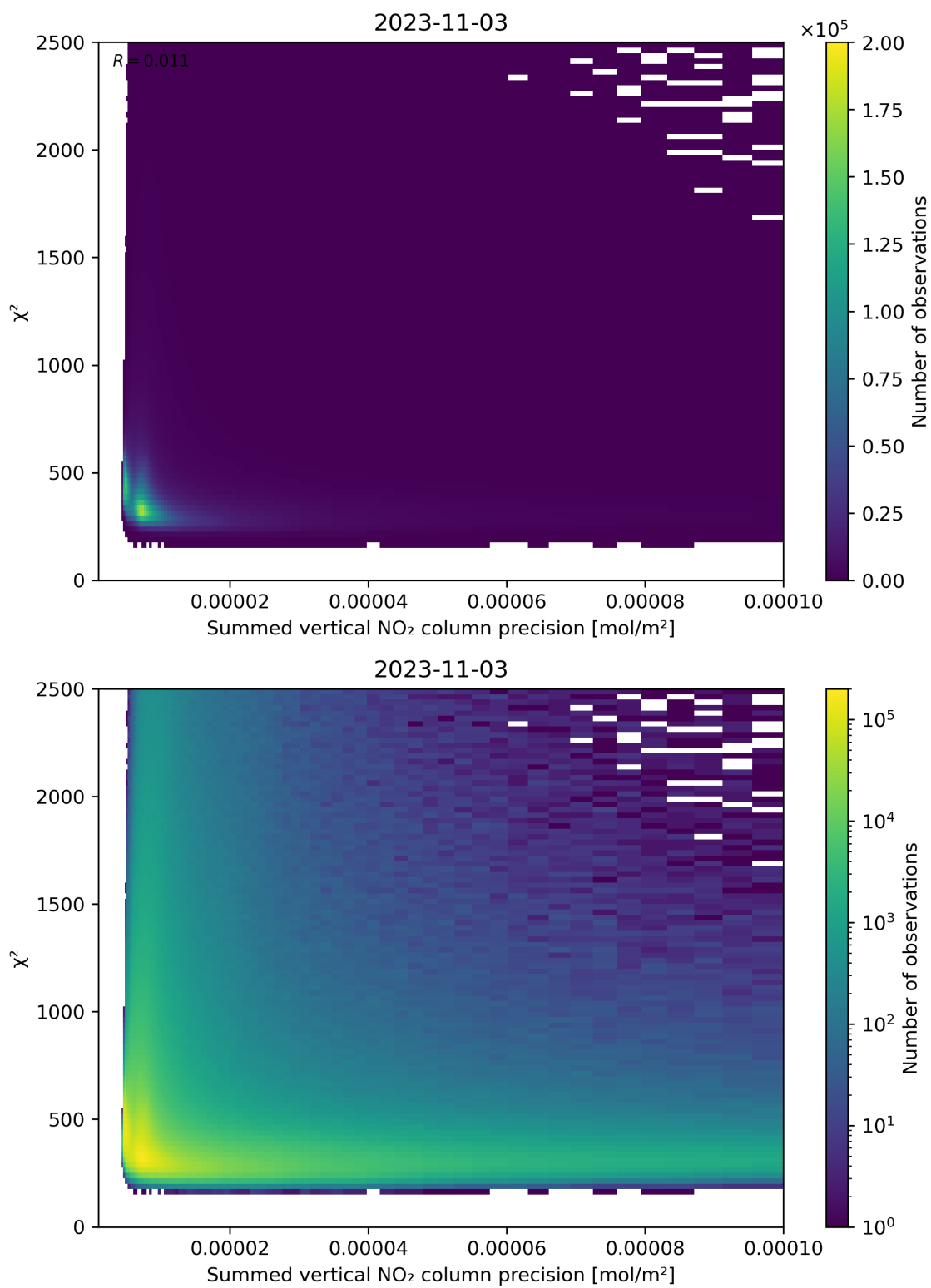
Figure 107: Scatter density plot of “Summed vertical NO 2 column precision” against “ \chi^2 ” for 2023-11-02 to 2023-11-04.
