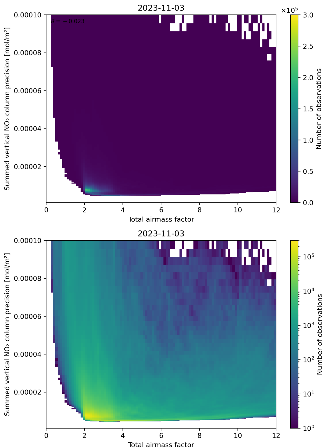
Figure 66: Scatter density plot of “Total airmass factor” against “Summed vertical NO 2 column precision” for 2023-11-02 to 2023-11-04.
