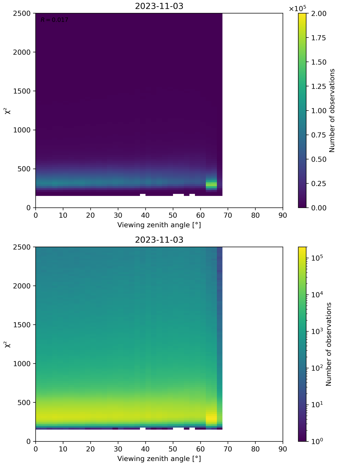
Figure 162: Scatter density plot of “Viewing zenith angle” against “ \chi^2 ” for 2023-11-02 to 2023-11-04.
