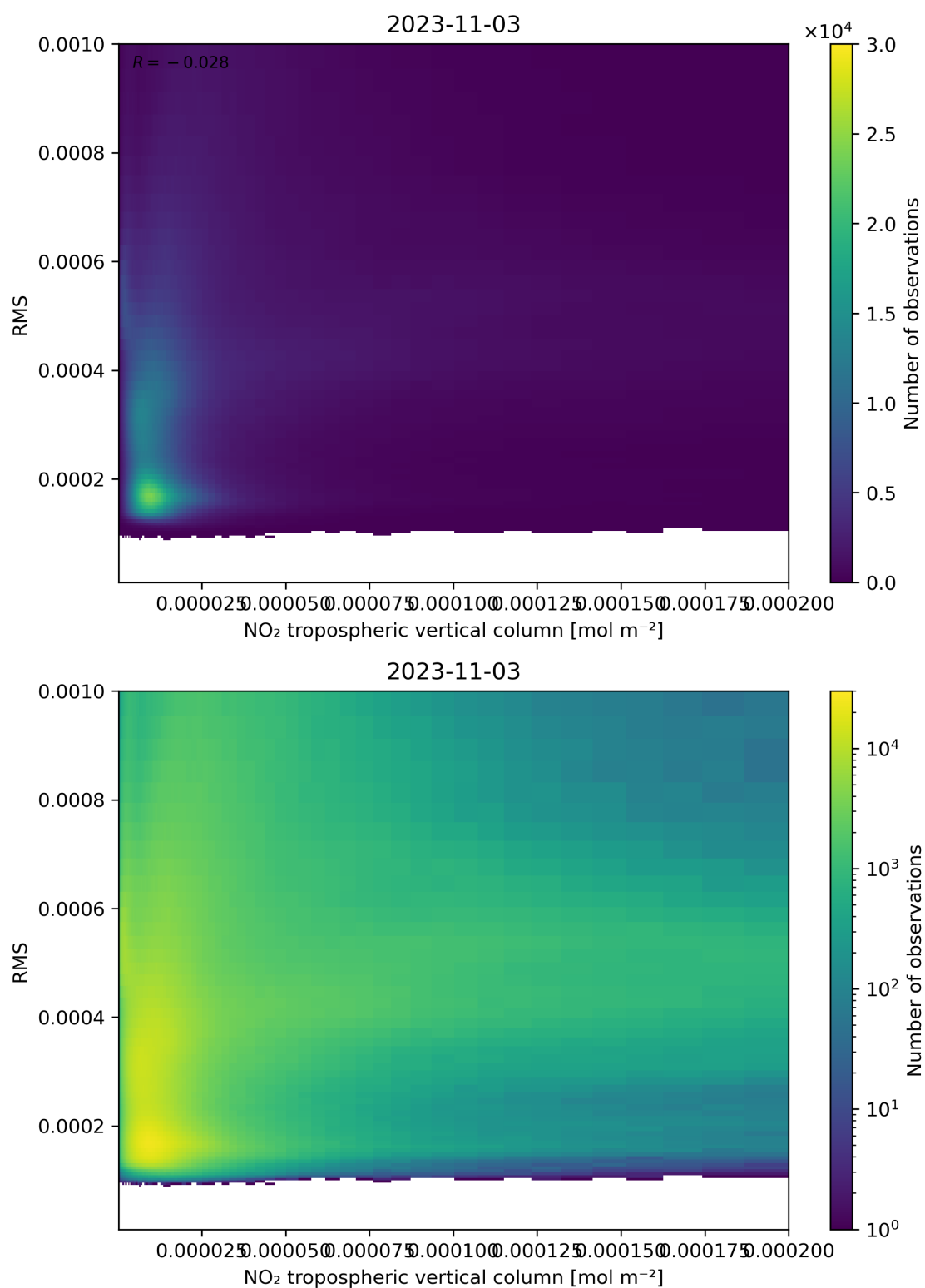
Figure 142: Scatter density plot of “NO 2 tropospheric vertical column” against “RMS” for 2023-11-02 to 2023-11-04.
