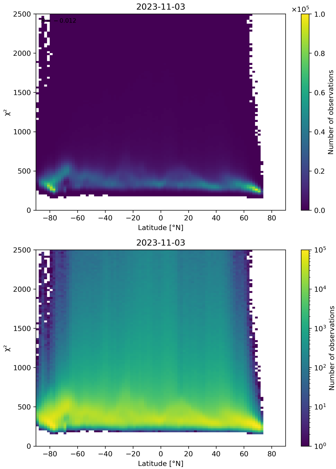
Figure 86: Scatter density plot of “Latitude” against “ \chi^2 ” for 2023-11-02 to 2023-11-04.
