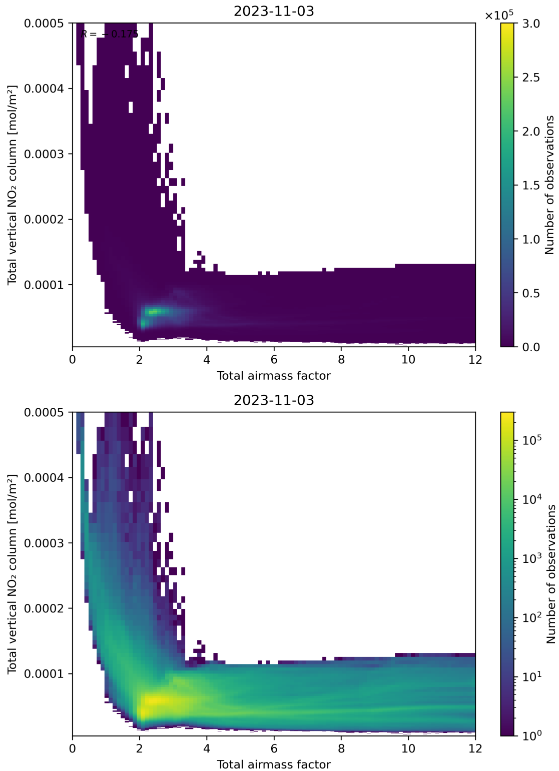
Figure 67: Scatter density plot of “Total airmass factor” against “Total vertical NO 2 column” for 2023-11-02 to 2023-11-04.
