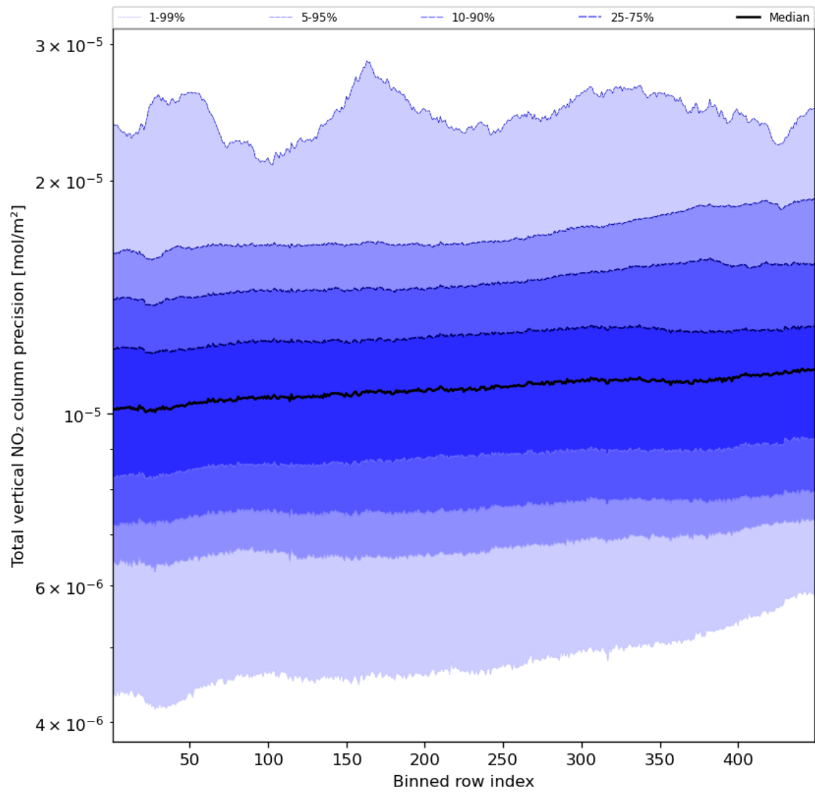
Figure 56: Along track statistics of “Total vertical NO 2 column precision” for 2023-11-02 to 2023-11-04
