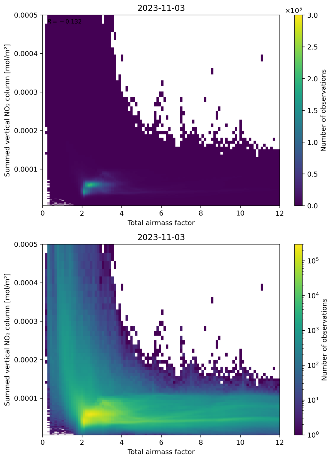
Figure 65: Scatter density plot of “Total airmass factor” against “Summed vertical NO 2 column” for 2023-11-02 to 2023-11-04.
