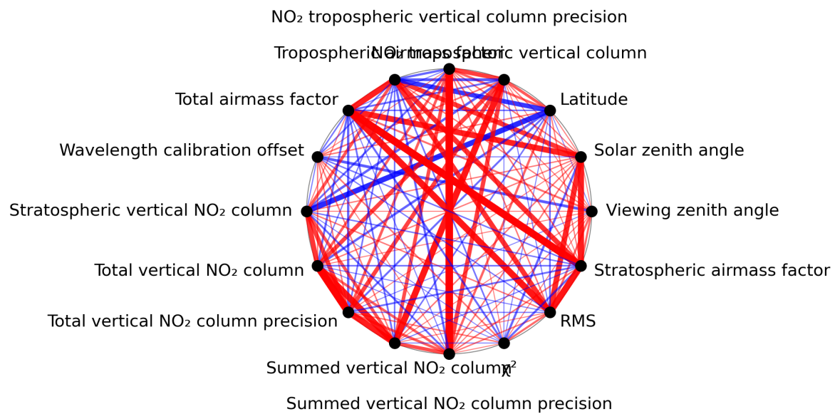
Figure 1: Map of correlation graph for 2023-11-02 to 2023-11-04.
