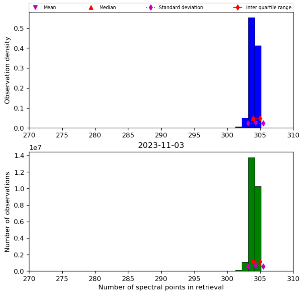
Figure 33: Histogram of “Number of spectral points in retrieval” for 2023-11-02 to 2023-11-04
