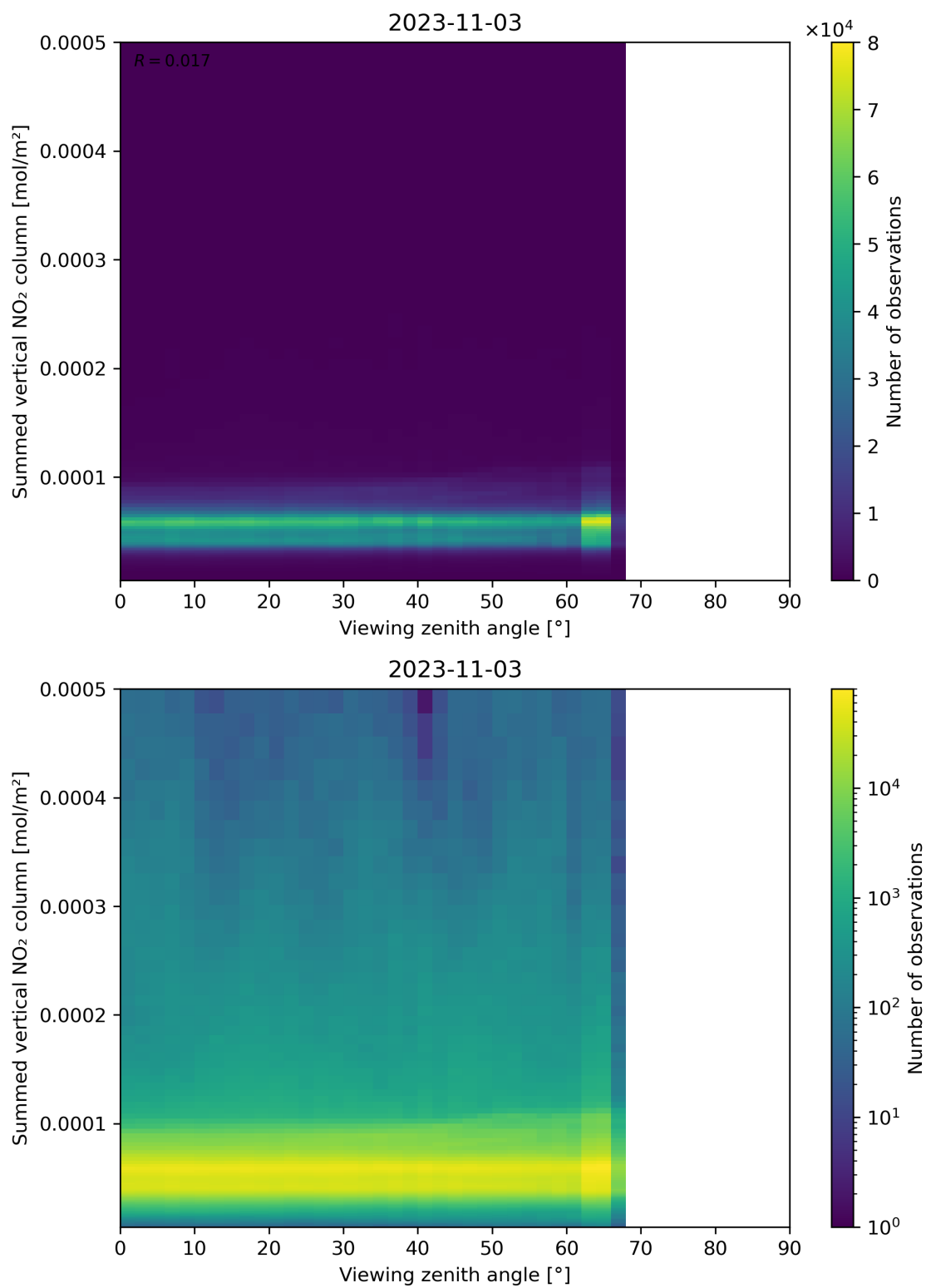
Figure 165: Scatter density plot of “Viewing zenith angle” against “Summed vertical NO 2 column” for 2023-11-02 to 2023-11-04.
