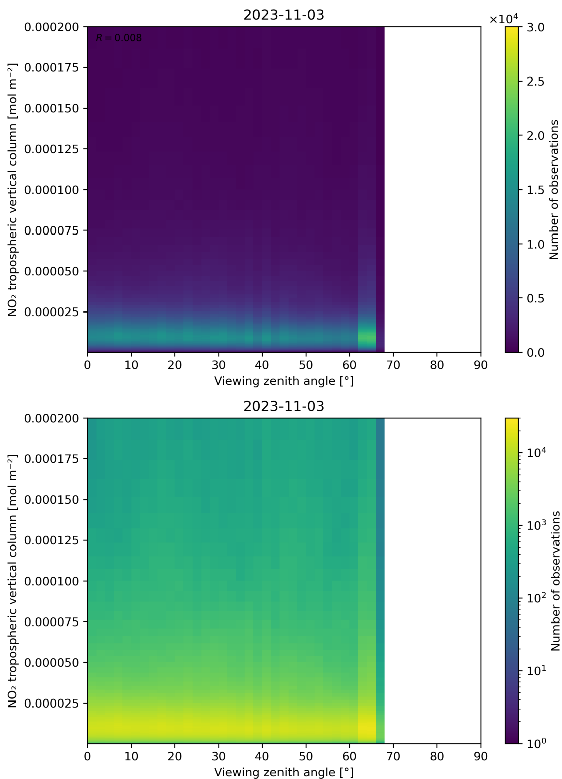
Figure 169: Scatter density plot of “Viewing zenith angle” against “NO 2 tropospheric vertical column” for 2023-11-02 to 2023-11-04.
