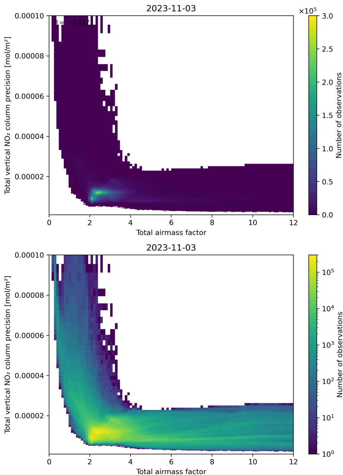
Figure 68: Scatter density plot of “Total airmass factor” against “Total vertical NO 2 column precision” for 2023-11-02 to 2023-11-04.
