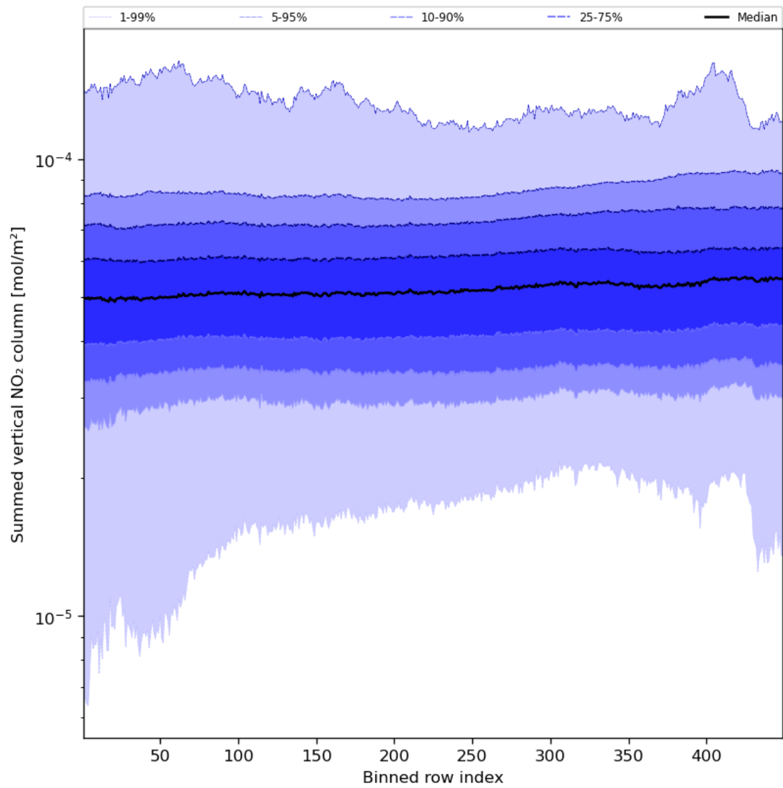
Figure 57: Along track statistics of “Summed vertical NO 2 column” for 2023-11-02 to 2023-11-04
