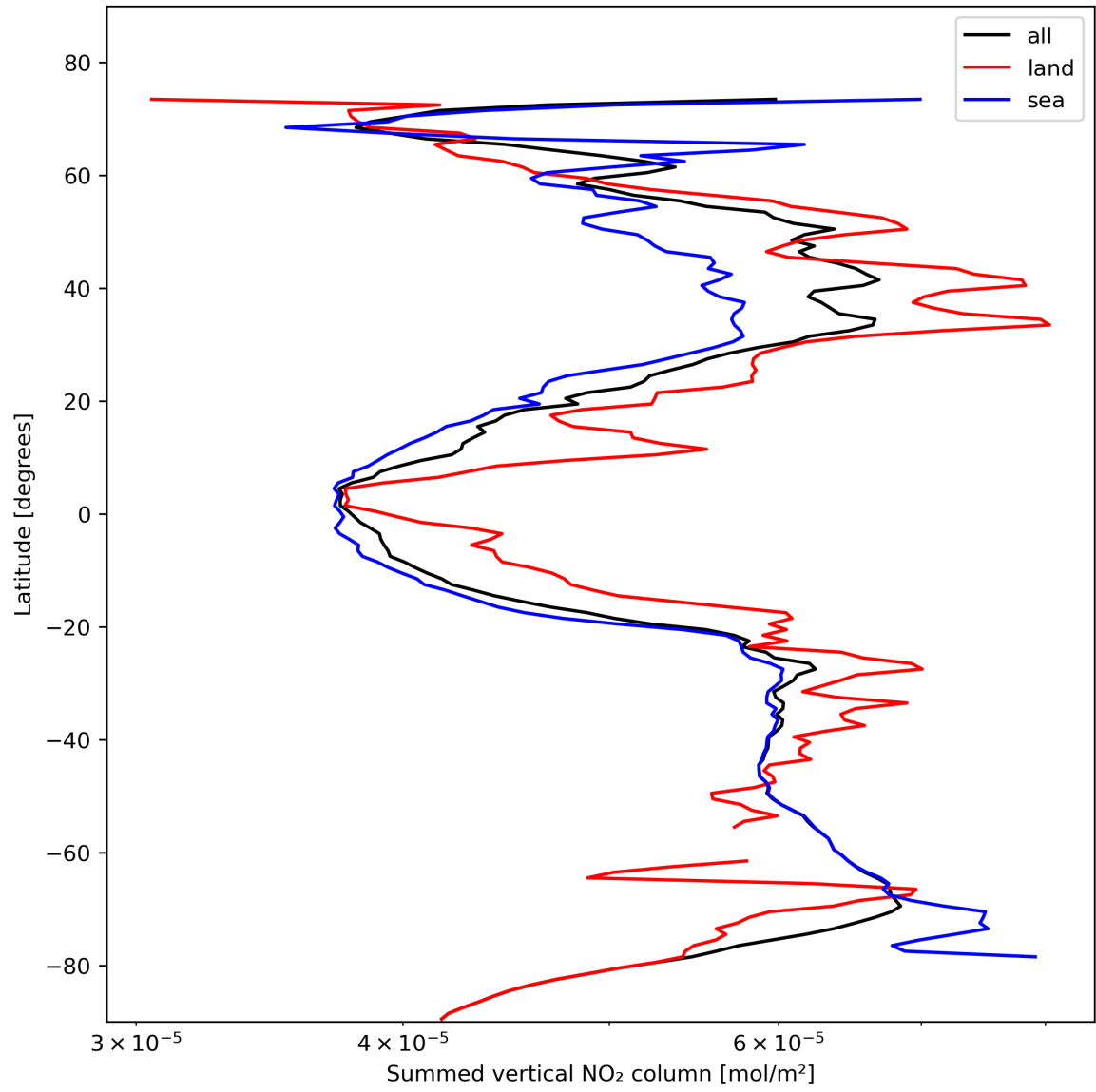
Figure 23: Zonal average of “Summed vertical NO 2 column” for 2023-11-02 to 2023-11-04.
