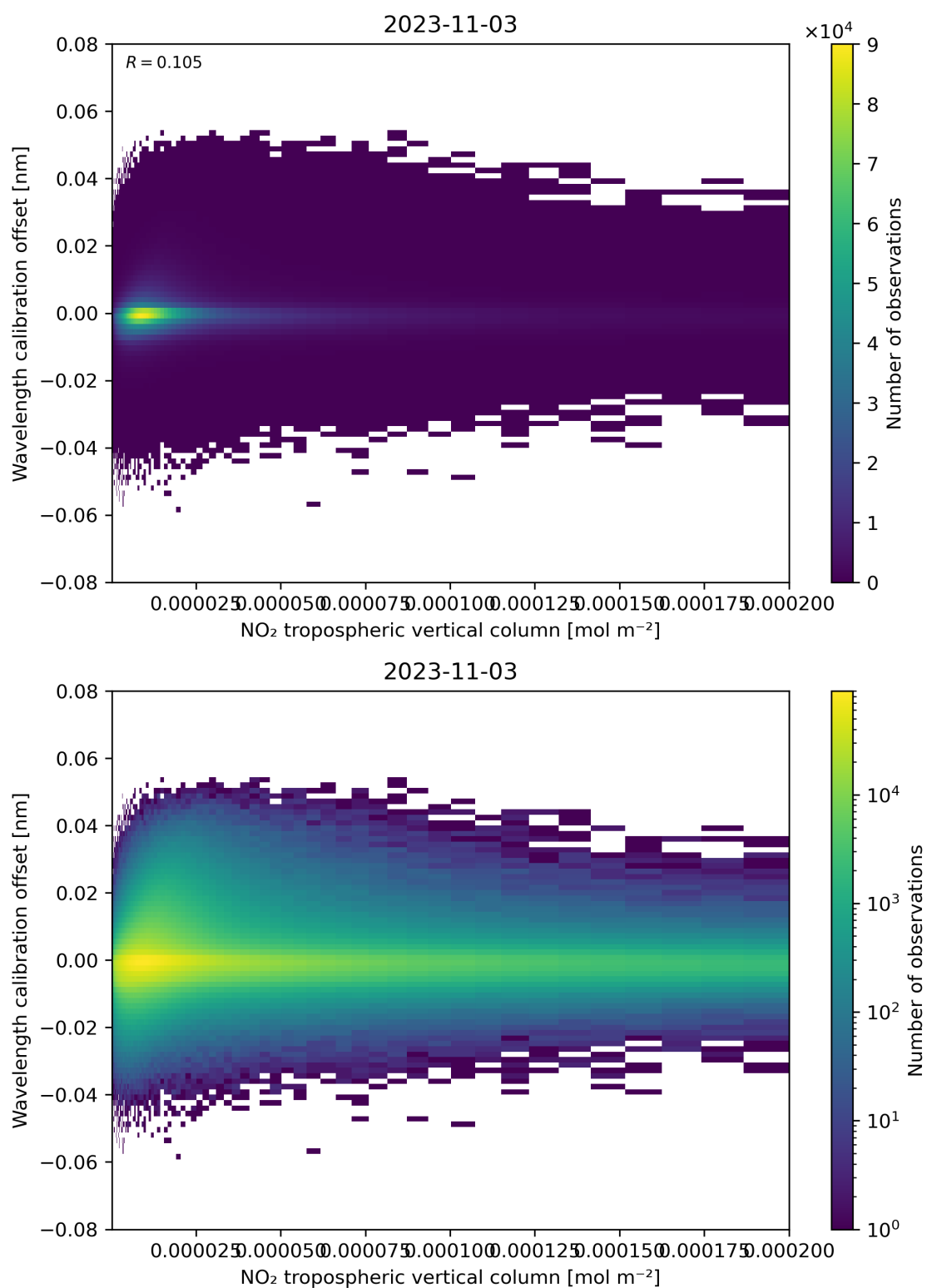
Figure 143: Scatter density plot of “NO 2 tropospheric vertical column” against “Wavelength calibration offset” for 2023-11-02 to 2023-11-04.
