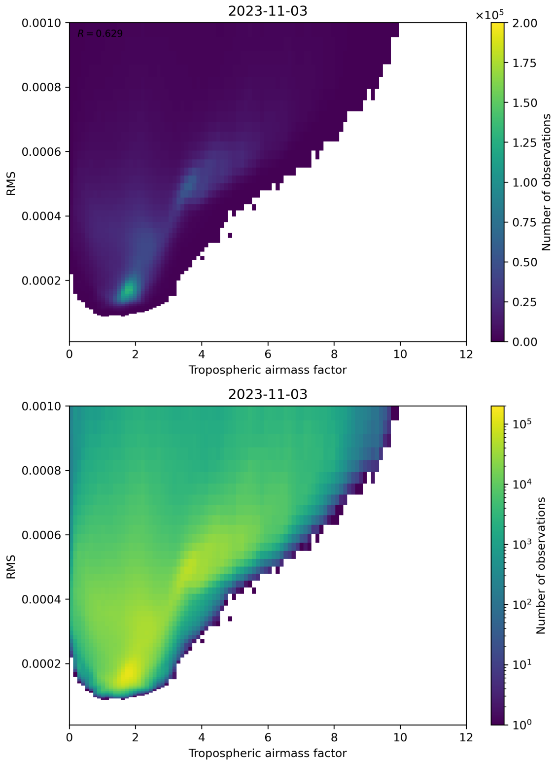
Figure 79: Scatter density plot of “Tropospheric airmass factor” against “RMS” for 2023-11-02 to 2023-11-04.
