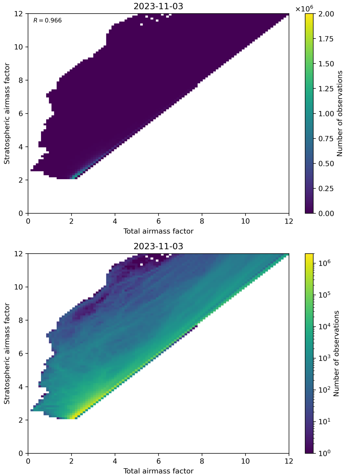
Figure 62: Scatter density plot of “Total airmass factor” against “Stratospheric airmass factor” for 2023-11-02 to 2023-11-04.
