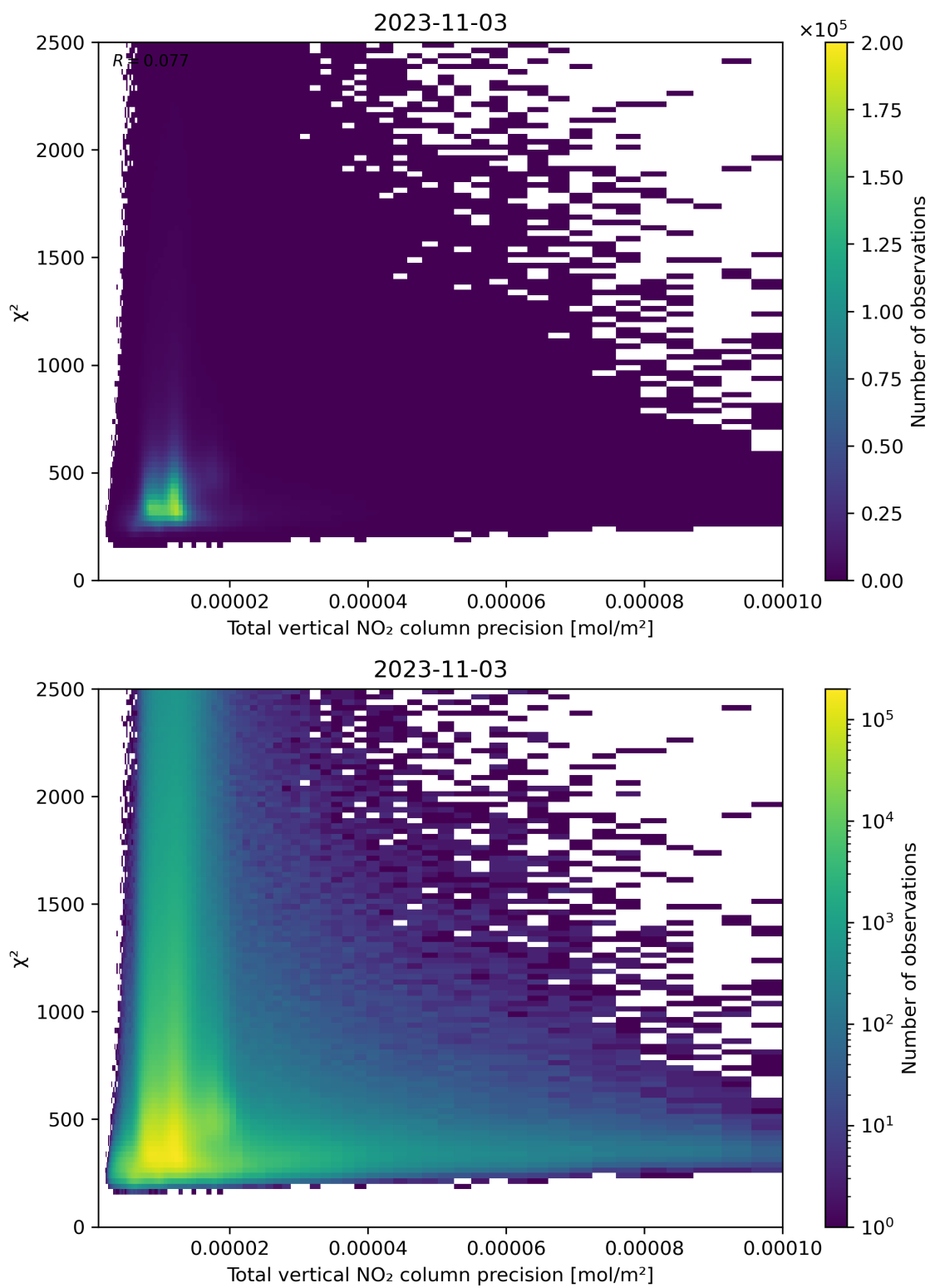
Figure 116: Scatter density plot of “Total vertical NO 2 column precision” against “ \chi^2 ” for 2023-11-02 to 2023-11-04.
