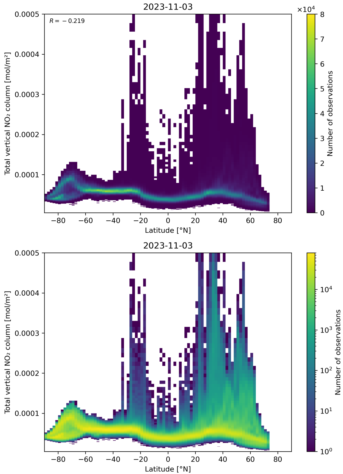
Figure 90: Scatter density plot of “Latitude” against “Total vertical NO 2 column” for 2023-11-02 to 2023-11-04.
