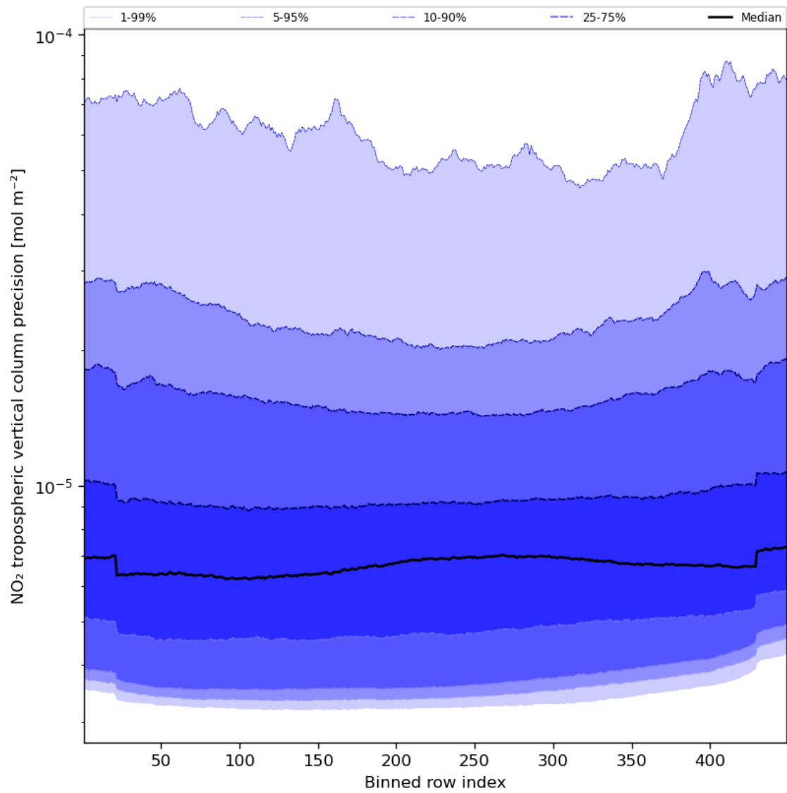
Figure 47: Along track statistics of “NO 2 tropospheric vertical column precision” for 2023-11-02 to 2023-11-04
