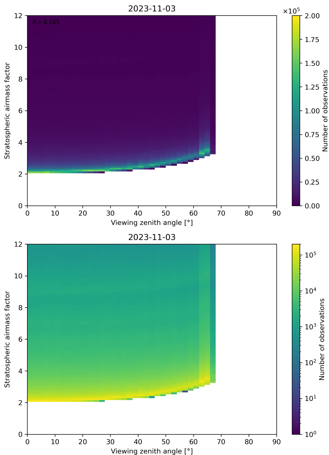
Figure 159: Scatter density plot of “Viewing zenith angle” against “Stratospheric airmass factor” for 2023-11-02 to 2023-11-04.
