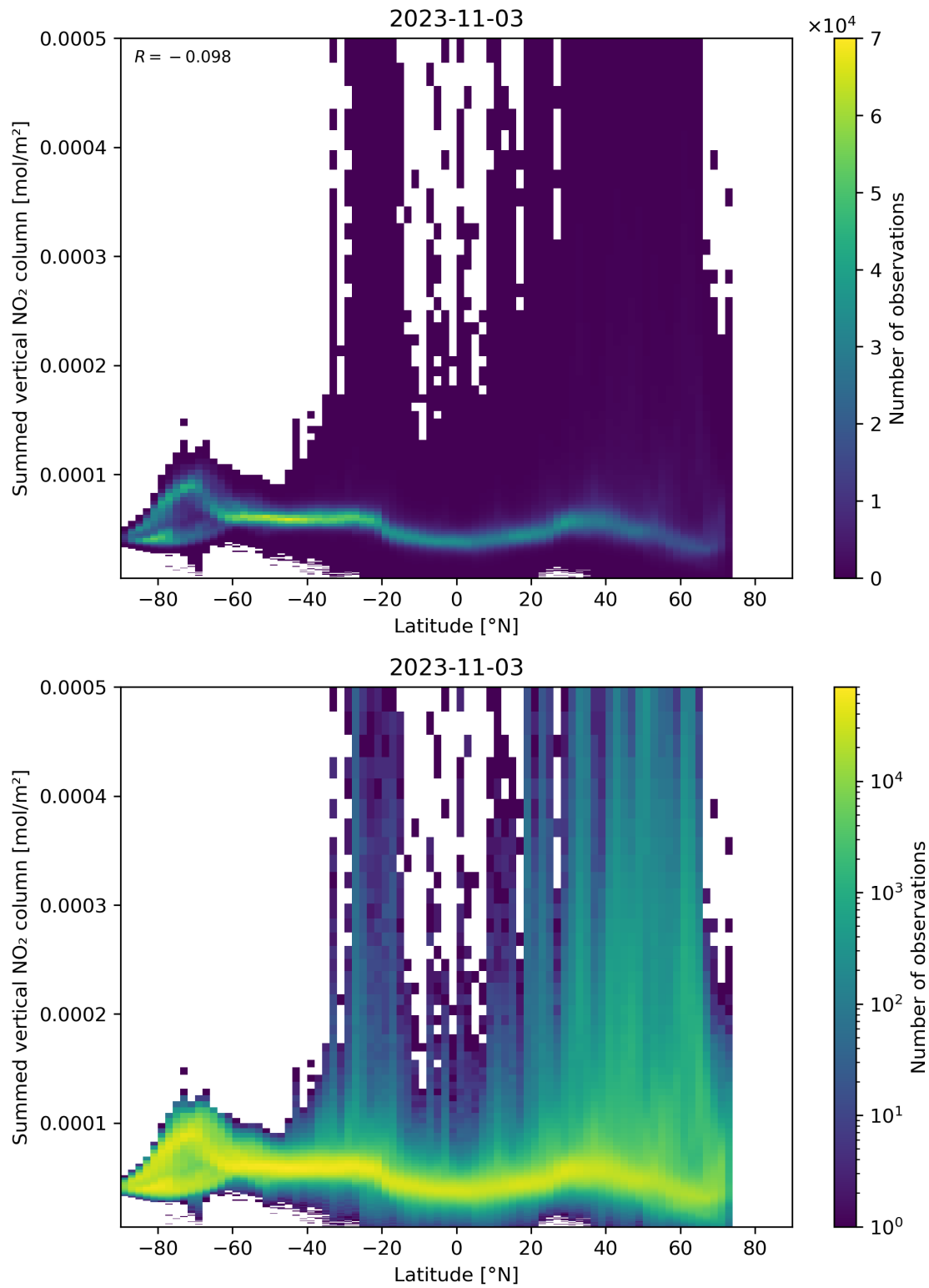
Figure 88: Scatter density plot of “Latitude” against “Summed vertical NO 2 column” for 2023-11-02 to 2023-11-04.
