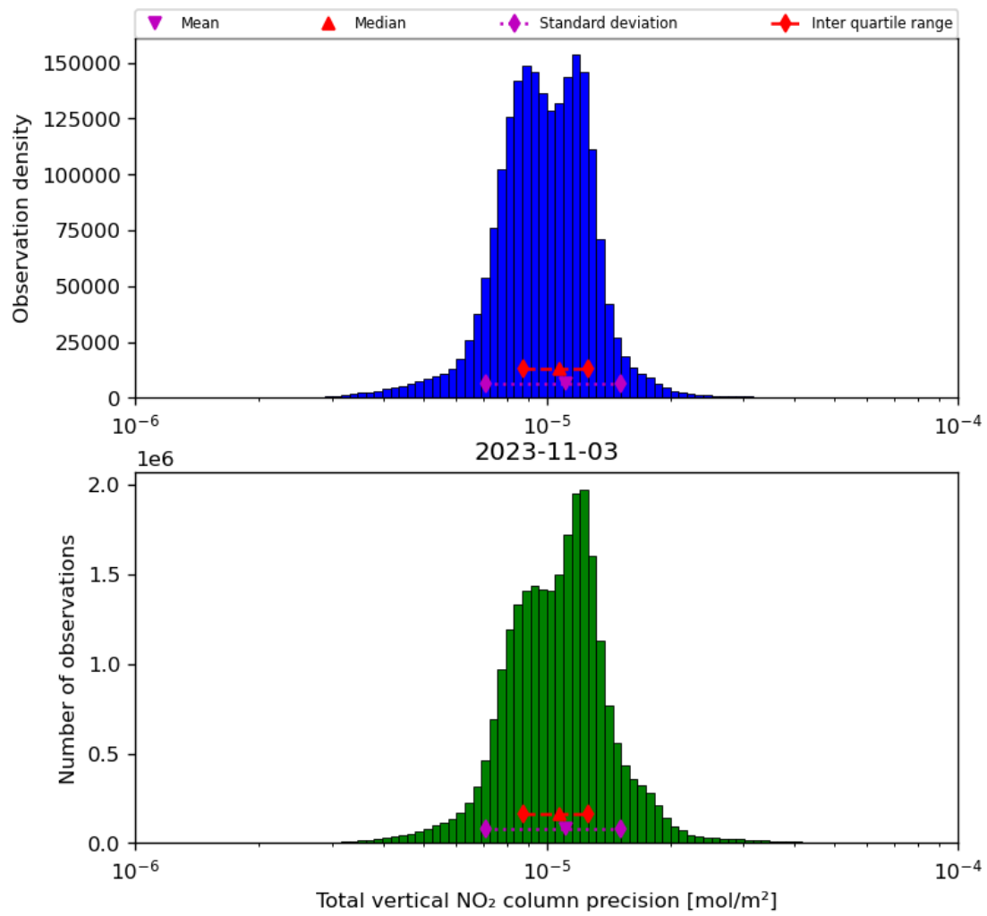
Figure 39: Histogram of "Total vertical NO 2 column precision" for 2023-11-02 to 2023-11-04
