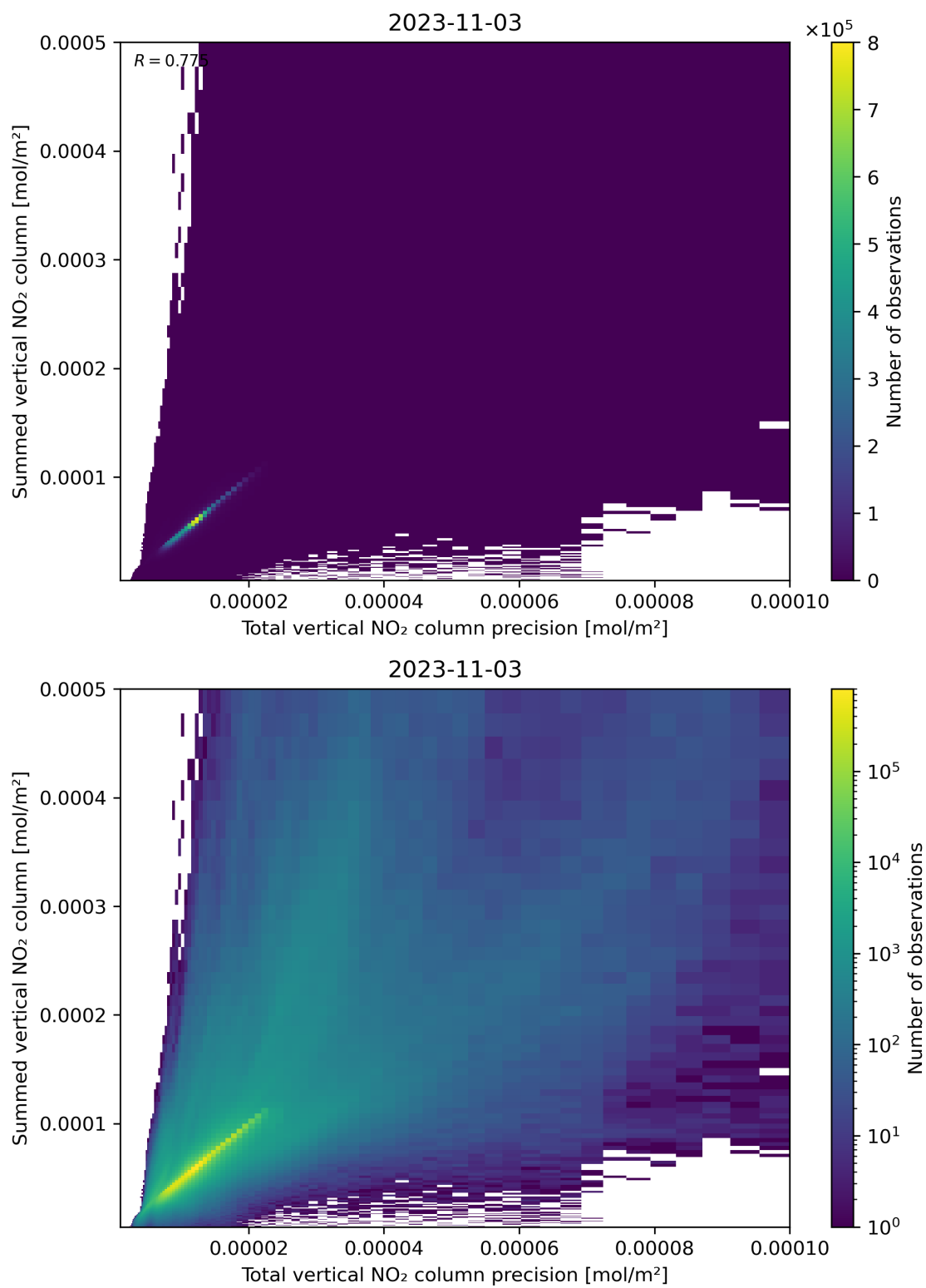
Figure 117: Scatter density plot of “Total vertical NO 2 column precision” against “Summed vertical NO 2 column” for 2023-11-02 to 2023-11-04.
