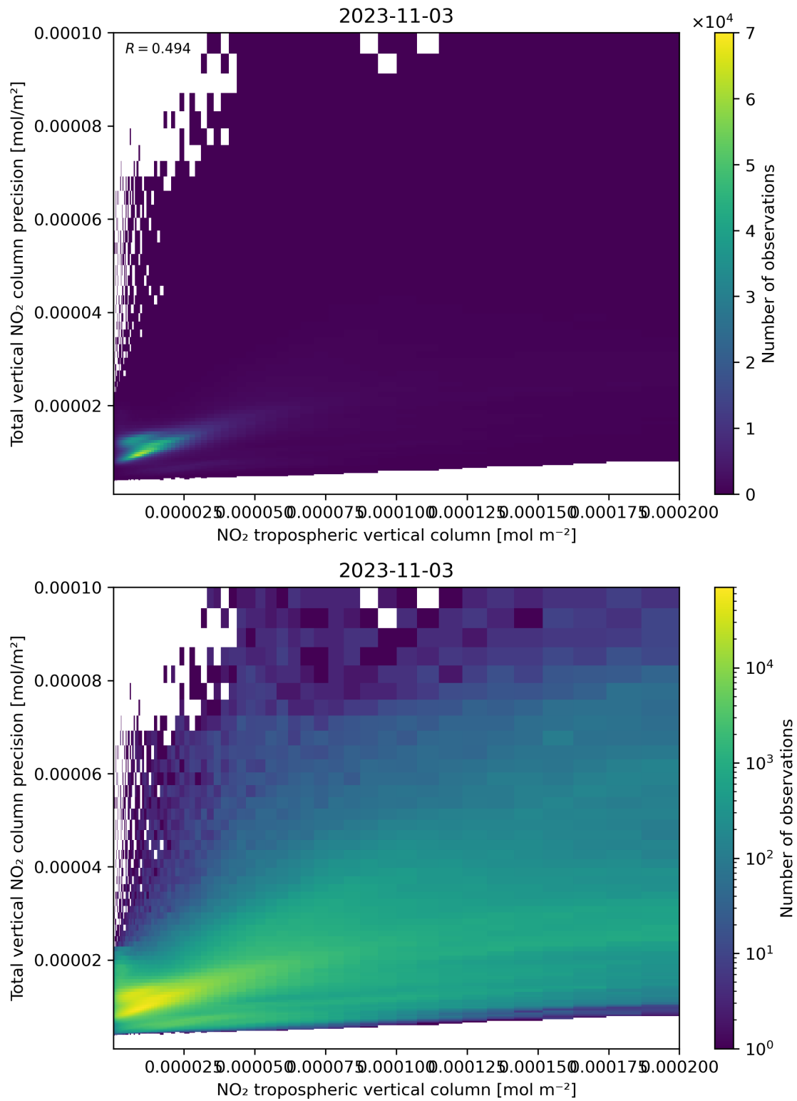
Figure 129: Scatter density plot of “NO 2 tropospheric vertical column” against “Total vertical NO 2 column precision” for 2023-11-02 to 2023-11-04.
