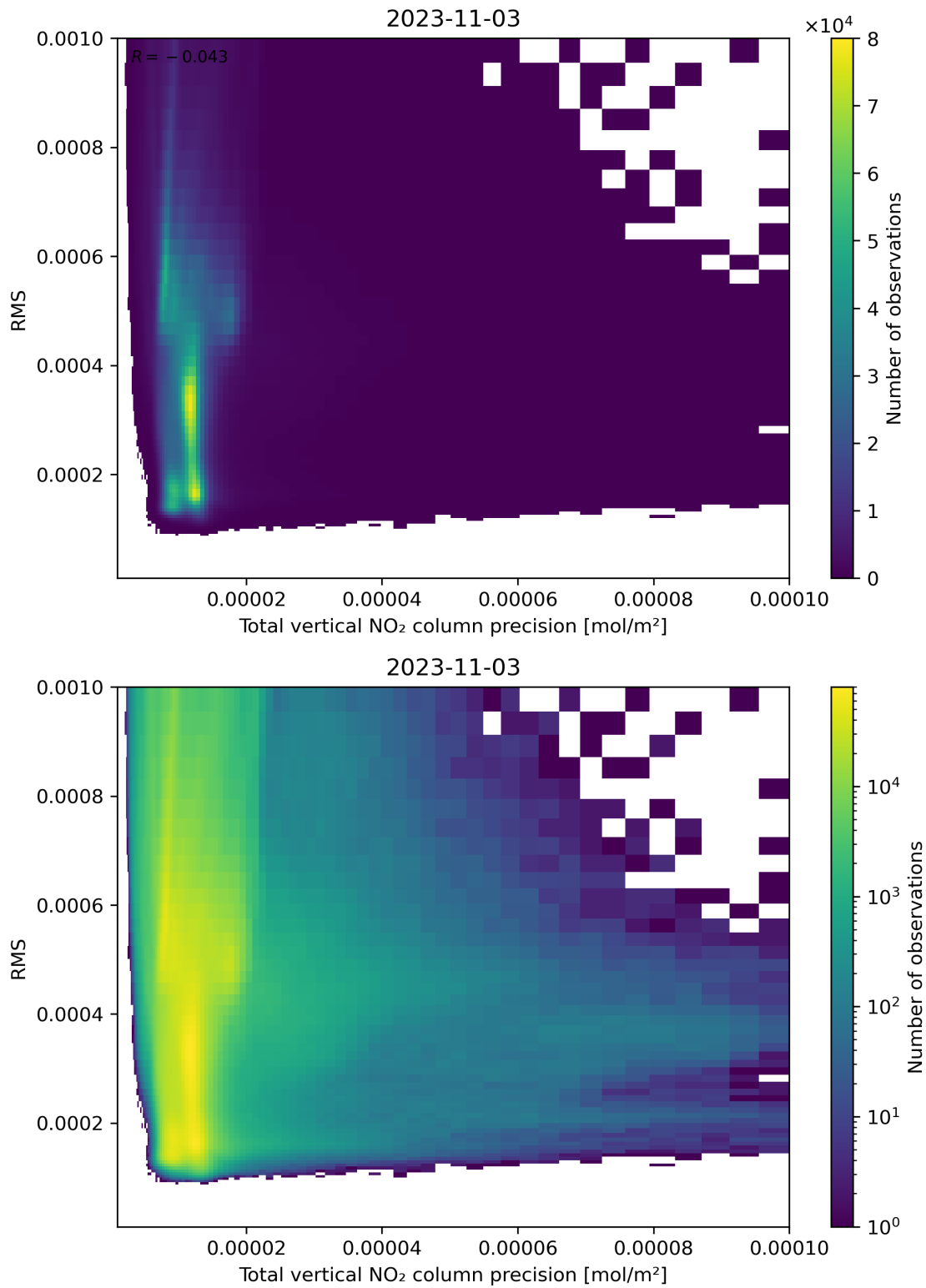
Figure 119: Scatter density plot of “Total vertical NO 2 column precision” against “RMS” for 2023-11-02 to 2023-11-04.
