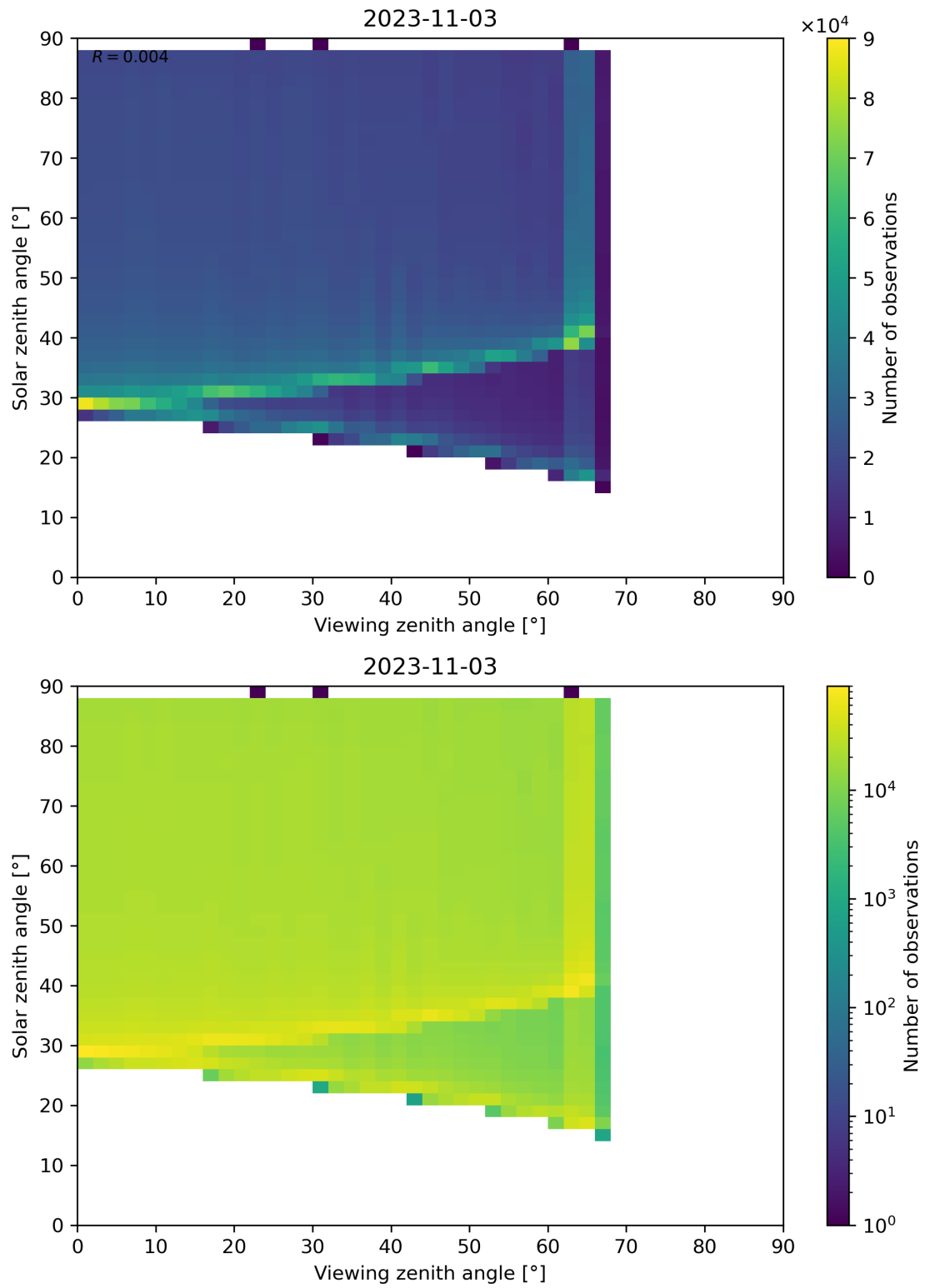
Figure 172: Scatter density plot of “Viewing zenith angle” against “Solar zenith angle” for 2023-11-02 to 2023-11-04.
