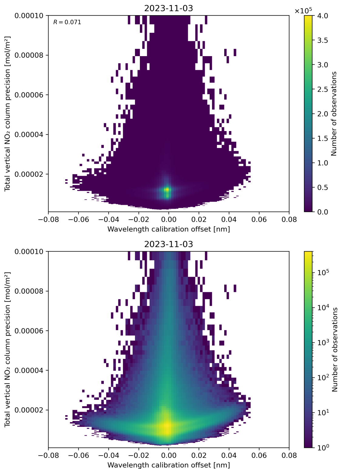
Figure 180: Scatter density plot of “Wavelength calibration offset” against “Total vertical NO 2 column precision” for 2023-11-02 to 2023-11-04.
