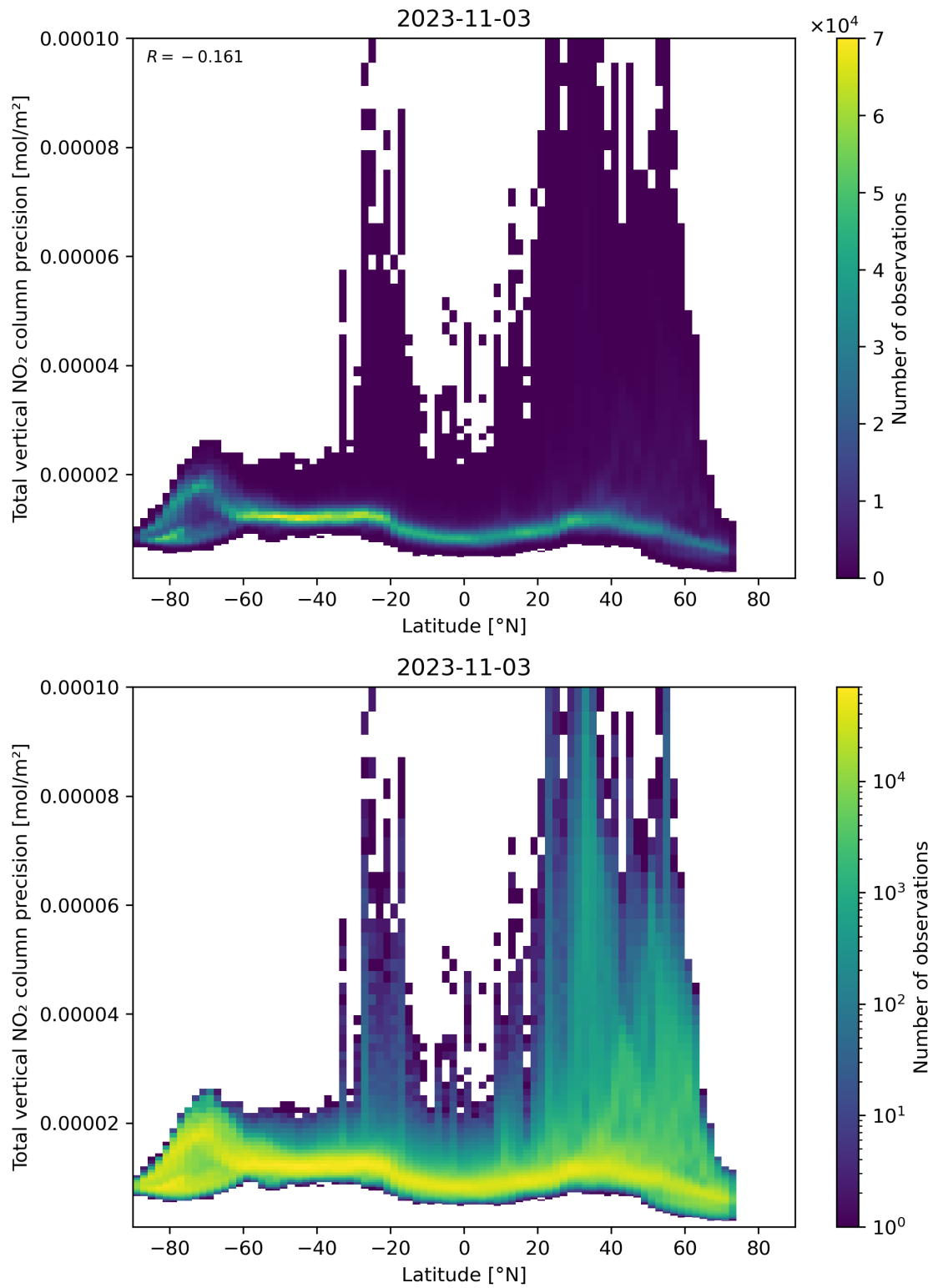
Figure 91: Scatter density plot of “Latitude” against “Total vertical NO 2 column precision” for 2023-11-02 to 2023-11-04.
