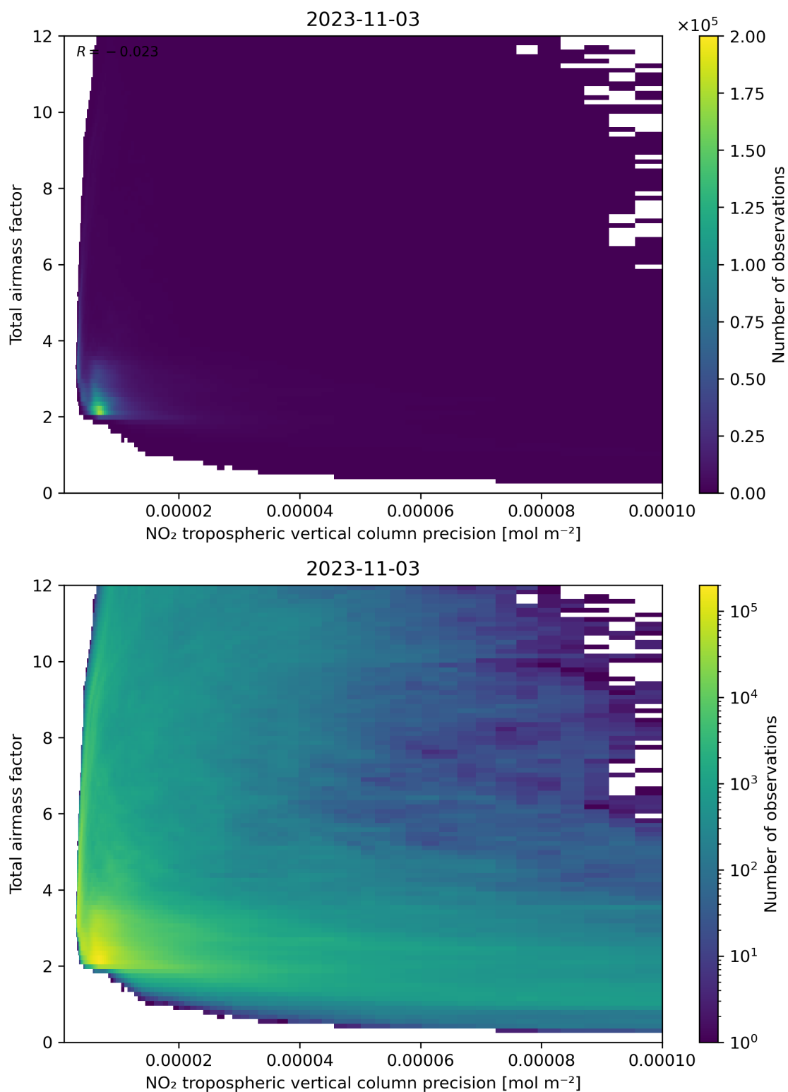
Figure 132: Scatter density plot of “NO 2 tropospheric vertical column precision” against “Total air mass factor” for 2023-11-02 to 2023-11-04.
