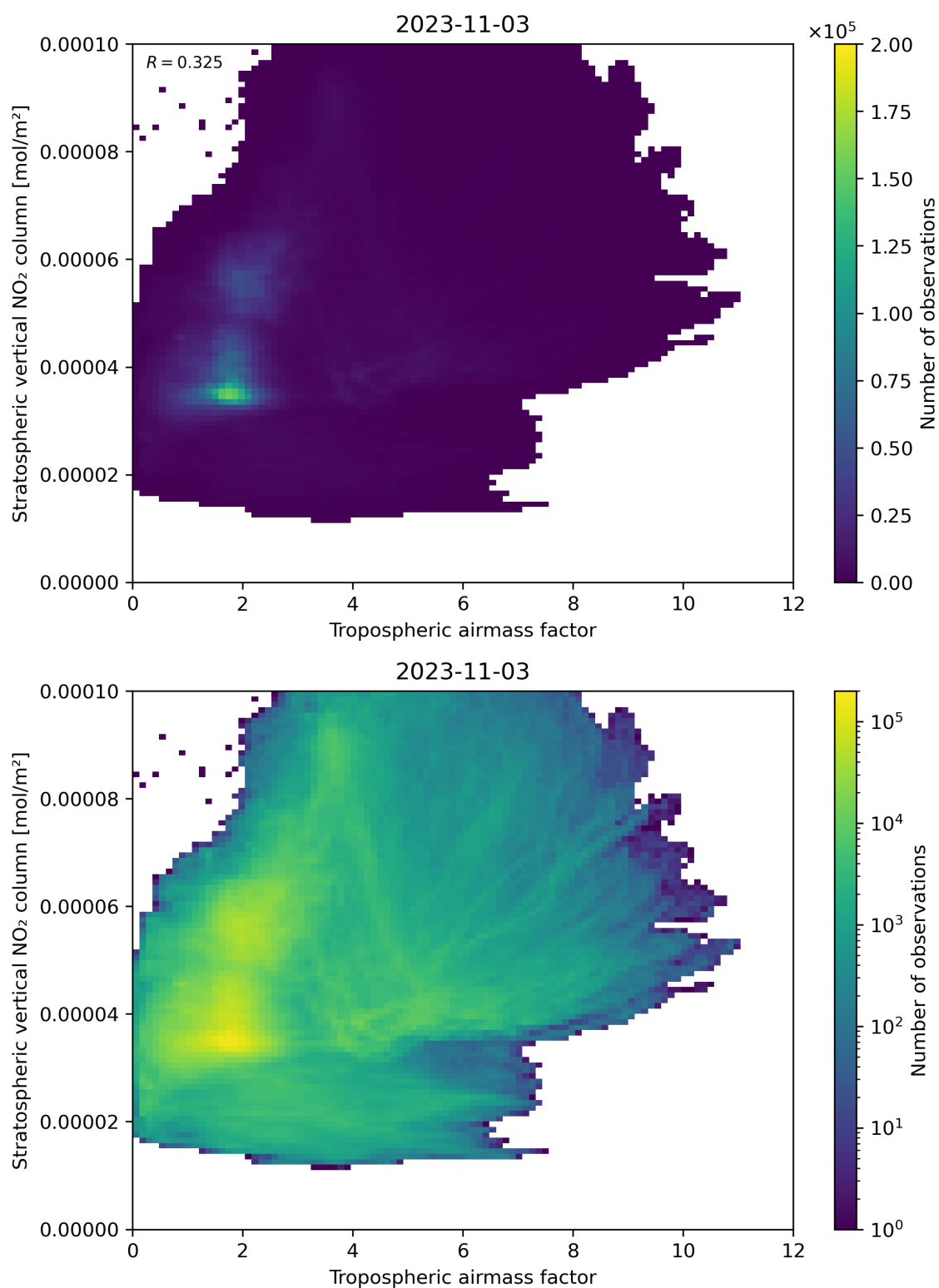
Figure 74: Scatter density plot of “Tropospheric air mass factor” against “Stratospheric vertical NO 2 column” for 2023-11-02 to 2023-11-04.
