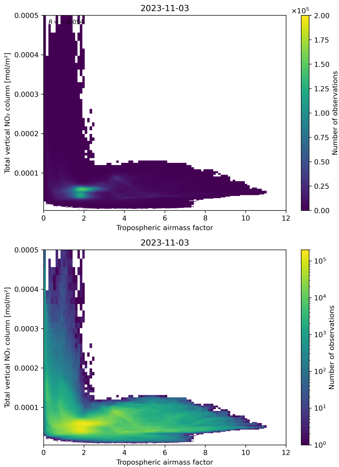
Figure 77: Scatter density plot of “Tropospheric airmass factor” against “Total vertical NO 2 column” for 2023-11-02 to 2023-11-04.
