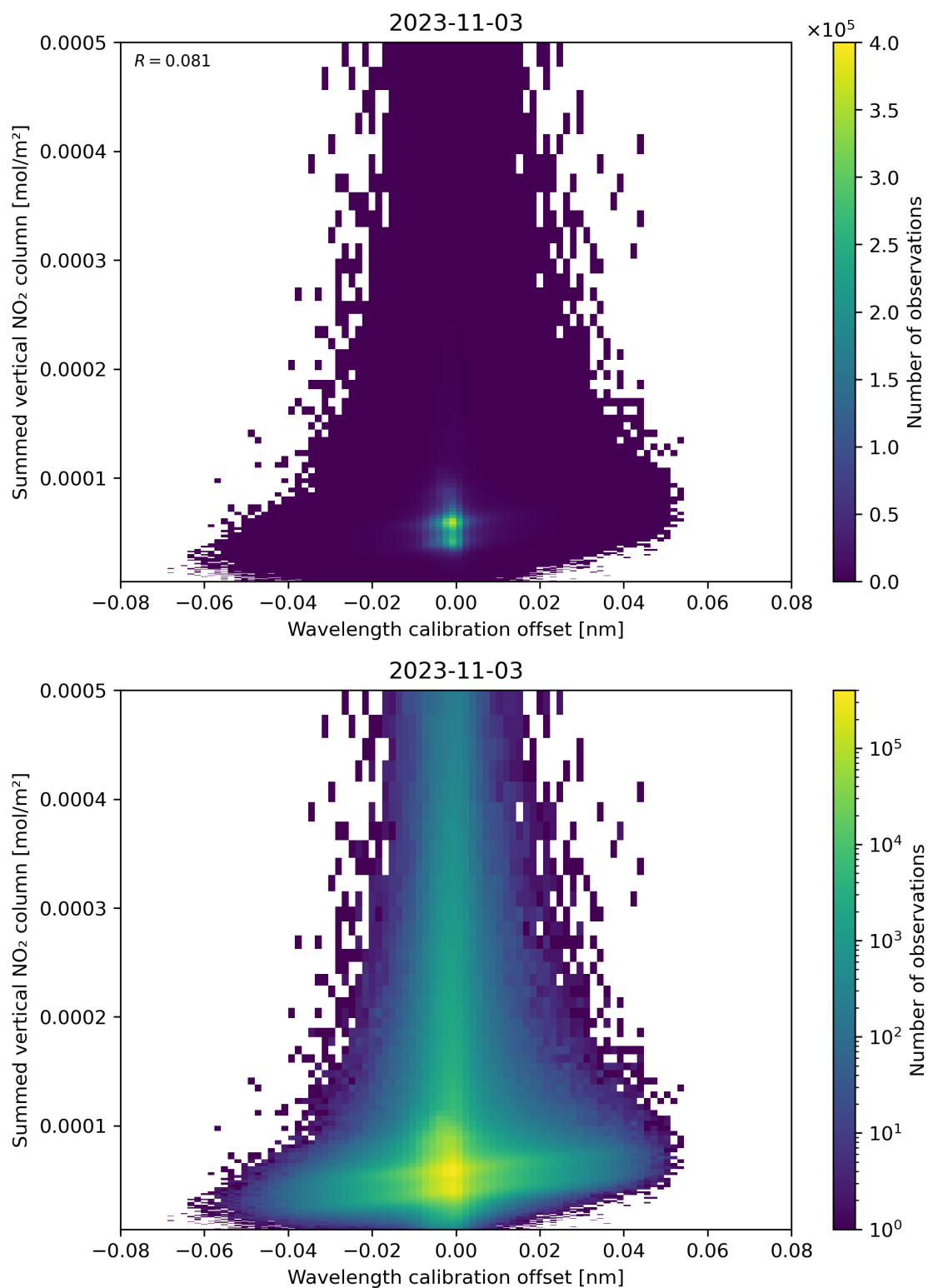
Figure 177: Scatter density plot of “Wavelength calibration offset” against “Summed vertical NO 2 column” for 2023-11-02 to 2023-11-04.
