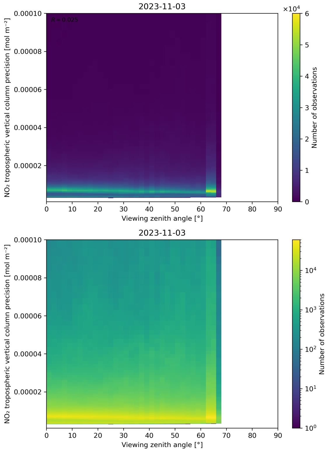
Figure 170: Scatter density plot of “Viewing zenith angle” against “NO 2 tropospheric vertical column precision” for 2023-11-02 to 2023-11-04.
