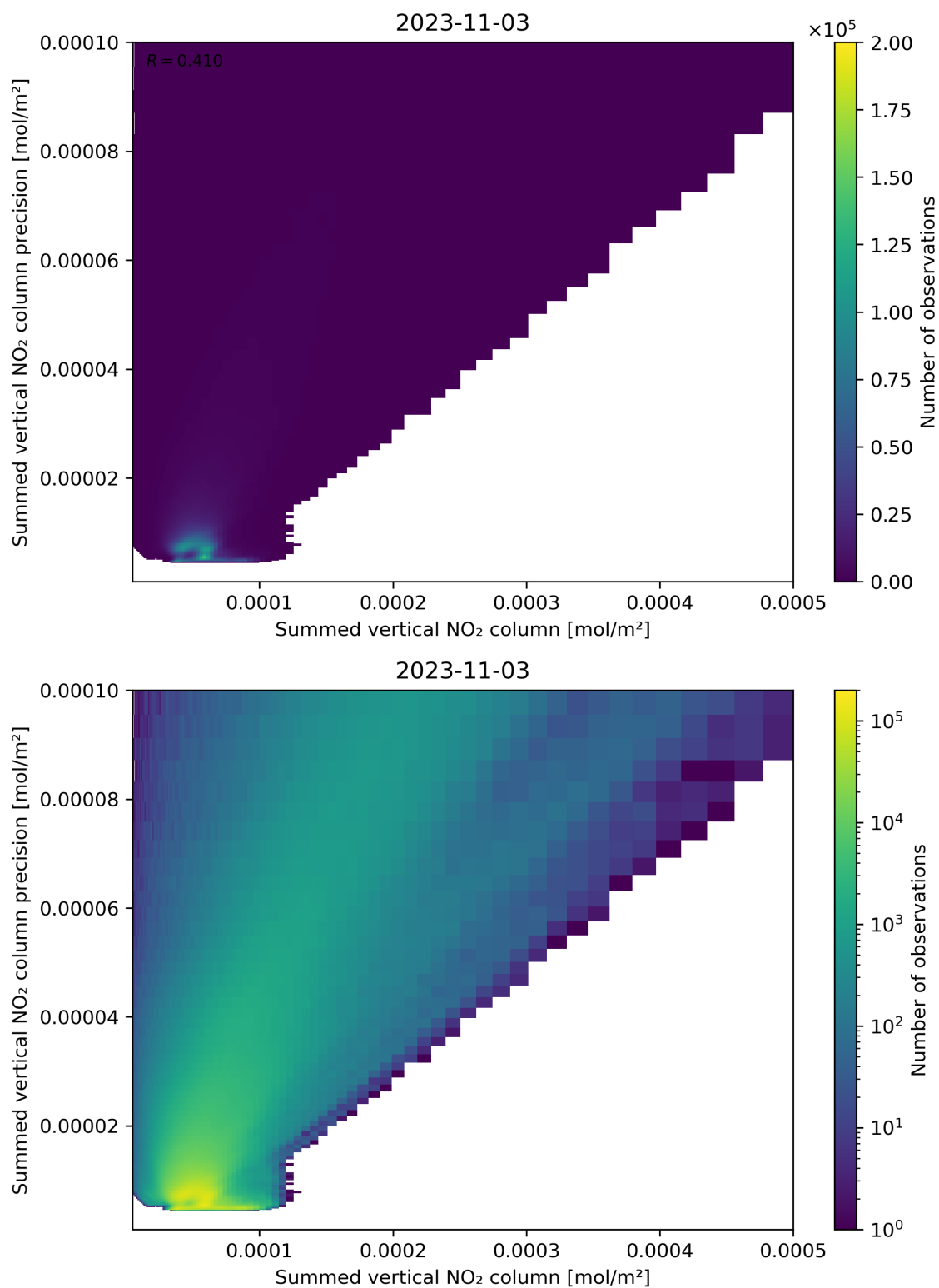
Figure 105: Scatter density plot of “Summed vertical NO 2 column” against “Summed vertical NO 2 column precision” for 2023-11-02 to 2023-11-04.
