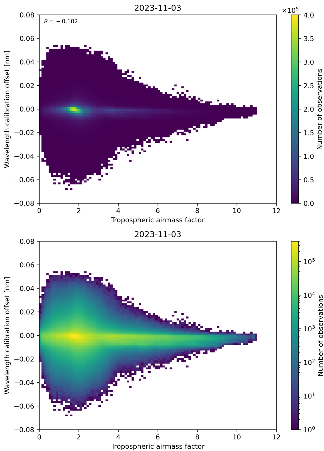
Figure 80: Scatter density plot of “Tropospheric airmass factor” against “Wavelength calibration offset” for 2023-11-02 to 2023-11-04.
