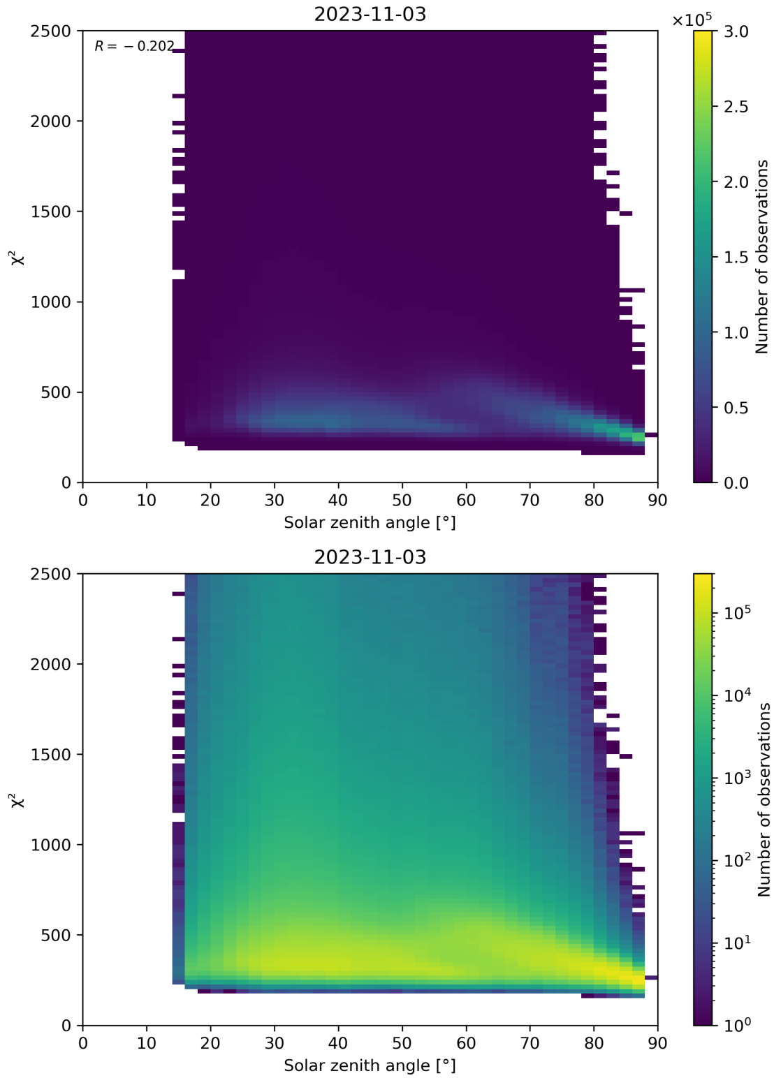
Figure 148: Scatter density plot of “Solar zenith angle” against “ \chi^2 ” for 2023-11-02 to 2023-11-04.
