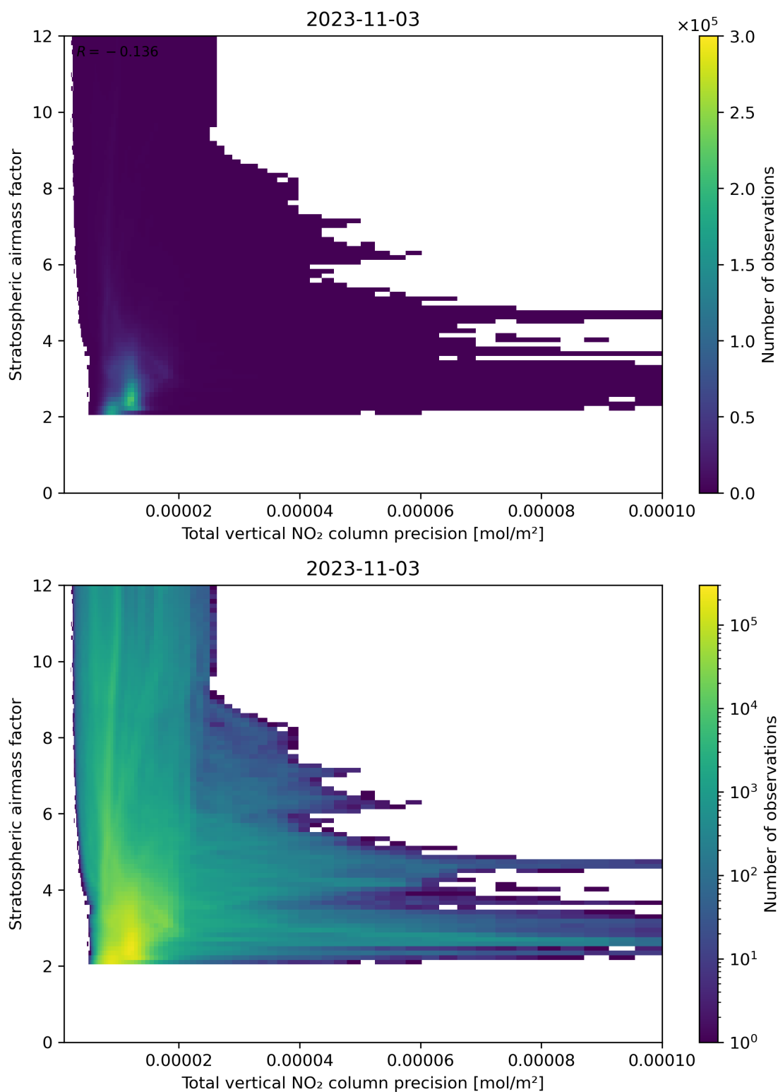
Figure 115: Scatter density plot of “Total vertical NO 2 column precision” against “Stratospheric air mass factor” for 2023-11-02 to 2023-11-04.
