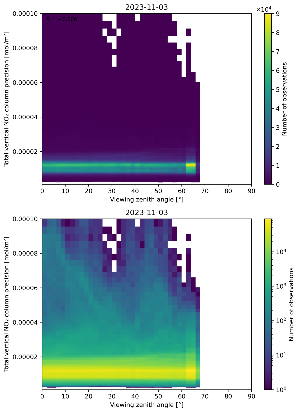
Figure 168: Scatter density plot of “Viewing zenith angle” against “Total vertical NO 2 column precision” for 2023-11-02 to 2023-11-04.
