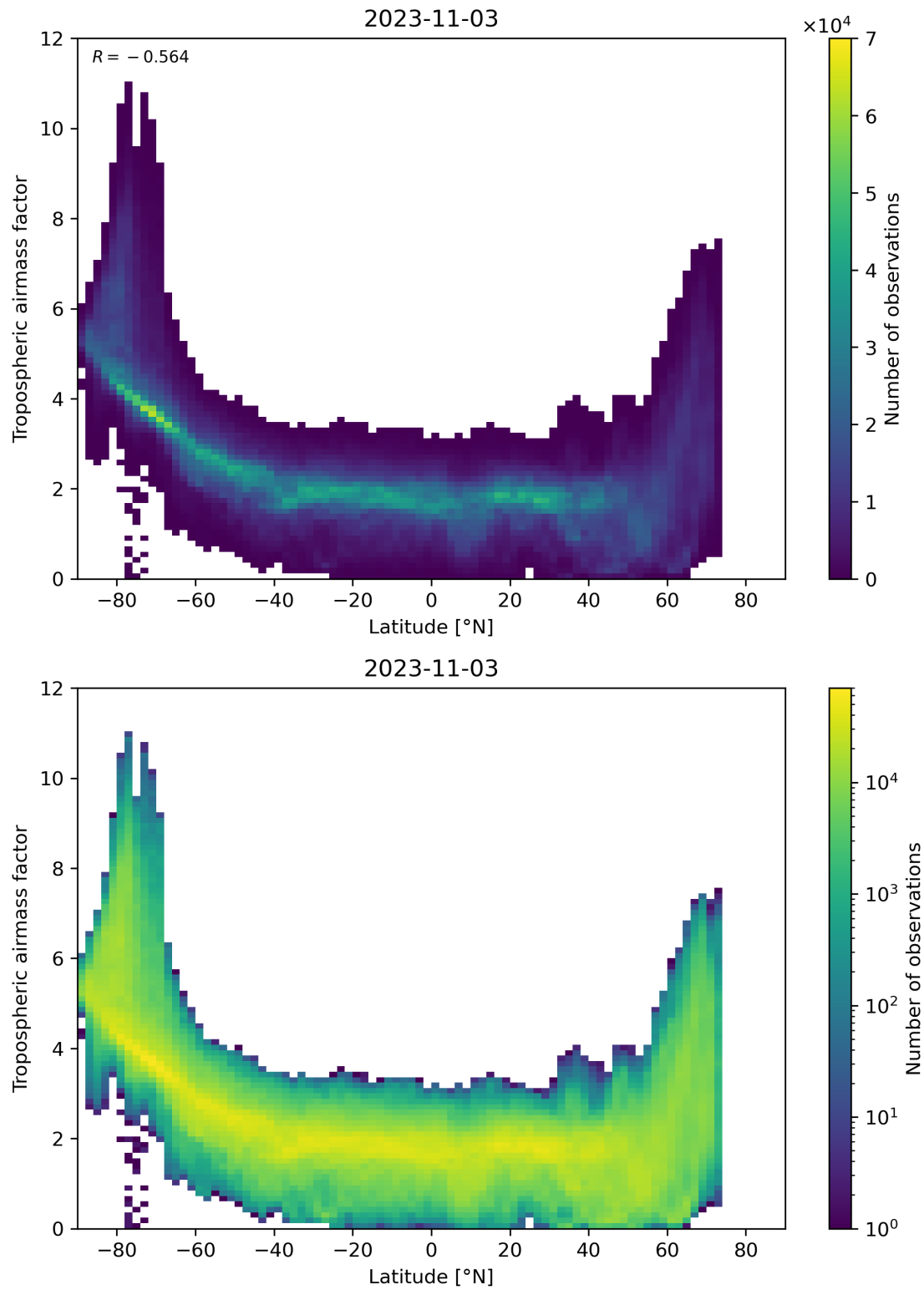
Figure 85: Scatter density plot of “Latitude” against “Tropospheric airmass factor” for 2023-11-02 to 2023-11-04.
