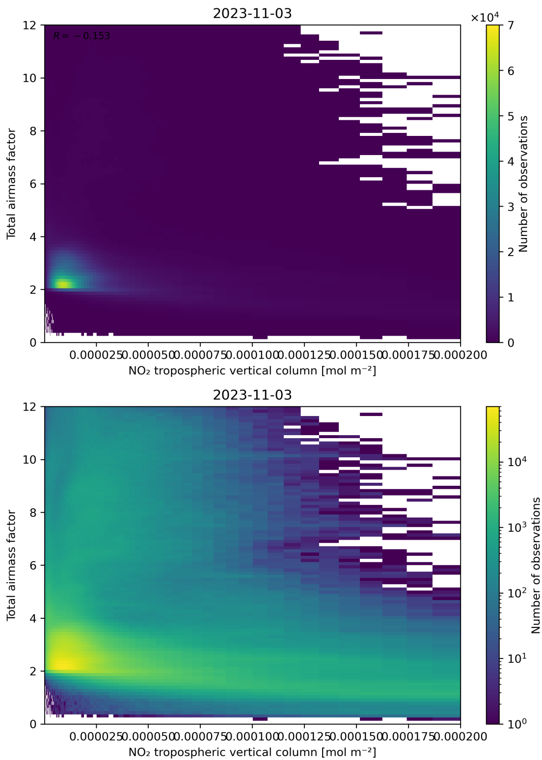
Figure 122: Scatter density plot of “NO 2 tropospheric vertical column” against “Total air mass factor” for 2023-11-02 to 2023-11-04.
