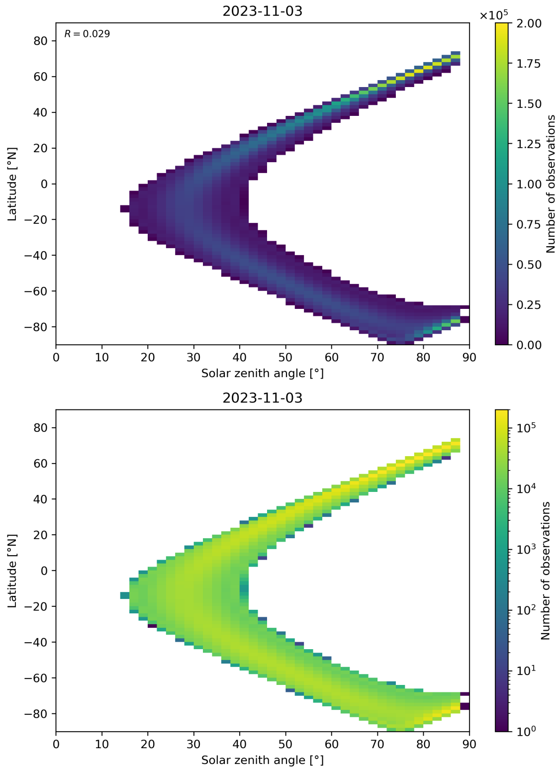
Figure 149: Scatter density plot of “Solar zenith angle” against “Latitude” for 2023-11-02 to 2023-11-04.
