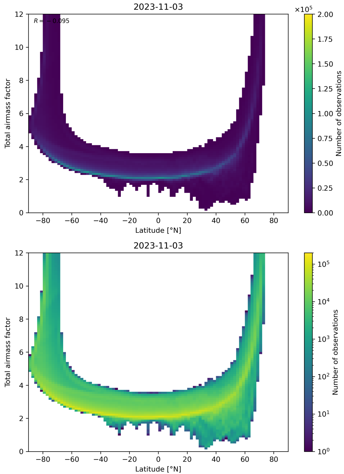
Figure 84: Scatter density plot of “Latitude” against “Total airmass factor” for 2023-11-02 to 2023-11-04.
