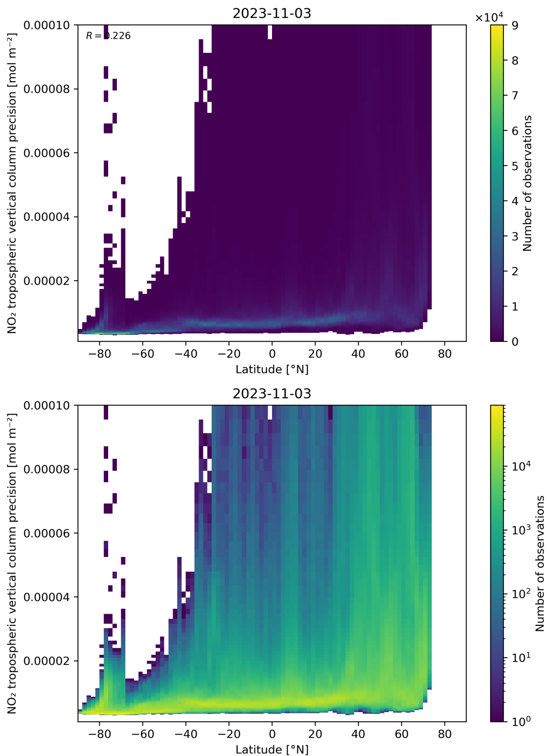
Figure 93: Scatter density plot of “Latitude” against “NO 2 tropospheric vertical column precision” for 2023-11-02 to 2023-11-04.
