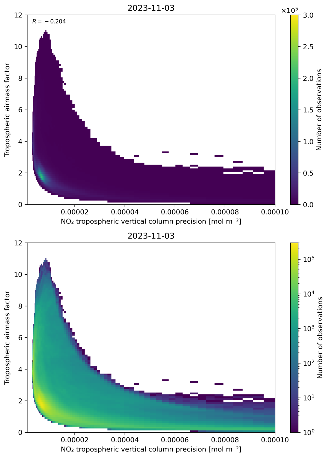
Figure 133: Scatter density plot of “NO 2 tropospheric vertical column precision” against “Tropospheric airmass factor” for 2023-11-02 to 2023-11-04.
