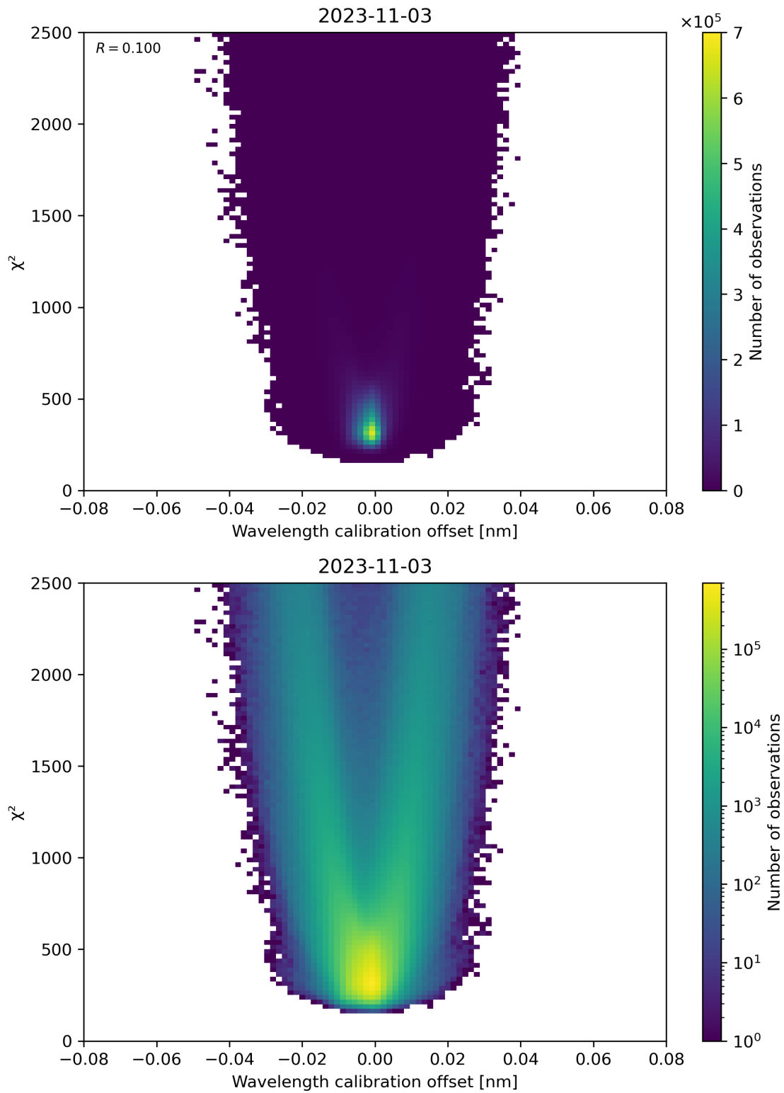
Figure 175: Scatter density plot of “Wavelength calibration offset” against “ \chi^2 ” for 2023-11-02 to 2023-11-04.
