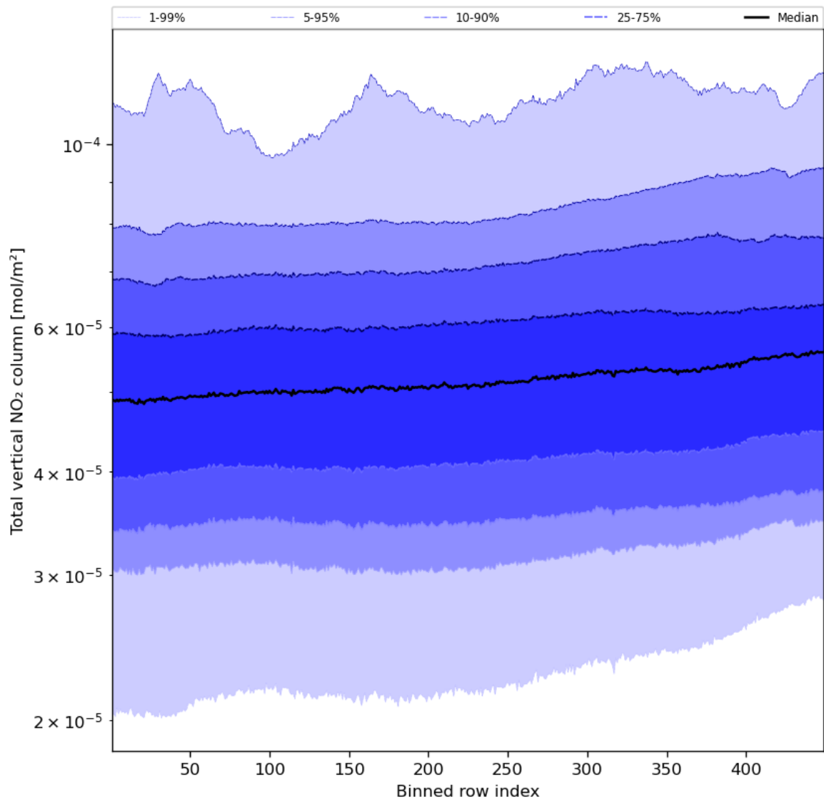
Figure 55: Along track statistics of “Total vertical NO 2 column” for 2023-11-02 to 2023-11-04
