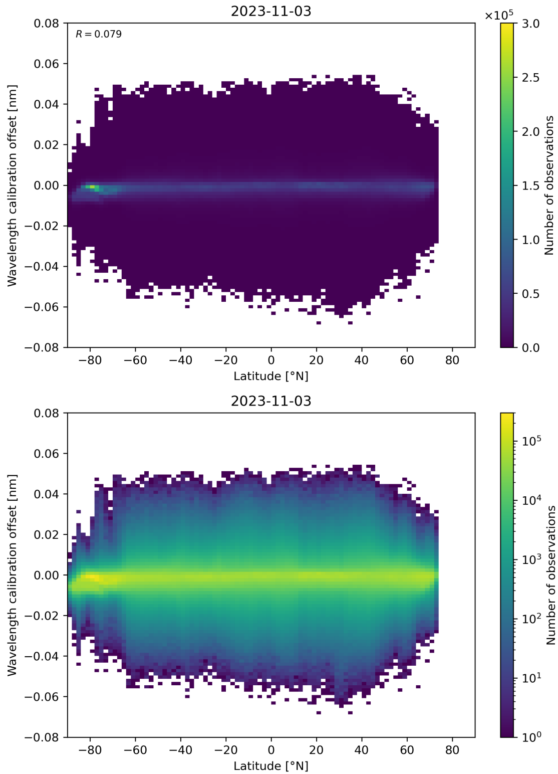
Figure 95: Scatter density plot of “Latitude” against “Wavelength calibration offset” for 2023-11-02 to 2023-11-04.
