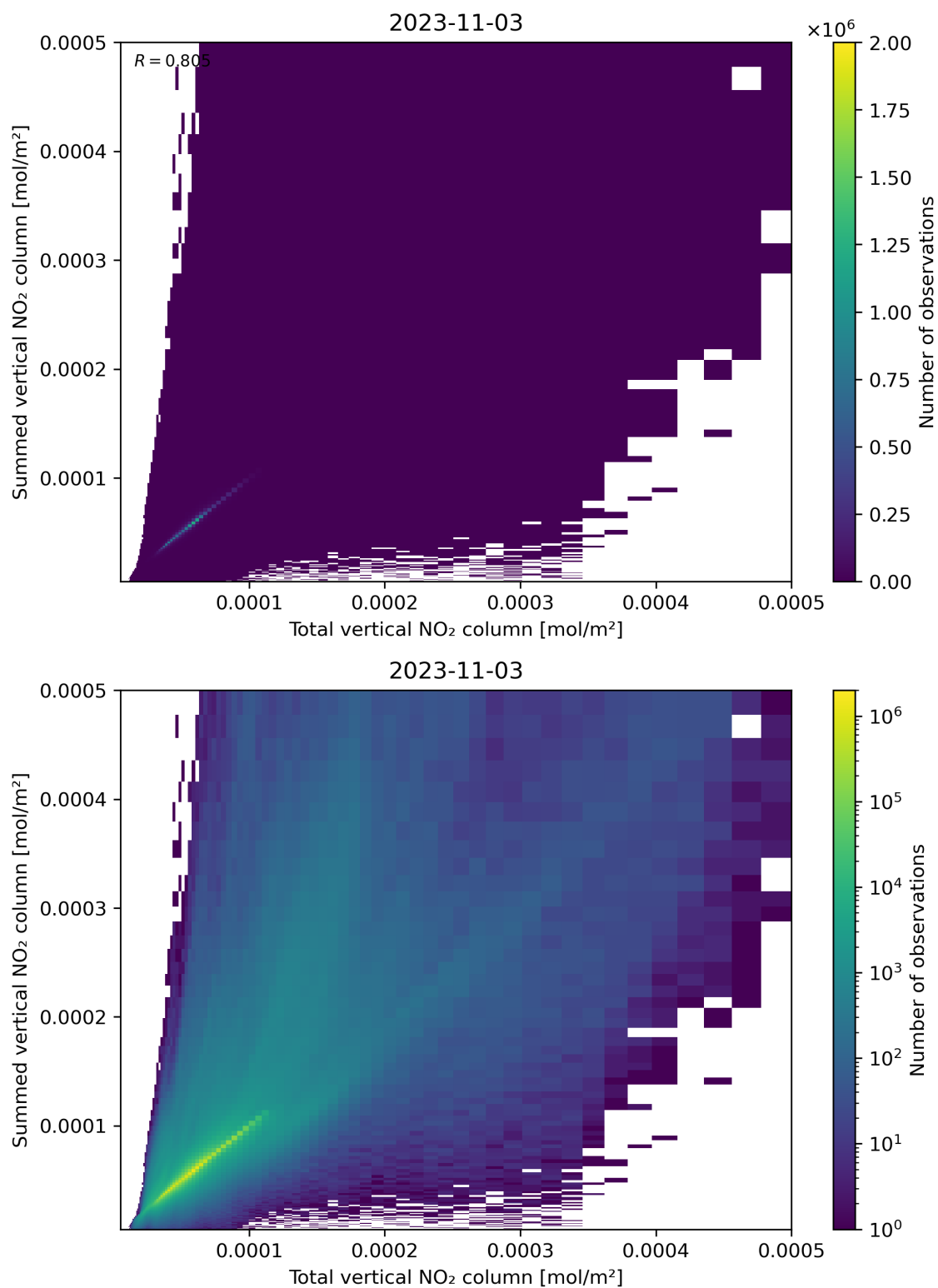
Figure 112: Scatter density plot of “Total vertical NO 2 column” against “Summed vertical NO 2 column” for 2023-11-02 to 2023-11-04.
