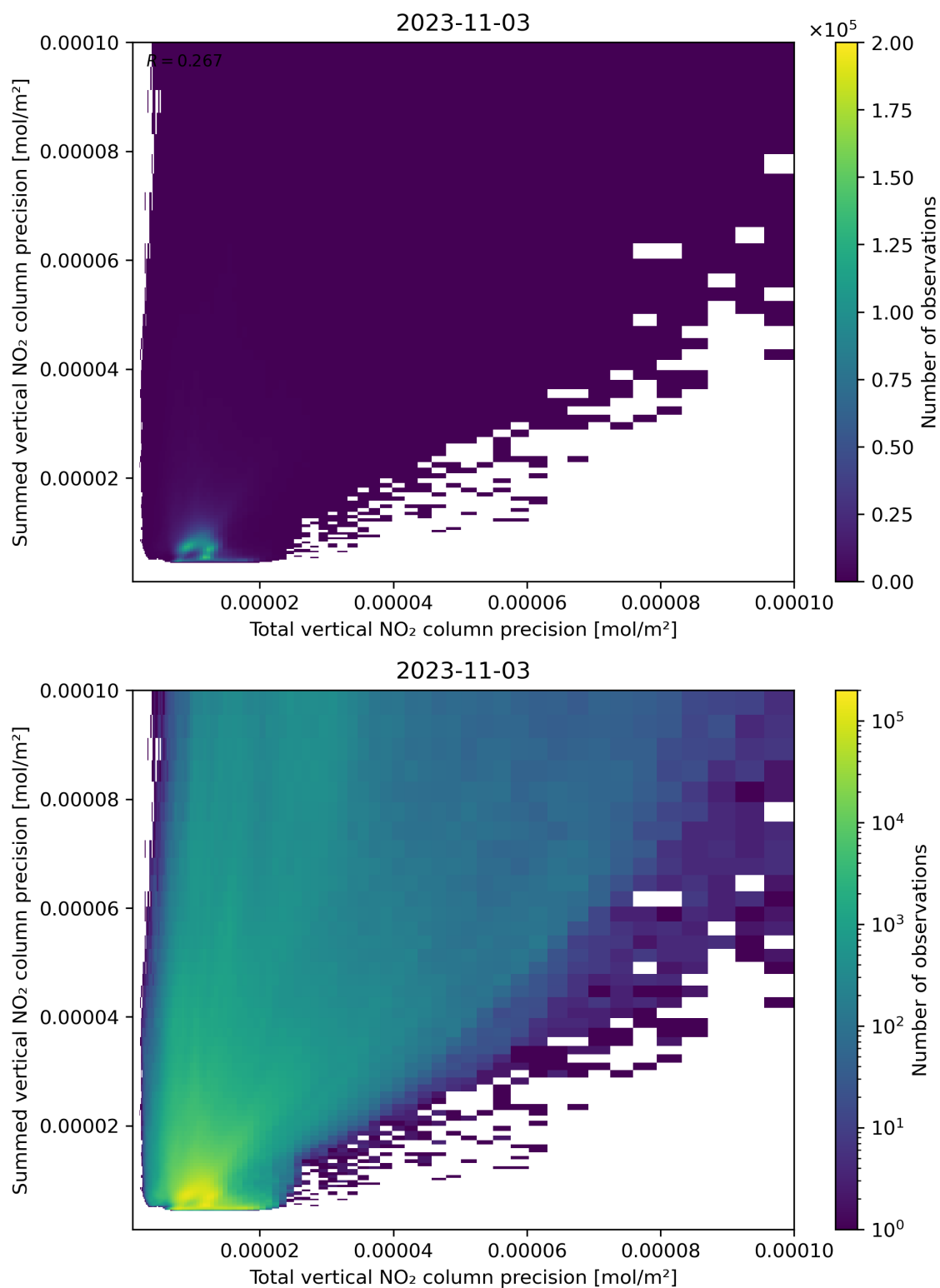
Figure 118: Scatter density plot of “Total vertical NO 2 column precision” against “Summed vertical NO 2 column precision” for 2023-11-02 to 2023-11-04.
