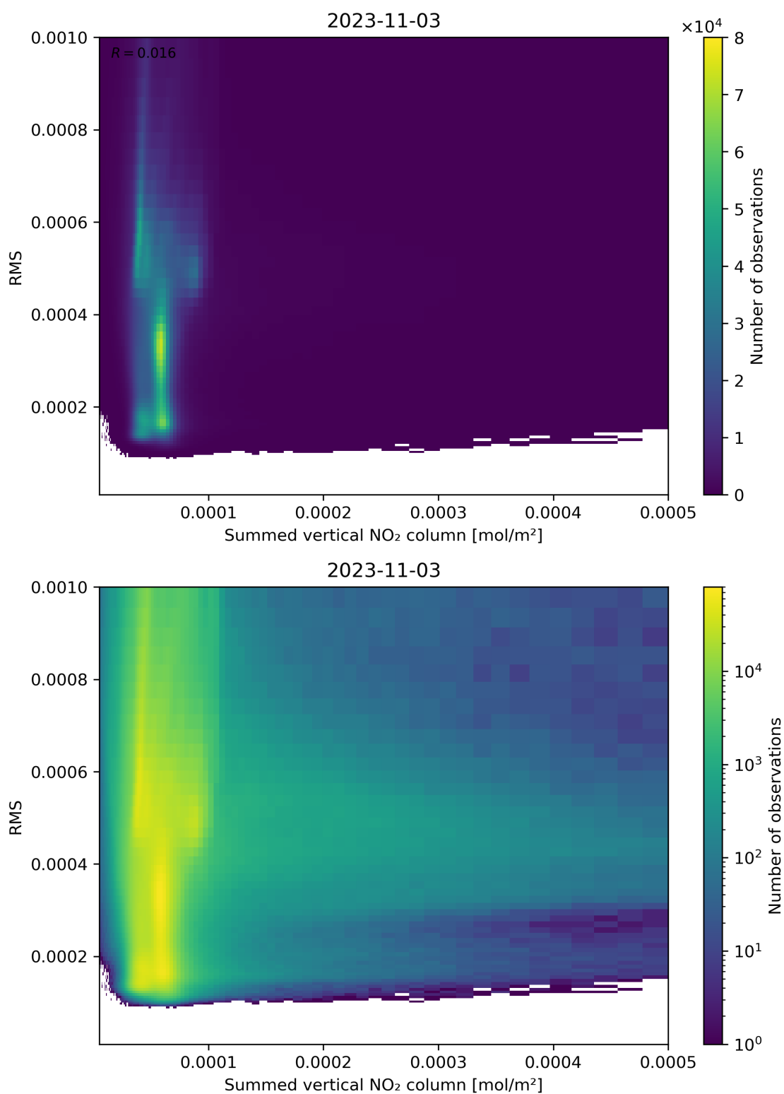
Figure 109: Scatter density plot of “Summed vertical NO 2 column” against “RMS” for 2023-11-02 to 2023-11-04.
