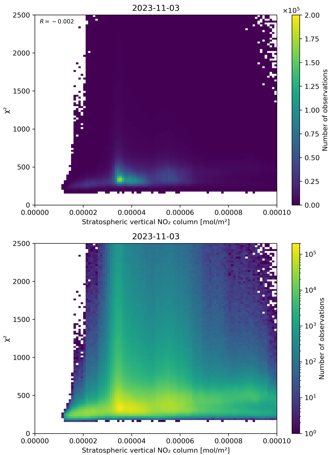
Figure 97: Scatter density plot of “Stratospheric vertical NO 2 column” against “ \chi^2 ” for 2023-11-02 to 2023-11-04.
