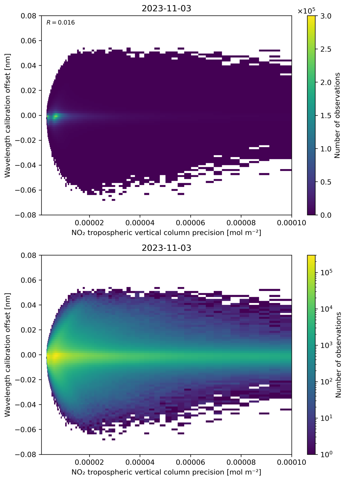
Figure 141: Scatter density plot of “NO 2 tropospheric vertical column precision” against “Wavelength calibration offset” for 2023-11-02 to 2023-11-04.
