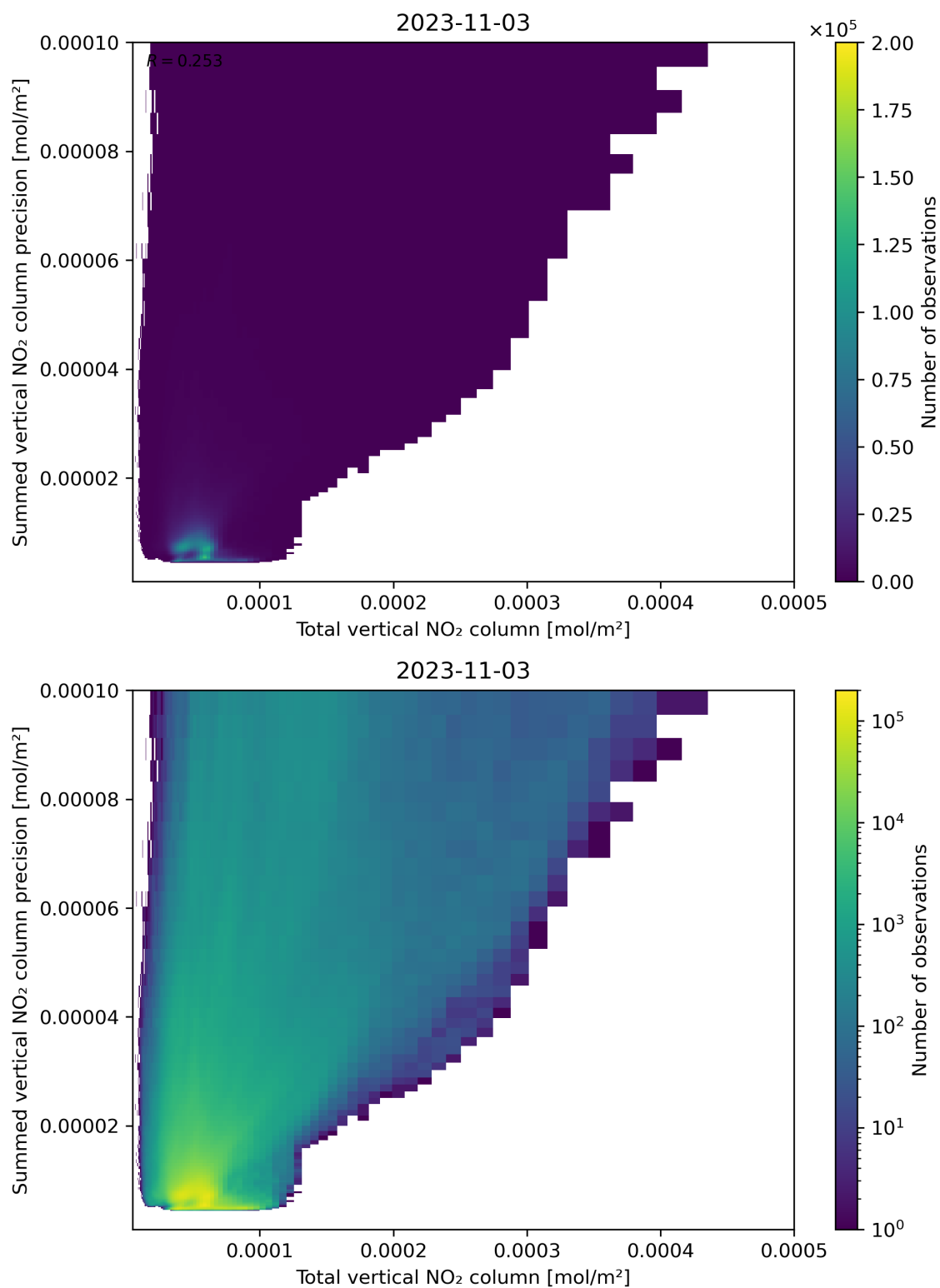
Figure 113: Scatter density plot of “Total vertical NO 2 column” against “Summed vertical NO 2 column precision” for 2023-11-02 to 2023-11-04.
