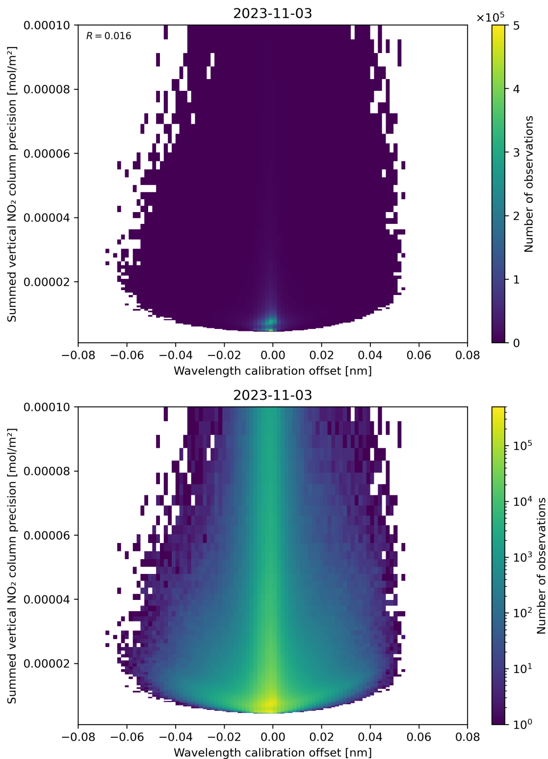
Figure 178: Scatter density plot of “Wavelength calibration offset” against “Summed vertical NO 2 column precision” for 2023-11-02 to 2023-11-04.
