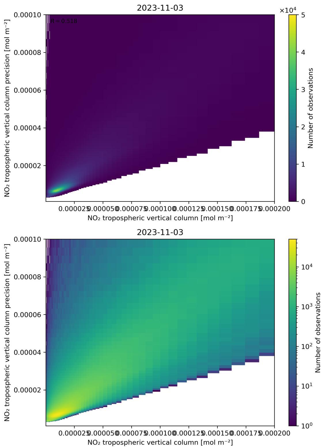
Figure 130: Scatter density plot of “NO 2 tropospheric vertical column” against “NO 2 tropospheric vertical column precision” for 2023-11-02 to 2023-11-04.
