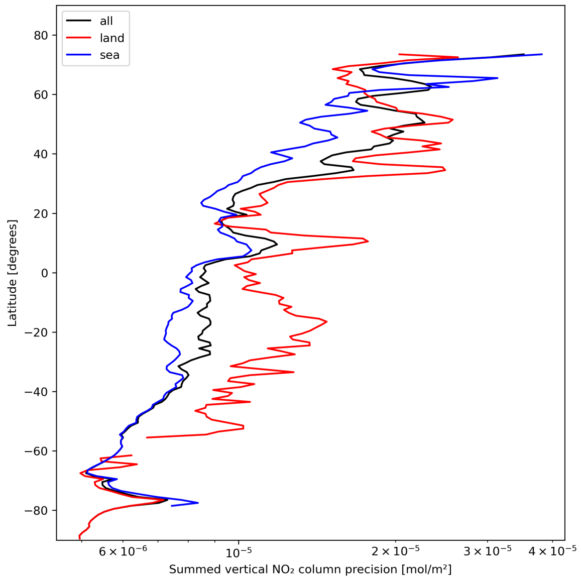
Figure 24: Zonal average of “Summed vertical NO 2 column precision” for 2023-11-02 to 2023-11-04.
