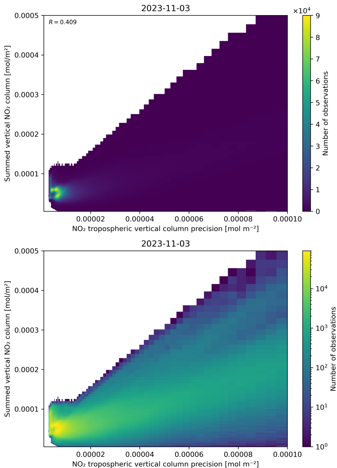
Figure 136: Scatter density plot of “NO 2 tropospheric vertical column precision” against “Summed vertical NO 2 column” for 2023-11-02 to 2023-11-04.
