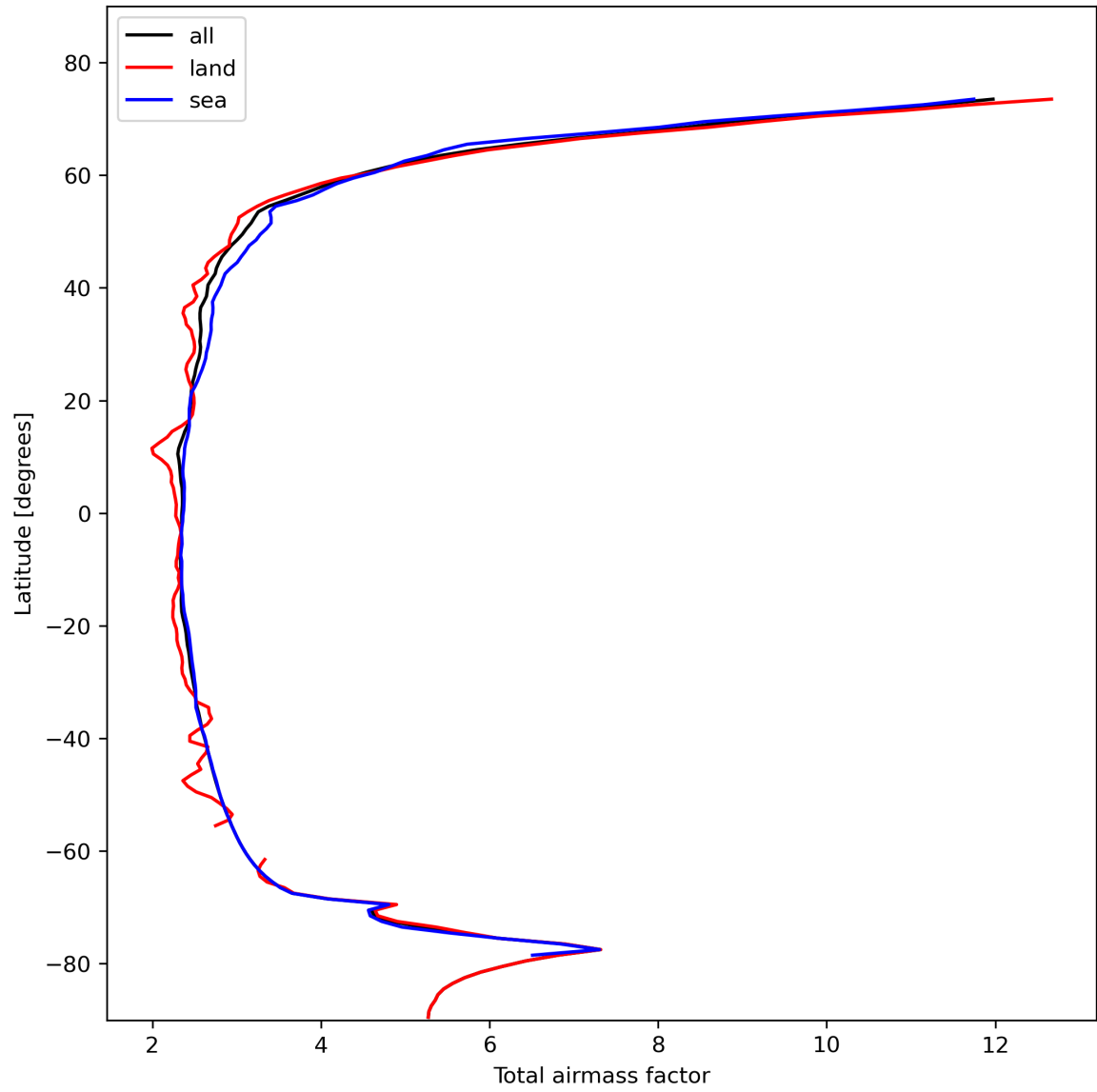
Figure 15: Zonal average of “Total airmass factor” for 2023-11-02 to 2023-11-04.
