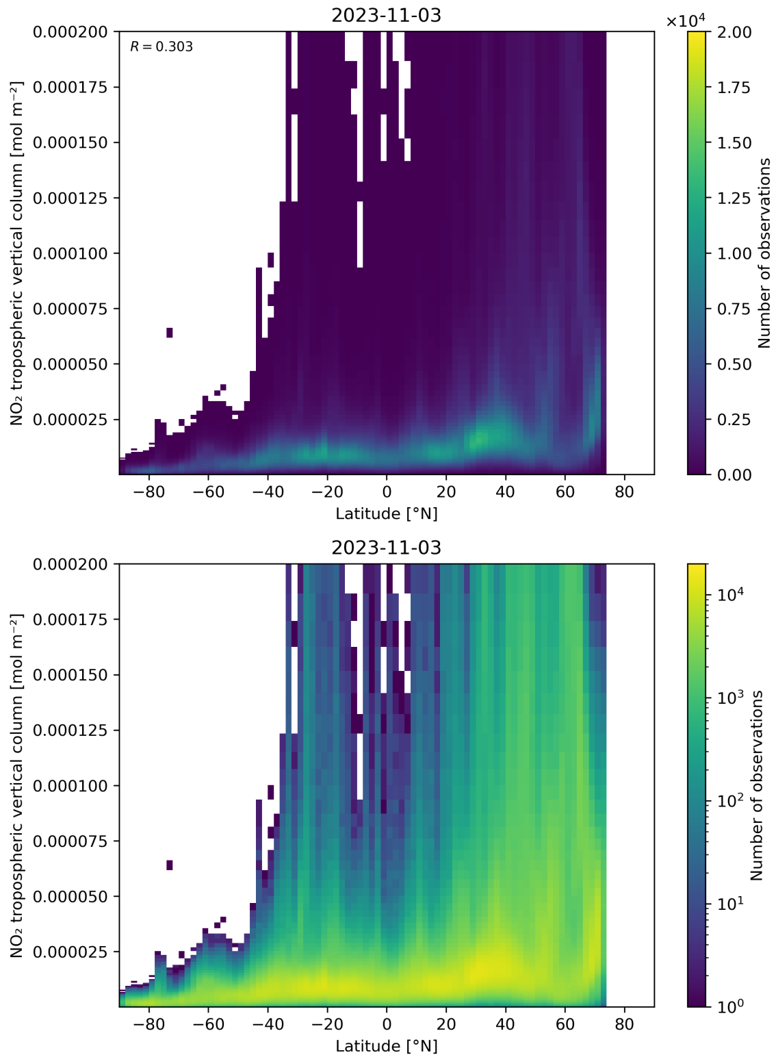
Figure 92: Scatter density plot of “Latitude” against “NO 2 tropospheric vertical column” for 2023-11-02 to 2023-11-04.
