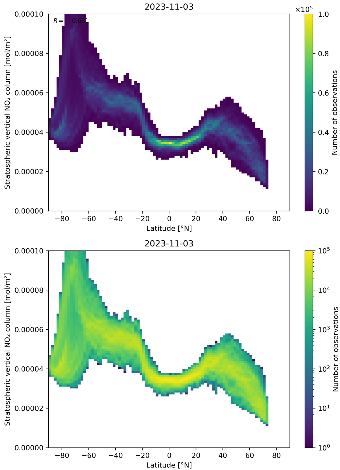
Figure 87: Scatter density plot of “Latitude” against “Stratospheric vertical NO 2 column” for 2023-11-02 to 2023-11-04.
