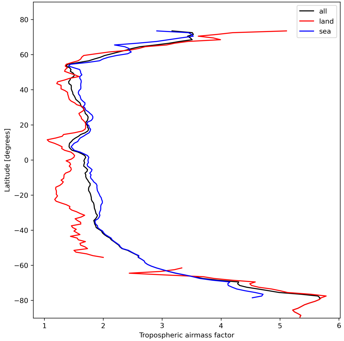
Figure 14: Zonal average of “Tropospheric airmass factor” for 2023-11-02 to 2023-11-04.
