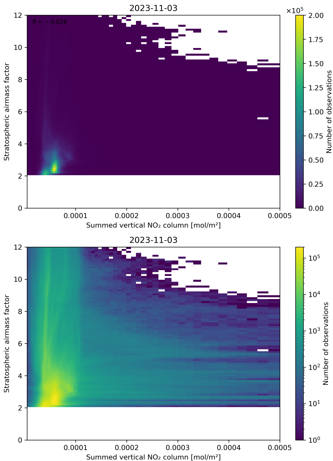
Figure 103: Scatter density plot of “Summed vertical NO 2 column” against “Stratospheric air mass factor” for 2023-11-02 to 2023-11-04.
