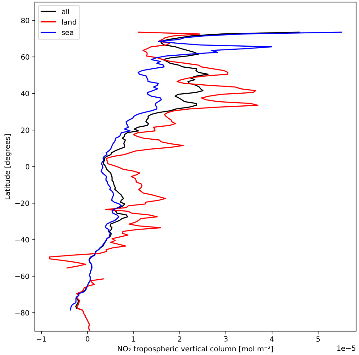
Figure 12: Zonal average of “NO 2 tropospheric vertical column” for 2023-11-02 to 2023-11-04.
