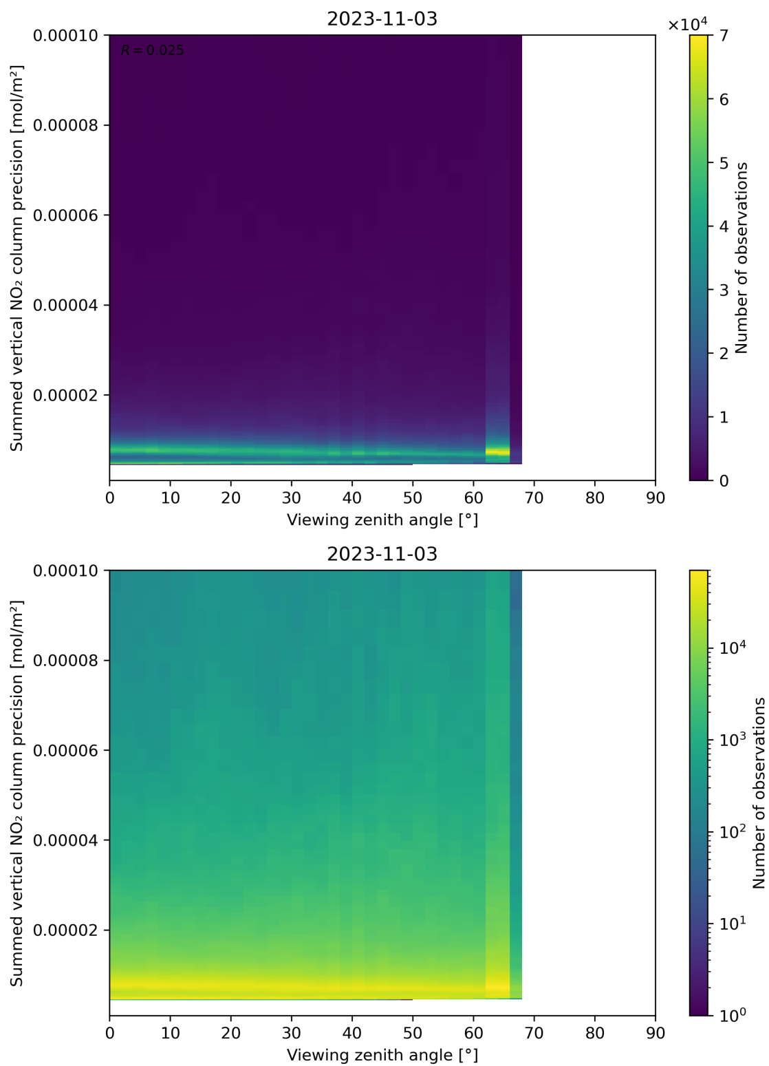
Figure 166: Scatter density plot of “Viewing zenith angle” against “Summed vertical NO 2 column precision” for 2023-11-02 to 2023-11-04.
