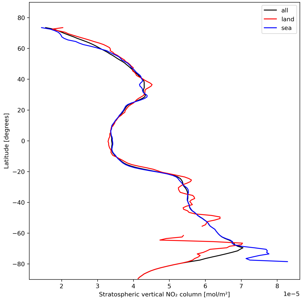
Figure 19: Zonal average of “Stratospheric vertical NO 2 column” for 2023-11-02 to 2023-11-04.
