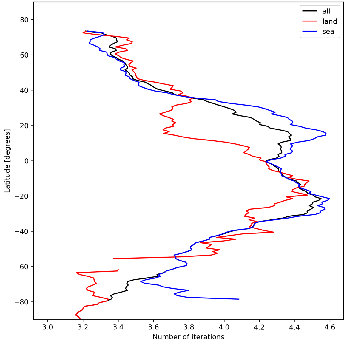
Figure 17: Zonal average of “Number of iterations” for 2023-11-02 to 2023-11-04.
