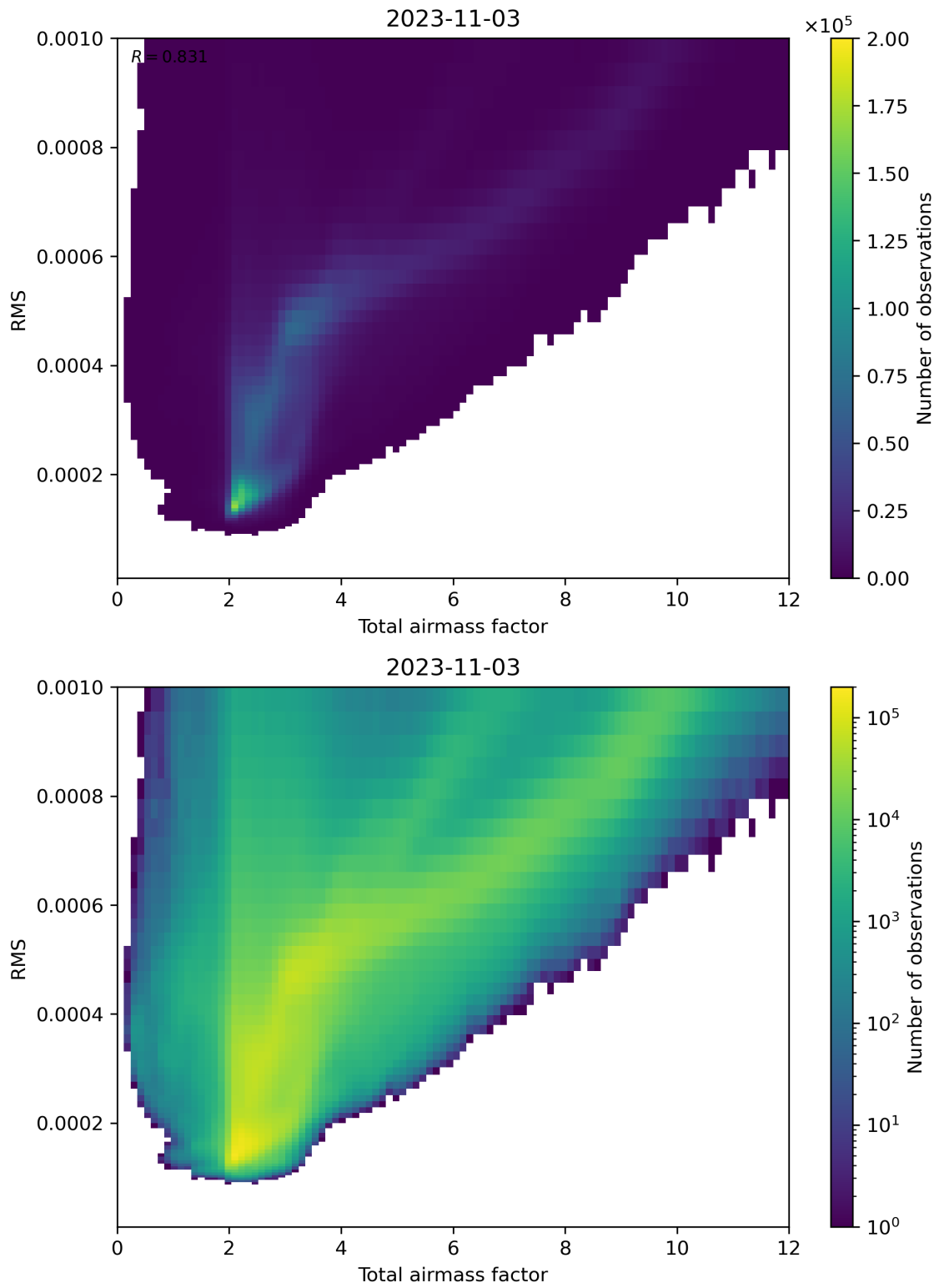
Figure 69: Scatter density plot of “Total airmass factor” against “RMS” for 2023-11-02 to 2023-11-04.
