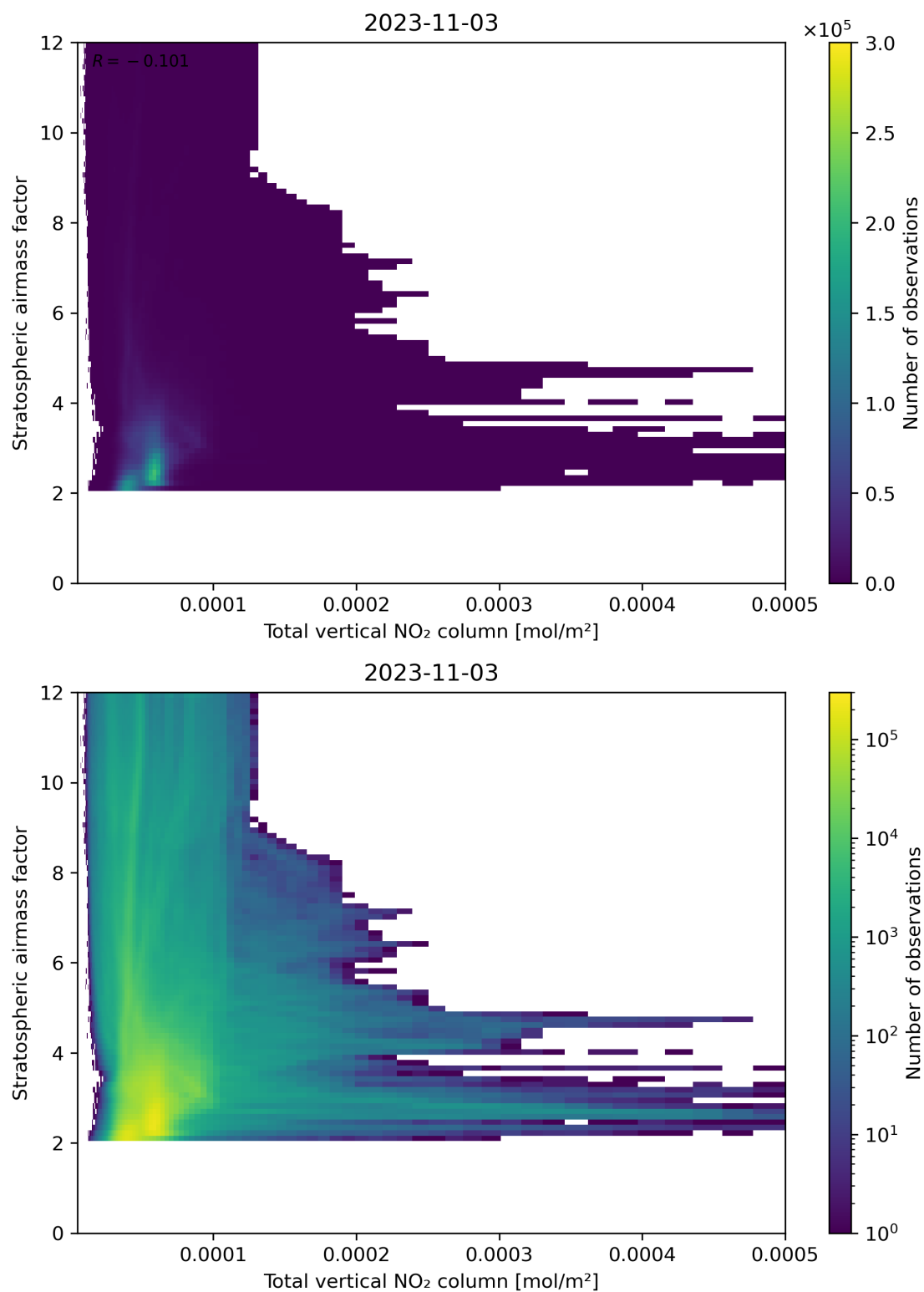
Figure 110: Scatter density plot of “Total vertical NO 2 column” against “Stratospheric air mass factor” for 2023-11-02 to 2023-11-04.
