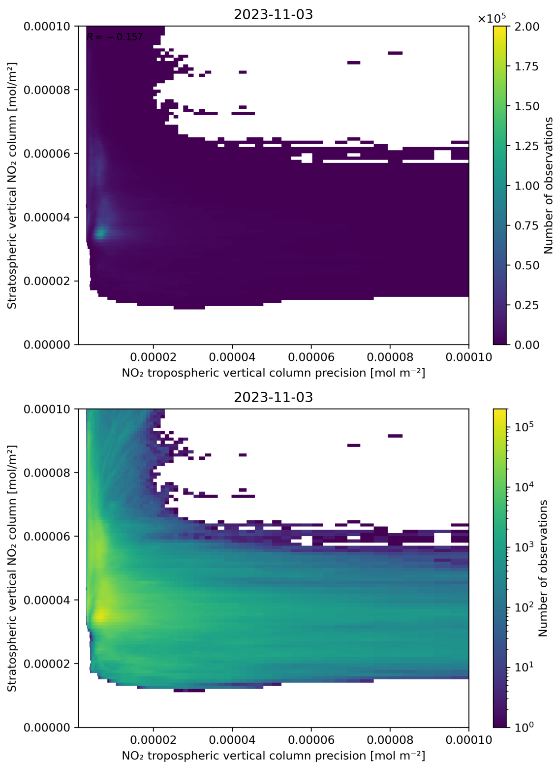
Figure 135: Scatter density plot of “NO 2 tropospheric vertical column precision” against “Stratospheric vertical NO 2 column” for 2023-11-02 to 2023-11-04.
