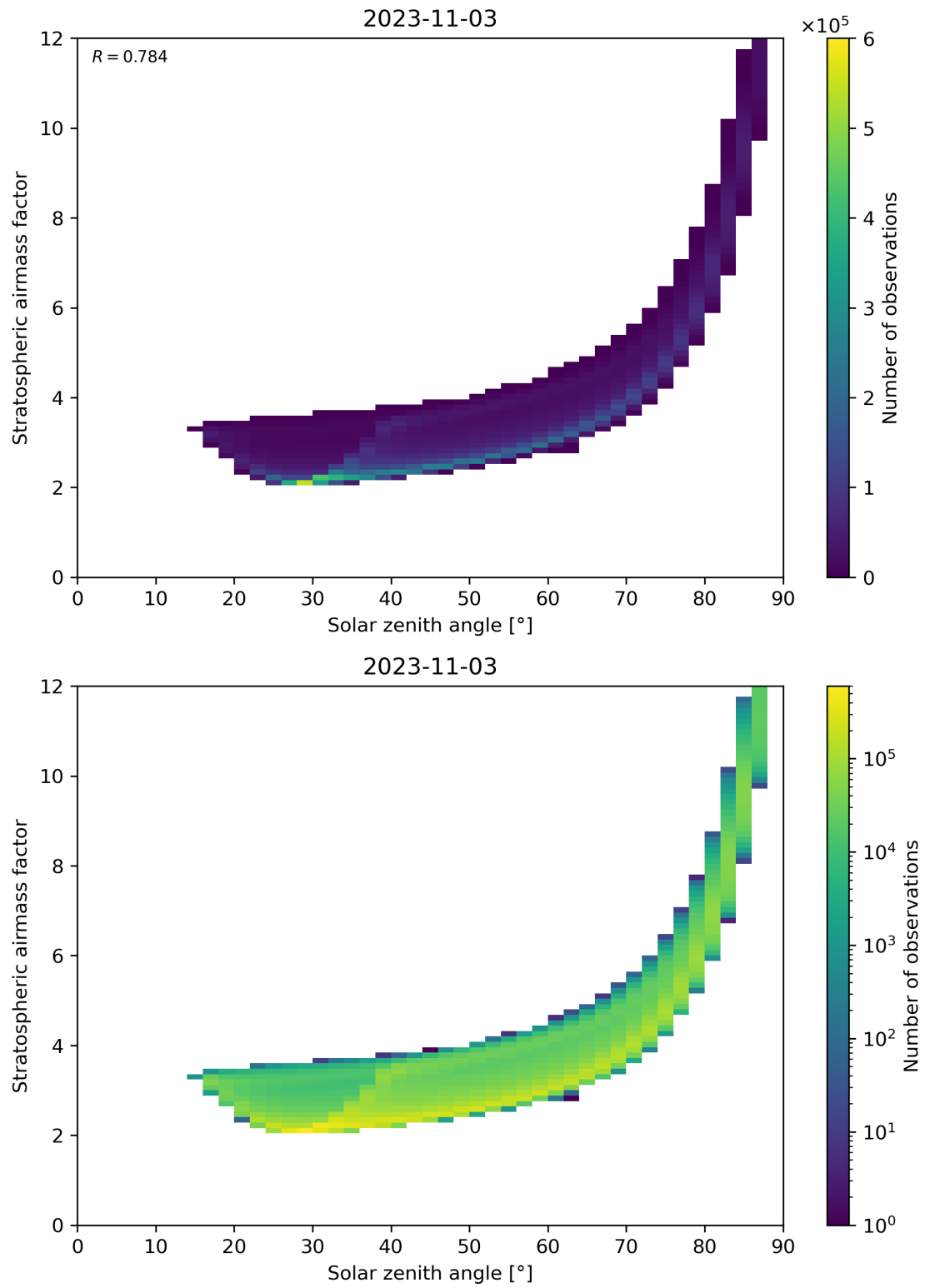
Figure 145: Scatter density plot of “Solar zenith angle” against “Stratospheric airmass factor” for 2023-11-02 to 2023-11-04.
