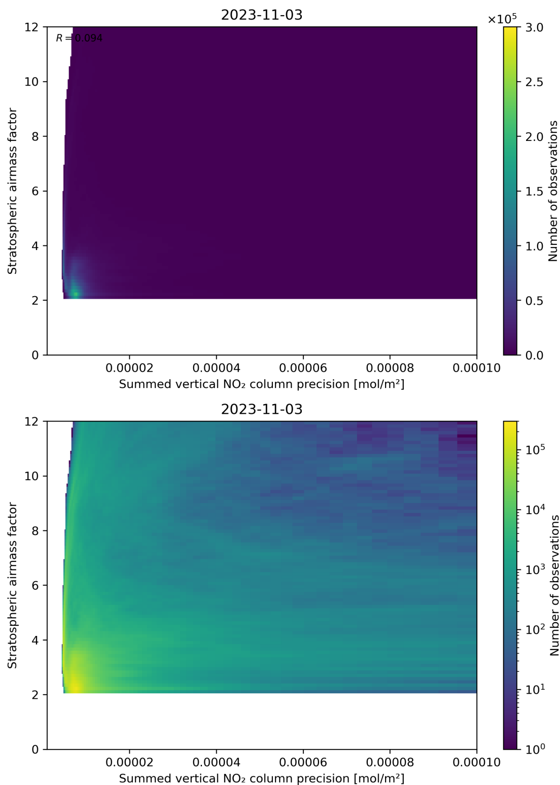
Figure 106: Scatter density plot of “Summed vertical NO 2 column precision” against “Stratospheric airmass factor” for 2023-11-02 to 2023-11-04.
