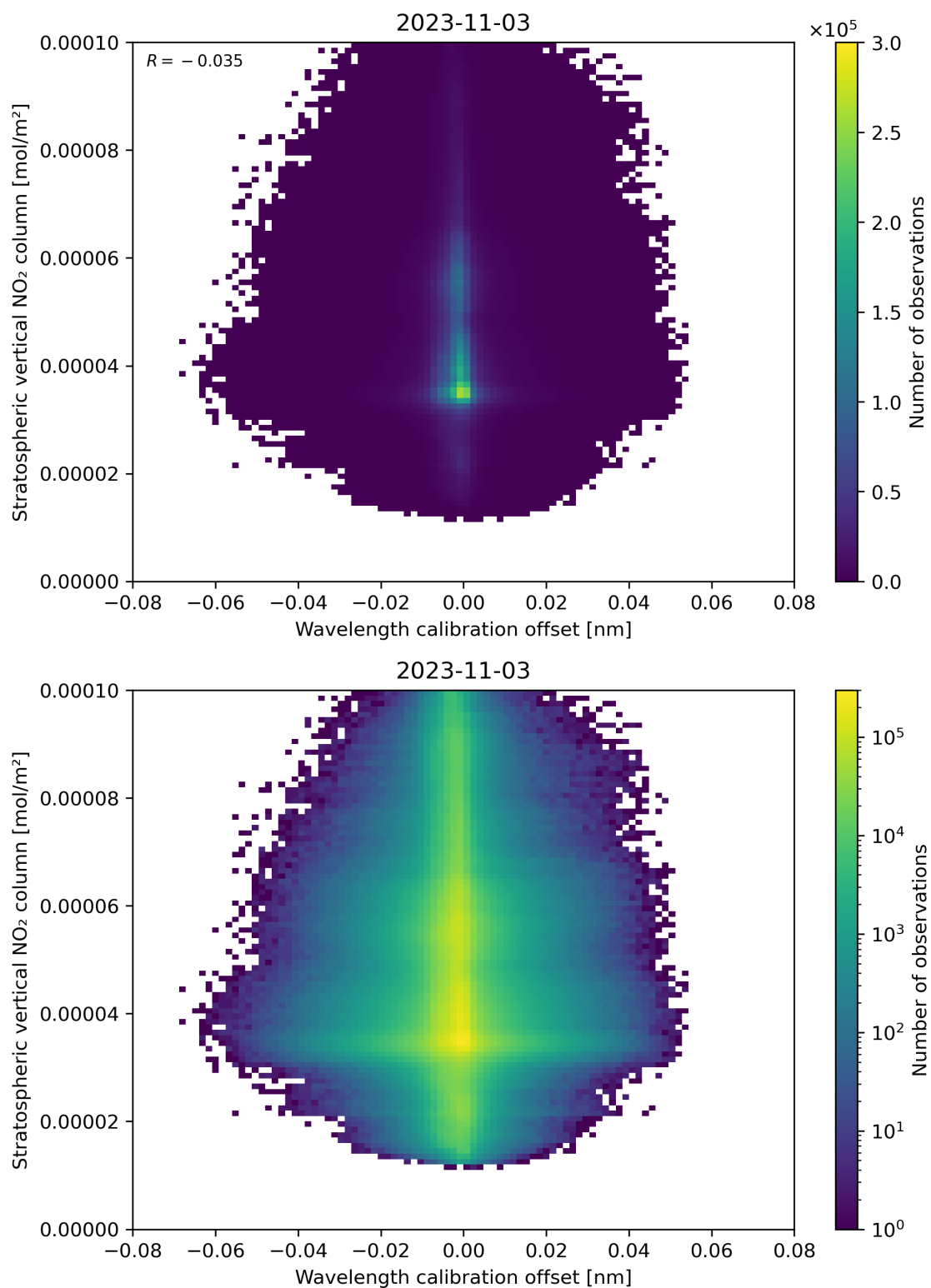
Figure 176: Scatter density plot of “Wavelength calibration offset” against “Stratospheric vertical NO 2 column” for 2023-11-02 to 2023-11-04.
