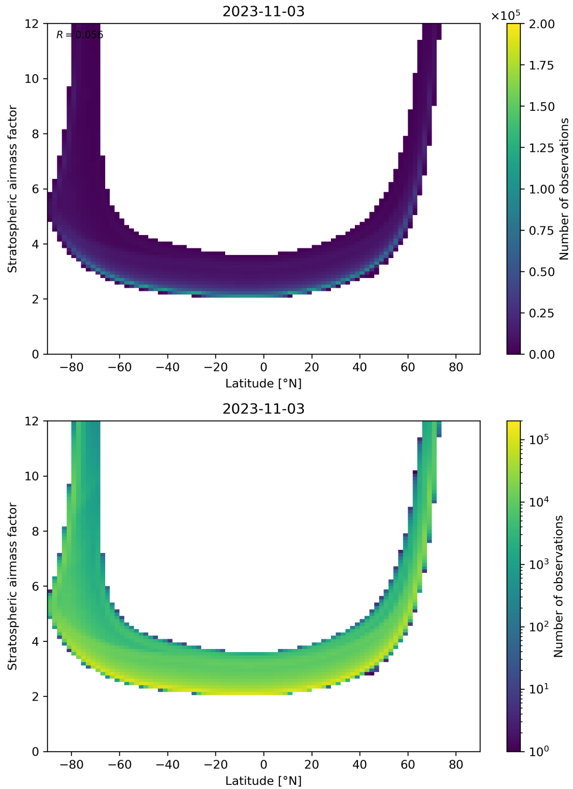
Figure 83: Scatter density plot of “Latitude” against “Stratospheric airmass factor” for 2023-11-02 to 2023-11-04.
