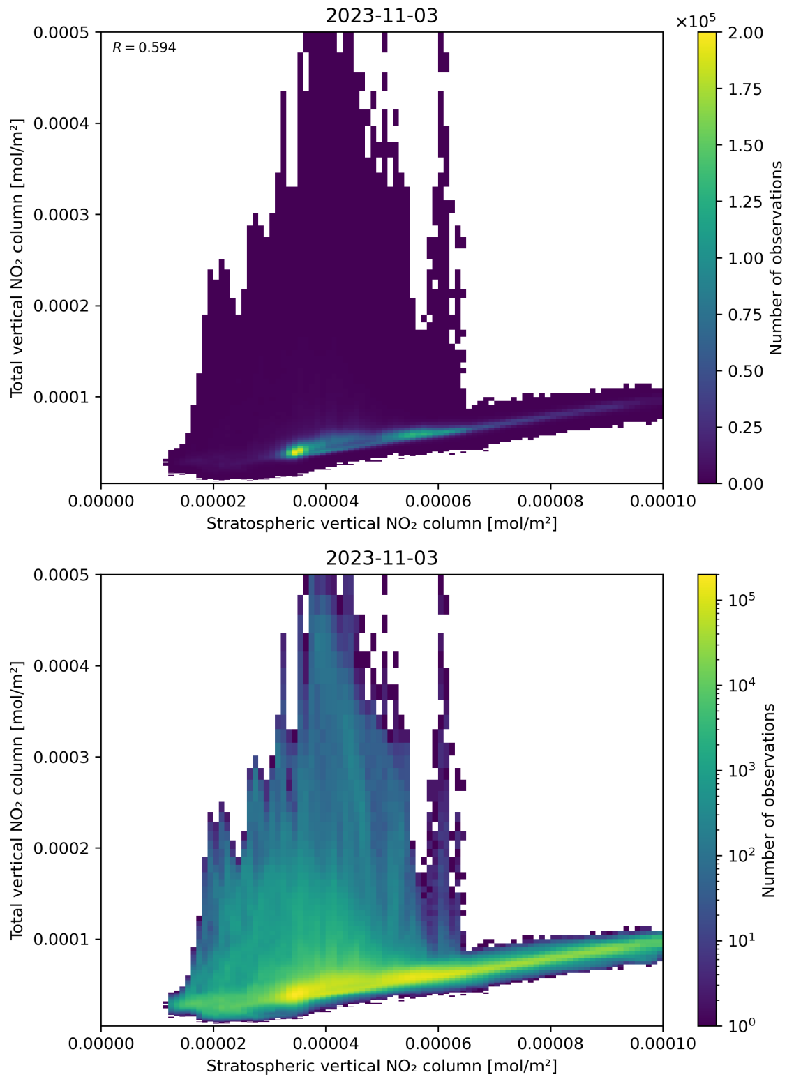
Figure 100: Scatter density plot of “Stratospheric vertical NO 2 column” against “Total vertical NO 2 column” for 2023-11-02 to 2023-11-04.
