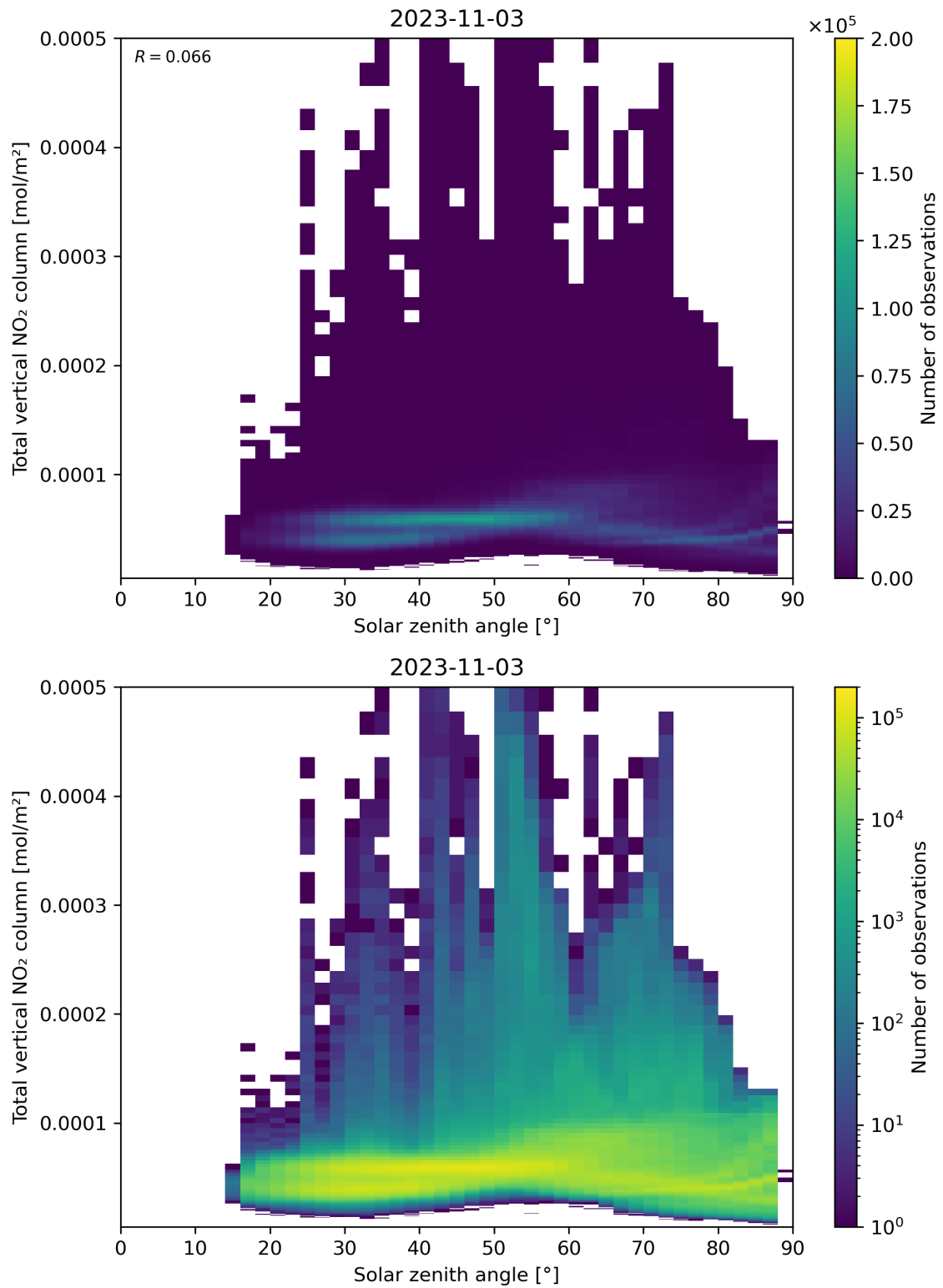
Figure 153: Scatter density plot of “Solar zenith angle” against “Total vertical NO 2 column” for 2023-11-02 to 2023-11-04.
