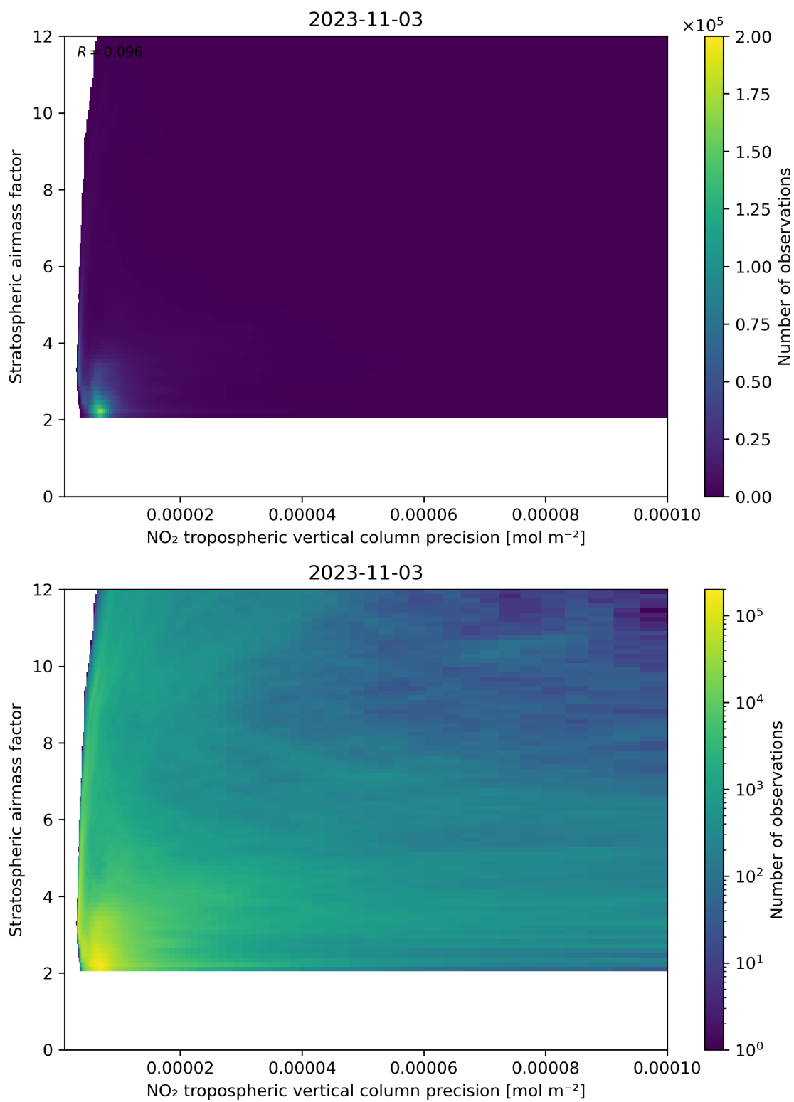
Figure 131: Scatter density plot of “NO 2 tropospheric vertical column precision” against “Stratospheric airmass factor” for 2023-11-02 to 2023-11-04.
