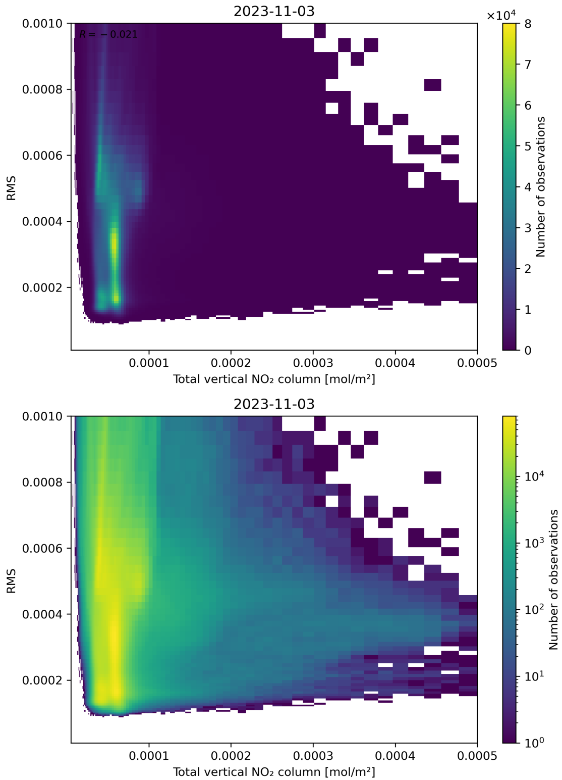
Figure 120: Scatter density plot of “Total vertical NO 2 column” against “RMS” for 2023-11-02 to 2023-11-04.
