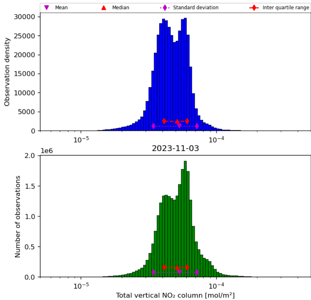
Figure 38: Histogram of “Total vertical NO 2 column” for 2023-11-02 to 2023-11-04
