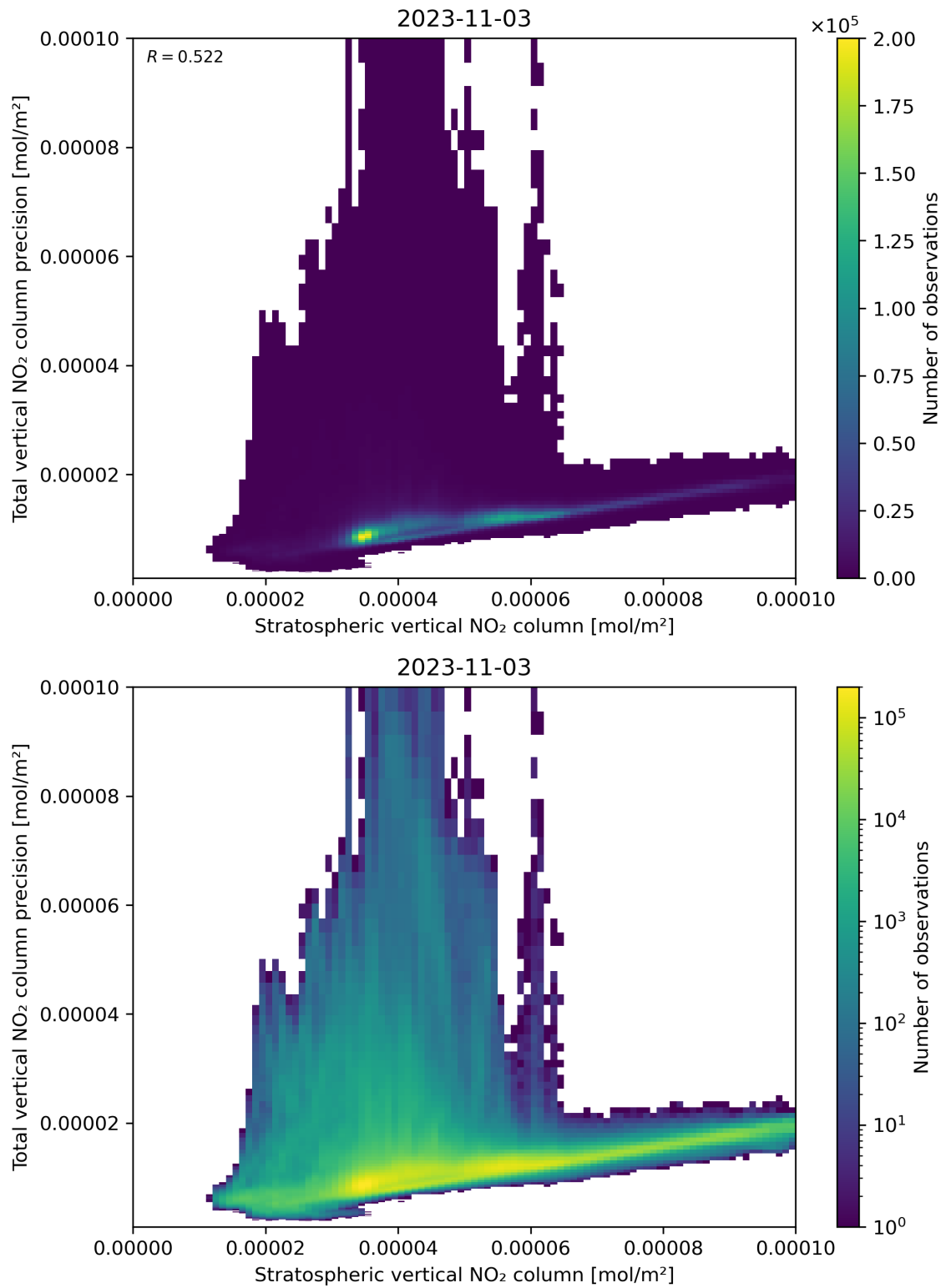
Figure 101: Scatter density plot of “Stratospheric vertical NO 2 column” against “Total vertical NO 2 column precision” for 2023-11-02 to 2023-11-04.
