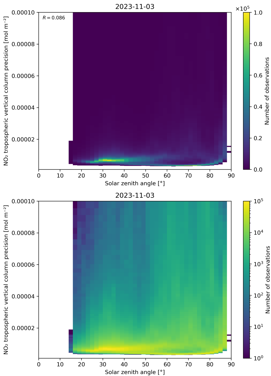
Figure 156: Scatter density plot of “Solar zenith angle” against “NO 2 tropospheric vertical column precision” for 2023-11-02 to 2023-11-04.
