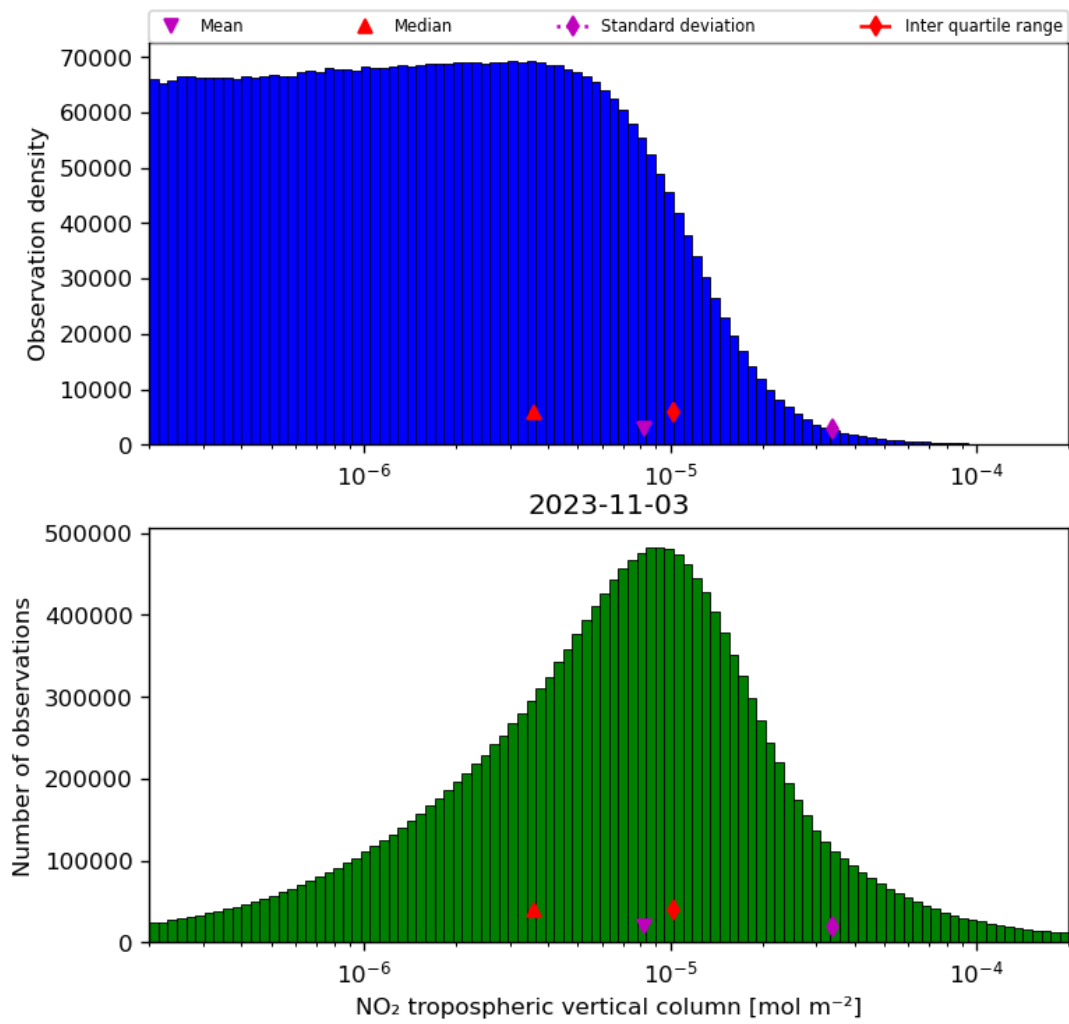
Figure 29: Histogram of “NO 2 tropospheric vertical column” for 2023-11-02 to 2023-11-04
