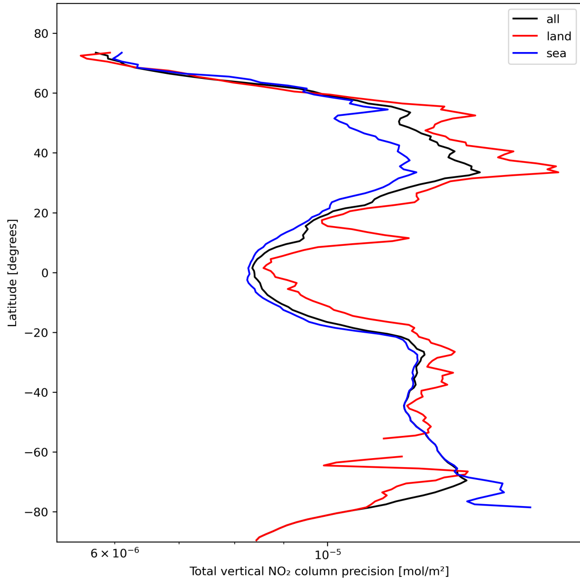
Figure 22: Zonal average of “Total vertical NO 2 column precision” for 2023-11-02 to 2023-11-04.
