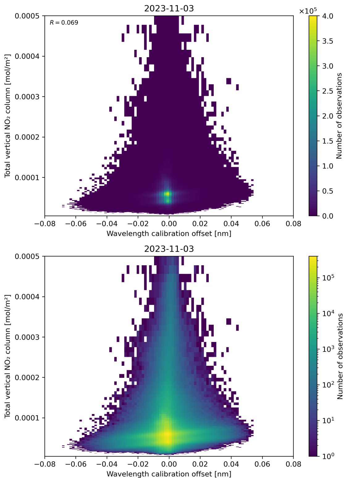
Figure 179: Scatter density plot of “Wavelength calibration offset” against “Total vertical NO 2 column” for 2023-11-02 to 2023-11-04.
