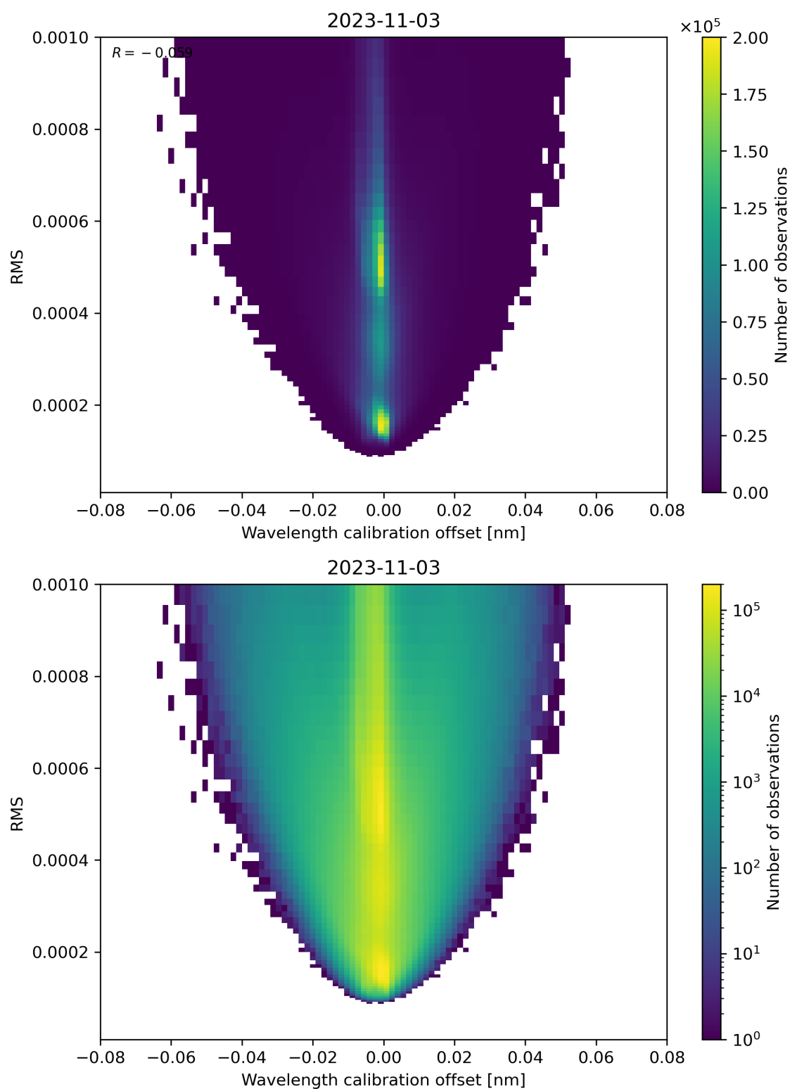
Figure 181: Scatter density plot of “Wavelength calibration offset” against “RMS” for 2023-11-02 to 2023-11-04.
