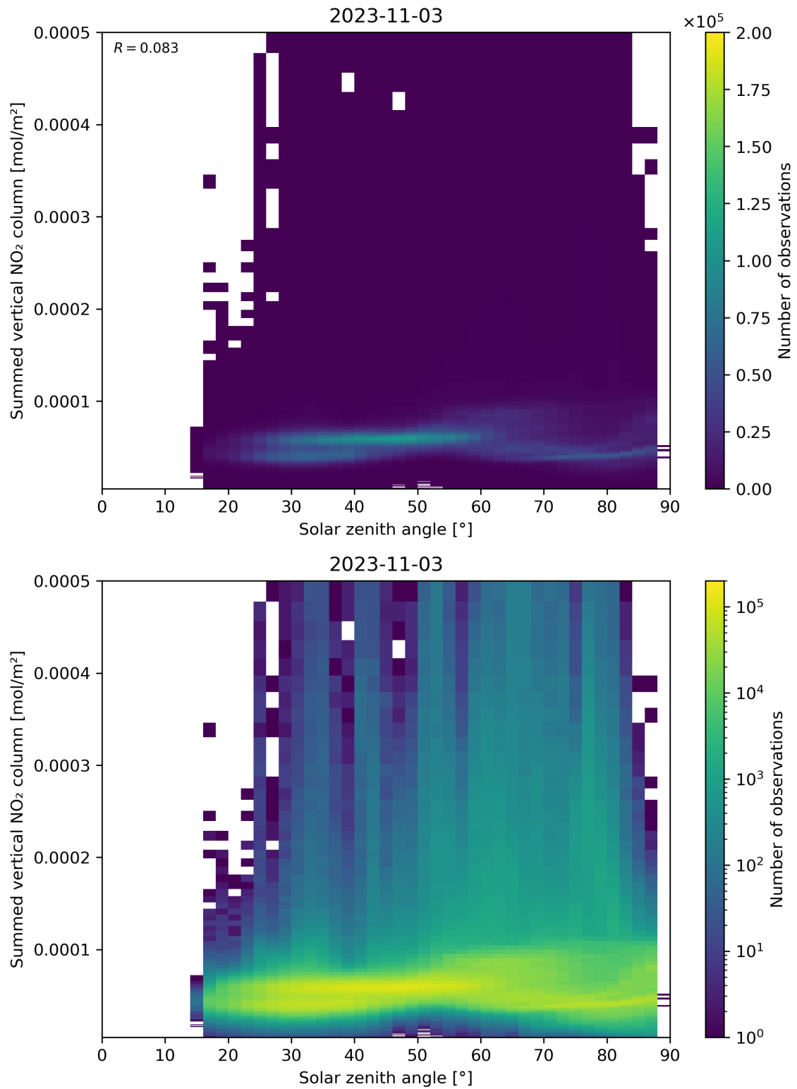
Figure 151: Scatter density plot of “Solar zenith angle” against “Summed vertical NO 2 column” for 2023-11-02 to 2023-11-04.
