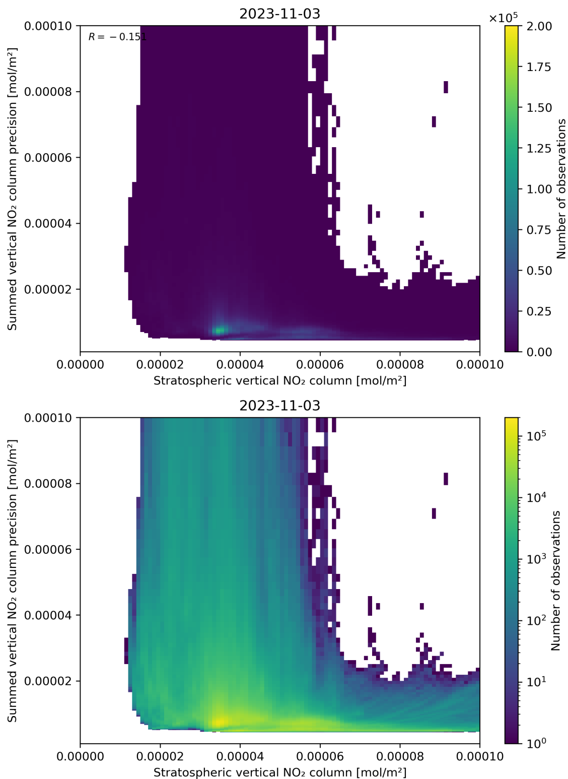
Figure 99: Scatter density plot of “Stratospheric vertical NO 2 column” against “Summed vertical NO 2 column precision” for 2023-11-02 to 2023-11-04.
