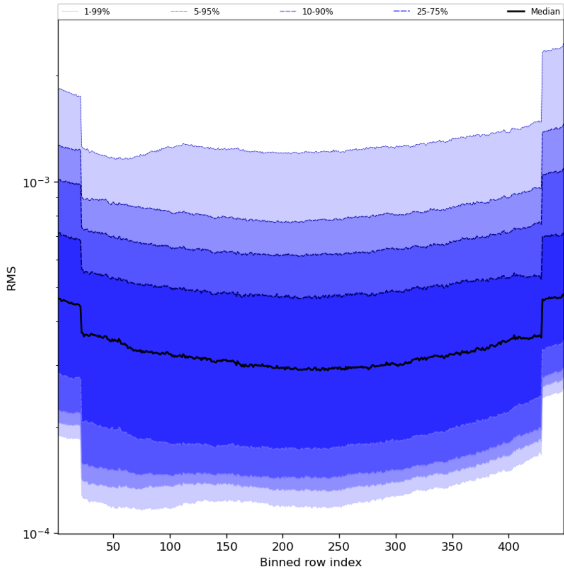
Figure 60: Along track statistics of “RMS” for 2023-11-02 to 2023-11-04
