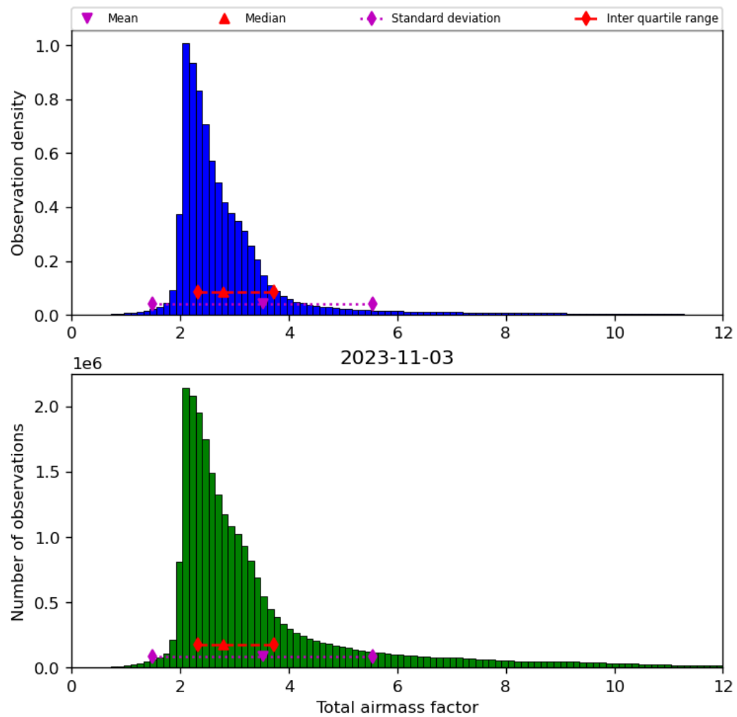
Figure 32: Histogram of “Total airmass factor” for 2023-11-02 to 2023-11-04
