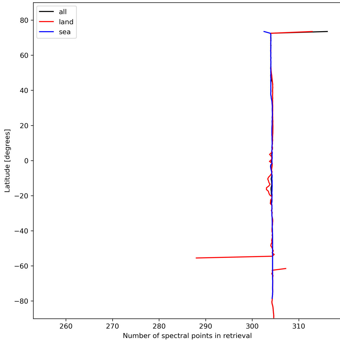
Figure 16: Zonal average of “Number of spectral points in retrieval” for 2023-11-02 to 2023-11-04.
