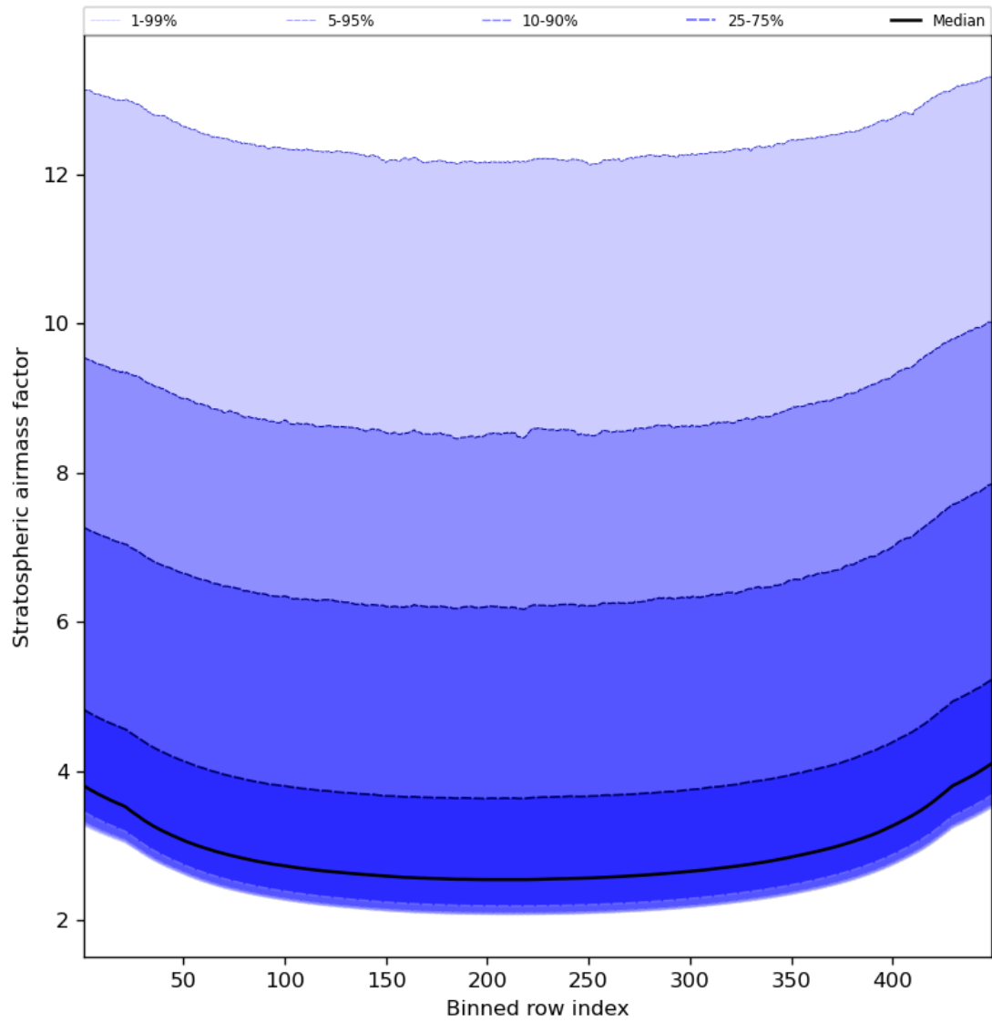
Figure 61: Along track statistics of “Stratospheric airmass factor” for 2023-11-02 to 2023-11-04
