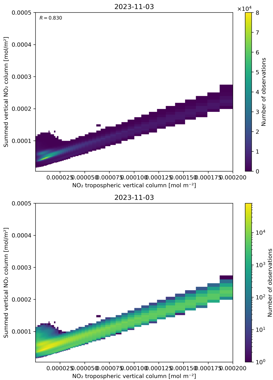
Figure 126: Scatter density plot of “NO 2 tropospheric vertical column” against “Summed vertical NO 2 column” for 2023-11-02 to 2023-11-04.
