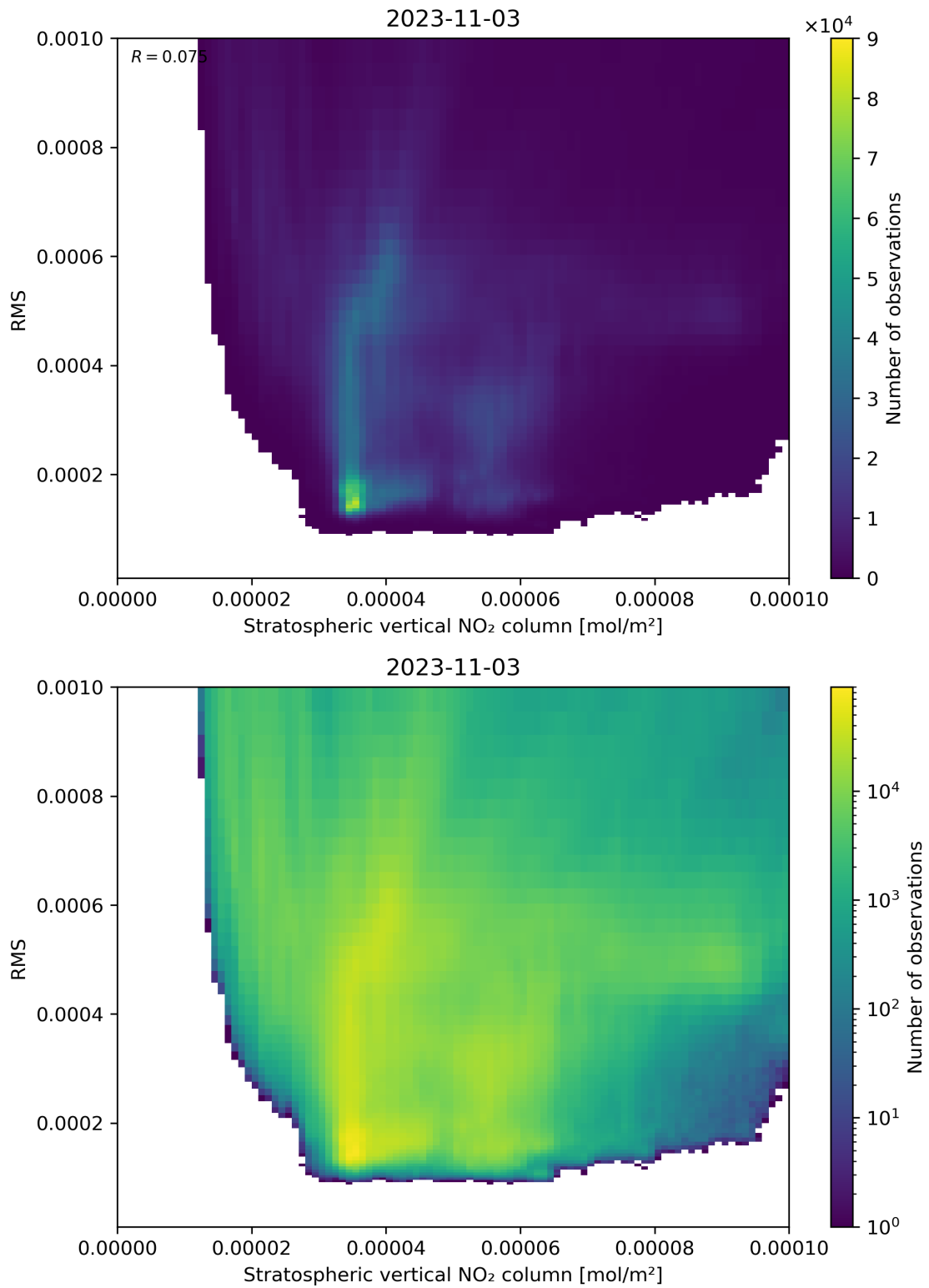
Figure 102: Scatter density plot of “Stratospheric vertical NO 2 column” against “RMS” for 2023-11-02 to 2023-11-04.
