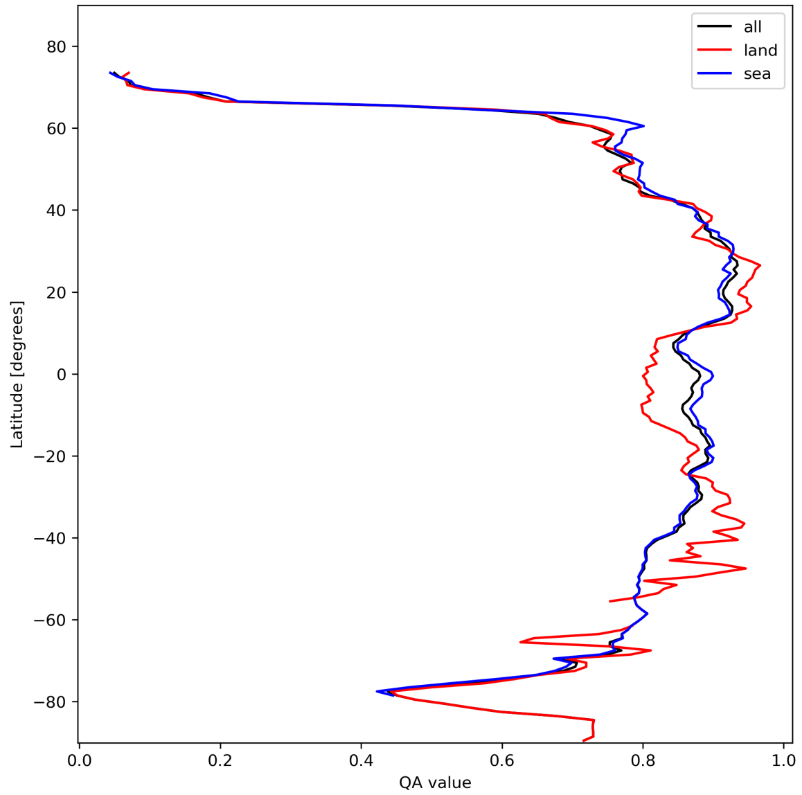
Figure 11: Zonal average of “QA value” for 2023-11-02 to 2023-11-04.
