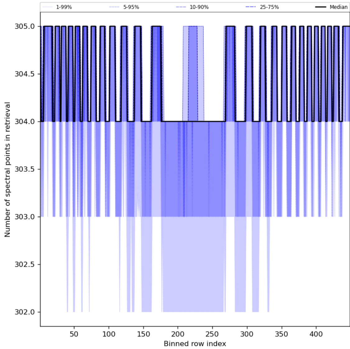
Figure 50: Along track statistics of “Number of spectral points in retrieval” for 2023-11-02 to 2023-11-04
