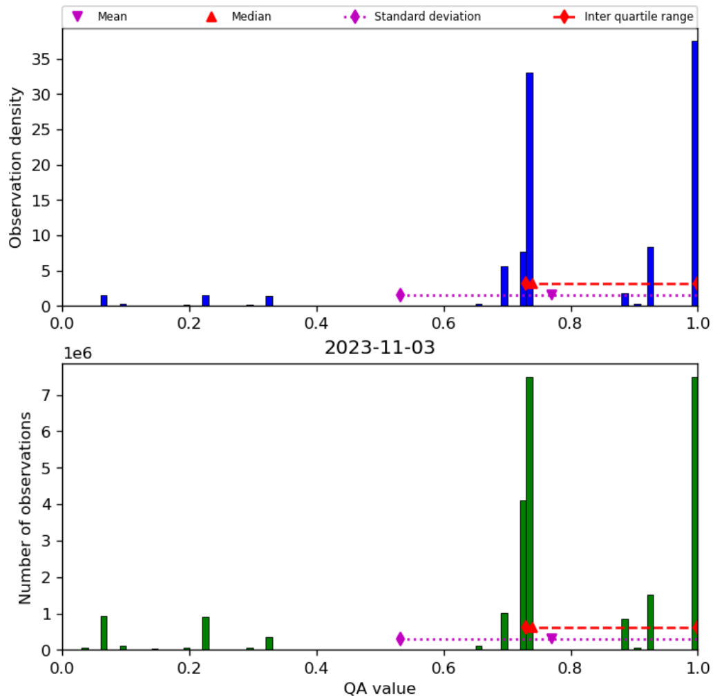
Figure 28: Histogram of “QA value” for 2023-11-02 to 2023-11-04
