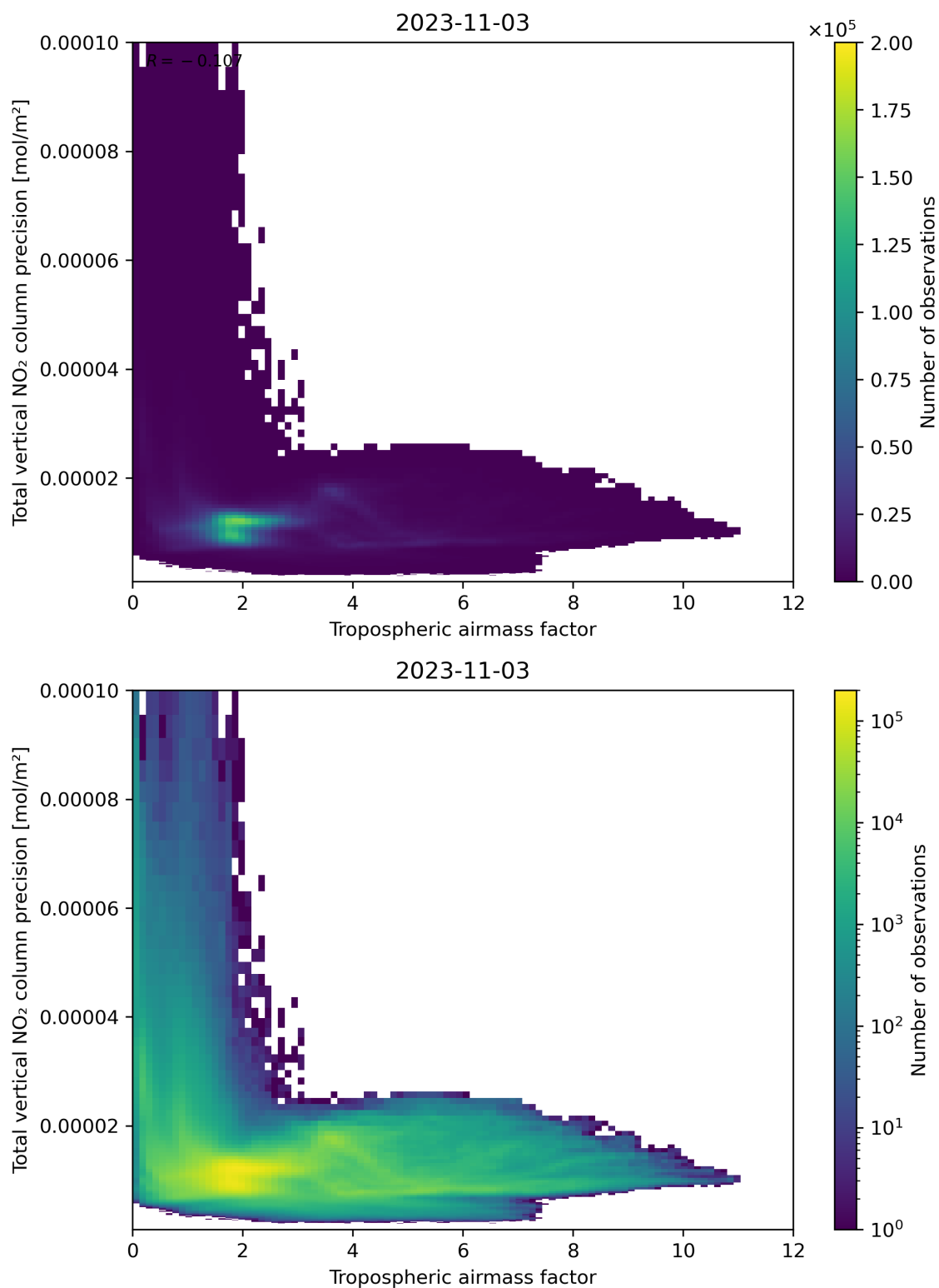
Figure 78: Scatter density plot of “Tropospheric air mass factor” against “Total vertical NO 2 column precision” for 2023-11-02 to 2023-11-04.
