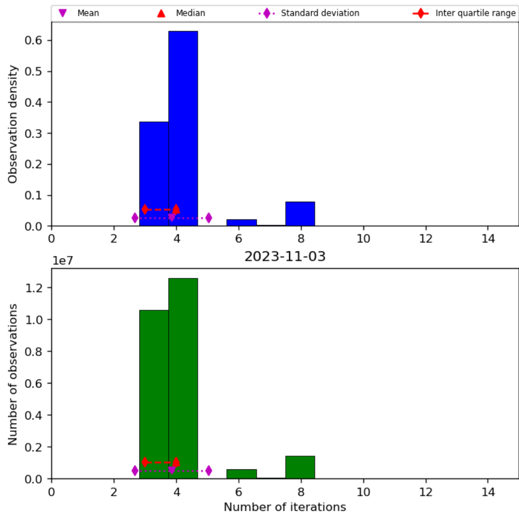
Figure 34: Histogram of “Number of iterations” for 2023-11-02 to 2023-11-04
