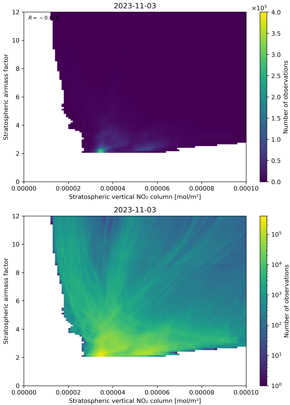
Figure 96: Scatter density plot of “Stratospheric vertical NO 2 column” against “Stratospheric airmass factor” for 2023-11-02 to 2023-11-04.
