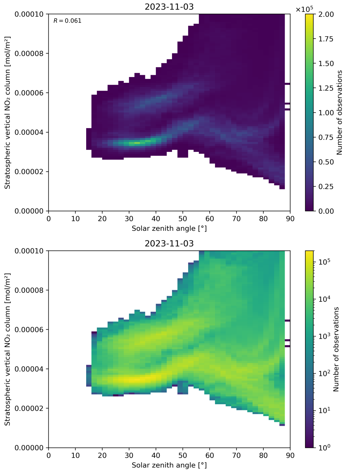
Figure 150: Scatter density plot of “Solar zenith angle” against “Stratospheric vertical NO 2 column” for 2023-11-02 to 2023-11-04.
