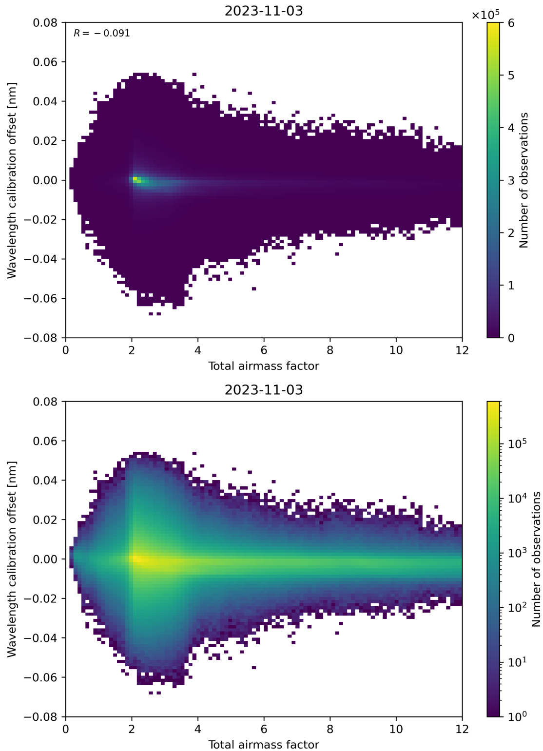
Figure 70: Scatter density plot of “Total airmass factor” against “Wavelength calibration offset” for 2023-11-02 to 2023-11-04.
