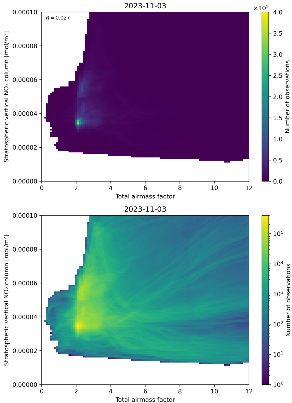
Figure 64: Scatter density plot of “Total airmass factor” against “Stratospheric vertical NO 2 column” for 2023-11-02 to 2023-11-04.
