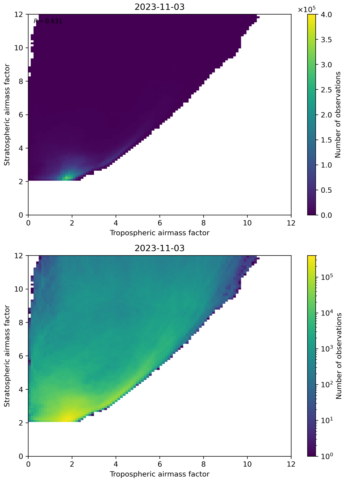
Figure 71: Scatter density plot of “Tropospheric airmass factor” against “Stratospheric airmass factor” for 2023-11-02 to 2023-11-04.
