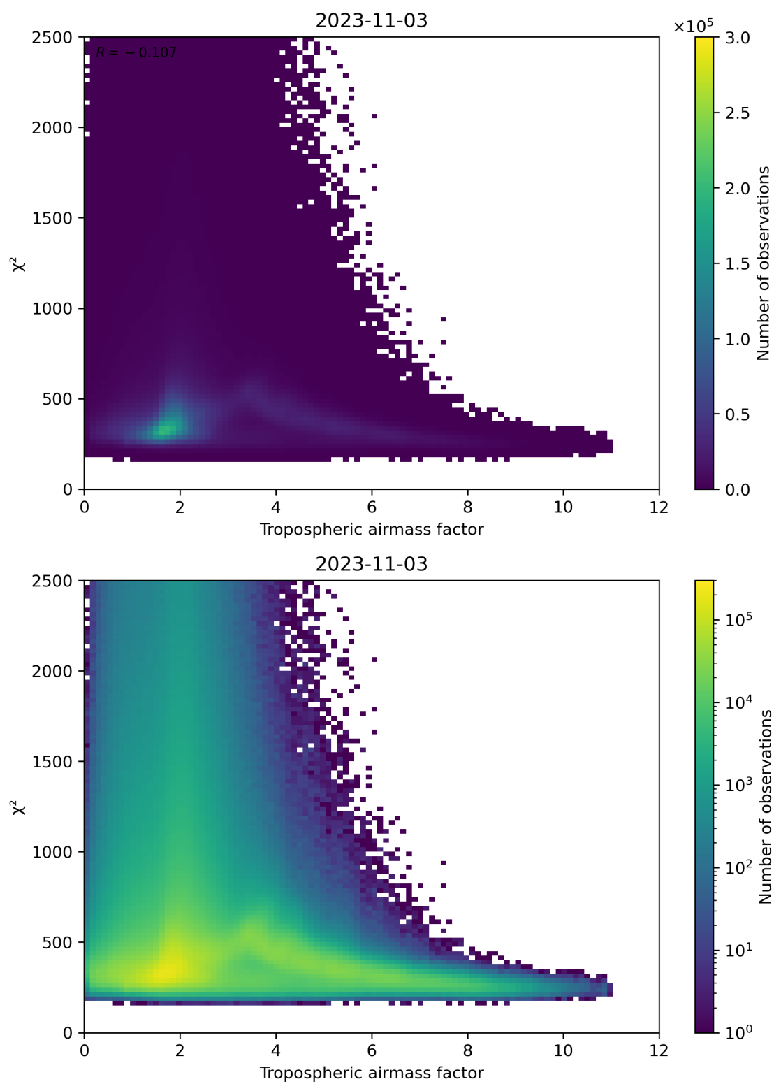
Figure 73: Scatter density plot of “Tropospheric airmass factor” against “ \chi^2 ” for 2023-11-02 to 2023-11-04.
