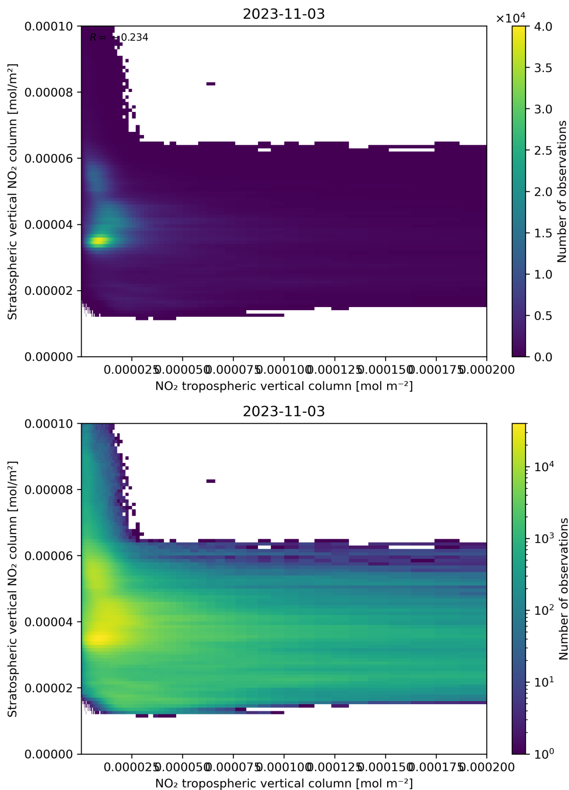
Figure 125: Scatter density plot of “NO 2 tropospheric vertical column” against “Stratospheric vertical NO 2 column” for 2023-11-02 to 2023-11-04.
