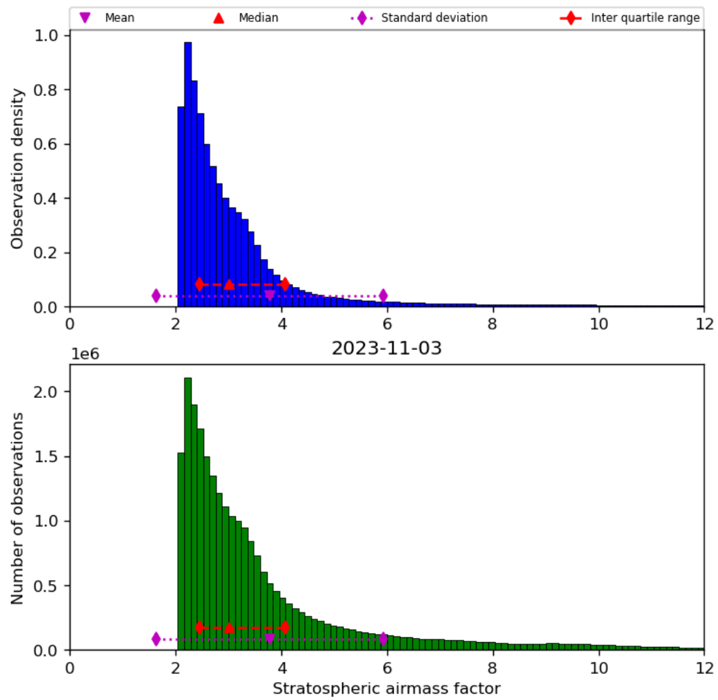
Figure 44: Histogram of “Stratospheric airmass factor” for 2023-11-02 to 2023-11-04
