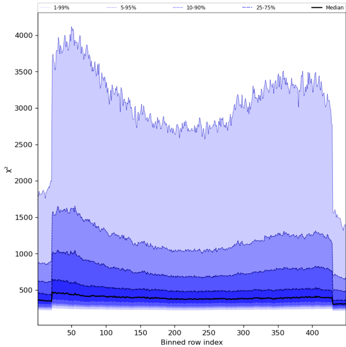
Figure 59: Along track statistics of “ \chi^2 ” for 2023-11-02 to 2023-11-04
