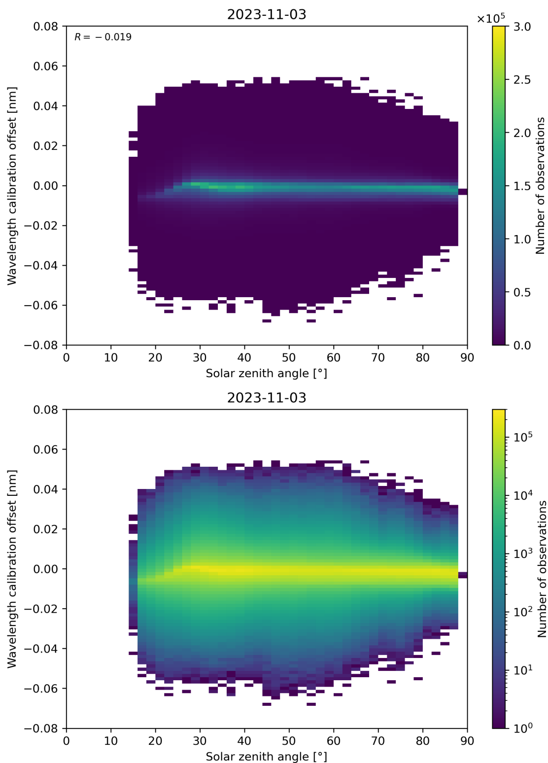
Figure 158: Scatter density plot of “Solar zenith angle” against “Wavelength calibration offset” for 2023-11-02 to 2023-11-04.
