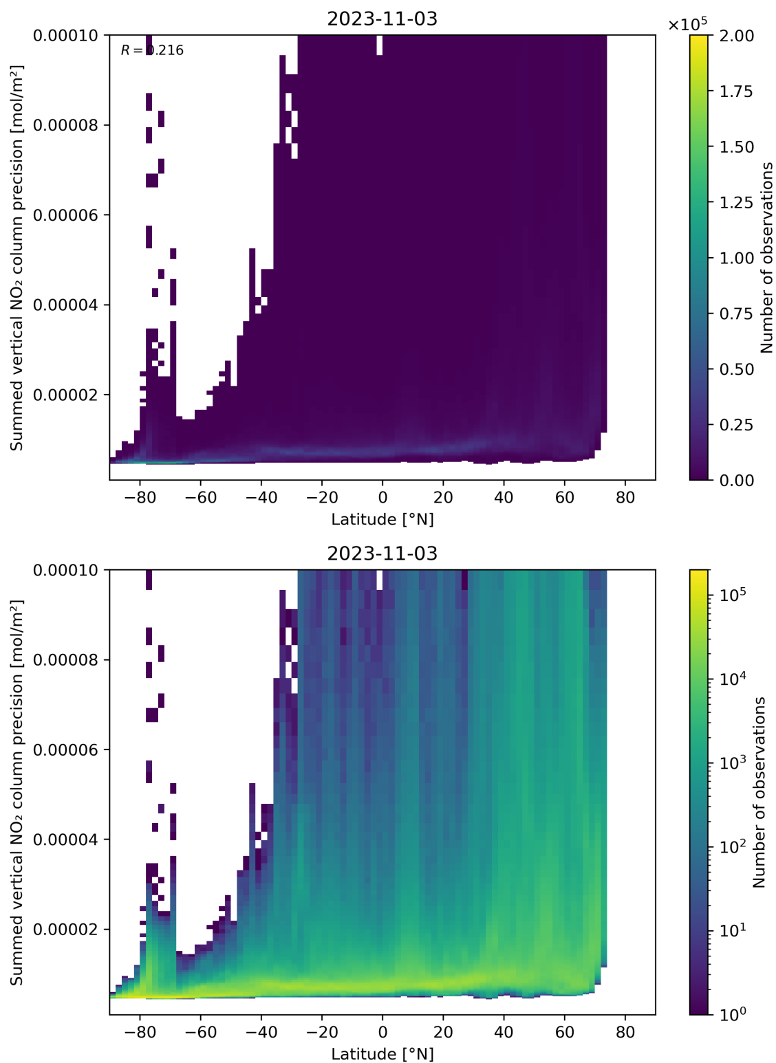
Figure 89: Scatter density plot of “Latitude” against “Summed vertical NO 2 column precision” for 2023-11-02 to 2023-11-04.
