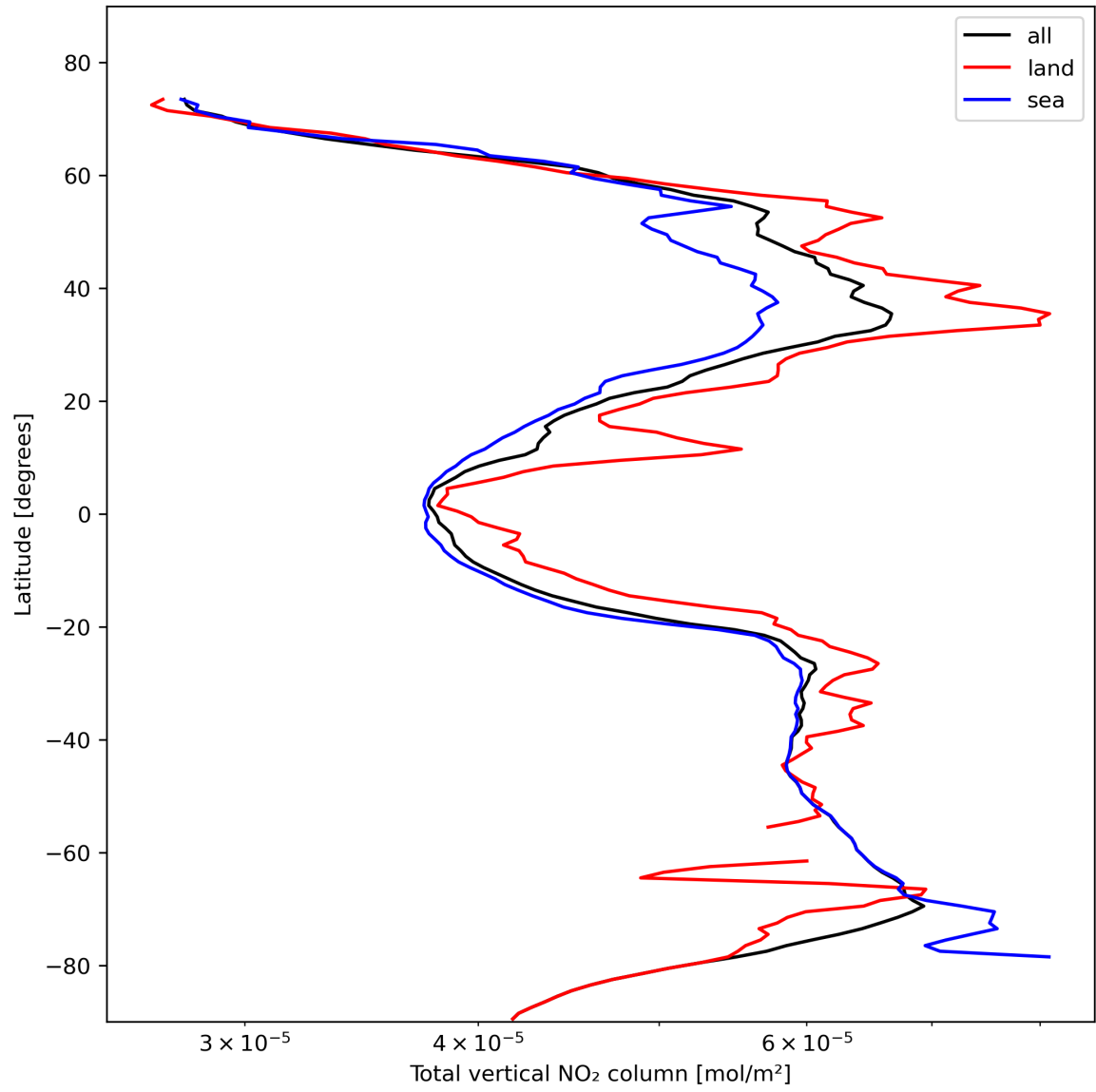
Figure 21: Zonal average of “Total vertical NO 2 column” for 2023-11-02 to 2023-11-04.
