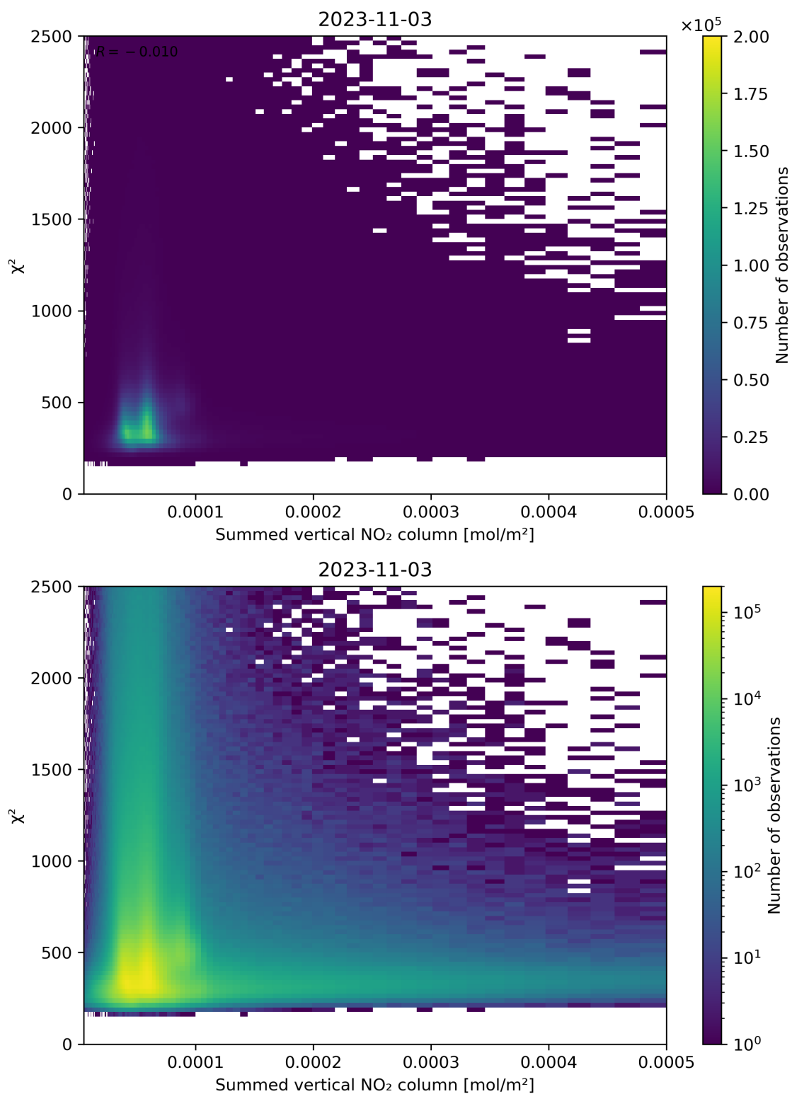
Figure 104: Scatter density plot of “Summed vertical NO 2 column” against “ \chi^2 ” for 2023-11-02 to 2023-11-04.
