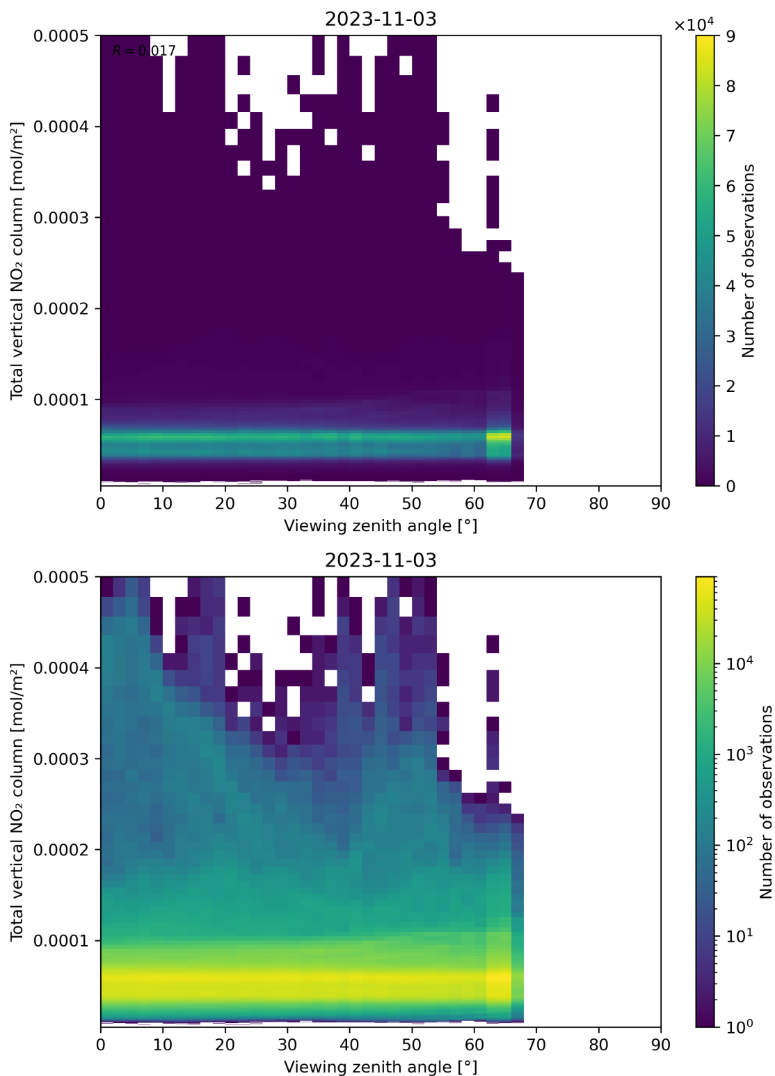
Figure 167: Scatter density plot of “Viewing zenith angle” against “Total vertical NO 2 column” for 2023-11-02 to 2023-11-04.
