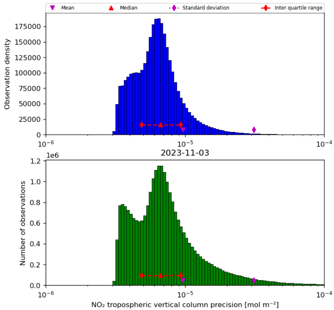
Figure 30: Histogram of “NO 2 tropospheric vertical column precision” for 2023-11-02 to 2023-11-04
