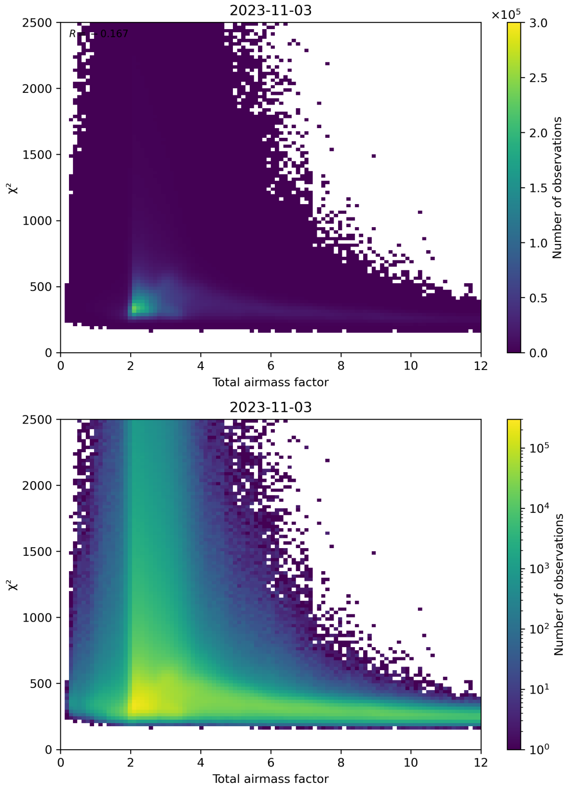
Figure 63: Scatter density plot of “Total airmass factor” against “ \chi^2 ” for 2023-11-02 to 2023-11-04.
