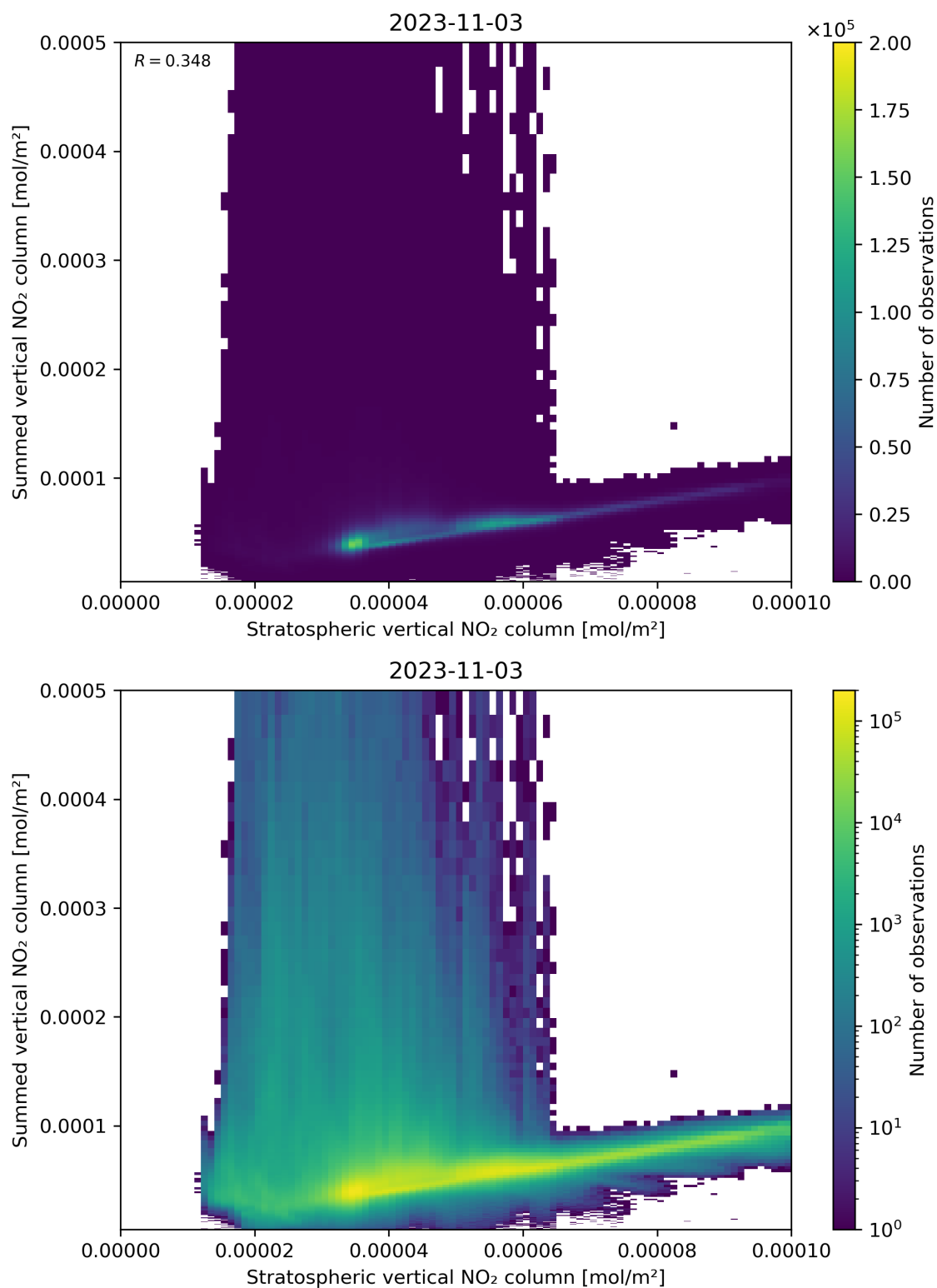
Figure 98: Scatter density plot of “Stratospheric vertical NO 2 column” against “Summed vertical NO 2 column” for 2023-11-02 to 2023-11-04.
