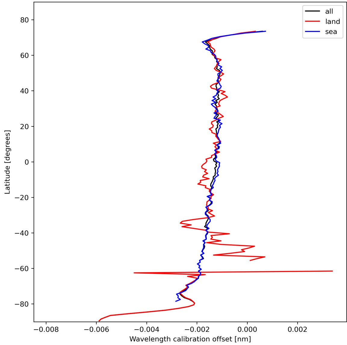
Figure 18: Zonal average of “Wavelength calibration offset” for 2023-11-02 to 2023-11-04.
