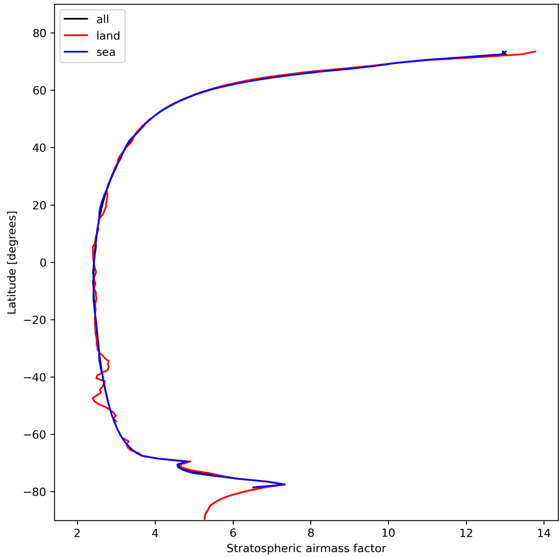
Figure 27: Zonal average of “Stratospheric airmass factor” for 2023-11-02 to 2023-11-04.
