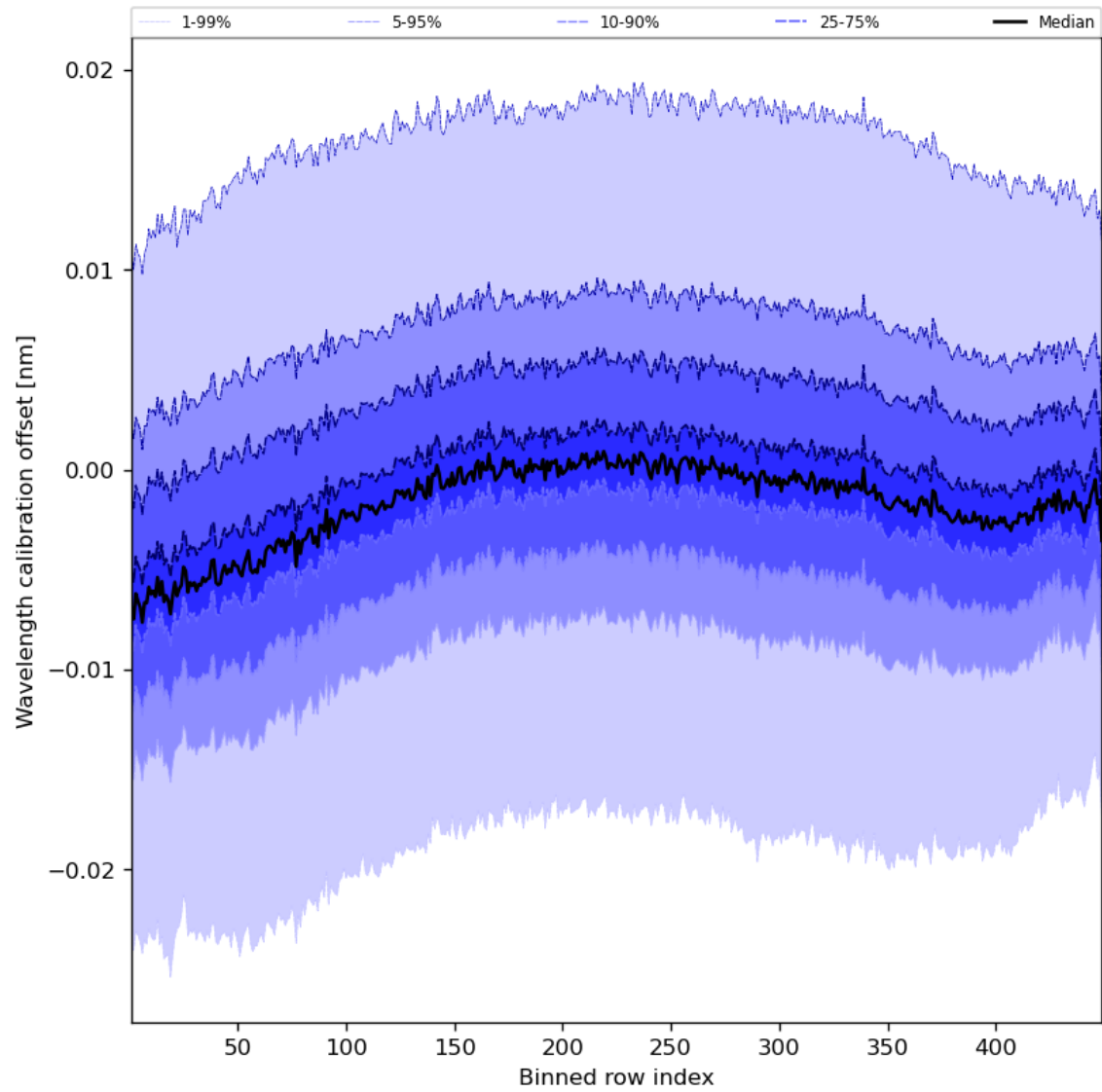
Figure 52: Along track statistics of “Wavelength calibration offset” for 2023-11-02 to 2023-11-04
