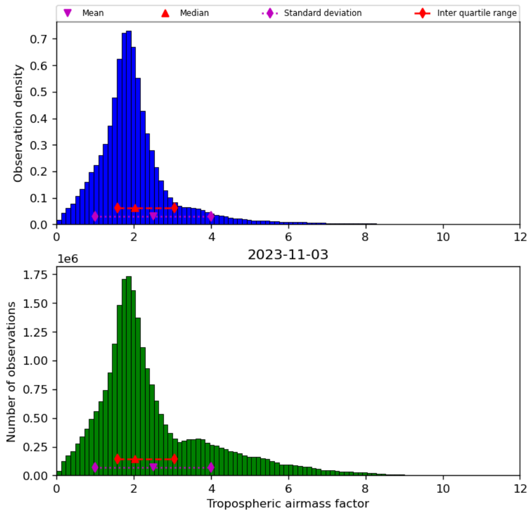
Figure 31: Histogram of “Tropospheric airmass factor” for 2023-11-02 to 2023-11-04
