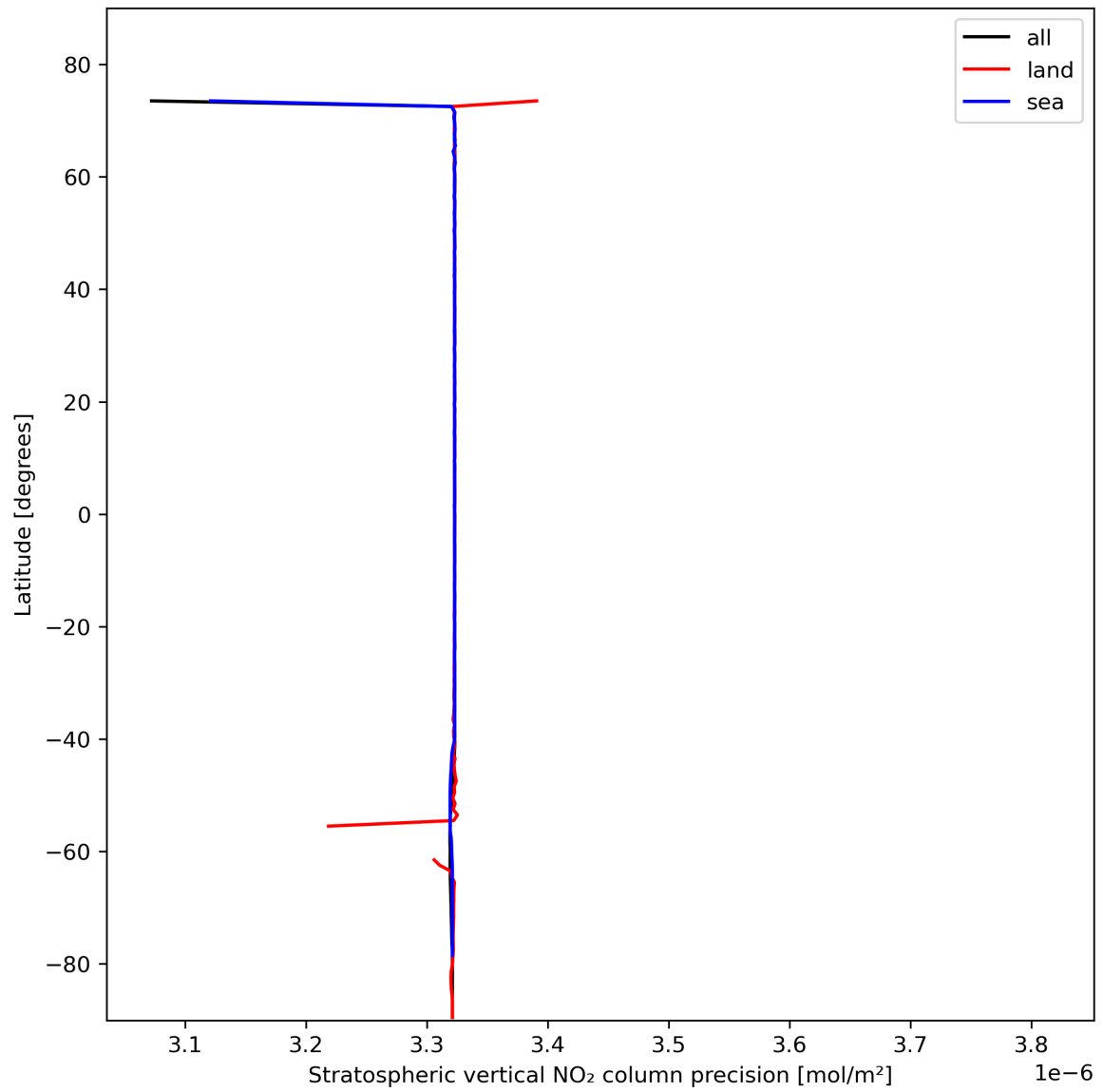
Figure 20: Zonal average of “Stratospheric vertical NO 2 column precision” for 2023-11-02 to 2023-11-04.
