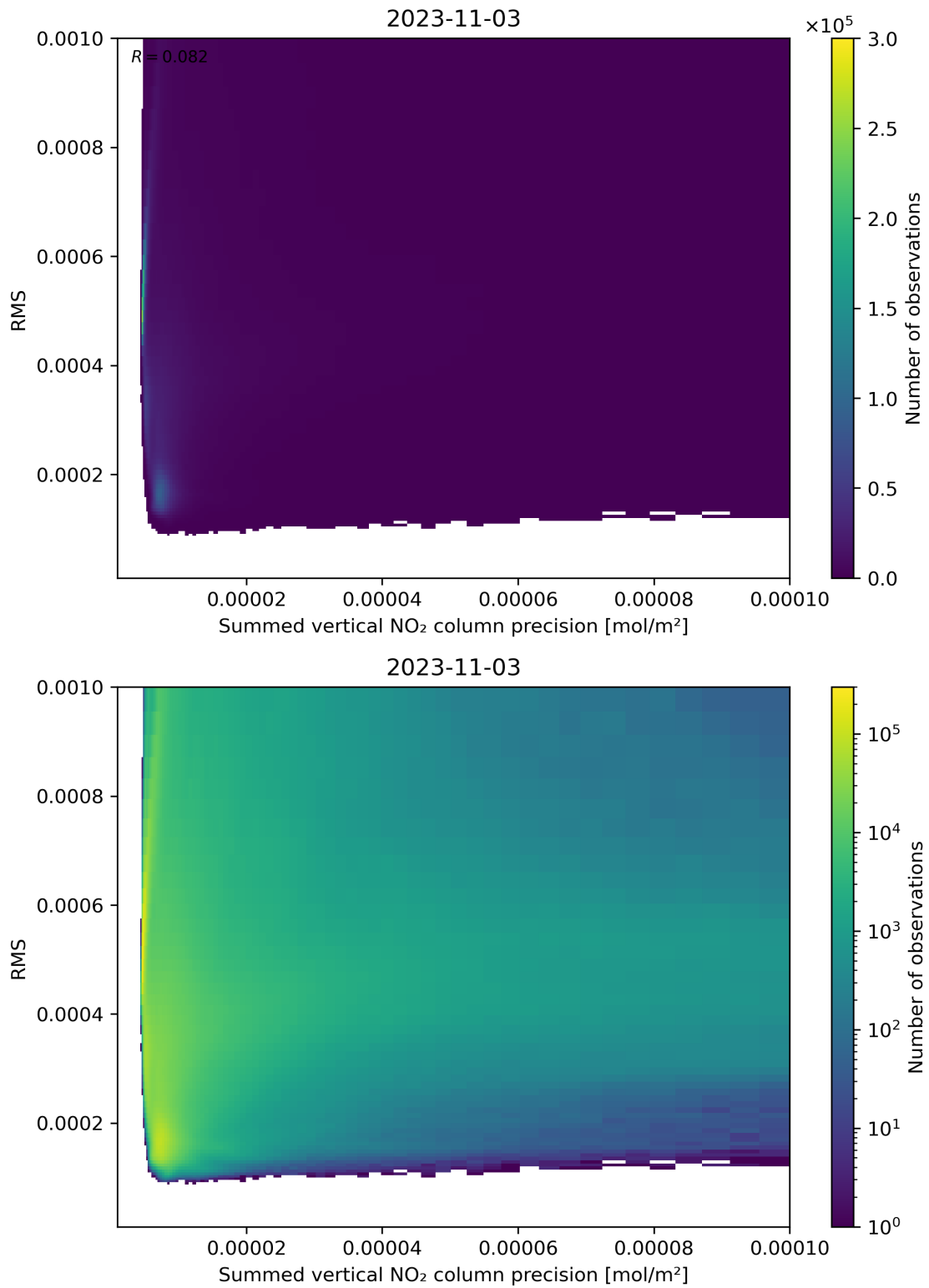
Figure 108: Scatter density plot of “Summed vertical NO 2 column precision” against “RMS” for 2023-11-02 to 2023-11-04.
