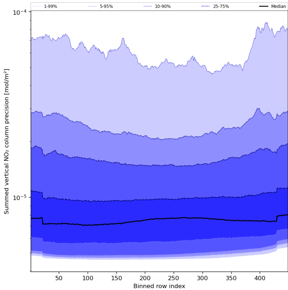
Figure 58: Along track statistics of “Summed vertical NO 2 column precision” for 2023-11-02 to 2023-11-04
