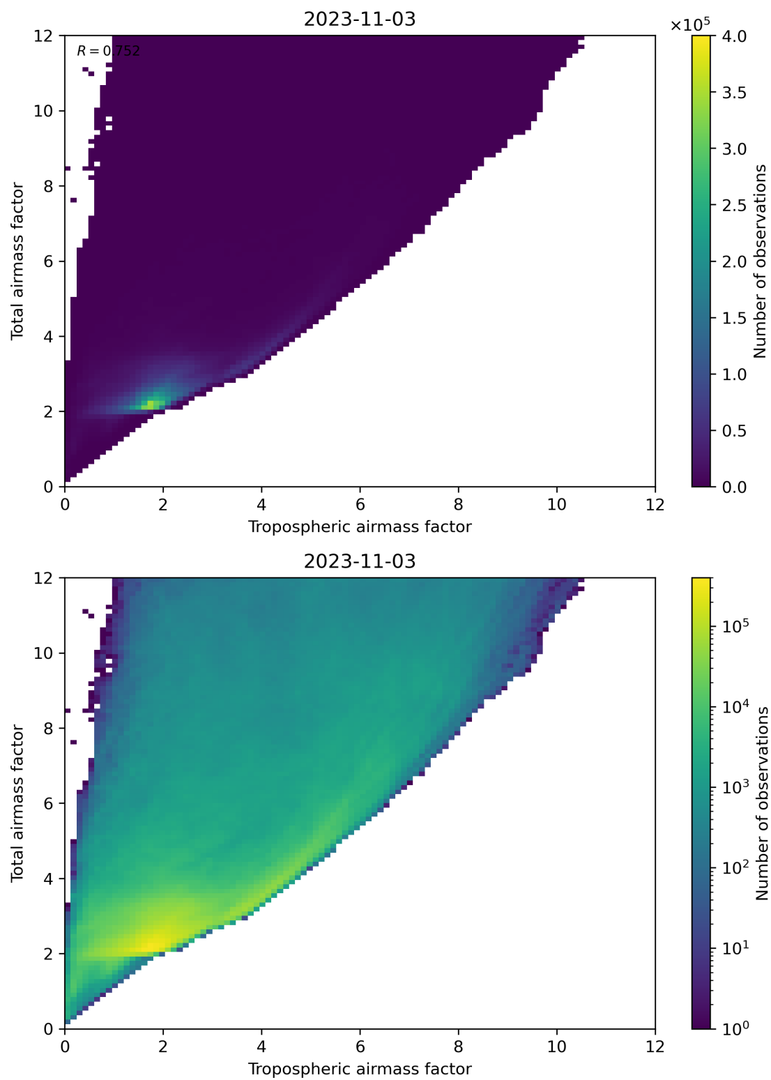
Figure 72: Scatter density plot of “Tropospheric airmass factor” against “Total airmass factor” for 2023-11-02 to 2023-11-04.
