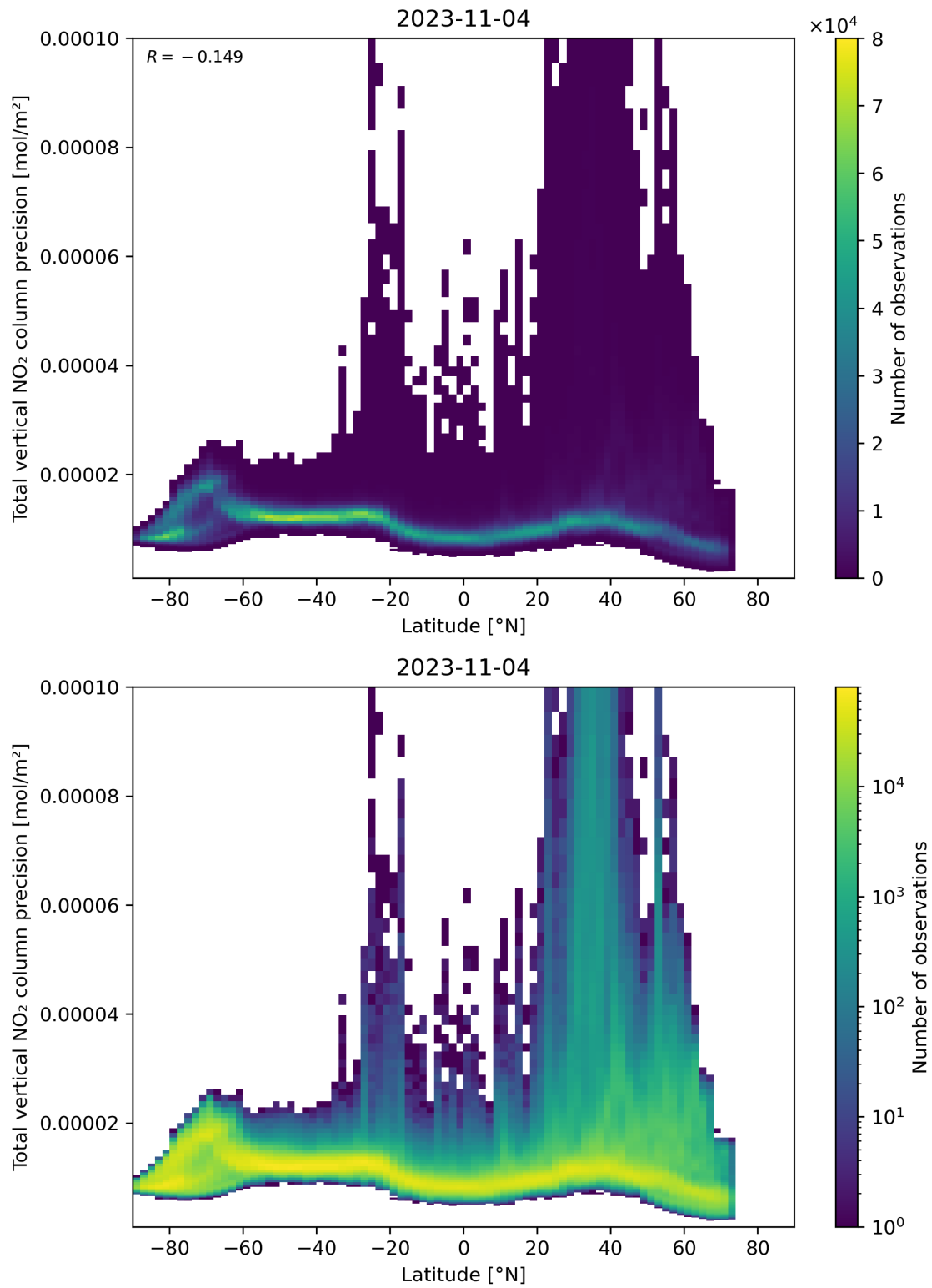
Figure 91: Scatter density plot of “Latitude” against “Total vertical NO 2 column precision” for 2023-11-03 to 2023-11-05.
