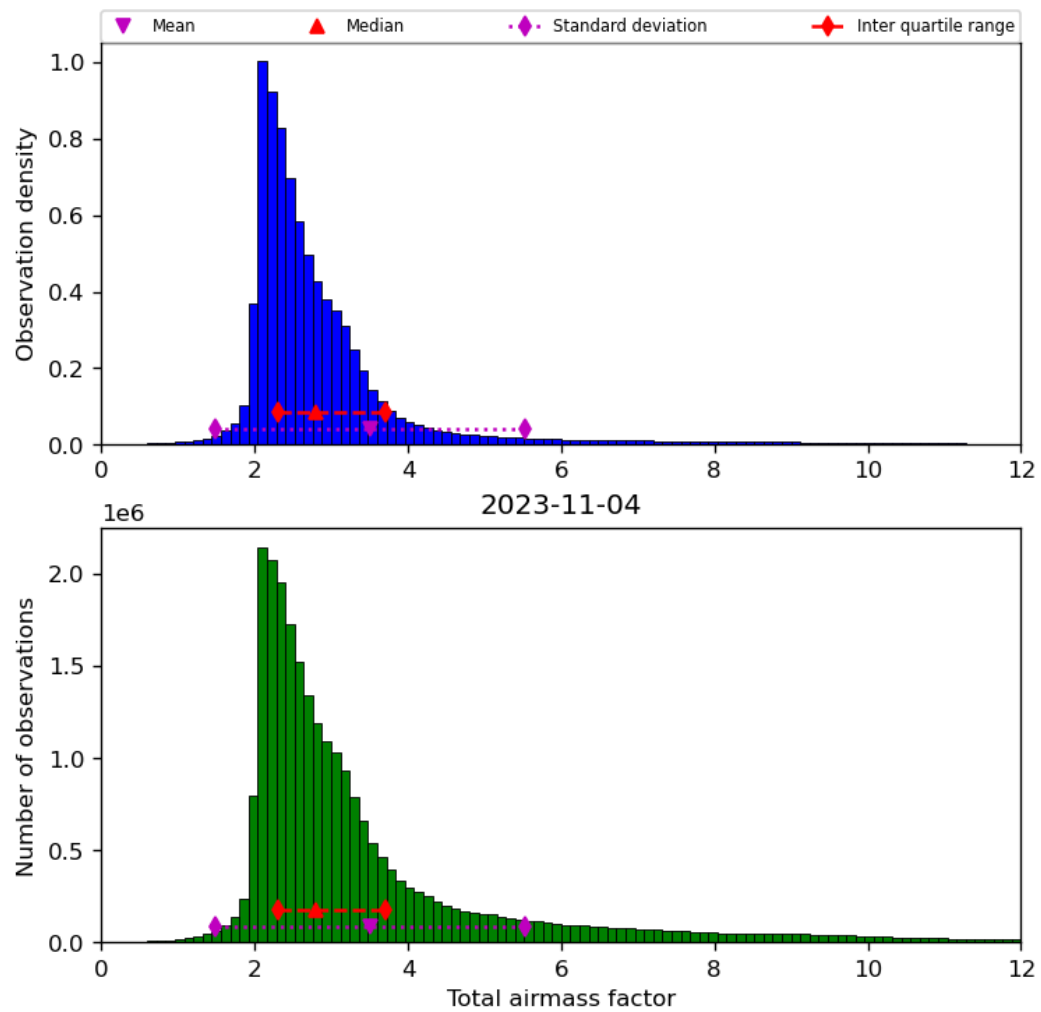
Figure 32: Histogram of “Total airmass factor” for 2023-11-03 to 2023-11-05
