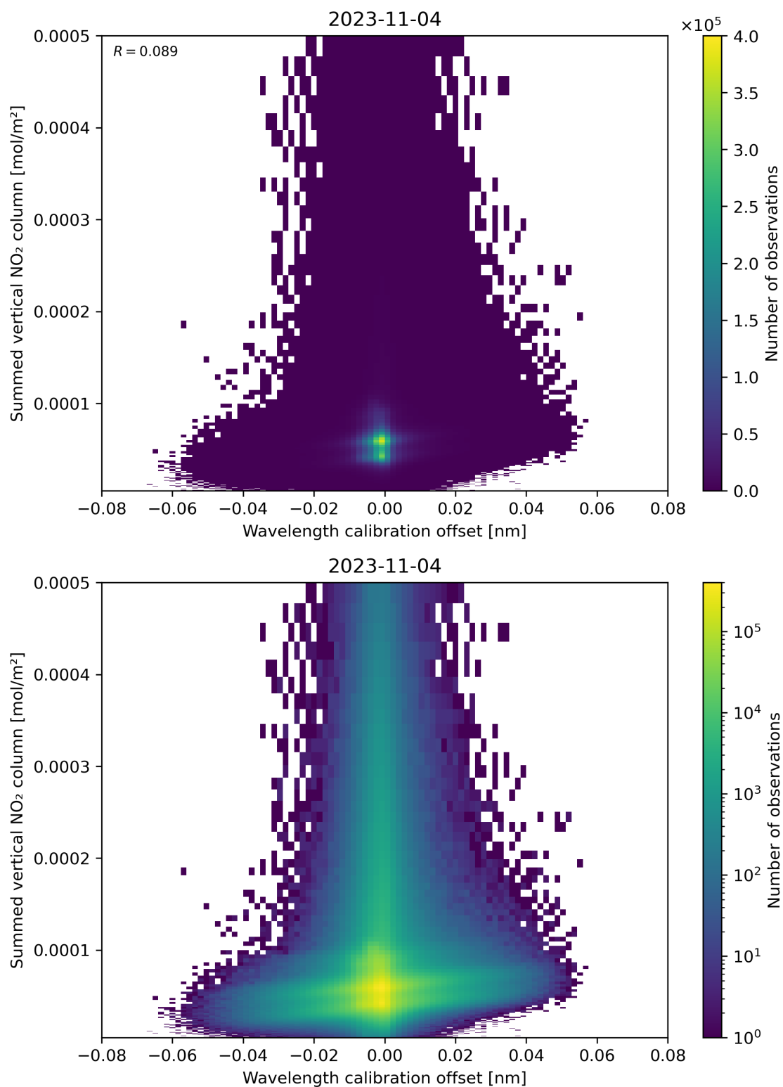
Figure 177: Scatter density plot of “Wavelength calibration offset” against “Summed vertical NO 2 column” for 2023-11-03 to 2023-11-05.
