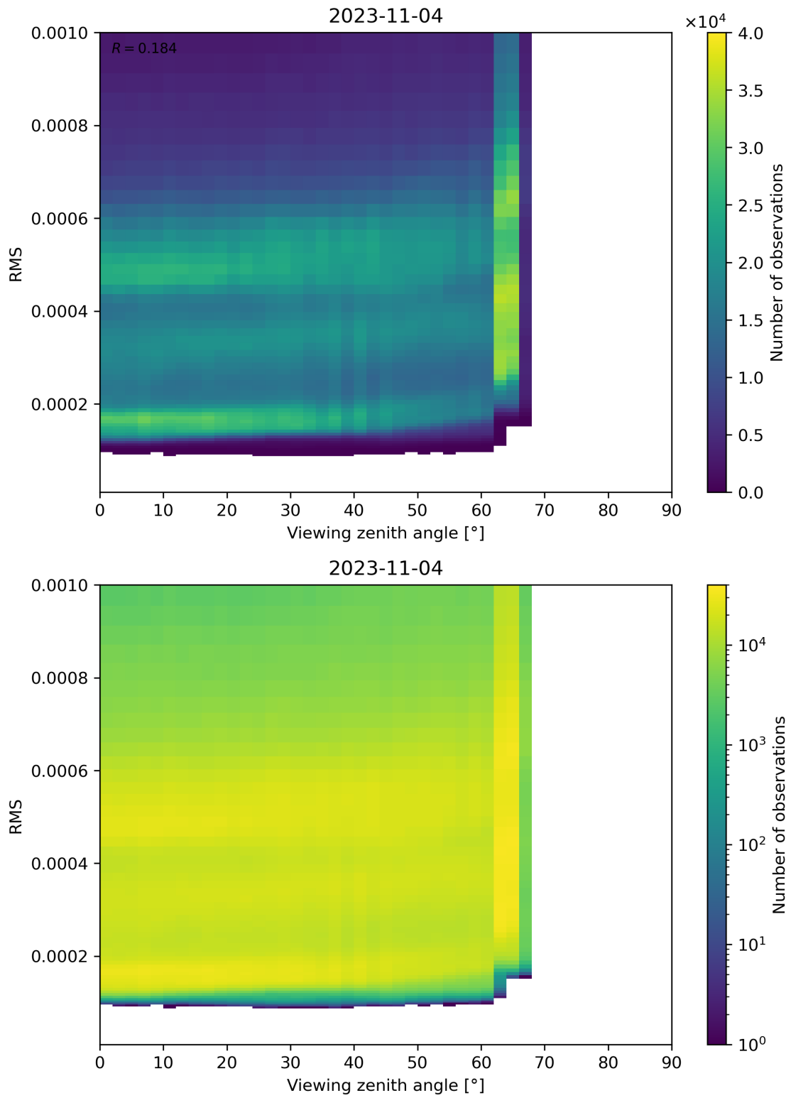
Figure 171: Scatter density plot of “Viewing zenith angle” against “RMS” for 2023-11-03 to 2023-11-05.
