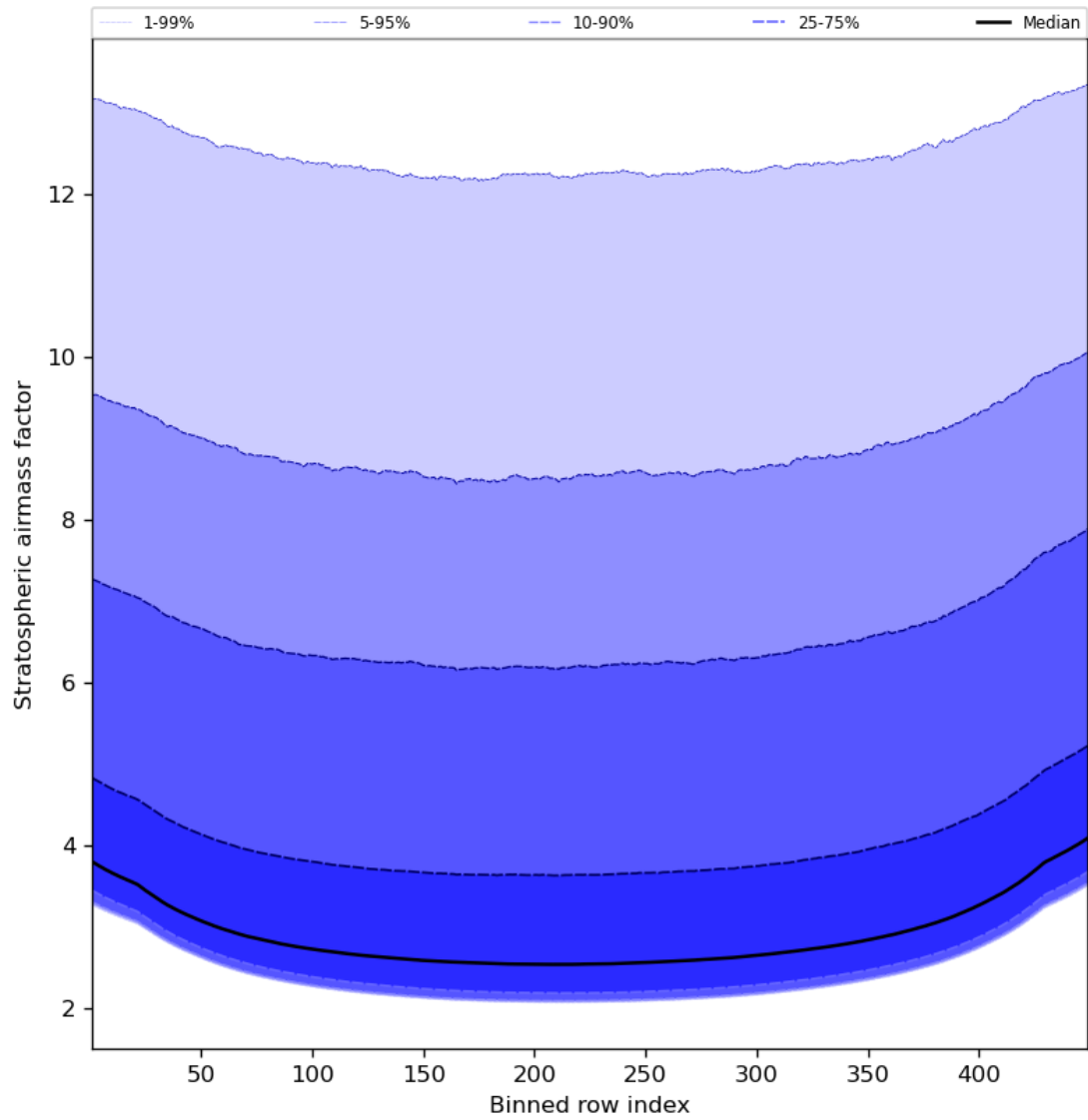
Figure 61: Along track statistics of “Stratospheric airmass factor” for 2023-11-03 to 2023-11-05
