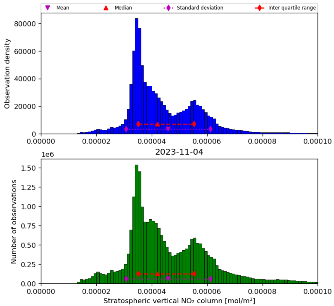
Figure 36: Histogram of “Stratospheric vertical NO 2 column” for 2023-11-03 to 2023-11-05
