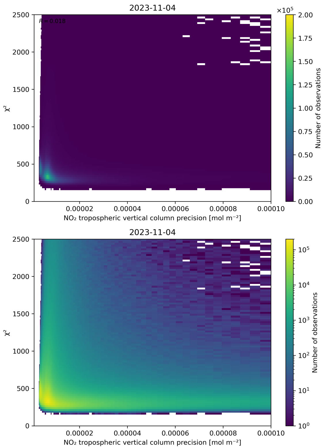
Figure 134: Scatter density plot of “NO 2 tropospheric vertical column precision” against “ \chi^2 ” for 2023-11-03 to 2023-11-05.
