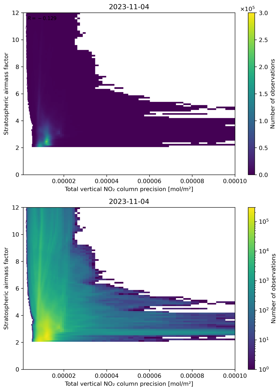
Figure 115: Scatter density plot of “Total vertical NO 2 column precision” against “Stratospheric air mass factor” for 2023-11-03 to 2023-11-05.
