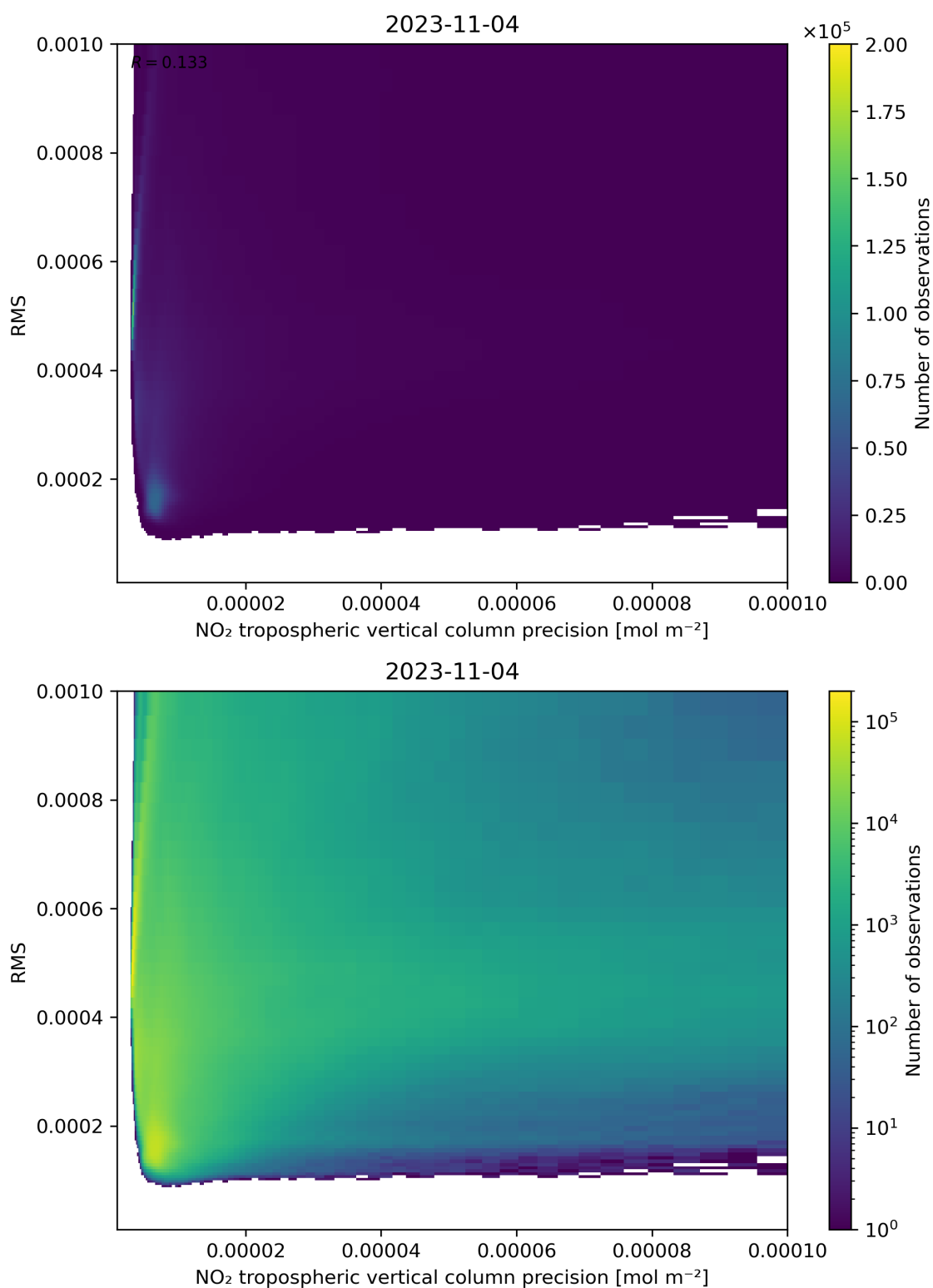
Figure 140: Scatter density plot of “NO 2 tropospheric vertical column precision” against “RMS” for 2023-11-03 to 2023-11-05.
