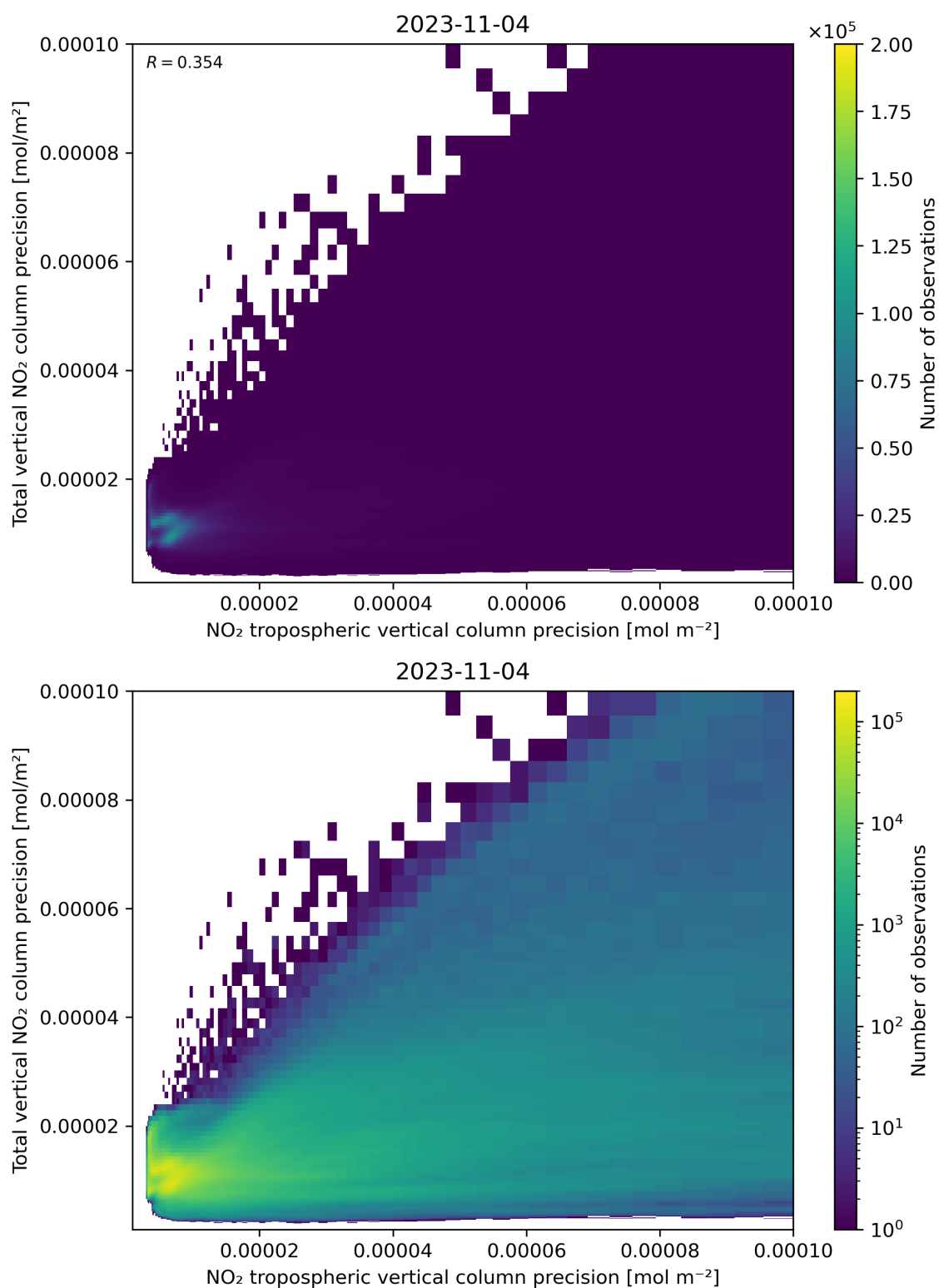
Figure 139: Scatter density plot of “NO 2 tropospheric vertical column precision” against “Total vertical NO 2 column precision” for 2023-11-03 to 2023-11-05.
