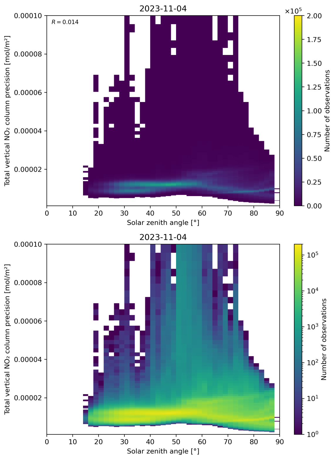
Figure 154: Scatter density plot of “Solar zenith angle” against “Total vertical NO 2 column precision” for 2023-11-03 to 2023-11-05.
