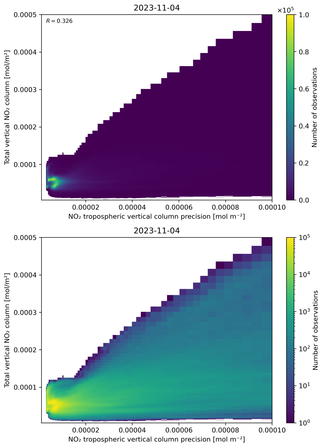
Figure 138: Scatter density plot of “NO 2 tropospheric vertical column precision” against “Total vertical NO 2 column” for 2023-11-03 to 2023-11-05.
