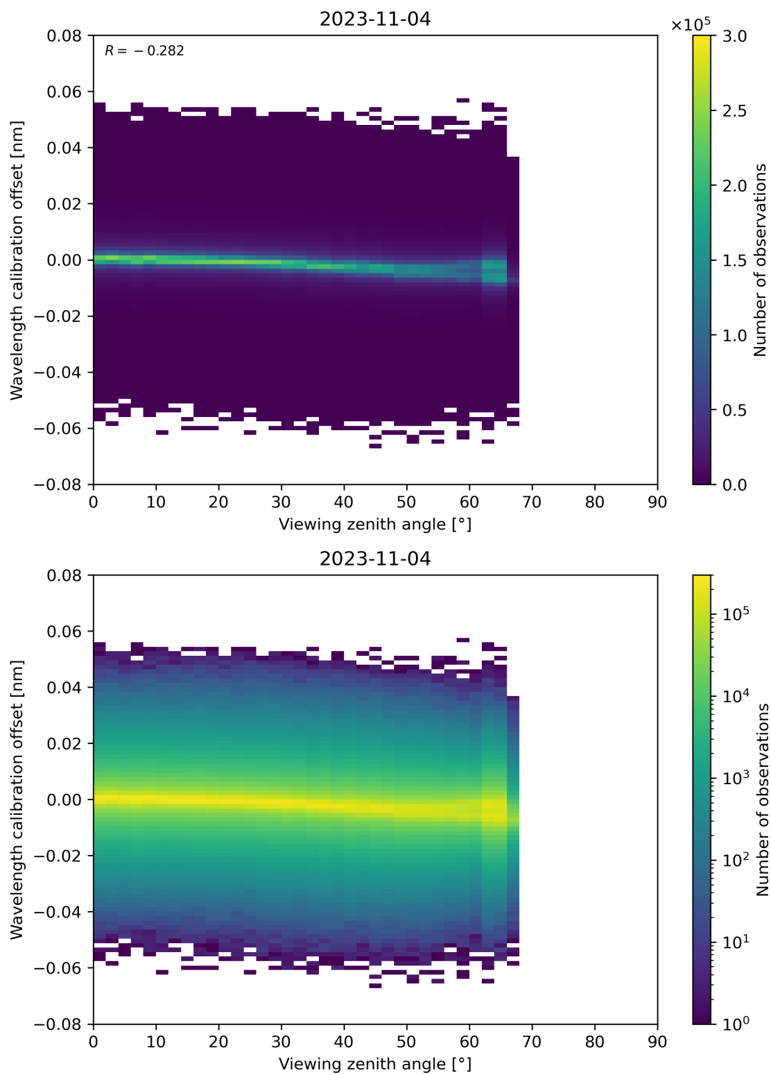
Figure 173: Scatter density plot of “Viewing zenith angle” against “Wavelength calibration offset” for 2023-11-03 to 2023-11-05.
