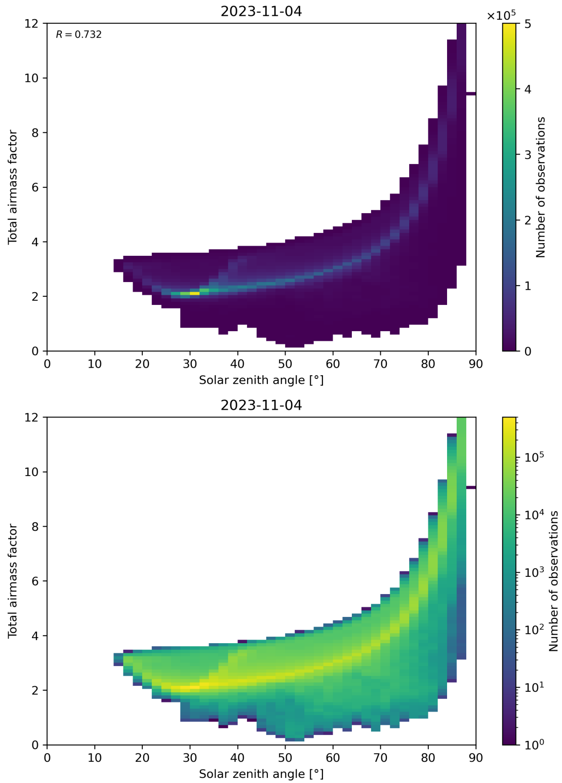
Figure 146: Scatter density plot of “Solar zenith angle” against “Total air mass factor” for 2023-11-03 to 2023-11-05.
