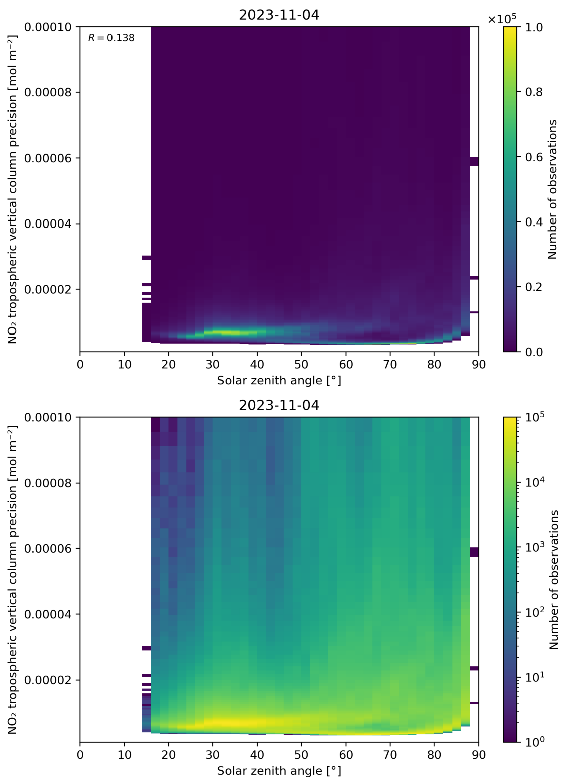
Figure 156: Scatter density plot of “Solar zenith angle” against “NO 2 tropospheric vertical column precision” for 2023-11-03 to 2023-11-05.
