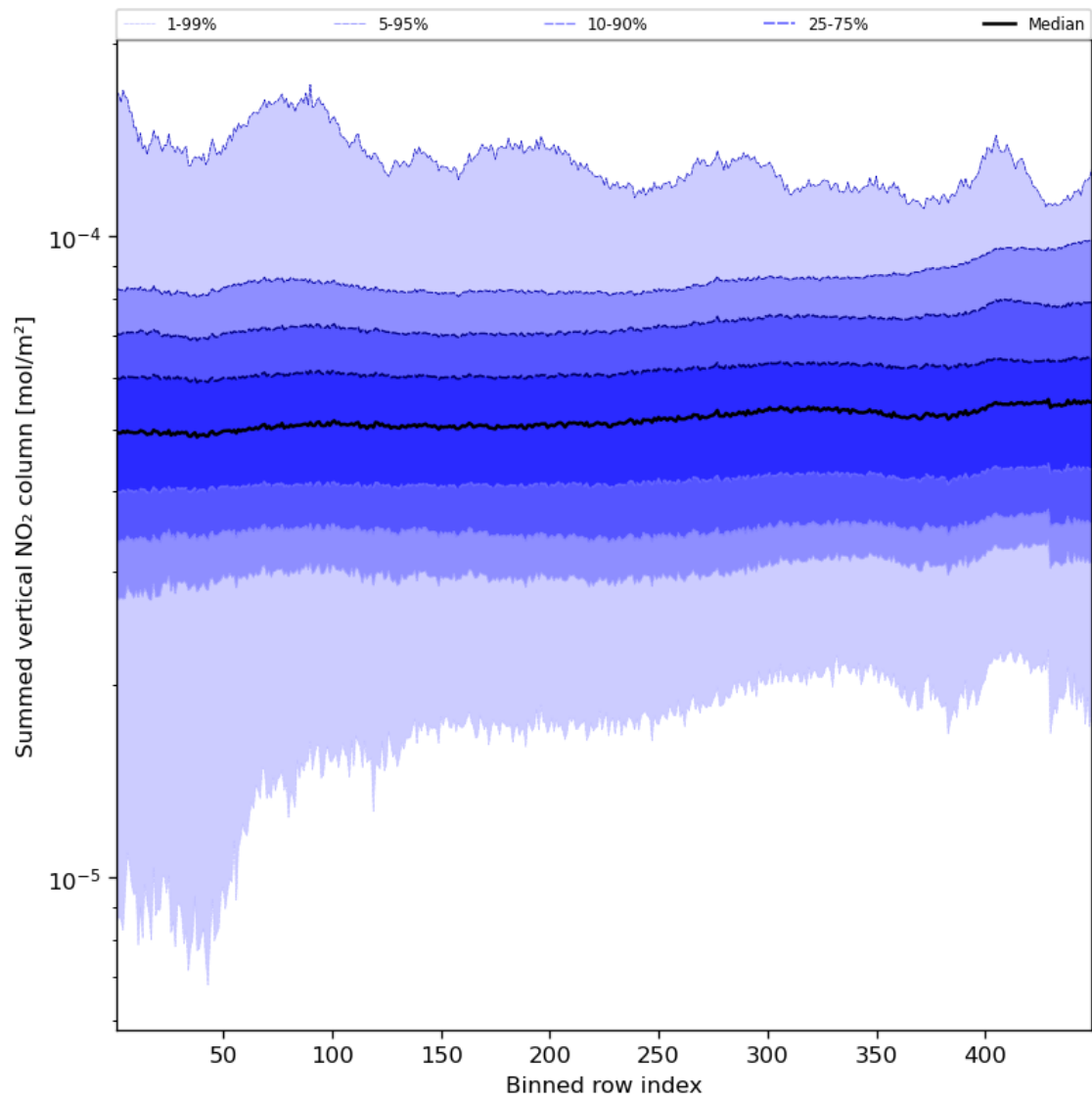
Figure 57: Along track statistics of “Summed vertical NO 2 column” for 2023-11-03 to 2023-11-05
