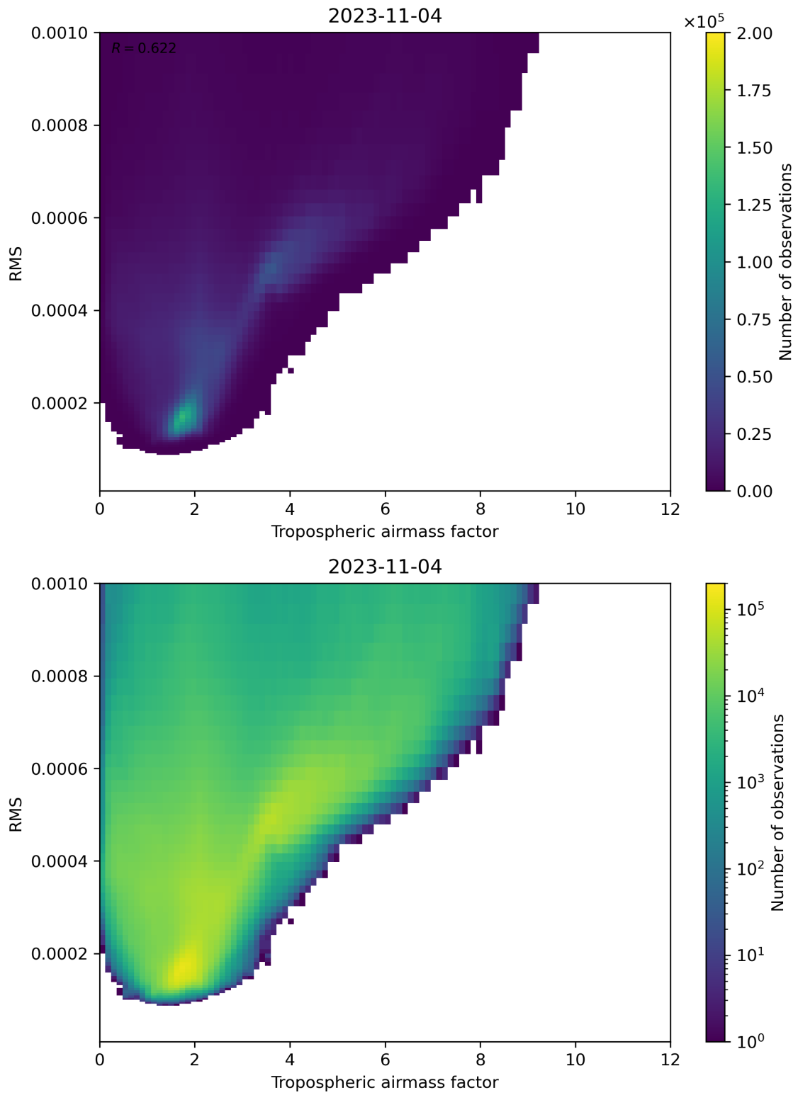
Figure 79: Scatter density plot of “Tropospheric airmass factor” against “RMS” for 2023-11-03 to 2023-11-05.
