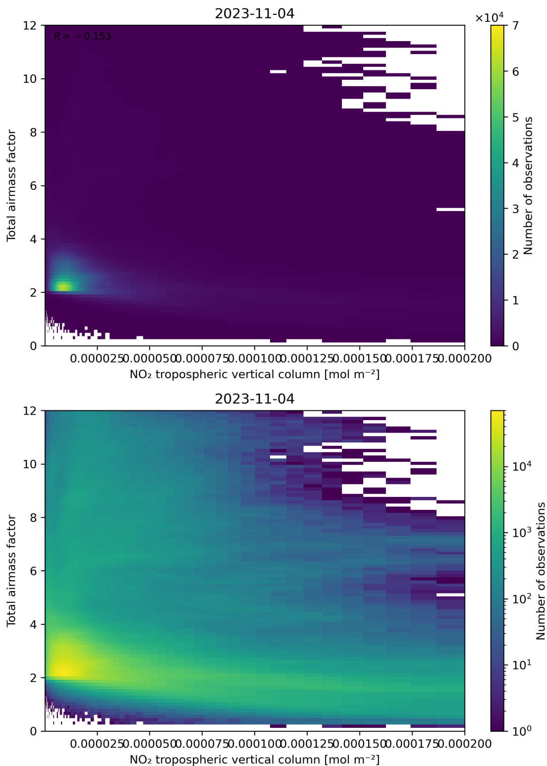
Figure 122: Scatter density plot of “NO 2 tropospheric vertical column” against “Total air mass factor” for 2023-11-03 to 2023-11-05.
