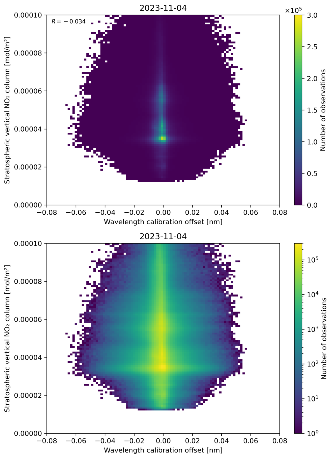
Figure 176: Scatter density plot of “Wavelength calibration offset” against “Stratospheric vertical NO 2 column” for 2023-11-03 to 2023-11-05.
