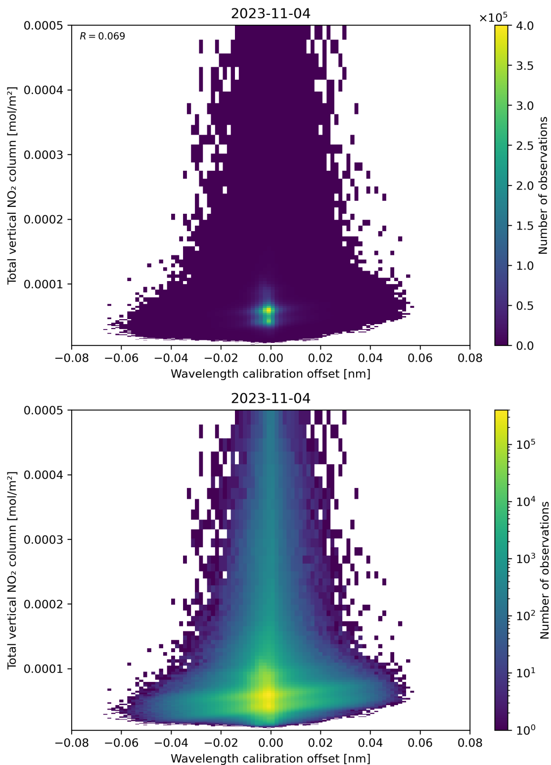
Figure 179: Scatter density plot of “Wavelength calibration offset” against “Total vertical NO 2 column” for 2023-11-03 to 2023-11-05.
