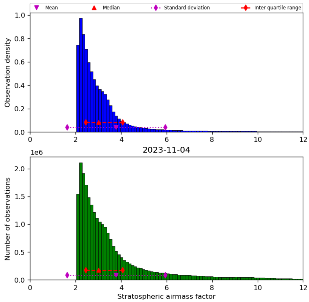
Figure 44: Histogram of “Stratospheric airmass factor” for 2023-11-03 to 2023-11-05
