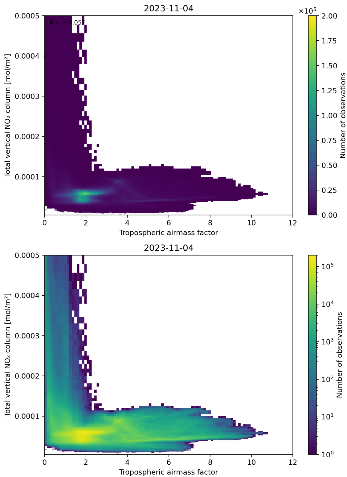
Figure 77: Scatter density plot of “Tropospheric airmass factor” against “Total vertical NO 2 column” for 2023-11-03 to 2023-11-05.
