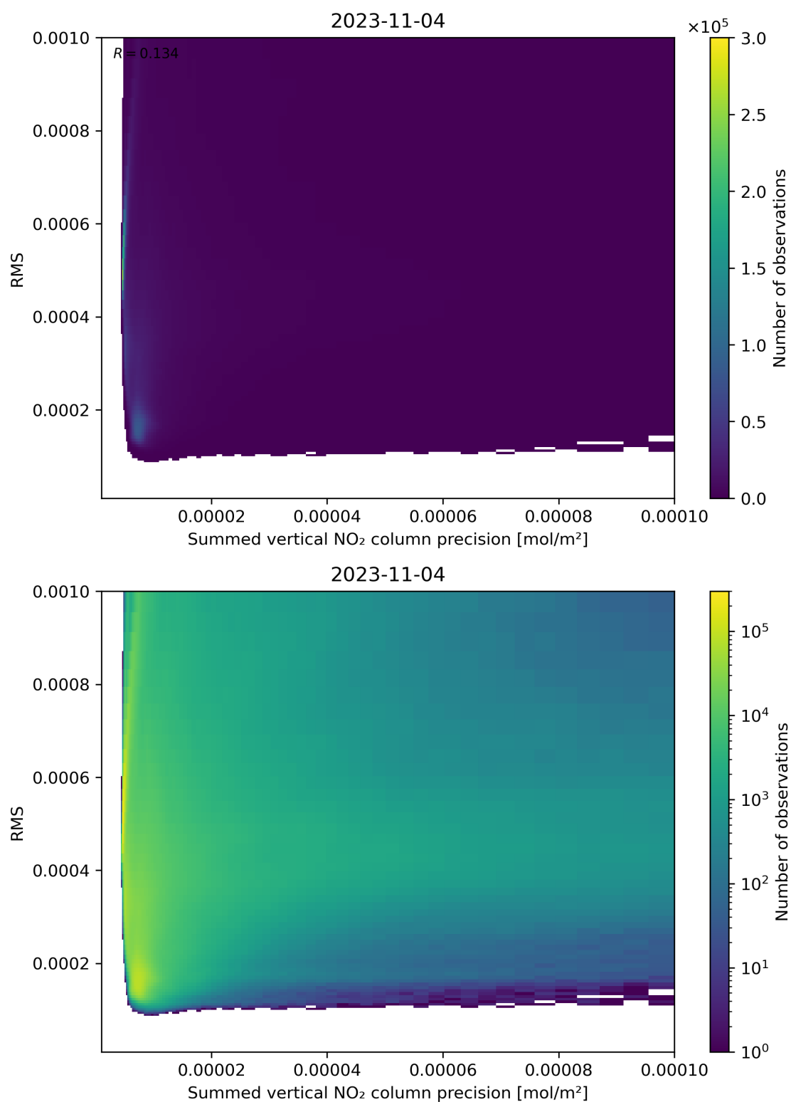
Figure 108: Scatter density plot of “Summed vertical NO 2 column precision” against “RMS” for 2023-11-03 to 2023-11-05.
