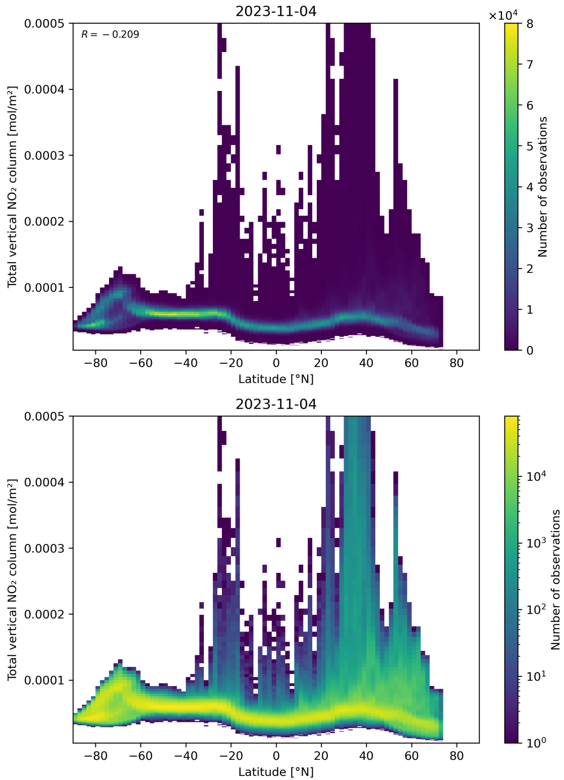
Figure 90: Scatter density plot of “Latitude” against “Total vertical NO 2 column” for 2023-11-03 to 2023-11-05.
