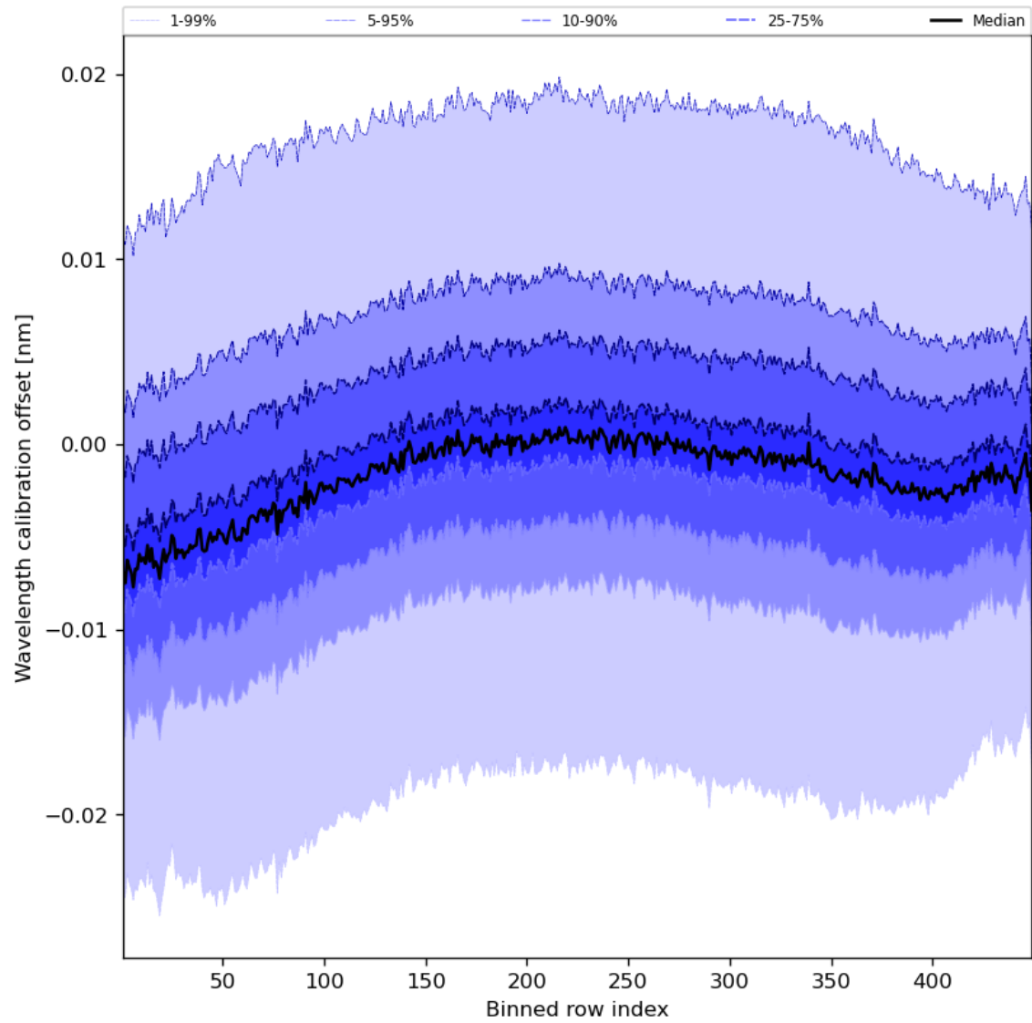
Figure 52: Along track statistics of “Wavelength calibration offset” for 2023-11-03 to 2023-11-05
