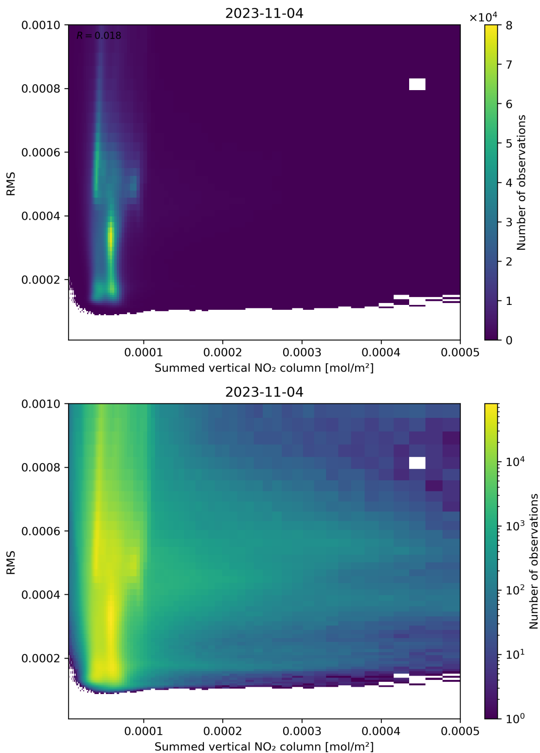
Figure 109: Scatter density plot of “Summed vertical NO 2 column” against “RMS” for 2023-11-03 to 2023-11-05.
