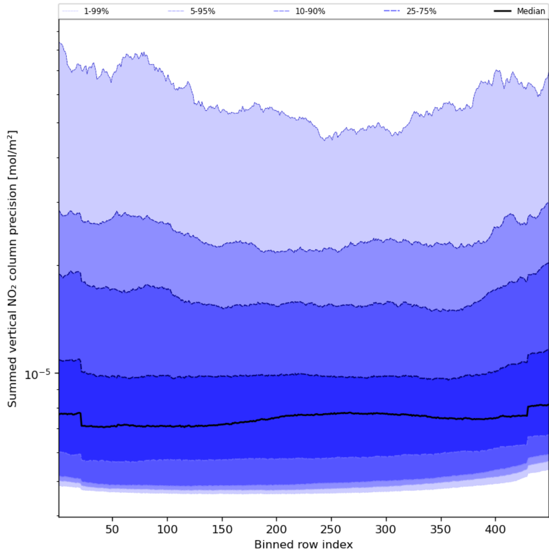
Figure 58: Along track statistics of “Summed vertical NO 2 column precision” for 2023-11-03 to 2023-11-05
