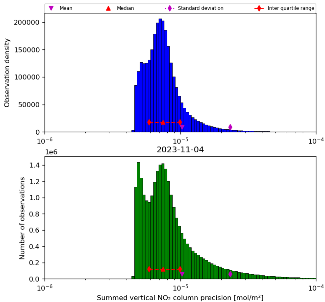
Figure 41: Histogram of “Summed vertical NO 2 column precision” for 2023-11-03 to 2023-11-05
