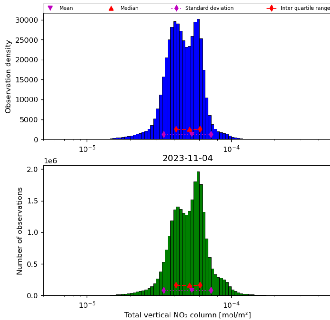
Figure 38: Histogram of “Total vertical NO 2 column” for 2023-11-03 to 2023-11-05
