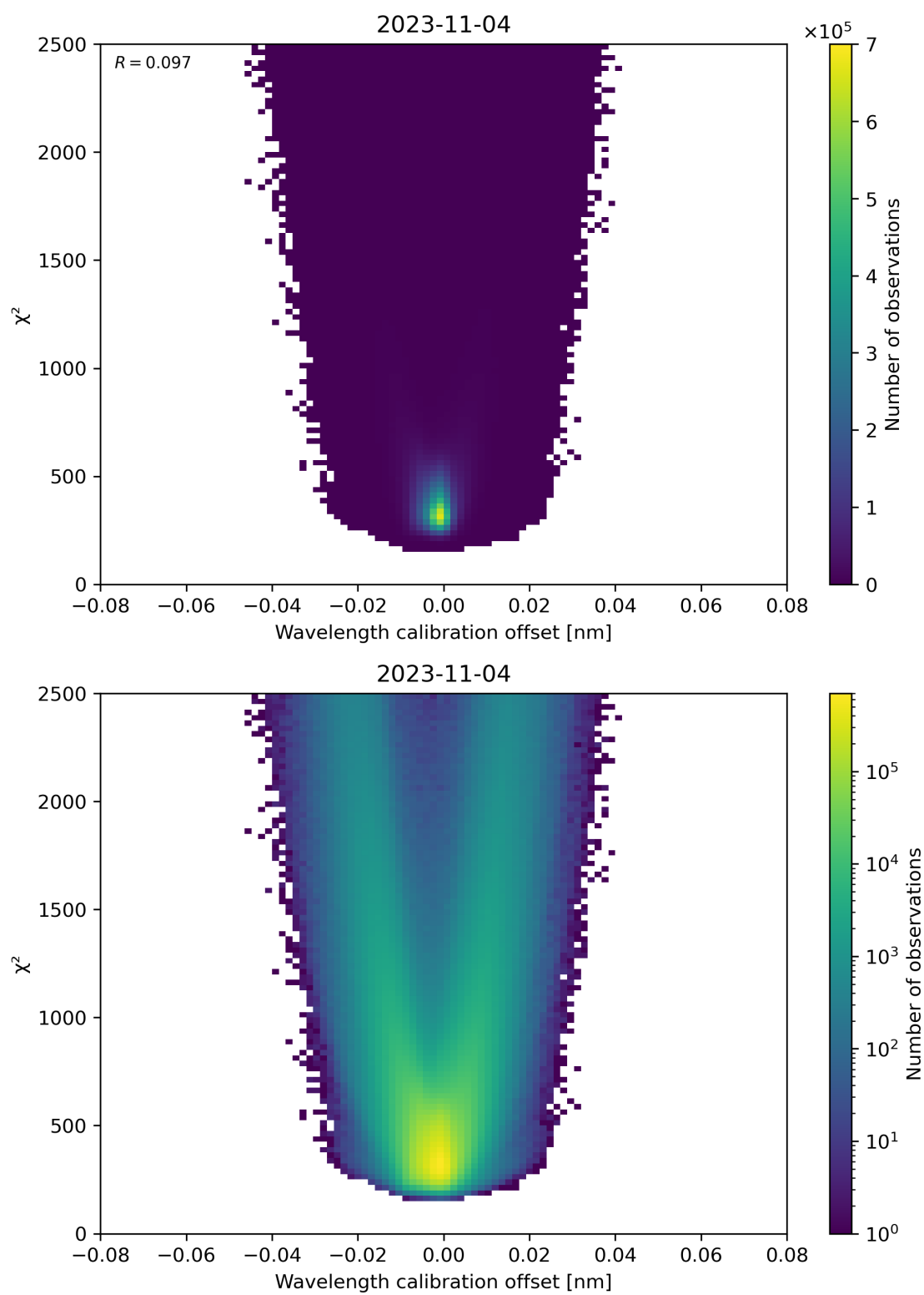
Figure 175: Scatter density plot of “Wavelength calibration offset” against “ \chi^2 ” for 2023-11-03 to 2023-11-05.
