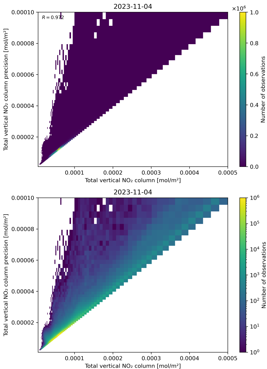
Figure 114: Scatter density plot of “Total vertical NO 2 column” against “Total vertical NO 2 column precision” for 2023-11-03 to 2023-11-05.
