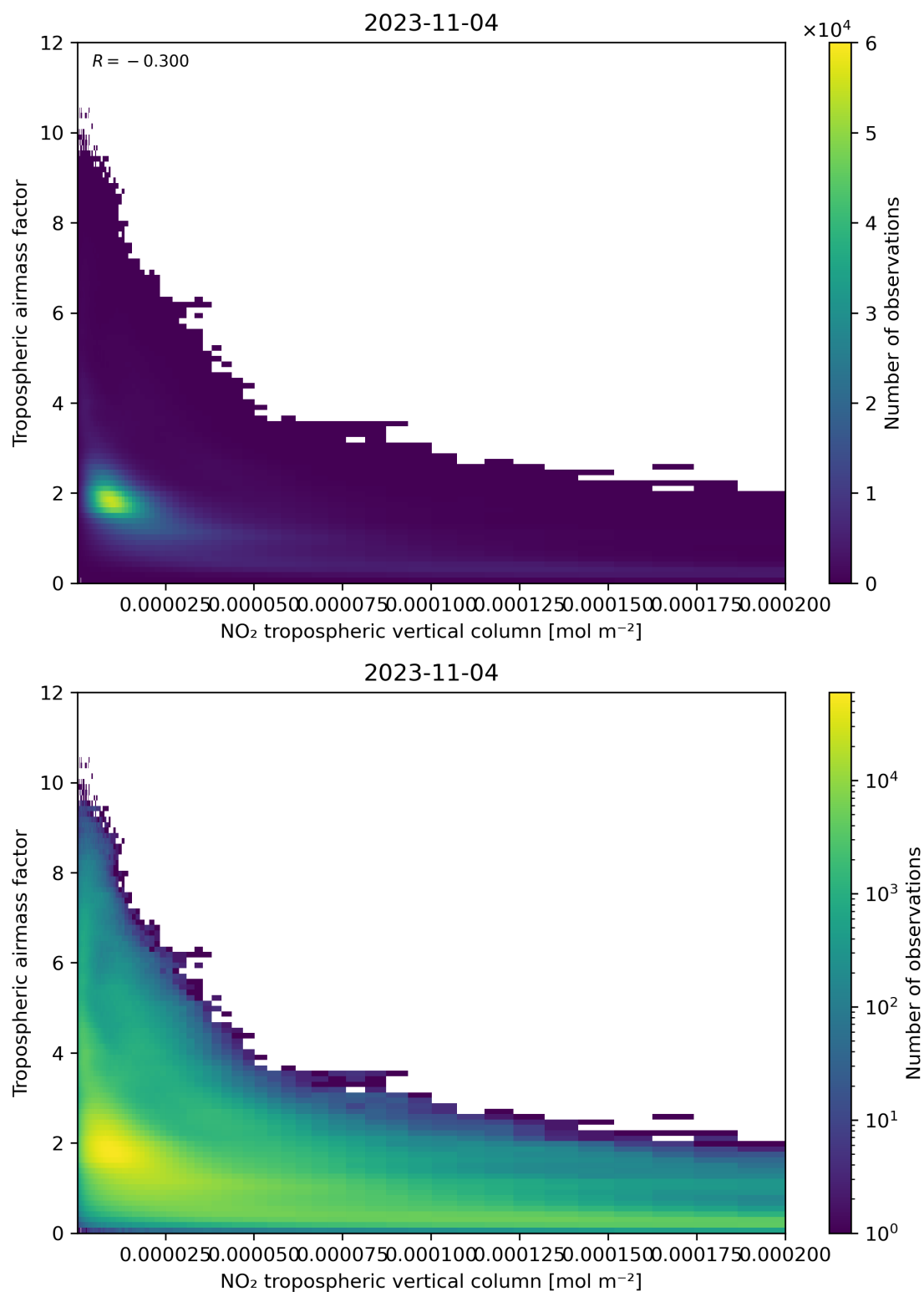
Figure 123: Scatter density plot of “NO 2 tropospheric vertical column” against “Tropospheric airmass factor” for 2023-11-03 to 2023-11-05.
