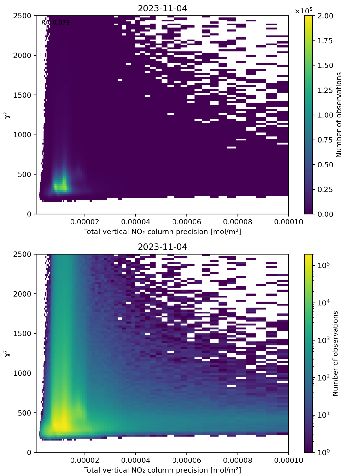
Figure 116: Scatter density plot of “Total vertical NO 2 column precision” against “ \chi^2 ” for 2023-11-03 to 2023-11-05.
