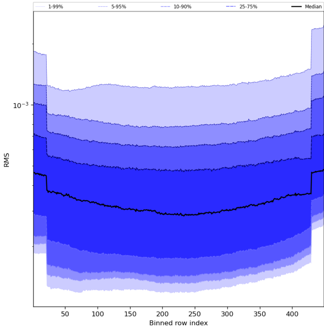
Figure 60: Along track statistics of “RMS” for 2023-11-03 to 2023-11-05
