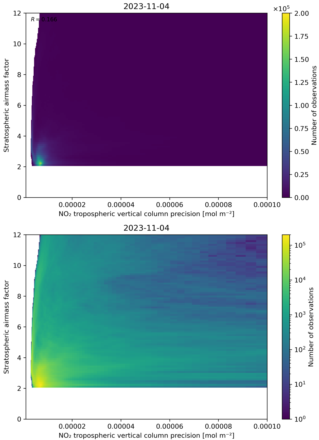
Figure 131: Scatter density plot of “NO 2 tropospheric vertical column precision” against “Stratospheric airmass factor” for 2023-11-03 to 2023-11-05.
