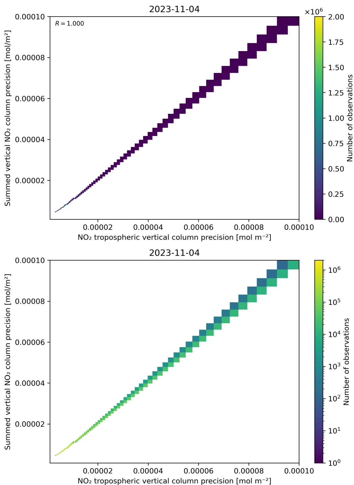
Figure 137: Scatter density plot of “NO 2 tropospheric vertical column precision” against “Summed vertical NO 2 column precision” for 2023-11-03 to 2023-11-05.
