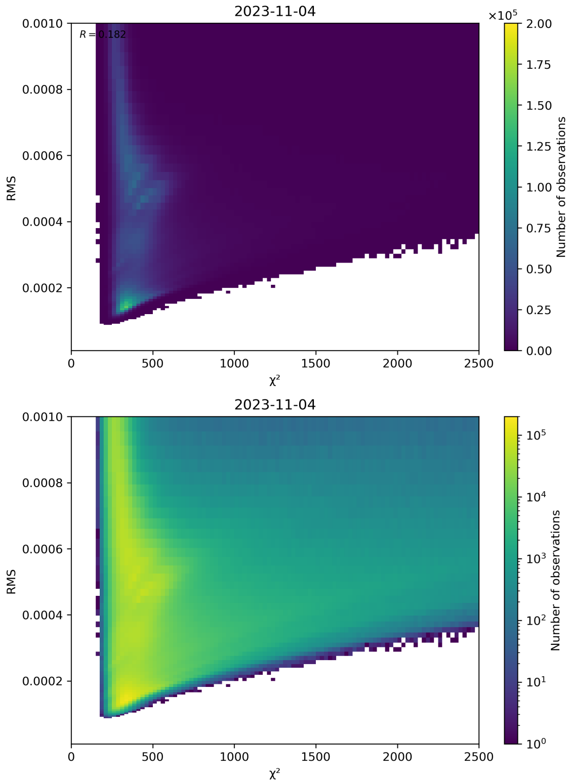
Figure 82: Scatter density plot of “ \chi^2 ” against “RMS” for 2023-11-03 to 2023-11-05.
