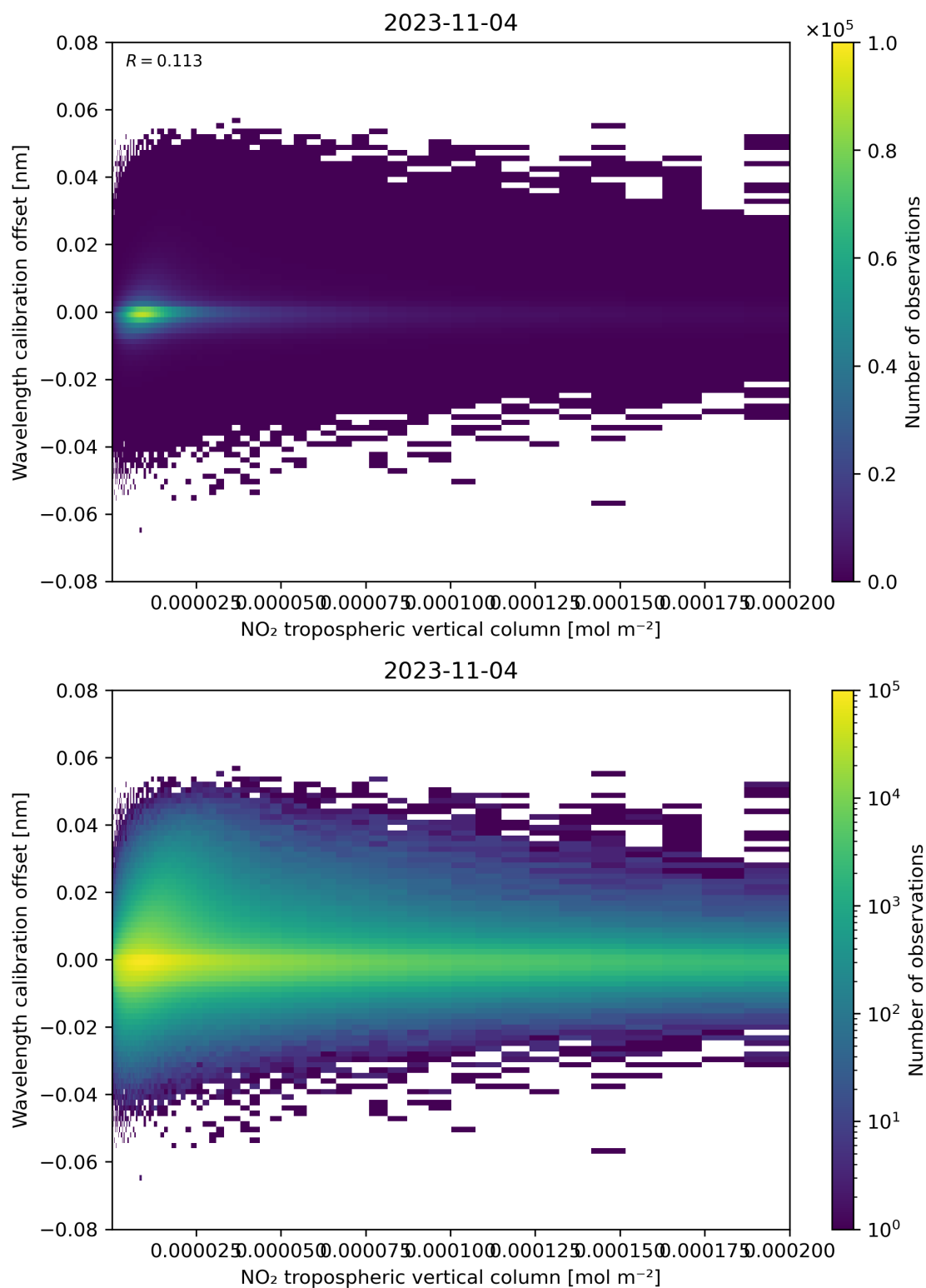
Figure 143: Scatter density plot of “NO 2 tropospheric vertical column” against “Wavelength calibration offset” for 2023-11-03 to 2023-11-05.
