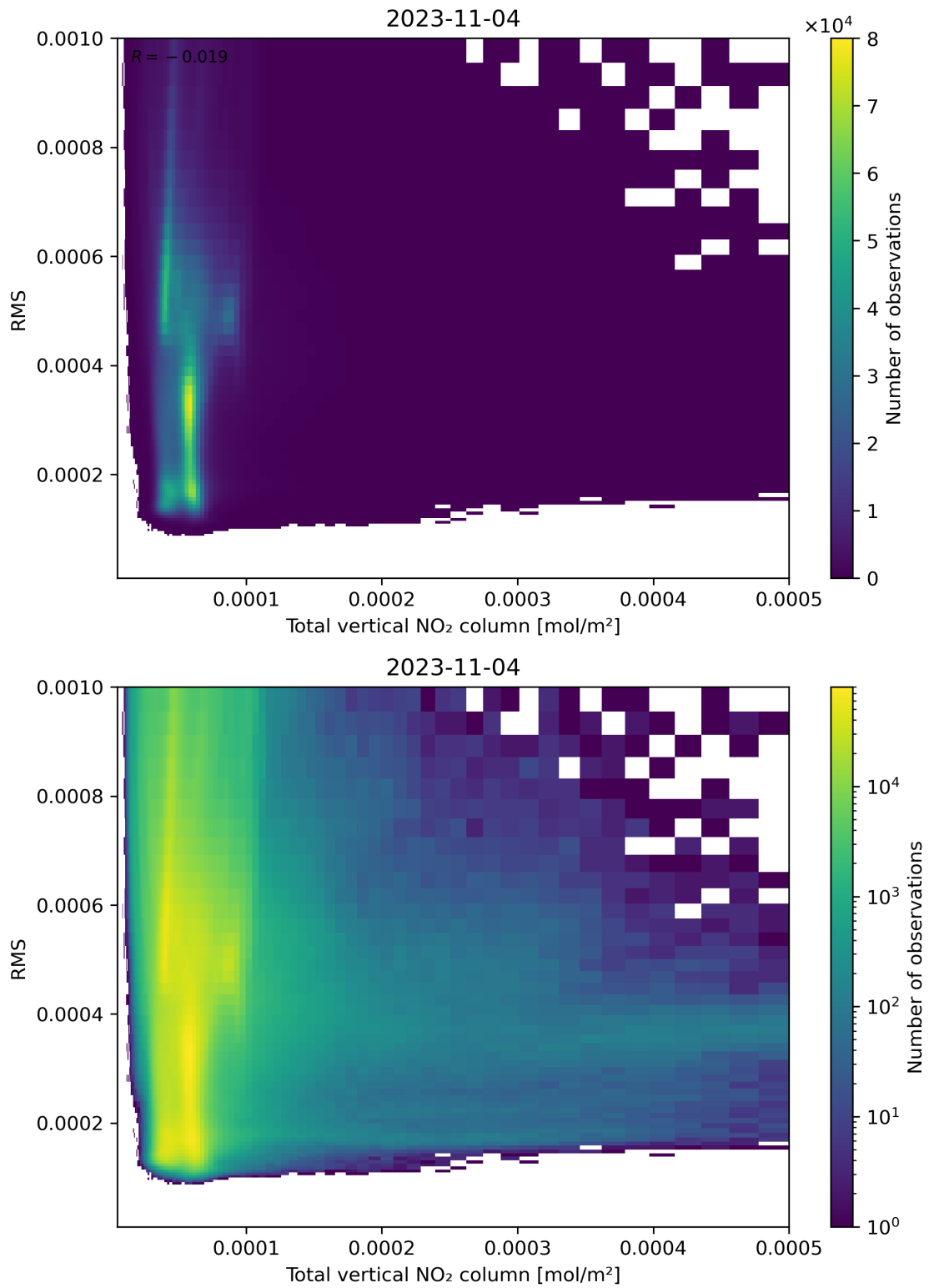
Figure 120: Scatter density plot of “Total vertical NO 2 column” against “RMS” for 2023-11-03 to 2023-11-05.
