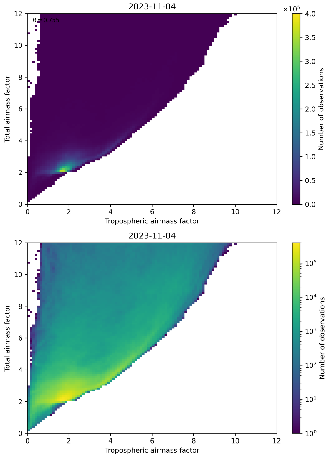
Figure 72: Scatter density plot of “Tropospheric airmass factor” against “Total airmass factor” for 2023-11-03 to 2023-11-05.
