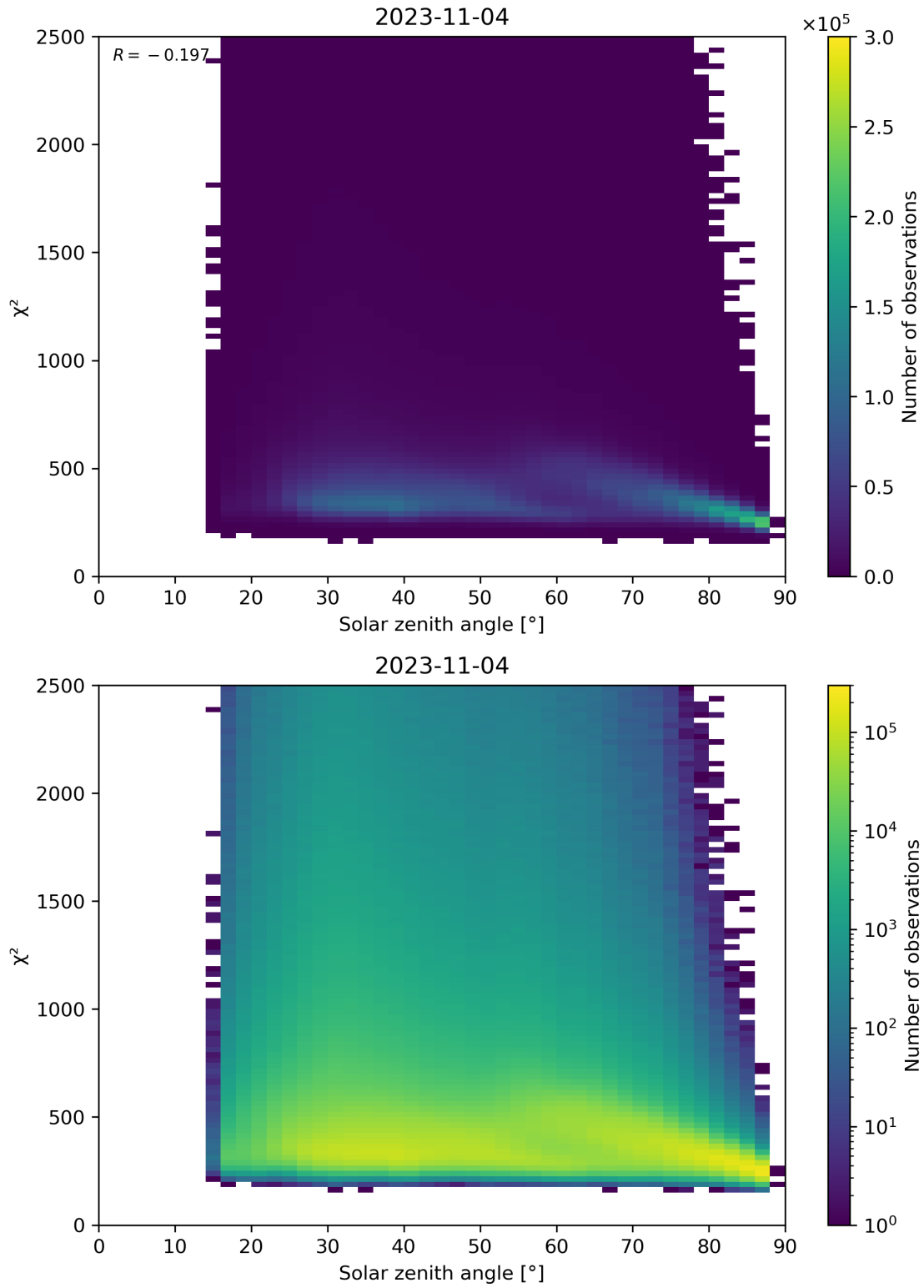
Figure 148: Scatter density plot of “Solar zenith angle” against “ \chi^2 ” for 2023-11-03 to 2023-11-05.
