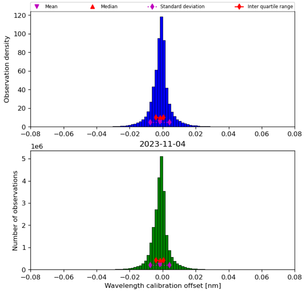
Figure 35: Histogram of “Wavelength calibration offset” for 2023-11-03 to 2023-11-05
