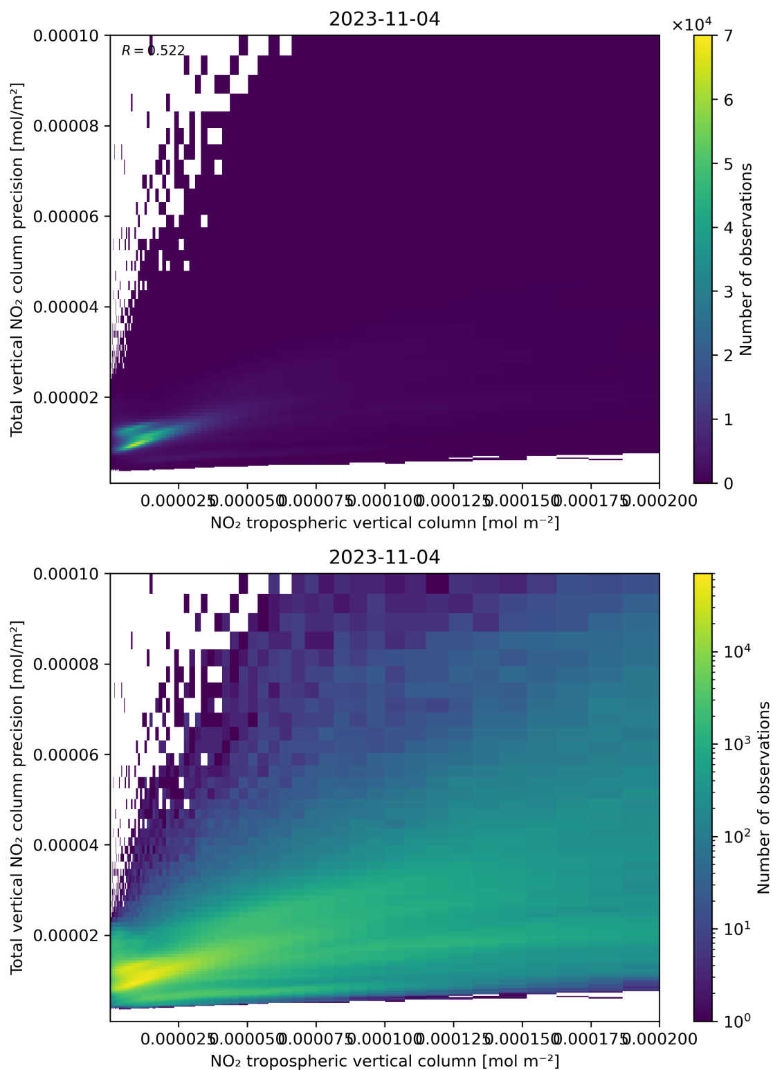
Figure 129: Scatter density plot of “NO 2 tropospheric vertical column” against “Total vertical NO 2 column precision” for 2023-11-03 to 2023-11-05.
