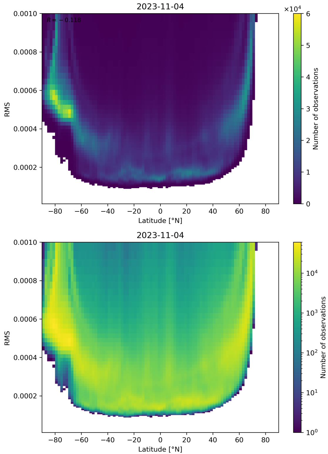
Figure 94: Scatter density plot of “Latitude” against “RMS” for 2023-11-03 to 2023-11-05.
