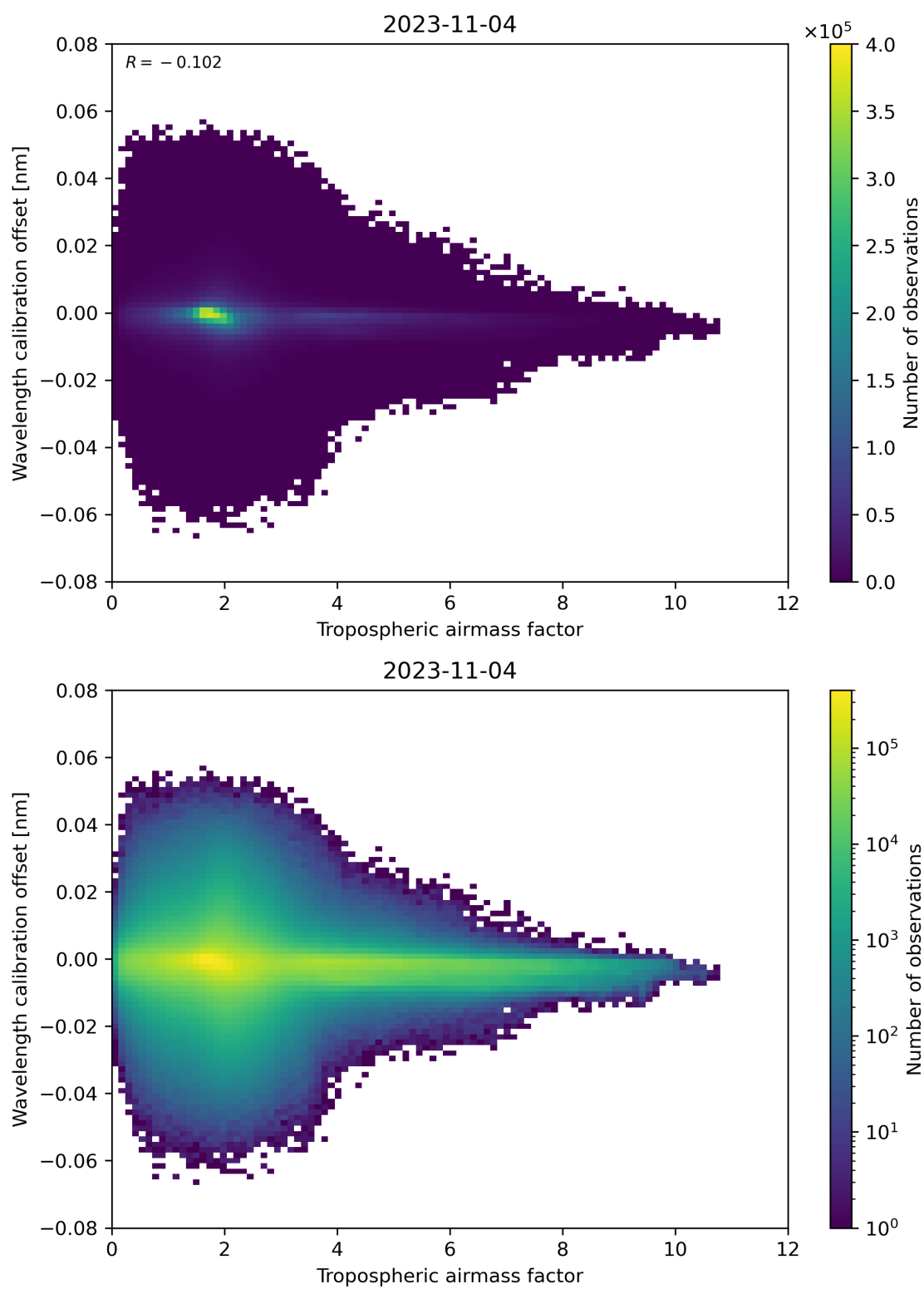
Figure 80: Scatter density plot of “Tropospheric airmass factor” against “Wavelength calibration offset” for 2023-11-03 to 2023-11-05.
