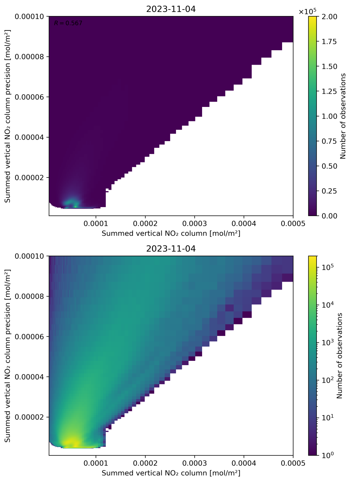
Figure 105: Scatter density plot of “Summed vertical NO 2 column” against “Summed vertical NO 2 column precision” for 2023-11-03 to 2023-11-05.
