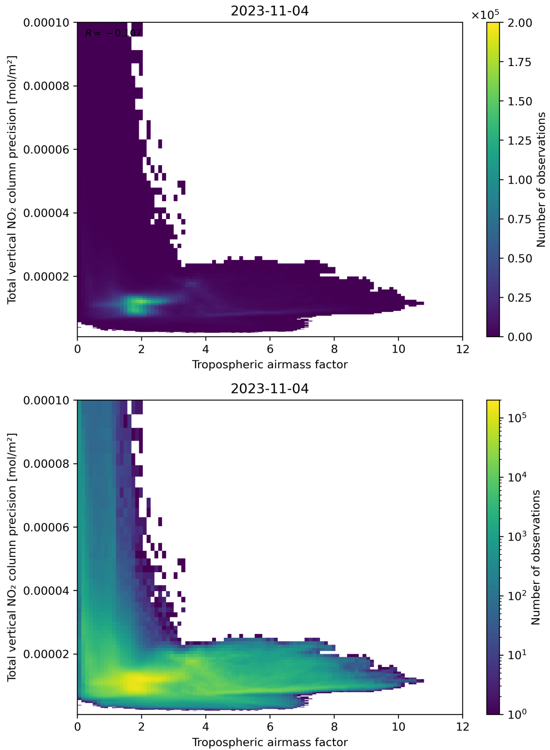
Figure 78: Scatter density plot of “Tropospheric air mass factor” against “Total vertical NO 2 column precision” for 2023-11-03 to 2023-11-05.
