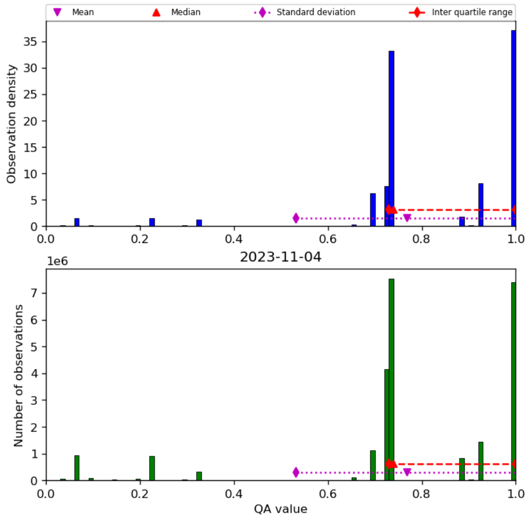
Figure 28: Histogram of “QA value” for 2023-11-03 to 2023-11-05
