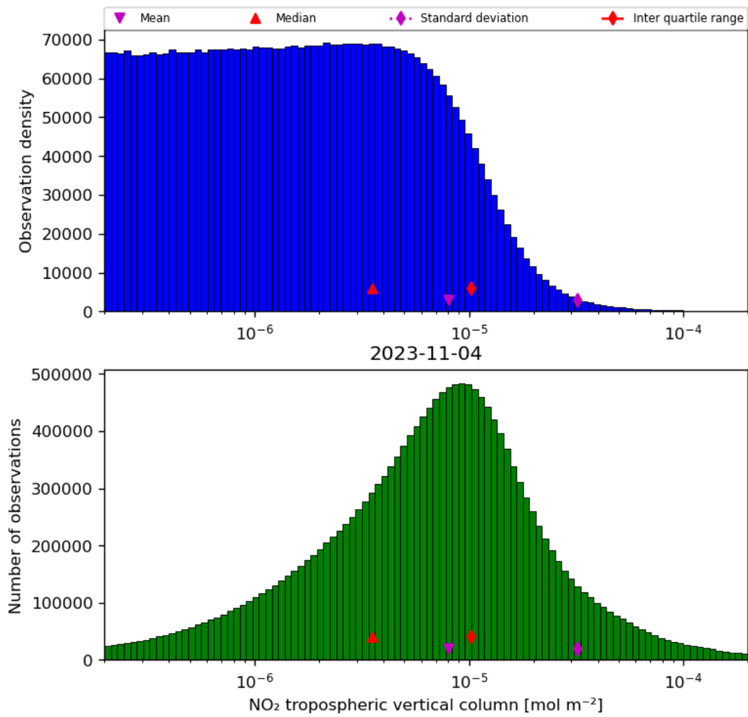
Figure 29: Histogram of “NO 2 tropospheric vertical column” for 2023-11-03 to 2023-11-05
