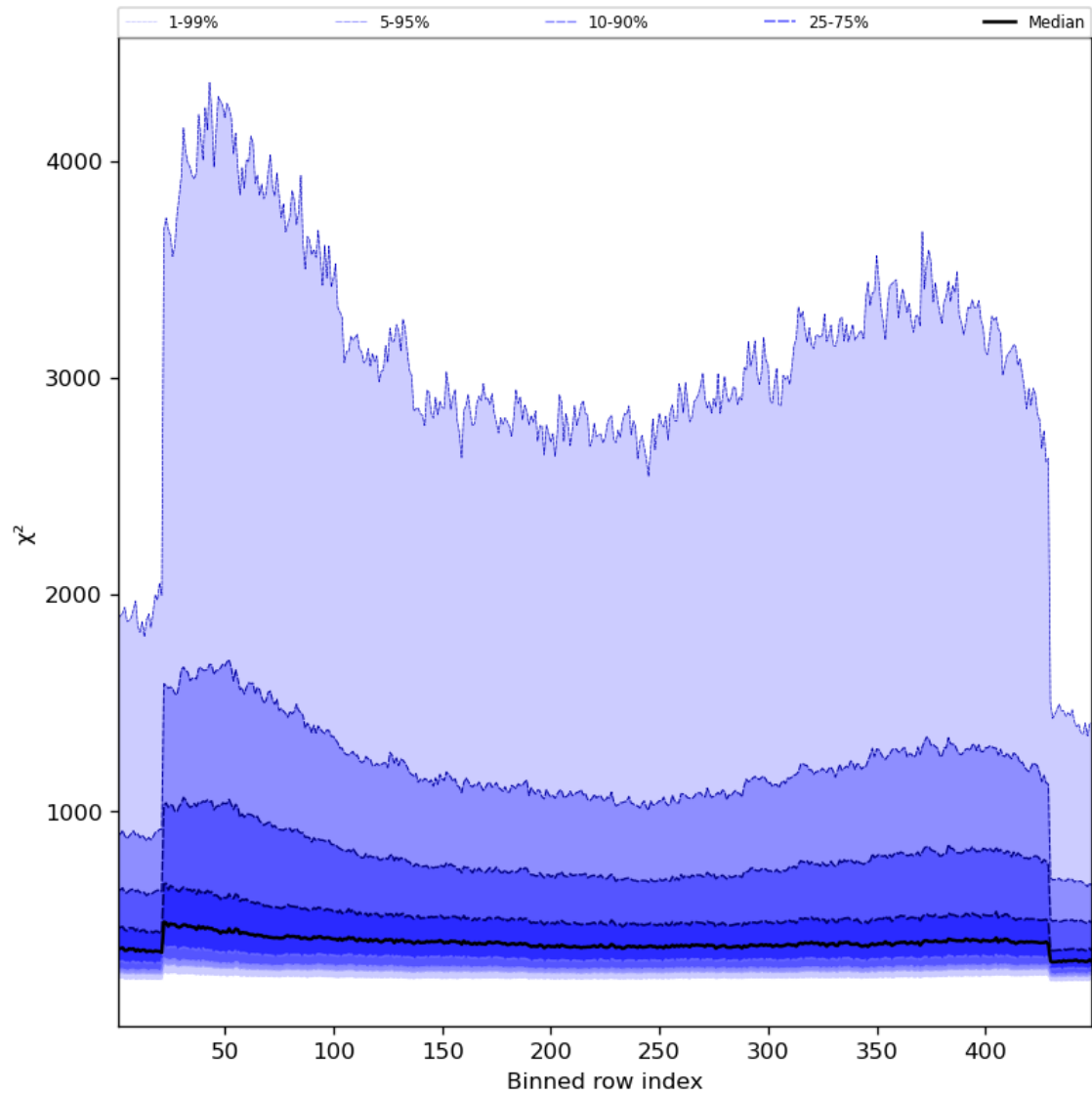
Figure 59: Along track statistics of “ \chi^2 ” for 2023-11-03 to 2023-11-05
