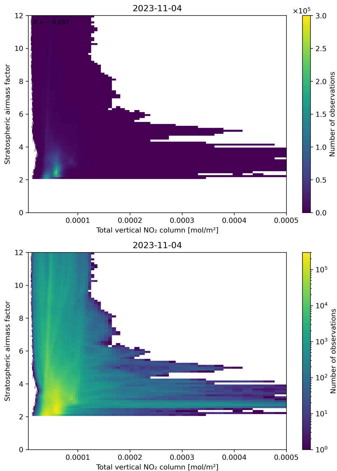
Figure 110: Scatter density plot of “Total vertical NO 2 column” against “Stratospheric airmass factor” for 2023-11-03 to 2023-11-05.
