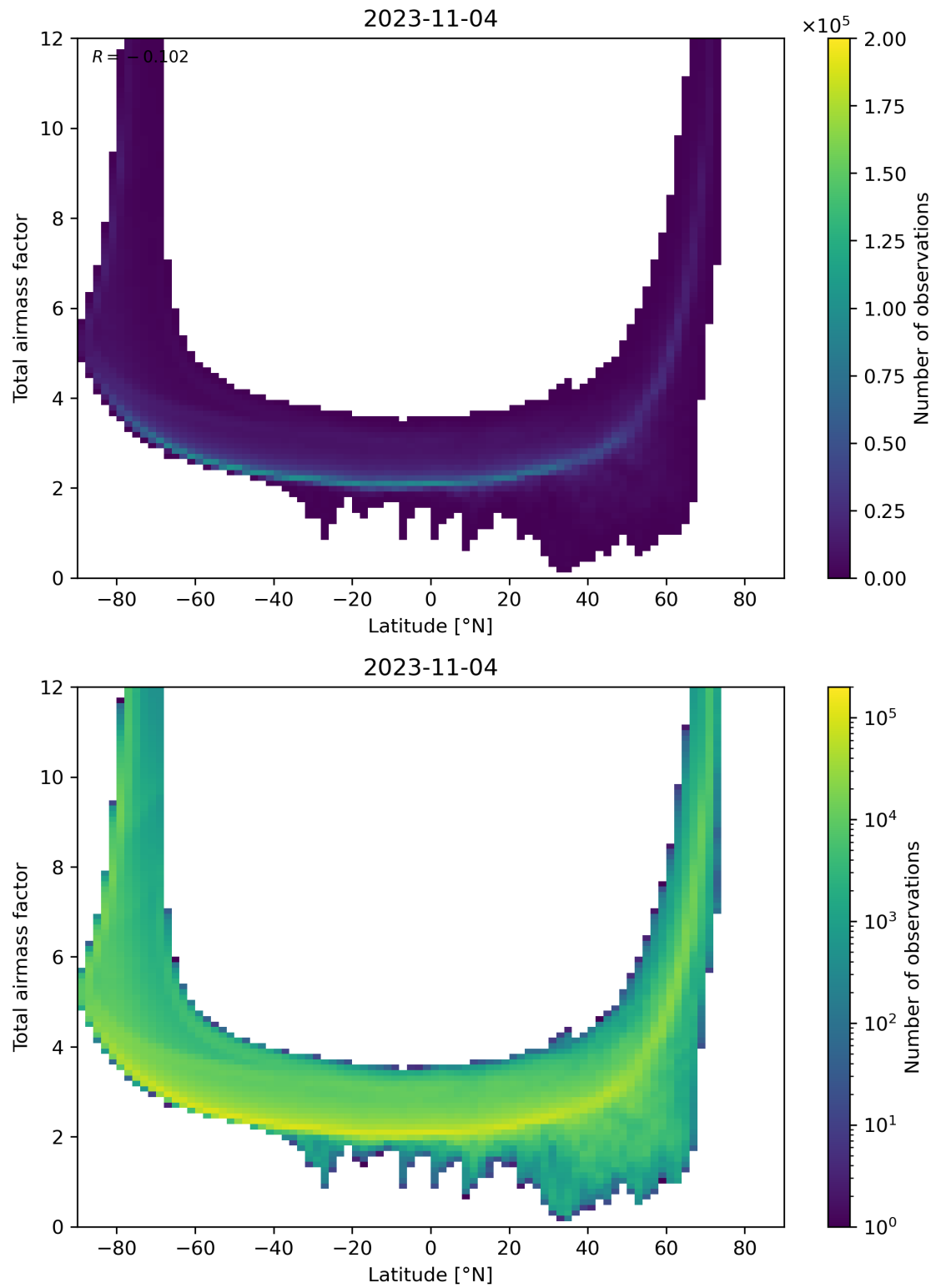
Figure 84: Scatter density plot of “Latitude” against “Total airmass factor” for 2023-11-03 to 2023-11-05.
