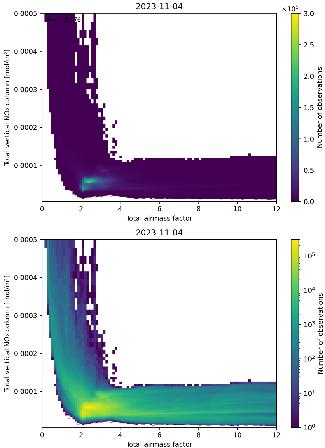
Figure 67: Scatter density plot of “Total airmass factor” against “Total vertical NO 2 column” for 2023-11-03 to 2023-11-05.
