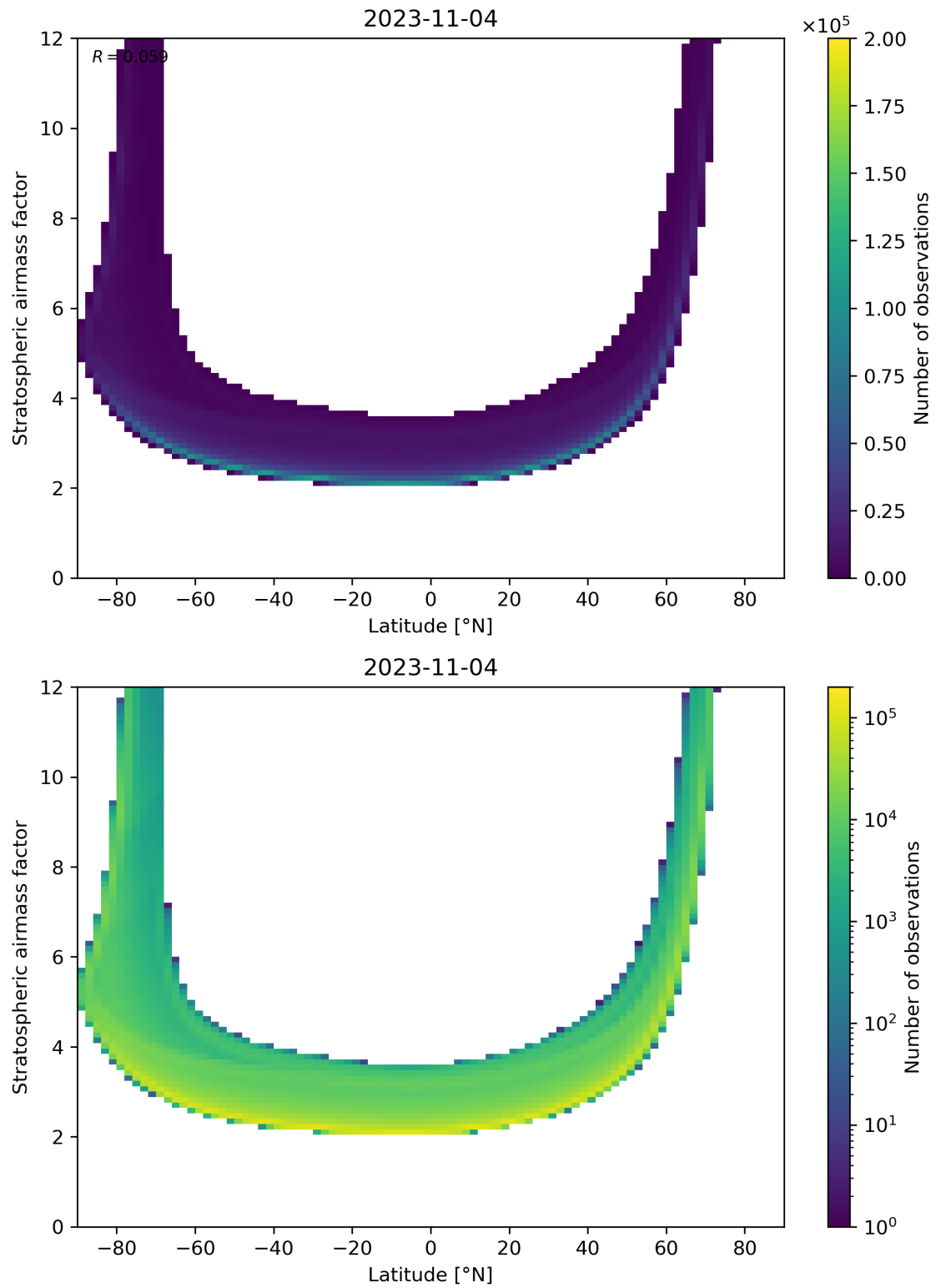
Figure 83: Scatter density plot of “Latitude” against “Stratospheric airmass factor” for 2023-11-03 to 2023-11-05.
