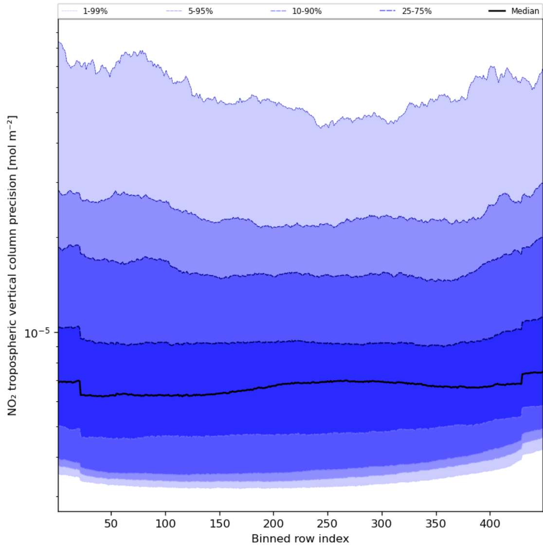
Figure 47: Along track statistics of “NO 2 tropospheric vertical column precision” for 2023-11-03 to 2023-11-05
