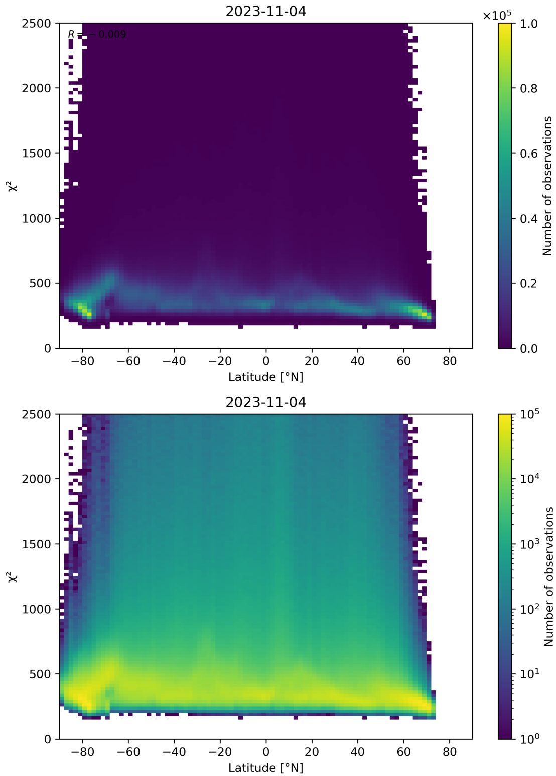
Figure 86: Scatter density plot of “Latitude” against “ \chi^2 ” for 2023-11-03 to 2023-11-05.
