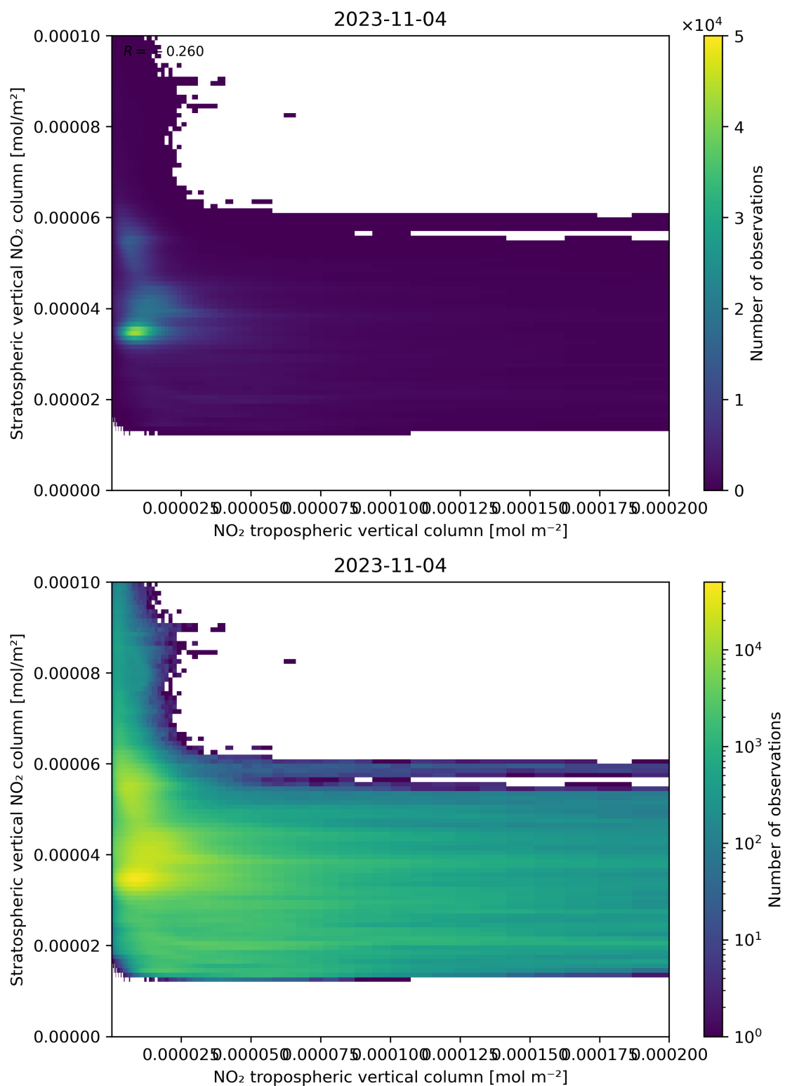
Figure 125: Scatter density plot of “NO 2 tropospheric vertical column” against “Stratospheric vertical NO 2 column” for 2023-11-03 to 2023-11-05.
