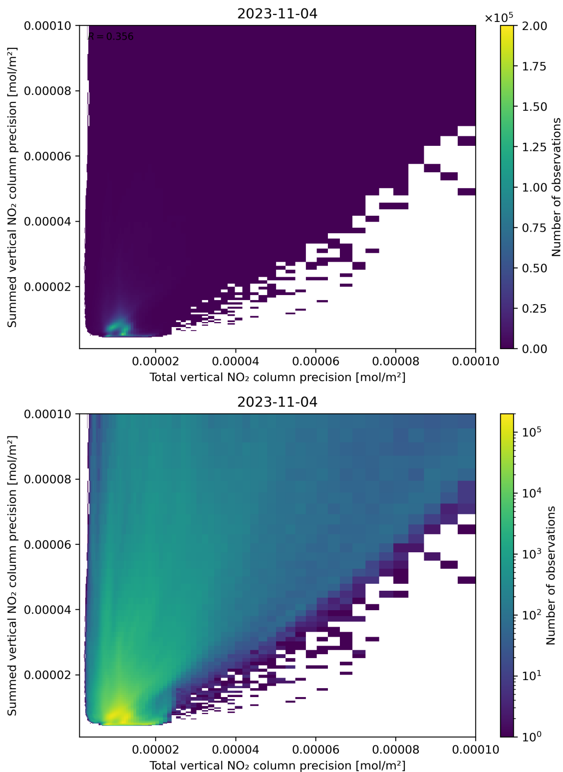
Figure 118: Scatter density plot of “Total vertical NO 2 column precision” against “Summed vertical NO 2 column precision” for 2023-11-03 to 2023-11-05.
