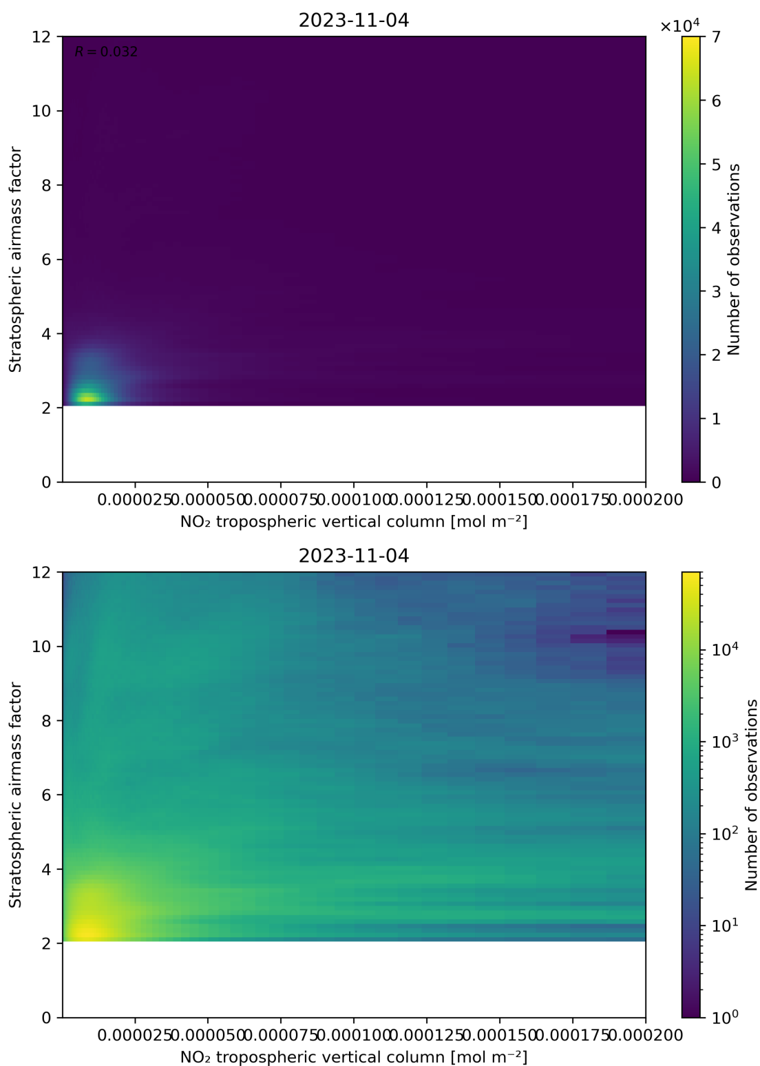
Figure 121: Scatter density plot of “NO 2 tropospheric vertical column” against “Stratospheric airmass factor” for 2023-11-03 to 2023-11-05.
