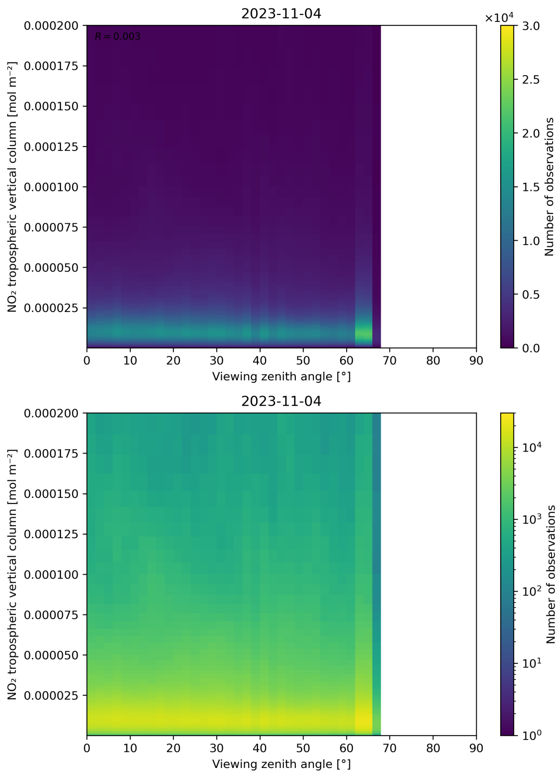
Figure 169: Scatter density plot of “Viewing zenith angle” against “NO 2 tropospheric vertical column” for 2023-11-03 to 2023-11-05.
