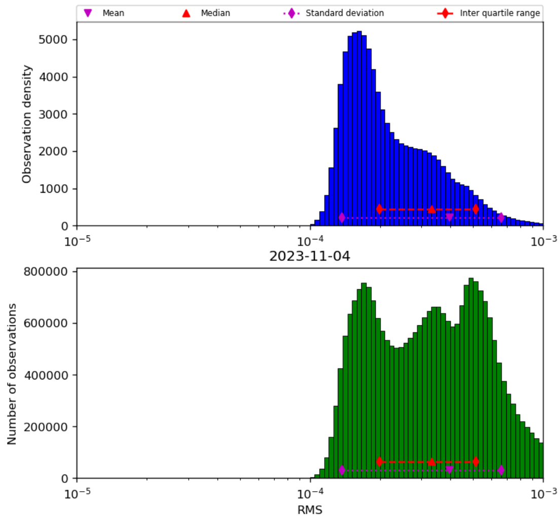
Figure 43: Histogram of “RMS” for 2023-11-03 to 2023-11-05
