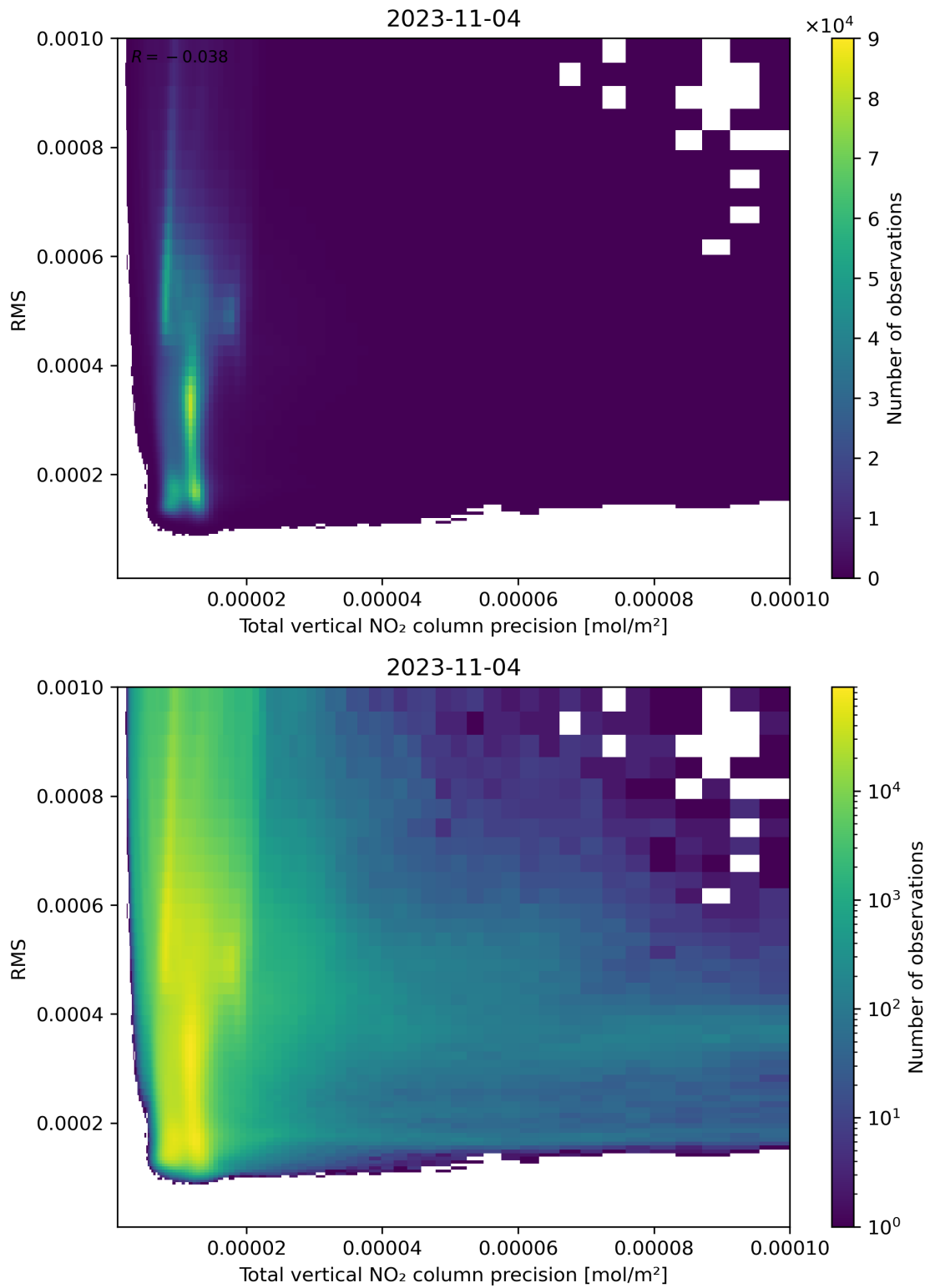
Figure 119: Scatter density plot of “Total vertical NO 2 column precision” against “RMS” for 2023-11-03 to 2023-11-05.
