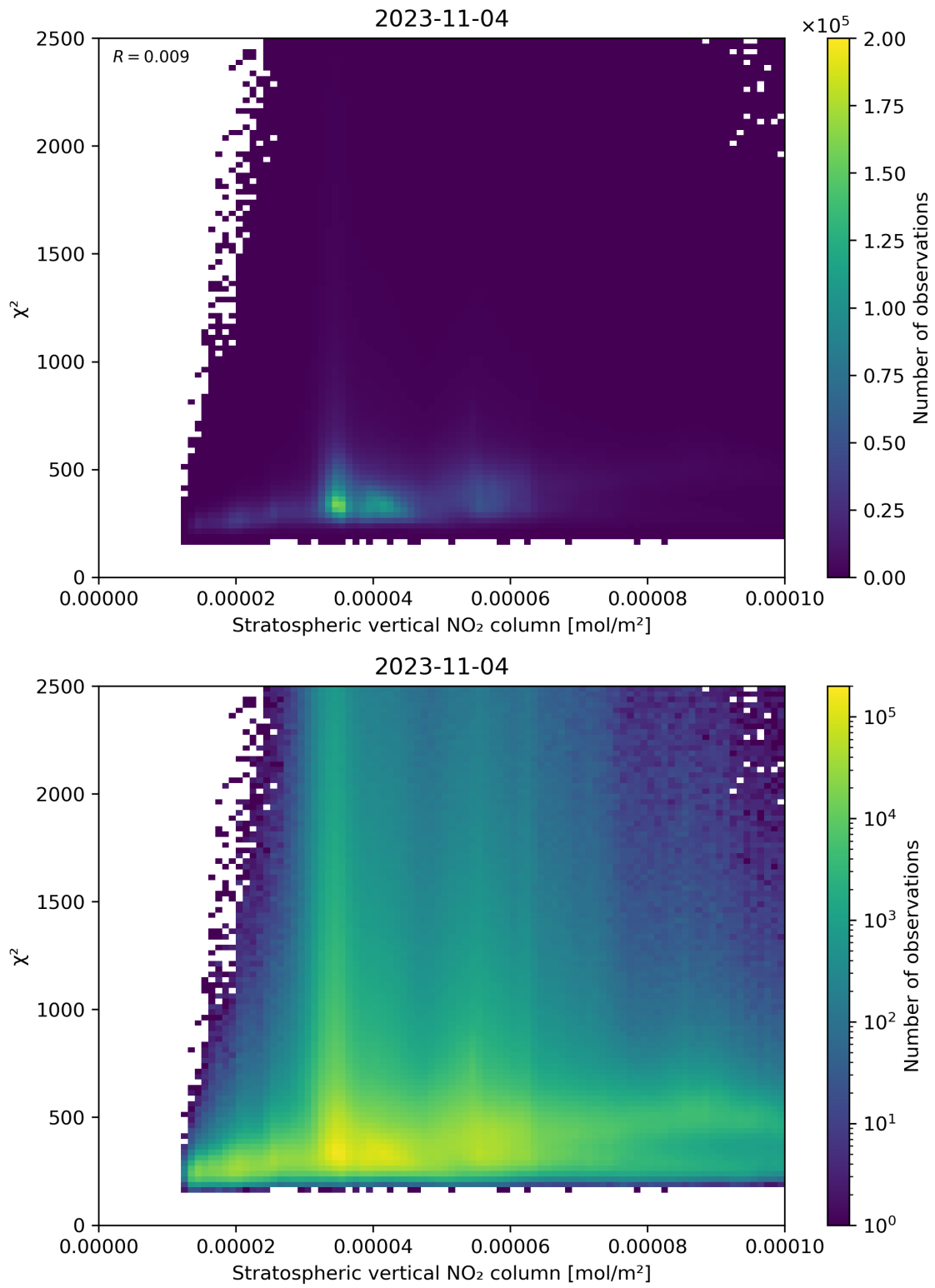
Figure 97: Scatter density plot of “Stratospheric vertical NO 2 column” against “ \chi^2 ” for 2023-11-03 to 2023-11-05.
