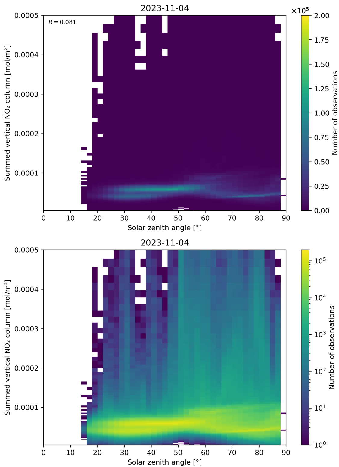
Figure 151: Scatter density plot of “Solar zenith angle” against “Summed vertical NO 2 column” for 2023-11-03 to 2023-11-05.
