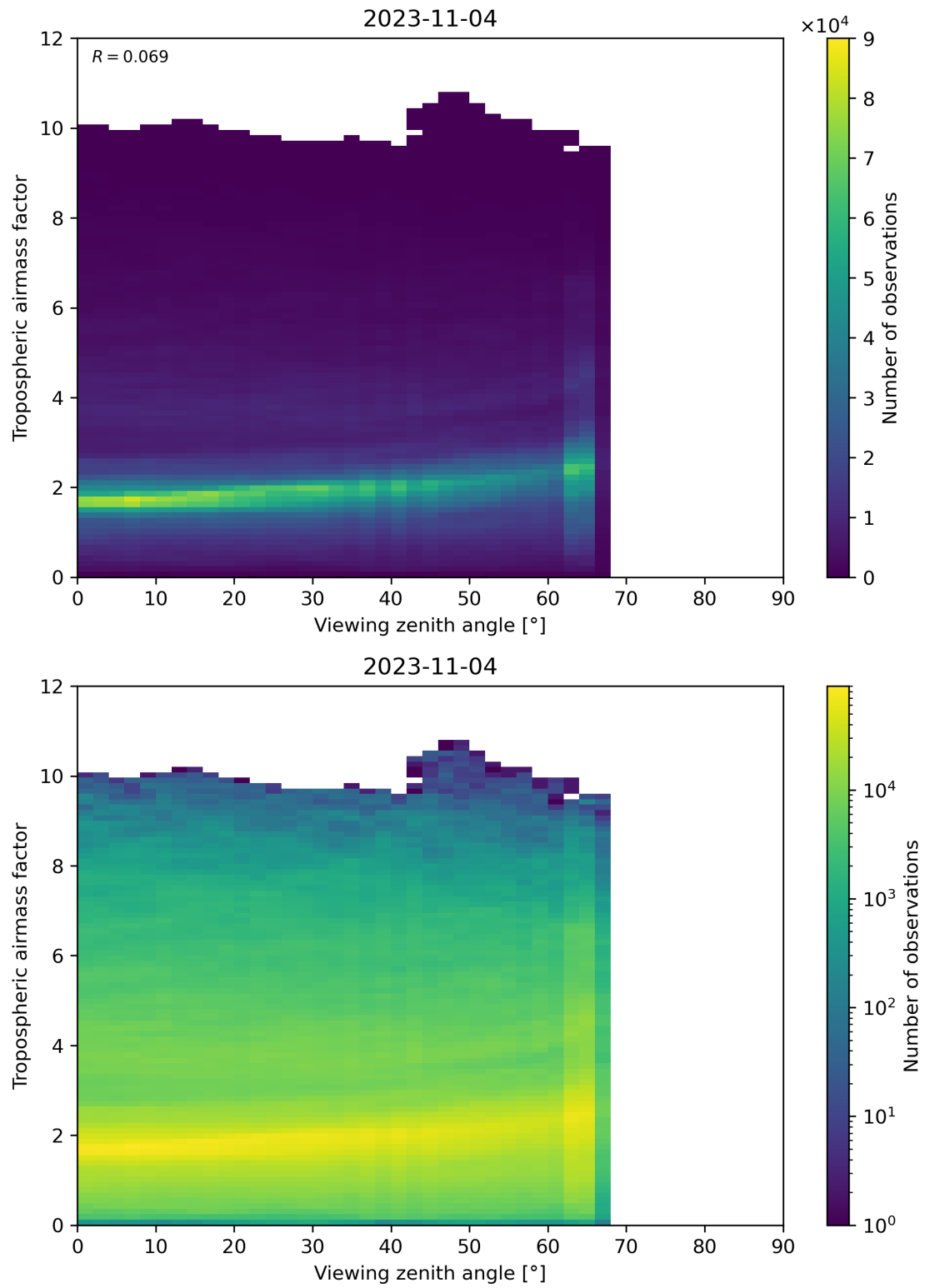
Figure 161: Scatter density plot of “Viewing zenith angle” against “Tropospheric airmass factor” for 2023-11-03 to 2023-11-05.
