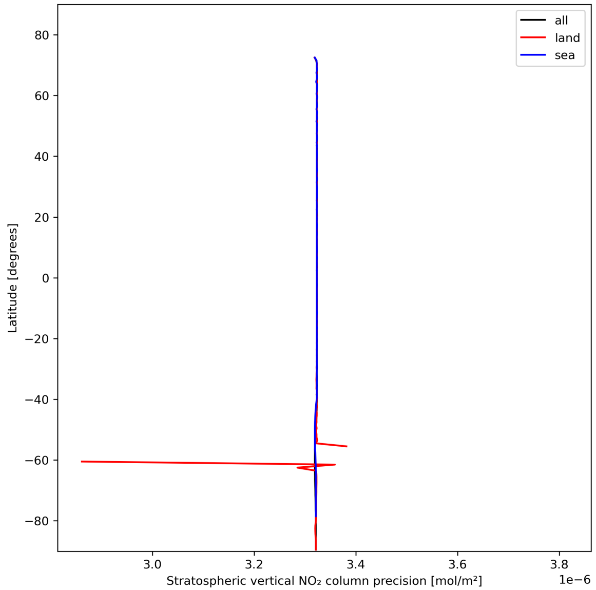
Figure 20: Zonal average of “Stratospheric vertical NO 2 column precision” for 2023-11-03 to 2023-11-05.
