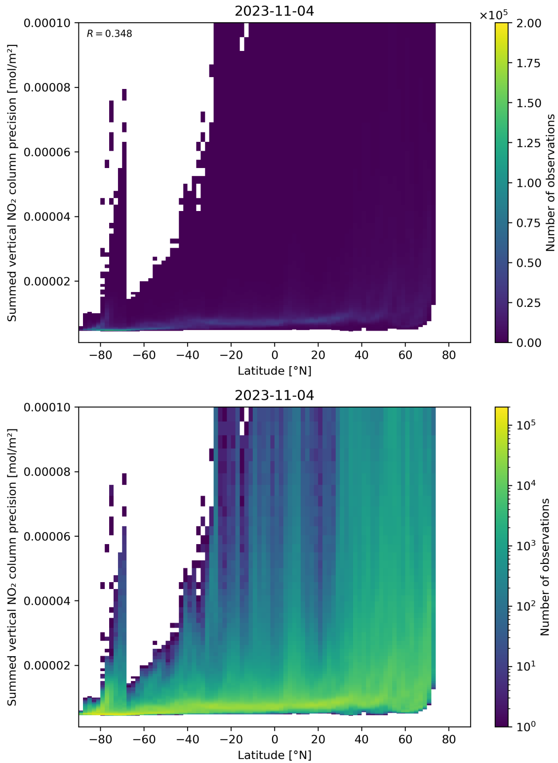
Figure 89: Scatter density plot of “Latitude” against “Summed vertical NO 2 column precision” for 2023-11-03 to 2023-11-05.
