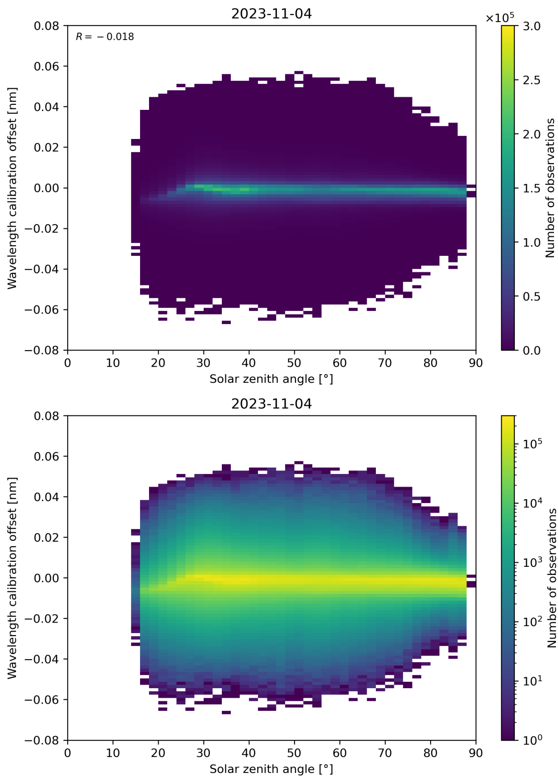
Figure 158: Scatter density plot of “Solar zenith angle” against “Wavelength calibration offset” for 2023-11-03 to 2023-11-05.
