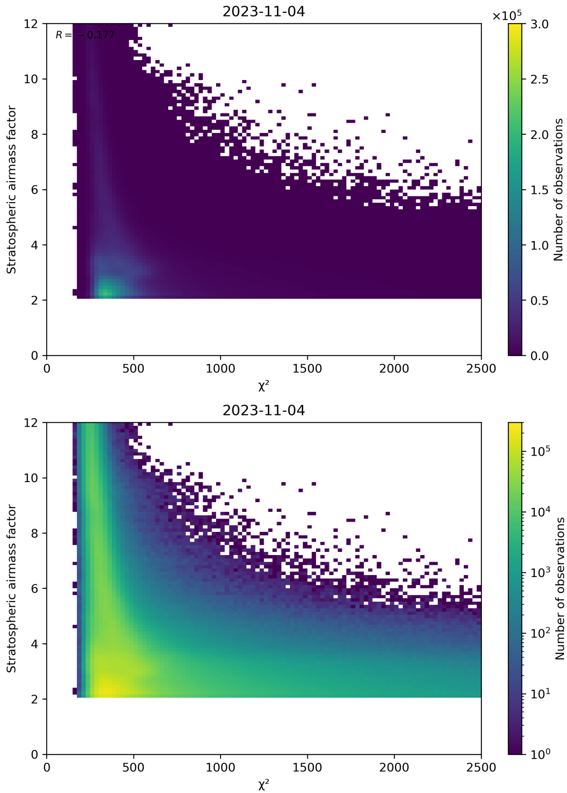
Figure 81: Scatter density plot of “ \chi^2 ” against “Stratospheric airmass factor” for 2023-11-03 to 2023-11-05.
