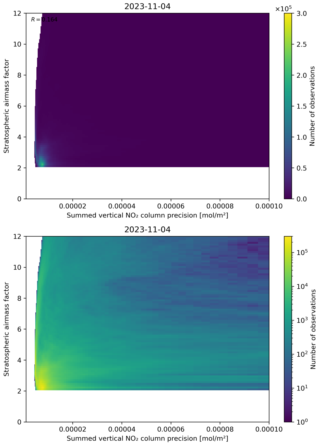
Figure 106: Scatter density plot of “Summed vertical NO 2 column precision” against “Stratospheric airmass factor” for 2023-11-03 to 2023-11-05.
