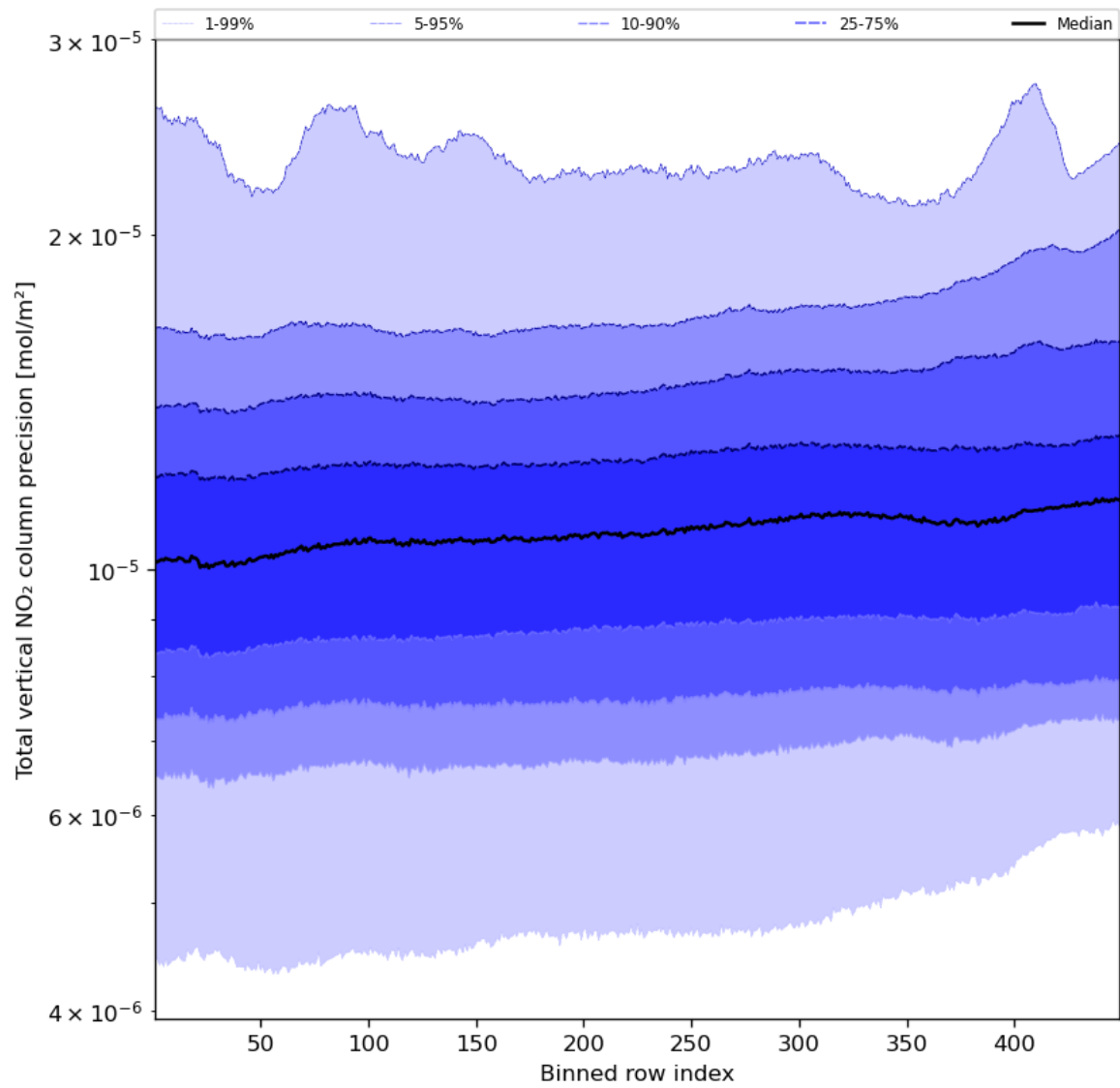
Figure 56: Along track statistics of “Total vertical NO 2 column precision” for 2023-11-03 to 2023-11-05
