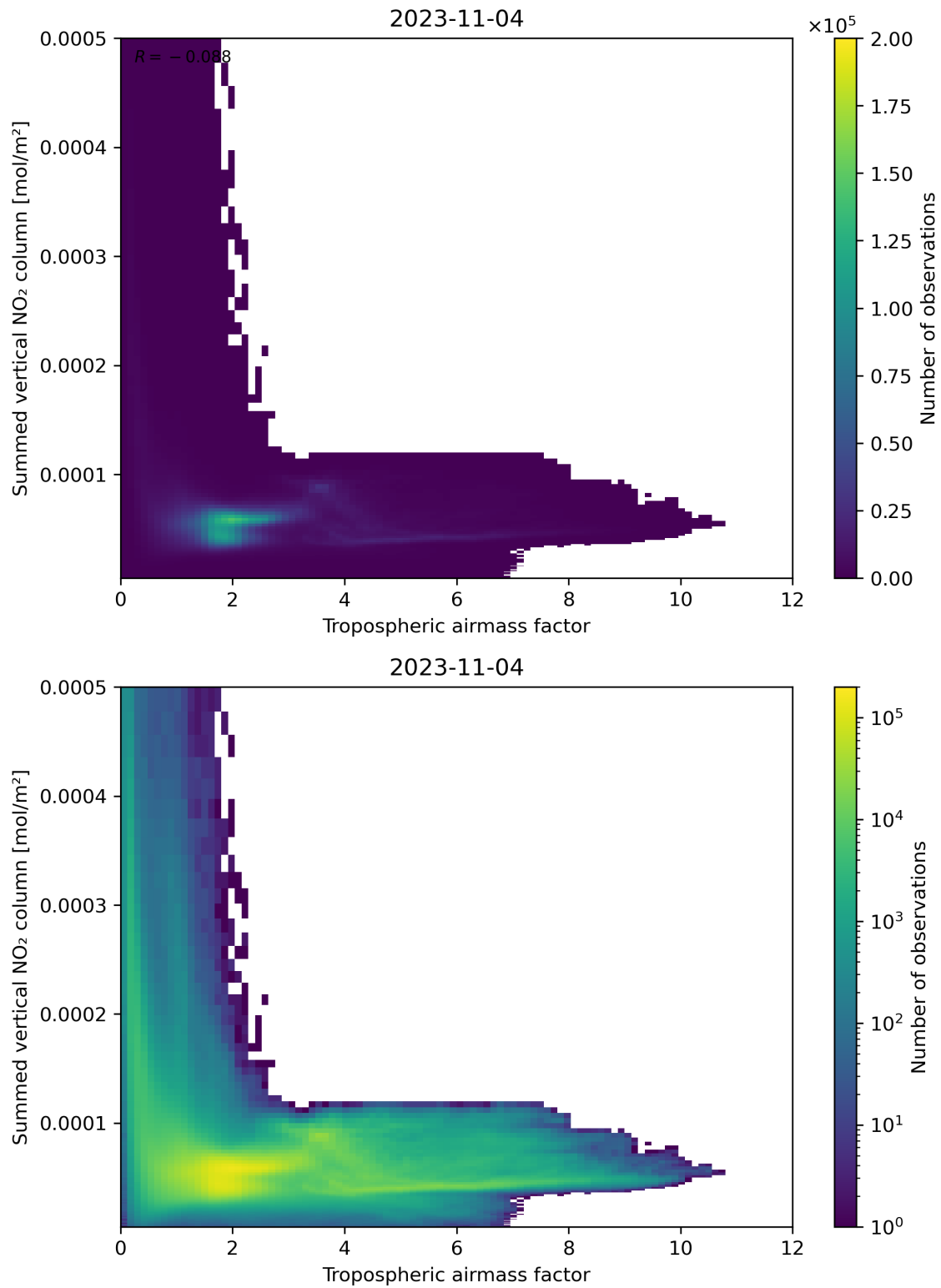
Figure 75: Scatter density plot of “Tropospheric airmass factor” against “Summed vertical NO 2 column” for 2023-11-03 to 2023-11-05.
