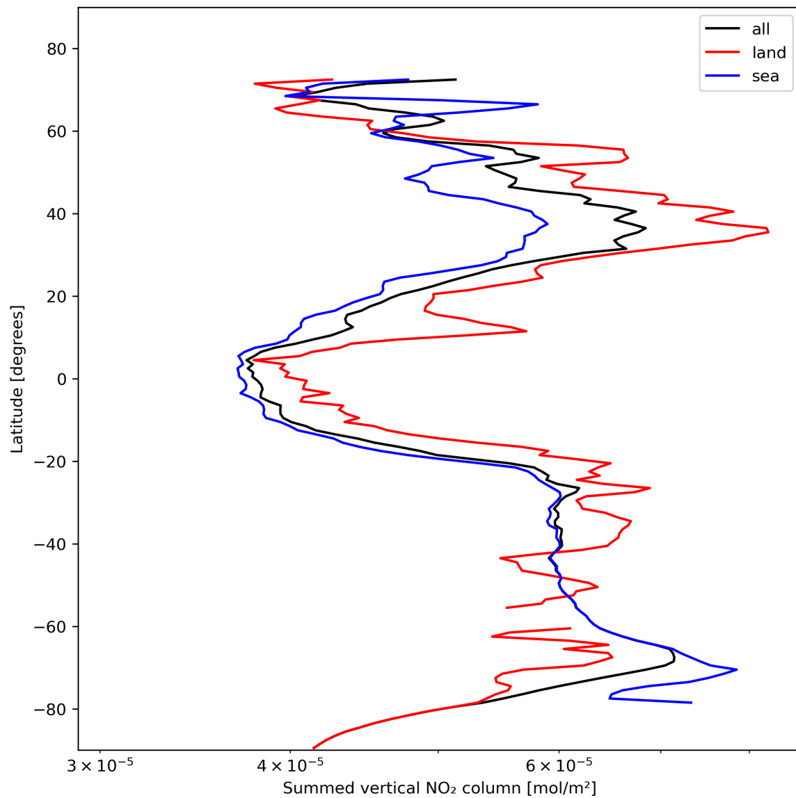
Figure 23: Zonal average of “Summed vertical NO 2 column” for 2023-11-03 to 2023-11-05.
