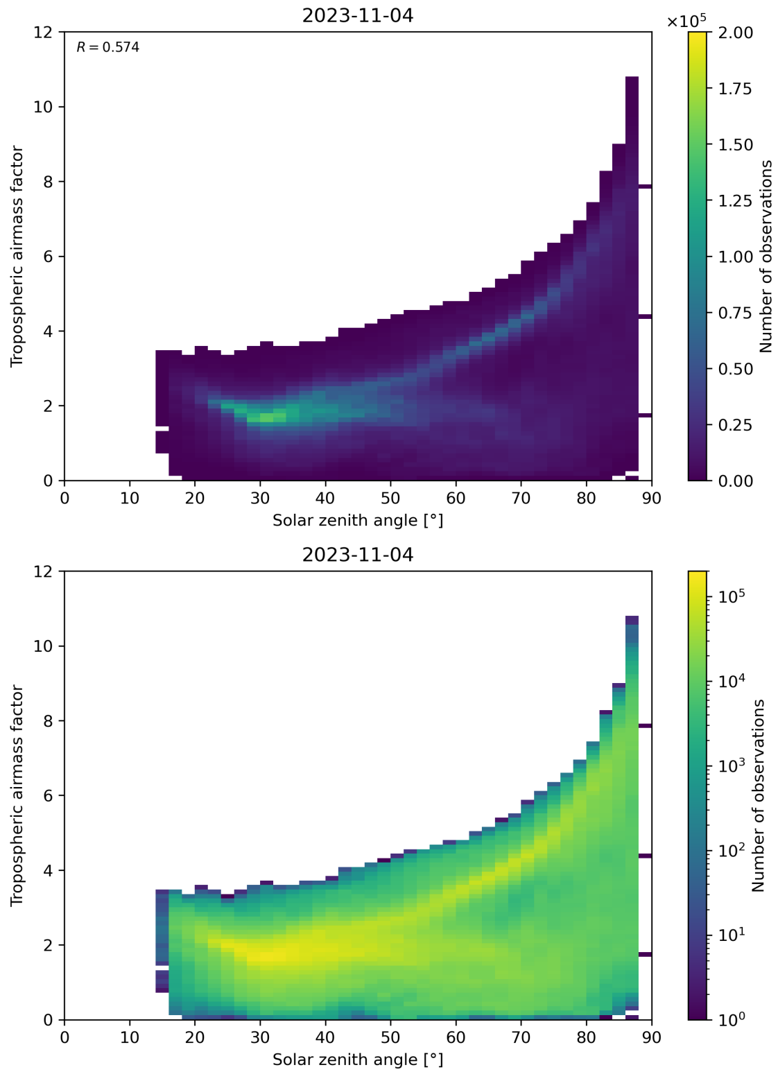
Figure 147: Scatter density plot of “Solar zenith angle” against “Tropospheric airmass factor” for 2023-11-03 to 2023-11-05.
