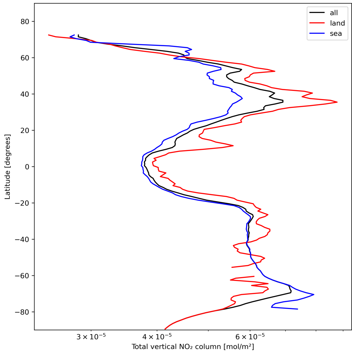
Figure 21: Zonal average of “Total vertical NO 2 column” for 2023-11-03 to 2023-11-05.
