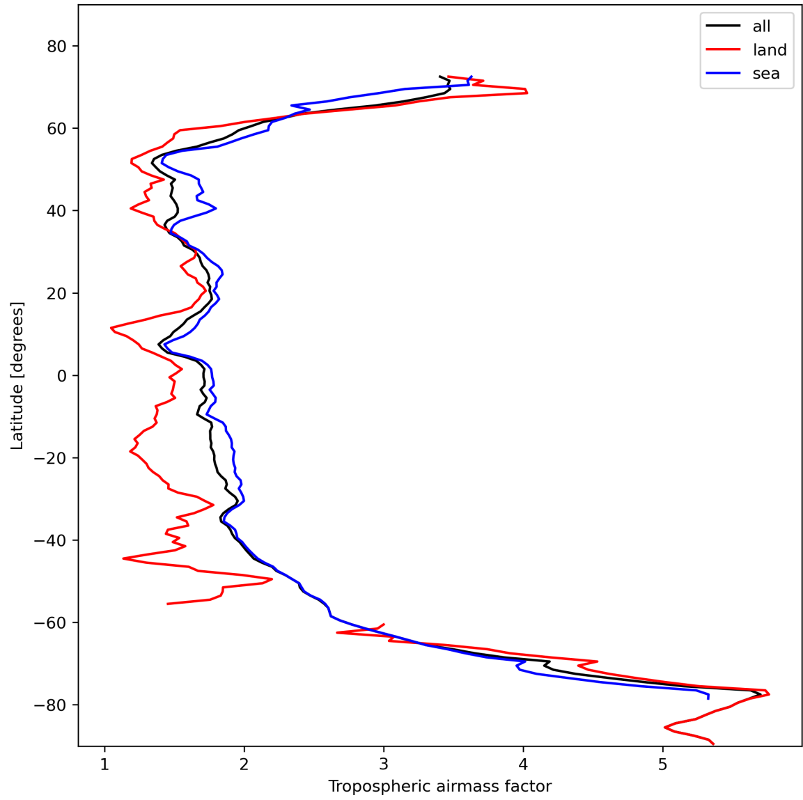
Figure 14: Zonal average of “Tropospheric airmass factor” for 2023-11-03 to 2023-11-05.
