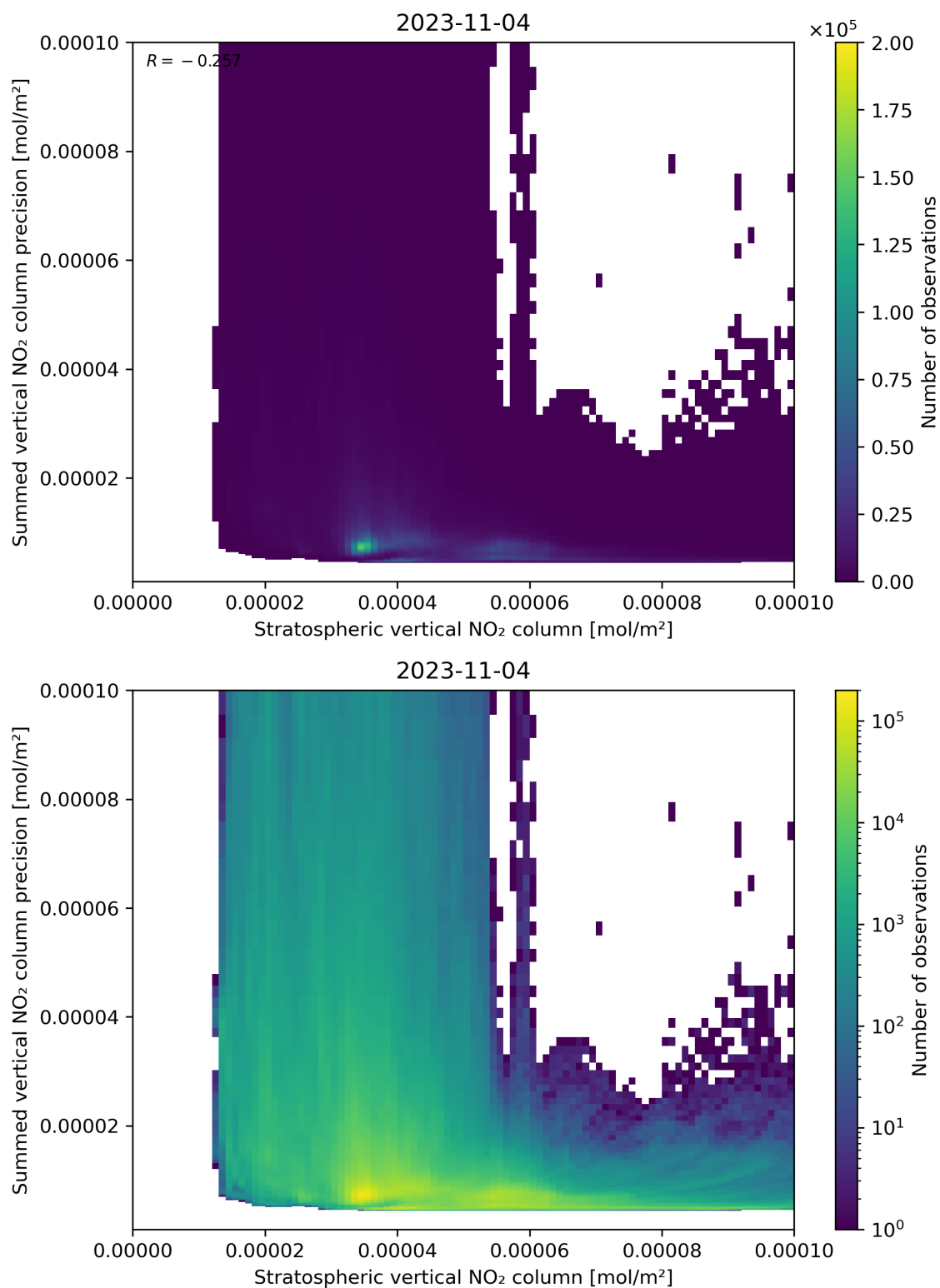
Figure 99: Scatter density plot of “Stratospheric vertical NO 2 column” against “Summed vertical NO 2 column precision” for 2023-11-03 to 2023-11-05.
