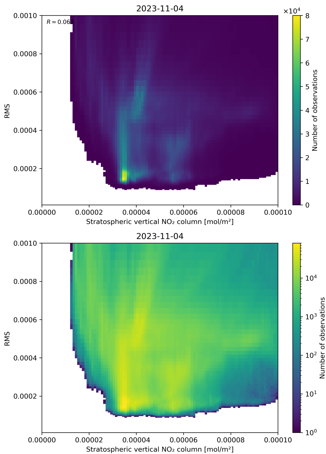
Figure 102: Scatter density plot of “Stratospheric vertical NO 2 column” against “RMS” for 2023-11-03 to 2023-11-05.
