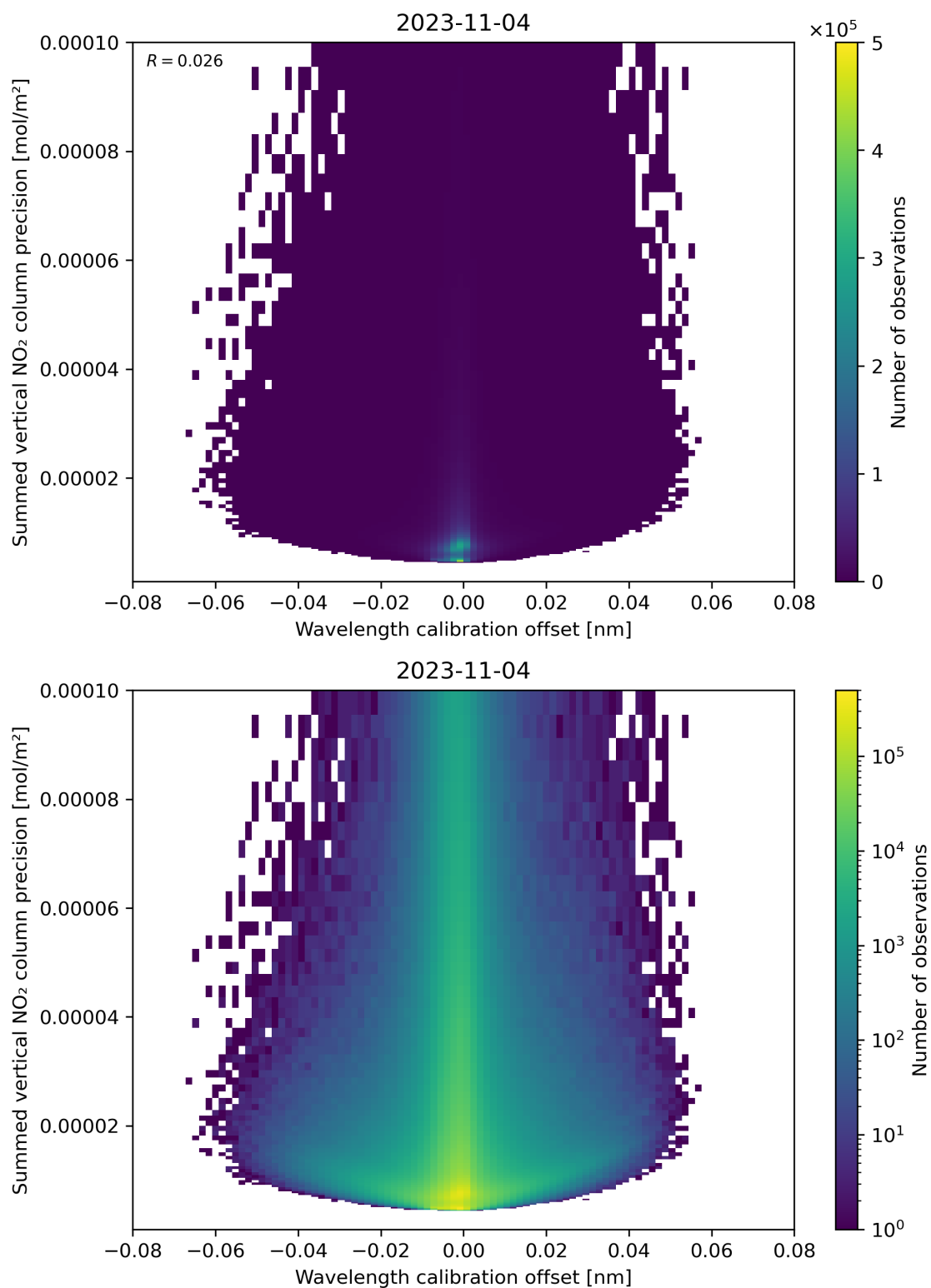
Figure 178: Scatter density plot of “Wavelength calibration offset” against “Summed vertical NO 2 column precision” for 2023-11-03 to 2023-11-05.
