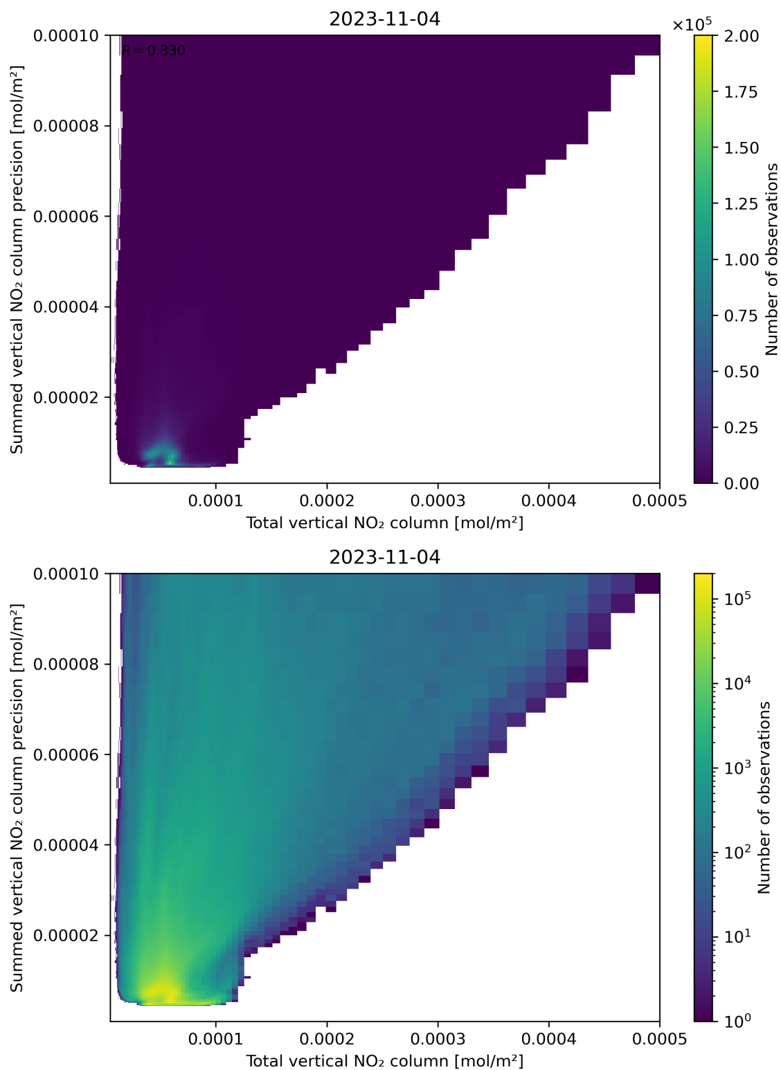
Figure 113: Scatter density plot of “Total vertical NO 2 column” against “Summed vertical NO 2 column precision” for 2023-11-03 to 2023-11-05.
