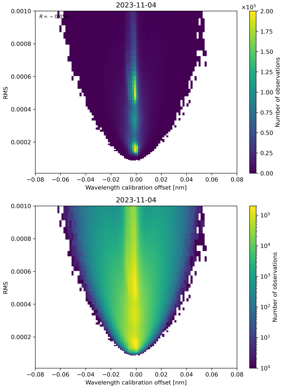
Figure 181: Scatter density plot of “Wavelength calibration offset” against “RMS” for 2023-11-03 to 2023-11-05.
