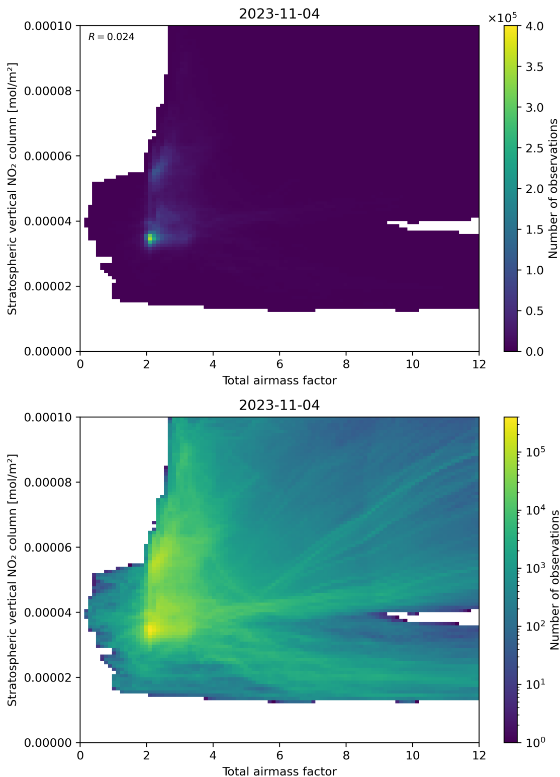
Figure 64: Scatter density plot of “Total airmass factor” against “Stratospheric vertical NO 2 column” for 2023-11-03 to 2023-11-05.
