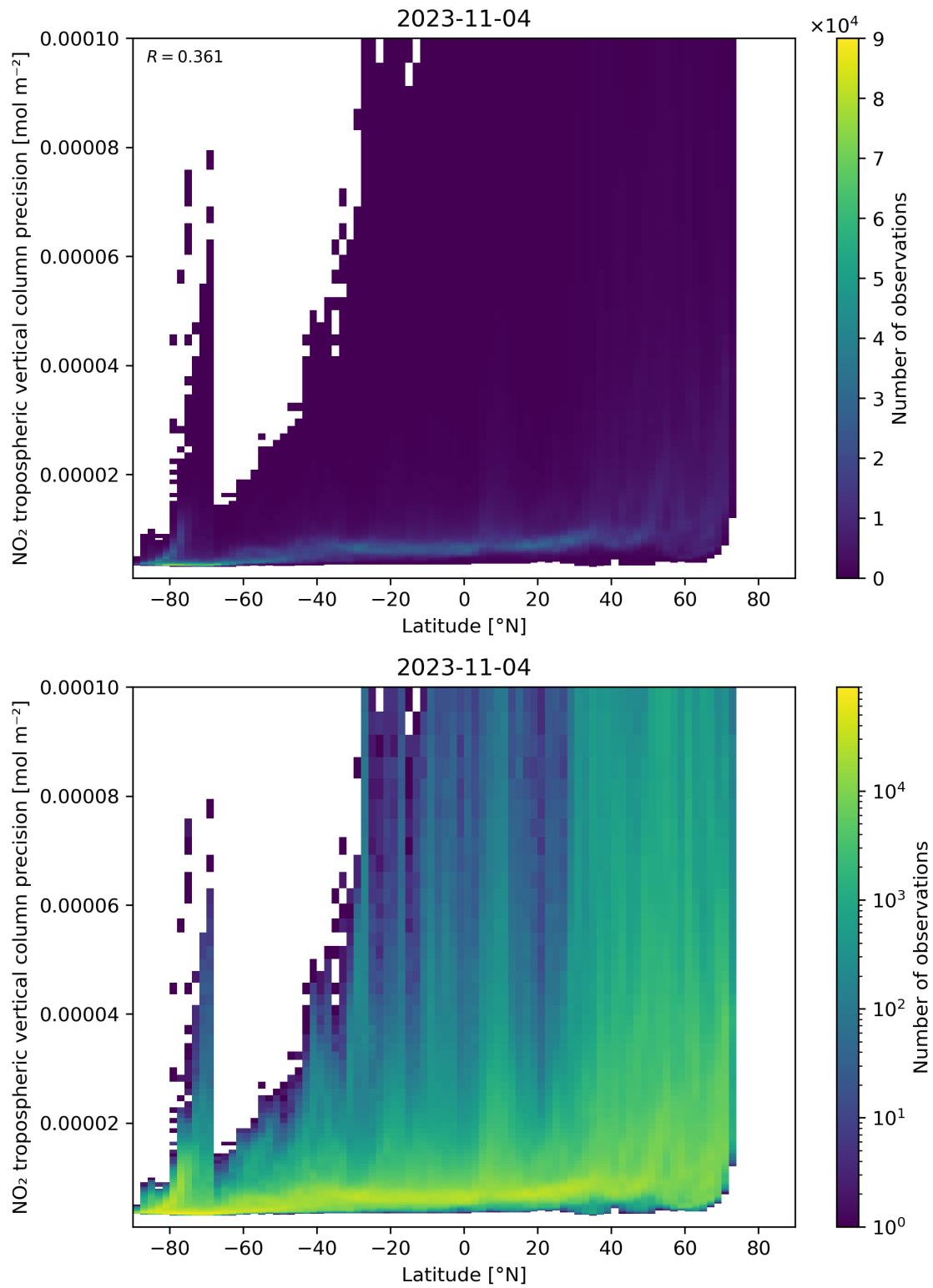
Figure 93: Scatter density plot of “Latitude” against “NO 2 tropospheric vertical column precision” for 2023-11-03 to 2023-11-05.
