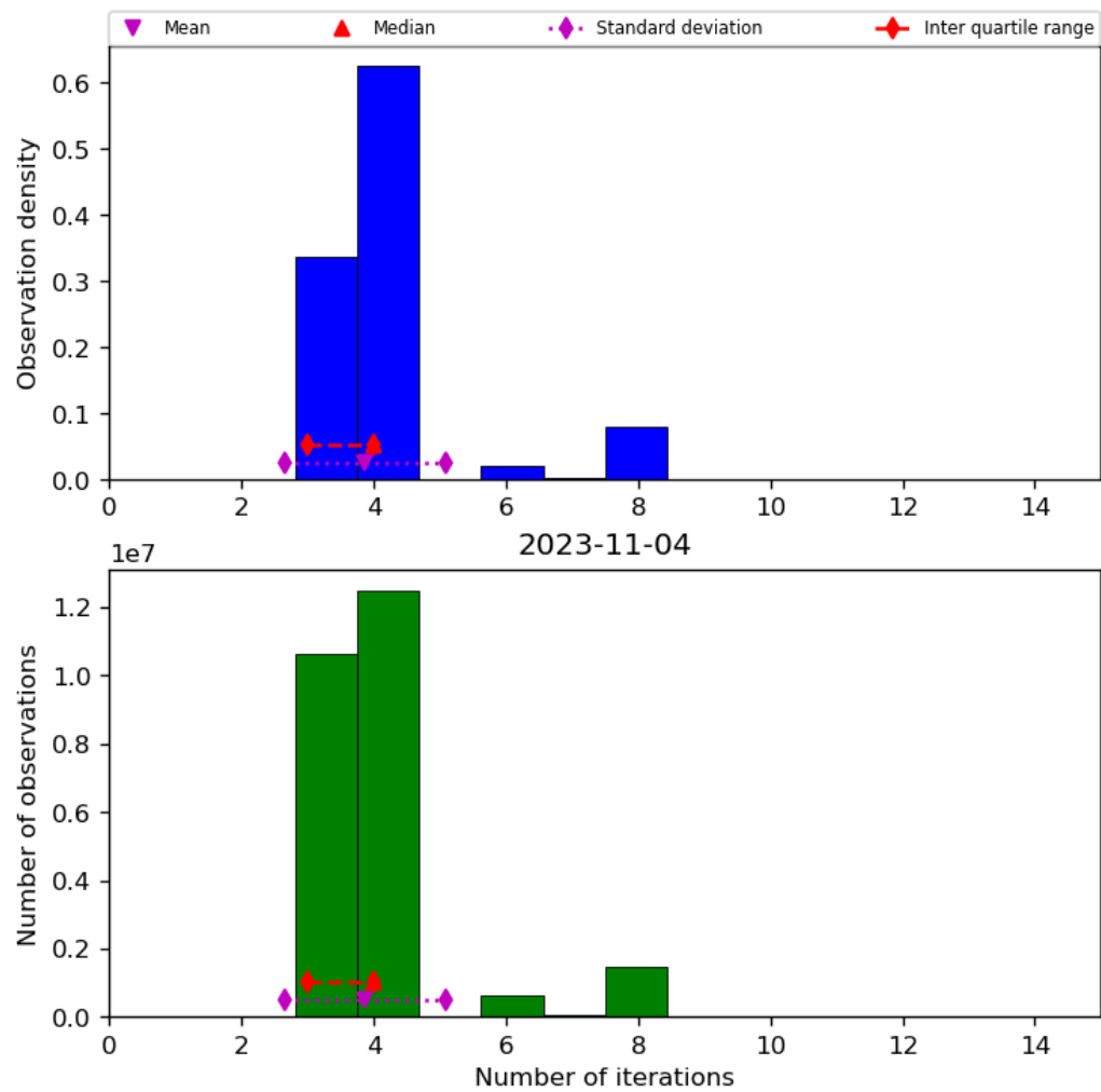
Figure 34: Histogram of “Number of iterations” for 2023-11-03 to 2023-11-05
