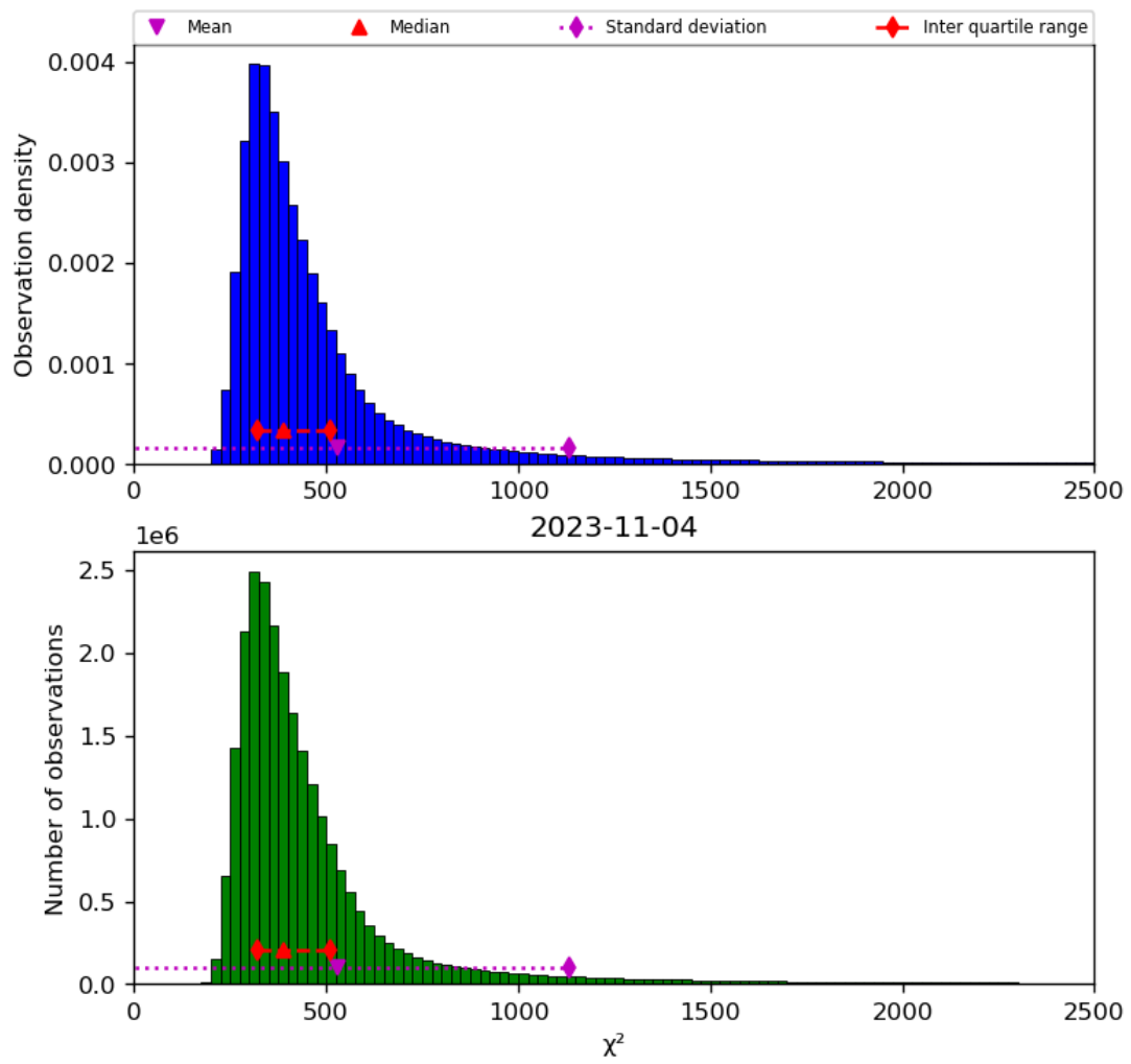
Figure 42: Histogram of “ \chi^2 ” for 2023-11-03 to 2023-11-05
