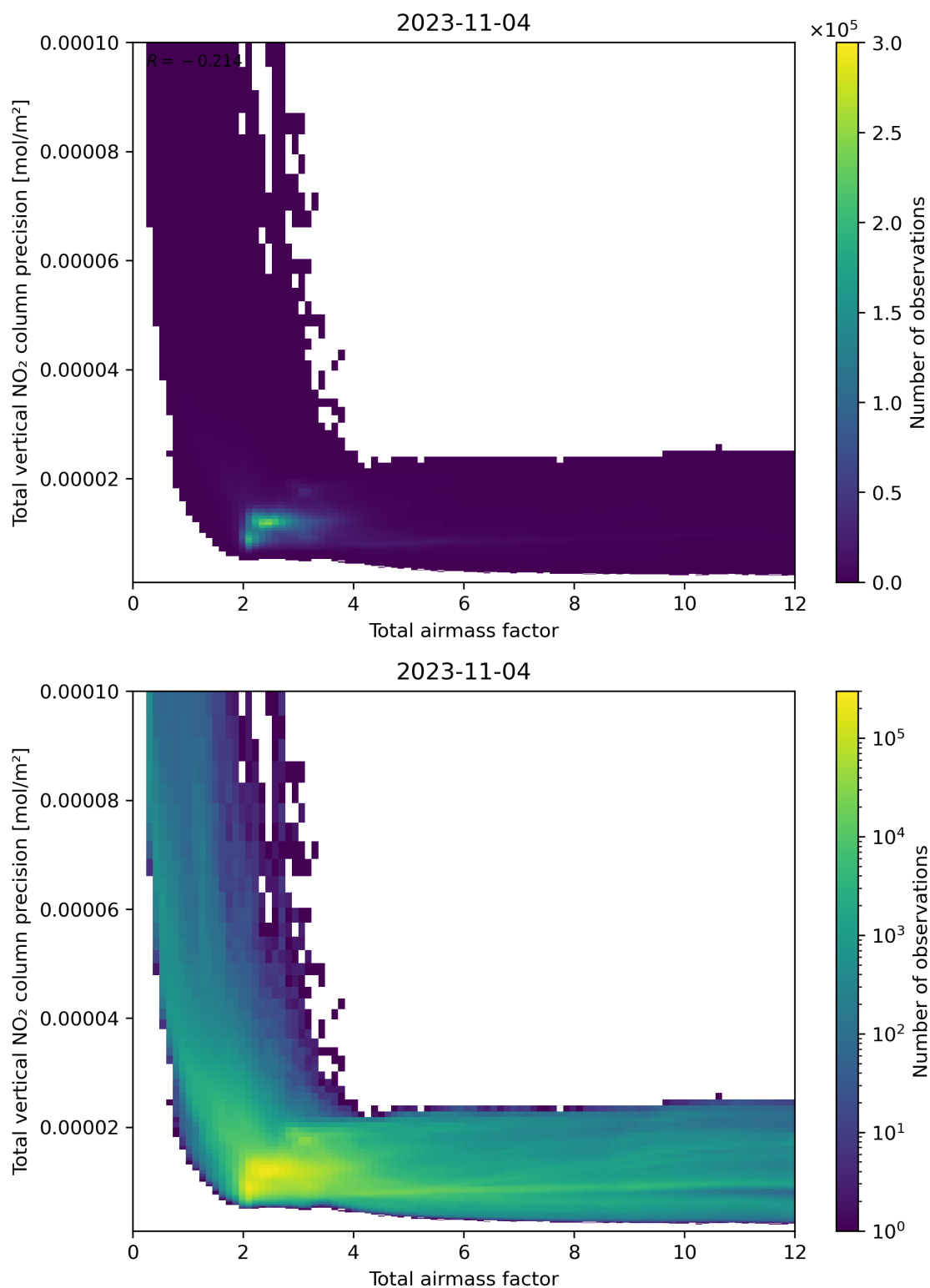
Figure 68: Scatter density plot of “Total airmass factor” against “Total vertical NO 2 column precision” for 2023-11-03 to 2023-11-05.
