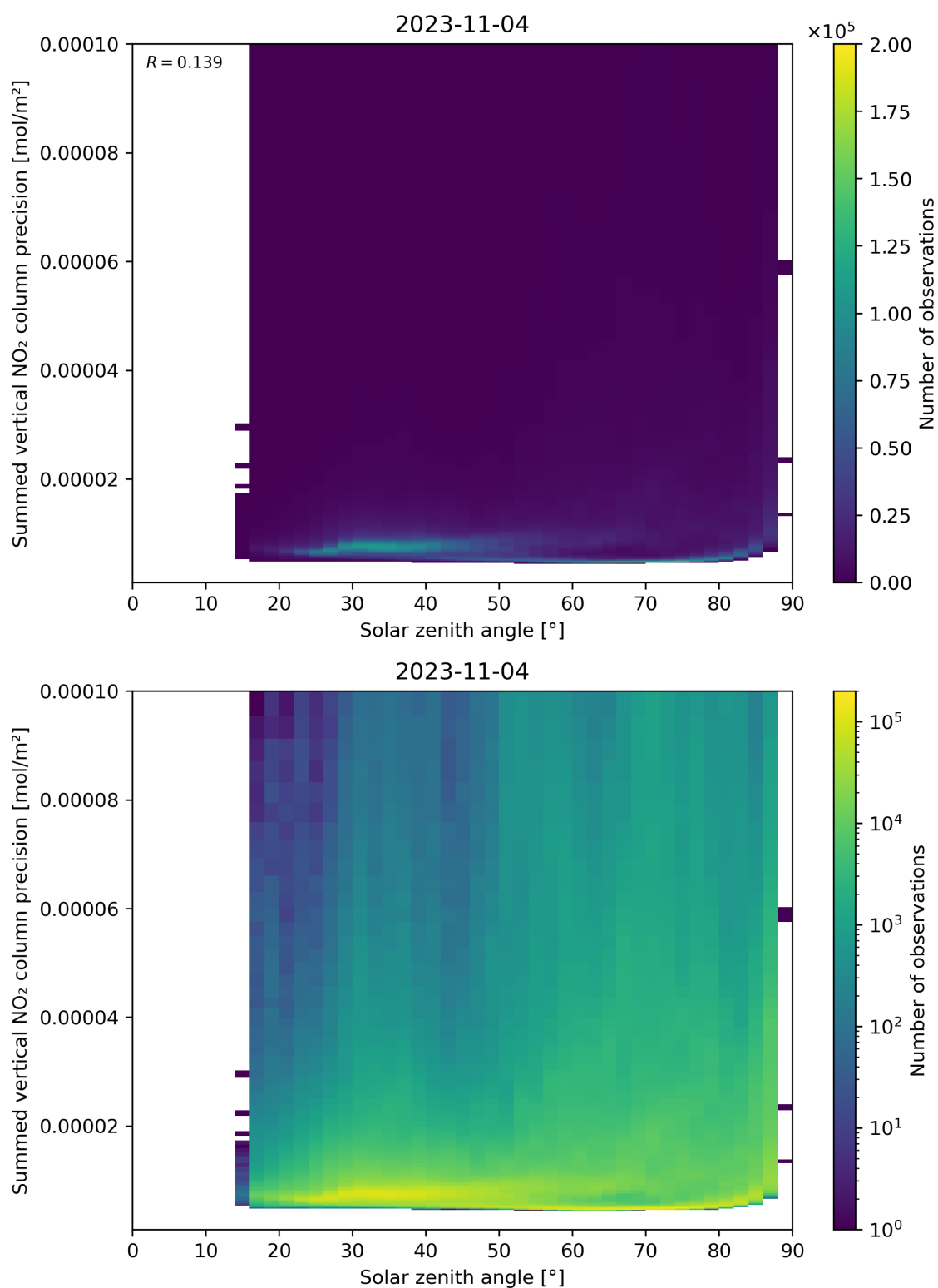
Figure 152: Scatter density plot of “Solar zenith angle” against “Summed vertical NO 2 column precision” for 2023-11-03 to 2023-11-05.
