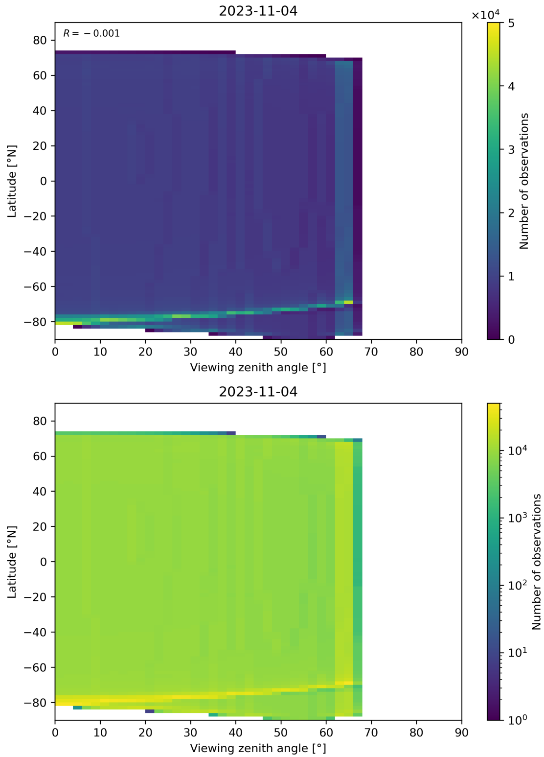
Figure 163: Scatter density plot of “Viewing zenith angle” against “Latitude” for 2023-11-03 to 2023-11-05.
