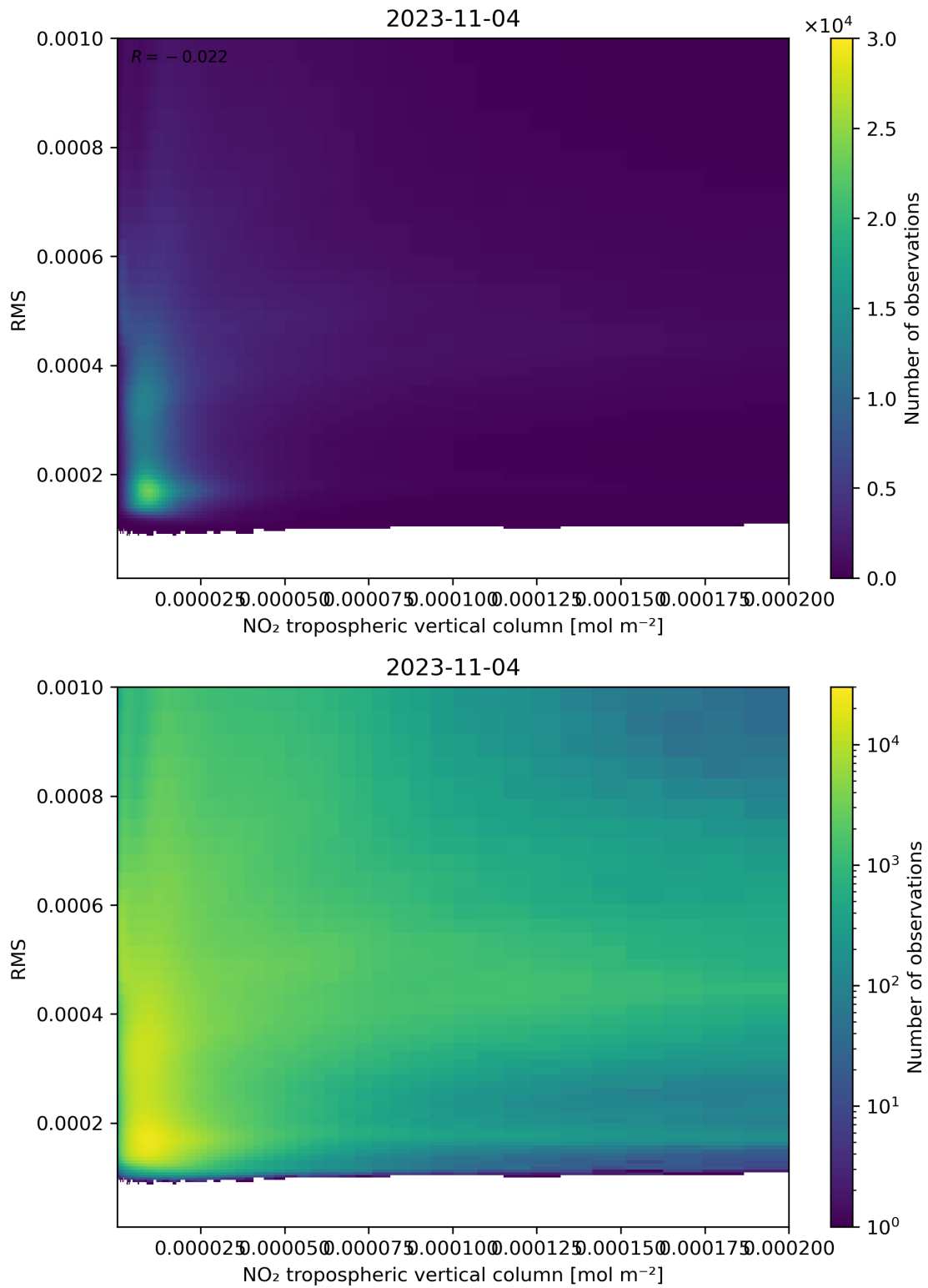
Figure 142: Scatter density plot of “NO 2 tropospheric vertical column” against “RMS” for 2023-11-03 to 2023-11-05.
