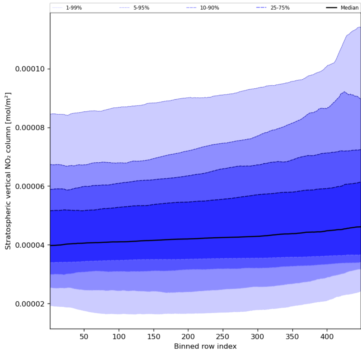
Figure 53: Along track statistics of “Stratospheric vertical NO 2 column” for 2023-11-03 to 2023-11-05
