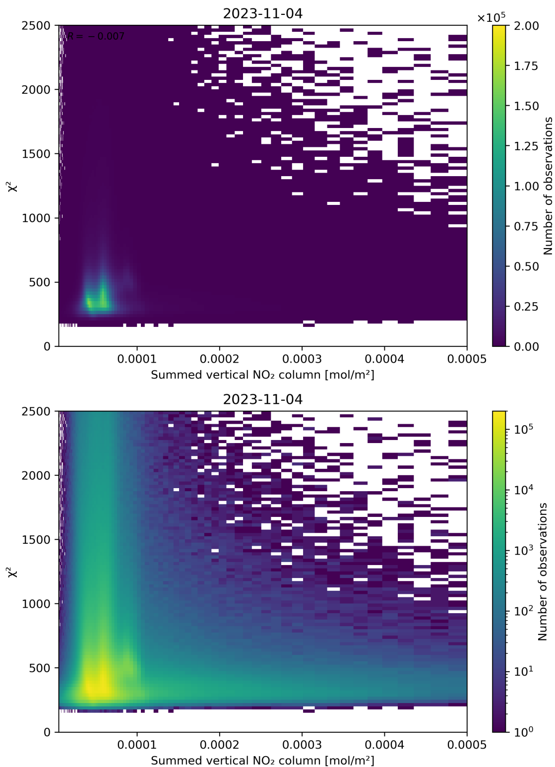
Figure 104: Scatter density plot of “Summed vertical NO 2 column” against “ \chi^2 ” for 2023-11-03 to 2023-11-05.
