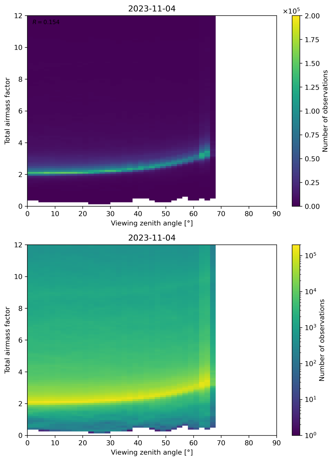
Figure 160: Scatter density plot of “Viewing zenith angle” against “Total airmass factor” for 2023-11-03 to 2023-11-05.
