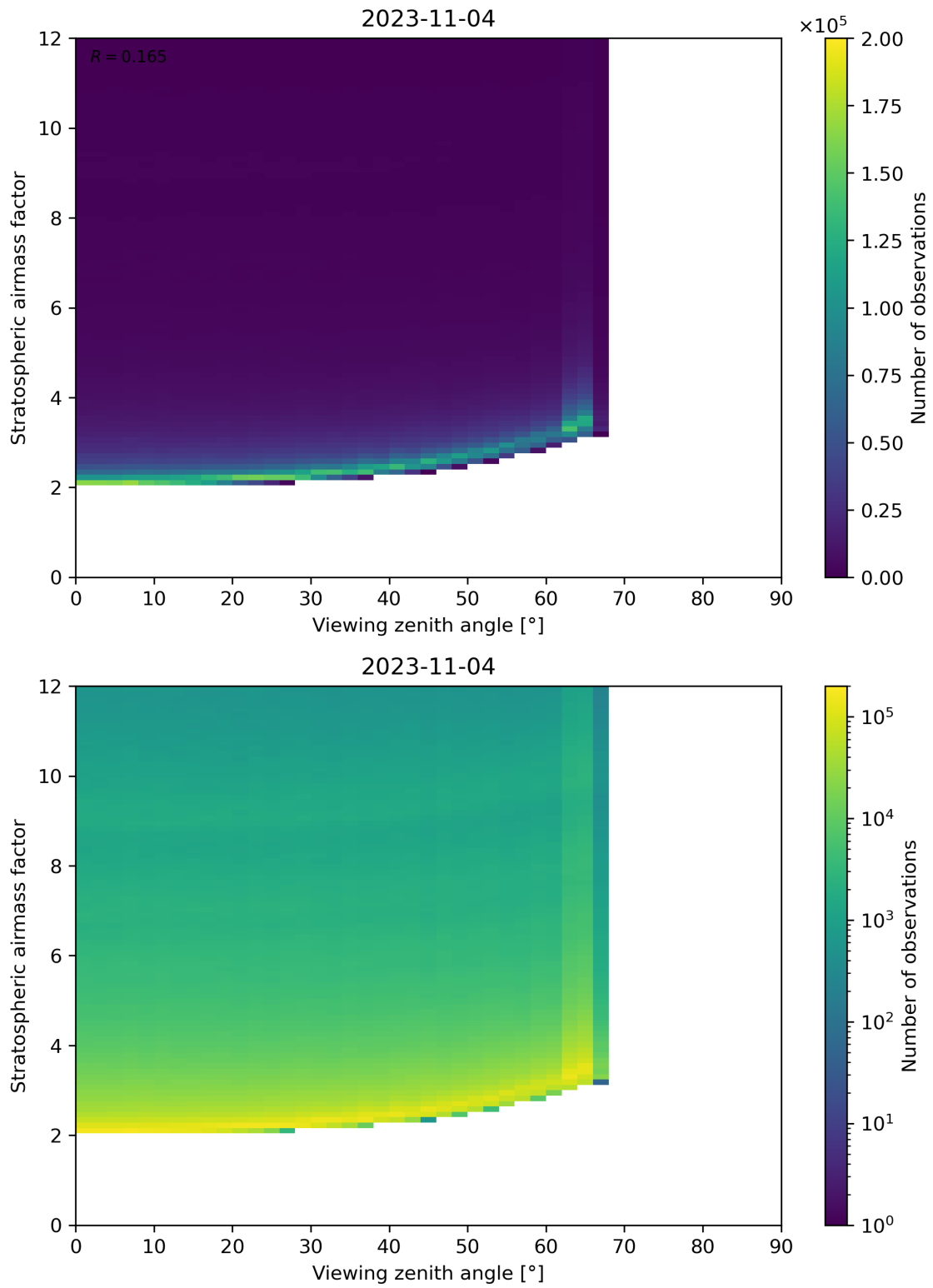
Figure 159: Scatter density plot of “Viewing zenith angle” against “Stratospheric airmass factor” for 2023-11-03 to 2023-11-05.
