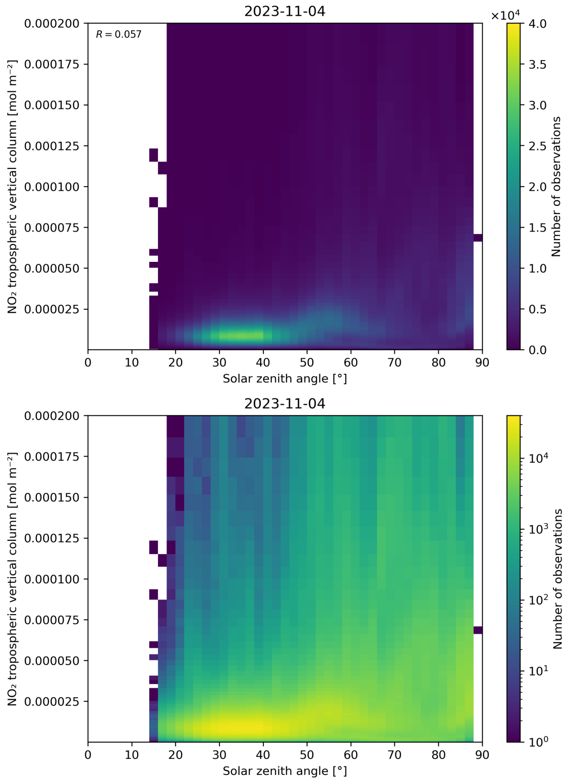
Figure 155: Scatter density plot of “Solar zenith angle” against “NO 2 tropospheric vertical column” for 2023-11-03 to 2023-11-05.
