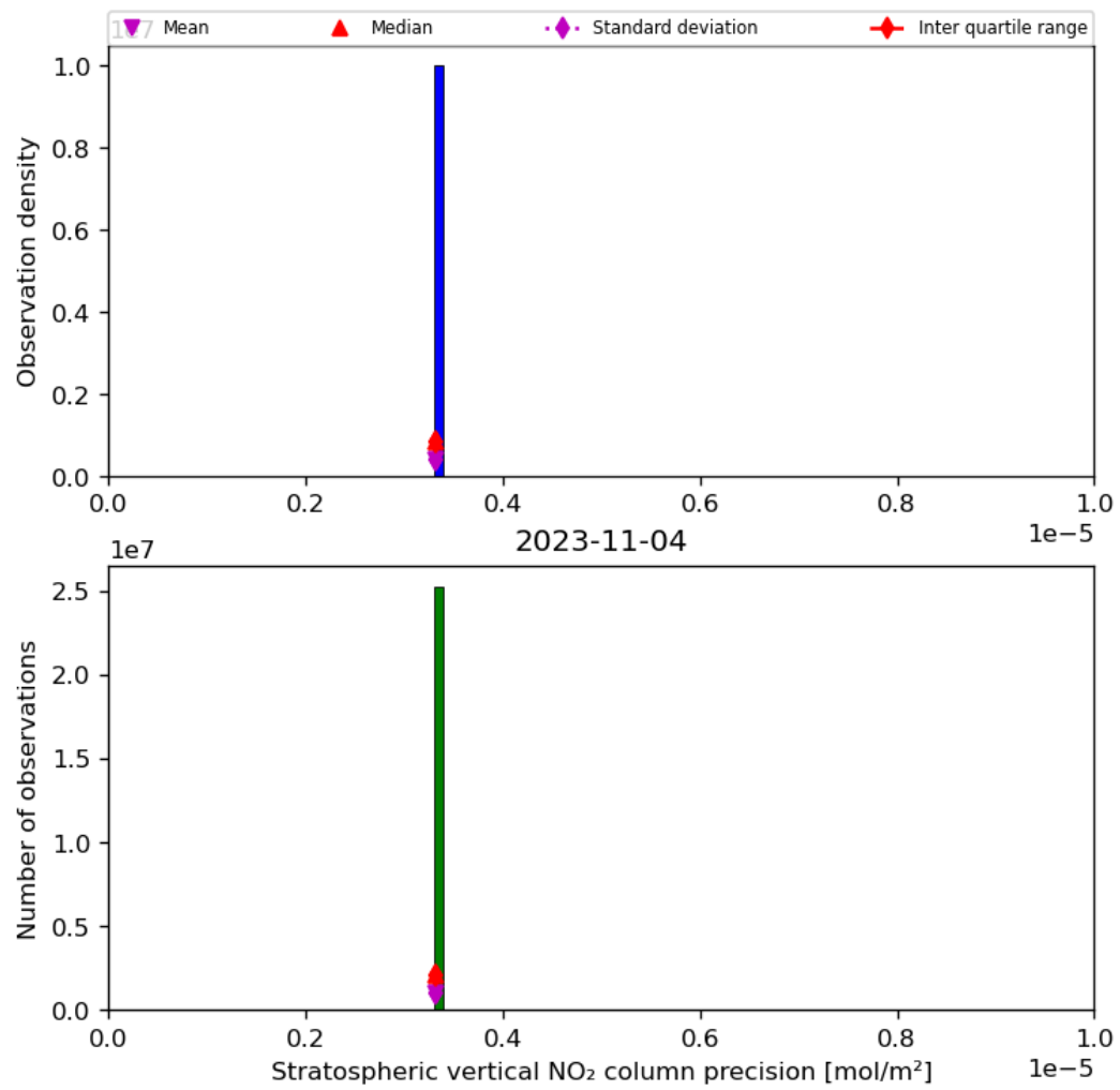
Figure 37: Histogram of “Stratospheric vertical NO 2 column precision” for 2023-11-03 to 2023-11-05
