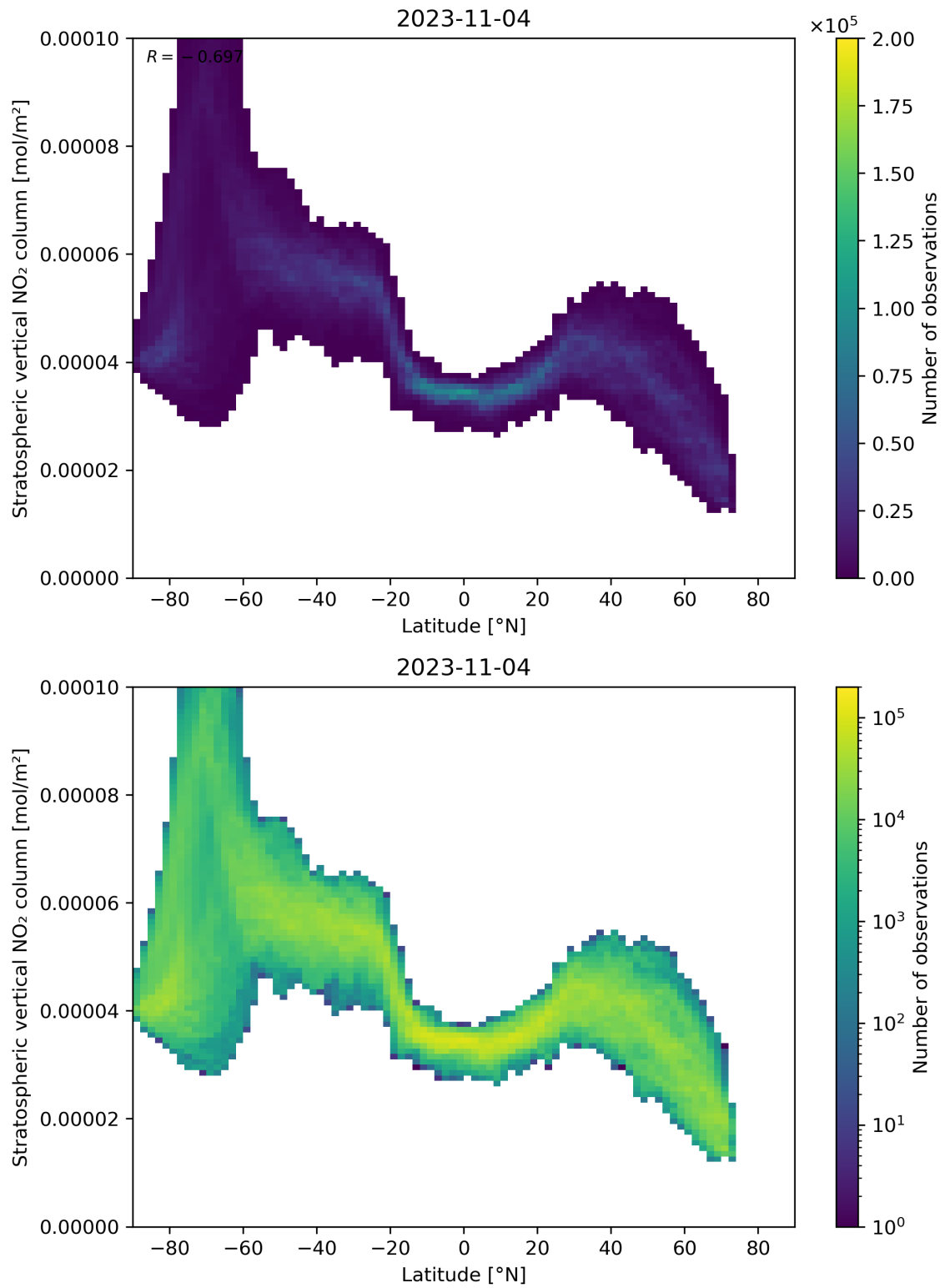
Figure 87: Scatter density plot of “Latitude” against “Stratospheric vertical NO 2 column” for 2023-11-03 to 2023-11-05.
