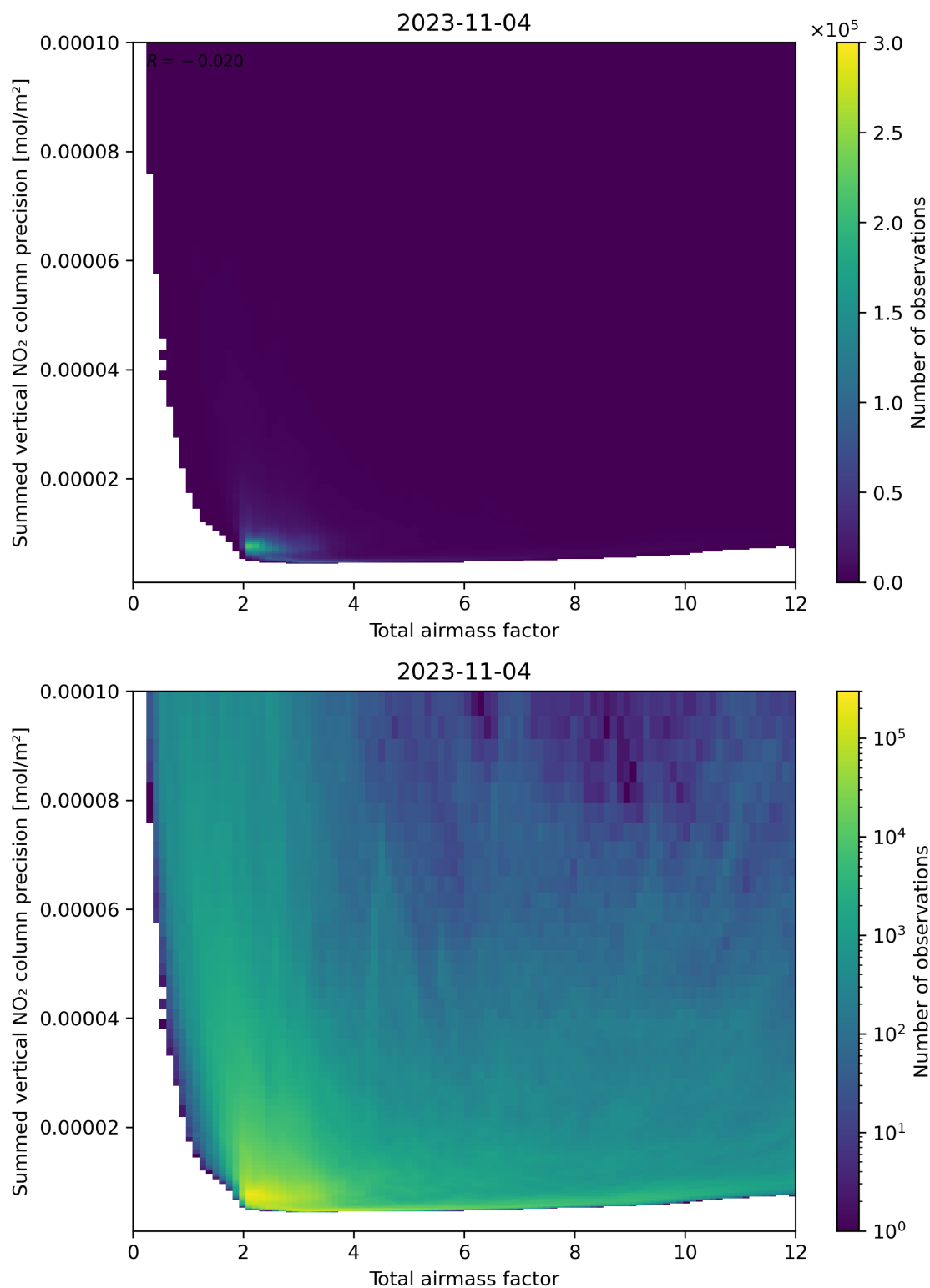
Figure 66: Scatter density plot of “Total airmass factor” against “Summed vertical NO 2 column precision” for 2023-11-03 to 2023-11-05.
