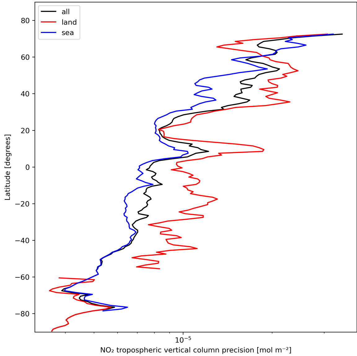
Figure 13: Zonal average of “NO 2 tropospheric vertical column precision” for 2023-11-03 to 2023-11-05.
