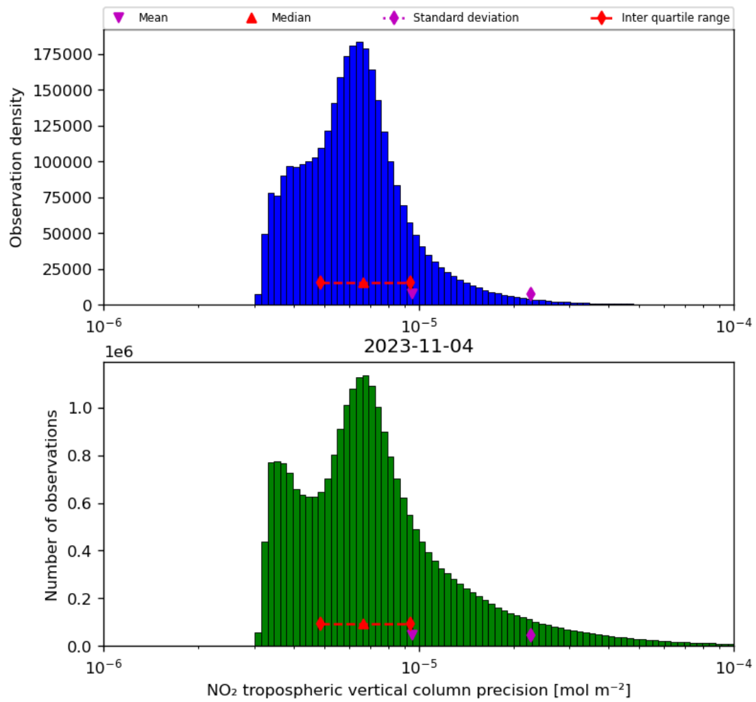
Figure 30: Histogram of “NO 2 tropospheric vertical column precision” for 2023-11-03 to 2023-11-05
