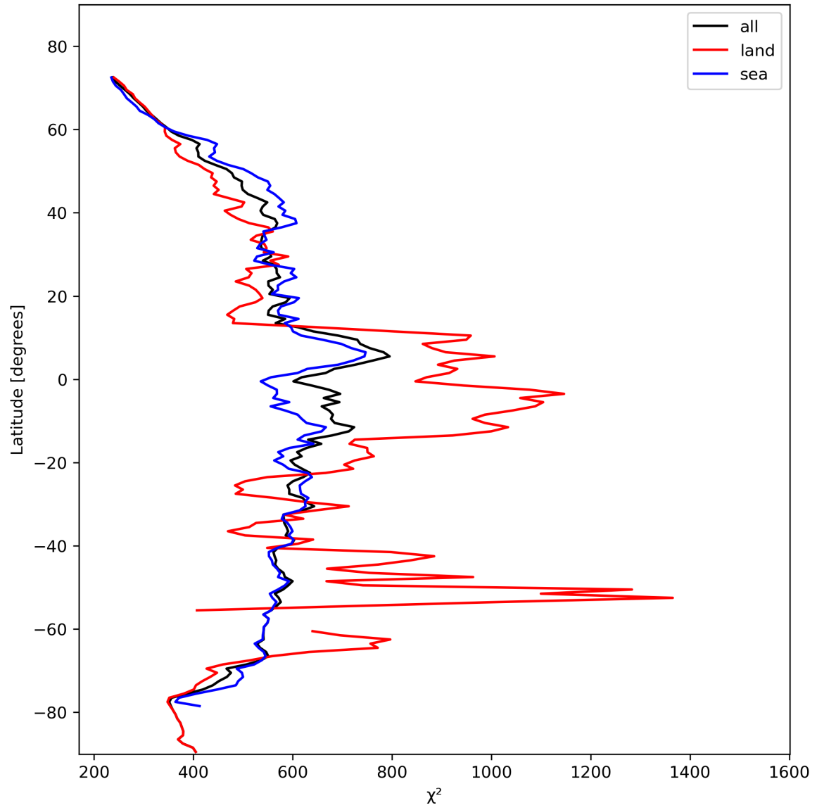
Figure 25: Zonal average of “ \chi^2 ” for 2023-11-03 to 2023-11-05.
