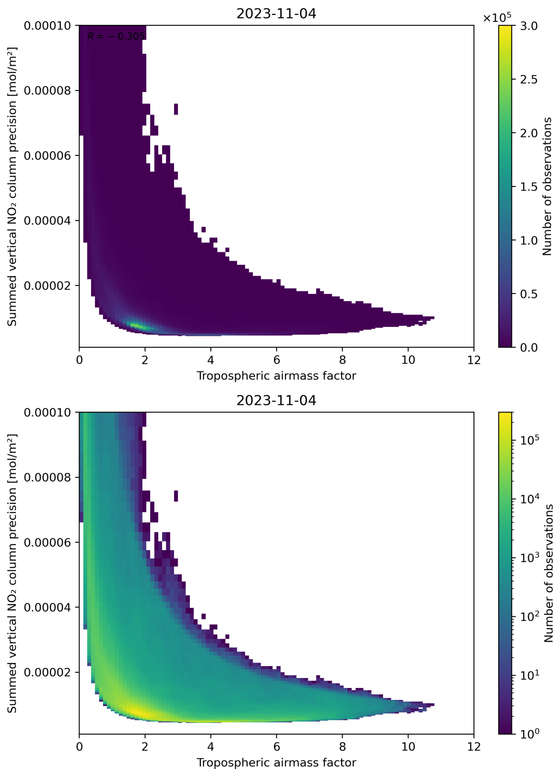
Figure 76: Scatter density plot of “Tropospheric air mass factor” against “Summed vertical NO 2 column precision” for 2023-11-03 to 2023-11-05.
