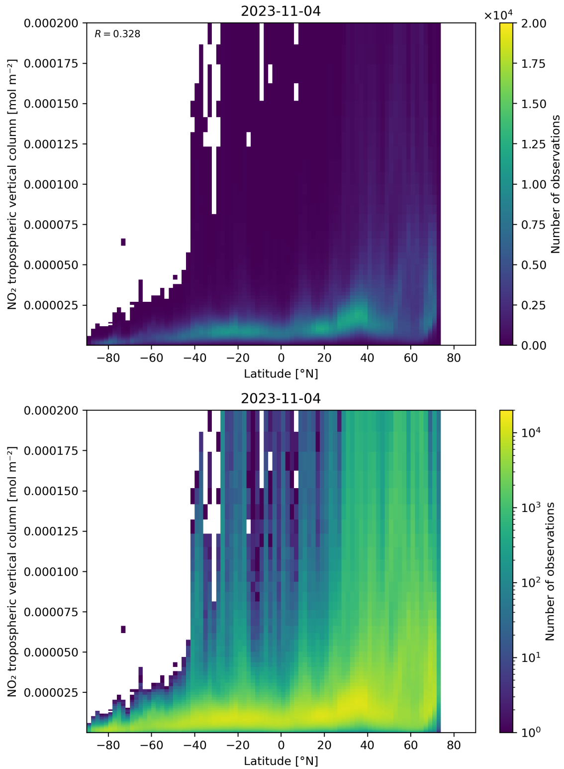
Figure 92: Scatter density plot of “Latitude” against “NO 2 tropospheric vertical column” for 2023-11-03 to 2023-11-05.
