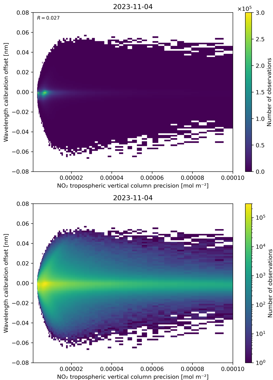
Figure 141: Scatter density plot of “NO 2 tropospheric vertical column precision” against “Wavelength calibration offset” for 2023-11-03 to 2023-11-05.
