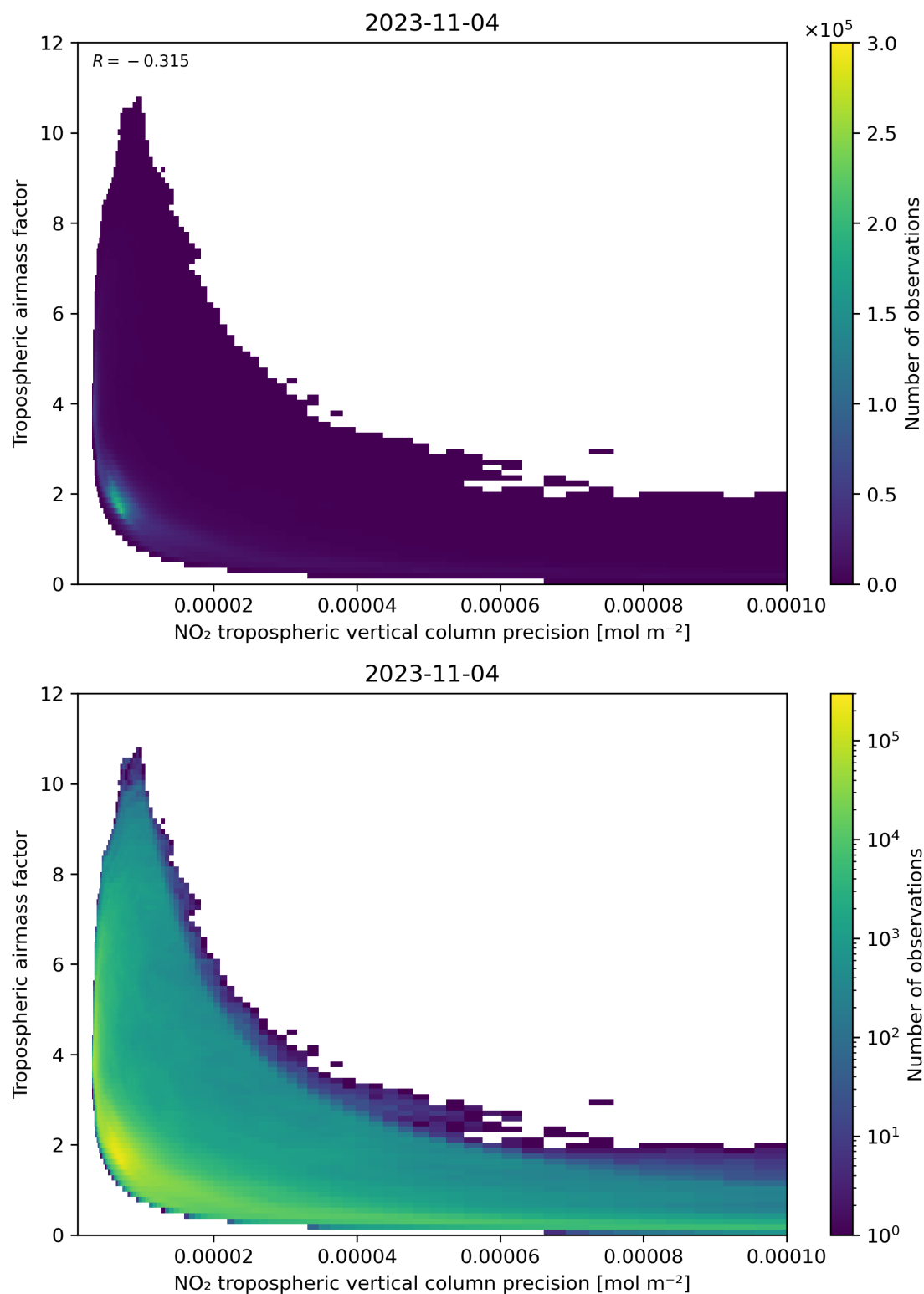
Figure 133: Scatter density plot of “NO 2 tropospheric vertical column precision” against “Tropospheric airmass factor” for 2023-11-03 to 2023-11-05.
