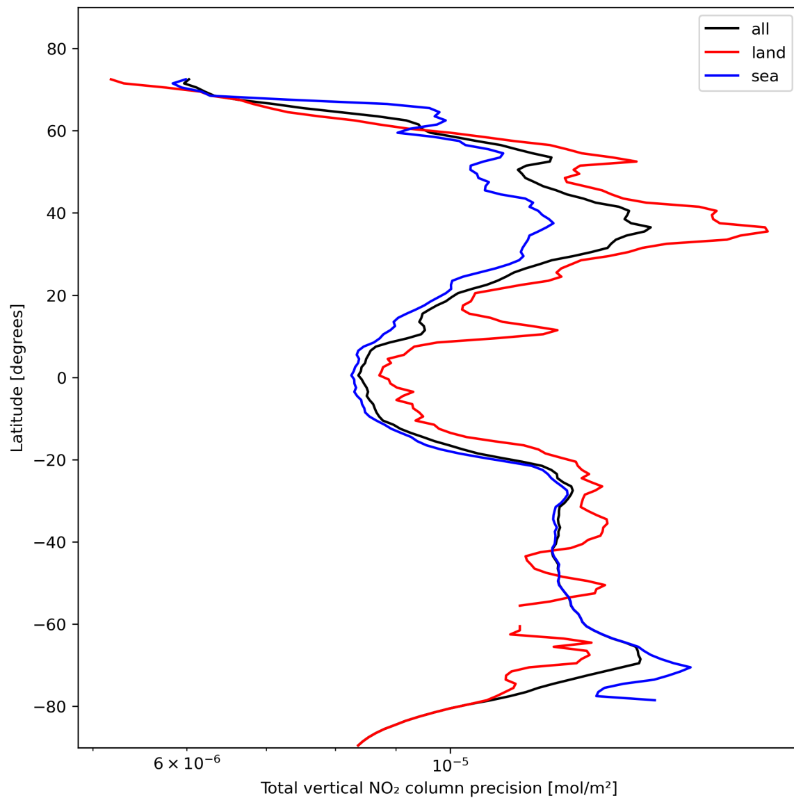
Figure 22: Zonal average of “Total vertical NO 2 column precision” for 2023-11-03 to 2023-11-05.
