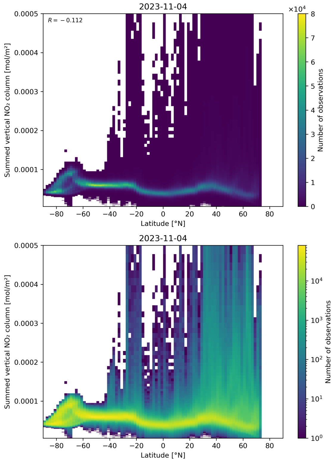
Figure 88: Scatter density plot of “Latitude” against “Summed vertical NO 2 column” for 2023-11-03 to 2023-11-05.
