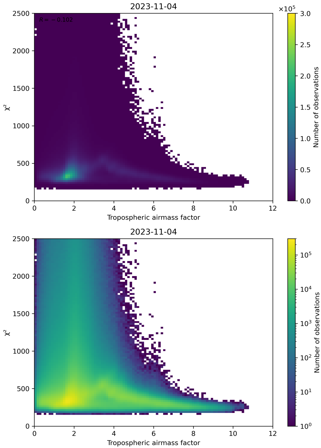
Figure 73: Scatter density plot of “Tropospheric airmass factor” against “ \chi^2 ” for 2023-11-03 to 2023-11-05.
