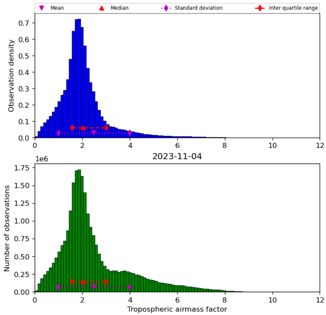
Figure 31: Histogram of “Tropospheric airmass factor” for 2023-11-03 to 2023-11-05
