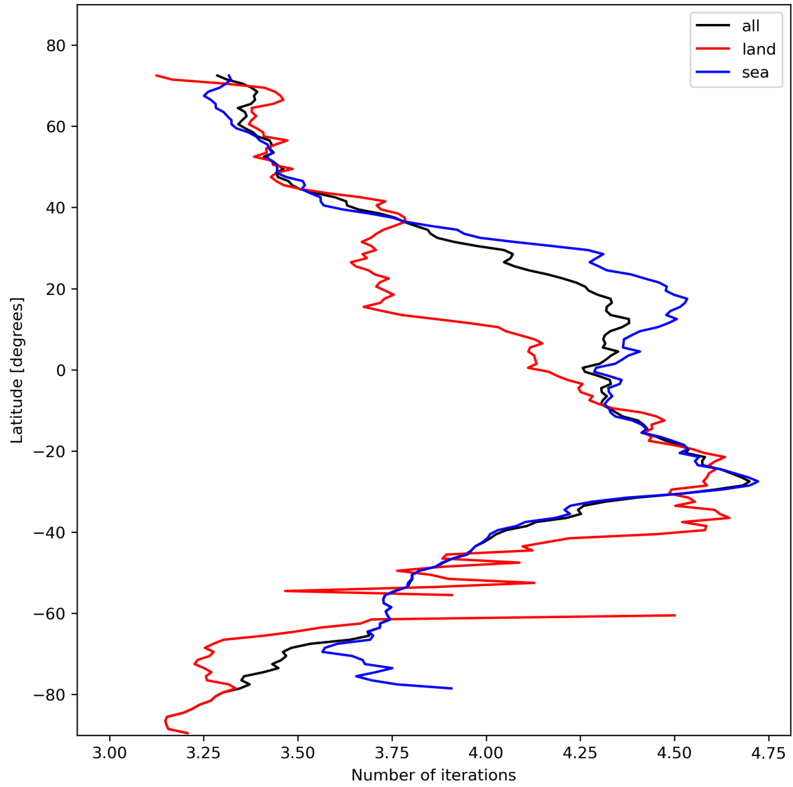
Figure 17: Zonal average of “Number of iterations” for 2023-11-03 to 2023-11-05.
