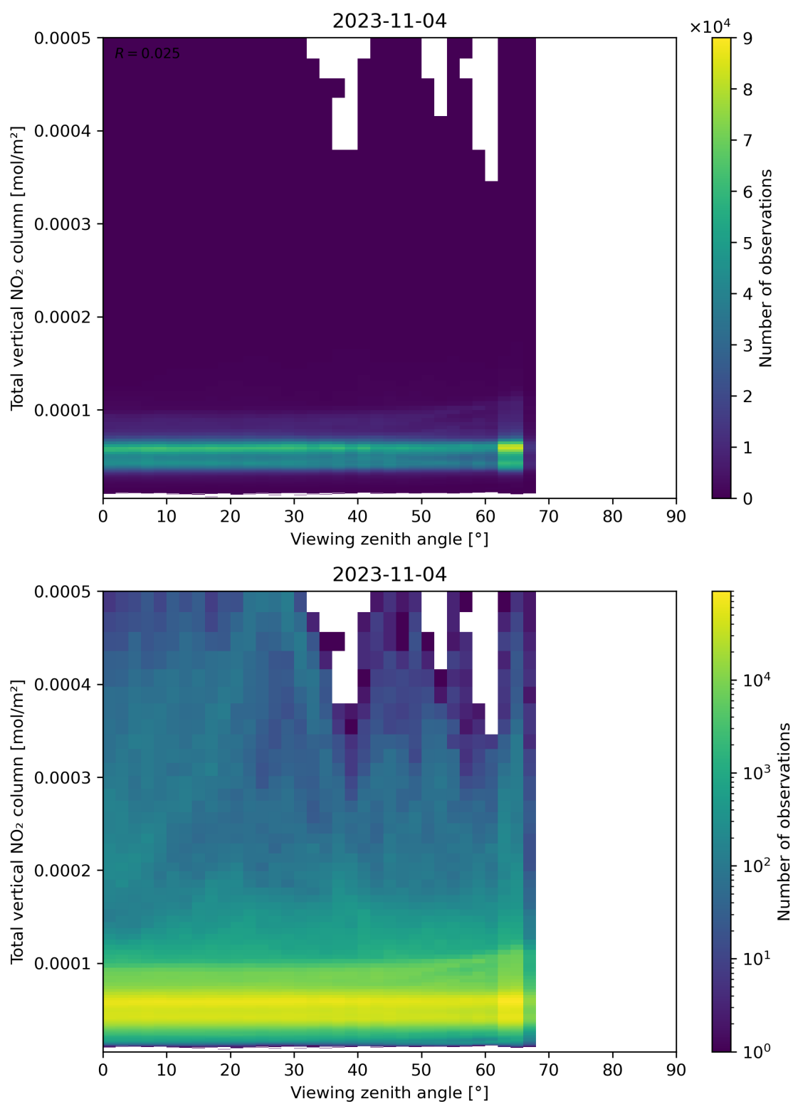
Figure 167: Scatter density plot of “Viewing zenith angle” against “Total vertical NO 2 column” for 2023-11-03 to 2023-11-05.
