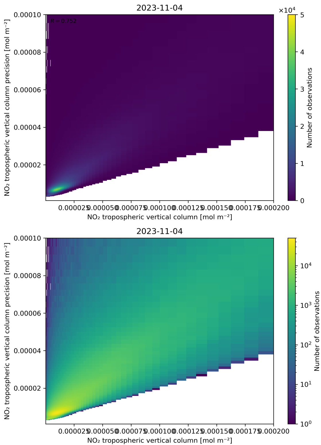
Figure 130: Scatter density plot of “NO 2 tropospheric vertical column” against “NO 2 tropospheric vertical column precision” for 2023-11-03 to 2023-11-05.
