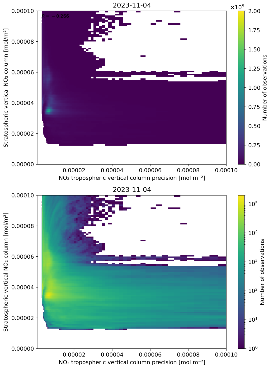
Figure 135: Scatter density plot of “NO 2 tropospheric vertical column precision” against “Stratospheric vertical NO 2 column” for 2023-11-03 to 2023-11-05.
