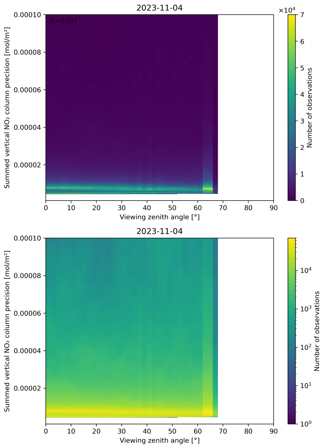
Figure 166: Scatter density plot of “Viewing zenith angle” against “Summed vertical NO 2 column precision” for 2023-11-03 to 2023-11-05.
