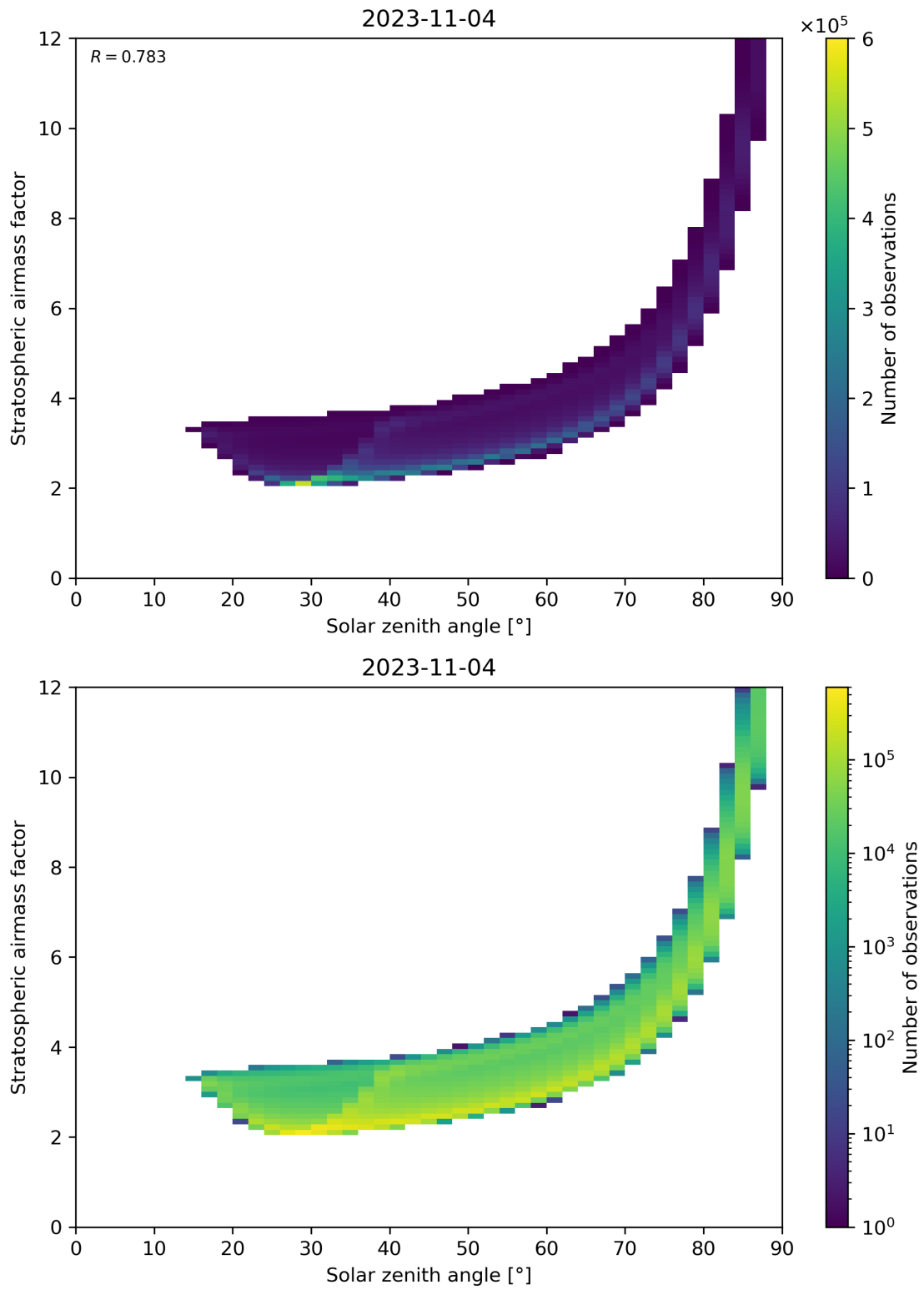
Figure 145: Scatter density plot of “Solar zenith angle” against “Stratospheric airmass factor” for 2023-11-03 to 2023-11-05.
