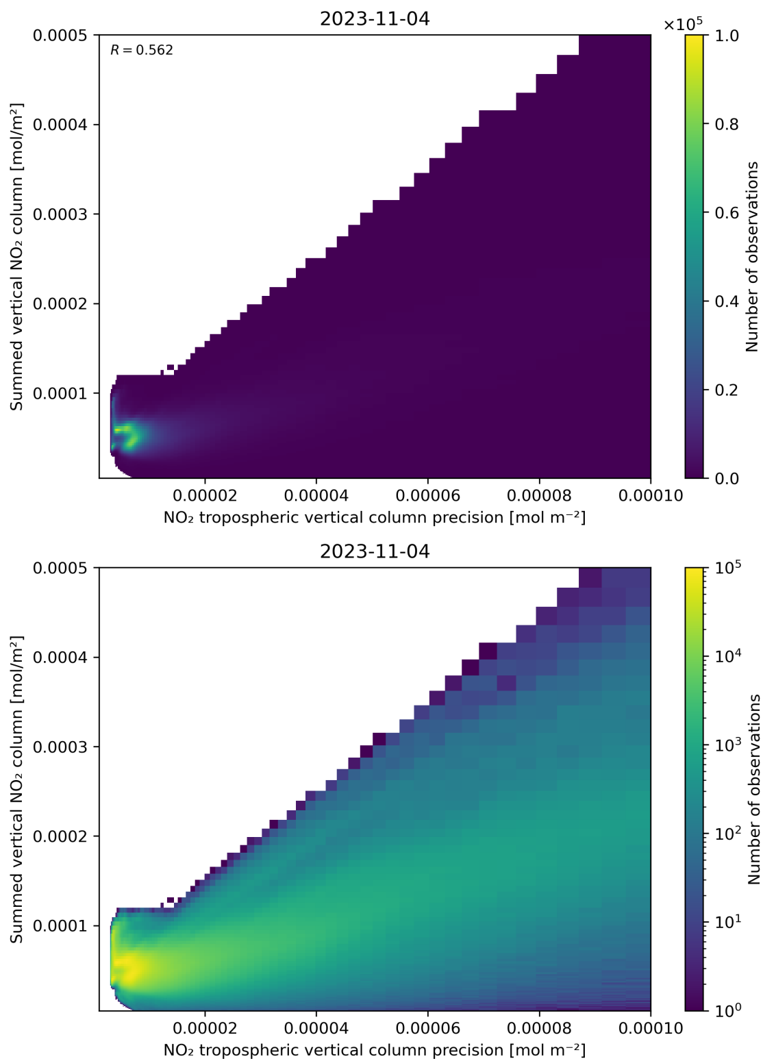
Figure 136: Scatter density plot of “NO 2 tropospheric vertical column precision” against “Summed vertical NO 2 column” for 2023-11-03 to 2023-11-05.
