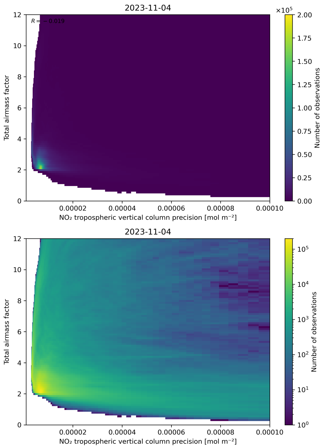
Figure 132: Scatter density plot of “NO 2 tropospheric vertical column precision” against “Total air mass factor” for 2023-11-03 to 2023-11-05.
