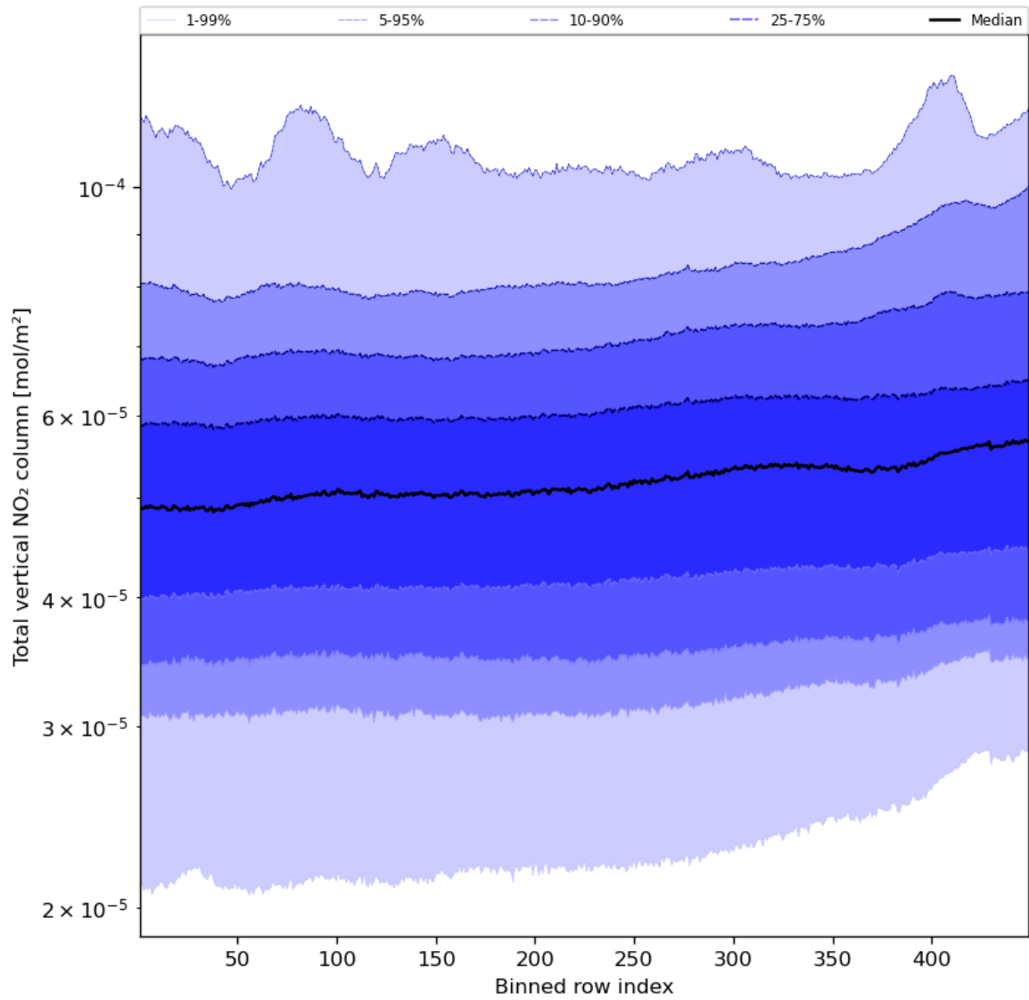
Figure 55: Along track statistics of “Total vertical NO 2 column” for 2023-11-03 to 2023-11-05
