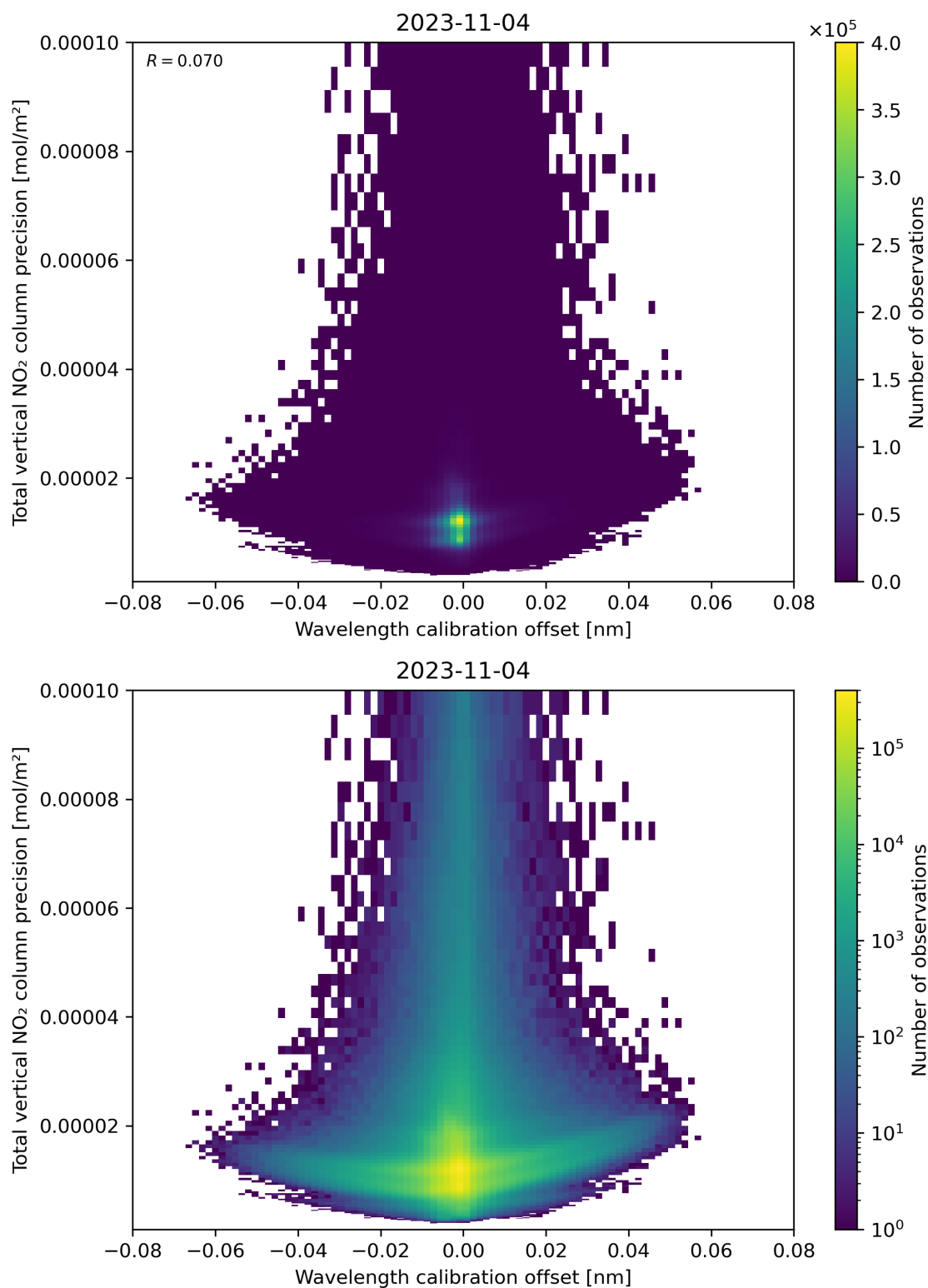
Figure 180: Scatter density plot of “Wavelength calibration offset” against “Total vertical NO 2 column precision” for 2023-11-03 to 2023-11-05.
