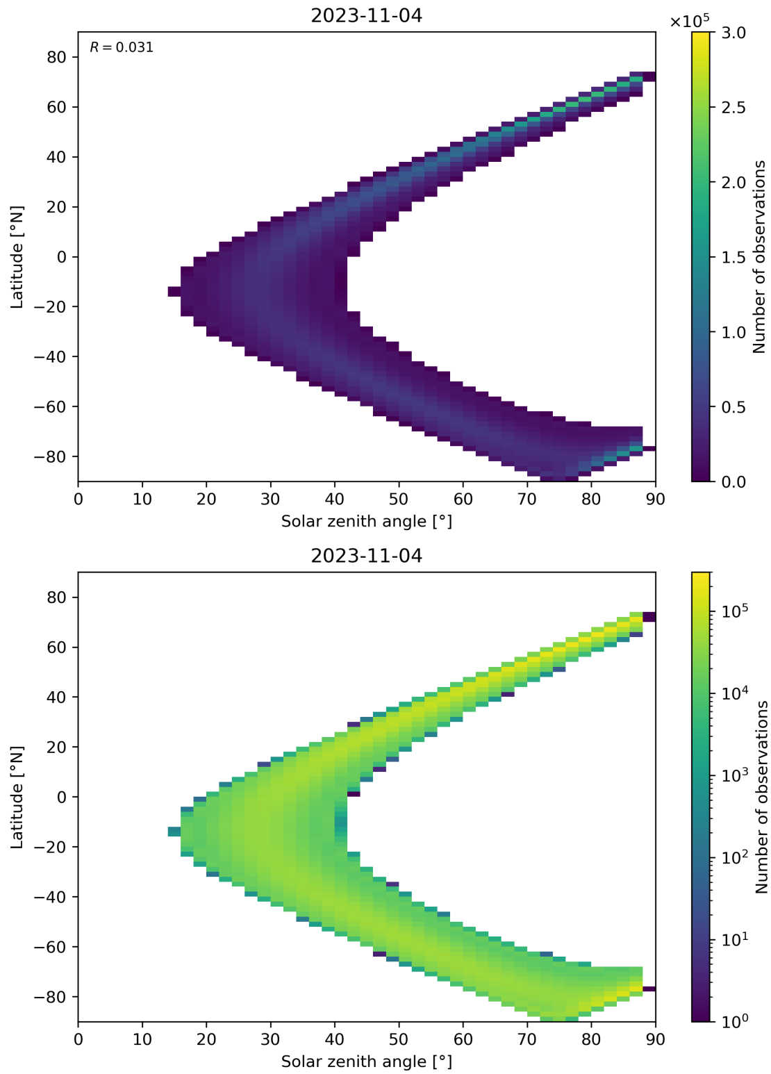
Figure 149: Scatter density plot of “Solar zenith angle” against “Latitude” for 2023-11-03 to 2023-11-05.
