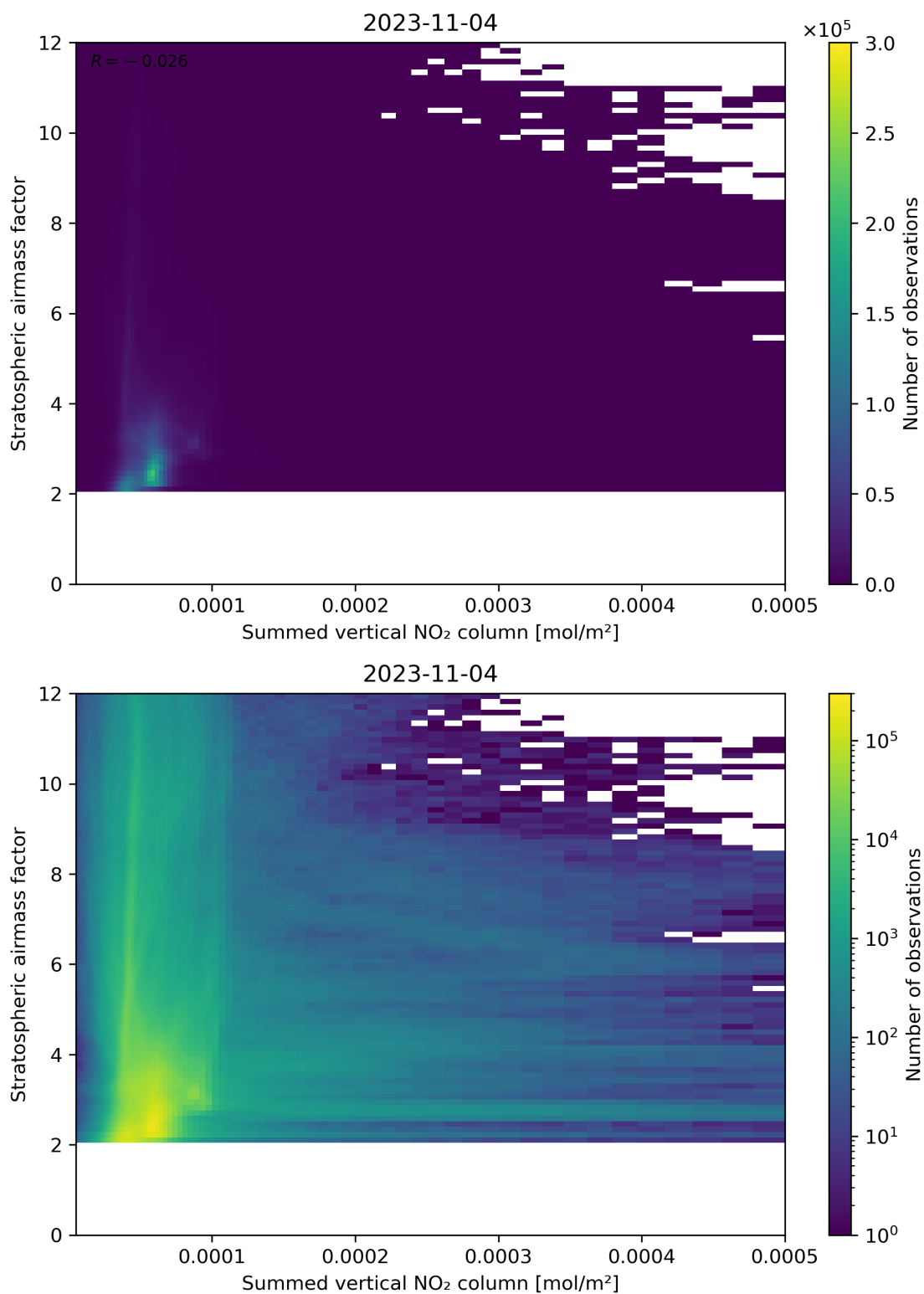
Figure 103: Scatter density plot of “Summed vertical NO 2 column” against “Stratospheric airmass factor” for 2023-11-03 to 2023-11-05.
