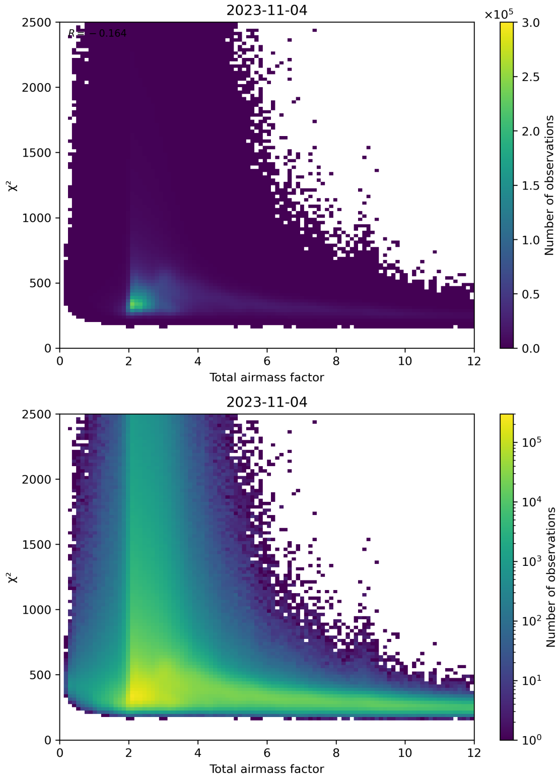
Figure 63: Scatter density plot of “Total airmass factor” against “ \chi^2 ” for 2023-11-03 to 2023-11-05.
