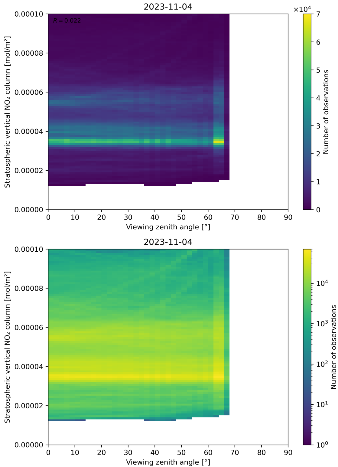
Figure 164: Scatter density plot of “Viewing zenith angle” against “Stratospheric vertical NO 2 column” for 2023-11-03 to 2023-11-05.
