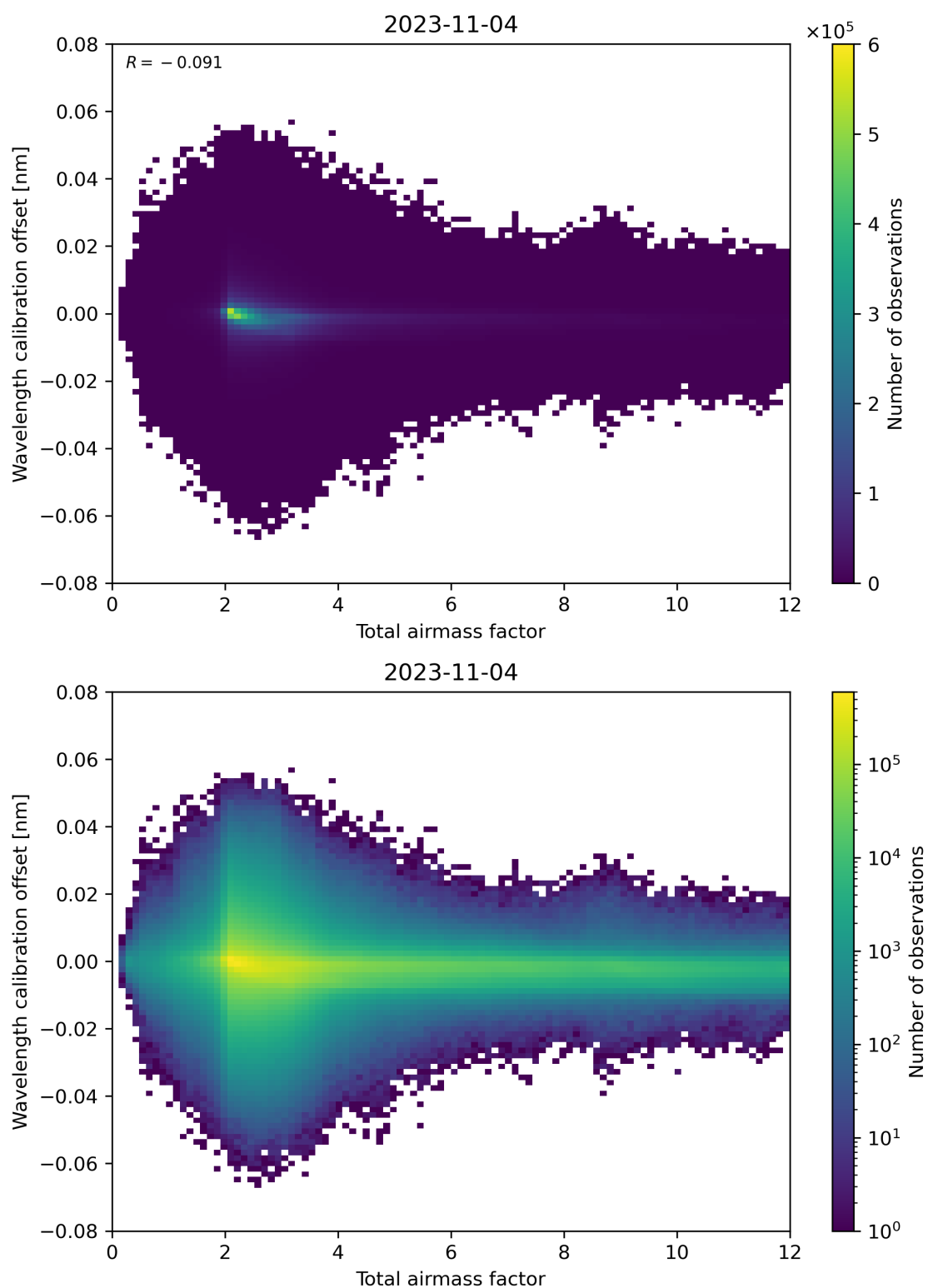
Figure 70: Scatter density plot of “Total airmass factor” against “Wavelength calibration offset” for 2023-11-03 to 2023-11-05.
