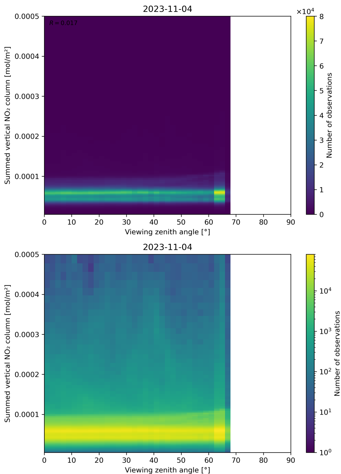
Figure 165: Scatter density plot of “Viewing zenith angle” against “Summed vertical NO 2 column” for 2023-11-03 to 2023-11-05.
