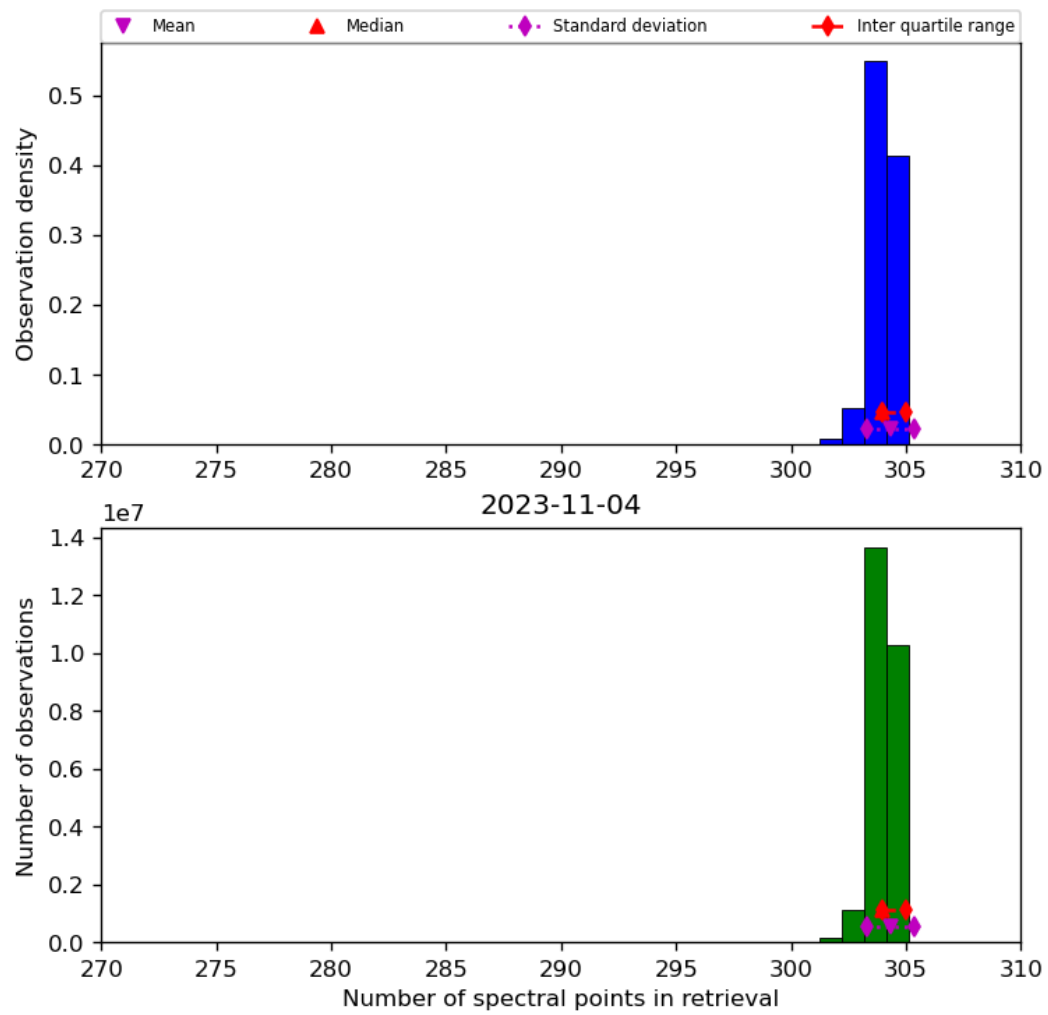
Figure 33: Histogram of “Number of spectral points in retrieval” for 2023-11-03 to 2023-11-05
