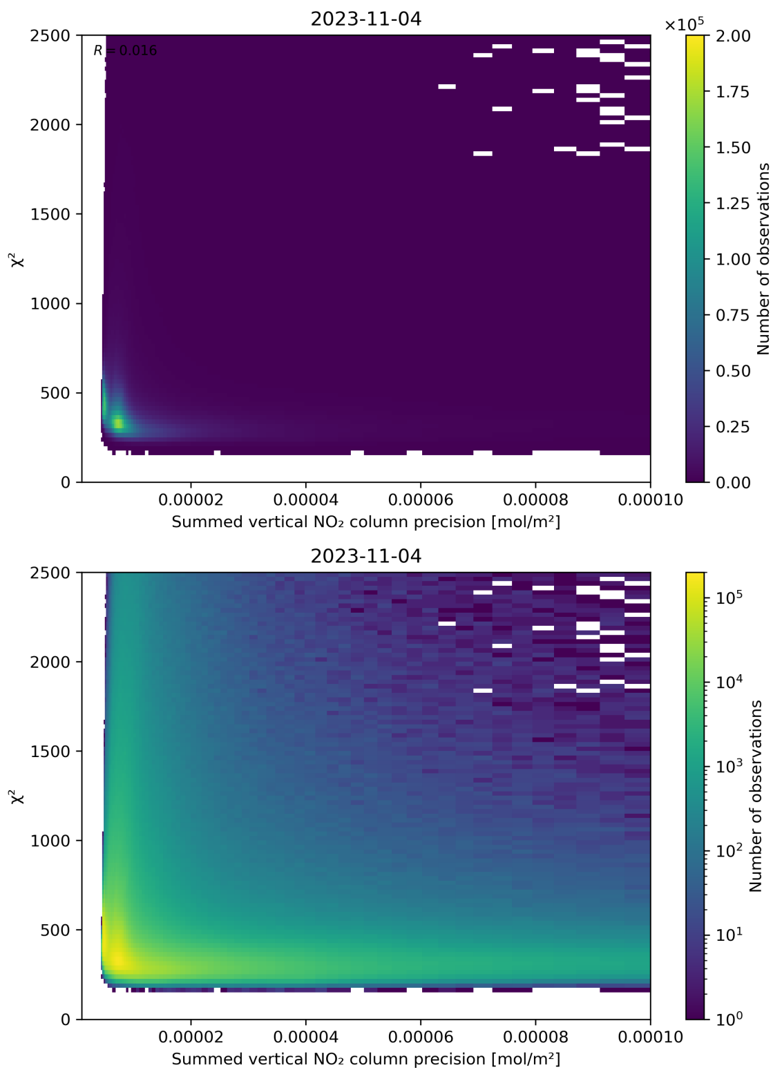
Figure 107: Scatter density plot of “Summed vertical NO 2 column precision” against “ \chi^2 ” for 2023-11-03 to 2023-11-05.
