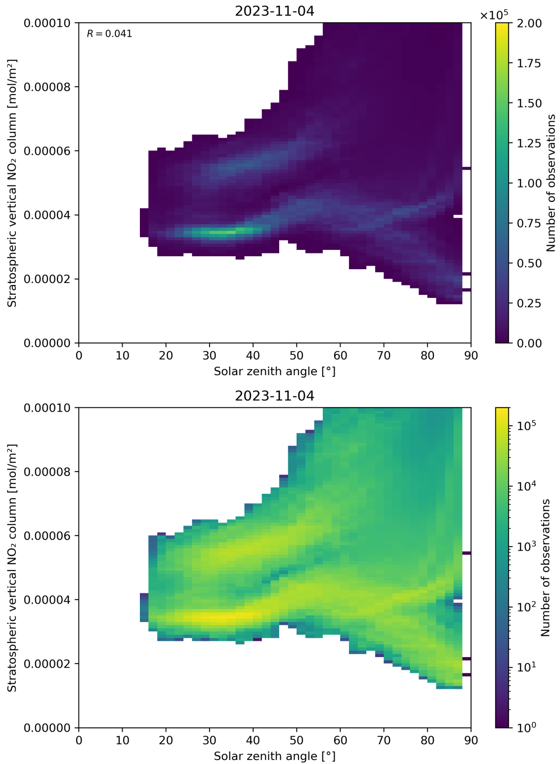
Figure 150: Scatter density plot of “Solar zenith angle” against “Stratospheric vertical NO 2 column” for 2023-11-03 to 2023-11-05.
