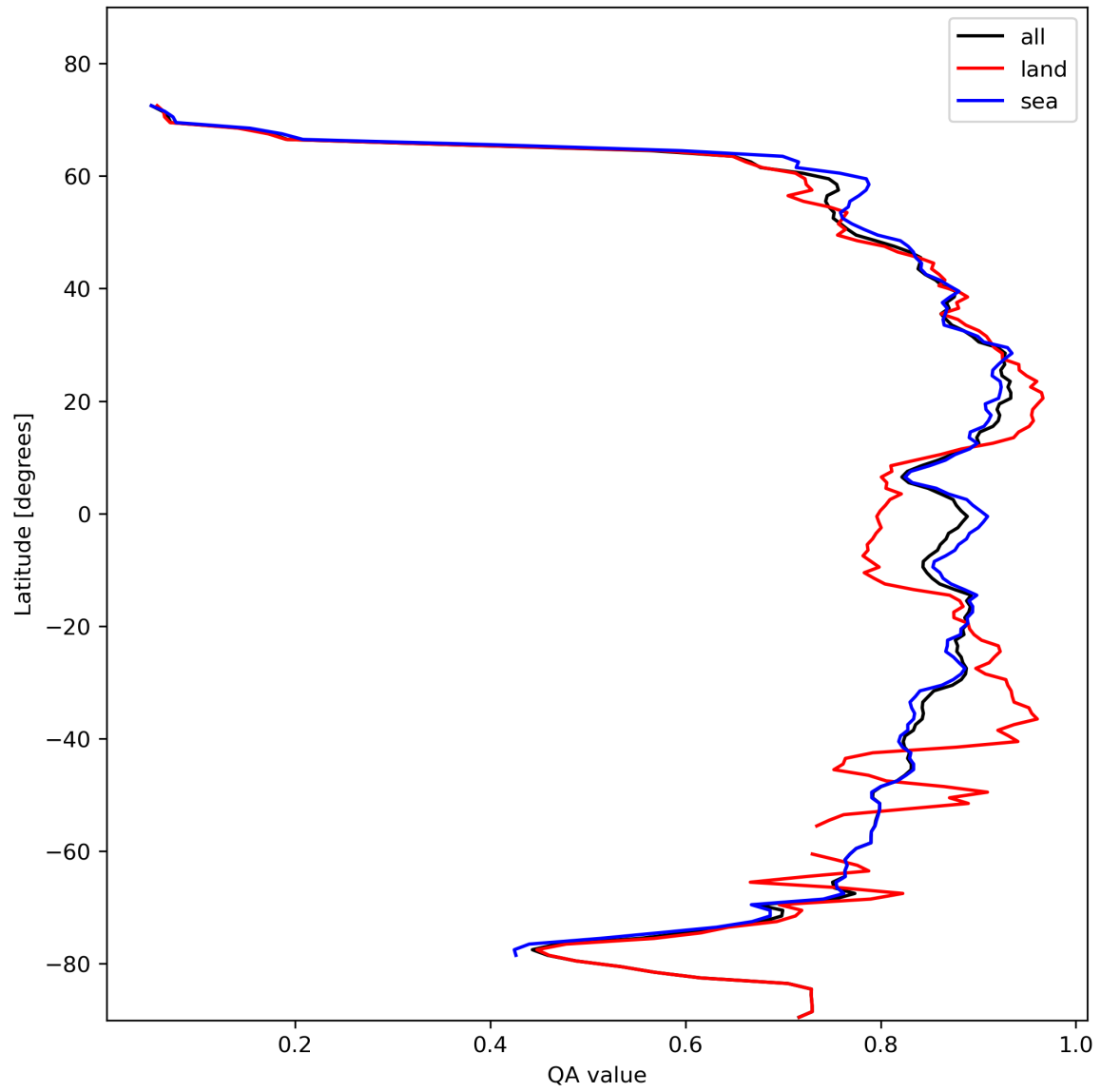
Figure 11: Zonal average of “QA value” for 2023-11-03 to 2023-11-05.
