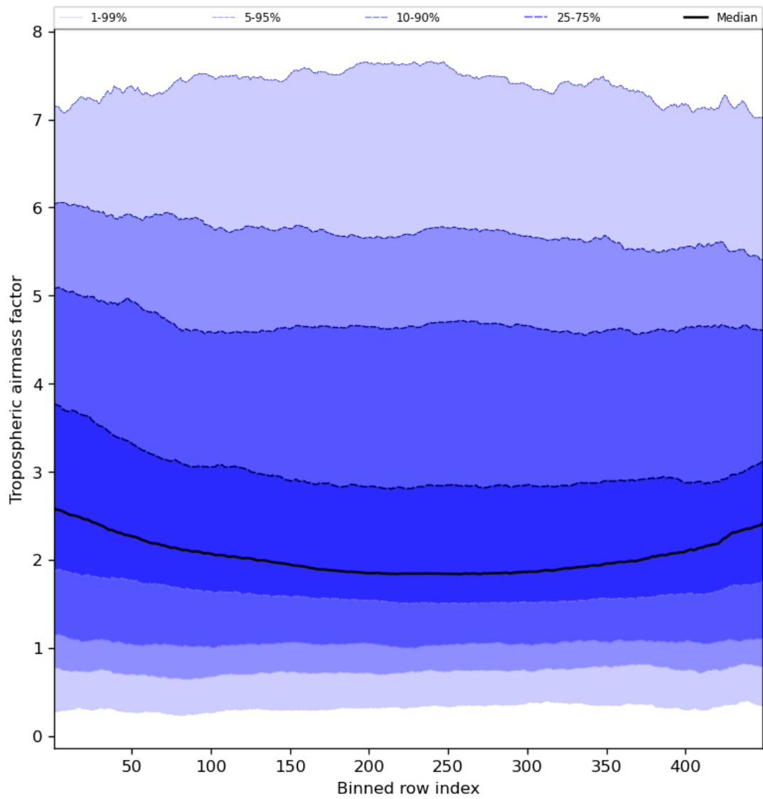
Figure 48: Along track statistics of “Tropospheric air mass factor” for 2023-11-03 to 2023-11-05
