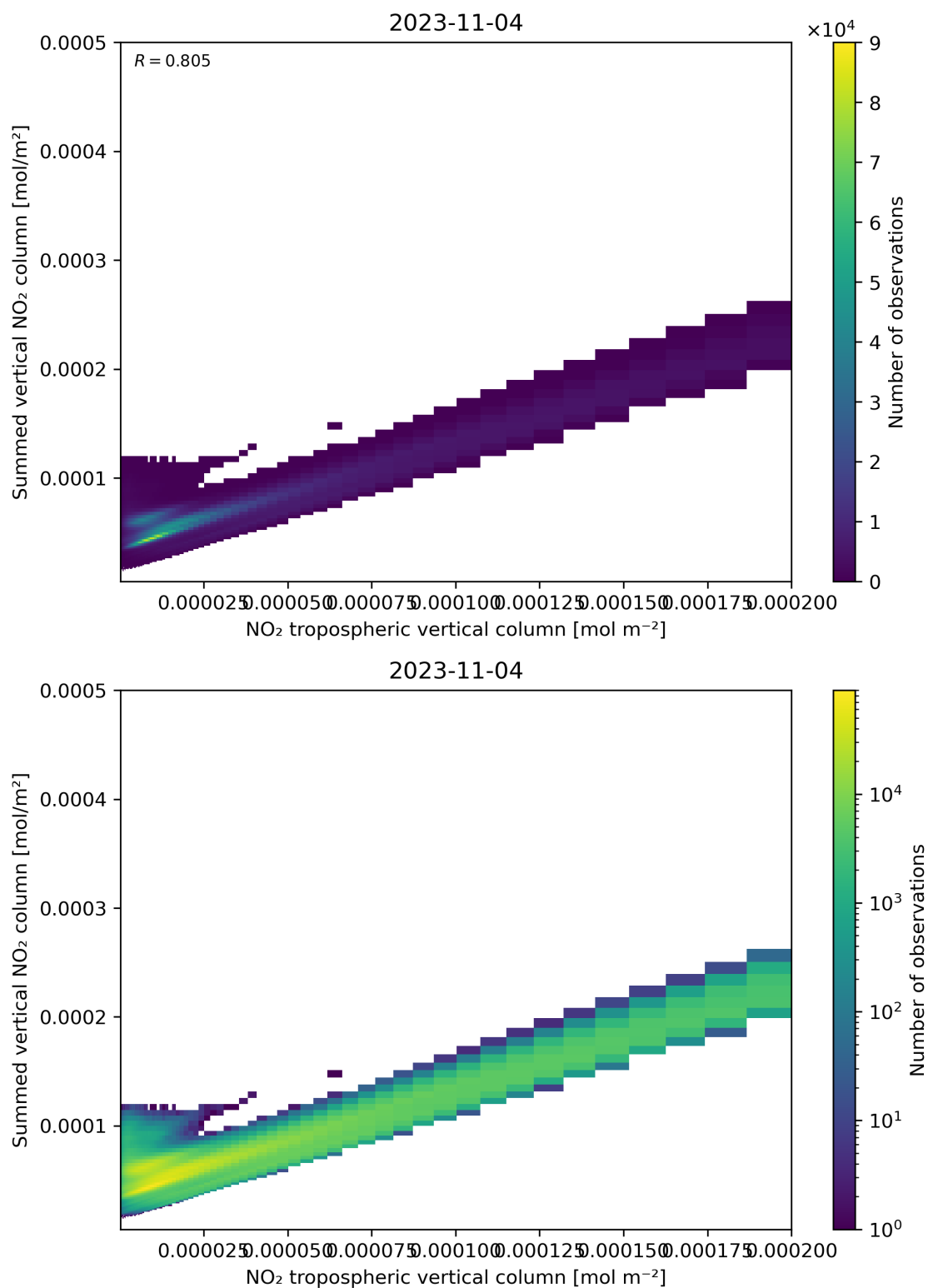
Figure 126: Scatter density plot of “NO 2 tropospheric vertical column” against “Summed vertical NO 2 column” for 2023-11-03 to 2023-11-05.
