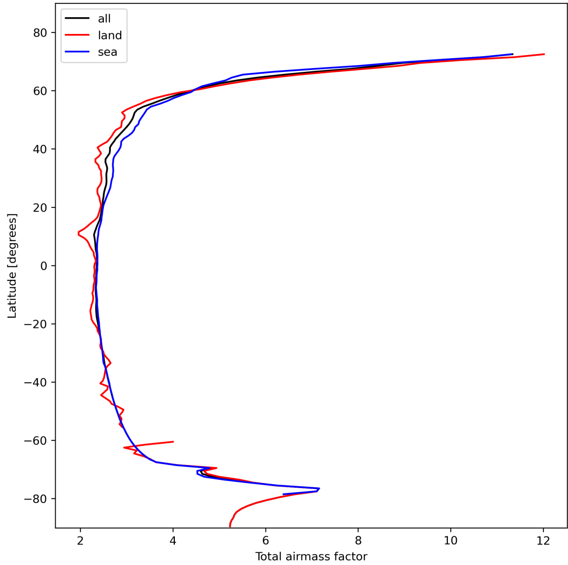
Figure 15: Zonal average of “Total airmass factor” for 2023-11-03 to 2023-11-05.
