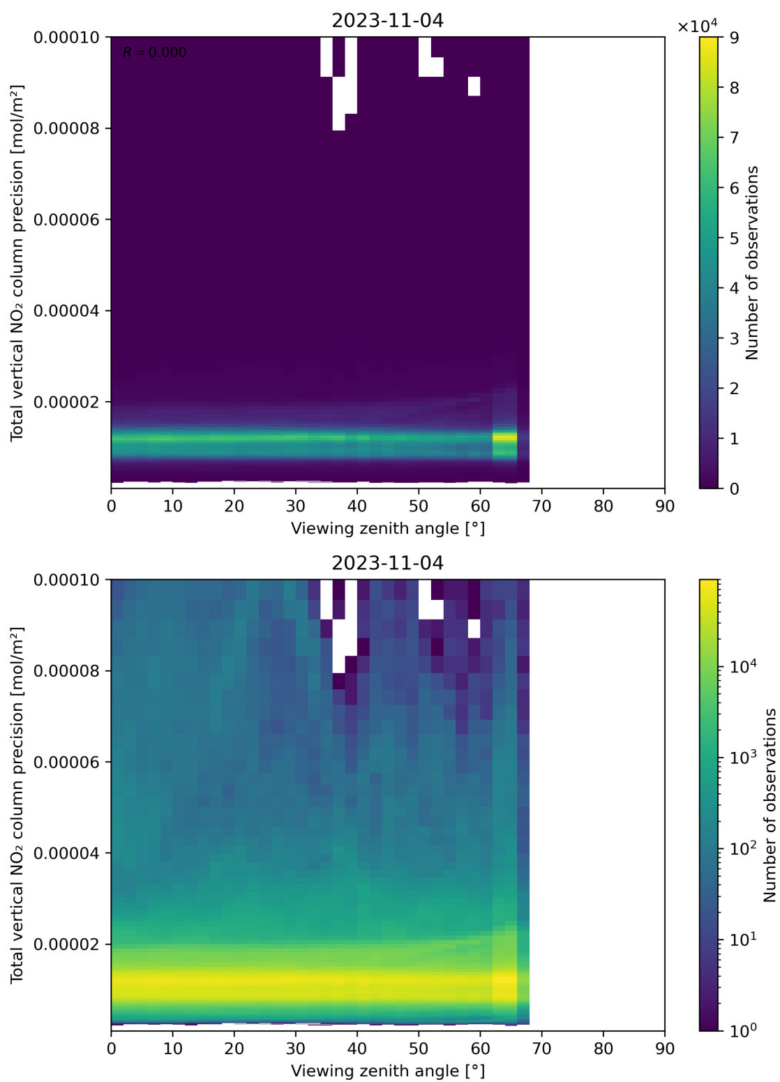
Figure 168: Scatter density plot of “Viewing zenith angle” against “Total vertical NO 2 column precision” for 2023-11-03 to 2023-11-05.
