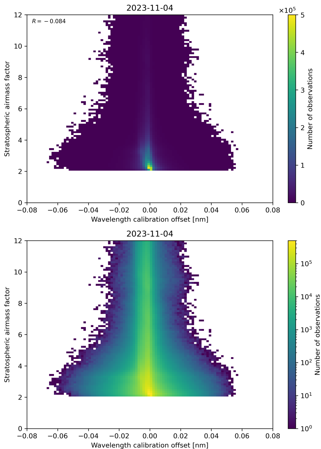
Figure 174: Scatter density plot of “Wavelength calibration offset” against “Stratospheric airmass factor” for 2023-11-03 to 2023-11-05.
