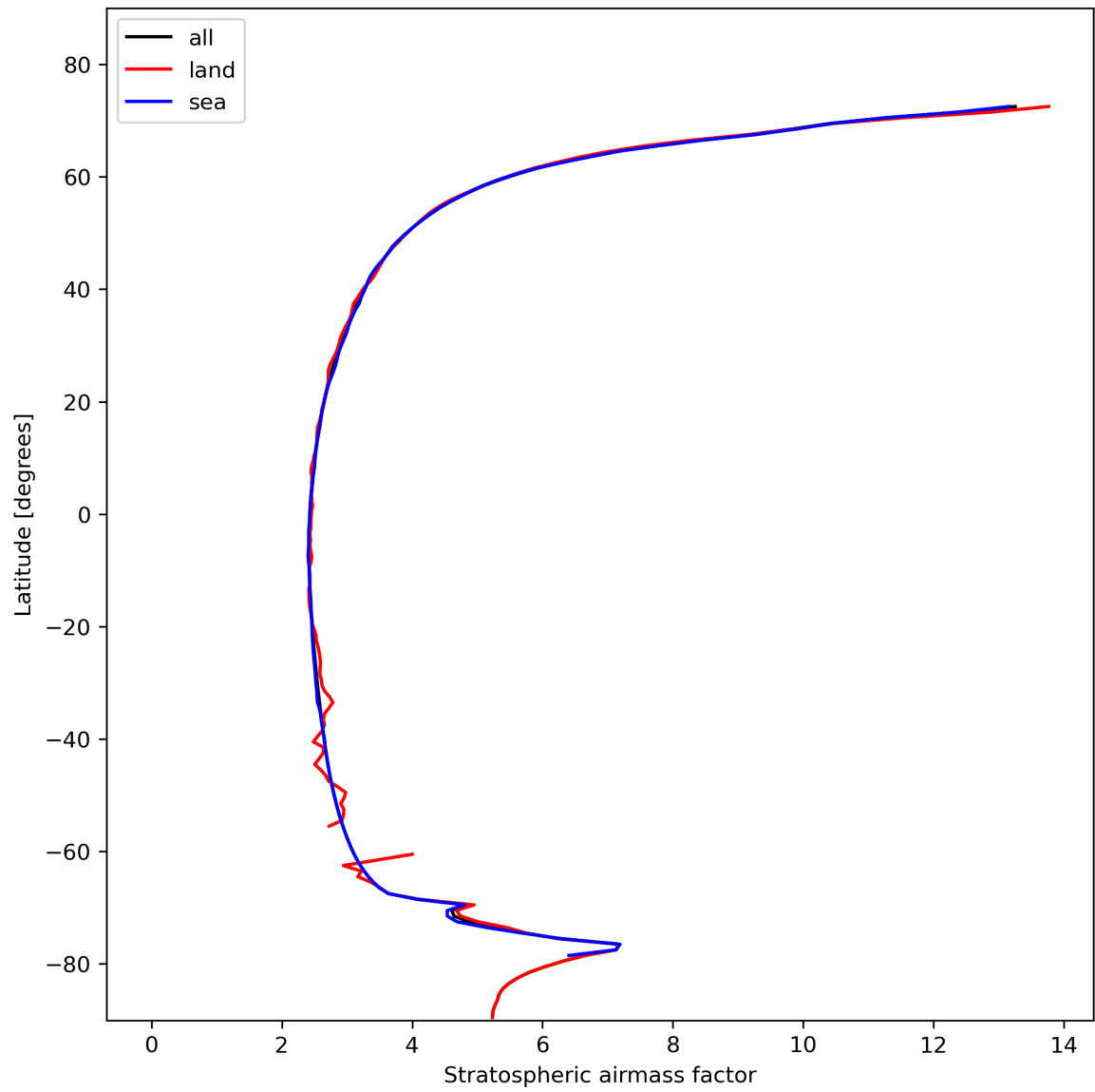
Figure 27: Zonal average of “Stratospheric airmass factor” for 2023-11-03 to 2023-11-05.
