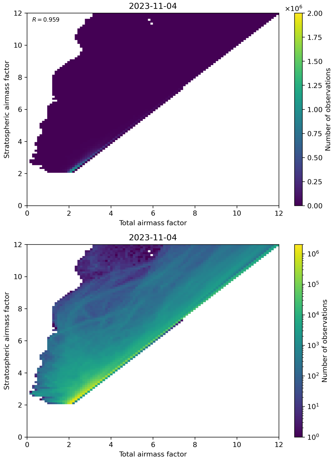
Figure 62: Scatter density plot of “Total airmass factor” against “Stratospheric airmass factor” for 2023-11-03 to 2023-11-05.
