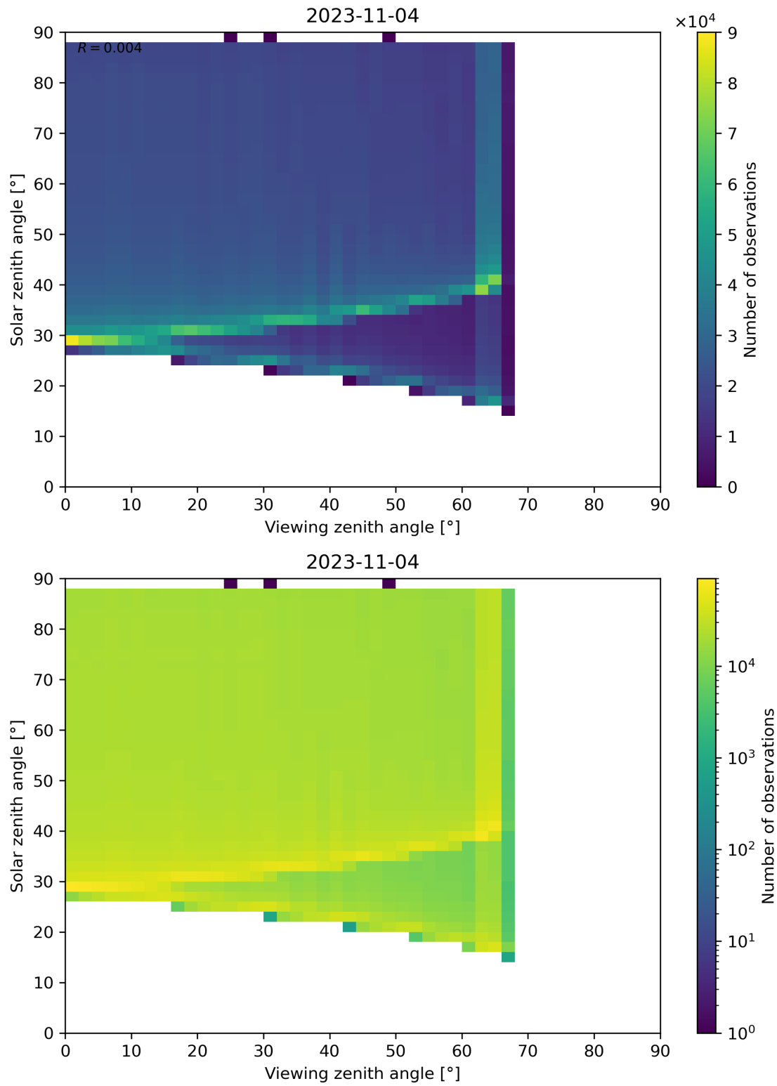
Figure 172: Scatter density plot of “Viewing zenith angle” against “Solar zenith angle” for 2023-11-03 to 2023-11-05.
