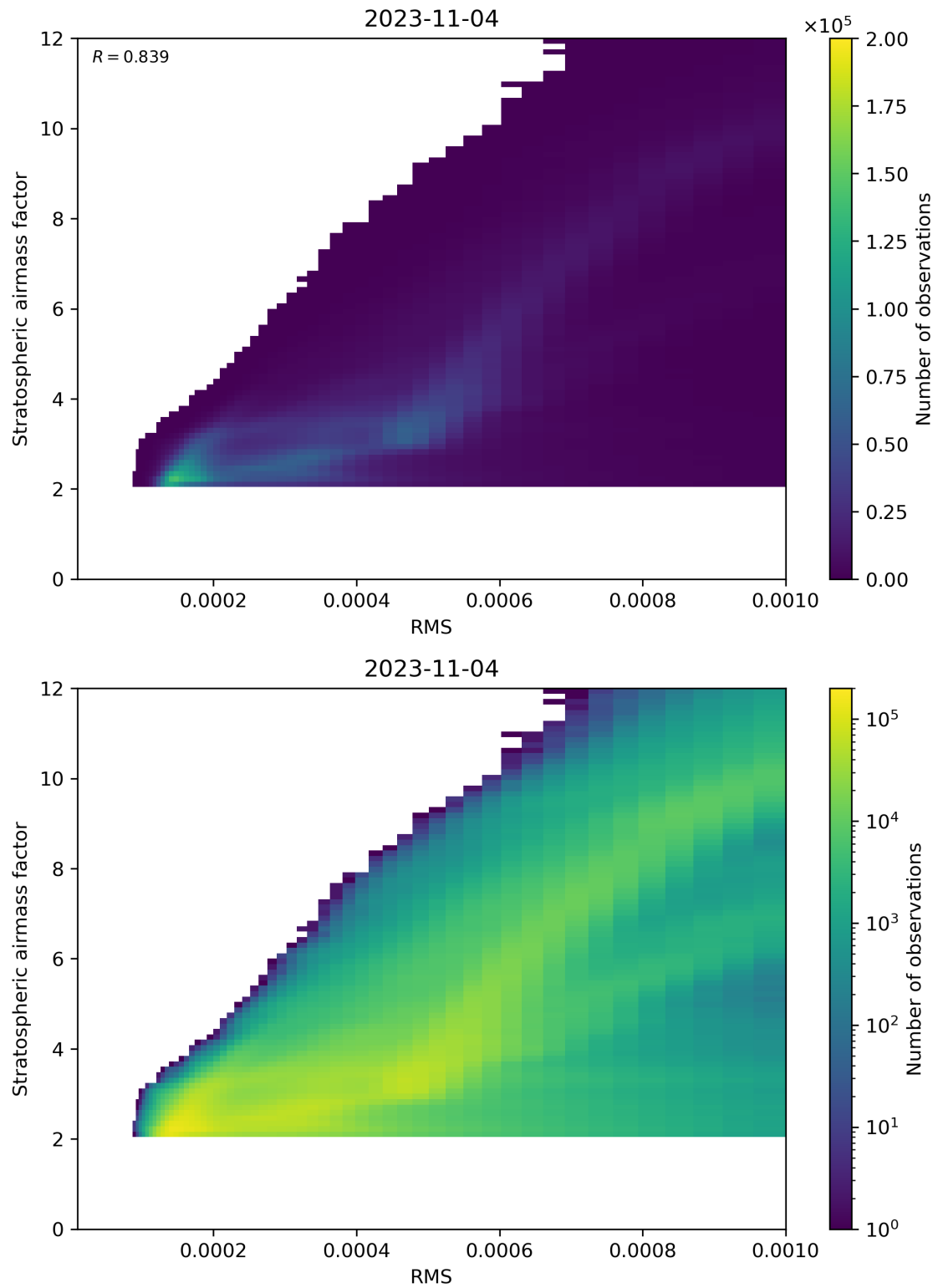
Figure 144: Scatter density plot of “RMS” against “Stratospheric airmass factor” for 2023-11-03 to 2023-11-05.
