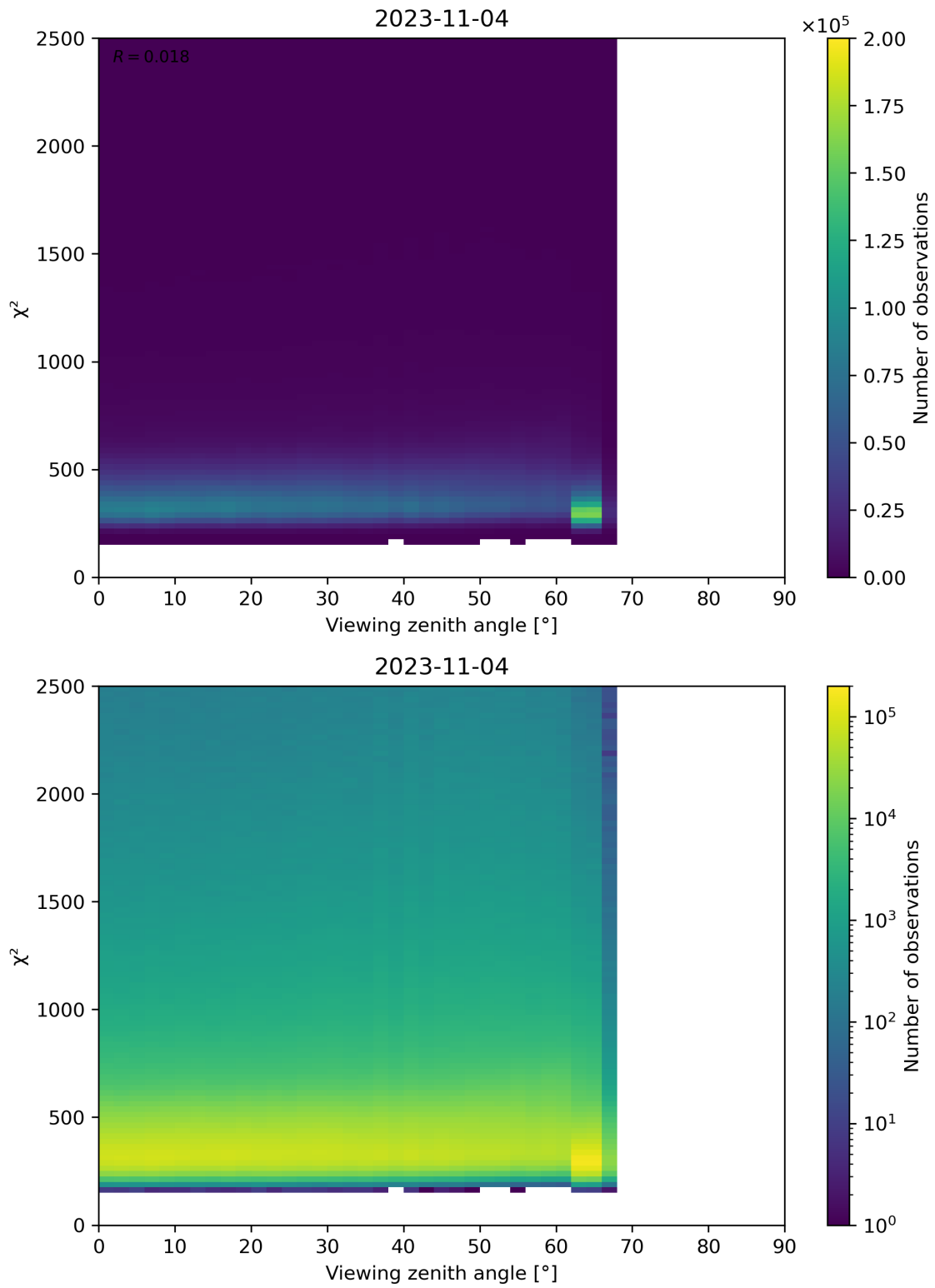
Figure 162: Scatter density plot of “Viewing zenith angle” against “ \chi^2 ” for 2023-11-03 to 2023-11-05.
