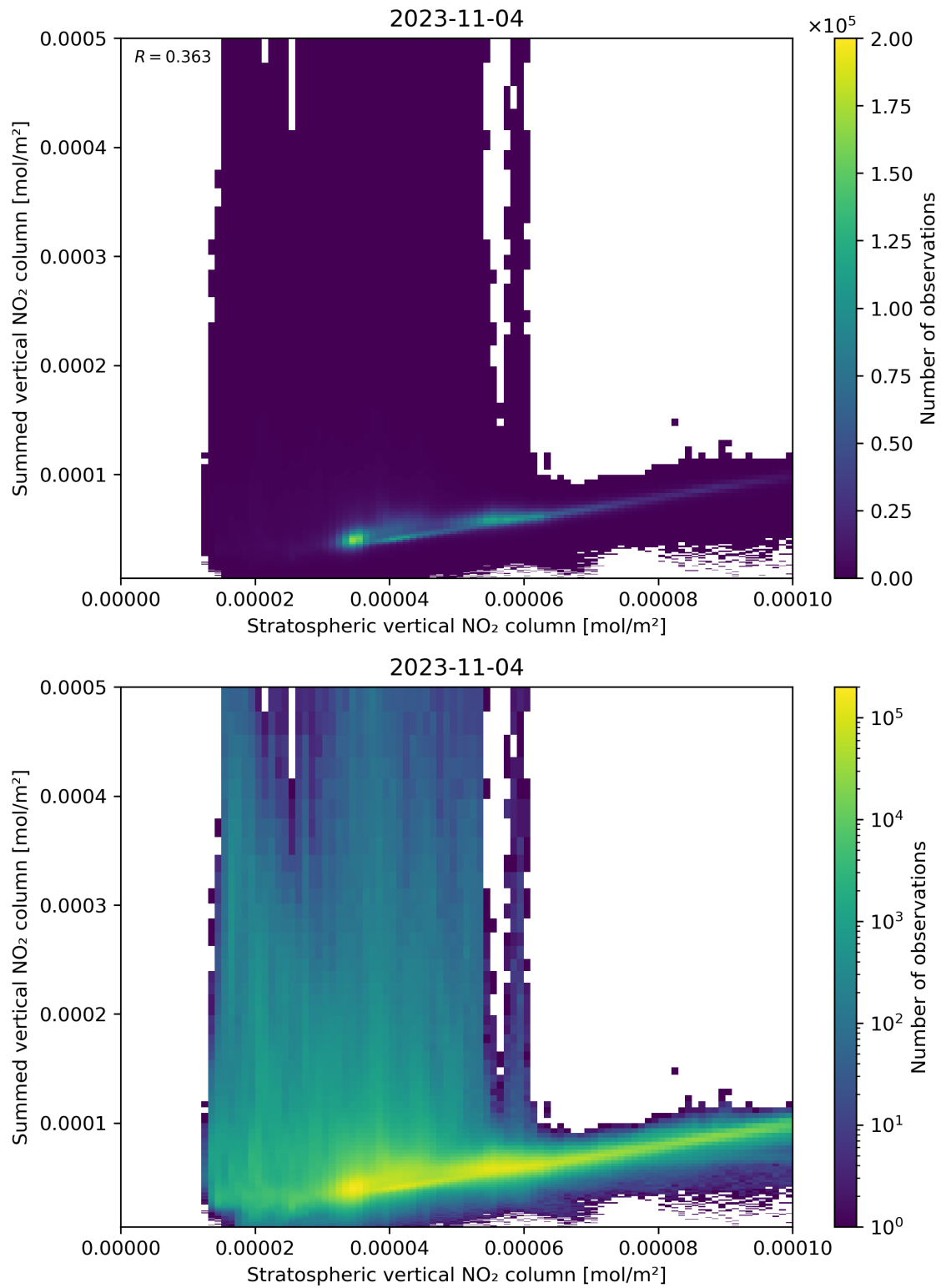
Figure 98: Scatter density plot of “Stratospheric vertical NO 2 column” against “Summed vertical NO 2 column” for 2023-11-03 to 2023-11-05.
