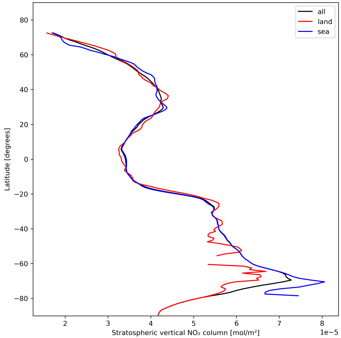
Figure 19: Zonal average of “Stratospheric vertical NO 2 column” for 2023-11-03 to 2023-11-05.
