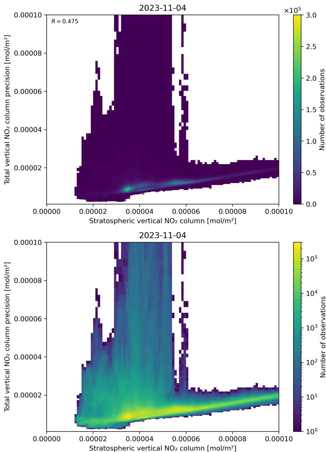
Figure 101: Scatter density plot of “Stratospheric vertical NO 2 column” against “Total vertical NO 2 column precision” for 2023-11-03 to 2023-11-05.
