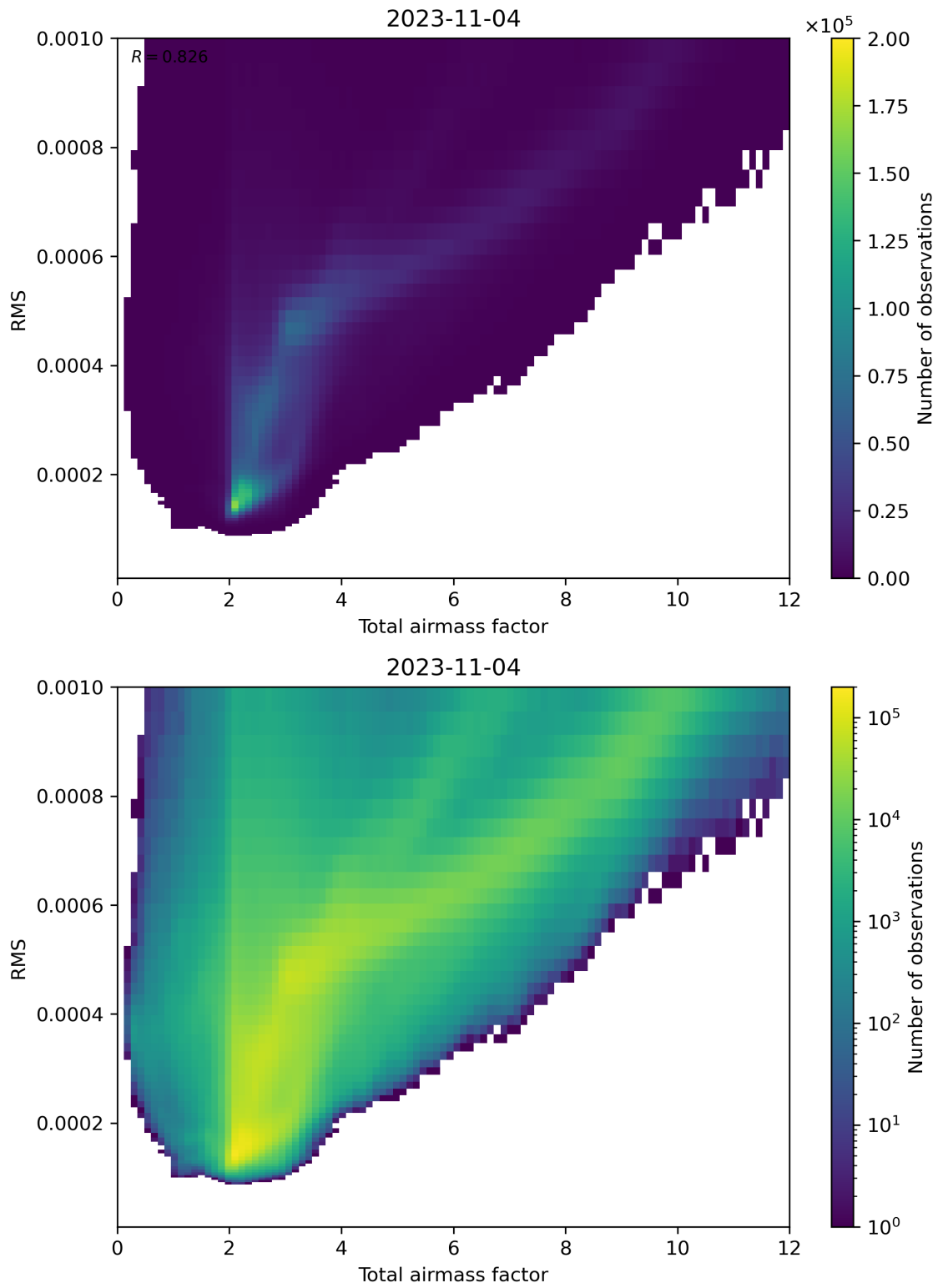
Figure 69: Scatter density plot of “Total airmass factor” against “RMS” for 2023-11-03 to 2023-11-05.
