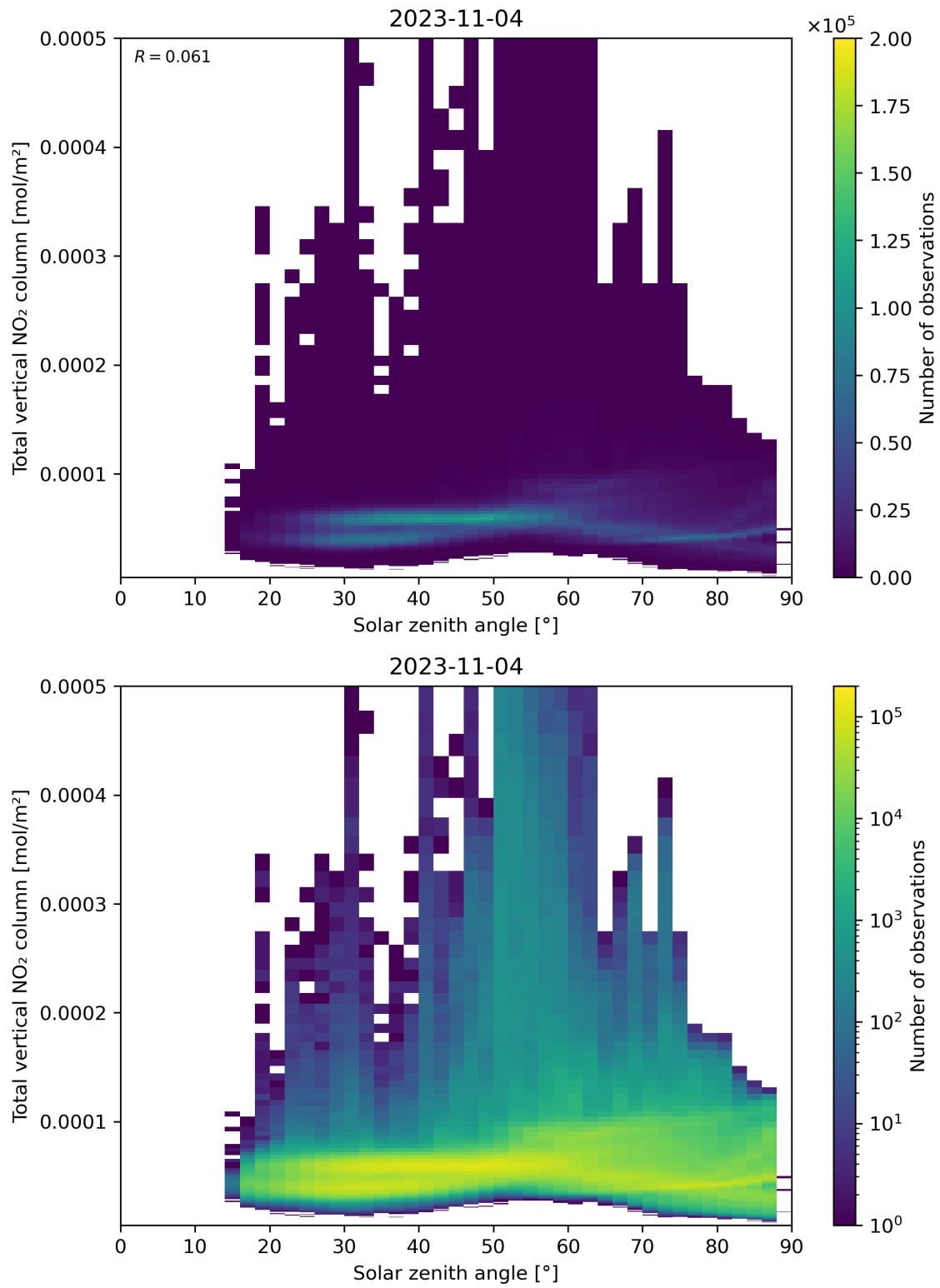
Figure 153: Scatter density plot of “Solar zenith angle” against “Total vertical NO 2 column” for 2023-11-03 to 2023-11-05.
