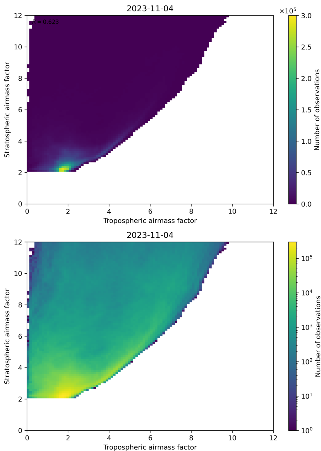
Figure 71: Scatter density plot of “Tropospheric airmass factor” against “Stratospheric airmass factor” for 2023-11-03 to 2023-11-05.
