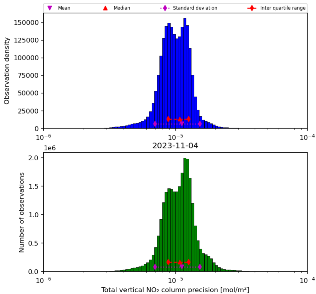
Figure 39: Histogram of "Total vertical NO 2 column precision" for 2023-11-03 to 2023-11-05
