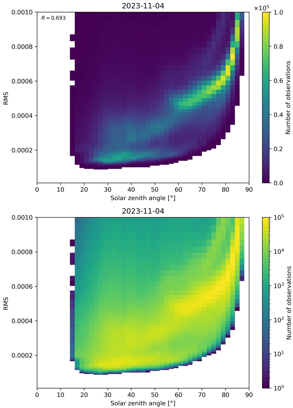
Figure 157: Scatter density plot of “Solar zenith angle” against “RMS” for 2023-11-03 to 2023-11-05.
