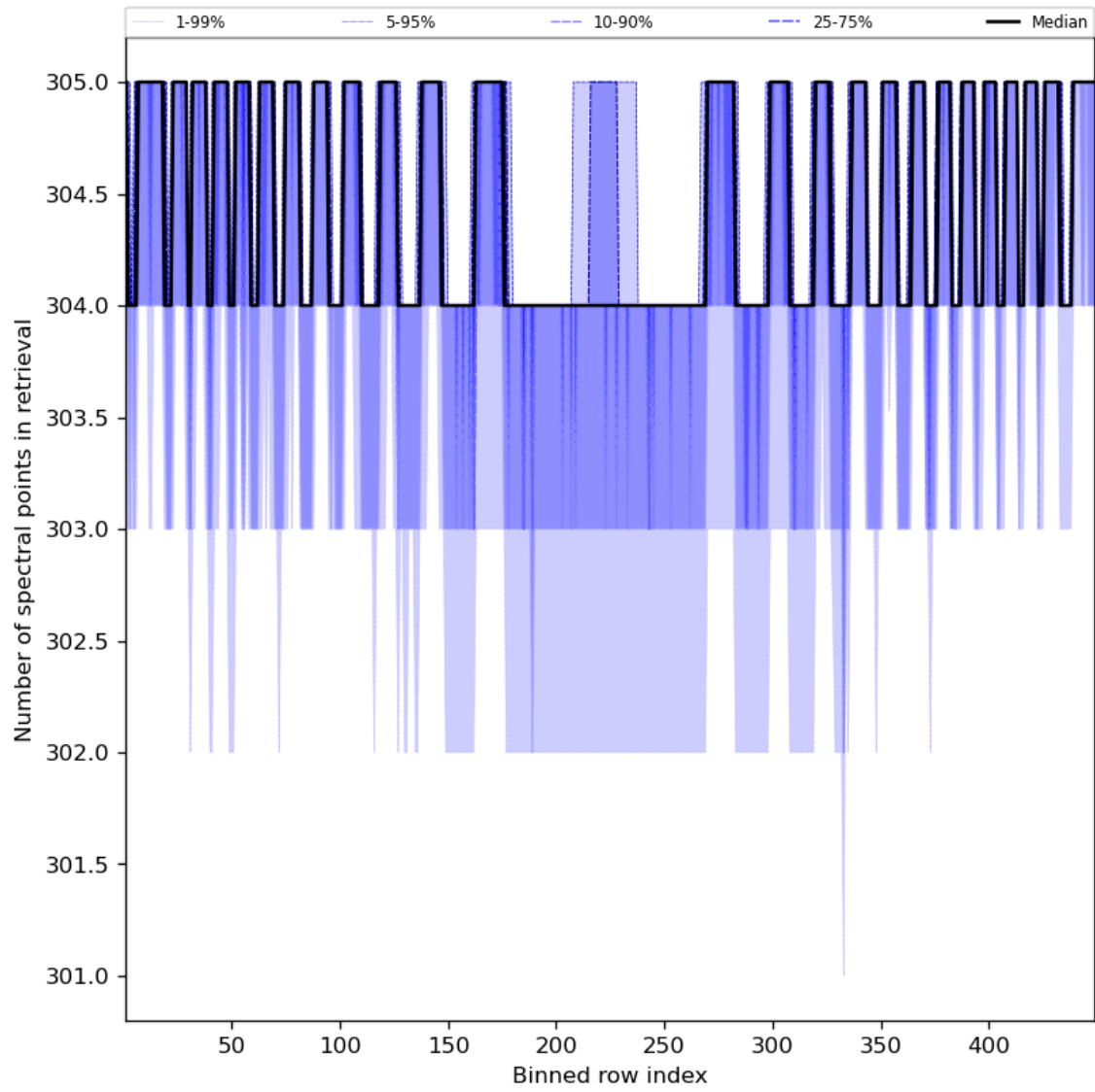
Figure 50: Along track statistics of “Number of spectral points in retrieval” for 2023-11-03 to 2023-11-05
