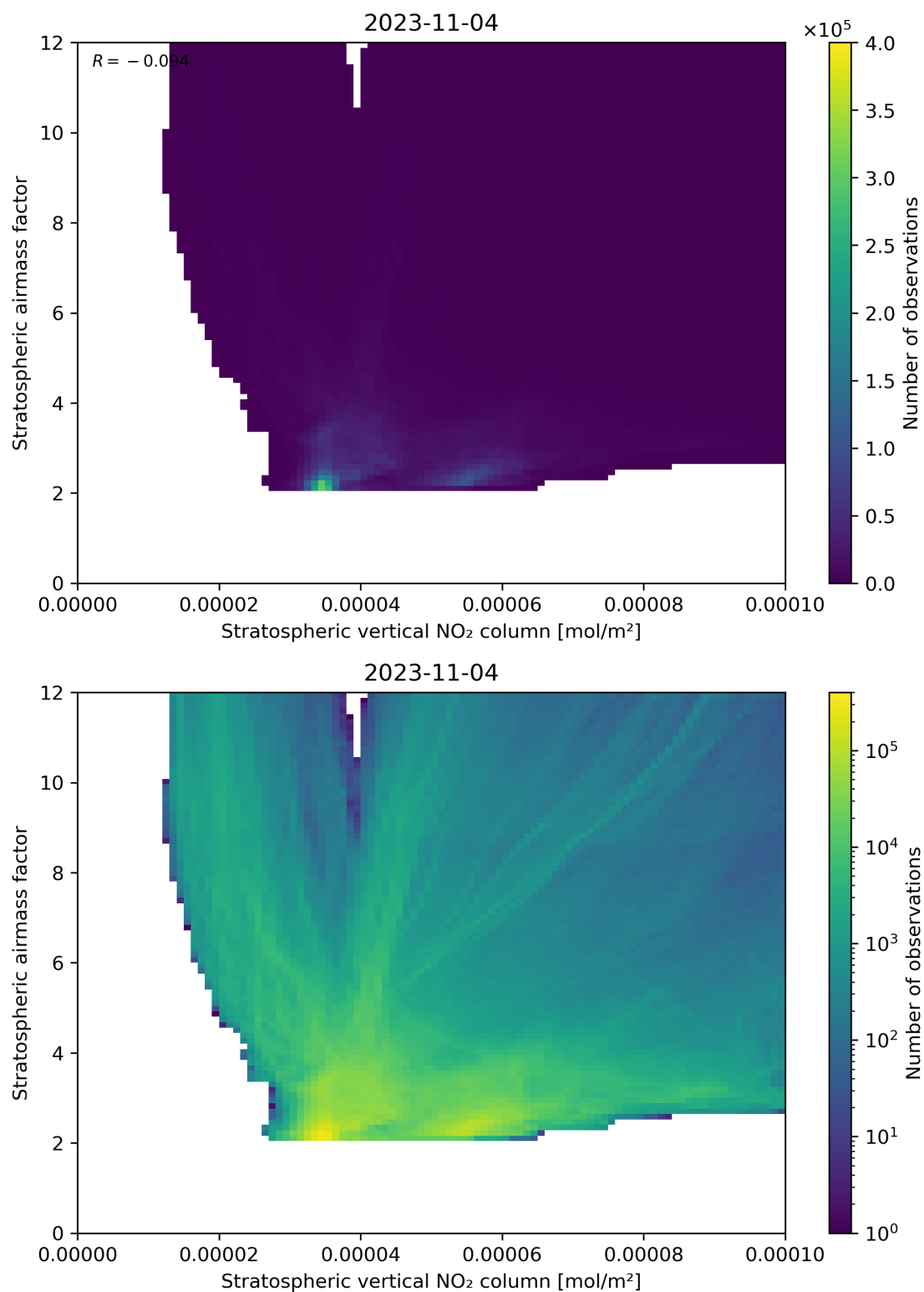
Figure 96: Scatter density plot of “Stratospheric vertical NO 2 column” against “Stratospheric airmass factor” for 2023-11-03 to 2023-11-05.
