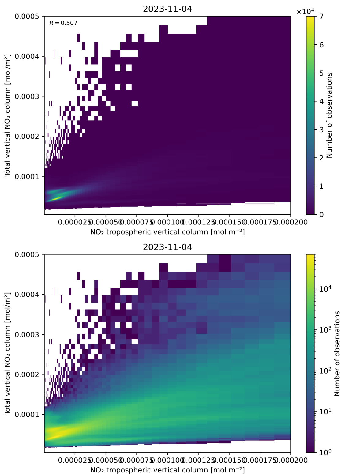
Figure 128: Scatter density plot of “NO 2 tropospheric vertical column” against “Total vertical NO 2 column” for 2023-11-03 to 2023-11-05.
