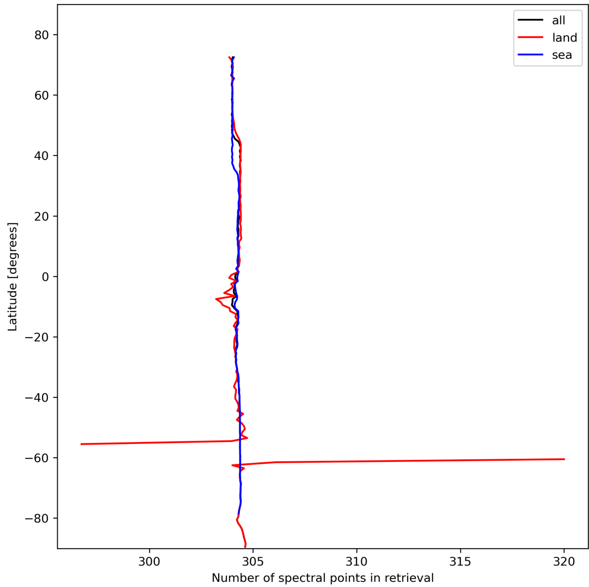
Figure 16: Zonal average of “Number of spectral points in retrieval” for 2023-11-03 to 2023-11-05.
