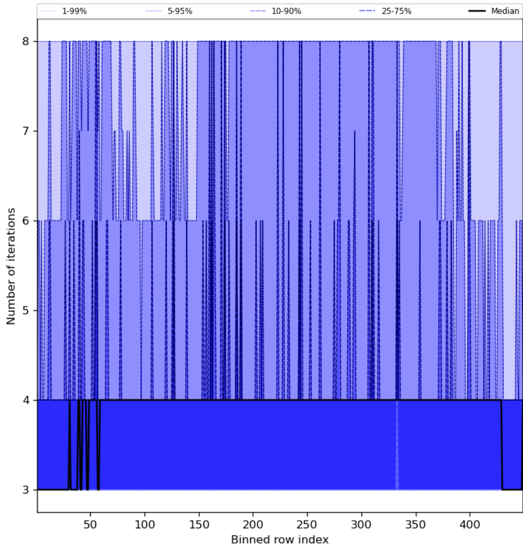
Figure 51: Along track statistics of “Number of iterations” for 2023-11-03 to 2023-11-05
