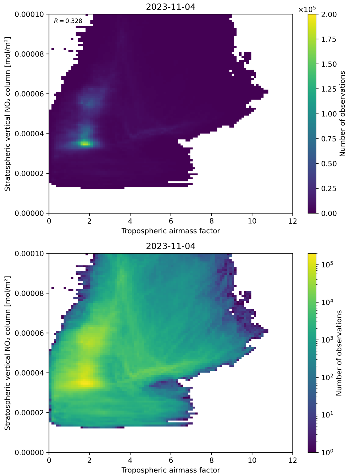
Figure 74: Scatter density plot of “Tropospheric air mass factor” against “Stratospheric vertical NO 2 column” for 2023-11-03 to 2023-11-05.
