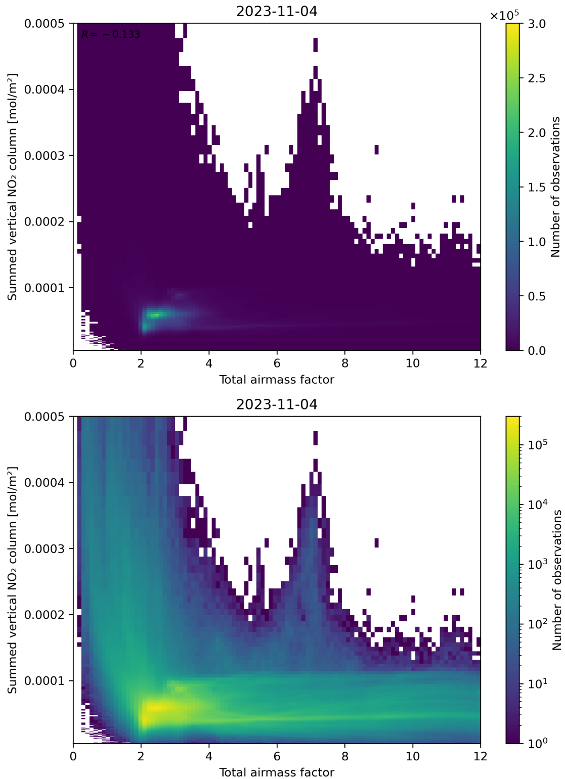
Figure 65: Scatter density plot of “Total airmass factor” against “Summed vertical NO 2 column” for 2023-11-03 to 2023-11-05.
