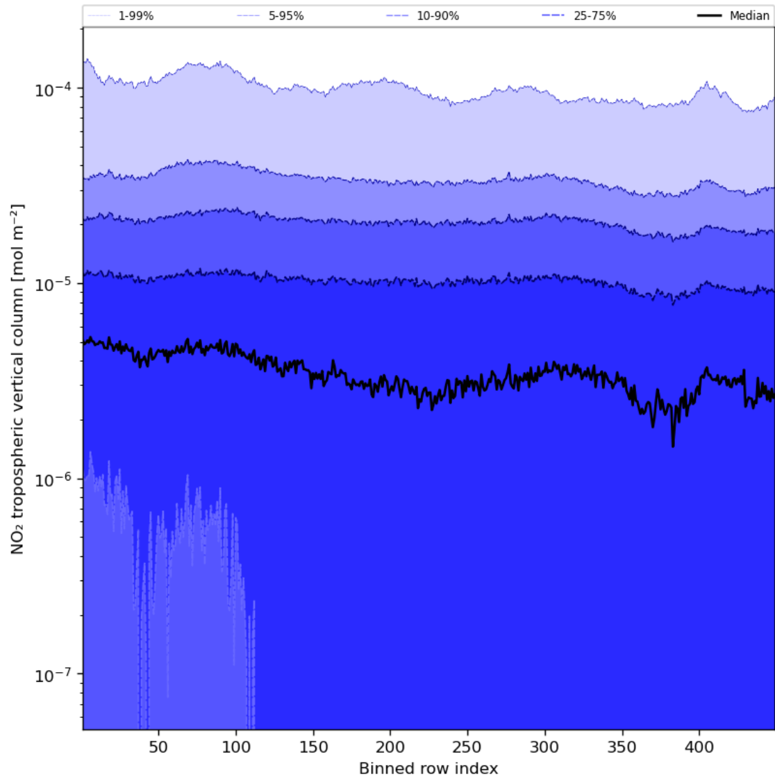
Figure 46: Along track statistics of “NO 2 tropospheric vertical column” for 2023-11-03 to 2023-11-05
