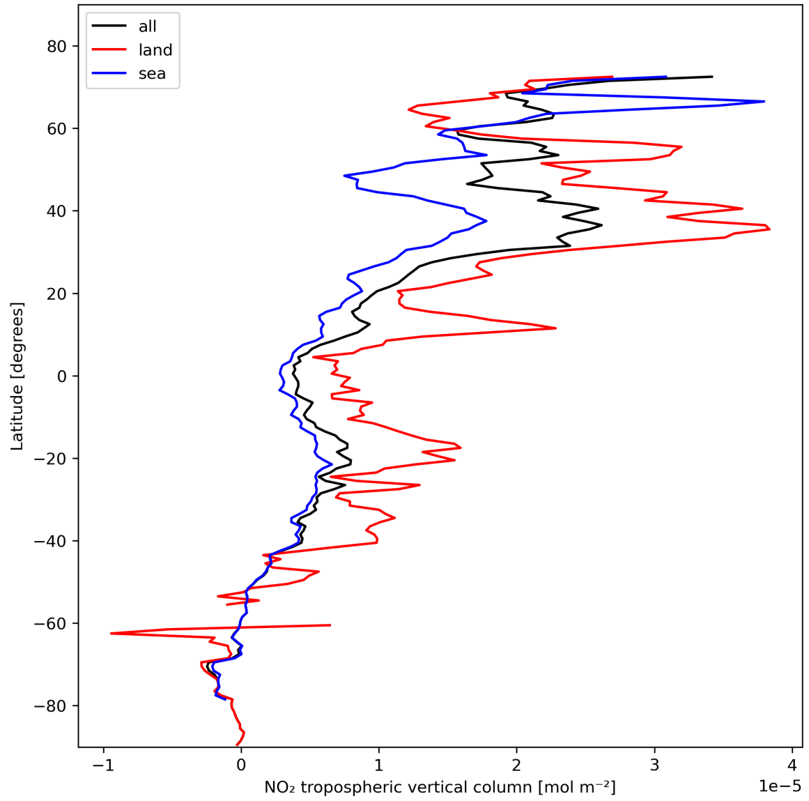
Figure 12: Zonal average of “NO 2 tropospheric vertical column” for 2023-11-03 to 2023-11-05.
