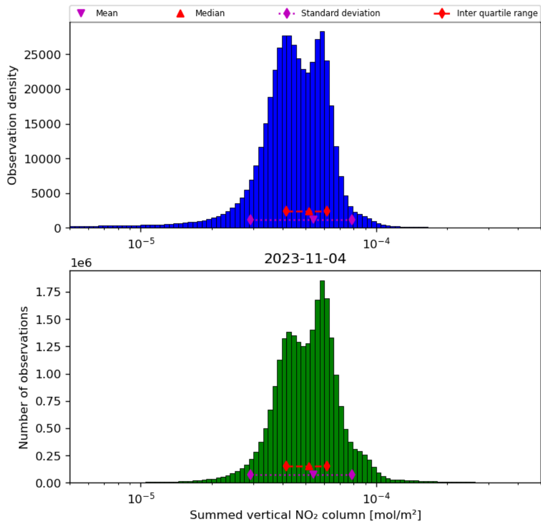
Figure 40: Histogram of “Summed vertical NO 2 column” for 2023-11-03 to 2023-11-05
