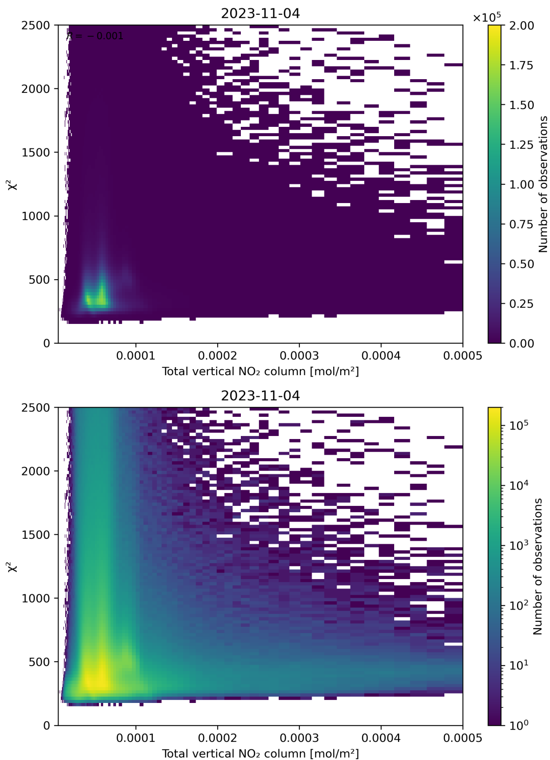
Figure 111: Scatter density plot of “Total vertical NO 2 column” against “ \chi^2 ” for 2023-11-03 to 2023-11-05.
