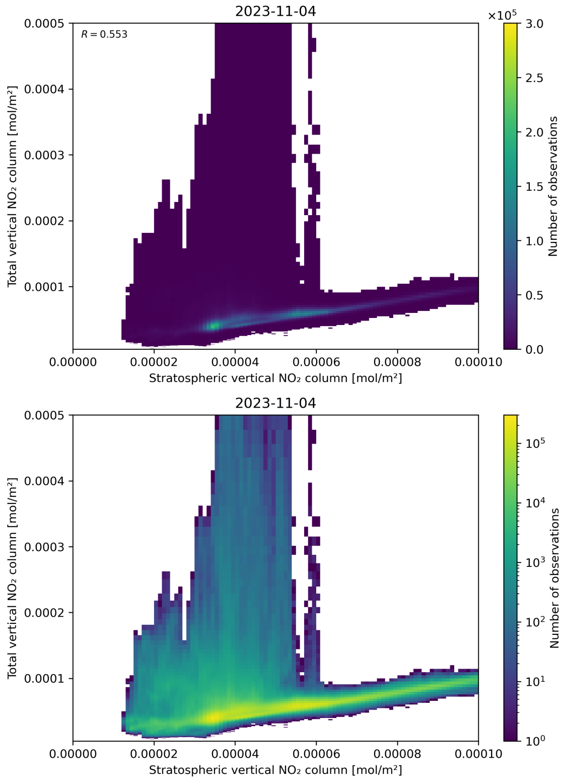
Figure 100: Scatter density plot of “Stratospheric vertical NO 2 column” against “Total vertical NO 2 column” for 2023-11-03 to 2023-11-05.
