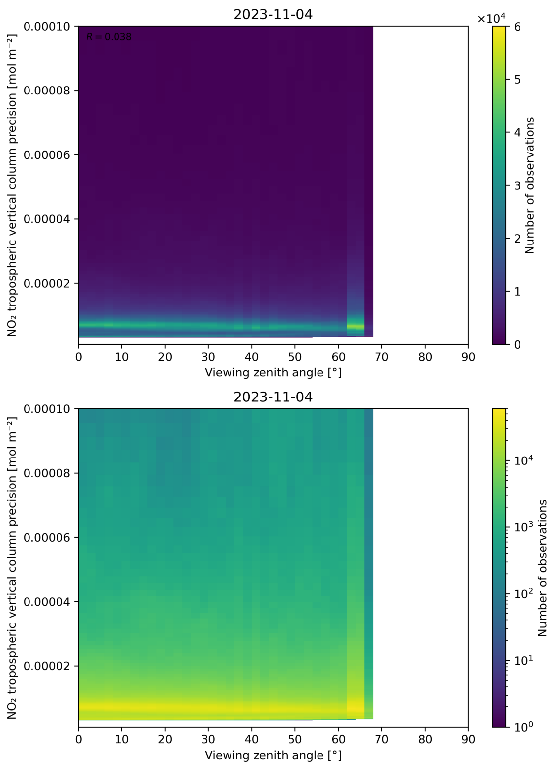
Figure 170: Scatter density plot of “Viewing zenith angle” against “NO 2 tropospheric vertical column precision” for 2023-11-03 to 2023-11-05.
