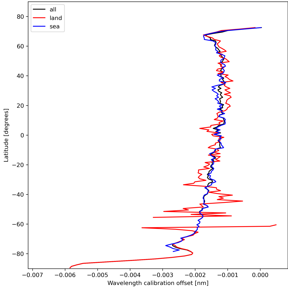
Figure 18: Zonal average of “Wavelength calibration offset” for 2023-11-03 to 2023-11-05.
