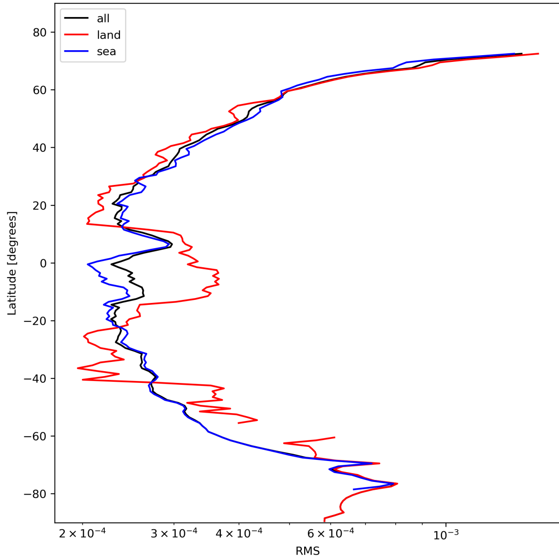
Figure 26: Zonal average of “RMS” for 2023-11-03 to 2023-11-05.
