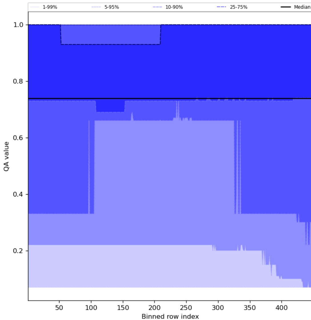
Figure 45: Along track statistics of “QA value” for 2023-11-03 to 2023-11-05
