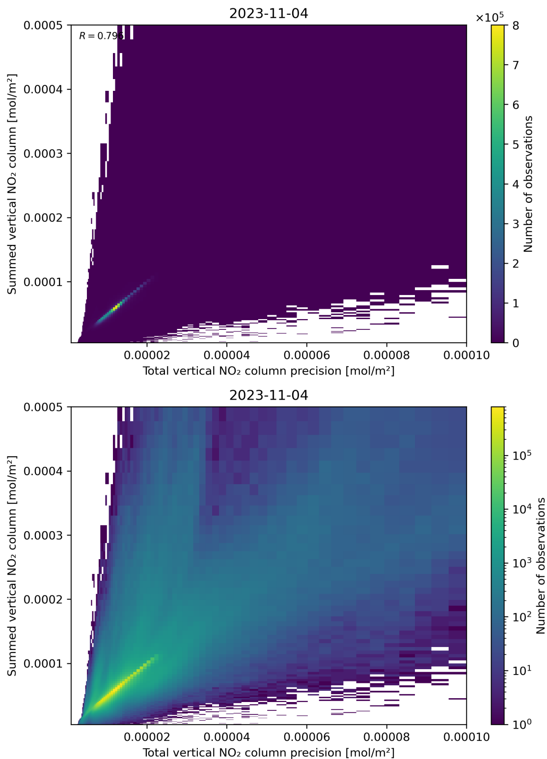
Figure 117: Scatter density plot of “Total vertical NO 2 column precision” against “Summed vertical NO 2 column” for 2023-11-03 to 2023-11-05.
