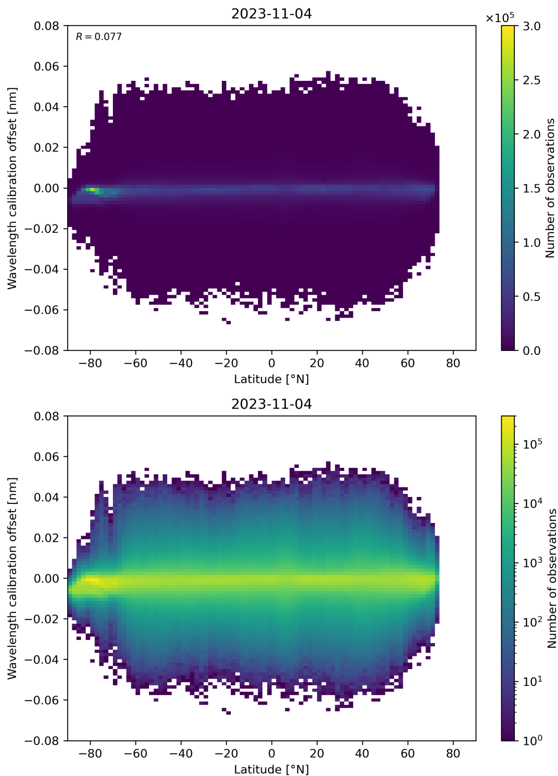
Figure 95: Scatter density plot of “Latitude” against “Wavelength calibration offset” for 2023-11-03 to 2023-11-05.
