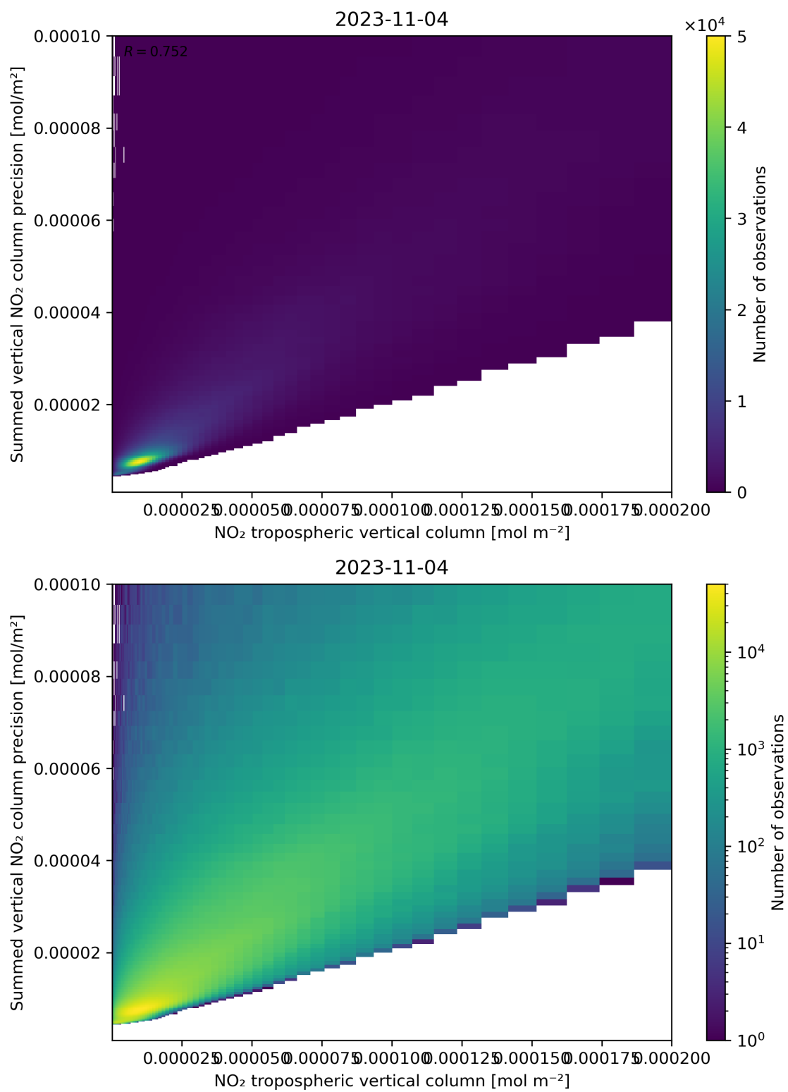
Figure 127: Scatter density plot of “NO 2 tropospheric vertical column” against “Summed vertical NO 2 column precision” for 2023-11-03 to 2023-11-05.
