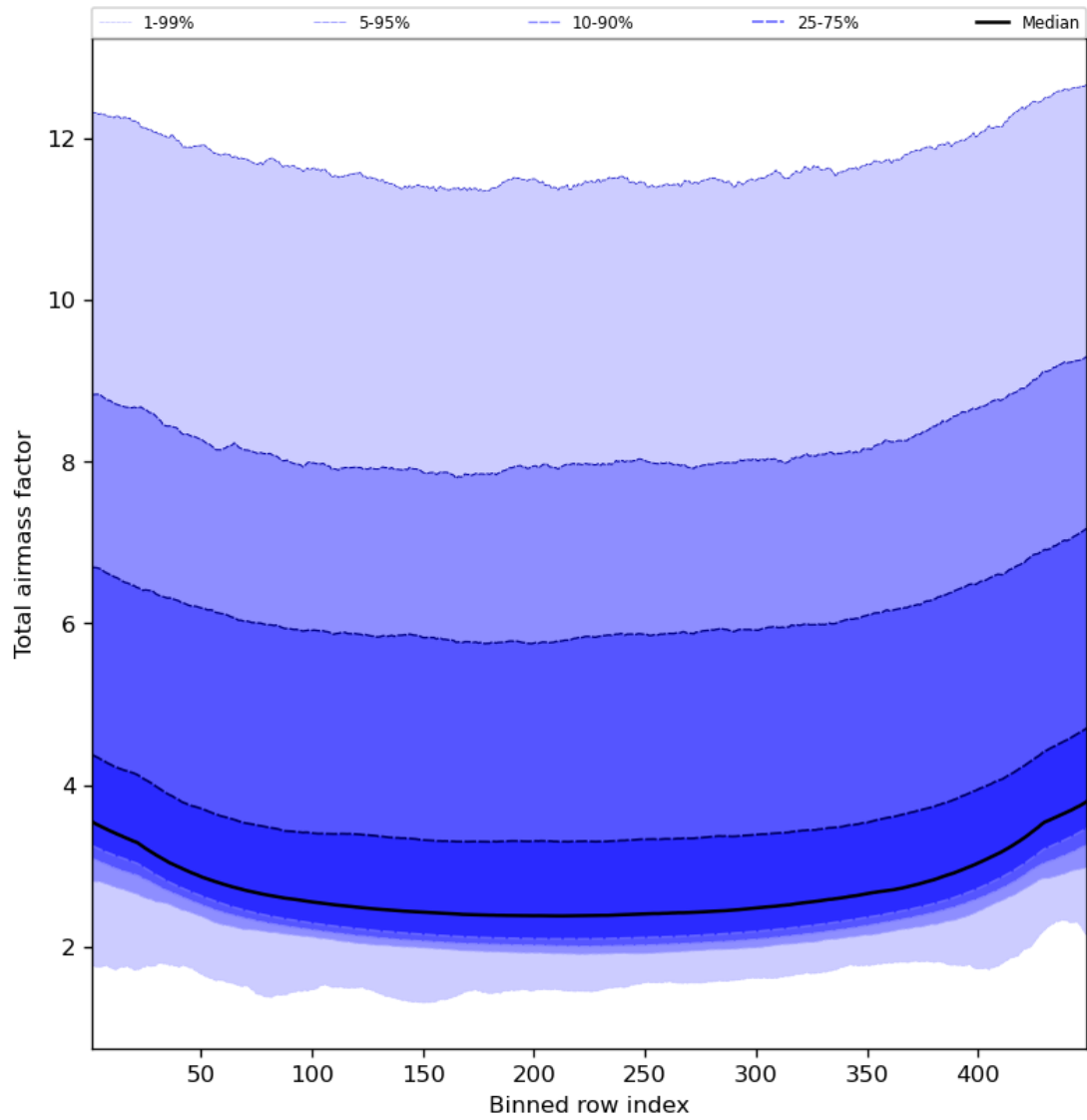
Figure 49: Along track statistics of “Total airmass factor” for 2023-11-03 to 2023-11-05
