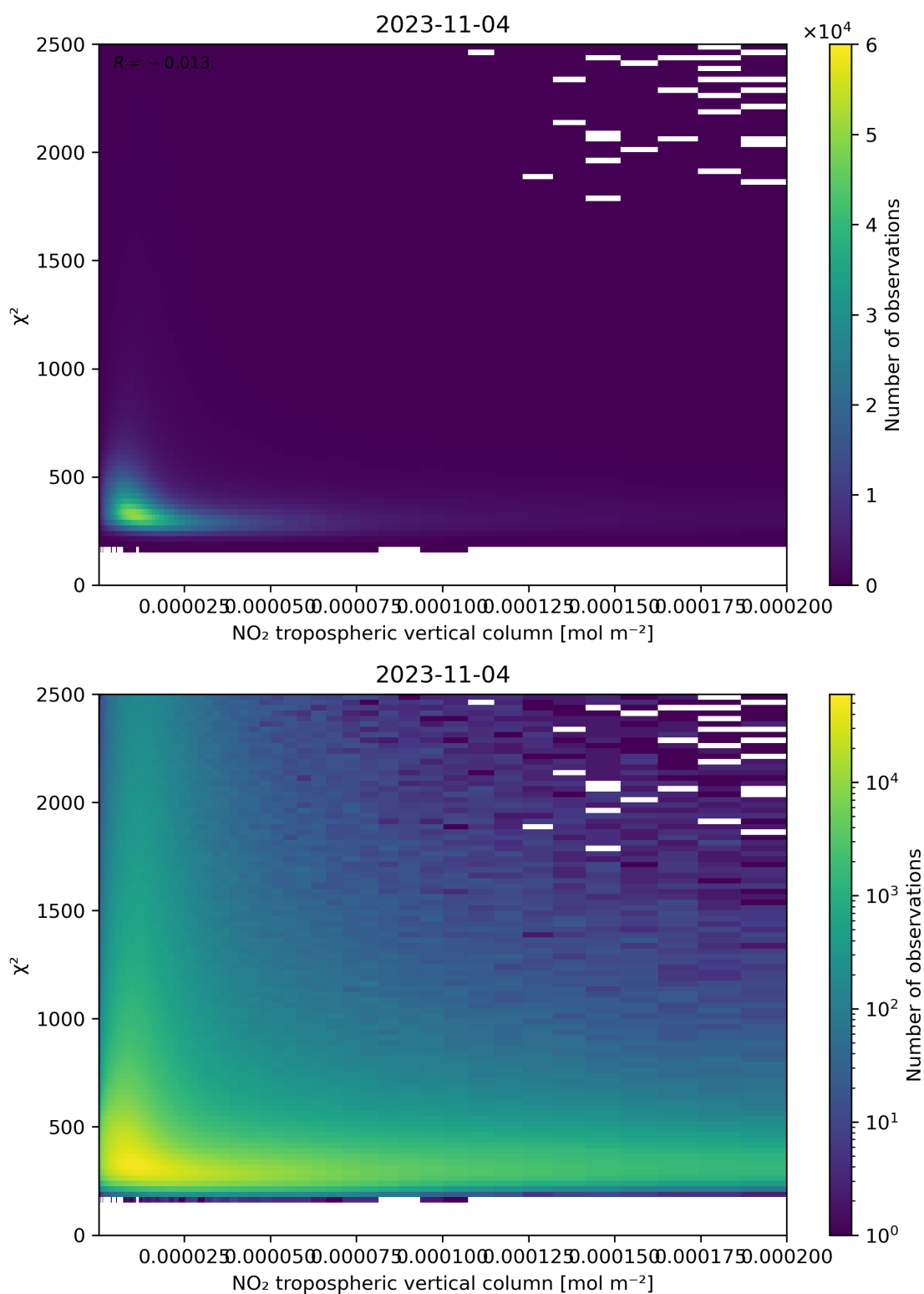
Figure 124: Scatter density plot of “NO 2 tropospheric vertical column” against “ \chi^2 ” for 2023-11-03 to 2023-11-05.
