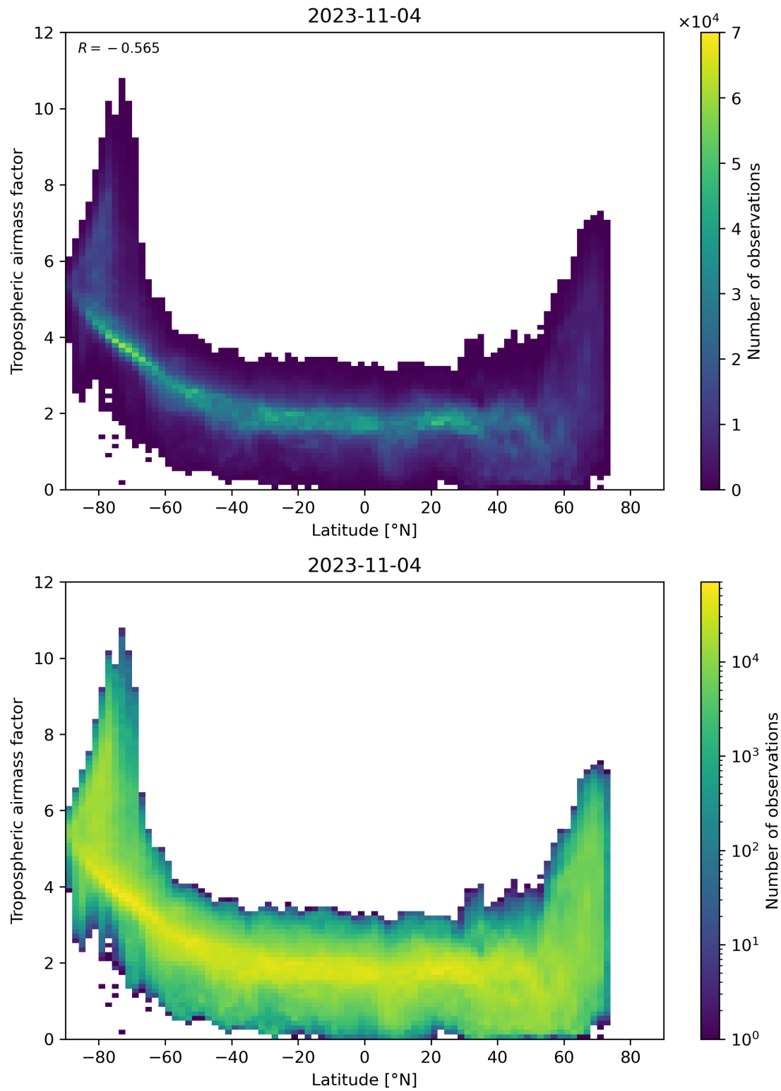
Figure 85: Scatter density plot of “Latitude” against “Tropospheric airmass factor” for 2023-11-03 to 2023-11-05.
