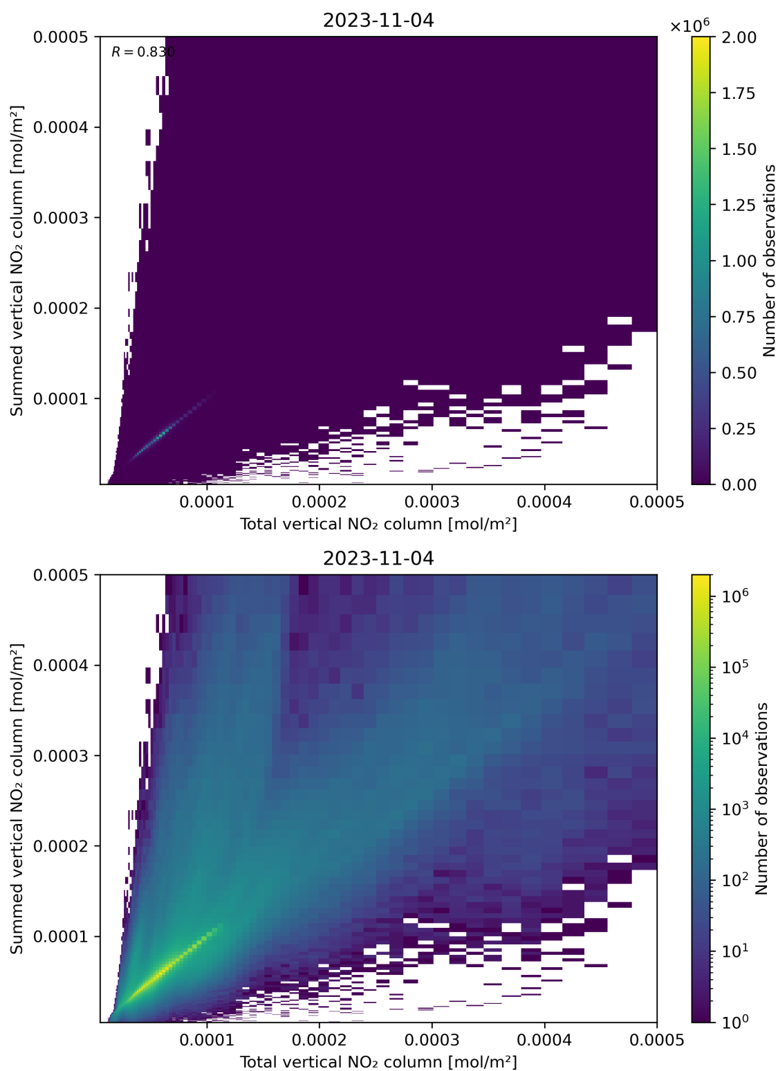
Figure 112: Scatter density plot of “Total vertical NO 2 column” against “Summed vertical NO 2 column” for 2023-11-03 to 2023-11-05.
