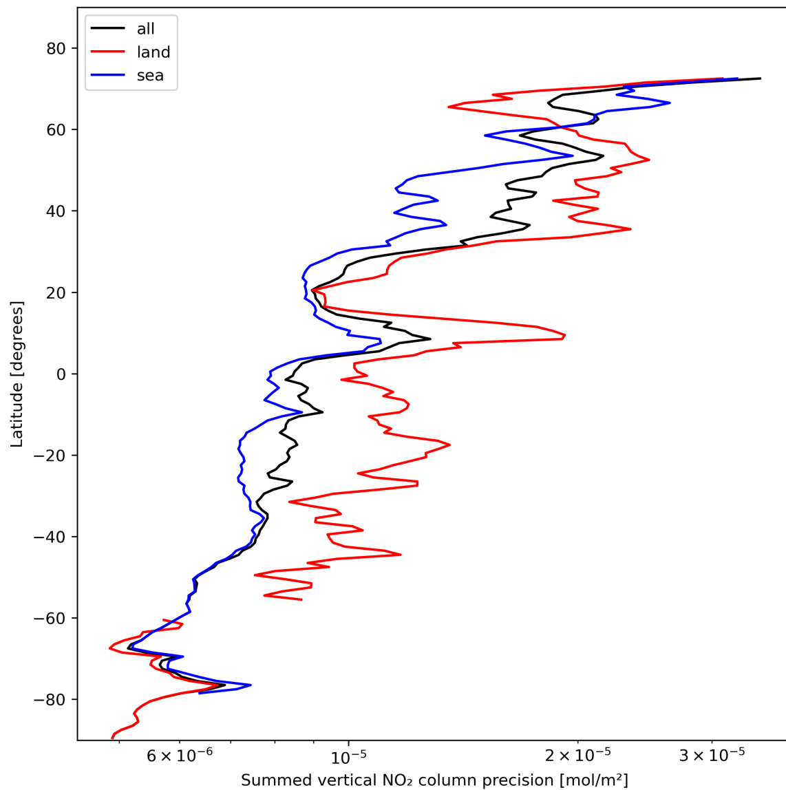
Figure 24: Zonal average of “Summed vertical NO 2 column precision” for 2023-11-03 to 2023-11-05.
