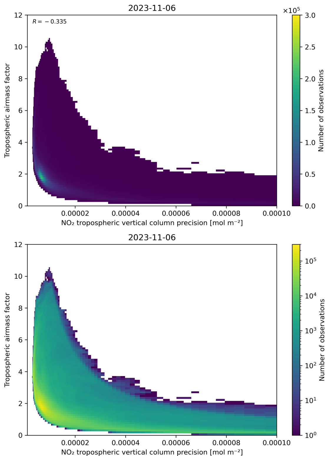
Figure 133: Scatter density plot of “NO 2 tropospheric vertical column precision” against “Tropospheric airmass factor” for 2023-11-05 to 2023-11-07.
