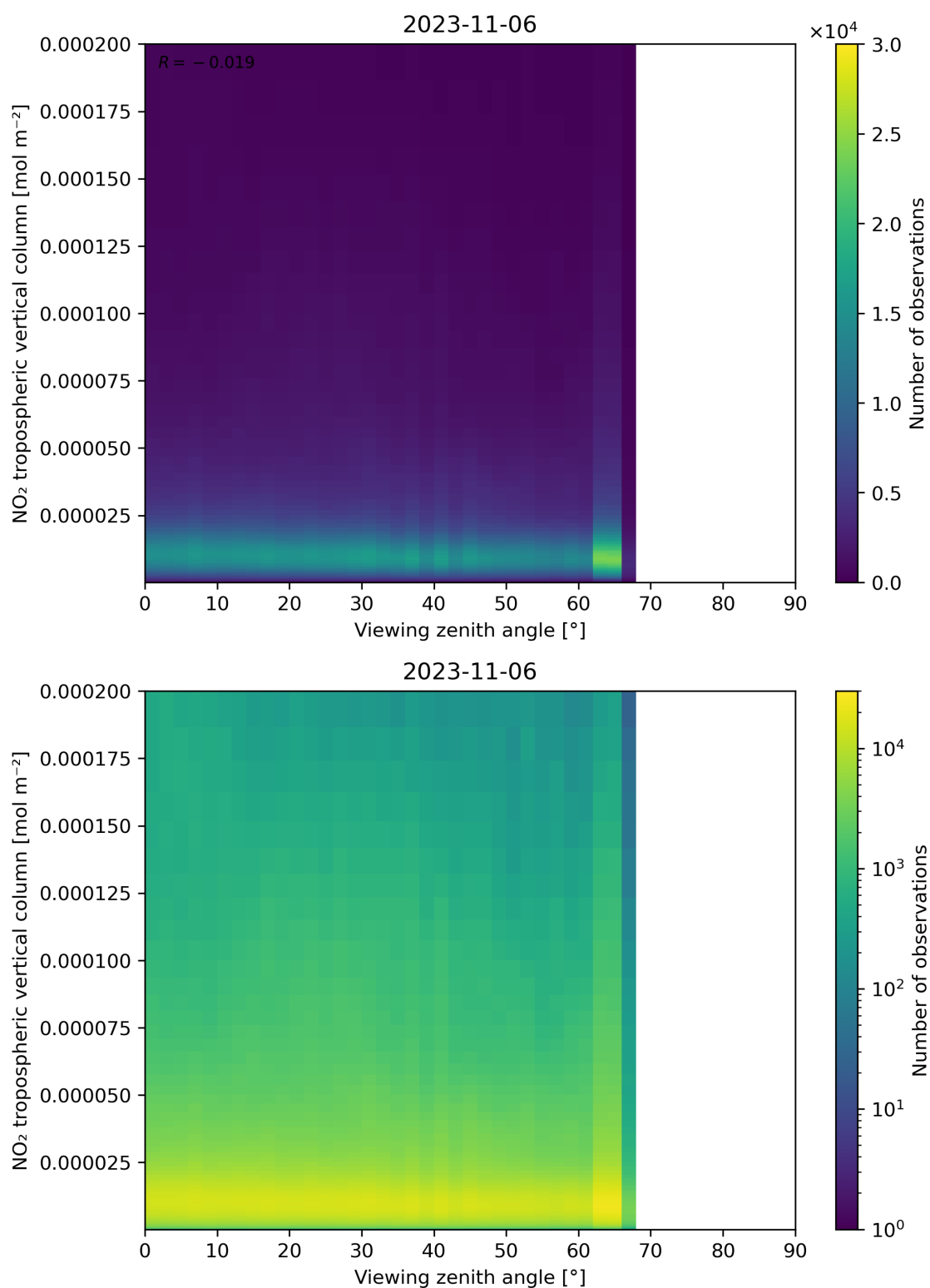
Figure 169: Scatter density plot of “Viewing zenith angle” against “NO 2 tropospheric vertical column” for 2023-11-05 to 2023-11-07.
