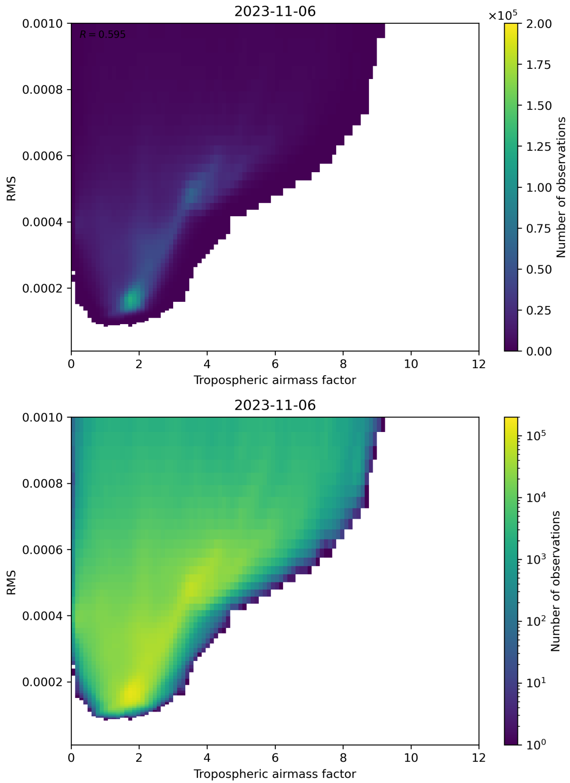
Figure 79: Scatter density plot of “Tropospheric airmass factor” against “RMS” for 2023-11-05 to 2023-11-07.
