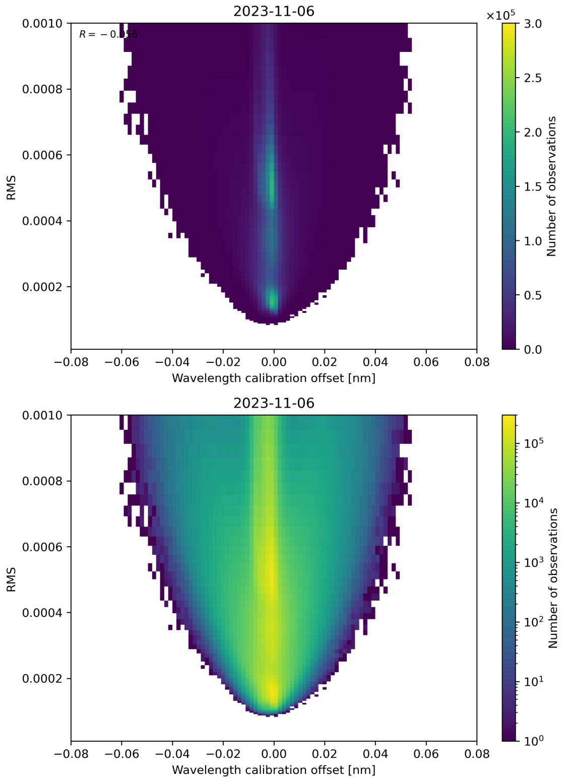
Figure 181: Scatter density plot of “Wavelength calibration offset” against “RMS” for 2023-11-05 to 2023-11-07.
