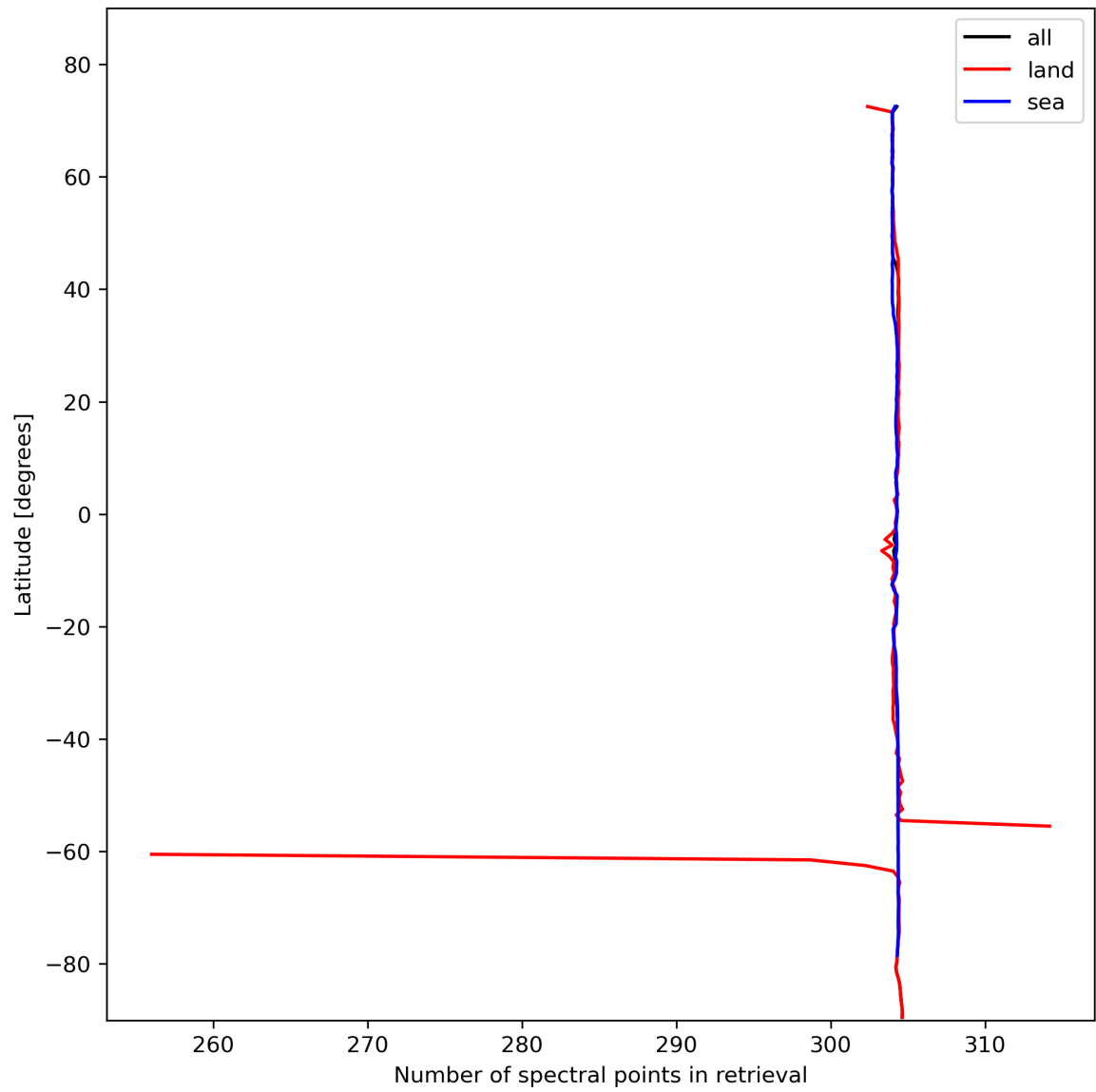
Figure 16: Zonal average of “Number of spectral points in retrieval” for 2023-11-05 to 2023-11-07.
