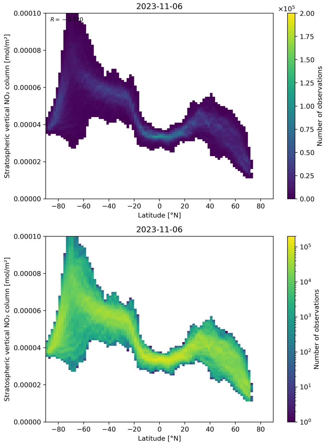
Figure 87: Scatter density plot of “Latitude” against “Stratospheric vertical NO 2 column” for 2023-11-05 to 2023-11-07.
