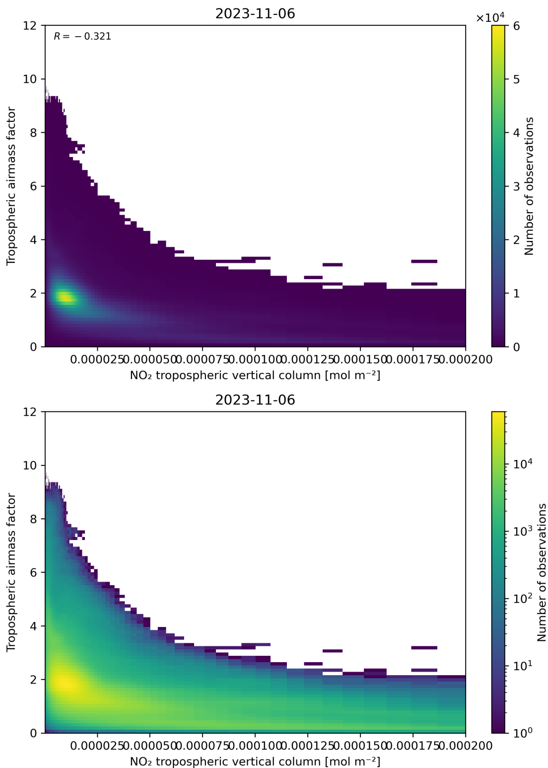
Figure 123: Scatter density plot of “NO 2 tropospheric vertical column” against “Tropospheric airmass factor” for 2023-11-05 to 2023-11-07.
