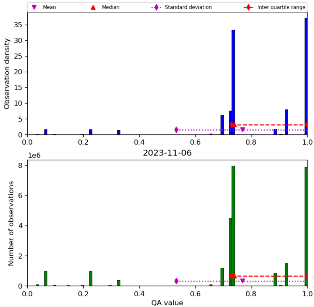
Figure 28: Histogram of “QA value” for 2023-11-05 to 2023-11-07
