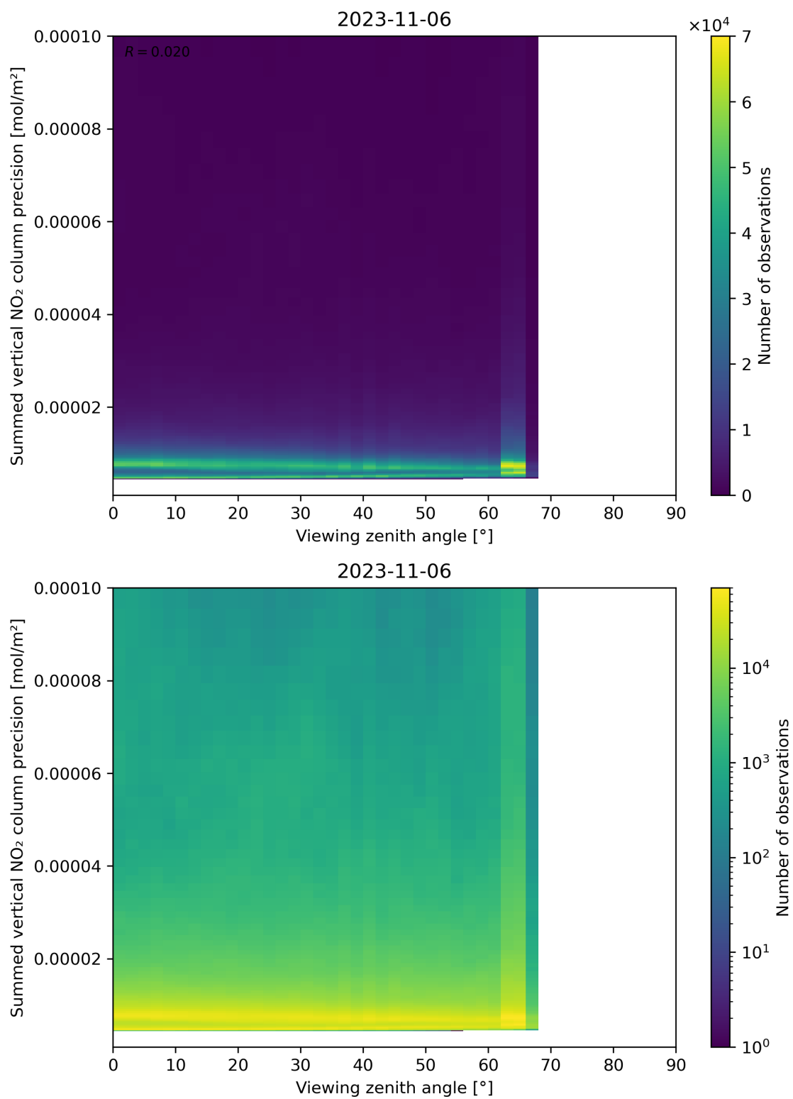
Figure 166: Scatter density plot of “Viewing zenith angle” against “Summed vertical NO 2 column precision” for 2023-11-05 to 2023-11-07.
