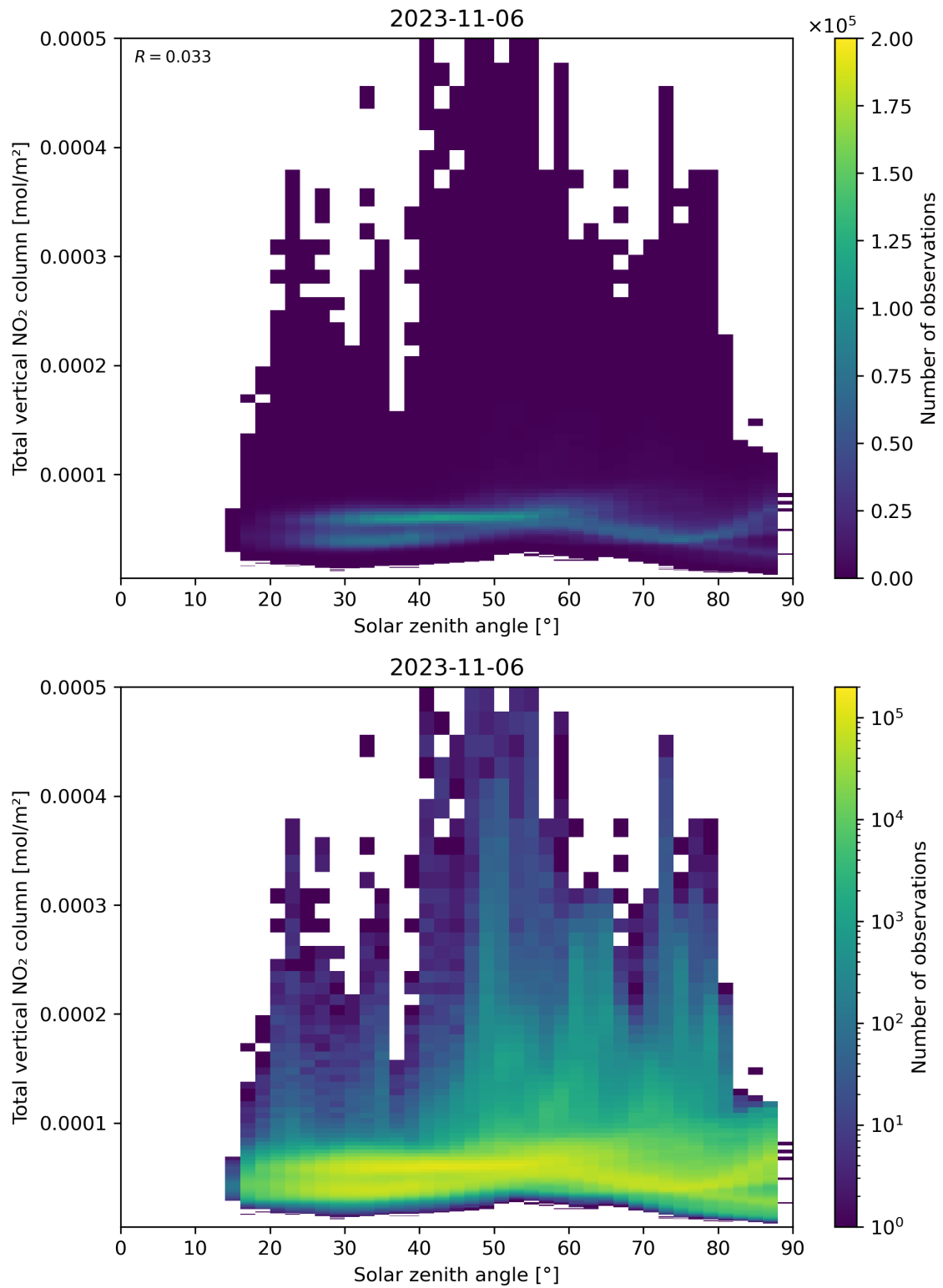
Figure 153: Scatter density plot of “Solar zenith angle” against “Total vertical NO 2 column” for 2023-11-05 to 2023-11-07.
