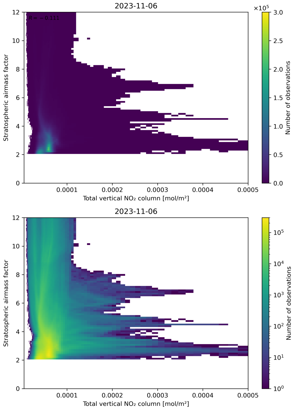
Figure 110: Scatter density plot of “Total vertical NO 2 column” against “Stratospheric air mass factor” for 2023-11-05 to 2023-11-07.
