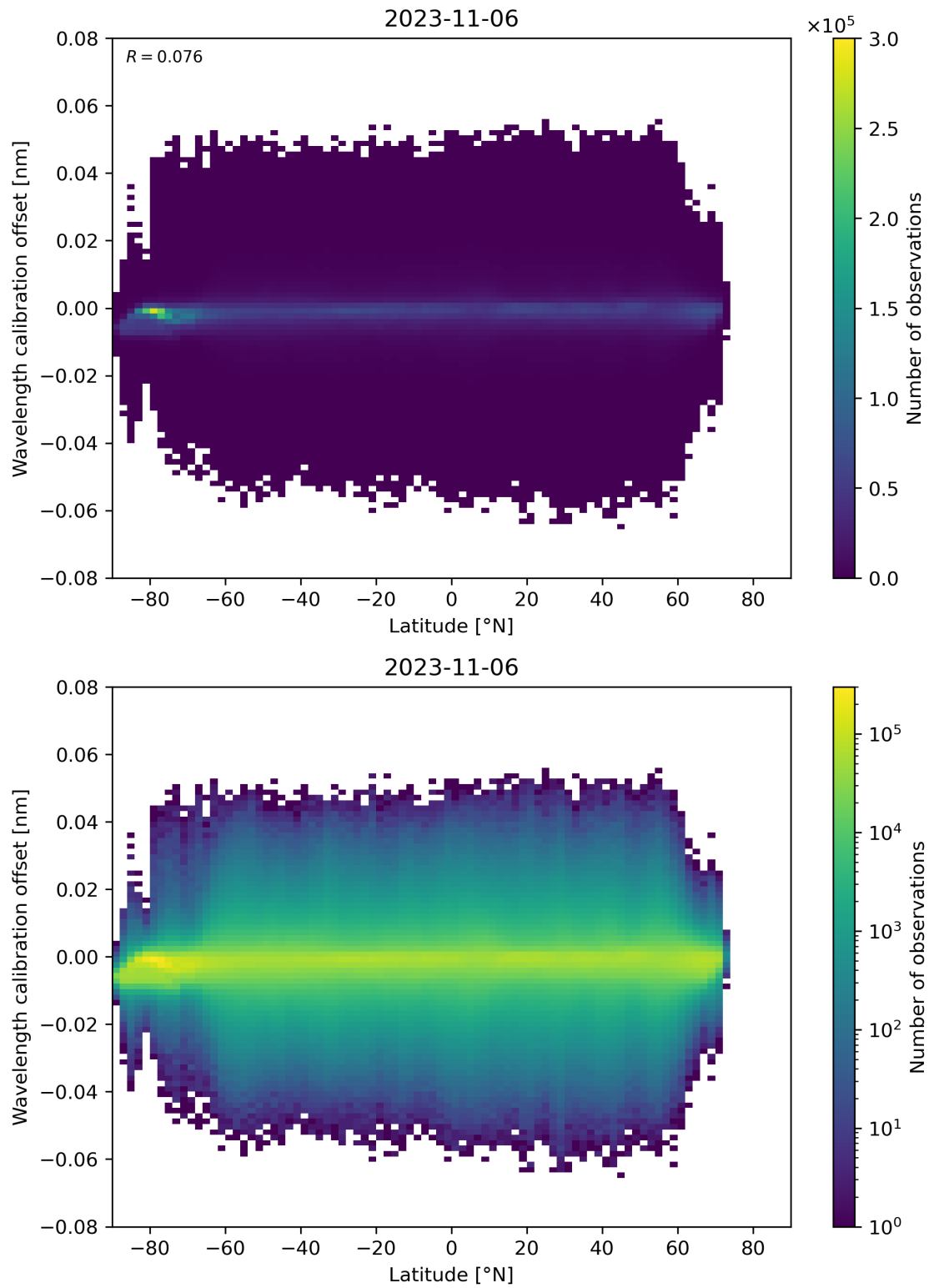
Figure 95: Scatter density plot of “Latitude” against “Wavelength calibration offset” for 2023-11-05 to 2023-11-07.
