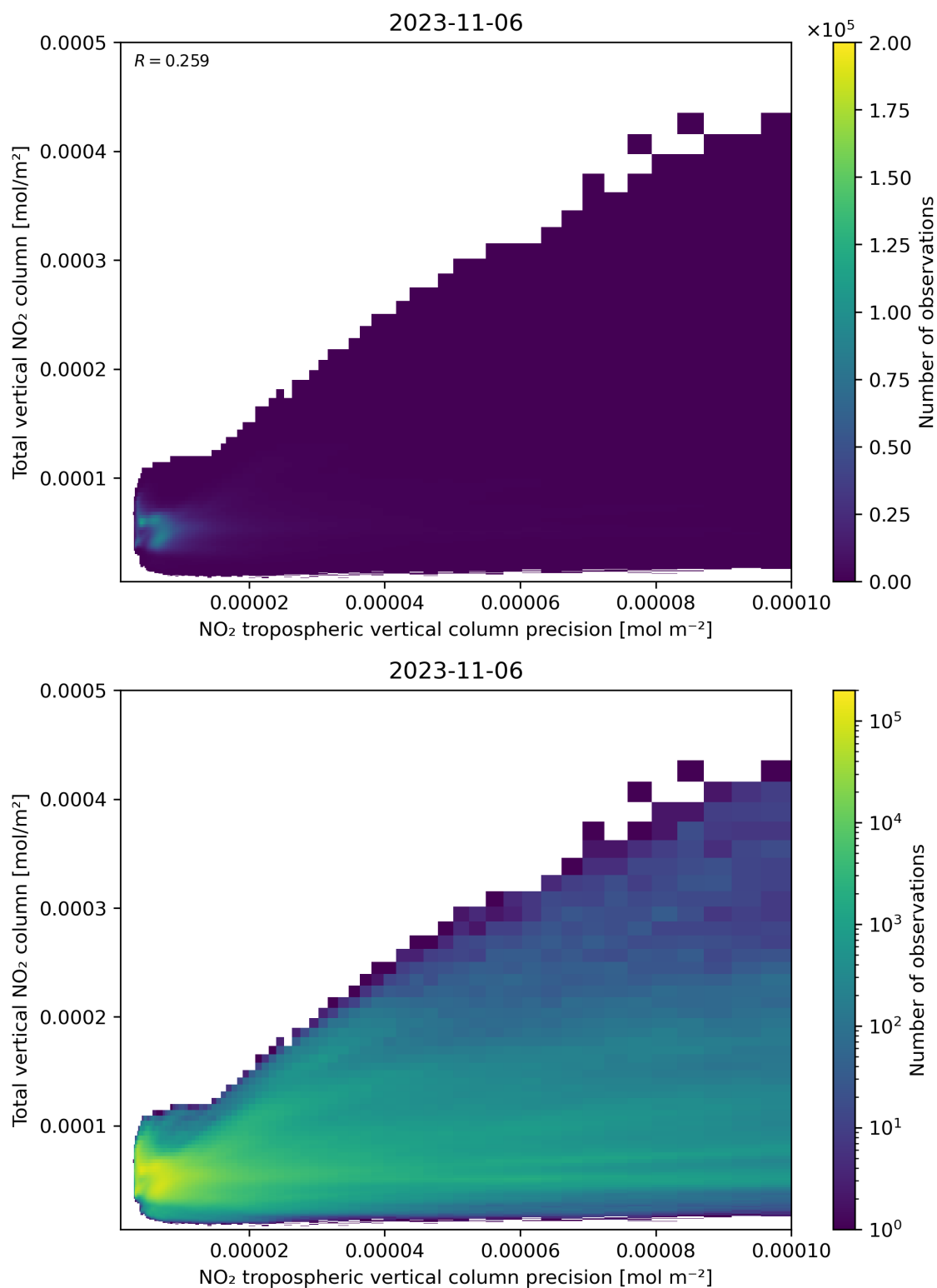
Figure 138: Scatter density plot of “NO 2 tropospheric vertical column precision” against “Total vertical NO 2 column” for 2023-11-05 to 2023-11-07.
