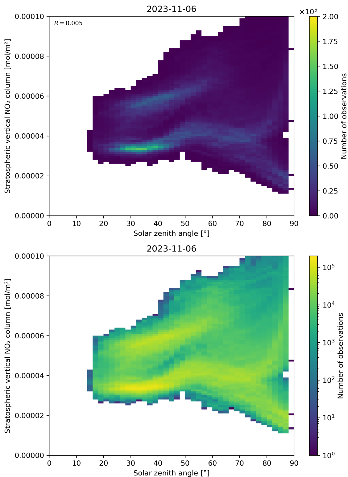
Figure 150: Scatter density plot of “Solar zenith angle” against “Stratospheric vertical \text{NO}_2 column” for 2023-11-05 to 2023-11-07.
