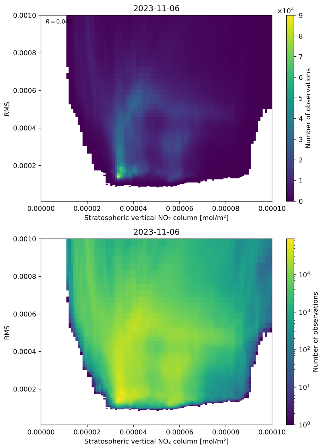
Figure 102: Scatter density plot of “Stratospheric vertical NO 2 column” against “RMS” for 2023-11-05 to 2023-11-07.
