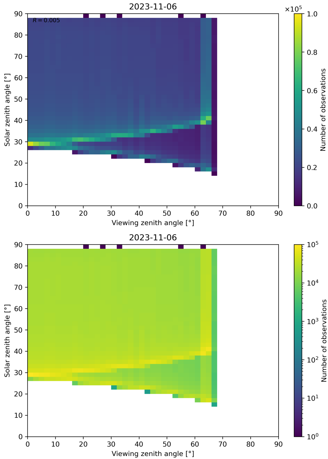
Figure 172: Scatter density plot of “Viewing zenith angle” against “Solar zenith angle” for 2023-11-05 to 2023-11-07.
