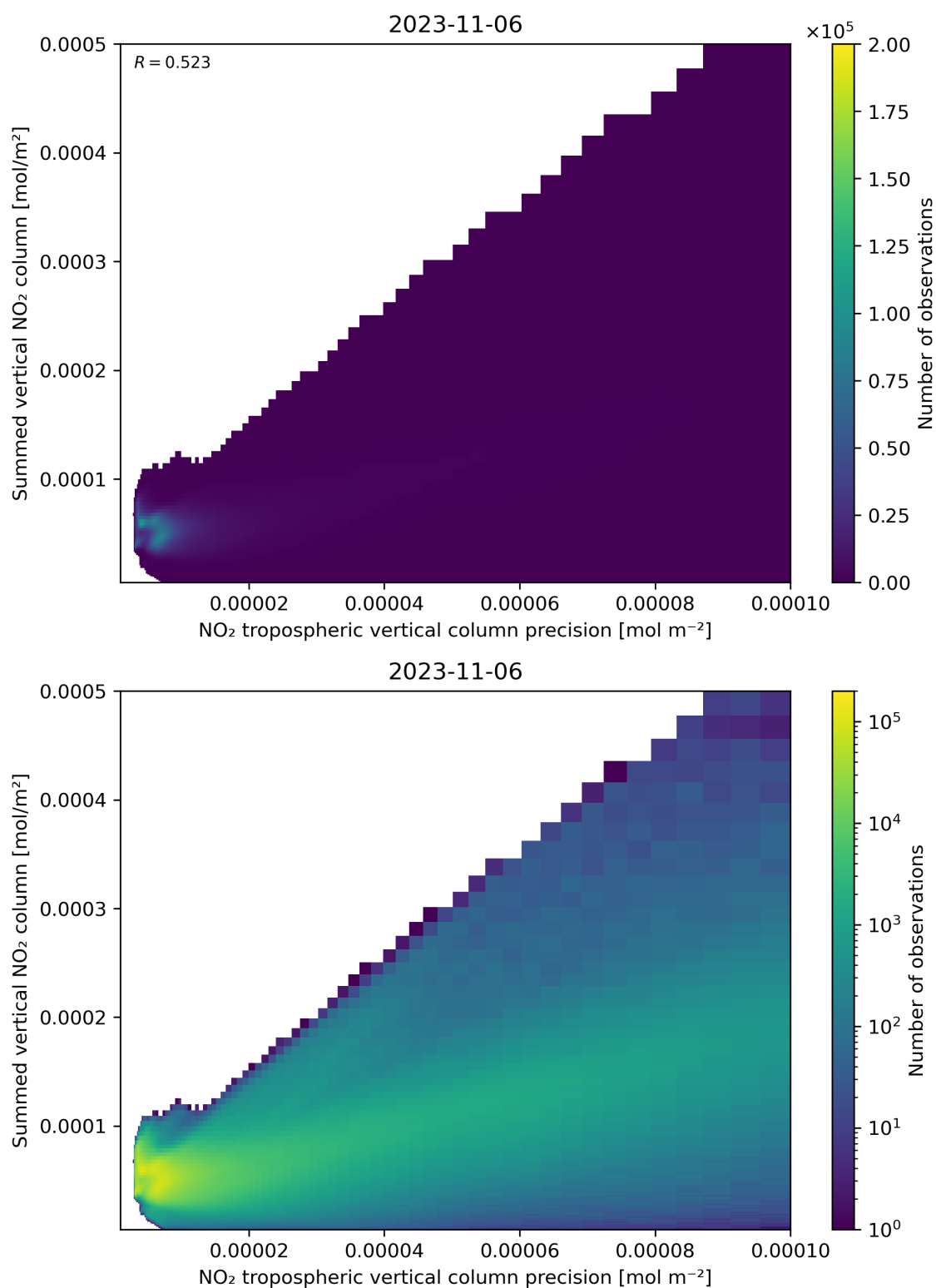
Figure 136: Scatter density plot of “NO 2 tropospheric vertical column precision” against “Summed vertical NO 2 column” for 2023-11-05 to 2023-11-07.
