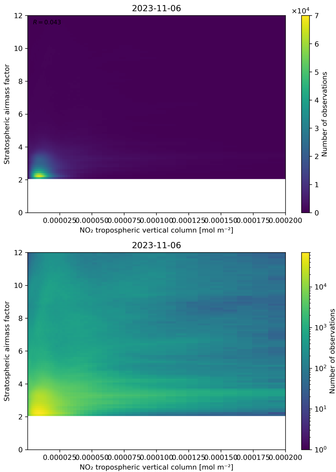
Figure 121: Scatter density plot of “NO 2 tropospheric vertical column” against “Stratospheric airmass factor” for 2023-11-05 to 2023-11-07.
