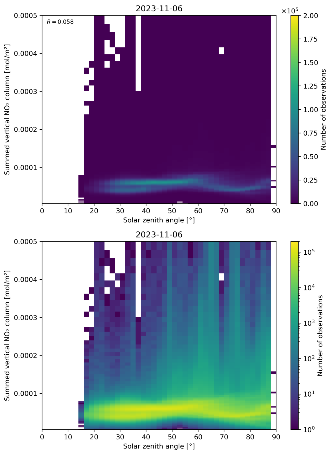
Figure 151: Scatter density plot of “Solar zenith angle” against “Summed vertical NO 2 column” for 2023-11-05 to 2023-11-07.
