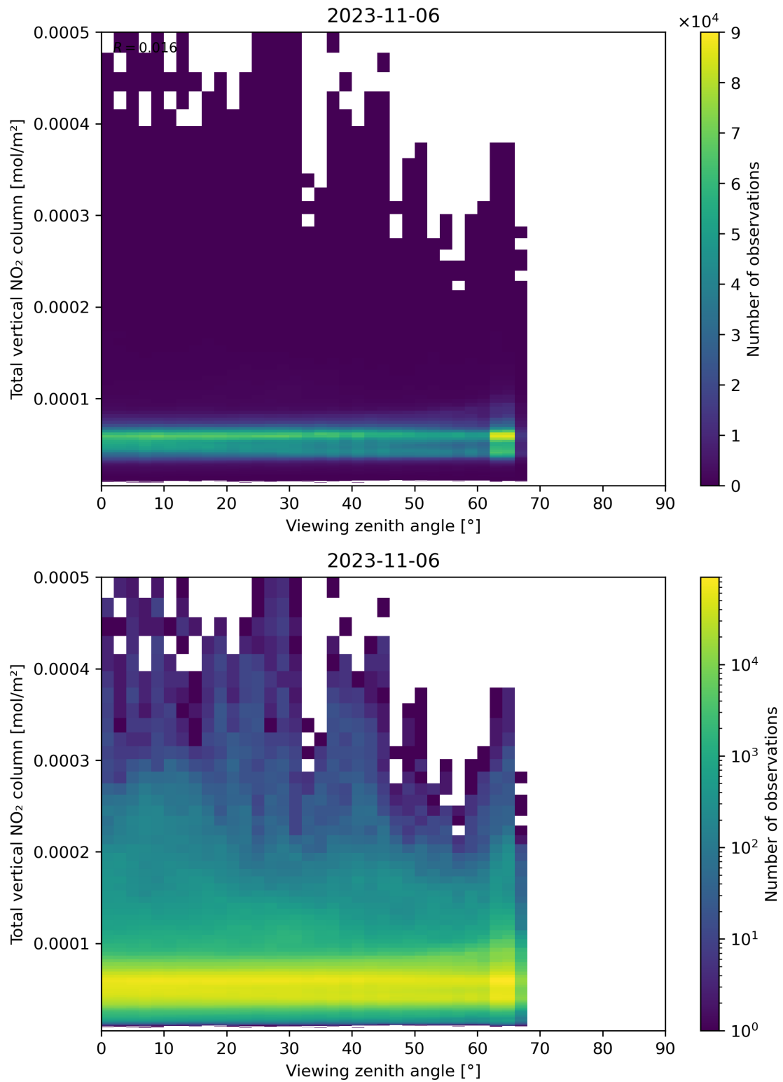
Figure 167: Scatter density plot of “Viewing zenith angle” against “Total vertical NO 2 column” for 2023-11-05 to 2023-11-07.
