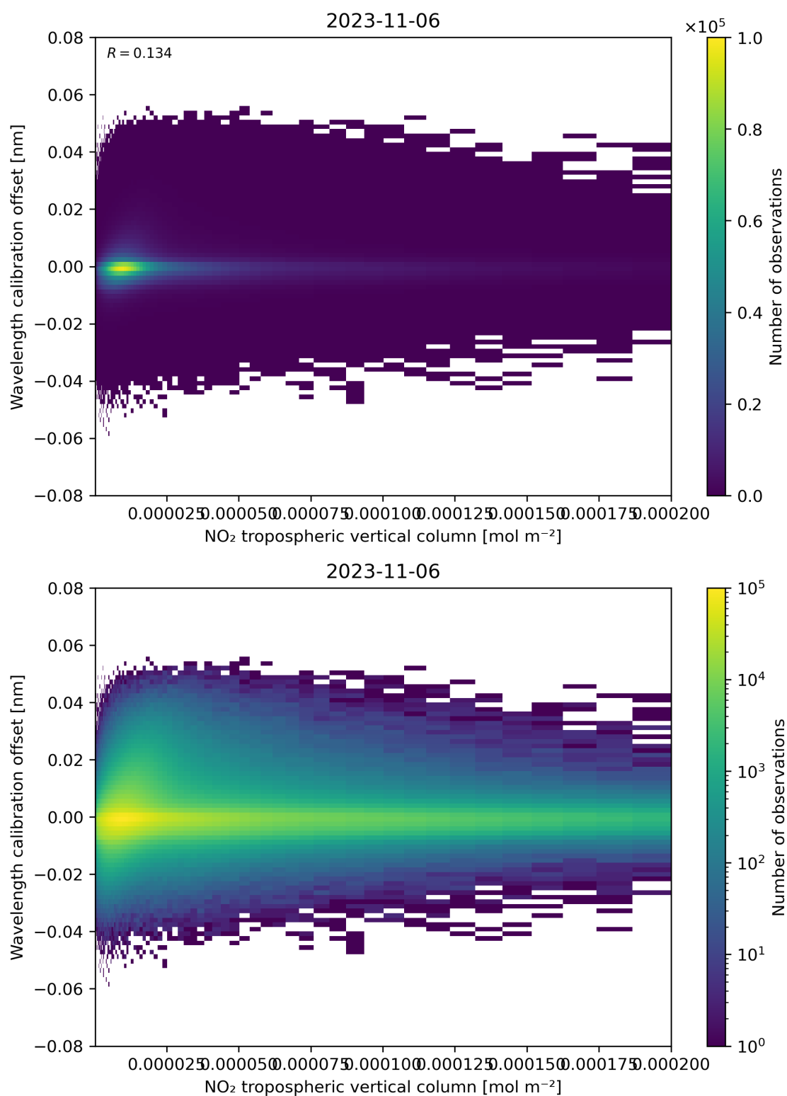
Figure 143: Scatter density plot of “NO 2 tropospheric vertical column” against “Wavelength calibration offset” for 2023-11-05 to 2023-11-07.
