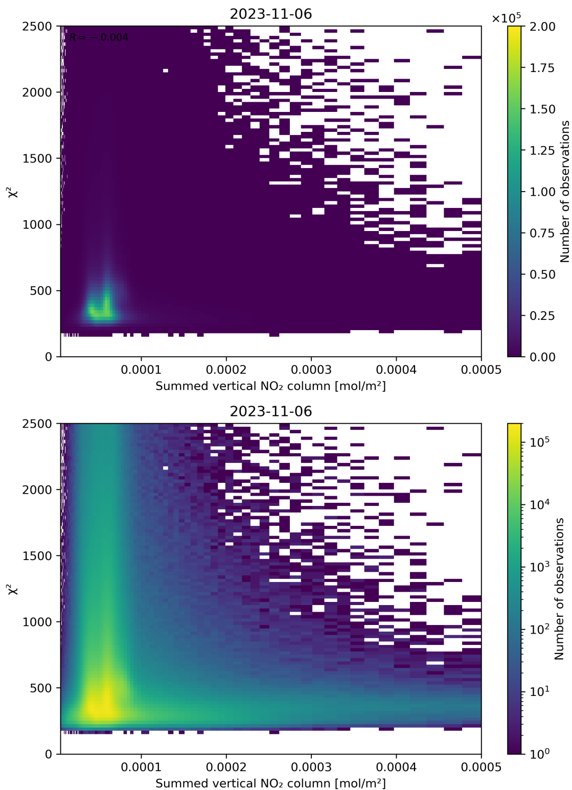
Figure 104: Scatter density plot of “Summed vertical NO 2 column” against “ \chi^2 ” for 2023-11-05 to 2023-11-07.
