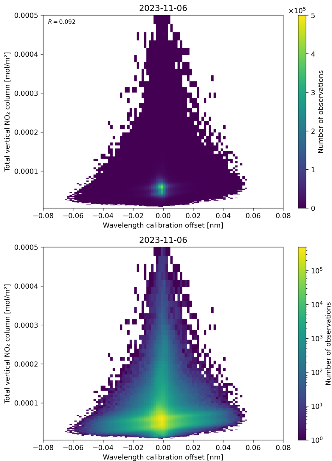
Figure 179: Scatter density plot of “Wavelength calibration offset” against “Total vertical NO 2 column” for 2023-11-05 to 2023-11-07.
