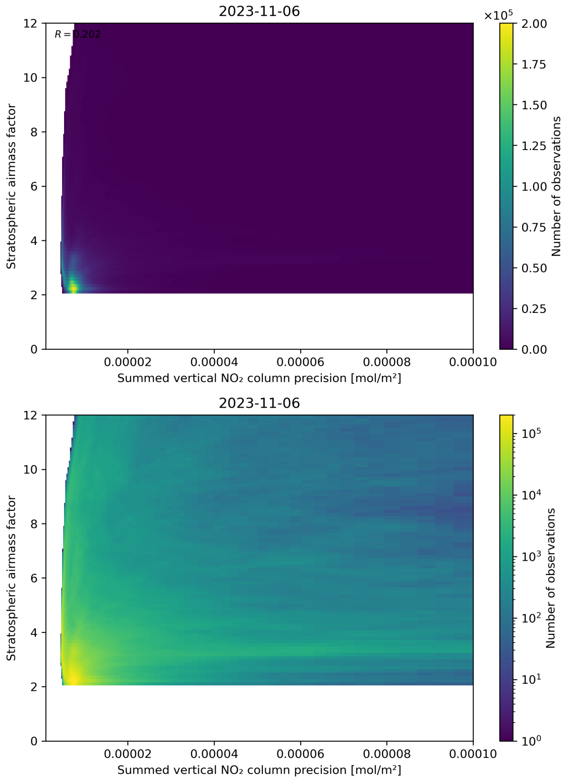
Figure 106: Scatter density plot of “Summed vertical NO 2 column precision” against “Stratospheric airmass factor” for 2023-11-05 to 2023-11-07.
