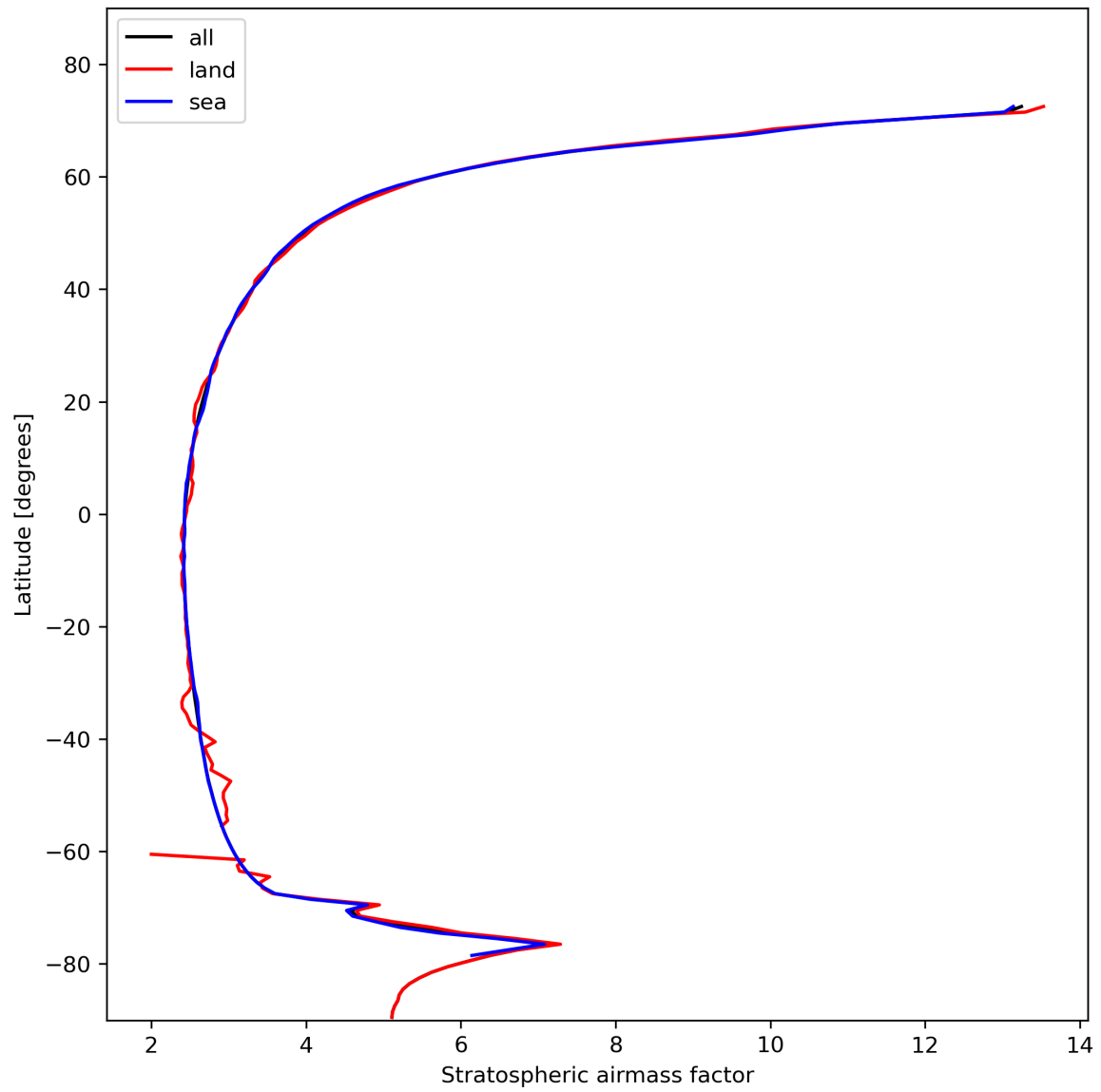
Figure 27: Zonal average of “Stratospheric airmass factor” for 2023-11-05 to 2023-11-07.
