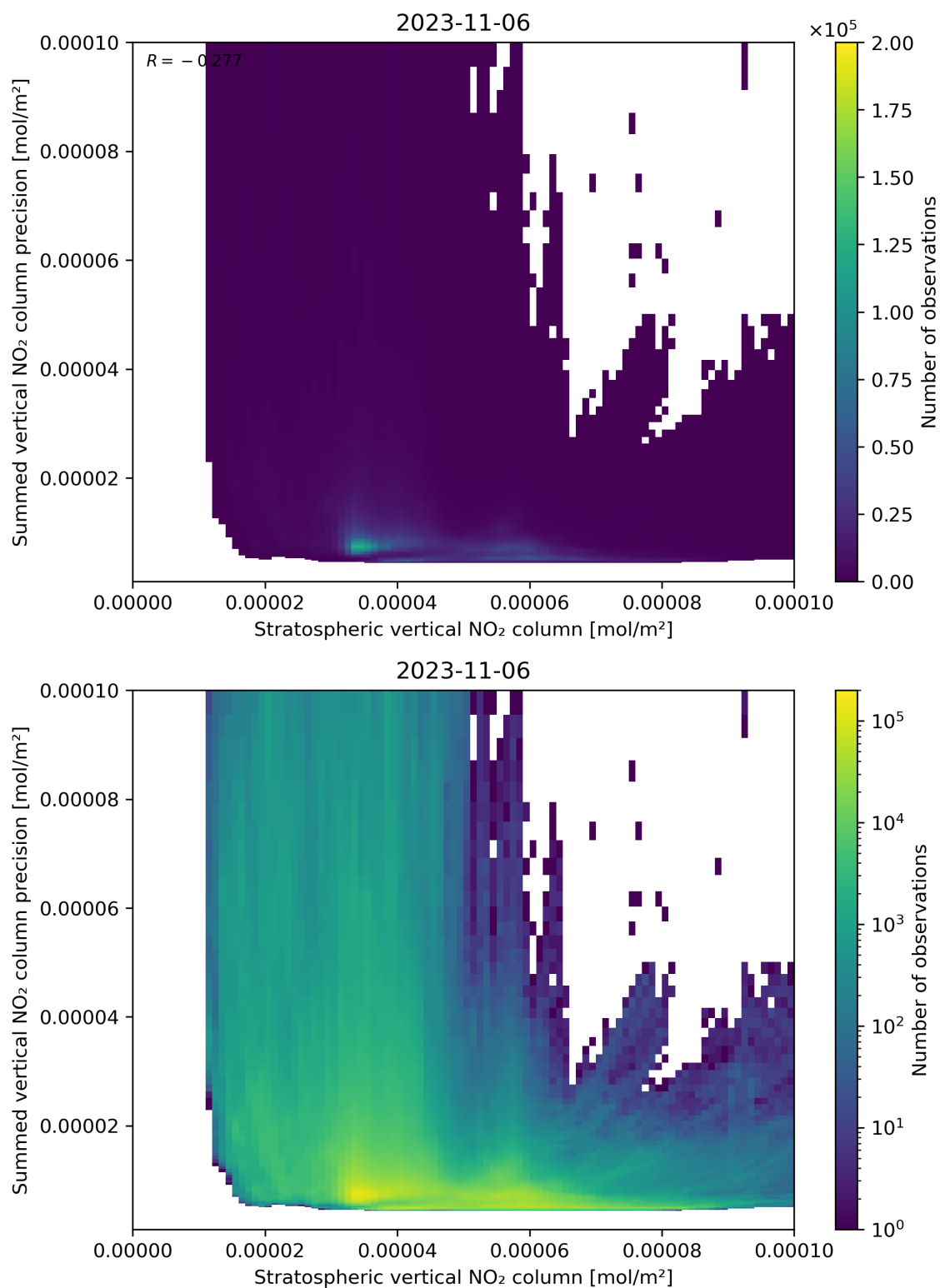
Figure 99: Scatter density plot of “Stratospheric vertical NO 2 column” against “Summed vertical NO 2 column precision” for 2023-11-05 to 2023-11-07.
