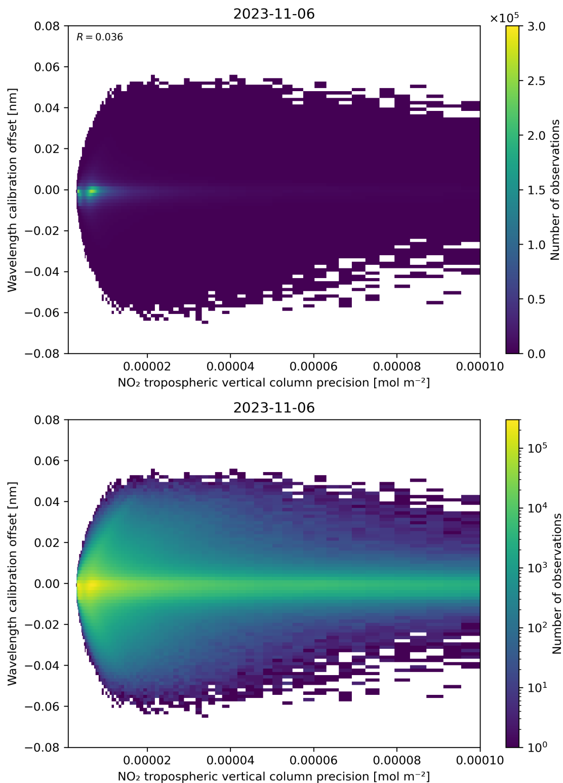
Figure 141: Scatter density plot of “NO 2 tropospheric vertical column precision” against “Wavelength calibration offset” for 2023-11-05 to 2023-11-07.
