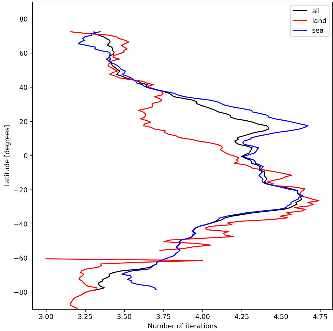
Figure 17: Zonal average of “Number of iterations” for 2023-11-05 to 2023-11-07.
