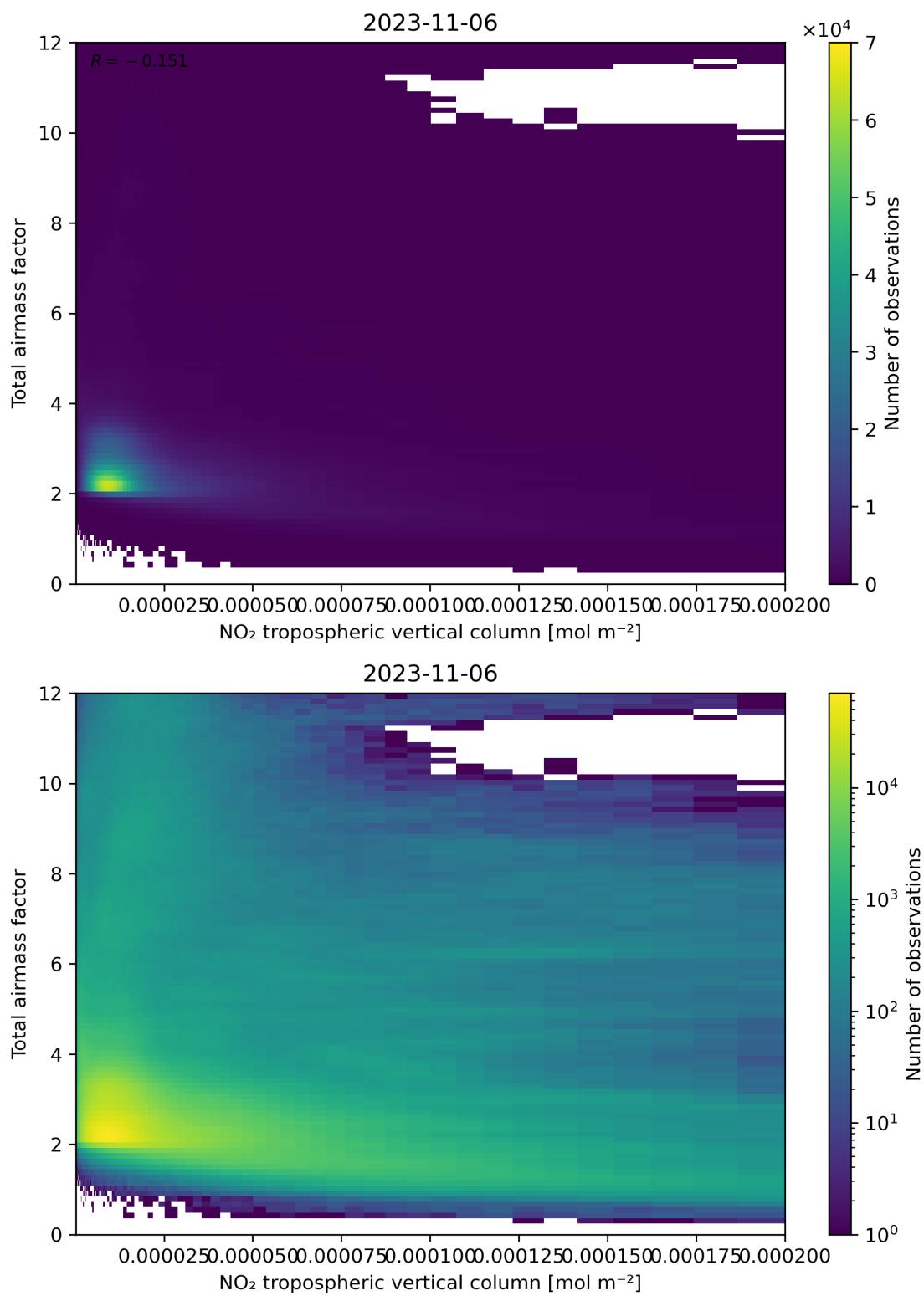
Figure 122: Scatter density plot of “NO 2 tropospheric vertical column” against “Total air mass factor” for 2023-11-05 to 2023-11-07.
