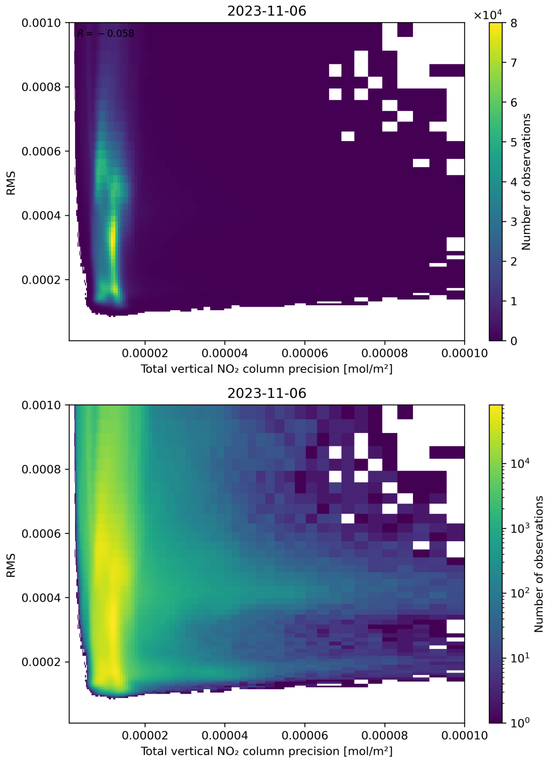
Figure 119: Scatter density plot of “Total vertical NO 2 column precision” against “RMS” for 2023-11-05 to 2023-11-07.
