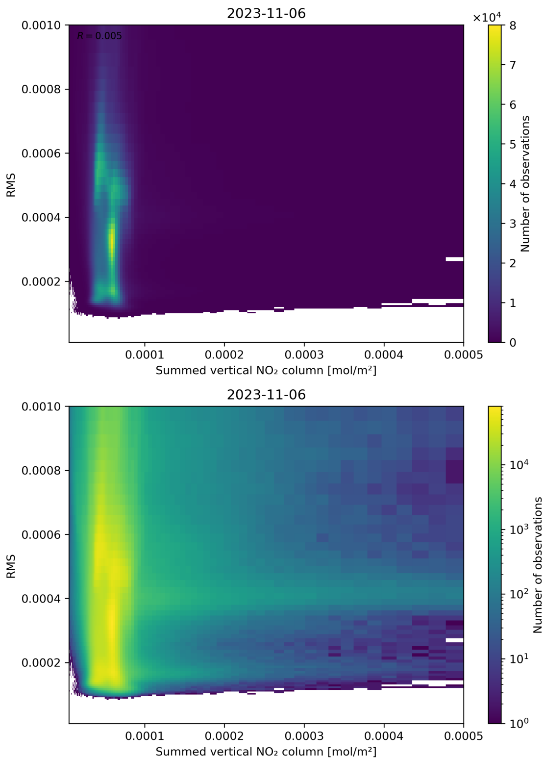
Figure 109: Scatter density plot of “Summed vertical NO 2 column” against “RMS” for 2023-11-05 to 2023-11-07.
