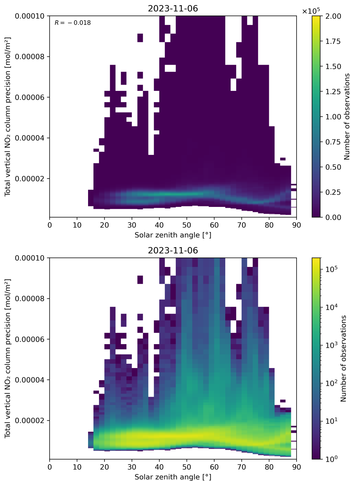
Figure 154: Scatter density plot of “Solar zenith angle” against “Total vertical NO 2 column precision” for 2023-11-05 to 2023-11-07.
