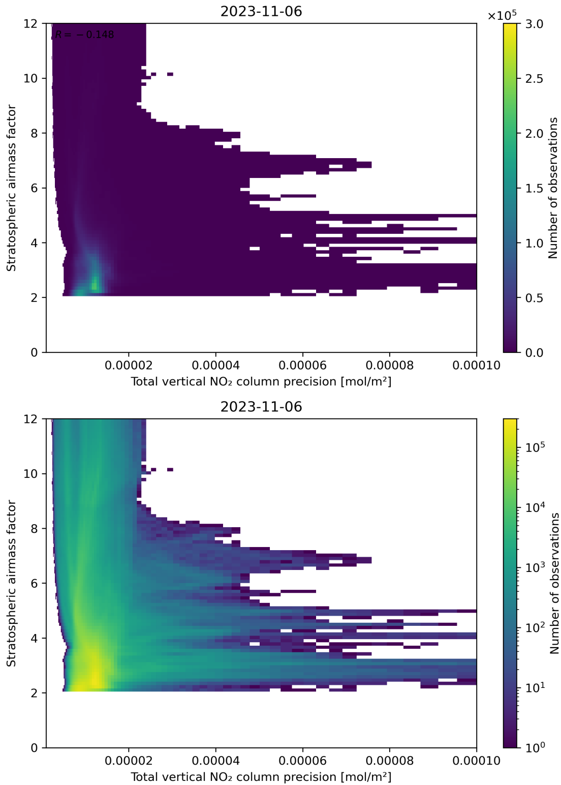
Figure 115: Scatter density plot of “Total vertical NO 2 column precision” against “Stratospheric airmass factor” for 2023-11-05 to 2023-11-07.
