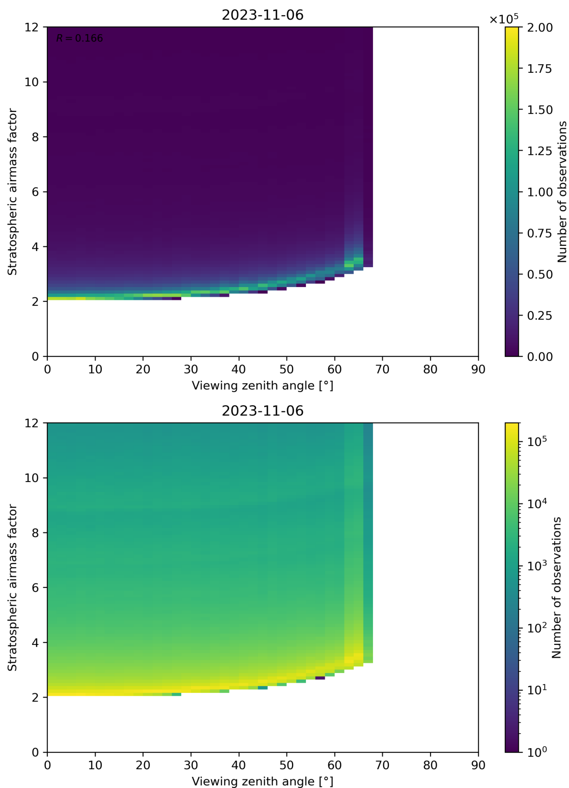
Figure 159: Scatter density plot of “Viewing zenith angle” against “Stratospheric airmass factor” for 2023-11-05 to 2023-11-07.
