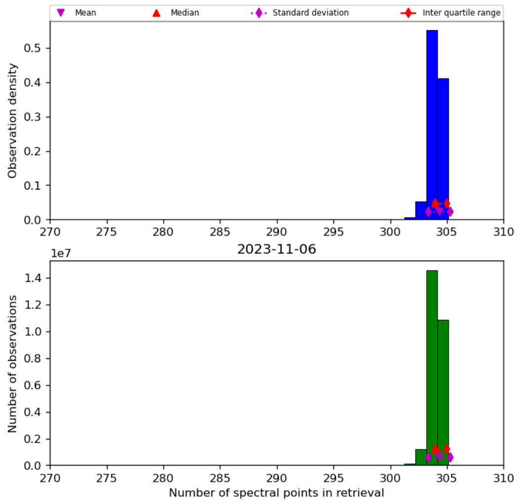
Figure 33: Histogram of “Number of spectral points in retrieval” for 2023-11-05 to 2023-11-07
