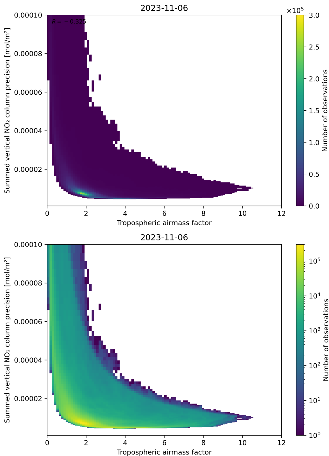
Figure 76: Scatter density plot of “Tropospheric air mass factor” against “Summed vertical NO 2 column precision” for 2023-11-05 to 2023-11-07.
