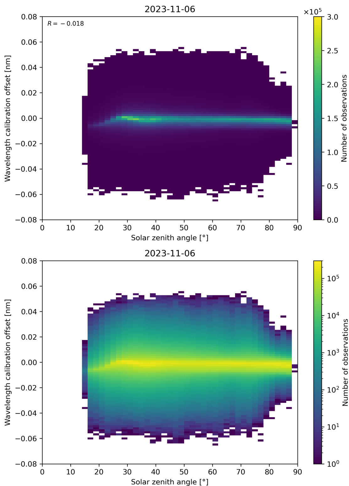
Figure 158: Scatter density plot of “Solar zenith angle” against “Wavelength calibration offset” for 2023-11-05 to 2023-11-07.
