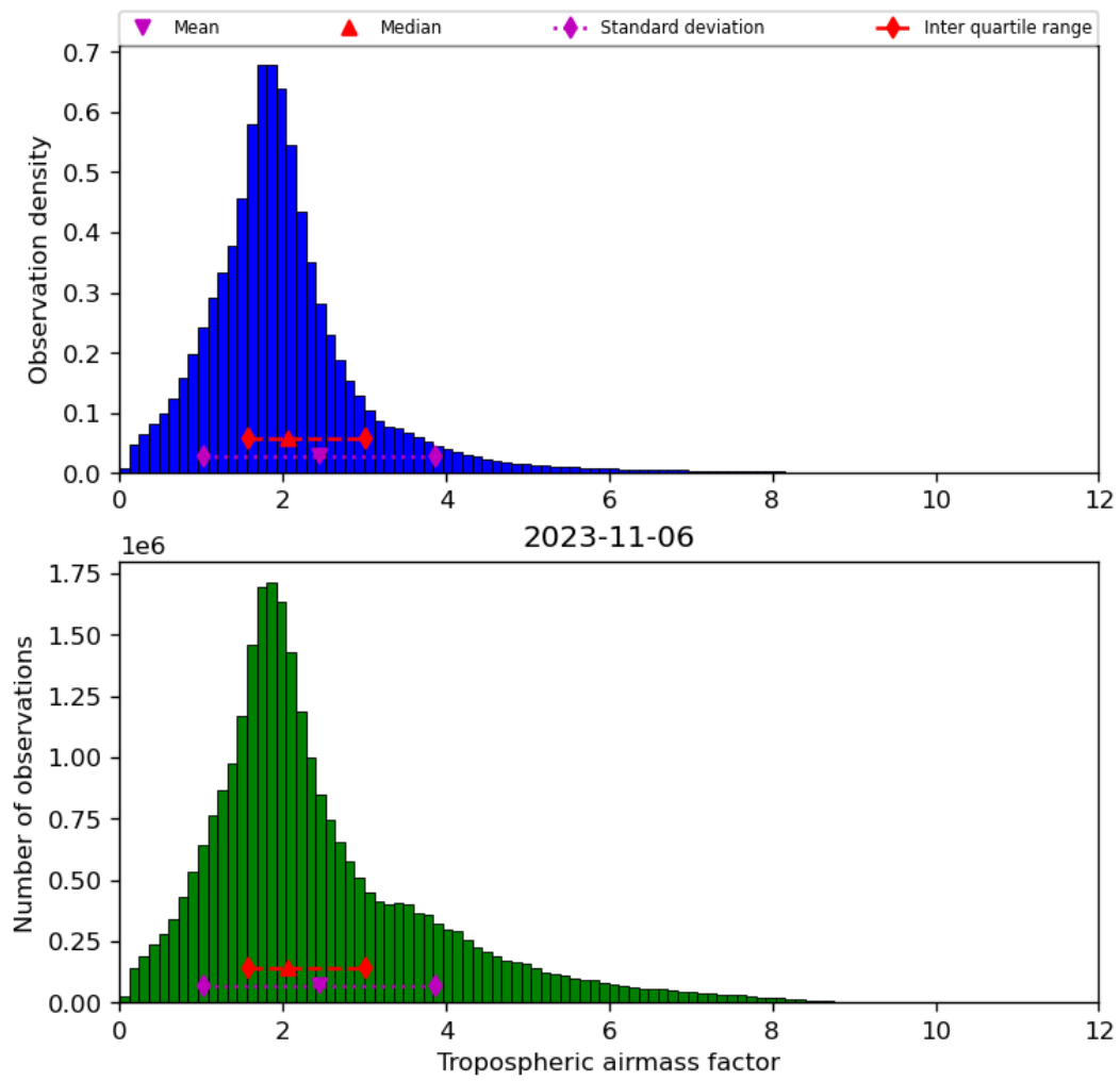
Figure 31: Histogram of “Tropospheric airmass factor” for 2023-11-05 to 2023-11-07
