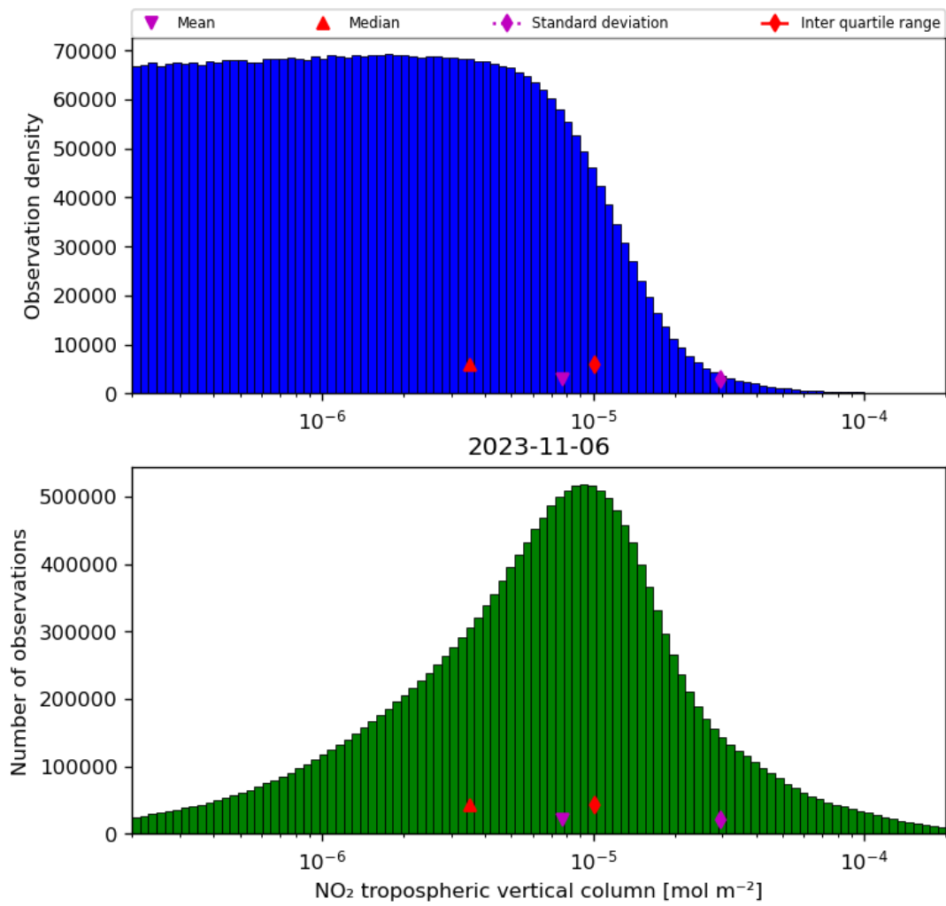
Figure 29: Histogram of “NO 2 tropospheric vertical column” for 2023-11-05 to 2023-11-07
