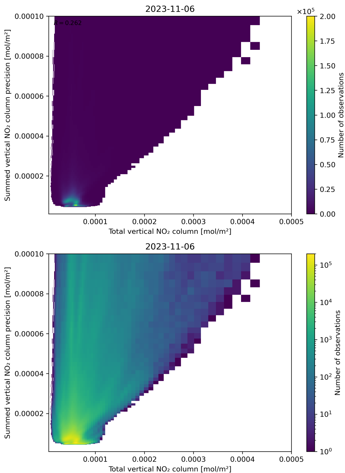
Figure 113: Scatter density plot of “Total vertical NO 2 column” against “Summed vertical NO 2 column precision” for 2023-11-05 to 2023-11-07.
