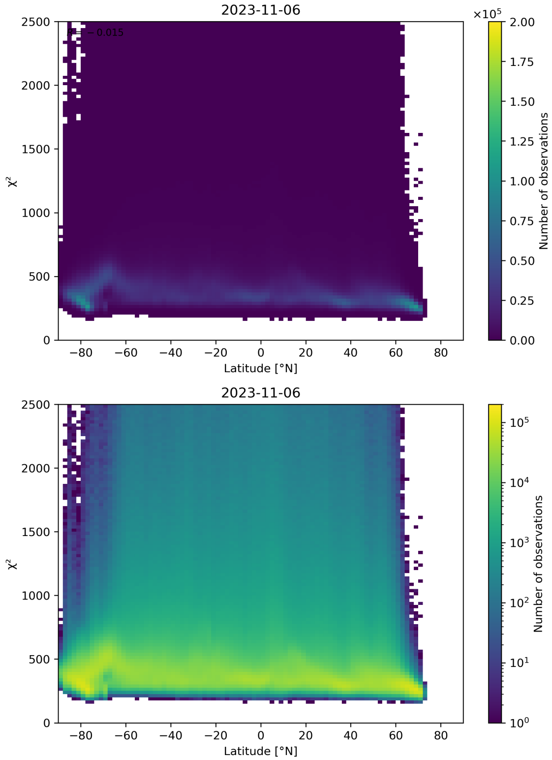
Figure 86: Scatter density plot of “Latitude” against “ \chi^2 ” for 2023-11-05 to 2023-11-07.
