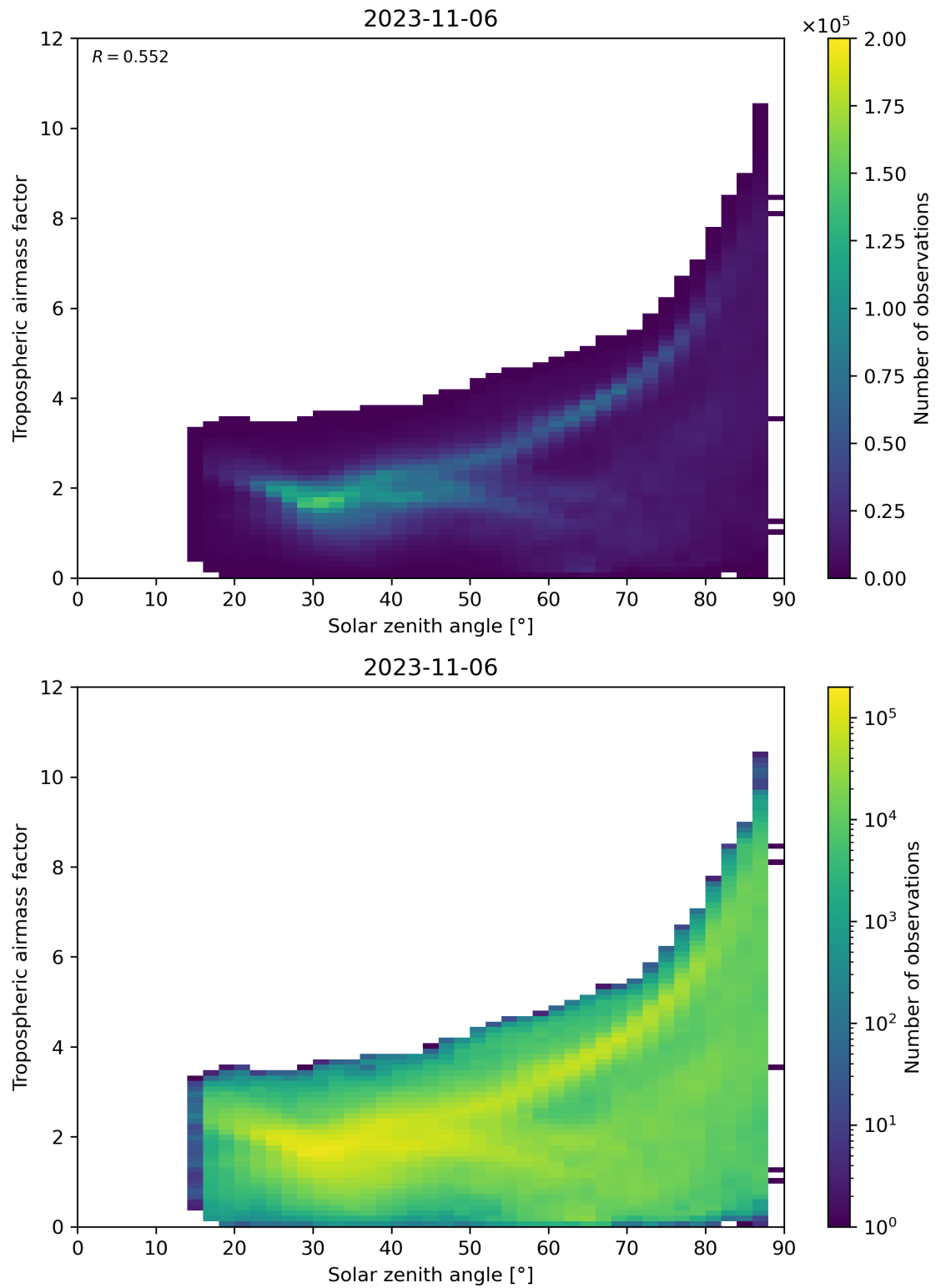
Figure 147: Scatter density plot of “Solar zenith angle” against “Tropospheric airmass factor” for 2023-11-05 to 2023-11-07.
