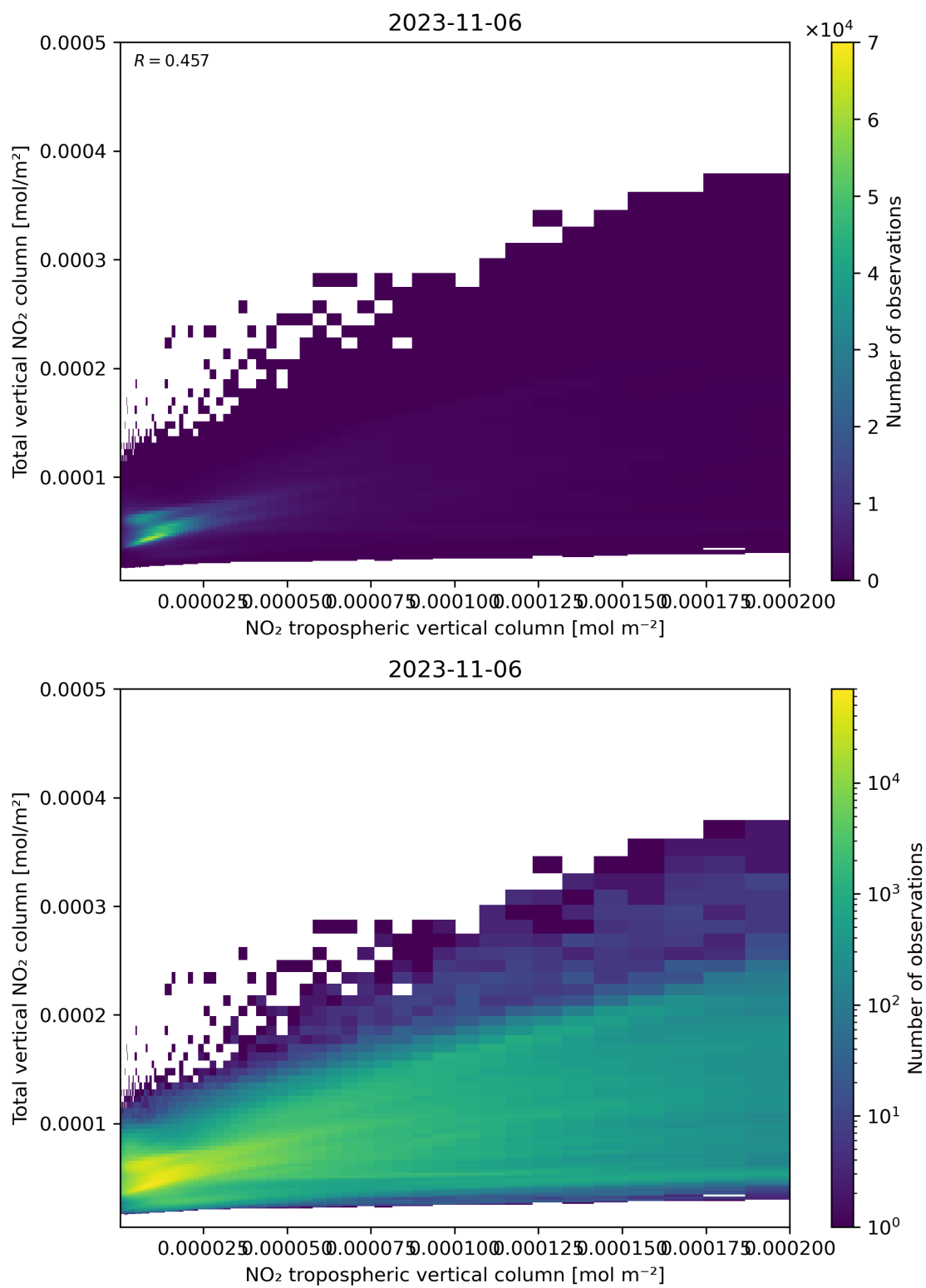
Figure 128: Scatter density plot of “NO 2 tropospheric vertical column” against “Total vertical NO 2 column” for 2023-11-05 to 2023-11-07.
