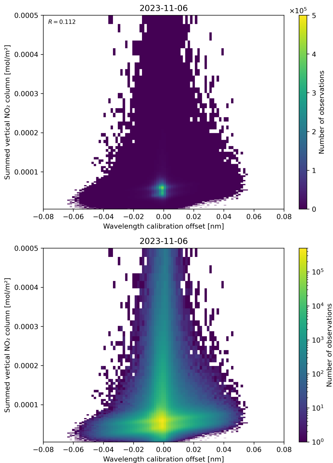
Figure 177: Scatter density plot of “Wavelength calibration offset” against “Summed vertical NO 2 column” for 2023-11-05 to 2023-11-07.
