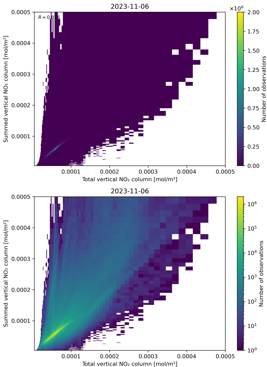
Figure 112: Scatter density plot of “Total vertical NO 2 column” against “Summed vertical NO 2 column” for 2023-11-05 to 2023-11-07.
