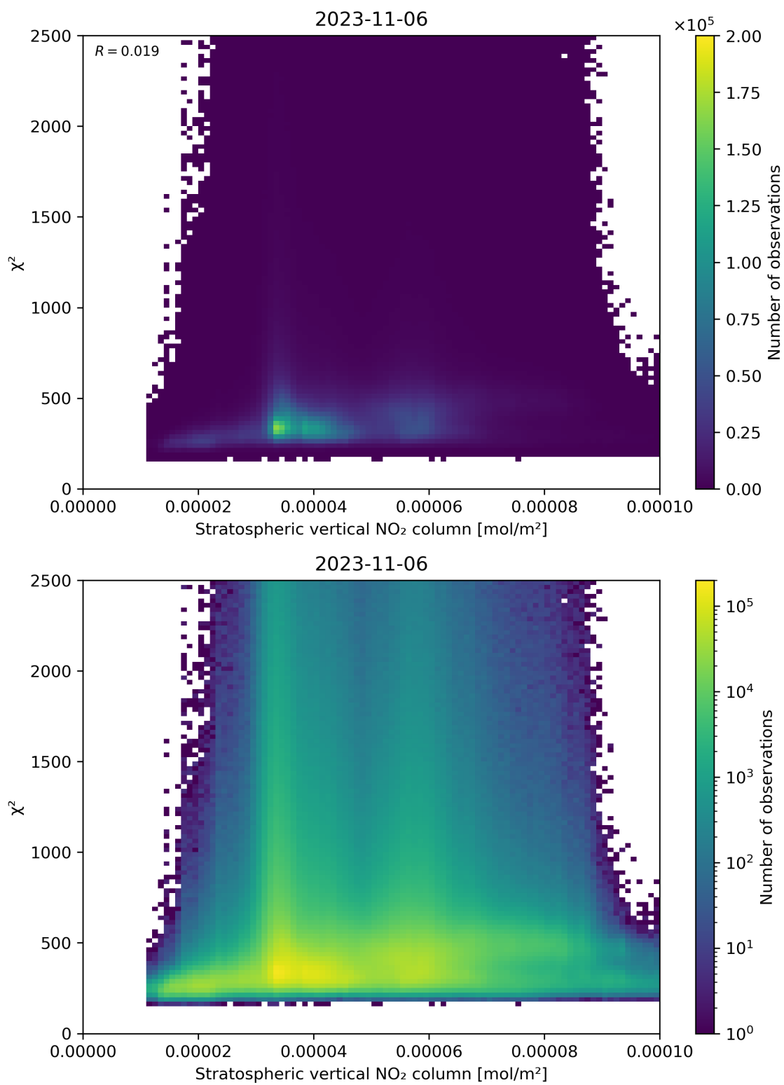
Figure 97: Scatter density plot of “Stratospheric vertical NO 2 column” against “ \chi^2 ” for 2023-11-05 to 2023-11-07.
