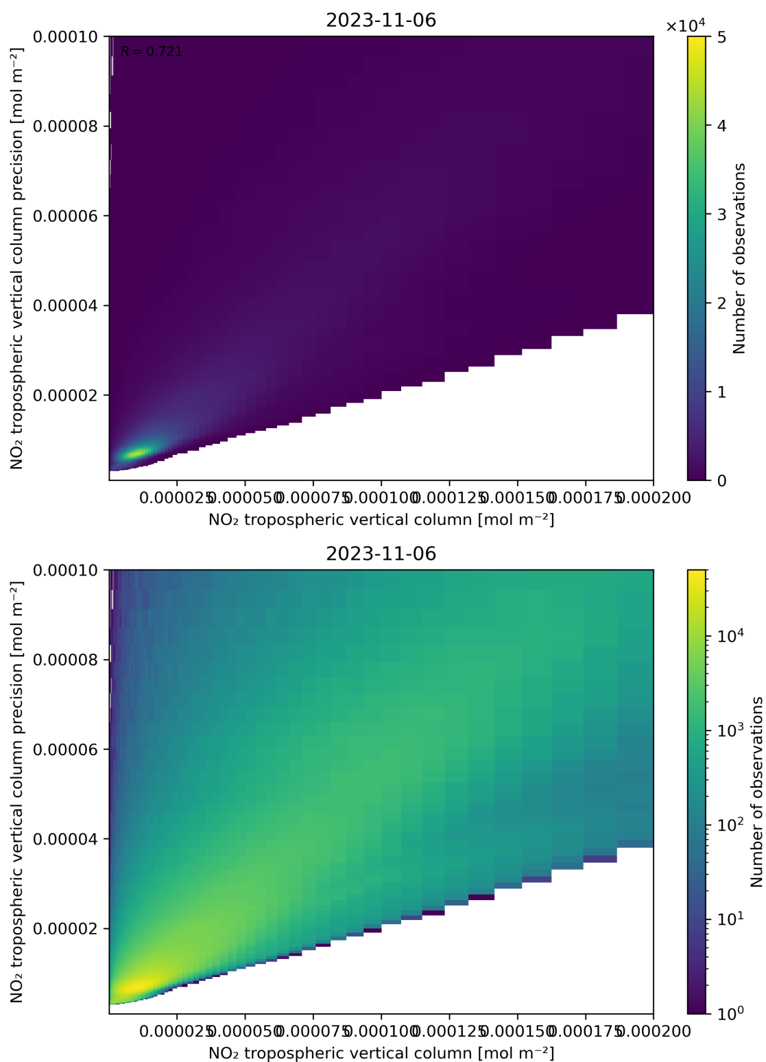
Figure 130: Scatter density plot of “NO 2 tropospheric vertical column” against “NO 2 tropospheric vertical column precision” for 2023-11-05 to 2023-11-07.
