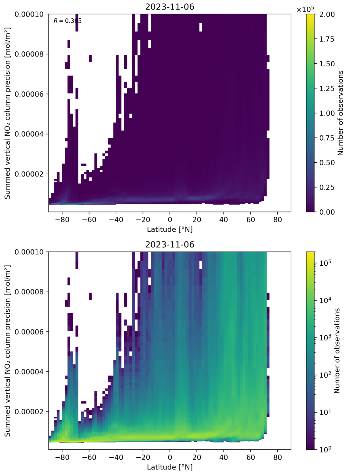
Figure 89: Scatter density plot of “Latitude” against “Summed vertical NO 2 column precision” for 2023-11-05 to 2023-11-07.
