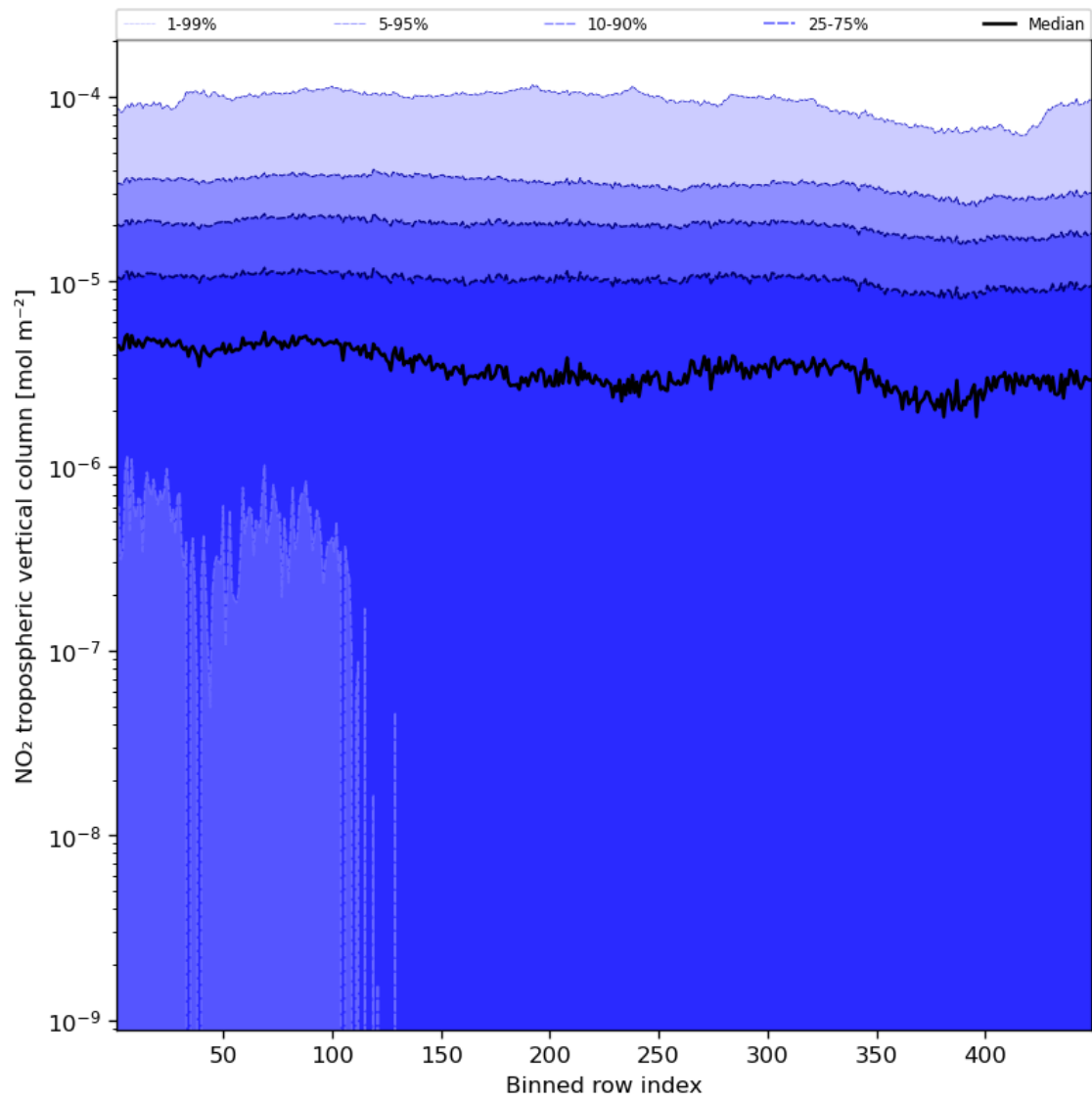
Figure 46: Along track statistics of “NO 2 tropospheric vertical column” for 2023-11-05 to 2023-11-07
