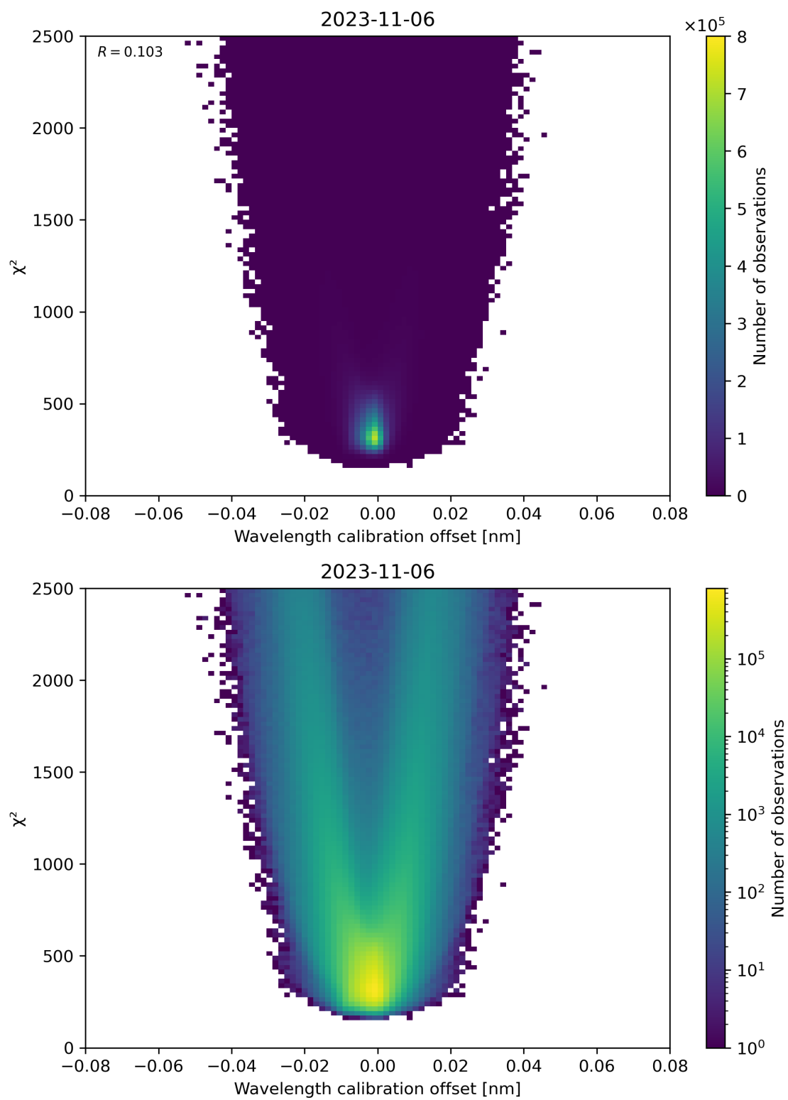
Figure 175: Scatter density plot of “Wavelength calibration offset” against “ \chi^2 ” for 2023-11-05 to 2023-11-07.
