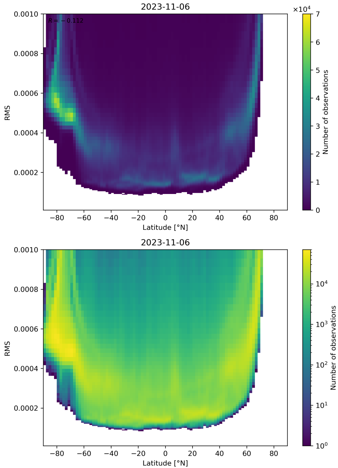
Figure 94: Scatter density plot of “Latitude” against “RMS” for 2023-11-05 to 2023-11-07.
