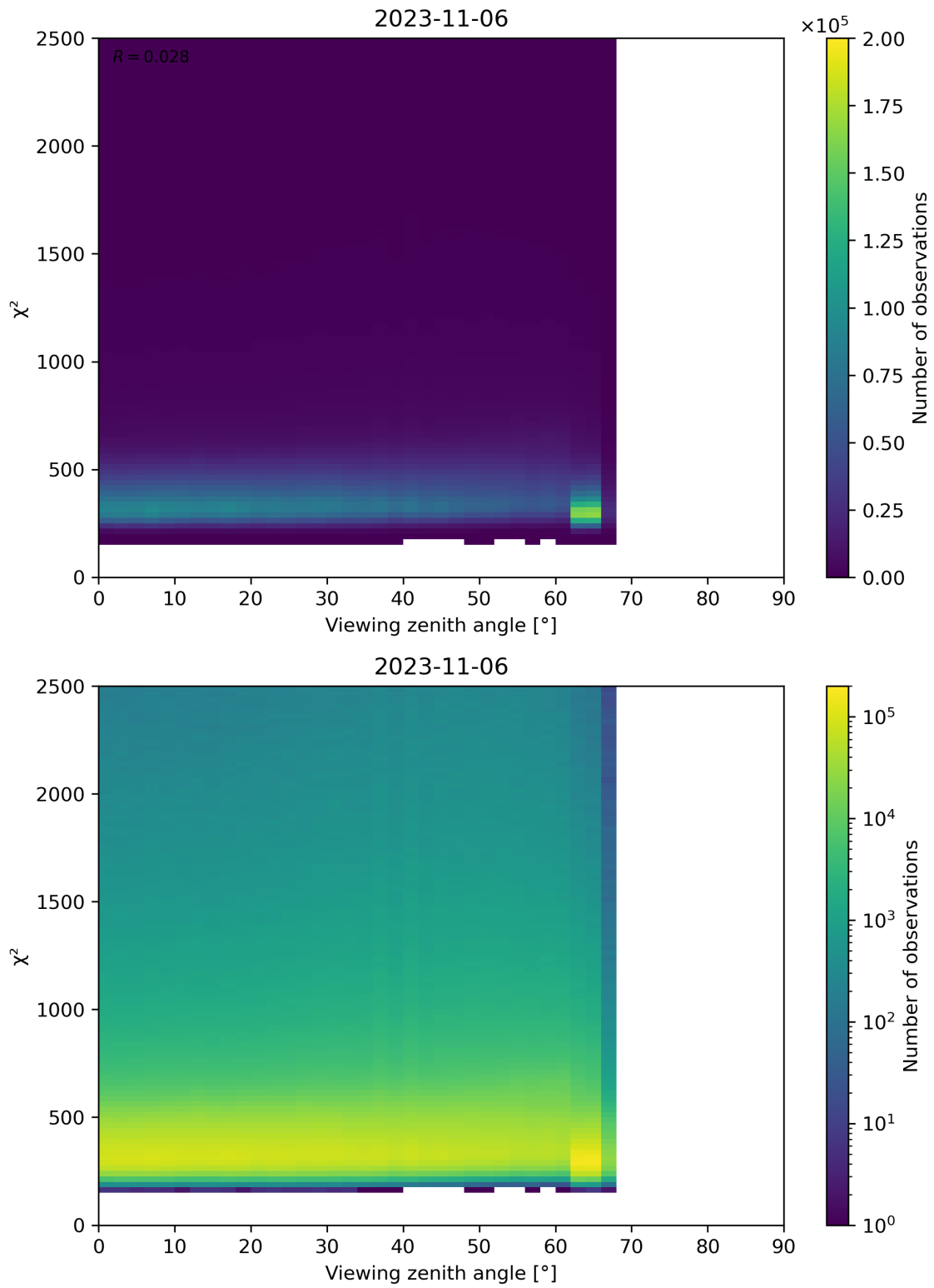
Figure 162: Scatter density plot of “Viewing zenith angle” against “ \chi^2 ” for 2023-11-05 to 2023-11-07.
