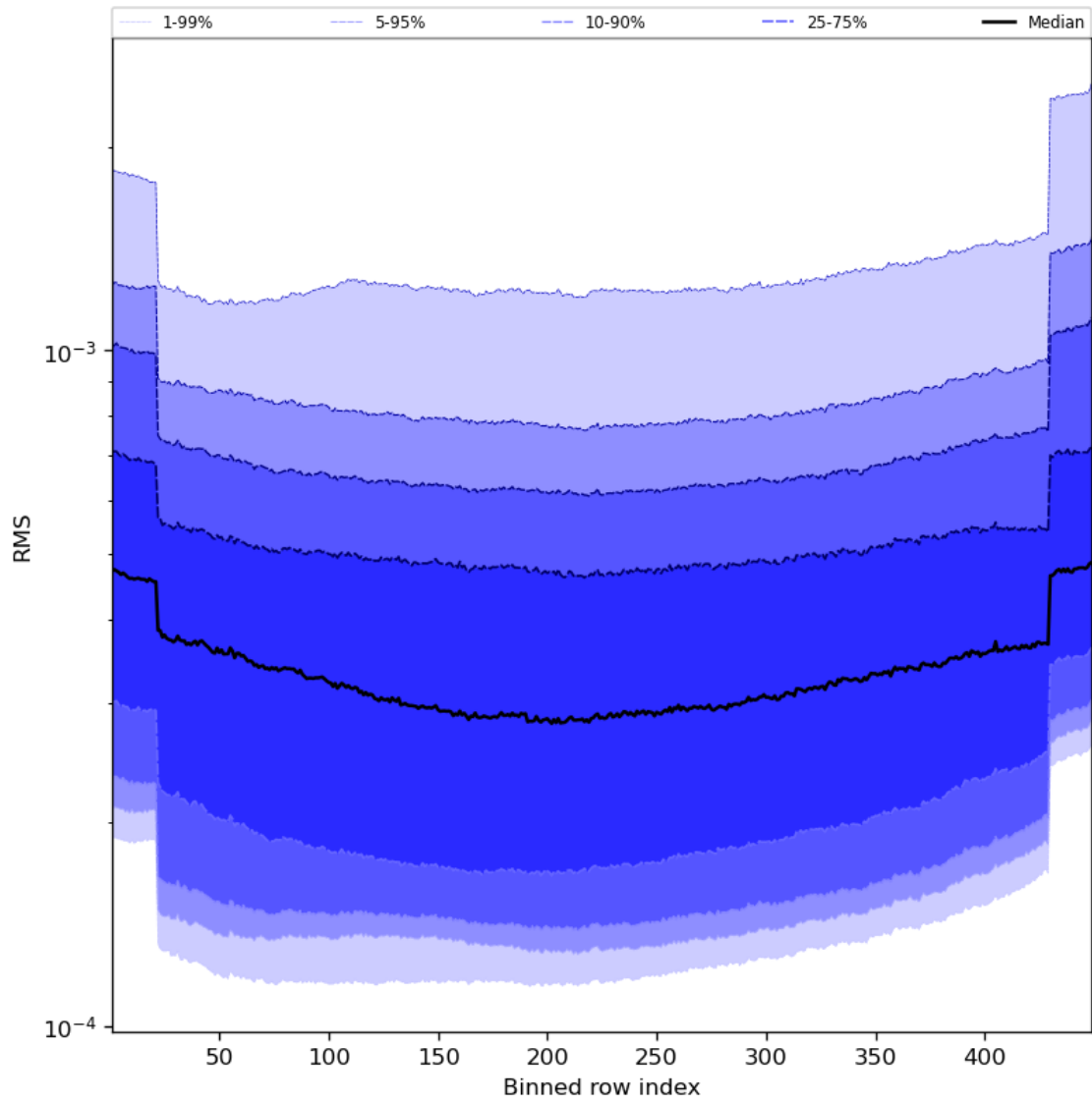
Figure 60: Along track statistics of “RMS” for 2023-11-05 to 2023-11-07
