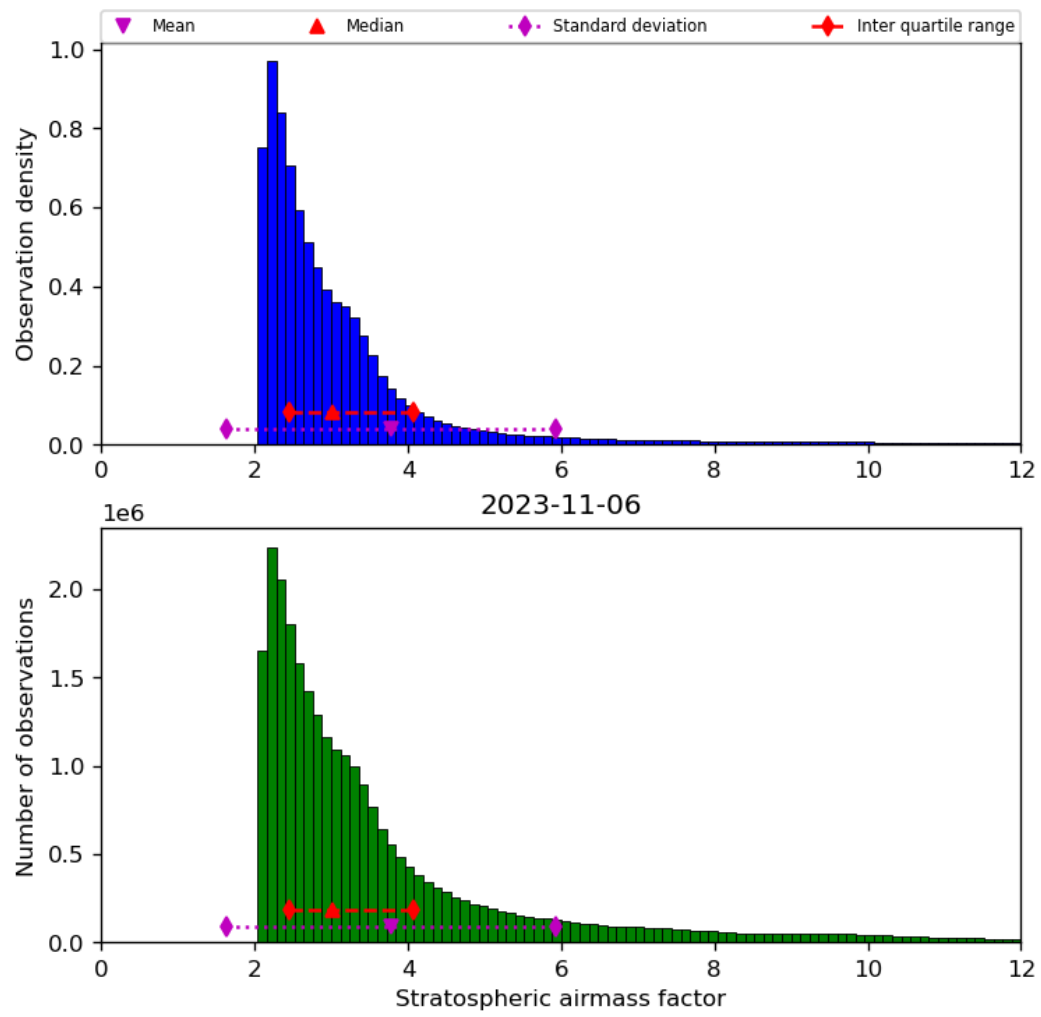
Figure 44: Histogram of “Stratospheric airmass factor” for 2023-11-05 to 2023-11-07
