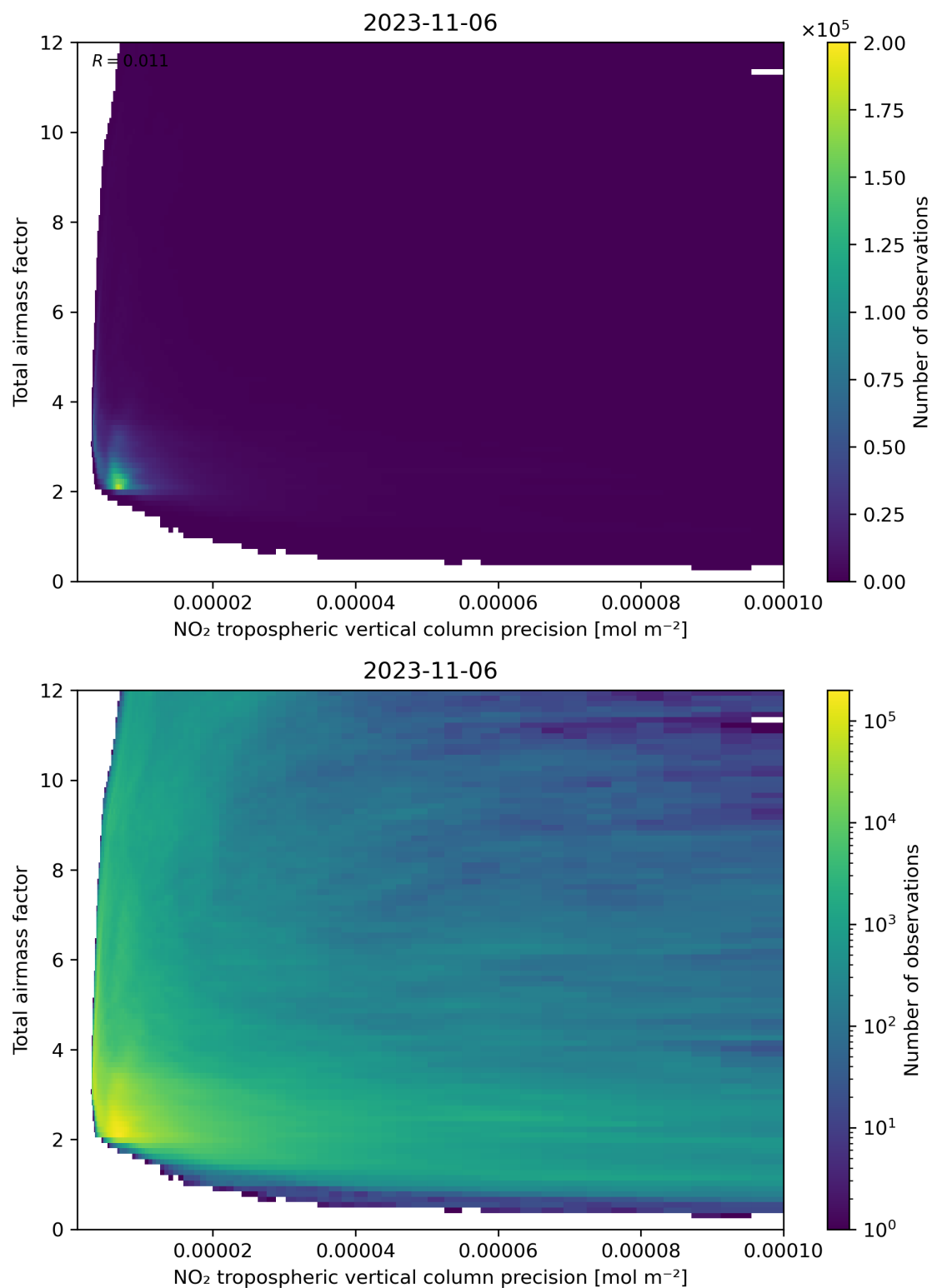
Figure 132: Scatter density plot of “NO 2 tropospheric vertical column precision” against “Total air mass factor” for 2023-11-05 to 2023-11-07.
