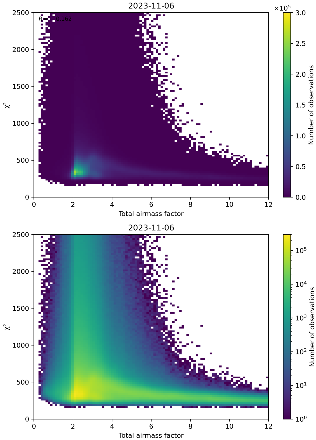
Figure 63: Scatter density plot of “Total airmass factor” against “ \chi^2 ” for 2023-11-05 to 2023-11-07.
