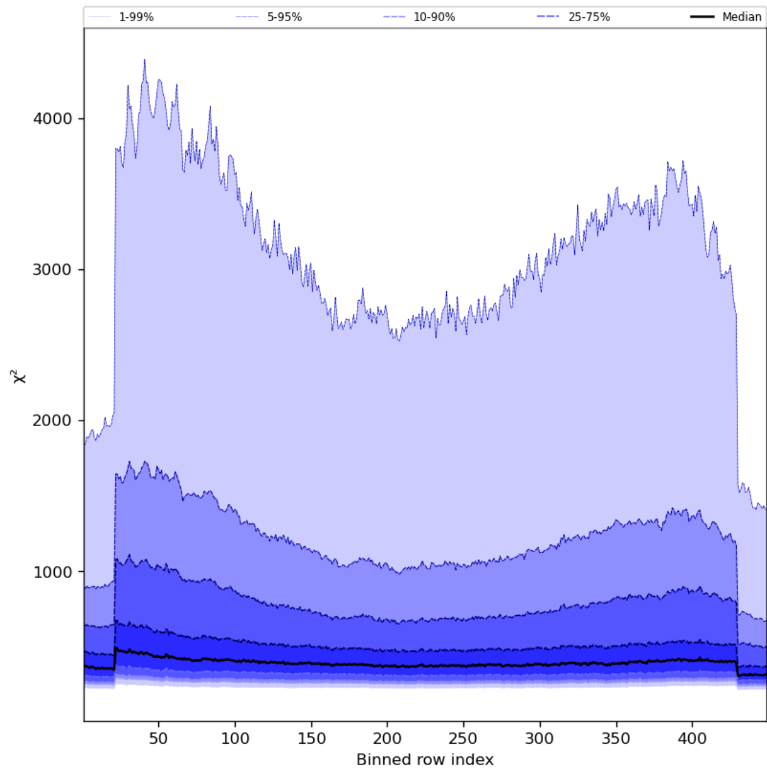
Figure 59: Along track statistics of “ \chi^2 ” for 2023-11-05 to 2023-11-07
