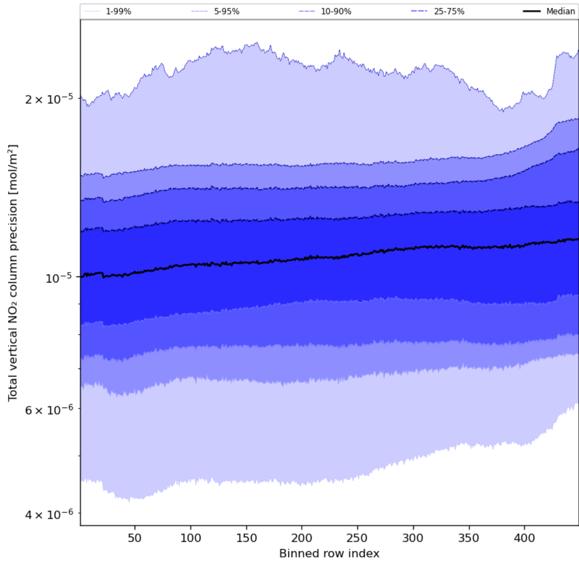
Figure 56: Along track statistics of “Total vertical NO 2 column precision” for 2023-11-05 to 2023-11-07
