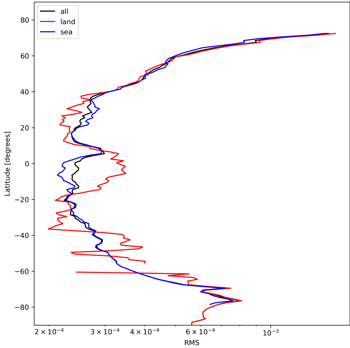
Figure 26: Zonal average of “RMS” for 2023-11-05 to 2023-11-07.
