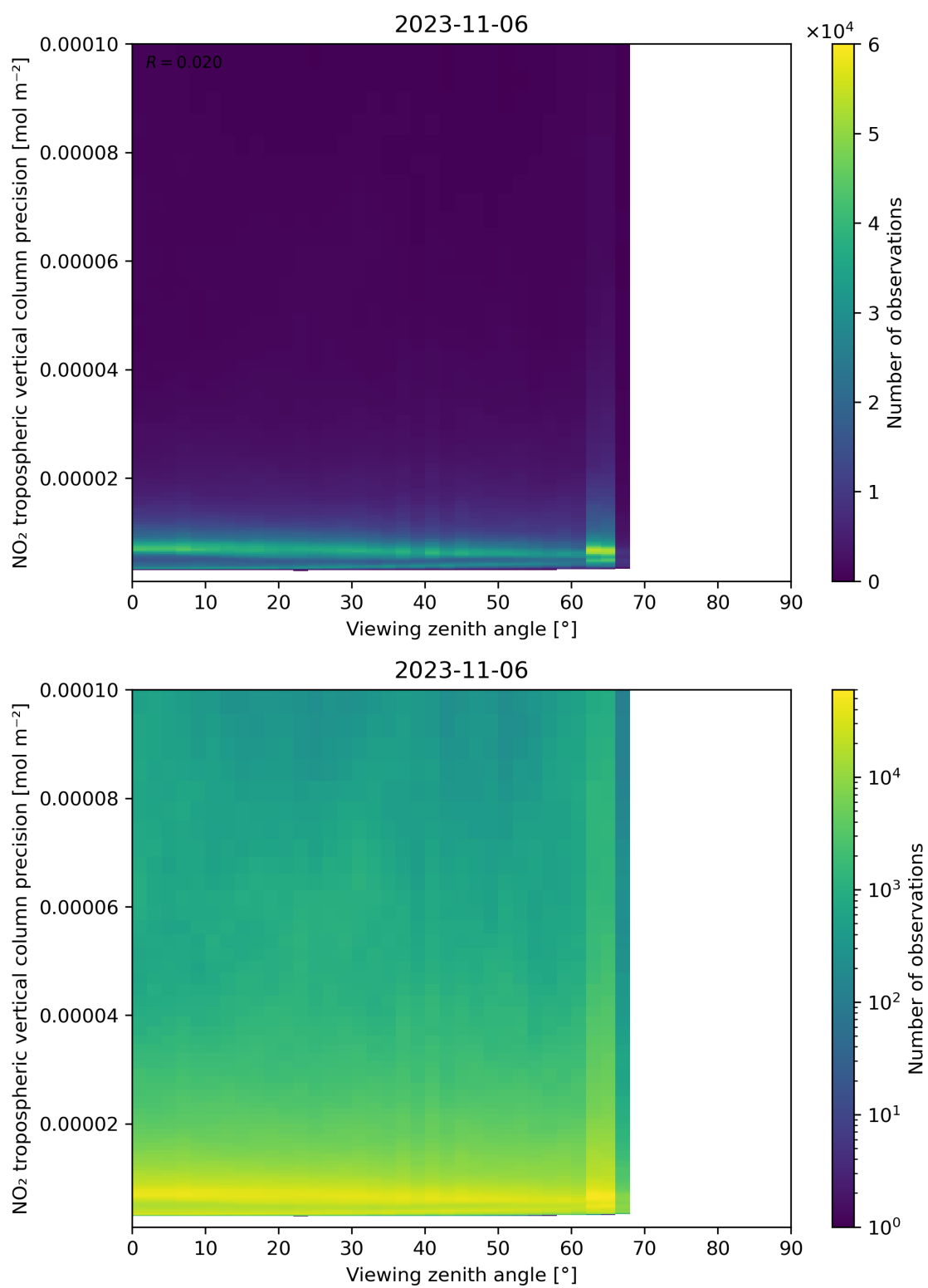
Figure 170: Scatter density plot of “Viewing zenith angle” against “NO 2 tropospheric vertical column precision” for 2023-11-05 to 2023-11-07.
