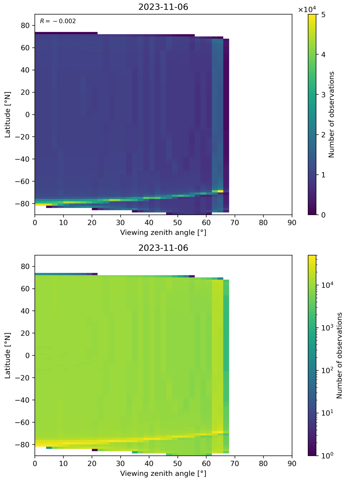
Figure 163: Scatter density plot of “Viewing zenith angle” against “Latitude” for 2023-11-05 to 2023-11-07.
