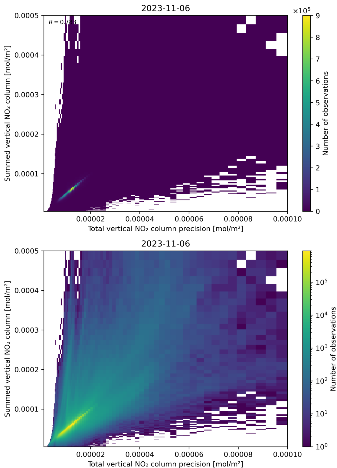
Figure 117: Scatter density plot of “Total vertical NO 2 column precision” against “Summed vertical NO 2 column” for 2023-11-05 to 2023-11-07.
