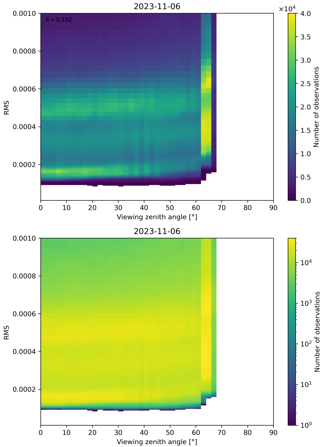
Figure 171: Scatter density plot of “Viewing zenith angle” against “RMS” for 2023-11-05 to 2023-11-07.
