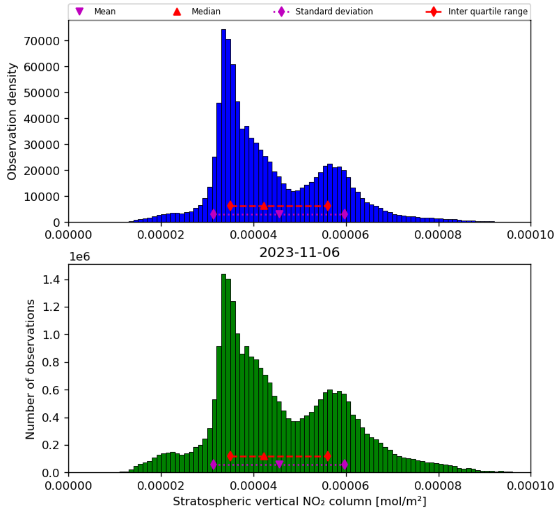
Figure 36: Histogram of “Stratospheric vertical NO 2 column” for 2023-11-05 to 2023-11-07
