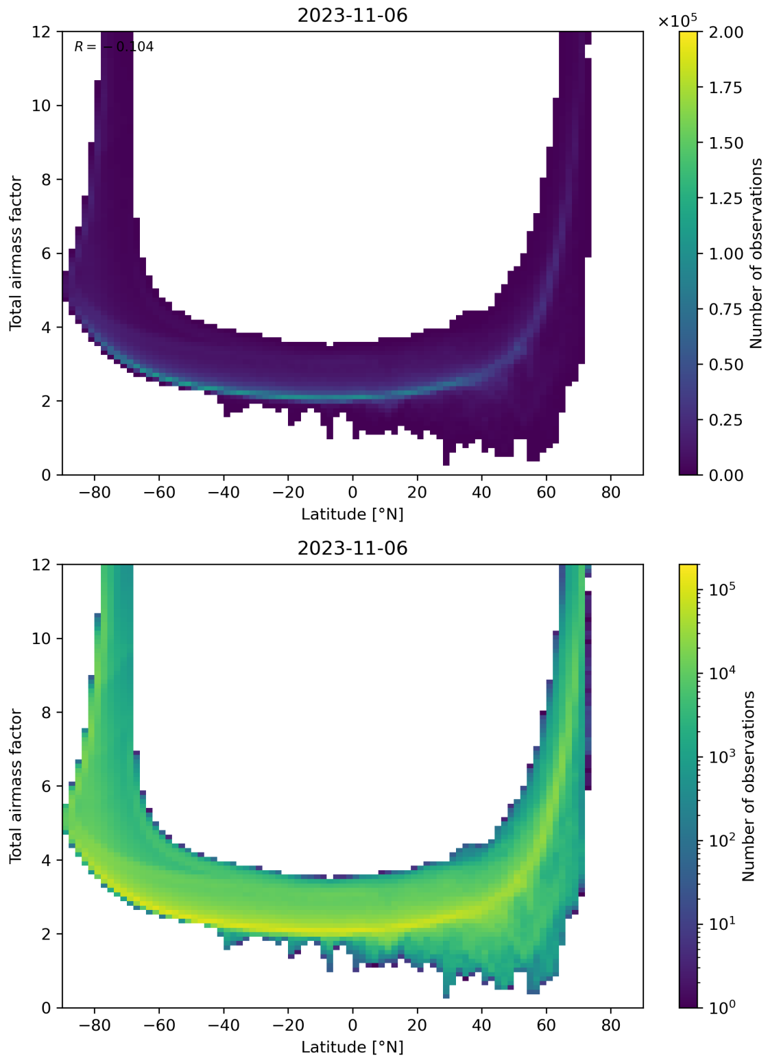
Figure 84: Scatter density plot of “Latitude” against “Total airmass factor” for 2023-11-05 to 2023-11-07.
