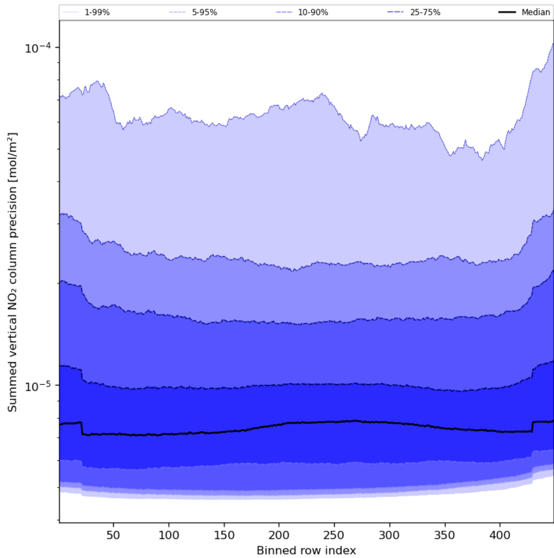
Figure 58: Along track statistics of “Summed vertical NO 2 column precision” for 2023-11-05 to 2023-11-07
