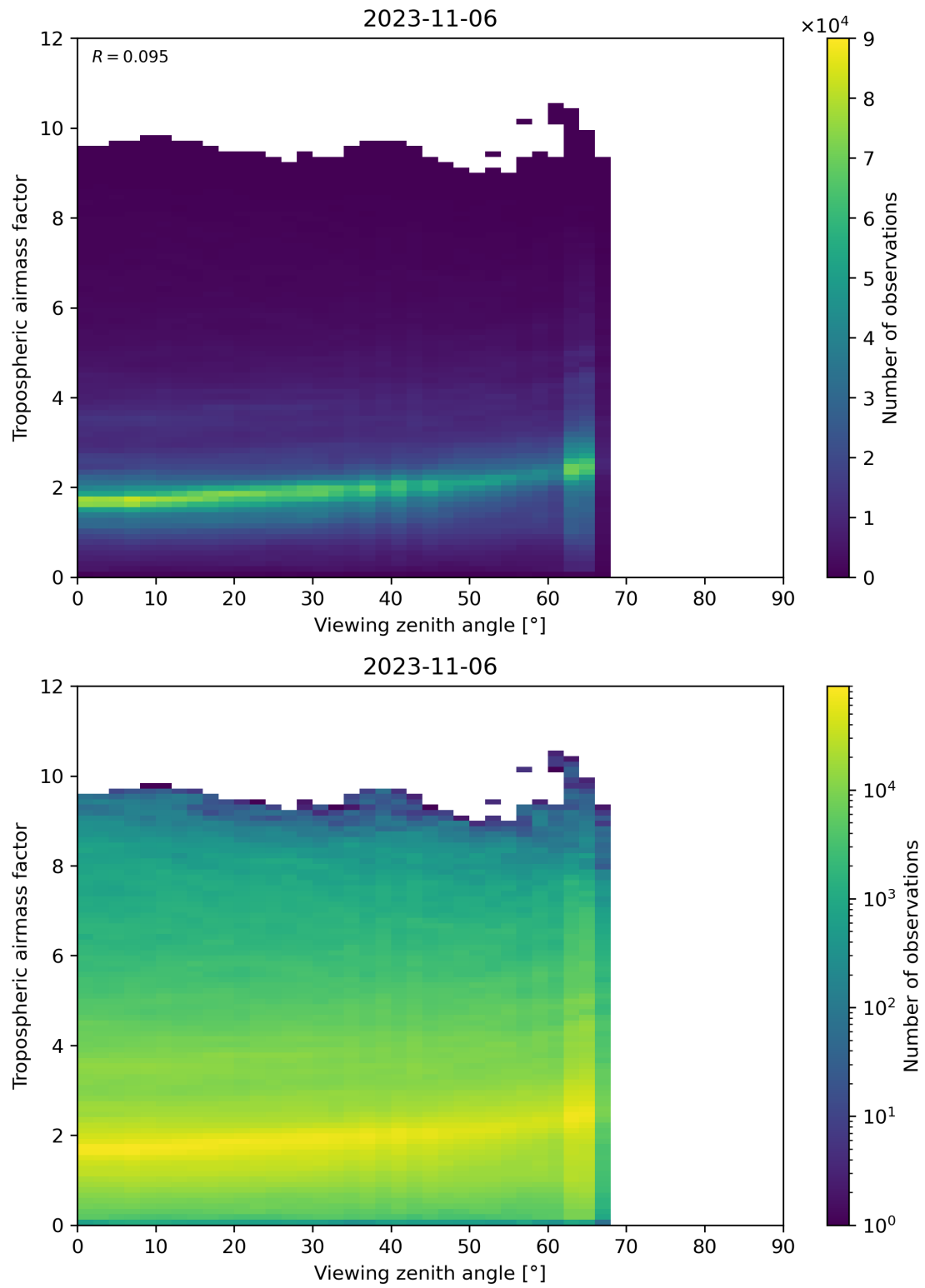
Figure 161: Scatter density plot of “Viewing zenith angle” against “Tropospheric airmass factor” for 2023-11-05 to 2023-11-07.
