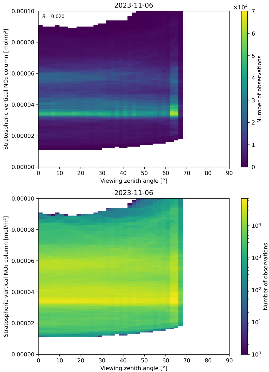
Figure 164: Scatter density plot of “Viewing zenith angle” against “Stratospheric vertical NO 2 column” for 2023-11-05 to 2023-11-07.
