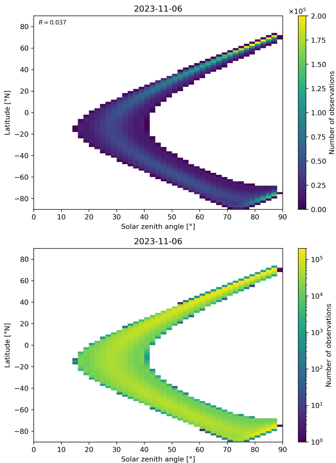
Figure 149: Scatter density plot of “Solar zenith angle” against “Latitude” for 2023-11-05 to 2023-11-07.
