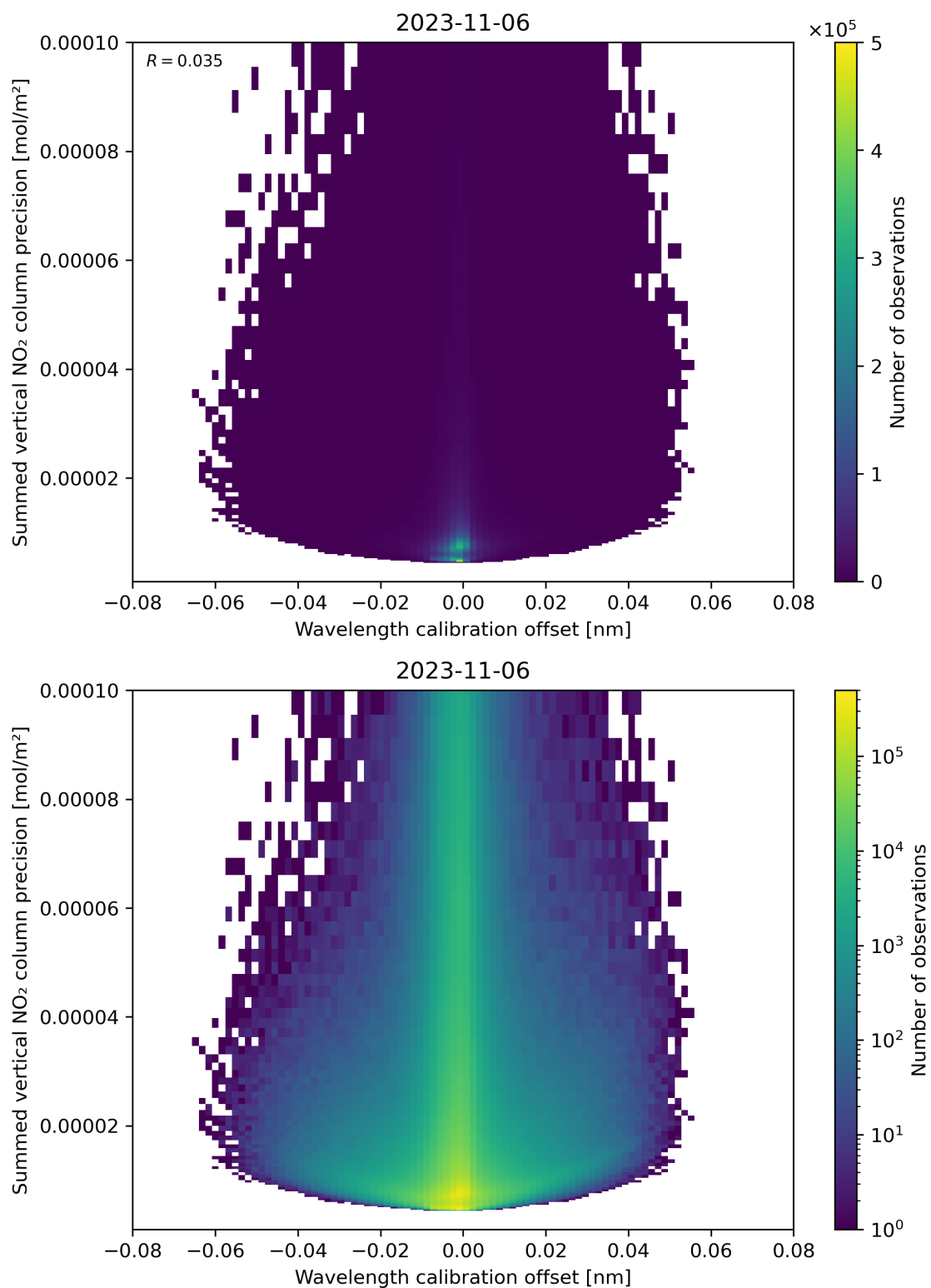
Figure 178: Scatter density plot of “Wavelength calibration offset” against “Summed vertical NO 2 column precision” for 2023-11-05 to 2023-11-07.
