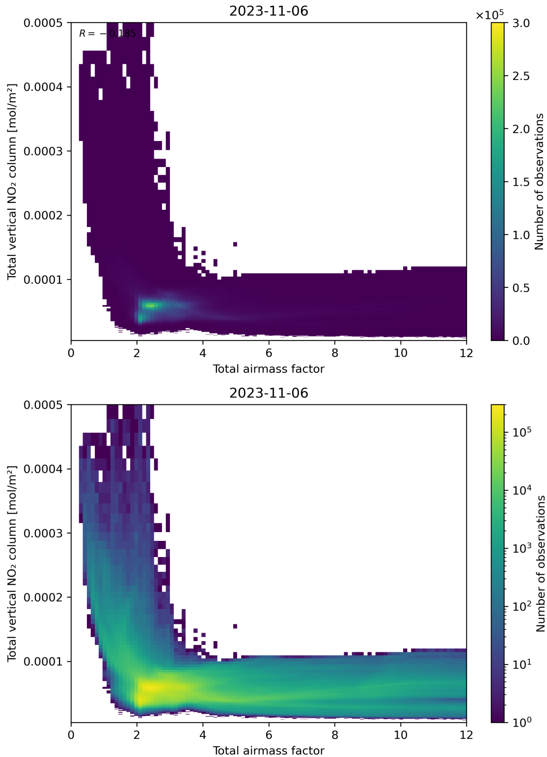
Figure 67: Scatter density plot of “Total airmass factor” against “Total vertical NO 2 column” for 2023-11-05 to 2023-11-07.
