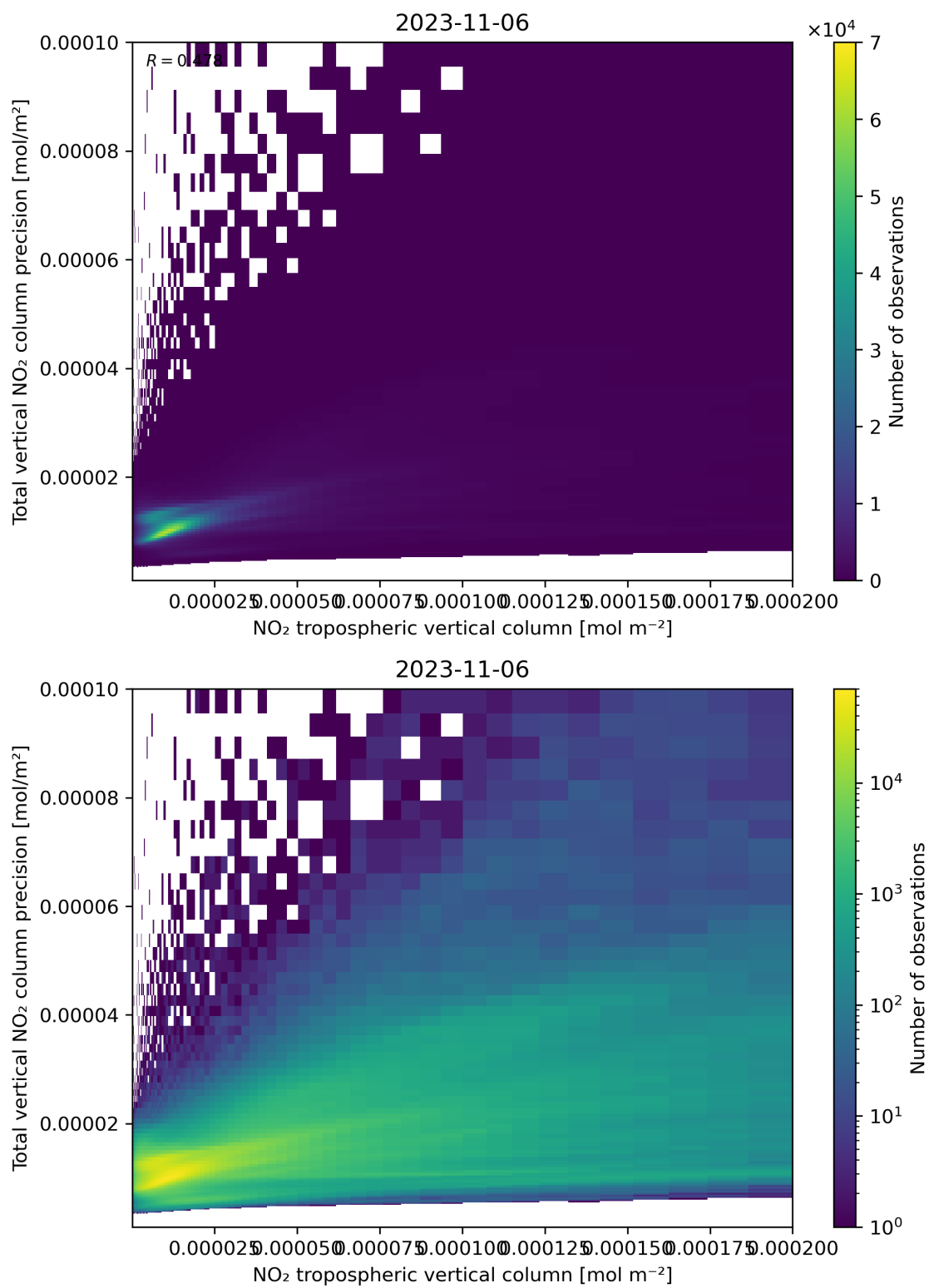
Figure 129: Scatter density plot of “NO 2 tropospheric vertical column” against “Total vertical NO 2 column precision” for 2023-11-05 to 2023-11-07.
