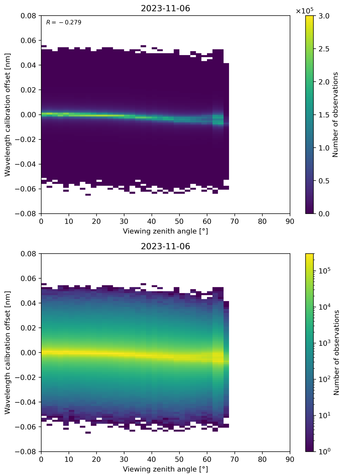
Figure 173: Scatter density plot of “Viewing zenith angle” against “Wavelength calibration offset” for 2023-11-05 to 2023-11-07.
