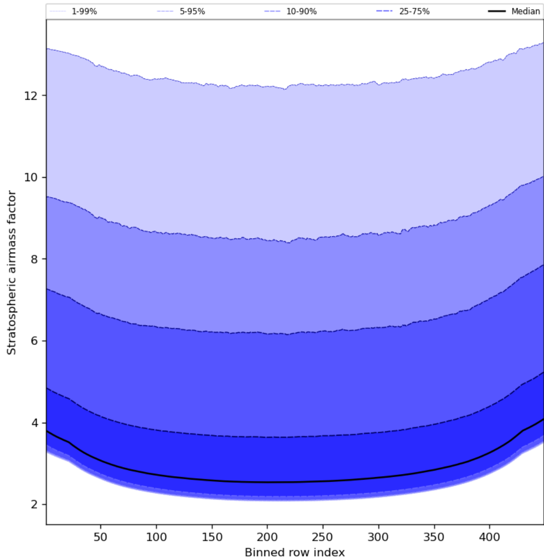
Figure 61: Along track statistics of “Stratospheric airmass factor” for 2023-11-05 to 2023-11-07
