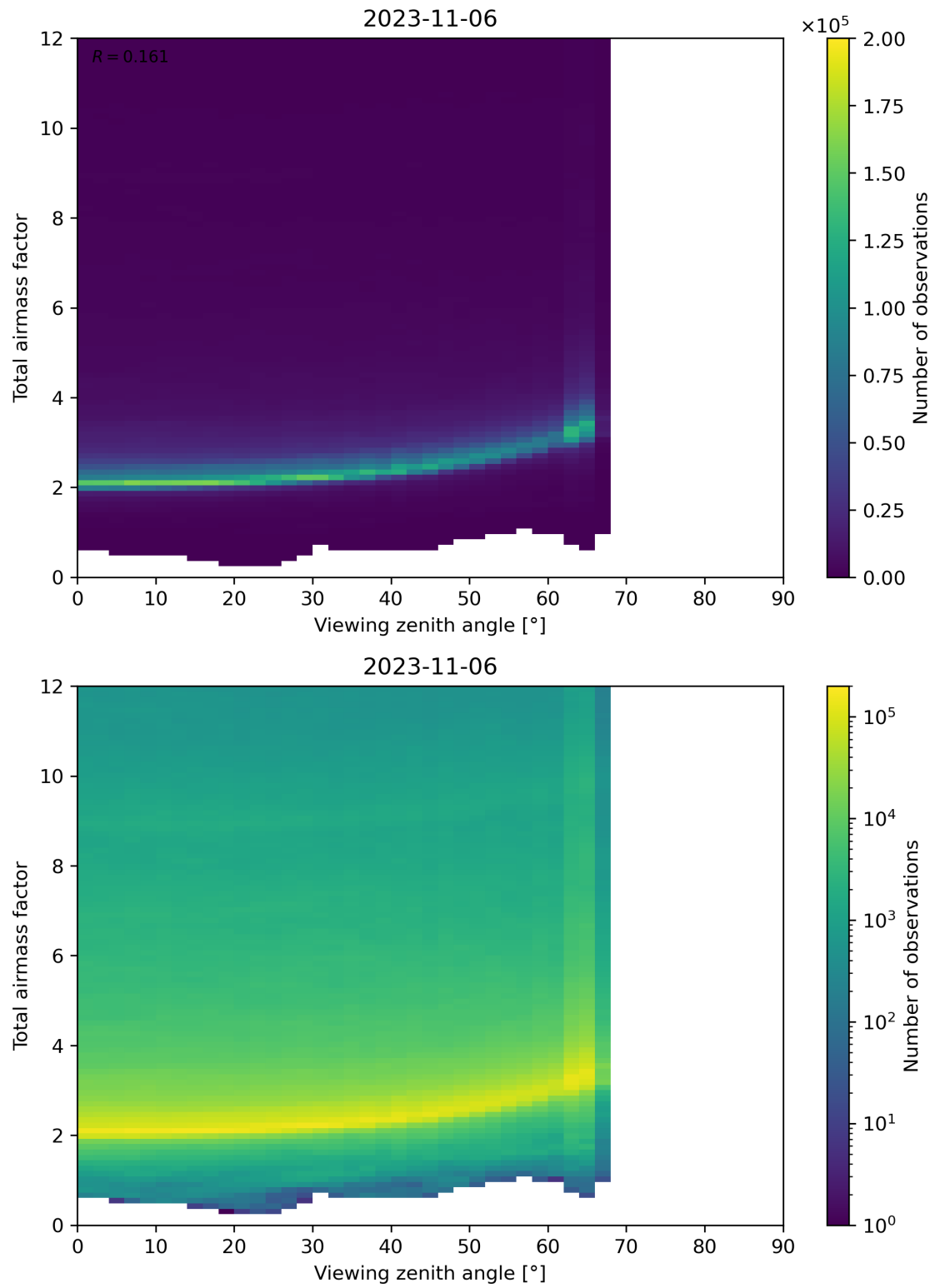
Figure 160: Scatter density plot of “Viewing zenith angle” against “Total airmass factor” for 2023-11-05 to 2023-11-07.
