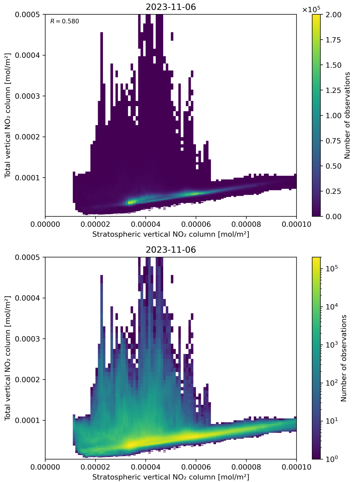
Figure 100: Scatter density plot of “Stratospheric vertical NO 2 column” against “Total vertical NO 2 column” for 2023-11-05 to 2023-11-07.
