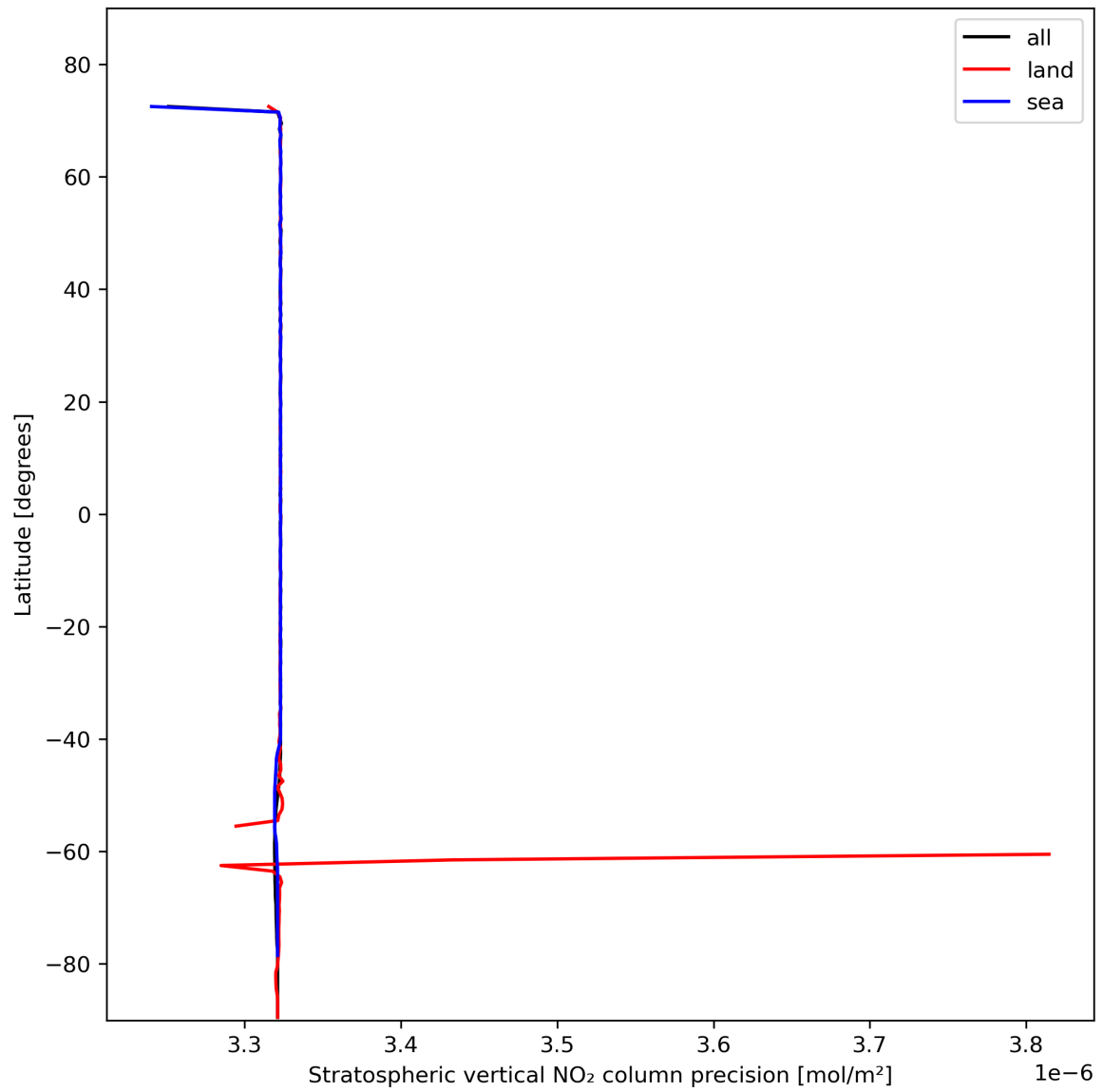
Figure 20: Zonal average of “Stratospheric vertical NO 2 column precision” for 2023-11-05 to 2023-11-07.
