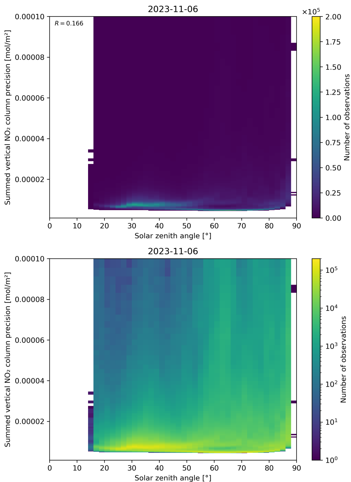
Figure 152: Scatter density plot of “Solar zenith angle” against “Summed vertical NO 2 column precision” for 2023-11-05 to 2023-11-07.
