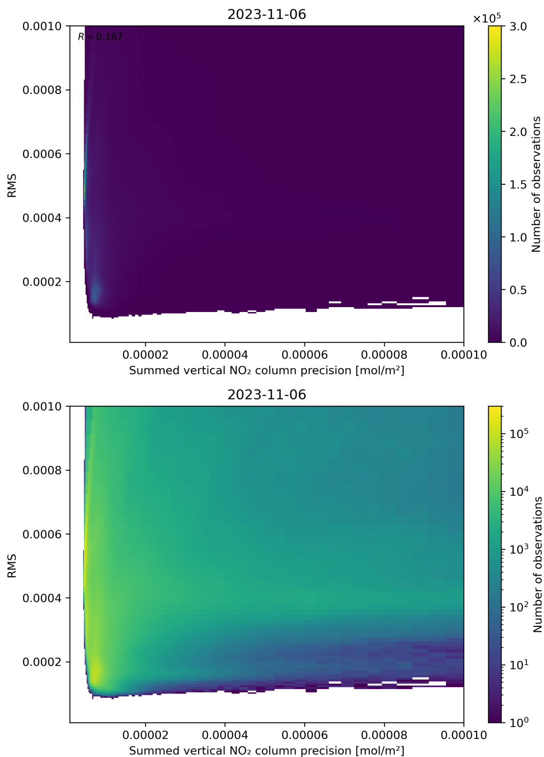
Figure 108: Scatter density plot of “Summed vertical NO 2 column precision” against “RMS” for 2023-11-05 to 2023-11-07.
