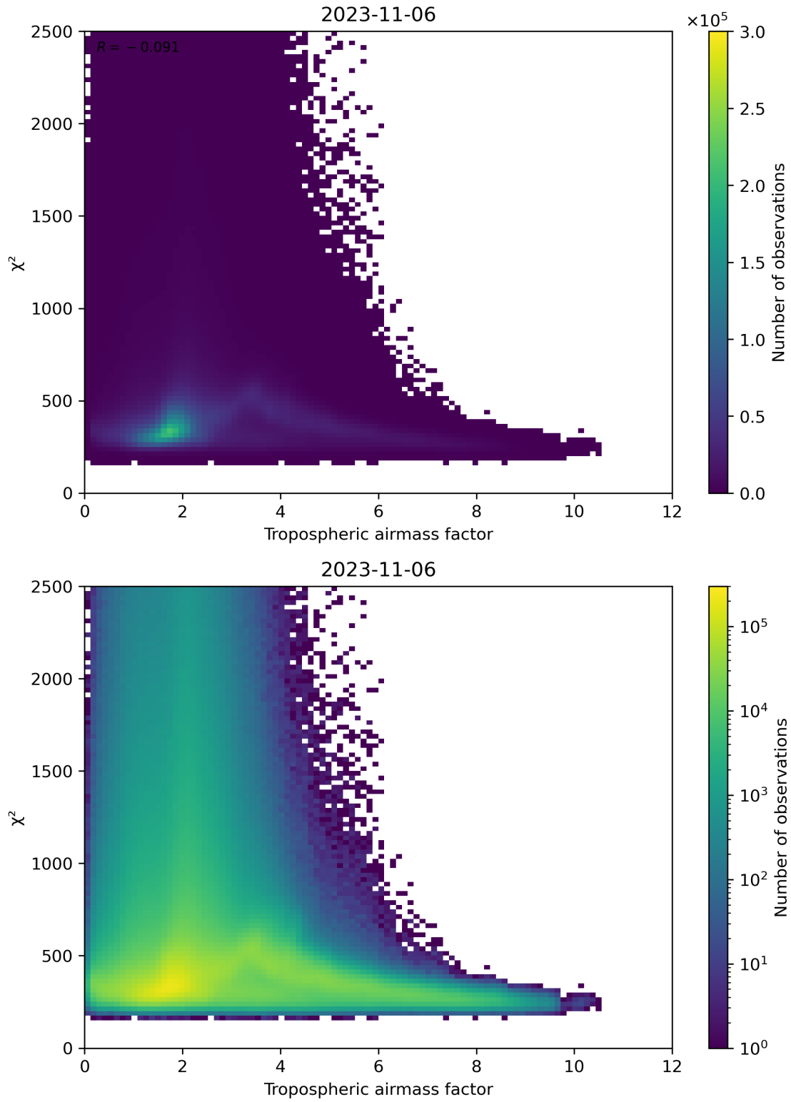
Figure 73: Scatter density plot of “Tropospheric airmass factor” against “ \chi^2 ” for 2023-11-05 to 2023-11-07.
