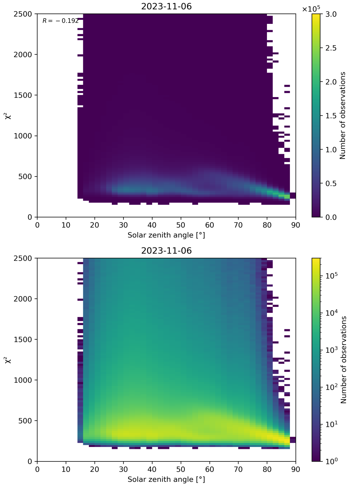
Figure 148: Scatter density plot of “Solar zenith angle” against “ \chi^2 ” for 2023-11-05 to 2023-11-07.
