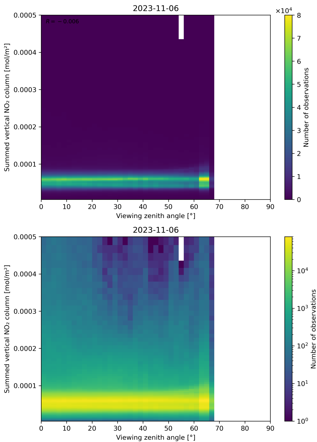
Figure 165: Scatter density plot of “Viewing zenith angle” against “Summed vertical NO 2 column” for 2023-11-05 to 2023-11-07.
