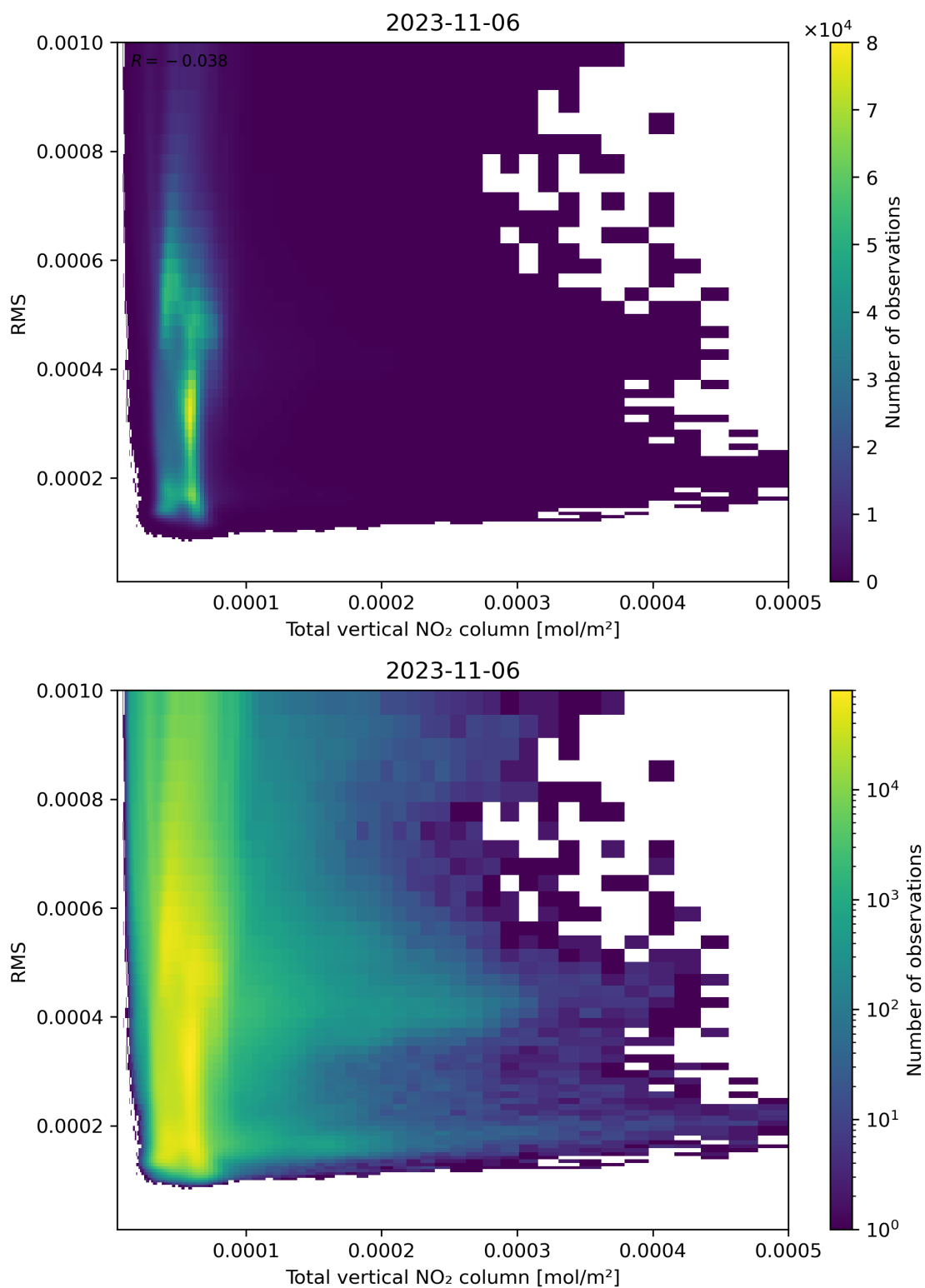
Figure 120: Scatter density plot of “Total vertical NO 2 column” against “RMS” for 2023-11-05 to 2023-11-07.
