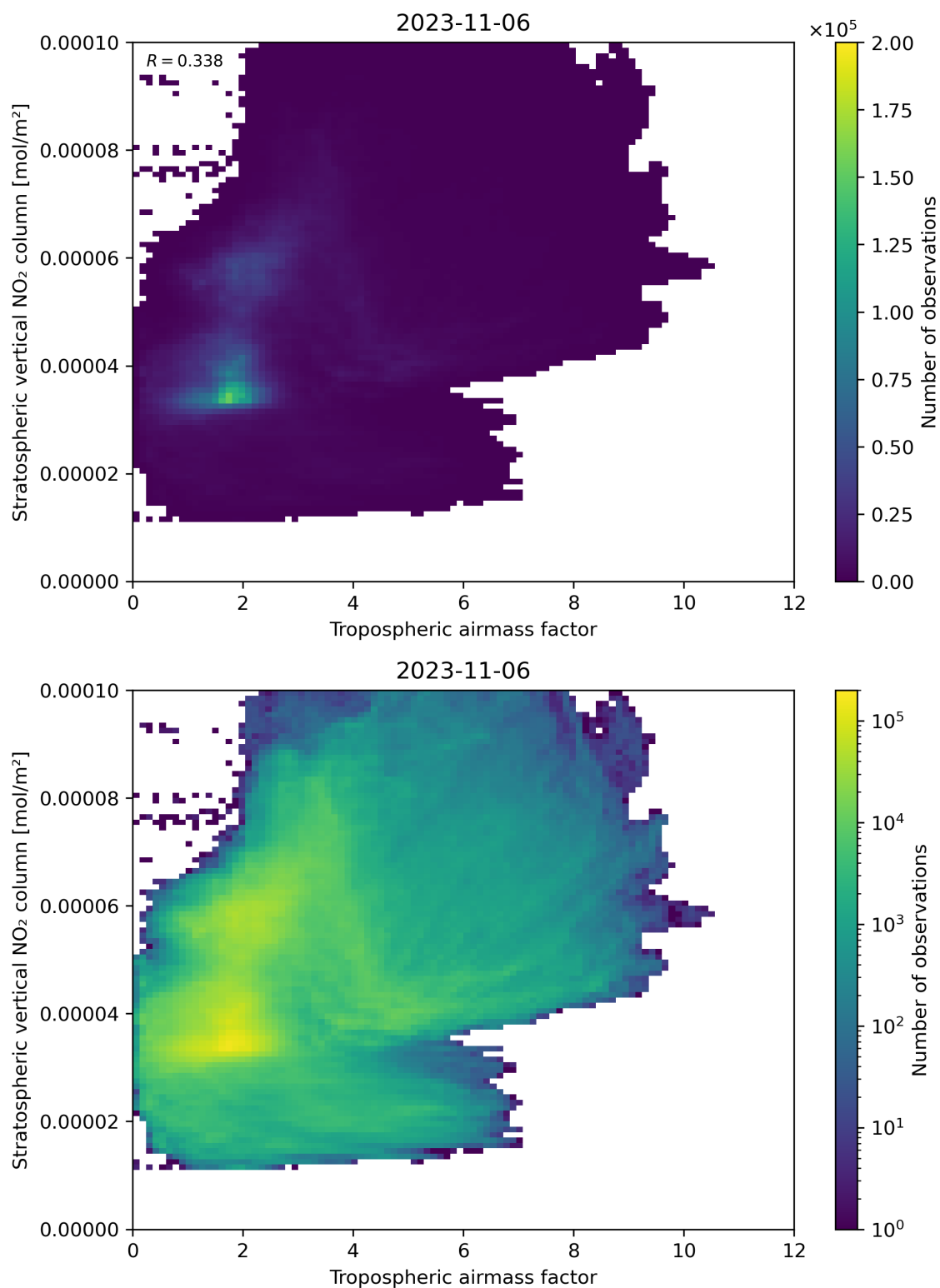
Figure 74: Scatter density plot of “Tropospheric airmass factor” against “Stratospheric vertical NO 2 column” for 2023-11-05 to 2023-11-07.
