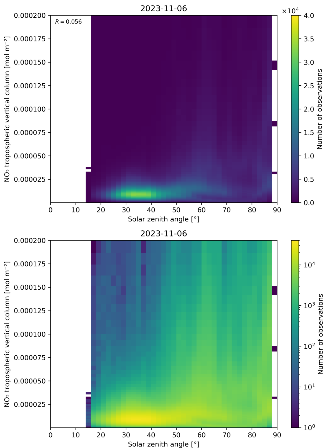
Figure 155: Scatter density plot of “Solar zenith angle” against “NO 2 tropospheric vertical column” for 2023-11-05 to 2023-11-07.
