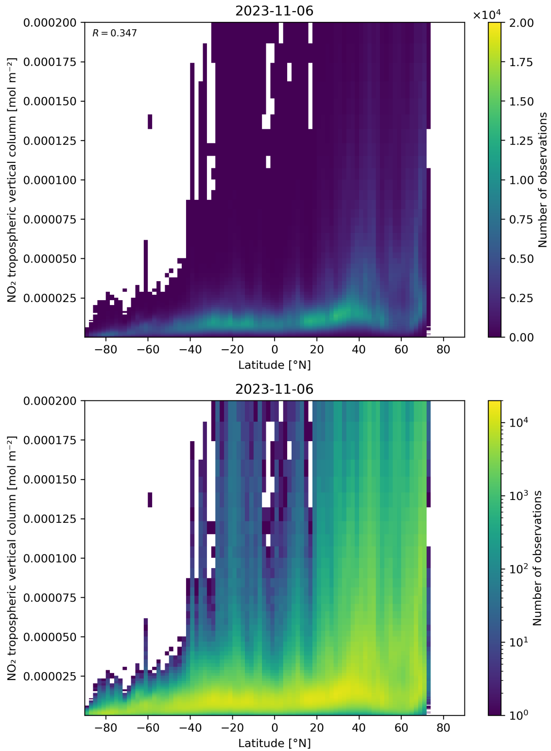
Figure 92: Scatter density plot of “Latitude” against “NO 2 tropospheric vertical column” for 2023-11-05 to 2023-11-07.
