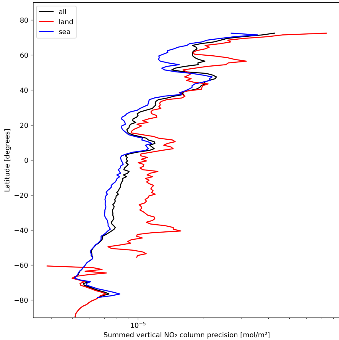
Figure 24: Zonal average of “Summed vertical NO 2 column precision” for 2023-11-05 to 2023-11-07.
