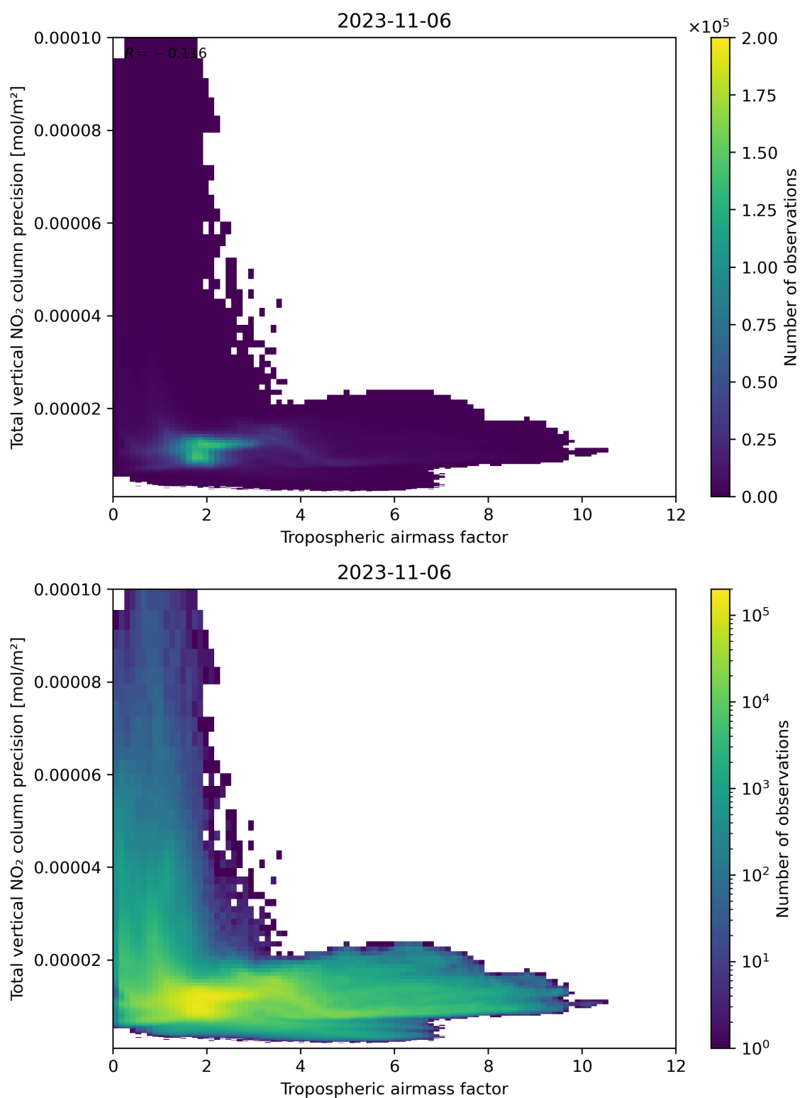
Figure 78: Scatter density plot of “Tropospheric air mass factor” against “Total vertical NO 2 column precision” for 2023-11-05 to 2023-11-07.
