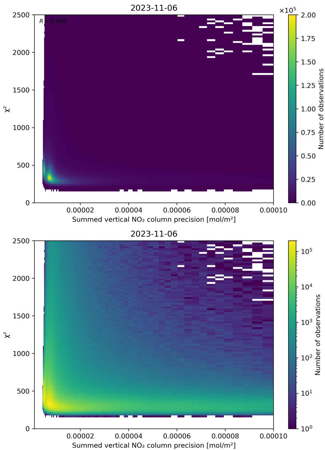
Figure 107: Scatter density plot of “Summed vertical NO 2 column precision” against “ \chi^2 ” for 2023-11-05 to 2023-11-07.
