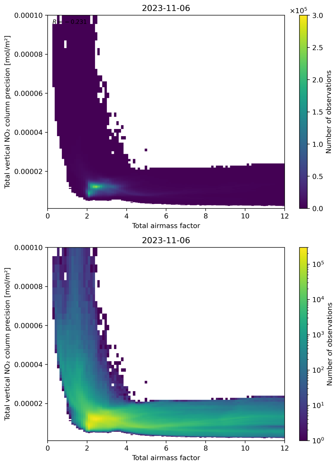
Figure 68: Scatter density plot of “Total airmass factor” against “Total vertical NO 2 column precision” for 2023-11-05 to 2023-11-07.
