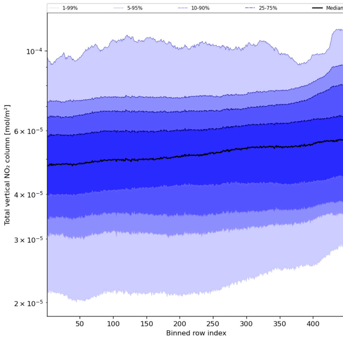
Figure 55: Along track statistics of “Total vertical NO 2 column” for 2023-11-05 to 2023-11-07
