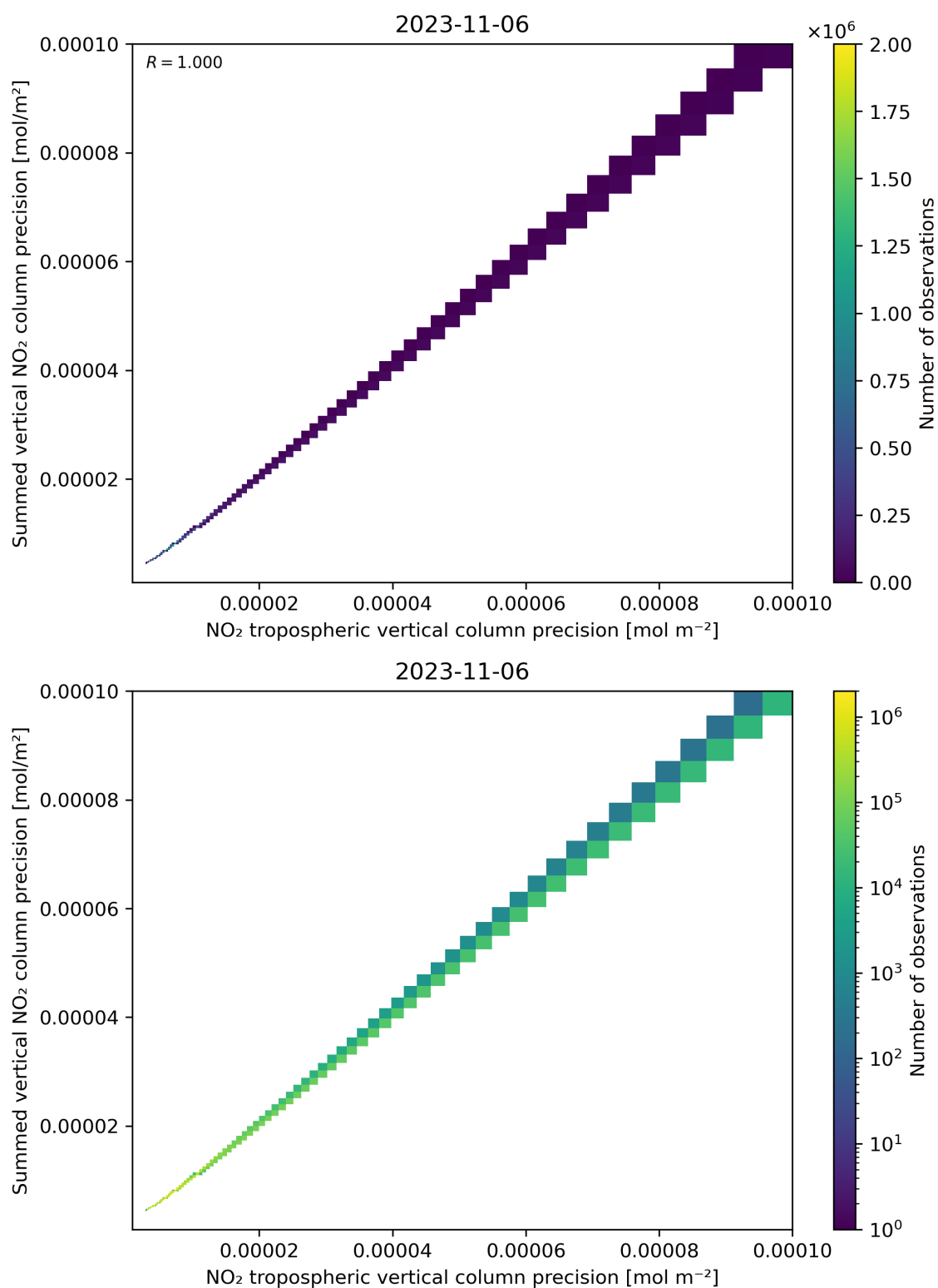
Figure 137: Scatter density plot of “NO 2 tropospheric vertical column precision” against “Summed vertical NO 2 column precision” for 2023-11-05 to 2023-11-07.
