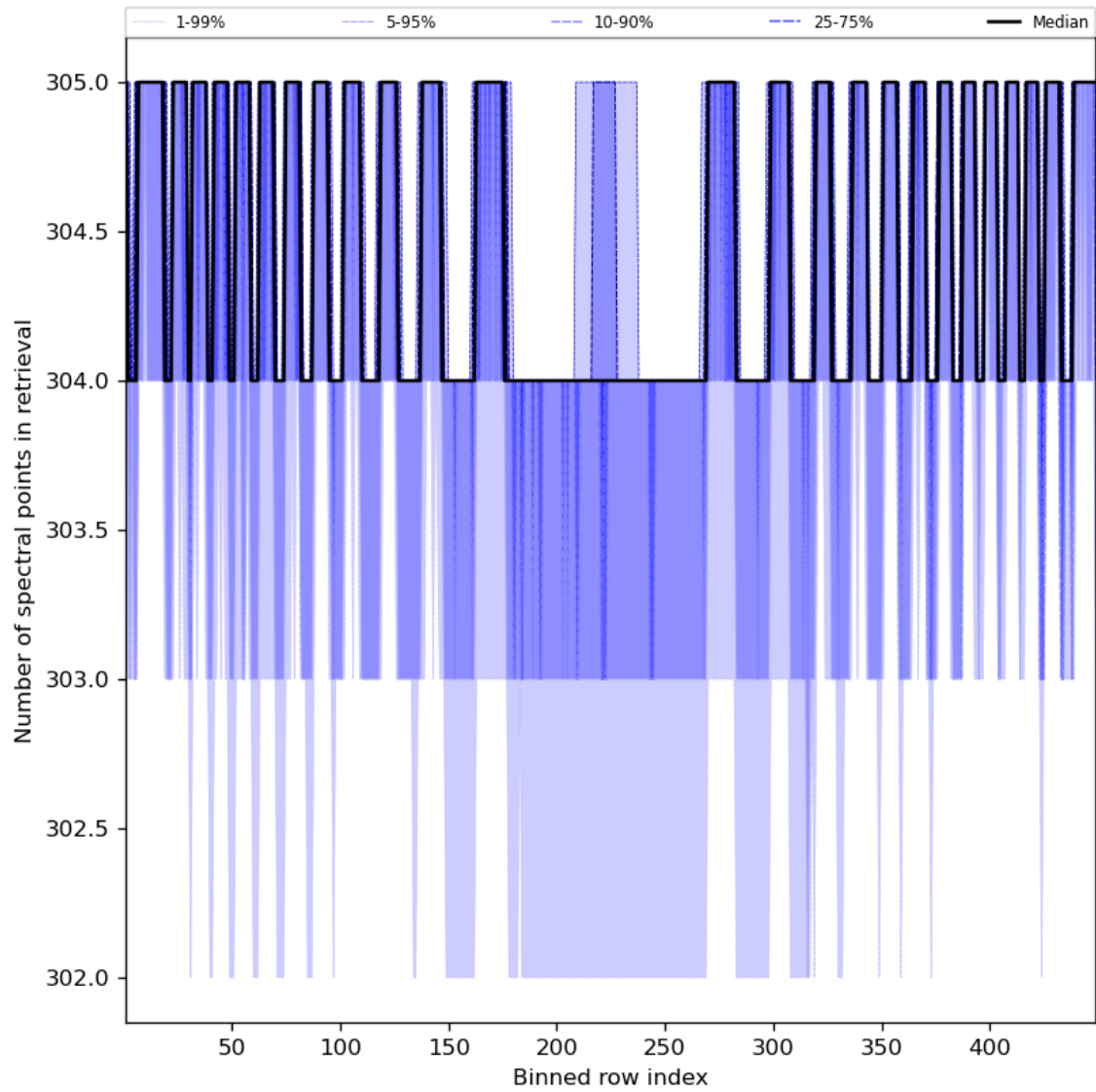
Figure 50: Along track statistics of “Number of spectral points in retrieval” for 2023-11-05 to 2023-11-07
