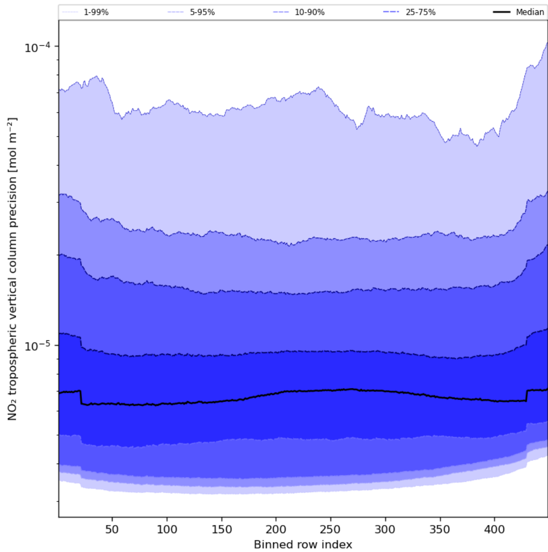
Figure 47: Along track statistics of “NO 2 tropospheric vertical column precision” for 2023-11-05 to 2023-11-07
