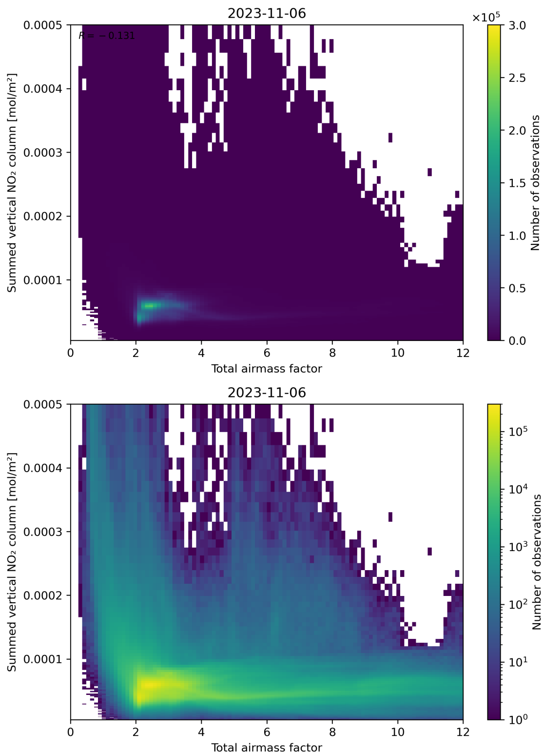
Figure 65: Scatter density plot of “Total airmass factor” against “Summed vertical NO 2 column” for 2023-11-05 to 2023-11-07.
