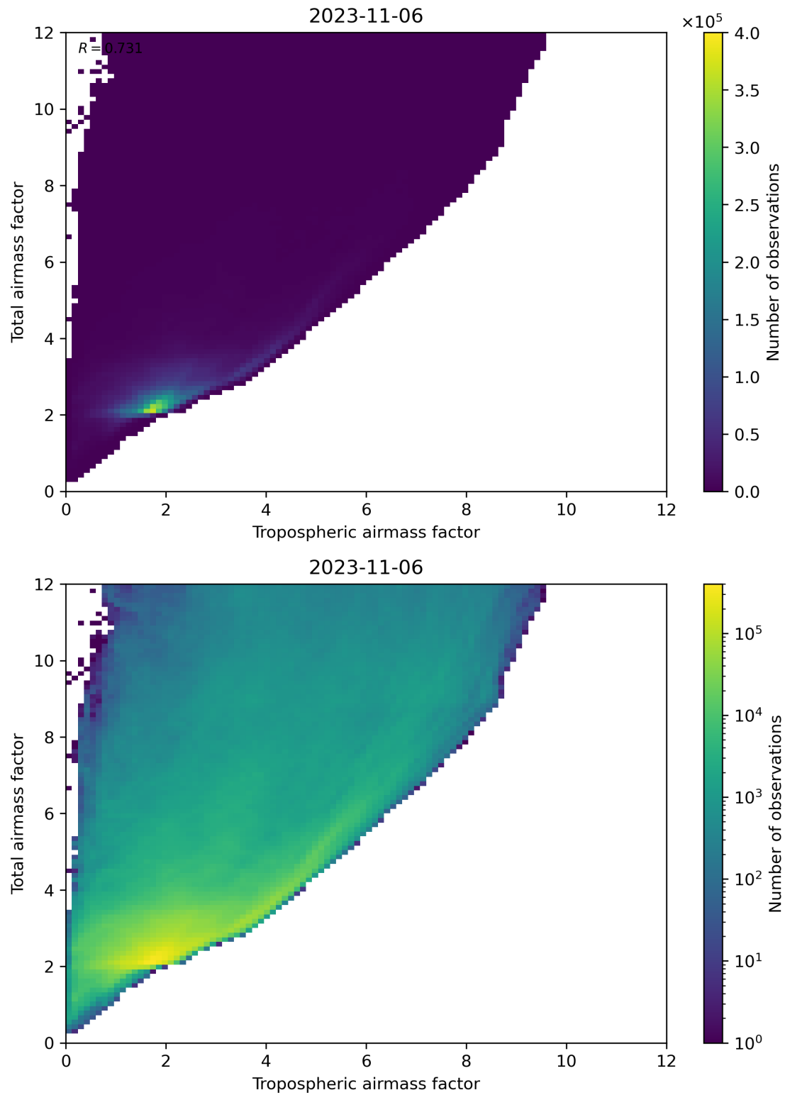
Figure 72: Scatter density plot of “Tropospheric airmass factor” against “Total airmass factor” for 2023-11-05 to 2023-11-07.
