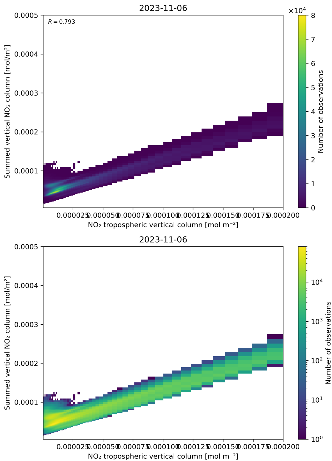
Figure 126: Scatter density plot of “NO 2 tropospheric vertical column” against “Summed vertical NO 2 column” for 2023-11-05 to 2023-11-07.
