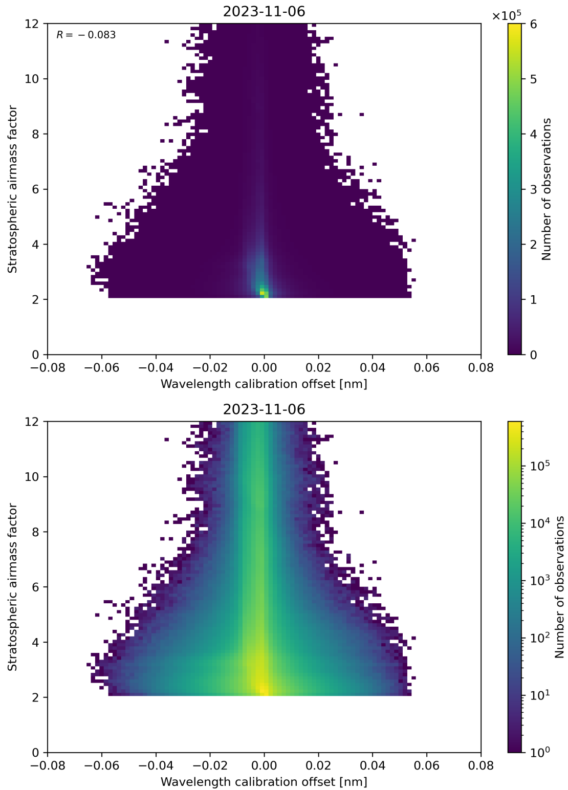
Figure 174: Scatter density plot of “Wavelength calibration offset” against “Stratospheric air mass factor” for 2023-11-05 to 2023-11-07.
