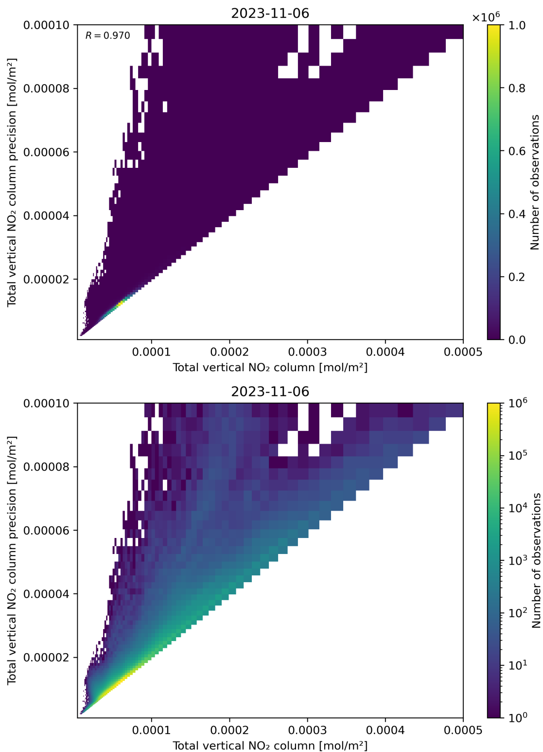
Figure 114: Scatter density plot of “Total vertical NO 2 column” against “Total vertical NO 2 column precision” for 2023-11-05 to 2023-11-07.
