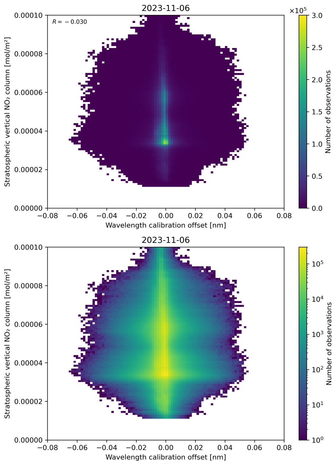
Figure 176: Scatter density plot of “Wavelength calibration offset” against “Stratospheric vertical NO 2 column” for 2023-11-05 to 2023-11-07.
