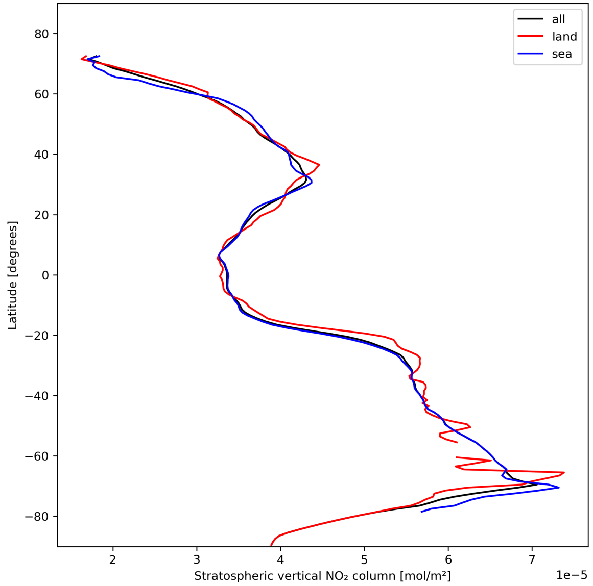
Figure 19: Zonal average of “Stratospheric vertical NO 2 column” for 2023-11-05 to 2023-11-07.
