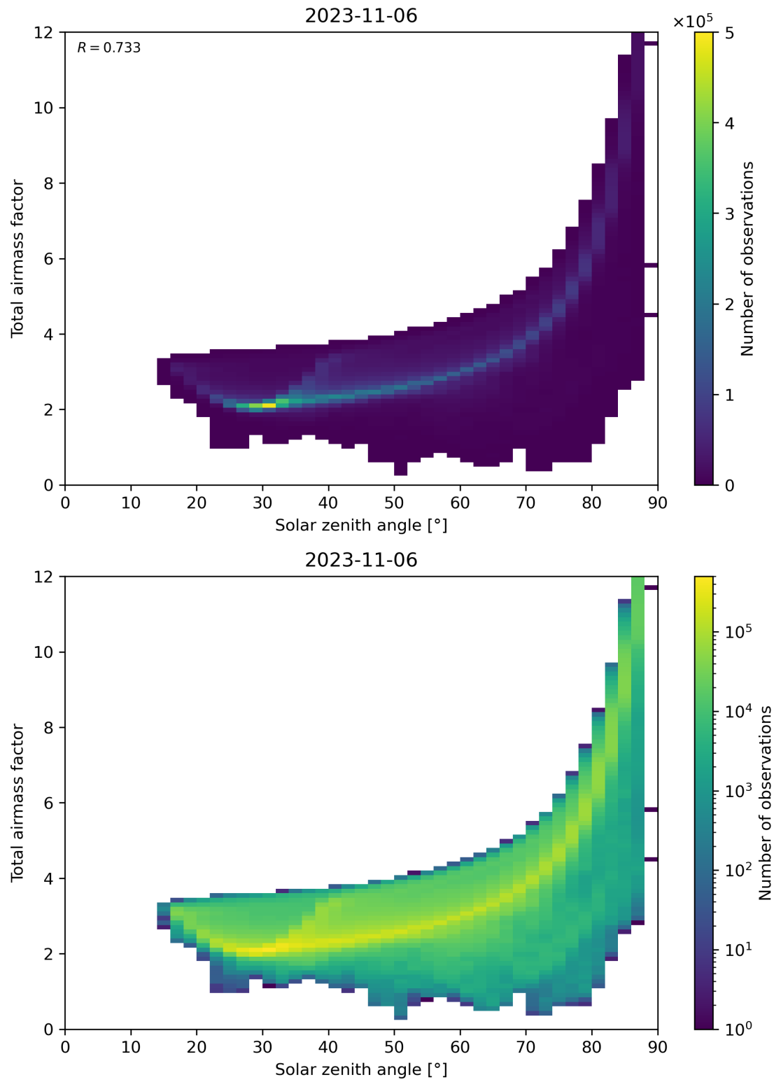
Figure 146: Scatter density plot of “Solar zenith angle” against “Total air mass factor” for 2023-11-05 to 2023-11-07.
