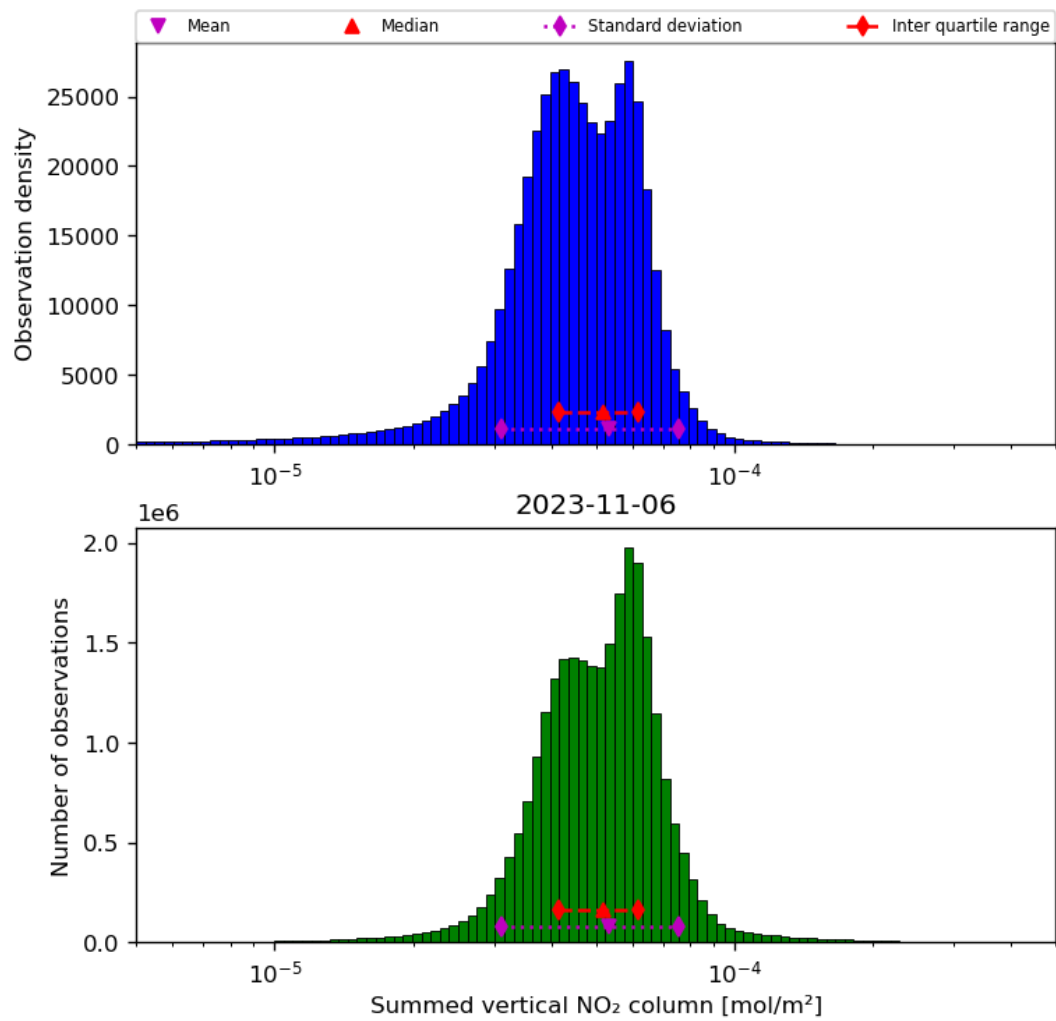
Figure 40: Histogram of “Summed vertical NO 2 column” for 2023-11-05 to 2023-11-07
