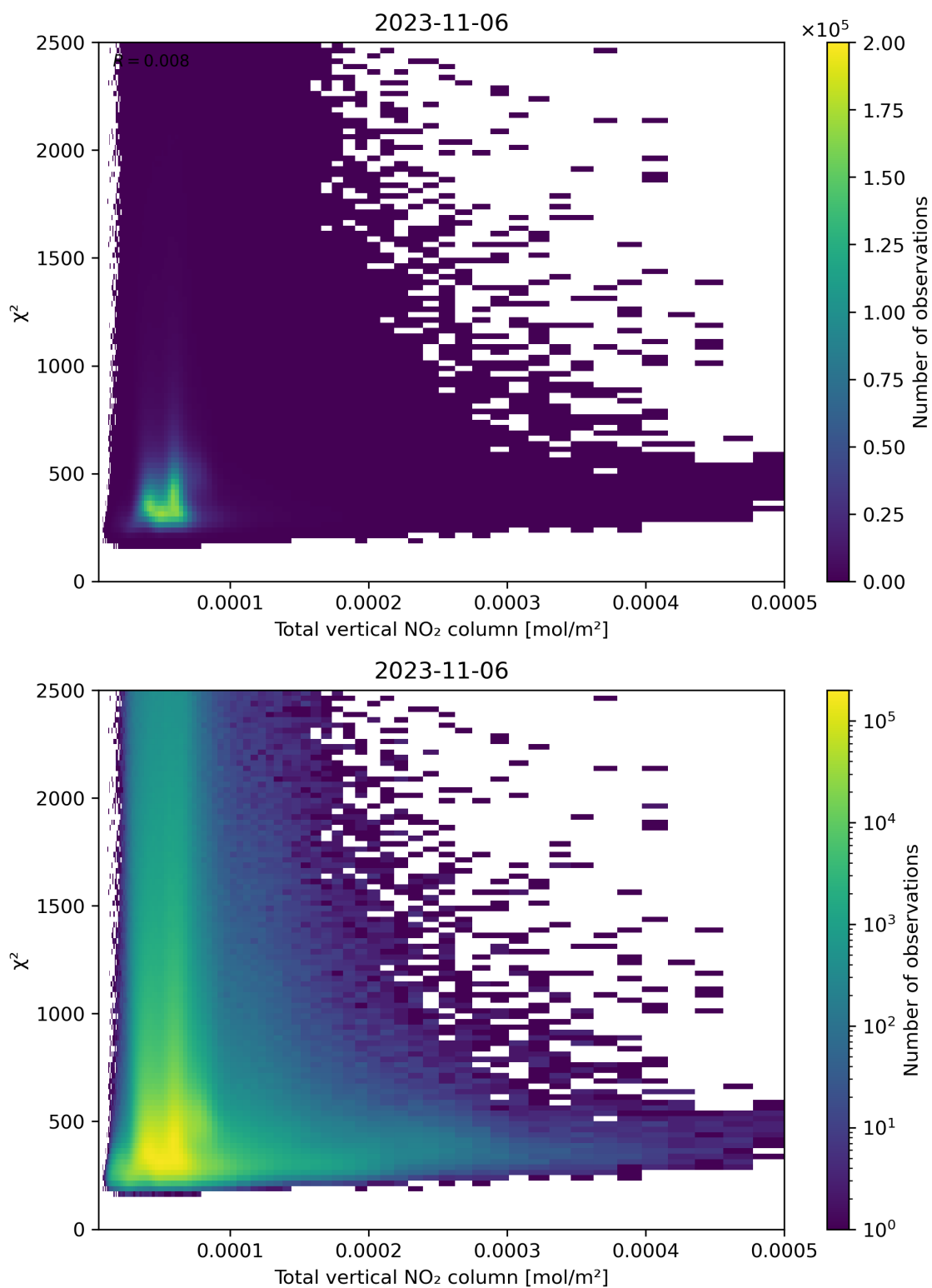
Figure 111: Scatter density plot of “Total vertical NO 2 column” against “ \chi^2 ” for 2023-11-05 to 2023-11-07.
