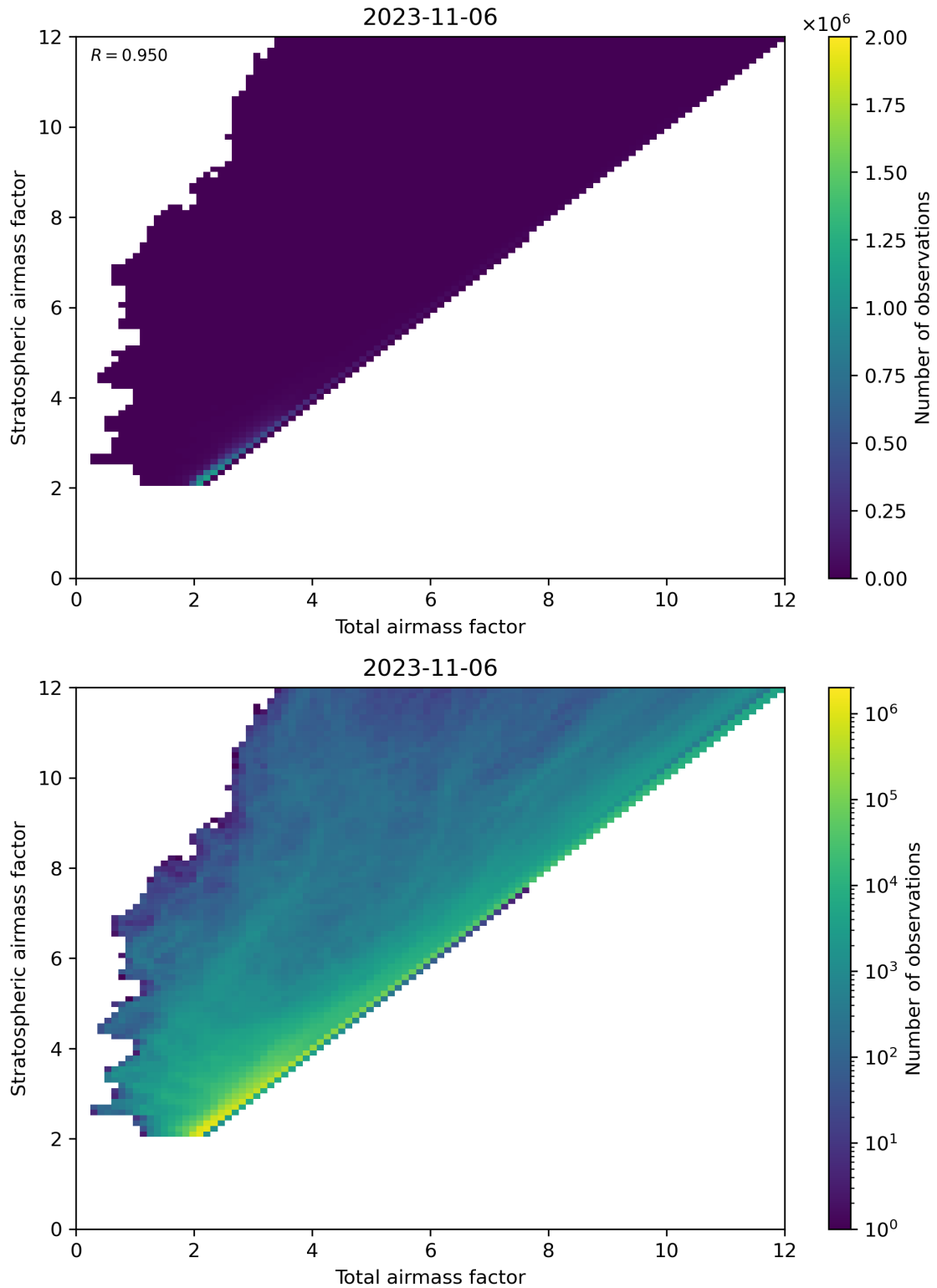
Figure 62: Scatter density plot of “Total airmass factor” against “Stratospheric airmass factor” for 2023-11-05 to 2023-11-07.
