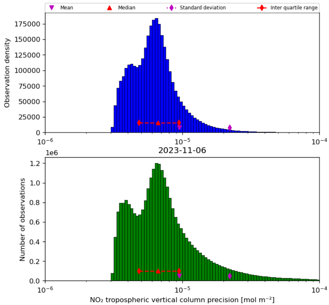
Figure 30: Histogram of “NO 2 tropospheric vertical column precision” for 2023-11-05 to 2023-11-07
