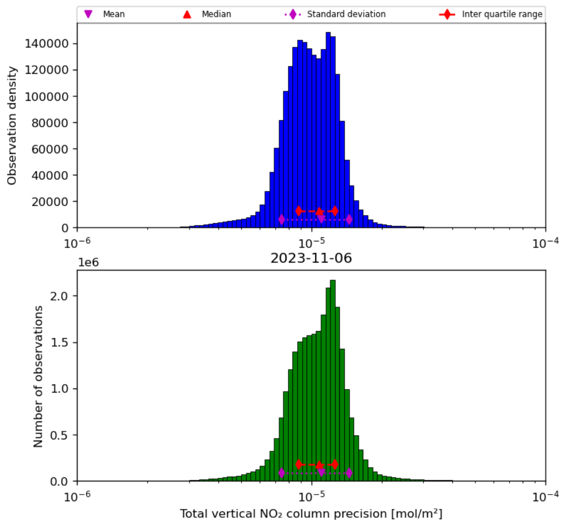
Figure 39: Histogram of "Total vertical NO 2 column precision" for 2023-11-05 to 2023-11-07
