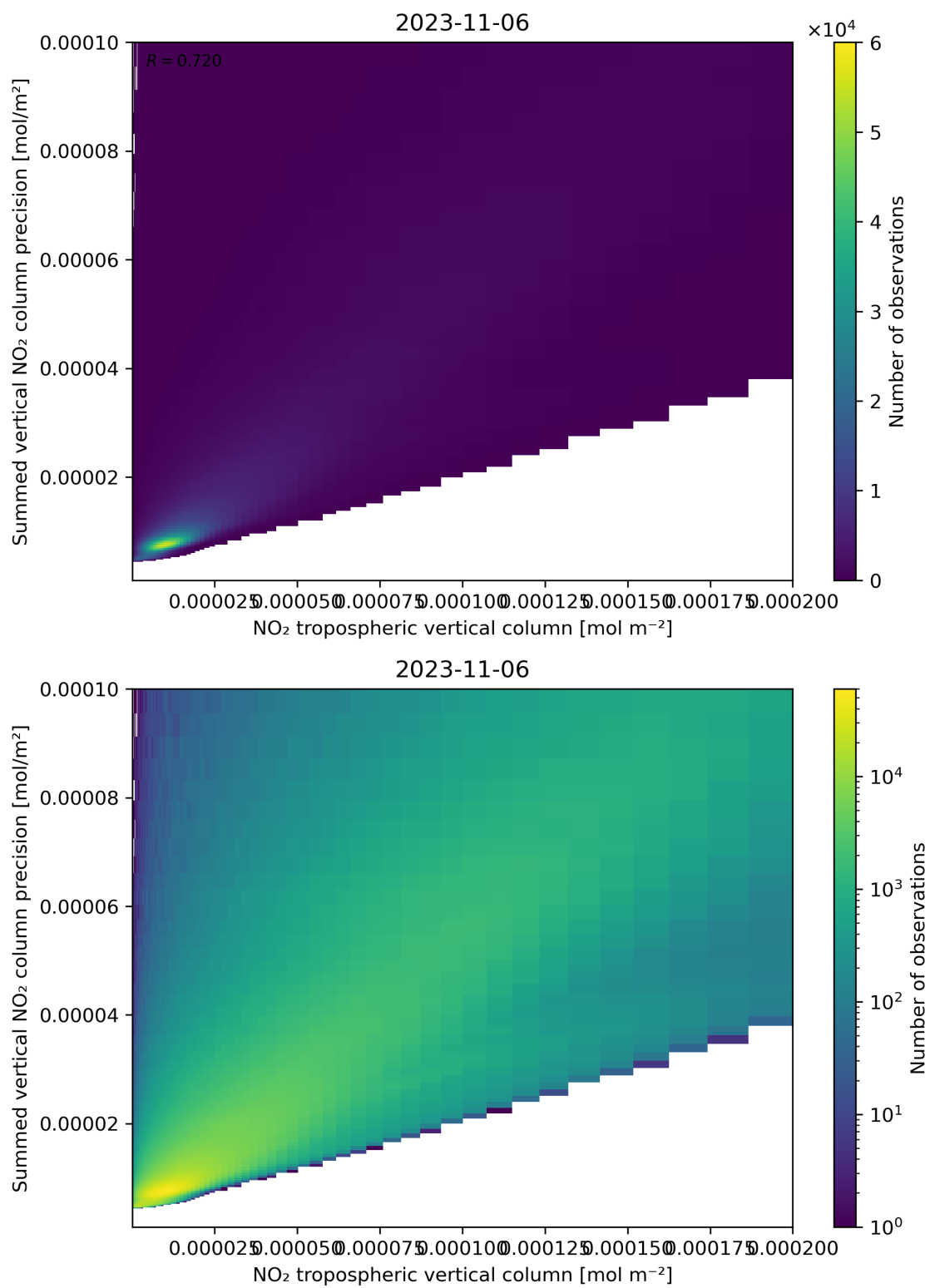
Figure 127: Scatter density plot of “NO 2 tropospheric vertical column” against “Summed vertical NO 2 column precision” for 2023-11-05 to 2023-11-07.
