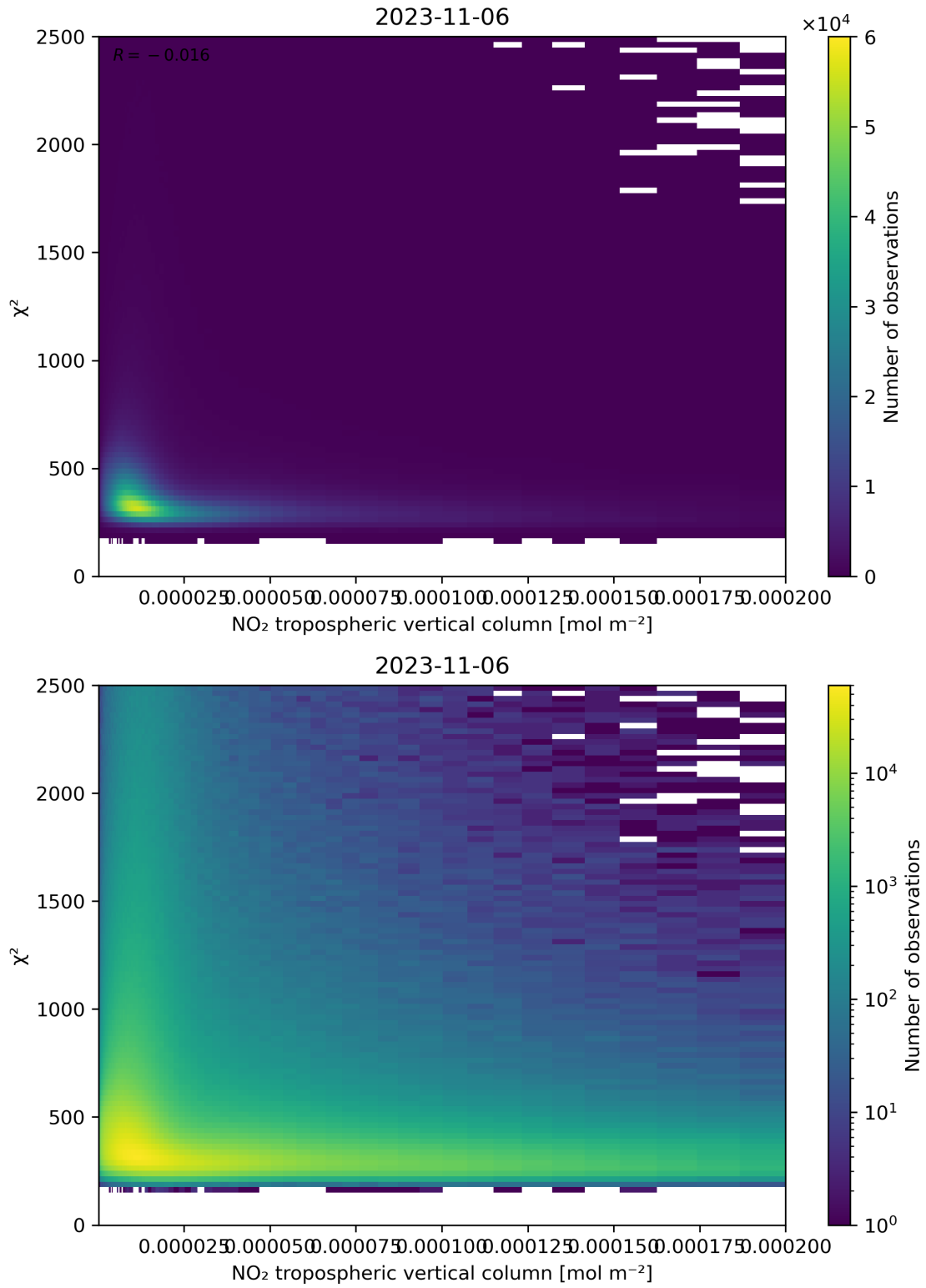
Figure 124: Scatter density plot of “NO 2 tropospheric vertical column” against “ \chi^2 ” for 2023-11-05 to 2023-11-07.
