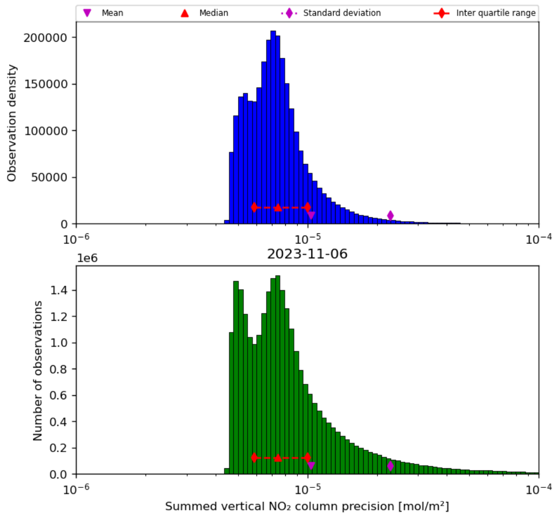
Figure 41: Histogram of "Summed vertical NO 2 column precision" for 2023-11-05 to 2023-11-07
