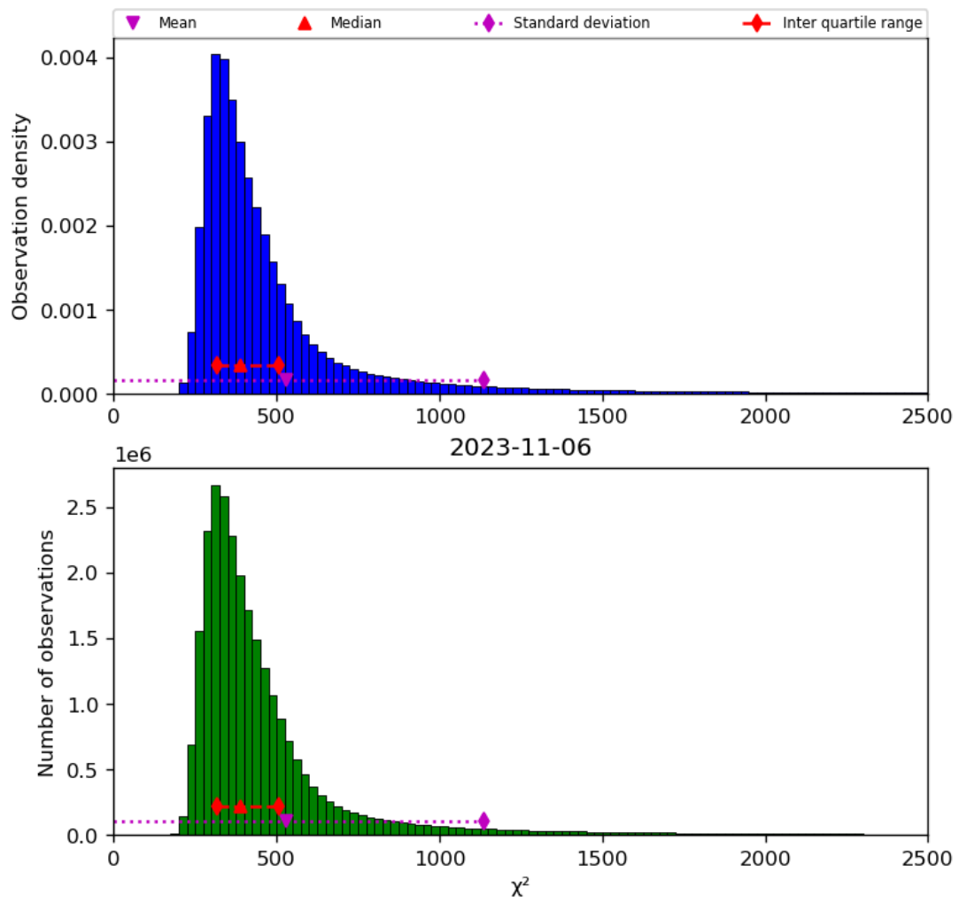
Figure 42: Histogram of “ \chi^2 ” for 2023-11-05 to 2023-11-07
