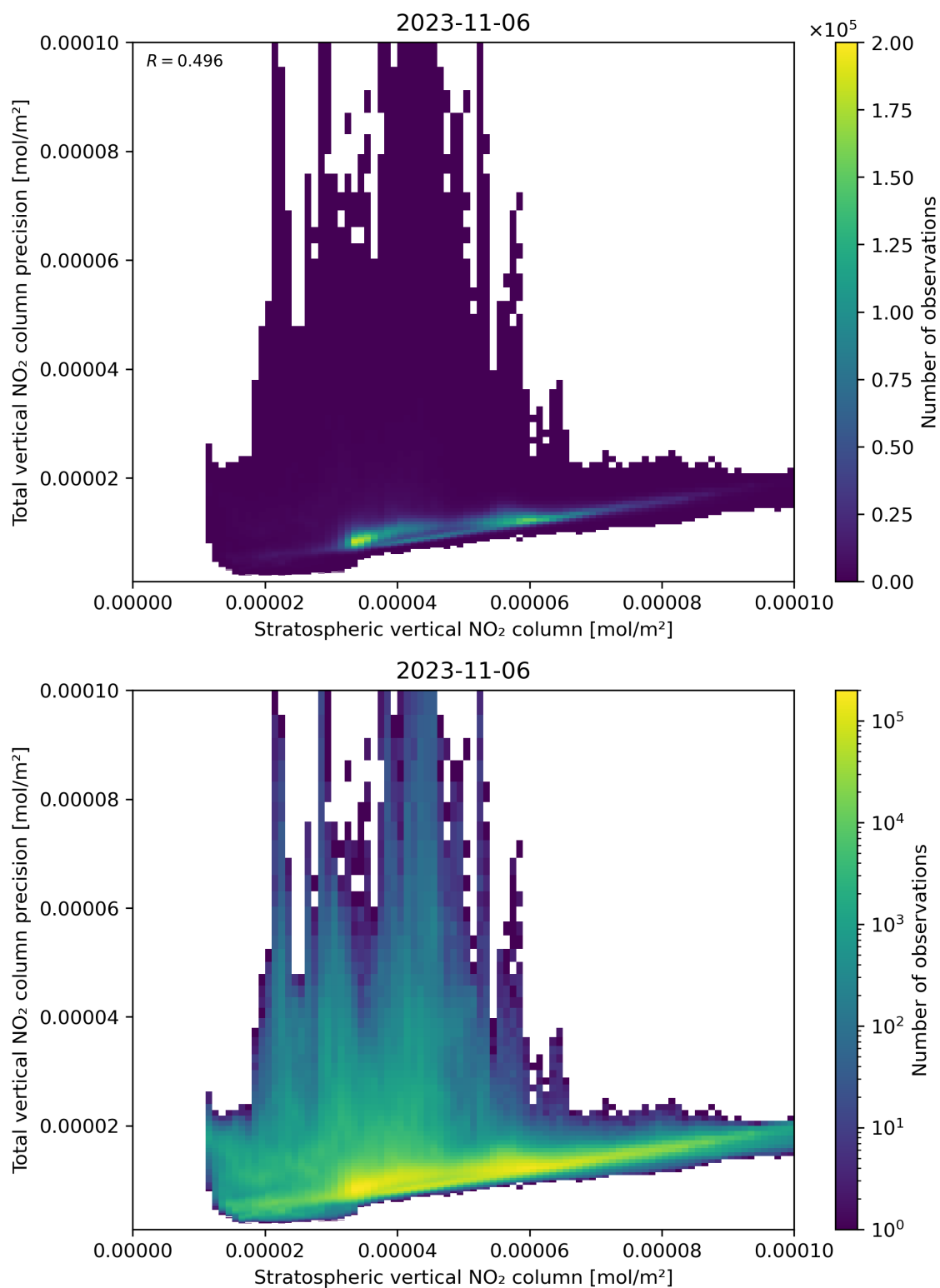
Figure 101: Scatter density plot of “Stratospheric vertical NO 2 column” against “Total vertical NO 2 column precision” for 2023-11-05 to 2023-11-07.
