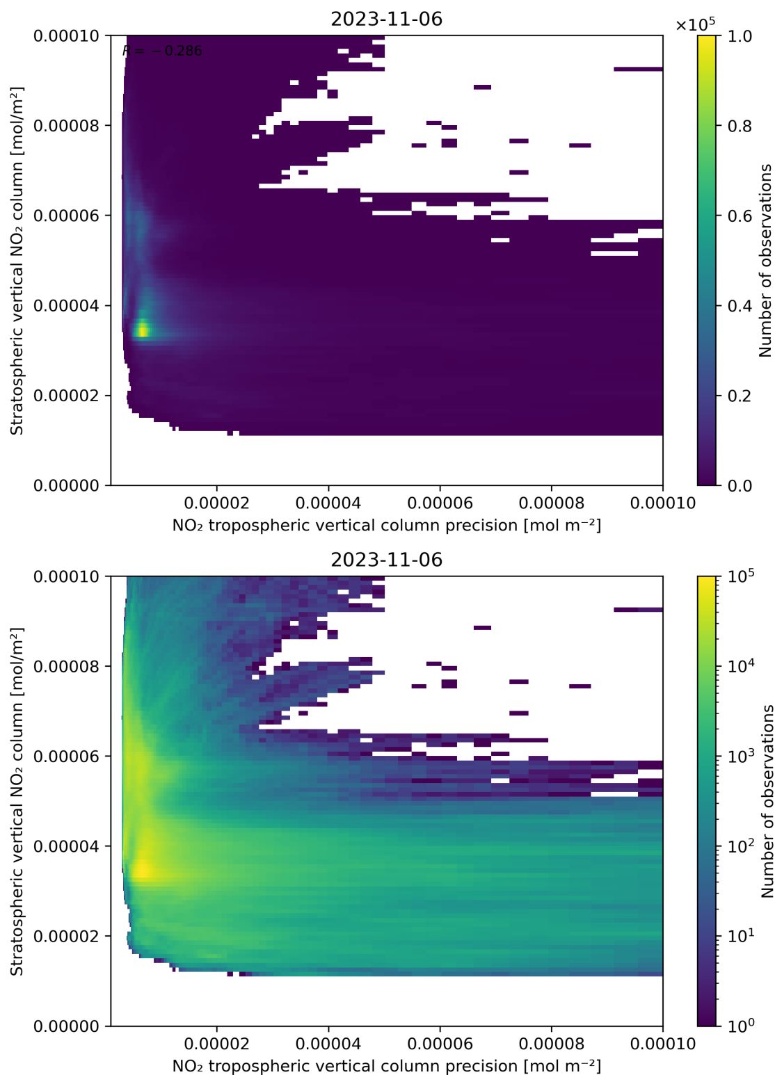
Figure 135: Scatter density plot of “NO 2 tropospheric vertical column precision” against “Stratospheric vertical NO 2 column” for 2023-11-05 to 2023-11-07.
