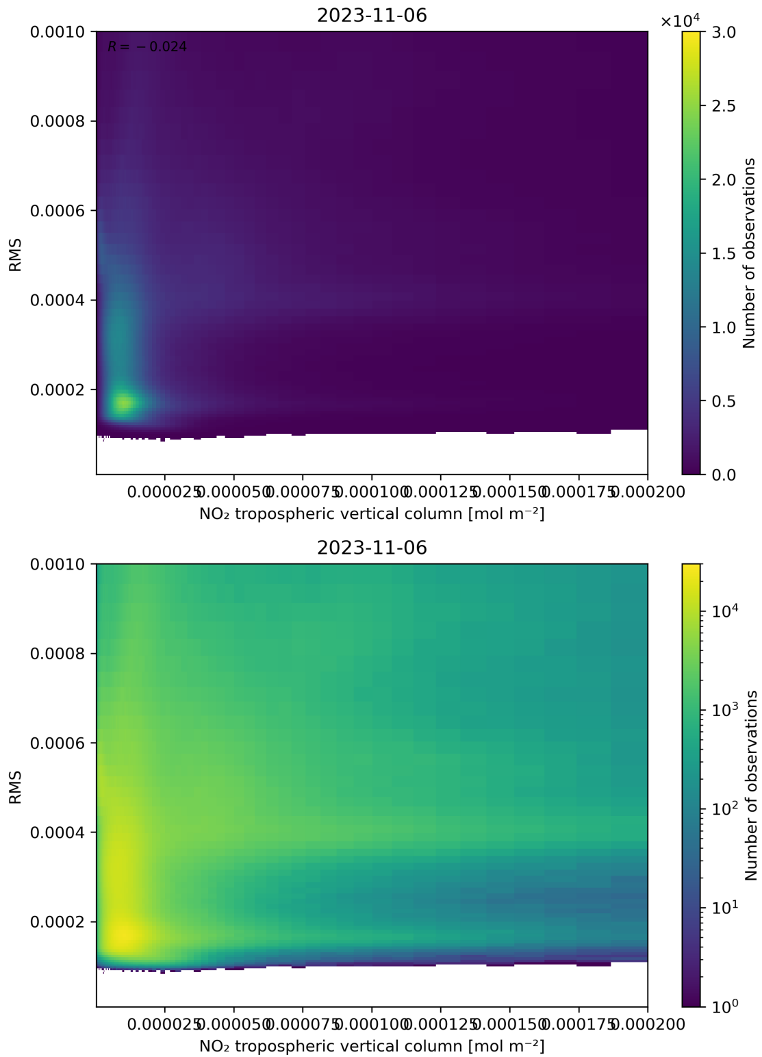
Figure 142: Scatter density plot of “NO 2 tropospheric vertical column” against “RMS” for 2023-11-05 to 2023-11-07.
