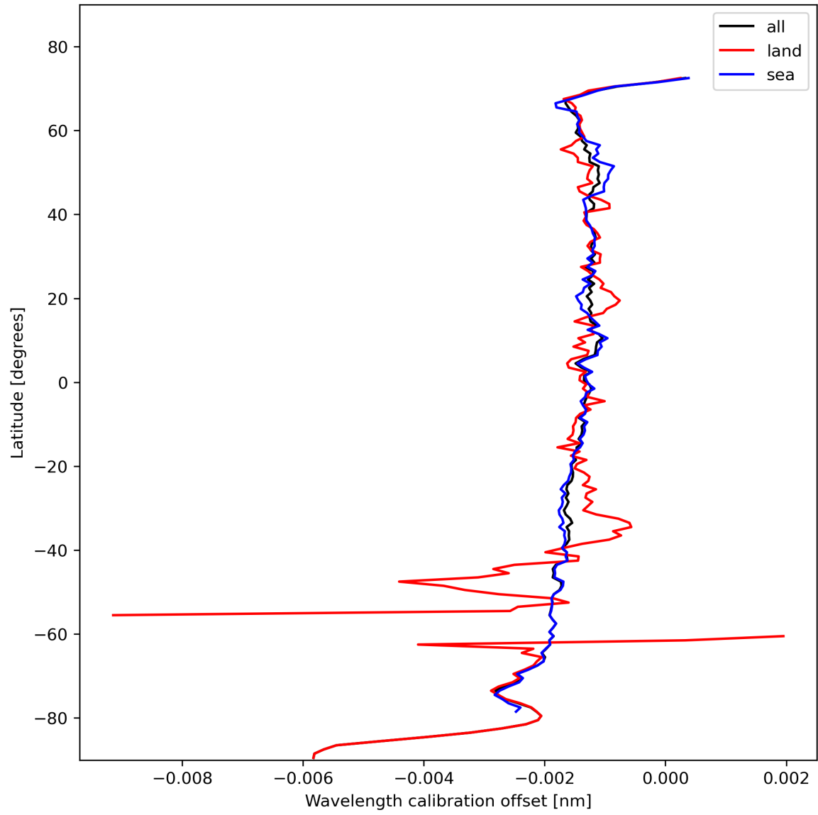
Figure 18: Zonal average of “Wavelength calibration offset” for 2023-11-05 to 2023-11-07.
