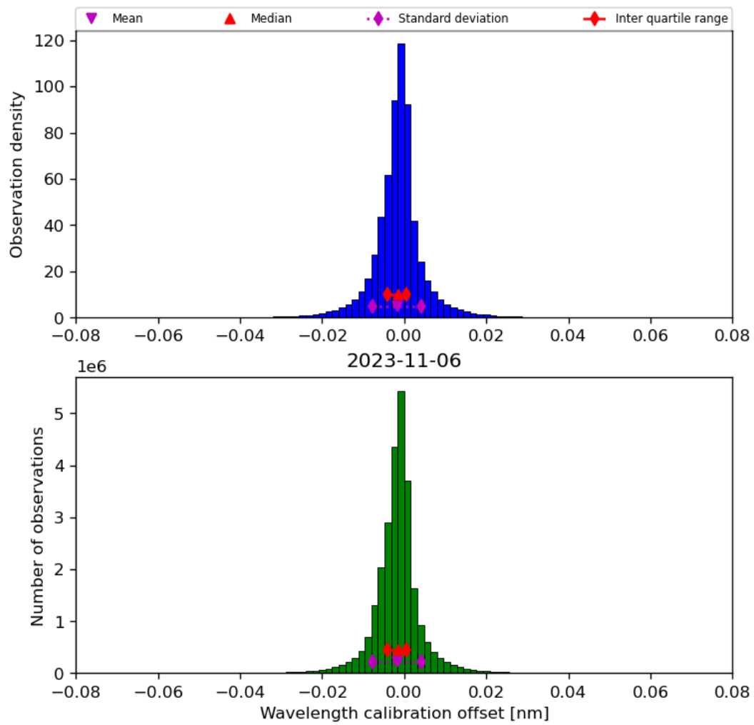
Figure 35: Histogram of “Wavelength calibration offset” for 2023-11-05 to 2023-11-07
