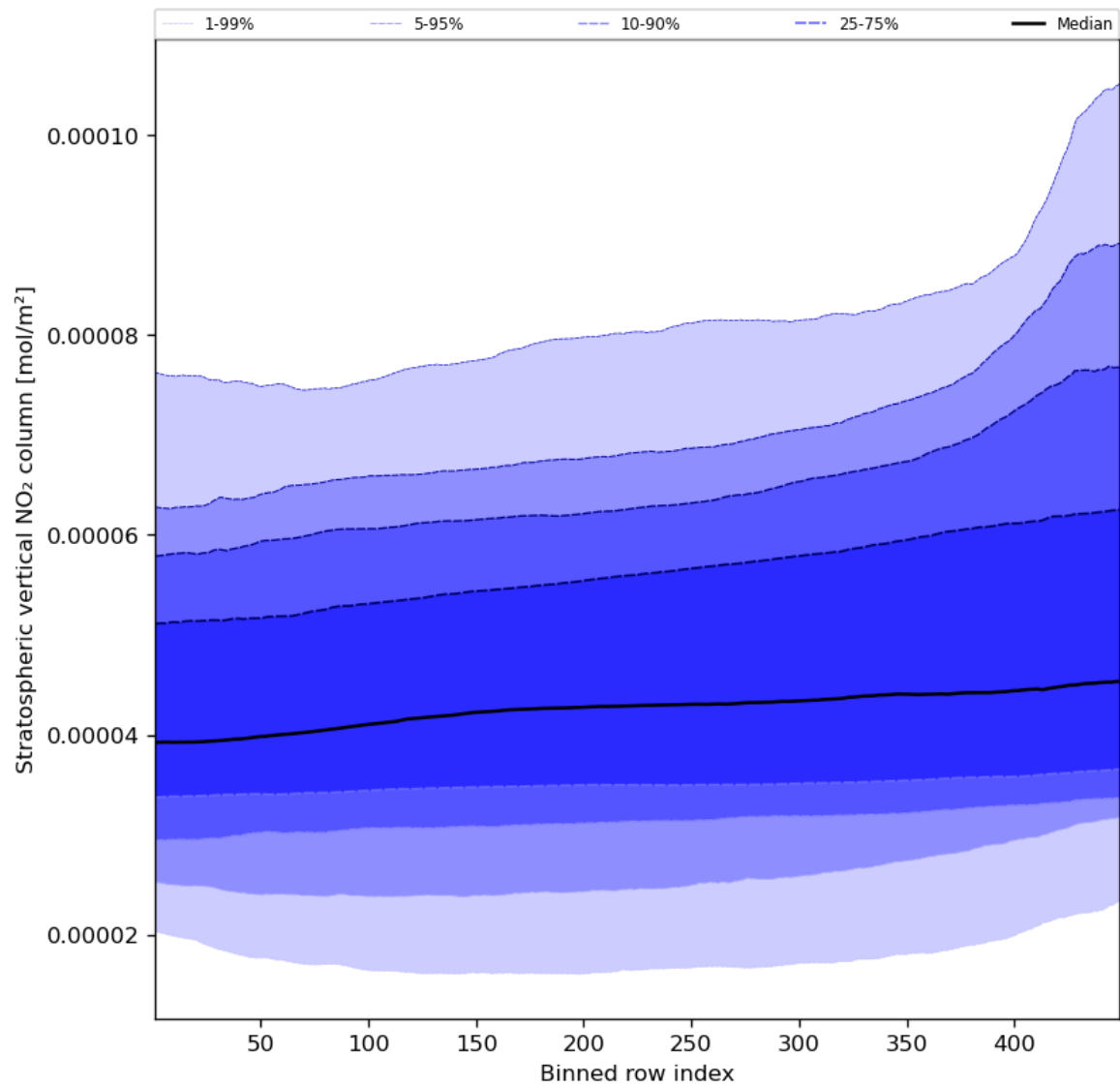
Figure 53: Along track statistics of “Stratospheric vertical NO 2 column” for 2023-11-05 to 2023-11-07
