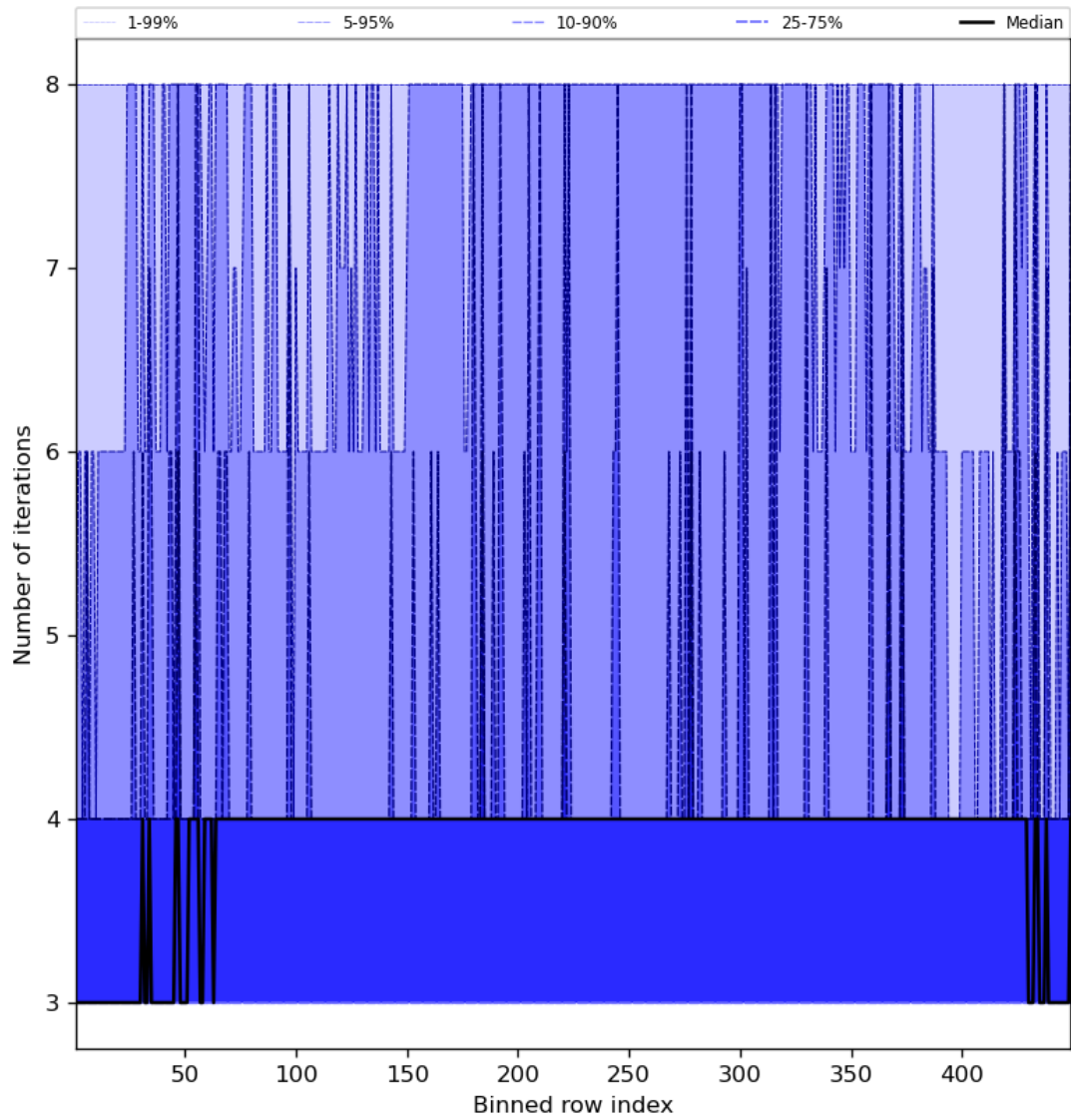
Figure 51: Along track statistics of "Number of iterations" for 2023-11-05 to 2023-11-07
