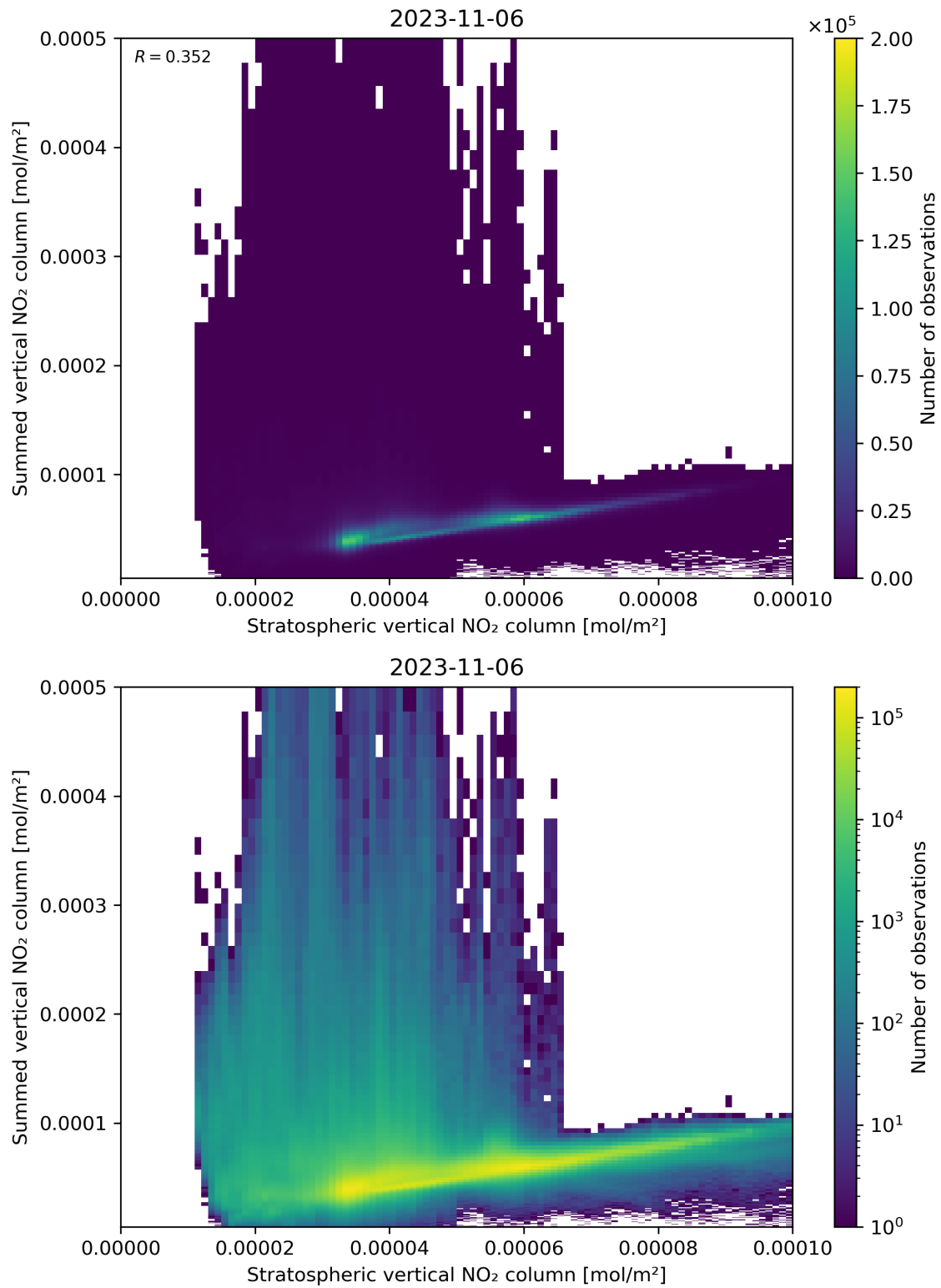
Figure 98: Scatter density plot of “Stratospheric vertical NO 2 column” against “Summed vertical NO 2 column” for 2023-11-05 to 2023-11-07.
