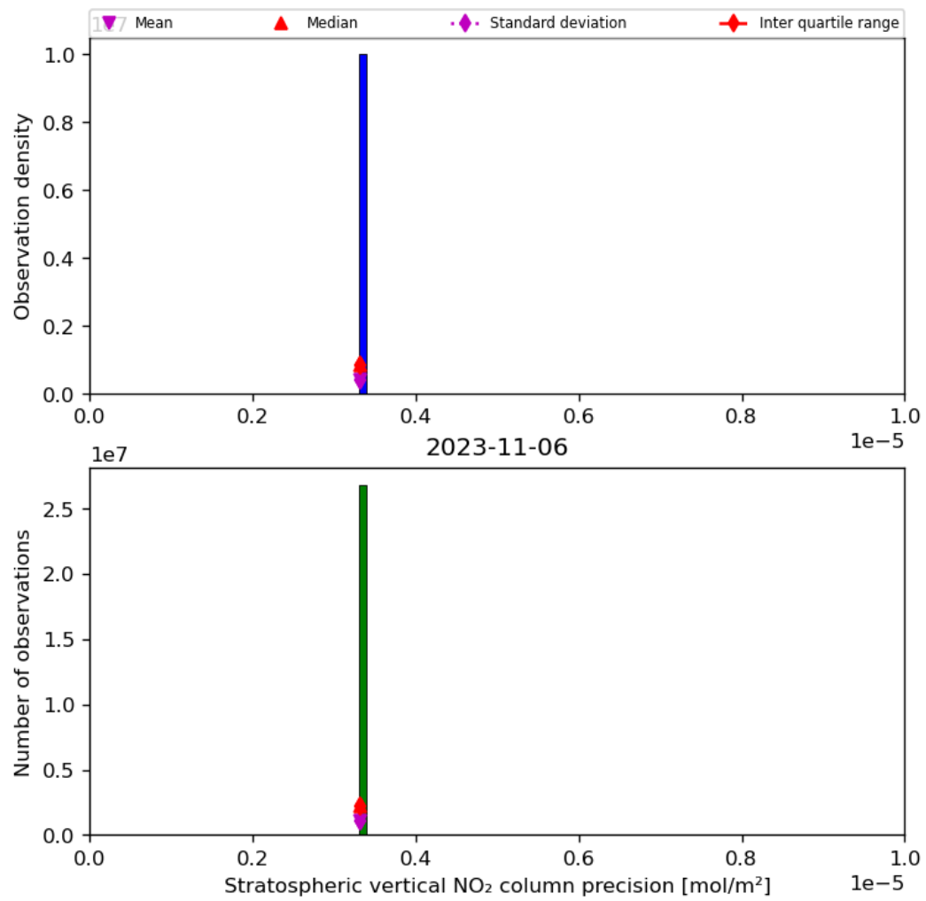
Figure 37: Histogram of “Stratospheric vertical NO 2 column precision” for 2023-11-05 to 2023-11-07
