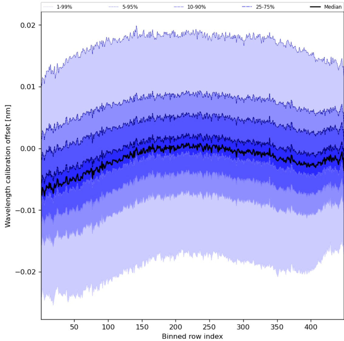
Figure 52: Along track statistics of “Wavelength calibration offset” for 2023-11-05 to 2023-11-07
