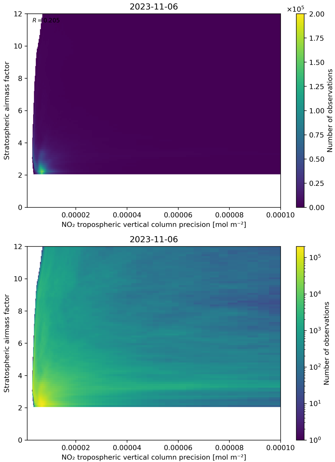
Figure 131: Scatter density plot of “NO 2 tropospheric vertical column precision” against “Stratospheric airmass factor” for 2023-11-05 to 2023-11-07.
