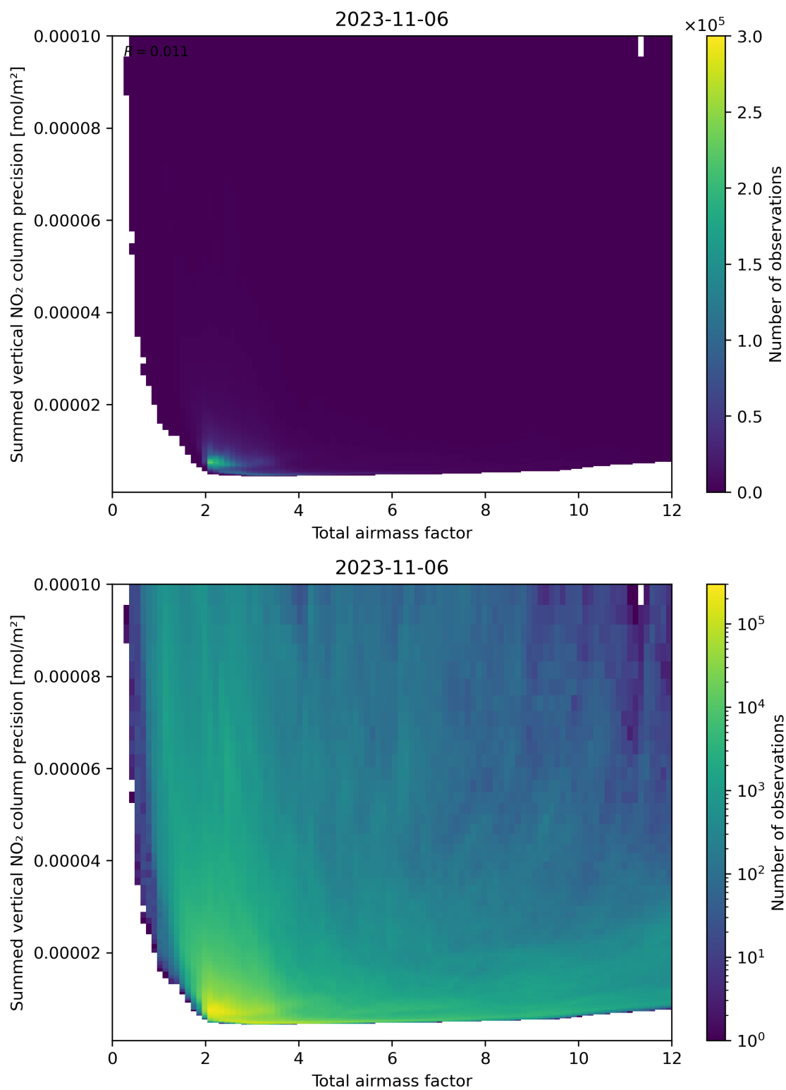
Figure 66: Scatter density plot of “Total airmass factor” against “Summed vertical NO 2 column precision” for 2023-11-05 to 2023-11-07.
