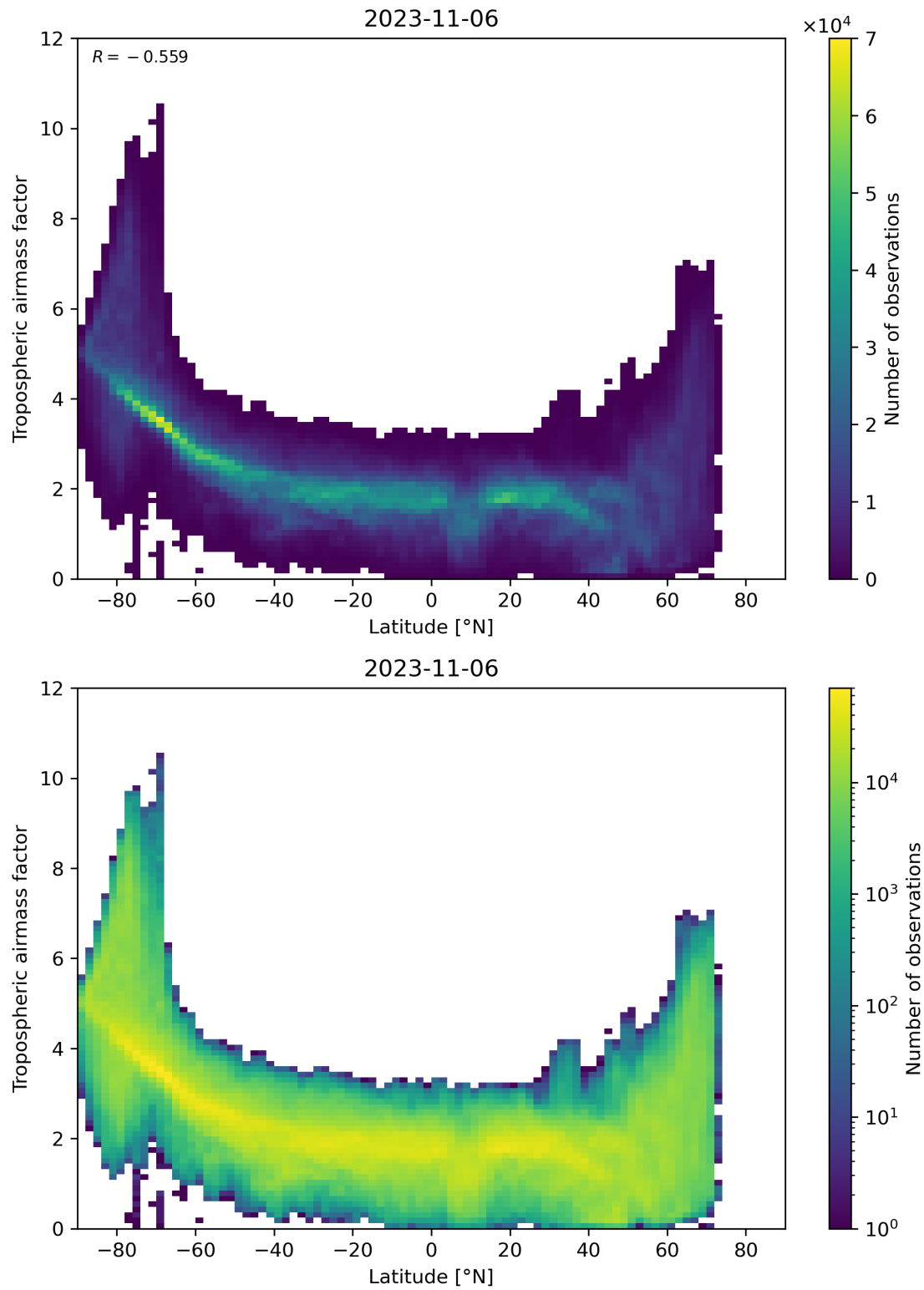
Figure 85: Scatter density plot of “Latitude” against “Tropospheric air mass factor” for 2023-11-05 to 2023-11-07.
