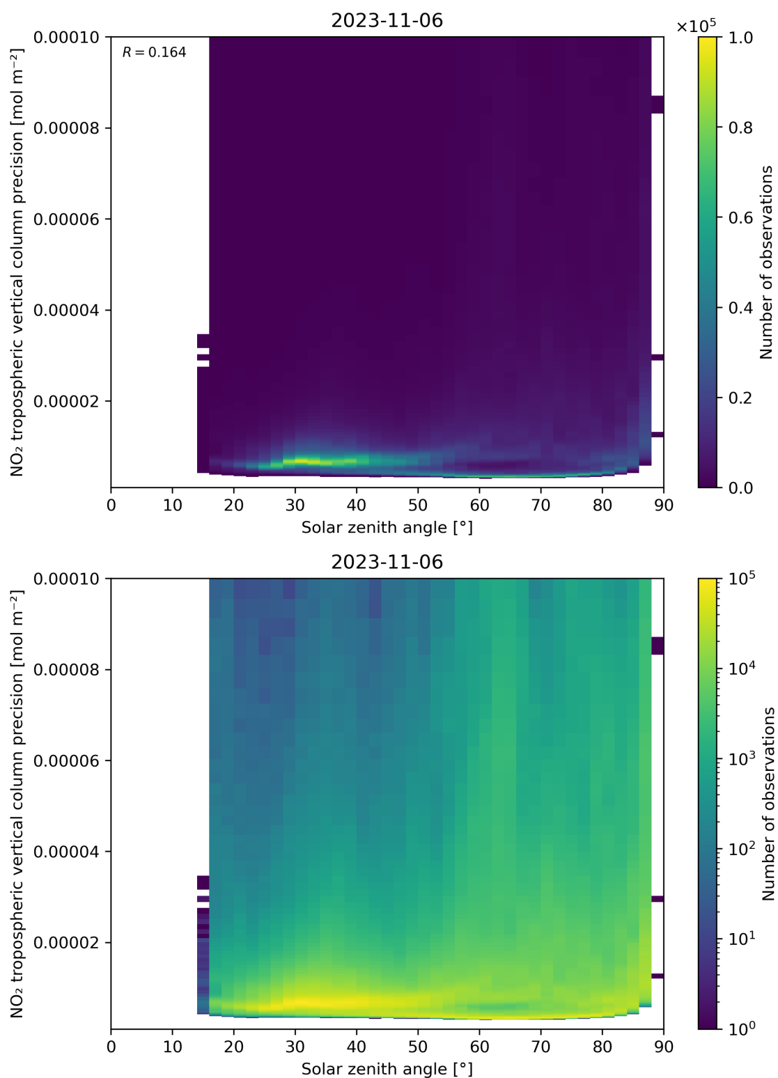
Figure 156: Scatter density plot of “Solar zenith angle” against “NO 2 tropospheric vertical column precision” for 2023-11-05 to 2023-11-07.
