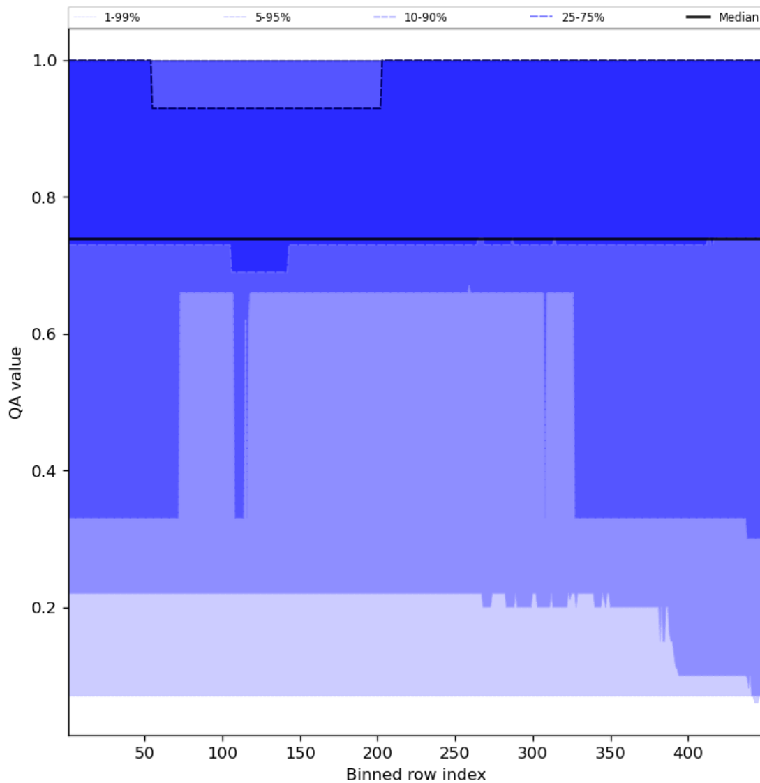
Figure 45: Along track statistics of “QA value” for 2023-11-05 to 2023-11-07
