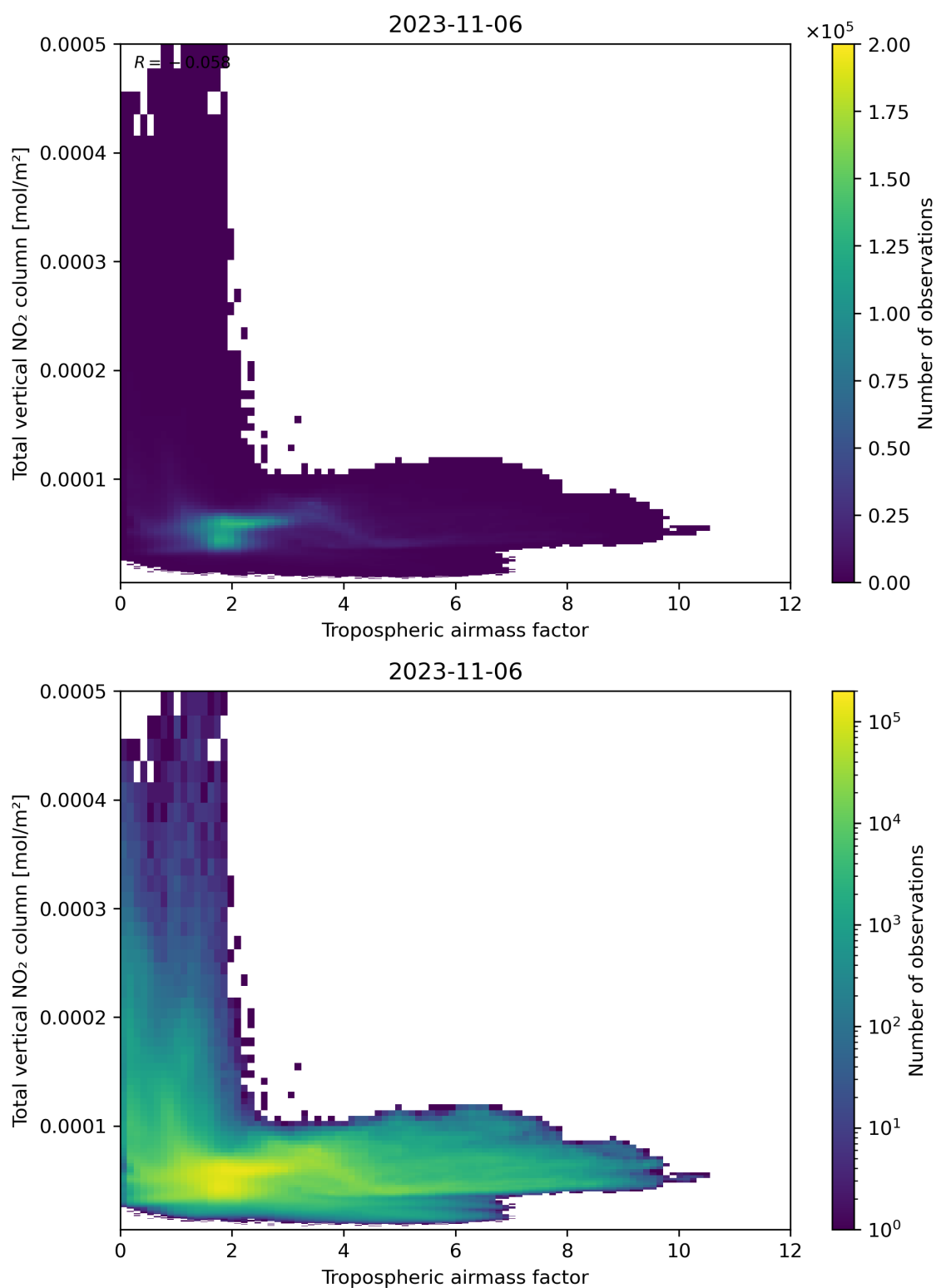
Figure 77: Scatter density plot of “Tropospheric airmass factor” against “Total vertical NO 2 column” for 2023-11-05 to 2023-11-07.
