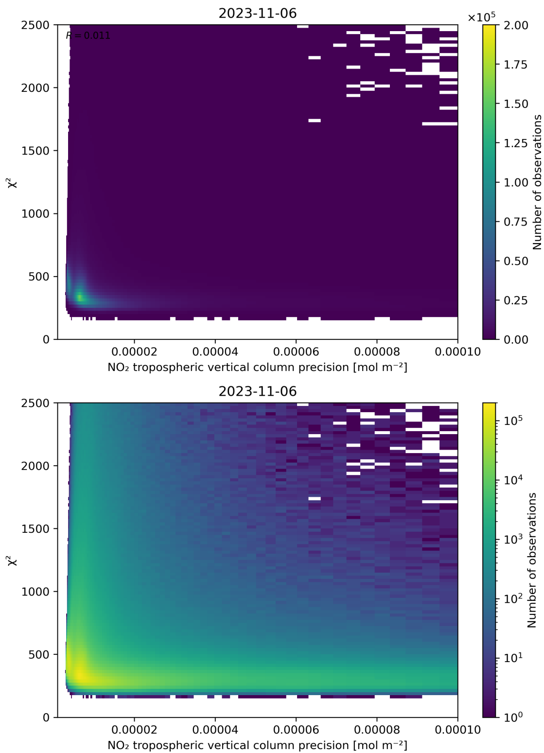
Figure 134: Scatter density plot of “NO 2 tropospheric vertical column precision” against “ \chi^2 ” for 2023-11-05 to 2023-11-07.
