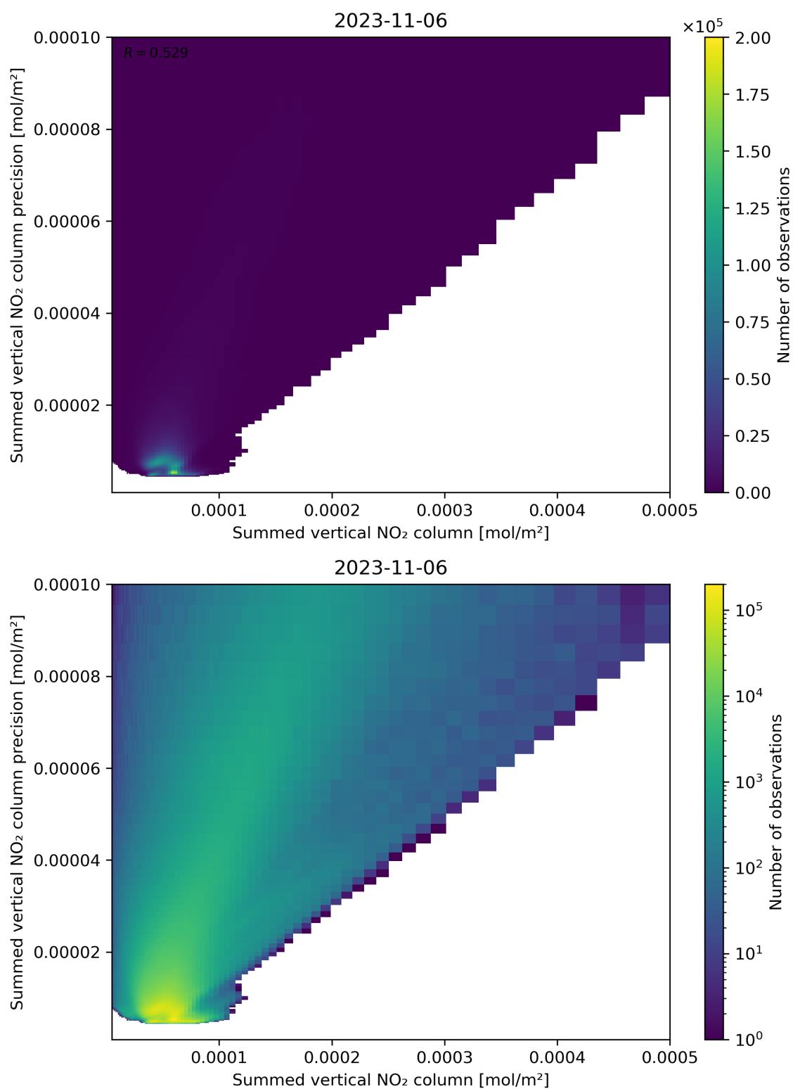
Figure 105: Scatter density plot of “Summed vertical NO 2 column” against “Summed vertical NO 2 column precision” for 2023-11-05 to 2023-11-07.
