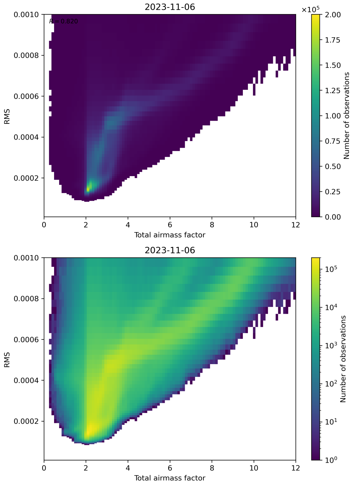
Figure 69: Scatter density plot of “Total airmass factor” against “RMS” for 2023-11-05 to 2023-11-07.
