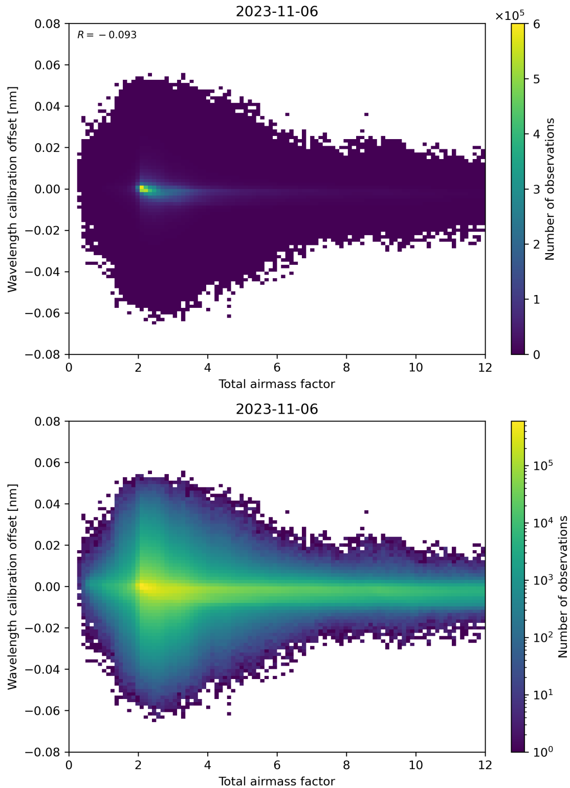
Figure 70: Scatter density plot of “Total airmass factor” against “Wavelength calibration offset” for 2023-11-05 to 2023-11-07.
