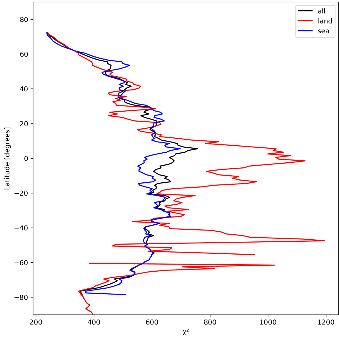
Figure 25: Zonal average of “ \chi^2 ” for 2023-11-05 to 2023-11-07.
