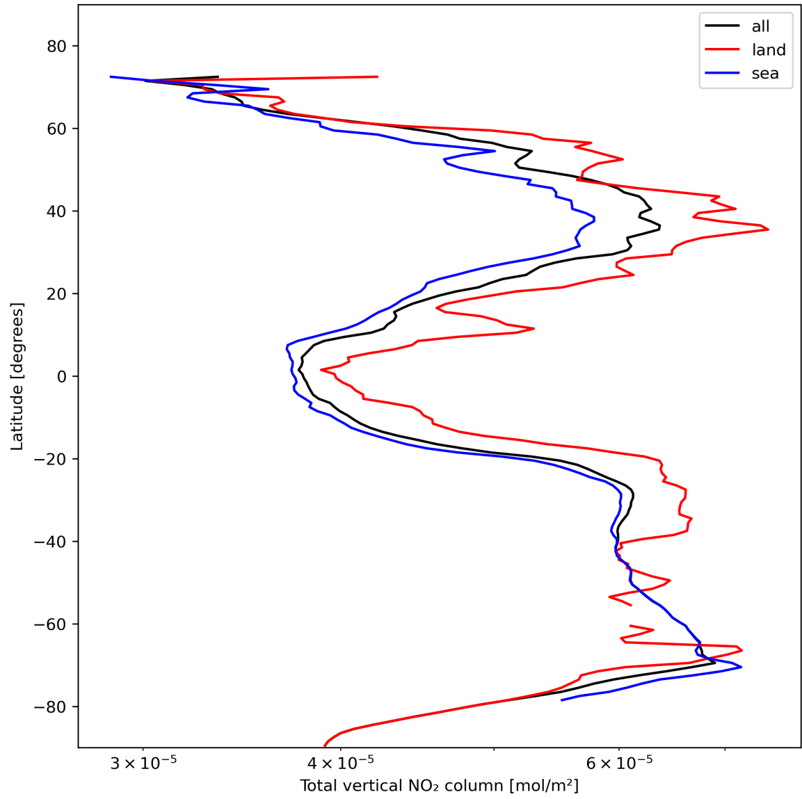
Figure 21: Zonal average of “Total vertical NO 2 column” for 2023-11-05 to 2023-11-07.
