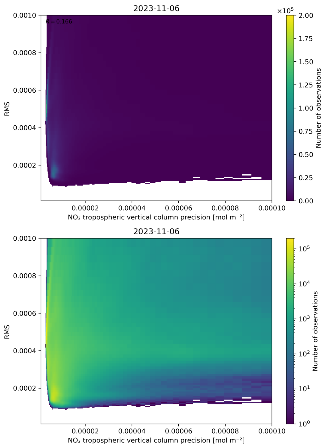
Figure 140: Scatter density plot of “NO 2 tropospheric vertical column precision” against “RMS” for 2023-11-05 to 2023-11-07.
