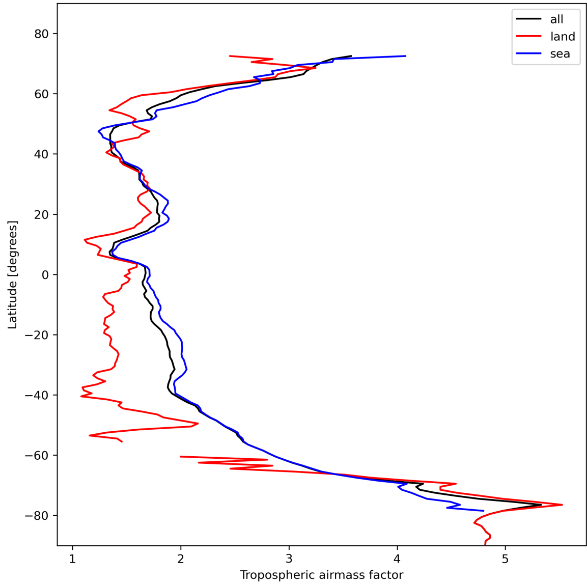
Figure 14: Zonal average of “Tropospheric airmass factor” for 2023-11-05 to 2023-11-07.
