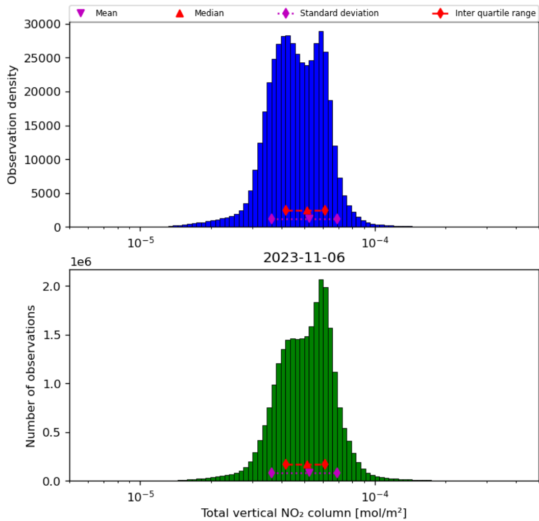
Figure 38: Histogram of “Total vertical NO 2 column” for 2023-11-05 to 2023-11-07
