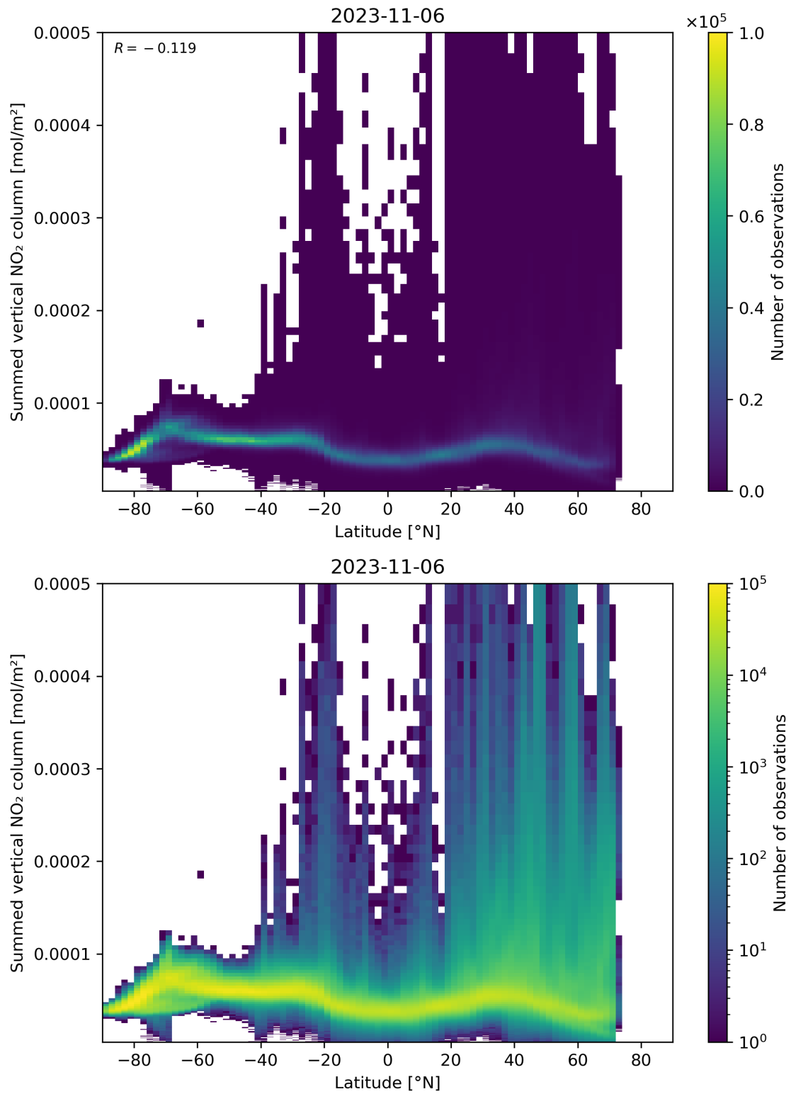
Figure 88: Scatter density plot of “Latitude” against “Summed vertical NO 2 column” for 2023-11-05 to 2023-11-07.
