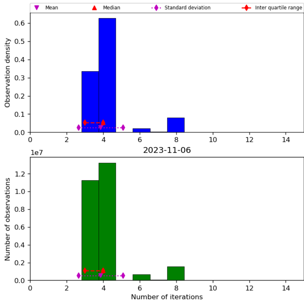
Figure 34: Histogram of "Number of iterations" for 2023-11-05 to 2023-11-07
