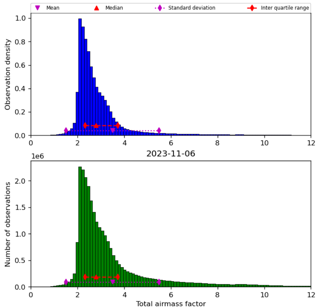
Figure 32: Histogram of “Total airmass factor” for 2023-11-05 to 2023-11-07
