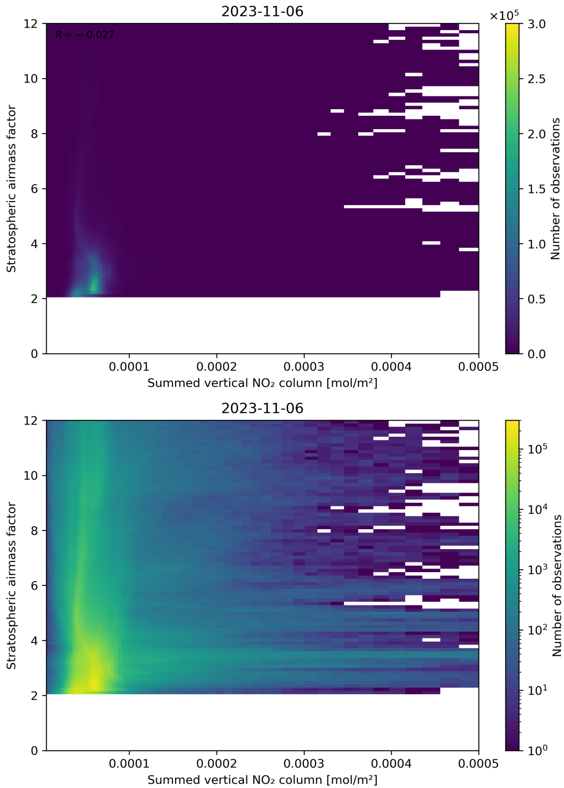
Figure 103: Scatter density plot of “Summed vertical NO 2 column” against “Stratospheric airmass factor” for 2023-11-05 to 2023-11-07.
