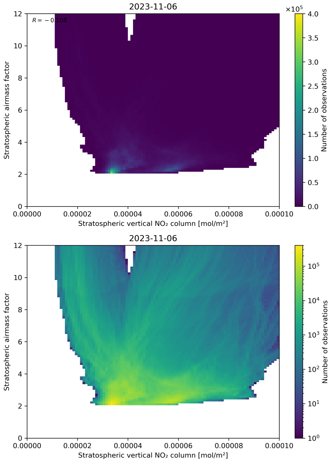
Figure 96: Scatter density plot of “Stratospheric vertical NO 2 column” against “Stratospheric airmass factor” for 2023-11-05 to 2023-11-07.
