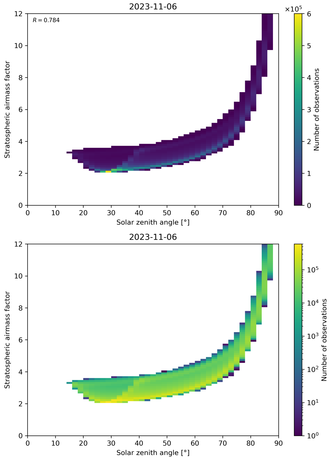
Figure 145: Scatter density plot of “Solar zenith angle” against “Stratospheric airmass factor” for 2023-11-05 to 2023-11-07.
