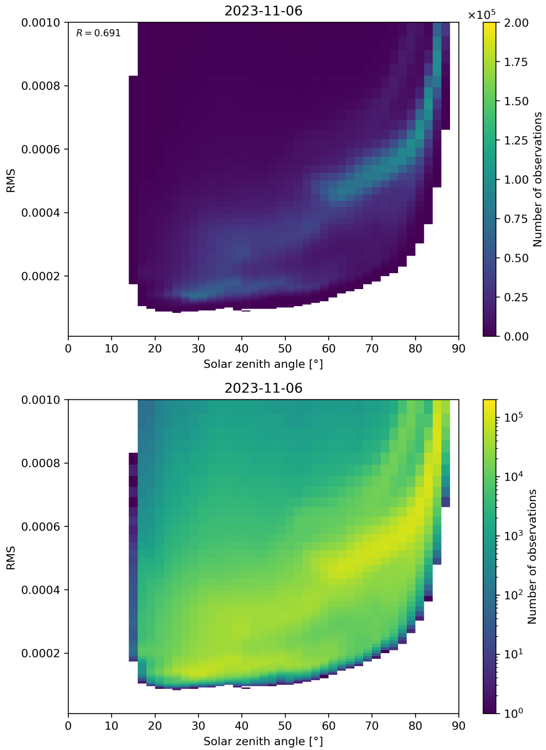
Figure 157: Scatter density plot of “Solar zenith angle” against “RMS” for 2023-11-05 to 2023-11-07.
