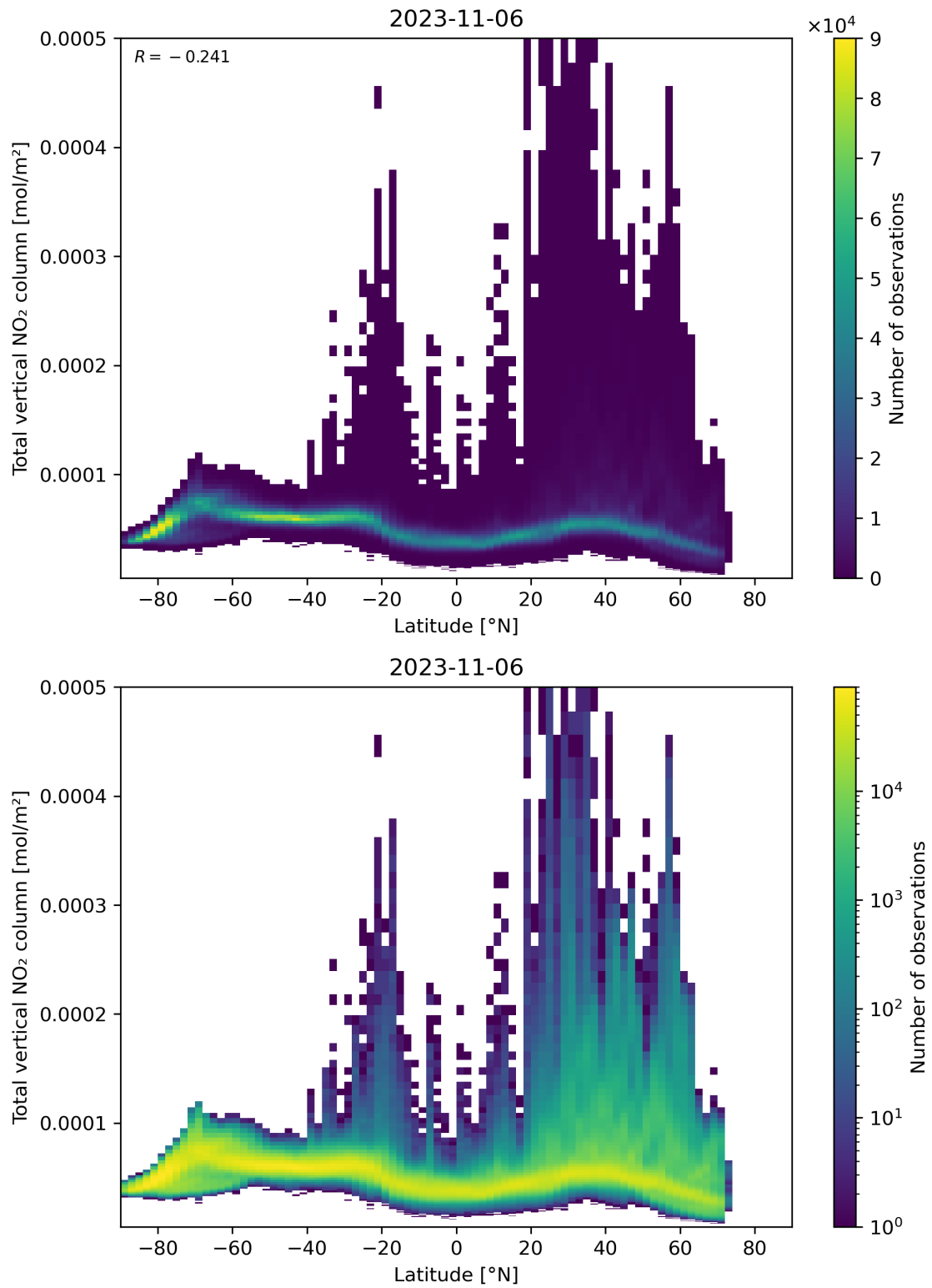
Figure 90: Scatter density plot of “Latitude” against “Total vertical NO 2 column” for 2023-11-05 to 2023-11-07.
