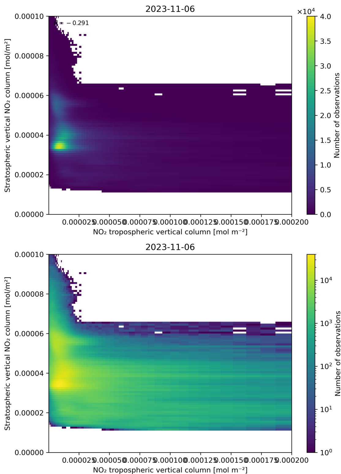
Figure 125: Scatter density plot of “NO 2 tropospheric vertical column” against “Stratospheric vertical NO 2 column” for 2023-11-05 to 2023-11-07.
