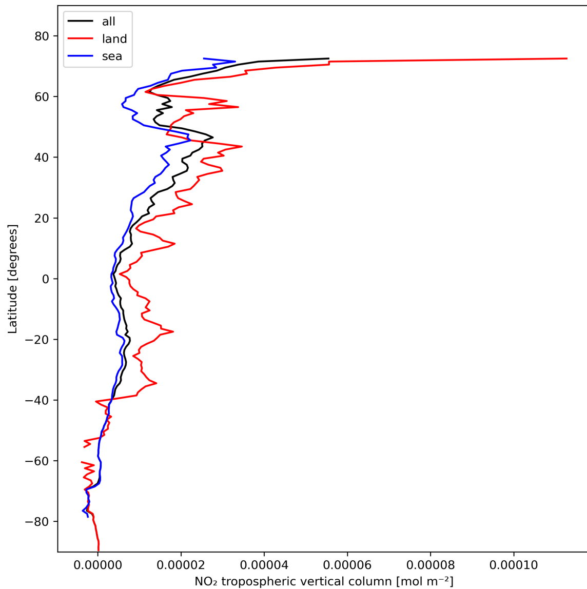
Figure 12: Zonal average of “NO 2 tropospheric vertical column” for 2023-11-05 to 2023-11-07.
