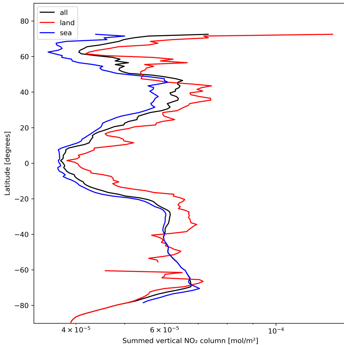
Figure 23: Zonal average of “Summed vertical NO 2 column” for 2023-11-05 to 2023-11-07.
