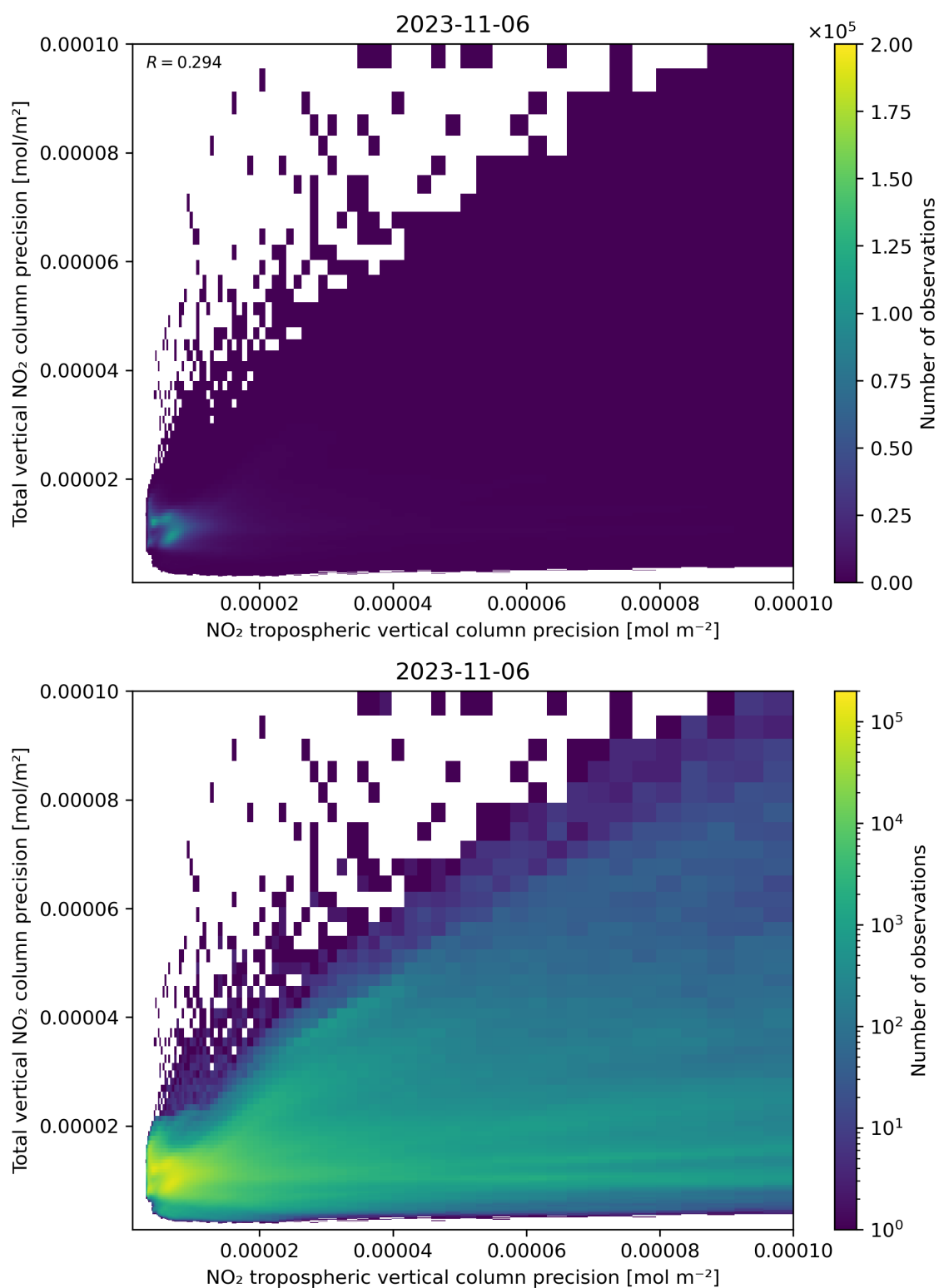
Figure 139: Scatter density plot of “NO 2 tropospheric vertical column precision” against “Total vertical NO 2 column precision” for 2023-11-05 to 2023-11-07.
