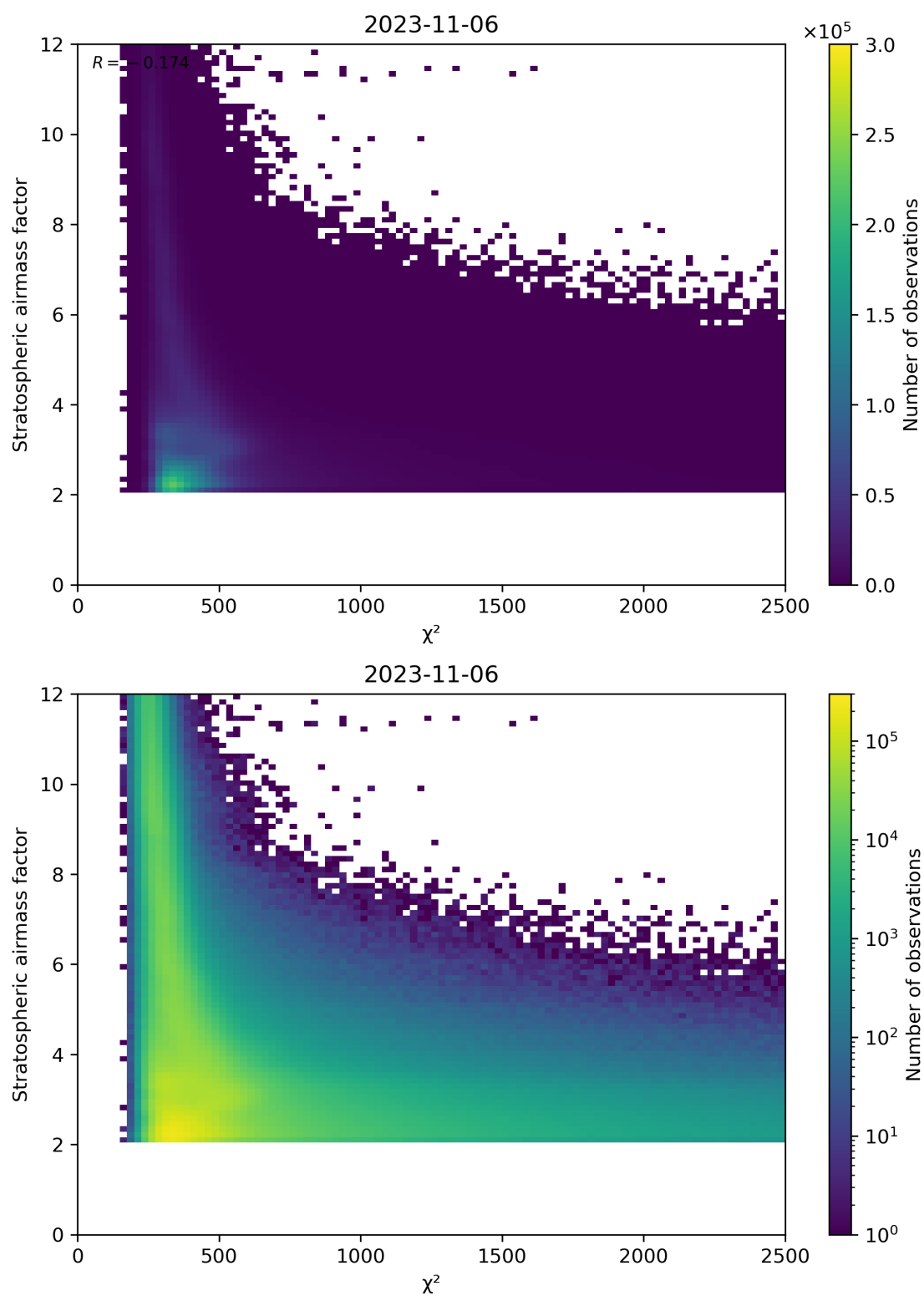
Figure 81: Scatter density plot of “ \chi^2 ” against “Stratospheric airmass factor” for 2023-11-05 to 2023-11-07.
