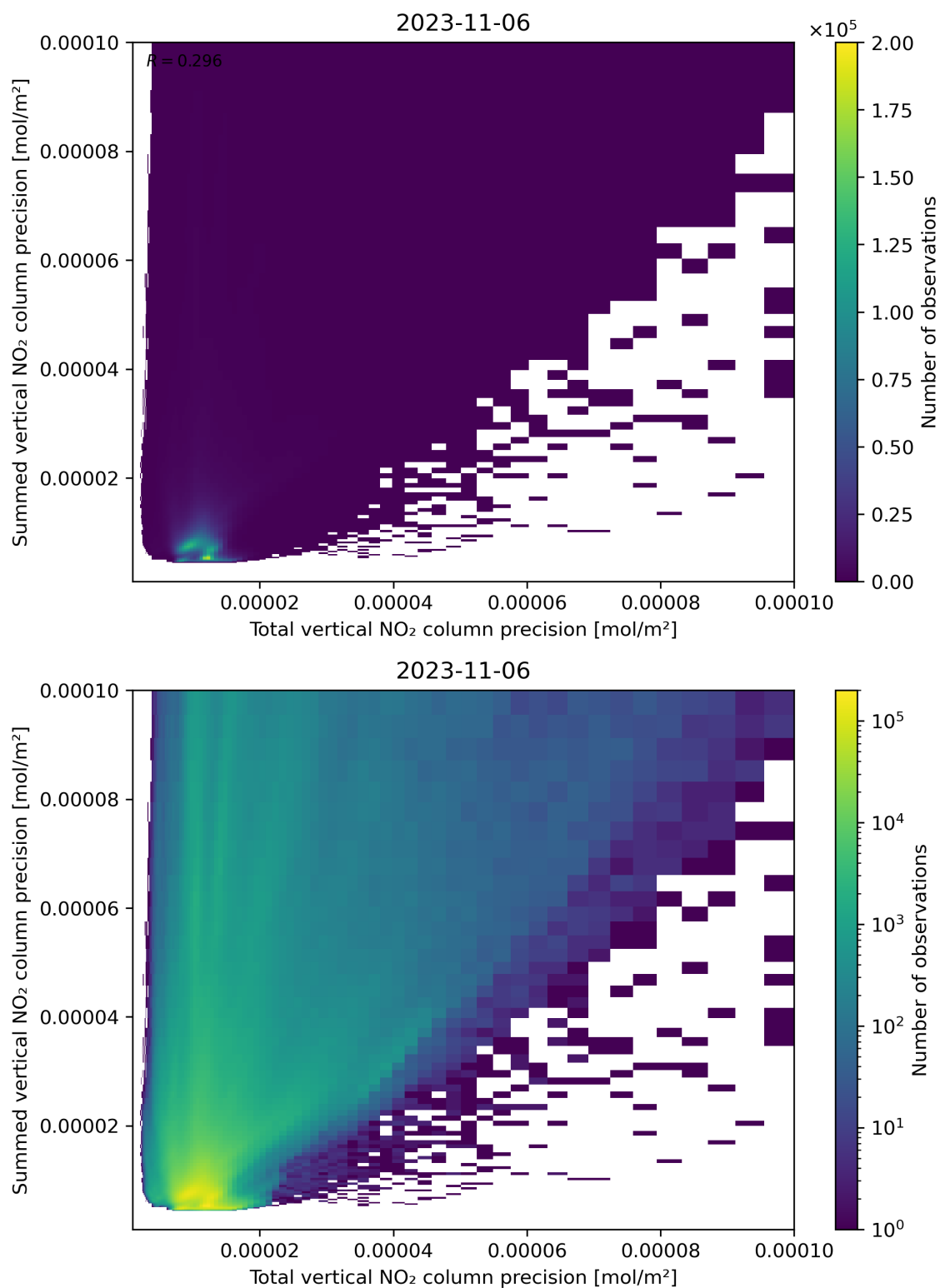
Figure 118: Scatter density plot of “Total vertical NO 2 column precision” against “Summed vertical NO 2 column precision” for 2023-11-05 to 2023-11-07.
