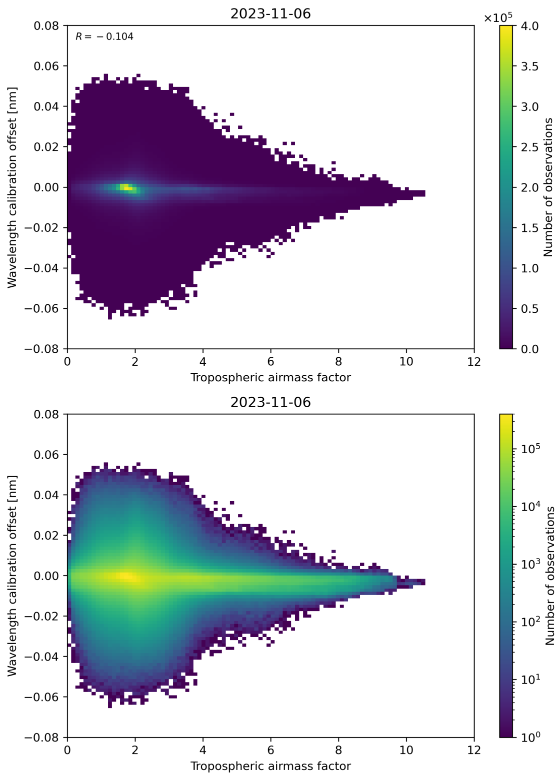
Figure 80: Scatter density plot of “Tropospheric airmass factor” against “Wavelength calibration offset” for 2023-11-05 to 2023-11-07.
