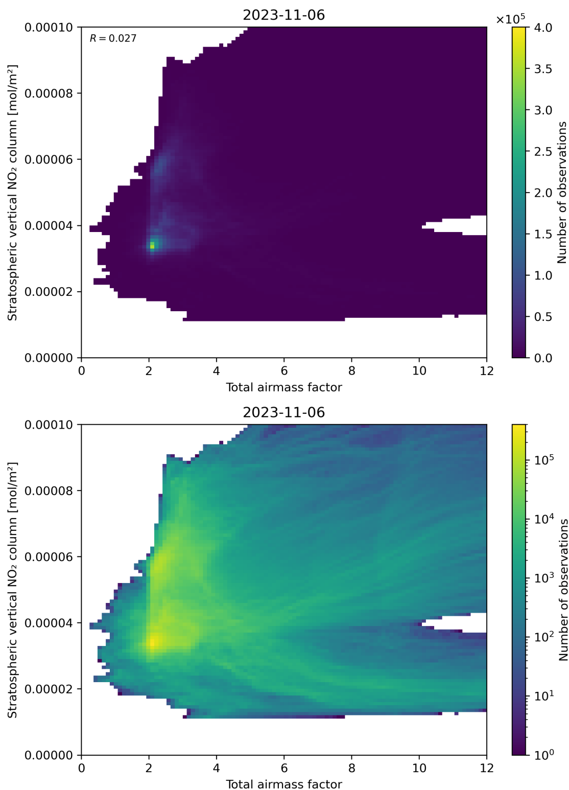
Figure 64: Scatter density plot of “Total airmass factor” against “Stratospheric vertical NO 2 column” for 2023-11-05 to 2023-11-07.
