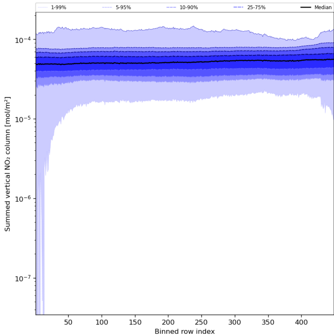
Figure 57: Along track statistics of “Summed vertical NO 2 column” for 2023-11-05 to 2023-11-07
