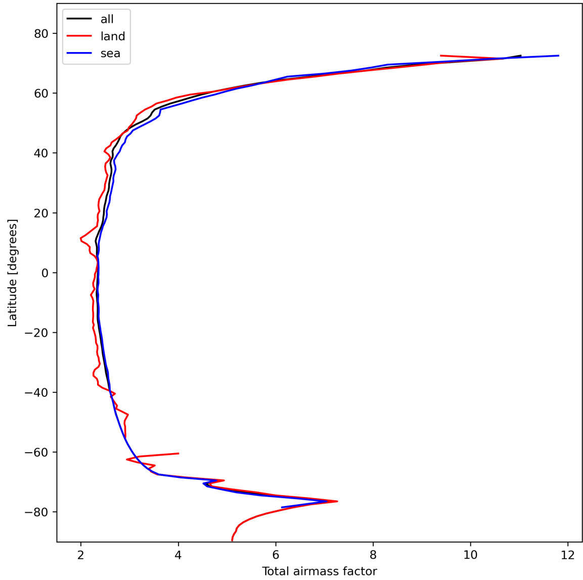
Figure 15: Zonal average of “Total airmass factor” for 2023-11-05 to 2023-11-07.
