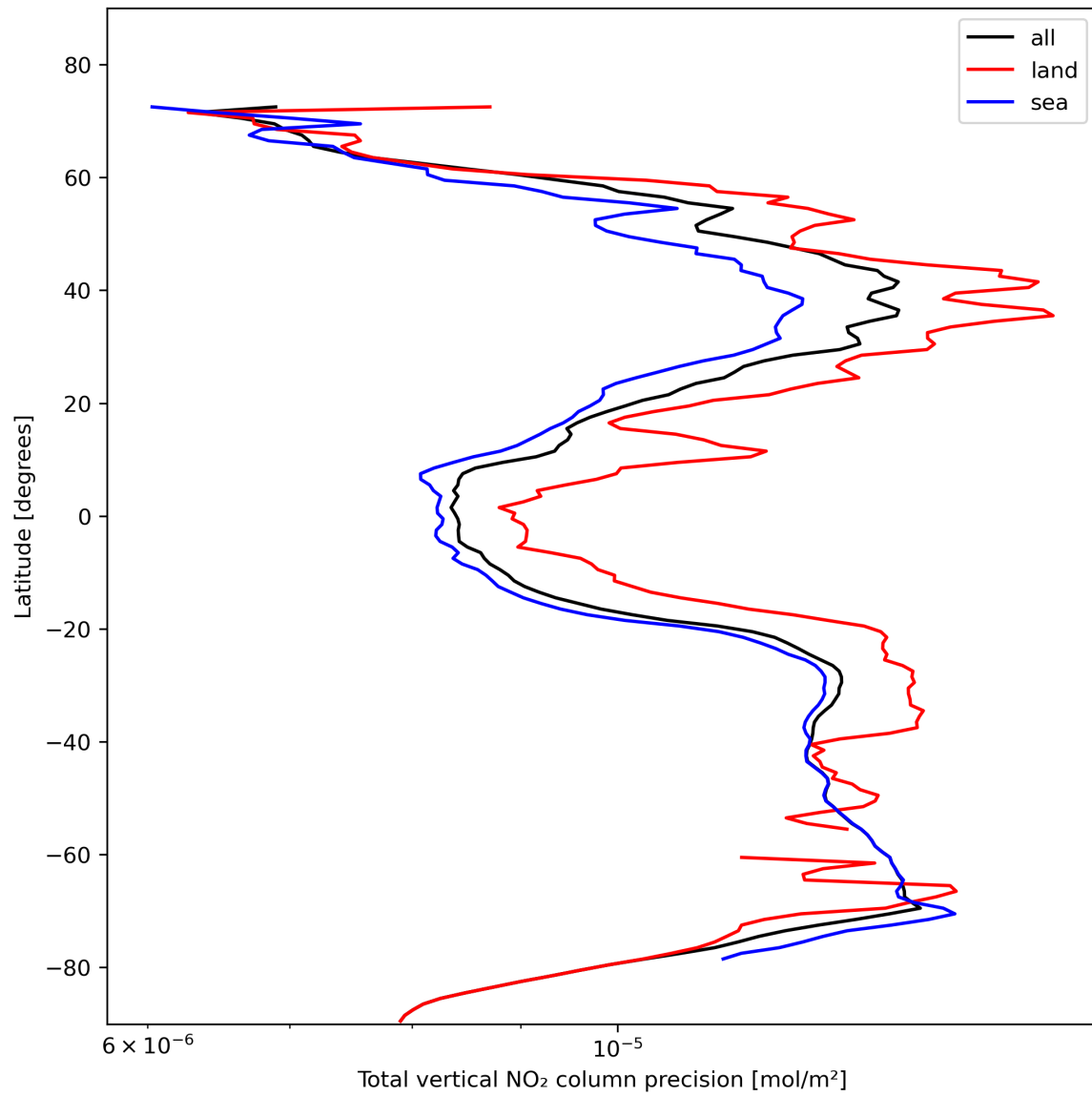
Figure 22: Zonal average of “Total vertical NO 2 column precision” for 2023-11-05 to 2023-11-07.
