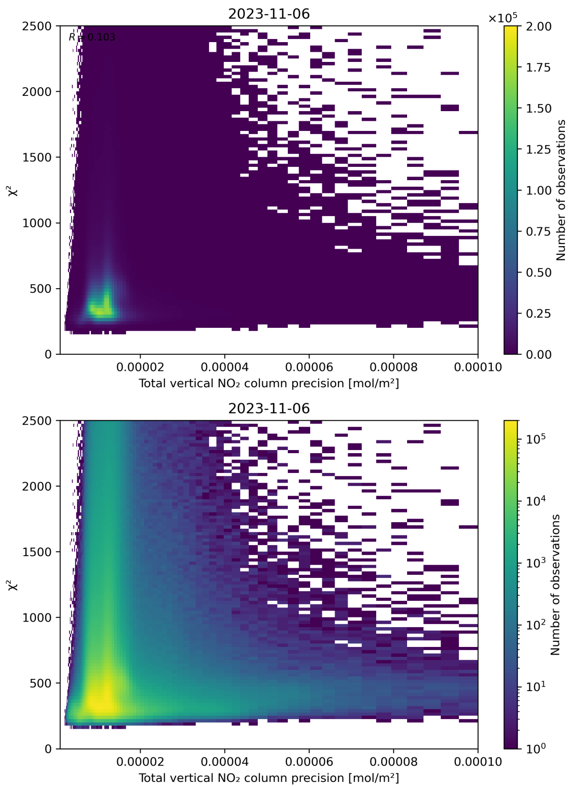
Figure 116: Scatter density plot of “Total vertical NO 2 column precision” against “ \chi^2 ” for 2023-11-05 to 2023-11-07.
