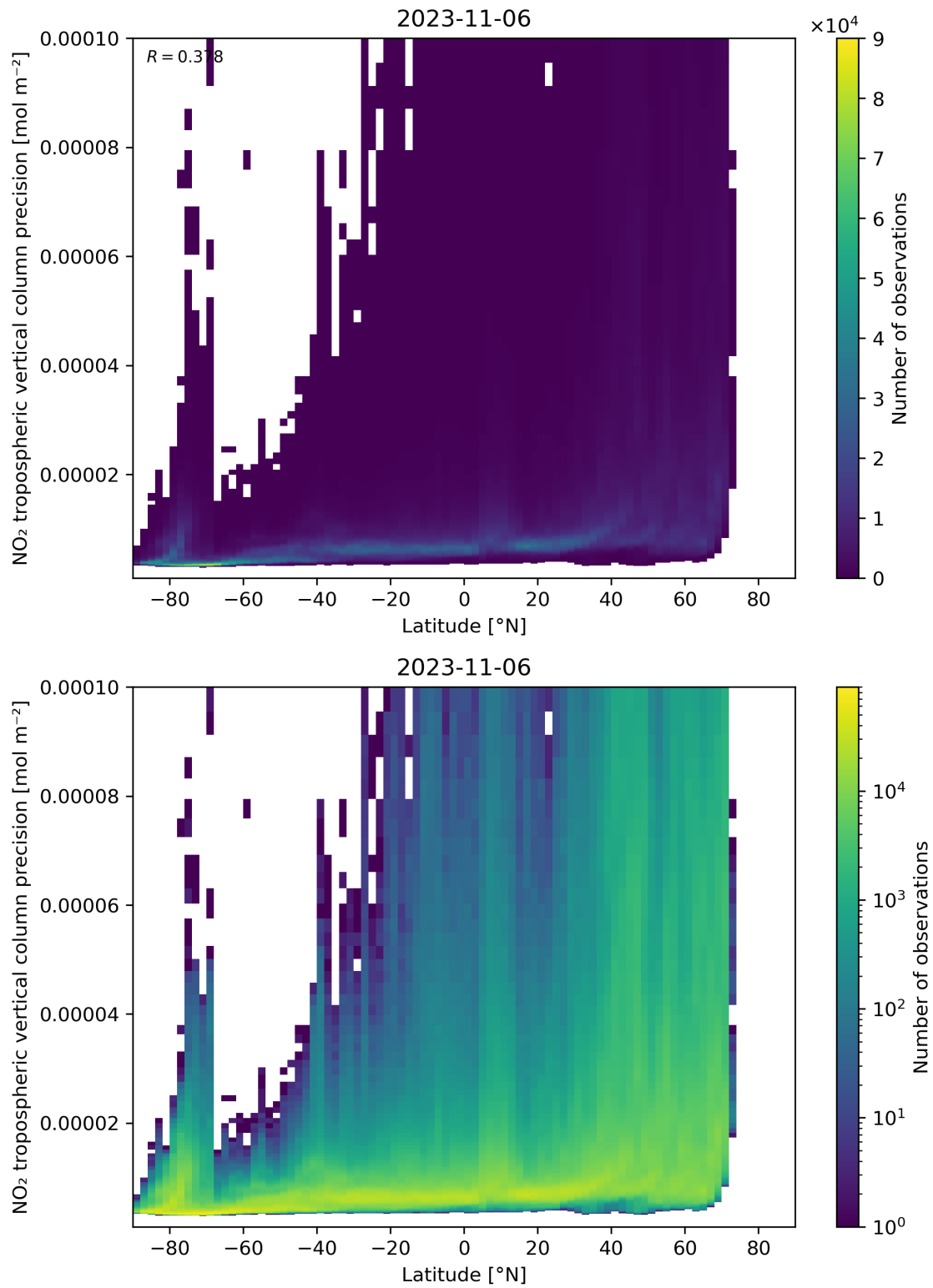
Figure 93: Scatter density plot of “Latitude” against “NO 2 tropospheric vertical column precision” for 2023-11-05 to 2023-11-07.
