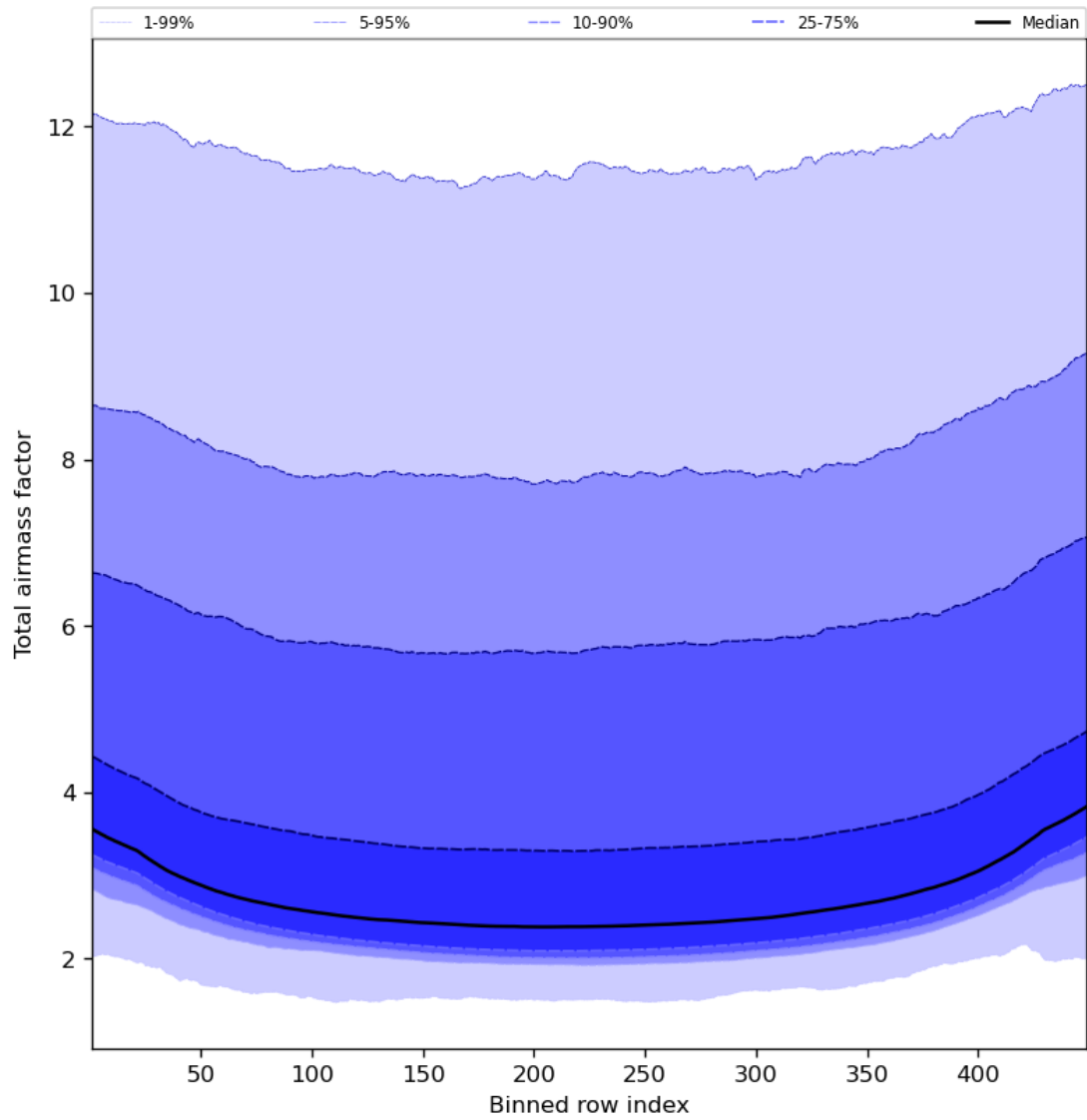
Figure 49: Along track statistics of “Total airmass factor” for 2023-11-05 to 2023-11-07
