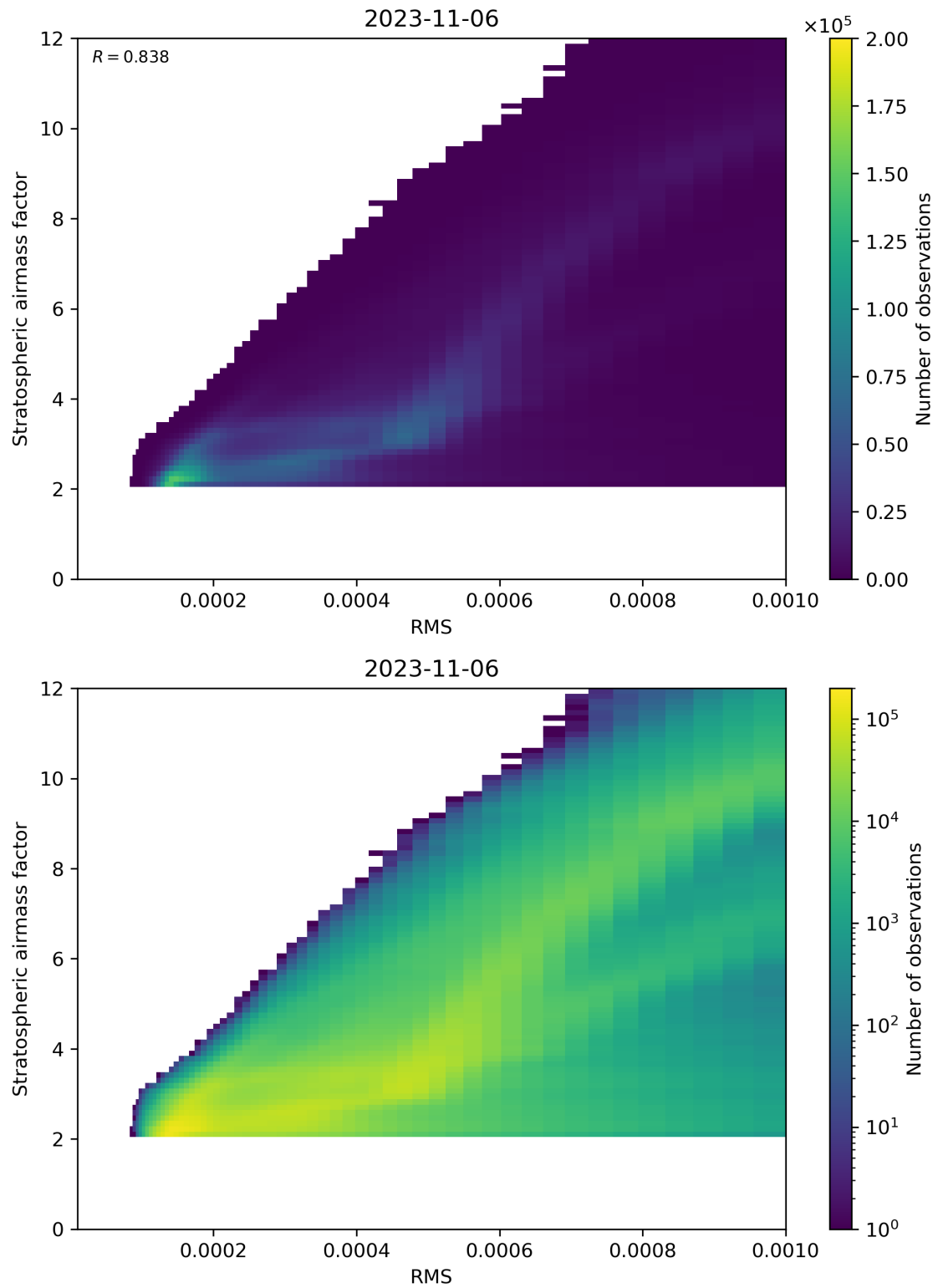
Figure 144: Scatter density plot of “RMS” against “Stratospheric airmass factor” for 2023-11-05 to 2023-11-07.
