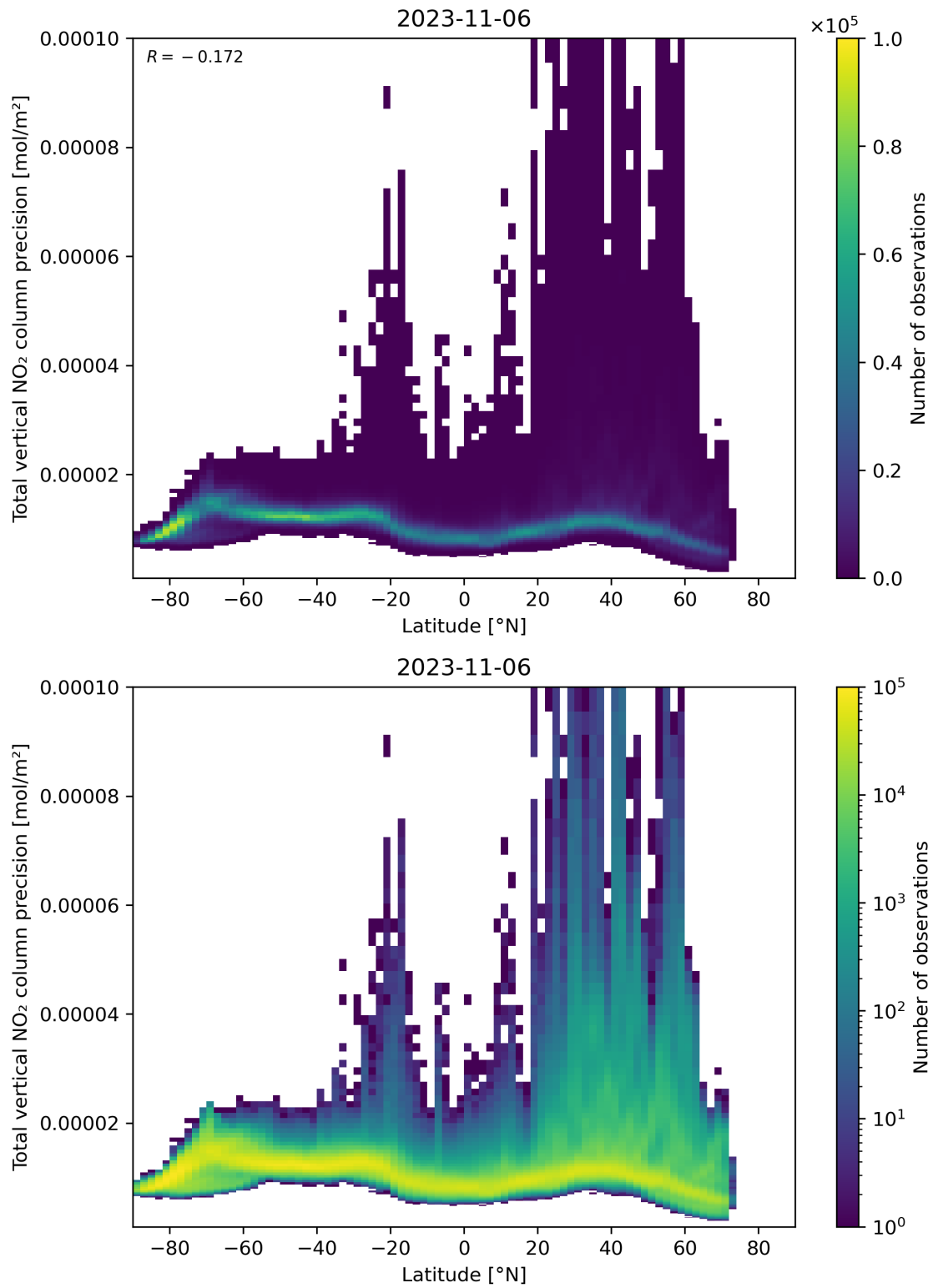
Figure 91: Scatter density plot of “Latitude” against “Total vertical NO 2 column precision” for 2023-11-05 to 2023-11-07.
