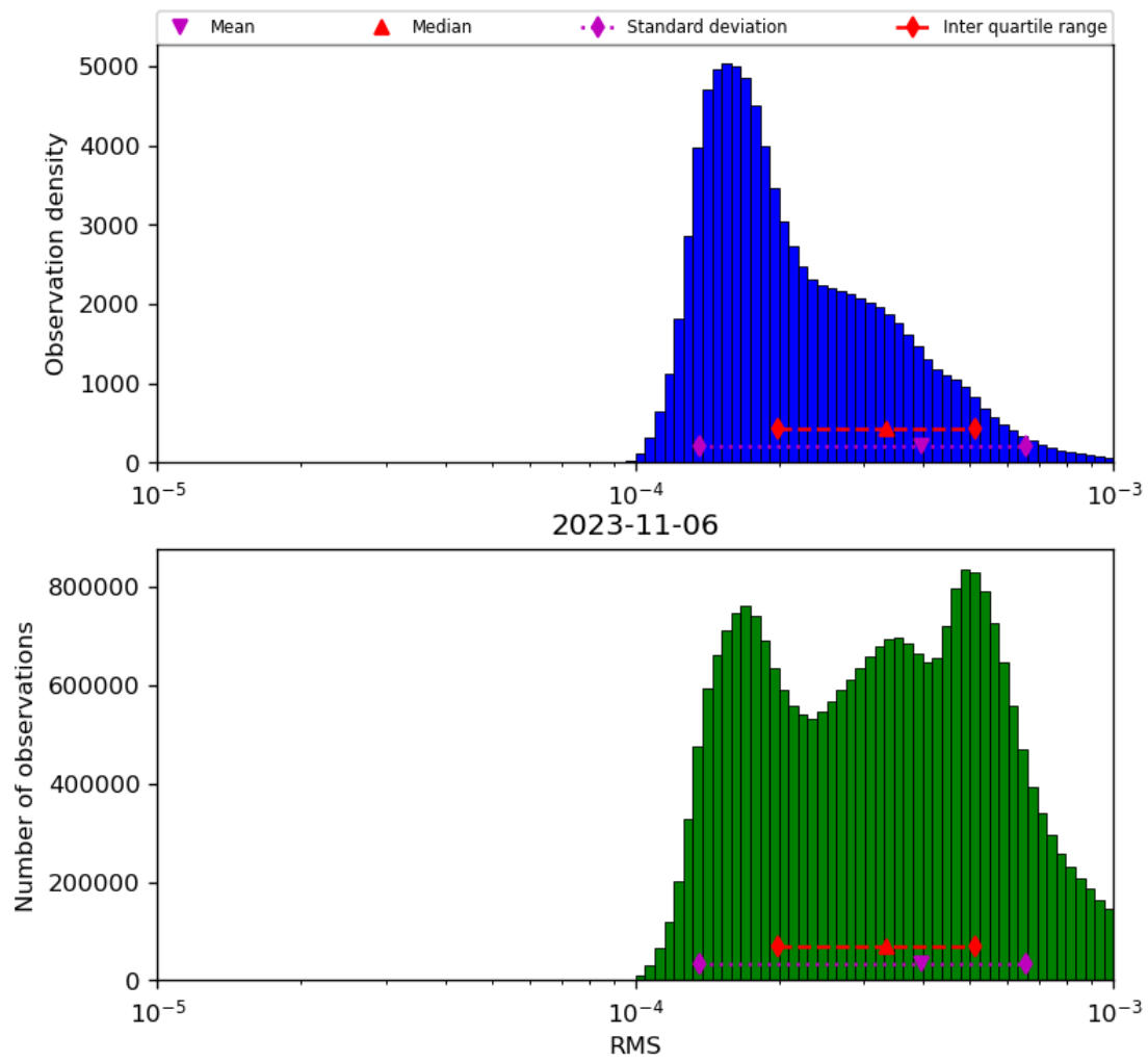
Figure 43: Histogram of “RMS” for 2023-11-05 to 2023-11-07
