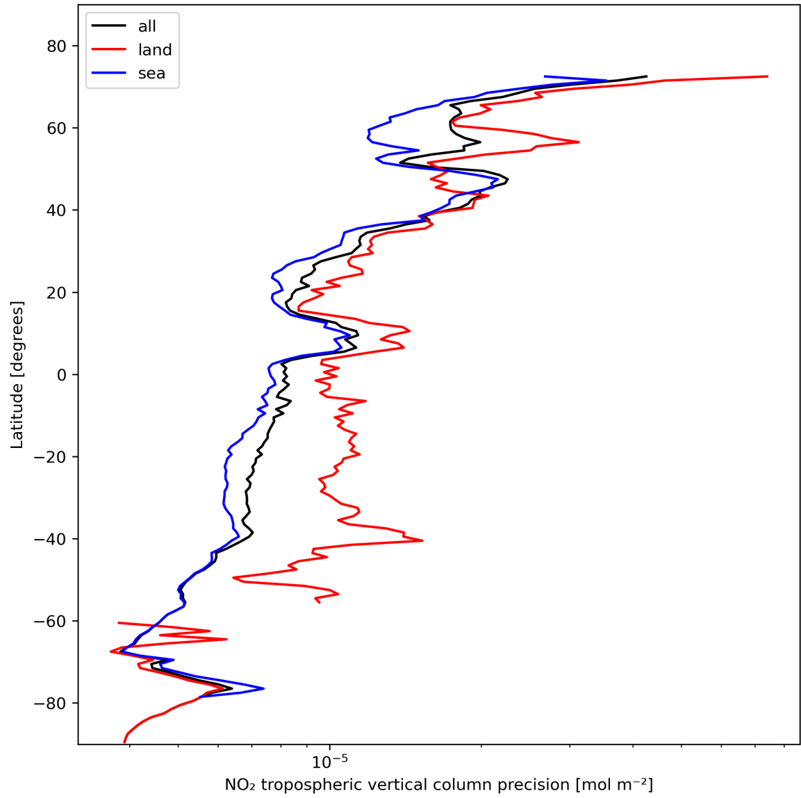
Figure 13: Zonal average of “NO 2 tropospheric vertical column precision” for 2023-11-05 to 2023-11-07.
