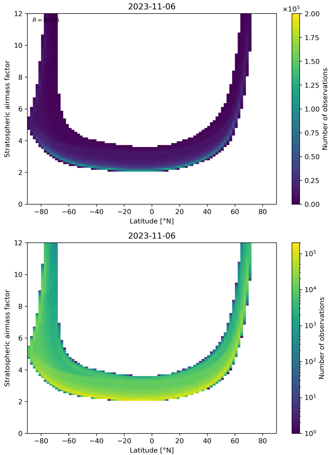
Figure 83: Scatter density plot of “Latitude” against “Stratospheric air mass factor” for 2023-11-05 to 2023-11-07.
