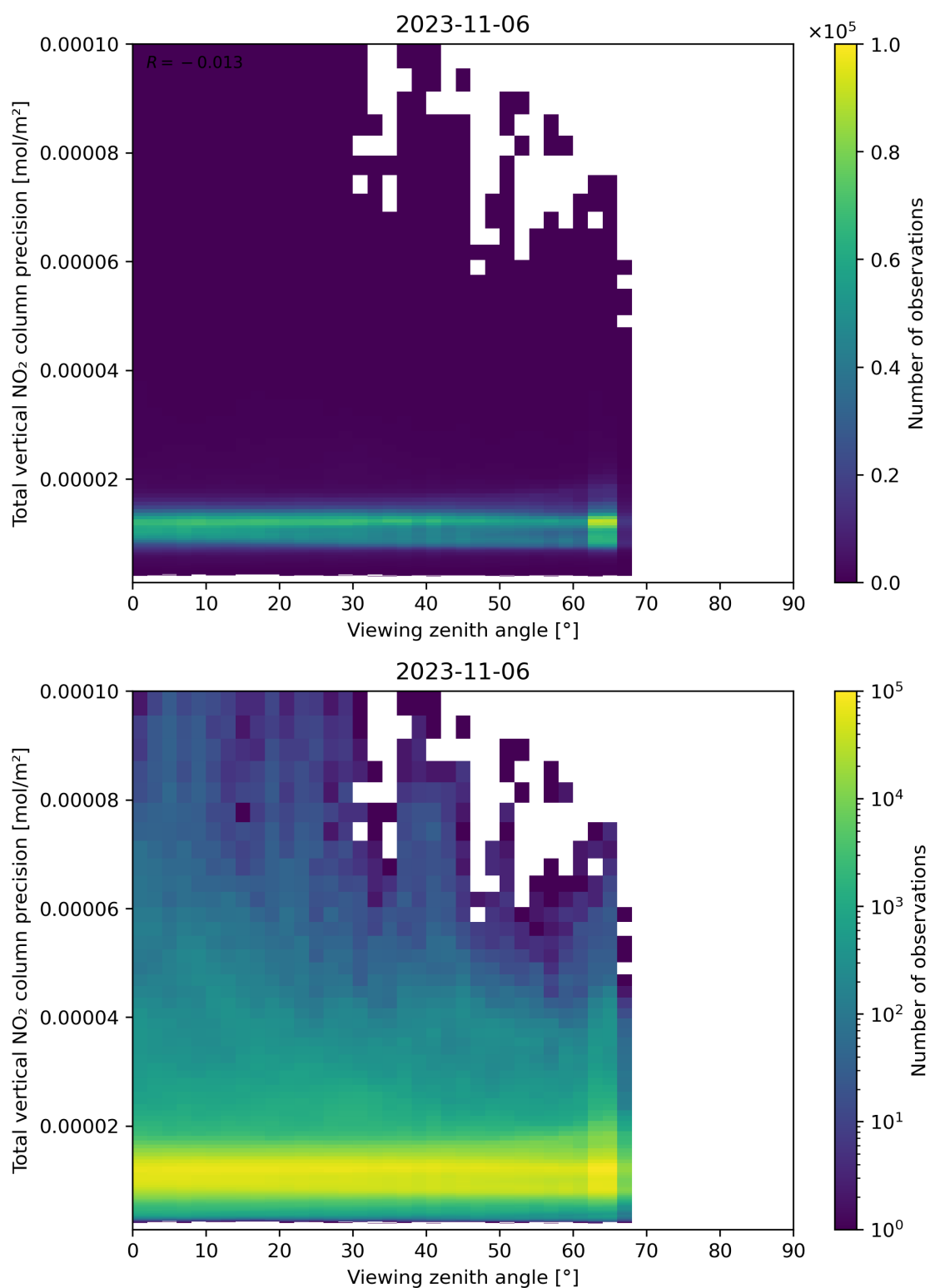
Figure 168: Scatter density plot of “Viewing zenith angle” against “Total vertical NO 2 column precision” for 2023-11-05 to 2023-11-07.
