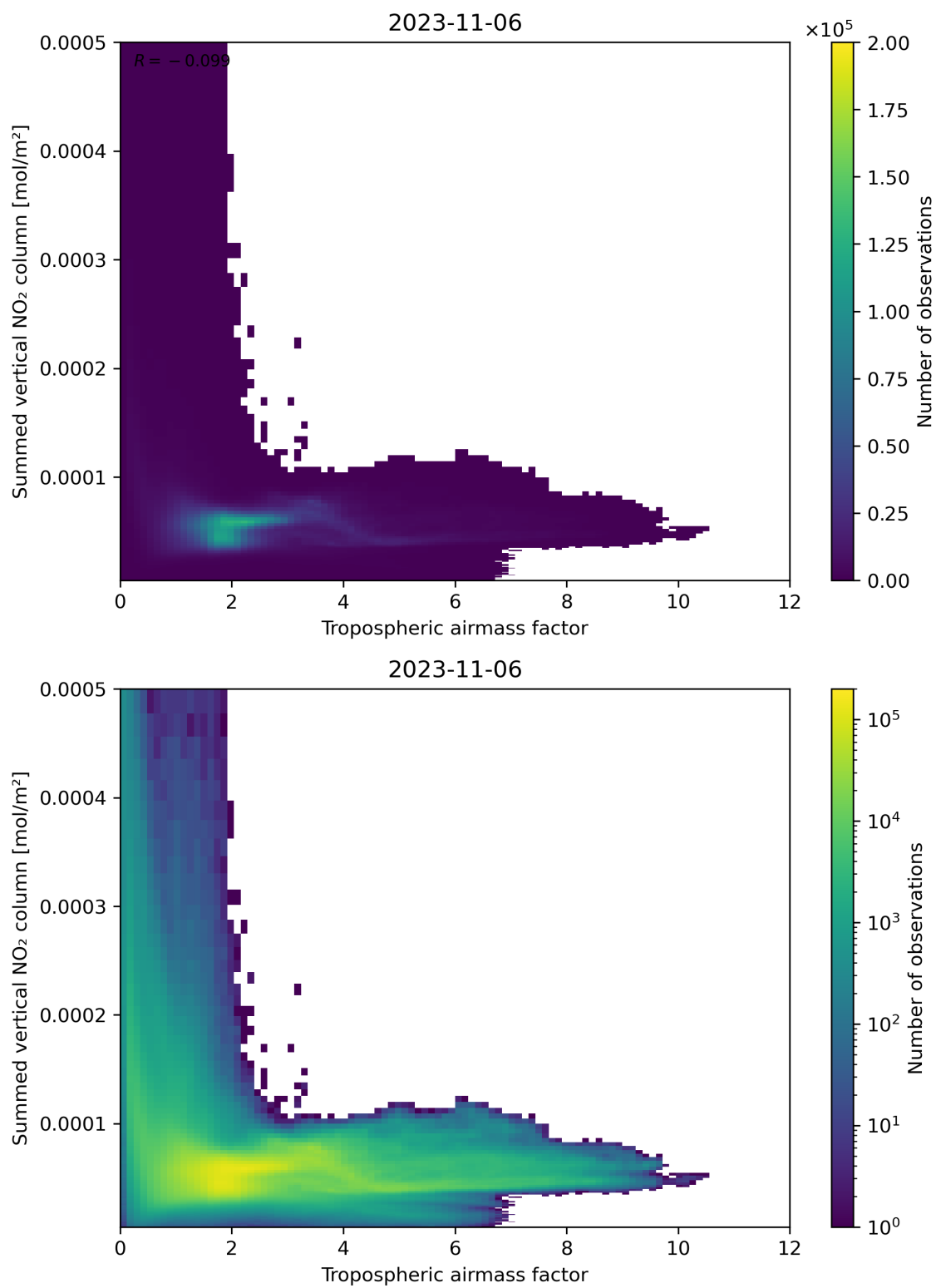
Figure 75: Scatter density plot of “Tropospheric airmass factor” against “Summed vertical NO 2 column” for 2023-11-05 to 2023-11-07.
