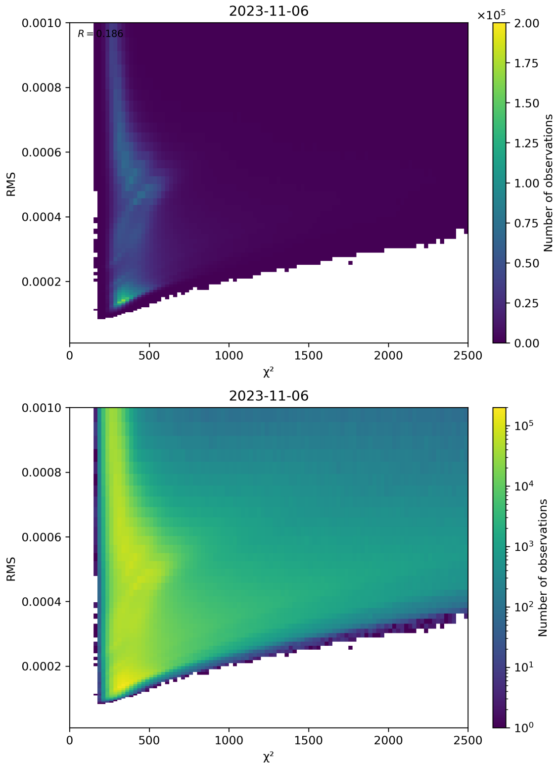
Figure 82: Scatter density plot of “ \chi^2 ” against “RMS” for 2023-11-05 to 2023-11-07.
