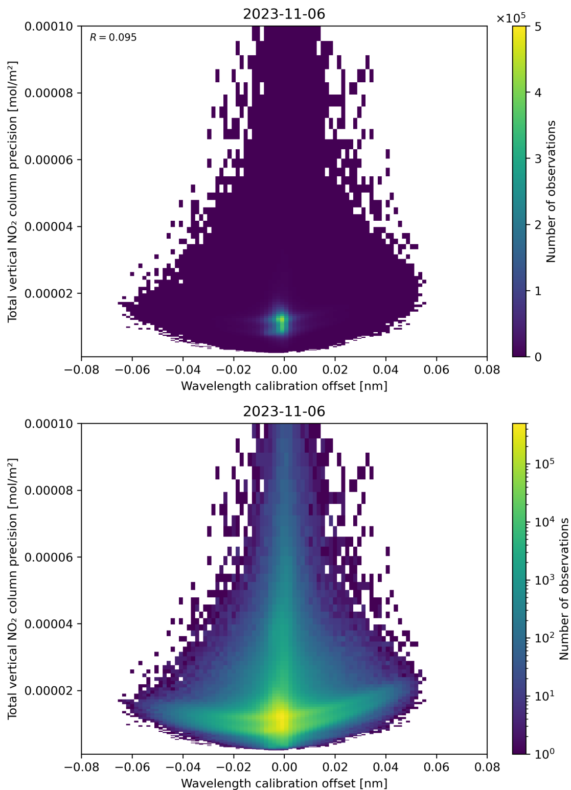
Figure 180: Scatter density plot of “Wavelength calibration offset” against “Total vertical NO 2 column precision” for 2023-11-05 to 2023-11-07.
