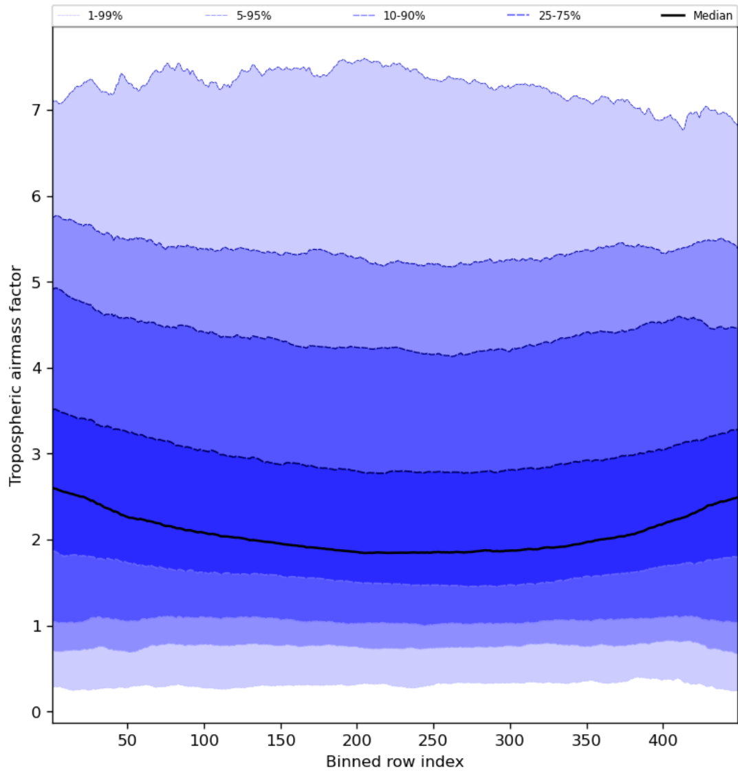
Figure 48: Along track statistics of “Tropospheric airmass factor” for 2023-11-05 to 2023-11-07
