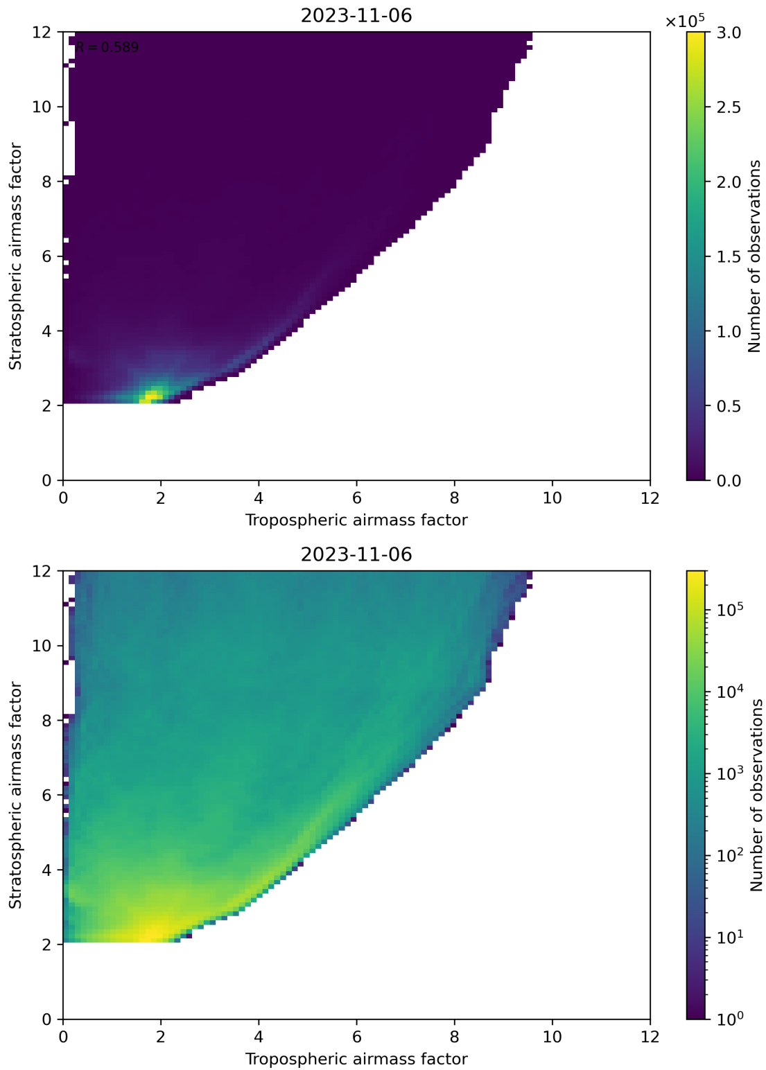
Figure 71: Scatter density plot of “Tropospheric airmass factor” against “Stratospheric airmass factor” for 2023-11-05 to 2023-11-07.
