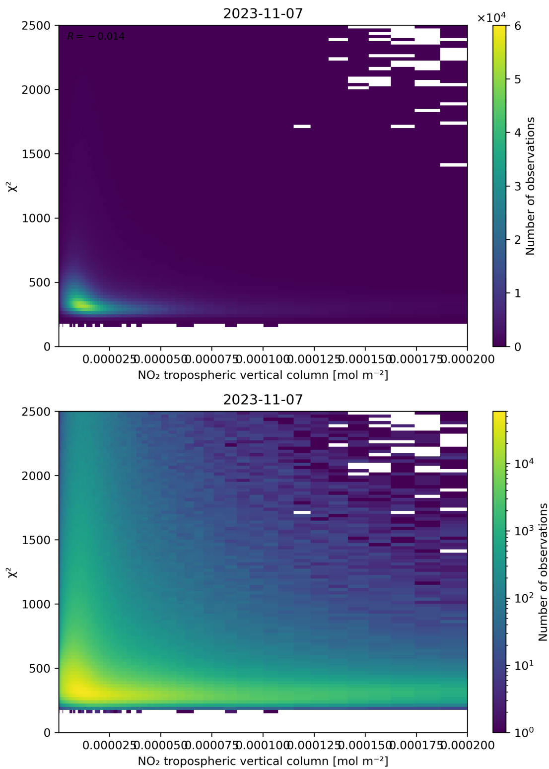
Figure 124: Scatter density plot of “NO 2 tropospheric vertical column” against “ \chi^2 ” for 2023-11-07 to 2023-11-08.
