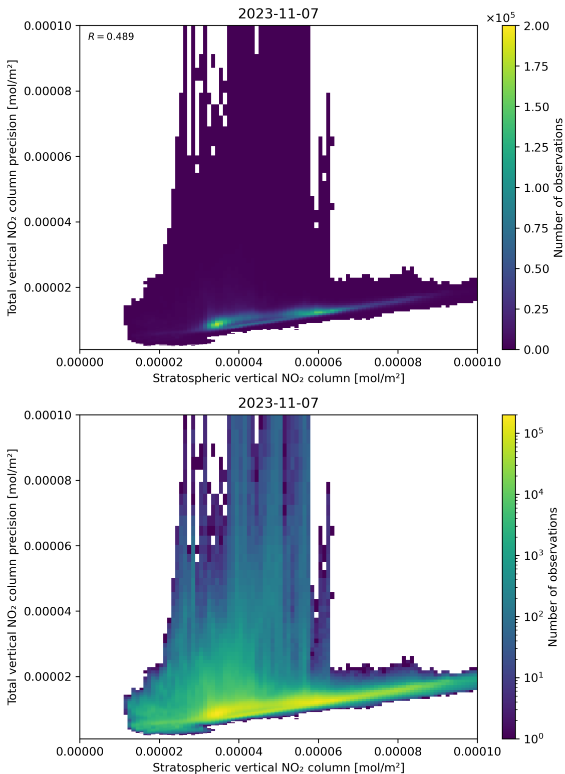
Figure 101: Scatter density plot of “Stratospheric vertical NO 2 column” against “Total vertical NO 2 column precision” for 2023-11-07 to 2023-11-08.
