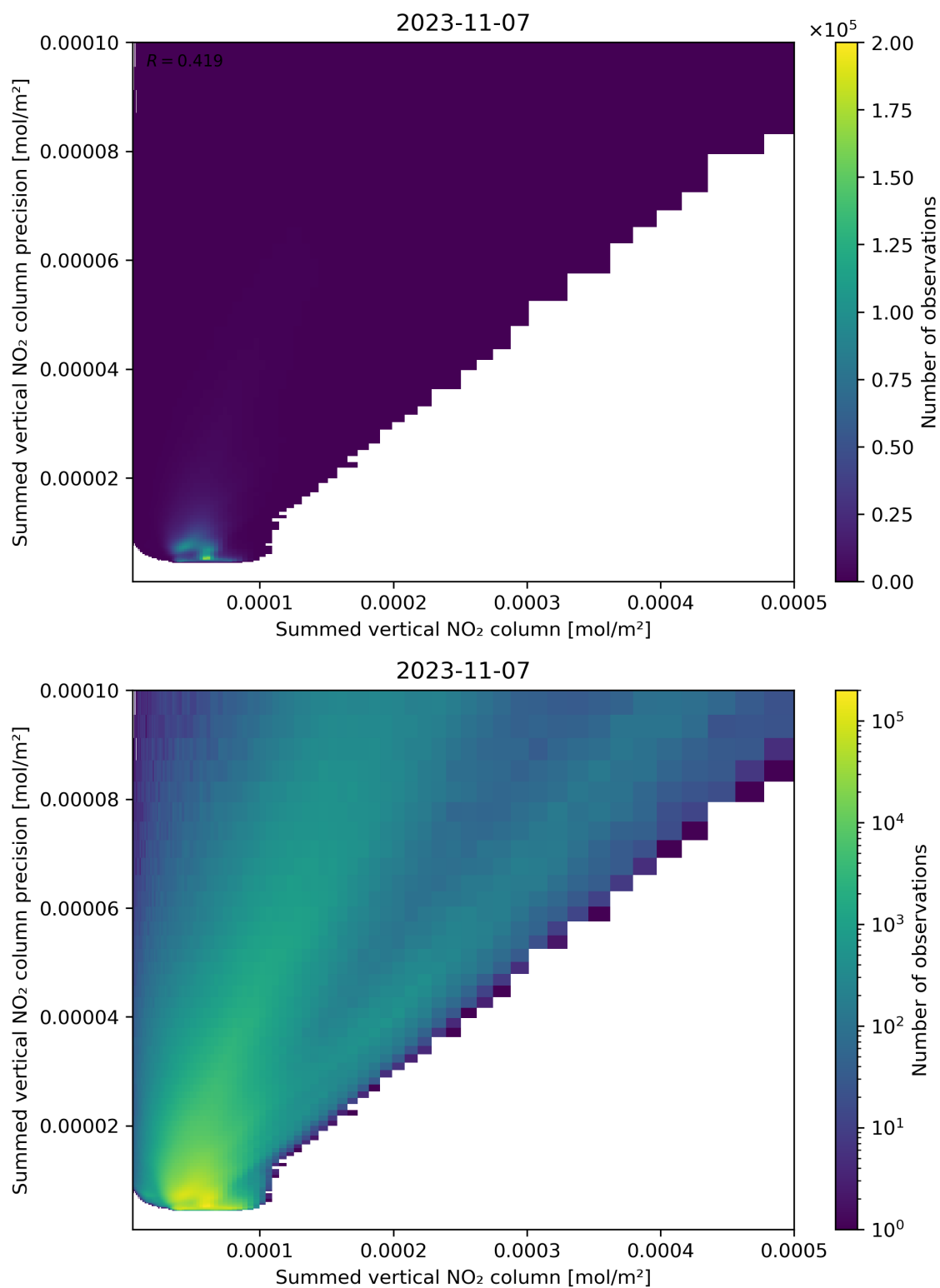
Figure 105: Scatter density plot of “Summed vertical NO 2 column” against “Summed vertical NO 2 column precision” for 2023-11-07 to 2023-11-08.
