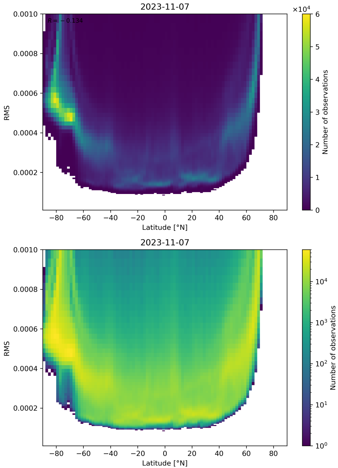
Figure 94: Scatter density plot of “Latitude” against “RMS” for 2023-11-07 to 2023-11-08.
