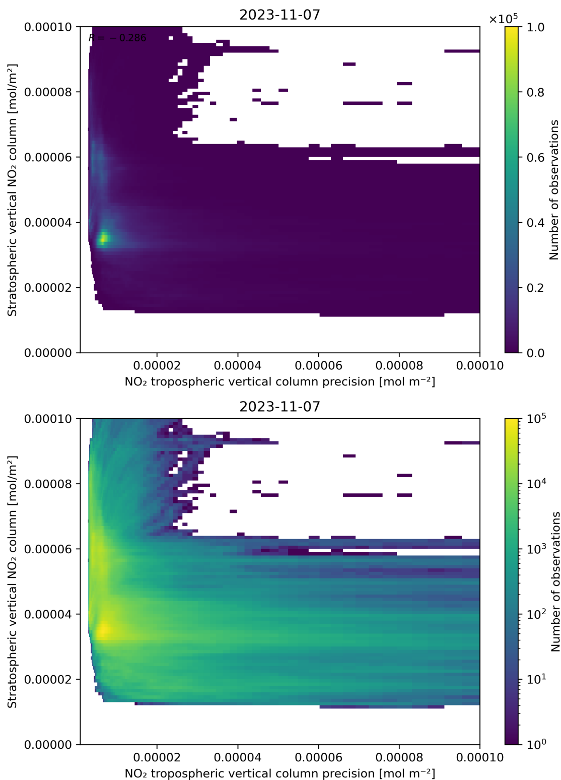
Figure 135: Scatter density plot of “ \text{NO}_2 tropospheric vertical column precision” against “Stratospheric vertical \text{NO}_2 column” for 2023-11-07 to 2023-11-08.
