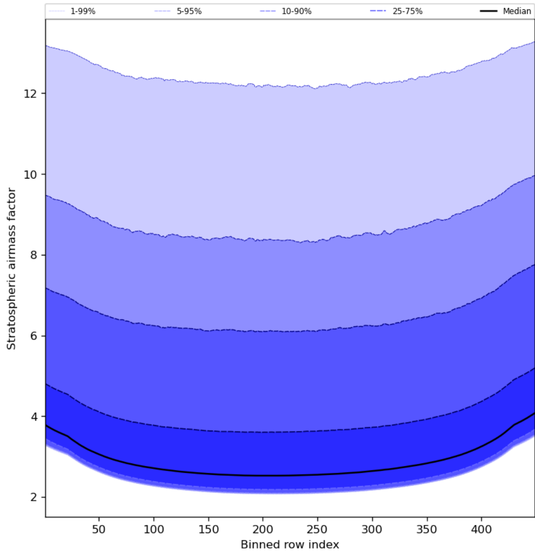
Figure 61: Along track statistics of “Stratospheric airmass factor” for 2023-11-07 to 2023-11-08
