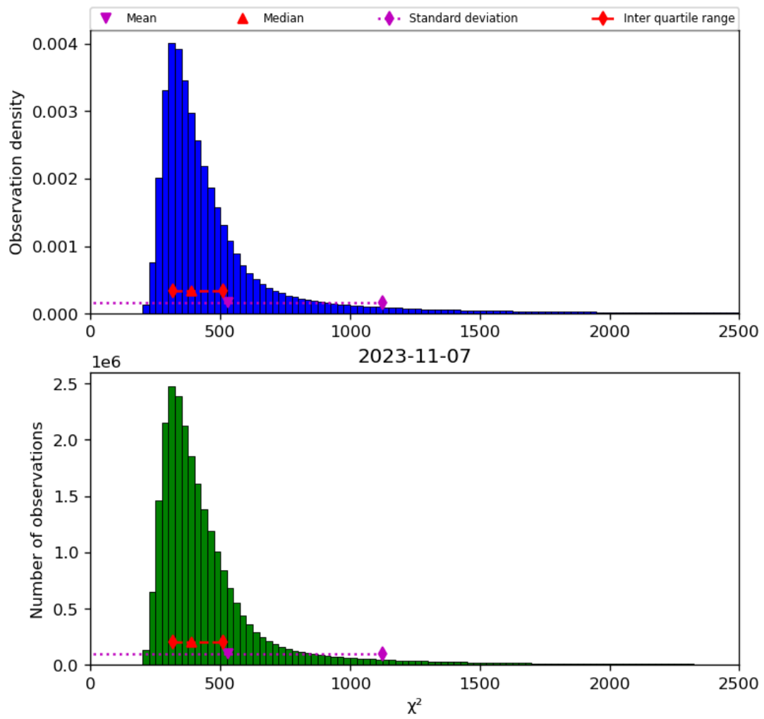
Figure 42: Histogram of “ \chi^2 ” for 2023-11-07 to 2023-11-08
