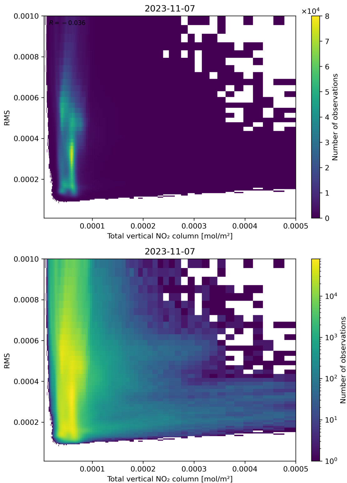
Figure 120: Scatter density plot of “Total vertical NO 2 column” against “RMS” for 2023-11-07 to 2023-11-08.
