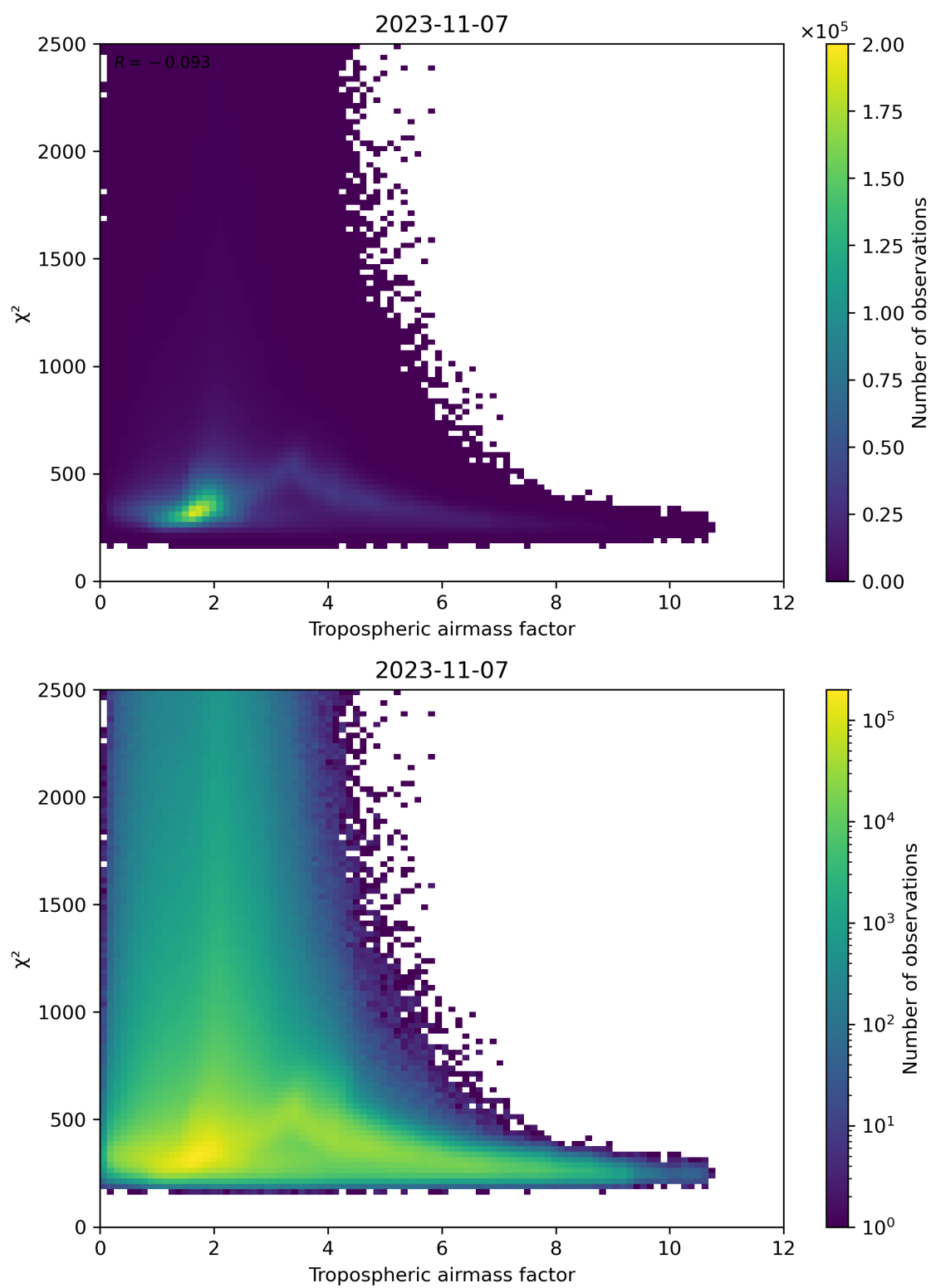
Figure 73: Scatter density plot of “Tropospheric airmass factor” against “ \chi^2 ” for 2023-11-07 to 2023-11-08.
