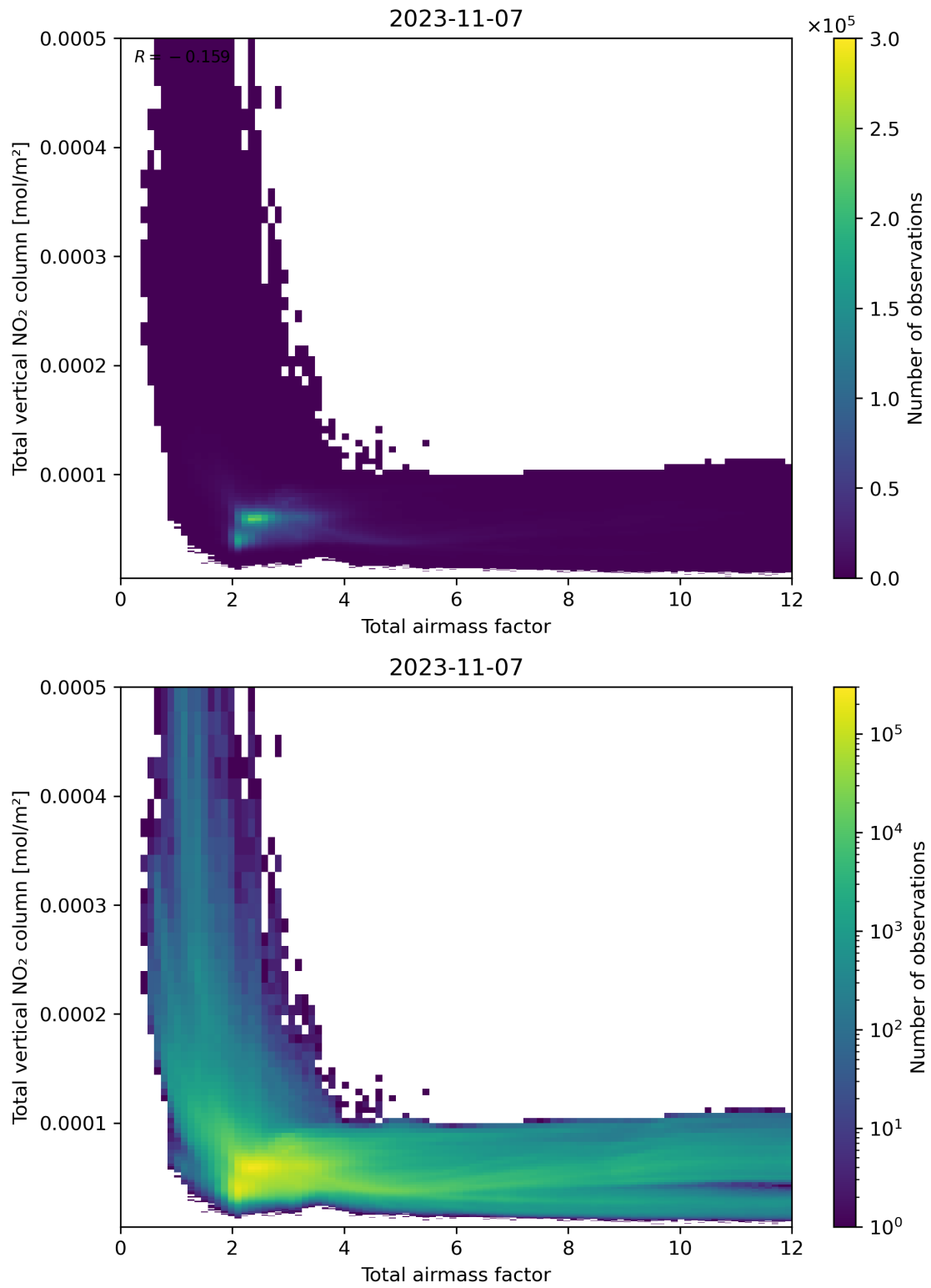
Figure 67: Scatter density plot of “Total air mass factor” against “Total vertical NO 2 column” for 2023-11-07 to 2023-11-08.
