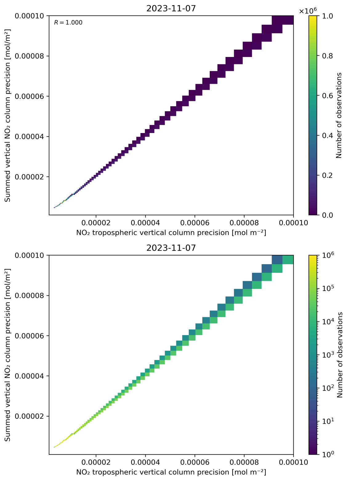
Figure 137: Scatter density plot of “NO 2 tropospheric vertical column precision” against “Summed vertical NO 2 column precision” for 2023-11-07 to 2023-11-08.
