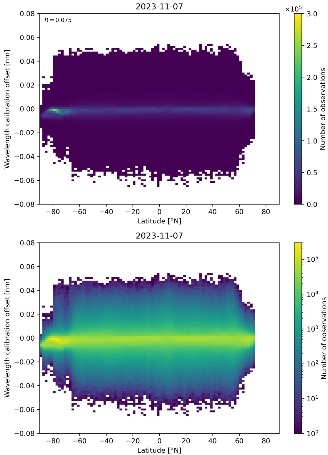
Figure 95: Scatter density plot of “Latitude” against “Wavelength calibration offset” for 2023-11-07 to 2023-11-08.
