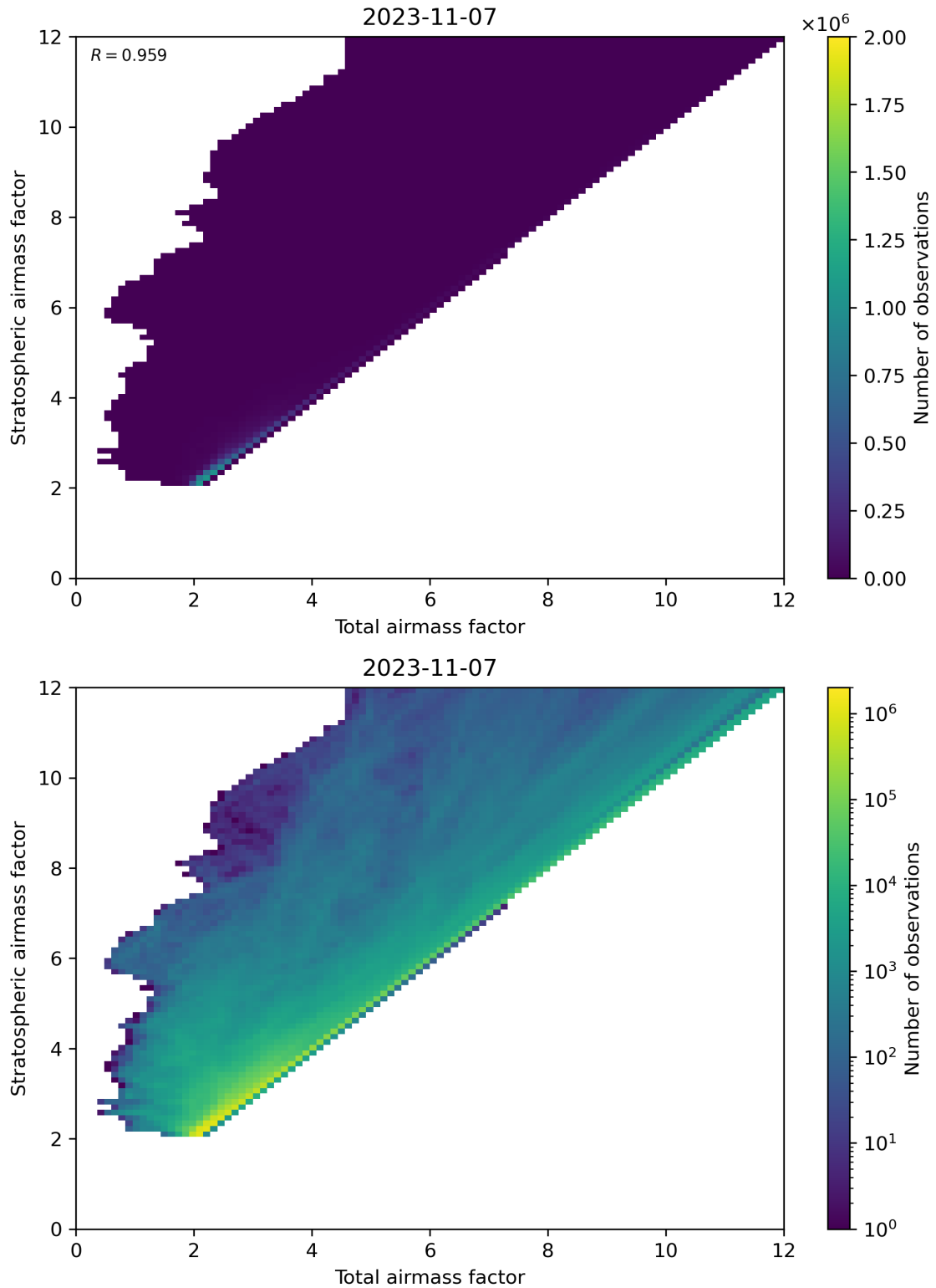
Figure 62: Scatter density plot of “Total airmass factor” against “Stratospheric airmass factor” for 2023-11-07 to 2023-11-08.
