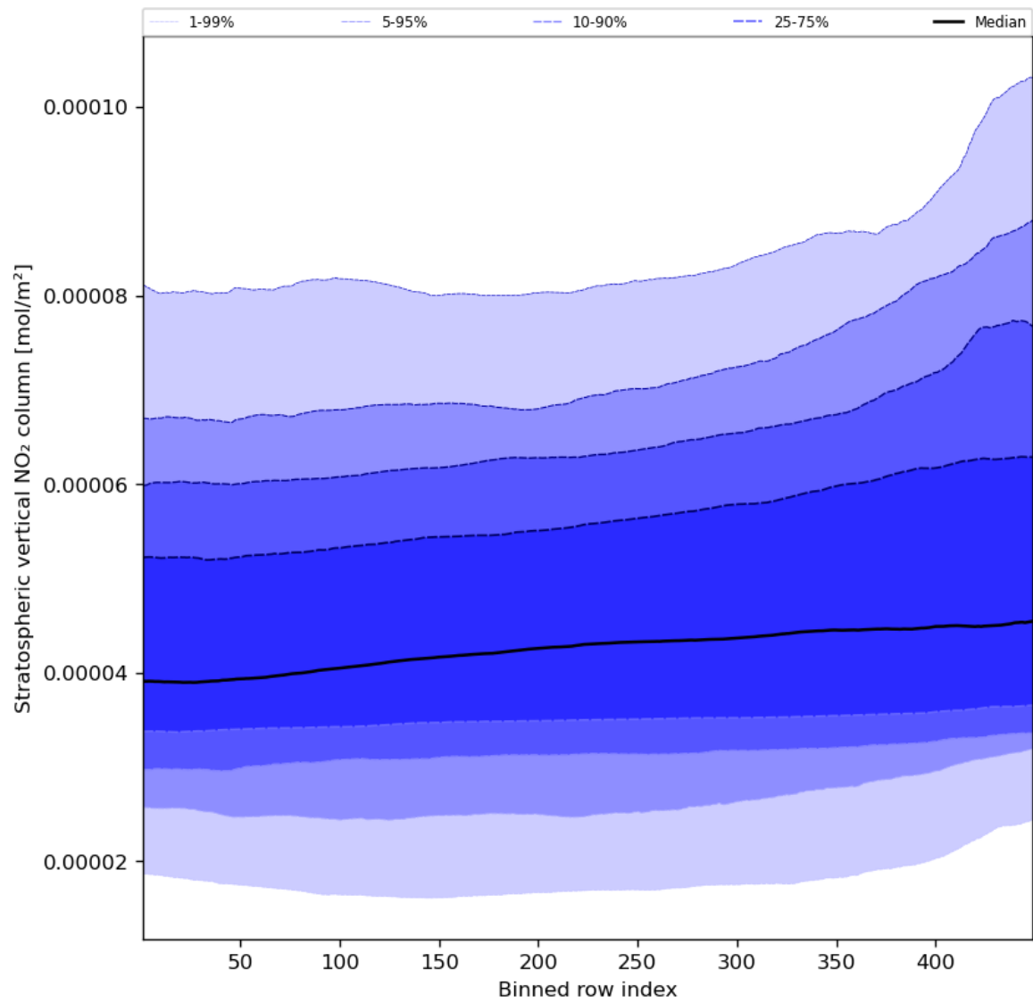
Figure 53: Along track statistics of “Stratospheric vertical NO 2 column” for 2023-11-07 to 2023-11-08
