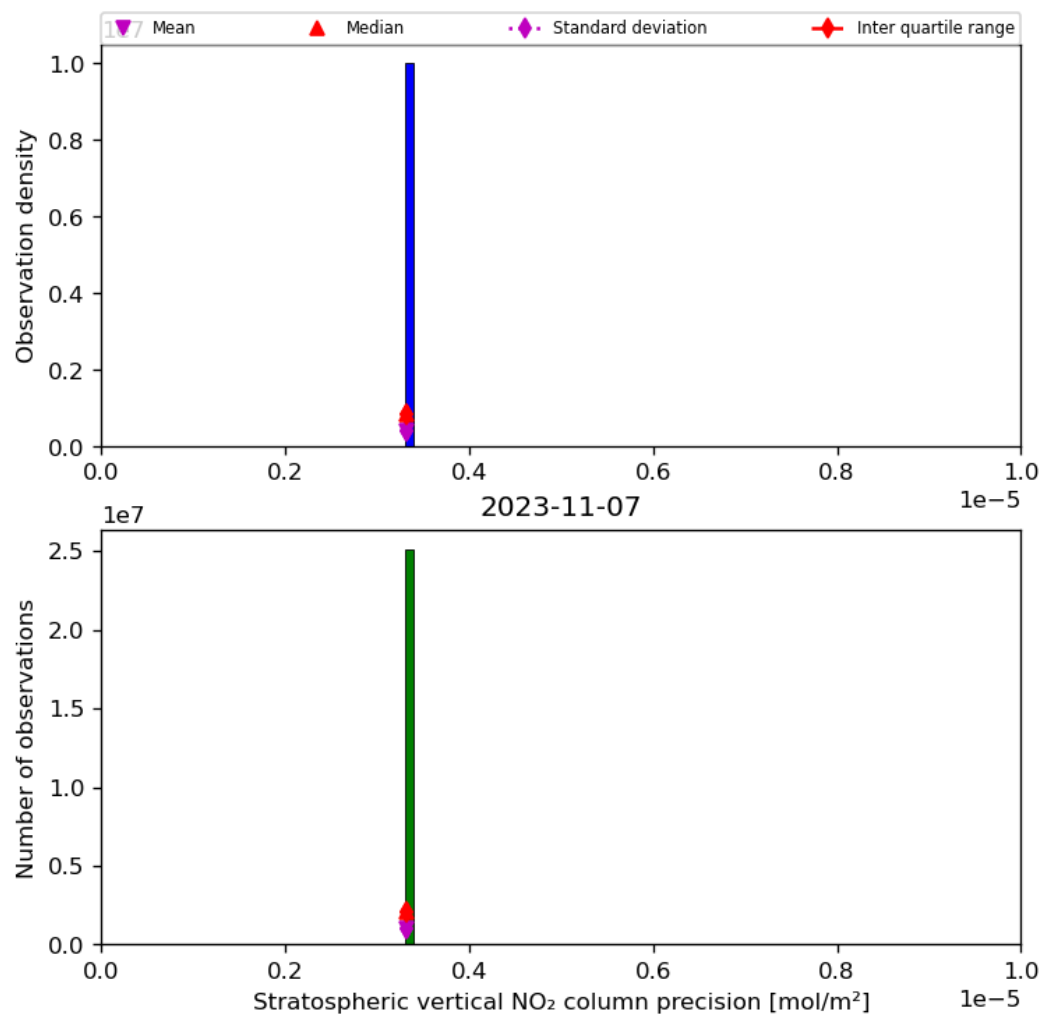
Figure 37: Histogram of “Stratospheric vertical NO 2 column precision” for 2023-11-07 to 2023-11-08
