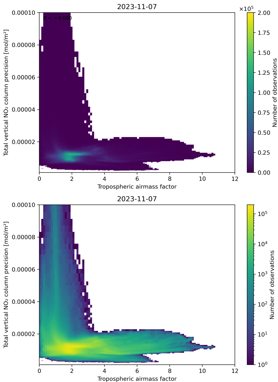
Figure 78: Scatter density plot of “Tropospheric air mass factor” against “Total vertical NO 2 column precision” for 2023-11-07 to 2023-11-08.
