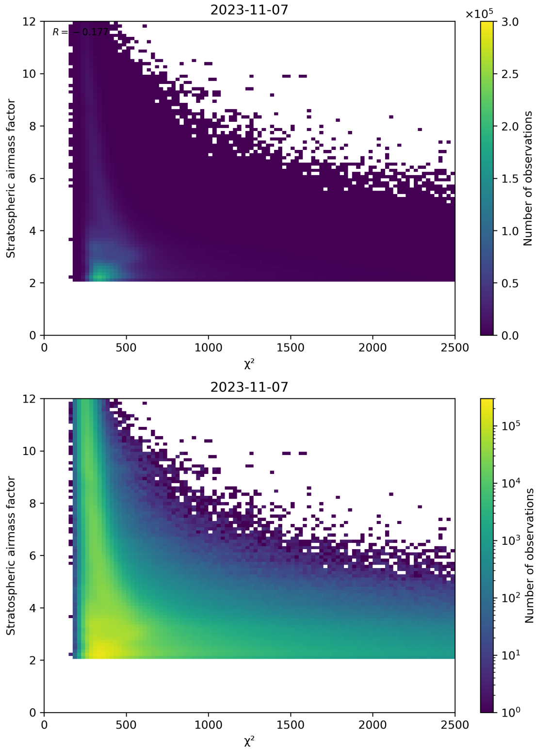
Figure 81: Scatter density plot of “ \chi^2 ” against “Stratospheric airmass factor” for 2023-11-07 to 2023-11-08.
