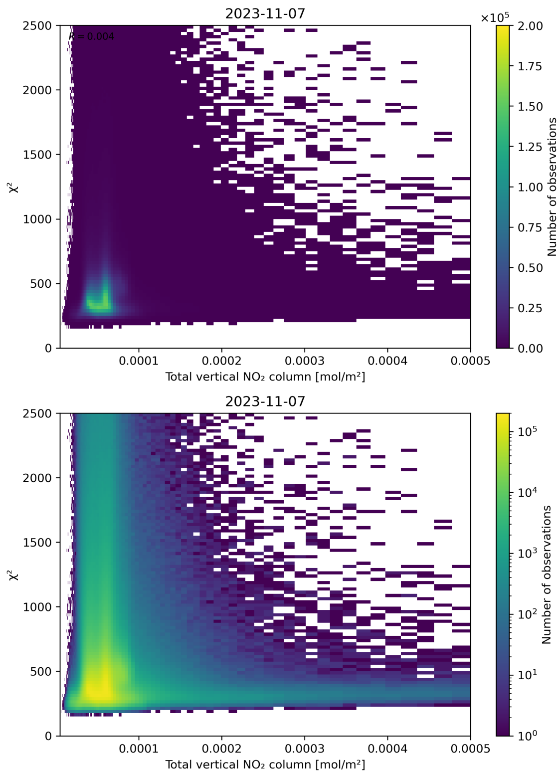
Figure 111: Scatter density plot of “Total vertical NO 2 column” against “ \chi^2 ” for 2023-11-07 to 2023-11-08.
