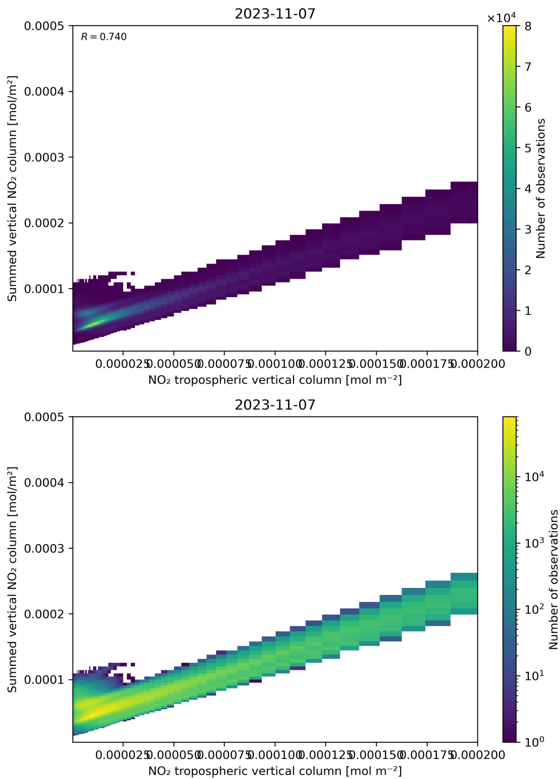
Figure 126: Scatter density plot of “NO 2 tropospheric vertical column” against “Summed vertical NO 2 column” for 2023-11-07 to 2023-11-08.
