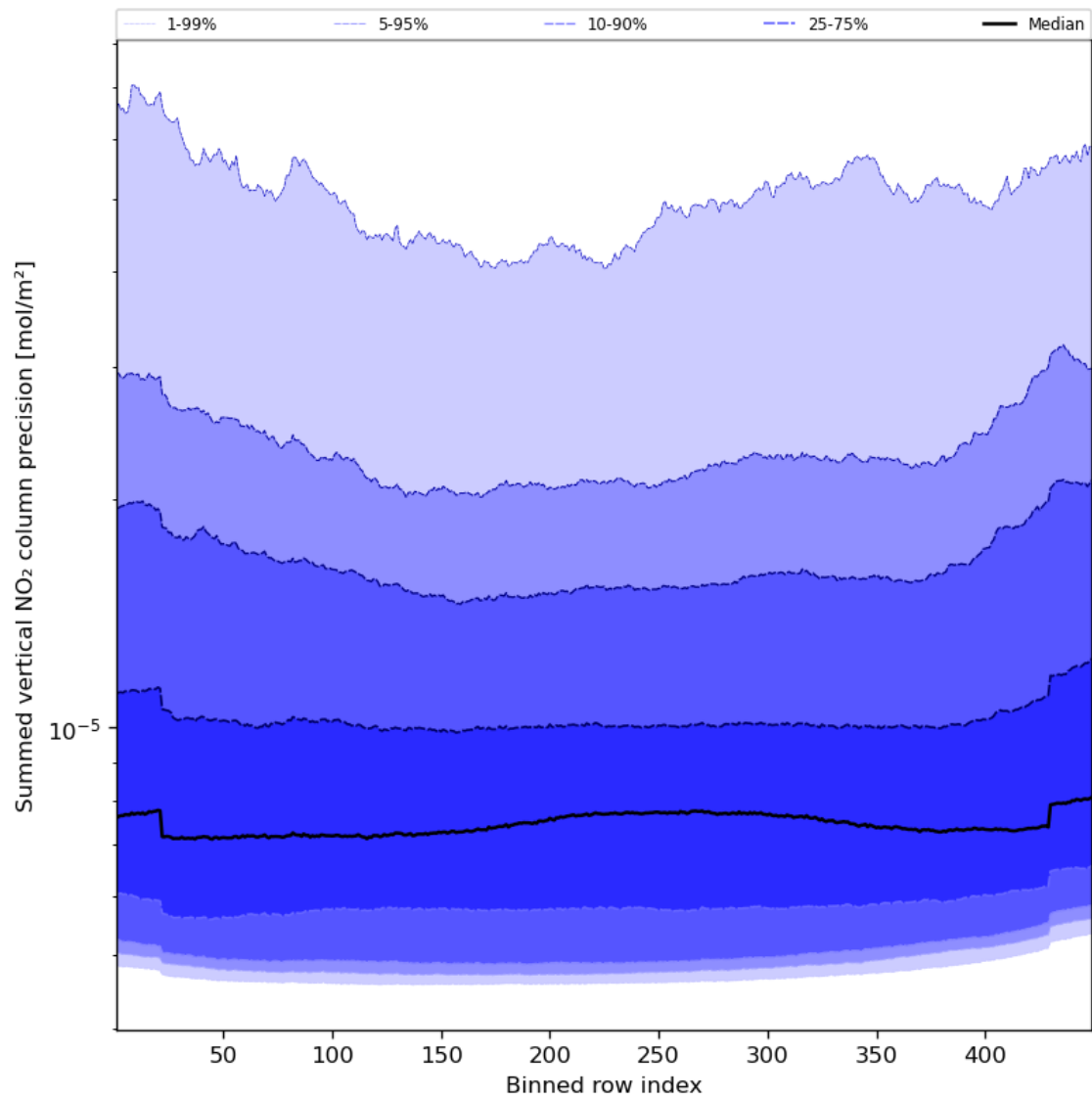
Figure 58: Along track statistics of “Summed vertical NO 2 column precision” for 2023-11-07 to 2023-11-08
