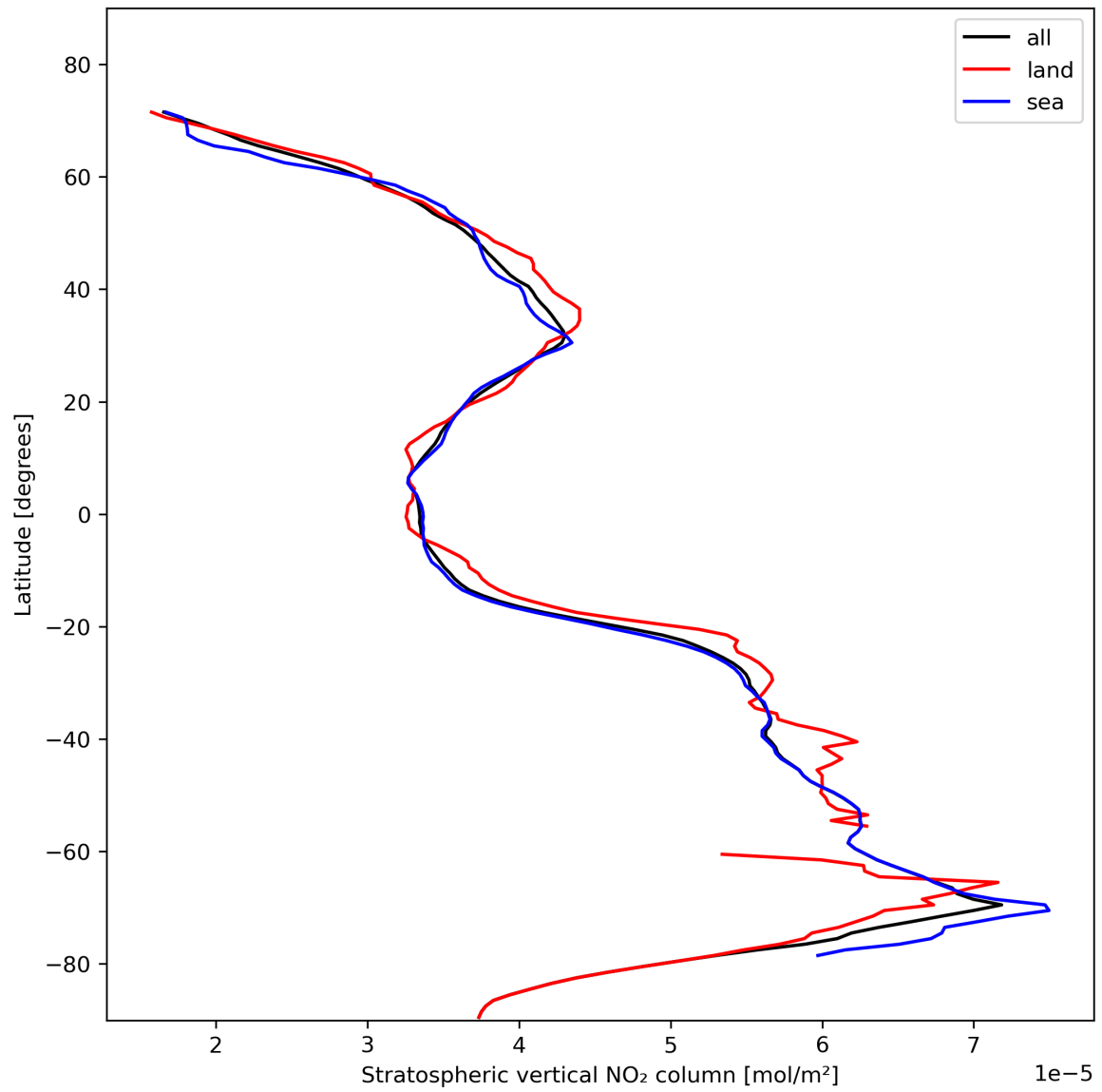
Figure 19: Zonal average of “Stratospheric vertical NO 2 column” for 2023-11-07 to 2023-11-08.
