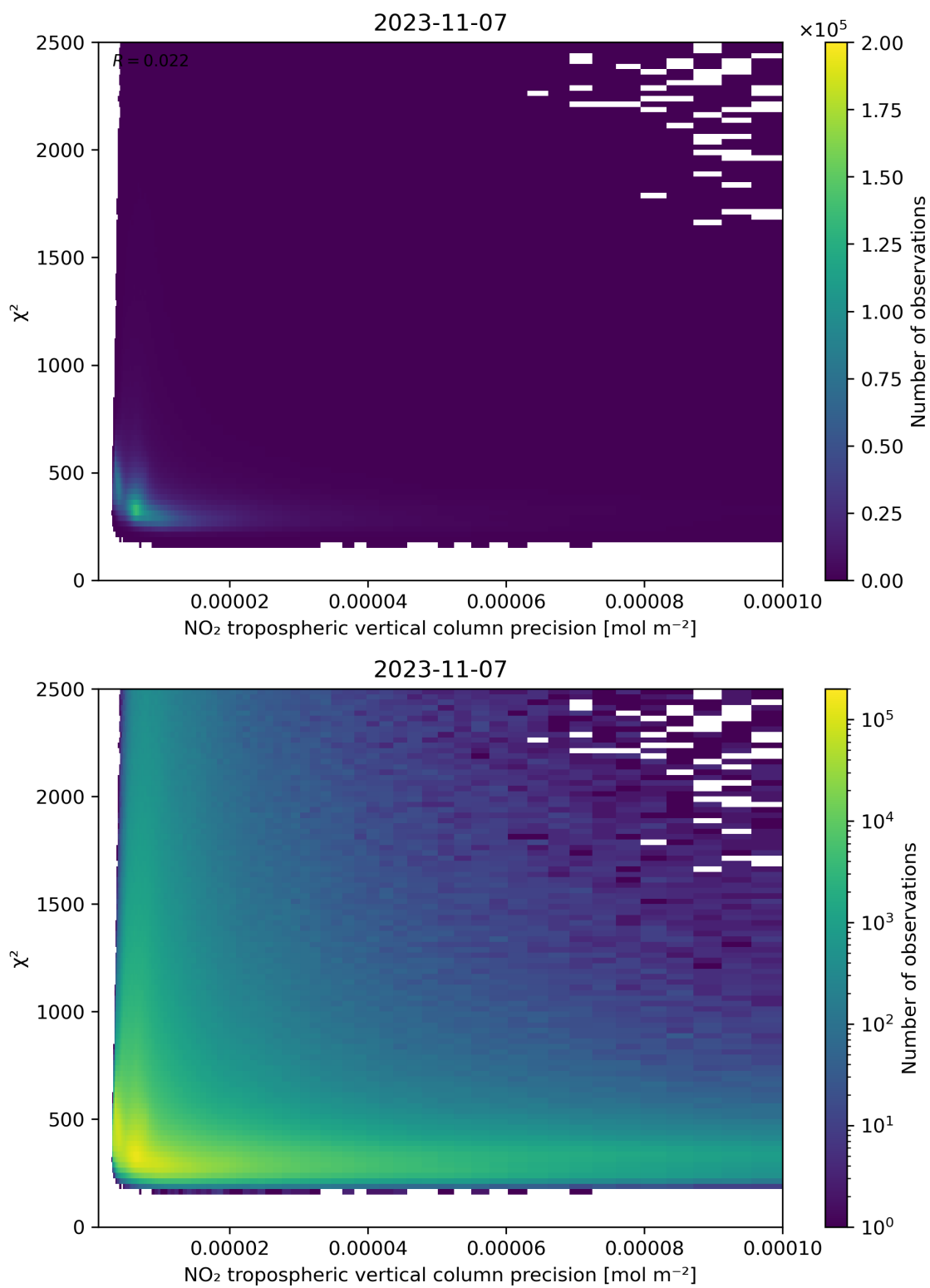
Figure 134: Scatter density plot of “NO 2 tropospheric vertical column precision” against “ \chi^2 ” for 2023-11-07 to 2023-11-08.
