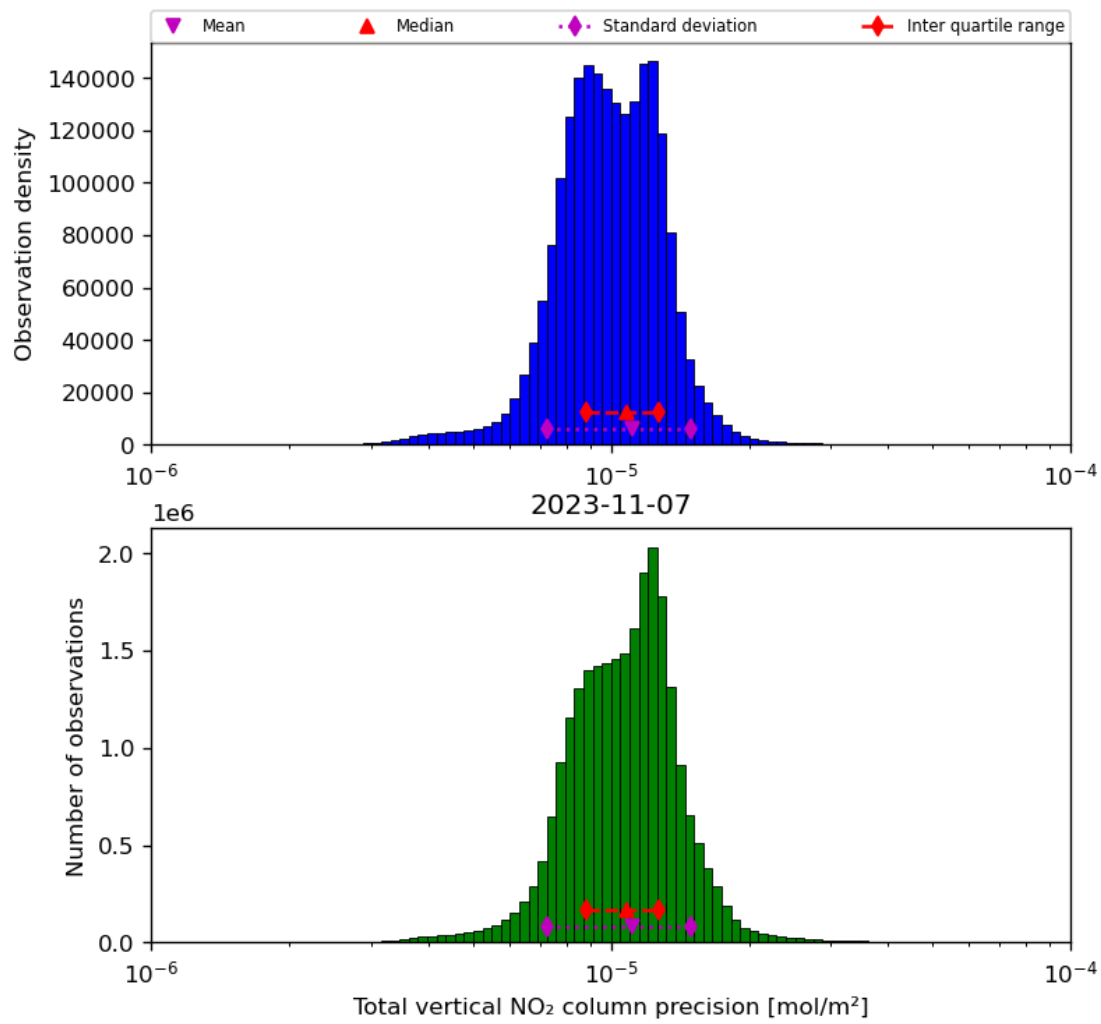
Figure 39: Histogram of "Total vertical NO 2 column precision" for 2023-11-07 to 2023-11-08
