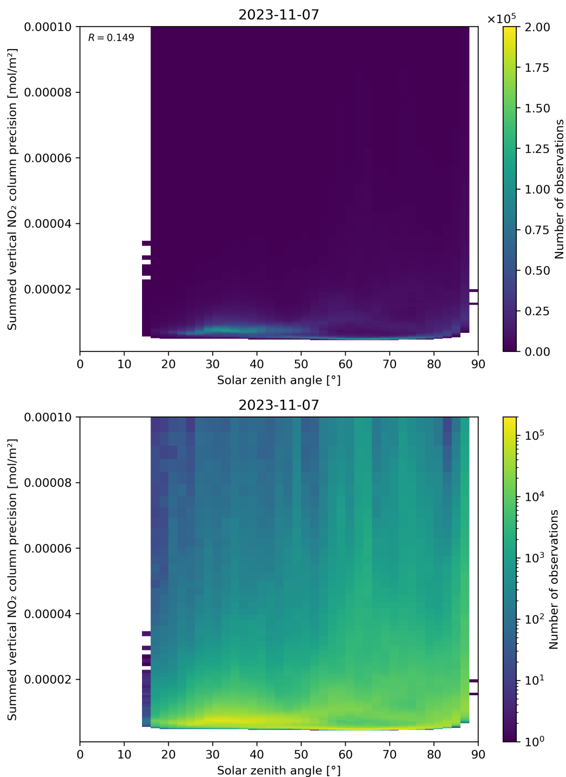
Figure 152: Scatter density plot of “Solar zenith angle” against “Summed vertical NO 2 column precision” for 2023-11-07 to 2023-11-08.
