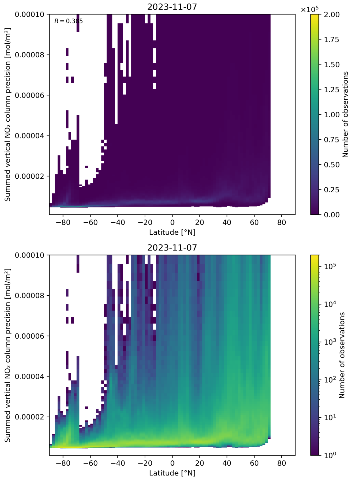
Figure 89: Scatter density plot of “Latitude” against “Summed vertical NO 2 column precision” for 2023-11-07 to 2023-11-08.
