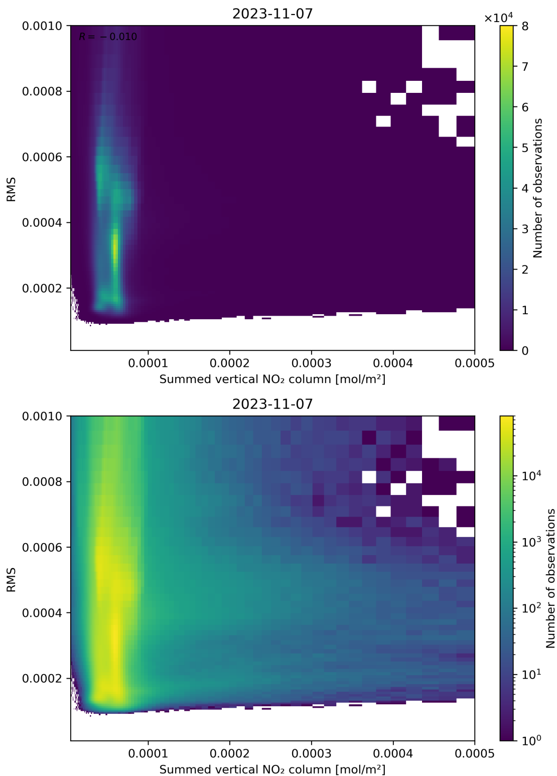
Figure 109: Scatter density plot of “Summed vertical NO 2 column” against “RMS” for 2023-11-07 to 2023-11-08.
