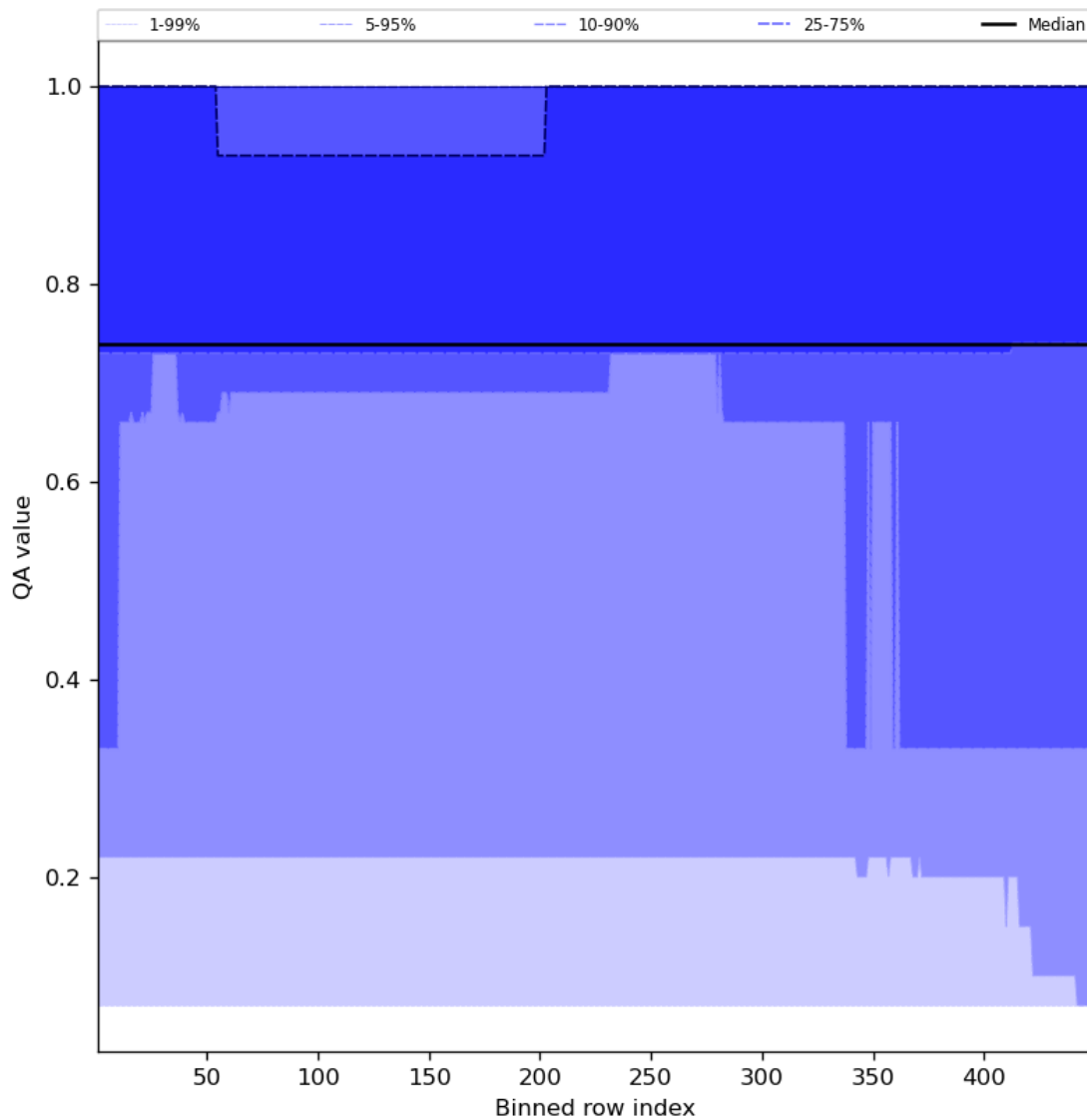
Figure 45: Along track statistics of “QA value” for 2023-11-07 to 2023-11-08
