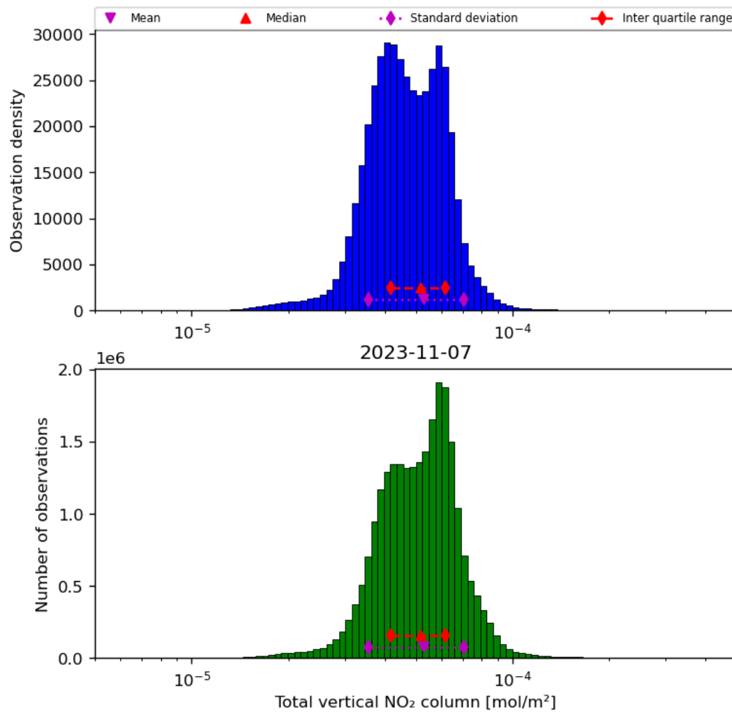
Figure 38: Histogram of “Total vertical NO 2 column” for 2023-11-07 to 2023-11-08
