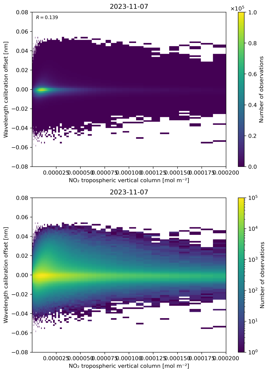
Figure 143: Scatter density plot of “NO 2 tropospheric vertical column” against “Wavelength calibration offset” for 2023-11-07 to 2023-11-08.
