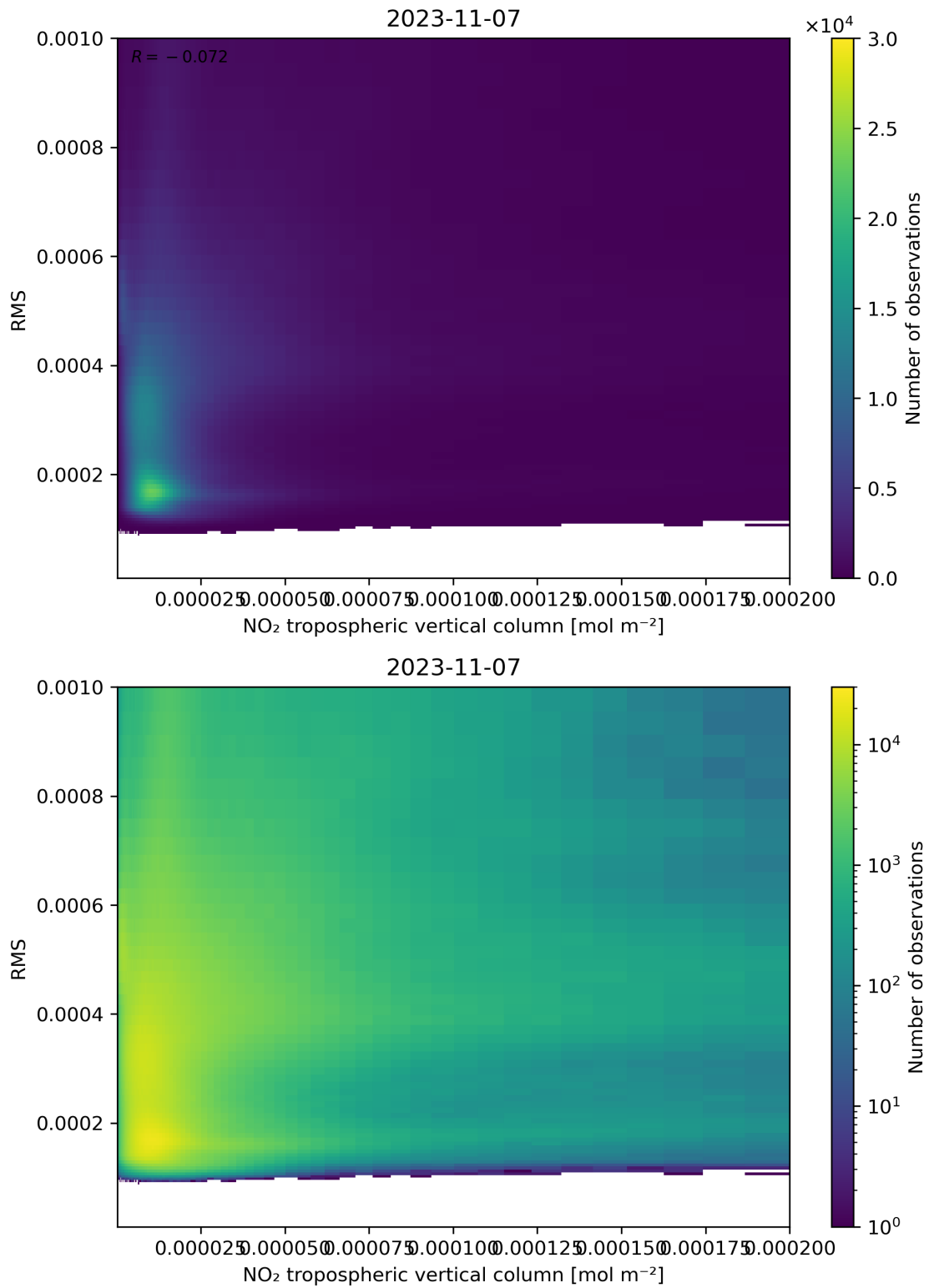
Figure 142: Scatter density plot of “NO 2 tropospheric vertical column” against “RMS” for 2023-11-07 to 2023-11-08.
