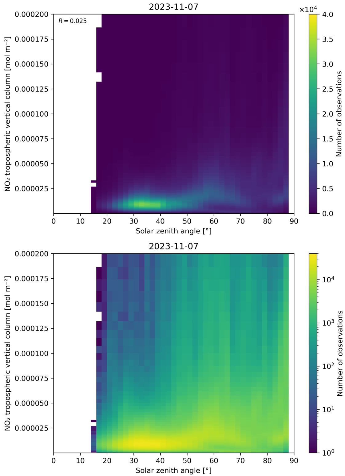
Figure 155: Scatter density plot of “Solar zenith angle” against “NO 2 tropospheric vertical column” for 2023-11-07 to 2023-11-08.
