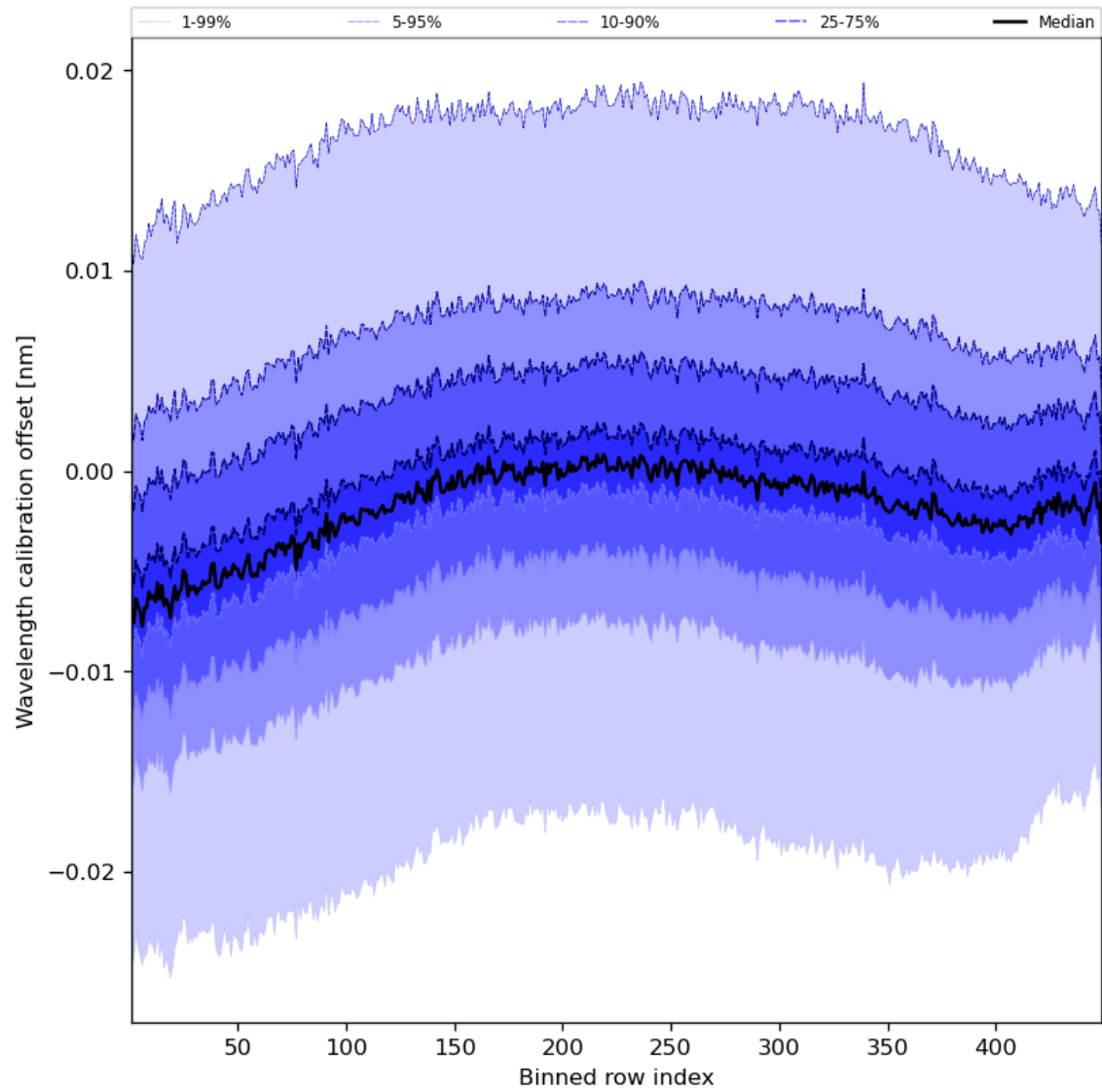
Figure 52: Along track statistics of “Wavelength calibration offset” for 2023-11-07 to 2023-11-08
