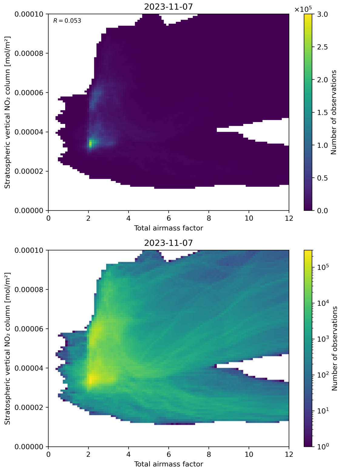
Figure 64: Scatter density plot of “Total airmass factor” against “Stratospheric vertical NO 2 column” for 2023-11-07 to 2023-11-08.
