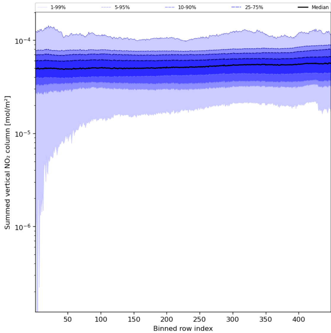
Figure 57: Along track statistics of “Summed vertical NO 2 column” for 2023-11-07 to 2023-11-08
