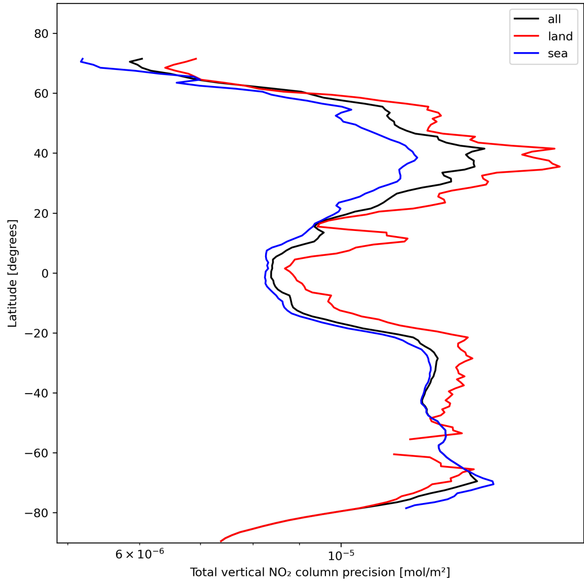
Figure 22: Zonal average of “Total vertical NO 2 column precision” for 2023-11-07 to 2023-11-08.
