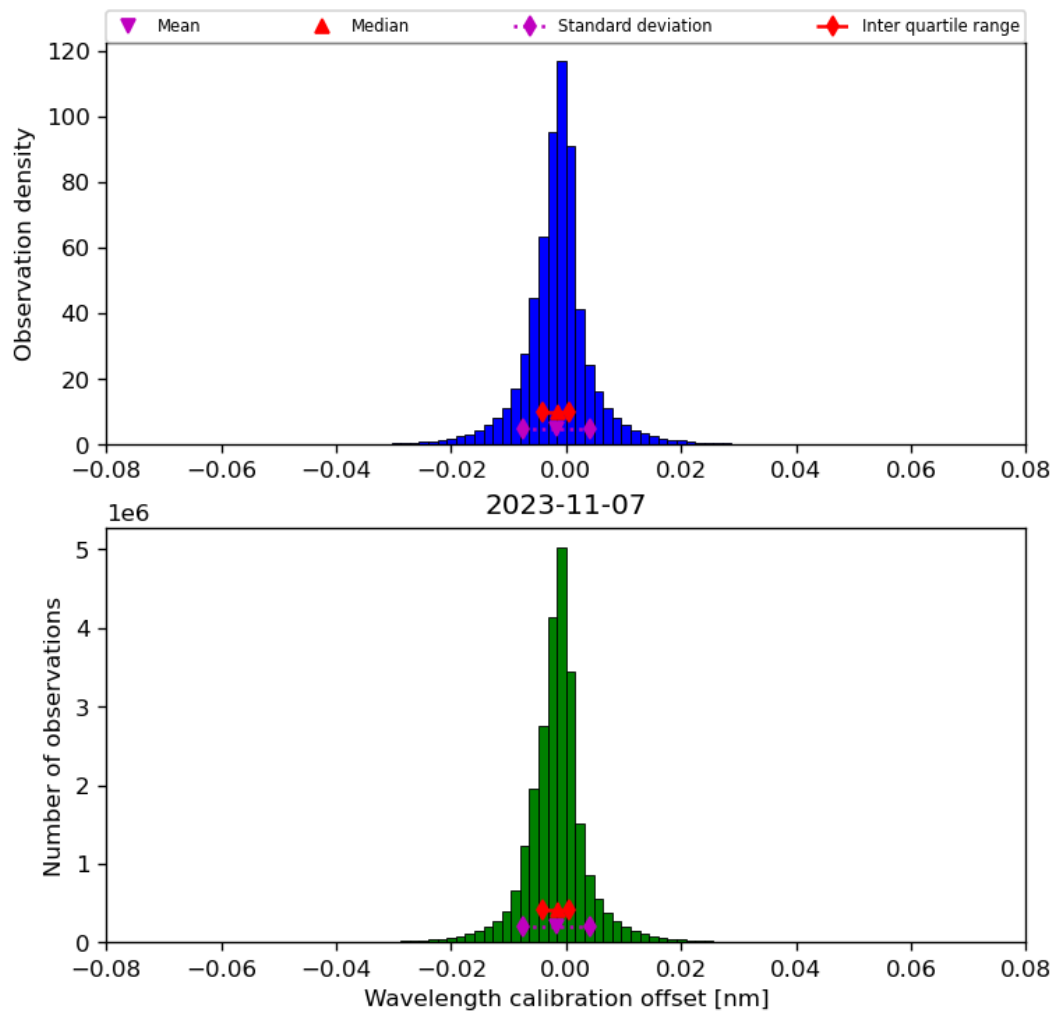
Figure 35: Histogram of “Wavelength calibration offset” for 2023-11-07 to 2023-11-08
