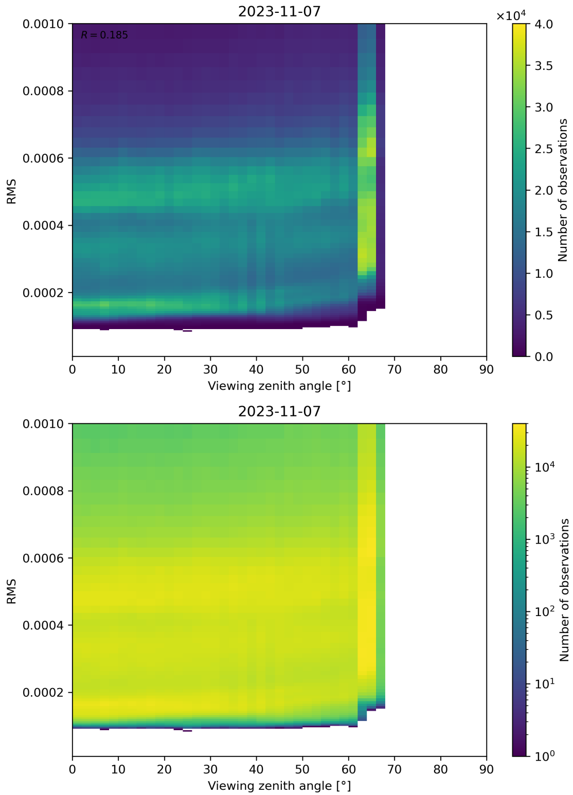
Figure 171: Scatter density plot of “Viewing zenith angle” against “RMS” for 2023-11-07 to 2023-11-08.
