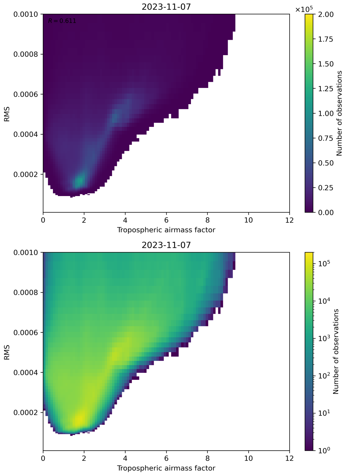
Figure 79: Scatter density plot of “Tropospheric airmass factor” against “RMS” for 2023-11-07 to 2023-11-08.
