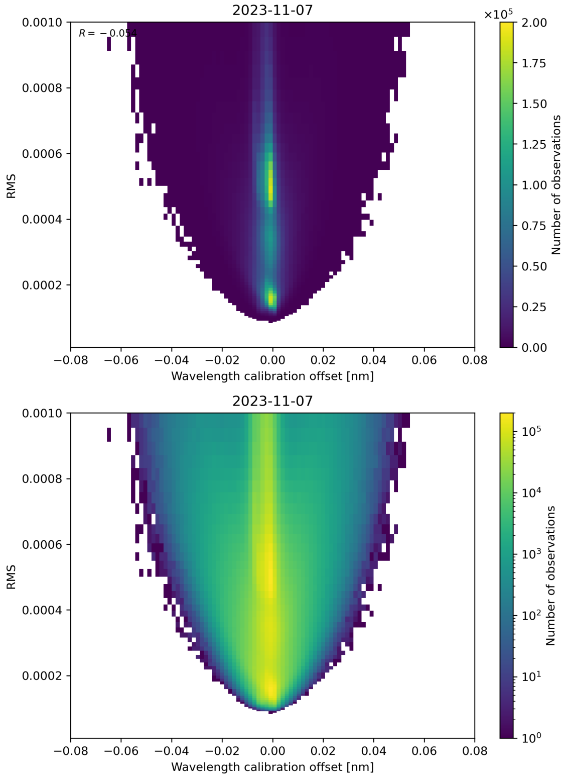
Figure 181: Scatter density plot of “Wavelength calibration offset” against “RMS” for 2023-11-07 to 2023-11-08.
