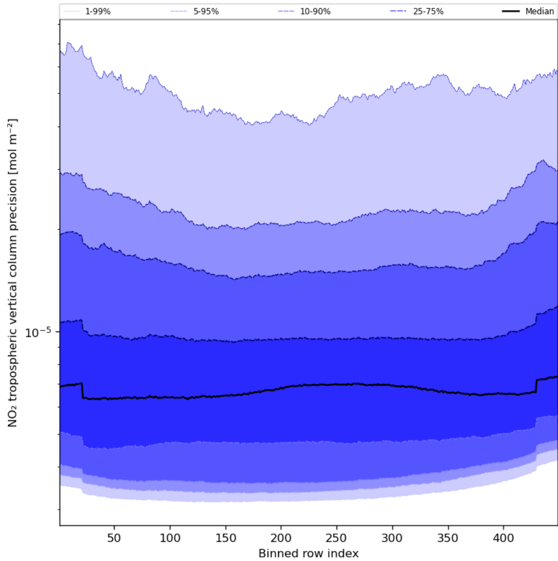
Figure 47: Along track statistics of “NO 2 tropospheric vertical column precision” for 2023-11-07 to 2023-11-08
