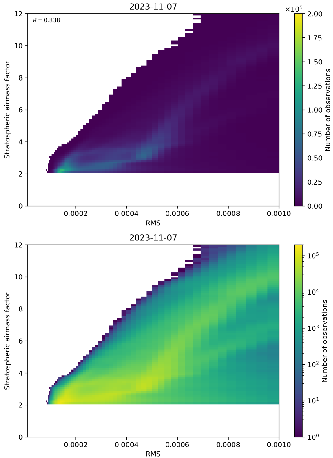
Figure 144: Scatter density plot of “RMS” against “Stratospheric airmass factor” for 2023-11-07 to 2023-11-08.
