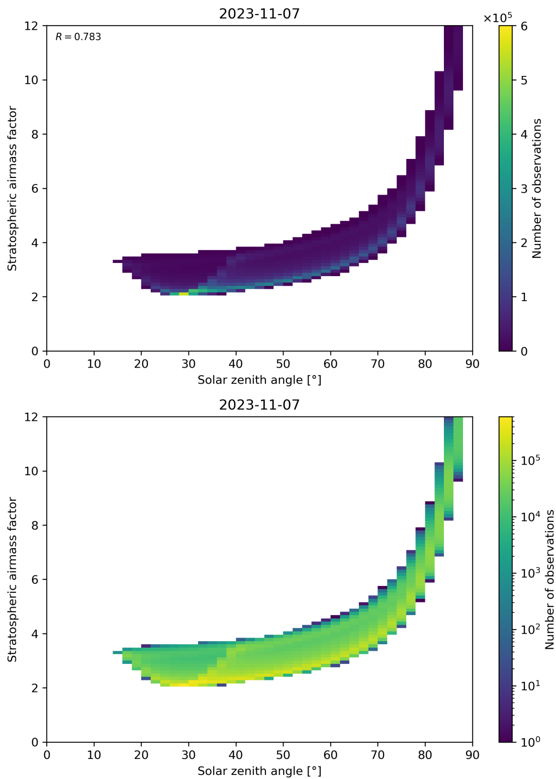
Figure 145: Scatter density plot of “Solar zenith angle” against “Stratospheric airmass factor” for 2023-11-07 to 2023-11-08.
