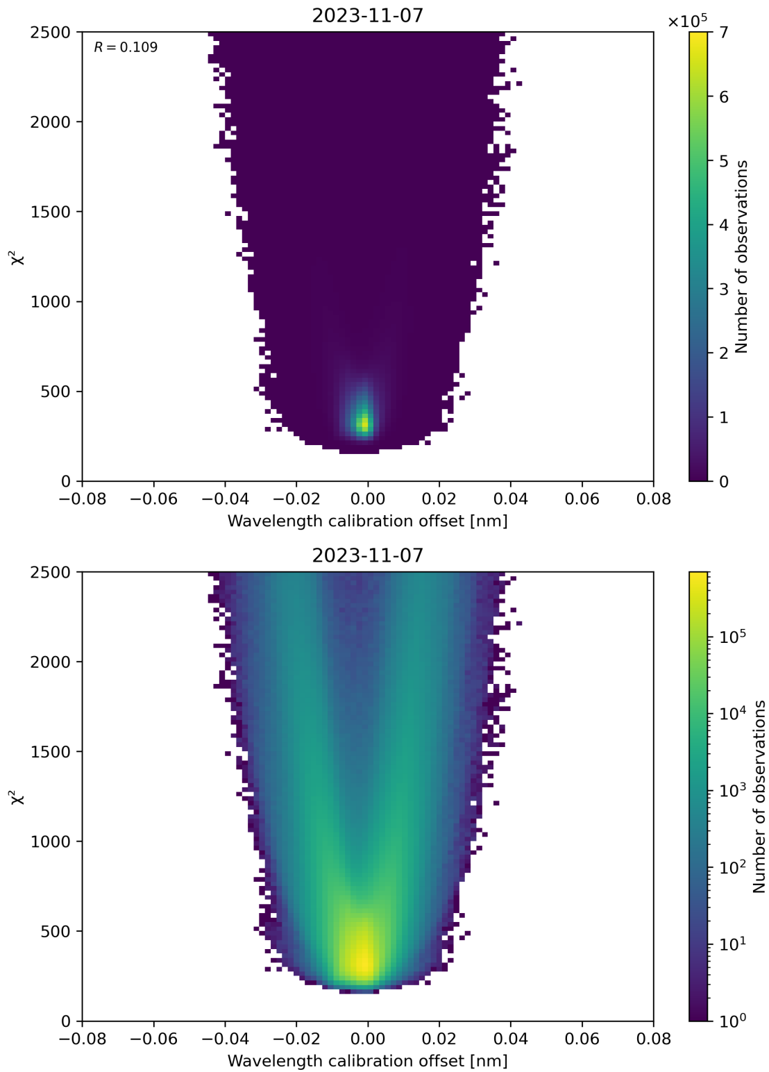
Figure 175: Scatter density plot of “Wavelength calibration offset” against “ \chi^2 ” for 2023-11-07 to 2023-11-08.
