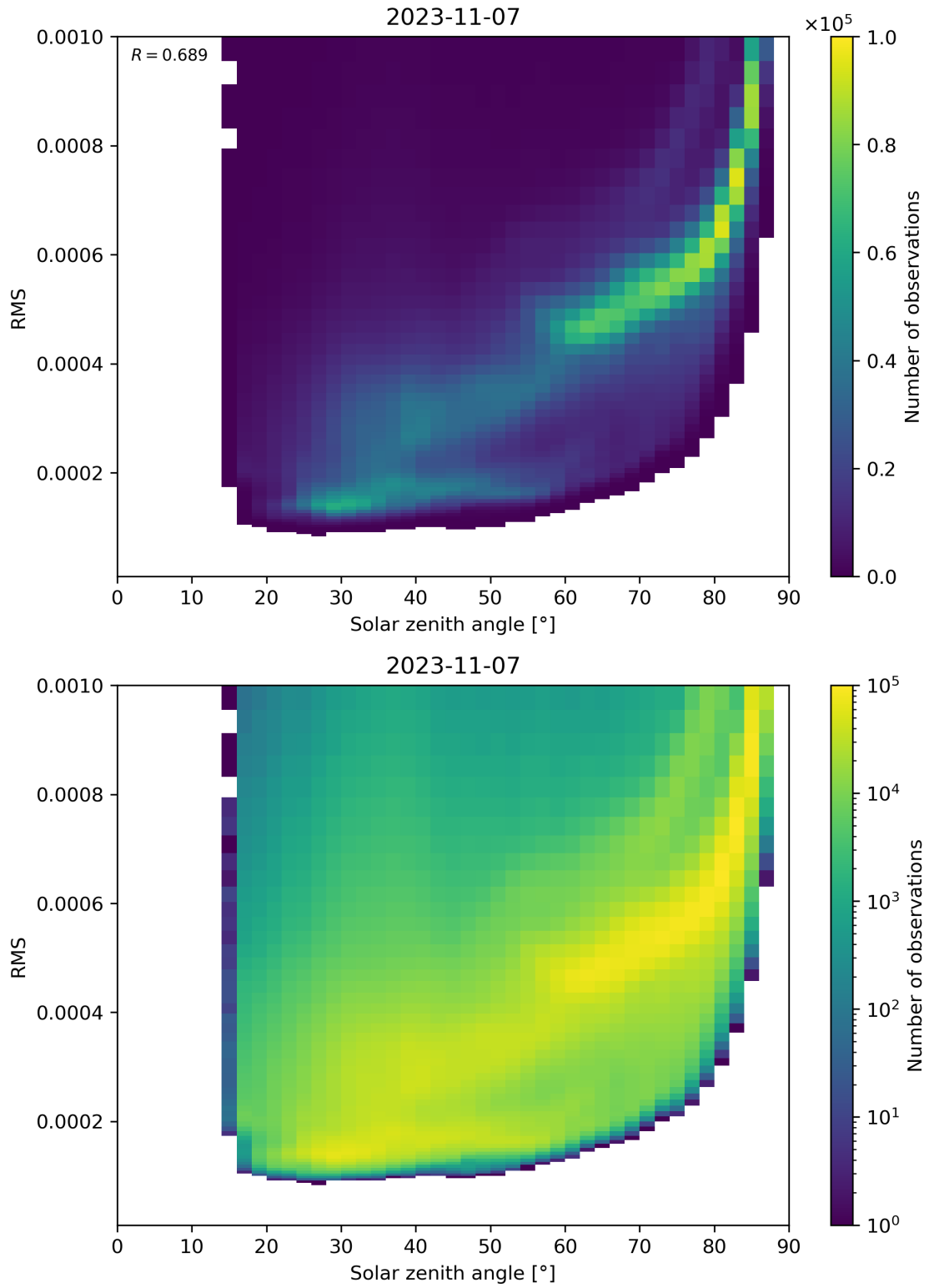
Figure 157: Scatter density plot of “Solar zenith angle” against “RMS” for 2023-11-07 to 2023-11-08.
