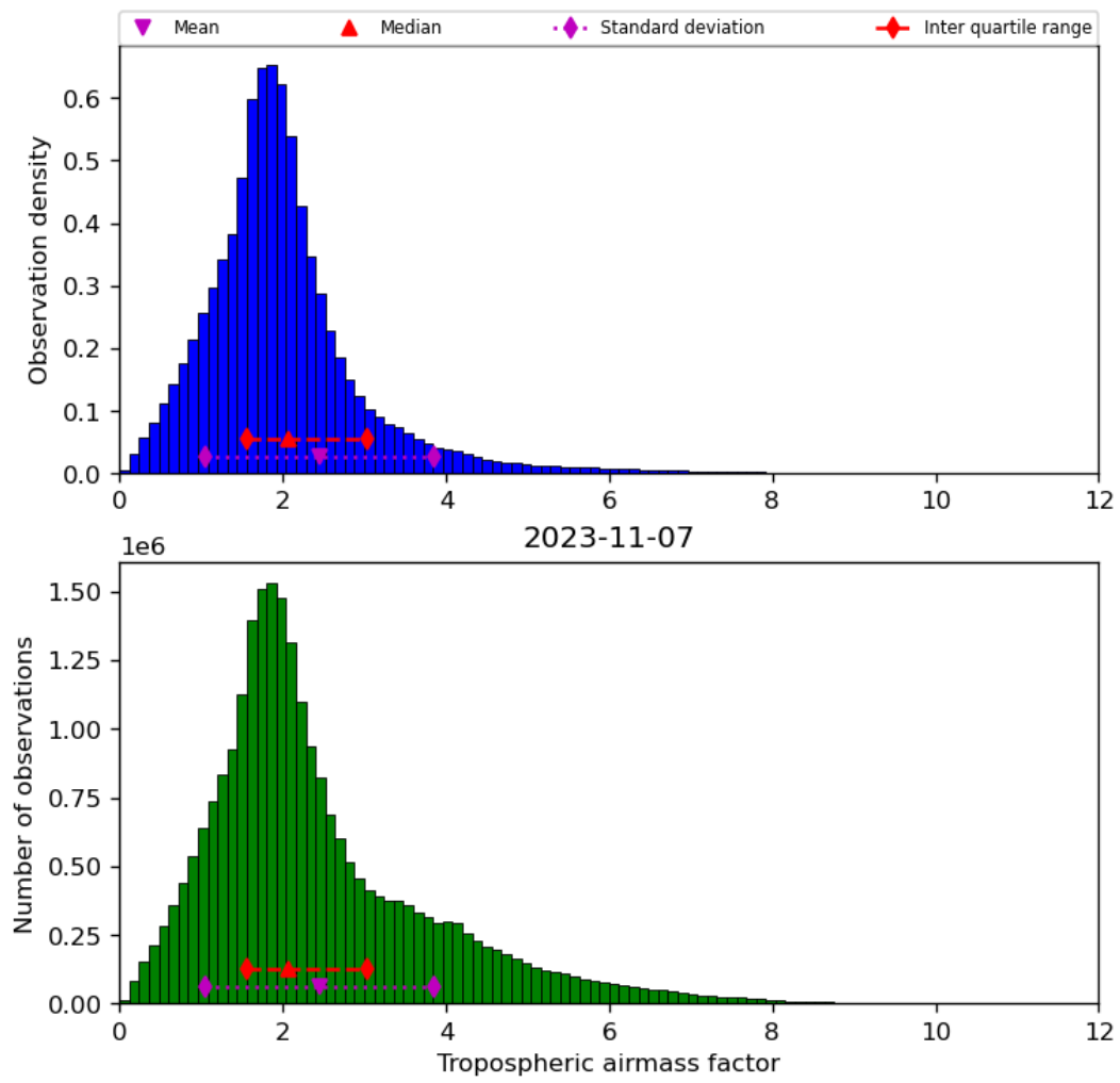
Figure 31: Histogram of “Tropospheric airmass factor” for 2023-11-07 to 2023-11-08
