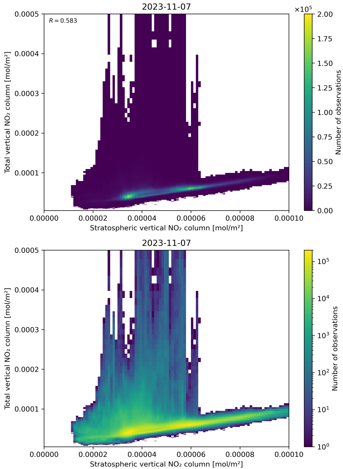
Figure 100: Scatter density plot of “Stratospheric vertical NO 2 column” against “Total vertical NO 2 column” for 2023-11-07 to 2023-11-08.
