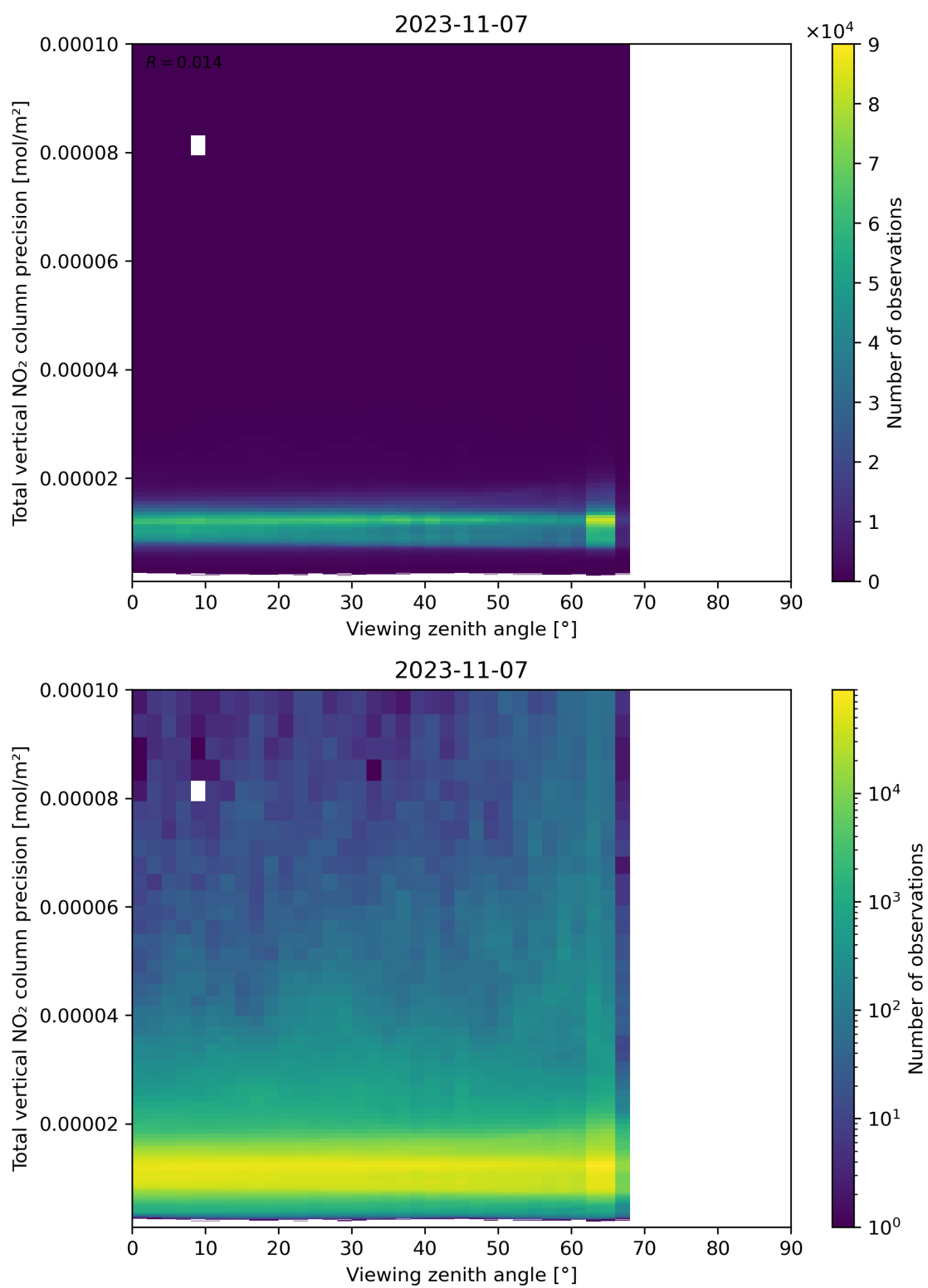
Figure 168: Scatter density plot of “Viewing zenith angle” against “Total vertical NO 2 column precision” for 2023-11-07 to 2023-11-08.
