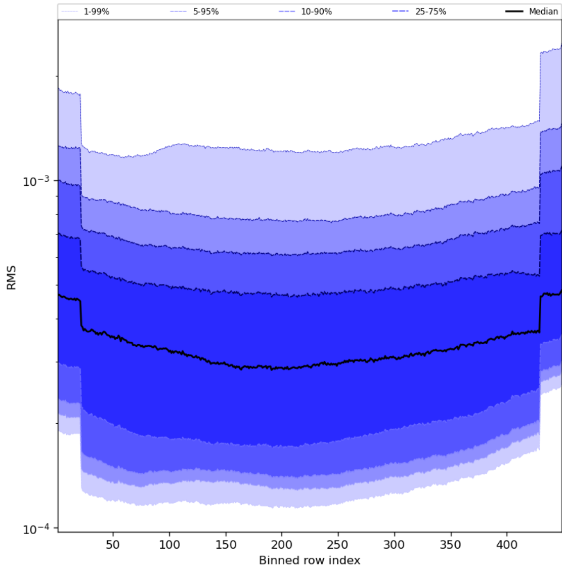
Figure 60: Along track statistics of “RMS” for 2023-11-07 to 2023-11-08
