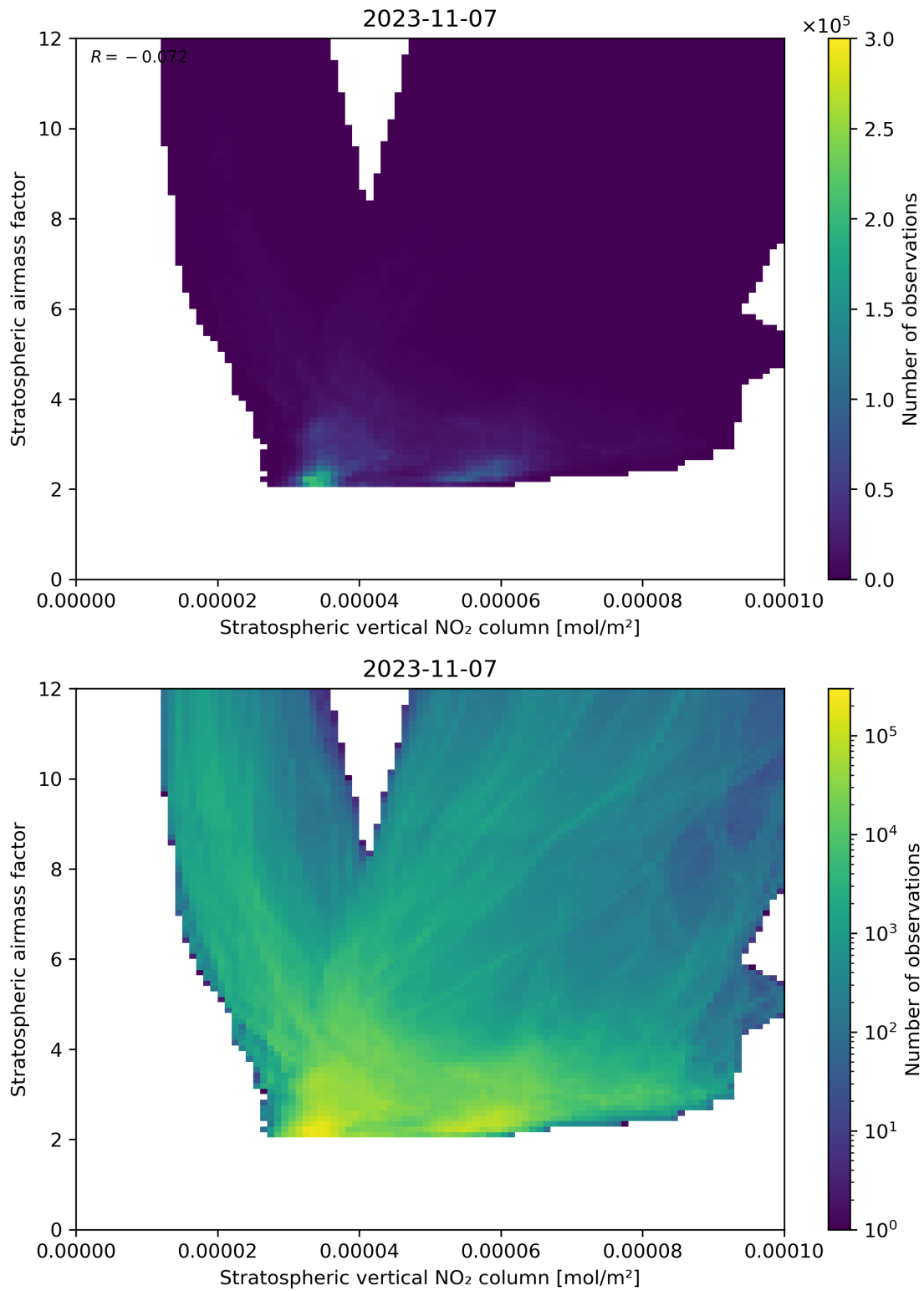
Figure 96: Scatter density plot of “Stratospheric vertical NO 2 column” against “Stratospheric airmass factor” for 2023-11-07 to 2023-11-08.
