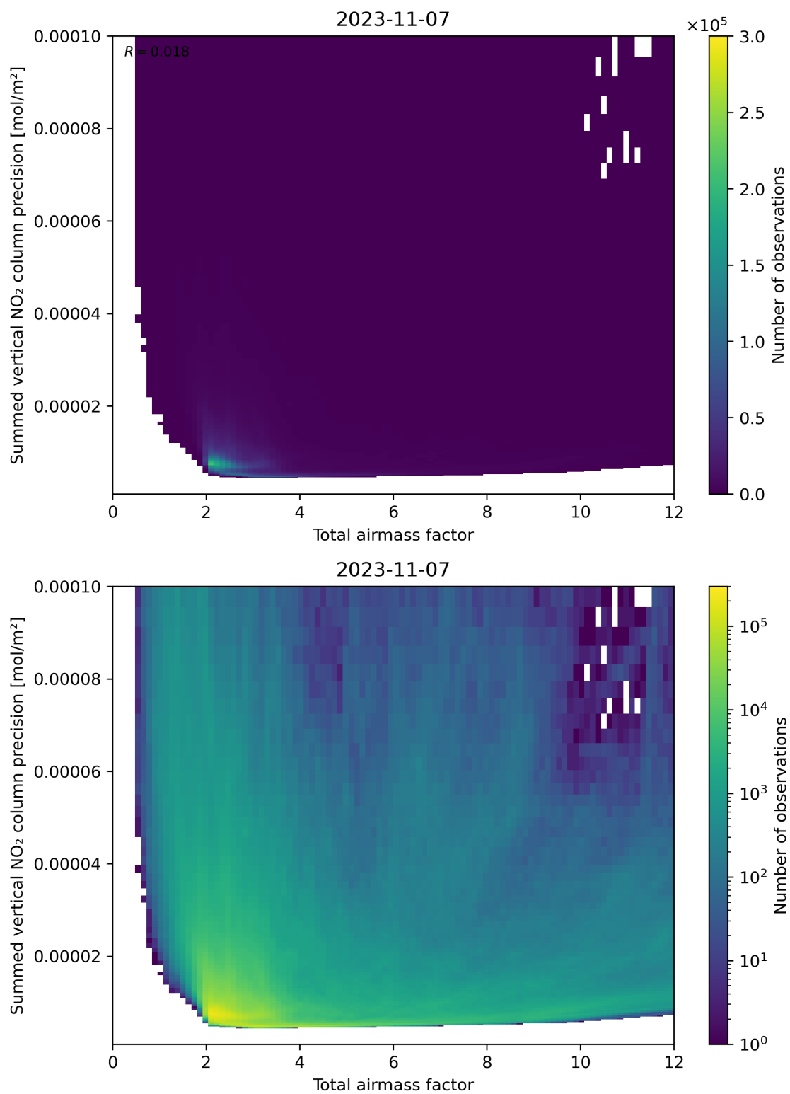
Figure 66: Scatter density plot of “Total airmass factor” against “Summed vertical NO 2 column precision” for 2023-11-07 to 2023-11-08.
