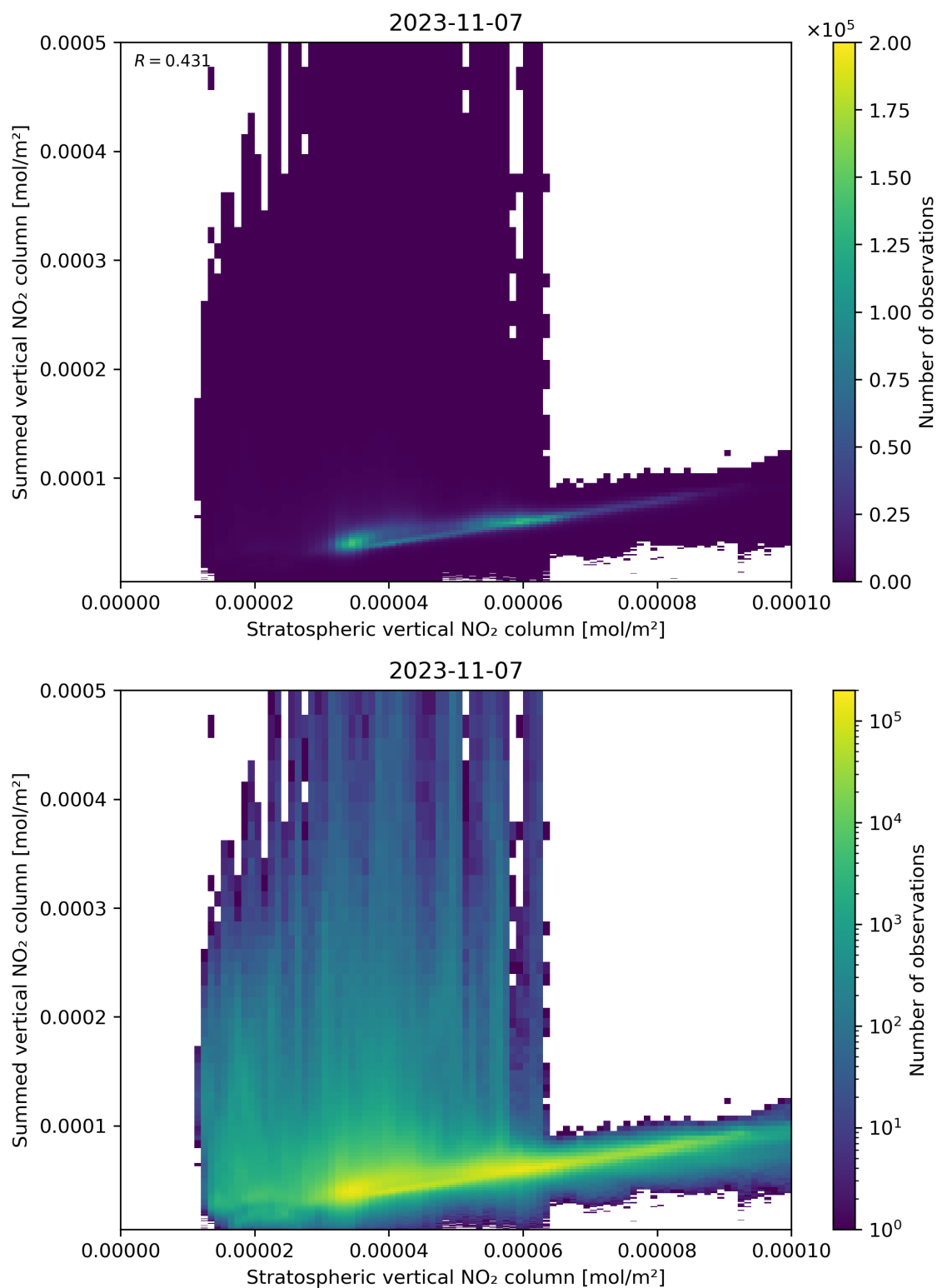
Figure 98: Scatter density plot of “Stratospheric vertical NO 2 column” against “Summed vertical NO 2 column” for 2023-11-07 to 2023-11-08.
