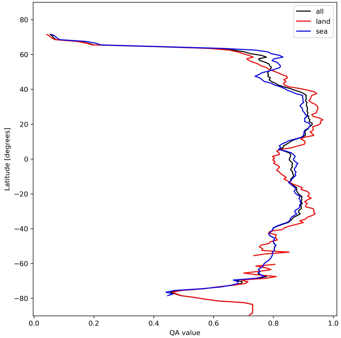
Figure 11: Zonal average of “QA value” for 2023-11-07 to 2023-11-08.
