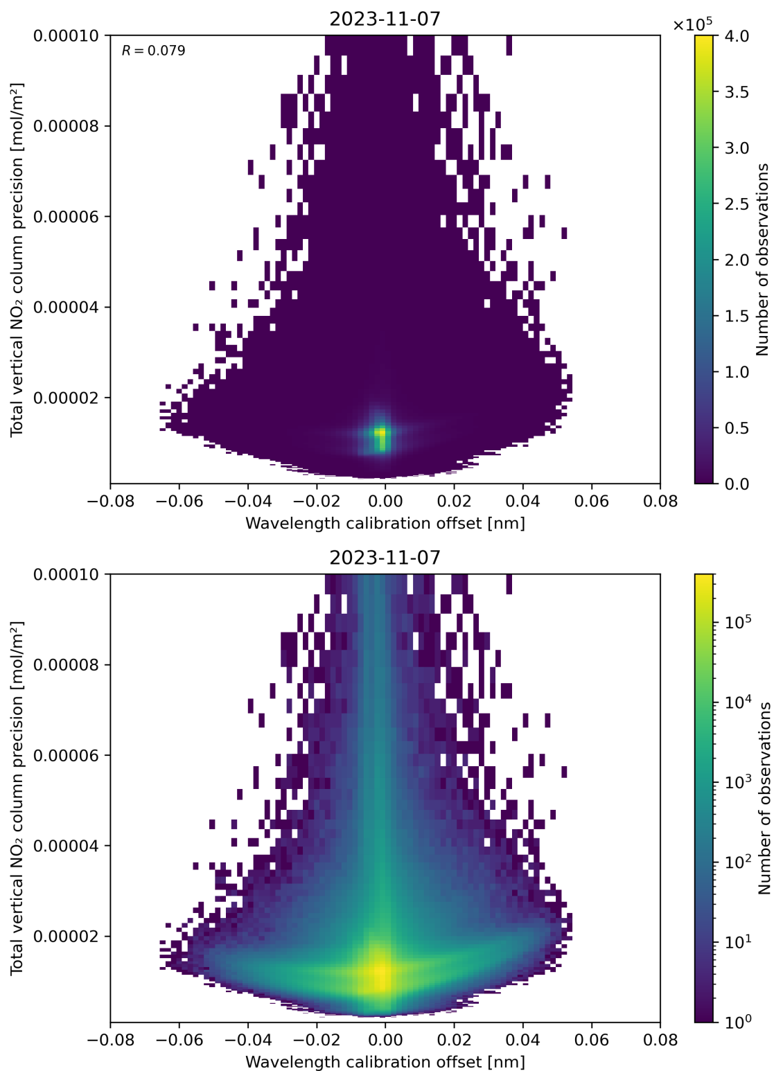
Figure 180: Scatter density plot of “Wavelength calibration offset” against “Total vertical NO 2 column precision” for 2023-11-07 to 2023-11-08.
