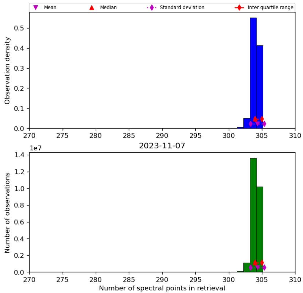
Figure 33: Histogram of “Number of spectral points in retrieval” for 2023-11-07 to 2023-11-08
