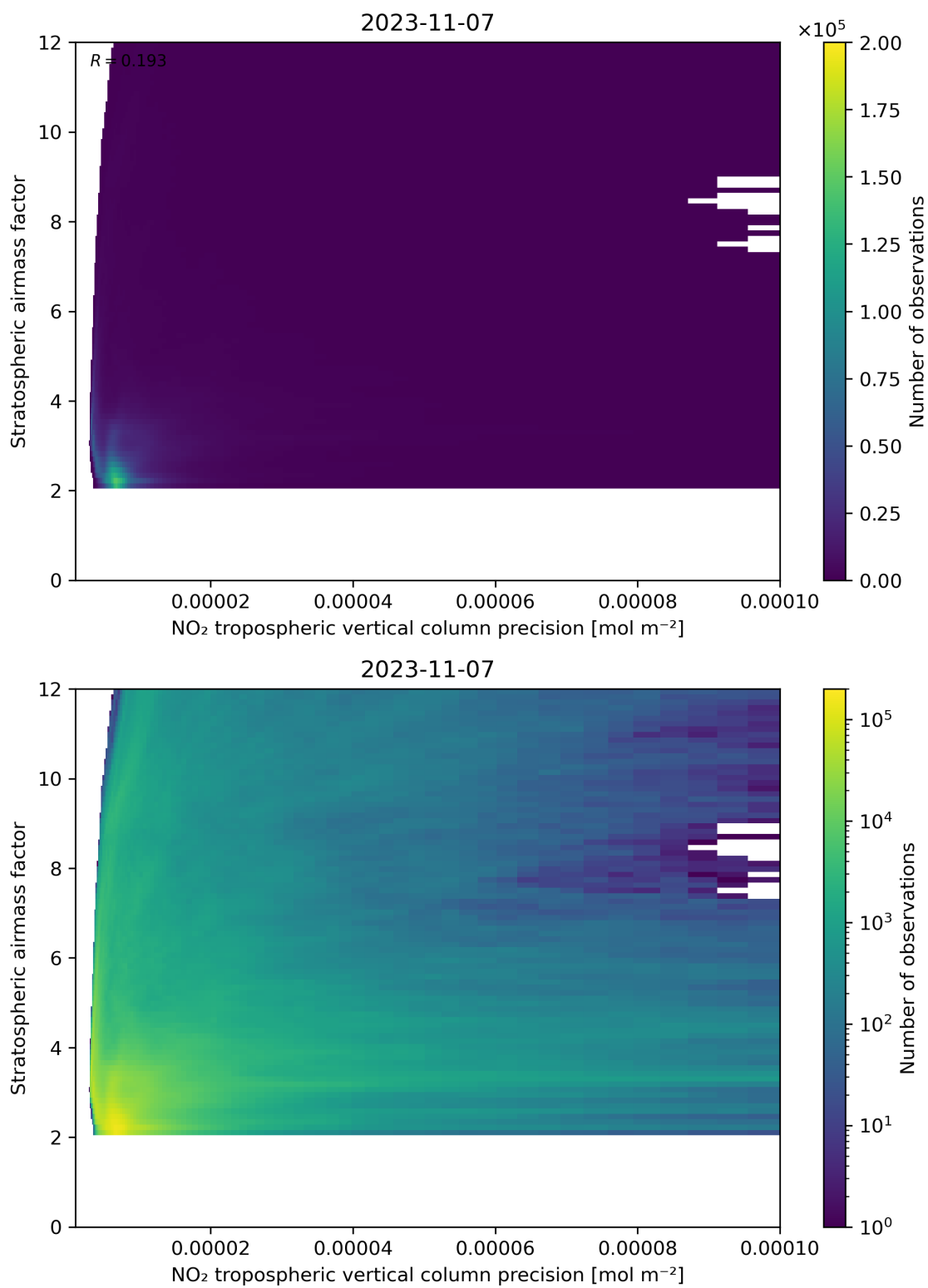
Figure 131: Scatter density plot of “NO 2 tropospheric vertical column precision” against “Stratospheric airmass factor” for 2023-11-07 to 2023-11-08.
