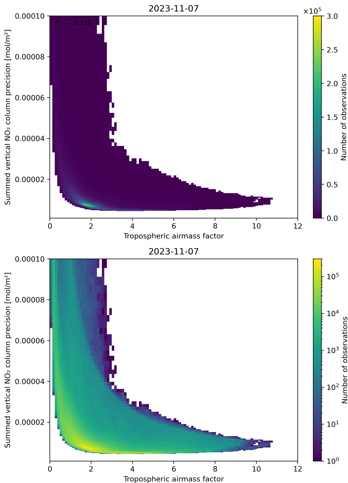
Figure 76: Scatter density plot of “Tropospheric air mass factor” against “Summed vertical NO 2 column precision” for 2023-11-07 to 2023-11-08.
