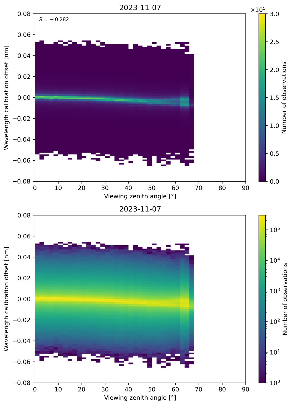
Figure 173: Scatter density plot of “Viewing zenith angle” against “Wavelength calibration offset” for 2023-11-07 to 2023-11-08.
