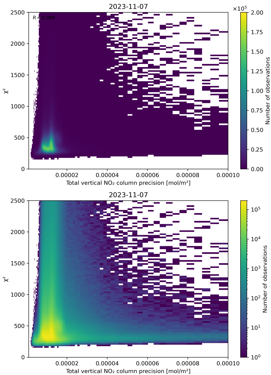
Figure 116: Scatter density plot of “Total vertical NO 2 column precision” against “ \chi^2 ” for 2023-11-07 to 2023-11-08.
