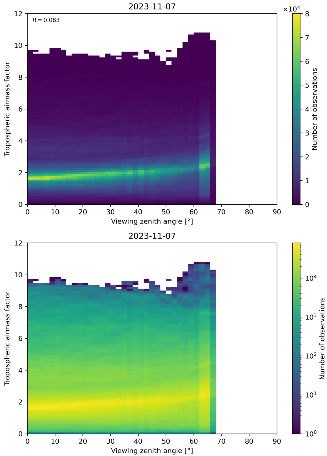
Figure 161: Scatter density plot of “Viewing zenith angle” against “Tropospheric airmass factor” for 2023-11-07 to 2023-11-08.
