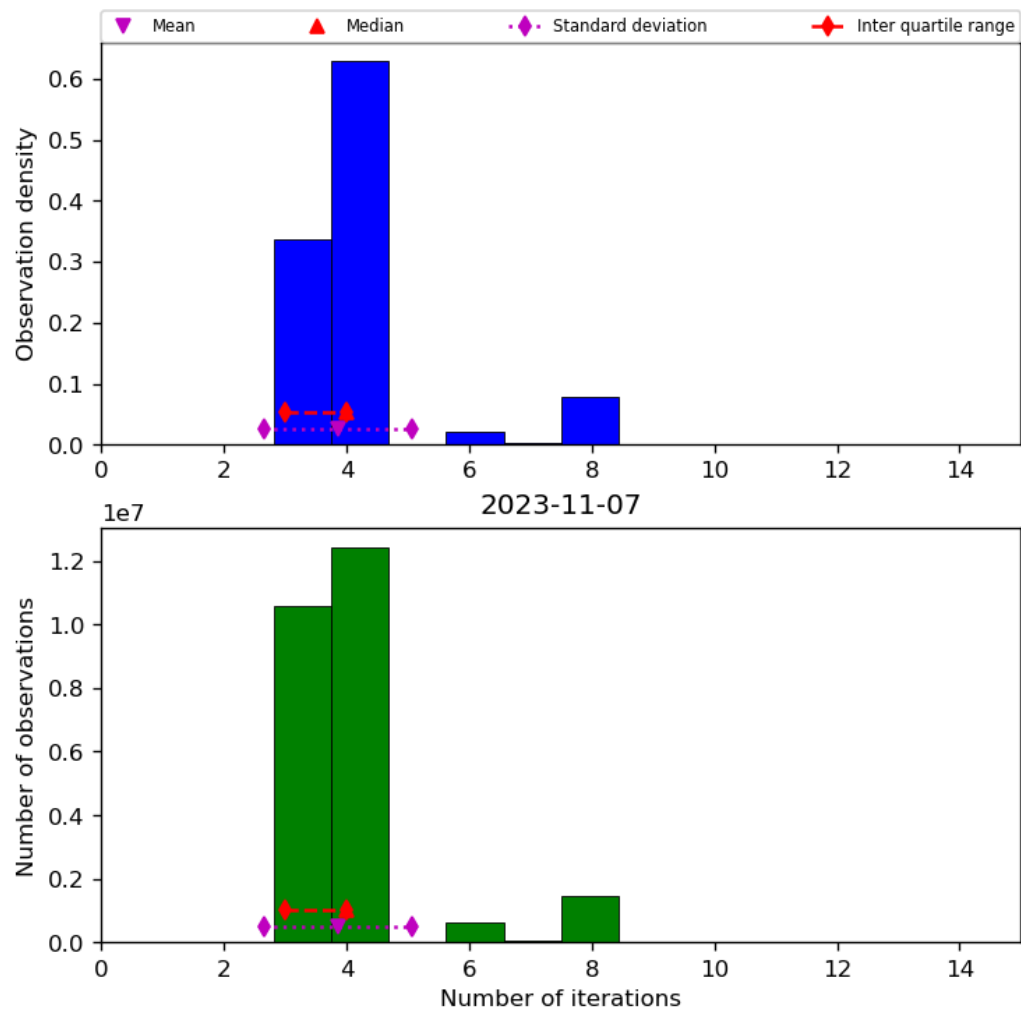
Figure 34: Histogram of “Number of iterations” for 2023-11-07 to 2023-11-08
