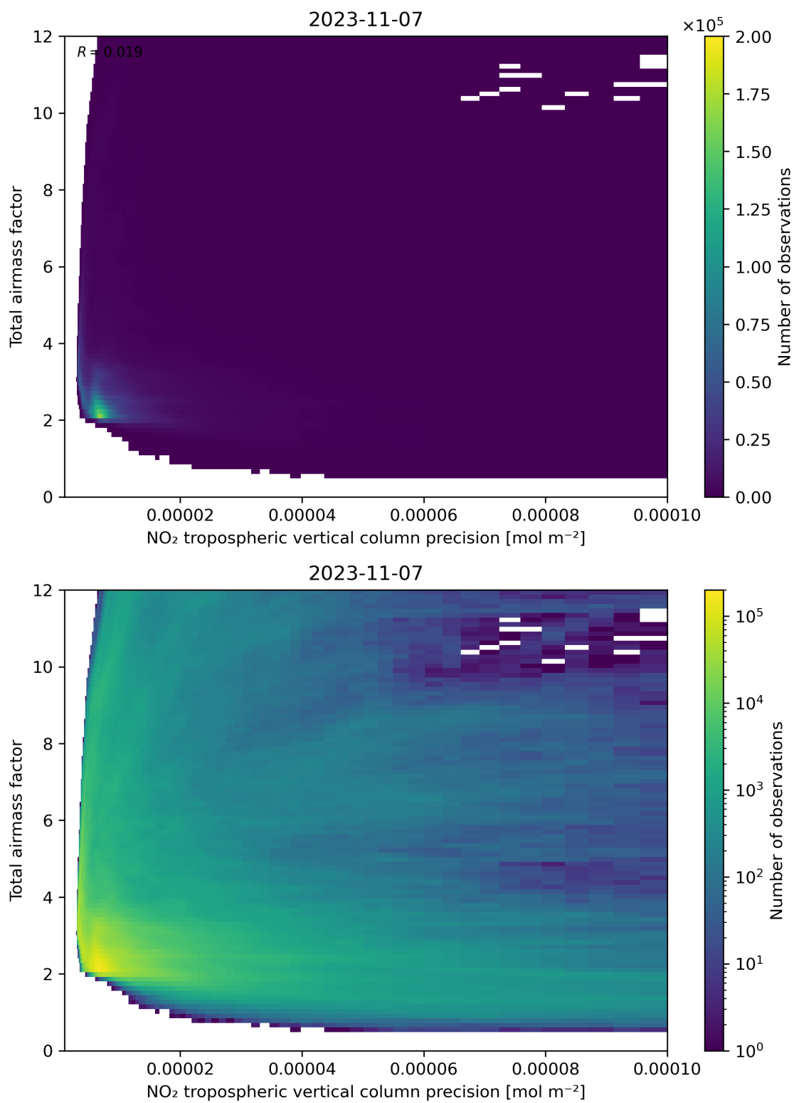
Figure 132: Scatter density plot of “NO 2 tropospheric vertical column precision” against “Total air mass factor” for 2023-11-07 to 2023-11-08.
