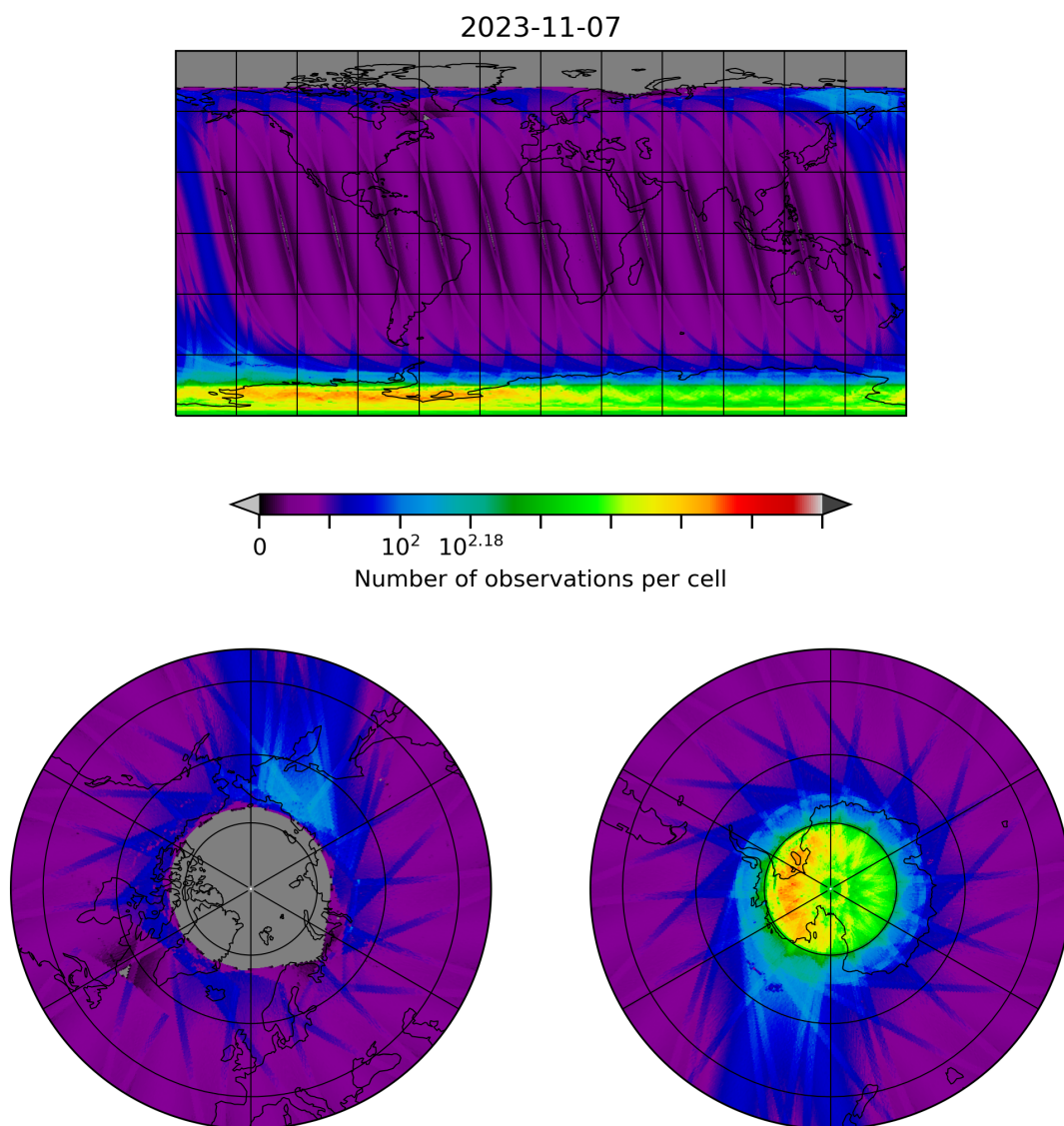
Figure 10: Map of the number of observations for 2023-11-07 to 2023-11-08
