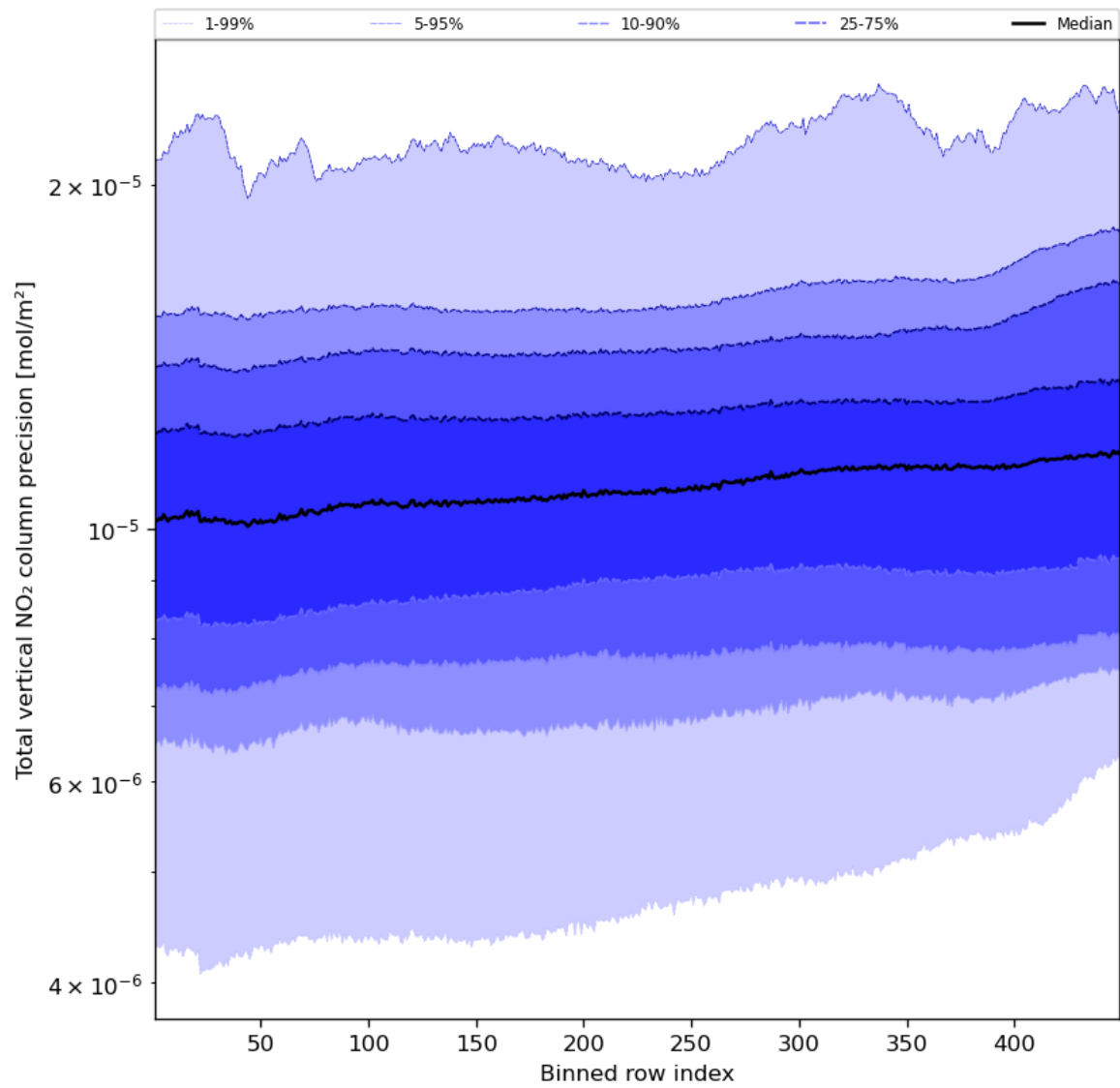
Figure 56: Along track statistics of "Total vertical NO 2 column precision" for 2023-11-07 to 2023-11-08
