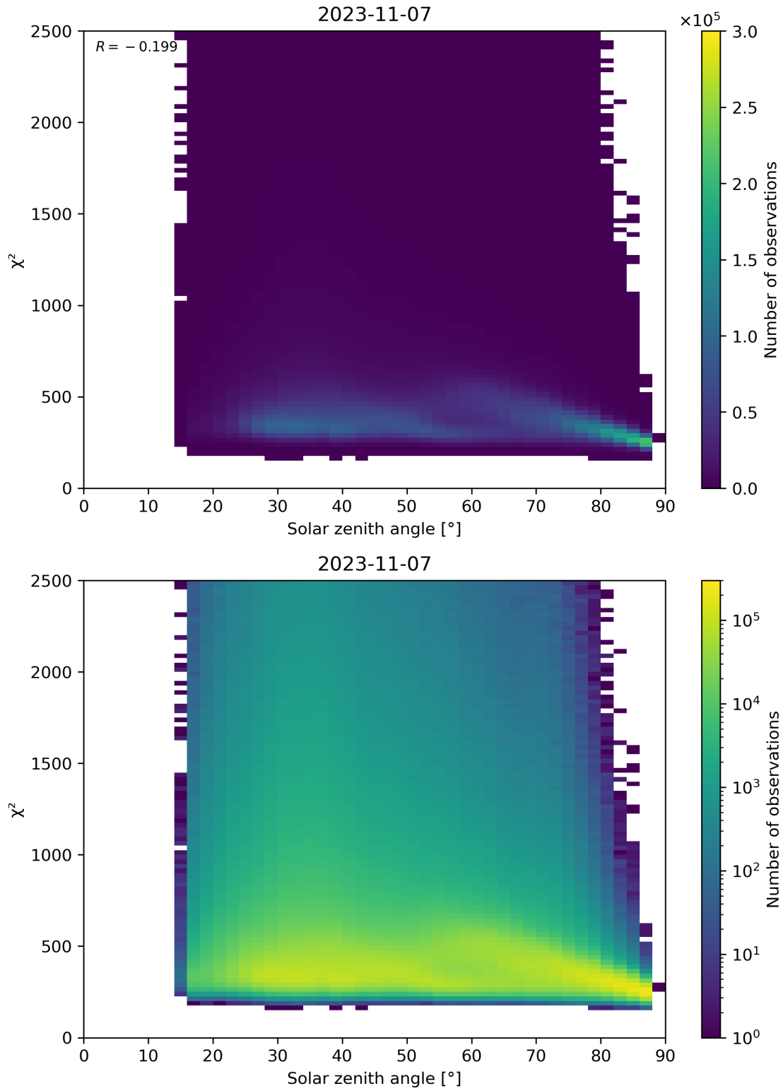
Figure 148: Scatter density plot of “Solar zenith angle” against “ \chi^2 ” for 2023-11-07 to 2023-11-08.
