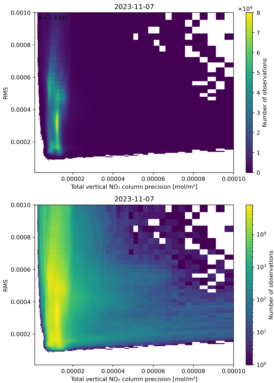
Figure 119: Scatter density plot of “Total vertical NO 2 column precision” against “RMS” for 2023-11-07 to 2023-11-08.
