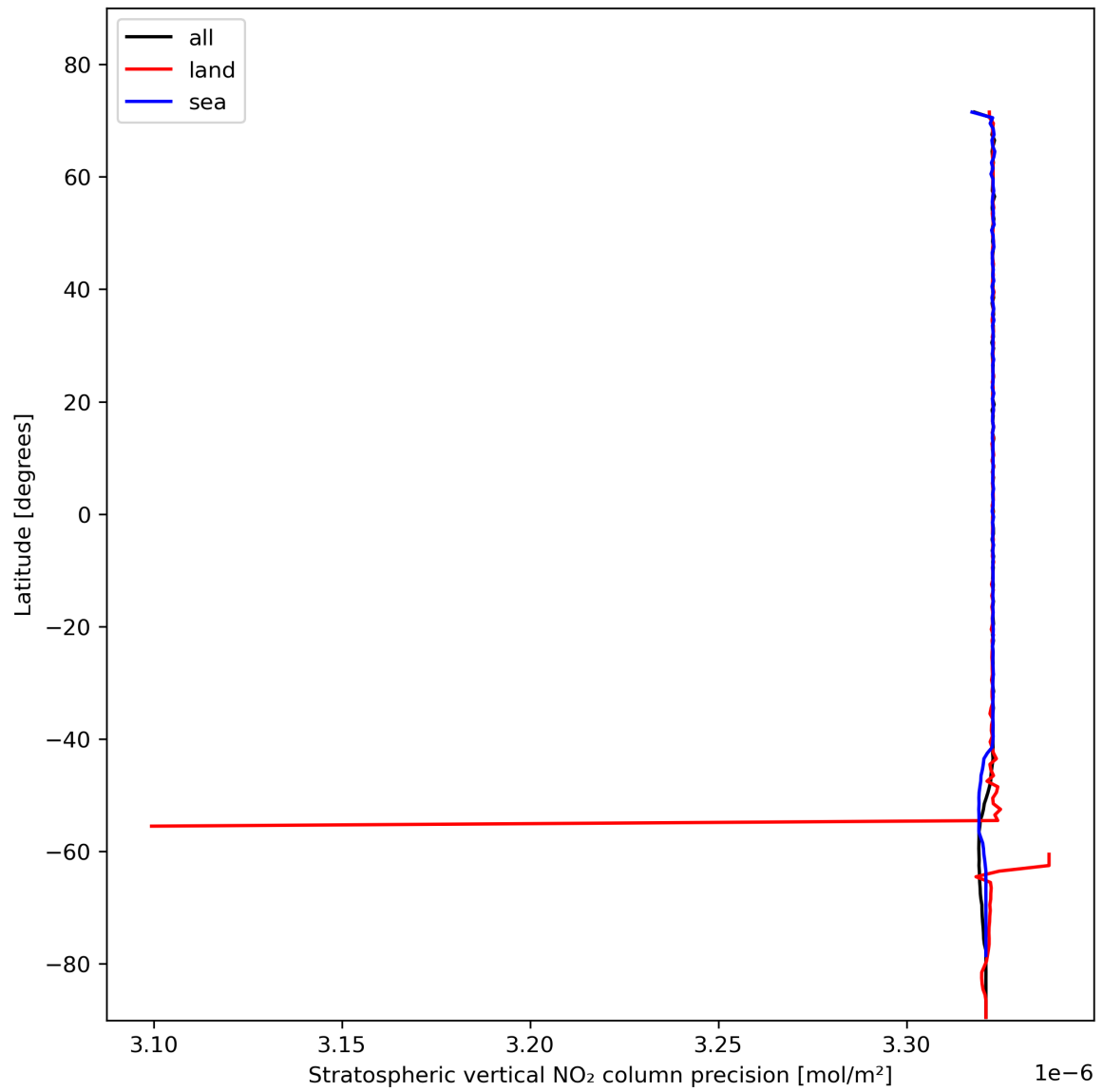
Figure 20: Zonal average of “Stratospheric vertical NO 2 column precision” for 2023-11-07 to 2023-11-08.
