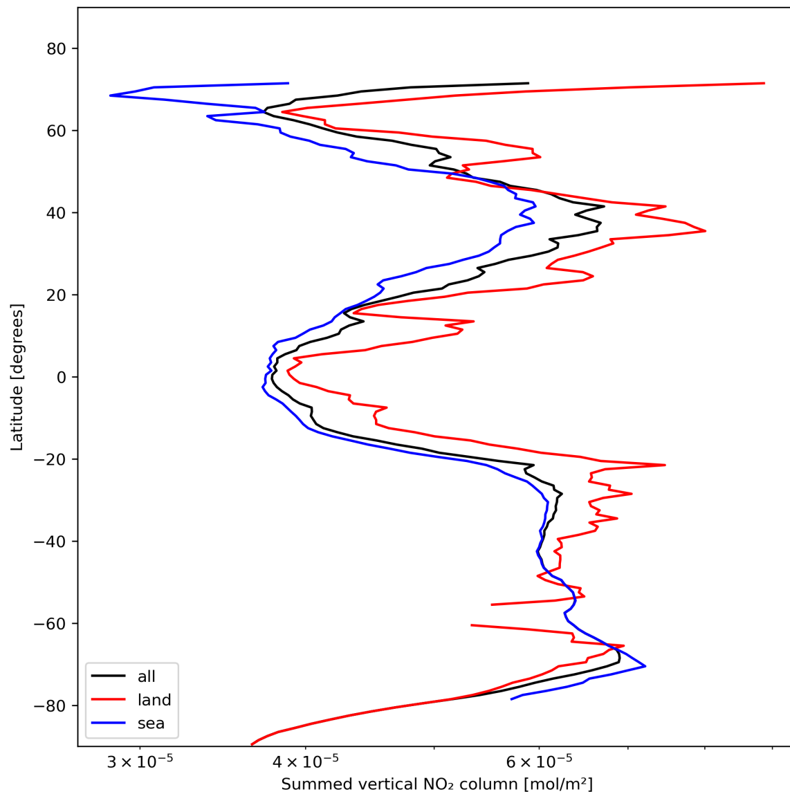
Figure 23: Zonal average of “Summed vertical NO 2 column” for 2023-11-07 to 2023-11-08.
