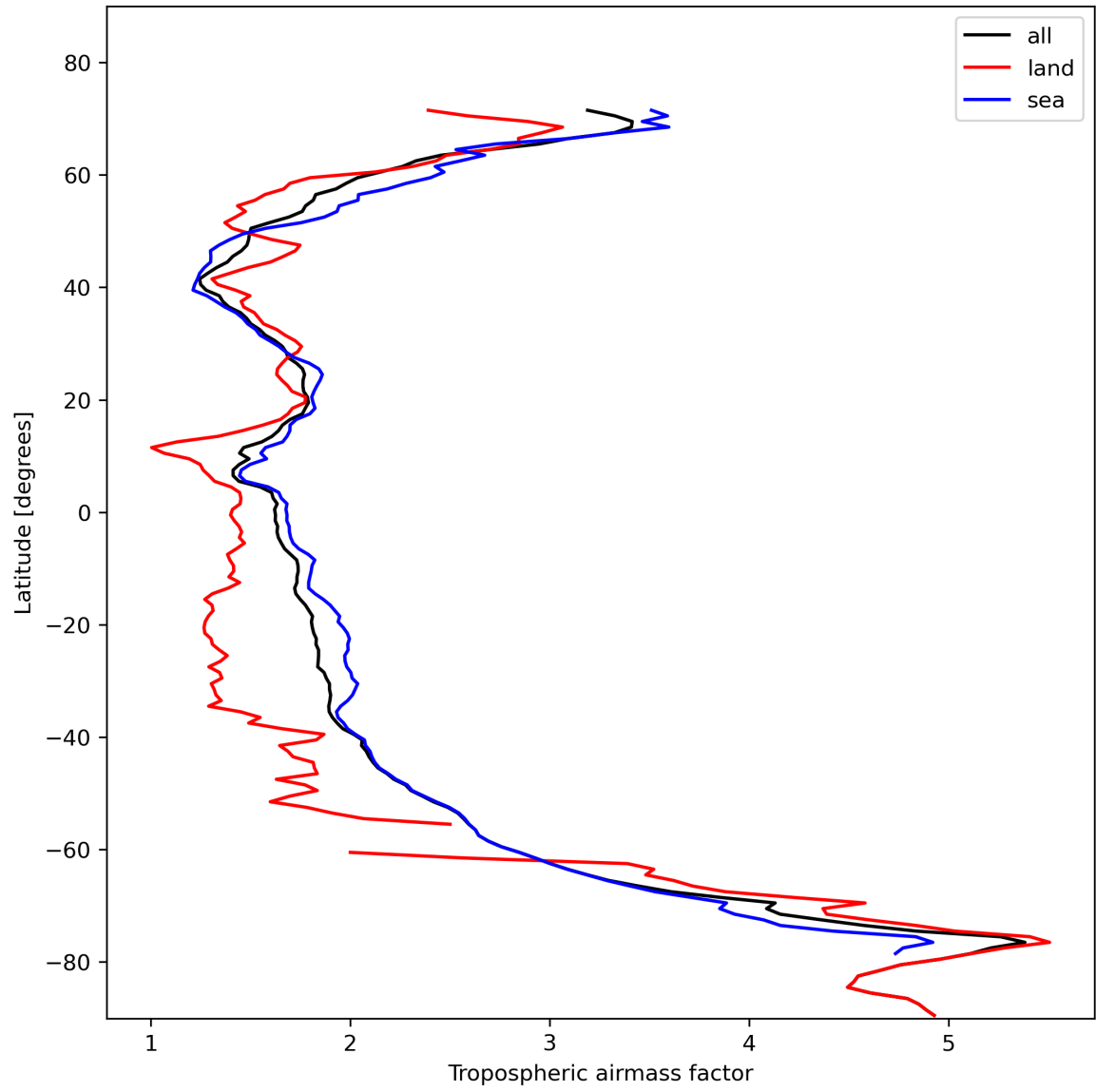
Figure 14: Zonal average of “Tropospheric airmass factor” for 2023-11-07 to 2023-11-08.
