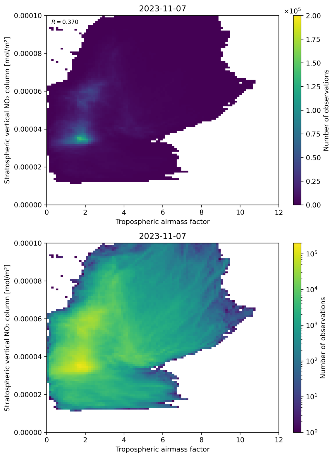
Figure 74: Scatter density plot of “Tropospheric air mass factor” against “Stratospheric vertical NO 2 column” for 2023-11-07 to 2023-11-08.
