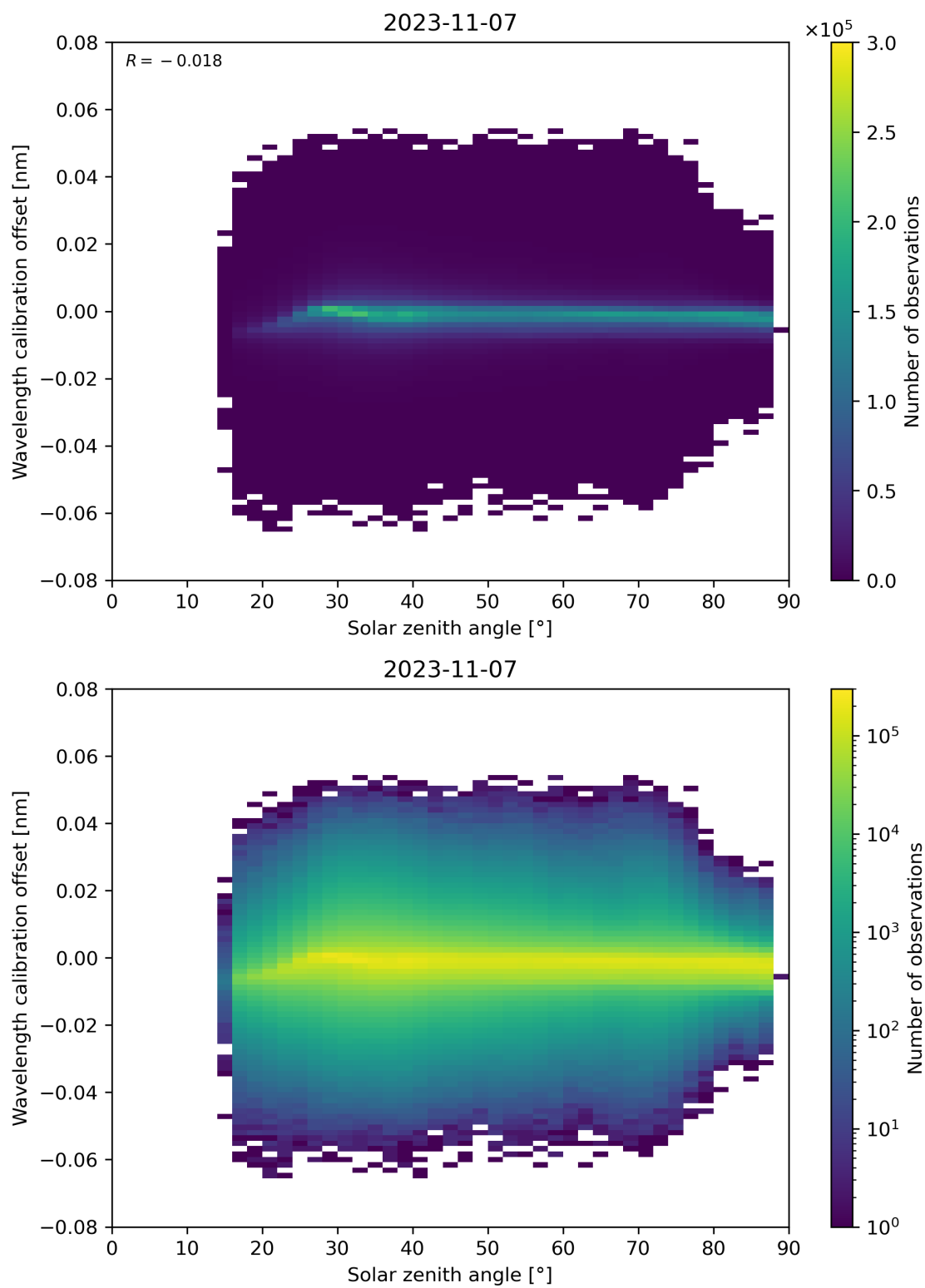
Figure 158: Scatter density plot of “Solar zenith angle” against “Wavelength calibration offset” for 2023-11-07 to 2023-11-08.
