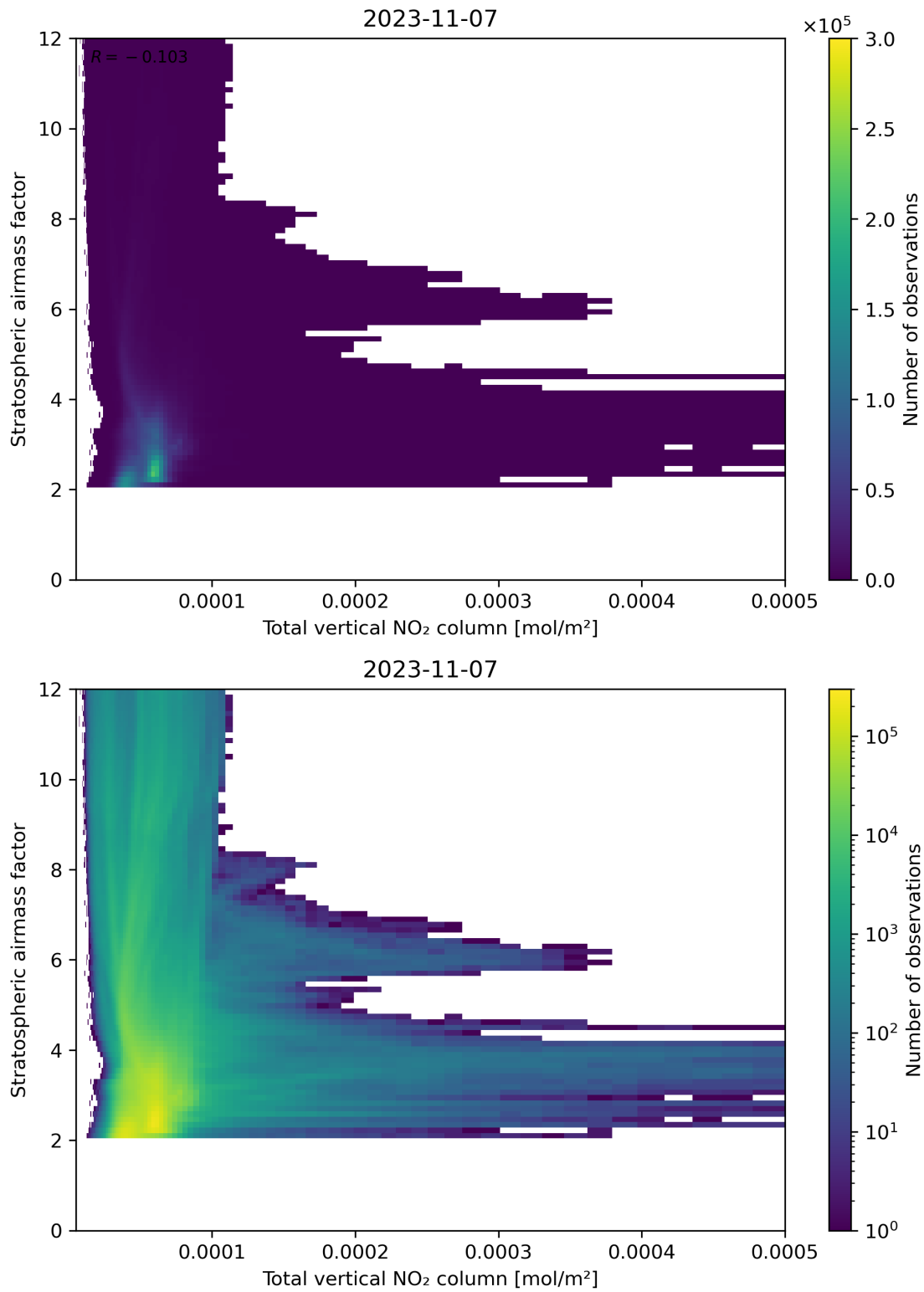
Figure 110: Scatter density plot of “Total vertical NO 2 column” against “Stratospheric airmass factor” for 2023-11-07 to 2023-11-08.
