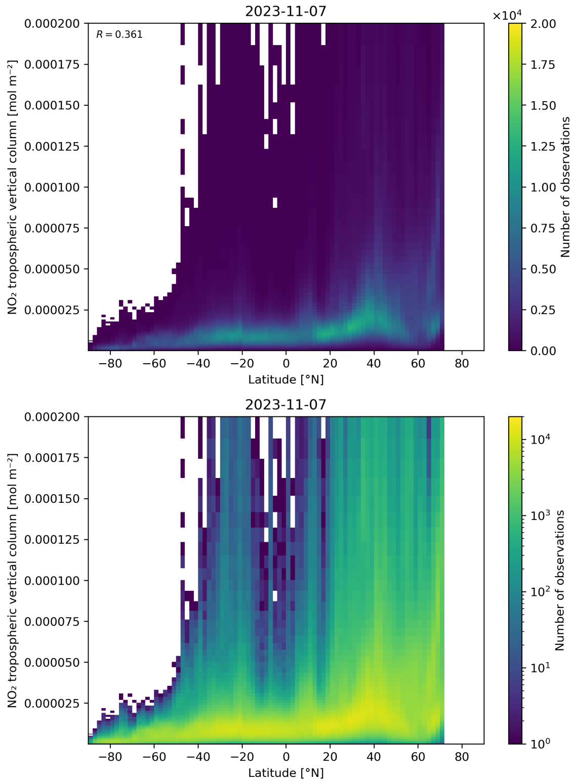
Figure 92: Scatter density plot of “Latitude” against “NO 2 tropospheric vertical column” for 2023-11-07 to 2023-11-08.
