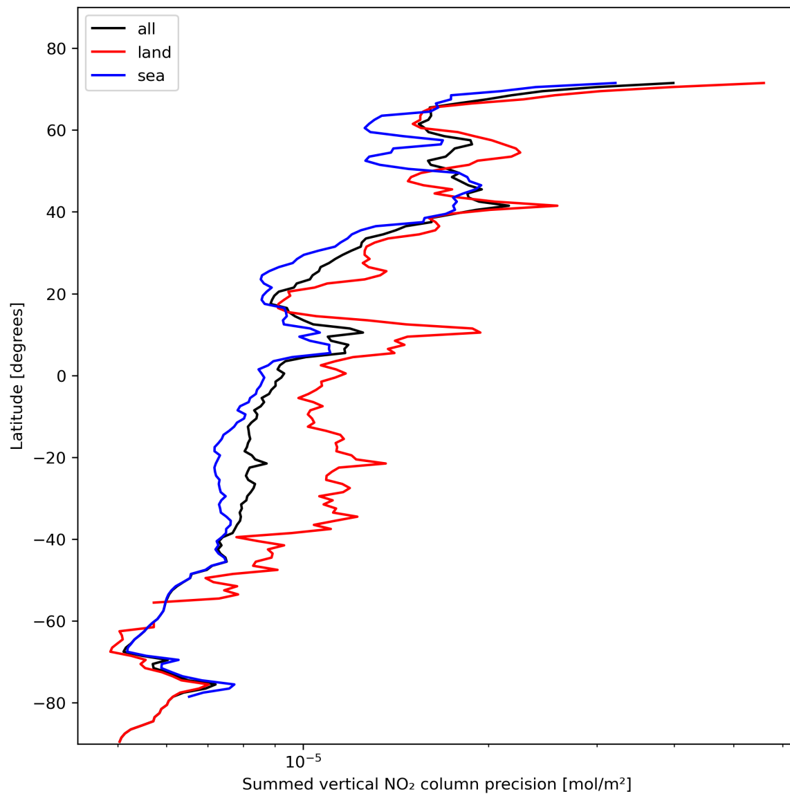
Figure 24: Zonal average of “Summed vertical NO 2 column precision” for 2023-11-07 to 2023-11-08.
