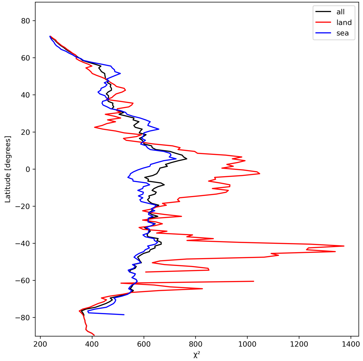
Figure 25: Zonal average of “ \chi^2 ” for 2023-11-07 to 2023-11-08.
