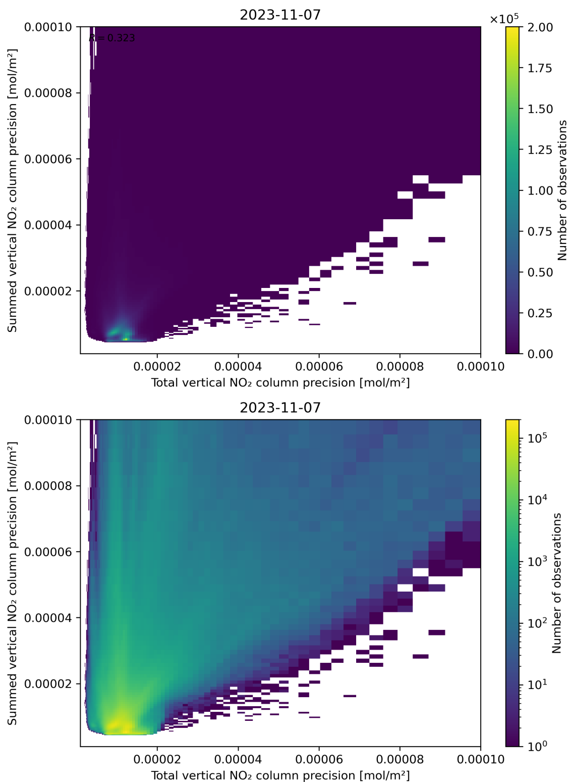
Figure 118: Scatter density plot of “Total vertical NO 2 column precision” against “Summed vertical NO 2 column precision” for 2023-11-07 to 2023-11-08.
