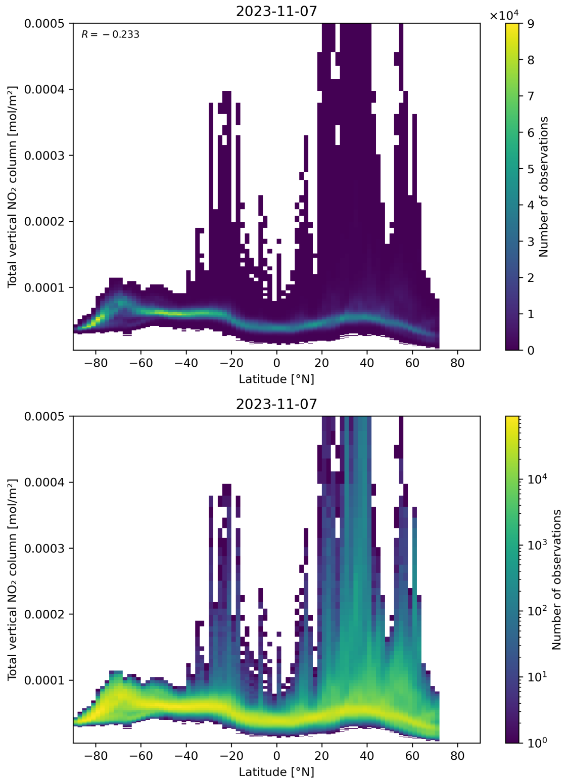
Figure 90: Scatter density plot of “Latitude” against “Total vertical NO 2 column” for 2023-11-07 to 2023-11-08.
