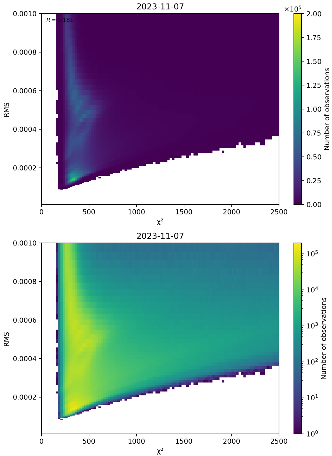
Figure 82: Scatter density plot of “ \chi^2 ” against “RMS” for 2023-11-07 to 2023-11-08.
