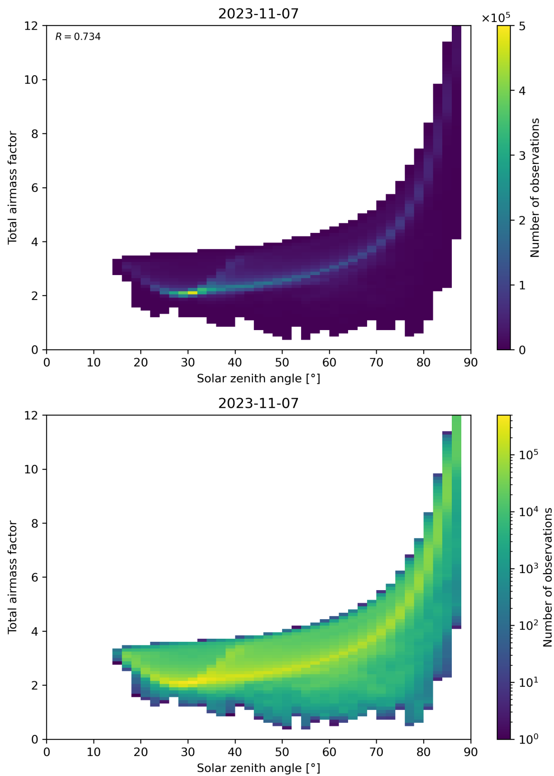
Figure 146: Scatter density plot of “Solar zenith angle” against “Total air mass factor” for 2023-11-07 to 2023-11-08.
