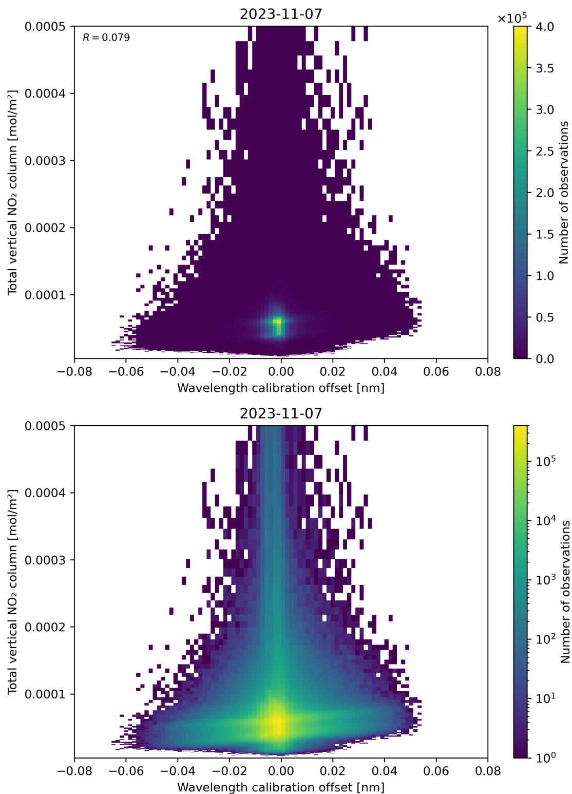
Figure 179: Scatter density plot of “Wavelength calibration offset” against “Total vertical NO 2 column” for 2023-11-07 to 2023-11-08.
