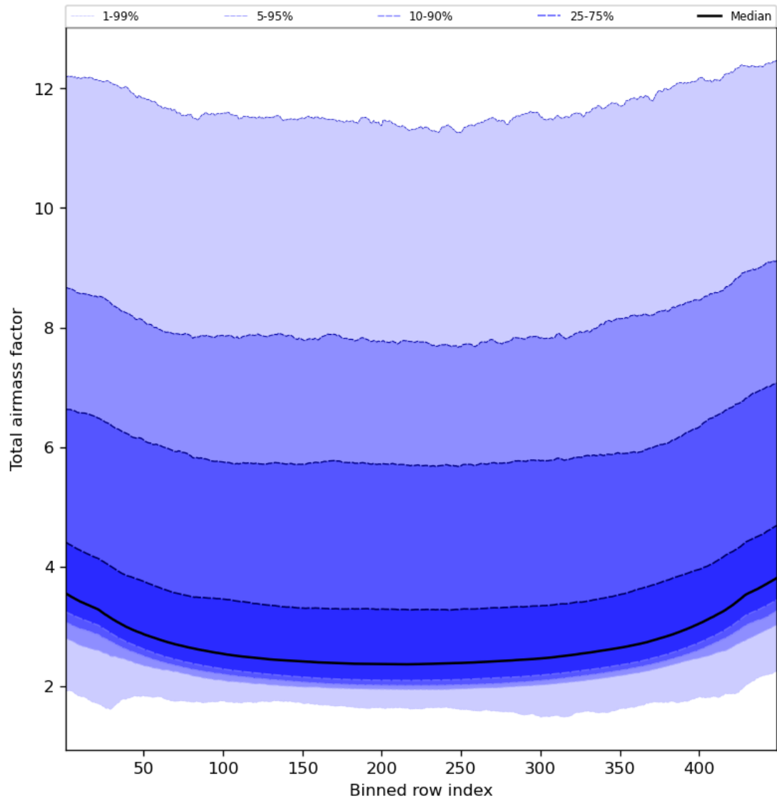
Figure 49: Along track statistics of “Total airmass factor” for 2023-11-07 to 2023-11-08
