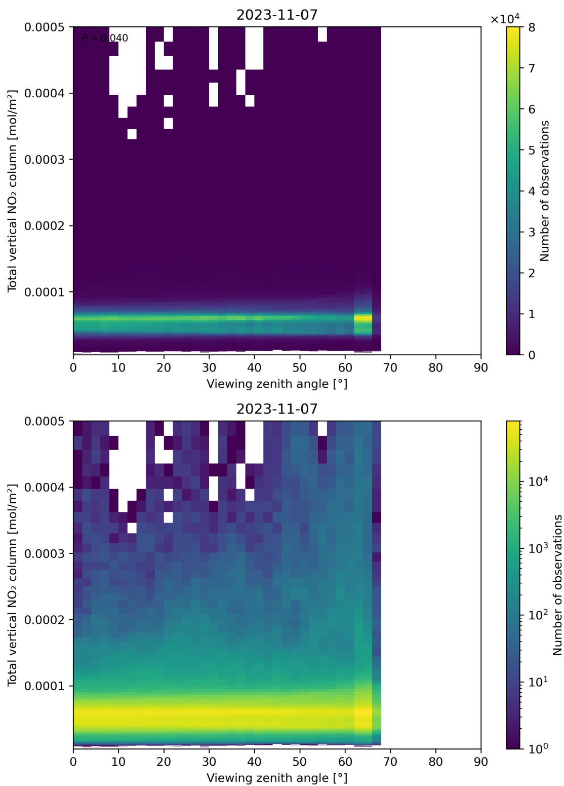
Figure 167: Scatter density plot of “Viewing zenith angle” against “Total vertical NO 2 column” for 2023-11-07 to 2023-11-08.
