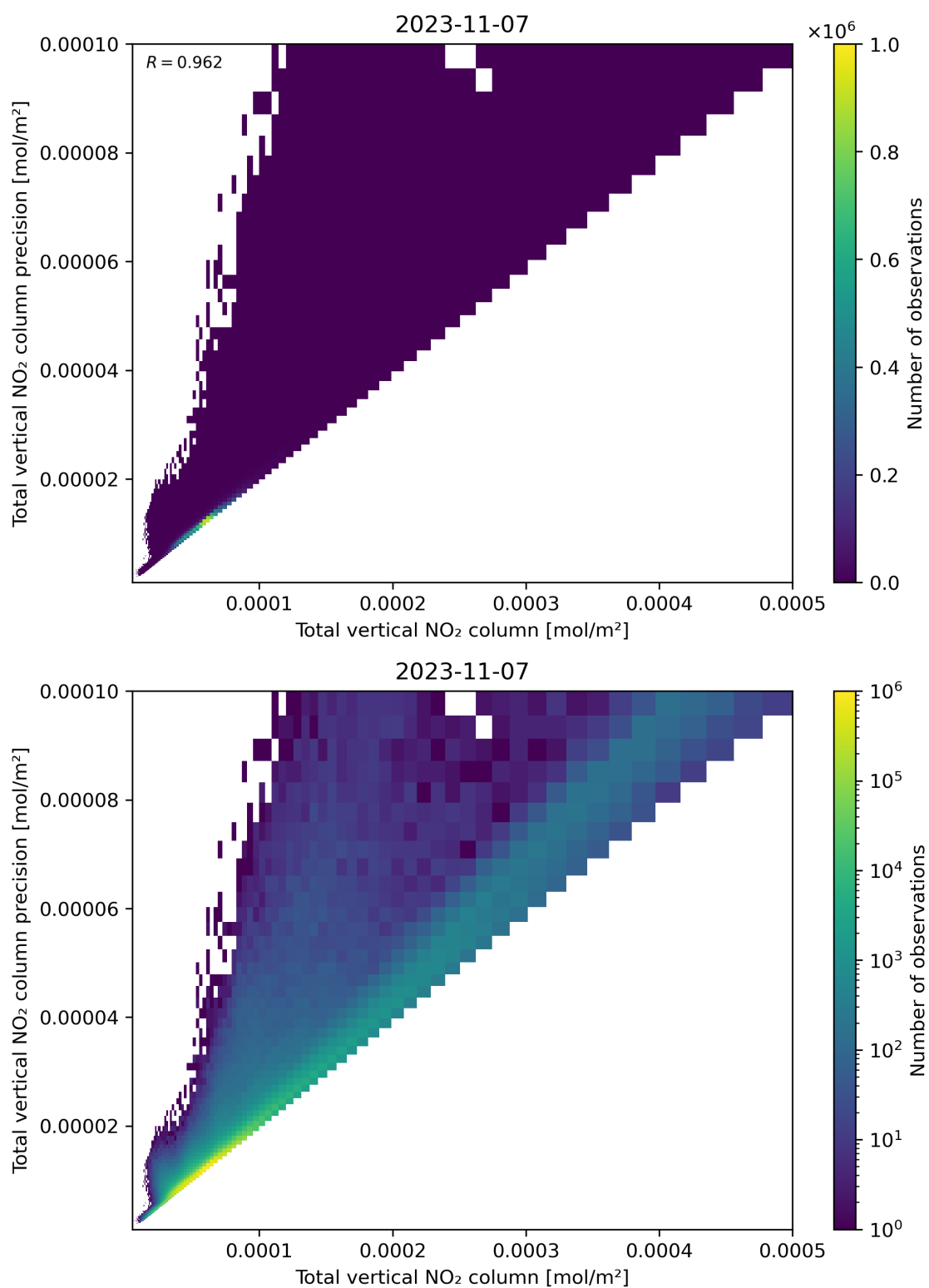
Figure 114: Scatter density plot of “Total vertical NO 2 column” against “Total vertical NO 2 column precision” for 2023-11-07 to 2023-11-08.
