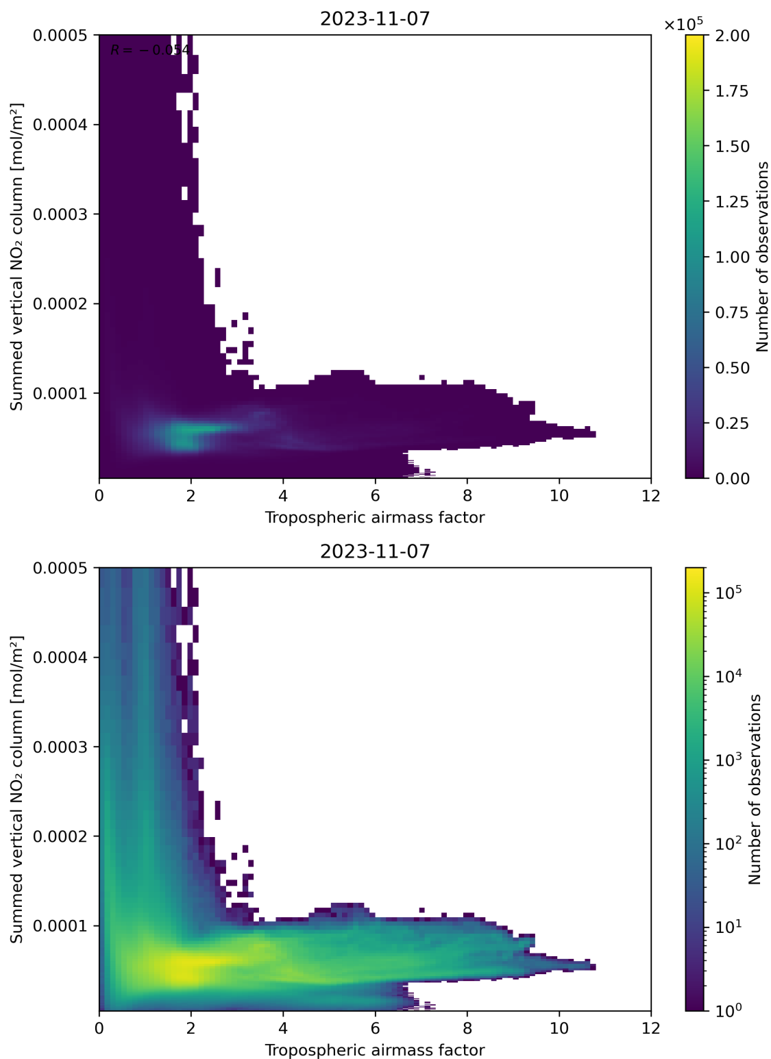
Figure 75: Scatter density plot of “Tropospheric airmass factor” against “Summed vertical NO 2 column” for 2023-11-07 to 2023-11-08.
