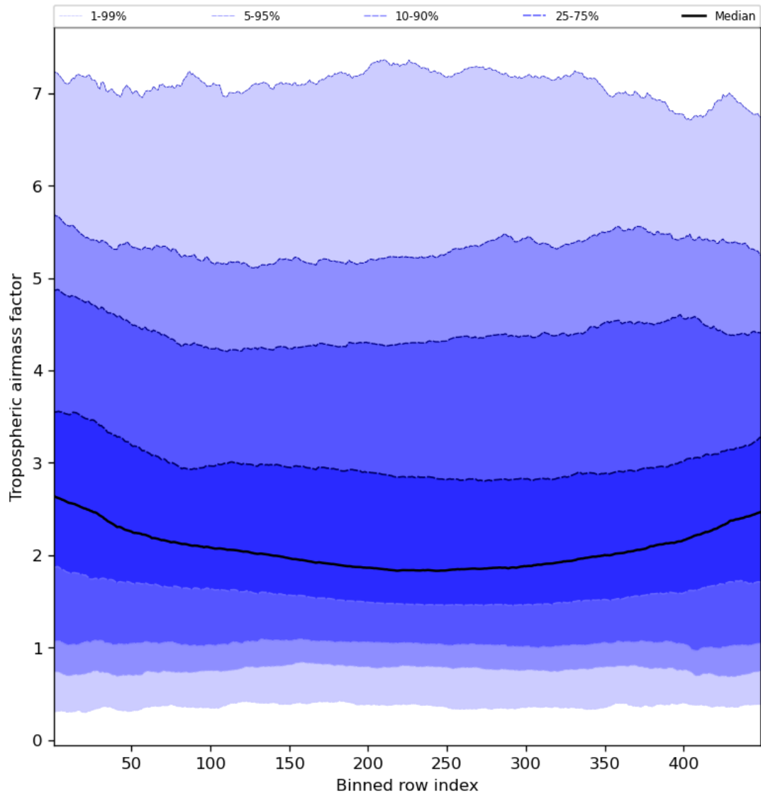
Figure 48: Along track statistics of “Tropospheric airmass factor” for 2023-11-07 to 2023-11-08
