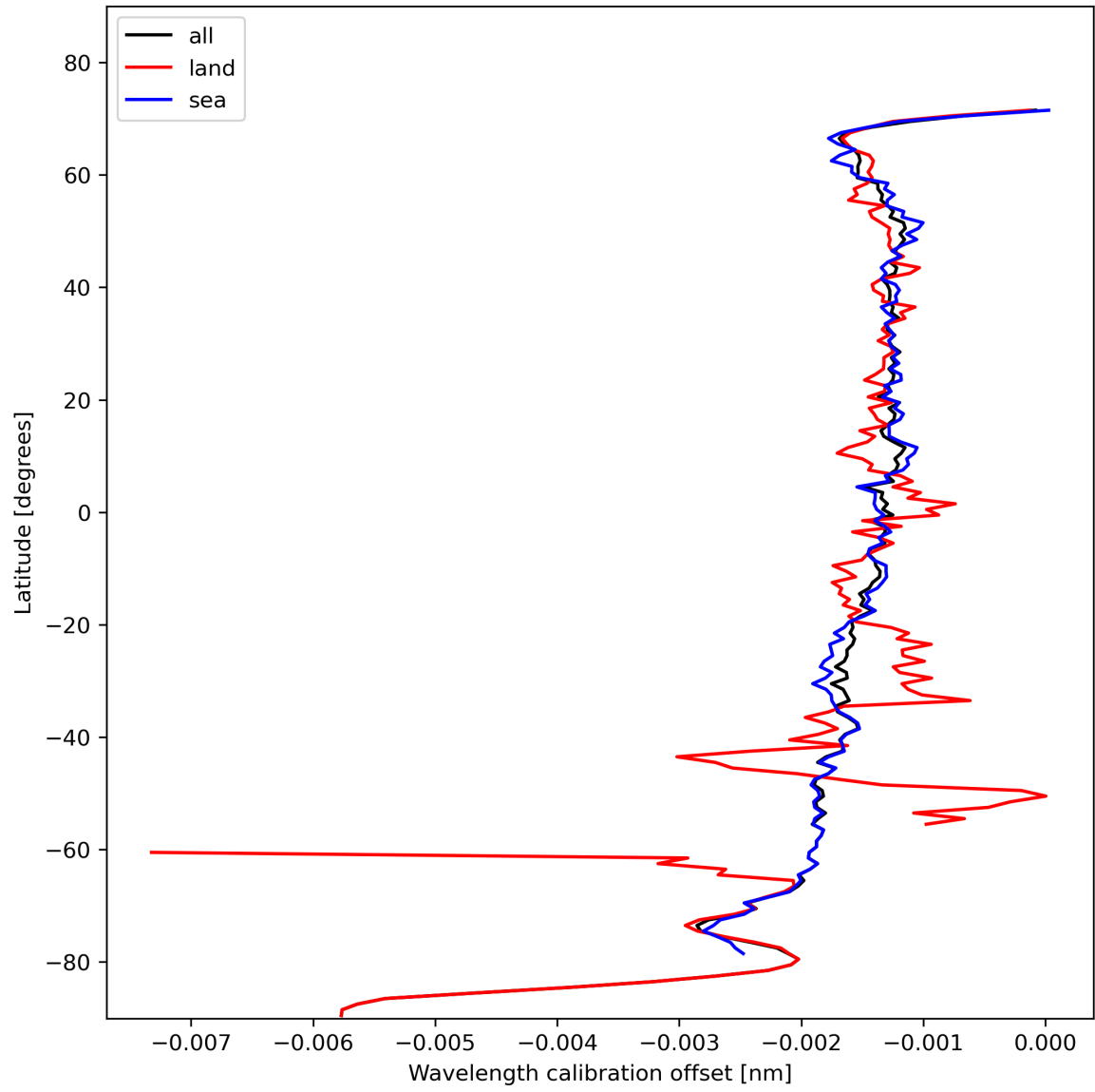
Figure 18: Zonal average of “Wavelength calibration offset” for 2023-11-07 to 2023-11-08.
