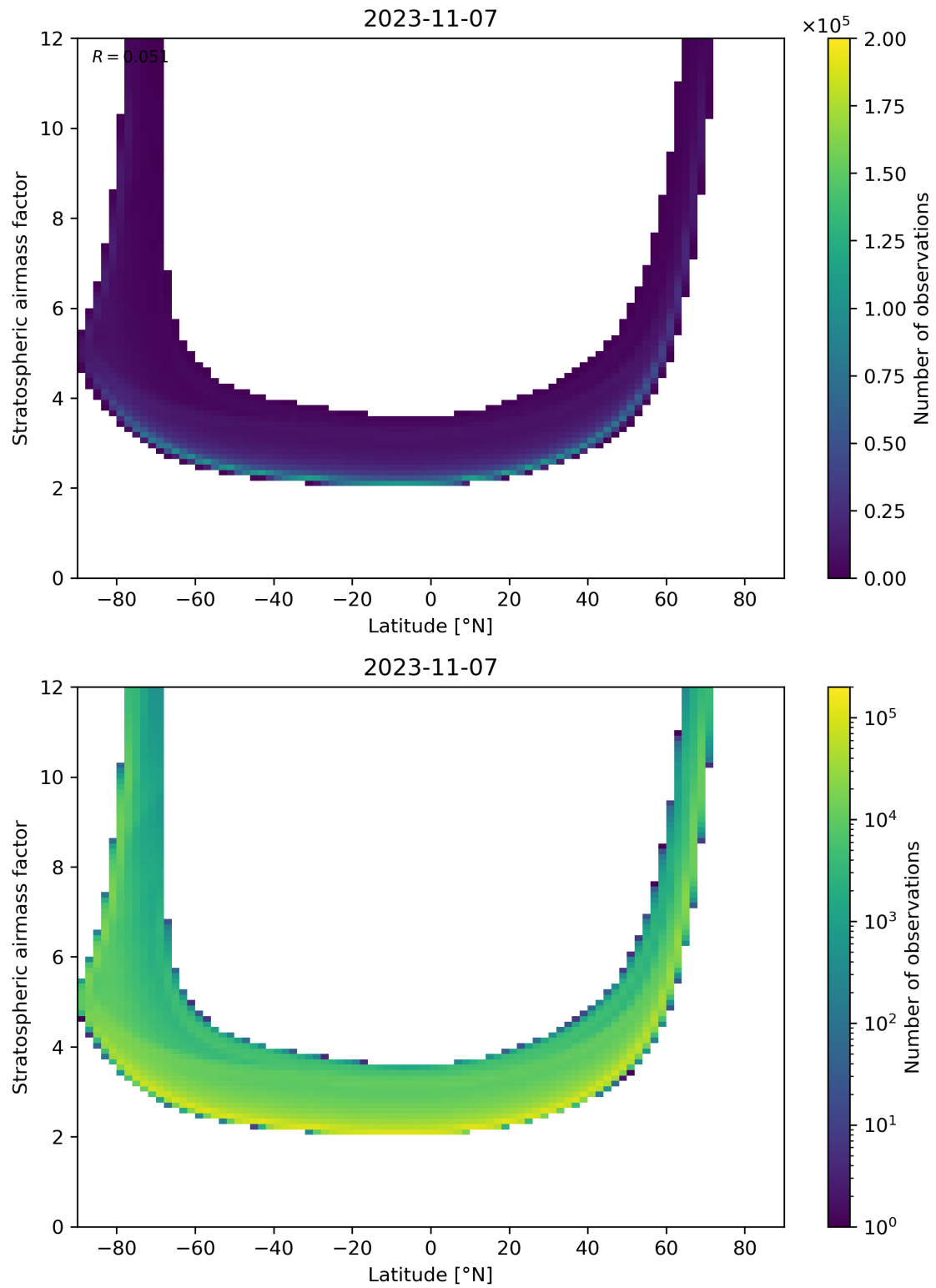
Figure 83: Scatter density plot of “Latitude” against “Stratospheric air mass factor” for 2023-11-07 to 2023-11-08.
