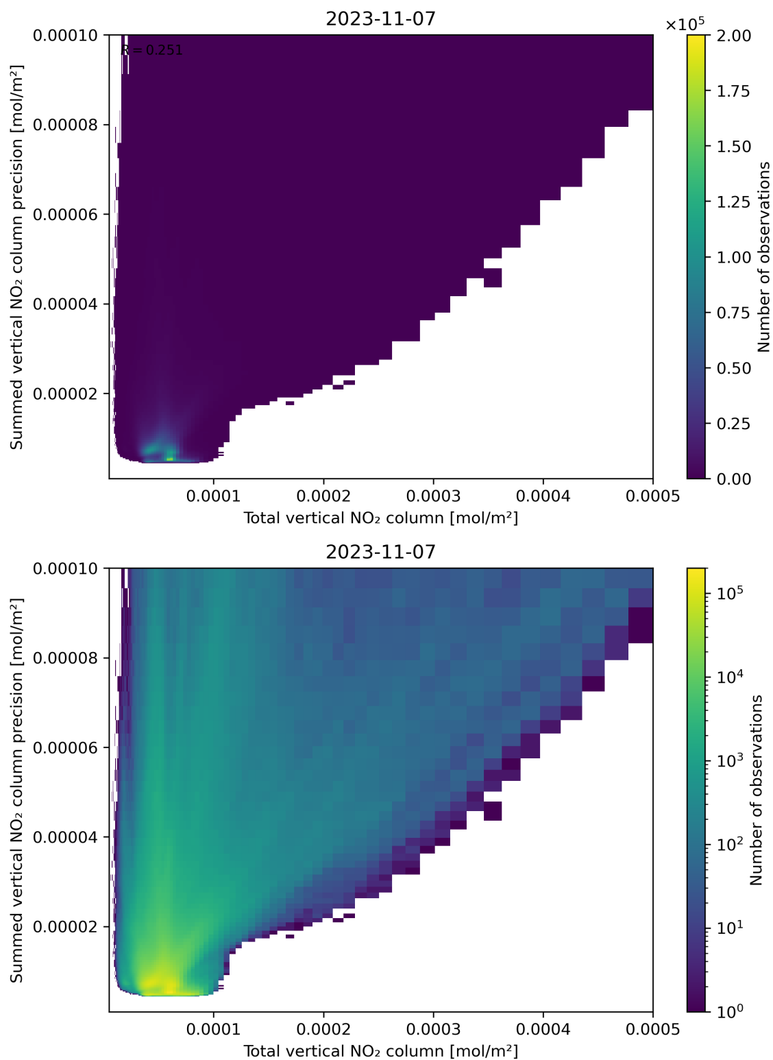
Figure 113: Scatter density plot of “Total vertical NO 2 column” against “Summed vertical NO 2 column precision” for 2023-11-07 to 2023-11-08.
