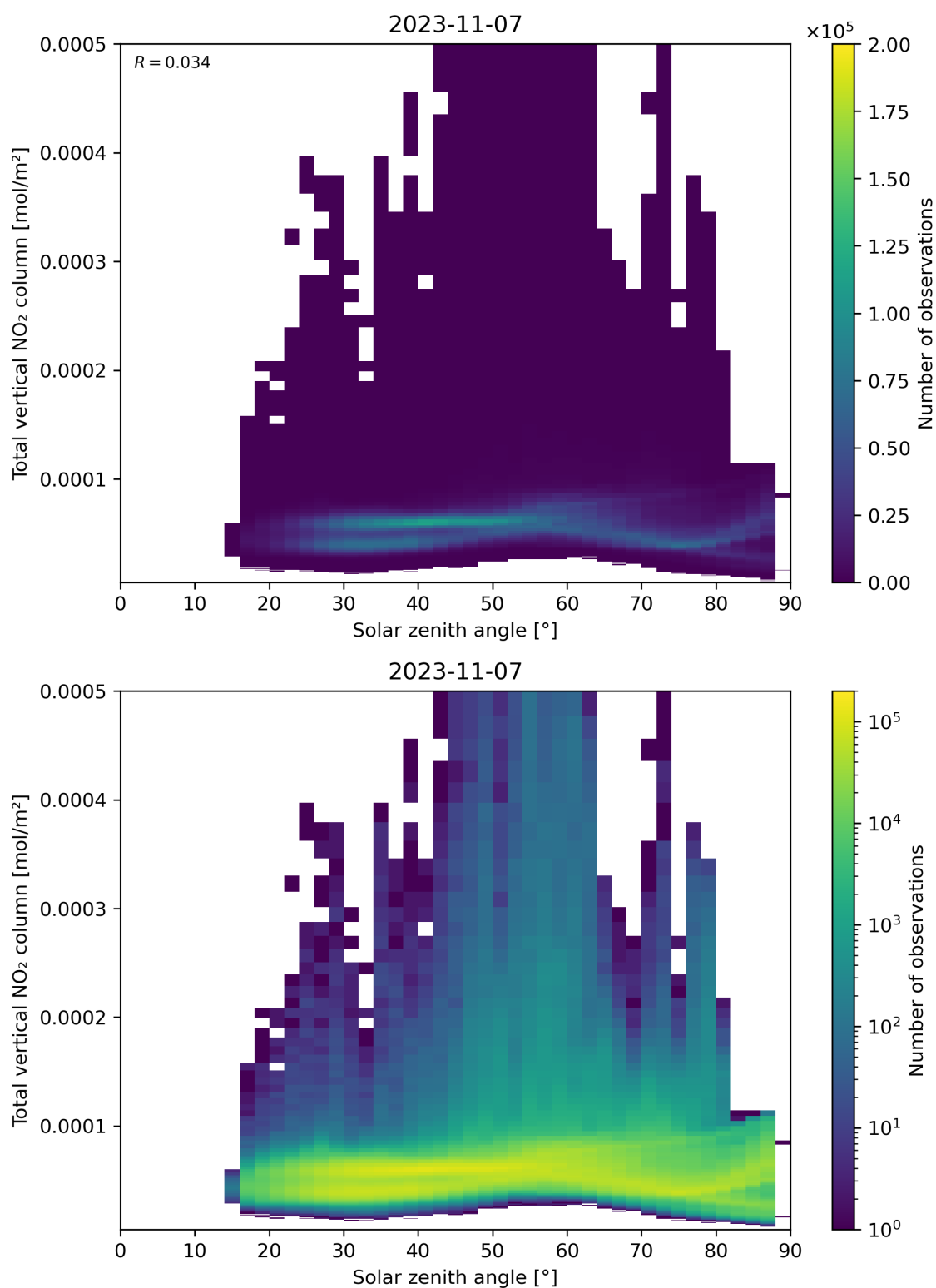
Figure 153: Scatter density plot of “Solar zenith angle” against “Total vertical NO 2 column” for 2023-11-07 to 2023-11-08.
