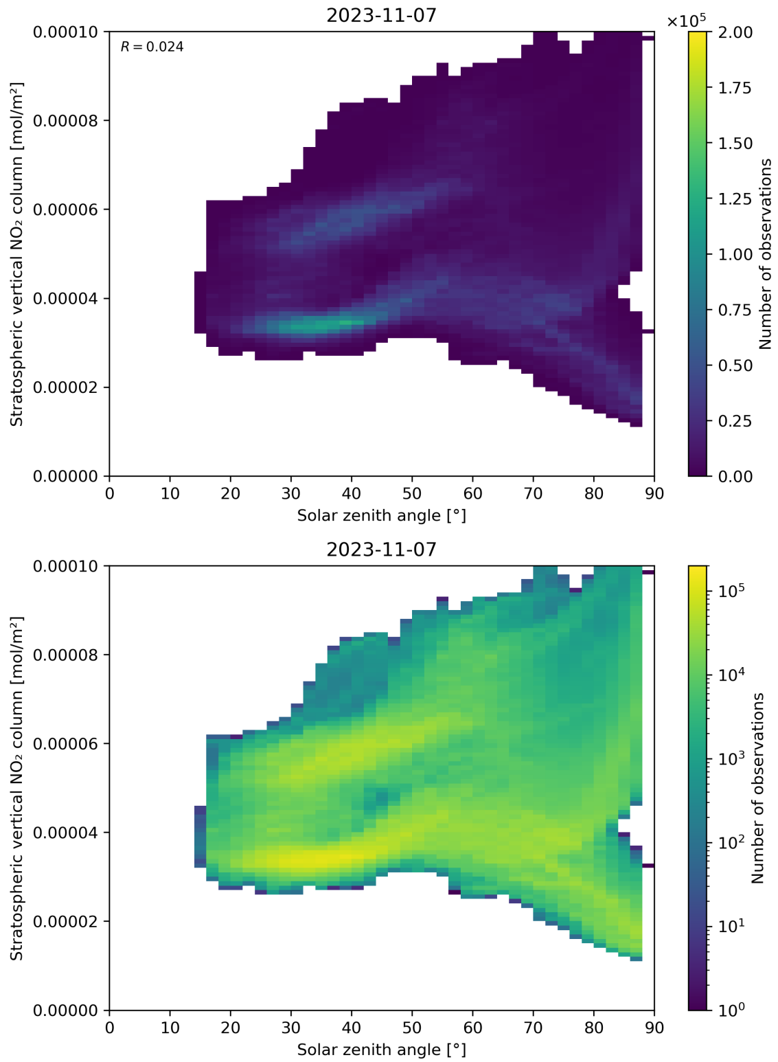
Figure 150: Scatter density plot of “Solar zenith angle” against “Stratospheric vertical NO 2 column” for 2023-11-07 to 2023-11-08.
