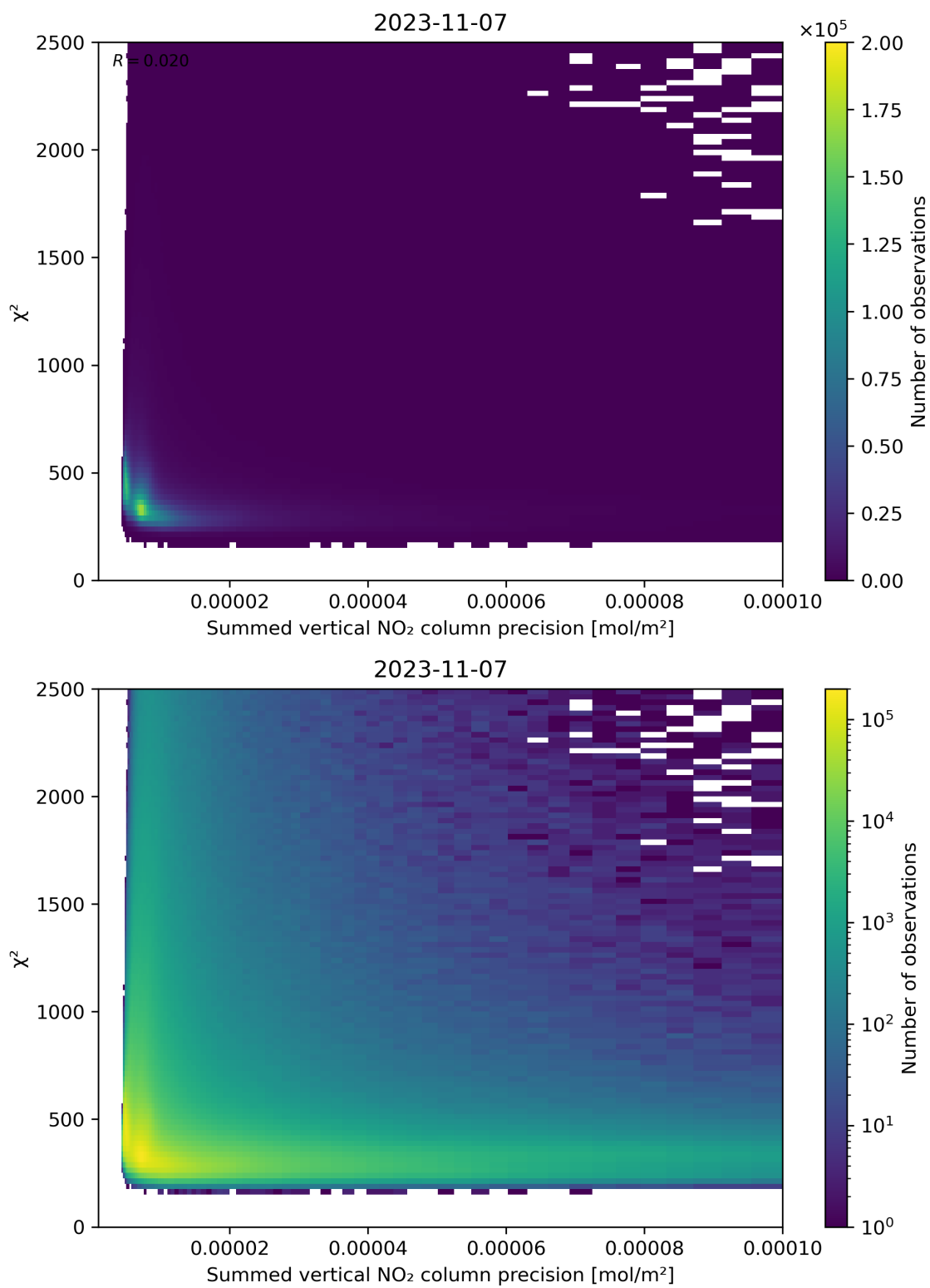
Figure 107: Scatter density plot of “Summed vertical NO 2 column precision” against “ \chi^2 ” for 2023-11-07 to 2023-11-08.
