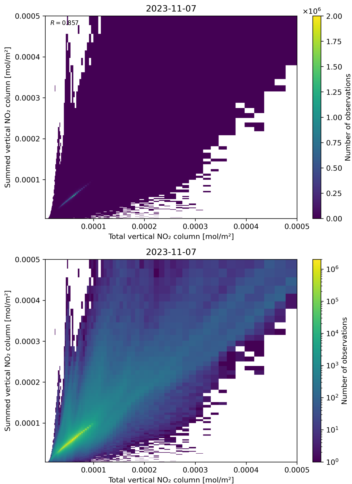
Figure 112: Scatter density plot of “Total vertical NO 2 column” against “Summed vertical NO 2 column” for 2023-11-07 to 2023-11-08.
