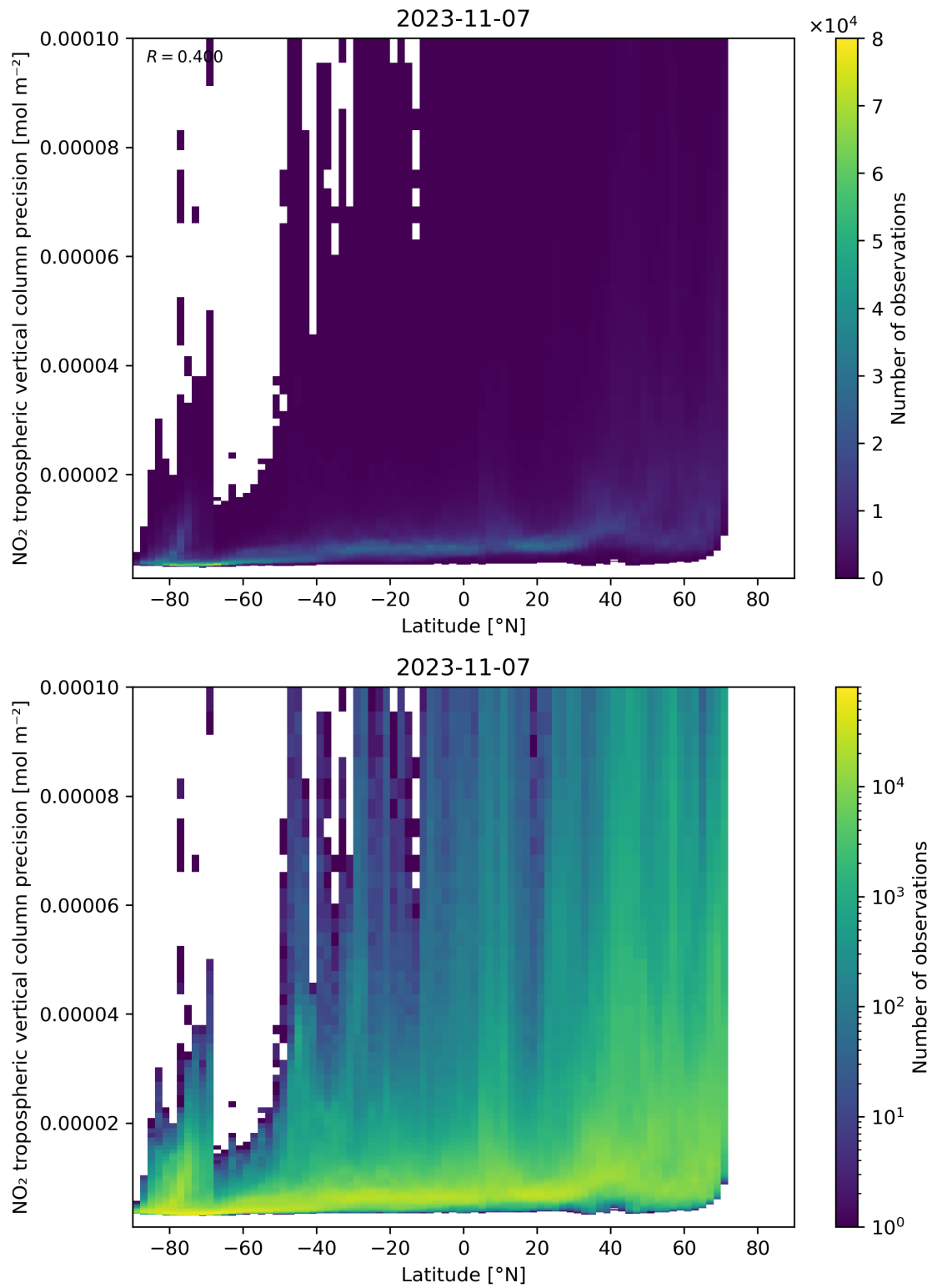
Figure 93: Scatter density plot of “Latitude” against “NO 2 tropospheric vertical column precision” for 2023-11-07 to 2023-11-08.
