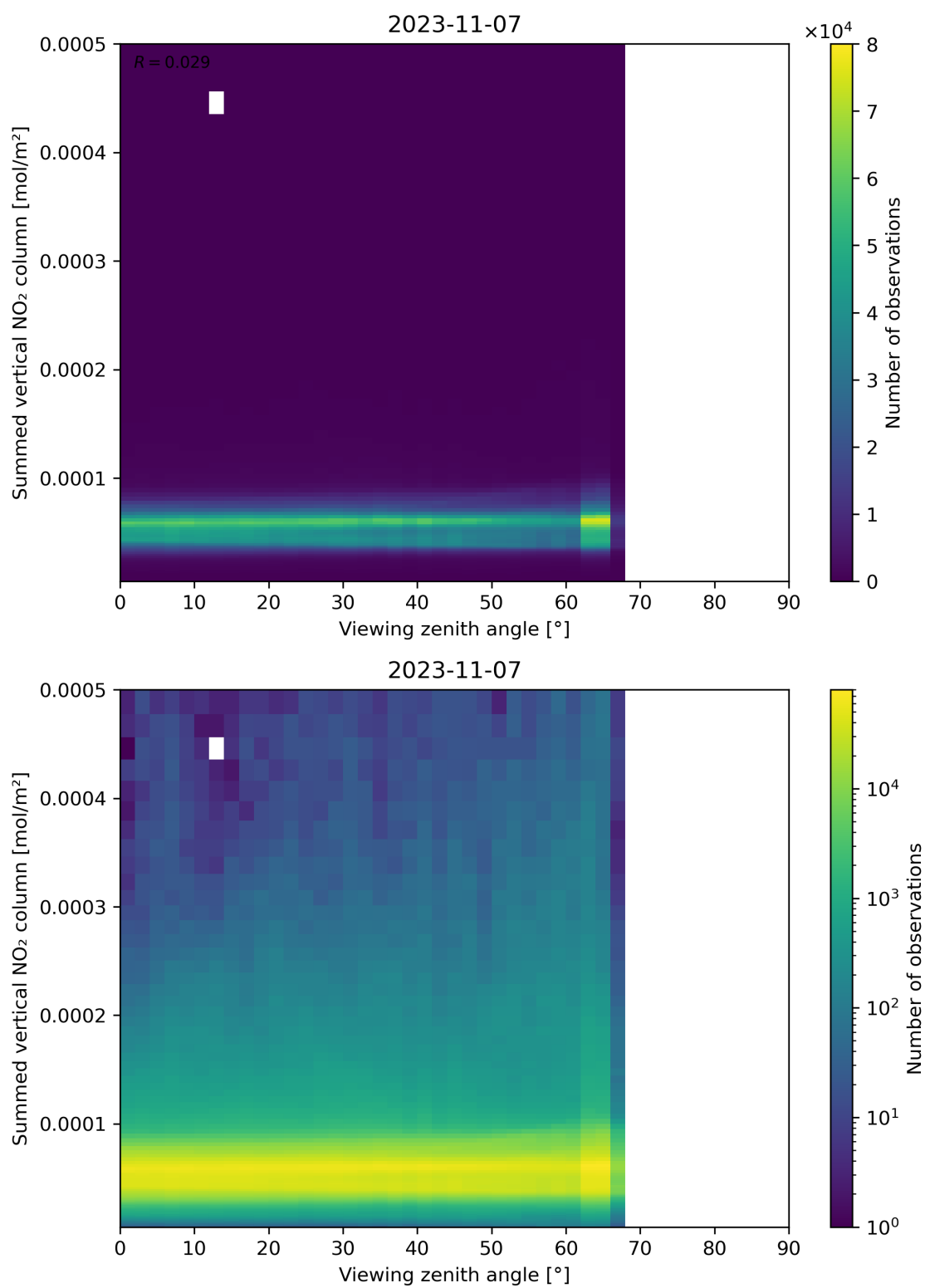
Figure 165: Scatter density plot of “Viewing zenith angle” against “Summed vertical NO 2 column” for 2023-11-07 to 2023-11-08.
