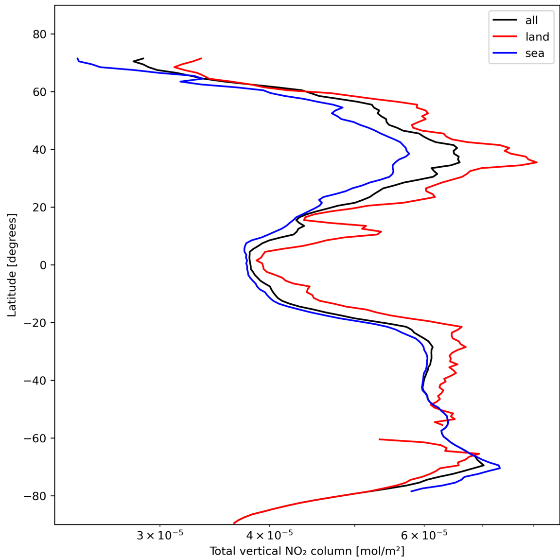
Figure 21: Zonal average of “Total vertical NO 2 column” for 2023-11-07 to 2023-11-08.
