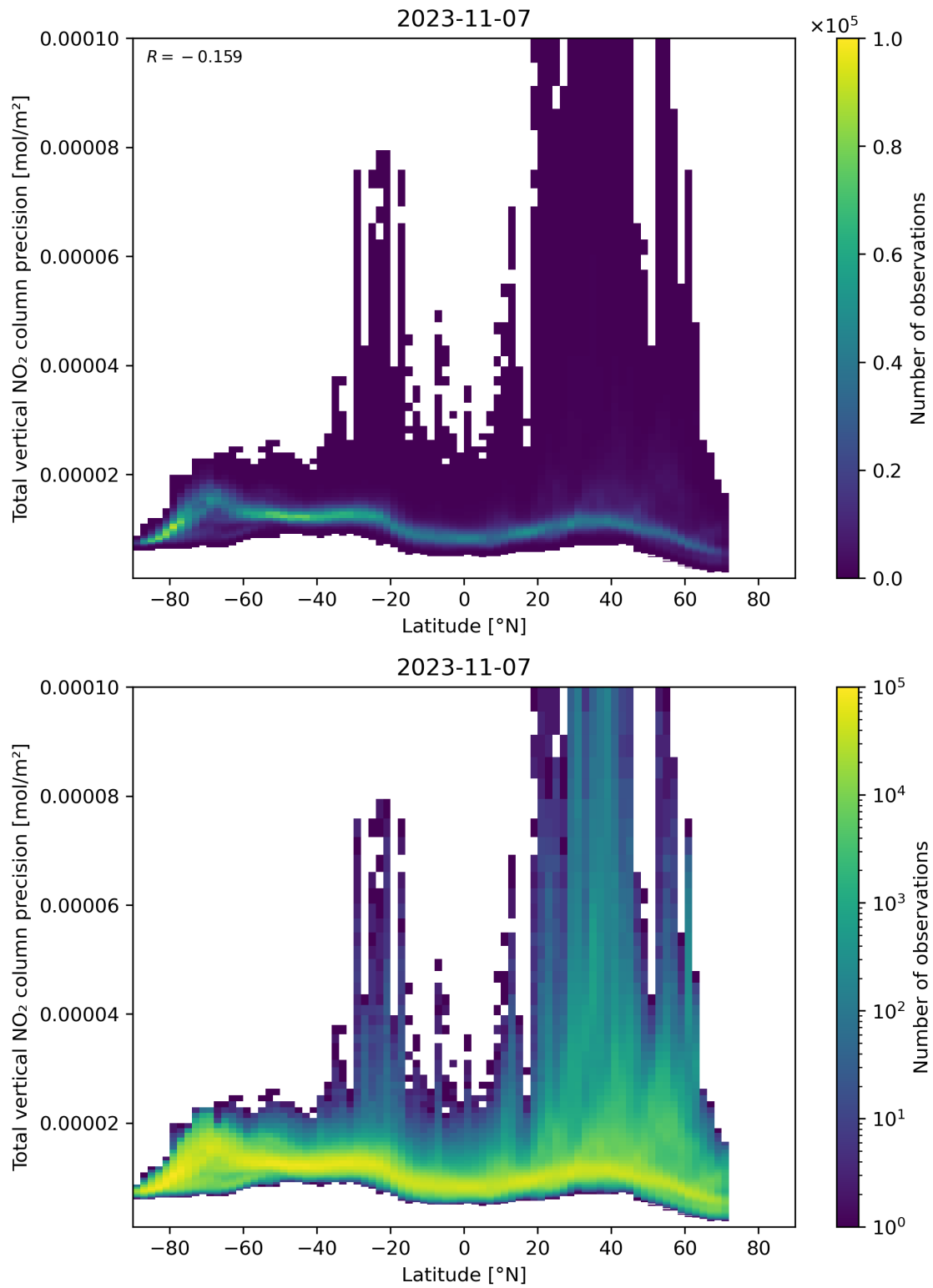
Figure 91: Scatter density plot of “Latitude” against “Total vertical NO 2 column precision” for 2023-11-07 to 2023-11-08.
