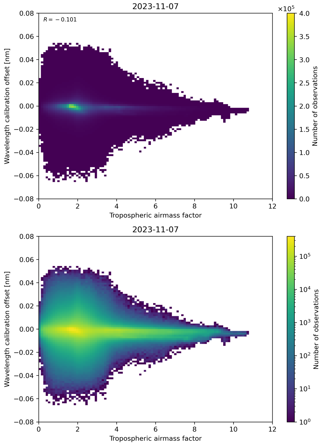
Figure 80: Scatter density plot of “Tropospheric airmass factor” against “Wavelength calibration offset” for 2023-11-07 to 2023-11-08.
