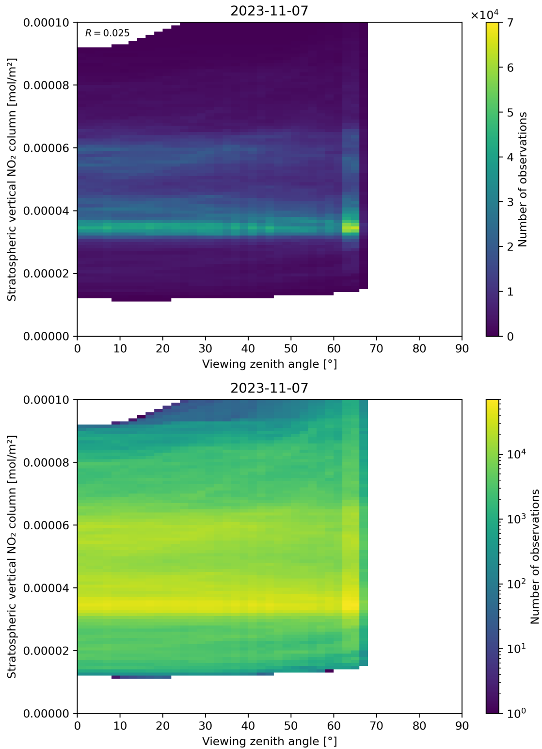
Figure 164: Scatter density plot of “Viewing zenith angle” against “Stratospheric vertical NO 2 column” for 2023-11-07 to 2023-11-08.
