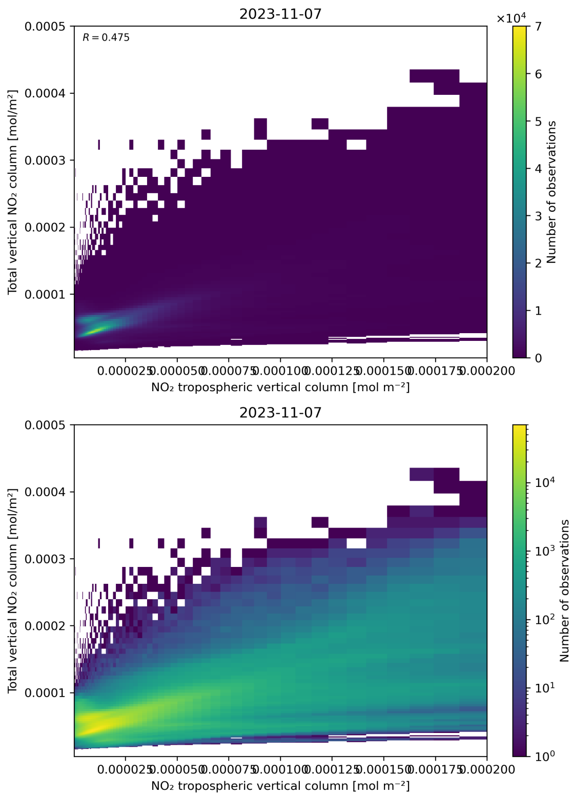
Figure 128: Scatter density plot of “NO 2 tropospheric vertical column” against “Total vertical NO 2 column” for 2023-11-07 to 2023-11-08.
