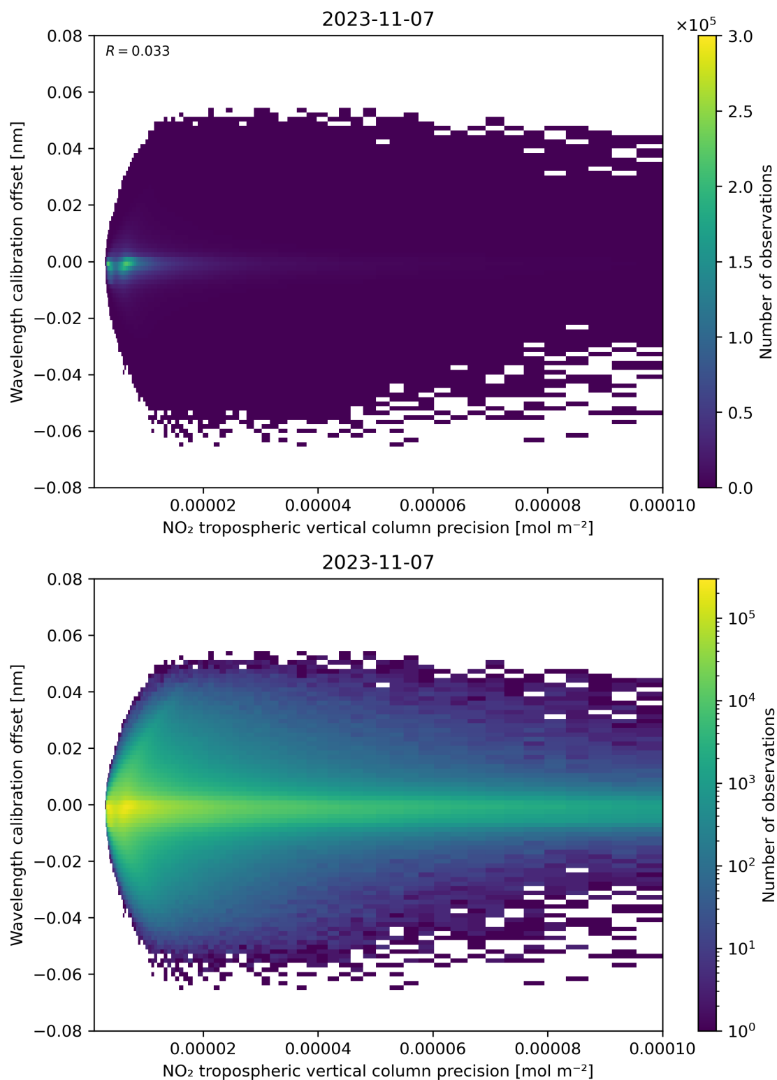
Figure 141: Scatter density plot of “NO 2 tropospheric vertical column precision” against “Wavelength calibration offset” for 2023-11-07 to 2023-11-08.
