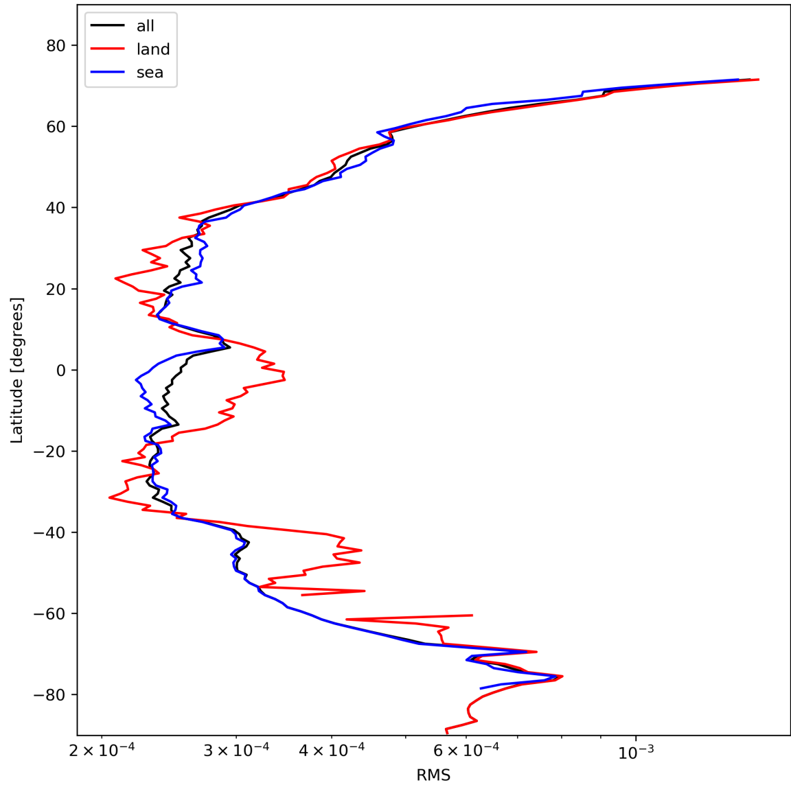
Figure 26: Zonal average of “RMS” for 2023-11-07 to 2023-11-08.
