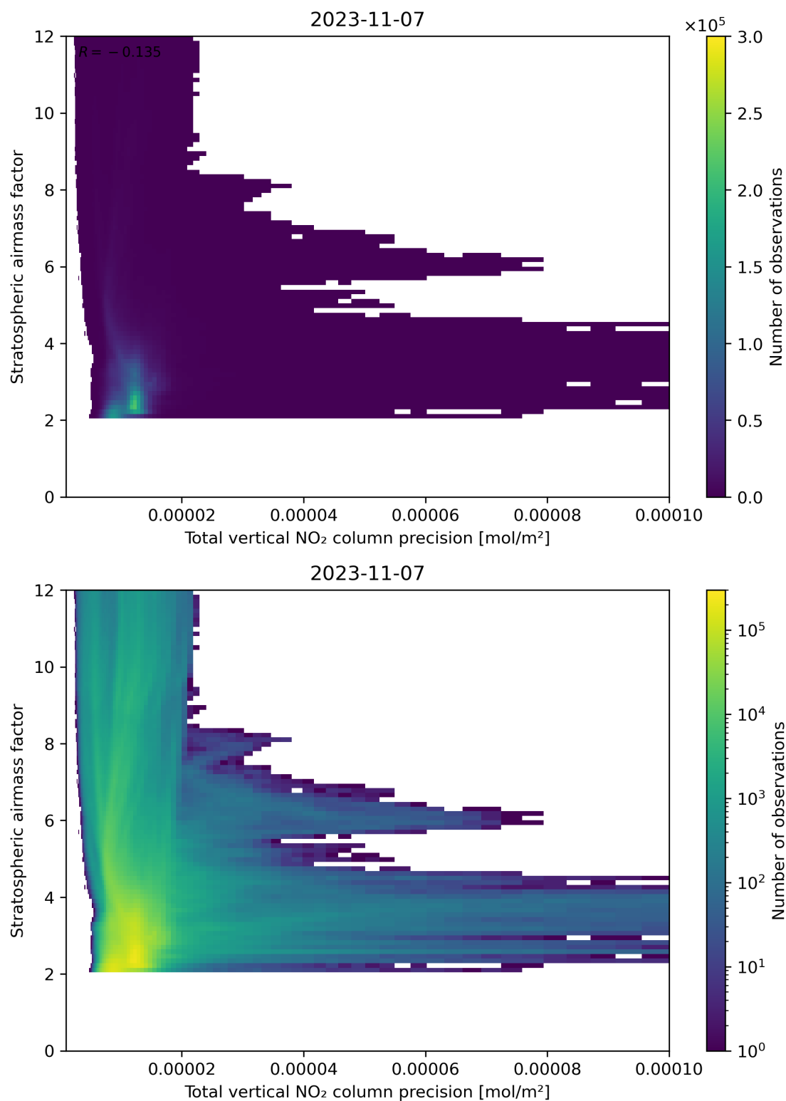
Figure 115: Scatter density plot of “Total vertical NO 2 column precision” against “Stratospheric airmass factor” for 2023-11-07 to 2023-11-08.
