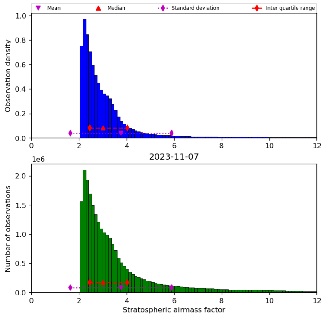
Figure 44: Histogram of “Stratospheric airmass factor” for 2023-11-07 to 2023-11-08
