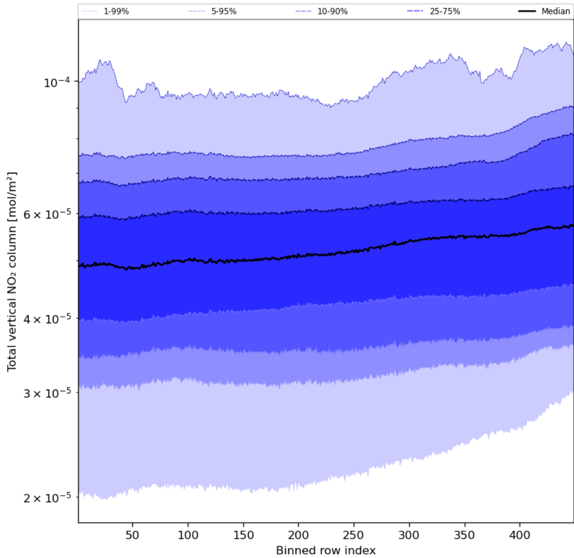
Figure 55: Along track statistics of “Total vertical NO 2 column” for 2023-11-07 to 2023-11-08
