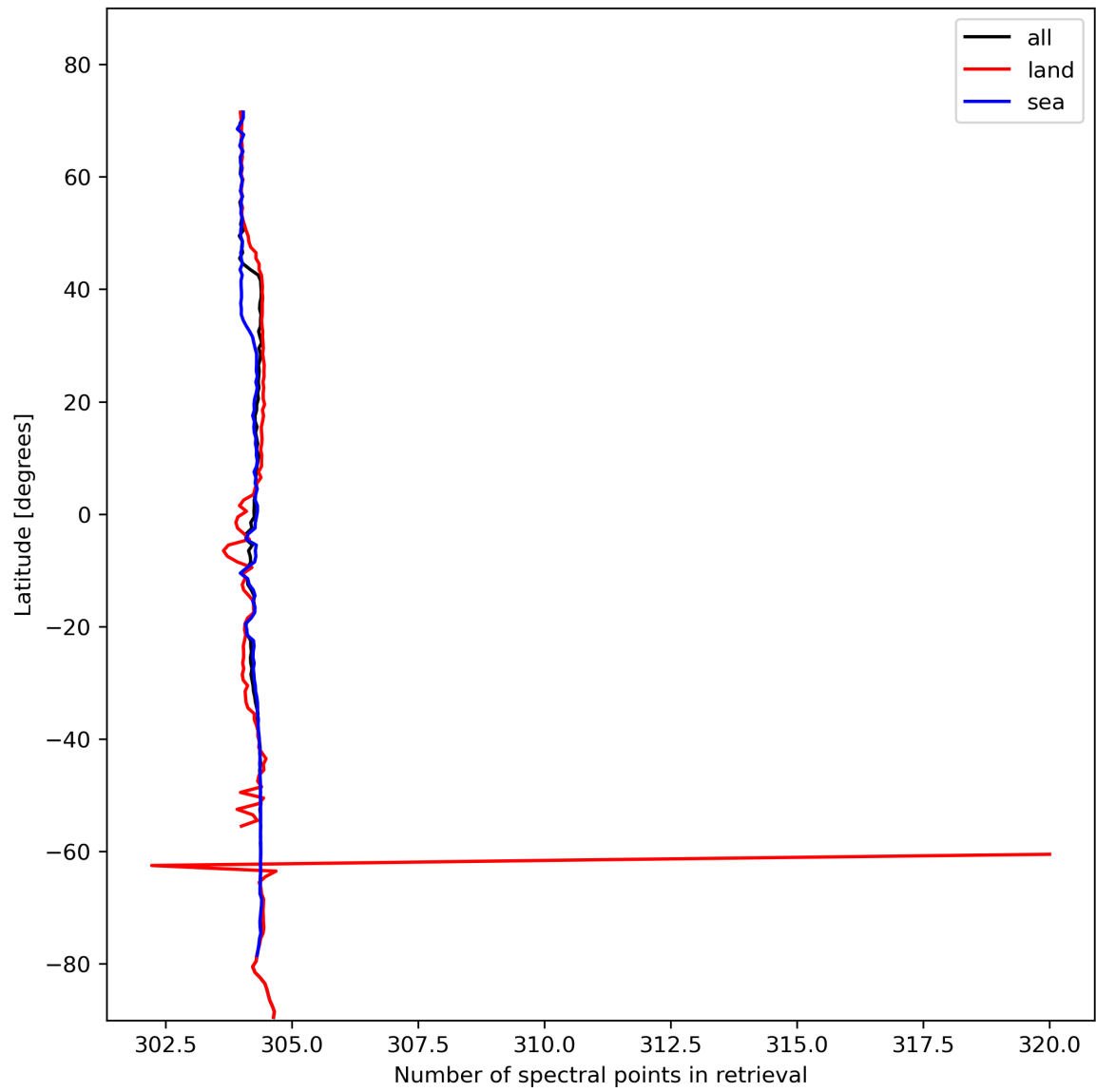
Figure 16: Zonal average of “Number of spectral points in retrieval” for 2023-11-07 to 2023-11-08.
