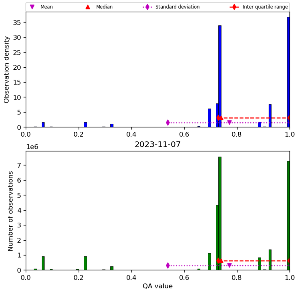
Figure 28: Histogram of “QA value” for 2023-11-07 to 2023-11-08
