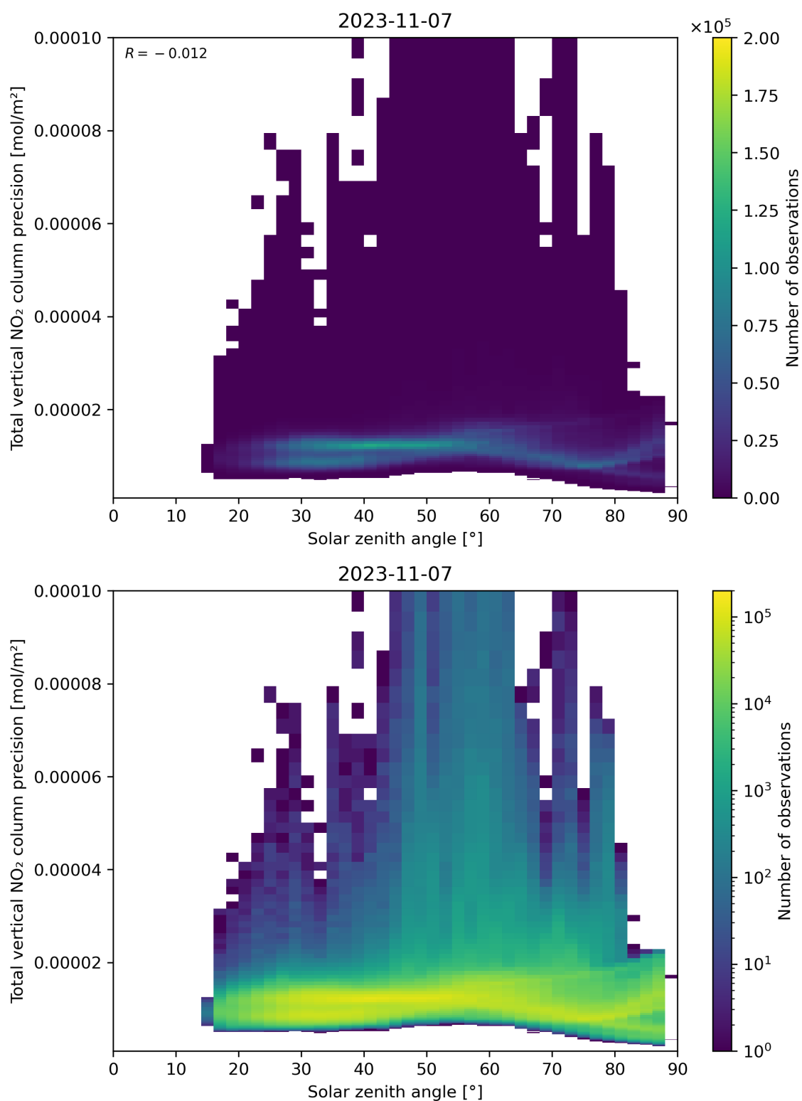
Figure 154: Scatter density plot of “Solar zenith angle” against “Total vertical NO 2 column precision” for 2023-11-07 to 2023-11-08.
