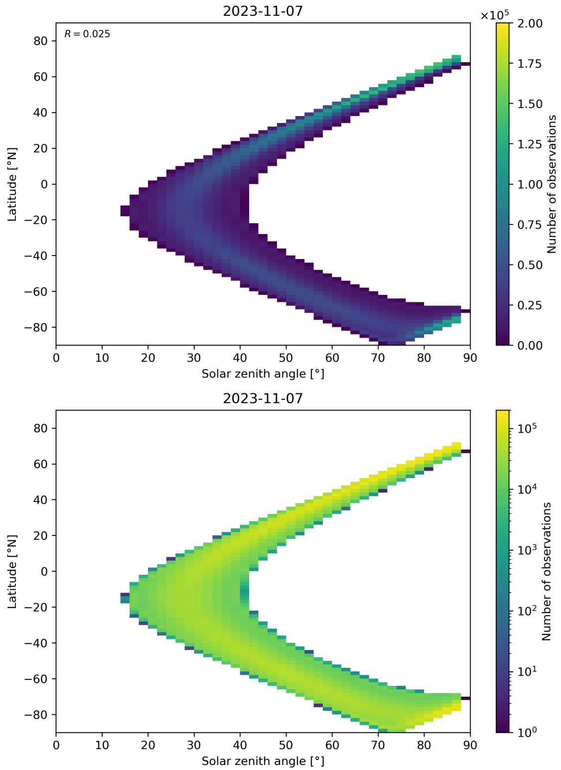
Figure 149: Scatter density plot of “Solar zenith angle” against “Latitude” for 2023-11-07 to 2023-11-08.
