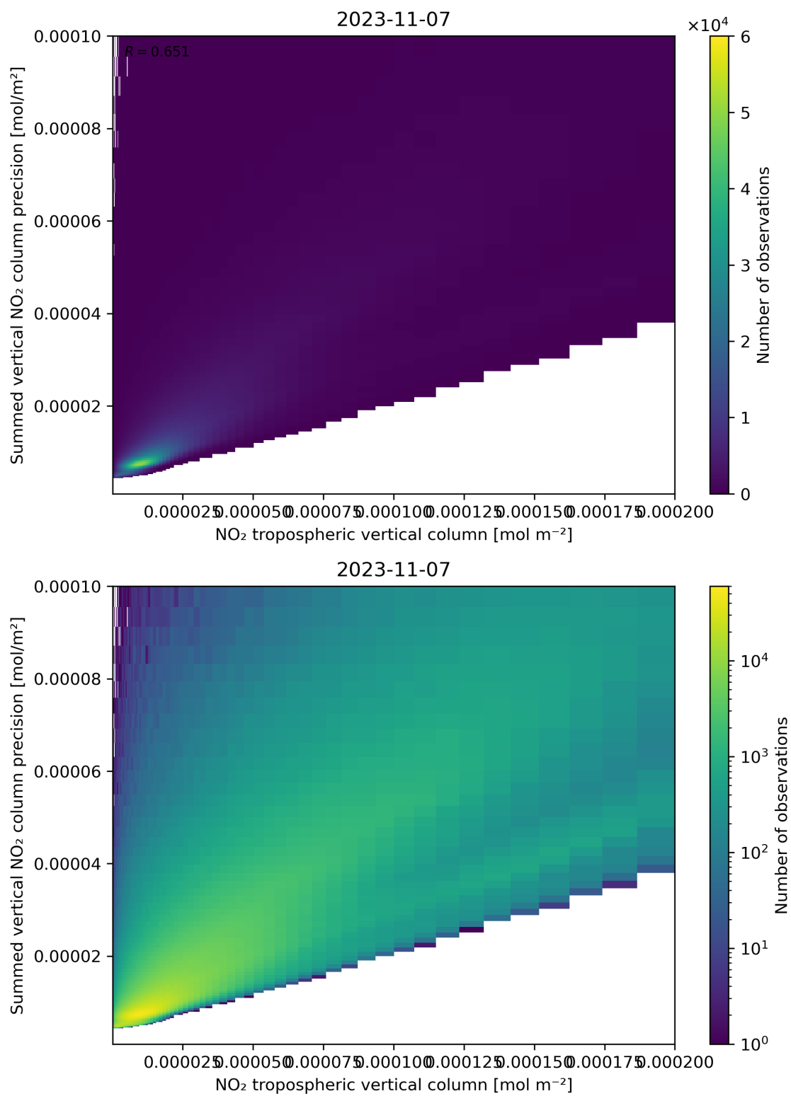
Figure 127: Scatter density plot of “NO 2 tropospheric vertical column” against “Summed vertical NO 2 column precision” for 2023-11-07 to 2023-11-08.
