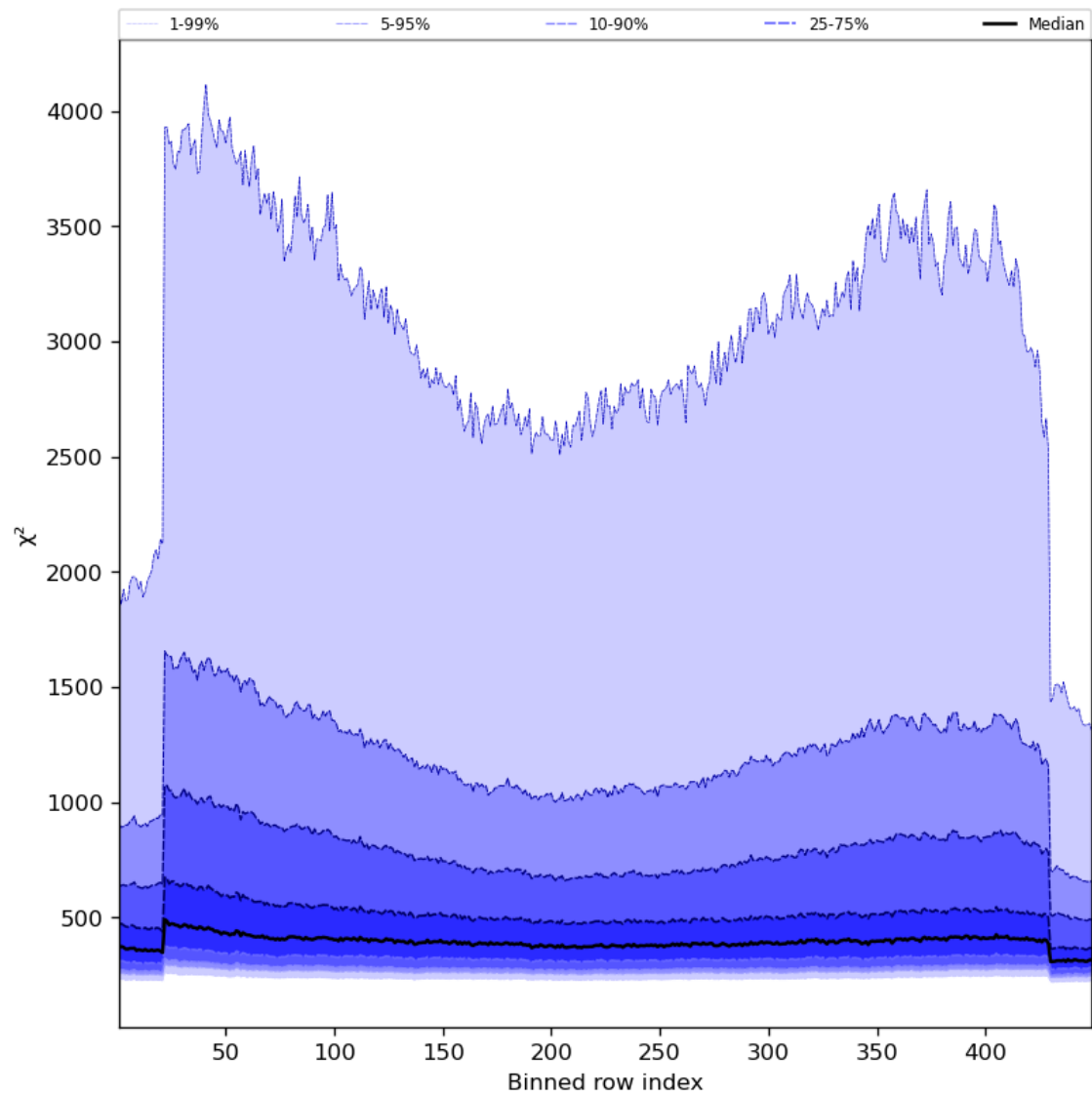
Figure 59: Along track statistics of “ \chi^2 ” for 2023-11-07 to 2023-11-08
