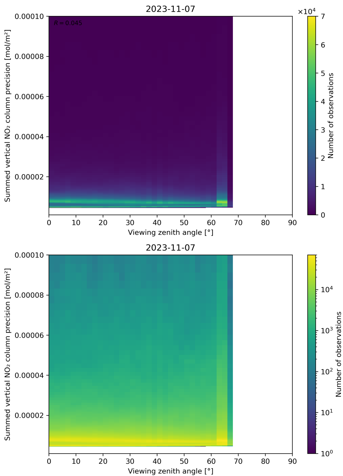
Figure 166: Scatter density plot of “Viewing zenith angle” against “Summed vertical NO 2 column precision” for 2023-11-07 to 2023-11-08.
