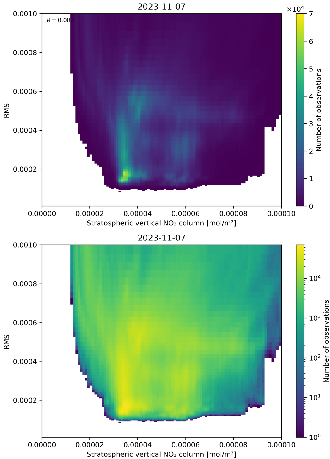
Figure 102: Scatter density plot of “Stratospheric vertical NO 2 column” against “RMS” for 2023-11-07 to 2023-11-08.
