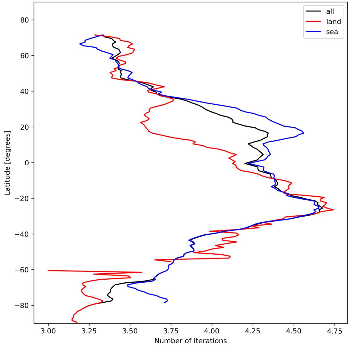
Figure 17: Zonal average of “Number of iterations” for 2023-11-07 to 2023-11-08.
