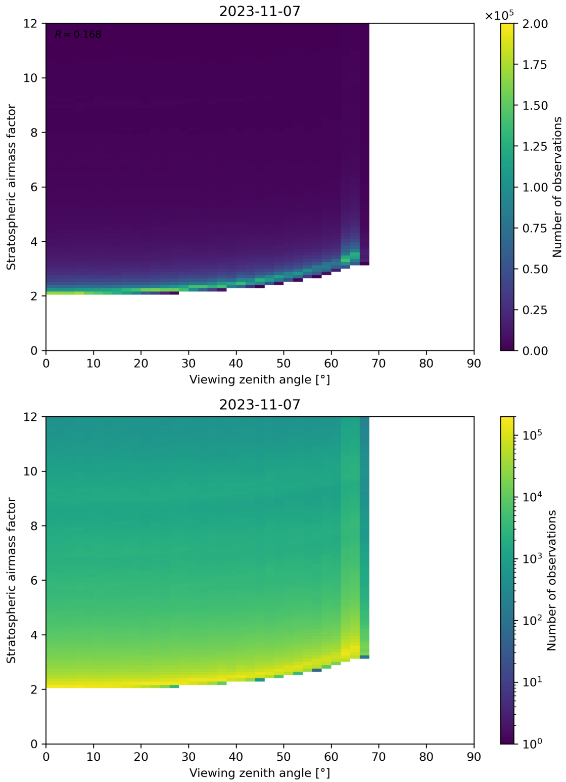
Figure 159: Scatter density plot of “Viewing zenith angle” against “Stratospheric airmass factor” for 2023-11-07 to 2023-11-08.
