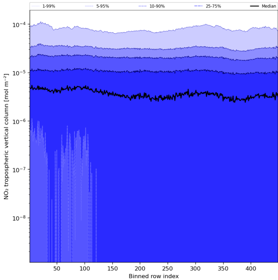
Figure 46: Along track statistics of “NO 2 tropospheric vertical column” for 2023-11-07 to 2023-11-08
