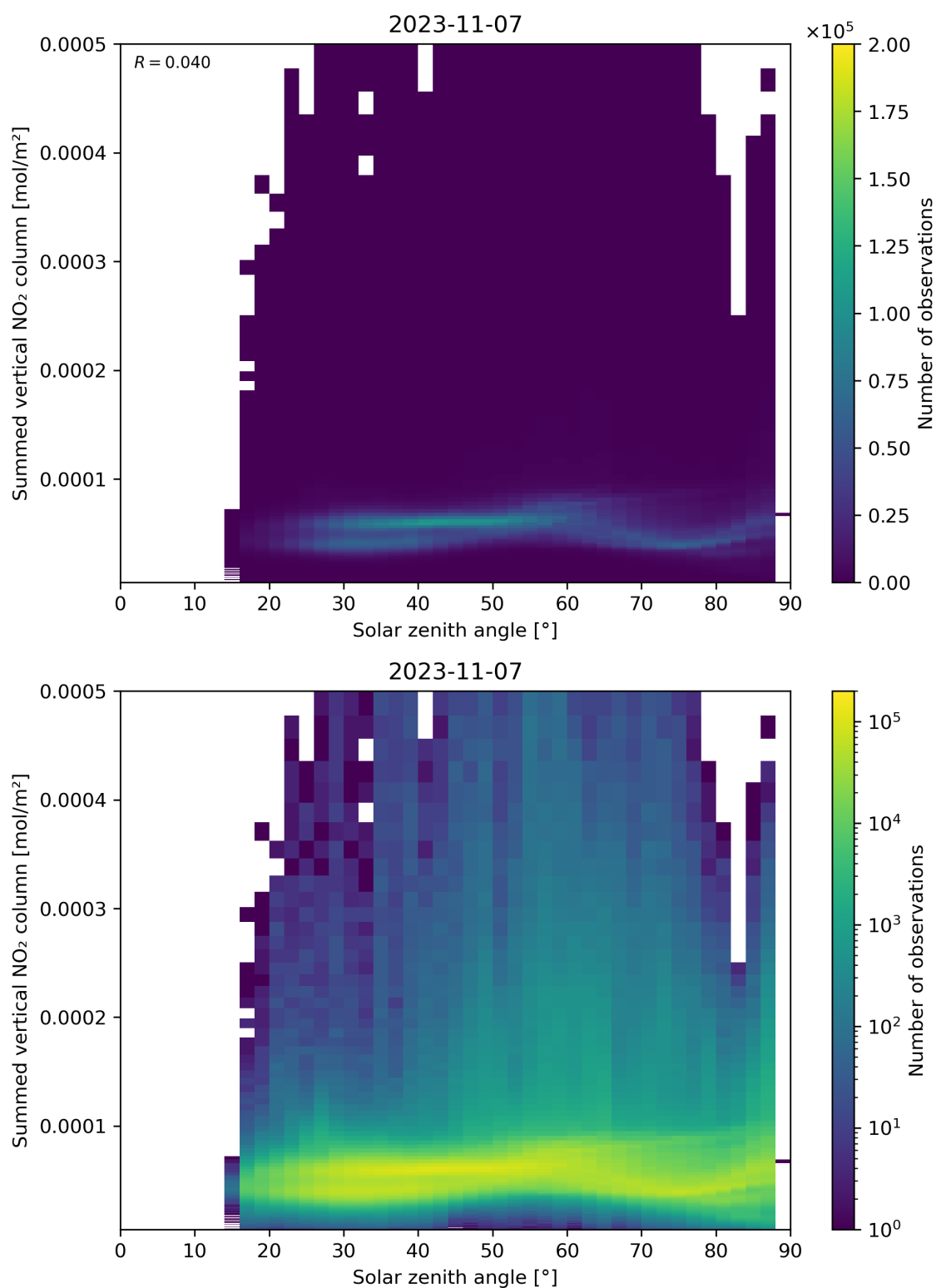
Figure 151: Scatter density plot of “Solar zenith angle” against “Summed vertical NO 2 column” for 2023-11-07 to 2023-11-08.
