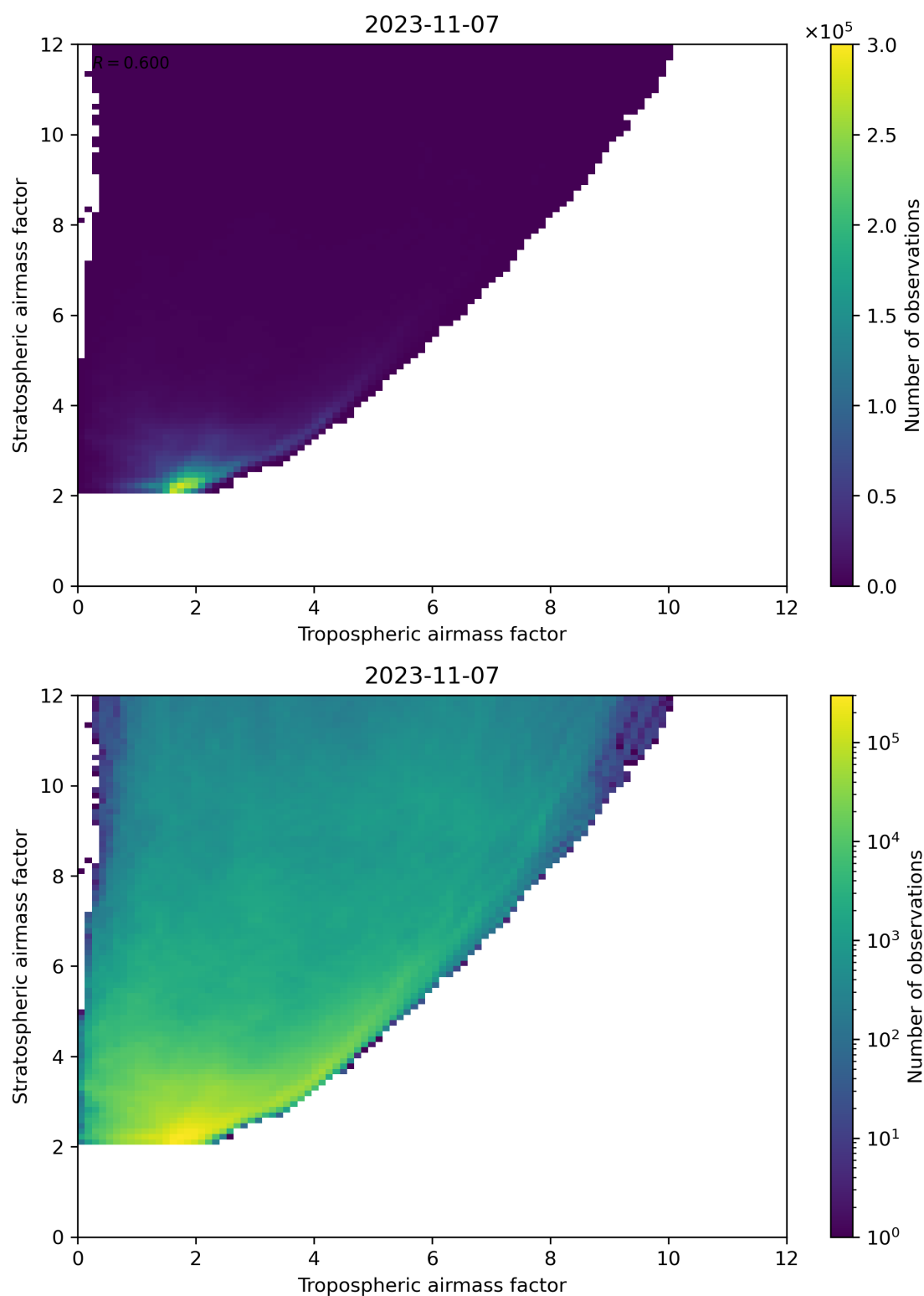
Figure 71: Scatter density plot of “Tropospheric airmass factor” against “Stratospheric airmass factor” for 2023-11-07 to 2023-11-08.
