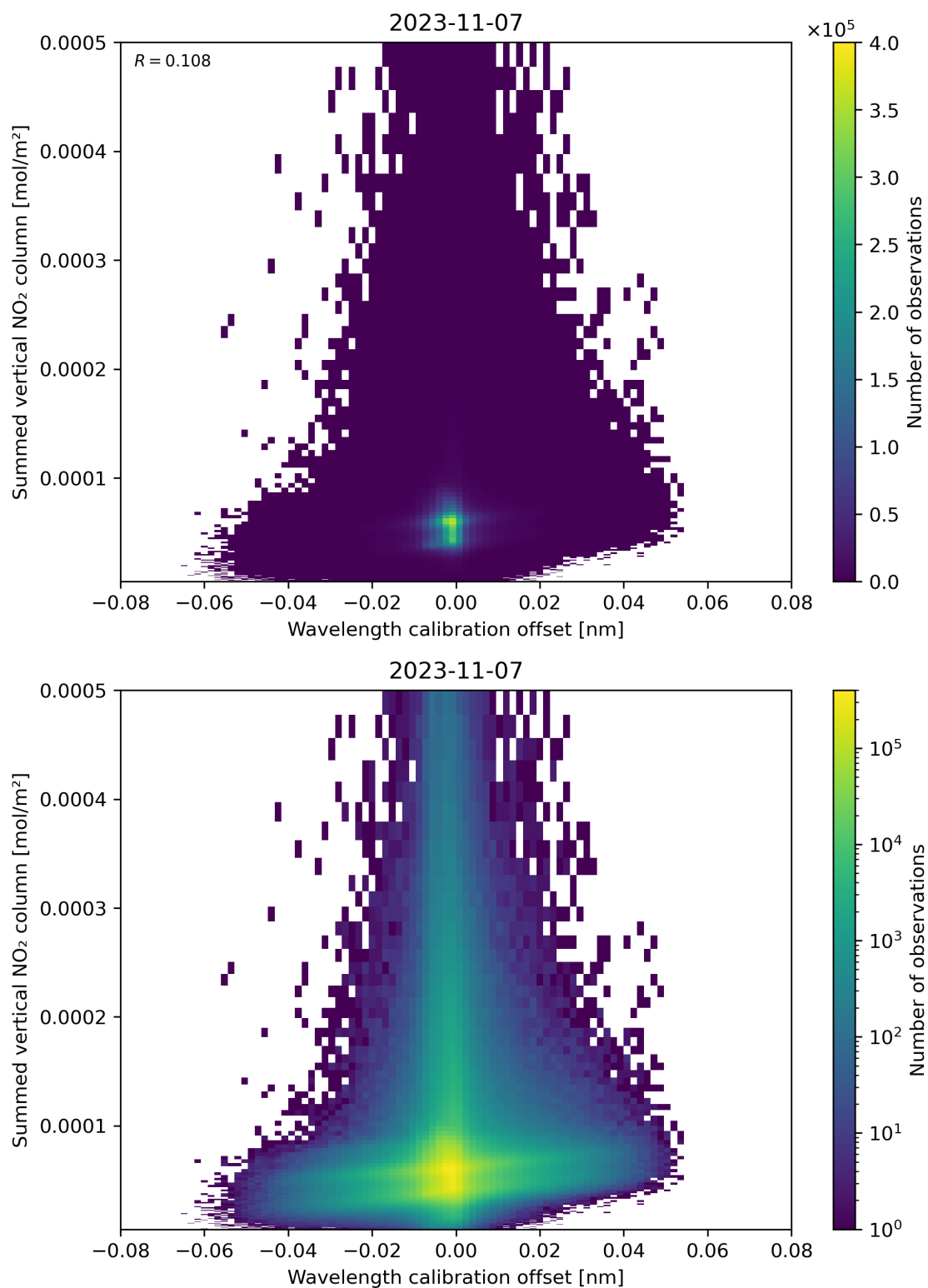
Figure 177: Scatter density plot of “Wavelength calibration offset” against “Summed vertical NO 2 column” for 2023-11-07 to 2023-11-08.
