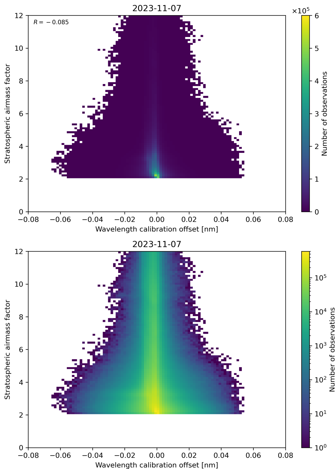
Figure 174: Scatter density plot of “Wavelength calibration offset” against “Stratospheric airmass factor” for 2023-11-07 to 2023-11-08.
