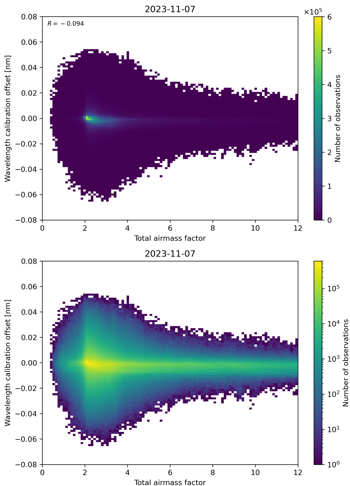
Figure 70: Scatter density plot of “Total airmass factor” against “Wavelength calibration offset” for 2023-11-07 to 2023-11-08.
