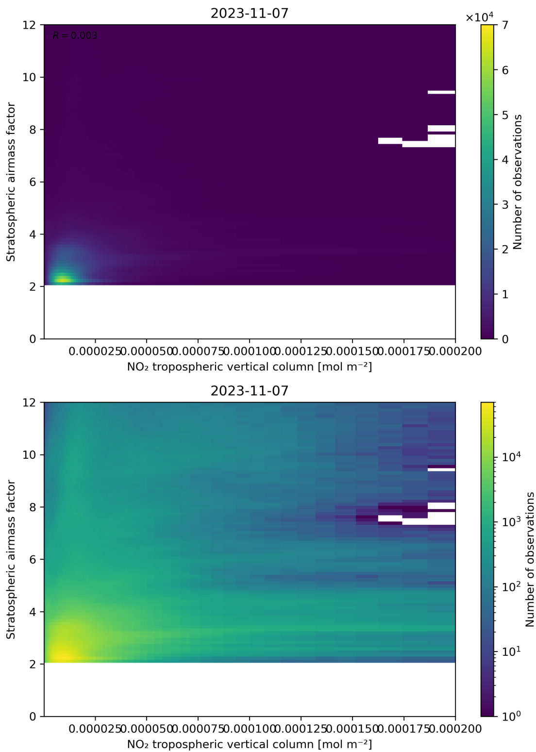
Figure 121: Scatter density plot of “NO 2 tropospheric vertical column” against “Stratospheric air mass factor” for 2023-11-07 to 2023-11-08.
