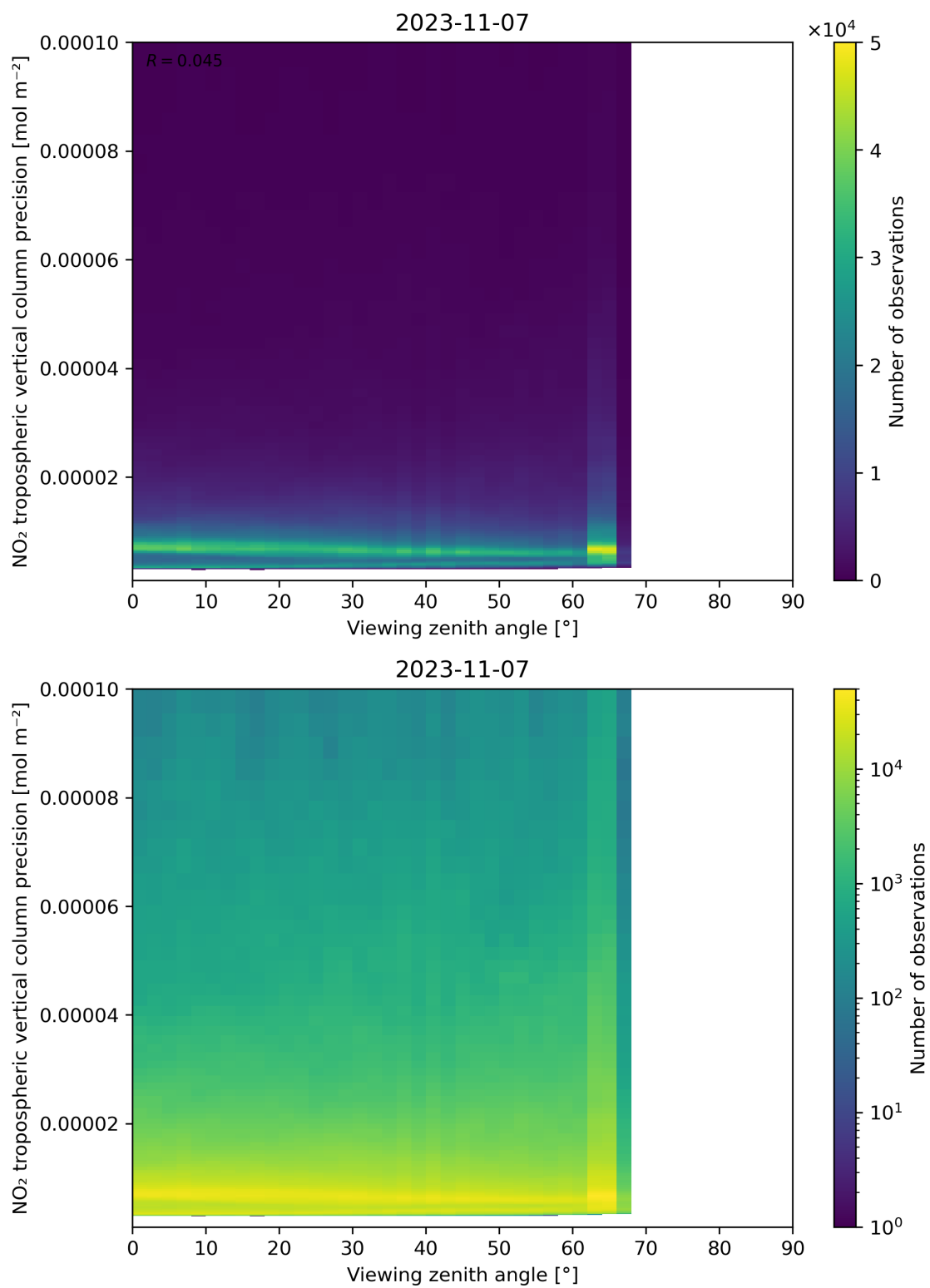
Figure 170: Scatter density plot of “Viewing zenith angle” against “NO 2 tropospheric vertical column precision” for 2023-11-07 to 2023-11-08.
