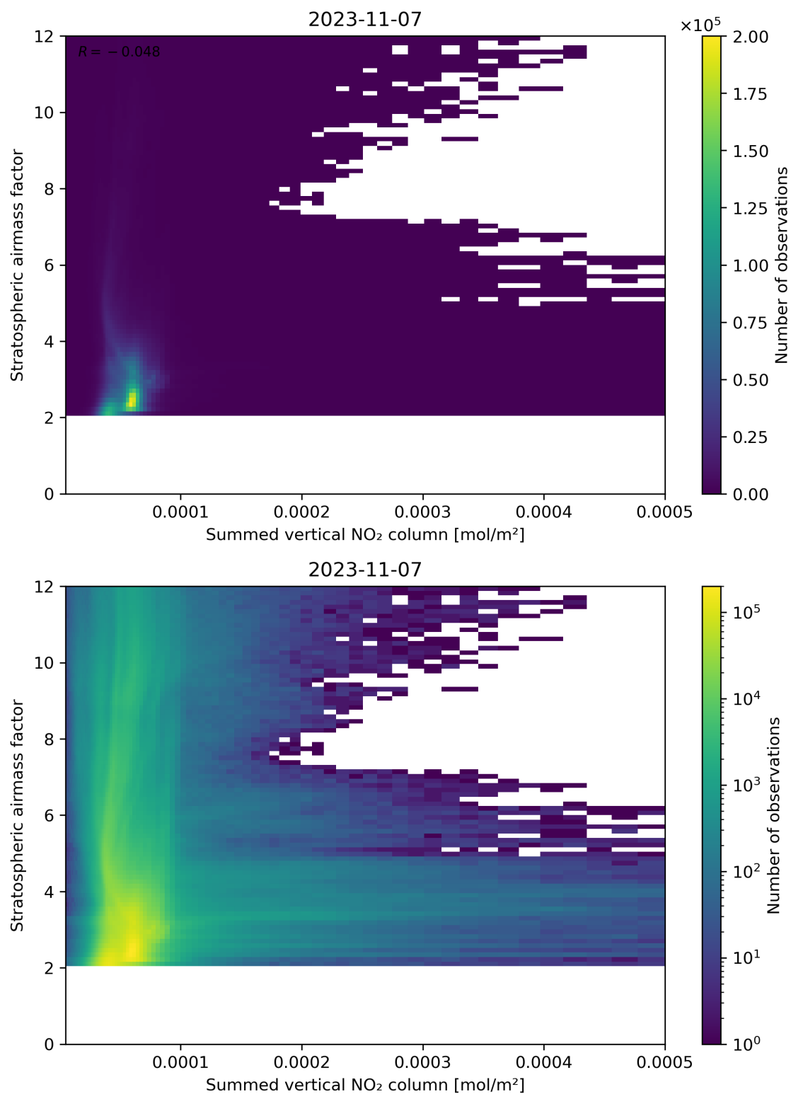
Figure 103: Scatter density plot of “Summed vertical NO 2 column” against “Stratospheric air mass factor” for 2023-11-07 to 2023-11-08.
