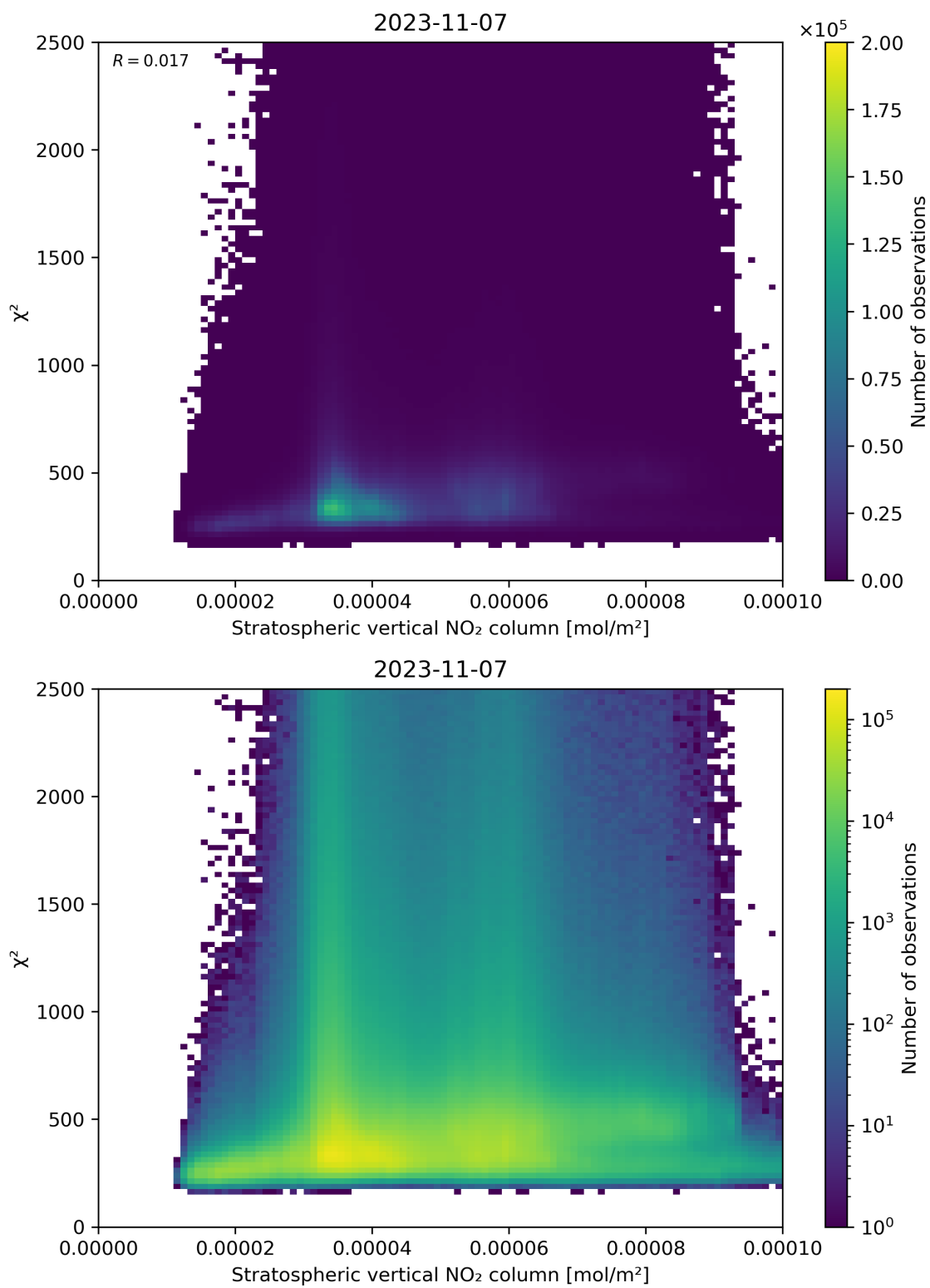
Figure 97: Scatter density plot of “Stratospheric vertical NO 2 column” against “ \chi^2 ” for 2023-11-07 to 2023-11-08.
