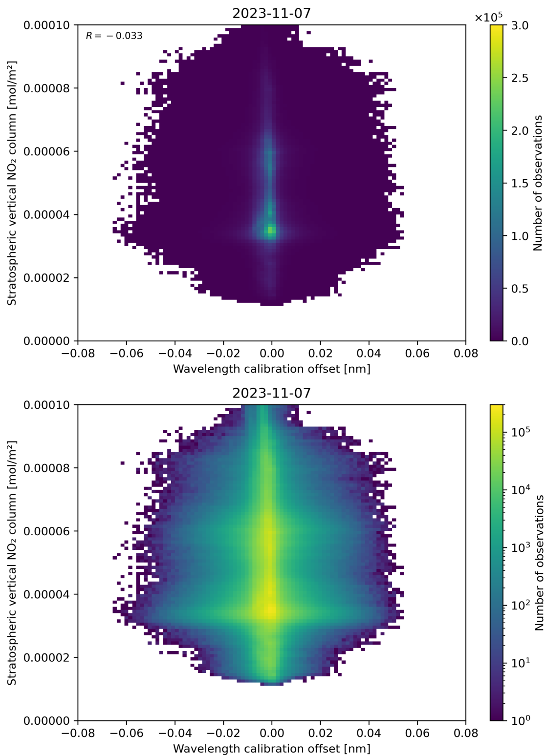
Figure 176: Scatter density plot of “Wavelength calibration offset” against “Stratospheric vertical NO 2 column” for 2023-11-07 to 2023-11-08.
