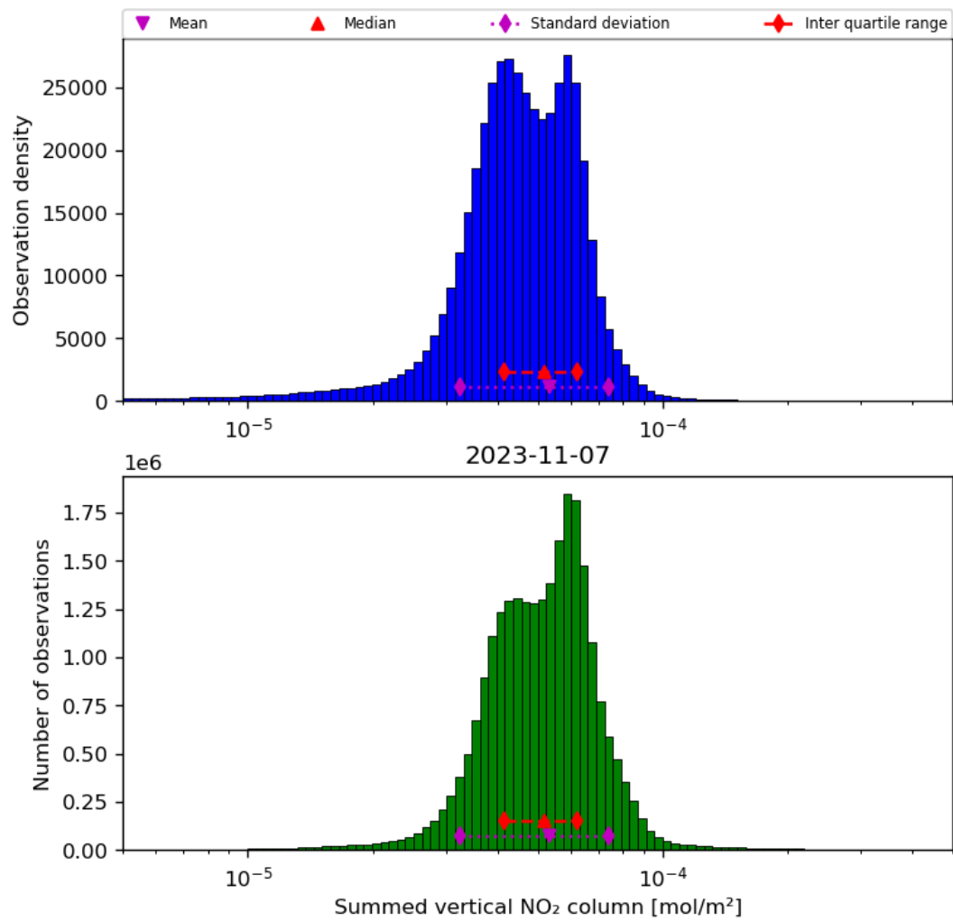
Figure 40: Histogram of “Summed vertical NO 2 column” for 2023-11-07 to 2023-11-08
