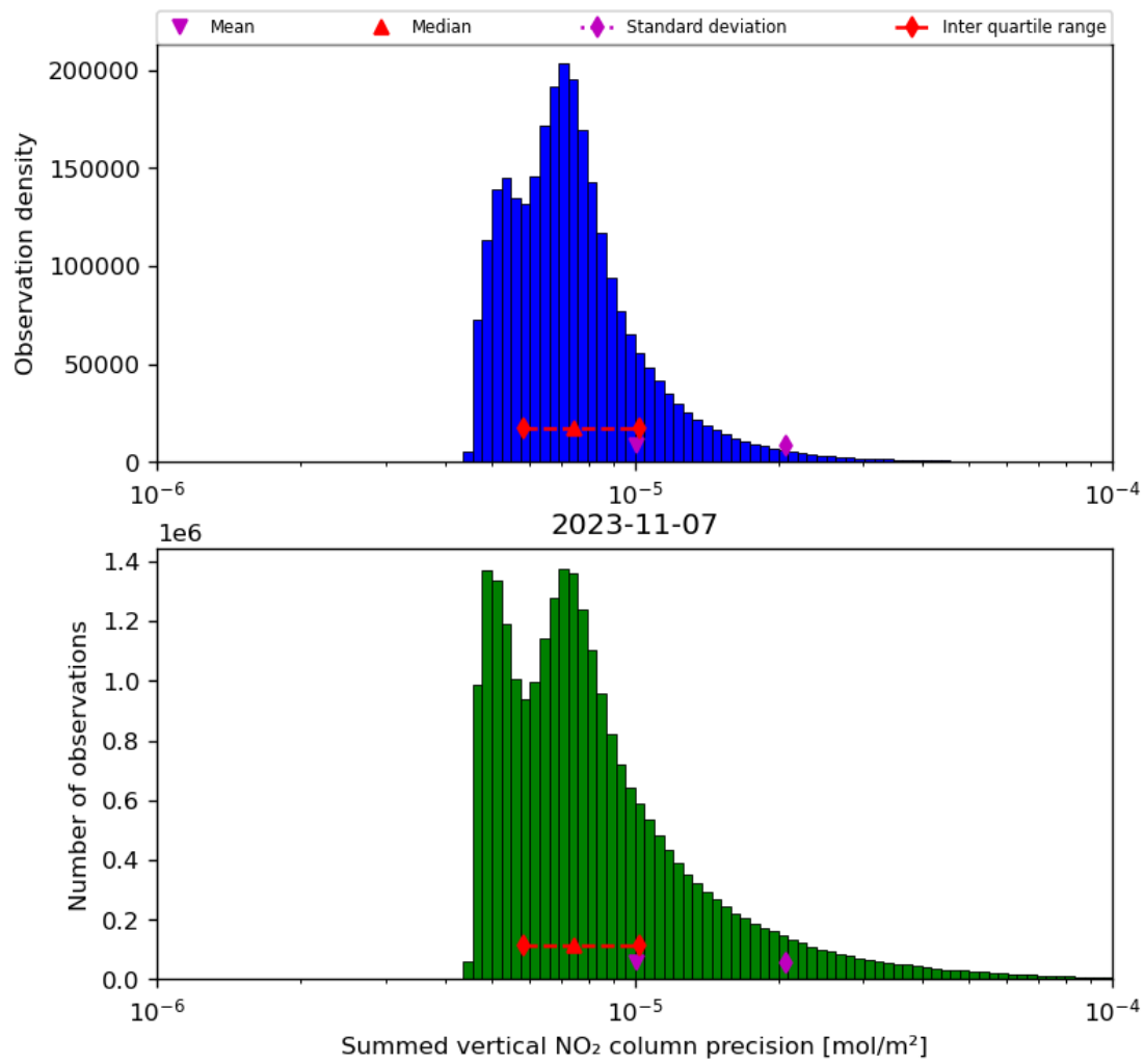
Figure 41: Histogram of "Summed vertical NO 2 column precision" for 2023-11-07 to 2023-11-08
