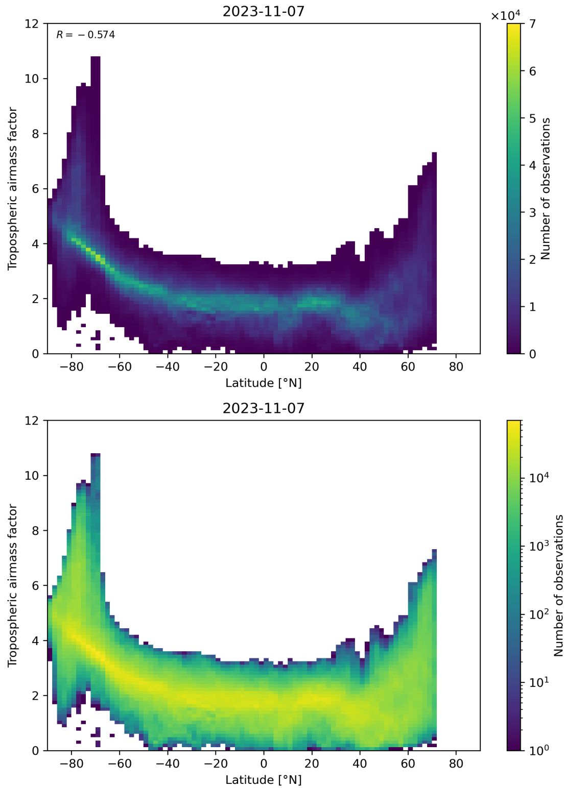
Figure 85: Scatter density plot of “Latitude” against “Tropospheric airmass factor” for 2023-11-07 to 2023-11-08.
