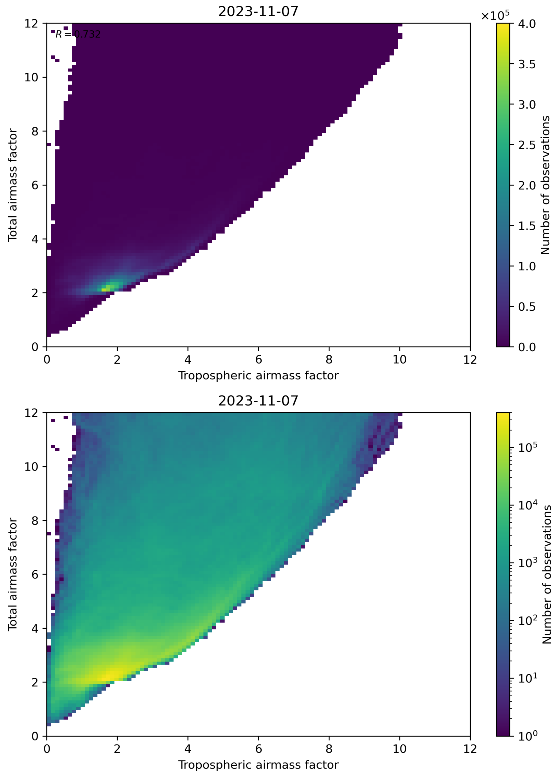
Figure 72: Scatter density plot of “Tropospheric airmass factor” against “Total airmass factor” for 2023-11-07 to 2023-11-08.
