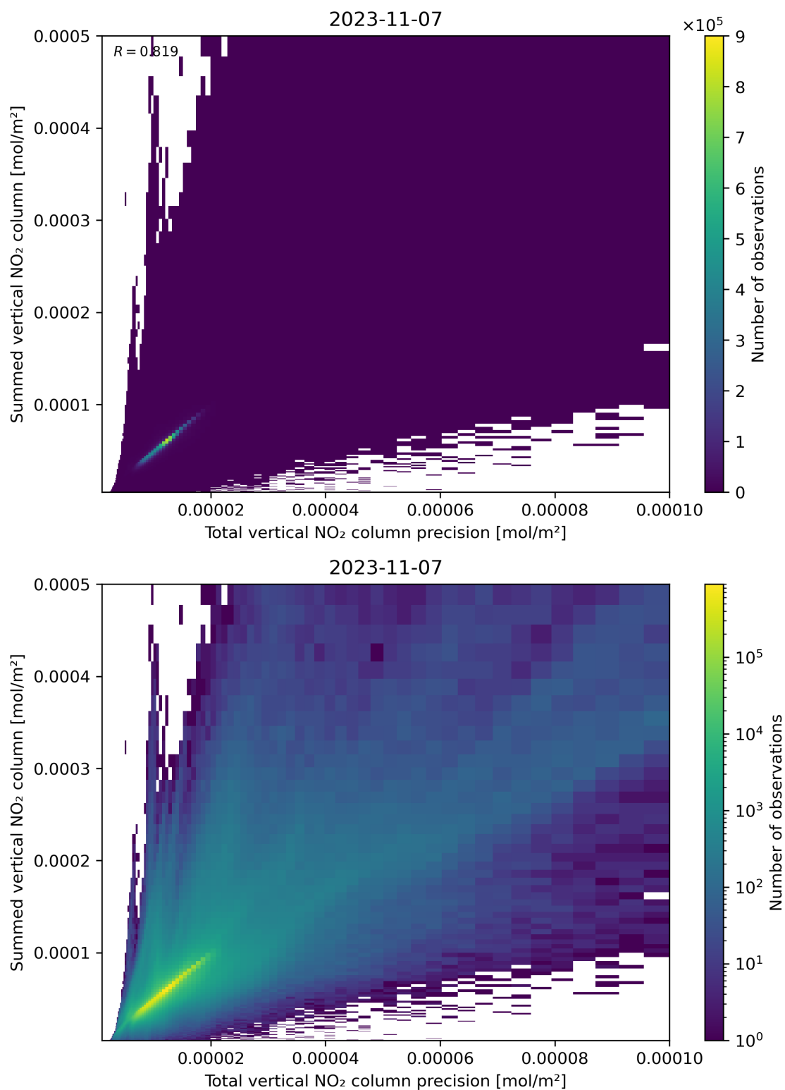
Figure 117: Scatter density plot of “Total vertical NO 2 column precision” against “Summed vertical NO 2 column” for 2023-11-07 to 2023-11-08.
