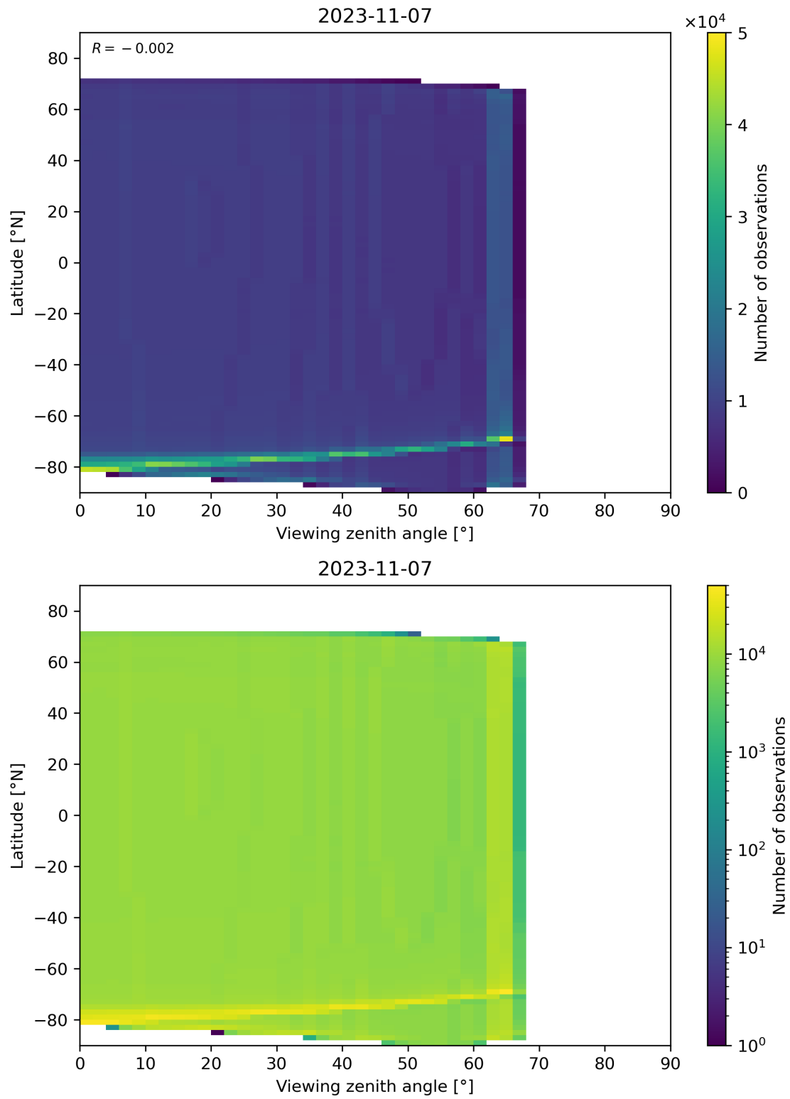
Figure 163: Scatter density plot of “Viewing zenith angle” against “Latitude” for 2023-11-07 to 2023-11-08.
