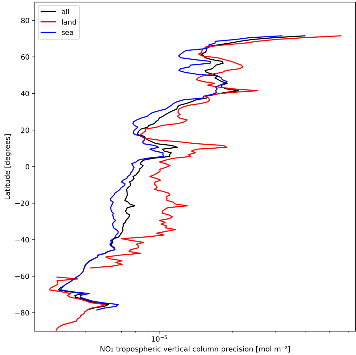
Figure 13: Zonal average of “NO 2 tropospheric vertical column precision” for 2023-11-07 to 2023-11-08.
