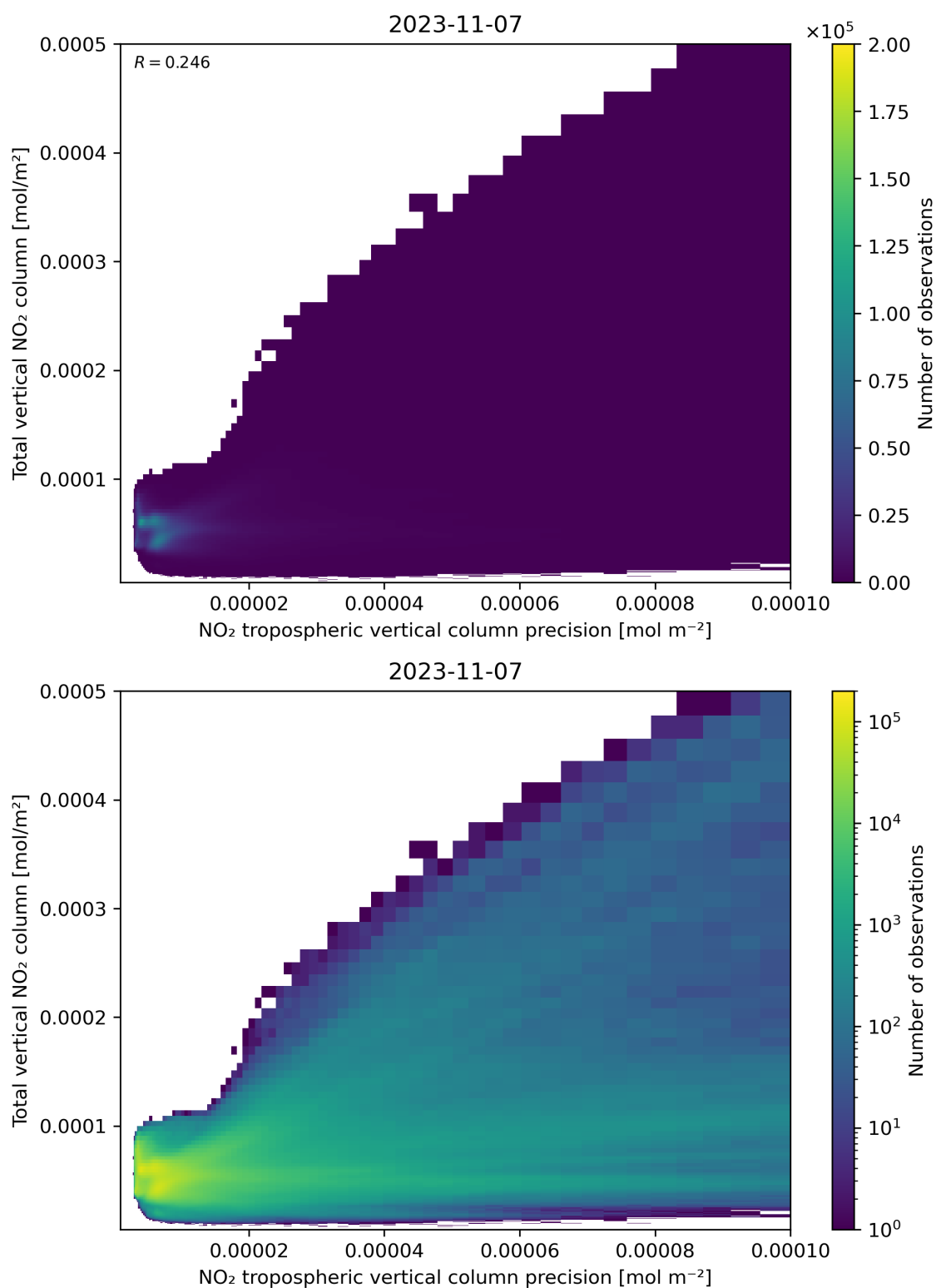
Figure 138: Scatter density plot of “NO 2 tropospheric vertical column precision” against “Total vertical NO 2 column” for 2023-11-07 to 2023-11-08.
