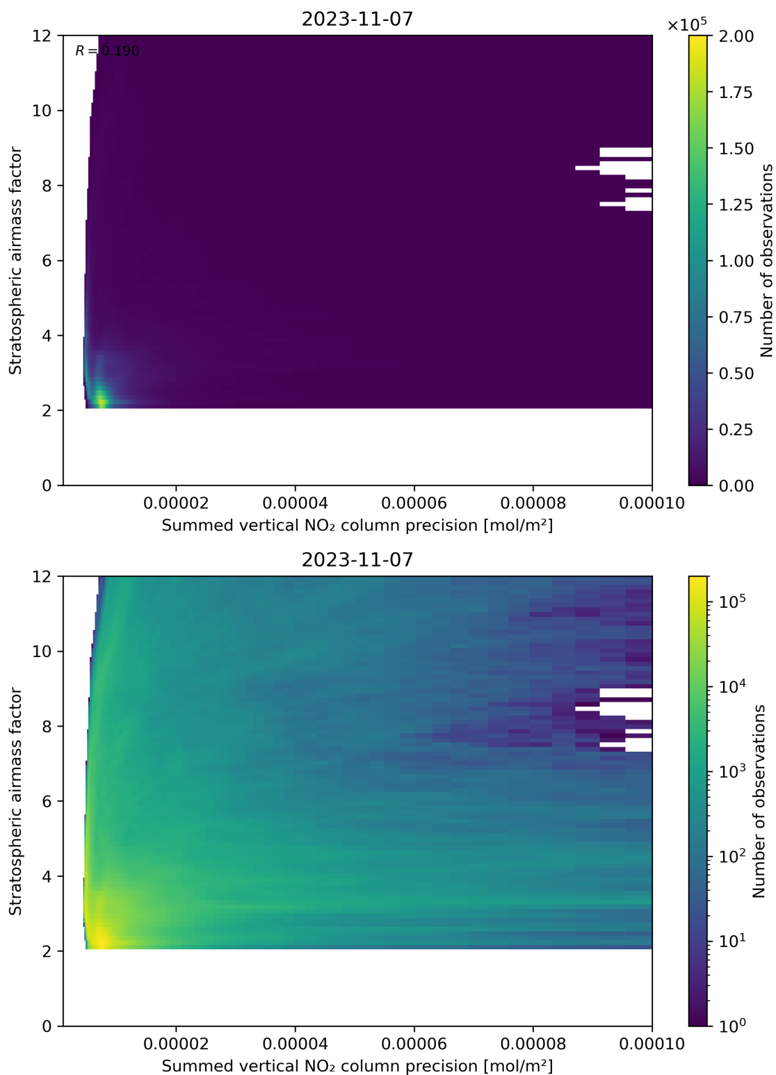
Figure 106: Scatter density plot of “Summed vertical NO 2 column precision” against “Stratospheric airmass factor” for 2023-11-07 to 2023-11-08.
