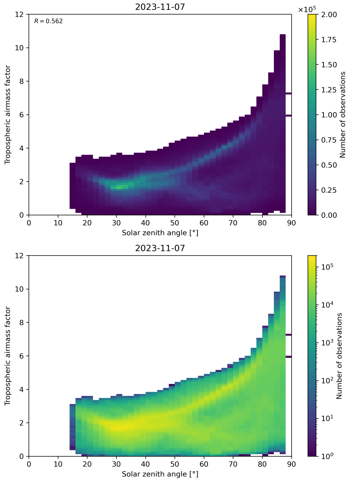
Figure 147: Scatter density plot of “Solar zenith angle” against “Tropospheric airmass factor” for 2023-11-07 to 2023-11-08.
