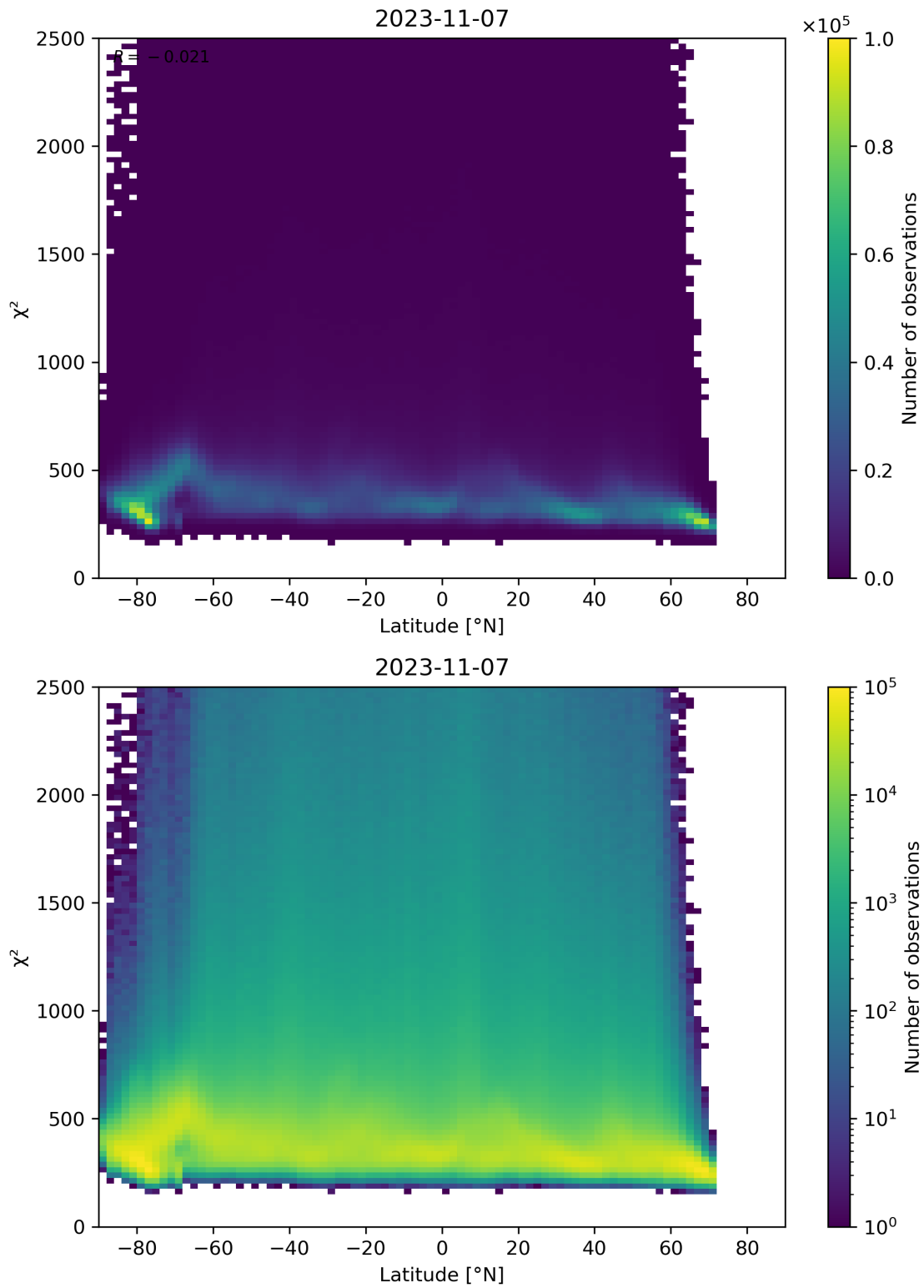
Figure 86: Scatter density plot of “Latitude” against “ \chi^2 ” for 2023-11-07 to 2023-11-08.
