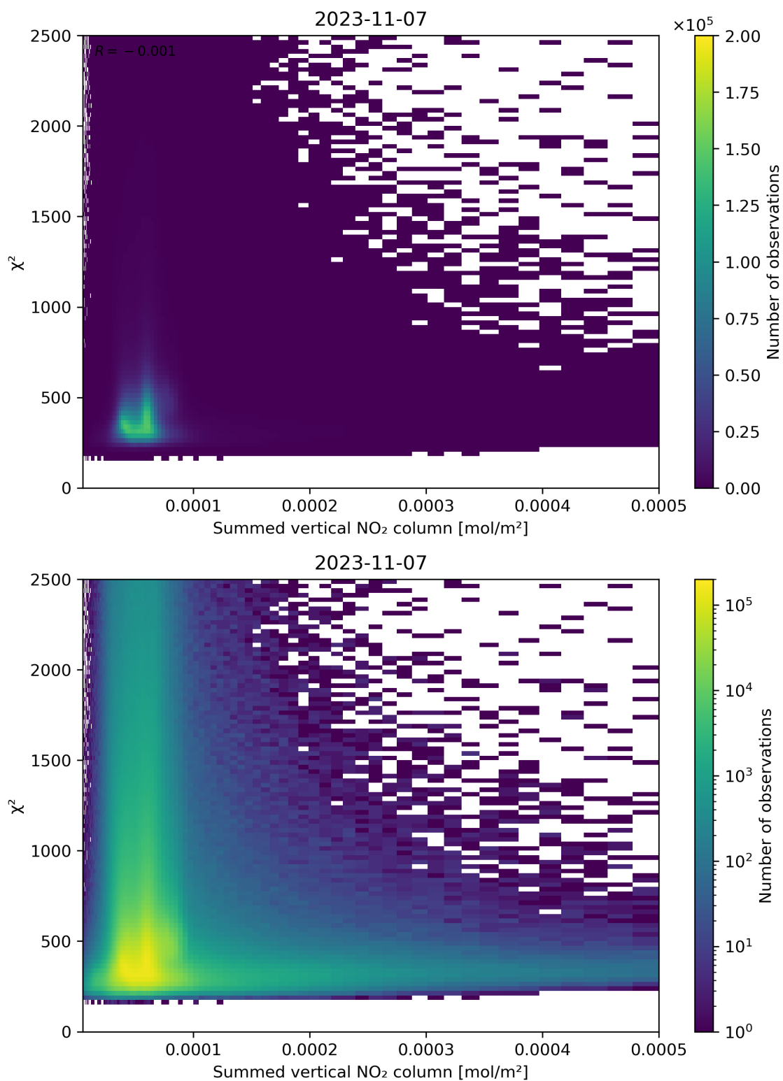
Figure 104: Scatter density plot of “Summed vertical NO 2 column” against “ \chi^2 ” for 2023-11-07 to 2023-11-08.
