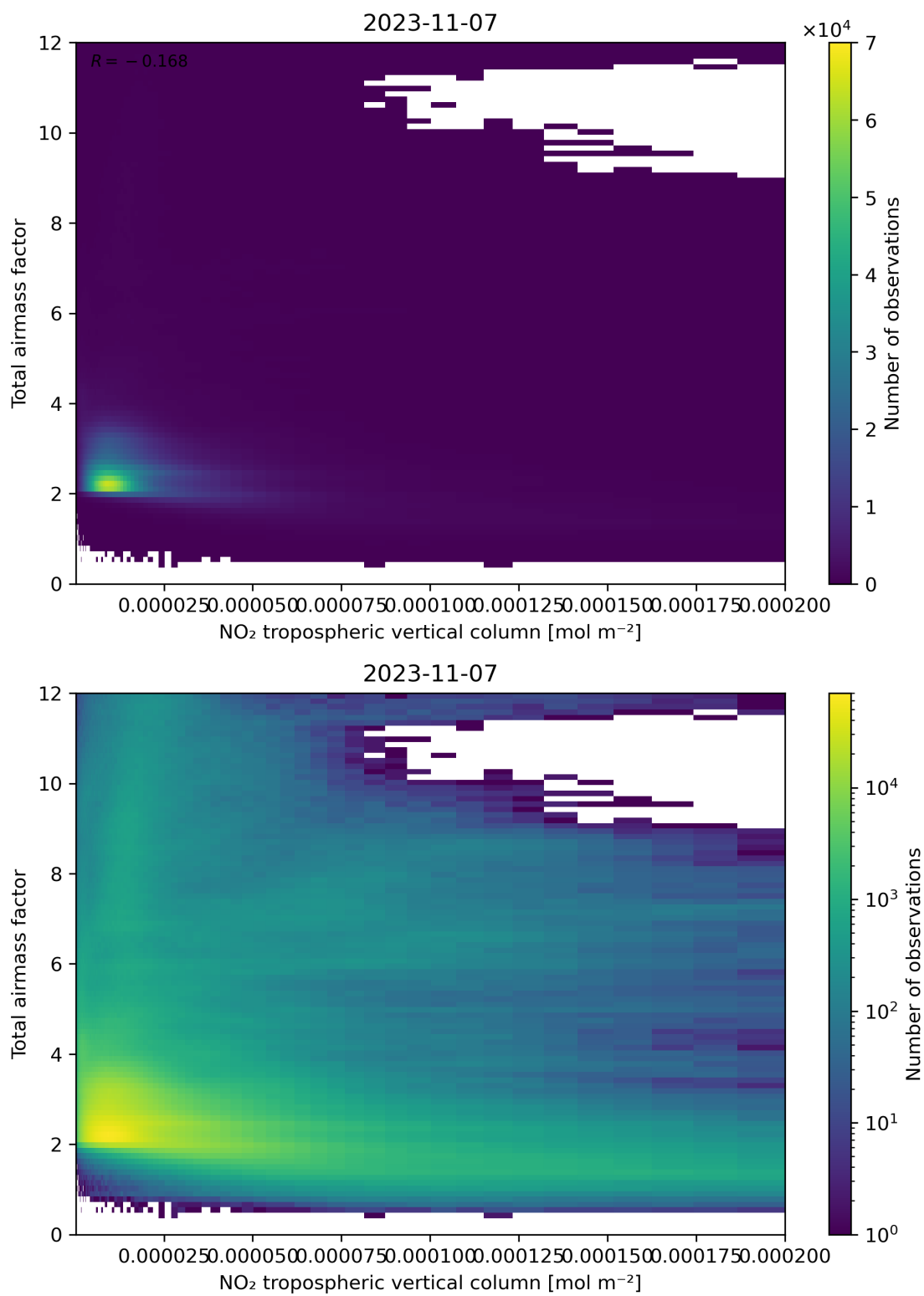
Figure 122: Scatter density plot of “NO 2 tropospheric vertical column” against “Total air mass factor” for 2023-11-07 to 2023-11-08.
