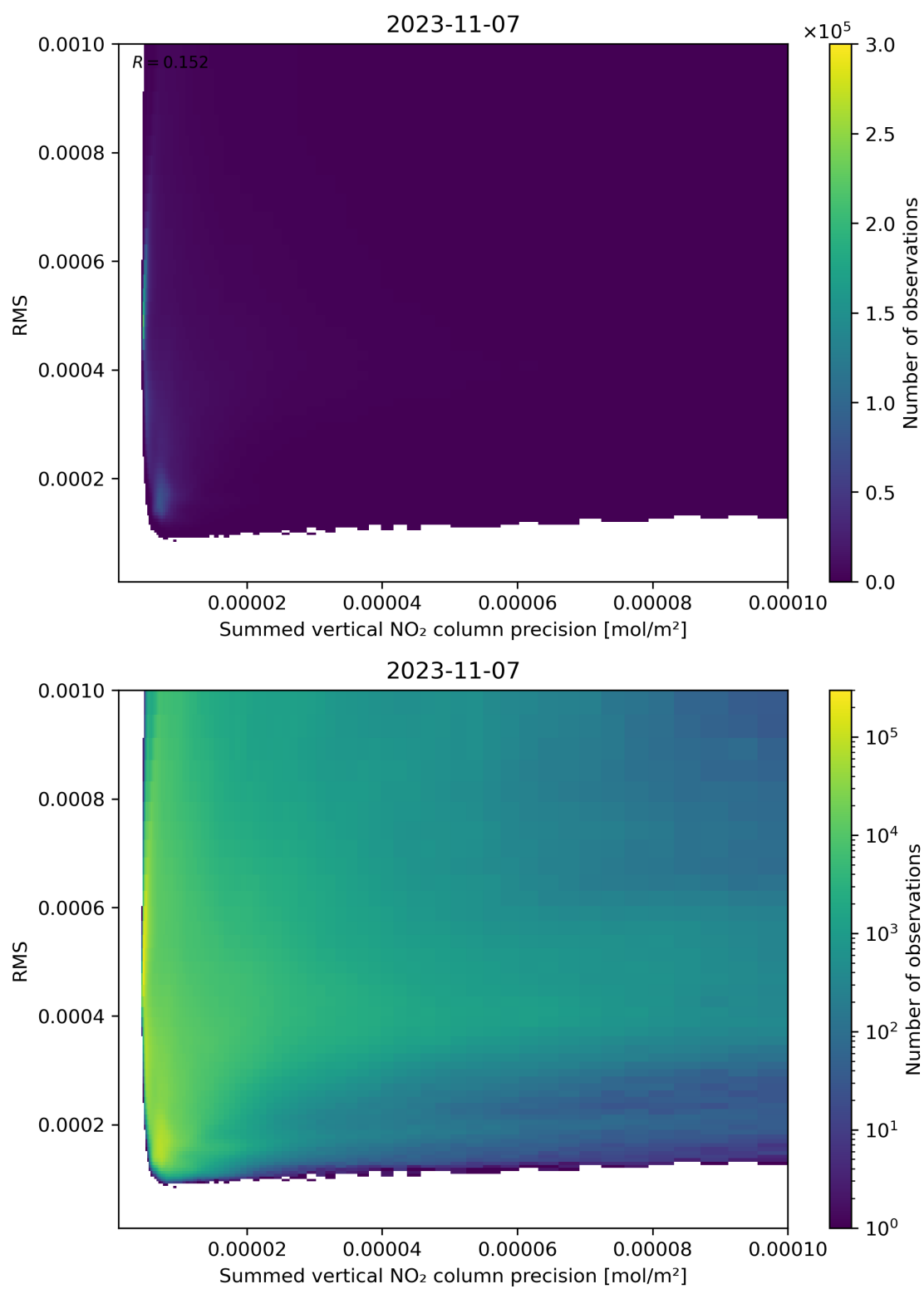
Figure 108: Scatter density plot of “Summed vertical NO 2 column precision” against “RMS” for 2023-11-07 to 2023-11-08.
