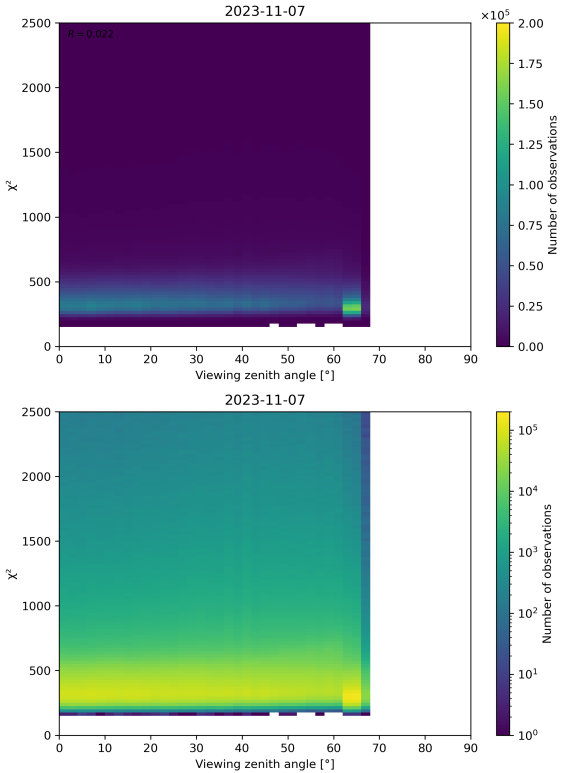
Figure 162: Scatter density plot of “Viewing zenith angle” against “ \chi^2 ” for 2023-11-07 to 2023-11-08.
