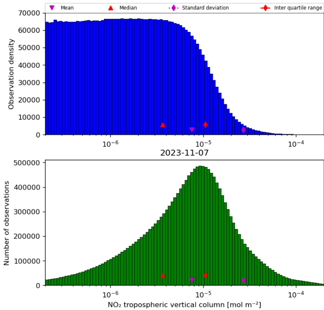
Figure 29: Histogram of “NO 2 tropospheric vertical column” for 2023-11-07 to 2023-11-08
