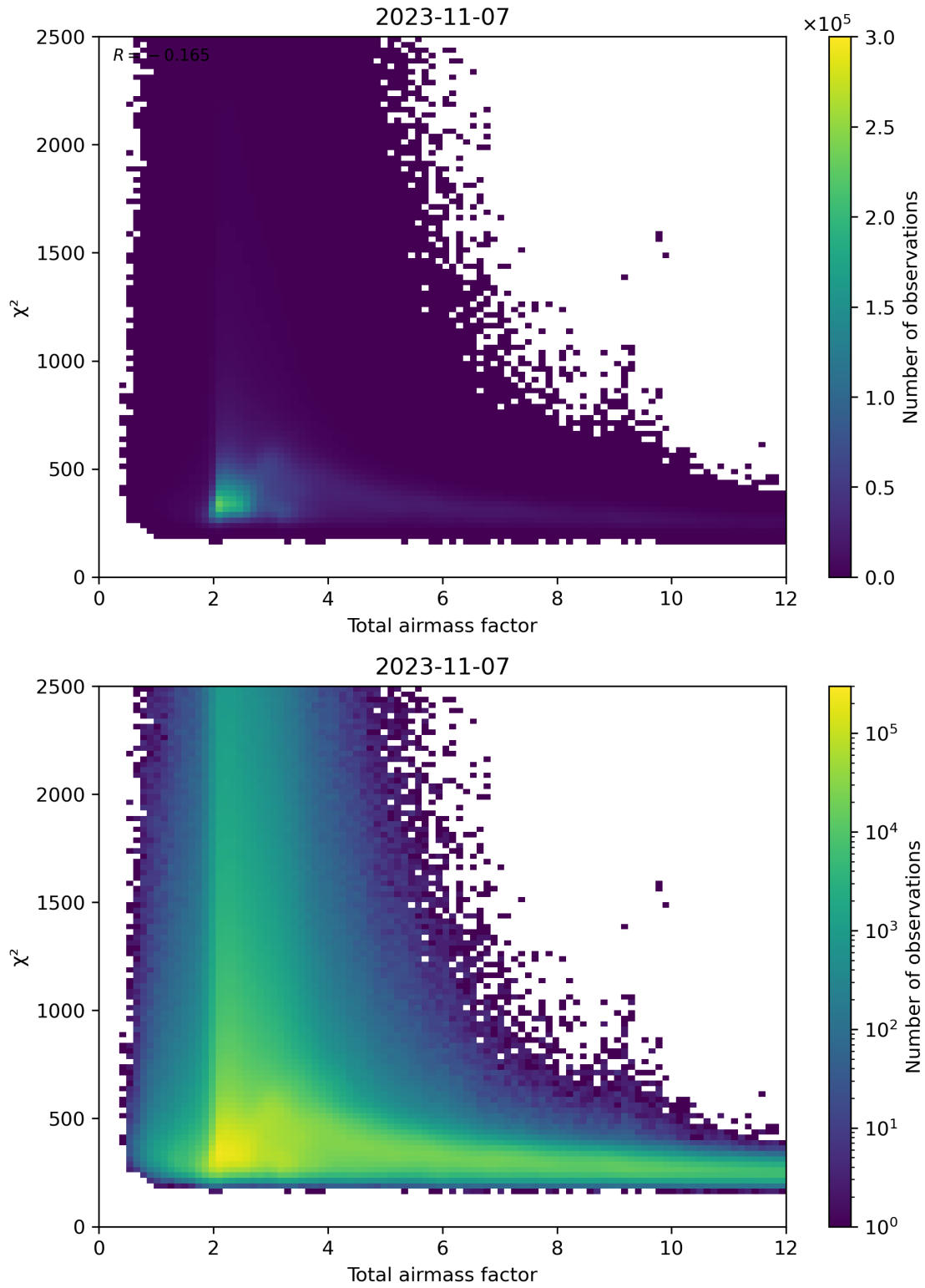
Figure 63: Scatter density plot of “Total airmass factor” against “ \chi^2 ” for 2023-11-07 to 2023-11-08.
