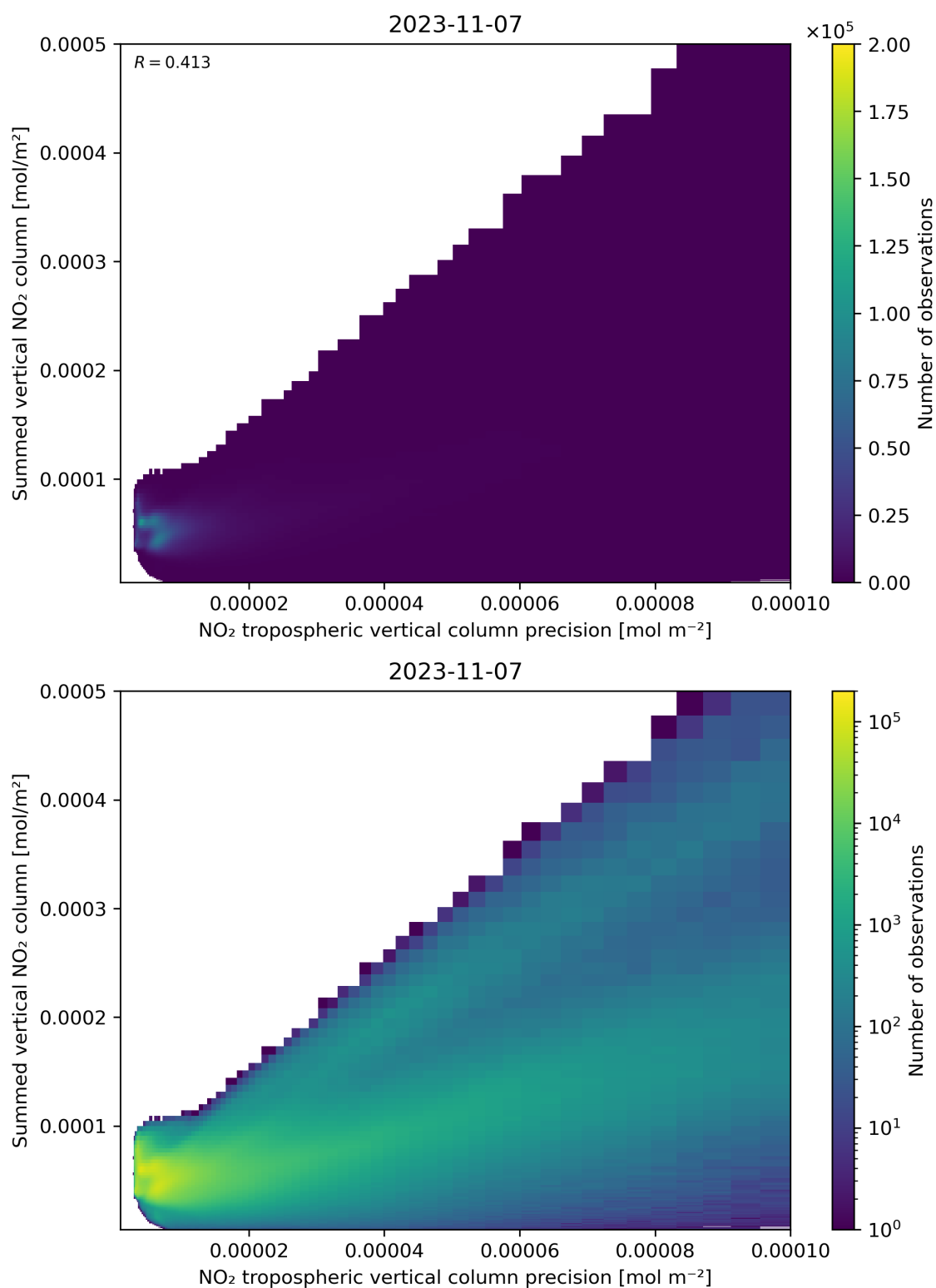
Figure 136: Scatter density plot of “NO 2 tropospheric vertical column precision” against “Summed vertical NO 2 column” for 2023-11-07 to 2023-11-08.
