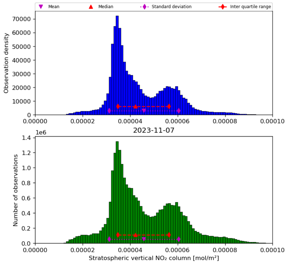
Figure 36: Histogram of “Stratospheric vertical NO 2 column” for 2023-11-07 to 2023-11-08
