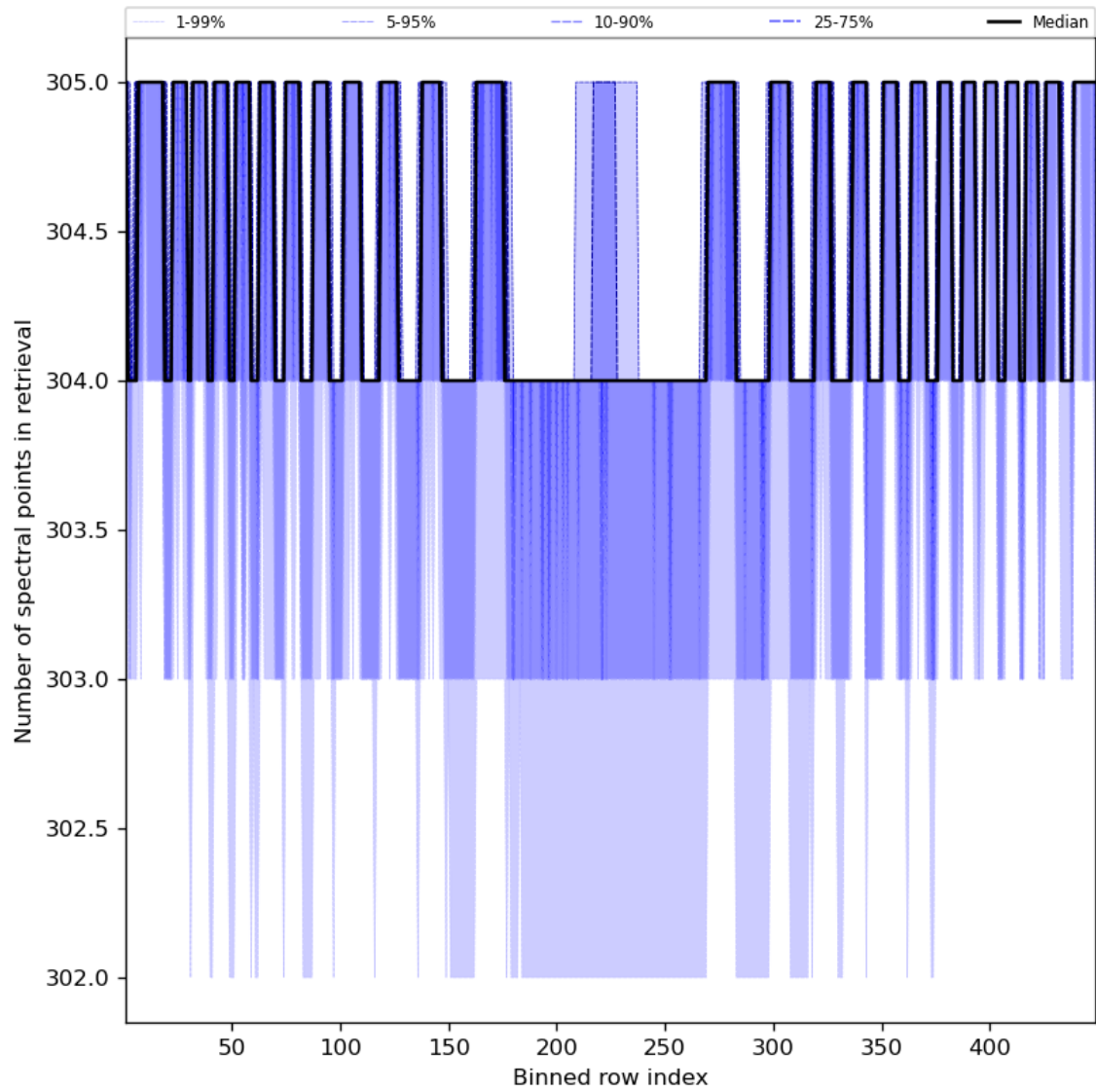
Figure 50: Along track statistics of “Number of spectral points in retrieval” for 2023-11-07 to 2023-11-08
