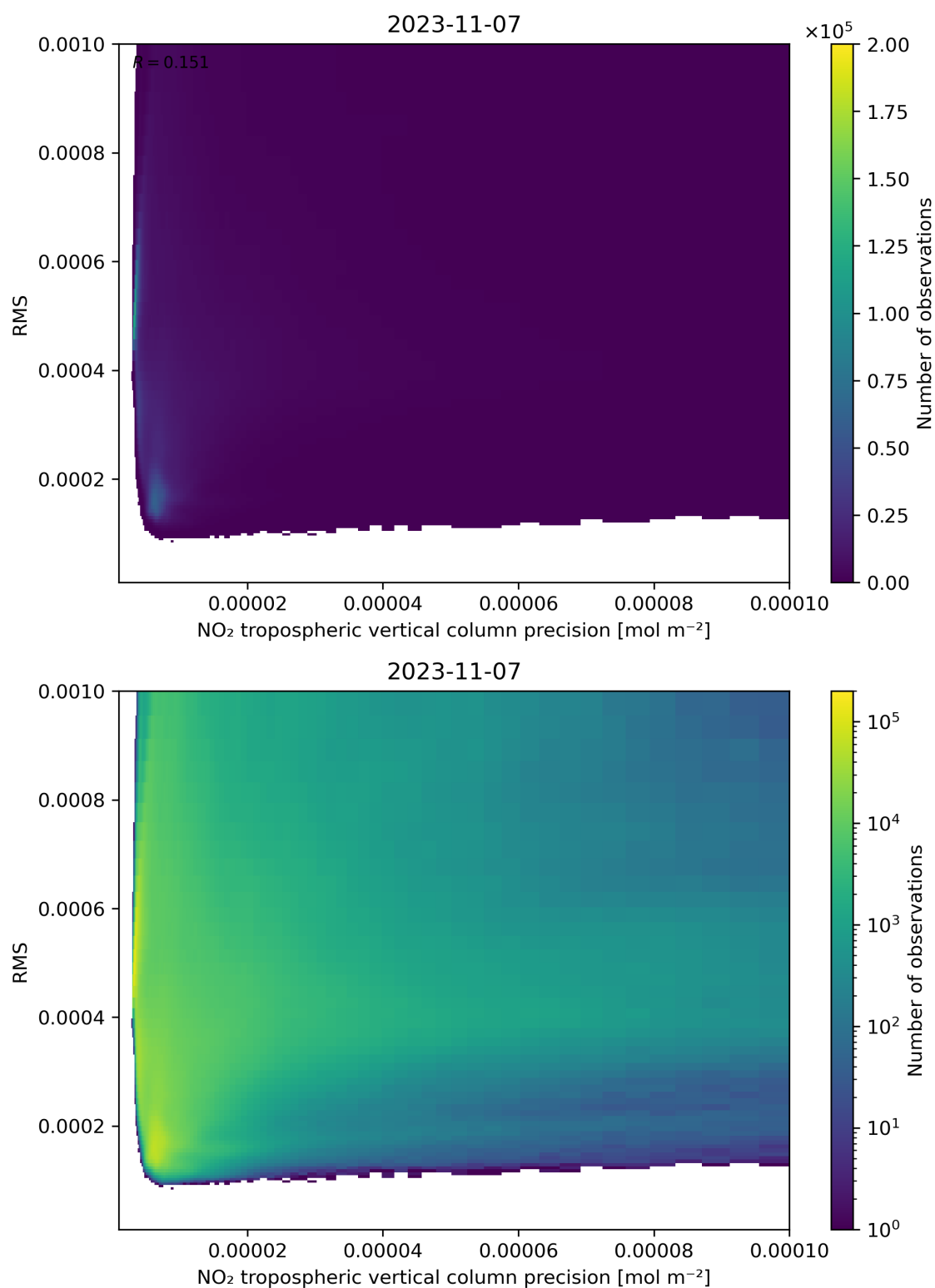
Figure 140: Scatter density plot of “NO 2 tropospheric vertical column precision” against “RMS” for 2023-11-07 to 2023-11-08.
