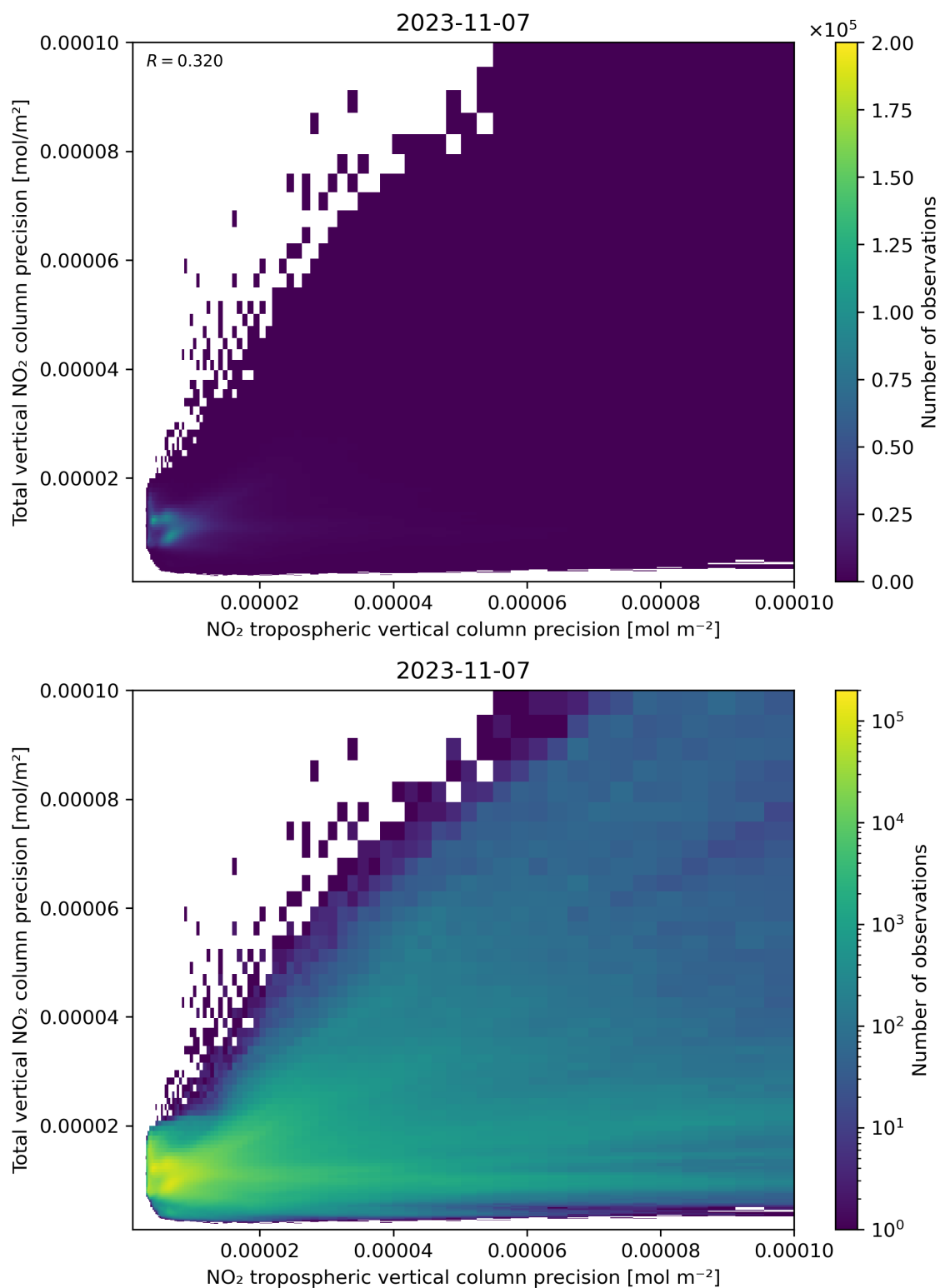
Figure 139: Scatter density plot of “NO 2 tropospheric vertical column precision” against “Total vertical NO 2 column precision” for 2023-11-07 to 2023-11-08.
