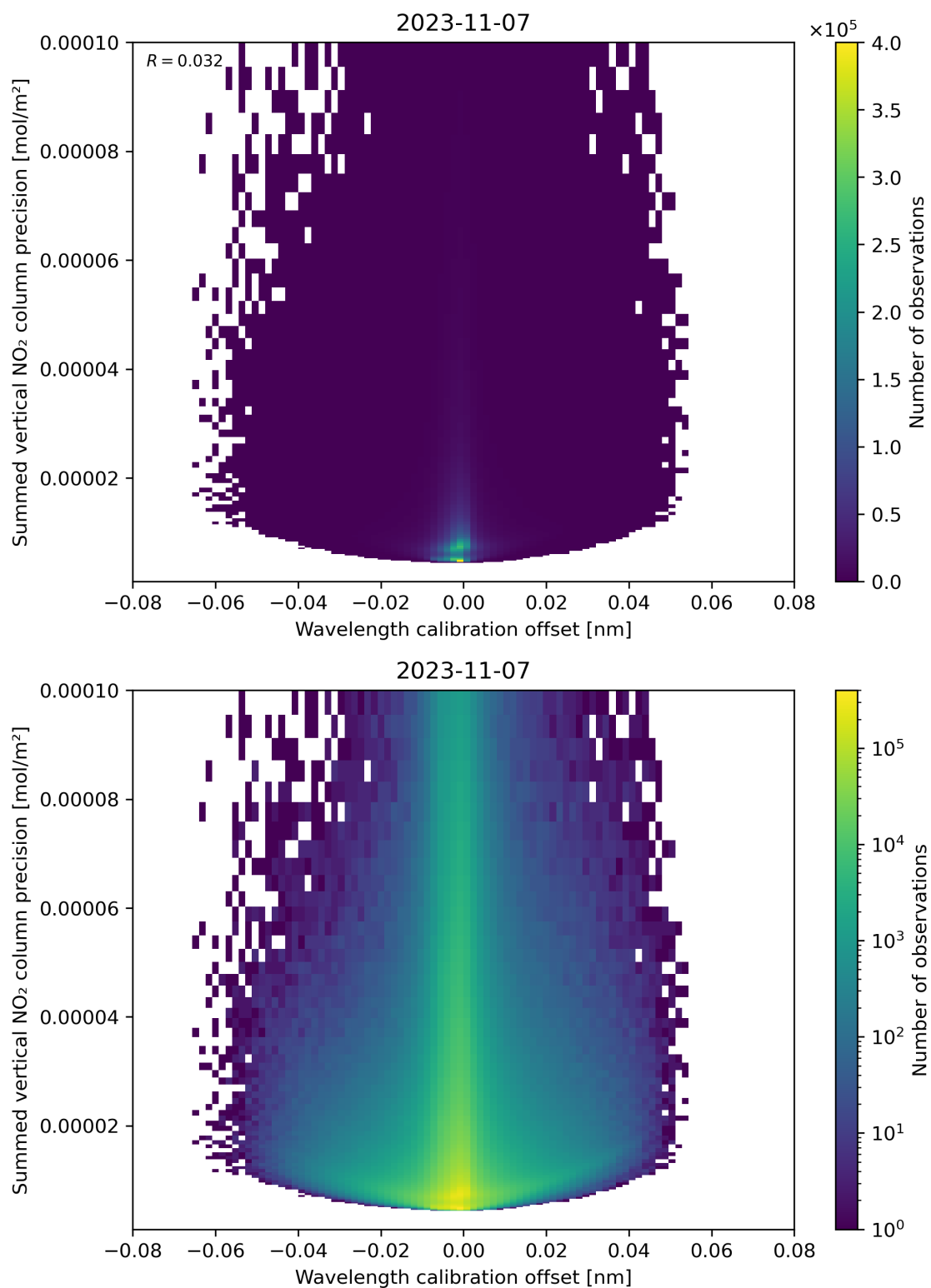
Figure 178: Scatter density plot of “Wavelength calibration offset” against “Summed vertical NO 2 column precision” for 2023-11-07 to 2023-11-08.
