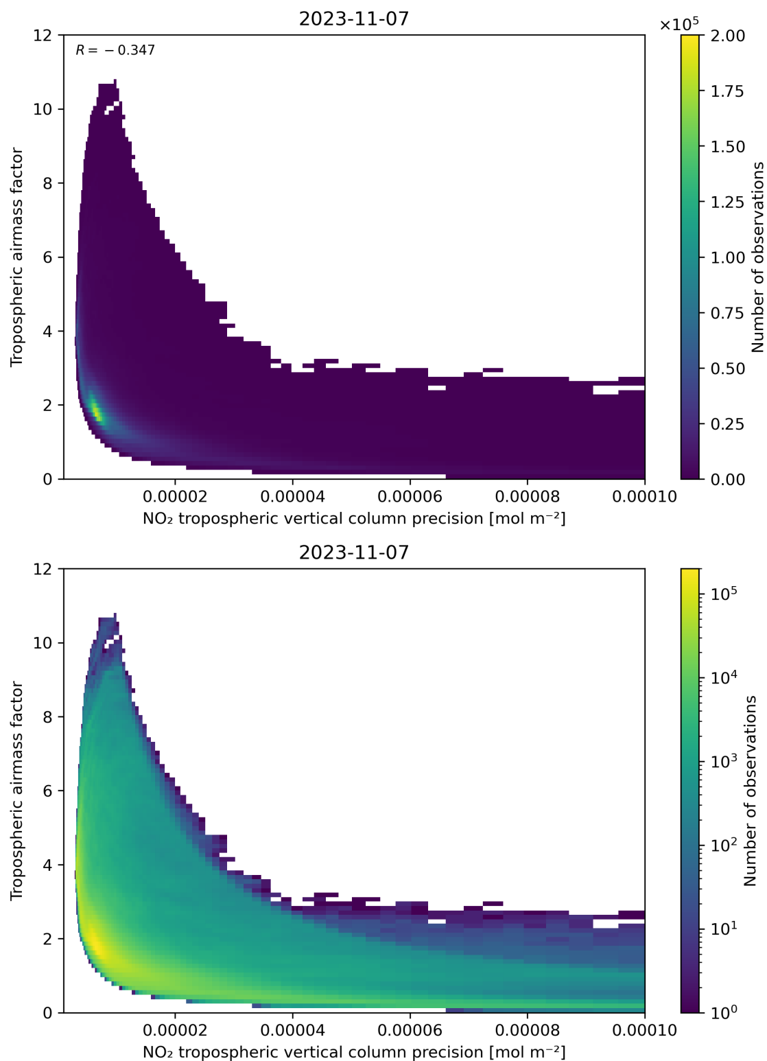
Figure 133: Scatter density plot of “NO 2 tropospheric vertical column precision” against “Tropospheric airmass factor” for 2023-11-07 to 2023-11-08.
