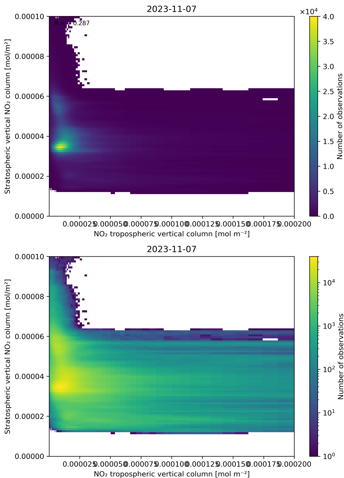
Figure 125: Scatter density plot of “NO 2 tropospheric vertical column” against “Stratospheric vertical NO 2 column” for 2023-11-07 to 2023-11-08.
