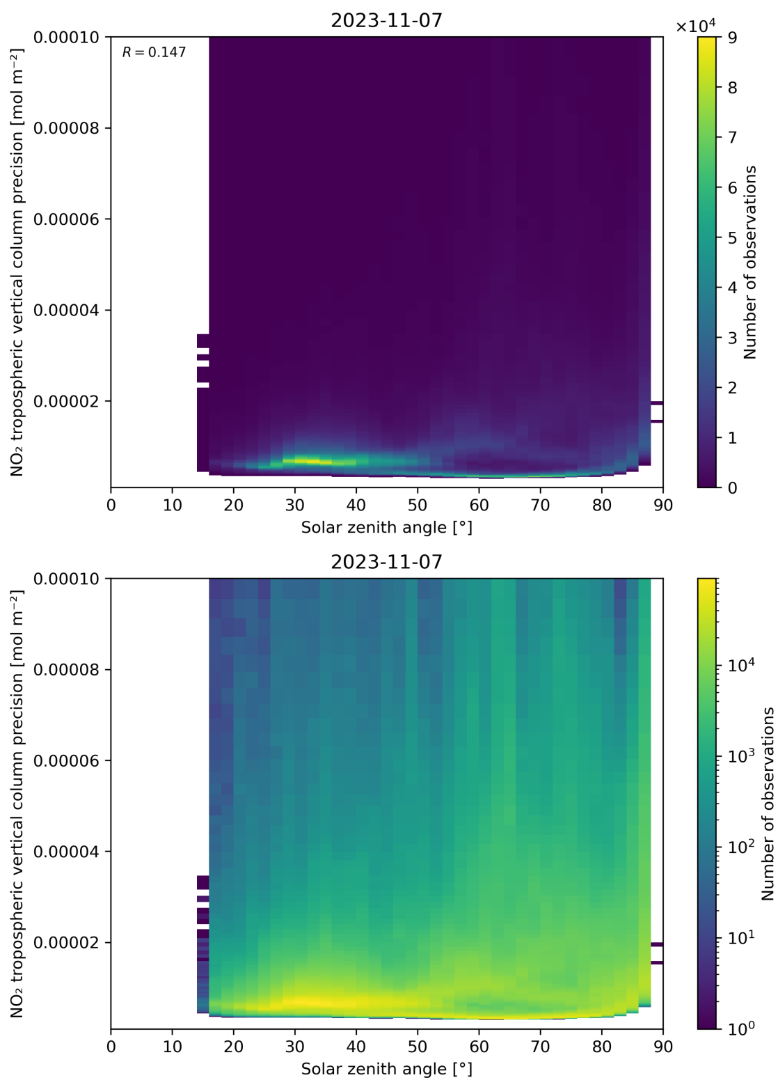
Figure 156: Scatter density plot of “Solar zenith angle” against “NO 2 tropospheric vertical column precision” for 2023-11-07 to 2023-11-08.
