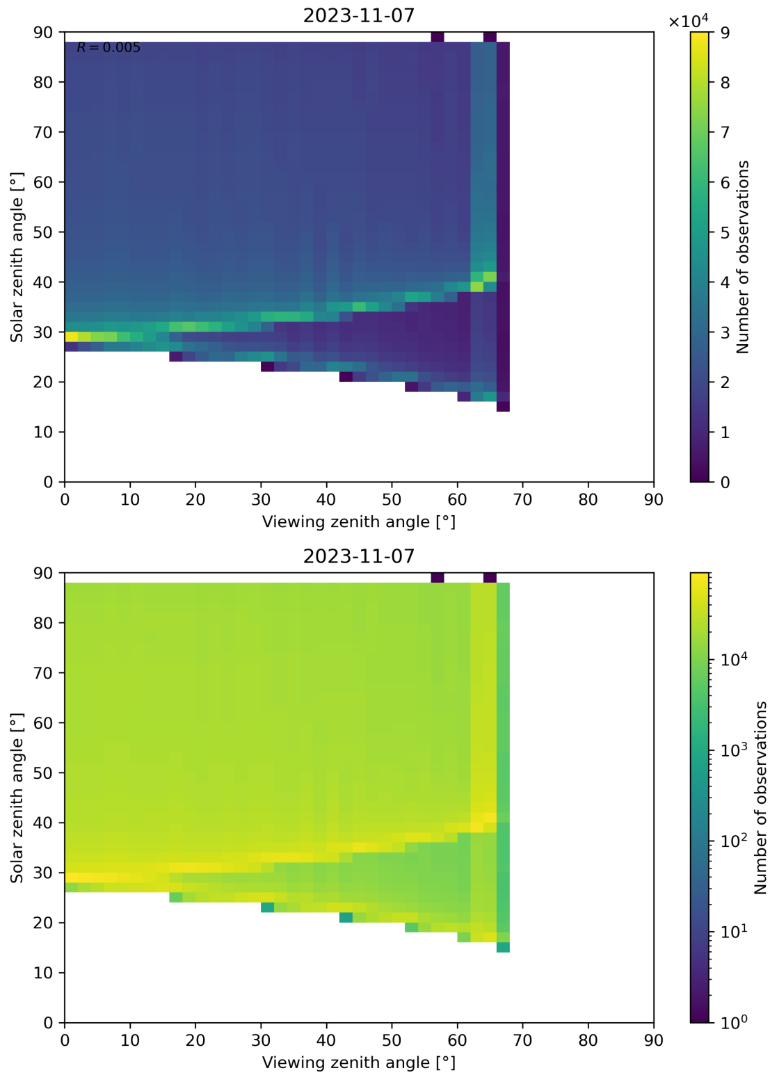
Figure 172: Scatter density plot of “Viewing zenith angle” against “Solar zenith angle” for 2023-11-07 to 2023-11-08.
