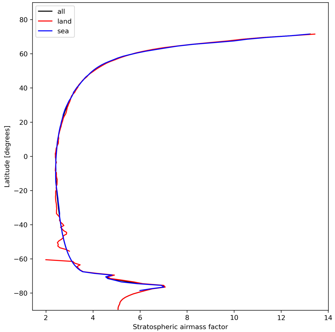
Figure 27: Zonal average of “Stratospheric airmass factor” for 2023-11-07 to 2023-11-08.
