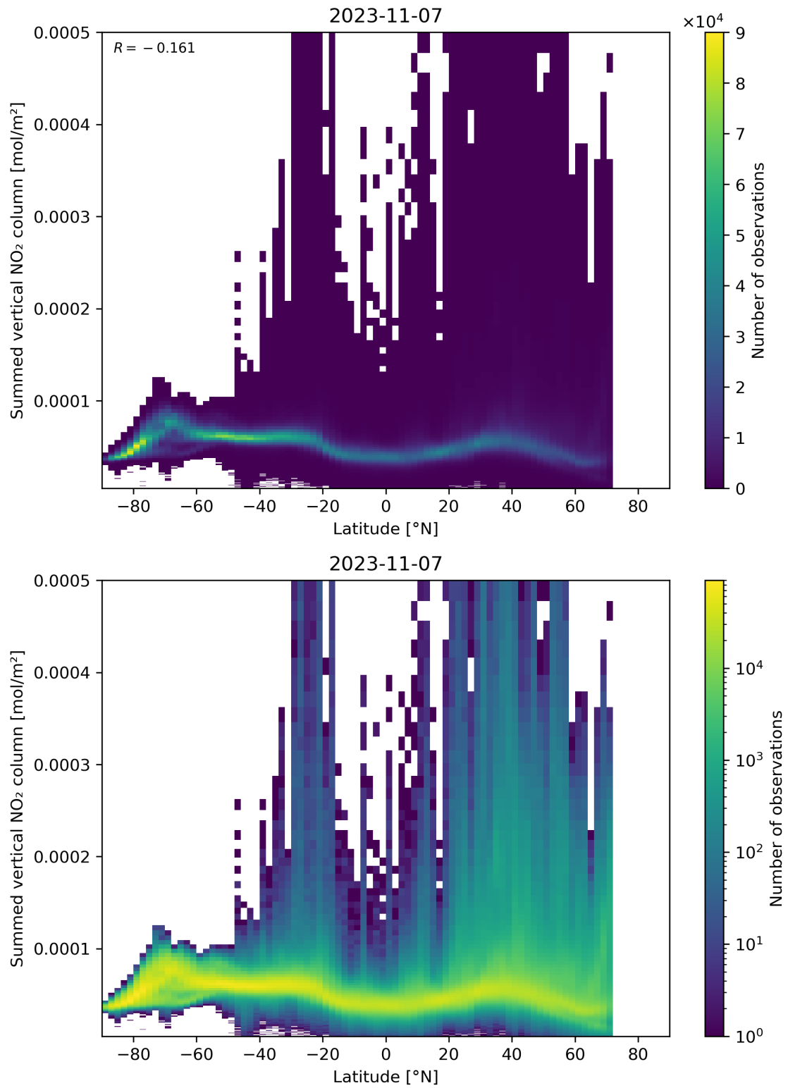
Figure 88: Scatter density plot of “Latitude” against “Summed vertical NO 2 column” for 2023-11-07 to 2023-11-08.
