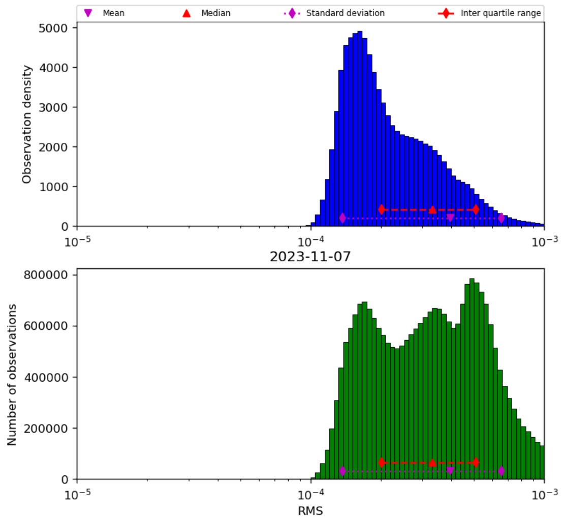
Figure 43: Histogram of “RMS” for 2023-11-07 to 2023-11-08
