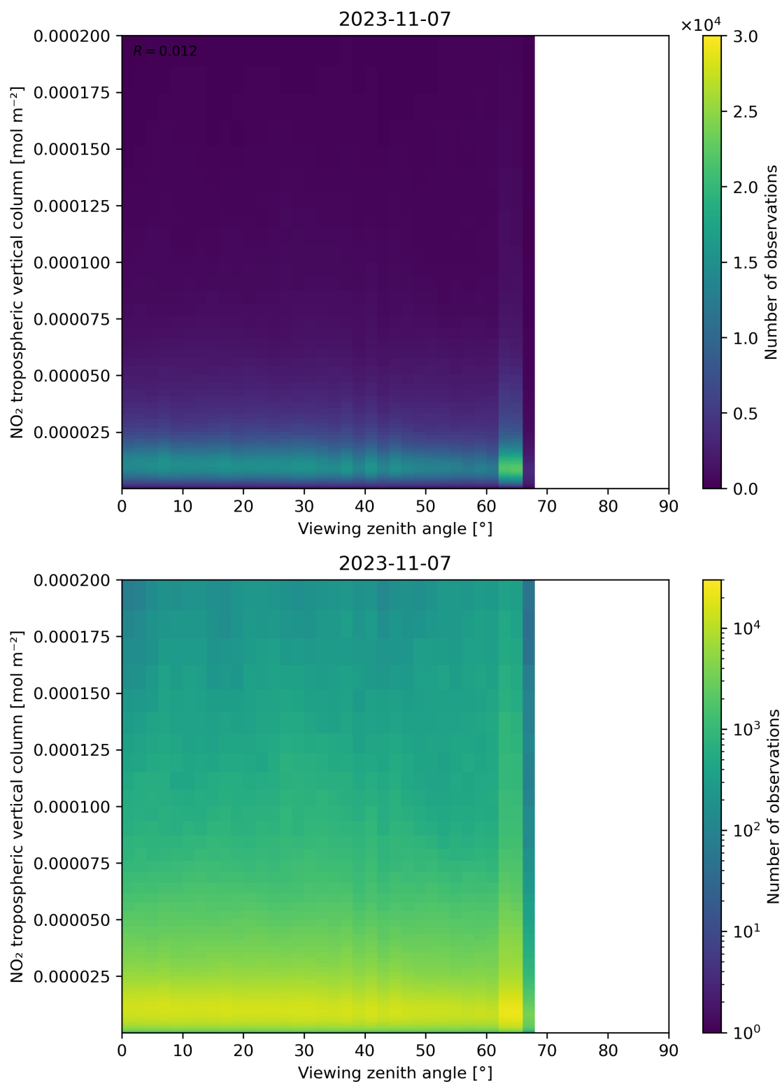
Figure 169: Scatter density plot of “Viewing zenith angle” against “NO 2 tropospheric vertical column” for 2023-11-07 to 2023-11-08.
