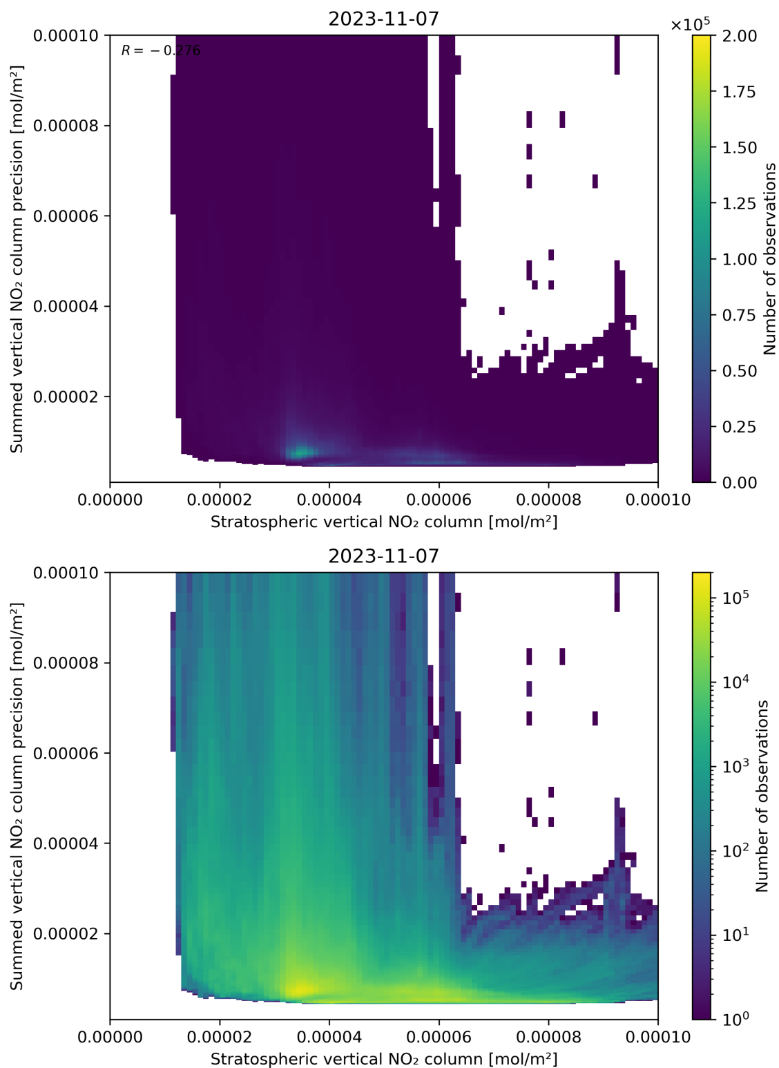
Figure 99: Scatter density plot of “Stratospheric vertical NO 2 column” against “Summed vertical NO 2 column precision” for 2023-11-07 to 2023-11-08.
