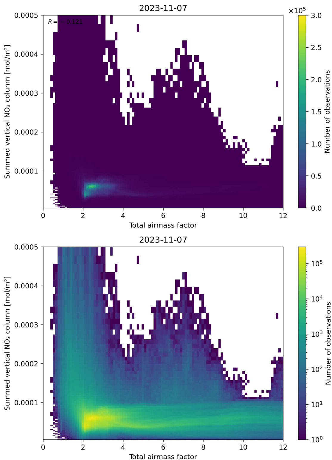
Figure 65: Scatter density plot of “Total airmass factor” against “Summed vertical NO 2 column” for 2023-11-07 to 2023-11-08.
