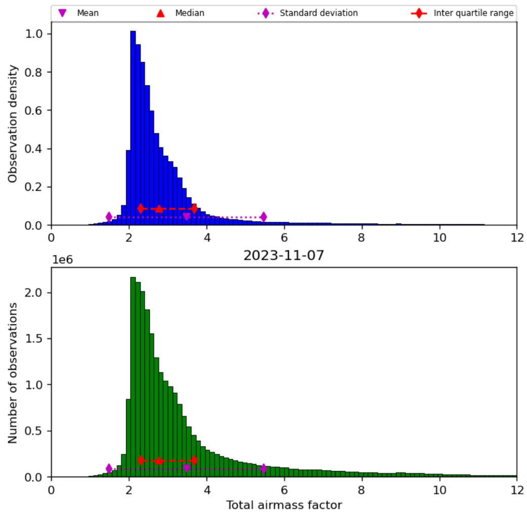
Figure 32: Histogram of “Total airmass factor” for 2023-11-07 to 2023-11-08
