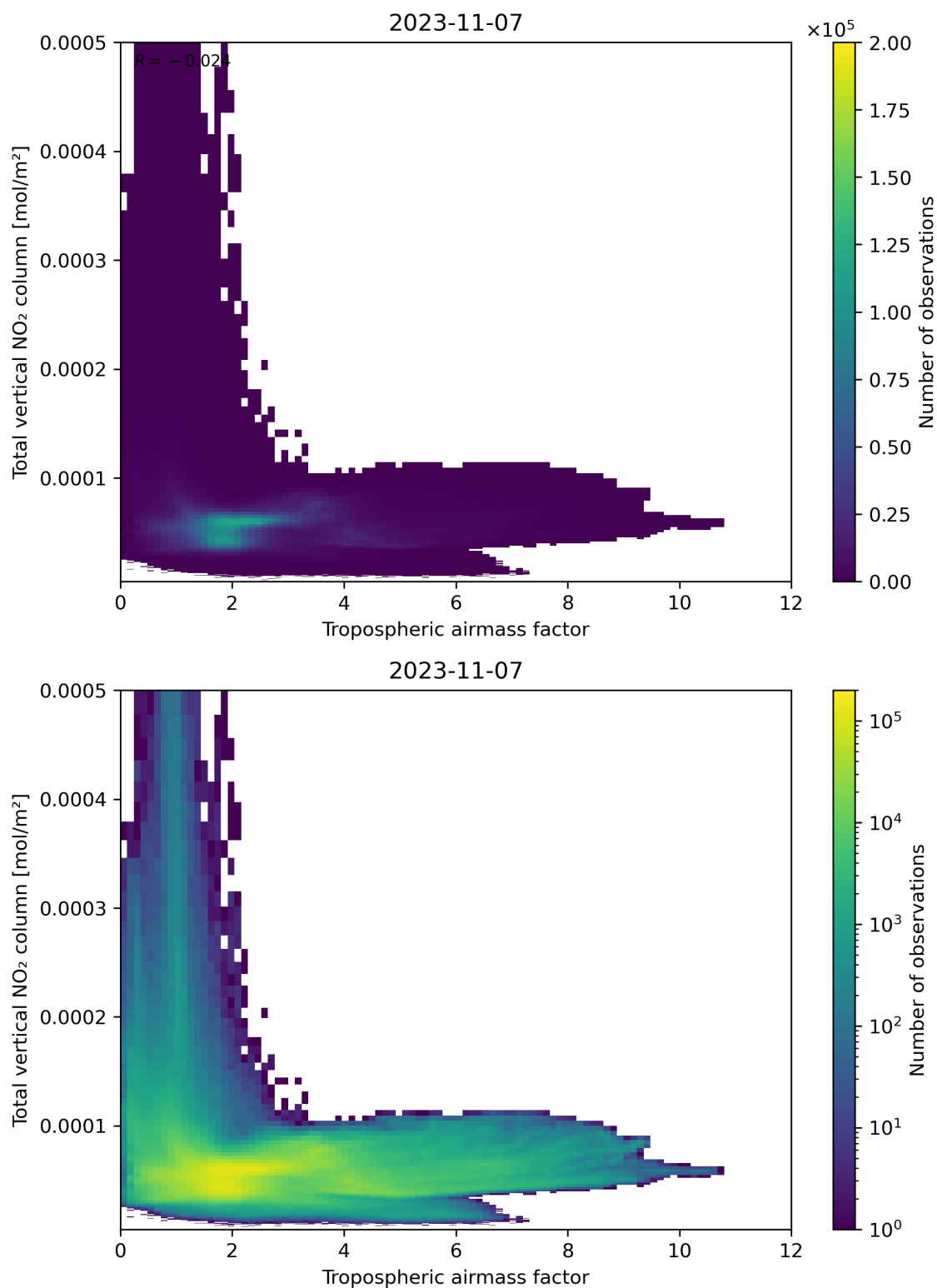
Figure 77: Scatter density plot of “Tropospheric airmass factor” against “Total vertical NO 2 column” for 2023-11-07 to 2023-11-08.
