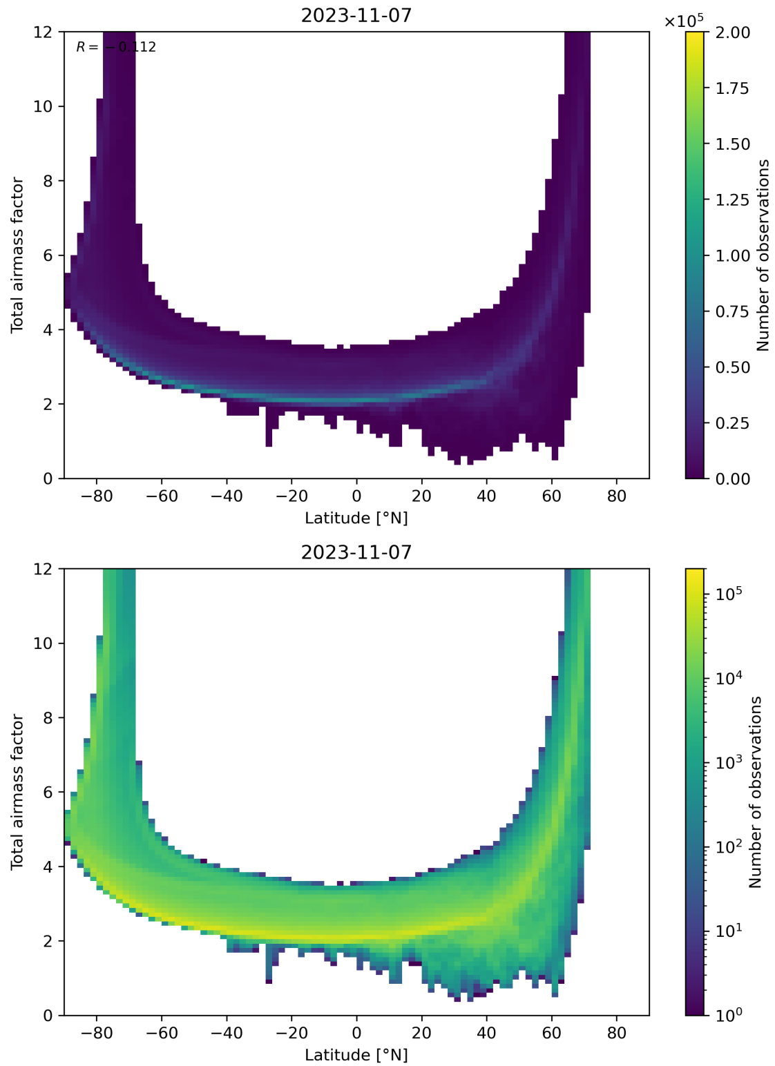
Figure 84: Scatter density plot of “Latitude” against “Total airmass factor” for 2023-11-07 to 2023-11-08.
