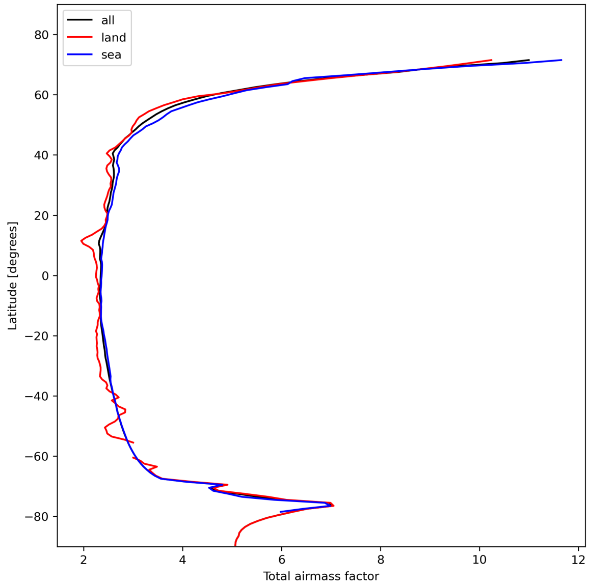
Figure 15: Zonal average of “Total airmass factor” for 2023-11-07 to 2023-11-08.
