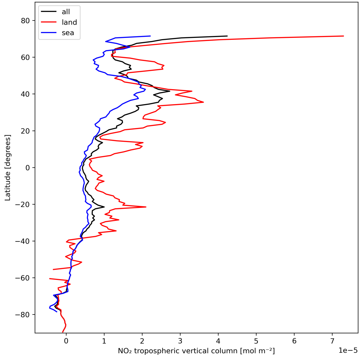
Figure 12: Zonal average of “NO 2 tropospheric vertical column” for 2023-11-07 to 2023-11-08.
