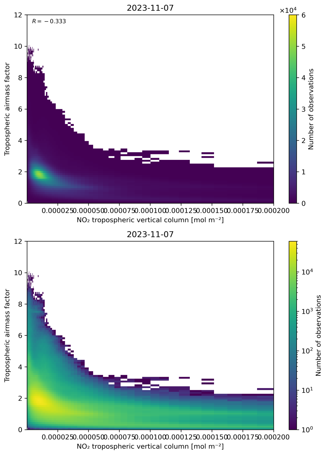
Figure 123: Scatter density plot of “NO 2 tropospheric vertical column” against “Tropospheric airmass factor” for 2023-11-07 to 2023-11-08.
