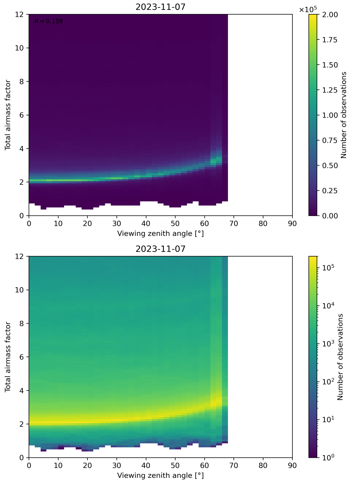
Figure 160: Scatter density plot of “Viewing zenith angle” against “Total airmass factor” for 2023-11-07 to 2023-11-08.
