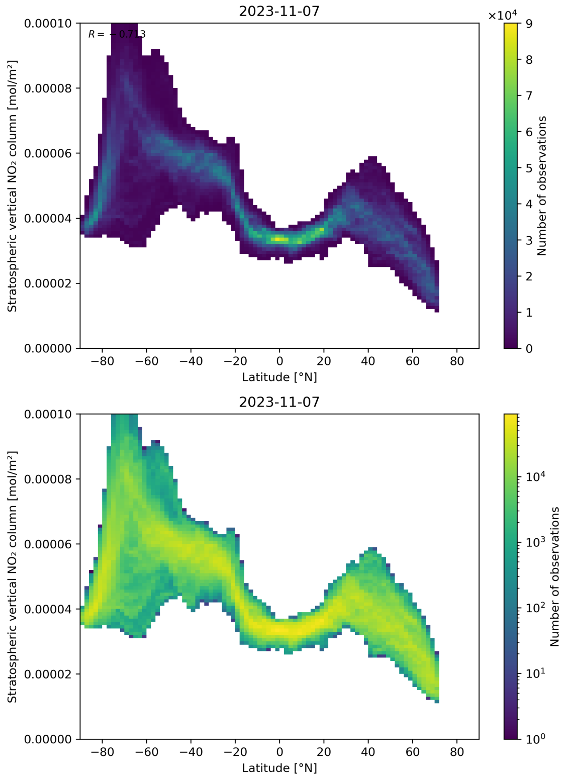
Figure 87: Scatter density plot of “Latitude” against “Stratospheric vertical NO 2 column” for 2023-11-07 to 2023-11-08.
