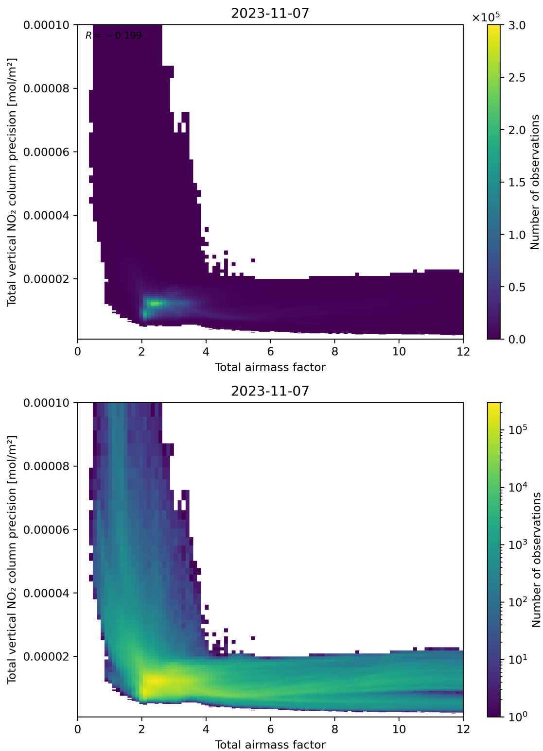
Figure 68: Scatter density plot of “Total airmass factor” against “Total vertical NO 2 column precision” for 2023-11-07 to 2023-11-08.
