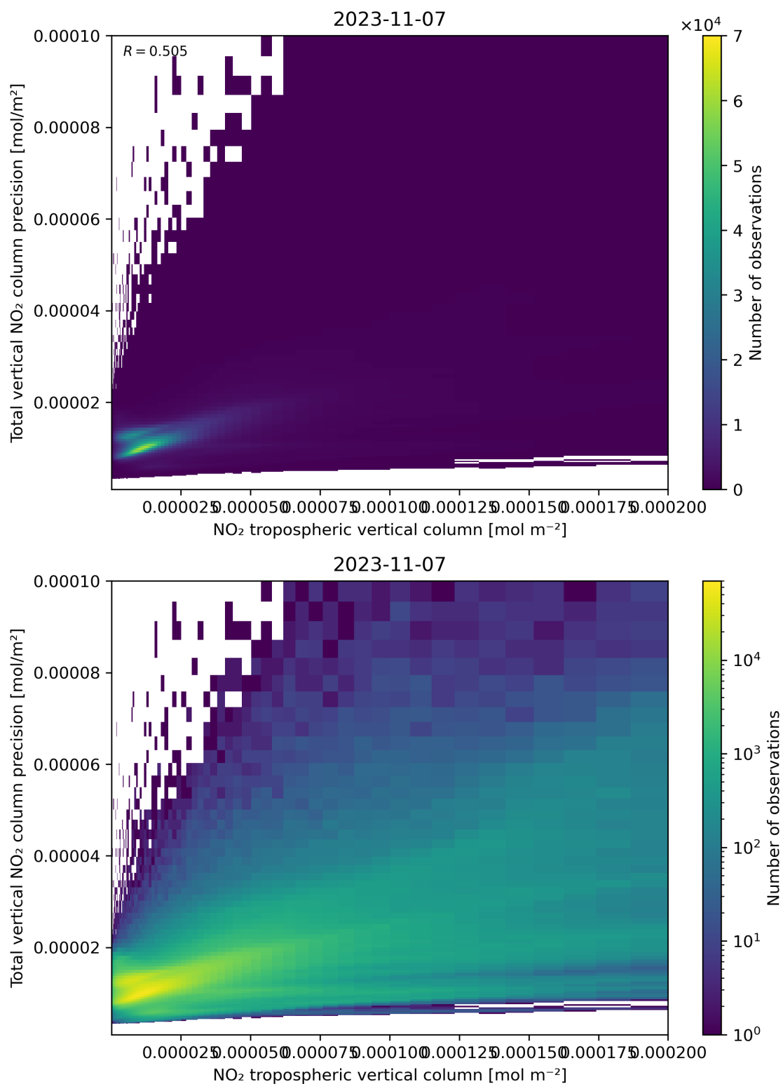
Figure 129: Scatter density plot of “NO 2 tropospheric vertical column” against “Total vertical NO 2 column precision” for 2023-11-07 to 2023-11-08.
