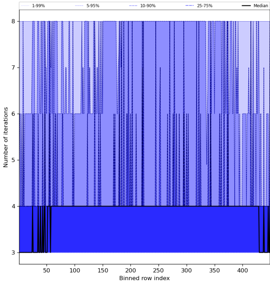
Figure 51: Along track statistics of “Number of iterations” for 2023-11-07 to 2023-11-08
