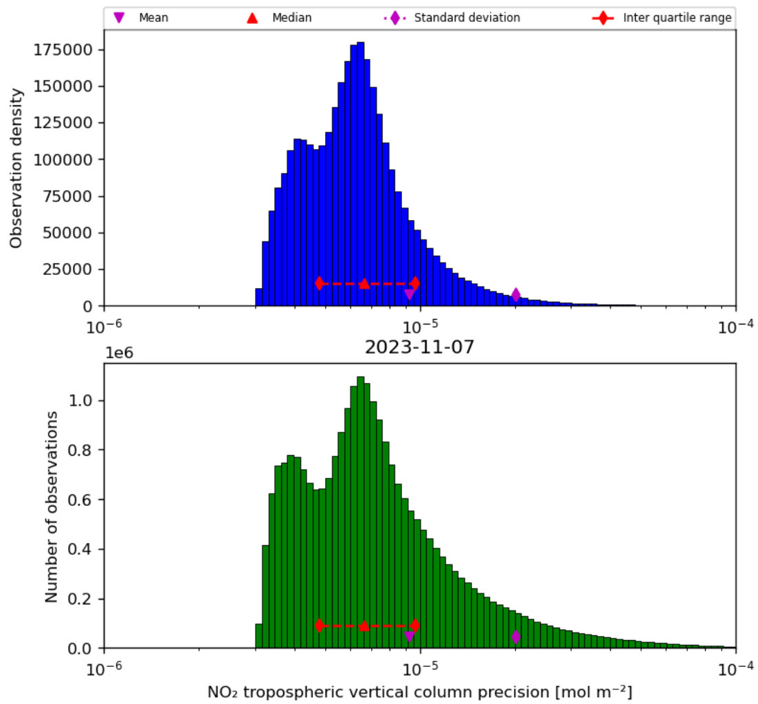
Figure 30: Histogram of “NO 2 tropospheric vertical column precision” for 2023-11-07 to 2023-11-08
