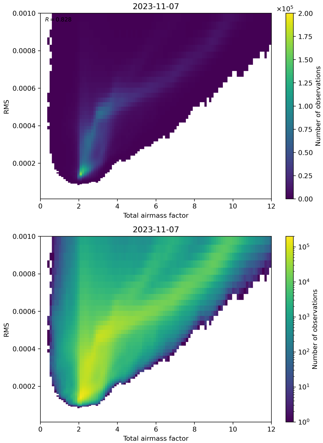
Figure 69: Scatter density plot of “Total airmass factor” against “RMS” for 2023-11-07 to 2023-11-08.
