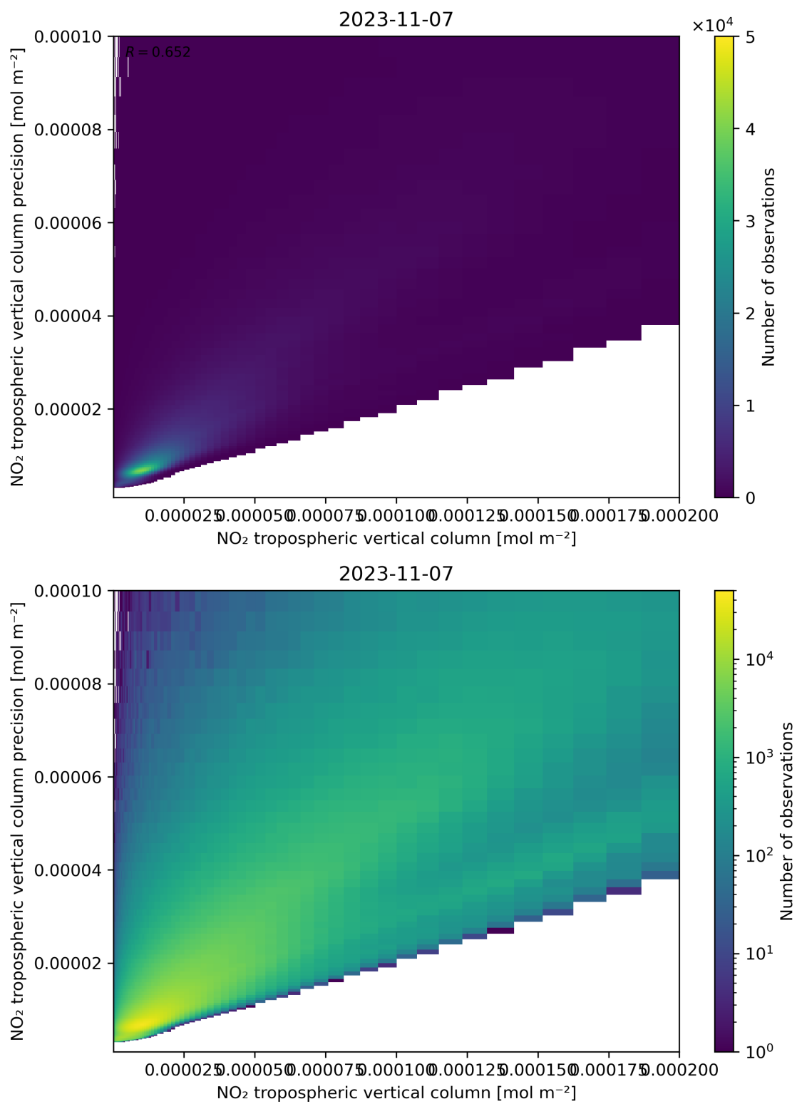
Figure 130: Scatter density plot of “NO 2 tropospheric vertical column” against “NO 2 tropospheric vertical column precision” for 2023-11-07 to 2023-11-08.
