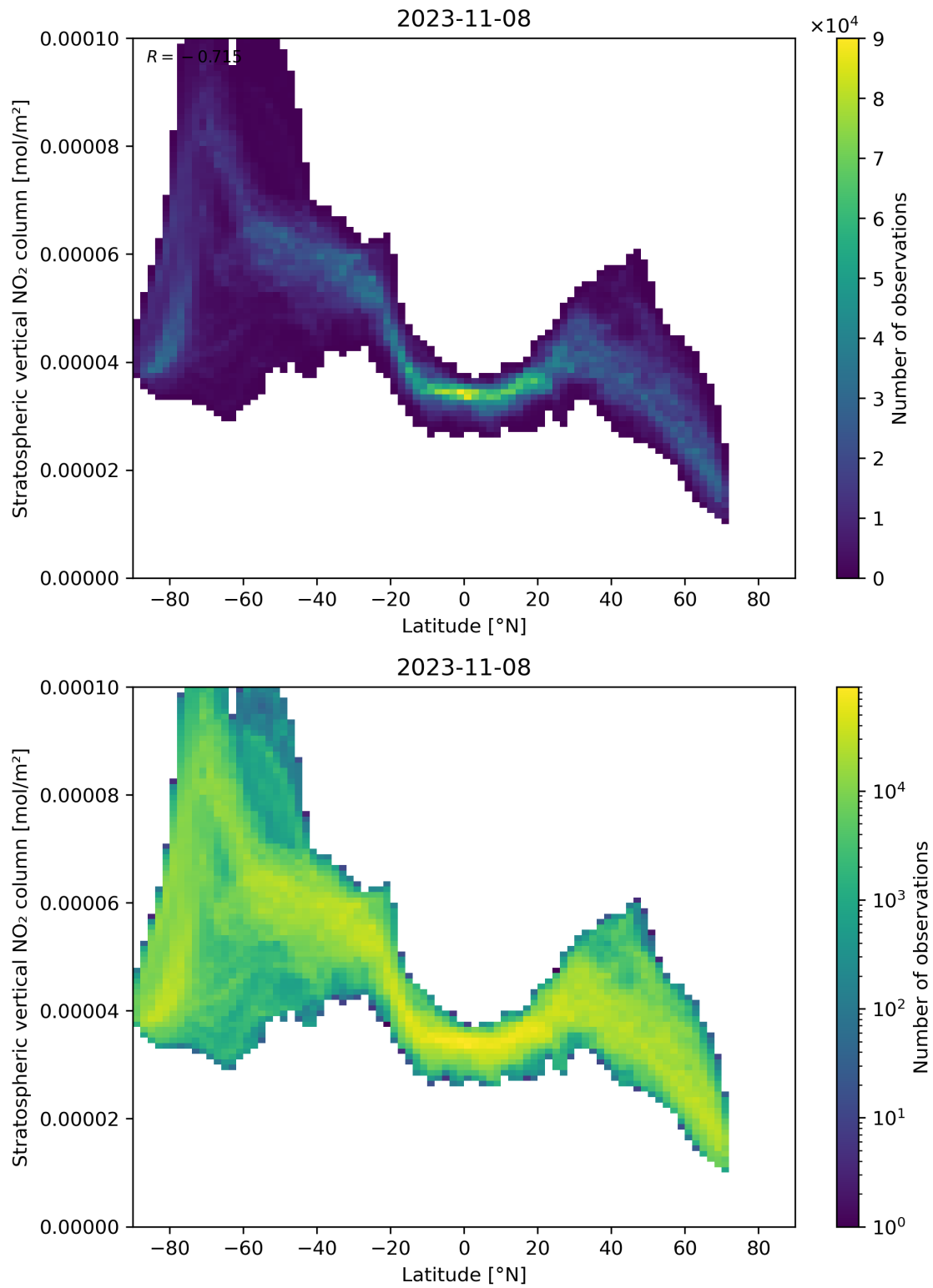
Figure 87: Scatter density plot of “Latitude” against “Stratospheric vertical NO 2 column” for 2023-11-07 to 2023-11-09.
