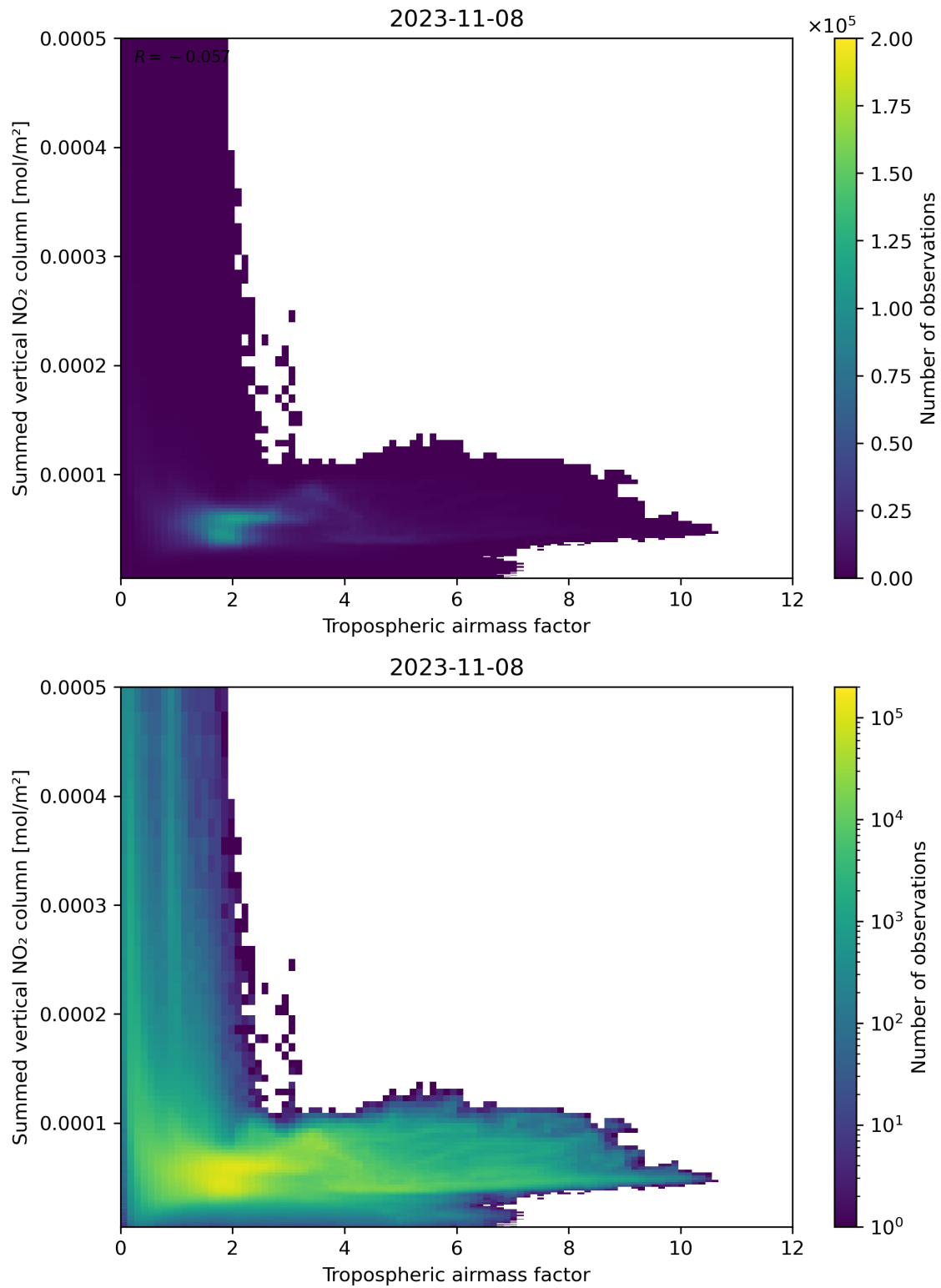
Figure 75: Scatter density plot of “Tropospheric airmass factor” against “Summed vertical NO 2 column” for 2023-11-07 to 2023-11-09.
