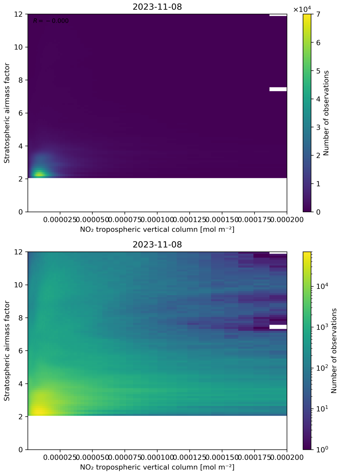
Figure 121: Scatter density plot of “NO 2 tropospheric vertical column” against “Stratospheric air mass factor” for 2023-11-07 to 2023-11-09.
