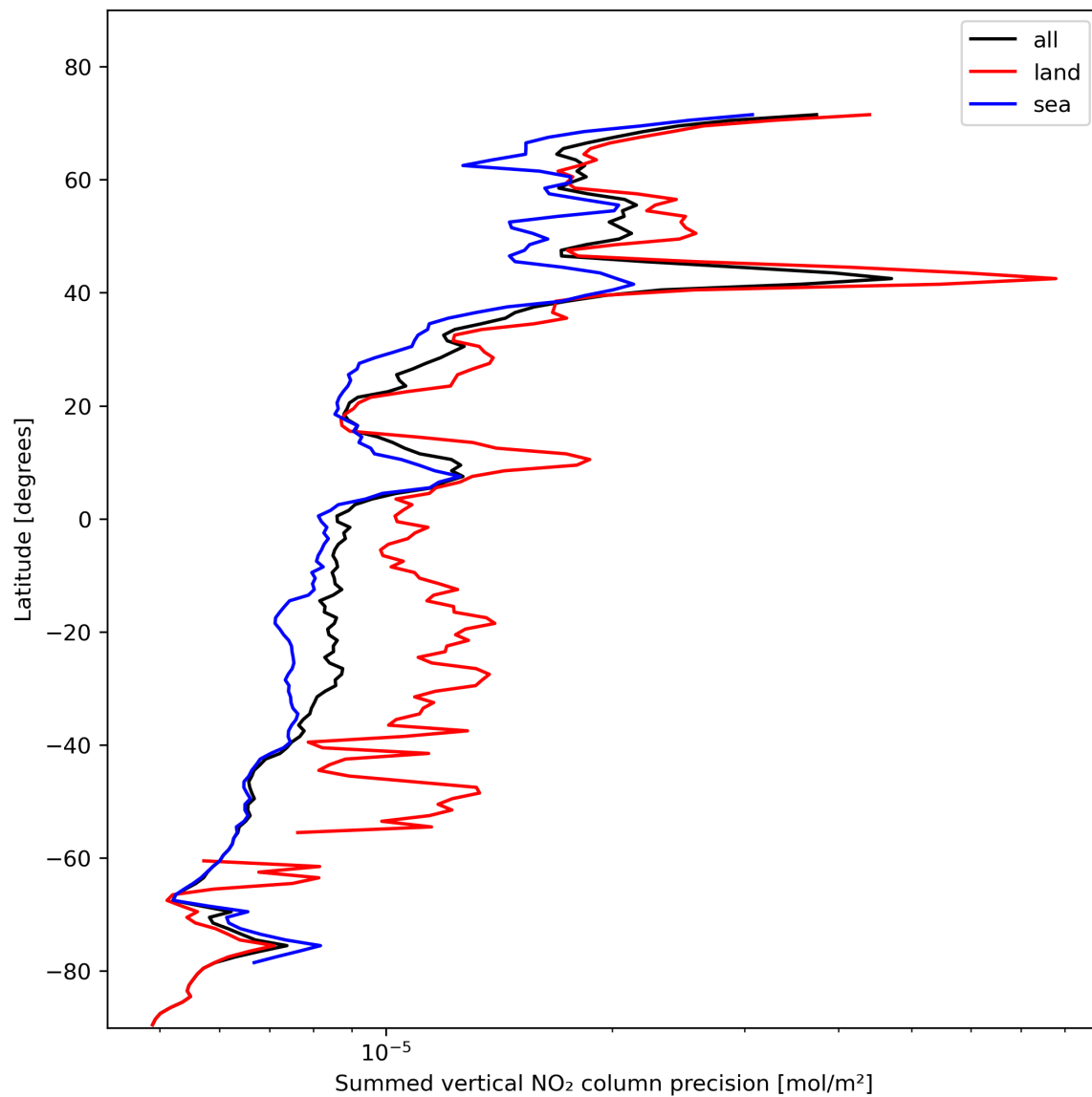
Figure 24: Zonal average of “Summed vertical NO 2 column precision” for 2023-11-07 to 2023-11-09.
