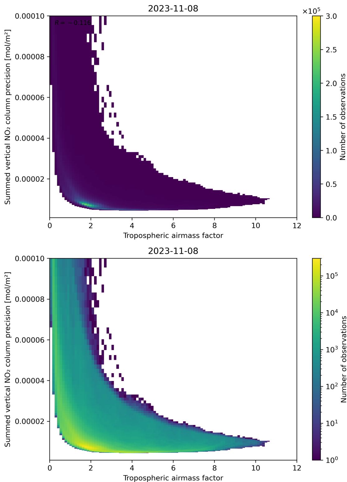
Figure 76: Scatter density plot of “Tropospheric air mass factor” against “Summed vertical NO 2 column precision” for 2023-11-07 to 2023-11-09.
