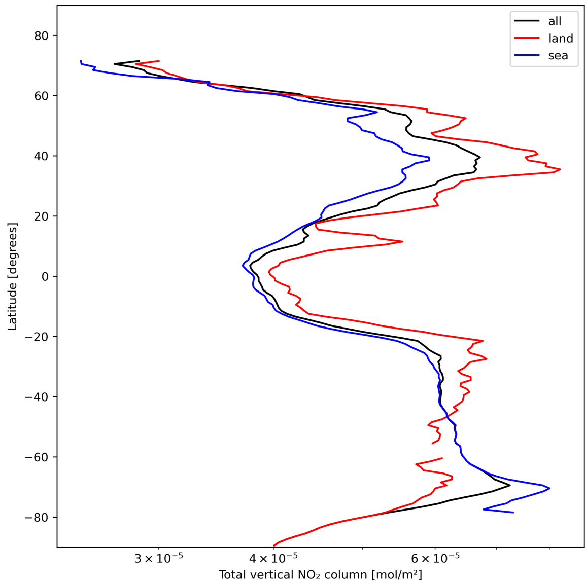
Figure 21: Zonal average of “Total vertical NO 2 column” for 2023-11-07 to 2023-11-09.
