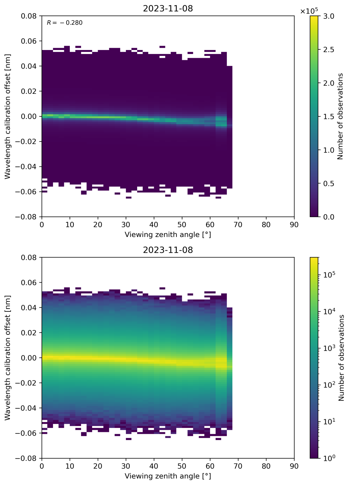
Figure 173: Scatter density plot of “Viewing zenith angle” against “Wavelength calibration offset” for 2023-11-07 to 2023-11-09.
