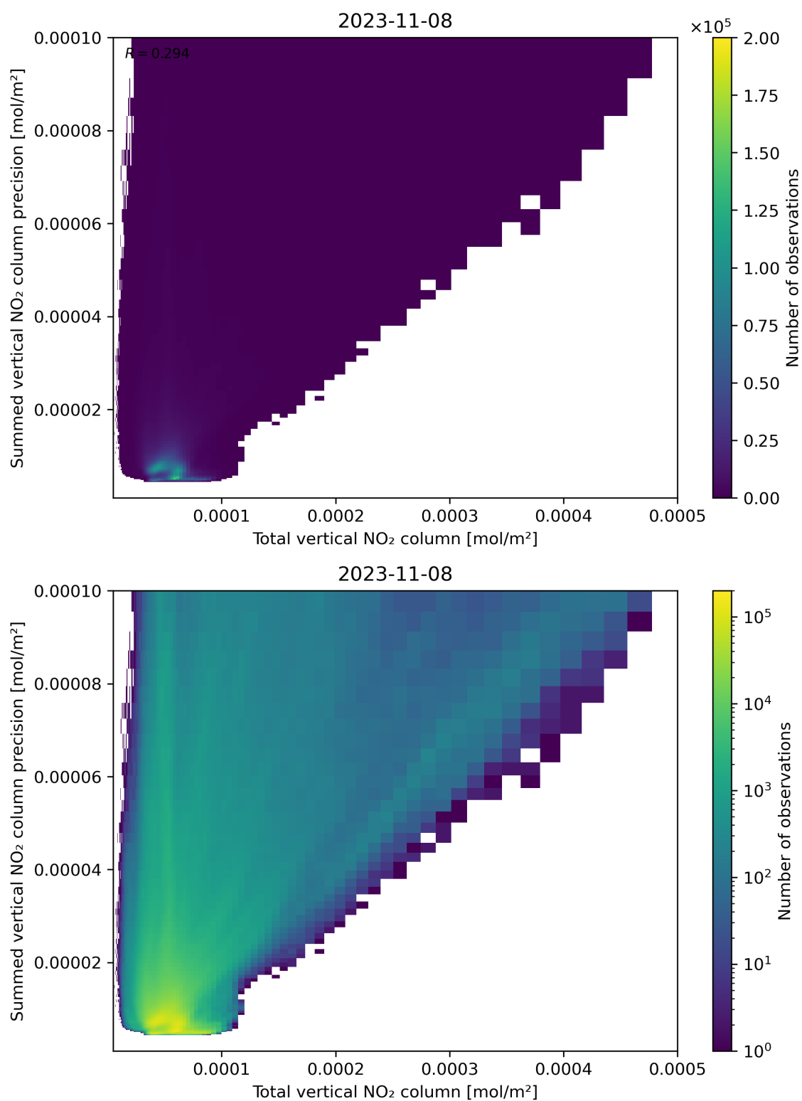
Figure 113: Scatter density plot of “Total vertical NO 2 column” against “Summed vertical NO 2 column precision” for 2023-11-07 to 2023-11-09.
