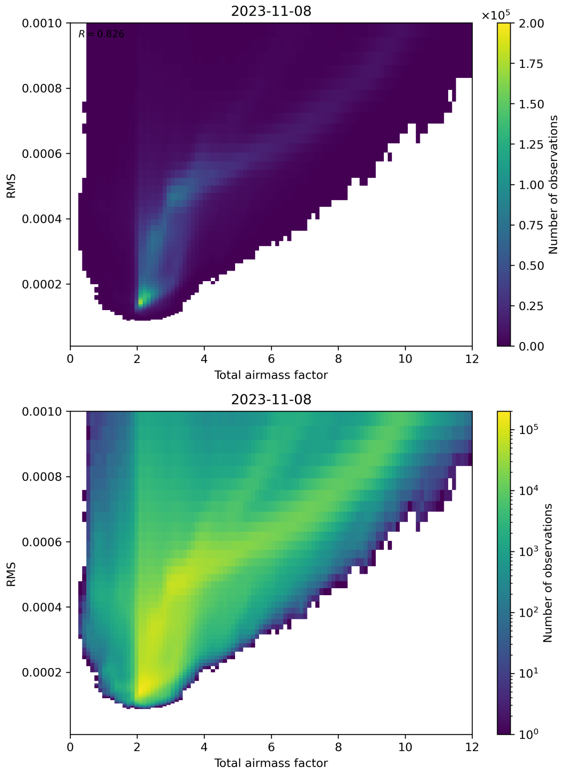
Figure 69: Scatter density plot of “Total airmass factor” against “RMS” for 2023-11-07 to 2023-11-09.
