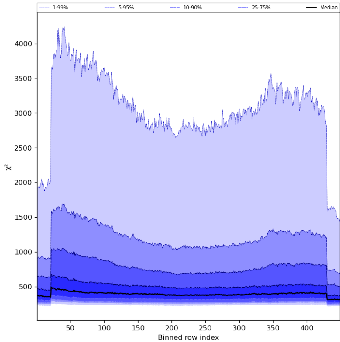
Figure 59: Along track statistics of “ \chi^2 ” for 2023-11-07 to 2023-11-09
