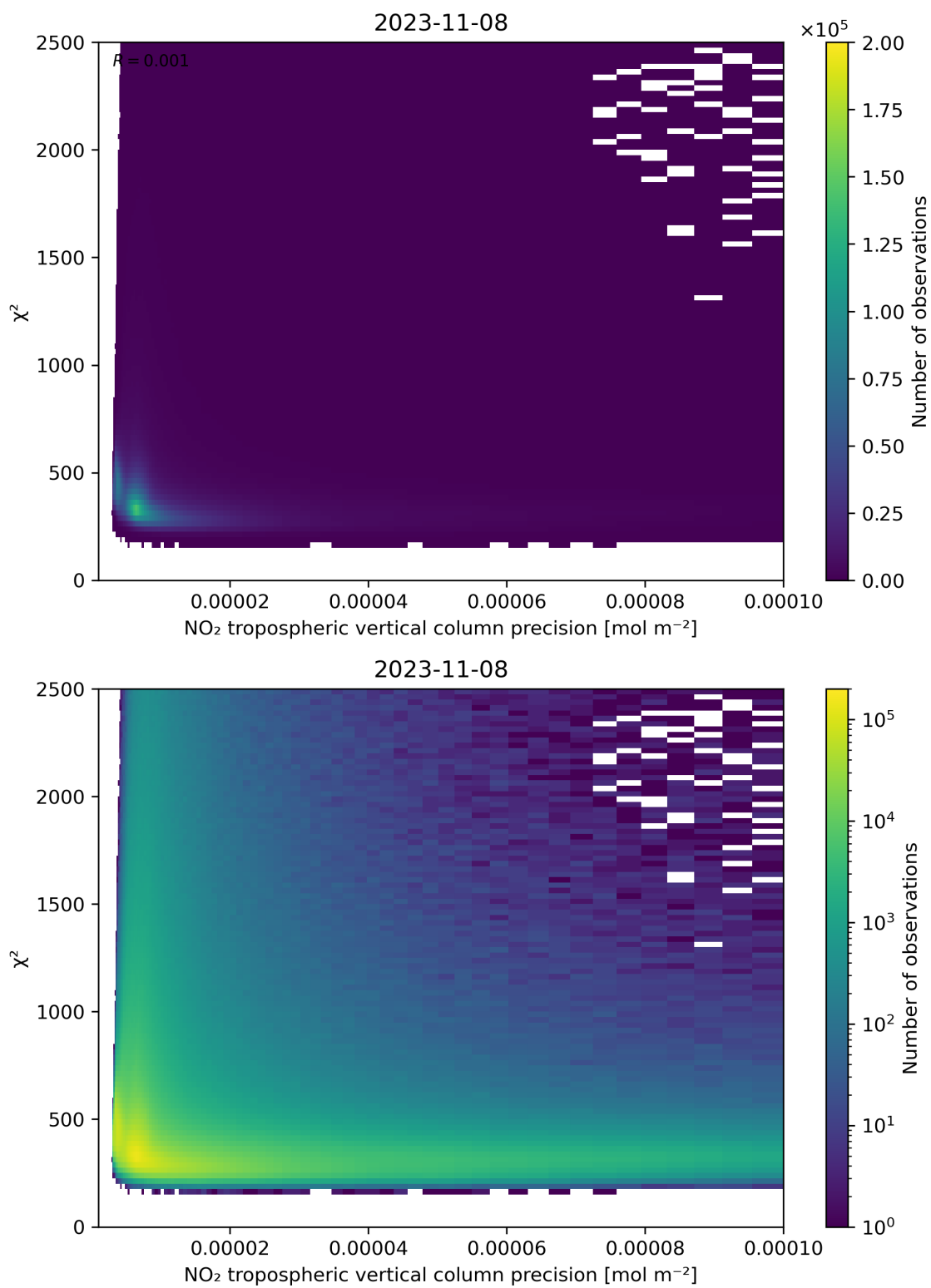
Figure 134: Scatter density plot of “NO 2 tropospheric vertical column precision” against “ \chi^2 ” for 2023-11-07 to 2023-11-09.
