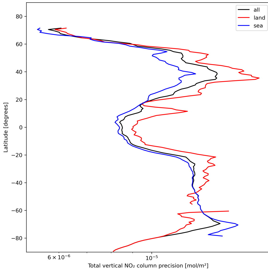
Figure 22: Zonal average of “Total vertical NO 2 column precision” for 2023-11-07 to 2023-11-09.
