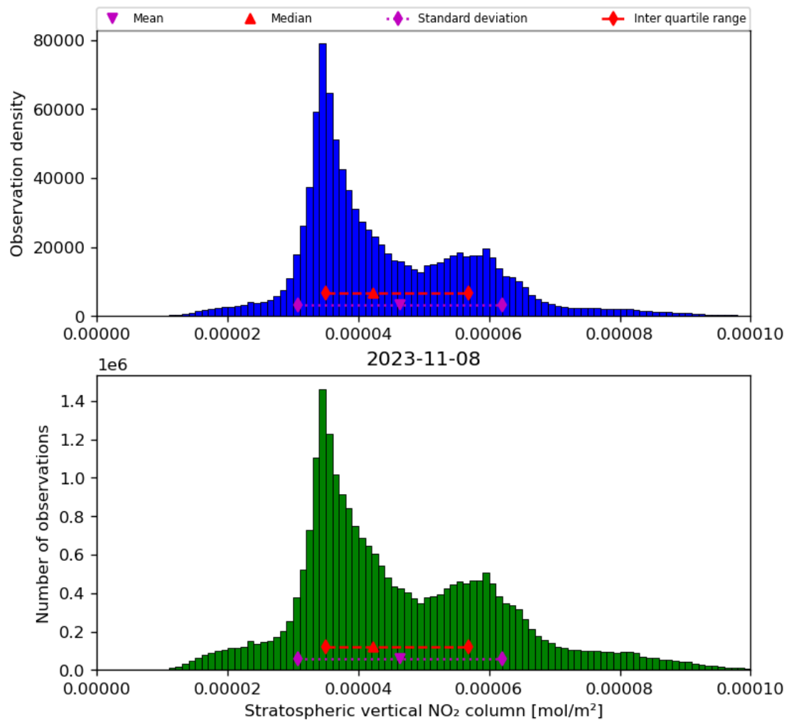
Figure 36: Histogram of “Stratospheric vertical NO 2 column” for 2023-11-07 to 2023-11-09
