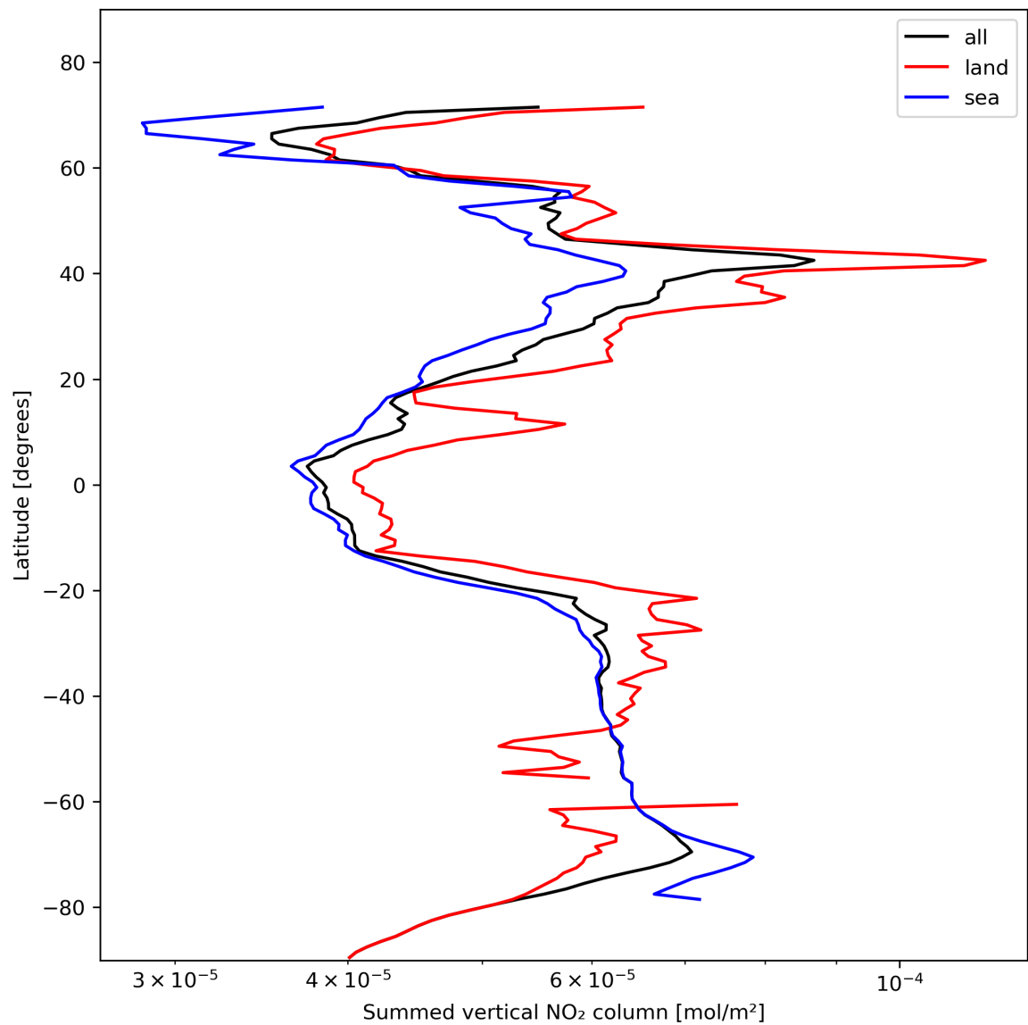
Figure 23: Zonal average of “Summed vertical NO 2 column” for 2023-11-07 to 2023-11-09.
