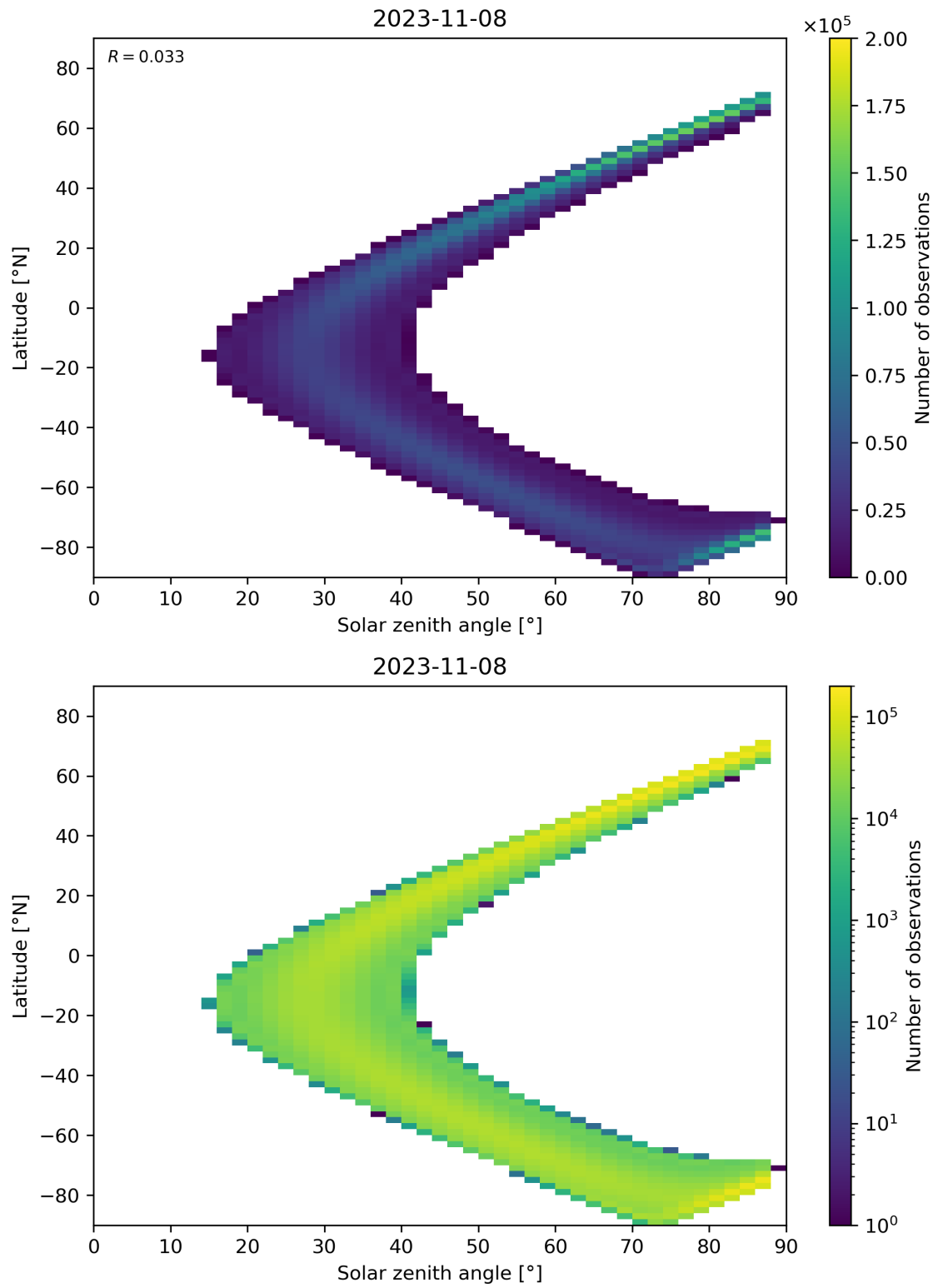
Figure 149: Scatter density plot of “Solar zenith angle” against “Latitude” for 2023-11-07 to 2023-11-09.
