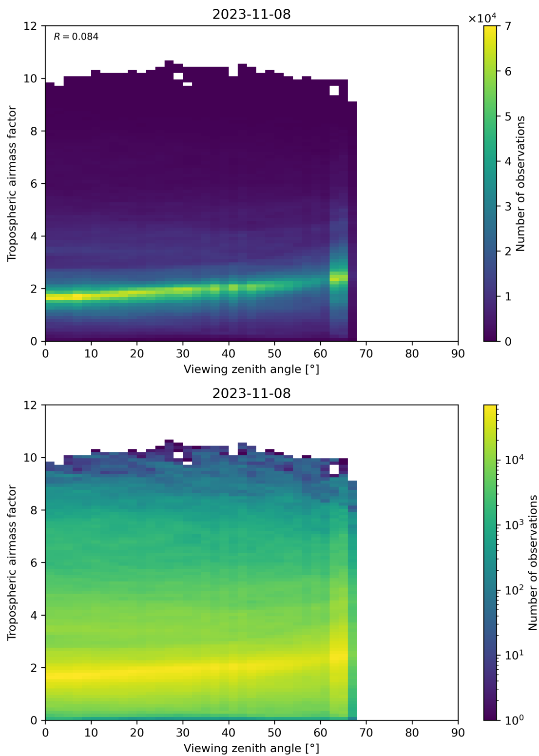
Figure 161: Scatter density plot of “Viewing zenith angle” against “Tropospheric airmass factor” for 2023-11-07 to 2023-11-09.
