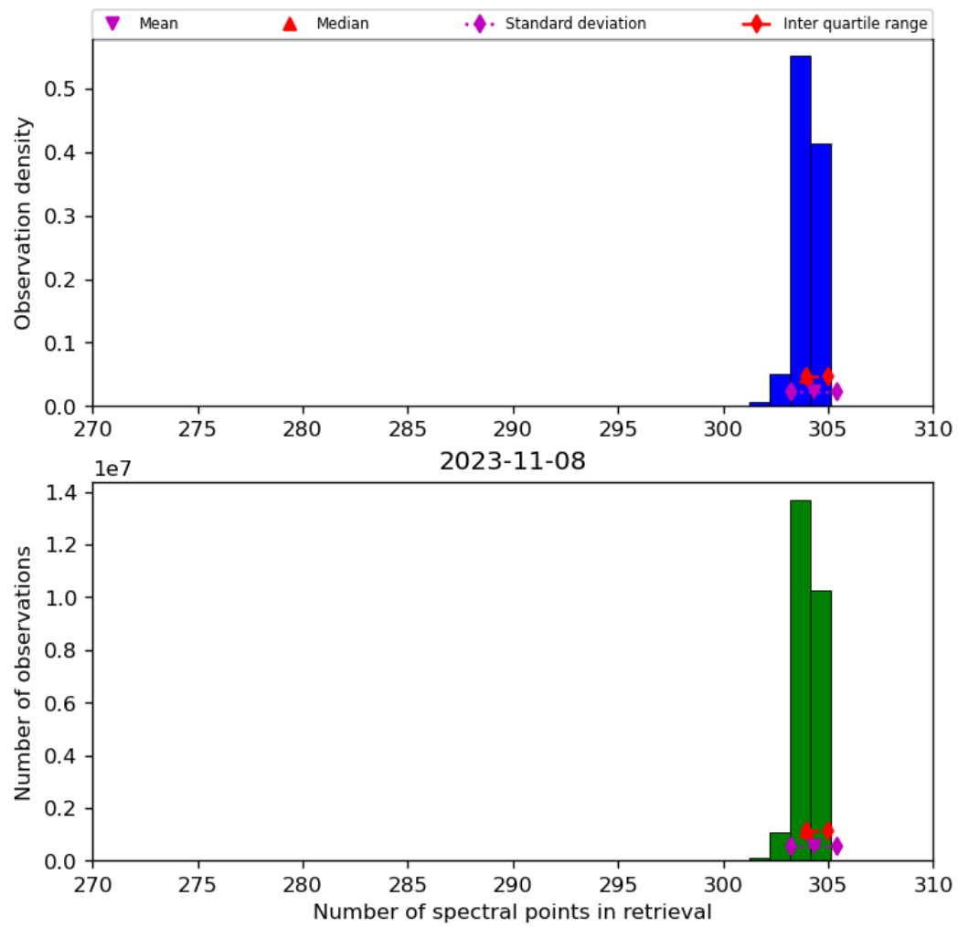
Figure 33: Histogram of “Number of spectral points in retrieval” for 2023-11-07 to 2023-11-09
