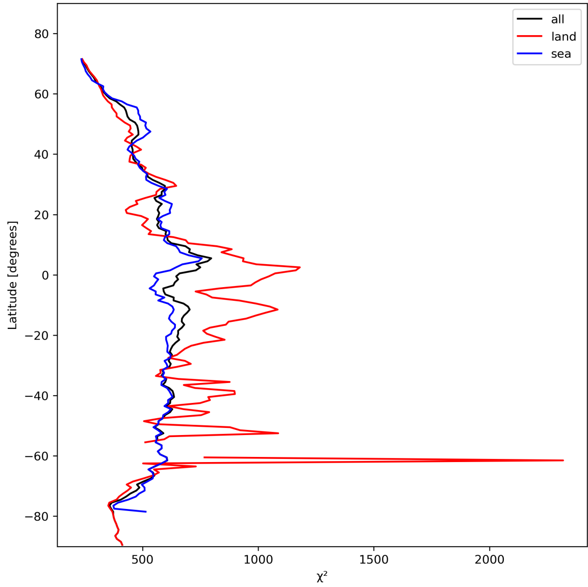
Figure 25: Zonal average of “ \chi^2 ” for 2023-11-07 to 2023-11-09.
