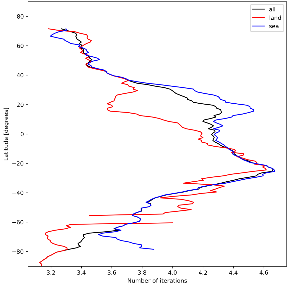
Figure 17: Zonal average of “Number of iterations” for 2023-11-07 to 2023-11-09.
