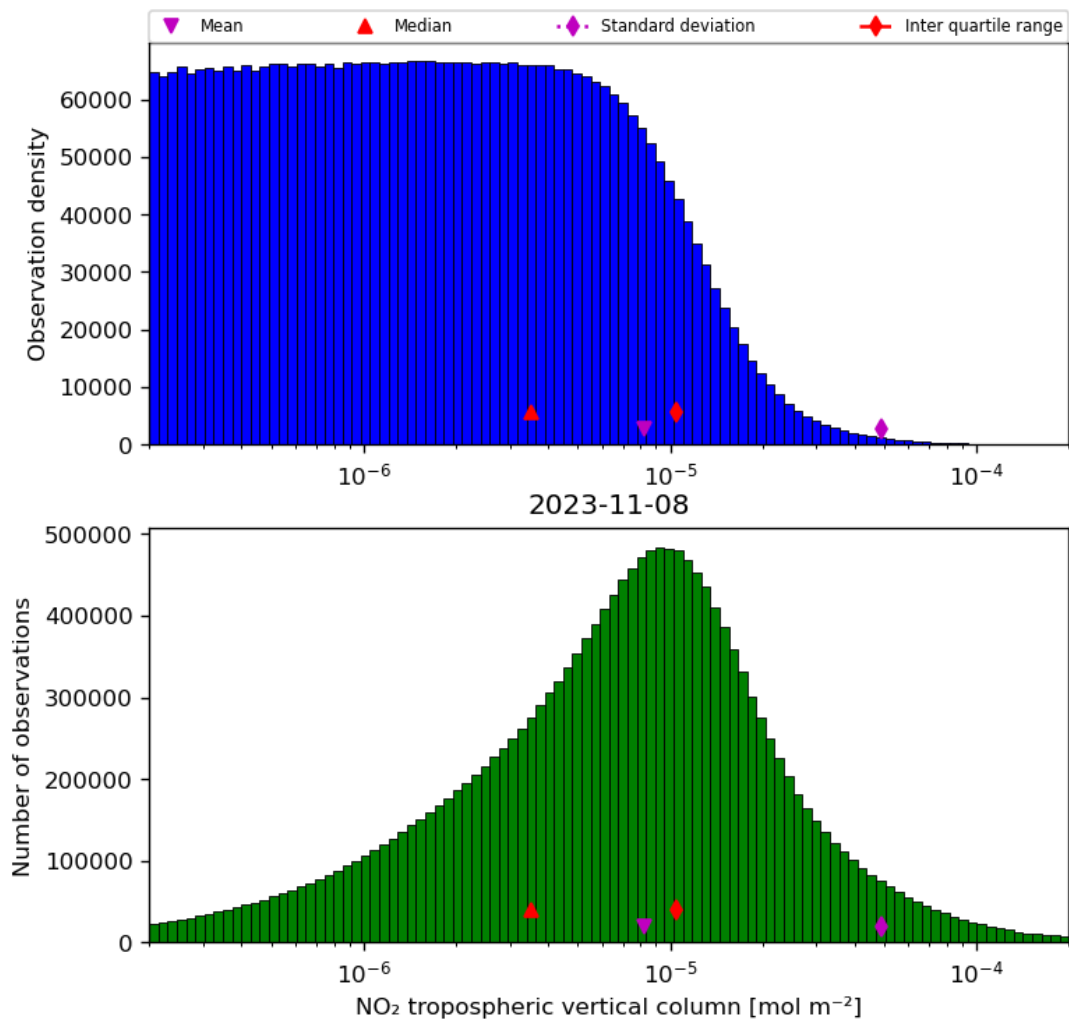
Figure 29: Histogram of “NO 2 tropospheric vertical column” for 2023-11-07 to 2023-11-09
