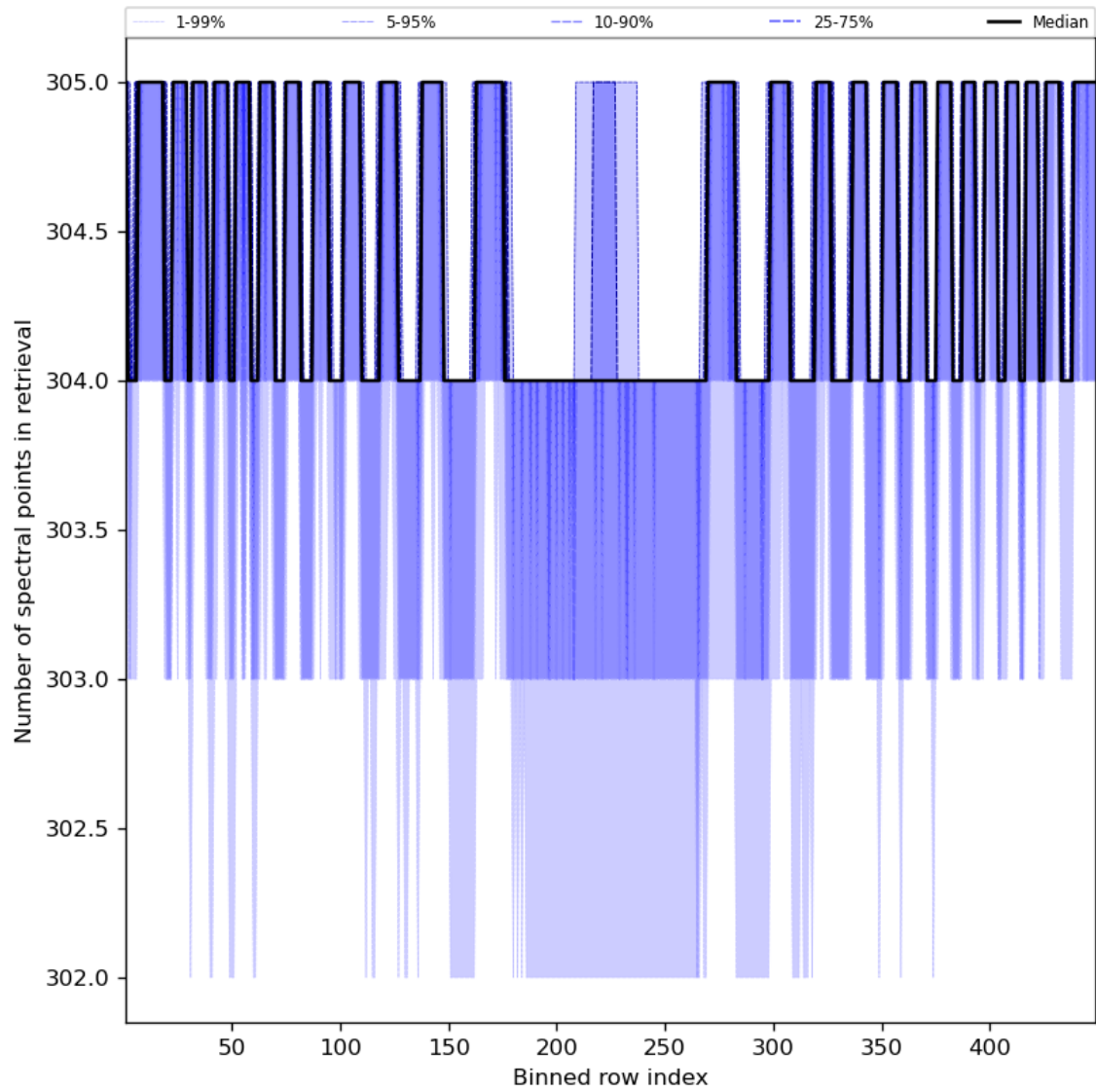
Figure 50: Along track statistics of “Number of spectral points in retrieval” for 2023-11-07 to 2023-11-09
