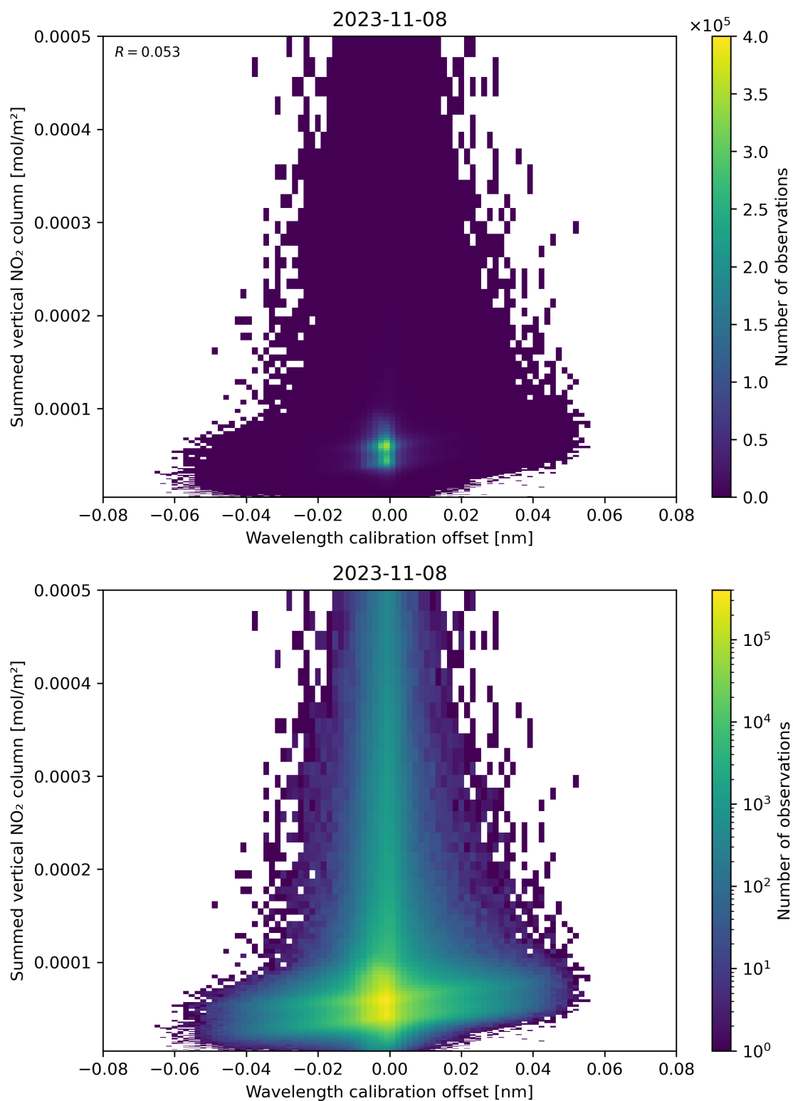
Figure 177: Scatter density plot of “Wavelength calibration offset” against “Summed vertical NO 2 column” for 2023-11-07 to 2023-11-09.
