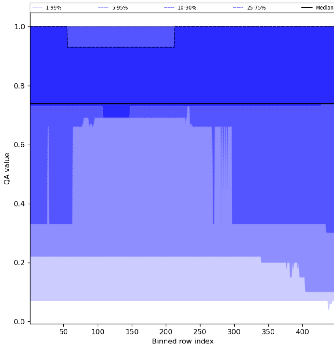
Figure 45: Along track statistics of “QA value” for 2023-11-07 to 2023-11-09
