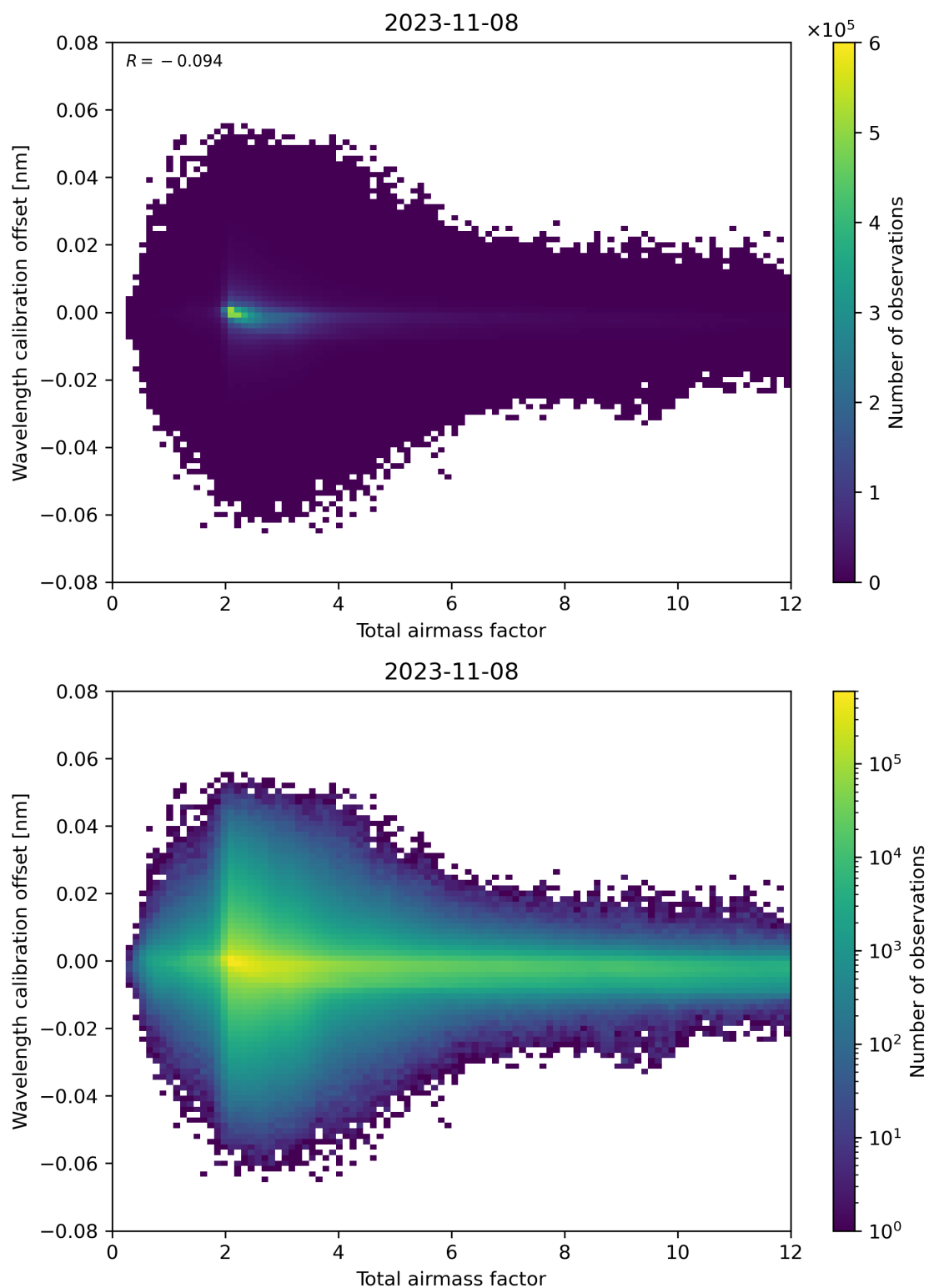
Figure 70: Scatter density plot of “Total airmass factor” against “Wavelength calibration offset” for 2023-11-07 to 2023-11-09.
