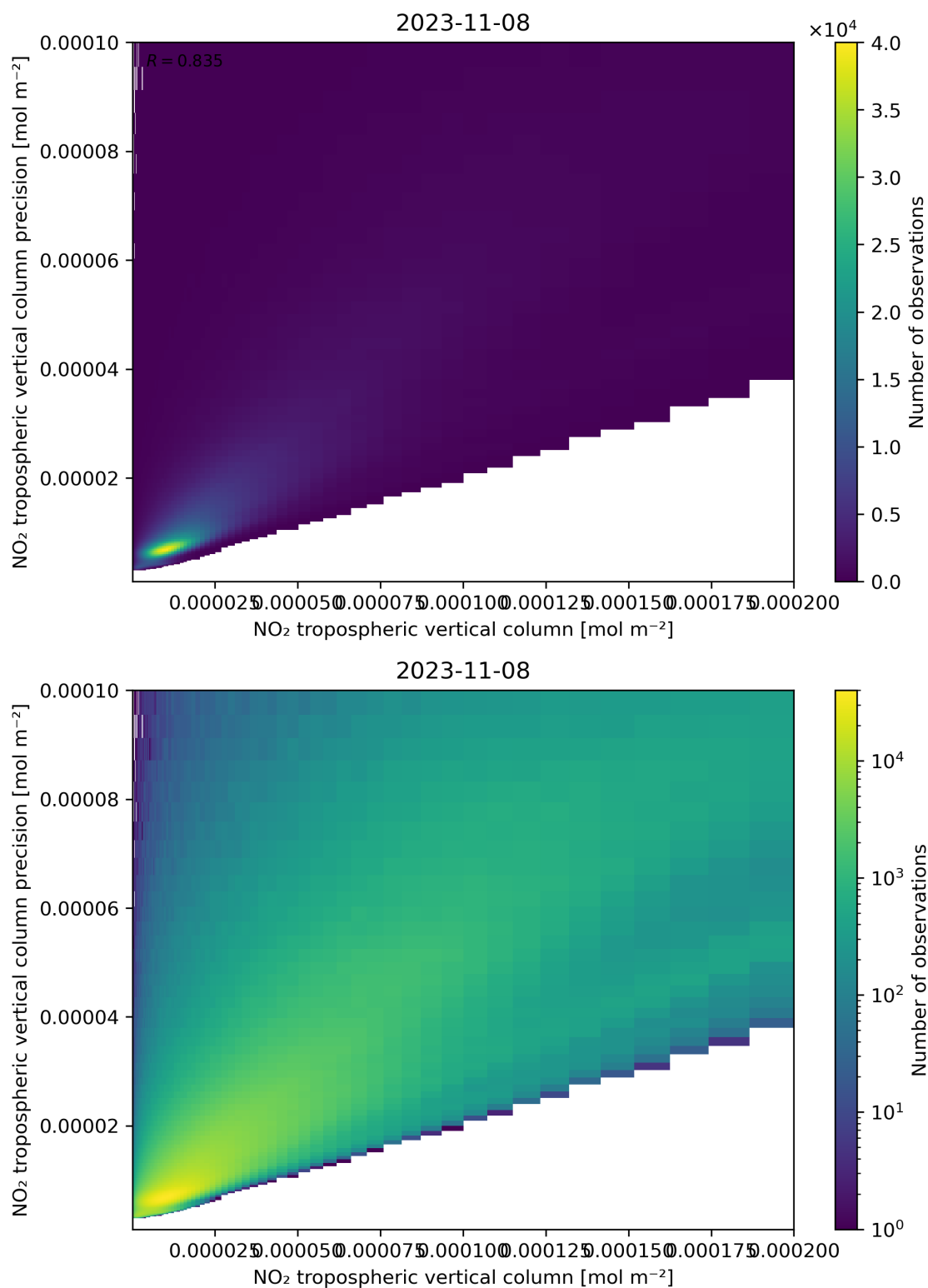
Figure 130: Scatter density plot of “NO 2 tropospheric vertical column” against “NO 2 tropospheric vertical column precision” for 2023-11-07 to 2023-11-09.
