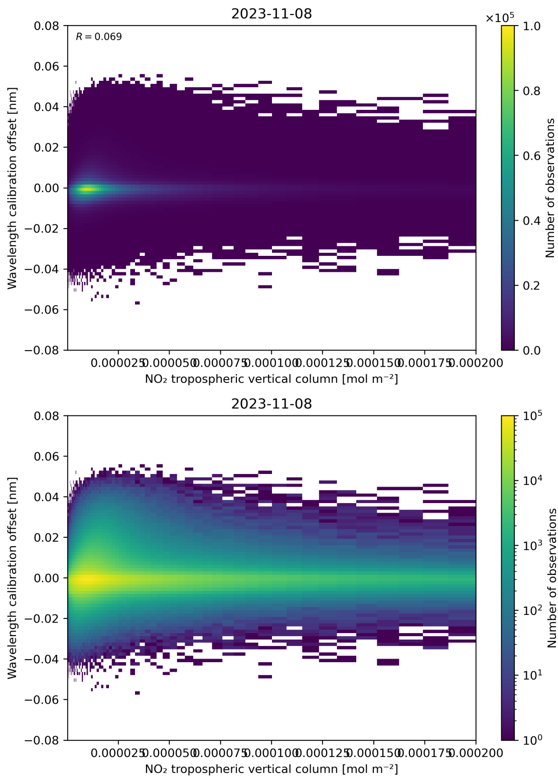
Figure 143: Scatter density plot of “NO 2 tropospheric vertical column” against “Wavelength calibration offset” for 2023-11-07 to 2023-11-09.
