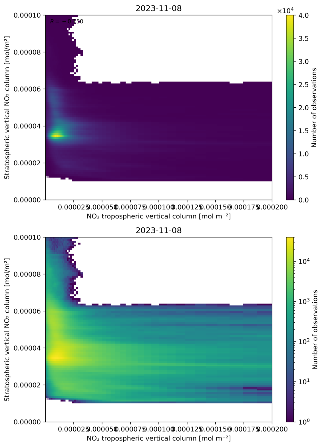
Figure 125: Scatter density plot of “NO 2 tropospheric vertical column” against “Stratospheric vertical NO 2 column” for 2023-11-07 to 2023-11-09.
