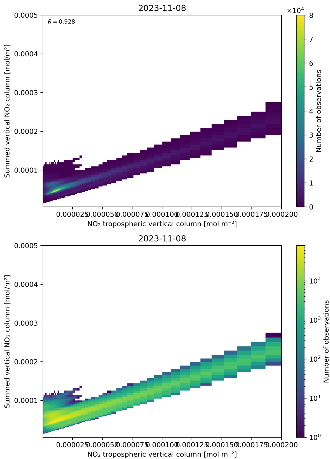
Figure 126: Scatter density plot of “NO 2 tropospheric vertical column” against “Summed vertical NO 2 column” for 2023-11-07 to 2023-11-09.
