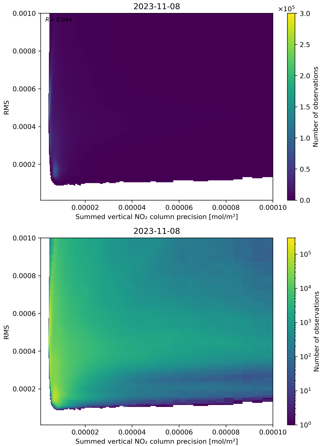
Figure 108: Scatter density plot of “Summed vertical NO 2 column precision” against “RMS” for 2023-11-07 to 2023-11-09.
