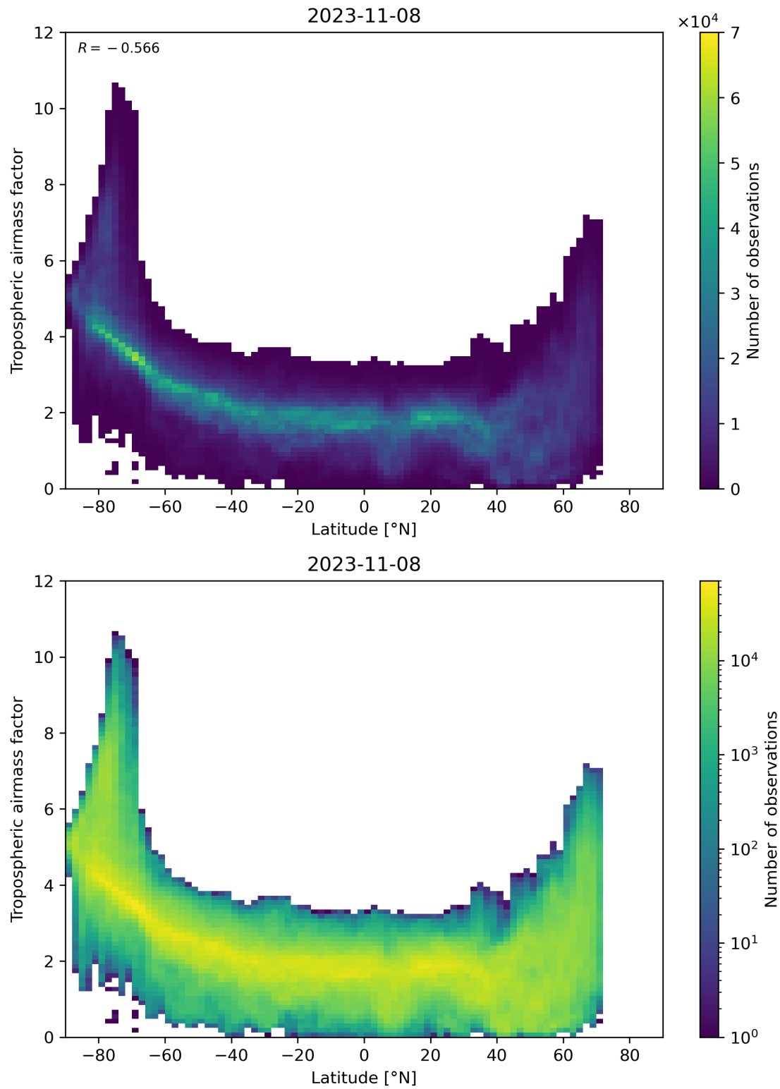
Figure 85: Scatter density plot of “Latitude” against “Tropospheric airmass factor” for 2023-11-07 to 2023-11-09.
