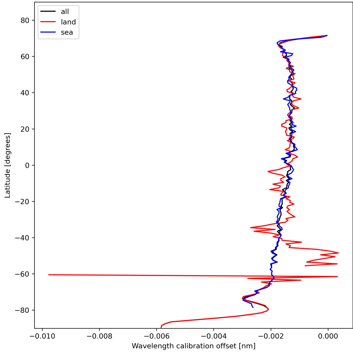
Figure 18: Zonal average of “Wavelength calibration offset” for 2023-11-07 to 2023-11-09.
