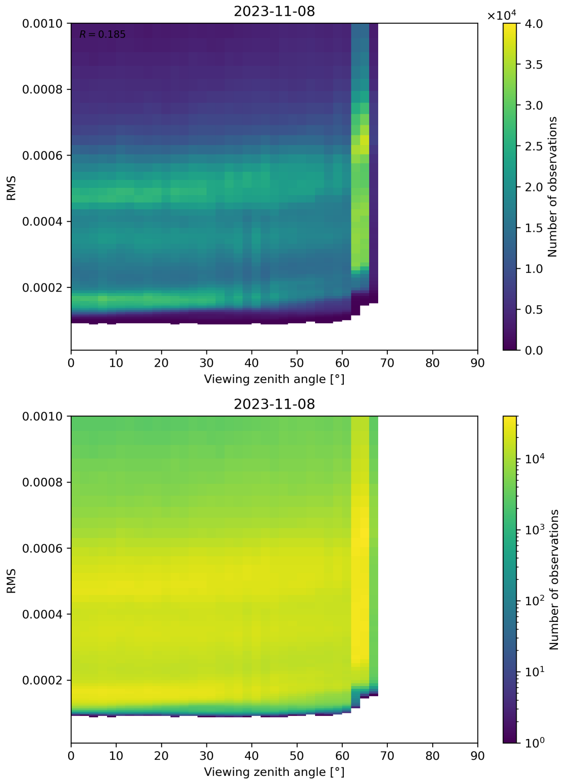
Figure 171: Scatter density plot of “Viewing zenith angle” against “RMS” for 2023-11-07 to 2023-11-09.
