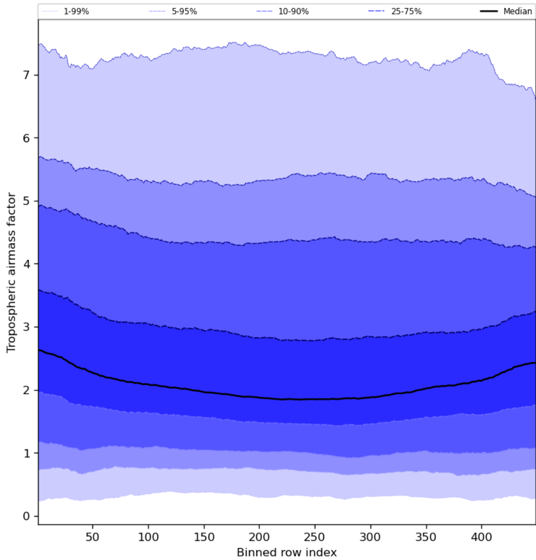
Figure 48: Along track statistics of “Tropospheric airmass factor” for 2023-11-07 to 2023-11-09
