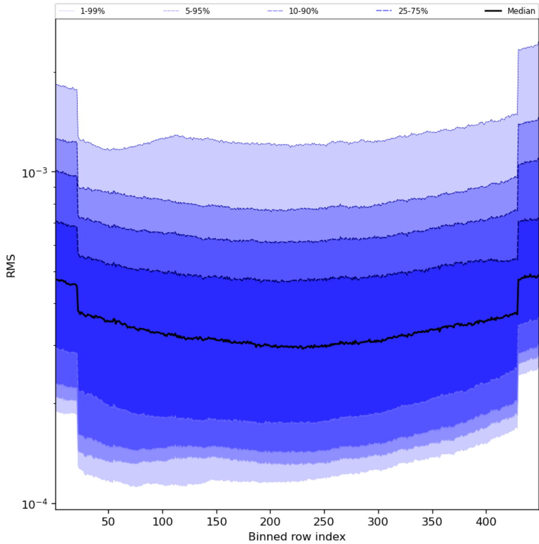
Figure 60: Along track statistics of “RMS” for 2023-11-07 to 2023-11-09
