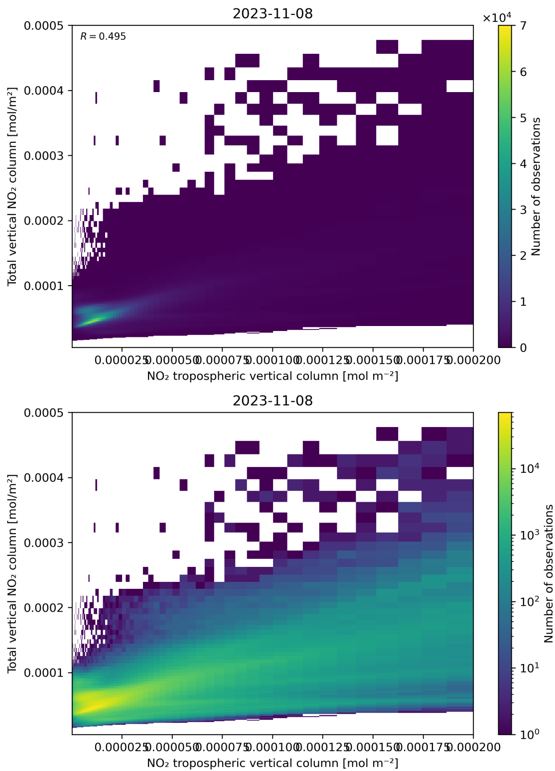
Figure 128: Scatter density plot of “NO 2 tropospheric vertical column” against “Total vertical NO 2 column” for 2023-11-07 to 2023-11-09.
