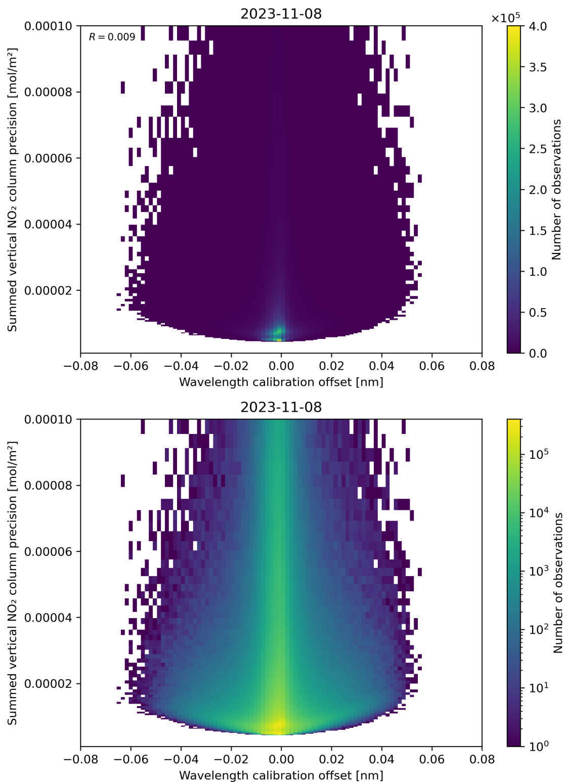
Figure 178: Scatter density plot of “Wavelength calibration offset” against “Summed vertical NO 2 column precision” for 2023-11-07 to 2023-11-09.
