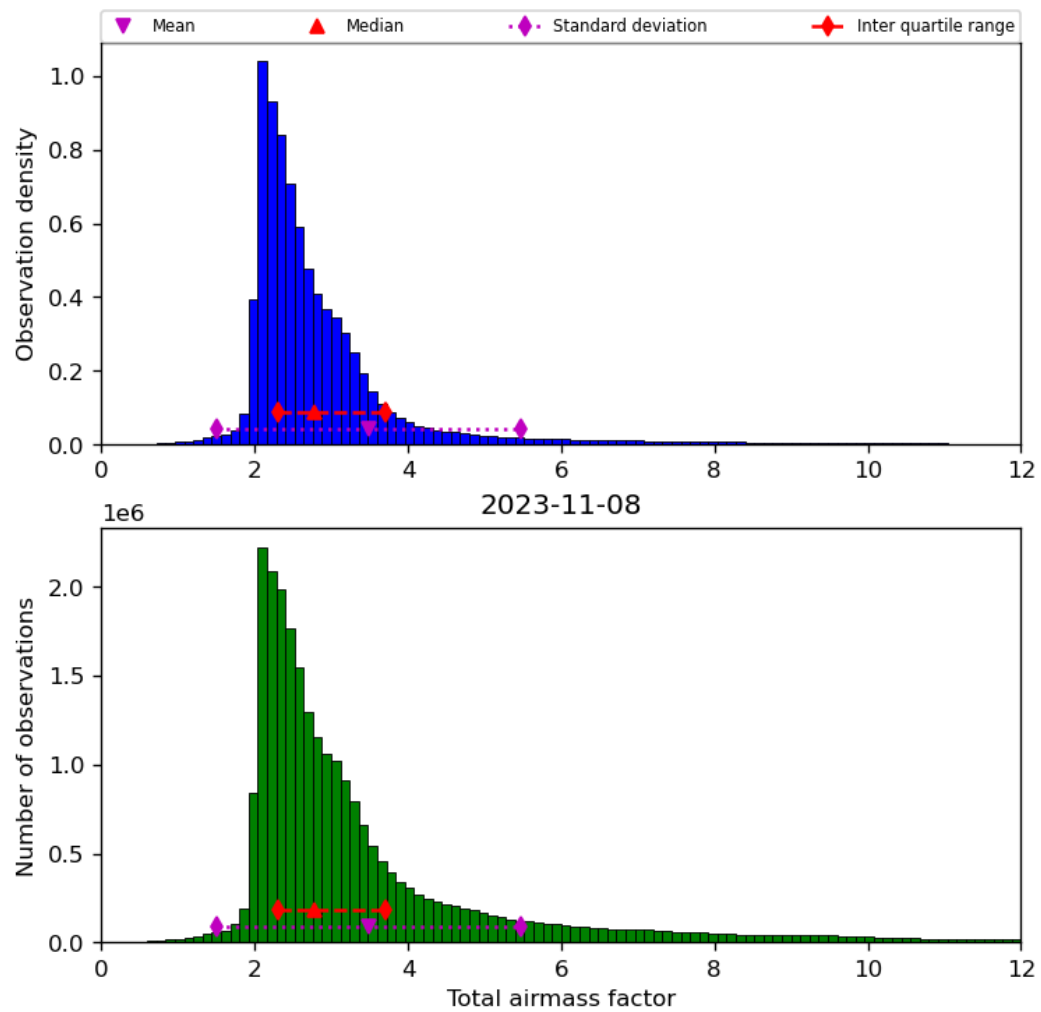
Figure 32: Histogram of “Total airmass factor” for 2023-11-07 to 2023-11-09
