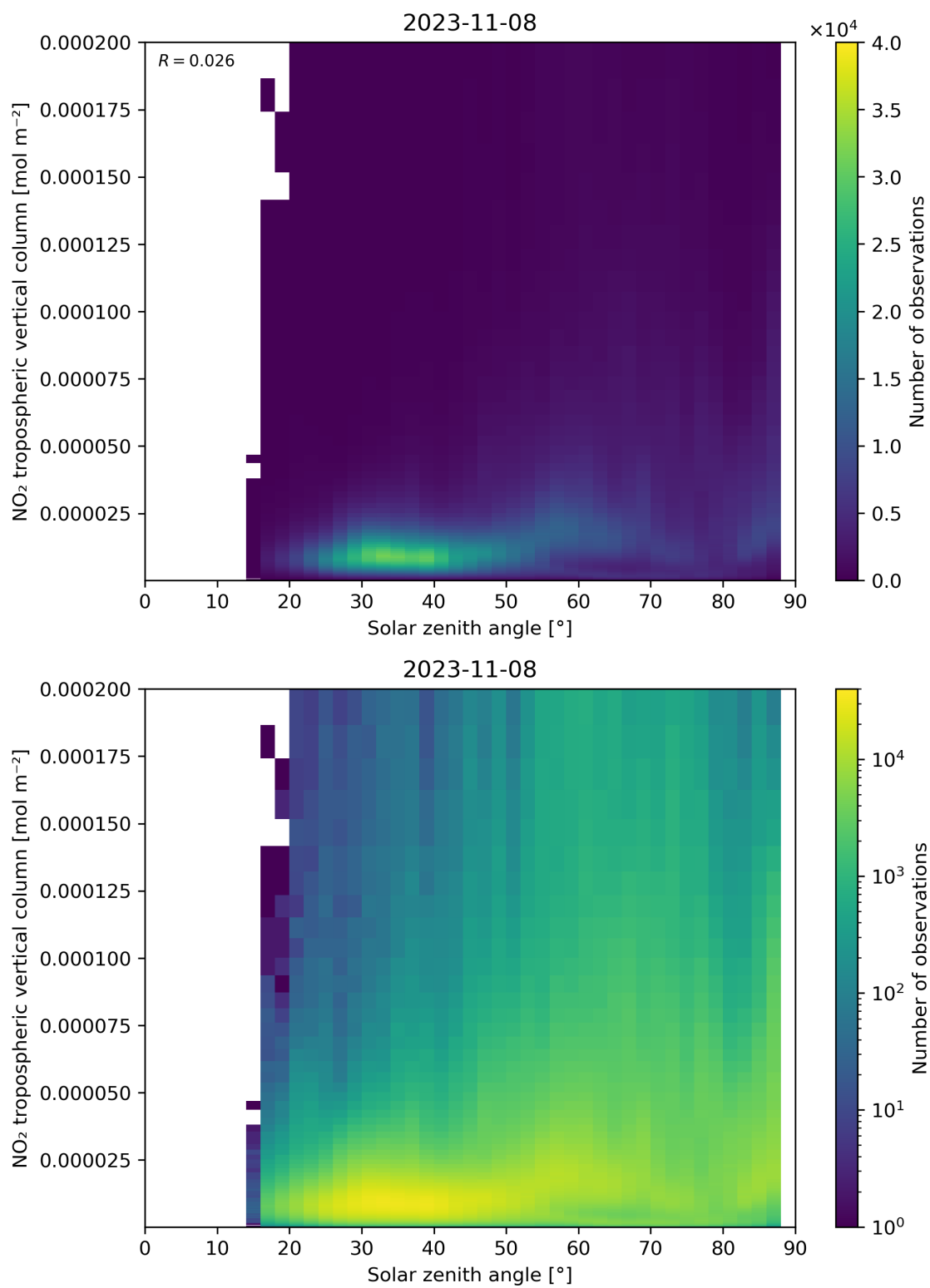
Figure 155: Scatter density plot of “Solar zenith angle” against “NO 2 tropospheric vertical column” for 2023-11-07 to 2023-11-09.
