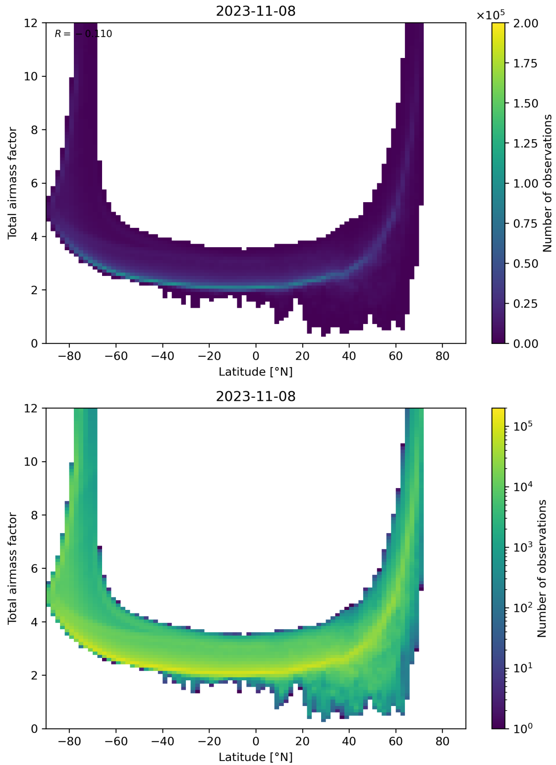
Figure 84: Scatter density plot of “Latitude” against “Total airmass factor” for 2023-11-07 to 2023-11-09.
