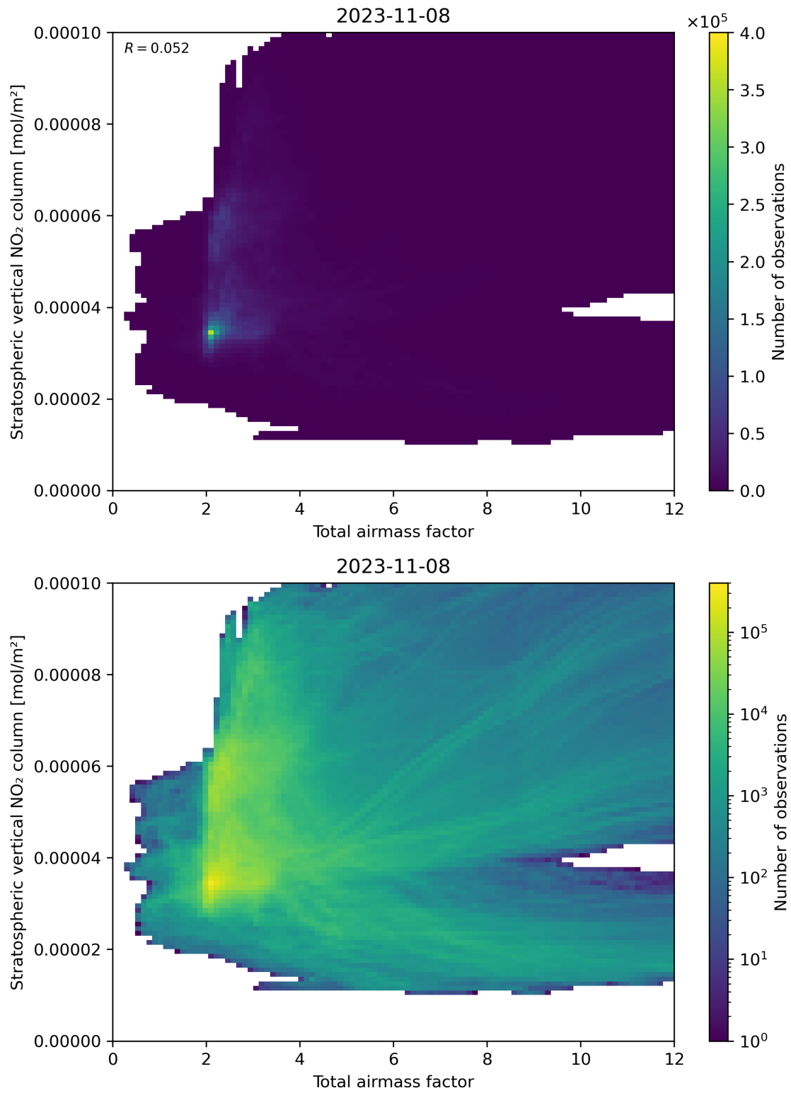
Figure 64: Scatter density plot of “Total airmass factor” against “Stratospheric vertical NO 2 column” for 2023-11-07 to 2023-11-09.
