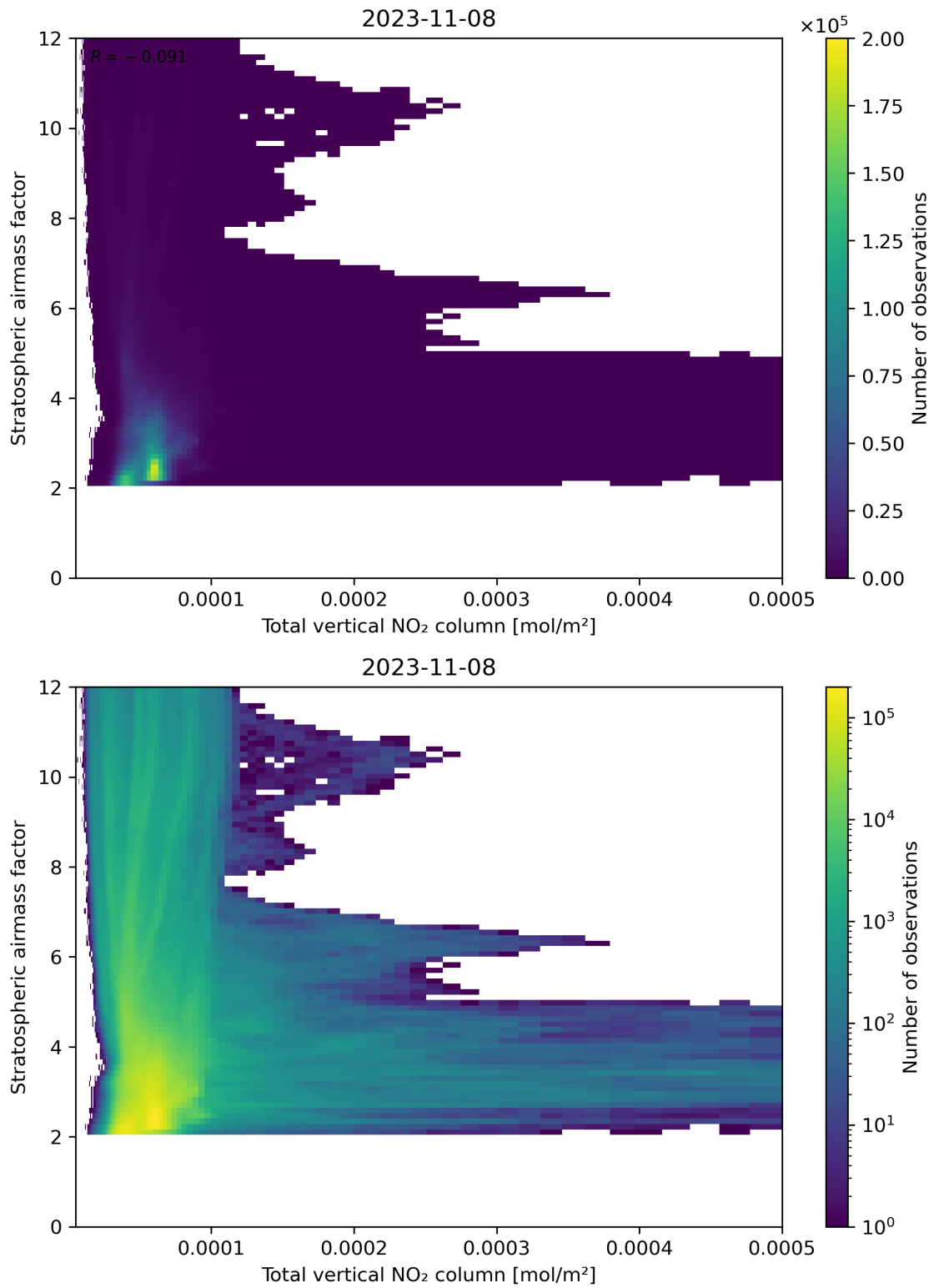
Figure 110: Scatter density plot of “Total vertical NO 2 column” against “Stratospheric air mass factor” for 2023-11-07 to 2023-11-09.
