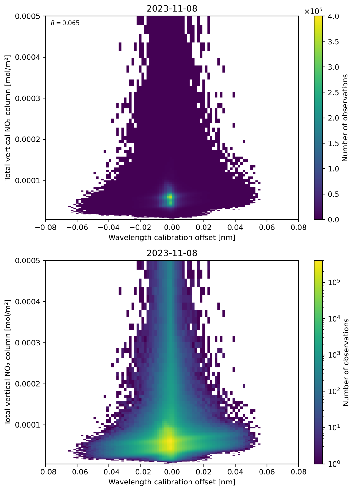
Figure 179: Scatter density plot of “Wavelength calibration offset” against “Total vertical NO 2 column” for 2023-11-07 to 2023-11-09.
