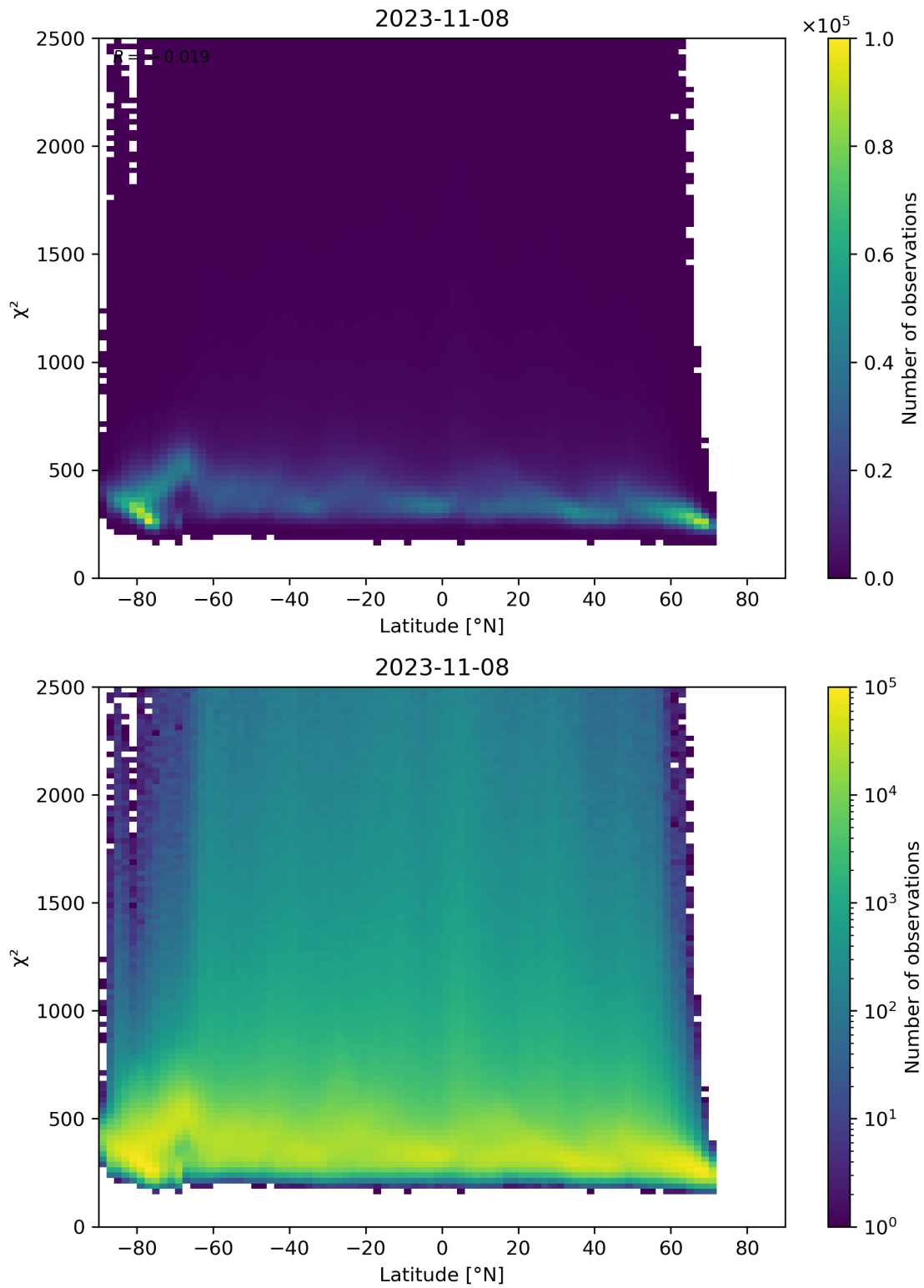
Figure 86: Scatter density plot of “Latitude” against “ \chi^2 ” for 2023-11-07 to 2023-11-09.
