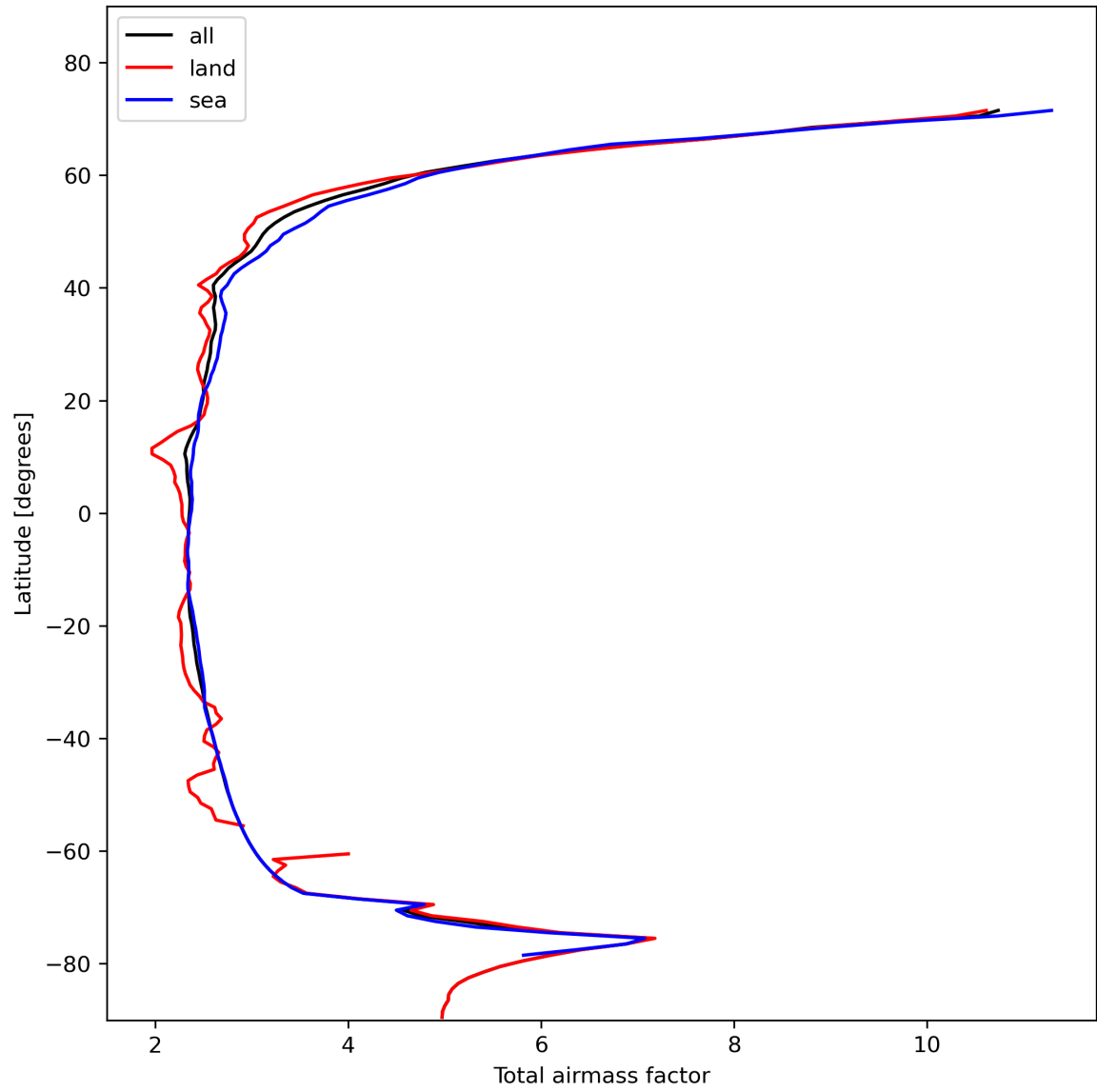
Figure 15: Zonal average of “Total airmass factor” for 2023-11-07 to 2023-11-09.
