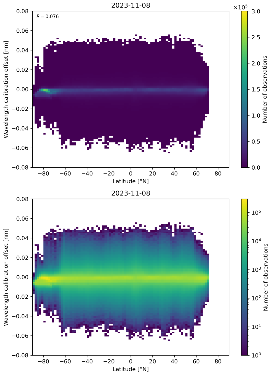
Figure 95: Scatter density plot of “Latitude” against “Wavelength calibration offset” for 2023-11-07 to 2023-11-09.
