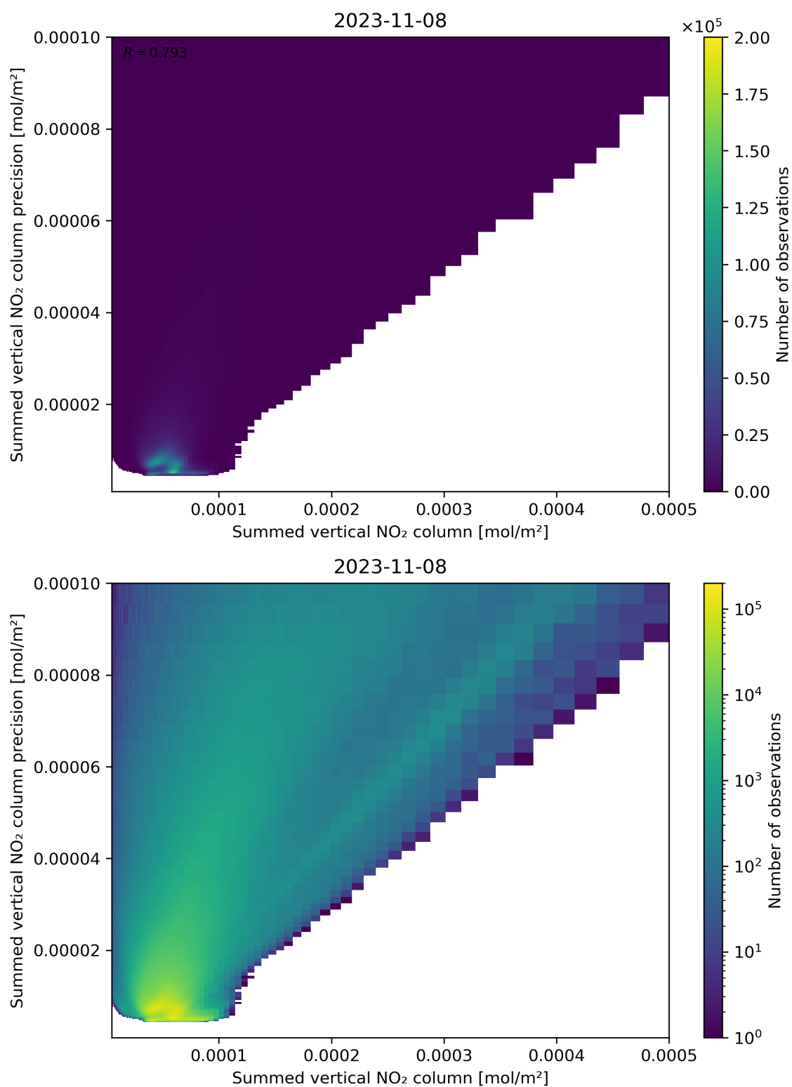
Figure 105: Scatter density plot of “Summed vertical NO 2 column” against “Summed vertical NO 2 column precision” for 2023-11-07 to 2023-11-09.
