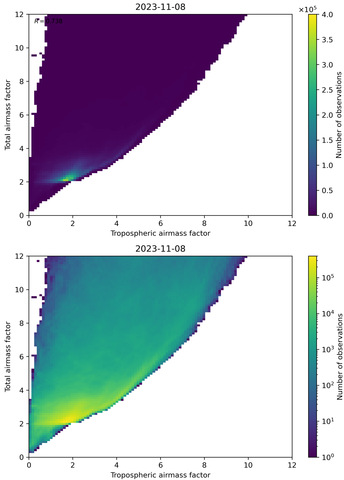
Figure 72: Scatter density plot of “Tropospheric airmass factor” against “Total airmass factor” for 2023-11-07 to 2023-11-09.
