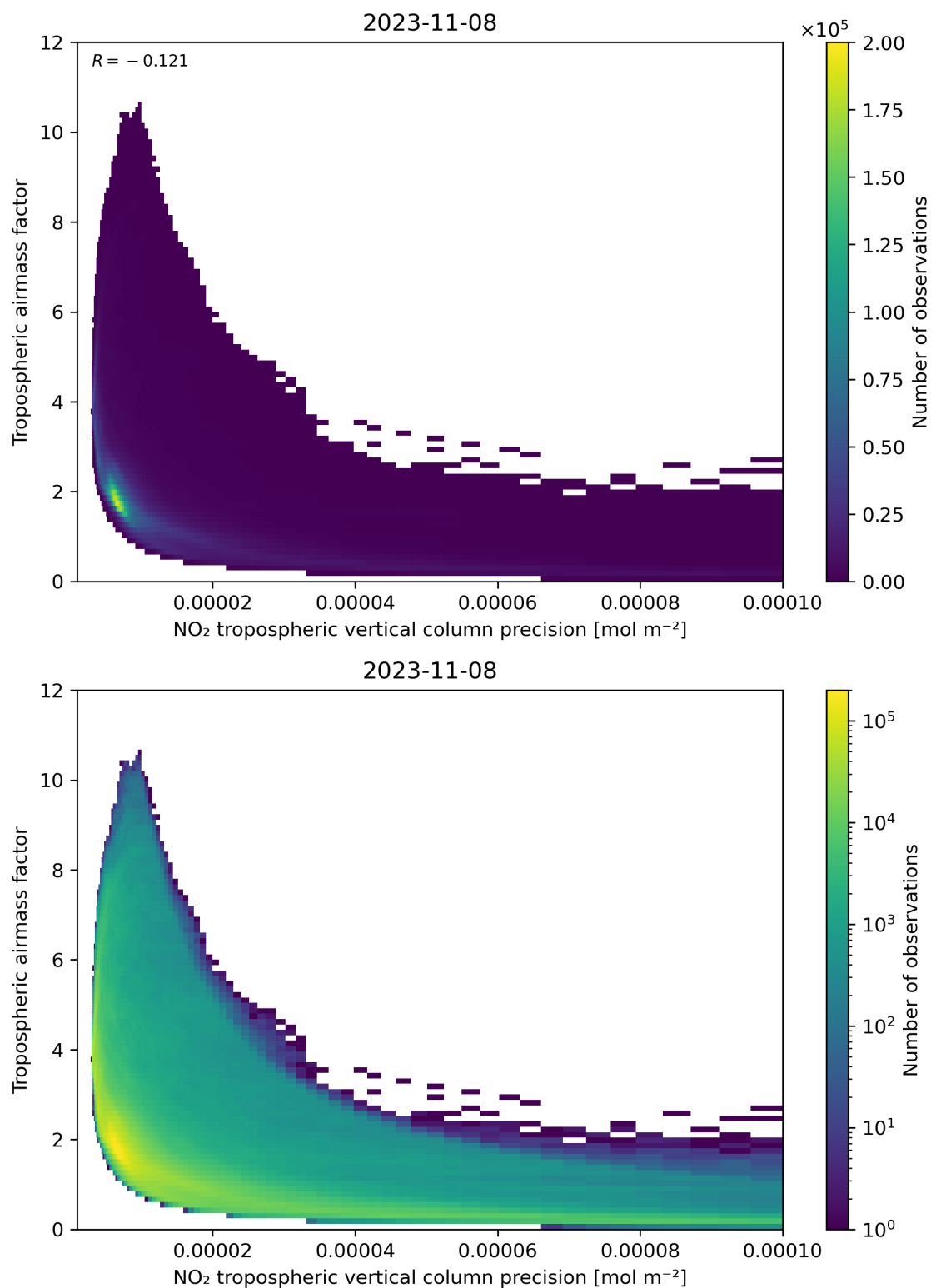
Figure 133: Scatter density plot of “NO 2 tropospheric vertical column precision” against “Tropospheric airmass factor” for 2023-11-07 to 2023-11-09.
