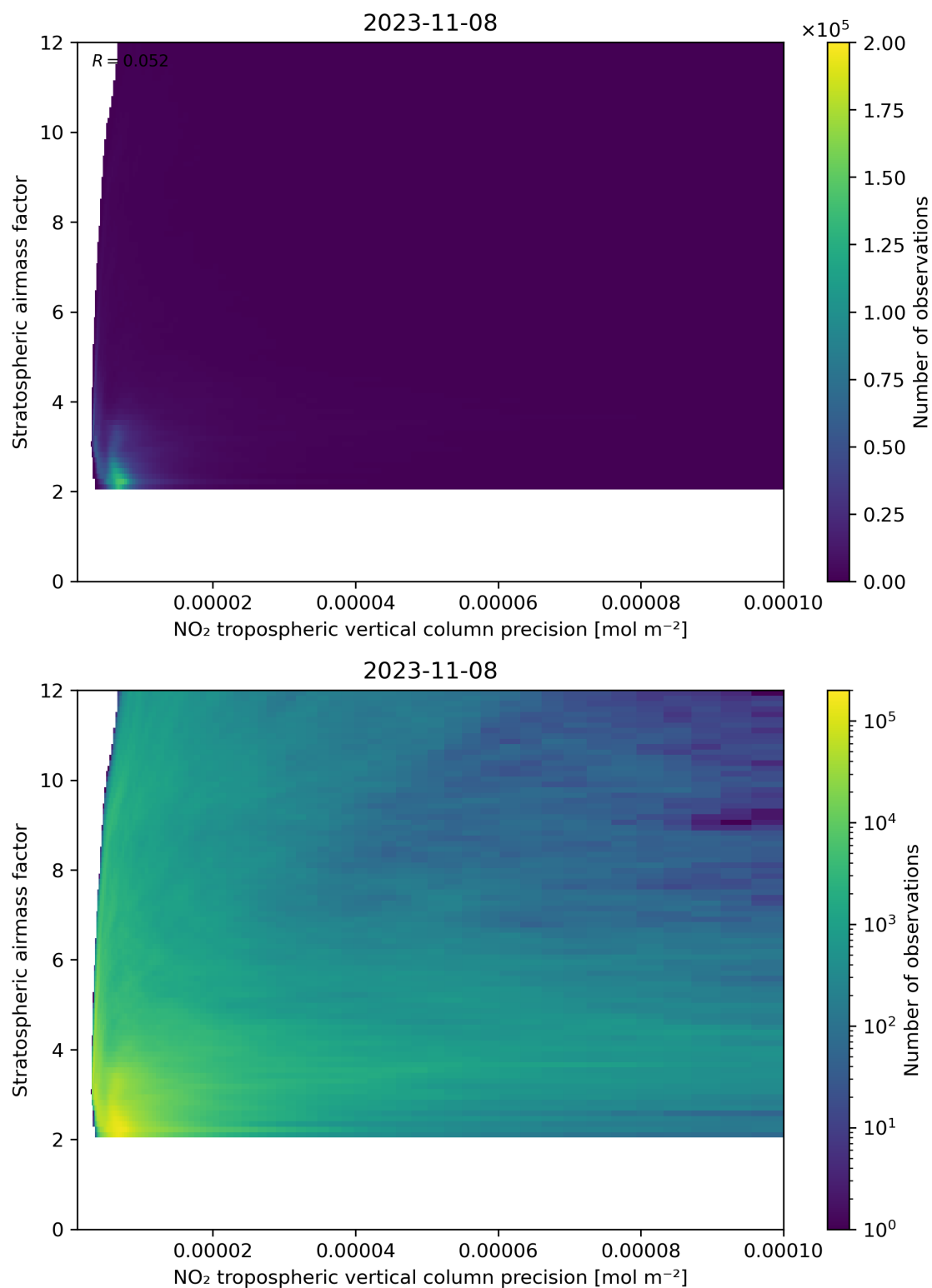
Figure 131: Scatter density plot of “NO 2 tropospheric vertical column precision” against “Stratospheric airmass factor” for 2023-11-07 to 2023-11-09.
