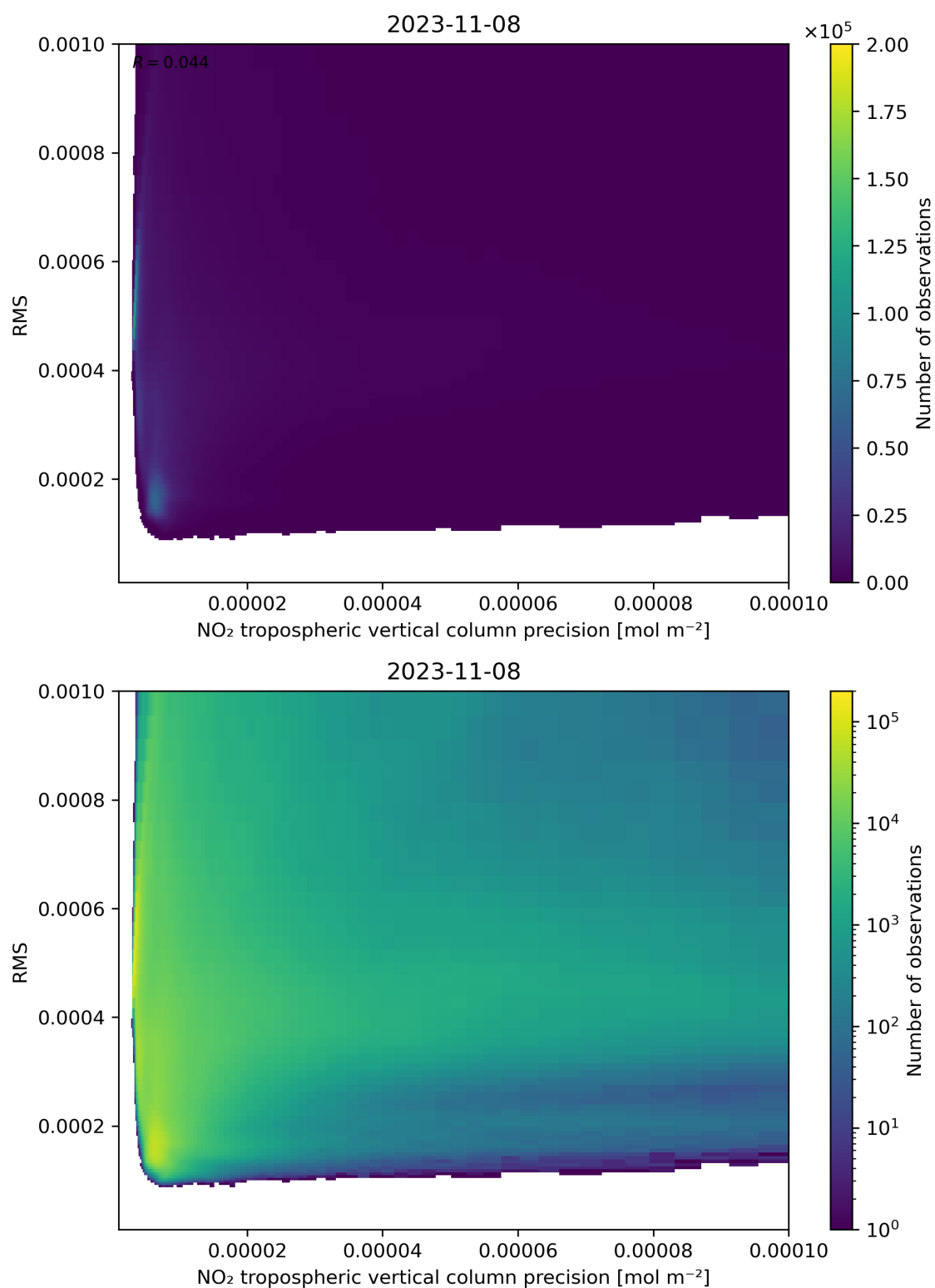
Figure 140: Scatter density plot of “NO 2 tropospheric vertical column precision” against “RMS” for 2023-11-07 to 2023-11-09.
