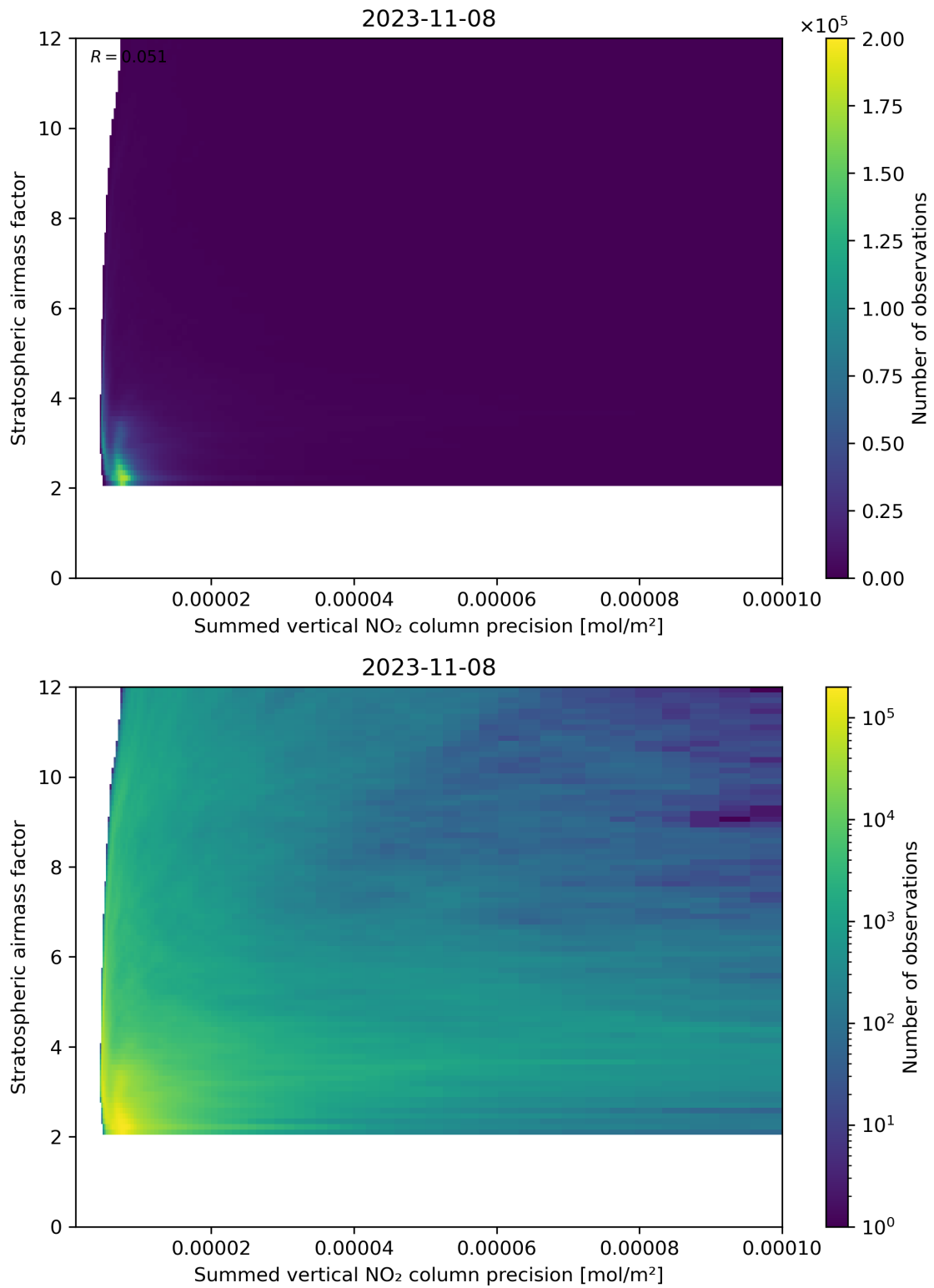
Figure 106: Scatter density plot of “Summed vertical NO 2 column precision” against “Stratospheric airmass factor” for 2023-11-07 to 2023-11-09.
