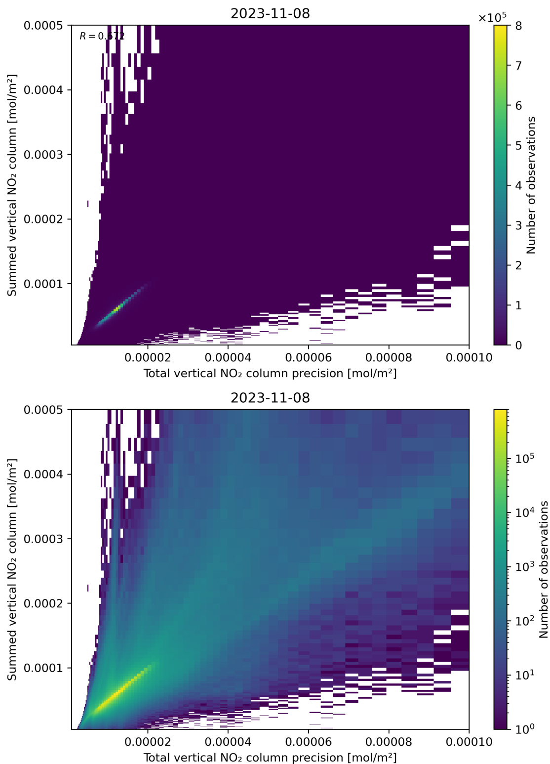
Figure 117: Scatter density plot of “Total vertical NO 2 column precision” against “Summed vertical NO 2 column” for 2023-11-07 to 2023-11-09.
