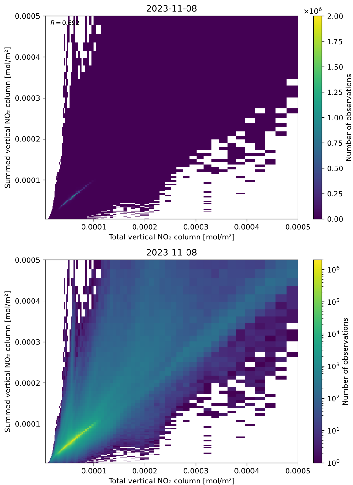
Figure 112: Scatter density plot of “Total vertical NO 2 column” against “Summed vertical NO 2 column” for 2023-11-07 to 2023-11-09.
