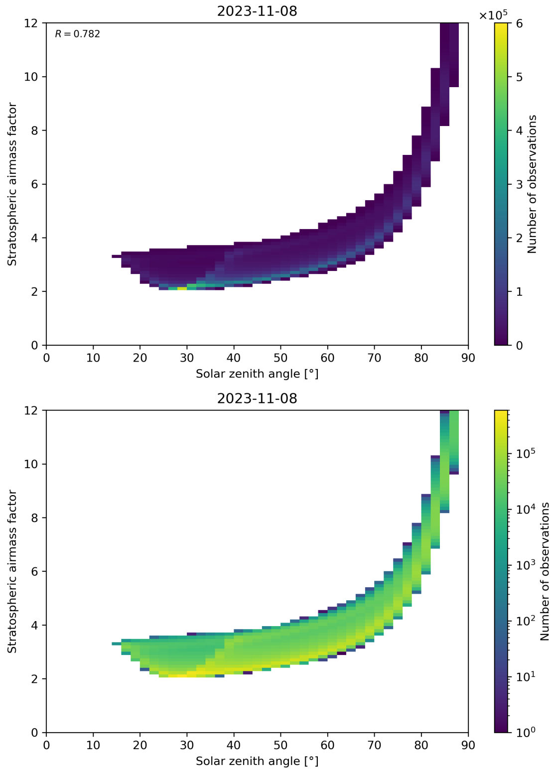
Figure 145: Scatter density plot of “Solar zenith angle” against “Stratospheric airmass factor” for 2023-11-07 to 2023-11-09.
