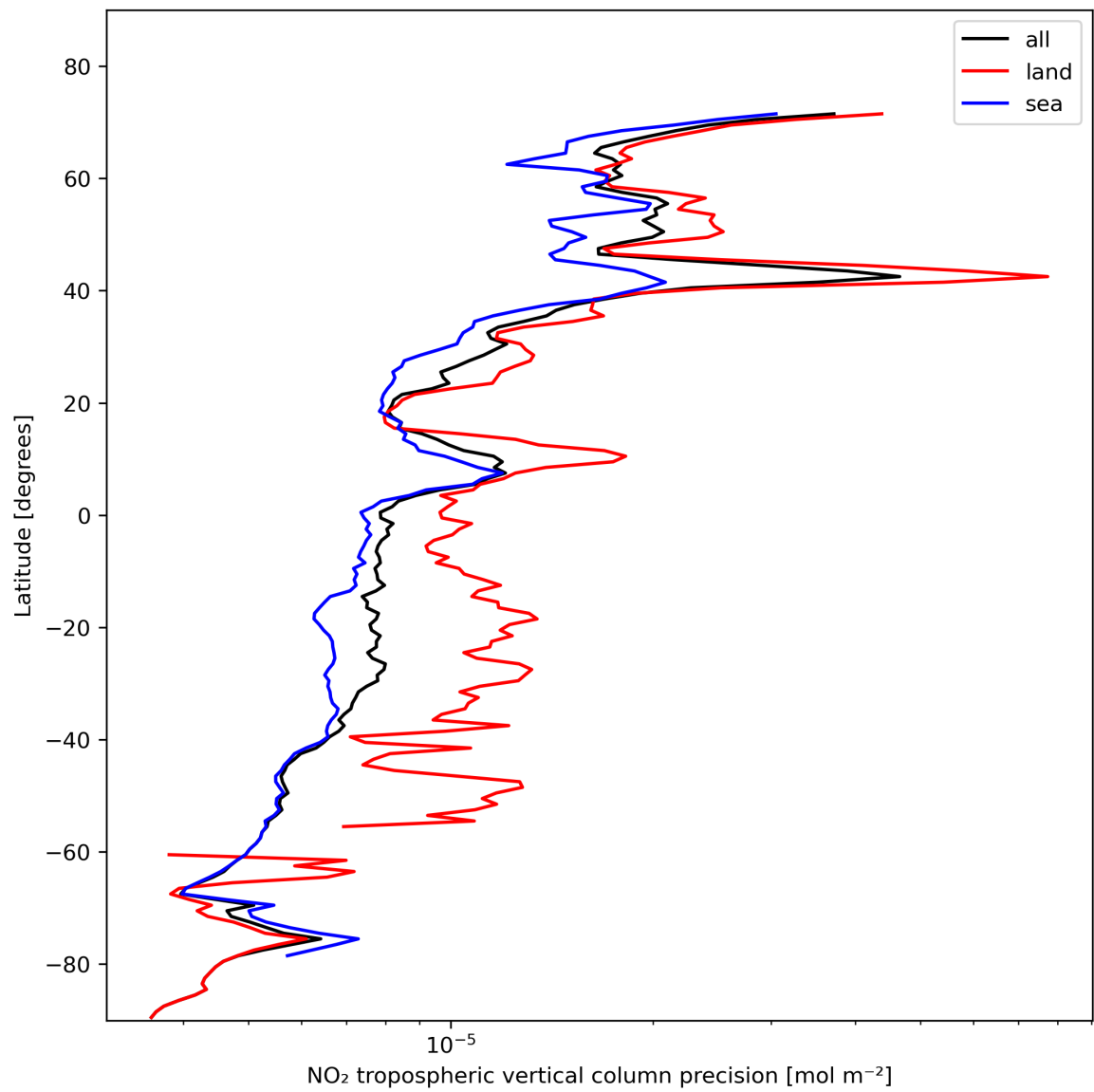
Figure 13: Zonal average of “NO 2 tropospheric vertical column precision” for 2023-11-07 to 2023-11-09.
