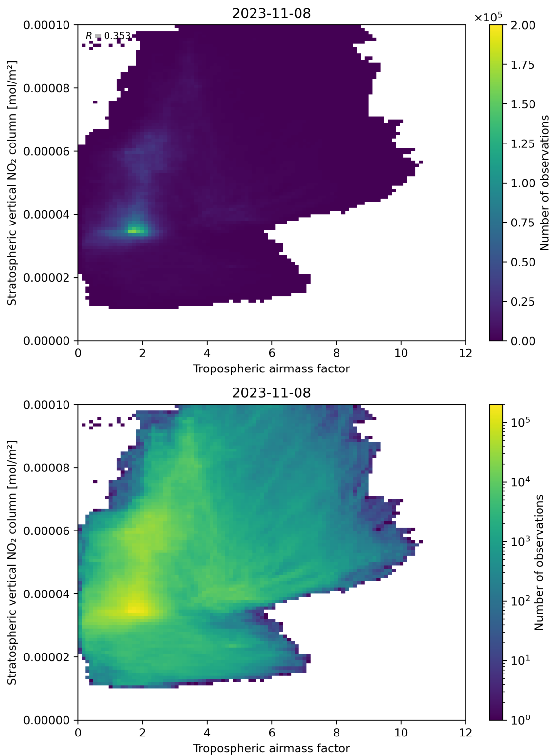
Figure 74: Scatter density plot of “Tropospheric airmass factor” against “Stratospheric vertical NO 2 column” for 2023-11-07 to 2023-11-09.
