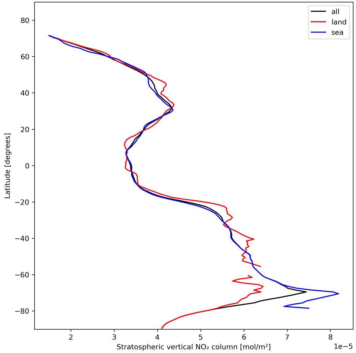
Figure 19: Zonal average of “Stratospheric vertical NO 2 column” for 2023-11-07 to 2023-11-09.
