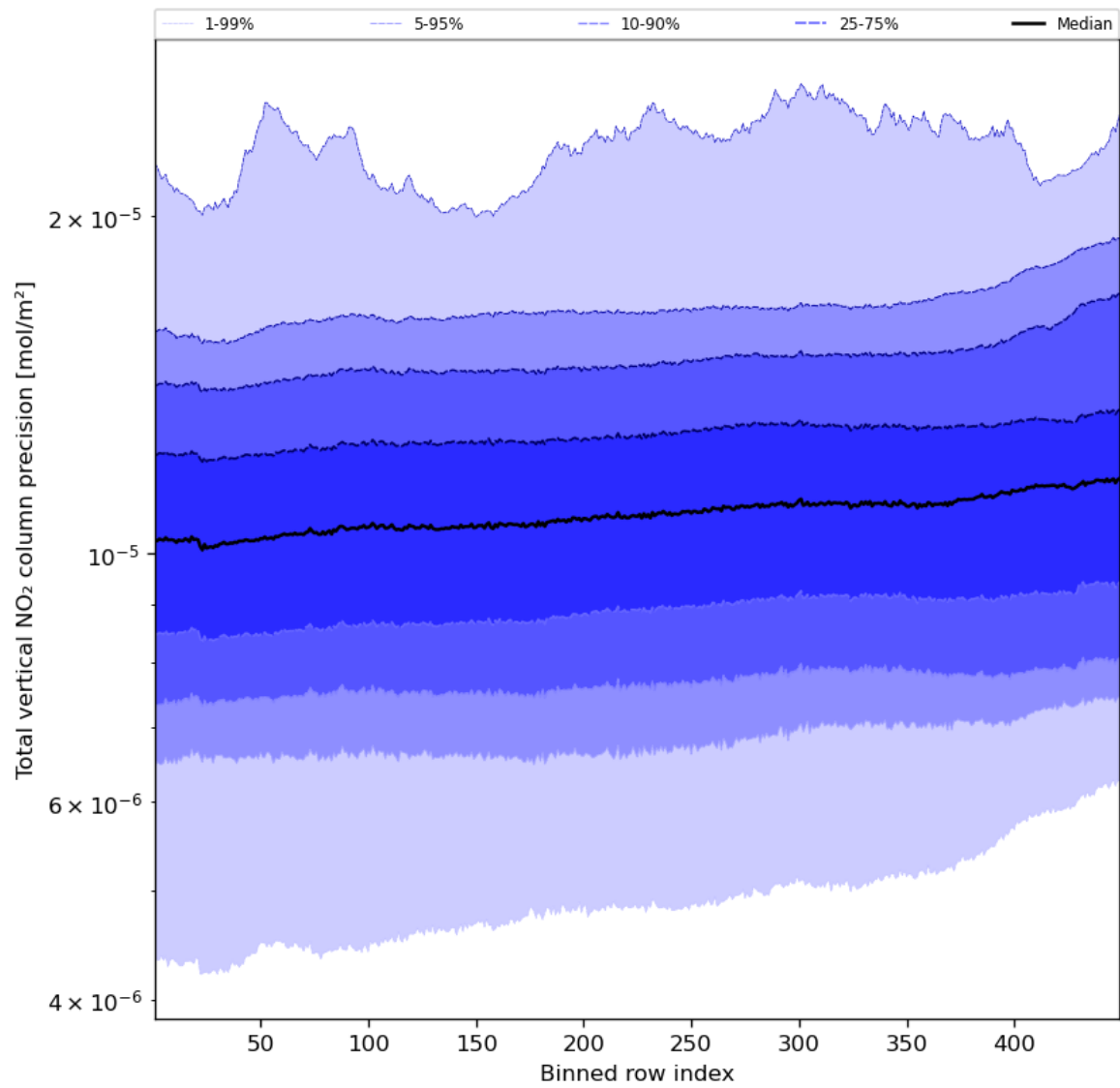
Figure 56: Along track statistics of “Total vertical NO 2 column precision” for 2023-11-07 to 2023-11-09
