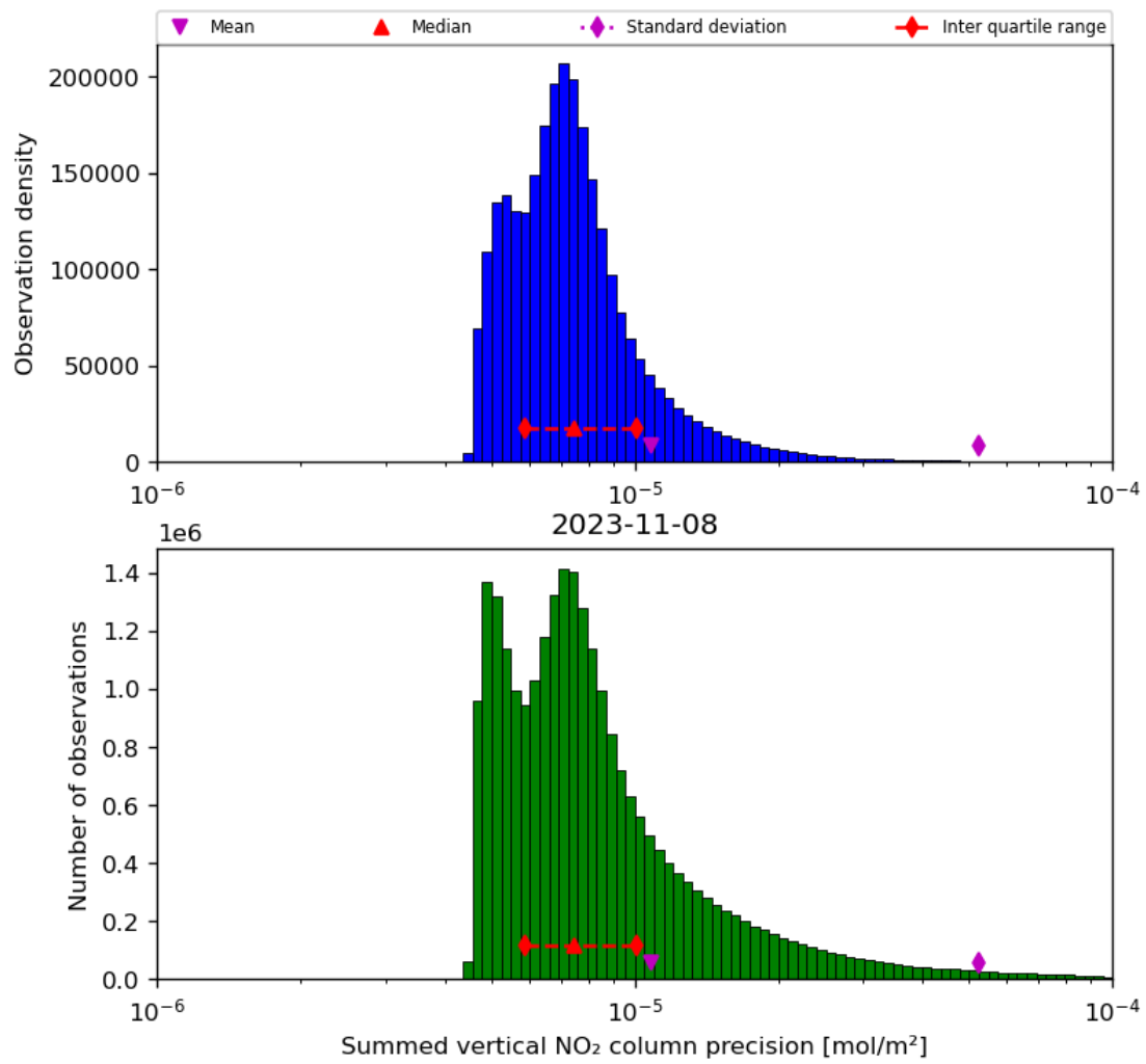
Figure 41: Histogram of "Summed vertical NO 2 column precision" for 2023-11-07 to 2023-11-09
