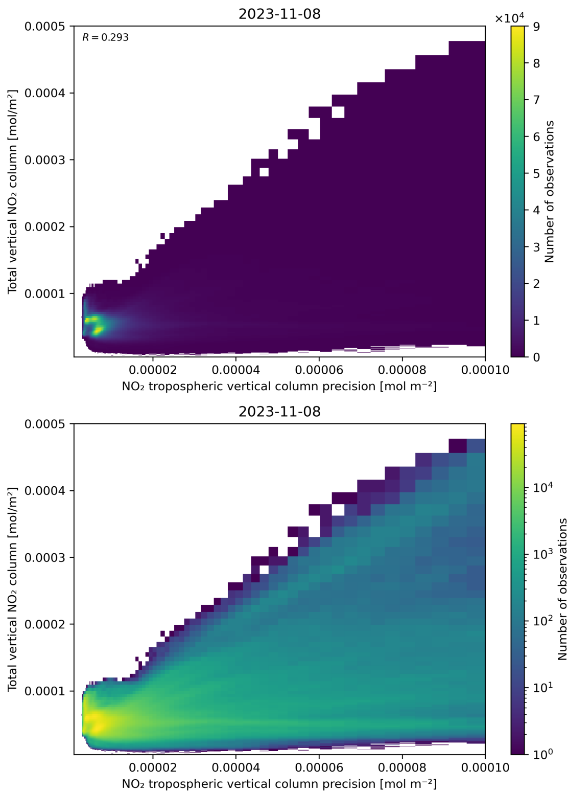
Figure 138: Scatter density plot of “NO 2 tropospheric vertical column precision” against “Total vertical NO 2 column” for 2023-11-07 to 2023-11-09.
