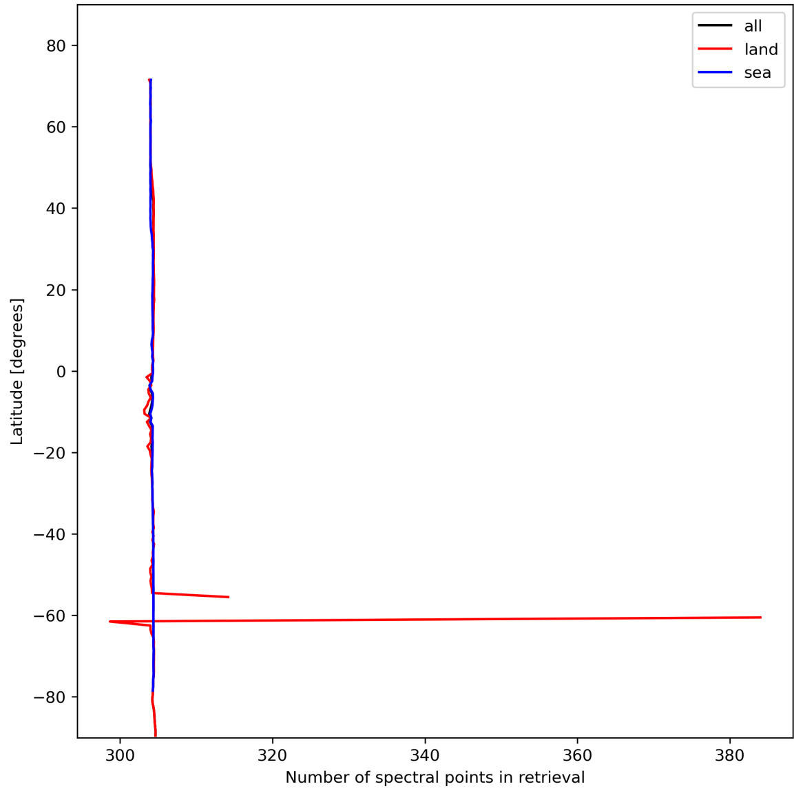
Figure 16: Zonal average of “Number of spectral points in retrieval” for 2023-11-07 to 2023-11-09.
