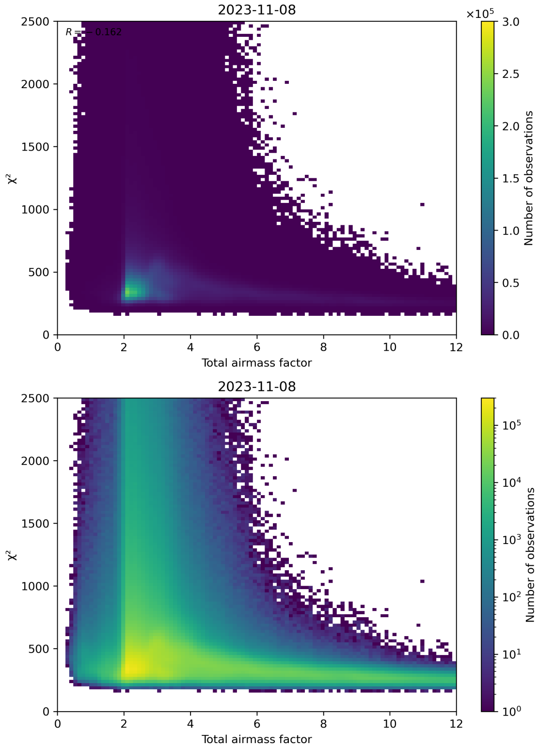
Figure 63: Scatter density plot of “Total airmass factor” against “ \chi^2 ” for 2023-11-07 to 2023-11-09.
