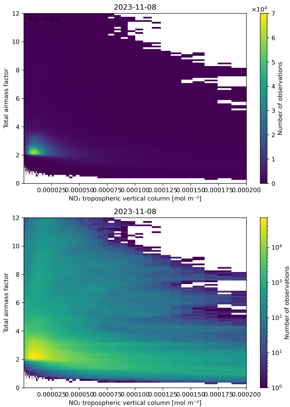
Figure 122: Scatter density plot of “NO 2 tropospheric vertical column” against “Total air mass factor” for 2023-11-07 to 2023-11-09.
