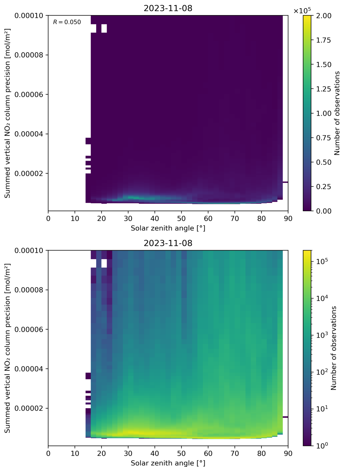
Figure 152: Scatter density plot of “Solar zenith angle” against “Summed vertical NO 2 column precision” for 2023-11-07 to 2023-11-09.
