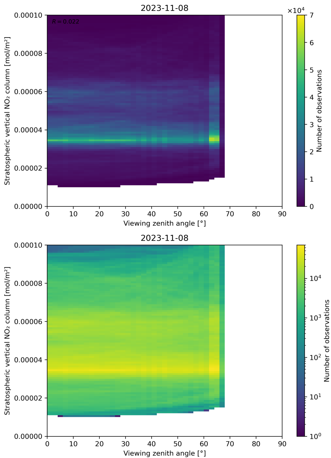
Figure 164: Scatter density plot of “Viewing zenith angle” against “Stratospheric vertical NO 2 column” for 2023-11-07 to 2023-11-09.
