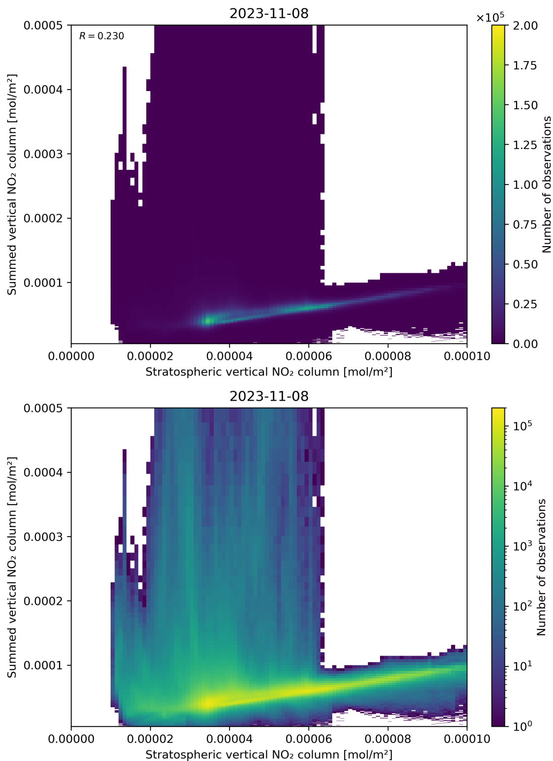
Figure 98: Scatter density plot of “Stratospheric vertical NO 2 column” against “Summed vertical NO 2 column” for 2023-11-07 to 2023-11-09.
