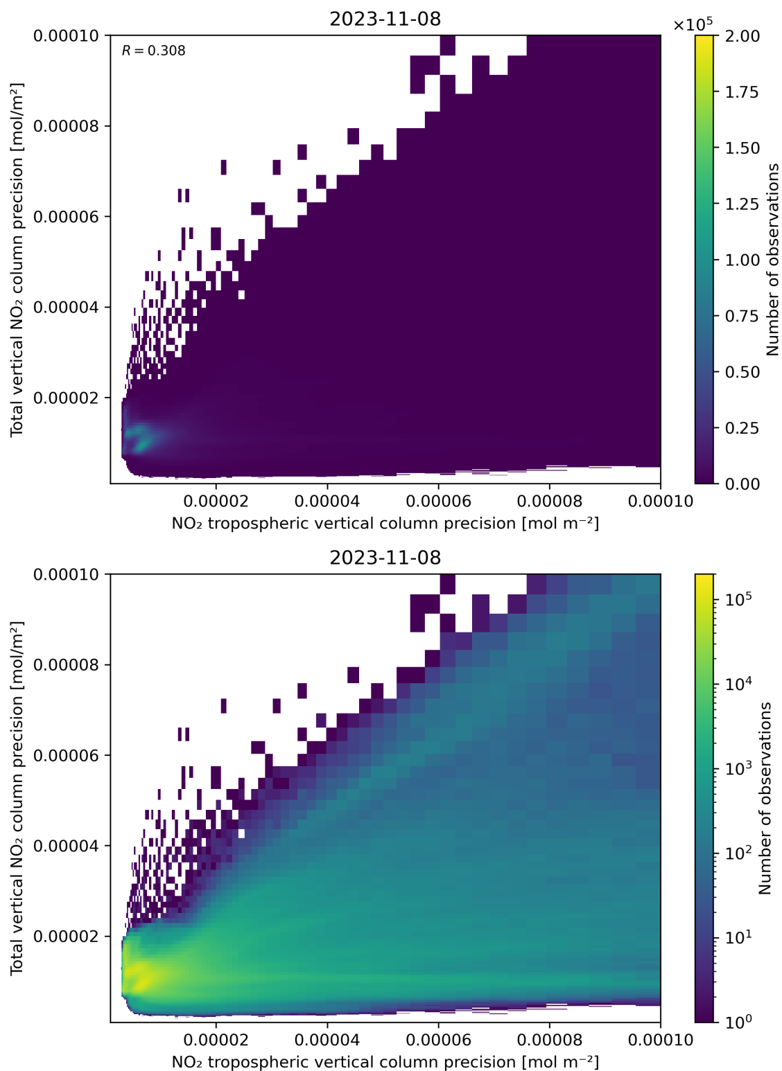
Figure 139: Scatter density plot of “NO 2 tropospheric vertical column precision” against “Total vertical NO 2 column precision” for 2023-11-07 to 2023-11-09.
