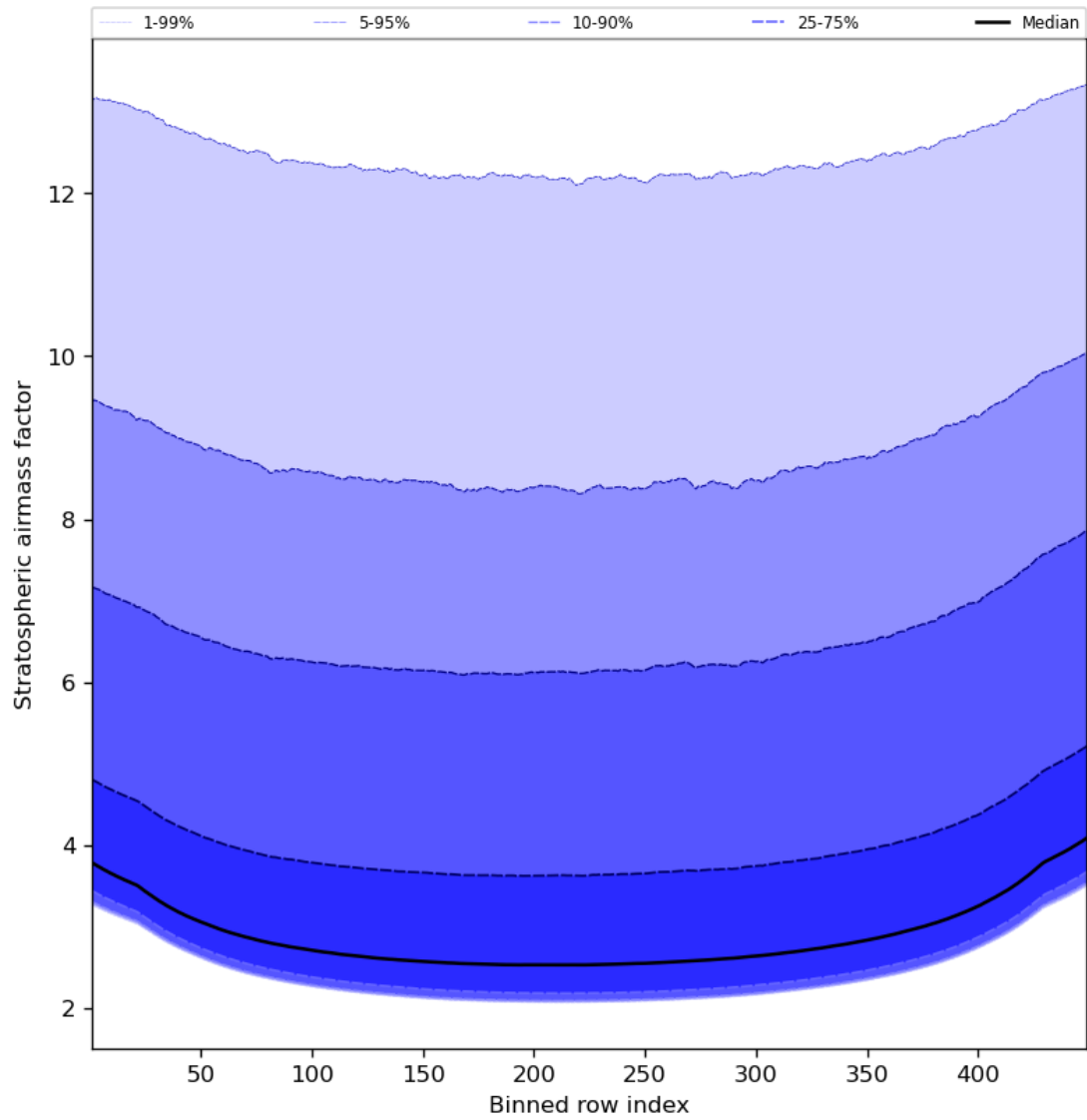
Figure 61: Along track statistics of “Stratospheric airmass factor” for 2023-11-07 to 2023-11-09
