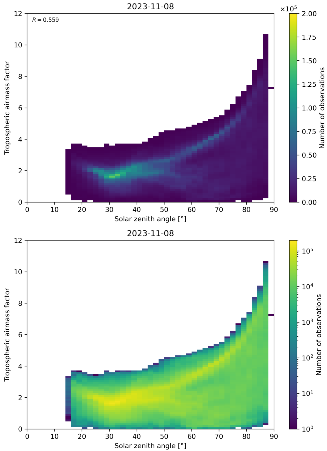
Figure 147: Scatter density plot of “Solar zenith angle” against “Tropospheric airmass factor” for 2023-11-07 to 2023-11-09.
