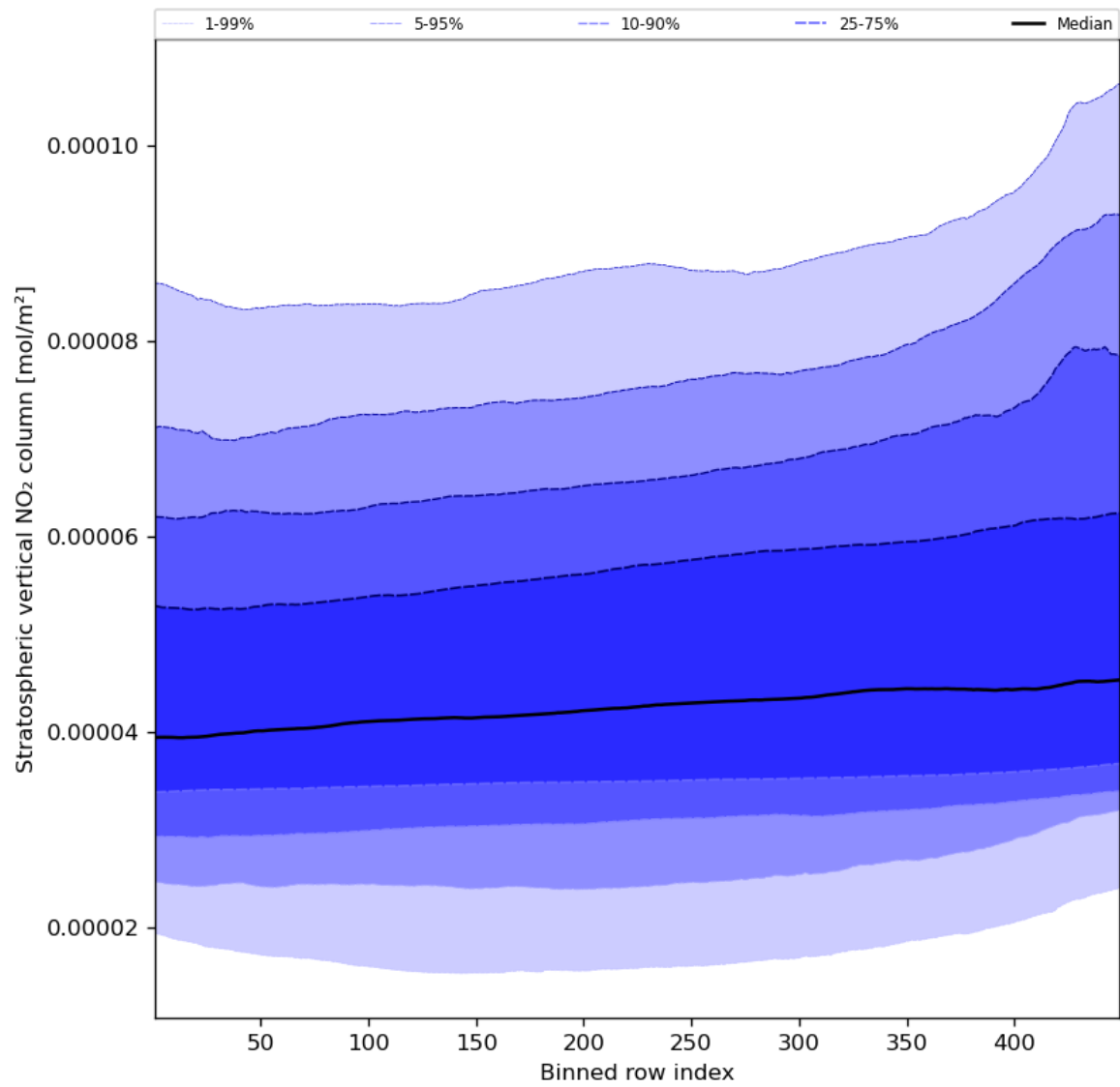
Figure 53: Along track statistics of “Stratospheric vertical NO 2 column” for 2023-11-07 to 2023-11-09
