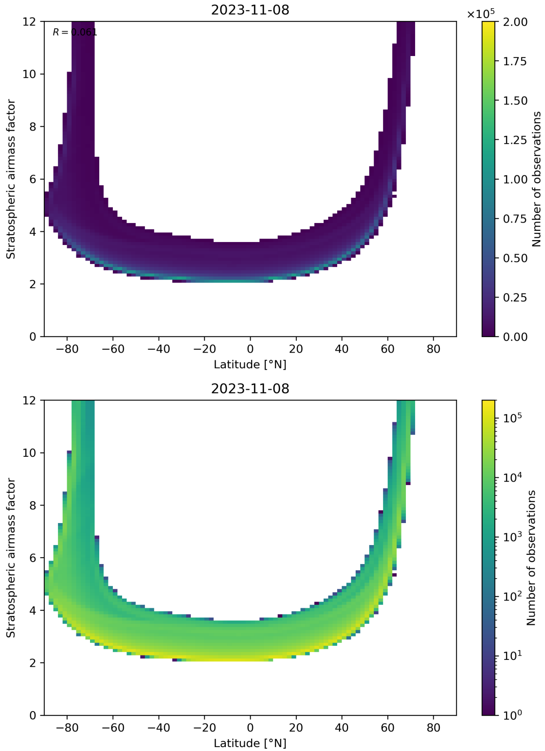
Figure 83: Scatter density plot of “Latitude” against “Stratospheric airmass factor” for 2023-11-07 to 2023-11-09.
