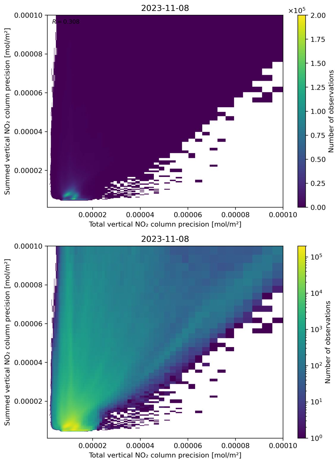
Figure 118: Scatter density plot of “Total vertical NO 2 column precision” against “Summed vertical NO 2 column precision” for 2023-11-07 to 2023-11-09.
