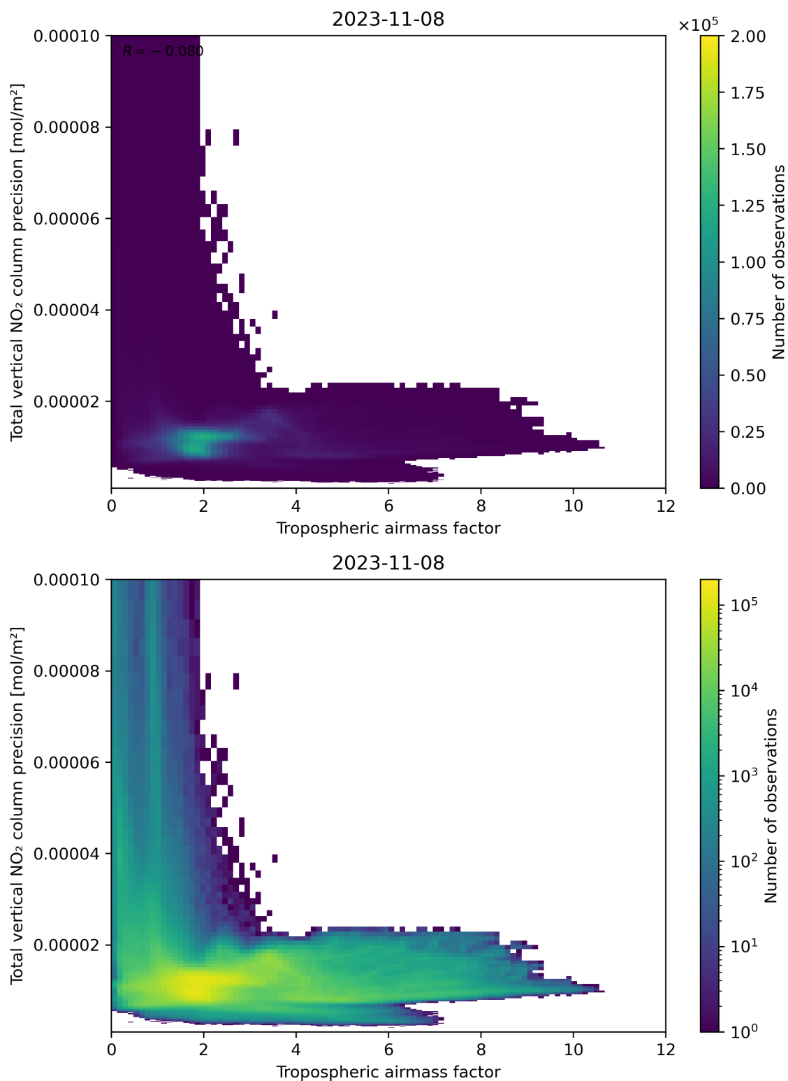
Figure 78: Scatter density plot of “Tropospheric air mass factor” against “Total vertical NO 2 column precision” for 2023-11-07 to 2023-11-09.
