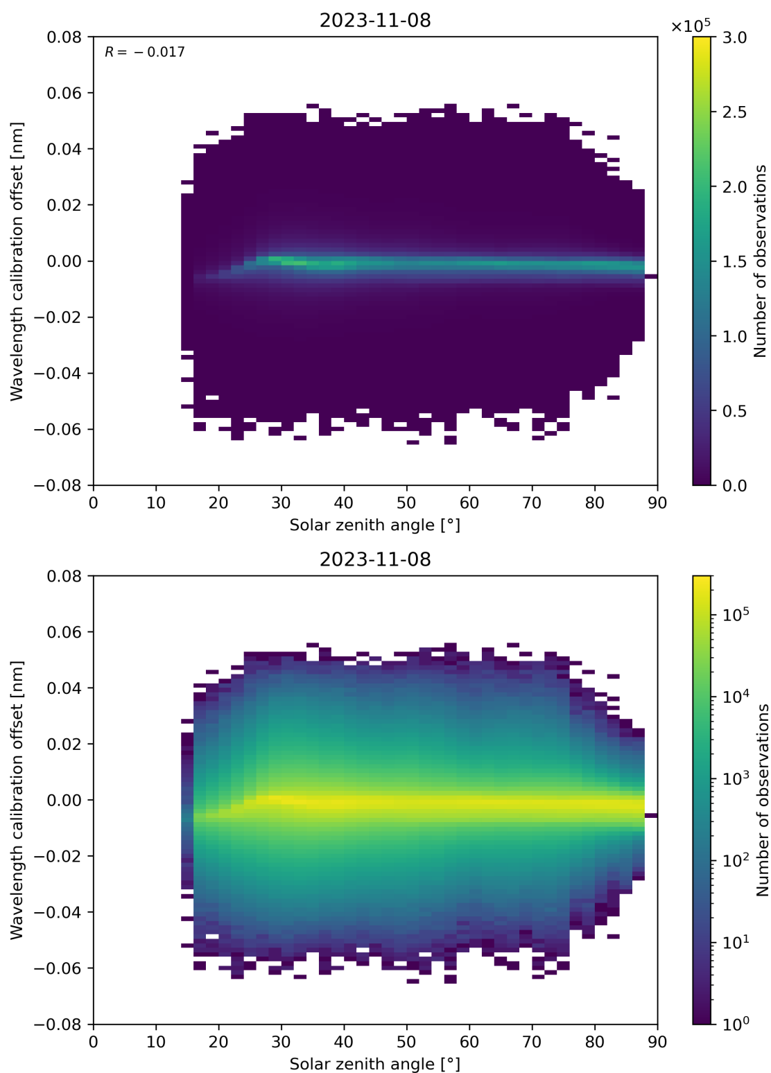
Figure 158: Scatter density plot of “Solar zenith angle” against “Wavelength calibration offset” for 2023-11-07 to 2023-11-09.
