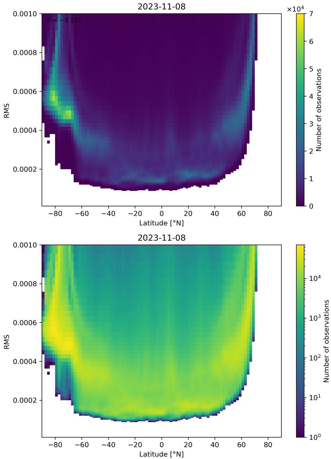
Figure 94: Scatter density plot of “Latitude” against “RMS” for 2023-11-07 to 2023-11-09.
