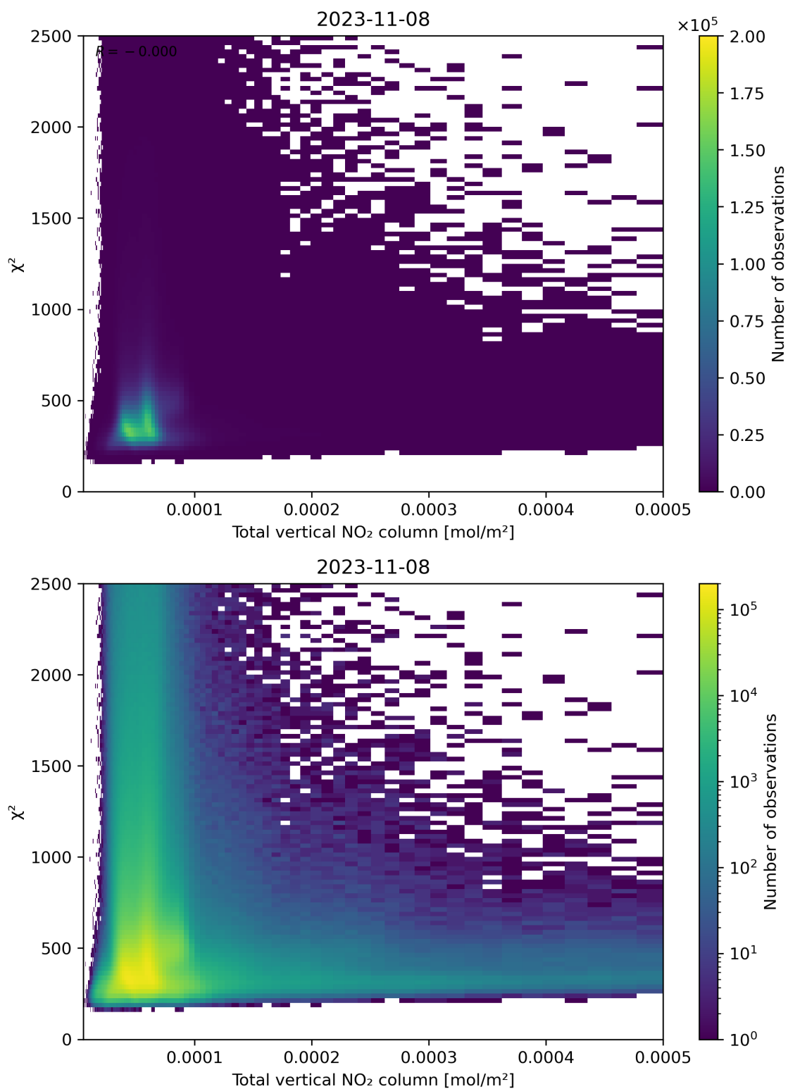
Figure 111: Scatter density plot of “Total vertical NO 2 column” against “ \chi^2 ” for 2023-11-07 to 2023-11-09.
