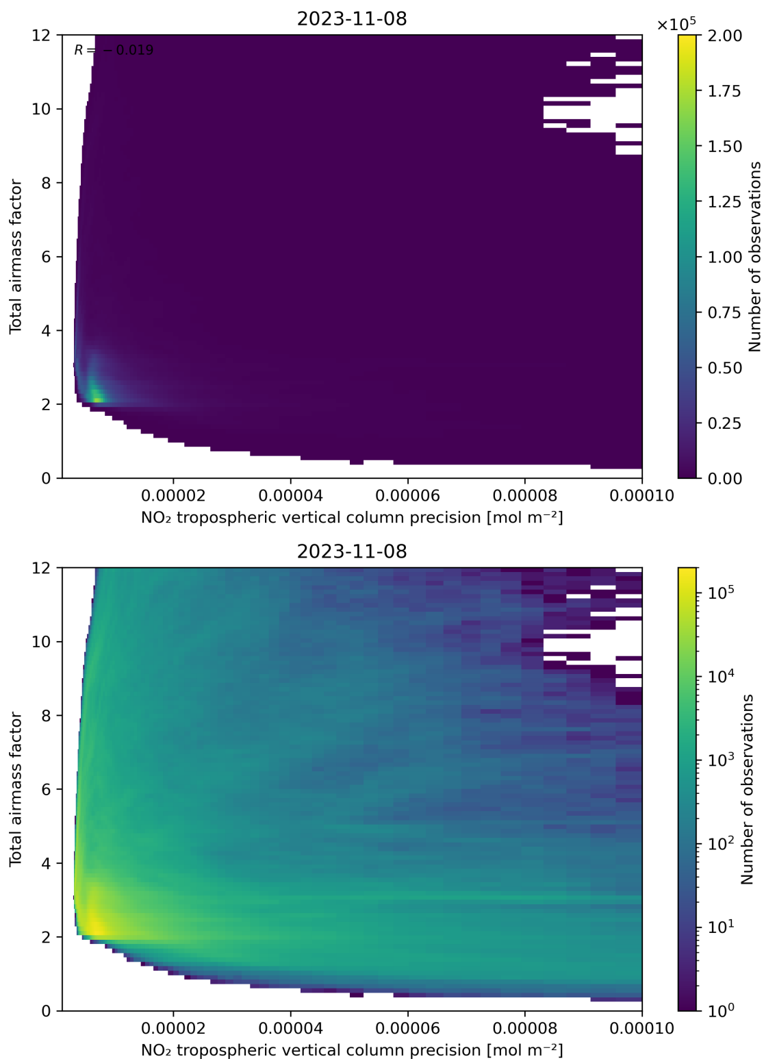
Figure 132: Scatter density plot of “NO 2 tropospheric vertical column precision” against “Total airmass factor” for 2023-11-07 to 2023-11-09.
