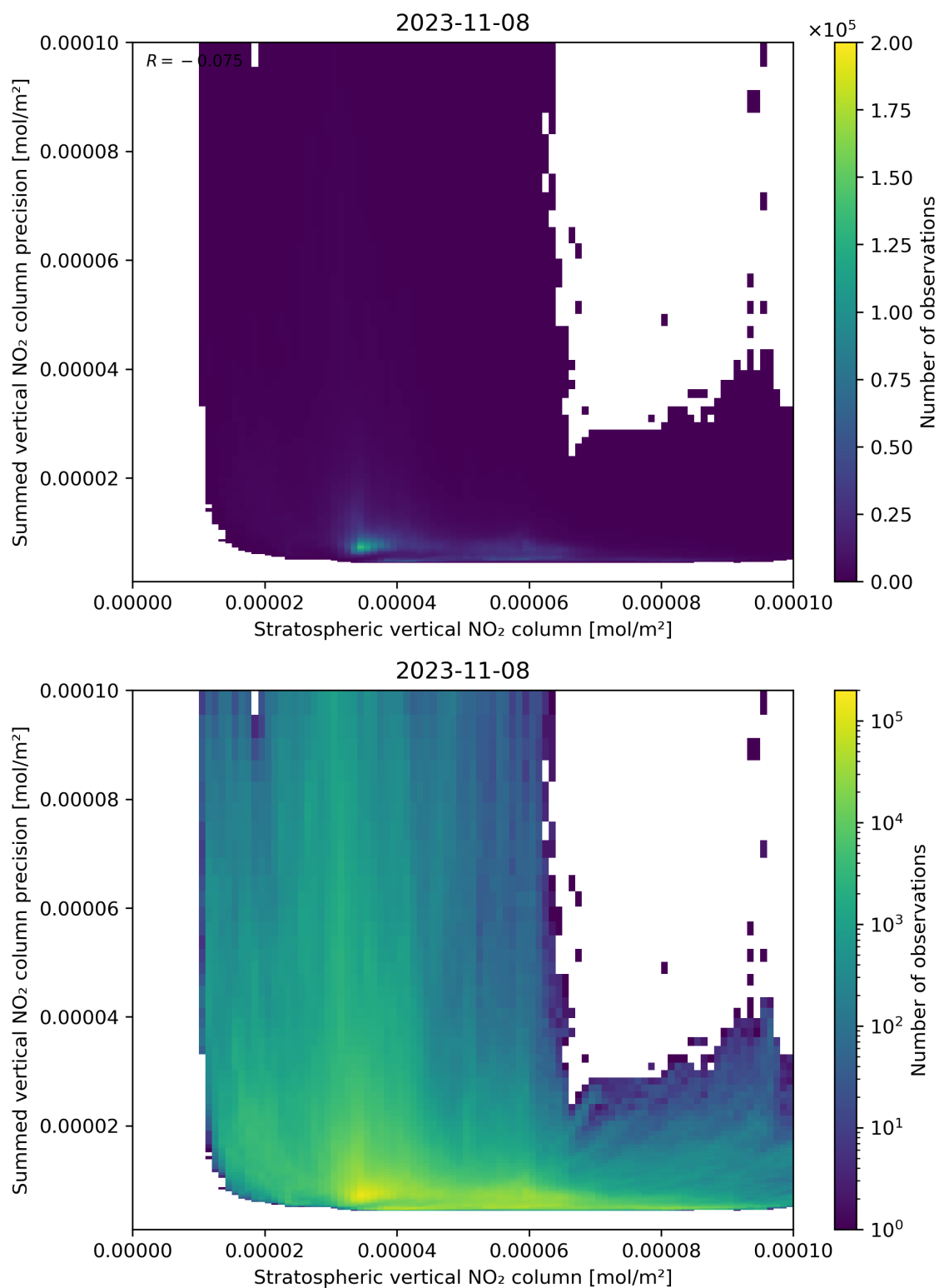
Figure 99: Scatter density plot of “Stratospheric vertical NO 2 column” against “Summed vertical NO 2 column precision” for 2023-11-07 to 2023-11-09.
