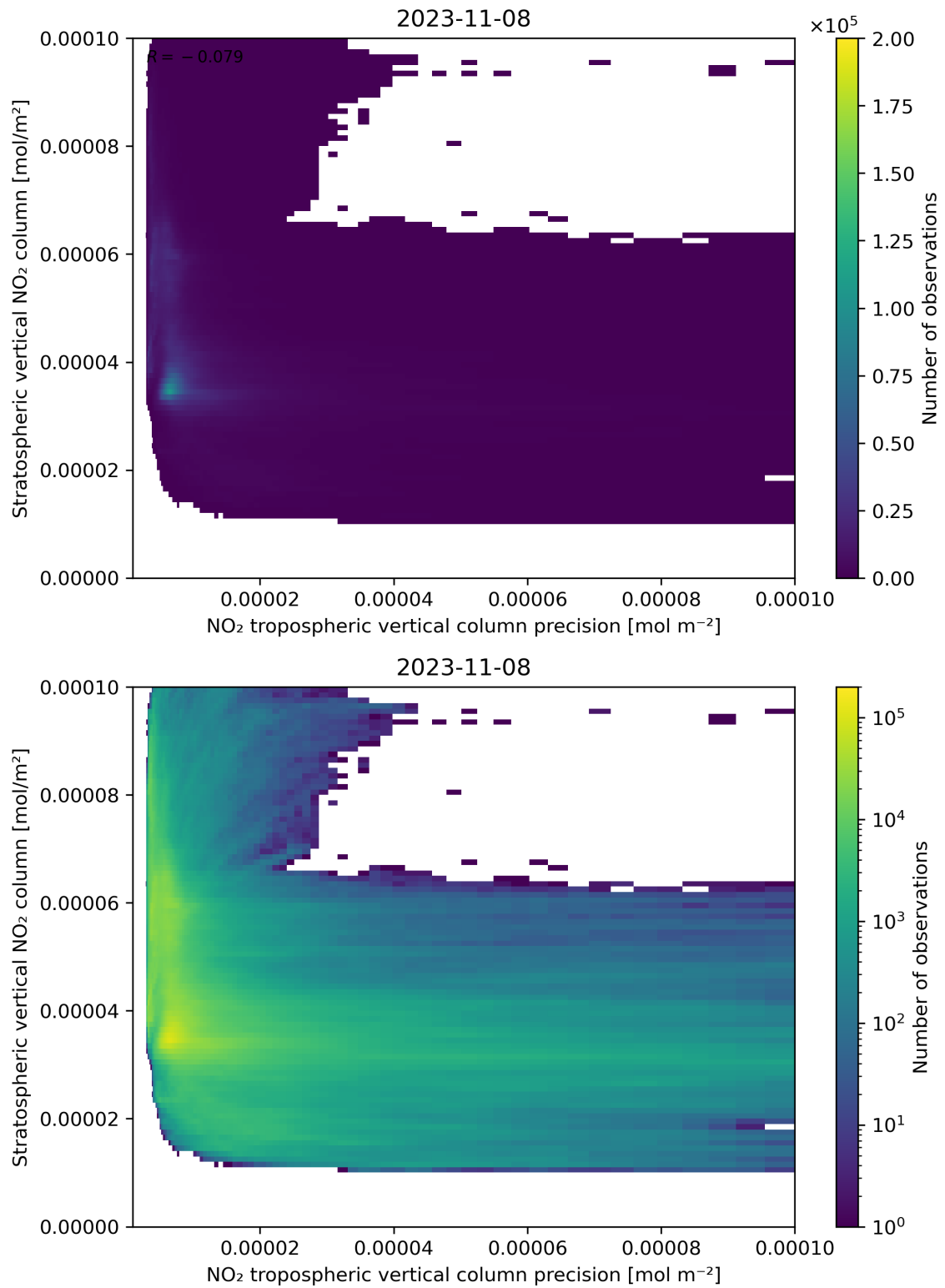
Figure 135: Scatter density plot of “NO 2 tropospheric vertical column precision” against “Stratospheric vertical NO 2 column” for 2023-11-07 to 2023-11-09.
