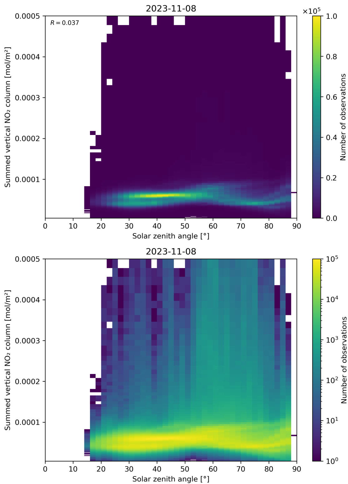
Figure 151: Scatter density plot of “Solar zenith angle” against “Summed vertical NO 2 column” for 2023-11-07 to 2023-11-09.
