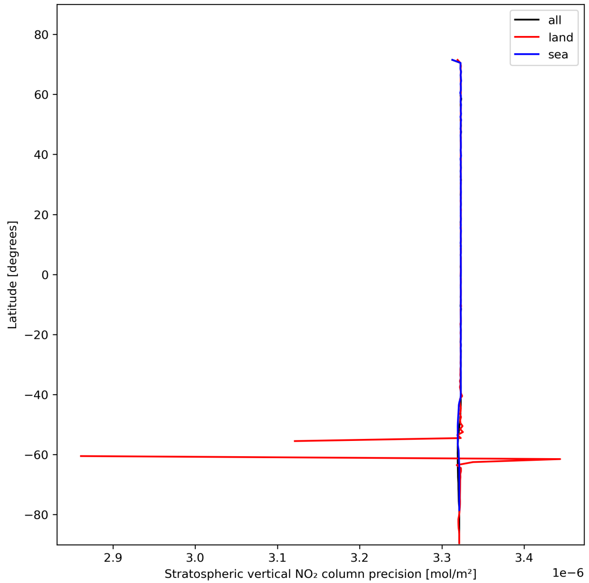
Figure 20: Zonal average of “Stratospheric vertical NO 2 column precision” for 2023-11-07 to 2023-11-09.
