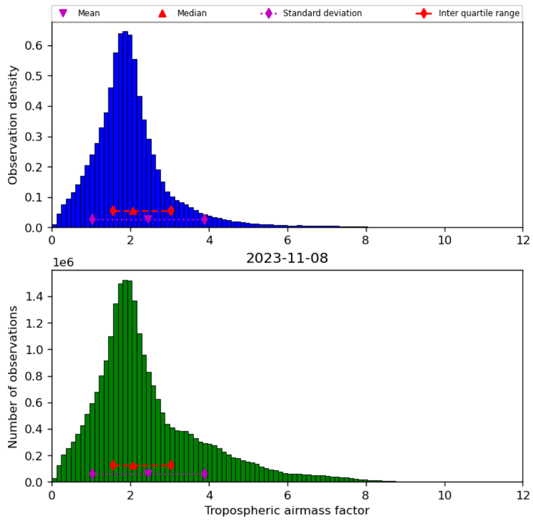
Figure 31: Histogram of “Tropospheric airmass factor” for 2023-11-07 to 2023-11-09
