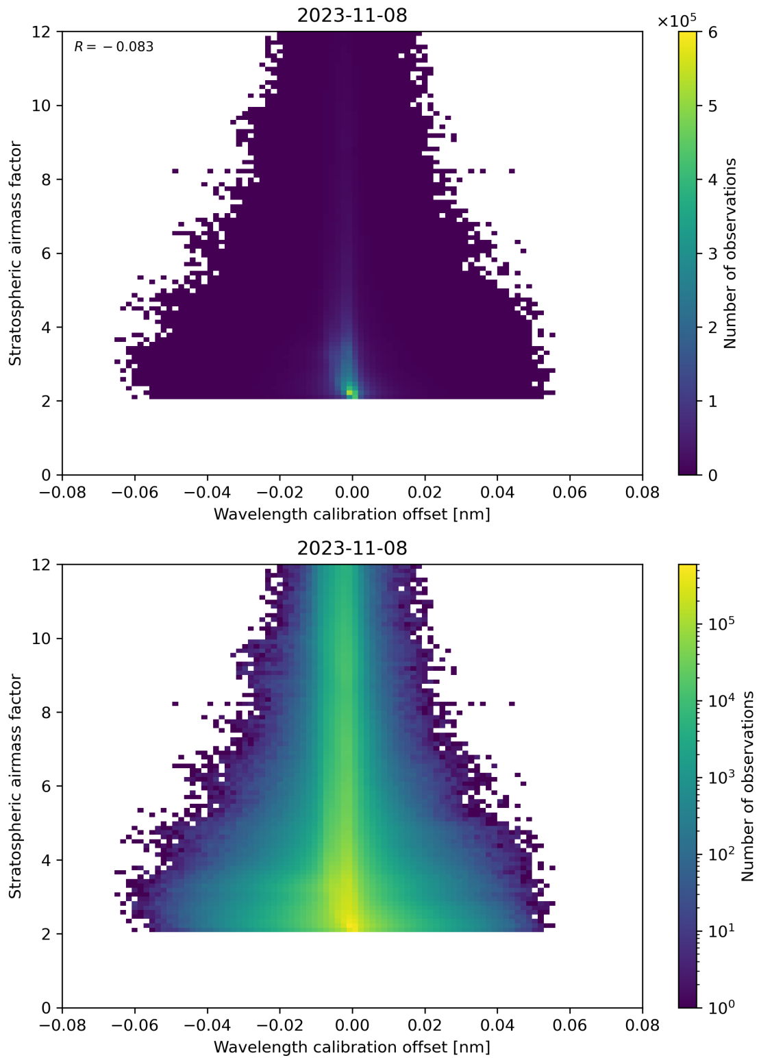
Figure 174: Scatter density plot of “Wavelength calibration offset” against “Stratospheric airmass factor” for 2023-11-07 to 2023-11-09.
