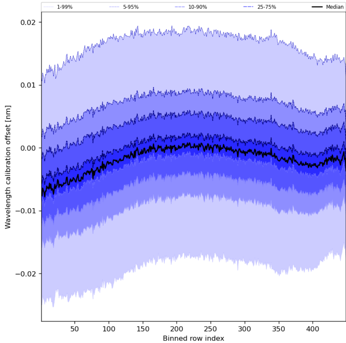
Figure 52: Along track statistics of “Wavelength calibration offset” for 2023-11-07 to 2023-11-09
