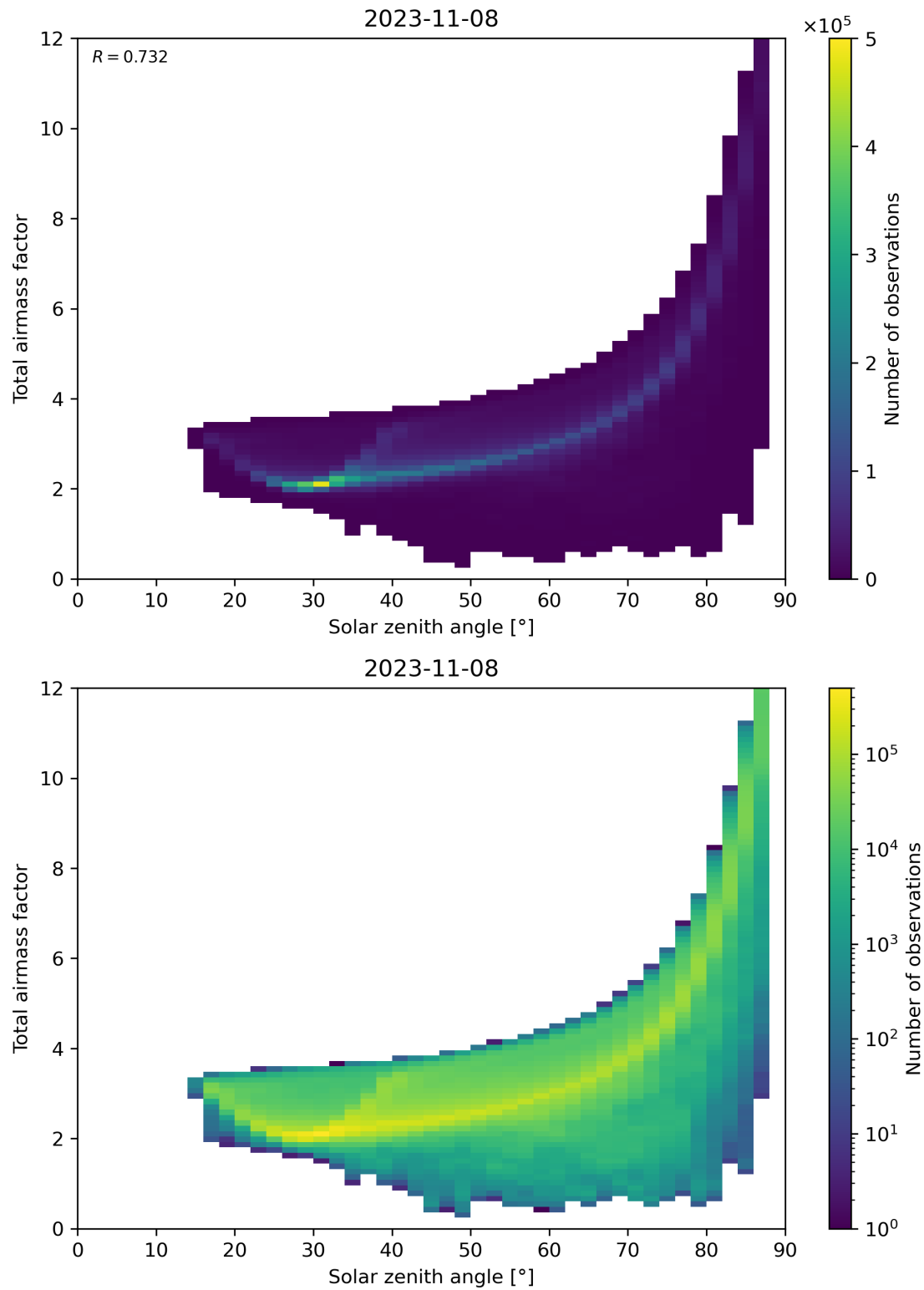
Figure 146: Scatter density plot of “Solar zenith angle” against “Total air mass factor” for 2023-11-07 to 2023-11-09.
