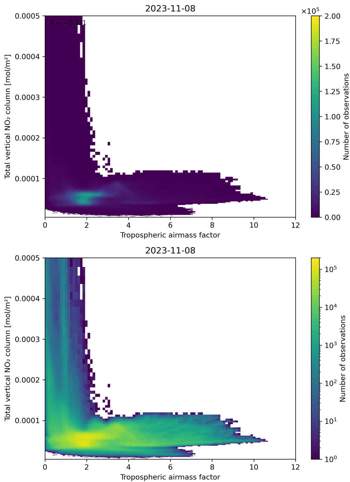
Figure 77: Scatter density plot of “Tropospheric airmass factor” against “Total vertical NO 2 column” for 2023-11-07 to 2023-11-09.
