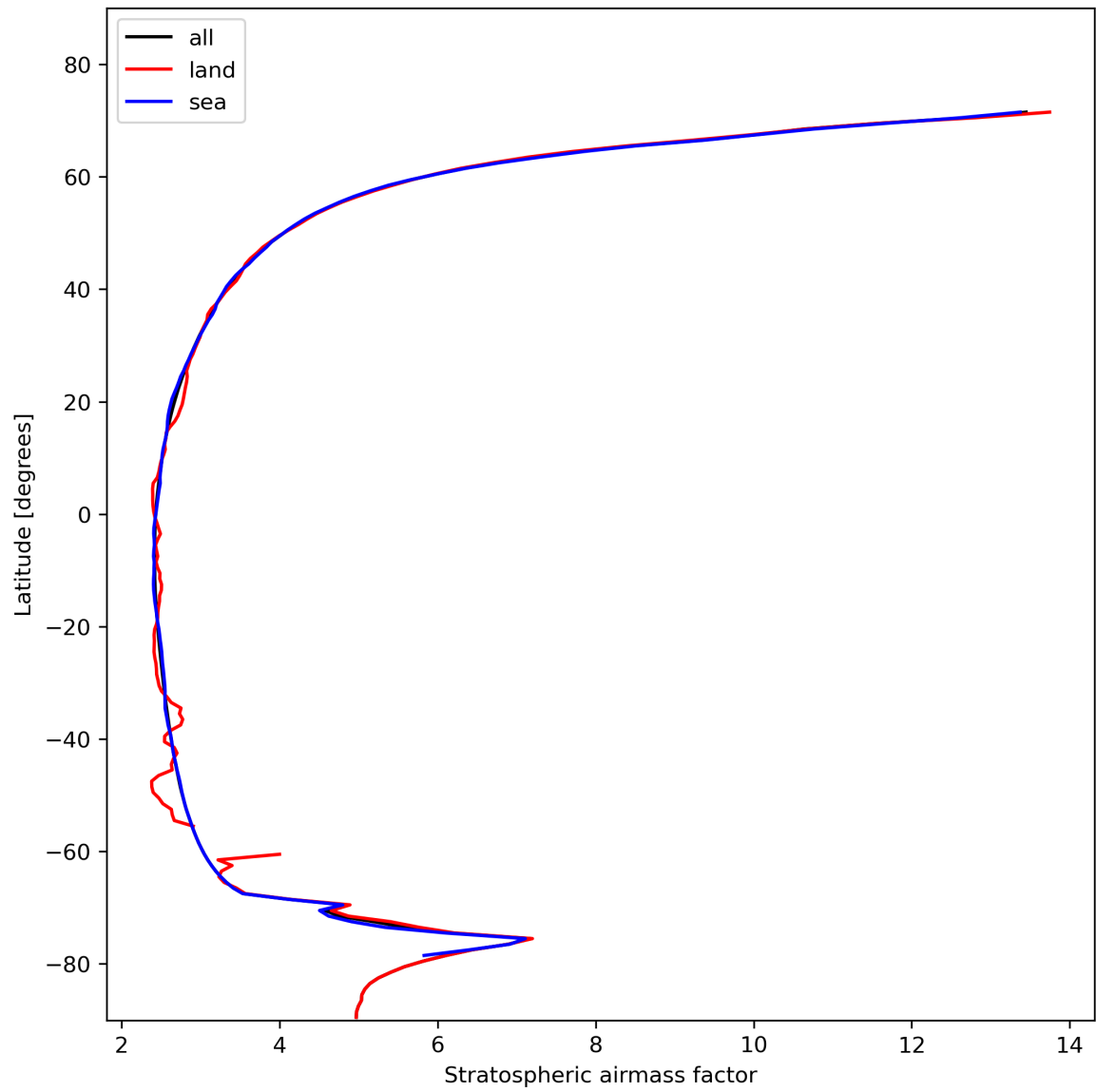
Figure 27: Zonal average of “Stratospheric air mass factor” for 2023-11-07 to 2023-11-09.
