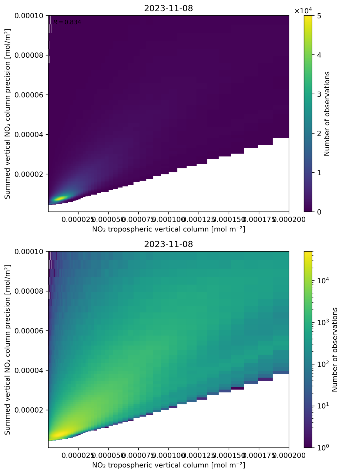
Figure 127: Scatter density plot of “NO 2 tropospheric vertical column” against “Summed vertical NO 2 column precision” for 2023-11-07 to 2023-11-09.
