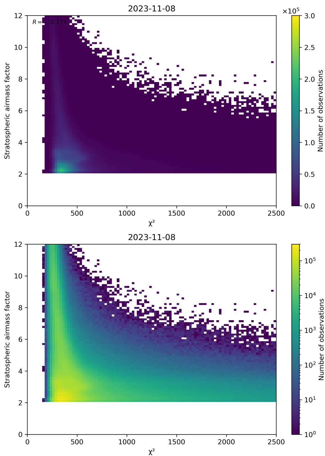
Figure 81: Scatter density plot of “ \chi^2 ” against “Stratospheric airmass factor” for 2023-11-07 to 2023-11-09.
