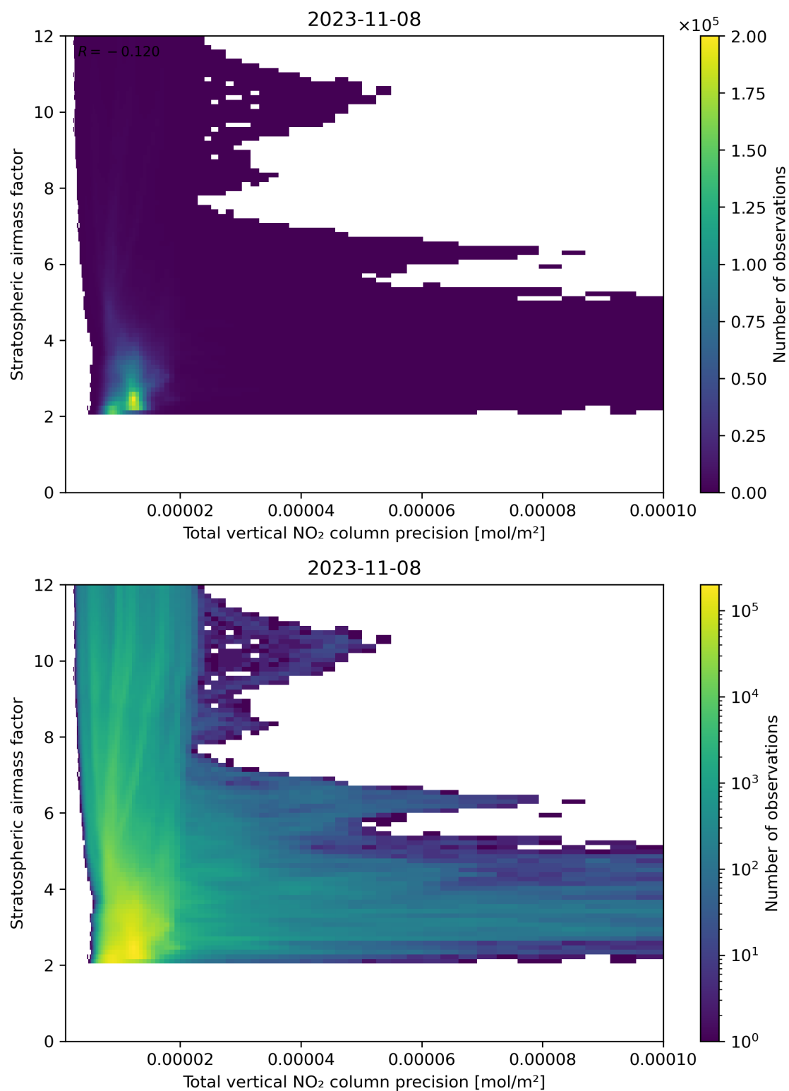
Figure 115: Scatter density plot of “Total vertical NO 2 column precision” against “Stratospheric air mass factor” for 2023-11-07 to 2023-11-09.
