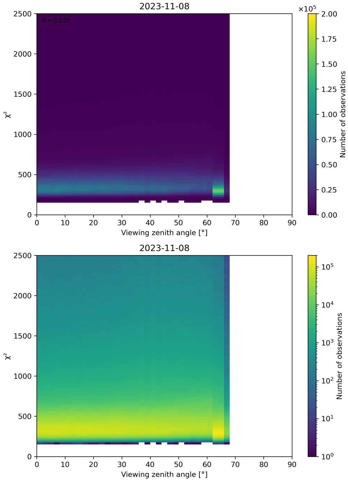
Figure 162: Scatter density plot of “Viewing zenith angle” against “ \chi^2 ” for 2023-11-07 to 2023-11-09.
