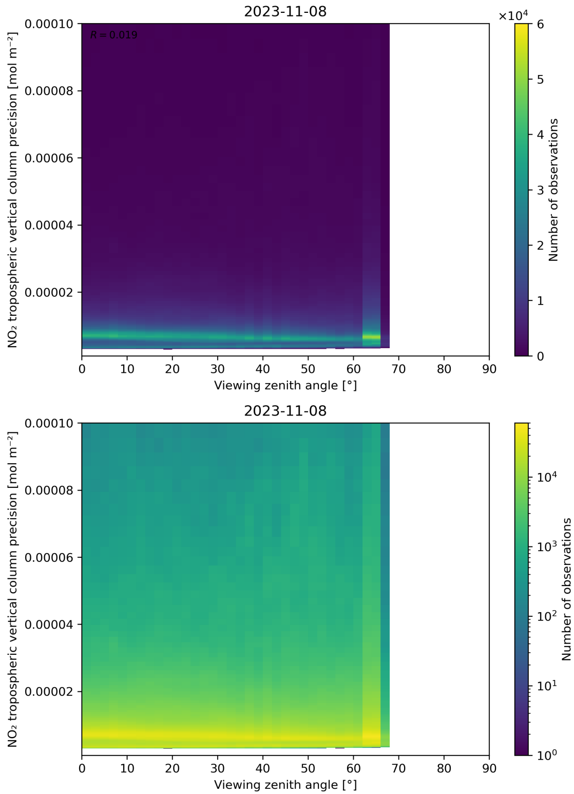
Figure 170: Scatter density plot of “Viewing zenith angle” against “NO 2 tropospheric vertical column precision” for 2023-11-07 to 2023-11-09.
