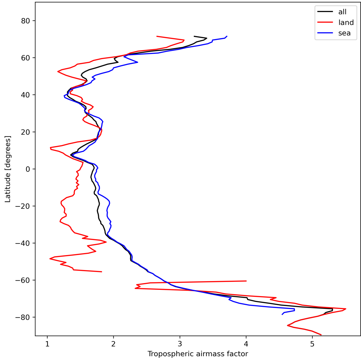
Figure 14: Zonal average of “Tropospheric airmass factor” for 2023-11-07 to 2023-11-09.
