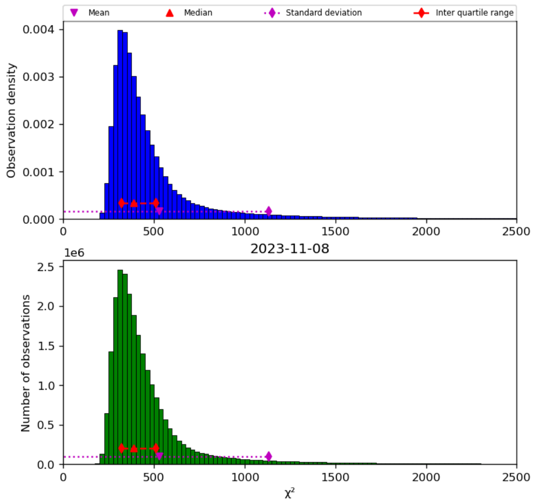
Figure 42: Histogram of “ \chi^2 ” for 2023-11-07 to 2023-11-09
