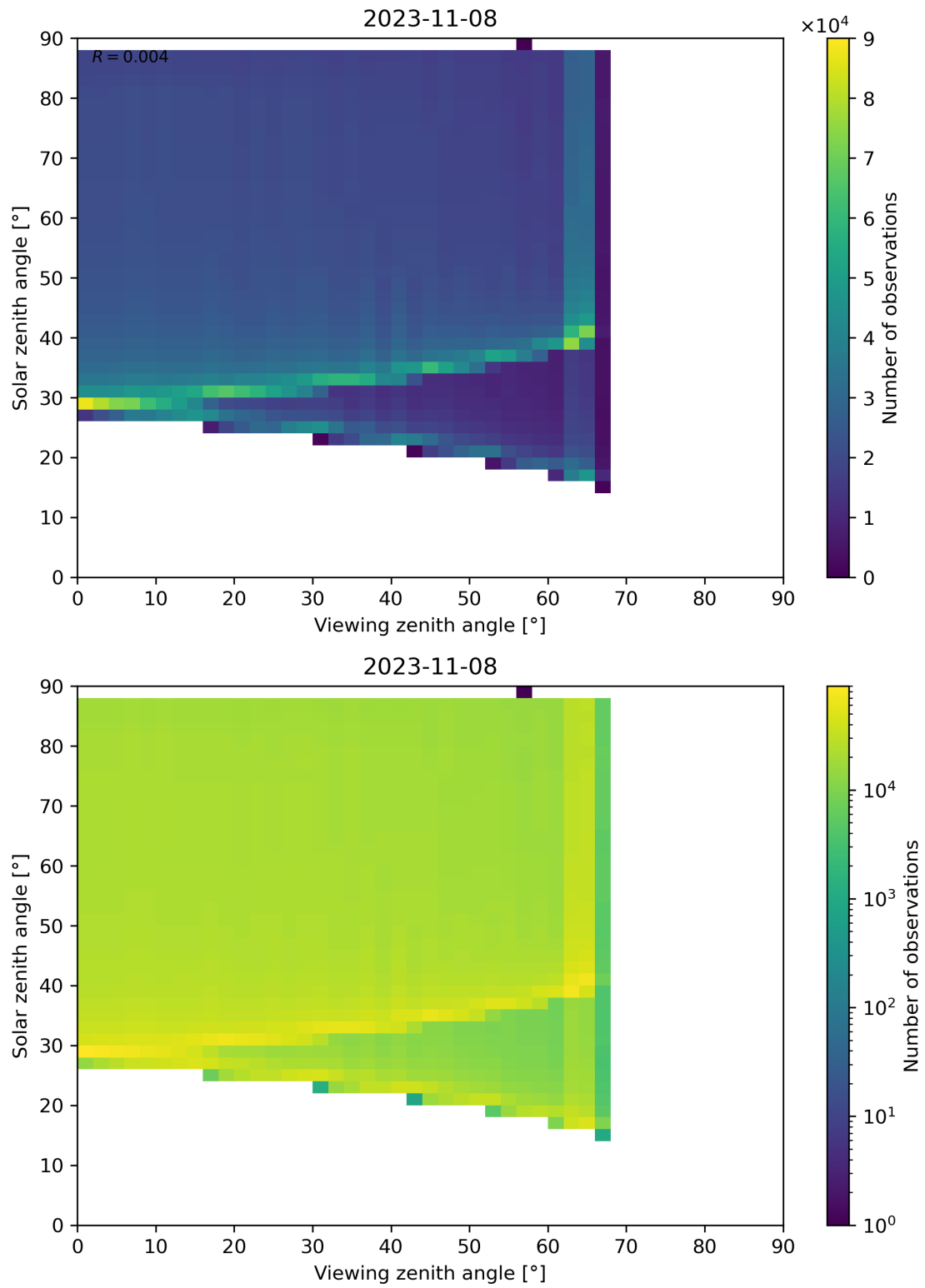
Figure 172: Scatter density plot of “Viewing zenith angle” against “Solar zenith angle” for 2023-11-07 to 2023-11-09.
