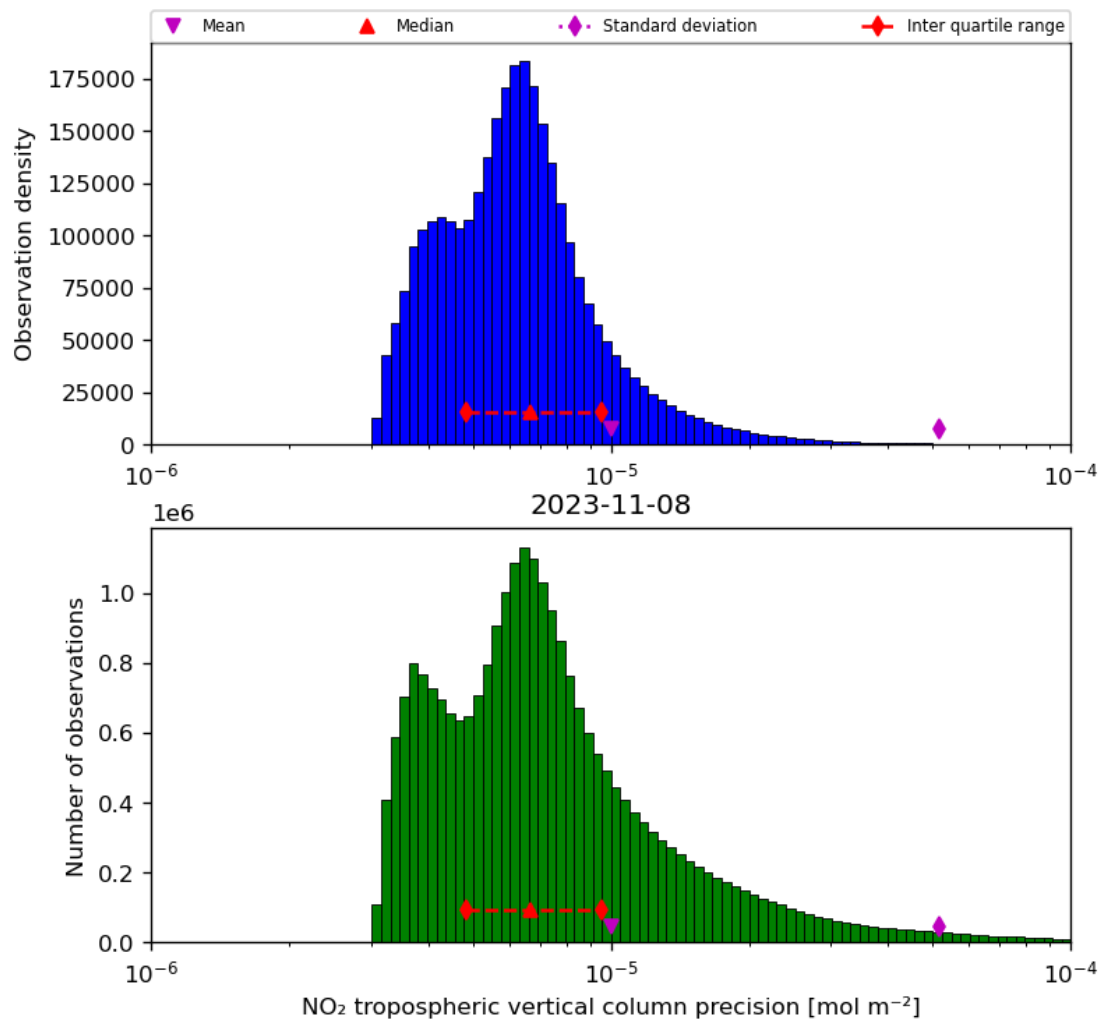
Figure 30: Histogram of “NO 2 tropospheric vertical column precision” for 2023-11-07 to 2023-11-09
