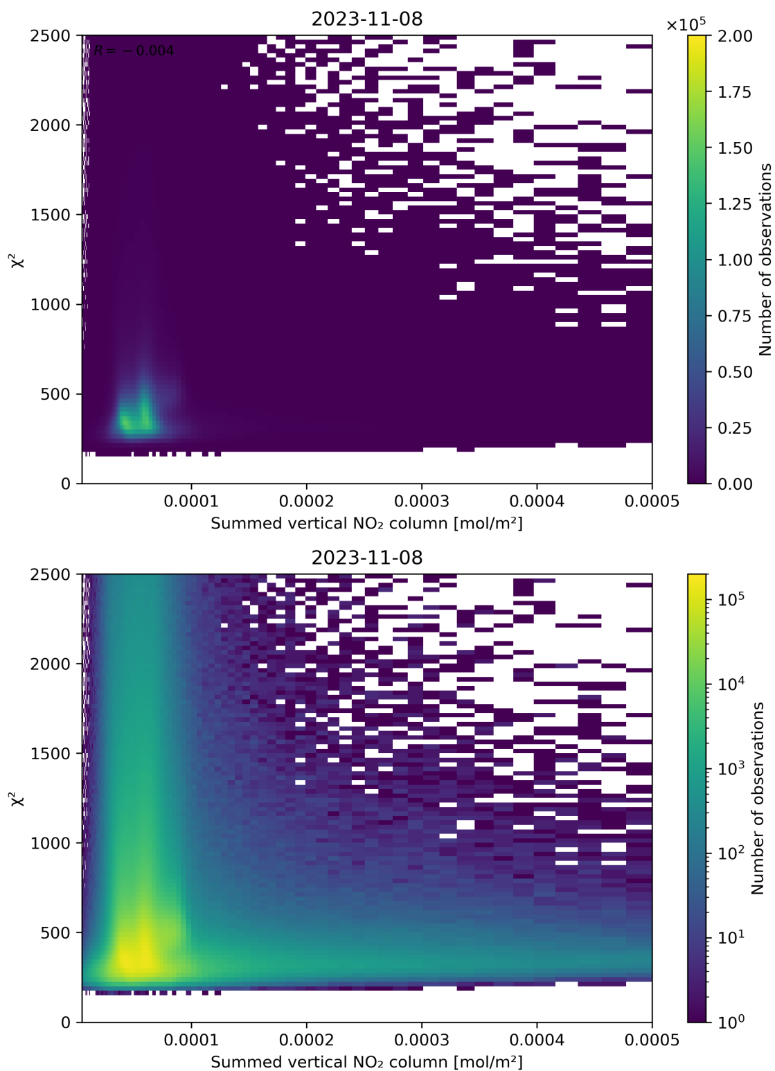
Figure 104: Scatter density plot of “Summed vertical NO 2 column” against “ \chi^2 ” for 2023-11-07 to 2023-11-09.
