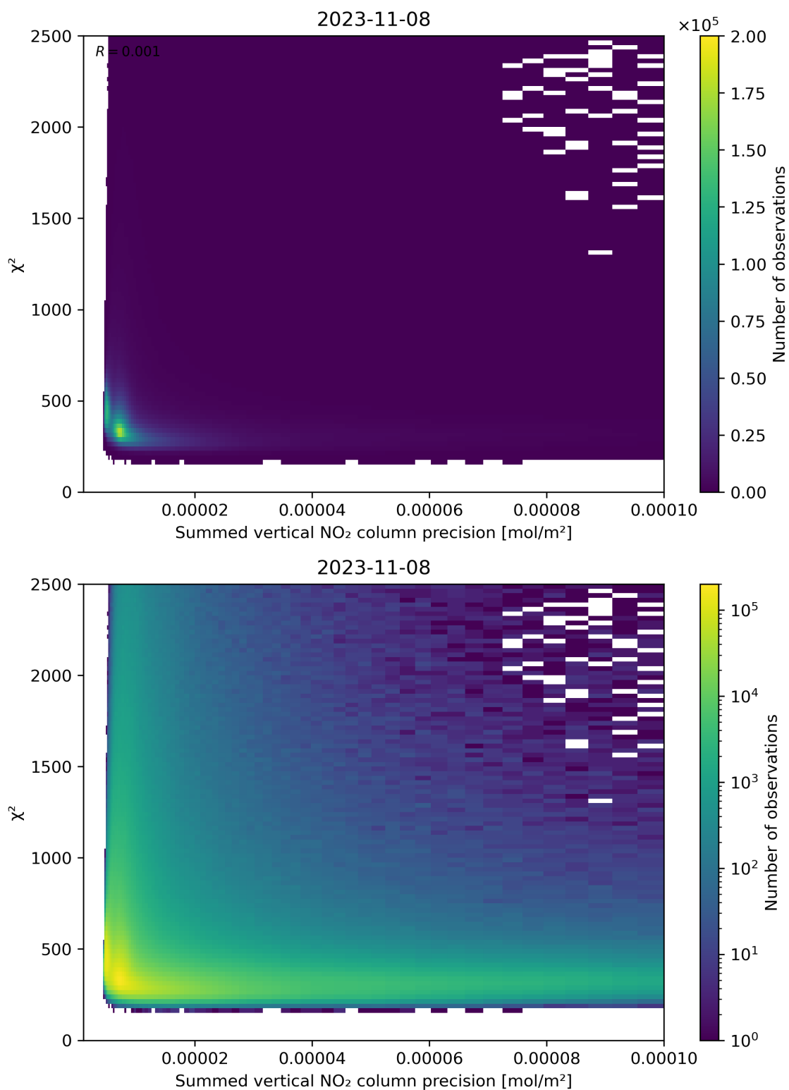
Figure 107: Scatter density plot of “Summed vertical NO 2 column precision” against “ \chi^2 ” for 2023-11-07 to 2023-11-09.
