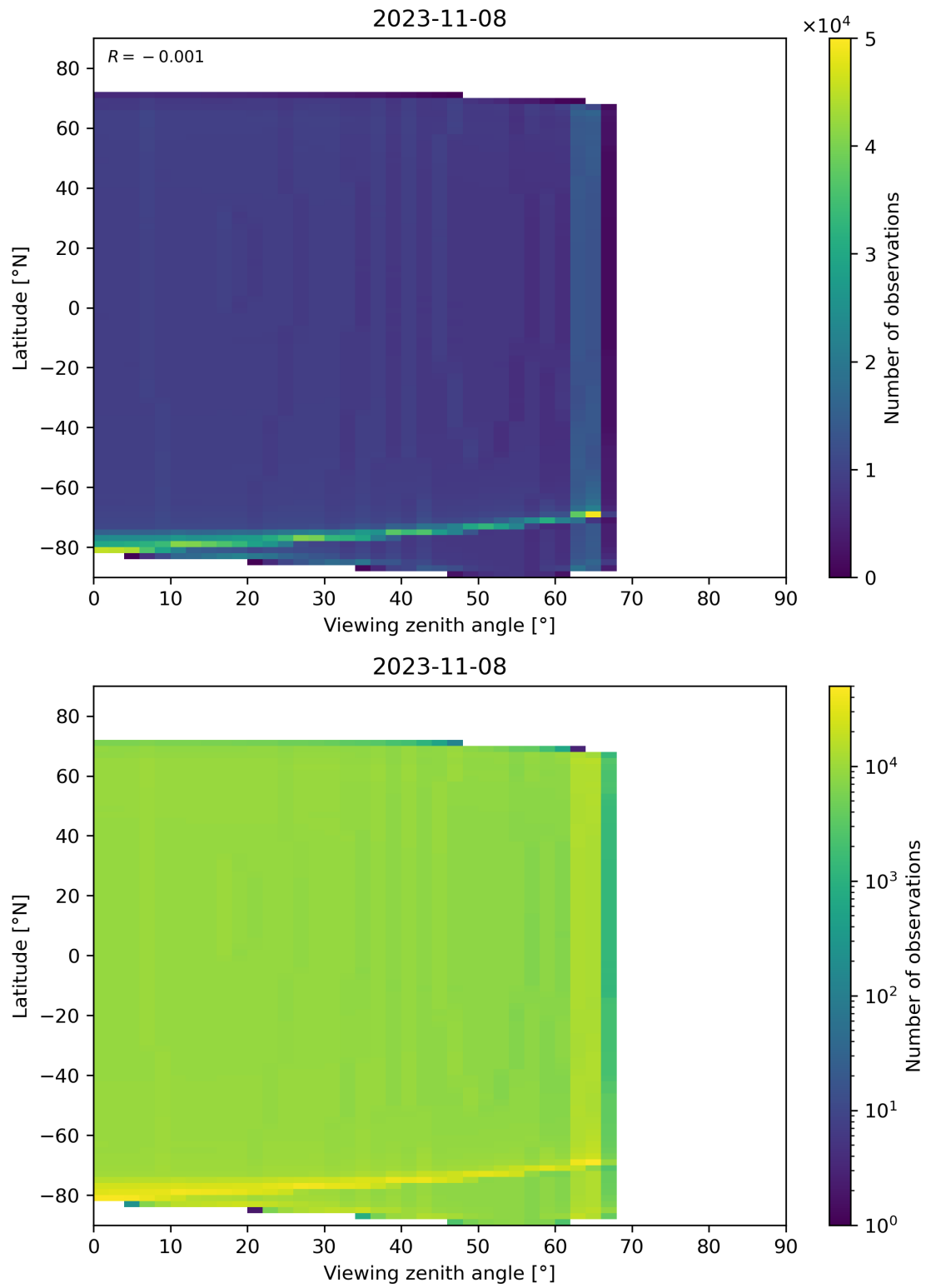
Figure 163: Scatter density plot of “Viewing zenith angle” against “Latitude” for 2023-11-07 to 2023-11-09.
