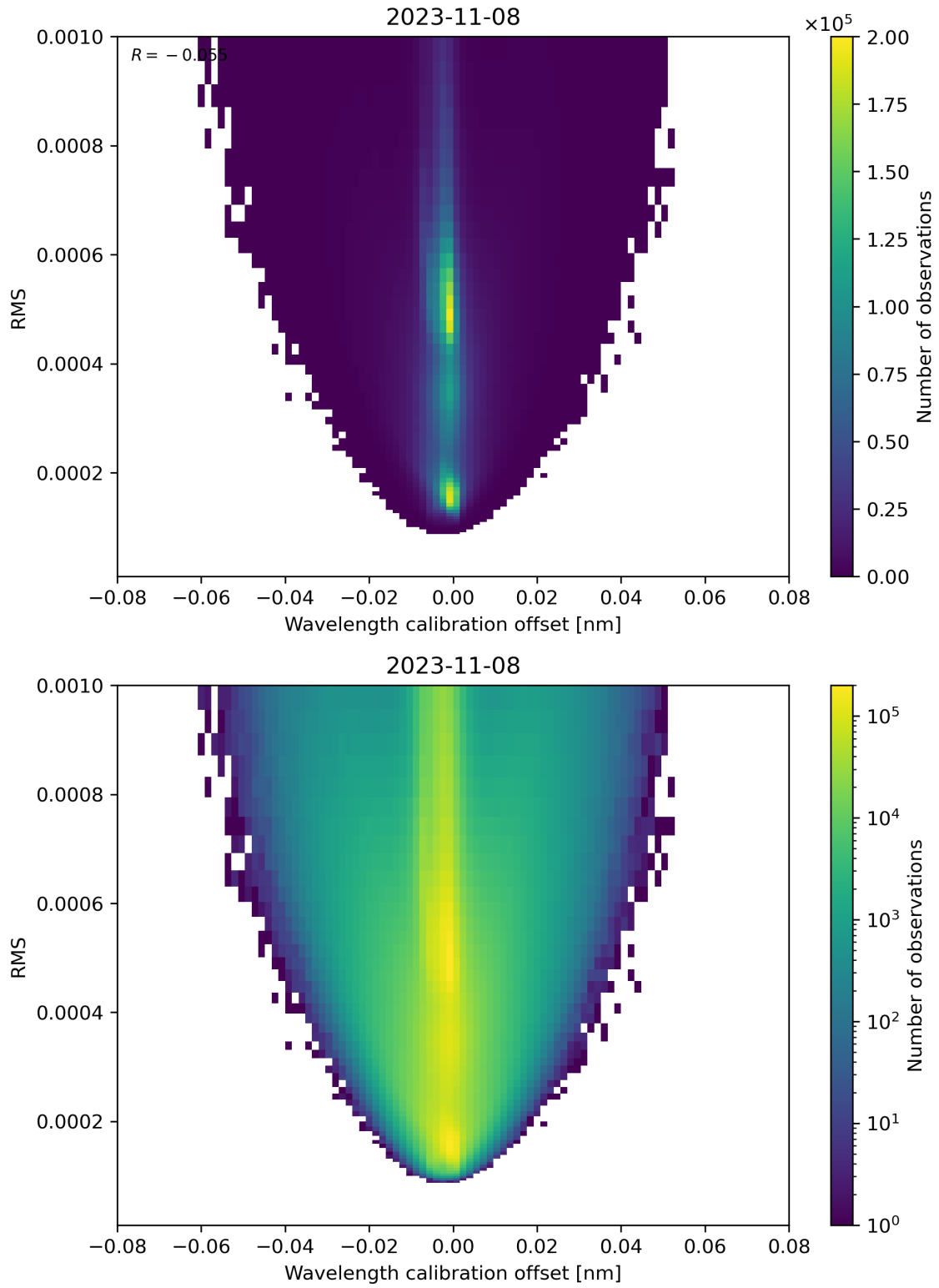
Figure 181: Scatter density plot of “Wavelength calibration offset” against “RMS” for 2023-11-07 to 2023-11-09.
