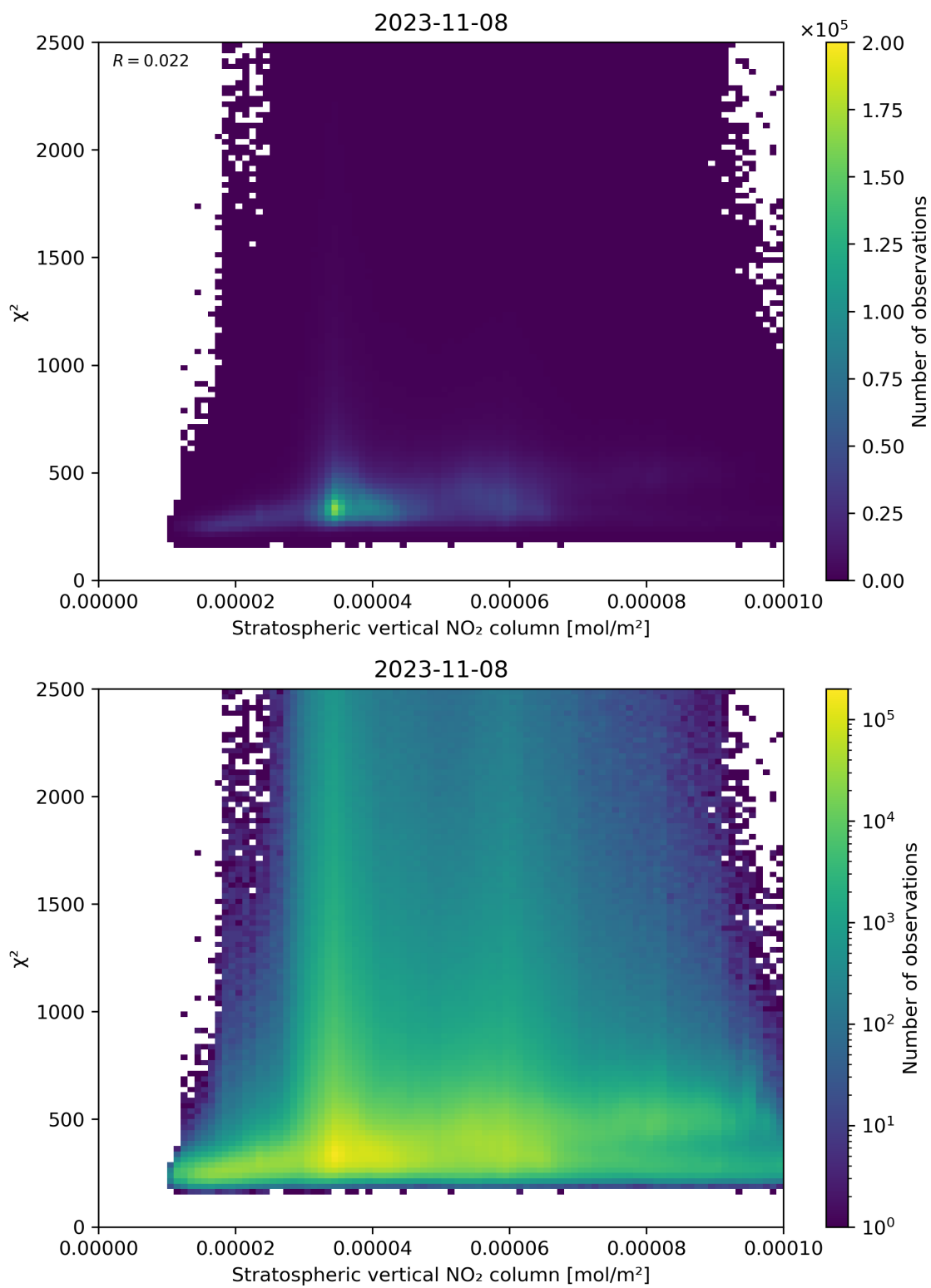
Figure 97: Scatter density plot of “Stratospheric vertical NO 2 column” against “ \chi^2 ” for 2023-11-07 to 2023-11-09.
