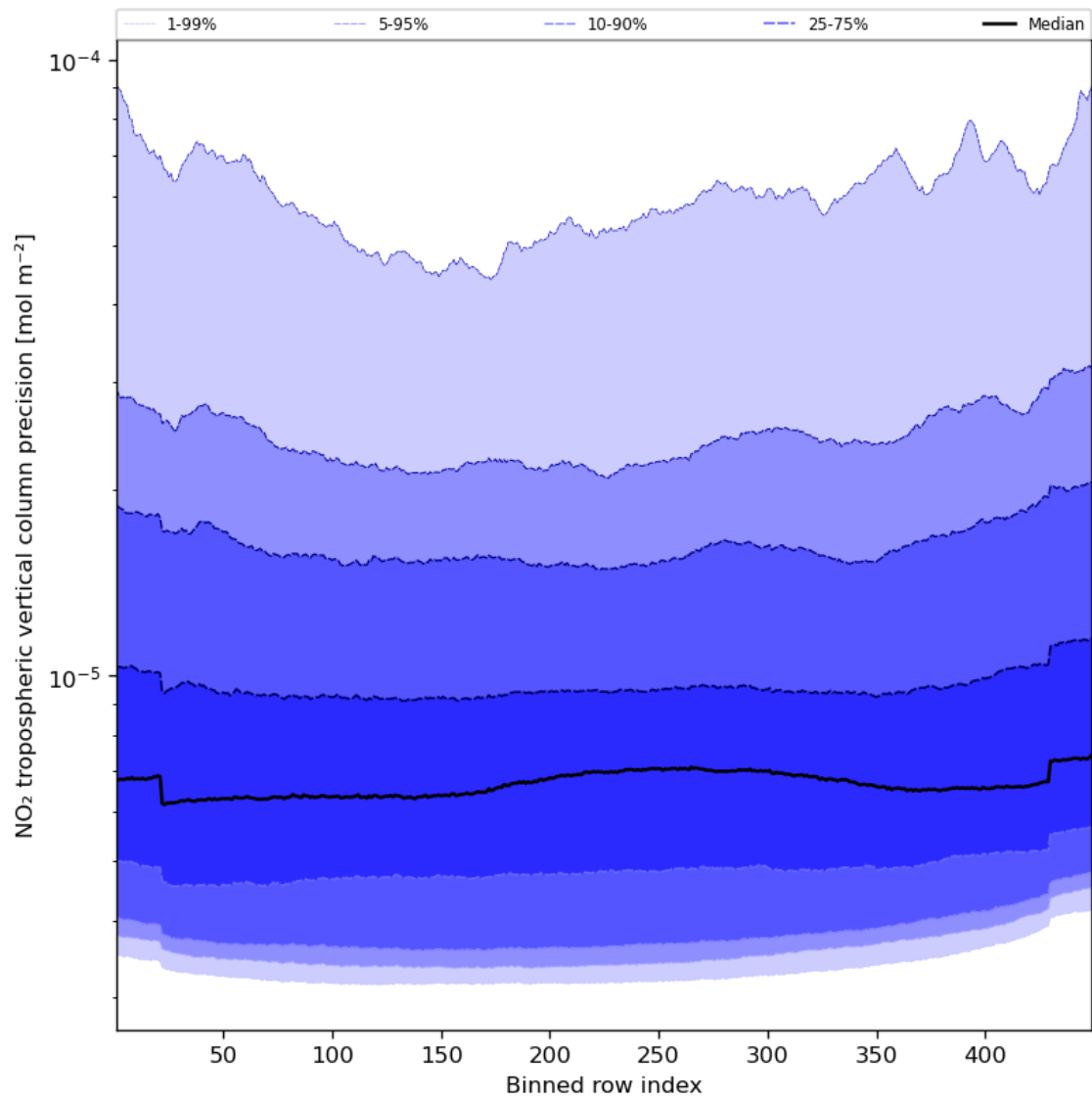
Figure 47: Along track statistics of “NO 2 tropospheric vertical column precision” for 2023-11-07 to 2023-11-09
