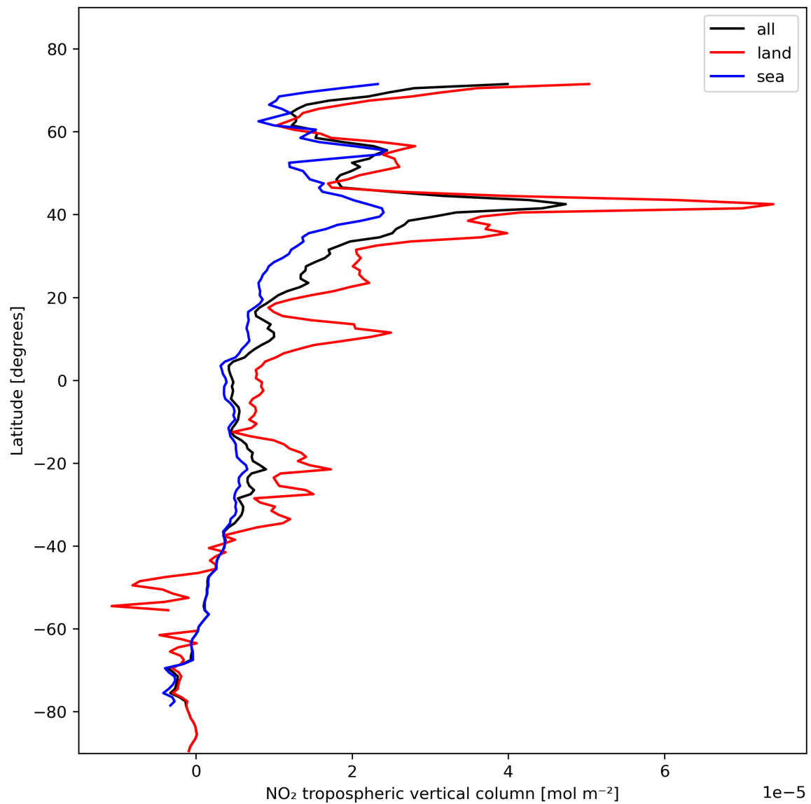
Figure 12: Zonal average of “NO 2 tropospheric vertical column” for 2023-11-07 to 2023-11-09.
