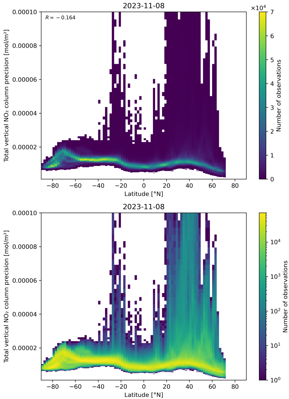
Figure 91: Scatter density plot of “Latitude” against “Total vertical NO 2 column precision” for 2023-11-07 to 2023-11-09.
