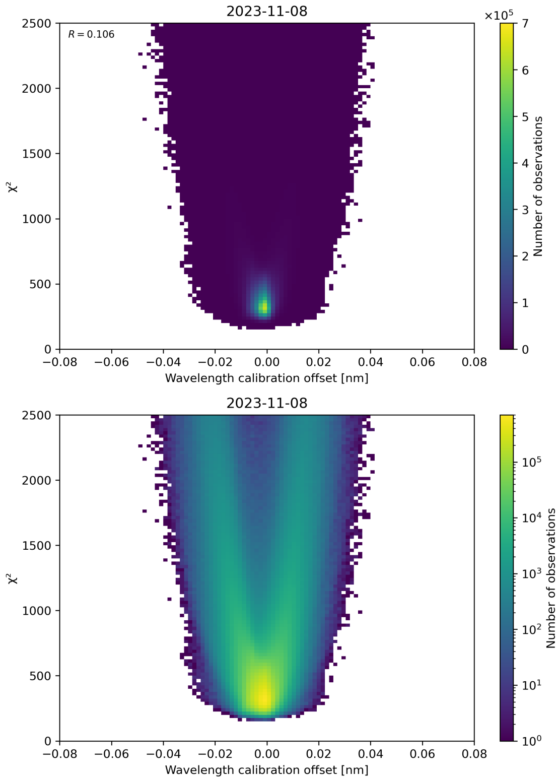
Figure 175: Scatter density plot of “Wavelength calibration offset” against “ \chi^2 ” for 2023-11-07 to 2023-11-09.
