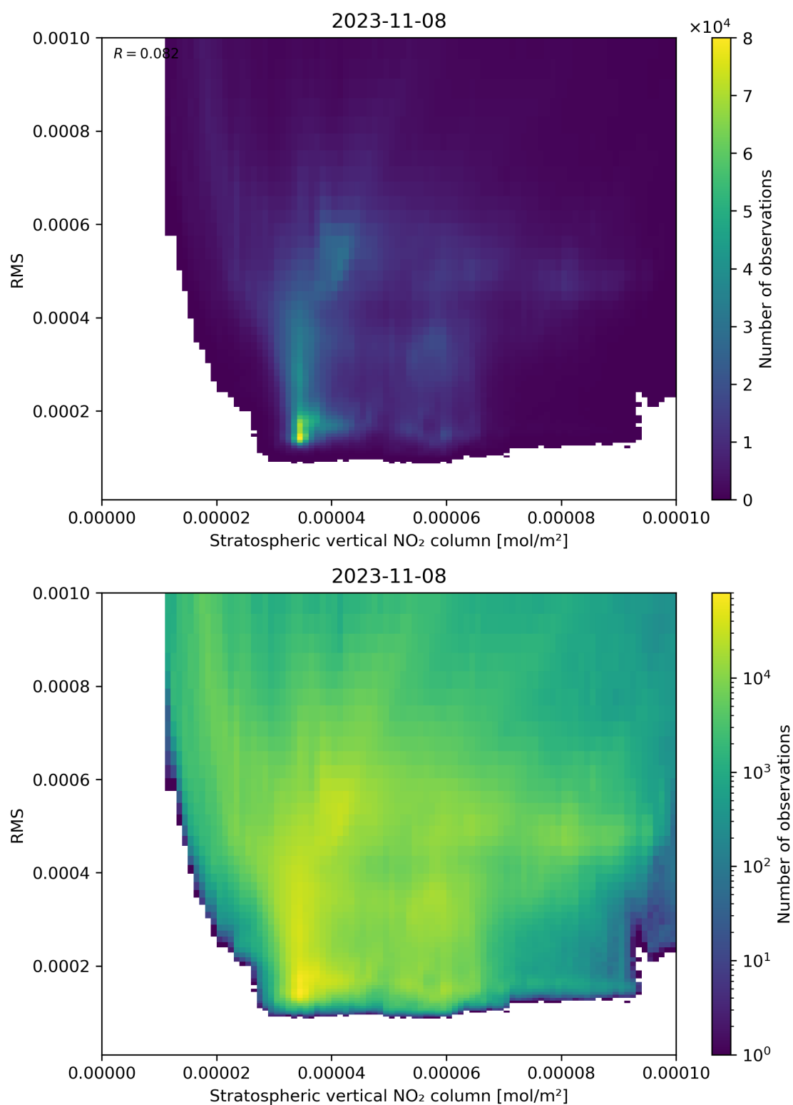
Figure 102: Scatter density plot of “Stratospheric vertical NO 2 column” against “RMS” for 2023-11-07 to 2023-11-09.
