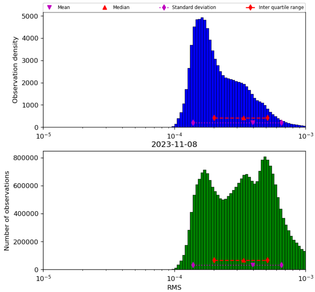
Figure 43: Histogram of “RMS” for 2023-11-07 to 2023-11-09
