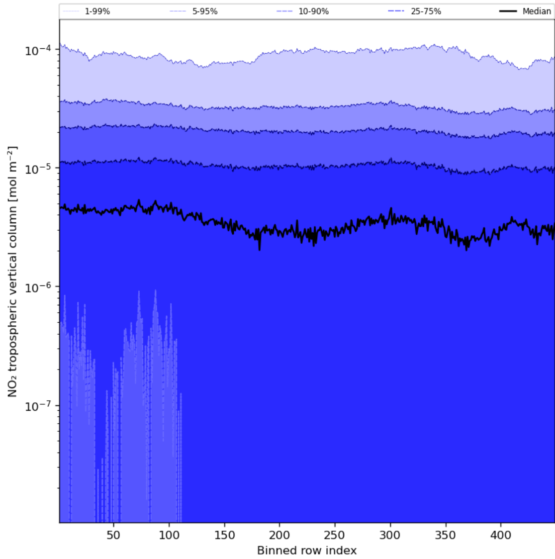
Figure 46: Along track statistics of “NO 2 tropospheric vertical column” for 2023-11-07 to 2023-11-09
