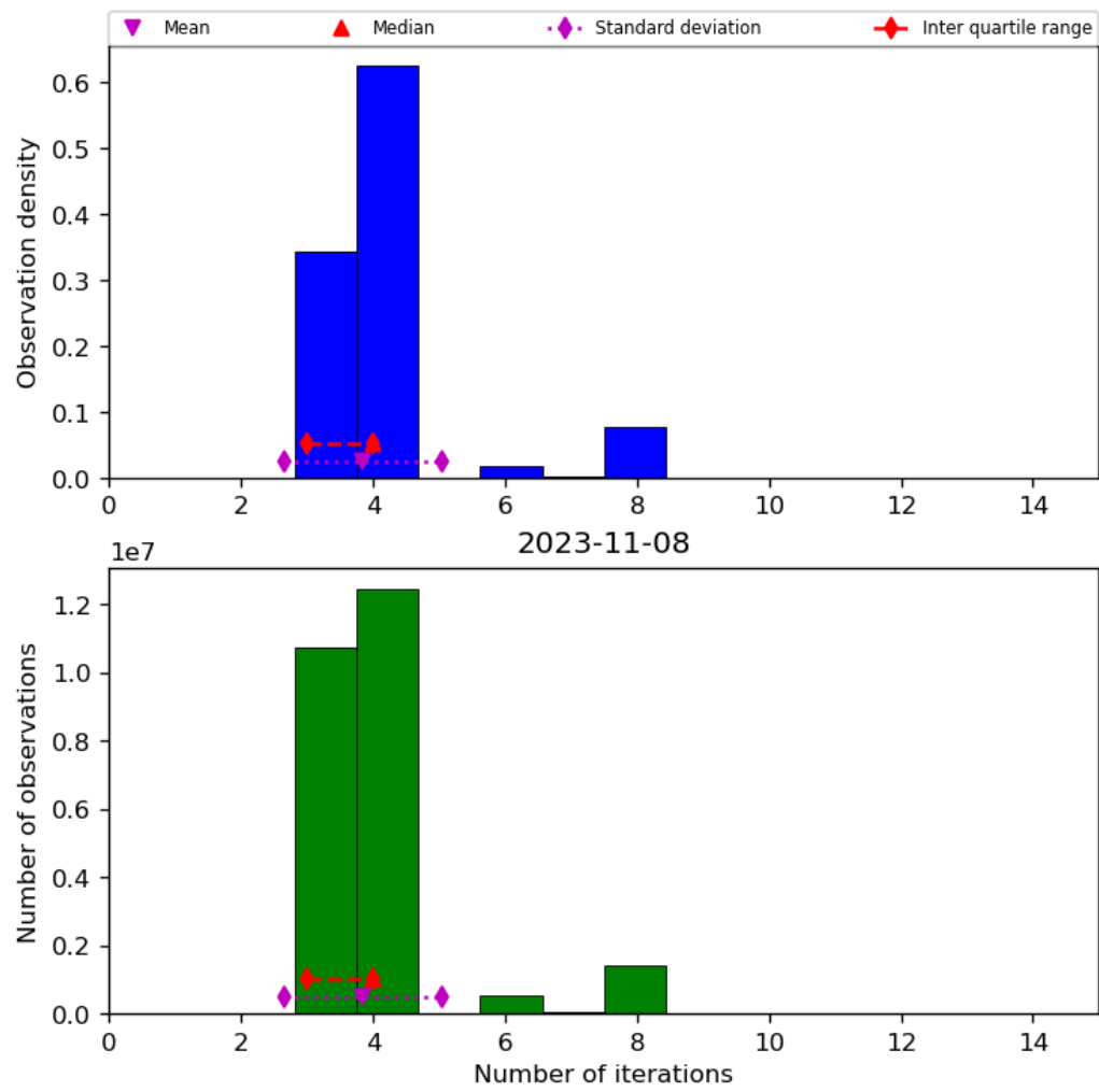
Figure 34: Histogram of “Number of iterations” for 2023-11-07 to 2023-11-09
