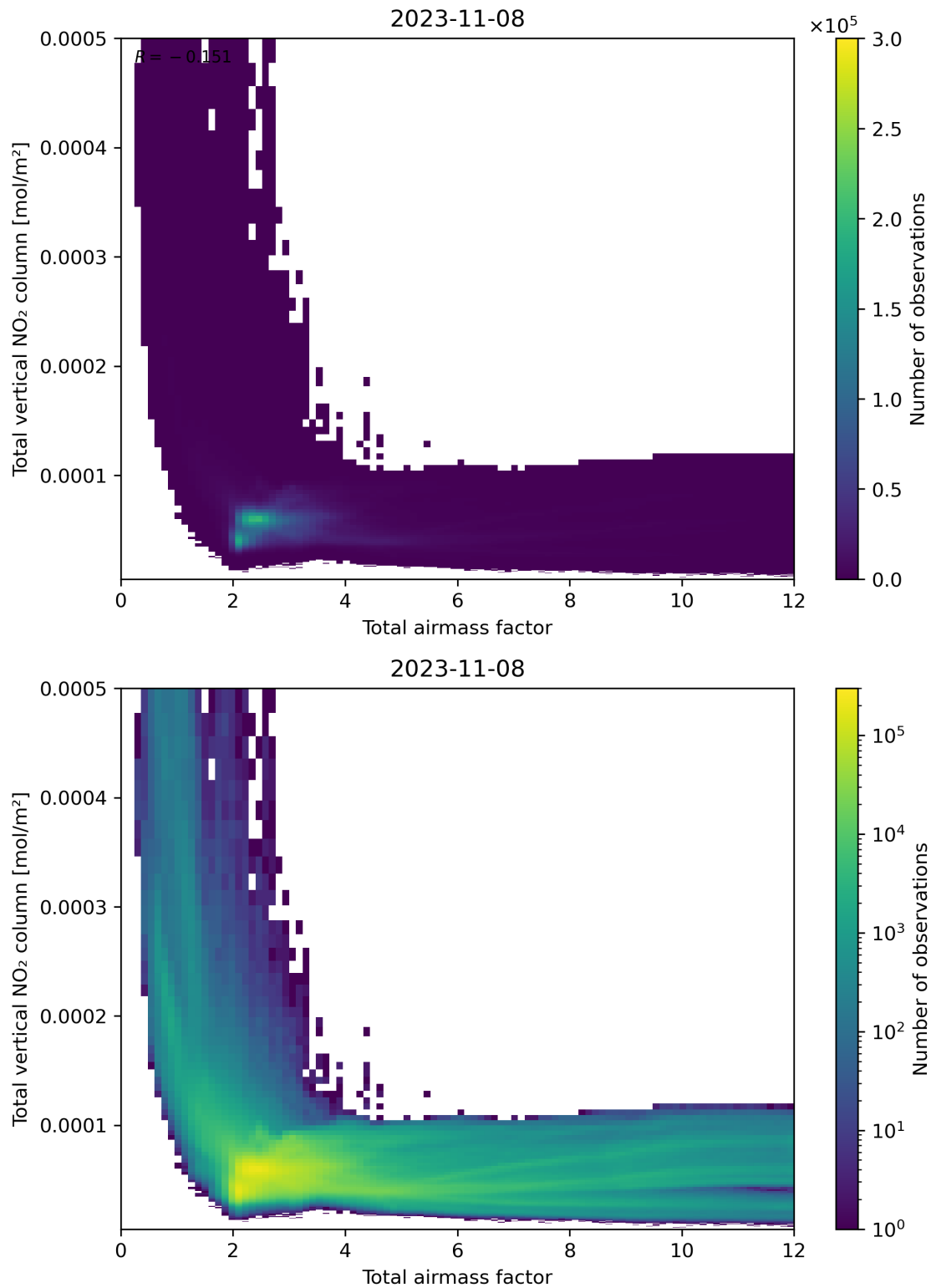
Figure 67: Scatter density plot of “Total airmass factor” against “Total vertical NO 2 column” for 2023-11-07 to 2023-11-09.
