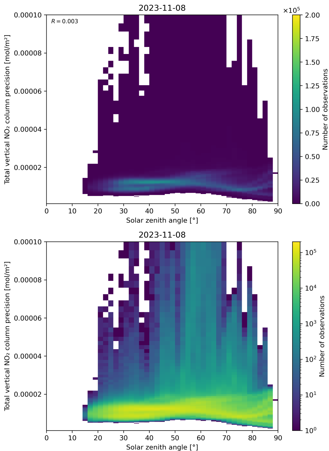
Figure 154: Scatter density plot of “Solar zenith angle” against “Total vertical NO 2 column precision” for 2023-11-07 to 2023-11-09.
