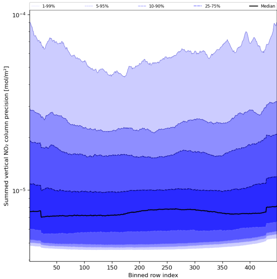
Figure 58: Along track statistics of “Summed vertical NO 2 column precision” for 2023-11-07 to 2023-11-09
