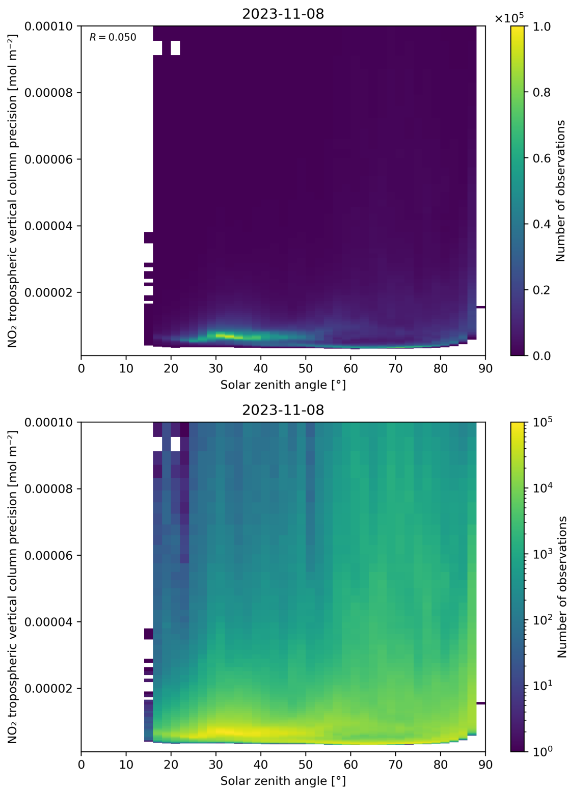
Figure 156: Scatter density plot of “Solar zenith angle” against “NO 2 tropospheric vertical column precision” for 2023-11-07 to 2023-11-09.
