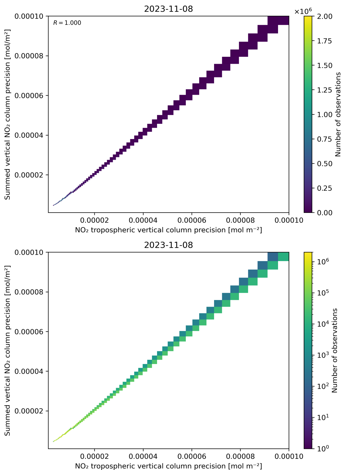
Figure 137: Scatter density plot of “NO 2 tropospheric vertical column precision” against “Summed vertical NO 2 column precision” for 2023-11-07 to 2023-11-09.
