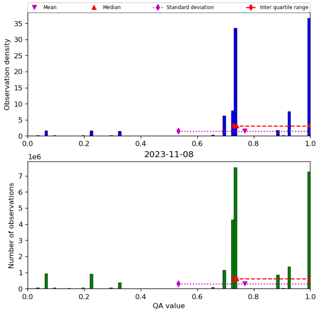
Figure 28: Histogram of “QA value” for 2023-11-07 to 2023-11-09
