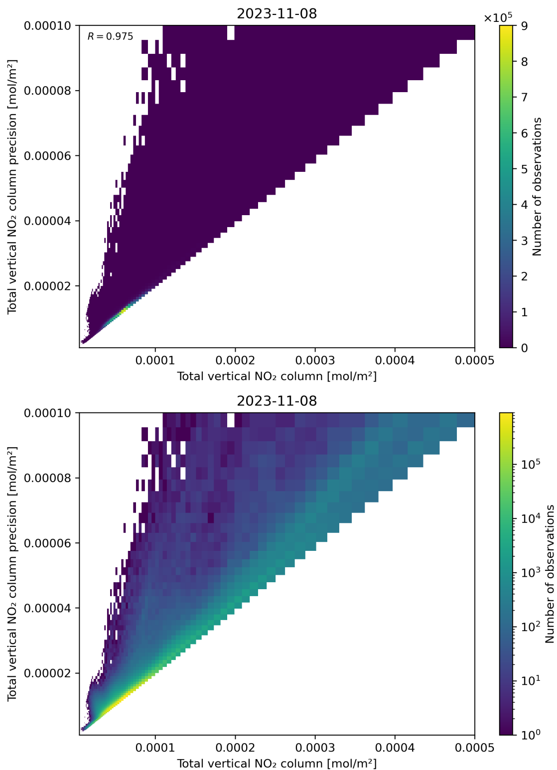
Figure 114: Scatter density plot of “Total vertical NO 2 column” against “Total vertical NO 2 column precision” for 2023-11-07 to 2023-11-09.
