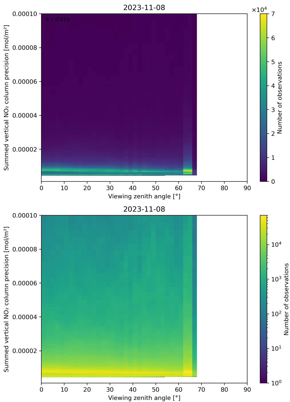
Figure 166: Scatter density plot of “Viewing zenith angle” against “Summed vertical NO 2 column precision” for 2023-11-07 to 2023-11-09.
