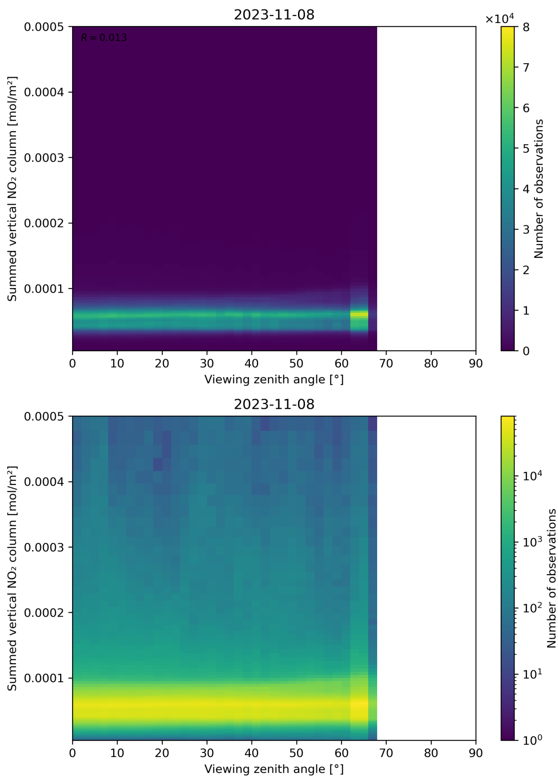
Figure 165: Scatter density plot of “Viewing zenith angle” against “Summed vertical NO 2 column” for 2023-11-07 to 2023-11-09.
