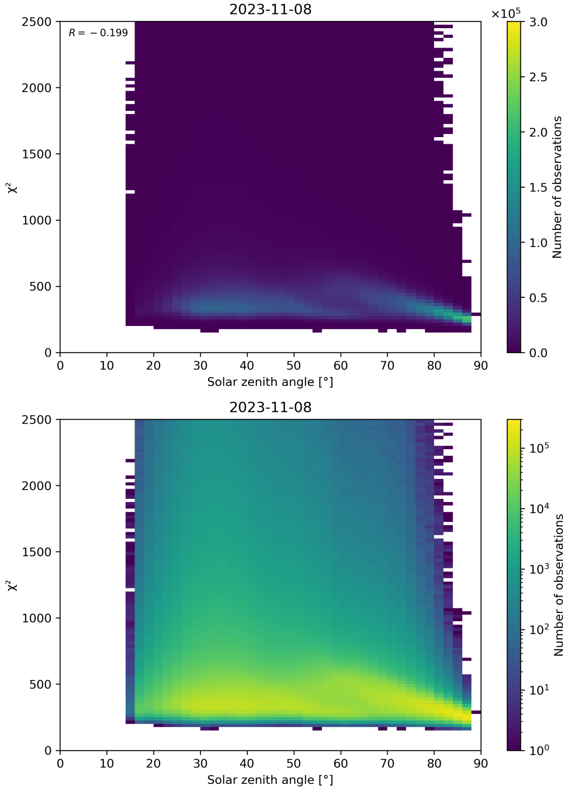
Figure 148: Scatter density plot of “Solar zenith angle” against “ \chi^2 ” for 2023-11-07 to 2023-11-09.
