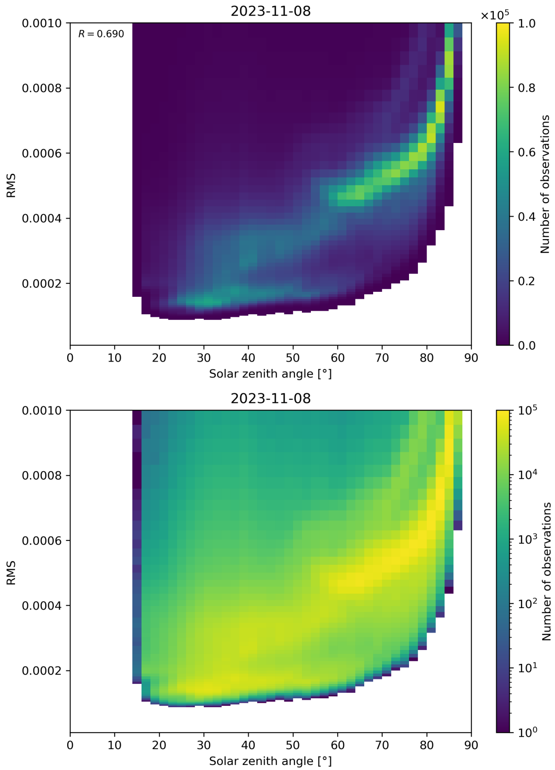
Figure 157: Scatter density plot of “Solar zenith angle” against “RMS” for 2023-11-07 to 2023-11-09.
