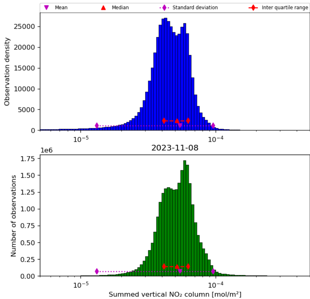
Figure 40: Histogram of “Summed vertical NO 2 column” for 2023-11-07 to 2023-11-09
