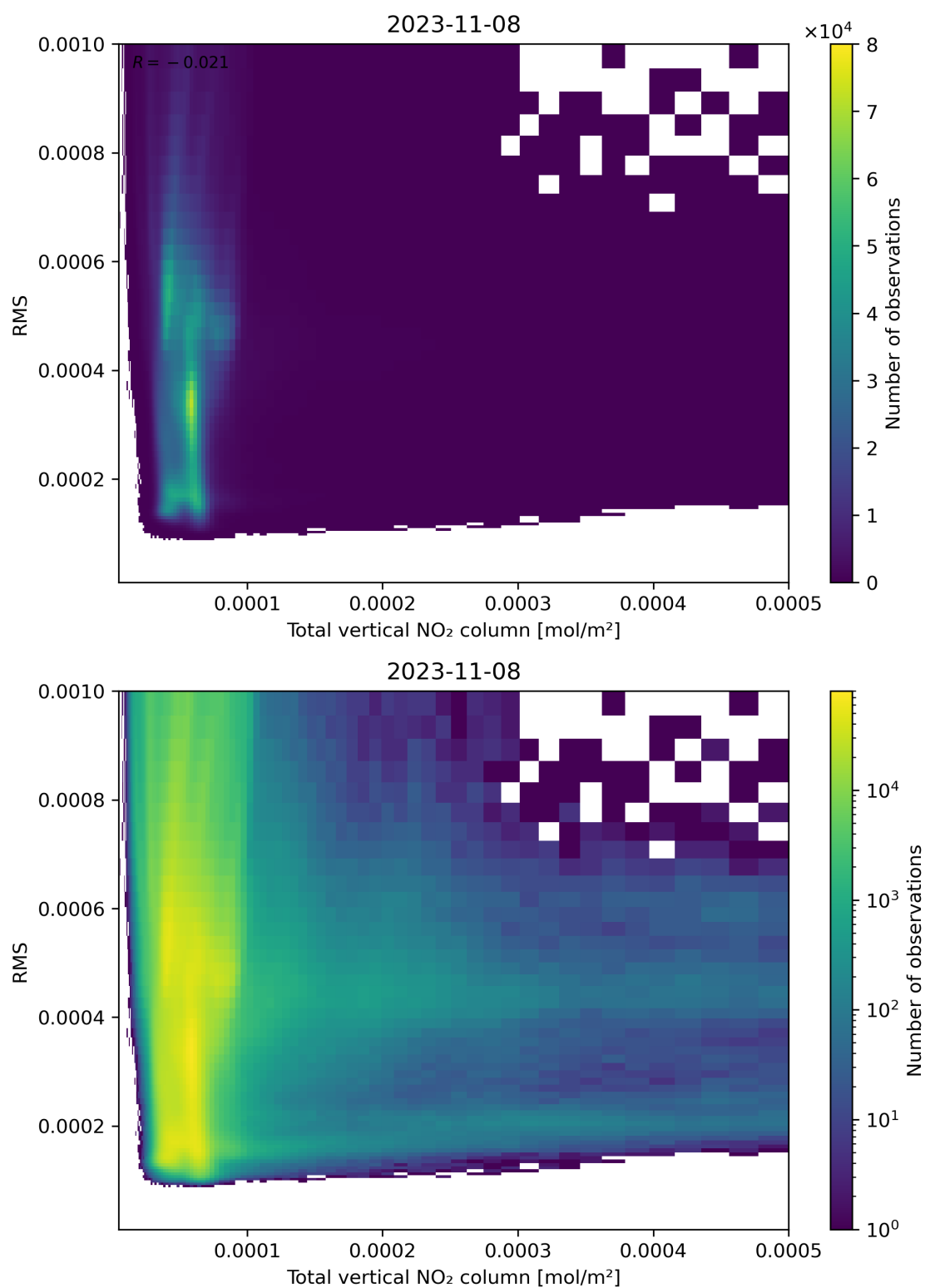
Figure 120: Scatter density plot of “Total vertical NO 2 column” against “RMS” for 2023-11-07 to 2023-11-09.
