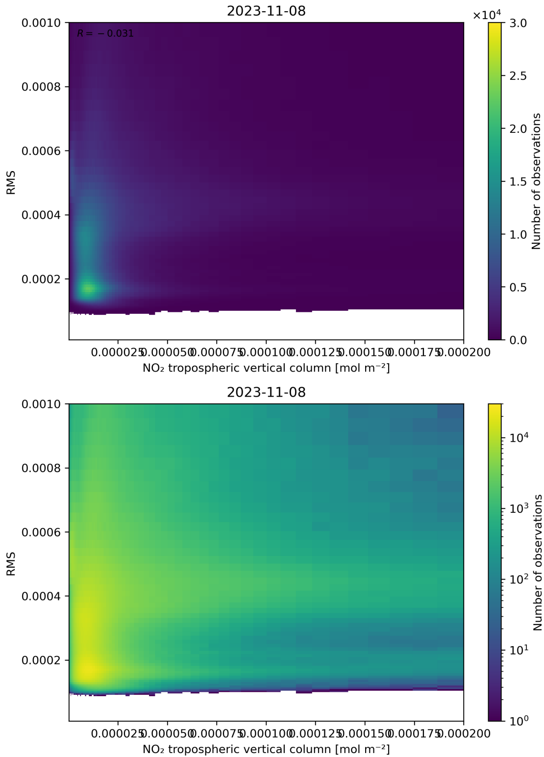
Figure 142: Scatter density plot of “NO 2 tropospheric vertical column” against “RMS” for 2023-11-07 to 2023-11-09.
