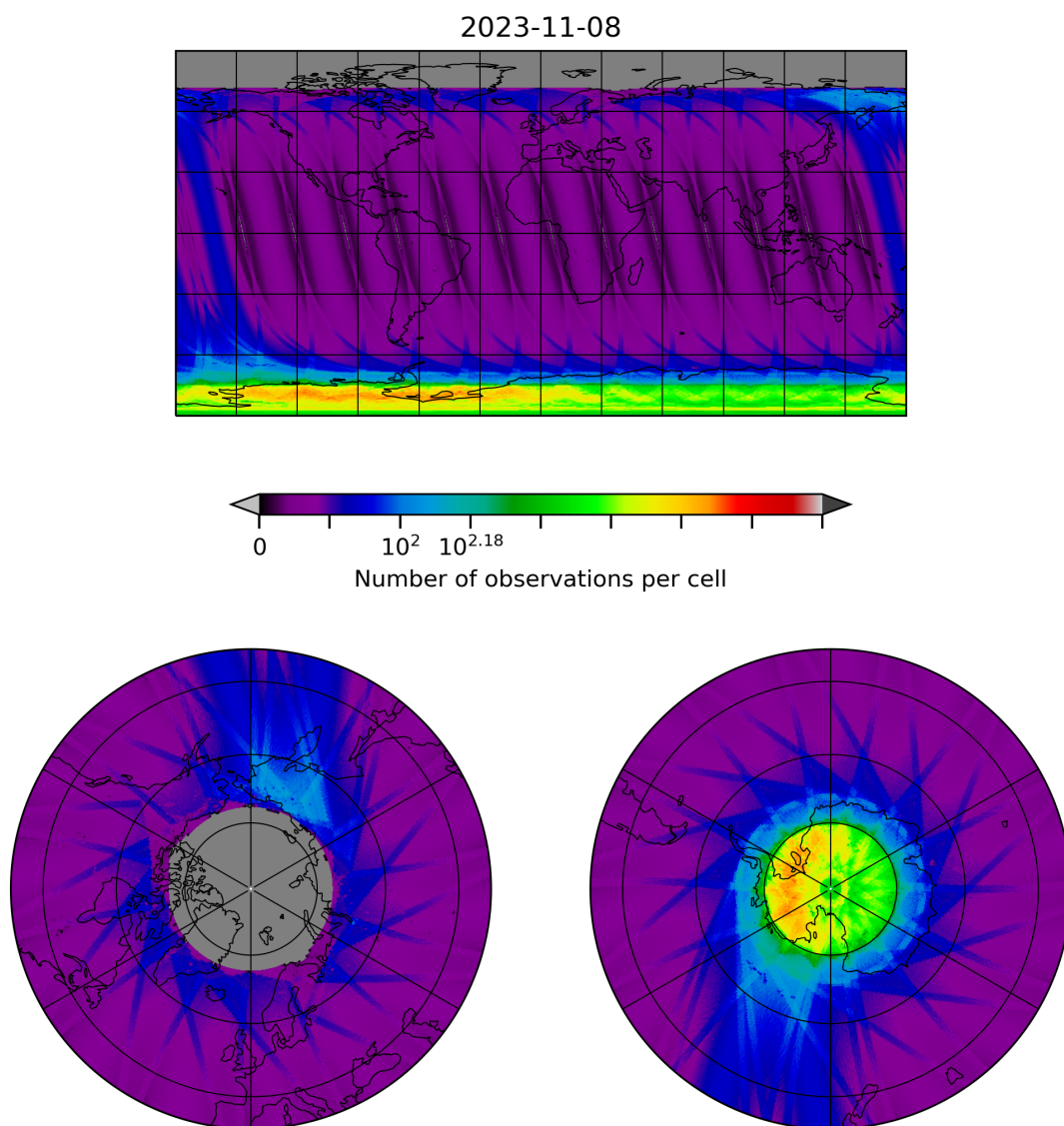
Figure 10: Map of the number of observations for 2023-11-07 to 2023-11-09
