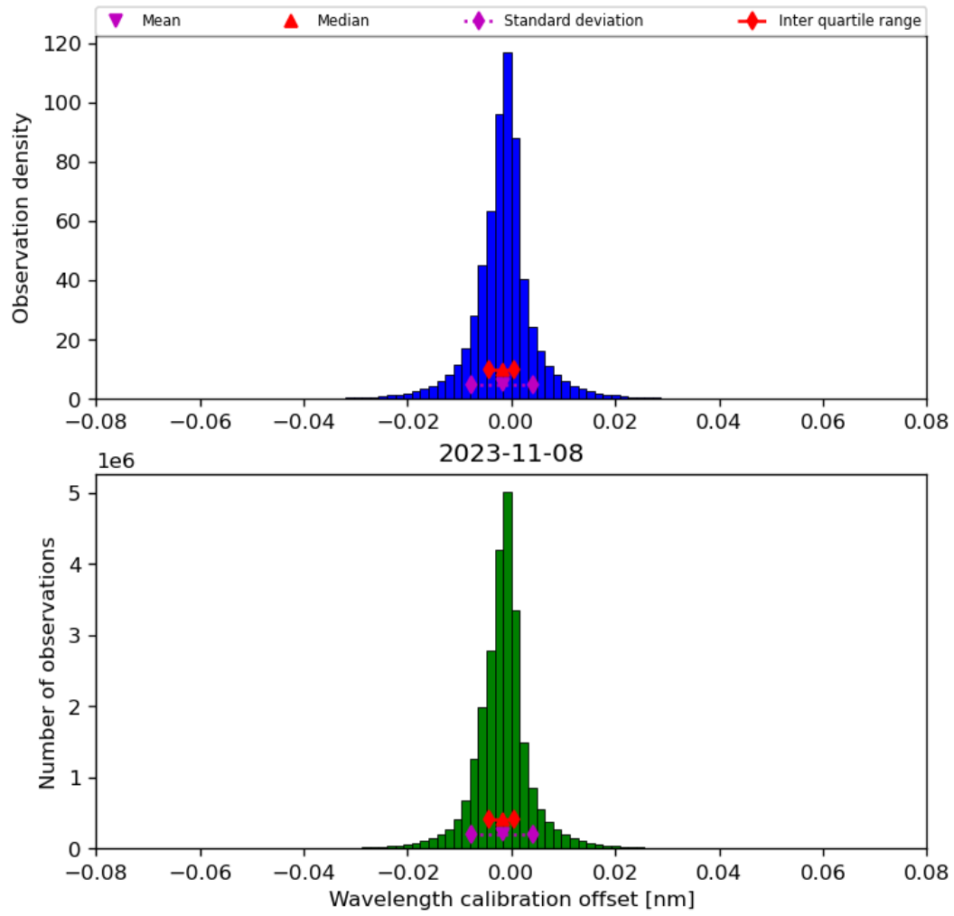
Figure 35: Histogram of “Wavelength calibration offset” for 2023-11-07 to 2023-11-09
