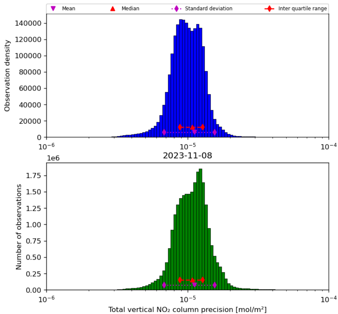
Figure 39: Histogram of “Total vertical NO 2 column precision” for 2023-11-07 to 2023-11-09
