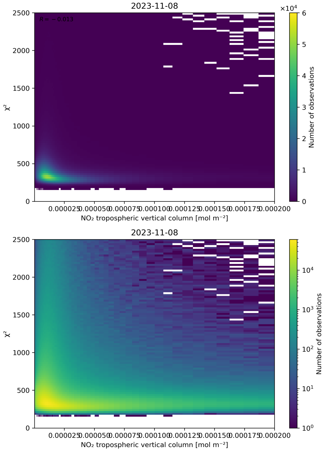
Figure 124: Scatter density plot of “NO 2 tropospheric vertical column” against “ \chi^2 ” for 2023-11-07 to 2023-11-09.
