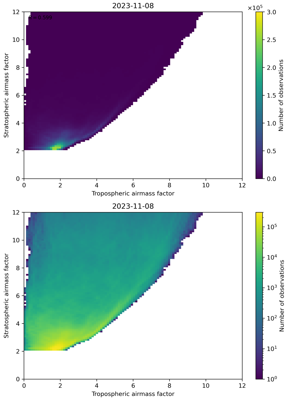
Figure 71: Scatter density plot of “Tropospheric airmass factor” against “Stratospheric airmass factor” for 2023-11-07 to 2023-11-09.
