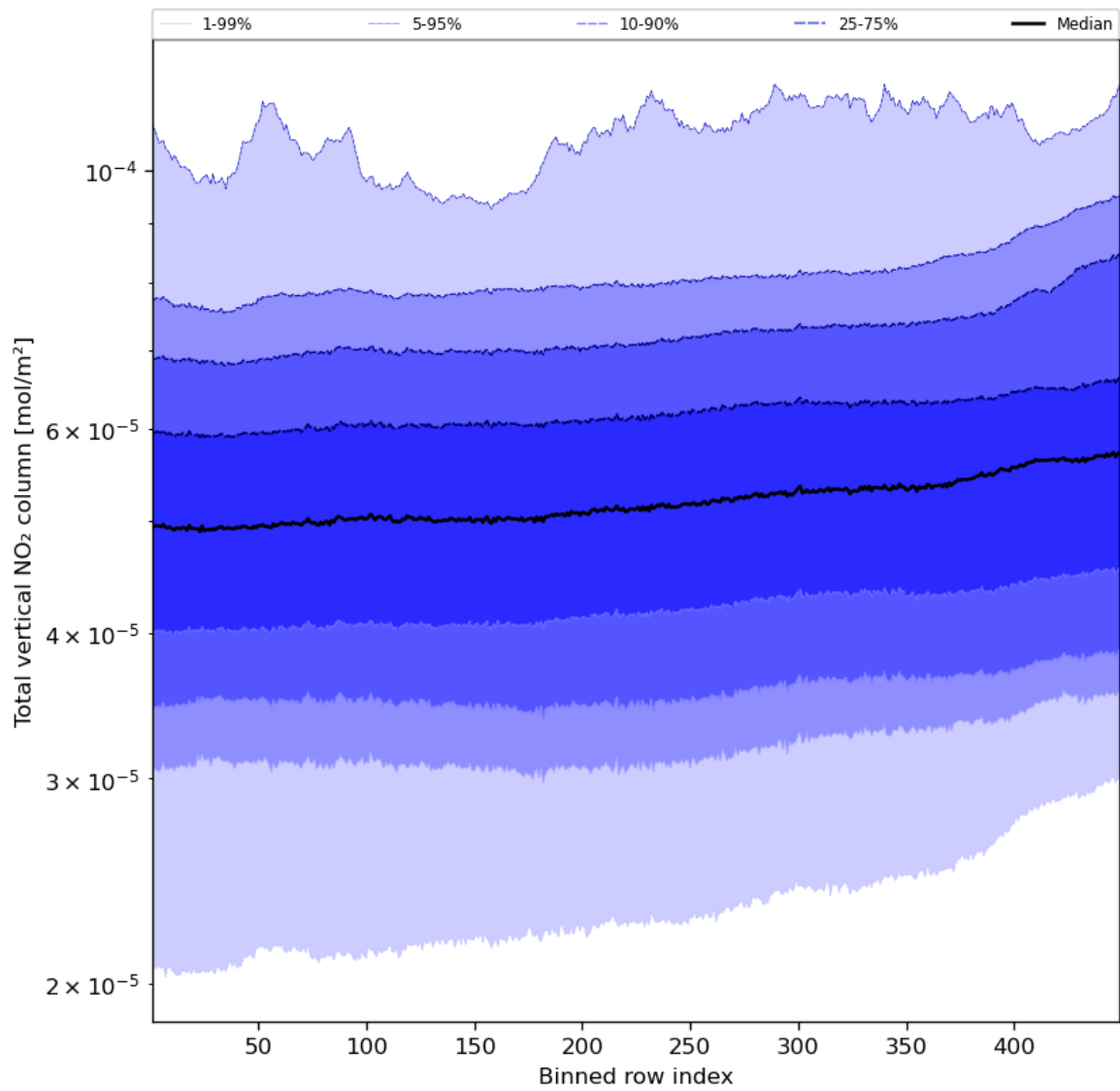
Figure 55: Along track statistics of “Total vertical NO 2 column” for 2023-11-07 to 2023-11-09
