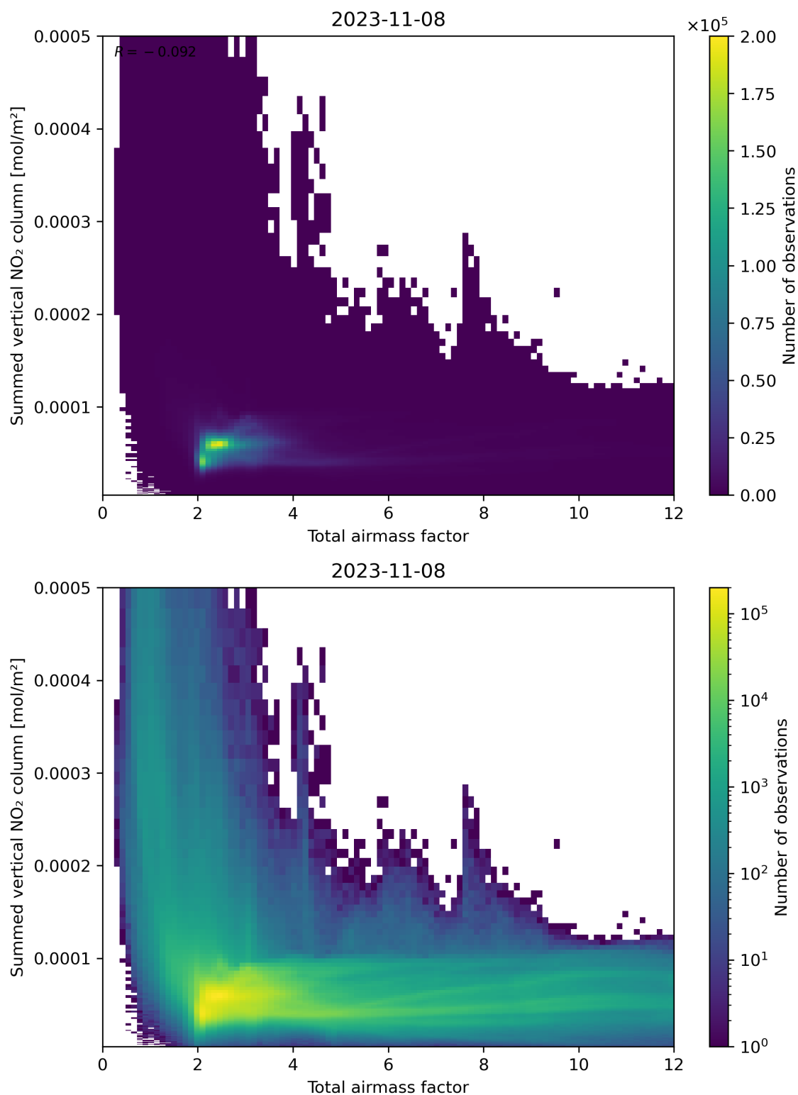
Figure 65: Scatter density plot of “Total airmass factor” against “Summed vertical NO 2 column” for 2023-11-07 to 2023-11-09.
