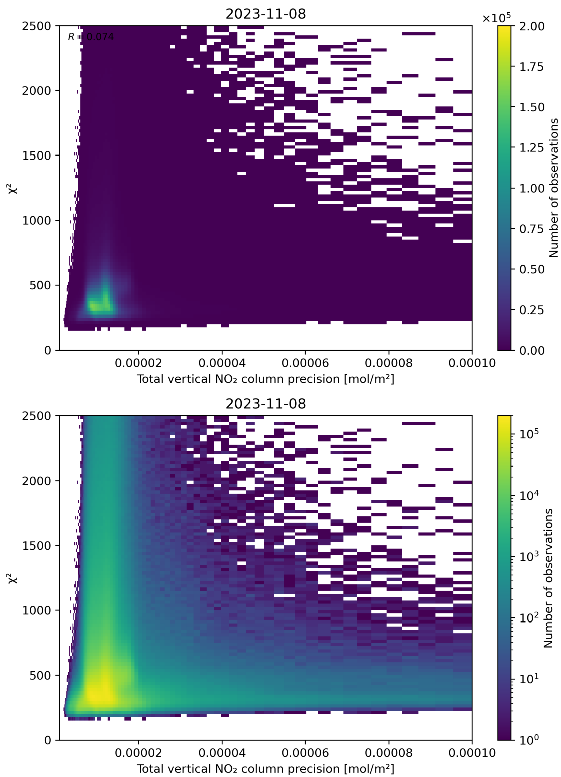
Figure 116: Scatter density plot of “Total vertical NO 2 column precision” against “ \chi^2 ” for 2023-11-07 to 2023-11-09.
