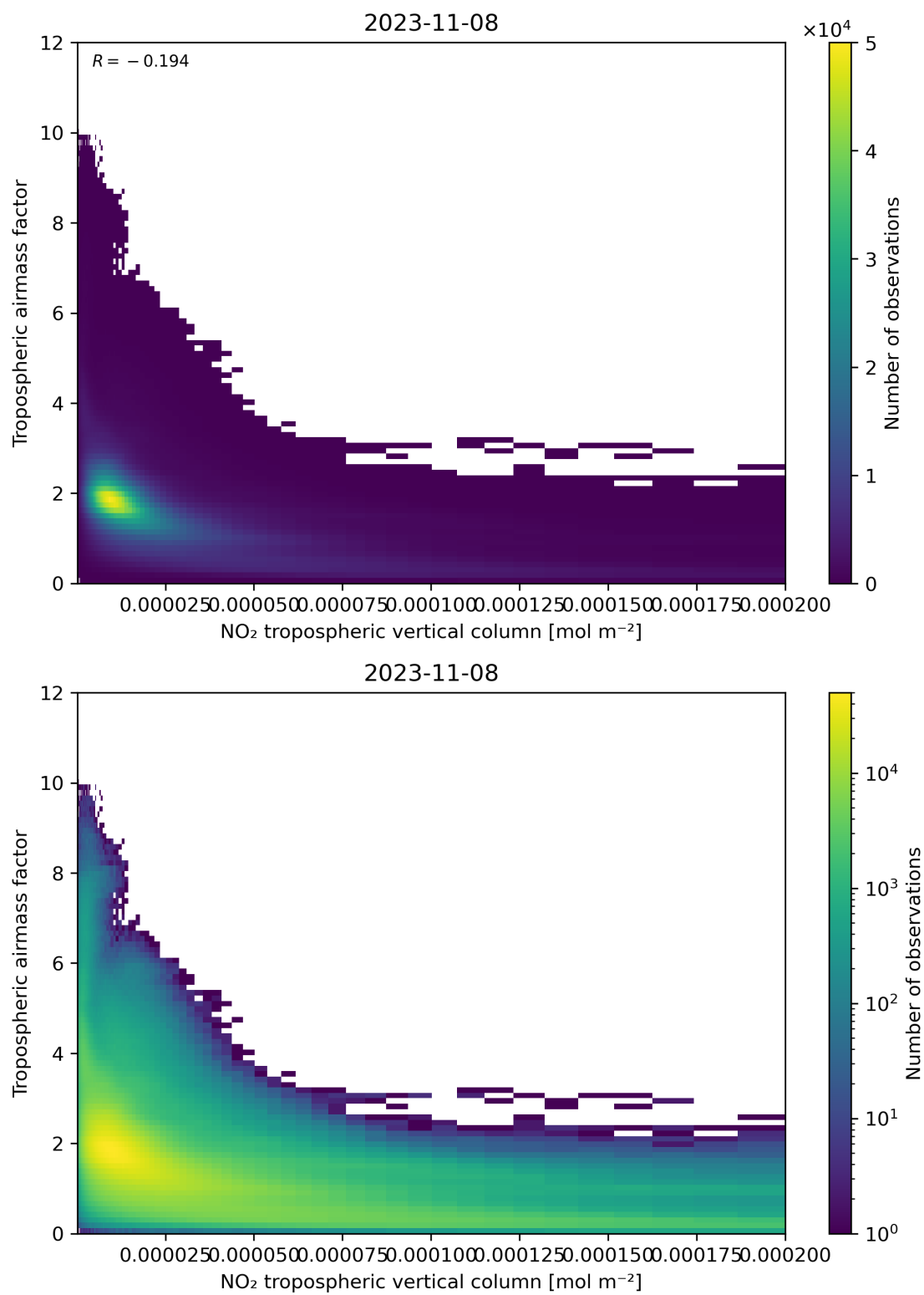
Figure 123: Scatter density plot of “NO 2 tropospheric vertical column” against “Tropospheric airmass factor” for 2023-11-07 to 2023-11-09.
