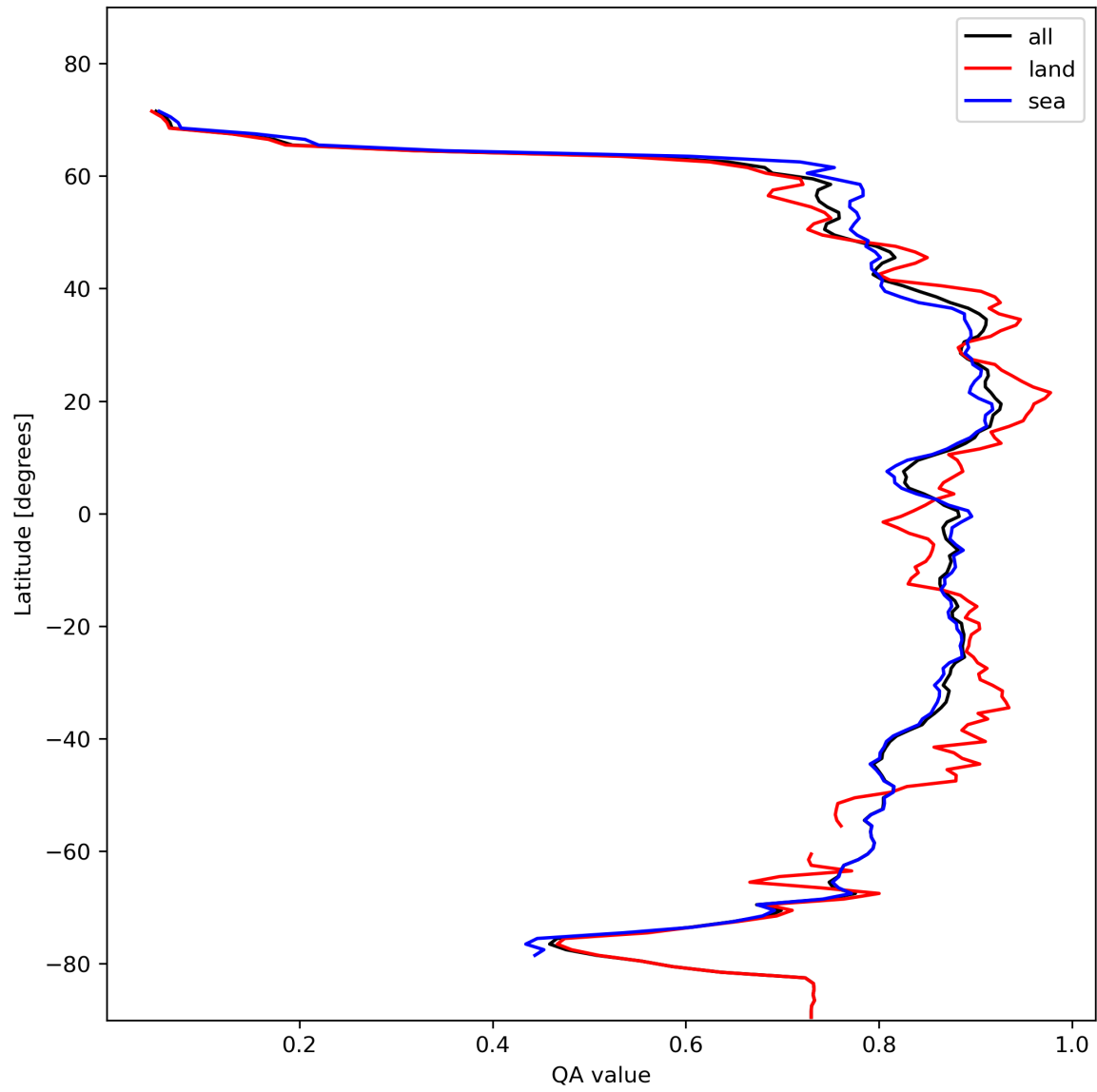
Figure 11: Zonal average of “QA value” for 2023-11-07 to 2023-11-09.
