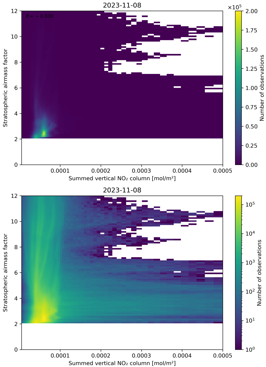
Figure 103: Scatter density plot of “Summed vertical NO 2 column” against “Stratospheric air mass factor” for 2023-11-07 to 2023-11-09.
