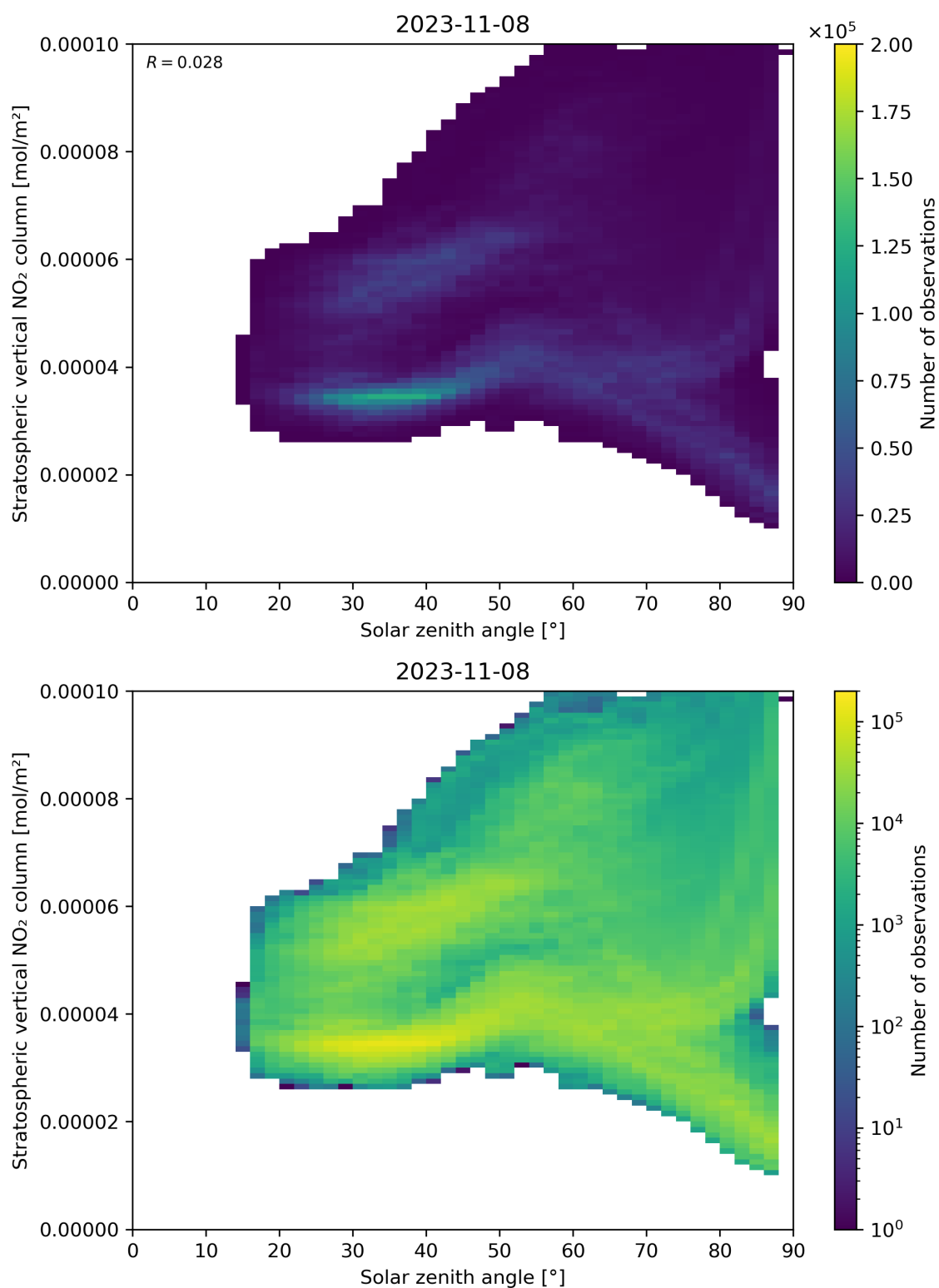
Figure 150: Scatter density plot of “Solar zenith angle” against “Stratospheric vertical NO 2 column” for 2023-11-07 to 2023-11-09.
