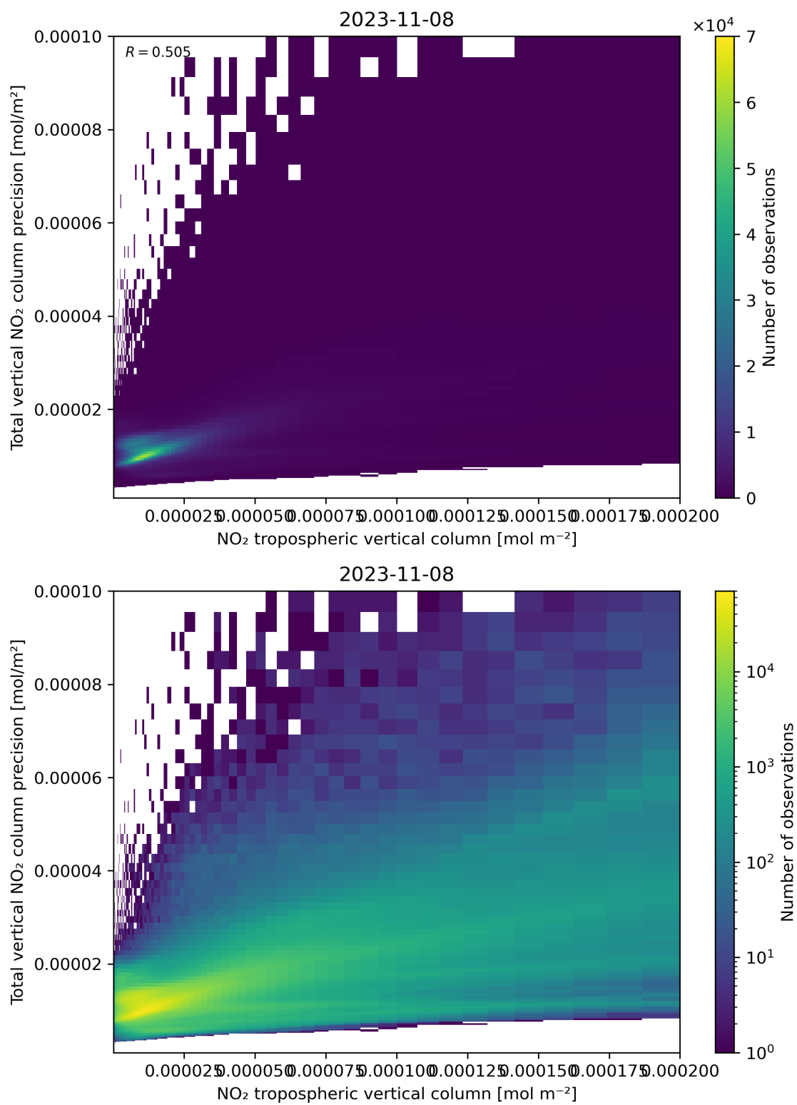
Figure 129: Scatter density plot of “NO 2 tropospheric vertical column” against “Total vertical NO 2 column precision” for 2023-11-07 to 2023-11-09.
