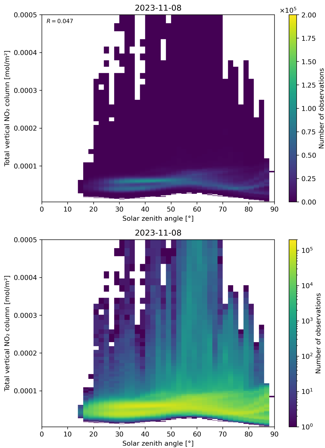
Figure 153: Scatter density plot of “Solar zenith angle” against “Total vertical NO 2 column” for 2023-11-07 to 2023-11-09.
