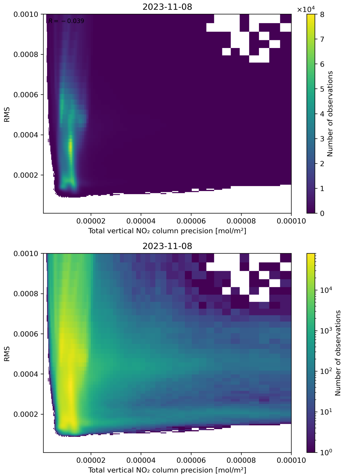
Figure 119: Scatter density plot of “Total vertical NO 2 column precision” against “RMS” for 2023-11-07 to 2023-11-09.
