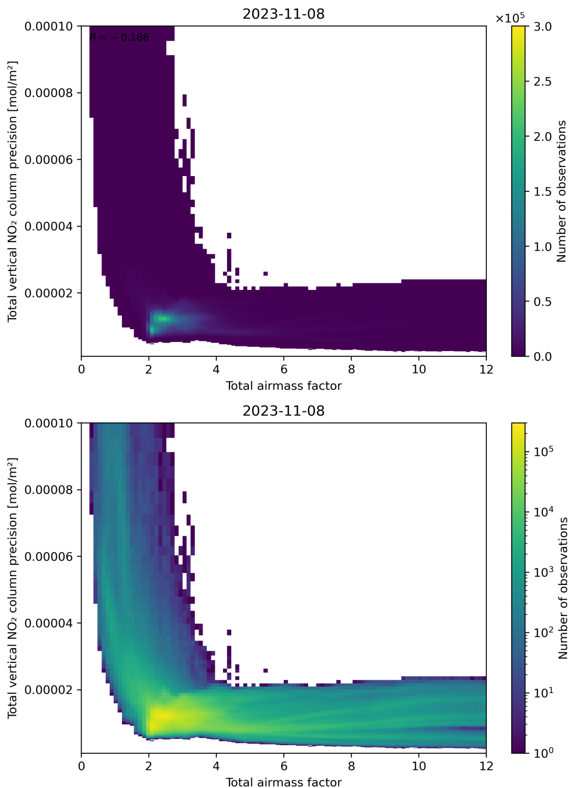
Figure 68: Scatter density plot of “Total airmass factor” against “Total vertical NO 2 column precision” for 2023-11-07 to 2023-11-09.
