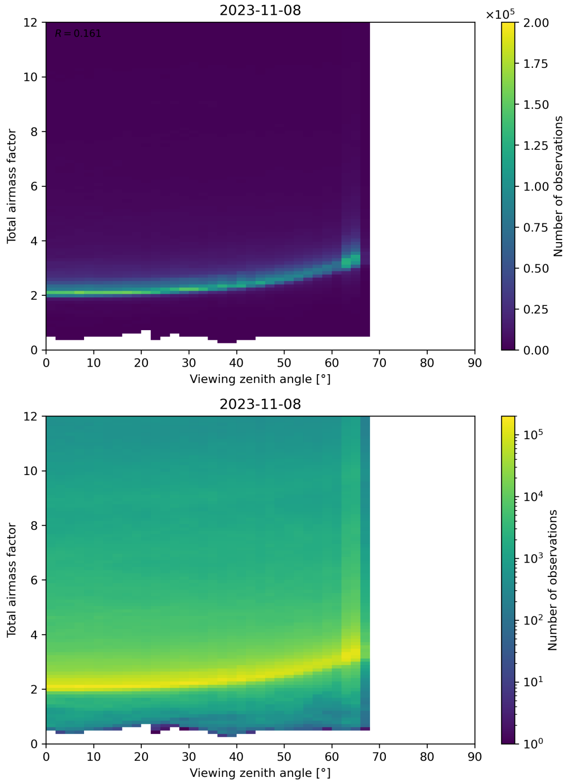
Figure 160: Scatter density plot of “Viewing zenith angle” against “Total airmass factor” for 2023-11-07 to 2023-11-09.
