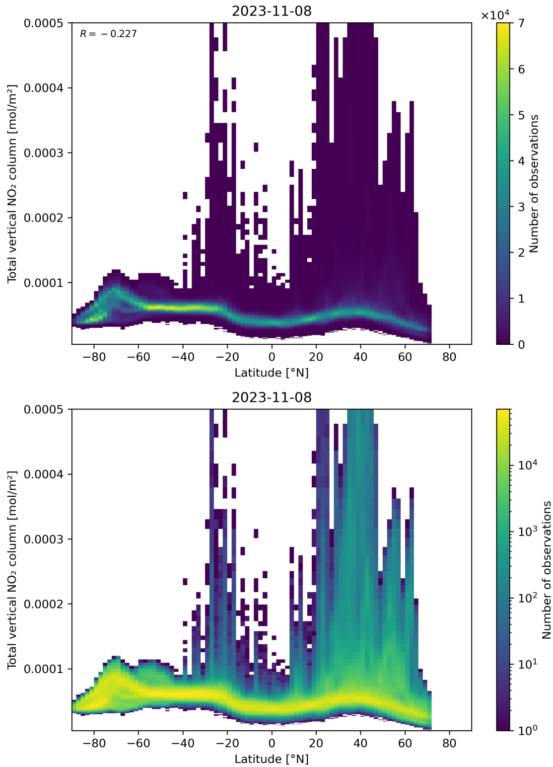
Figure 90: Scatter density plot of “Latitude” against “Total vertical NO 2 column” for 2023-11-07 to 2023-11-09.
