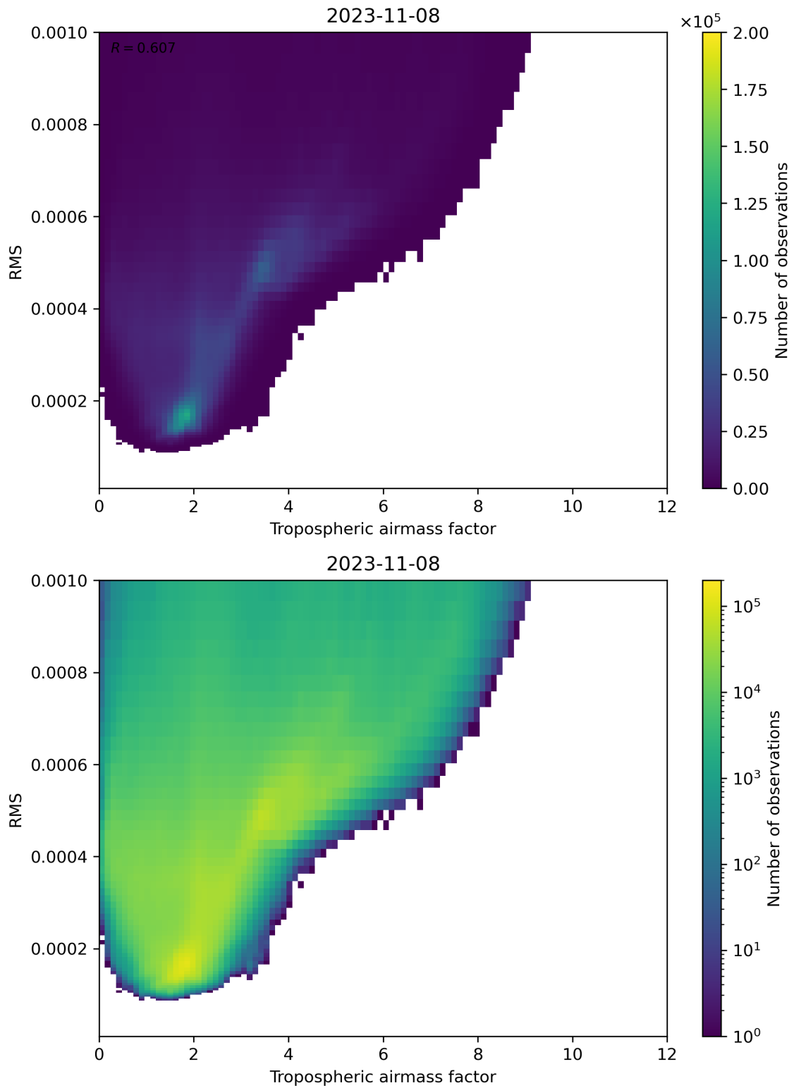
Figure 79: Scatter density plot of “Tropospheric airmass factor” against “RMS” for 2023-11-07 to 2023-11-09.
