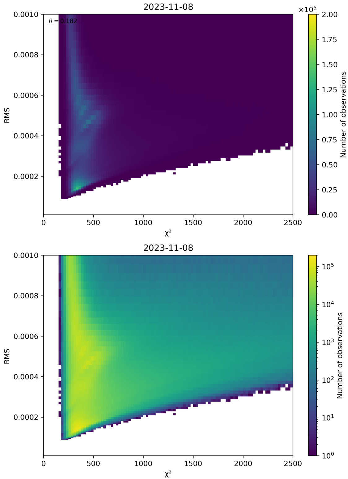
Figure 82: Scatter density plot of “ \chi^2 ” against “RMS” for 2023-11-07 to 2023-11-09.
