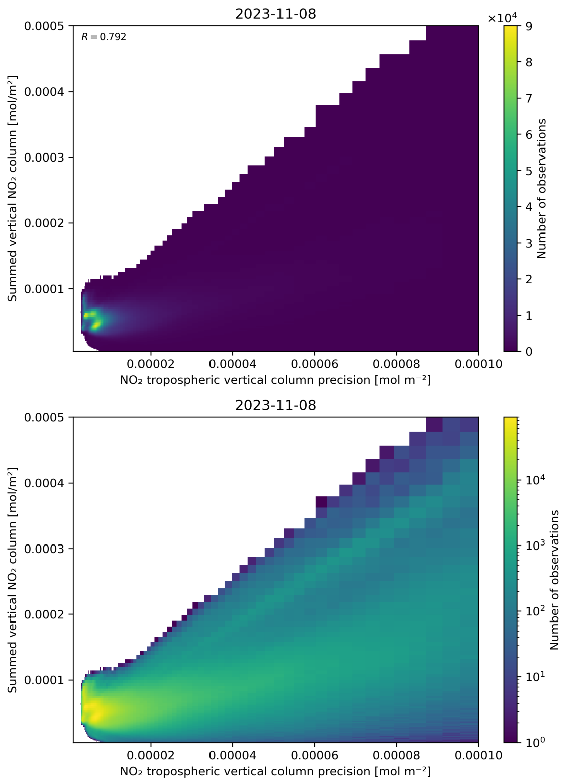
Figure 136: Scatter density plot of “NO 2 tropospheric vertical column precision” against “Summed vertical NO 2 column” for 2023-11-07 to 2023-11-09.
