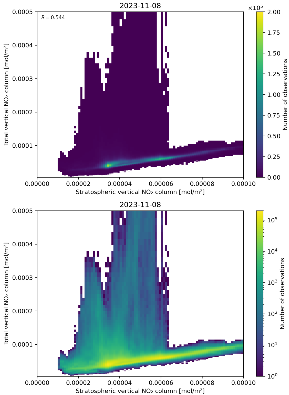
Figure 100: Scatter density plot of “Stratospheric vertical NO 2 column” against “Total vertical NO 2 column” for 2023-11-07 to 2023-11-09.
