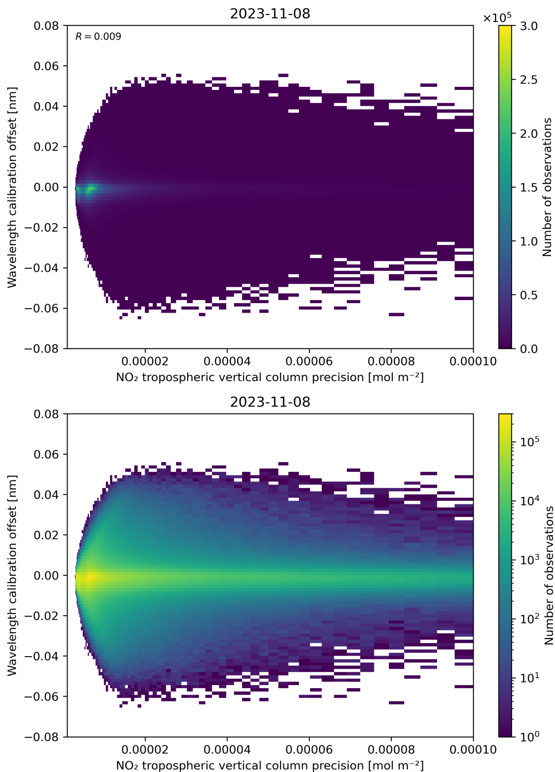
Figure 141: Scatter density plot of “NO 2 tropospheric vertical column precision” against “Wavelength calibration offset” for 2023-11-07 to 2023-11-09.
