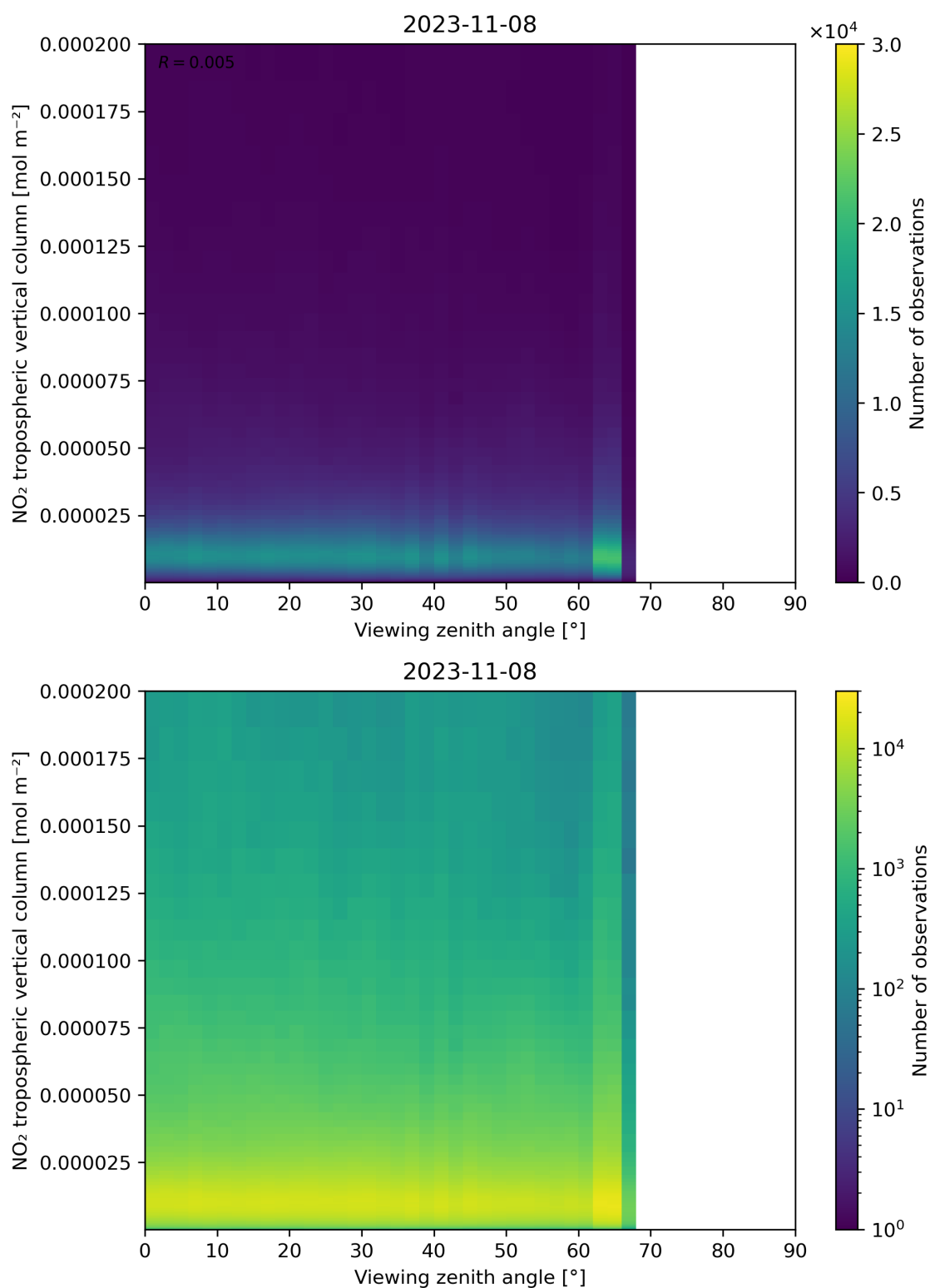
Figure 169: Scatter density plot of “Viewing zenith angle” against “NO 2 tropospheric vertical column” for 2023-11-07 to 2023-11-09.
