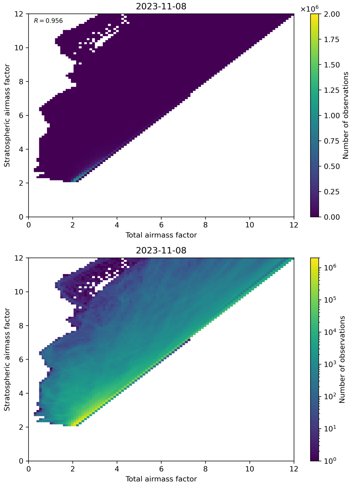
Figure 62: Scatter density plot of “Total airmass factor” against “Stratospheric airmass factor” for 2023-11-07 to 2023-11-09.
