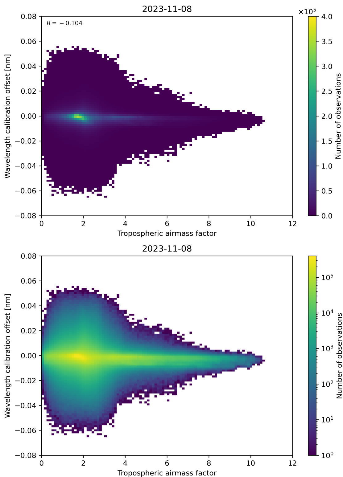
Figure 80: Scatter density plot of “Tropospheric airmass factor” against “Wavelength calibration offset” for 2023-11-07 to 2023-11-09.
