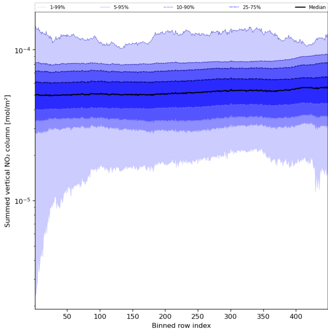
Figure 57: Along track statistics of “Summed vertical NO 2 column” for 2023-11-07 to 2023-11-09
