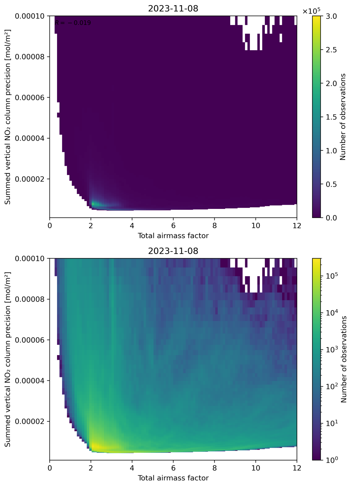
Figure 66: Scatter density plot of “Total airmass factor” against “Summed vertical NO 2 column precision” for 2023-11-07 to 2023-11-09.
