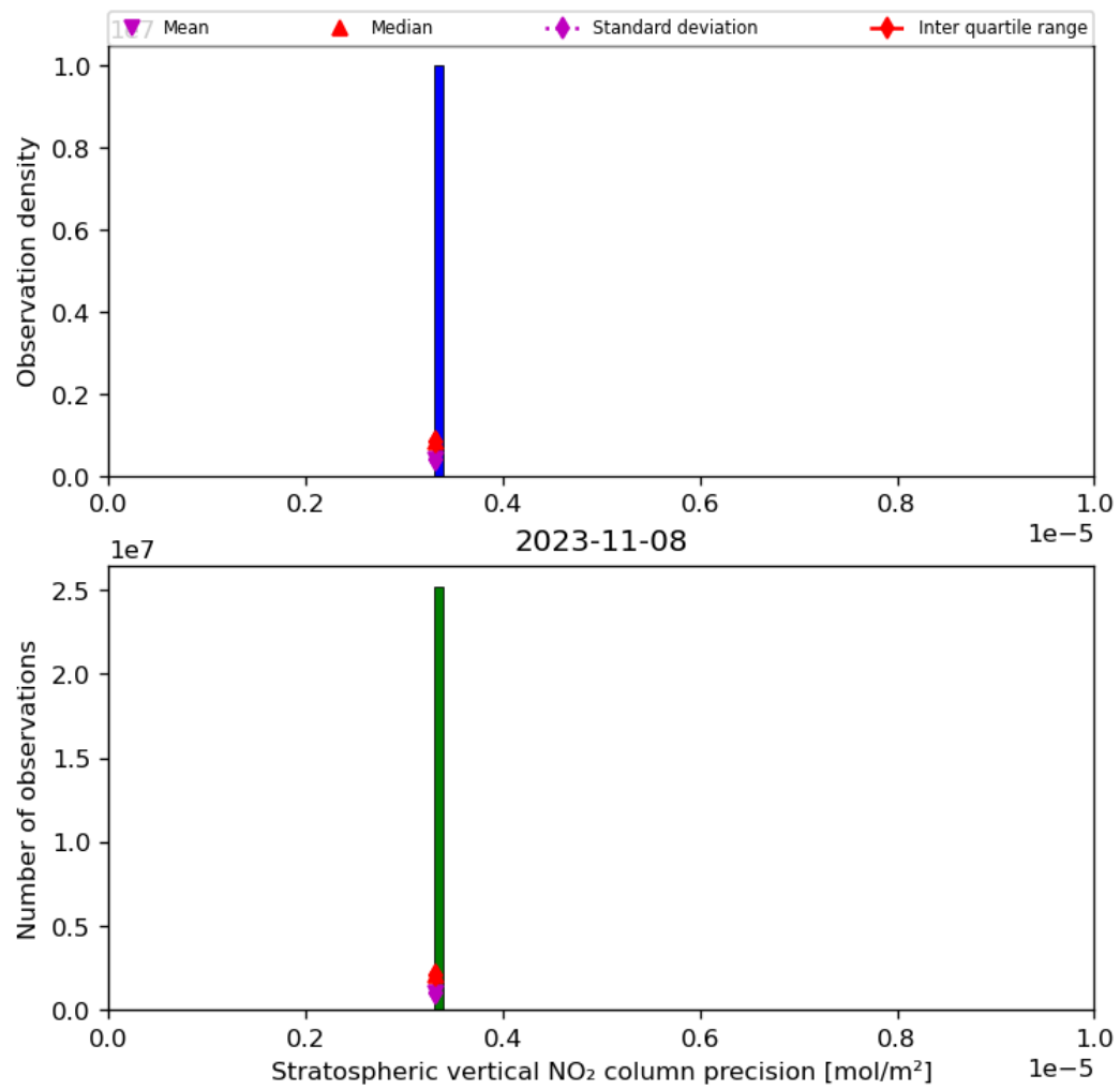
Figure 37: Histogram of “Stratospheric vertical NO 2 column precision” for 2023-11-07 to 2023-11-09
