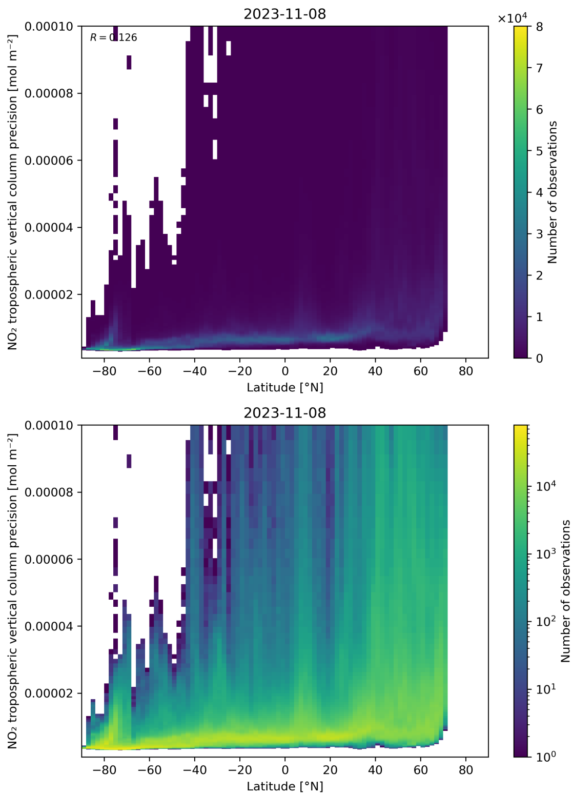
Figure 93: Scatter density plot of “Latitude” against “NO 2 tropospheric vertical column precision” for 2023-11-07 to 2023-11-09.
