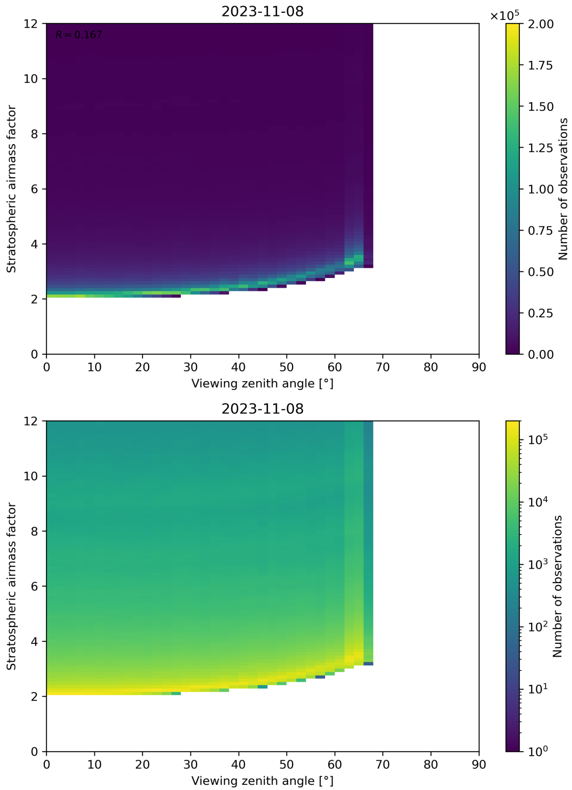
Figure 159: Scatter density plot of “Viewing zenith angle” against “Stratospheric airmass factor” for 2023-11-07 to 2023-11-09.
