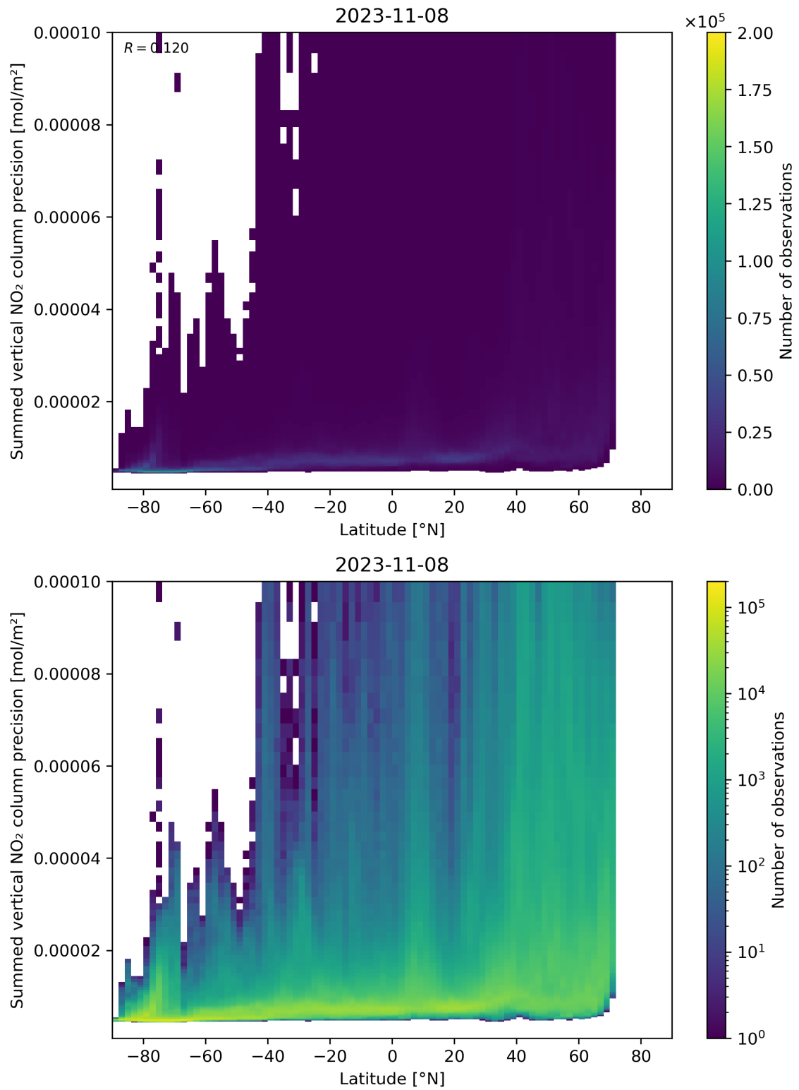
Figure 89: Scatter density plot of “Latitude” against “Summed vertical NO 2 column precision” for 2023-11-07 to 2023-11-09.
