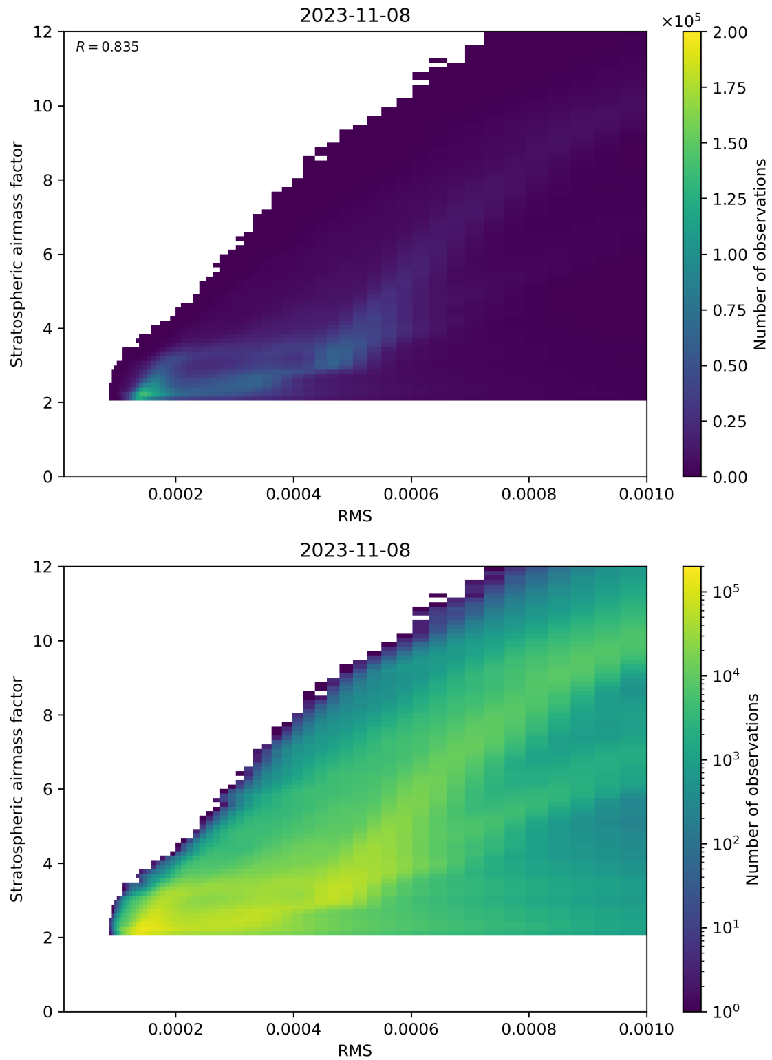
Figure 144: Scatter density plot of “RMS” against “Stratospheric airmass factor” for 2023-11-07 to 2023-11-09.
