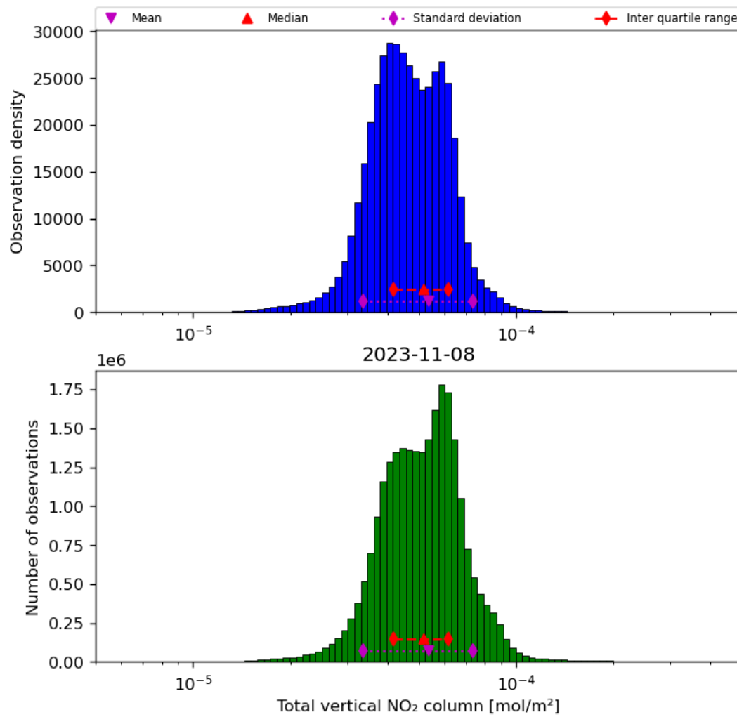
Figure 38: Histogram of “Total vertical NO 2 column” for 2023-11-07 to 2023-11-09
