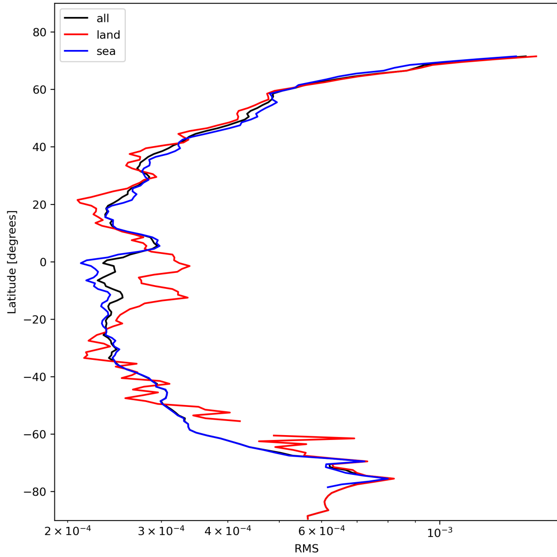
Figure 26: Zonal average of “RMS” for 2023-11-07 to 2023-11-09.
