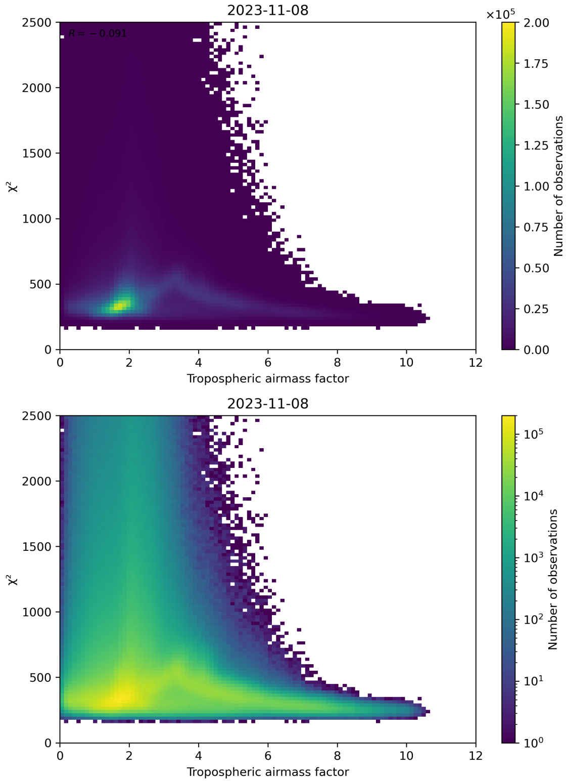
Figure 73: Scatter density plot of “Tropospheric airmass factor” against “ \chi^2 ” for 2023-11-07 to 2023-11-09.
