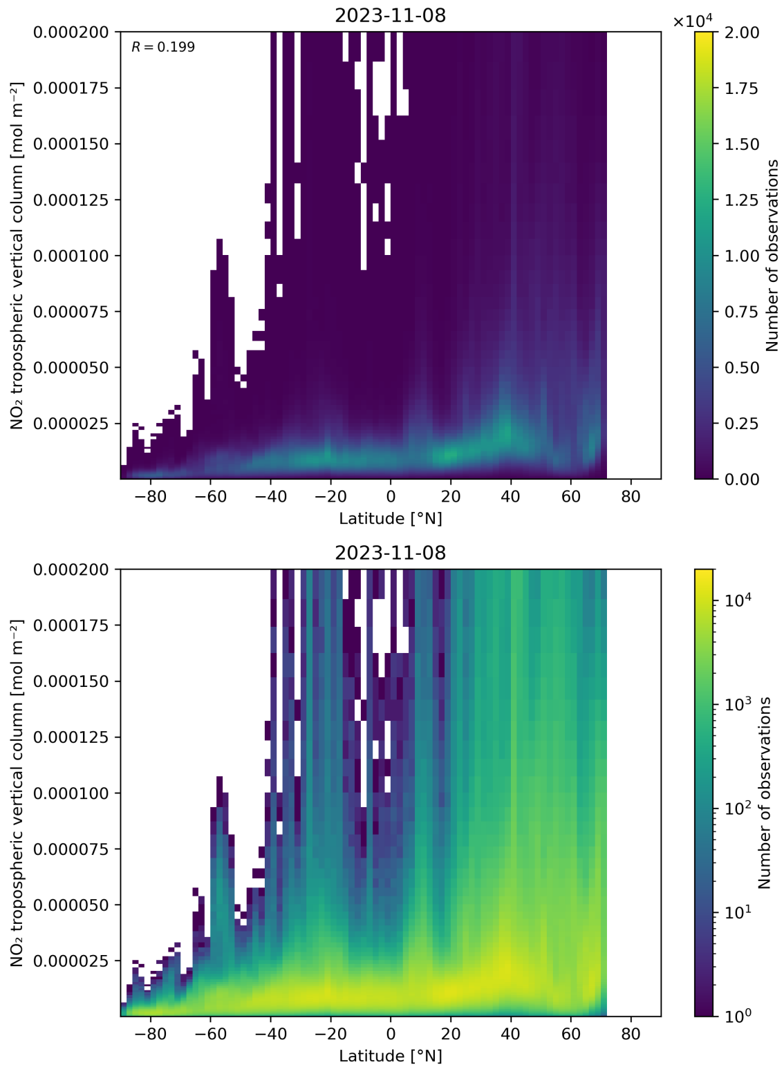
Figure 92: Scatter density plot of “Latitude” against “NO 2 tropospheric vertical column” for 2023-11-07 to 2023-11-09.
