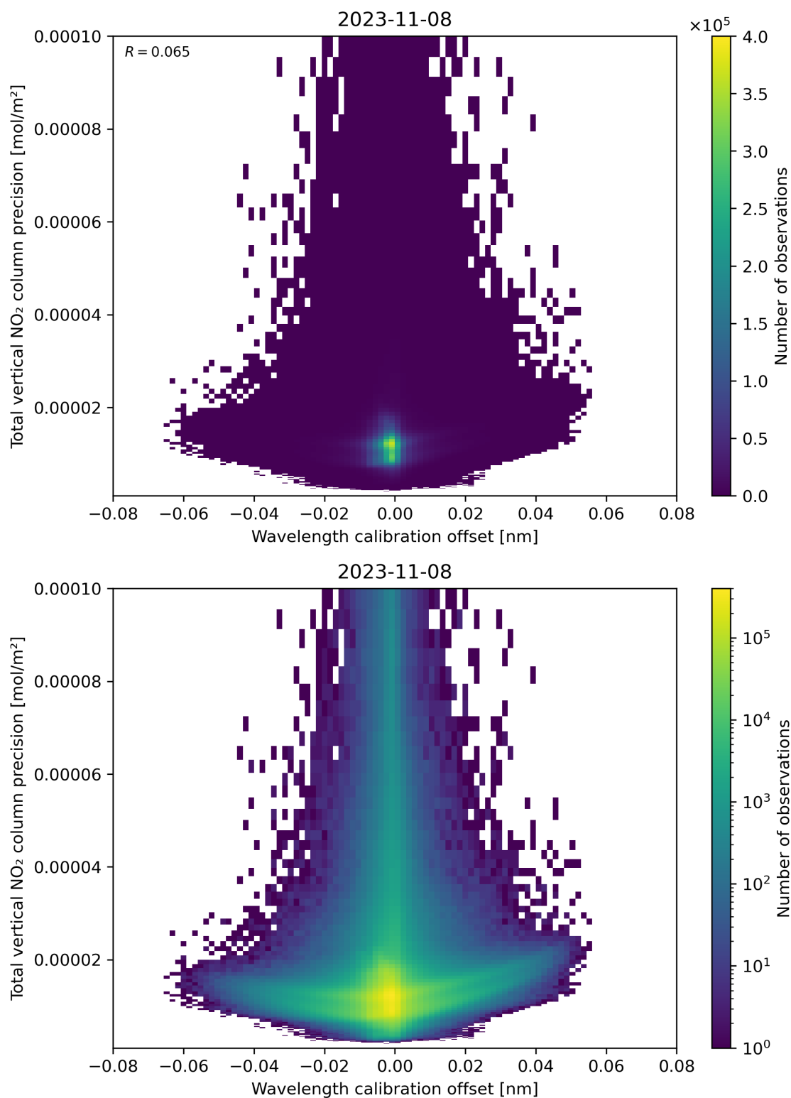
Figure 180: Scatter density plot of “Wavelength calibration offset” against “Total vertical NO 2 column precision” for 2023-11-07 to 2023-11-09.
