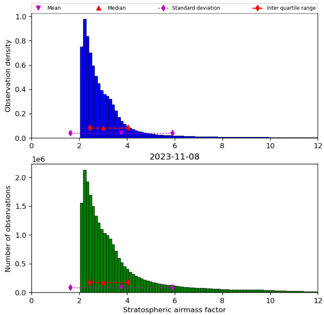
Figure 44: Histogram of “Stratospheric airmass factor” for 2023-11-07 to 2023-11-09
