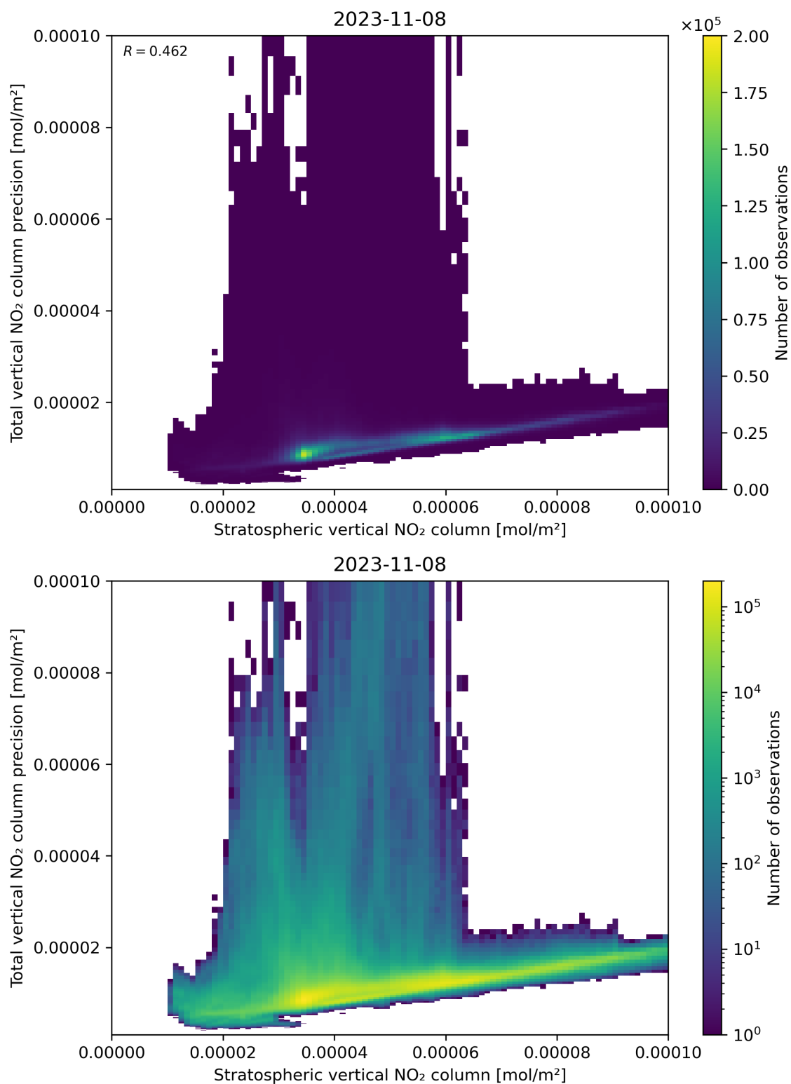
Figure 101: Scatter density plot of “Stratospheric vertical NO 2 column” against “Total vertical NO 2 column precision” for 2023-11-07 to 2023-11-09.
