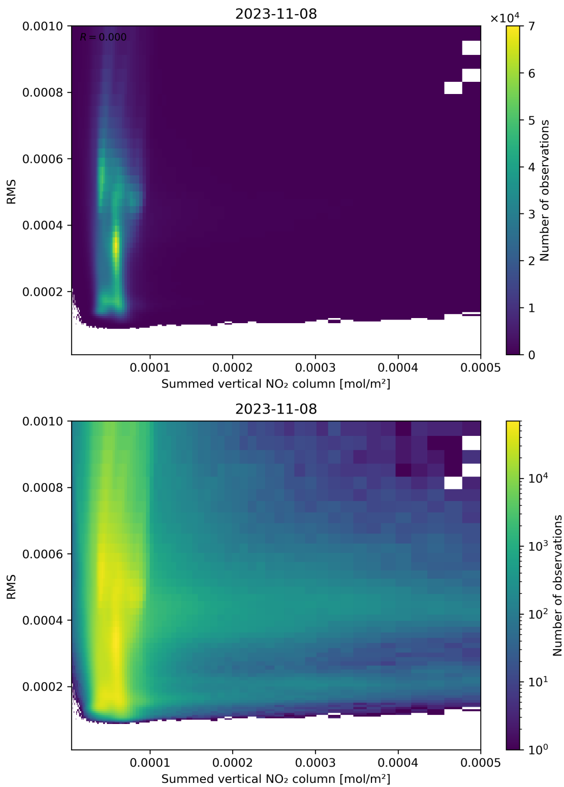
Figure 109: Scatter density plot of “Summed vertical NO 2 column” against “RMS” for 2023-11-07 to 2023-11-09.
