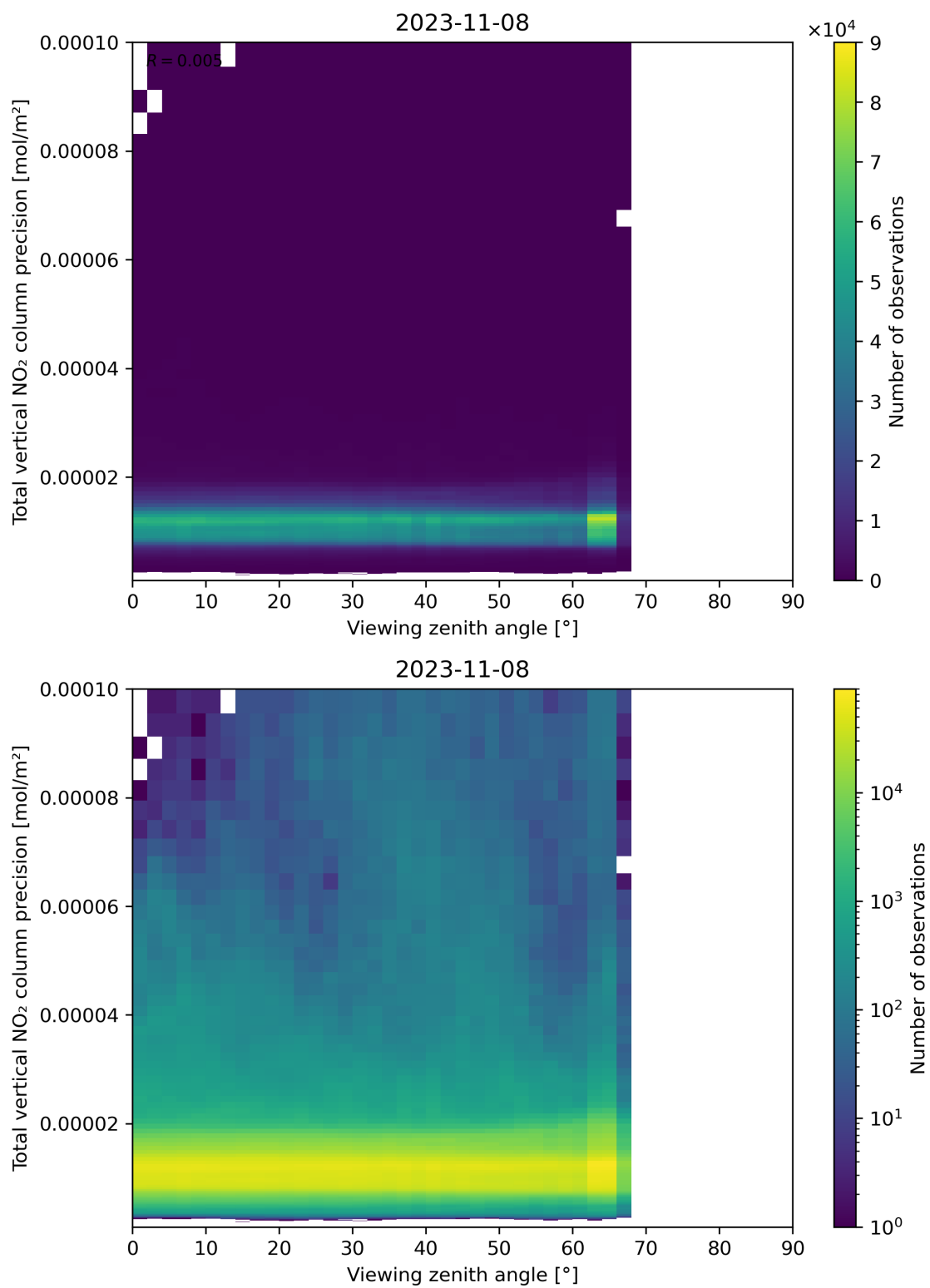
Figure 168: Scatter density plot of “Viewing zenith angle” against “Total vertical NO 2 column precision” for 2023-11-07 to 2023-11-09.
