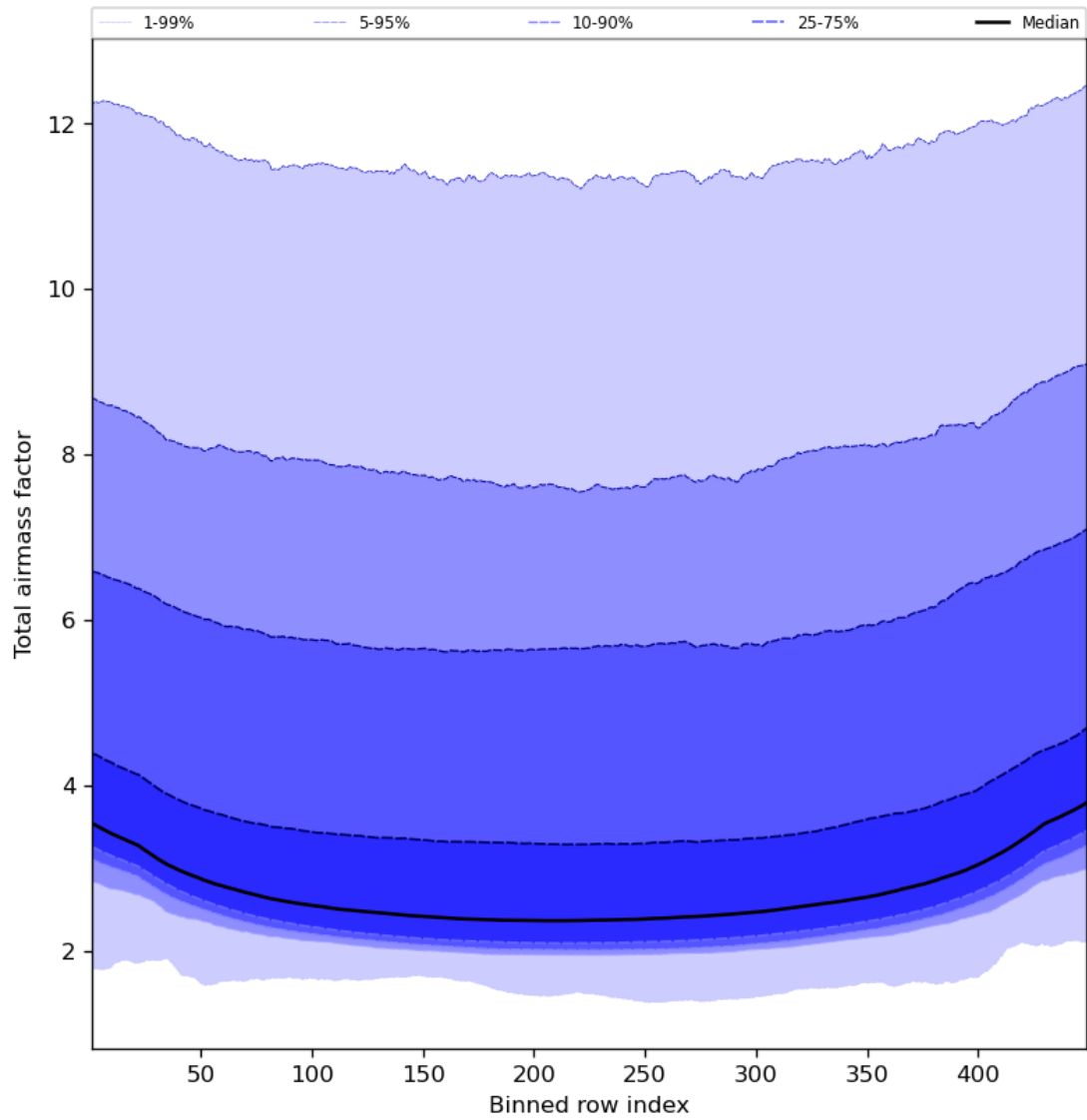
Figure 49: Along track statistics of “Total airmass factor” for 2023-11-07 to 2023-11-09
