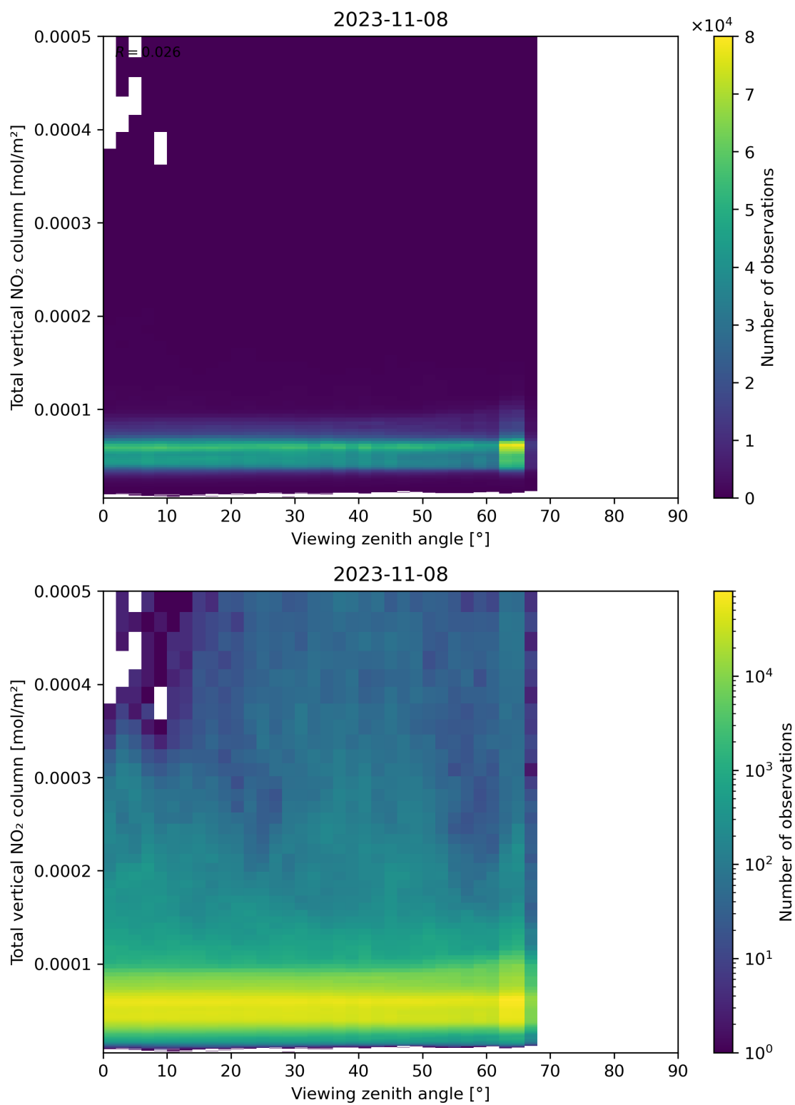
Figure 167: Scatter density plot of “Viewing zenith angle” against “Total vertical NO 2 column” for 2023-11-07 to 2023-11-09.
