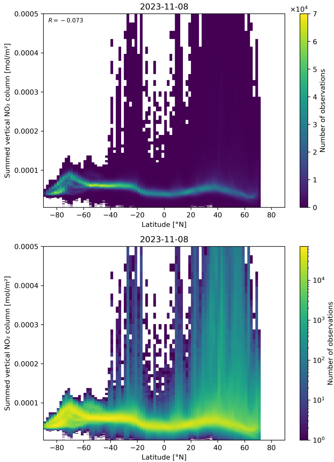
Figure 88: Scatter density plot of “Latitude” against “Summed vertical NO 2 column” for 2023-11-07 to 2023-11-09.
