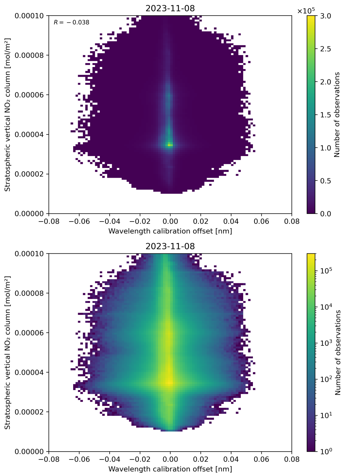
Figure 176: Scatter density plot of “Wavelength calibration offset” against “Stratospheric vertical NO 2 column” for 2023-11-07 to 2023-11-09.
