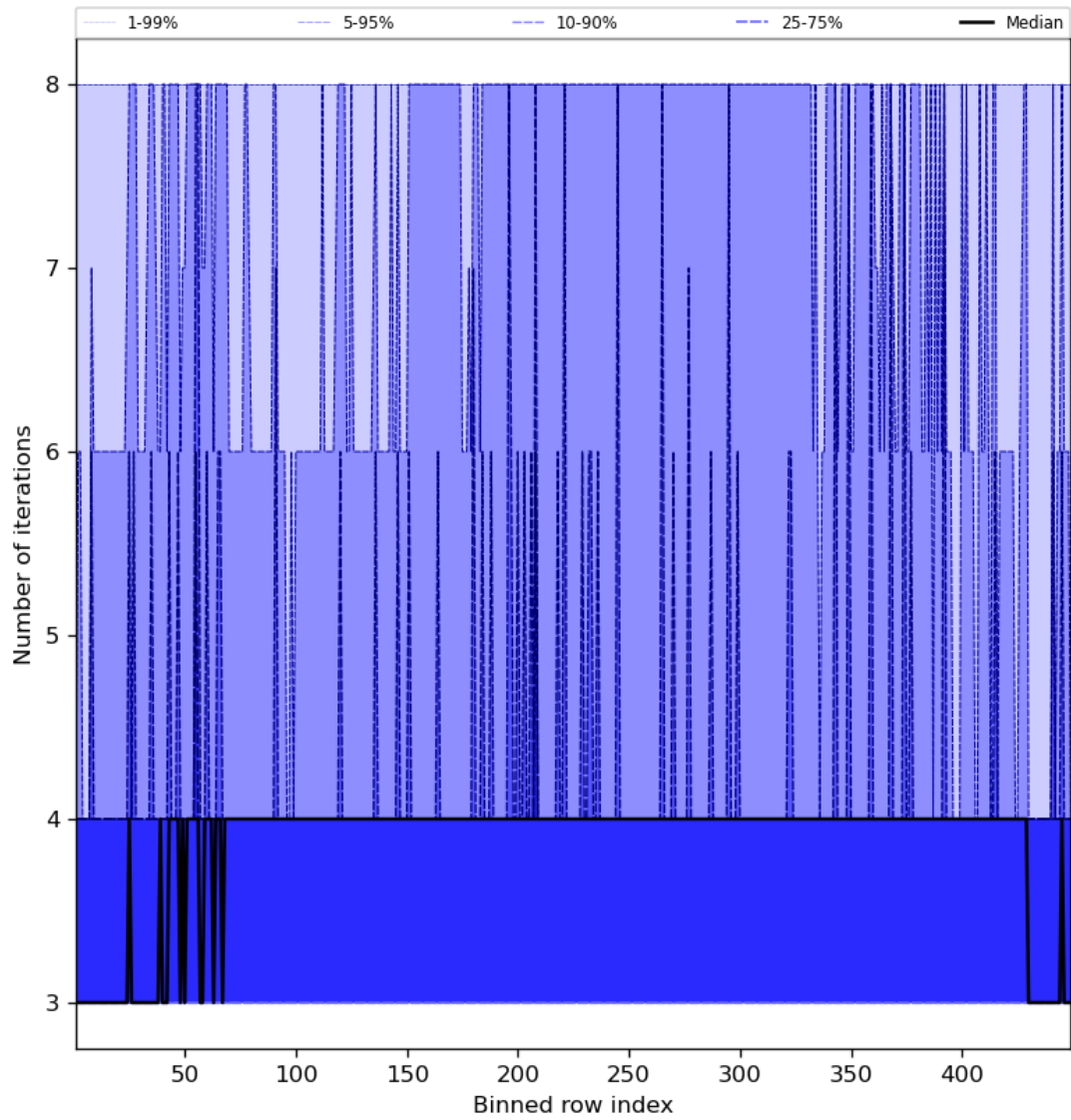
Figure 51: Along track statistics of “Number of iterations” for 2023-11-07 to 2023-11-09
