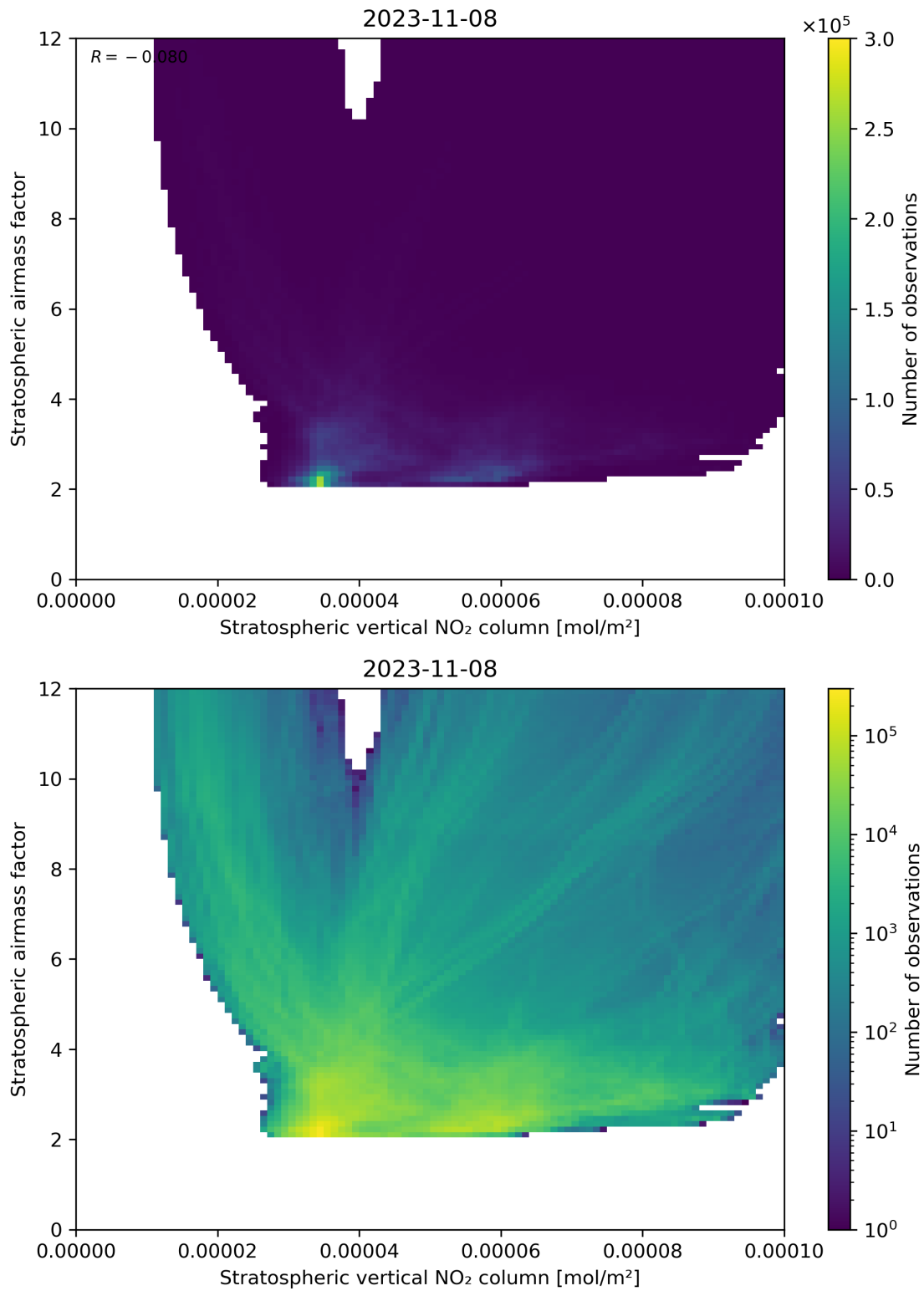
Figure 96: Scatter density plot of “Stratospheric vertical NO 2 column” against “Stratospheric airmass factor” for 2023-11-07 to 2023-11-09.
