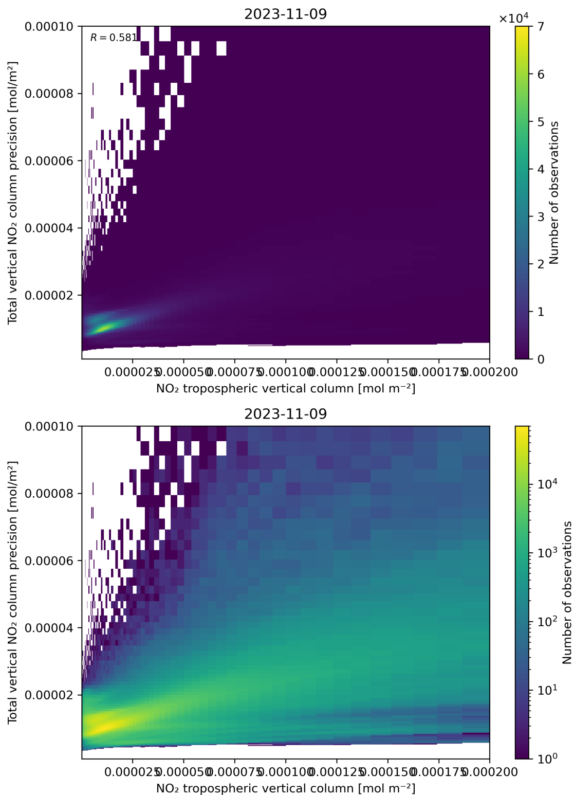
Figure 129: Scatter density plot of “NO 2 tropospheric vertical column” against “Total vertical NO 2 column precision” for 2023-11-08 to 2023-11-10.
