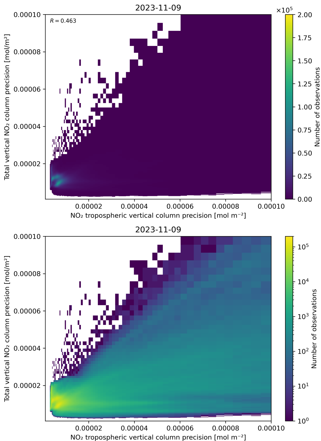
Figure 139: Scatter density plot of “NO 2 tropospheric vertical column precision” against “Total vertical NO 2 column precision” for 2023-11-08 to 2023-11-10.
