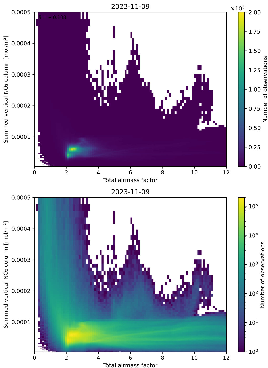
Figure 65: Scatter density plot of “Total airmass factor” against “Summed vertical NO 2 column” for 2023-11-08 to 2023-11-10.
