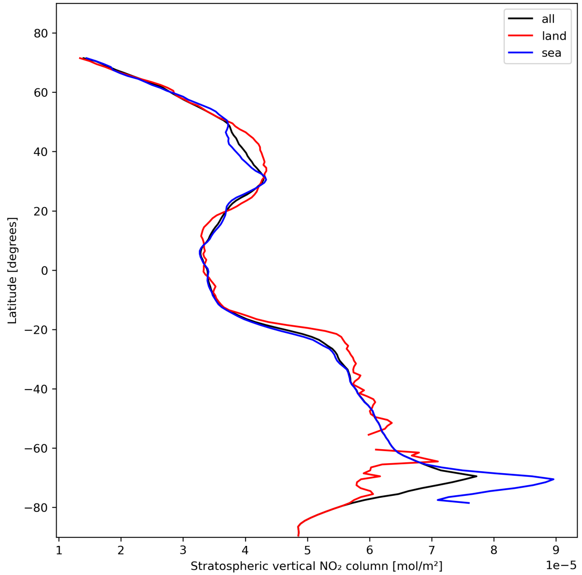
Figure 19: Zonal average of “Stratospheric vertical NO 2 column” for 2023-11-08 to 2023-11-10.
