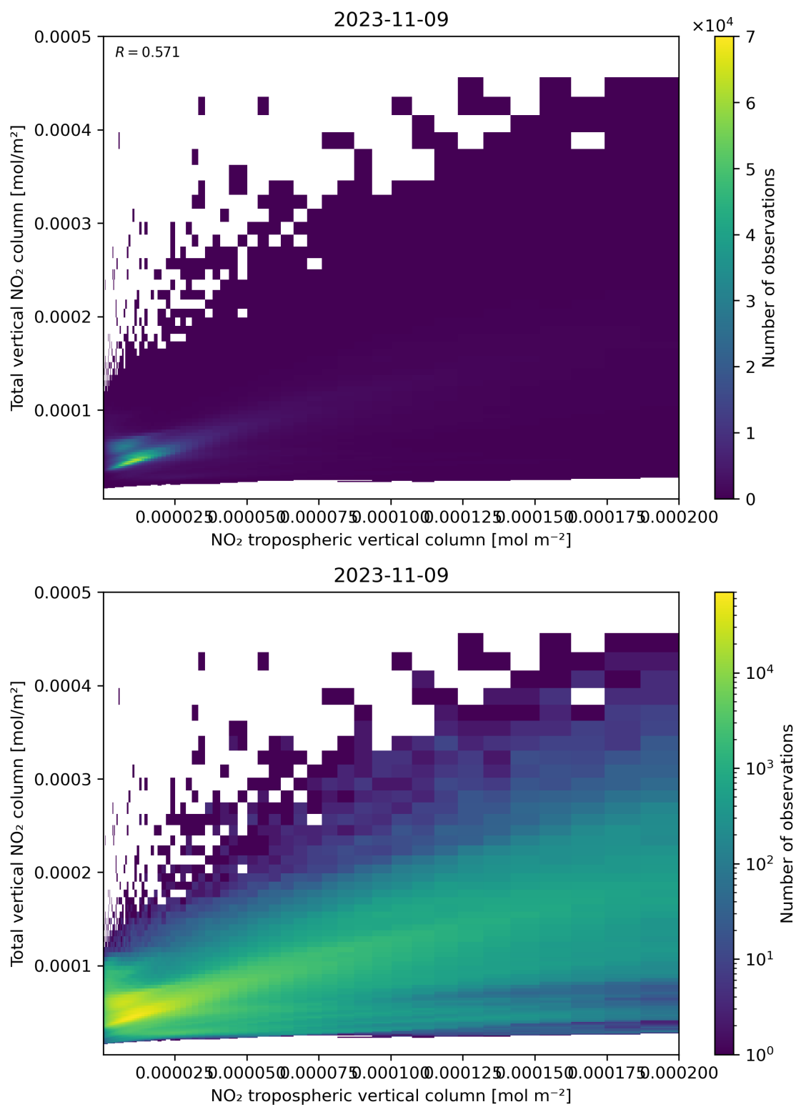
Figure 128: Scatter density plot of “NO 2 tropospheric vertical column” against “Total vertical NO 2 column” for 2023-11-08 to 2023-11-10.
