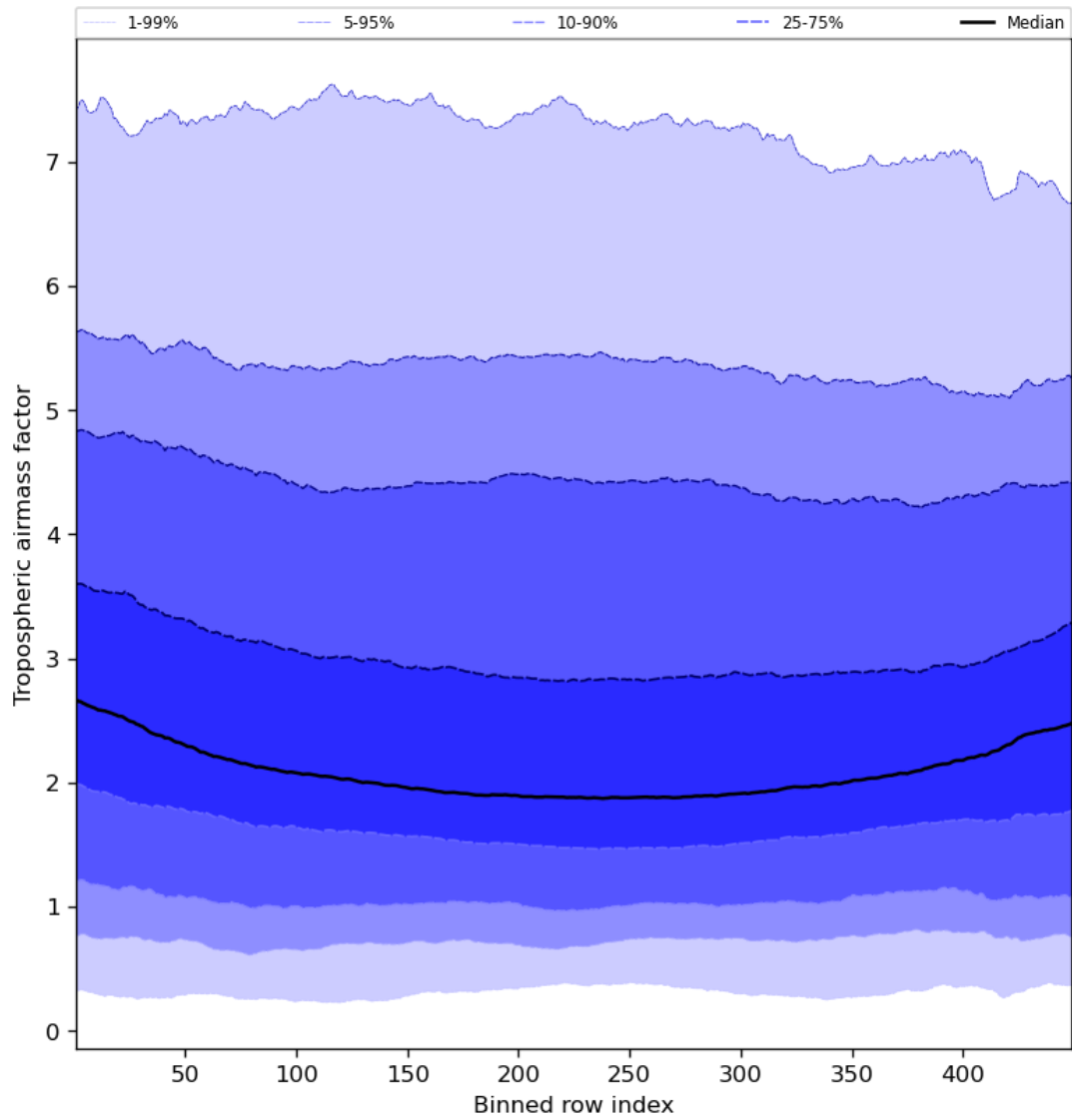
Figure 48: Along track statistics of “Tropospheric airmass factor” for 2023-11-08 to 2023-11-10
