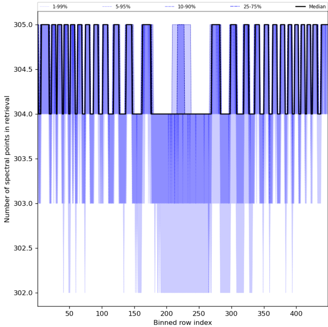
Figure 50: Along track statistics of “Number of spectral points in retrieval” for 2023-11-08 to 2023-11-10
