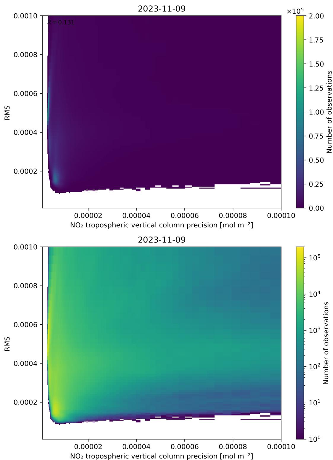
Figure 140: Scatter density plot of “NO 2 tropospheric vertical column precision” against “RMS” for 2023-11-08 to 2023-11-10.
