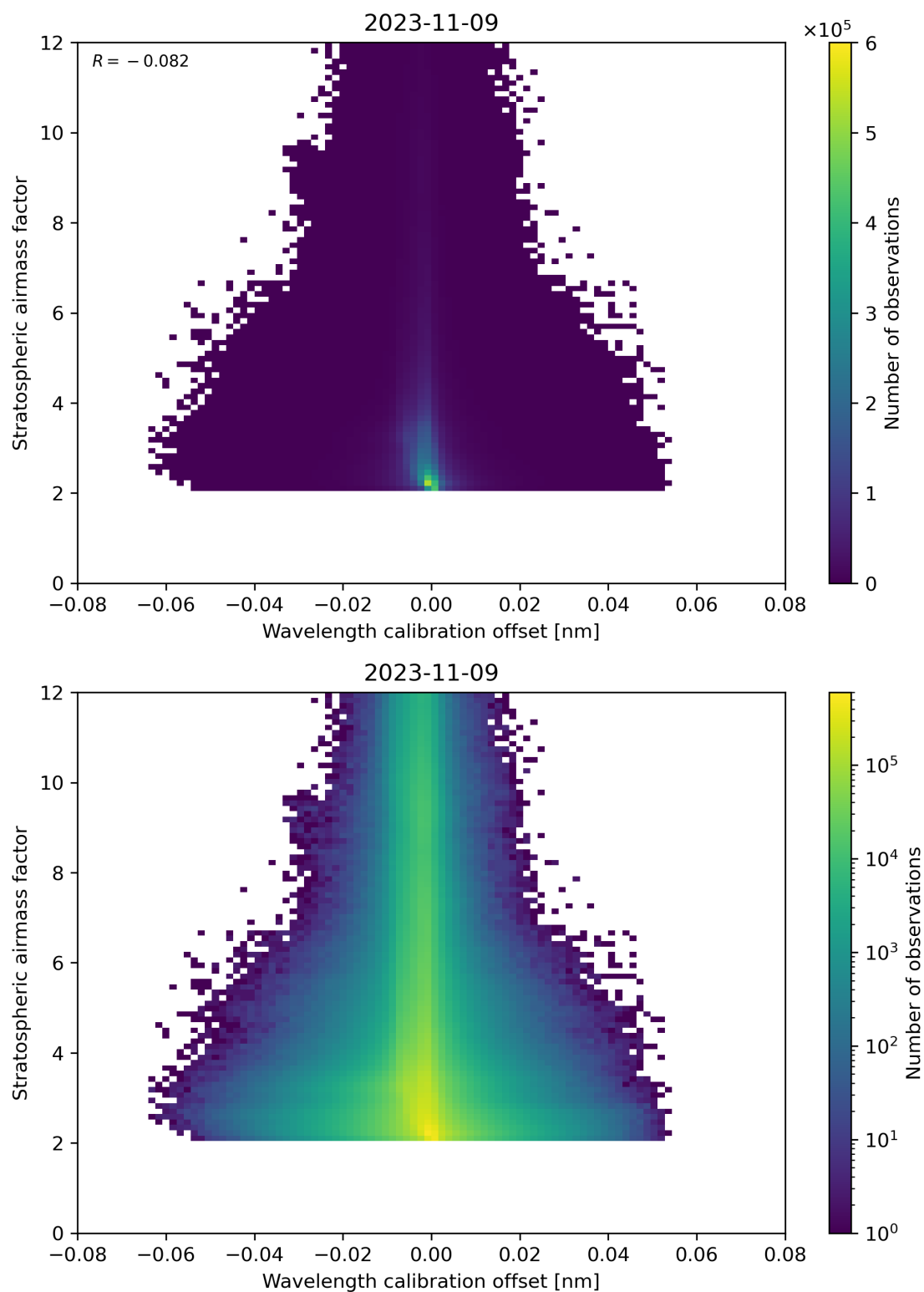
Figure 174: Scatter density plot of “Wavelength calibration offset” against “Stratospheric airmass factor” for 2023-11-08 to 2023-11-10.
