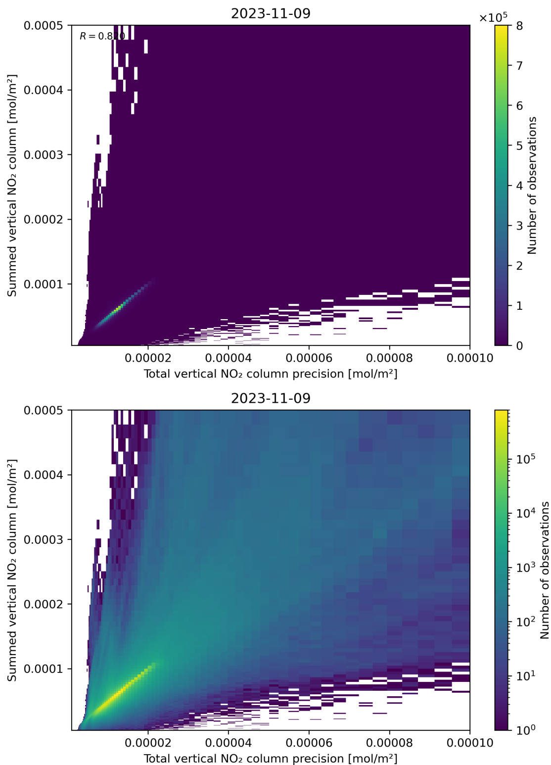
Figure 117: Scatter density plot of “Total vertical NO 2 column precision” against “Summed vertical NO 2 column” for 2023-11-08 to 2023-11-10.
