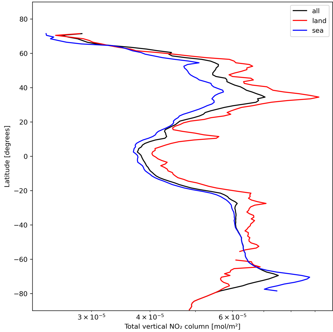
Figure 21: Zonal average of “Total vertical NO 2 column” for 2023-11-08 to 2023-11-10.
