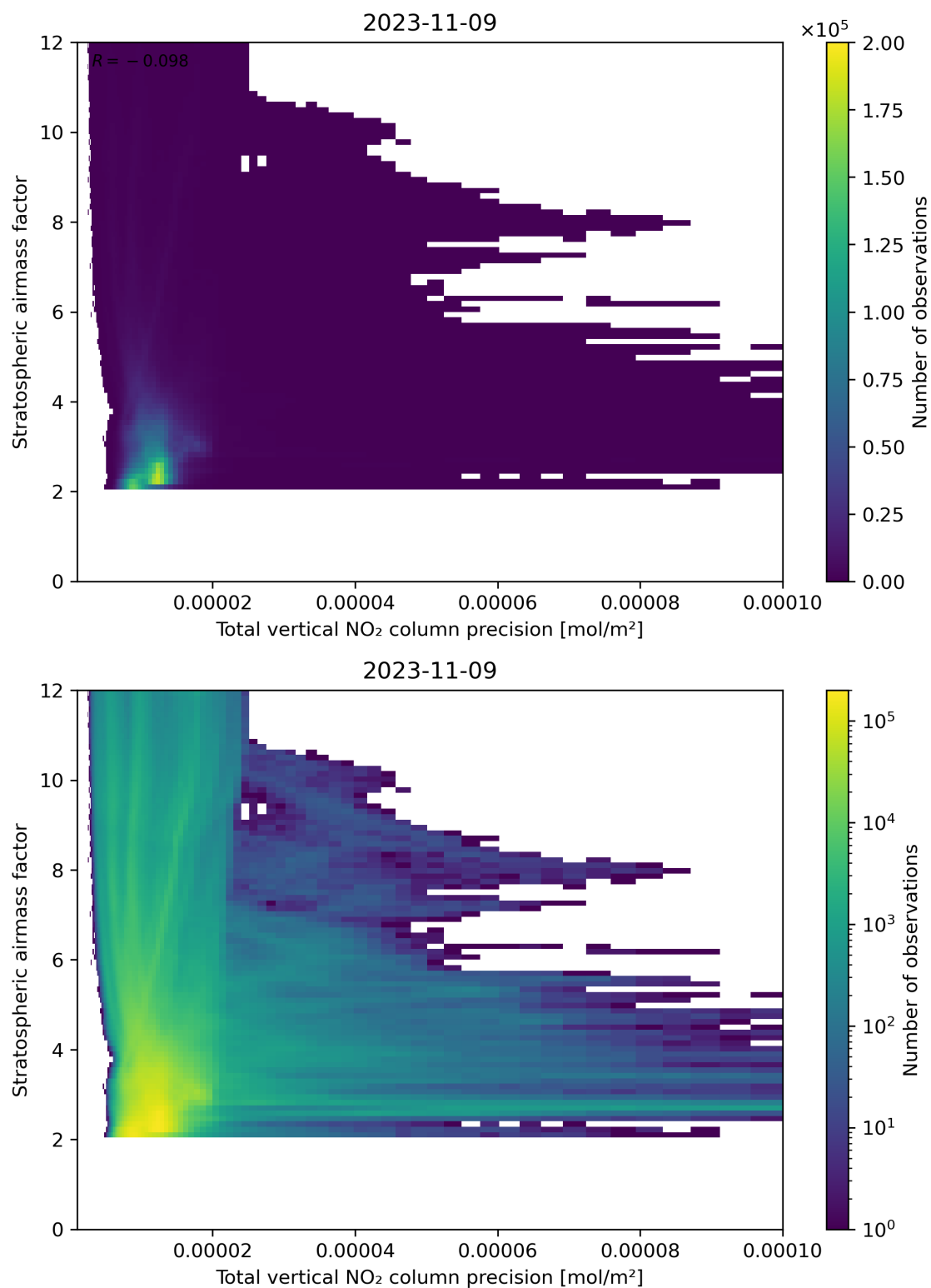
Figure 115: Scatter density plot of “Total vertical NO 2 column precision” against “Stratospheric air mass factor” for 2023-11-08 to 2023-11-10.
