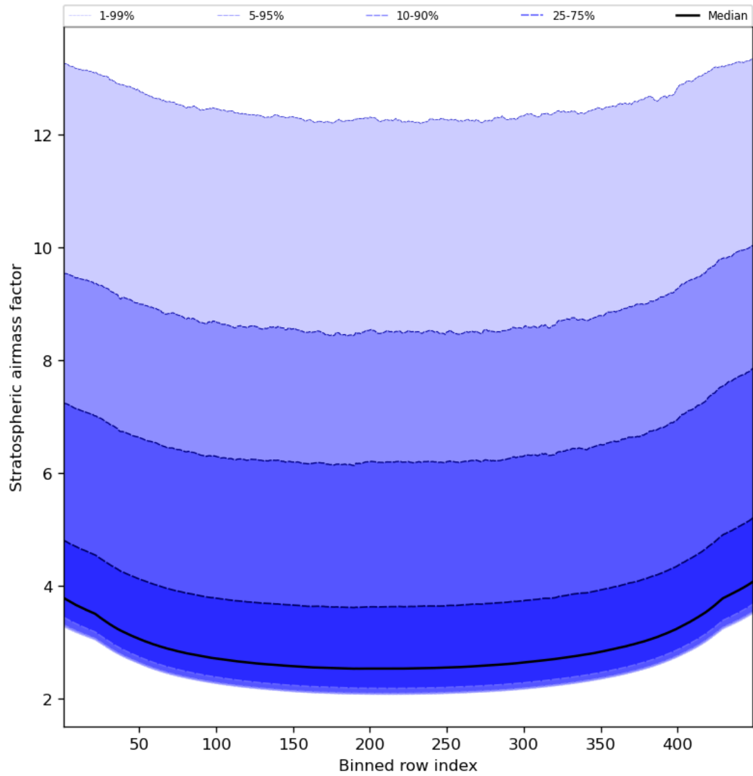
Figure 61: Along track statistics of “Stratospheric air mass factor” for 2023-11-08 to 2023-11-10
