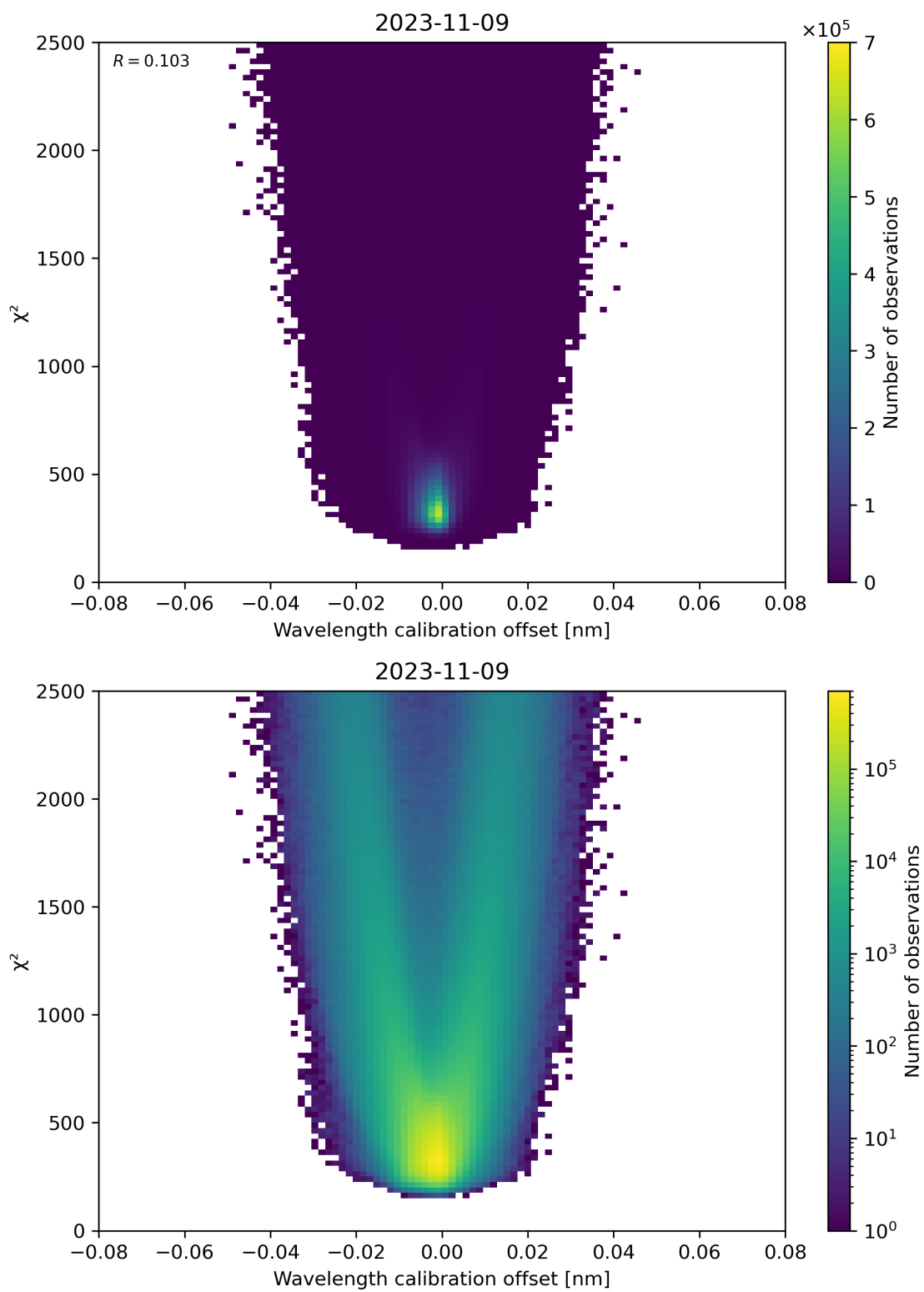
Figure 175: Scatter density plot of “Wavelength calibration offset” against “ \chi^2 ” for 2023-11-08 to 2023-11-10.
