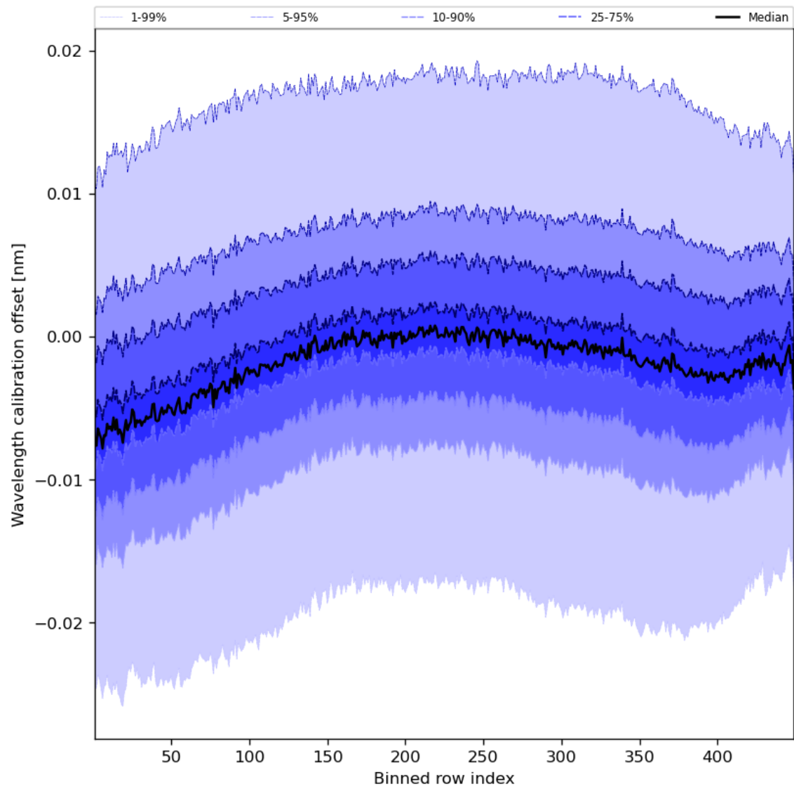
Figure 52: Along track statistics of “Wavelength calibration offset” for 2023-11-08 to 2023-11-10
