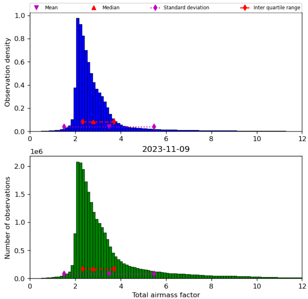
Figure 32: Histogram of “Total airmass factor” for 2023-11-08 to 2023-11-10
