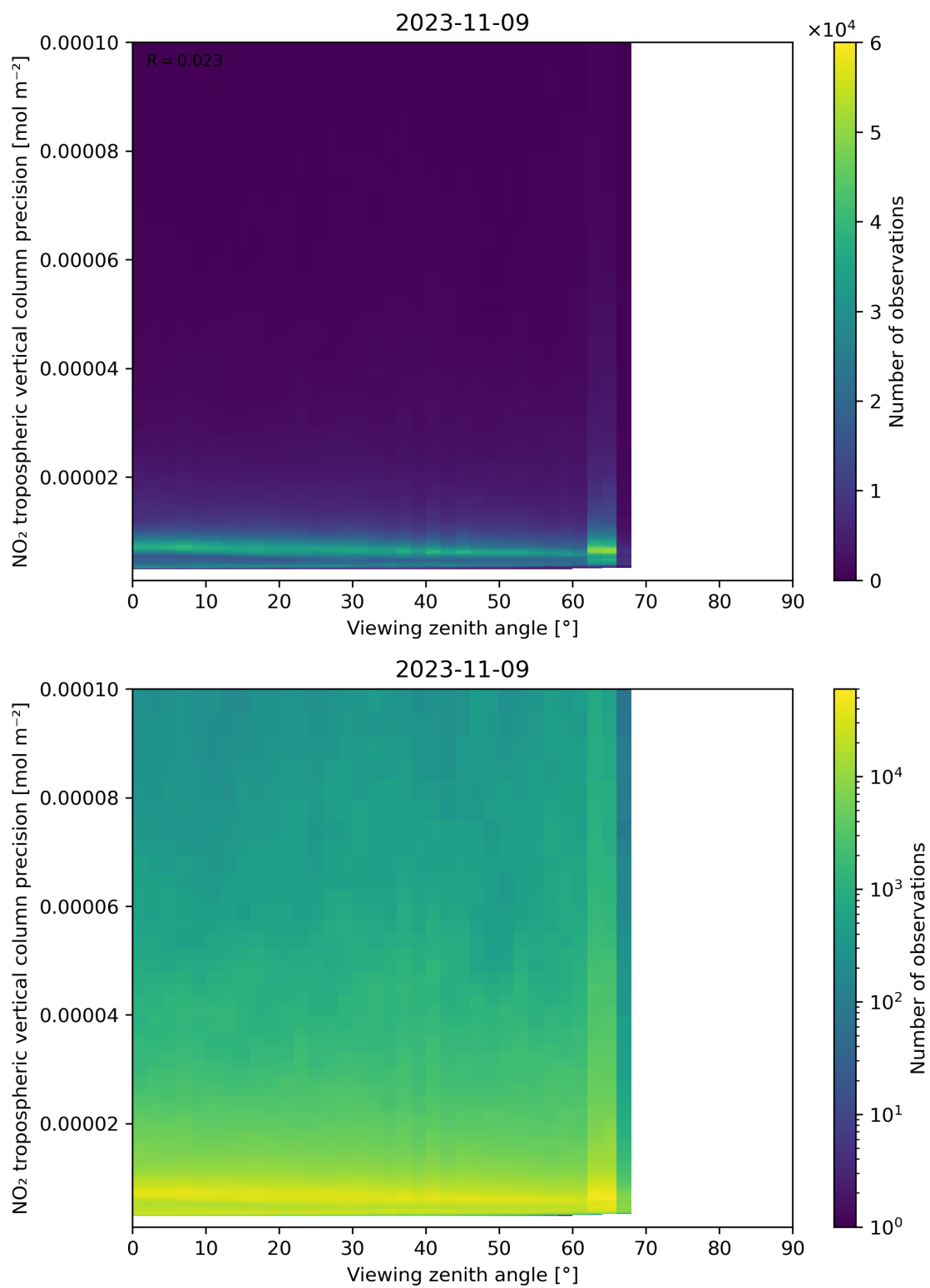
Figure 170: Scatter density plot of “Viewing zenith angle” against “NO 2 tropospheric vertical column precision” for 2023-11-08 to 2023-11-10.
