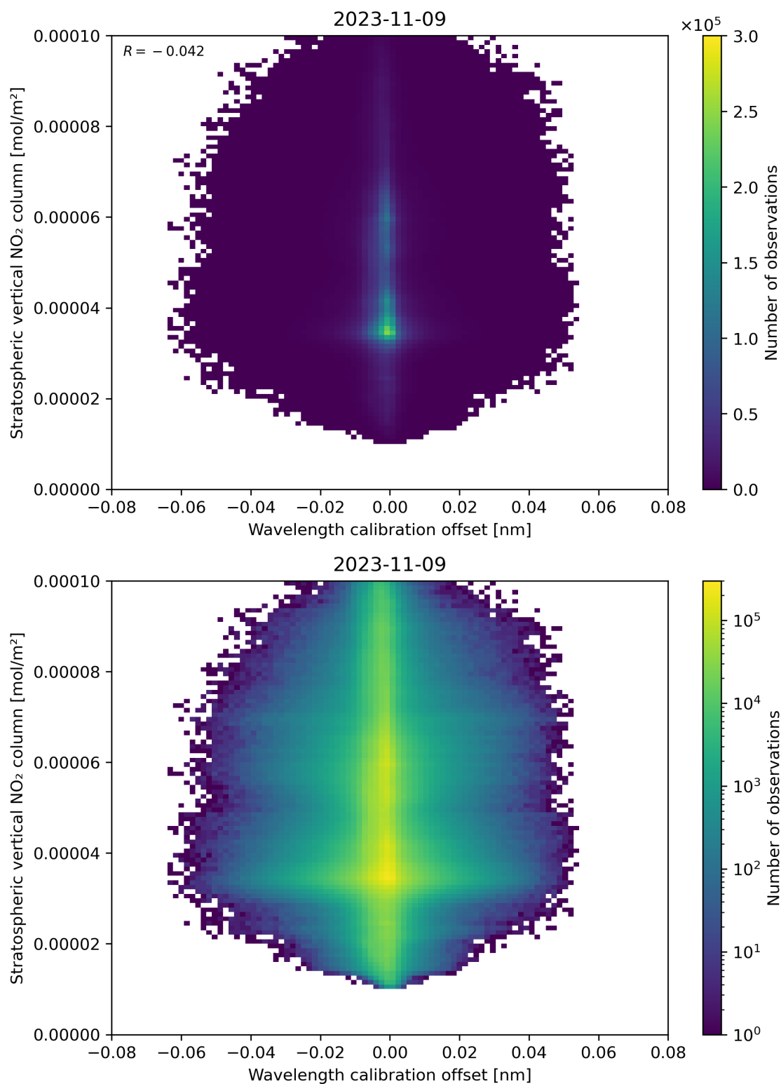
Figure 176: Scatter density plot of “Wavelength calibration offset” against “Stratospheric vertical NO 2 column” for 2023-11-08 to 2023-11-10.
