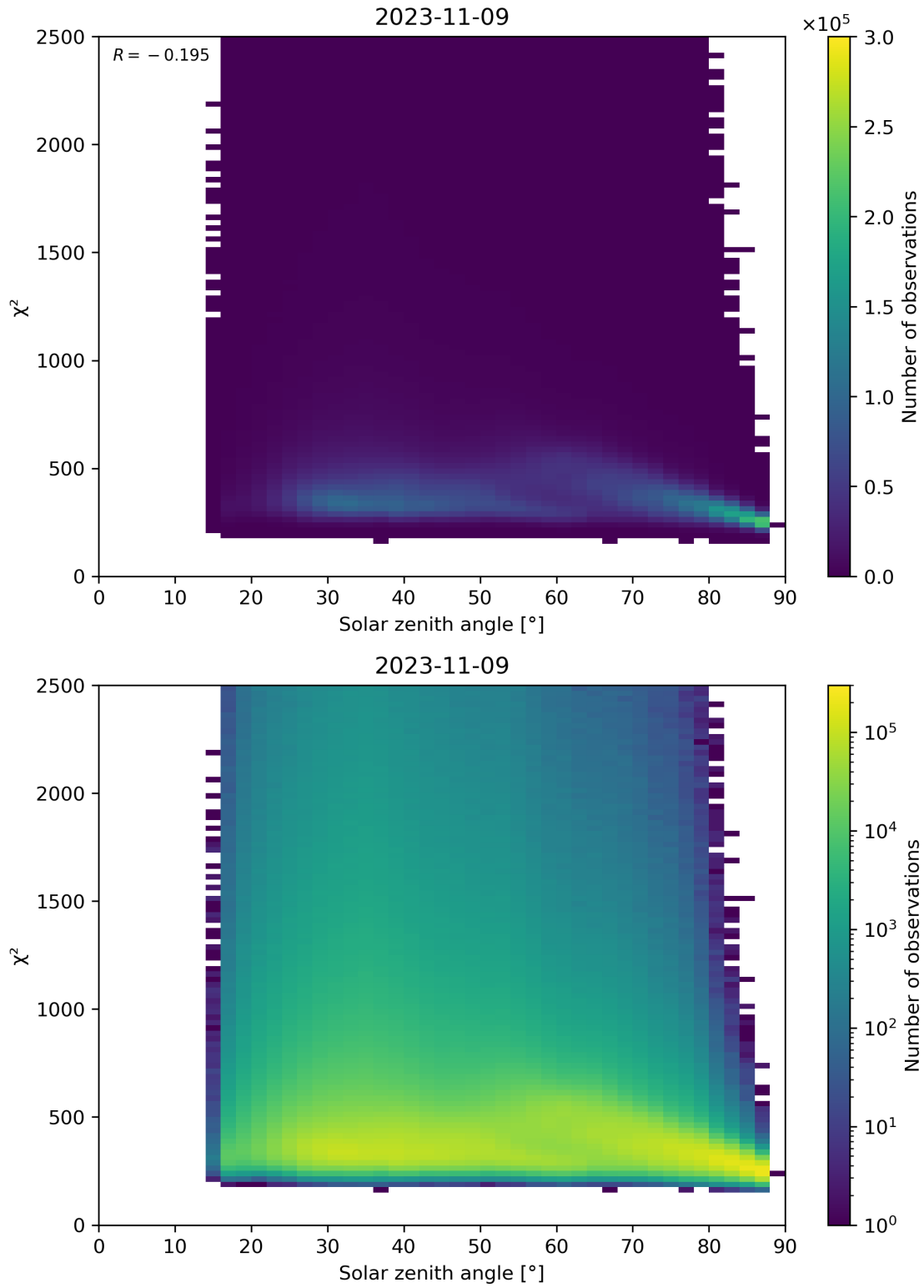
Figure 148: Scatter density plot of “Solar zenith angle” against “ \chi^2 ” for 2023-11-08 to 2023-11-10.
