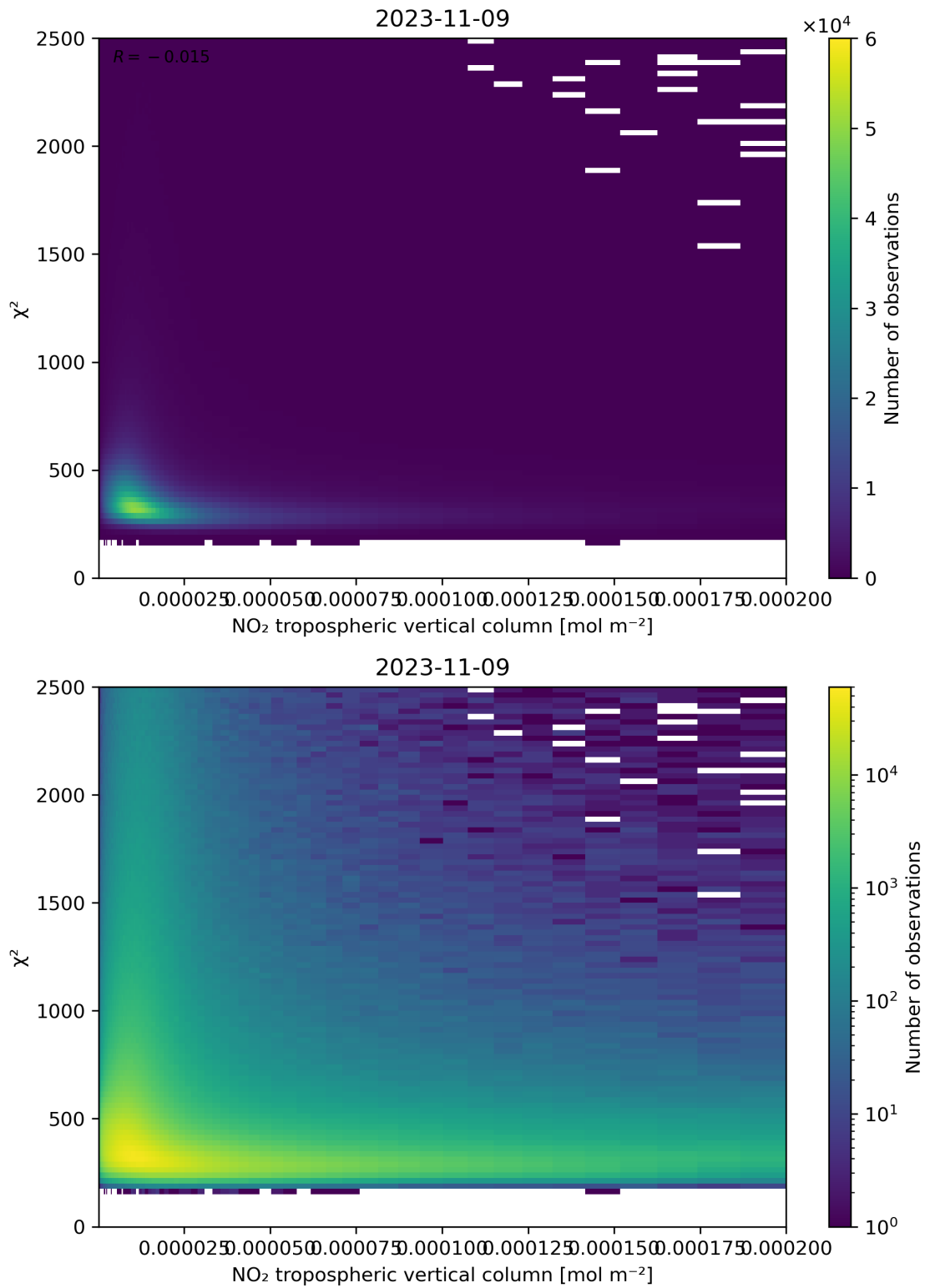
Figure 124: Scatter density plot of “NO 2 tropospheric vertical column” against “ \chi^2 ” for 2023-11-08 to 2023-11-10.
