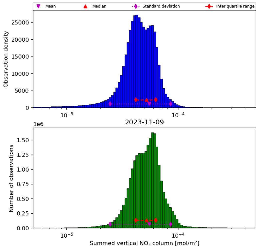
Figure 40: Histogram of “Summed vertical NO 2 column” for 2023-11-08 to 2023-11-10
