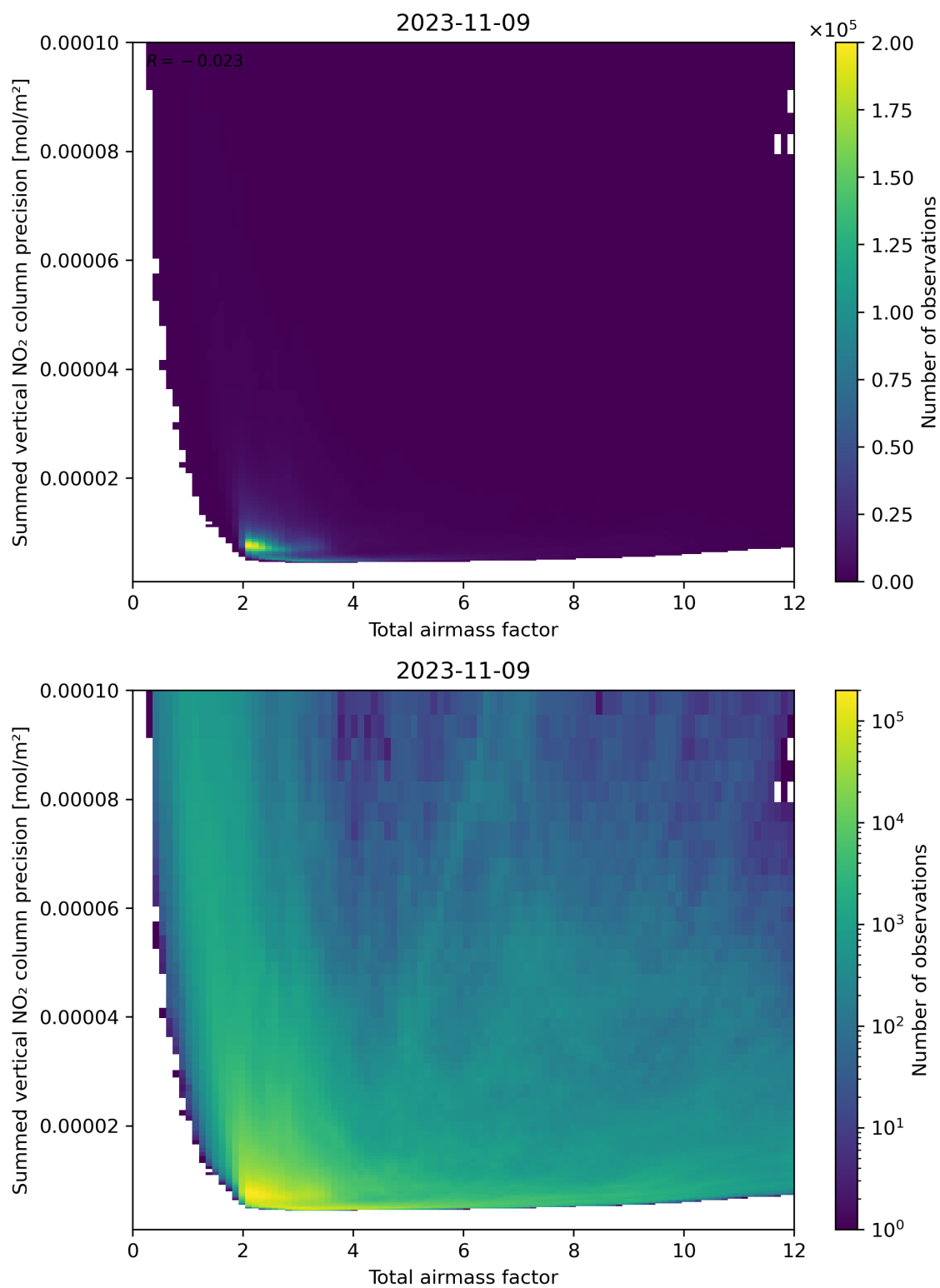
Figure 66: Scatter density plot of “Total airmass factor” against “Summed vertical NO 2 column precision” for 2023-11-08 to 2023-11-10.
