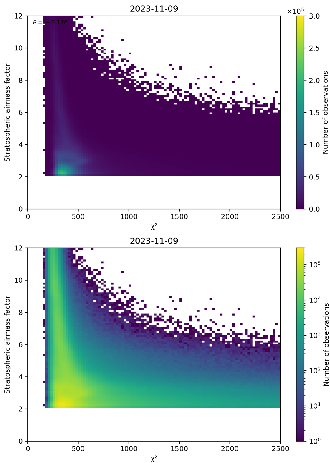
Figure 81: Scatter density plot of “ \chi^2 ” against “Stratospheric airmass factor” for 2023-11-08 to 2023-11-10.
