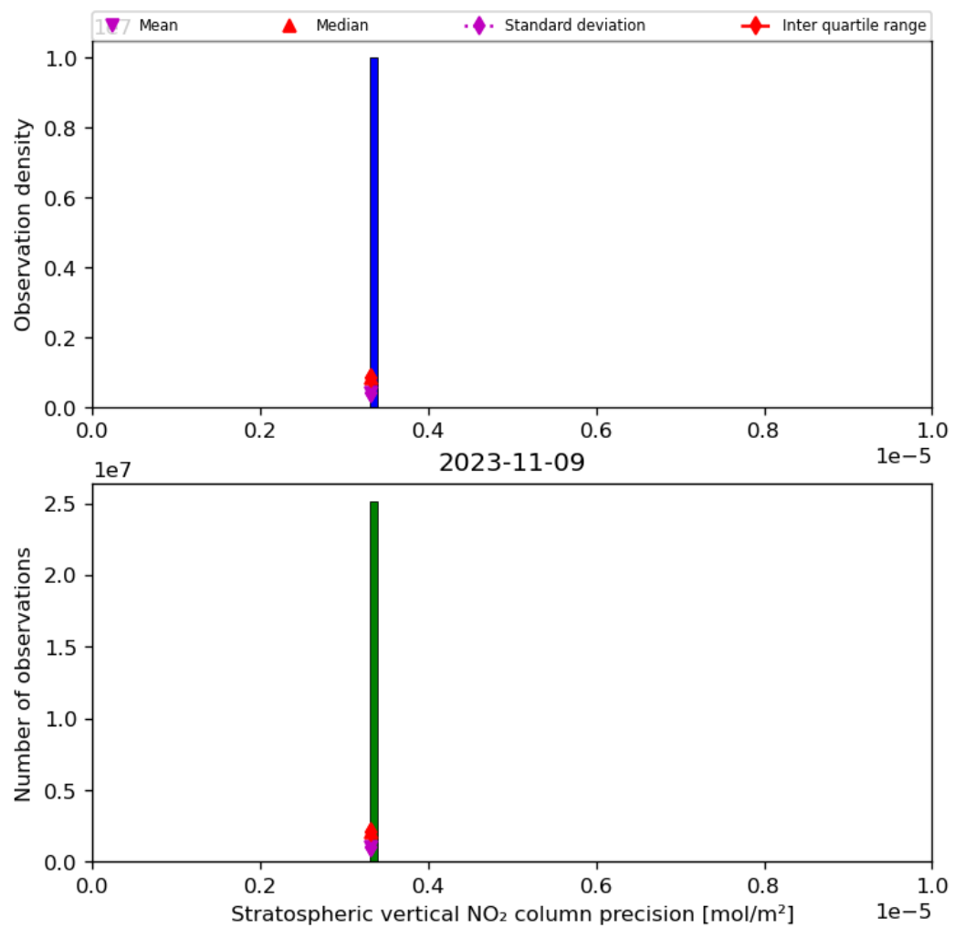
Figure 37: Histogram of “Stratospheric vertical NO 2 column precision” for 2023-11-08 to 2023-11-10
