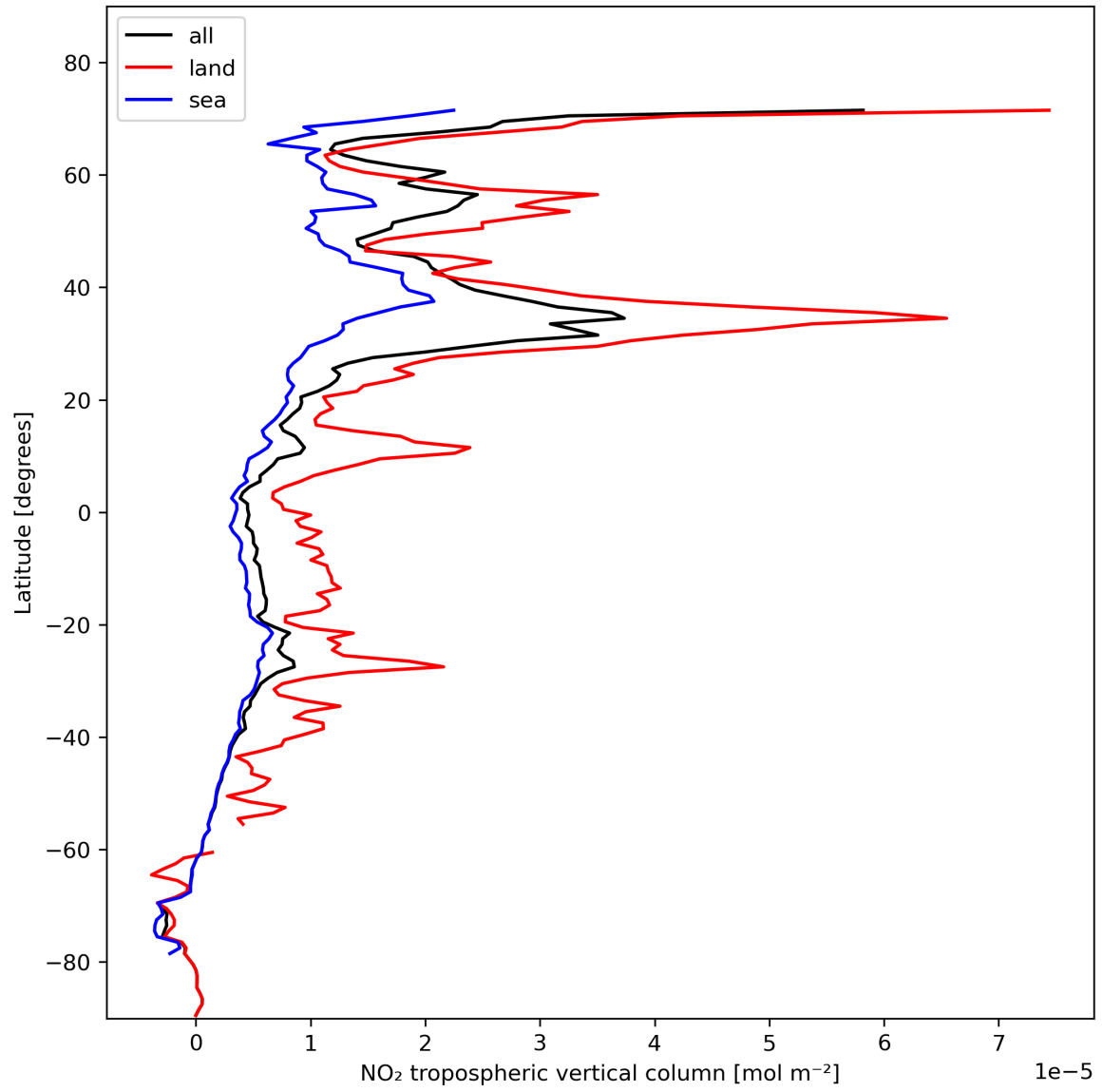
Figure 12: Zonal average of “NO 2 tropospheric vertical column” for 2023-11-08 to 2023-11-10.
