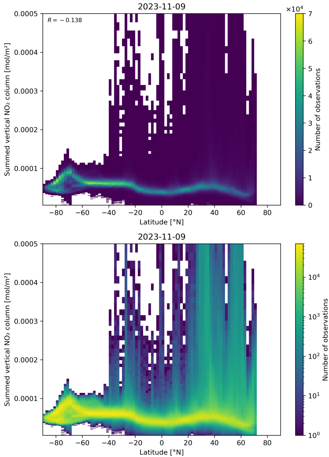
Figure 88: Scatter density plot of “Latitude” against “Summed vertical NO 2 column” for 2023-11-08 to 2023-11-10.
