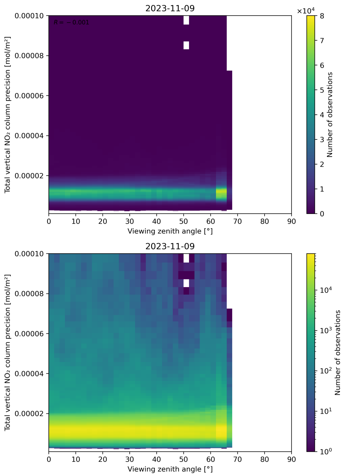
Figure 168: Scatter density plot of “Viewing zenith angle” against “Total vertical NO 2 column precision” for 2023-11-08 to 2023-11-10.
