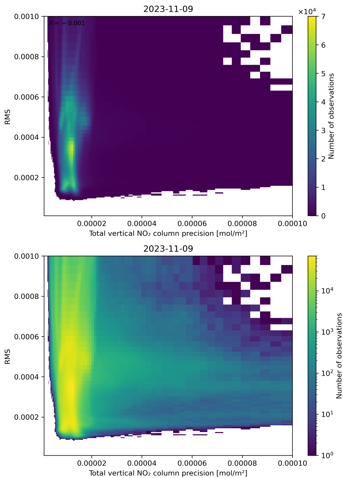
Figure 119: Scatter density plot of “Total vertical NO 2 column precision” against “RMS” for 2023-11-08 to 2023-11-10.
