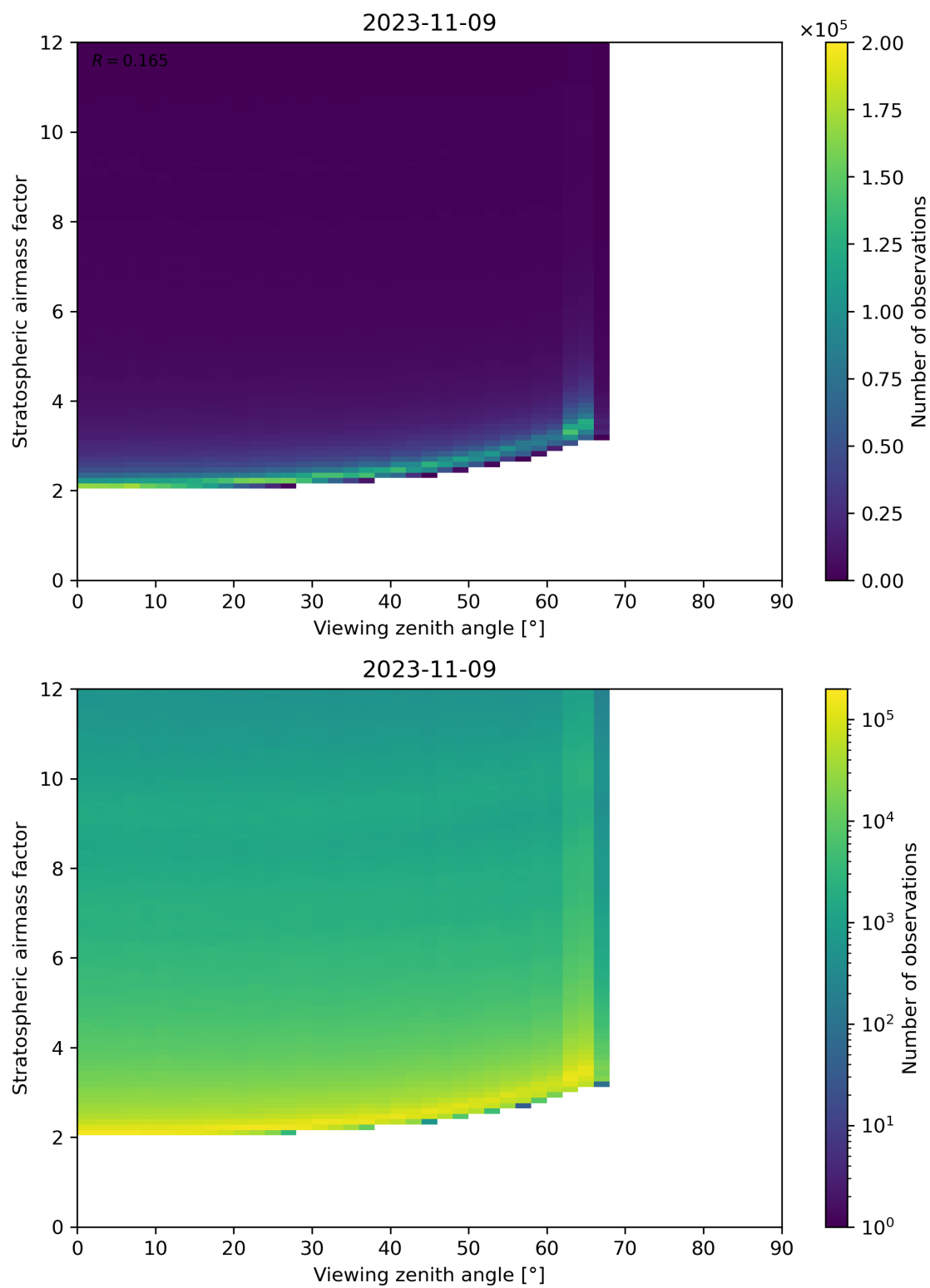
Figure 159: Scatter density plot of “Viewing zenith angle” against “Stratospheric airmass factor” for 2023-11-08 to 2023-11-10.
