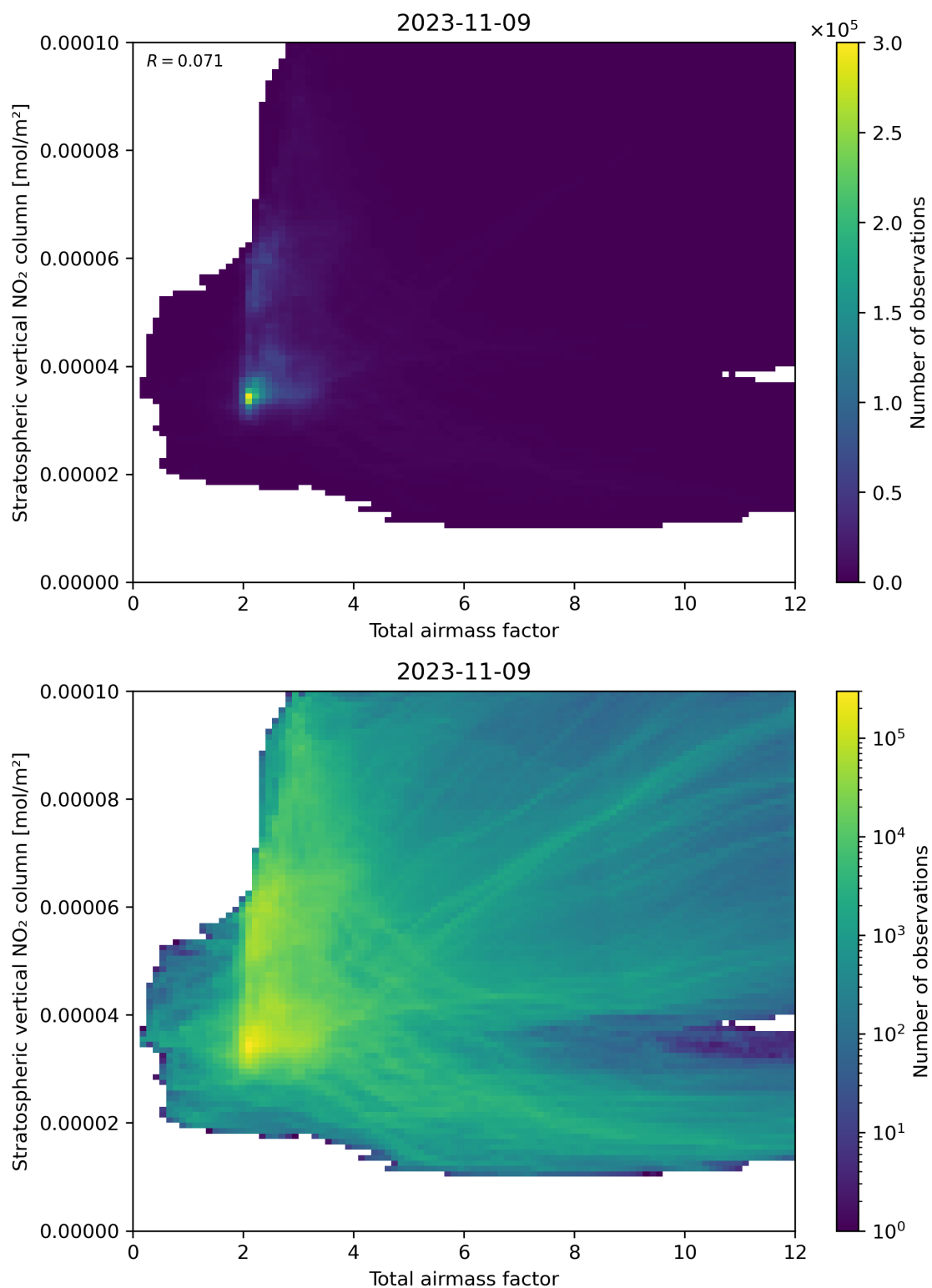
Figure 64: Scatter density plot of “Total airmass factor” against “Stratospheric vertical NO 2 column” for 2023-11-08 to 2023-11-10.
