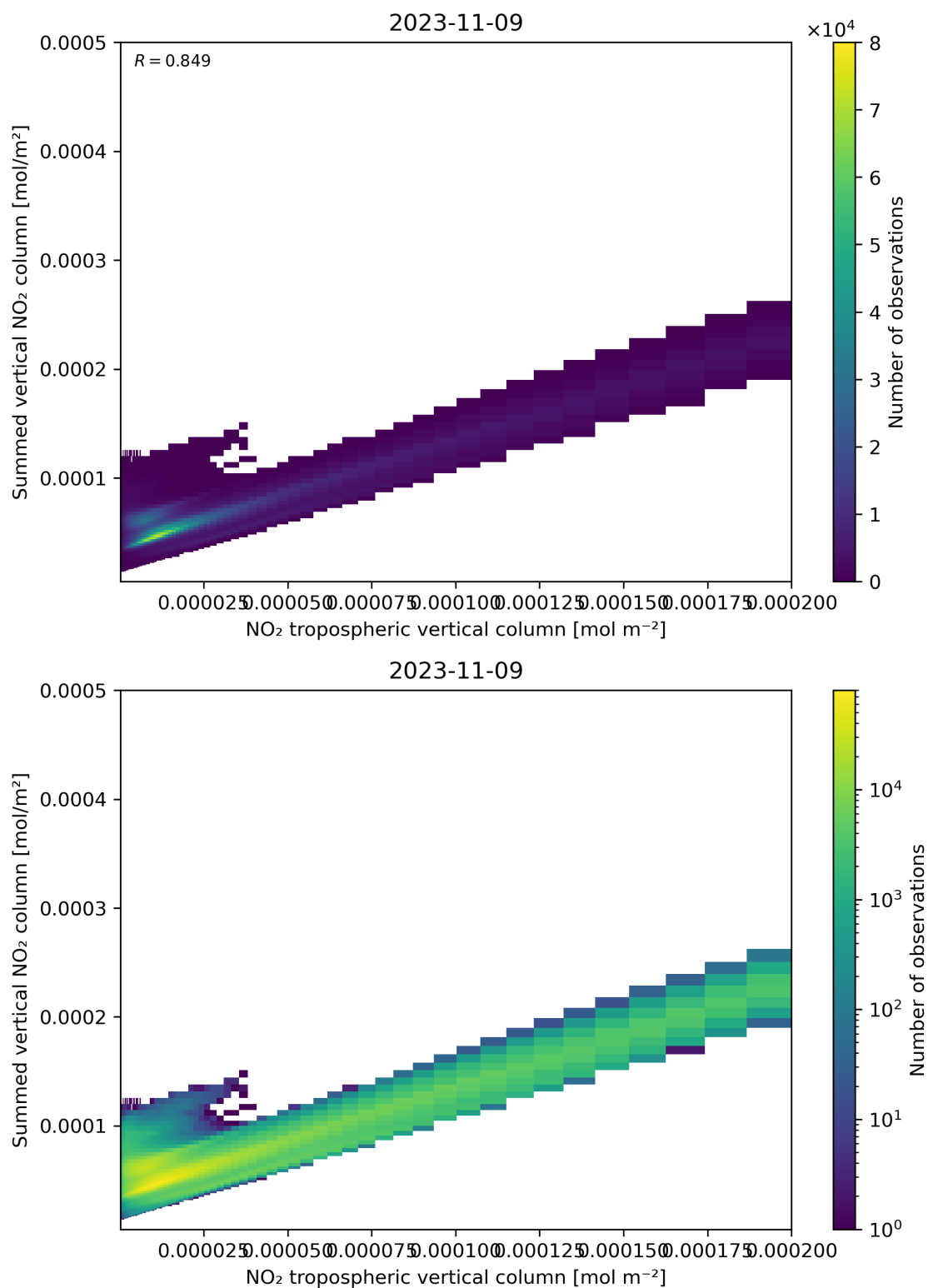
Figure 126: Scatter density plot of “NO 2 tropospheric vertical column” against “Summed vertical NO 2 column” for 2023-11-08 to 2023-11-10.
