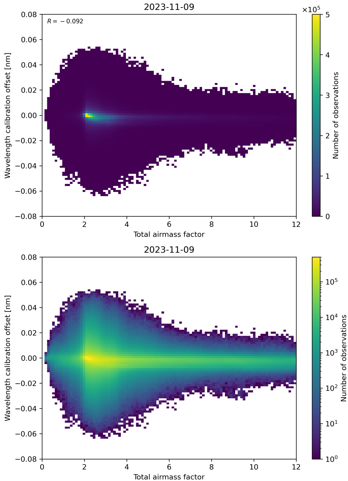
Figure 70: Scatter density plot of “Total airmass factor” against “Wavelength calibration offset” for 2023-11-08 to 2023-11-10.
