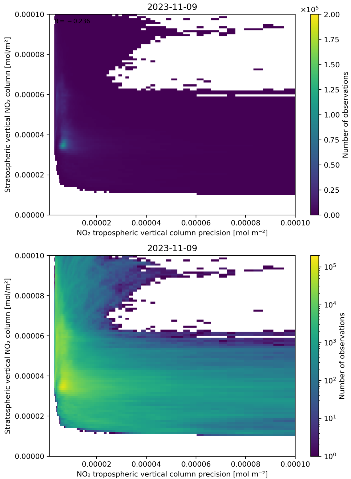
Figure 135: Scatter density plot of “NO 2 tropospheric vertical column precision” against “Stratospheric vertical NO 2 column” for 2023-11-08 to 2023-11-10.
