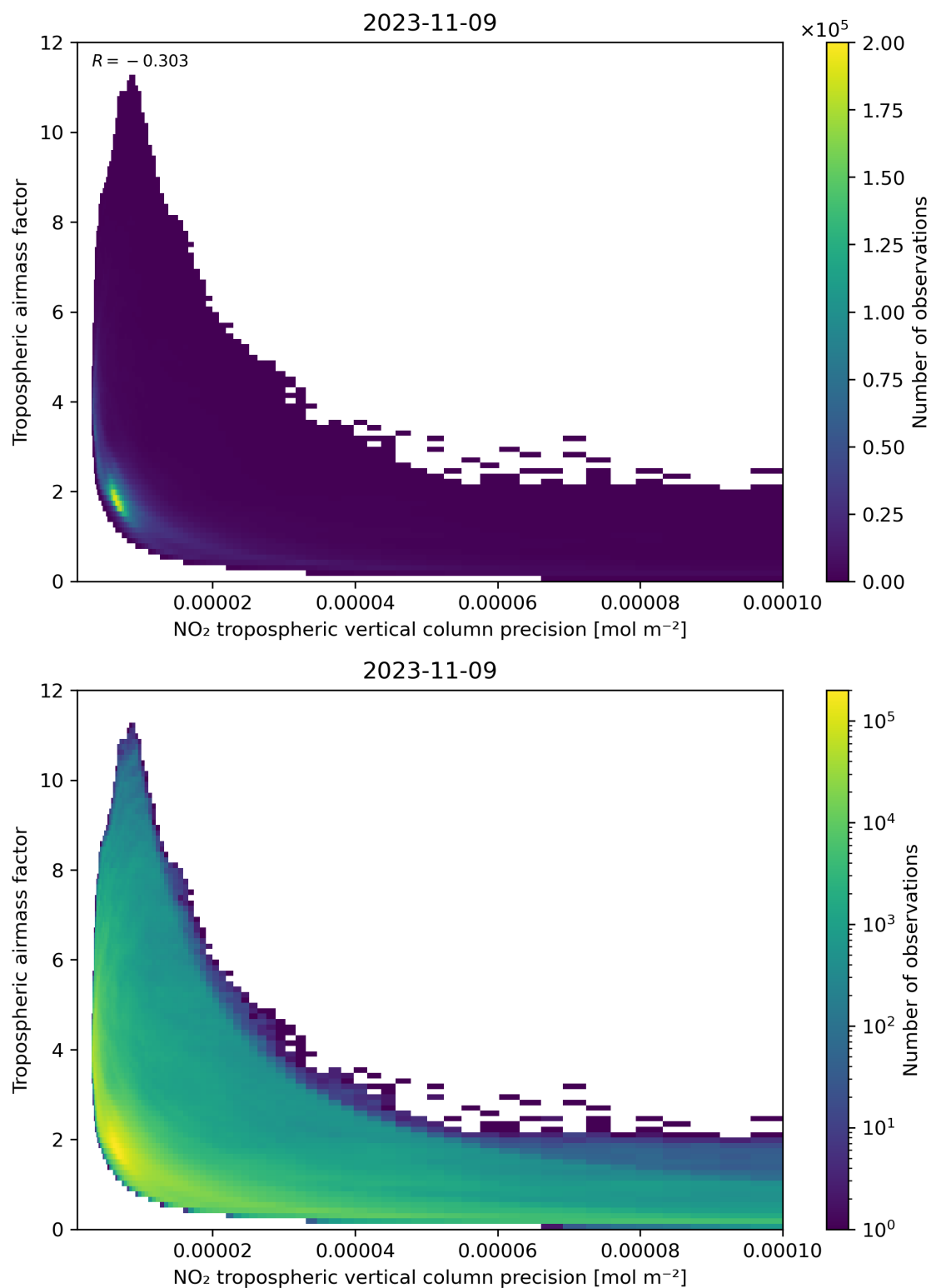
Figure 133: Scatter density plot of “NO 2 tropospheric vertical column precision” against “Tropospheric airmass factor” for 2023-11-08 to 2023-11-10.
