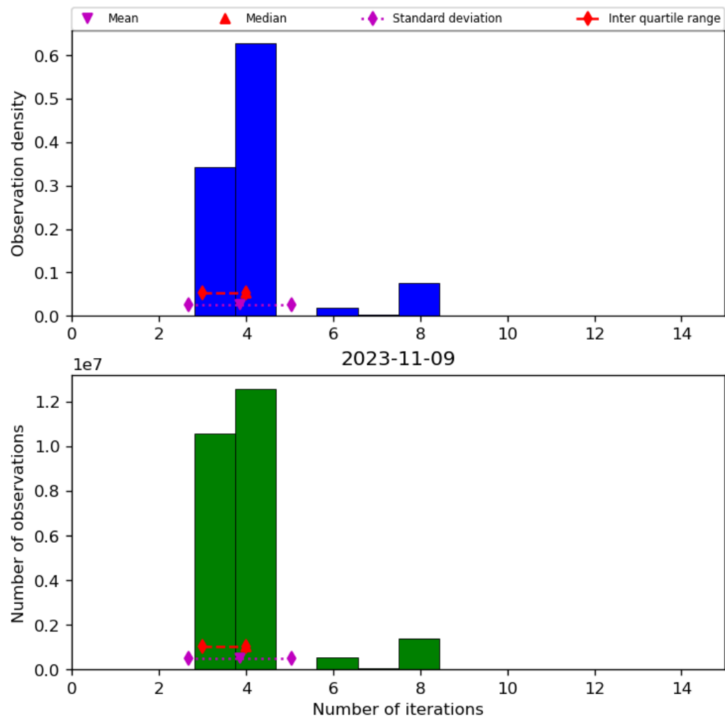
Figure 34: Histogram of “Number of iterations” for 2023-11-08 to 2023-11-10
