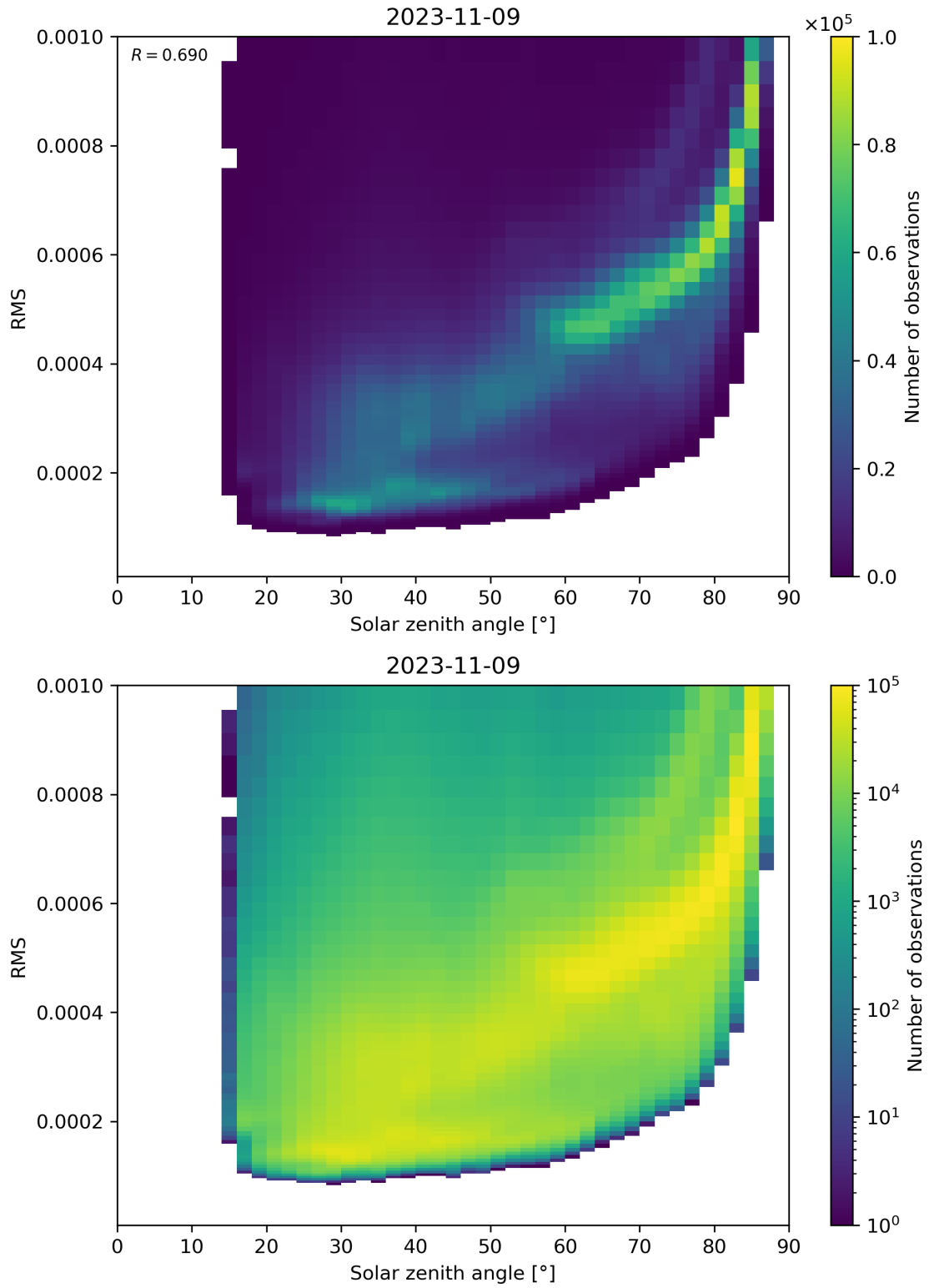
Figure 157: Scatter density plot of “Solar zenith angle” against “RMS” for 2023-11-08 to 2023-11-10.
