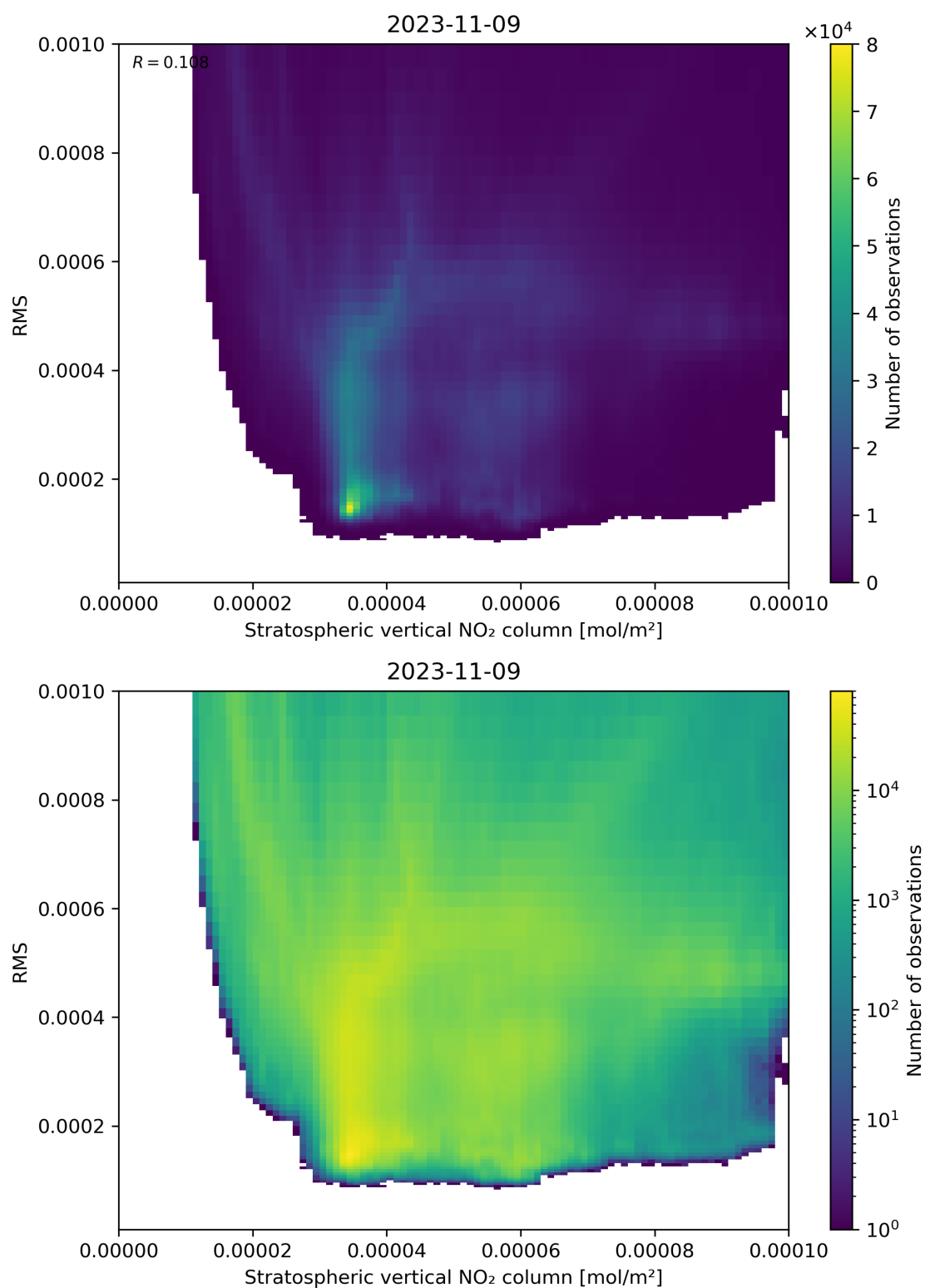
Figure 102: Scatter density plot of “Stratospheric vertical NO 2 column” against “RMS” for 2023-11-08 to 2023-11-10.
