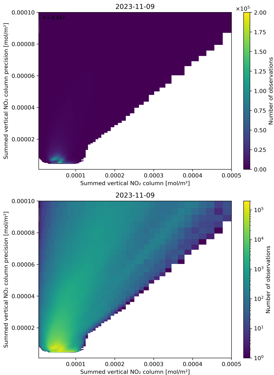
Figure 105: Scatter density plot of “Summed vertical NO 2 column” against “Summed vertical NO 2 column precision” for 2023-11-08 to 2023-11-10.
