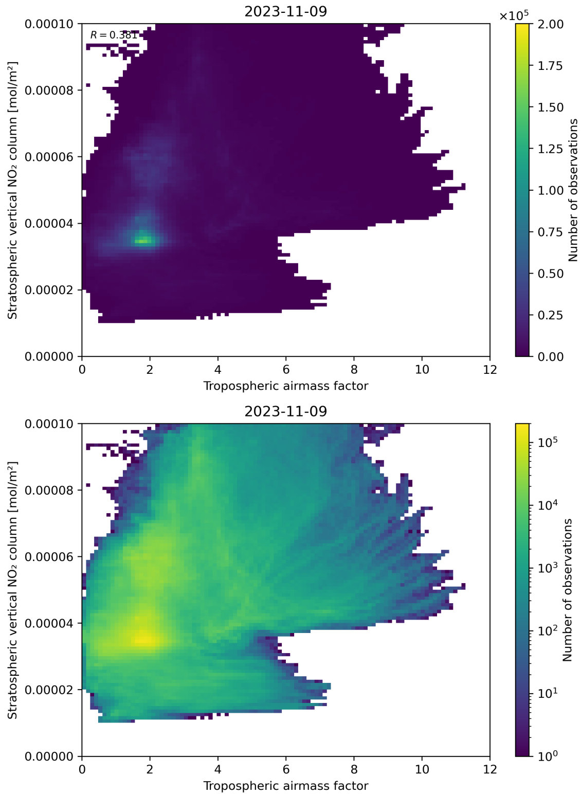
Figure 74: Scatter density plot of “Tropospheric air mass factor” against “Stratospheric vertical NO 2 column” for 2023-11-08 to 2023-11-10.
