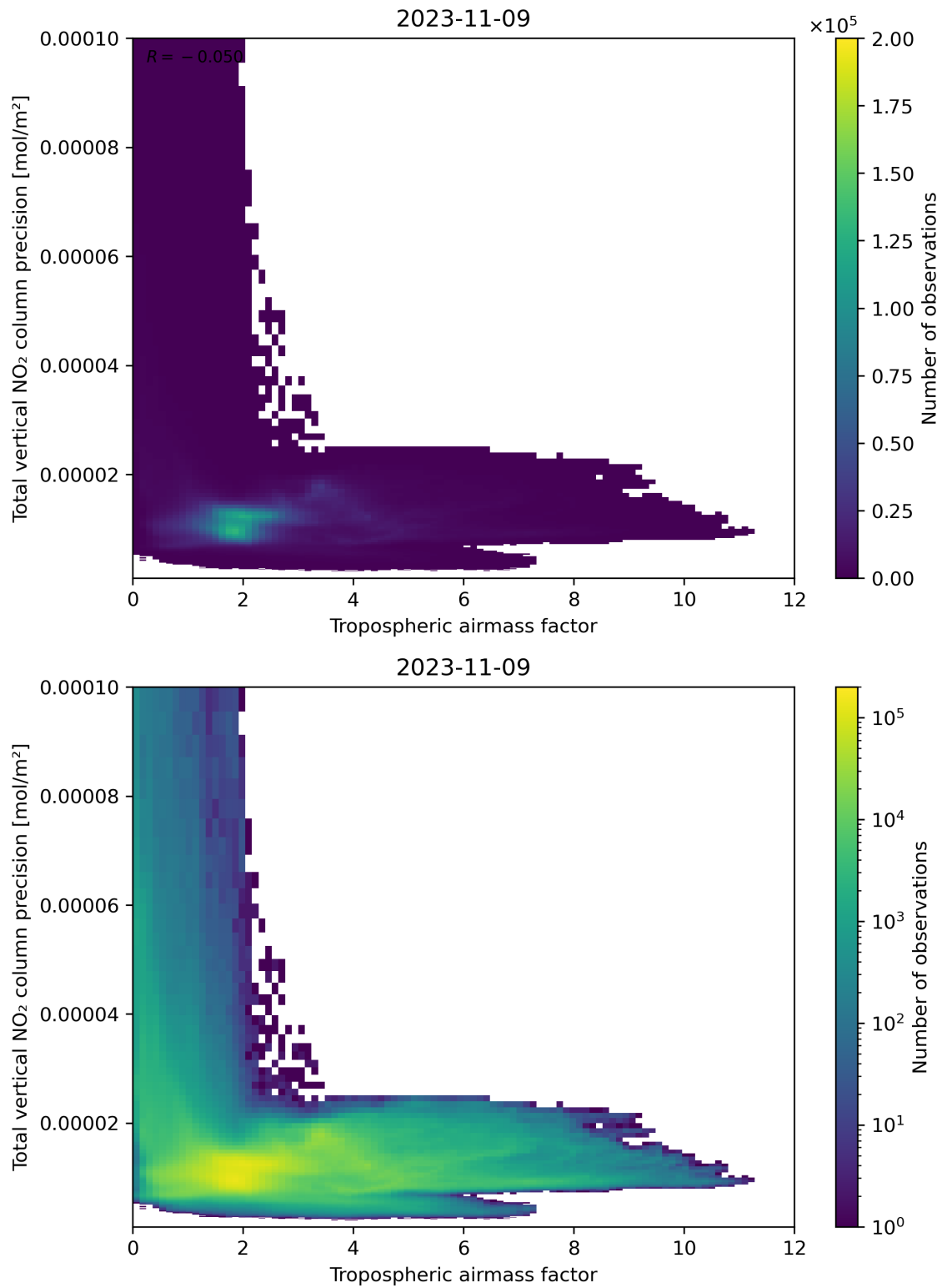
Figure 78: Scatter density plot of “Tropospheric airmass factor” against “Total vertical NO 2 column precision” for 2023-11-08 to 2023-11-10.
