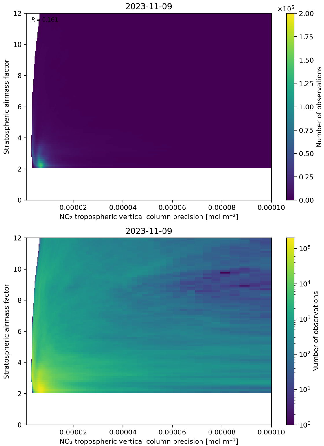
Figure 131: Scatter density plot of “NO 2 tropospheric vertical column precision” against “Stratospheric airmass factor” for 2023-11-08 to 2023-11-10.
