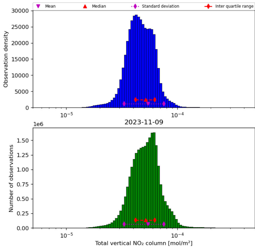
Figure 38: Histogram of “Total vertical NO 2 column” for 2023-11-08 to 2023-11-10
