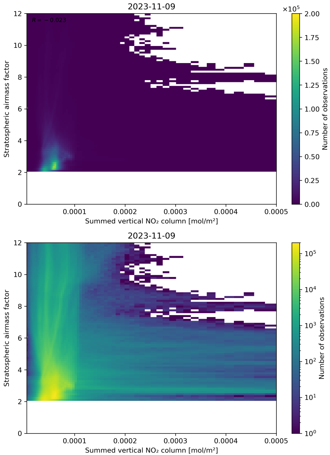
Figure 103: Scatter density plot of “Summed vertical NO 2 column” against “Stratospheric air mass factor” for 2023-11-08 to 2023-11-10.
