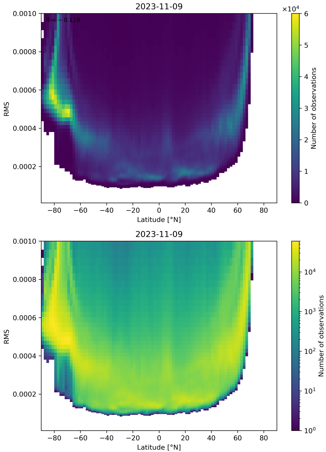
Figure 94: Scatter density plot of “Latitude” against “RMS” for 2023-11-08 to 2023-11-10.
