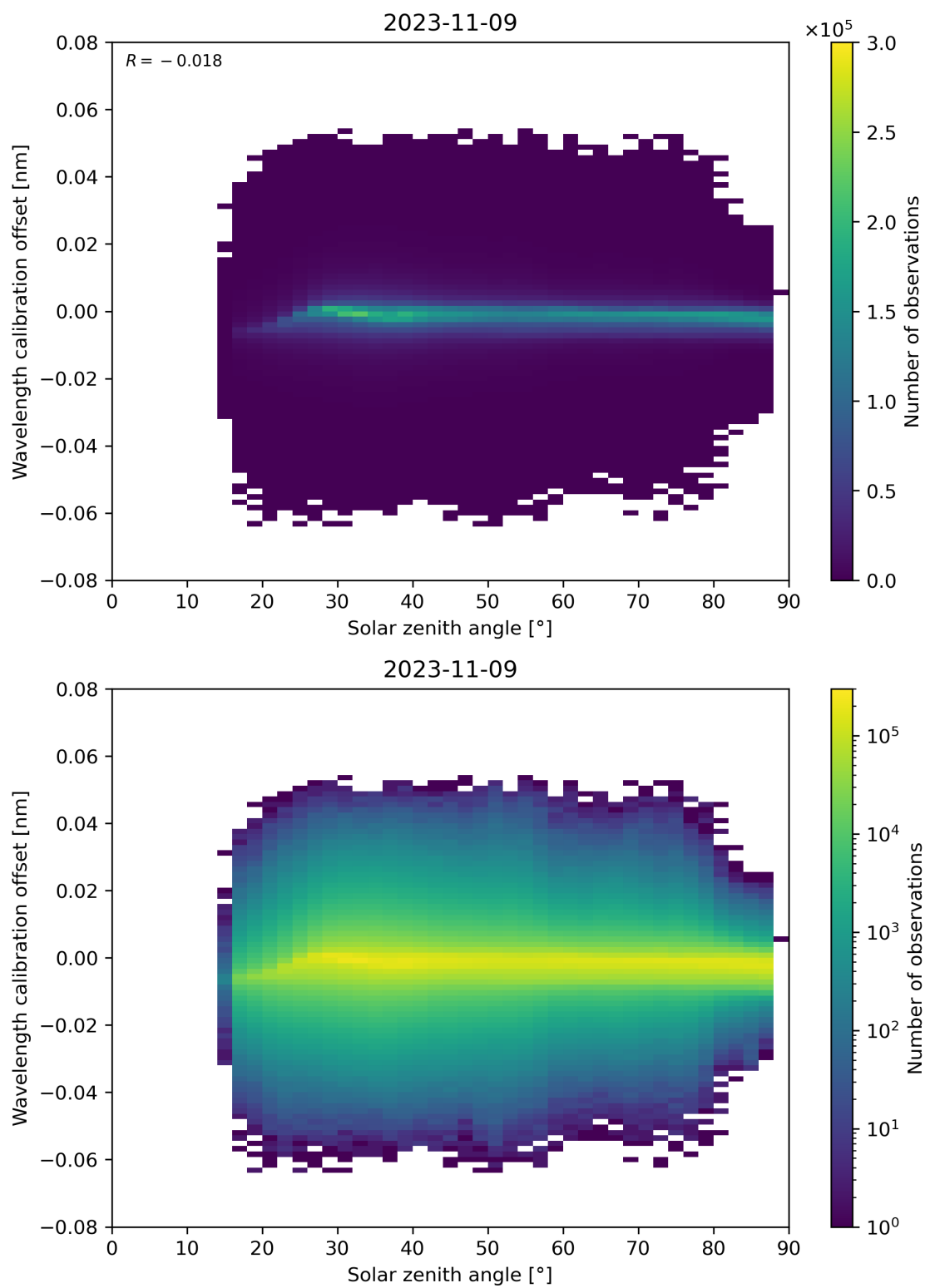
Figure 158: Scatter density plot of “Solar zenith angle” against “Wavelength calibration offset” for 2023-11-08 to 2023-11-10.
