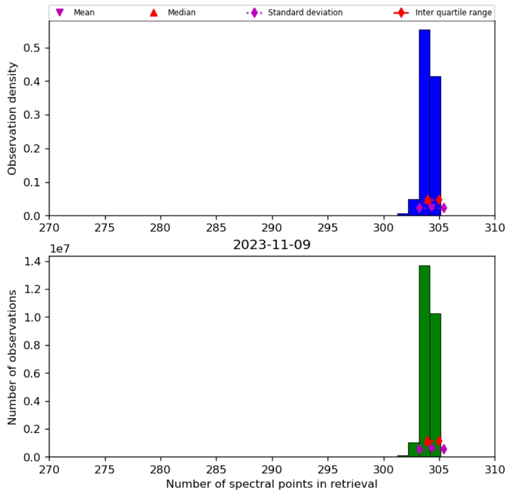
Figure 33: Histogram of “Number of spectral points in retrieval” for 2023-11-08 to 2023-11-10
