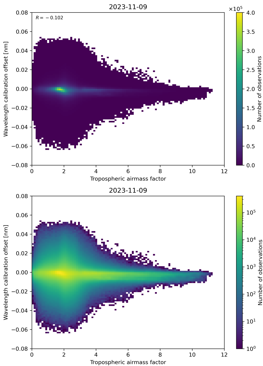
Figure 80: Scatter density plot of “Tropospheric airmass factor” against “Wavelength calibration offset” for 2023-11-08 to 2023-11-10.
