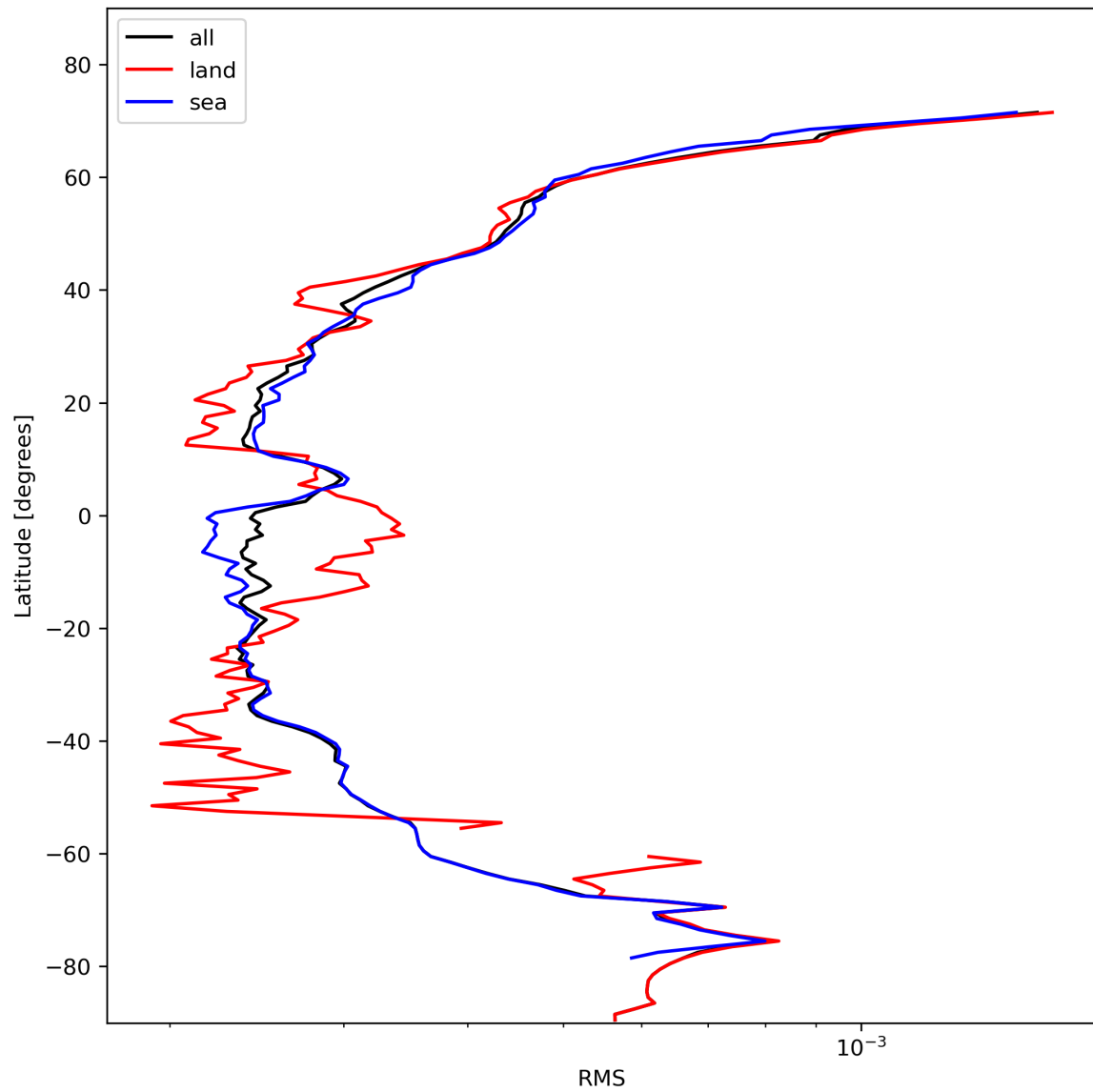
Figure 26: Zonal average of “RMS” for 2023-11-08 to 2023-11-10.
