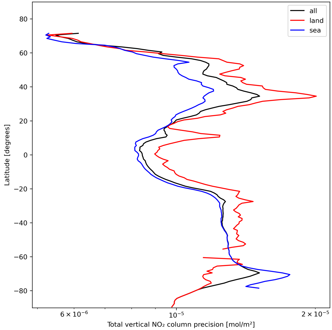
Figure 22: Zonal average of “Total vertical NO 2 column precision” for 2023-11-08 to 2023-11-10.
