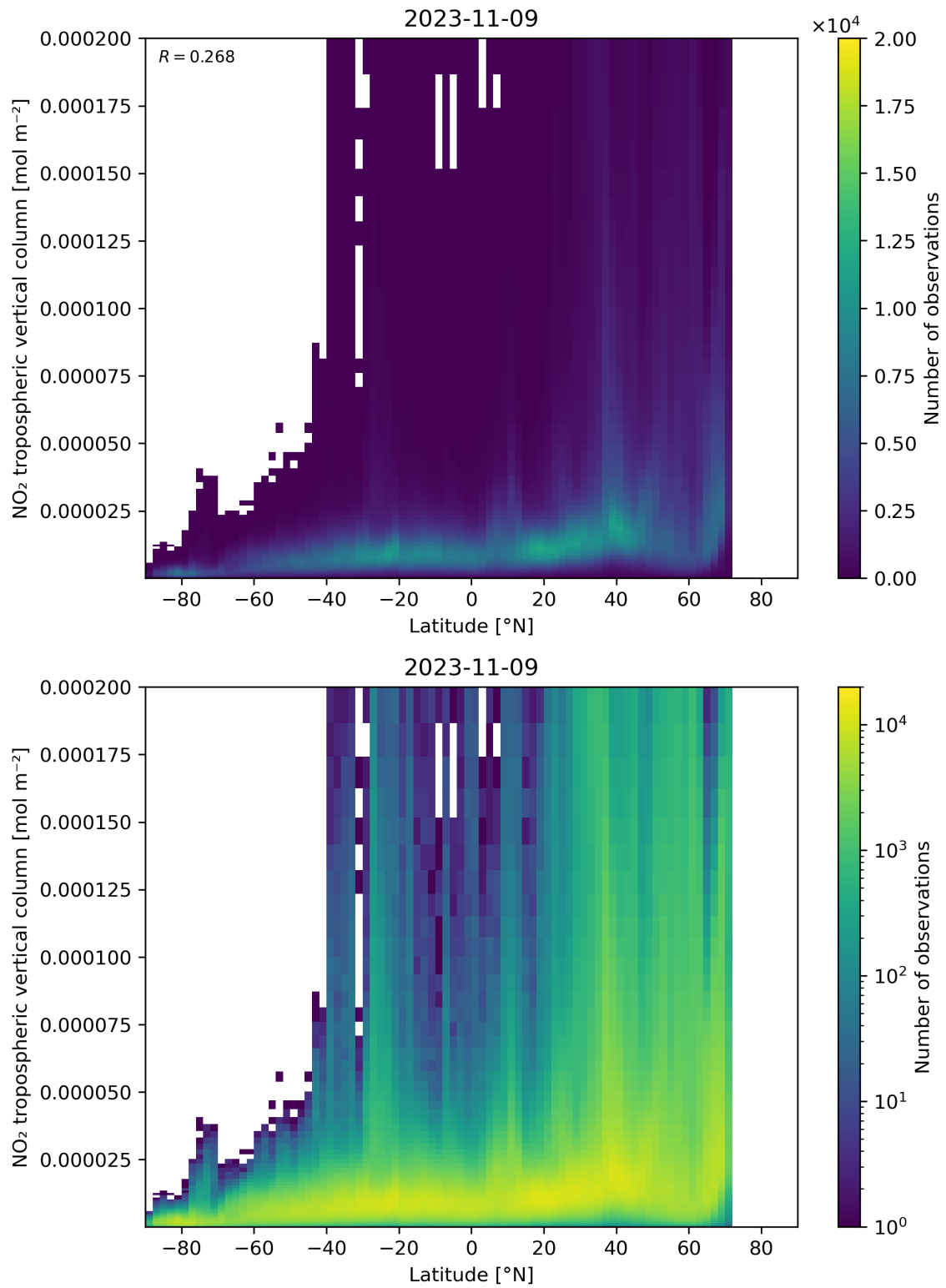
Figure 92: Scatter density plot of “Latitude” against “NO 2 tropospheric vertical column” for 2023-11-08 to 2023-11-10.
