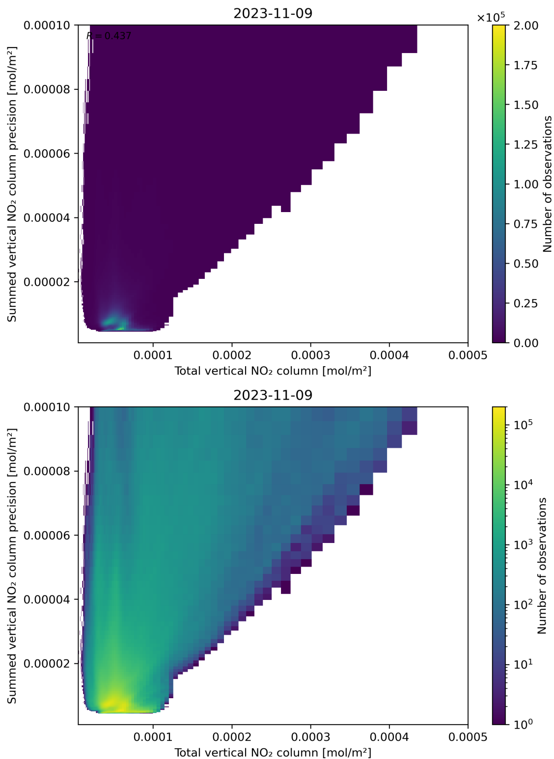
Figure 113: Scatter density plot of “Total vertical NO 2 column” against “Summed vertical NO 2 column precision” for 2023-11-08 to 2023-11-10.
