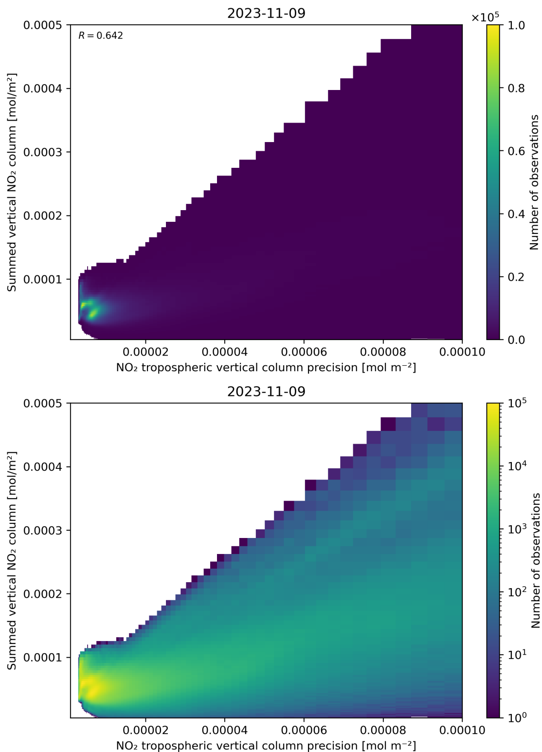
Figure 136: Scatter density plot of “NO 2 tropospheric vertical column precision” against “Summed vertical NO 2 column” for 2023-11-08 to 2023-11-10.
