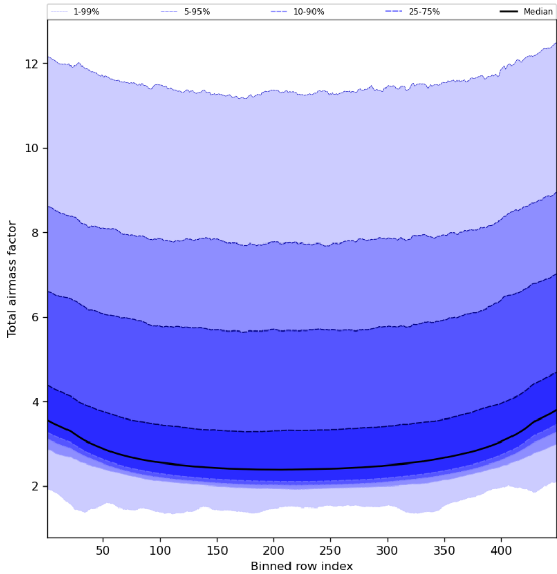
Figure 49: Along track statistics of “Total airmass factor” for 2023-11-08 to 2023-11-10
