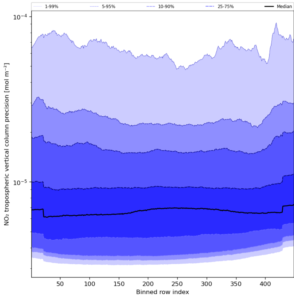
Figure 47: Along track statistics of “NO 2 tropospheric vertical column precision” for 2023-11-08 to 2023-11-10
