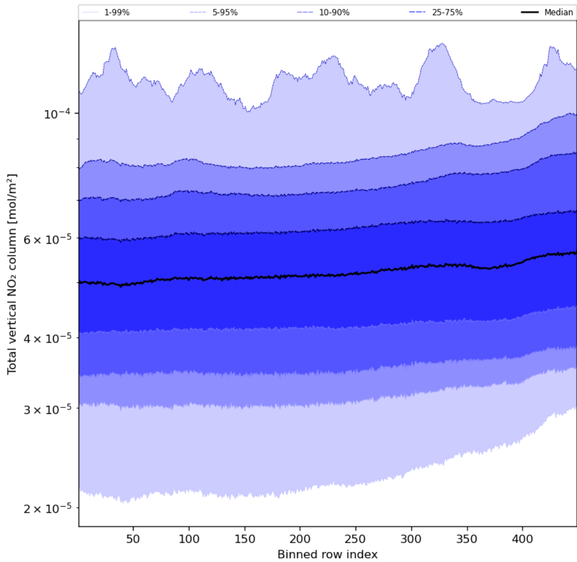
Figure 55: Along track statistics of “Total vertical NO 2 column” for 2023-11-08 to 2023-11-10
