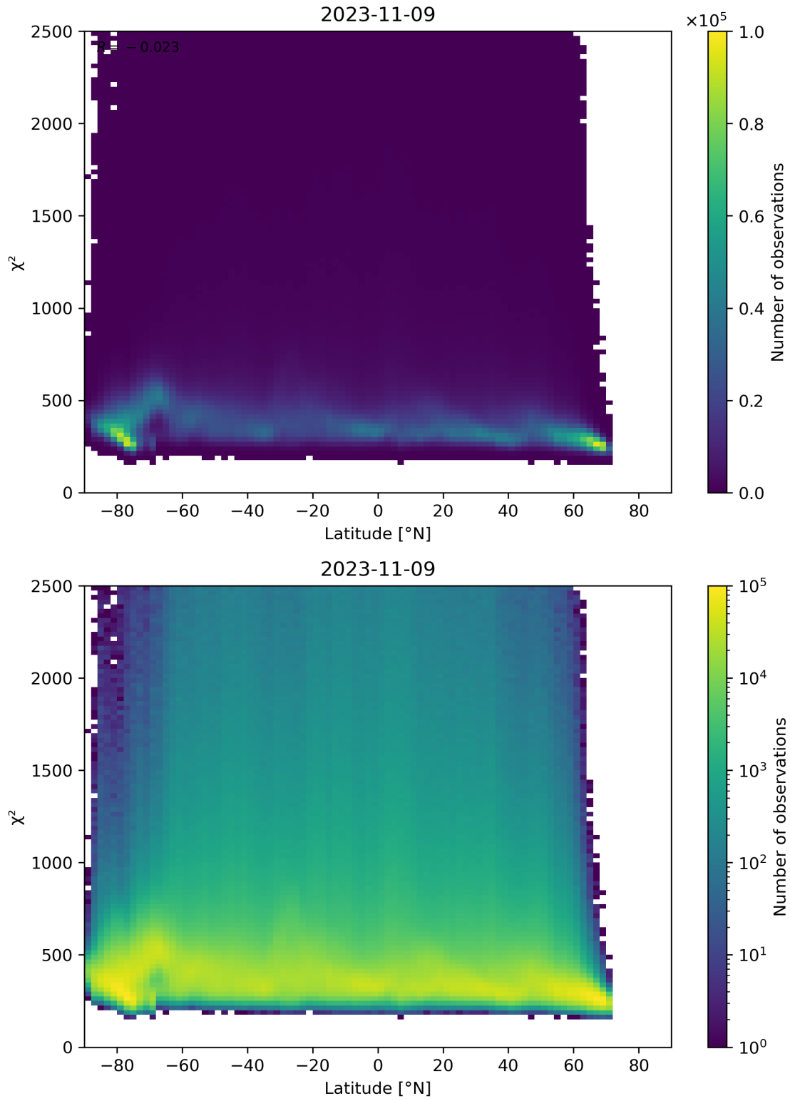
Figure 86: Scatter density plot of “Latitude” against “ \chi^2 ” for 2023-11-08 to 2023-11-10.
