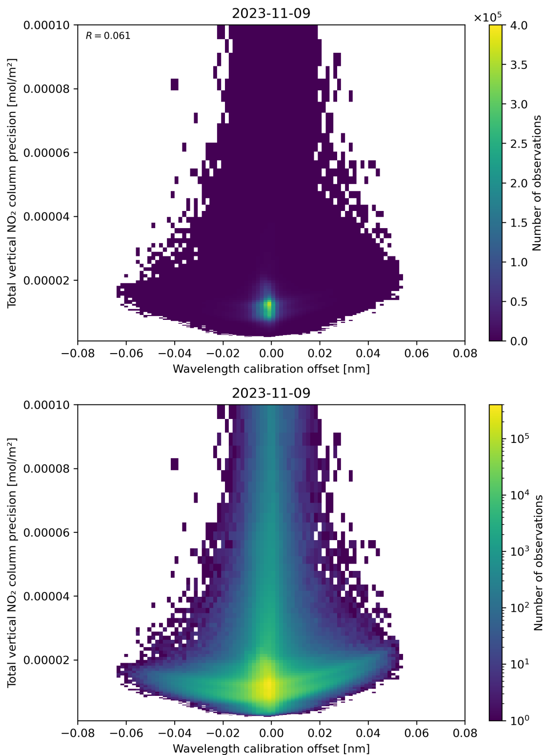
Figure 180: Scatter density plot of “Wavelength calibration offset” against “Total vertical NO 2 column precision” for 2023-11-08 to 2023-11-10.
