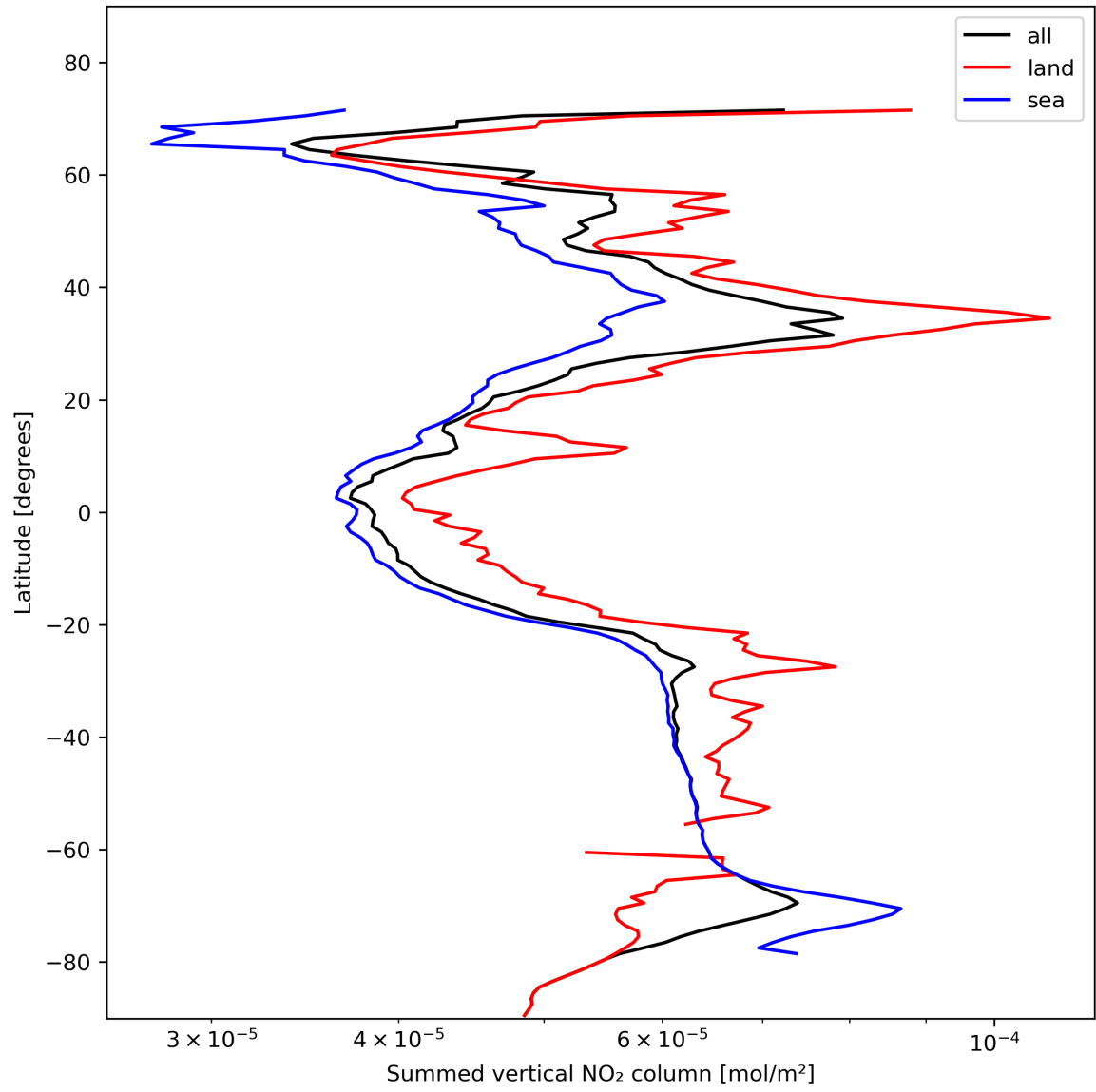
Figure 23: Zonal average of “Summed vertical NO 2 column” for 2023-11-08 to 2023-11-10.
