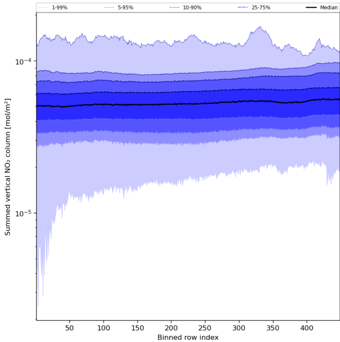
Figure 57: Along track statistics of “Summed vertical NO 2 column” for 2023-11-08 to 2023-11-10
