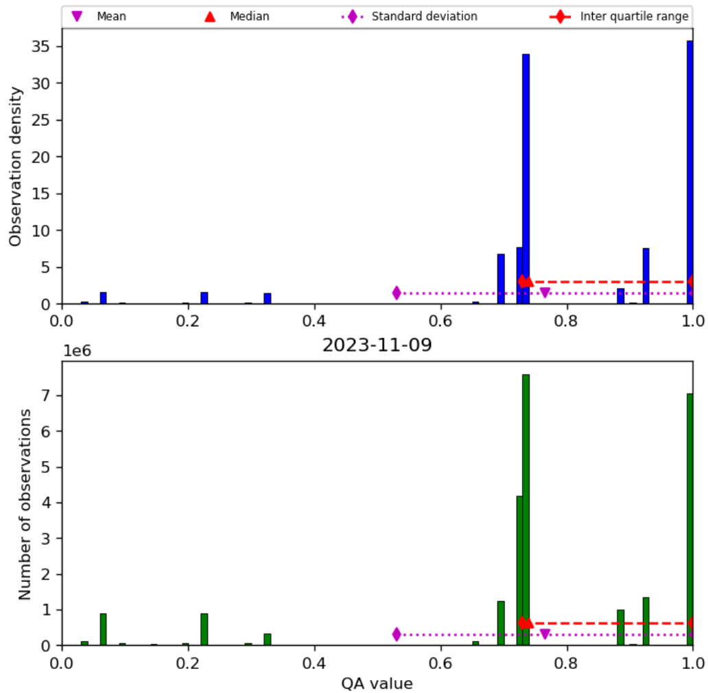
Figure 28: Histogram of “QA value” for 2023-11-08 to 2023-11-10
