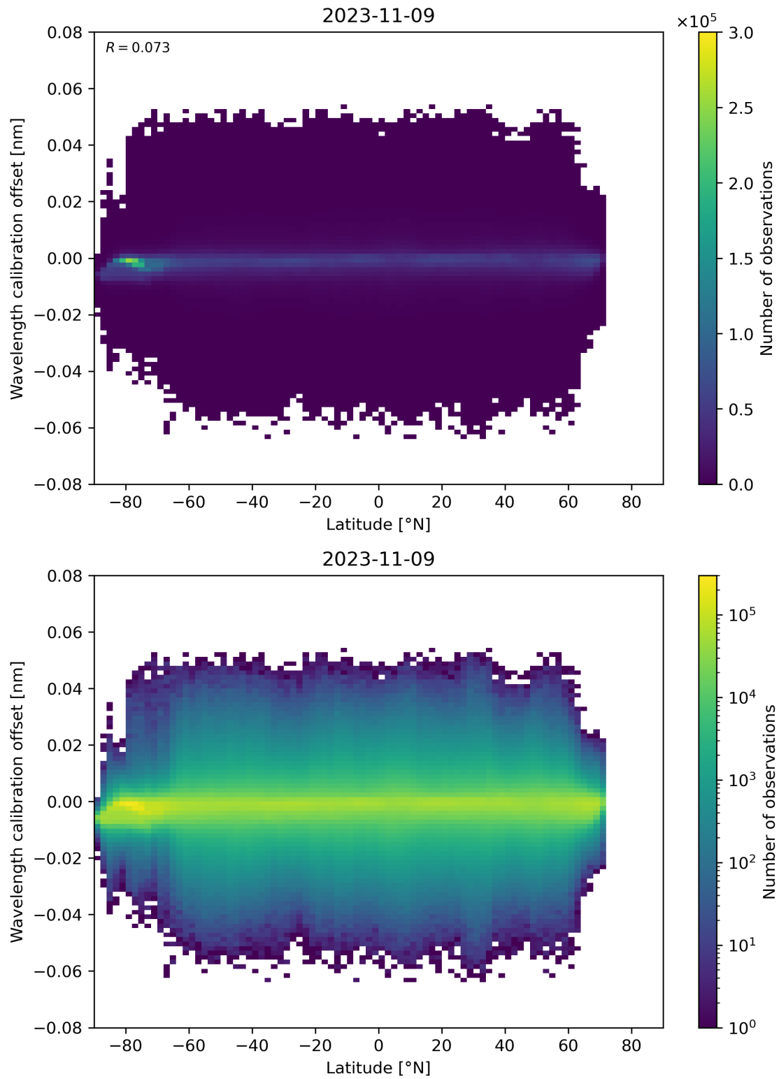
Figure 95: Scatter density plot of “Latitude” against “Wavelength calibration offset” for 2023-11-08 to 2023-11-10.
