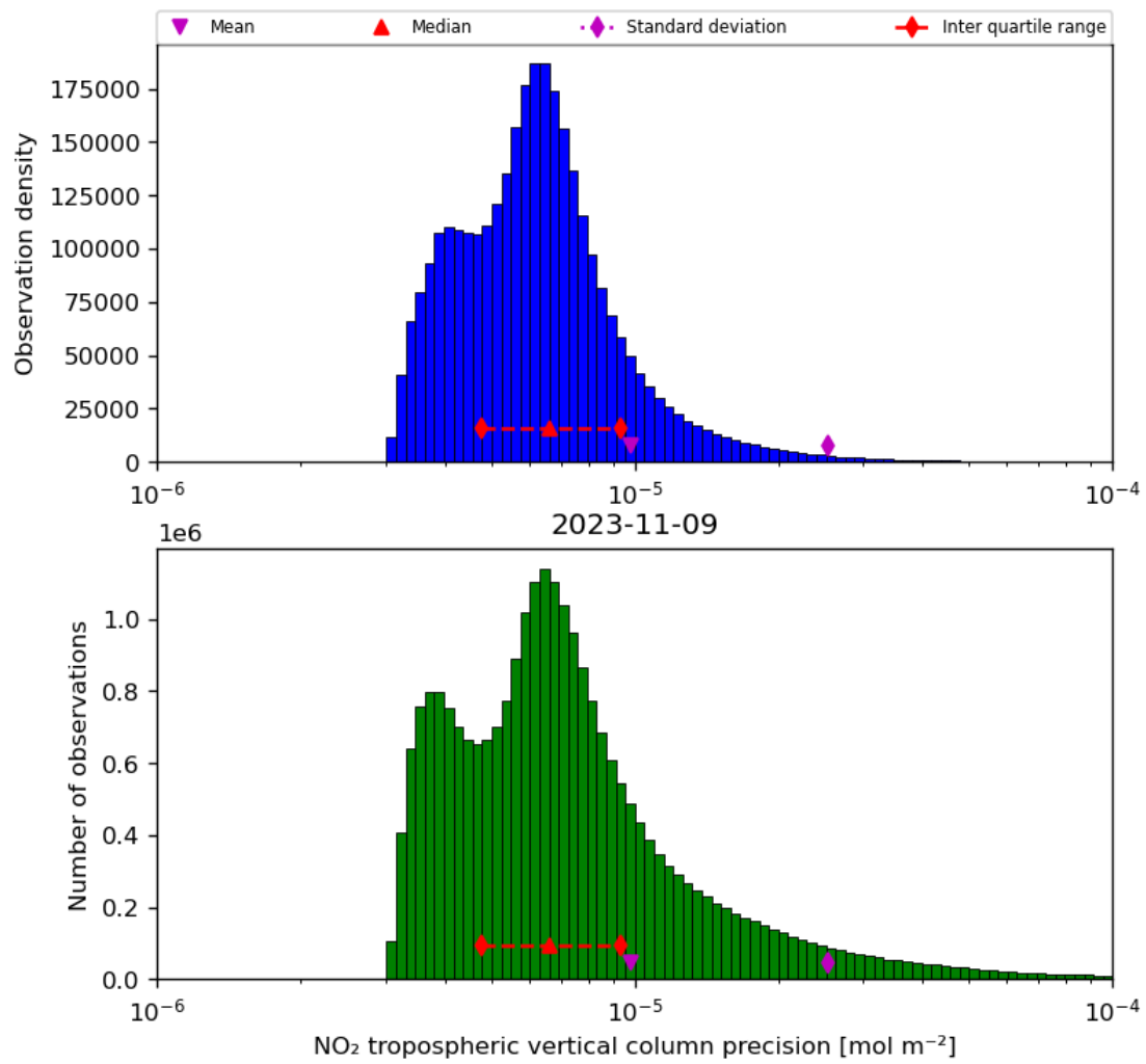
Figure 30: Histogram of “NO 2 tropospheric vertical column precision” for 2023-11-08 to 2023-11-10
