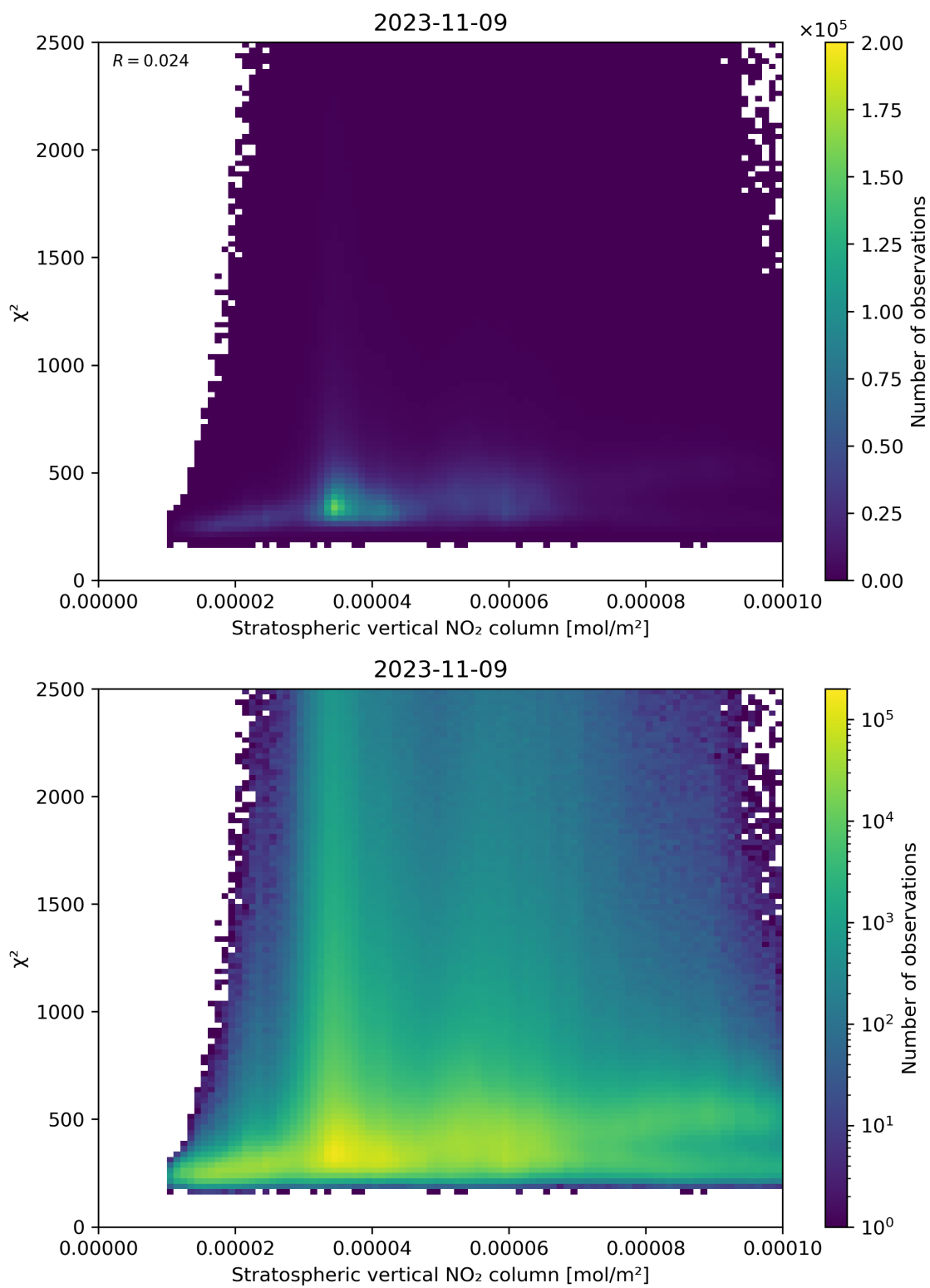
Figure 97: Scatter density plot of “Stratospheric vertical NO 2 column” against “ \chi^2 ” for 2023-11-08 to 2023-11-10.
