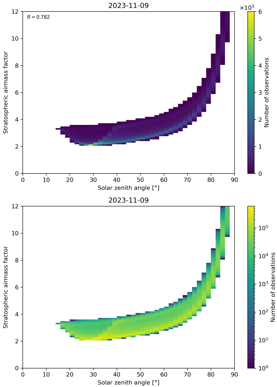
Figure 145: Scatter density plot of “Solar zenith angle” against “Stratospheric airmass factor” for 2023-11-08 to 2023-11-10.
