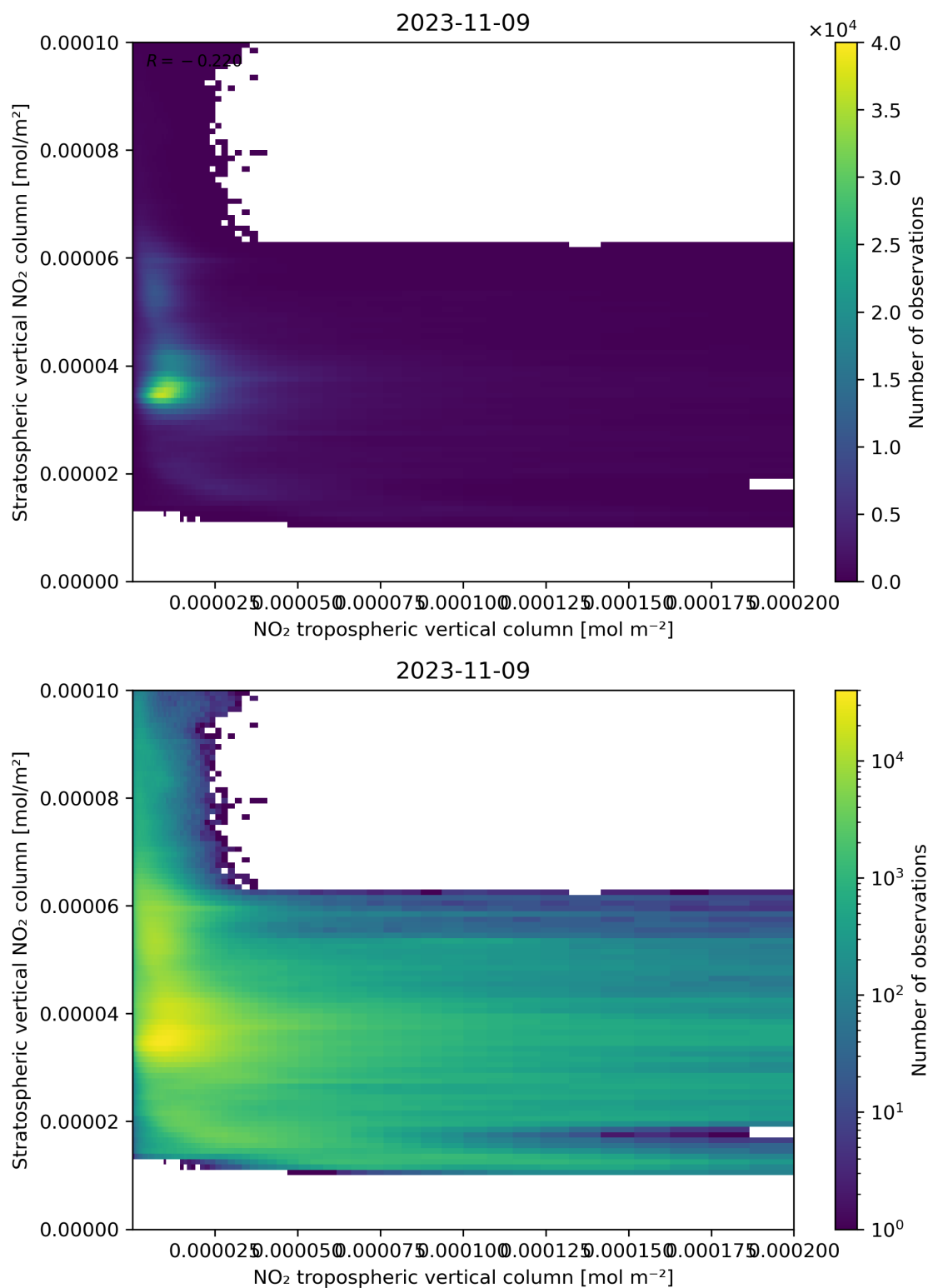
Figure 125: Scatter density plot of “NO 2 tropospheric vertical column” against “Stratospheric vertical NO 2 column” for 2023-11-08 to 2023-11-10.
