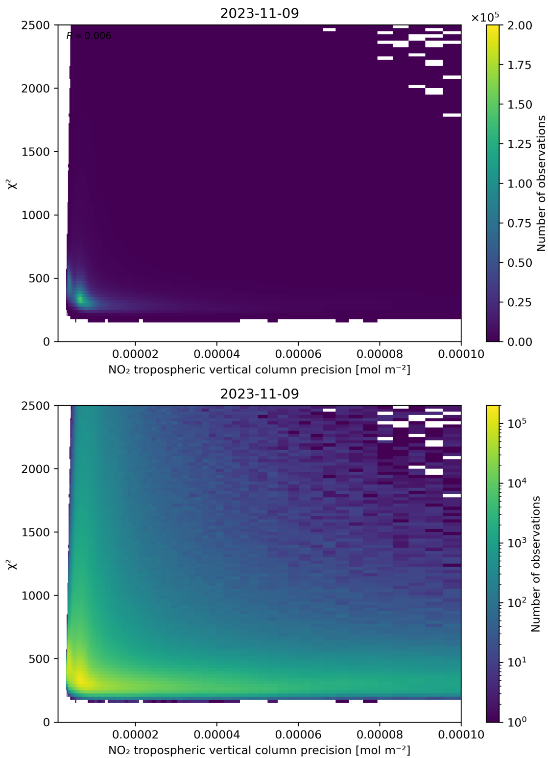
Figure 134: Scatter density plot of “NO 2 tropospheric vertical column precision” against “ \chi^2 ” for 2023-11-08 to 2023-11-10.
