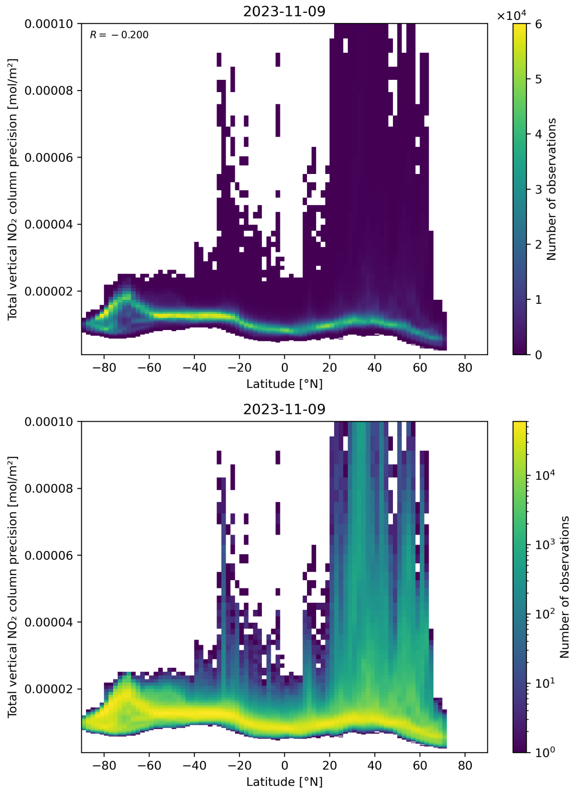
Figure 91: Scatter density plot of “Latitude” against “Total vertical NO 2 column precision” for 2023-11-08 to 2023-11-10.
