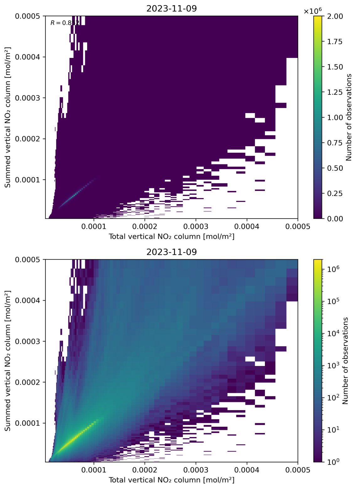
Figure 112: Scatter density plot of “Total vertical NO 2 column” against “Summed vertical NO 2 column” for 2023-11-08 to 2023-11-10.
