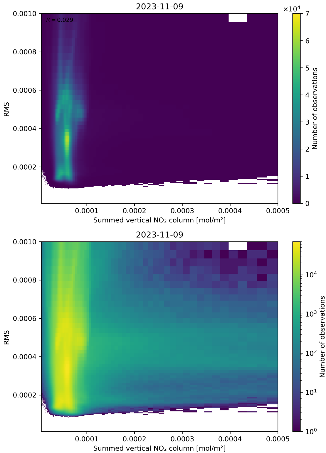
Figure 109: Scatter density plot of “Summed vertical NO 2 column” against “RMS” for 2023-11-08 to 2023-11-10.
