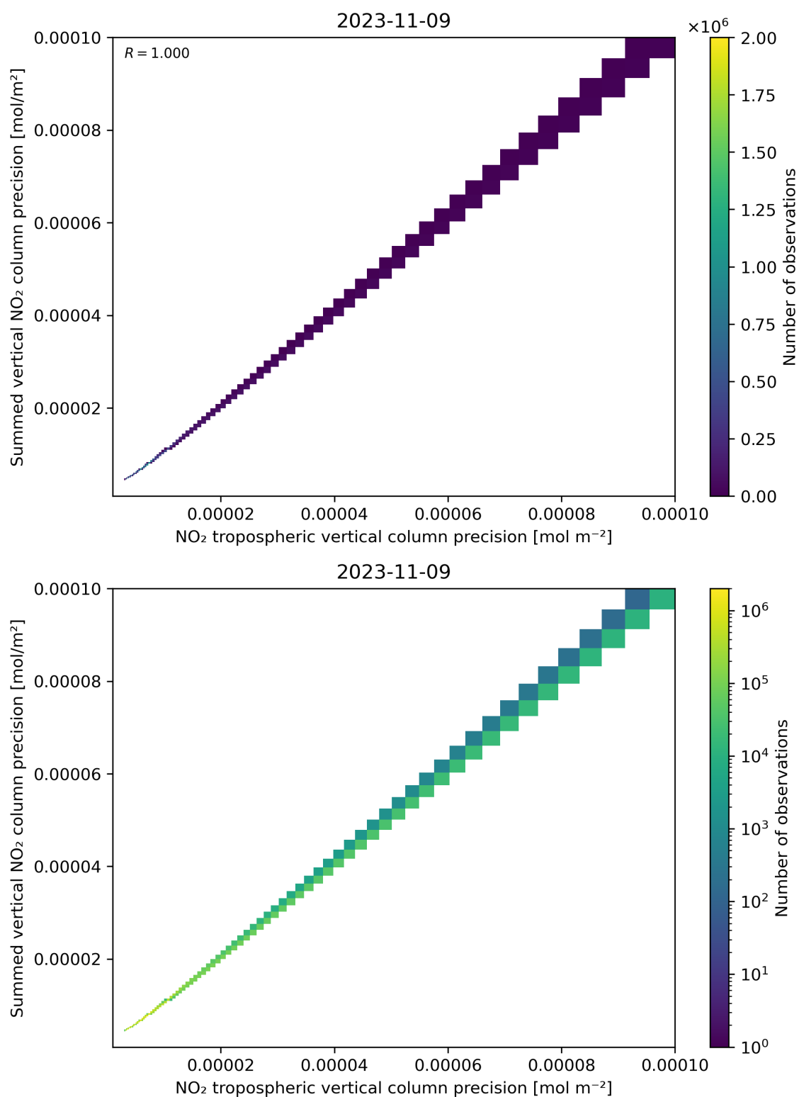
Figure 137: Scatter density plot of “NO 2 tropospheric vertical column precision” against “Summed vertical NO 2 column precision” for 2023-11-08 to 2023-11-10.
