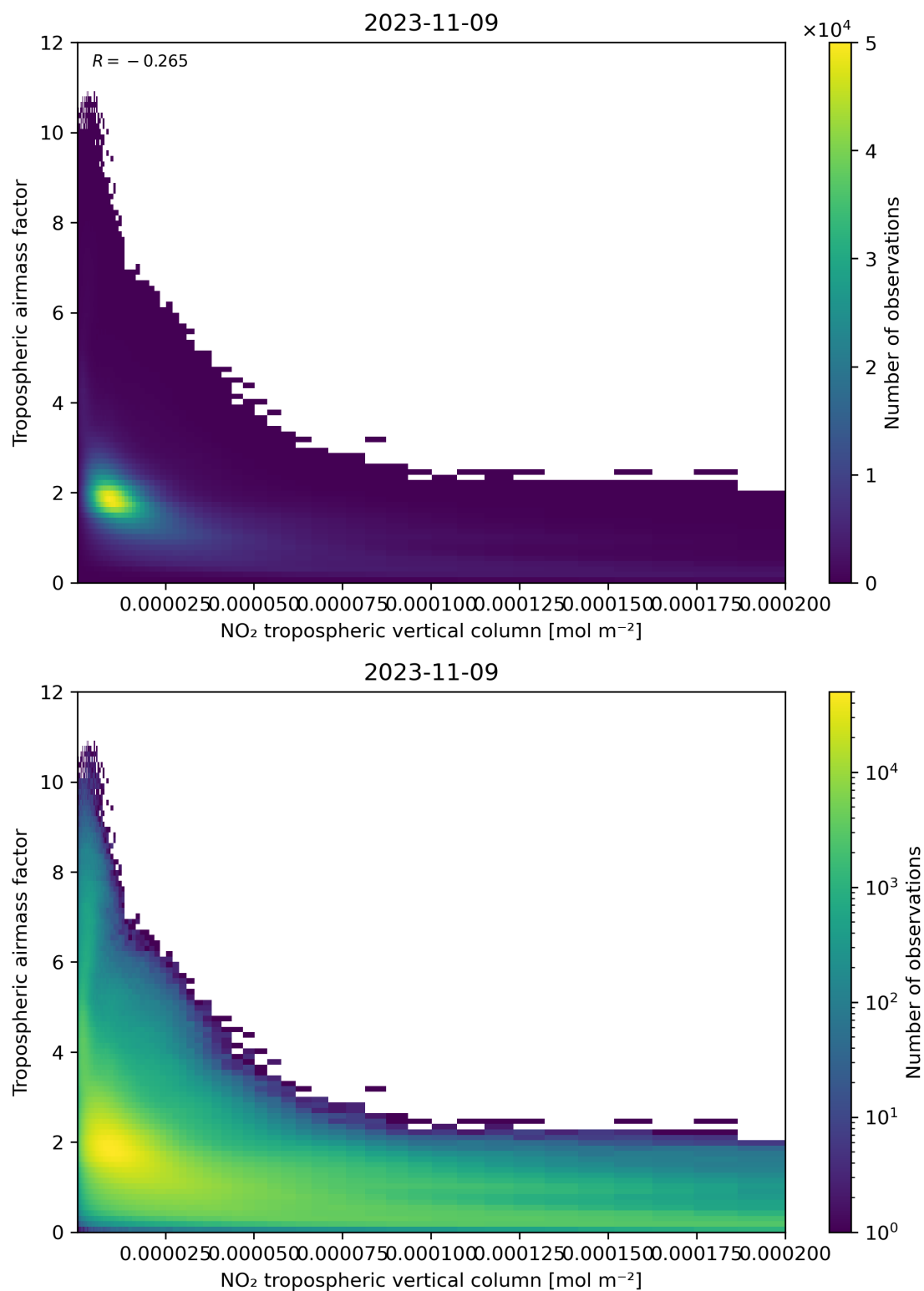
Figure 123: Scatter density plot of “NO 2 tropospheric vertical column” against “Tropospheric airmass factor” for 2023-11-08 to 2023-11-10.
