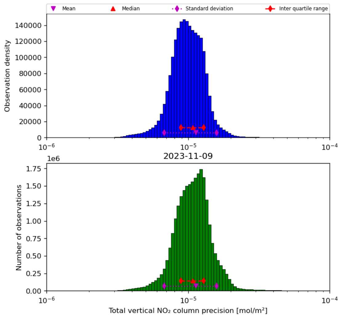
Figure 39: Histogram of “Total vertical NO 2 column precision” for 2023-11-08 to 2023-11-10
