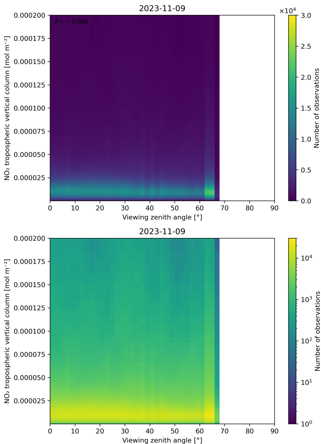
Figure 169: Scatter density plot of “Viewing zenith angle” against “NO 2 tropospheric vertical column” for 2023-11-08 to 2023-11-10.
