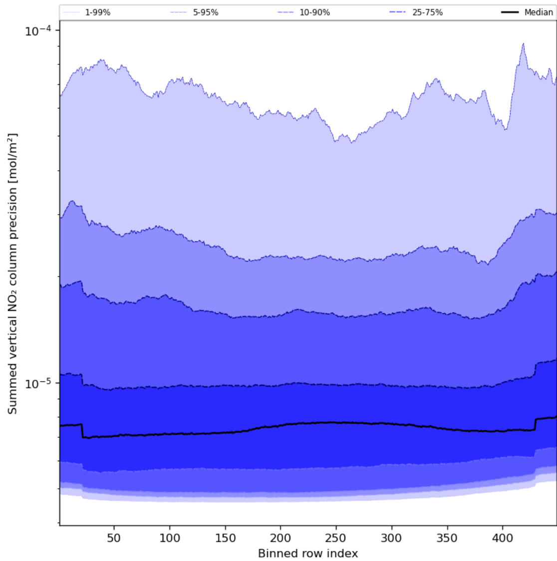
Figure 58: Along track statistics of “Summed vertical NO 2 column precision” for 2023-11-08 to 2023-11-10
