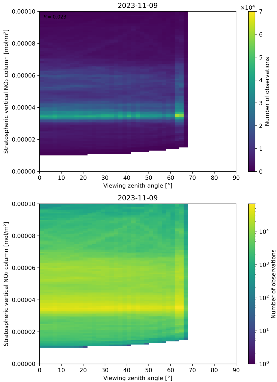
Figure 164: Scatter density plot of “Viewing zenith angle” against “Stratospheric vertical NO 2 column” for 2023-11-08 to 2023-11-10.
