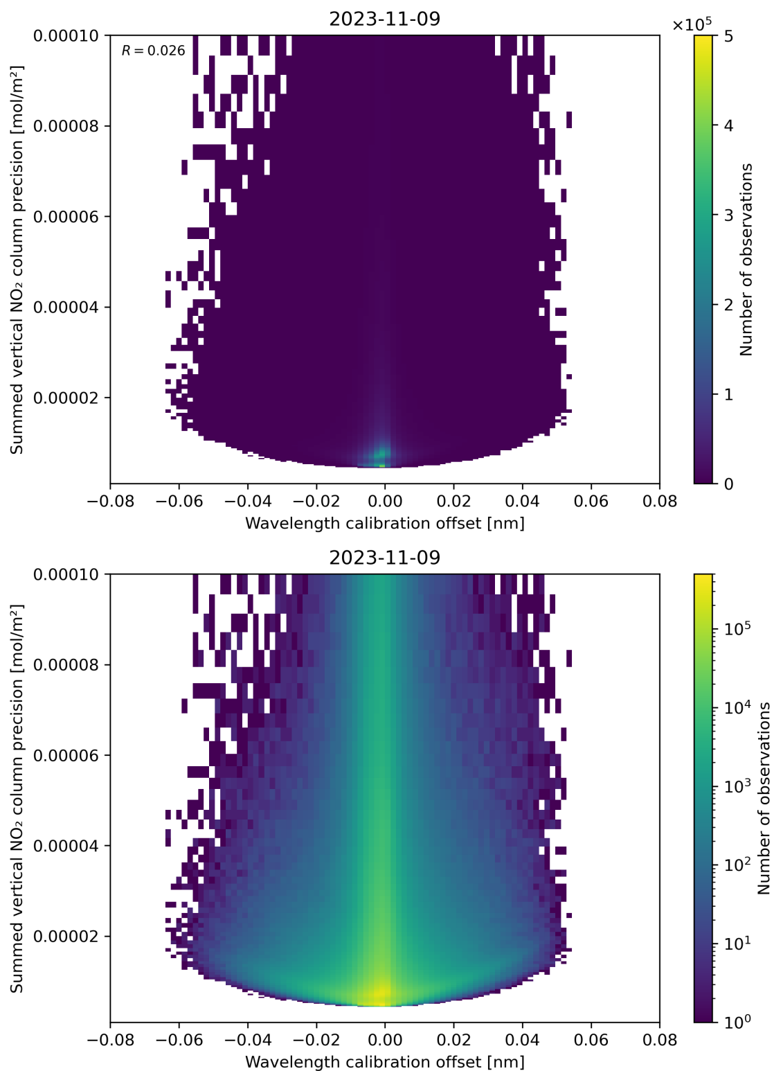
Figure 178: Scatter density plot of “Wavelength calibration offset” against “Summed vertical NO 2 column precision” for 2023-11-08 to 2023-11-10.
