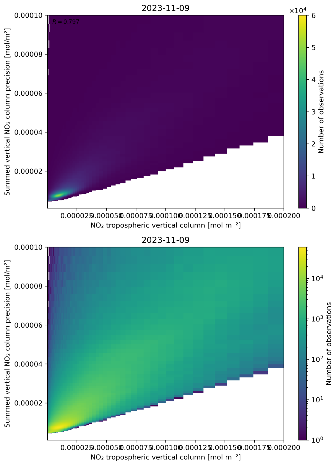
Figure 127: Scatter density plot of “NO 2 tropospheric vertical column” against “Summed vertical NO 2 column precision” for 2023-11-08 to 2023-11-10.
