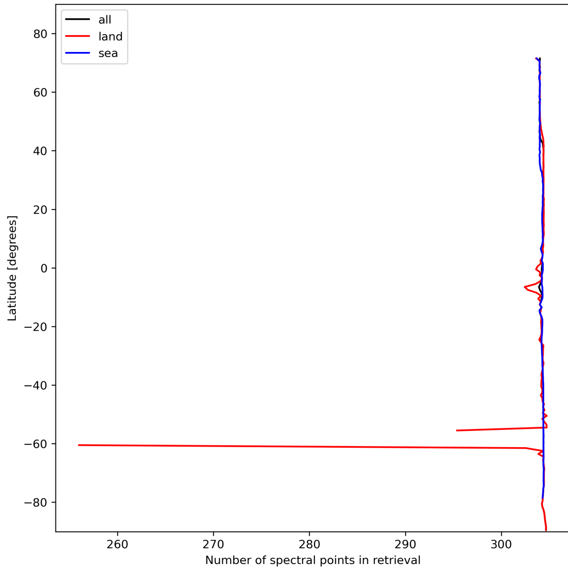
Figure 16: Zonal average of “Number of spectral points in retrieval” for 2023-11-08 to 2023-11-10.
