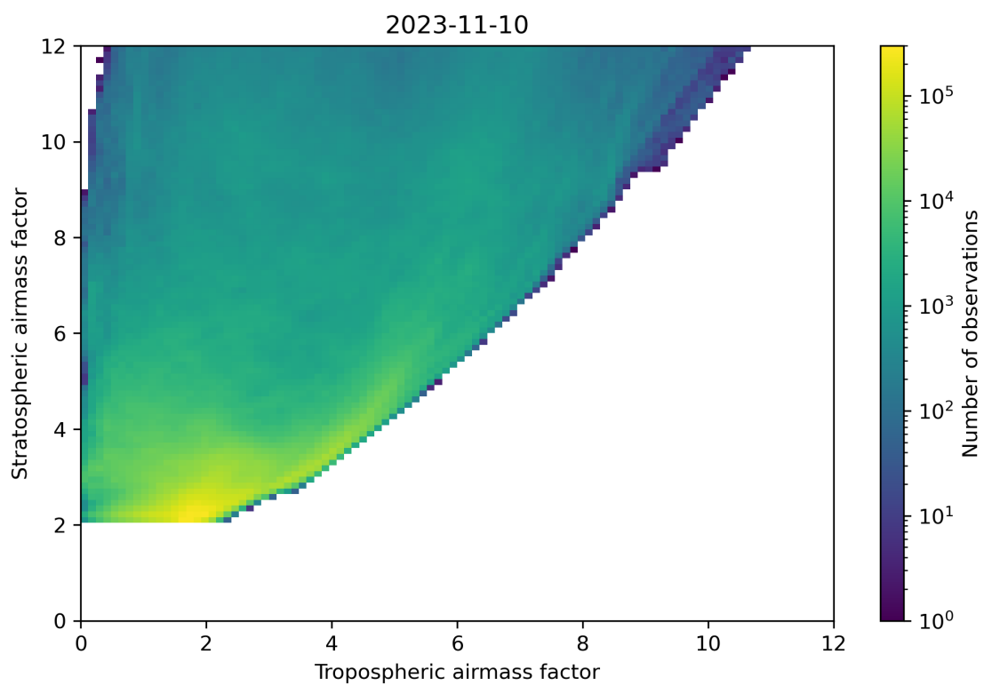
Figure 71: Scatter density plot of “Tropospheric airmass factor” against “Stratospheric airmass factor” for 2023-11-09 to 2023-11-11.
