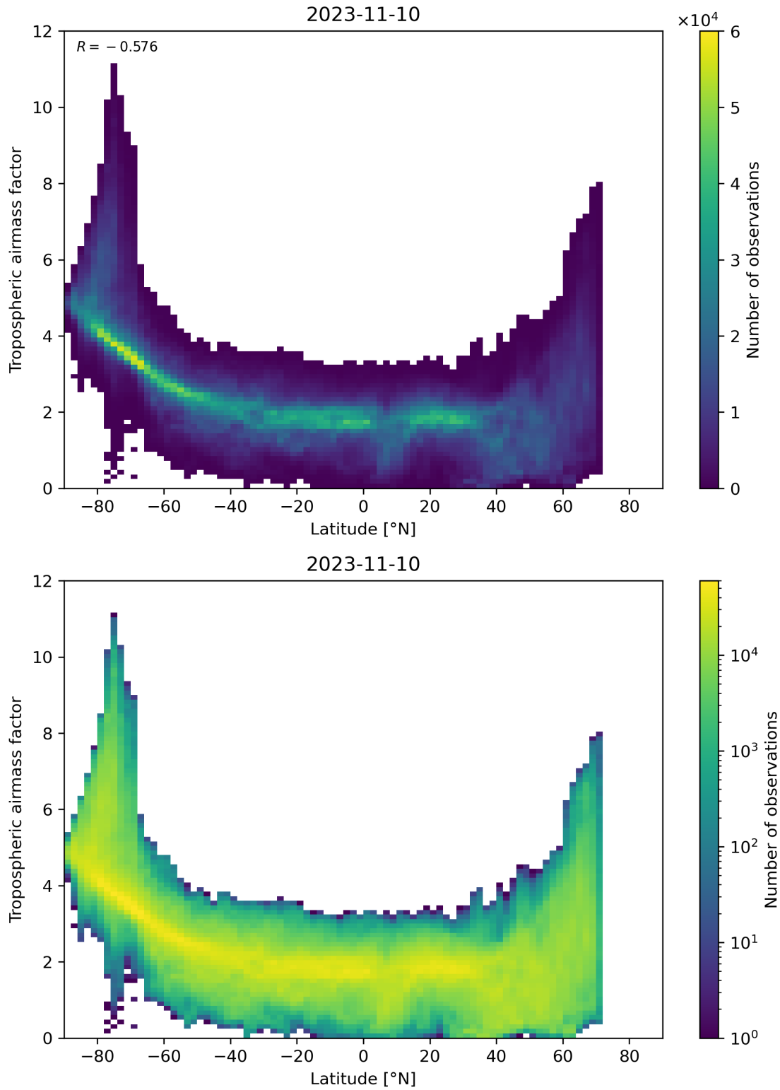
Figure 85: Scatter density plot of “Latitude” against “Tropospheric airmass factor” for 2023-11-09 to 2023-11-11.
