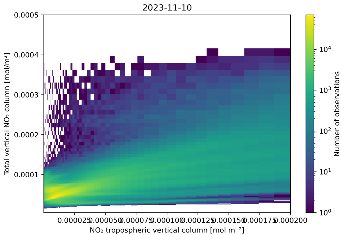
Figure 128: Scatter density plot of “NO 2 tropospheric vertical column” against “Total vertical NO 2 column” for 2023-11-09 to 2023-11-11.
