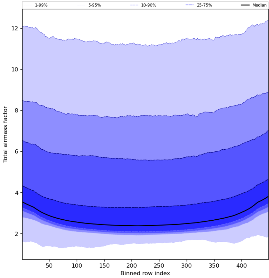
Figure 49: Along track statistics of “Total airmass factor” for 2023-11-09 to 2023-11-11
