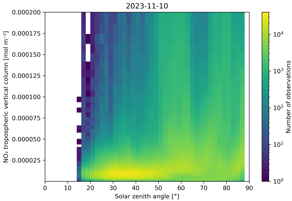
Figure 155: Scatter density plot of “Solar zenith angle” against “NO 2 tropospheric vertical column” for 2023-11-09 to 2023-11-11.
