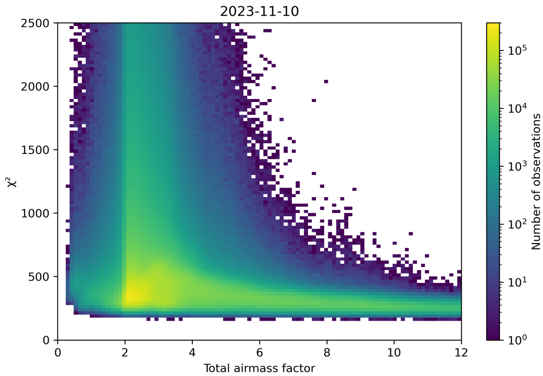
Figure 63: Scatter density plot of “Total airmass factor” against “ \chi^2 ” for 2023-11-09 to 2023-11-11.
