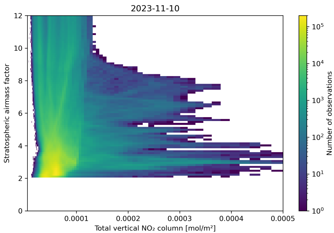
Figure 110: Scatter density plot of “Total vertical NO 2 column” against “Stratospheric airmass factor” for 2023-11-09 to 2023-11-11.
