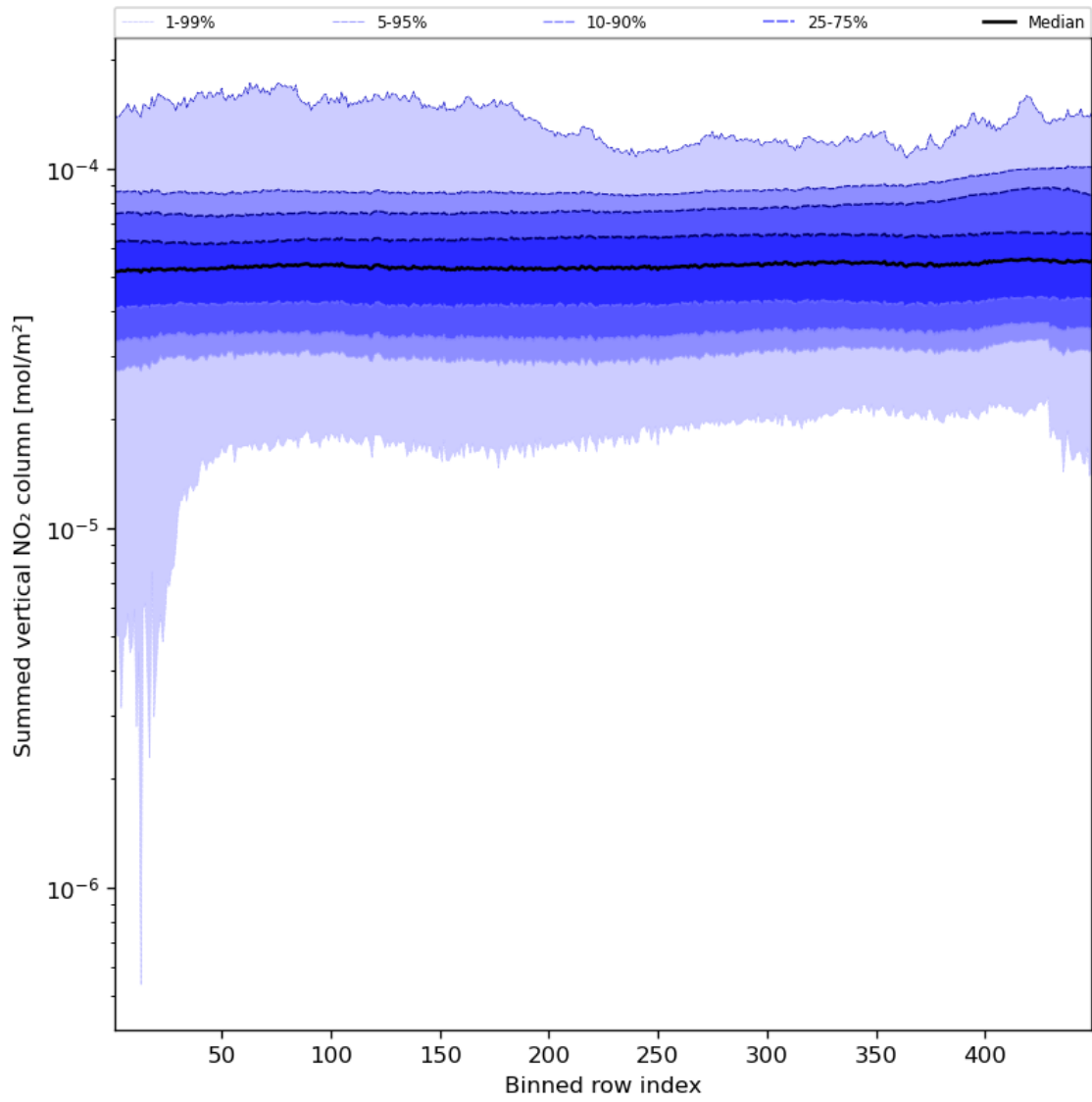
Figure 57: Along track statistics of “Summed vertical NO 2 column” for 2023-11-09 to 2023-11-11
