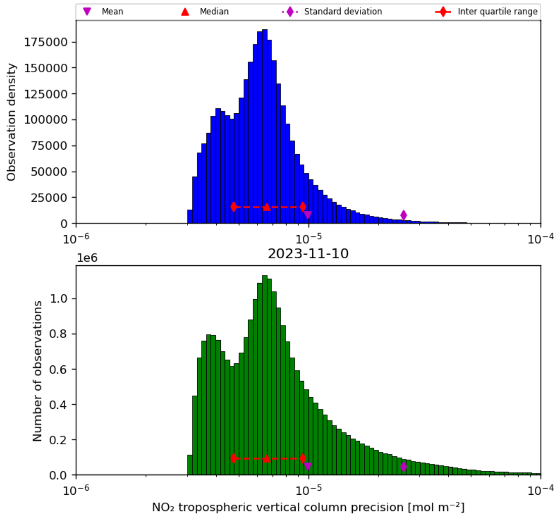
Figure 30: Histogram of “NO 2 tropospheric vertical column precision” for 2023-11-09 to 2023-11-11
