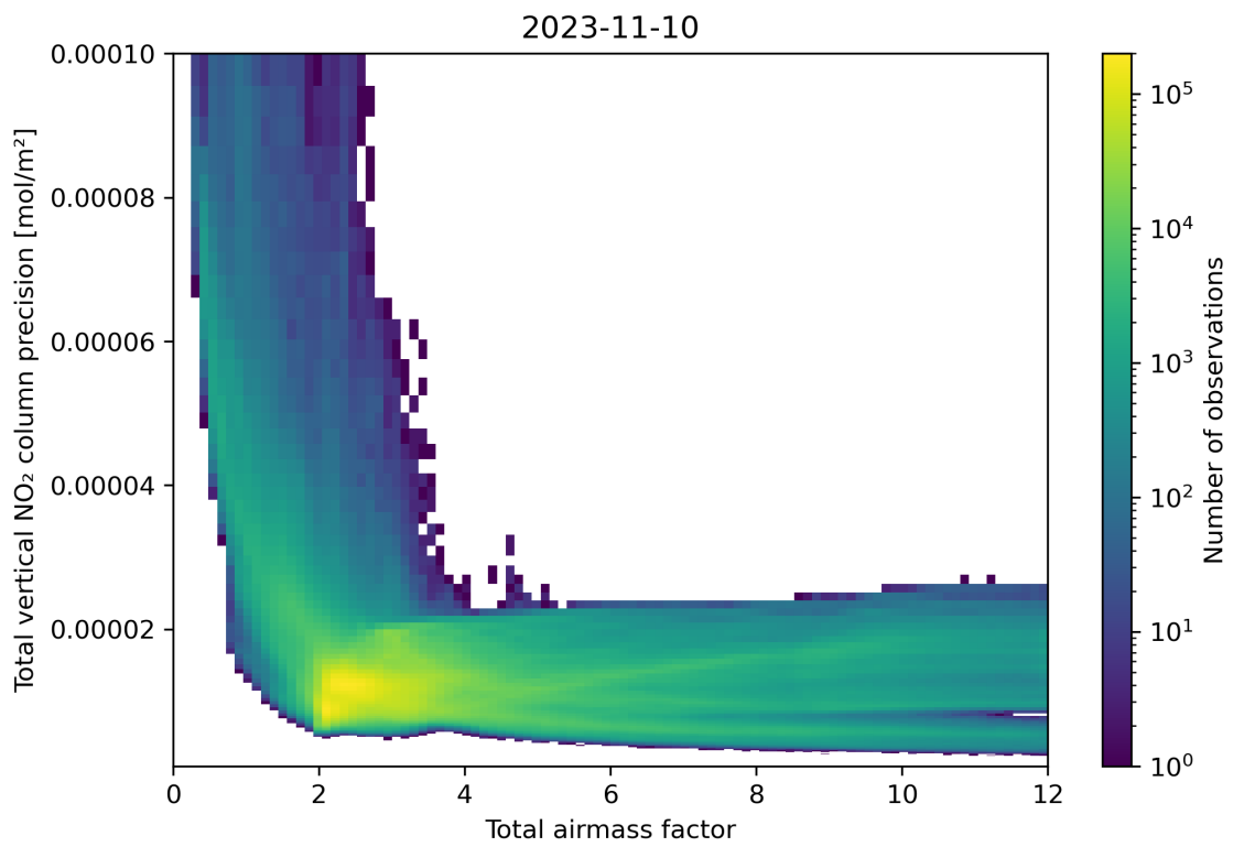
Figure 68: Scatter density plot of “Total airmass factor” against “Total vertical NO 2 column precision” for 2023-11-09 to 2023-11-11.
