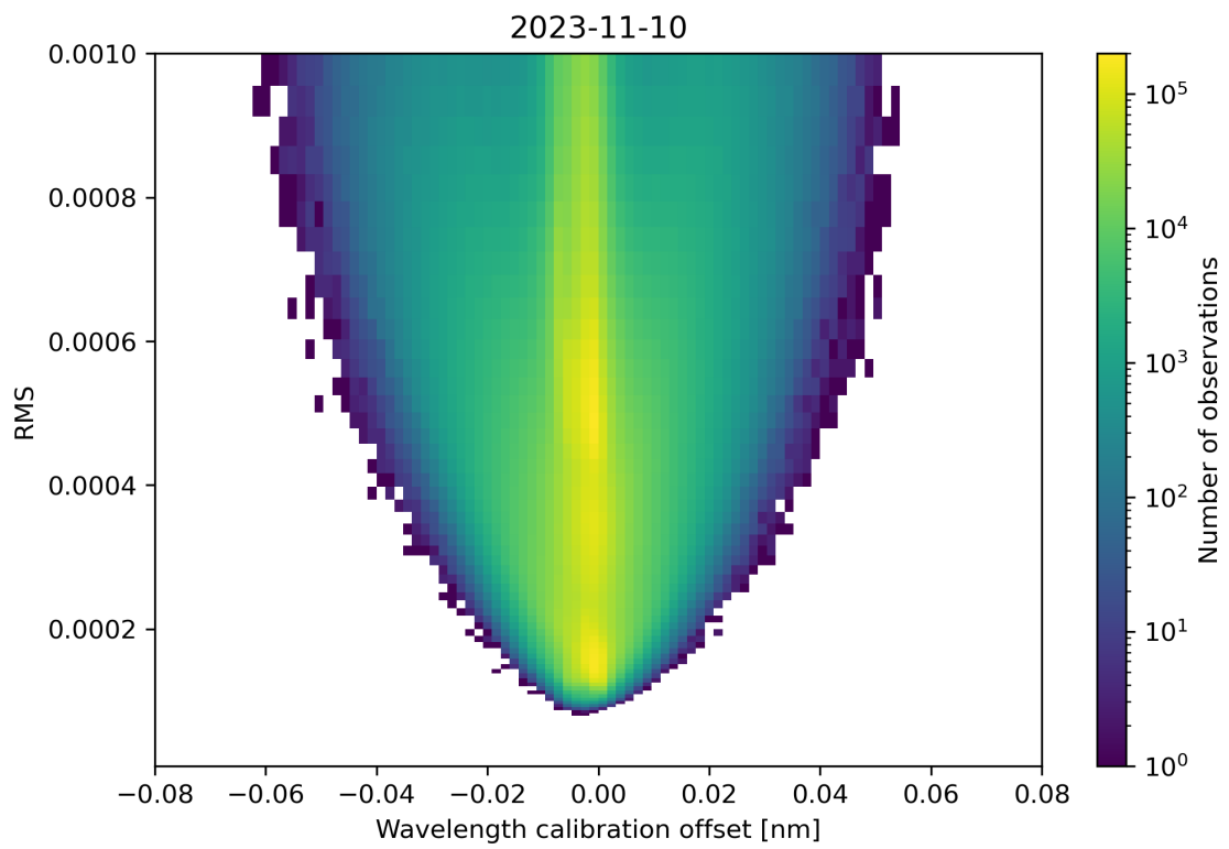
Figure 181: Scatter density plot of “Wavelength calibration offset” against “RMS” for 2023-11-09 to 2023-11-11.
