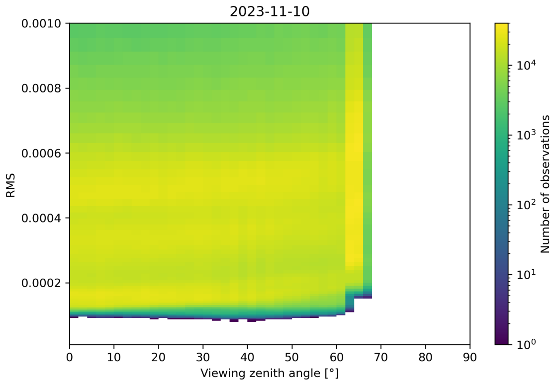
Figure 171: Scatter density plot of “Viewing zenith angle” against “RMS” for 2023-11-09 to 2023-11-11.
