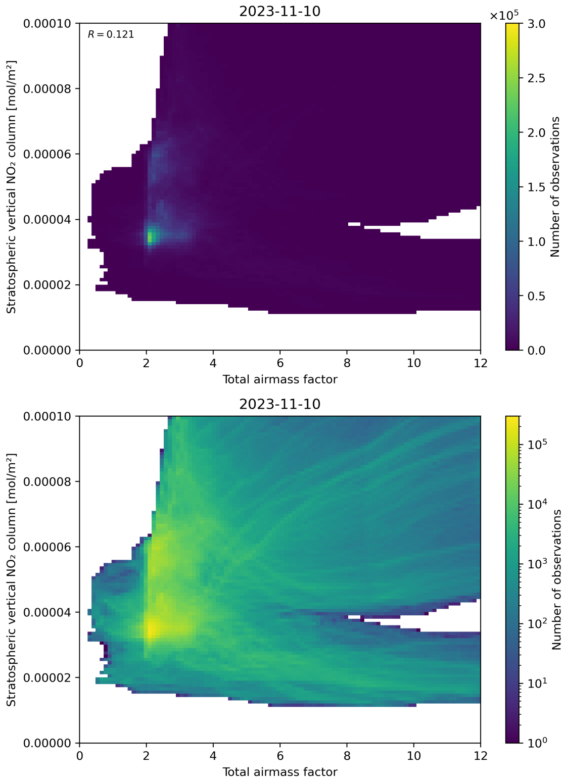
Figure 64: Scatter density plot of “Total airmass factor” against “Stratospheric vertical NO 2 column” for 2023-11-09 to 2023-11-11.
