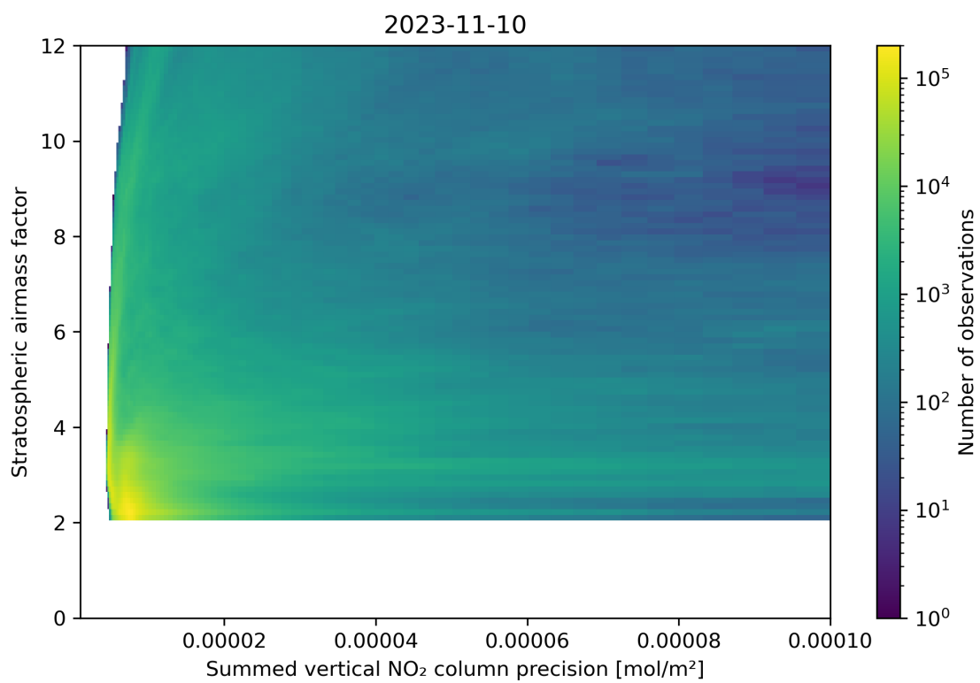
Figure 106: Scatter density plot of “Summed vertical NO 2 column precision” against “Stratospheric airmass factor” for 2023-11-09 to 2023-11-11.
