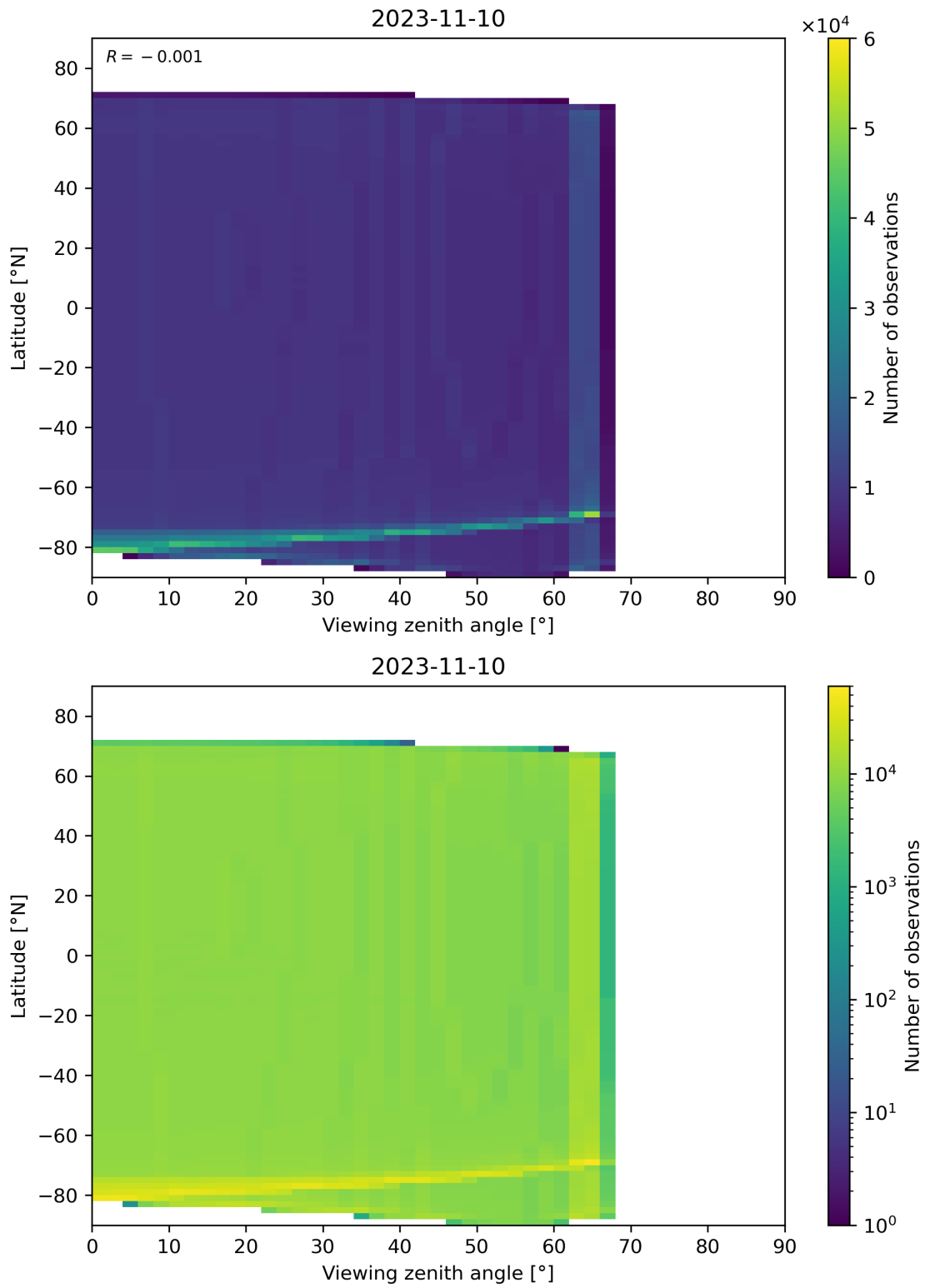
Figure 163: Scatter density plot of “Viewing zenith angle” against “Latitude” for 2023-11-09 to 2023-11-11.
