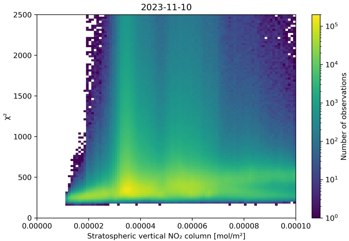
Figure 97: Scatter density plot of “Stratospheric vertical NO 2 column” against “ \chi^2 ” for 2023-11-09 to 2023-11-11.
