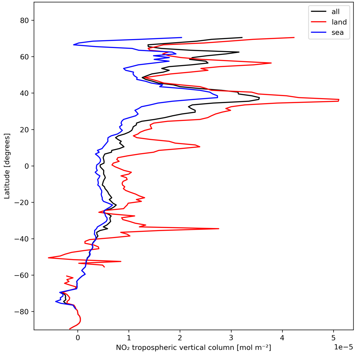
Figure 12: Zonal average of “NO 2 tropospheric vertical column” for 2023-11-09 to 2023-11-11.
