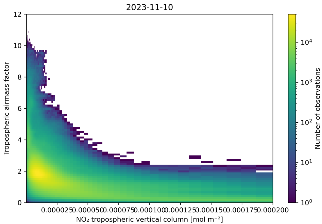
Figure 123: Scatter density plot of “NO 2 tropospheric vertical column” against “Tropospheric airmass factor” for 2023-11-09 to 2023-11-11.
