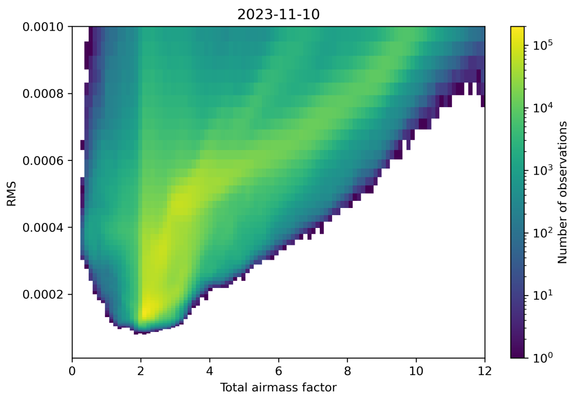
Figure 69: Scatter density plot of “Total airmass factor” against “RMS” for 2023-11-09 to 2023-11-11.
