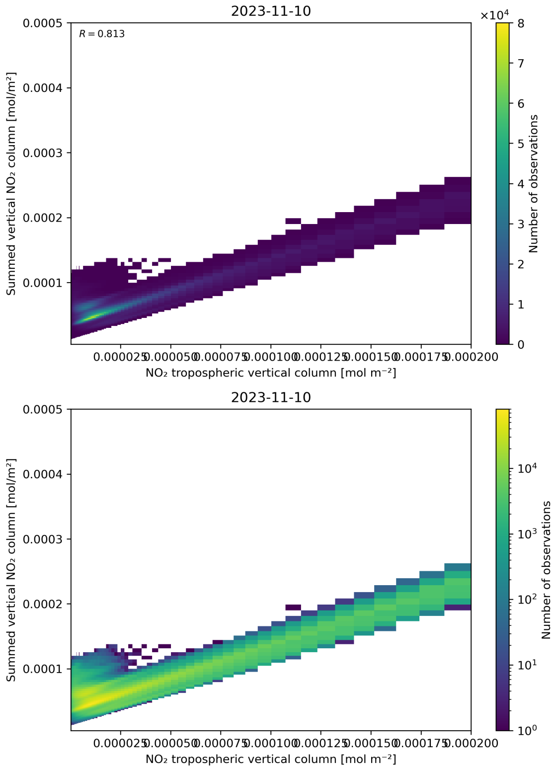
Figure 126: Scatter density plot of “NO 2 tropospheric vertical column” against “Summed vertical NO 2 column” for 2023-11-09 to 2023-11-11.
