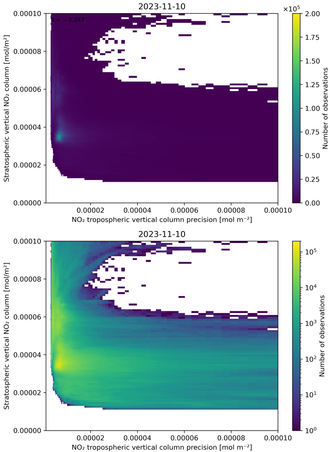
Figure 135: Scatter density plot of “NO 2 tropospheric vertical column precision” against “Stratospheric vertical NO 2 column” for 2023-11-09 to 2023-11-11.
