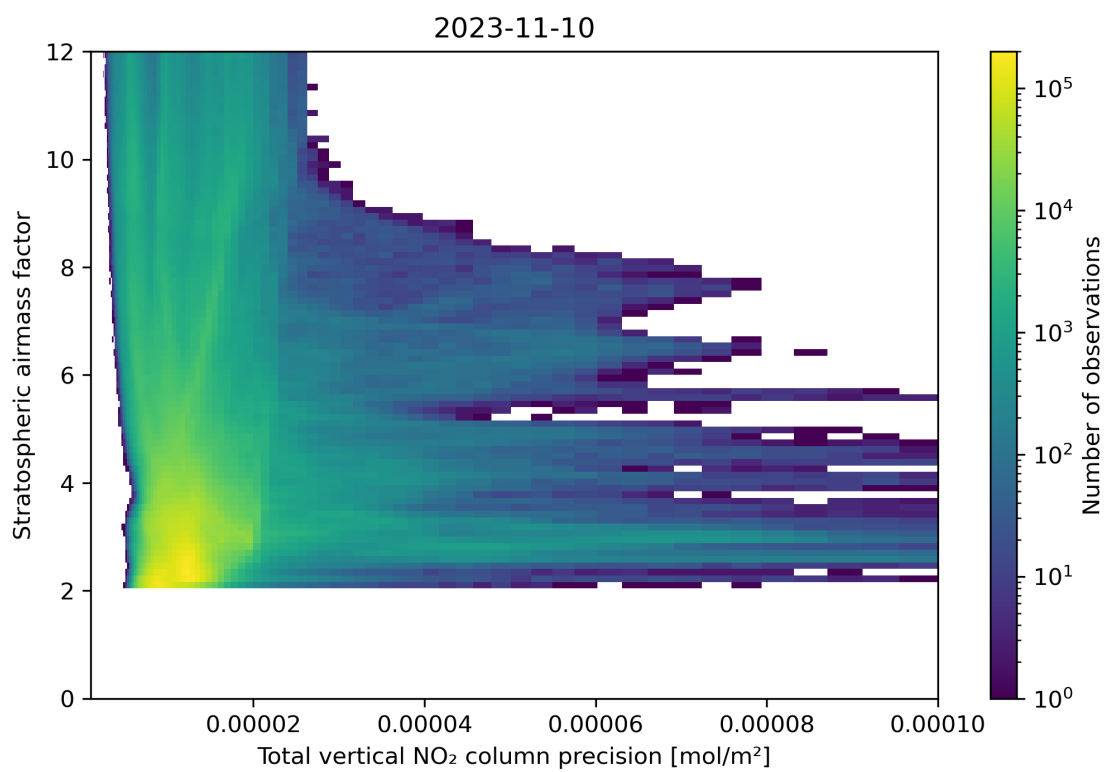
Figure 115: Scatter density plot of “Total vertical NO 2 column precision” against “Stratospheric airmass factor” for 2023-11-09 to 2023-11-11.
