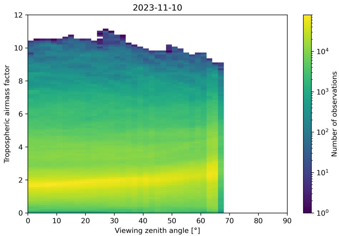
Figure 161: Scatter density plot of “Viewing zenith angle” against “Tropospheric airmass factor” for 2023-11-09 to 2023-11-11.
