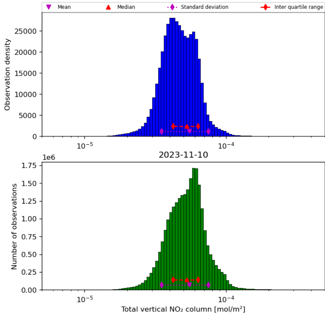
Figure 38: Histogram of “Total vertical NO 2 column” for 2023-11-09 to 2023-11-11
