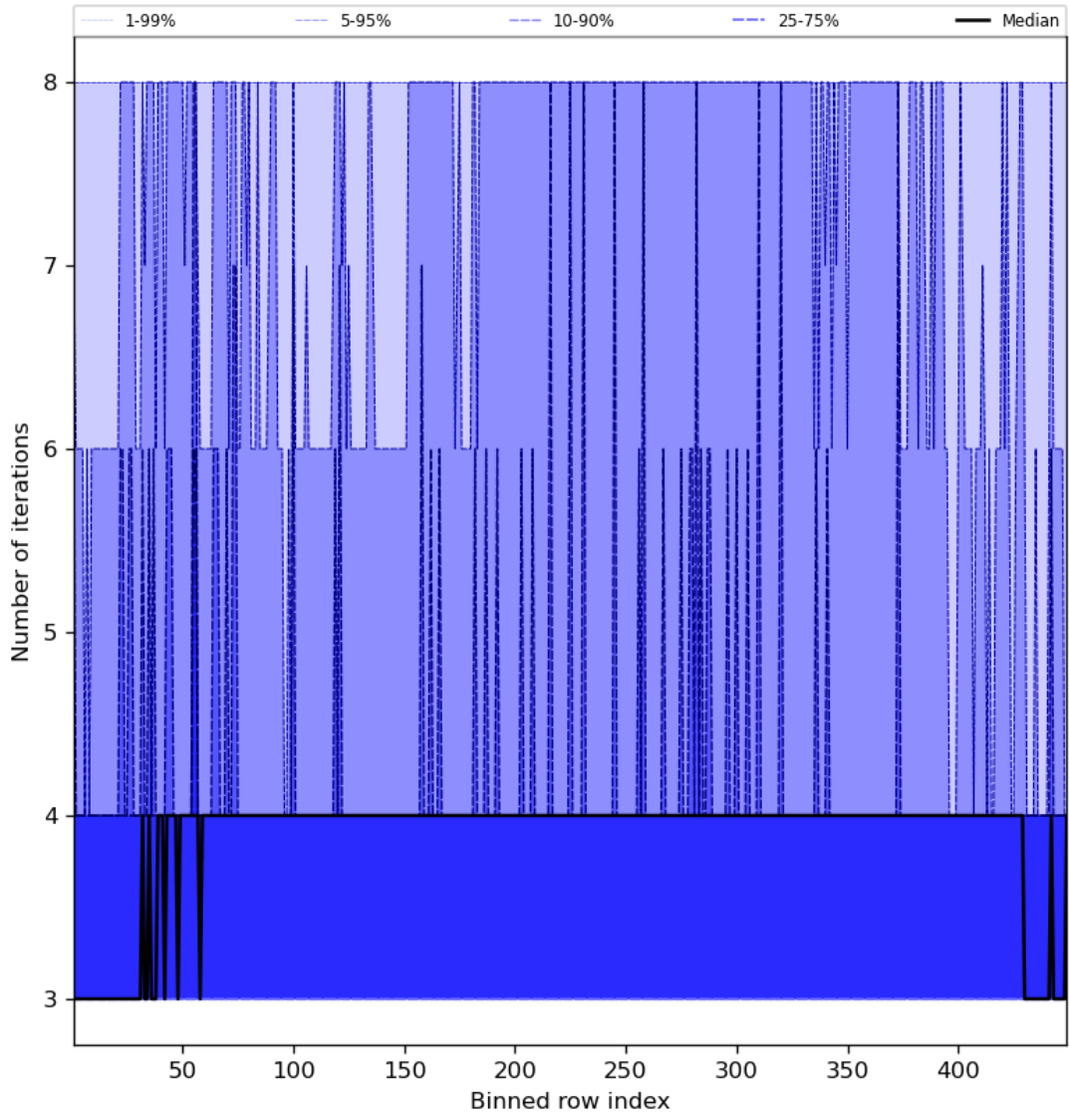
Figure 51: Along track statistics of “Number of iterations” for 2023-11-09 to 2023-11-11
