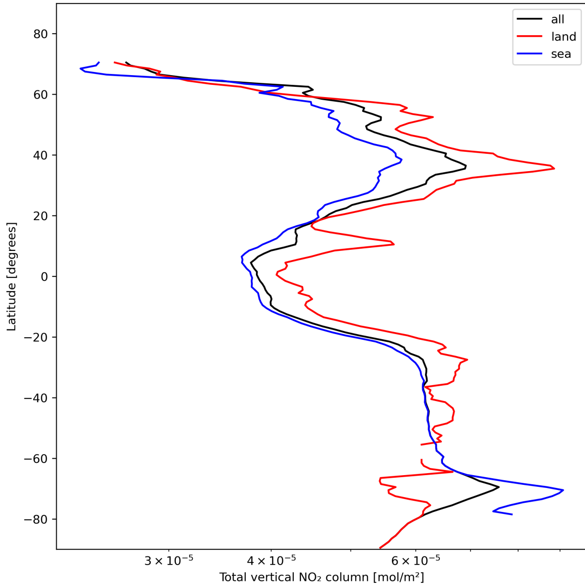
Figure 21: Zonal average of “Total vertical NO 2 column” for 2023-11-09 to 2023-11-11.
