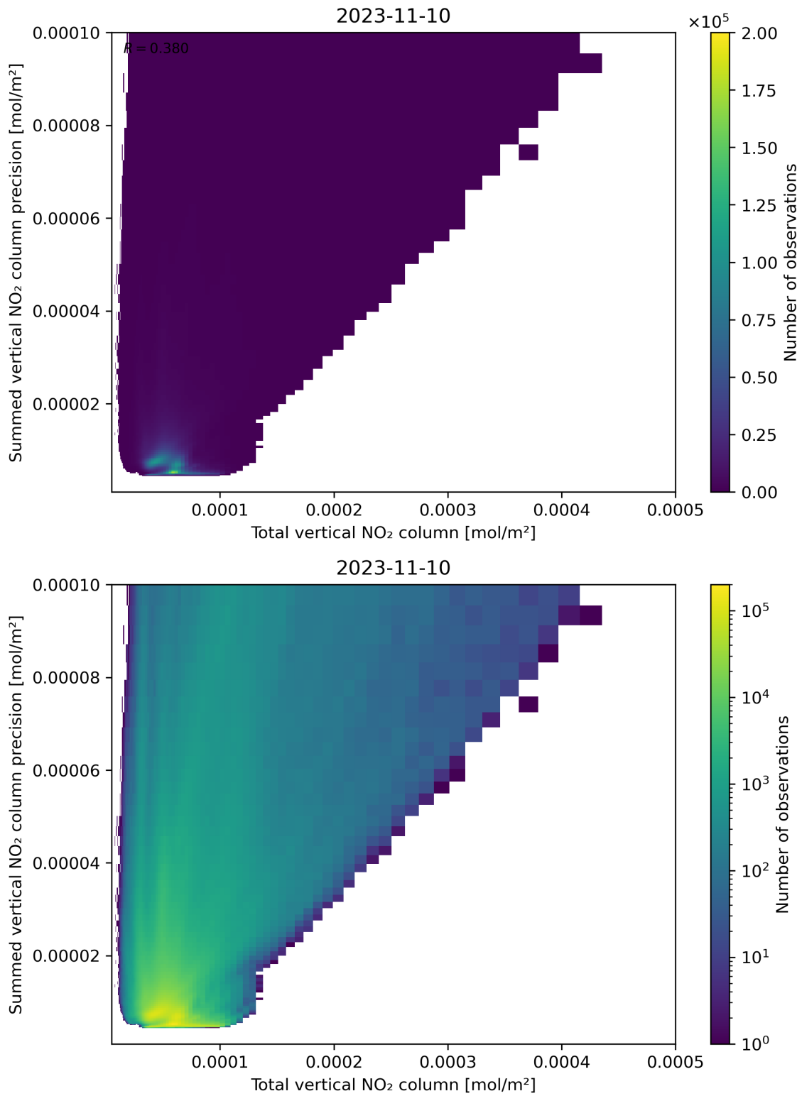
Figure 113: Scatter density plot of “Total vertical NO 2 column” against “Summed vertical NO 2 column precision” for 2023-11-09 to 2023-11-11.
