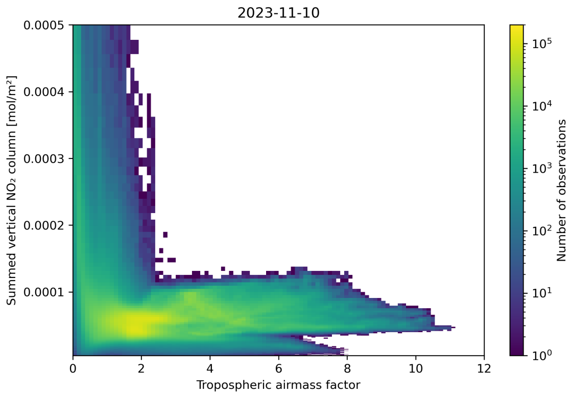
Figure 75: Scatter density plot of “Tropospheric airmass factor” against “Summed vertical NO 2 column” for 2023-11-09 to 2023-11-11.
