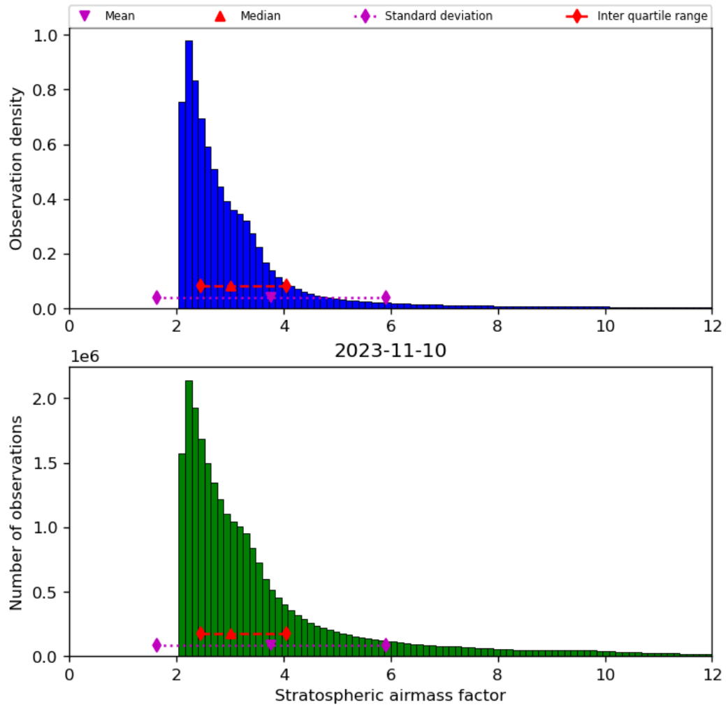
Figure 44: Histogram of “Stratospheric airmass factor” for 2023-11-09 to 2023-11-11
