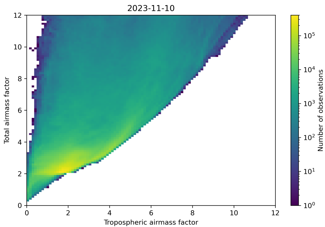
Figure 72: Scatter density plot of “Tropospheric airmass factor” against “Total airmass factor” for 2023-11-09 to 2023-11-11.
