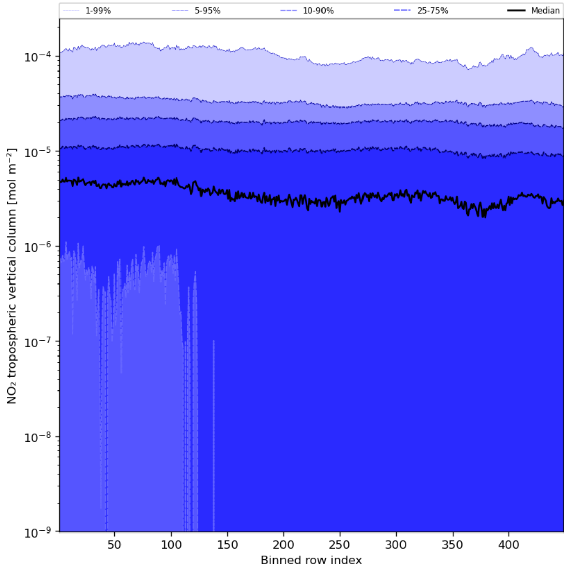
Figure 46: Along track statistics of “NO 2 tropospheric vertical column” for 2023-11-09 to 2023-11-11
