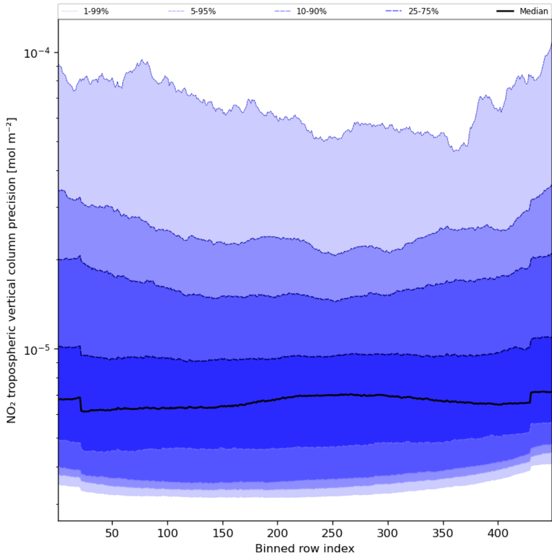
Figure 47: Along track statistics of “NO 2 tropospheric vertical column precision” for 2023-11-09 to 2023-11-11
