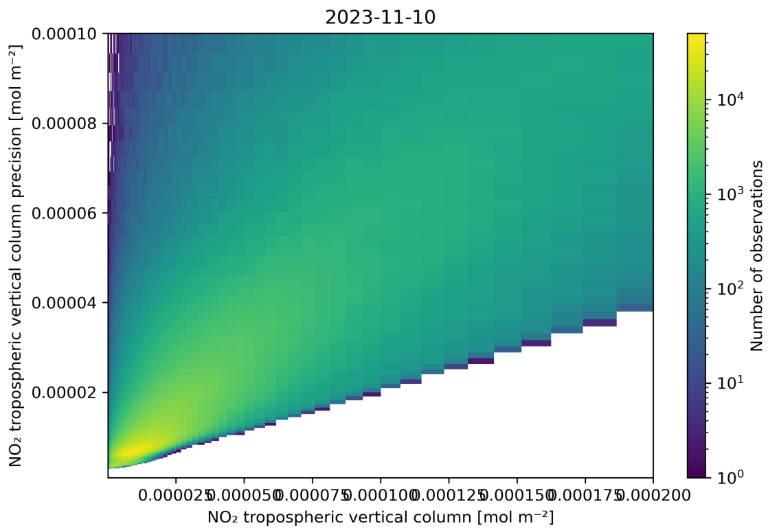
Figure 130: Scatter density plot of “NO 2 tropospheric vertical column” against “NO 2 tropospheric vertical column precision” for 2023-11-09 to 2023-11-11.
