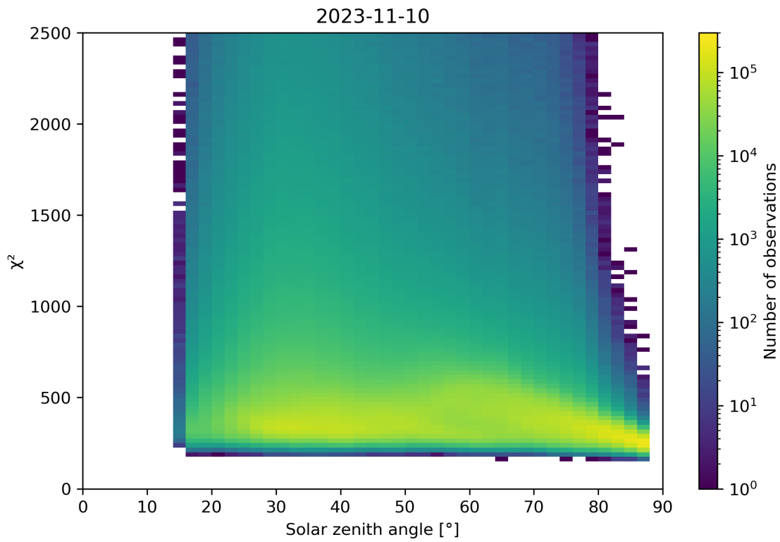
Figure 148: Scatter density plot of “Solar zenith angle” against “ \chi^2 ” for 2023-11-09 to 2023-11-11.
