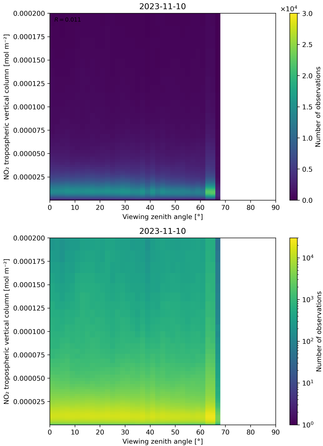
Figure 169: Scatter density plot of “Viewing zenith angle” against “NO 2 tropospheric vertical column” for 2023-11-09 to 2023-11-11.
