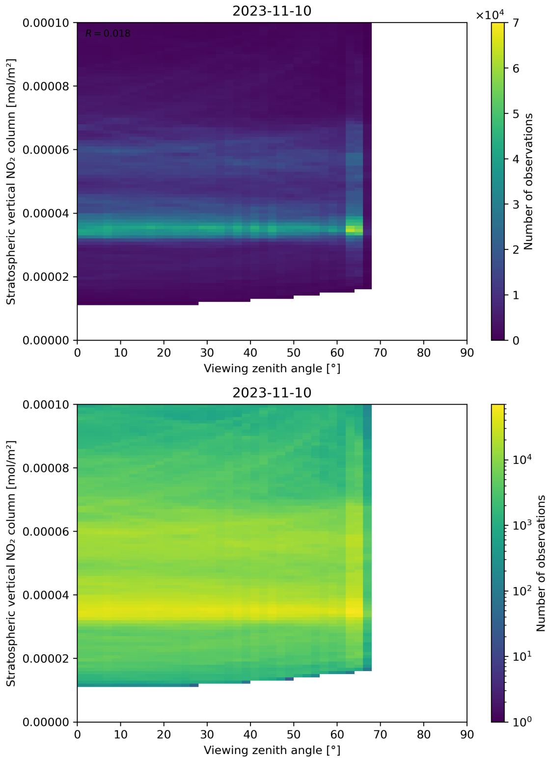
Figure 164: Scatter density plot of “Viewing zenith angle” against “Stratospheric vertical NO 2 column” for 2023-11-09 to 2023-11-11.
