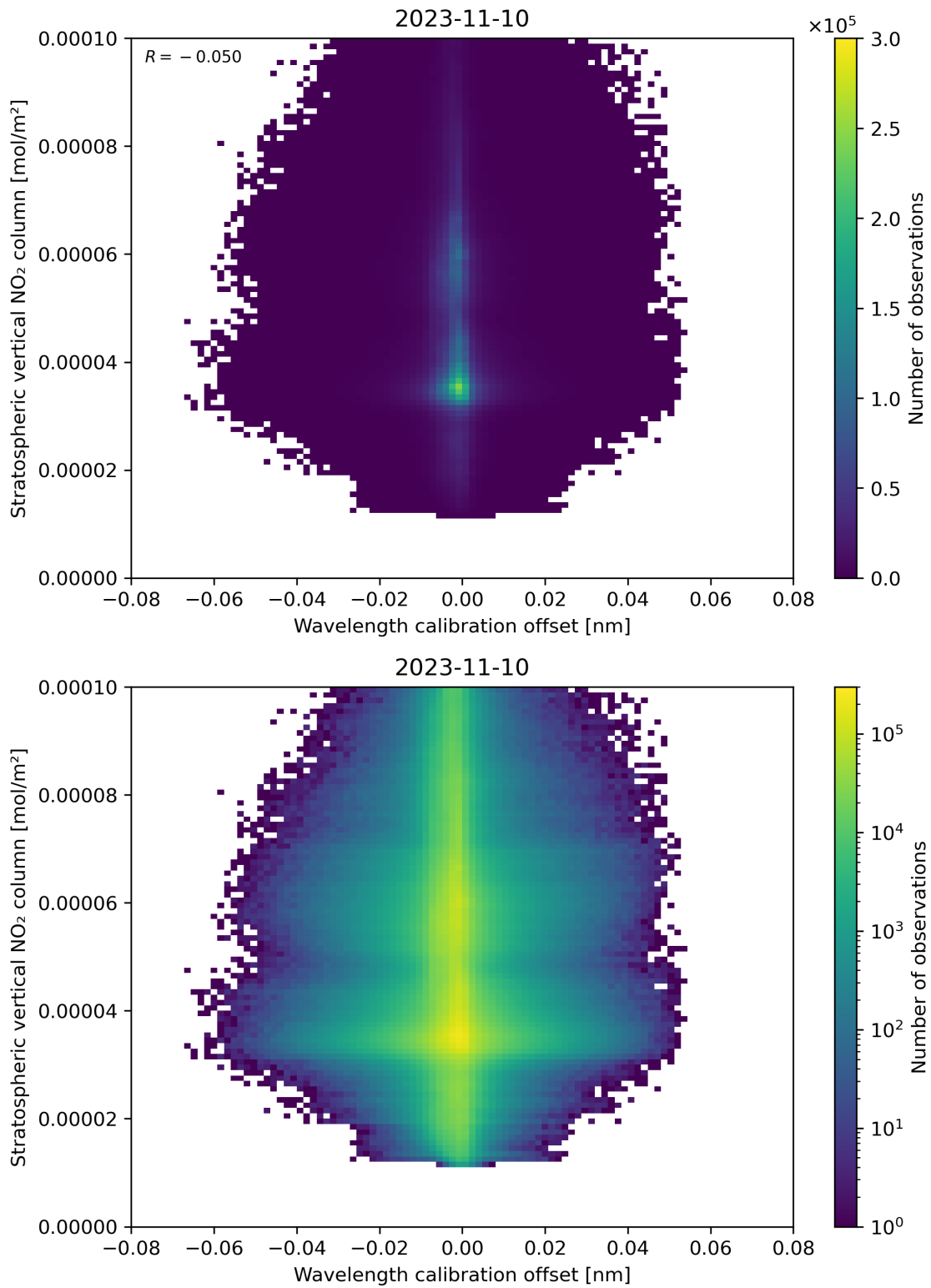
Figure 176: Scatter density plot of “Wavelength calibration offset” against “Stratospheric vertical NO 2 column” for 2023-11-09 to 2023-11-11.
