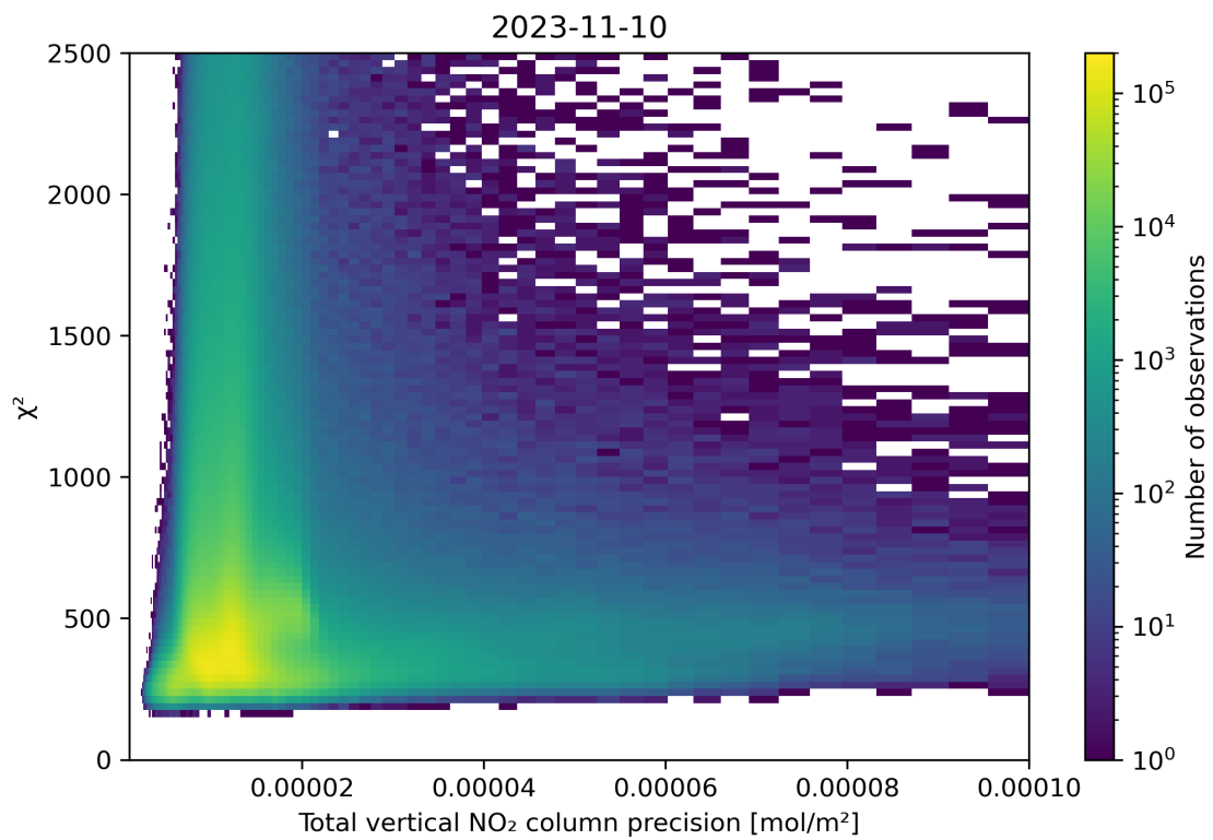
Figure 116: Scatter density plot of “Total vertical NO 2 column precision” against “ \chi^2 ” for 2023-11-09 to 2023-11-11.
