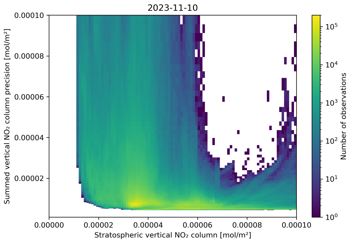
Figure 99: Scatter density plot of “Stratospheric vertical NO 2 column” against “Summed vertical NO 2 column precision” for 2023-11-09 to 2023-11-11.
