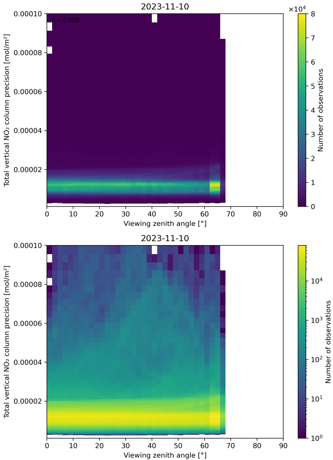
Figure 168: Scatter density plot of “Viewing zenith angle” against “Total vertical NO 2 column precision” for 2023-11-09 to 2023-11-11.
