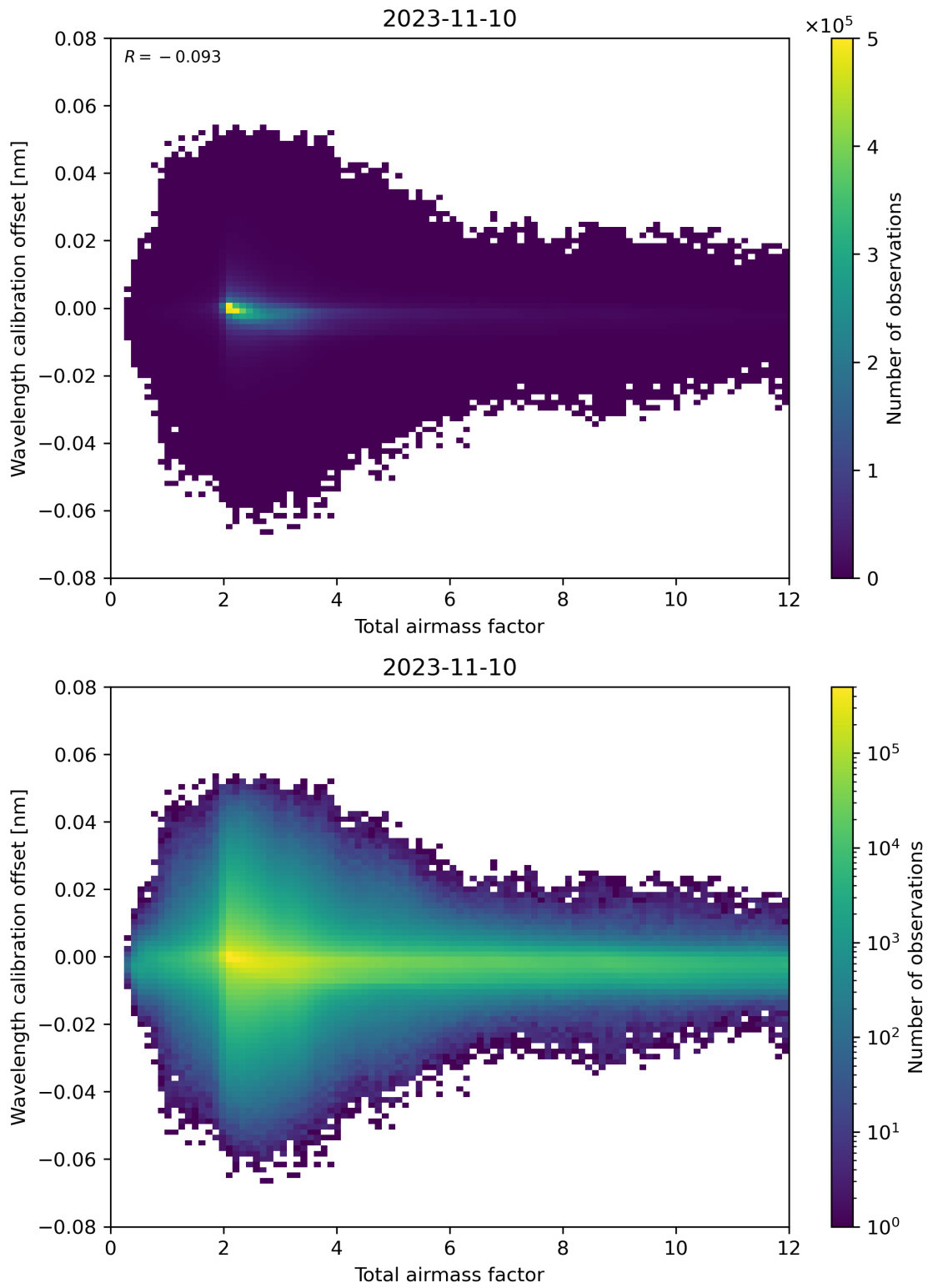
Figure 70: Scatter density plot of “Total airmass factor” against “Wavelength calibration offset” for 2023-11-09 to 2023-11-11.
