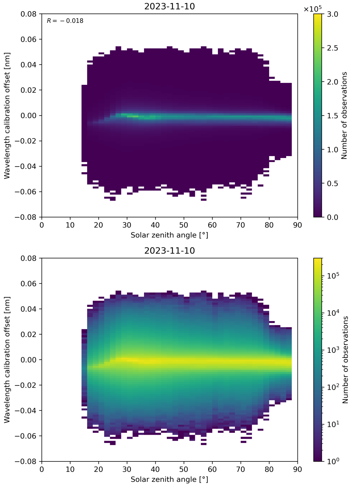
Figure 158: Scatter density plot of “Solar zenith angle” against “Wavelength calibration offset” for 2023-11-09 to 2023-11-11.
