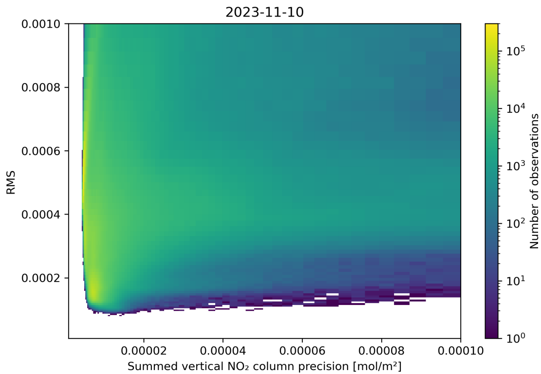
Figure 108: Scatter density plot of “Summed vertical NO 2 column precision” against “RMS” for 2023-11-09 to 2023-11-11.
