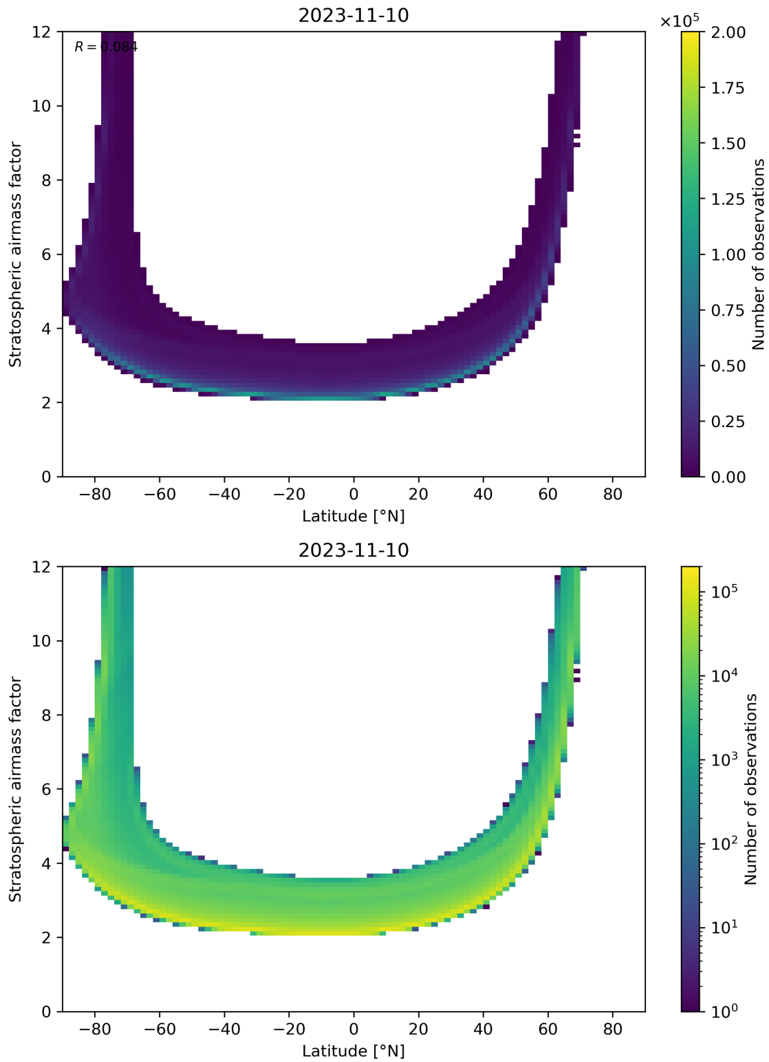
Figure 83: Scatter density plot of “Latitude” against “Stratospheric airmass factor” for 2023-11-09 to 2023-11-11.
