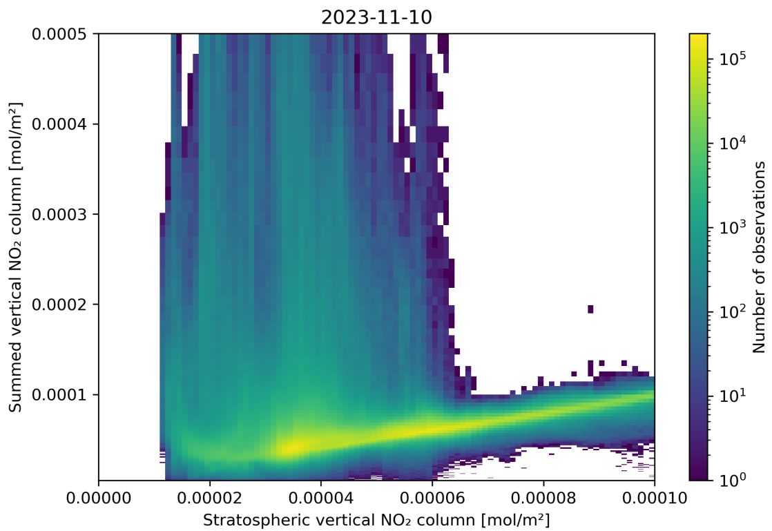
Figure 98: Scatter density plot of “Stratospheric vertical NO 2 column” against “Summed vertical NO 2 column” for 2023-11-09 to 2023-11-11.
