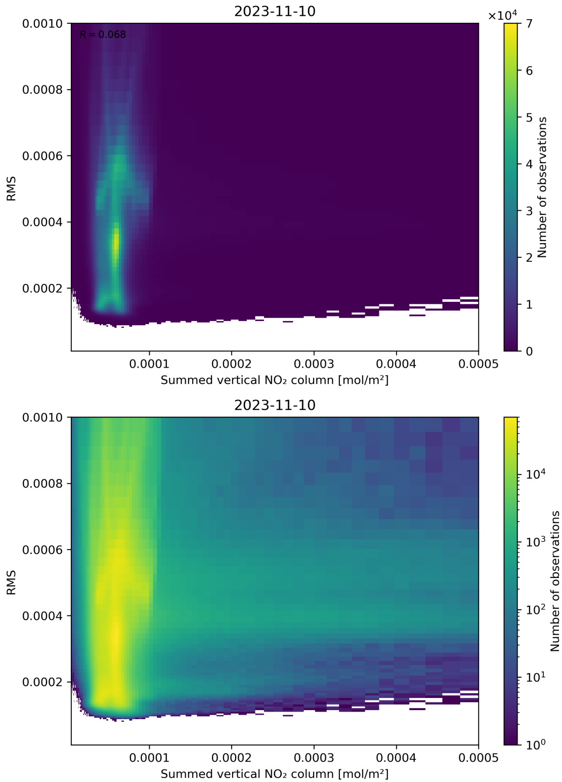
Figure 109: Scatter density plot of “Summed vertical NO 2 column” against “RMS” for 2023-11-09 to 2023-11-11.
