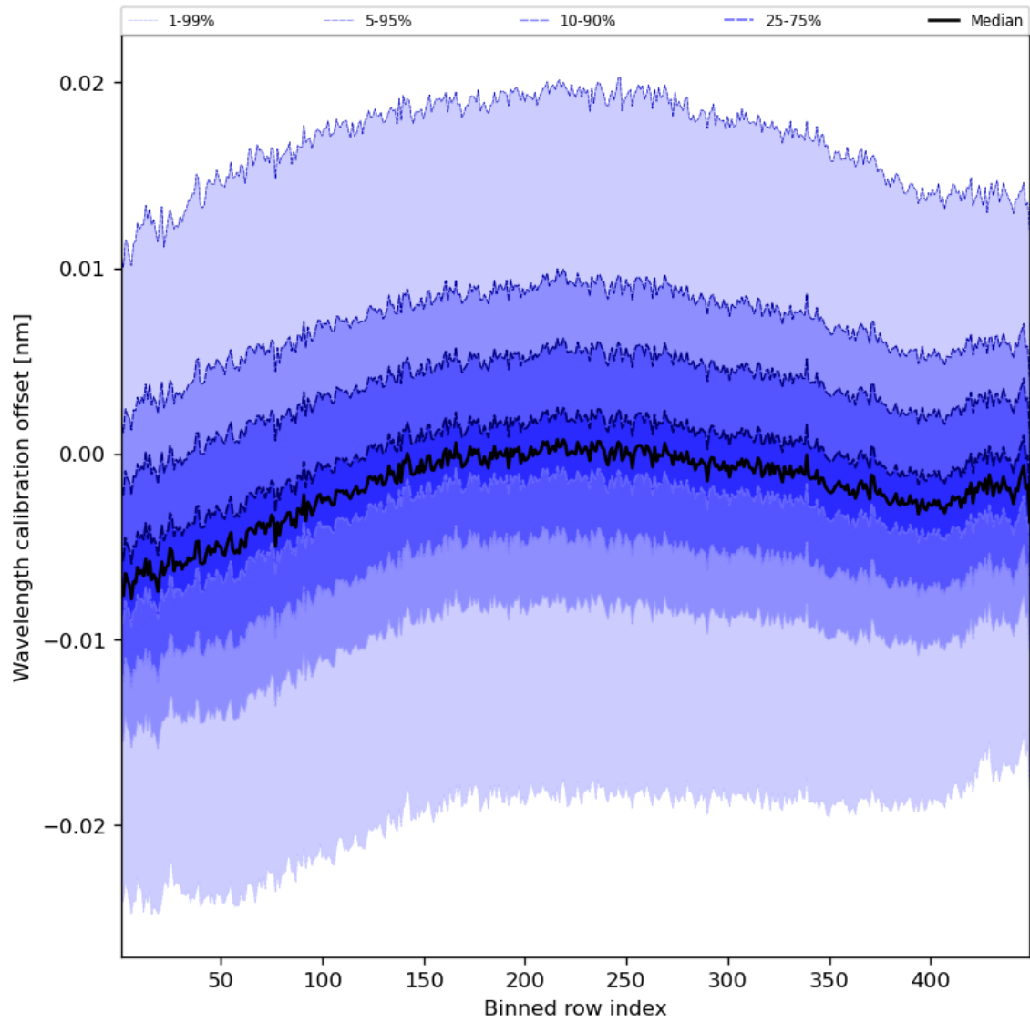
Figure 52: Along track statistics of “Wavelength calibration offset” for 2023-11-09 to 2023-11-11
