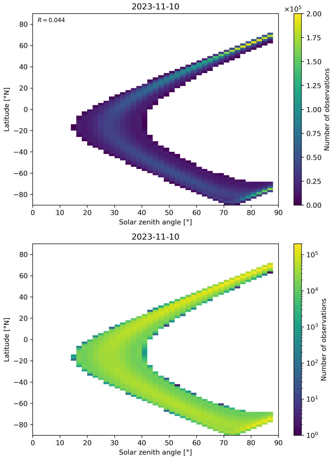
Figure 149: Scatter density plot of “Solar zenith angle” against “Latitude” for 2023-11-09 to 2023-11-11.
