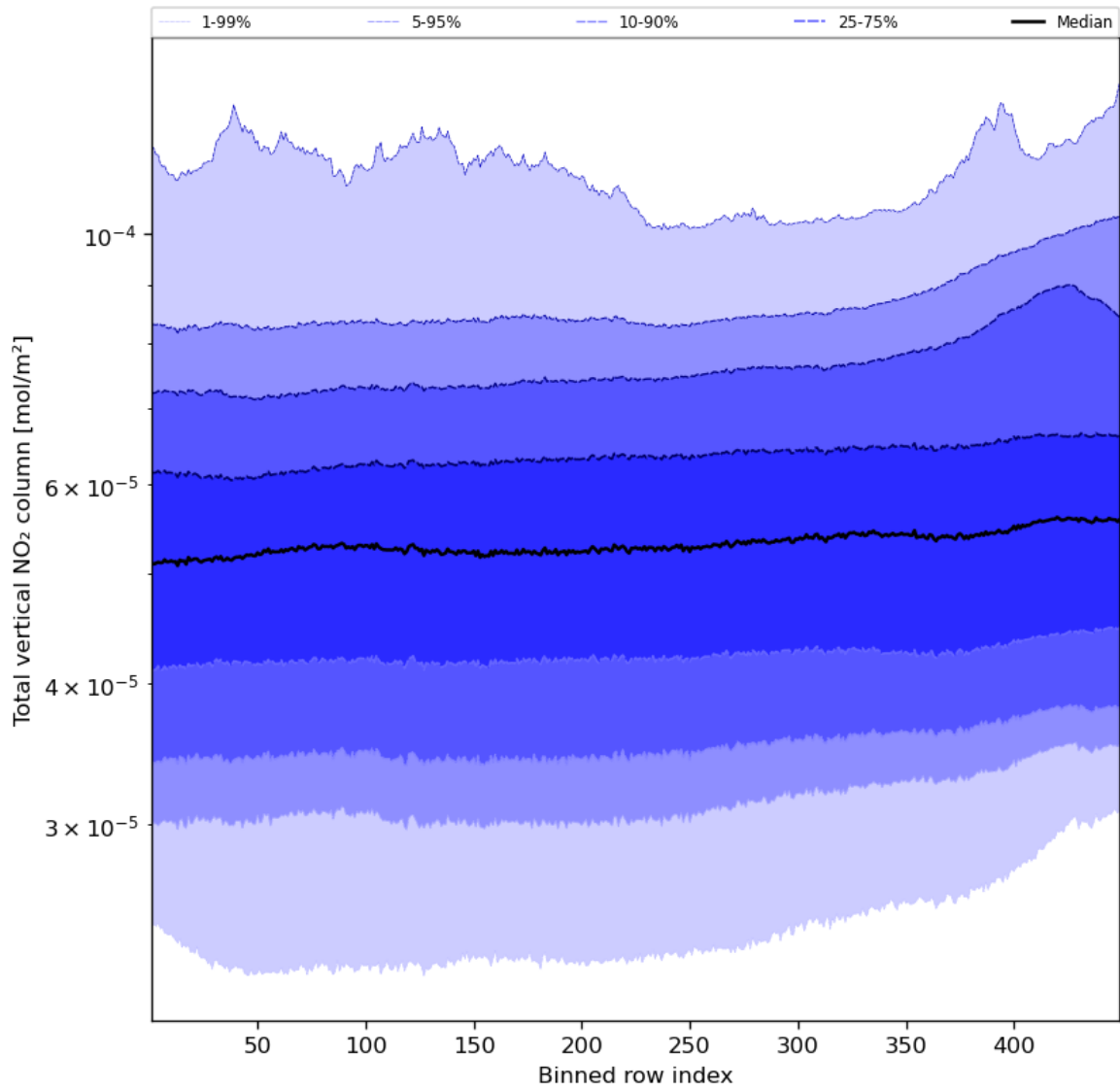
Figure 55: Along track statistics of “Total vertical NO 2 column” for 2023-11-09 to 2023-11-11
