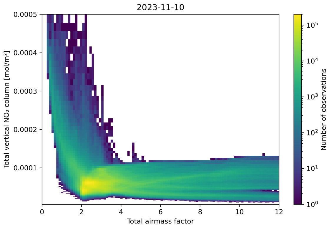
Figure 67: Scatter density plot of “Total airmass factor” against “Total vertical NO 2 column” for 2023-11-09 to 2023-11-11.
