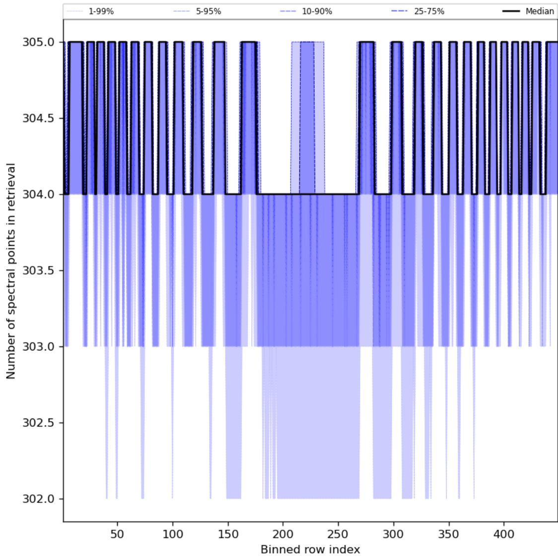
Figure 50: Along track statistics of “Number of spectral points in retrieval” for 2023-11-09 to 2023-11-11
