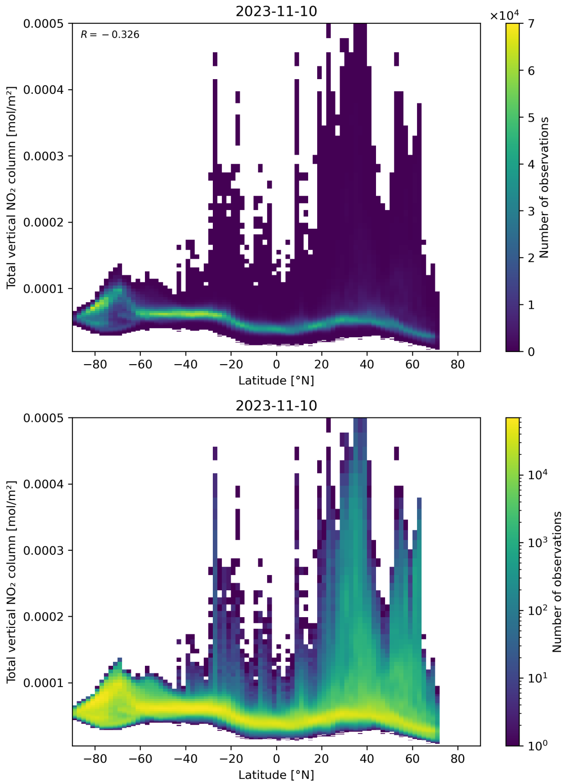
Figure 90: Scatter density plot of “Latitude” against “Total vertical NO 2 column” for 2023-11-09 to 2023-11-11.
