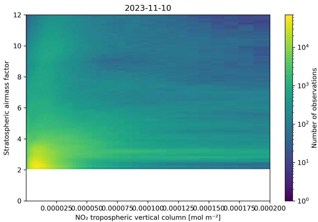
Figure 121: Scatter density plot of “NO 2 tropospheric vertical column” against “Stratospheric airmass factor” for 2023-11-09 to 2023-11-11.
