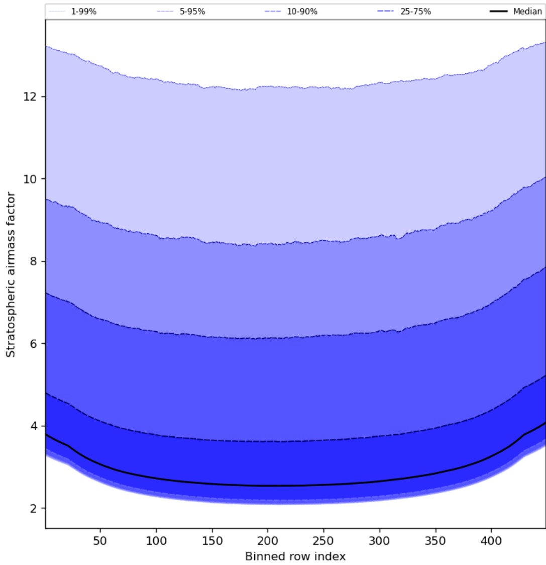
Figure 61: Along track statistics of “Stratospheric air mass factor” for 2023-11-09 to 2023-11-11
