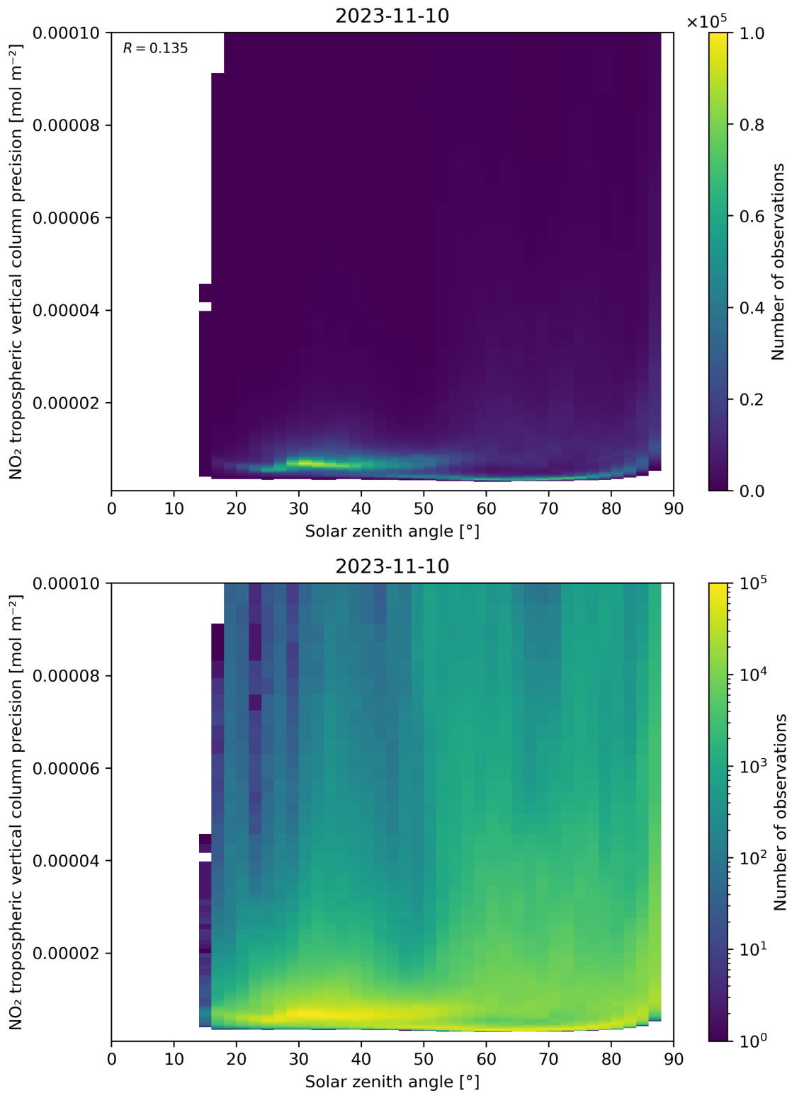
Figure 156: Scatter density plot of “Solar zenith angle” against “NO 2 tropospheric vertical column precision” for 2023-11-09 to 2023-11-11.
