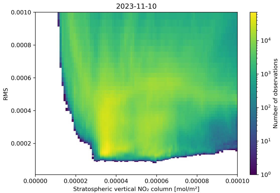
Figure 102: Scatter density plot of “Stratospheric vertical NO 2 column” against “RMS” for 2023-11-09 to 2023-11-11.
