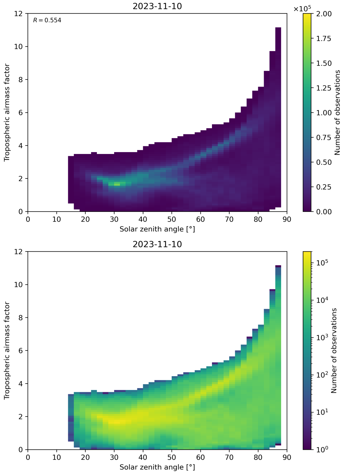
Figure 147: Scatter density plot of “Solar zenith angle” against “Tropospheric airmass factor” for 2023-11-09 to 2023-11-11.
