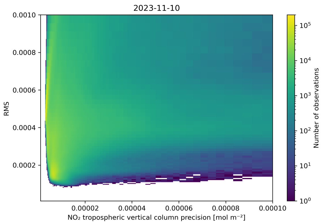
Figure 140: Scatter density plot of “NO 2 tropospheric vertical column precision” against “RMS” for 2023-11-09 to 2023-11-11.
