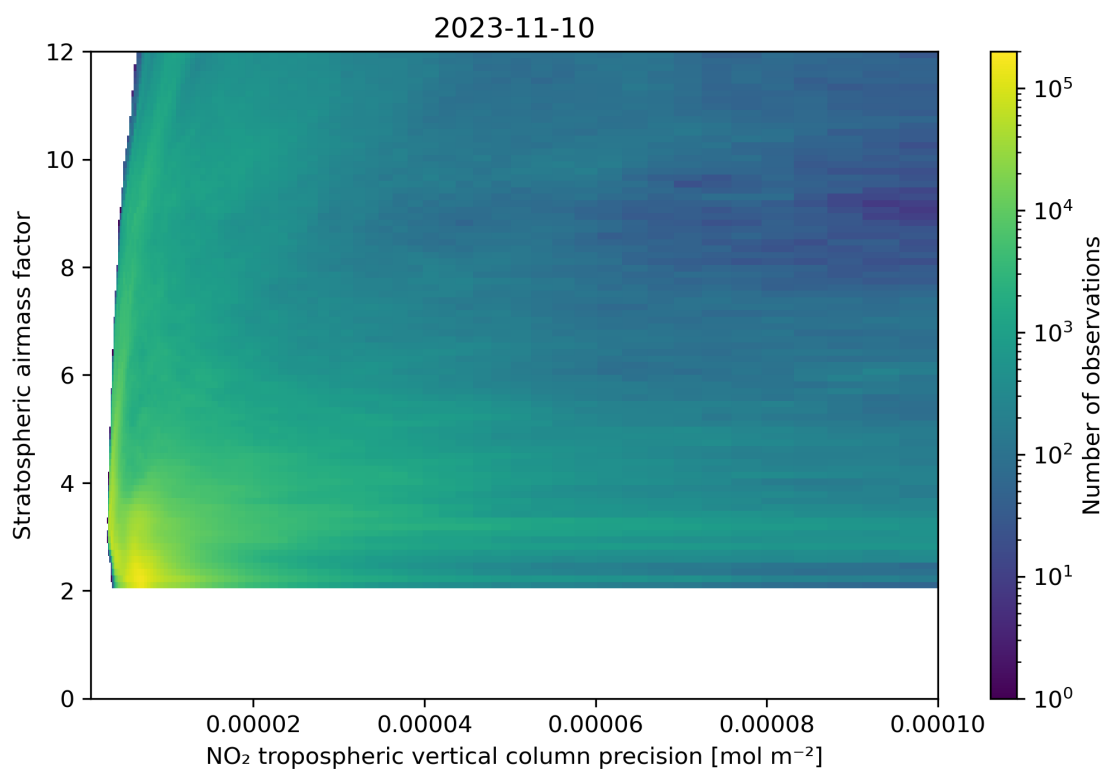
Figure 131: Scatter density plot of “NO 2 tropospheric vertical column precision” against “Stratospheric airmass factor” for 2023-11-09 to 2023-11-11.
