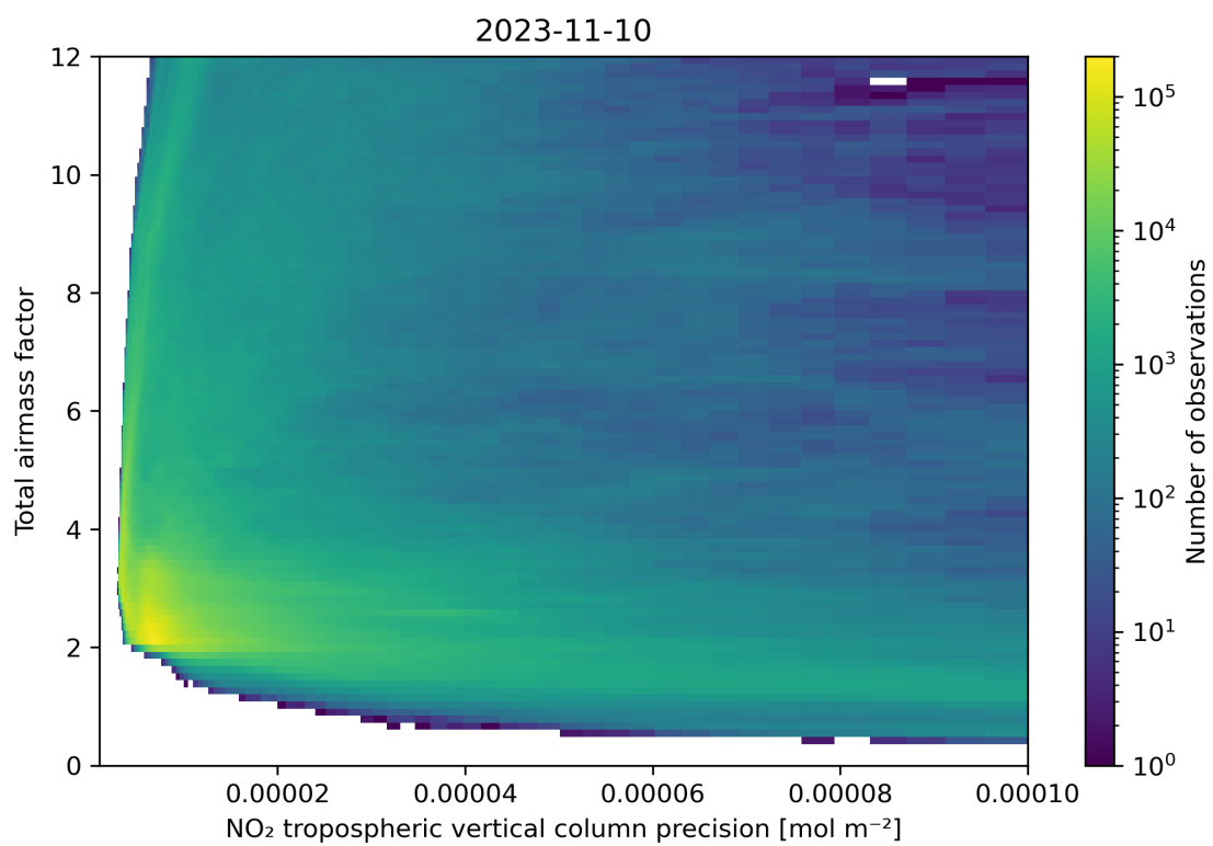
Figure 132: Scatter density plot of “NO 2 tropospheric vertical column precision” against “Total airmass factor” for 2023-11-09 to 2023-11-11.
