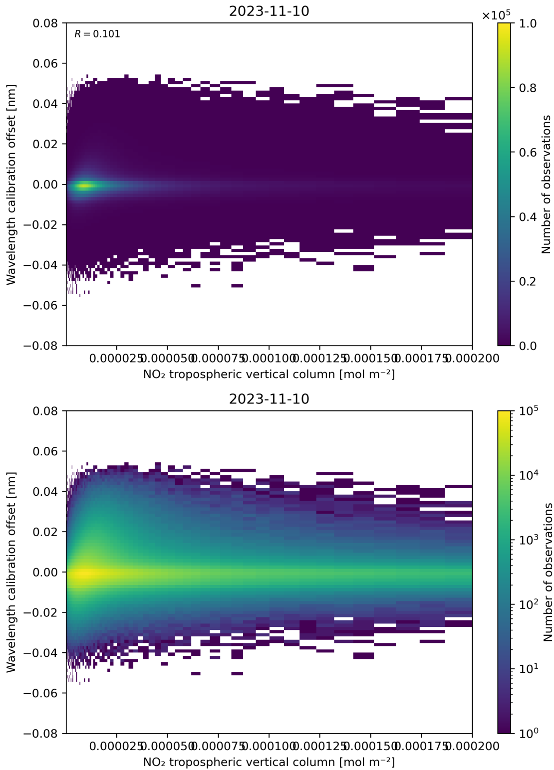
Figure 143: Scatter density plot of “NO 2 tropospheric vertical column” against “Wavelength calibration offset” for 2023-11-09 to 2023-11-11.
