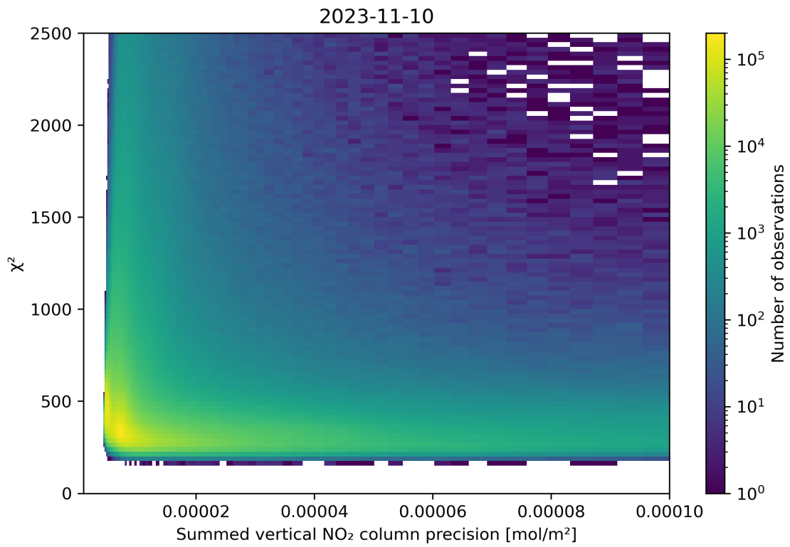
Figure 107: Scatter density plot of “Summed vertical NO 2 column precision” against “ \chi^2 ” for 2023-11-09 to 2023-11-11.
