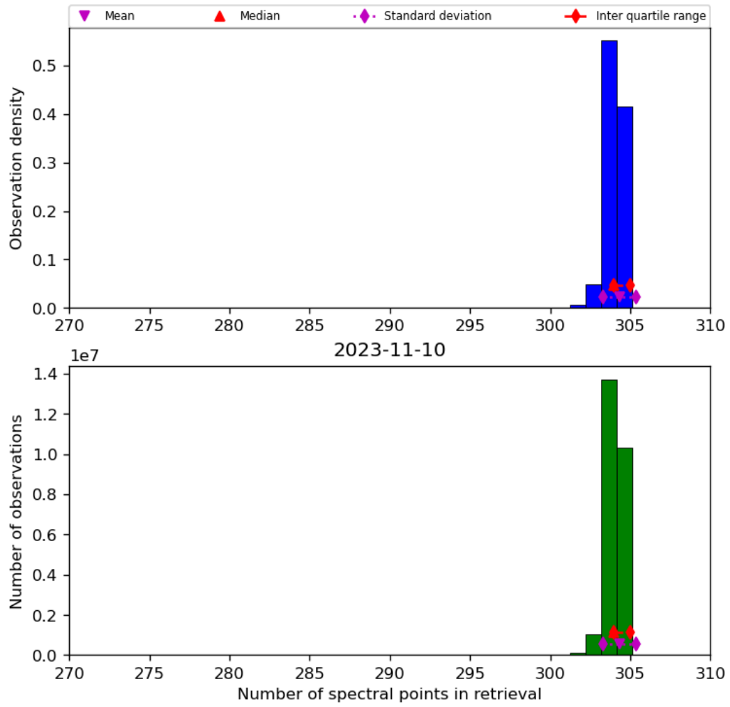
Figure 33: Histogram of “Number of spectral points in retrieval” for 2023-11-09 to 2023-11-11
