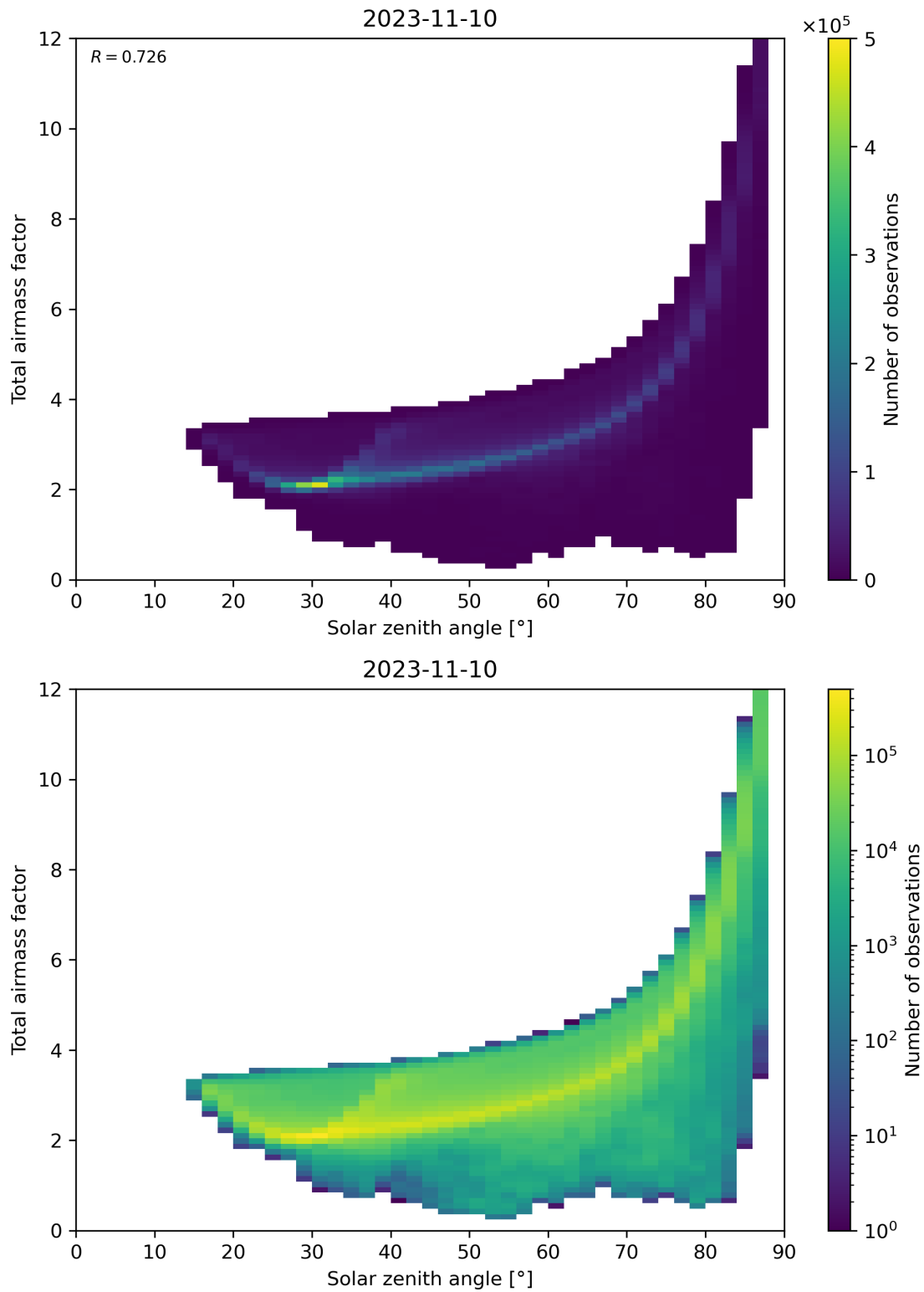
Figure 146: Scatter density plot of “Solar zenith angle” against “Total airmass factor” for 2023-11-09 to 2023-11-11.
