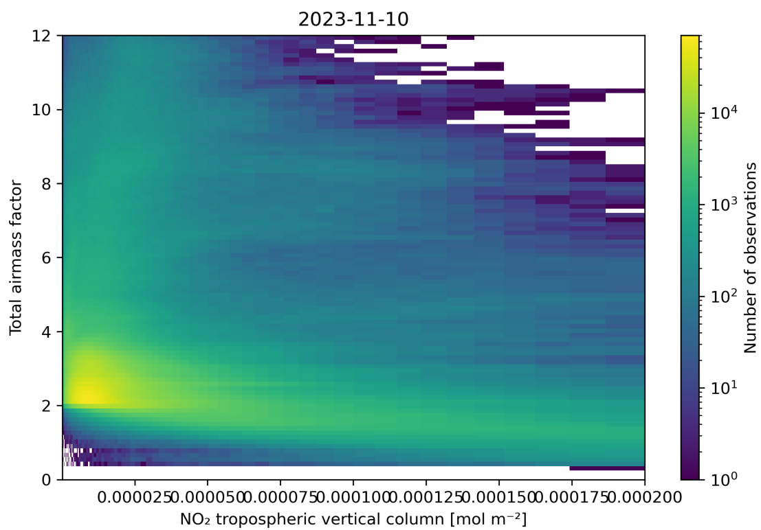
Figure 122: Scatter density plot of “NO 2 tropospheric vertical column” against “Total airmass factor” for 2023-11-09 to 2023-11-11.
