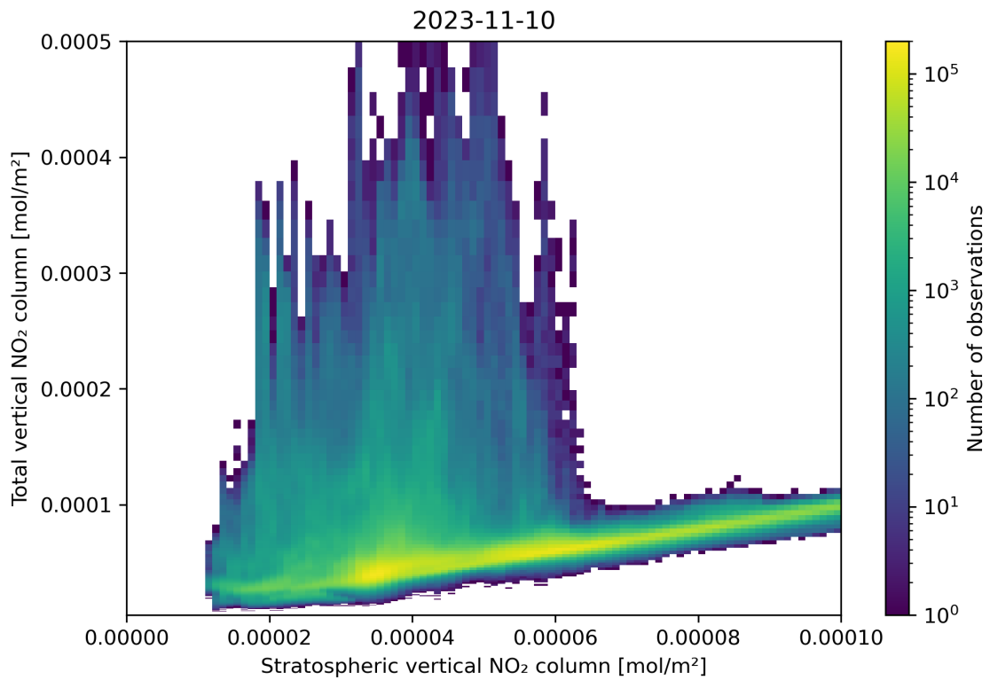
Figure 100: Scatter density plot of “Stratospheric vertical NO 2 column” against “Total vertical NO 2 column” for 2023-11-09 to 2023-11-11.
