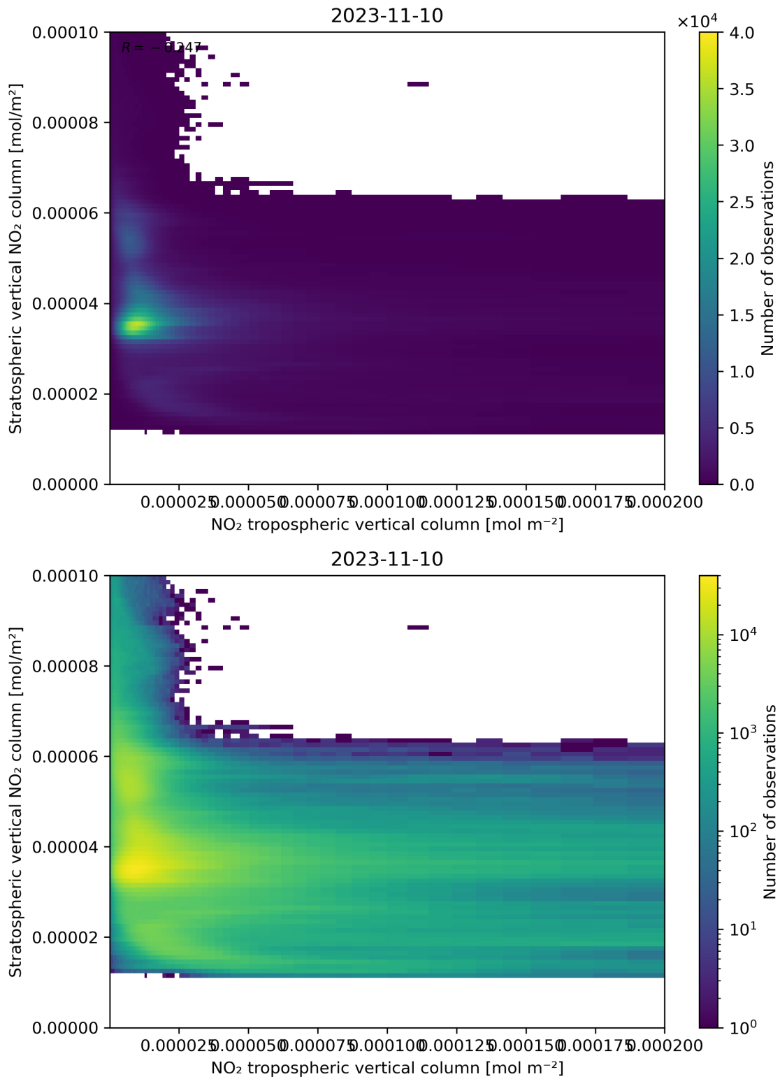
Figure 125: Scatter density plot of “NO 2 tropospheric vertical column” against “Stratospheric vertical NO 2 column” for 2023-11-09 to 2023-11-11.
