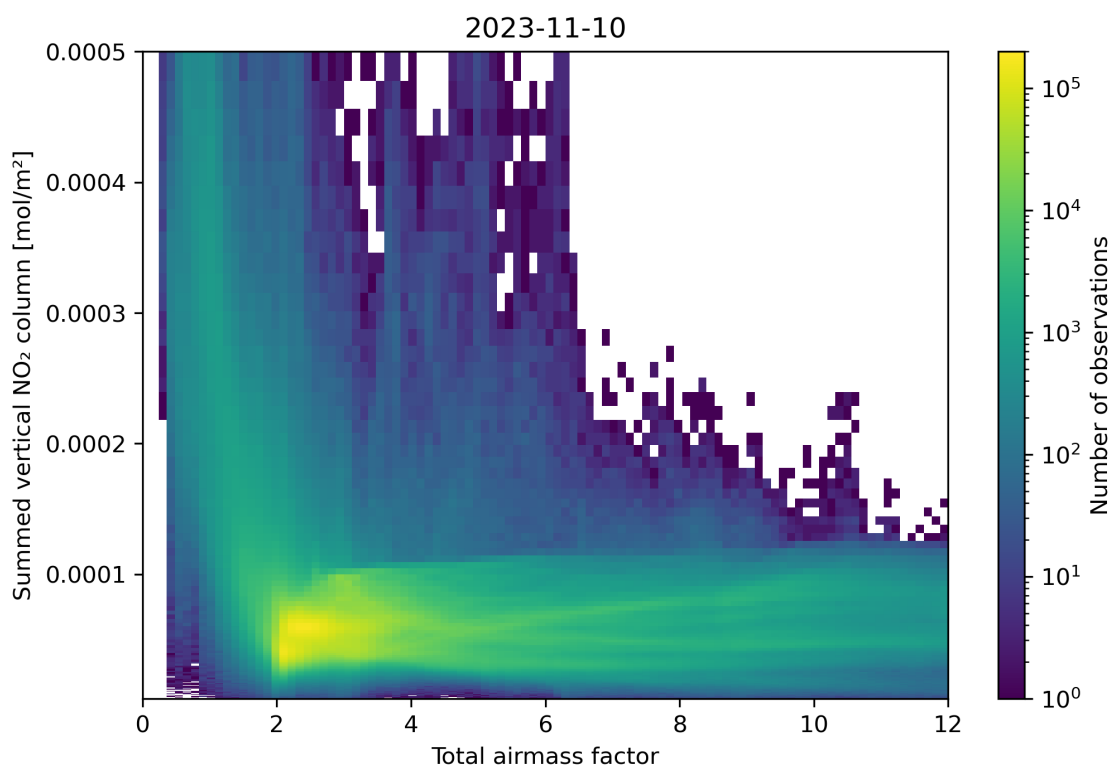
Figure 65: Scatter density plot of “Total airmass factor” against “Summed vertical NO 2 column” for 2023-11-09 to 2023-11-11.
