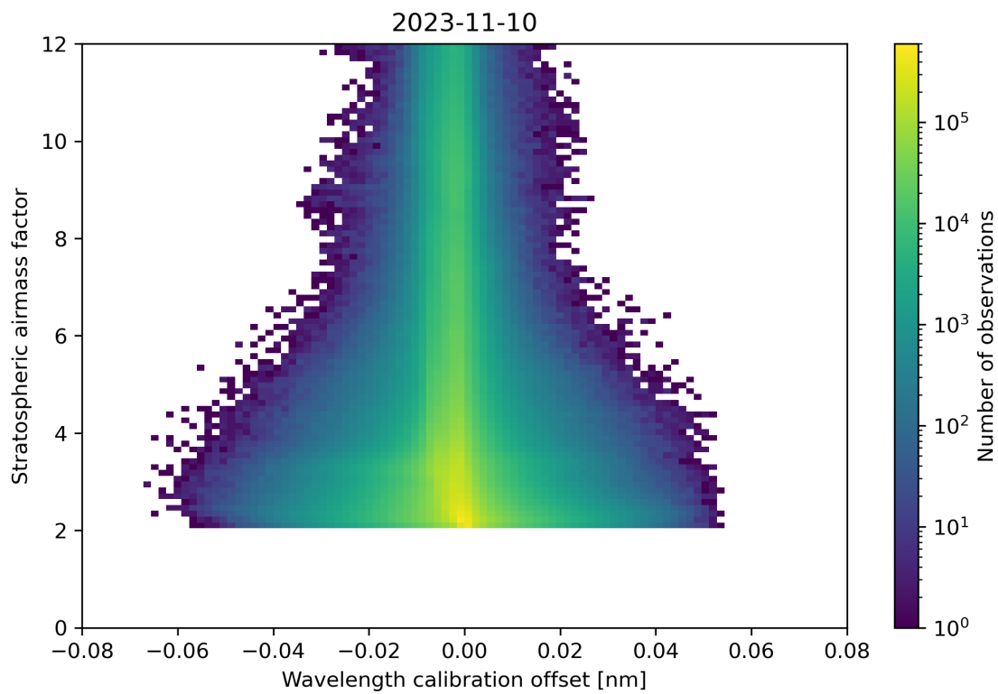
Figure 174: Scatter density plot of “Wavelength calibration offset” against “Stratospheric airmass factor” for 2023-11-09 to 2023-11-11.
