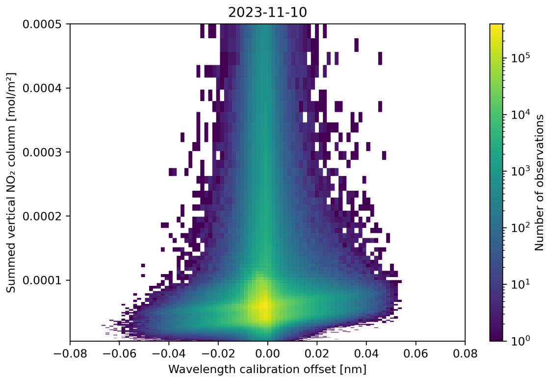
Figure 177: Scatter density plot of “Wavelength calibration offset” against “Summed vertical NO 2 column” for 2023-11-09 to 2023-11-11.
