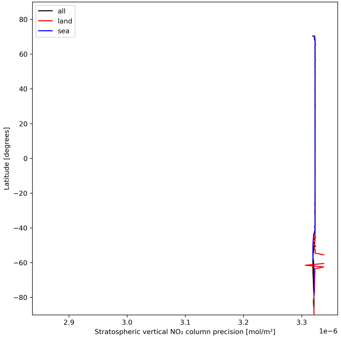
Figure 20: Zonal average of “Stratospheric vertical NO 2 column precision” for 2023-11-09 to 2023-11-11.
