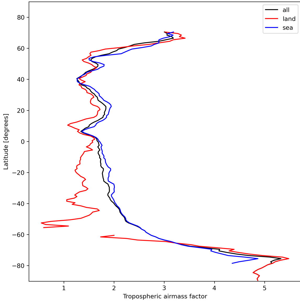
Figure 14: Zonal average of “Tropospheric airmass factor” for 2023-11-09 to 2023-11-11.
