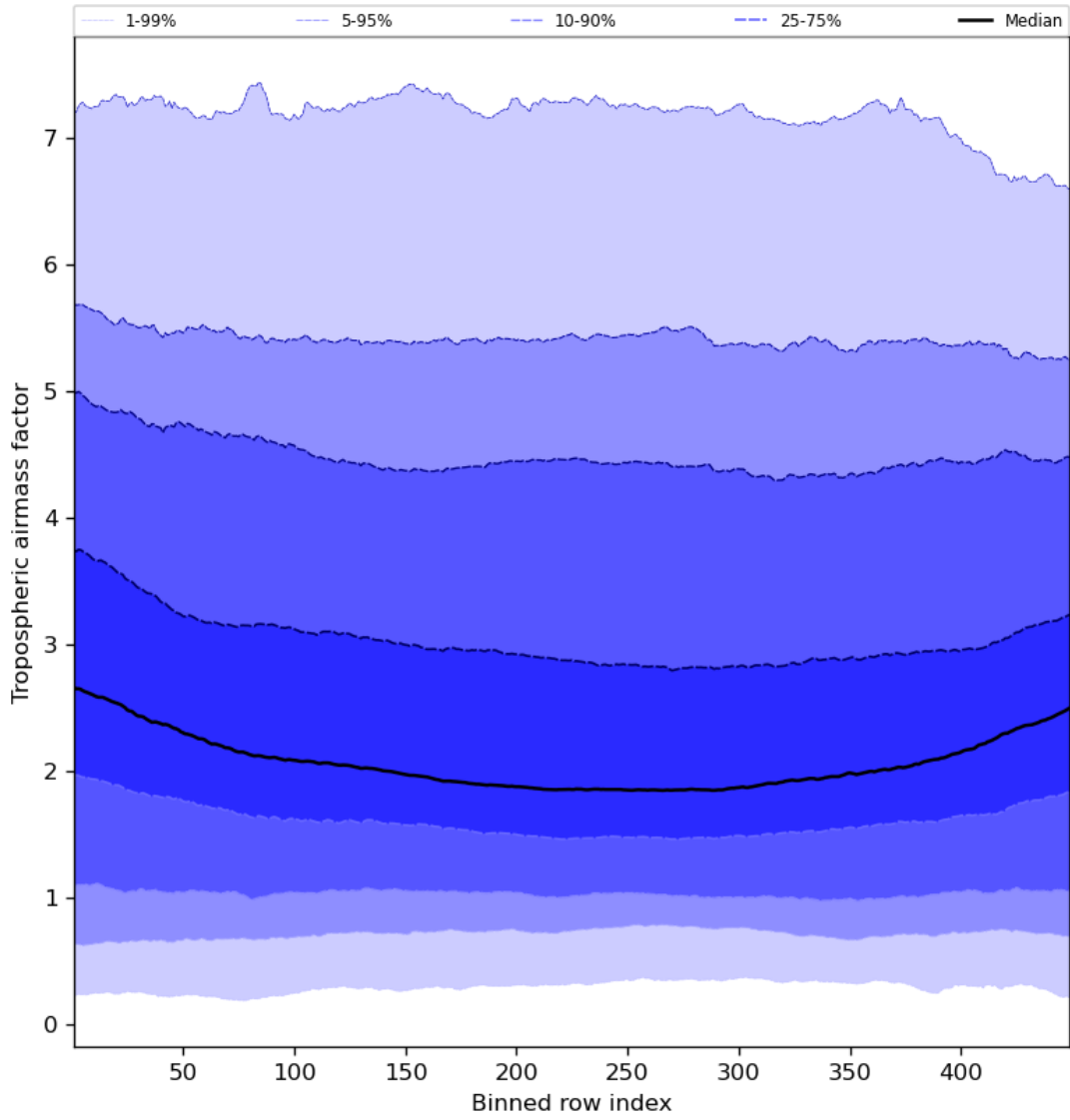
Figure 48: Along track statistics of “Tropospheric airmass factor” for 2023-11-09 to 2023-11-11
