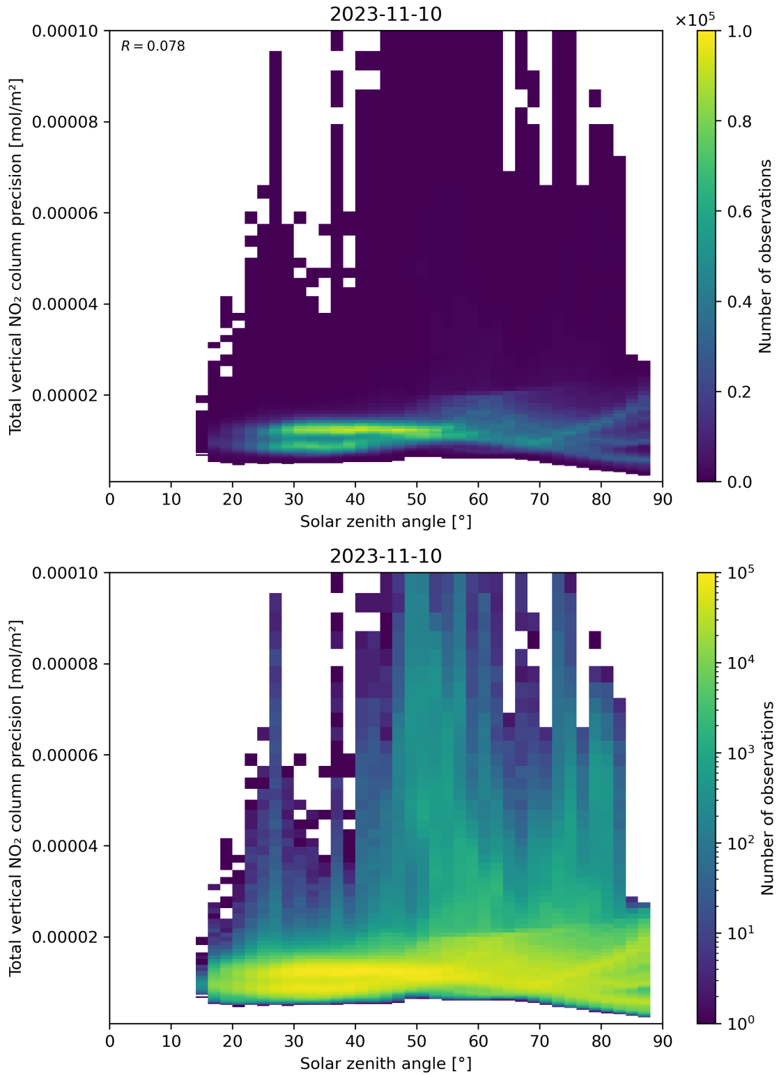
Figure 154: Scatter density plot of “Solar zenith angle” against “Total vertical NO 2 column precision” for 2023-11-09 to 2023-11-11.
