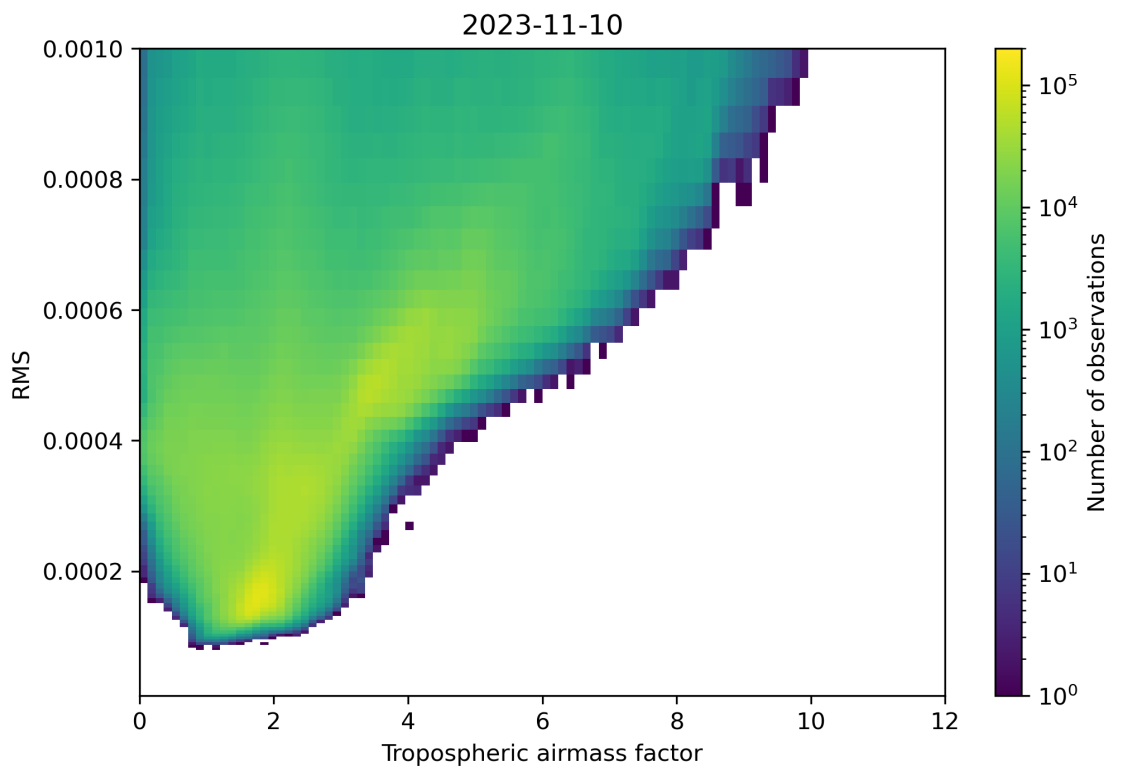
Figure 79: Scatter density plot of “Tropospheric airmass factor” against “RMS” for 2023-11-09 to 2023-11-11.
