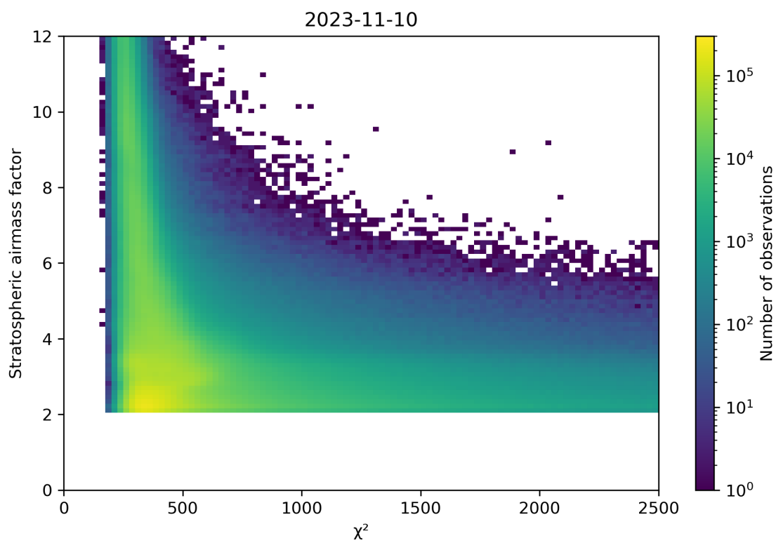
Figure 81: Scatter density plot of “ \chi^2 ” against “Stratospheric airmass factor” for 2023-11-09 to 2023-11-11.
