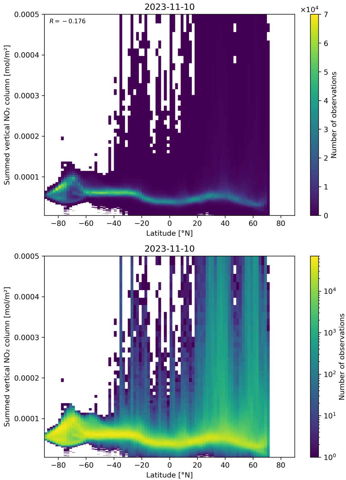
Figure 88: Scatter density plot of “Latitude” against “Summed vertical NO 2 column” for 2023-11-09 to 2023-11-11.
