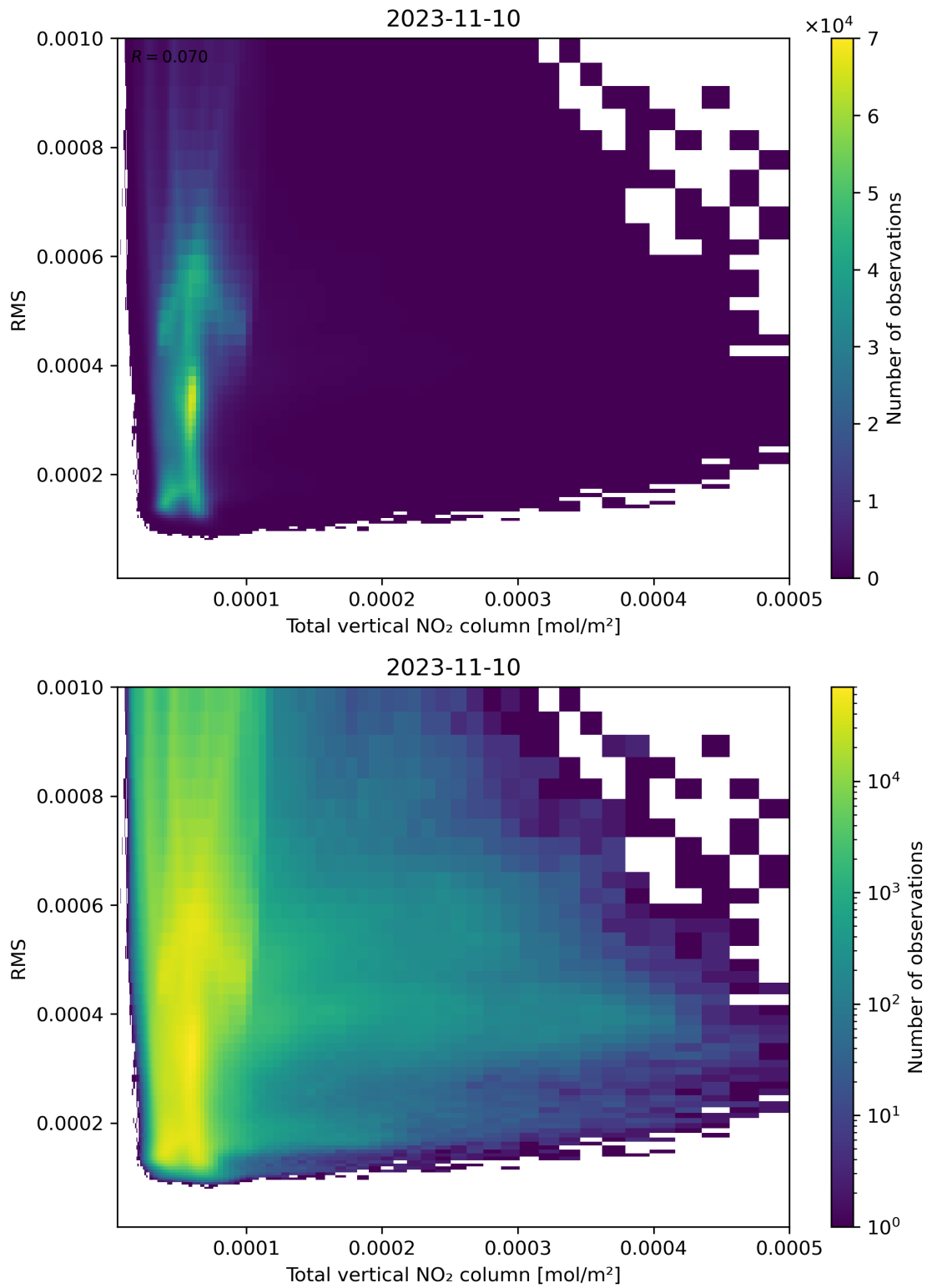
Figure 120: Scatter density plot of “Total vertical NO 2 column” against “RMS” for 2023-11-09 to 2023-11-11.
