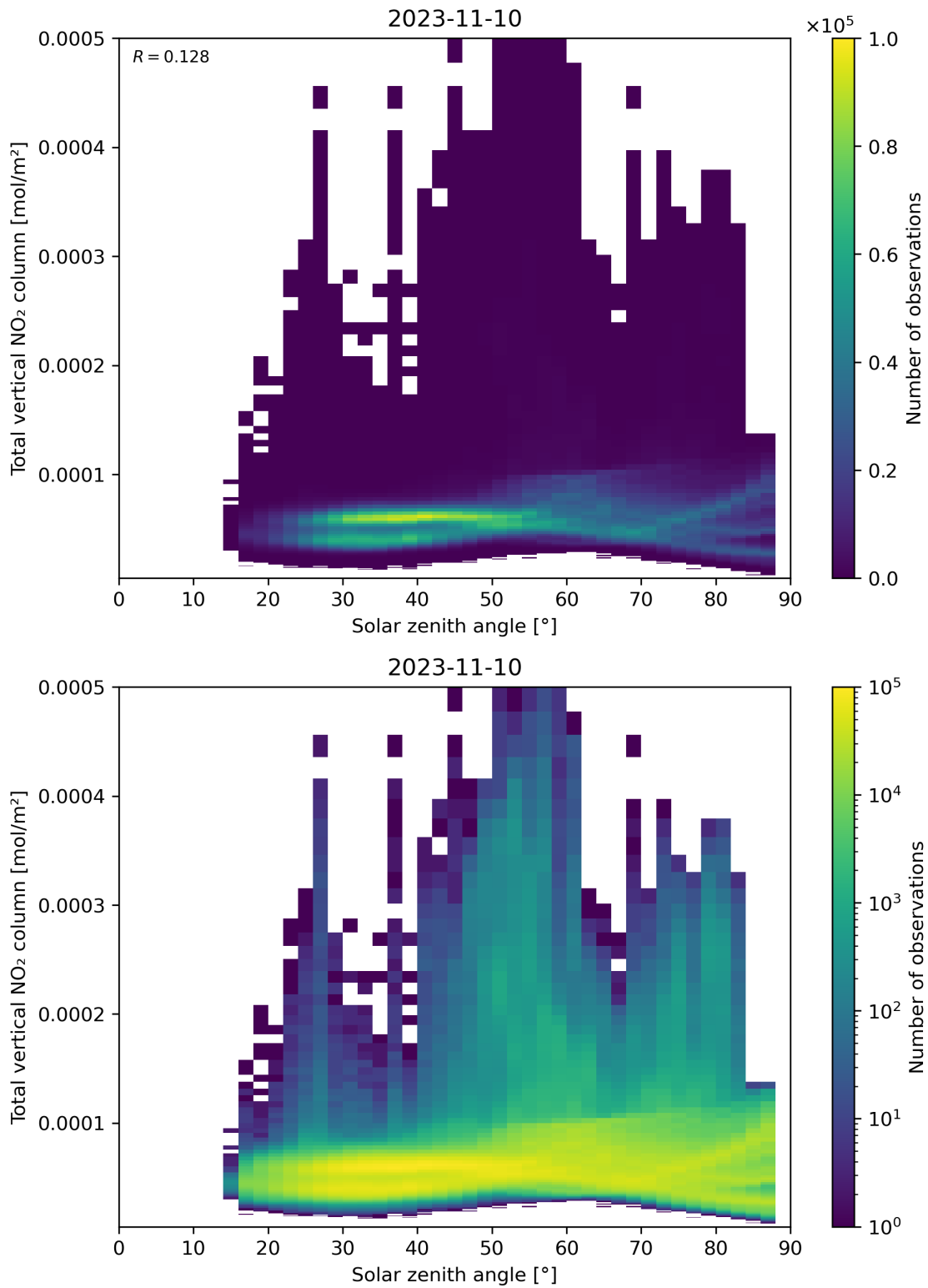
Figure 153: Scatter density plot of “Solar zenith angle” against “Total vertical NO 2 column” for 2023-11-09 to 2023-11-11.
