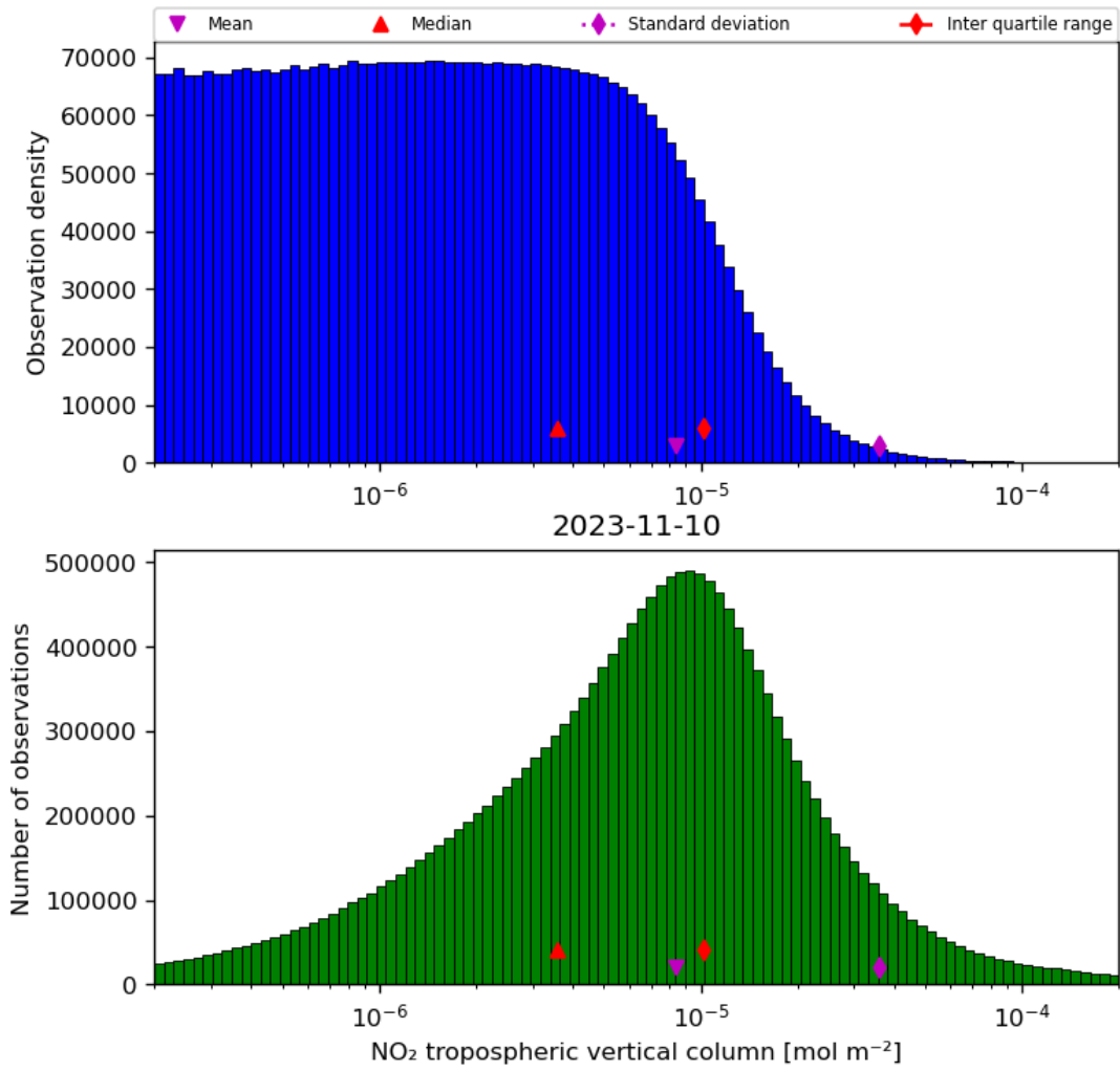
Figure 29: Histogram of “NO 2 tropospheric vertical column” for 2023-11-09 to 2023-11-11
