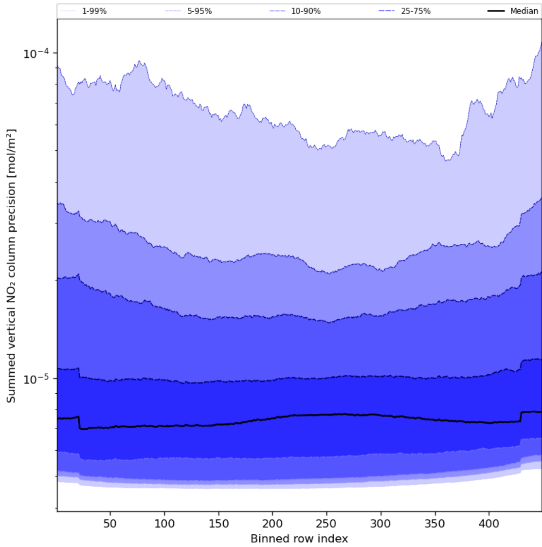
Figure 58: Along track statistics of “Summed vertical NO 2 column precision” for 2023-11-09 to 2023-11-11
