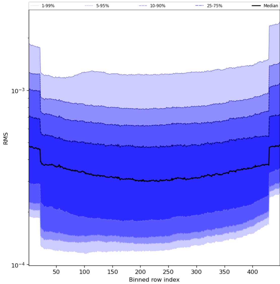
Figure 60: Along track statistics of “RMS” for 2023-11-09 to 2023-11-11
