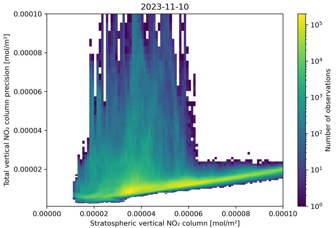
Figure 101: Scatter density plot of “Stratospheric vertical NO 2 column” against “Total vertical NO 2 column precision” for 2023-11-09 to 2023-11-11.
