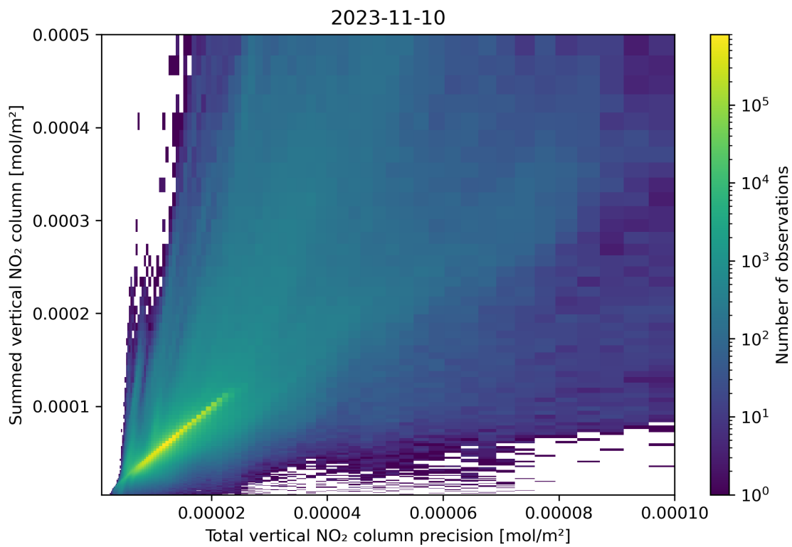
Figure 117: Scatter density plot of “Total vertical NO 2 column precision” against “Summed vertical NO 2 column” for 2023-11-09 to 2023-11-11.
