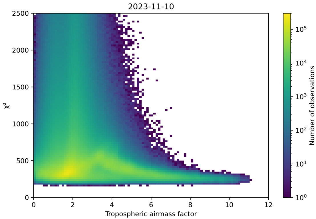
Figure 73: Scatter density plot of “Tropospheric airmass factor” against “ \chi^2 ” for 2023-11-09 to 2023-11-11.
