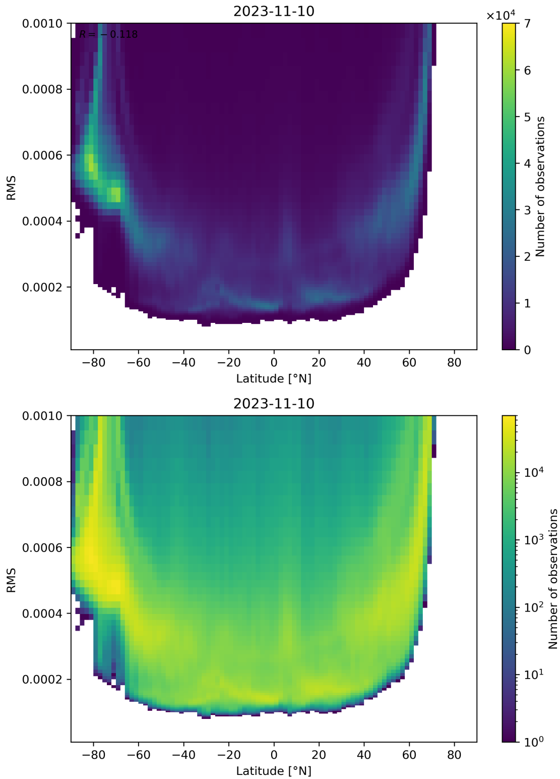
Figure 94: Scatter density plot of “Latitude” against “RMS” for 2023-11-09 to 2023-11-11.
