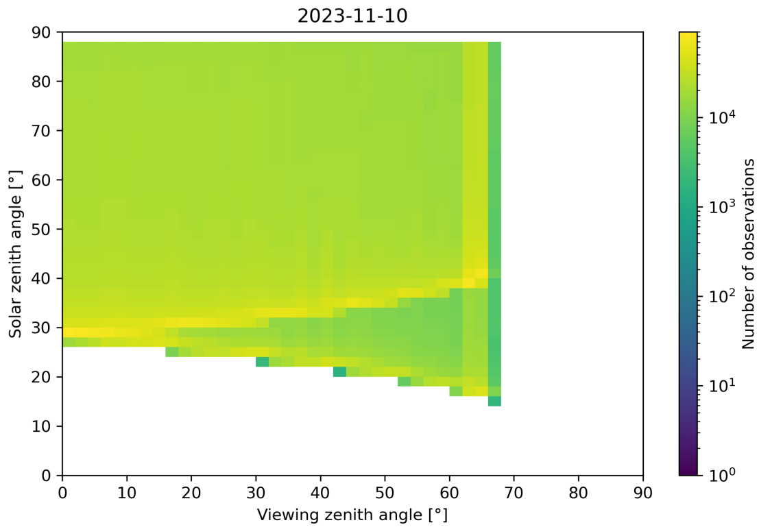
Figure 172: Scatter density plot of “Viewing zenith angle” against “Solar zenith angle” for 2023-11-09 to 2023-11-11.
