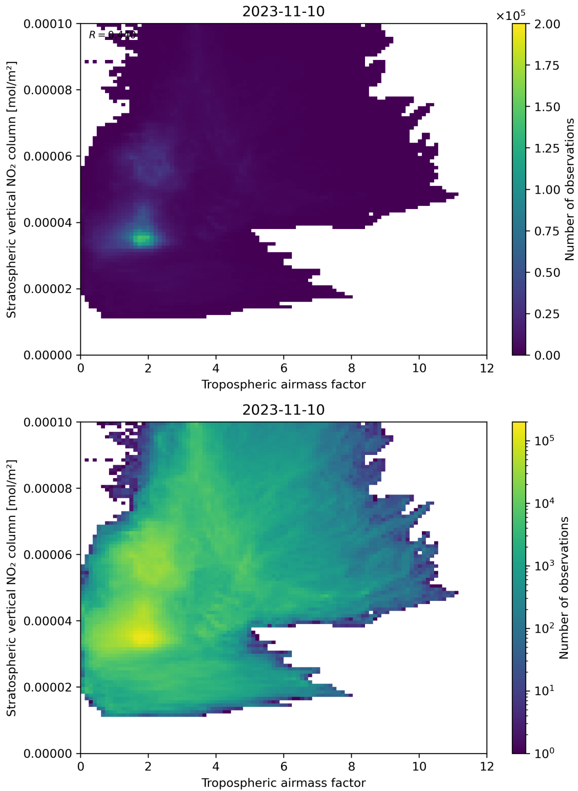
Figure 74: Scatter density plot of “Tropospheric airmass factor” against “Stratospheric vertical NO 2 column” for 2023-11-09 to 2023-11-11.
