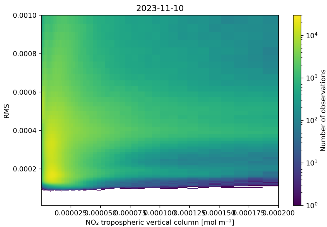
Figure 142: Scatter density plot of “NO 2 tropospheric vertical column” against “RMS” for 2023-11-09 to 2023-11-11.
