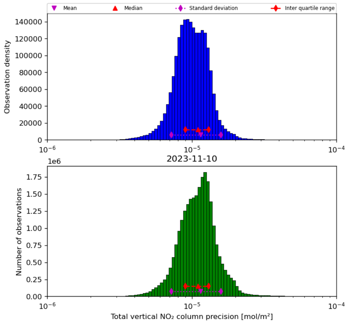
Figure 39: Histogram of “Total vertical NO 2 column precision” for 2023-11-09 to 2023-11-11
