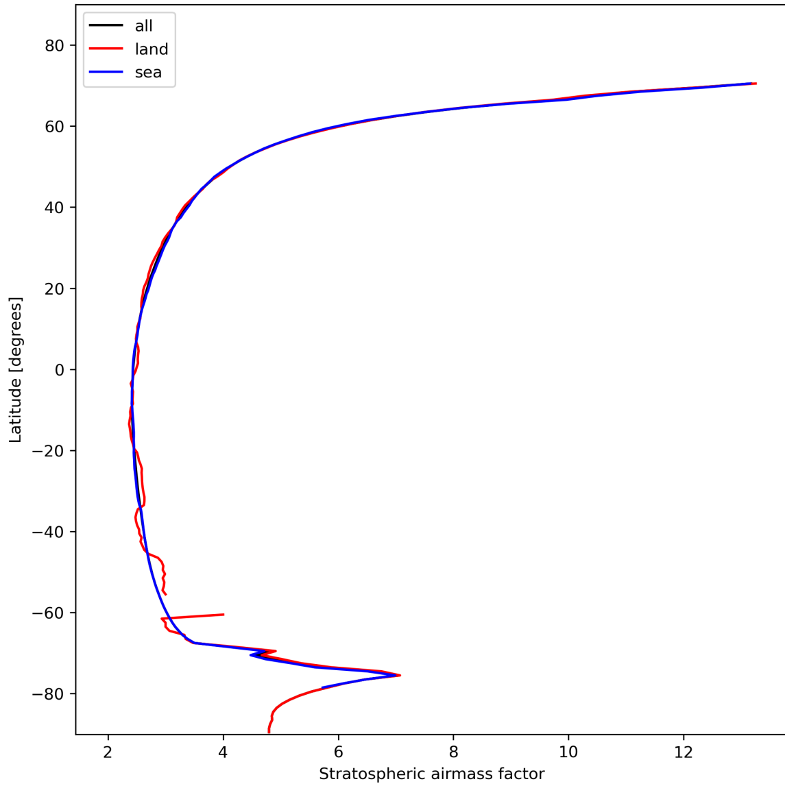
Figure 27: Zonal average of “Stratospheric air mass factor” for 2023-11-09 to 2023-11-11.
