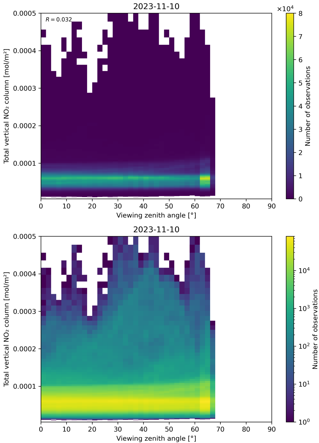
Figure 167: Scatter density plot of “Viewing zenith angle” against “Total vertical NO 2 column” for 2023-11-09 to 2023-11-11.
