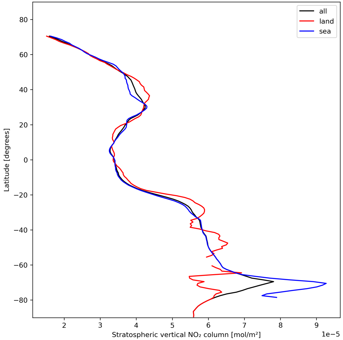
Figure 19: Zonal average of “Stratospheric vertical NO 2 column” for 2023-11-09 to 2023-11-11.
