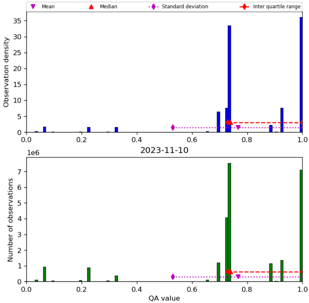
Figure 28: Histogram of “QA value” for 2023-11-09 to 2023-11-11
