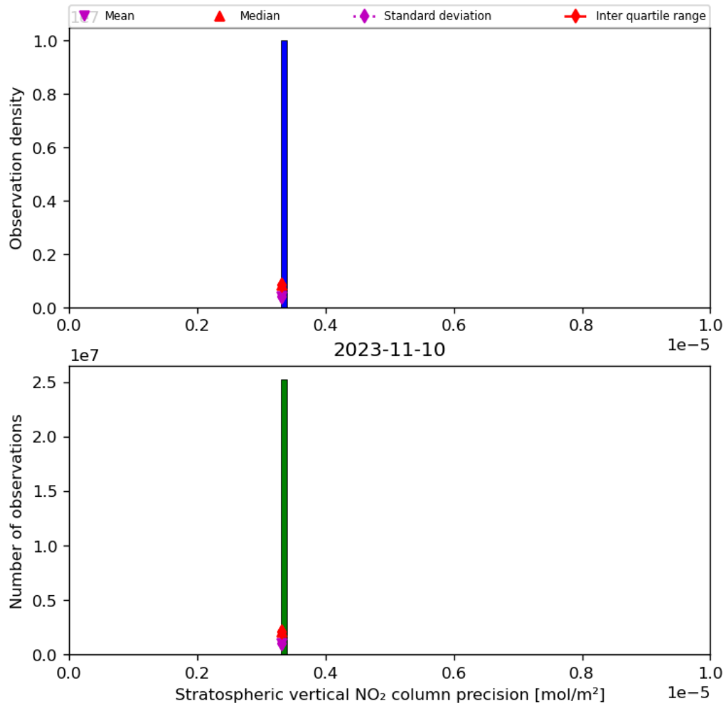
Figure 37: Histogram of “Stratospheric vertical NO 2 column precision” for 2023-11-09 to 2023-11-11
