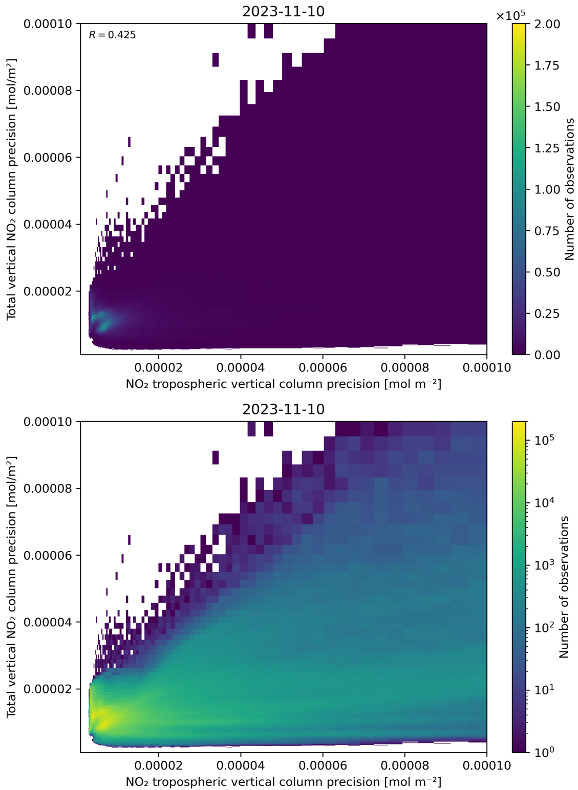
Figure 139: Scatter density plot of “NO 2 tropospheric vertical column precision” against “Total vertical NO 2 column precision” for 2023-11-09 to 2023-11-11.
