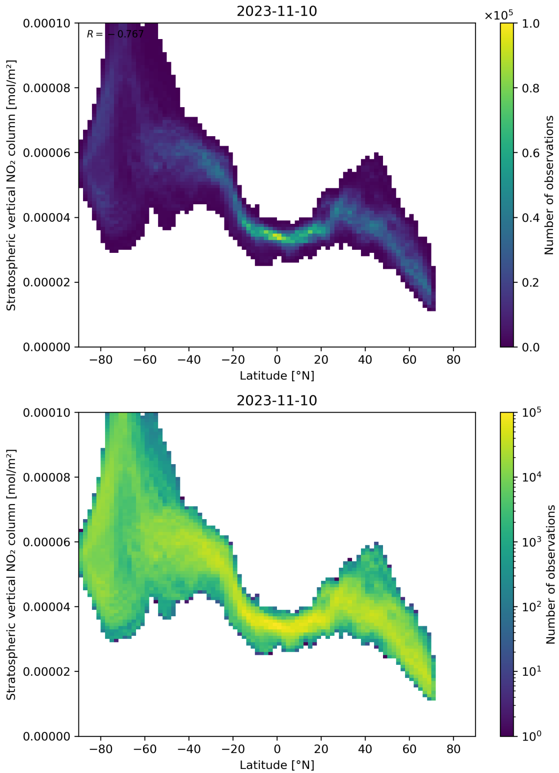
Figure 87: Scatter density plot of “Latitude” against “Stratospheric vertical NO 2 column” for 2023-11-09 to 2023-11-11.
