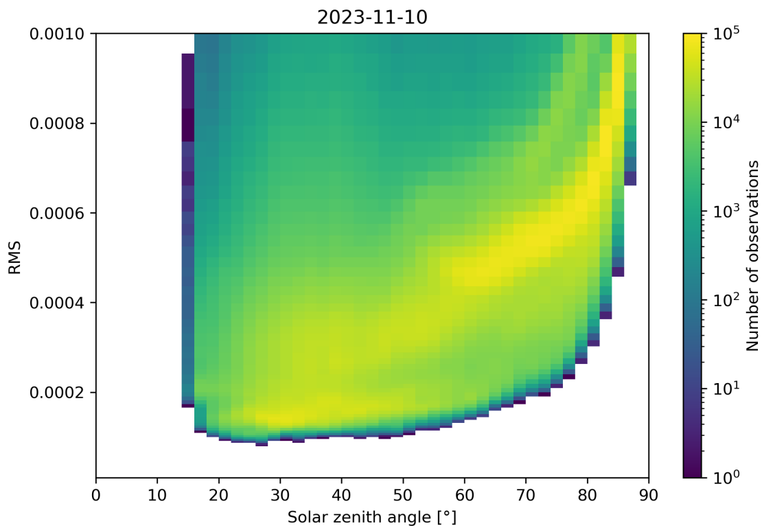
Figure 157: Scatter density plot of “Solar zenith angle” against “RMS” for 2023-11-09 to 2023-11-11.
