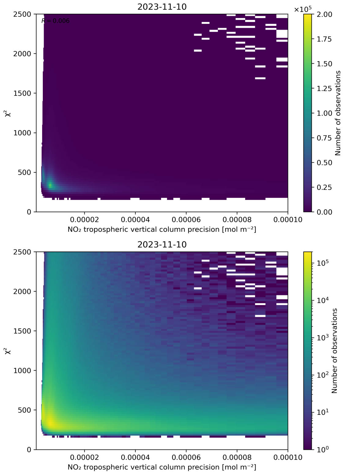
Figure 134: Scatter density plot of “NO 2 tropospheric vertical column precision” against “ \chi^2 ” for 2023-11-09 to 2023-11-11.
