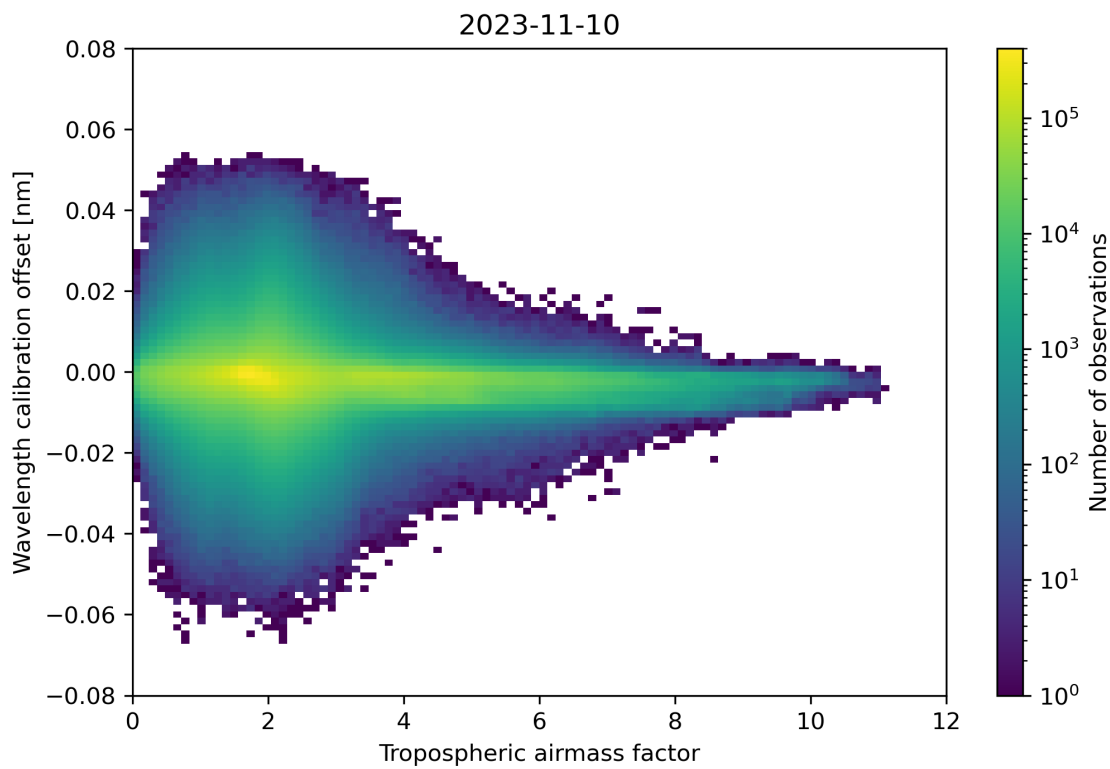
Figure 80: Scatter density plot of “Tropospheric airmass factor” against “Wavelength calibration offset” for 2023-11-09 to 2023-11-11.
