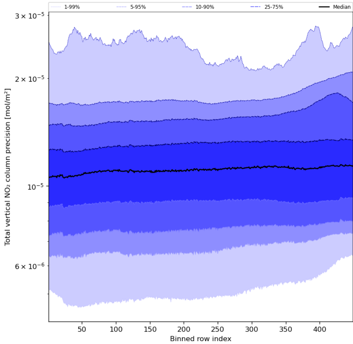
Figure 56: Along track statistics of “Total vertical NO 2 column precision” for 2023-11-09 to 2023-11-11
