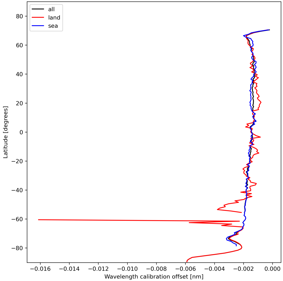
Figure 18: Zonal average of “Wavelength calibration offset” for 2023-11-09 to 2023-11-11.
