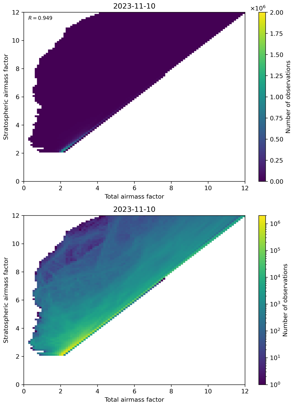
Figure 62: Scatter density plot of “Total airmass factor” against “Stratospheric airmass factor” for 2023-11-09 to 2023-11-11.
