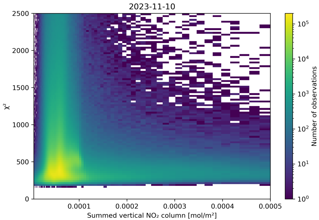
Figure 104: Scatter density plot of “Summed vertical NO 2 column” against “ \chi^2 ” for 2023-11-09 to 2023-11-11.
