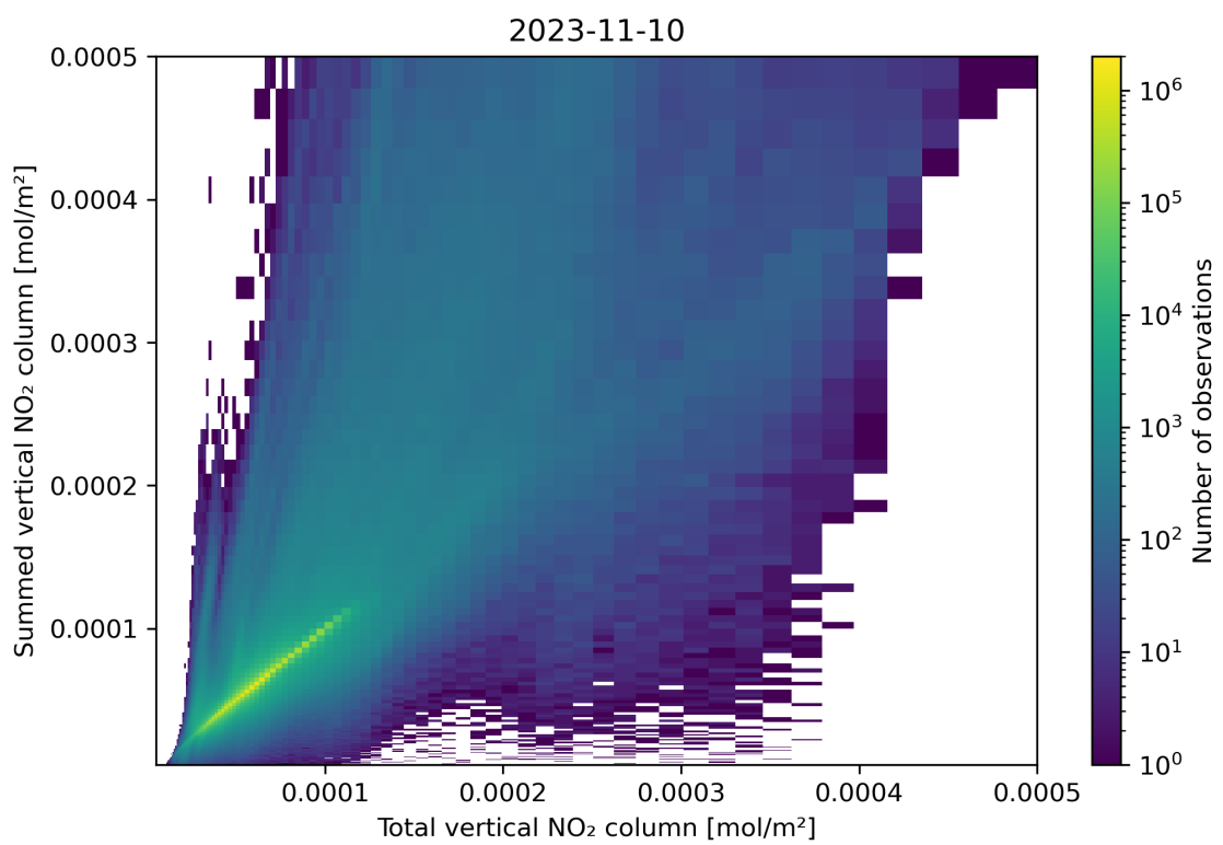
Figure 112: Scatter density plot of “Total vertical NO 2 column” against “Summed vertical NO 2 column” for 2023-11-09 to 2023-11-11.
