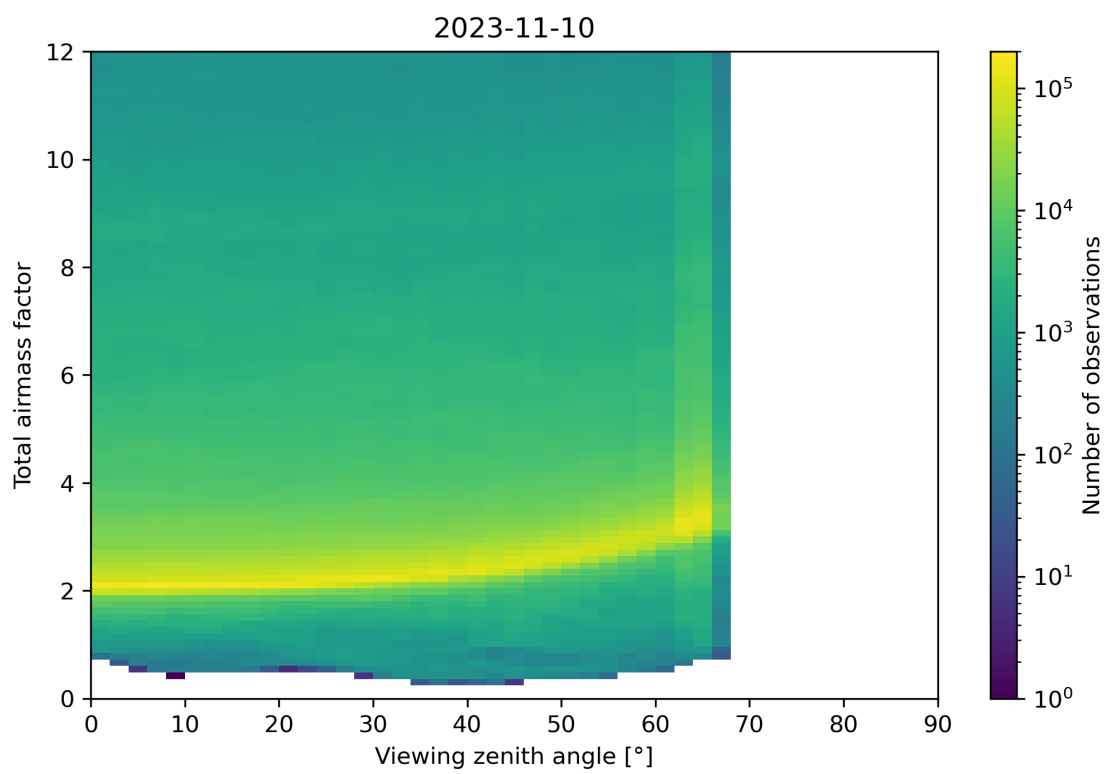
Figure 160: Scatter density plot of “Viewing zenith angle” against “Total airmass factor” for 2023-11-09 to 2023-11-11.
