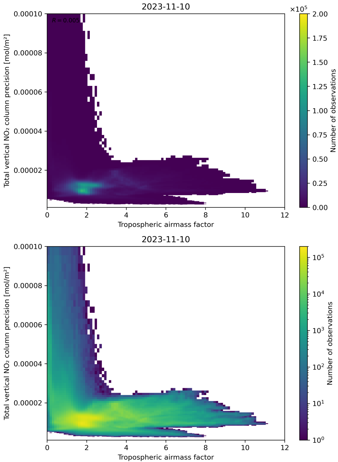
Figure 78: Scatter density plot of “Tropospheric airmass factor” against “Total vertical NO 2 column precision” for 2023-11-09 to 2023-11-11.
