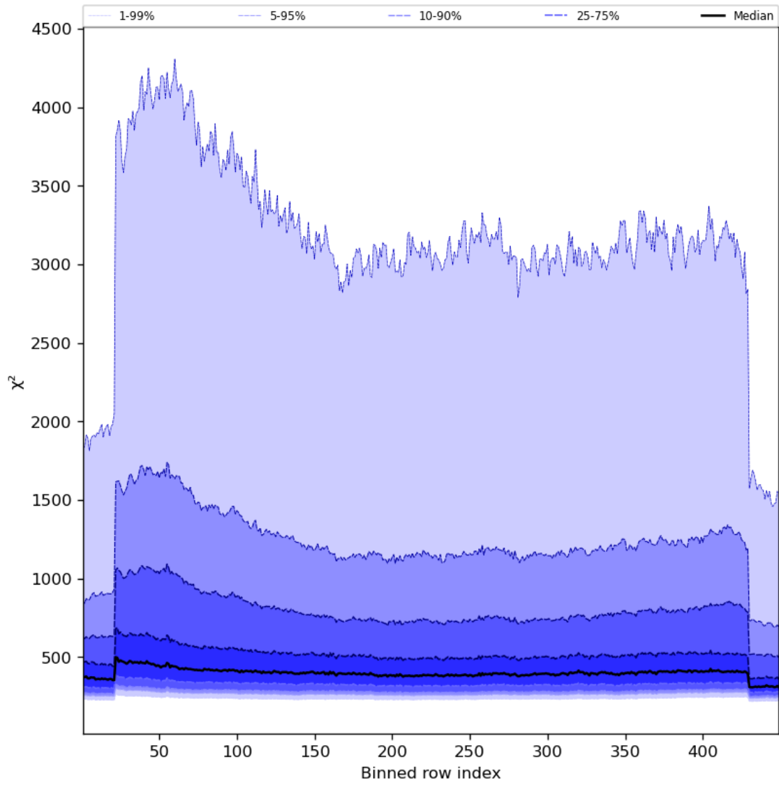
Figure 59: Along track statistics of “ \chi^2 ” for 2023-11-09 to 2023-11-11
