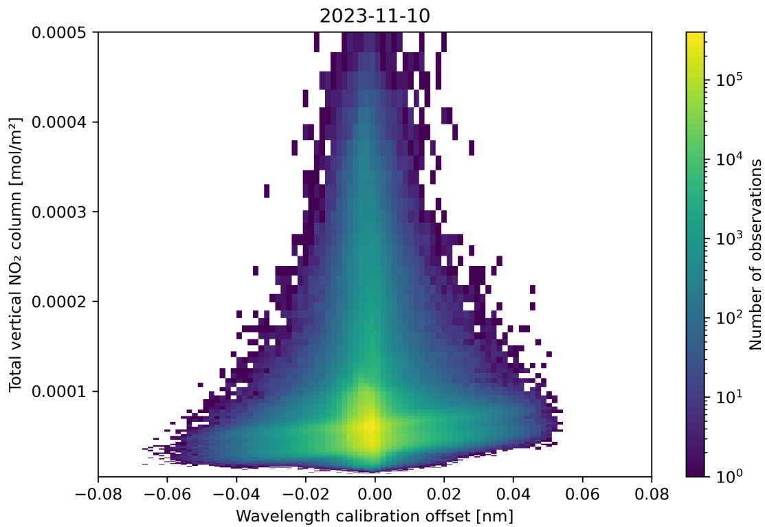
Figure 179: Scatter density plot of “Wavelength calibration offset” against “Total vertical NO 2 column” for 2023-11-09 to 2023-11-11.
