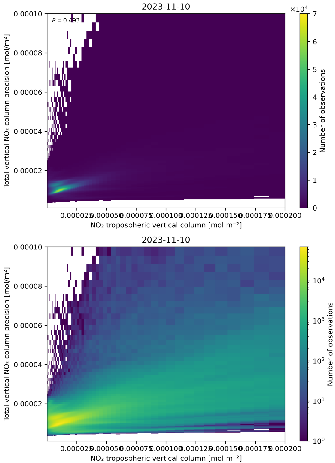
Figure 129: Scatter density plot of “NO 2 tropospheric vertical column” against “Total vertical NO 2 column precision” for 2023-11-09 to 2023-11-11.
