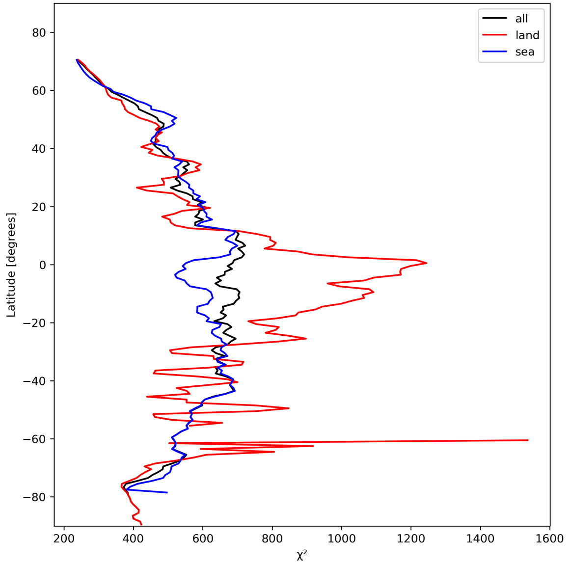
Figure 25: Zonal average of " \chi^2 " for 2023-11-09 to 2023-11-11.
