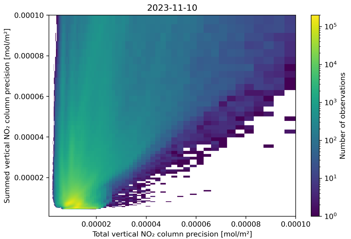
Figure 118: Scatter density plot of “Total vertical NO 2 column precision” against “Summed vertical NO 2 column precision” for 2023-11-09 to 2023-11-11.
