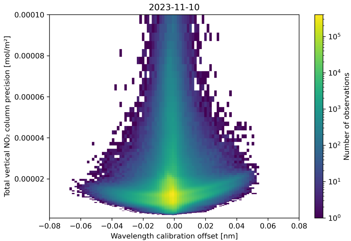
Figure 180: Scatter density plot of “Wavelength calibration offset” against “Total vertical NO 2 column precision” for 2023-11-09 to 2023-11-11.
