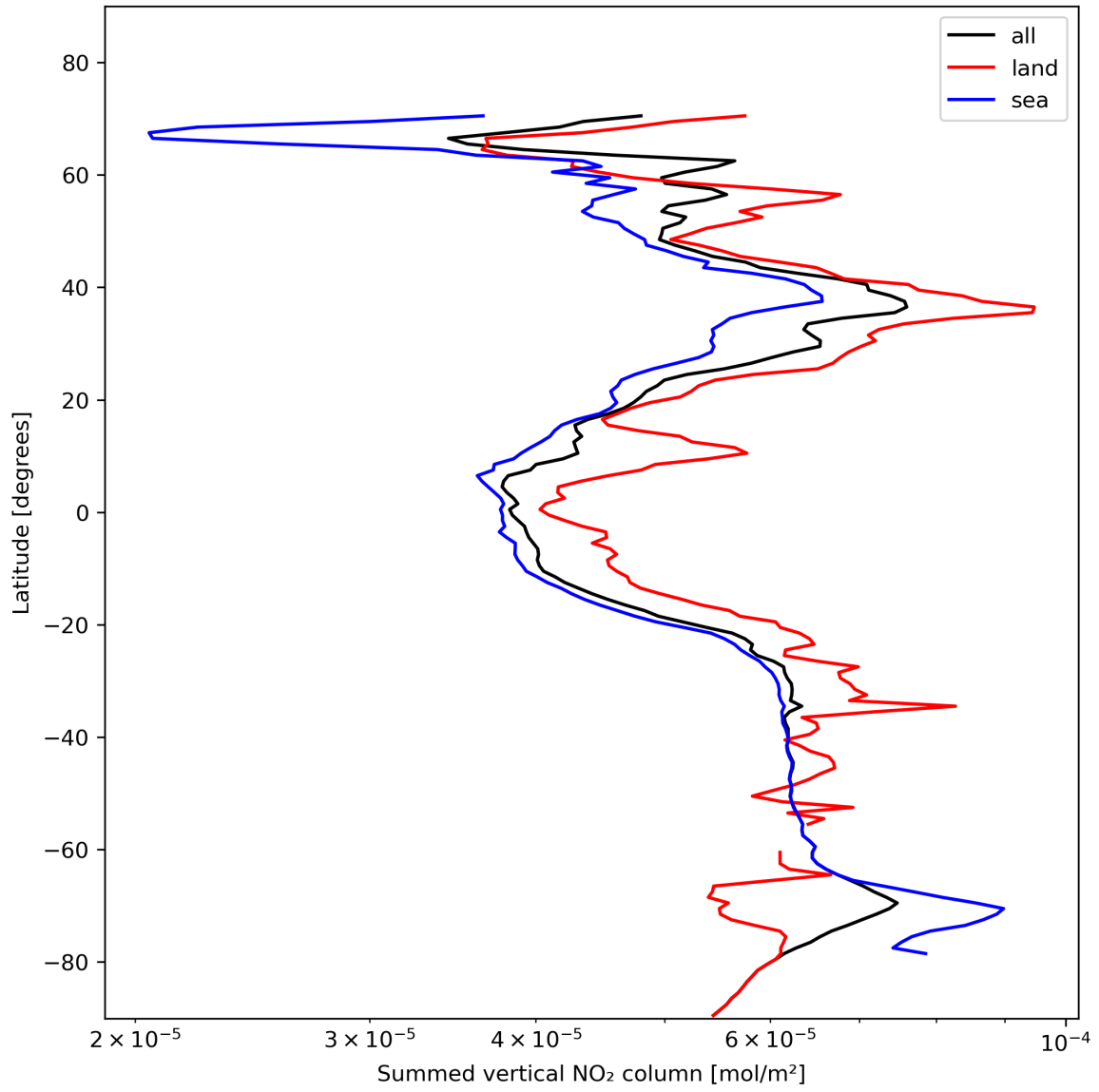
Figure 23: Zonal average of “Summed vertical NO 2 column” for 2023-11-09 to 2023-11-11.
