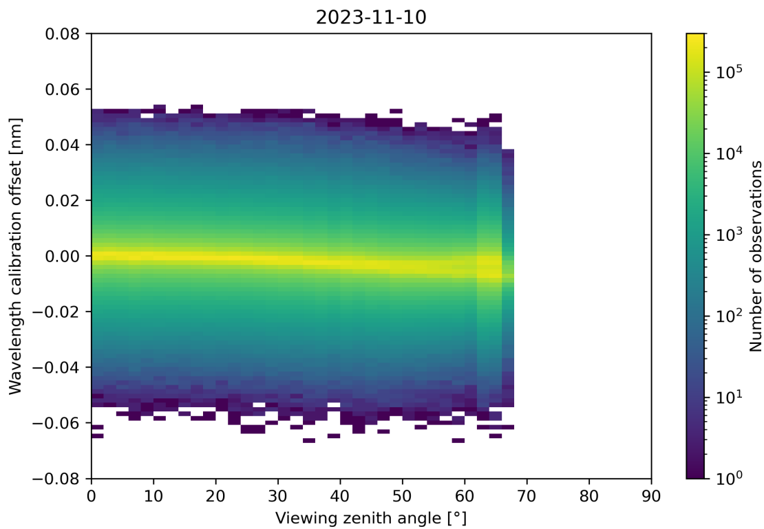
Figure 173: Scatter density plot of “Viewing zenith angle” against “Wavelength calibration offset” for 2023-11-09 to 2023-11-11.
