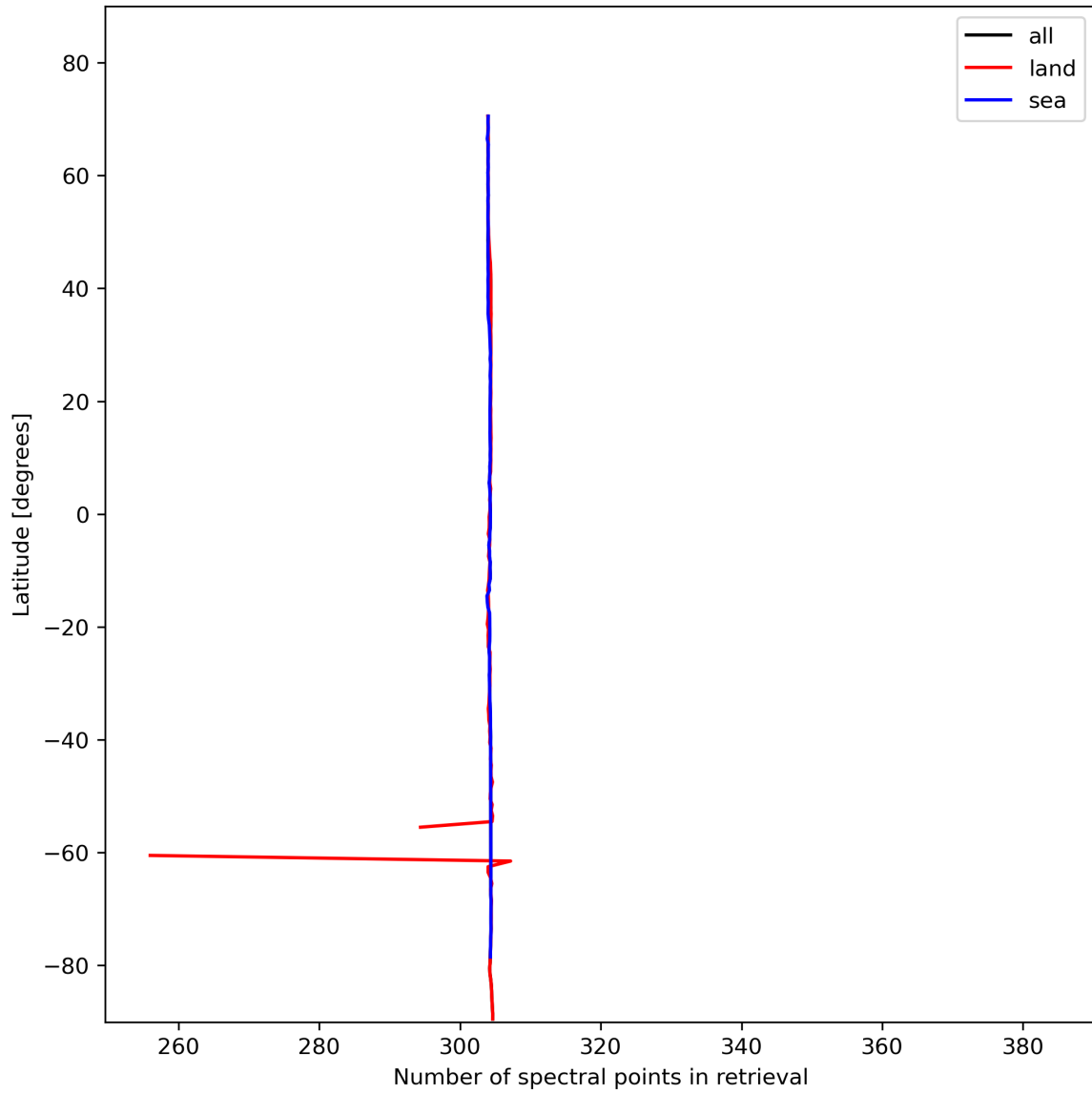
Figure 16: Zonal average of “Number of spectral points in retrieval” for 2023-11-09 to 2023-11-11.
