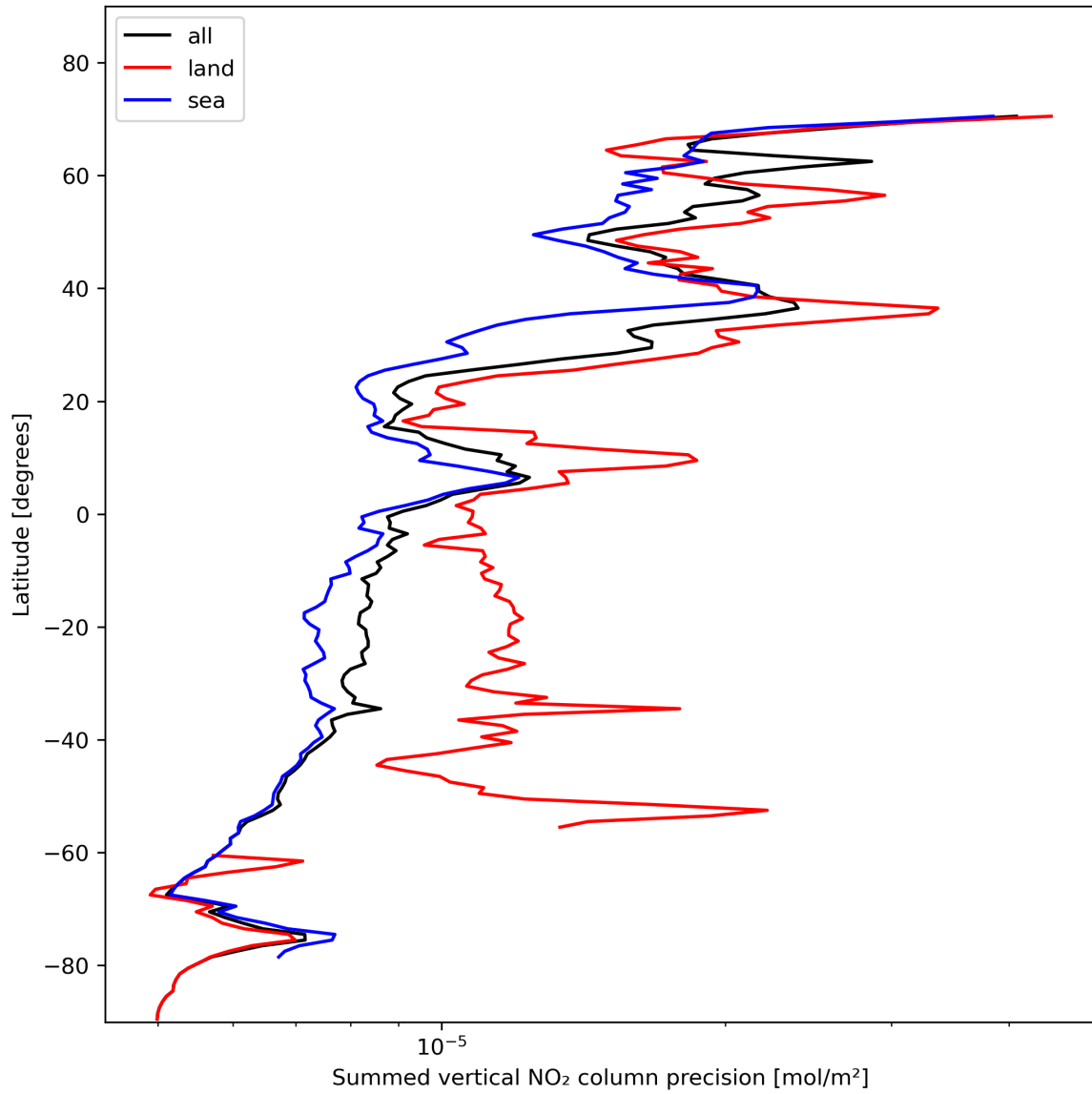
Figure 24: Zonal average of “Summed vertical NO 2 column precision” for 2023-11-09 to 2023-11-11.
