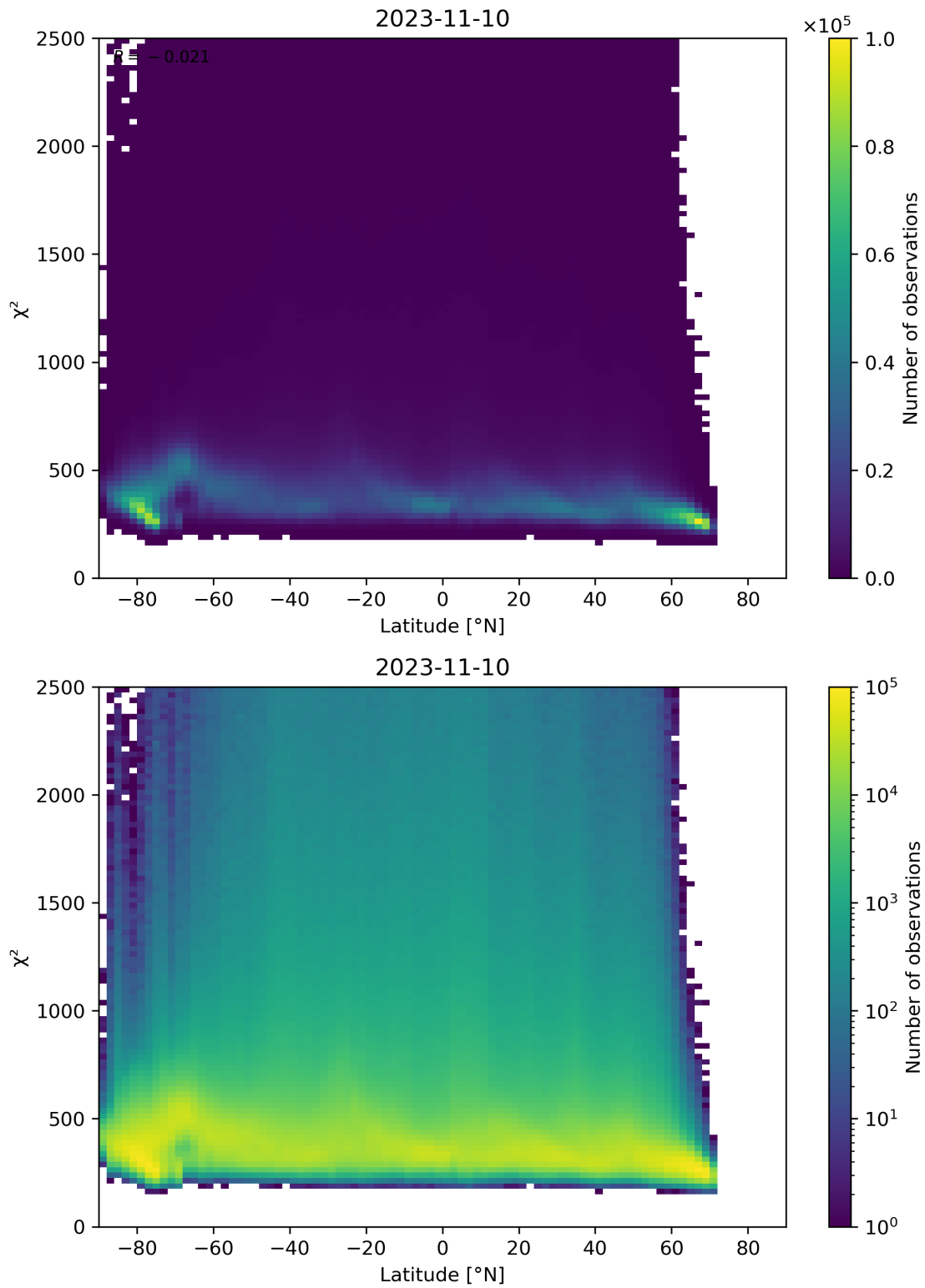
Figure 86: Scatter density plot of “Latitude” against “ \chi^2 ” for 2023-11-09 to 2023-11-11.
