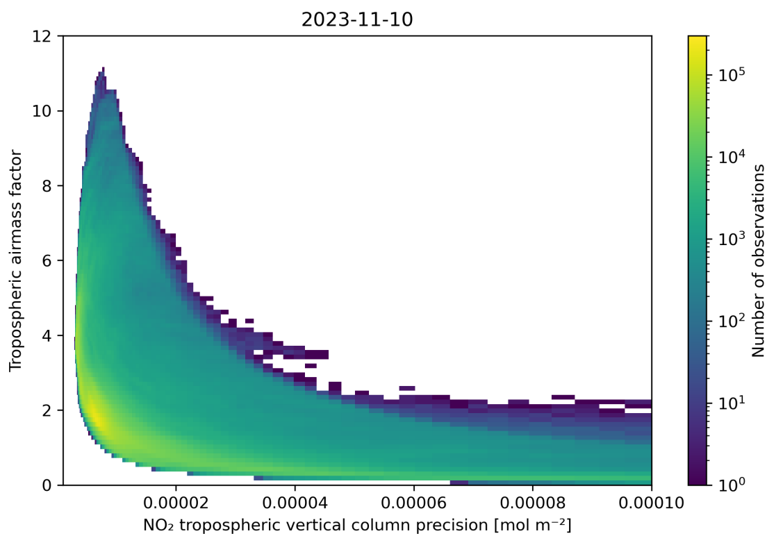
Figure 133: Scatter density plot of “NO 2 tropospheric vertical column precision” against “Tropospheric air mass factor” for 2023-11-09 to 2023-11-11.
