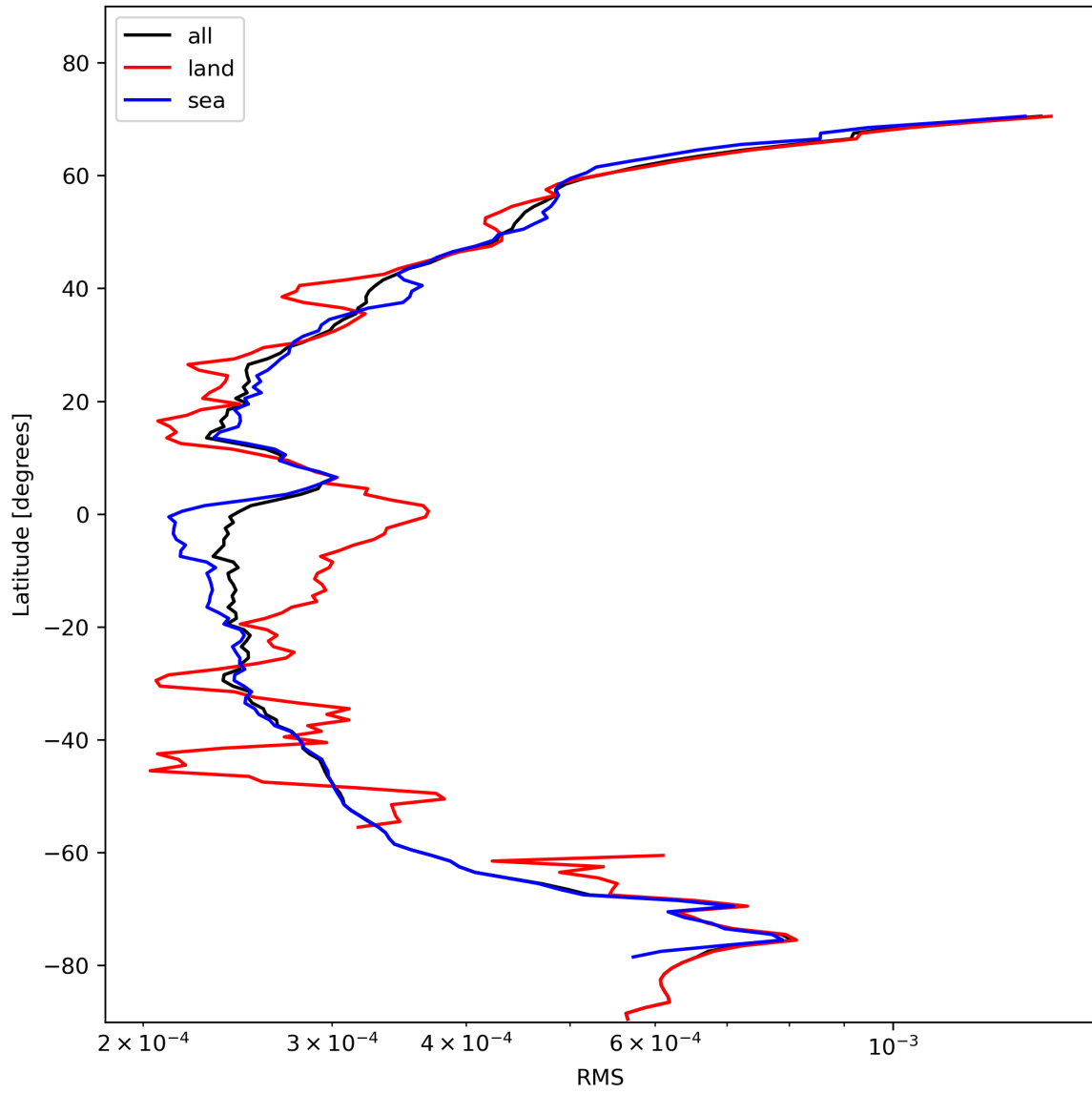
Figure 26: Zonal average of “RMS” for 2023-11-09 to 2023-11-11.
