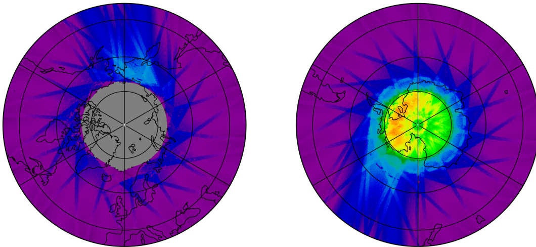
Figure 10: Map of the number of observations for 2023-11-09 to 2023-11-11
