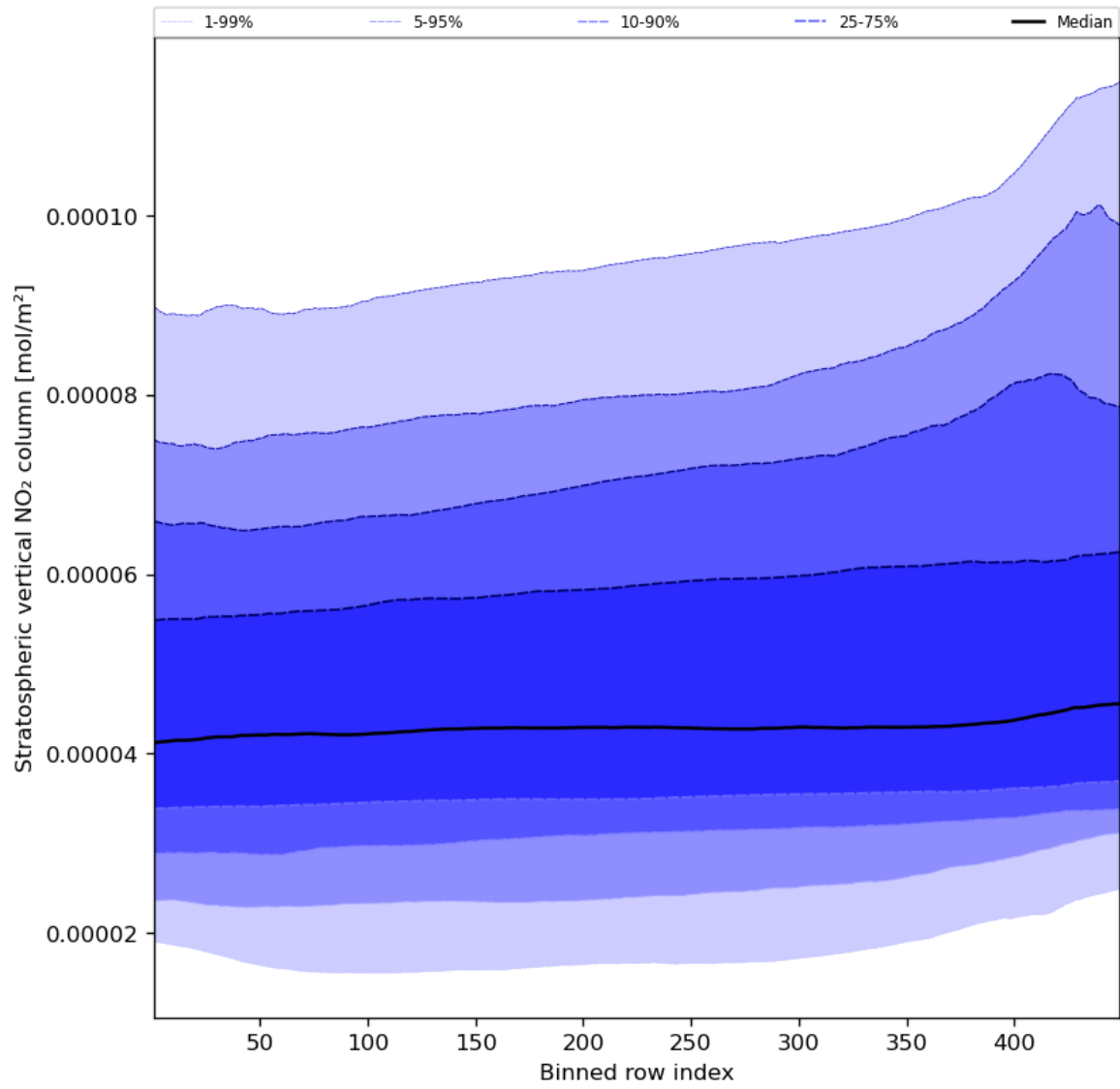
Figure 53: Along track statistics of “Stratospheric vertical NO 2 column” for 2023-11-09 to 2023-11-11
