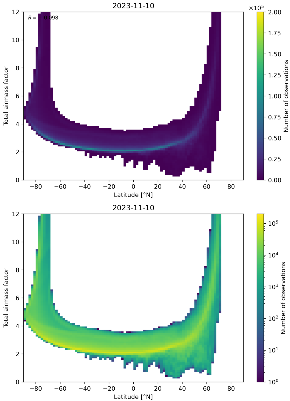
Figure 84: Scatter density plot of “Latitude” against “Total airmass factor” for 2023-11-09 to 2023-11-11.
