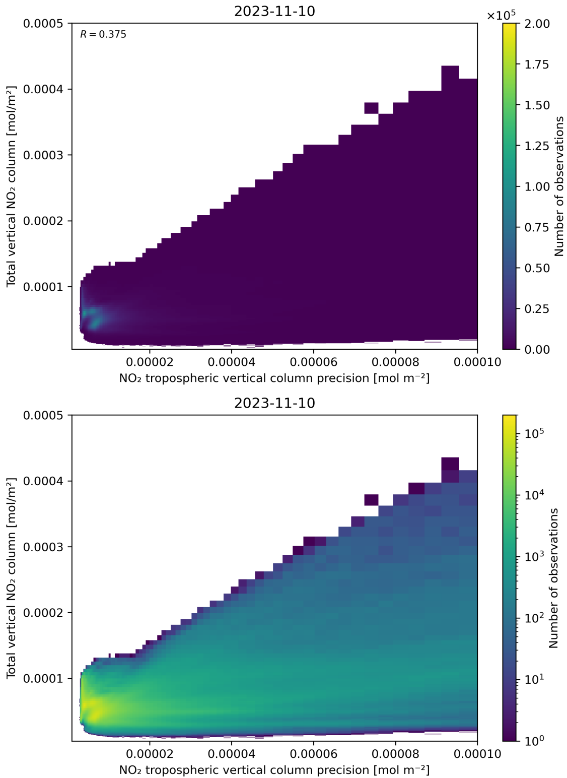
Figure 138: Scatter density plot of “NO 2 tropospheric vertical column precision” against “Total vertical NO 2 column” for 2023-11-09 to 2023-11-11.
