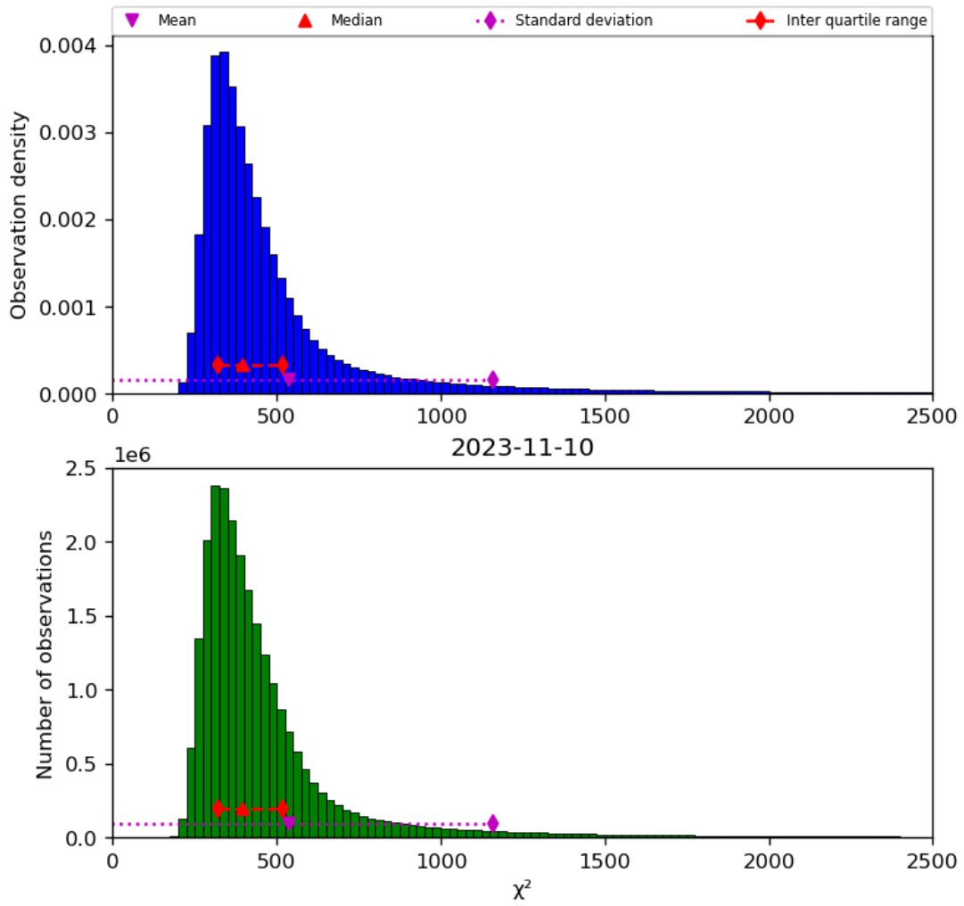
Figure 42: Histogram of “ \chi^2 ” for 2023-11-09 to 2023-11-11
