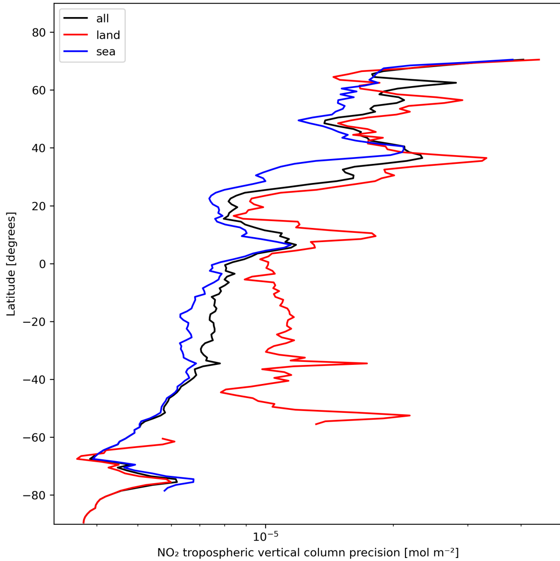
Figure 13: Zonal average of “NO 2 tropospheric vertical column precision” for 2023-11-09 to 2023-11-11.
