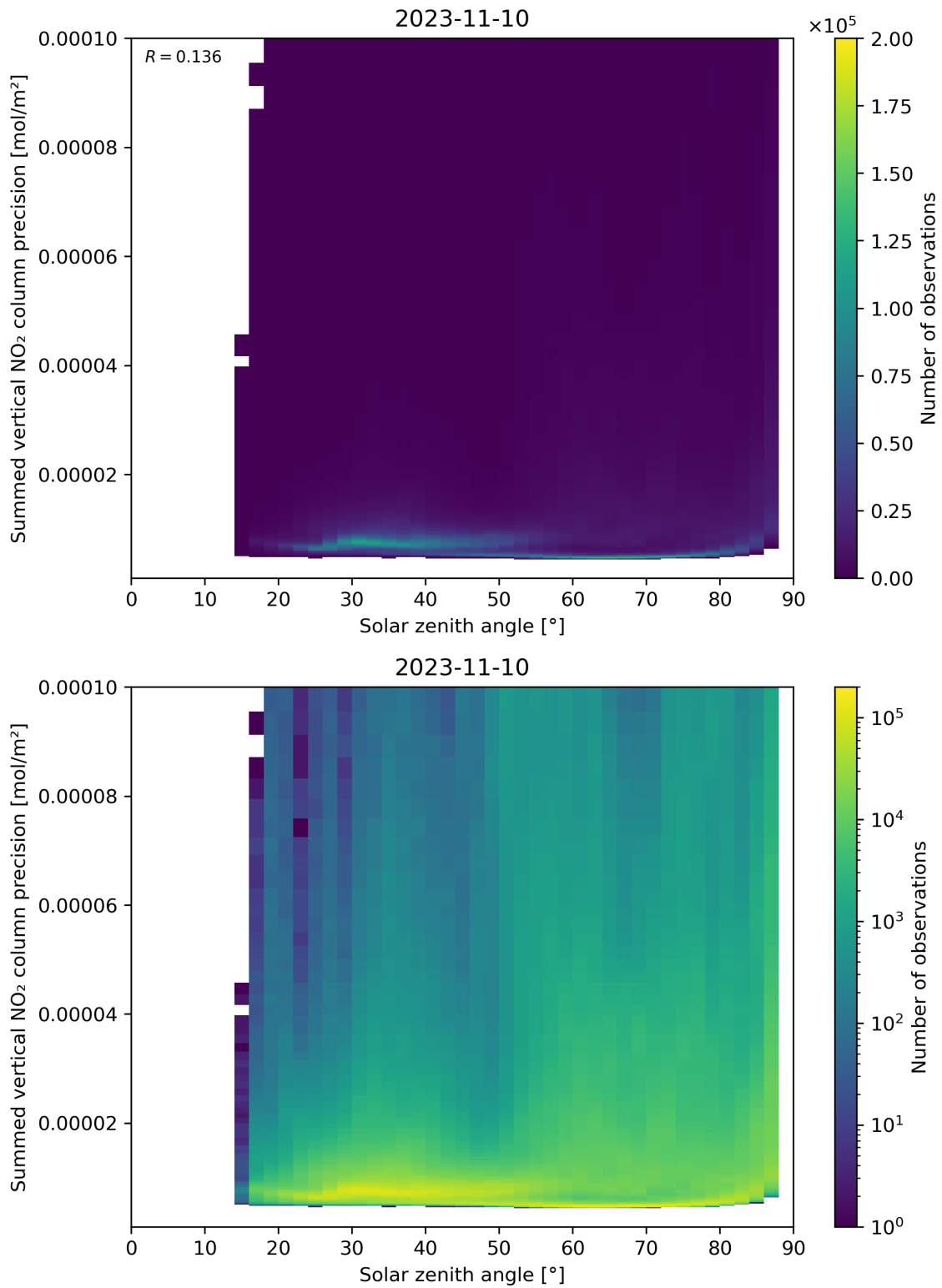
Figure 152: Scatter density plot of “Solar zenith angle” against “Summed vertical NO 2 column precision” for 2023-11-09 to 2023-11-11.
