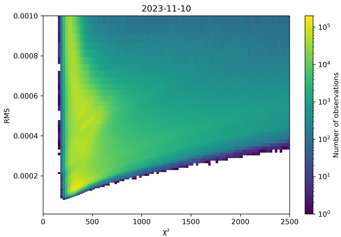
Figure 82: Scatter density plot of " \chi^2 " against "RMS" for 2023-11-09 to 2023-11-11.
