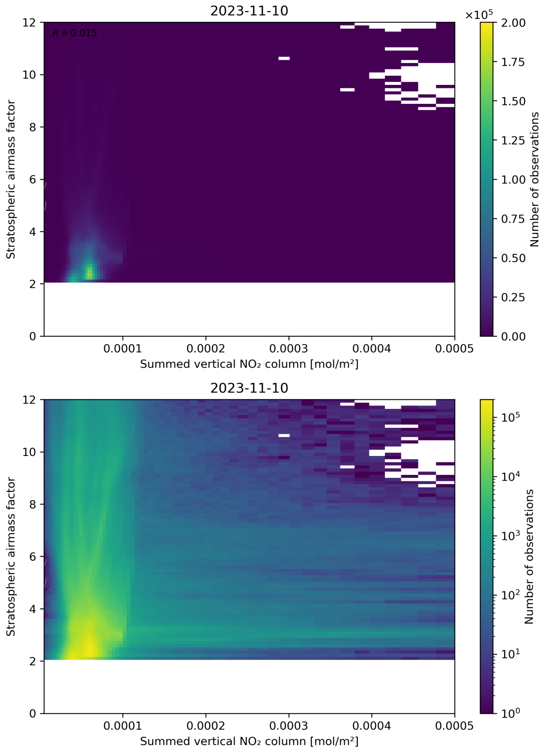
Figure 103: Scatter density plot of “Summed vertical NO 2 column” against “Stratospheric airmass factor” for 2023-11-09 to 2023-11-11.
