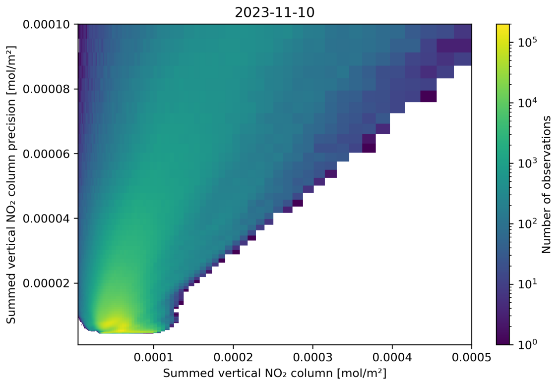
Figure 105: Scatter density plot of “Summed vertical NO 2 column” against “Summed vertical NO 2 column precision” for 2023-11-09 to 2023-11-11.
