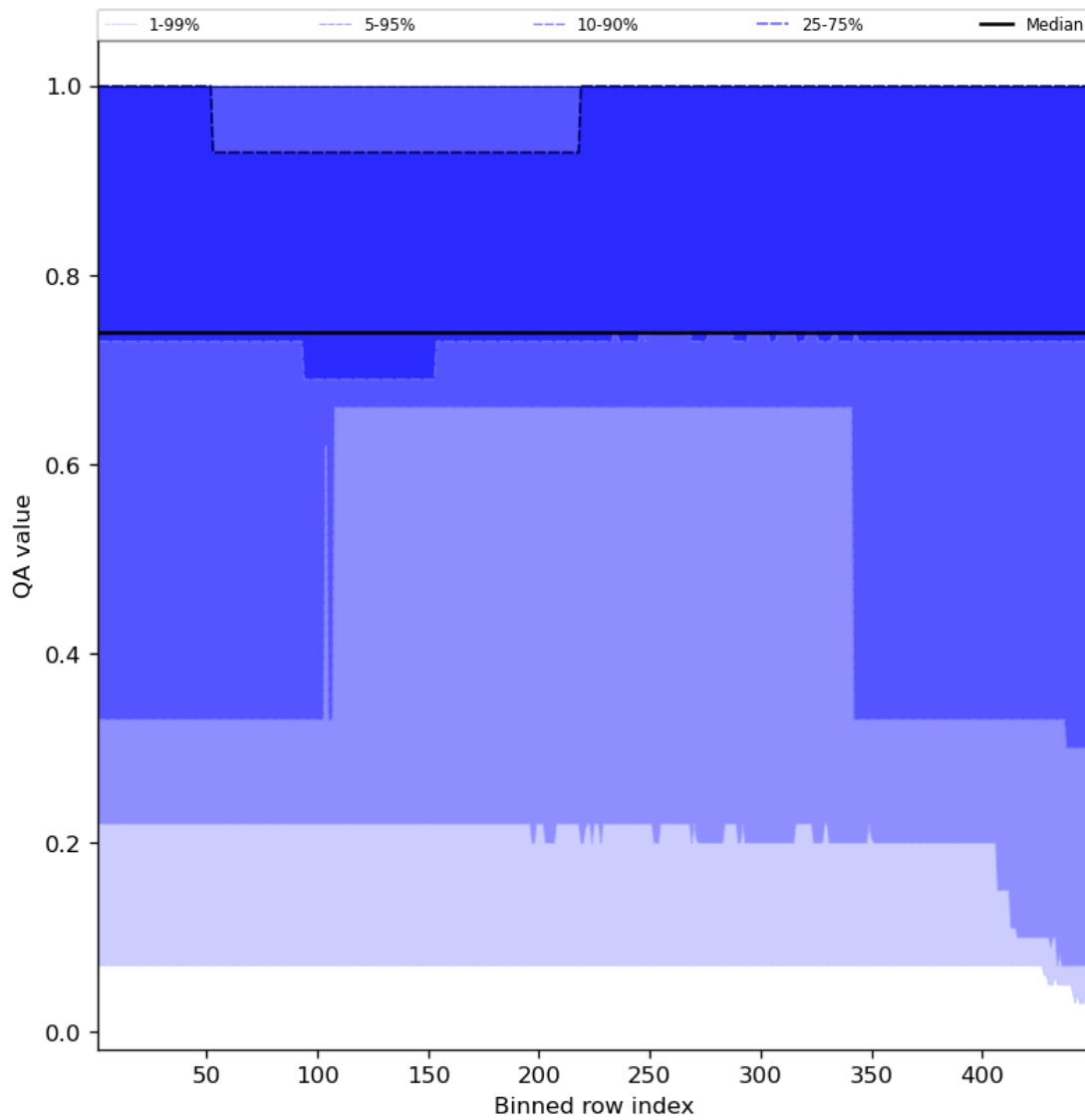
Figure 45: Along track statistics of "QA value" for 2023-11-09 to 2023-11-11
