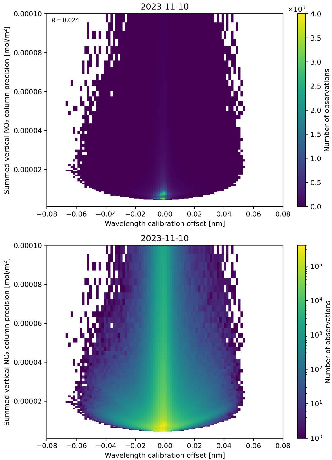
Figure 178: Scatter density plot of “Wavelength calibration offset” against “Summed vertical NO 2 column precision” for 2023-11-09 to 2023-11-11.
