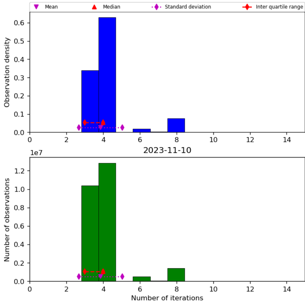
Figure 34: Histogram of “Number of iterations” for 2023-11-09 to 2023-11-11
