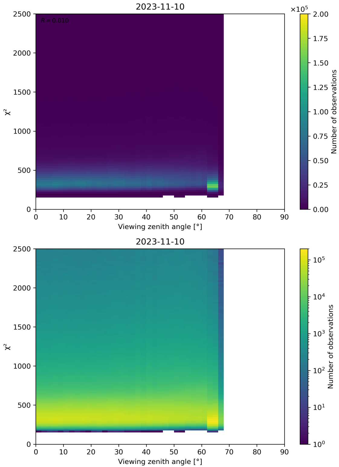
Figure 162: Scatter density plot of “Viewing zenith angle” against “ \chi^2 ” for 2023-11-09 to 2023-11-11.
