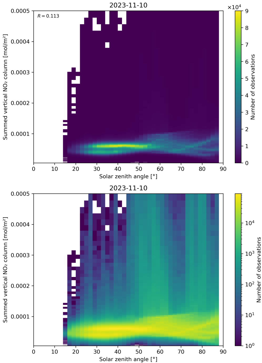
Figure 151: Scatter density plot of “Solar zenith angle” against “Summed vertical NO 2 column” for 2023-11-09 to 2023-11-11.
