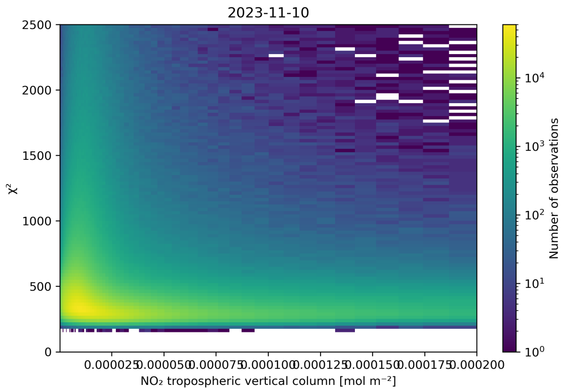
Figure 124: Scatter density plot of “NO 2 tropospheric vertical column” against “ \chi^2 ” for 2023-11-09 to 2023-11-11.
