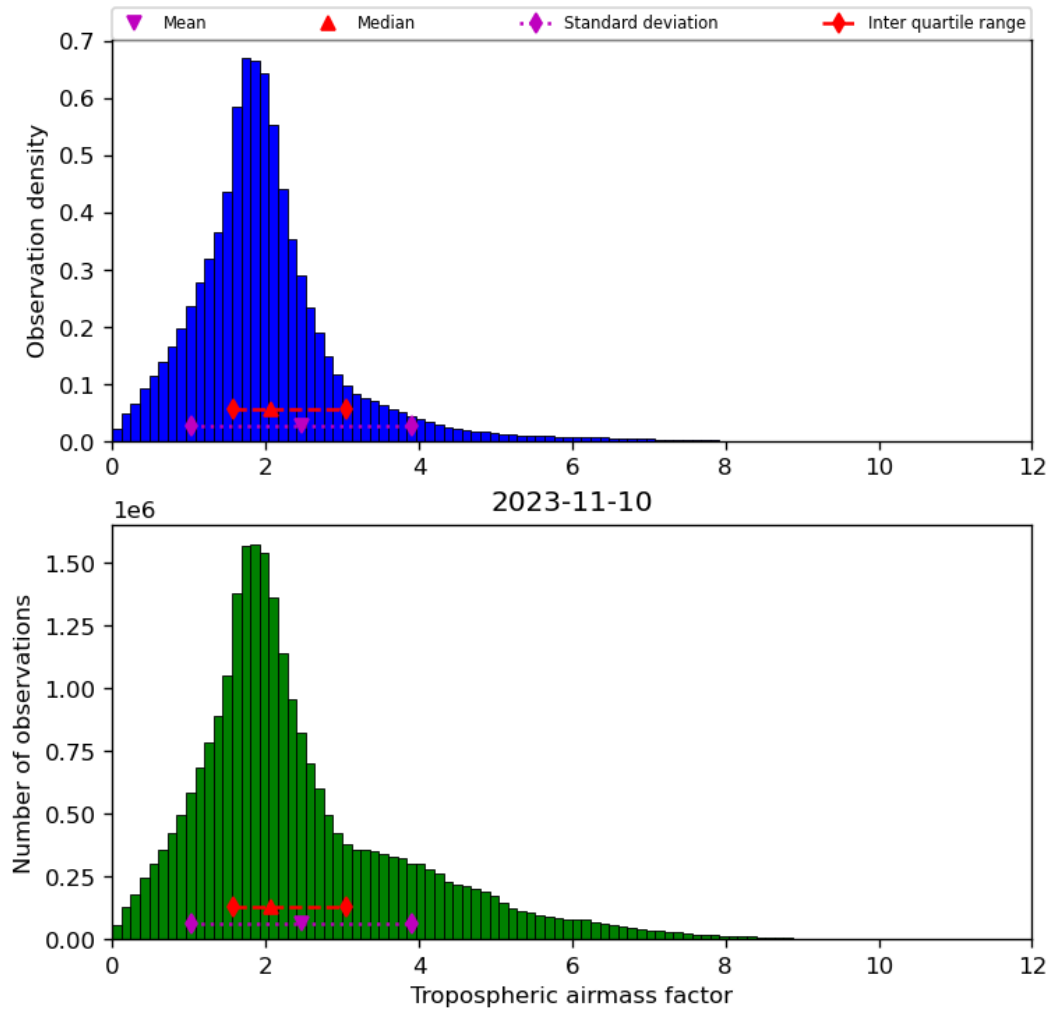
Figure 31: Histogram of “Tropospheric airmass factor” for 2023-11-09 to 2023-11-11
