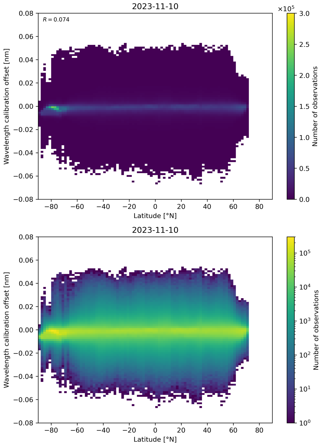
Figure 95: Scatter density plot of “Latitude” against “Wavelength calibration offset” for 2023-11-09 to 2023-11-11.
