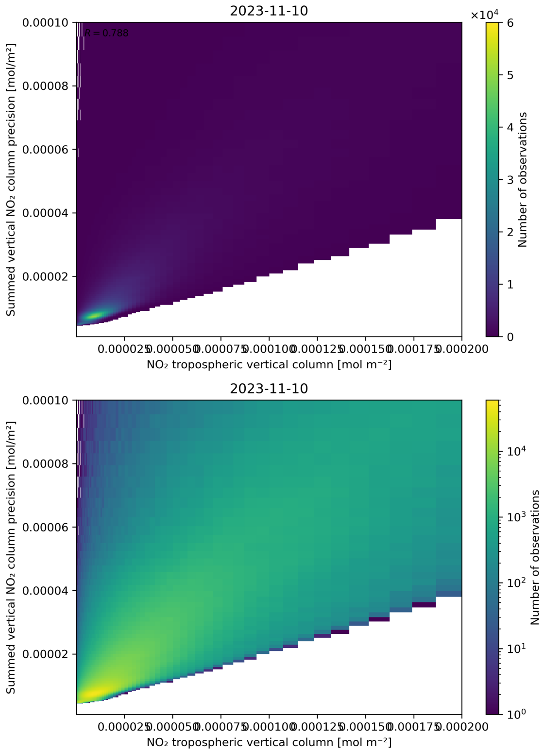
Figure 127: Scatter density plot of “NO 2 tropospheric vertical column” against “Summed vertical NO 2 column precision” for 2023-11-09 to 2023-11-11.
