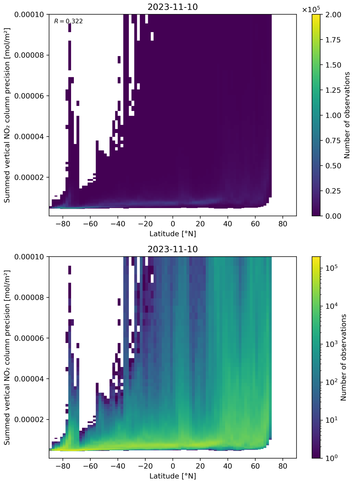
Figure 89: Scatter density plot of “Latitude” against “Summed vertical NO 2 column precision” for 2023-11-09 to 2023-11-11.
