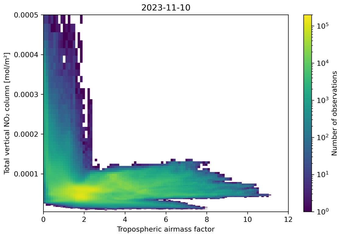
Figure 77: Scatter density plot of “Tropospheric airmass factor” against “Total vertical NO 2 column” for 2023-11-09 to 2023-11-11.
