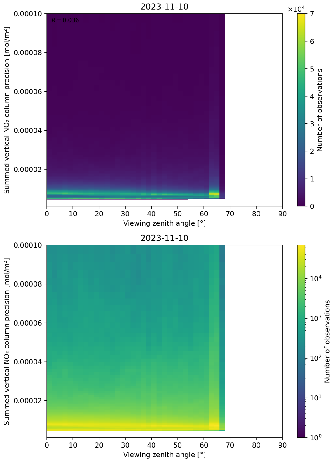
Figure 166: Scatter density plot of “Viewing zenith angle” against “Summed vertical NO 2 column precision” for 2023-11-09 to 2023-11-11.
