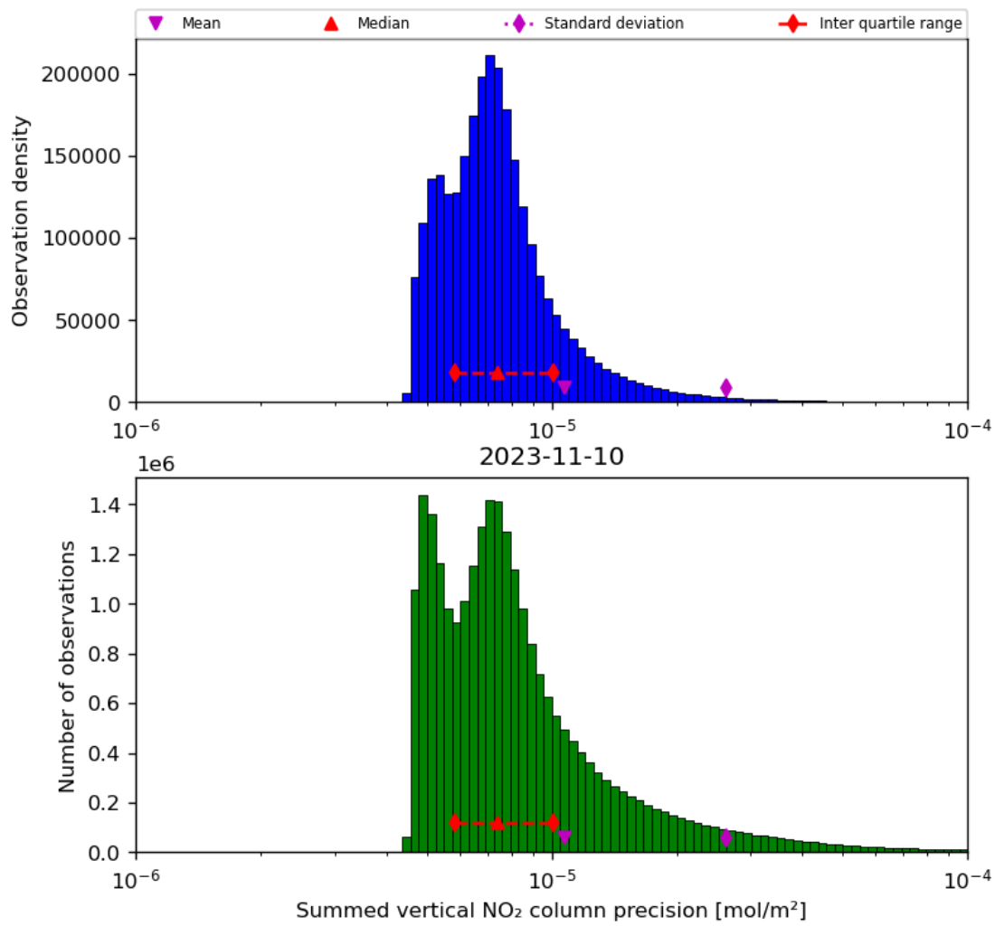
Figure 41: Histogram of “Summed vertical NO 2 column precision” for 2023-11-09 to 2023-11-11
