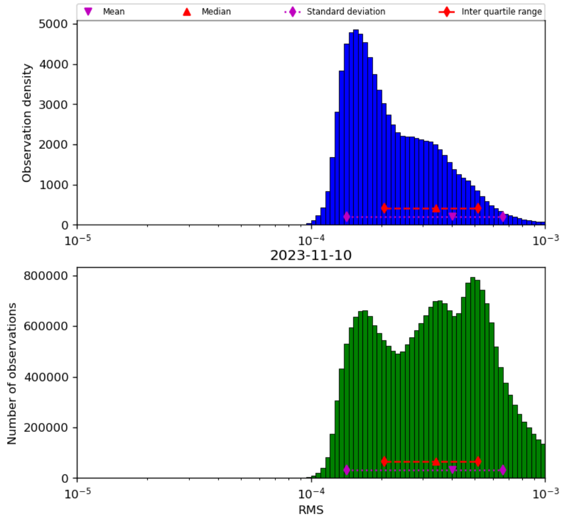
Figure 43: Histogram of “RMS” for 2023-11-09 to 2023-11-11
