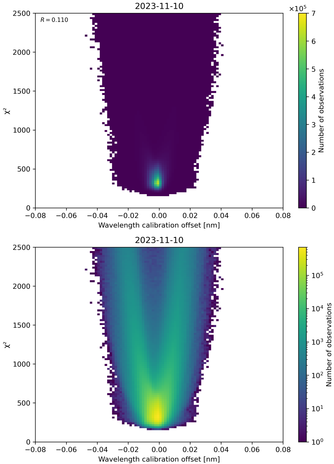
Figure 175: Scatter density plot of “Wavelength calibration offset” against “ \chi^2 ” for 2023-11-09 to 2023-11-11.
