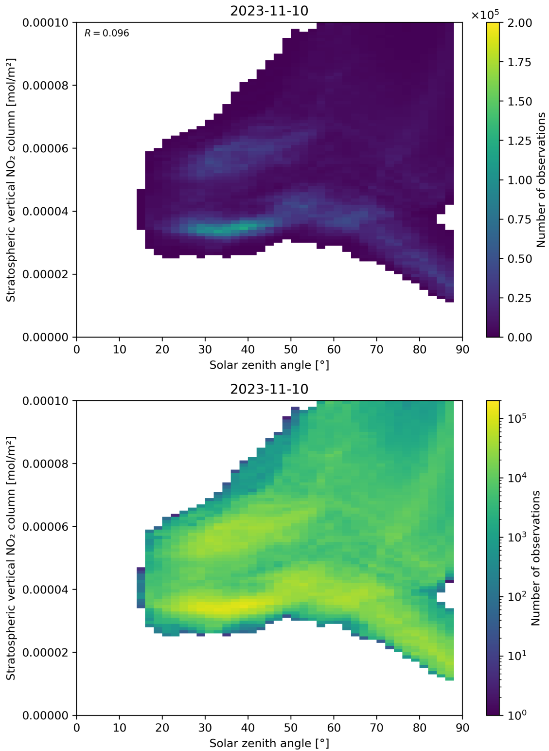
Figure 150: Scatter density plot of “Solar zenith angle” against “Stratospheric vertical NO 2 column” for 2023-11-09 to 2023-11-11.
