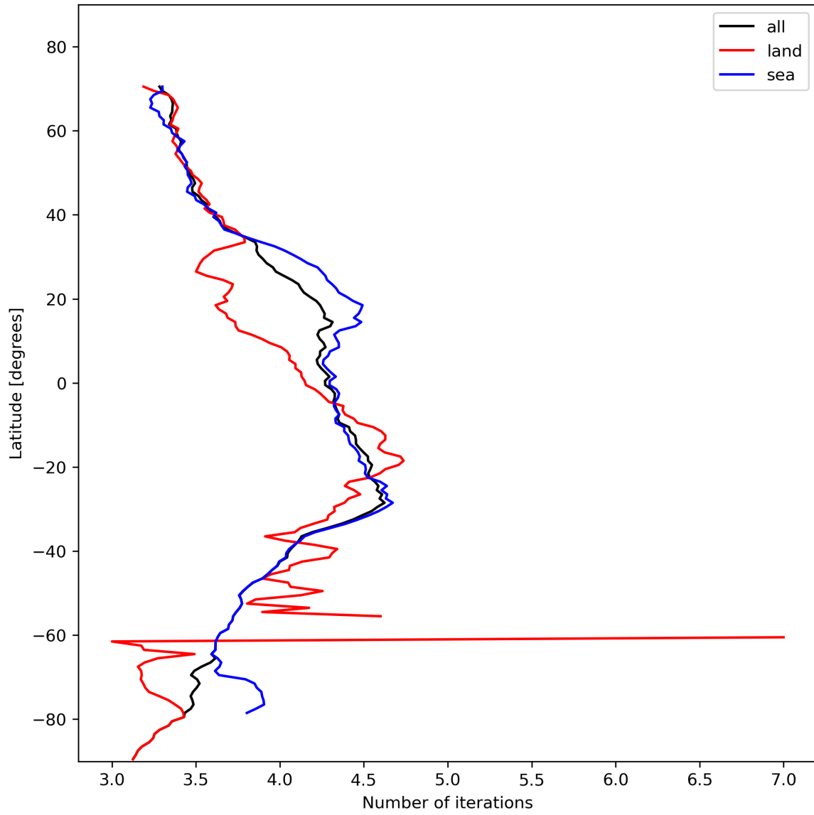
Figure 17: Zonal average of “Number of iterations” for 2023-11-09 to 2023-11-11.
