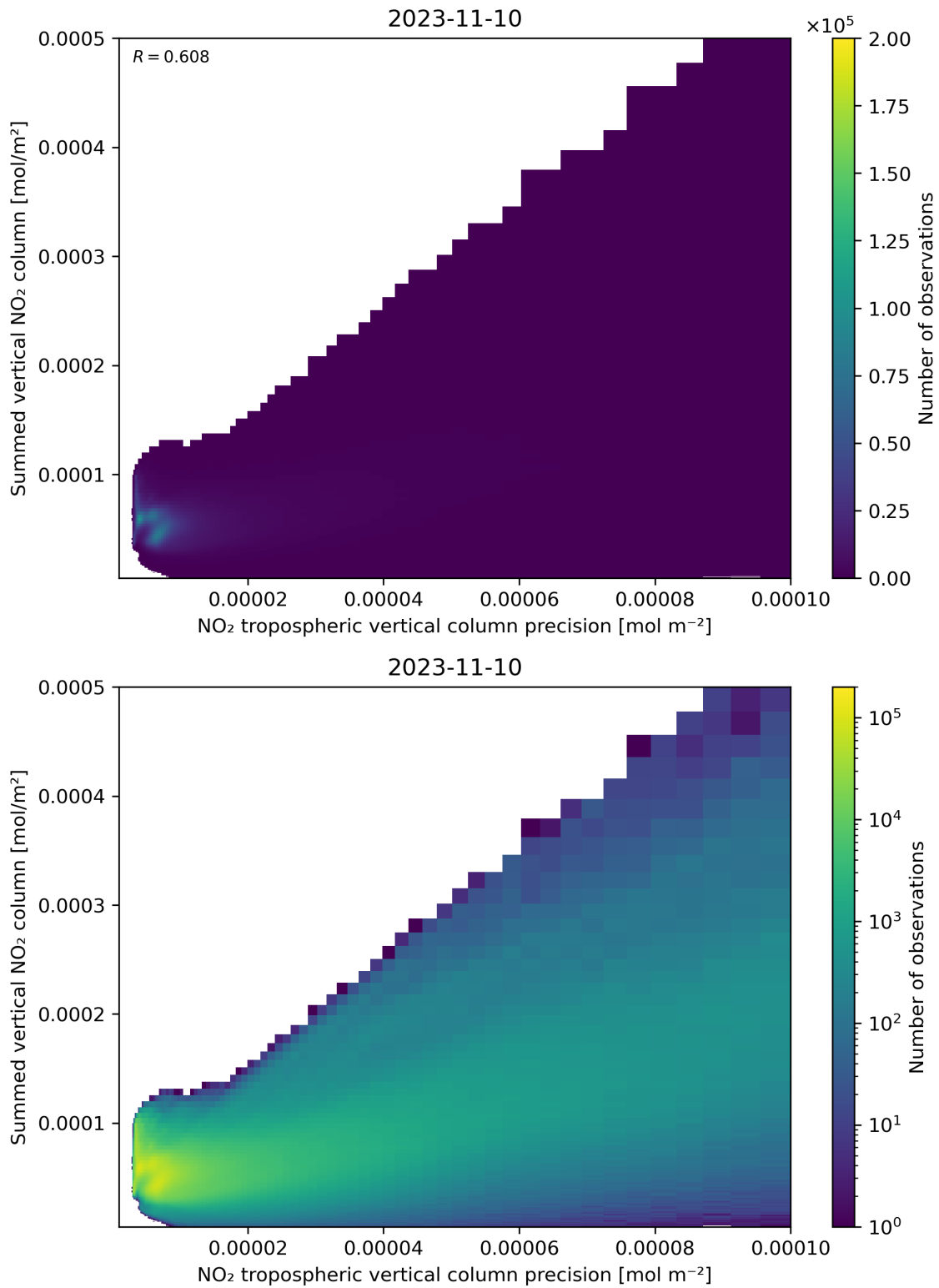
Figure 136: Scatter density plot of “NO 2 tropospheric vertical column precision” against “Summed vertical NO 2 column” for 2023-11-09 to 2023-11-11.
