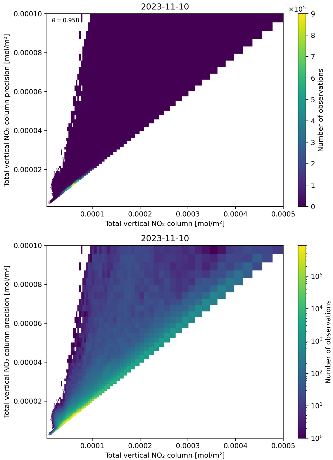
Figure 114: Scatter density plot of “Total vertical NO 2 column” against “Total vertical NO 2 column precision” for 2023-11-09 to 2023-11-11.
