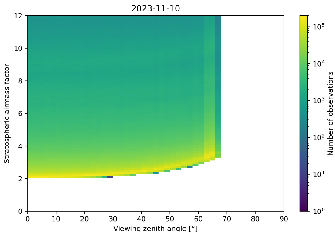
Figure 159: Scatter density plot of “Viewing zenith angle” against “Stratospheric airmass factor” for 2023-11-09 to 2023-11-11.
