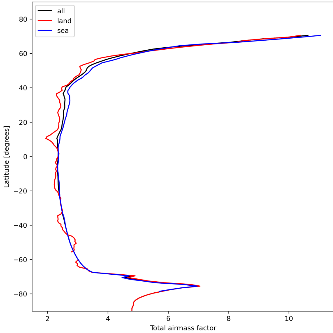
Figure 15: Zonal average of “Total airmass factor” for 2023-11-09 to 2023-11-11.
