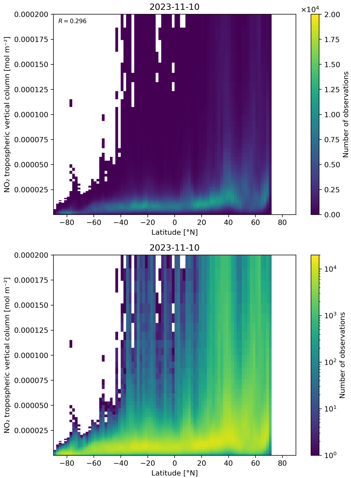
Figure 92: Scatter density plot of “Latitude” against “NO 2 tropospheric vertical column” for 2023-11-09 to 2023-11-11.
