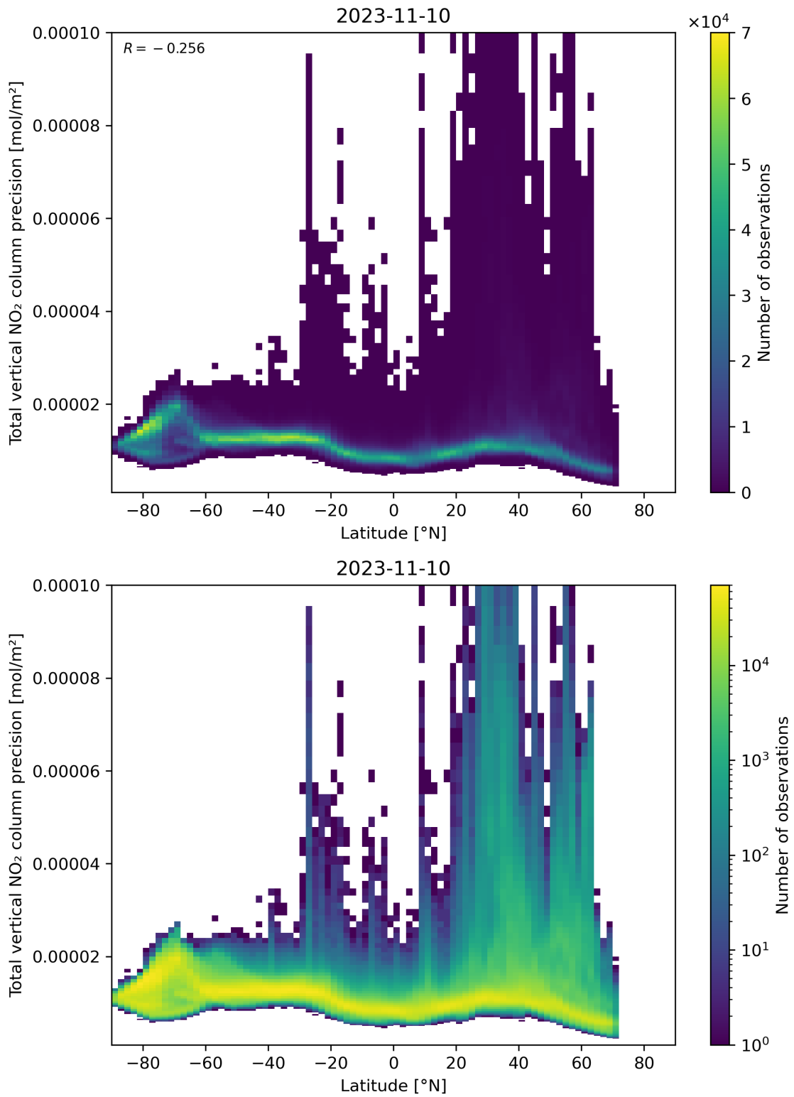
Figure 91: Scatter density plot of “Latitude” against “Total vertical NO 2 column precision” for 2023-11-09 to 2023-11-11.
