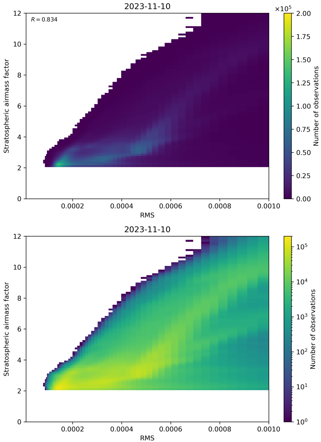
Figure 144: Scatter density plot of “RMS” against “Stratospheric airmass factor” for 2023-11-09 to 2023-11-11.
