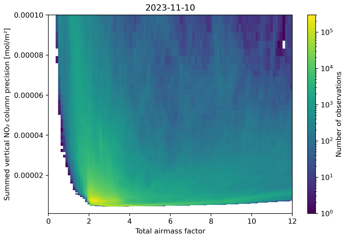
Figure 66: Scatter density plot of “Total airmass factor” against “Summed vertical NO 2 column precision” for 2023-11-09 to 2023-11-11.
