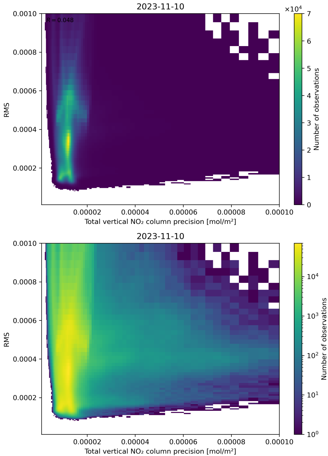
Figure 119: Scatter density plot of “Total vertical NO 2 column precision” against “RMS” for 2023-11-09 to 2023-11-11.
