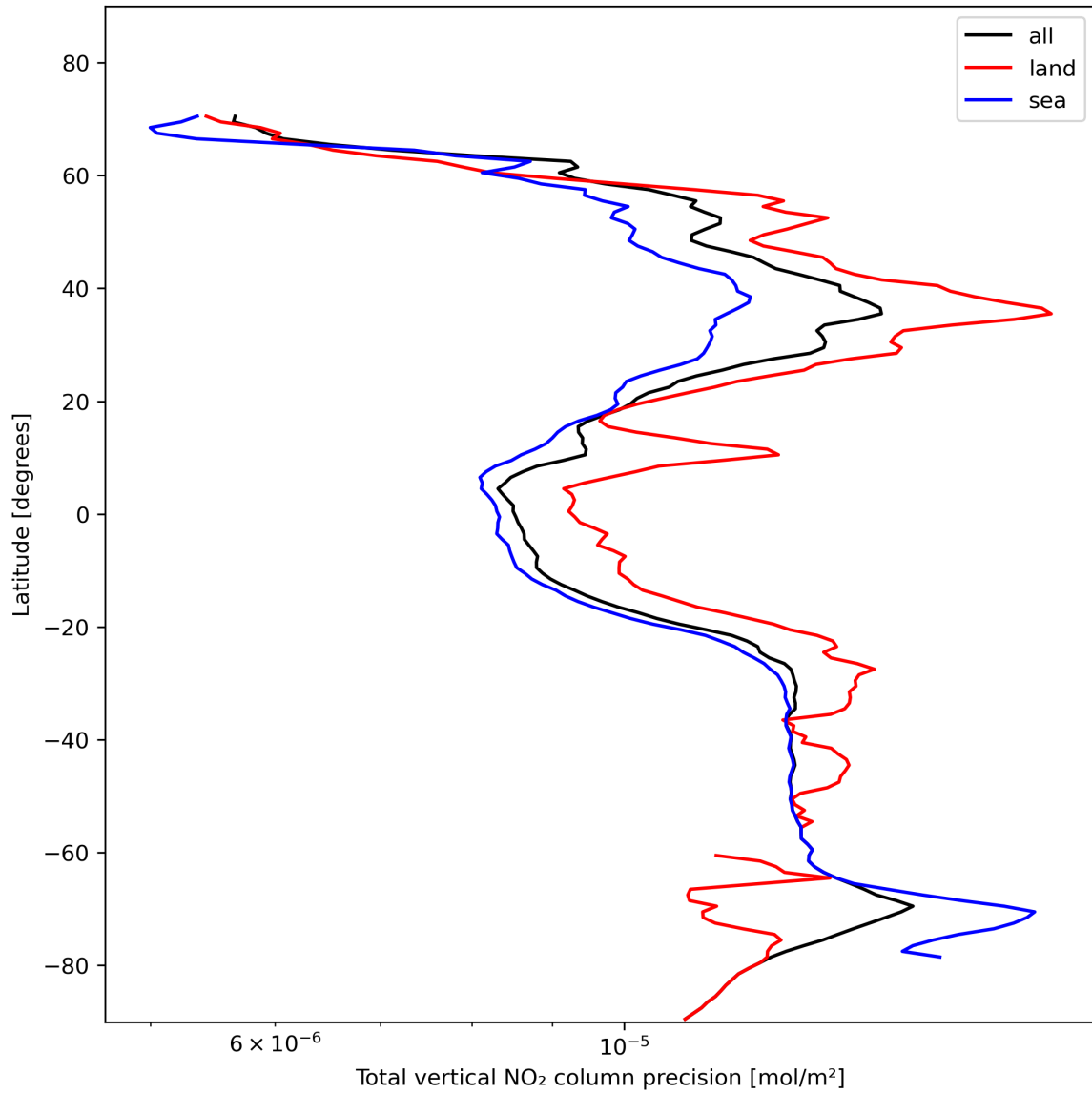
Figure 22: Zonal average of “Total vertical NO 2 column precision” for 2023-11-09 to 2023-11-11.
