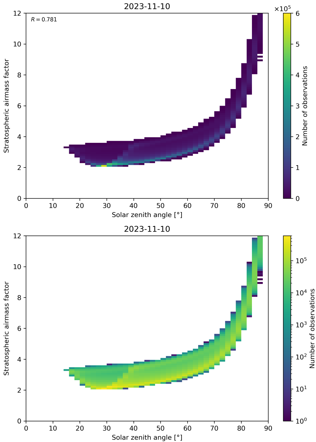
Figure 145: Scatter density plot of “Solar zenith angle” against “Stratospheric airmass factor” for 2023-11-09 to 2023-11-11.
