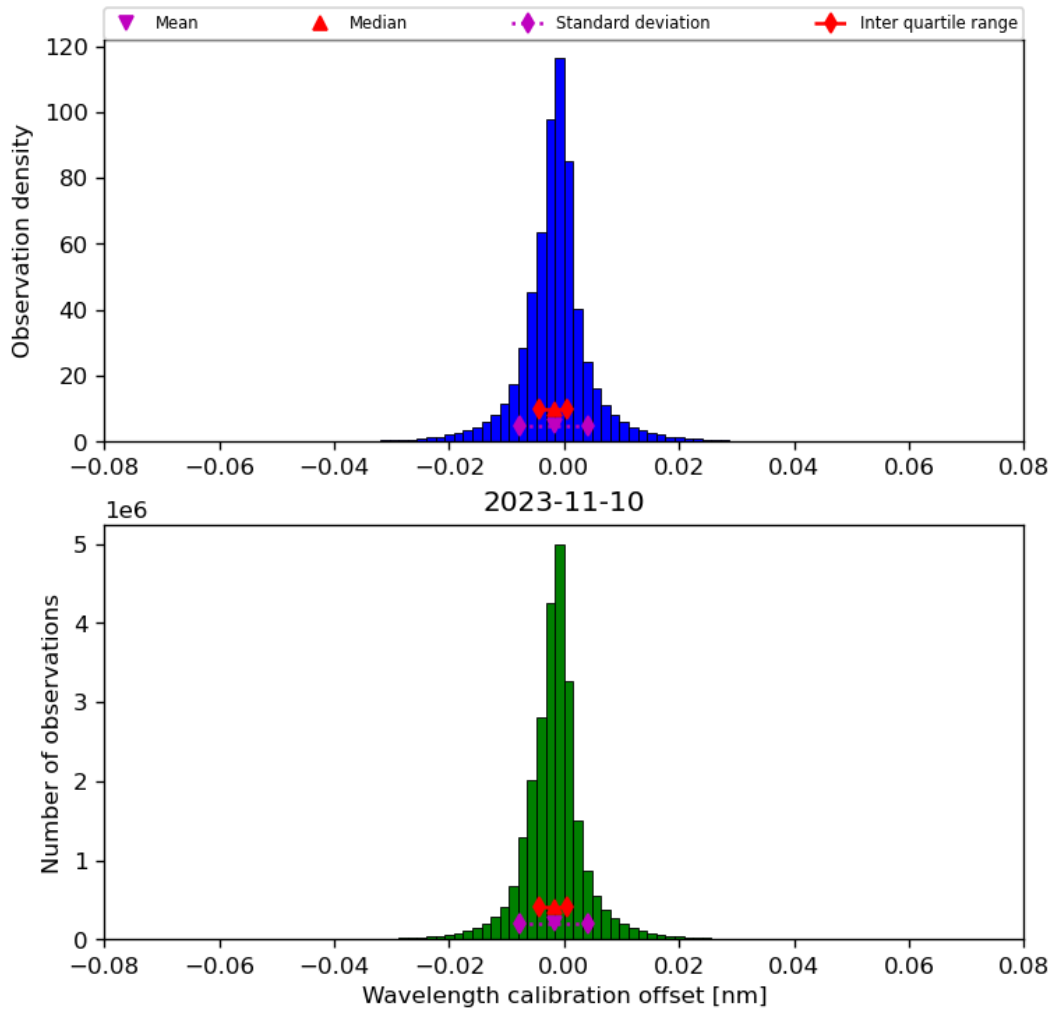
Figure 35: Histogram of “Wavelength calibration offset” for 2023-11-09 to 2023-11-11
