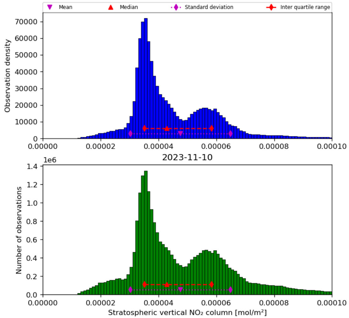
Figure 36: Histogram of “Stratospheric vertical NO 2 column” for 2023-11-09 to 2023-11-11
