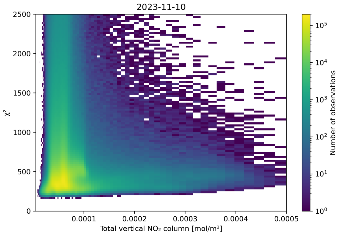
Figure 111: Scatter density plot of “Total vertical NO 2 column” against “ \chi^2 ” for 2023-11-09 to 2023-11-11.
