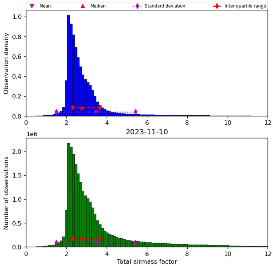
Figure 32: Histogram of “Total air mass factor” for 2023-11-09 to 2023-11-11
