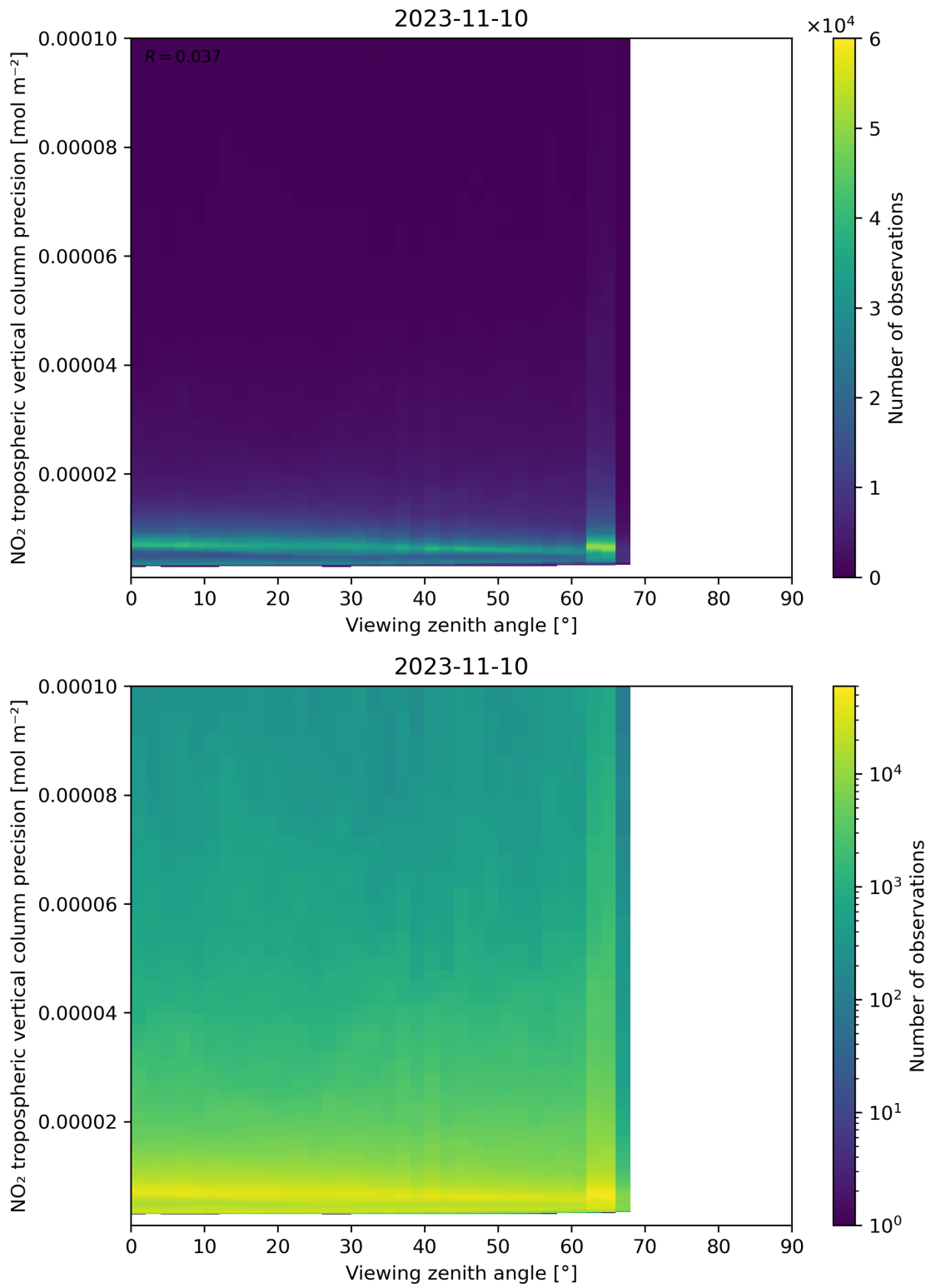
Figure 170: Scatter density plot of “Viewing zenith angle” against “NO 2 tropospheric vertical column precision” for 2023-11-09 to 2023-11-11.
