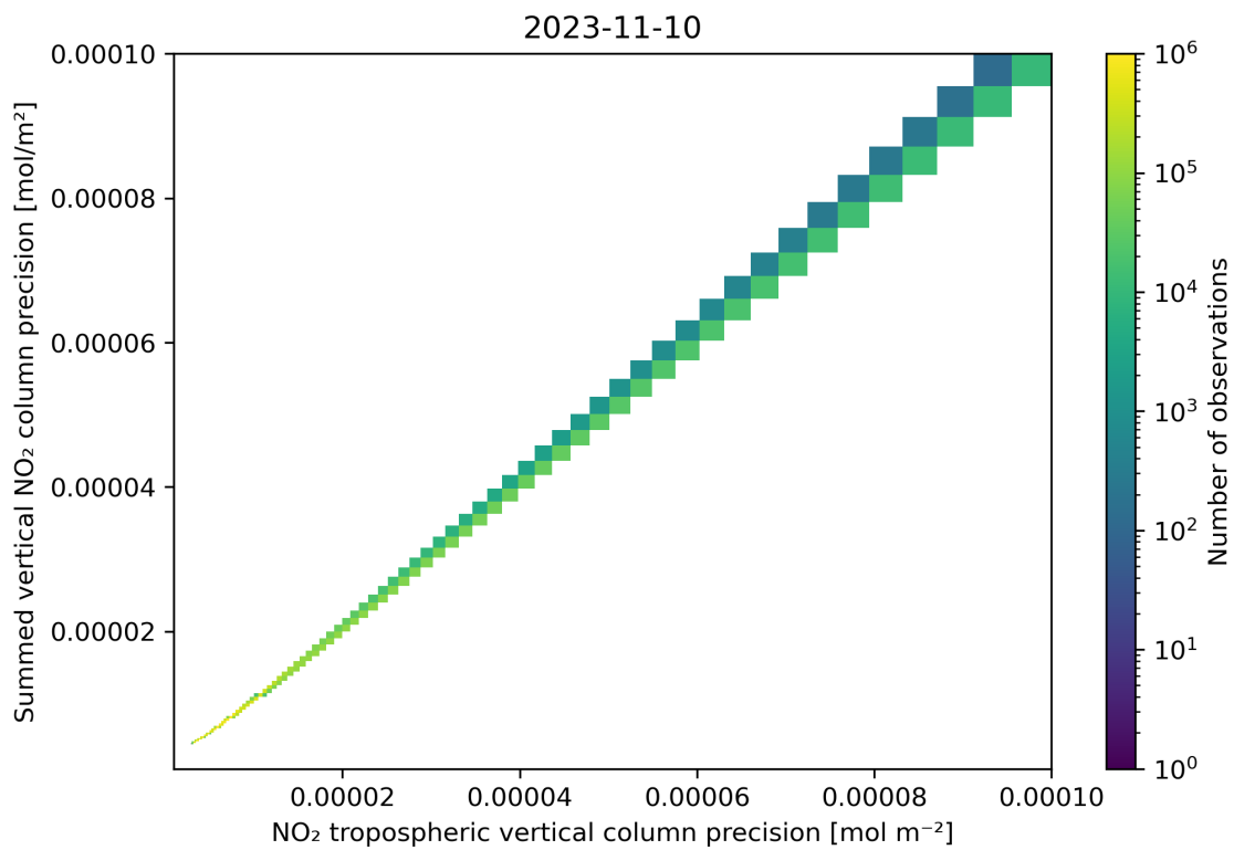
Figure 137: Scatter density plot of “NO 2 tropospheric vertical column precision” against “Summed vertical NO 2 column precision” for 2023-11-09 to 2023-11-11.
