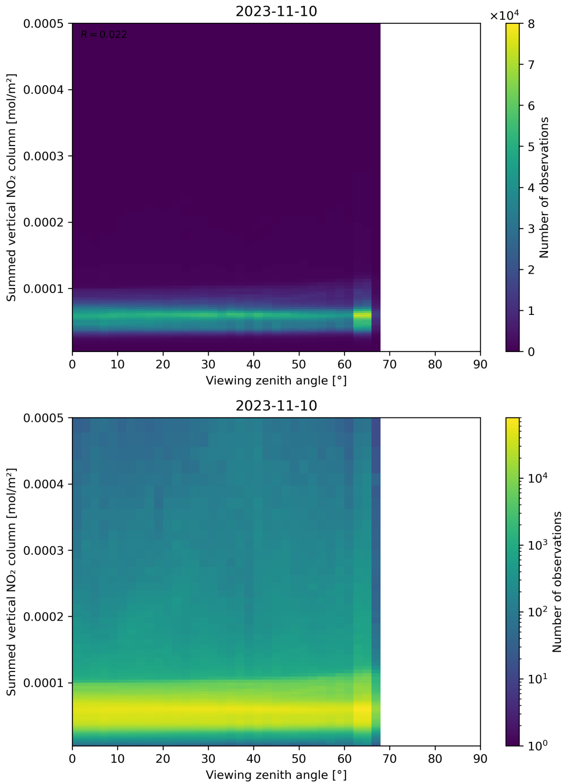
Figure 165: Scatter density plot of “Viewing zenith angle” against “Summed vertical NO 2 column” for 2023-11-09 to 2023-11-11.
