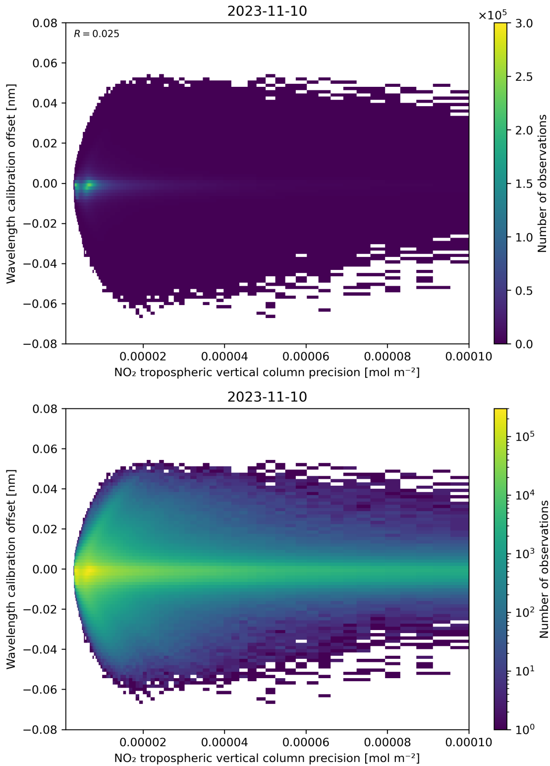
Figure 141: Scatter density plot of “NO 2 tropospheric vertical column precision” against “Wavelength calibration offset” for 2023-11-09 to 2023-11-11.
