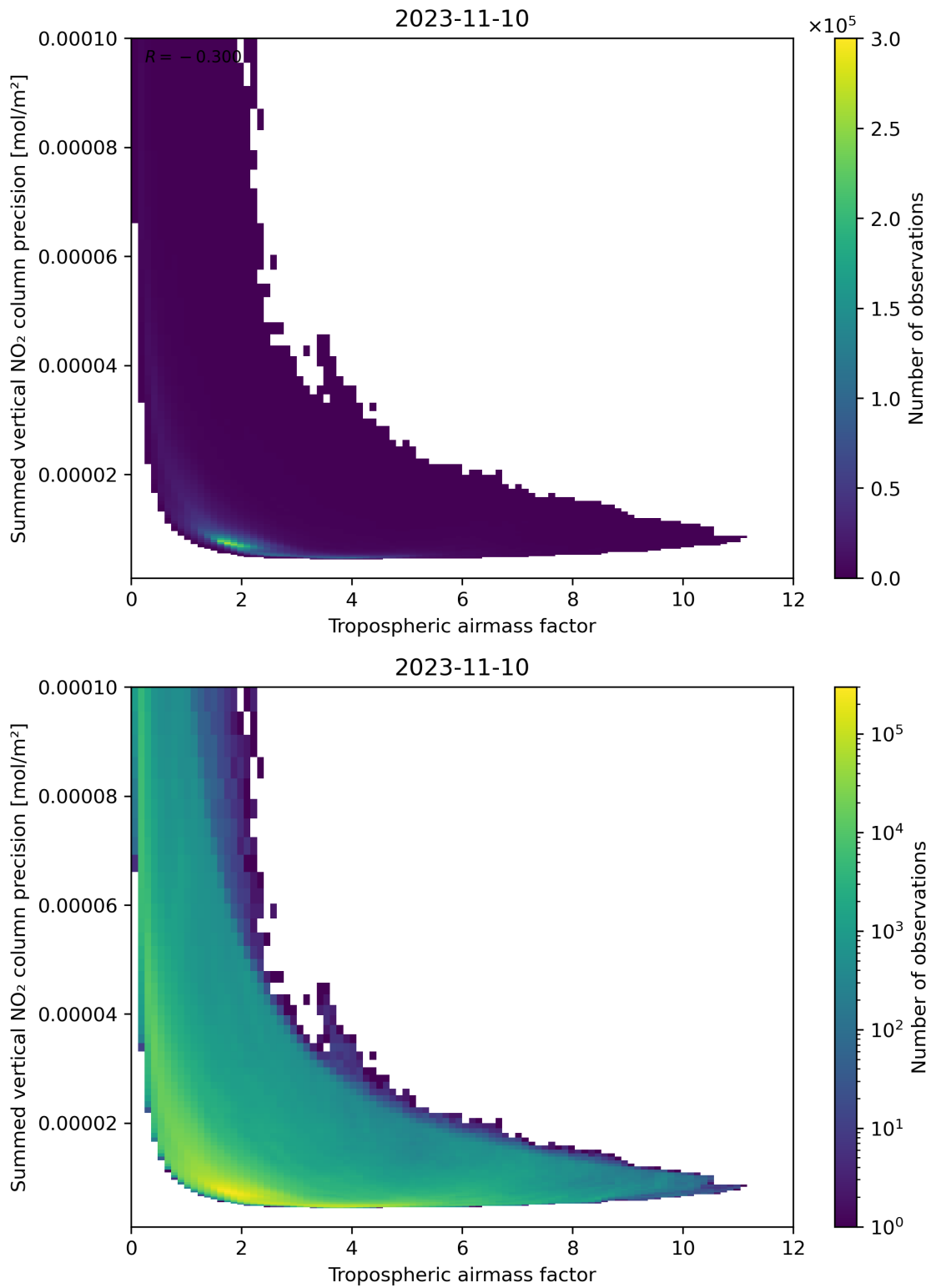
Figure 76: Scatter density plot of “Tropospheric airmass factor” against “Summed vertical NO 2 column precision” for 2023-11-09 to 2023-11-11.
