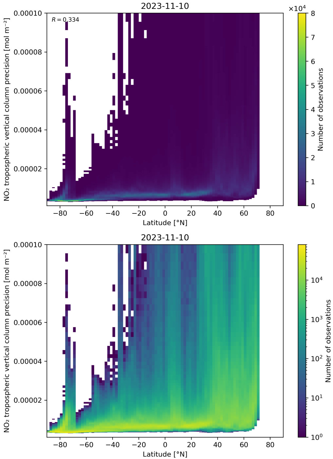
Figure 93: Scatter density plot of “Latitude” against “NO 2 tropospheric vertical column precision” for 2023-11-09 to 2023-11-11.
