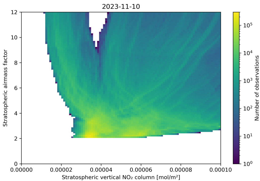
Figure 96: Scatter density plot of “Stratospheric vertical NO 2 column” against “Stratospheric airmass factor” for 2023-11-09 to 2023-11-11.
