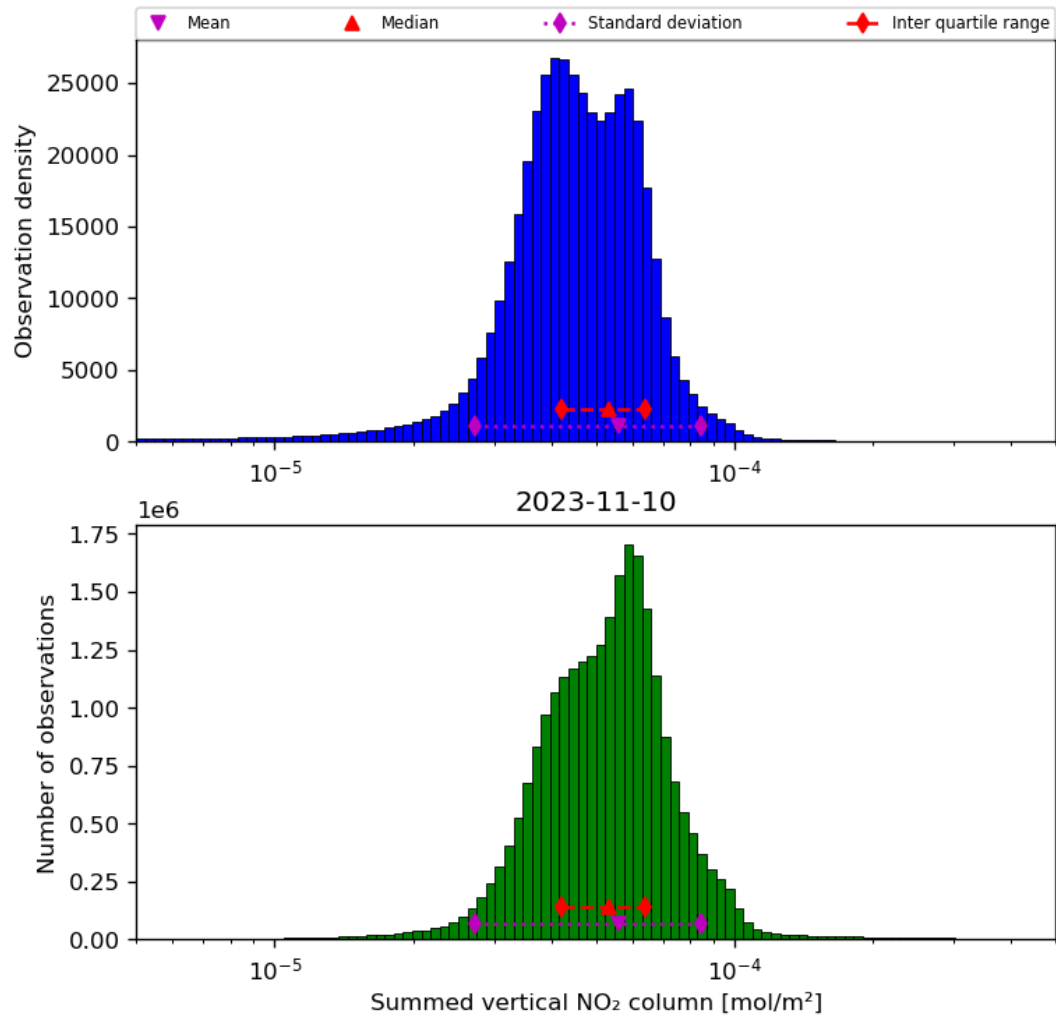
Figure 40: Histogram of “Summed vertical NO 2 column” for 2023-11-09 to 2023-11-11
